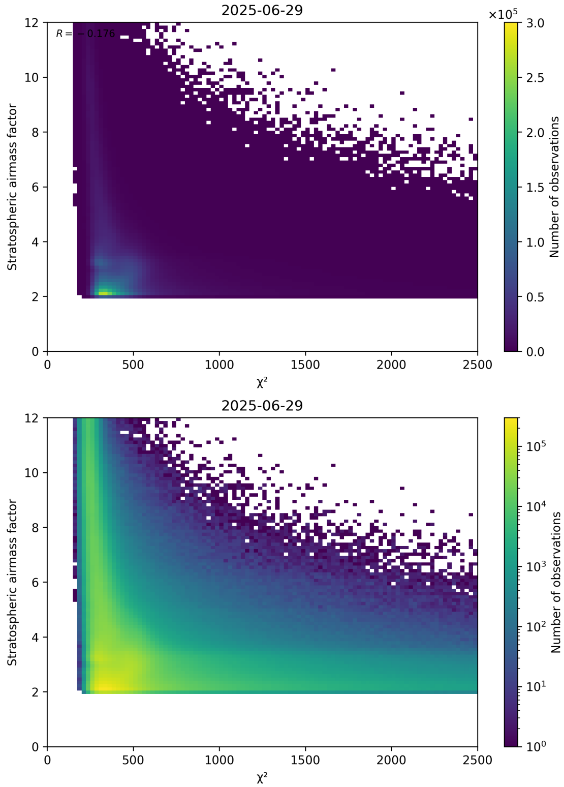
Figure 81: Scatter density plot of “ \chi^2 ” against “Stratospheric airmass factor” for 2025-06-28 to 2025-06-30.
