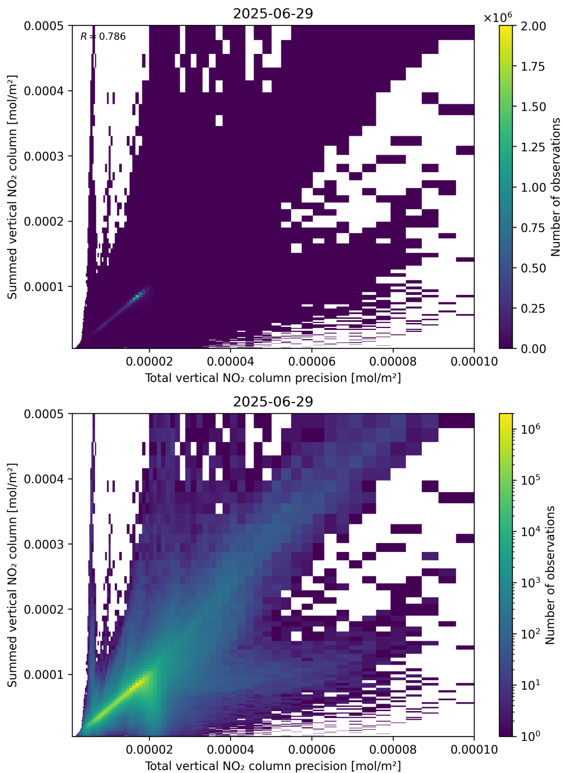
Figure 117: Scatter density plot of “Total vertical NO 2 column precision” against “Summed vertical NO 2 column” for 2025-06-28 to 2025-06-30.
