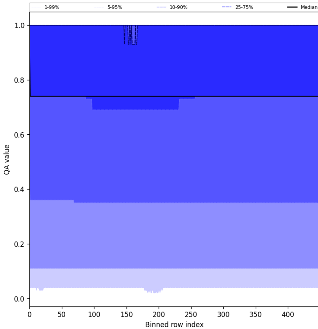
Figure 45: Along track statistics of “QA value” for 2025-06-28 to 2025-06-30
