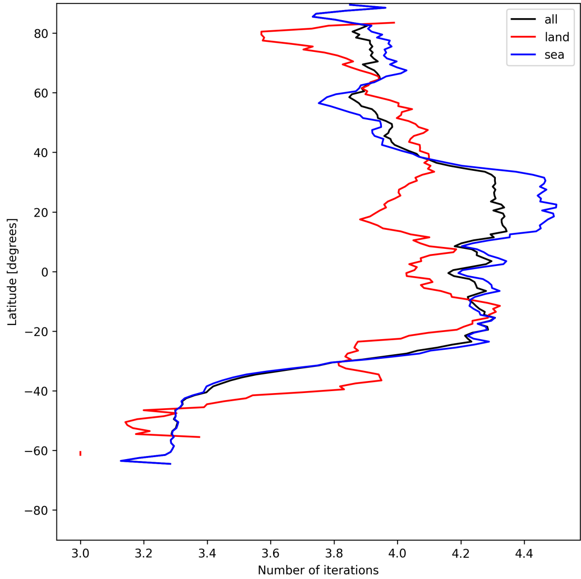
Figure 17: Zonal average of “Number of iterations” for 2025-06-28 to 2025-06-30.
