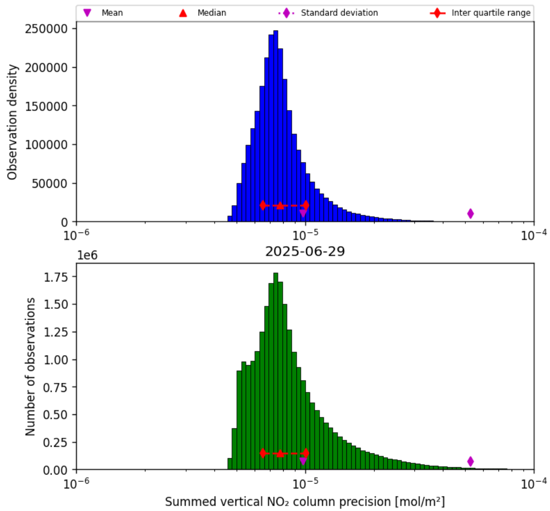
Figure 41: Histogram of "Summed vertical NO 2 column precision" for 2025-06-28 to 2025-06-30
