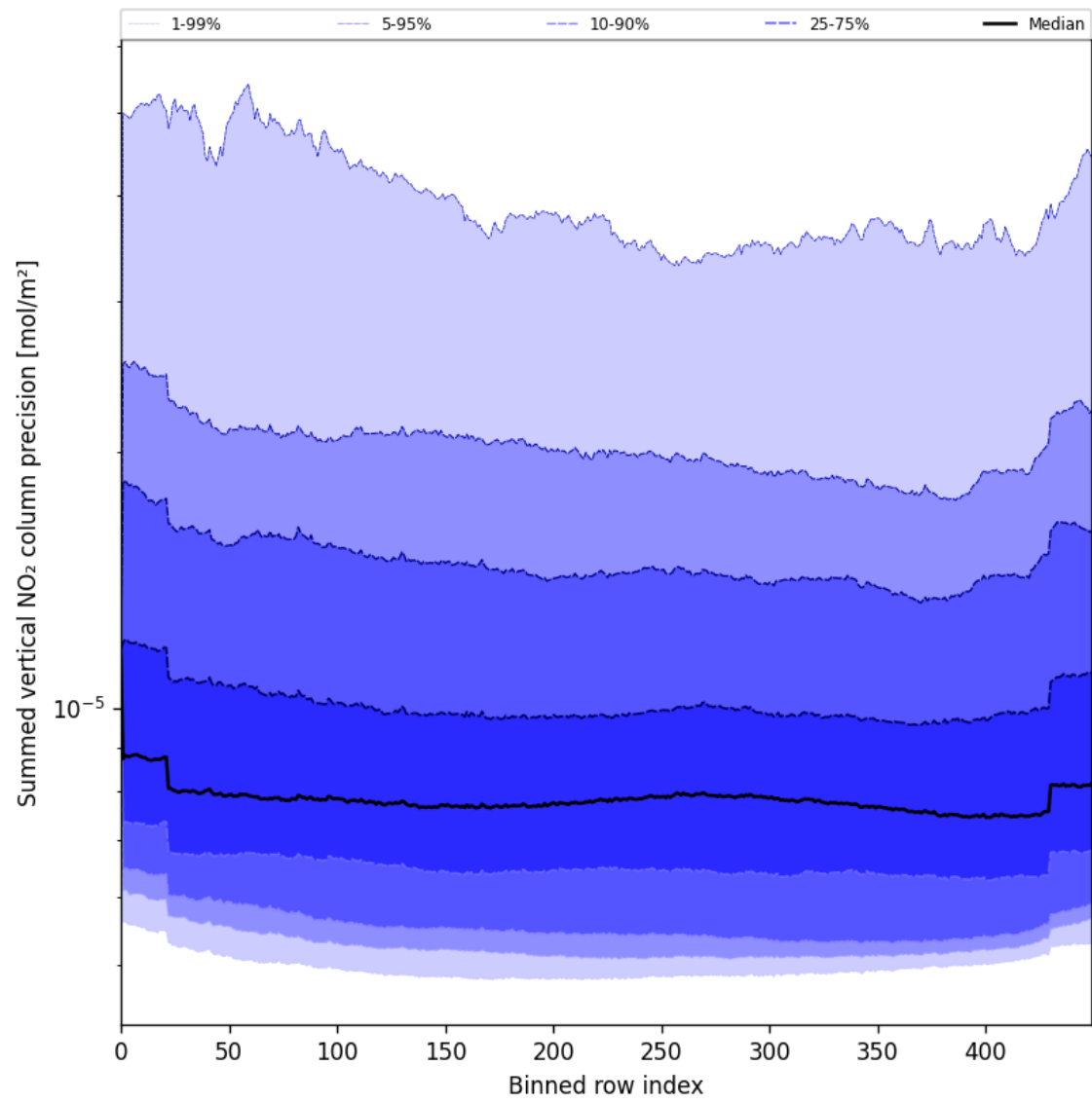
Figure 58: Along track statistics of “Summed vertical NO 2 column precision” for 2025-06-28 to 2025-06-30
