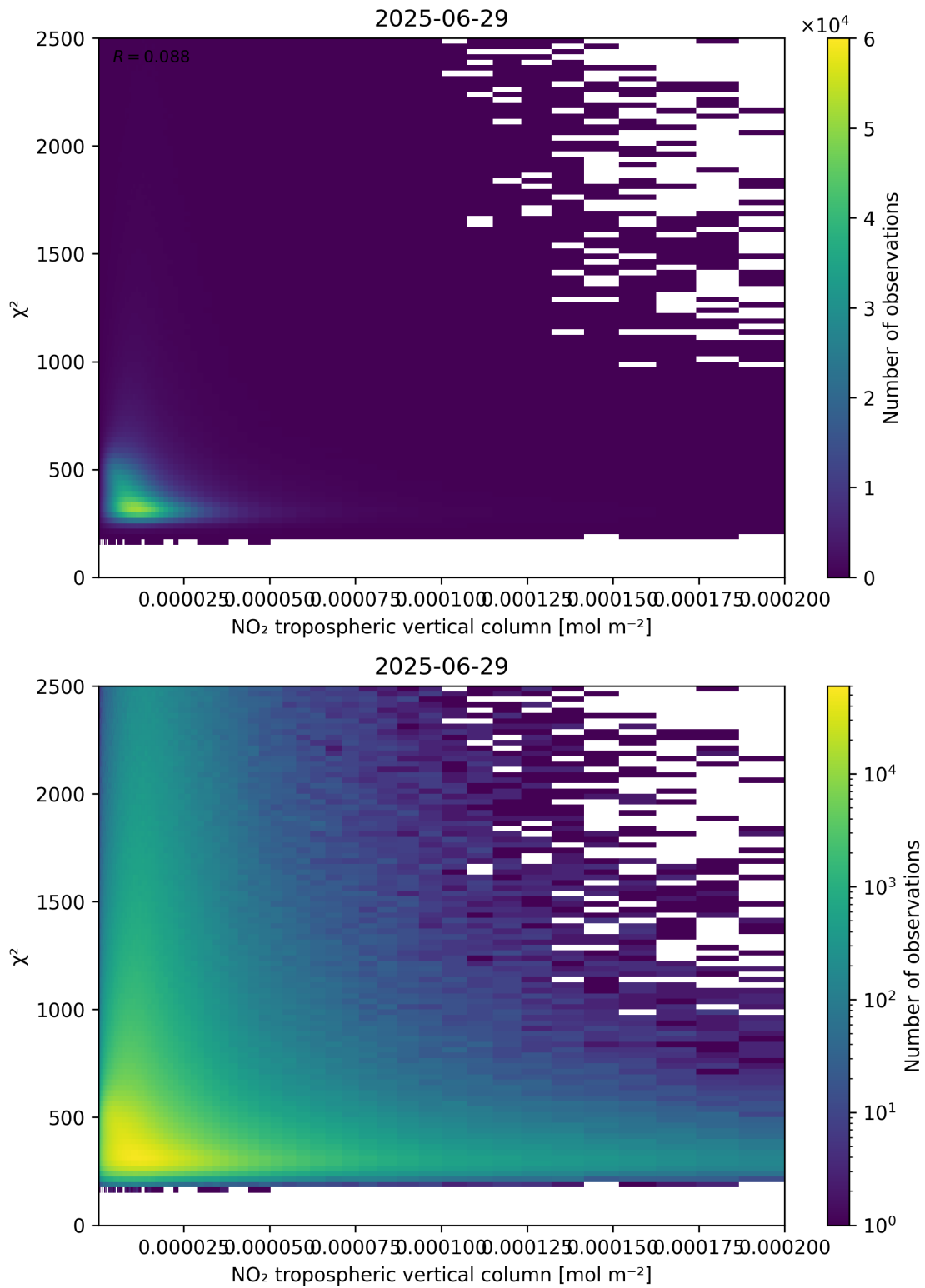
Figure 124: Scatter density plot of “NO 2 tropospheric vertical column” against “ \chi^2 ” for 2025-06-28 to 2025-06-30.
