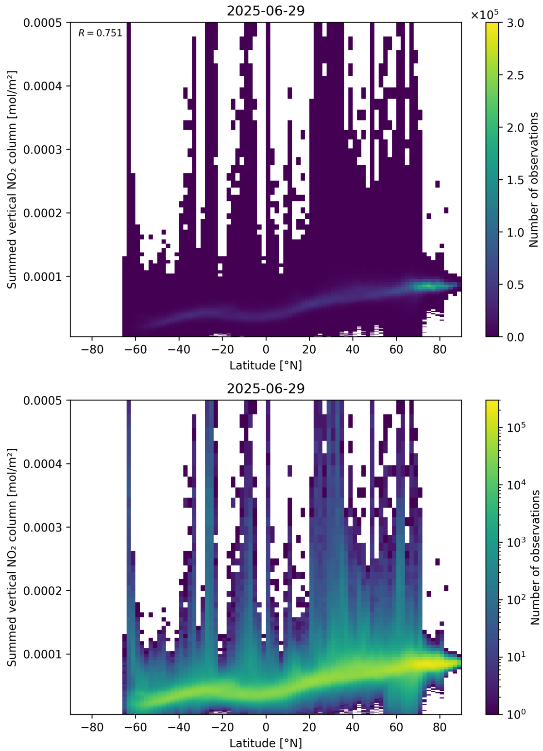
Figure 88: Scatter density plot of “Latitude” against “Summed vertical NO 2 column” for 2025-06-28 to 2025-06-30.
