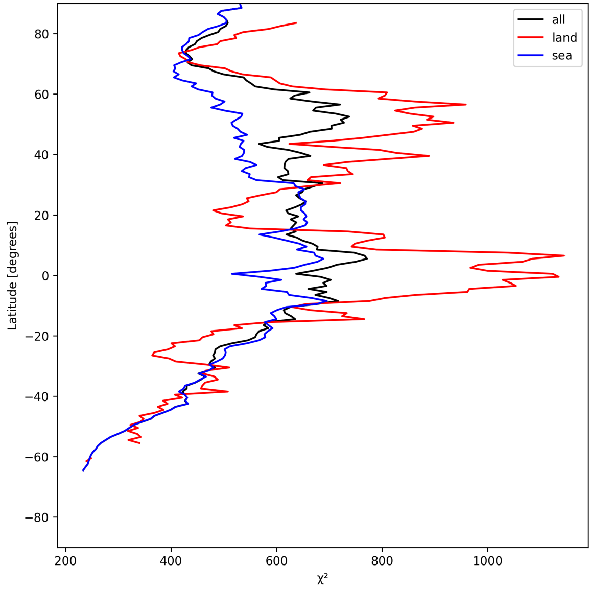
Figure 25: Zonal average of “ \chi^2 ” for 2025-06-28 to 2025-06-30.
