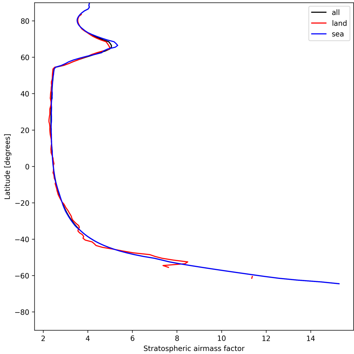
Figure 27: Zonal average of “Stratospheric airmass factor” for 2025-06-28 to 2025-06-30.
