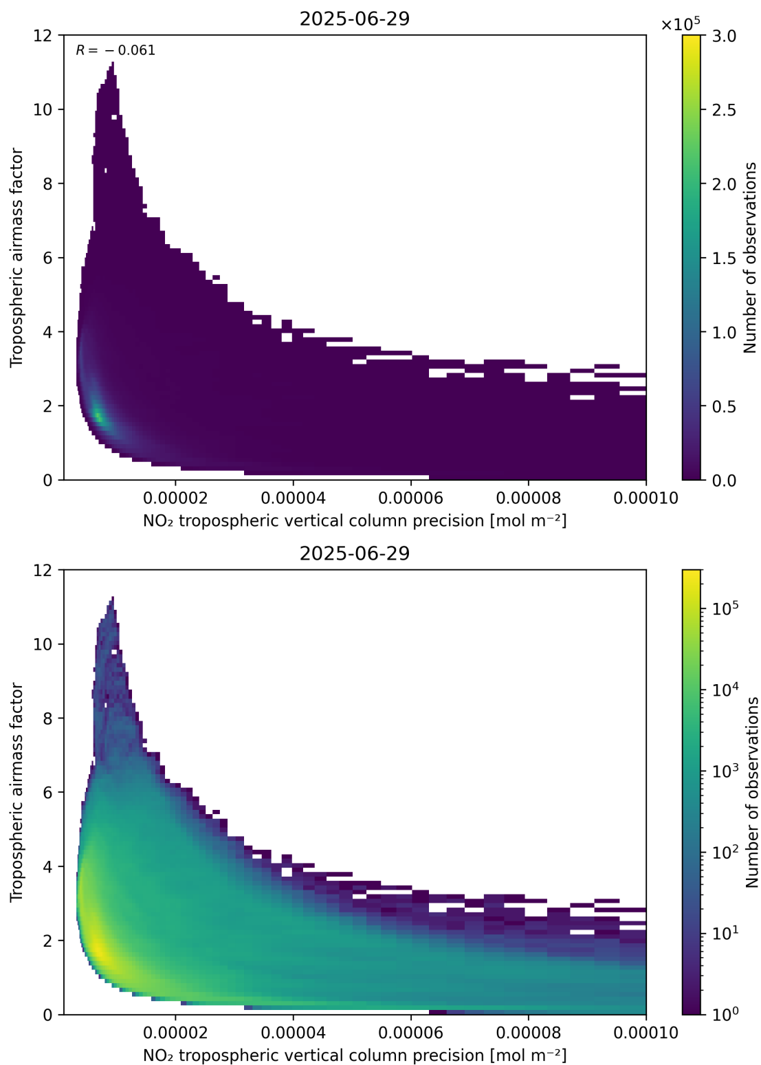
Figure 133: Scatter density plot of “NO 2 tropospheric vertical column precision” against “Tropospheric air mass factor” for 2025-06-28 to 2025-06-30.
