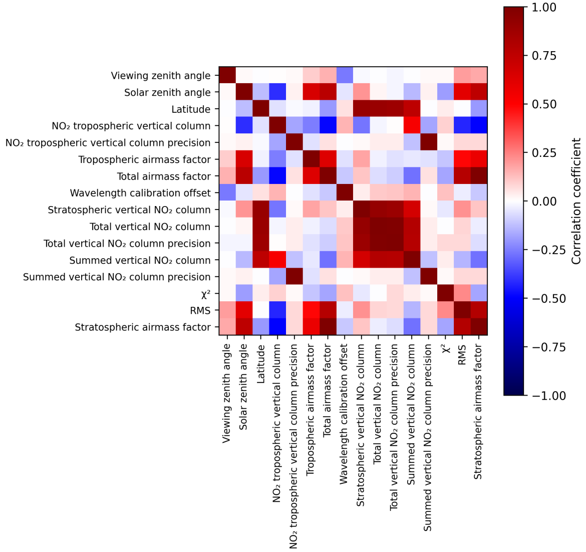
Figure 2: Map of correlation matrix for 2025-06-28 to 2025-06-30.
