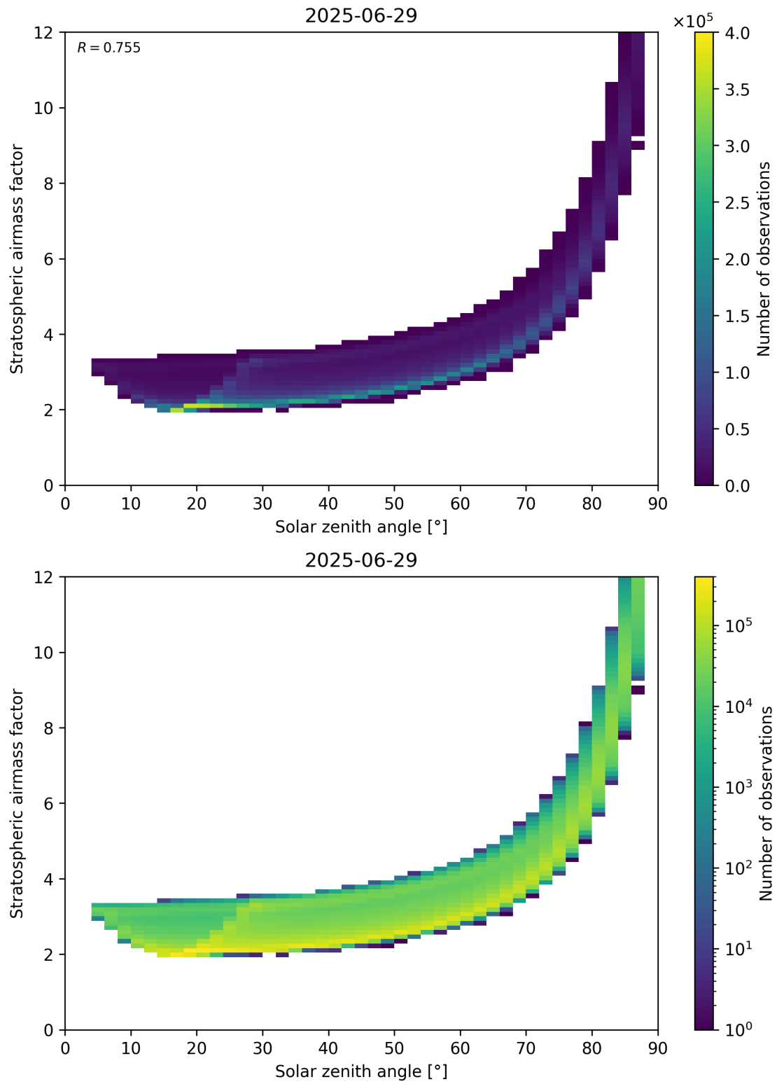
Figure 145: Scatter density plot of “Solar zenith angle” against “Stratospheric airmass factor” for 2025-06-28 to 2025-06-30.
