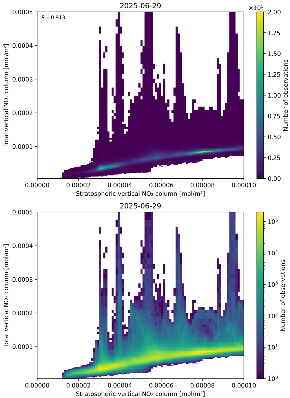
Figure 100: Scatter density plot of “Stratospheric vertical NO 2 column” against “Total vertical NO 2 column” for 2025-06-28 to 2025-06-30.
