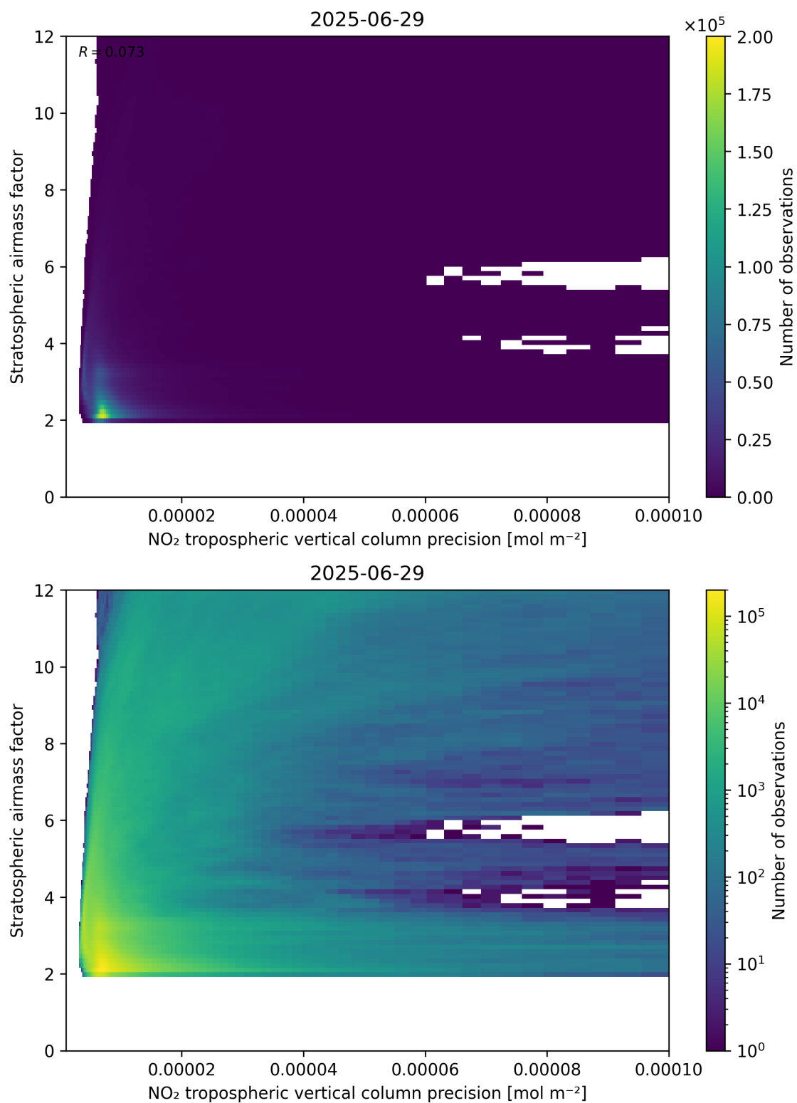
Figure 131: Scatter density plot of “NO 2 tropospheric vertical column precision” against “Stratospheric airmass factor” for 2025-06-28 to 2025-06-30.
