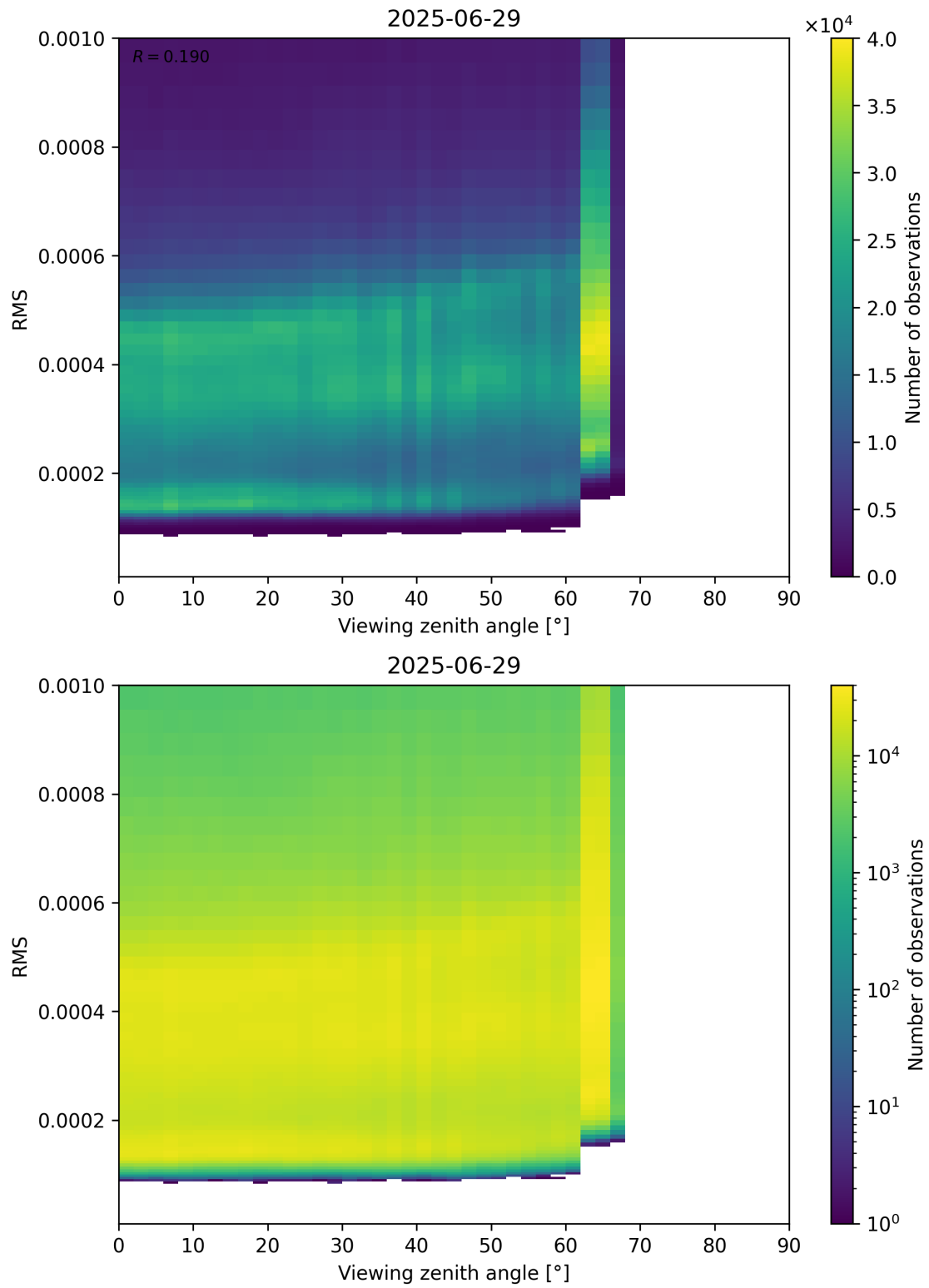
Figure 171: Scatter density plot of “Viewing zenith angle” against “RMS” for 2025-06-28 to 2025-06-30.
