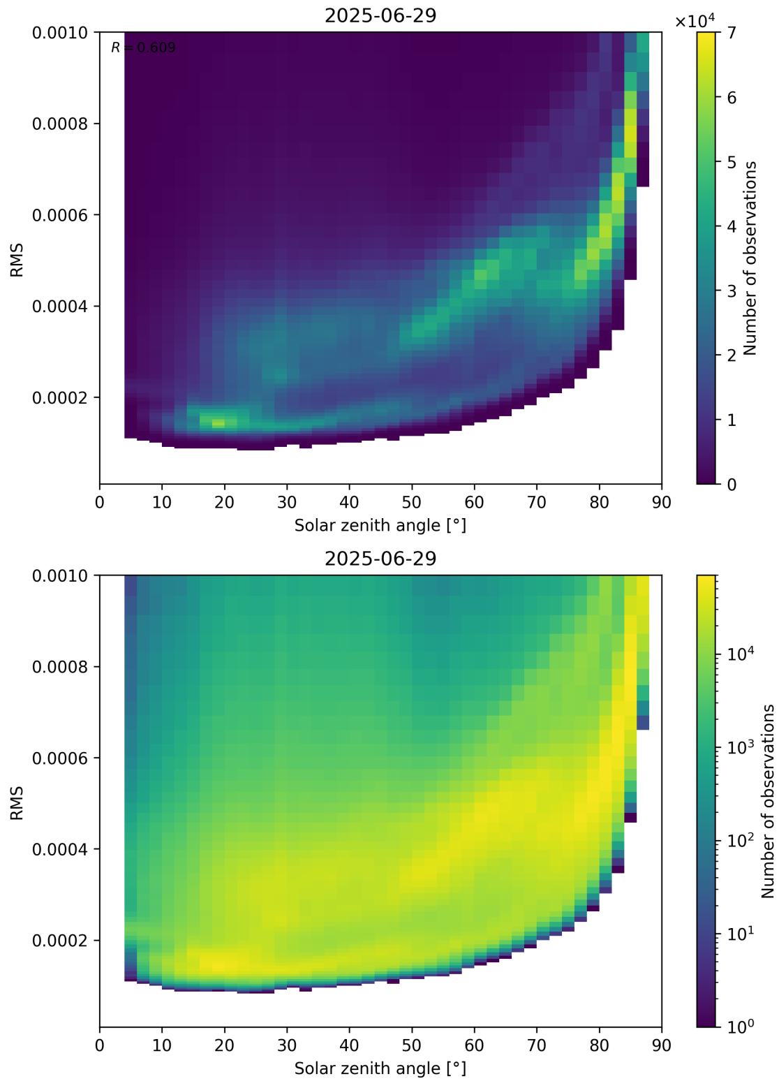
Figure 157: Scatter density plot of “Solar zenith angle” against “RMS” for 2025-06-28 to 2025-06-30.
