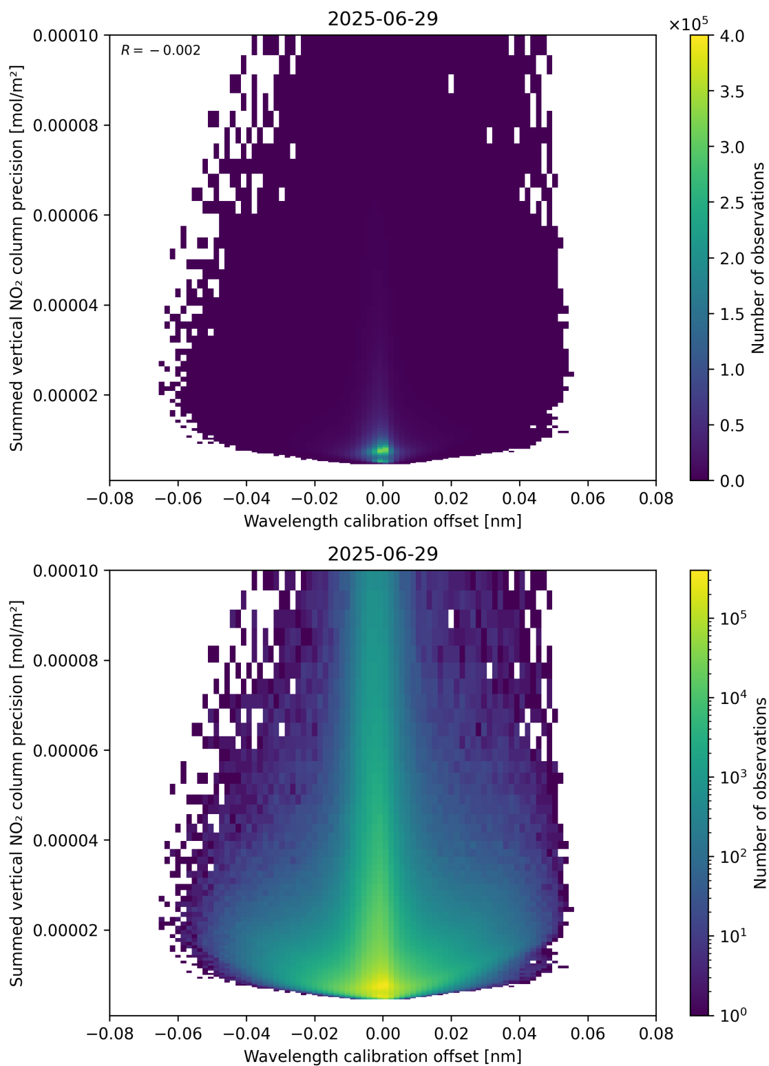
Figure 178: Scatter density plot of “Wavelength calibration offset” against “Summed vertical NO 2 column precision” for 2025-06-28 to 2025-06-30.
