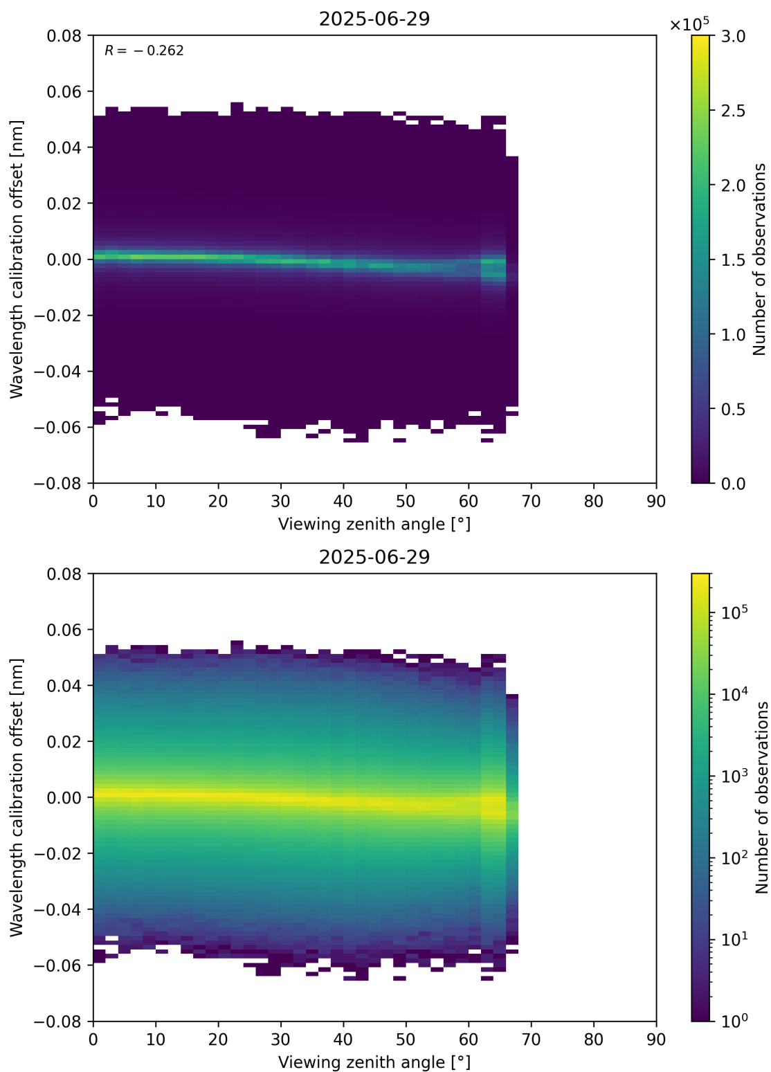
Figure 173: Scatter density plot of “Viewing zenith angle” against “Wavelength calibration offset” for 2025-06-28 to 2025-06-30.
