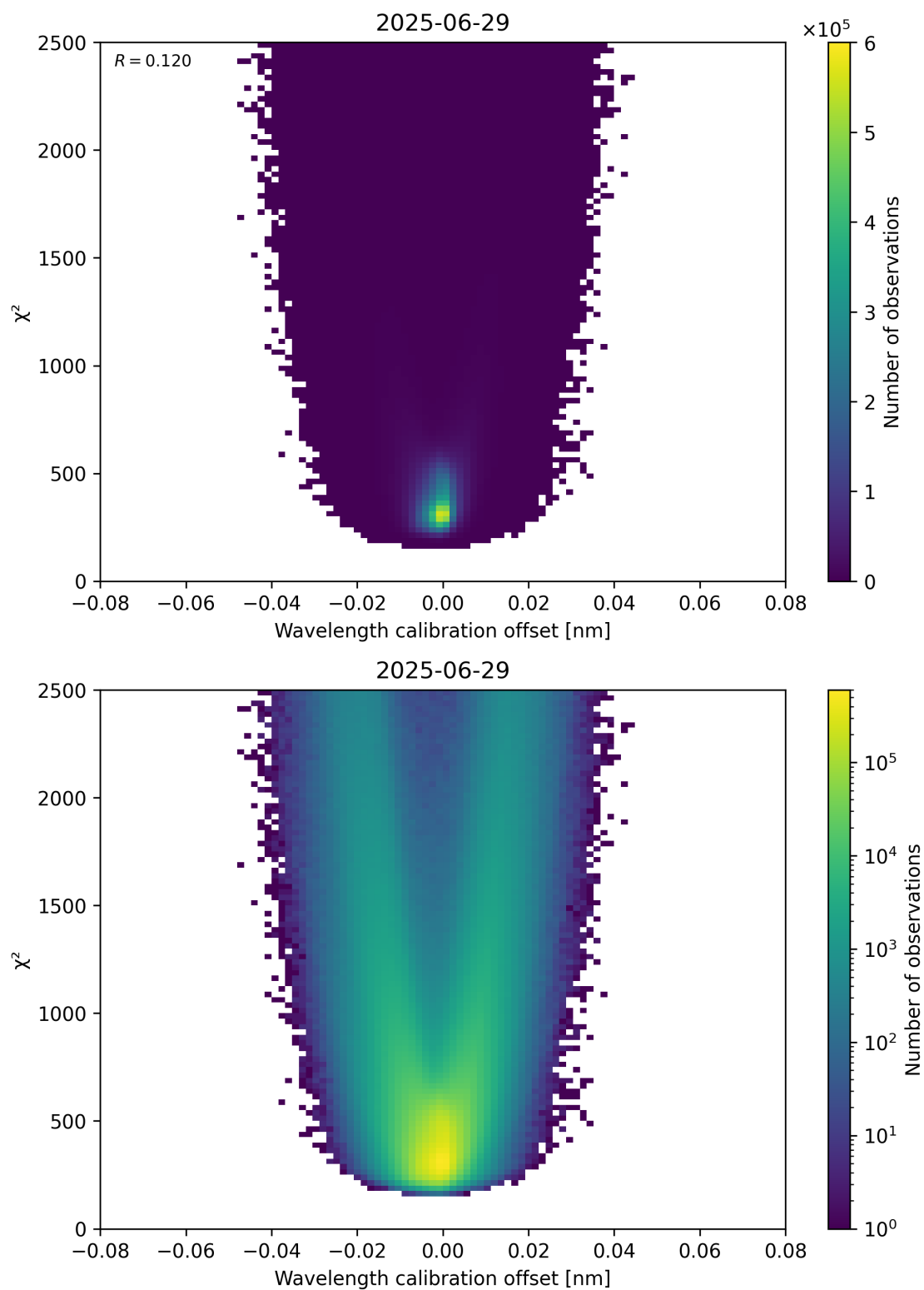
Figure 175: Scatter density plot of “Wavelength calibration offset” against “ \chi^2 ” for 2025-06-28 to 2025-06-30.
