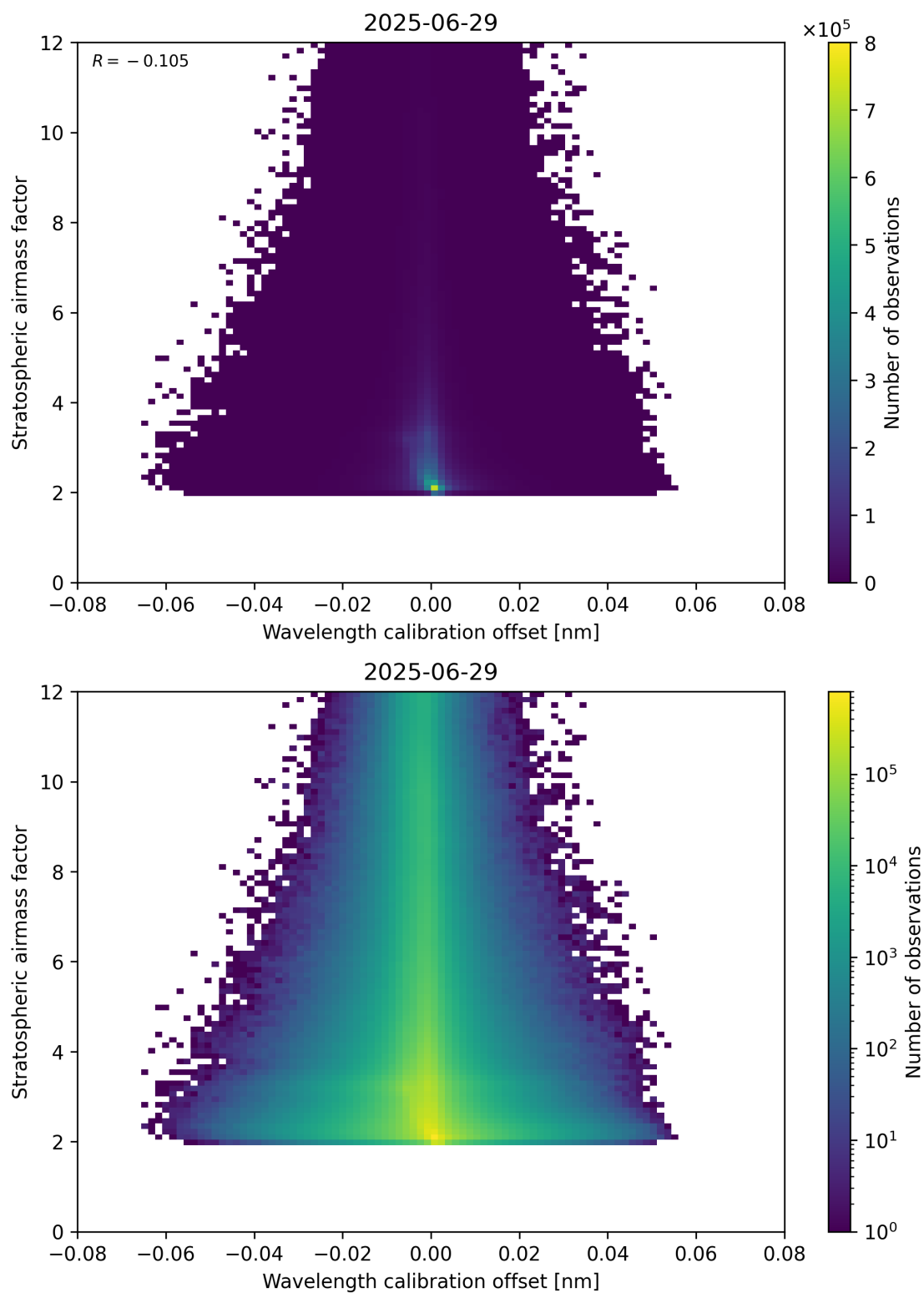
Figure 174: Scatter density plot of “Wavelength calibration offset” against “Stratospheric air mass factor” for 2025-06-28 to 2025-06-30.
