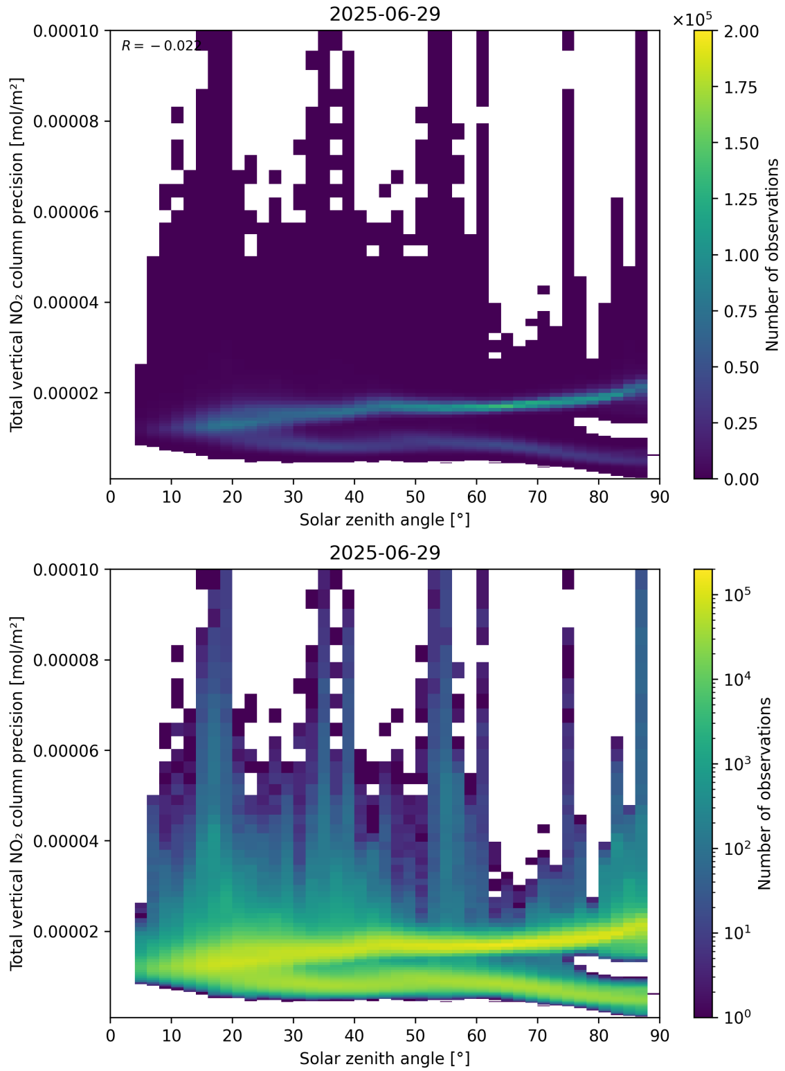
Figure 154: Scatter density plot of “Solar zenith angle” against “Total vertical NO 2 column precision” for 2025-06-28 to 2025-06-30.
