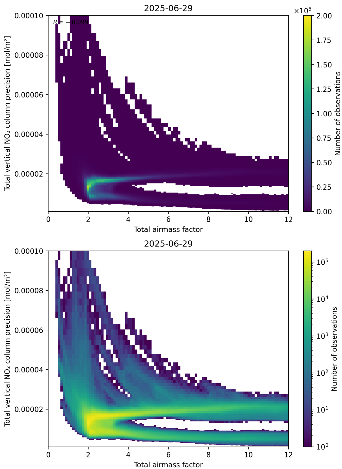
Figure 68: Scatter density plot of “Total airmass factor” against “Total vertical NO 2 column precision” for 2025-06-28 to 2025-06-30.
