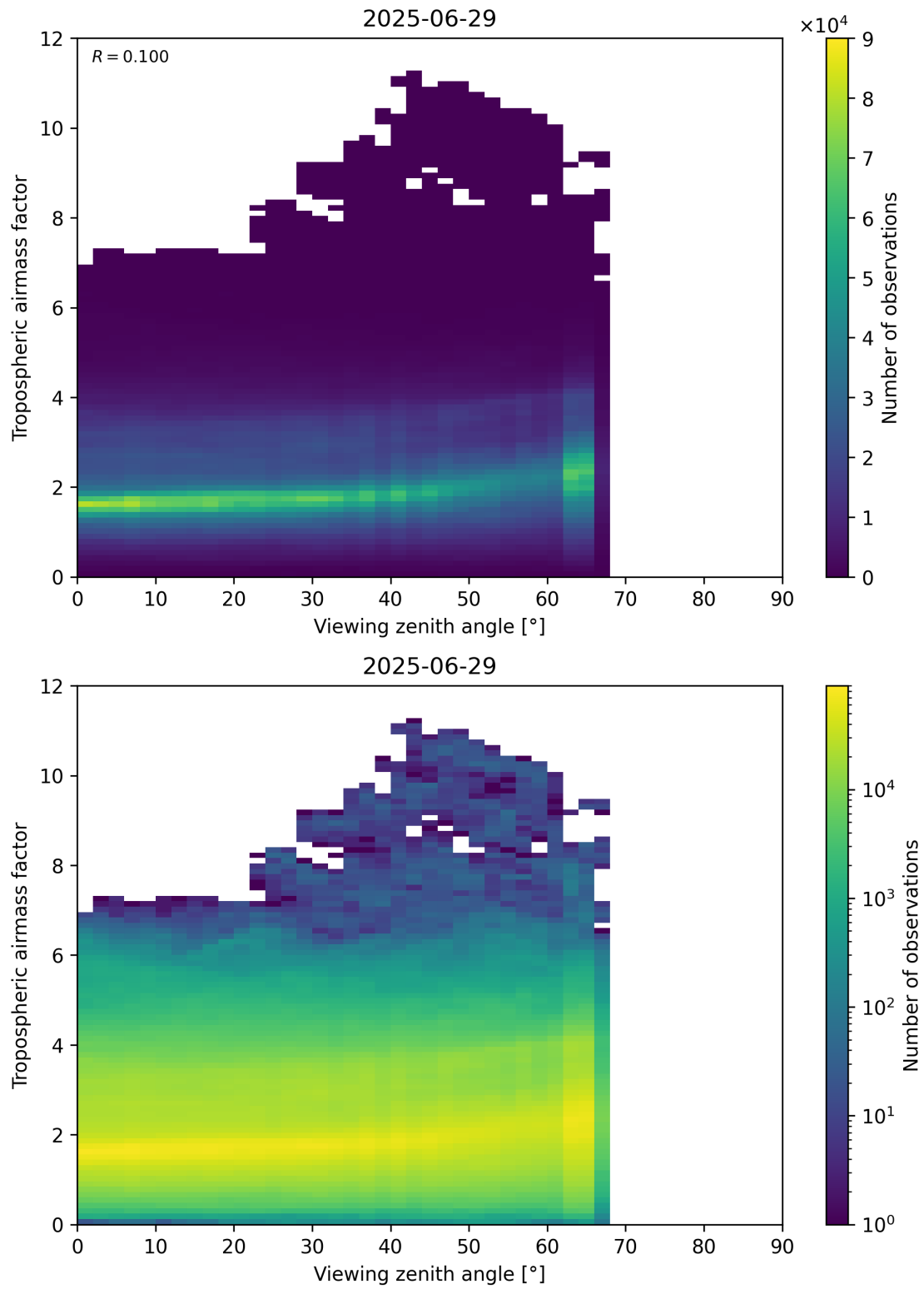
Figure 161: Scatter density plot of “Viewing zenith angle” against “Tropospheric airmass factor” for 2025-06-28 to 2025-06-30.
