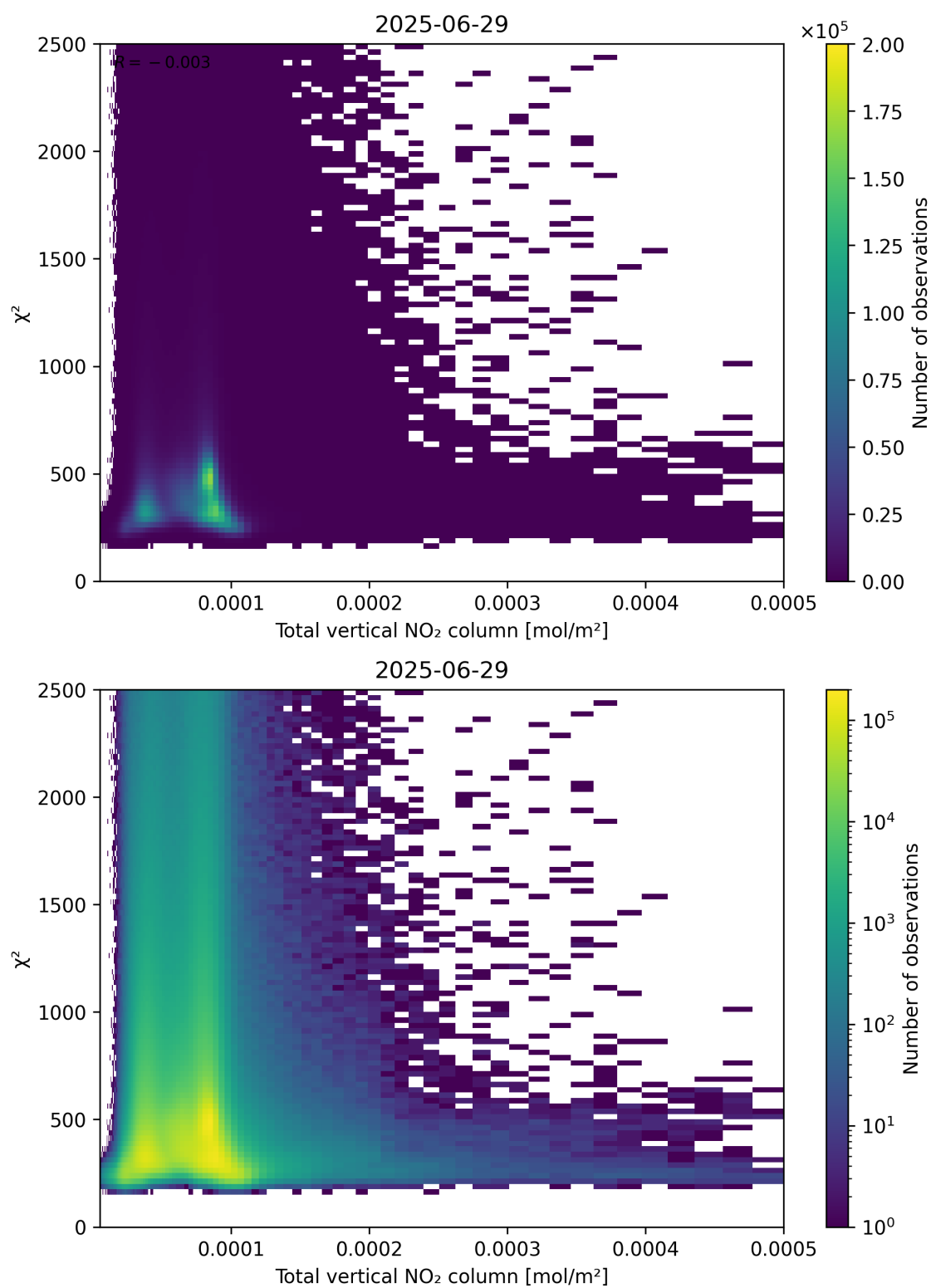
Figure 111: Scatter density plot of “Total vertical NO 2 column” against “ \chi^2 ” for 2025-06-28 to 2025-06-30.
