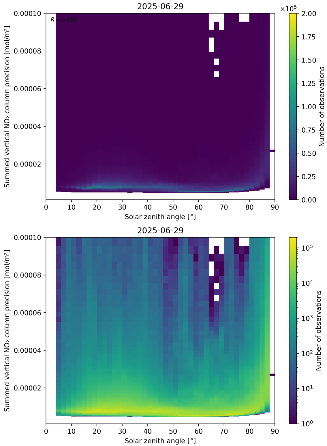
Figure 152: Scatter density plot of “Solar zenith angle” against “Summed vertical NO 2 column precision” for 2025-06-28 to 2025-06-30.
