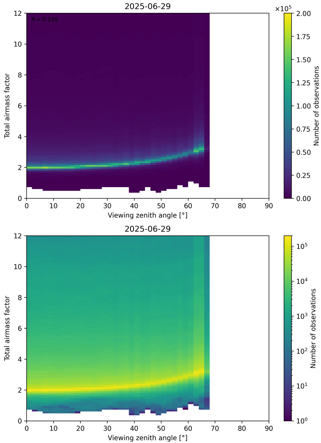
Figure 160: Scatter density plot of “Viewing zenith angle” against “Total airmass factor” for 2025-06-28 to 2025-06-30.
