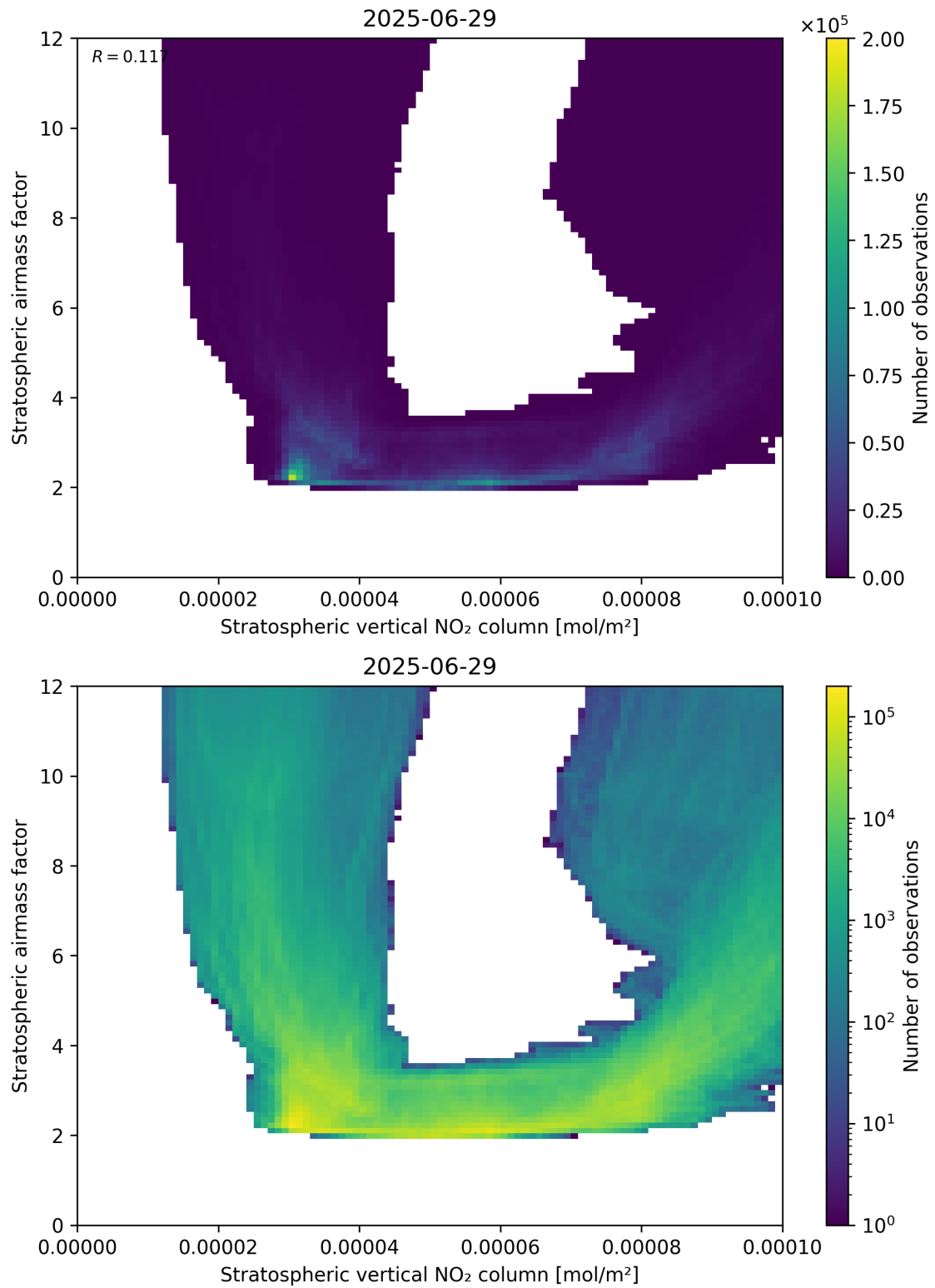
Figure 96: Scatter density plot of “Stratospheric vertical NO 2 column” against “Stratospheric airmass factor” for 2025-06-28 to 2025-06-30.
