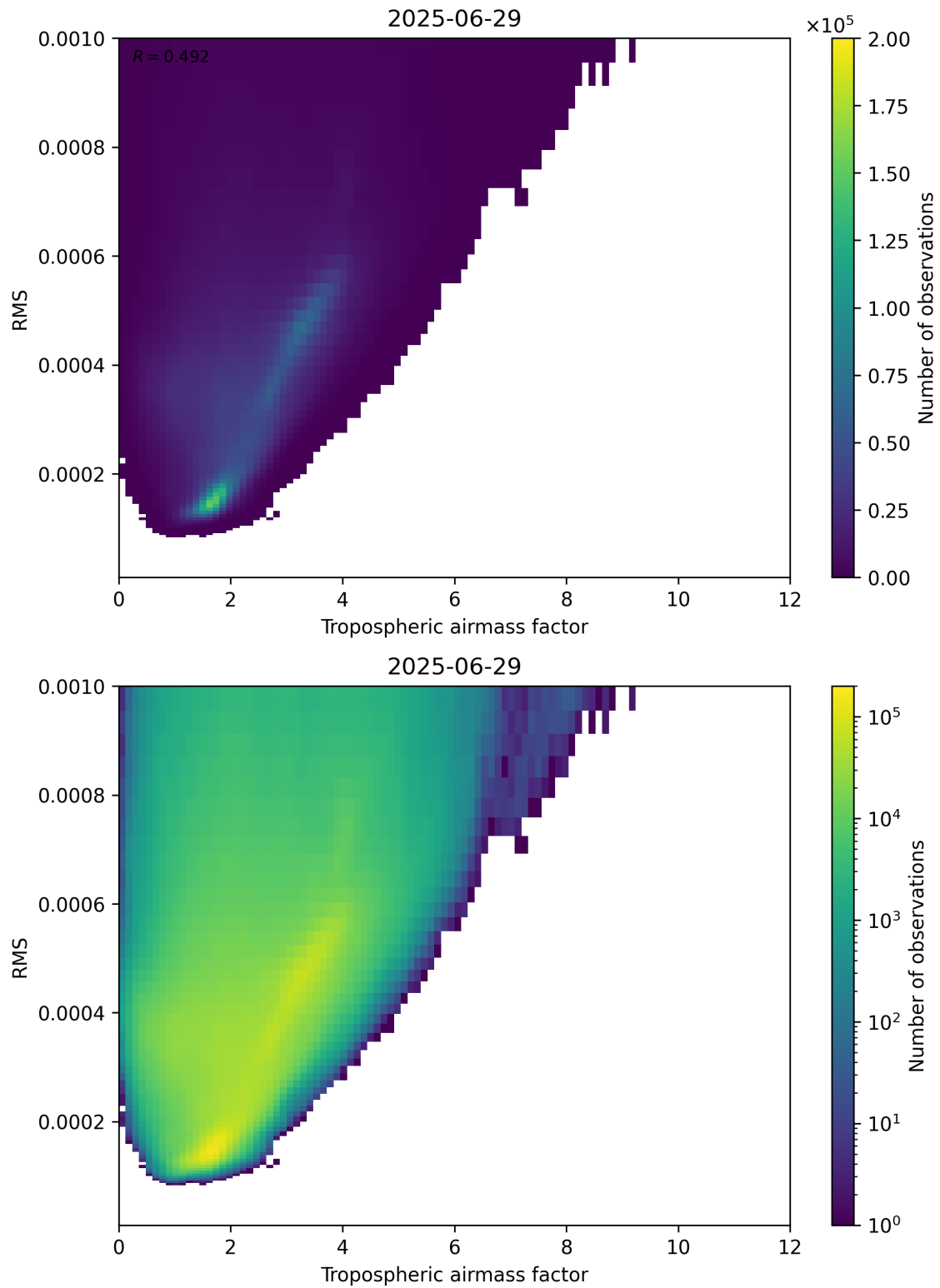
Figure 79: Scatter density plot of “Tropospheric airmass factor” against “RMS” for 2025-06-28 to 2025-06-30.
