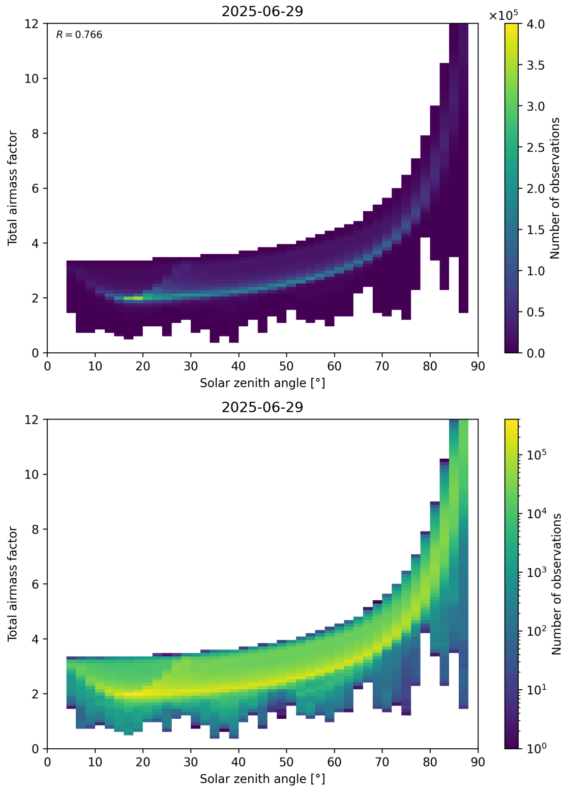
Figure 146: Scatter density plot of “Solar zenith angle” against “Total air mass factor” for 2025-06-28 to 2025-06-30.
