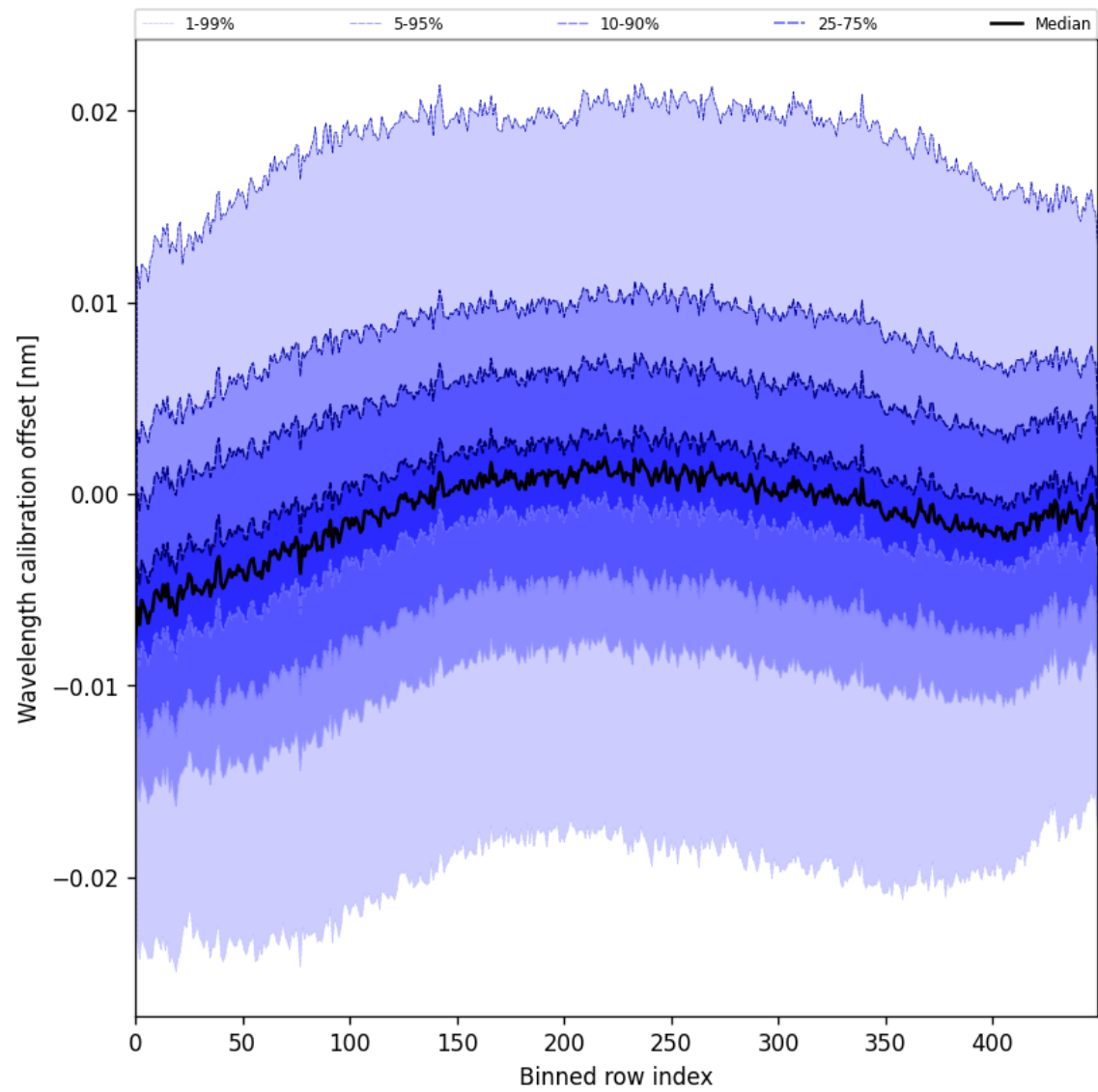
Figure 52: Along track statistics of “Wavelength calibration offset” for 2025-06-28 to 2025-06-30
