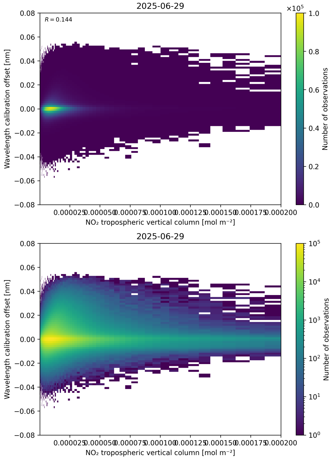
Figure 143: Scatter density plot of “NO 2 tropospheric vertical column” against “Wavelength calibration offset” for 2025-06-28 to 2025-06-30.
