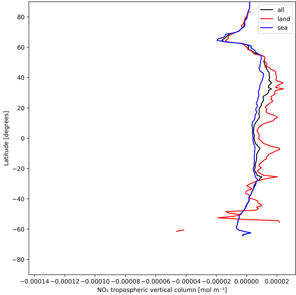
Figure 12: Zonal average of “NO 2 tropospheric vertical column” for 2025-06-28 to 2025-06-30.
