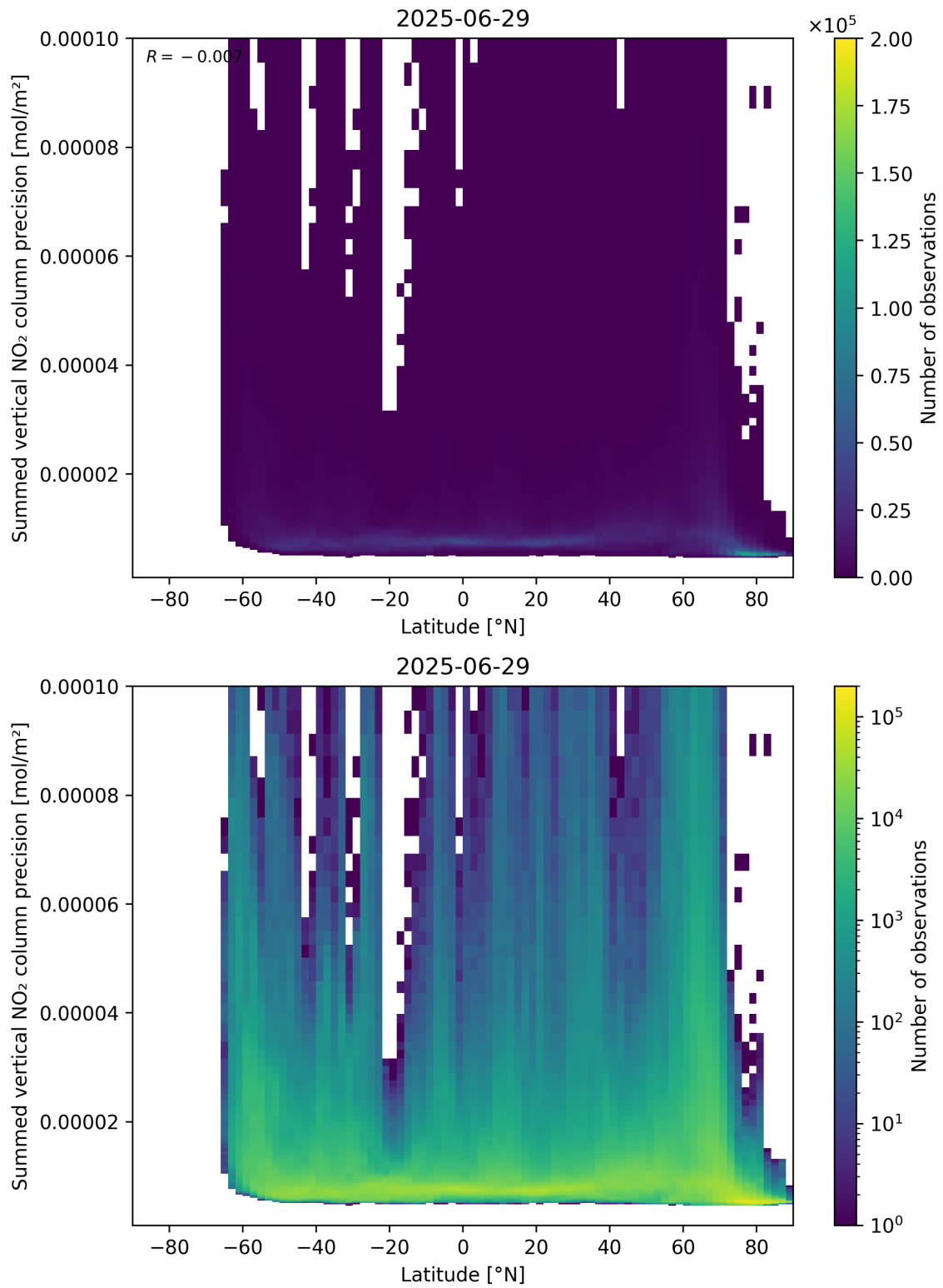
Figure 89: Scatter density plot of “Latitude” against “Summed vertical NO 2 column precision” for 2025-06-28 to 2025-06-30.
