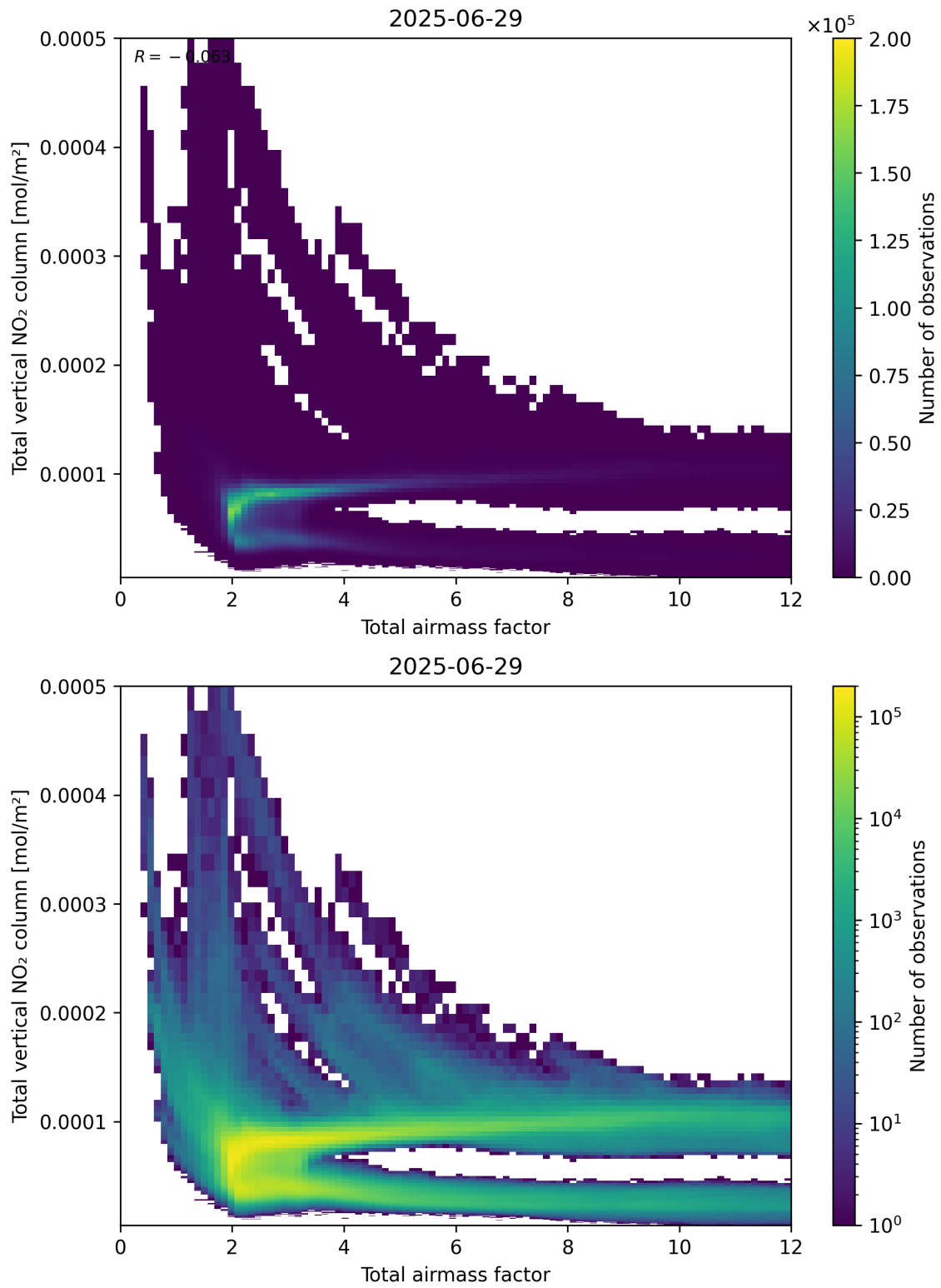
Figure 67: Scatter density plot of “Total airmass factor” against “Total vertical NO 2 column” for 2025-06-28 to 2025-06-30.
