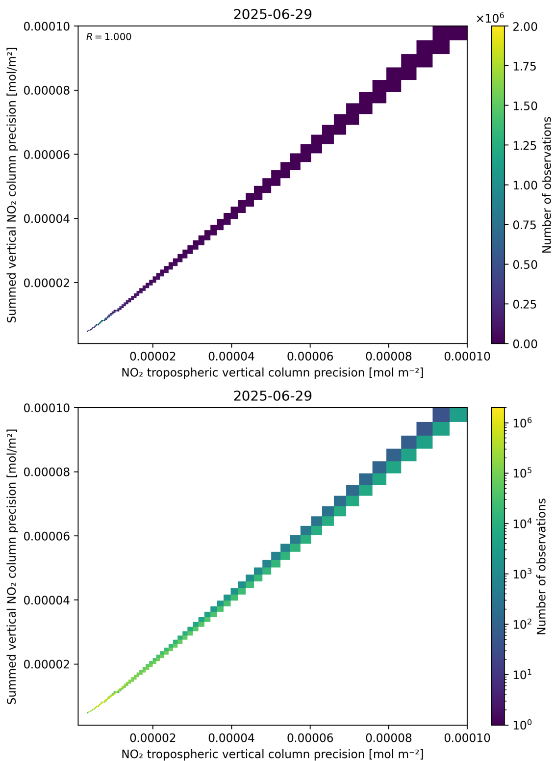
Figure 137: Scatter density plot of “NO 2 tropospheric vertical column precision” against “Summed vertical NO 2 column precision” for 2025-06-28 to 2025-06-30.
