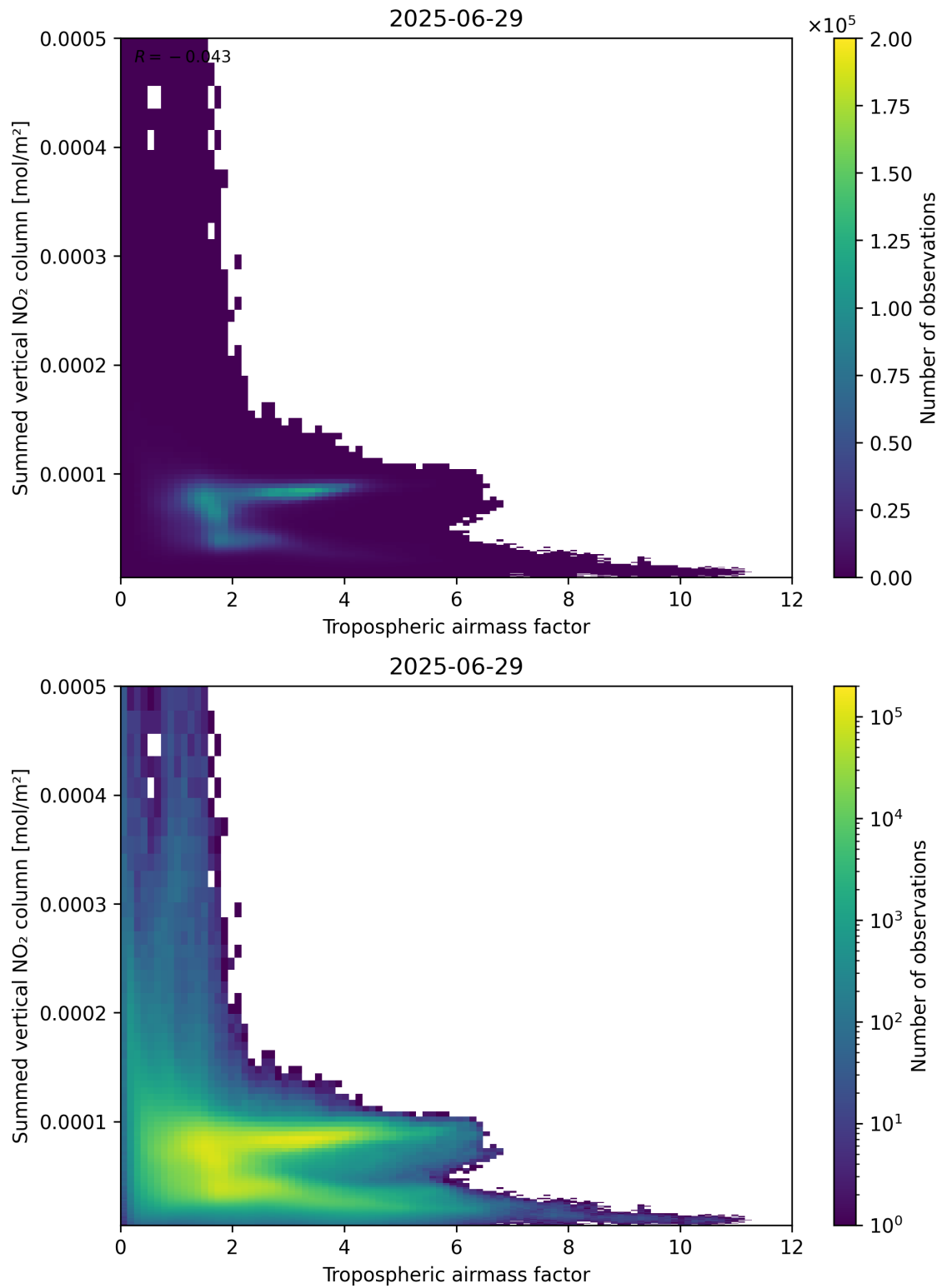
Figure 75: Scatter density plot of “Tropospheric airmass factor” against “Summed vertical NO 2 column” for 2025-06-28 to 2025-06-30.
