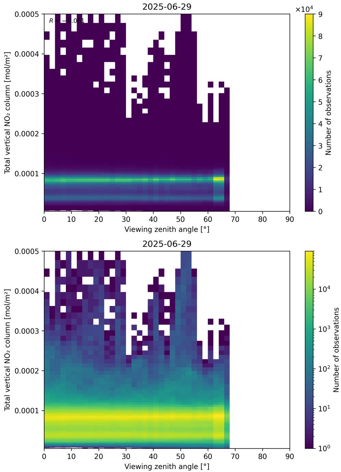
Figure 167: Scatter density plot of “Viewing zenith angle” against “Total vertical NO 2 column” for 2025-06-28 to 2025-06-30.
