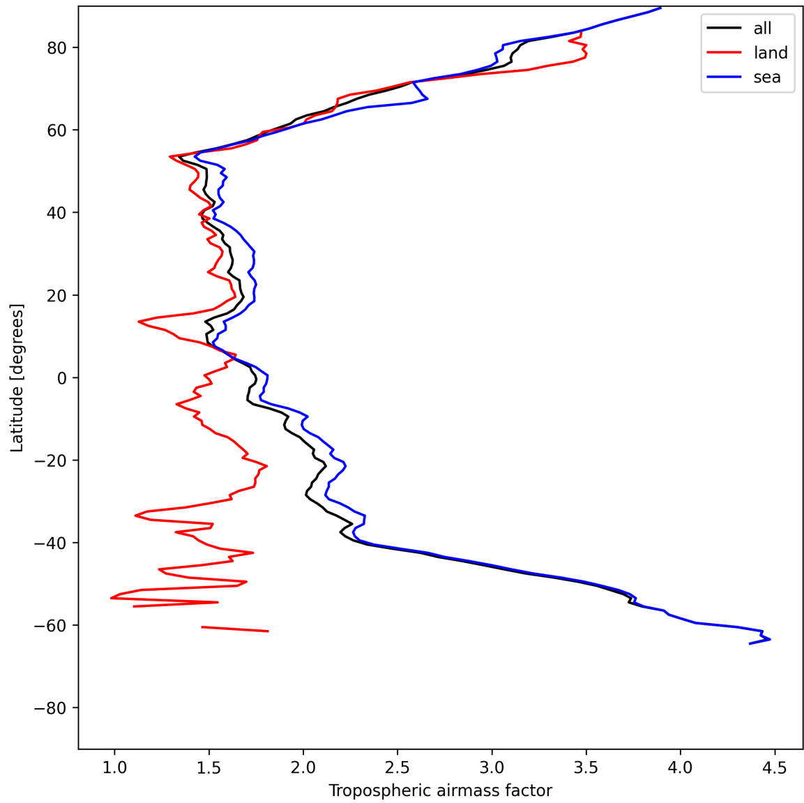
Figure 14: Zonal average of “Tropospheric airmass factor” for 2025-06-28 to 2025-06-30.
