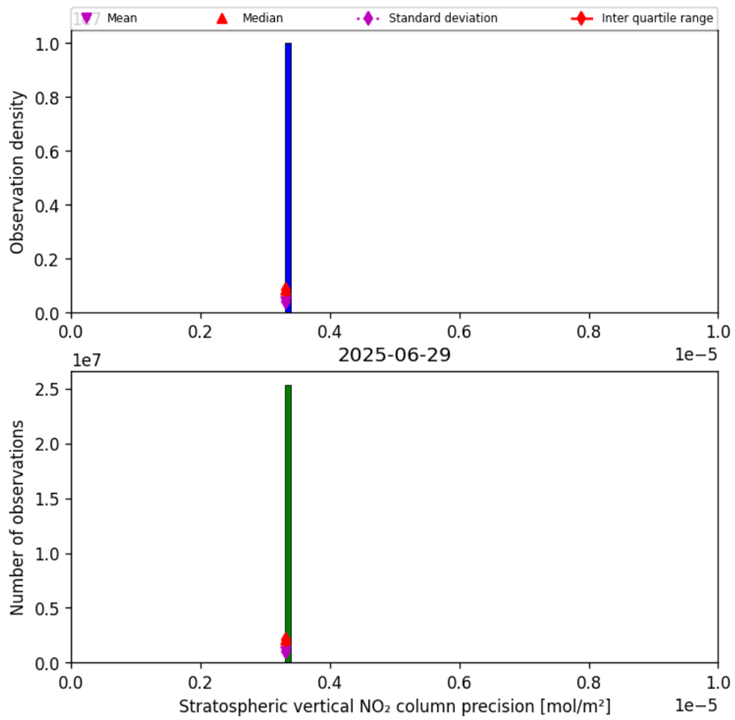
Figure 37: Histogram of “Stratospheric vertical NO 2 column precision” for 2025-06-28 to 2025-06-30
