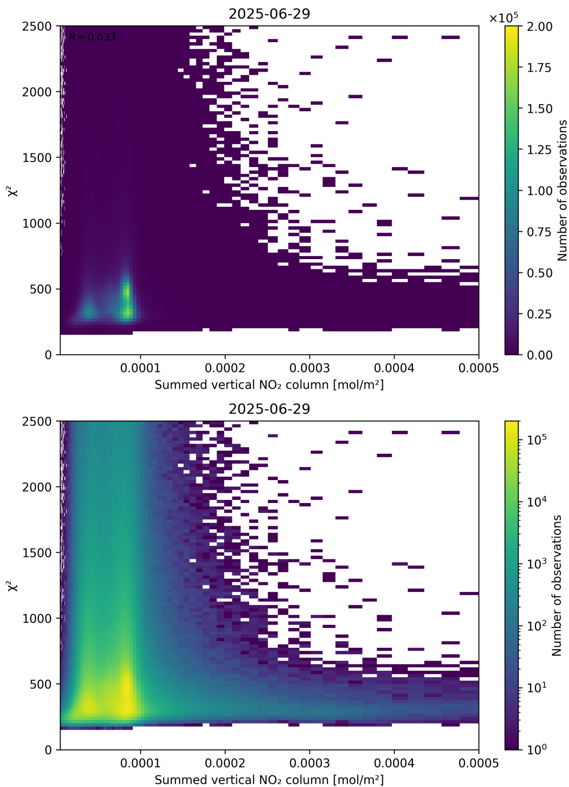
Figure 104: Scatter density plot of “Summed vertical NO 2 column” against “ \chi^2 ” for 2025-06-28 to 2025-06-30.
