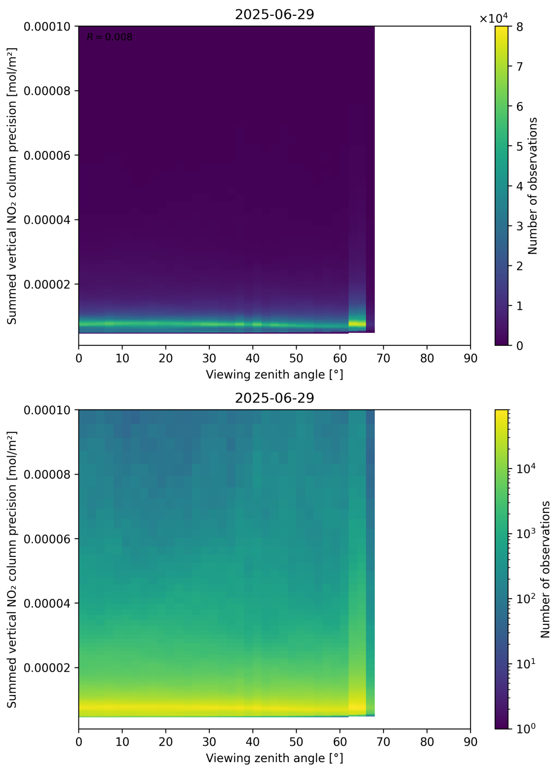
Figure 166: Scatter density plot of “Viewing zenith angle” against “Summed vertical NO 2 column precision” for 2025-06-28 to 2025-06-30.
