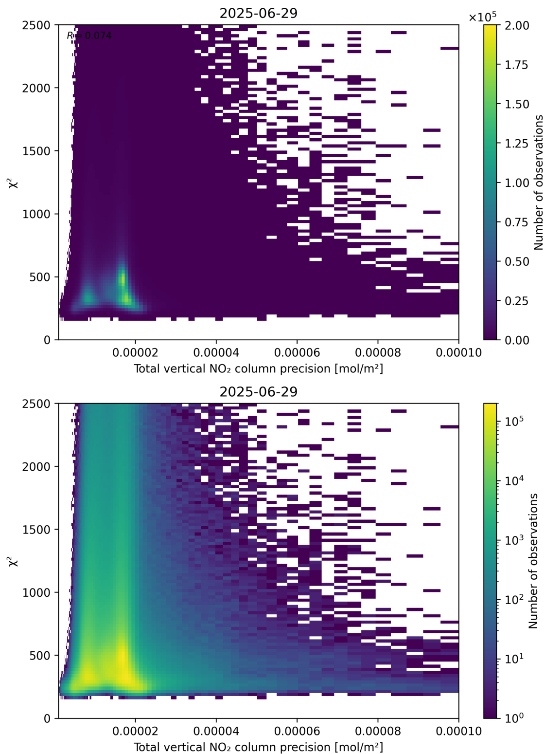
Figure 116: Scatter density plot of “Total vertical NO 2 column precision” against “ \chi^2 ” for 2025-06-28 to 2025-06-30.
