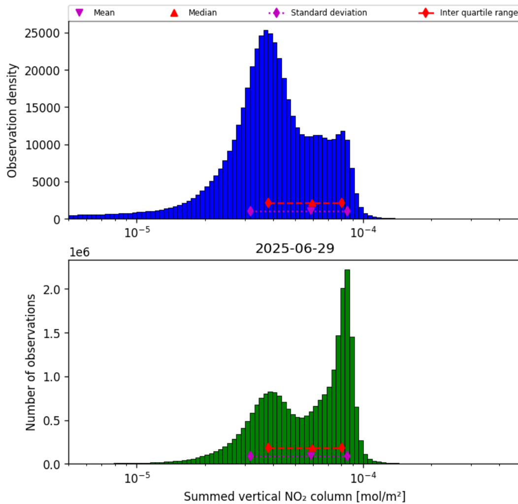
Figure 40: Histogram of “Summed vertical NO 2 column” for 2025-06-28 to 2025-06-30
