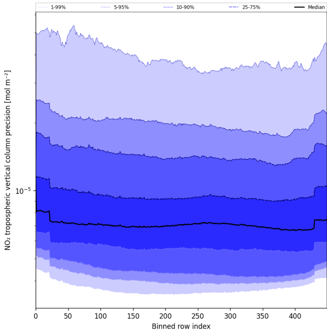
Figure 47: Along track statistics of “NO 2 tropospheric vertical column precision” for 2025-06-28 to 2025-06-30
