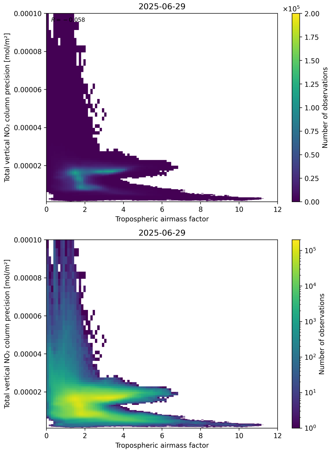
Figure 78: Scatter density plot of “Tropospheric airmass factor” against “Total vertical NO 2 column precision” for 2025-06-28 to 2025-06-30.
