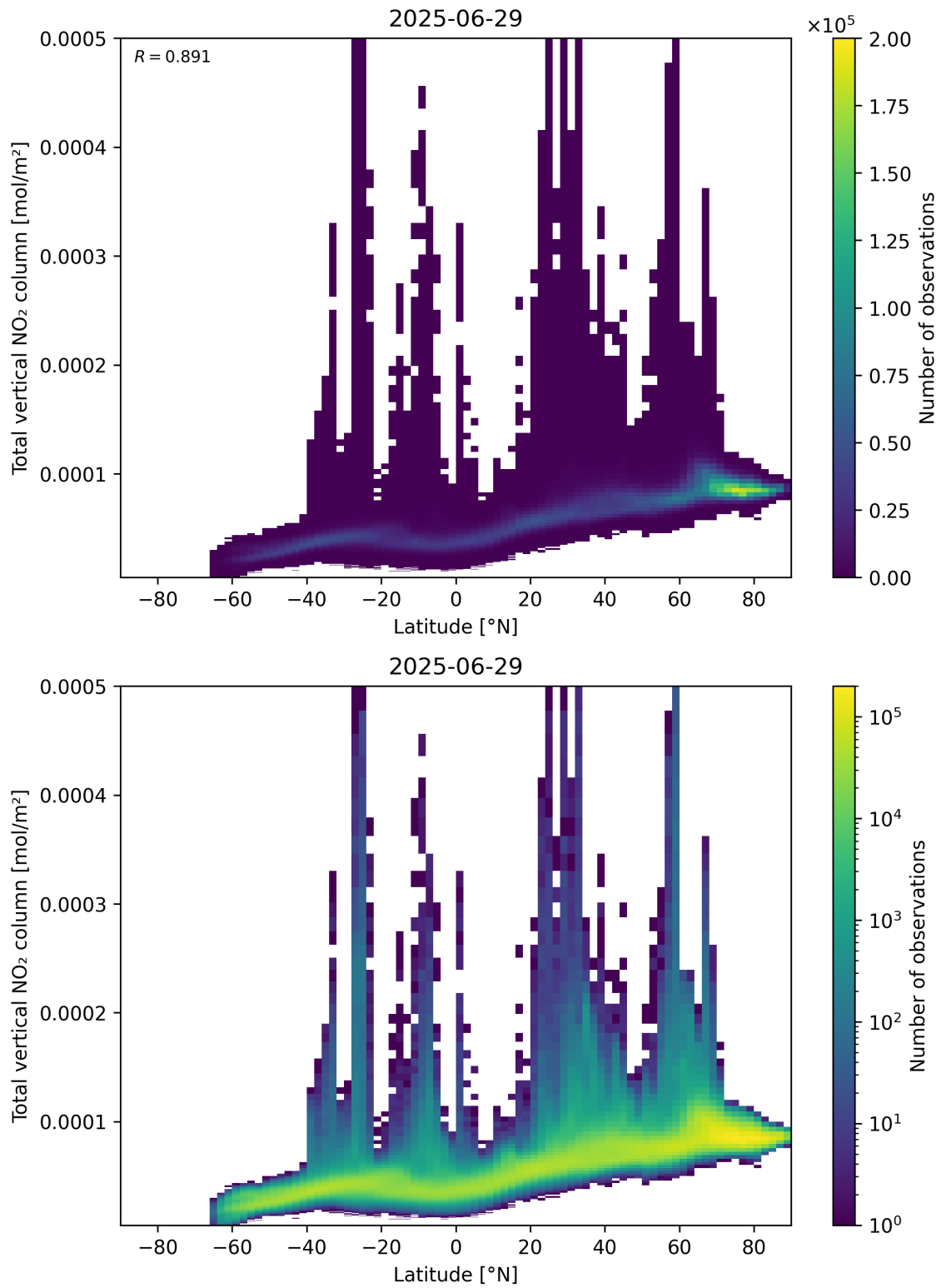
Figure 90: Scatter density plot of “Latitude” against “Total vertical NO 2 column” for 2025-06-28 to 2025-06-30.
