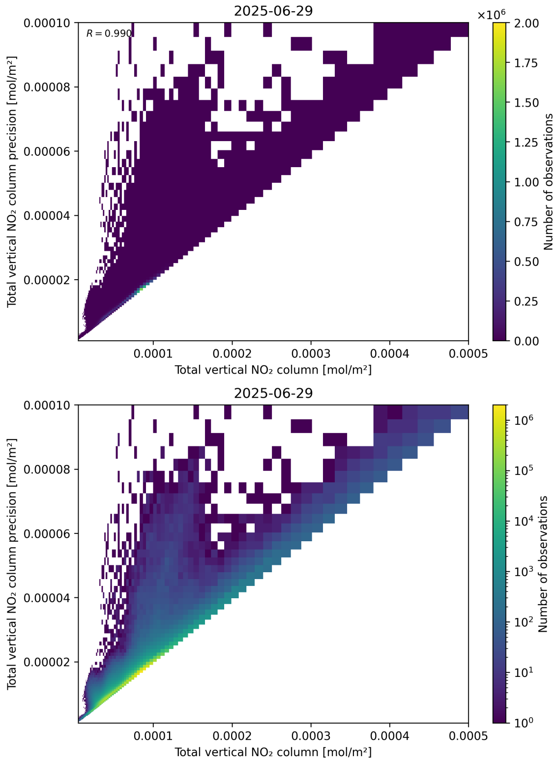
Figure 114: Scatter density plot of “Total vertical NO 2 column” against “Total vertical NO 2 column precision” for 2025-06-28 to 2025-06-30.
