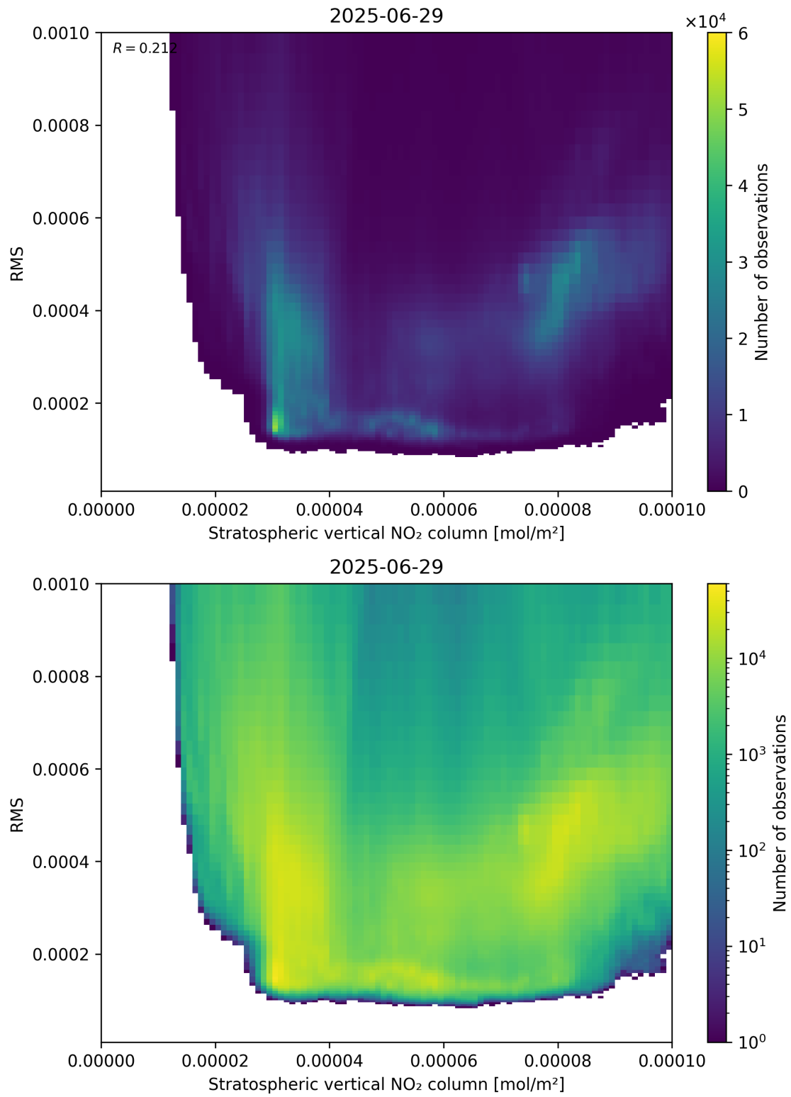
Figure 102: Scatter density plot of “Stratospheric vertical NO 2 column” against “RMS” for 2025-06-28 to 2025-06-30.
