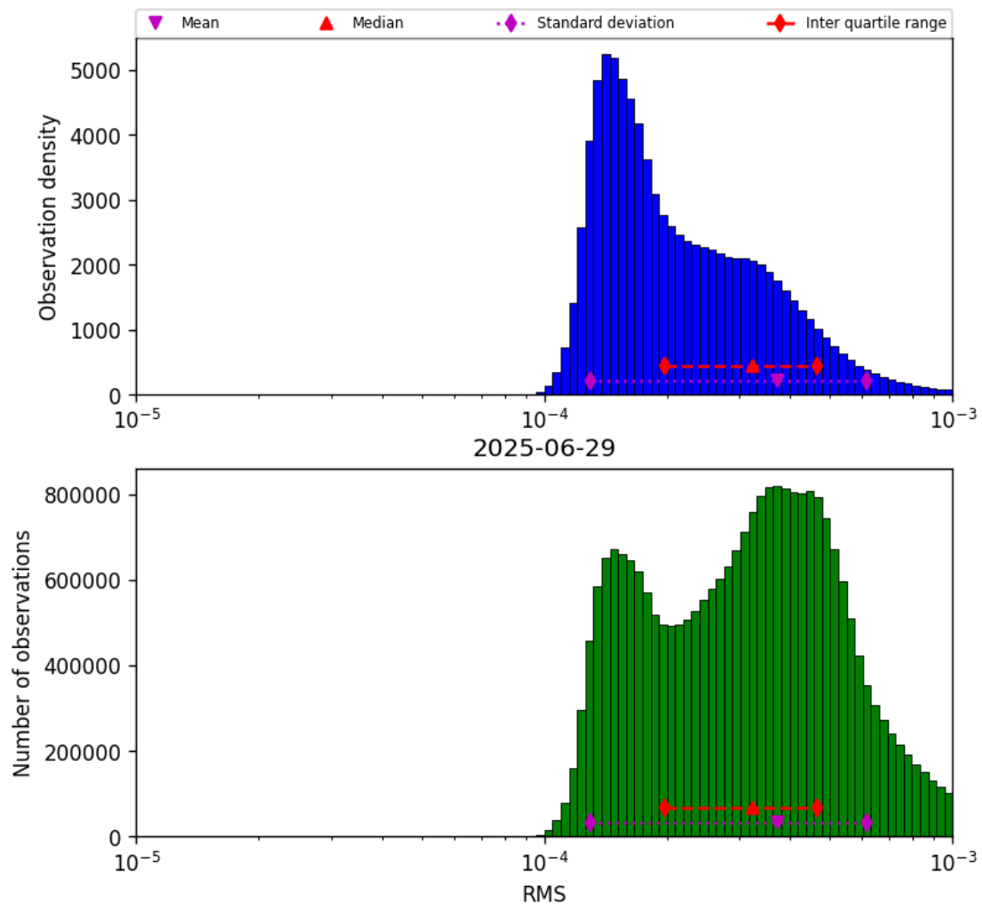
Figure 43: Histogram of “RMS” for 2025-06-28 to 2025-06-30
