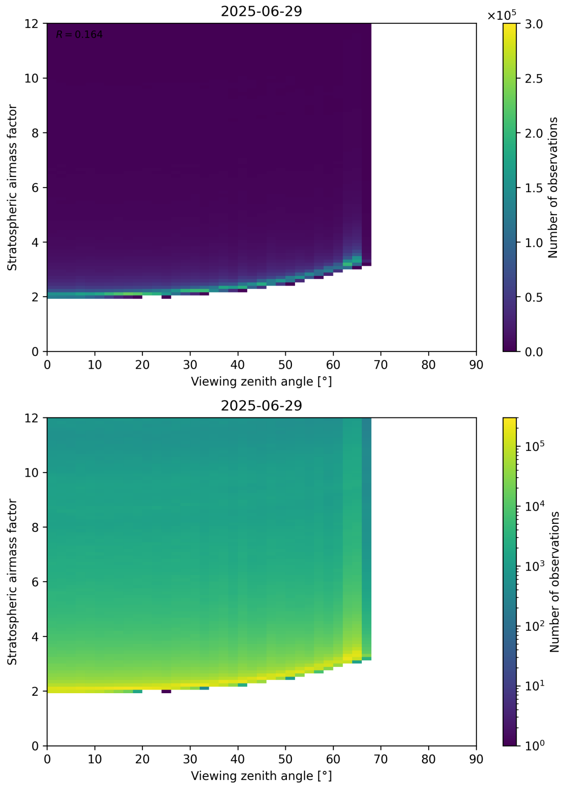
Figure 159: Scatter density plot of “Viewing zenith angle” against “Stratospheric airmass factor” for 2025-06-28 to 2025-06-30.
