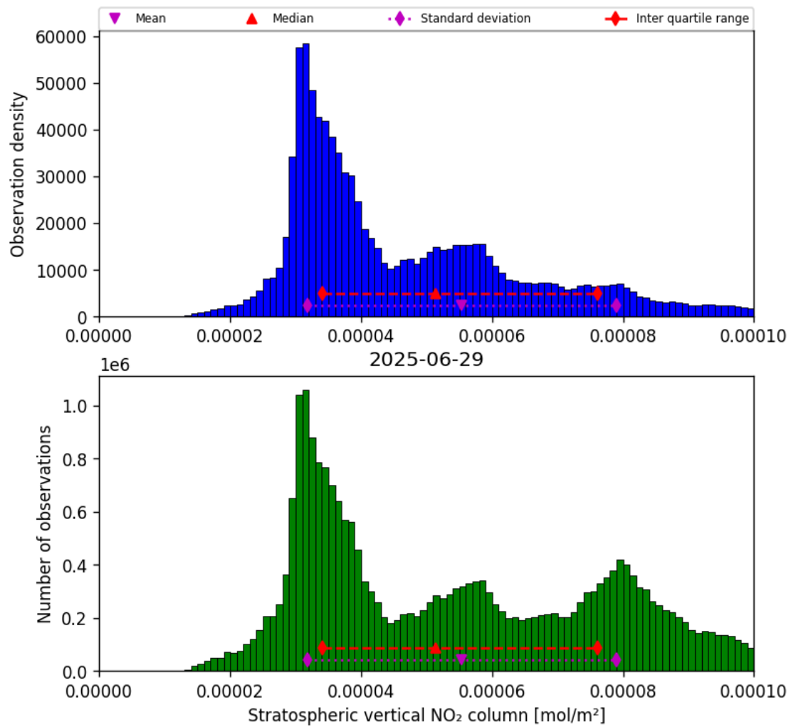
Figure 36: Histogram of “Stratospheric vertical NO 2 column” for 2025-06-28 to 2025-06-30
