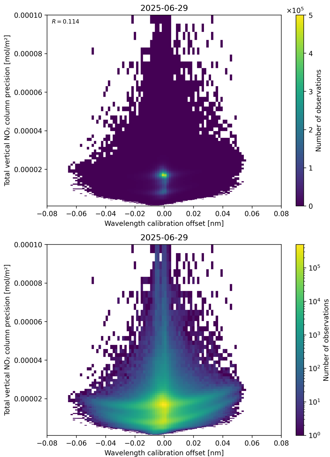
Figure 180: Scatter density plot of “Wavelength calibration offset” against “Total vertical NO 2 column precision” for 2025-06-28 to 2025-06-30.
