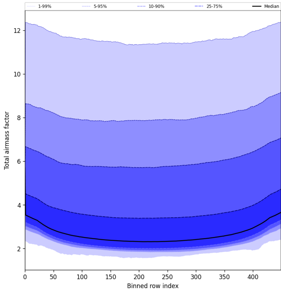
Figure 49: Along track statistics of “Total airmass factor” for 2025-06-28 to 2025-06-30
