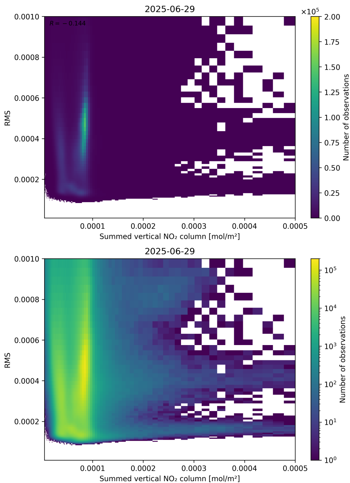
Figure 109: Scatter density plot of “Summed vertical NO 2 column” against “RMS” for 2025-06-28 to 2025-06-30.
