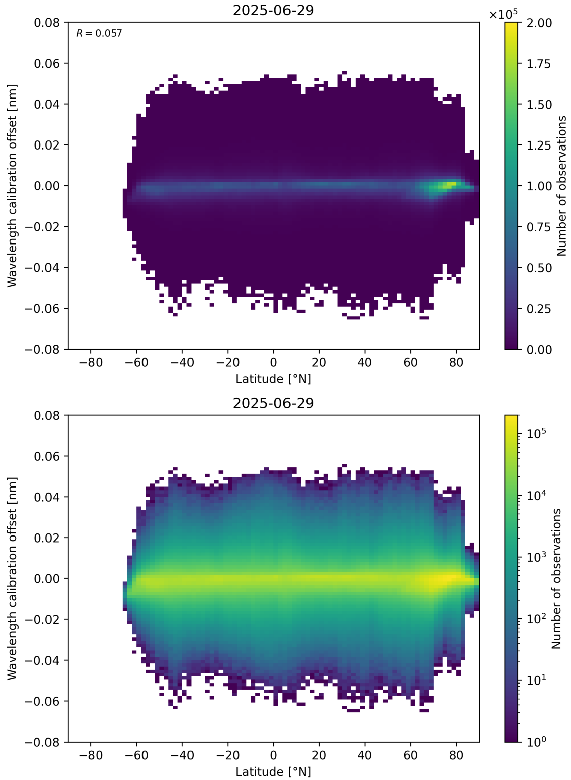
Figure 95: Scatter density plot of “Latitude” against “Wavelength calibration offset” for 2025-06-28 to 2025-06-30.
