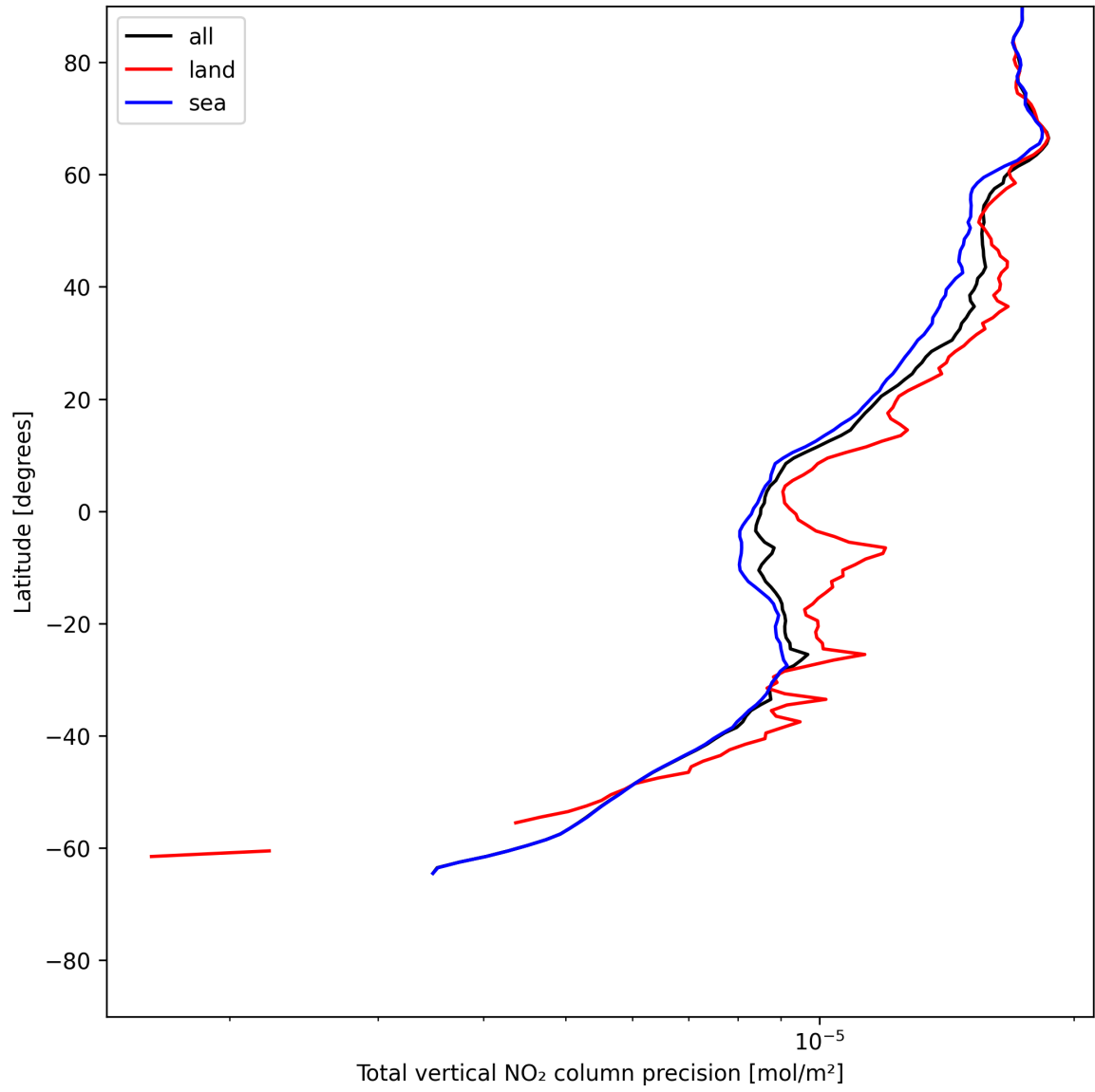
Figure 22: Zonal average of “Total vertical NO 2 column precision” for 2025-06-28 to 2025-06-30.
