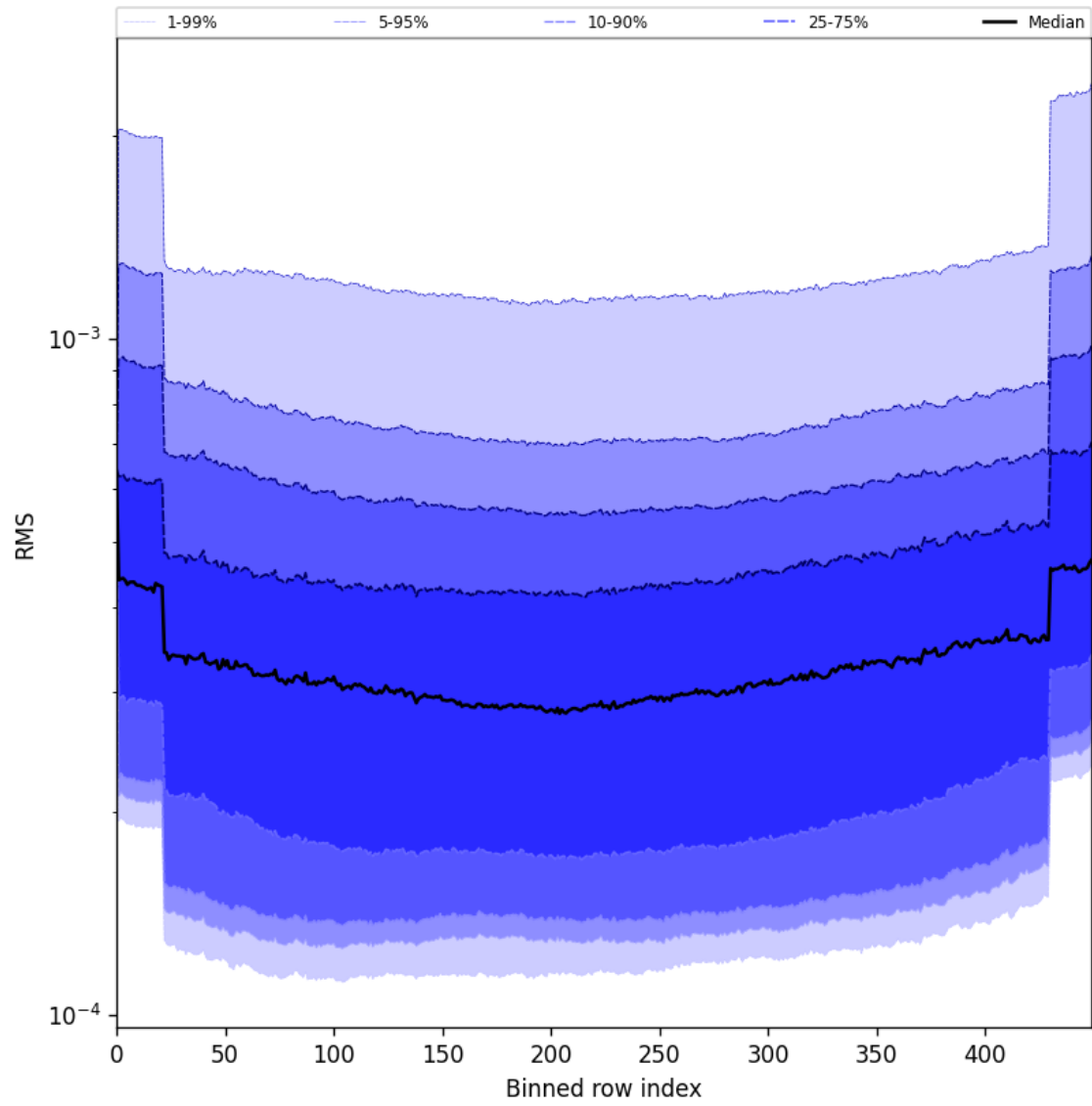
Figure 60: Along track statistics of “RMS” for 2025-06-28 to 2025-06-30
