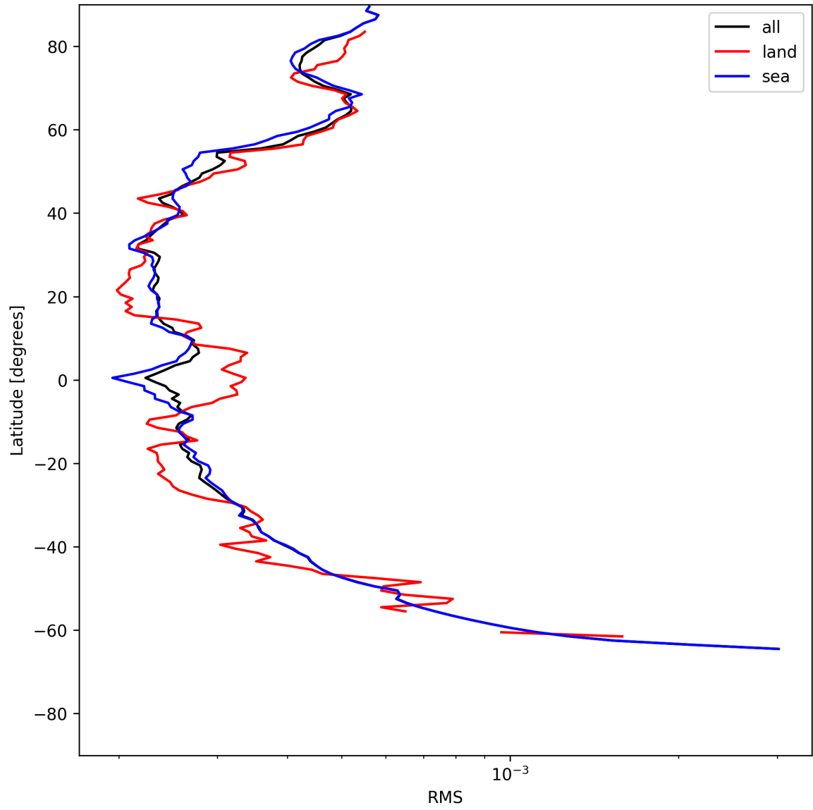
Figure 26: Zonal average of “RMS” for 2025-06-28 to 2025-06-30.
