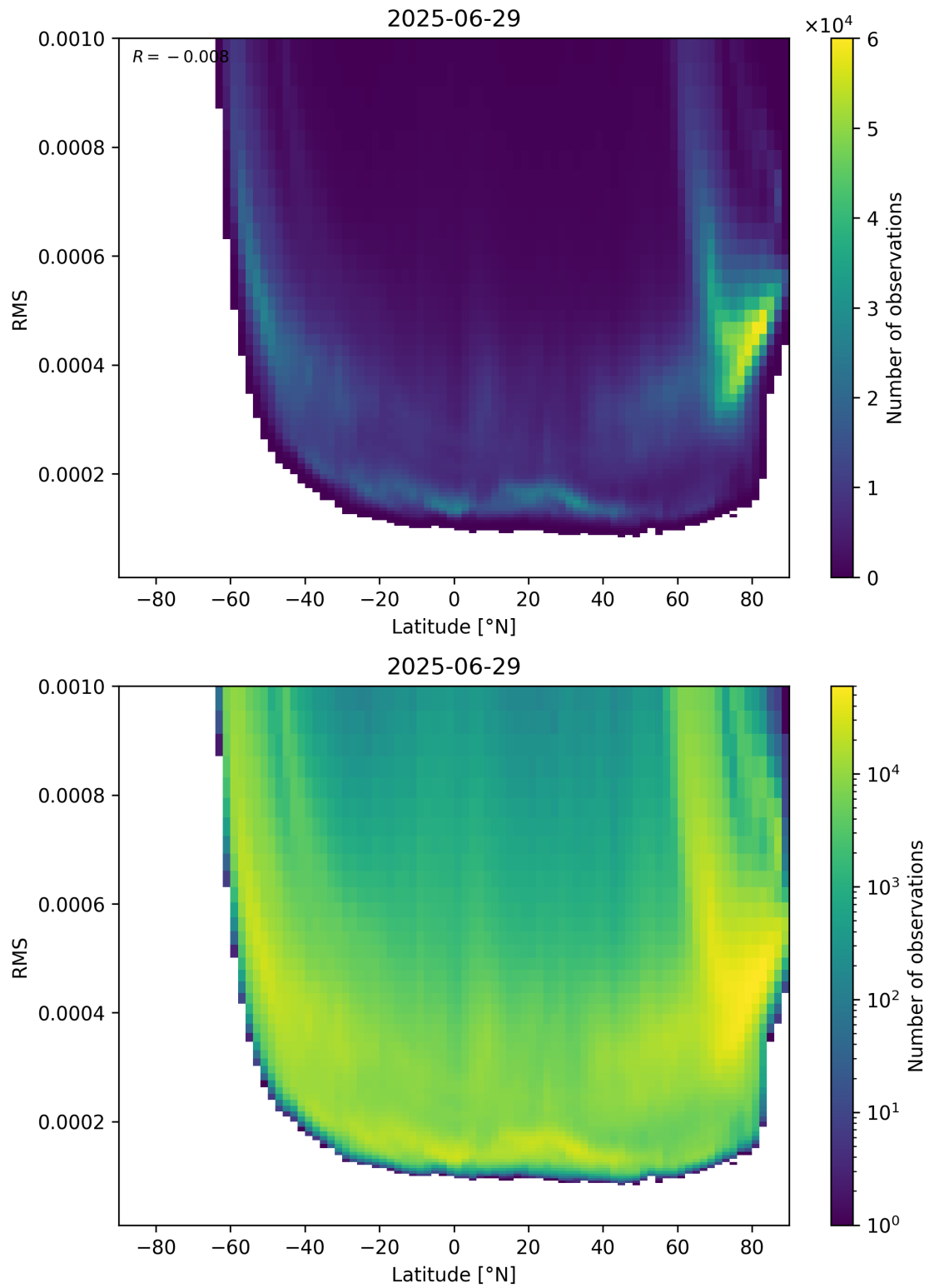
Figure 94: Scatter density plot of “Latitude” against “RMS” for 2025-06-28 to 2025-06-30.
