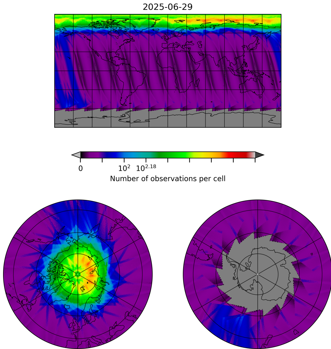
Figure 10: Map of the number of observations for 2025-06-28 to 2025-06-30
