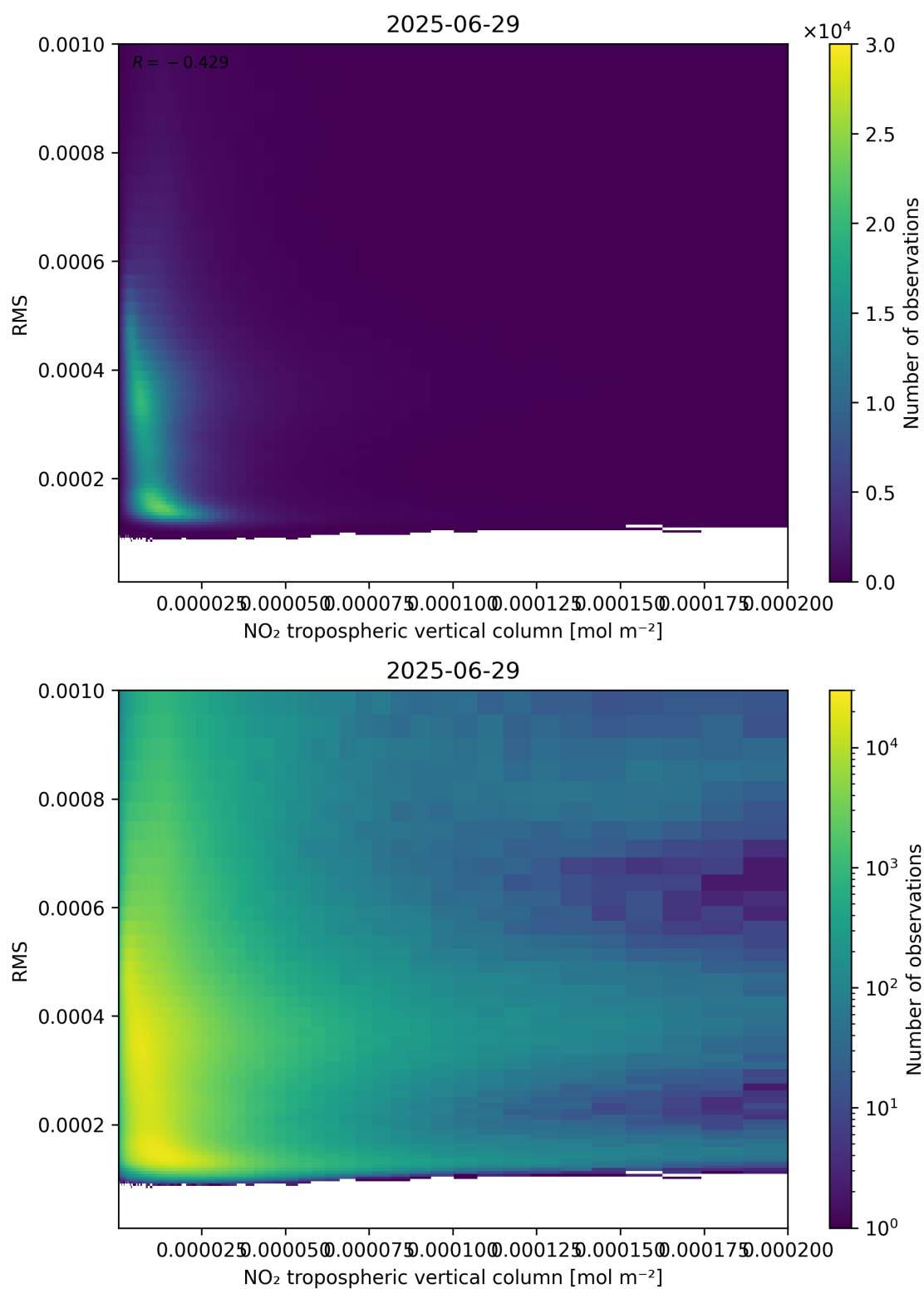
Figure 142: Scatter density plot of “NO 2 tropospheric vertical column” against “RMS” for 2025-06-28 to 2025-06-30.
