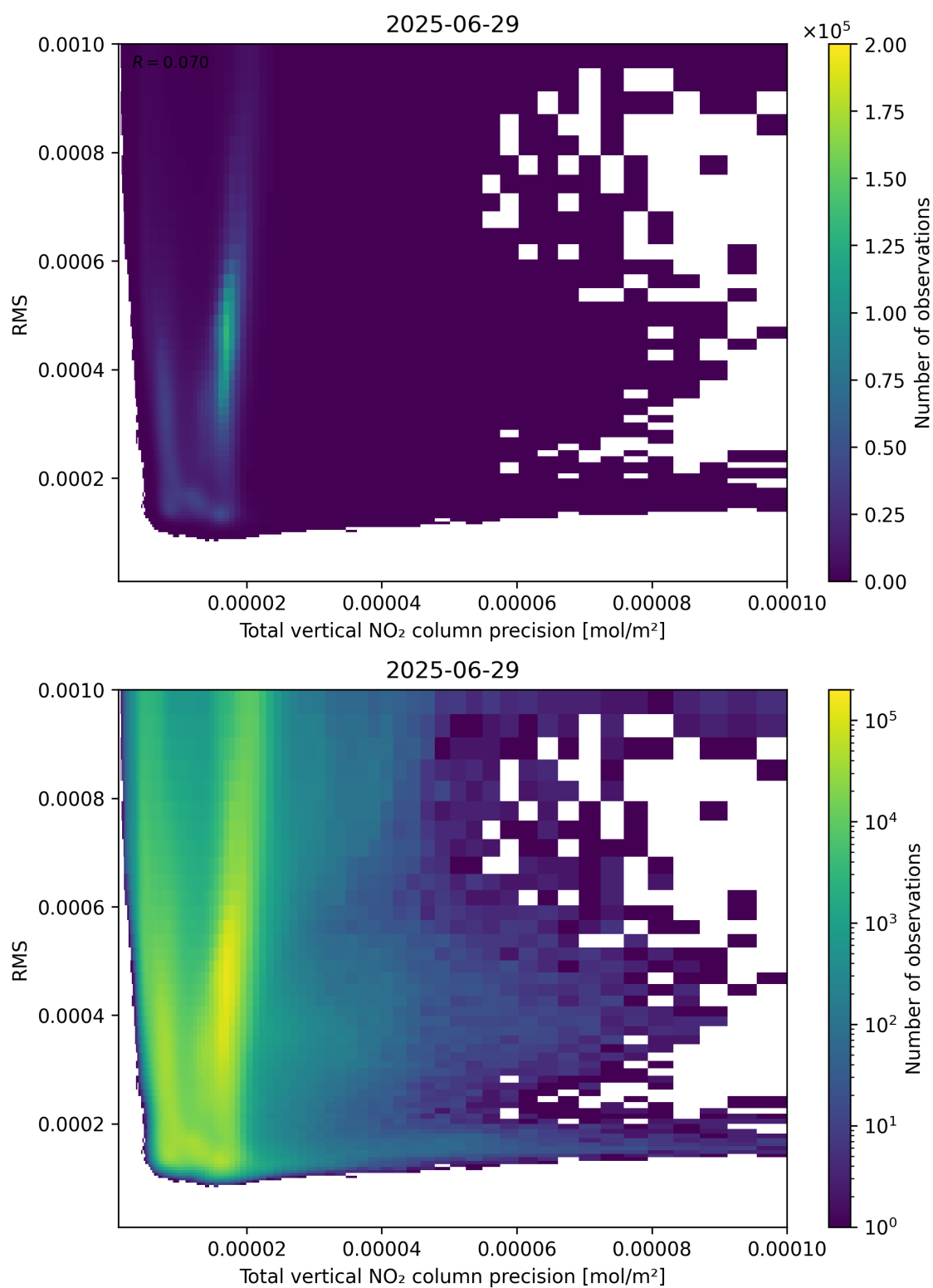
Figure 119: Scatter density plot of “Total vertical NO 2 column precision” against “RMS” for 2025-06-28 to 2025-06-30.
