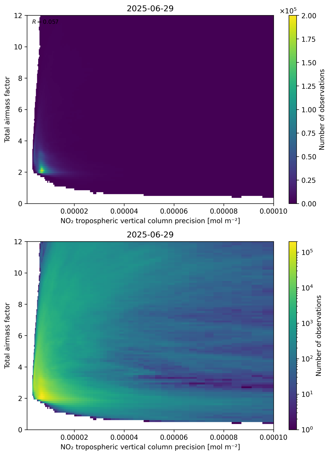
Figure 132: Scatter density plot of “NO 2 tropospheric vertical column precision” against “Total air mass factor” for 2025-06-28 to 2025-06-30.
