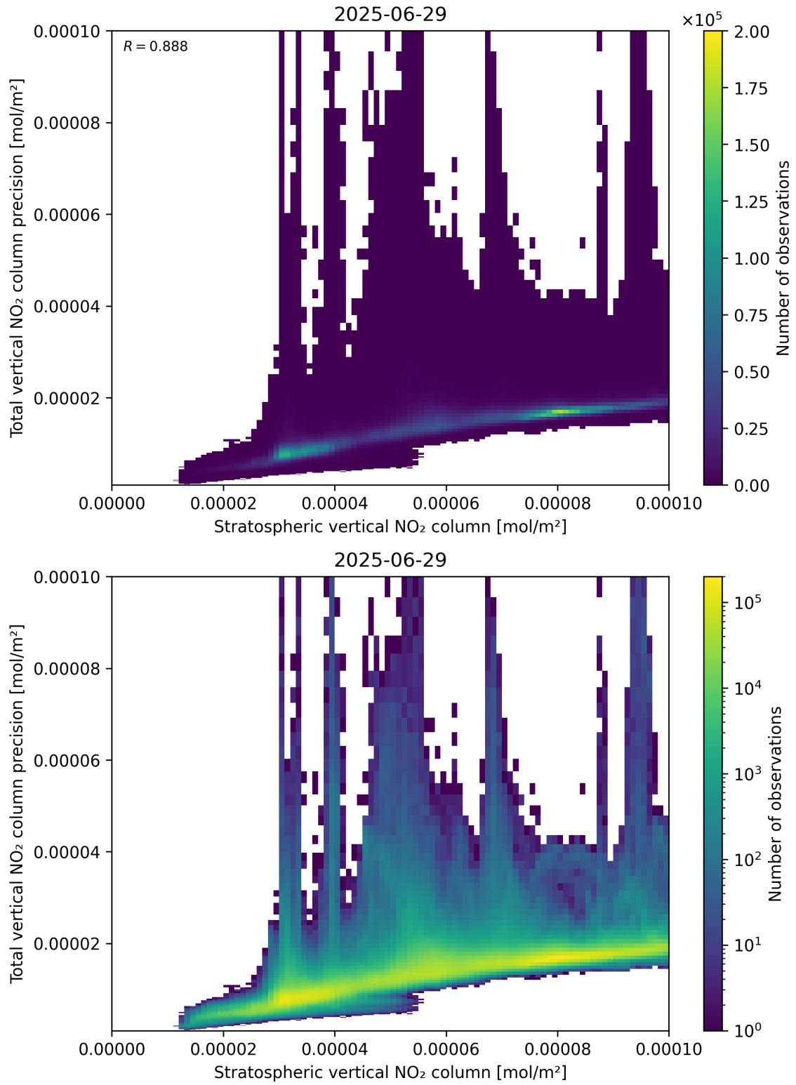
Figure 101: Scatter density plot of “Stratospheric vertical NO 2 column” against “Total vertical NO 2 column precision” for 2025-06-28 to 2025-06-30.
