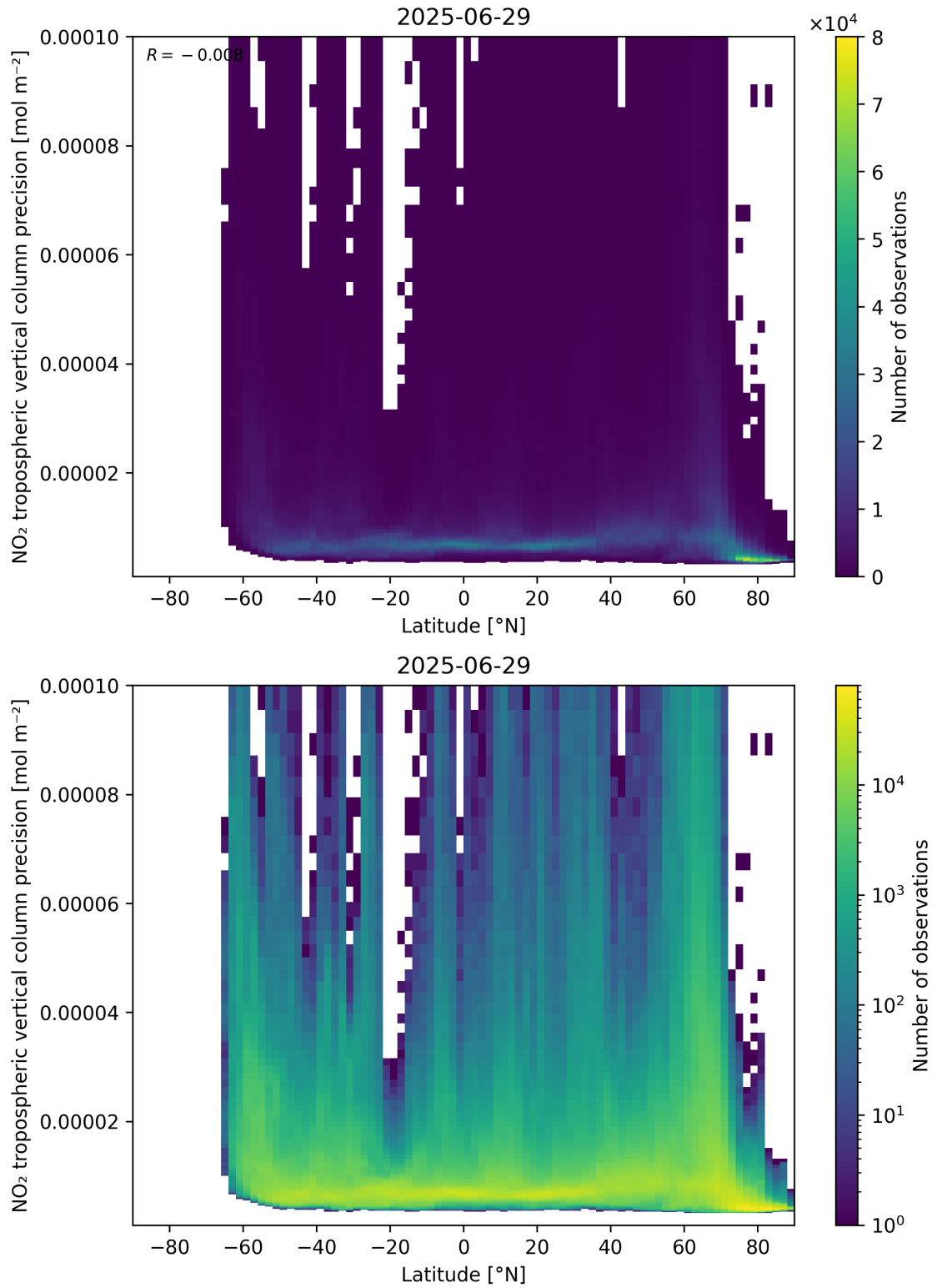
Figure 93: Scatter density plot of “Latitude” against “NO 2 tropospheric vertical column precision” for 2025-06-28 to 2025-06-30.
