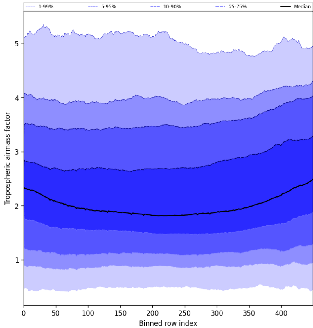
Figure 48: Along track statistics of “Tropospheric airmass factor” for 2025-06-28 to 2025-06-30
