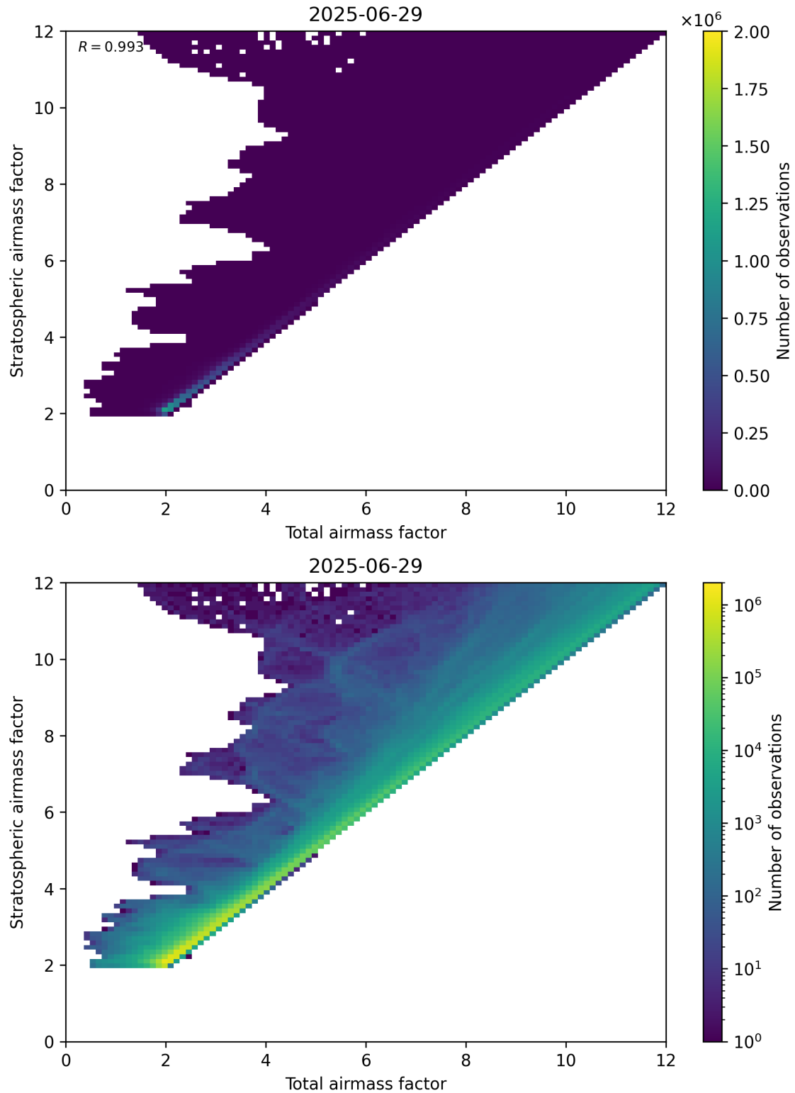
Figure 62: Scatter density plot of “Total airmass factor” against “Stratospheric airmass factor” for 2025-06-28 to 2025-06-30.
