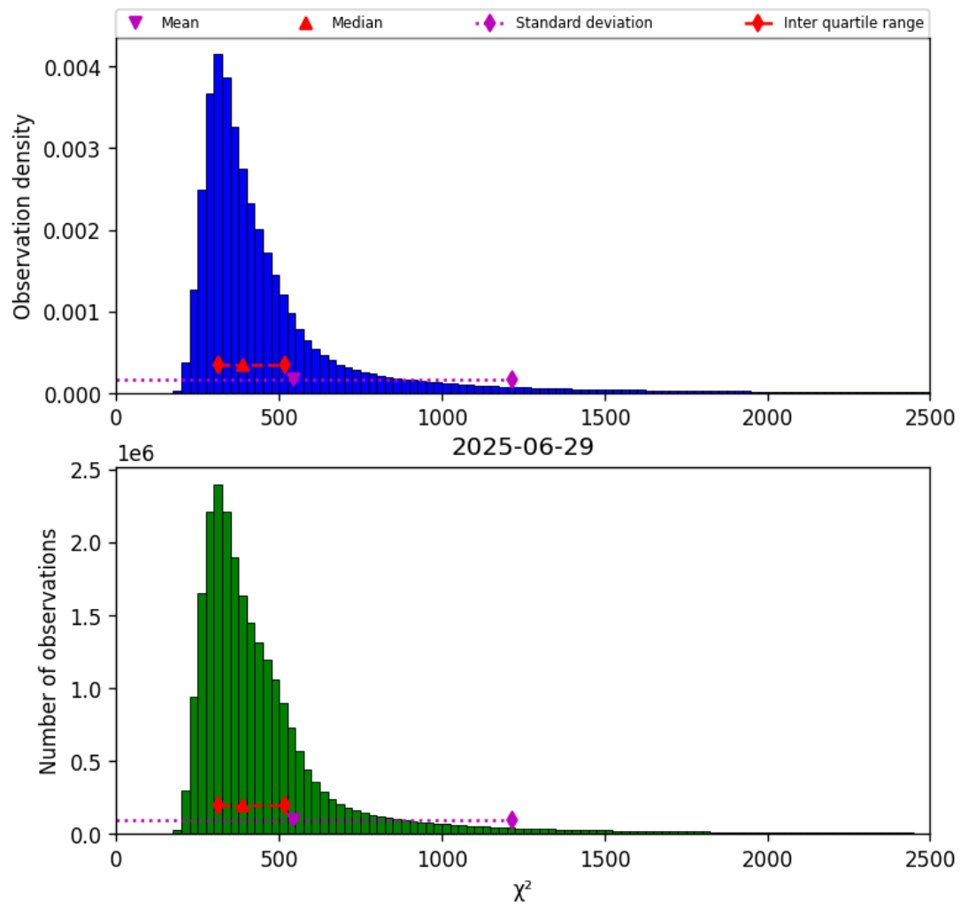
Figure 42: Histogram of “ \chi^2 ” for 2025-06-28 to 2025-06-30
