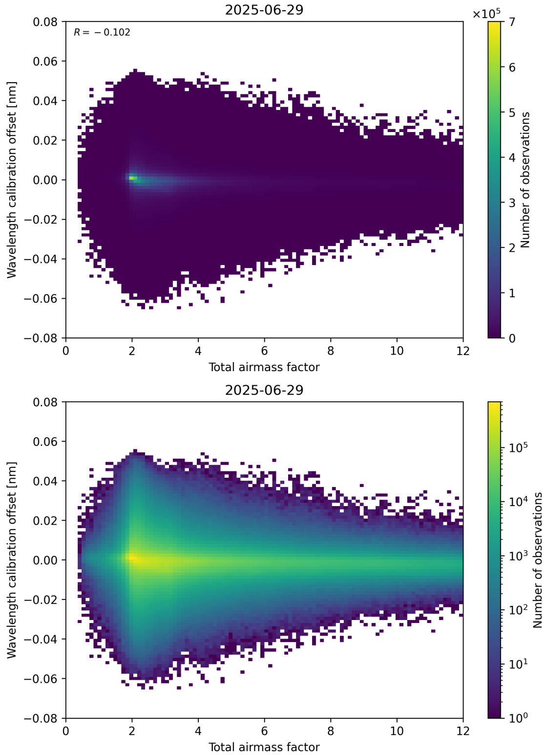
Figure 70: Scatter density plot of “Total airmass factor” against “Wavelength calibration offset” for 2025-06-28 to 2025-06-30.
