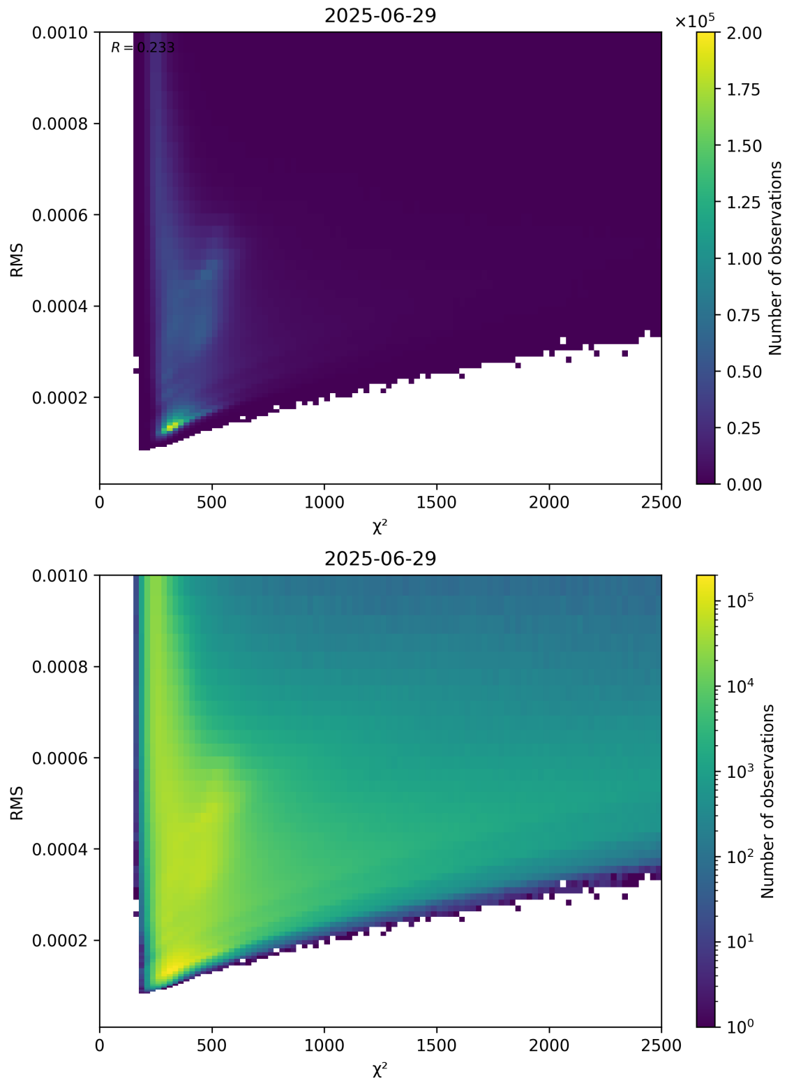
Figure 82: Scatter density plot of “ \chi^2 ” against “RMS” for 2025-06-28 to 2025-06-30.
