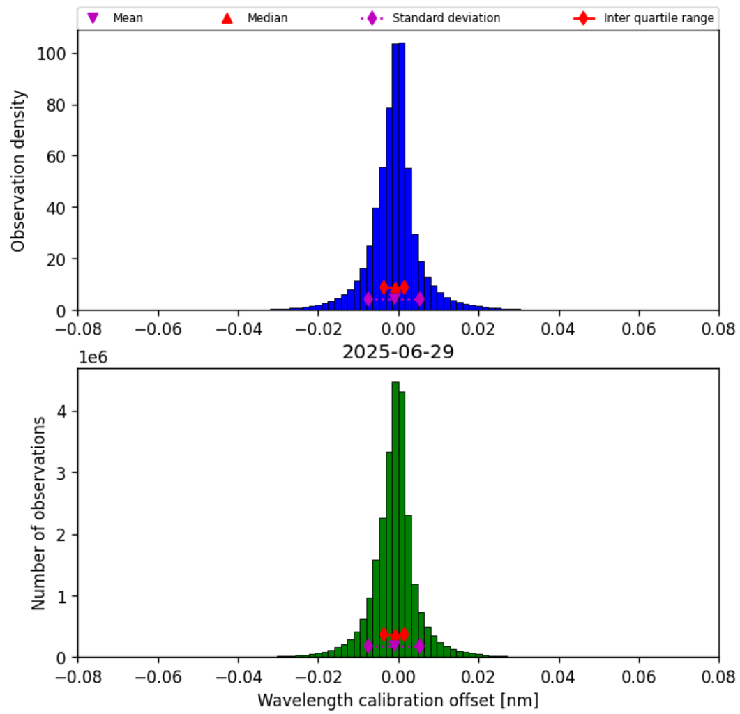
Figure 35: Histogram of “Wavelength calibration offset” for 2025-06-28 to 2025-06-30
