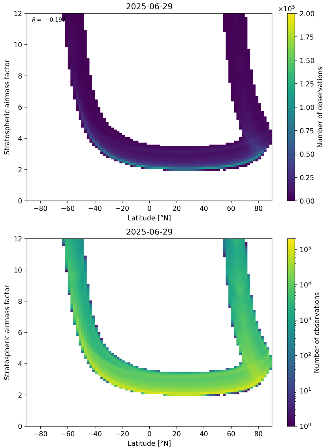
Figure 83: Scatter density plot of “Latitude” against “Stratospheric air mass factor” for 2025-06-28 to 2025-06-30.
