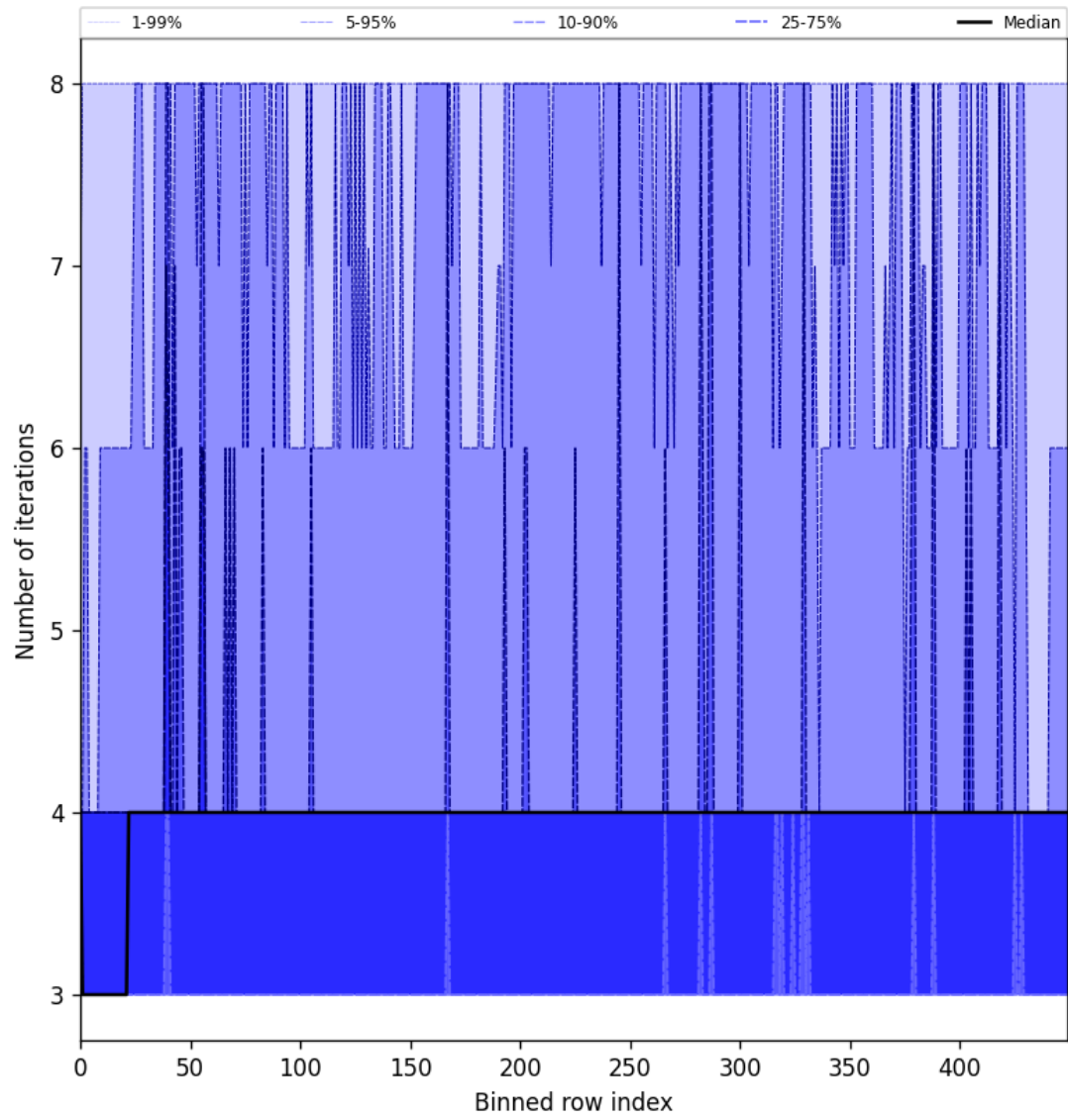
Figure 51: Along track statistics of “Number of iterations” for 2025-06-28 to 2025-06-30
