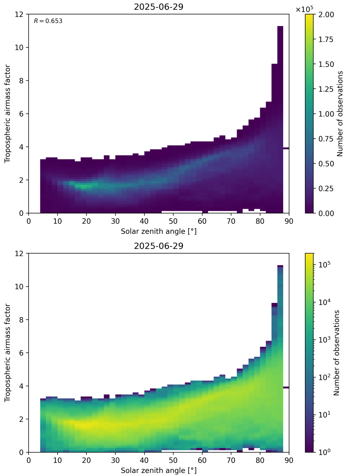
Figure 147: Scatter density plot of “Solar zenith angle” against “Tropospheric airmass factor” for 2025-06-28 to 2025-06-30.
