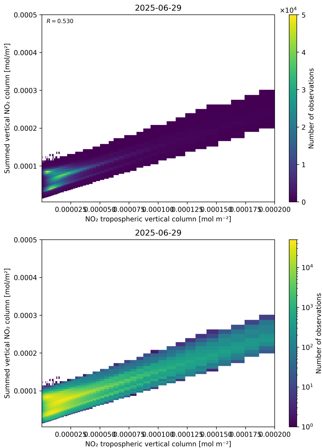
Figure 126: Scatter density plot of “NO 2 tropospheric vertical column” against “Summed vertical NO 2 column” for 2025-06-28 to 2025-06-30.
