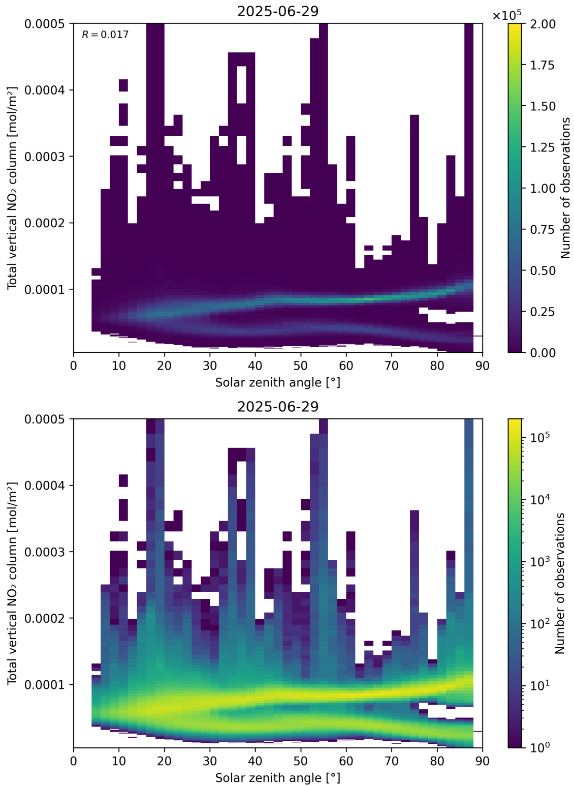
Figure 153: Scatter density plot of “Solar zenith angle” against “Total vertical NO 2 column” for 2025-06-28 to 2025-06-30.
