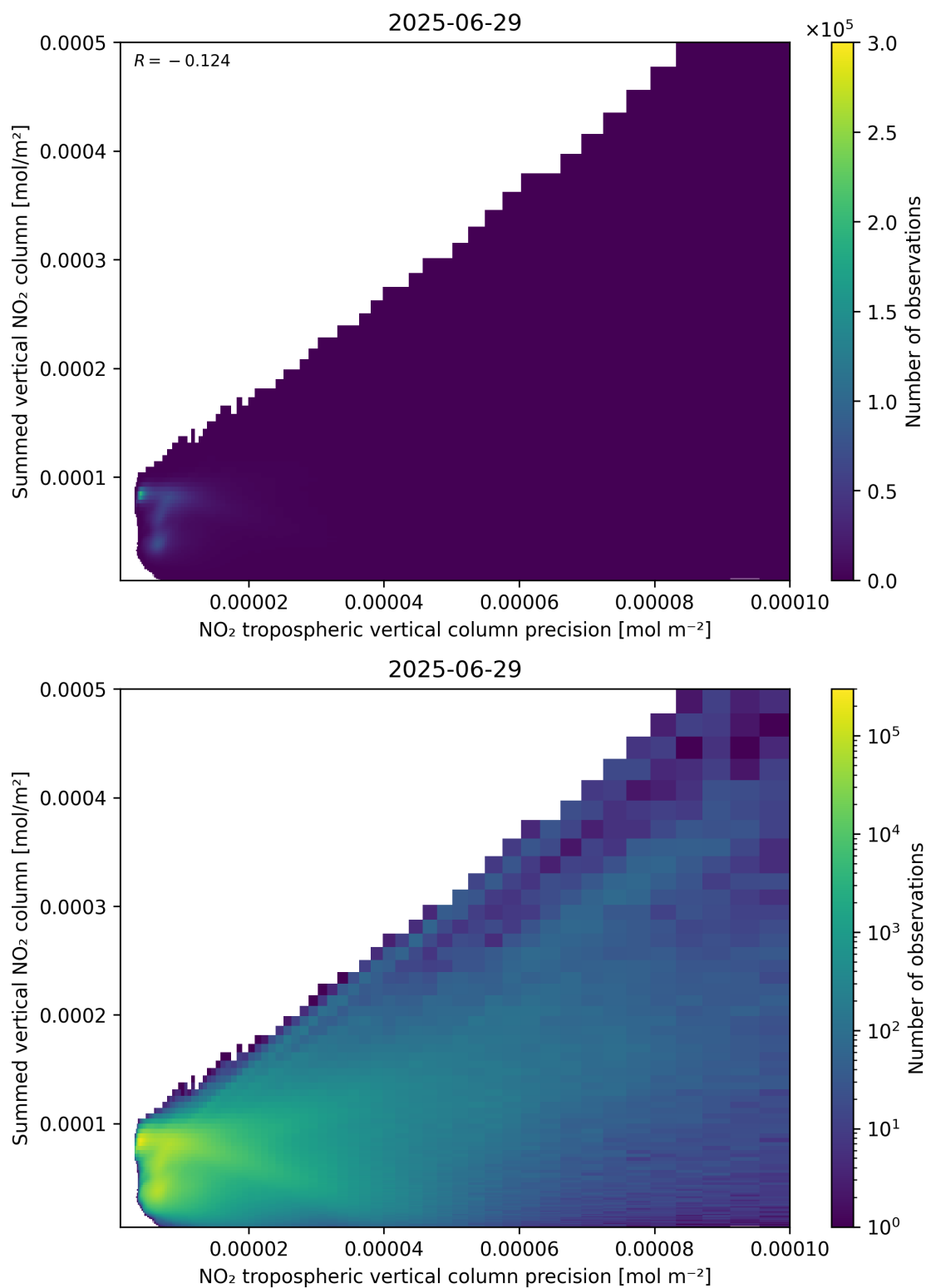
Figure 136: Scatter density plot of “NO 2 tropospheric vertical column precision” against “Summed vertical NO 2 column” for 2025-06-28 to 2025-06-30.
