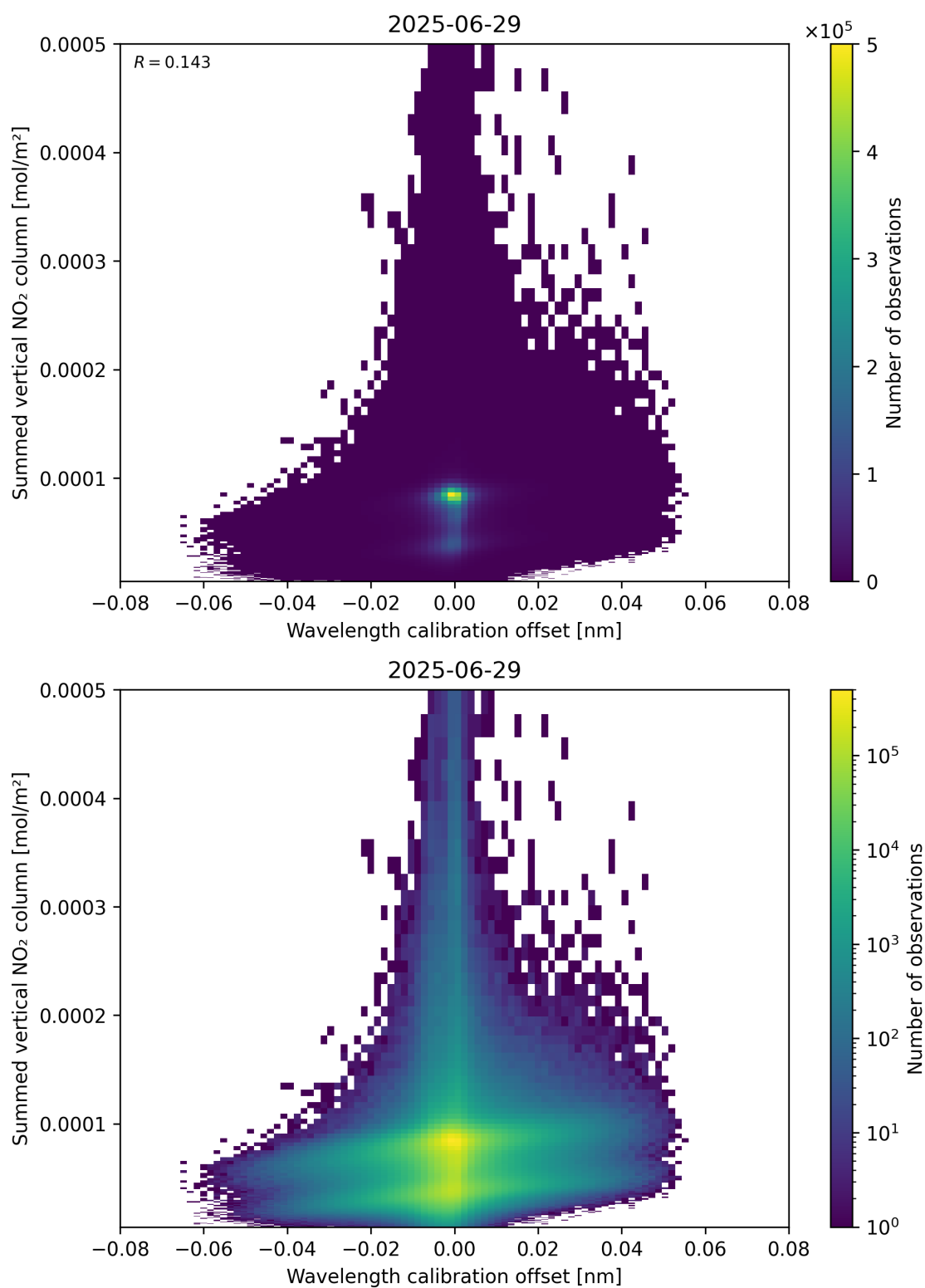
Figure 177: Scatter density plot of “Wavelength calibration offset” against “Summed vertical NO 2 column” for 2025-06-28 to 2025-06-30.
