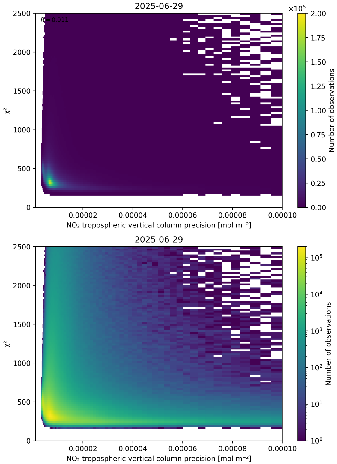
Figure 134: Scatter density plot of “NO 2 tropospheric vertical column precision” against “ \chi^2 ” for 2025-06-28 to 2025-06-30.
