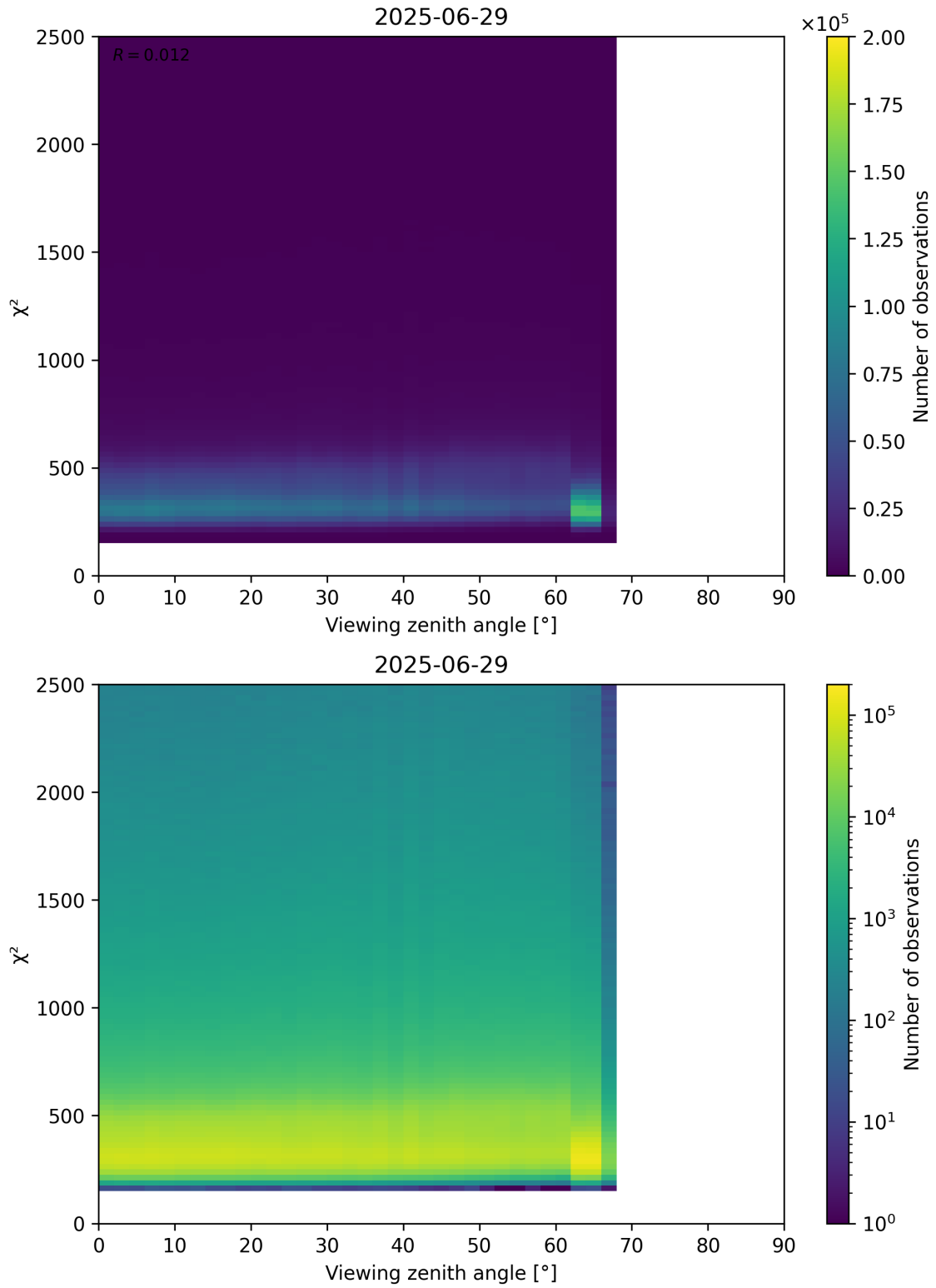
Figure 162: Scatter density plot of “Viewing zenith angle” against “ \chi^2 ” for 2025-06-28 to 2025-06-30.
