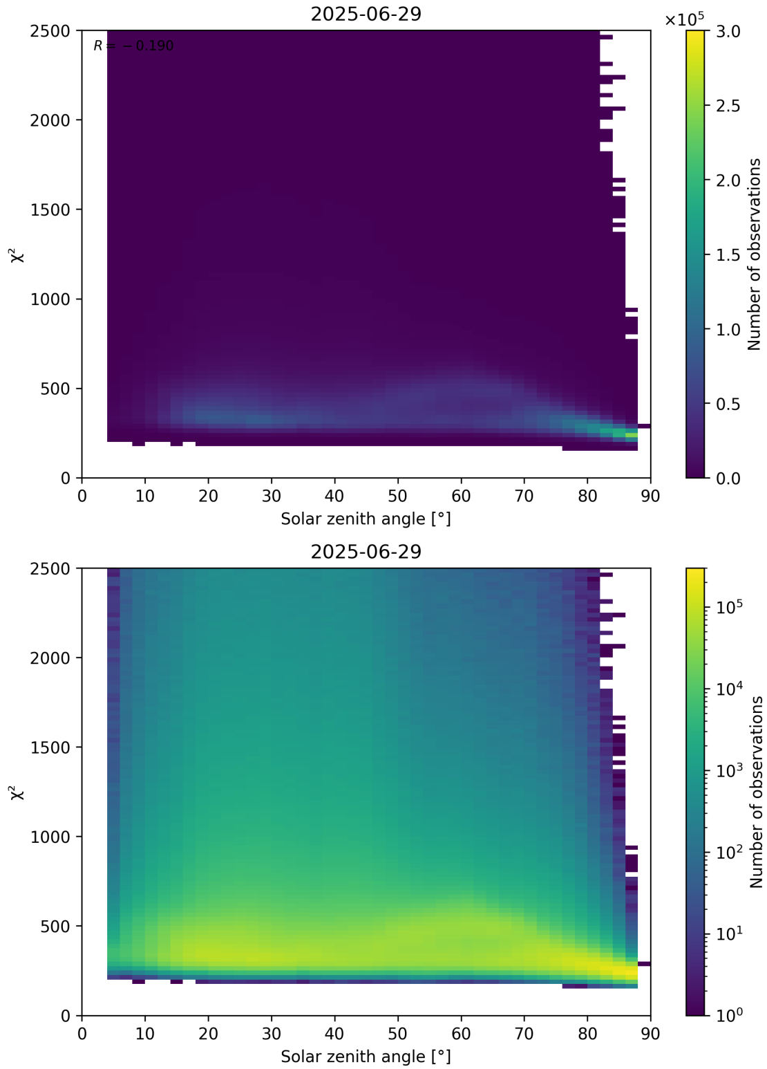
Figure 148: Scatter density plot of “Solar zenith angle” against “ \chi^2 ” for 2025-06-28 to 2025-06-30.
