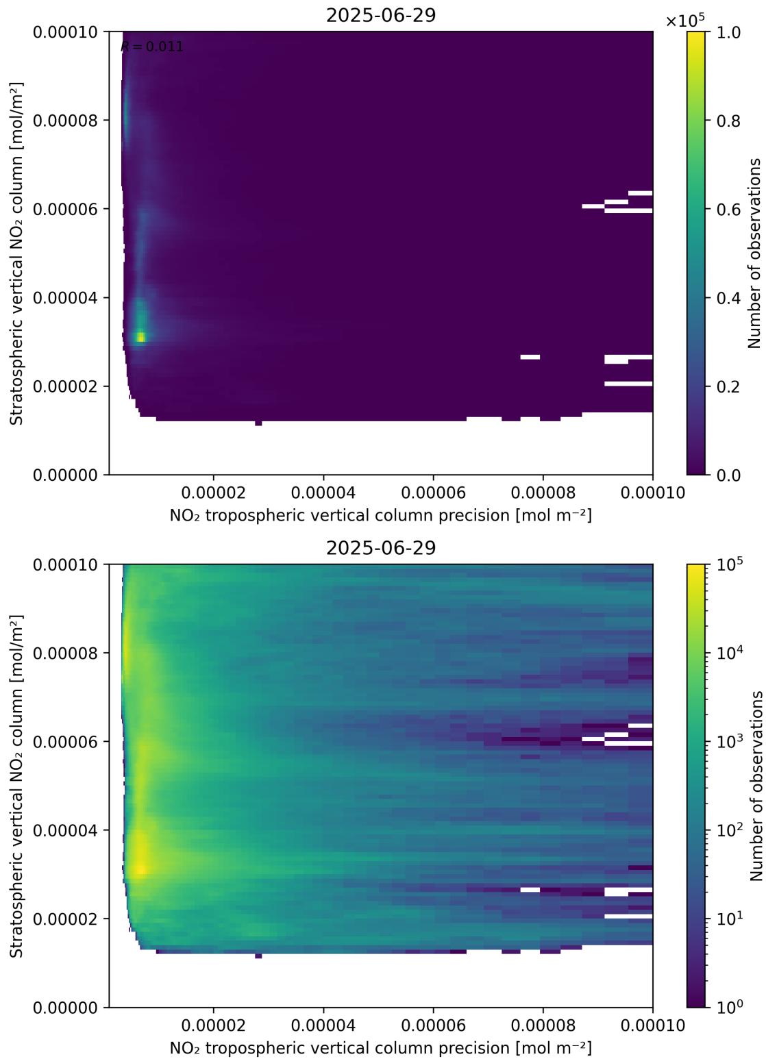
Figure 135: Scatter density plot of “NO 2 tropospheric vertical column precision” against “Stratospheric vertical NO 2 column” for 2025-06-28 to 2025-06-30.
