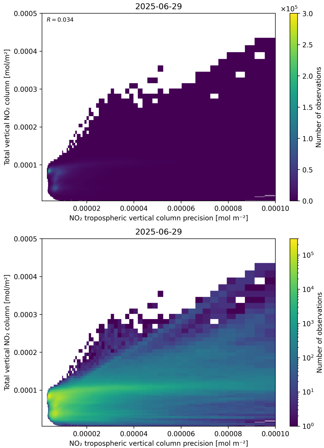
Figure 138: Scatter density plot of “NO 2 tropospheric vertical column precision” against “Total vertical NO 2 column” for 2025-06-28 to 2025-06-30.
