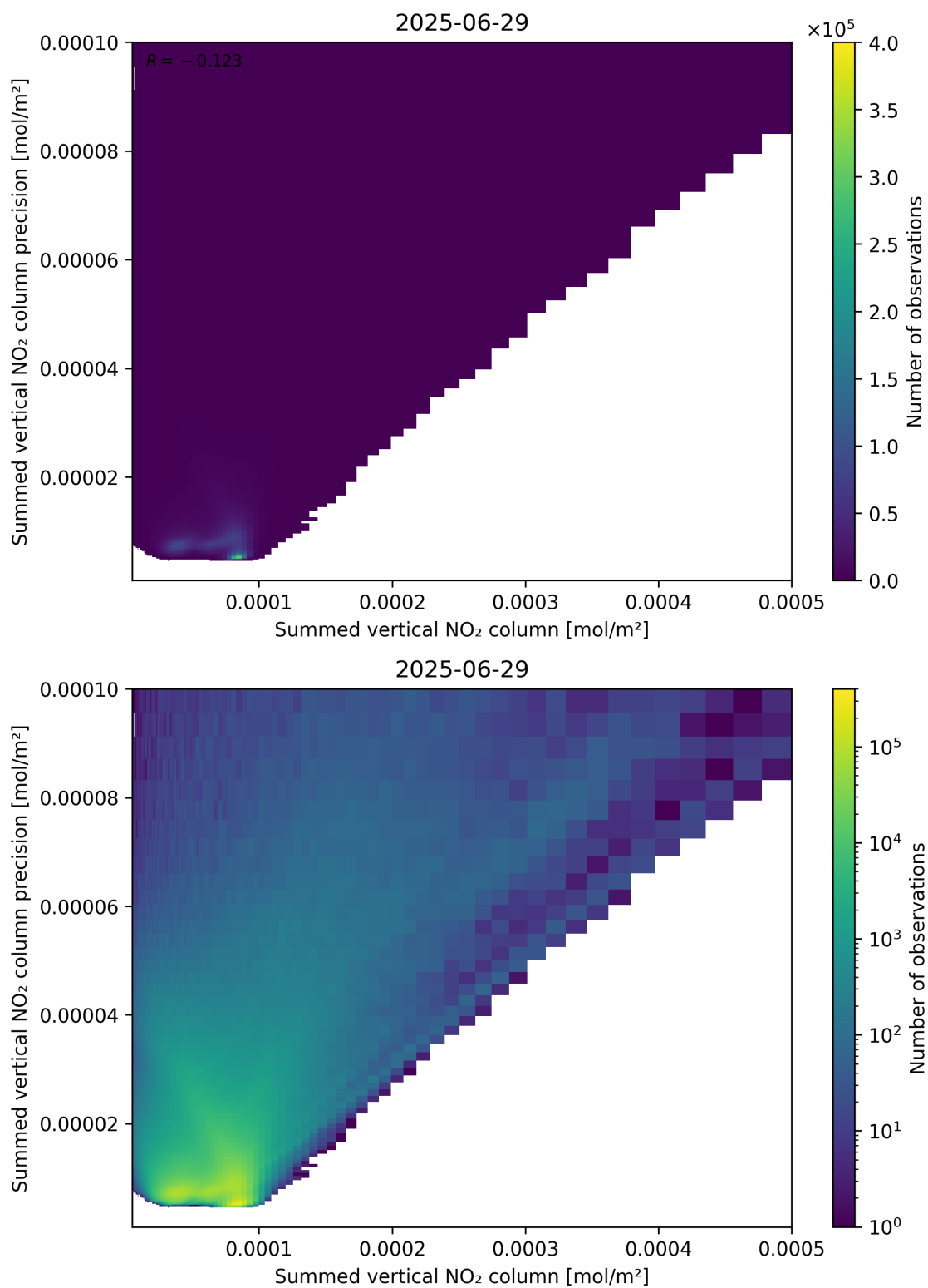
Figure 105: Scatter density plot of “Summed vertical NO 2 column” against “Summed vertical NO 2 column precision” for 2025-06-28 to 2025-06-30.
