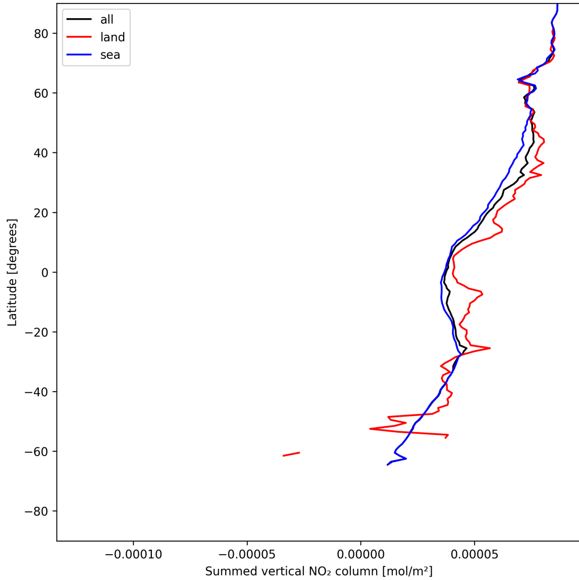
Figure 23: Zonal average of “Summed vertical NO 2 column” for 2025-06-28 to 2025-06-30.
