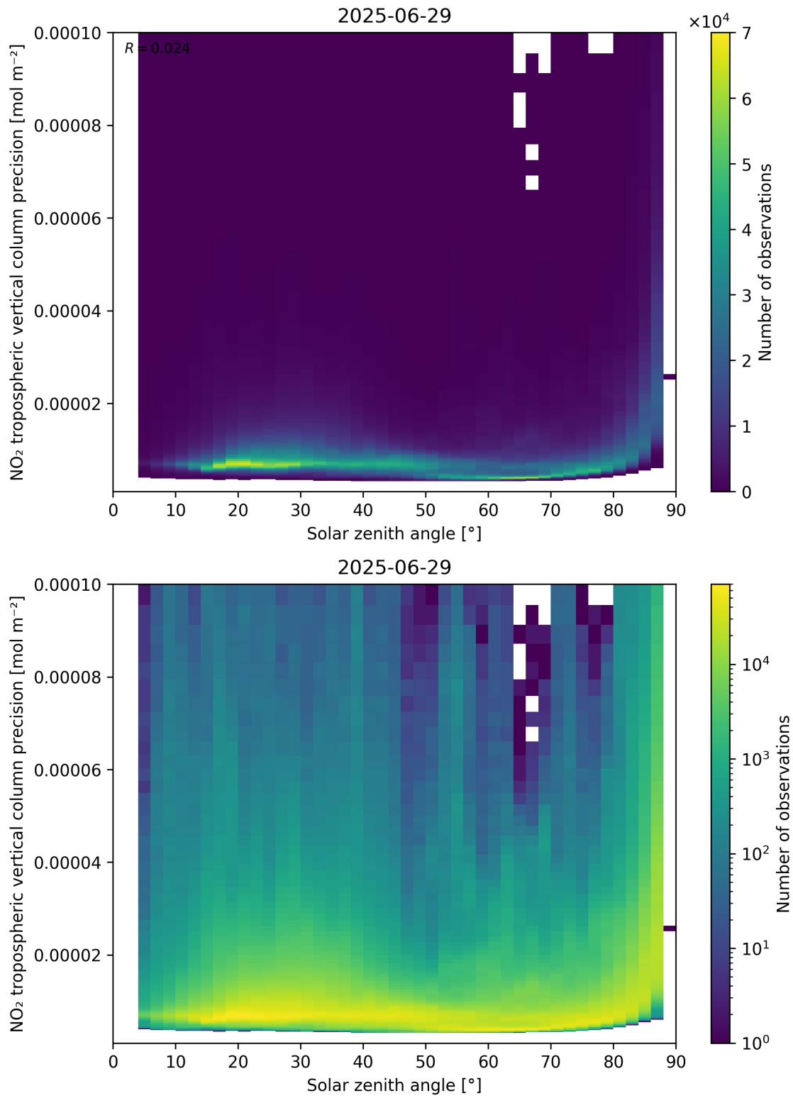
Figure 156: Scatter density plot of “Solar zenith angle” against “NO 2 tropospheric vertical column precision” for 2025-06-28 to 2025-06-30.
