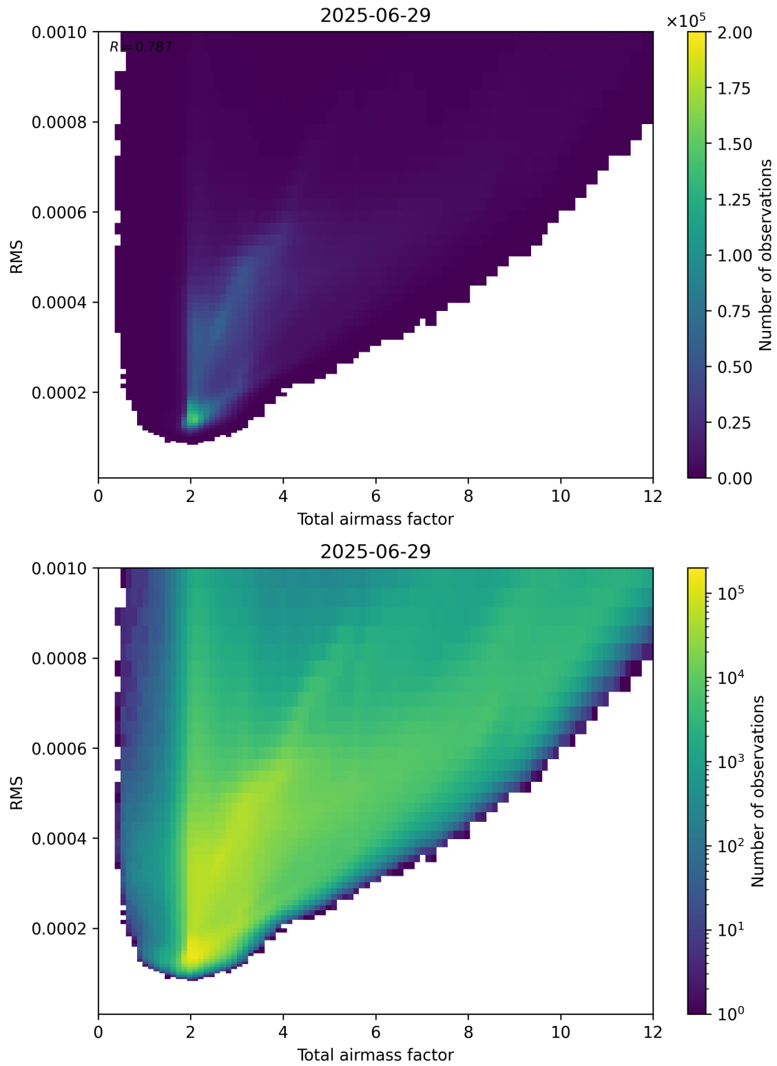
Figure 69: Scatter density plot of “Total airmass factor” against “RMS” for 2025-06-28 to 2025-06-30.
