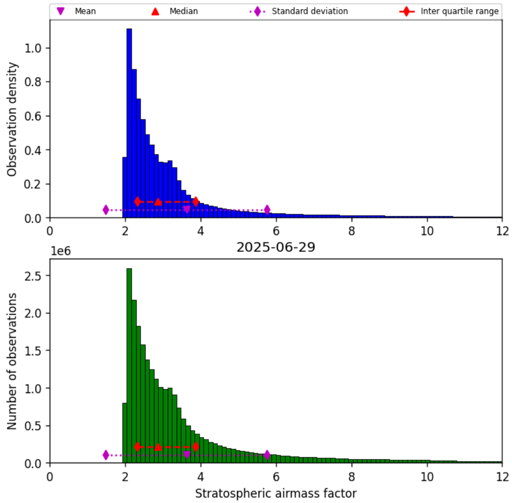
Figure 44: Histogram of “Stratospheric airmass factor” for 2025-06-28 to 2025-06-30
