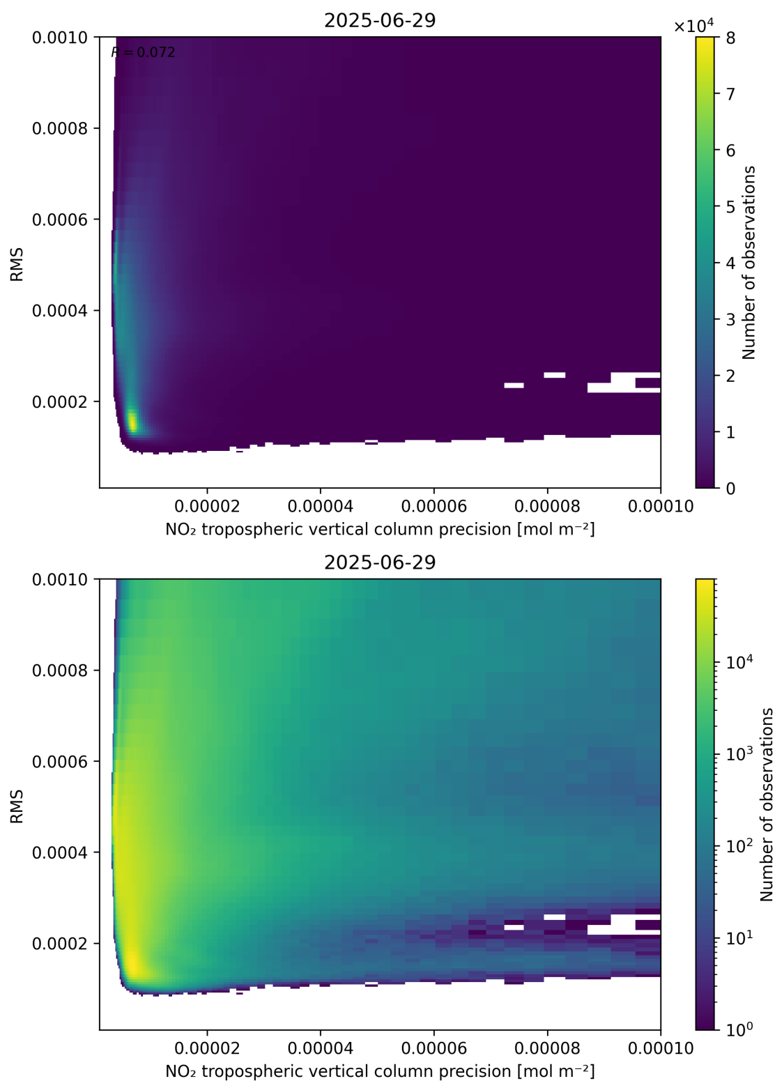
Figure 140: Scatter density plot of “NO 2 tropospheric vertical column precision” against “RMS” for 2025-06-28 to 2025-06-30.
