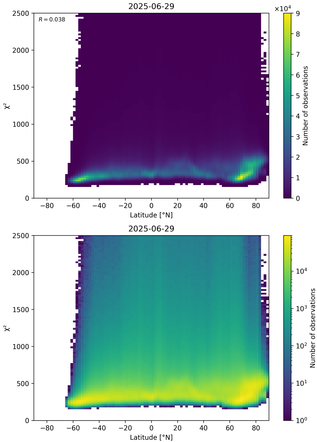
Figure 86: Scatter density plot of “Latitude” against “ \chi^2 ” for 2025-06-28 to 2025-06-30.
