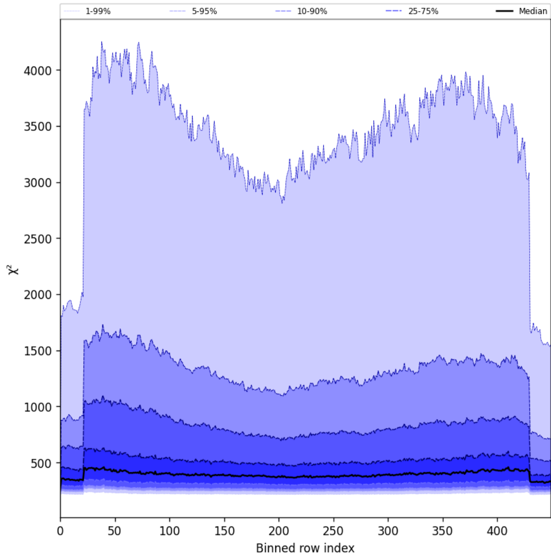
Figure 59: Along track statistics of “ \chi^2 ” for 2025-06-28 to 2025-06-30
