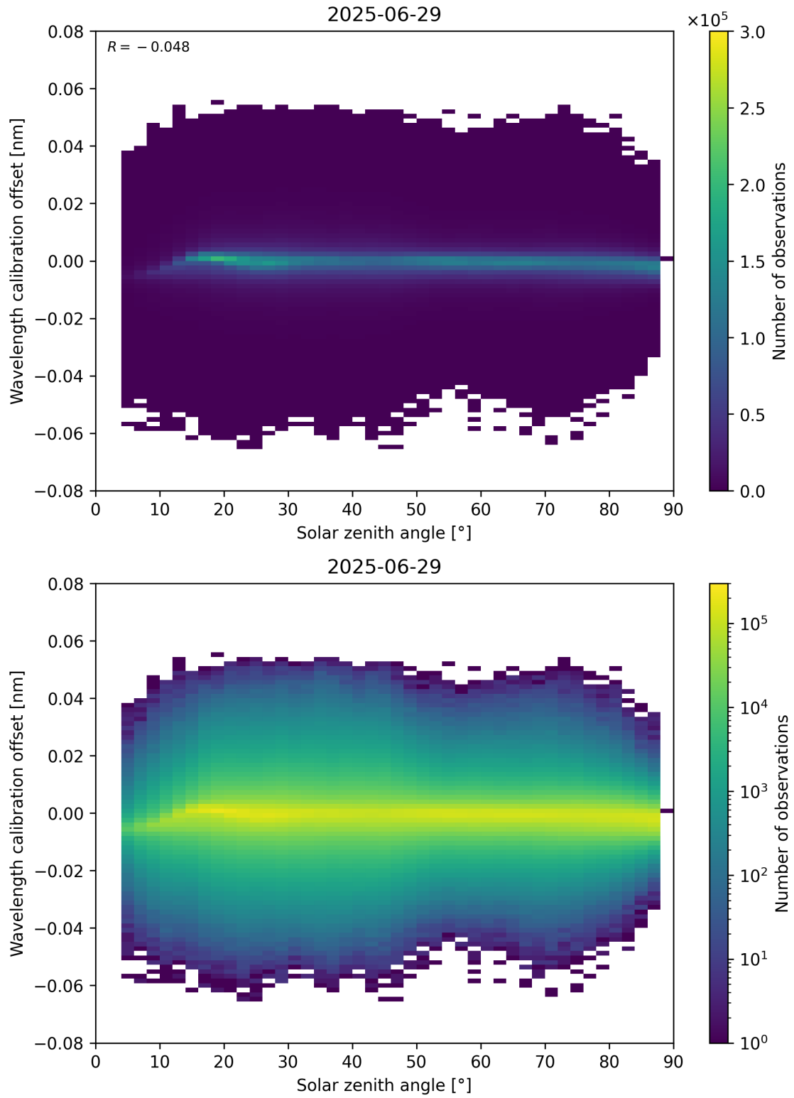
Figure 158: Scatter density plot of “Solar zenith angle” against “Wavelength calibration offset” for 2025-06-28 to 2025-06-30.
