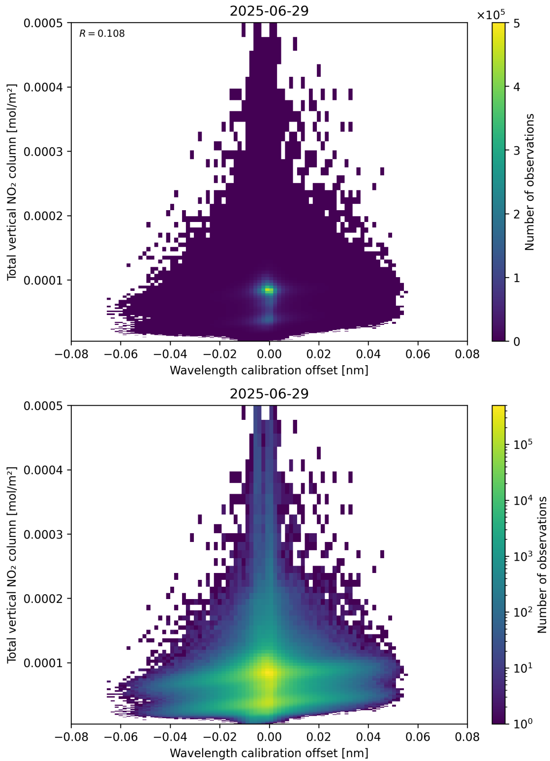
Figure 179: Scatter density plot of “Wavelength calibration offset” against “Total vertical NO 2 column” for 2025-06-28 to 2025-06-30.
