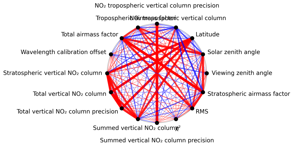
Figure 1: Map of correlation graph for 2025-06-28 to 2025-06-30.
