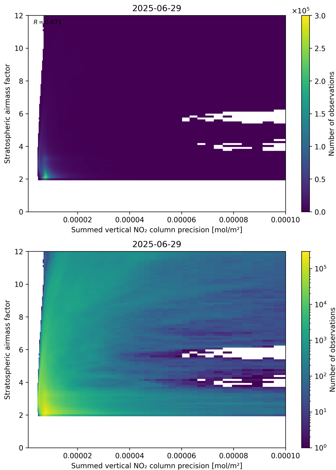
Figure 106: Scatter density plot of “Summed vertical NO 2 column precision” against “Stratospheric airmass factor” for 2025-06-28 to 2025-06-30.
