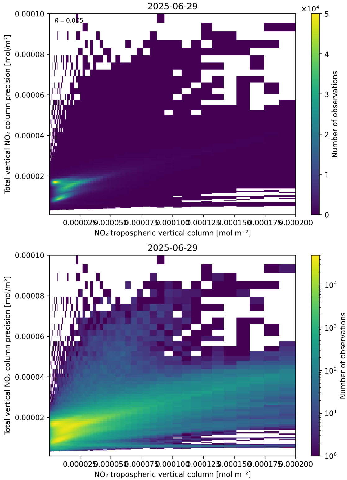
Figure 129: Scatter density plot of “NO 2 tropospheric vertical column” against “Total vertical NO 2 column precision” for 2025-06-28 to 2025-06-30.
