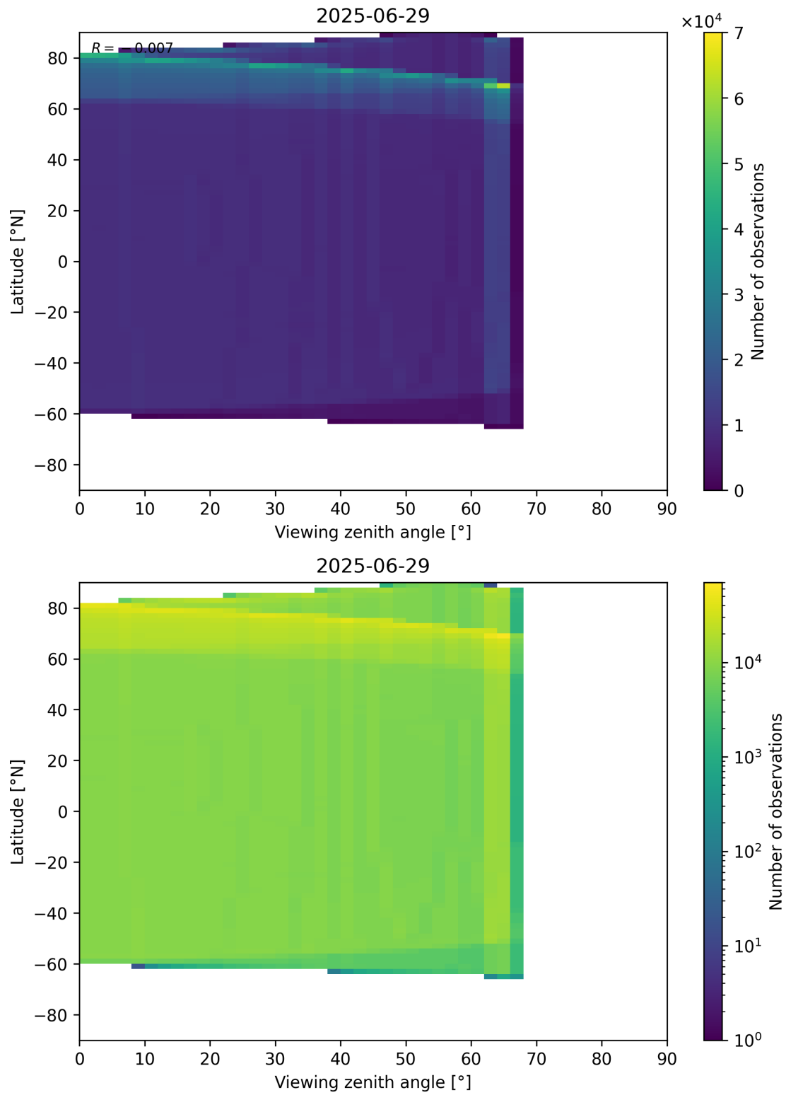
Figure 163: Scatter density plot of “Viewing zenith angle” against “Latitude” for 2025-06-28 to 2025-06-30.
