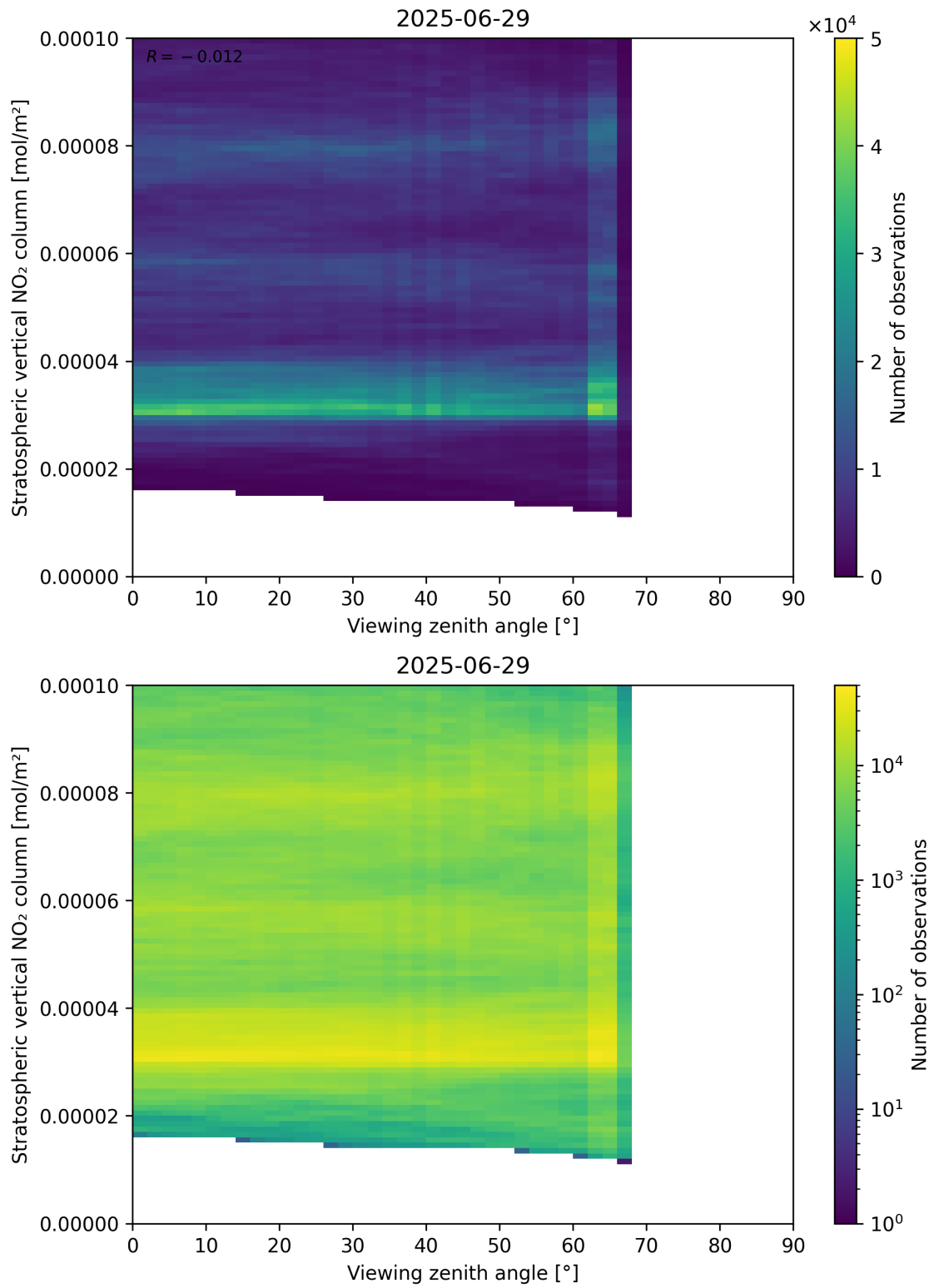
Figure 164: Scatter density plot of “Viewing zenith angle” against “Stratospheric vertical NO 2 column” for 2025-06-28 to 2025-06-30.
