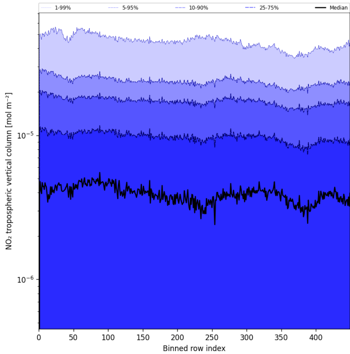
Figure 46: Along track statistics of “NO 2 tropospheric vertical column” for 2025-06-28 to 2025-06-30
