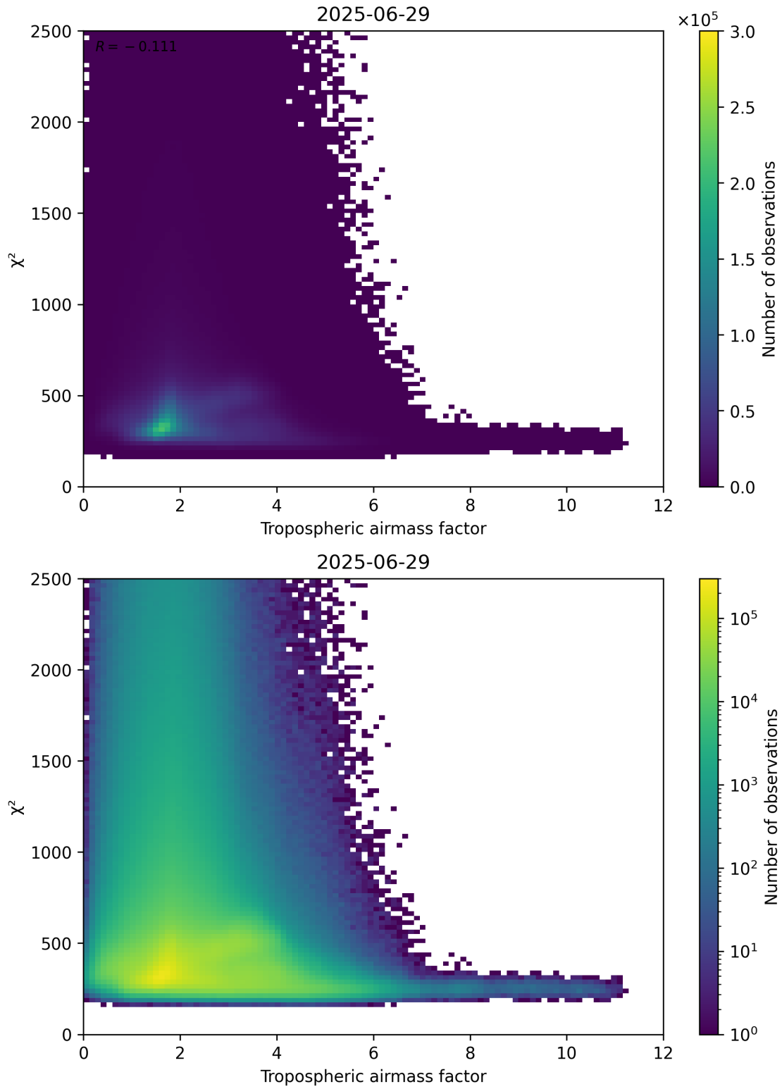
Figure 73: Scatter density plot of “Tropospheric airmass factor” against “ \chi^2 ” for 2025-06-28 to 2025-06-30.
