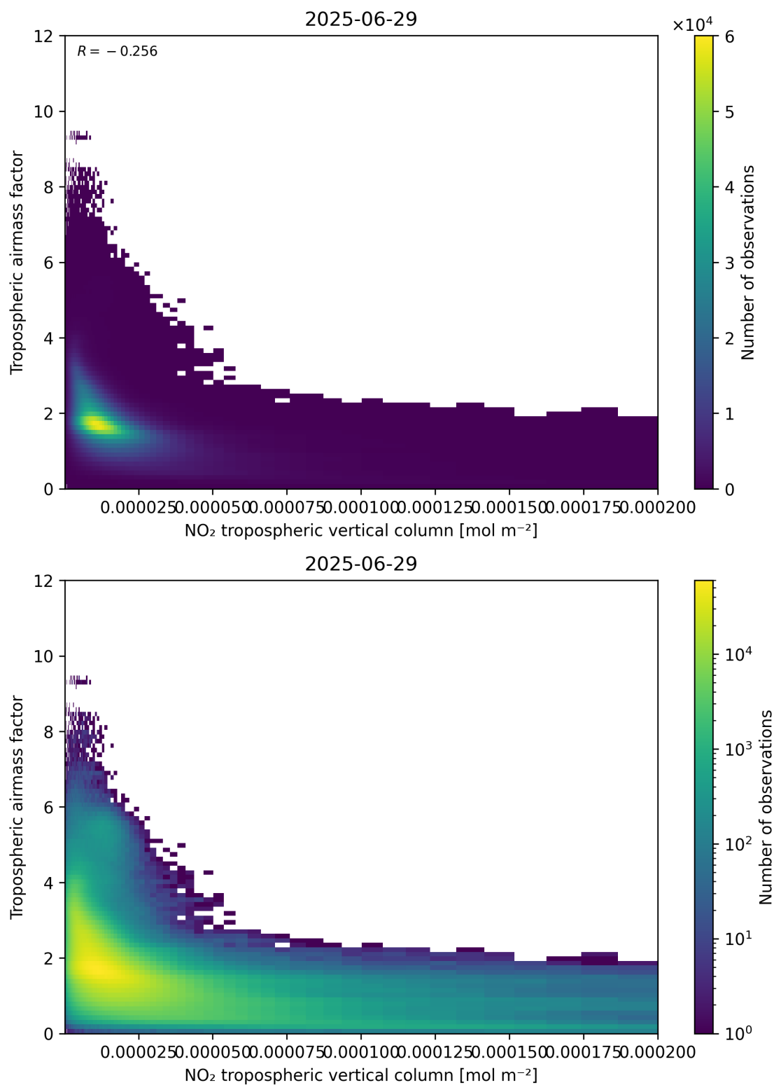
Figure 123: Scatter density plot of “NO 2 tropospheric vertical column” against “Tropospheric airmass factor” for 2025-06-28 to 2025-06-30.
