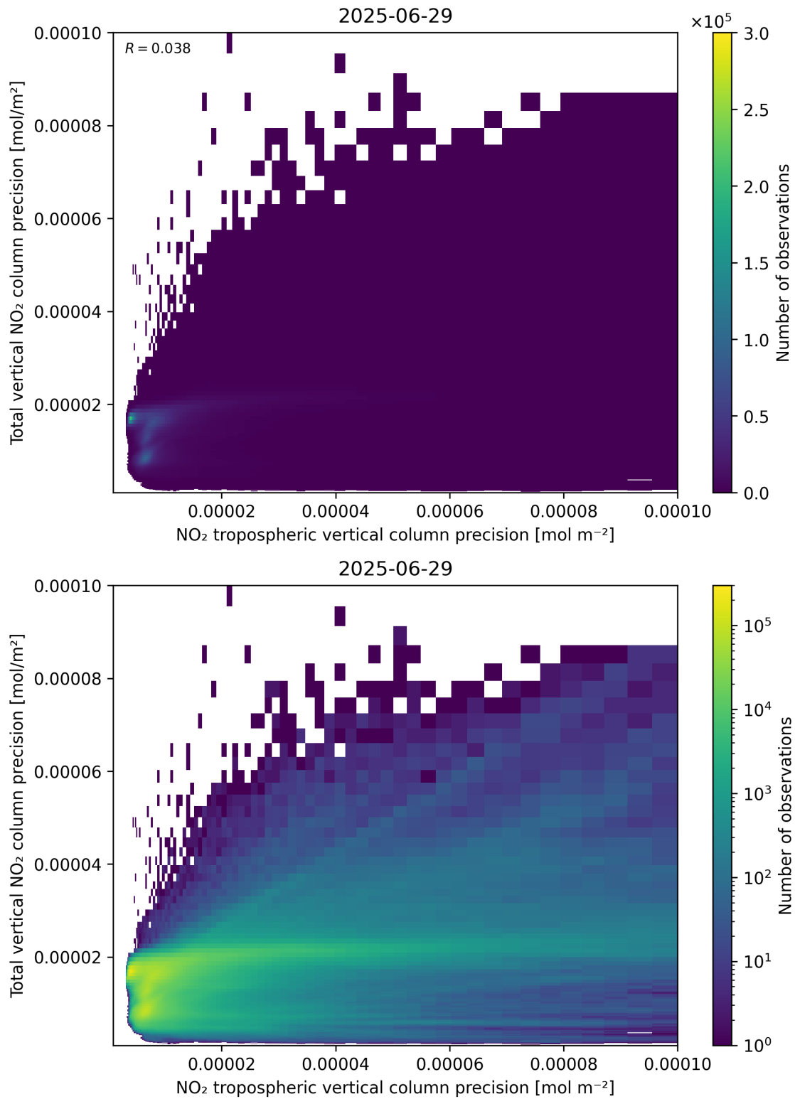
Figure 139: Scatter density plot of “NO 2 tropospheric vertical column precision” against “Total vertical NO 2 column precision” for 2025-06-28 to 2025-06-30.
