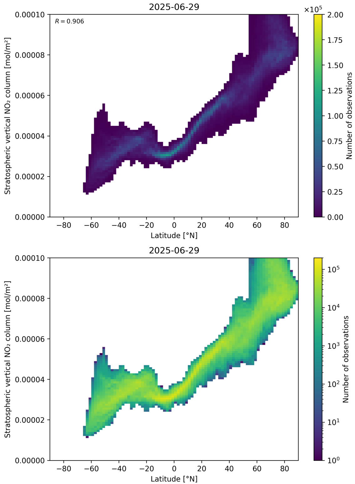
Figure 87: Scatter density plot of “Latitude” against “Stratospheric vertical \text{NO}_2 column” for 2025-06-28 to 2025-06-30.
