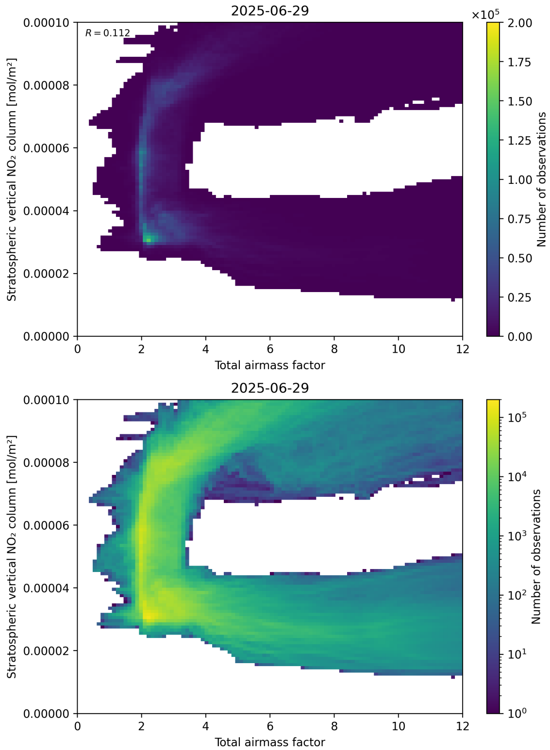
Figure 64: Scatter density plot of “Total airmass factor” against “Stratospheric vertical NO 2 column” for 2025-06-28 to 2025-06-30.
