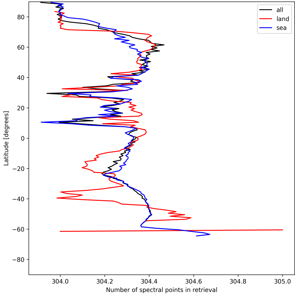
Figure 16: Zonal average of “Number of spectral points in retrieval” for 2025-06-28 to 2025-06-30.
