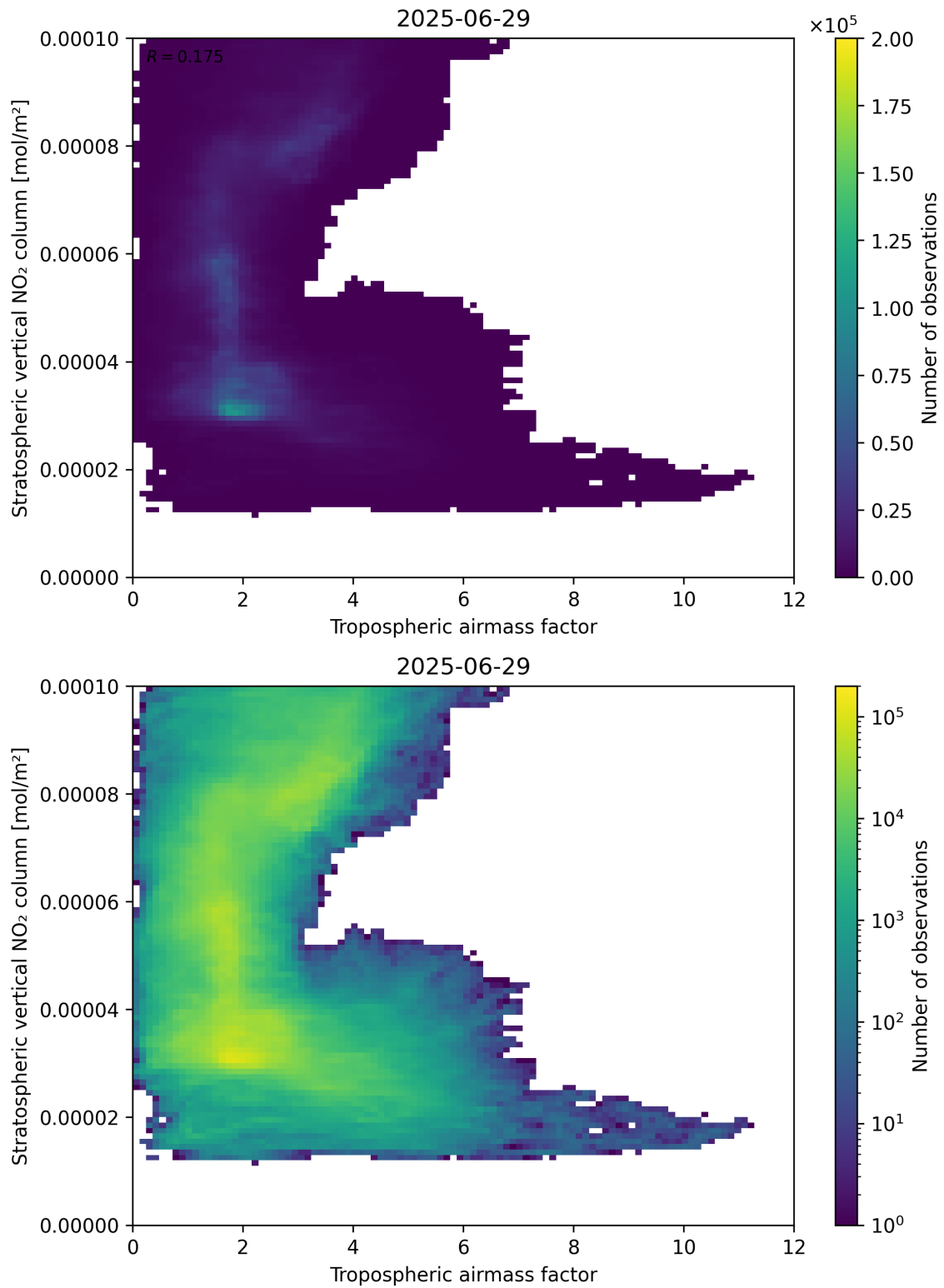
Figure 74: Scatter density plot of “Tropospheric airmass factor” against “Stratospheric vertical NO 2 column” for 2025-06-28 to 2025-06-30.
