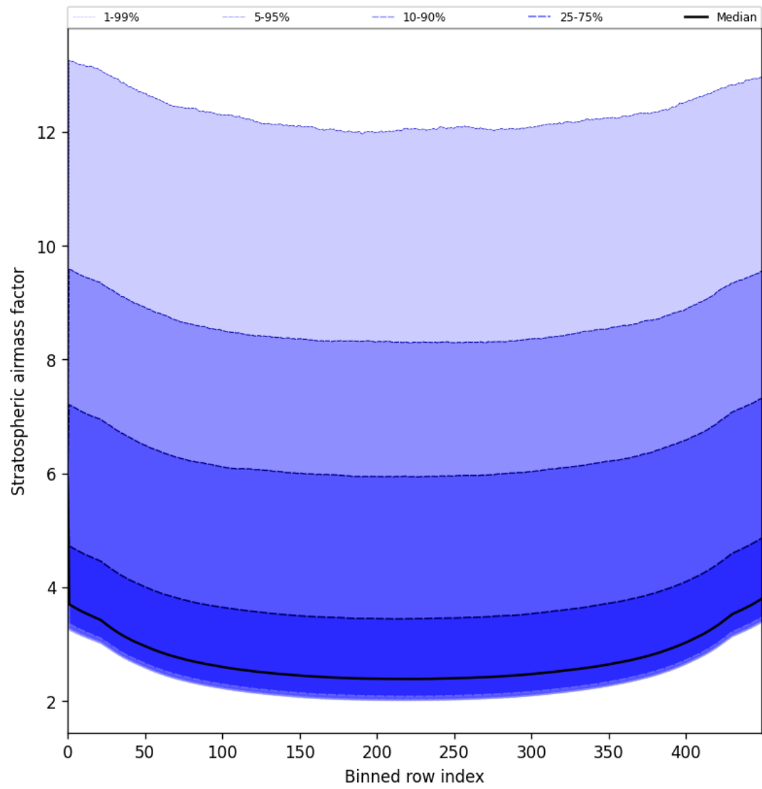
Figure 61: Along track statistics of “Stratospheric airmass factor” for 2025-06-28 to 2025-06-30
