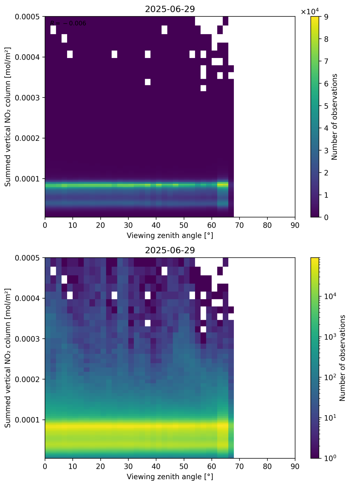
Figure 165: Scatter density plot of “Viewing zenith angle” against “Summed vertical NO 2 column” for 2025-06-28 to 2025-06-30.
