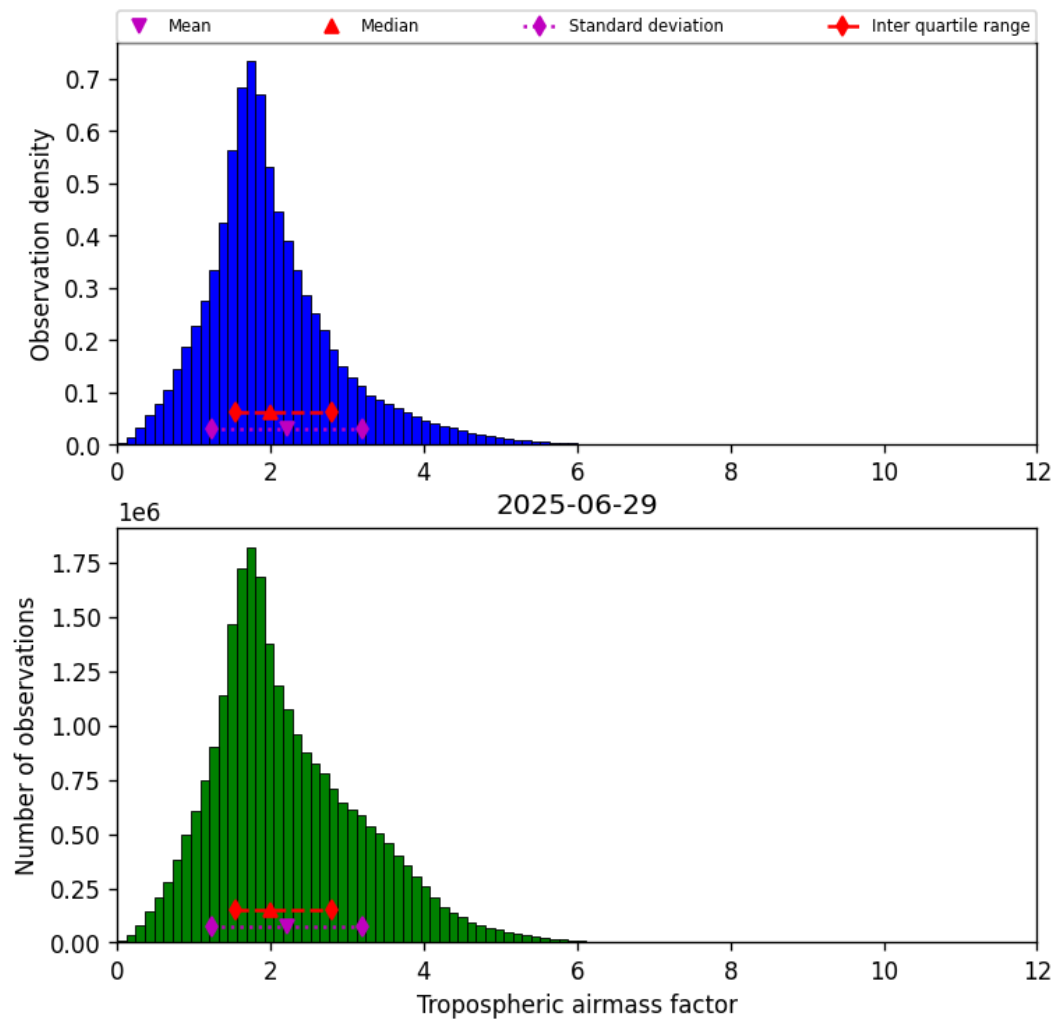
Figure 31: Histogram of “Tropospheric airmass factor” for 2025-06-28 to 2025-06-30
