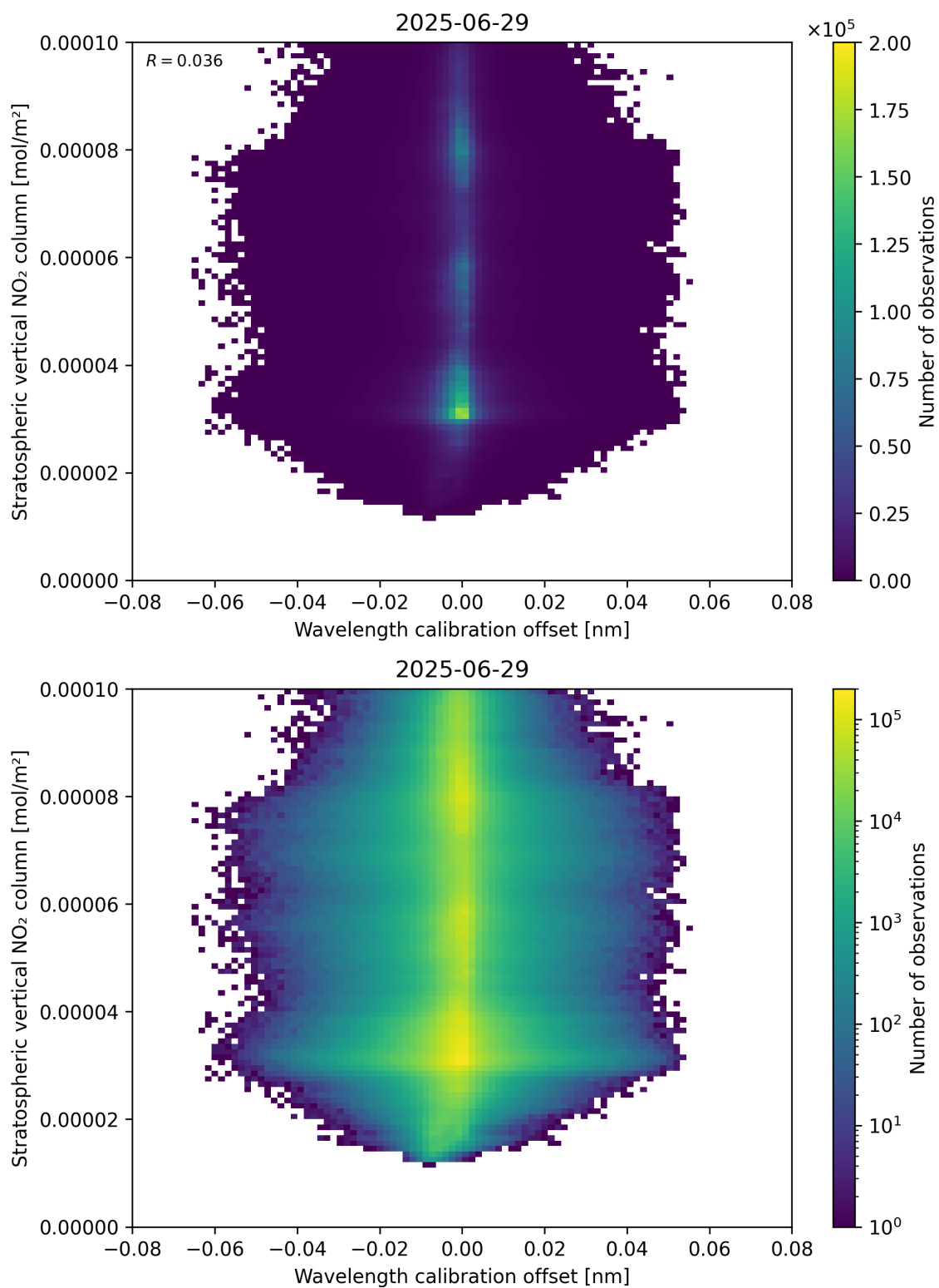
Figure 176: Scatter density plot of “Wavelength calibration offset” against “Stratospheric vertical NO 2 column” for 2025-06-28 to 2025-06-30.
