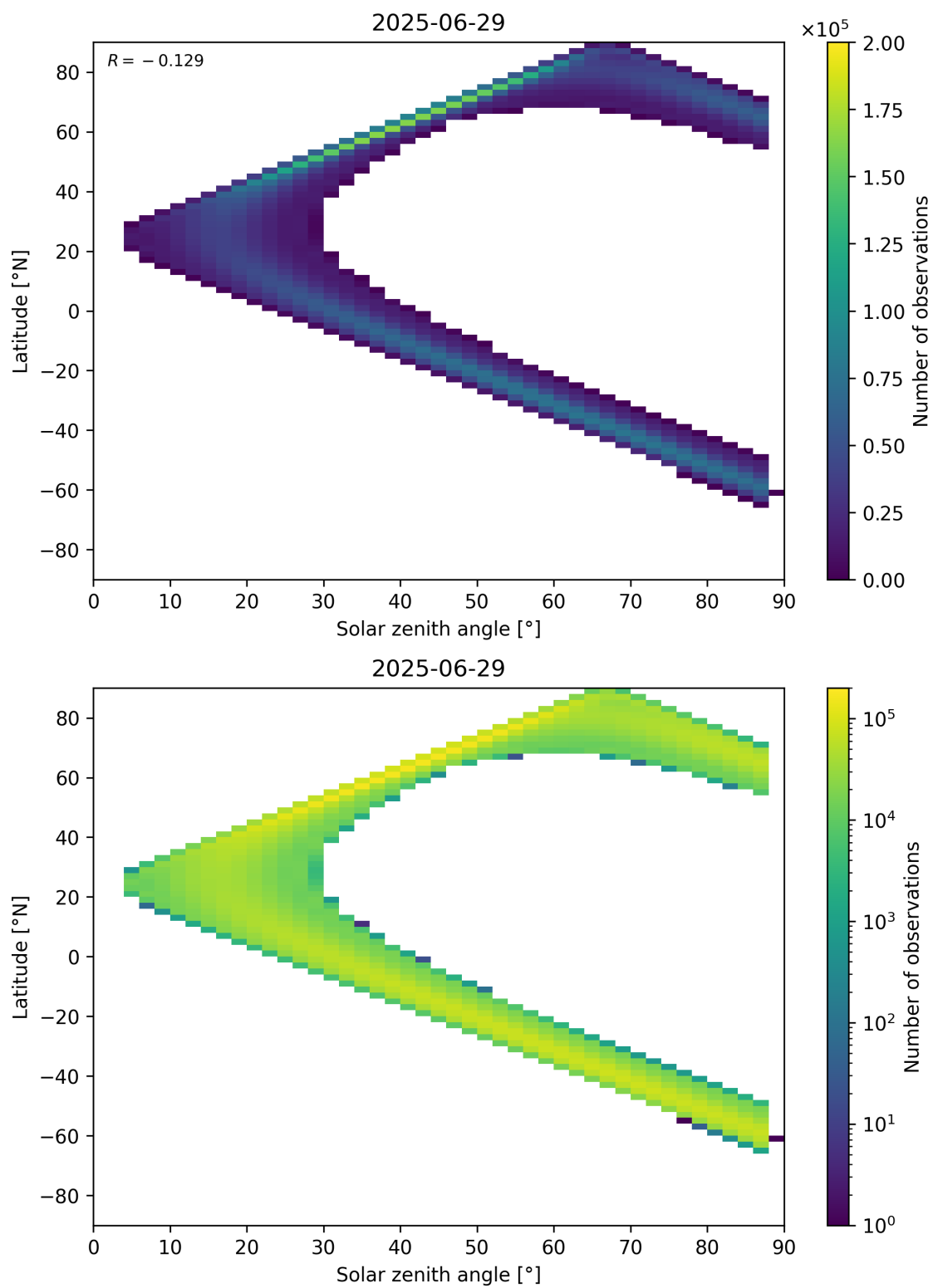
Figure 149: Scatter density plot of “Solar zenith angle” against “Latitude” for 2025-06-28 to 2025-06-30.
