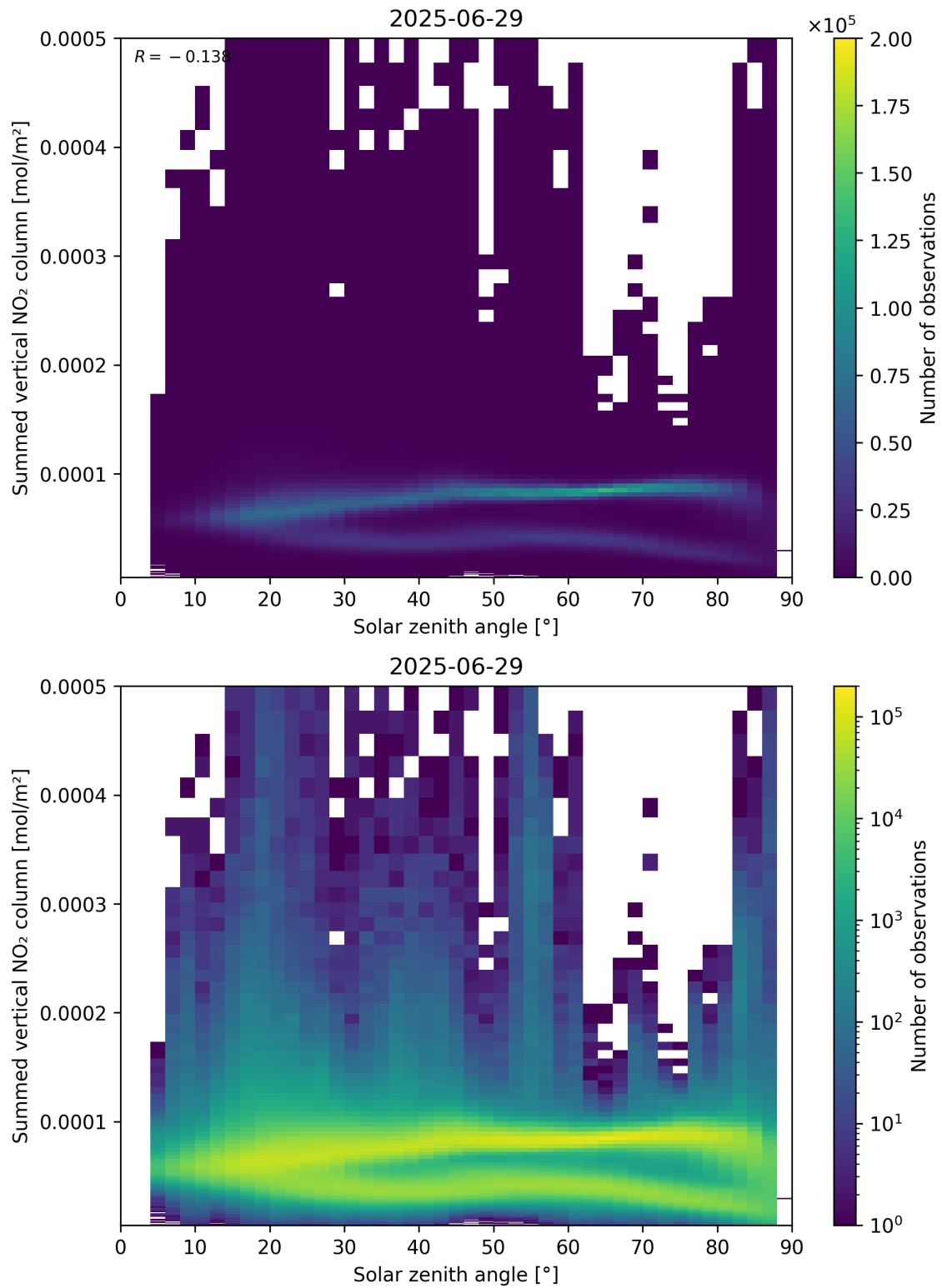
Figure 151: Scatter density plot of “Solar zenith angle” against “Summed vertical NO 2 column” for 2025-06-28 to 2025-06-30.
