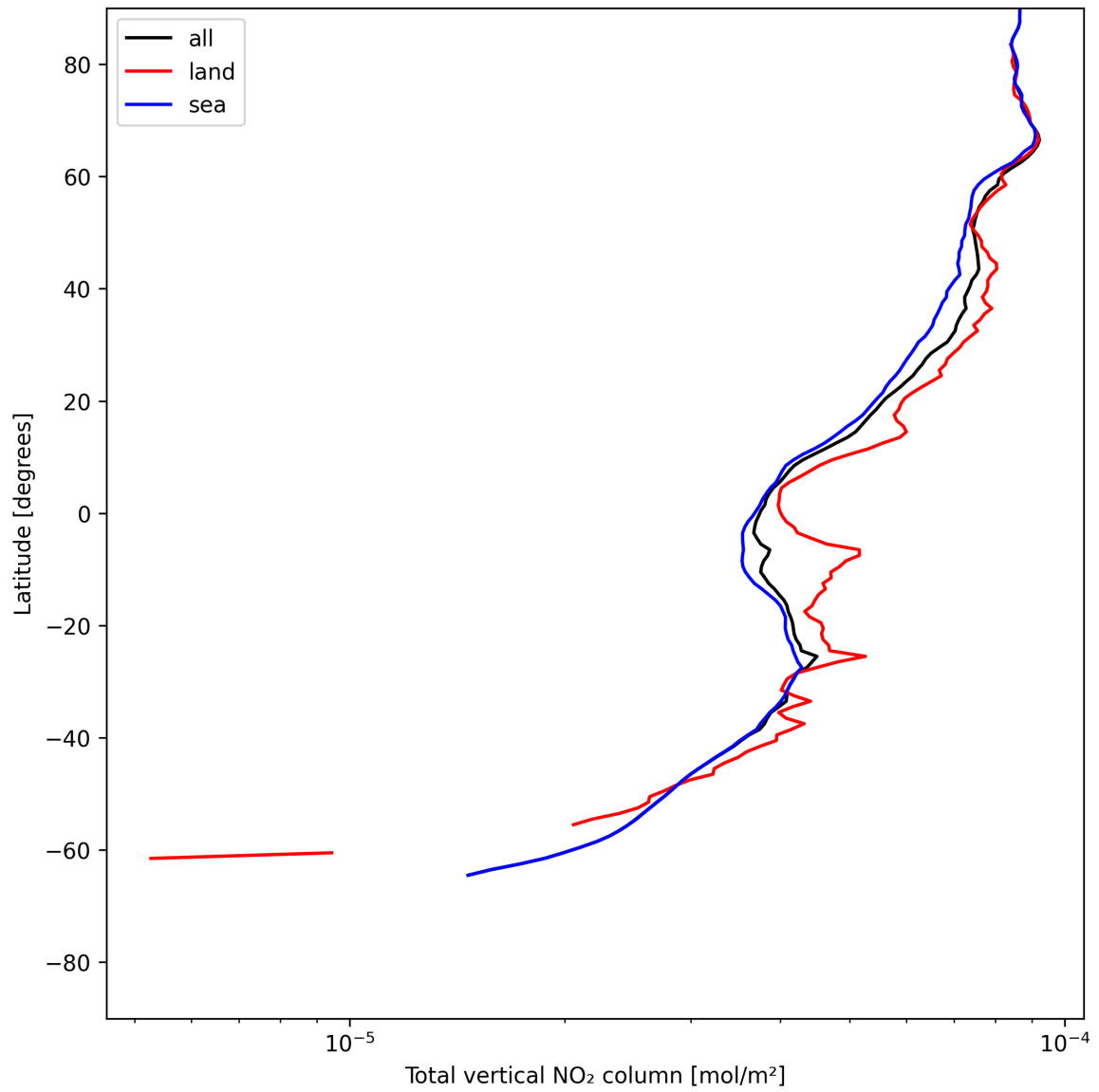
Figure 21: Zonal average of “Total vertical NO 2 column” for 2025-06-28 to 2025-06-30.
