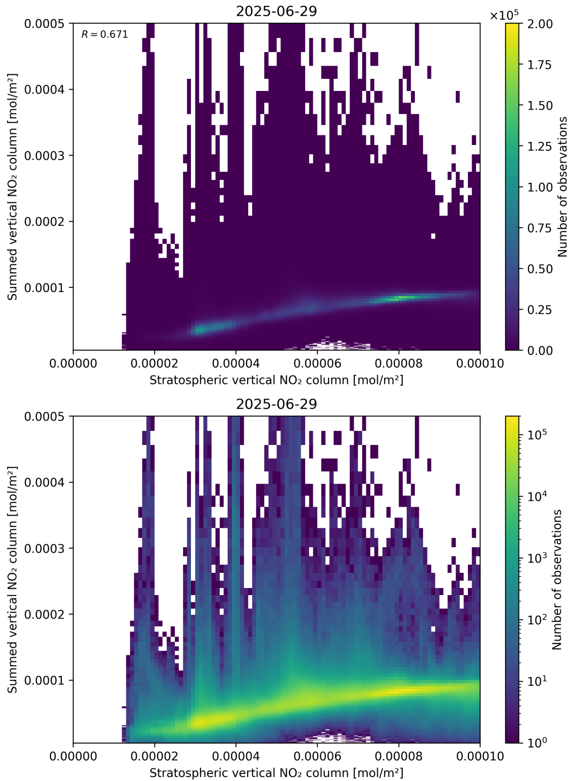
Figure 98: Scatter density plot of “Stratospheric vertical NO 2 column” against “Summed vertical NO 2 column” for 2025-06-28 to 2025-06-30.
