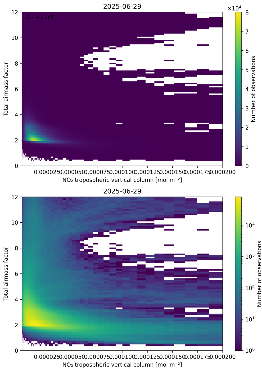
Figure 122: Scatter density plot of “NO 2 tropospheric vertical column” against “Total air mass factor” for 2025-06-28 to 2025-06-30.
