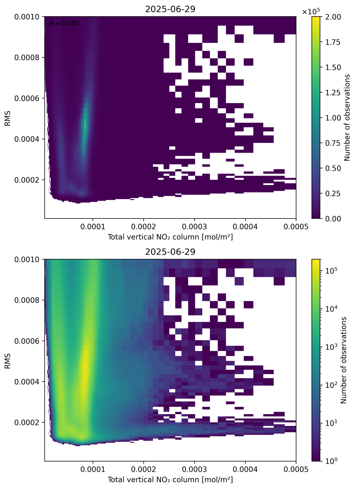
Figure 120: Scatter density plot of “Total vertical NO 2 column” against “RMS” for 2025-06-28 to 2025-06-30.
