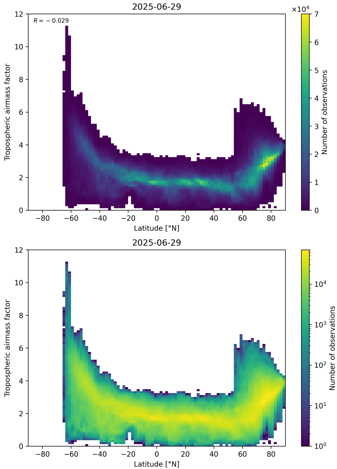
Figure 85: Scatter density plot of “Latitude” against “Tropospheric air mass factor” for 2025-06-28 to 2025-06-30.
