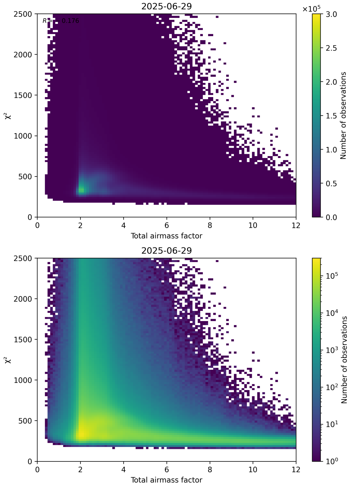
Figure 63: Scatter density plot of “Total airmass factor” against “ \chi^2 ” for 2025-06-28 to 2025-06-30.
