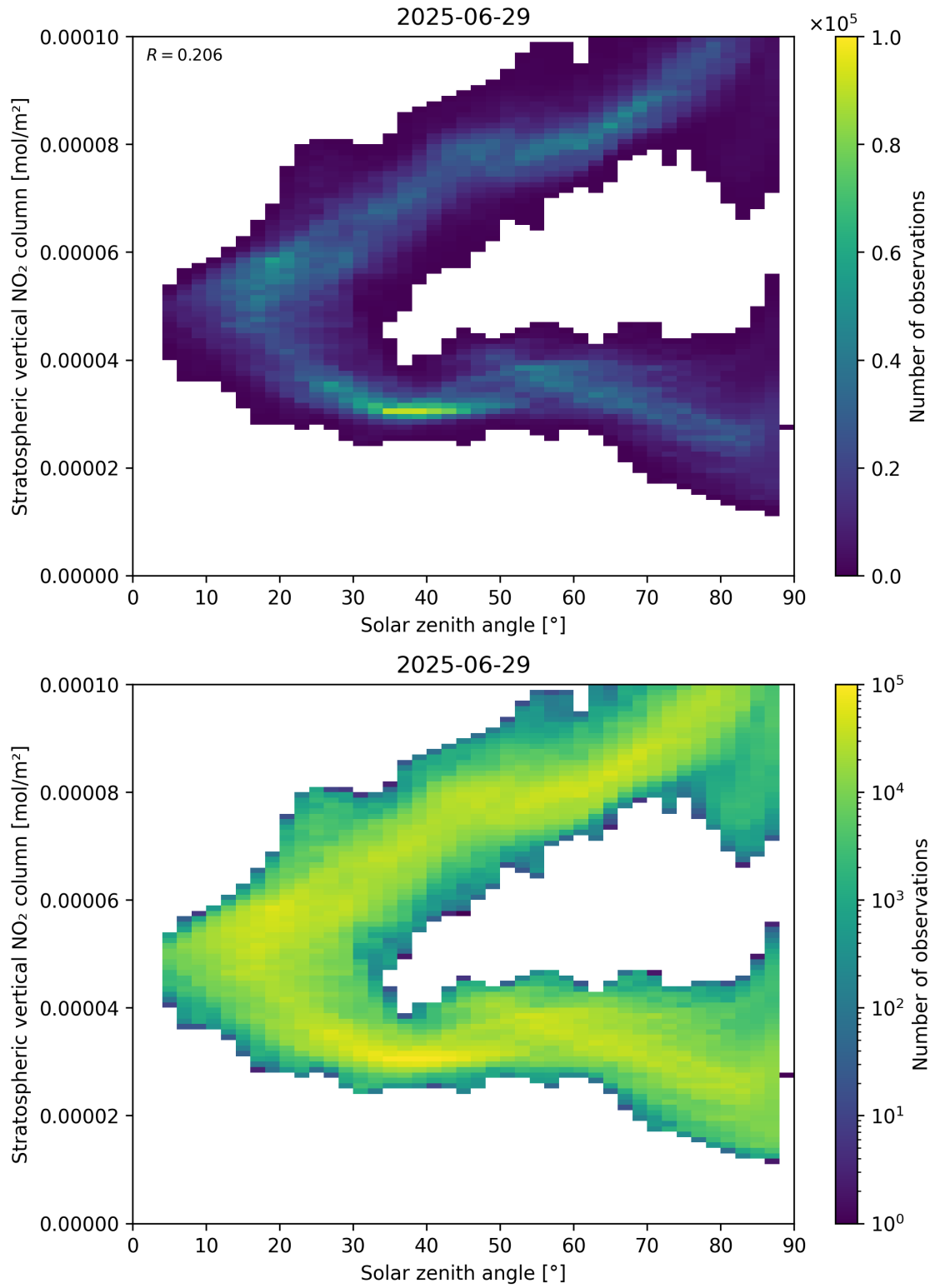
Figure 150: Scatter density plot of “Solar zenith angle” against “Stratospheric vertical NO 2 column” for 2025-06-28 to 2025-06-30.
