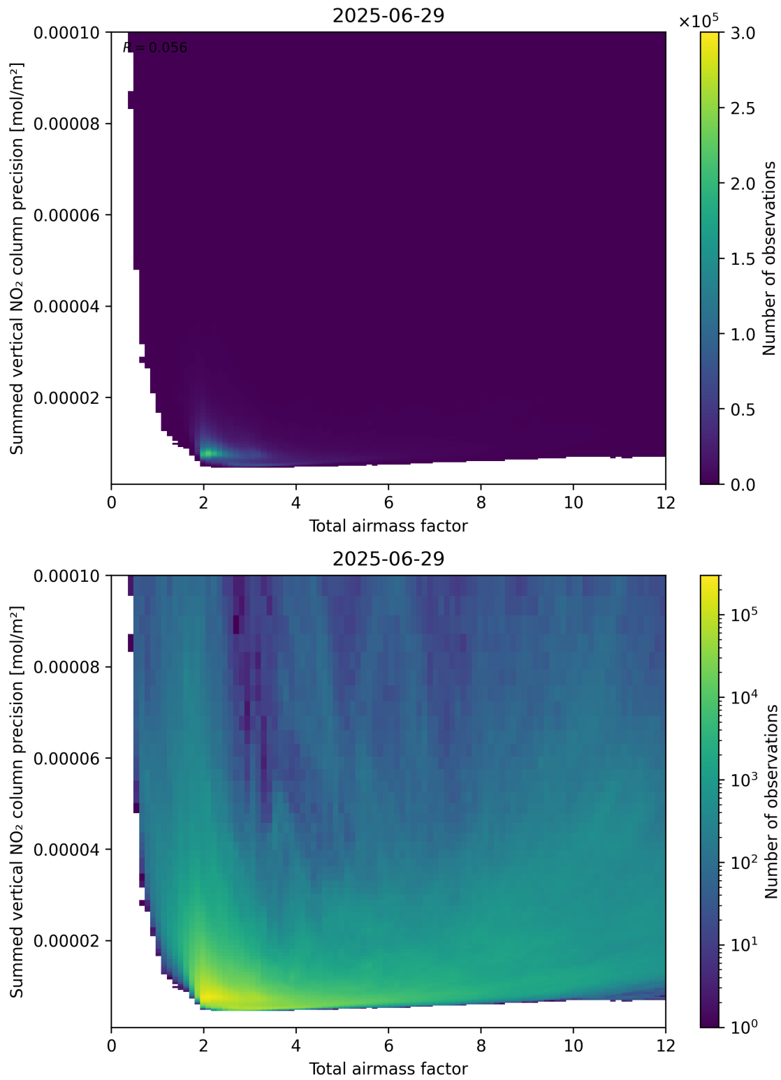
Figure 66: Scatter density plot of “Total airmass factor” against “Summed vertical NO 2 column precision” for 2025-06-28 to 2025-06-30.
