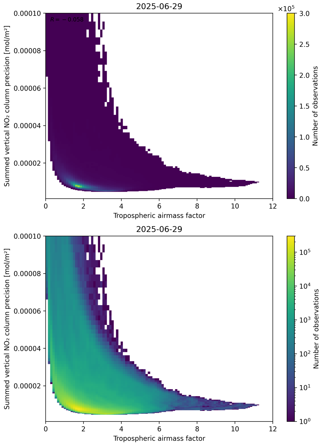
Figure 76: Scatter density plot of “Tropospheric air mass factor” against “Summed vertical NO 2 column precision” for 2025-06-28 to 2025-06-30.
