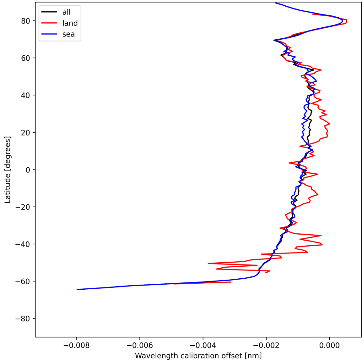
Figure 18: Zonal average of “Wavelength calibration offset” for 2025-06-28 to 2025-06-30.
