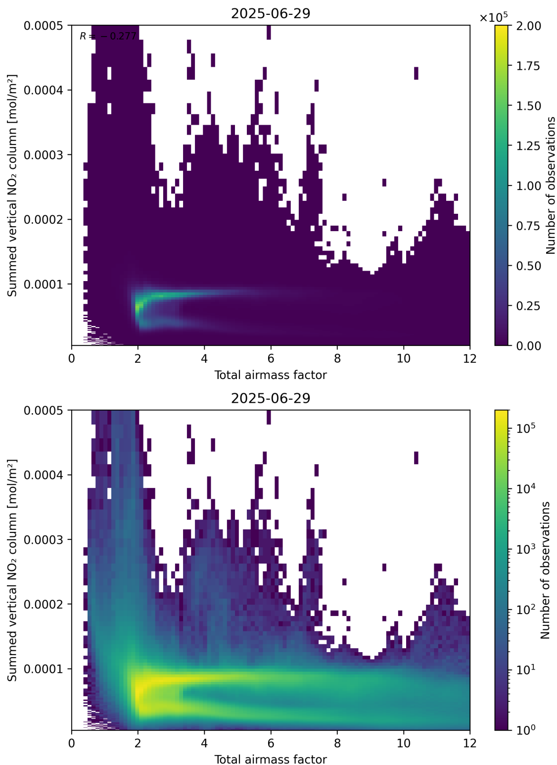
Figure 65: Scatter density plot of “Total airmass factor” against “Summed vertical NO 2 column” for 2025-06-28 to 2025-06-30.
