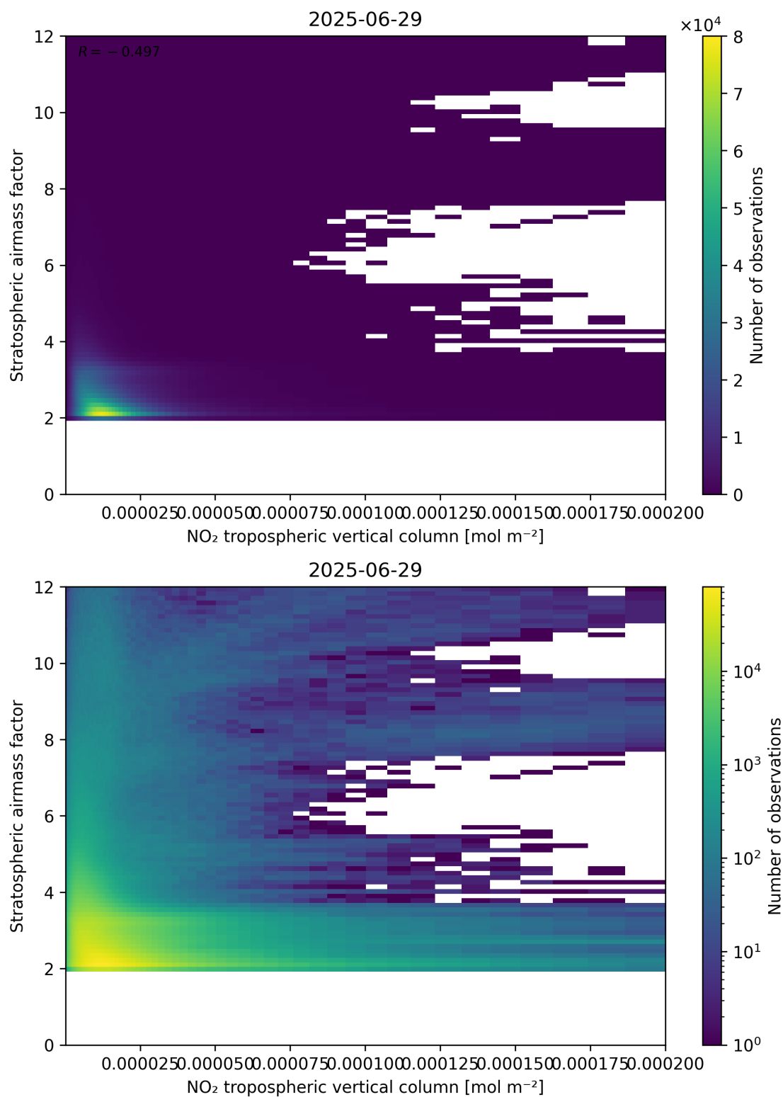
Figure 121: Scatter density plot of “NO 2 tropospheric vertical column” against “Stratospheric air mass factor” for 2025-06-28 to 2025-06-30.
