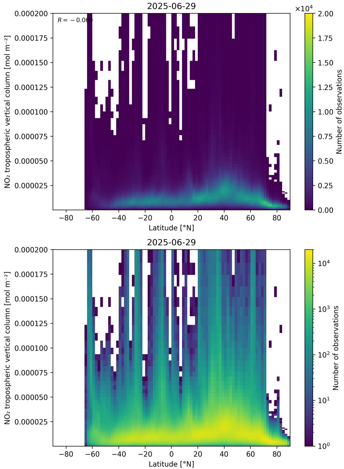
Figure 92: Scatter density plot of “Latitude” against “NO 2 tropospheric vertical column” for 2025-06-28 to 2025-06-30.
