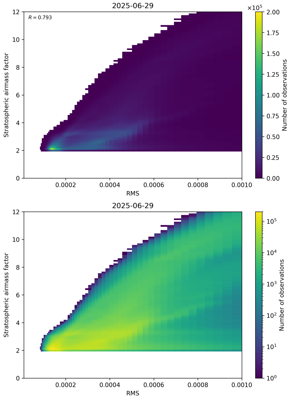
Figure 144: Scatter density plot of “RMS” against “Stratospheric airmass factor” for 2025-06-28 to 2025-06-30.
