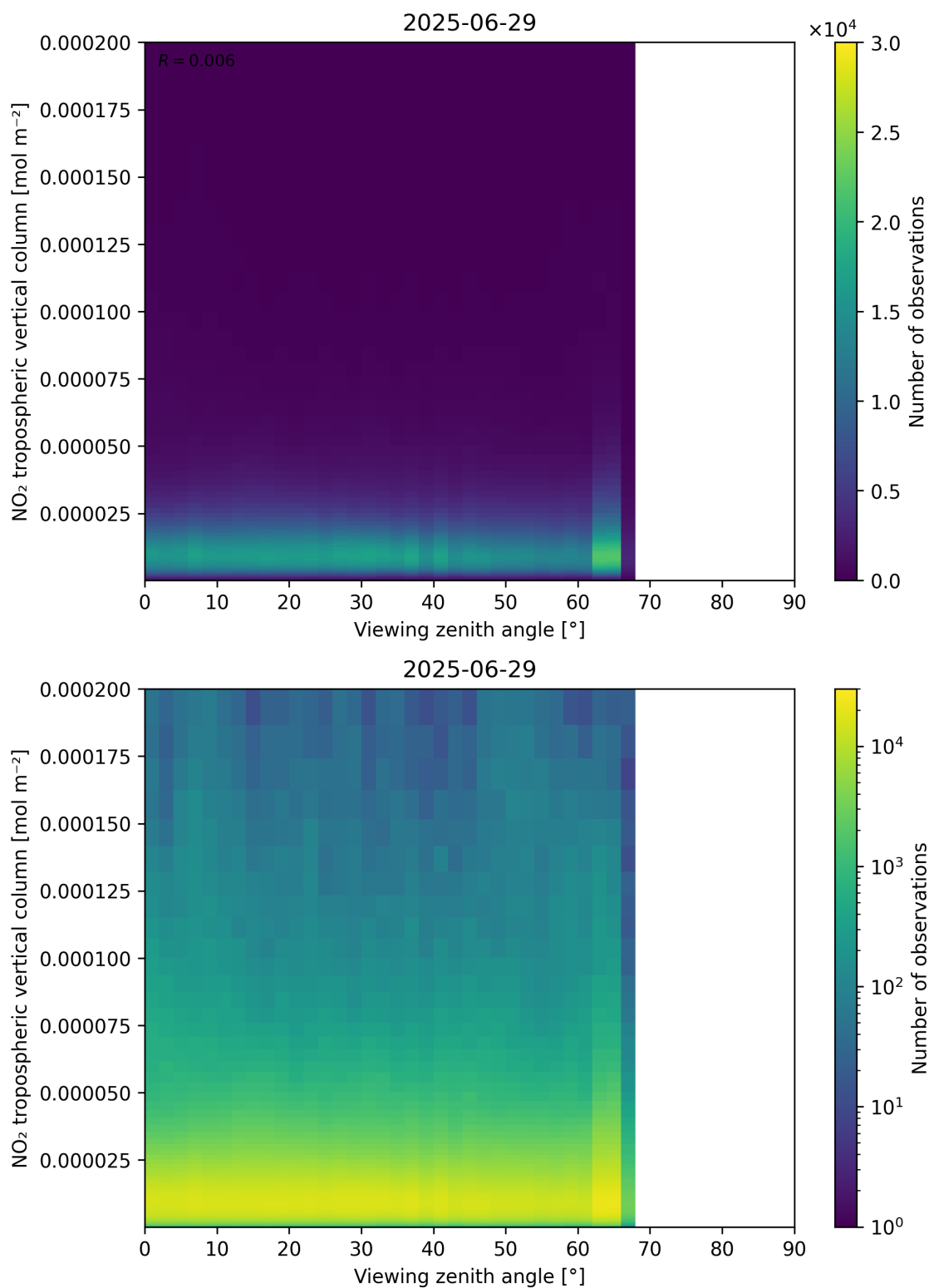
Figure 169: Scatter density plot of “Viewing zenith angle” against “NO 2 tropospheric vertical column” for 2025-06-28 to 2025-06-30.
