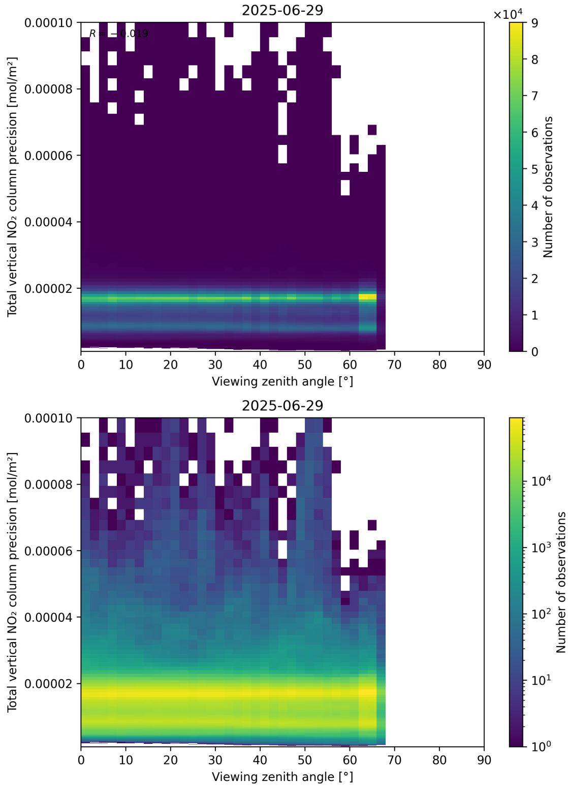
Figure 168: Scatter density plot of “Viewing zenith angle” against “Total vertical NO 2 column precision” for 2025-06-28 to 2025-06-30.
