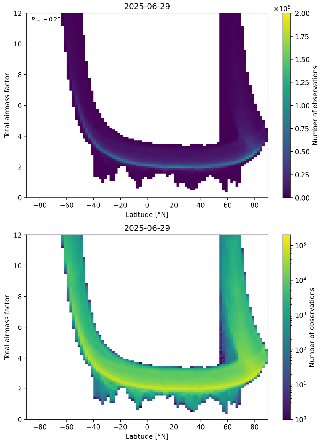
Figure 84: Scatter density plot of “Latitude” against “Total airmass factor” for 2025-06-28 to 2025-06-30.
