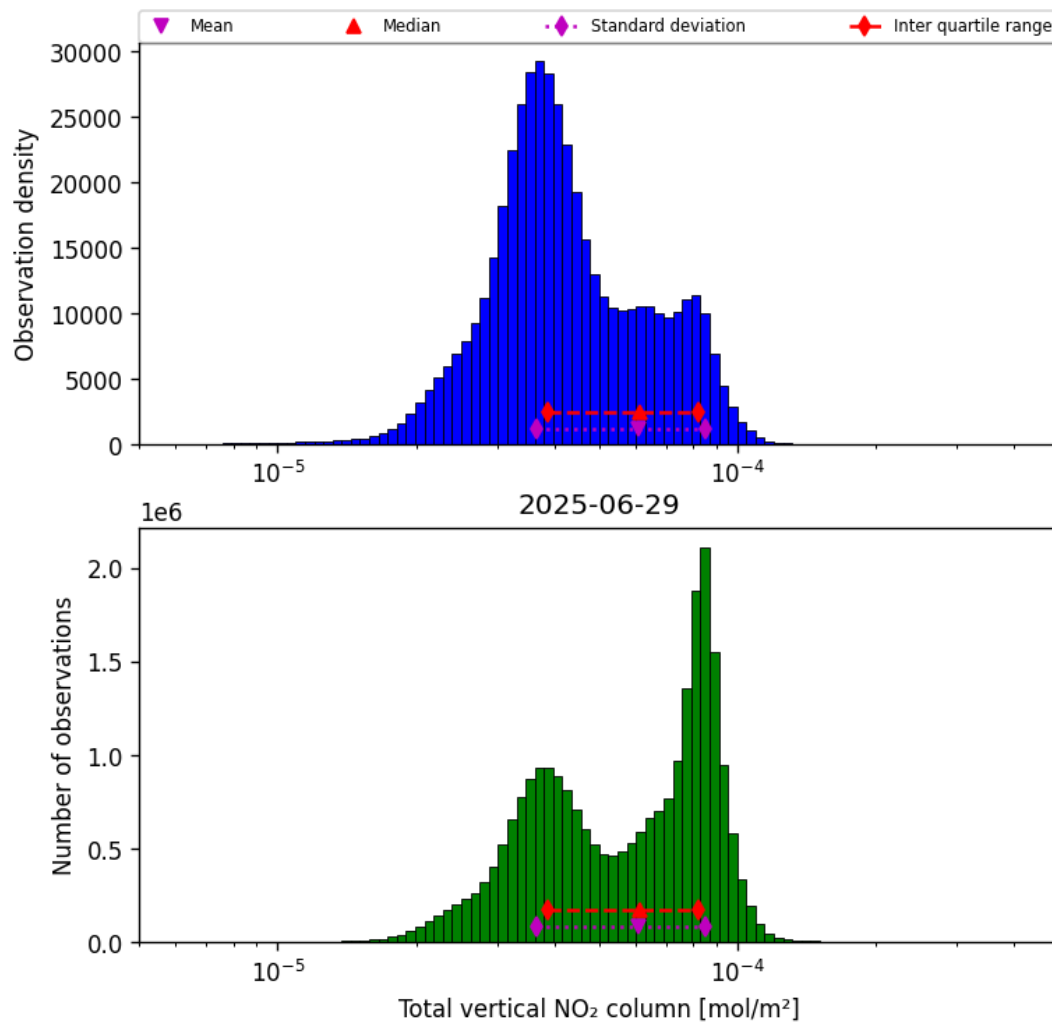
Figure 38: Histogram of “Total vertical NO 2 column” for 2025-06-28 to 2025-06-30
