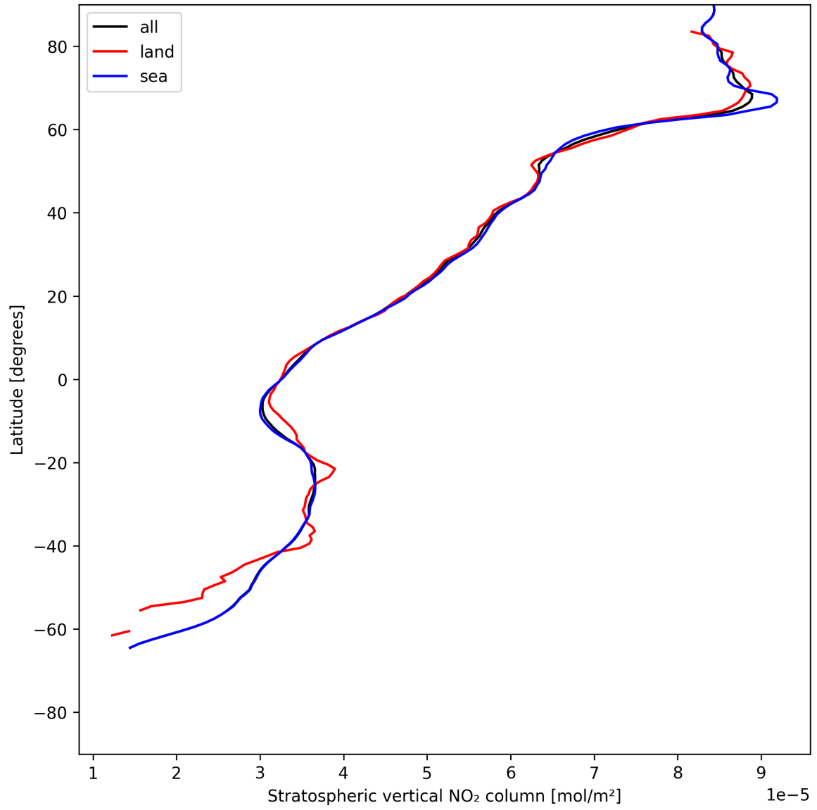
Figure 19: Zonal average of “Stratospheric vertical NO 2 column” for 2025-06-28 to 2025-06-30.
