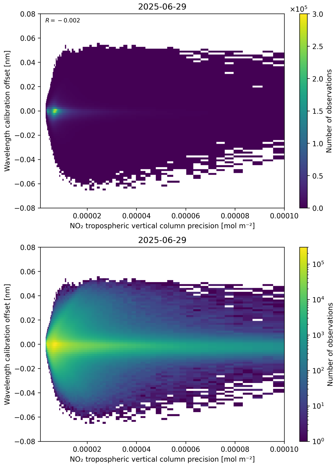
Figure 141: Scatter density plot of “NO 2 tropospheric vertical column precision” against “Wavelength calibration offset” for 2025-06-28 to 2025-06-30.
