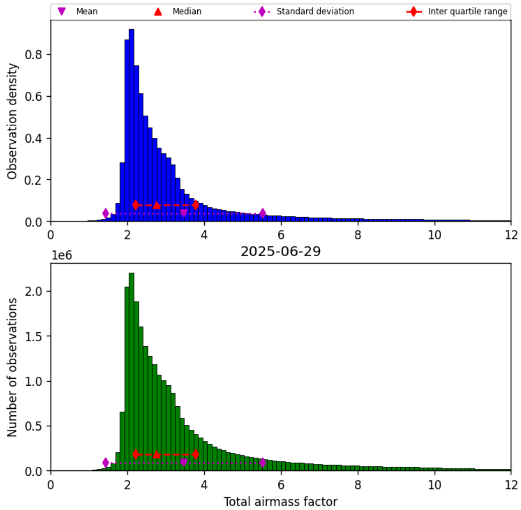
Figure 32: Histogram of “Total airmass factor” for 2025-06-28 to 2025-06-30
