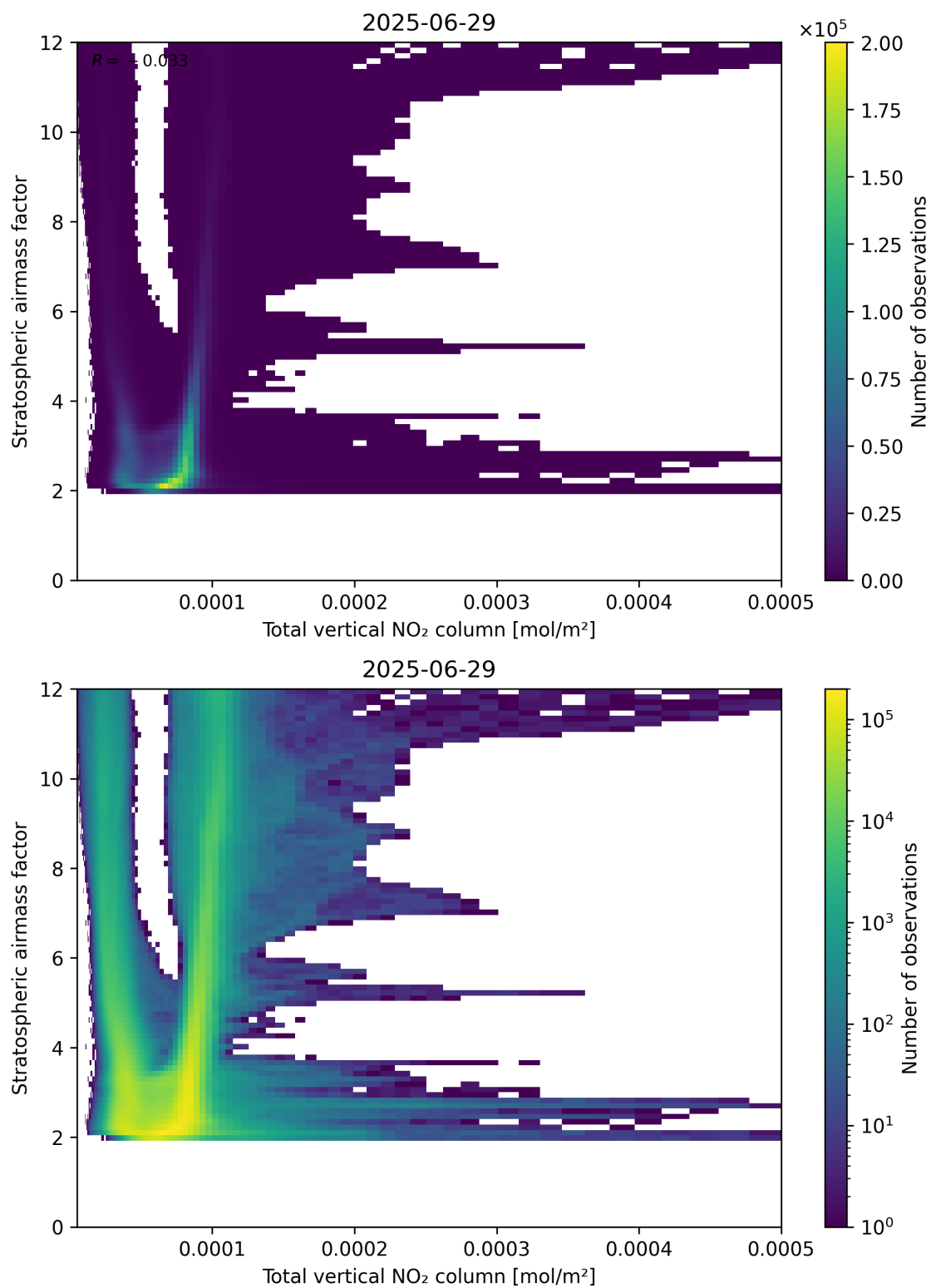
Figure 110: Scatter density plot of “Total vertical NO 2 column” against “Stratospheric airmass factor” for 2025-06-28 to 2025-06-30.
