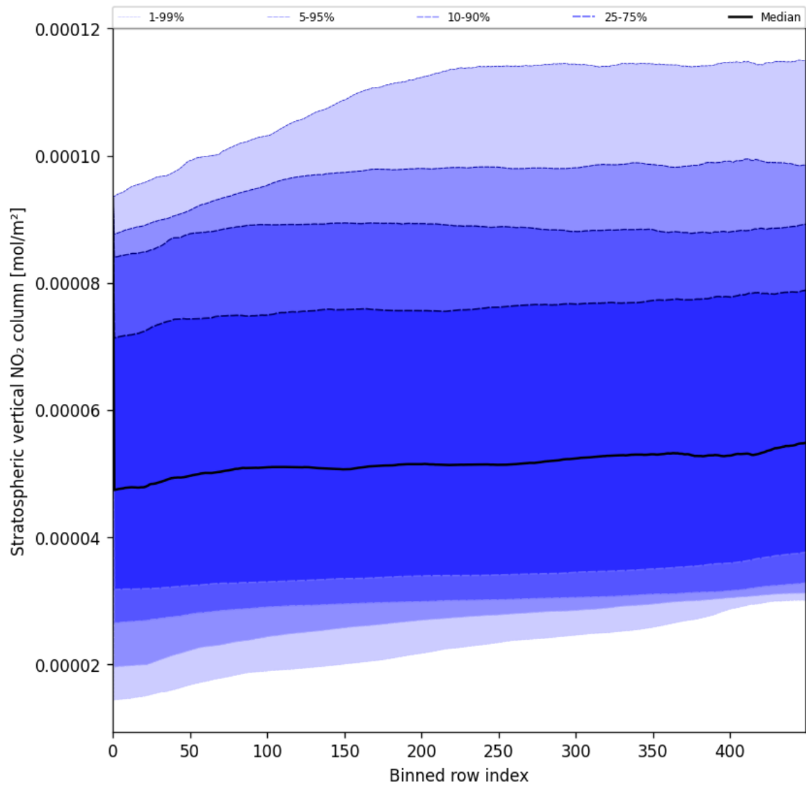
Figure 53: Along track statistics of “Stratospheric vertical NO 2 column” for 2025-06-28 to 2025-06-30
