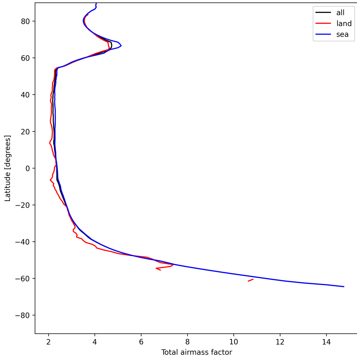
Figure 15: Zonal average of “Total airmass factor” for 2025-06-28 to 2025-06-30.
