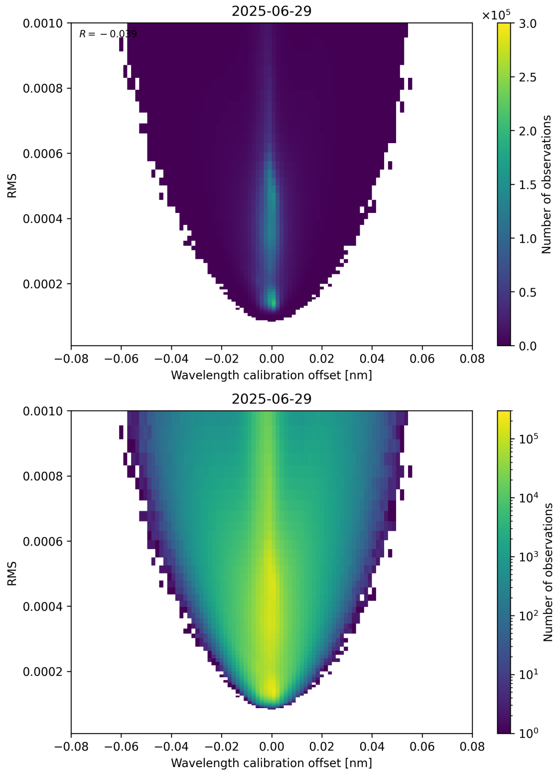
Figure 181: Scatter density plot of “Wavelength calibration offset” against “RMS” for 2025-06-28 to 2025-06-30.
