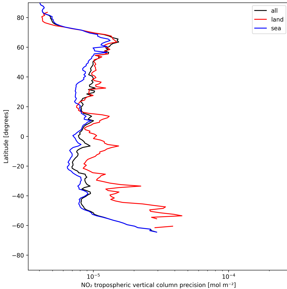
Figure 13: Zonal average of “NO 2 tropospheric vertical column precision” for 2025-06-28 to 2025-06-30.
