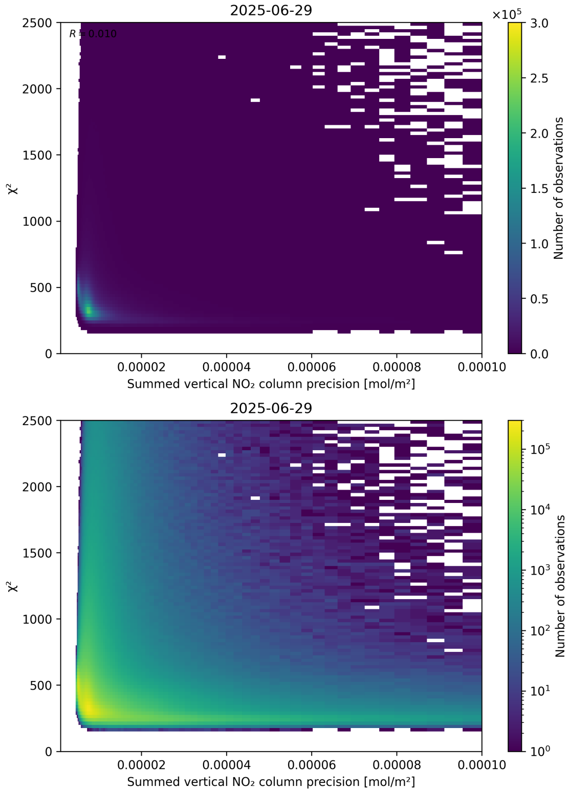
Figure 107: Scatter density plot of “Summed vertical NO 2 column precision” against “ \chi^2 ” for 2025-06-28 to 2025-06-30.
