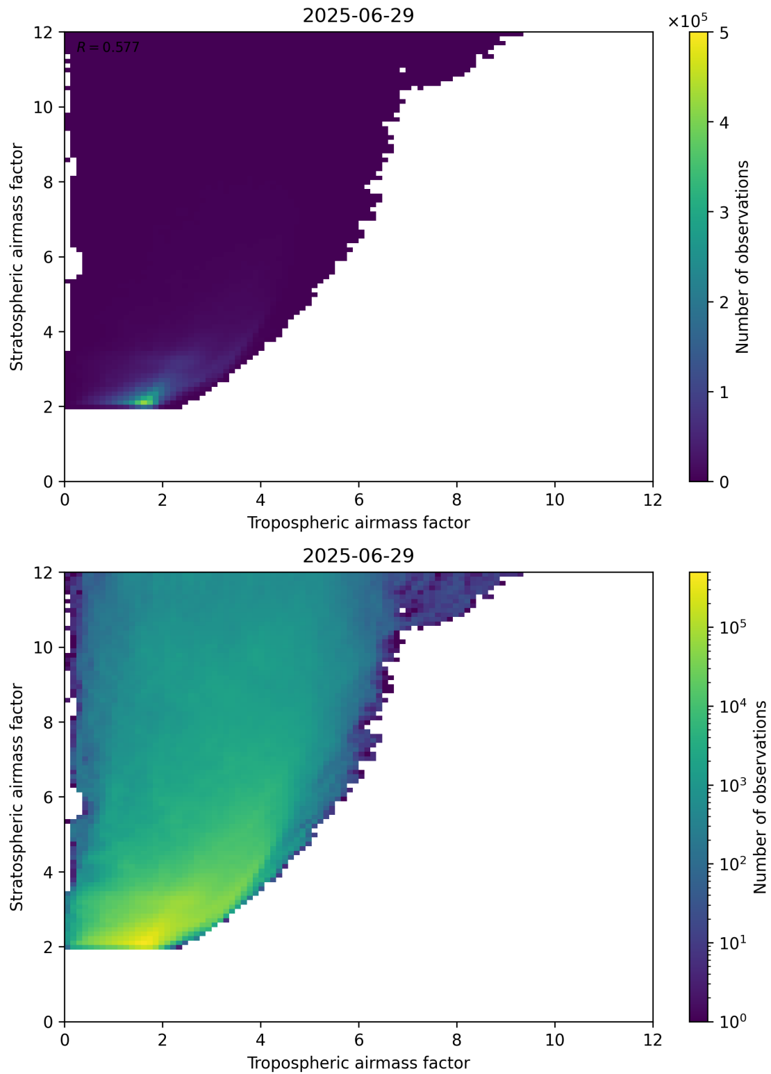
Figure 71: Scatter density plot of “Tropospheric airmass factor” against “Stratospheric airmass factor” for 2025-06-28 to 2025-06-30.
