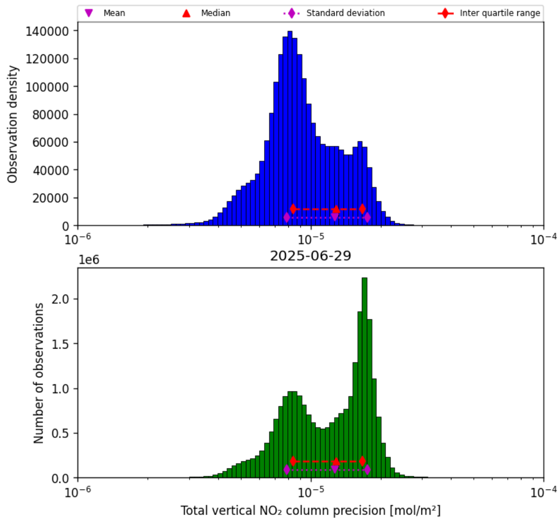
Figure 39: Histogram of "Total vertical NO 2 column precision" for 2025-06-28 to 2025-06-30
