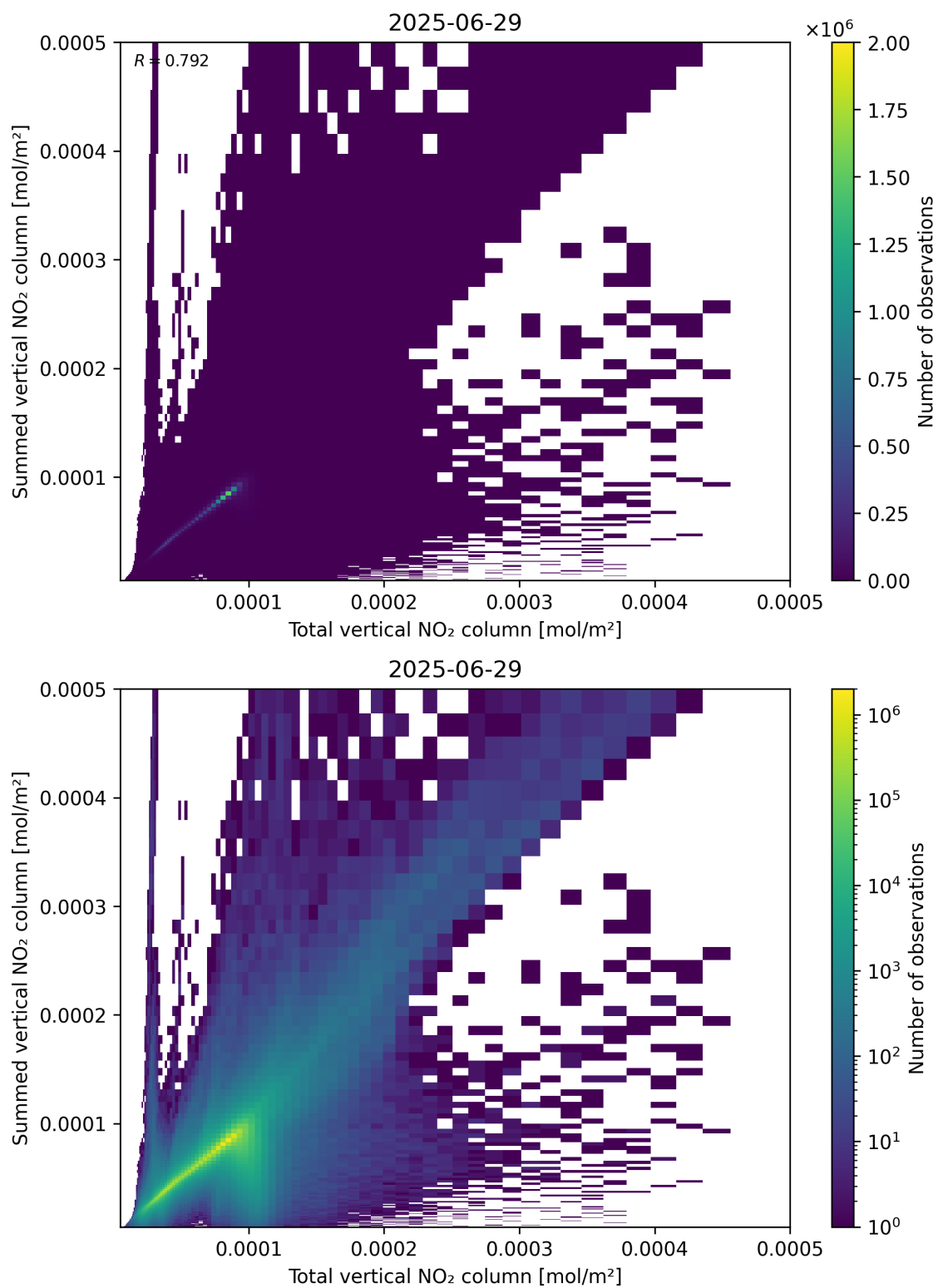
Figure 112: Scatter density plot of “Total vertical NO 2 column” against “Summed vertical NO 2 column” for 2025-06-28 to 2025-06-30.
