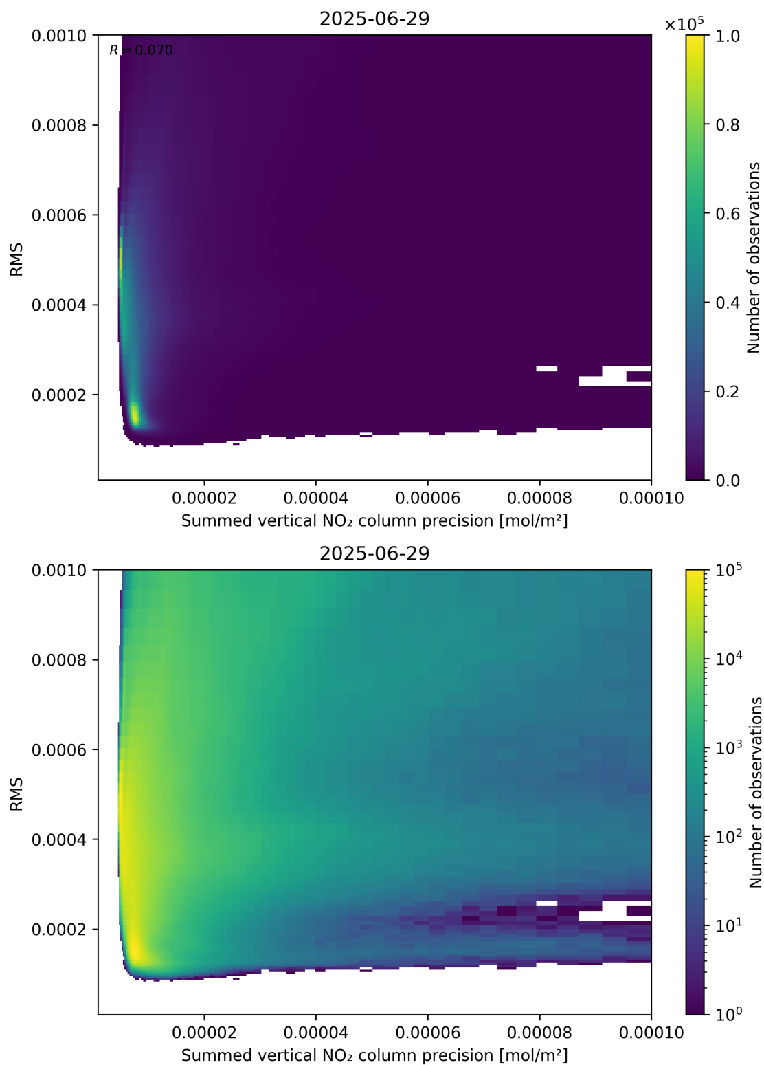
Figure 108: Scatter density plot of “Summed vertical NO 2 column precision” against “RMS” for 2025-06-28 to 2025-06-30.
