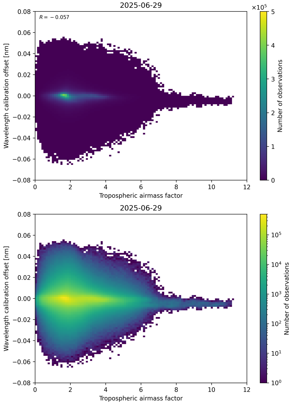
Figure 80: Scatter density plot of “Tropospheric airmass factor” against “Wavelength calibration offset” for 2025-06-28 to 2025-06-30.
