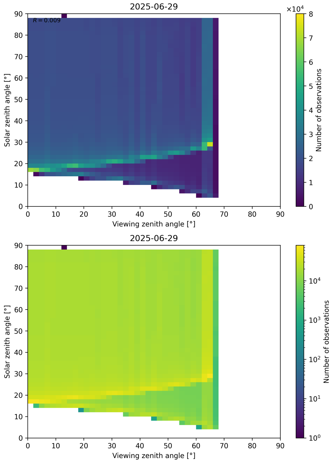
Figure 172: Scatter density plot of “Viewing zenith angle” against “Solar zenith angle” for 2025-06-28 to 2025-06-30.
