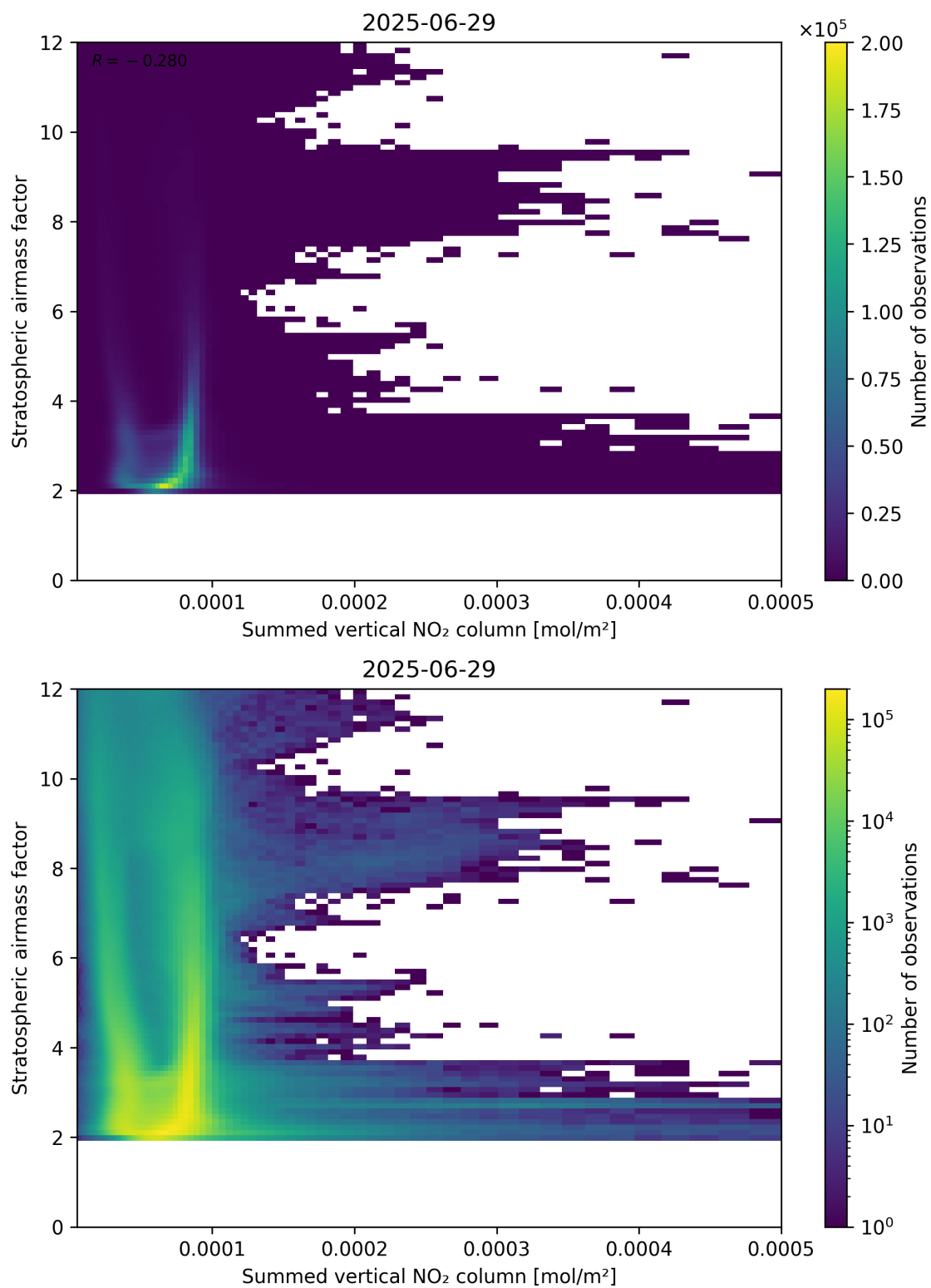
Figure 103: Scatter density plot of “Summed vertical NO 2 column” against “Stratospheric air mass factor” for 2025-06-28 to 2025-06-30.
