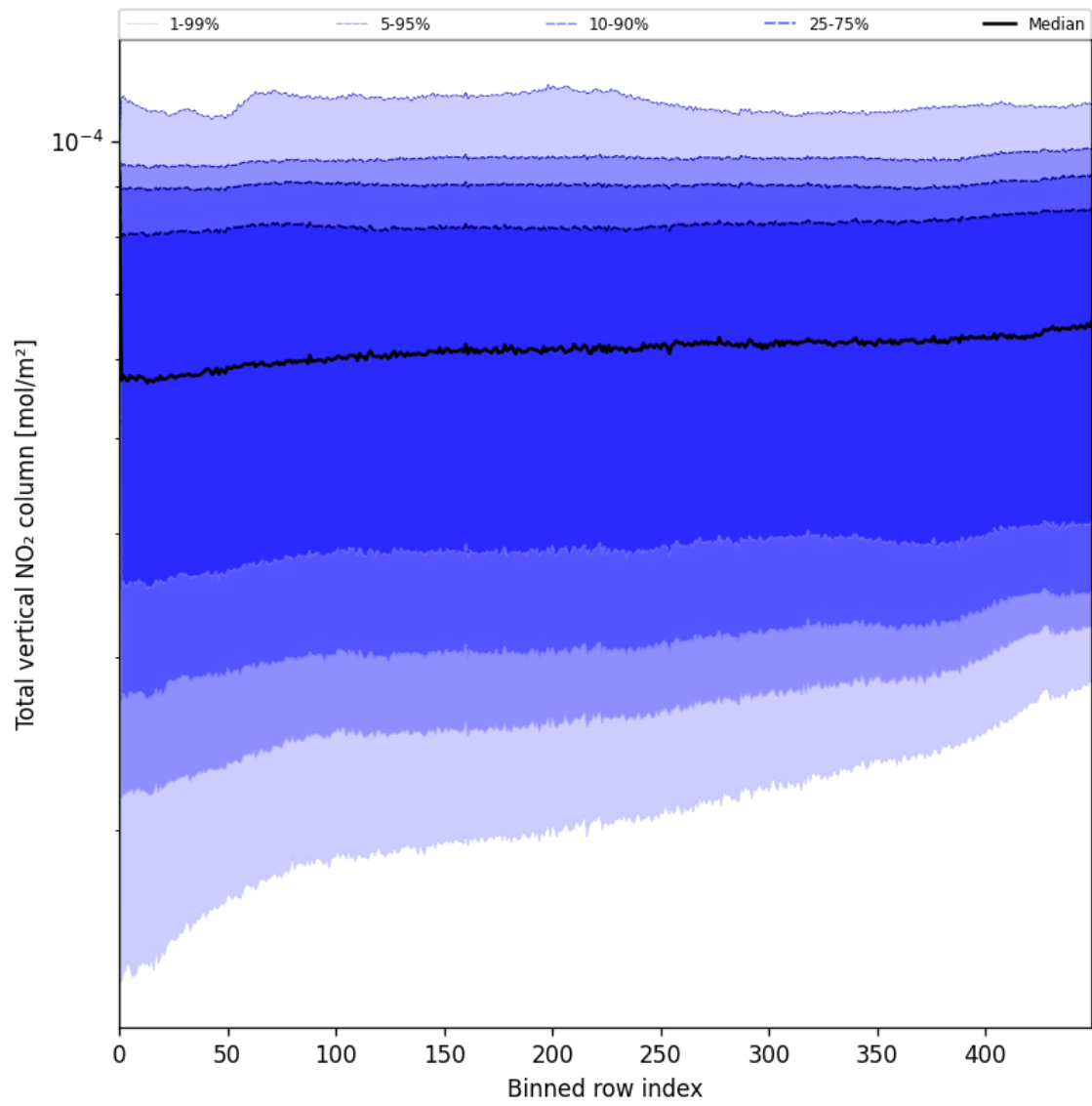
Figure 55: Along track statistics of “Total vertical NO 2 column” for 2025-06-28 to 2025-06-30
