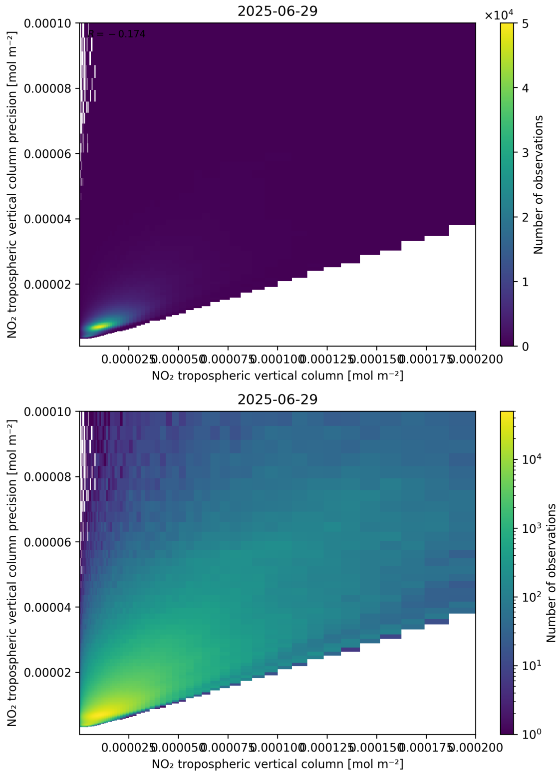
Figure 130: Scatter density plot of “NO 2 tropospheric vertical column” against “NO 2 tropospheric vertical column precision” for 2025-06-28 to 2025-06-30.
