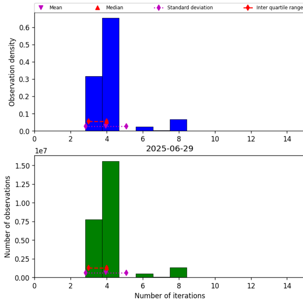
Figure 34: Histogram of “Number of iterations” for 2025-06-28 to 2025-06-30
