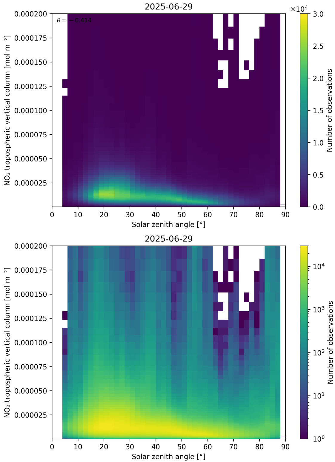
Figure 155: Scatter density plot of “Solar zenith angle” against “NO 2 tropospheric vertical column” for 2025-06-28 to 2025-06-30.
