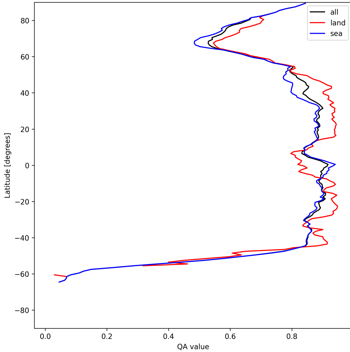
Figure 11: Zonal average of “QA value” for 2025-06-28 to 2025-06-30.
