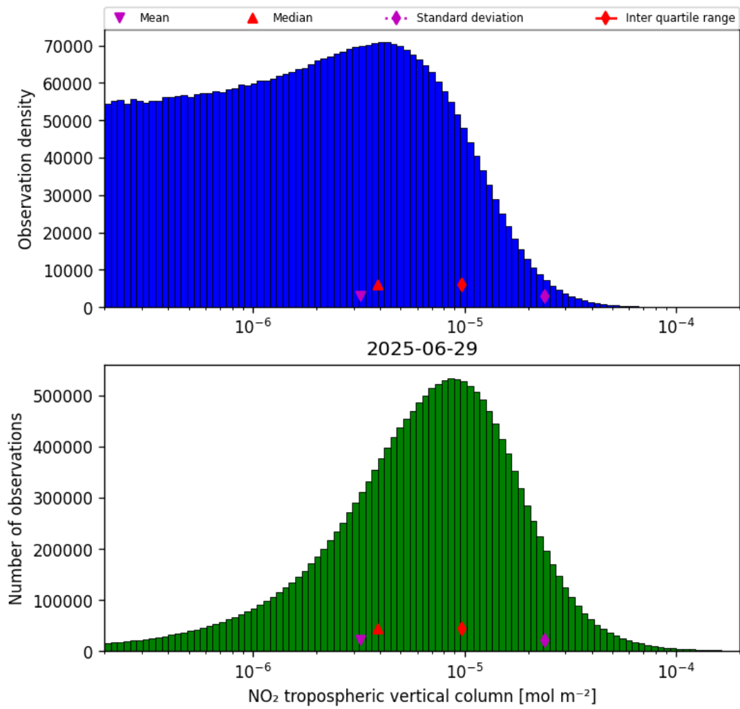
Figure 29: Histogram of “NO 2 tropospheric vertical column” for 2025-06-28 to 2025-06-30
