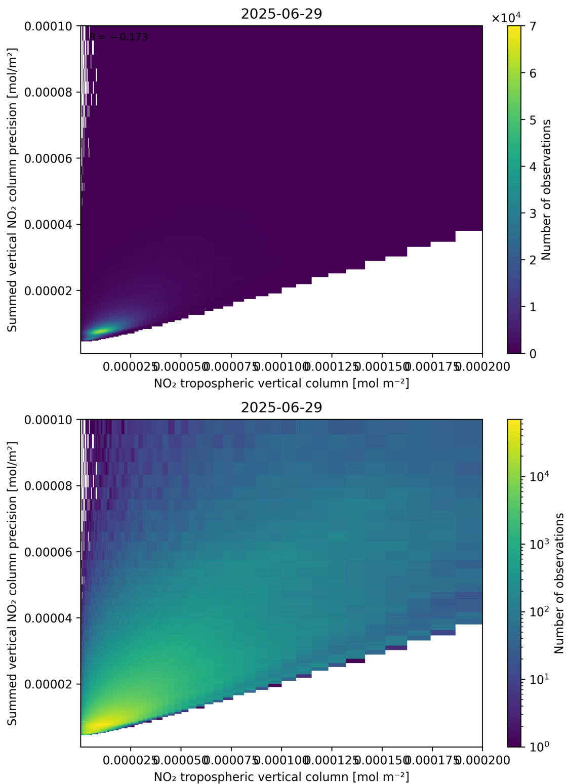
Figure 127: Scatter density plot of “NO 2 tropospheric vertical column” against “Summed vertical NO 2 column precision” for 2025-06-28 to 2025-06-30.
