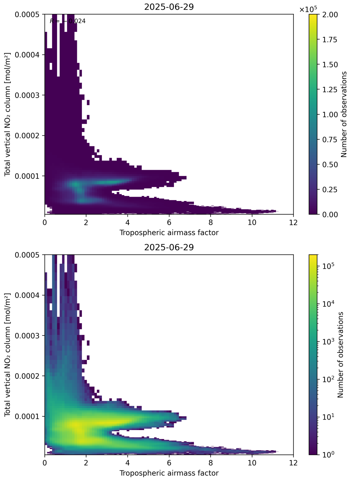
Figure 77: Scatter density plot of “Tropospheric airmass factor” against “Total vertical NO 2 column” for 2025-06-28 to 2025-06-30.
