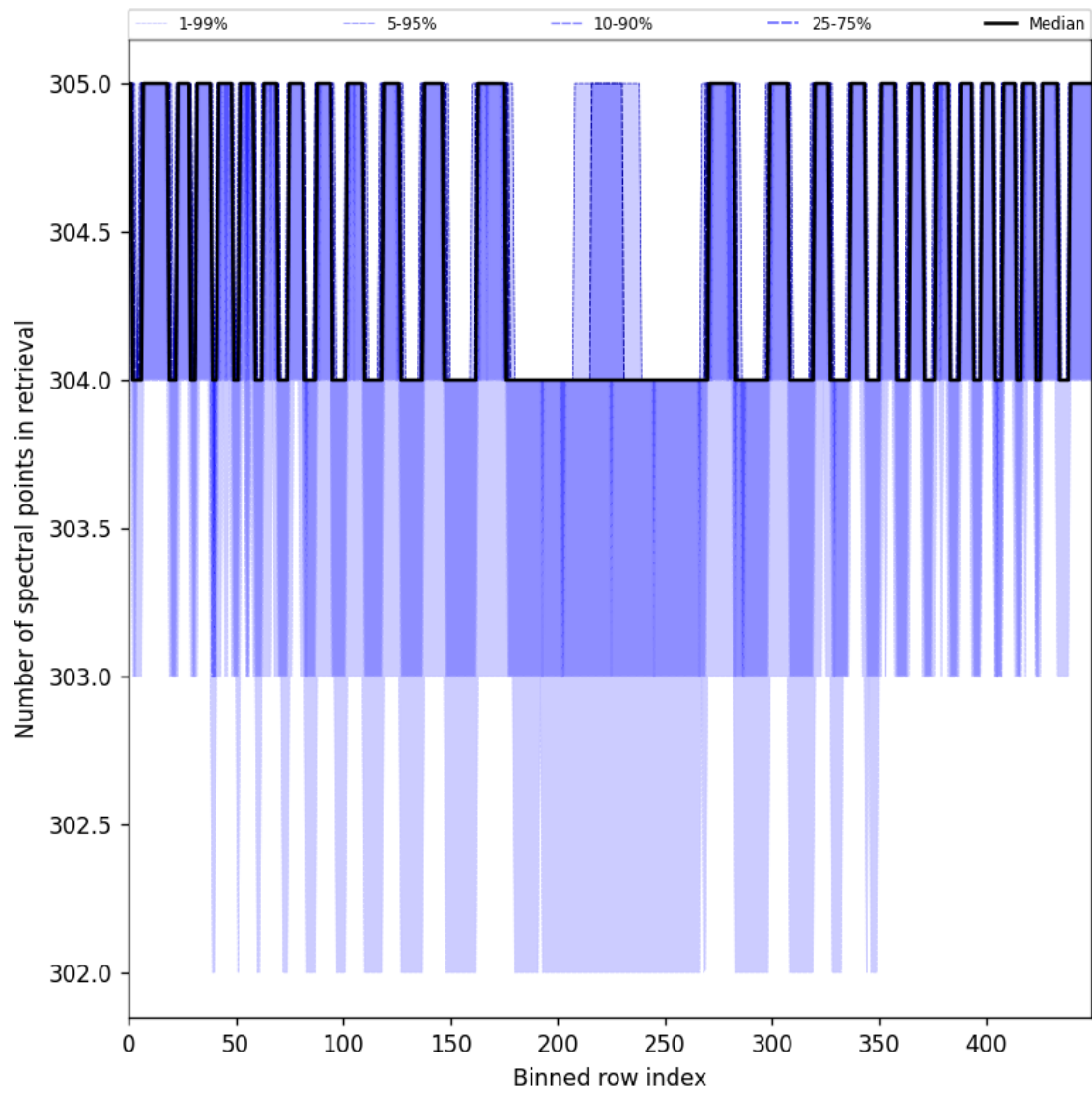
Figure 50: Along track statistics of “Number of spectral points in retrieval” for 2025-06-28 to 2025-06-30
