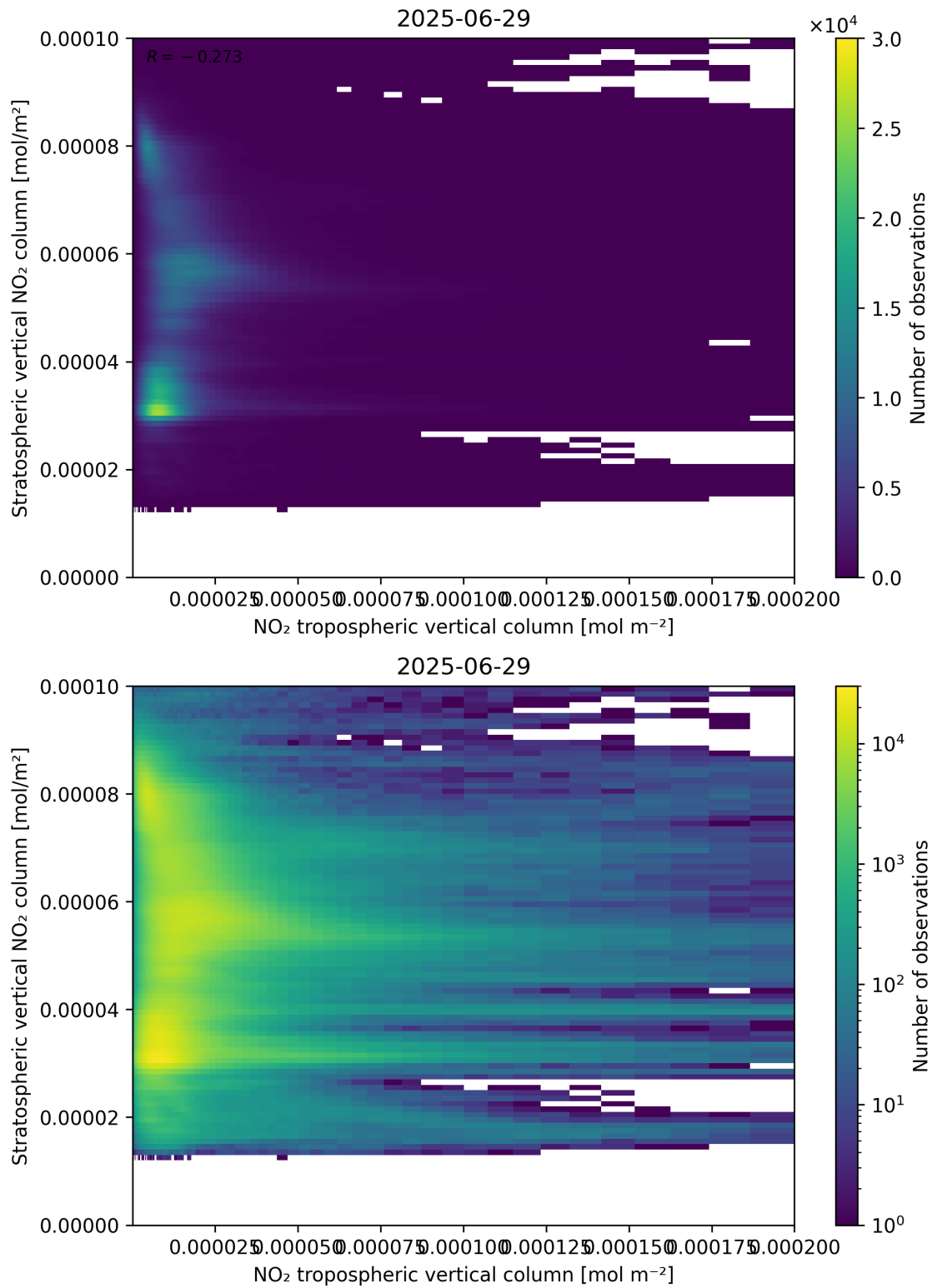
Figure 125: Scatter density plot of “NO 2 tropospheric vertical column” against “Stratospheric vertical NO 2 column” for 2025-06-28 to 2025-06-30.
