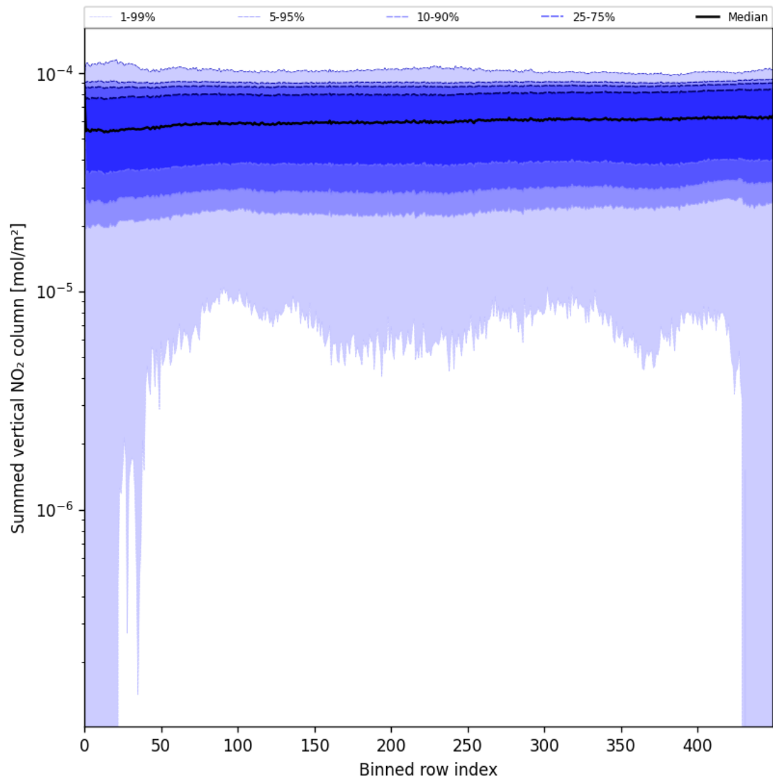
Figure 57: Along track statistics of “Summed vertical NO 2 column” for 2025-06-28 to 2025-06-30
