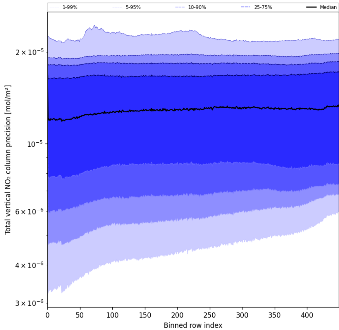
Figure 56: Along track statistics of “Total vertical NO 2 column precision” for 2025-06-28 to 2025-06-30
