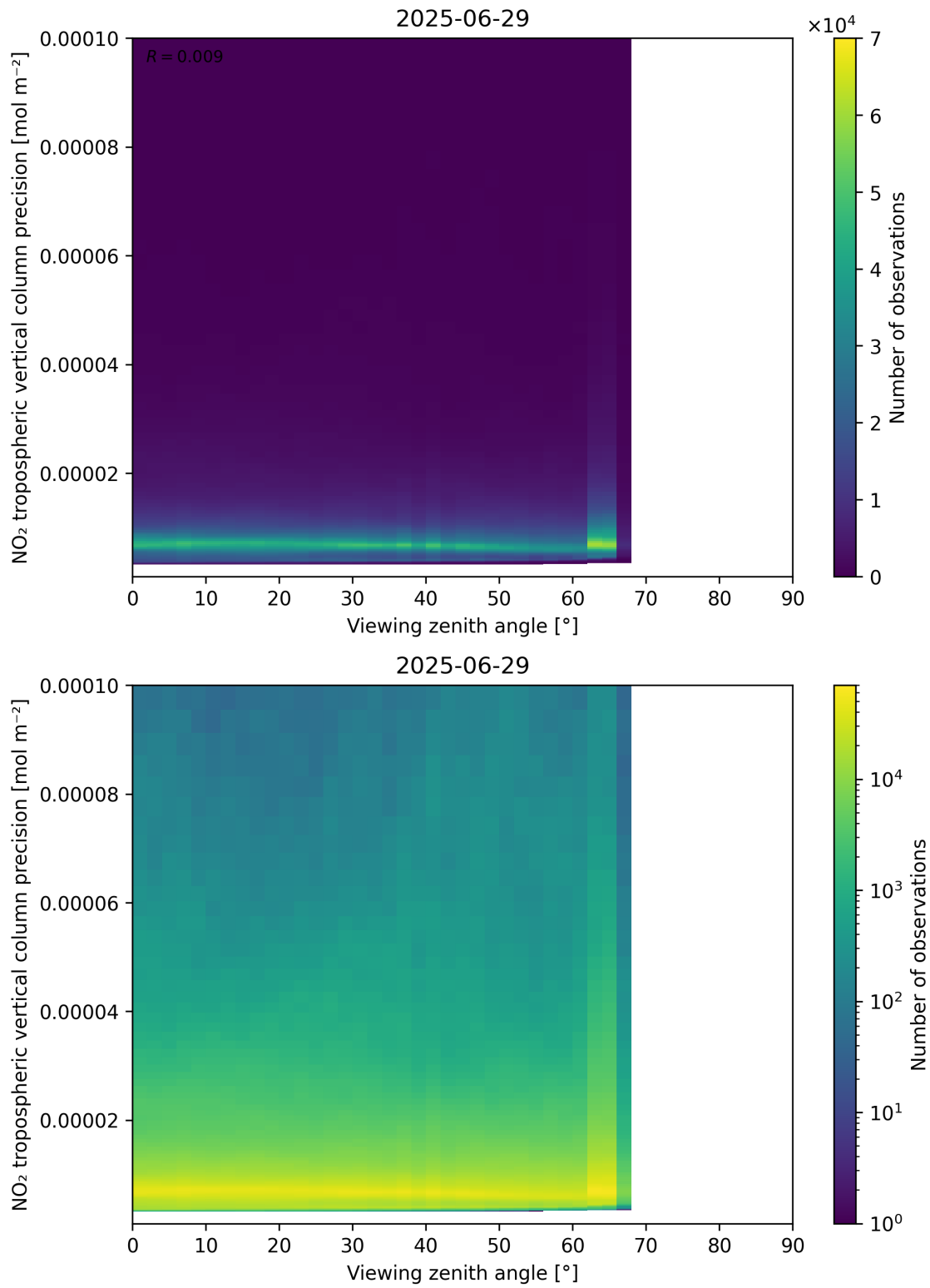
Figure 170: Scatter density plot of “Viewing zenith angle” against “NO 2 tropospheric vertical column precision” for 2025-06-28 to 2025-06-30.
