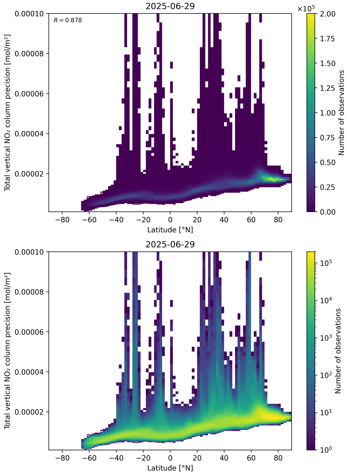
Figure 91: Scatter density plot of “Latitude” against “Total vertical NO 2 column precision” for 2025-06-28 to 2025-06-30.
