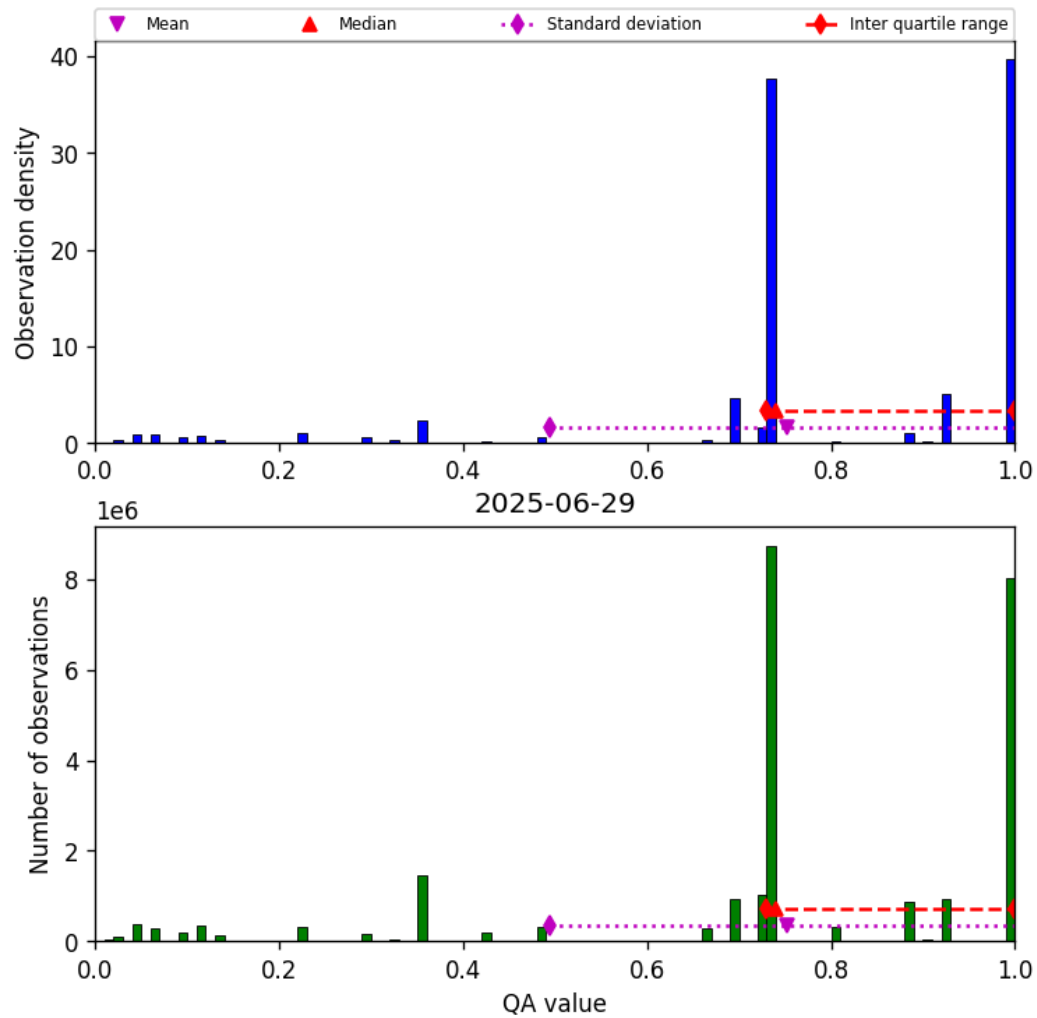
Figure 28: Histogram of “QA value” for 2025-06-28 to 2025-06-30
