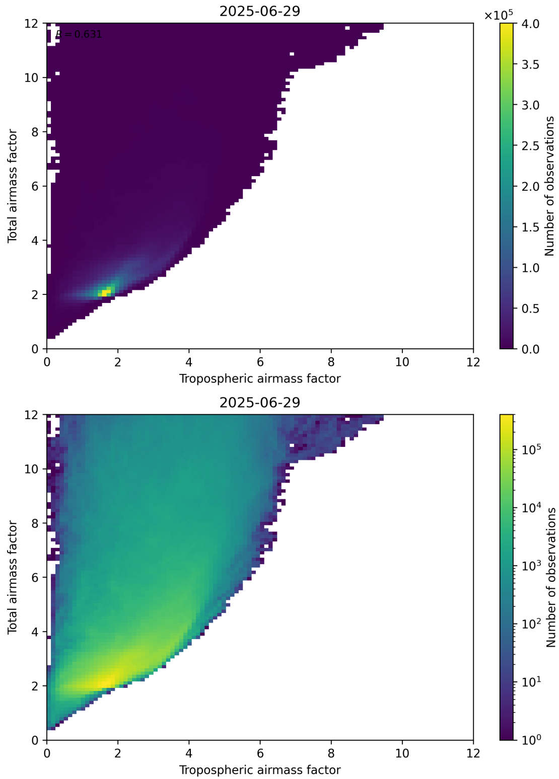
Figure 72: Scatter density plot of “Tropospheric airmass factor” against “Total airmass factor” for 2025-06-28 to 2025-06-30.
