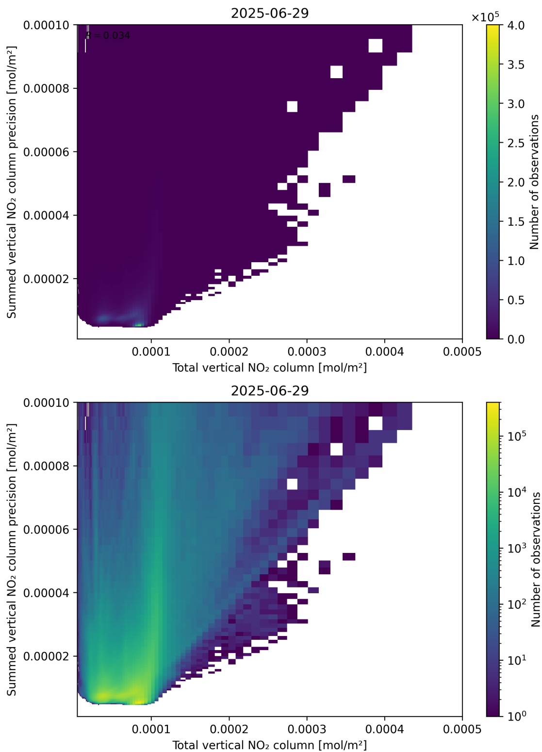
Figure 113: Scatter density plot of “Total vertical NO 2 column” against “Summed vertical NO 2 column precision” for 2025-06-28 to 2025-06-30.
