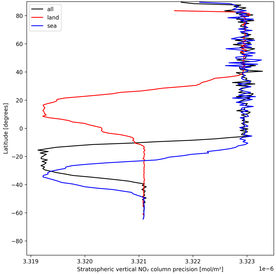
Figure 20: Zonal average of “Stratospheric vertical NO 2 column precision” for 2025-06-28 to 2025-06-30.
