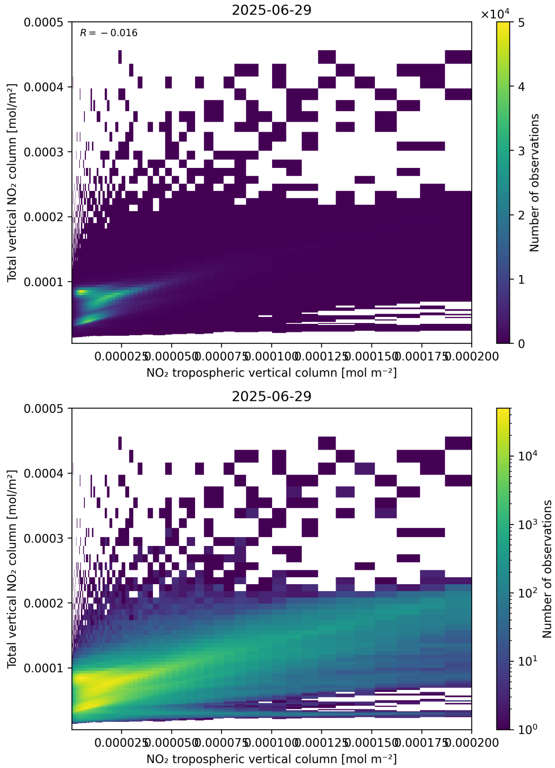
Figure 128: Scatter density plot of “NO 2 tropospheric vertical column” against “Total vertical NO 2 column” for 2025-06-28 to 2025-06-30.
