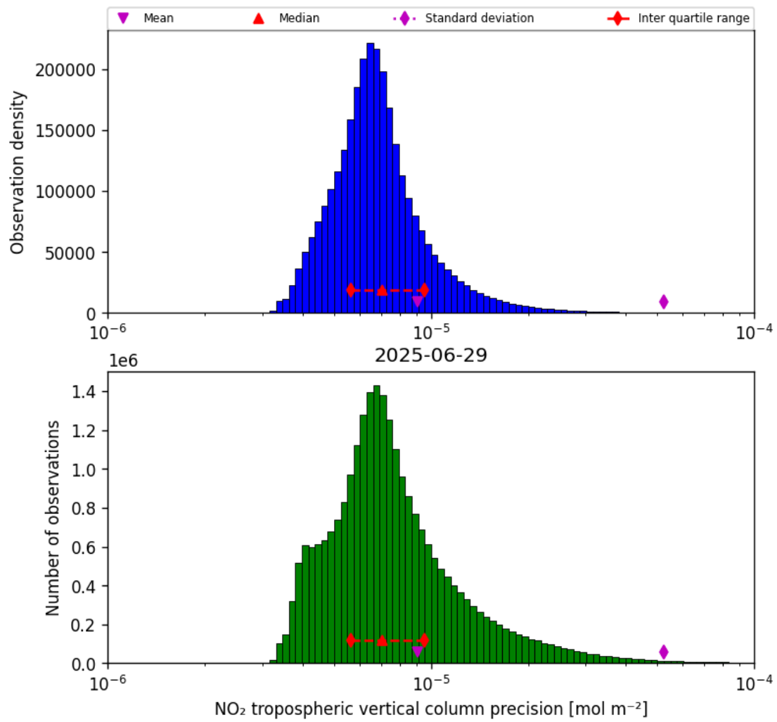
Figure 30: Histogram of “NO 2 tropospheric vertical column precision” for 2025-06-28 to 2025-06-30
