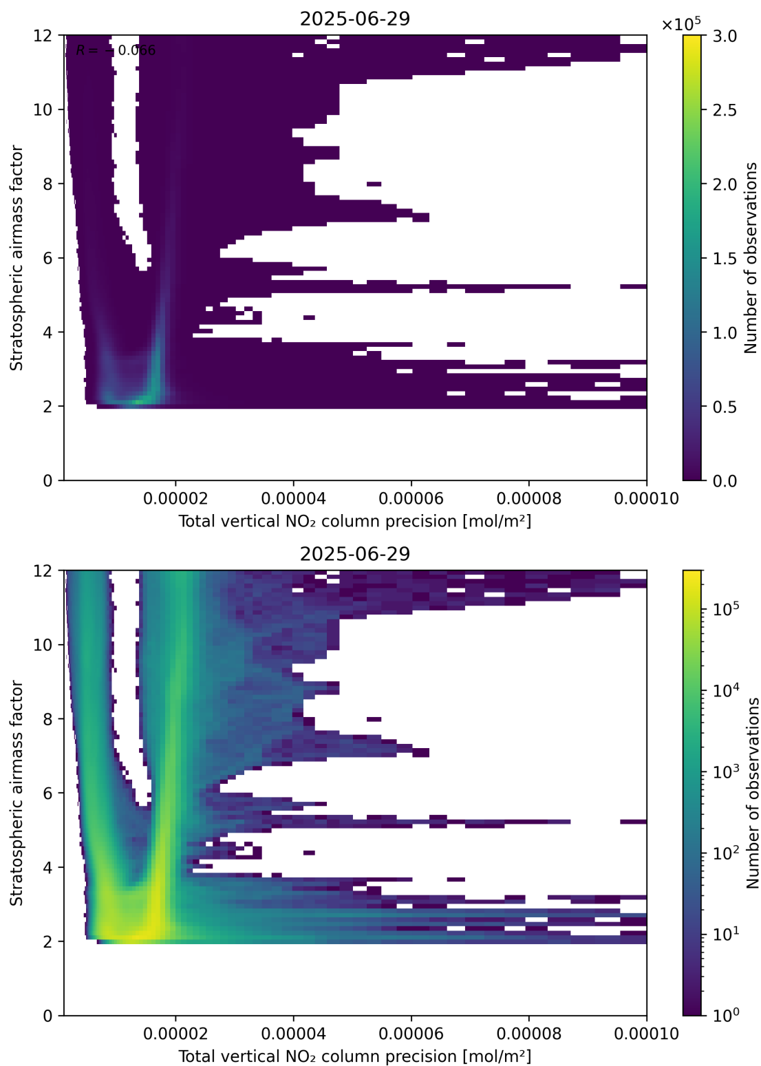
Figure 115: Scatter density plot of “Total vertical NO 2 column precision” against “Stratospheric air mass factor” for 2025-06-28 to 2025-06-30.
