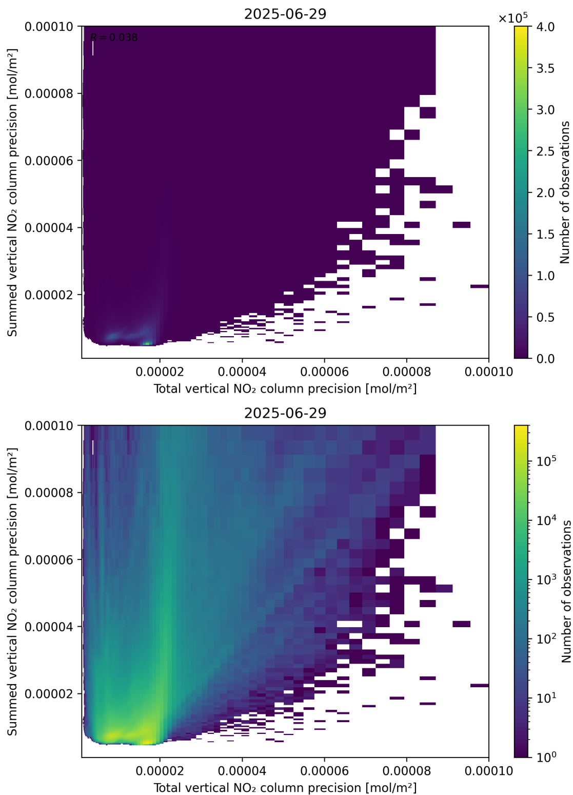
Figure 118: Scatter density plot of “Total vertical NO 2 column precision” against “Summed vertical NO 2 column precision” for 2025-06-28 to 2025-06-30.
