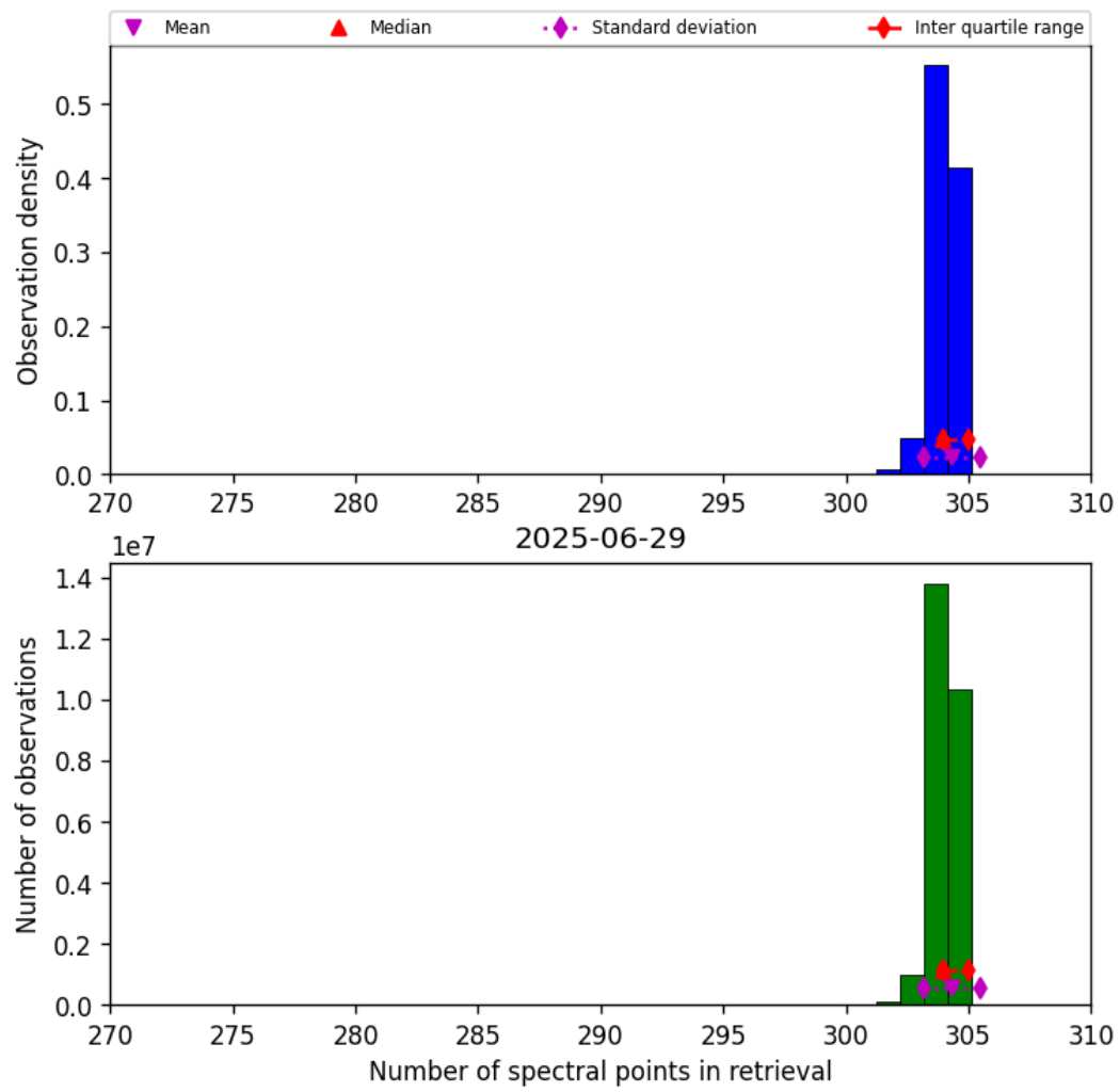
Figure 33: Histogram of “Number of spectral points in retrieval” for 2025-06-28 to 2025-06-30
