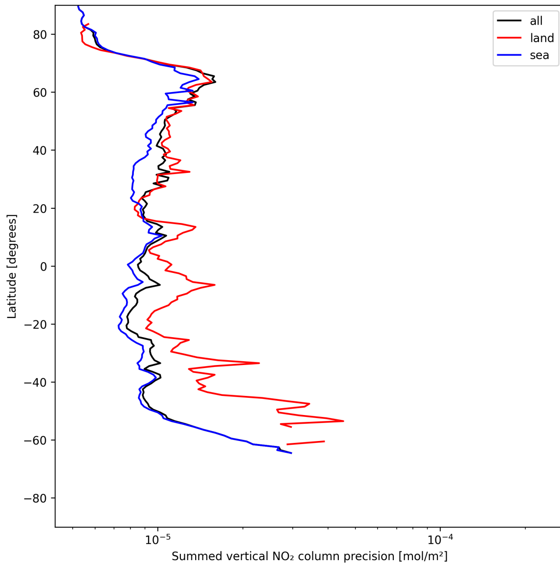
Figure 24: Zonal average of “Summed vertical NO 2 column precision” for 2025-06-28 to 2025-06-30.
