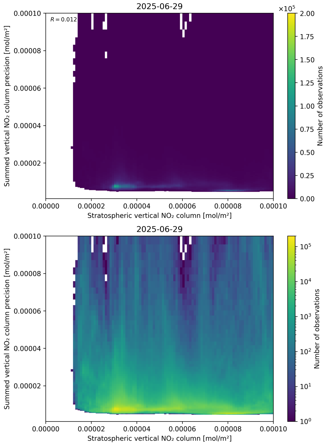
Figure 99: Scatter density plot of “Stratospheric vertical NO 2 column” against “Summed vertical NO 2 column precision” for 2025-06-28 to 2025-06-30.
