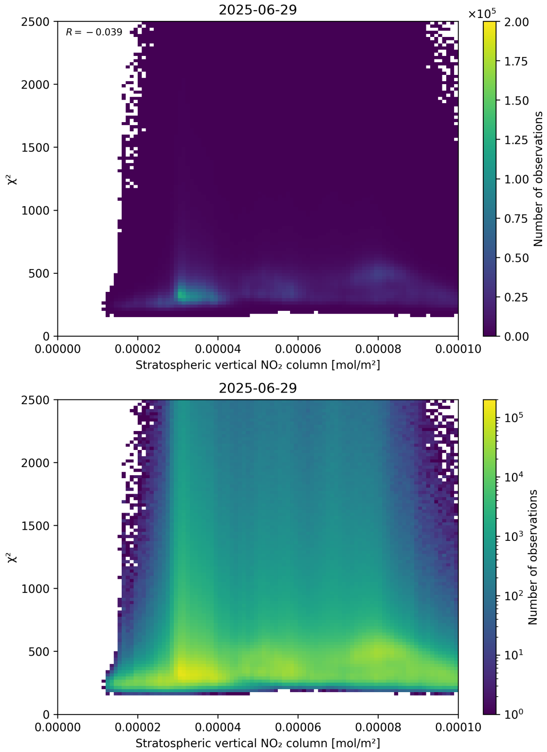
Figure 97: Scatter density plot of “Stratospheric vertical NO 2 column” against “ \chi^2 ” for 2025-06-28 to 2025-06-30.
