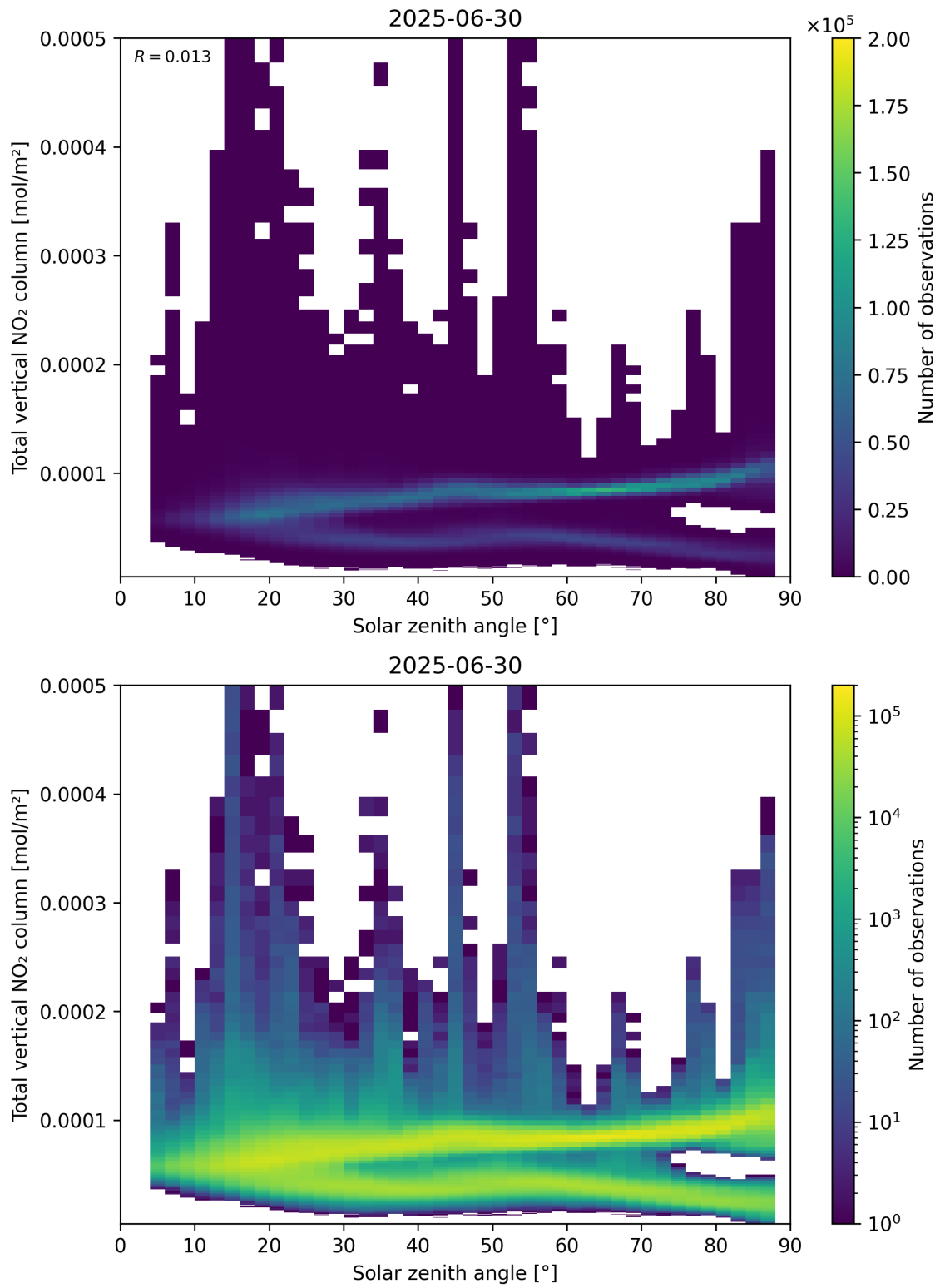
Figure 153: Scatter density plot of “Solar zenith angle” against “Total vertical NO 2 column” for 2025-06-29 to 2025-07-01.
