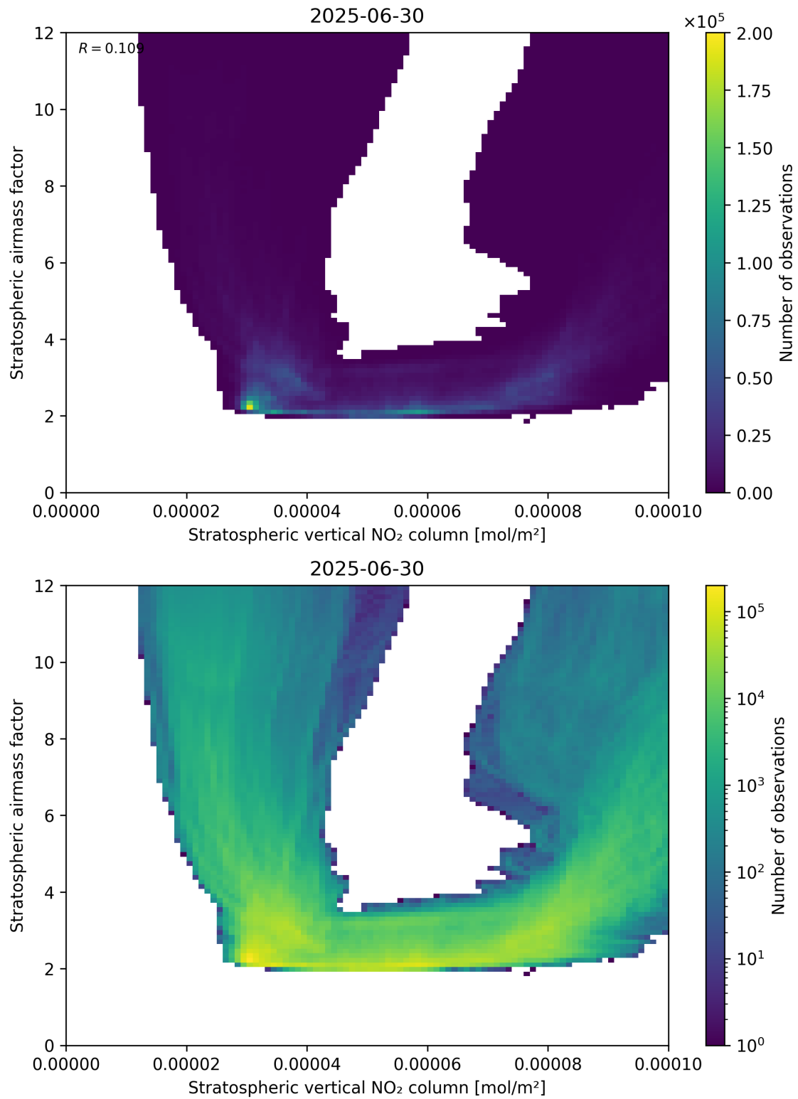
Figure 96: Scatter density plot of “Stratospheric vertical NO 2 column” against “Stratospheric airmass factor” for 2025-06-29 to 2025-07-01.
