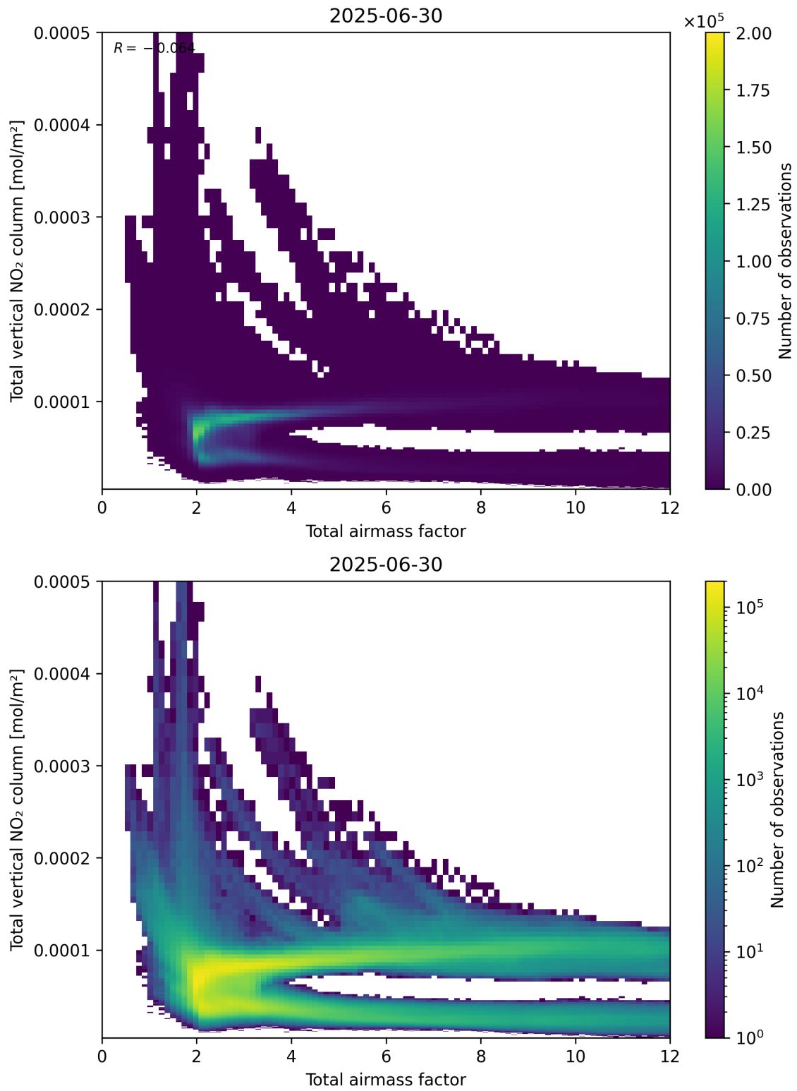
Figure 67: Scatter density plot of “Total airmass factor” against “Total vertical NO 2 column” for 2025-06-29 to 2025-07-01.
