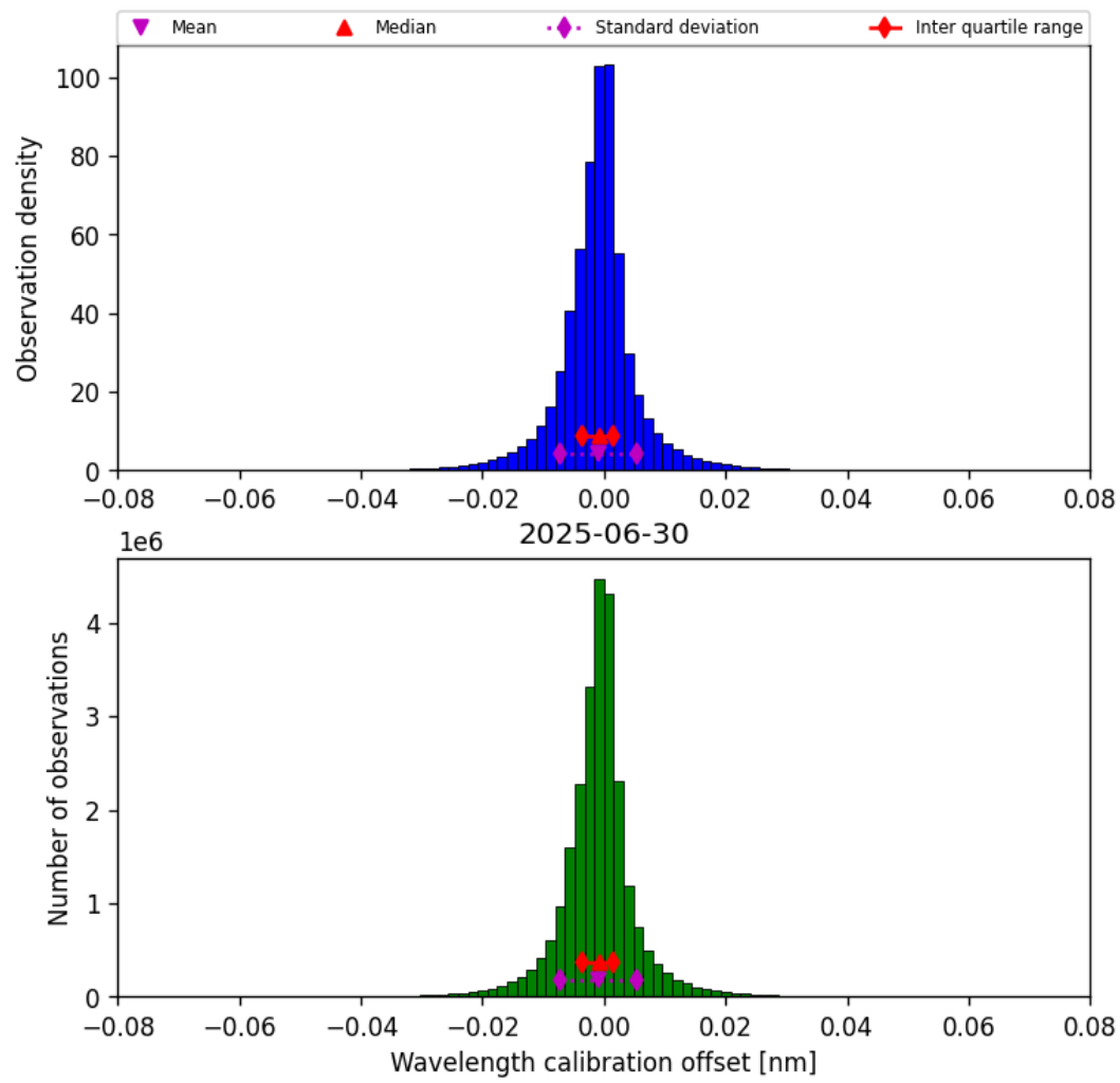
Figure 35: Histogram of “Wavelength calibration offset” for 2025-06-29 to 2025-07-01
