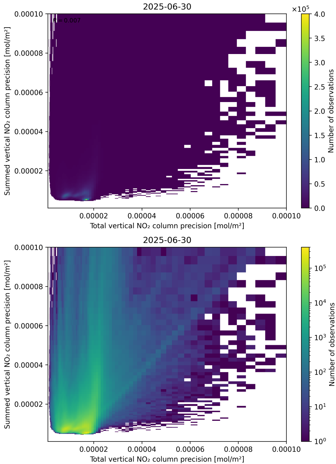
Figure 118: Scatter density plot of “Total vertical NO 2 column precision” against “Summed vertical NO 2 column precision” for 2025-06-29 to 2025-07-01.
