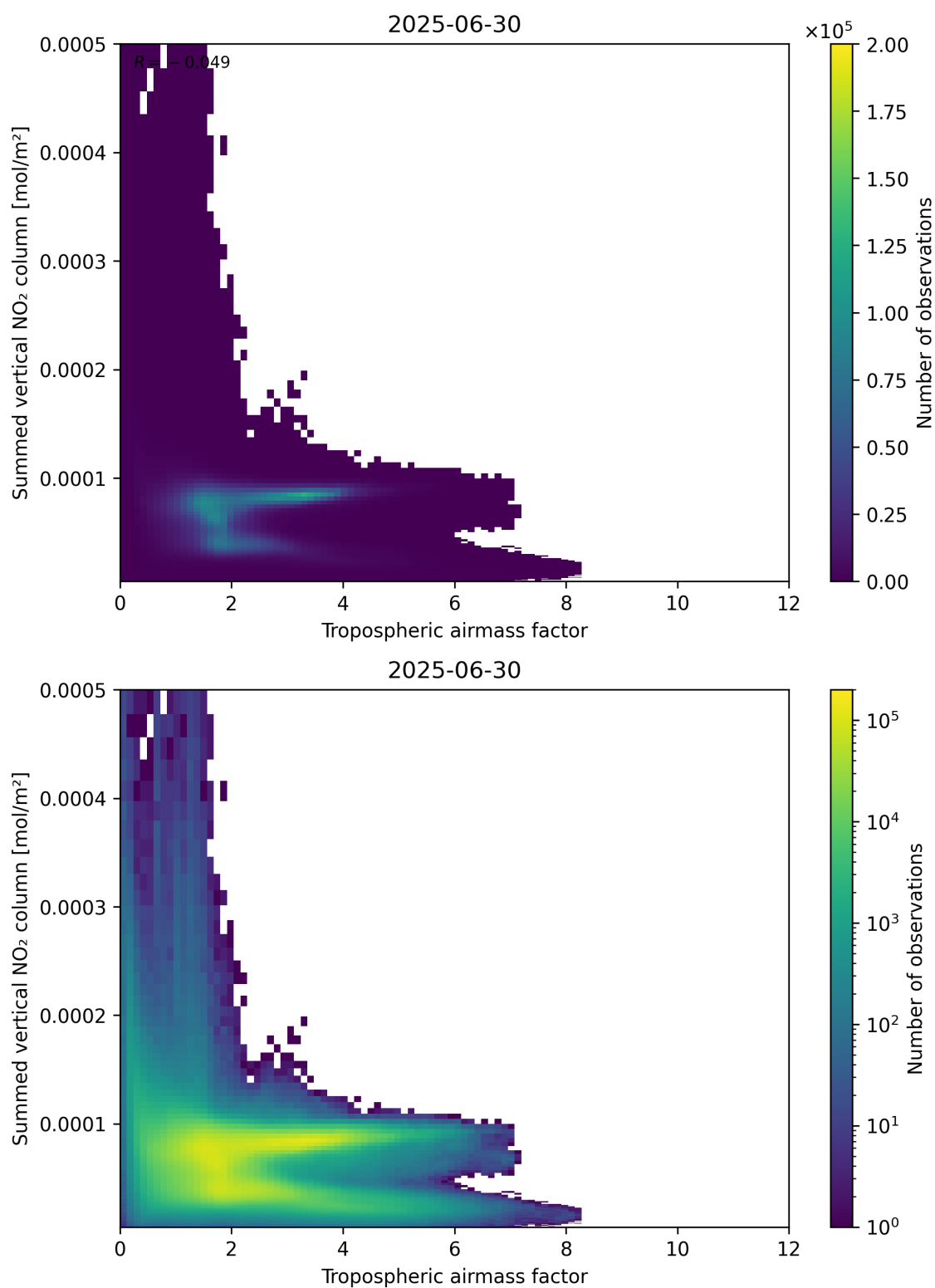
Figure 75: Scatter density plot of “Tropospheric airmass factor” against “Summed vertical NO 2 column” for 2025-06-29 to 2025-07-01.
