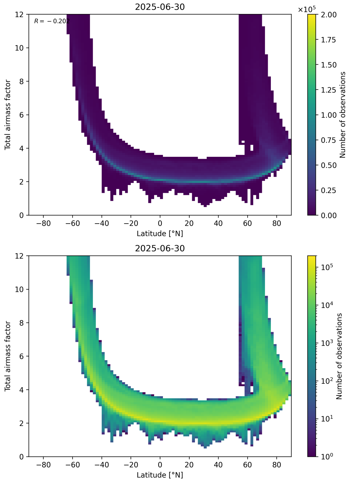
Figure 84: Scatter density plot of “Latitude” against “Total airmass factor” for 2025-06-29 to 2025-07-01.
