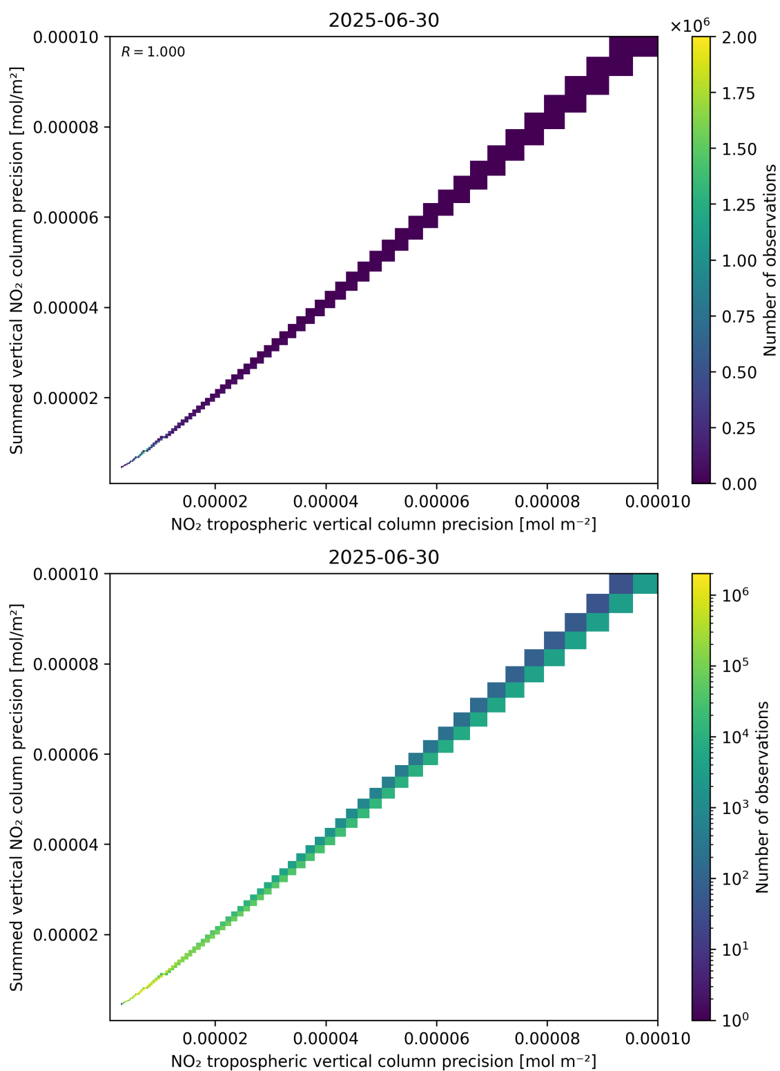
Figure 137: Scatter density plot of “NO 2 tropospheric vertical column precision” against “Summed vertical NO 2 column precision” for 2025-06-29 to 2025-07-01.
