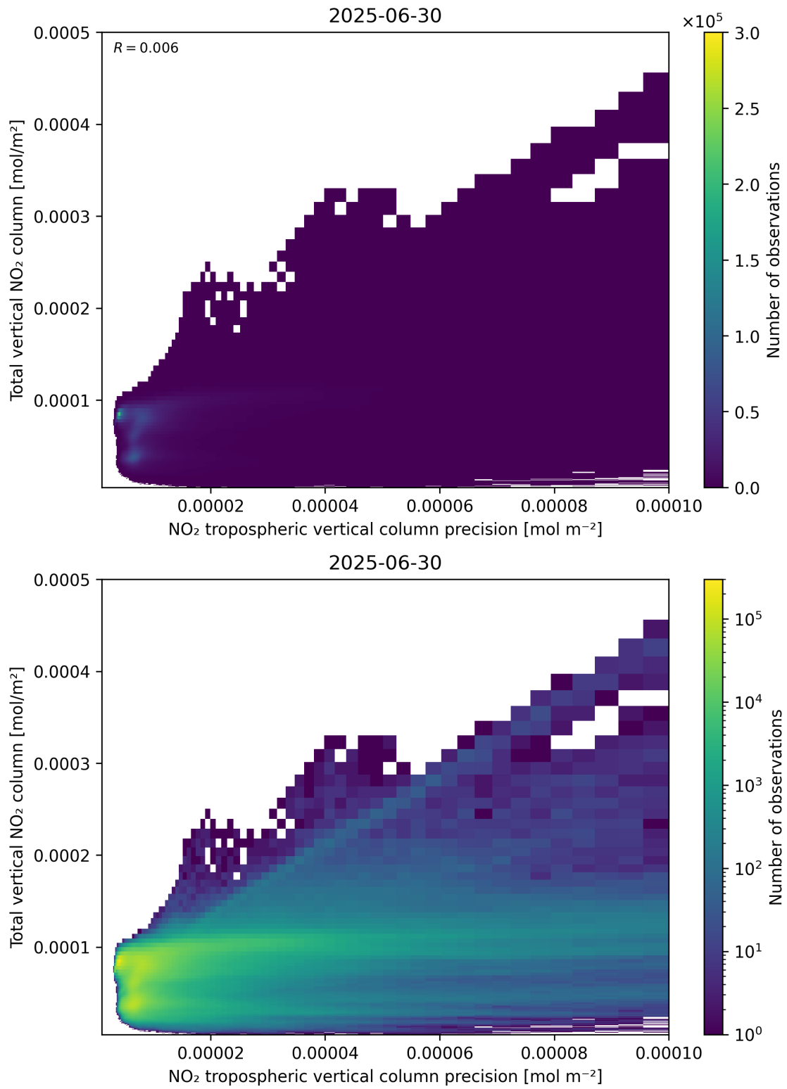
Figure 138: Scatter density plot of “NO 2 tropospheric vertical column precision” against “Total vertical NO 2 column” for 2025-06-29 to 2025-07-01.
