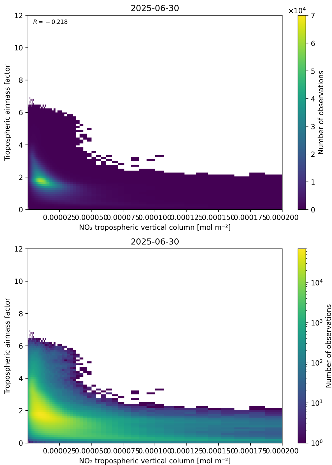
Figure 123: Scatter density plot of “NO 2 tropospheric vertical column” against “Tropospheric air mass factor” for 2025-06-29 to 2025-07-01.
