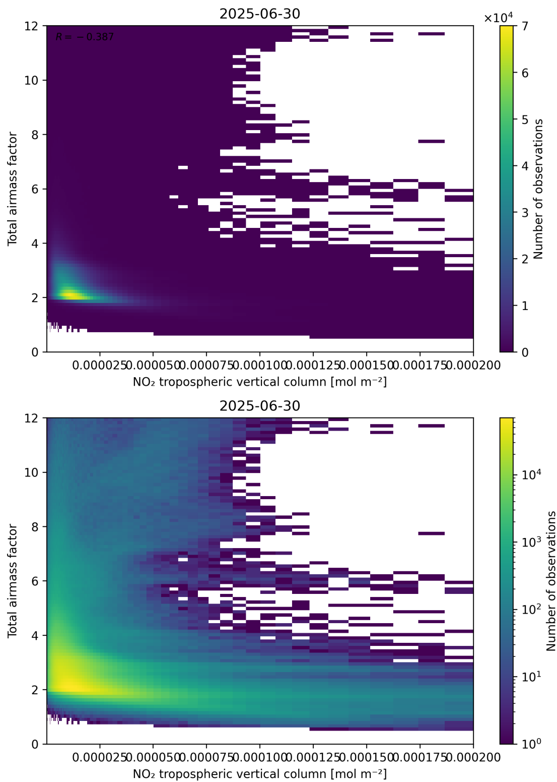
Figure 122: Scatter density plot of “NO 2 tropospheric vertical column” against “Total air mass factor” for 2025-06-29 to 2025-07-01.
