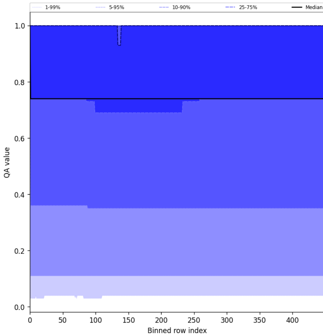
Figure 45: Along track statistics of “QA value” for 2025-06-29 to 2025-07-01
