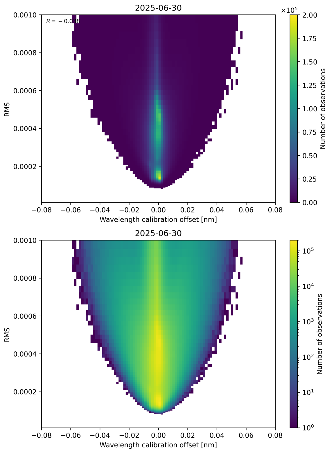
Figure 181: Scatter density plot of “Wavelength calibration offset” against “RMS” for 2025-06-29 to 2025-07-01.
