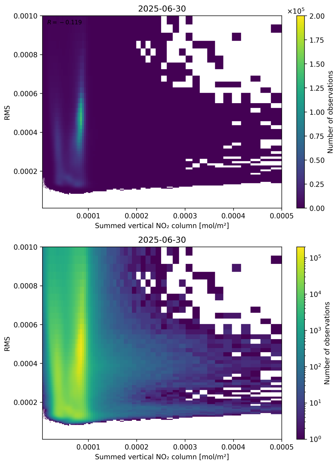
Figure 109: Scatter density plot of “Summed vertical NO 2 column” against “RMS” for 2025-06-29 to 2025-07-01.
