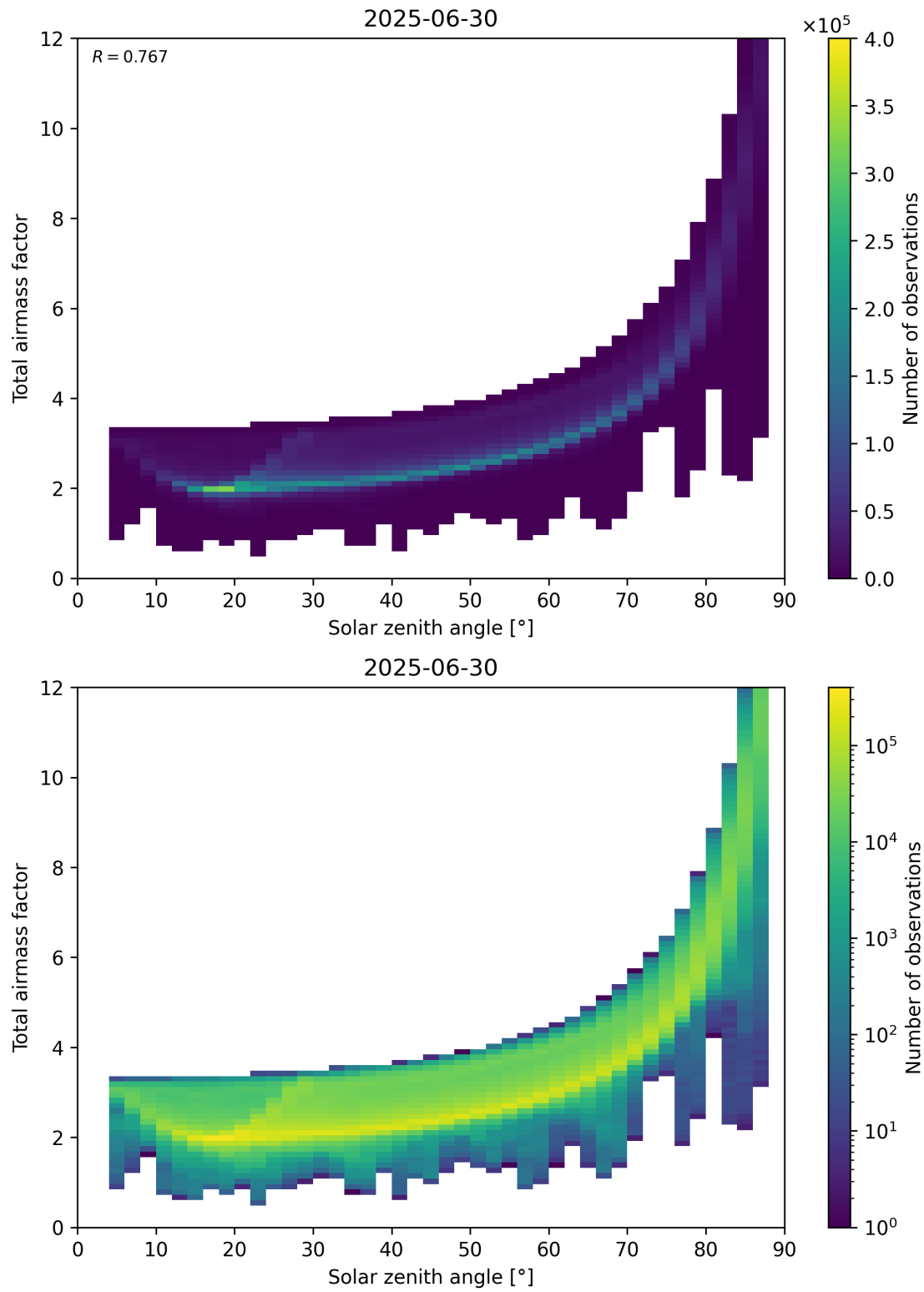
Figure 146: Scatter density plot of “Solar zenith angle” against “Total air mass factor” for 2025-06-29 to 2025-07-01.
