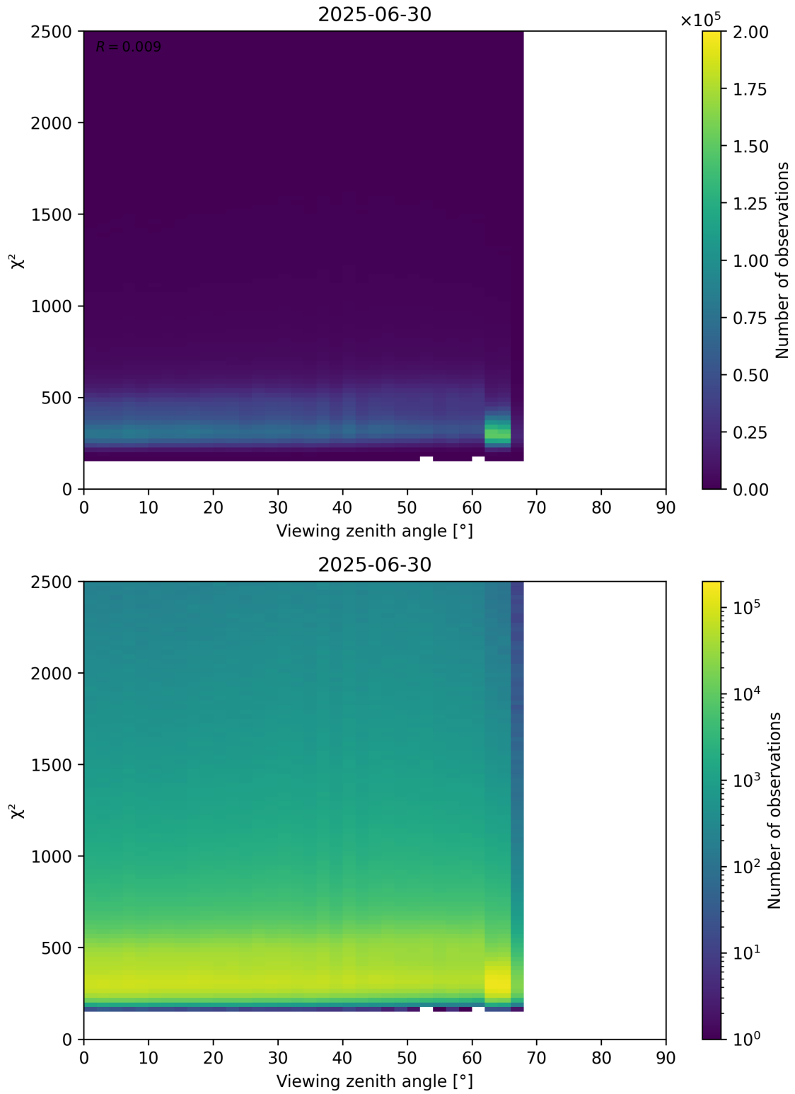
Figure 162: Scatter density plot of “Viewing zenith angle” against “ \chi^2 ” for 2025-06-29 to 2025-07-01.
