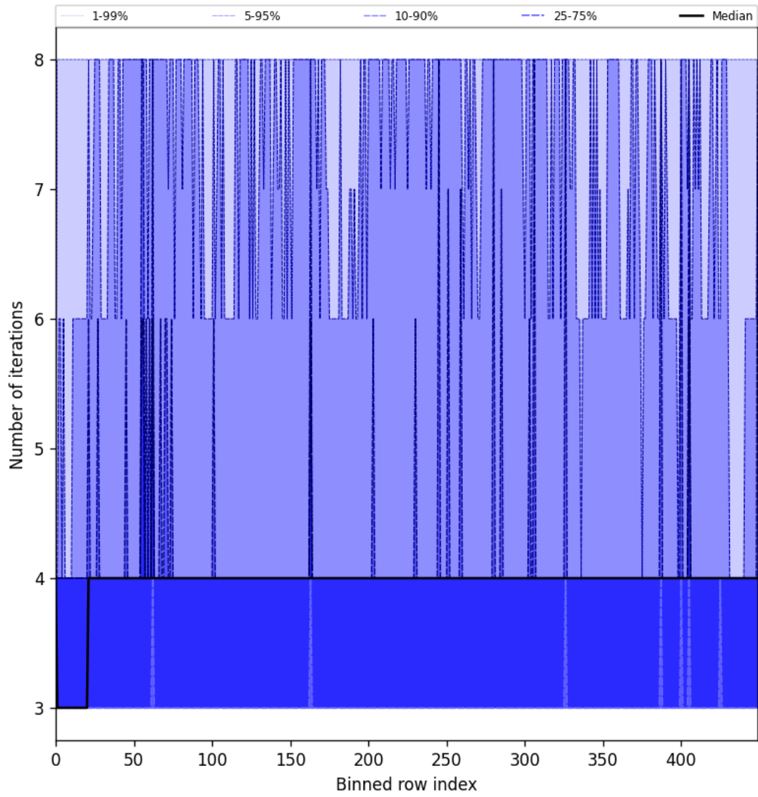
Figure 51: Along track statistics of “Number of iterations” for 2025-06-29 to 2025-07-01
