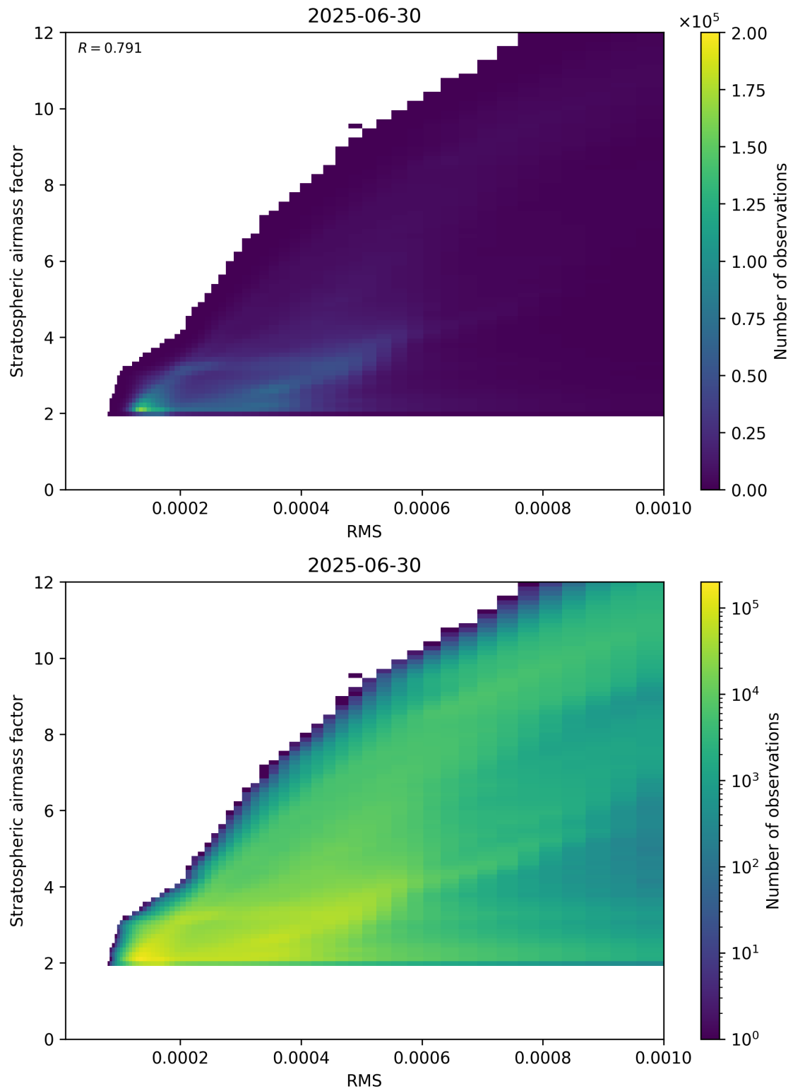
Figure 144: Scatter density plot of “RMS” against “Stratospheric airmass factor” for 2025-06-29 to 2025-07-01.
