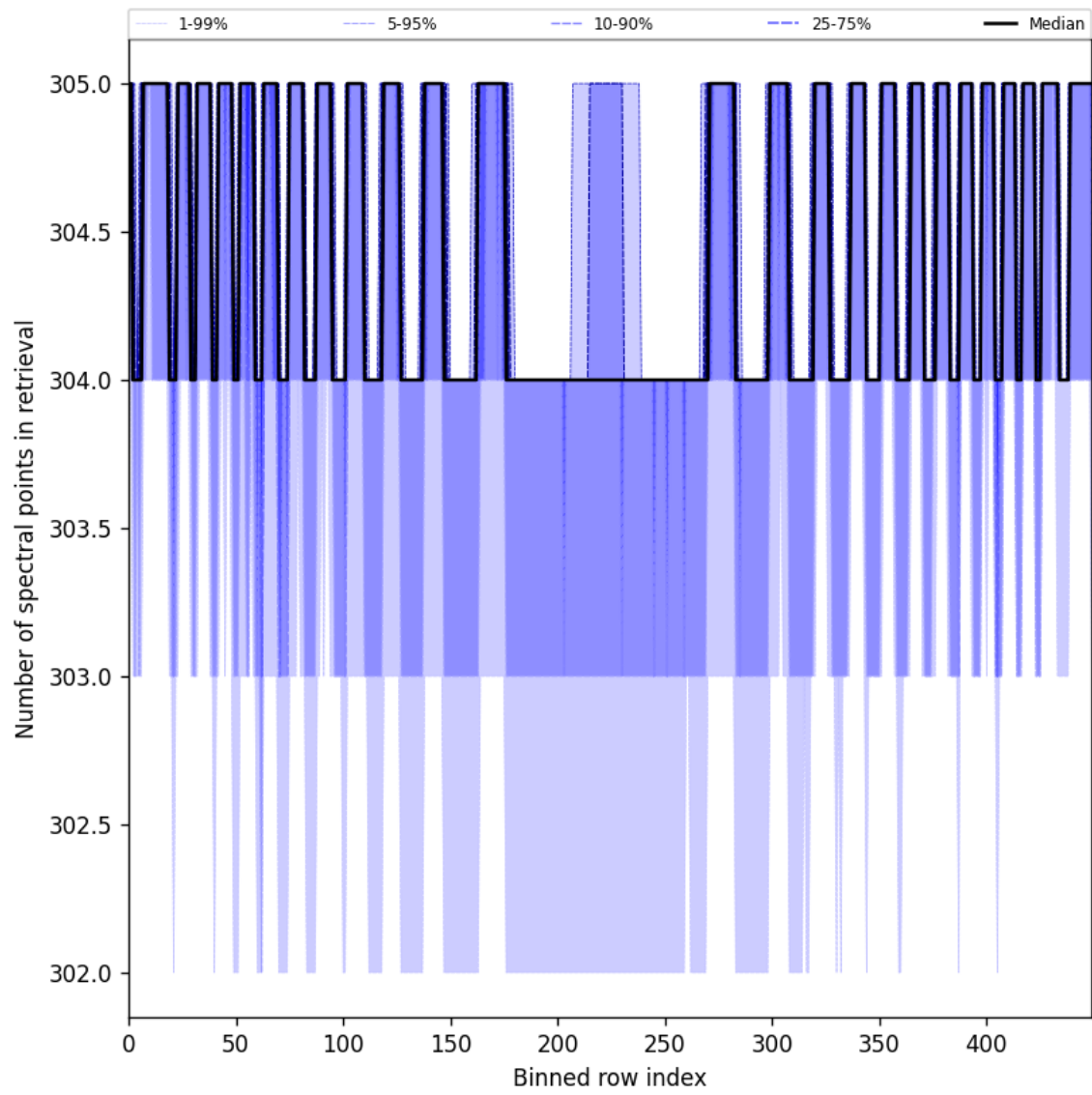
Figure 50: Along track statistics of “Number of spectral points in retrieval” for 2025-06-29 to 2025-07-01
