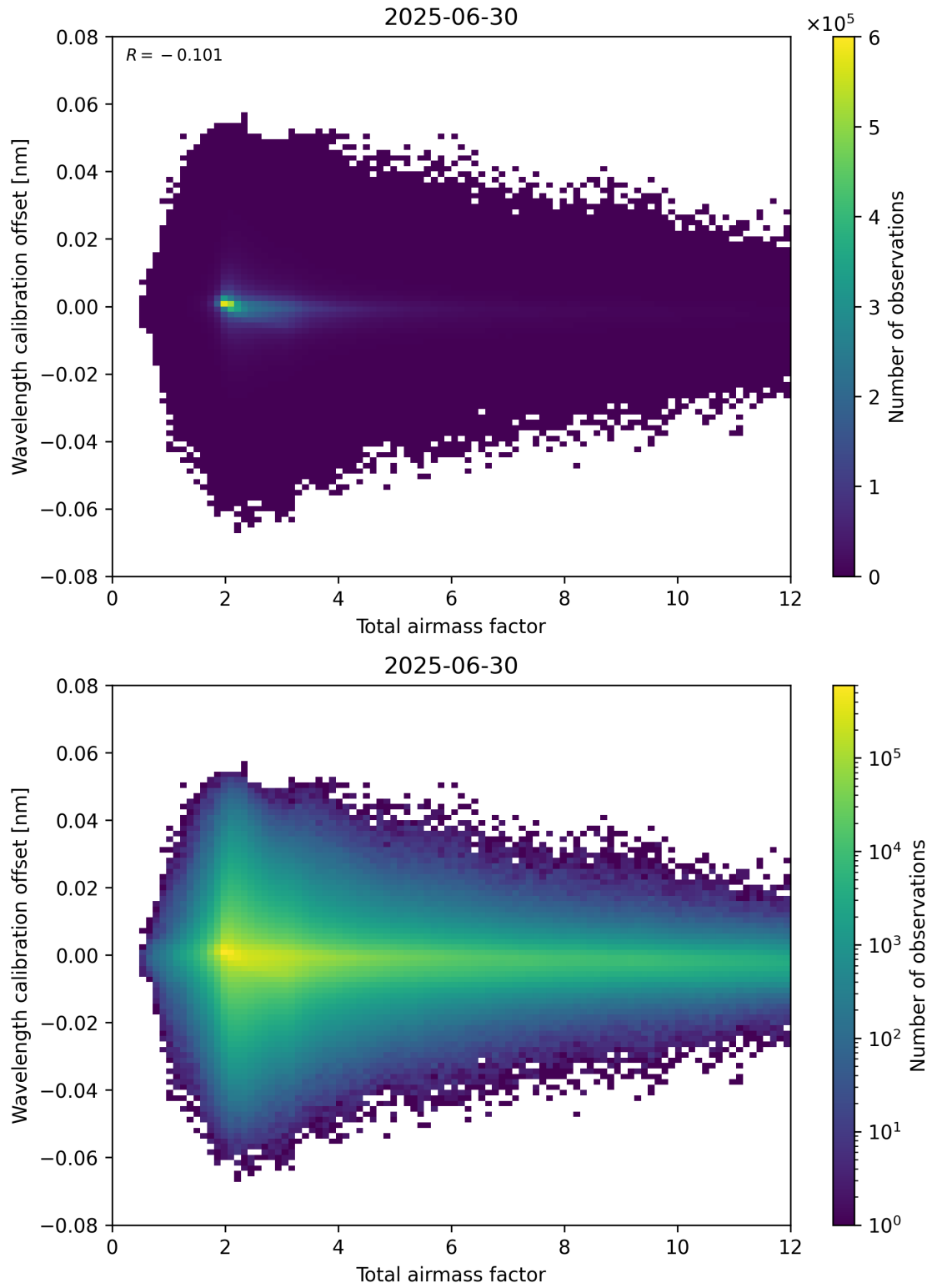
Figure 70: Scatter density plot of “Total airmass factor” against “Wavelength calibration offset” for 2025-06-29 to 2025-07-01.
