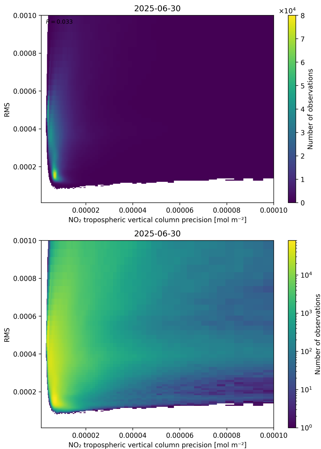
Figure 140: Scatter density plot of “NO 2 tropospheric vertical column precision” against “RMS” for 2025-06-29 to 2025-07-01.
