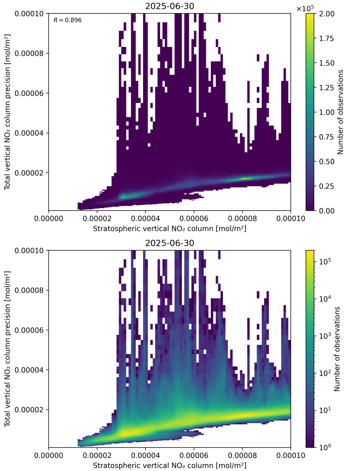
Figure 101: Scatter density plot of “Stratospheric vertical NO 2 column” against “Total vertical NO 2 column precision” for 2025-06-29 to 2025-07-01.
