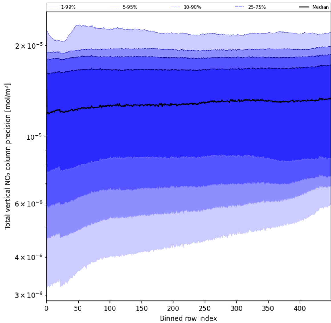
Figure 56: Along track statistics of “Total vertical NO 2 column precision” for 2025-06-29 to 2025-07-01
