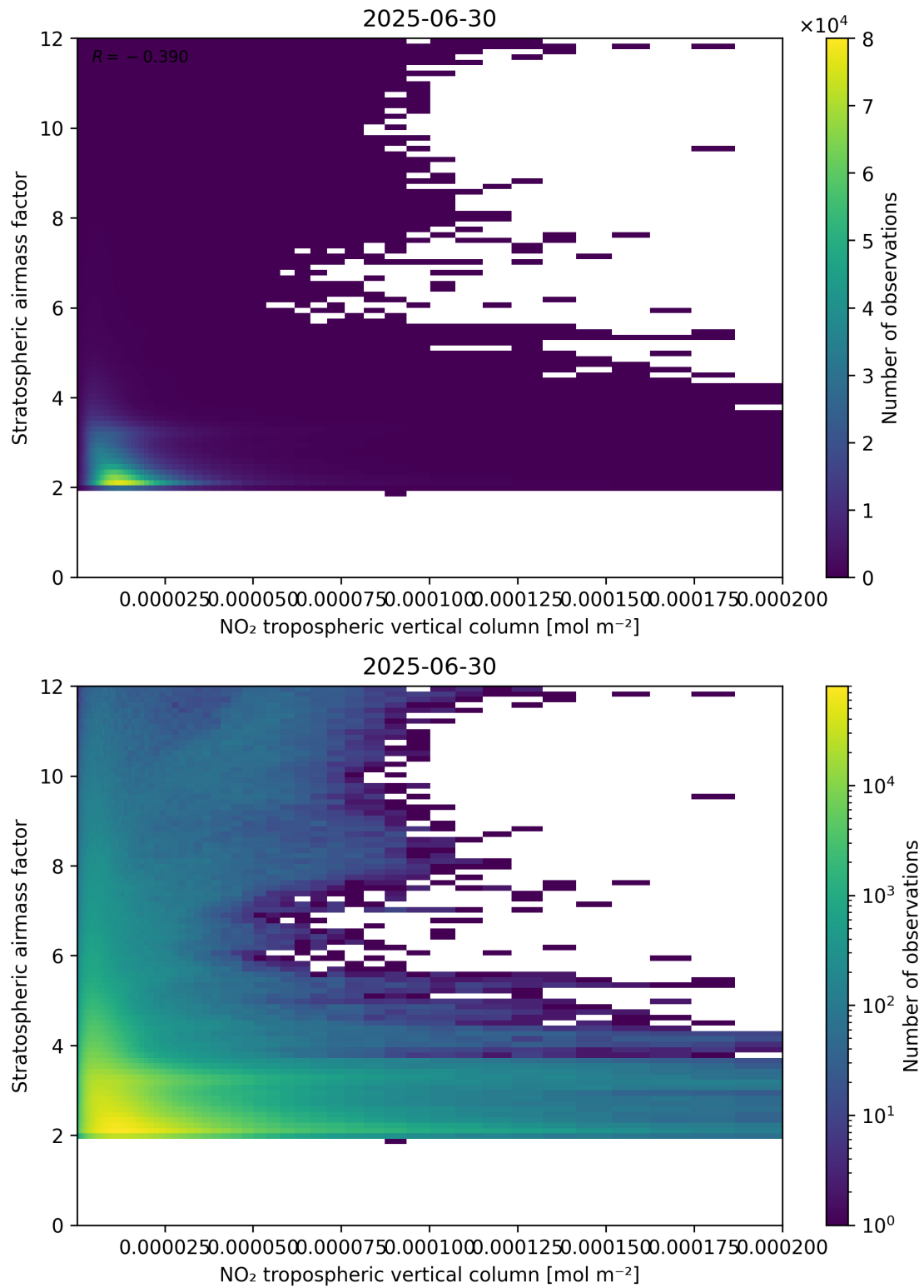
Figure 121: Scatter density plot of “NO 2 tropospheric vertical column” against “Stratospheric air mass factor” for 2025-06-29 to 2025-07-01.
