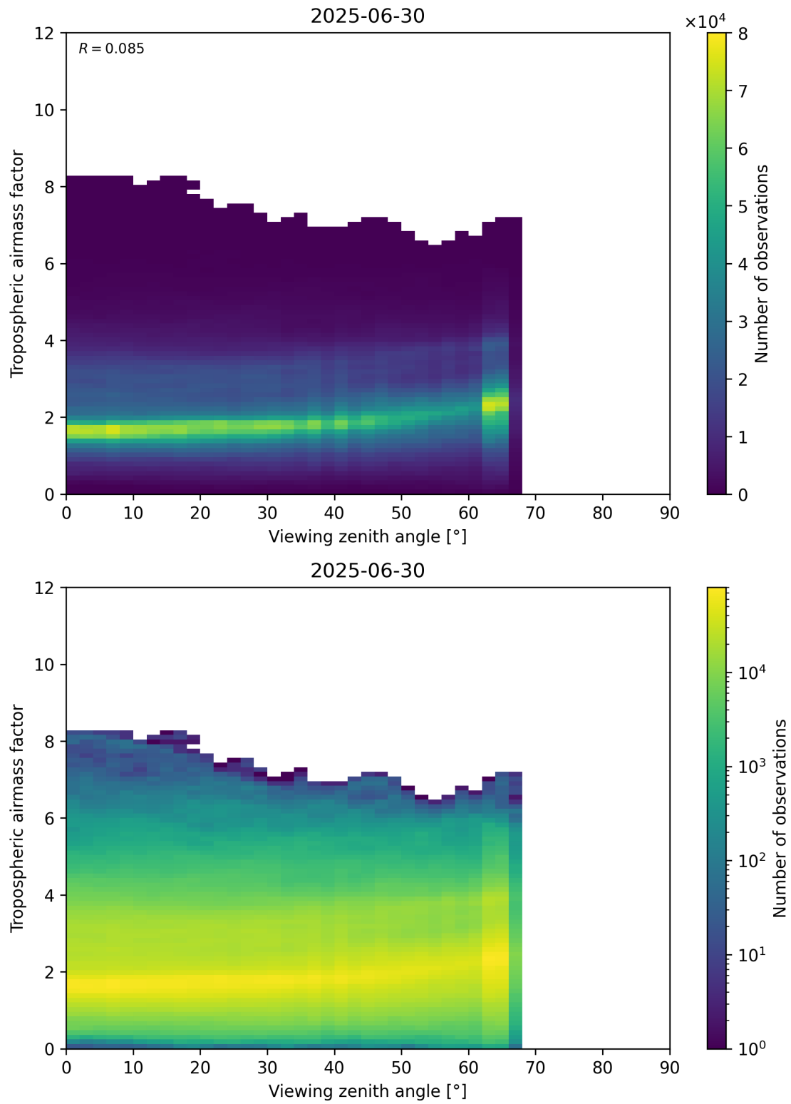
Figure 161: Scatter density plot of “Viewing zenith angle” against “Tropospheric airmass factor” for 2025-06-29 to 2025-07-01.
