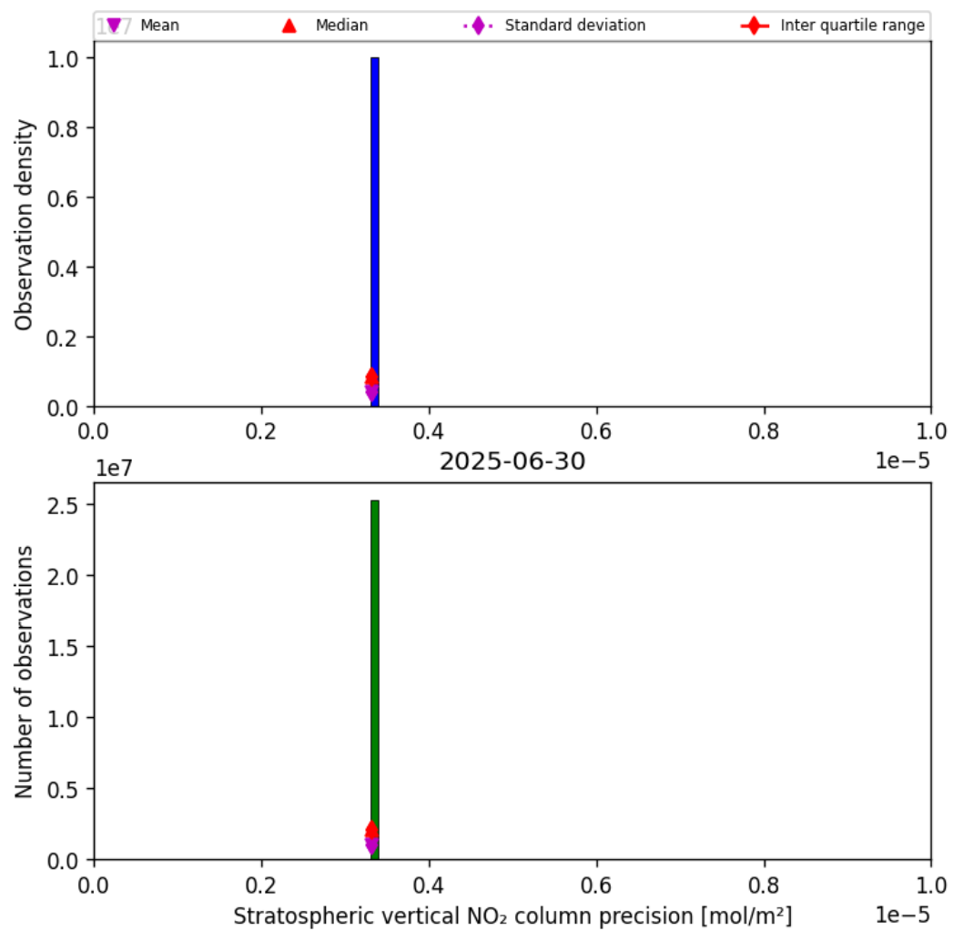
Figure 37: Histogram of “Stratospheric vertical NO 2 column precision” for 2025-06-29 to 2025-07-01
