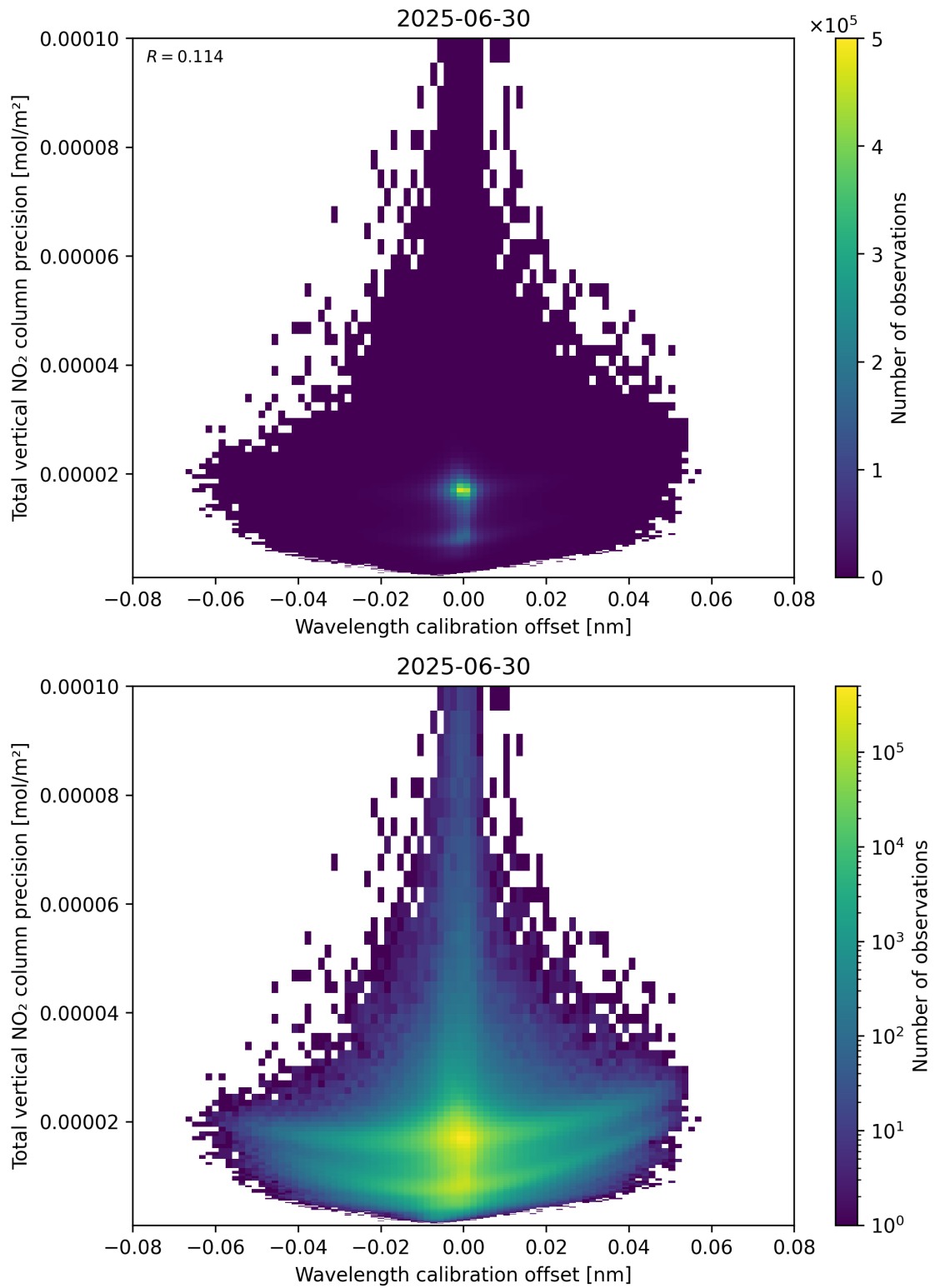
Figure 180: Scatter density plot of “Wavelength calibration offset” against “Total vertical NO 2 column precision” for 2025-06-29 to 2025-07-01.
