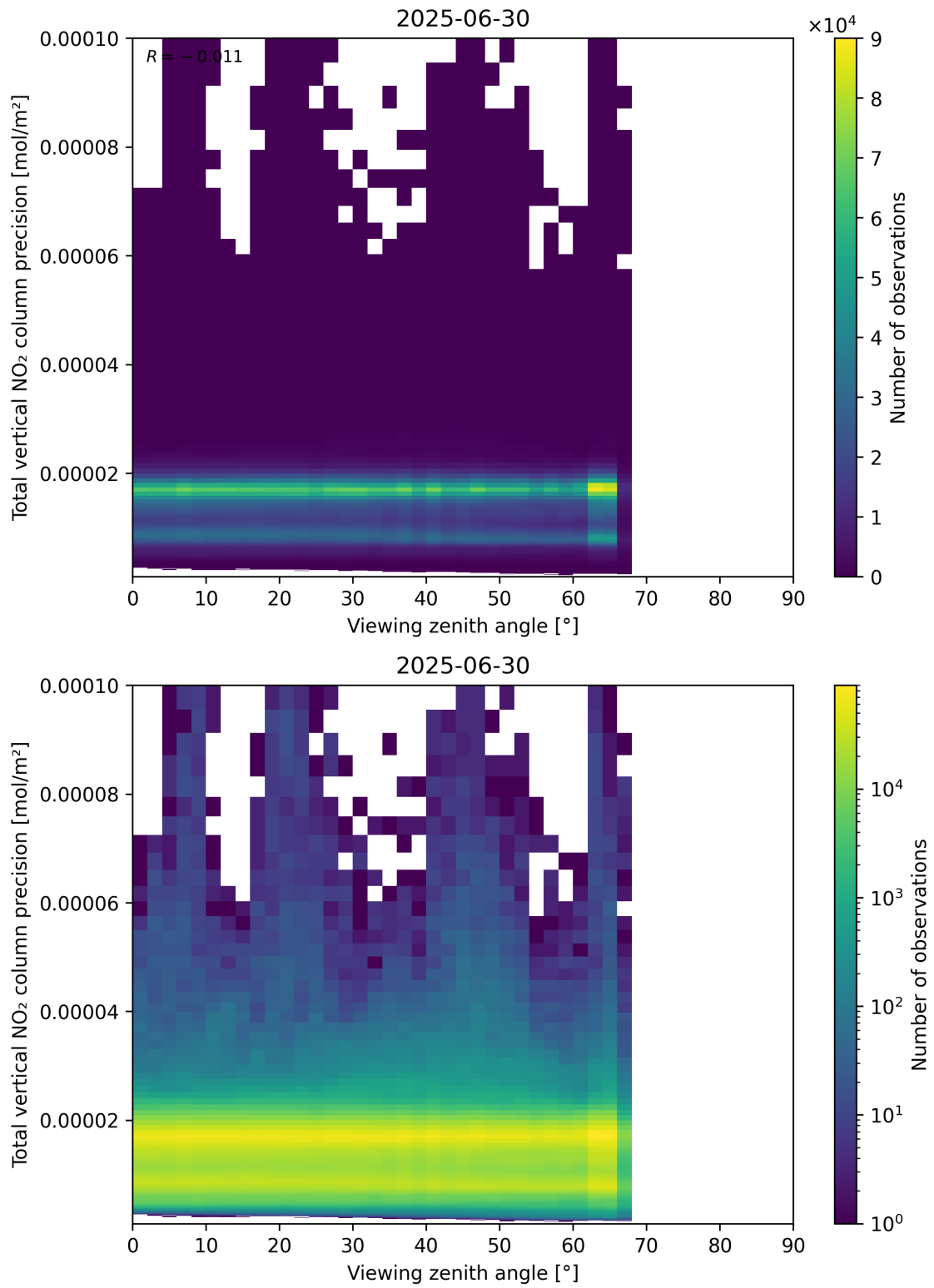
Figure 168: Scatter density plot of “Viewing zenith angle” against “Total vertical NO 2 column precision” for 2025-06-29 to 2025-07-01.
