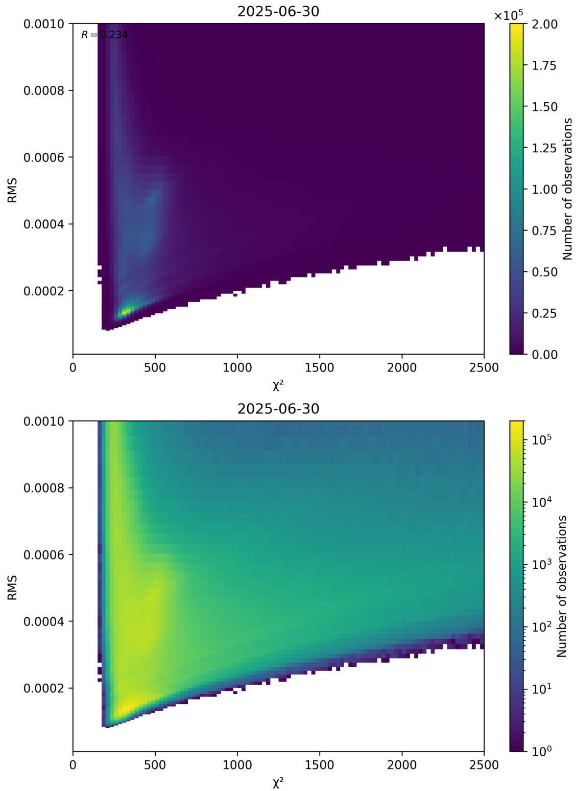
Figure 82: Scatter density plot of “ \chi^2 ” against “RMS” for 2025-06-29 to 2025-07-01.
