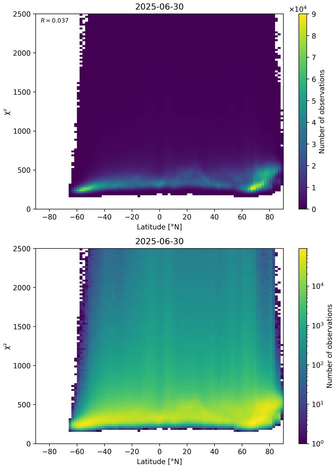
Figure 86: Scatter density plot of “Latitude” against “ \chi^2 ” for 2025-06-29 to 2025-07-01.
