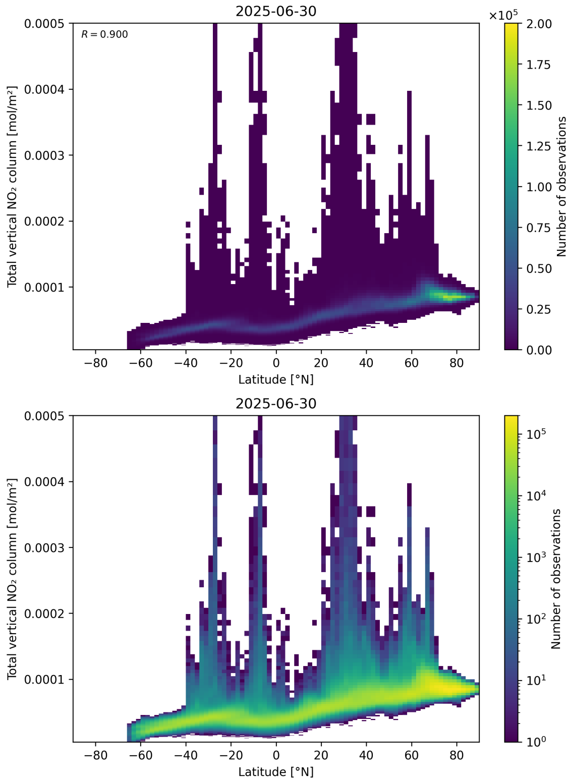
Figure 90: Scatter density plot of “Latitude” against “Total vertical NO 2 column” for 2025-06-29 to 2025-07-01.
