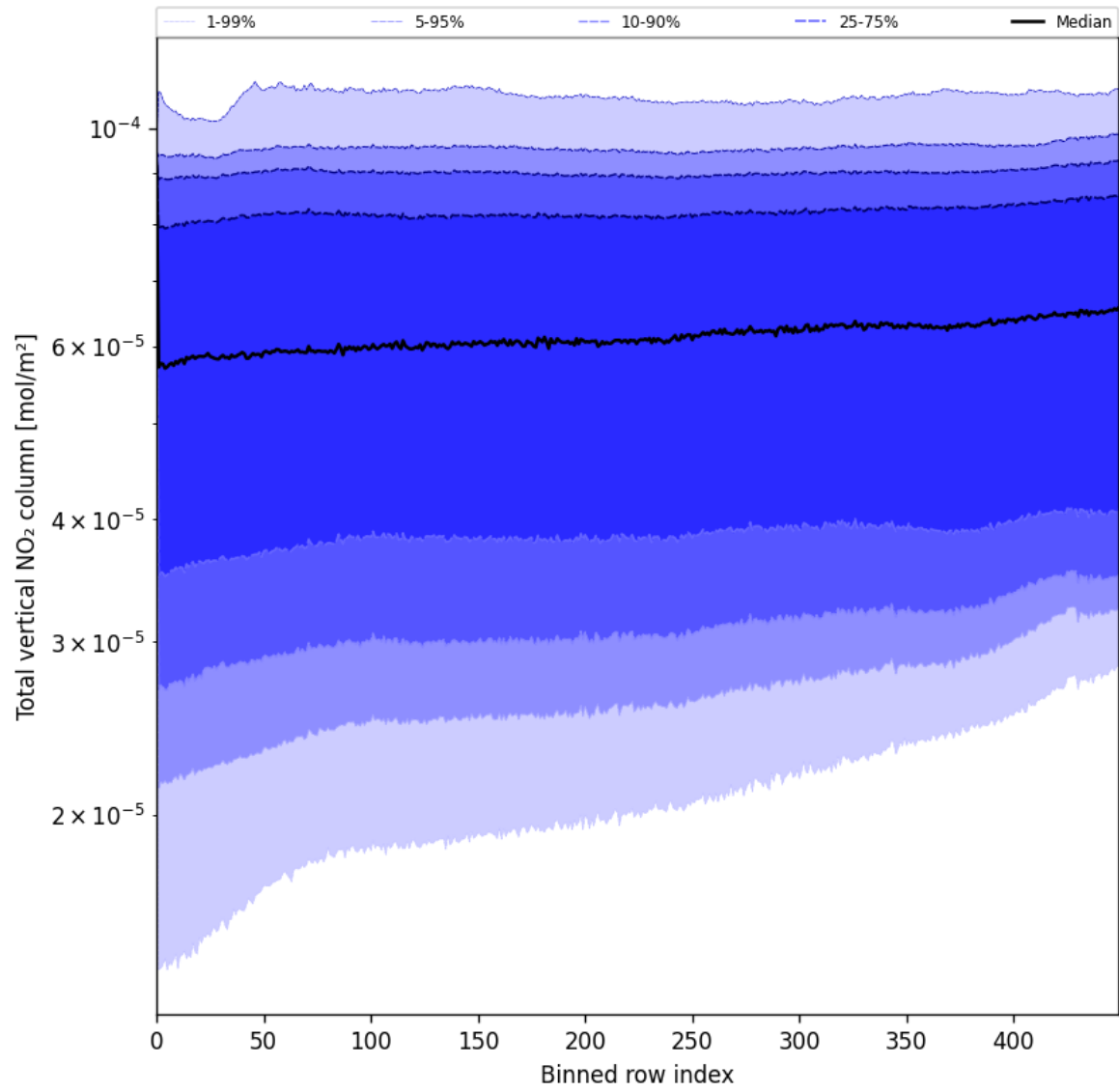
Figure 55: Along track statistics of “Total vertical NO 2 column” for 2025-06-29 to 2025-07-01
