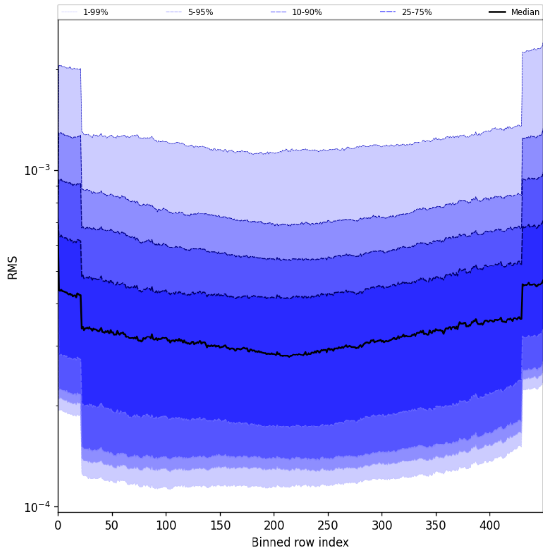
Figure 60: Along track statistics of “RMS” for 2025-06-29 to 2025-07-01
