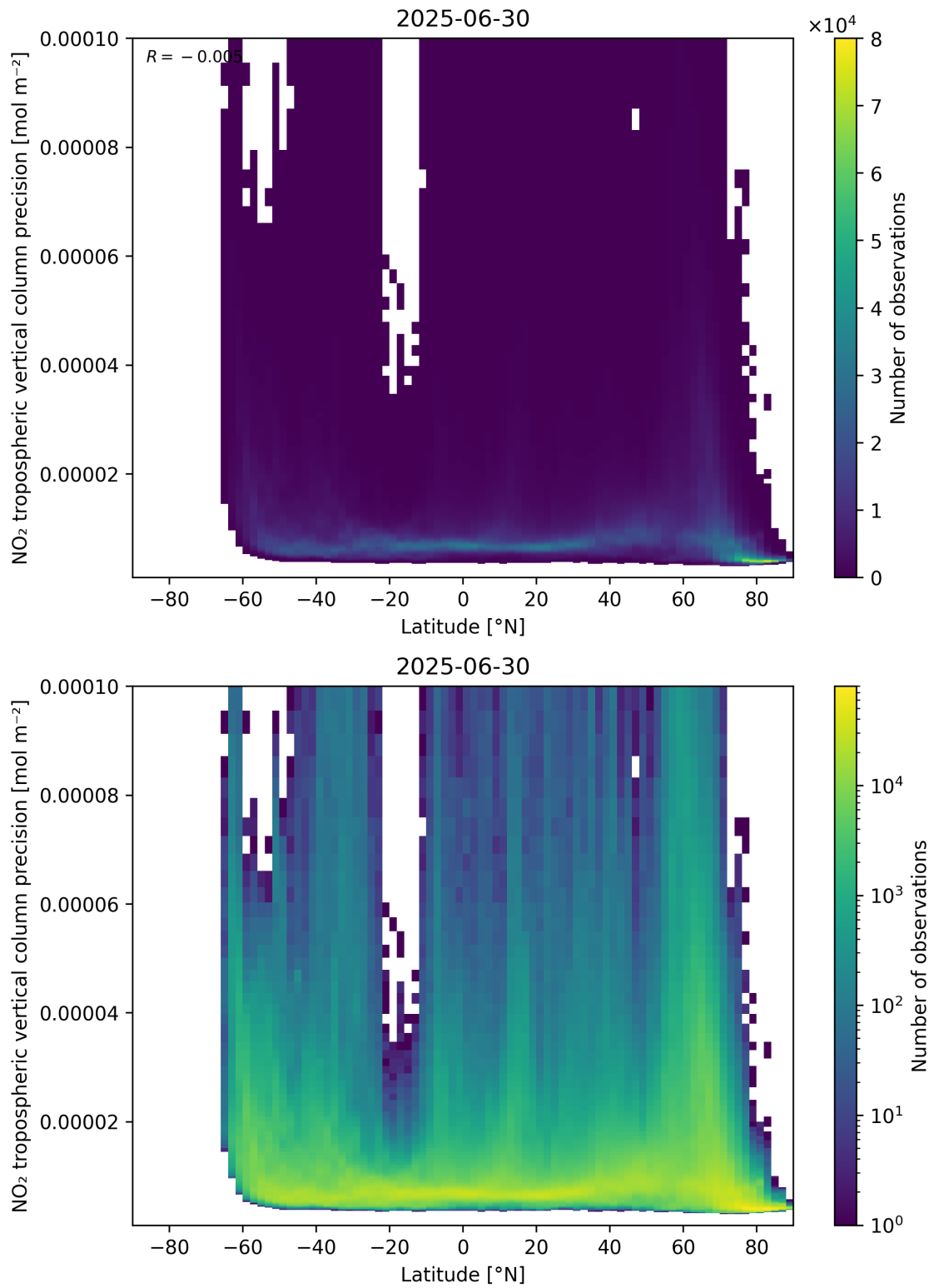
Figure 93: Scatter density plot of “Latitude” against “NO 2 tropospheric vertical column precision” for 2025-06-29 to 2025-07-01.
