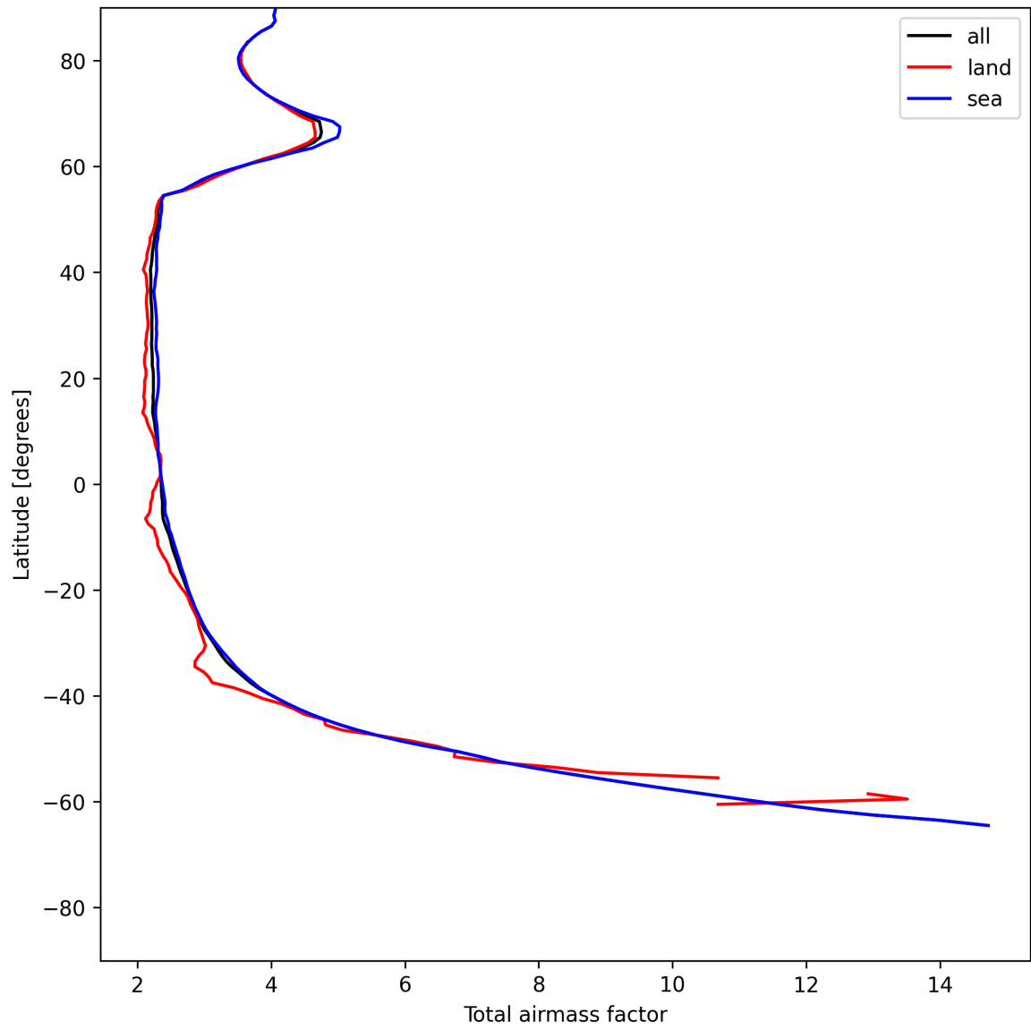
Figure 15: Zonal average of “Total airmass factor” for 2025-06-29 to 2025-07-01.
