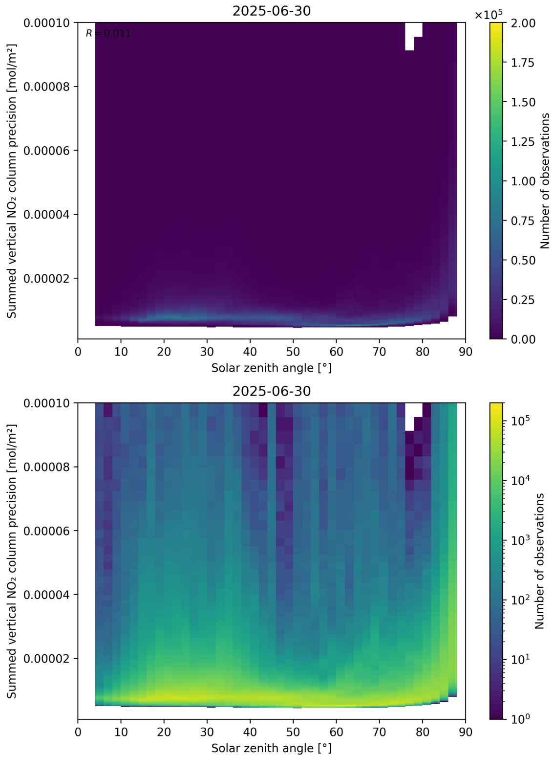
Figure 152: Scatter density plot of “Solar zenith angle” against “Summed vertical NO 2 column precision” for 2025-06-29 to 2025-07-01.
