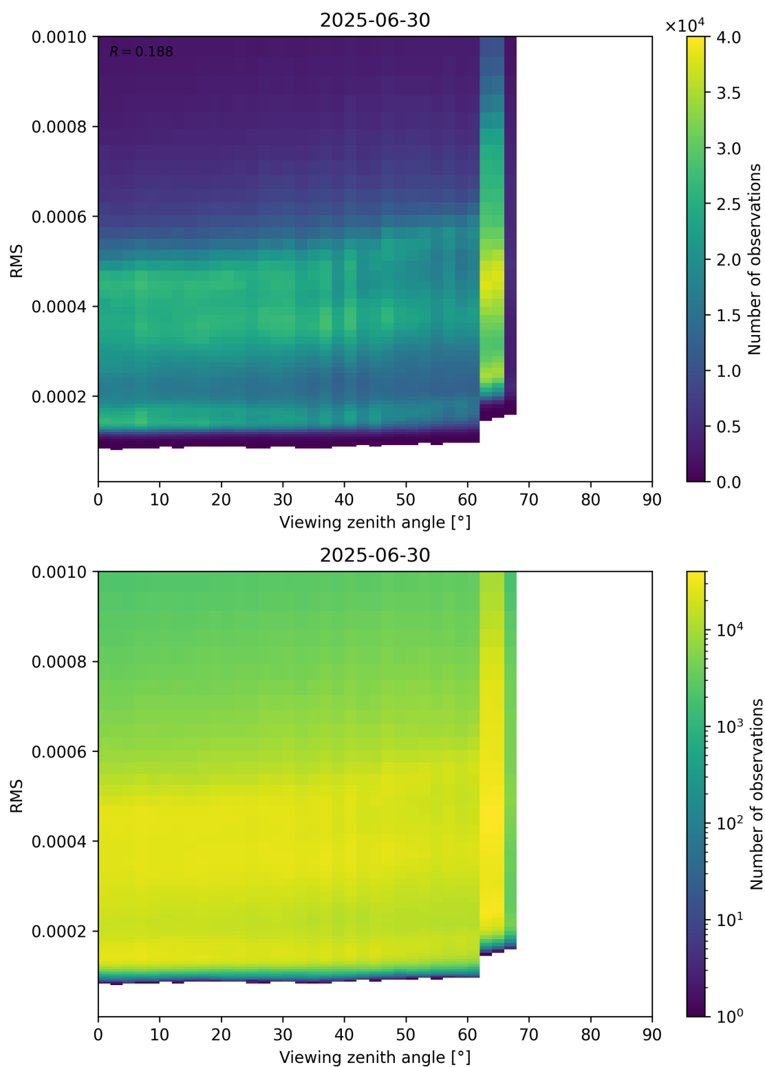
Figure 171: Scatter density plot of “Viewing zenith angle” against “RMS” for 2025-06-29 to 2025-07-01.
