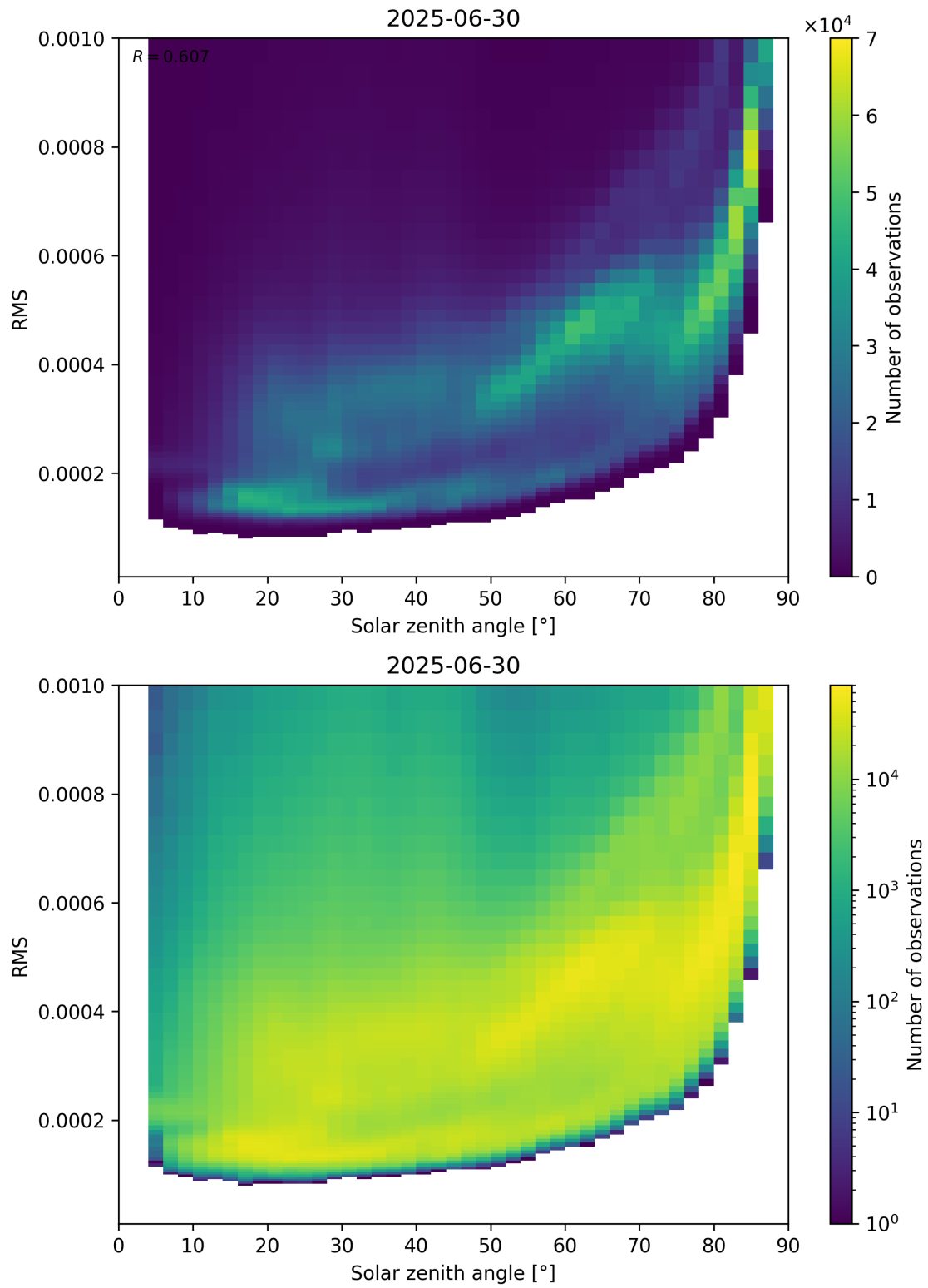
Figure 157: Scatter density plot of “Solar zenith angle” against “RMS” for 2025-06-29 to 2025-07-01.
