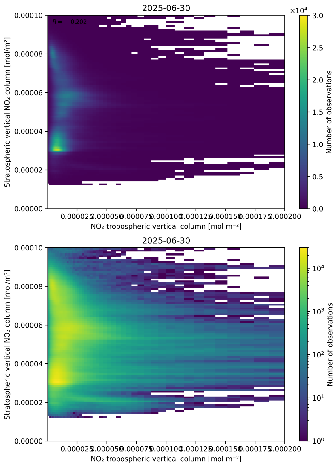
Figure 125: Scatter density plot of “NO 2 tropospheric vertical column” against “Stratospheric vertical NO 2 column” for 2025-06-29 to 2025-07-01.
