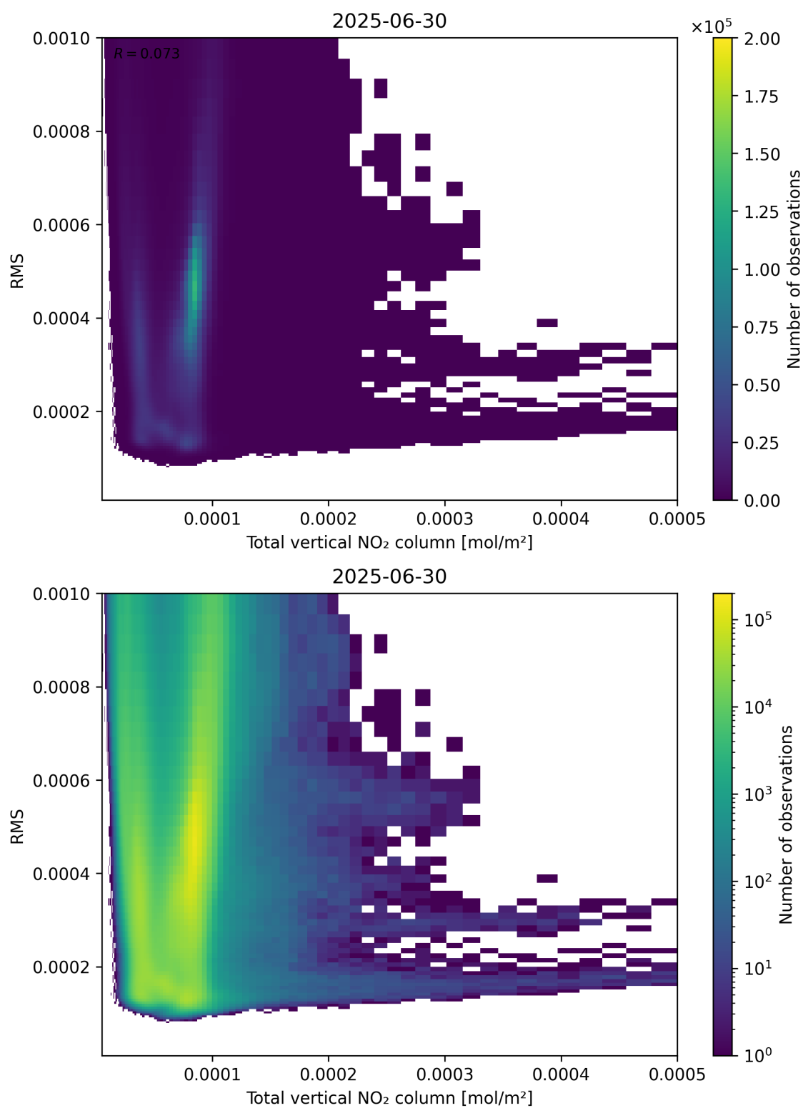
Figure 120: Scatter density plot of “Total vertical NO 2 column” against “RMS” for 2025-06-29 to 2025-07-01.
