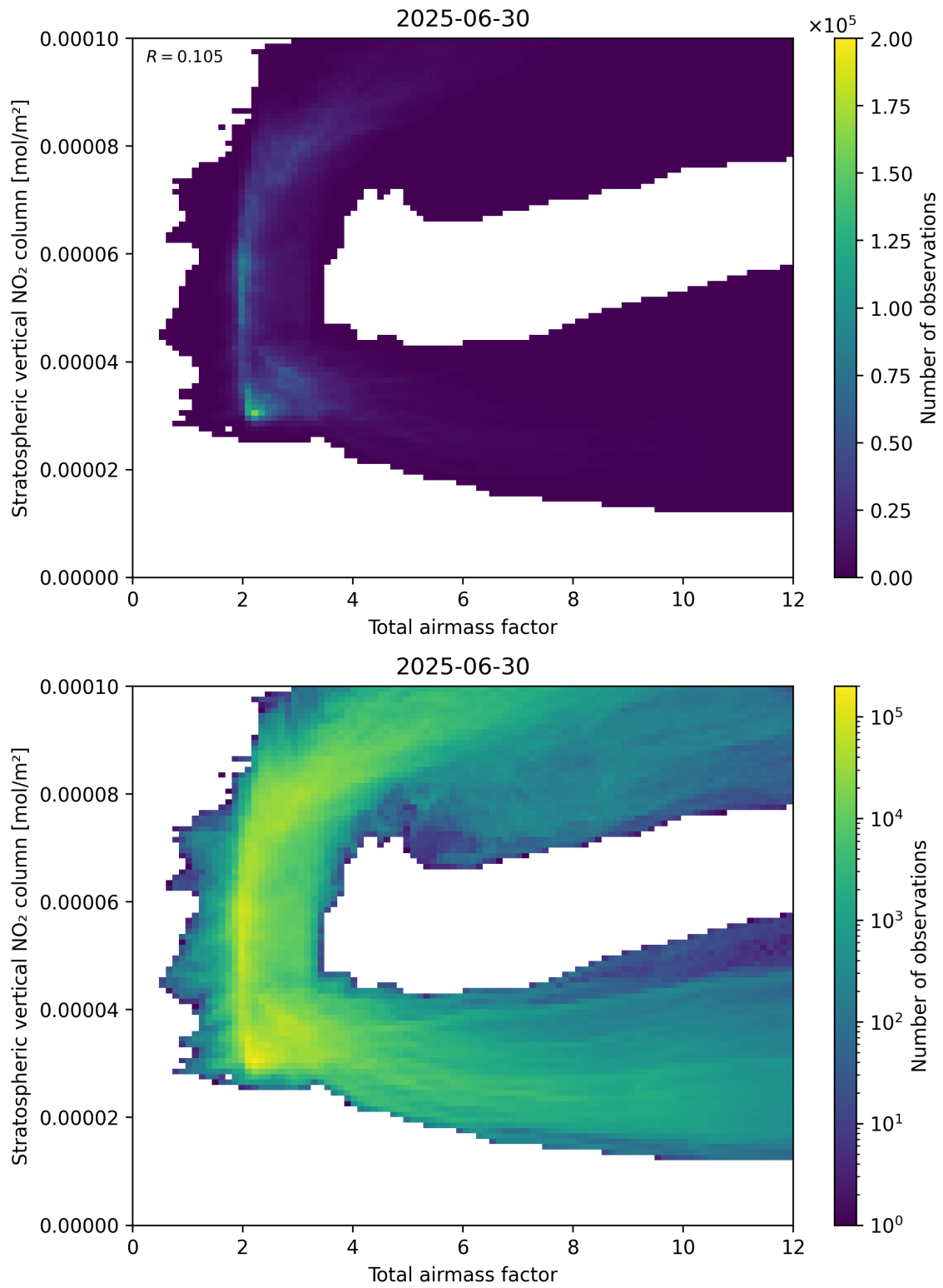
Figure 64: Scatter density plot of “Total airmass factor” against “Stratospheric vertical \text{NO}_2 column” for 2025-06-29 to 2025-07-01.
