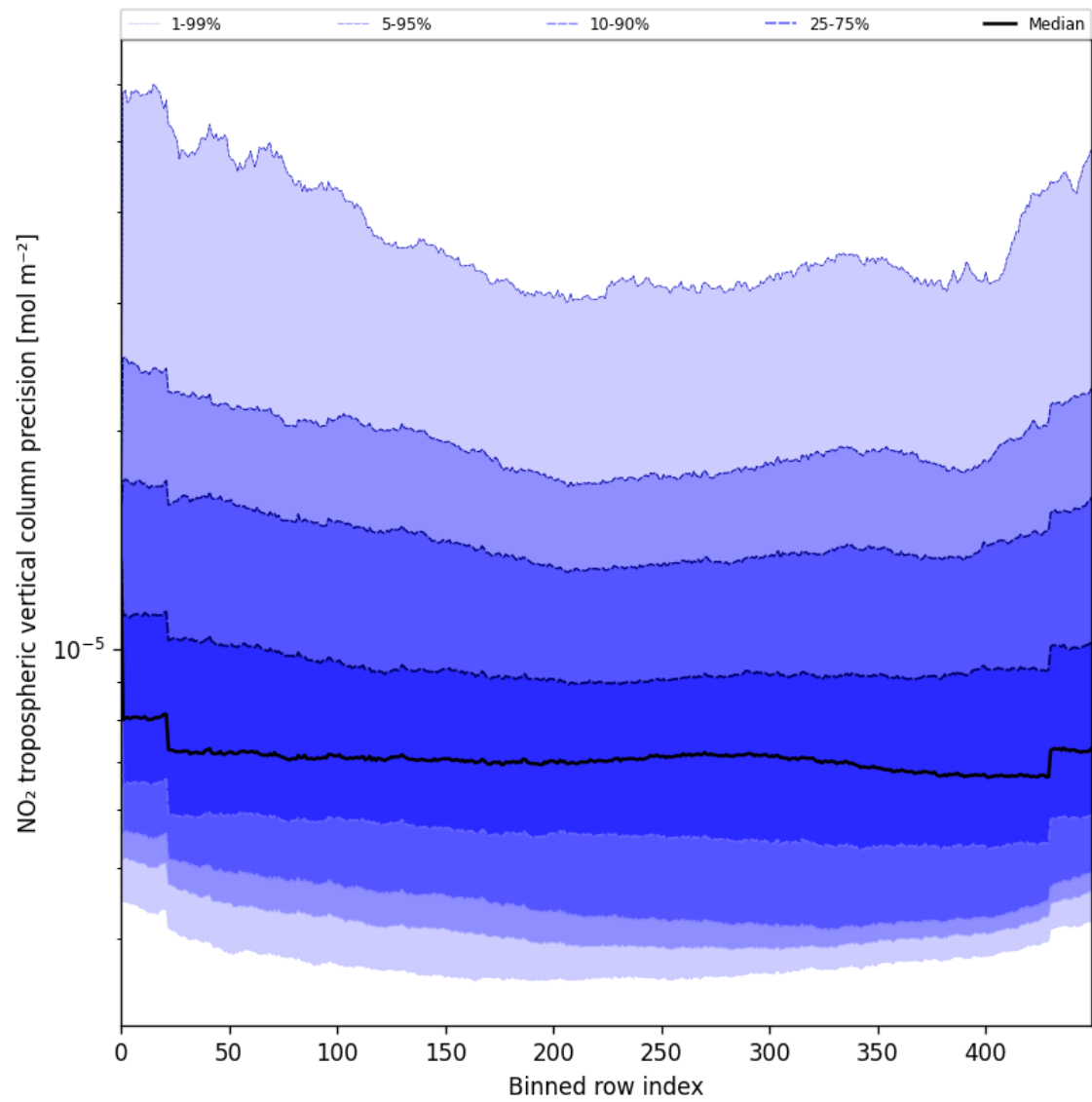
Figure 47: Along track statistics of “NO 2 tropospheric vertical column precision” for 2025-06-29 to 2025-07-01
