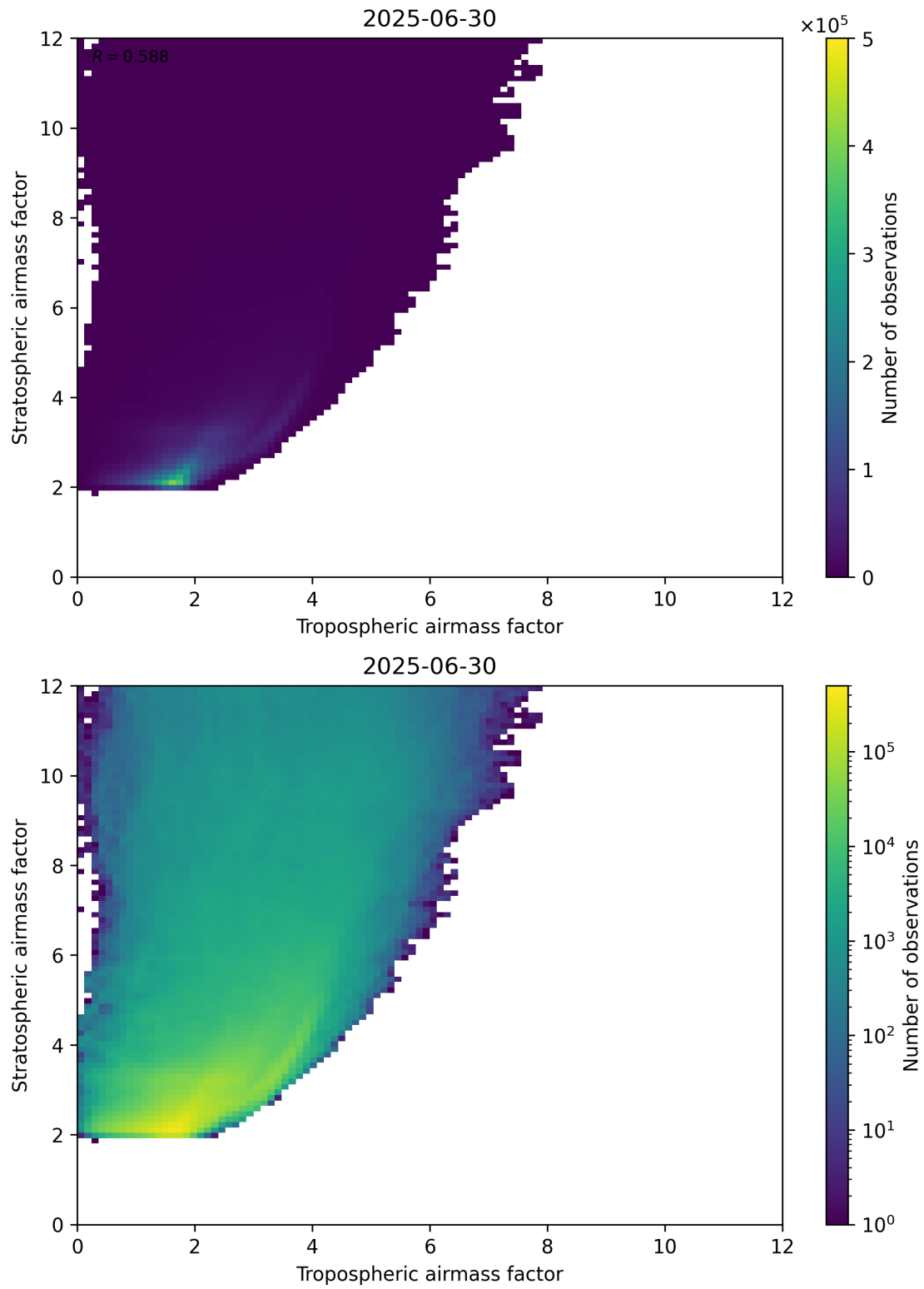
Figure 71: Scatter density plot of “Tropospheric airmass factor” against “Stratospheric airmass factor” for 2025-06-29 to 2025-07-01.
