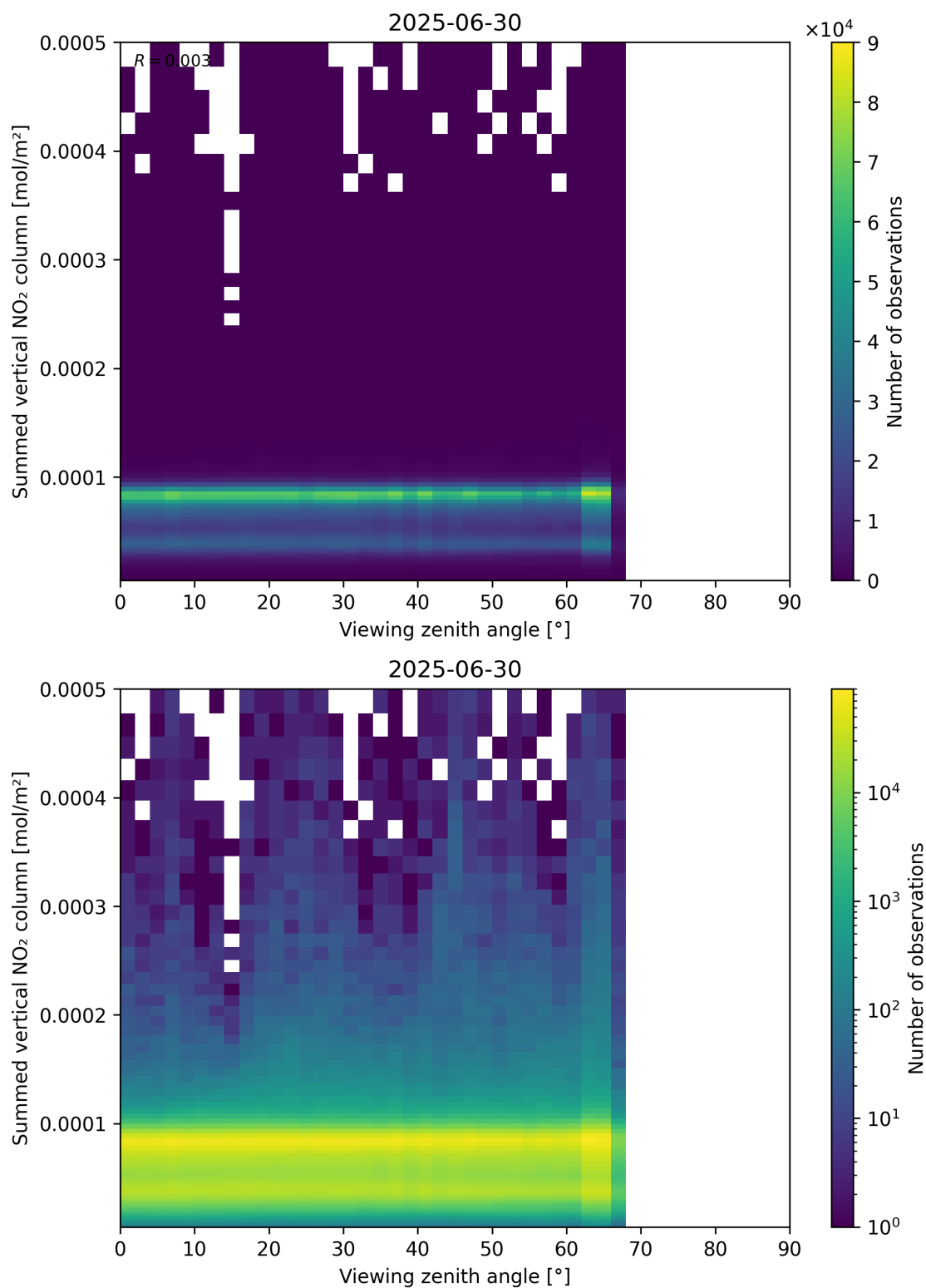
Figure 165: Scatter density plot of “Viewing zenith angle” against “Summed vertical NO 2 column” for 2025-06-29 to 2025-07-01.
