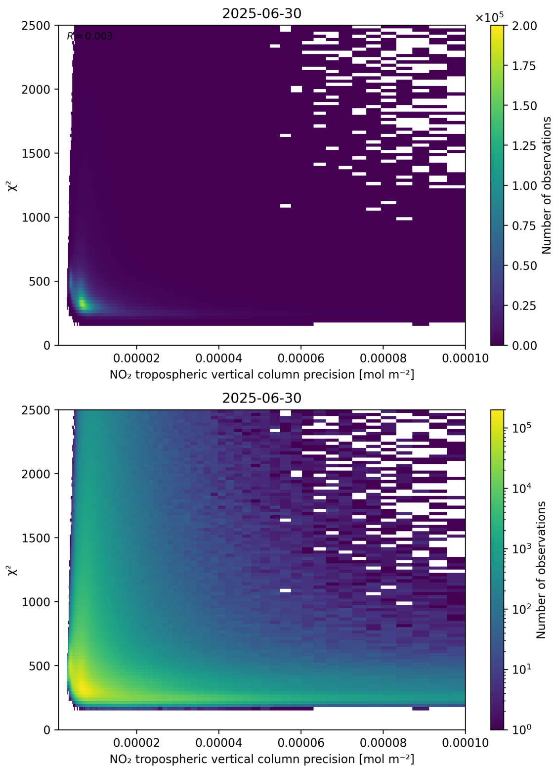
Figure 134: Scatter density plot of “NO 2 tropospheric vertical column precision” against “ \chi^2 ” for 2025-06-29 to 2025-07-01.
