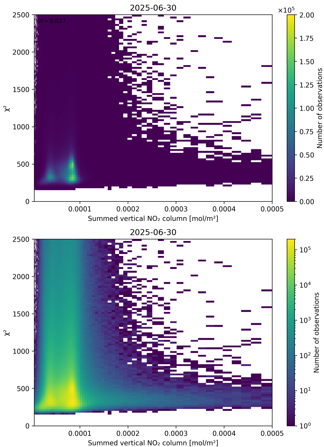
Figure 104: Scatter density plot of “Summed vertical NO 2 column” against “ \chi^2 ” for 2025-06-29 to 2025-07-01.
