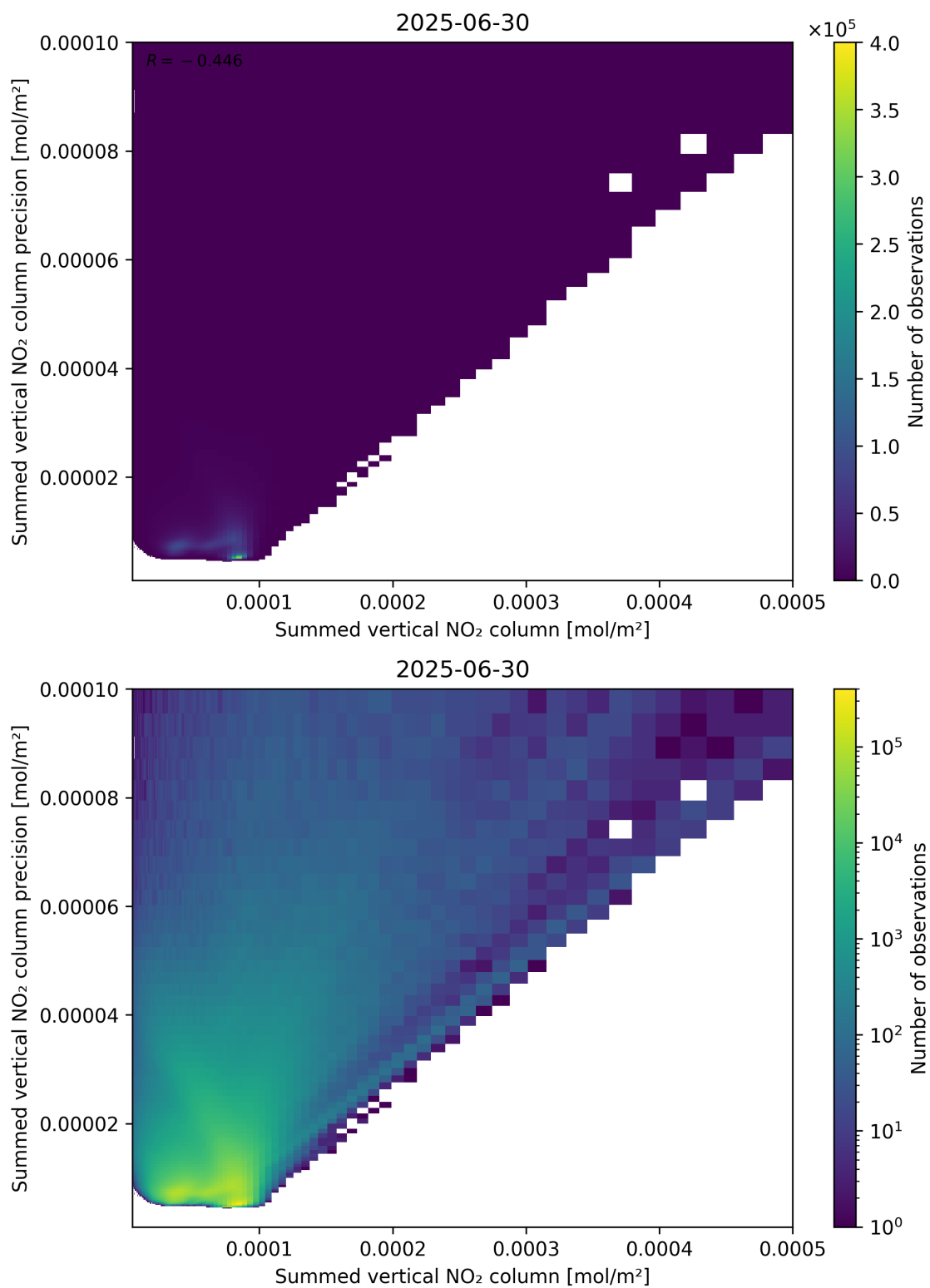
Figure 105: Scatter density plot of “Summed vertical NO 2 column” against “Summed vertical NO 2 column precision” for 2025-06-29 to 2025-07-01.
