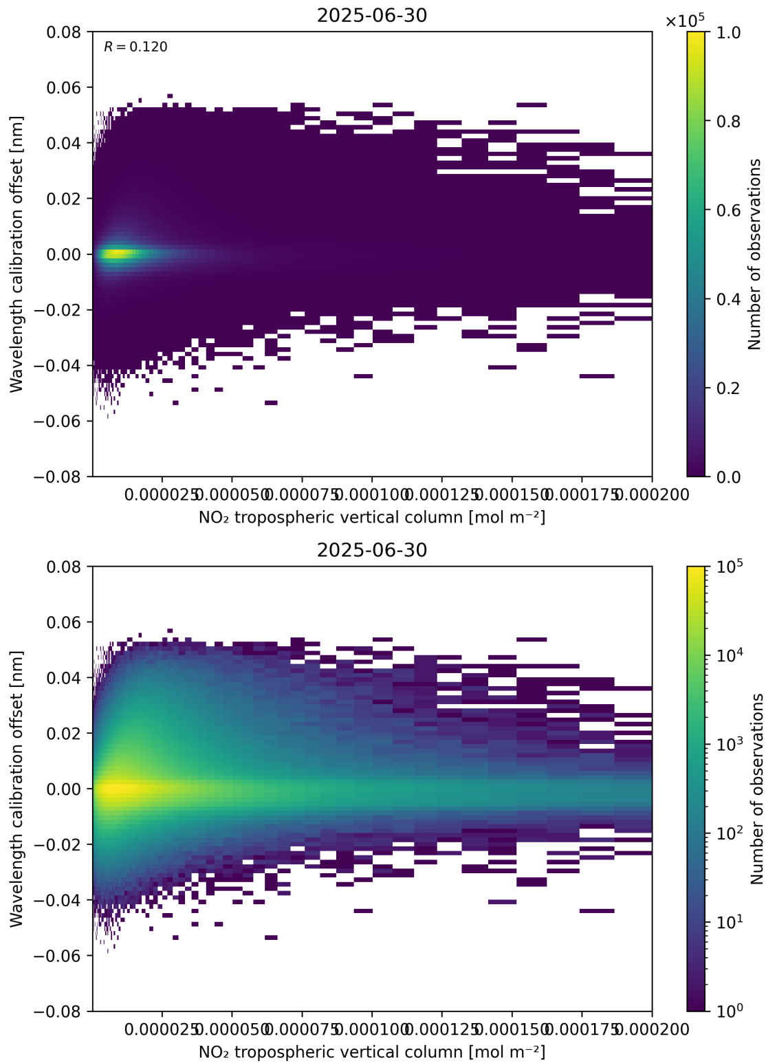
Figure 143: Scatter density plot of “NO 2 tropospheric vertical column” against “Wavelength calibration offset” for 2025-06-29 to 2025-07-01.
