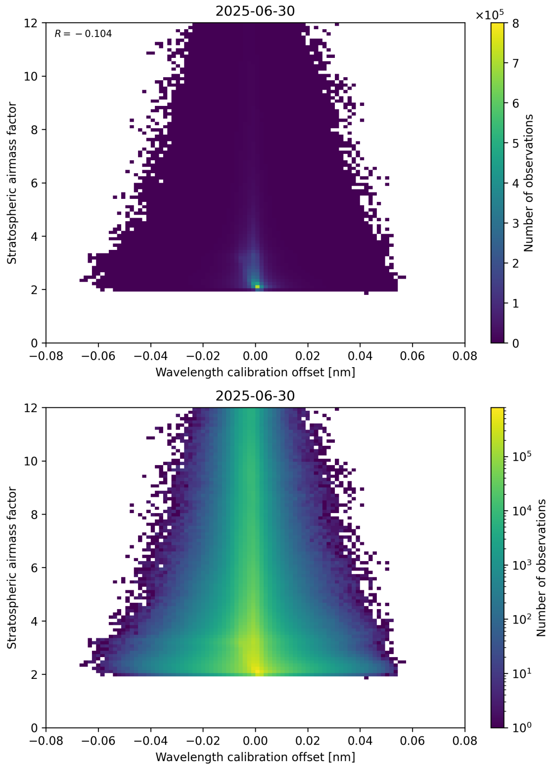
Figure 174: Scatter density plot of “Wavelength calibration offset” against “Stratospheric airmass factor” for 2025-06-29 to 2025-07-01.
