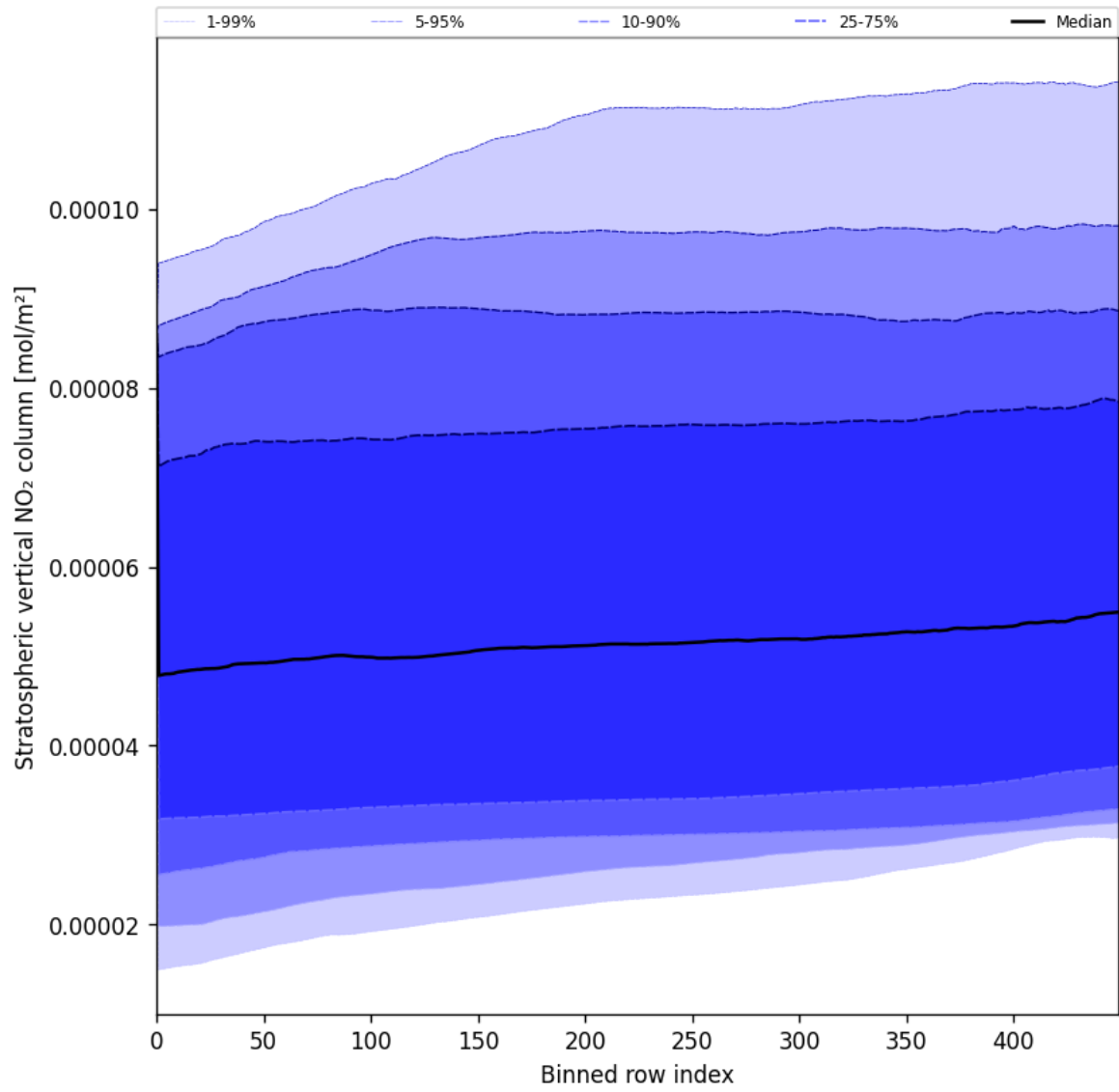
Figure 53: Along track statistics of “Stratospheric vertical NO 2 column” for 2025-06-29 to 2025-07-01
