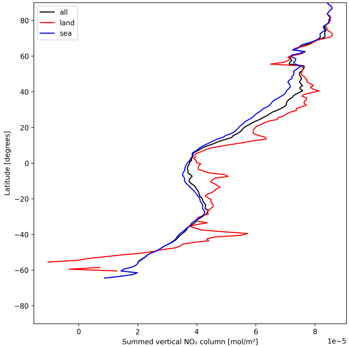
Figure 23: Zonal average of “Summed vertical NO 2 column” for 2025-06-29 to 2025-07-01.
