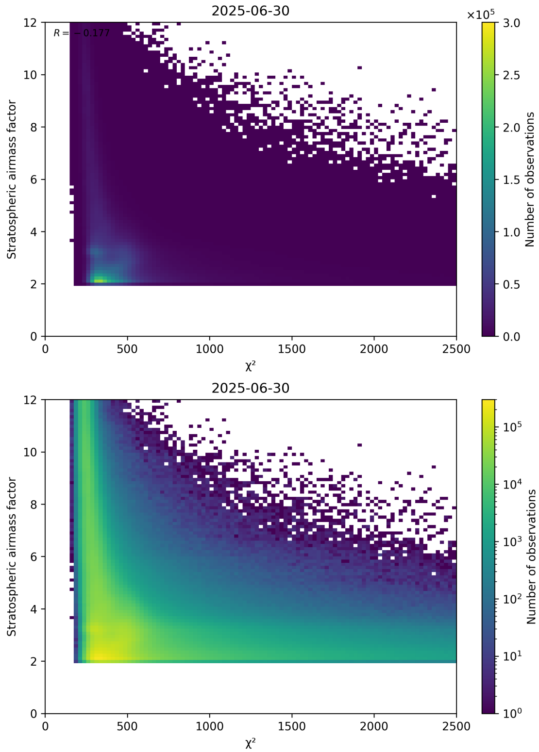
Figure 81: Scatter density plot of “ \chi^2 ” against “Stratospheric airmass factor” for 2025-06-29 to 2025-07-01.
