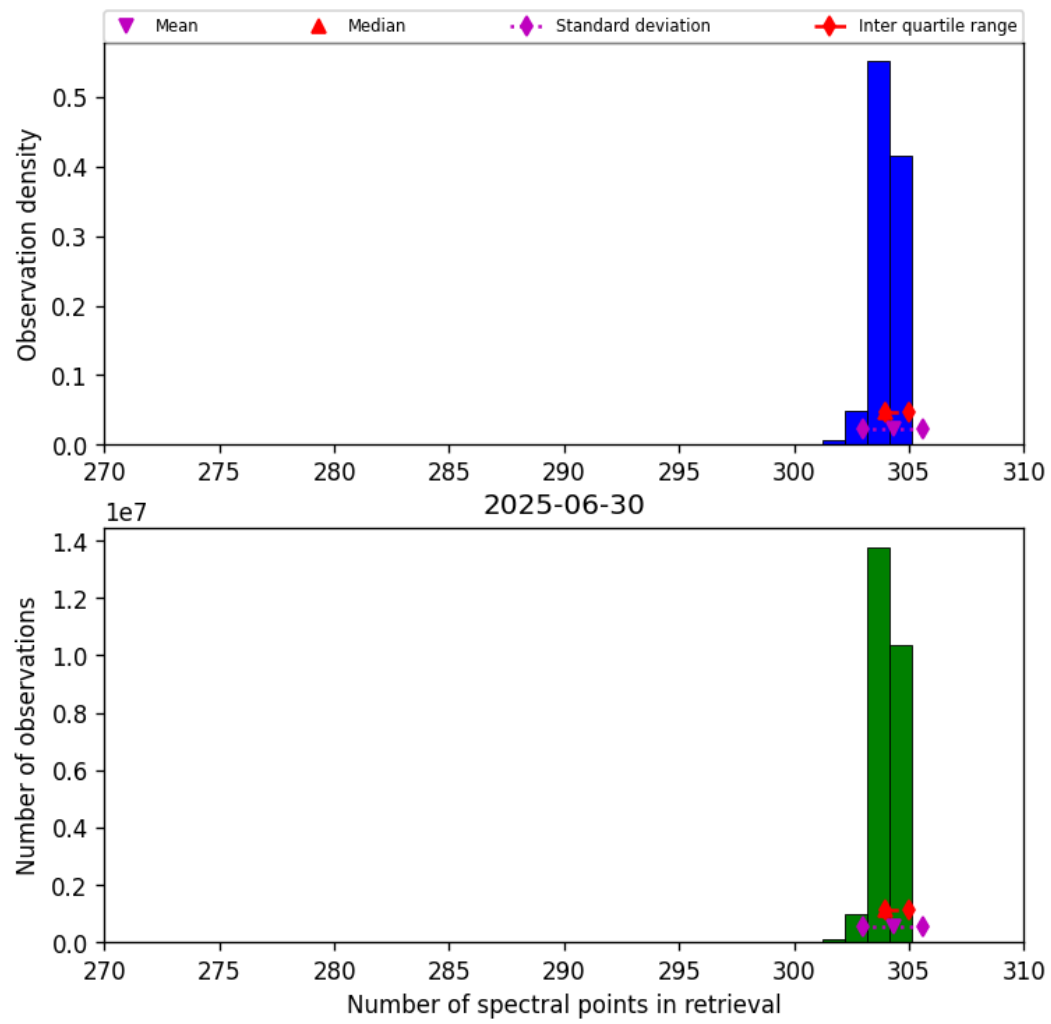
Figure 33: Histogram of “Number of spectral points in retrieval” for 2025-06-29 to 2025-07-01
