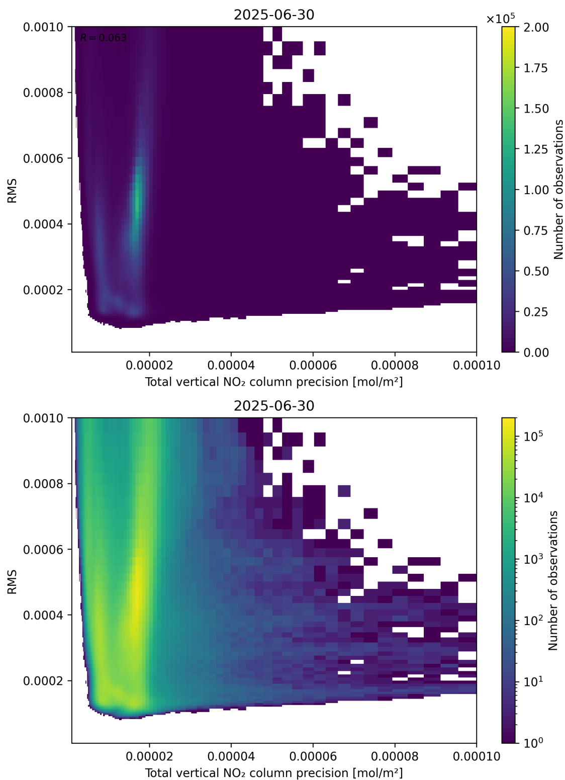
Figure 119: Scatter density plot of “Total vertical NO 2 column precision” against “RMS” for 2025-06-29 to 2025-07-01.
