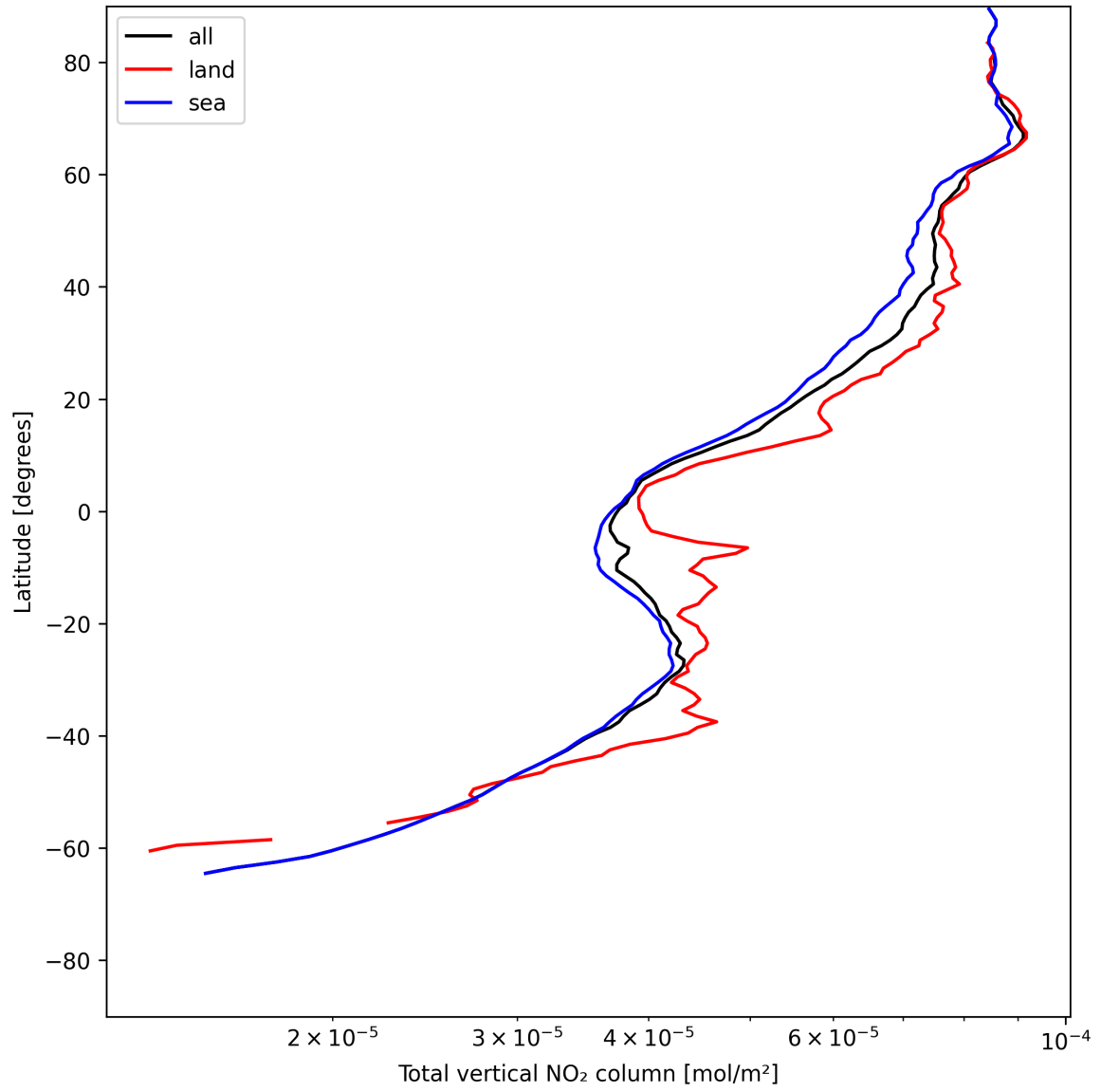
Figure 21: Zonal average of “Total vertical NO 2 column” for 2025-06-29 to 2025-07-01.
