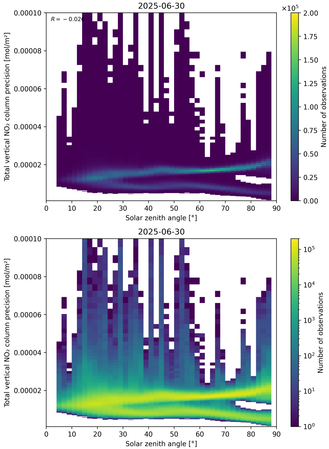
Figure 154: Scatter density plot of “Solar zenith angle” against “Total vertical NO 2 column precision” for 2025-06-29 to 2025-07-01.
