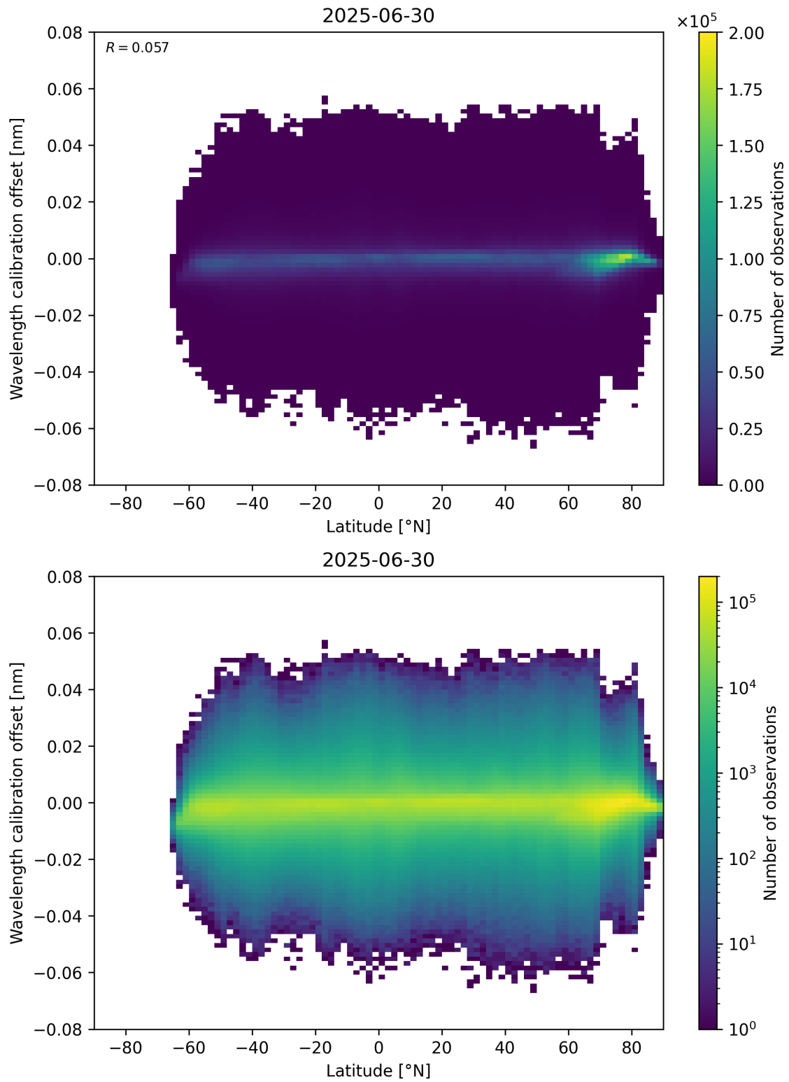
Figure 95: Scatter density plot of “Latitude” against “Wavelength calibration offset” for 2025-06-29 to 2025-07-01.
