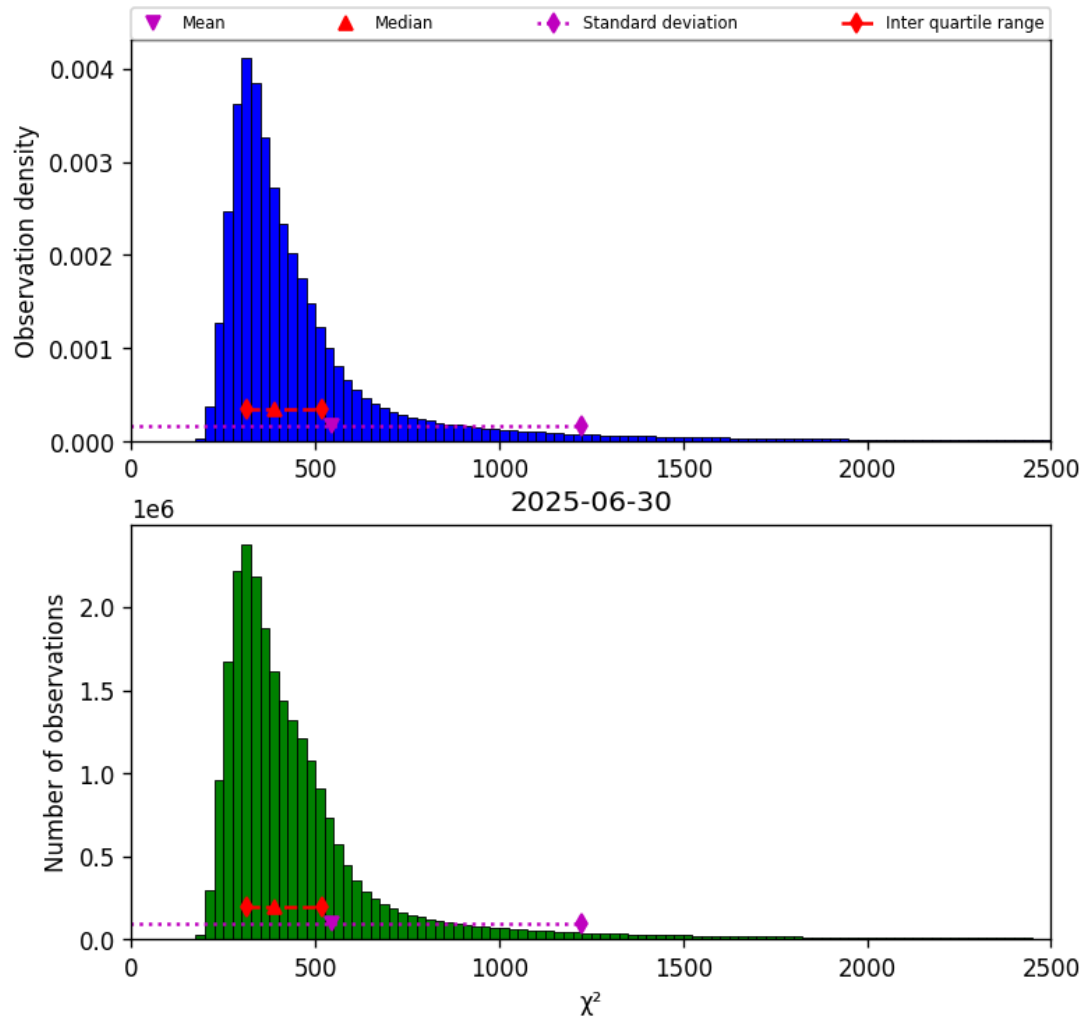
Figure 42: Histogram of “ \chi^2 ” for 2025-06-29 to 2025-07-01
