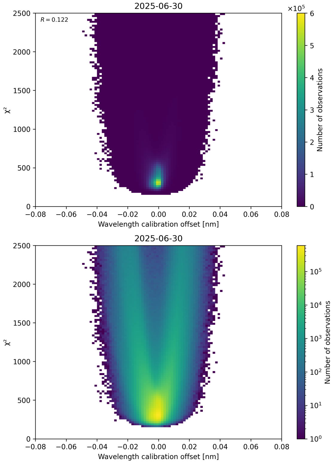
Figure 175: Scatter density plot of “Wavelength calibration offset” against “ \chi^2 ” for 2025-06-29 to 2025-07-01.
