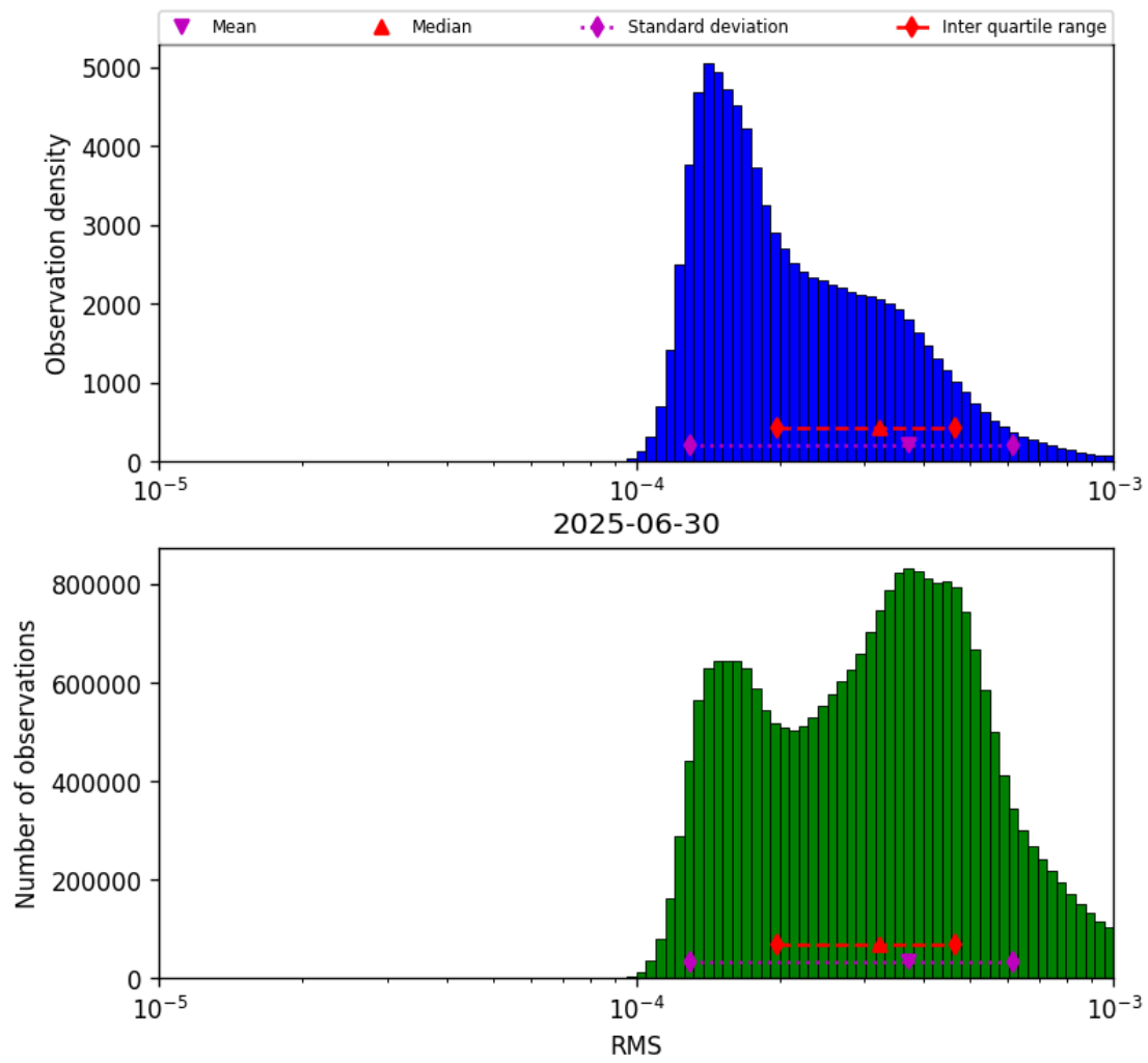
Figure 43: Histogram of “RMS” for 2025-06-29 to 2025-07-01
