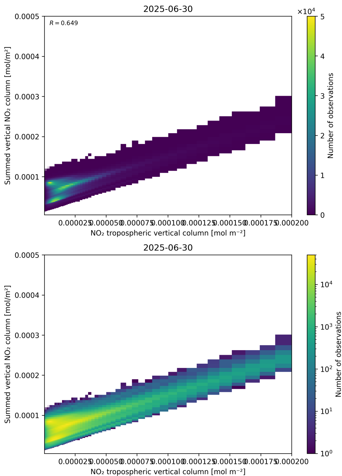
Figure 126: Scatter density plot of “NO 2 tropospheric vertical column” against “Summed vertical NO 2 column” for 2025-06-29 to 2025-07-01.
