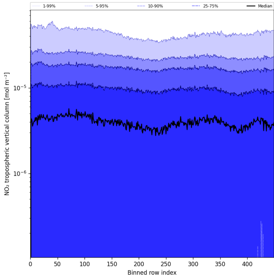
Figure 46: Along track statistics of “NO 2 tropospheric vertical column” for 2025-06-29 to 2025-07-01
