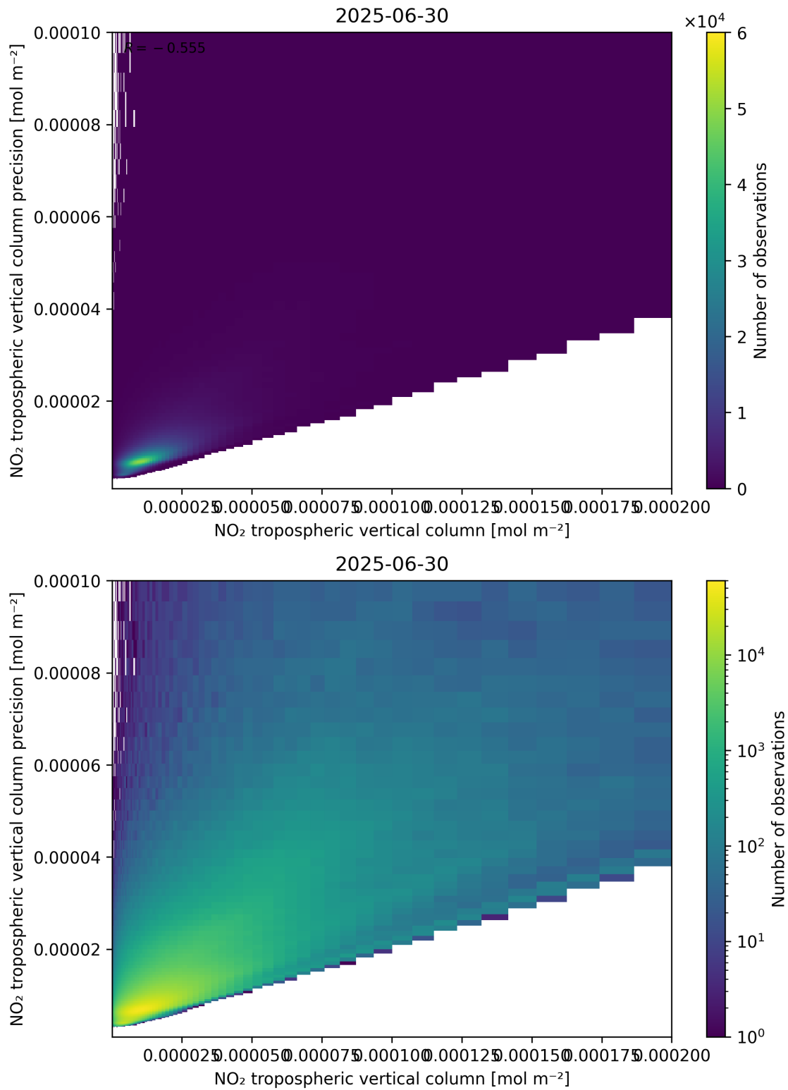
Figure 130: Scatter density plot of “NO 2 tropospheric vertical column” against “NO 2 tropospheric vertical column precision” for 2025-06-29 to 2025-07-01.
