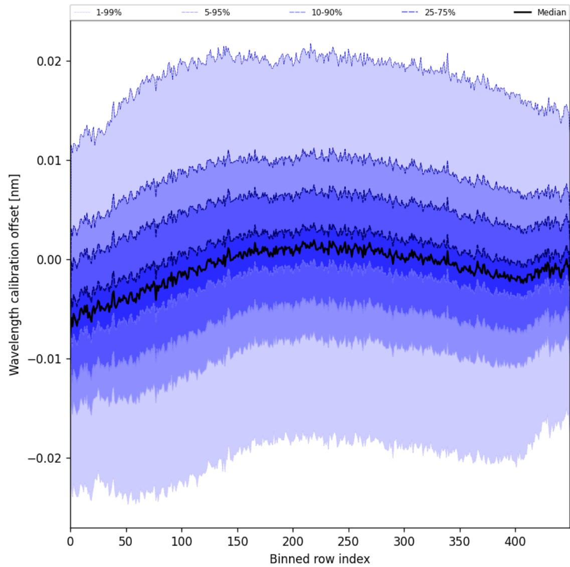
Figure 52: Along track statistics of “Wavelength calibration offset” for 2025-06-29 to 2025-07-01
