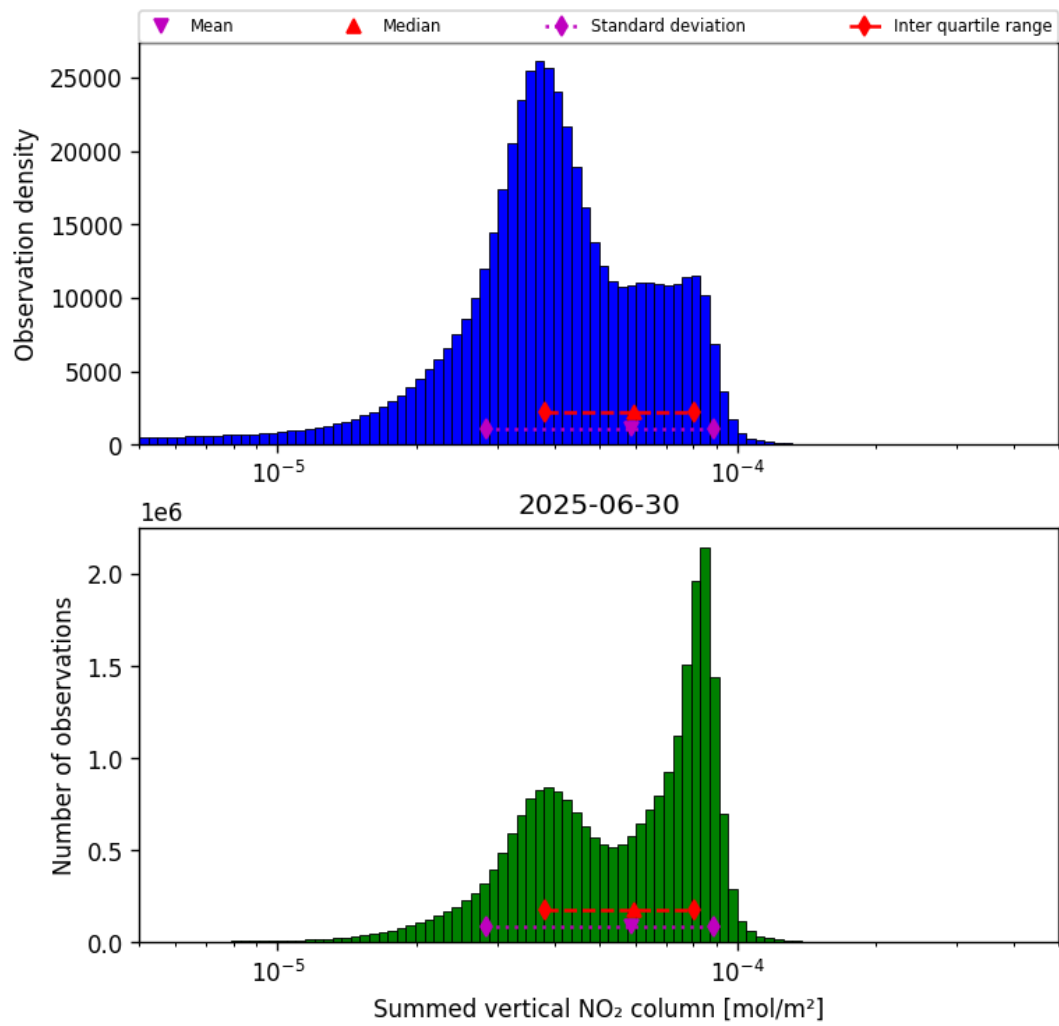
Figure 40: Histogram of “Summed vertical NO 2 column” for 2025-06-29 to 2025-07-01
