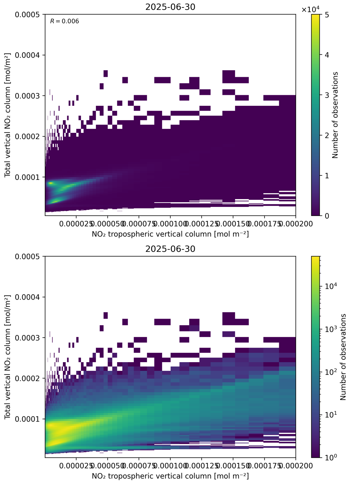
Figure 128: Scatter density plot of “NO 2 tropospheric vertical column” against “Total vertical NO 2 column” for 2025-06-29 to 2025-07-01.
