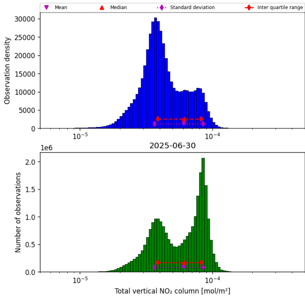
Figure 38: Histogram of “Total vertical NO 2 column” for 2025-06-29 to 2025-07-01
