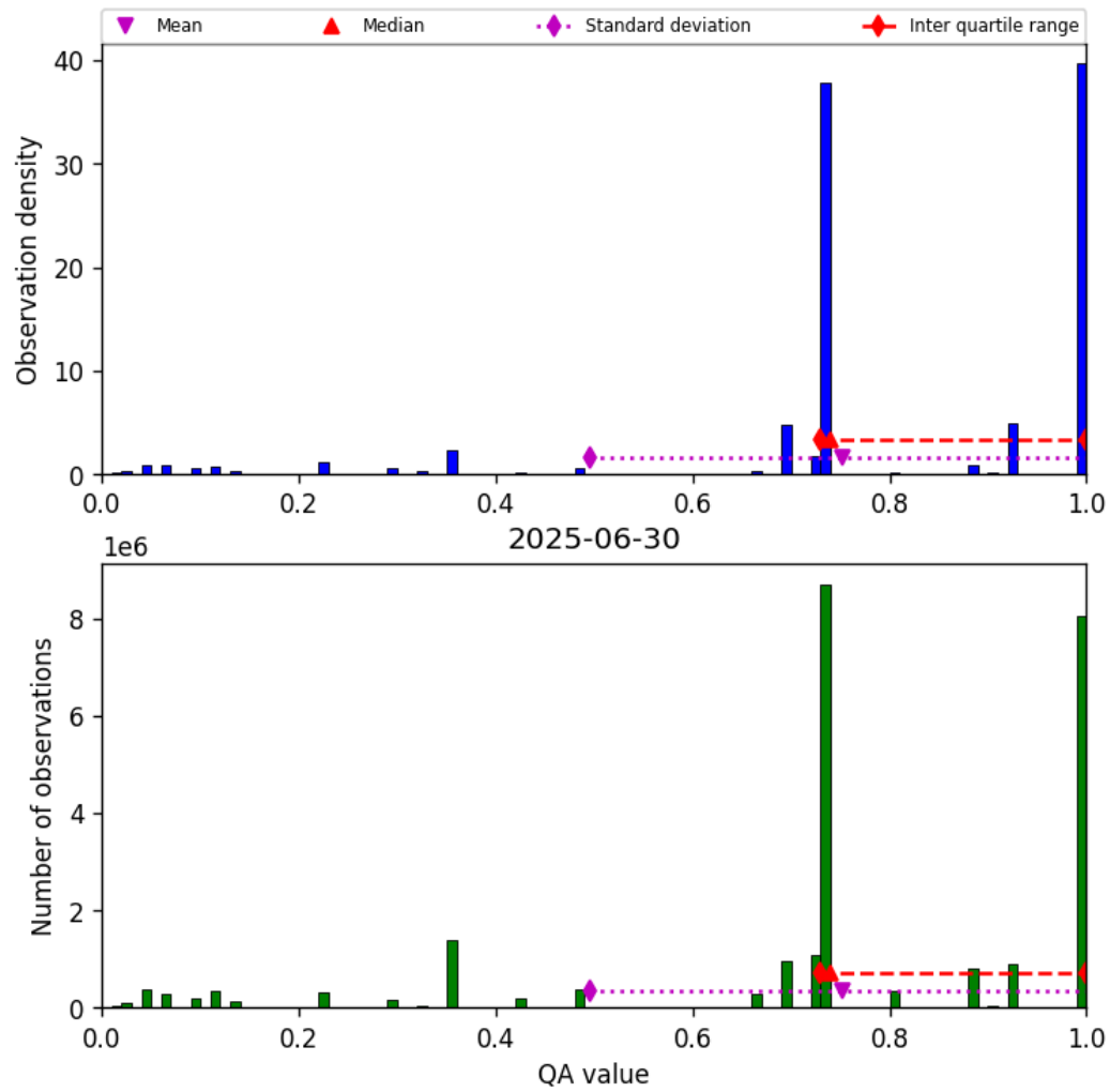
Figure 28: Histogram of “QA value” for 2025-06-29 to 2025-07-01
