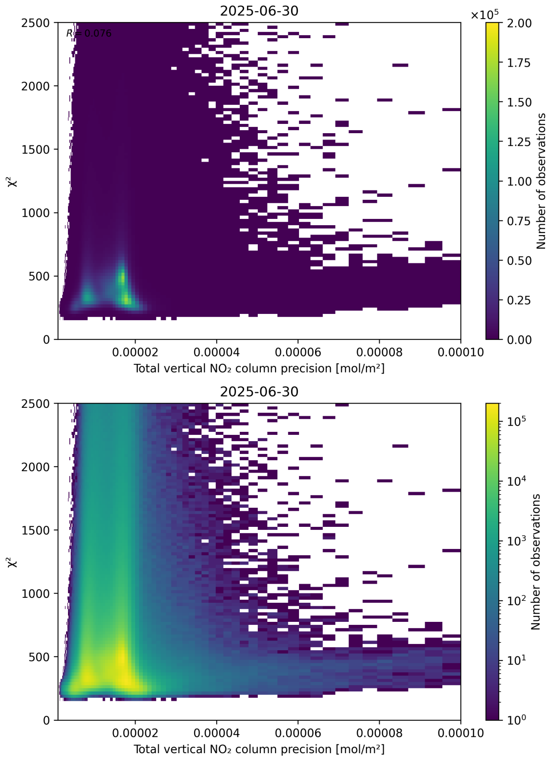
Figure 116: Scatter density plot of “Total vertical NO 2 column precision” against “ \chi^2 ” for 2025-06-29 to 2025-07-01.
