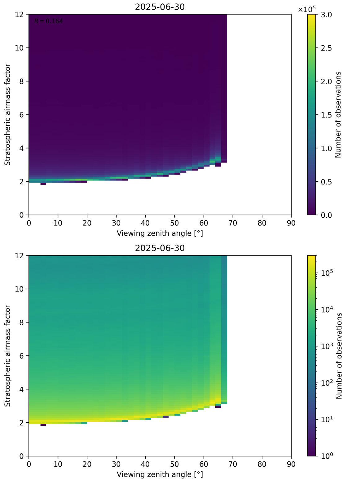
Figure 159: Scatter density plot of “Viewing zenith angle” against “Stratospheric airmass factor” for 2025-06-29 to 2025-07-01.
