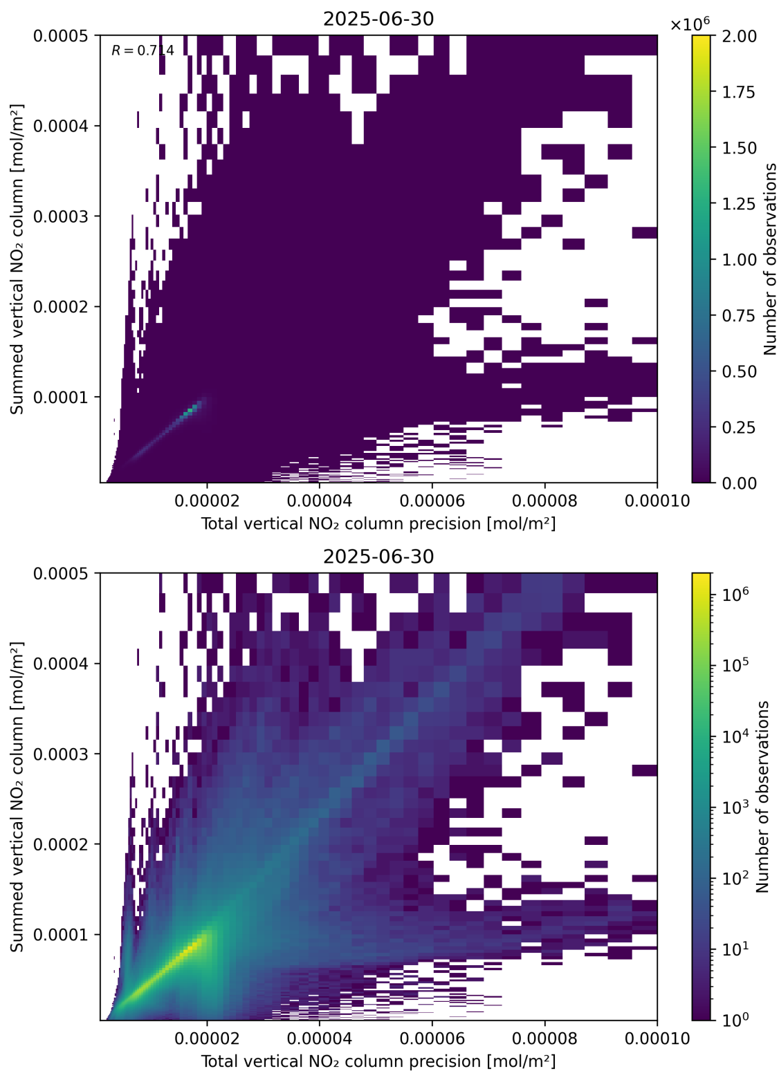
Figure 117: Scatter density plot of “Total vertical NO 2 column precision” against “Summed vertical NO 2 column” for 2025-06-29 to 2025-07-01.
