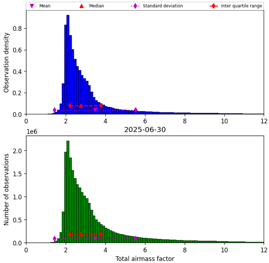
Figure 32: Histogram of “Total airmass factor” for 2025-06-29 to 2025-07-01
