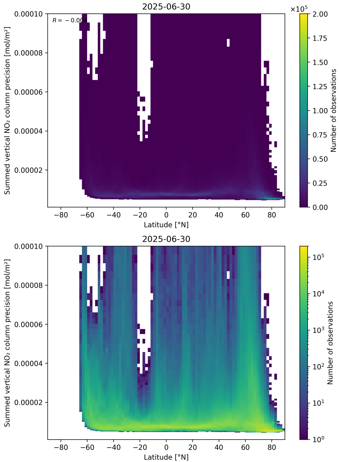
Figure 89: Scatter density plot of “Latitude” against “Summed vertical NO 2 column precision” for 2025-06-29 to 2025-07-01.
