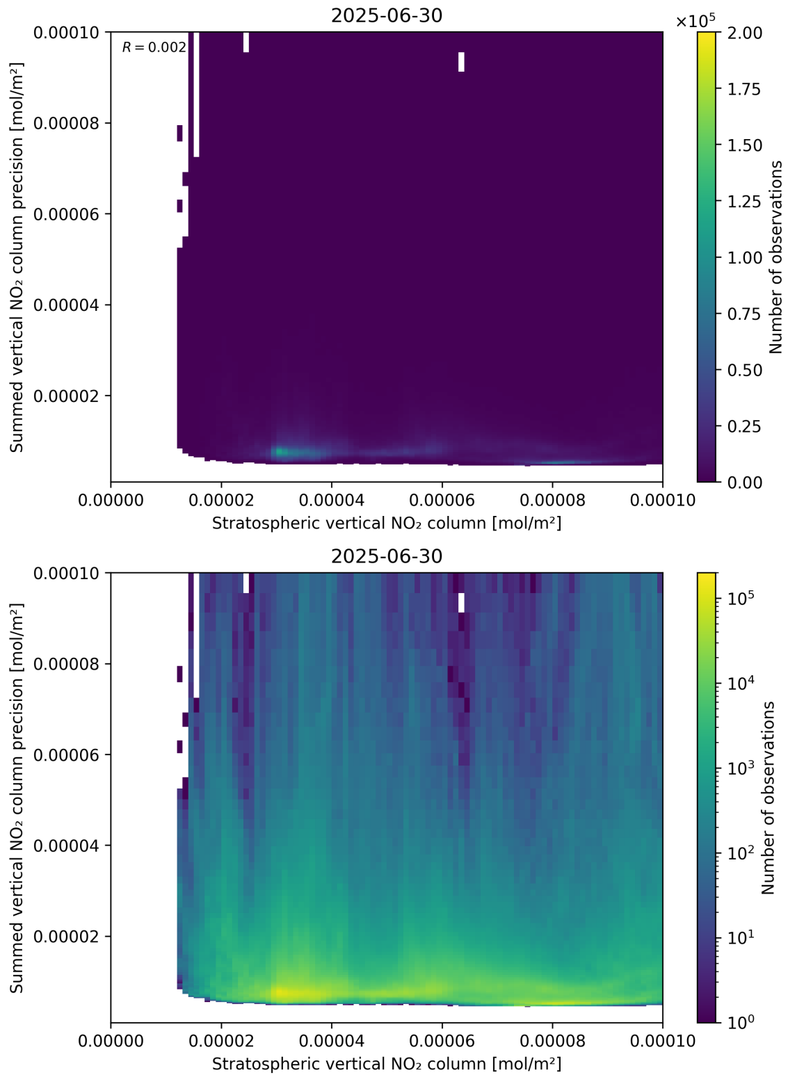
Figure 99: Scatter density plot of “Stratospheric vertical NO 2 column” against “Summed vertical NO 2 column precision” for 2025-06-29 to 2025-07-01.
