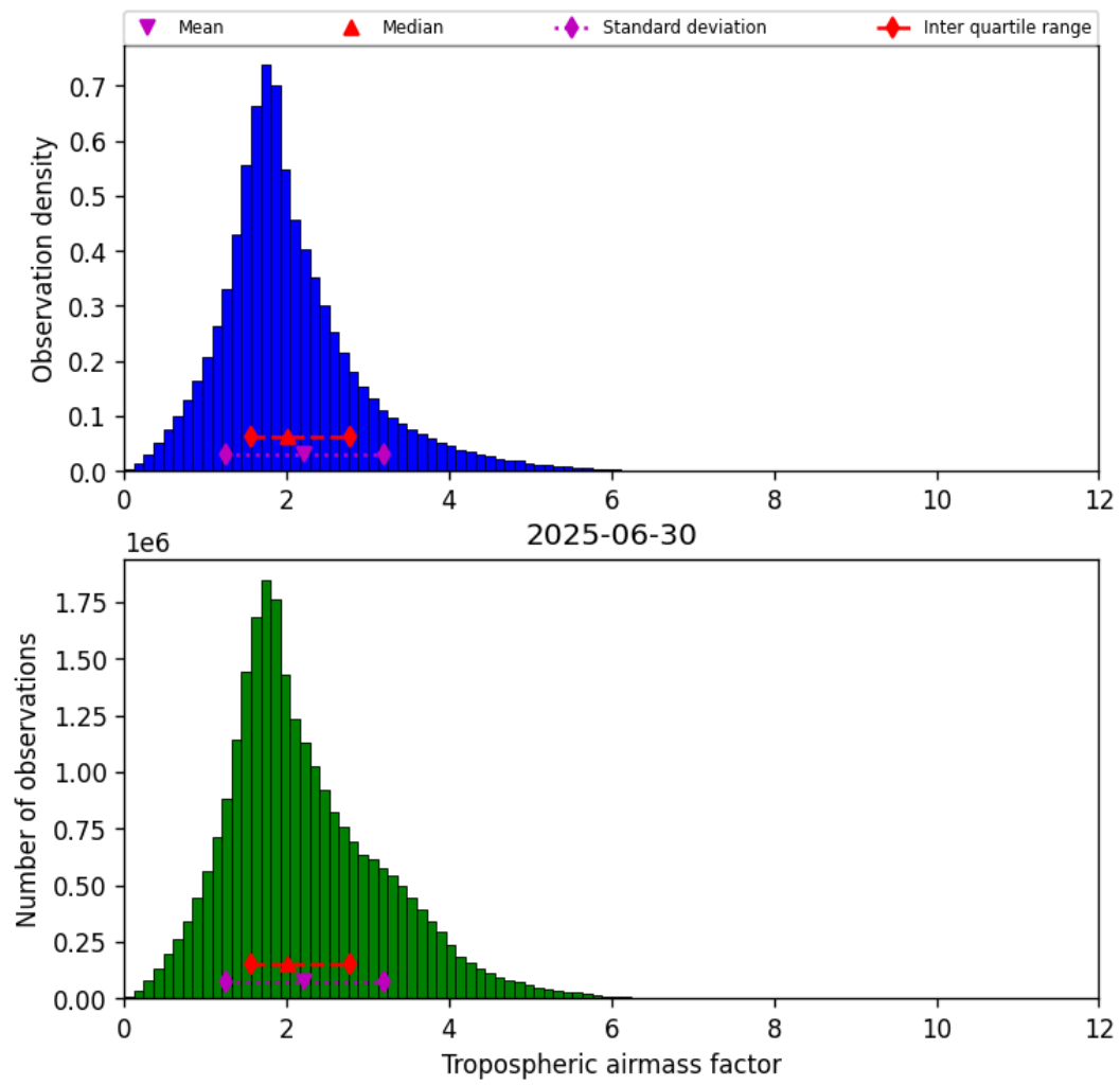
Figure 31: Histogram of “Tropospheric airmass factor” for 2025-06-29 to 2025-07-01
