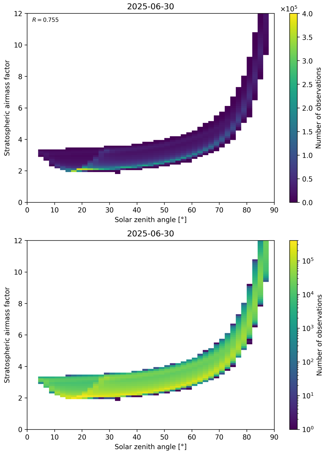
Figure 145: Scatter density plot of “Solar zenith angle” against “Stratospheric airmass factor” for 2025-06-29 to 2025-07-01.
