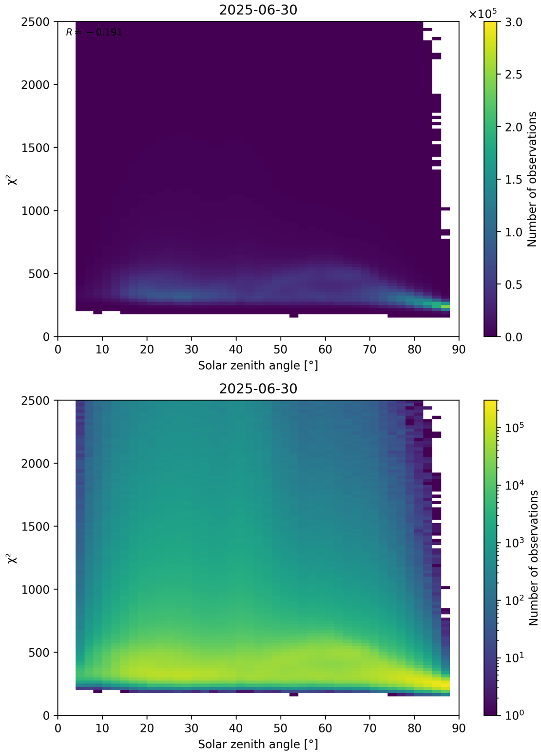
Figure 148: Scatter density plot of “Solar zenith angle” against “ \chi^2 ” for 2025-06-29 to 2025-07-01.
