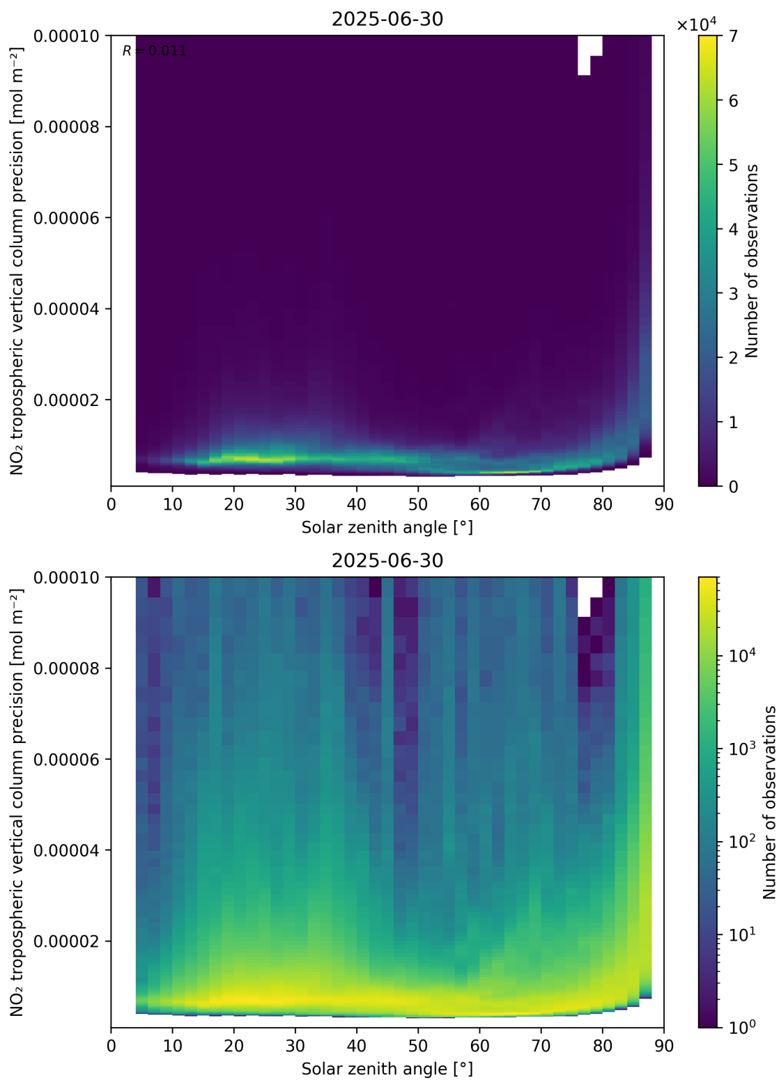
Figure 156: Scatter density plot of “Solar zenith angle” against “NO 2 tropospheric vertical column precision” for 2025-06-29 to 2025-07-01.
