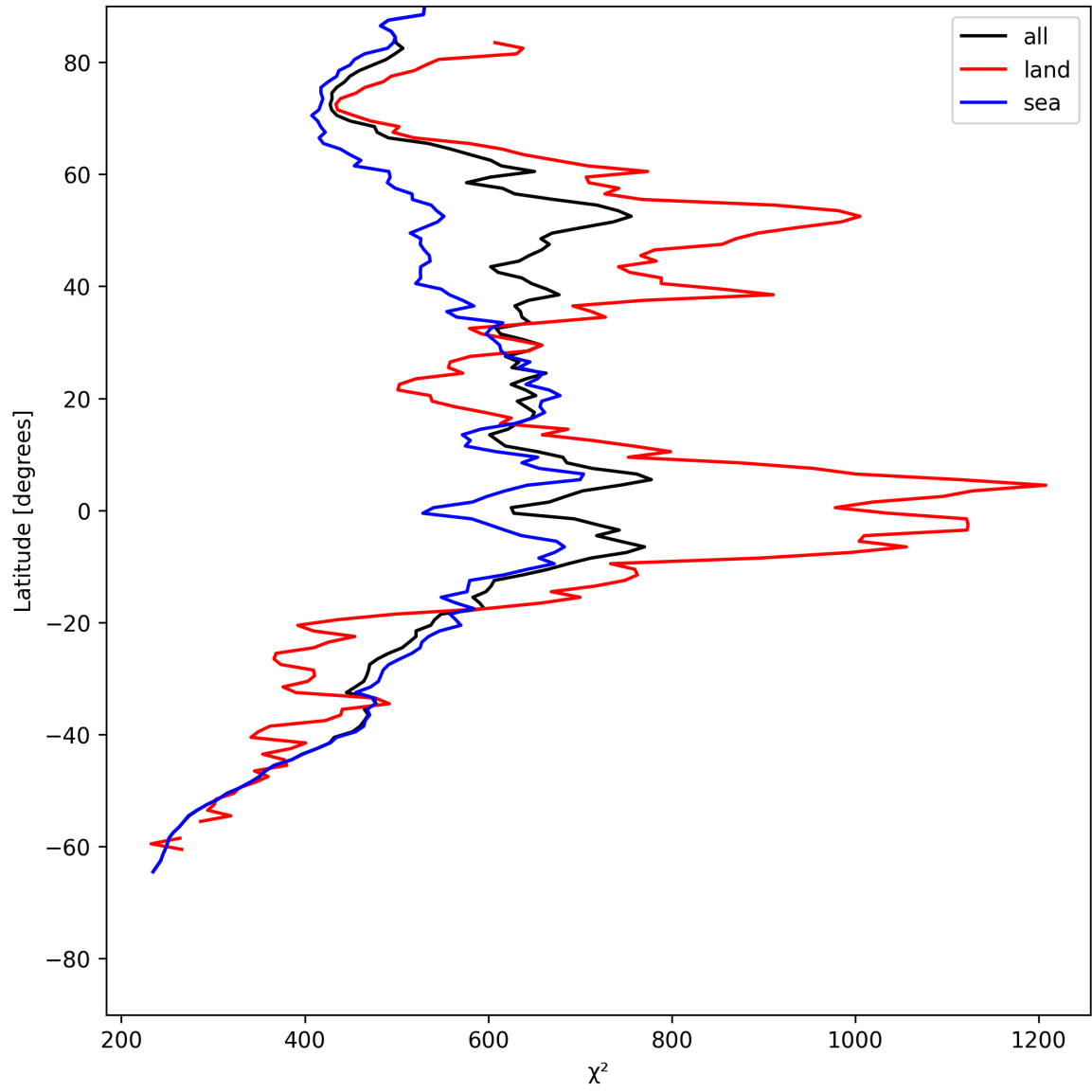
Figure 25: Zonal average of “ \chi^2 ” for 2025-06-29 to 2025-07-01.
