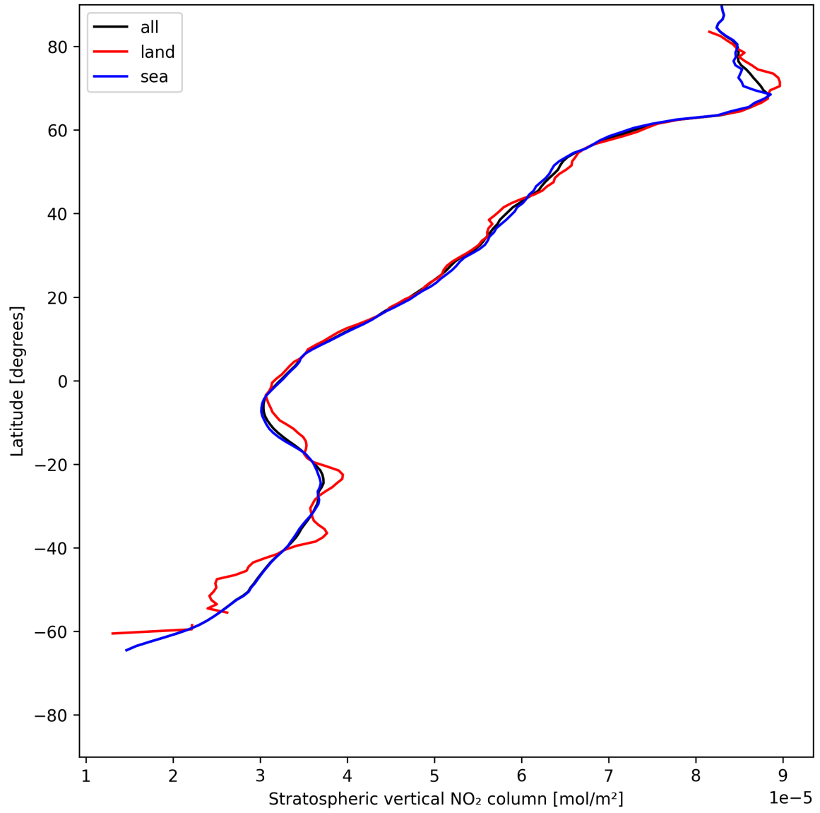
Figure 19: Zonal average of “Stratospheric vertical NO 2 column” for 2025-06-29 to 2025-07-01.
