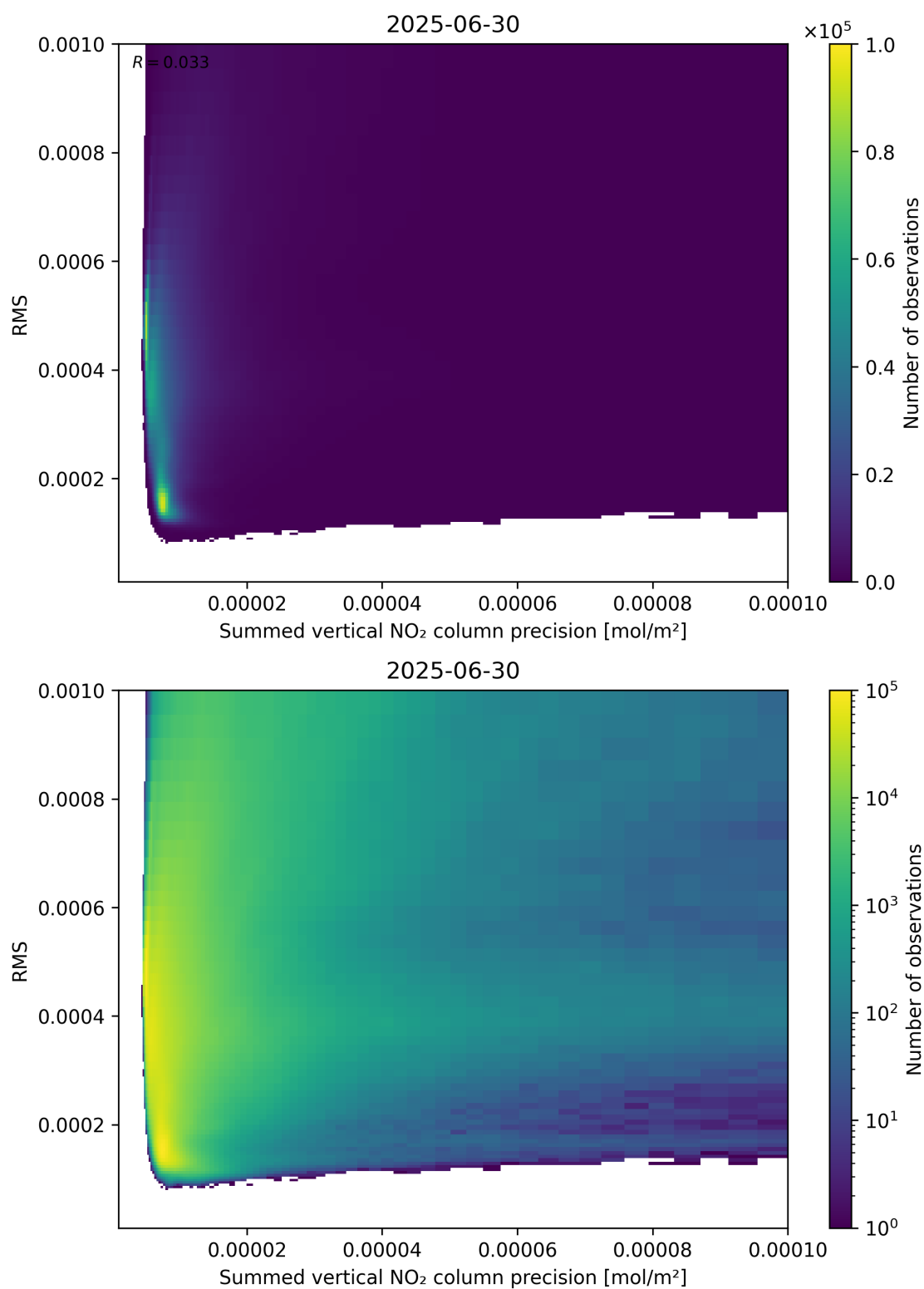
Figure 108: Scatter density plot of “Summed vertical NO 2 column precision” against “RMS” for 2025-06-29 to 2025-07-01.
