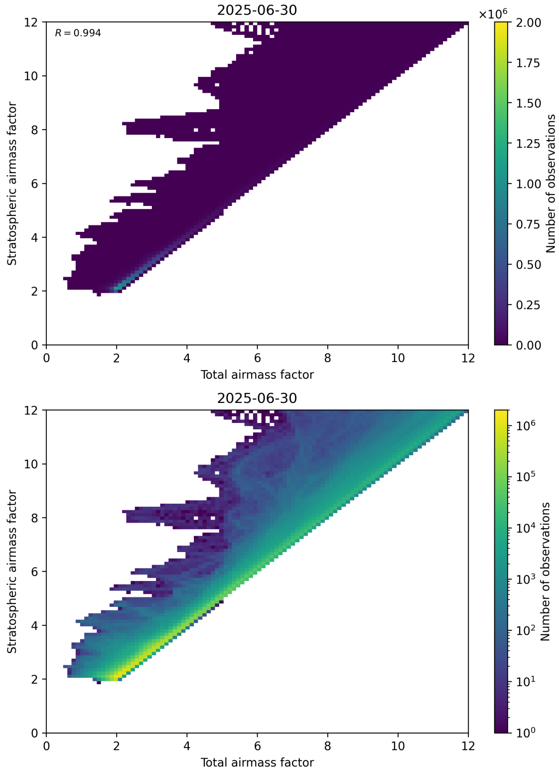
Figure 62: Scatter density plot of “Total airmass factor” against “Stratospheric airmass factor” for 2025-06-29 to 2025-07-01.
