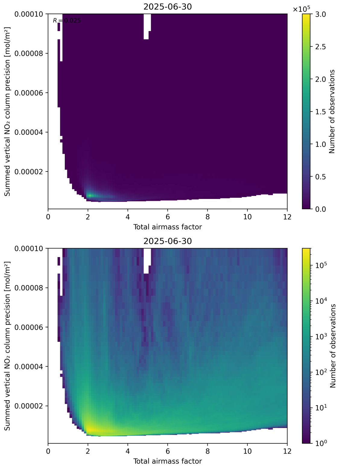
Figure 66: Scatter density plot of “Total airmass factor” against “Summed vertical NO 2 column precision” for 2025-06-29 to 2025-07-01.
