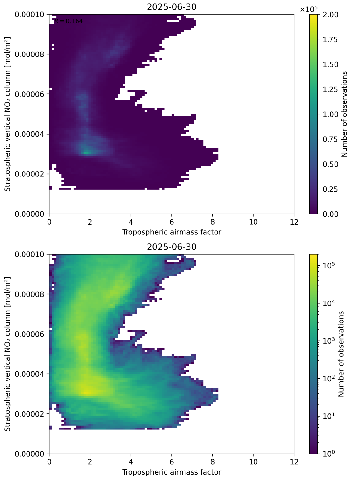
Figure 74: Scatter density plot of “Tropospheric airmass factor” against “Stratospheric vertical NO 2 column” for 2025-06-29 to 2025-07-01.
