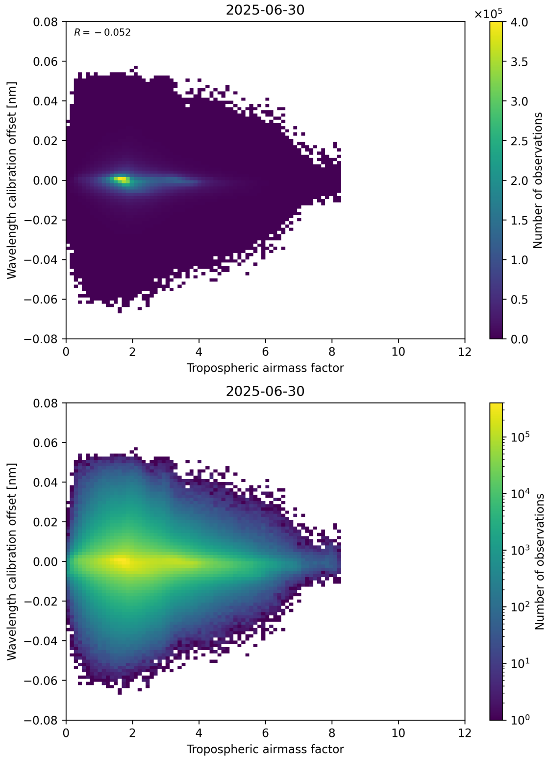
Figure 80: Scatter density plot of “Tropospheric airmass factor” against “Wavelength calibration offset” for 2025-06-29 to 2025-07-01.
