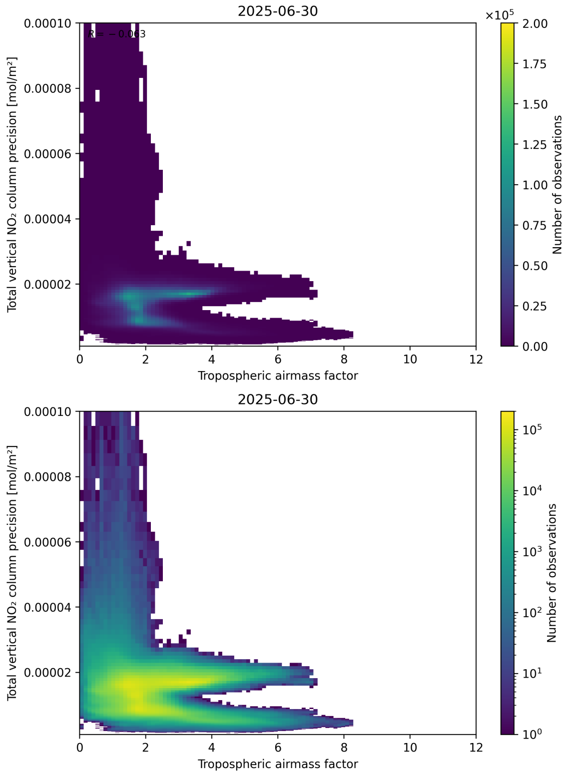
Figure 78: Scatter density plot of “Tropospheric air mass factor” against “Total vertical NO 2 column precision” for 2025-06-29 to 2025-07-01.
