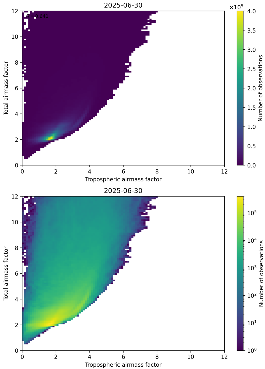
Figure 72: Scatter density plot of “Tropospheric airmass factor” against “Total airmass factor” for 2025-06-29 to 2025-07-01.
