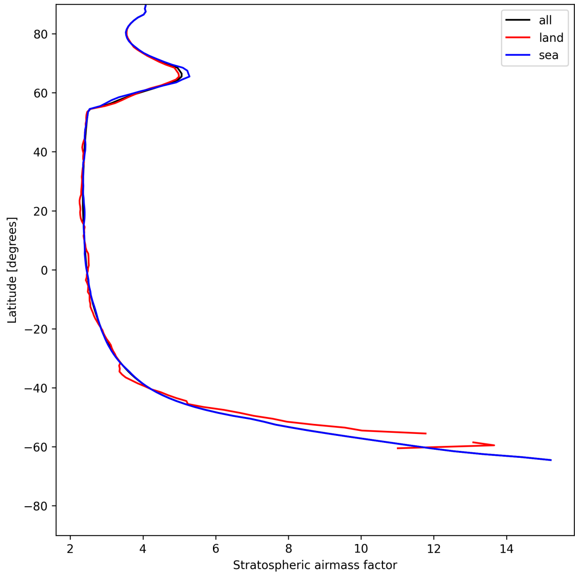
Figure 27: Zonal average of “Stratospheric air mass factor” for 2025-06-29 to 2025-07-01.
