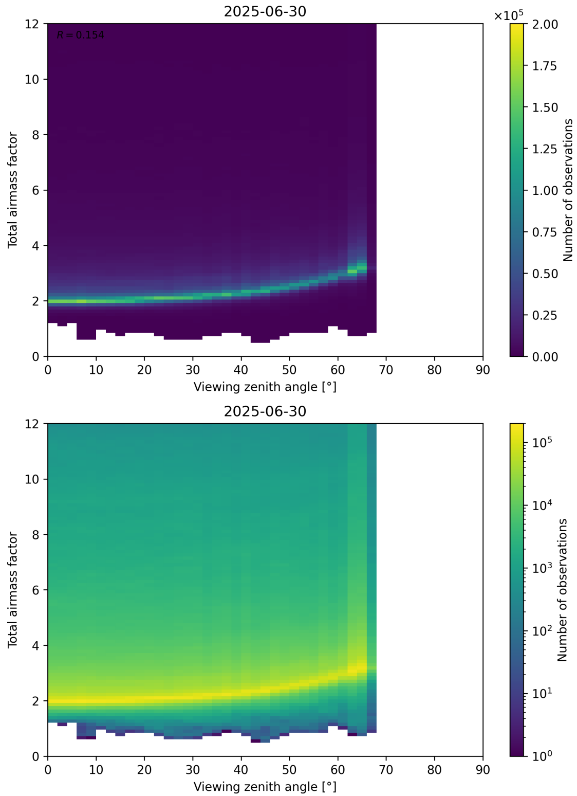
Figure 160: Scatter density plot of “Viewing zenith angle” against “Total airmass factor” for 2025-06-29 to 2025-07-01.
