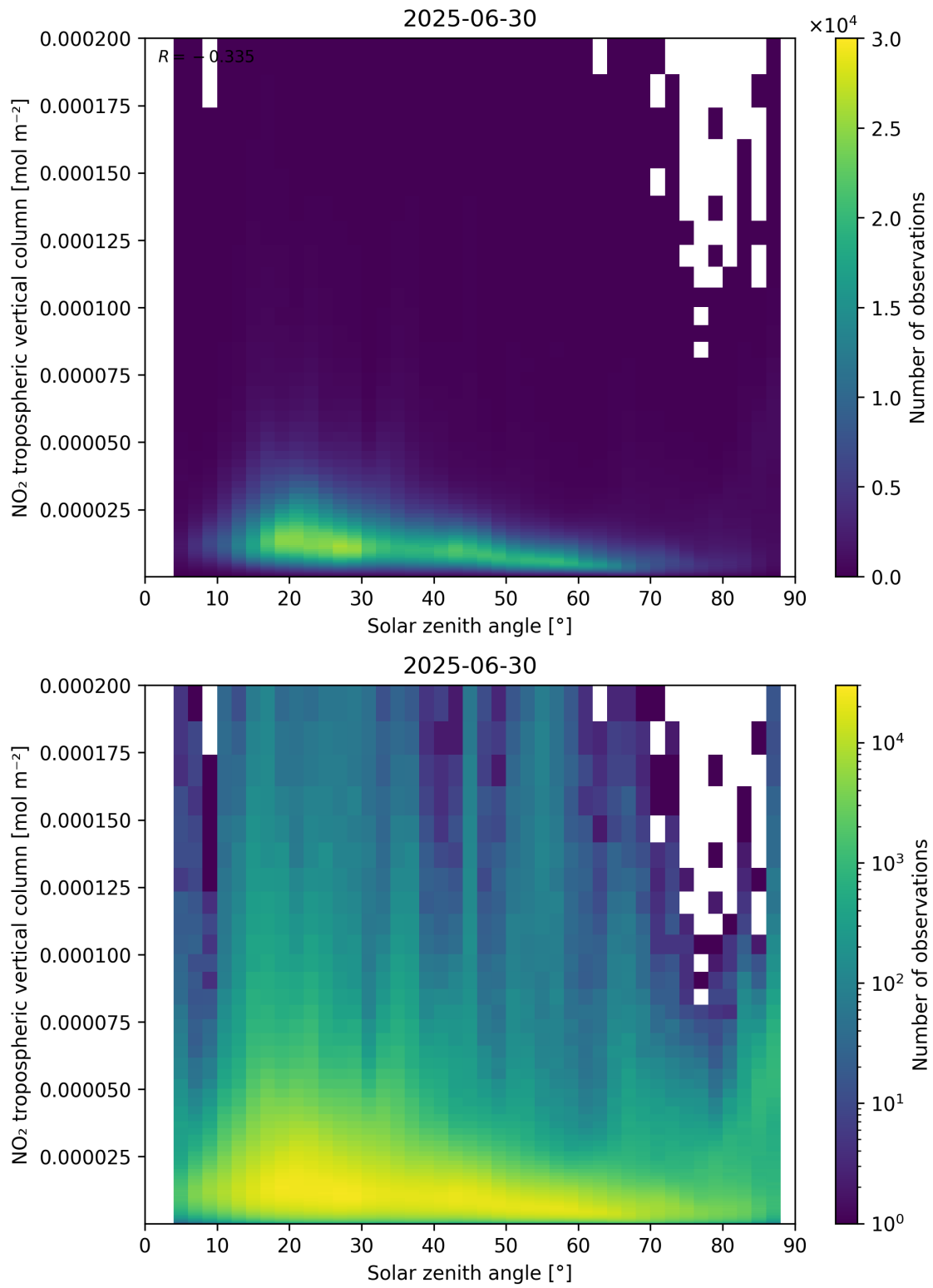
Figure 155: Scatter density plot of “Solar zenith angle” against “NO 2 tropospheric vertical column” for 2025-06-29 to 2025-07-01.
