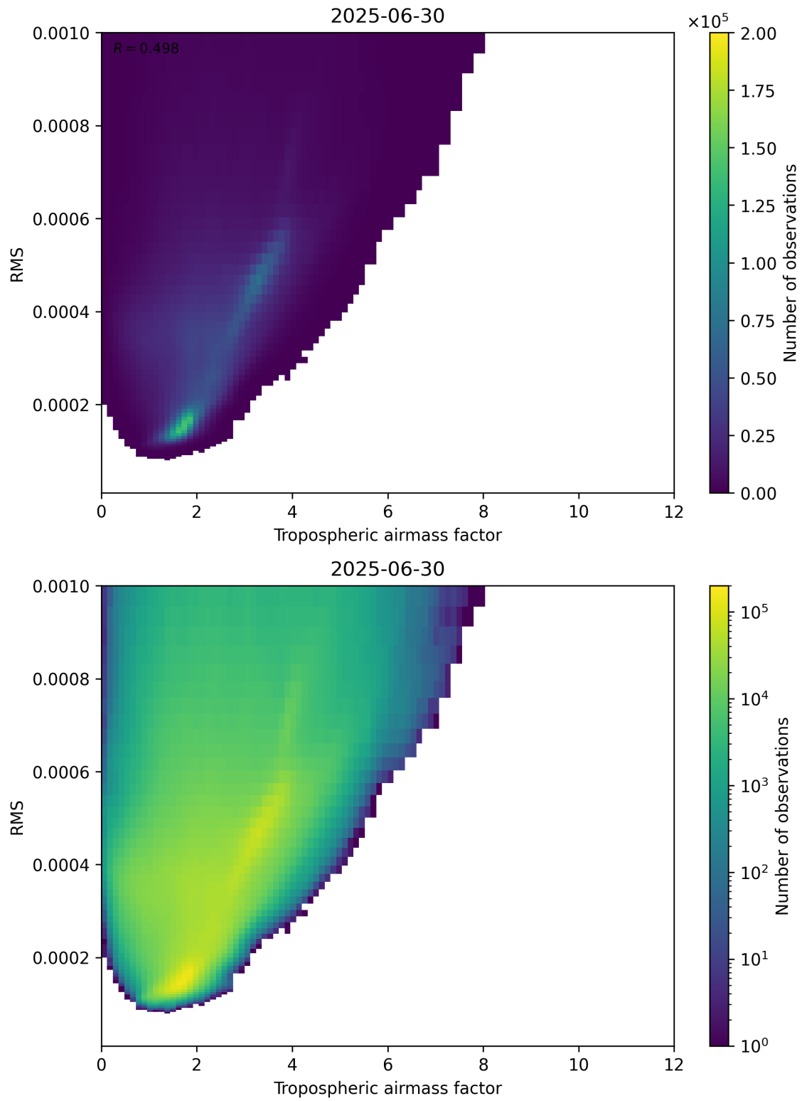
Figure 79: Scatter density plot of “Tropospheric airmass factor” against “RMS” for 2025-06-29 to 2025-07-01.
