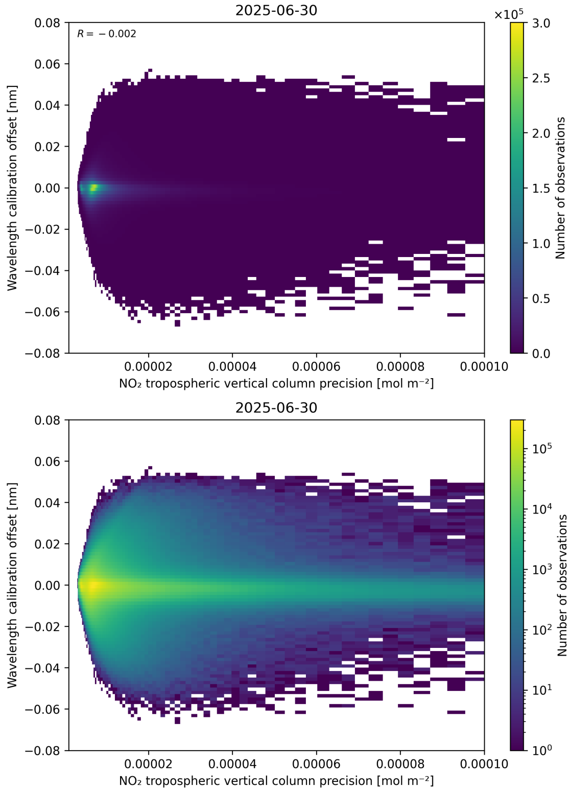
Figure 141: Scatter density plot of “NO 2 tropospheric vertical column precision” against “Wavelength calibration offset” for 2025-06-29 to 2025-07-01.
