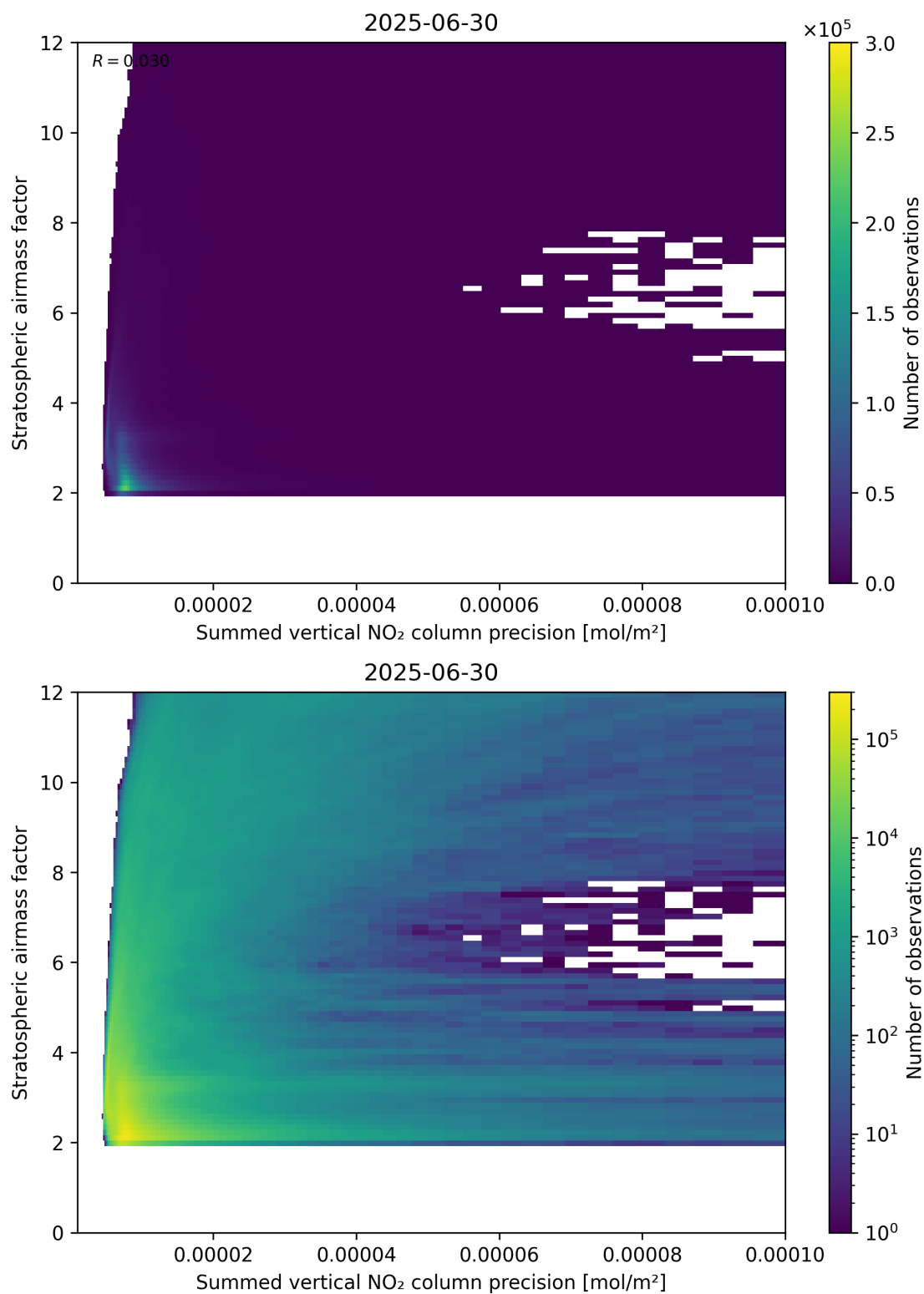
Figure 106: Scatter density plot of “Summed vertical NO 2 column precision” against “Stratospheric airmass factor” for 2025-06-29 to 2025-07-01.
