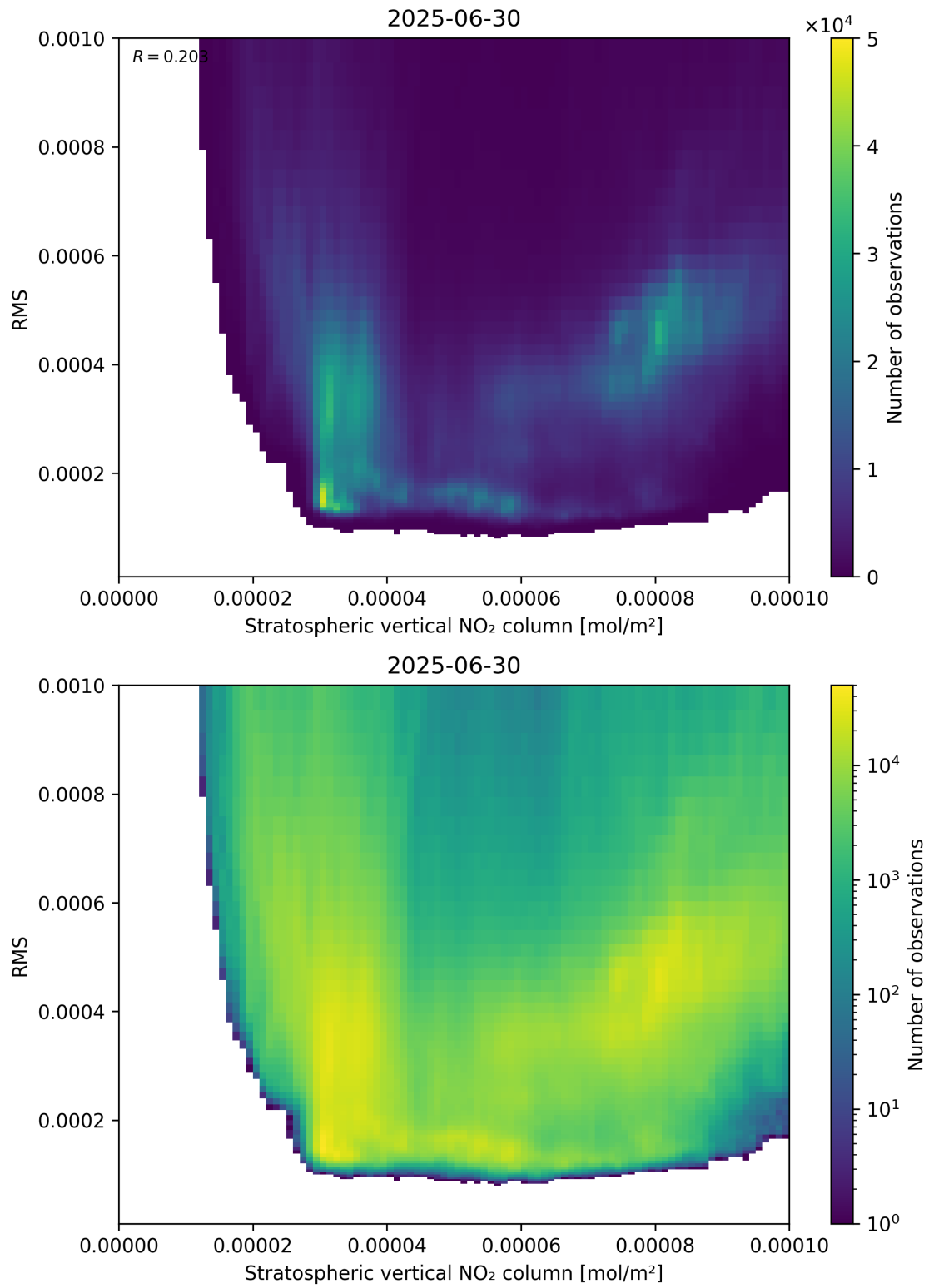
Figure 102: Scatter density plot of “Stratospheric vertical NO 2 column” against “RMS” for 2025-06-29 to 2025-07-01.
