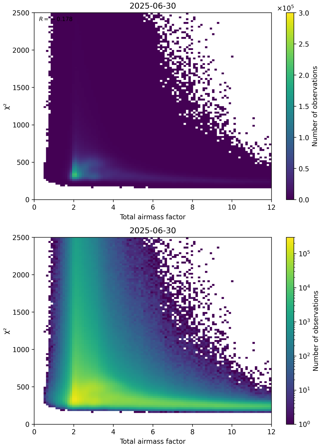
Figure 63: Scatter density plot of “Total airmass factor” against “ \chi^2 ” for 2025-06-29 to 2025-07-01.
