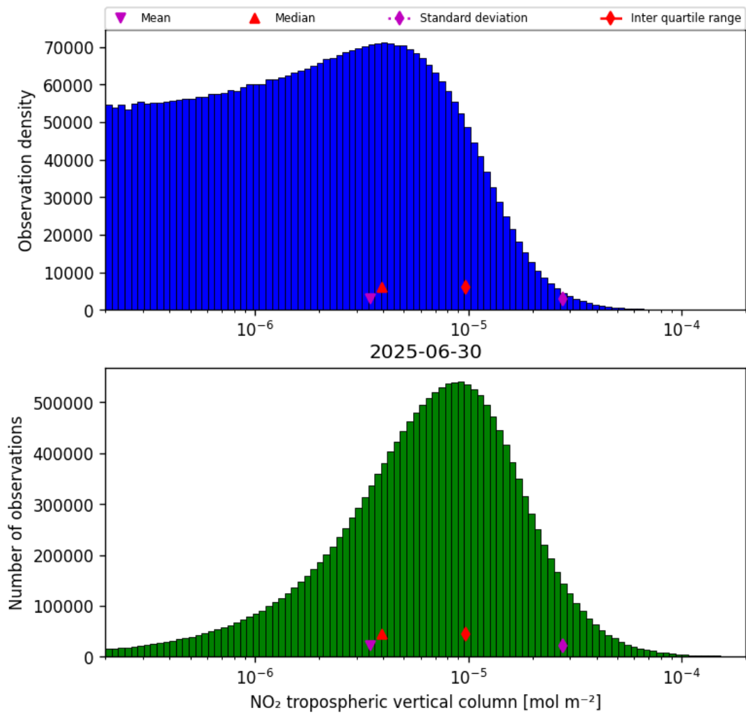
Figure 29: Histogram of “NO 2 tropospheric vertical column” for 2025-06-29 to 2025-07-01
