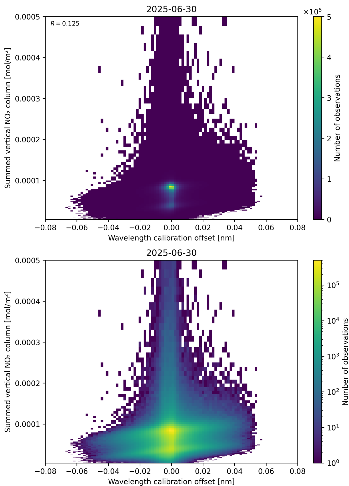
Figure 177: Scatter density plot of “Wavelength calibration offset” against “Summed vertical NO 2 column” for 2025-06-29 to 2025-07-01.
