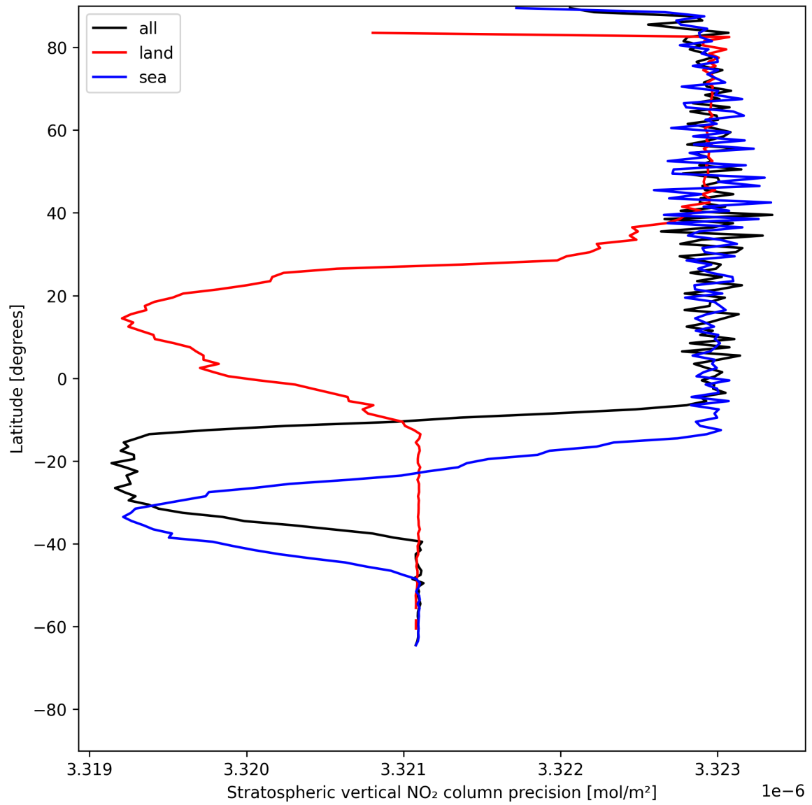
Figure 20: Zonal average of “Stratospheric vertical NO 2 column precision” for 2025-06-29 to 2025-07-01.
