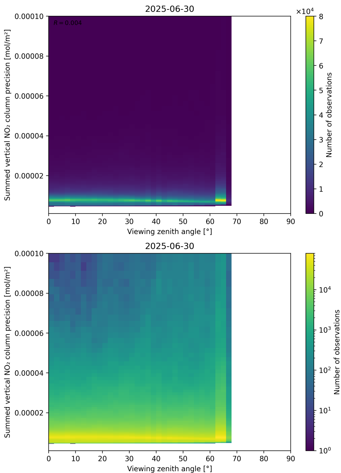
Figure 166: Scatter density plot of “Viewing zenith angle” against “Summed vertical NO 2 column precision” for 2025-06-29 to 2025-07-01.
