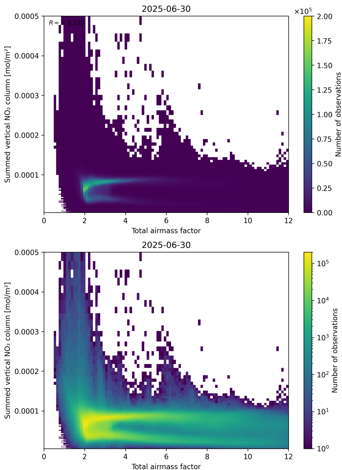
Figure 65: Scatter density plot of “Total airmass factor” against “Summed vertical NO 2 column” for 2025-06-29 to 2025-07-01.
