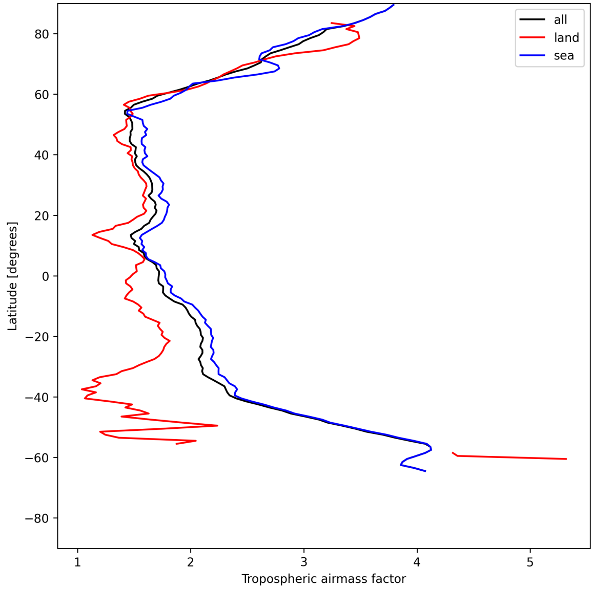
Figure 14: Zonal average of “Tropospheric airmass factor” for 2025-06-29 to 2025-07-01.
