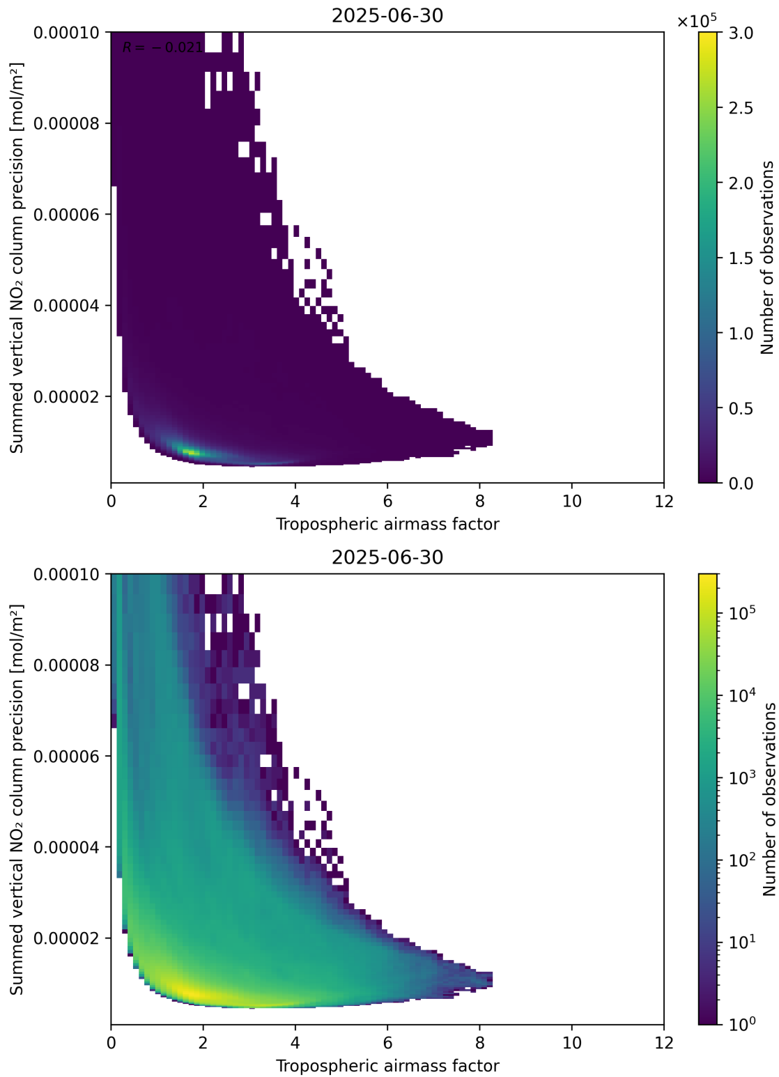
Figure 76: Scatter density plot of “Tropospheric air mass factor” against “Summed vertical NO 2 column precision” for 2025-06-29 to 2025-07-01.
