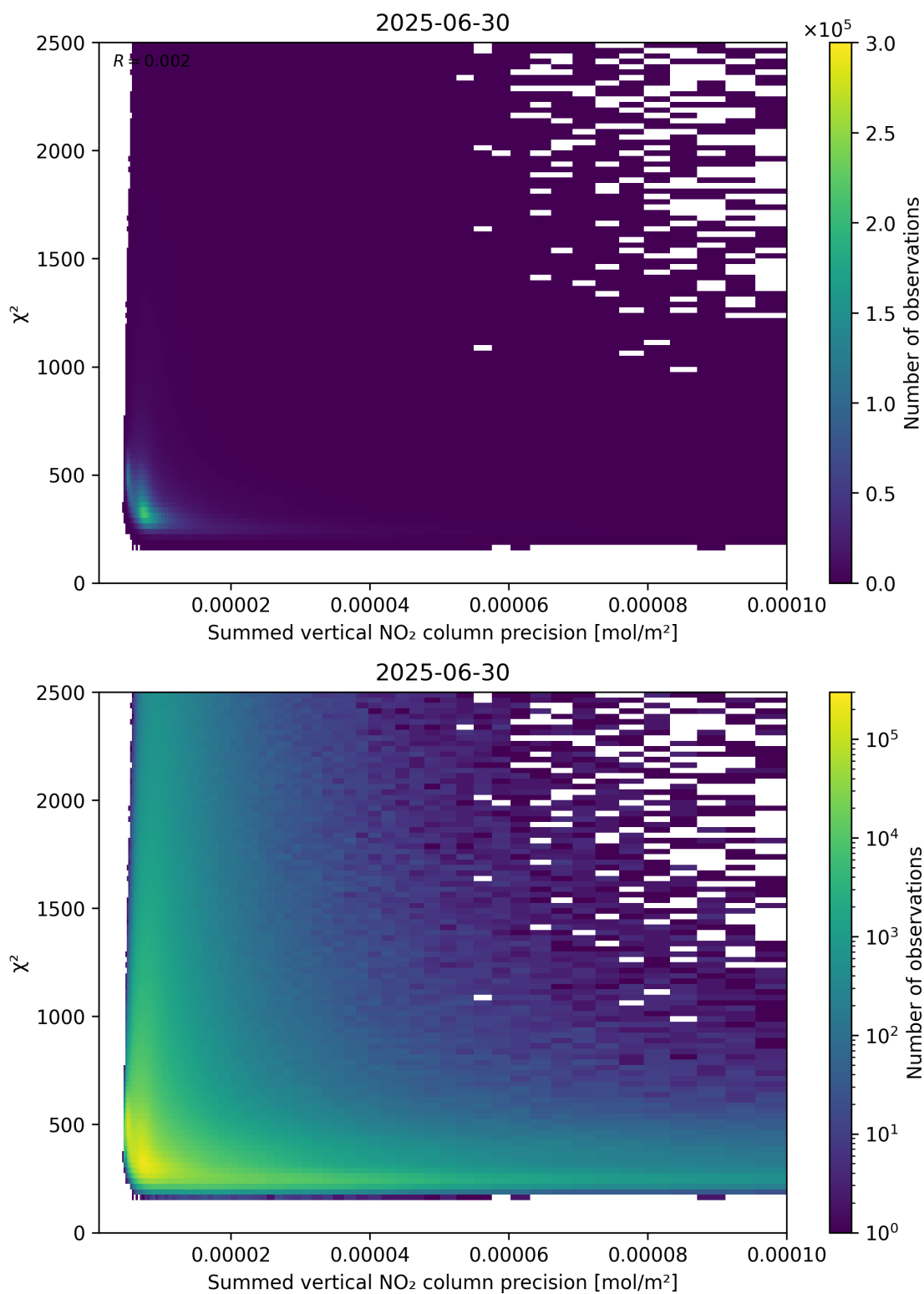
Figure 107: Scatter density plot of “Summed vertical NO 2 column precision” against “ \chi^2 ” for 2025-06-29 to 2025-07-01.
