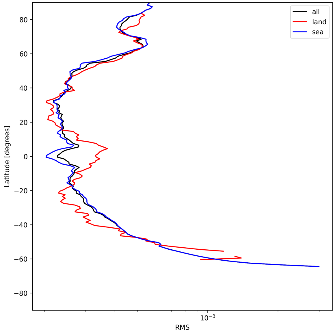
Figure 26: Zonal average of “RMS” for 2025-06-29 to 2025-07-01.
