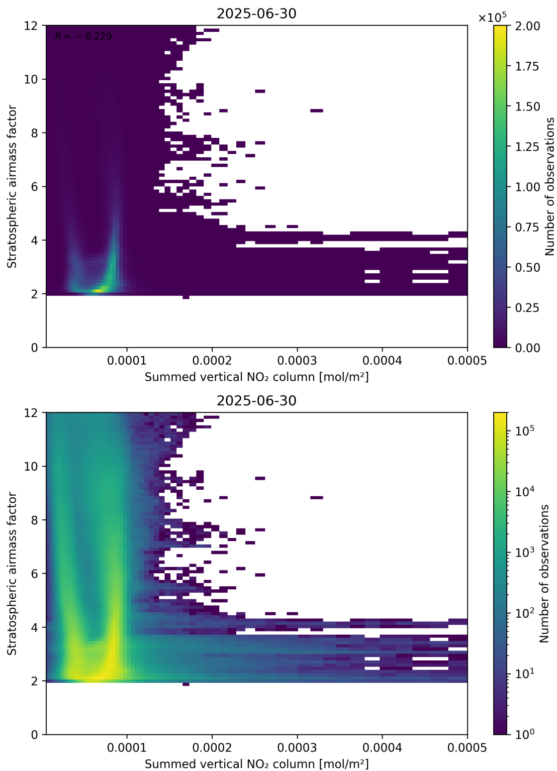
Figure 103: Scatter density plot of “Summed vertical NO 2 column” against “Stratospheric air mass factor” for 2025-06-29 to 2025-07-01.
