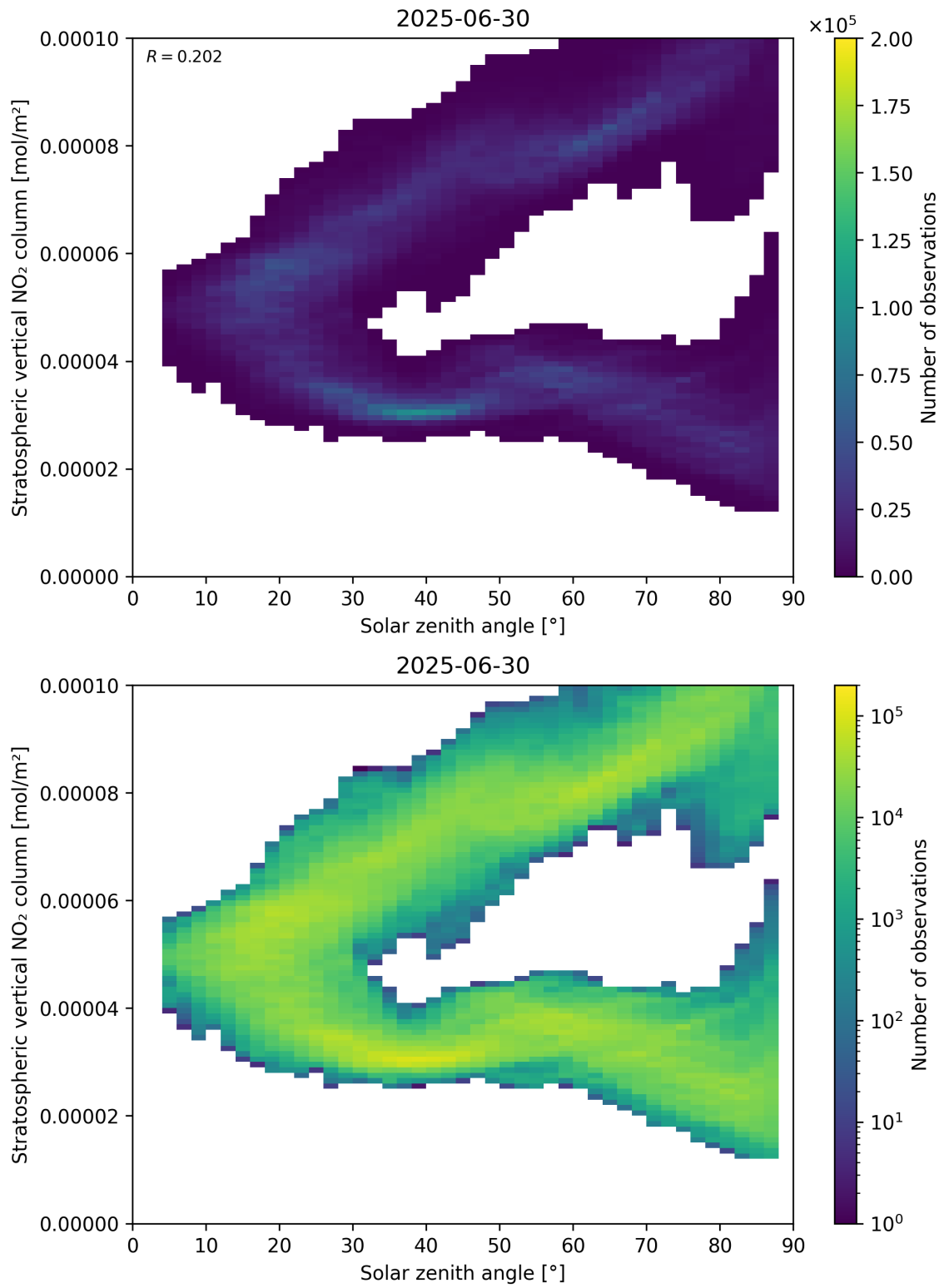
Figure 150: Scatter density plot of “Solar zenith angle” against “Stratospheric vertical NO 2 column” for 2025-06-29 to 2025-07-01.
