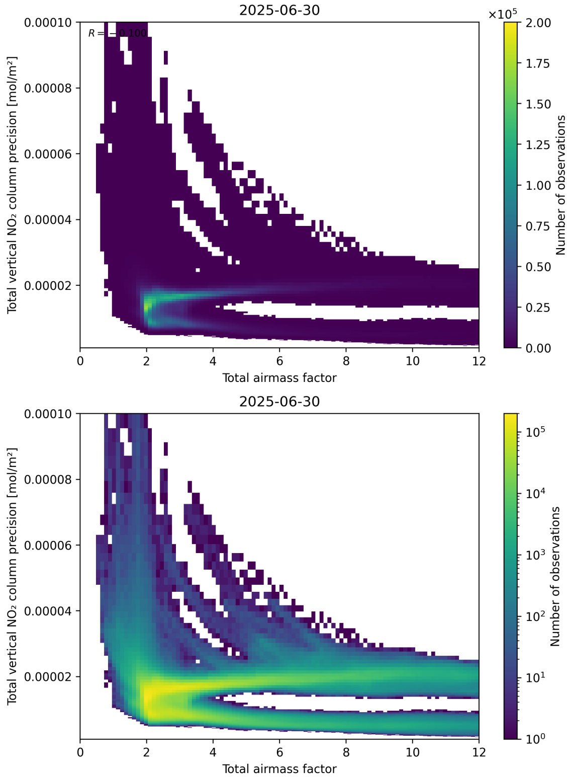
Figure 68: Scatter density plot of “Total airmass factor” against “Total vertical NO 2 column precision” for 2025-06-29 to 2025-07-01.
