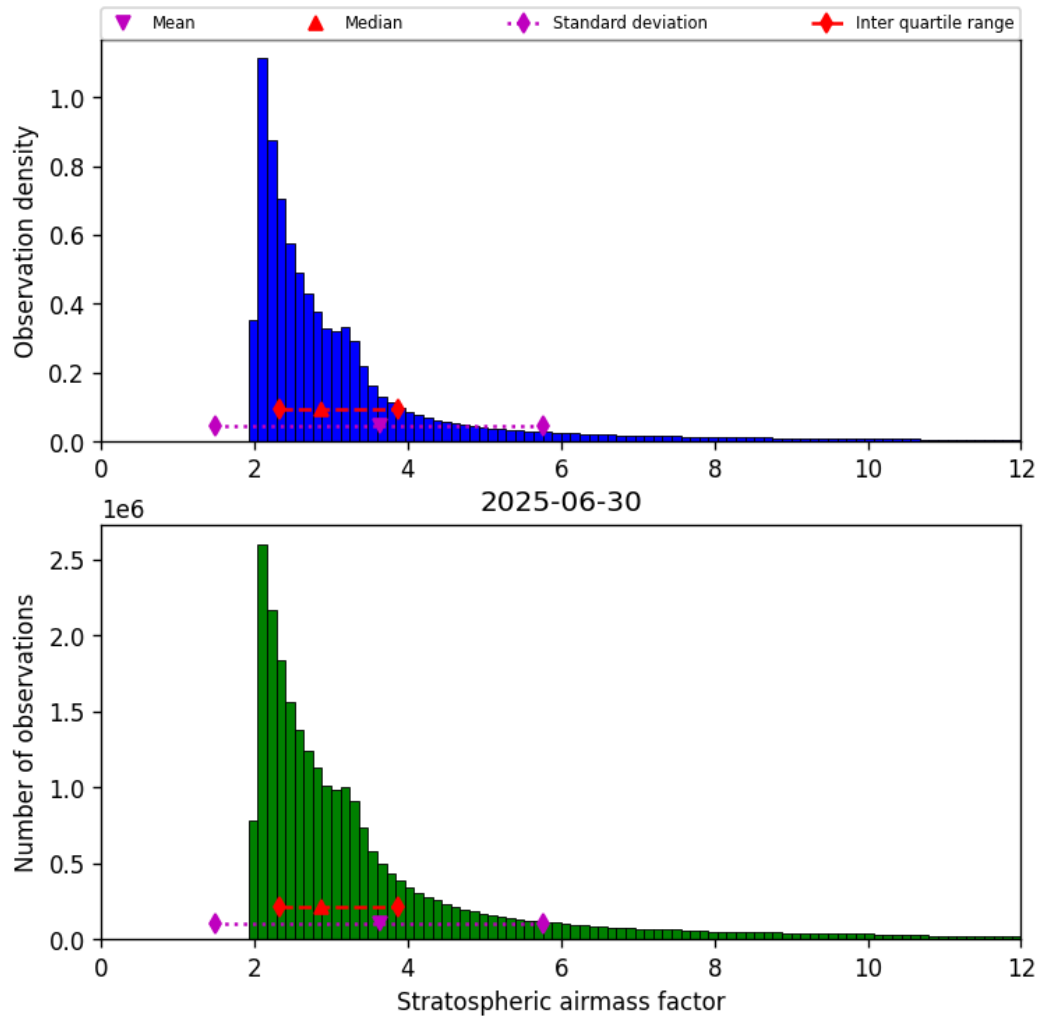
Figure 44: Histogram of “Stratospheric airmass factor” for 2025-06-29 to 2025-07-01
