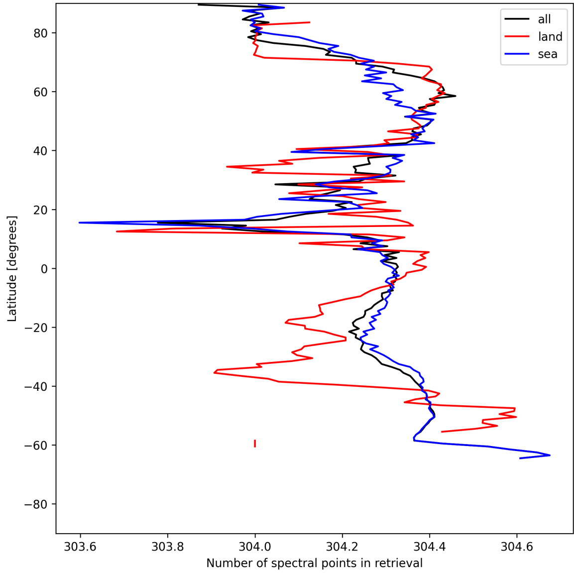
Figure 16: Zonal average of “Number of spectral points in retrieval” for 2025-06-29 to 2025-07-01.
