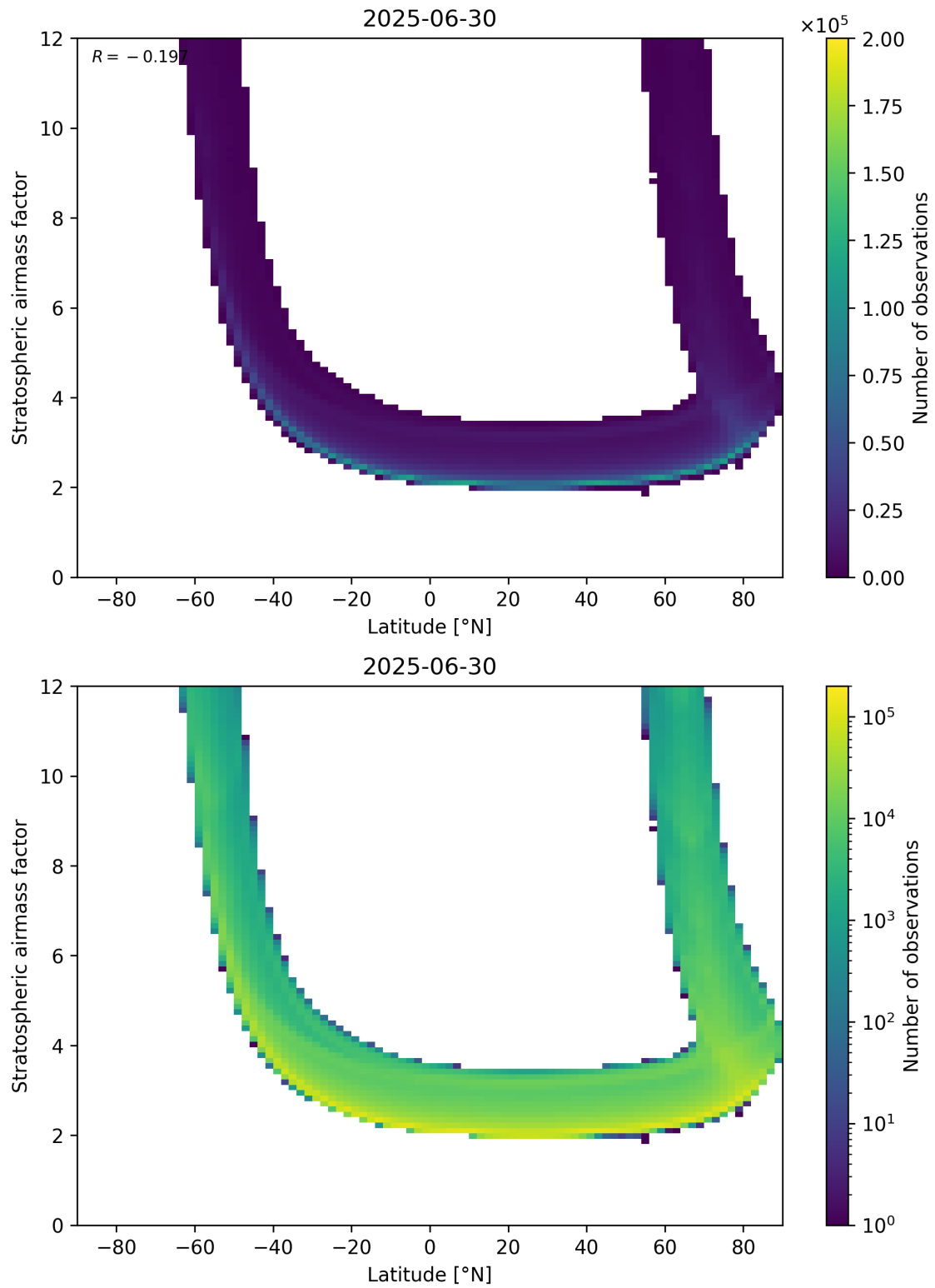
Figure 83: Scatter density plot of “Latitude” against “Stratospheric air mass factor” for 2025-06-29 to 2025-07-01.
