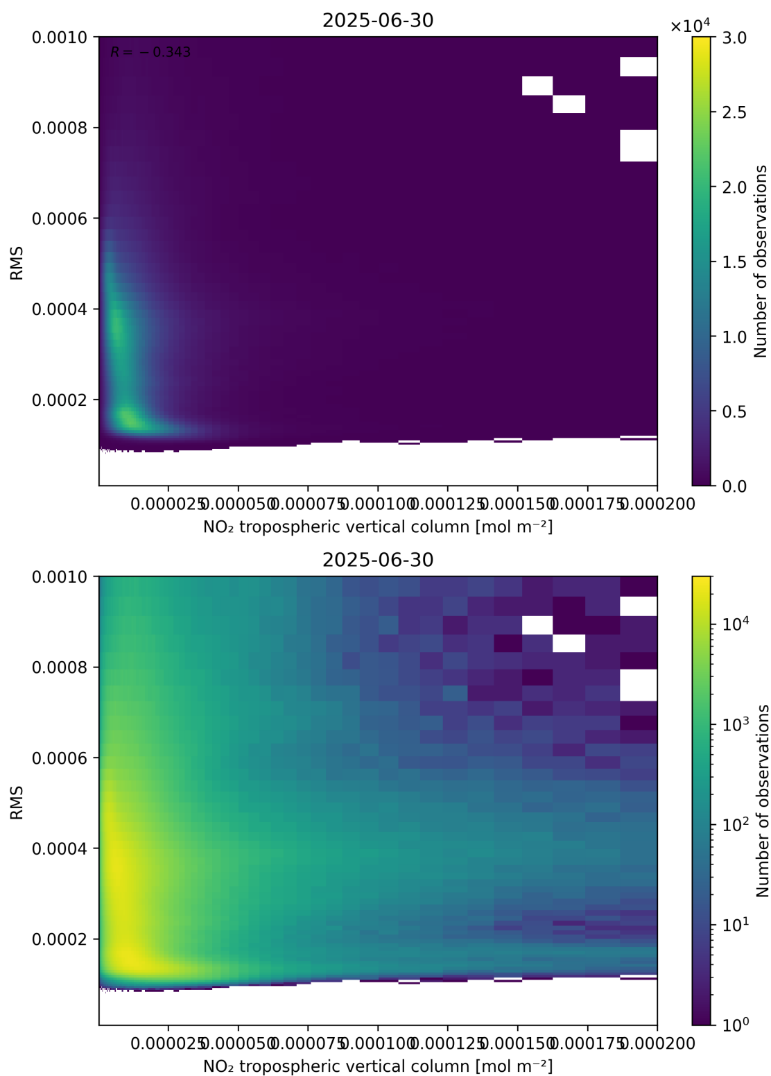
Figure 142: Scatter density plot of “NO 2 tropospheric vertical column” against “RMS” for 2025-06-29 to 2025-07-01.
