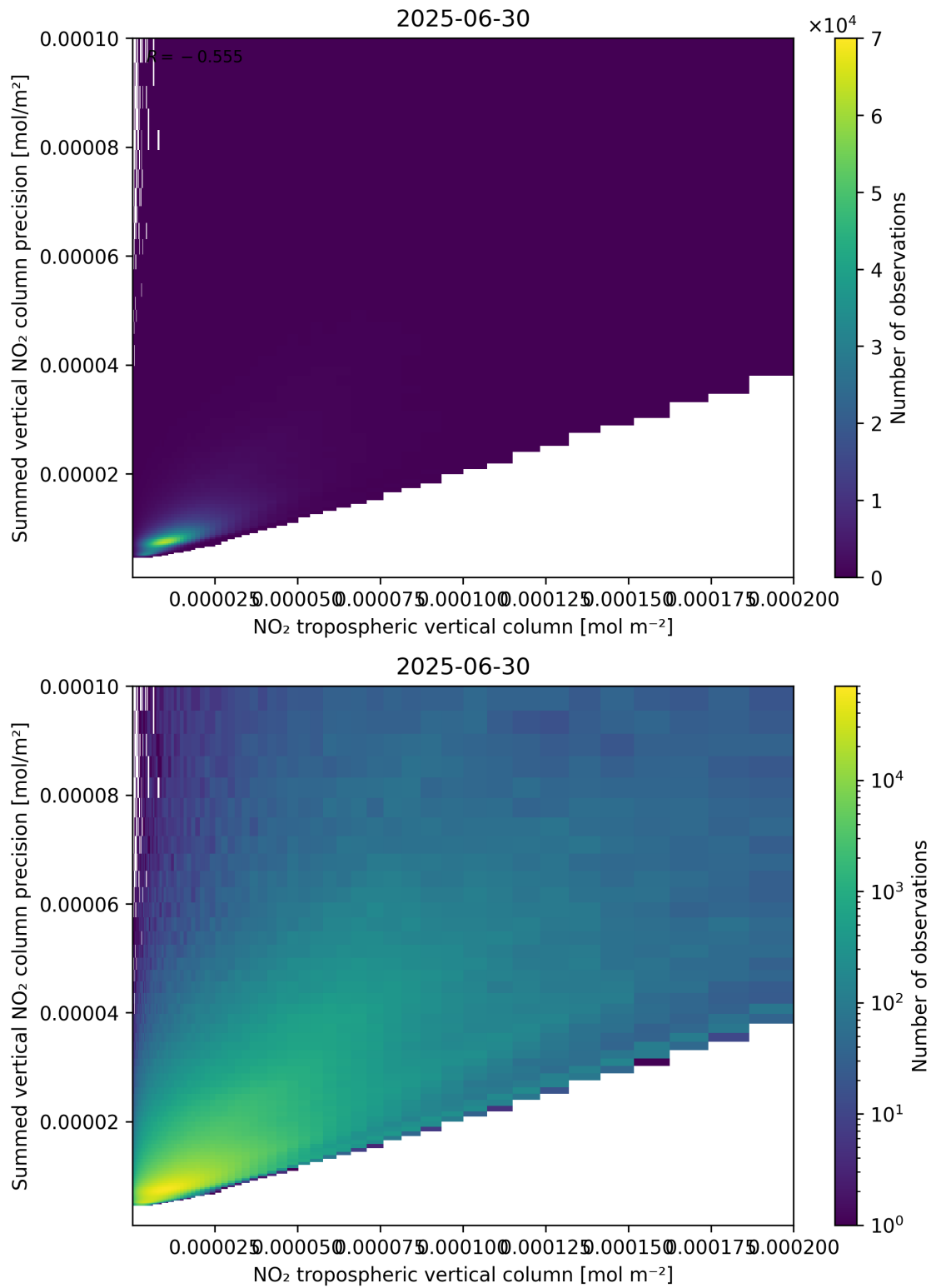
Figure 127: Scatter density plot of “NO 2 tropospheric vertical column” against “Summed vertical NO 2 column precision” for 2025-06-29 to 2025-07-01.
