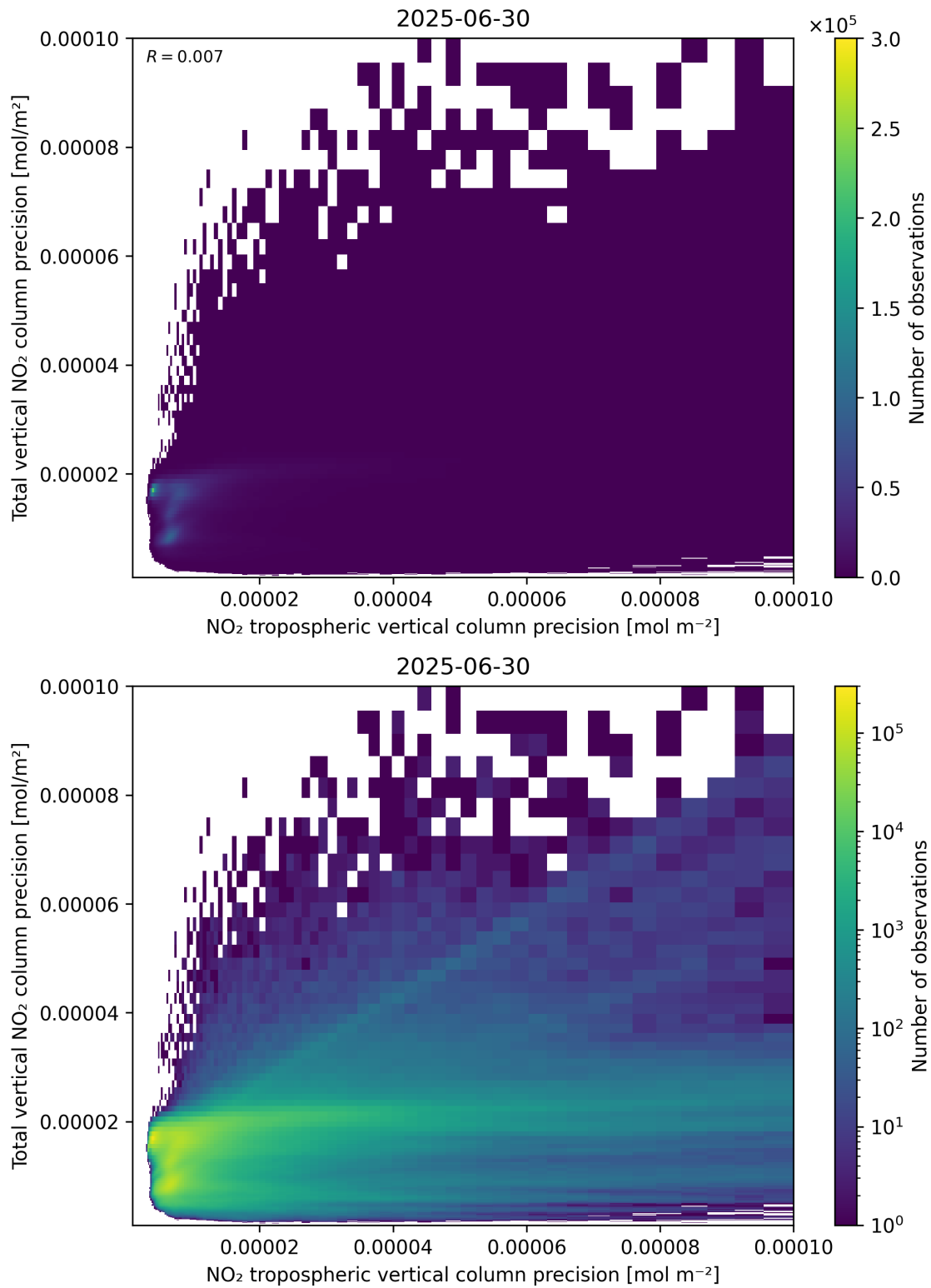
Figure 139: Scatter density plot of “NO 2 tropospheric vertical column precision” against “Total vertical NO 2 column precision” for 2025-06-29 to 2025-07-01.
