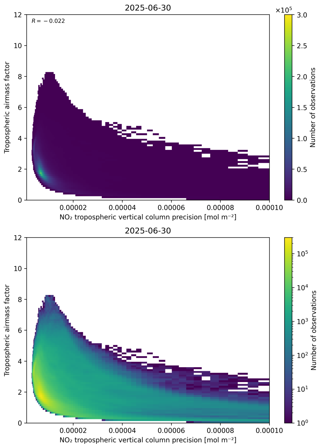
Figure 133: Scatter density plot of “NO 2 tropospheric vertical column precision” against “Tropospheric airmass factor” for 2025-06-29 to 2025-07-01.
