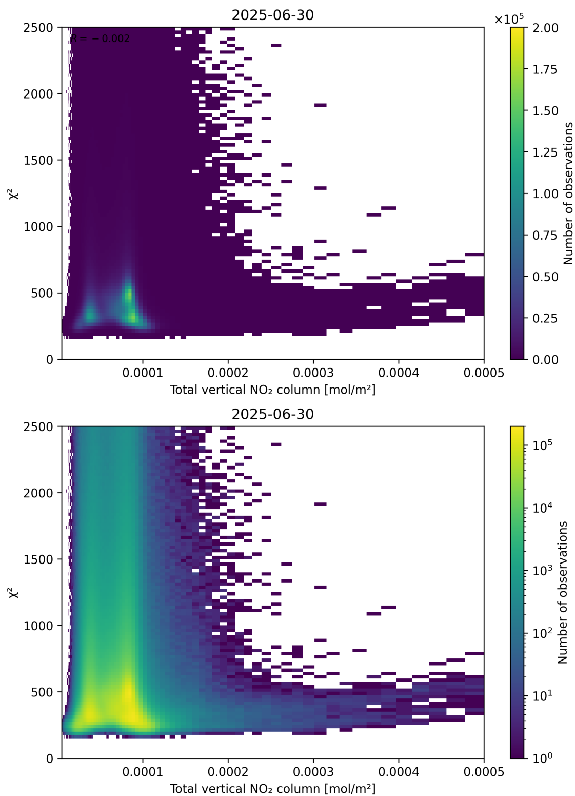
Figure 111: Scatter density plot of “Total vertical NO 2 column” against “ \chi^2 ” for 2025-06-29 to 2025-07-01.
