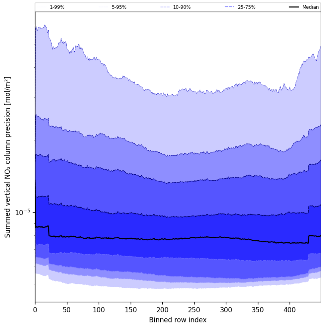
Figure 58: Along track statistics of “Summed vertical NO 2 column precision” for 2025-06-29 to 2025-07-01
