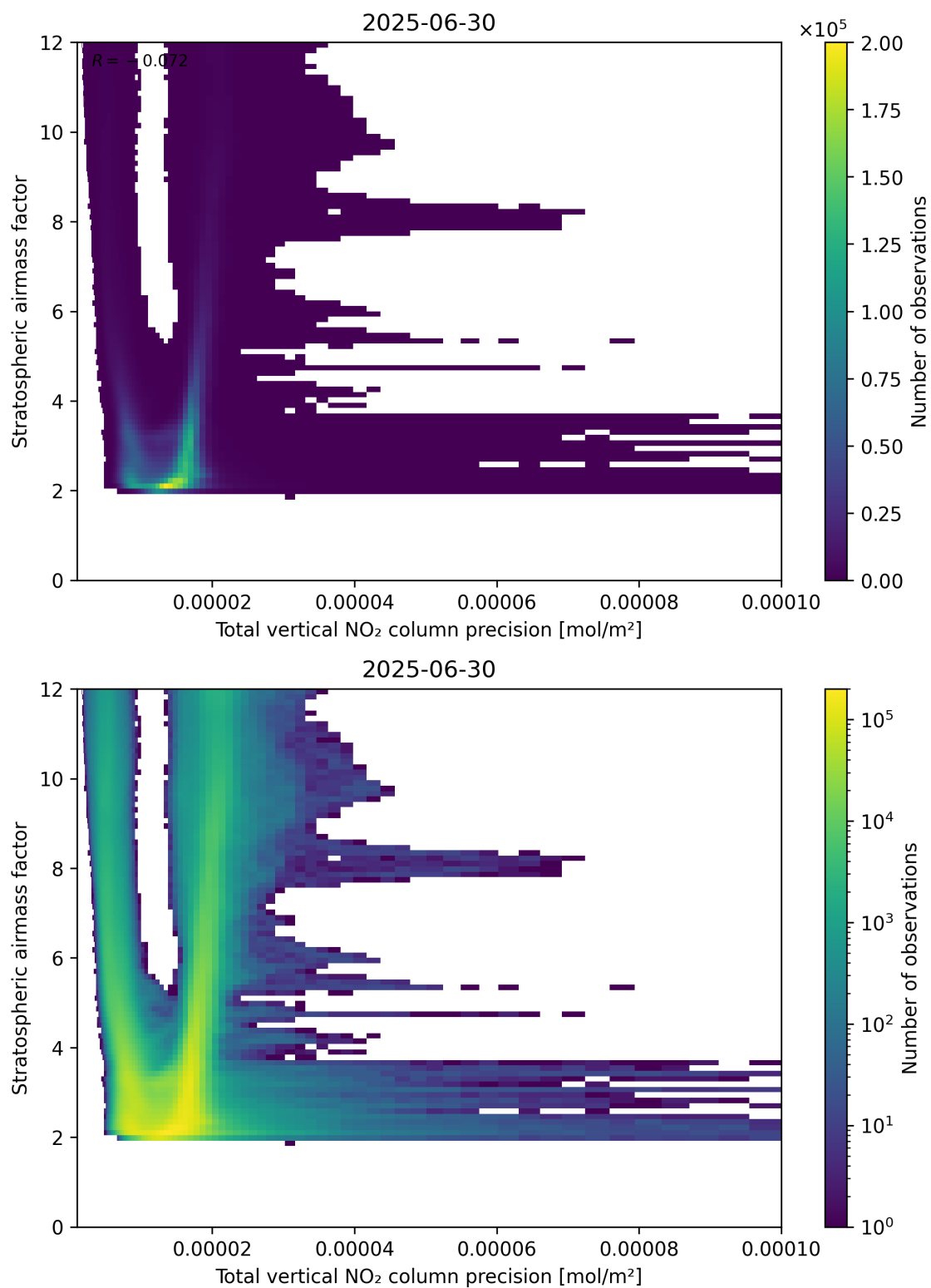
Figure 115: Scatter density plot of “Total vertical NO 2 column precision” against “Stratospheric air mass factor” for 2025-06-29 to 2025-07-01.
