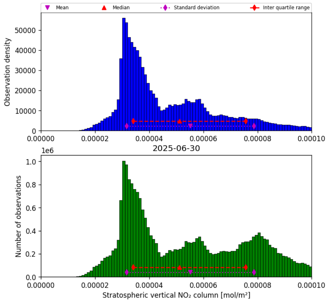
Figure 36: Histogram of “Stratospheric vertical NO 2 column” for 2025-06-29 to 2025-07-01
