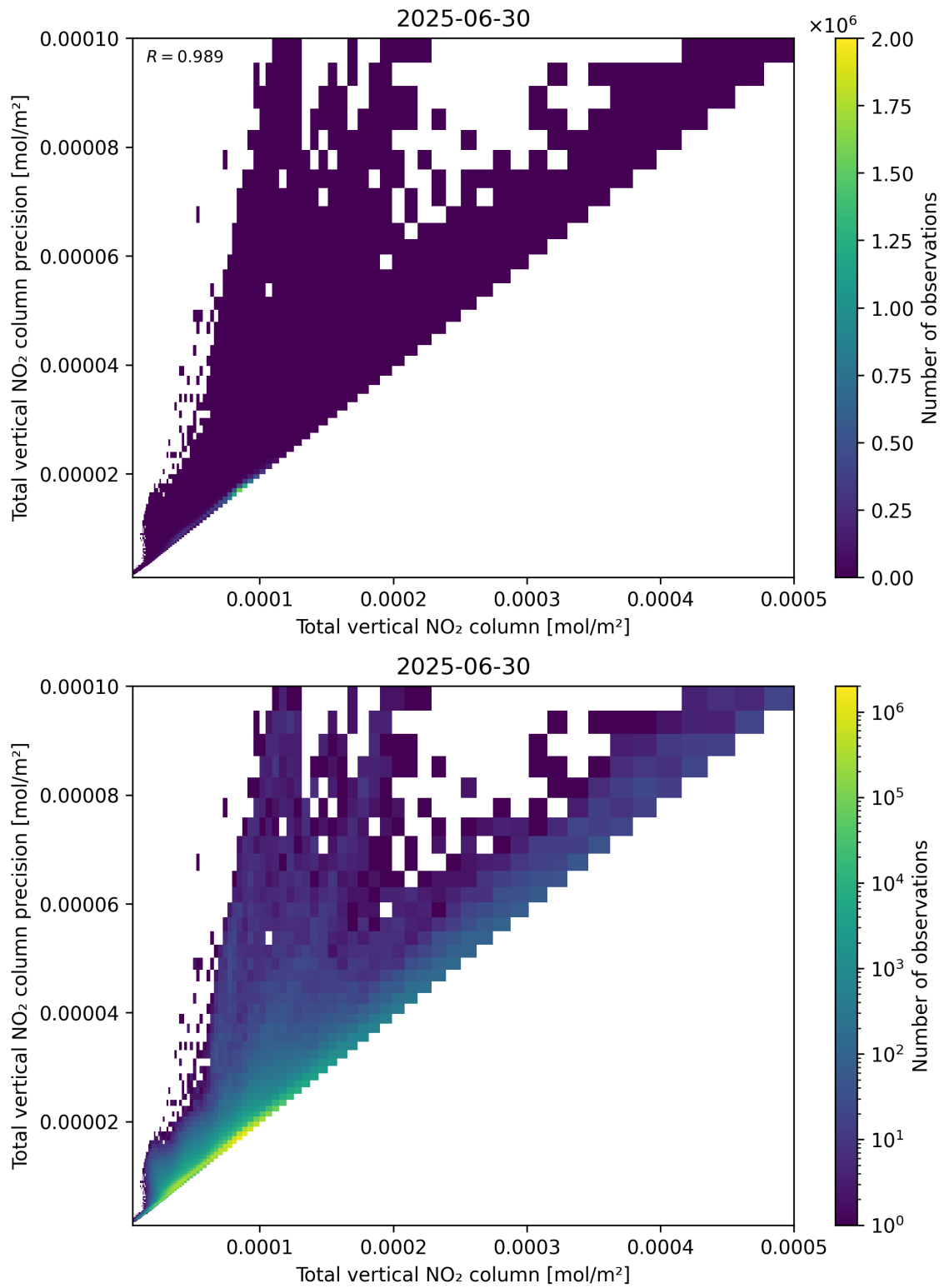
Figure 114: Scatter density plot of “Total vertical NO 2 column” against “Total vertical NO 2 column precision” for 2025-06-29 to 2025-07-01.
