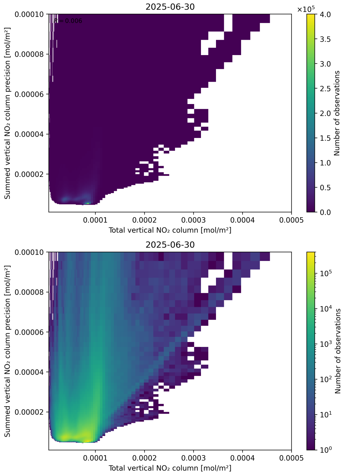
Figure 113: Scatter density plot of “Total vertical NO 2 column” against “Summed vertical NO 2 column precision” for 2025-06-29 to 2025-07-01.
