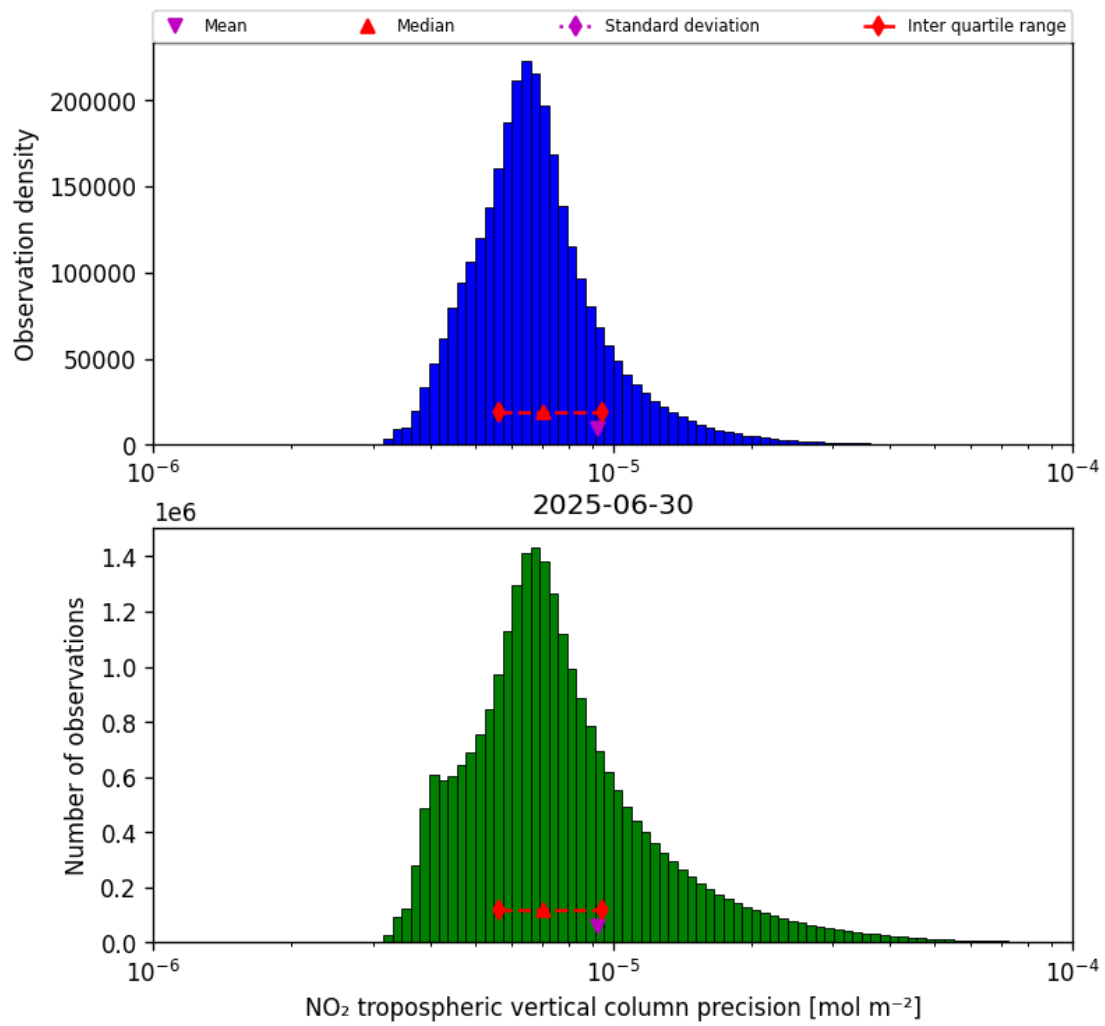
Figure 30: Histogram of “NO 2 tropospheric vertical column precision” for 2025-06-29 to 2025-07-01
