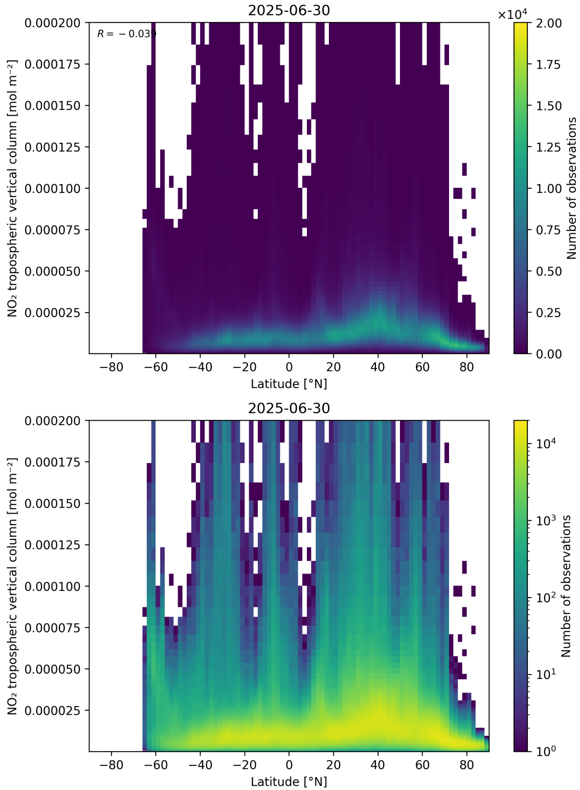
Figure 92: Scatter density plot of “Latitude” against “NO 2 tropospheric vertical column” for 2025-06-29 to 2025-07-01.
