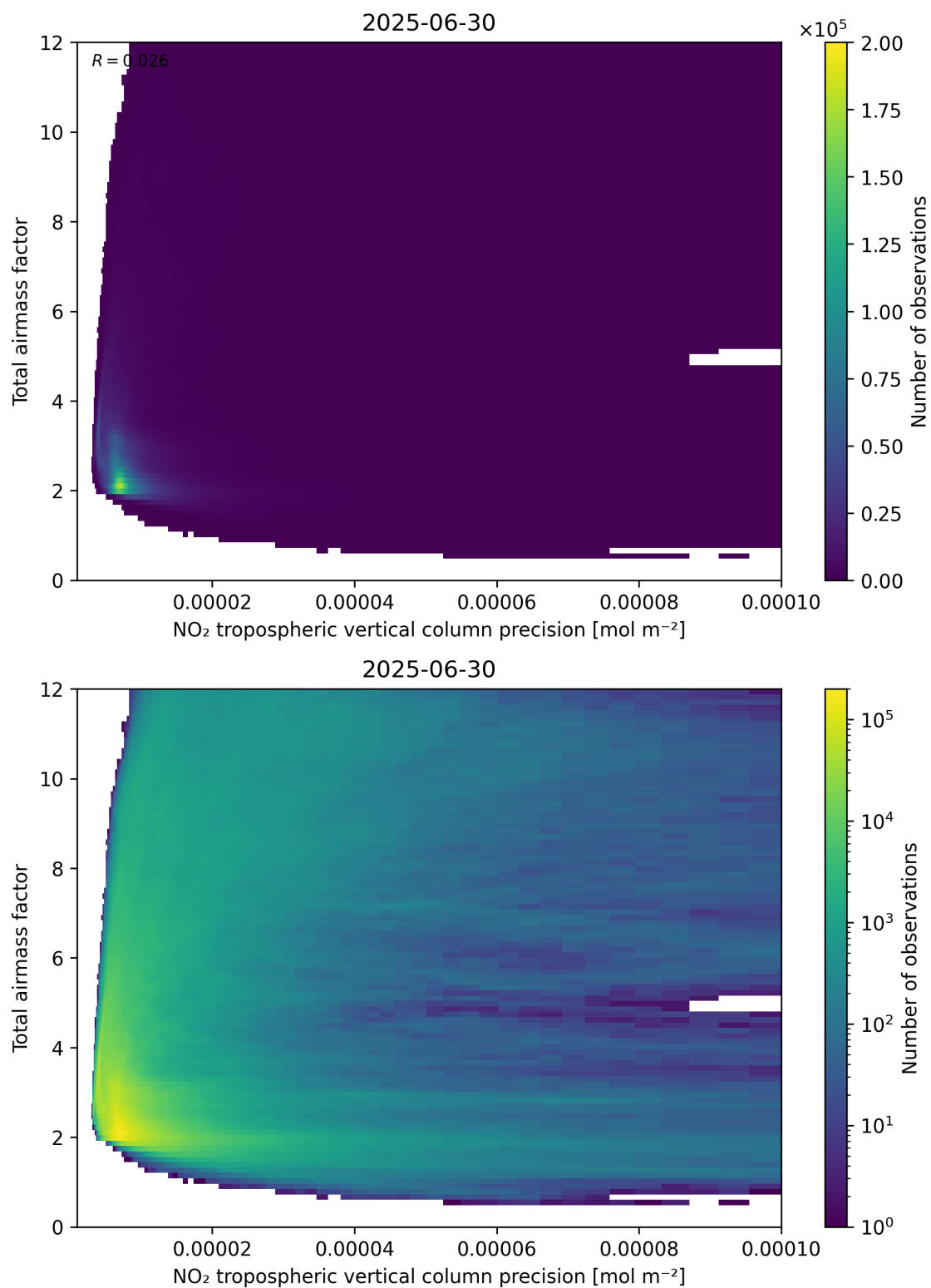
Figure 132: Scatter density plot of “NO 2 tropospheric vertical column precision” against “Total air mass factor” for 2025-06-29 to 2025-07-01.
