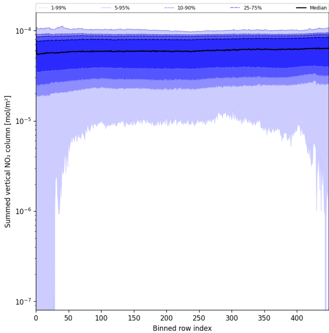
Figure 57: Along track statistics of “Summed vertical NO 2 column” for 2025-06-29 to 2025-07-01
