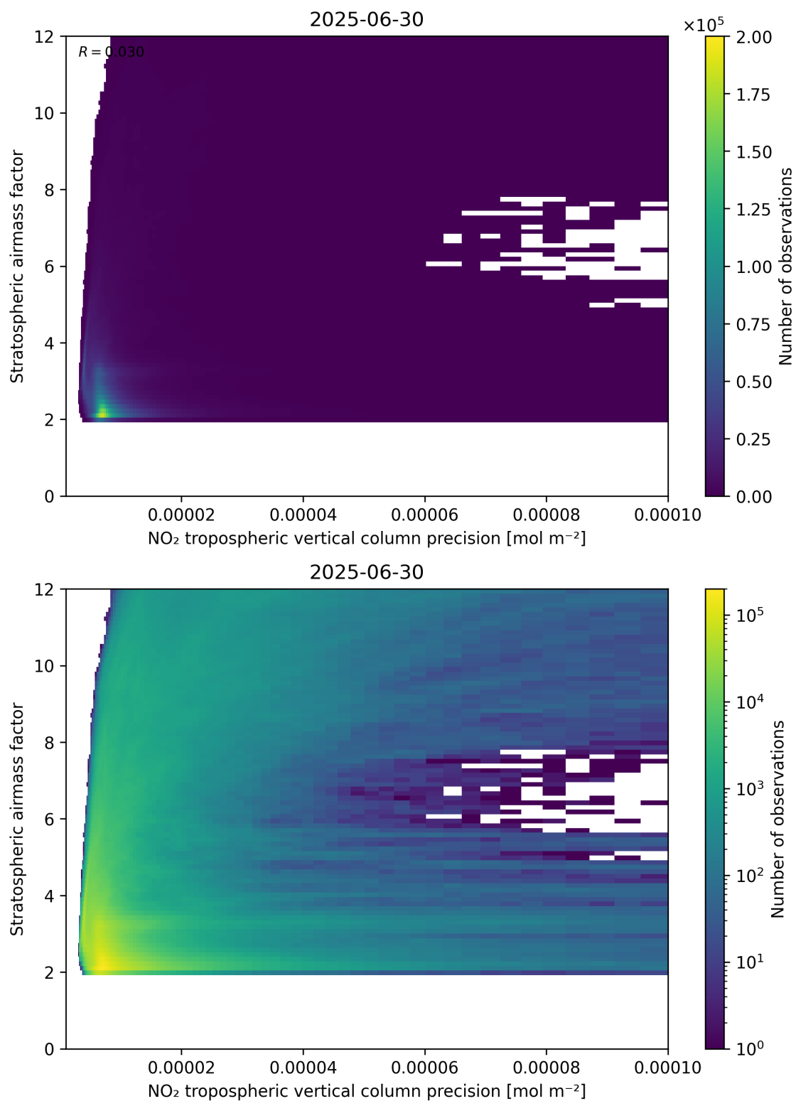
Figure 131: Scatter density plot of “NO 2 tropospheric vertical column precision” against “Stratospheric airmass factor” for 2025-06-29 to 2025-07-01.
