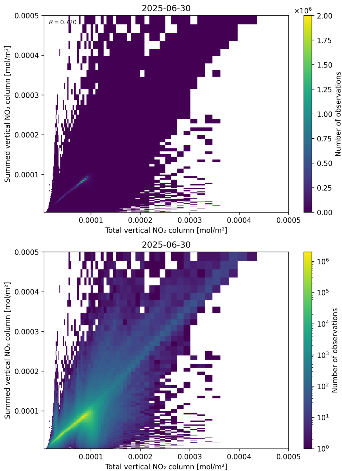
Figure 112: Scatter density plot of “Total vertical NO 2 column” against “Summed vertical NO 2 column” for 2025-06-29 to 2025-07-01.
