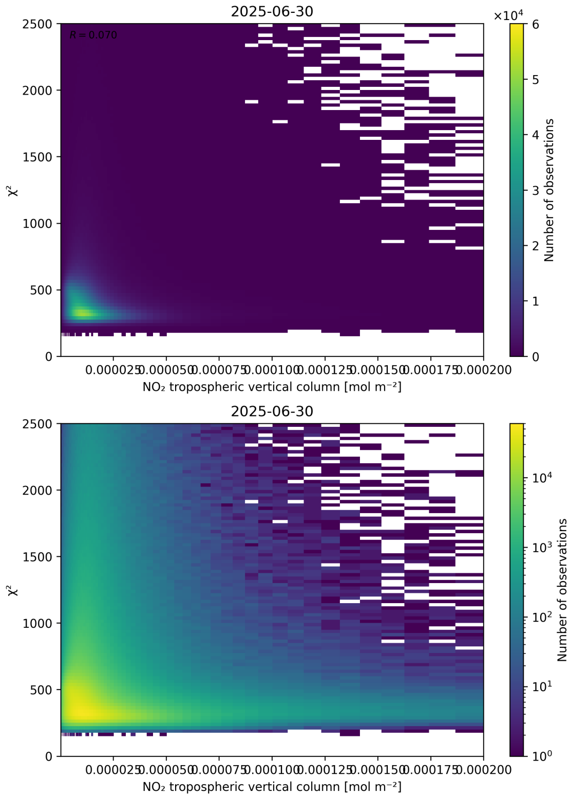
Figure 124: Scatter density plot of “NO 2 tropospheric vertical column” against “ \chi^2 ” for 2025-06-29 to 2025-07-01.
