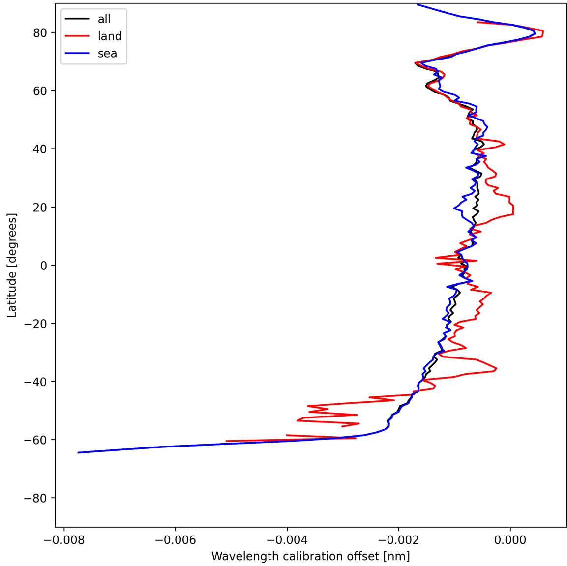
Figure 18: Zonal average of “Wavelength calibration offset” for 2025-06-29 to 2025-07-01.
