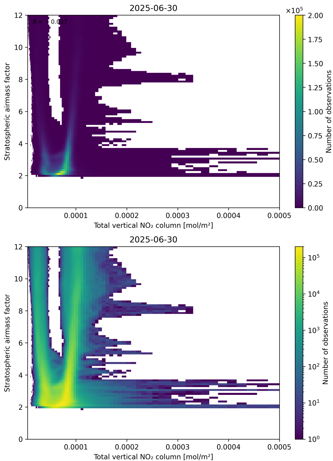
Figure 110: Scatter density plot of “Total vertical NO 2 column” against “Stratospheric airmass factor” for 2025-06-29 to 2025-07-01.
