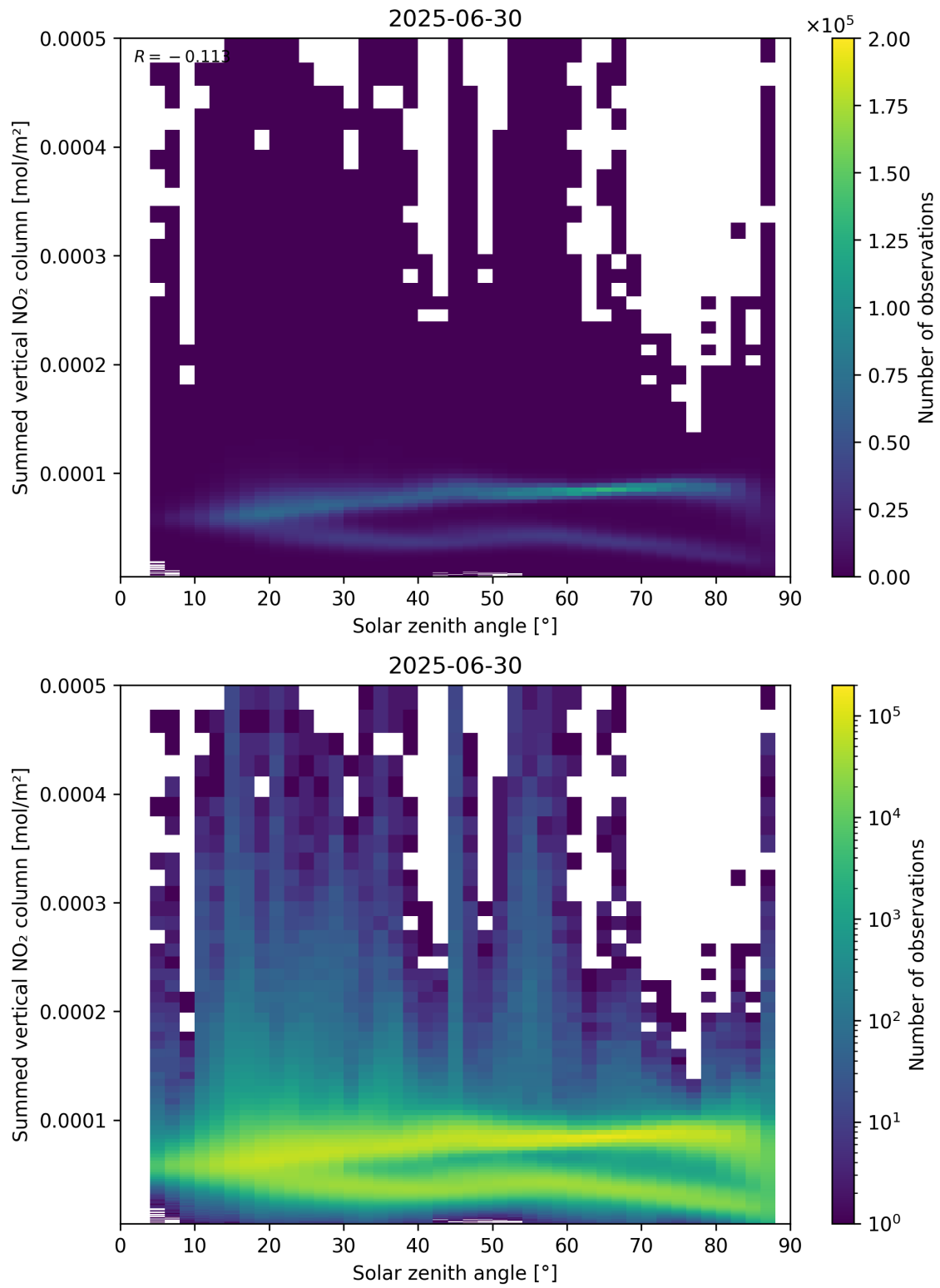
Figure 151: Scatter density plot of “Solar zenith angle” against “Summed vertical NO 2 column” for 2025-06-29 to 2025-07-01.
