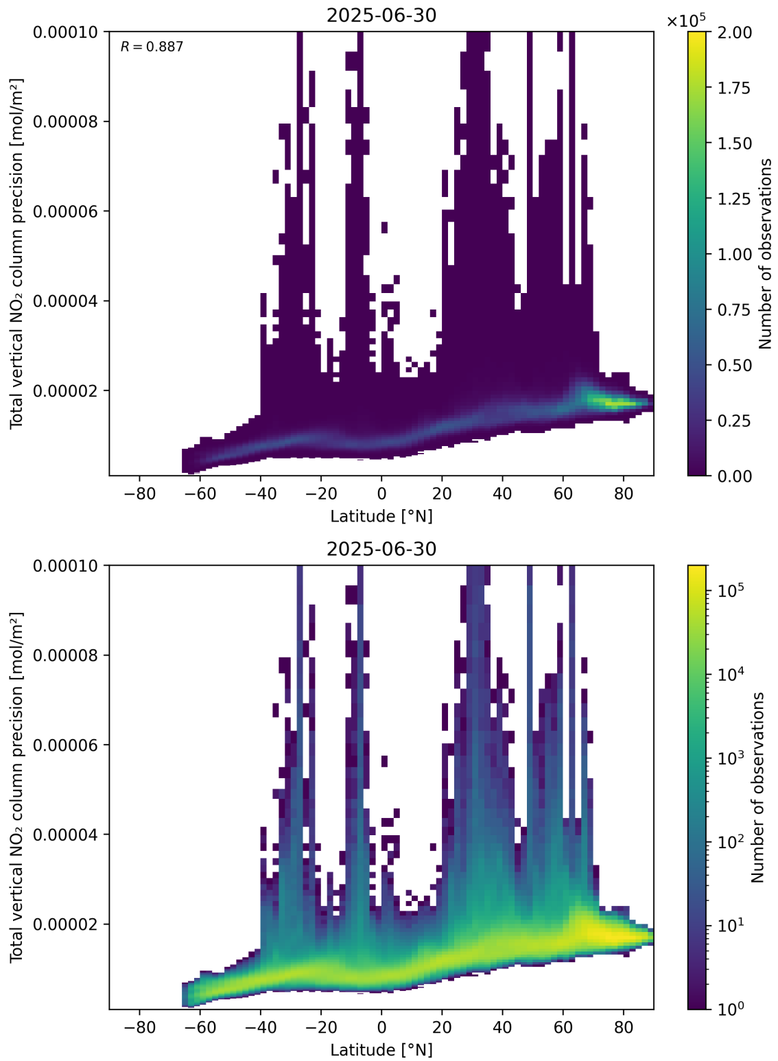
Figure 91: Scatter density plot of “Latitude” against “Total vertical NO 2 column precision” for 2025-06-29 to 2025-07-01.
