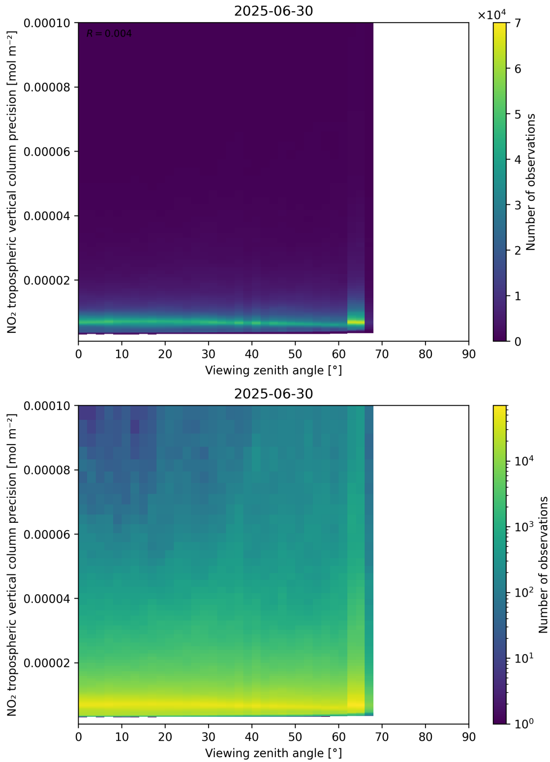
Figure 170: Scatter density plot of “Viewing zenith angle” against “NO 2 tropospheric vertical column precision” for 2025-06-29 to 2025-07-01.
