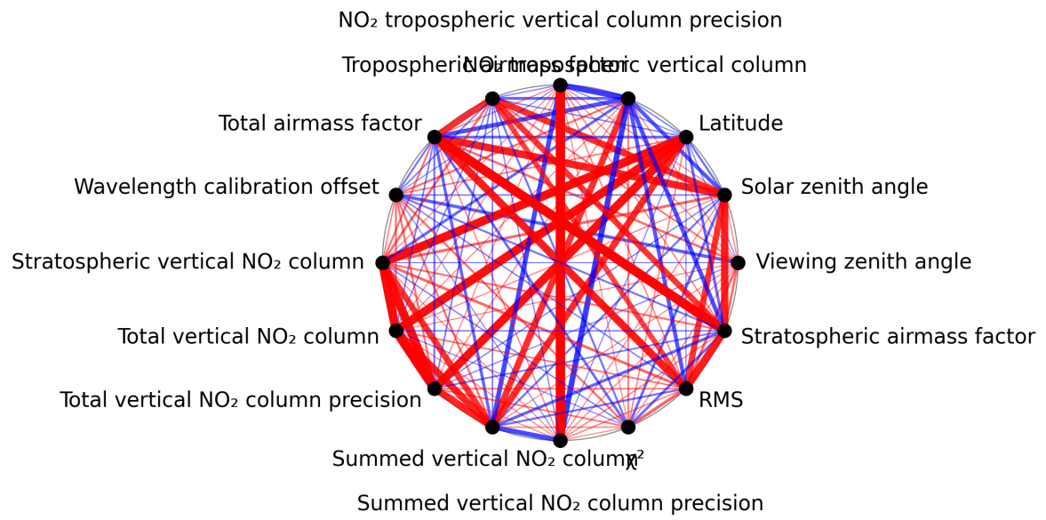
Figure 1: Map of correlation graph for 2025-06-29 to 2025-07-01.
