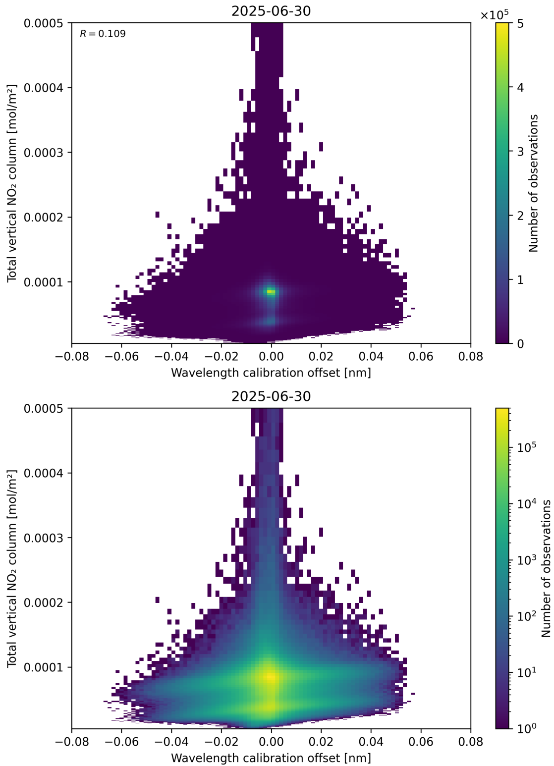
Figure 179: Scatter density plot of “Wavelength calibration offset” against “Total vertical NO 2 column” for 2025-06-29 to 2025-07-01.
