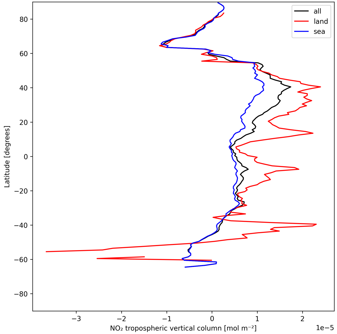
Figure 12: Zonal average of “NO 2 tropospheric vertical column” for 2025-06-29 to 2025-07-01.
