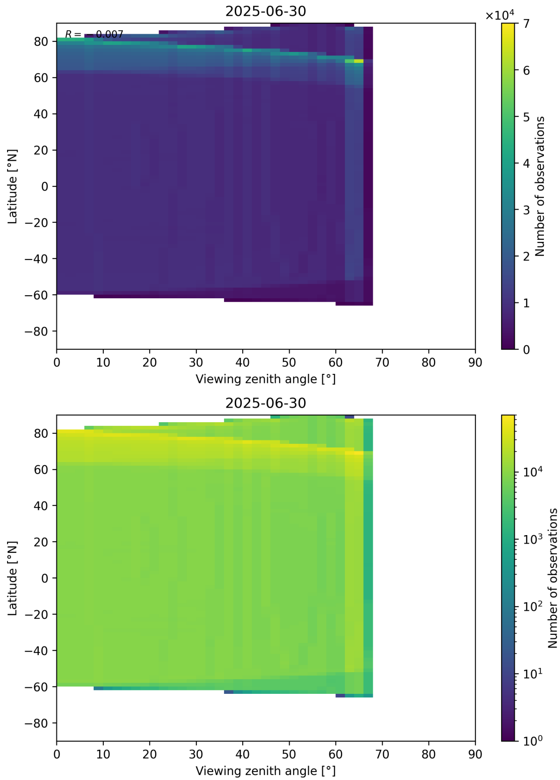
Figure 163: Scatter density plot of “Viewing zenith angle” against “Latitude” for 2025-06-29 to 2025-07-01.
