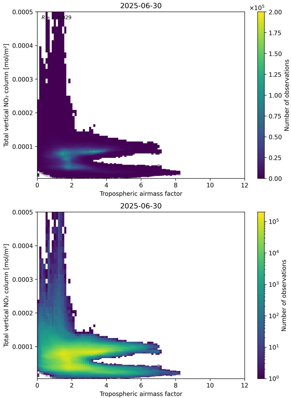
Figure 77: Scatter density plot of “Tropospheric airmass factor” against “Total vertical NO 2 column” for 2025-06-29 to 2025-07-01.
