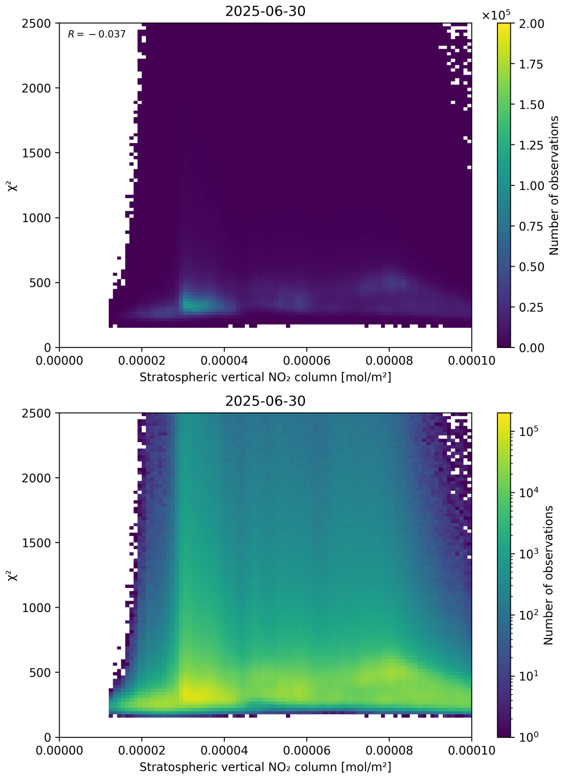
Figure 97: Scatter density plot of “Stratospheric vertical NO 2 column” against “ \chi^2 ” for 2025-06-29 to 2025-07-01.
