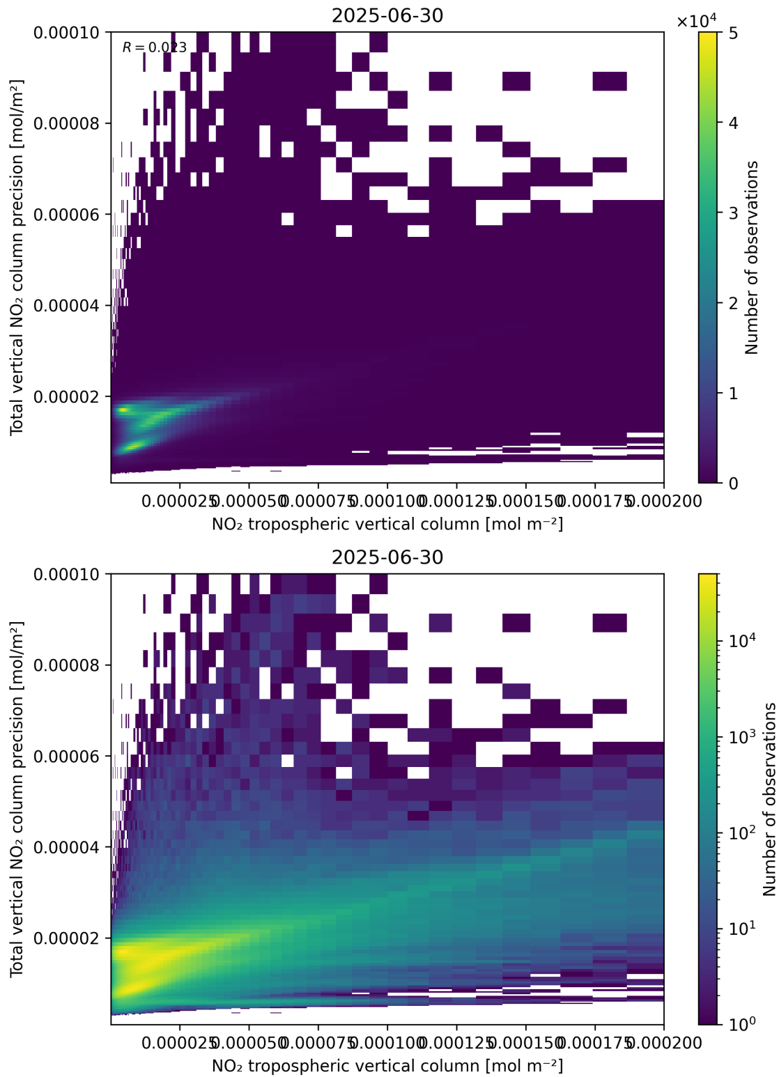
Figure 129: Scatter density plot of “NO 2 tropospheric vertical column” against “Total vertical NO 2 column precision” for 2025-06-29 to 2025-07-01.
