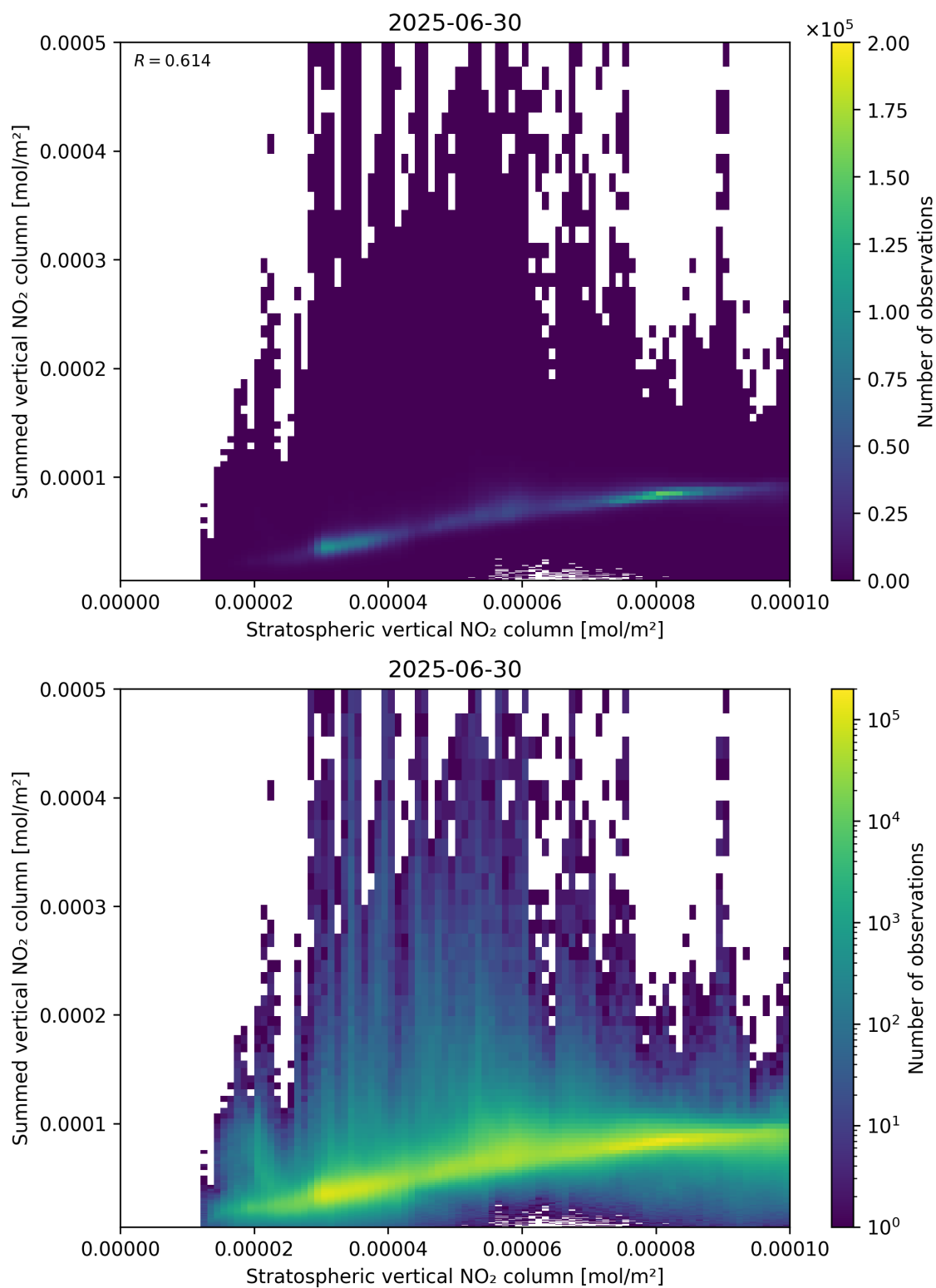
Figure 98: Scatter density plot of “Stratospheric vertical NO 2 column” against “Summed vertical NO 2 column” for 2025-06-29 to 2025-07-01.
