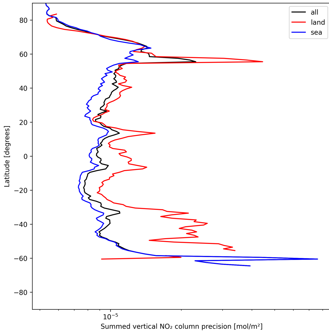
Figure 24: Zonal average of “Summed vertical NO 2 column precision” for 2025-06-29 to 2025-07-01.
