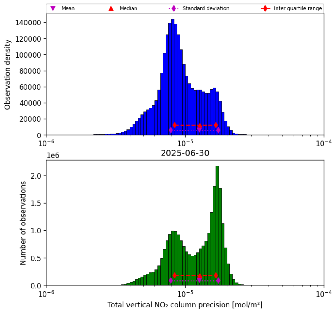
Figure 39: Histogram of “Total vertical NO 2 column precision” for 2025-06-29 to 2025-07-01
