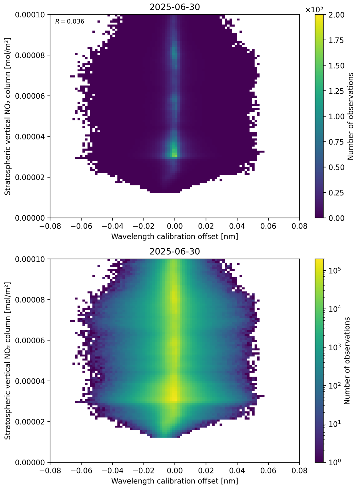
Figure 176: Scatter density plot of “Wavelength calibration offset” against “Stratospheric vertical NO 2 column” for 2025-06-29 to 2025-07-01.
