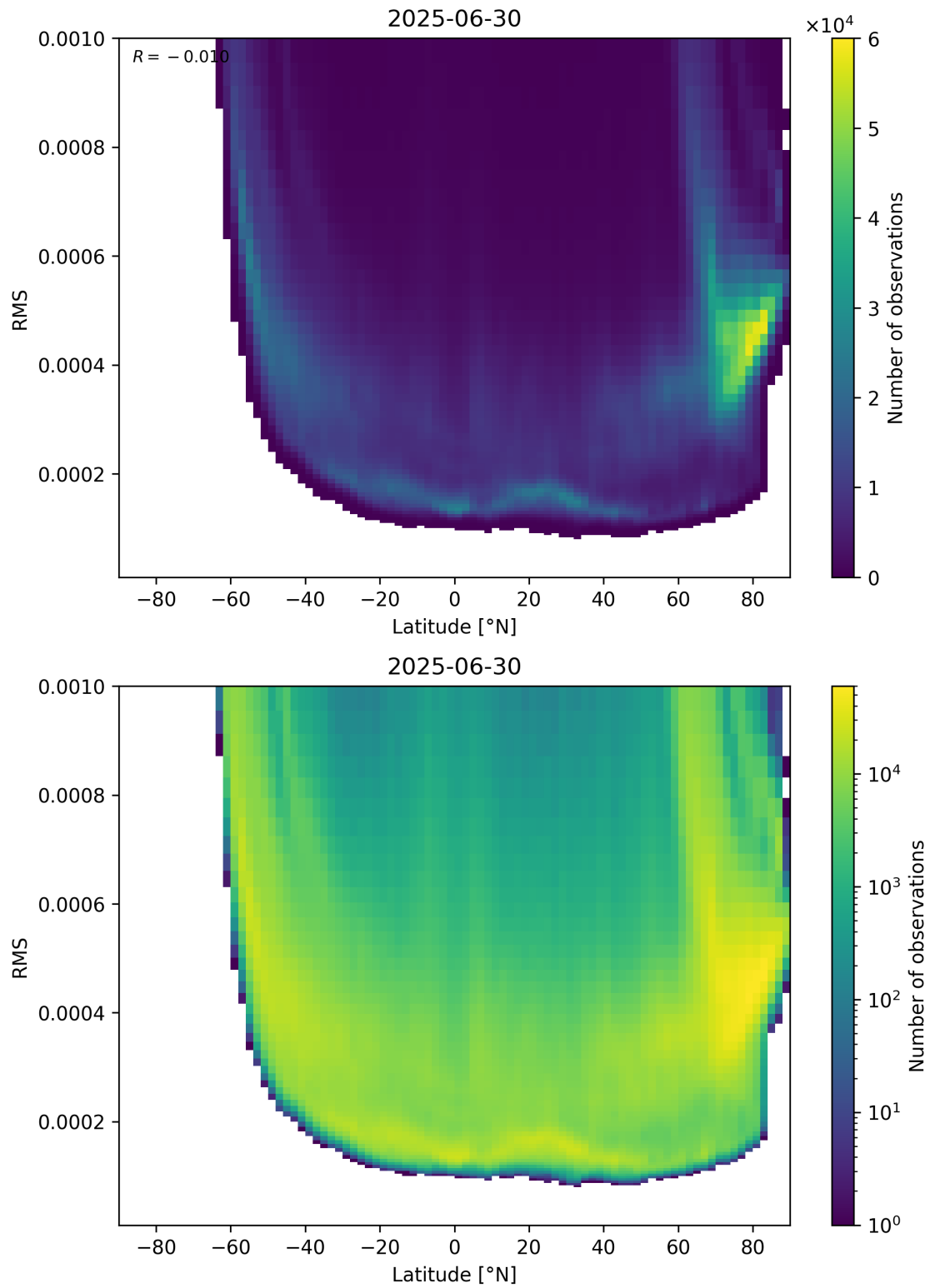
Figure 94: Scatter density plot of “Latitude” against “RMS” for 2025-06-29 to 2025-07-01.
