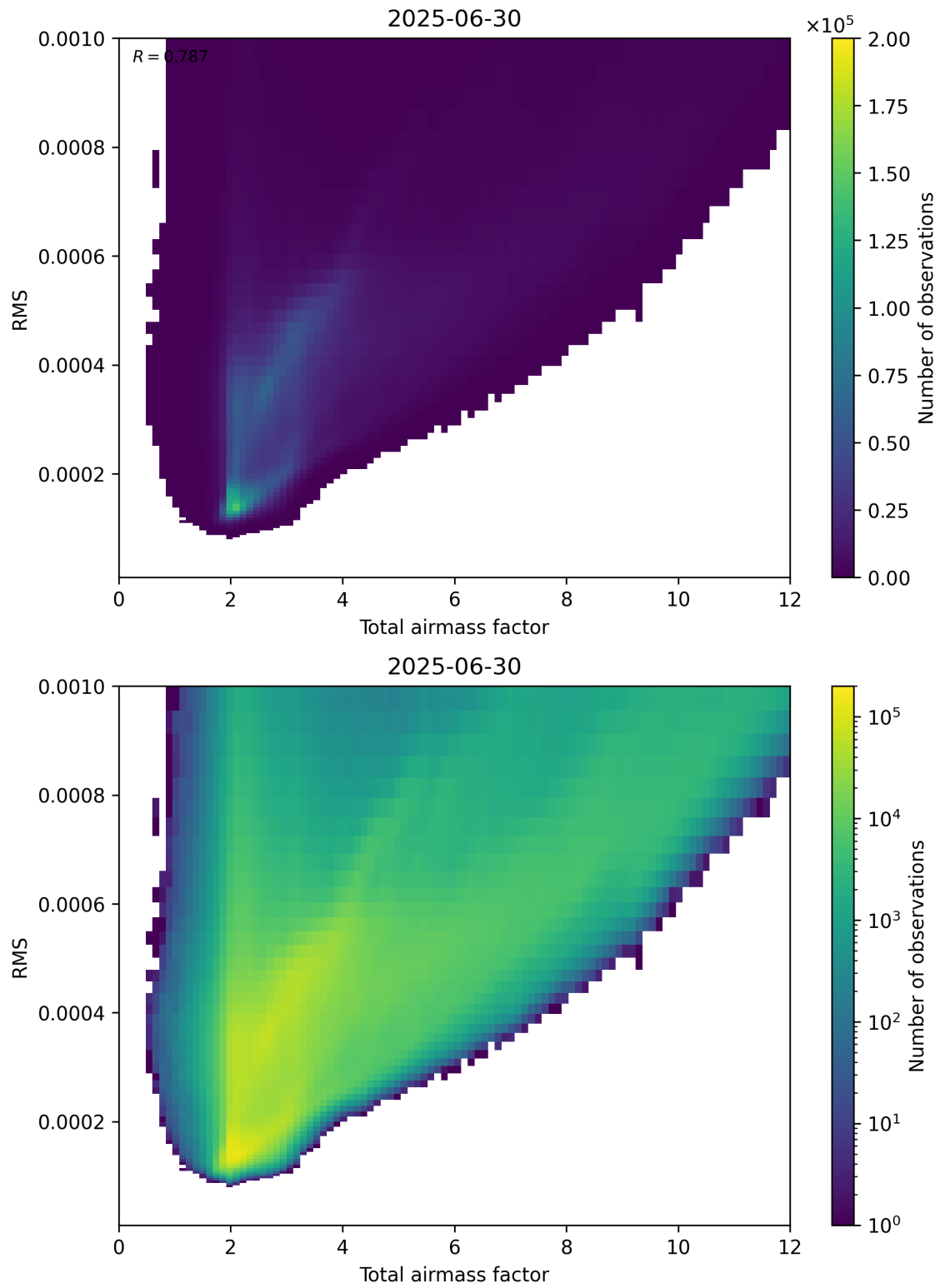
Figure 69: Scatter density plot of “Total airmass factor” against “RMS” for 2025-06-29 to 2025-07-01.
