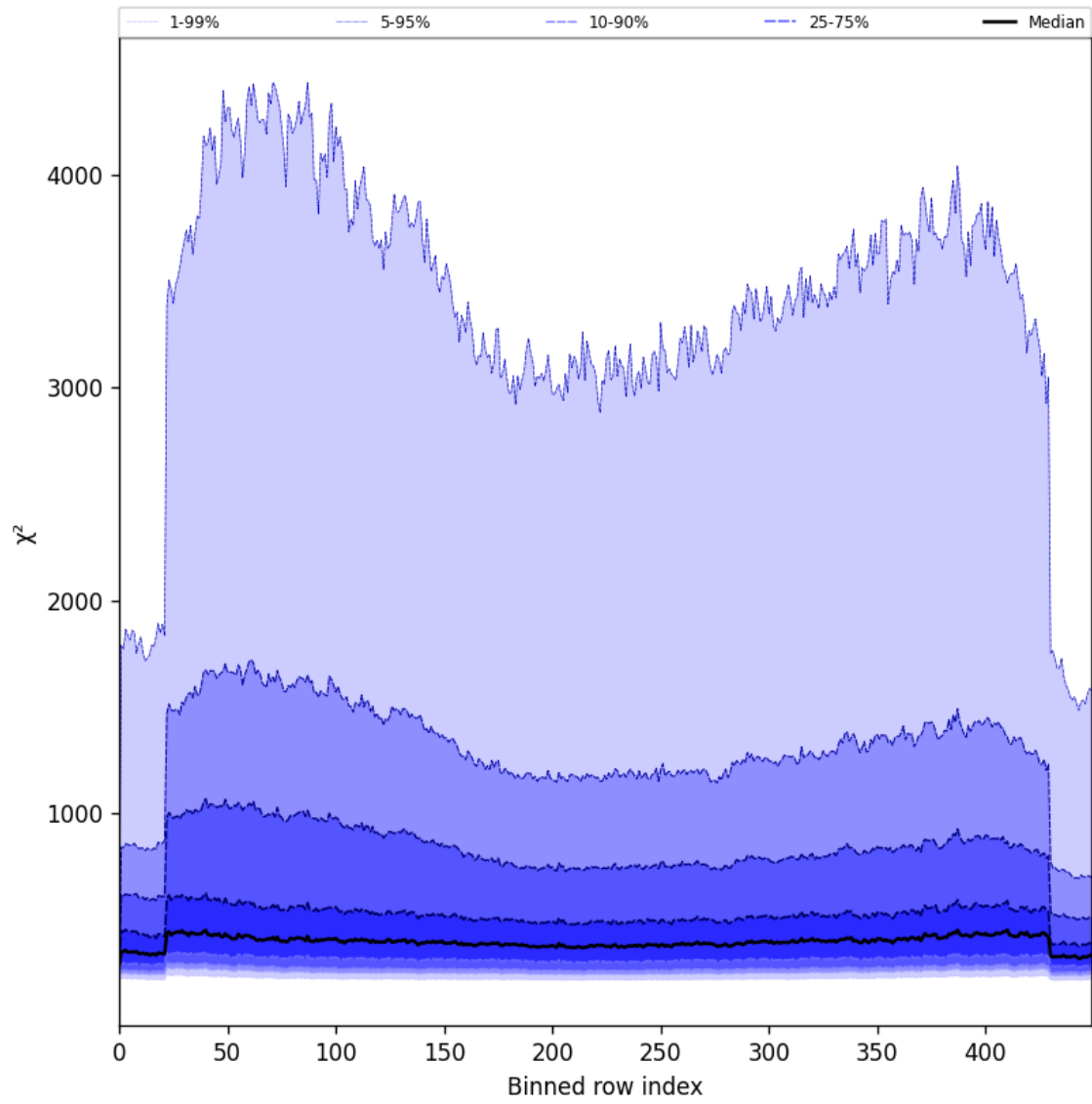
Figure 59: Along track statistics of “ \chi^2 ” for 2025-06-29 to 2025-07-01
