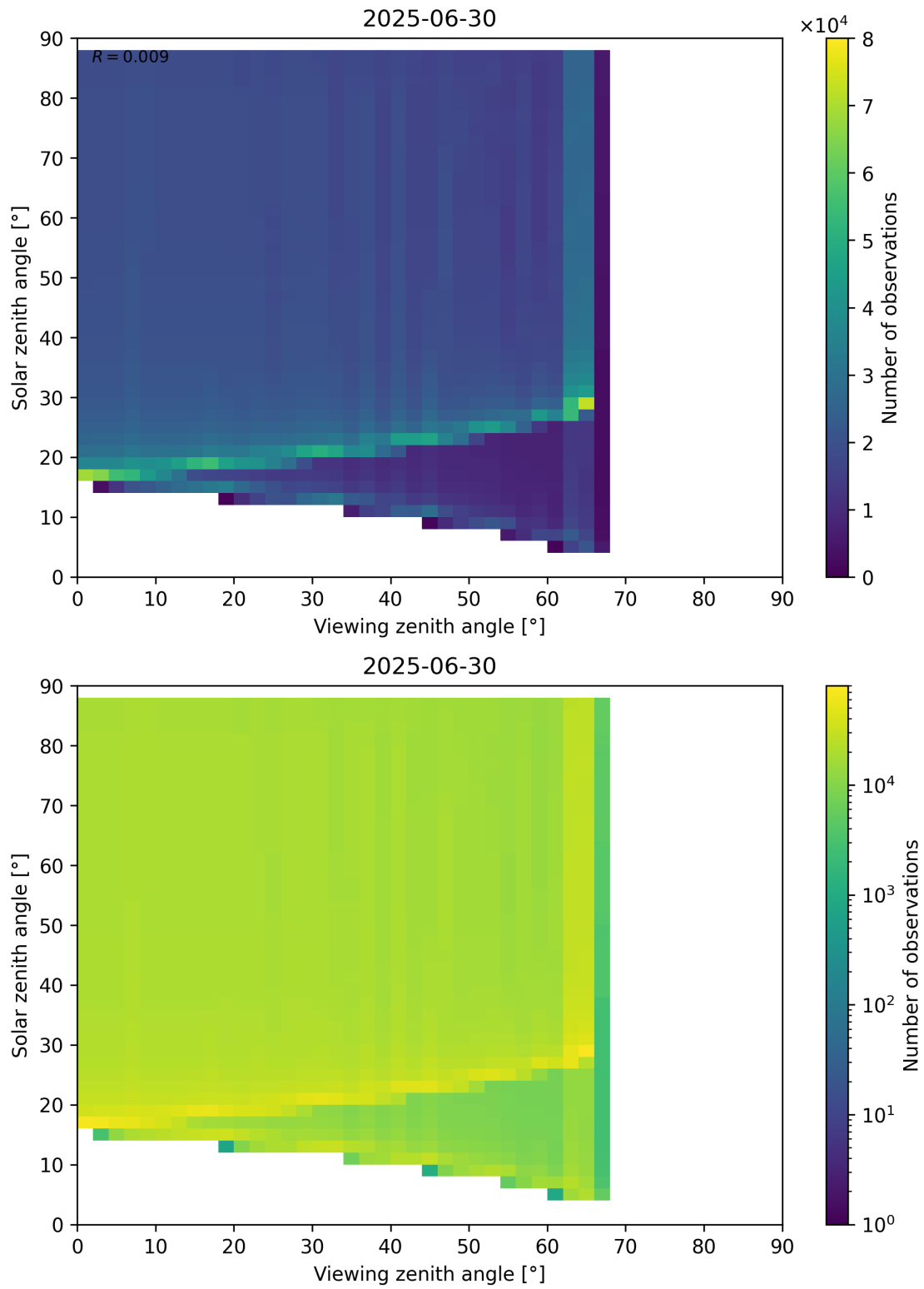
Figure 172: Scatter density plot of “Viewing zenith angle” against “Solar zenith angle” for 2025-06-29 to 2025-07-01.
