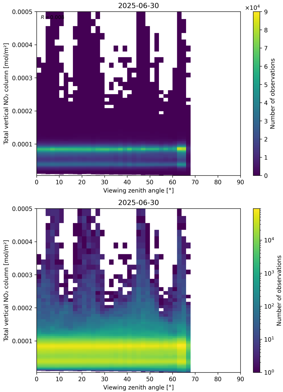
Figure 167: Scatter density plot of “Viewing zenith angle” against “Total vertical NO 2 column” for 2025-06-29 to 2025-07-01.
