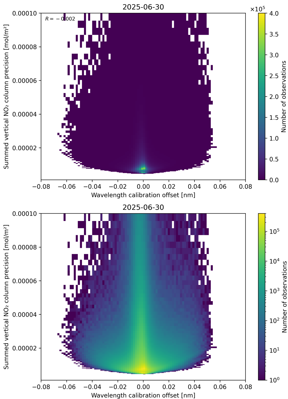
Figure 178: Scatter density plot of “Wavelength calibration offset” against “Summed vertical NO 2 column precision” for 2025-06-29 to 2025-07-01.
