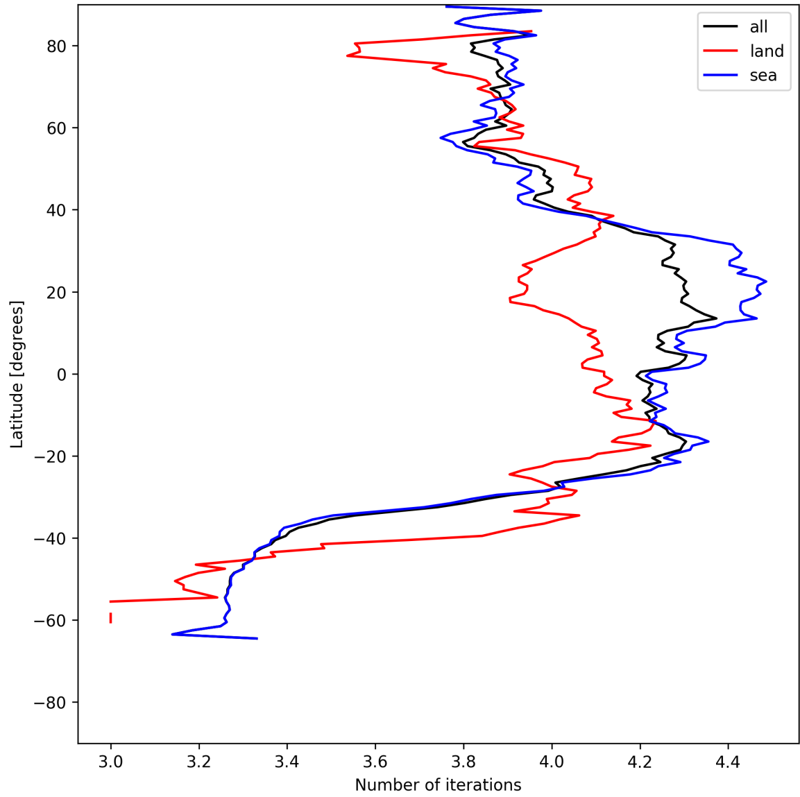
Figure 17: Zonal average of “Number of iterations” for 2025-06-29 to 2025-07-01.
