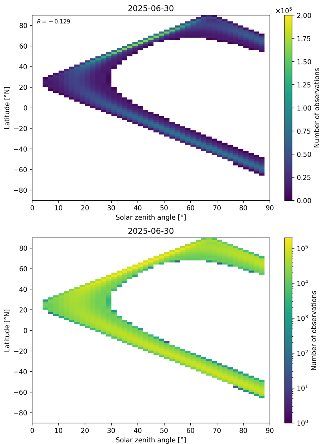
Figure 149: Scatter density plot of “Solar zenith angle” against “Latitude” for 2025-06-29 to 2025-07-01.
