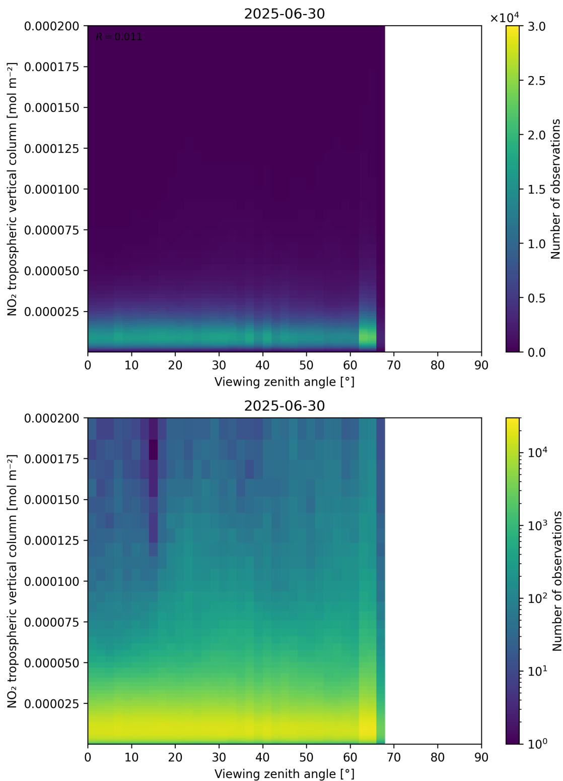
Figure 169: Scatter density plot of “Viewing zenith angle” against “NO 2 tropospheric vertical column” for 2025-06-29 to 2025-07-01.
