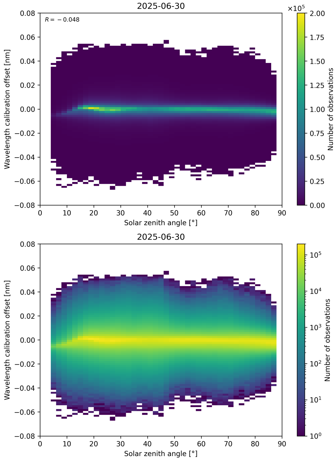
Figure 158: Scatter density plot of “Solar zenith angle” against “Wavelength calibration offset” for 2025-06-29 to 2025-07-01.
