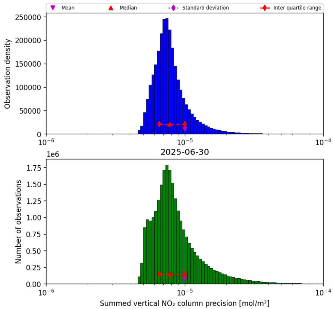
Figure 41: Histogram of "Summed vertical NO 2 column precision" for 2025-06-29 to 2025-07-01
