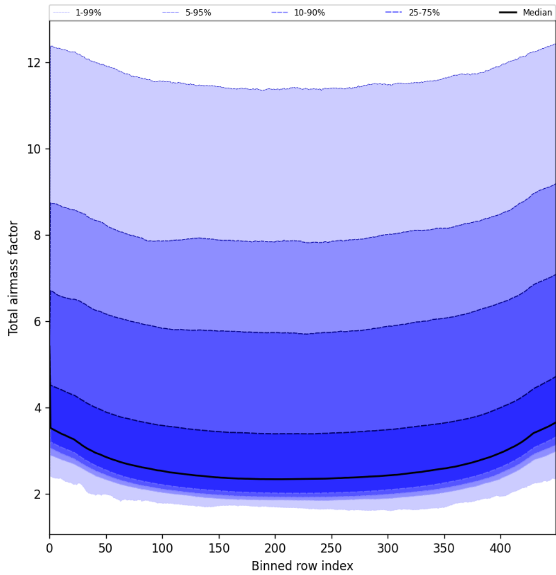
Figure 49: Along track statistics of “Total airmass factor” for 2025-06-29 to 2025-07-01
