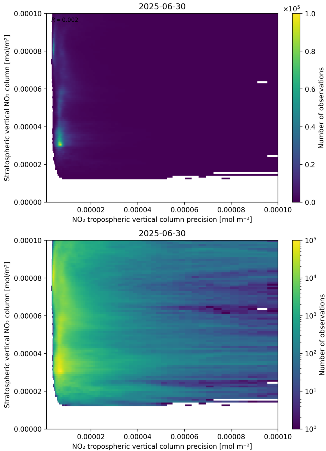
Figure 135: Scatter density plot of “NO 2 tropospheric vertical column precision” against “Stratospheric vertical NO 2 column” for 2025-06-29 to 2025-07-01.
