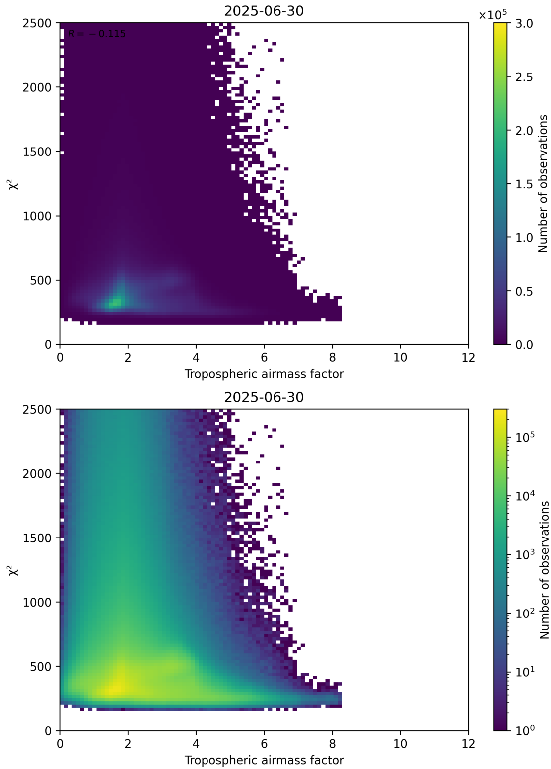
Figure 73: Scatter density plot of “Tropospheric airmass factor” against “ \chi^2 ” for 2025-06-29 to 2025-07-01.
