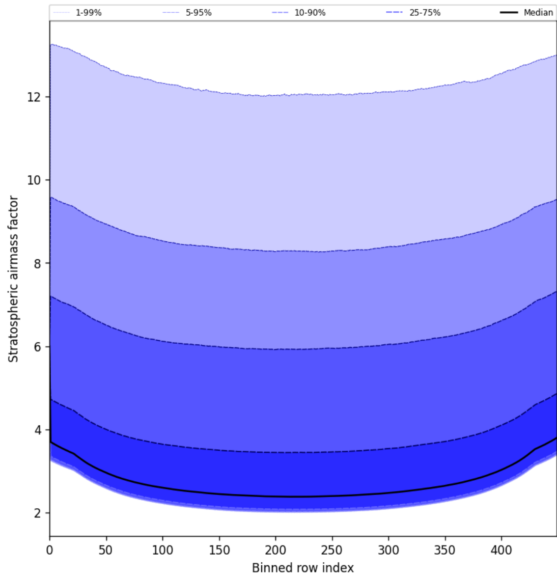
Figure 61: Along track statistics of “Stratospheric airmass factor” for 2025-06-29 to 2025-07-01
