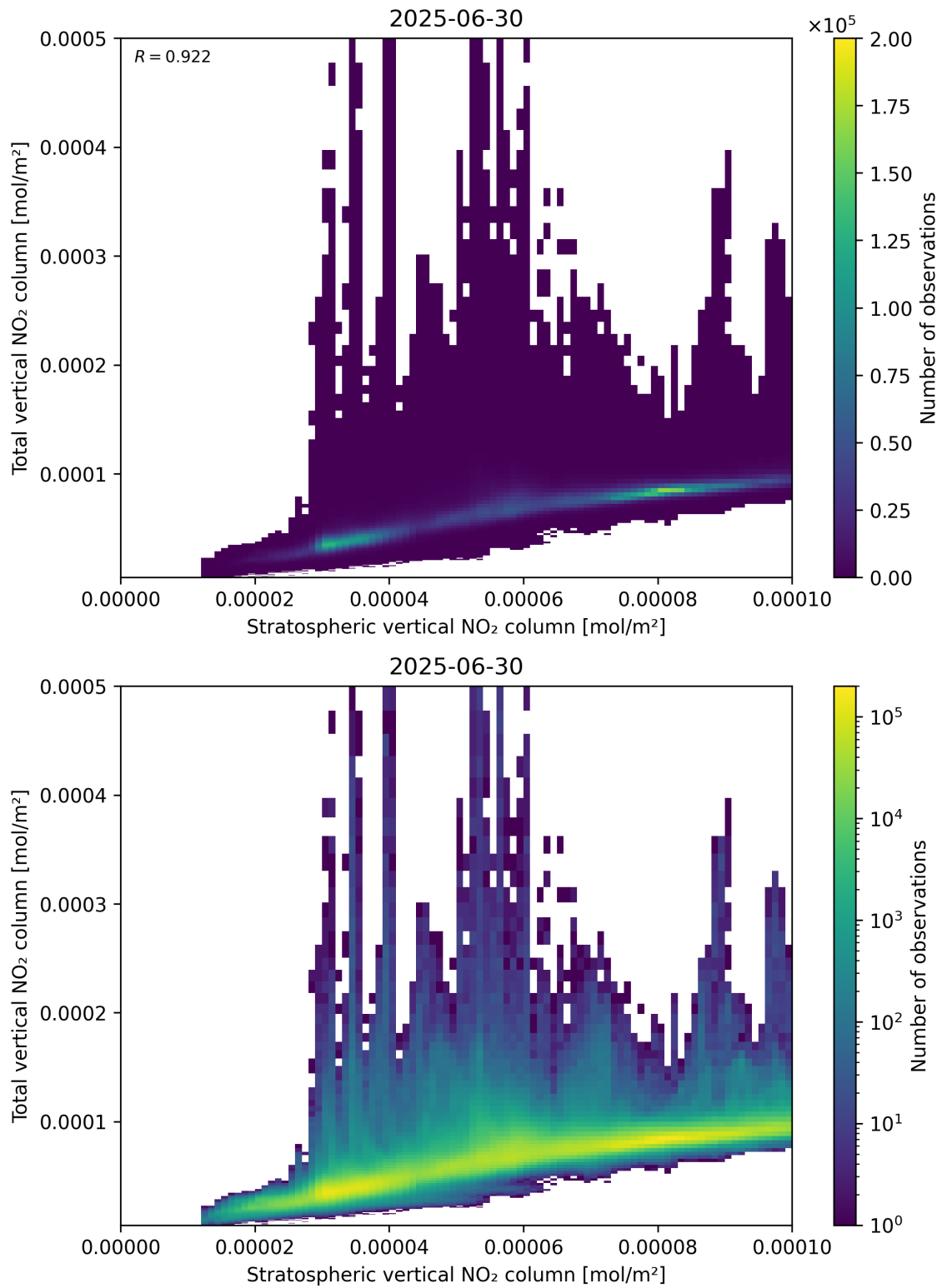
Figure 100: Scatter density plot of “Stratospheric vertical NO 2 column” against “Total vertical NO 2 column” for 2025-06-29 to 2025-07-01.
