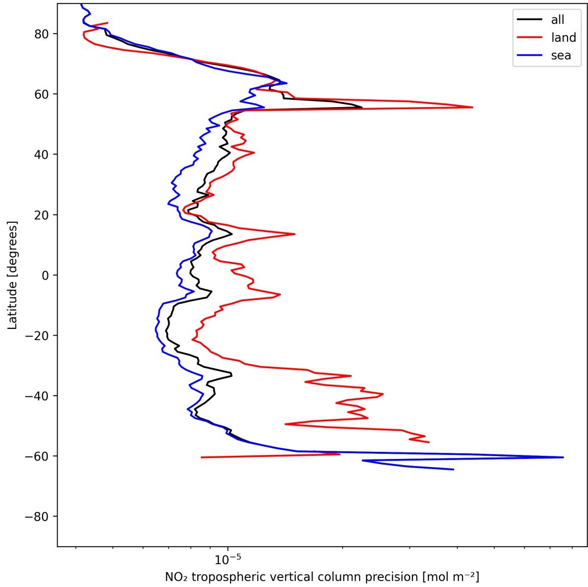
Figure 13: Zonal average of “NO 2 tropospheric vertical column precision” for 2025-06-29 to 2025-07-01.
