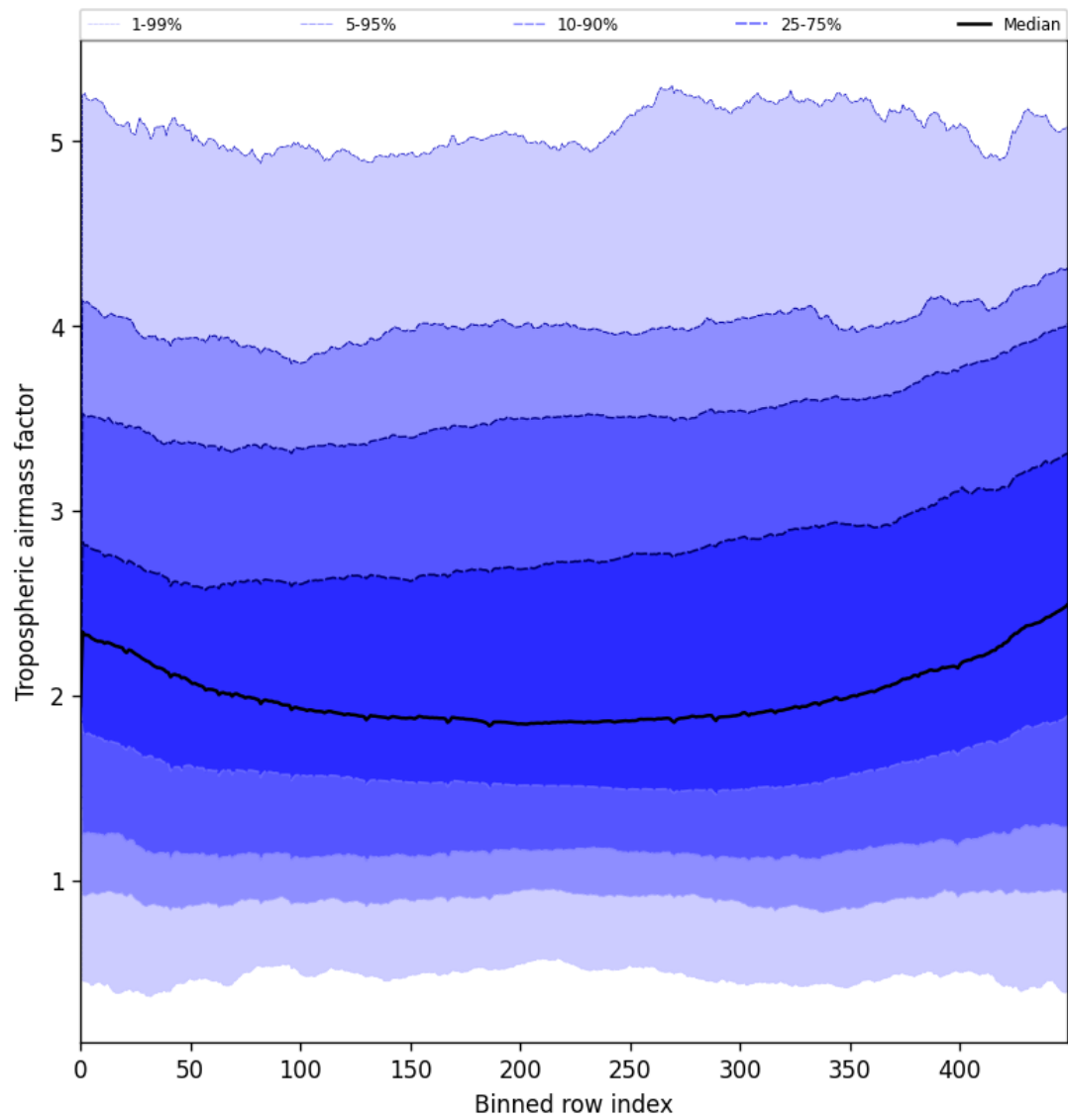
Figure 48: Along track statistics of “Tropospheric air mass factor” for 2025-06-29 to 2025-07-01
