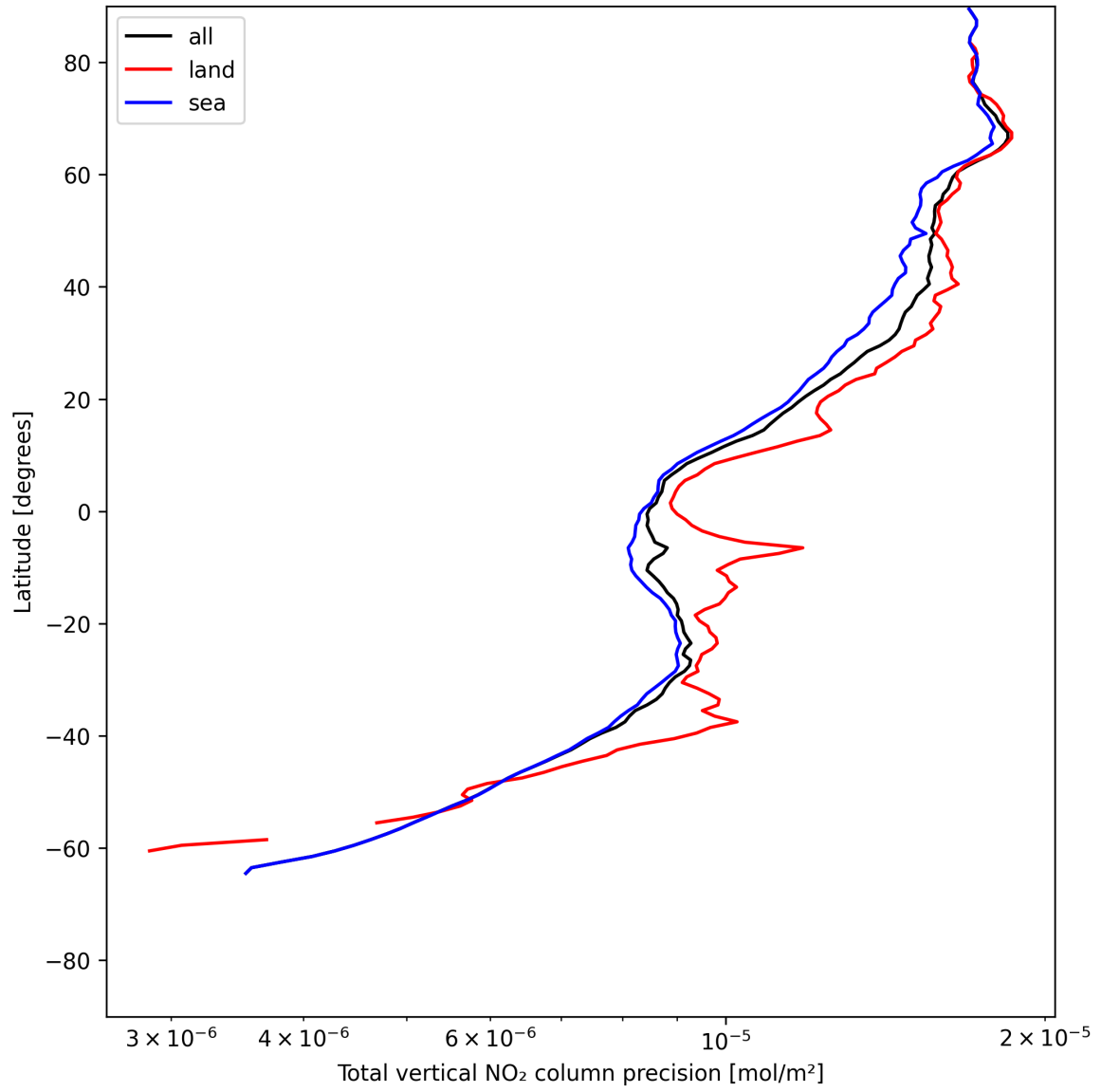
Figure 22: Zonal average of “Total vertical NO 2 column precision” for 2025-06-29 to 2025-07-01.
