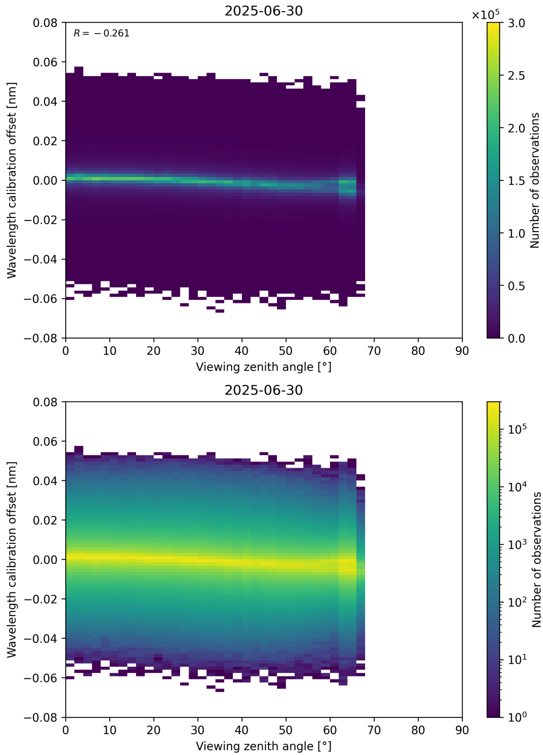
Figure 173: Scatter density plot of “Viewing zenith angle” against “Wavelength calibration offset” for 2025-06-29 to 2025-07-01.
