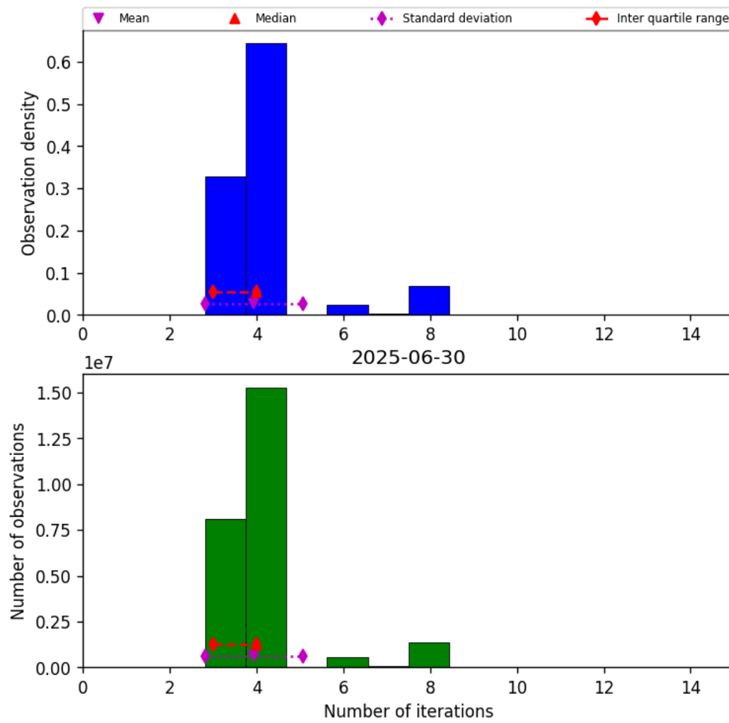
Figure 34: Histogram of "Number of iterations" for 2025-06-29 to 2025-07-01
