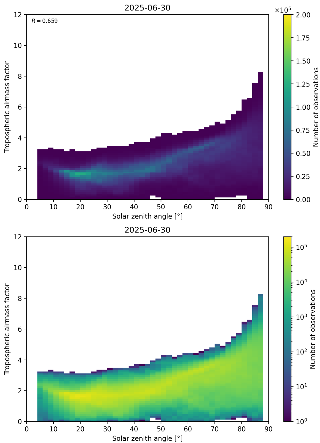
Figure 147: Scatter density plot of “Solar zenith angle” against “Tropospheric airmass factor” for 2025-06-29 to 2025-07-01.
