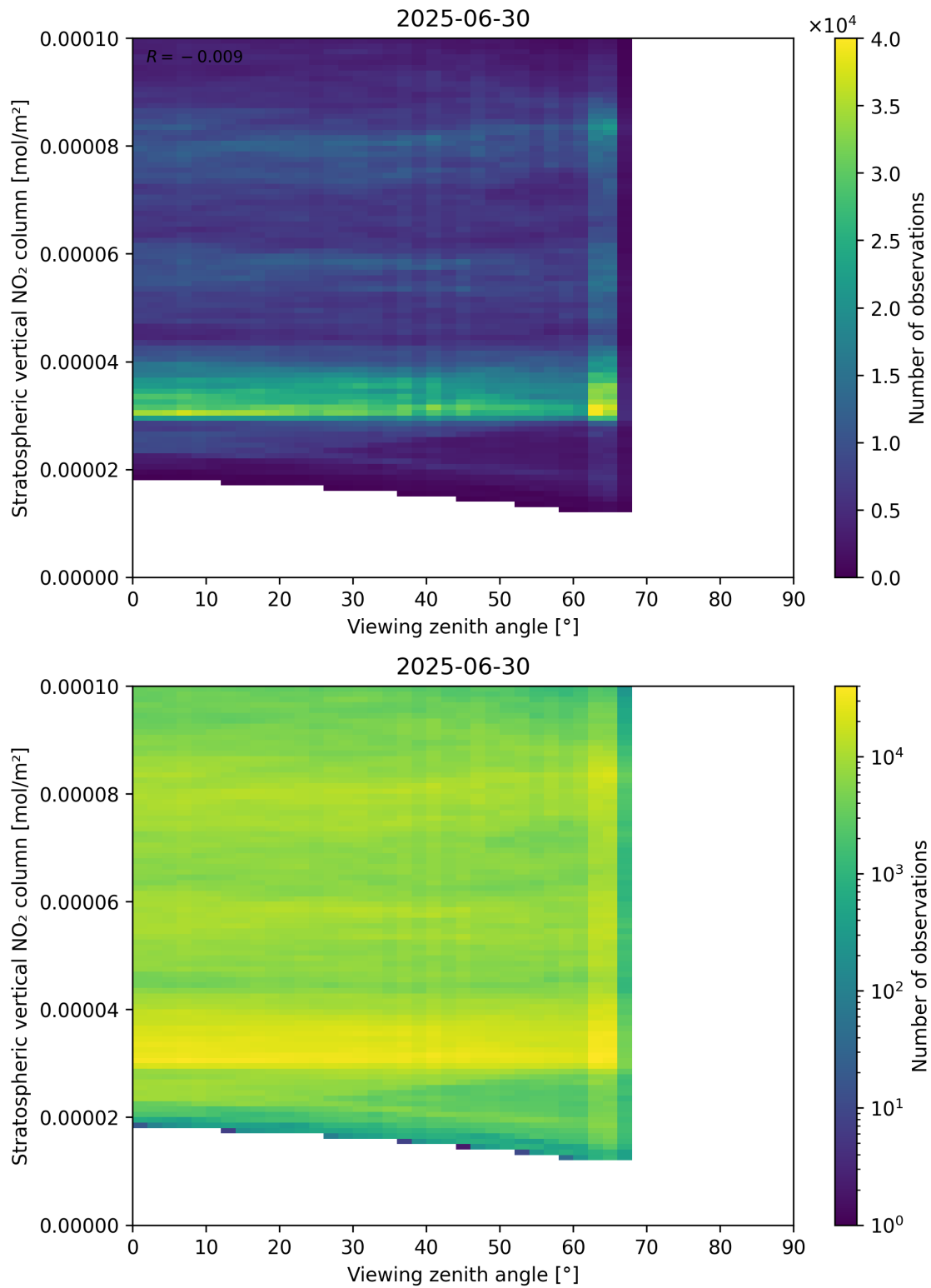
Figure 164: Scatter density plot of “Viewing zenith angle” against “Stratospheric vertical NO 2 column” for 2025-06-29 to 2025-07-01.
