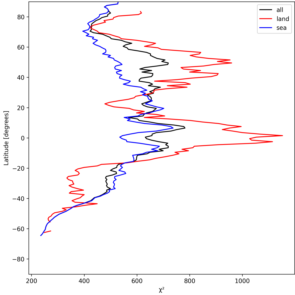
Figure 25: Zonal average of “ \chi^2 ” for 2025-06-30 to 2025-07-02.
