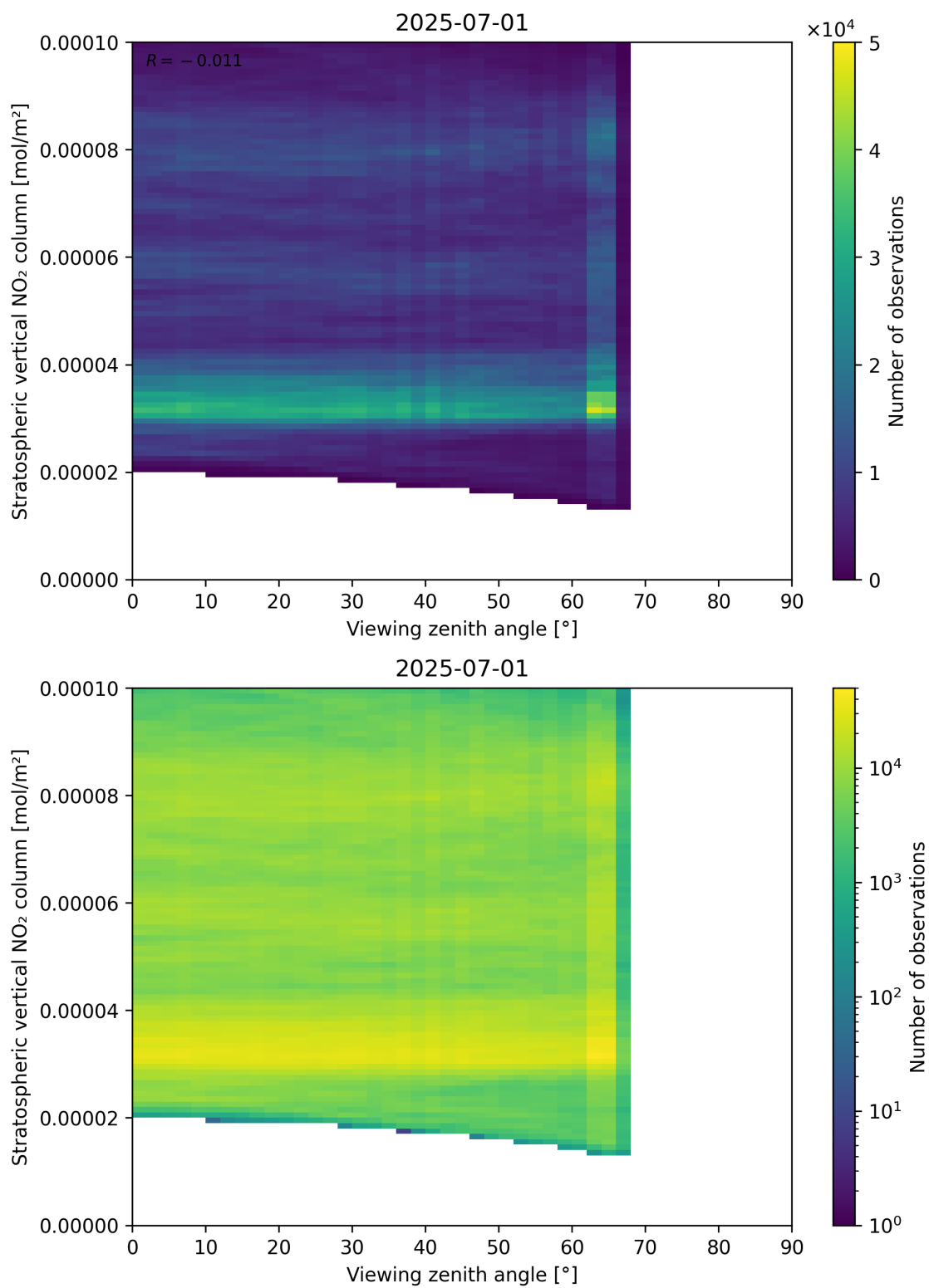
Figure 164: Scatter density plot of “Viewing zenith angle” against “Stratospheric vertical NO 2 column” for 2025-06-30 to 2025-07-02.
