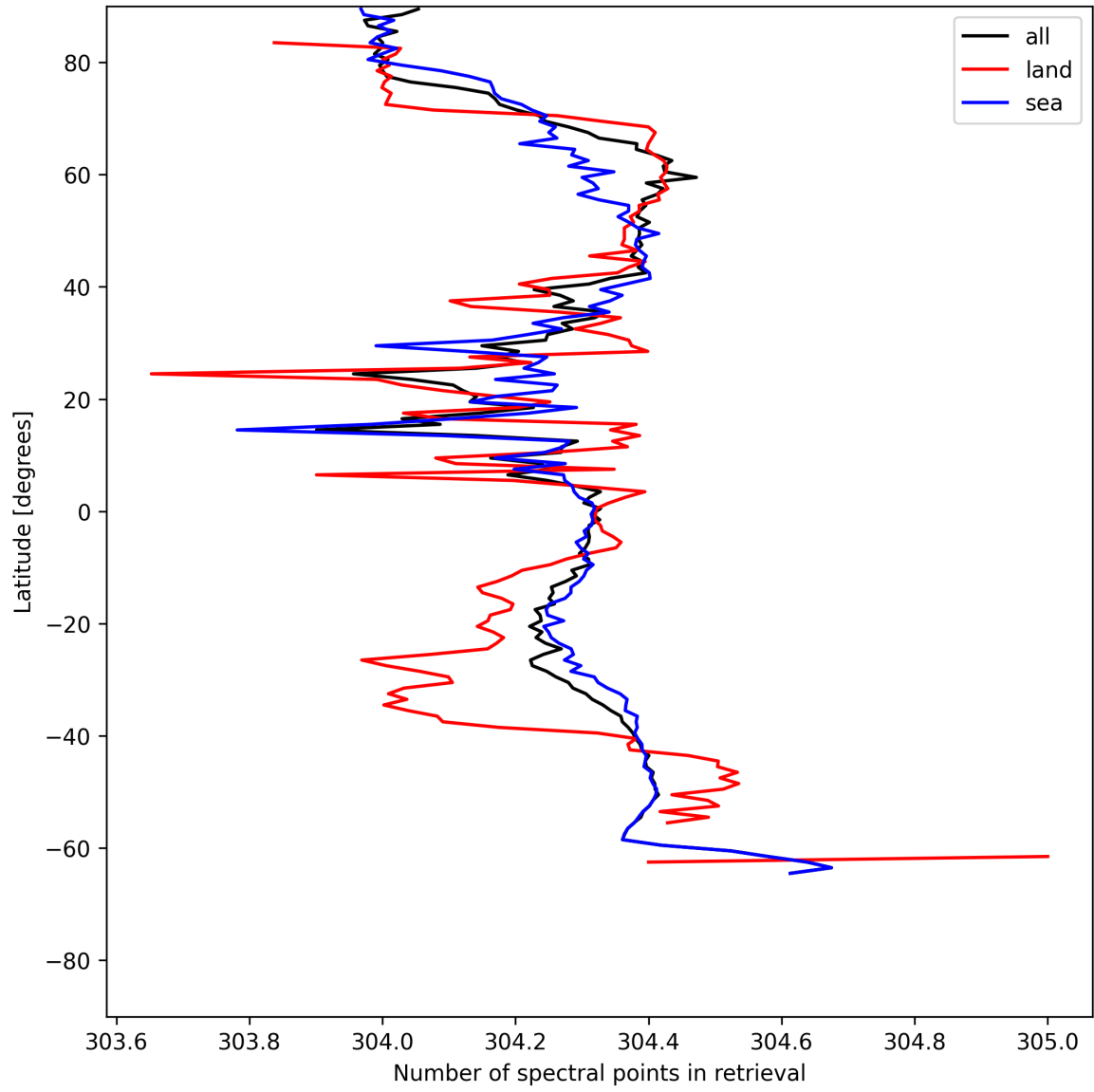
Figure 16: Zonal average of “Number of spectral points in retrieval” for 2025-06-30 to 2025-07-02.
