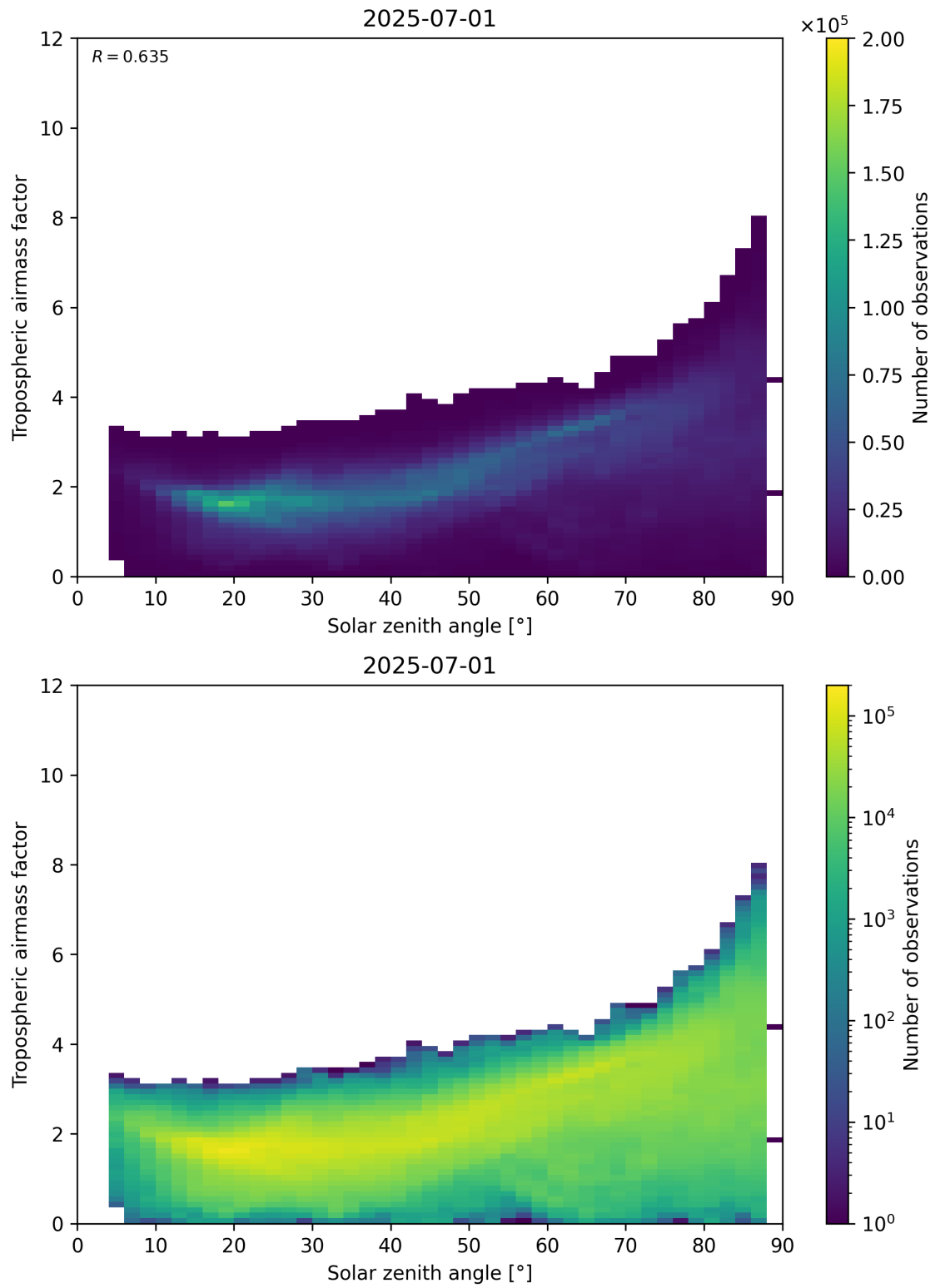
Figure 147: Scatter density plot of “Solar zenith angle” against “Tropospheric airmass factor” for 2025-06-30 to 2025-07-02.
