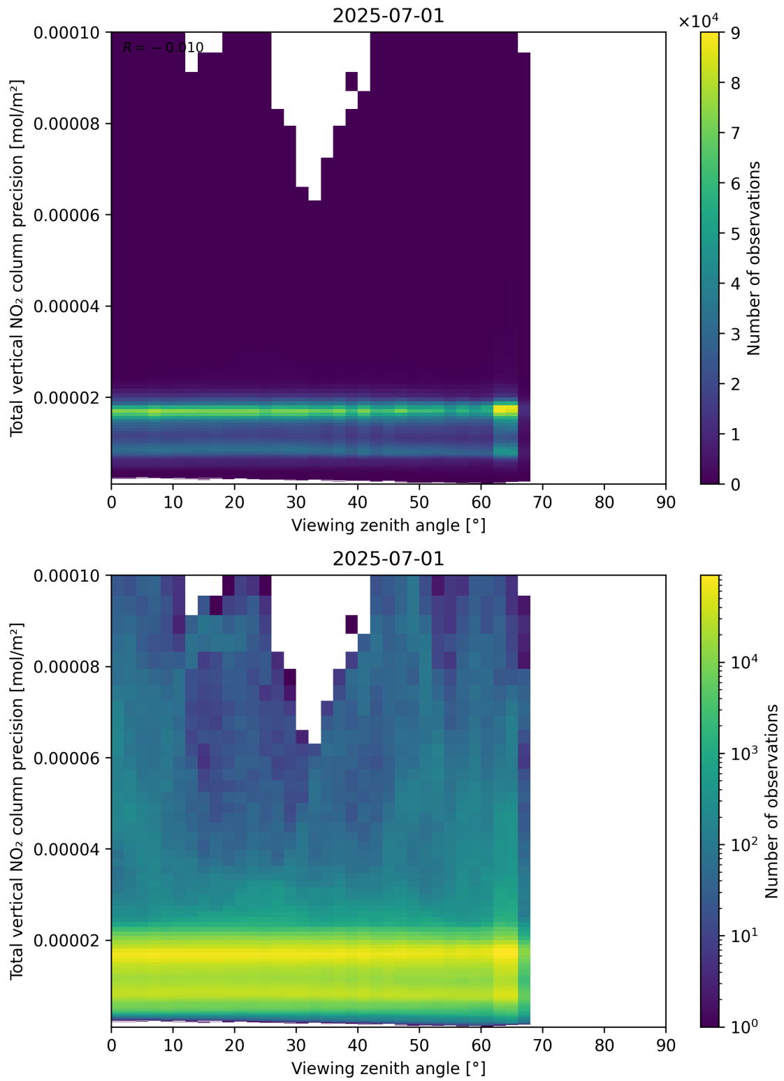
Figure 168: Scatter density plot of “Viewing zenith angle” against “Total vertical NO 2 column precision” for 2025-06-30 to 2025-07-02.
