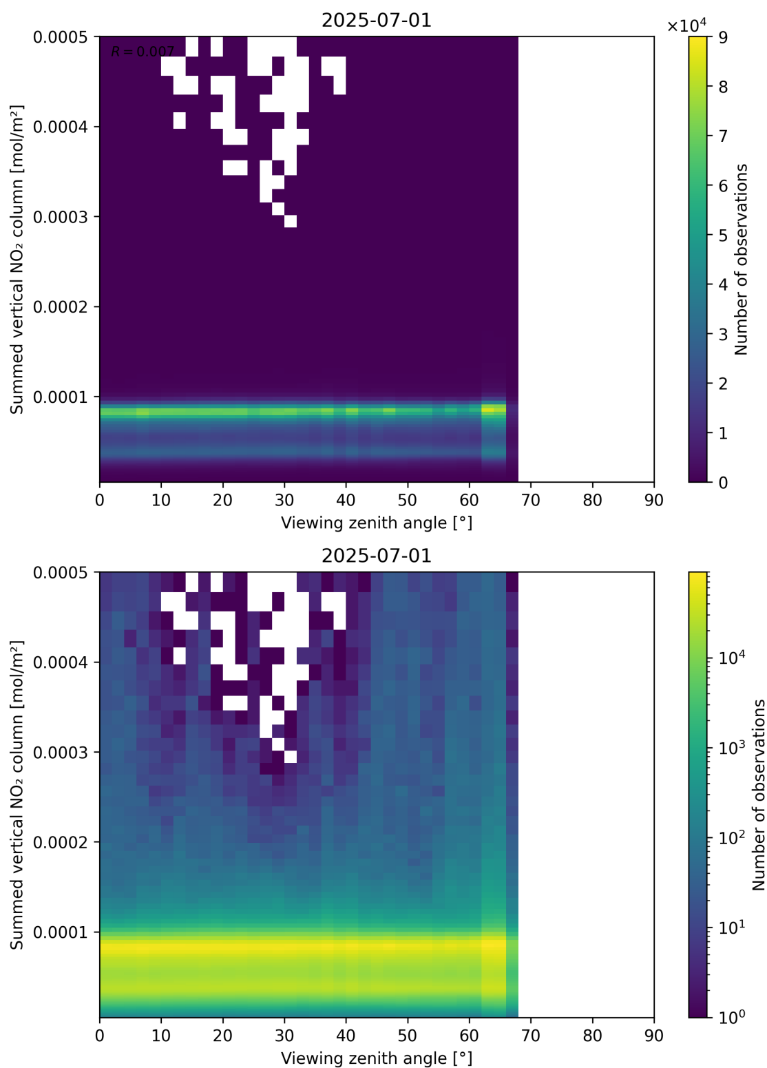
Figure 165: Scatter density plot of “Viewing zenith angle” against “Summed vertical NO 2 column” for 2025-06-30 to 2025-07-02.
