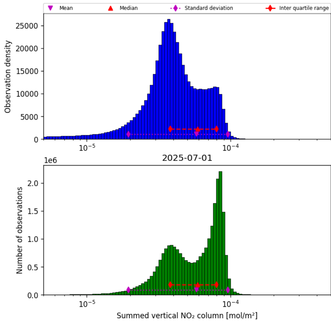
Figure 40: Histogram of “Summed vertical NO 2 column” for 2025-06-30 to 2025-07-02
