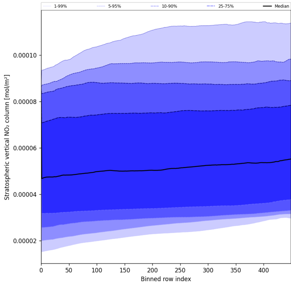
Figure 53: Along track statistics of “Stratospheric vertical NO 2 column” for 2025-06-30 to 2025-07-02
