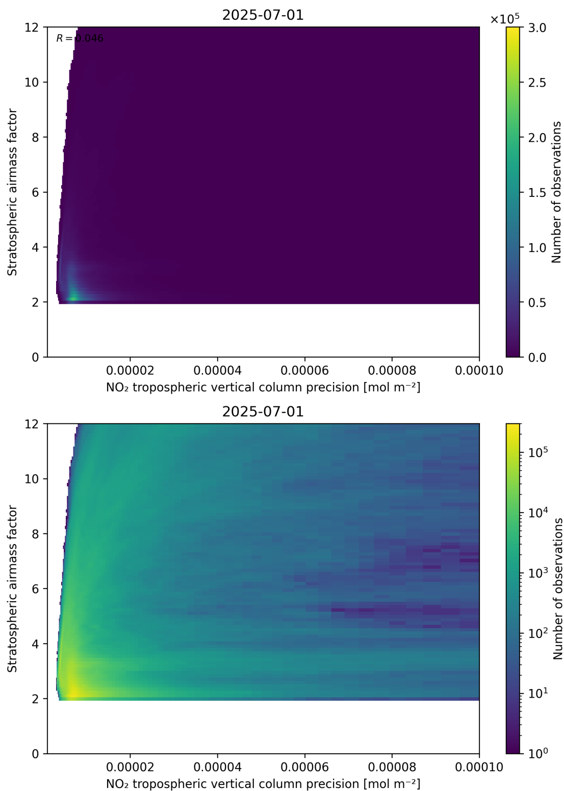
Figure 131: Scatter density plot of “NO 2 tropospheric vertical column precision” against “Stratospheric airmass factor” for 2025-06-30 to 2025-07-02.
