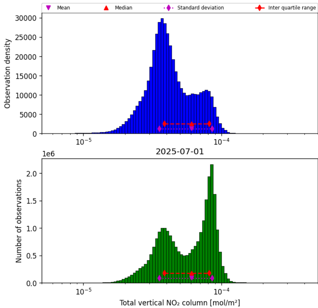
Figure 38: Histogram of “Total vertical NO 2 column” for 2025-06-30 to 2025-07-02
