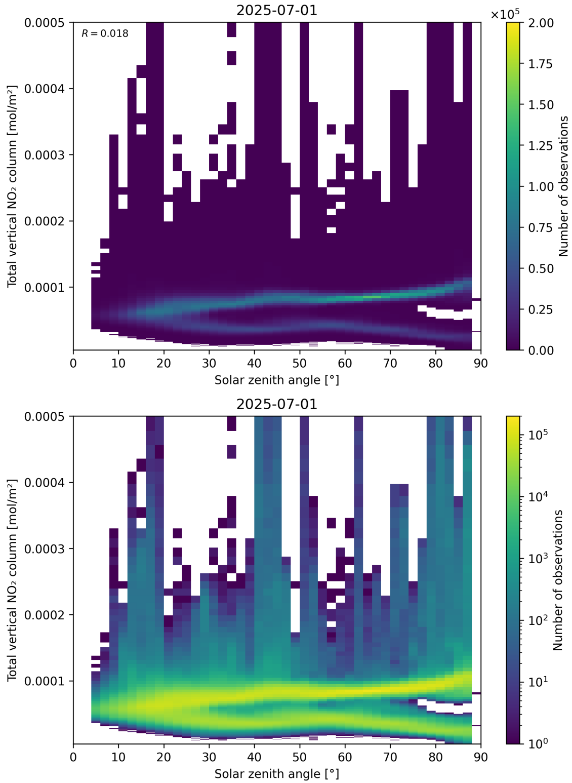
Figure 153: Scatter density plot of “Solar zenith angle” against “Total vertical NO 2 column” for 2025-06-30 to 2025-07-02.
