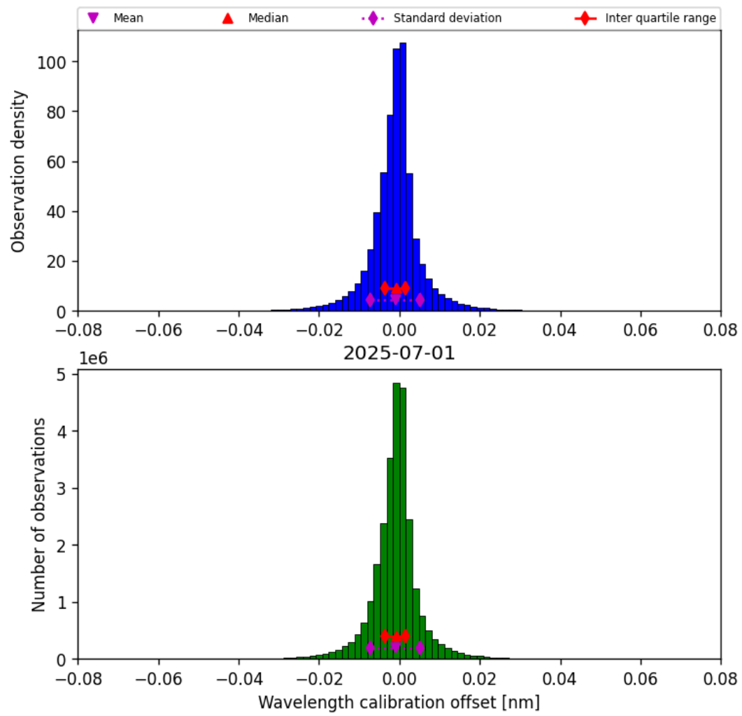
Figure 35: Histogram of "Wavelength calibration offset" for 2025-06-30 to 2025-07-02
