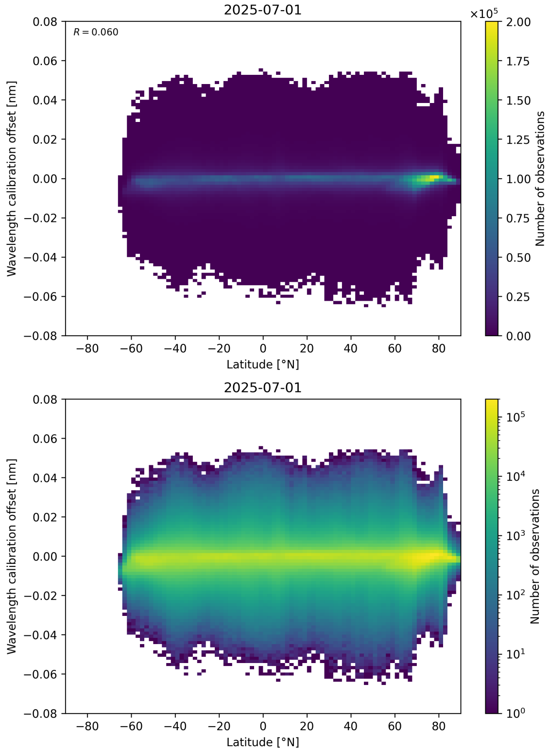
Figure 95: Scatter density plot of “Latitude” against “Wavelength calibration offset” for 2025-06-30 to 2025-07-02.
