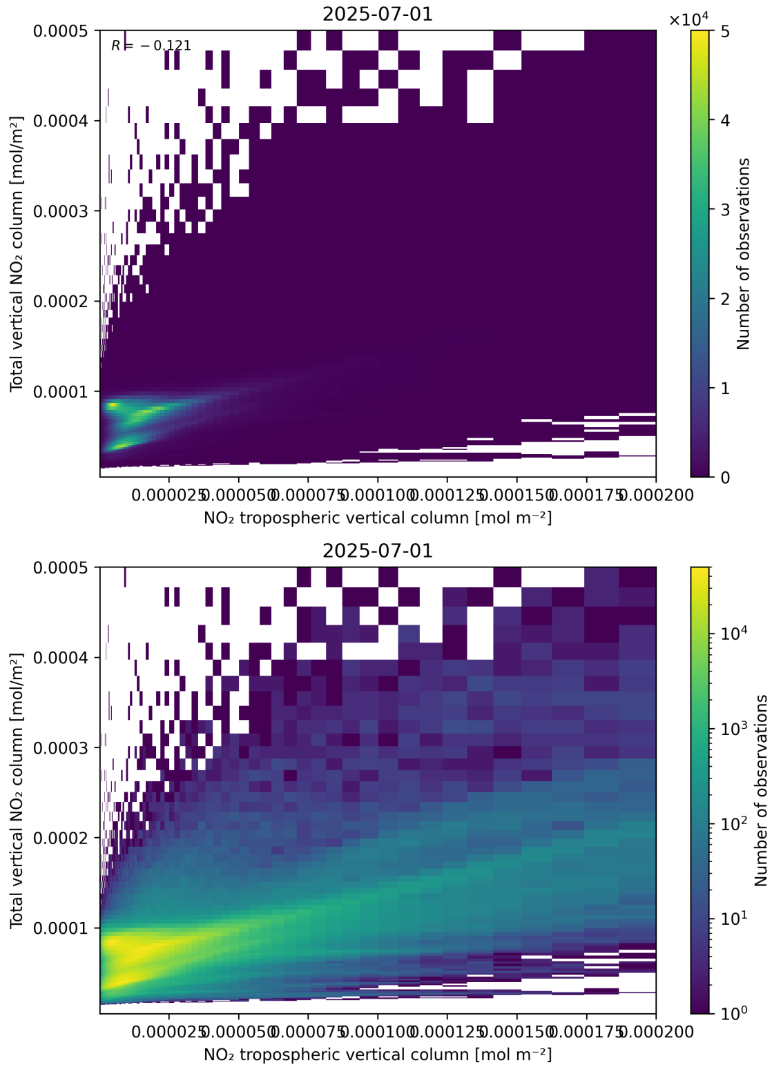
Figure 128: Scatter density plot of “NO 2 tropospheric vertical column” against “Total vertical NO 2 column” for 2025-06-30 to 2025-07-02.
