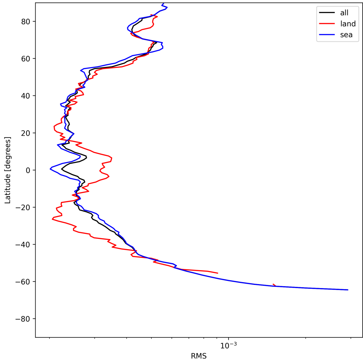
Figure 26: Zonal average of “RMS” for 2025-06-30 to 2025-07-02.
