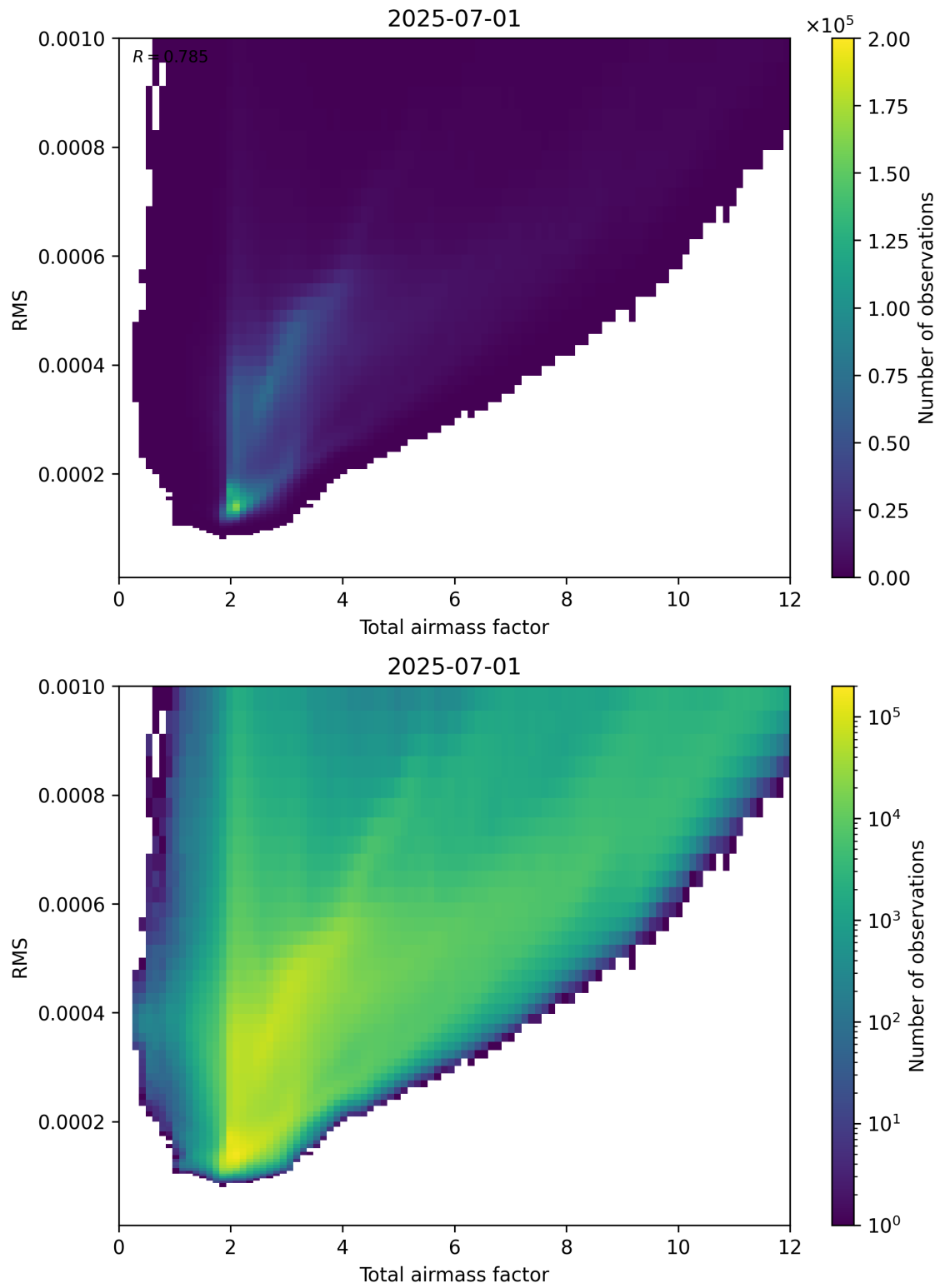
Figure 69: Scatter density plot of “Total airmass factor” against “RMS” for 2025-06-30 to 2025-07-02.
