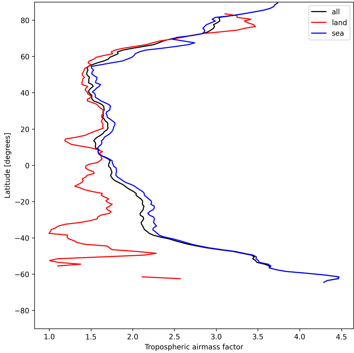
Figure 14: Zonal average of “Tropospheric airmass factor” for 2025-06-30 to 2025-07-02.
