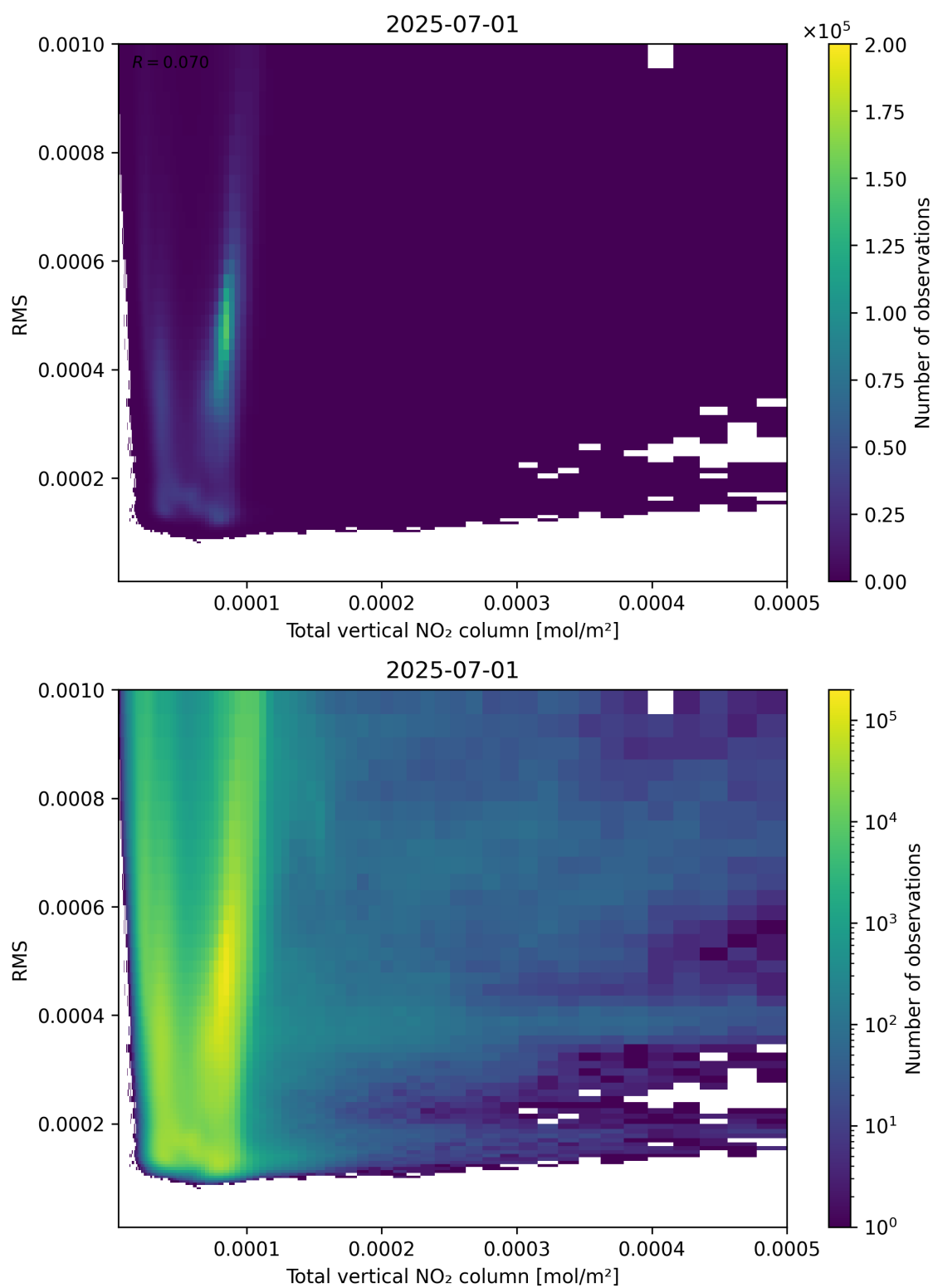
Figure 120: Scatter density plot of “Total vertical NO 2 column” against “RMS” for 2025-06-30 to 2025-07-02.
