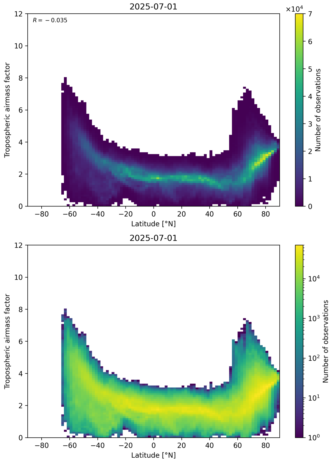
Figure 85: Scatter density plot of “Latitude” against “Tropospheric air mass factor” for 2025-06-30 to 2025-07-02.
