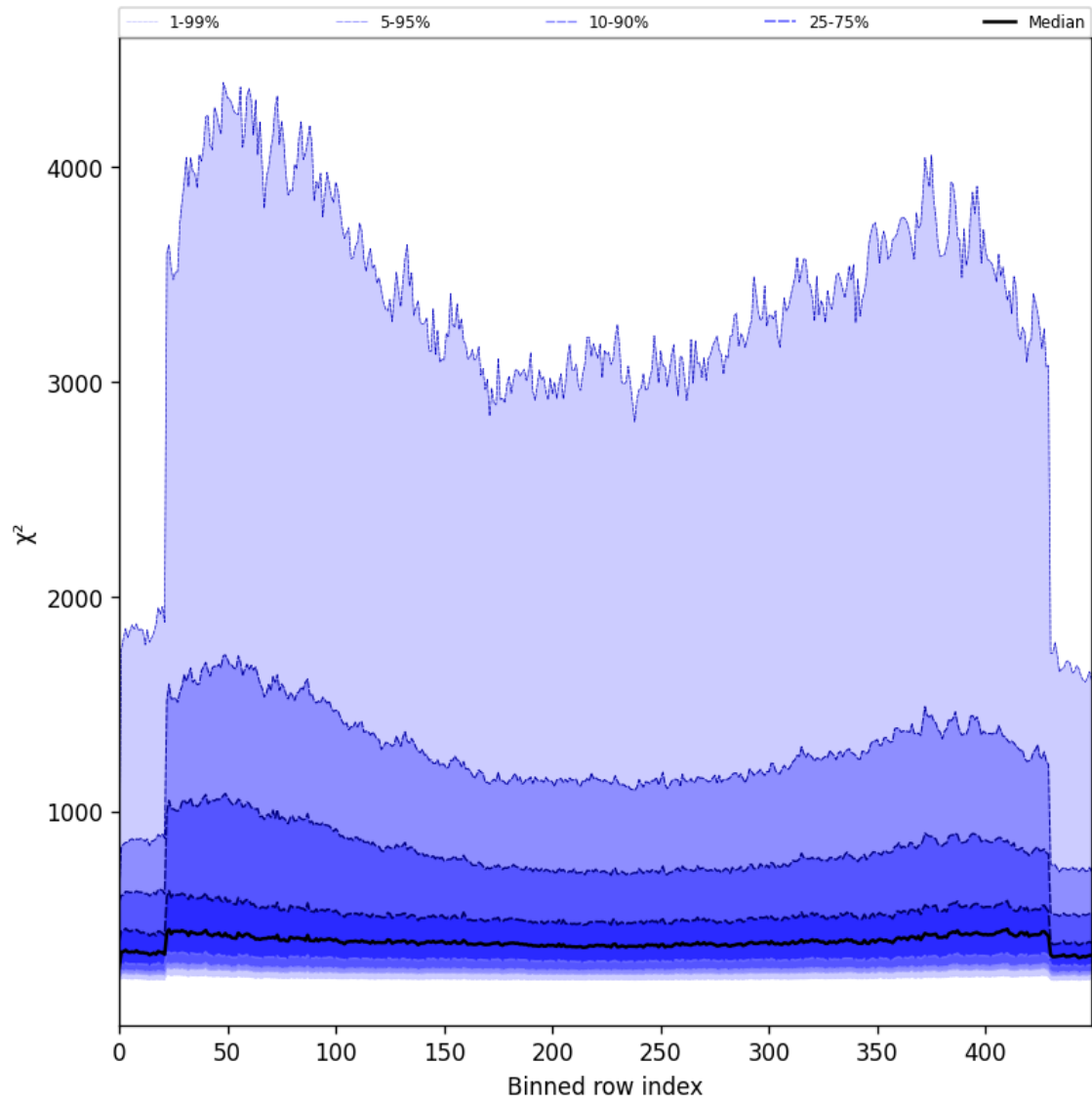
Figure 59: Along track statistics of “ \chi^2 ” for 2025-06-30 to 2025-07-02
