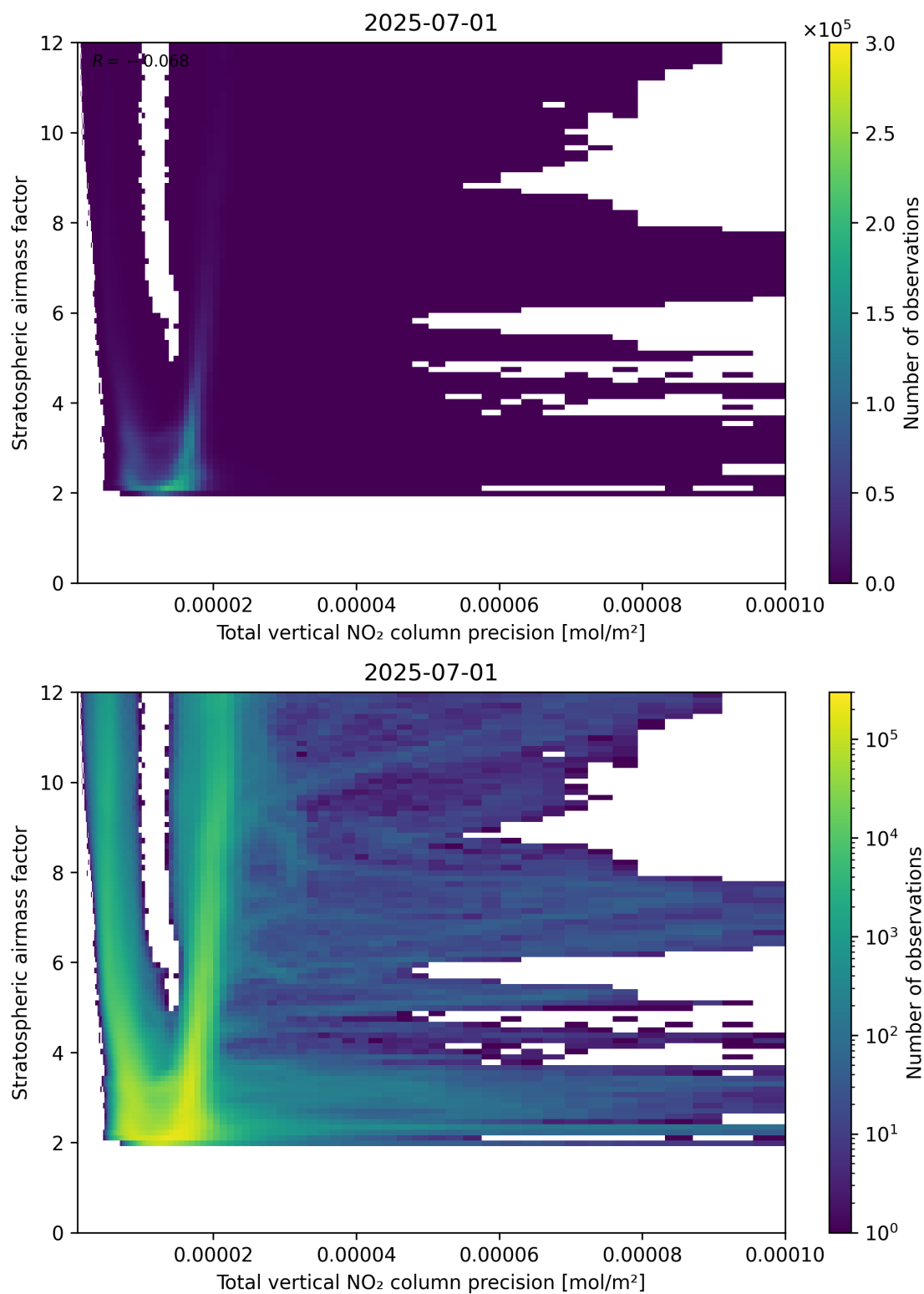
Figure 115: Scatter density plot of “Total vertical NO 2 column precision” against “Stratospheric air mass factor” for 2025-06-30 to 2025-07-02.
