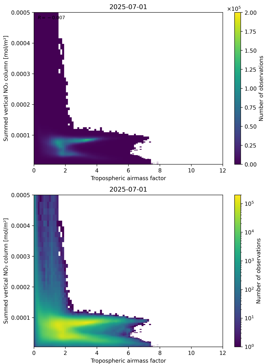
Figure 75: Scatter density plot of “Tropospheric airmass factor” against “Summed vertical NO 2 column” for 2025-06-30 to 2025-07-02.
