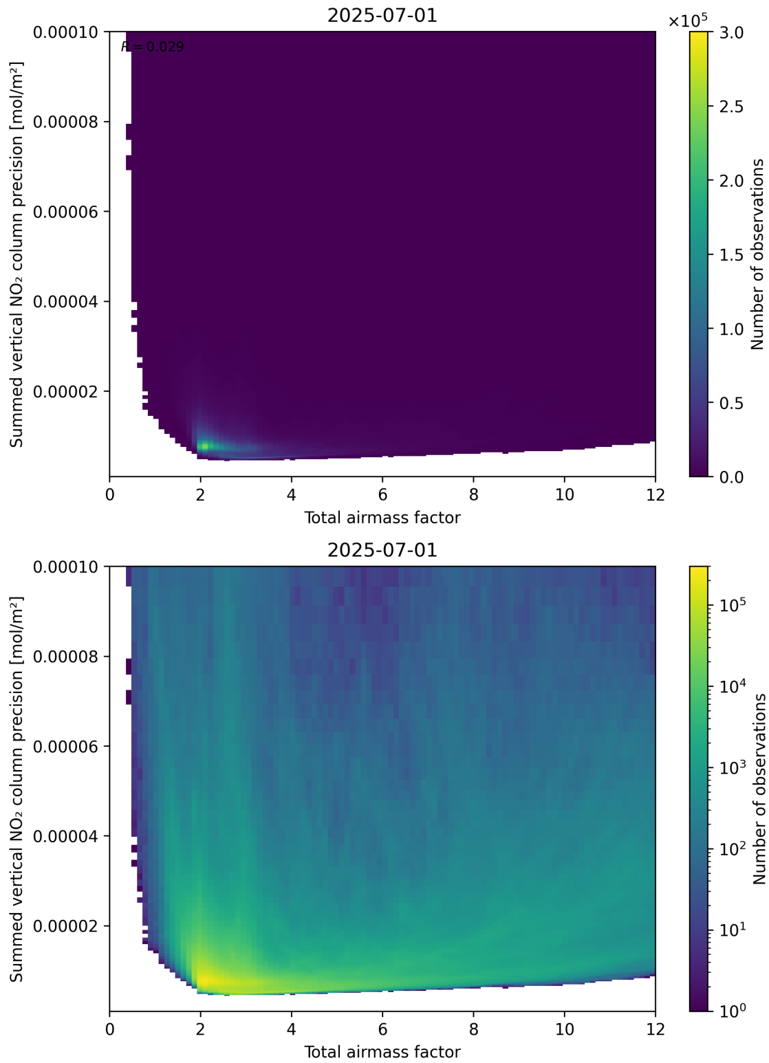
Figure 66: Scatter density plot of “Total airmass factor” against “Summed vertical NO 2 column precision” for 2025-06-30 to 2025-07-02.
