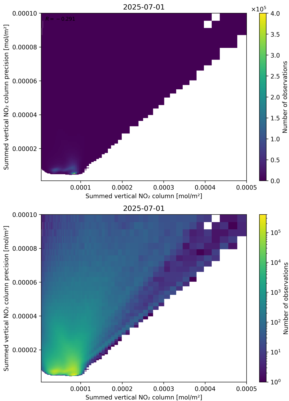
Figure 105: Scatter density plot of “Summed vertical NO 2 column” against “Summed vertical NO 2 column precision” for 2025-06-30 to 2025-07-02.
