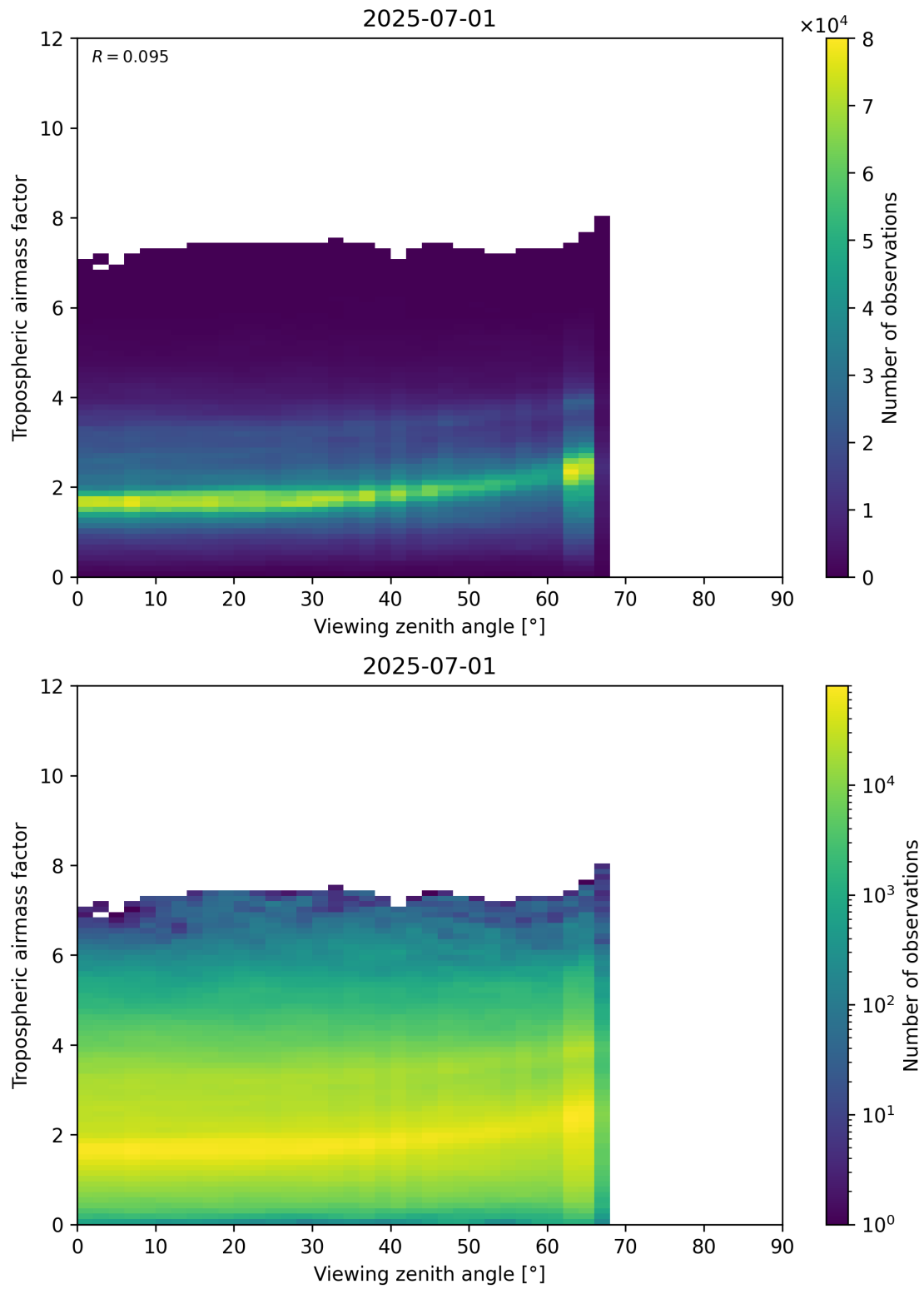
Figure 161: Scatter density plot of “Viewing zenith angle” against “Tropospheric airmass factor” for 2025-06-30 to 2025-07-02.
