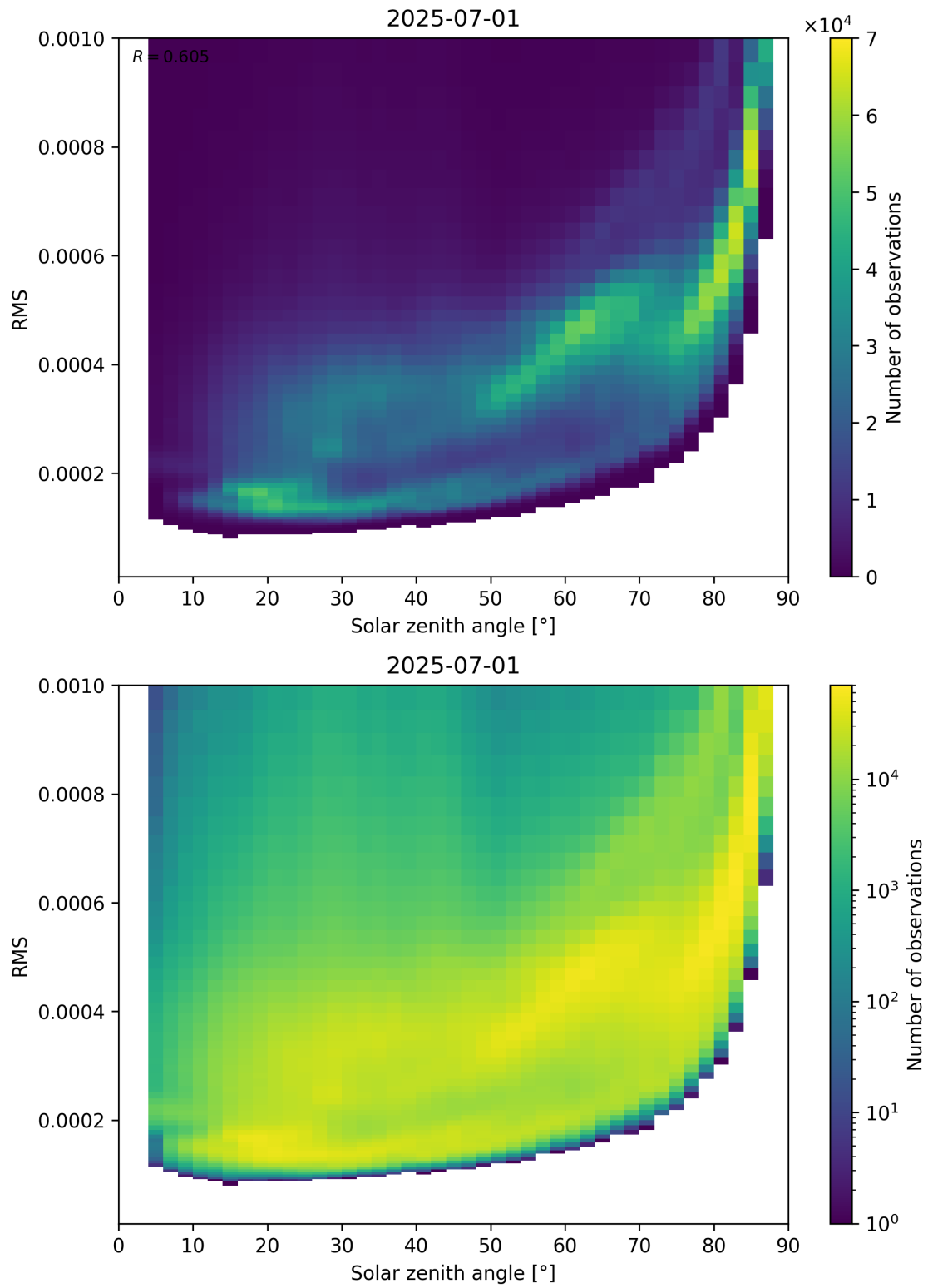
Figure 157: Scatter density plot of “Solar zenith angle” against “RMS” for 2025-06-30 to 2025-07-02.
