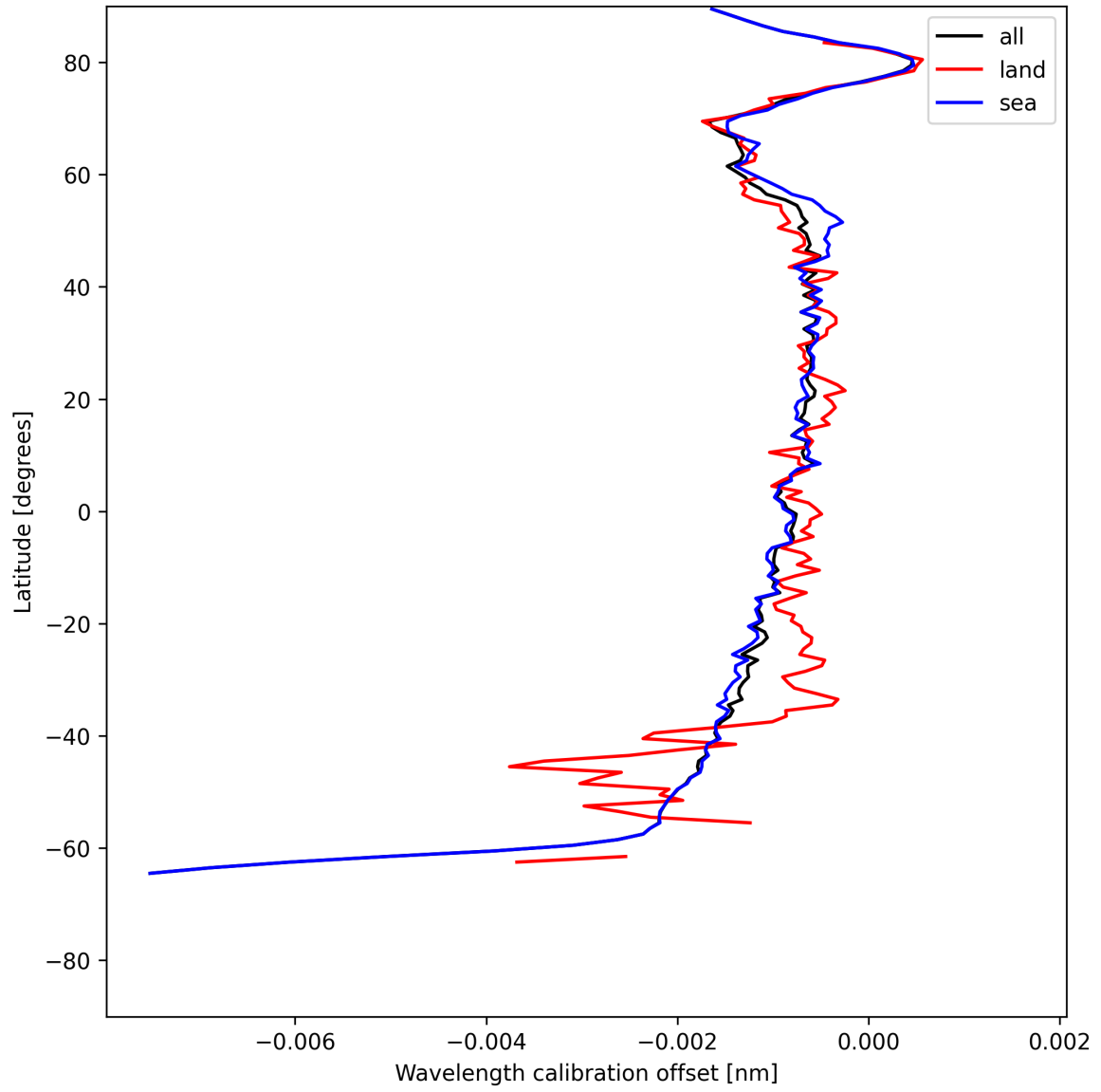
Figure 18: Zonal average of “Wavelength calibration offset” for 2025-06-30 to 2025-07-02.
