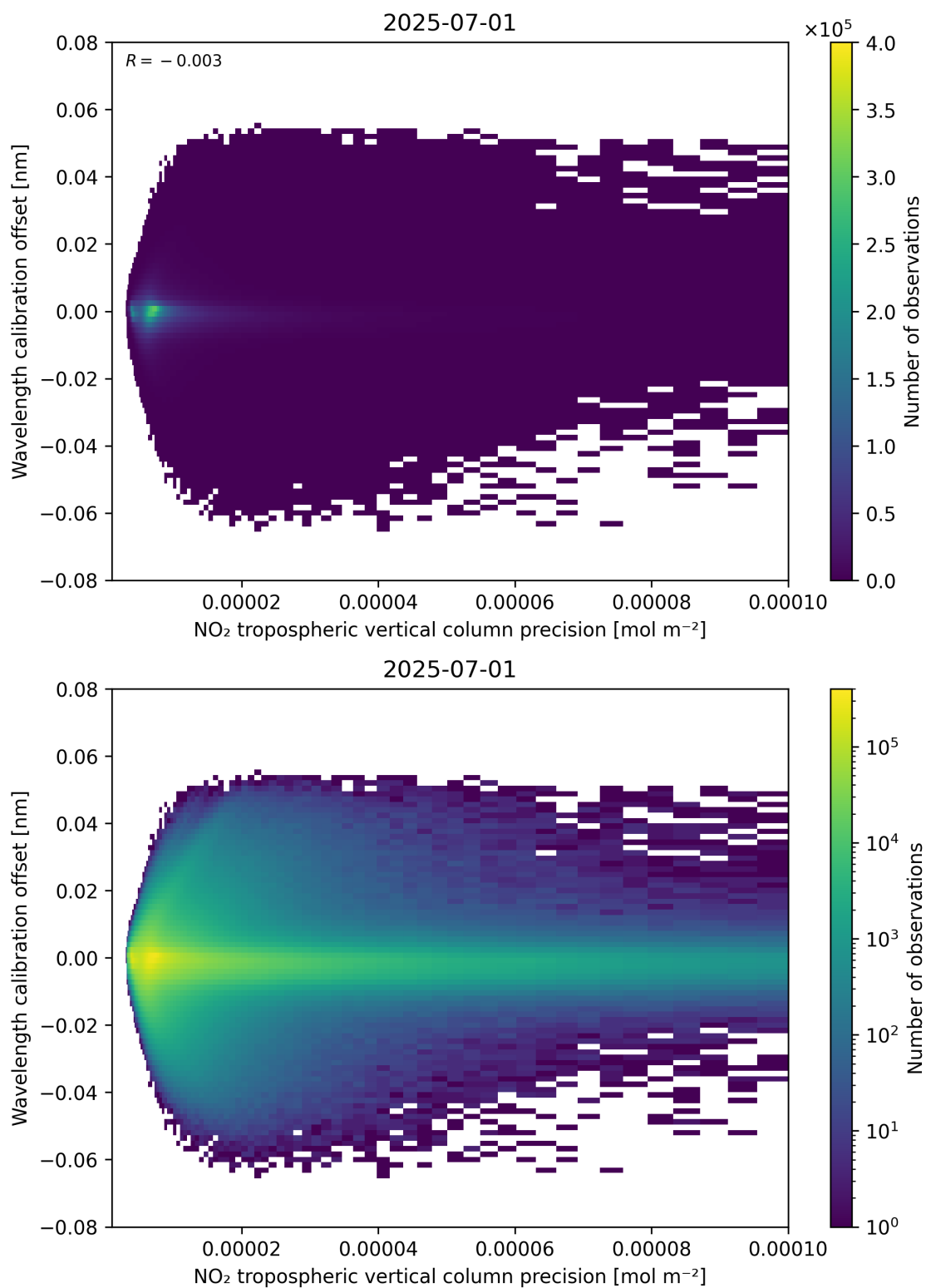
Figure 141: Scatter density plot of “NO 2 tropospheric vertical column precision” against “Wavelength calibration offset” for 2025-06-30 to 2025-07-02.
