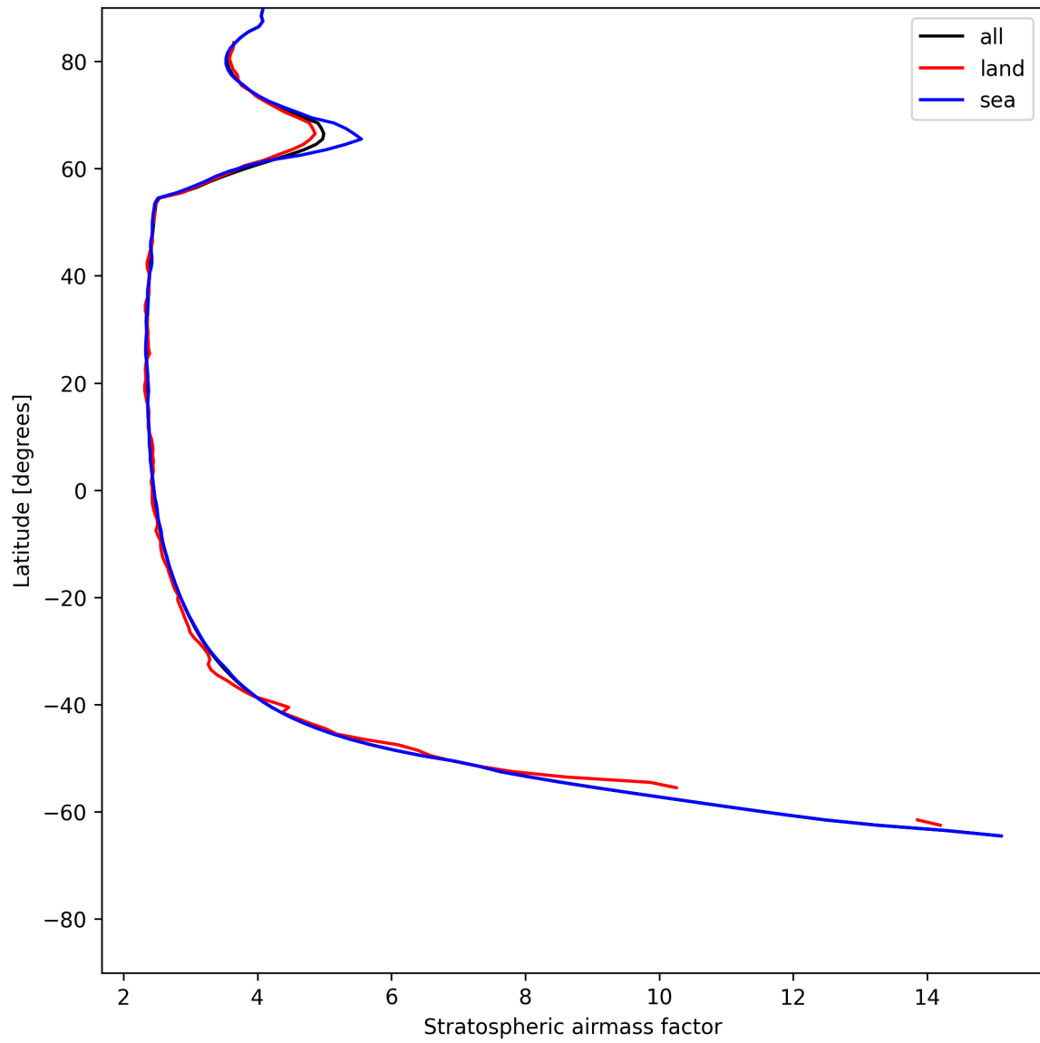
Figure 27: Zonal average of “Stratospheric airmass factor” for 2025-06-30 to 2025-07-02.
