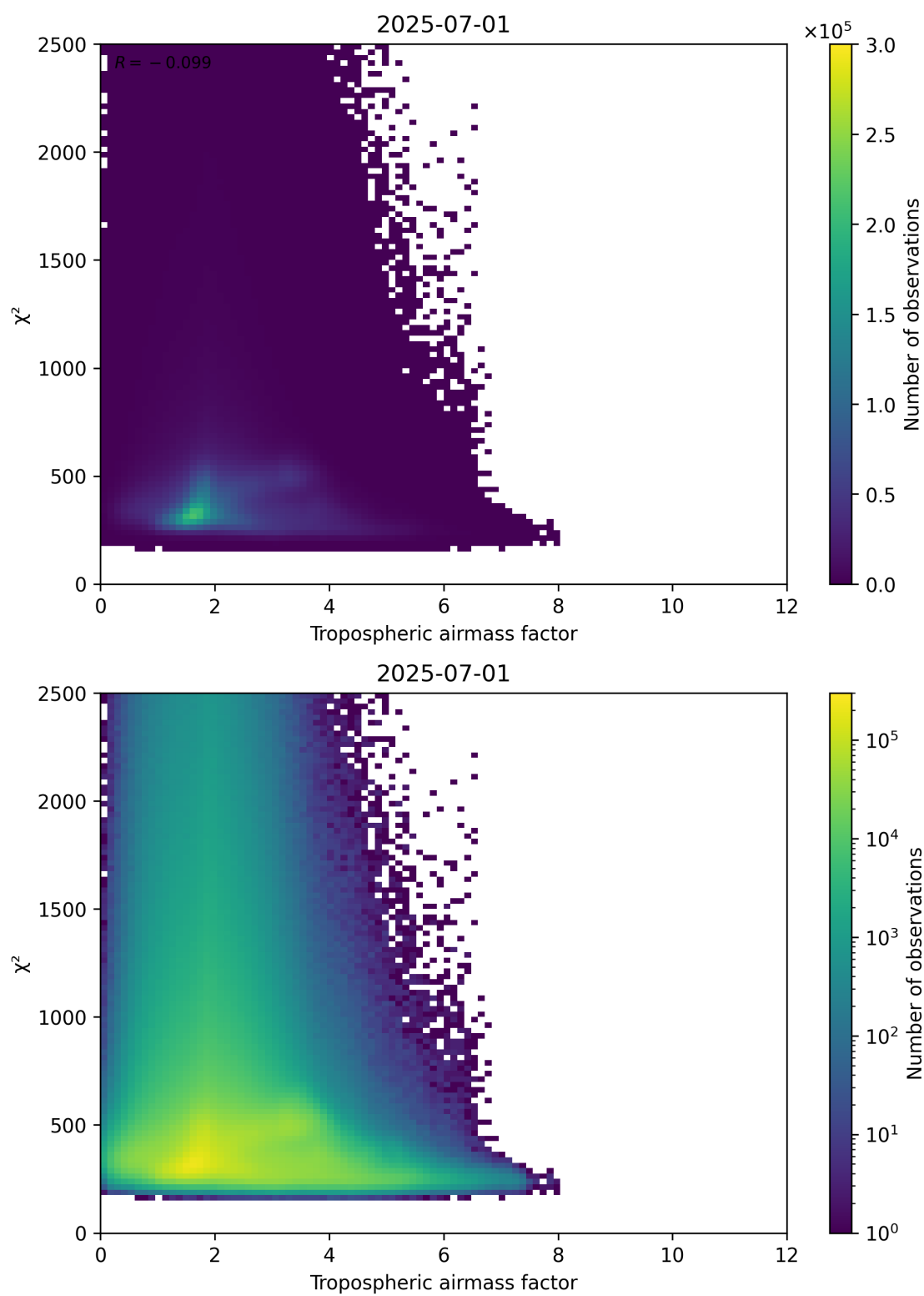
Figure 73: Scatter density plot of “Tropospheric airmass factor” against “ \chi^2 ” for 2025-06-30 to 2025-07-02.
