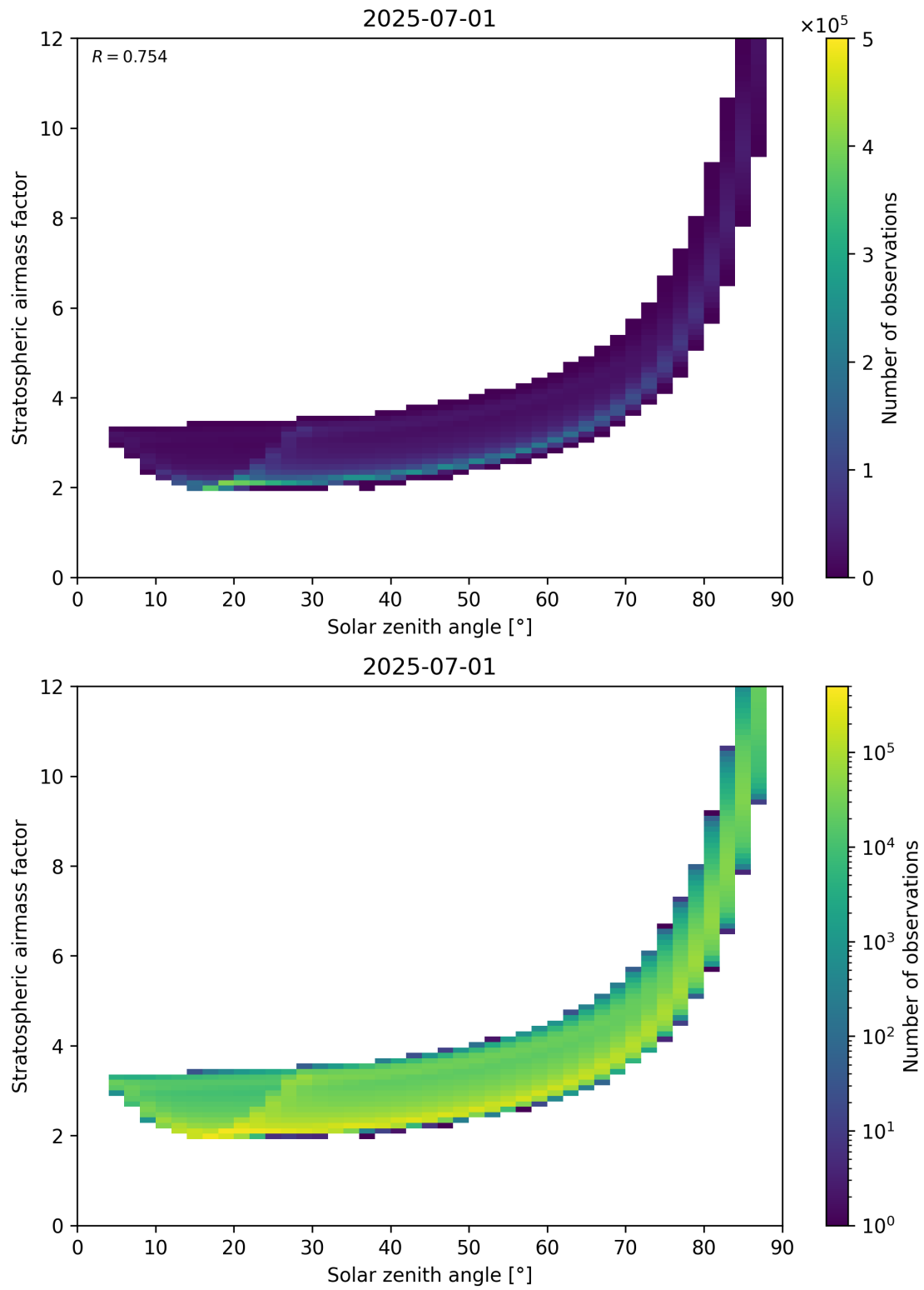
Figure 145: Scatter density plot of “Solar zenith angle” against “Stratospheric airmass factor” for 2025-06-30 to 2025-07-02.
