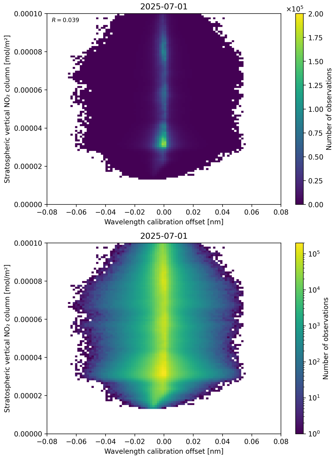
Figure 176: Scatter density plot of “Wavelength calibration offset” against “Stratospheric vertical NO 2 column” for 2025-06-30 to 2025-07-02.
