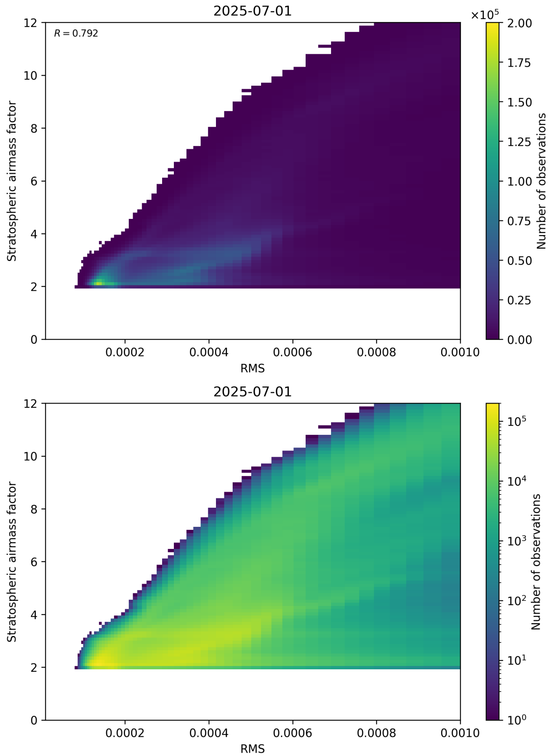
Figure 144: Scatter density plot of “RMS” against “Stratospheric airmass factor” for 2025-06-30 to 2025-07-02.
