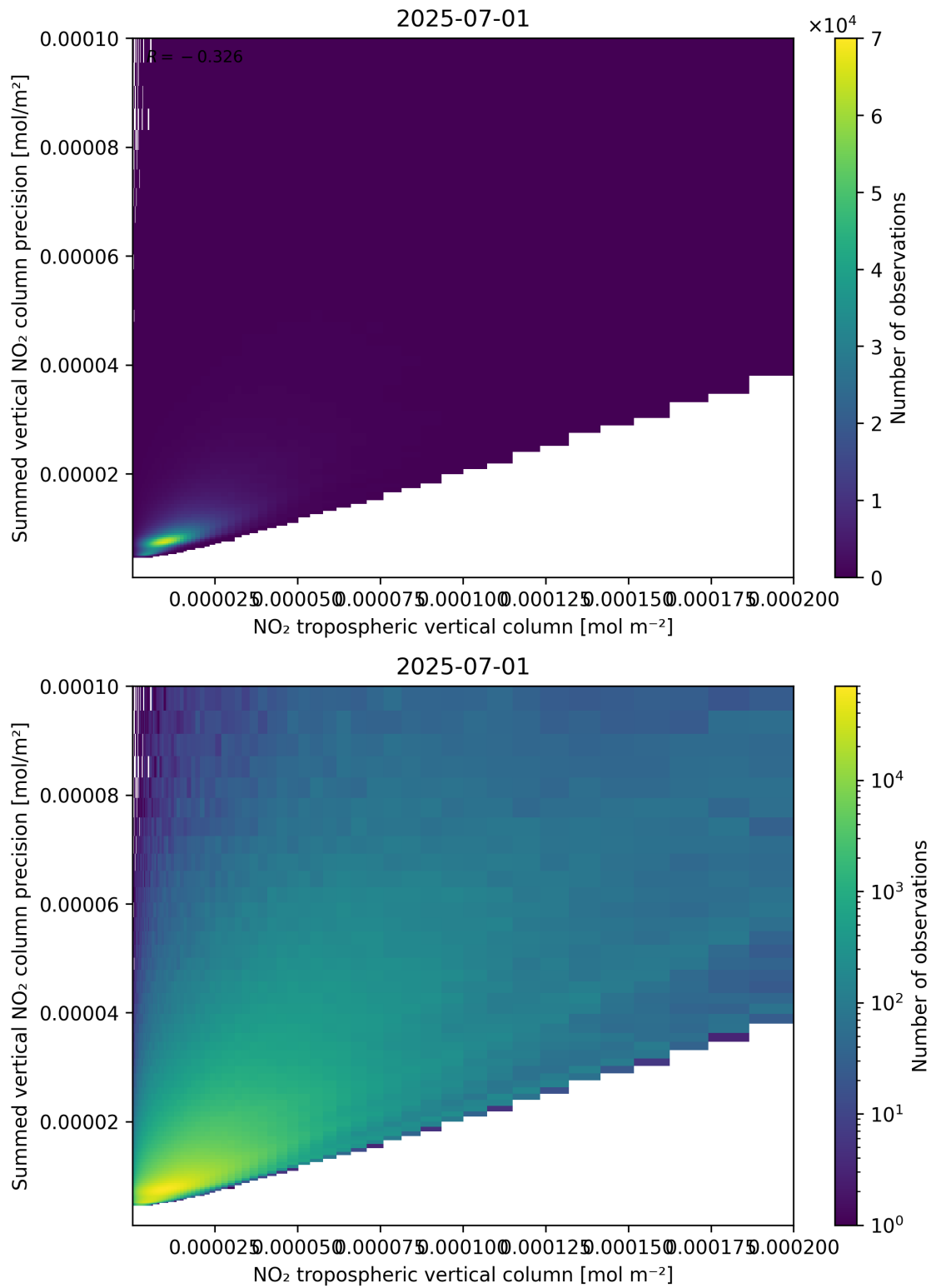
Figure 127: Scatter density plot of “NO 2 tropospheric vertical column” against “Summed vertical NO 2 column precision” for 2025-06-30 to 2025-07-02.
