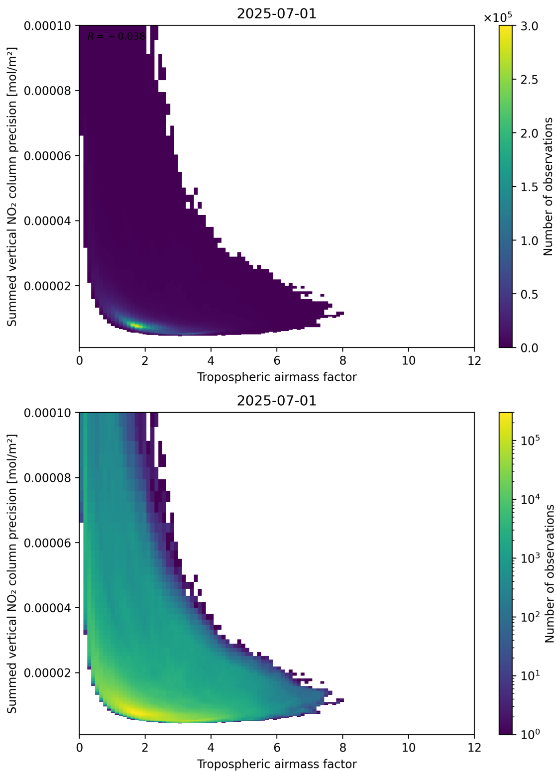
Figure 76: Scatter density plot of “Tropospheric air mass factor” against “Summed vertical NO 2 column precision” for 2025-06-30 to 2025-07-02.
