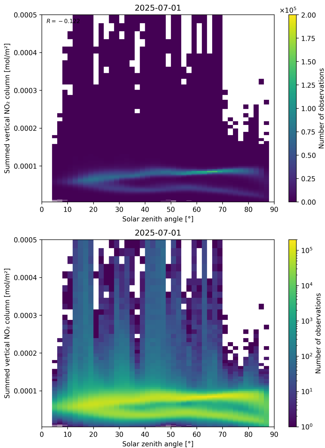
Figure 151: Scatter density plot of “Solar zenith angle” against “Summed vertical NO 2 column” for 2025-06-30 to 2025-07-02.
