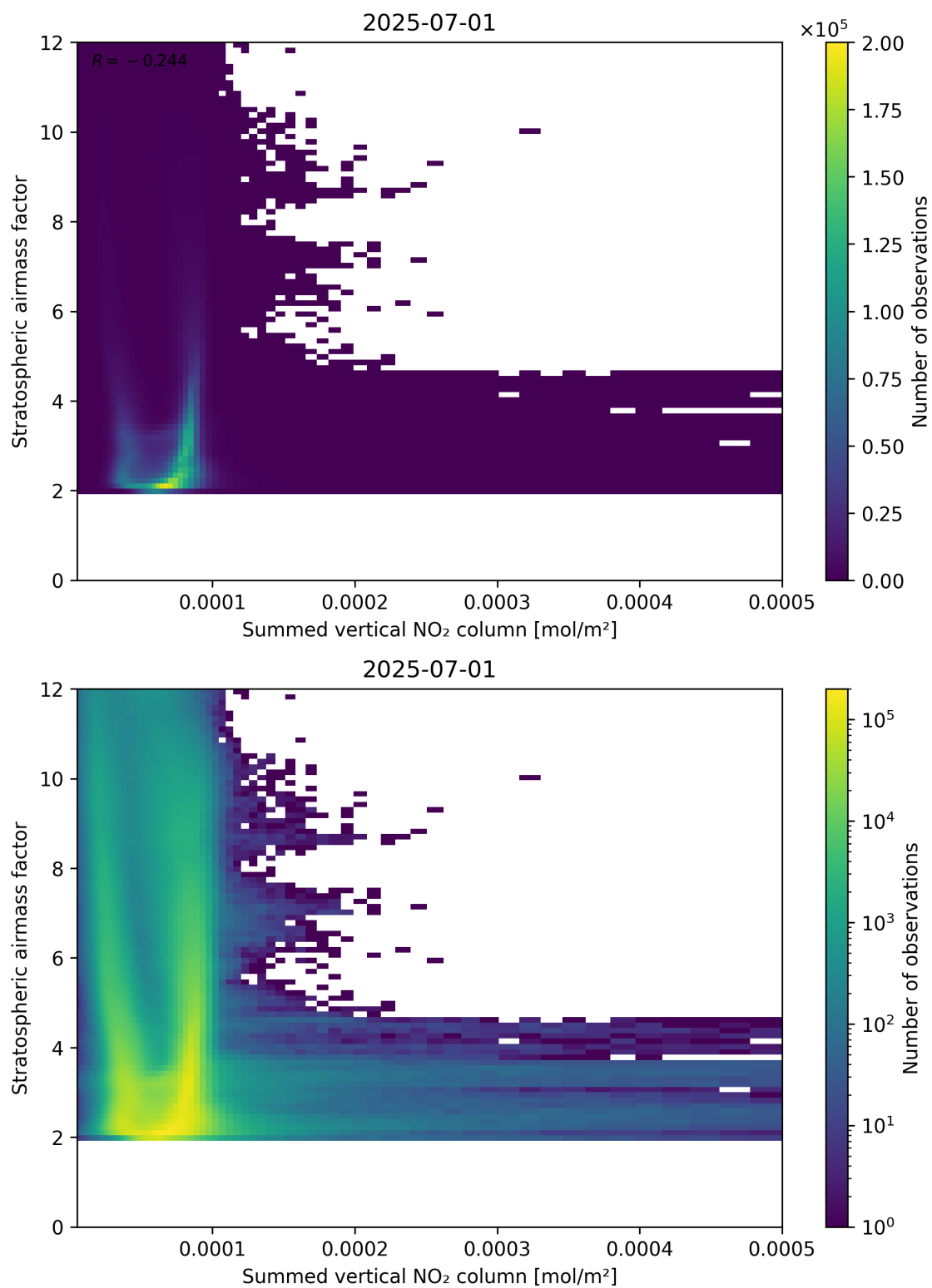
Figure 103: Scatter density plot of “Summed vertical NO 2 column” against “Stratospheric airmass factor” for 2025-06-30 to 2025-07-02.
