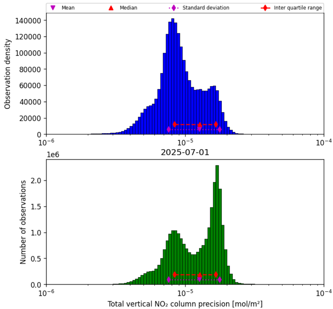
Figure 39: Histogram of “Total vertical NO 2 column precision” for 2025-06-30 to 2025-07-02
