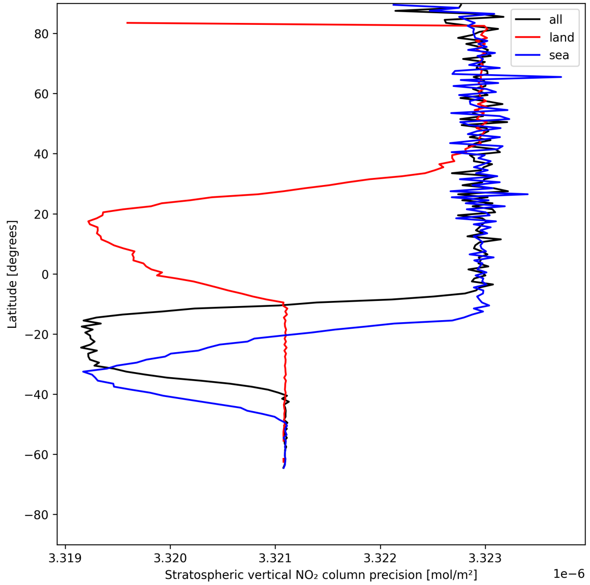
Figure 20: Zonal average of “Stratospheric vertical NO 2 column precision” for 2025-06-30 to 2025-07-02.
