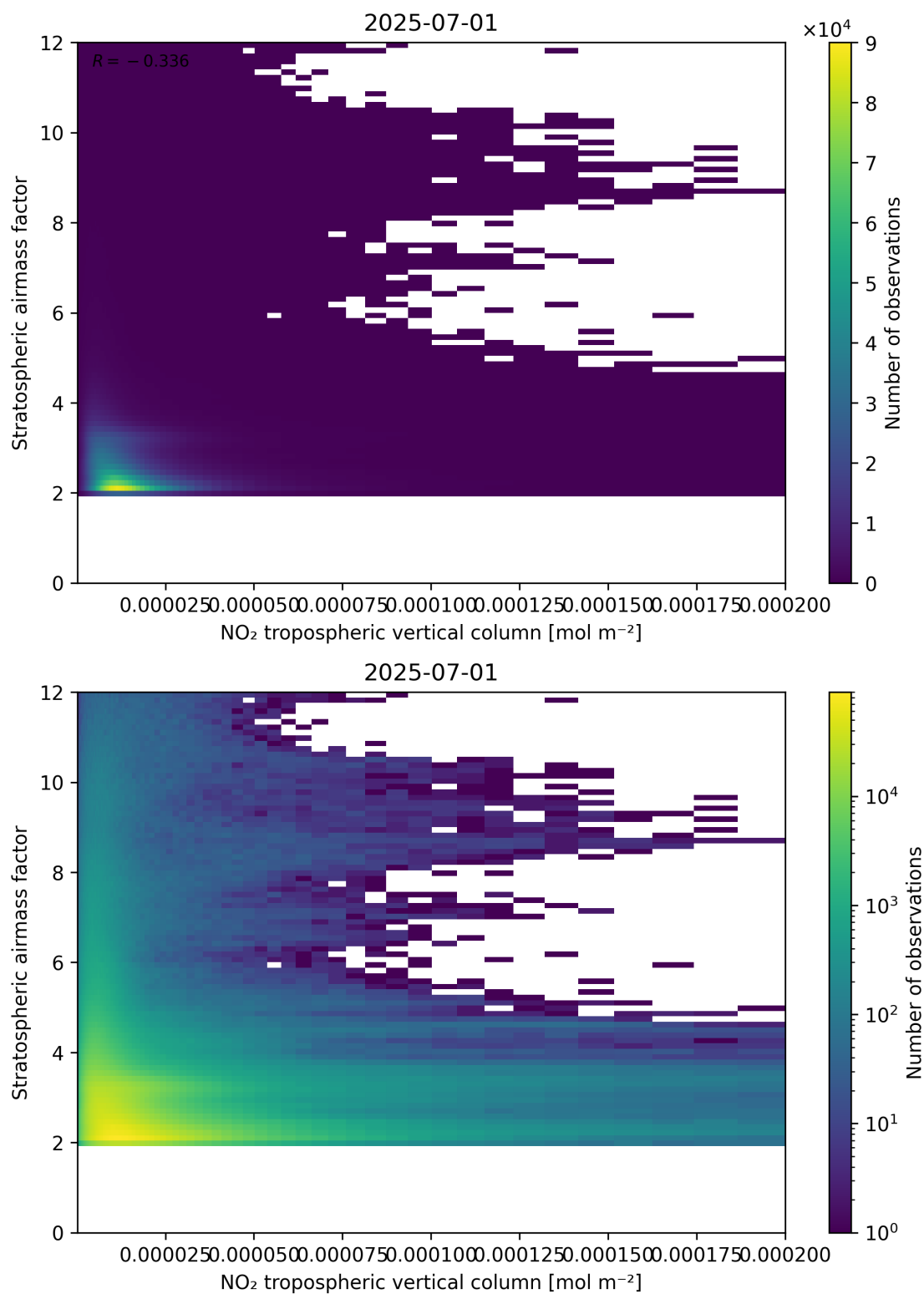
Figure 121: Scatter density plot of “NO 2 tropospheric vertical column” against “Stratospheric air mass factor” for 2025-06-30 to 2025-07-02.
