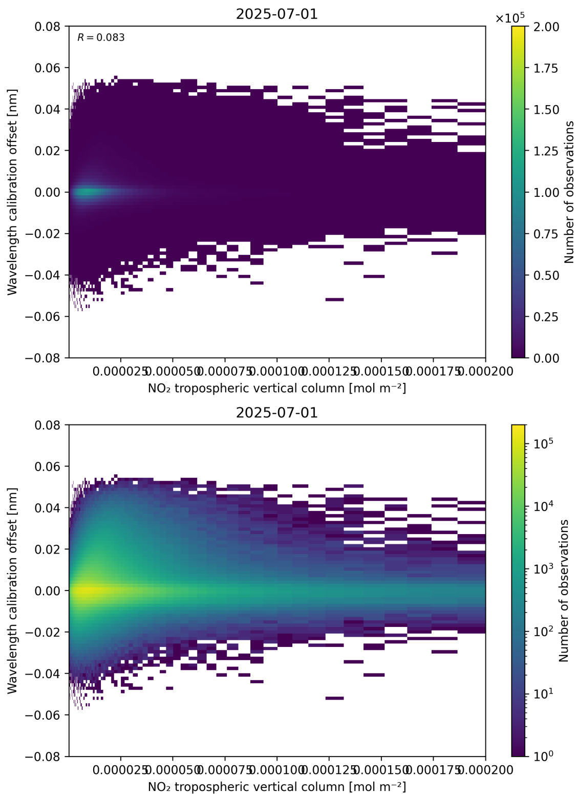
Figure 143: Scatter density plot of “NO 2 tropospheric vertical column” against “Wavelength calibration offset” for 2025-06-30 to 2025-07-02.
