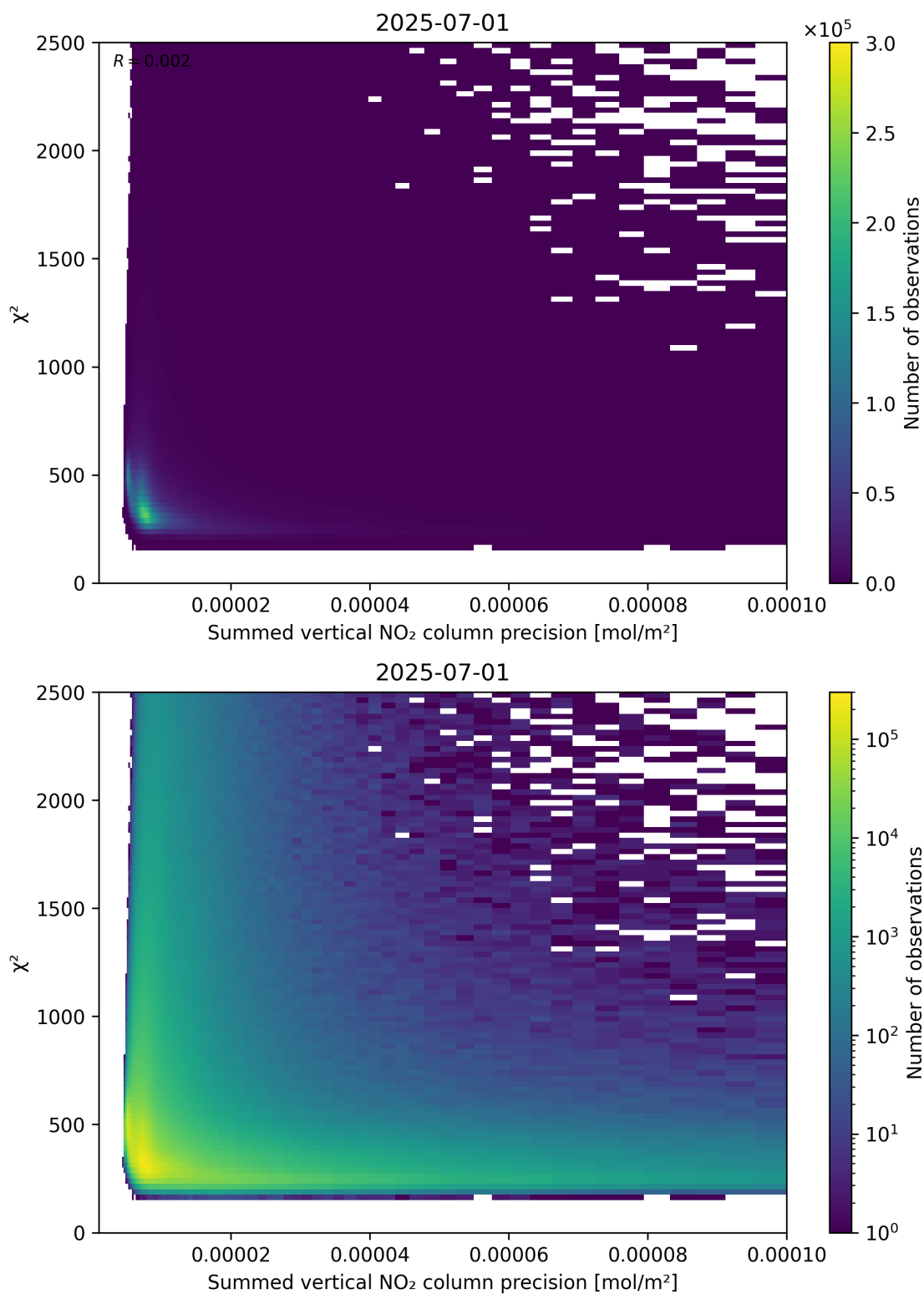
Figure 107: Scatter density plot of “Summed vertical NO 2 column precision” against “ \chi^2 ” for 2025-06-30 to 2025-07-02.
