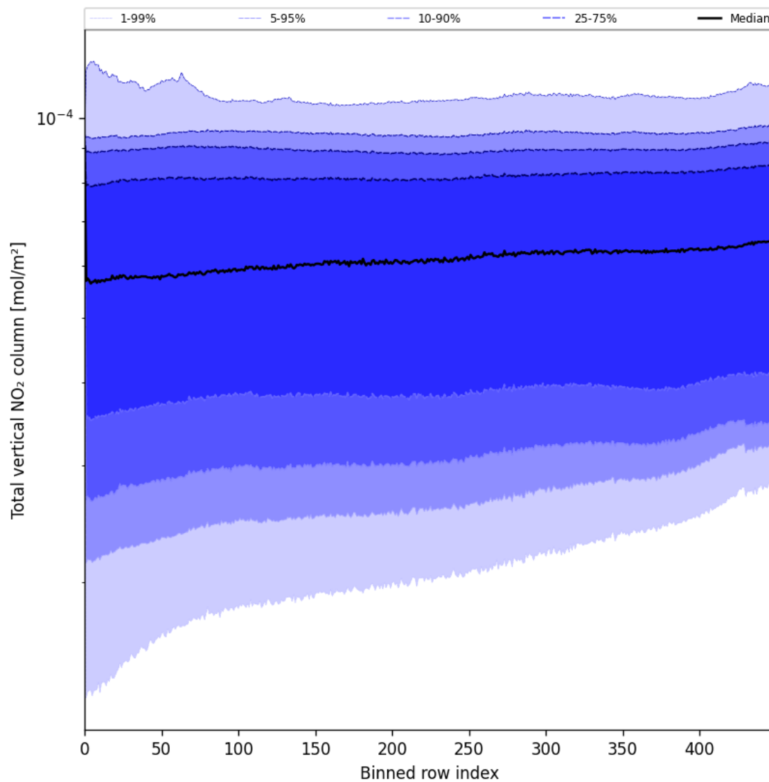
Figure 55: Along track statistics of “Total vertical NO 2 column” for 2025-06-30 to 2025-07-02
