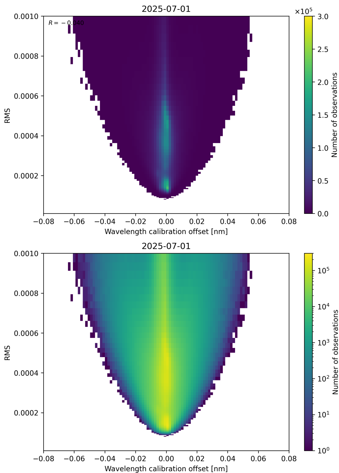
Figure 181: Scatter density plot of “Wavelength calibration offset” against “RMS” for 2025-06-30 to 2025-07-02.
