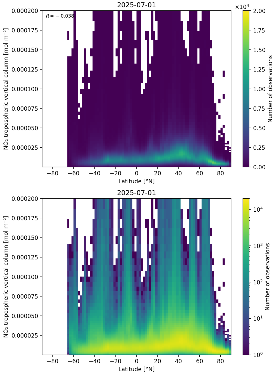
Figure 92: Scatter density plot of “Latitude” against “NO 2 tropospheric vertical column” for 2025-06-30 to 2025-07-02.
