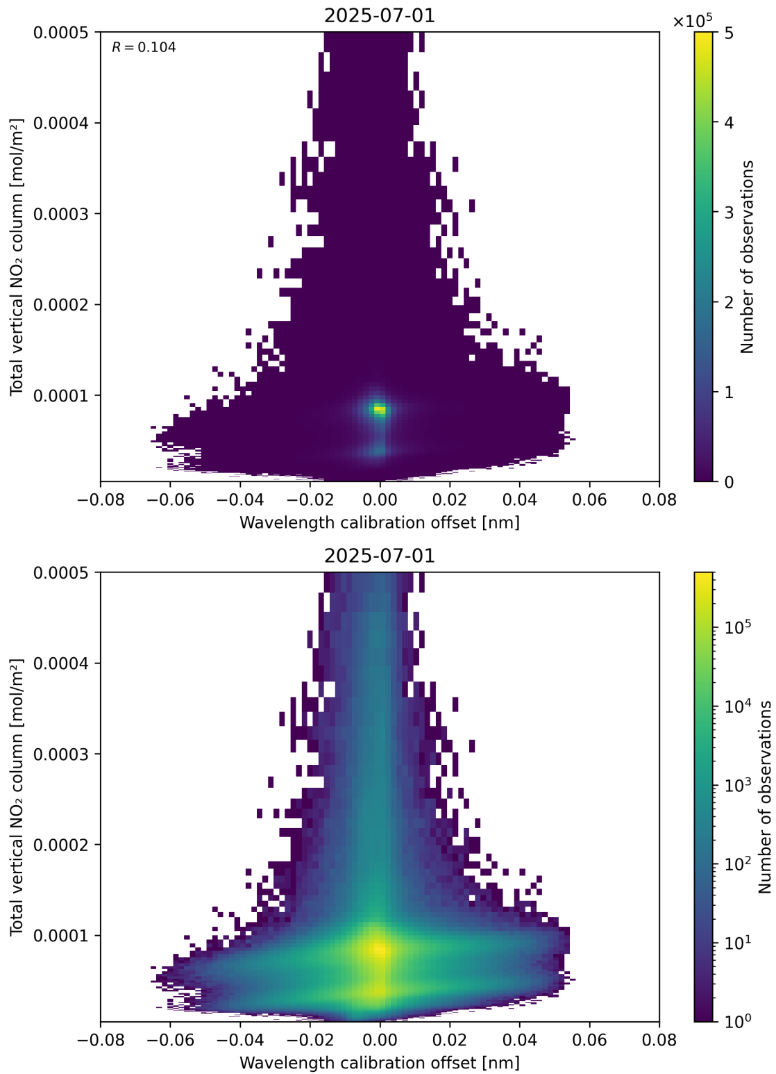
Figure 179: Scatter density plot of “Wavelength calibration offset” against “Total vertical NO 2 column” for 2025-06-30 to 2025-07-02.
