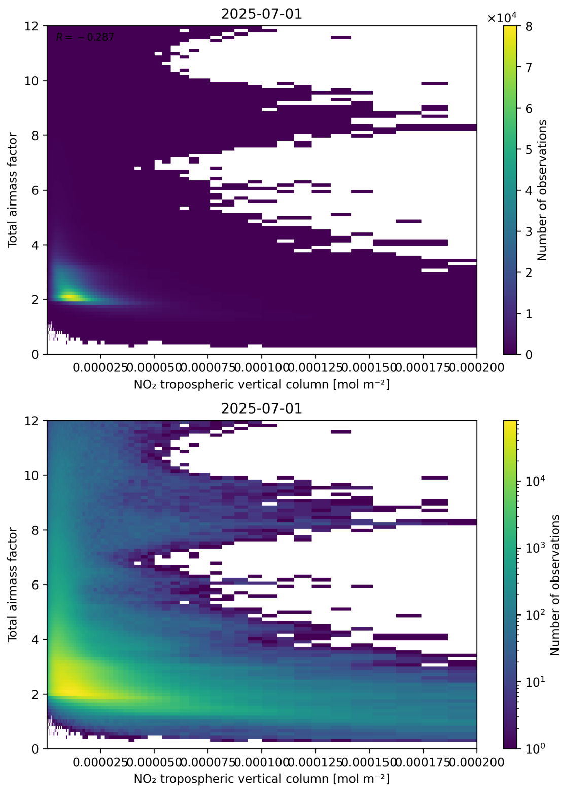
Figure 122: Scatter density plot of “NO 2 tropospheric vertical column” against “Total air mass factor” for 2025-06-30 to 2025-07-02.
