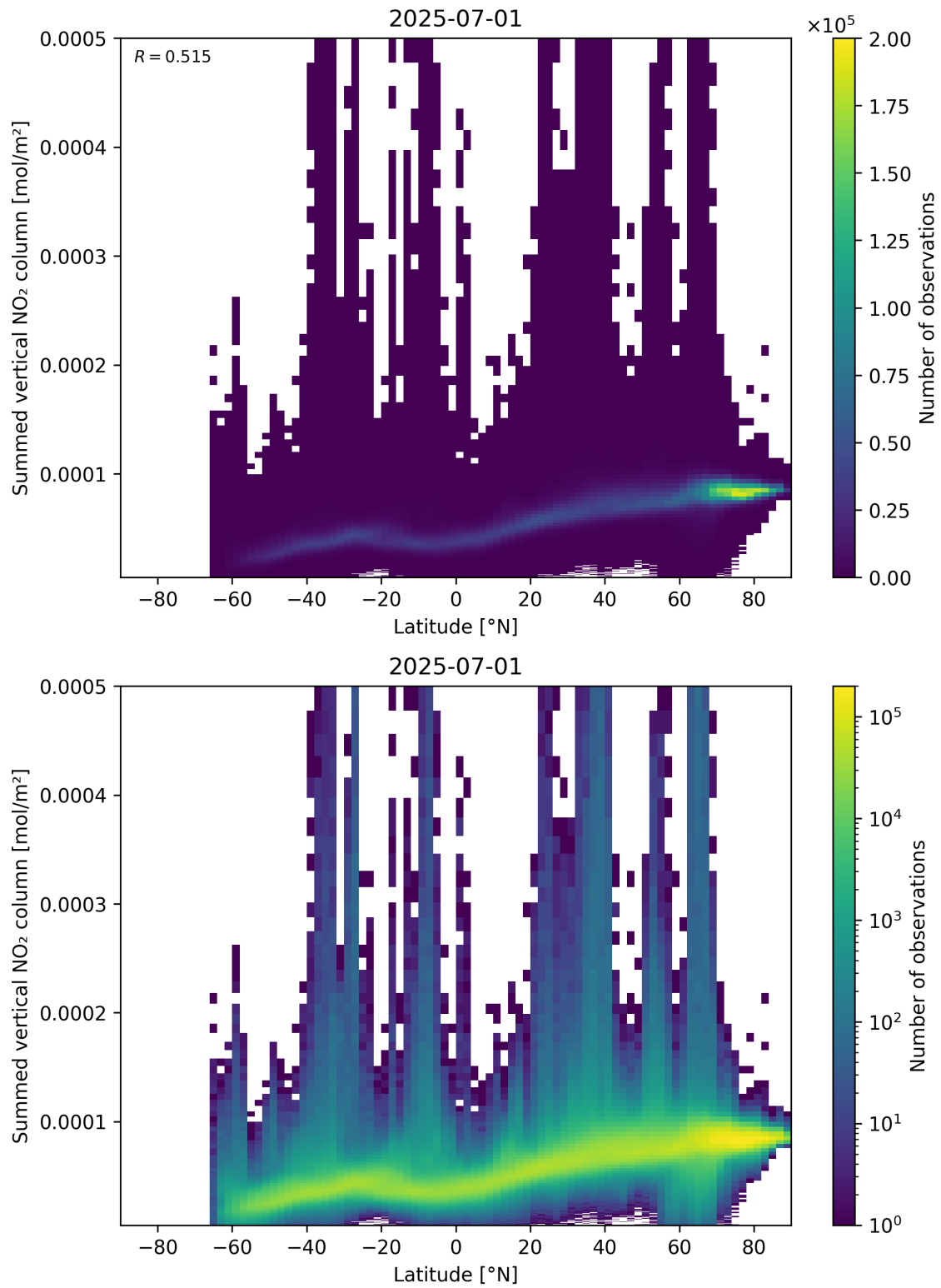
Figure 88: Scatter density plot of “Latitude” against “Summed vertical NO 2 column” for 2025-06-30 to 2025-07-02.
