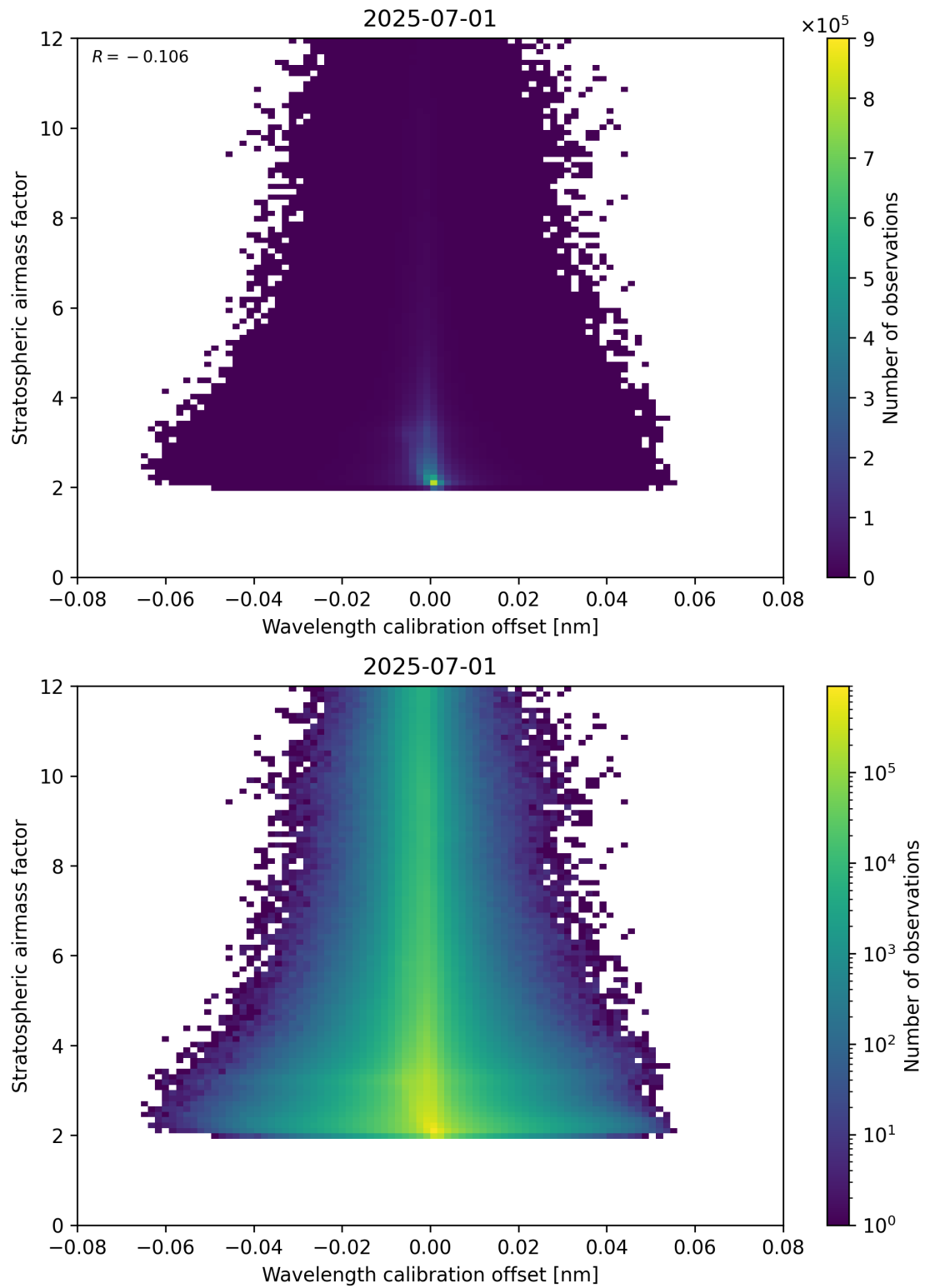
Figure 174: Scatter density plot of “Wavelength calibration offset” against “Stratospheric air mass factor” for 2025-06-30 to 2025-07-02.
