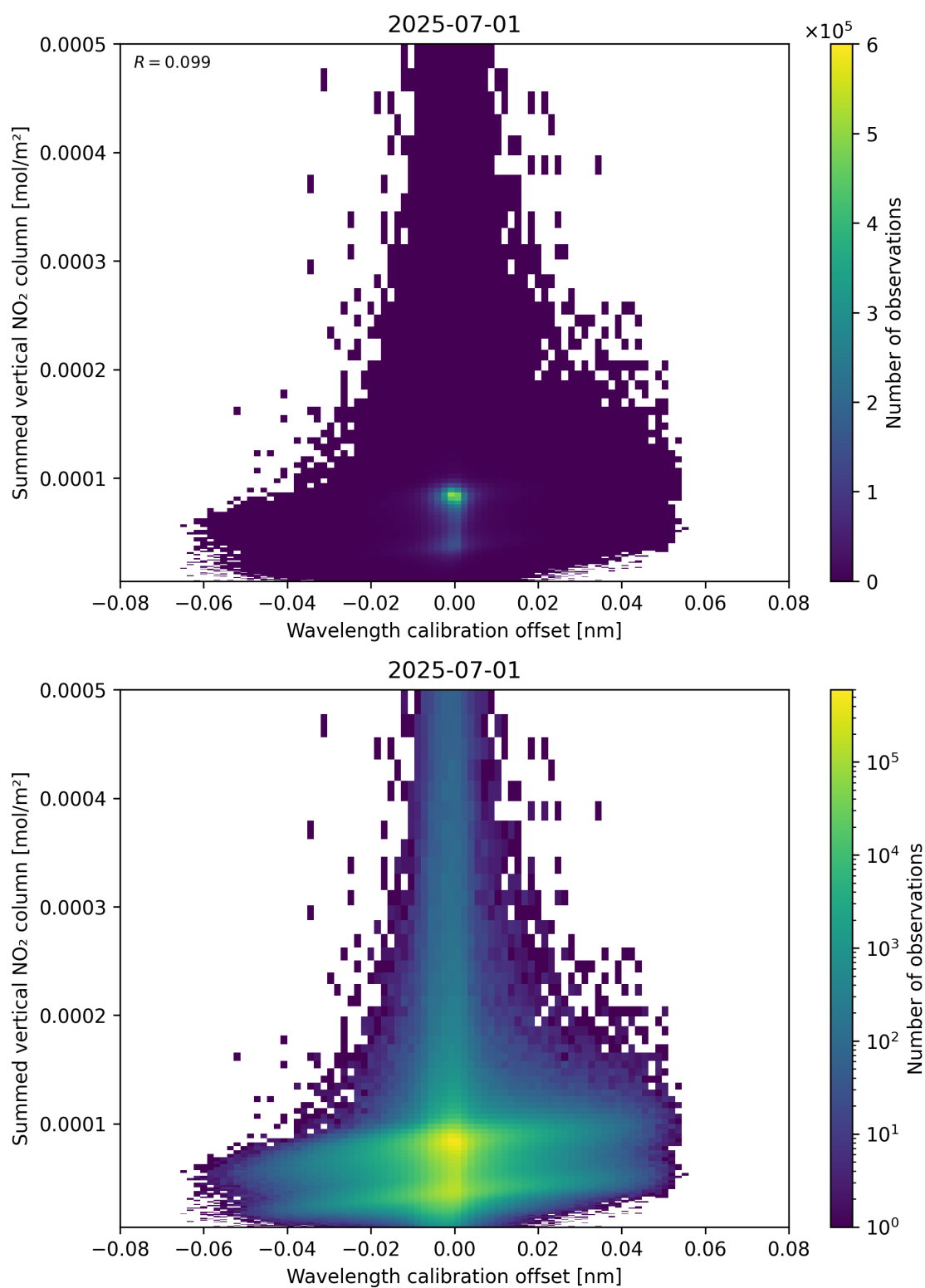
Figure 177: Scatter density plot of “Wavelength calibration offset” against “Summed vertical NO 2 column” for 2025-06-30 to 2025-07-02.
