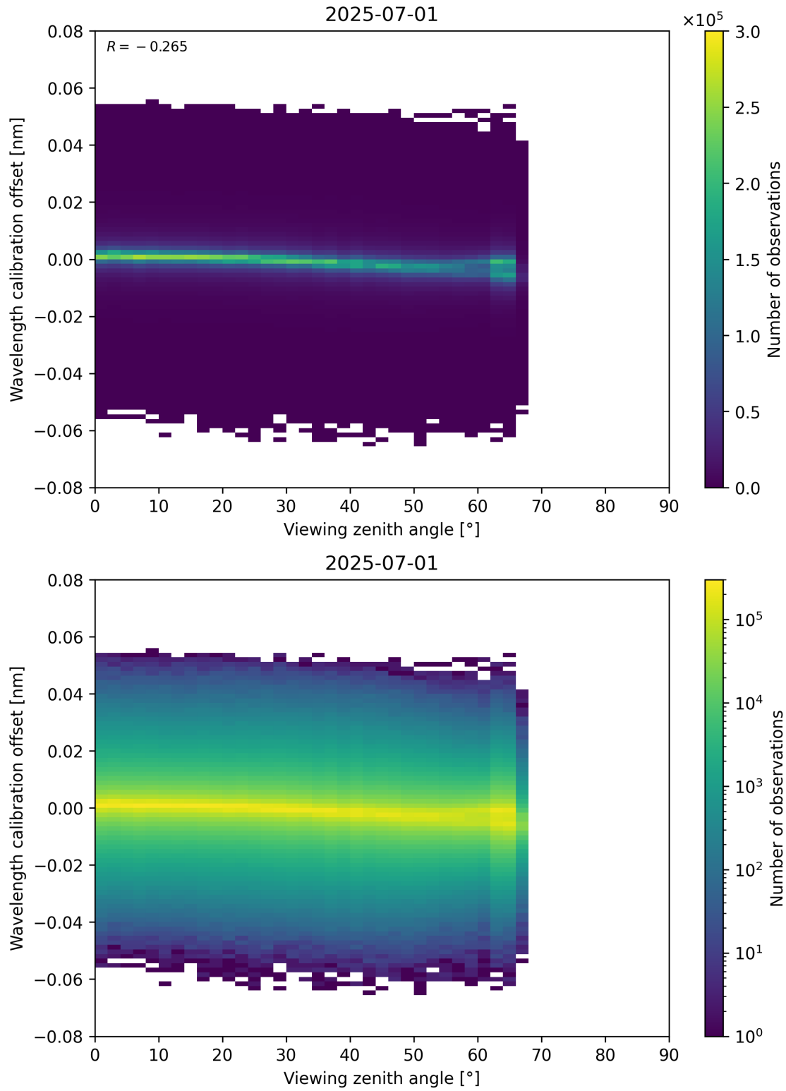
Figure 173: Scatter density plot of “Viewing zenith angle” against “Wavelength calibration offset” for 2025-06-30 to 2025-07-02.
