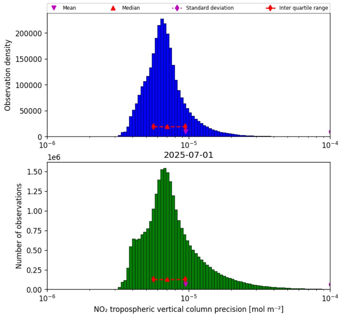
Figure 30: Histogram of “NO 2 tropospheric vertical column precision” for 2025-06-30 to 2025-07-02
