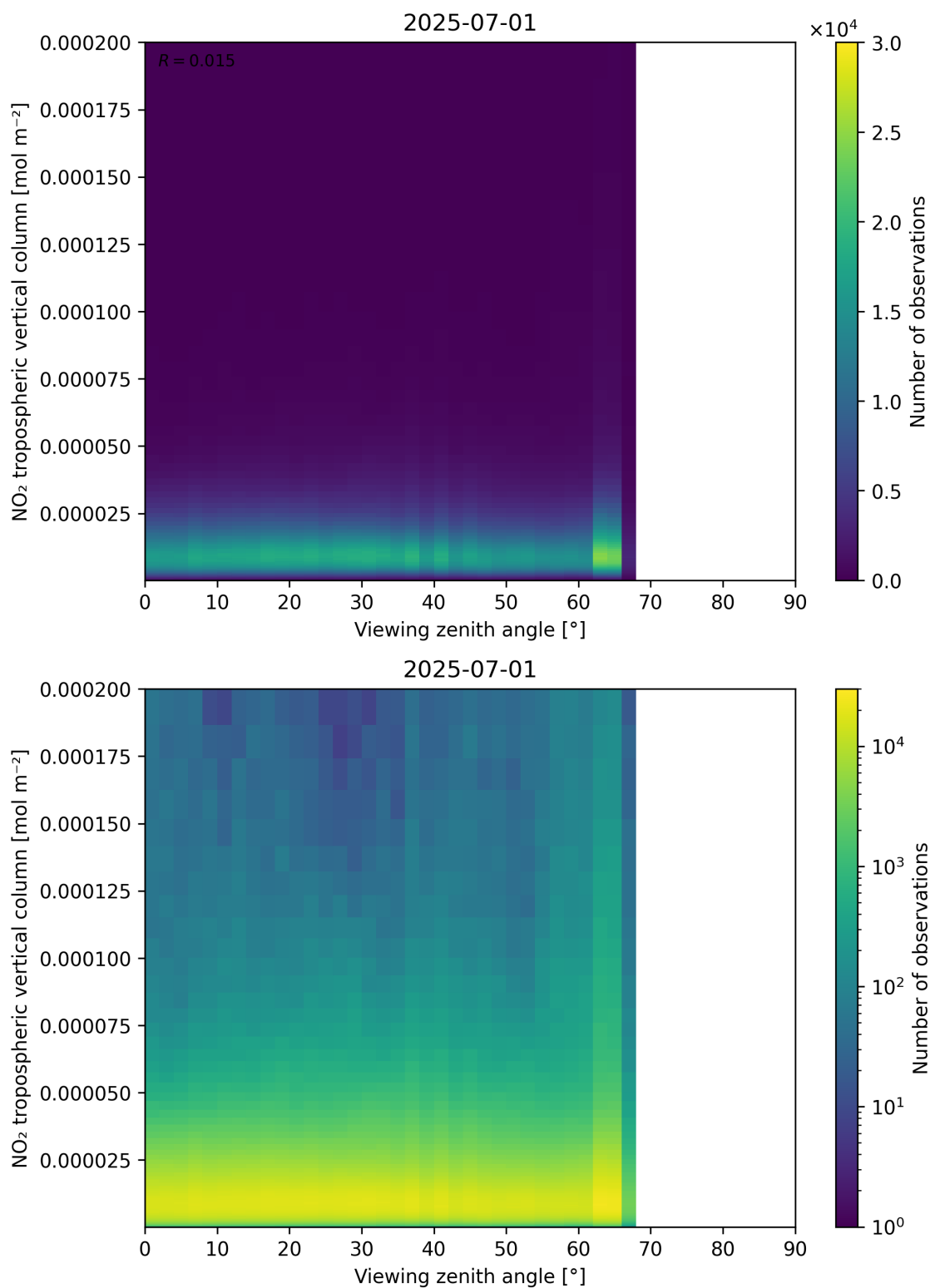
Figure 169: Scatter density plot of “Viewing zenith angle” against “NO 2 tropospheric vertical column” for 2025-06-30 to 2025-07-02.
