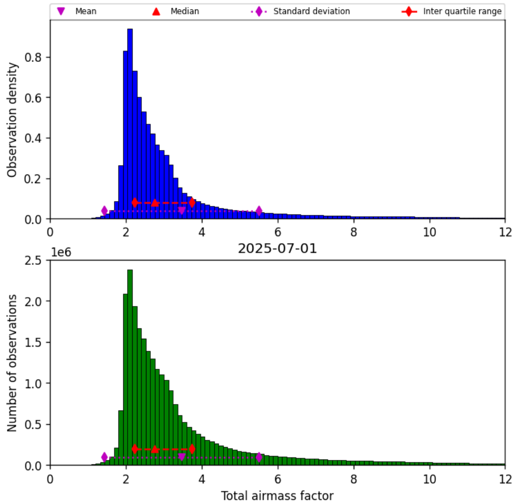
Figure 32: Histogram of “Total airmass factor” for 2025-06-30 to 2025-07-02
