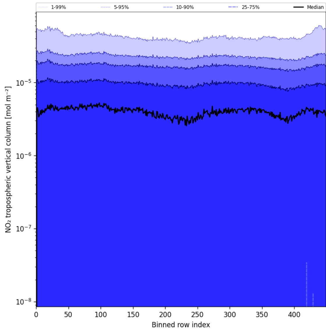
Figure 46: Along track statistics of “NO 2 tropospheric vertical column” for 2025-06-30 to 2025-07-02
