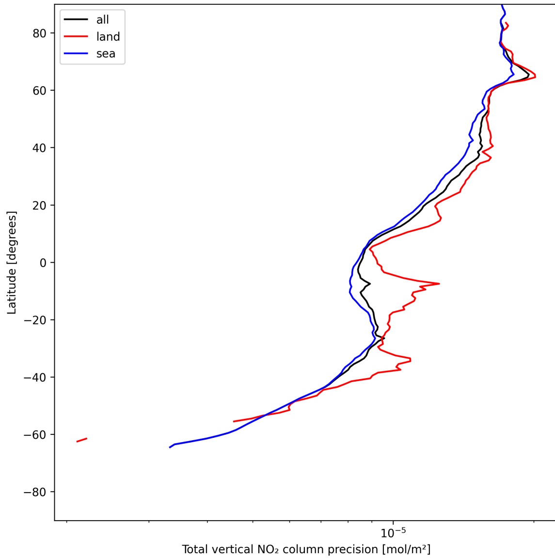
Figure 22: Zonal average of “Total vertical NO 2 column precision” for 2025-06-30 to 2025-07-02.
