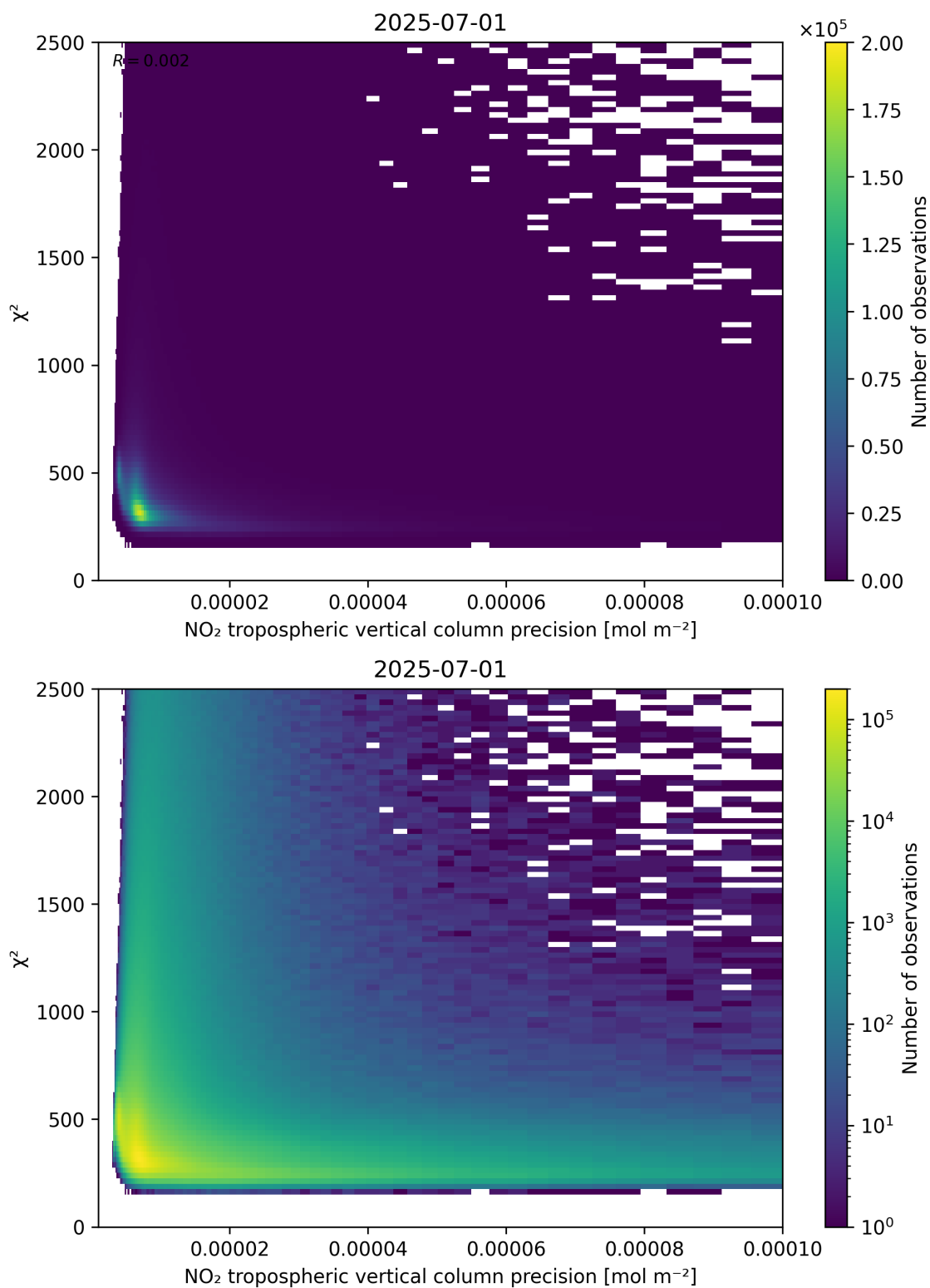
Figure 134: Scatter density plot of “NO 2 tropospheric vertical column precision” against “ \chi^2 ” for 2025-06-30 to 2025-07-02.
