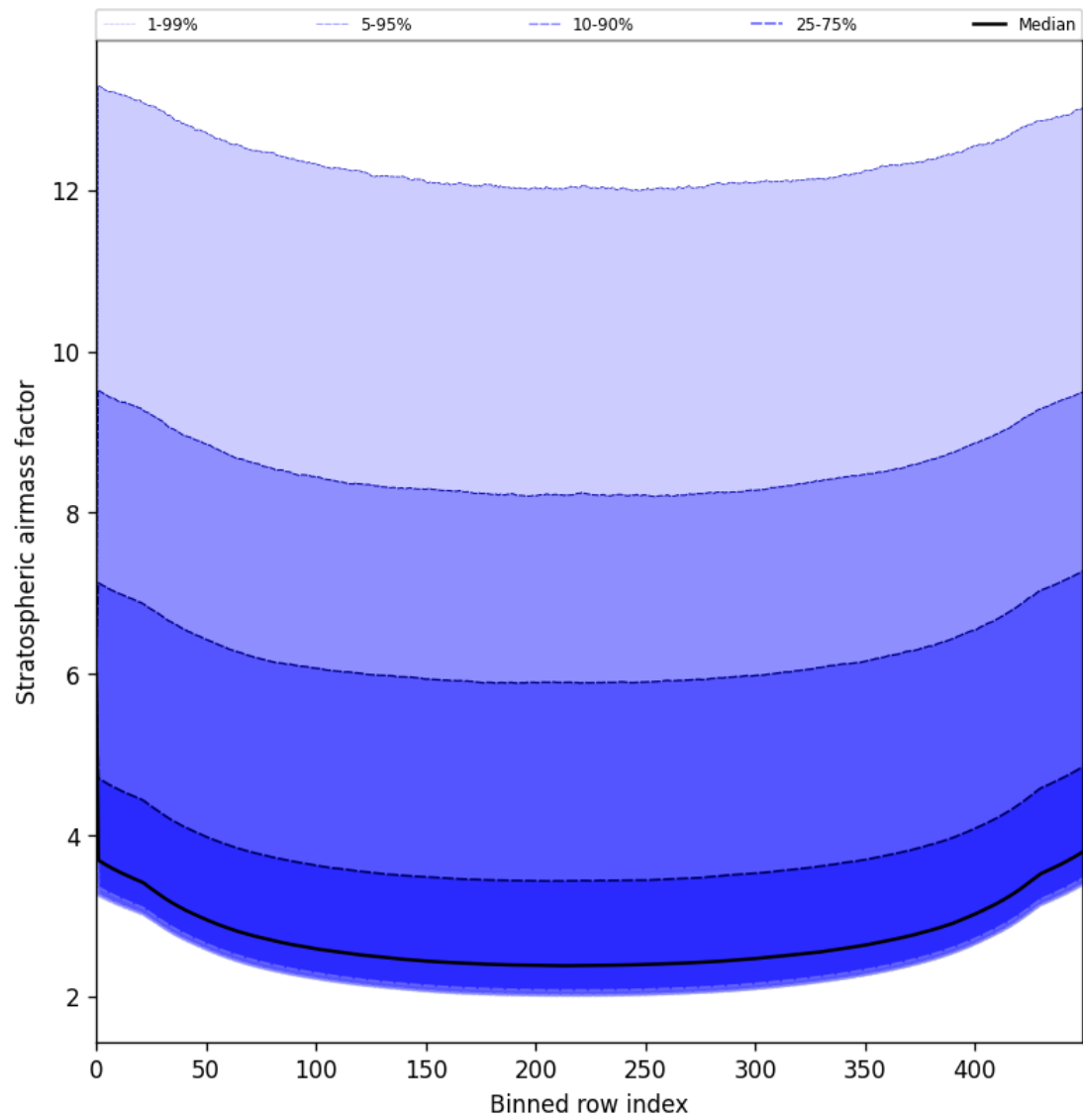
Figure 61: Along track statistics of “Stratospheric airmass factor” for 2025-06-30 to 2025-07-02
