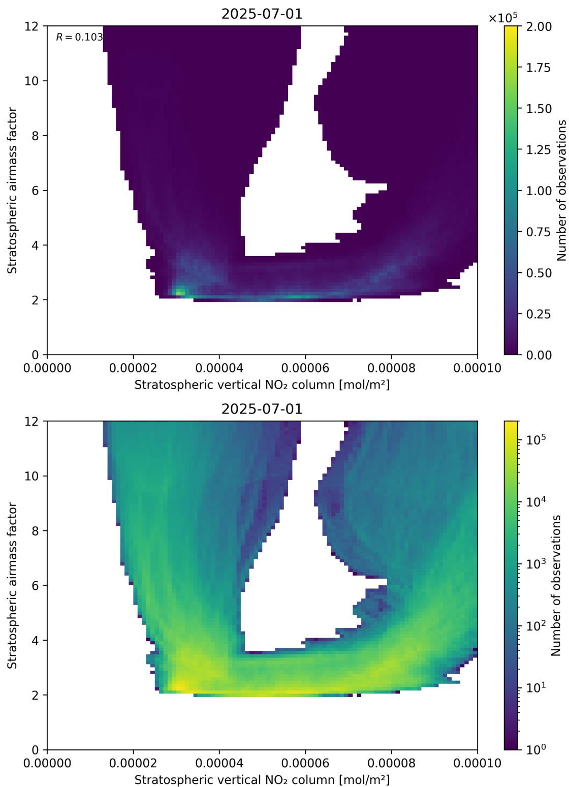
Figure 96: Scatter density plot of “Stratospheric vertical NO 2 column” against “Stratospheric airmass factor” for 2025-06-30 to 2025-07-02.
