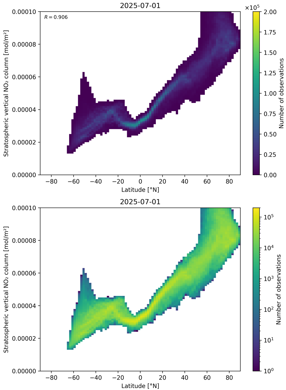
Figure 87: Scatter density plot of “Latitude” against “Stratospheric vertical NO 2 column” for 2025-06-30 to 2025-07-02.
