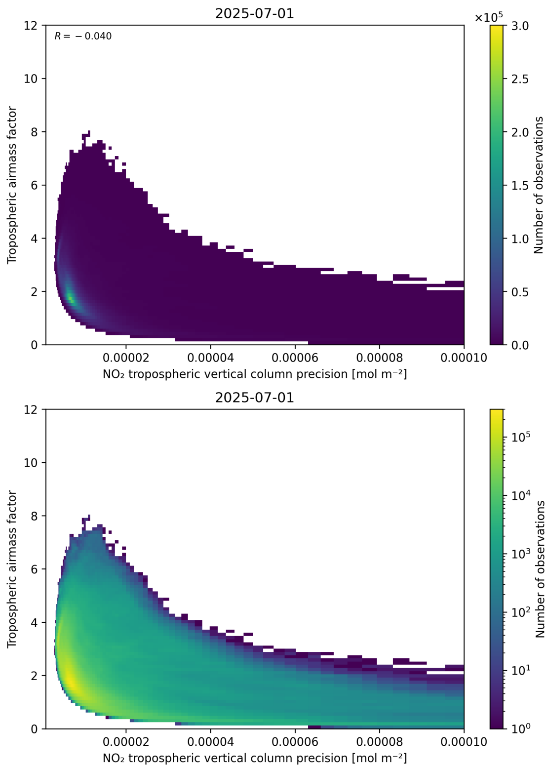
Figure 133: Scatter density plot of “NO 2 tropospheric vertical column precision” against “Tropospheric air mass factor” for 2025-06-30 to 2025-07-02.
