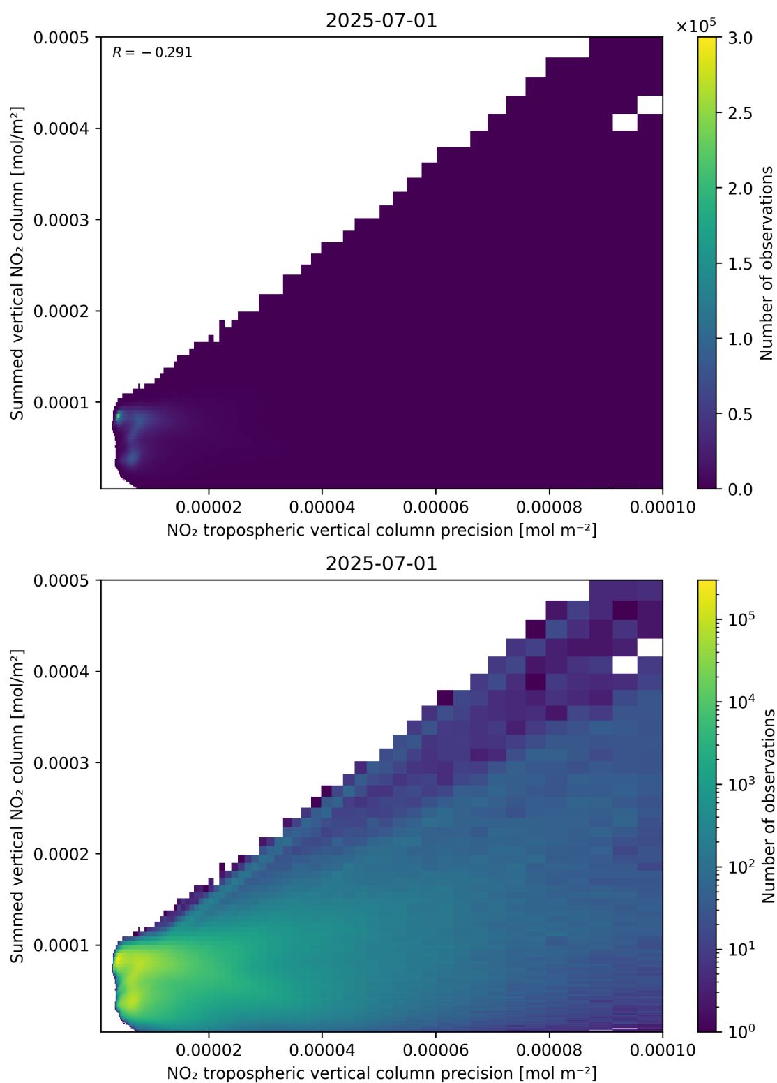
Figure 136: Scatter density plot of “NO 2 tropospheric vertical column precision” against “Summed vertical NO 2 column” for 2025-06-30 to 2025-07-02.
