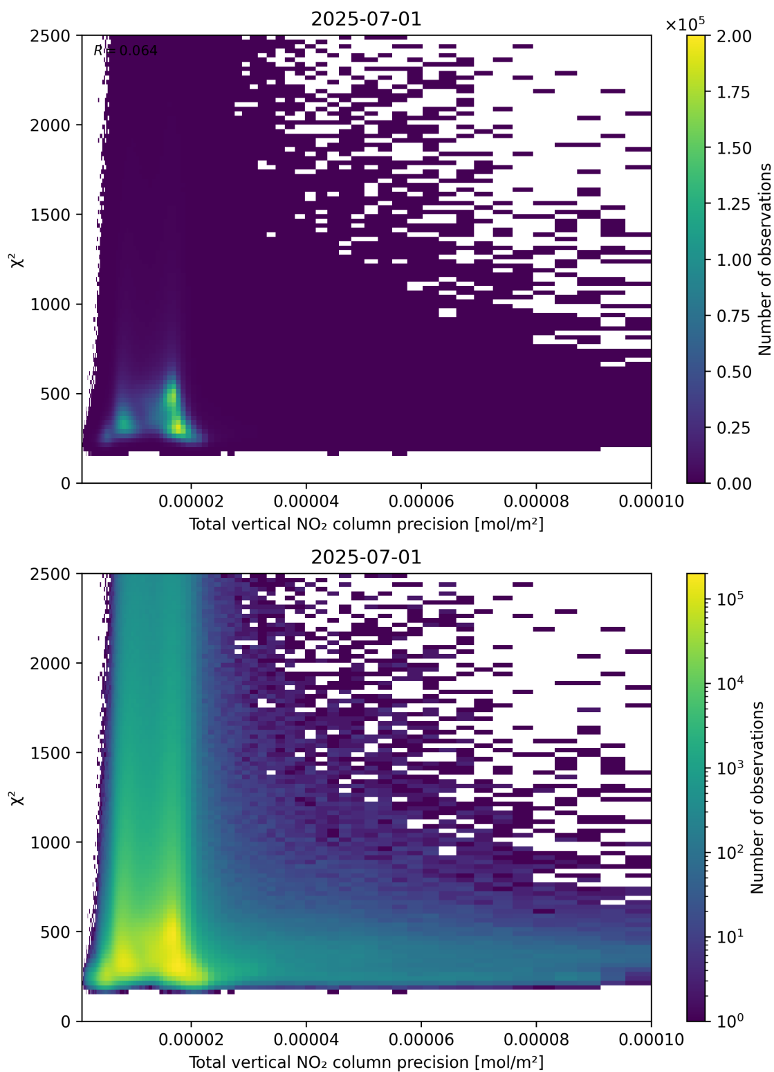
Figure 116: Scatter density plot of “Total vertical NO 2 column precision” against “ \chi^2 ” for 2025-06-30 to 2025-07-02.
