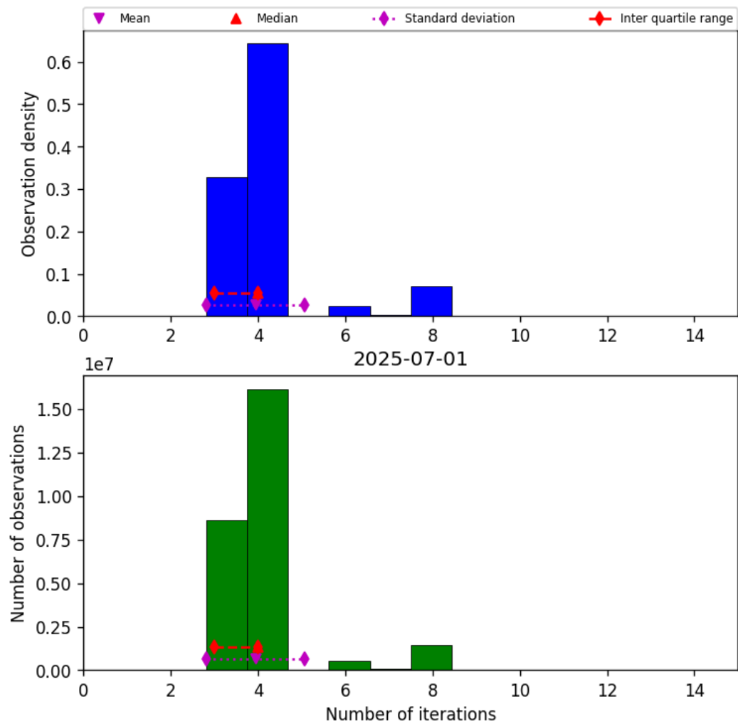
Figure 34: Histogram of "Number of iterations" for 2025-06-30 to 2025-07-02
