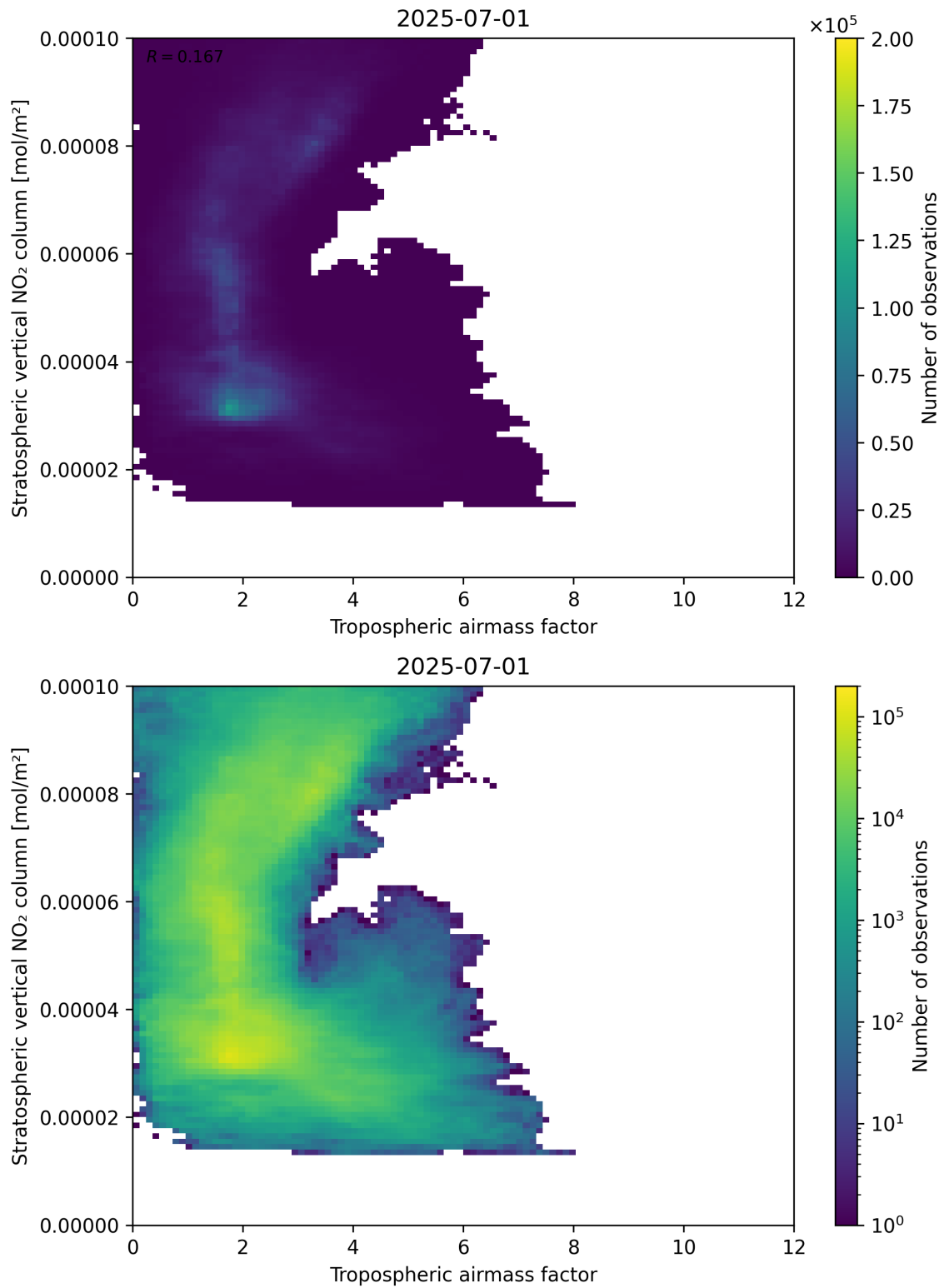
Figure 74: Scatter density plot of “Tropospheric air mass factor” against “Stratospheric vertical NO 2 column” for 2025-06-30 to 2025-07-02.
