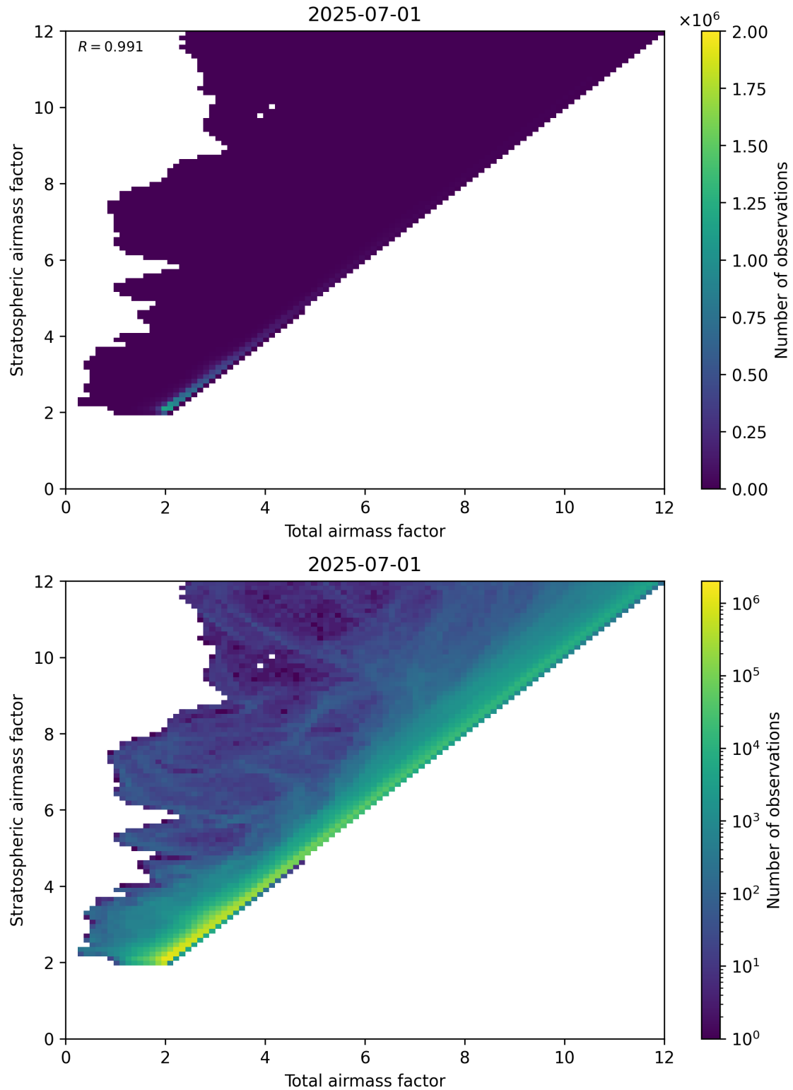
Figure 62: Scatter density plot of “Total airmass factor” against “Stratospheric airmass factor” for 2025-06-30 to 2025-07-02.
