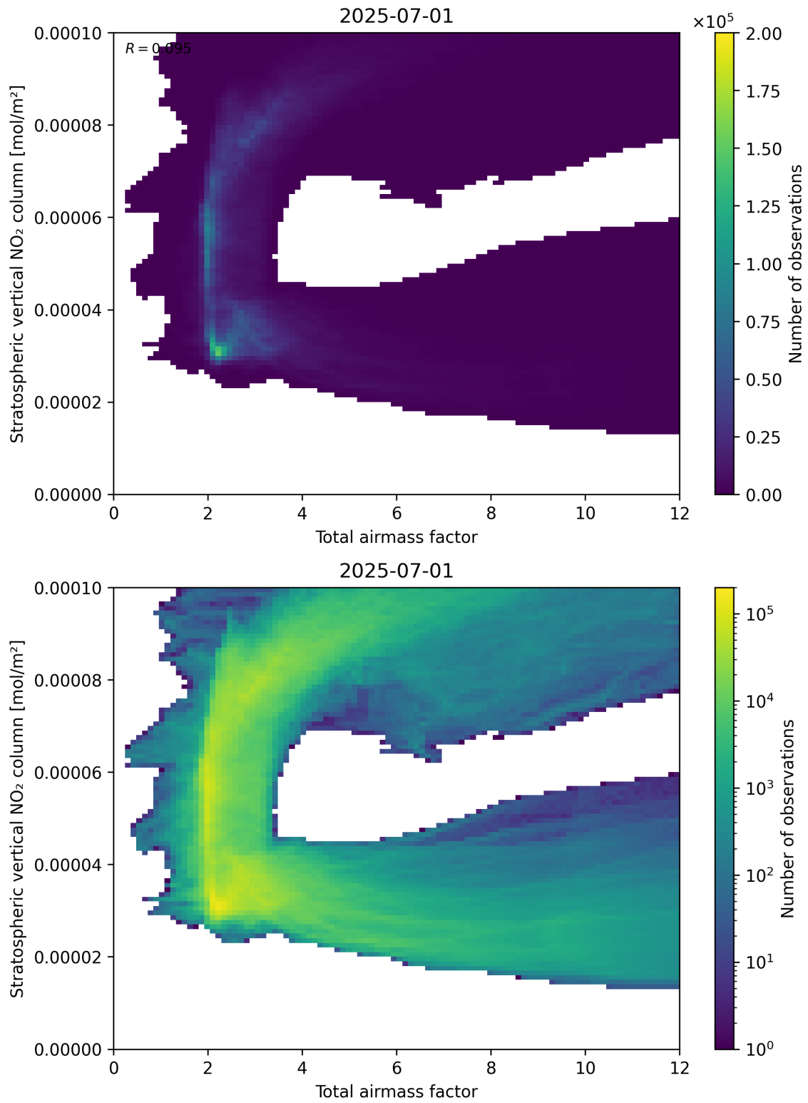
Figure 64: Scatter density plot of “Total airmass factor” against “Stratospheric vertical NO 2 column” for 2025-06-30 to 2025-07-02.
