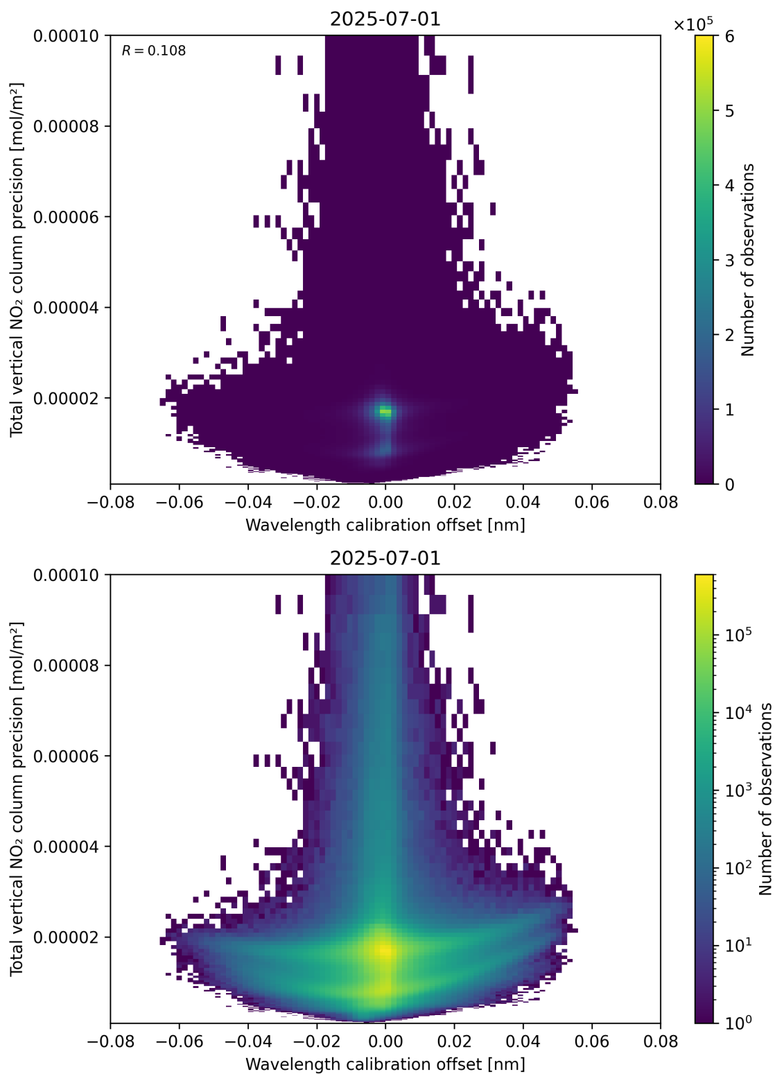
Figure 180: Scatter density plot of “Wavelength calibration offset” against “Total vertical NO 2 column precision” for 2025-06-30 to 2025-07-02.
