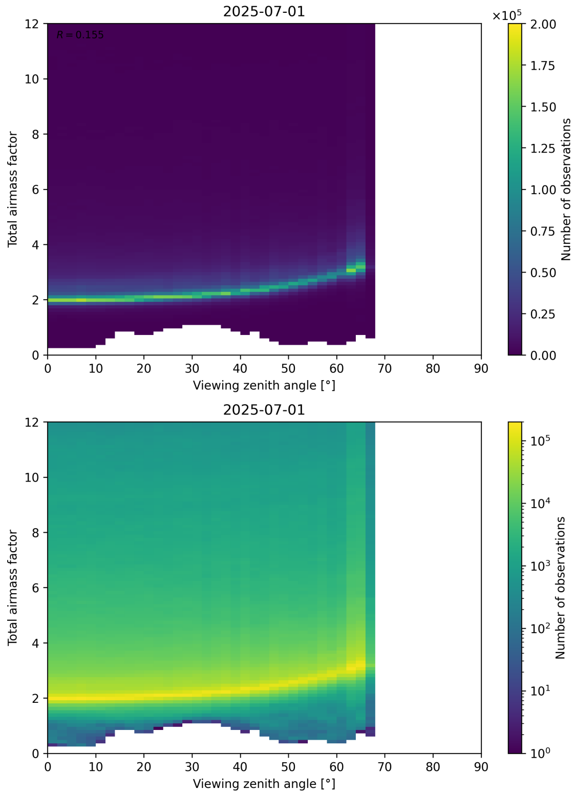
Figure 160: Scatter density plot of “Viewing zenith angle” against “Total airmass factor” for 2025-06-30 to 2025-07-02.
