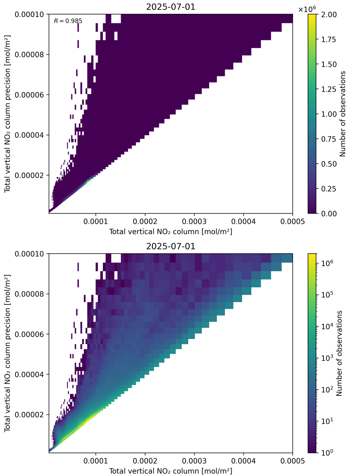
Figure 114: Scatter density plot of “Total vertical NO 2 column” against “Total vertical NO 2 column precision” for 2025-06-30 to 2025-07-02.
