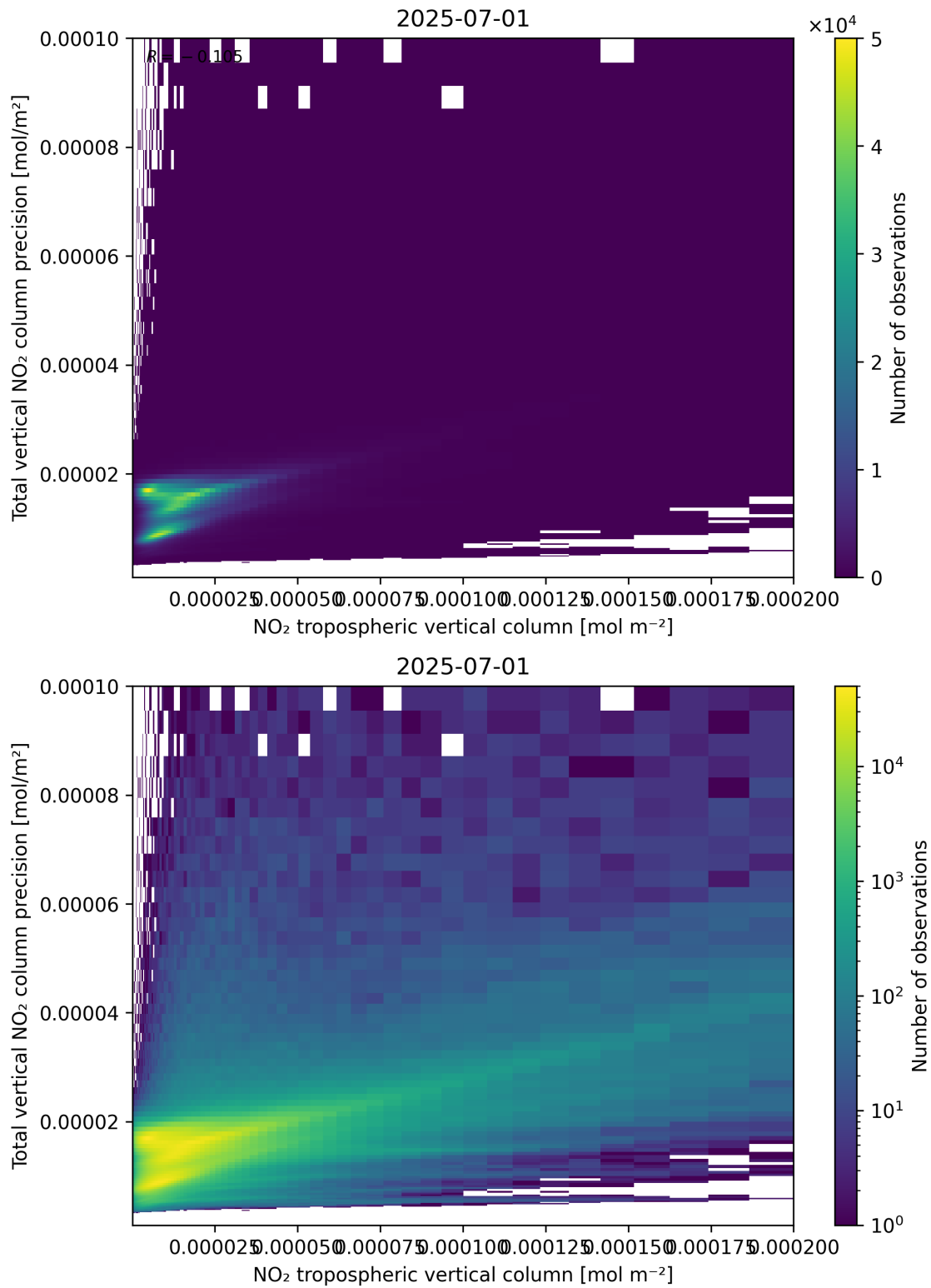
Figure 129: Scatter density plot of “NO 2 tropospheric vertical column” against “Total vertical NO 2 column precision” for 2025-06-30 to 2025-07-02.
