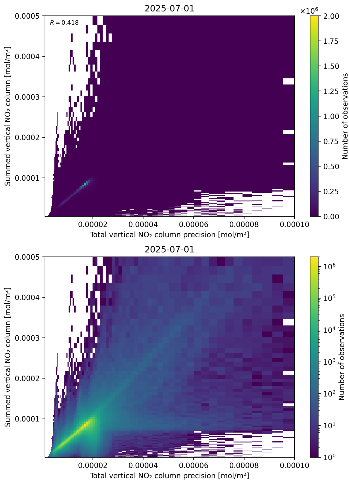
Figure 117: Scatter density plot of “Total vertical NO 2 column precision” against “Summed vertical NO 2 column” for 2025-06-30 to 2025-07-02.
