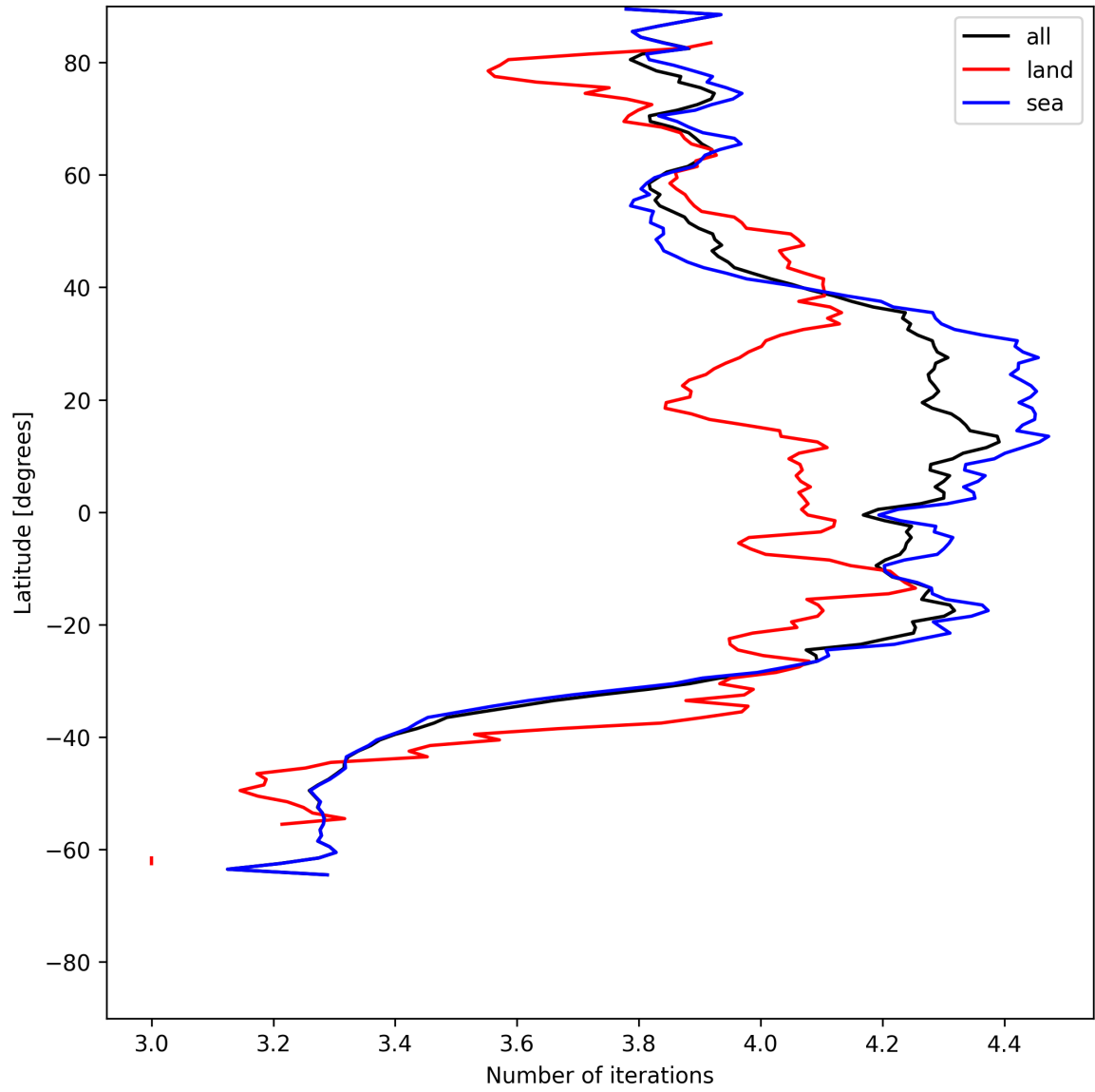
Figure 17: Zonal average of “Number of iterations” for 2025-06-30 to 2025-07-02.
