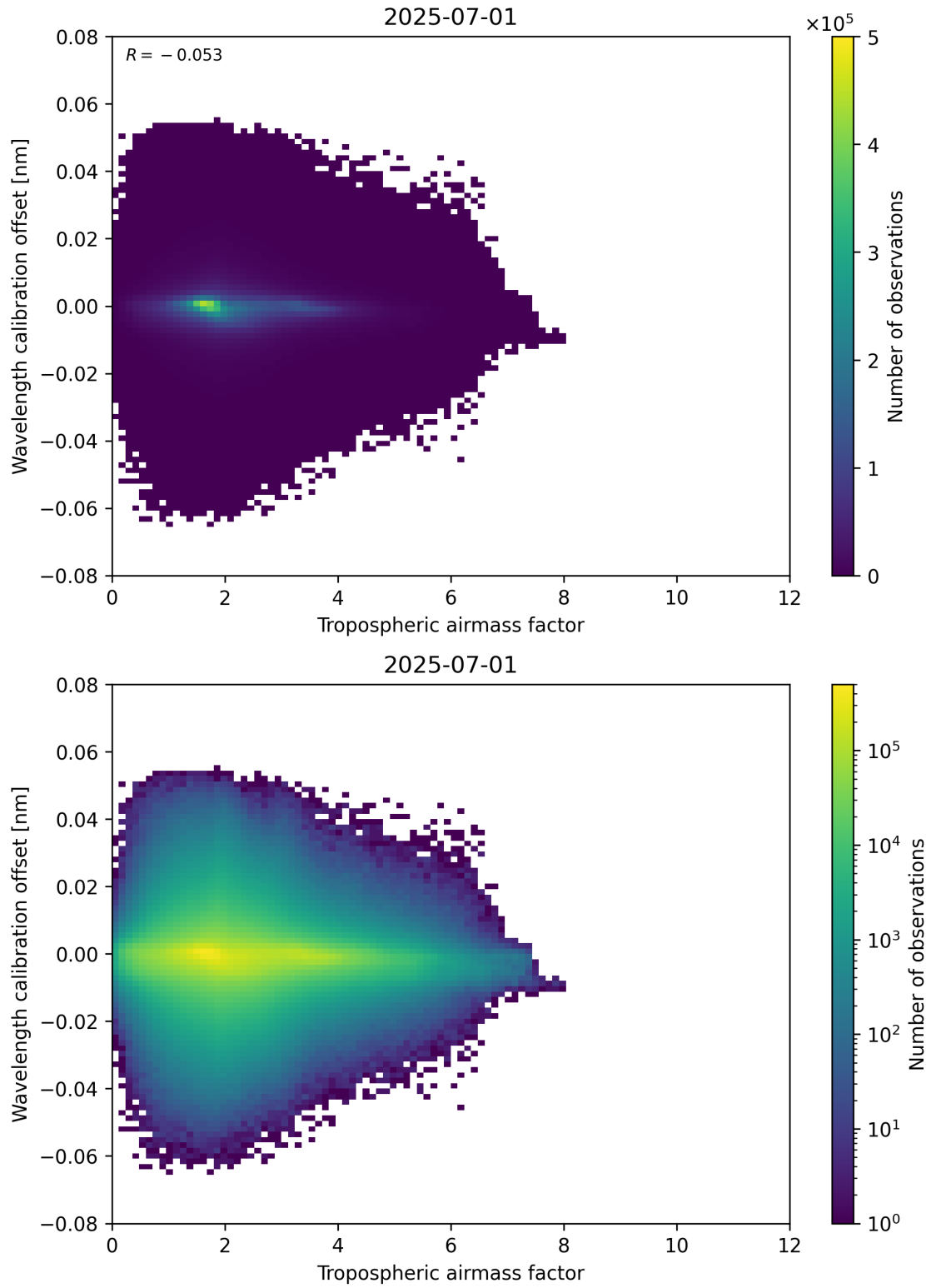
Figure 80: Scatter density plot of “Tropospheric airmass factor” against “Wavelength calibration offset” for 2025-06-30 to 2025-07-02.
