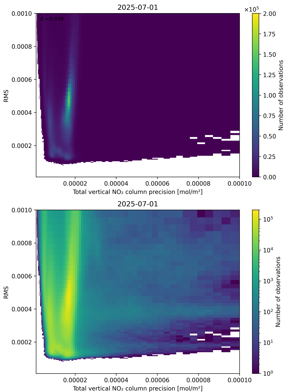
Figure 119: Scatter density plot of “Total vertical NO 2 column precision” against “RMS” for 2025-06-30 to 2025-07-02.
