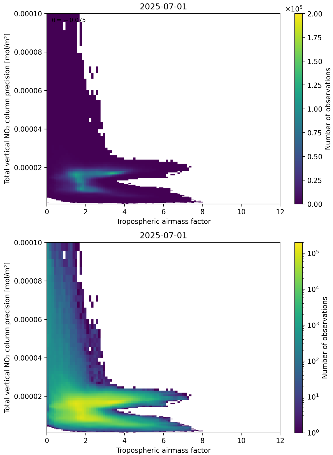
Figure 78: Scatter density plot of “Tropospheric air mass factor” against “Total vertical NO 2 column precision” for 2025-06-30 to 2025-07-02.
