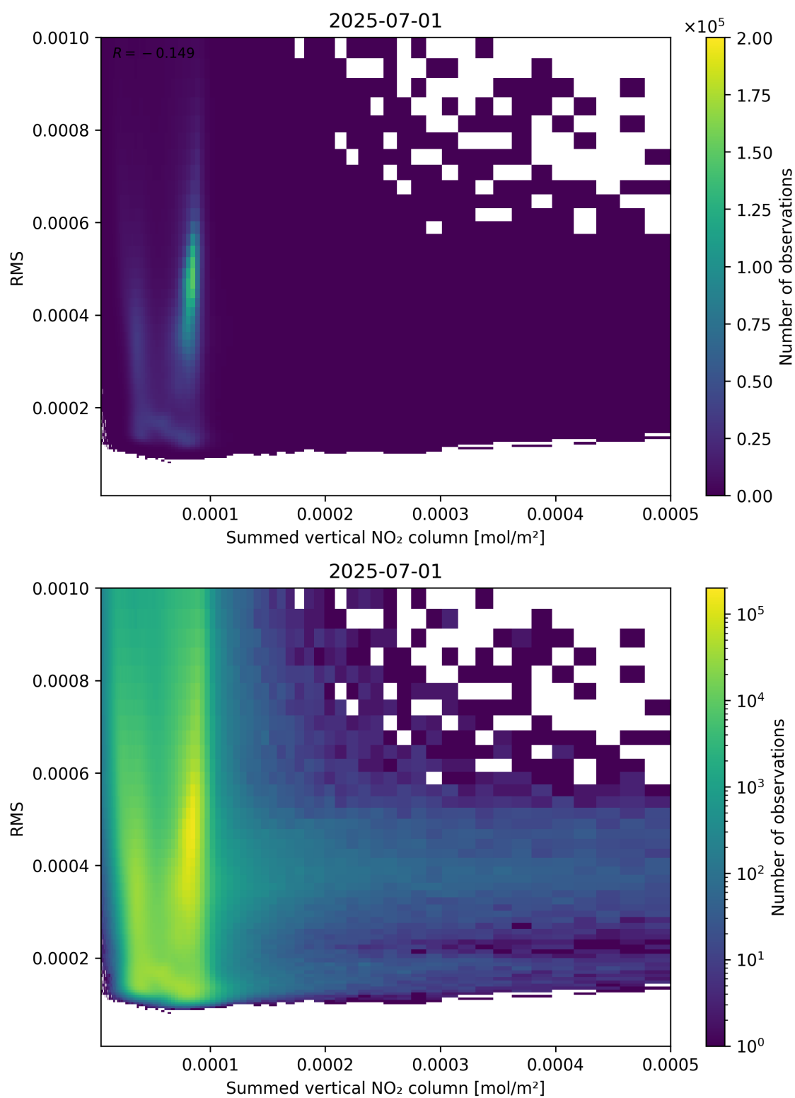
Figure 109: Scatter density plot of “Summed vertical NO 2 column” against “RMS” for 2025-06-30 to 2025-07-02.
