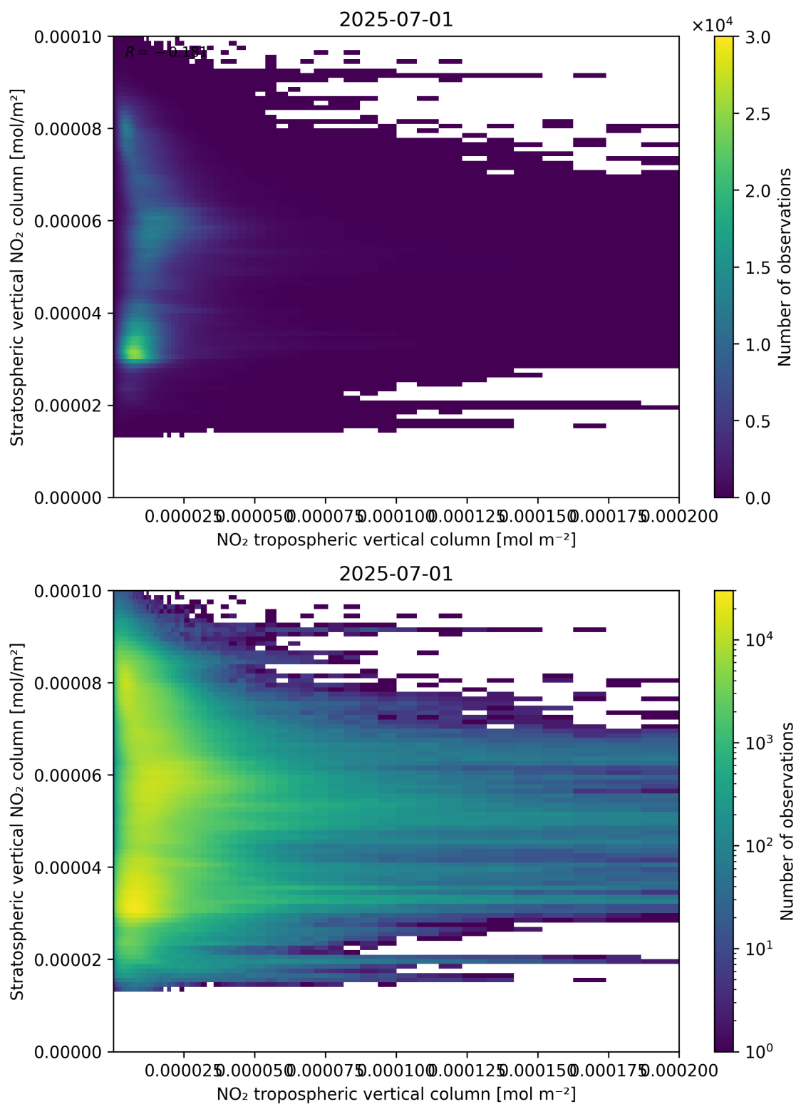
Figure 125: Scatter density plot of “NO 2 tropospheric vertical column” against “Stratospheric vertical NO 2 column” for 2025-06-30 to 2025-07-02.
