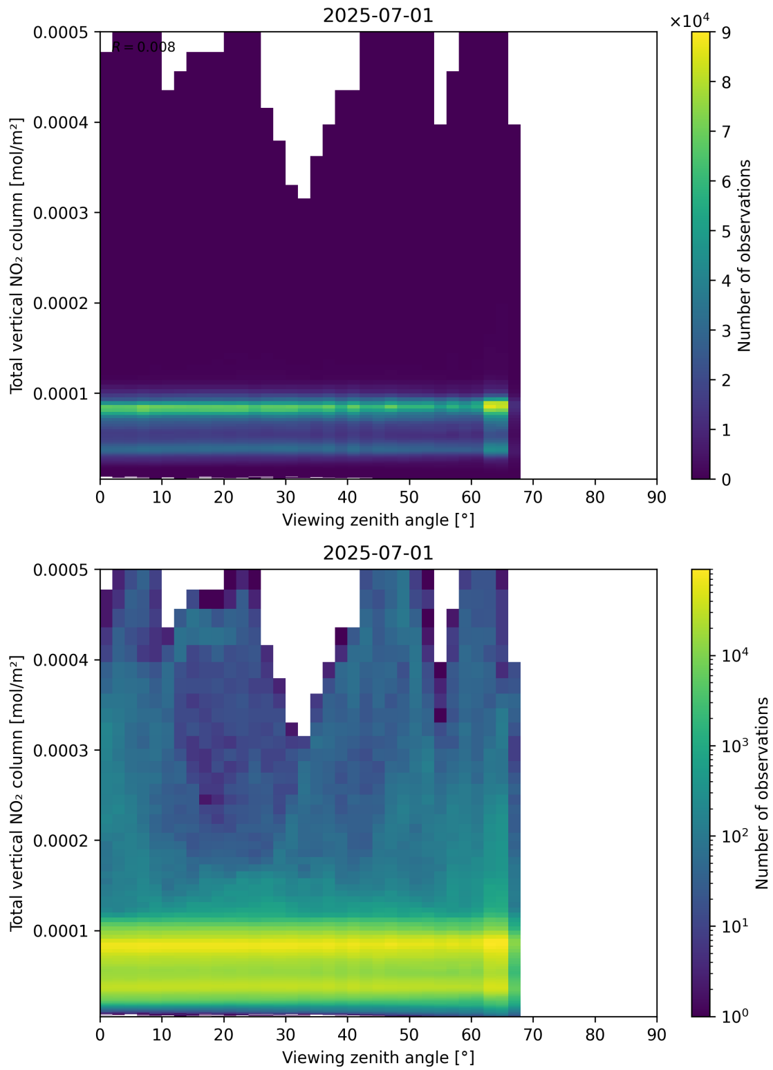
Figure 167: Scatter density plot of “Viewing zenith angle” against “Total vertical NO 2 column” for 2025-06-30 to 2025-07-02.
