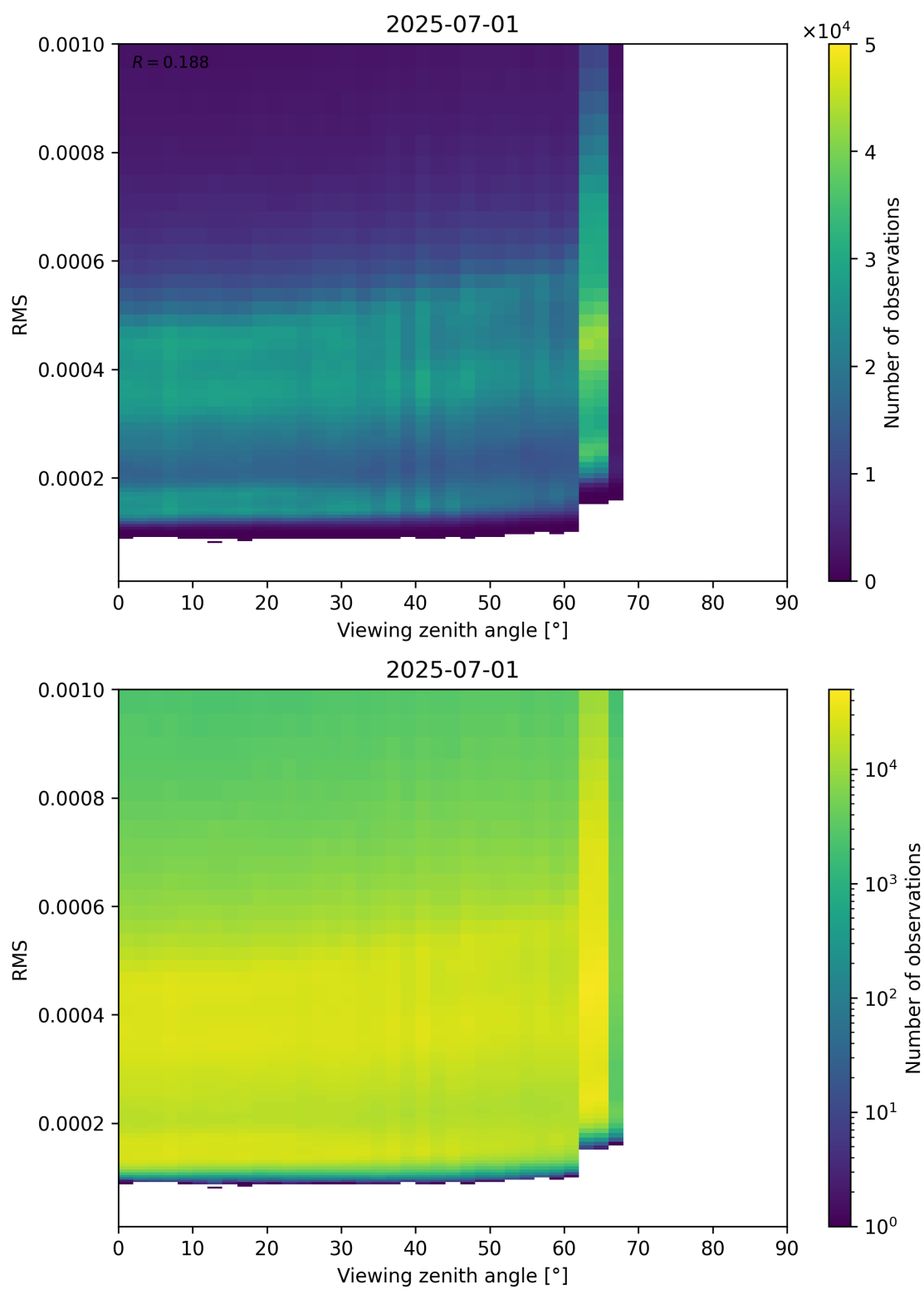
Figure 171: Scatter density plot of “Viewing zenith angle” against “RMS” for 2025-06-30 to 2025-07-02.
