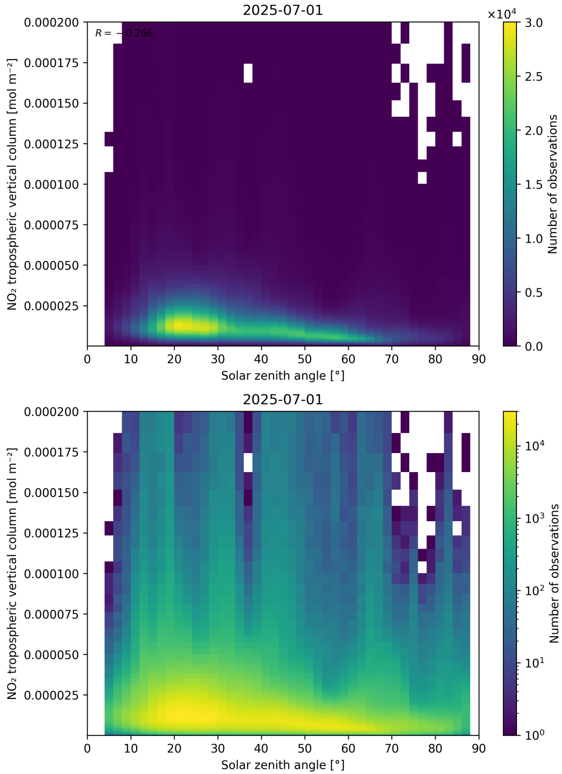
Figure 155: Scatter density plot of “Solar zenith angle” against “NO 2 tropospheric vertical column” for 2025-06-30 to 2025-07-02.
