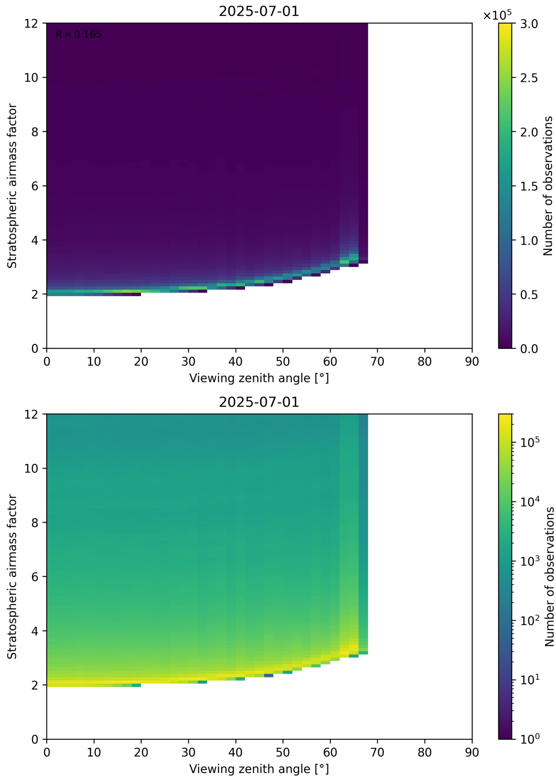
Figure 159: Scatter density plot of “Viewing zenith angle” against “Stratospheric airmass factor” for 2025-06-30 to 2025-07-02.
