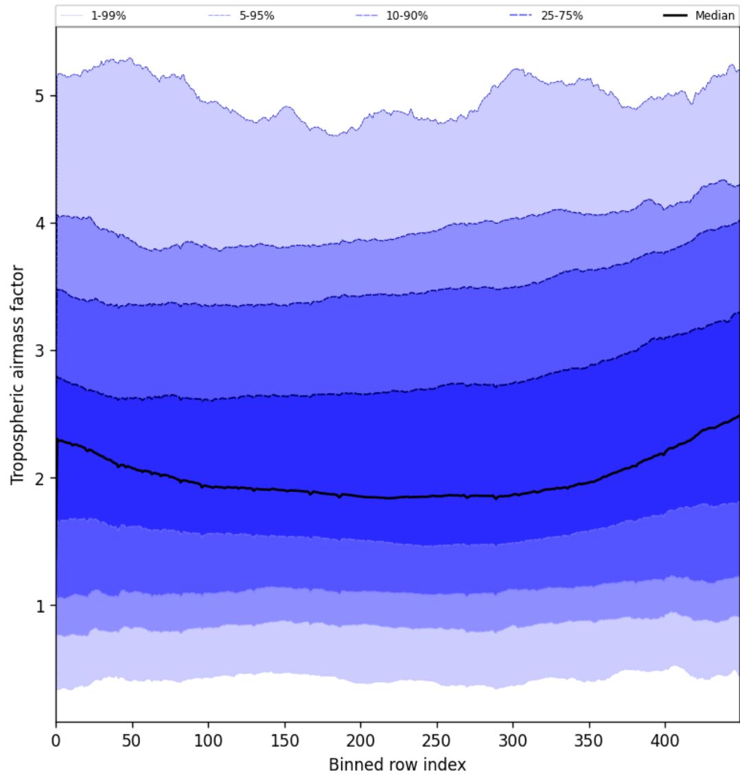
Figure 48: Along track statistics of “Tropospheric air mass factor” for 2025-06-30 to 2025-07-02
