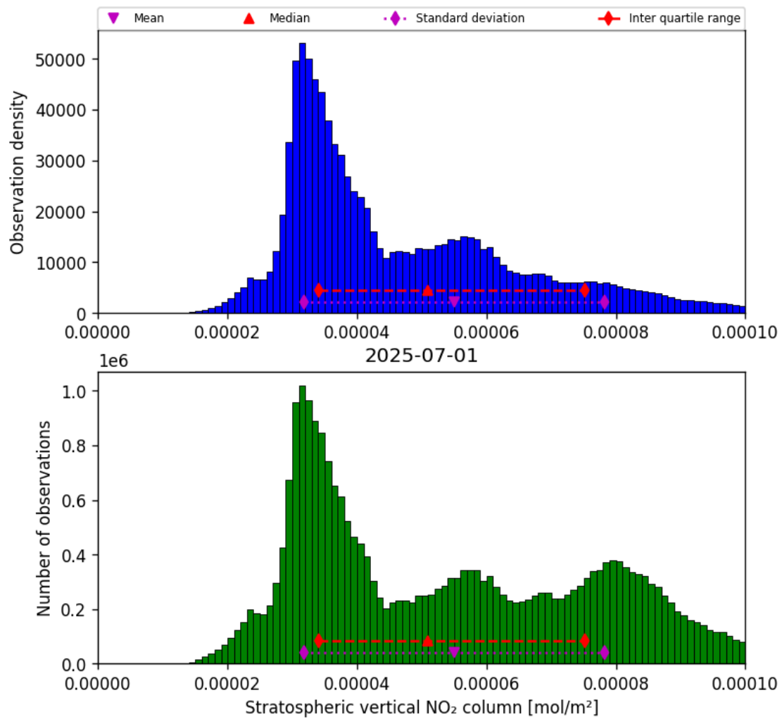
Figure 36: Histogram of “Stratospheric vertical NO 2 column” for 2025-06-30 to 2025-07-02
