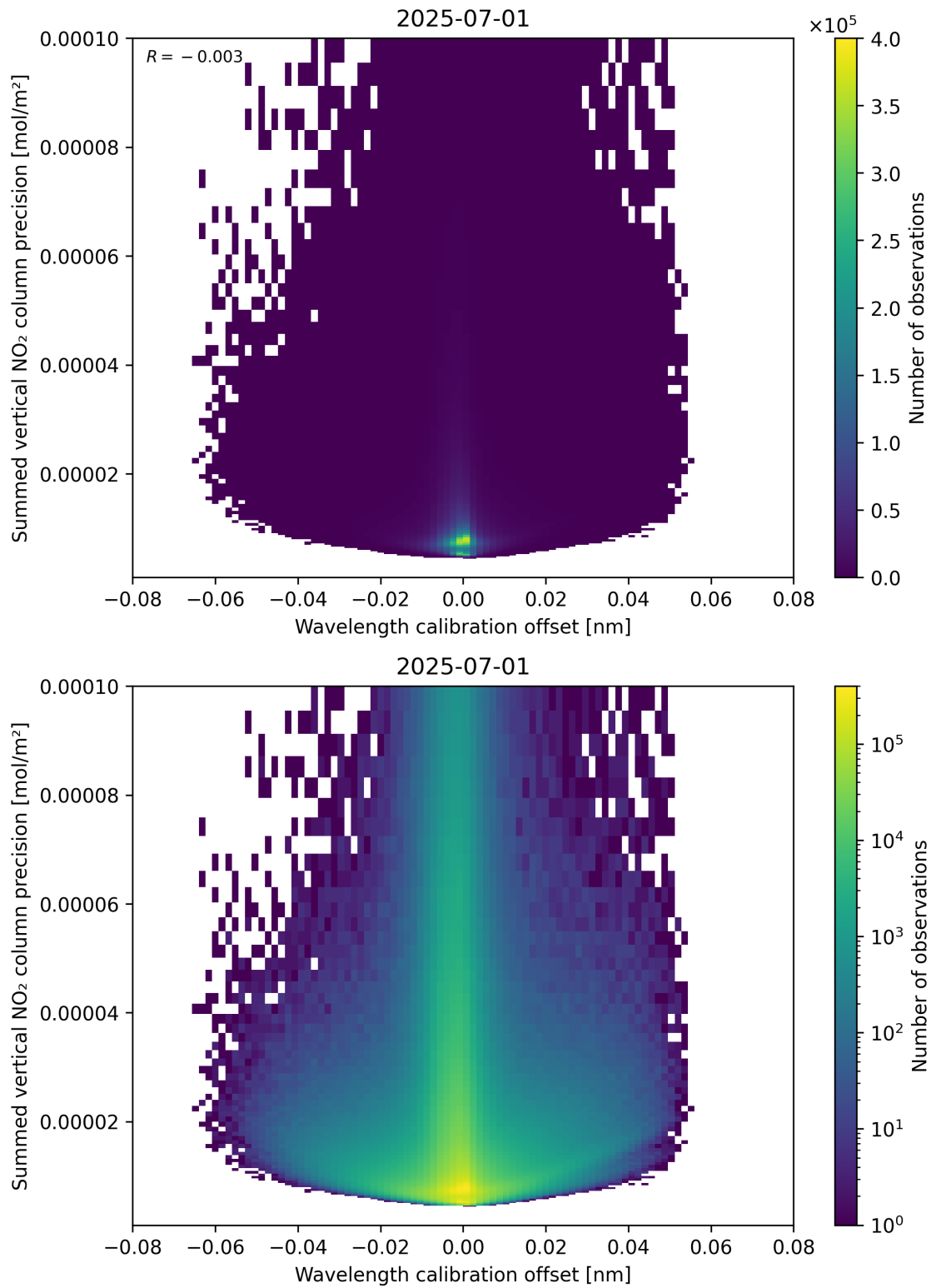
Figure 178: Scatter density plot of “Wavelength calibration offset” against “Summed vertical NO 2 column precision” for 2025-06-30 to 2025-07-02.
