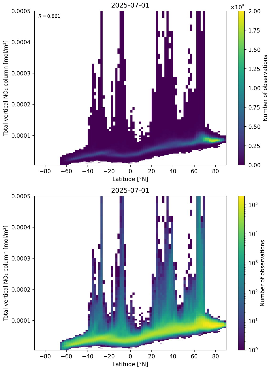
Figure 90: Scatter density plot of “Latitude” against “Total vertical NO 2 column” for 2025-06-30 to 2025-07-02.
