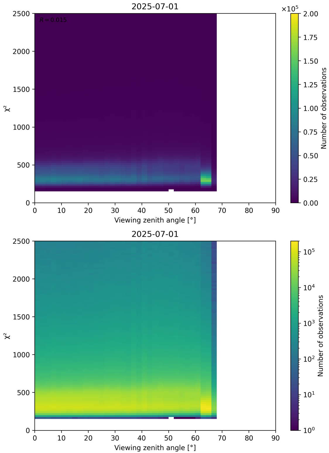
Figure 162: Scatter density plot of “Viewing zenith angle” against “ \chi^2 ” for 2025-06-30 to 2025-07-02.
