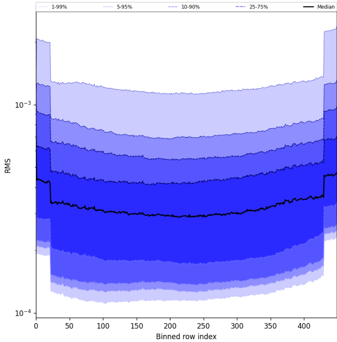
Figure 60: Along track statistics of “RMS” for 2025-06-30 to 2025-07-02
