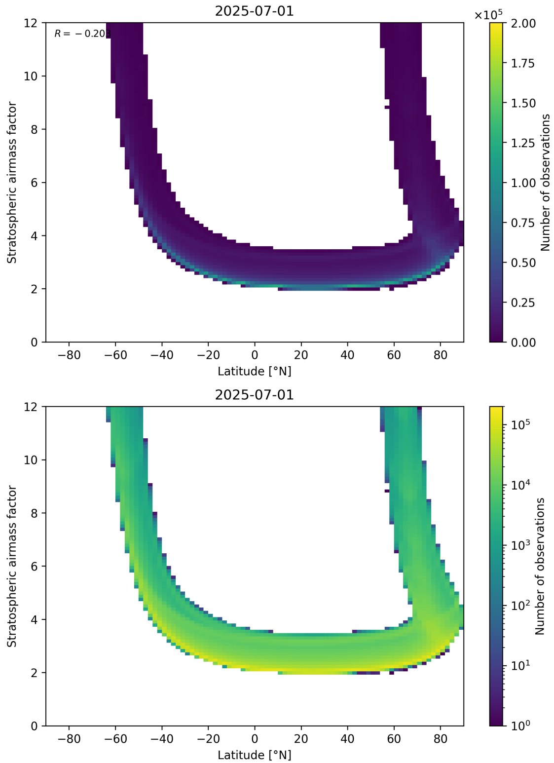
Figure 83: Scatter density plot of “Latitude” against “Stratospheric air mass factor” for 2025-06-30 to 2025-07-02.
