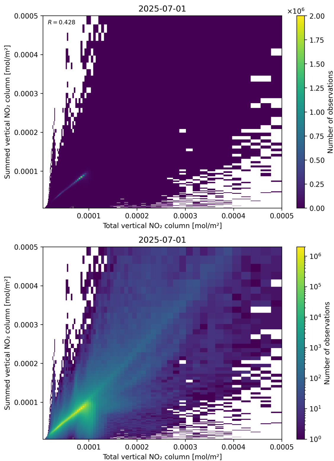
Figure 112: Scatter density plot of “Total vertical NO 2 column” against “Summed vertical NO 2 column” for 2025-06-30 to 2025-07-02.
