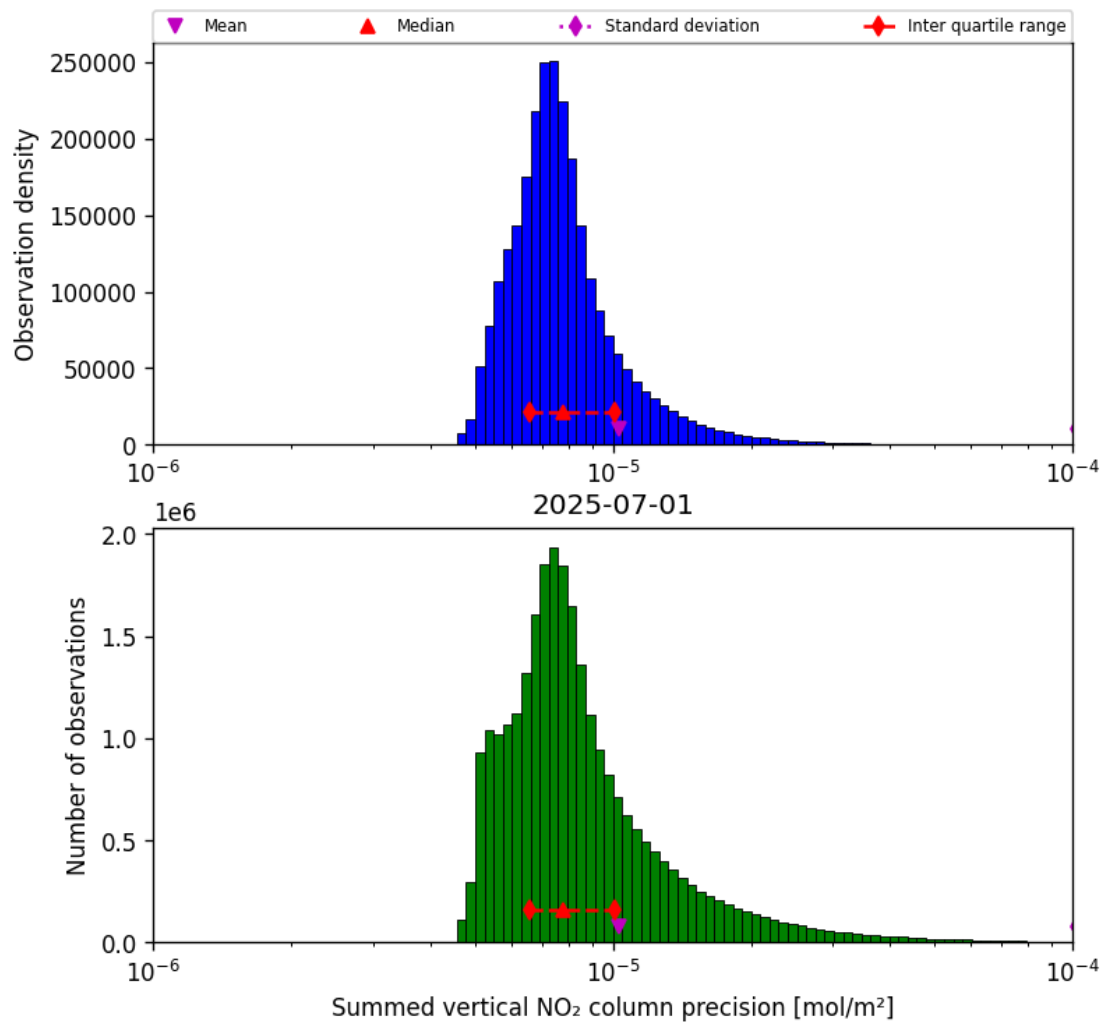
Figure 41: Histogram of "Summed vertical NO 2 column precision" for 2025-06-30 to 2025-07-02
