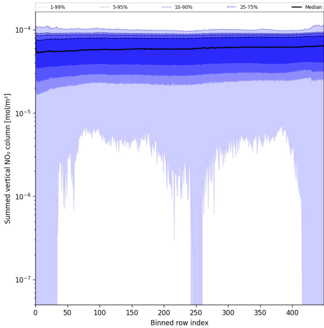
Figure 57: Along track statistics of “Summed vertical NO 2 column” for 2025-06-30 to 2025-07-02
