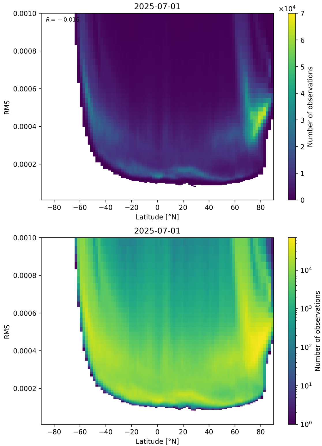
Figure 94: Scatter density plot of “Latitude” against “RMS” for 2025-06-30 to 2025-07-02.
