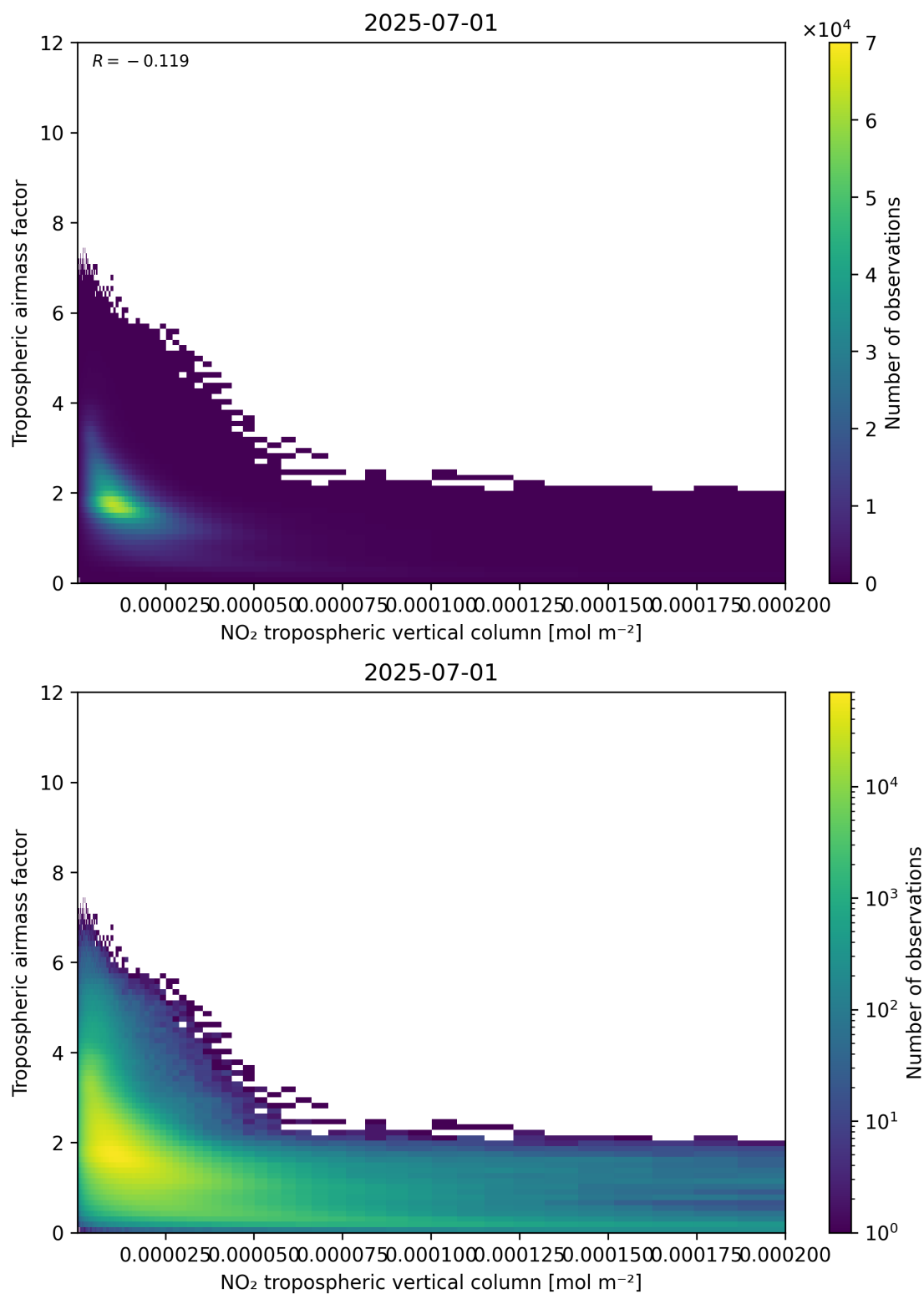
Figure 123: Scatter density plot of “NO 2 tropospheric vertical column” against “Tropospheric air mass factor” for 2025-06-30 to 2025-07-02.
