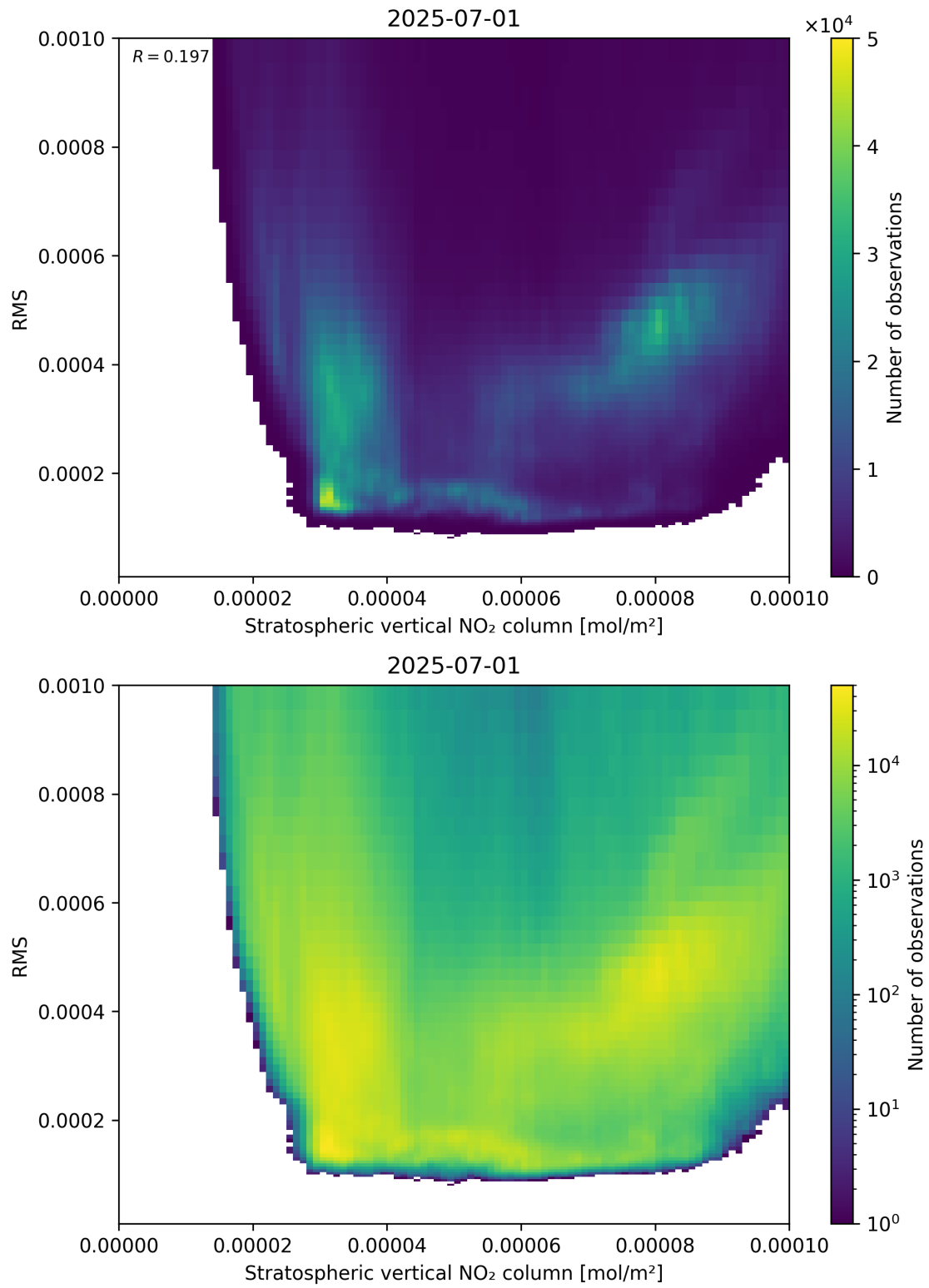
Figure 102: Scatter density plot of “Stratospheric vertical NO 2 column” against “RMS” for 2025-06-30 to 2025-07-02.
