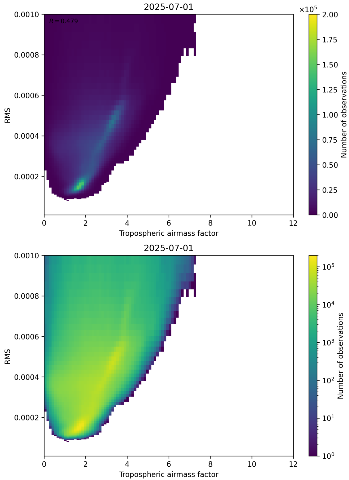
Figure 79: Scatter density plot of “Tropospheric airmass factor” against “RMS” for 2025-06-30 to 2025-07-02.
