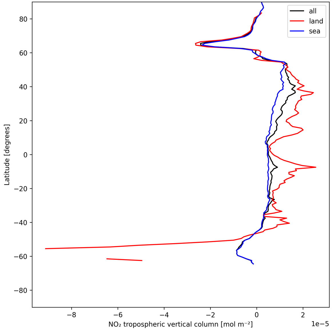
Figure 12: Zonal average of “NO 2 tropospheric vertical column” for 2025-06-30 to 2025-07-02.
