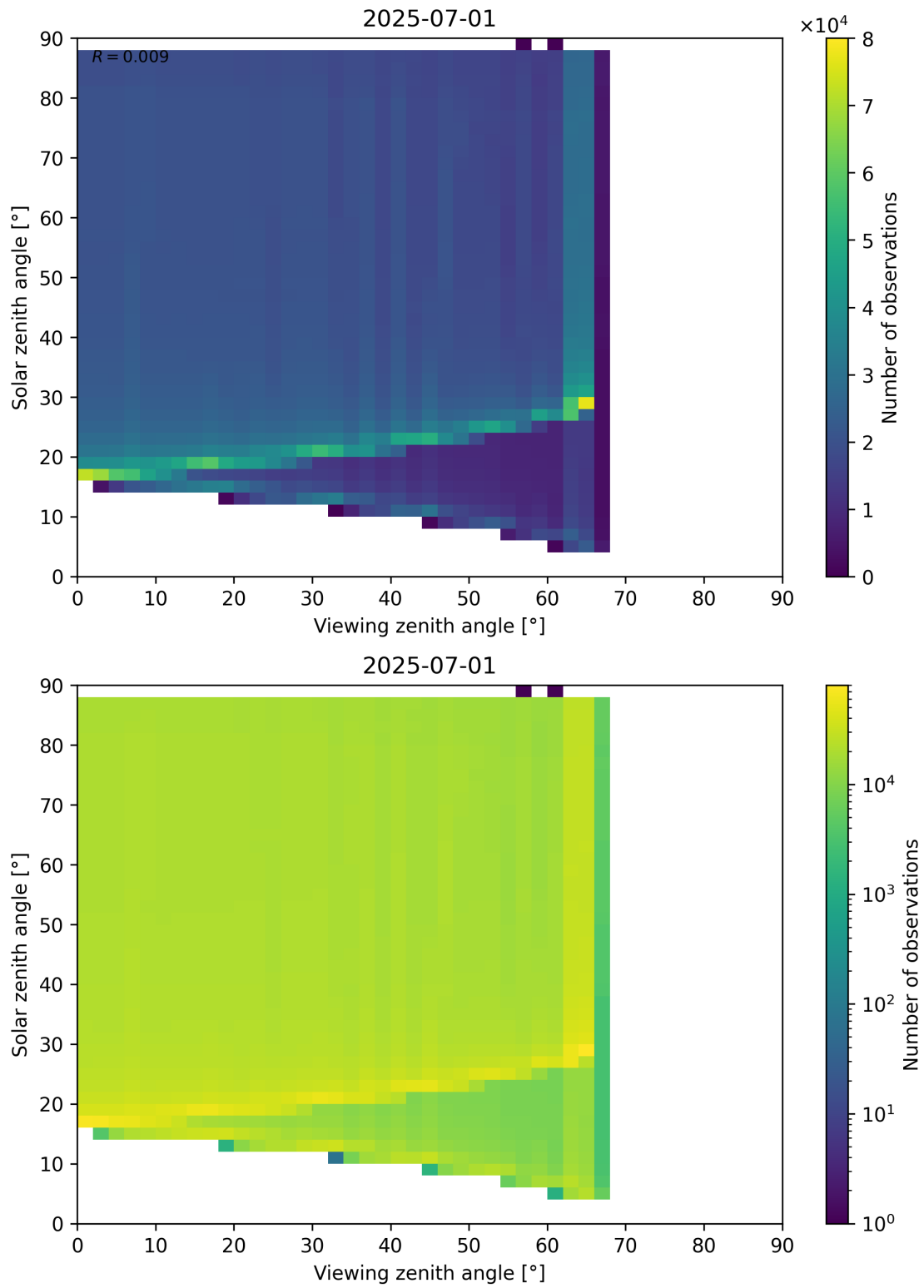
Figure 172: Scatter density plot of “Viewing zenith angle” against “Solar zenith angle” for 2025-06-30 to 2025-07-02.
