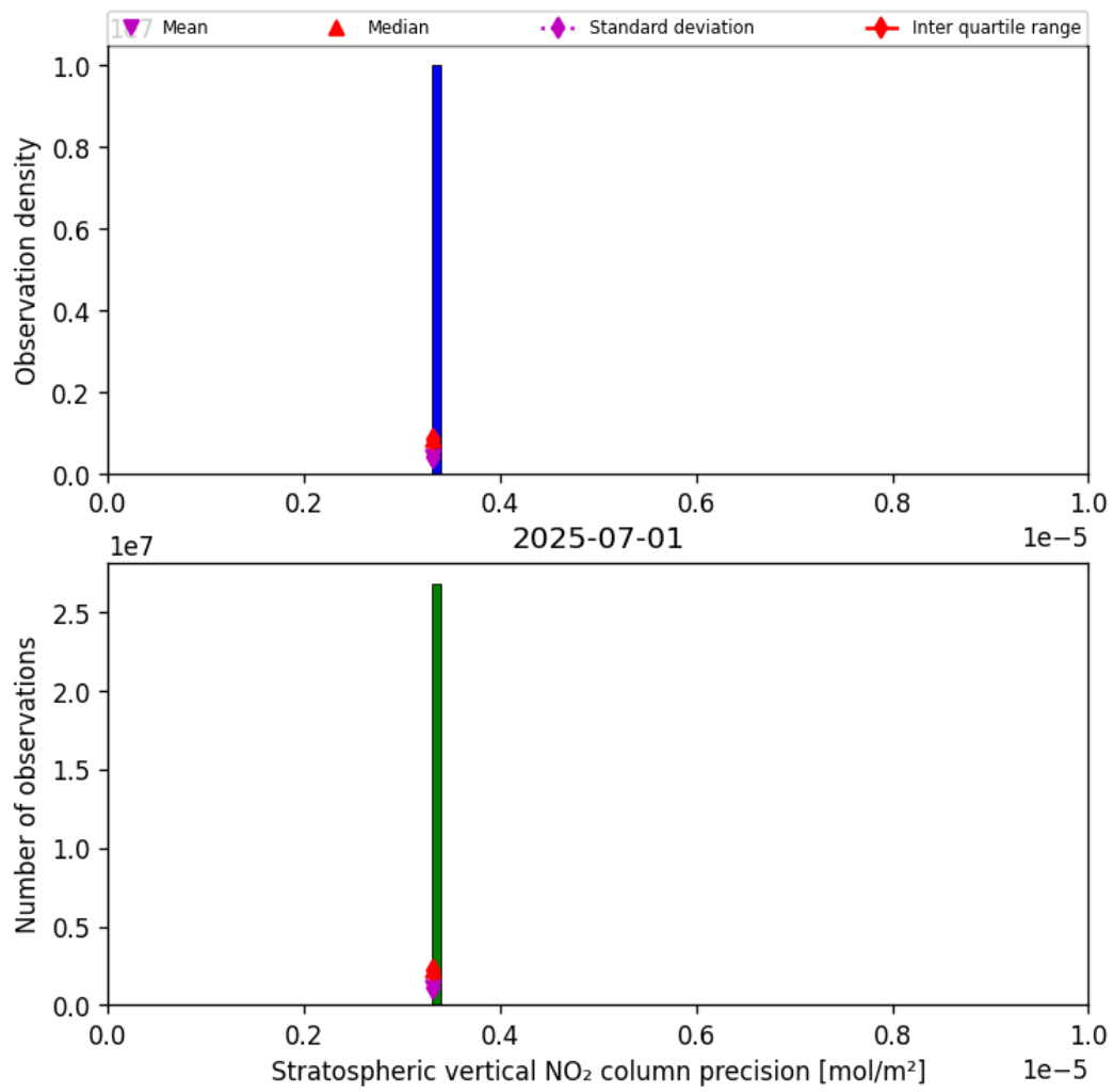
Figure 37: Histogram of “Stratospheric vertical NO 2 column precision” for 2025-06-30 to 2025-07-02
