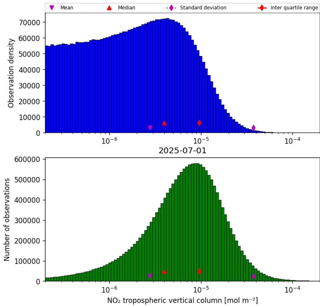
Figure 29: Histogram of “NO 2 tropospheric vertical column” for 2025-06-30 to 2025-07-02
