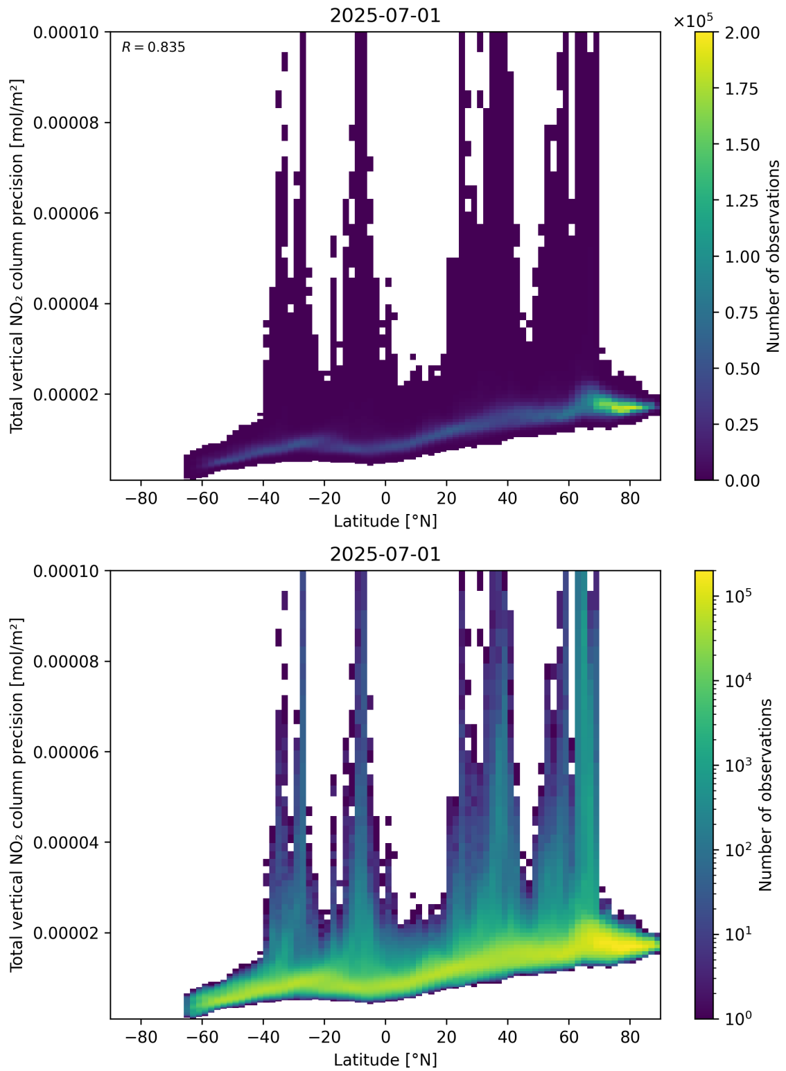
Figure 91: Scatter density plot of “Latitude” against “Total vertical NO 2 column precision” for 2025-06-30 to 2025-07-02.
