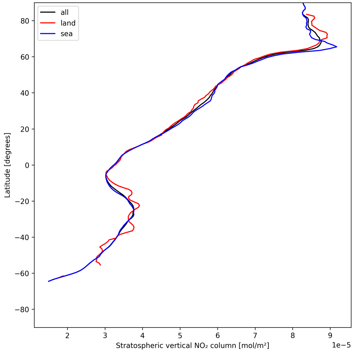
Figure 19: Zonal average of “Stratospheric vertical NO 2 column” for 2025-06-30 to 2025-07-02.
