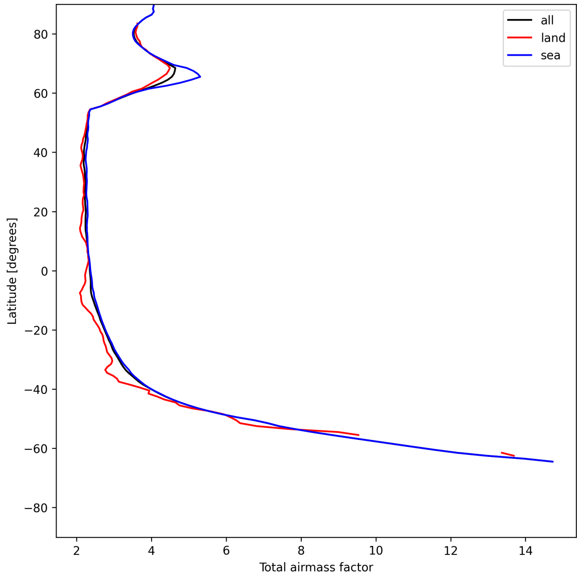
Figure 15: Zonal average of “Total airmass factor” for 2025-06-30 to 2025-07-02.
