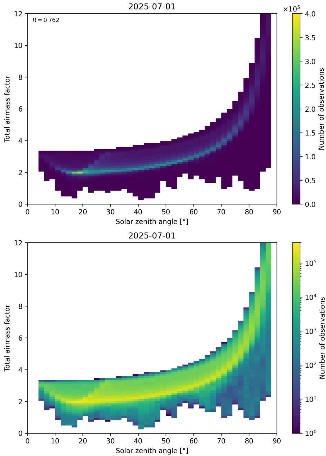
Figure 146: Scatter density plot of “Solar zenith angle” against “Total air mass factor” for 2025-06-30 to 2025-07-02.
