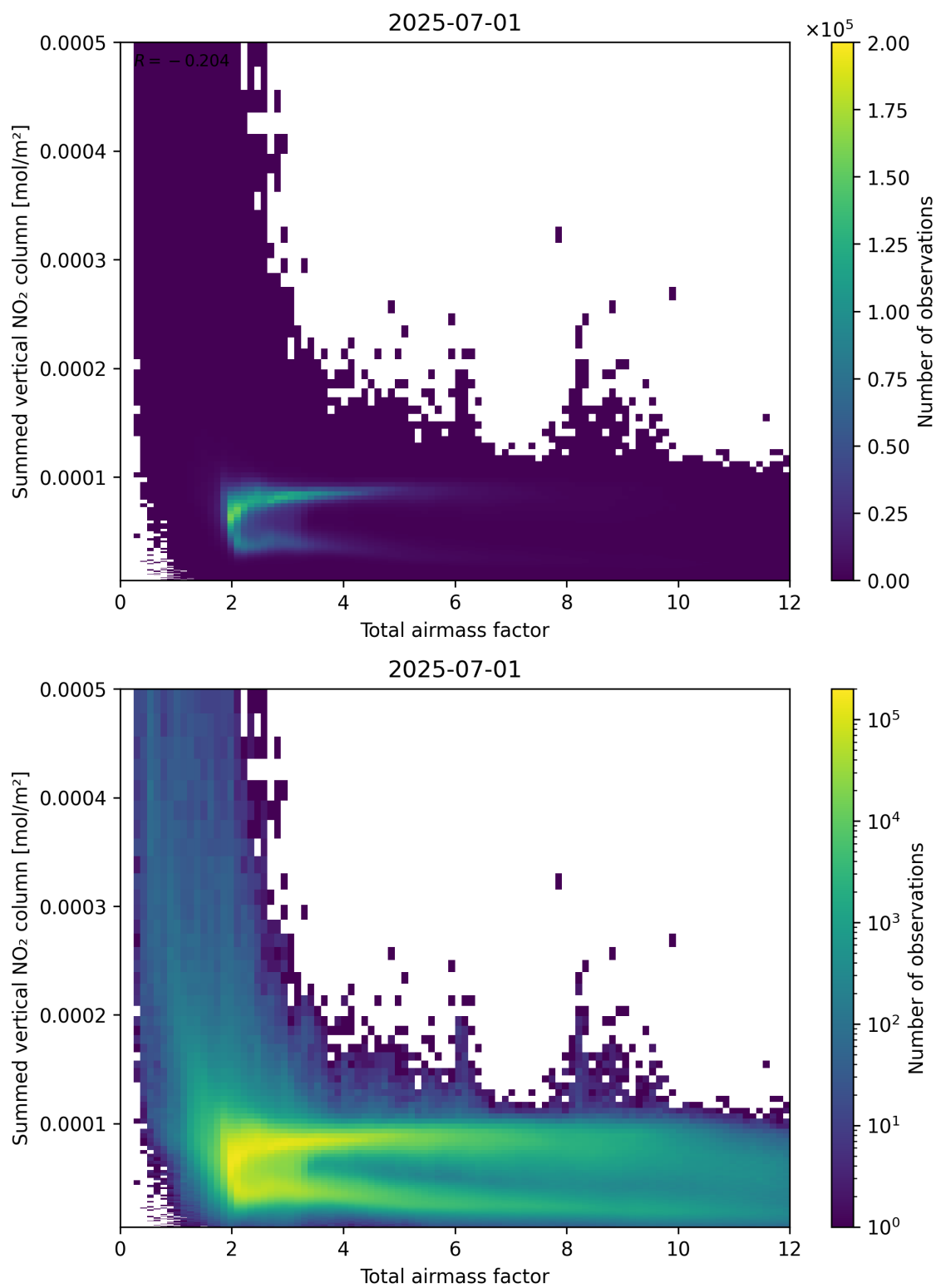
Figure 65: Scatter density plot of “Total airmass factor” against “Summed vertical NO 2 column” for 2025-06-30 to 2025-07-02.
