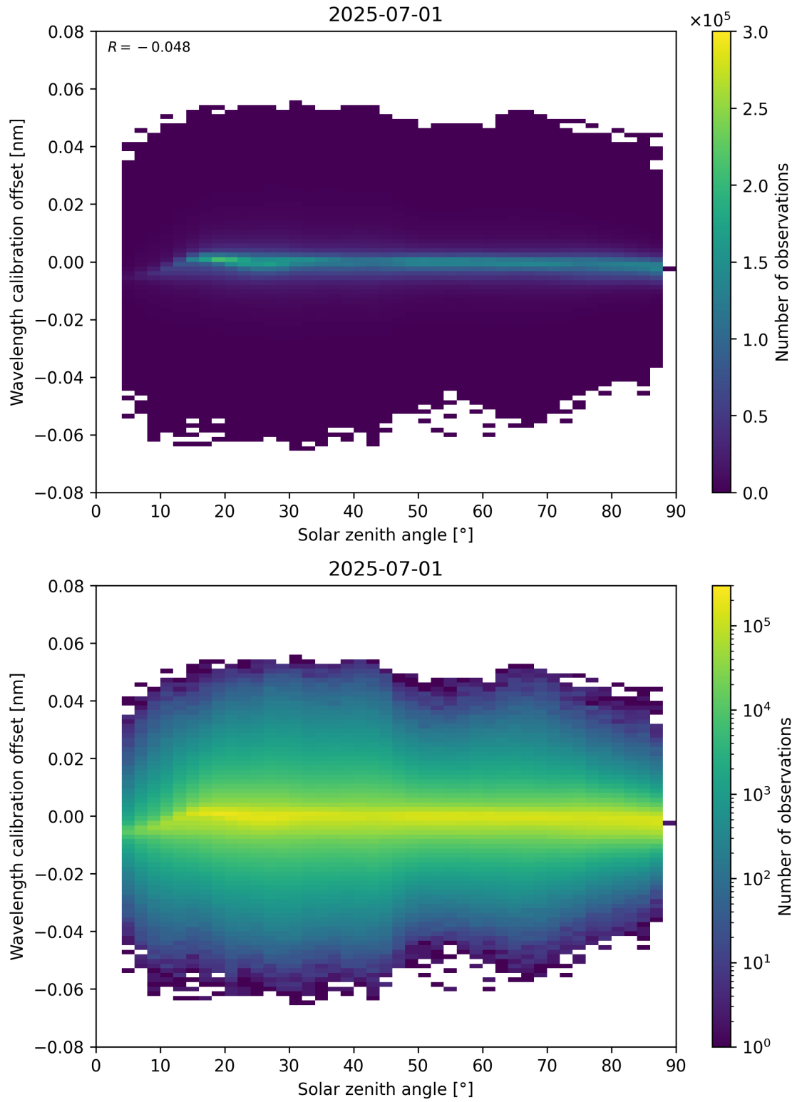
Figure 158: Scatter density plot of “Solar zenith angle” against “Wavelength calibration offset” for 2025-06-30 to 2025-07-02.
