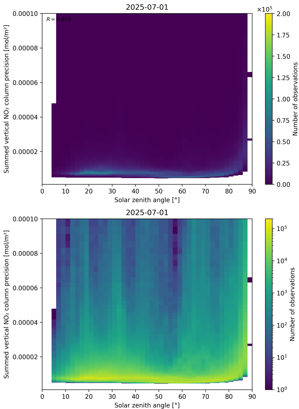
Figure 152: Scatter density plot of “Solar zenith angle” against “Summed vertical NO 2 column precision” for 2025-06-30 to 2025-07-02.
