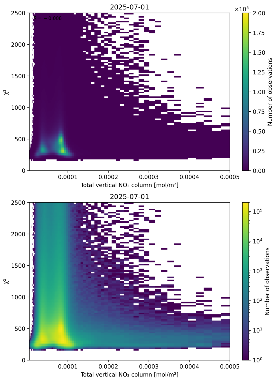
Figure 111: Scatter density plot of “Total vertical NO 2 column” against “ \chi^2 ” for 2025-06-30 to 2025-07-02.
