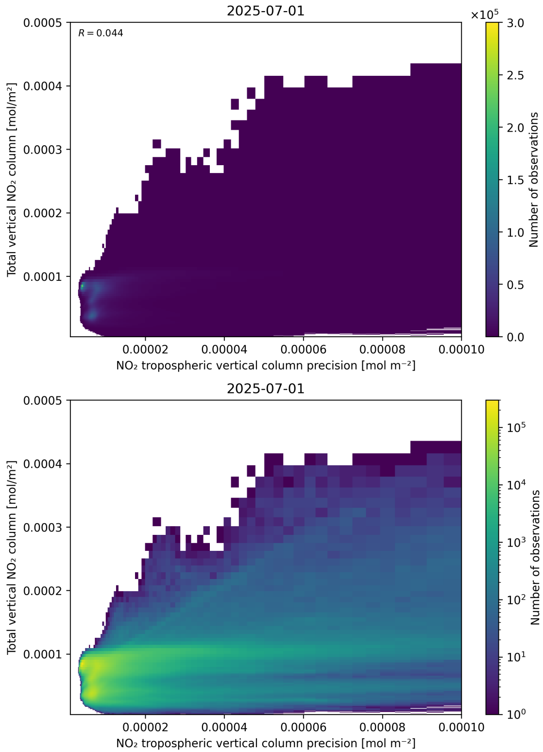
Figure 138: Scatter density plot of “NO 2 tropospheric vertical column precision” against “Total vertical NO 2 column” for 2025-06-30 to 2025-07-02.
