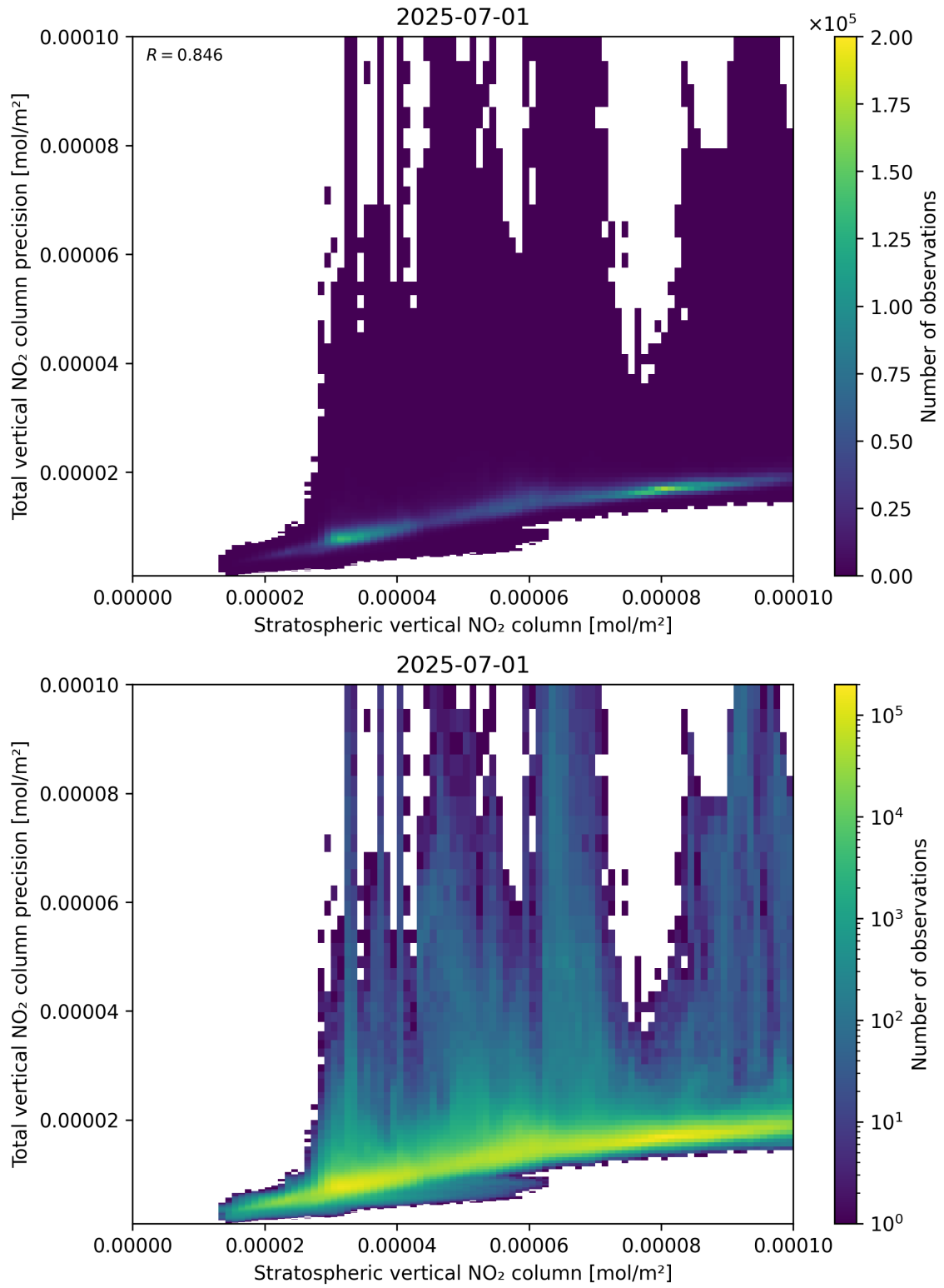
Figure 101: Scatter density plot of “Stratospheric vertical NO 2 column” against “Total vertical NO 2 column precision” for 2025-06-30 to 2025-07-02.
