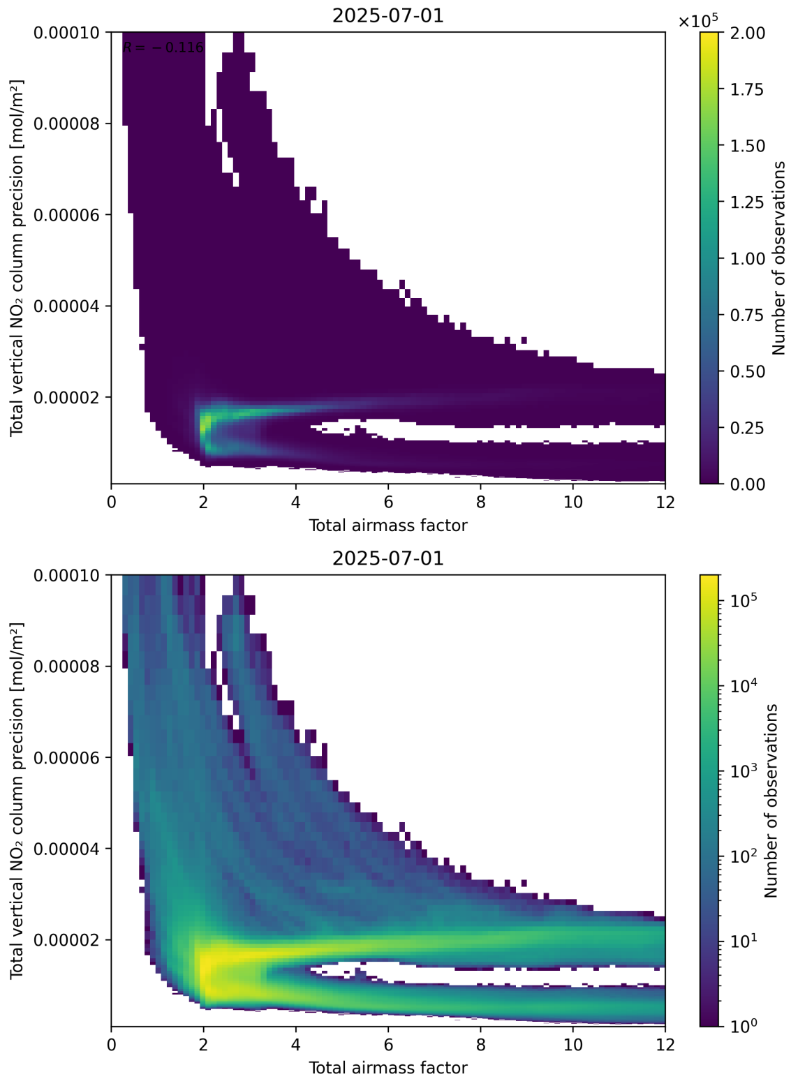
Figure 68: Scatter density plot of “Total airmass factor” against “Total vertical NO 2 column precision” for 2025-06-30 to 2025-07-02.
