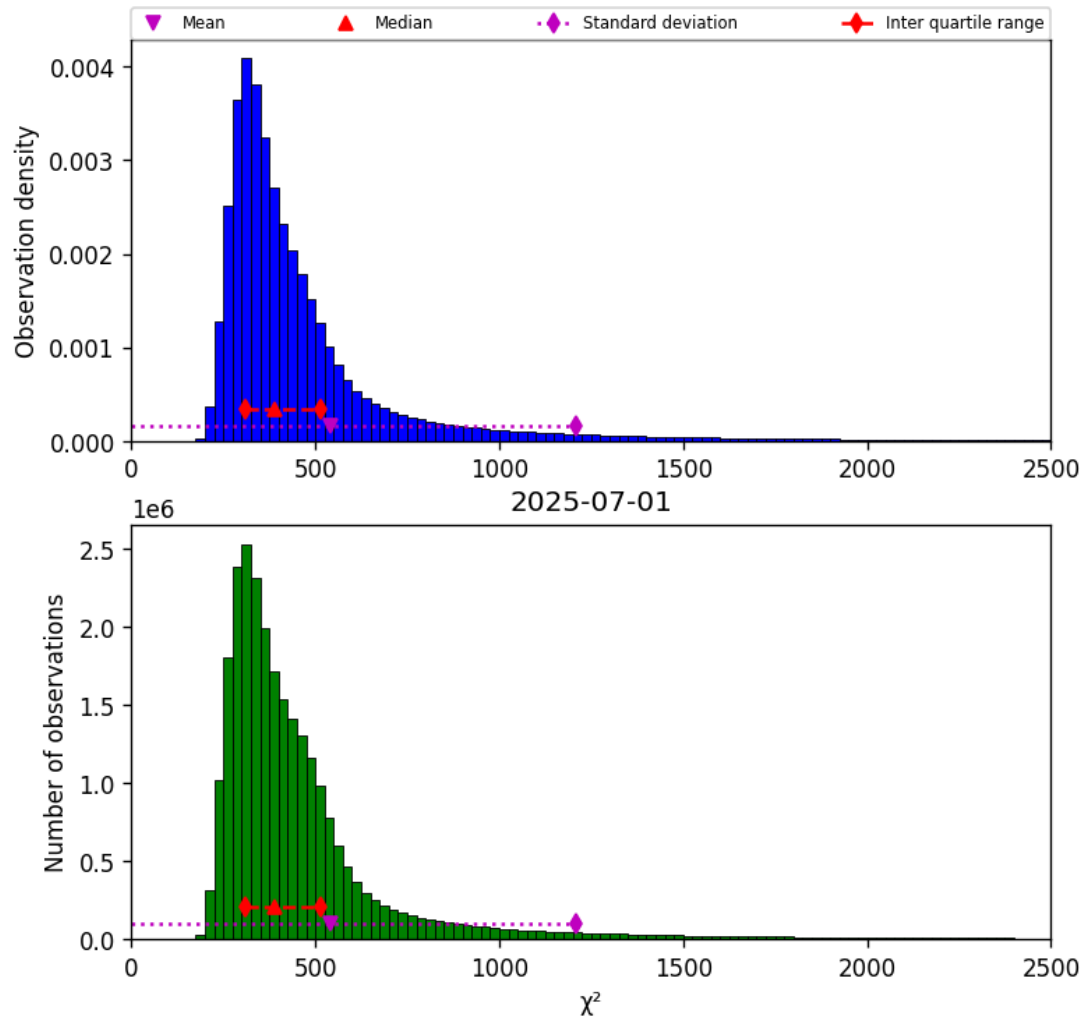
Figure 42: Histogram of " \chi^2 " for 2025-06-30 to 2025-07-02
