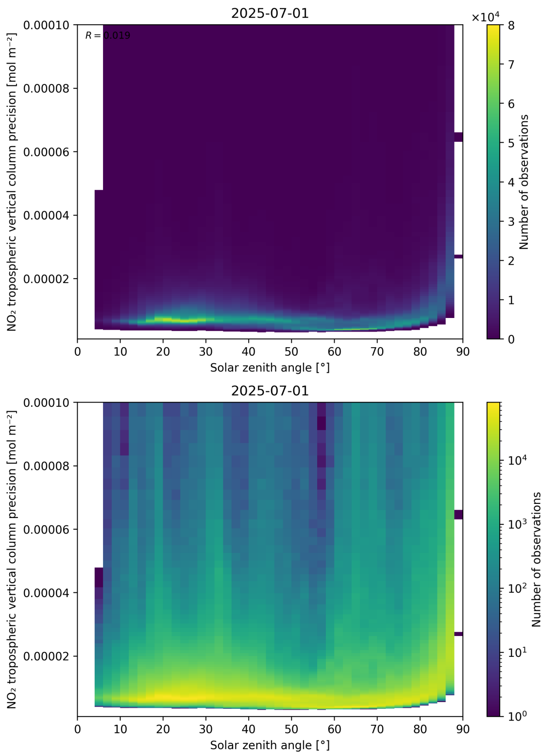
Figure 156: Scatter density plot of “Solar zenith angle” against “NO 2 tropospheric vertical column precision” for 2025-06-30 to 2025-07-02.
