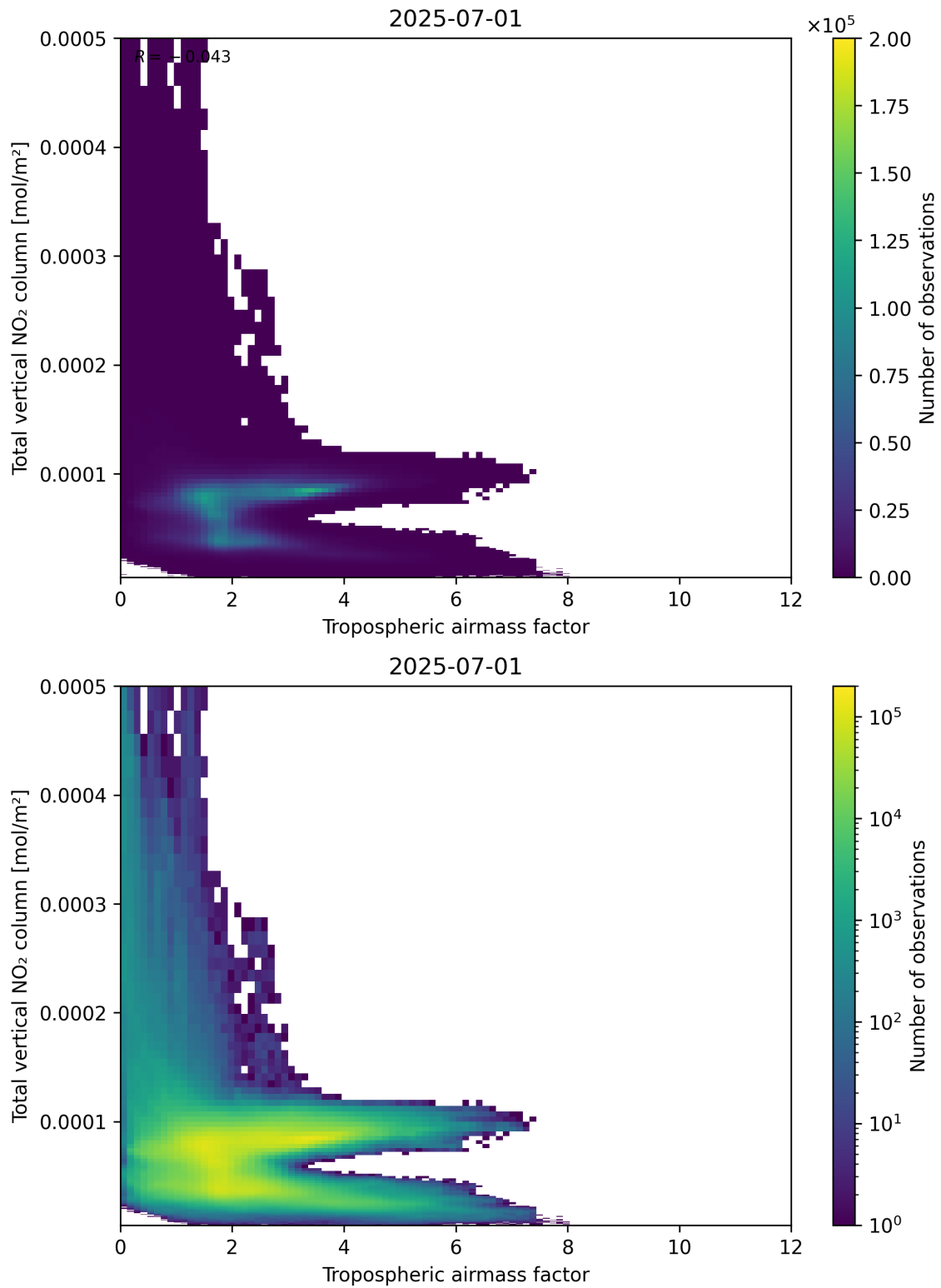
Figure 77: Scatter density plot of “Tropospheric airmass factor” against “Total vertical NO 2 column” for 2025-06-30 to 2025-07-02.
