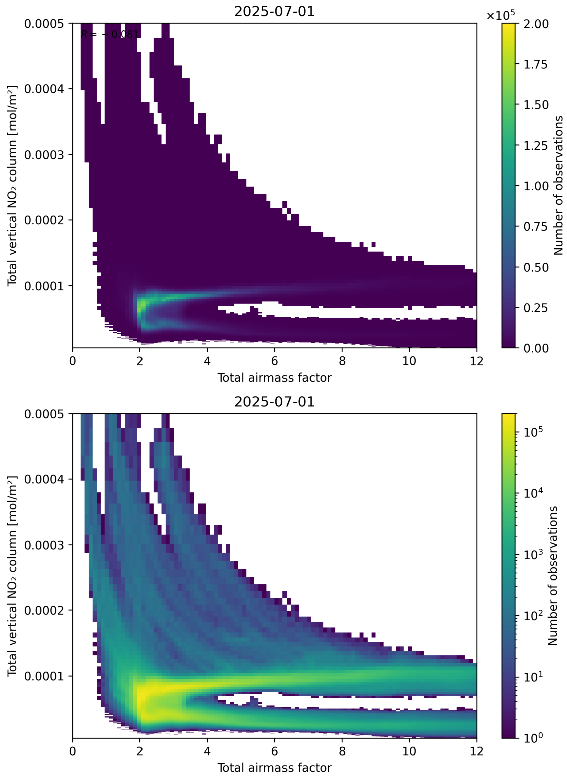
Figure 67: Scatter density plot of “Total airmass factor” against “Total vertical NO 2 column” for 2025-06-30 to 2025-07-02.
