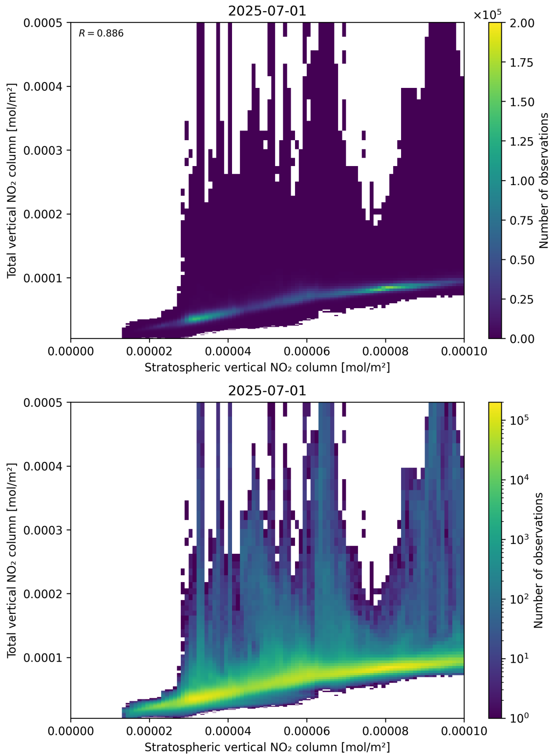
Figure 100: Scatter density plot of “Stratospheric vertical NO 2 column” against “Total vertical NO 2 column” for 2025-06-30 to 2025-07-02.
