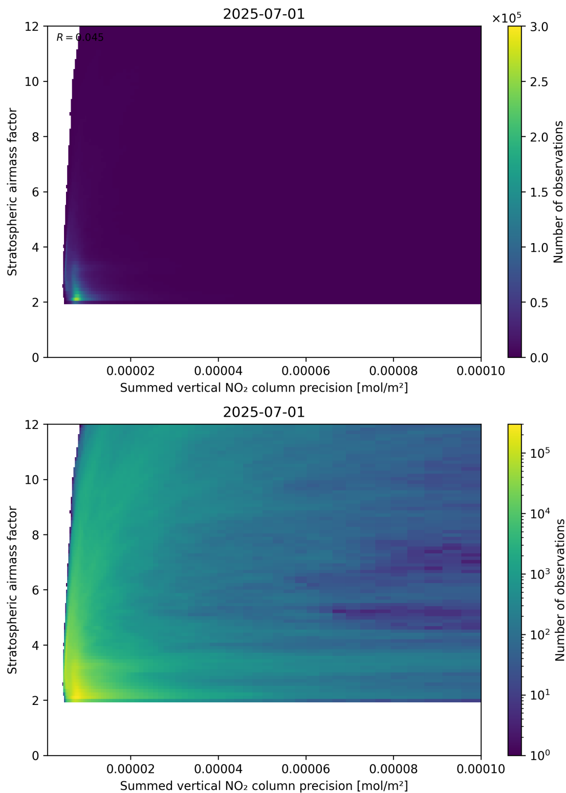
Figure 106: Scatter density plot of “Summed vertical NO 2 column precision” against “Stratospheric airmass factor” for 2025-06-30 to 2025-07-02.
