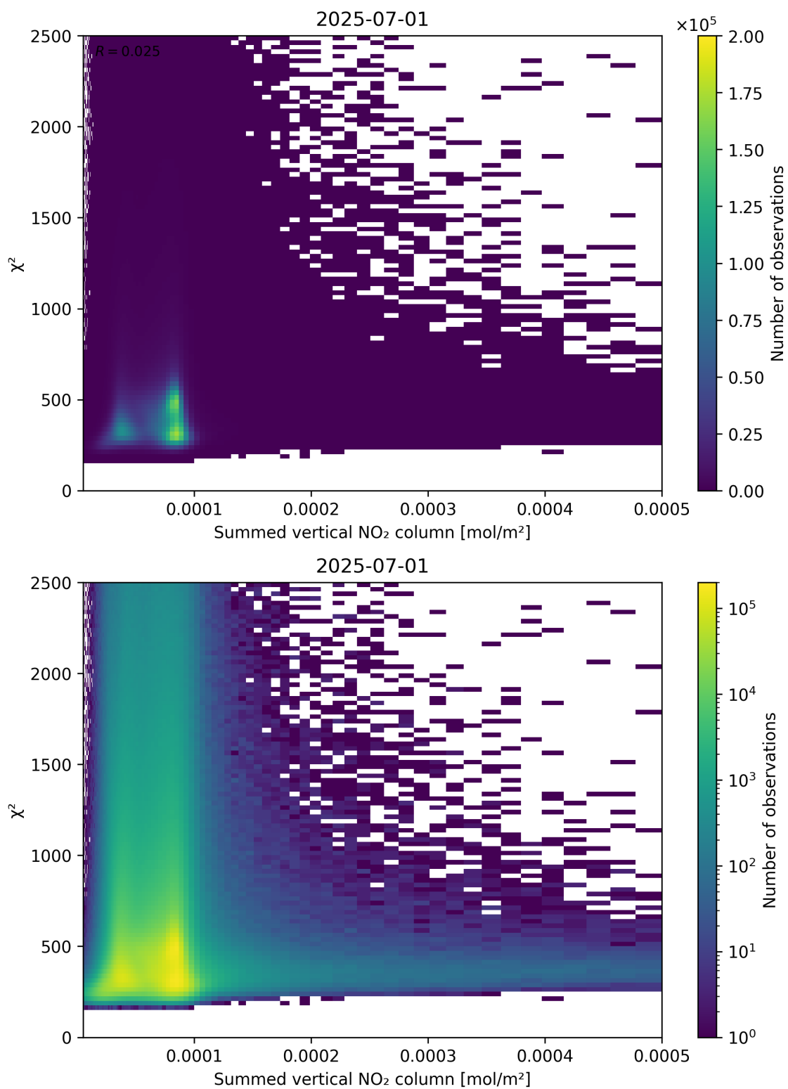
Figure 104: Scatter density plot of “Summed vertical NO 2 column” against “ \chi^2 ” for 2025-06-30 to 2025-07-02.
