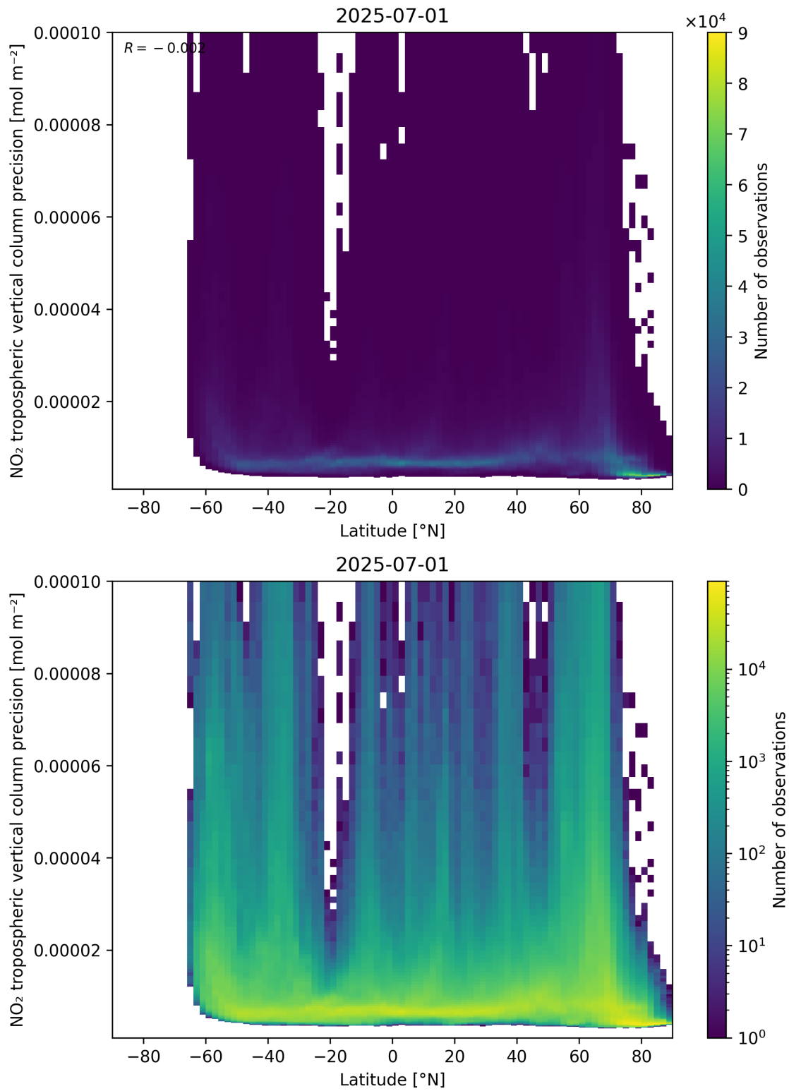
Figure 93: Scatter density plot of “Latitude” against “NO 2 tropospheric vertical column precision” for 2025-06-30 to 2025-07-02.
