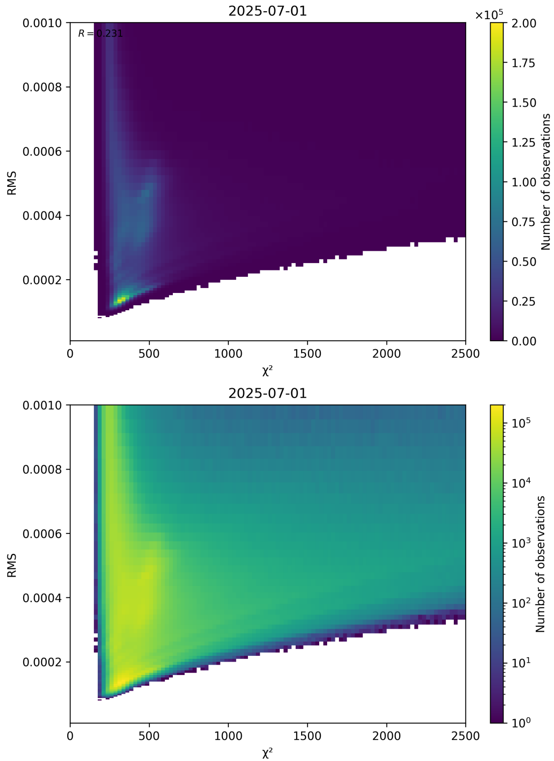
Figure 82: Scatter density plot of “ \chi^2 ” against “RMS” for 2025-06-30 to 2025-07-02.
