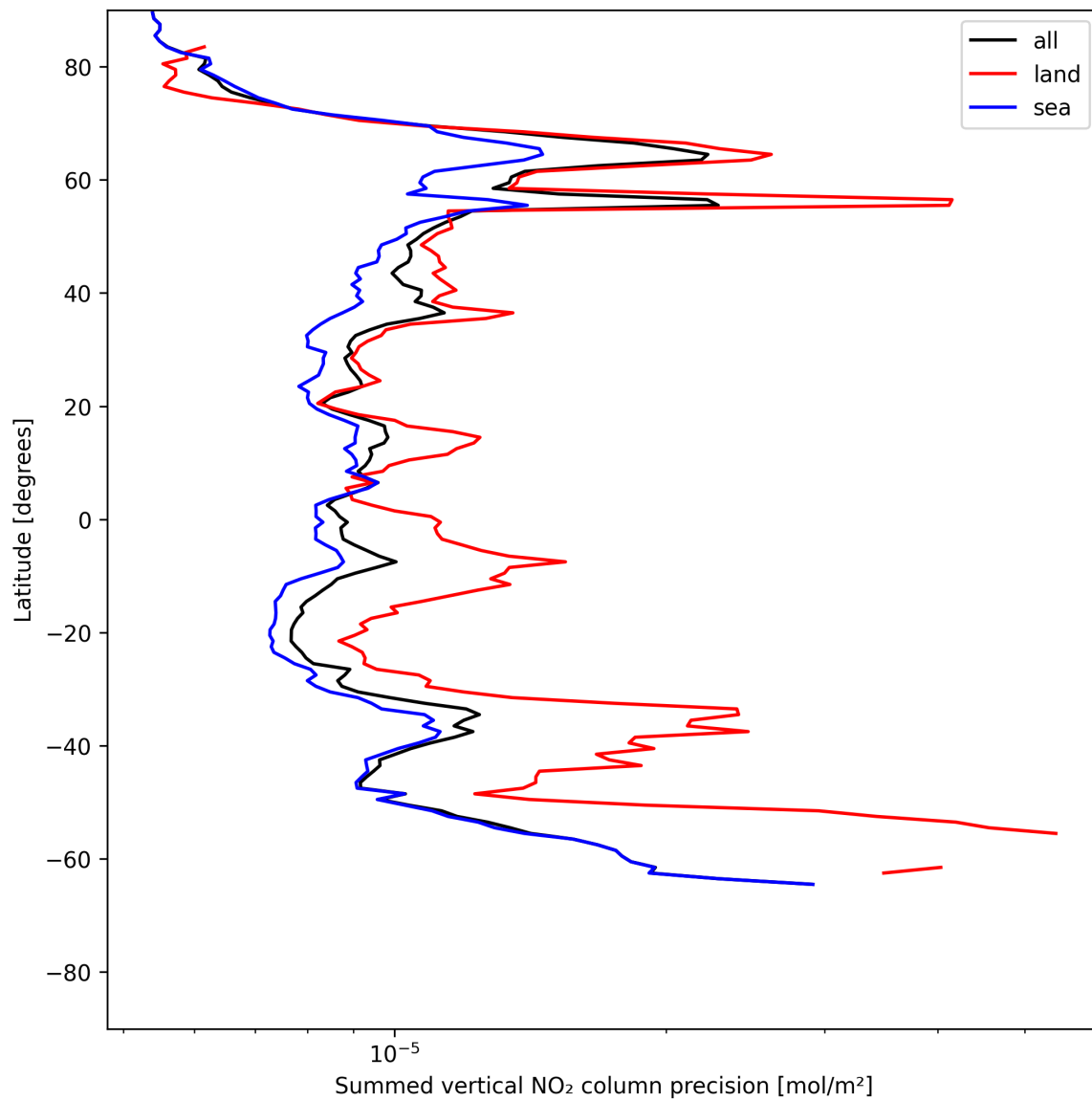
Figure 24: Zonal average of “Summed vertical NO 2 column precision” for 2025-06-30 to 2025-07-02.
