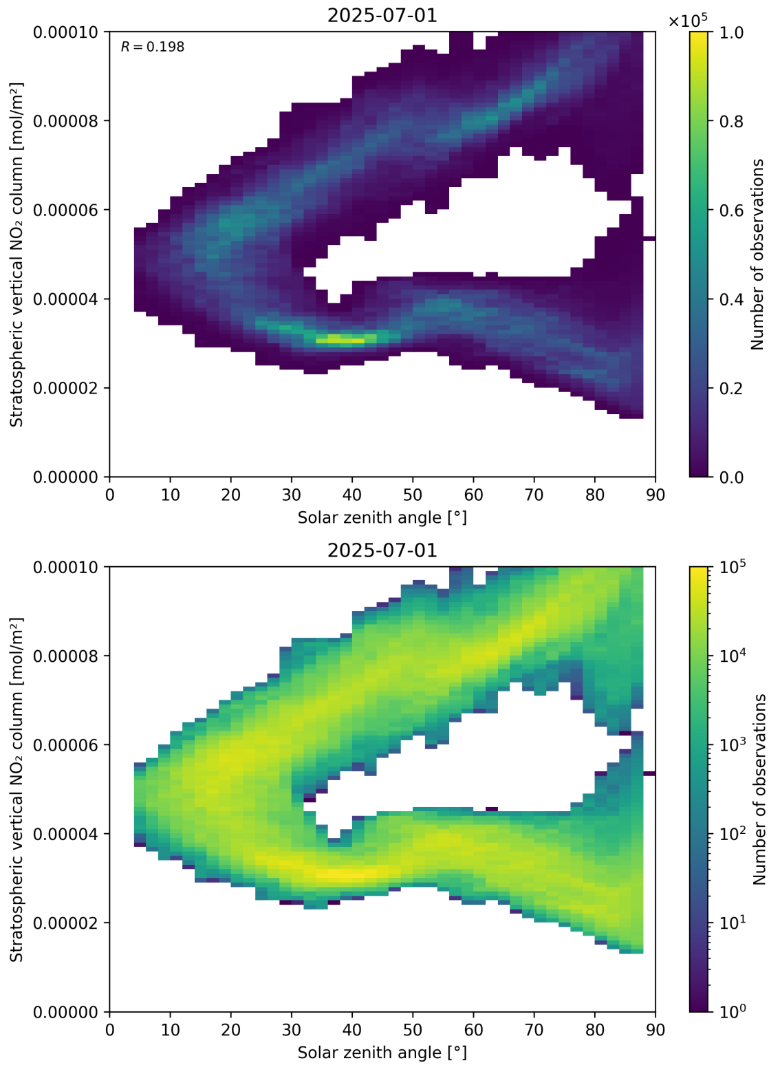
Figure 150: Scatter density plot of “Solar zenith angle” against “Stratospheric vertical NO 2 column” for 2025-06-30 to 2025-07-02.
