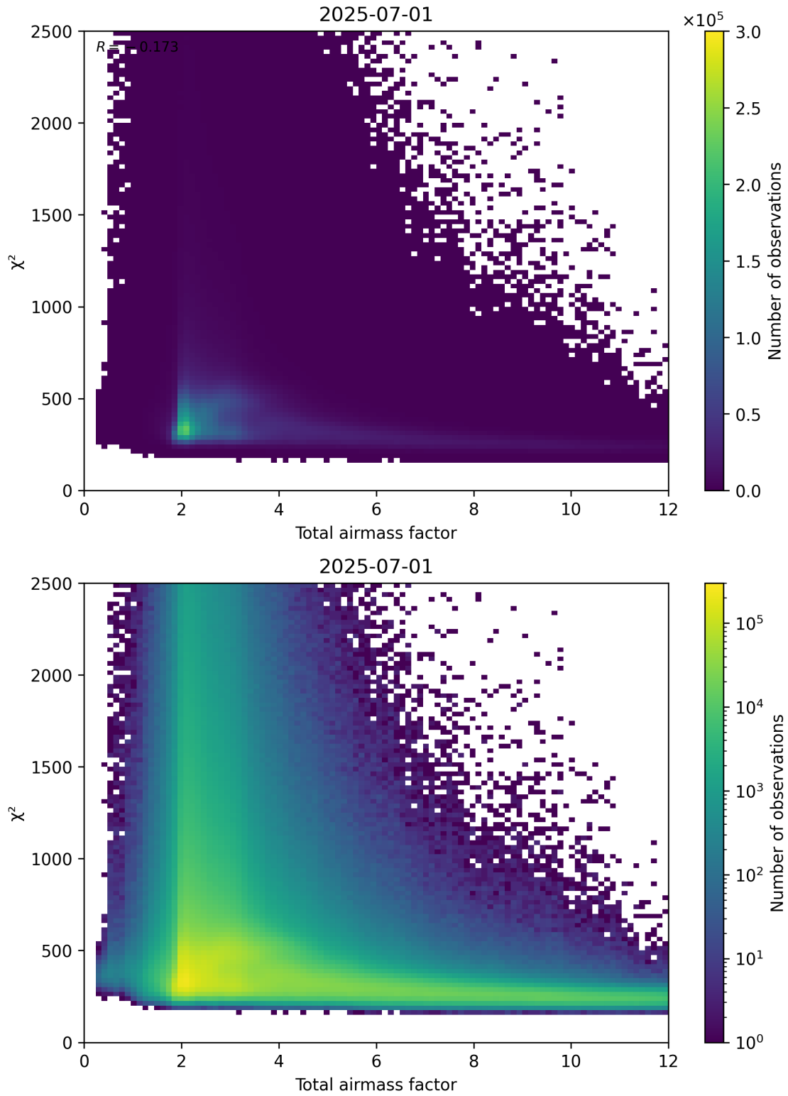
Figure 63: Scatter density plot of “Total airmass factor” against “ \chi^2 ” for 2025-06-30 to 2025-07-02.
