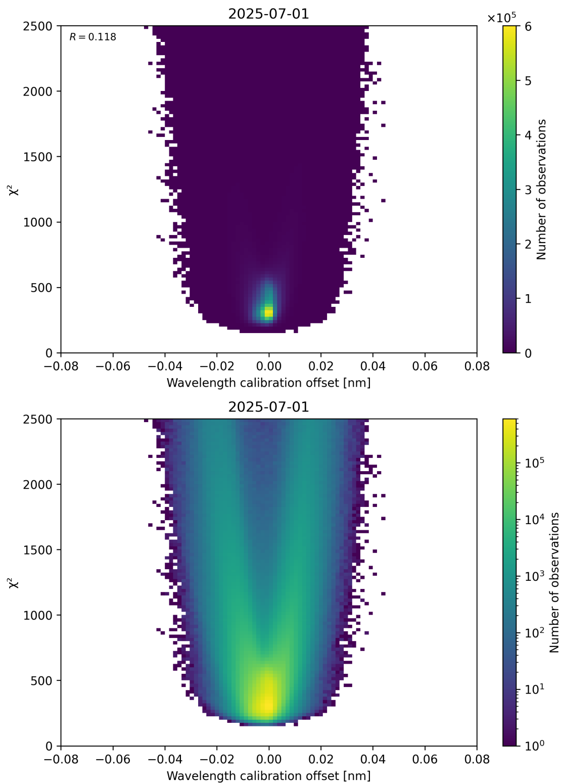
Figure 175: Scatter density plot of “Wavelength calibration offset” against “ \chi^2 ” for 2025-06-30 to 2025-07-02.
