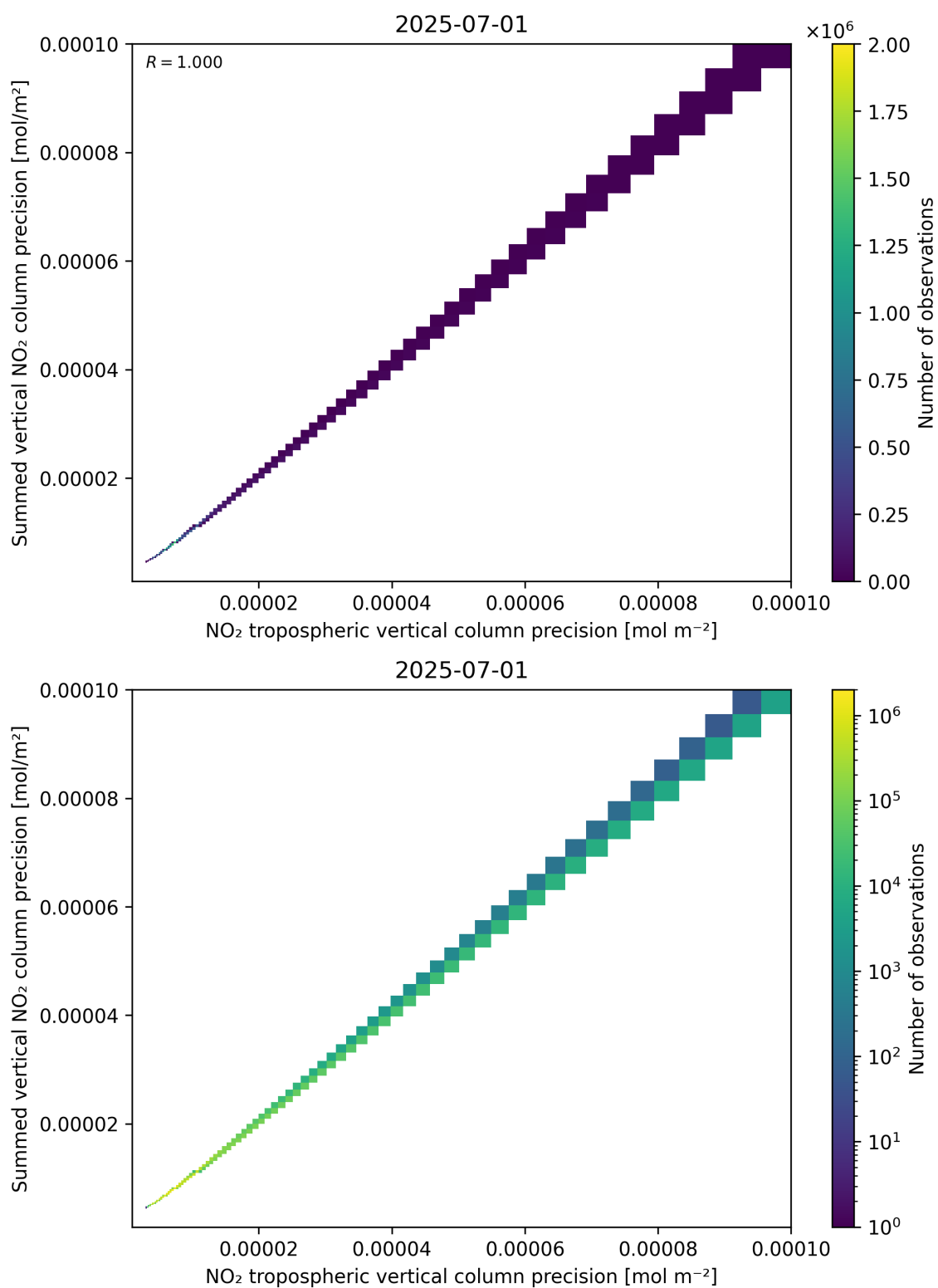
Figure 137: Scatter density plot of “NO 2 tropospheric vertical column precision” against “Summed vertical NO 2 column precision” for 2025-06-30 to 2025-07-02.
