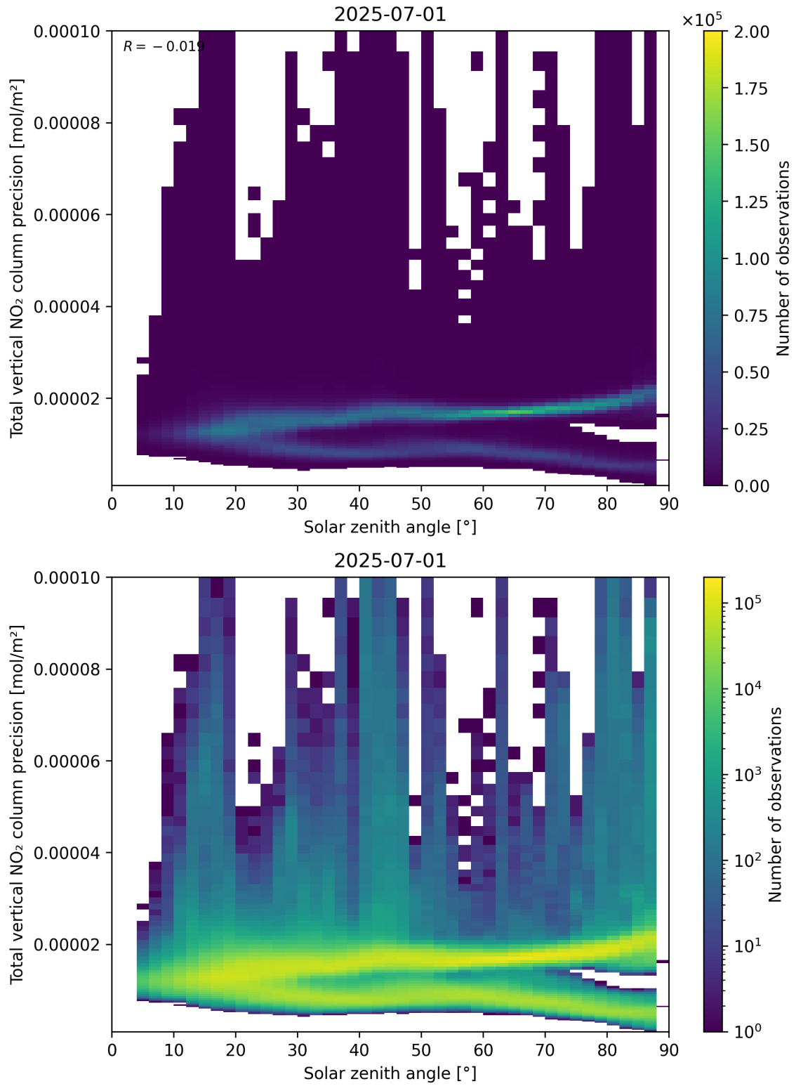
Figure 154: Scatter density plot of “Solar zenith angle” against “Total vertical NO 2 column precision” for 2025-06-30 to 2025-07-02.
