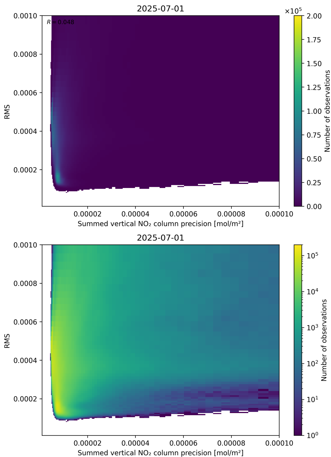
Figure 108: Scatter density plot of “Summed vertical NO 2 column precision” against “RMS” for 2025-06-30 to 2025-07-02.
