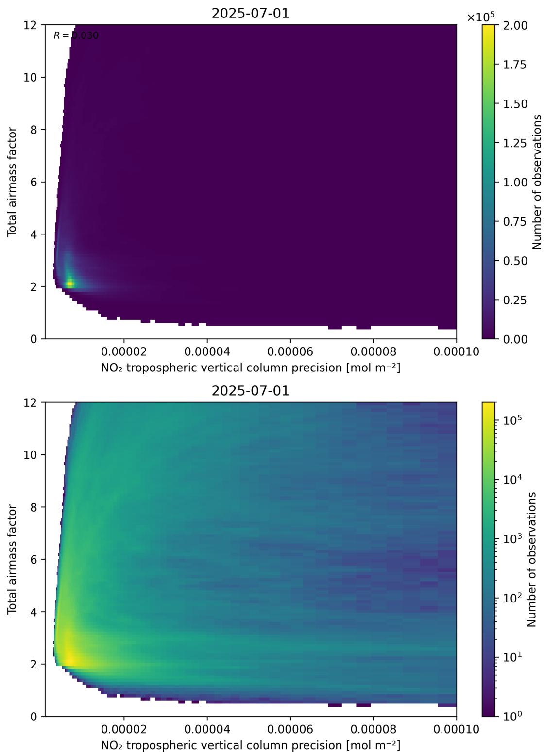
Figure 132: Scatter density plot of “NO 2 tropospheric vertical column precision” against “Total air mass factor” for 2025-06-30 to 2025-07-02.
