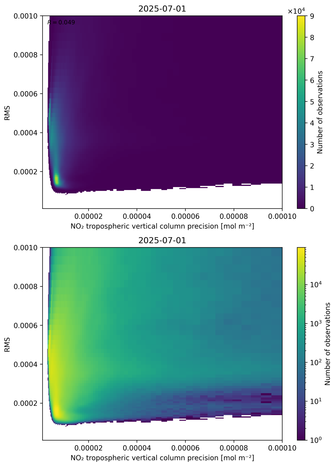
Figure 140: Scatter density plot of “NO 2 tropospheric vertical column precision” against “RMS” for 2025-06-30 to 2025-07-02.
