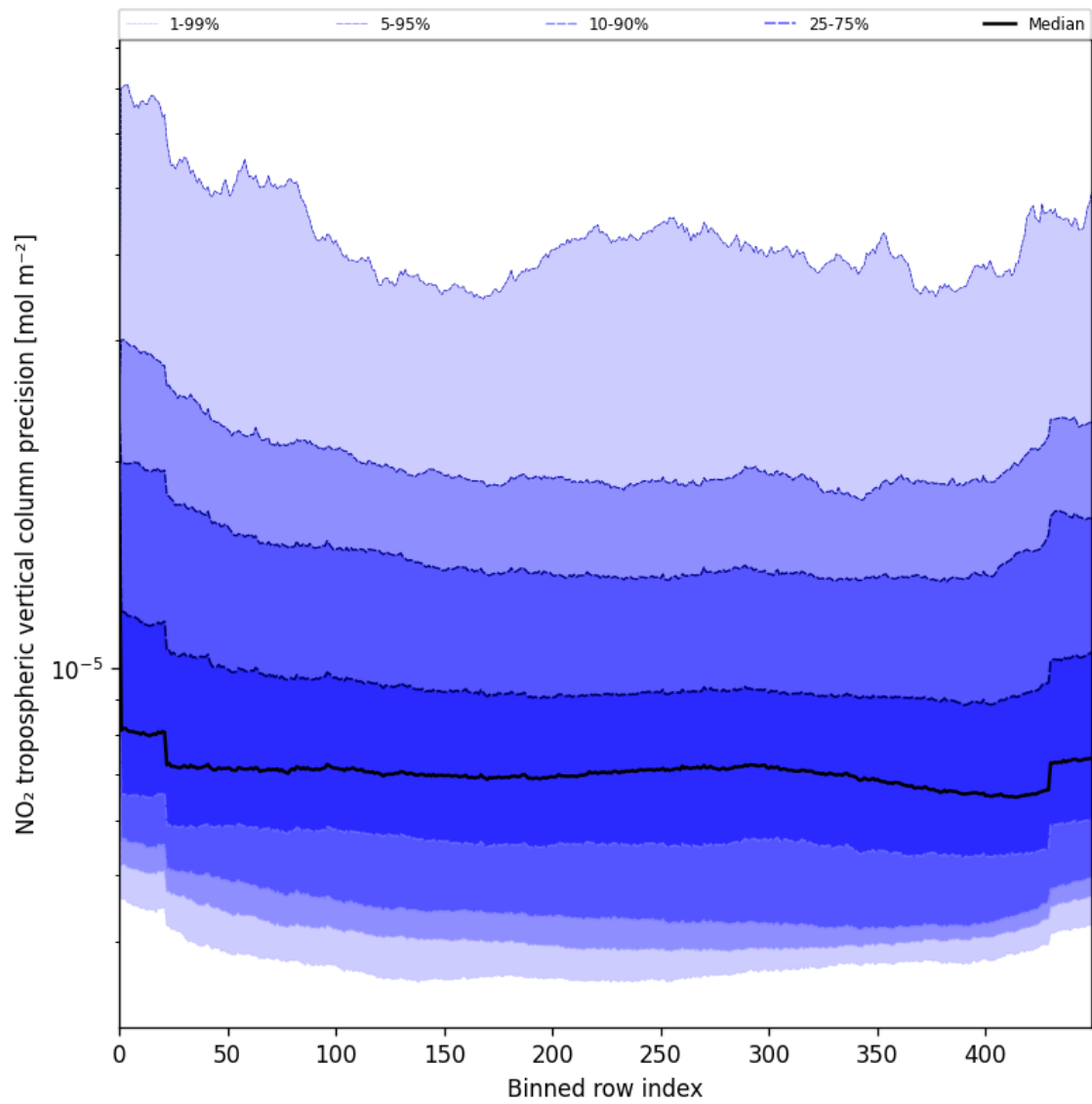
Figure 47: Along track statistics of “NO 2 tropospheric vertical column precision” for 2025-06-30 to 2025-07-02
