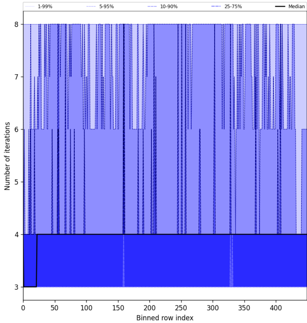
Figure 51: Along track statistics of "Number of iterations" for 2025-06-30 to 2025-07-02
