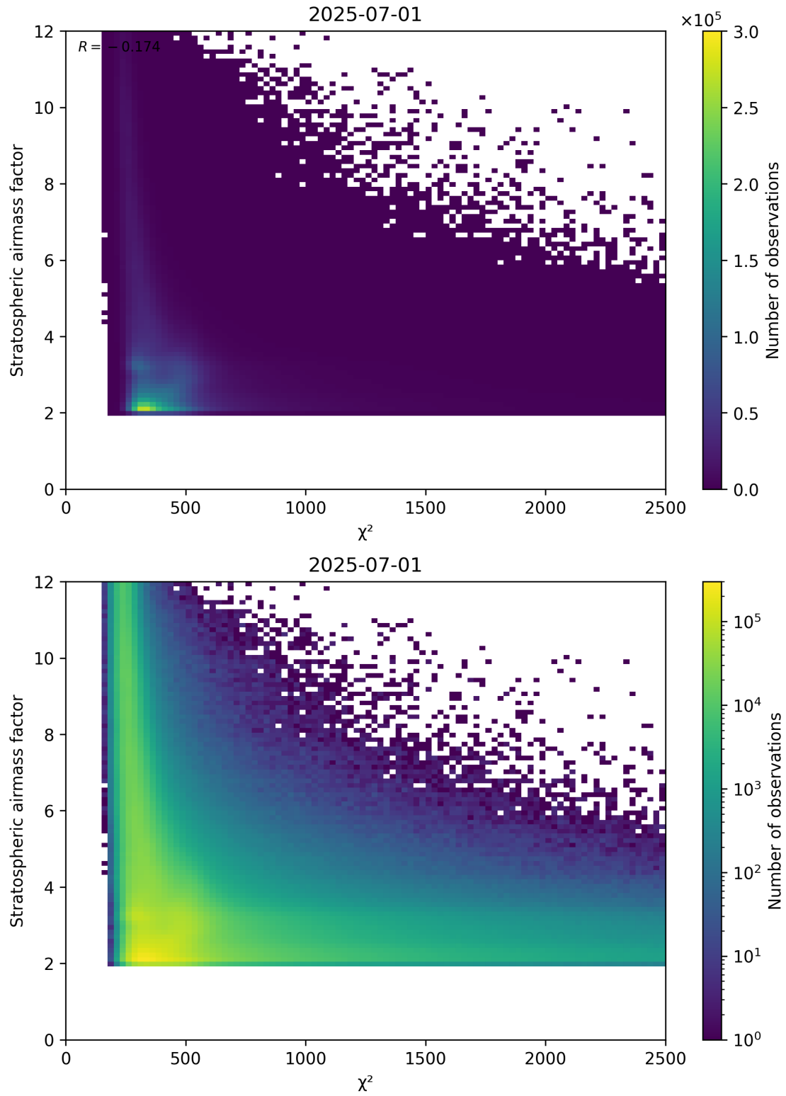
Figure 81: Scatter density plot of “ \chi^2 ” against “Stratospheric airmass factor” for 2025-06-30 to 2025-07-02.
