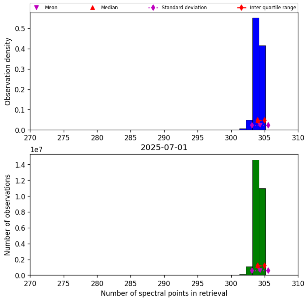
Figure 33: Histogram of “Number of spectral points in retrieval” for 2025-06-30 to 2025-07-02
