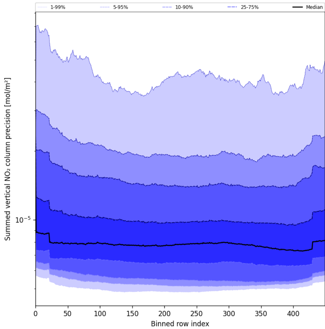
Figure 58: Along track statistics of “Summed vertical NO 2 column precision” for 2025-06-30 to 2025-07-02
