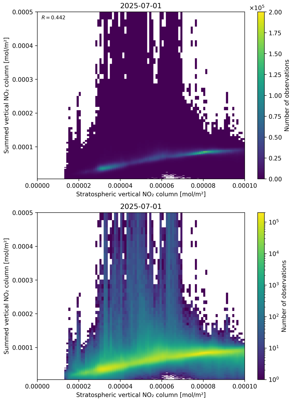
Figure 98: Scatter density plot of “Stratospheric vertical NO 2 column” against “Summed vertical NO 2 column” for 2025-06-30 to 2025-07-02.
