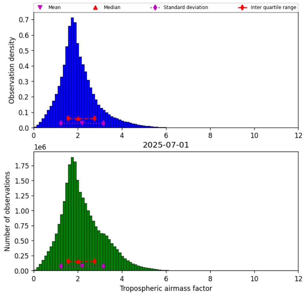
Figure 31: Histogram of “Tropospheric airmass factor” for 2025-06-30 to 2025-07-02
