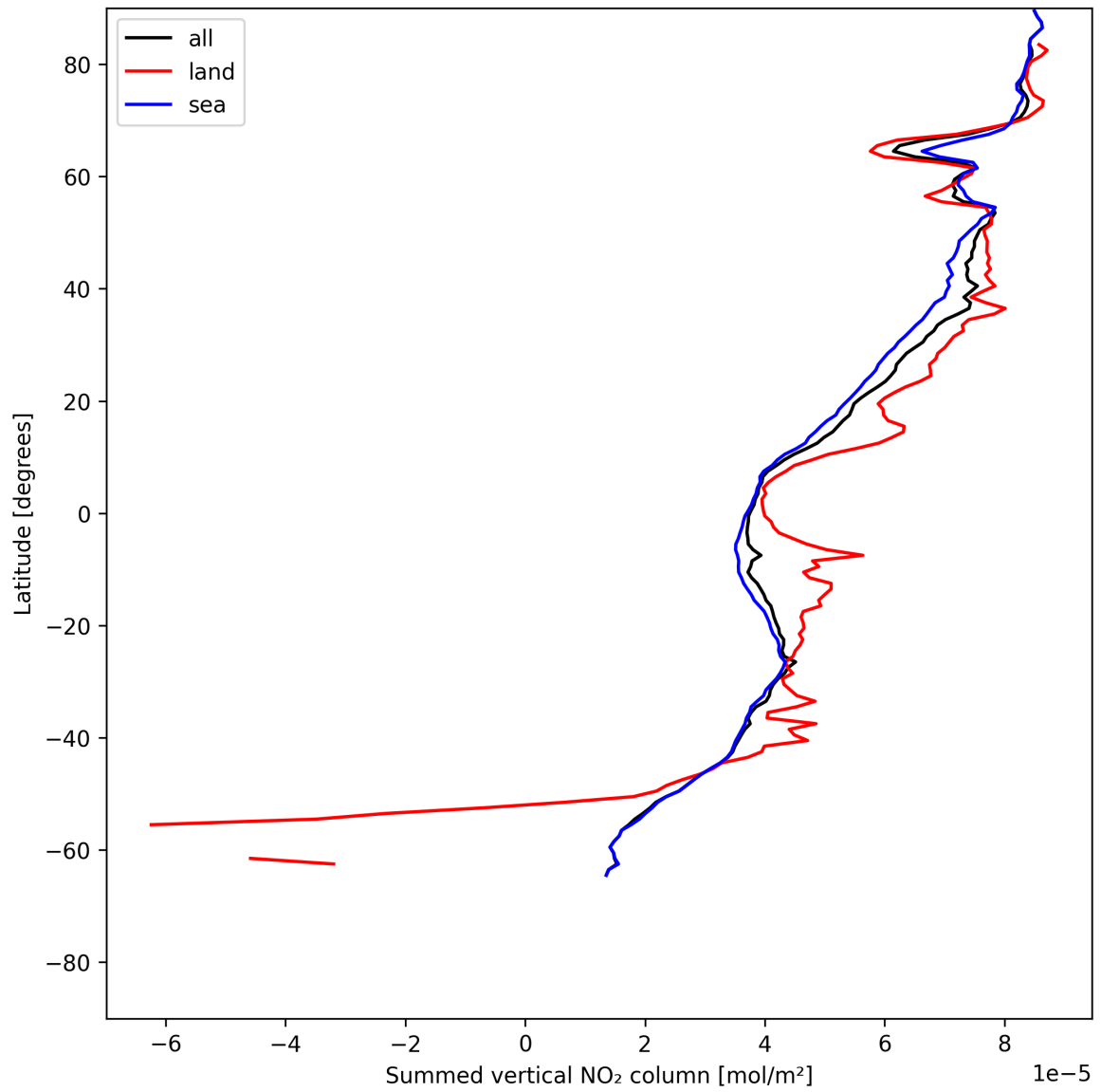
Figure 23: Zonal average of “Summed vertical NO 2 column” for 2025-06-30 to 2025-07-02.
