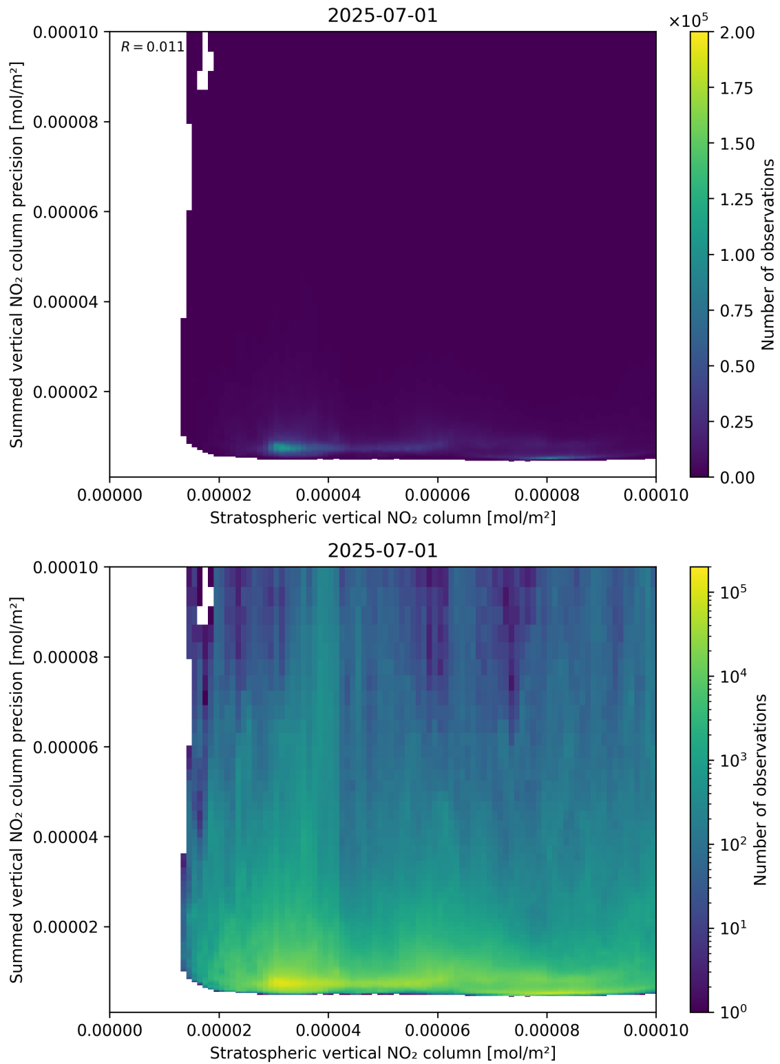
Figure 99: Scatter density plot of “Stratospheric vertical NO 2 column” against “Summed vertical NO 2 column precision” for 2025-06-30 to 2025-07-02.
