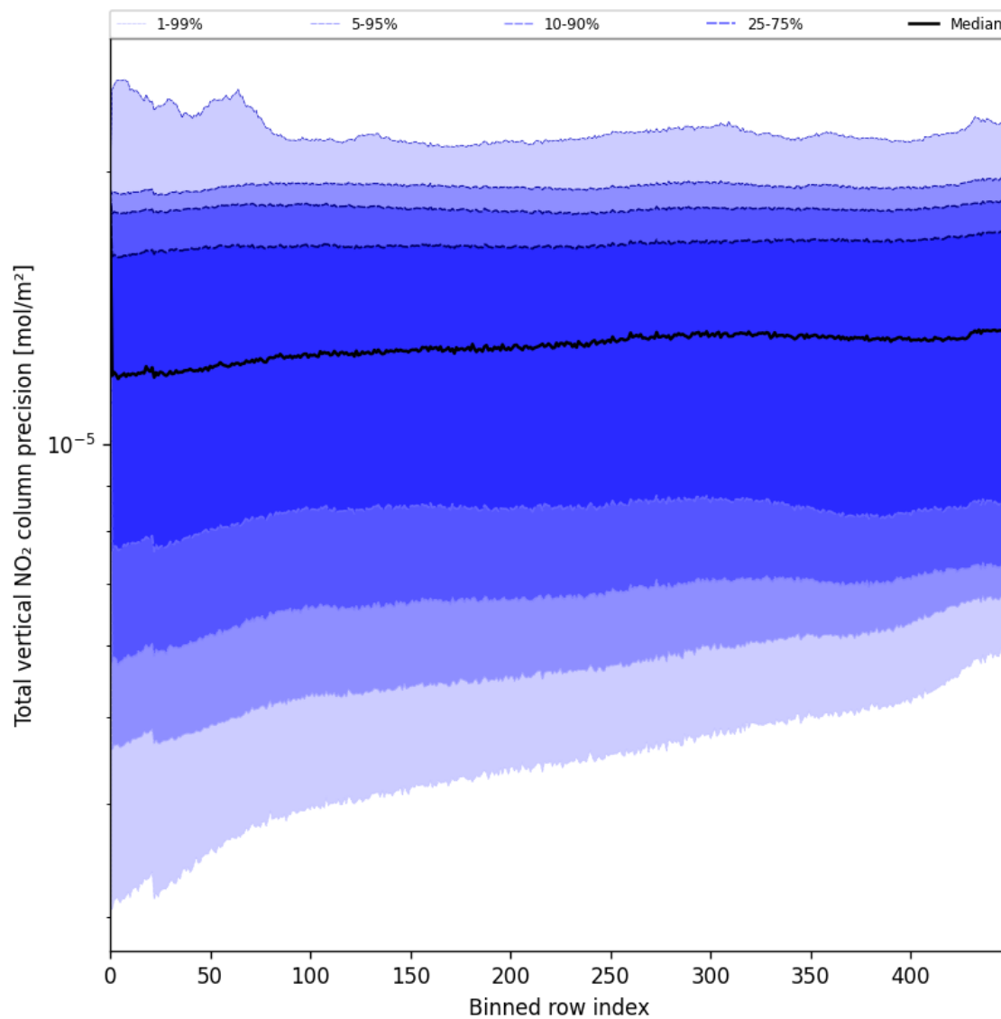
Figure 56: Along track statistics of “Total vertical NO 2 column precision” for 2025-06-30 to 2025-07-02
