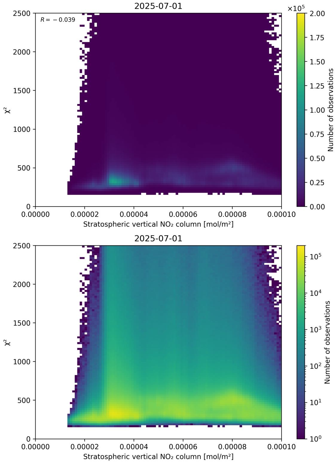
Figure 97: Scatter density plot of “Stratospheric vertical NO 2 column” against “ \chi^2 ” for 2025-06-30 to 2025-07-02.
