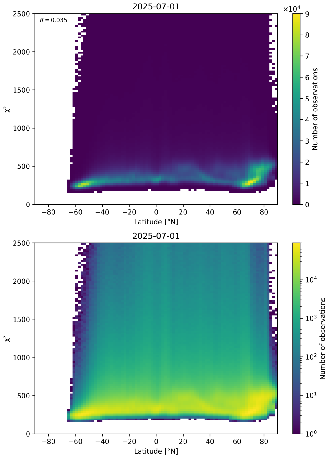
Figure 86: Scatter density plot of “Latitude” against “ \chi^2 ” for 2025-06-30 to 2025-07-02.
