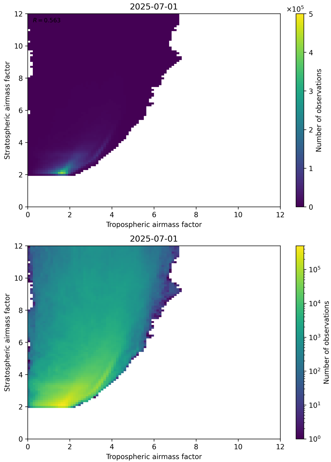
Figure 71: Scatter density plot of “Tropospheric airmass factor” against “Stratospheric airmass factor” for 2025-06-30 to 2025-07-02.
