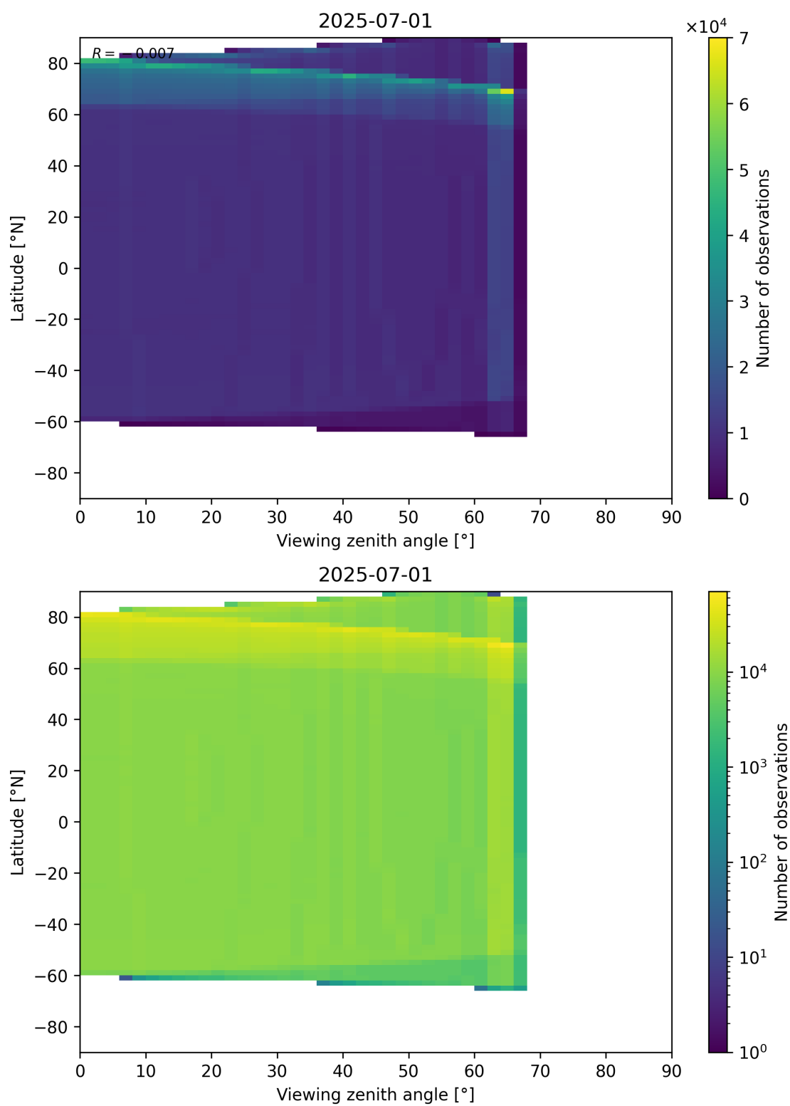
Figure 163: Scatter density plot of “Viewing zenith angle” against “Latitude” for 2025-06-30 to 2025-07-02.
