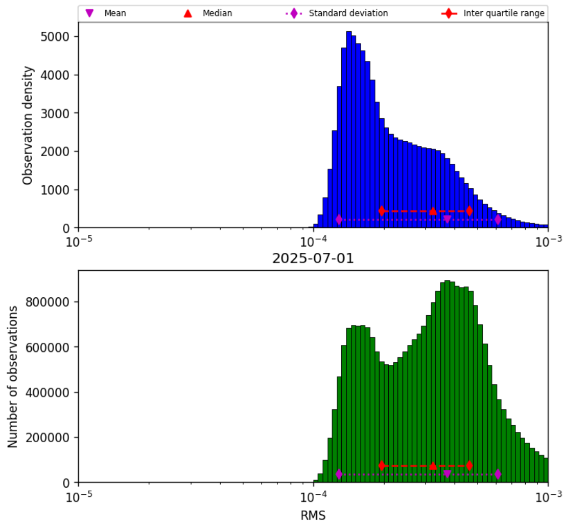
Figure 43: Histogram of “RMS” for 2025-06-30 to 2025-07-02
