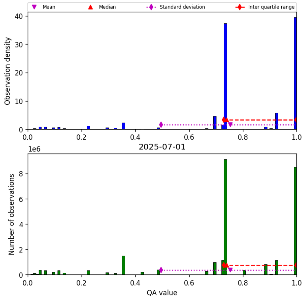
Figure 28: Histogram of “QA value” for 2025-06-30 to 2025-07-02
