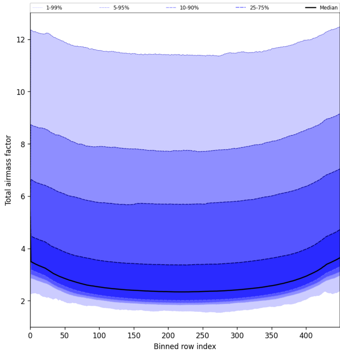
Figure 49: Along track statistics of “Total airmass factor” for 2025-06-30 to 2025-07-02
