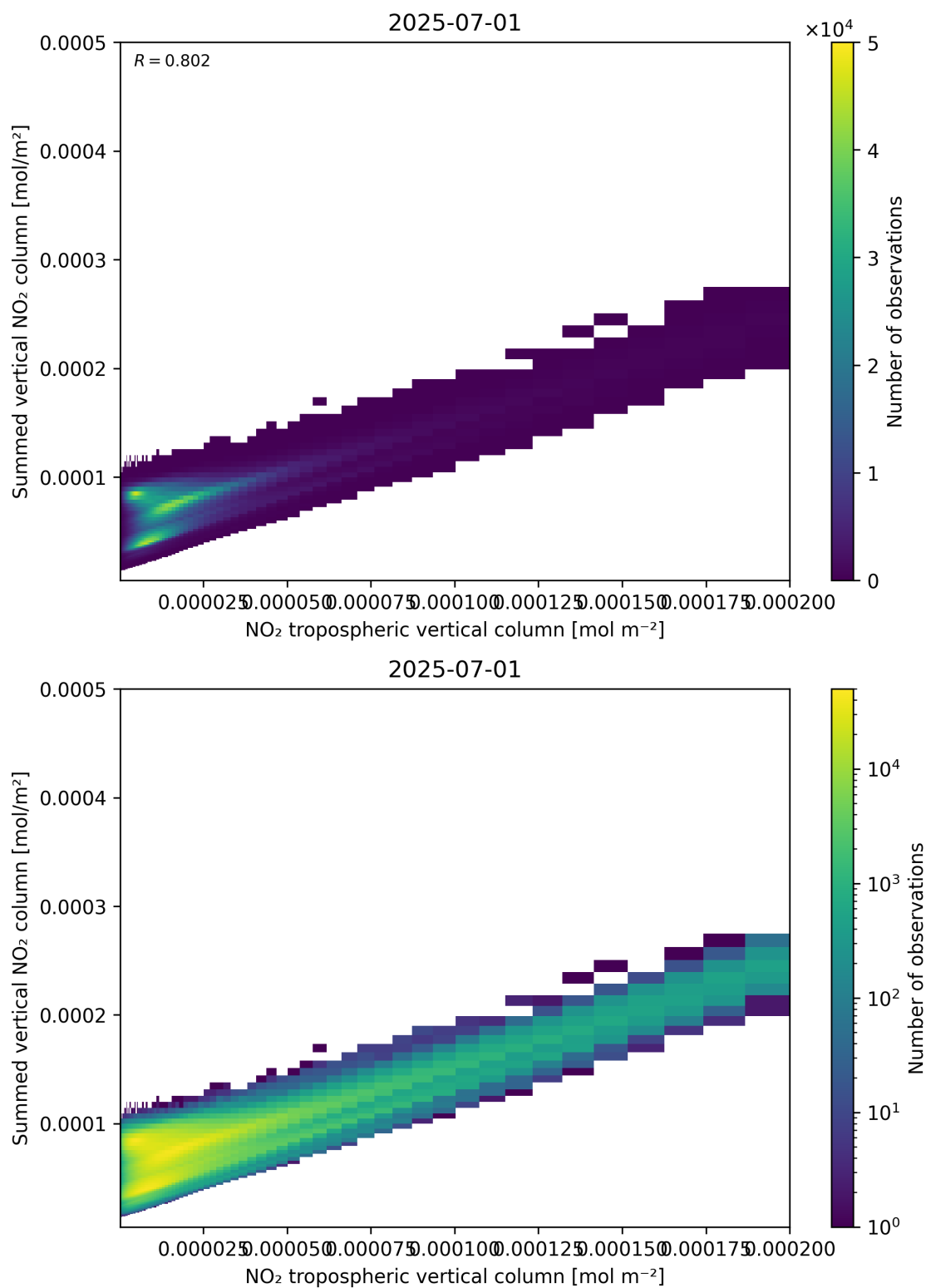
Figure 126: Scatter density plot of “NO 2 tropospheric vertical column” against “Summed vertical NO 2 column” for 2025-06-30 to 2025-07-02.
