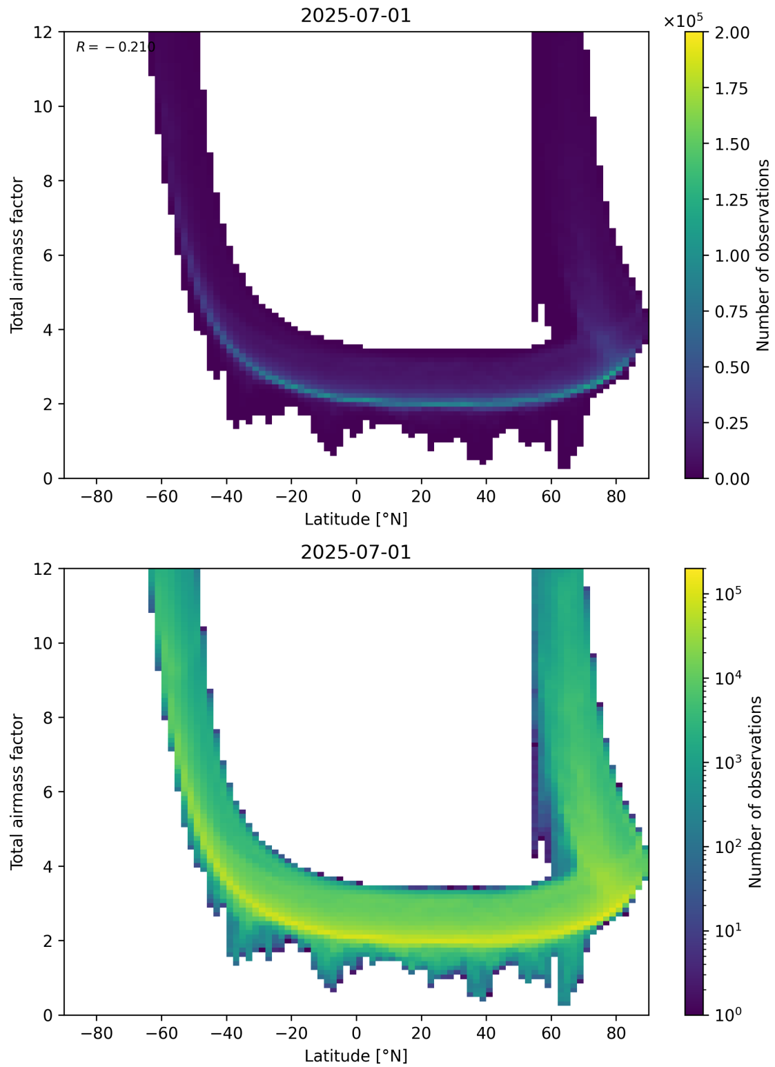
Figure 84: Scatter density plot of “Latitude” against “Total airmass factor” for 2025-06-30 to 2025-07-02.
