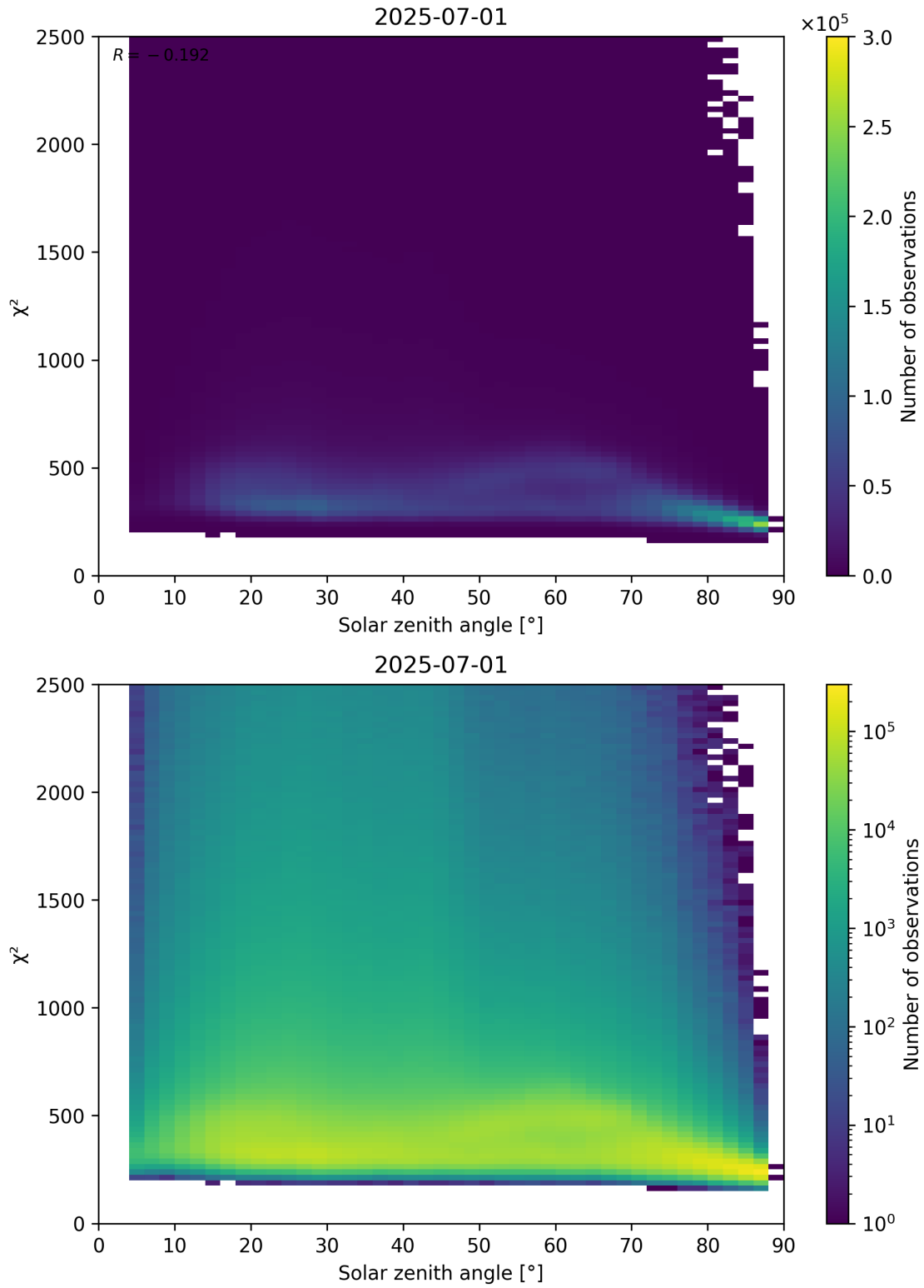
Figure 148: Scatter density plot of “Solar zenith angle” against “ \chi^2 ” for 2025-06-30 to 2025-07-02.
