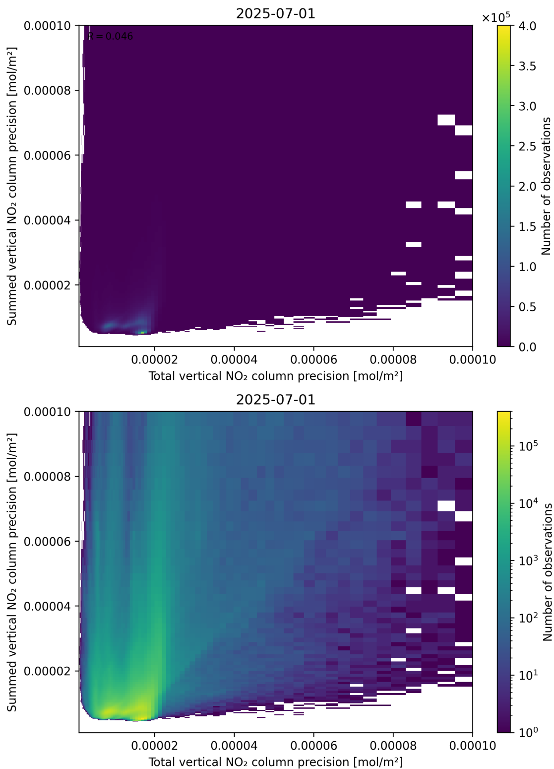
Figure 118: Scatter density plot of “Total vertical NO 2 column precision” against “Summed vertical NO 2 column precision” for 2025-06-30 to 2025-07-02.
