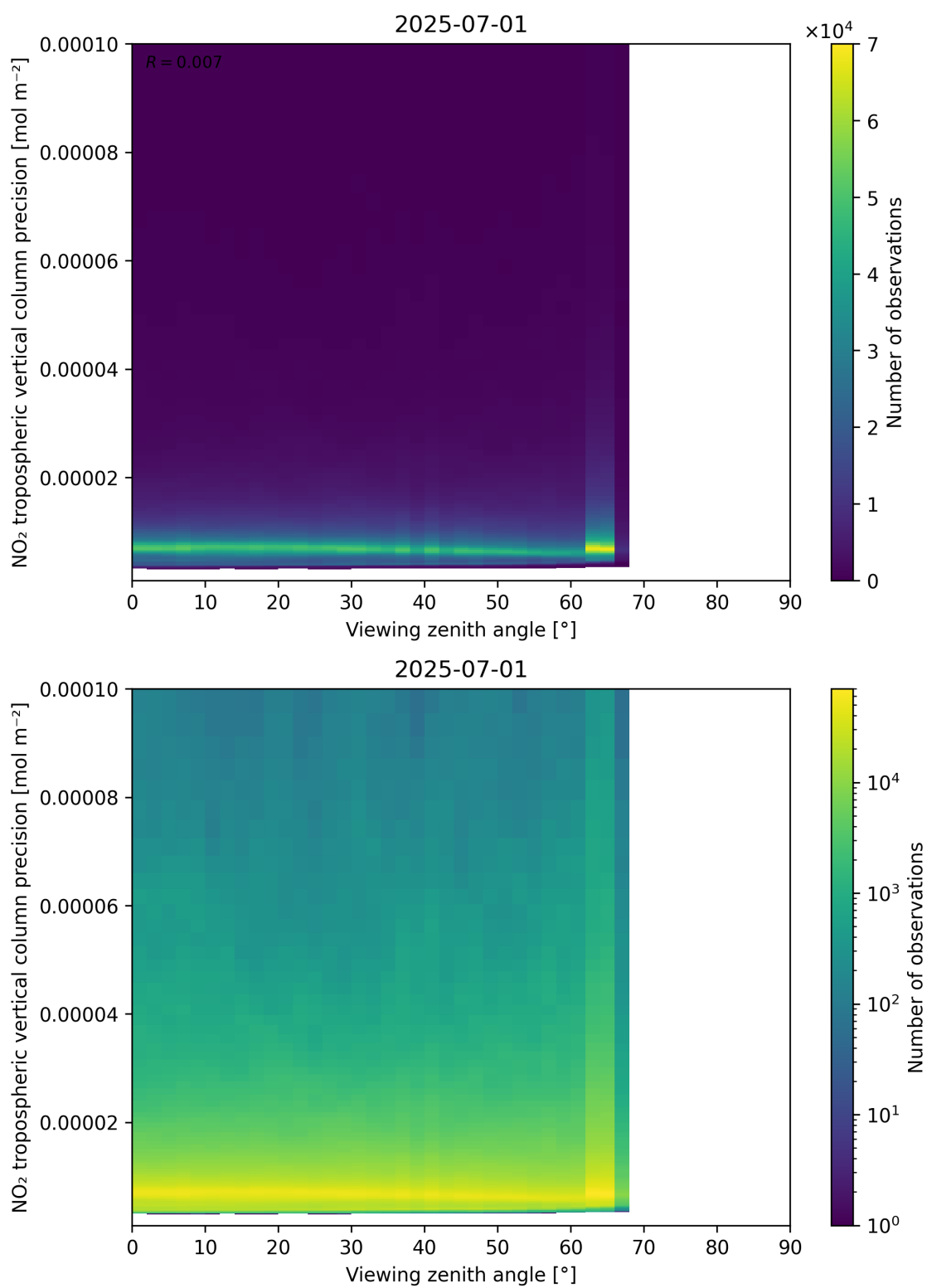
Figure 170: Scatter density plot of “Viewing zenith angle” against “NO 2 tropospheric vertical column precision” for 2025-06-30 to 2025-07-02.
