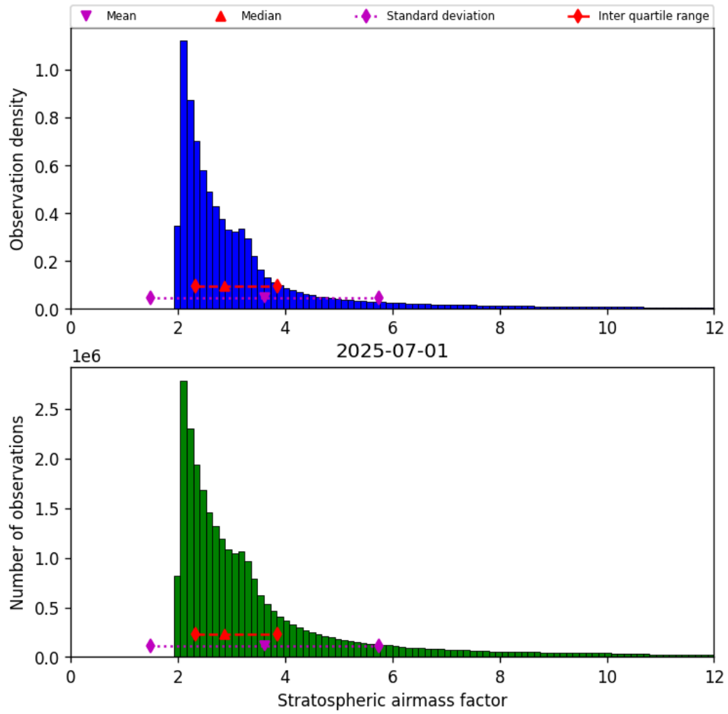
Figure 44: Histogram of “Stratospheric airmass factor” for 2025-06-30 to 2025-07-02
