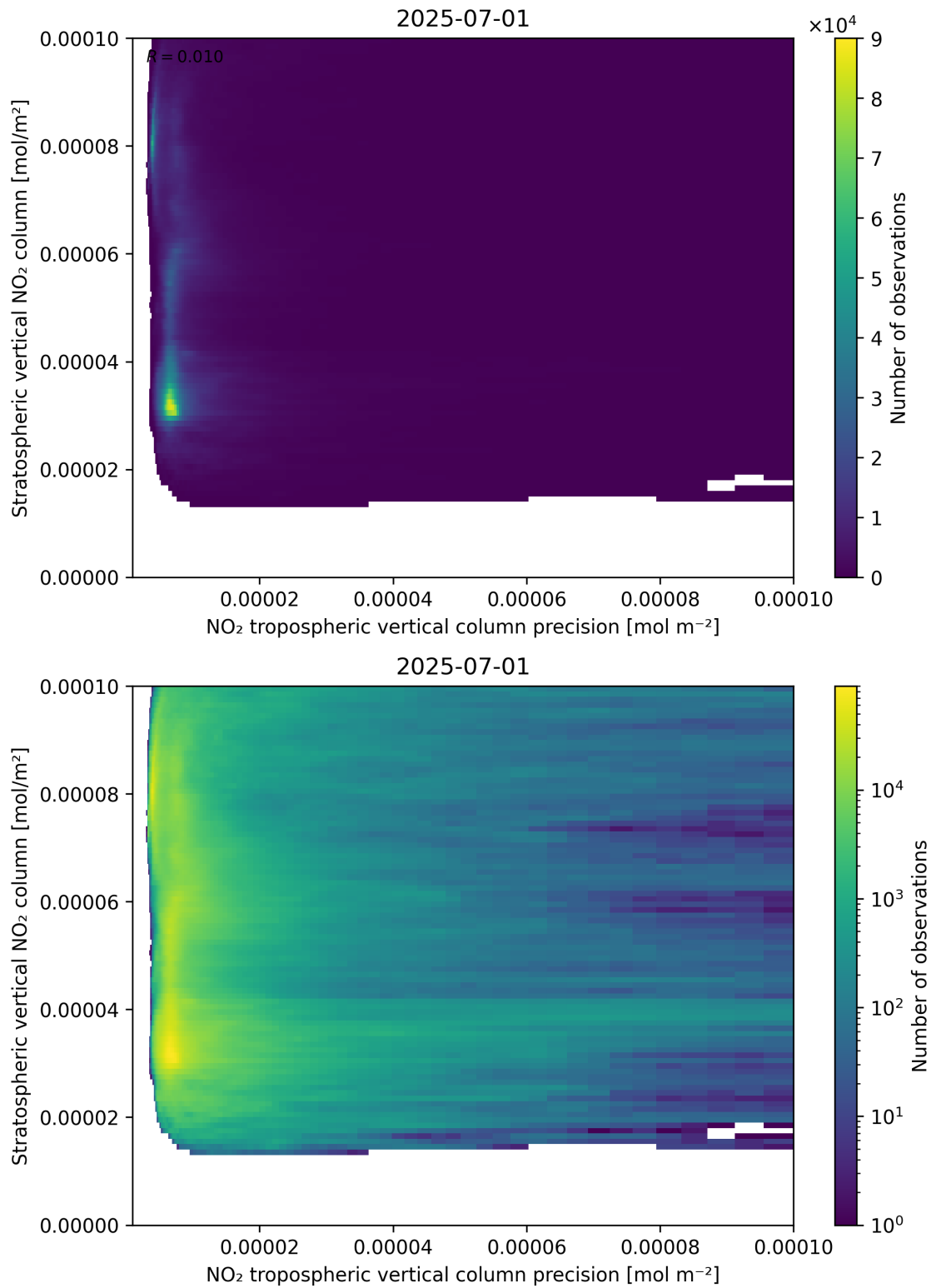
Figure 135: Scatter density plot of “NO 2 tropospheric vertical column precision” against “Stratospheric vertical NO 2 column” for 2025-06-30 to 2025-07-02.
