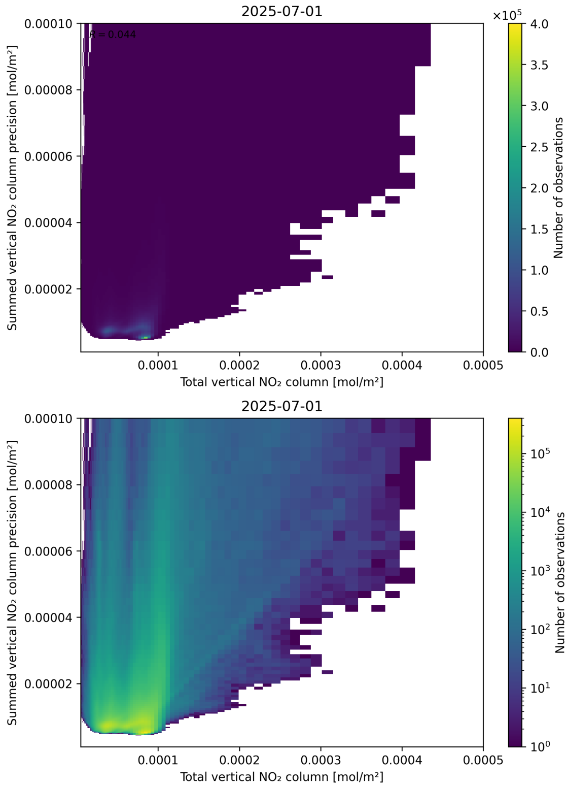
Figure 113: Scatter density plot of “Total vertical NO 2 column” against “Summed vertical NO 2 column precision” for 2025-06-30 to 2025-07-02.
