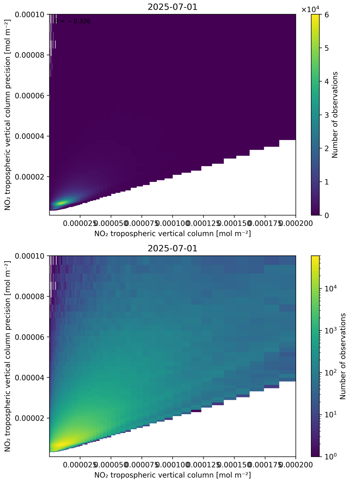
Figure 130: Scatter density plot of “NO 2 tropospheric vertical column” against “NO 2 tropospheric vertical column precision” for 2025-06-30 to 2025-07-02.
