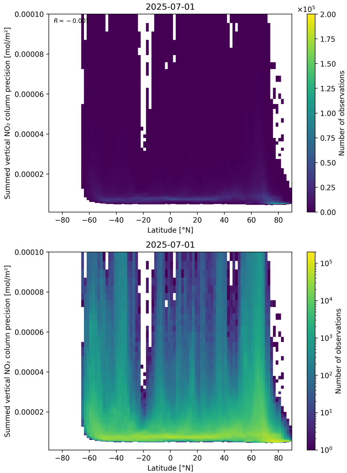
Figure 89: Scatter density plot of “Latitude” against “Summed vertical NO 2 column precision” for 2025-06-30 to 2025-07-02.
