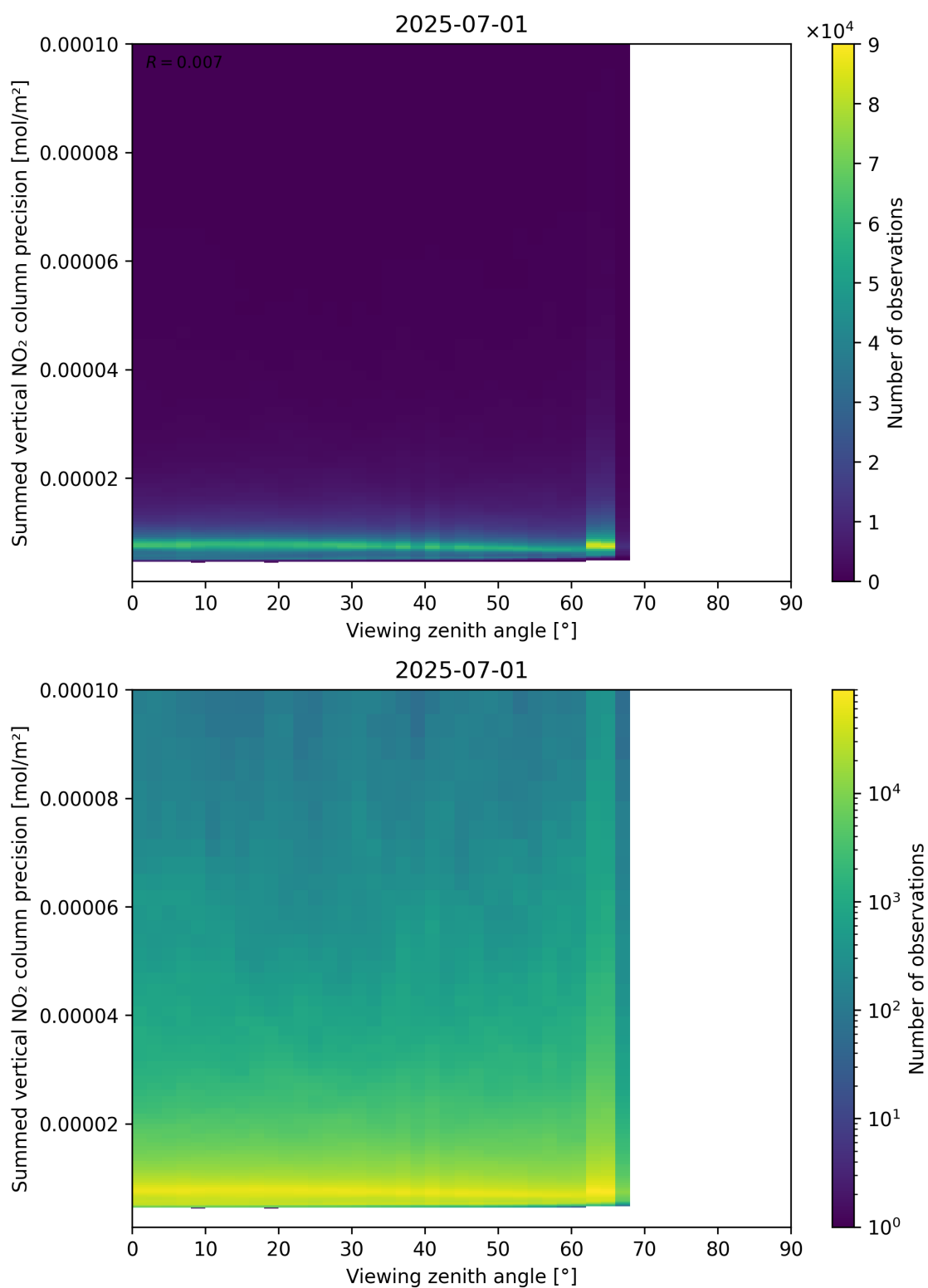
Figure 166: Scatter density plot of “Viewing zenith angle” against “Summed vertical NO 2 column precision” for 2025-06-30 to 2025-07-02.
