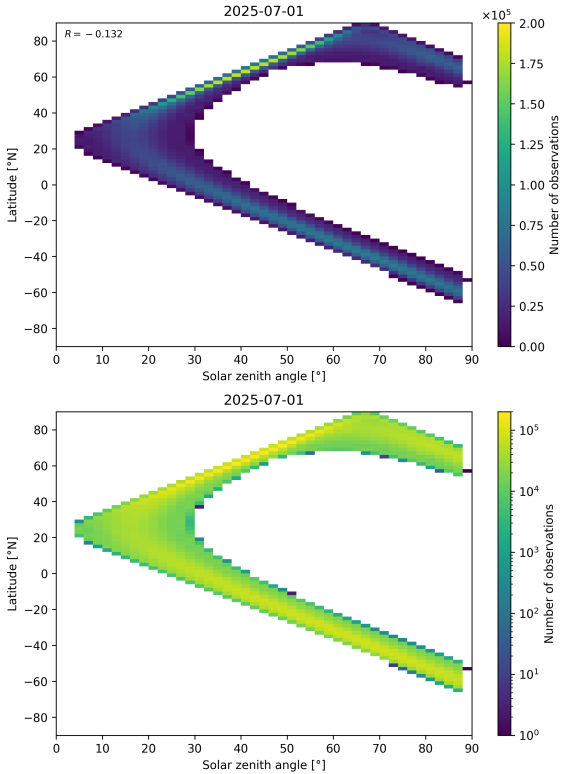
Figure 149: Scatter density plot of “Solar zenith angle” against “Latitude” for 2025-06-30 to 2025-07-02.
