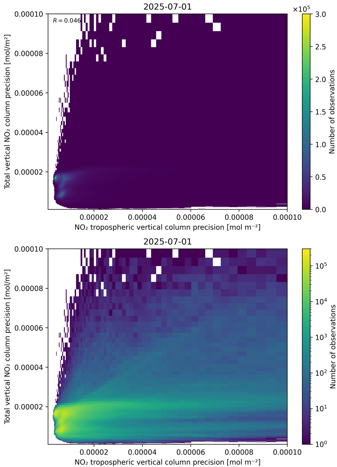
Figure 139: Scatter density plot of “NO 2 tropospheric vertical column precision” against “Total vertical NO 2 column precision” for 2025-06-30 to 2025-07-02.
