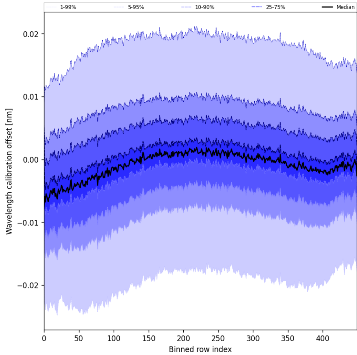
Figure 52: Along track statistics of “Wavelength calibration offset” for 2025-06-30 to 2025-07-02
