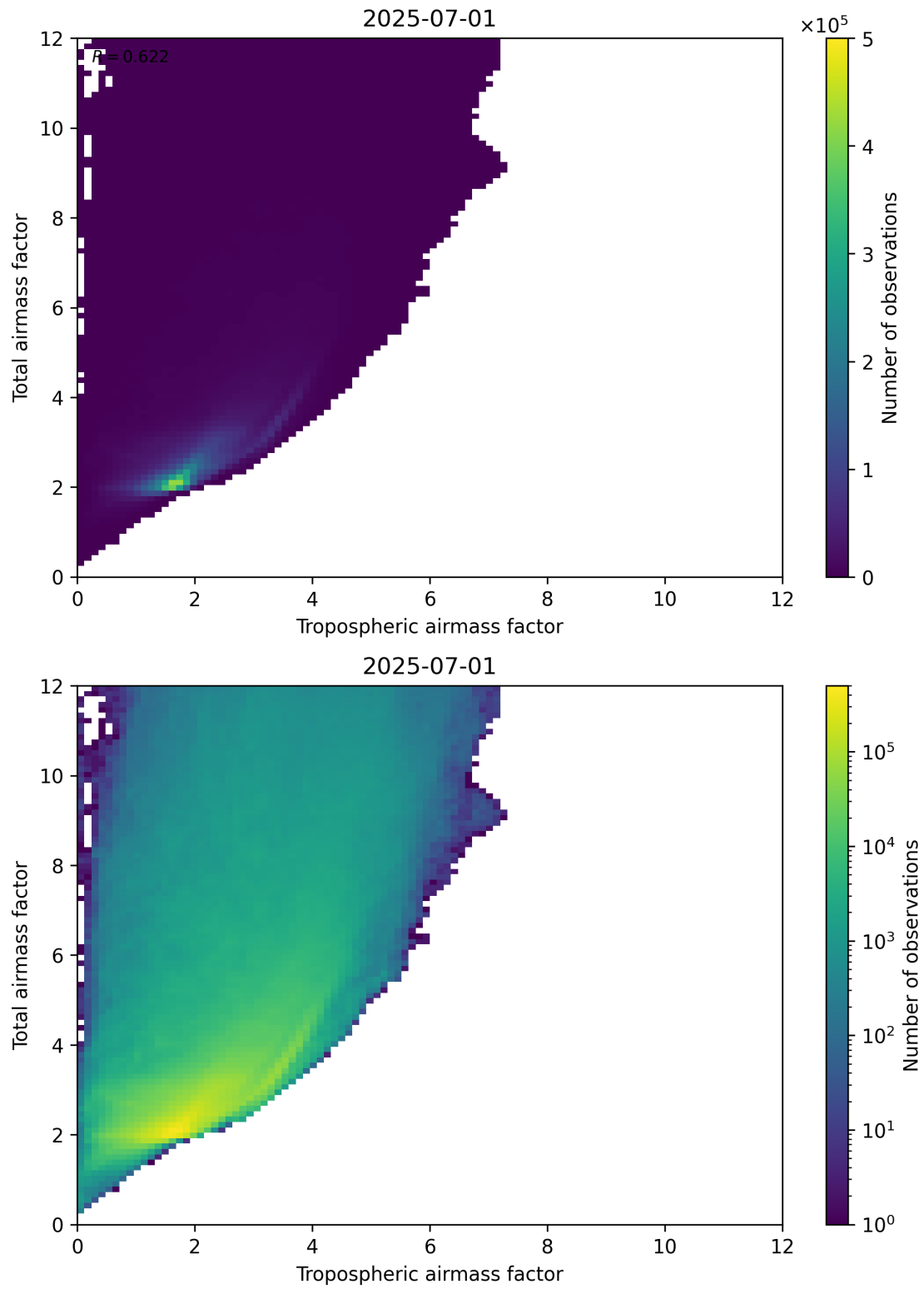
Figure 72: Scatter density plot of “Tropospheric airmass factor” against “Total airmass factor” for 2025-06-30 to 2025-07-02.
