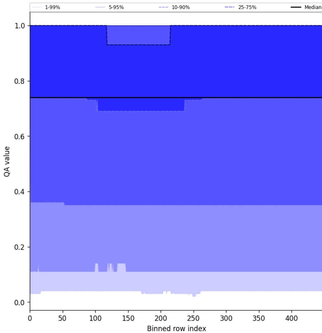
Figure 45: Along track statistics of “QA value” for 2025-06-30 to 2025-07-02
