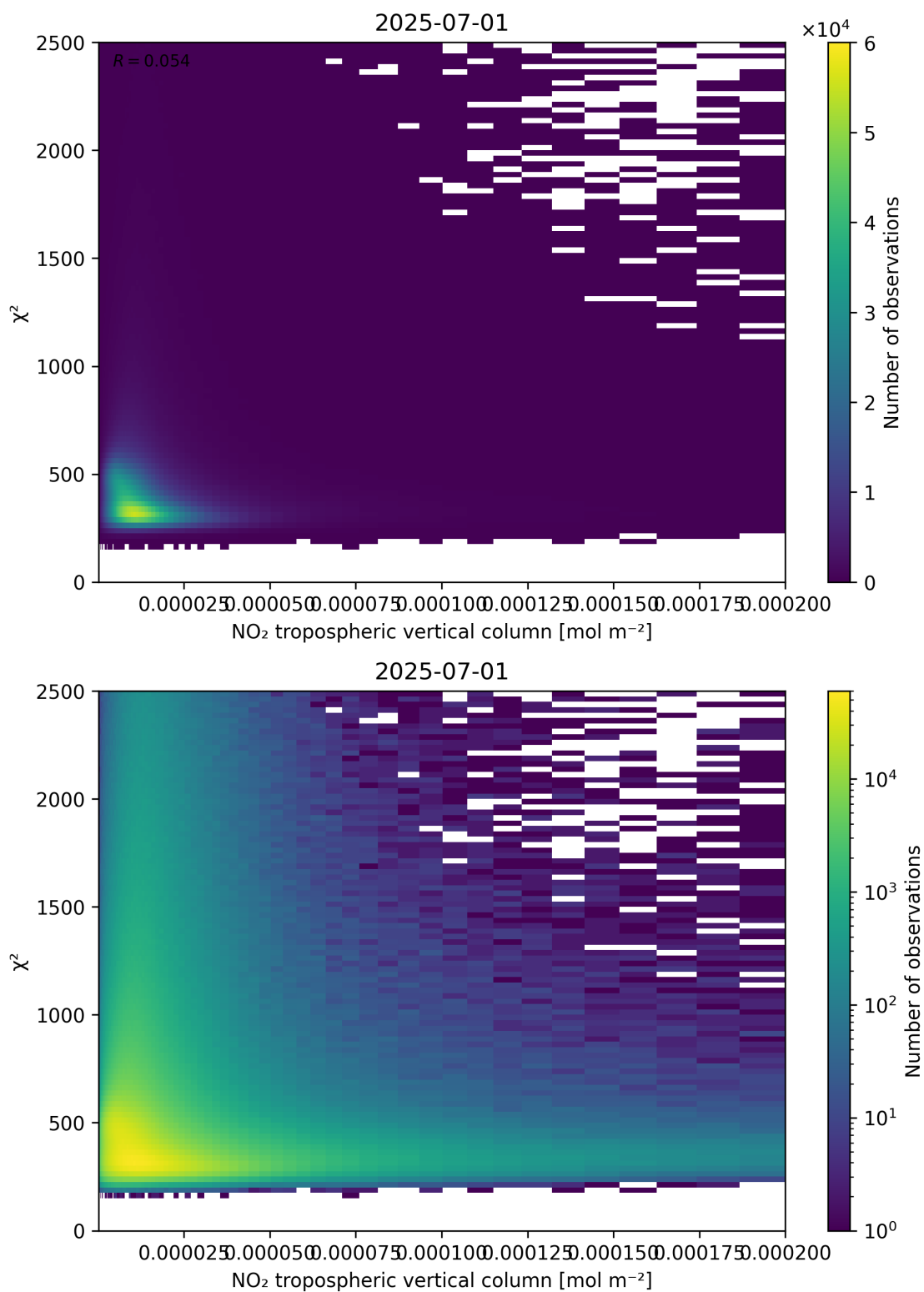
Figure 124: Scatter density plot of “NO 2 tropospheric vertical column” against “ \chi^2 ” for 2025-06-30 to 2025-07-02.
