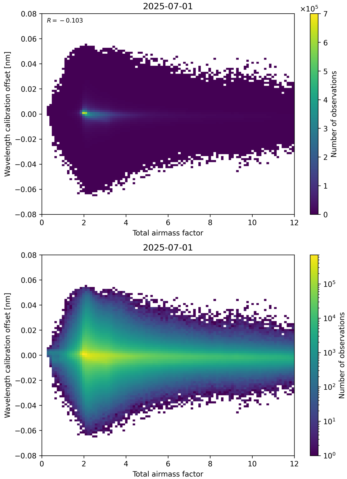
Figure 70: Scatter density plot of “Total airmass factor” against “Wavelength calibration offset” for 2025-06-30 to 2025-07-02.
