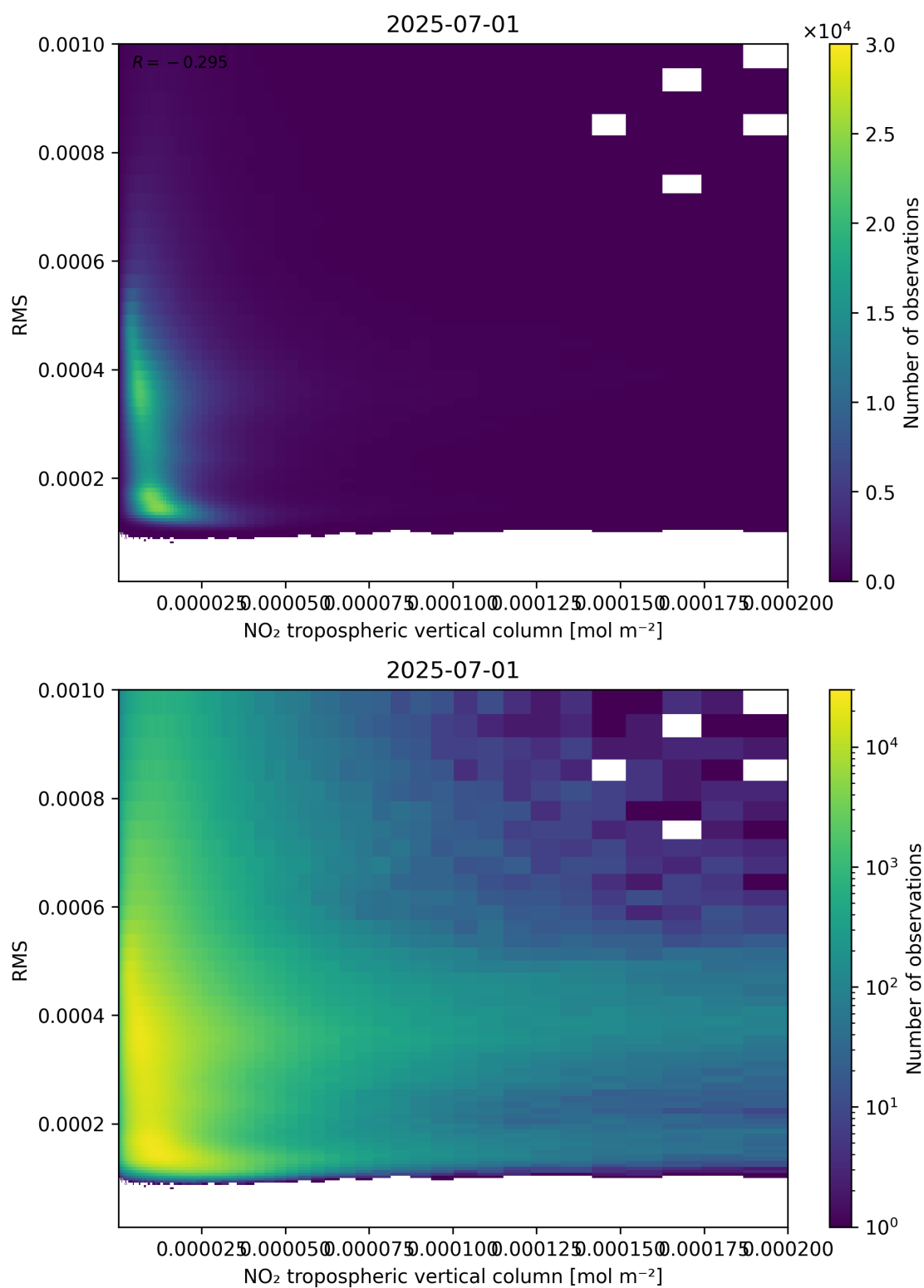
Figure 142: Scatter density plot of “NO 2 tropospheric vertical column” against “RMS” for 2025-06-30 to 2025-07-02.
