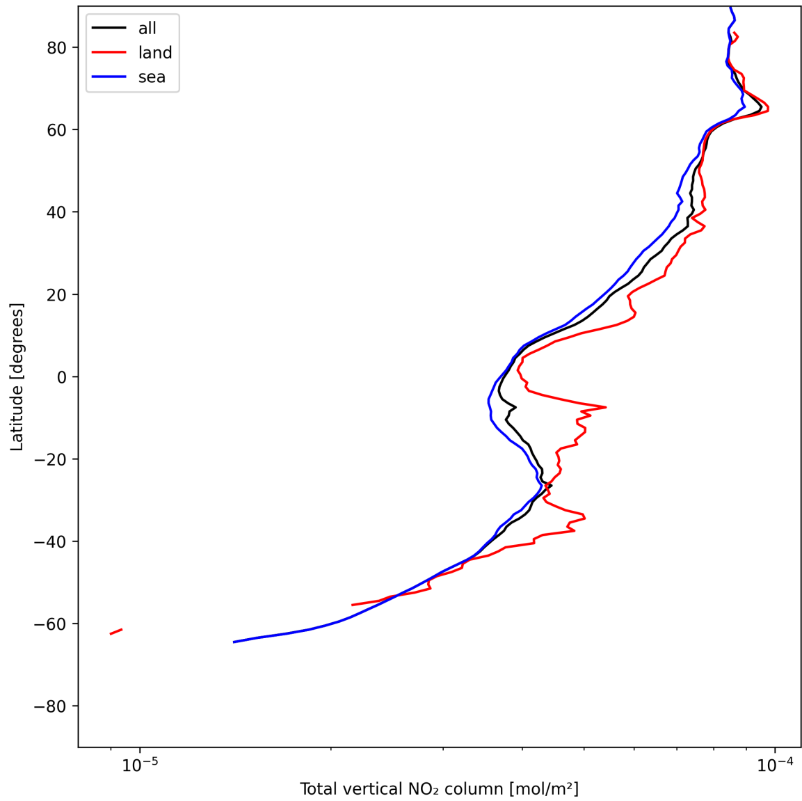
Figure 21: Zonal average of “Total vertical NO 2 column” for 2025-06-30 to 2025-07-02.
