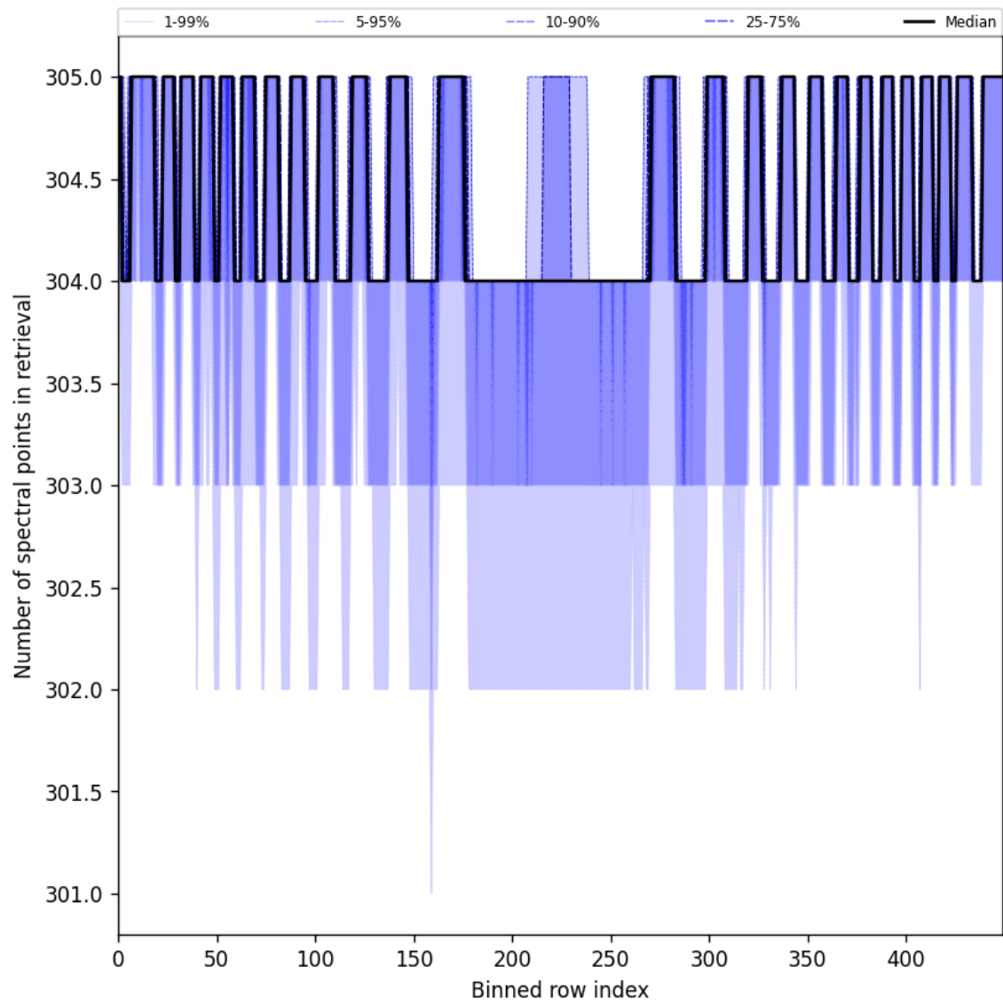
Figure 50: Along track statistics of “Number of spectral points in retrieval” for 2025-06-30 to 2025-07-02
