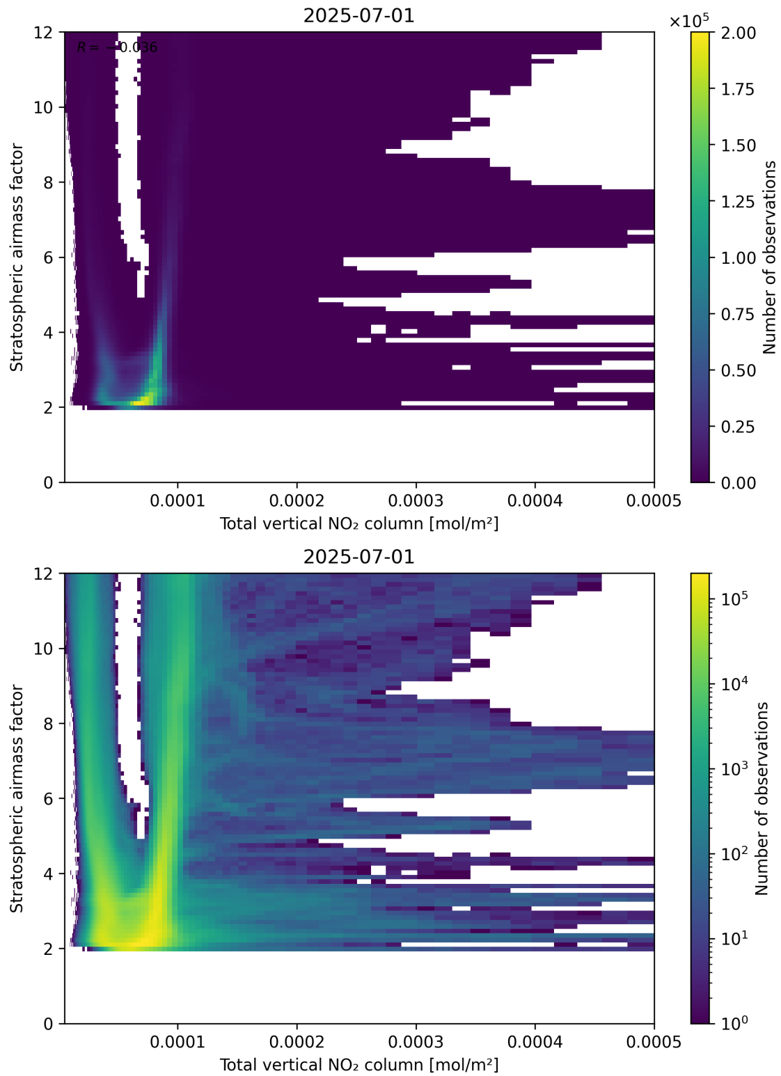
Figure 110: Scatter density plot of “Total vertical NO 2 column” against “Stratospheric airmass factor” for 2025-06-30 to 2025-07-02.
