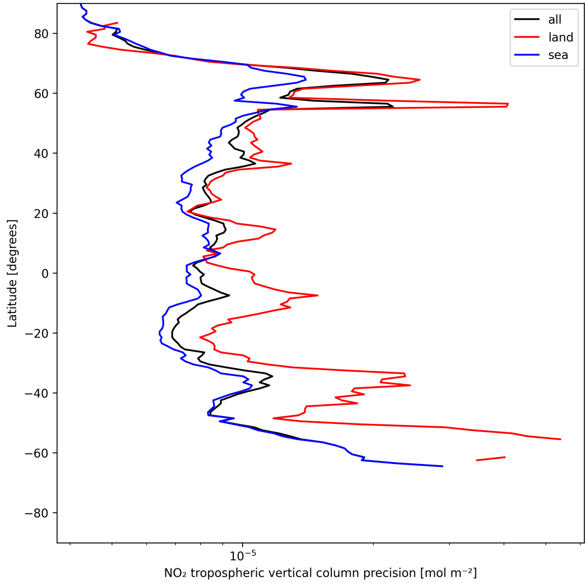
Figure 13: Zonal average of “NO 2 tropospheric vertical column precision” for 2025-06-30 to 2025-07-02.
