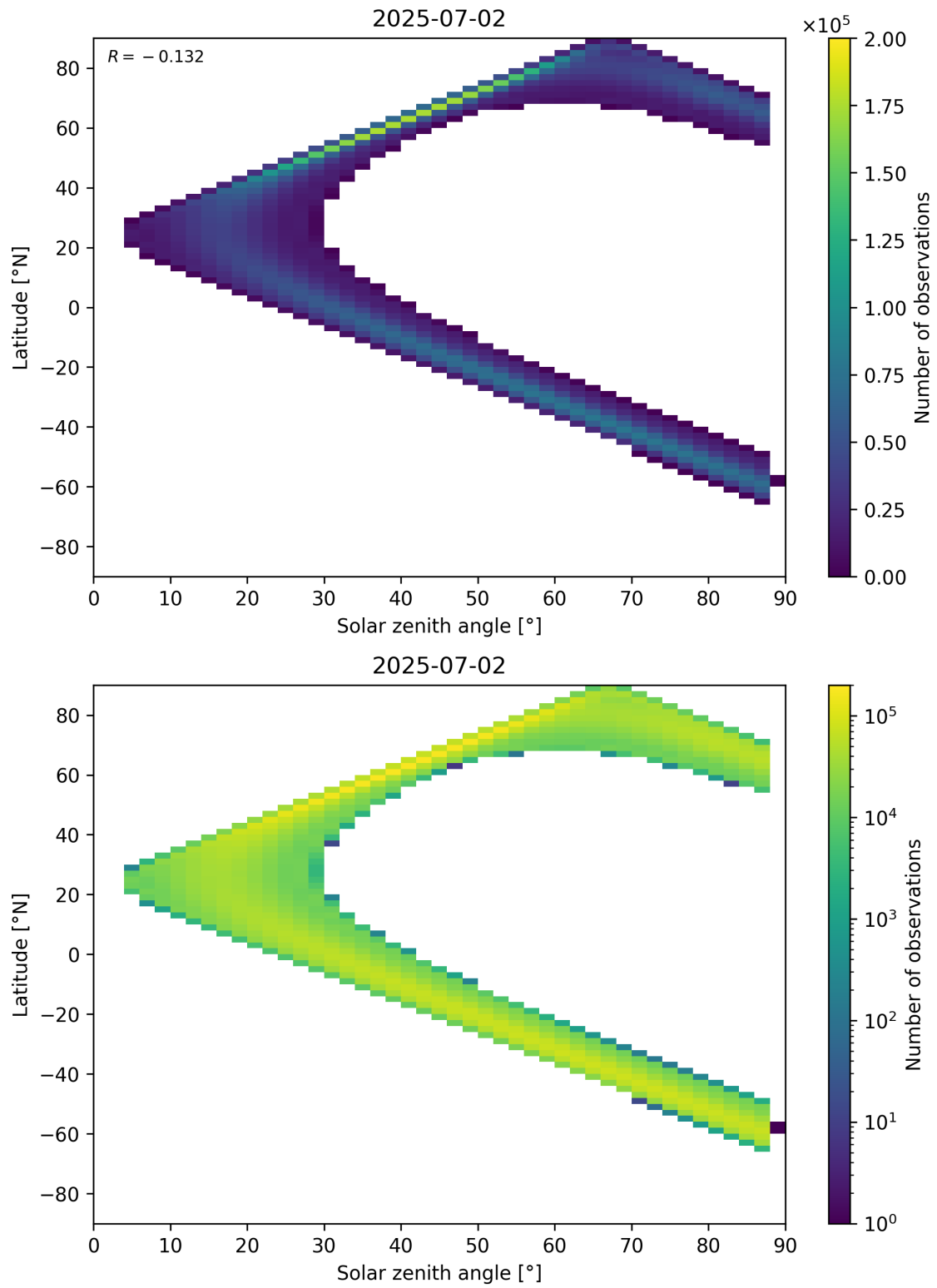
Figure 149: Scatter density plot of “Solar zenith angle” against “Latitude” for 2025-07-02 to 2025-07-03.
