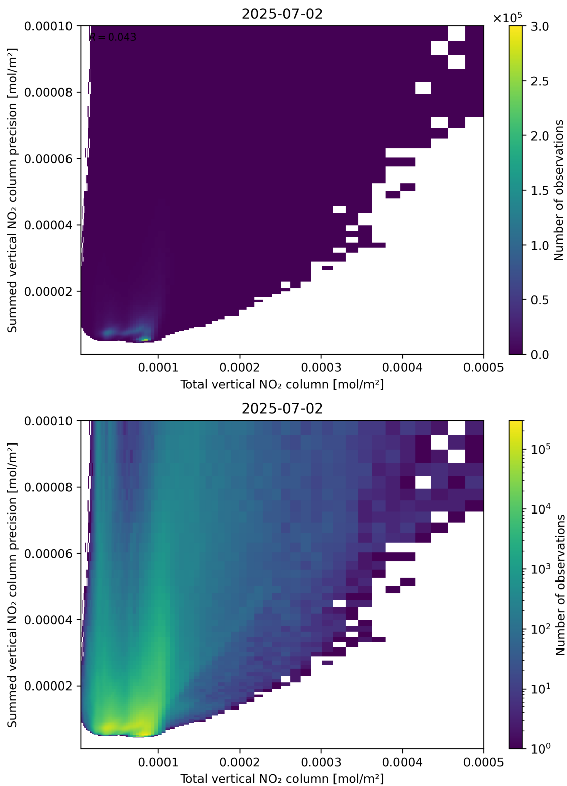
Figure 113: Scatter density plot of “Total vertical NO 2 column” against “Summed vertical NO 2 column precision” for 2025-07-02 to 2025-07-03.
