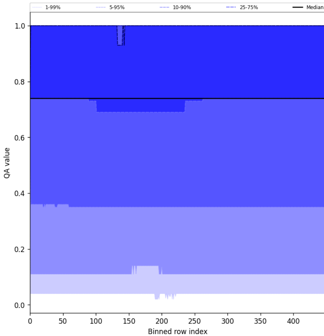
Figure 45: Along track statistics of “QA value” for 2025-07-02 to 2025-07-03
