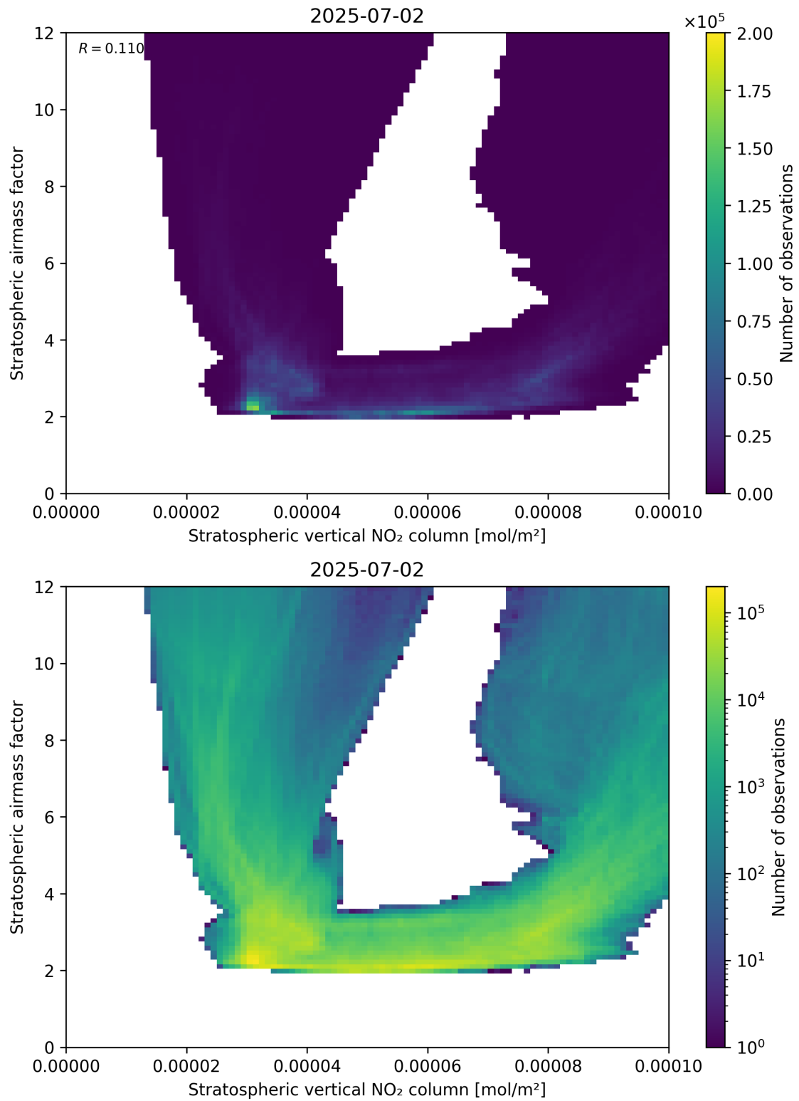
Figure 96: Scatter density plot of “Stratospheric vertical NO 2 column” against “Stratospheric airmass factor” for 2025-07-02 to 2025-07-03.
