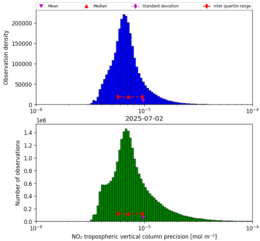
Figure 30: Histogram of “NO 2 tropospheric vertical column precision” for 2025-07-02 to 2025-07-03
