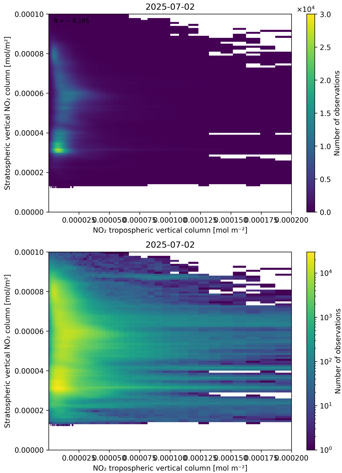
Figure 125: Scatter density plot of “NO 2 tropospheric vertical column” against “Stratospheric vertical NO 2 column” for 2025-07-02 to 2025-07-03.
