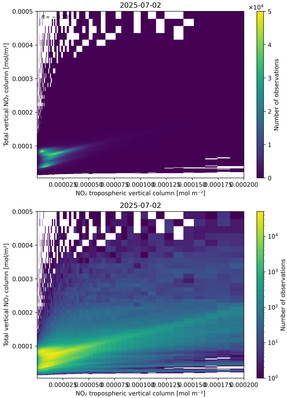
Figure 128: Scatter density plot of “NO 2 tropospheric vertical column” against “Total vertical NO 2 column” for 2025-07-02 to 2025-07-03.
