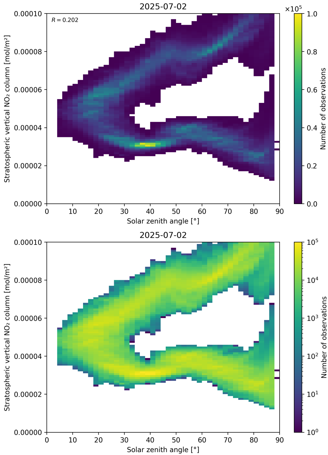
Figure 150: Scatter density plot of “Solar zenith angle” against “Stratospheric vertical NO 2 column” for 2025-07-02 to 2025-07-03.
