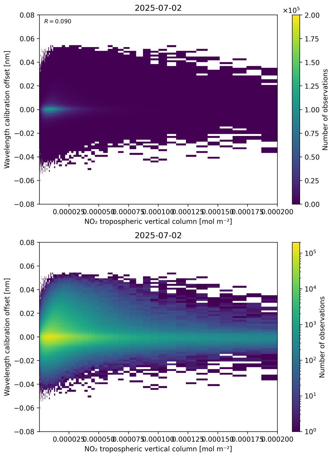
Figure 143: Scatter density plot of “NO 2 tropospheric vertical column” against “Wavelength calibration offset” for 2025-07-02 to 2025-07-03.
