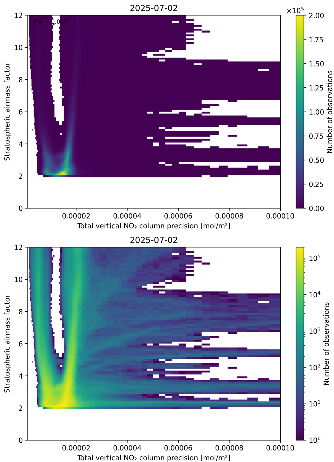
Figure 115: Scatter density plot of “Total vertical NO 2 column precision” against “Stratospheric air mass factor” for 2025-07-02 to 2025-07-03.
