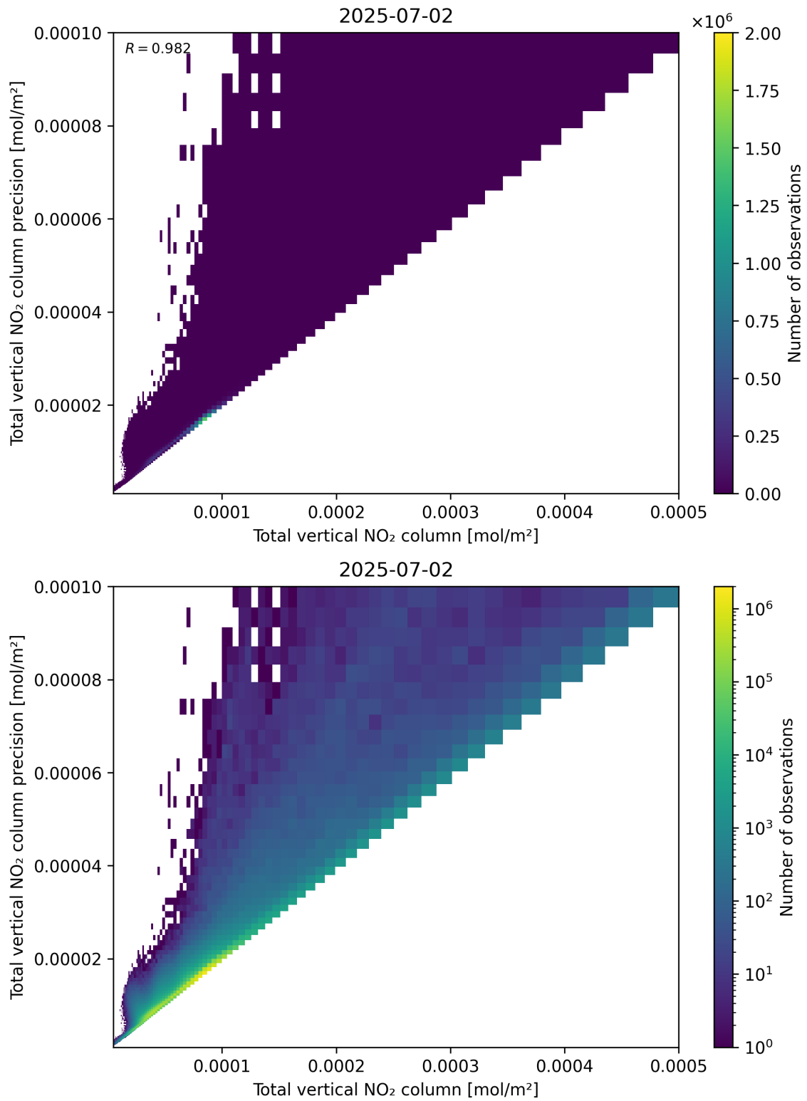
Figure 114: Scatter density plot of “Total vertical NO 2 column” against “Total vertical NO 2 column precision” for 2025-07-02 to 2025-07-03.
