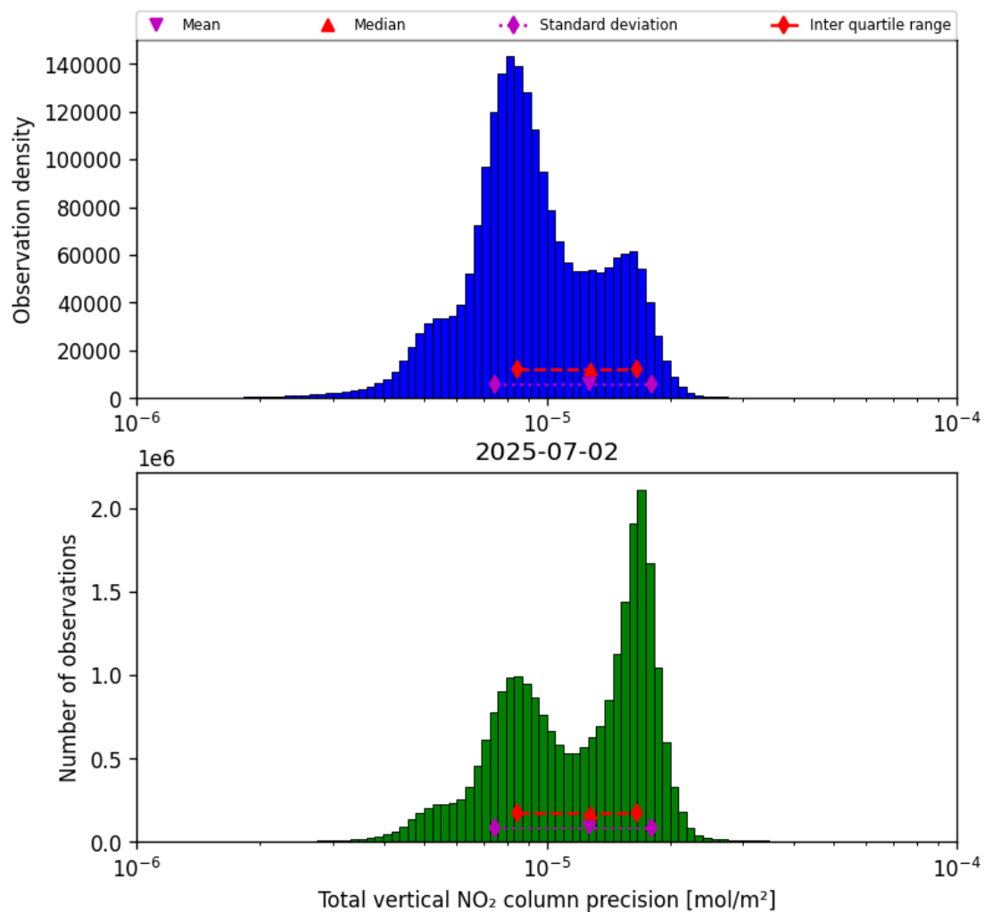
Figure 39: Histogram of “Total vertical NO 2 column precision” for 2025-07-02 to 2025-07-03
