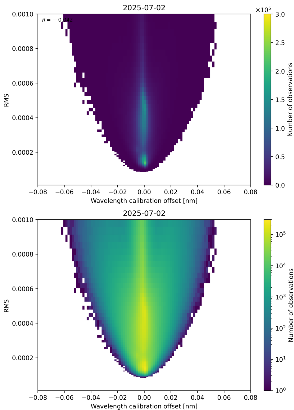
Figure 181: Scatter density plot of “Wavelength calibration offset” against “RMS” for 2025-07-02 to 2025-07-03.
