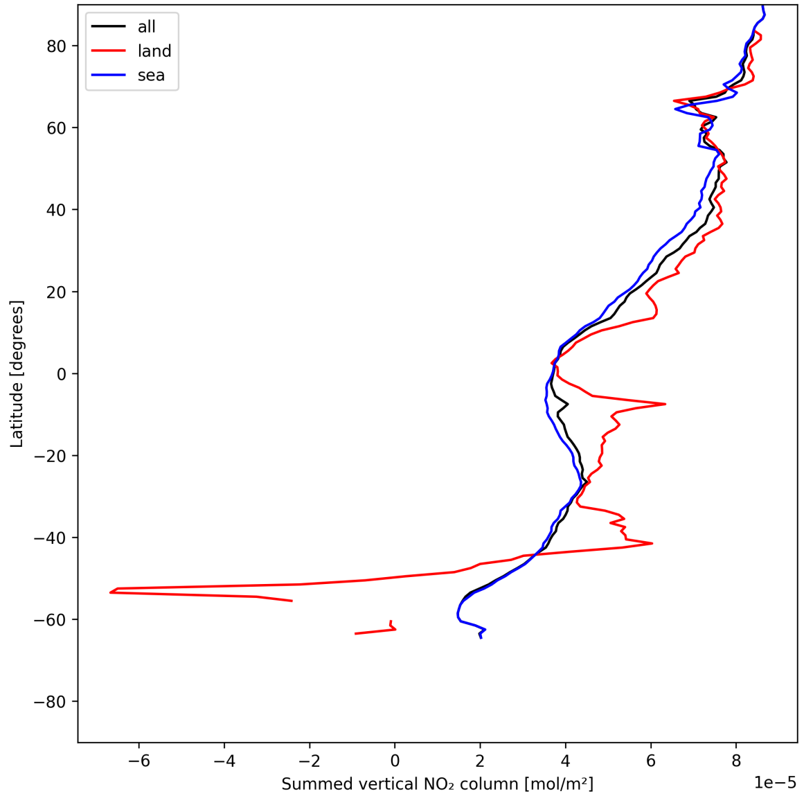
Figure 23: Zonal average of “Summed vertical NO 2 column” for 2025-07-02 to 2025-07-03.
