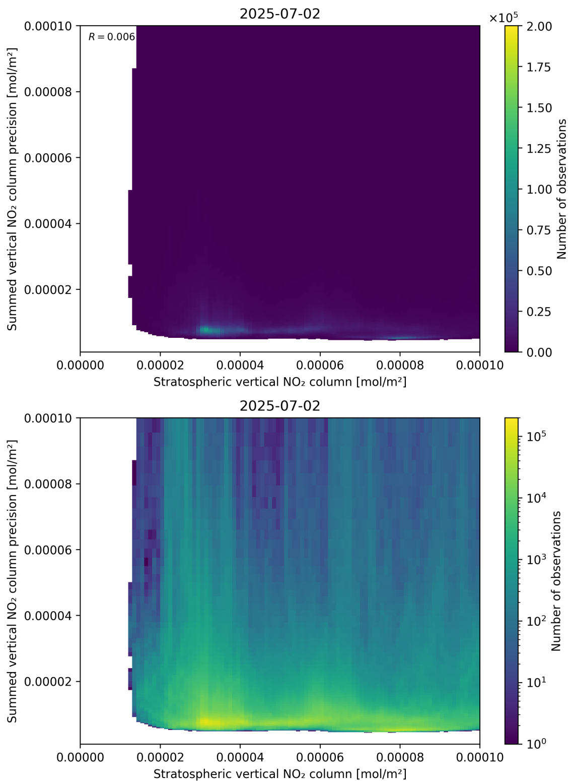
Figure 99: Scatter density plot of “Stratospheric vertical NO 2 column” against “Summed vertical NO 2 column precision” for 2025-07-02 to 2025-07-03.
