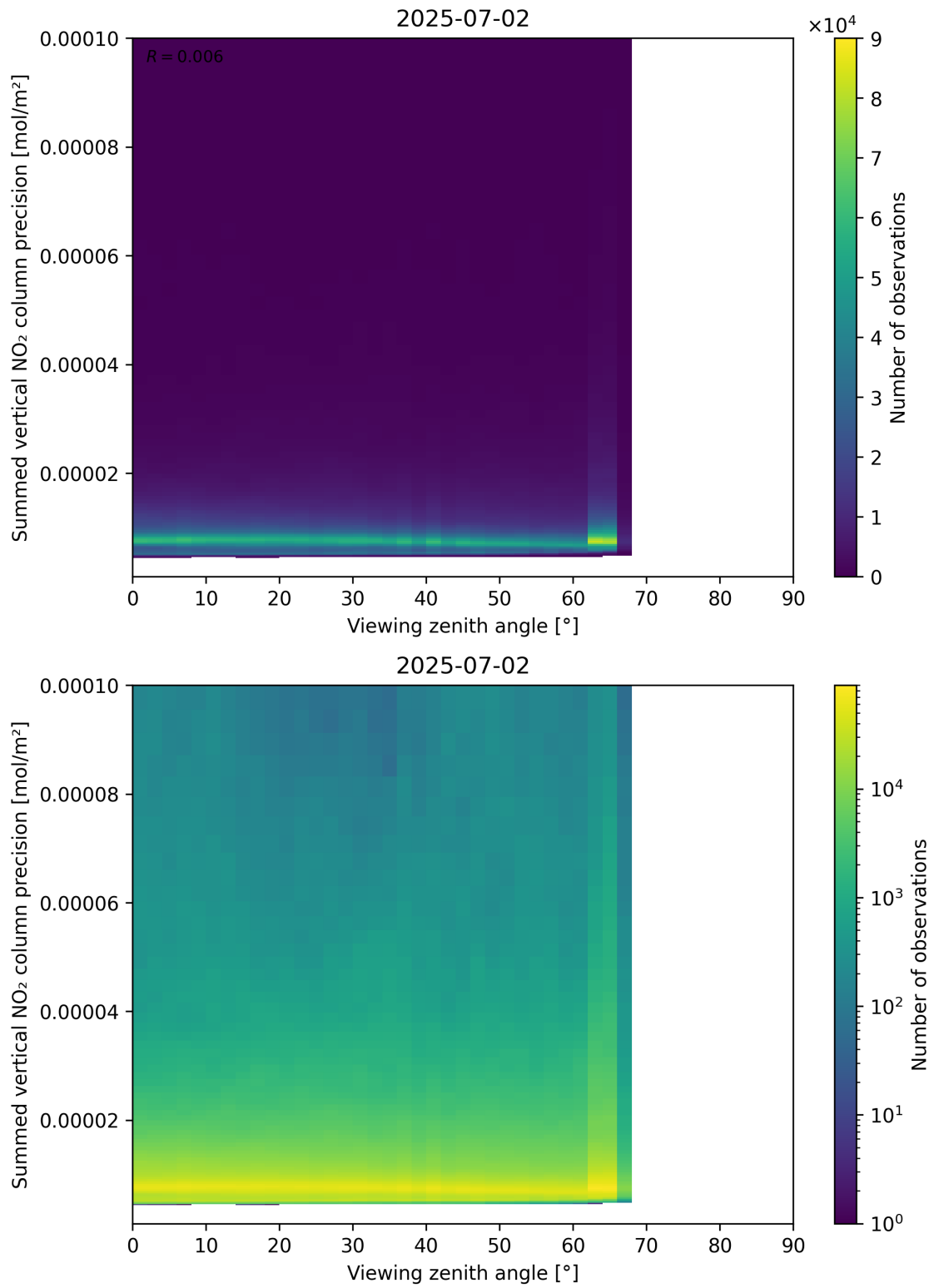
Figure 166: Scatter density plot of “Viewing zenith angle” against “Summed vertical NO 2 column precision” for 2025-07-02 to 2025-07-03.
