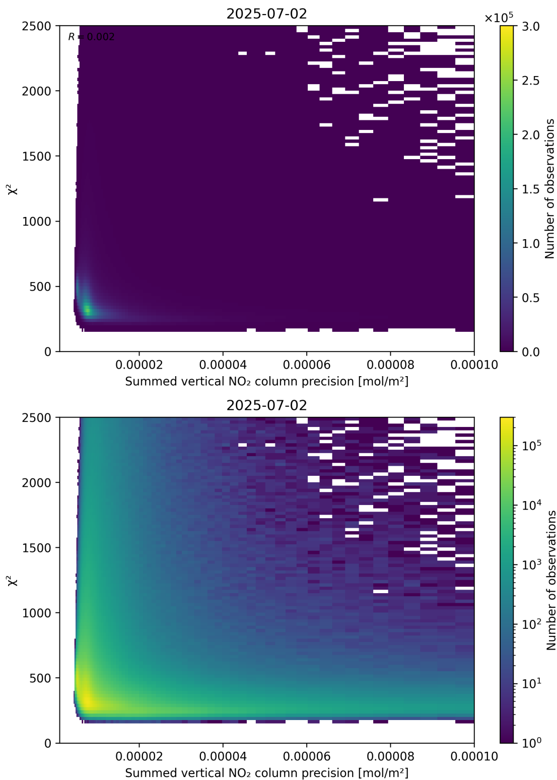
Figure 107: Scatter density plot of “Summed vertical NO 2 column precision” against “ \chi^2 ” for 2025-07-02 to 2025-07-03.
