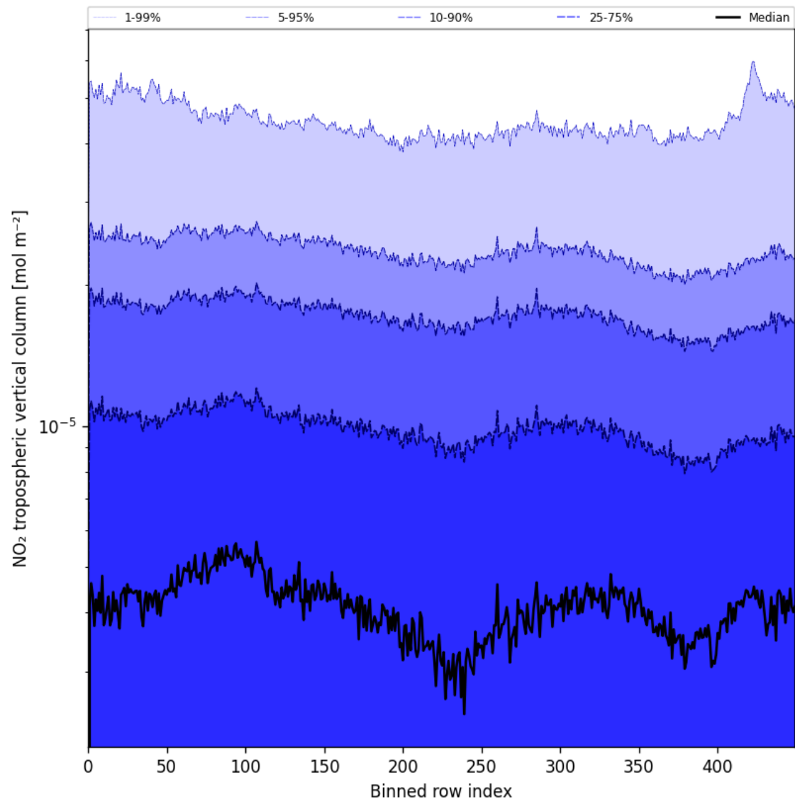
Figure 46: Along track statistics of “NO 2 tropospheric vertical column” for 2025-07-02 to 2025-07-03
