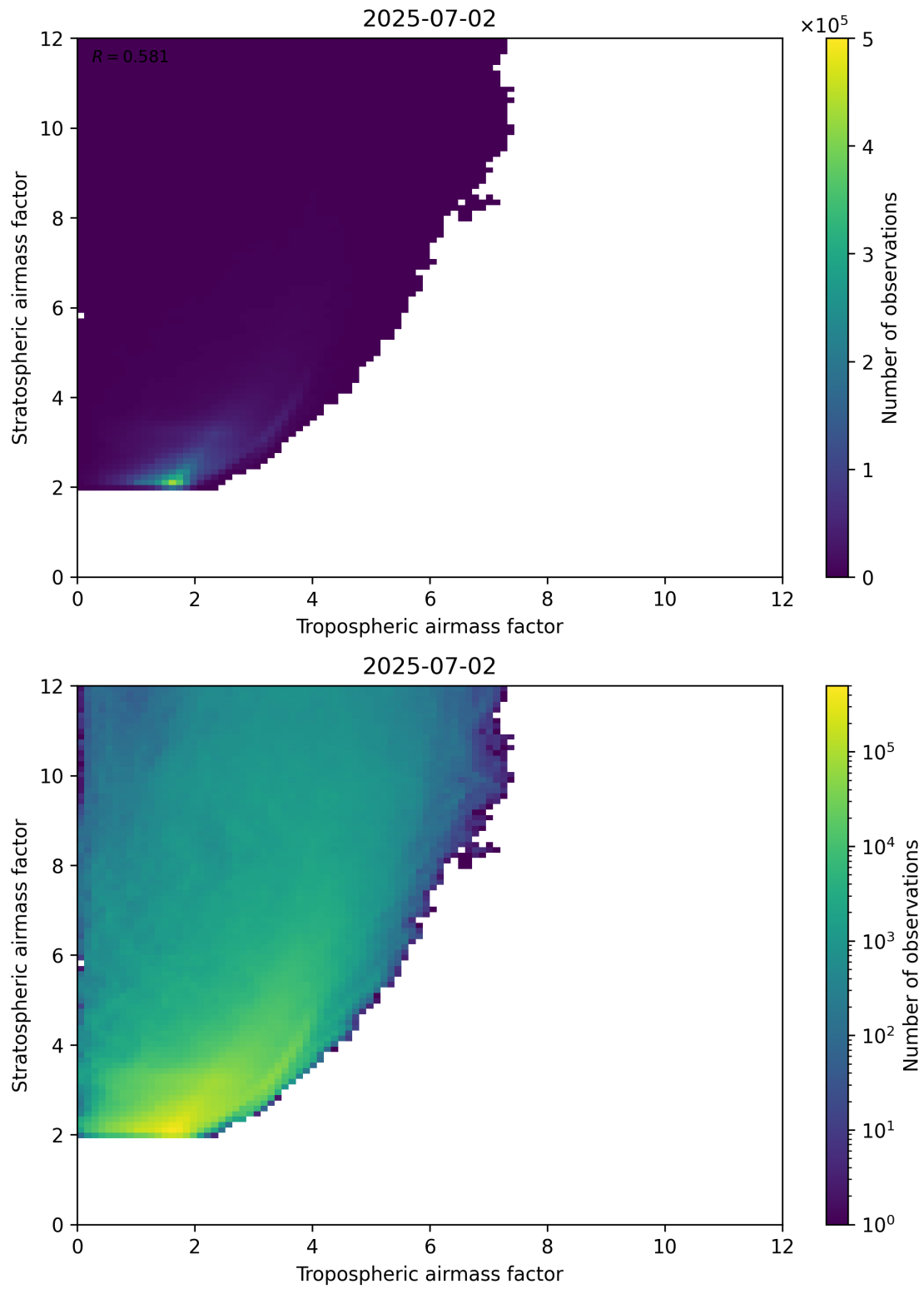
Figure 71: Scatter density plot of “Tropospheric airmass factor” against “Stratospheric airmass factor” for 2025-07-02 to 2025-07-03.
