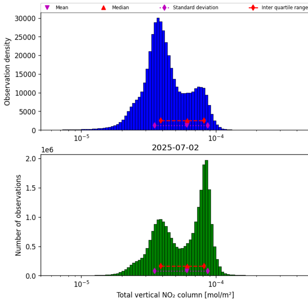
Figure 38: Histogram of “Total vertical NO 2 column” for 2025-07-02 to 2025-07-03
