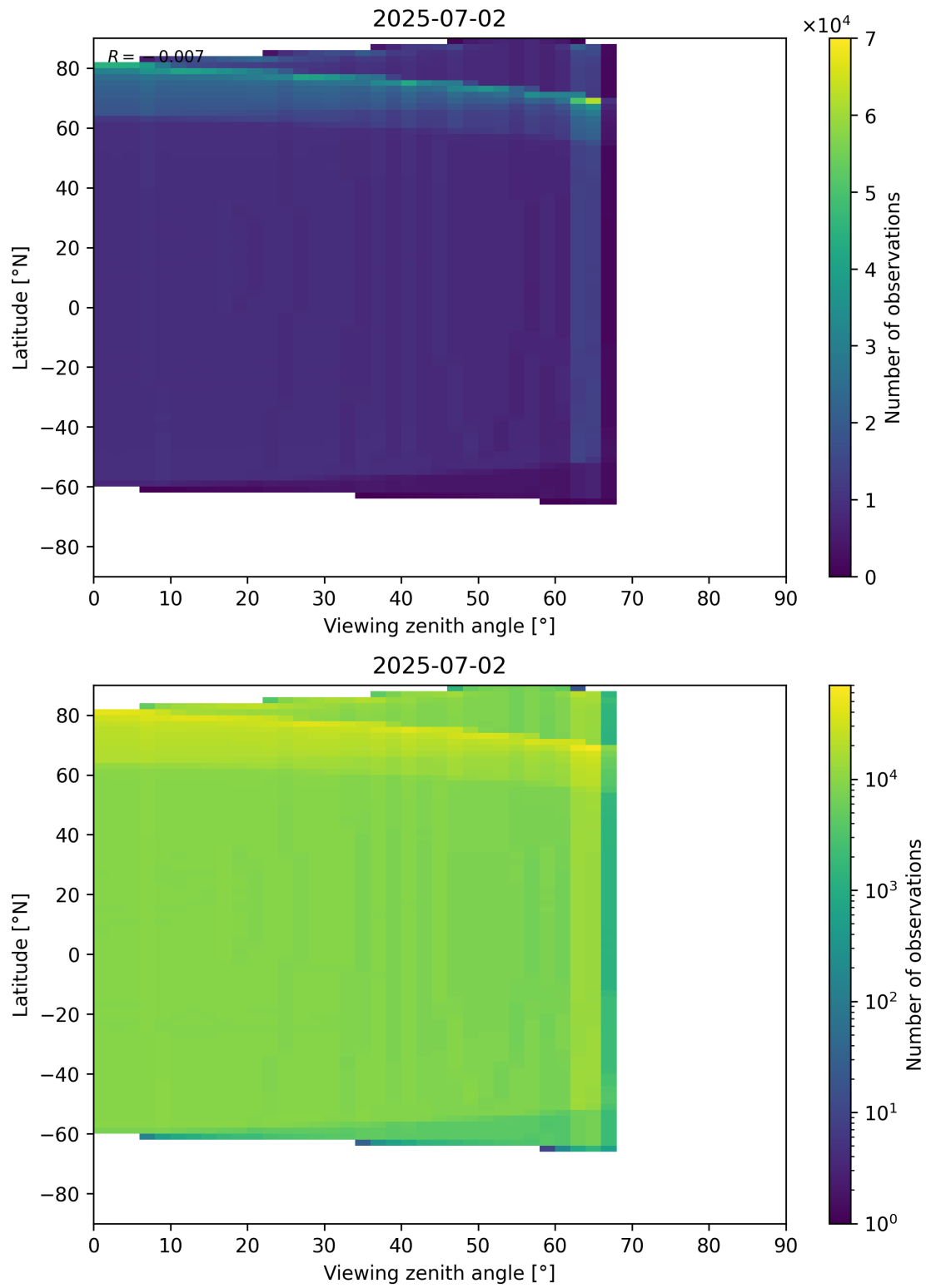
Figure 163: Scatter density plot of “Viewing zenith angle” against “Latitude” for 2025-07-02 to 2025-07-03.
