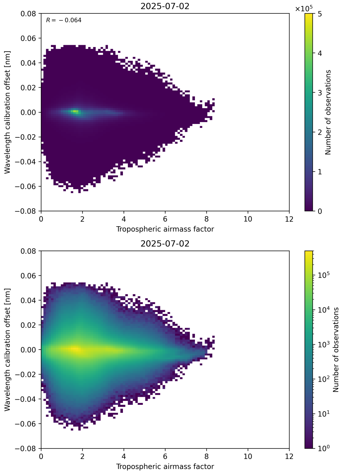
Figure 80: Scatter density plot of “Tropospheric airmass factor” against “Wavelength calibration offset” for 2025-07-02 to 2025-07-03.
