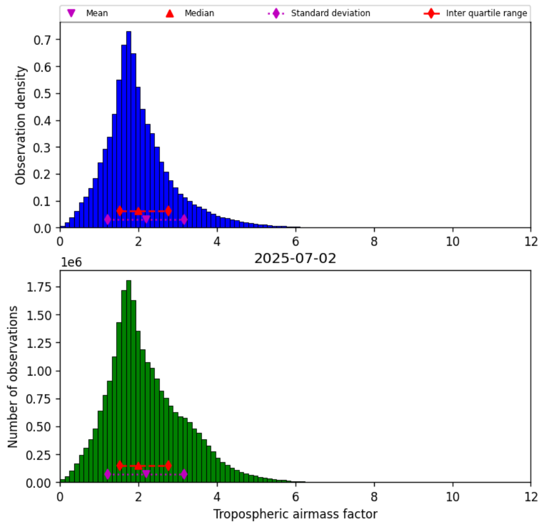
Figure 31: Histogram of “Tropospheric airmass factor” for 2025-07-02 to 2025-07-03
