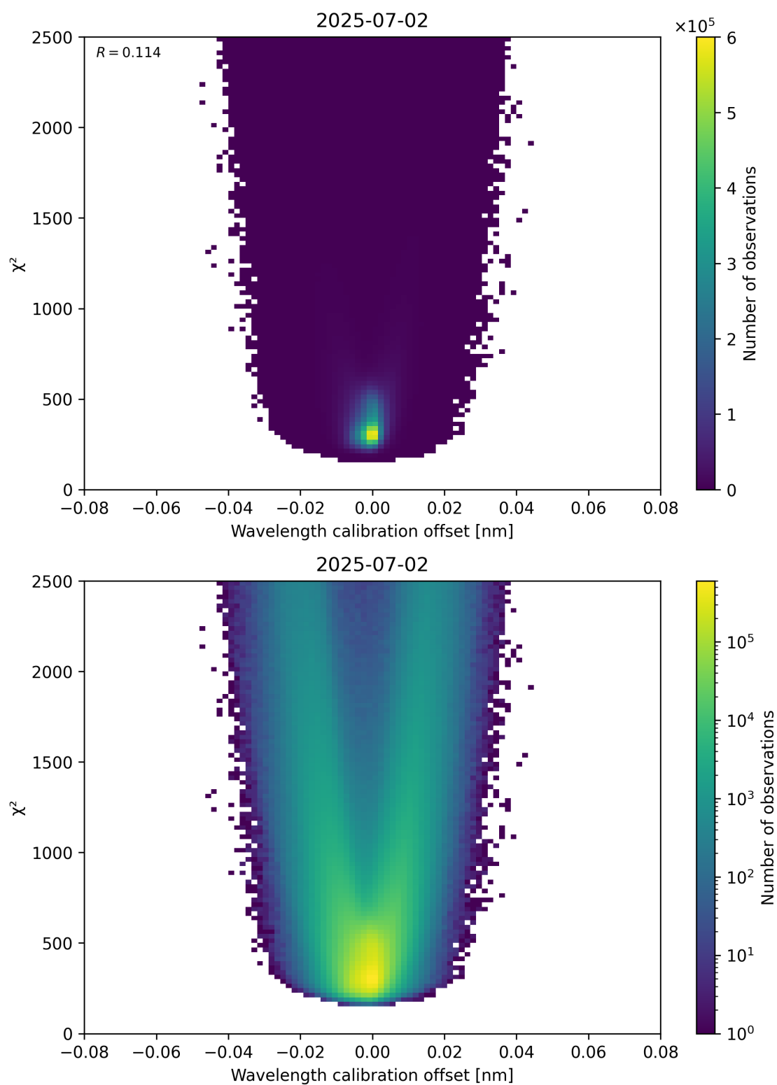
Figure 175: Scatter density plot of “Wavelength calibration offset” against “ \chi^2 ” for 2025-07-02 to 2025-07-03.
