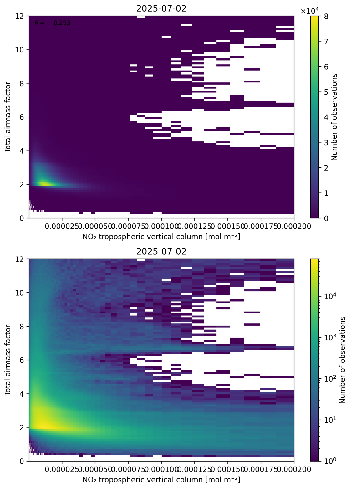
Figure 122: Scatter density plot of “NO 2 tropospheric vertical column” against “Total air mass factor” for 2025-07-02 to 2025-07-03.
