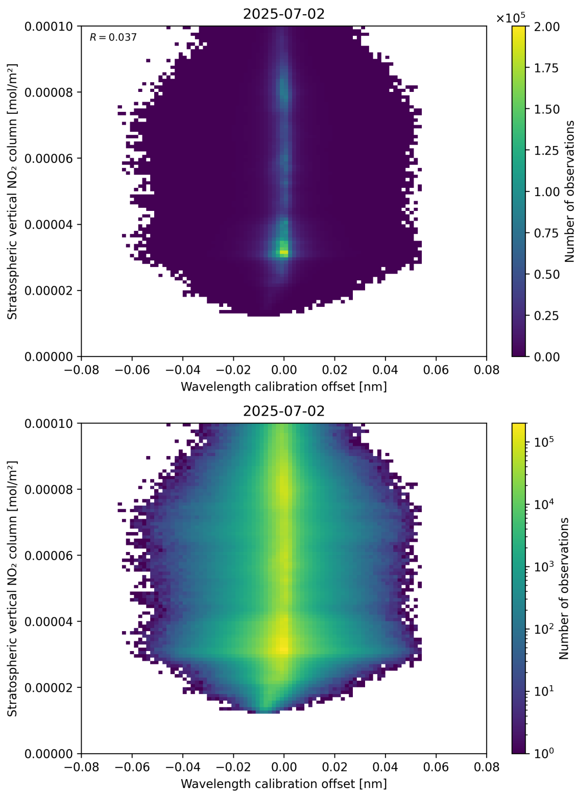
Figure 176: Scatter density plot of “Wavelength calibration offset” against “Stratospheric vertical NO 2 column” for 2025-07-02 to 2025-07-03.
