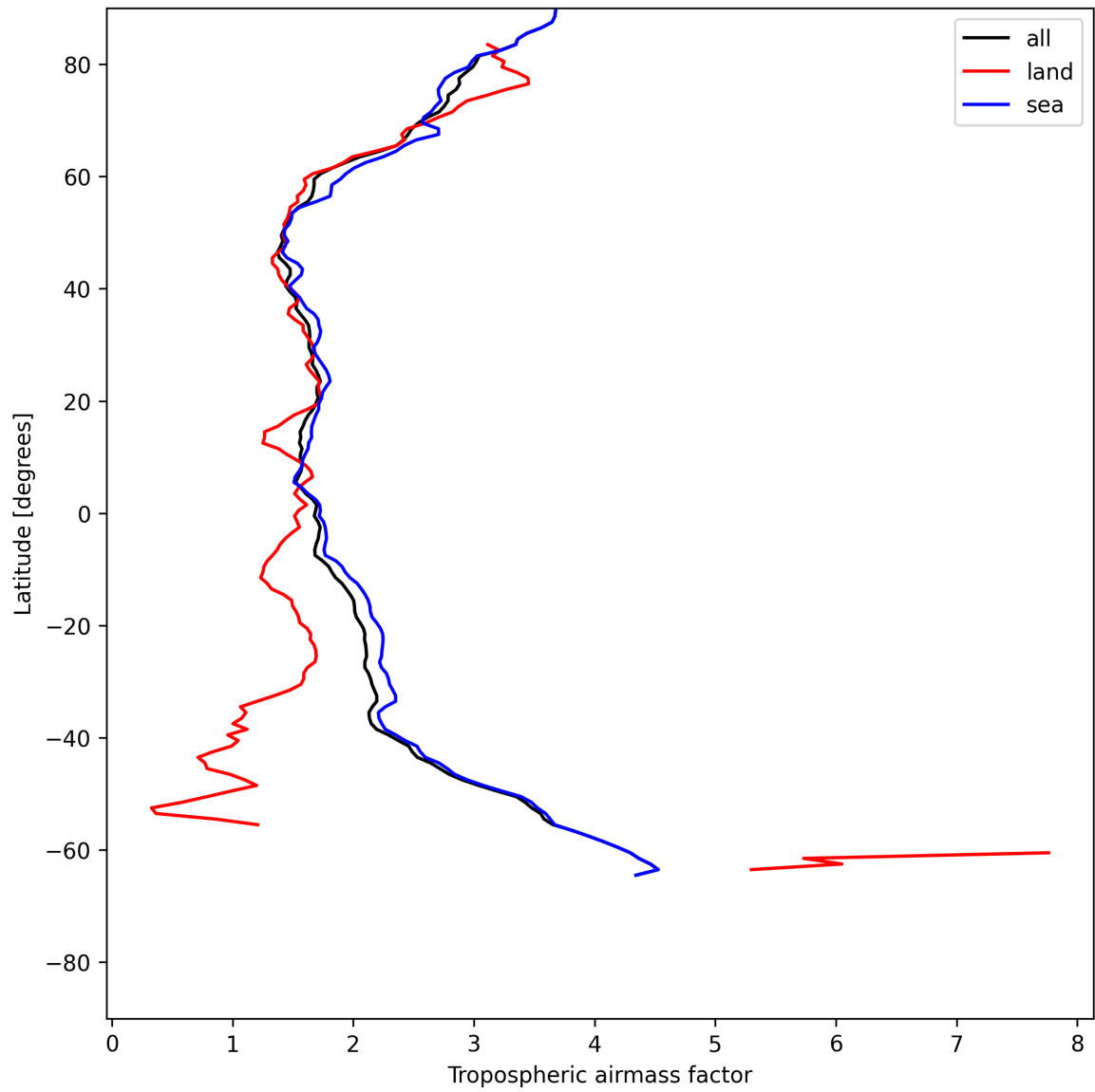
Figure 14: Zonal average of “Tropospheric air mass factor” for 2025-07-02 to 2025-07-03.
