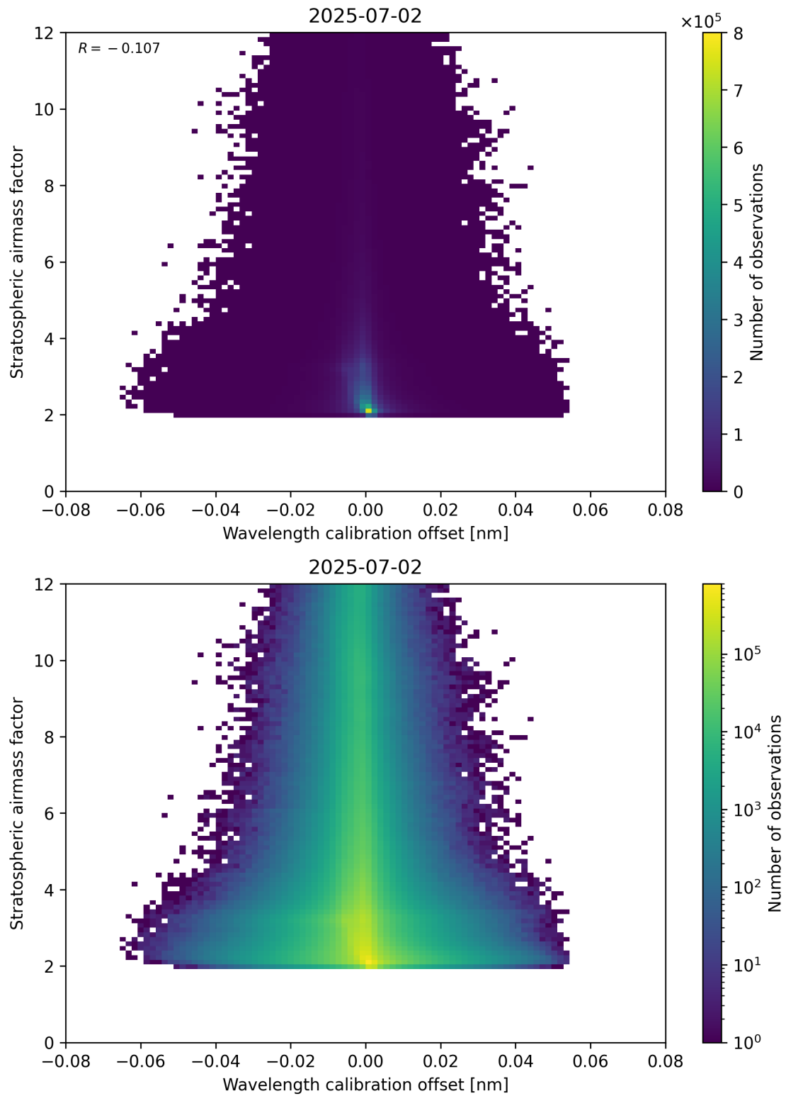
Figure 174: Scatter density plot of “Wavelength calibration offset” against “Stratospheric airmass factor” for 2025-07-02 to 2025-07-03.
