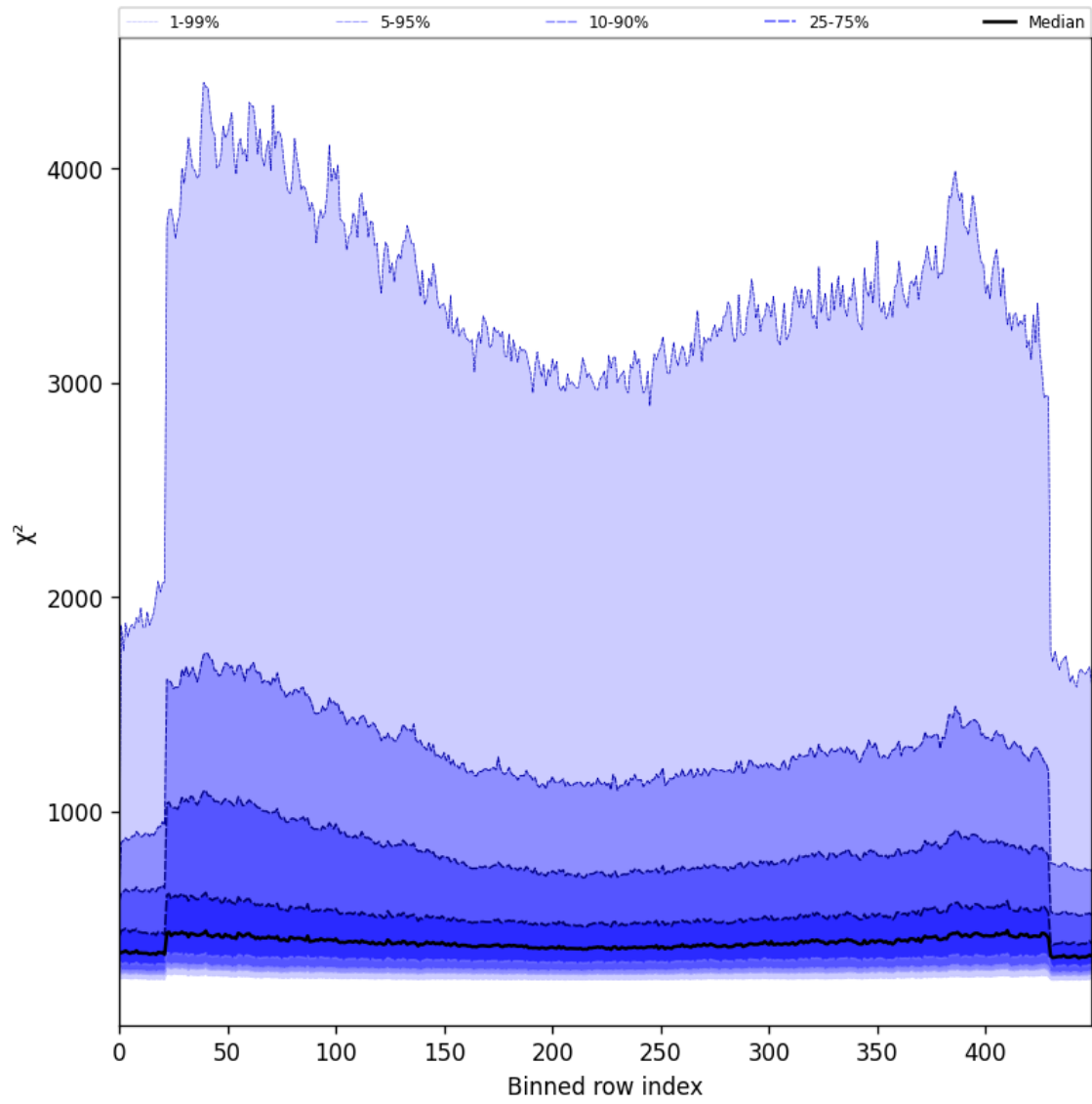
Figure 59: Along track statistics of “ \chi^2 ” for 2025-07-02 to 2025-07-03
