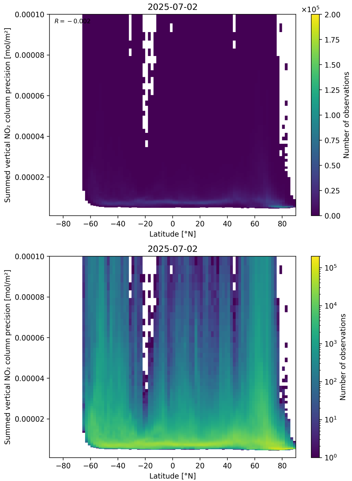
Figure 89: Scatter density plot of “Latitude” against “Summed vertical NO 2 column precision” for 2025-07-02 to 2025-07-03.
