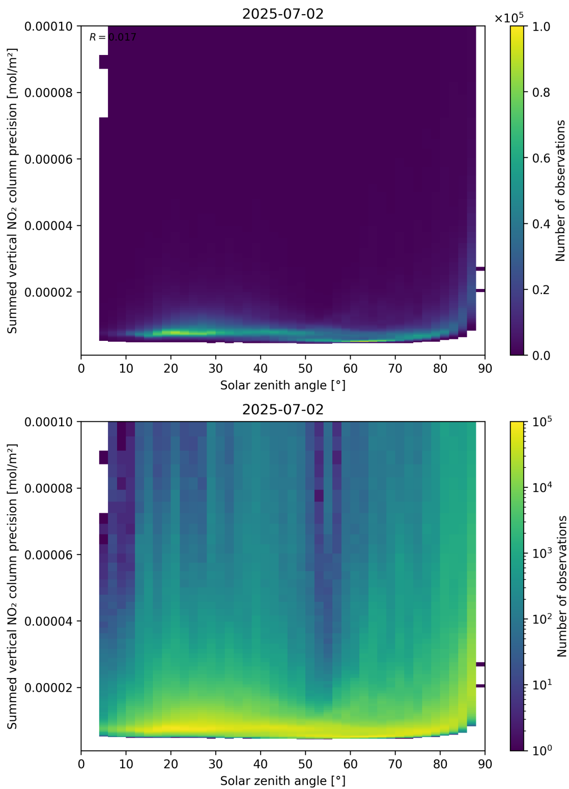
Figure 152: Scatter density plot of “Solar zenith angle” against “Summed vertical NO 2 column precision” for 2025-07-02 to 2025-07-03.
