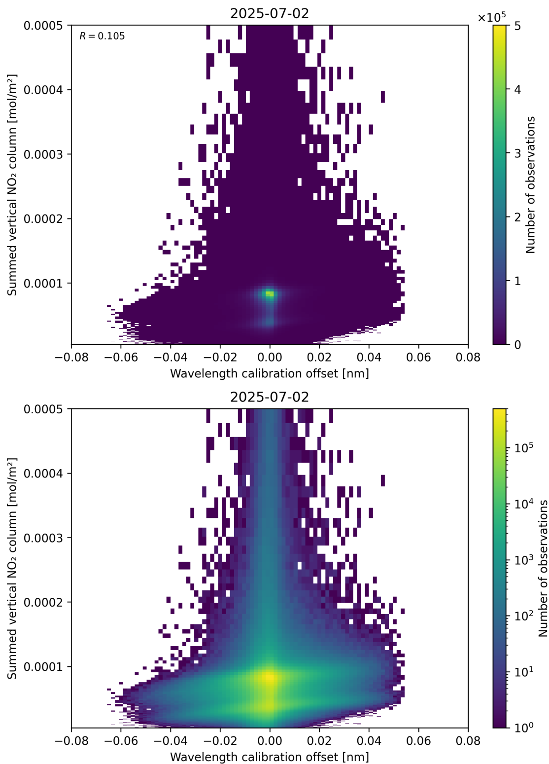
Figure 177: Scatter density plot of “Wavelength calibration offset” against “Summed vertical NO 2 column” for 2025-07-02 to 2025-07-03.
