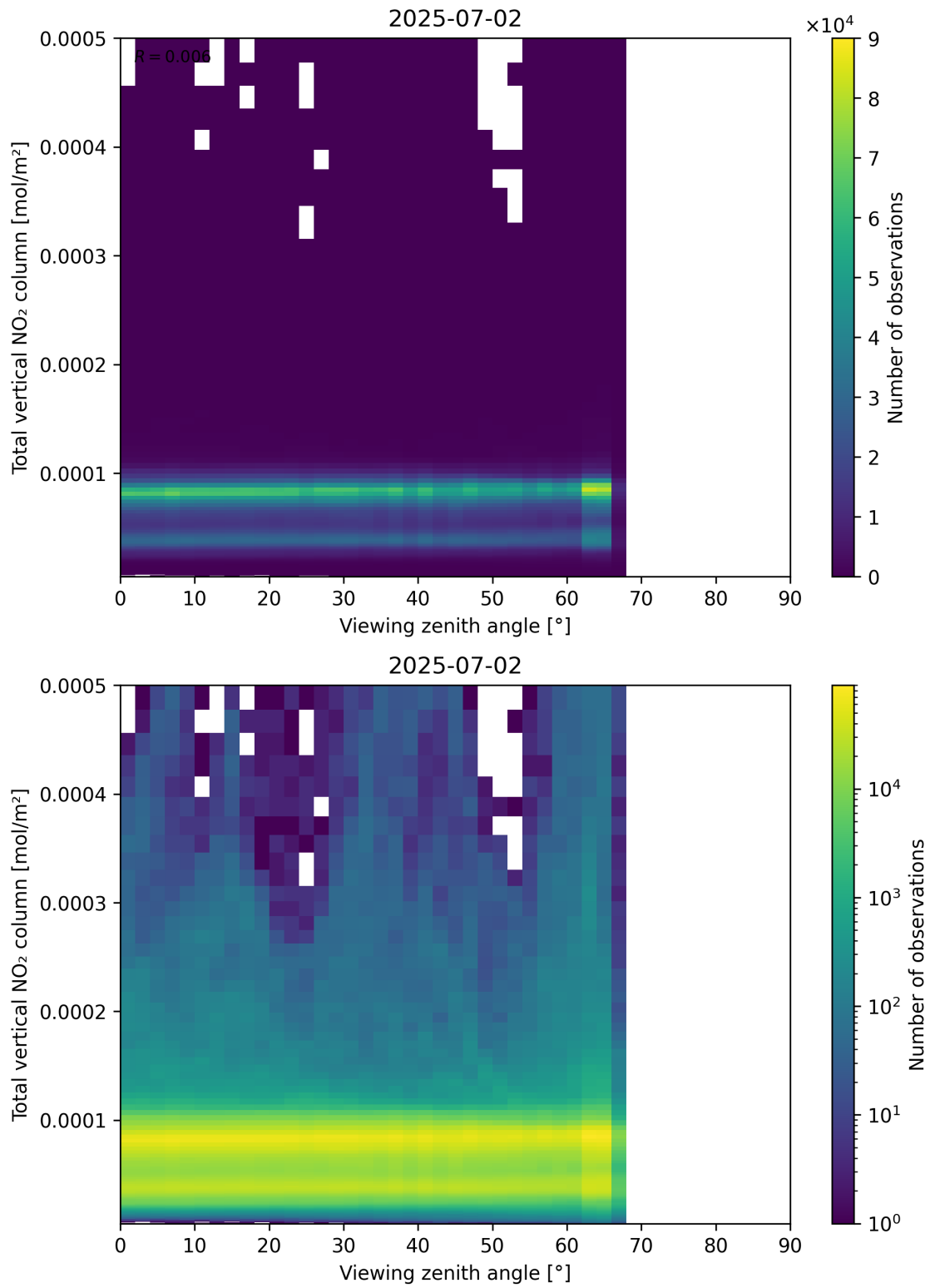
Figure 167: Scatter density plot of “Viewing zenith angle” against “Total vertical NO 2 column” for 2025-07-02 to 2025-07-03.
