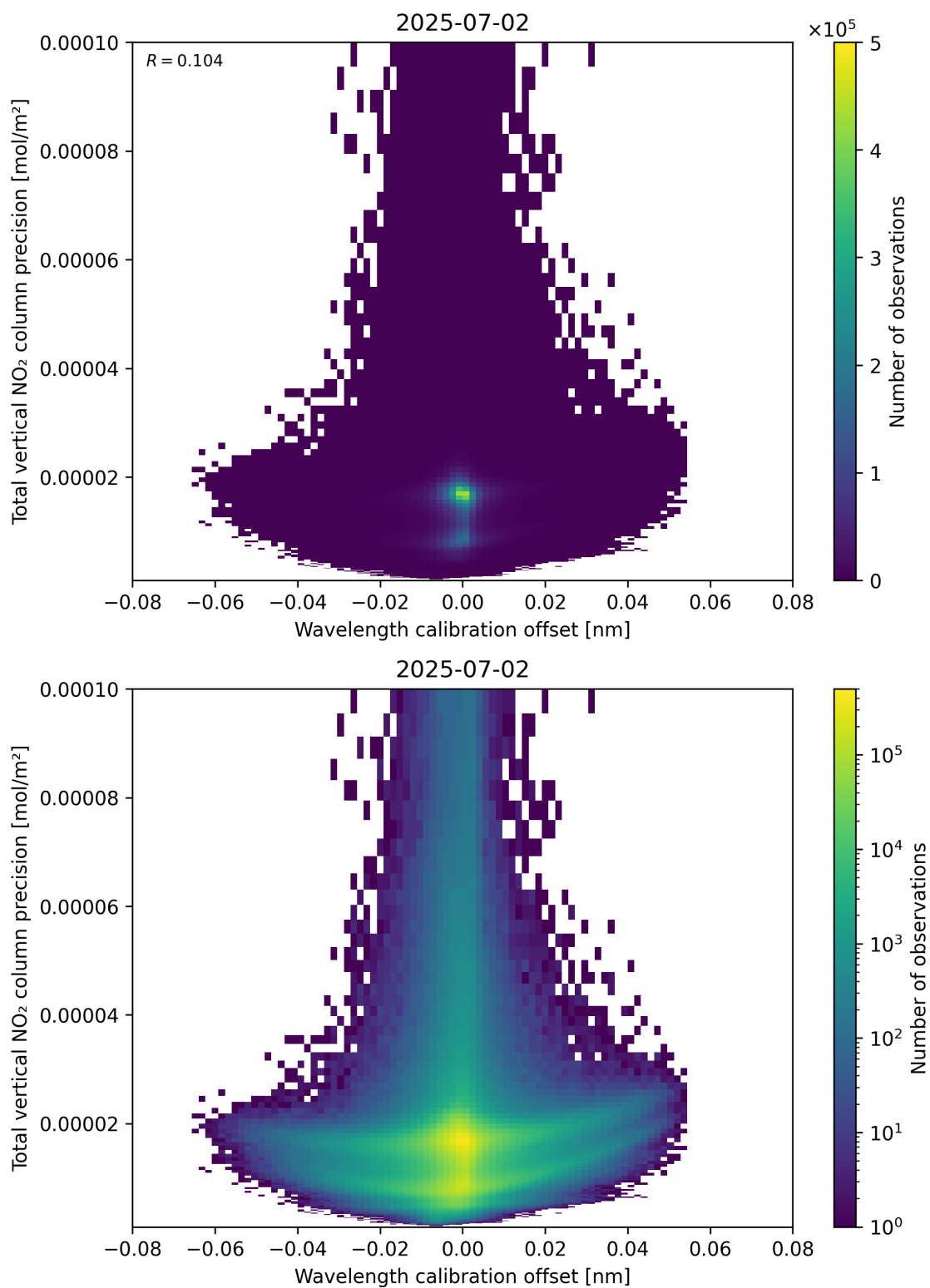
Figure 180: Scatter density plot of “Wavelength calibration offset” against “Total vertical NO 2 column precision” for 2025-07-02 to 2025-07-03.
