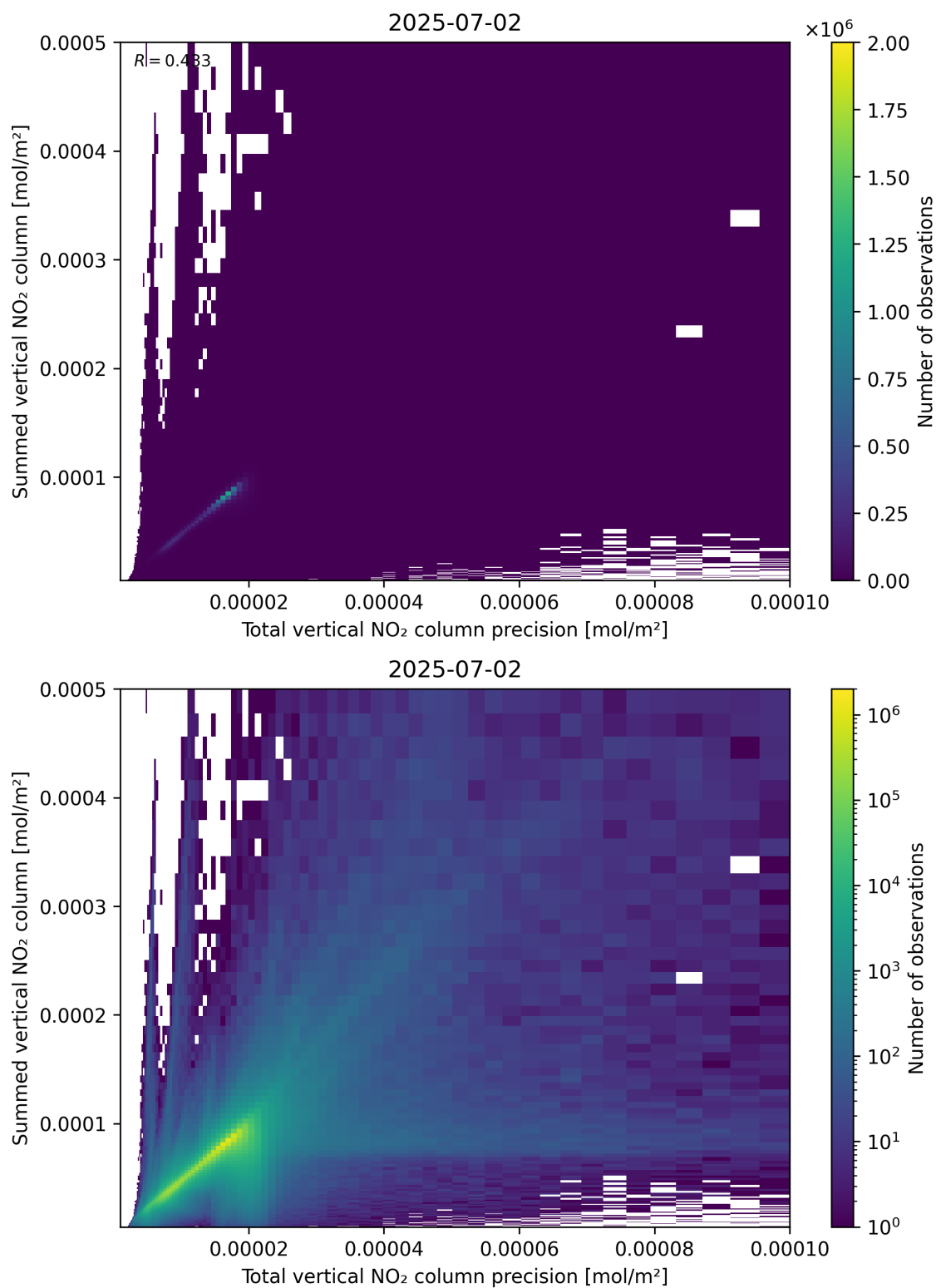
Figure 117: Scatter density plot of “Total vertical NO 2 column precision” against “Summed vertical NO 2 column” for 2025-07-02 to 2025-07-03.
