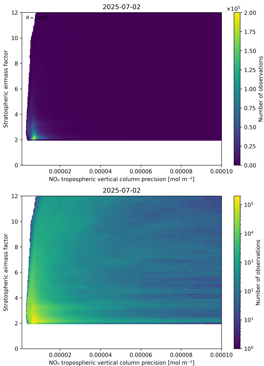
Figure 131: Scatter density plot of “NO 2 tropospheric vertical column precision” against “Stratospheric airmass factor” for 2025-07-02 to 2025-07-03.
