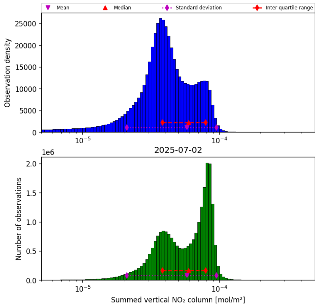
Figure 40: Histogram of “Summed vertical NO 2 column” for 2025-07-02 to 2025-07-03
