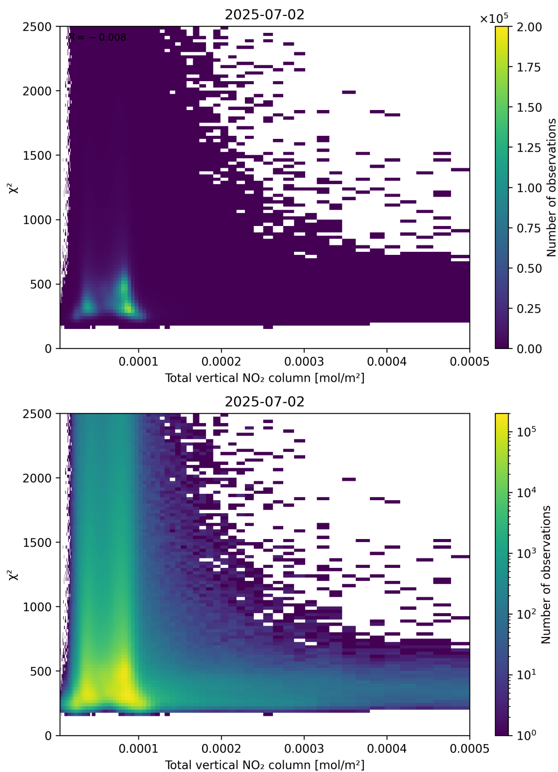
Figure 111: Scatter density plot of “Total vertical NO 2 column” against “ \chi^2 ” for 2025-07-02 to 2025-07-03.
