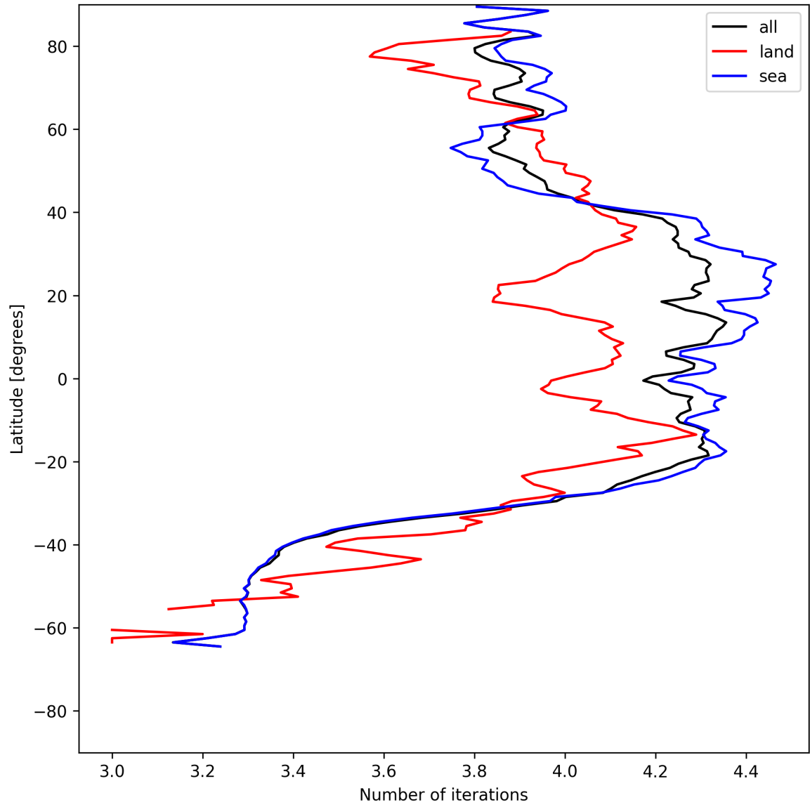
Figure 17: Zonal average of “Number of iterations” for 2025-07-02 to 2025-07-03.
