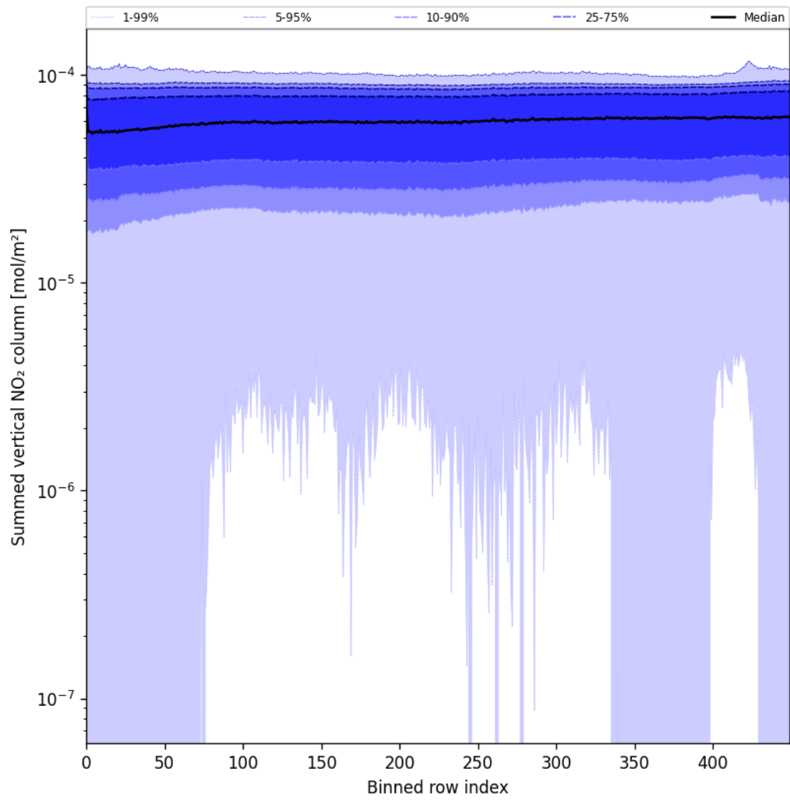
Figure 57: Along track statistics of “Summed vertical NO 2 column” for 2025-07-02 to 2025-07-03
