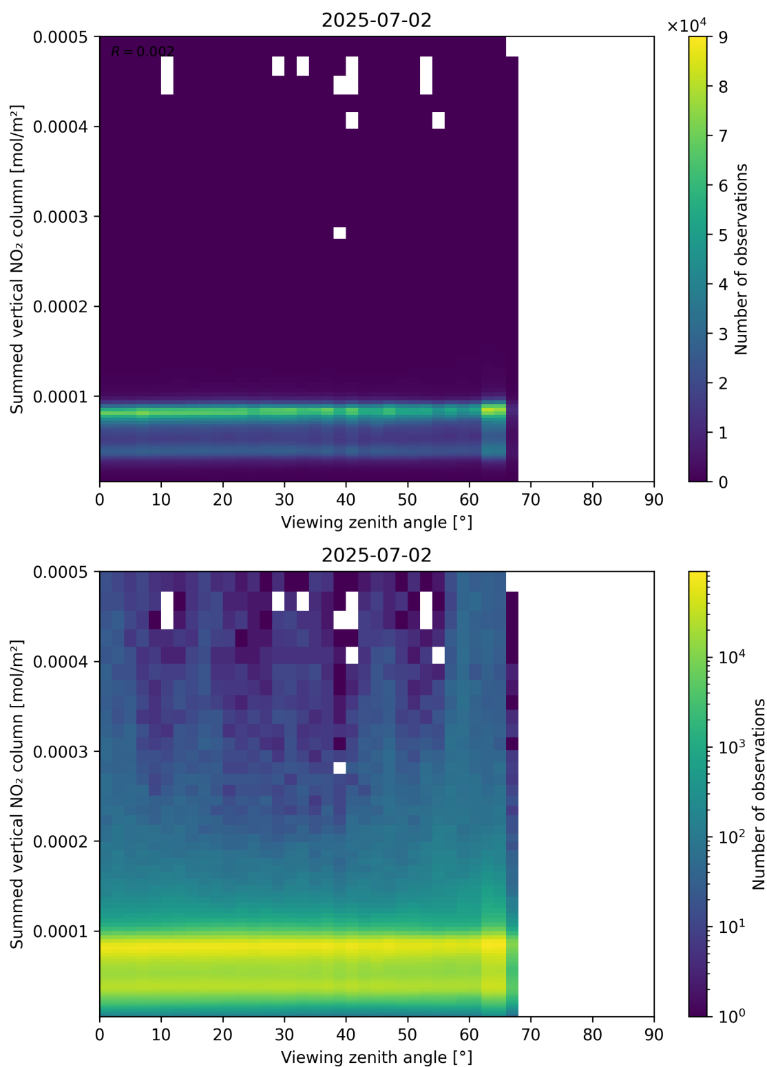
Figure 165: Scatter density plot of “Viewing zenith angle” against “Summed vertical NO 2 column” for 2025-07-02 to 2025-07-03.
