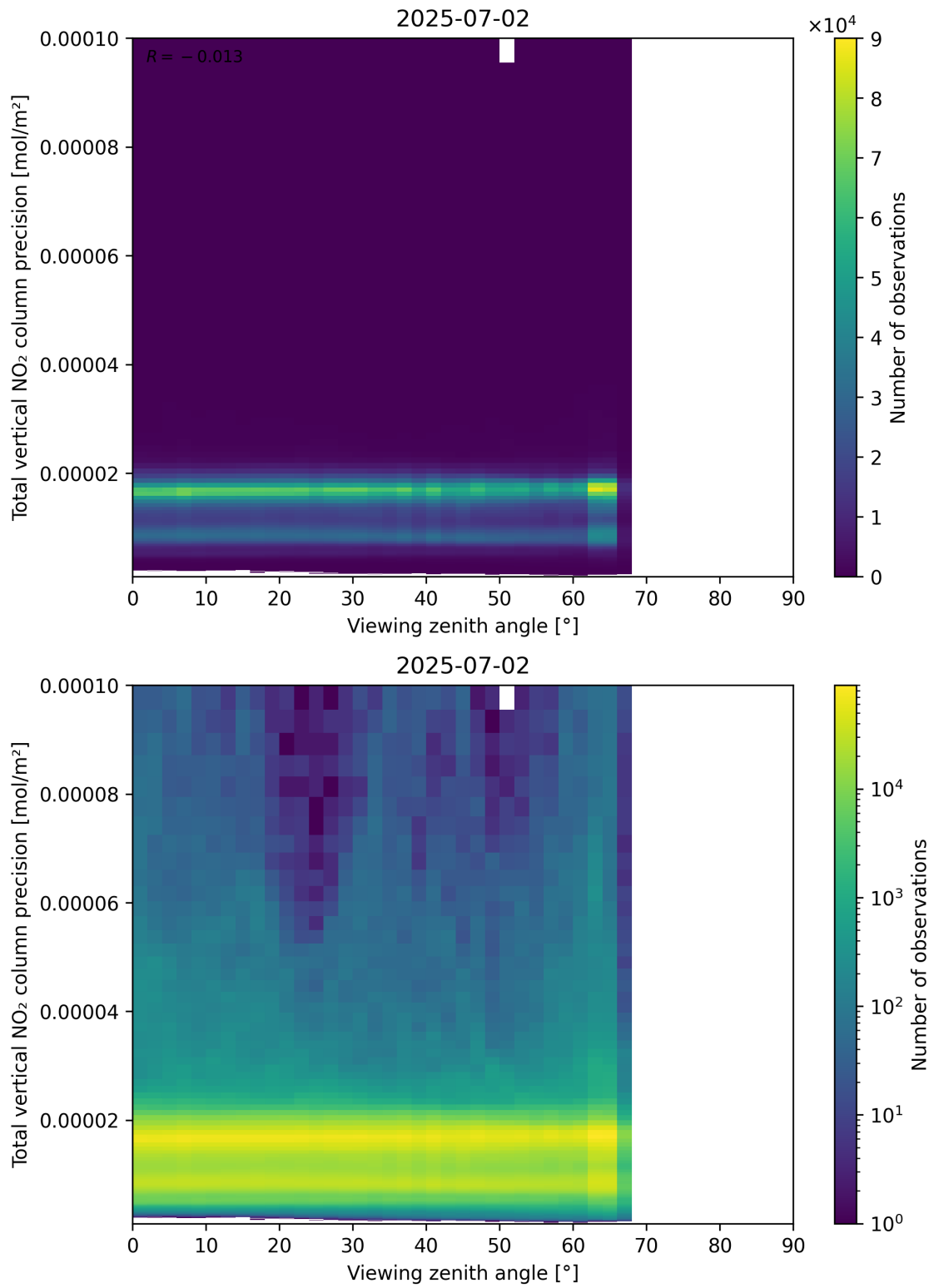
Figure 168: Scatter density plot of “Viewing zenith angle” against “Total vertical NO 2 column precision” for 2025-07-02 to 2025-07-03.
