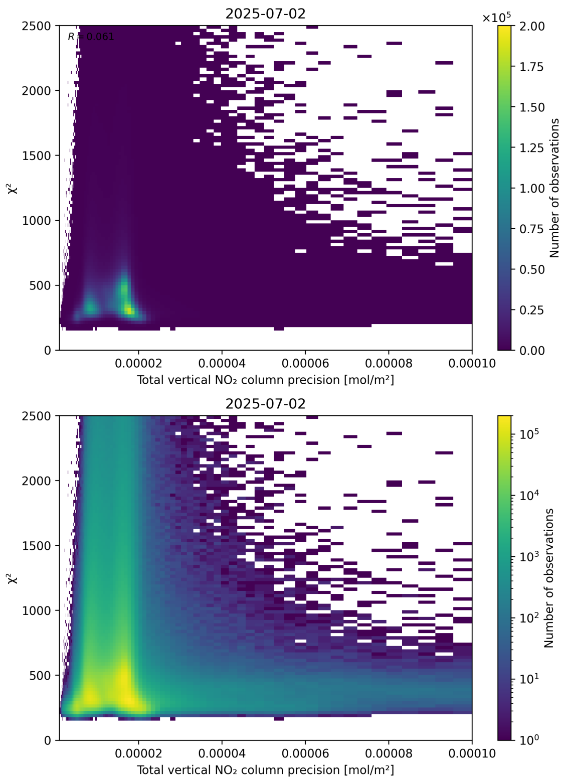
Figure 116: Scatter density plot of “Total vertical NO 2 column precision” against “ \chi^2 ” for 2025-07-02 to 2025-07-03.
