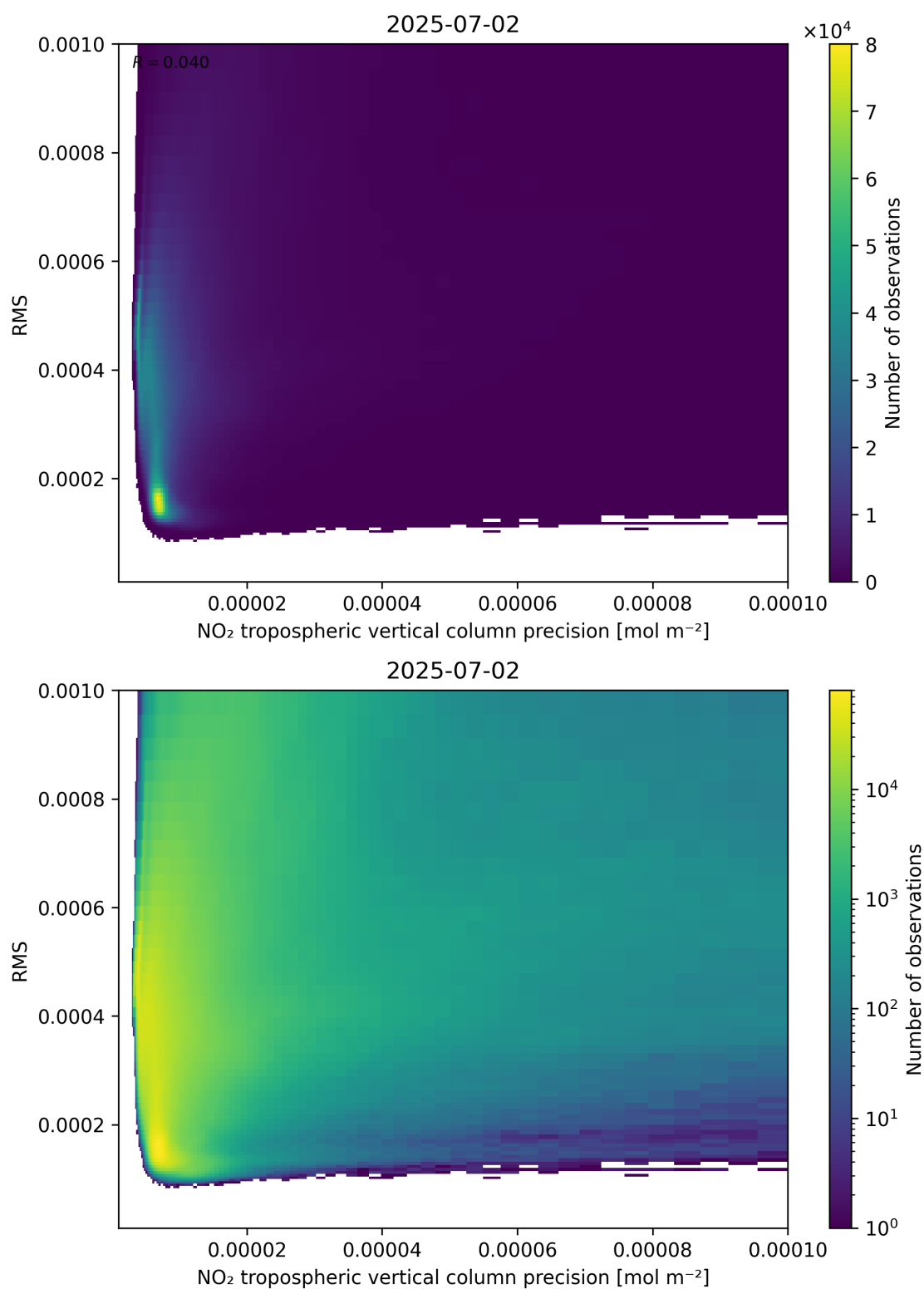
Figure 140: Scatter density plot of “NO 2 tropospheric vertical column precision” against “RMS” for 2025-07-02 to 2025-07-03.
