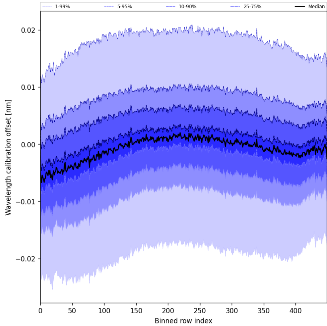
Figure 52: Along track statistics of “Wavelength calibration offset” for 2025-07-02 to 2025-07-03
