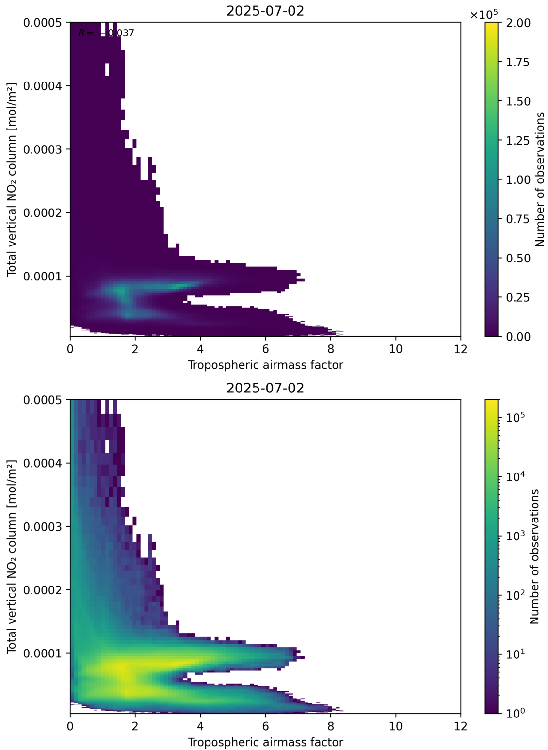
Figure 77: Scatter density plot of “Tropospheric airmass factor” against “Total vertical NO 2 column” for 2025-07-02 to 2025-07-03.
