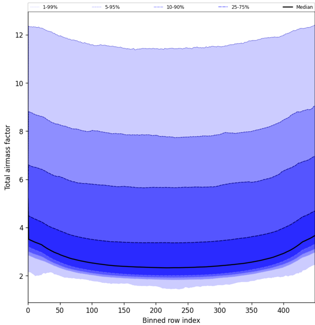
Figure 49: Along track statistics of “Total airmass factor” for 2025-07-02 to 2025-07-03
