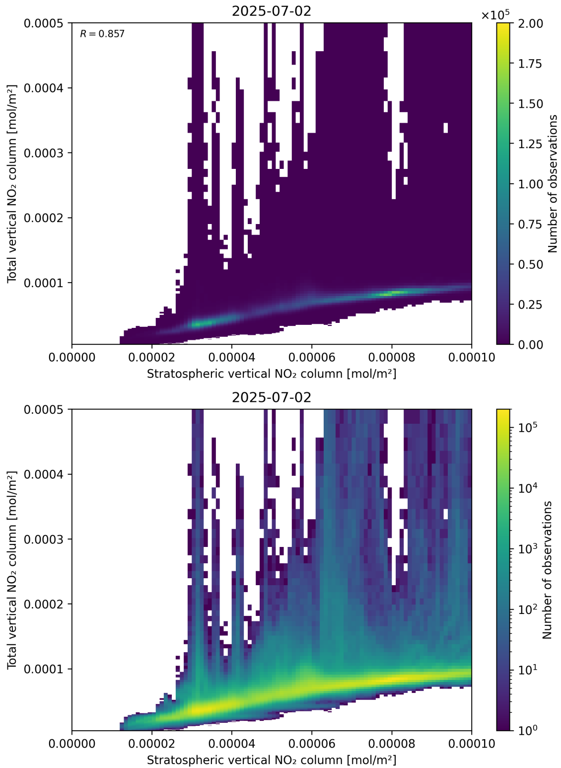
Figure 100: Scatter density plot of “Stratospheric vertical NO 2 column” against “Total vertical NO 2 column” for 2025-07-02 to 2025-07-03.
