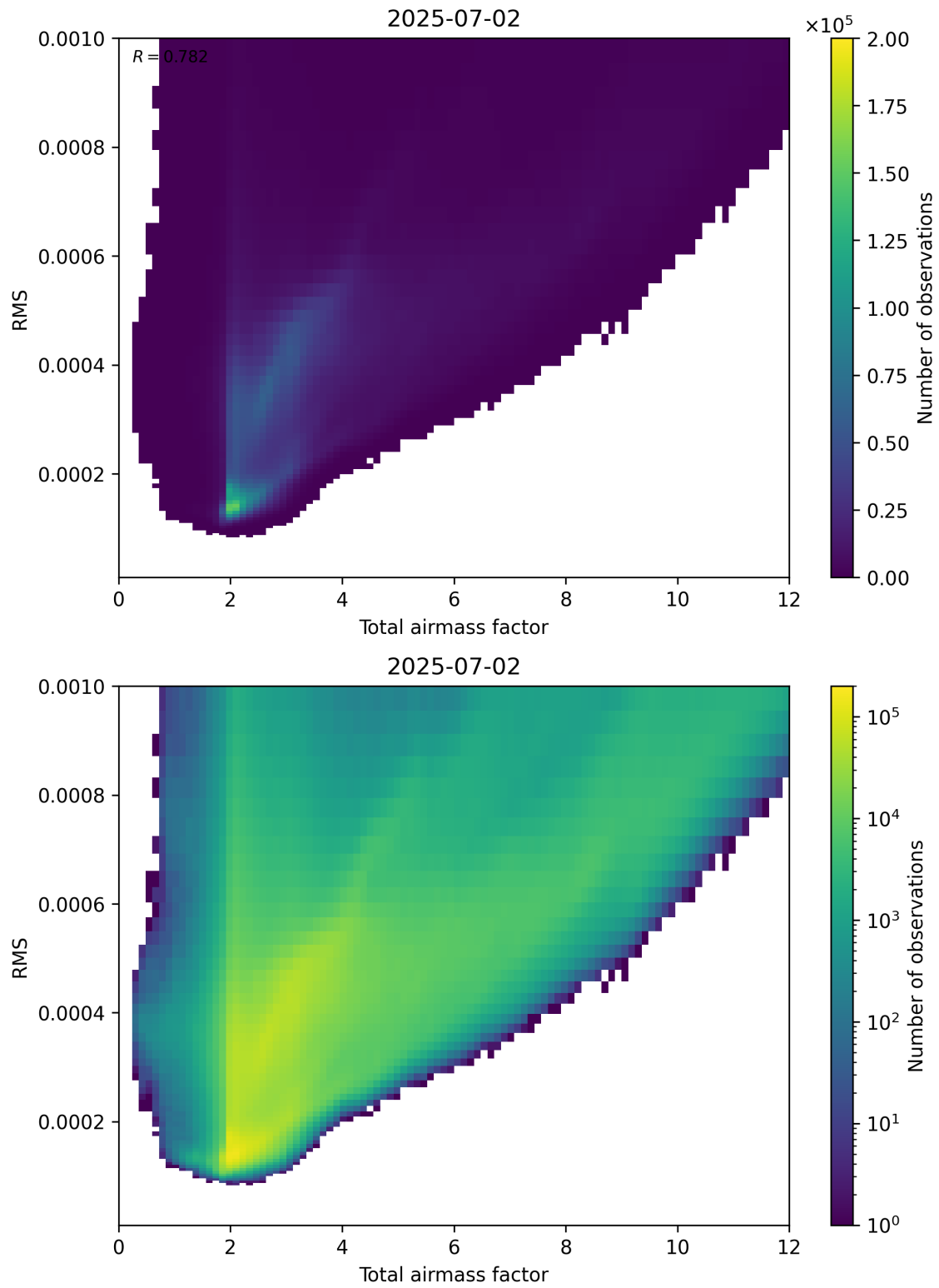
Figure 69: Scatter density plot of “Total airmass factor” against “RMS” for 2025-07-02 to 2025-07-03.
