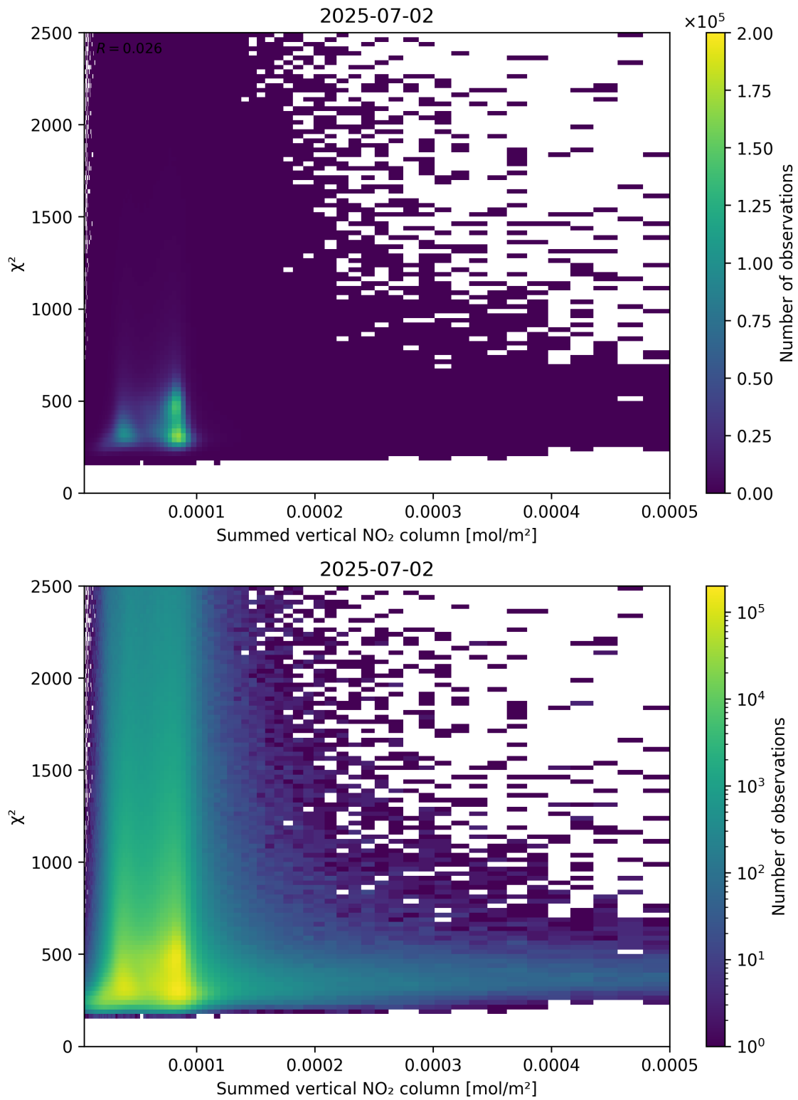
Figure 104: Scatter density plot of “Summed vertical NO 2 column” against “ \chi^2 ” for 2025-07-02 to 2025-07-03.
