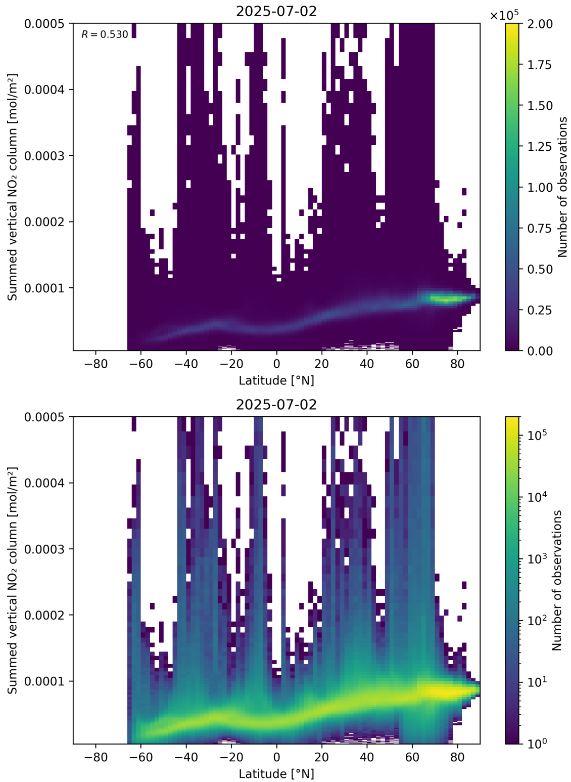
Figure 88: Scatter density plot of “Latitude” against “Summed vertical NO 2 column” for 2025-07-02 to 2025-07-03.
