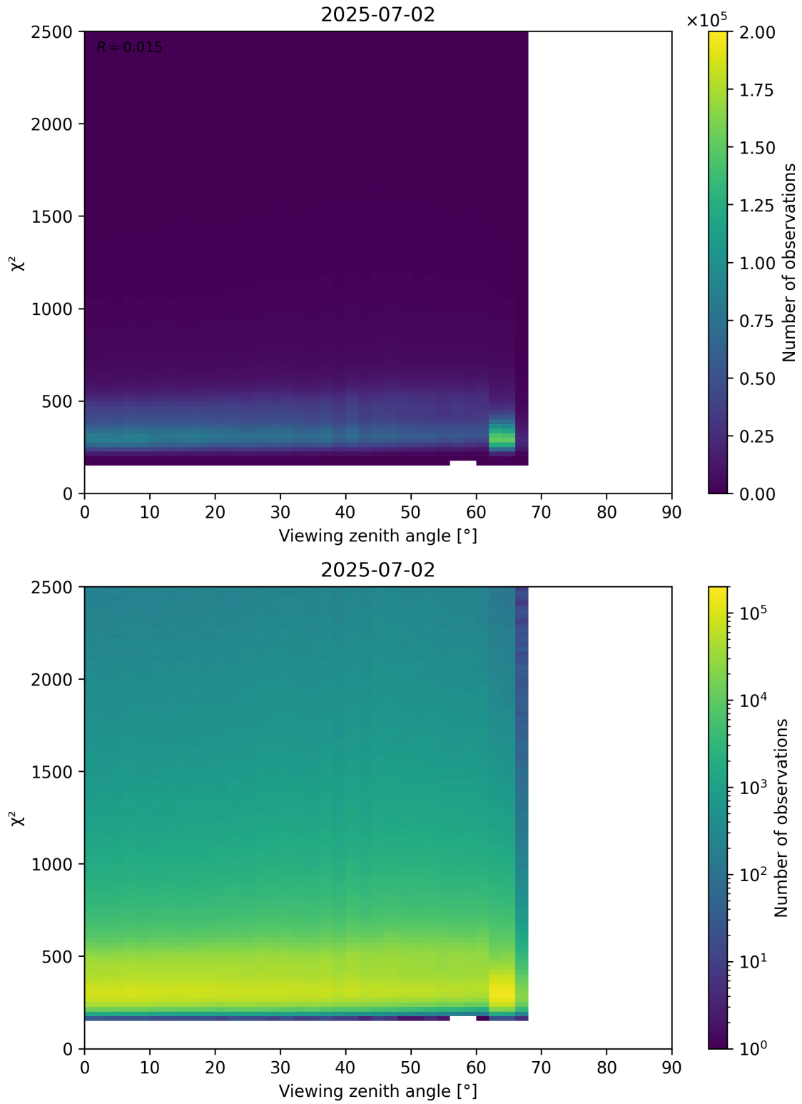
Figure 162: Scatter density plot of “Viewing zenith angle” against “ \chi^2 ” for 2025-07-02 to 2025-07-03.
