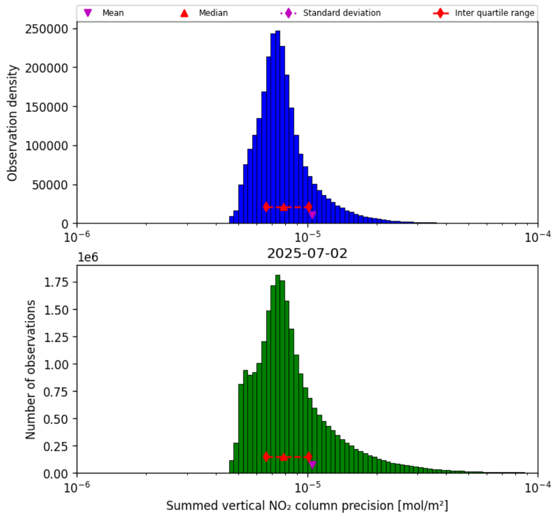
Figure 41: Histogram of "Summed vertical NO 2 column precision" for 2025-07-02 to 2025-07-03
