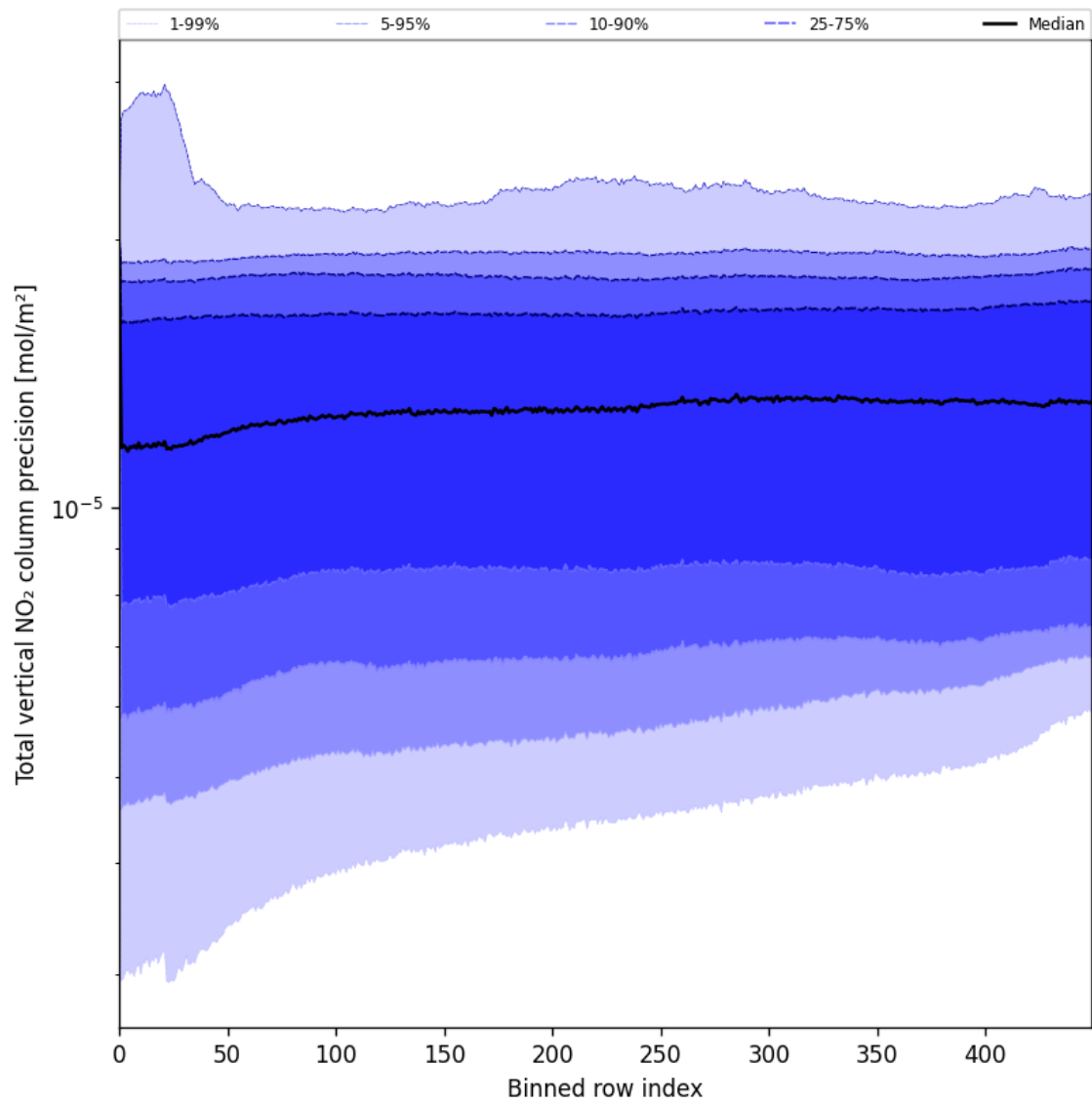
Figure 56: Along track statistics of “Total vertical NO 2 column precision” for 2025-07-02 to 2025-07-03
