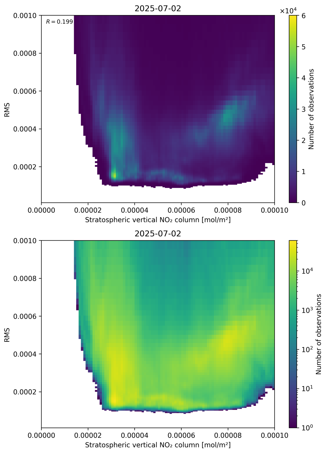
Figure 102: Scatter density plot of “Stratospheric vertical NO 2 column” against “RMS” for 2025-07-02 to 2025-07-03.
