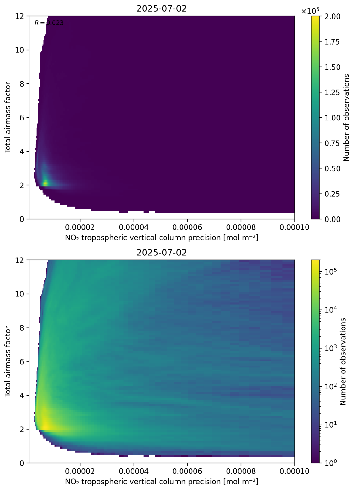
Figure 132: Scatter density plot of “NO 2 tropospheric vertical column precision” against “Total air mass factor” for 2025-07-02 to 2025-07-03.
