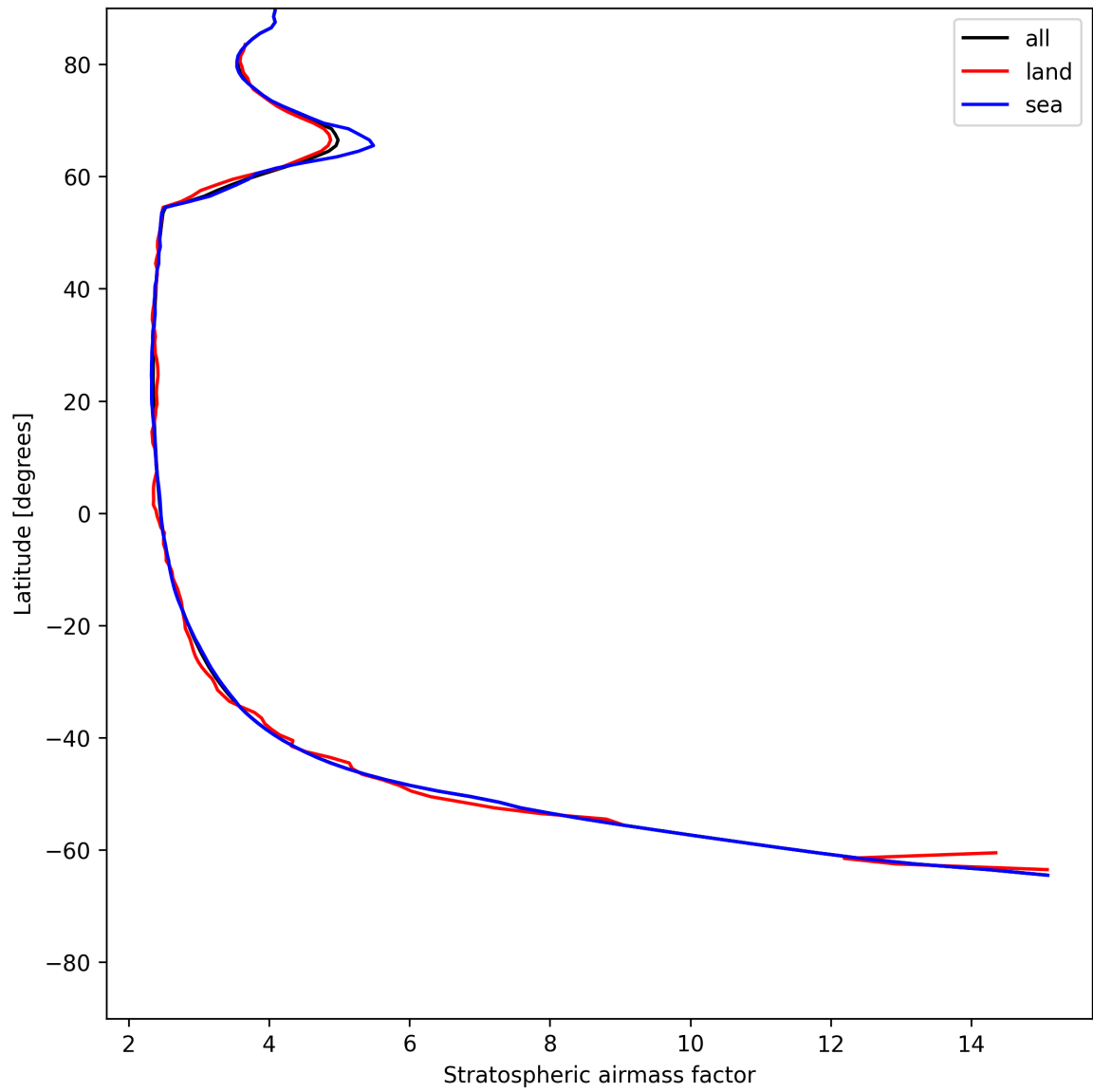
Figure 27: Zonal average of “Stratospheric airmass factor” for 2025-07-02 to 2025-07-03.
