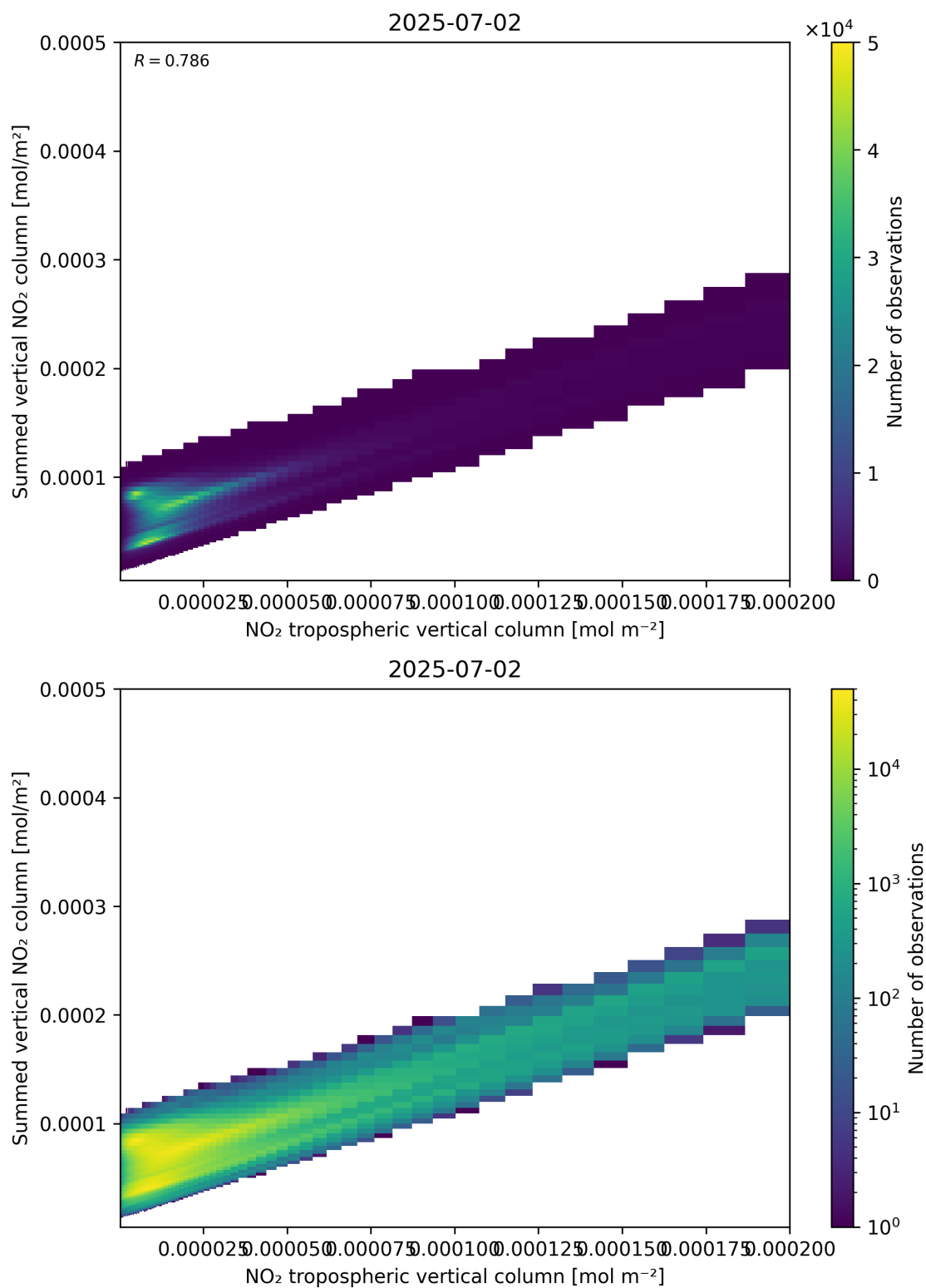
Figure 126: Scatter density plot of “NO 2 tropospheric vertical column” against “Summed vertical NO 2 column” for 2025-07-02 to 2025-07-03.
