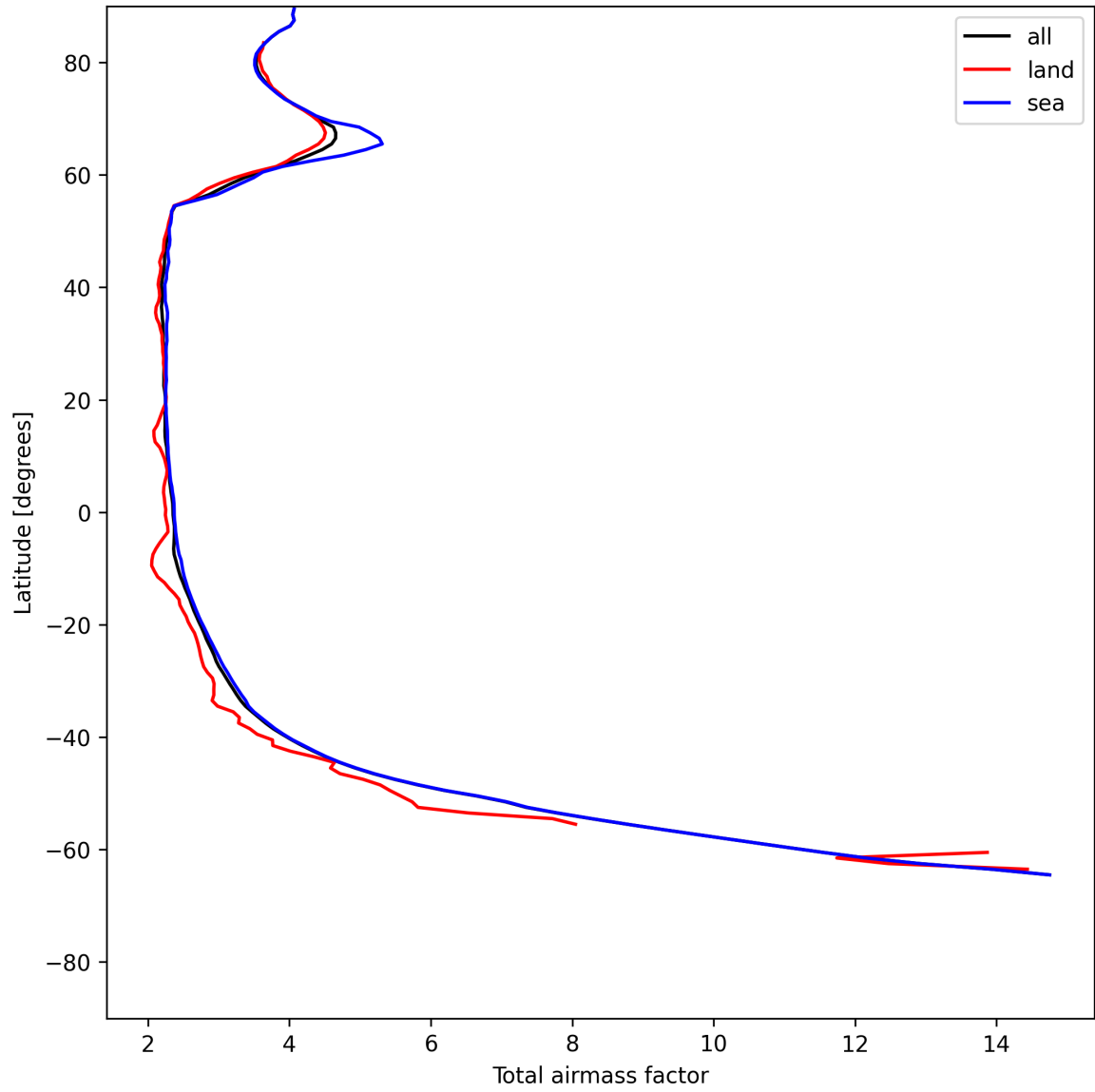
Figure 15: Zonal average of “Total airmass factor” for 2025-07-02 to 2025-07-03.
