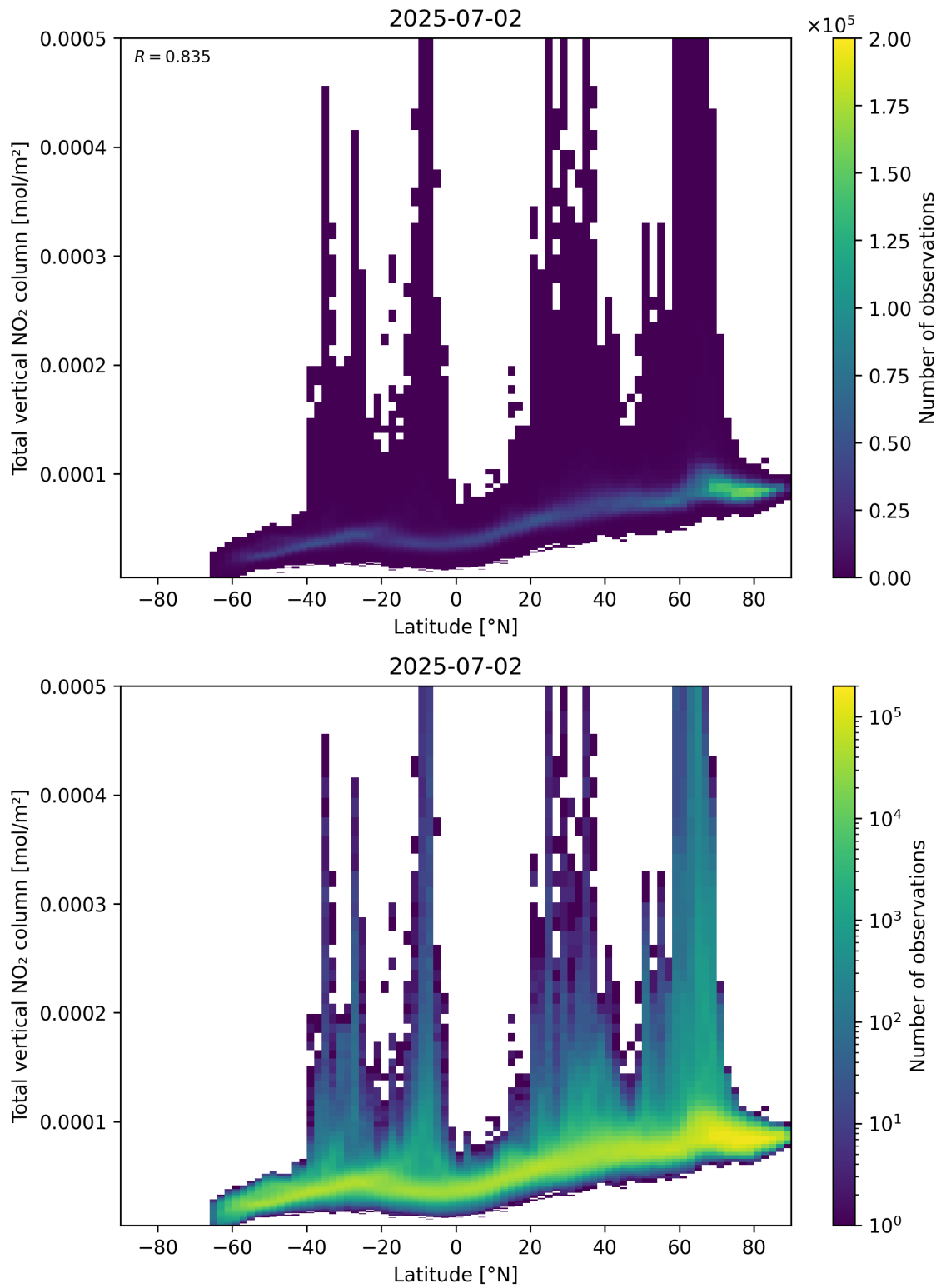
Figure 90: Scatter density plot of “Latitude” against “Total vertical NO 2 column” for 2025-07-02 to 2025-07-03.
