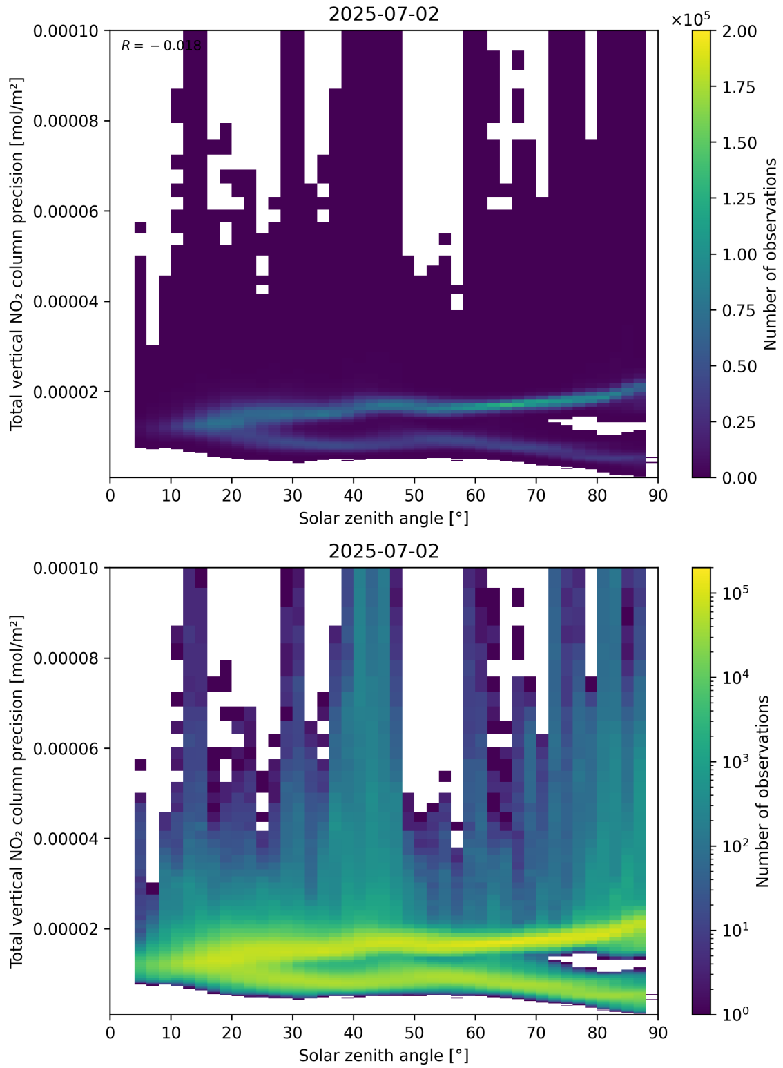
Figure 154: Scatter density plot of “Solar zenith angle” against “Total vertical NO 2 column precision” for 2025-07-02 to 2025-07-03.
