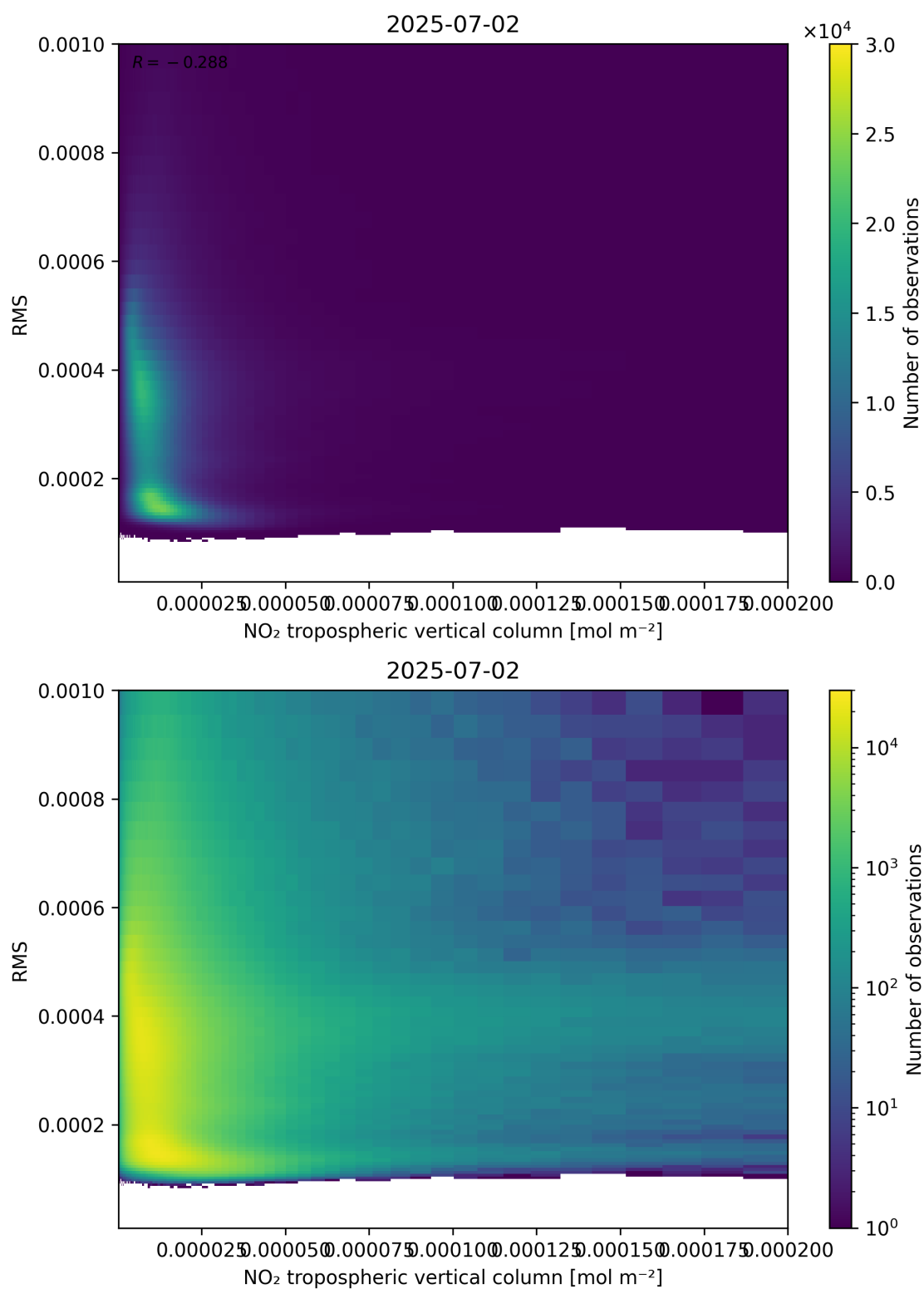
Figure 142: Scatter density plot of “NO 2 tropospheric vertical column” against “RMS” for 2025-07-02 to 2025-07-03.
