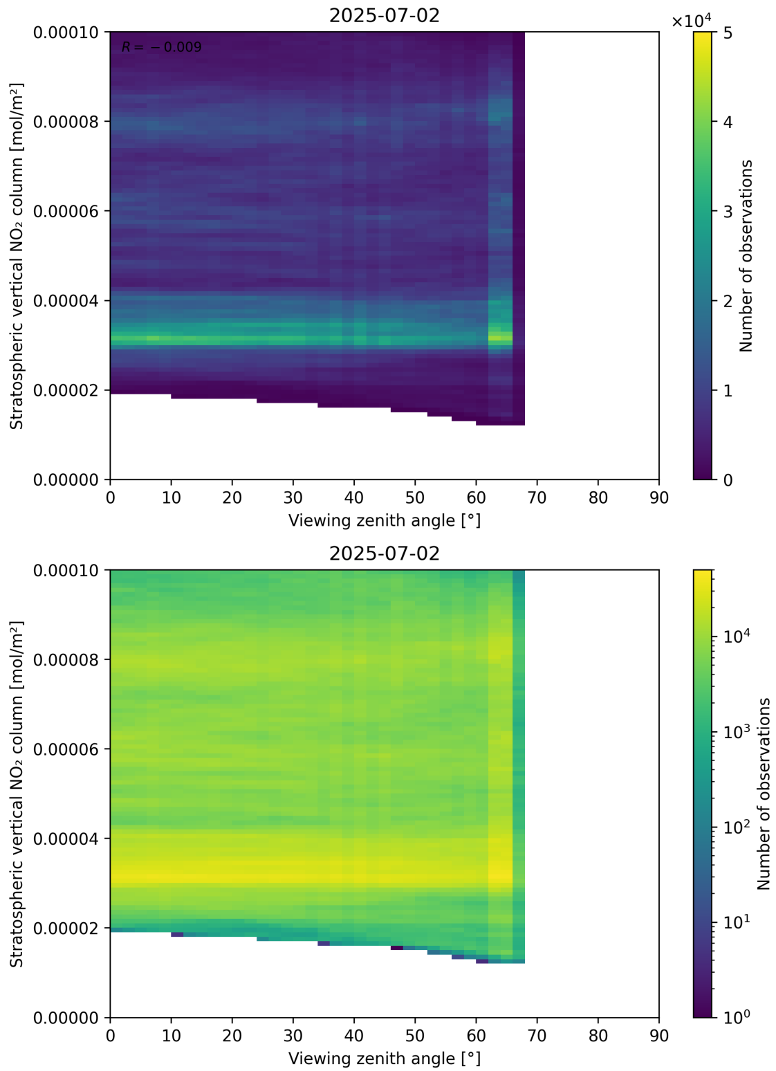
Figure 164: Scatter density plot of “Viewing zenith angle” against “Stratospheric vertical NO 2 column” for 2025-07-02 to 2025-07-03.
