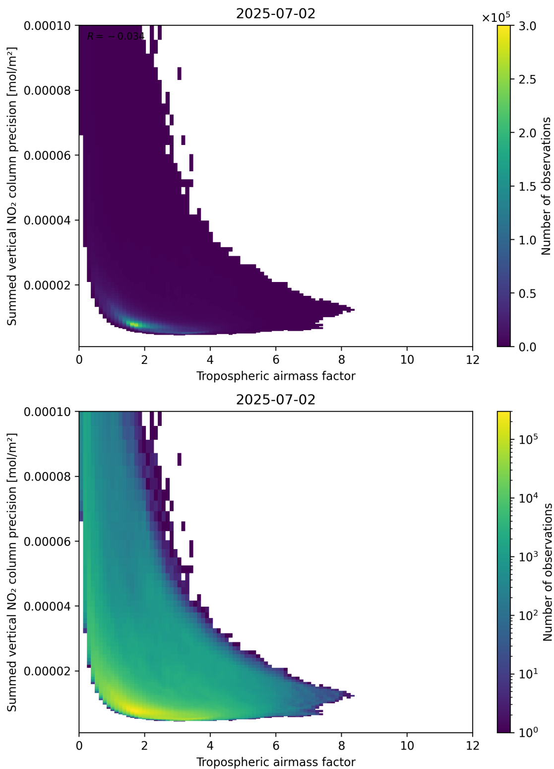
Figure 76: Scatter density plot of “Tropospheric air mass factor” against “Summed vertical NO 2 column precision” for 2025-07-02 to 2025-07-03.
