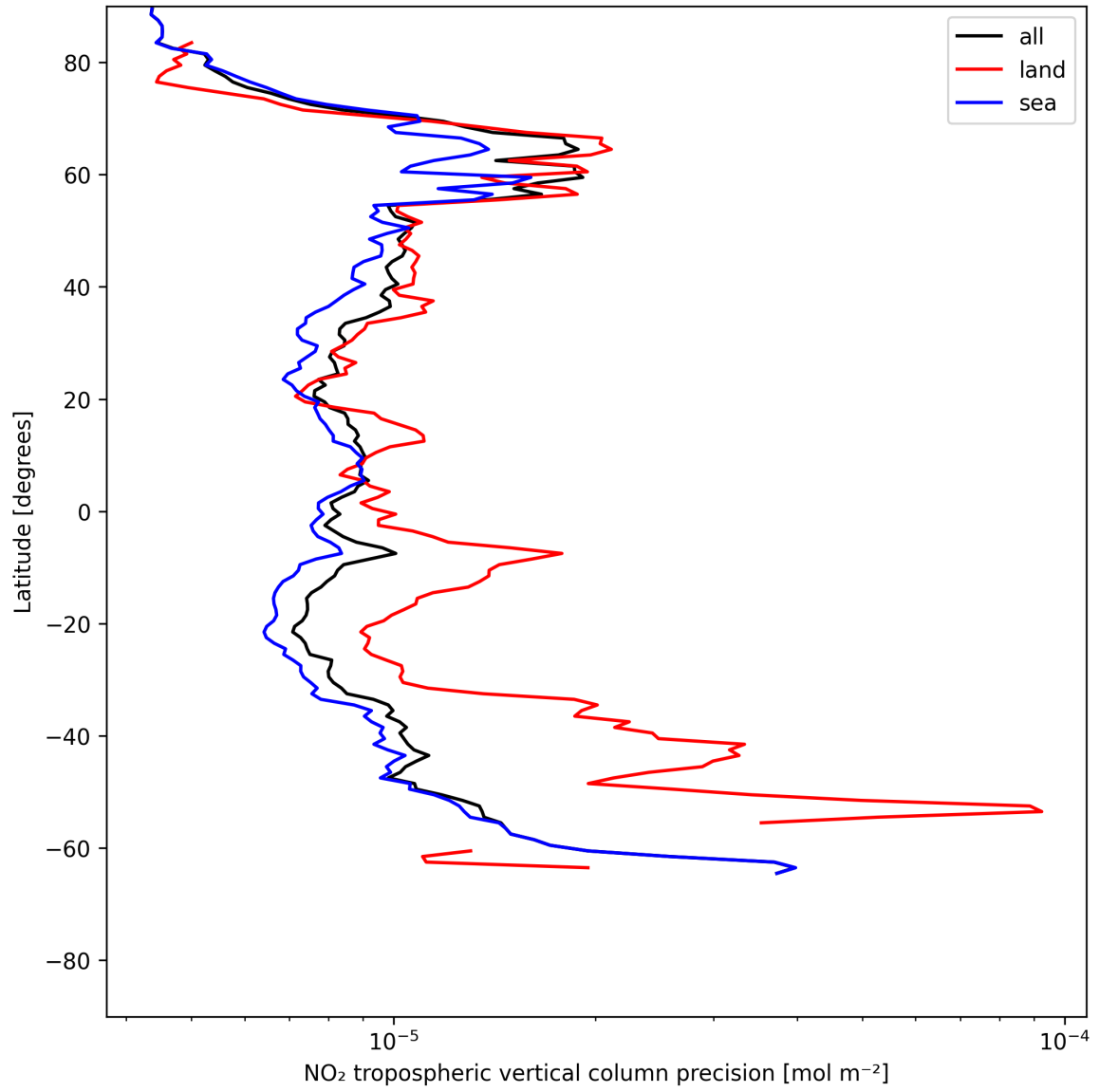
Figure 13: Zonal average of “NO 2 tropospheric vertical column precision” for 2025-07-02 to 2025-07-03.
