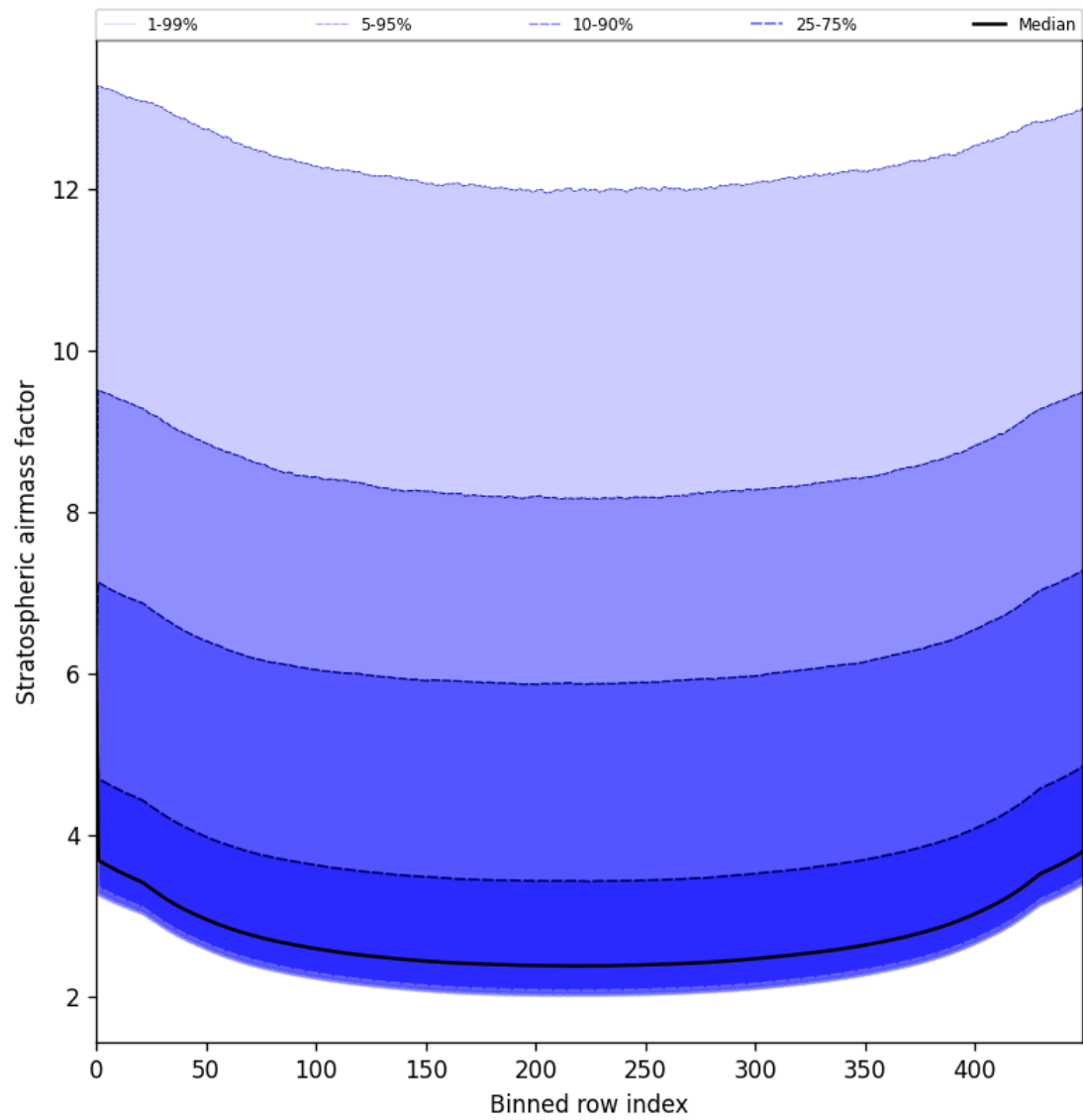
Figure 61: Along track statistics of “Stratospheric airmass factor” for 2025-07-02 to 2025-07-03
