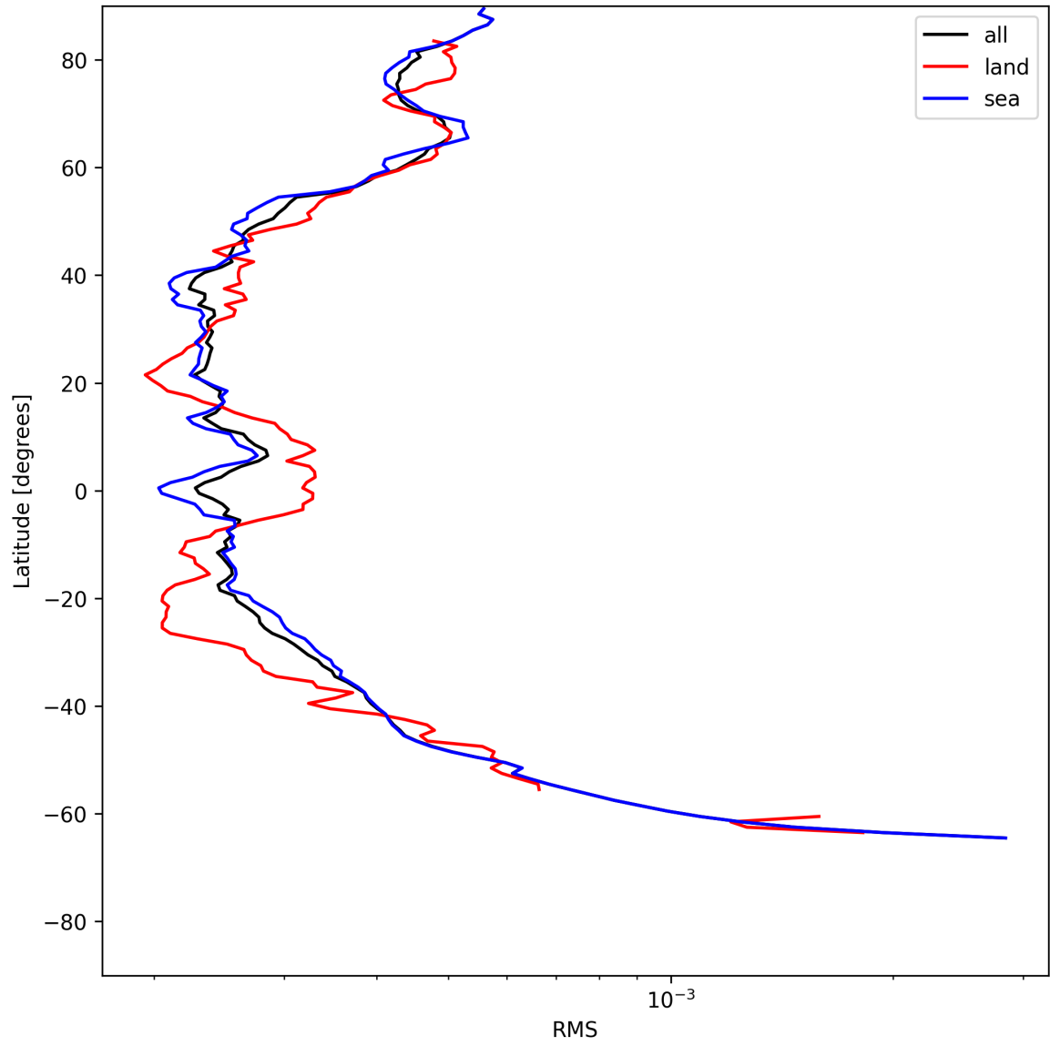
Figure 26: Zonal average of “RMS” for 2025-07-02 to 2025-07-03.
