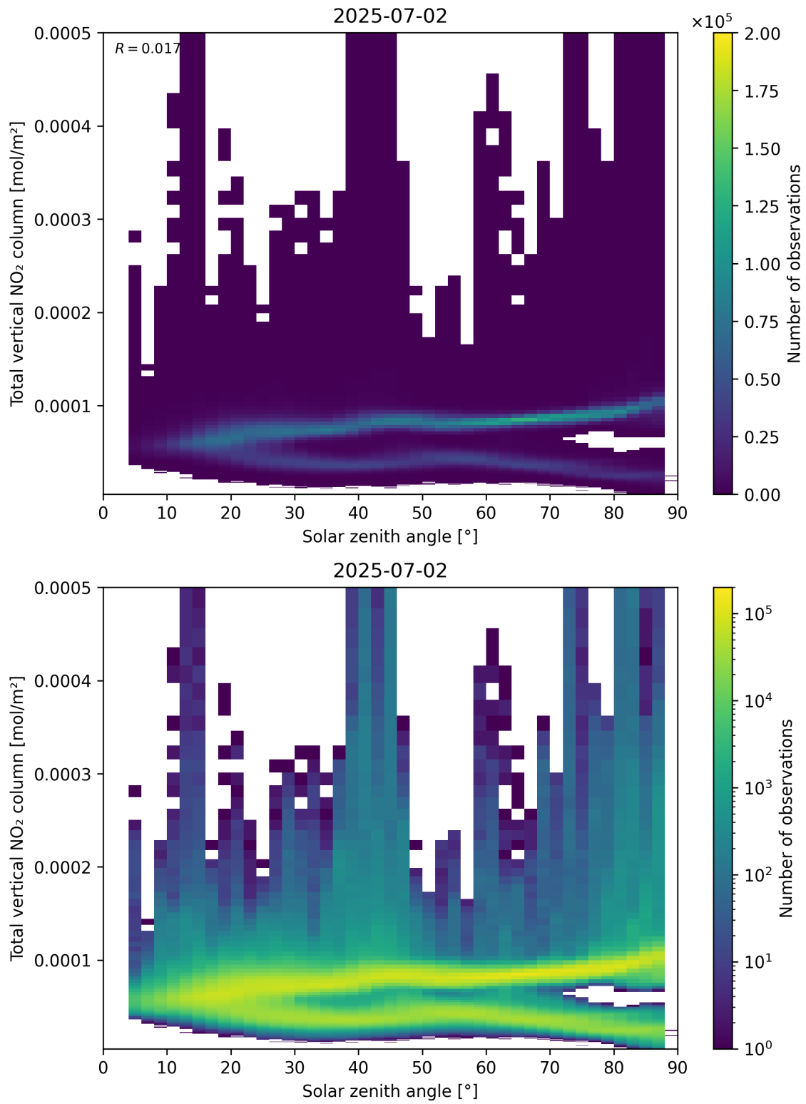
Figure 153: Scatter density plot of “Solar zenith angle” against “Total vertical NO 2 column” for 2025-07-02 to 2025-07-03.
