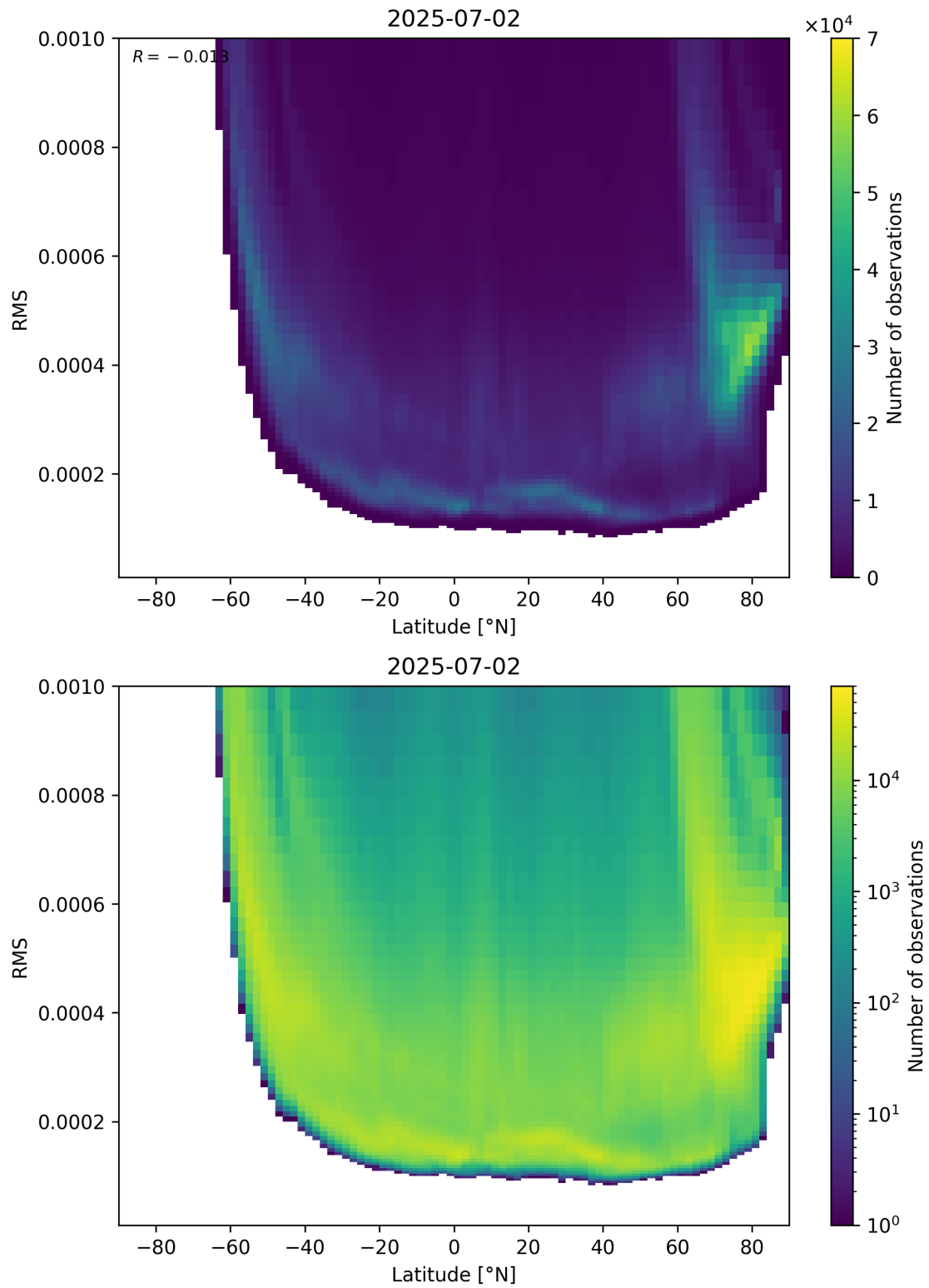
Figure 94: Scatter density plot of “Latitude” against “RMS” for 2025-07-02 to 2025-07-03.
