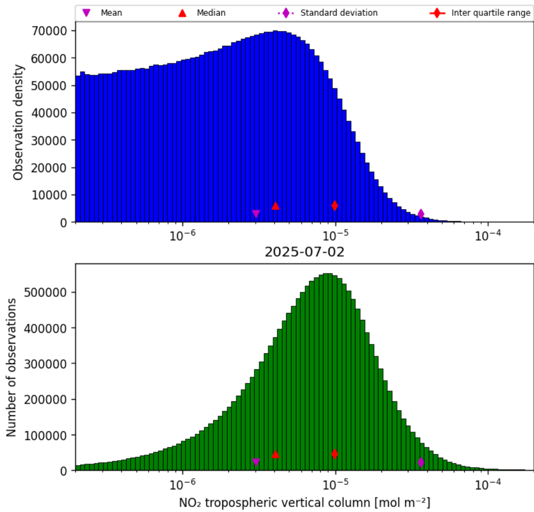
Figure 29: Histogram of “NO 2 tropospheric vertical column” for 2025-07-02 to 2025-07-03
