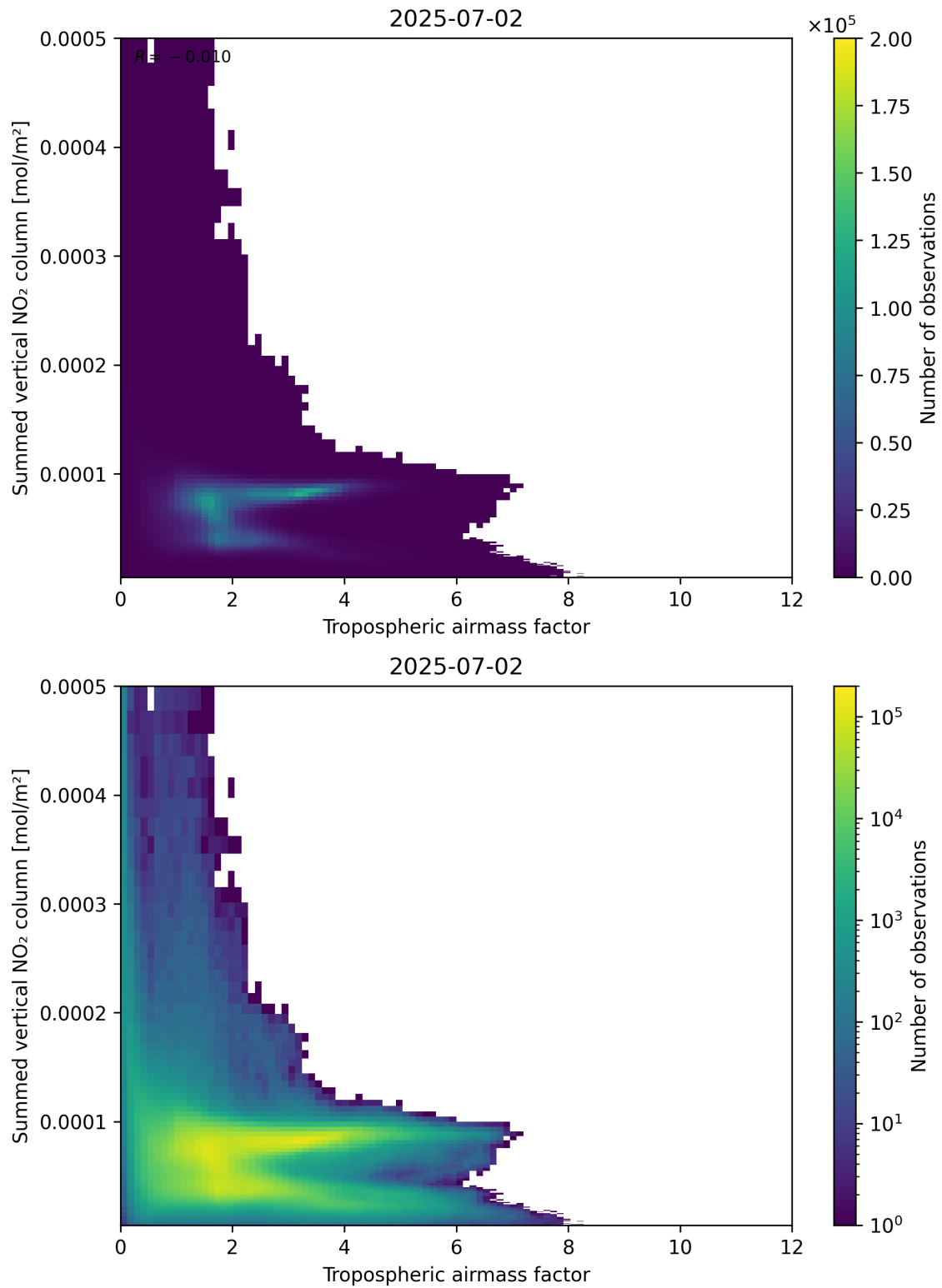
Figure 75: Scatter density plot of “Tropospheric airmass factor” against “Summed vertical NO 2 column” for 2025-07-02 to 2025-07-03.
