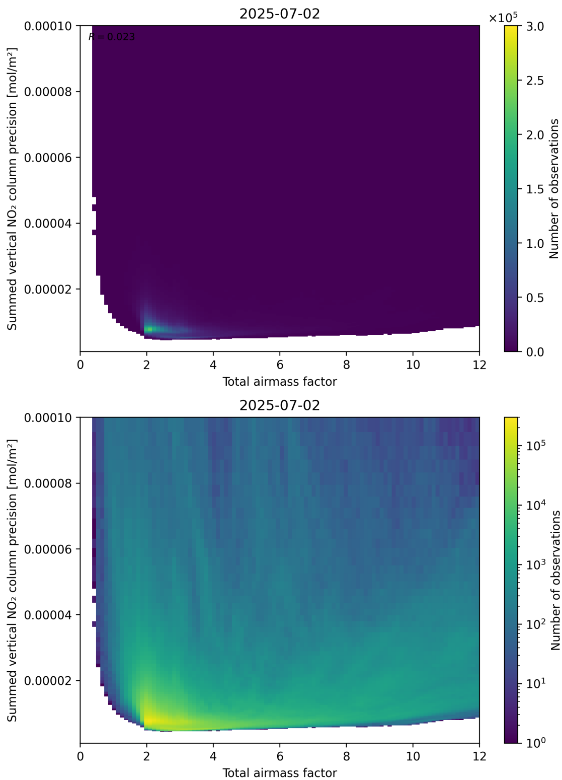
Figure 66: Scatter density plot of “Total airmass factor” against “Summed vertical NO 2 column precision” for 2025-07-02 to 2025-07-03.
