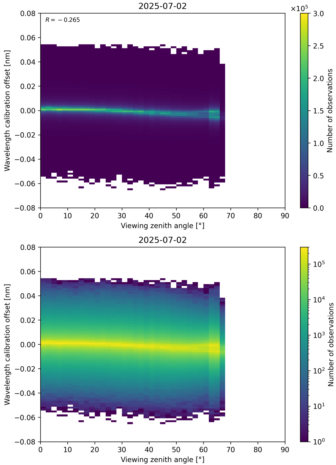
Figure 173: Scatter density plot of “Viewing zenith angle” against “Wavelength calibration offset” for 2025-07-02 to 2025-07-03.
