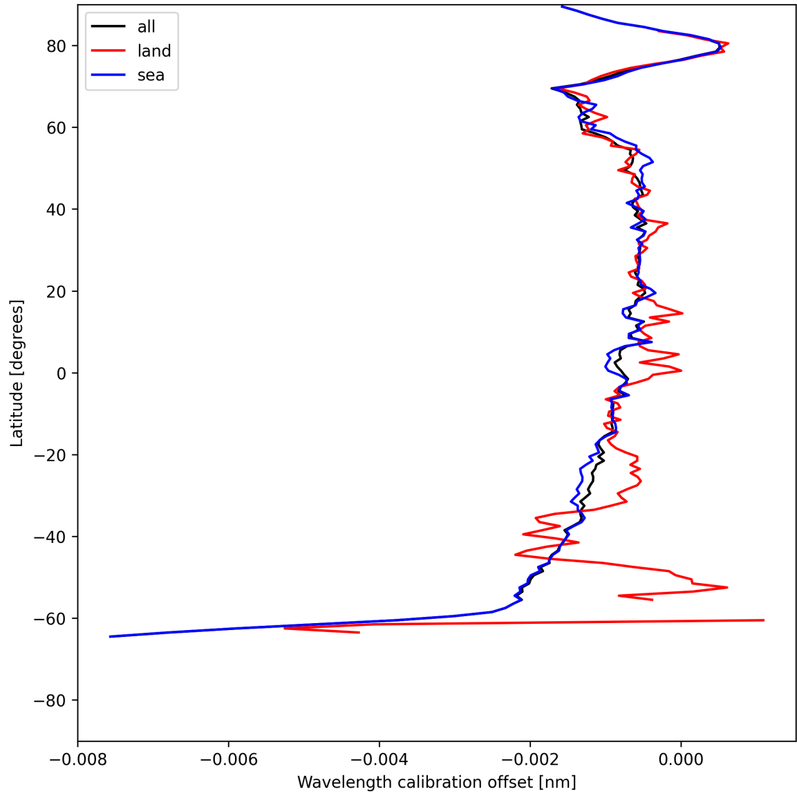
Figure 18: Zonal average of “Wavelength calibration offset” for 2025-07-02 to 2025-07-03.
