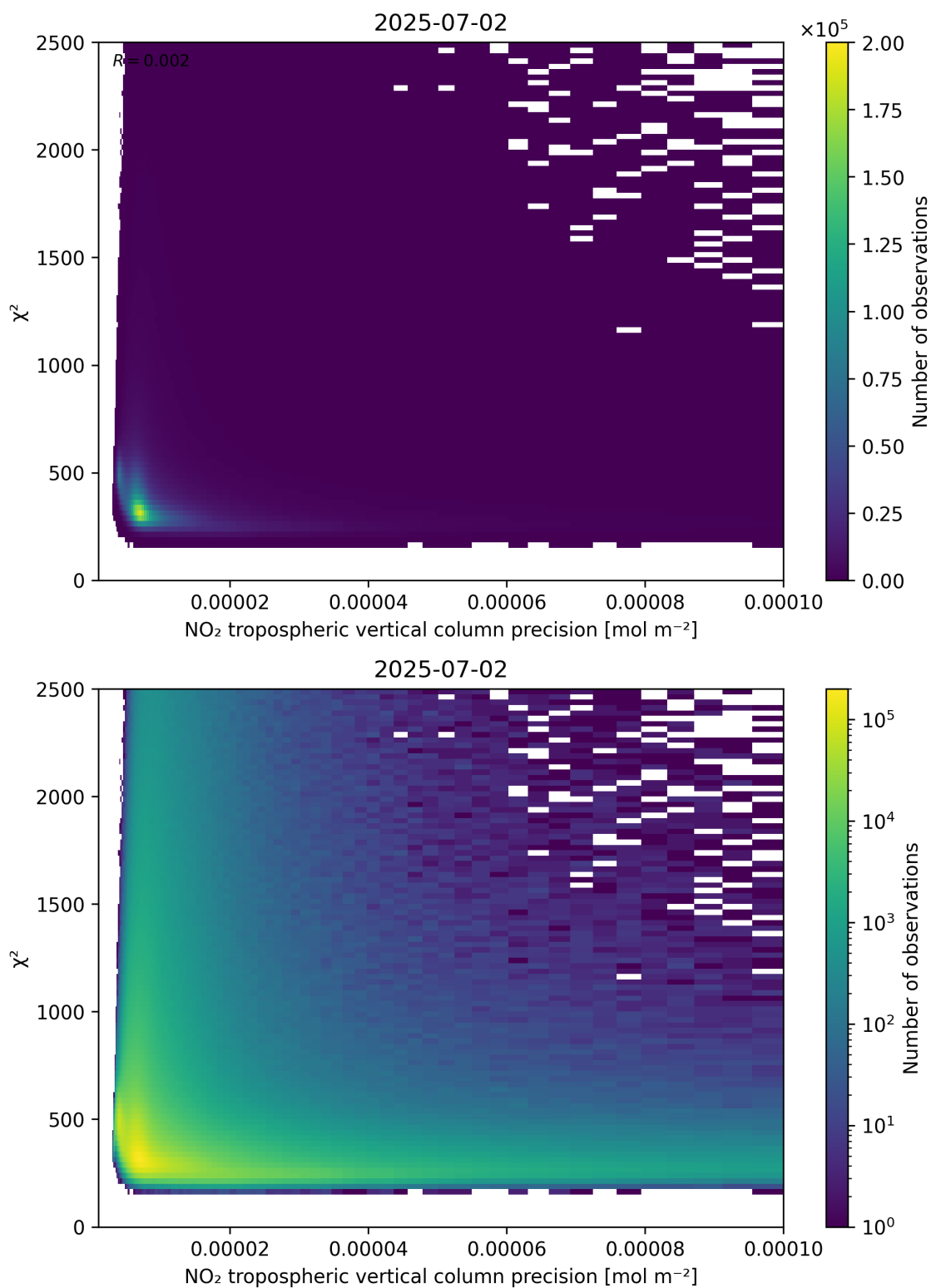
Figure 134: Scatter density plot of “NO 2 tropospheric vertical column precision” against “ \chi^2 ” for 2025-07-02 to 2025-07-03.
