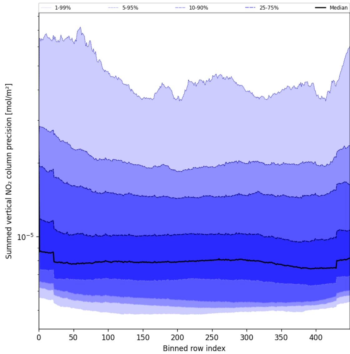
Figure 58: Along track statistics of “Summed vertical NO 2 column precision” for 2025-07-02 to 2025-07-03
