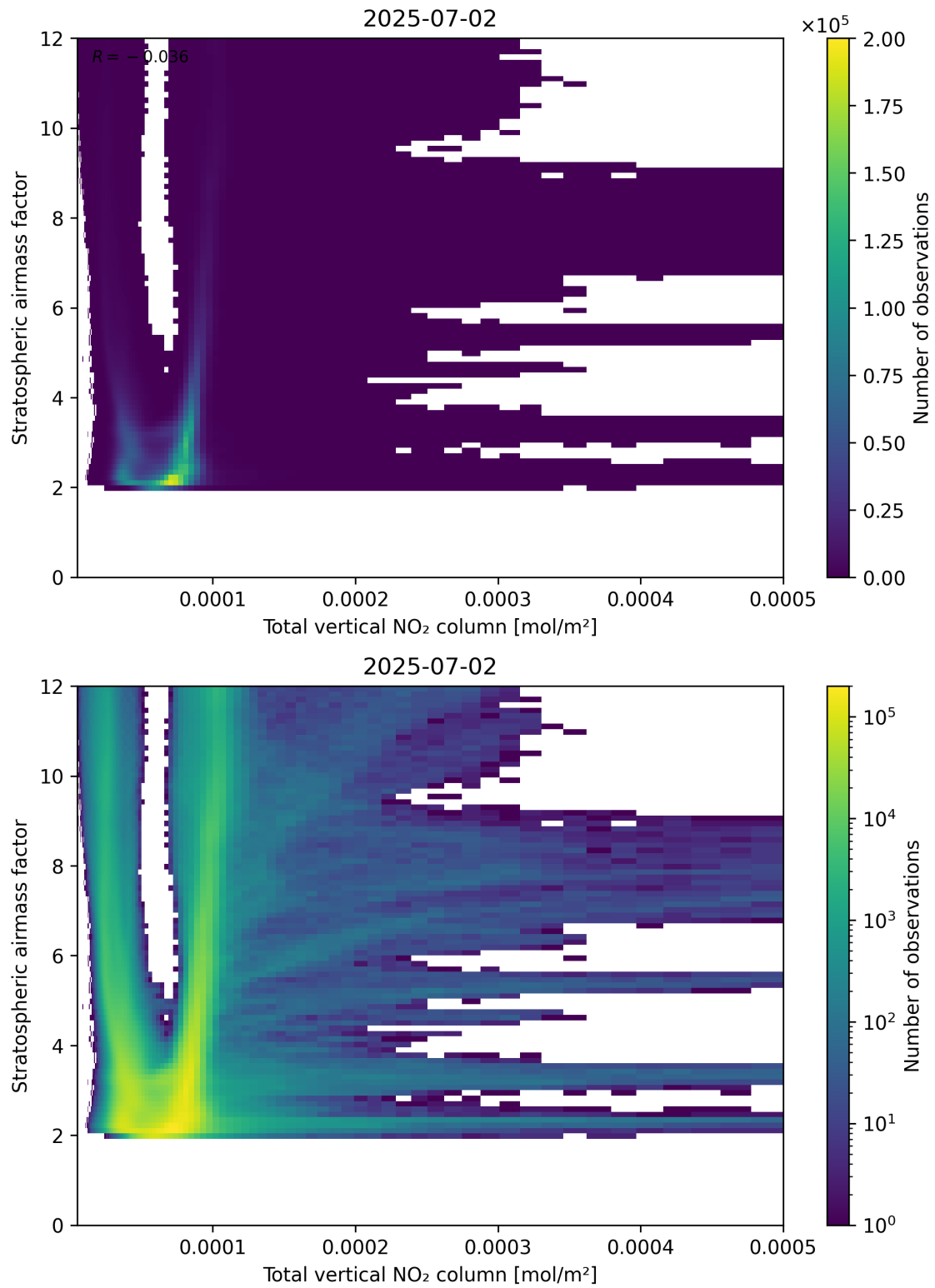
Figure 110: Scatter density plot of “Total vertical NO 2 column” against “Stratospheric airmass factor” for 2025-07-02 to 2025-07-03.
