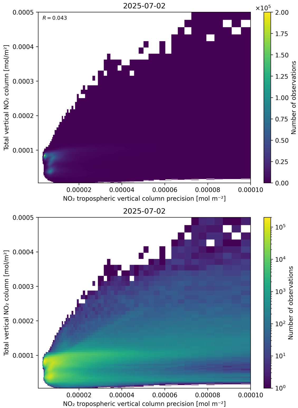
Figure 138: Scatter density plot of “NO 2 tropospheric vertical column precision” against “Total vertical NO 2 column” for 2025-07-02 to 2025-07-03.
