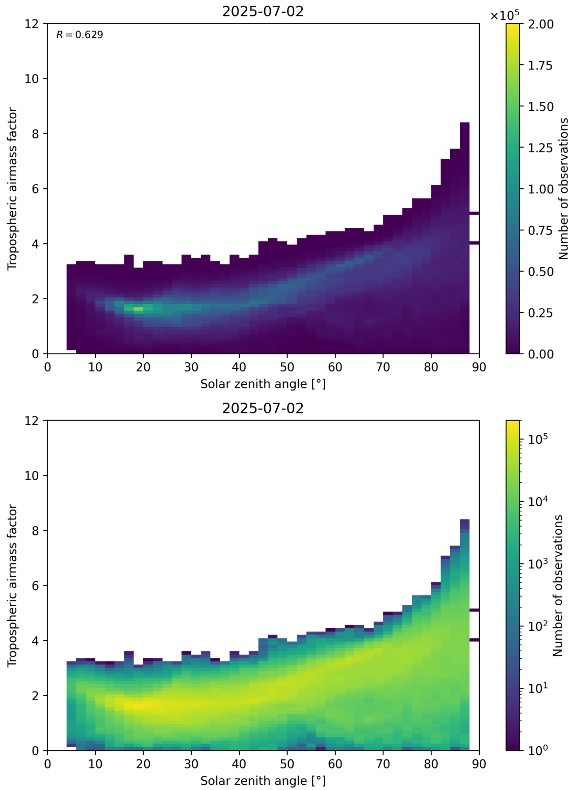
Figure 147: Scatter density plot of “Solar zenith angle” against “Tropospheric airmass factor” for 2025-07-02 to 2025-07-03.
