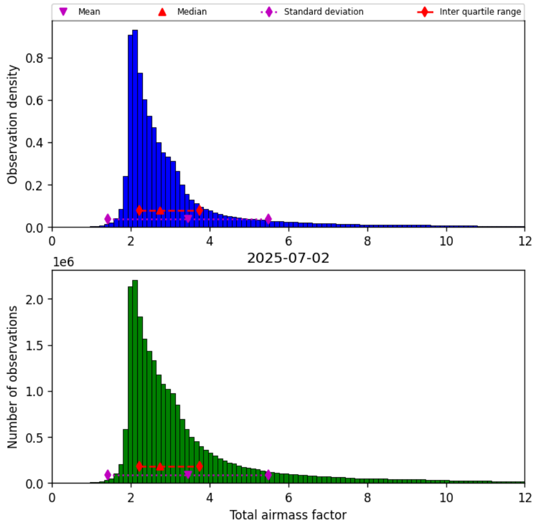
Figure 32: Histogram of “Total airmass factor” for 2025-07-02 to 2025-07-03
