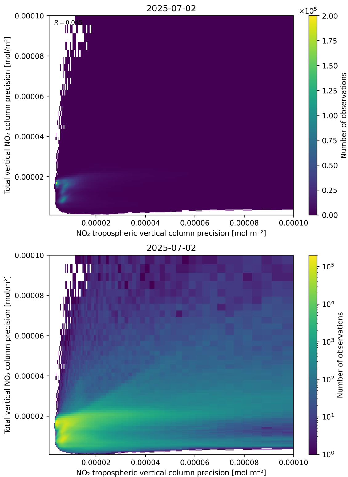
Figure 139: Scatter density plot of “NO 2 tropospheric vertical column precision” against “Total vertical NO 2 column precision” for 2025-07-02 to 2025-07-03.
