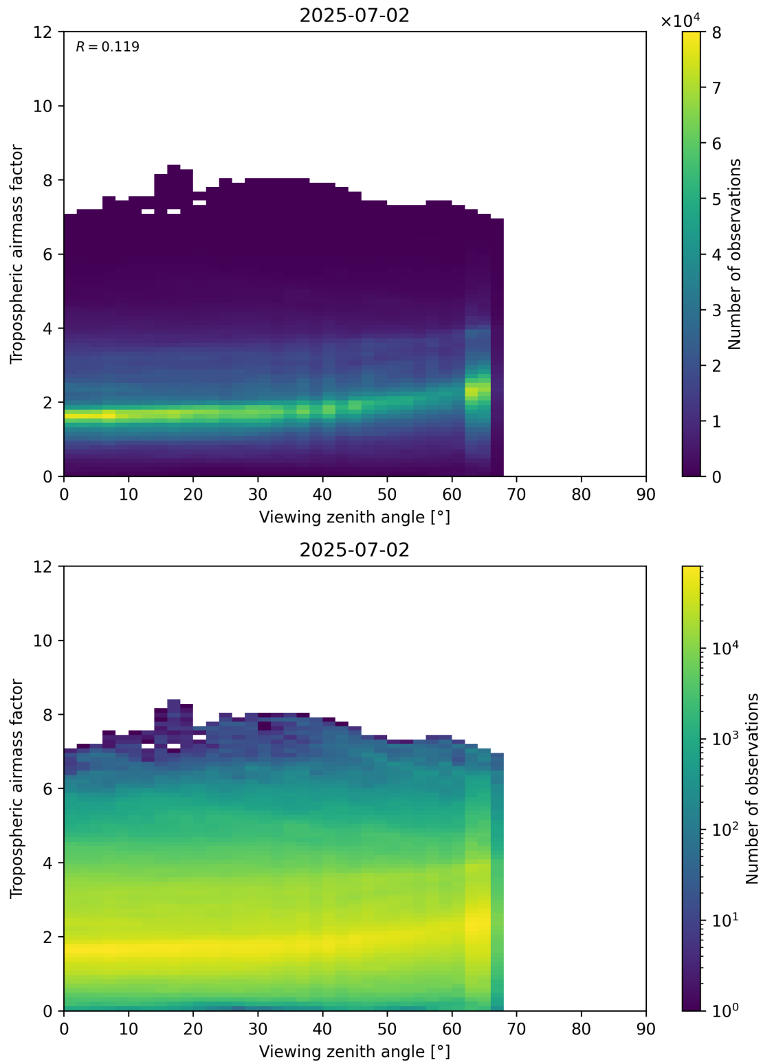
Figure 161: Scatter density plot of “Viewing zenith angle” against “Tropospheric airmass factor” for 2025-07-02 to 2025-07-03.
