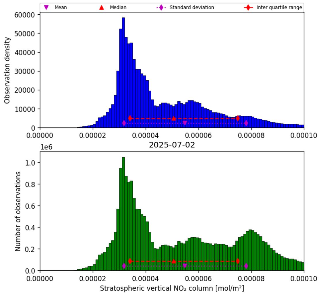
Figure 36: Histogram of “Stratospheric vertical NO 2 column” for 2025-07-02 to 2025-07-03
