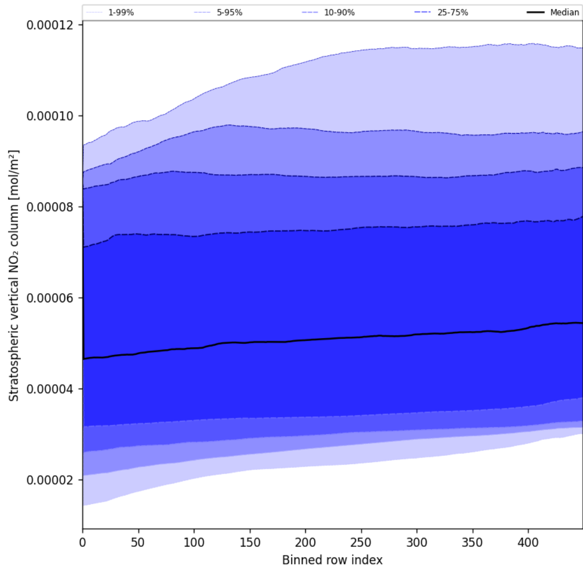
Figure 53: Along track statistics of “Stratospheric vertical NO 2 column” for 2025-07-02 to 2025-07-03
