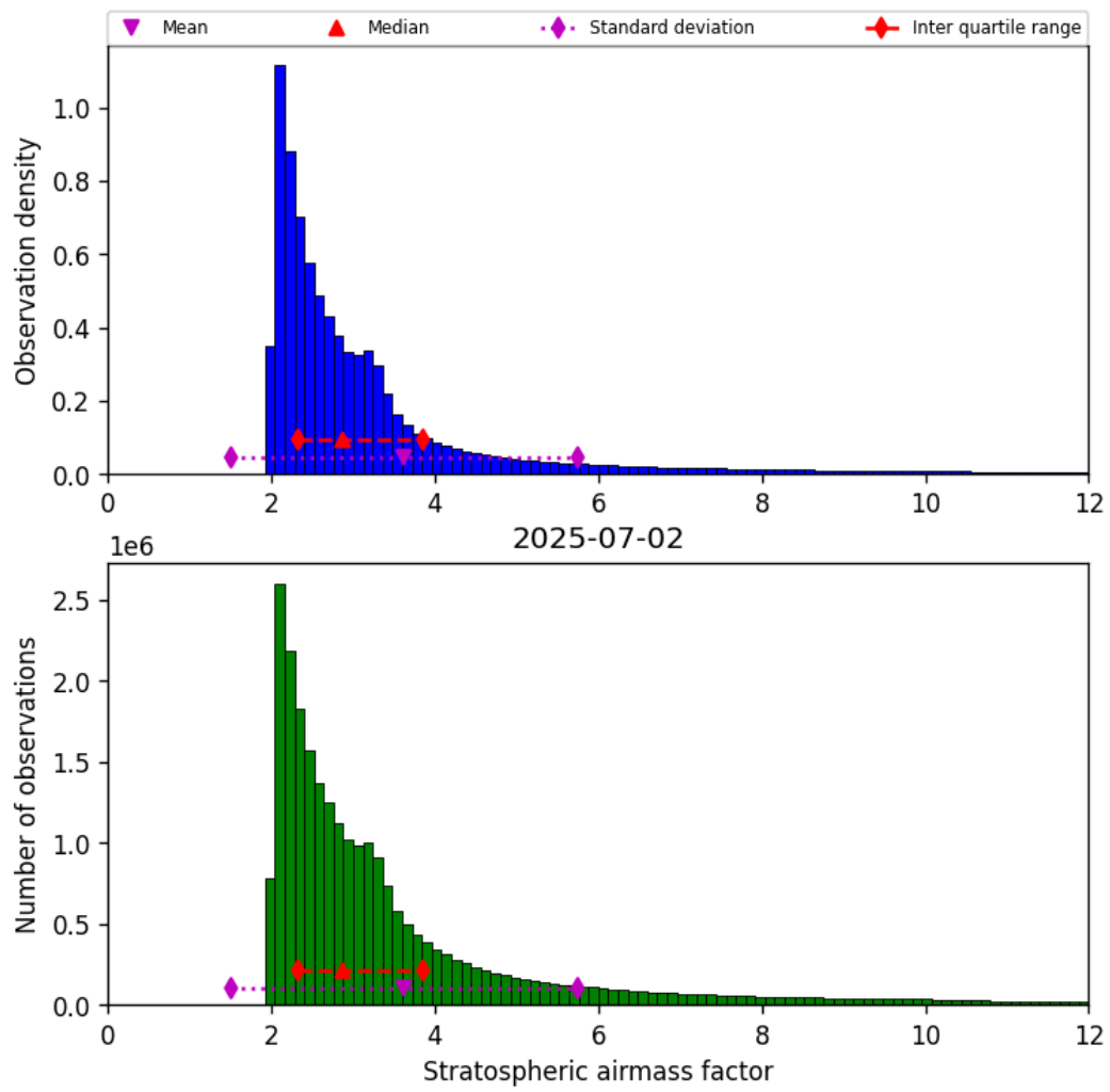
Figure 44: Histogram of “Stratospheric airmass factor” for 2025-07-02 to 2025-07-03
