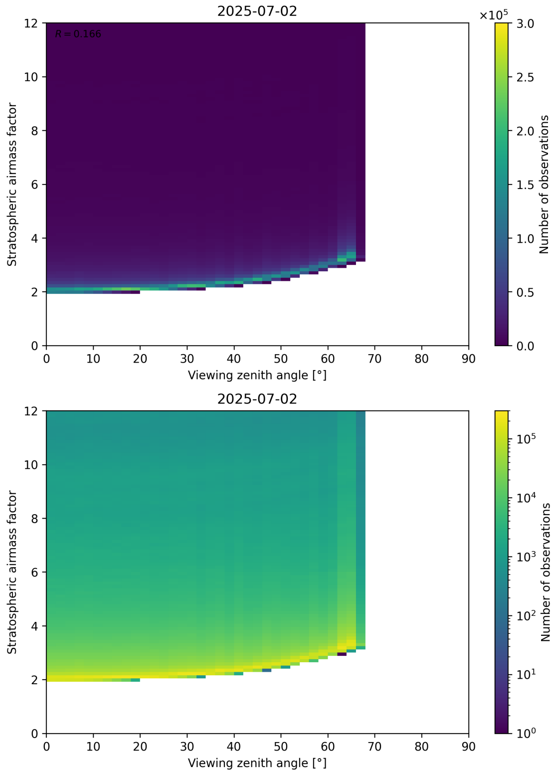
Figure 159: Scatter density plot of “Viewing zenith angle” against “Stratospheric airmass factor” for 2025-07-02 to 2025-07-03.
