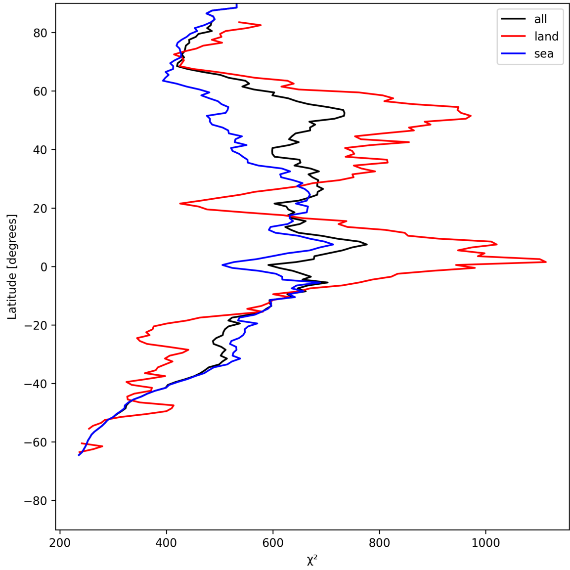
Figure 25: Zonal average of “ \chi^2 ” for 2025-07-02 to 2025-07-03.
