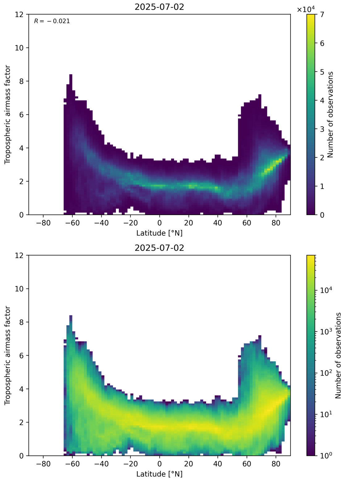
Figure 85: Scatter density plot of “Latitude” against “Tropospheric air mass factor” for 2025-07-02 to 2025-07-03.
