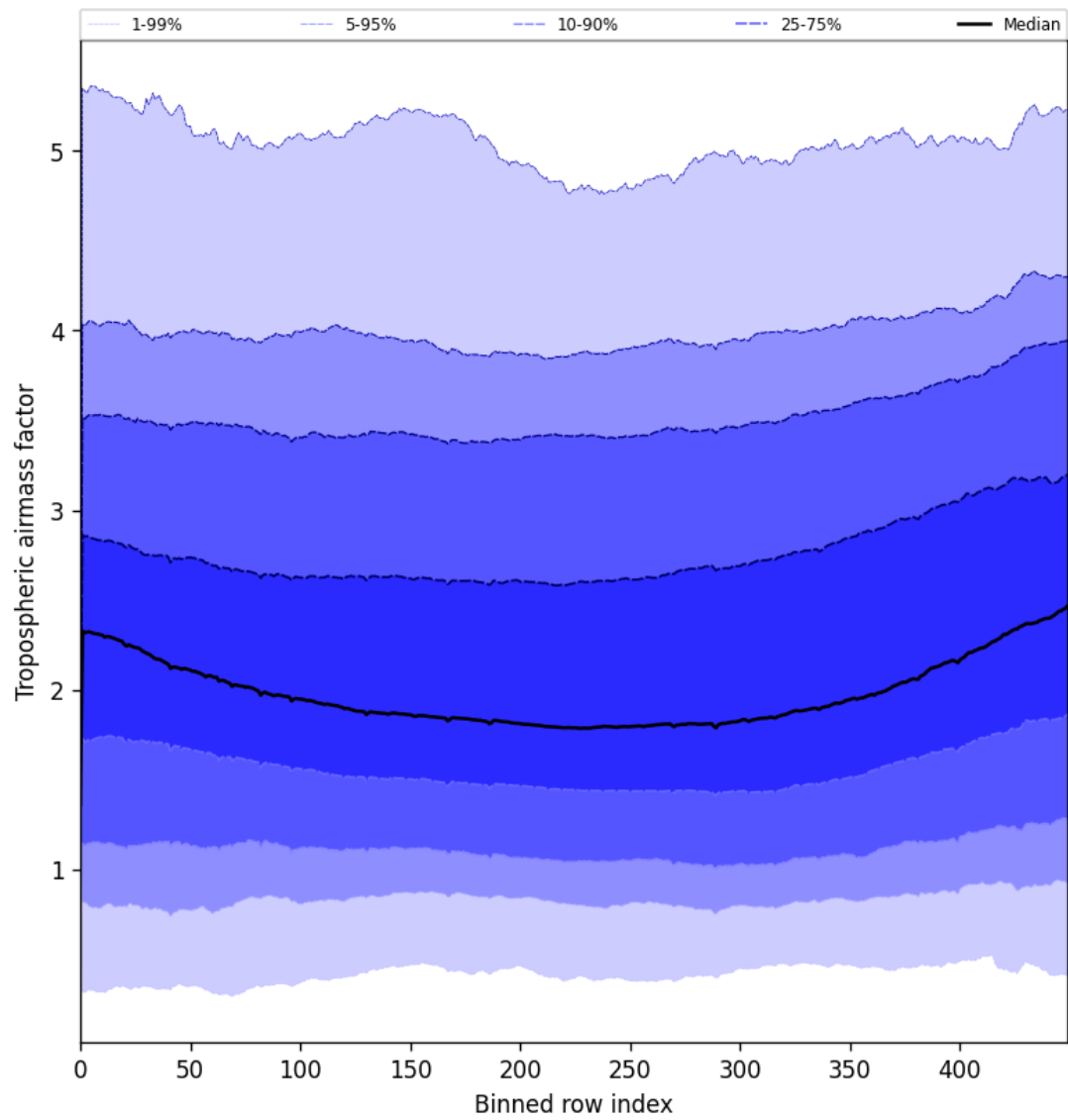
Figure 48: Along track statistics of “Tropospheric airmass factor” for 2025-07-02 to 2025-07-03
