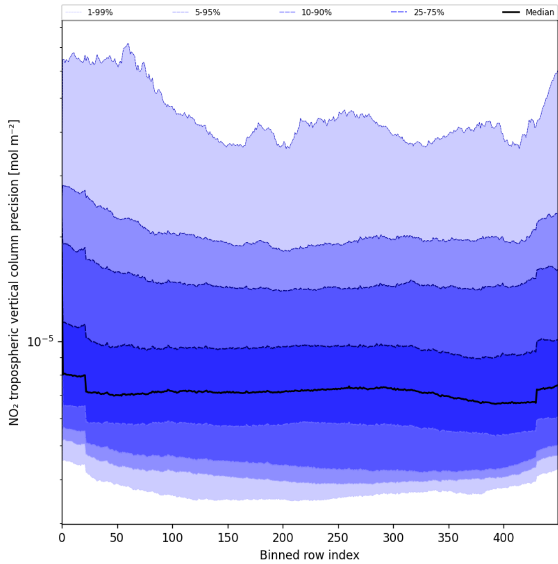
Figure 47: Along track statistics of “NO 2 tropospheric vertical column precision” for 2025-07-02 to 2025-07-03
