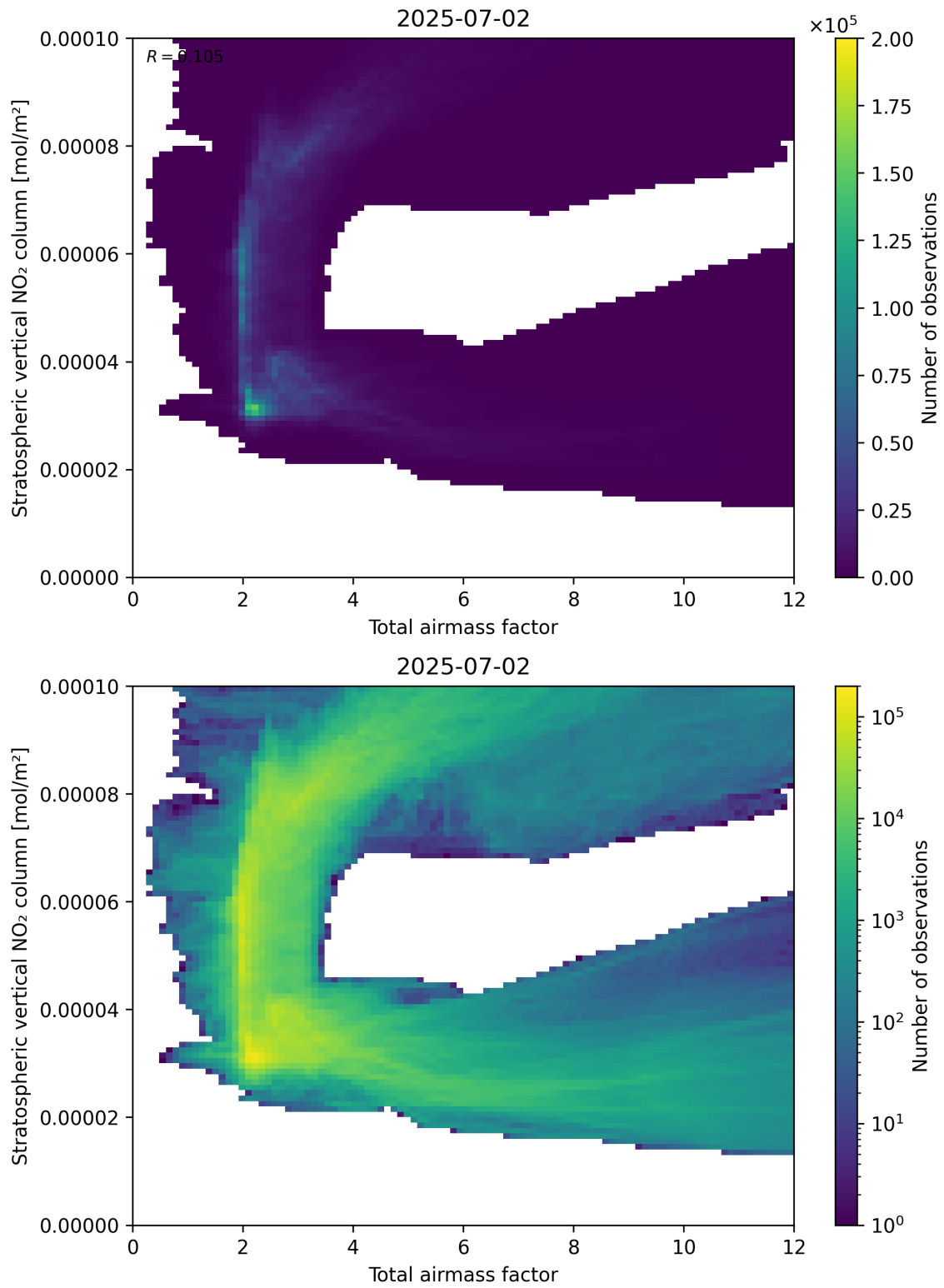
Figure 64: Scatter density plot of “Total airmass factor” against “Stratospheric vertical NO 2 column” for 2025-07-02 to 2025-07-03.
