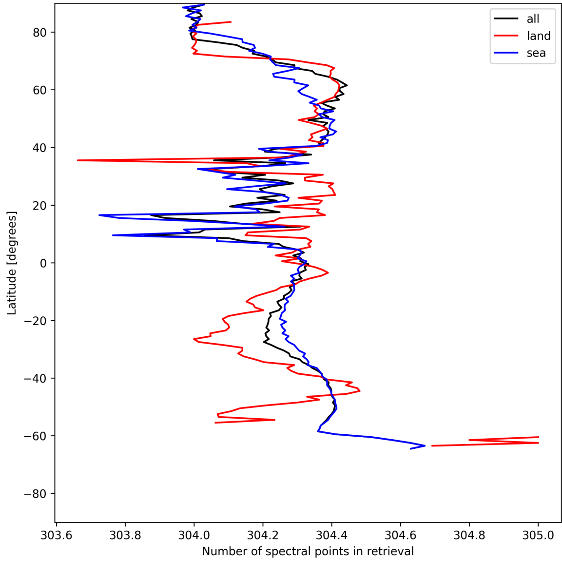
Figure 16: Zonal average of “Number of spectral points in retrieval” for 2025-07-02 to 2025-07-03.
