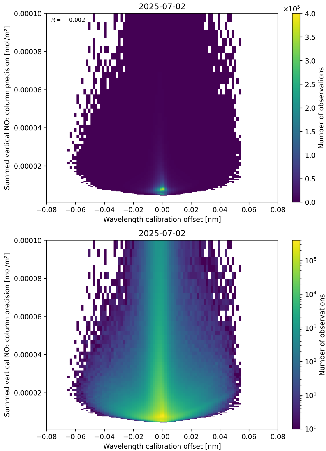
Figure 178: Scatter density plot of “Wavelength calibration offset” against “Summed vertical NO 2 column precision” for 2025-07-02 to 2025-07-03.
