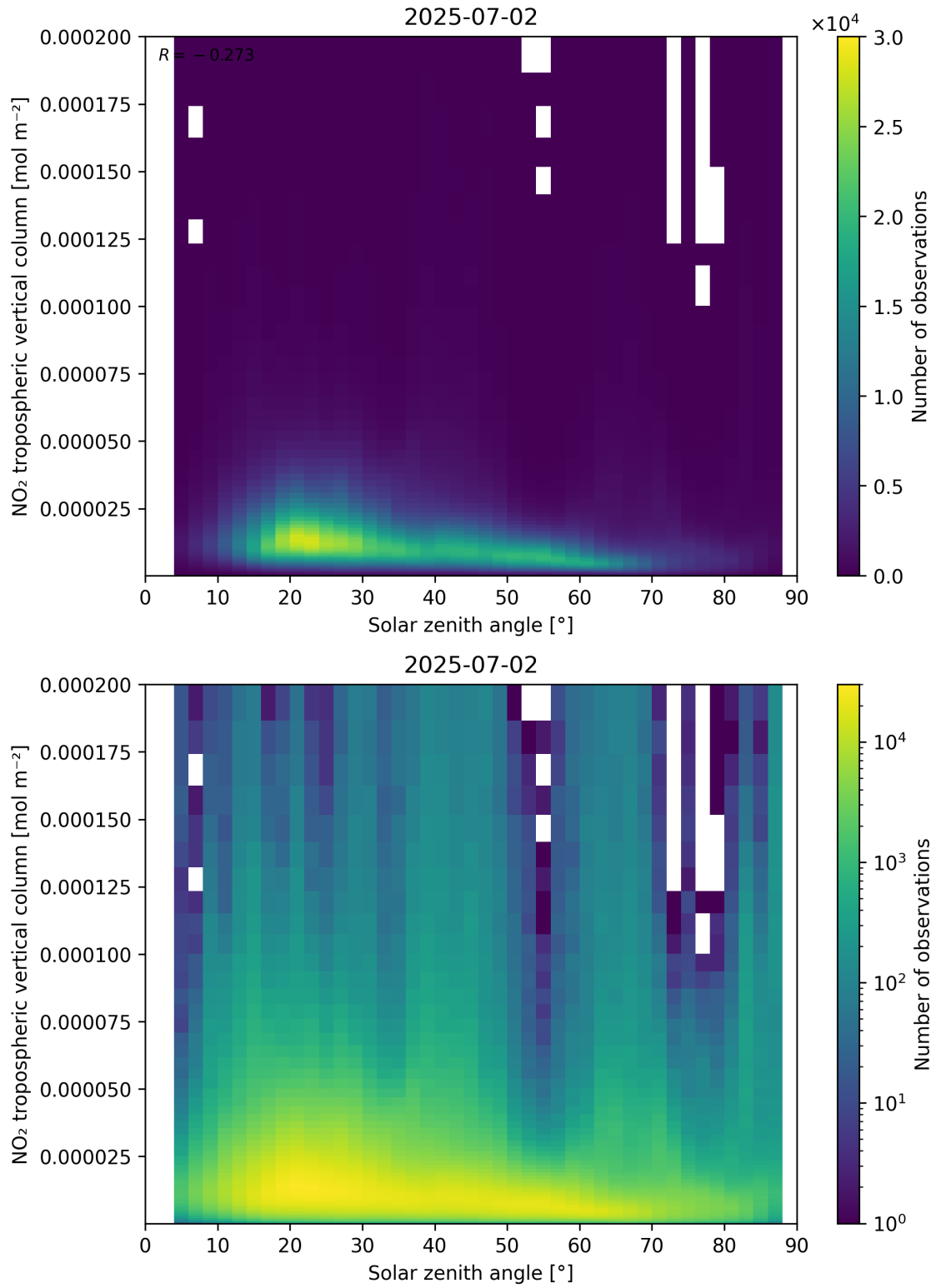
Figure 155: Scatter density plot of “Solar zenith angle” against “NO 2 tropospheric vertical column” for 2025-07-02 to 2025-07-03.
