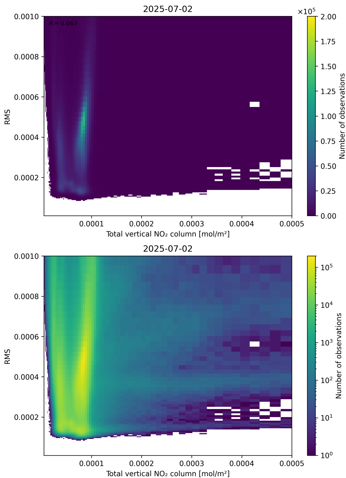
Figure 120: Scatter density plot of “Total vertical NO 2 column” against “RMS” for 2025-07-02 to 2025-07-03.
