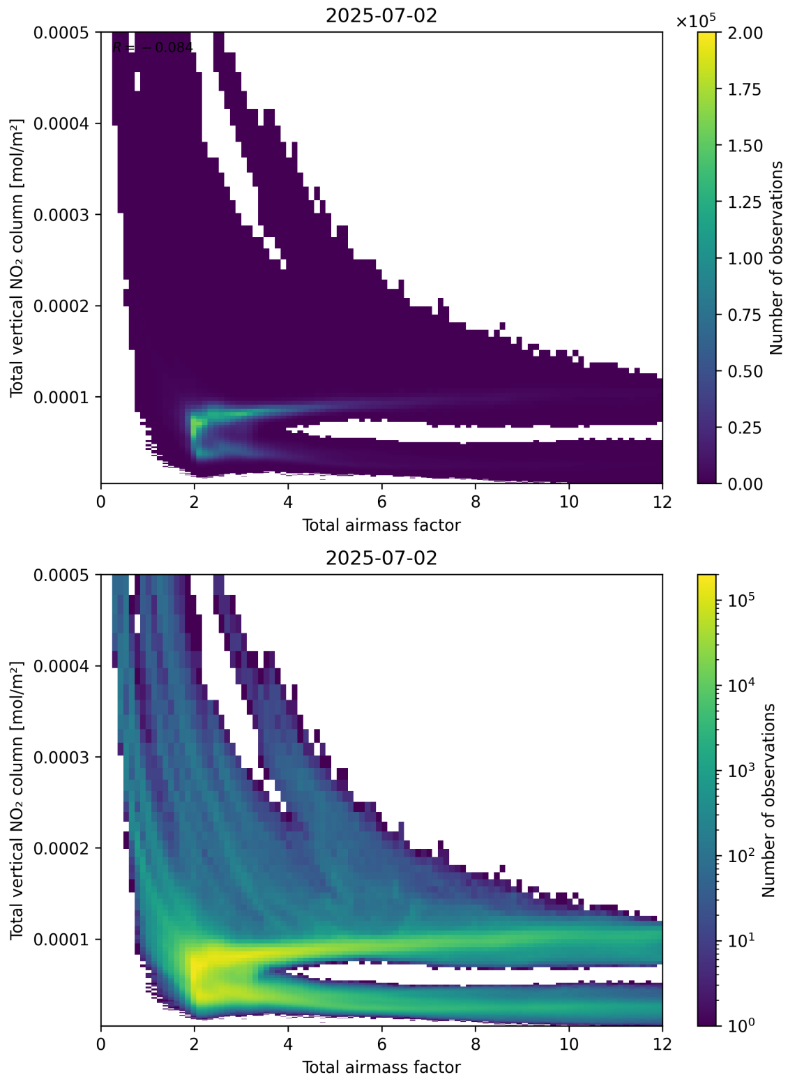
Figure 67: Scatter density plot of “Total airmass factor” against “Total vertical NO 2 column” for 2025-07-02 to 2025-07-03.
