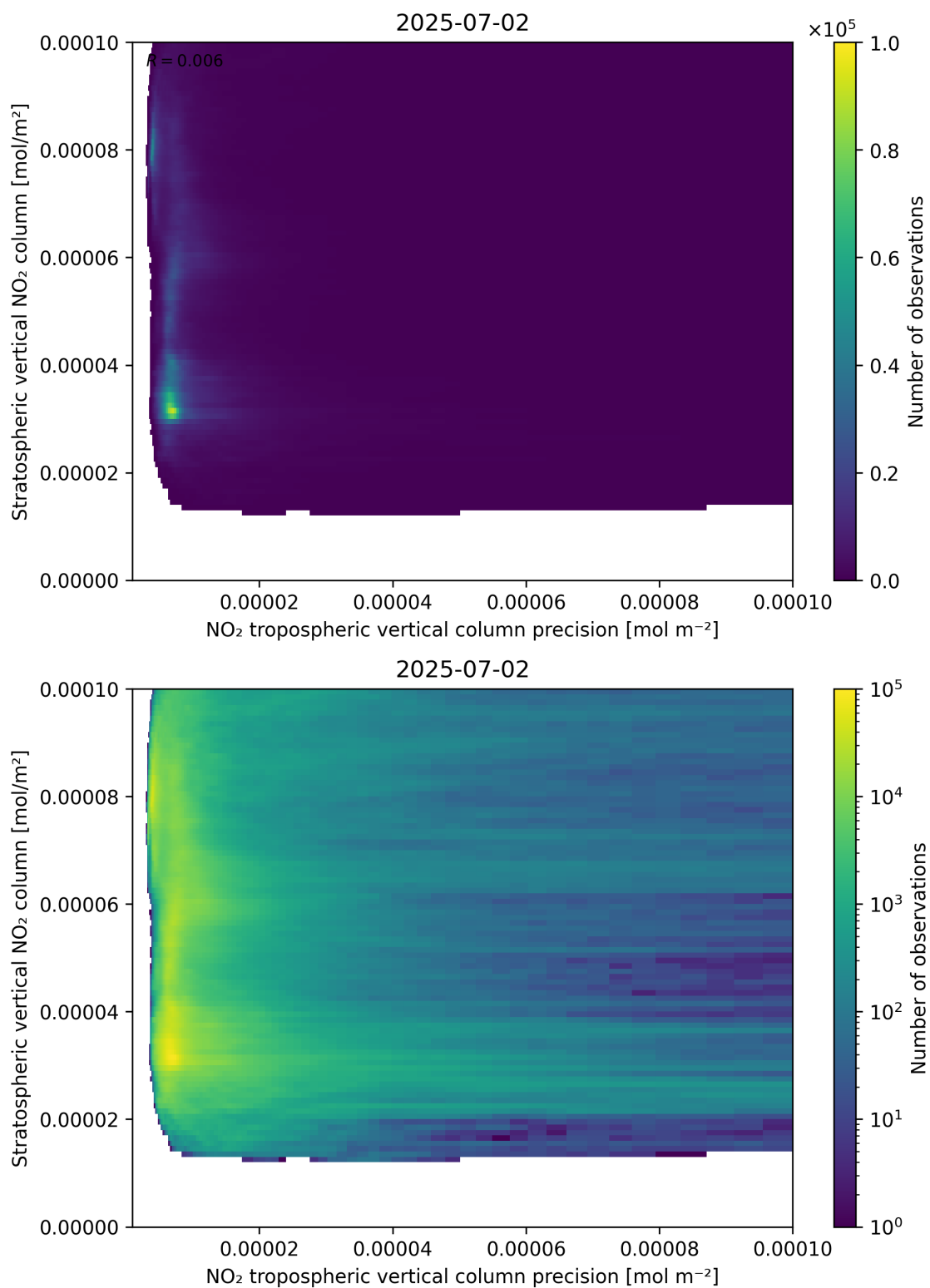
Figure 135: Scatter density plot of “NO 2 tropospheric vertical column precision” against “Stratospheric vertical NO 2 column” for 2025-07-02 to 2025-07-03.
