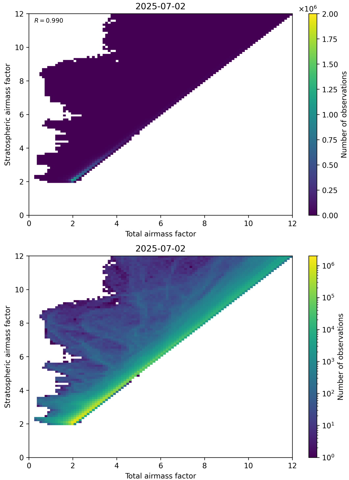
Figure 62: Scatter density plot of “Total airmass factor” against “Stratospheric airmass factor” for 2025-07-02 to 2025-07-03.
