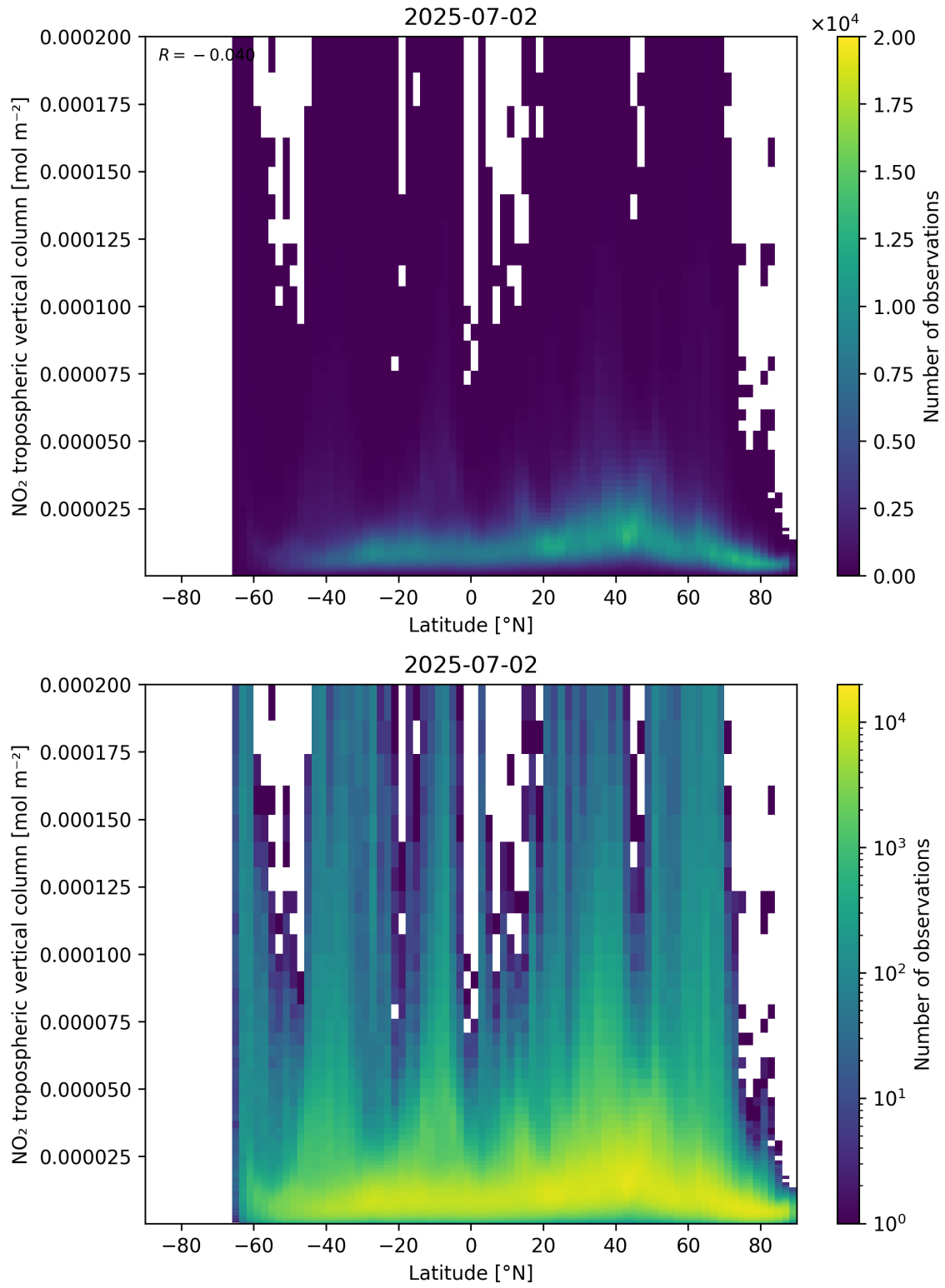
Figure 92: Scatter density plot of “Latitude” against “NO 2 tropospheric vertical column” for 2025-07-02 to 2025-07-03.
