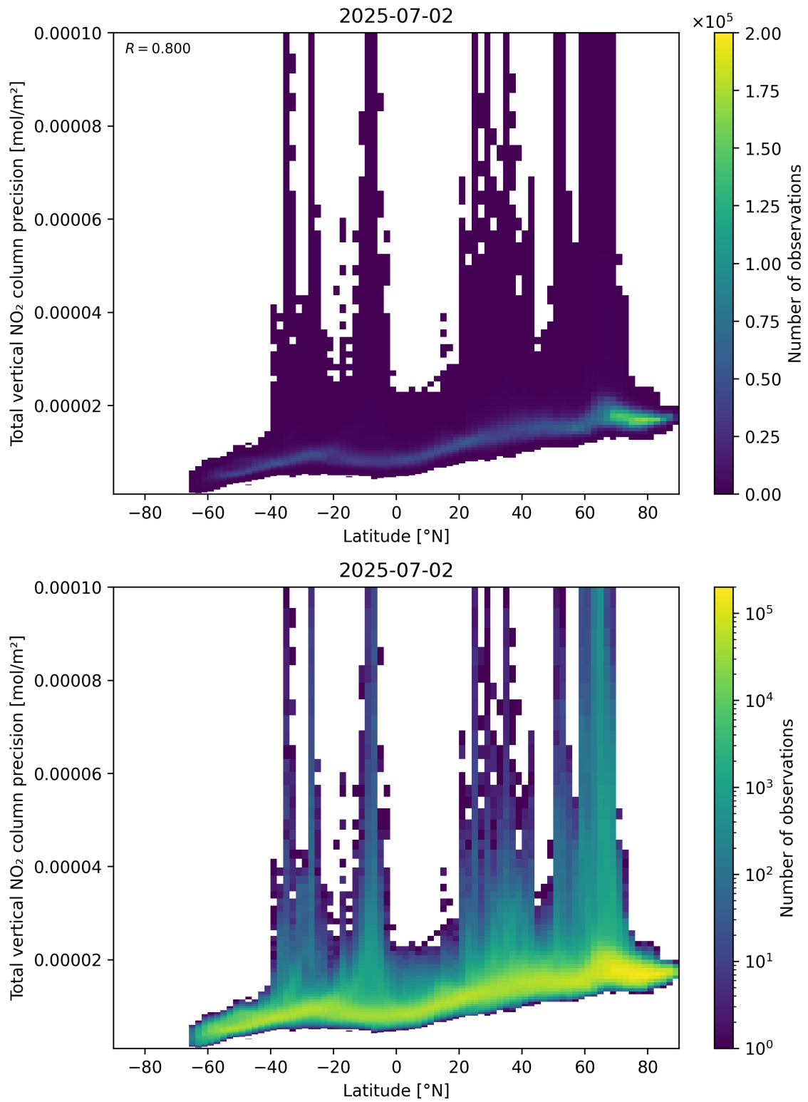
Figure 91: Scatter density plot of “Latitude” against “Total vertical NO 2 column precision” for 2025-07-02 to 2025-07-03.
