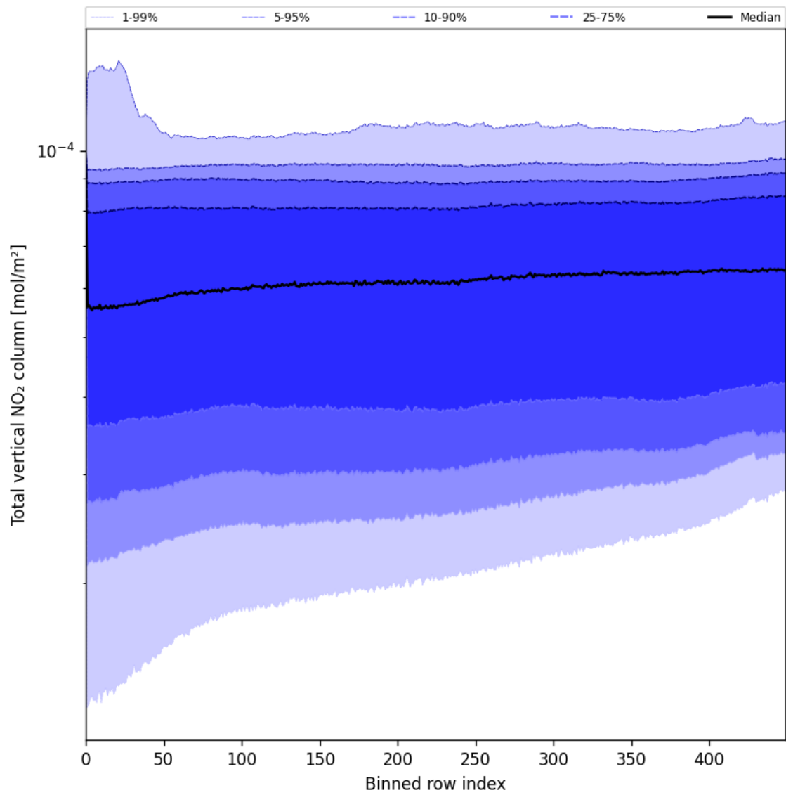
Figure 55: Along track statistics of “Total vertical NO 2 column” for 2025-07-02 to 2025-07-03
