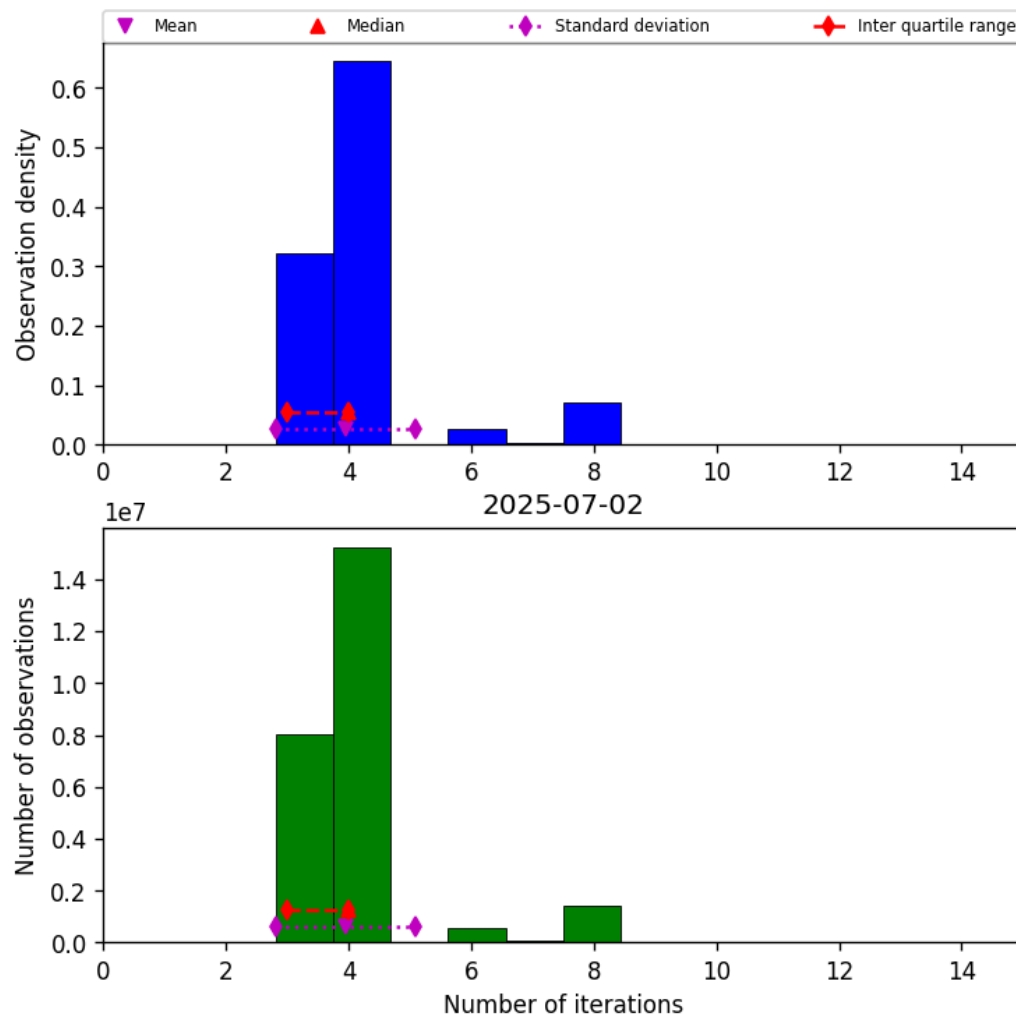
Figure 34: Histogram of “Number of iterations” for 2025-07-02 to 2025-07-03
