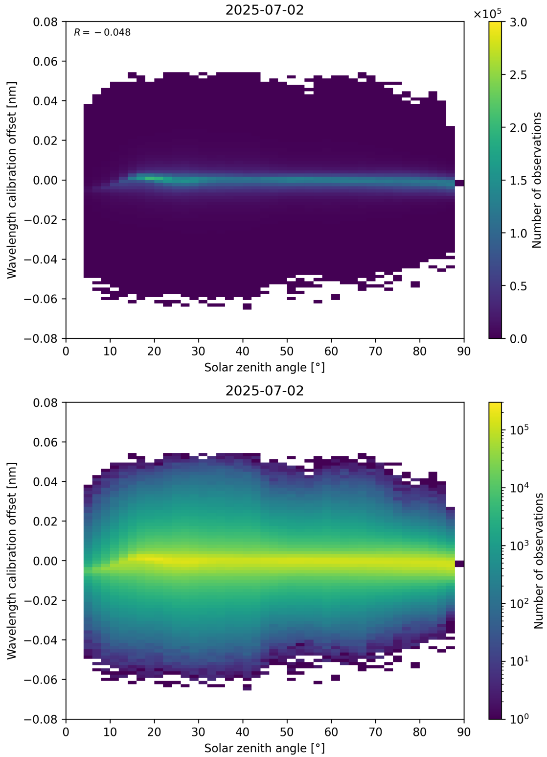
Figure 158: Scatter density plot of “Solar zenith angle” against “Wavelength calibration offset” for 2025-07-02 to 2025-07-03.
