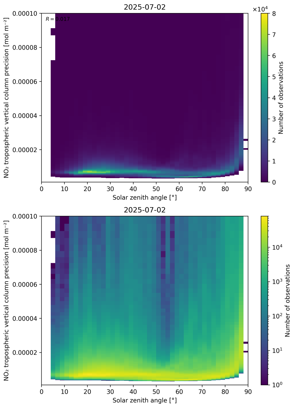
Figure 156: Scatter density plot of “Solar zenith angle” against “NO 2 tropospheric vertical column precision” for 2025-07-02 to 2025-07-03.
