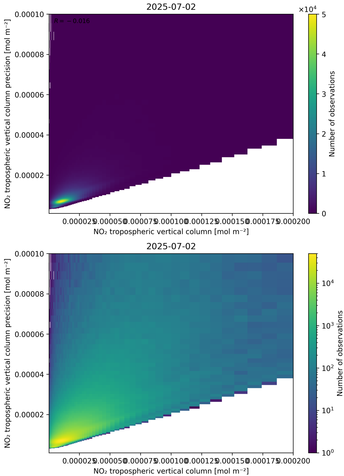
Figure 130: Scatter density plot of “NO 2 tropospheric vertical column” against “NO 2 tropospheric vertical column precision” for 2025-07-02 to 2025-07-03.
