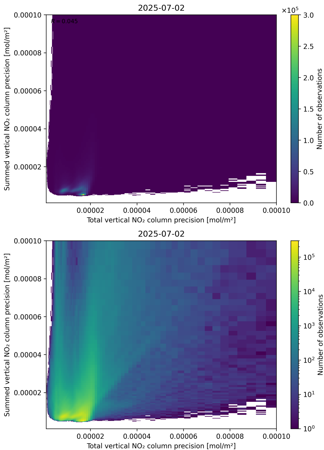
Figure 118: Scatter density plot of “Total vertical NO 2 column precision” against “Summed vertical NO 2 column precision” for 2025-07-02 to 2025-07-03.
