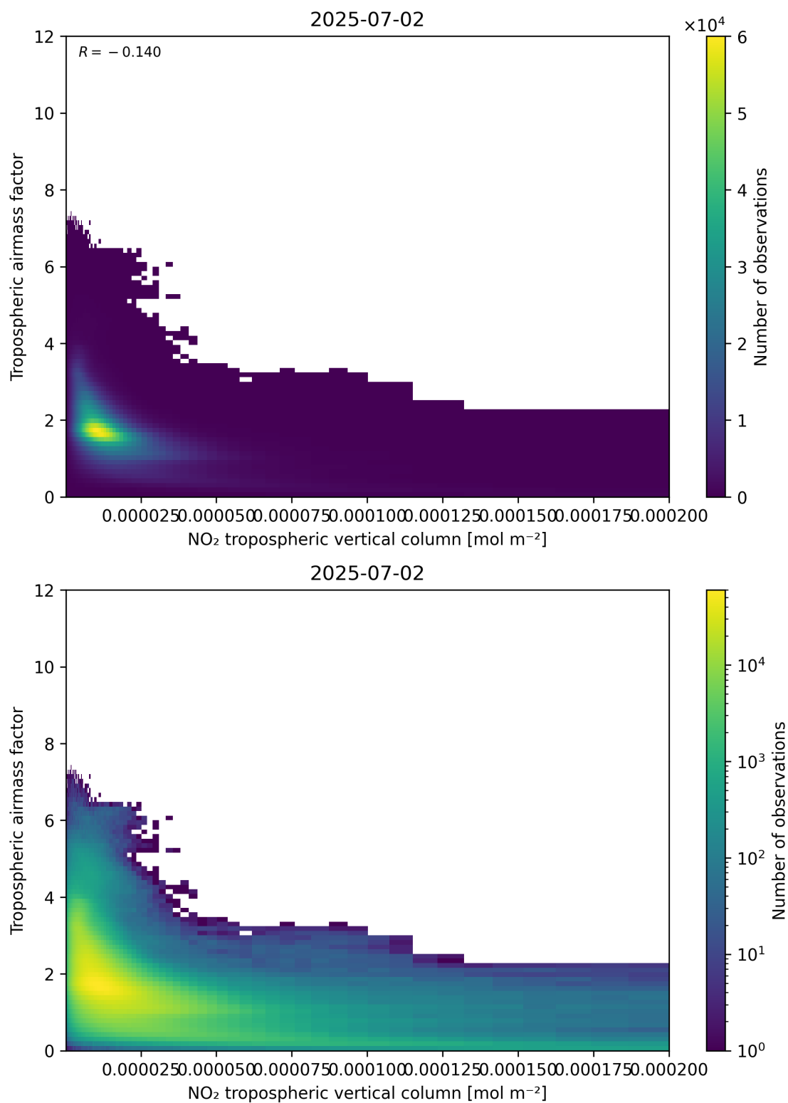
Figure 123: Scatter density plot of “NO 2 tropospheric vertical column” against “Tropospheric air mass factor” for 2025-07-02 to 2025-07-03.
