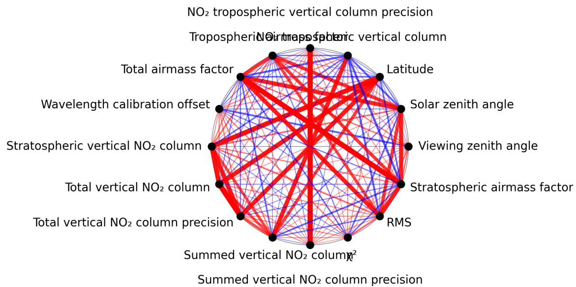
Figure 1: Map of correlation graph for 2025-07-02 to 2025-07-03.
