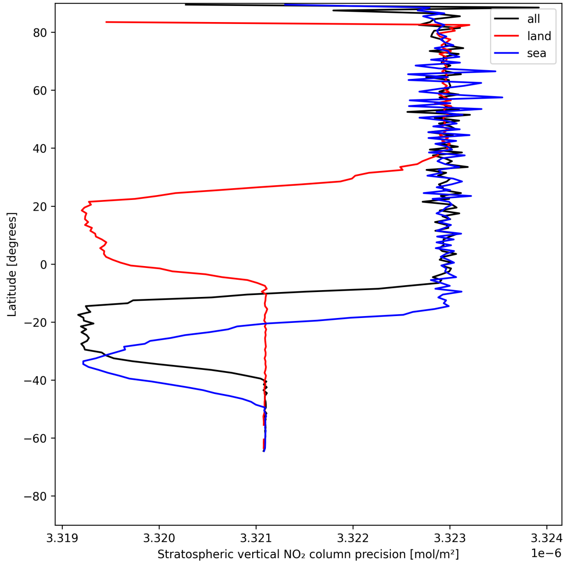
Figure 20: Zonal average of “Stratospheric vertical NO 2 column precision” for 2025-07-02 to 2025-07-03.
