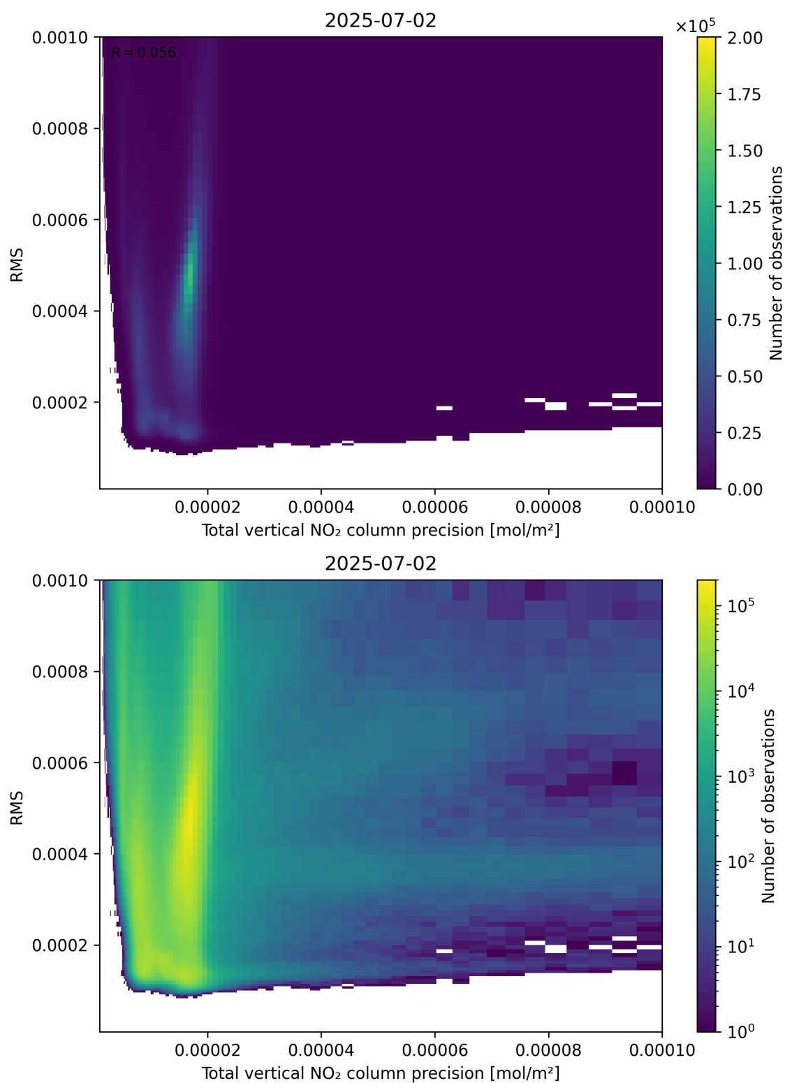
Figure 119: Scatter density plot of “Total vertical NO 2 column precision” against “RMS” for 2025-07-02 to 2025-07-03.
