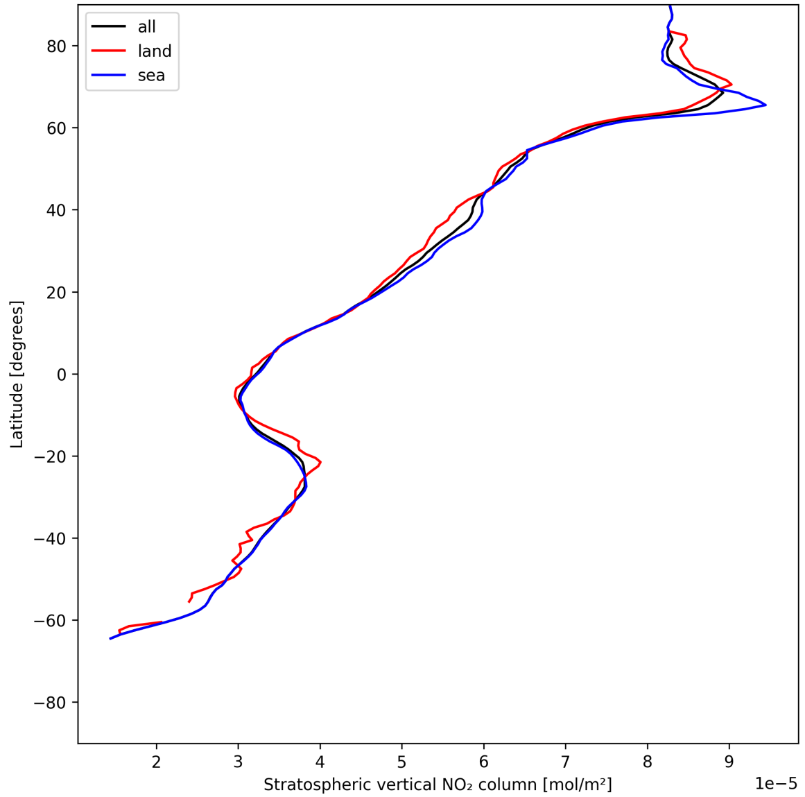
Figure 19: Zonal average of “Stratospheric vertical NO 2 column” for 2025-07-02 to 2025-07-03.
