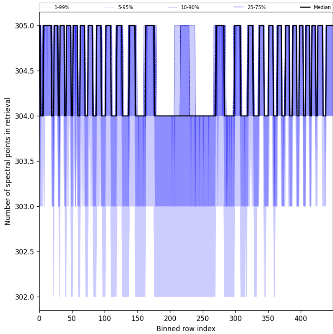
Figure 50: Along track statistics of “Number of spectral points in retrieval” for 2025-07-02 to 2025-07-03
