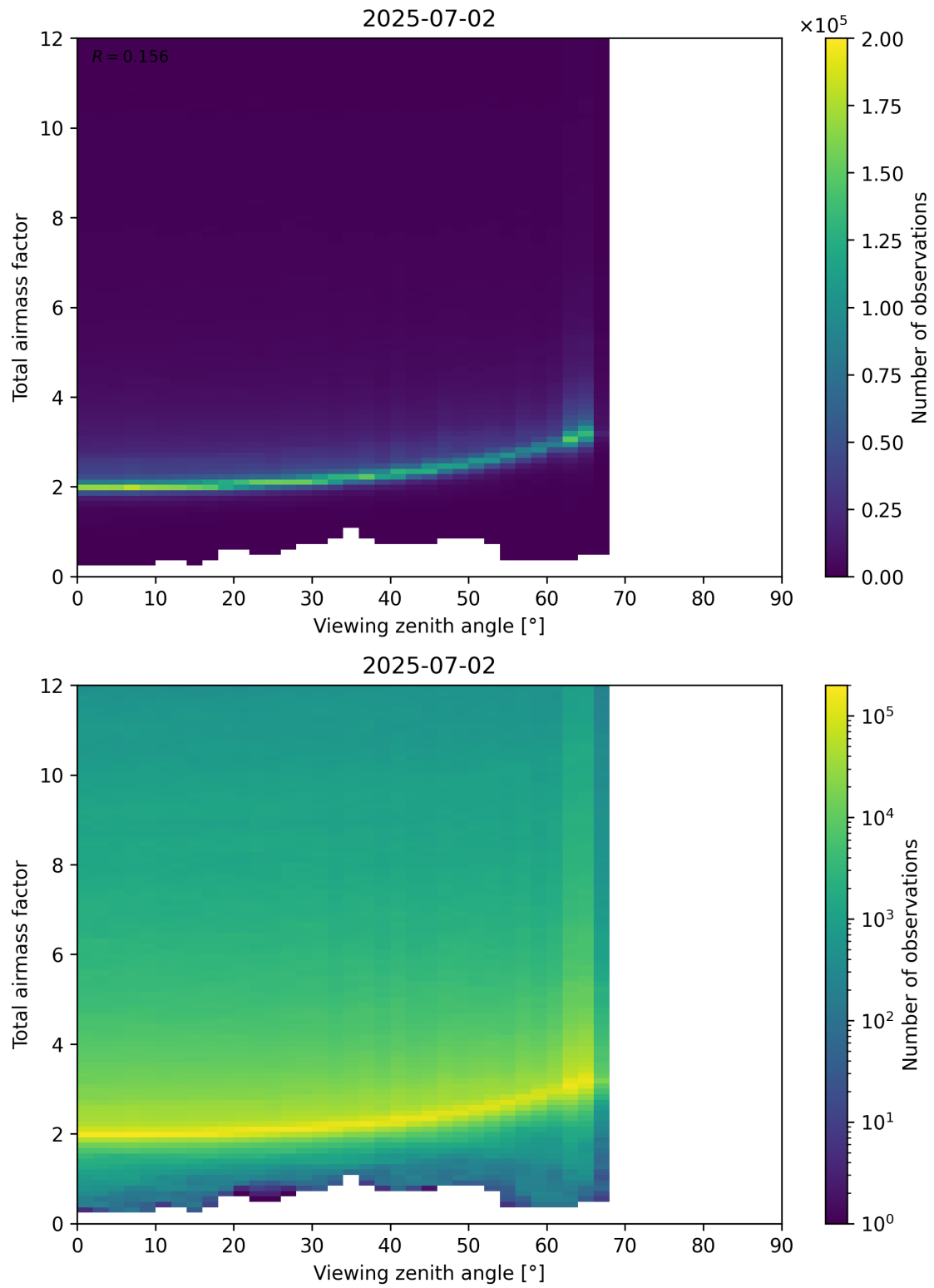
Figure 160: Scatter density plot of “Viewing zenith angle” against “Total airmass factor” for 2025-07-02 to 2025-07-03.
