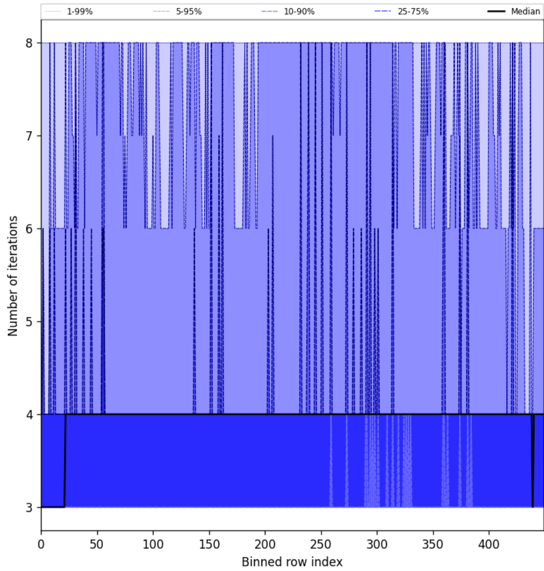
Figure 51: Along track statistics of “Number of iterations” for 2025-07-02 to 2025-07-03
