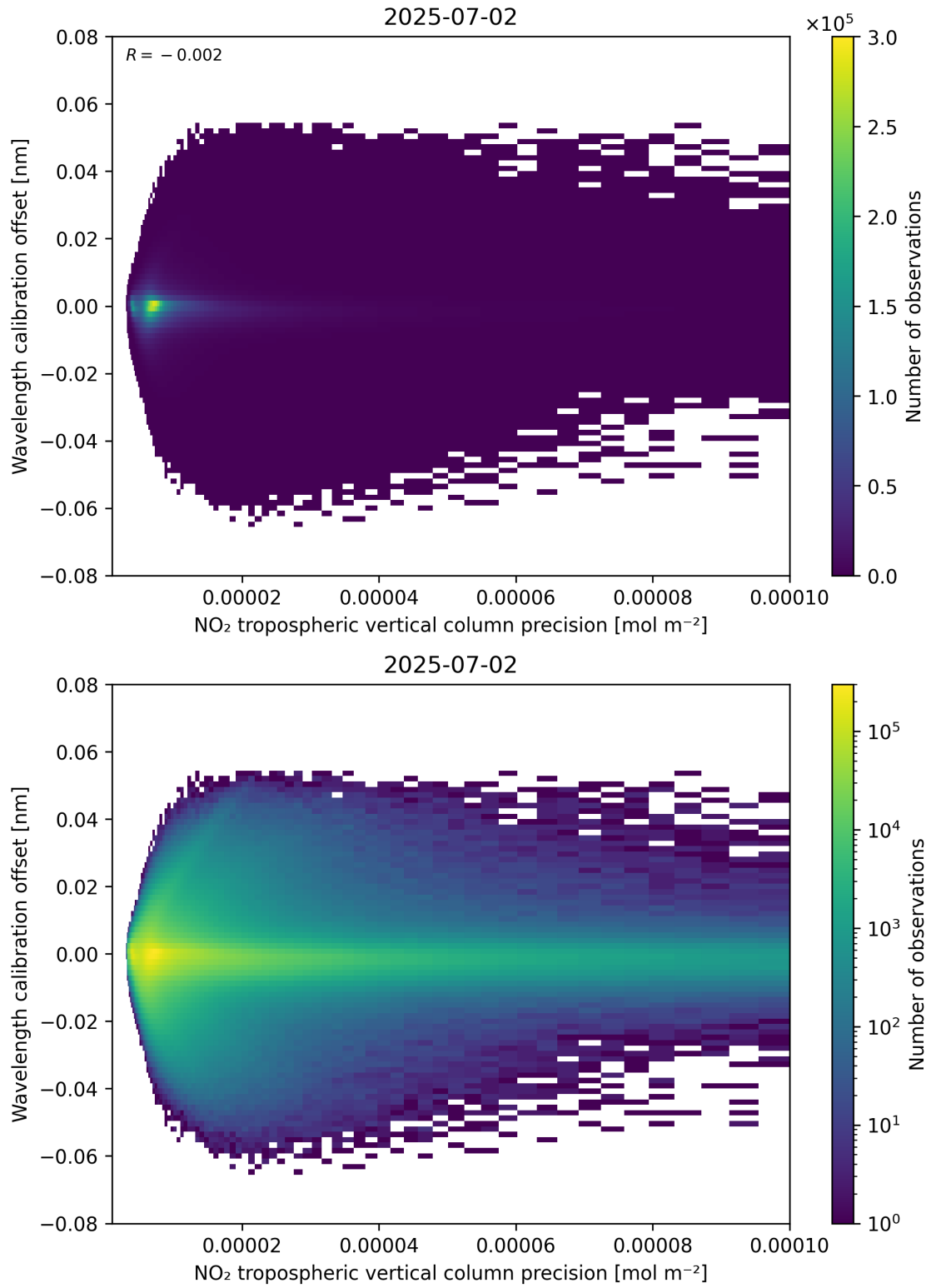
Figure 141: Scatter density plot of “NO 2 tropospheric vertical column precision” against “Wavelength calibration offset” for 2025-07-02 to 2025-07-03.
