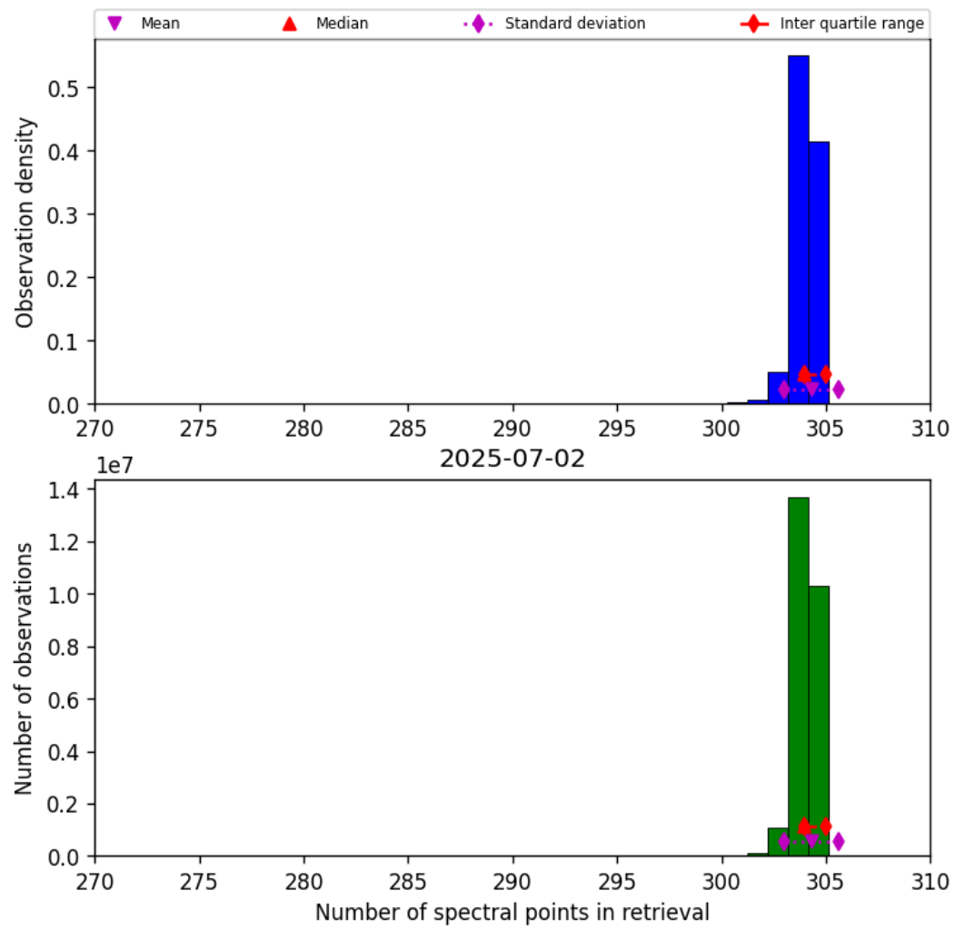
Figure 33: Histogram of “Number of spectral points in retrieval” for 2025-07-02 to 2025-07-03
