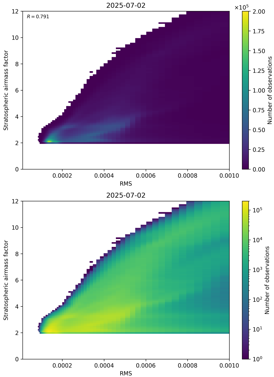
Figure 144: Scatter density plot of “RMS” against “Stratospheric airmass factor” for 2025-07-02 to 2025-07-03.
