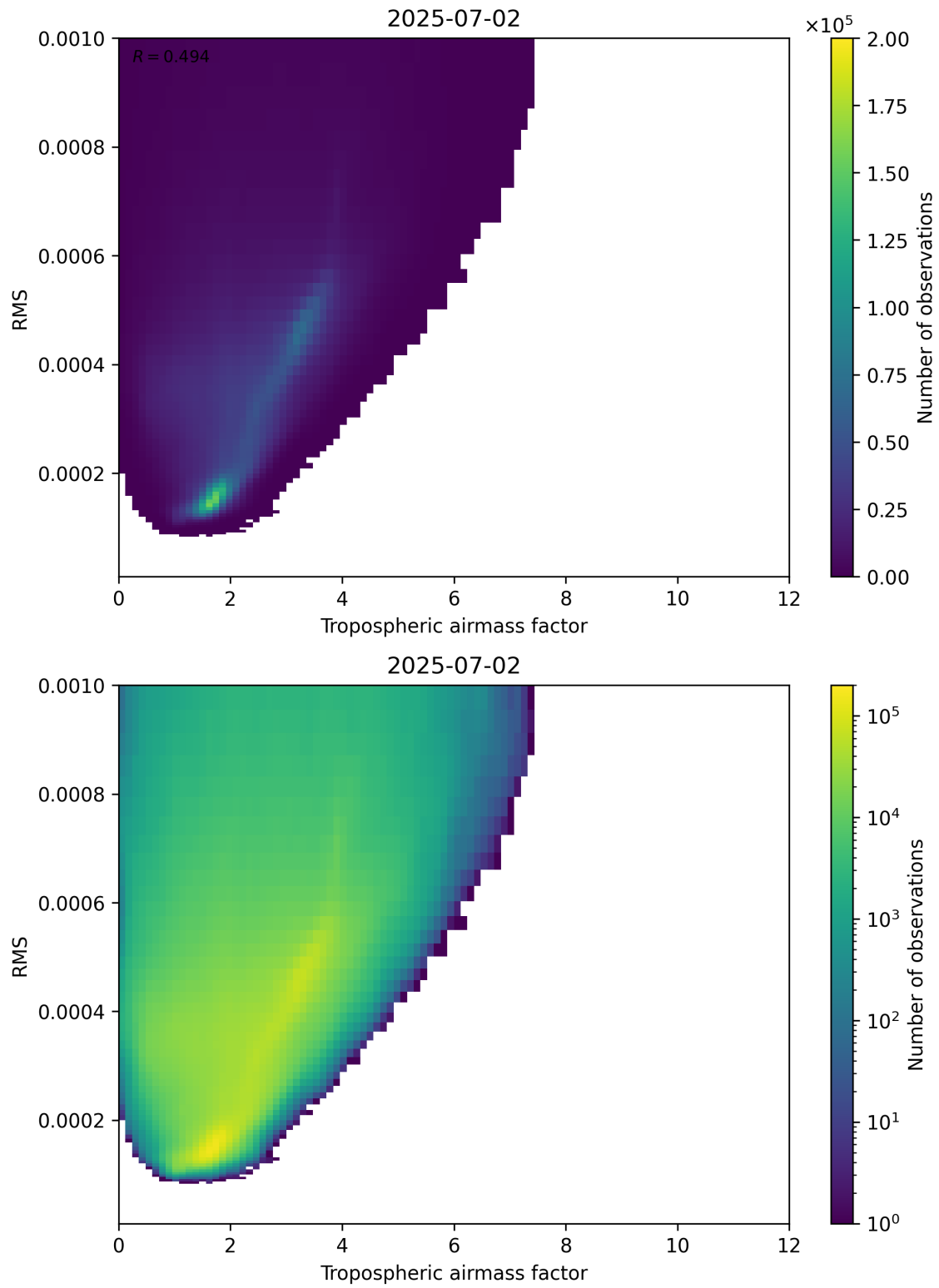
Figure 79: Scatter density plot of “Tropospheric airmass factor” against “RMS” for 2025-07-02 to 2025-07-03.
