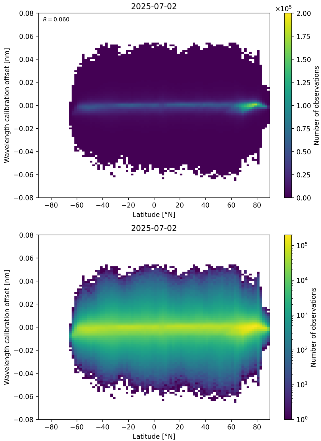
Figure 95: Scatter density plot of “Latitude” against “Wavelength calibration offset” for 2025-07-02 to 2025-07-03.
