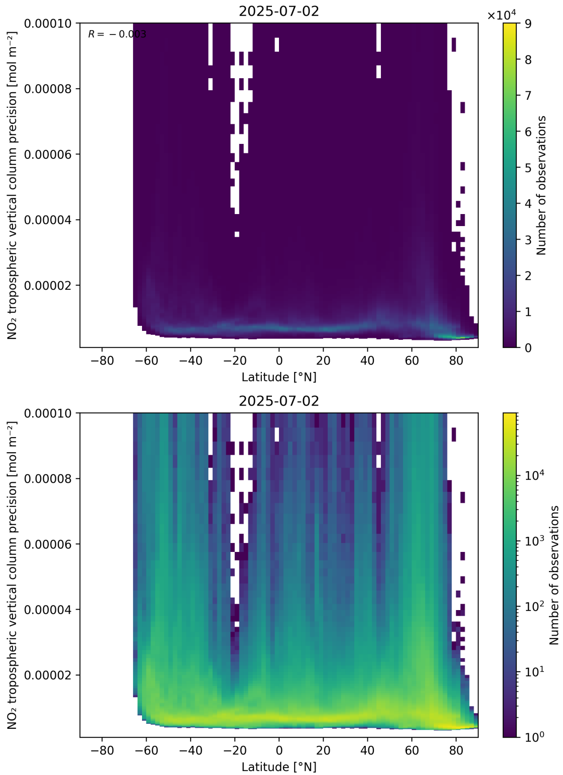
Figure 93: Scatter density plot of “Latitude” against “NO 2 tropospheric vertical column precision” for 2025-07-02 to 2025-07-03.
