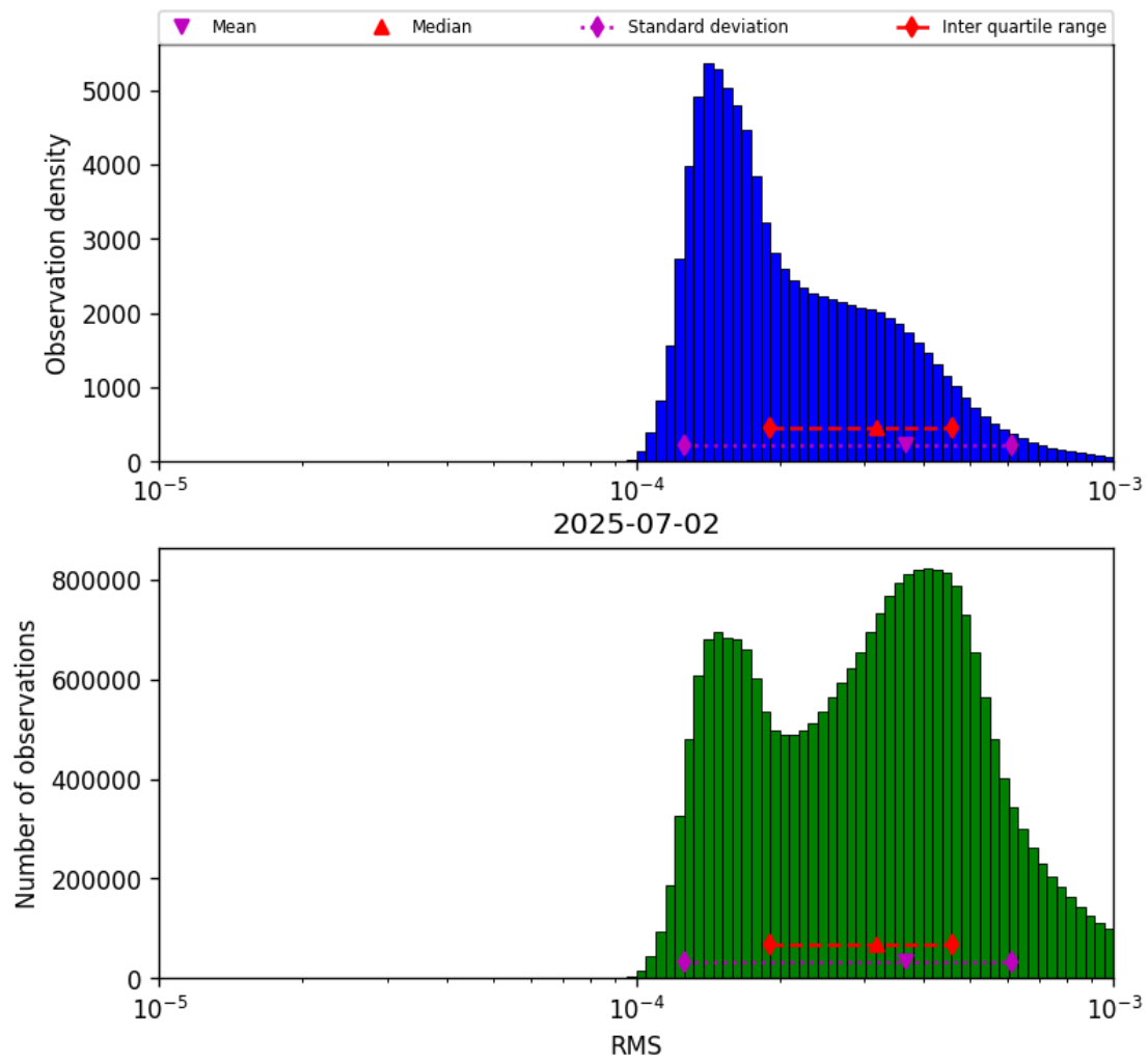
Figure 43: Histogram of “RMS” for 2025-07-02 to 2025-07-03
