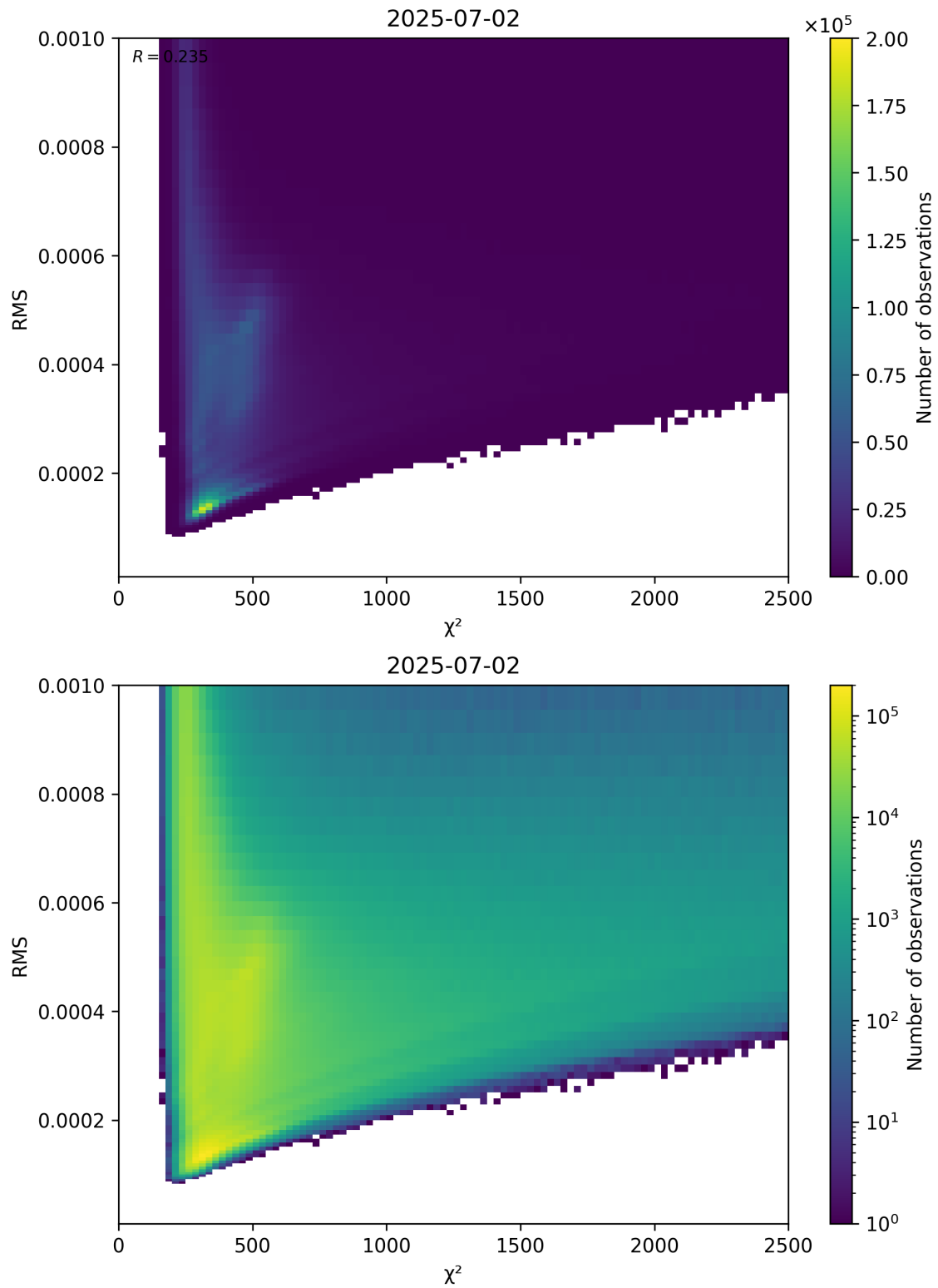
Figure 82: Scatter density plot of “ \chi^2 ” against “RMS” for 2025-07-02 to 2025-07-03.
