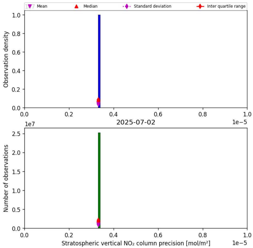
Figure 37: Histogram of “Stratospheric vertical NO 2 column precision” for 2025-07-02 to 2025-07-03
