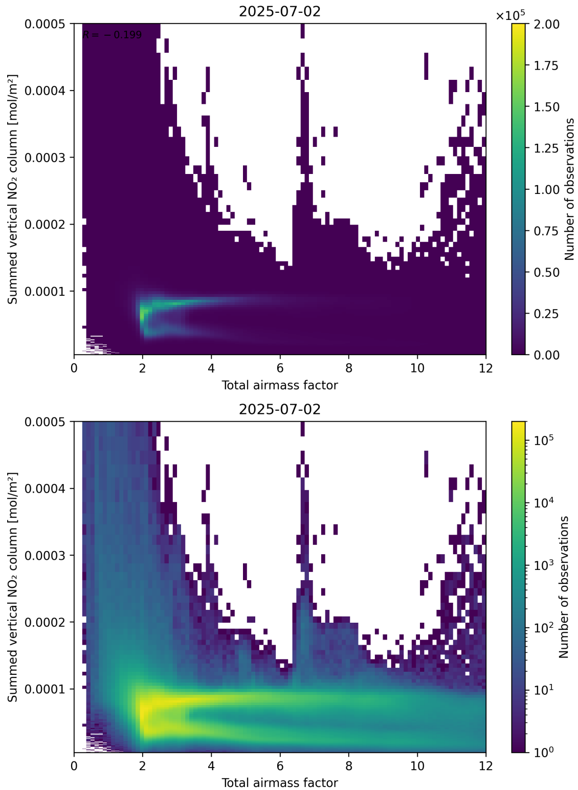
Figure 65: Scatter density plot of “Total airmass factor” against “Summed vertical NO 2 column” for 2025-07-02 to 2025-07-03.
