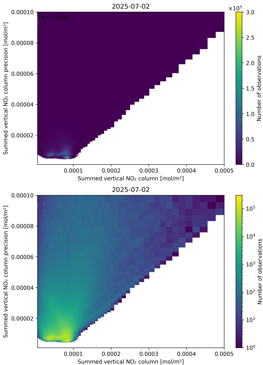
Figure 105: Scatter density plot of “Summed vertical NO 2 column” against “Summed vertical NO 2 column precision” for 2025-07-02 to 2025-07-03.
