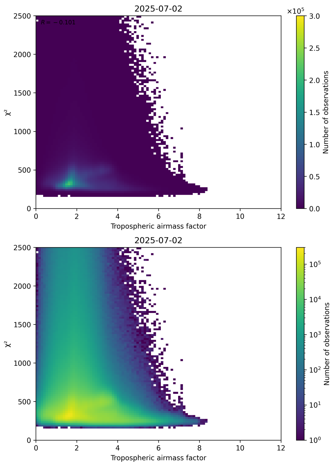
Figure 73: Scatter density plot of “Tropospheric airmass factor” against “ \chi^2 ” for 2025-07-02 to 2025-07-03.
