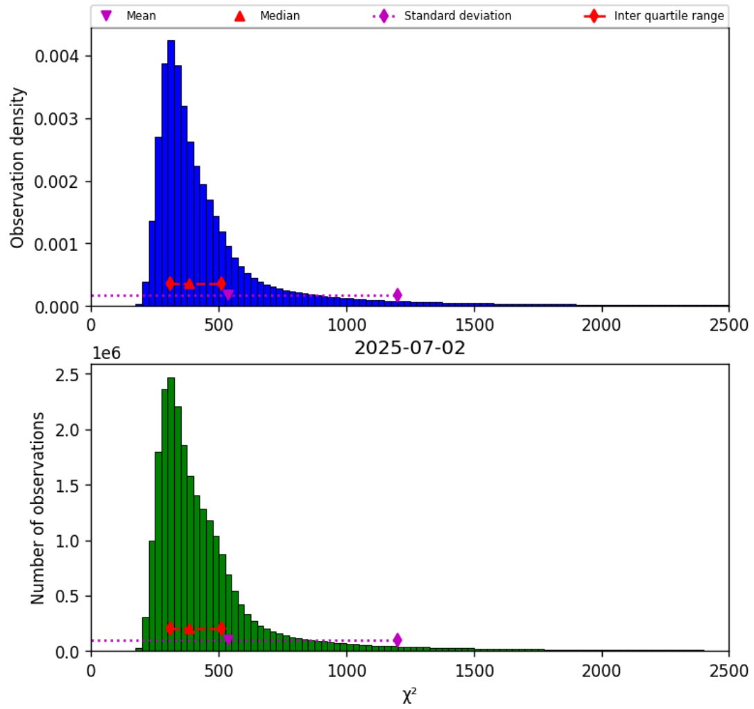
Figure 42: Histogram of “ \chi^2 ” for 2025-07-02 to 2025-07-03
