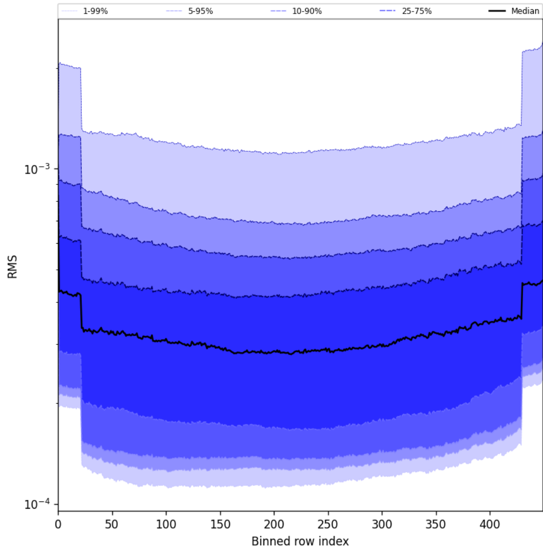
Figure 60: Along track statistics of “RMS” for 2025-07-02 to 2025-07-03
