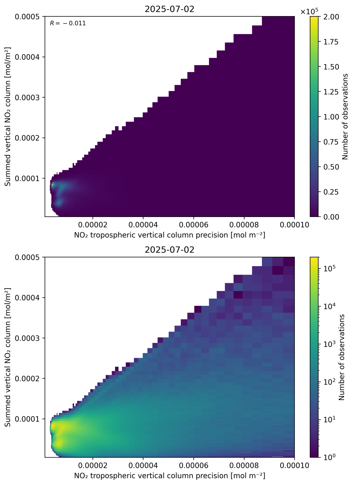
Figure 136: Scatter density plot of “NO 2 tropospheric vertical column precision” against “Summed vertical NO 2 column” for 2025-07-02 to 2025-07-03.
