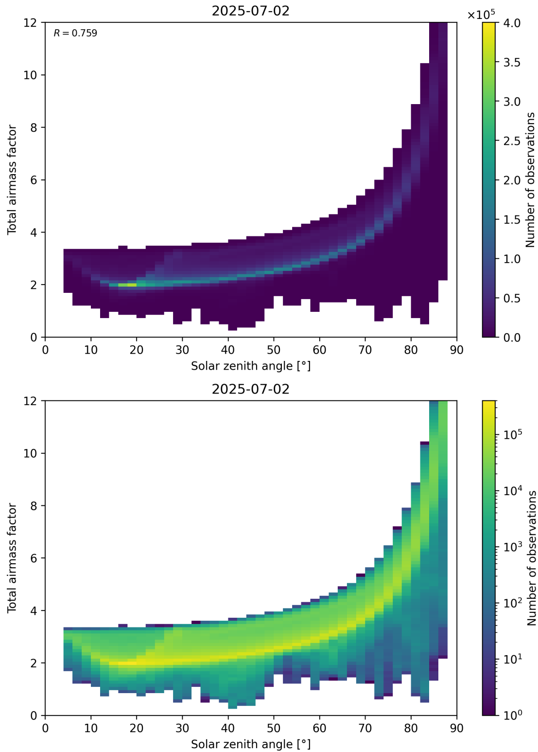
Figure 146: Scatter density plot of “Solar zenith angle” against “Total air mass factor” for 2025-07-02 to 2025-07-03.
