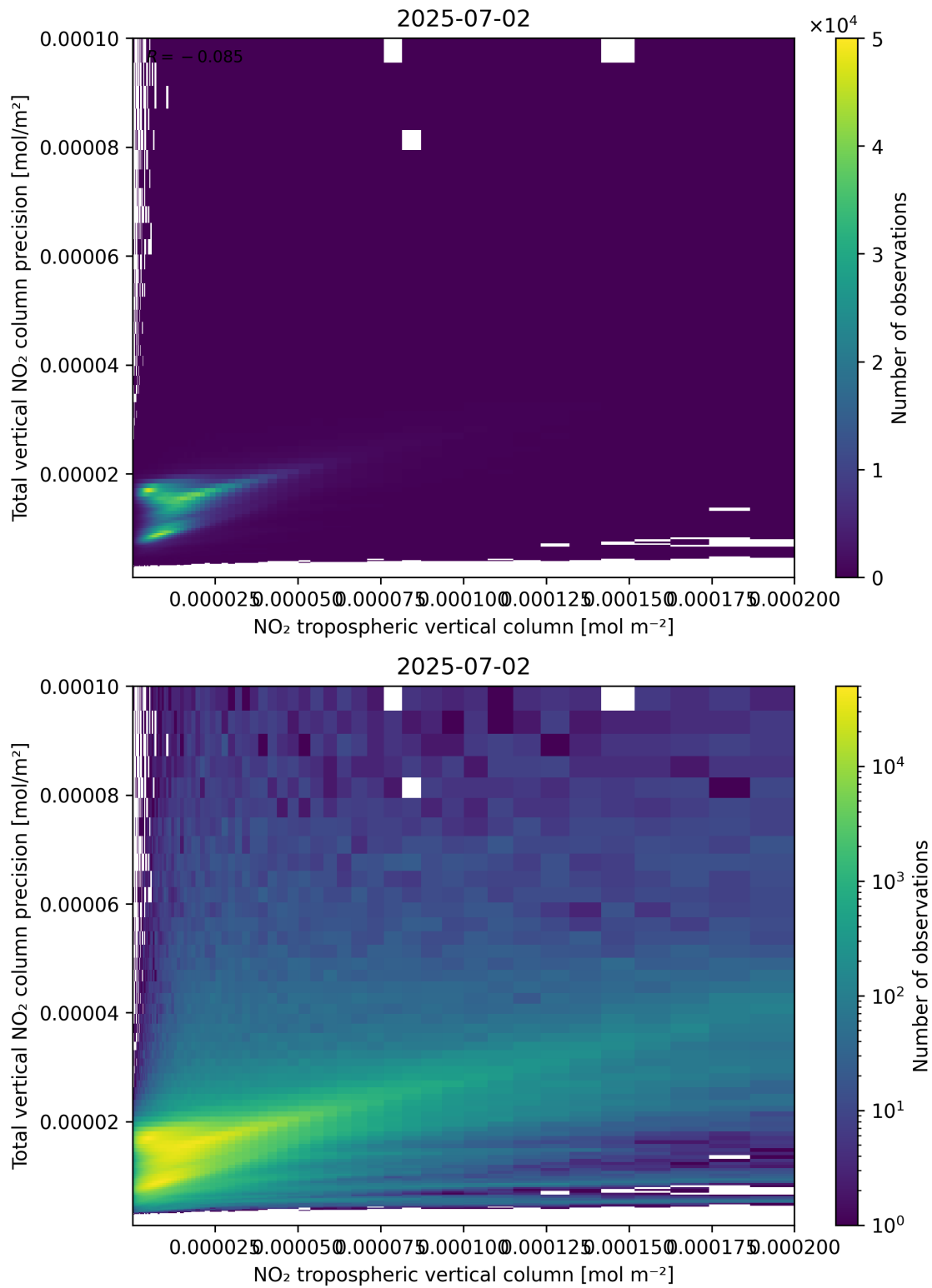
Figure 129: Scatter density plot of “NO 2 tropospheric vertical column” against “Total vertical NO 2 column precision” for 2025-07-02 to 2025-07-03.
