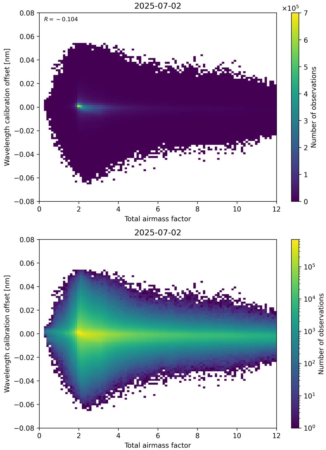
Figure 70: Scatter density plot of “Total airmass factor” against “Wavelength calibration offset” for 2025-07-02 to 2025-07-03.
