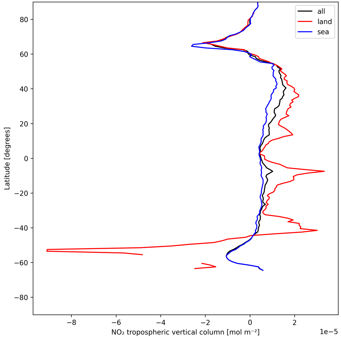
Figure 12: Zonal average of “NO 2 tropospheric vertical column” for 2025-07-02 to 2025-07-03.
