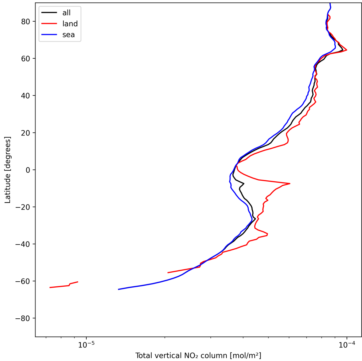
Figure 21: Zonal average of “Total vertical NO 2 column” for 2025-07-02 to 2025-07-03.
