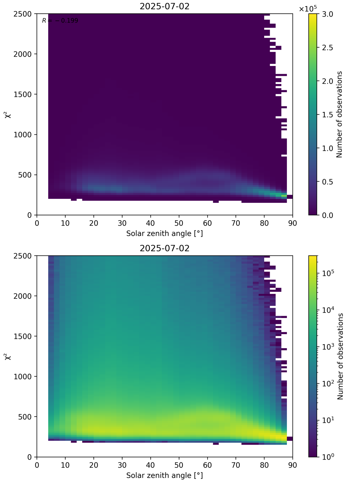
Figure 148: Scatter density plot of “Solar zenith angle” against “ \chi^2 ” for 2025-07-02 to 2025-07-03.
