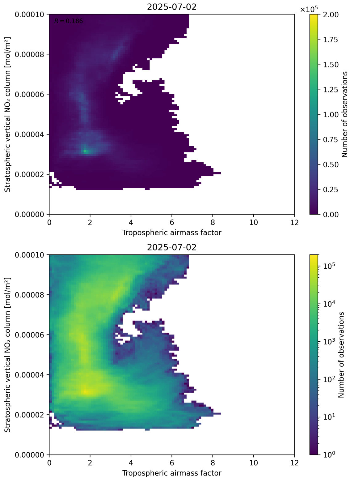
Figure 74: Scatter density plot of “Tropospheric air mass factor” against “Stratospheric vertical NO 2 column” for 2025-07-02 to 2025-07-03.
