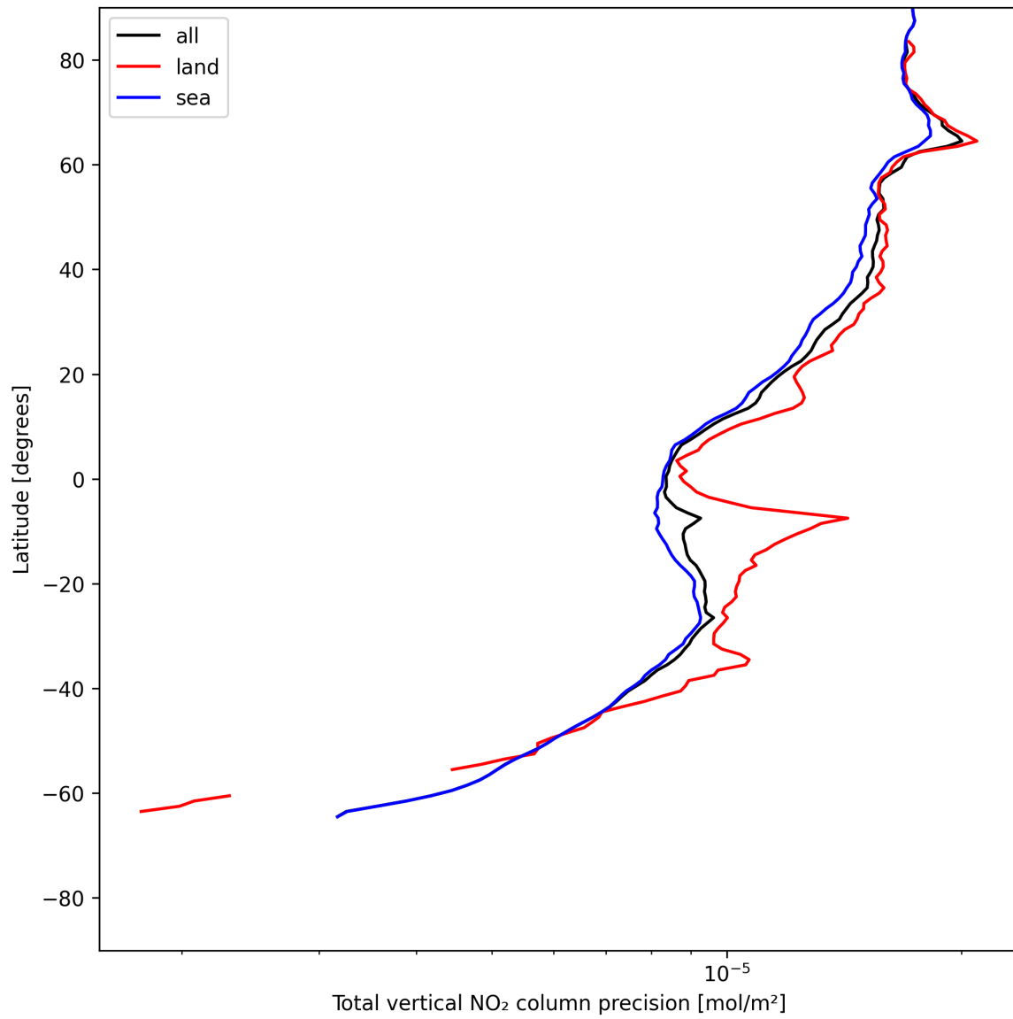
Figure 22: Zonal average of “Total vertical NO 2 column precision” for 2025-07-02 to 2025-07-03.
