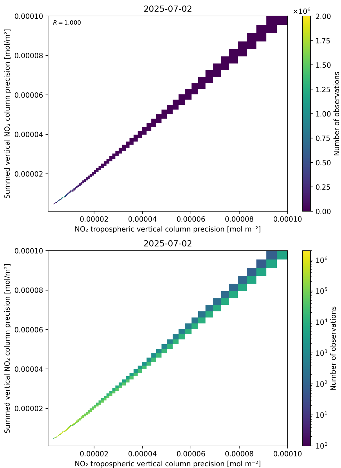
Figure 137: Scatter density plot of “NO 2 tropospheric vertical column precision” against “Summed vertical NO 2 column precision” for 2025-07-02 to 2025-07-03.
