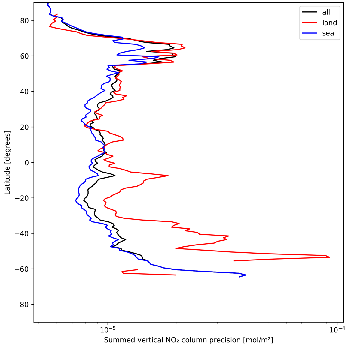
Figure 24: Zonal average of “Summed vertical NO 2 column precision” for 2025-07-02 to 2025-07-03.
