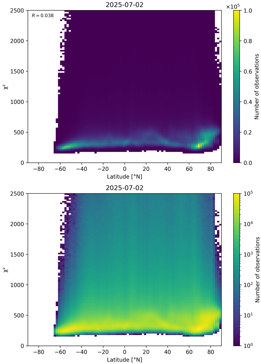
Figure 86: Scatter density plot of “Latitude” against “ \chi^2 ” for 2025-07-02 to 2025-07-03.
