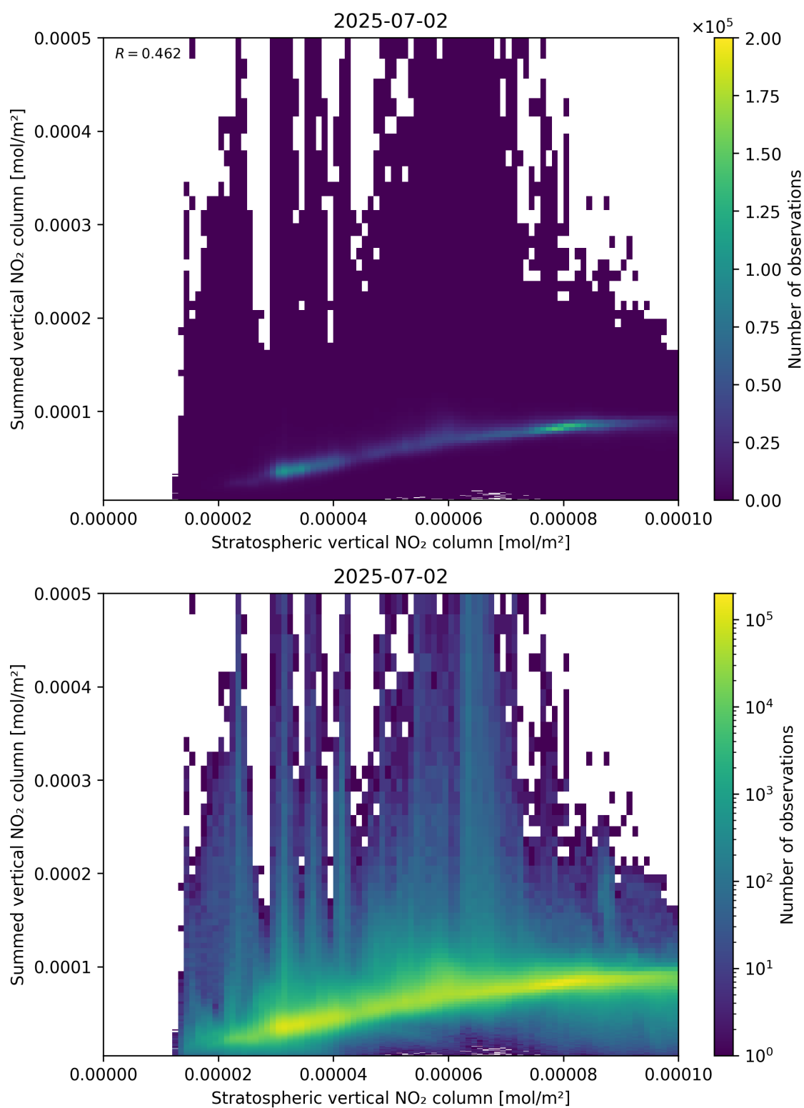
Figure 98: Scatter density plot of “Stratospheric vertical NO 2 column” against “Summed vertical NO 2 column” for 2025-07-02 to 2025-07-03.
