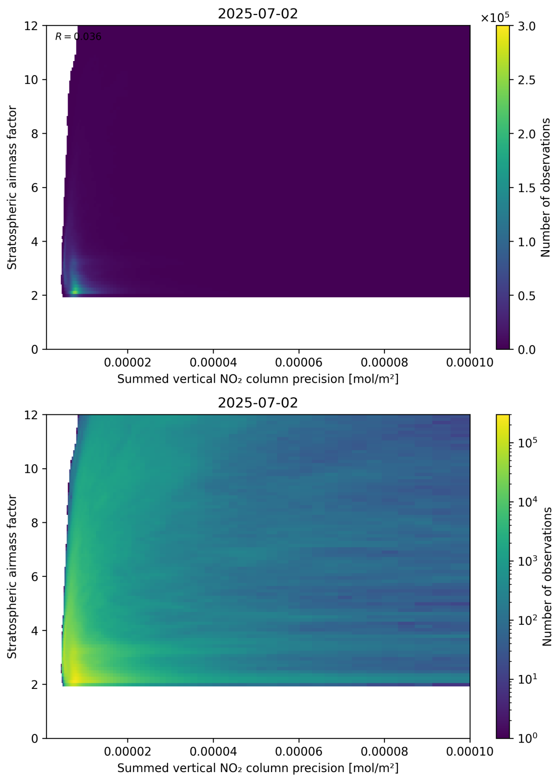
Figure 106: Scatter density plot of “Summed vertical NO 2 column precision” against “Stratospheric airmass factor” for 2025-07-02 to 2025-07-03.
