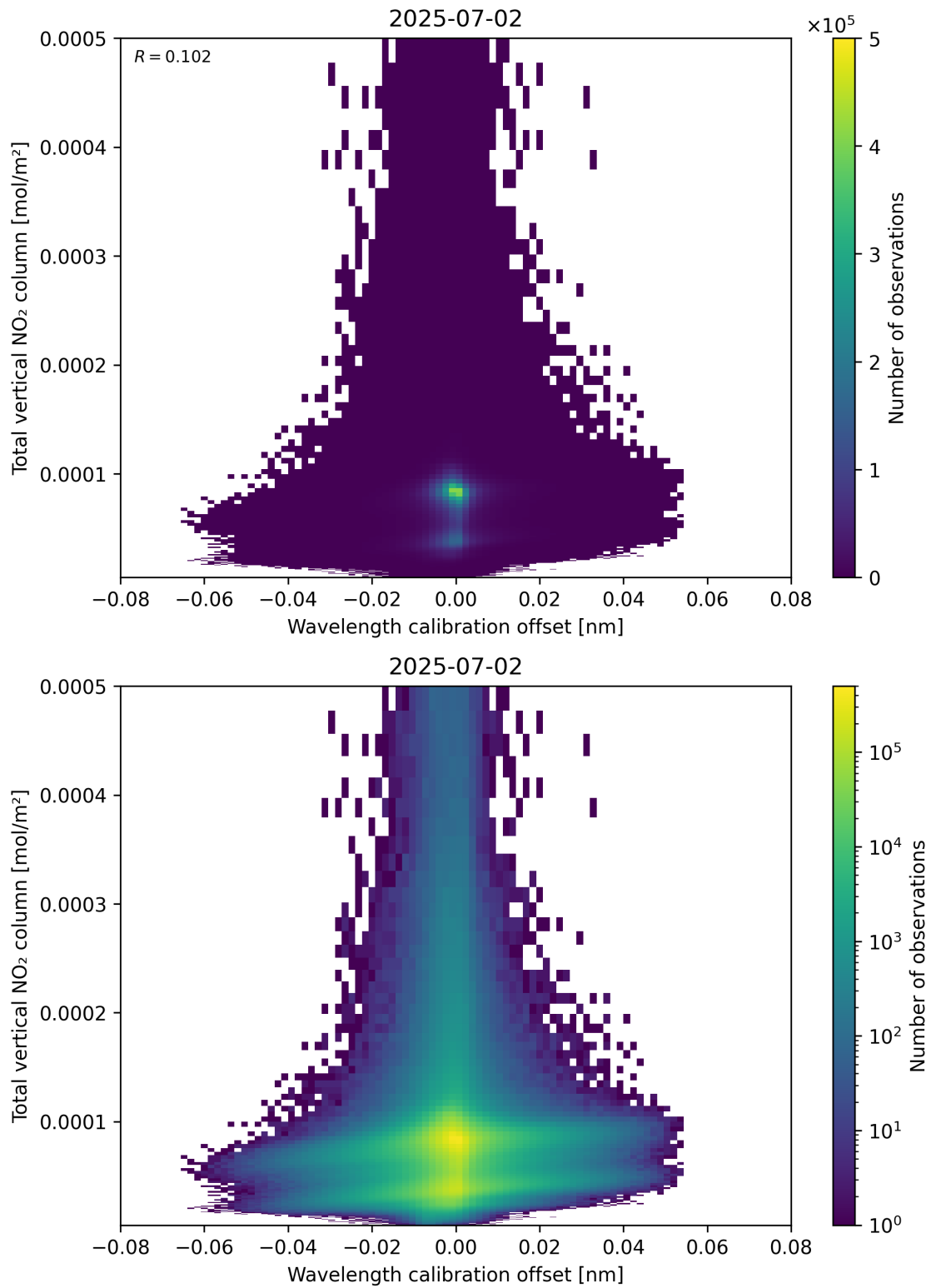
Figure 179: Scatter density plot of “Wavelength calibration offset” against “Total vertical NO 2 column” for 2025-07-02 to 2025-07-03.
