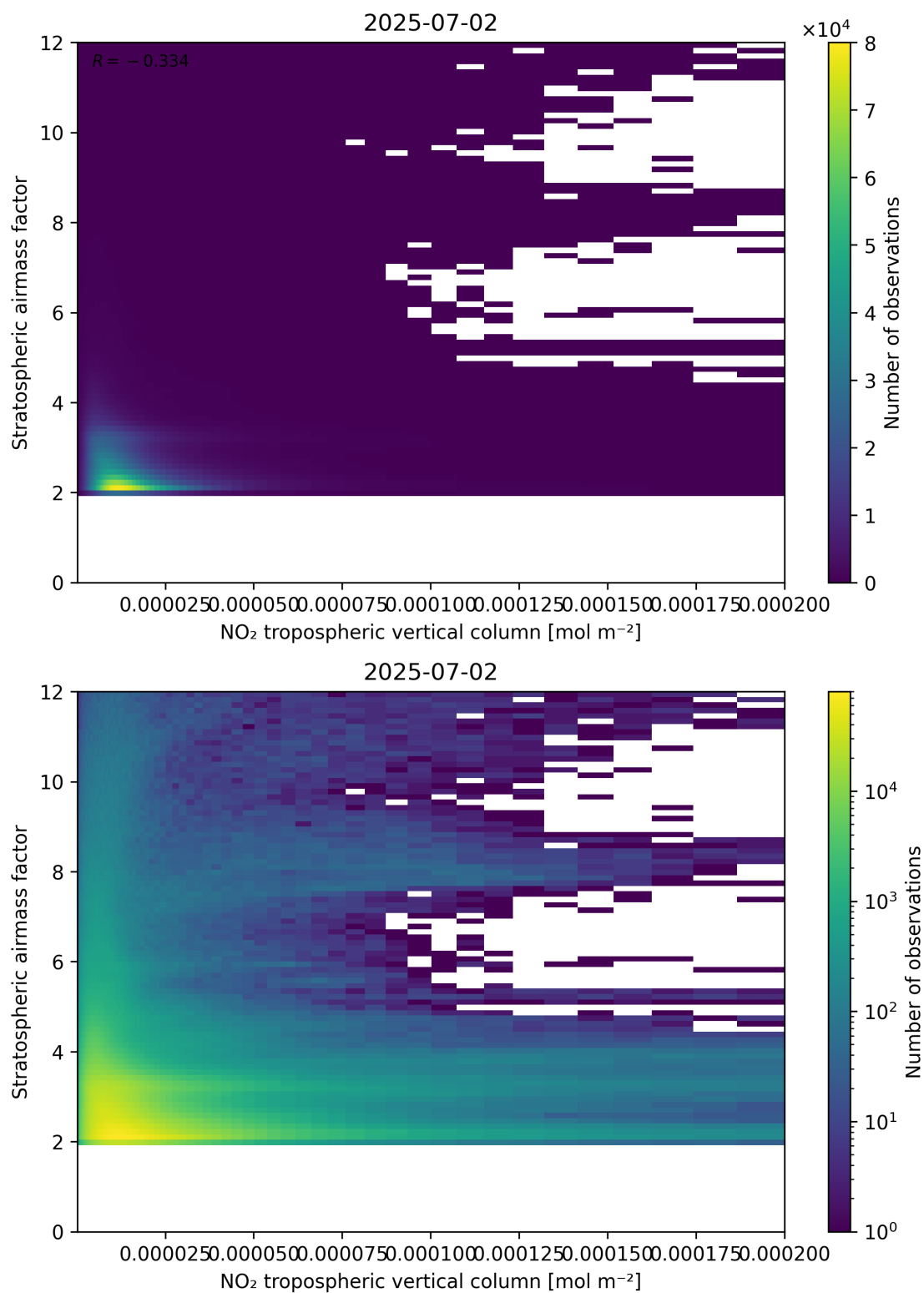
Figure 121: Scatter density plot of “NO 2 tropospheric vertical column” against “Stratospheric air mass factor” for 2025-07-02 to 2025-07-03.
