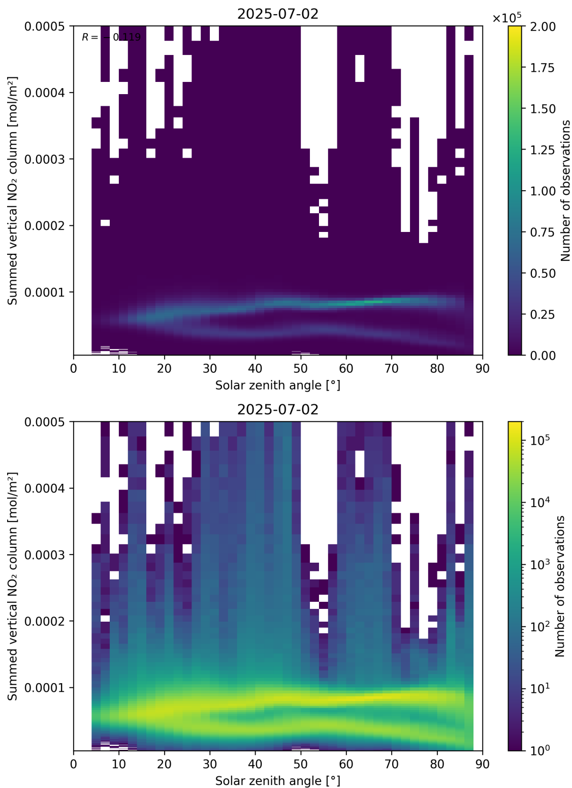
Figure 151: Scatter density plot of “Solar zenith angle” against “Summed vertical NO 2 column” for 2025-07-02 to 2025-07-03.
