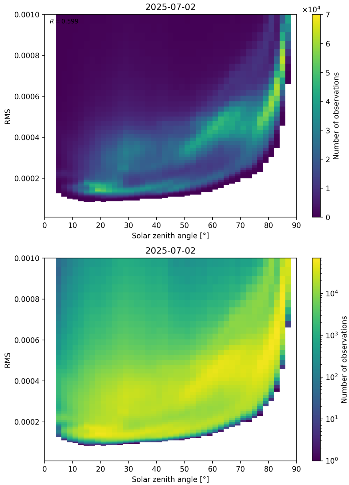
Figure 157: Scatter density plot of “Solar zenith angle” against “RMS” for 2025-07-02 to 2025-07-03.
