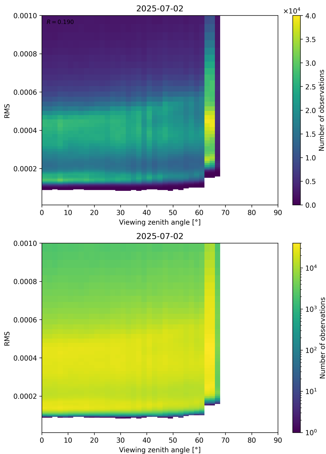
Figure 171: Scatter density plot of “Viewing zenith angle” against “RMS” for 2025-07-02 to 2025-07-03.
