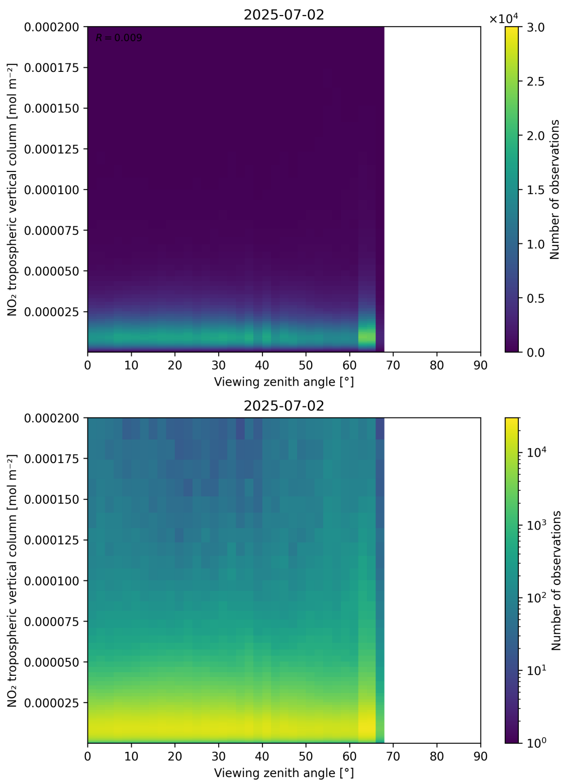
Figure 169: Scatter density plot of “Viewing zenith angle” against “NO 2 tropospheric vertical column” for 2025-07-02 to 2025-07-03.
