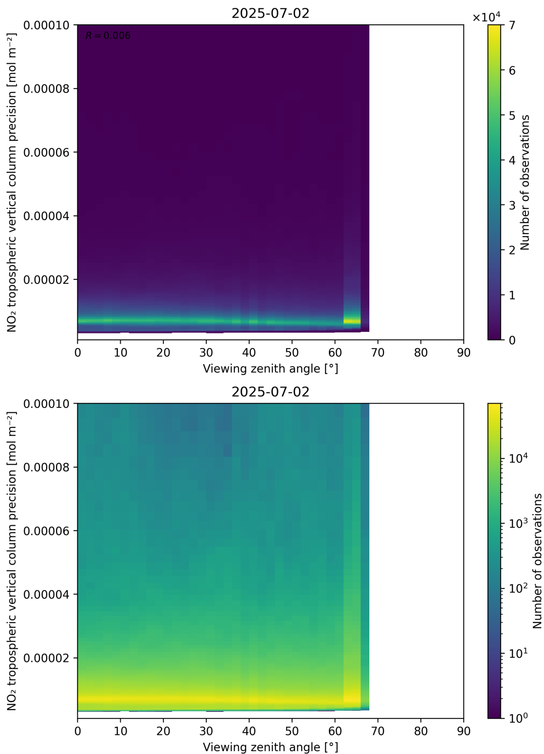
Figure 170: Scatter density plot of “Viewing zenith angle” against “NO 2 tropospheric vertical column precision” for 2025-07-02 to 2025-07-03.
