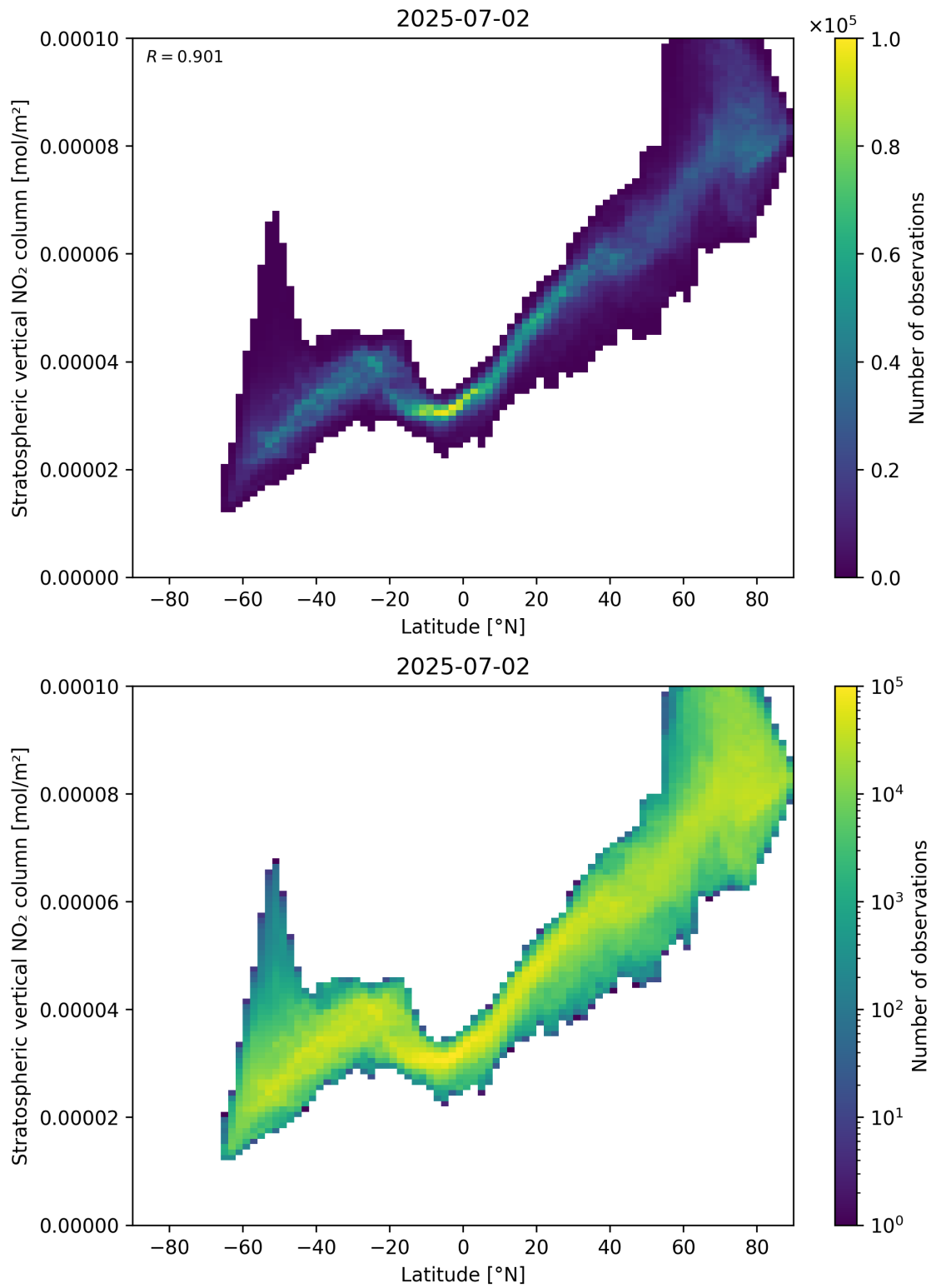
Figure 87: Scatter density plot of “Latitude” against “Stratospheric vertical \text{NO}_2 column” for 2025-07-02 to 2025-07-03.
