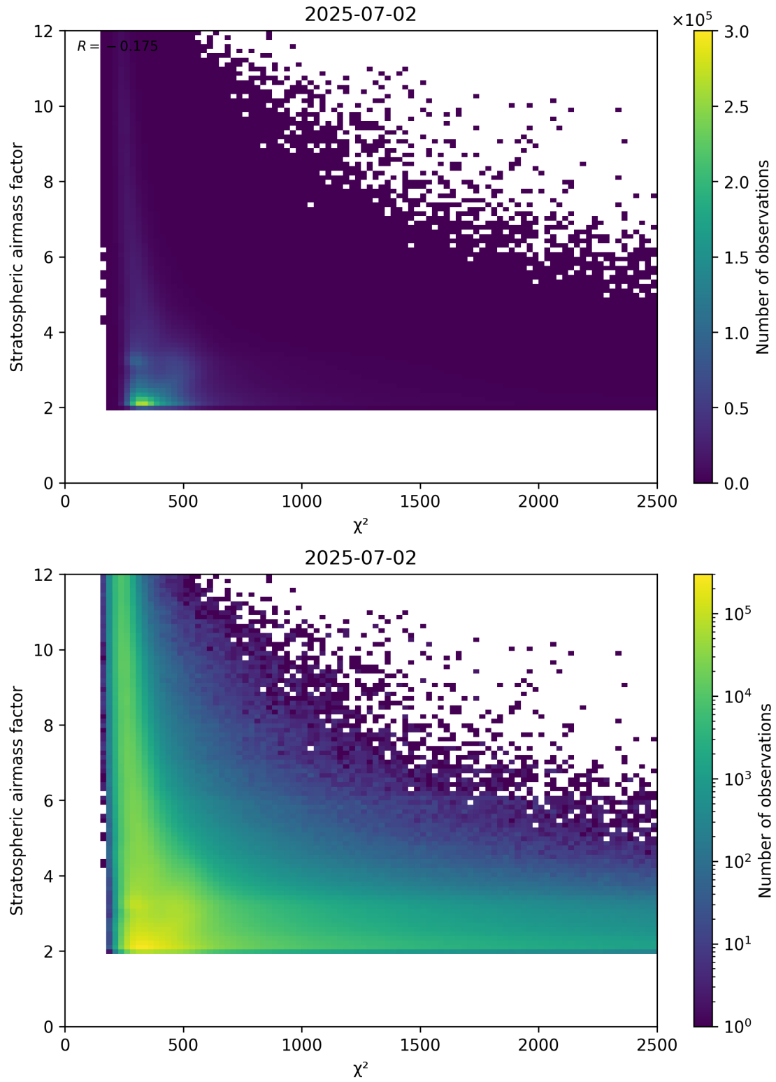
Figure 81: Scatter density plot of “ \chi^2 ” against “Stratospheric airmass factor” for 2025-07-02 to 2025-07-03.
