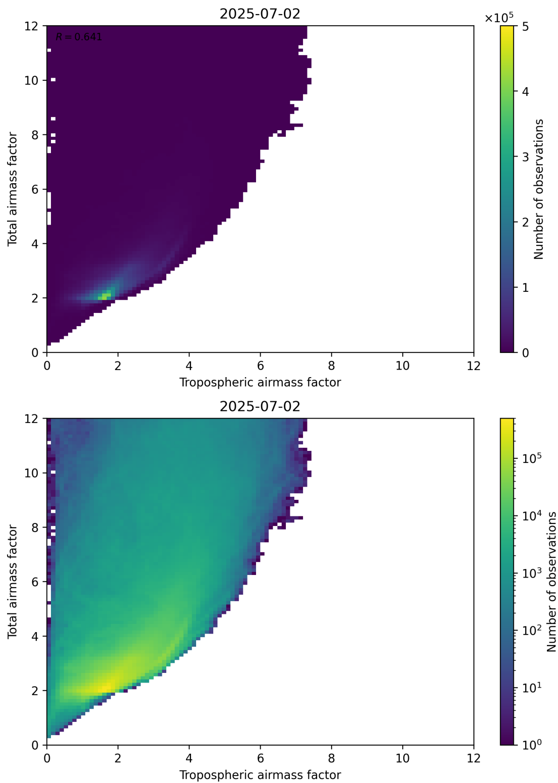
Figure 72: Scatter density plot of “Tropospheric airmass factor” against “Total airmass factor” for 2025-07-02 to 2025-07-03.
