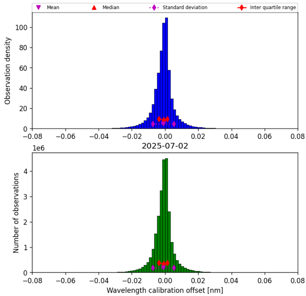
Figure 35: Histogram of “Wavelength calibration offset” for 2025-07-02 to 2025-07-03
