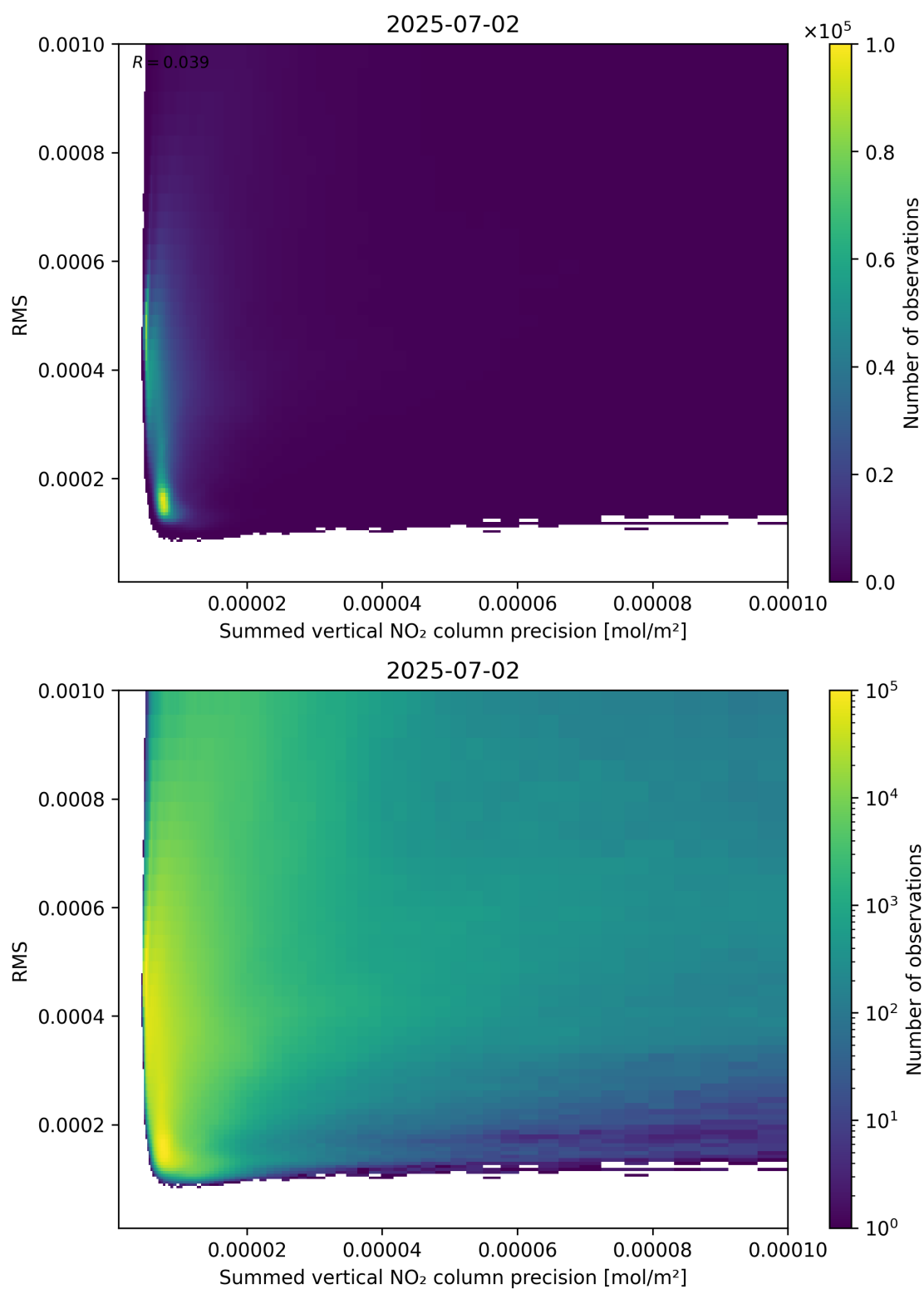
Figure 108: Scatter density plot of “Summed vertical NO 2 column precision” against “RMS” for 2025-07-02 to 2025-07-03.
