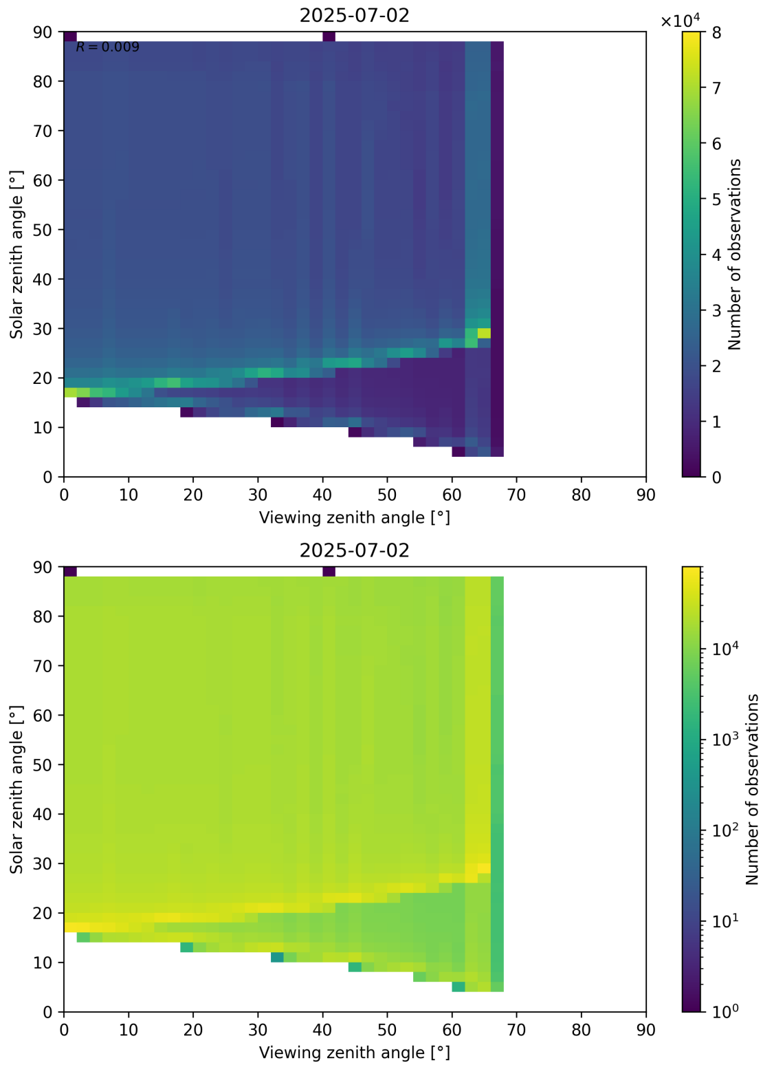
Figure 172: Scatter density plot of “Viewing zenith angle” against “Solar zenith angle” for 2025-07-02 to 2025-07-03.
