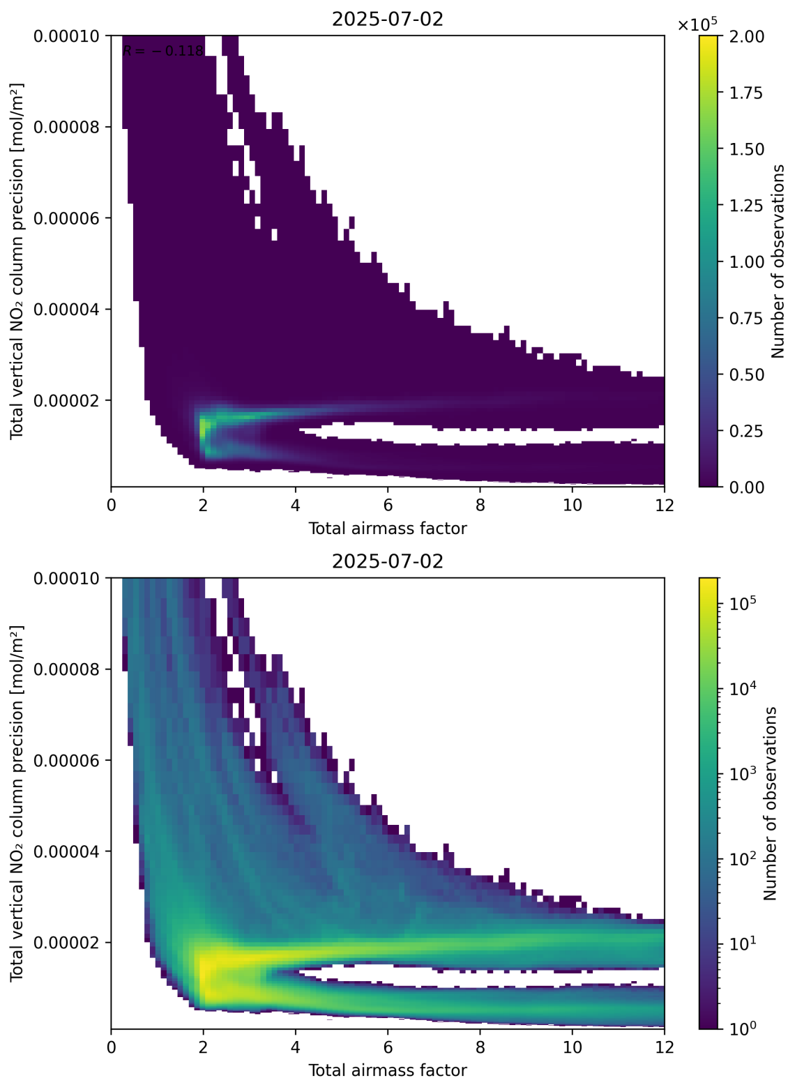
Figure 68: Scatter density plot of “Total airmass factor” against “Total vertical NO 2 column precision” for 2025-07-02 to 2025-07-03.
