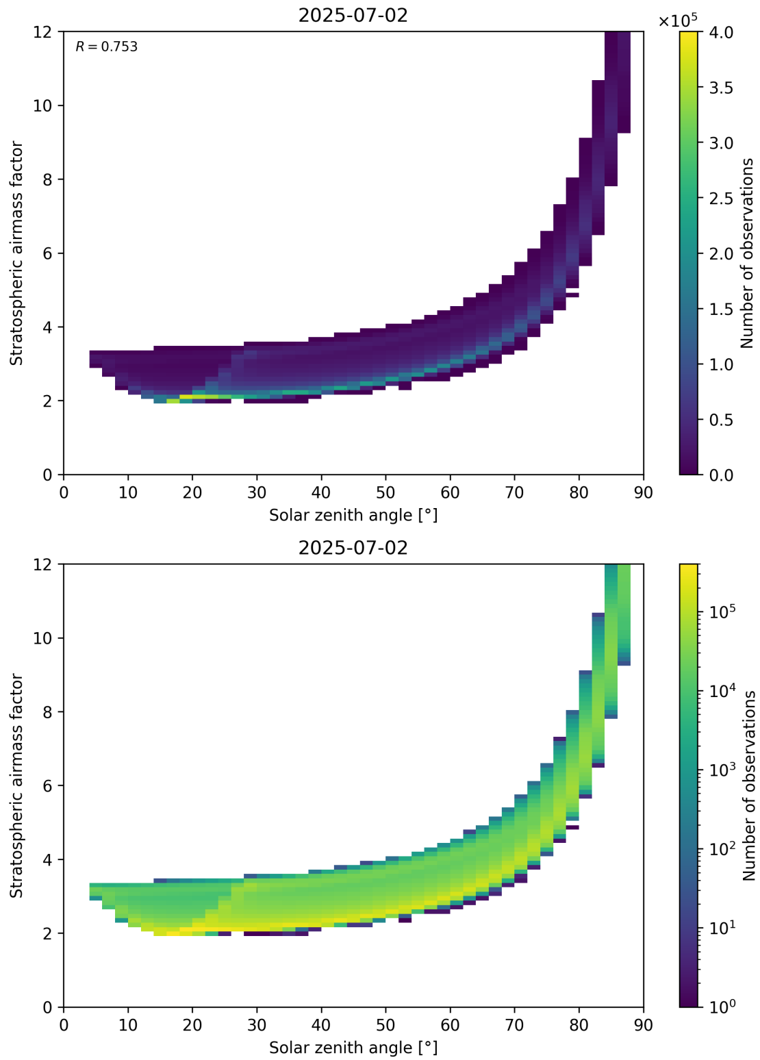
Figure 145: Scatter density plot of “Solar zenith angle” against “Stratospheric airmass factor” for 2025-07-02 to 2025-07-03.
