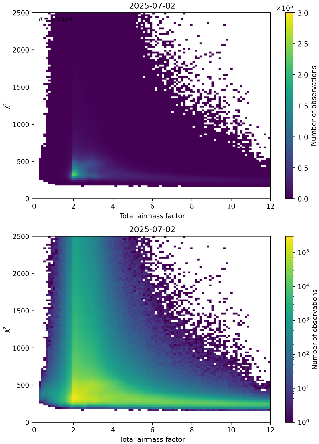
Figure 63: Scatter density plot of “Total airmass factor” against “ \chi^2 ” for 2025-07-02 to 2025-07-03.
