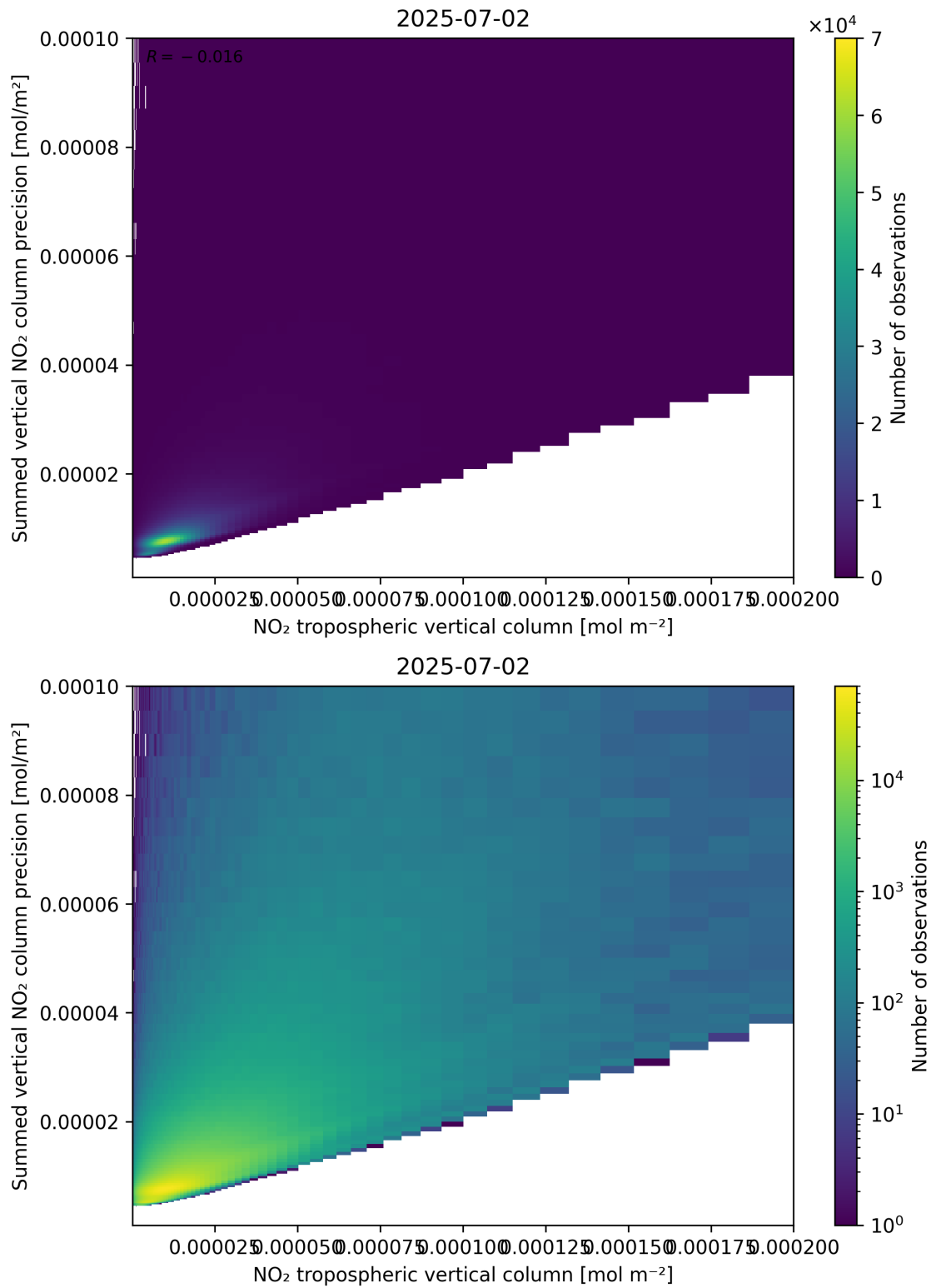
Figure 127: Scatter density plot of “NO 2 tropospheric vertical column” against “Summed vertical NO 2 column precision” for 2025-07-02 to 2025-07-03.
