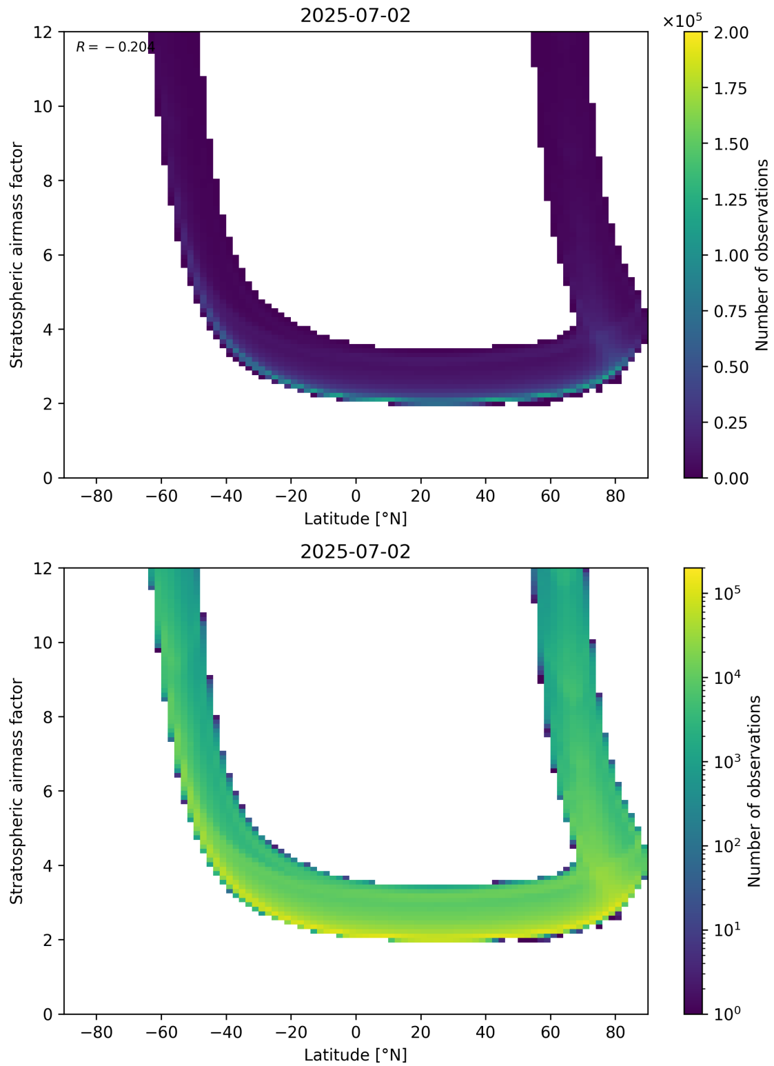
Figure 83: Scatter density plot of “Latitude” against “Stratospheric air mass factor” for 2025-07-02 to 2025-07-03.
