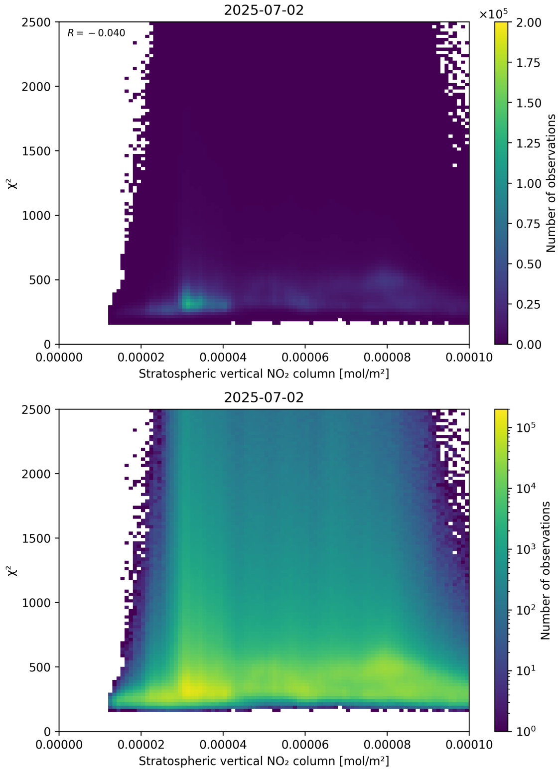
Figure 97: Scatter density plot of “Stratospheric vertical NO 2 column” against “ \chi^2 ” for 2025-07-02 to 2025-07-03.
