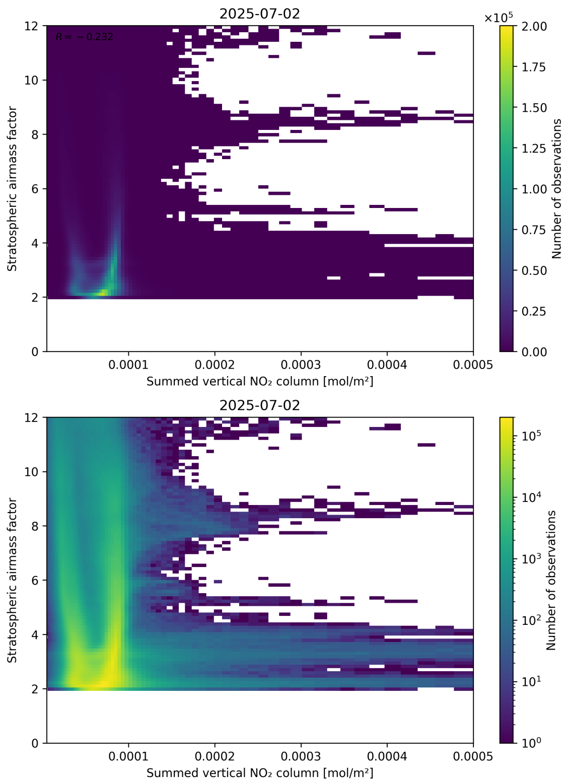
Figure 103: Scatter density plot of “Summed vertical NO 2 column” against “Stratospheric air mass factor” for 2025-07-02 to 2025-07-03.
