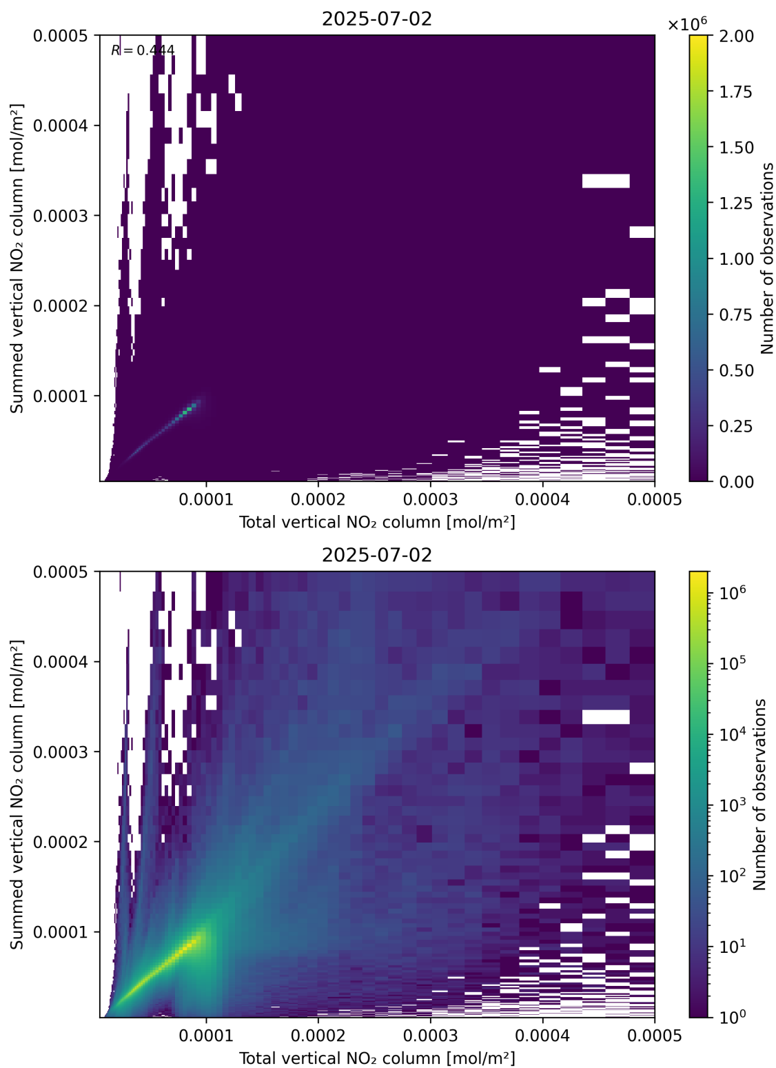
Figure 112: Scatter density plot of “Total vertical NO 2 column” against “Summed vertical NO 2 column” for 2025-07-02 to 2025-07-03.
