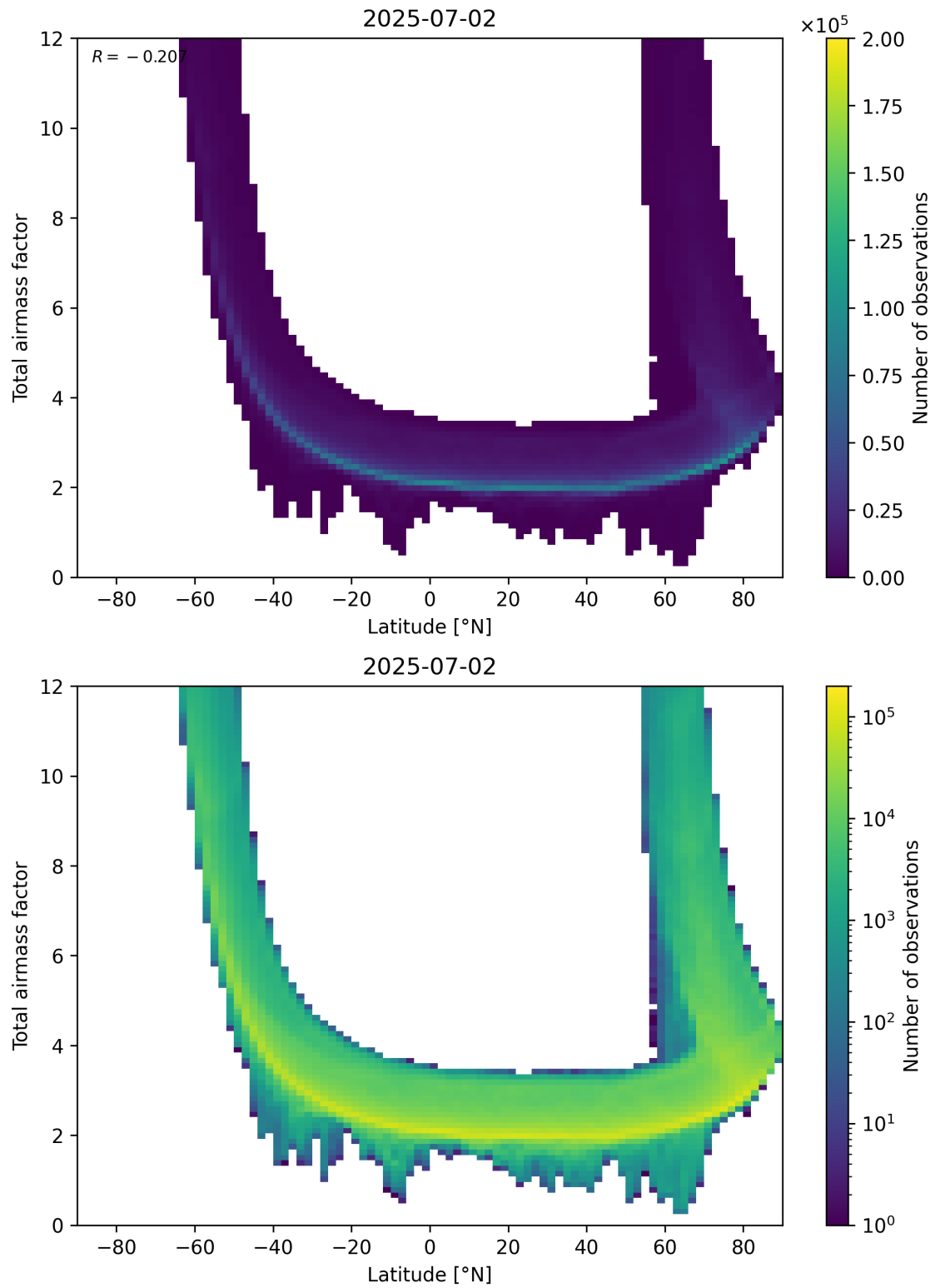
Figure 84: Scatter density plot of “Latitude” against “Total airmass factor” for 2025-07-02 to 2025-07-03.
