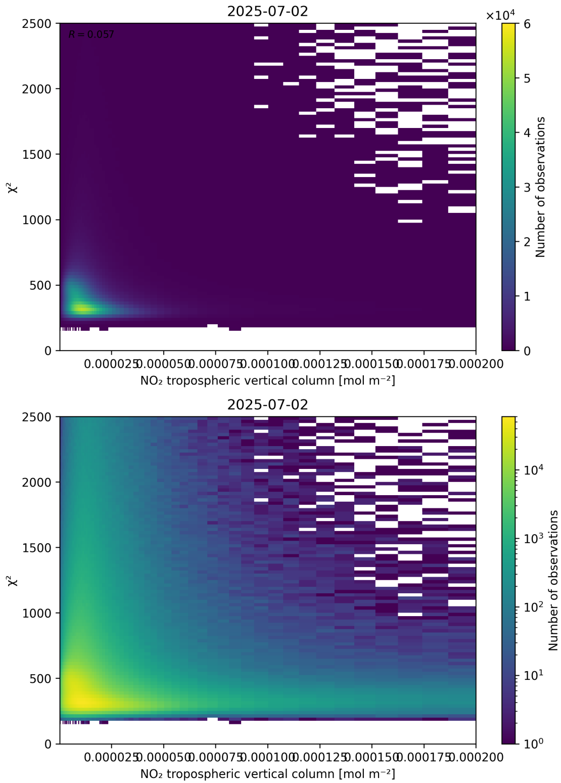
Figure 124: Scatter density plot of “NO 2 tropospheric vertical column” against “ \chi^2 ” for 2025-07-02 to 2025-07-03.
