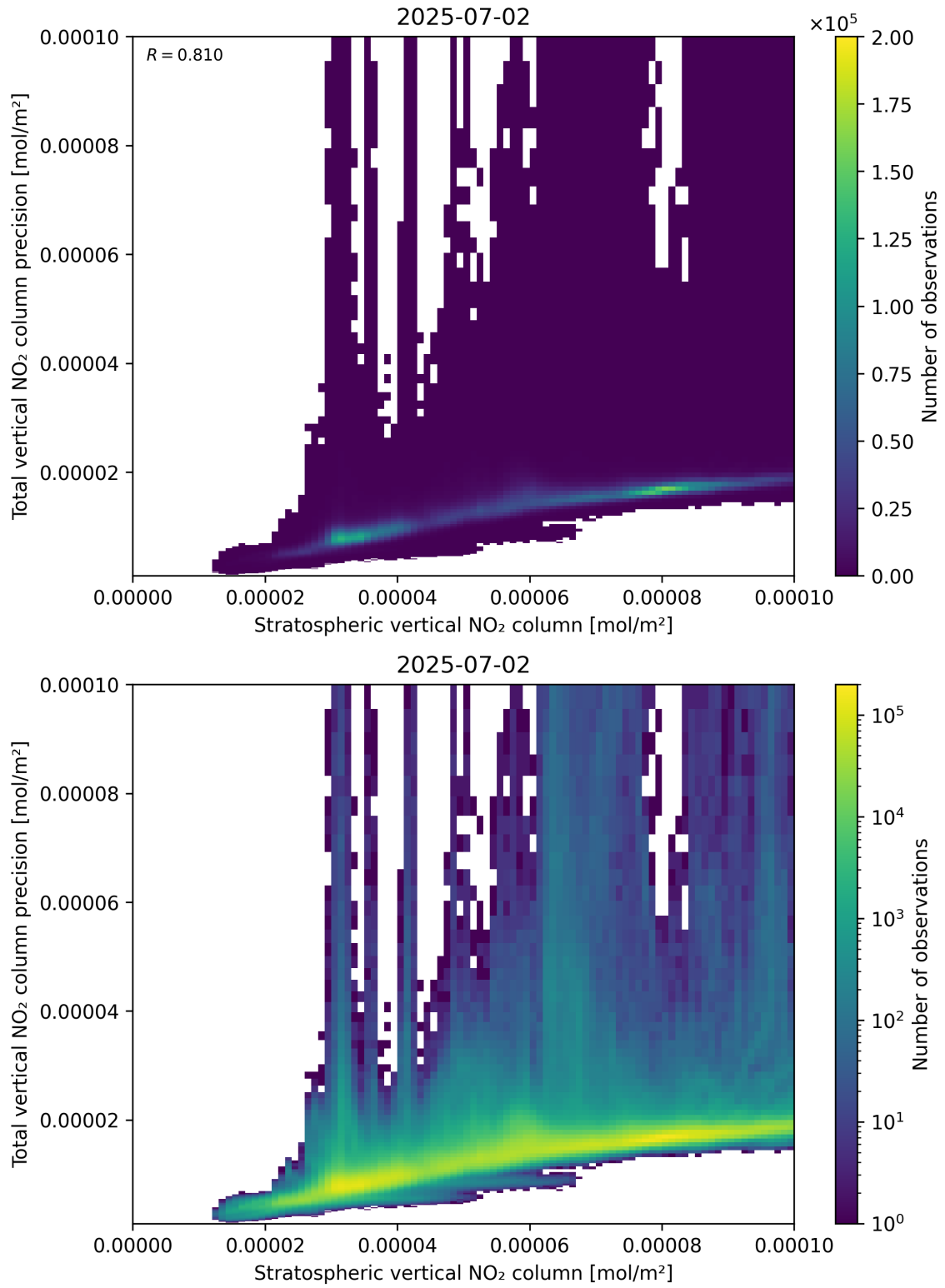
Figure 101: Scatter density plot of “Stratospheric vertical NO 2 column” against “Total vertical NO 2 column precision” for 2025-07-02 to 2025-07-03.
