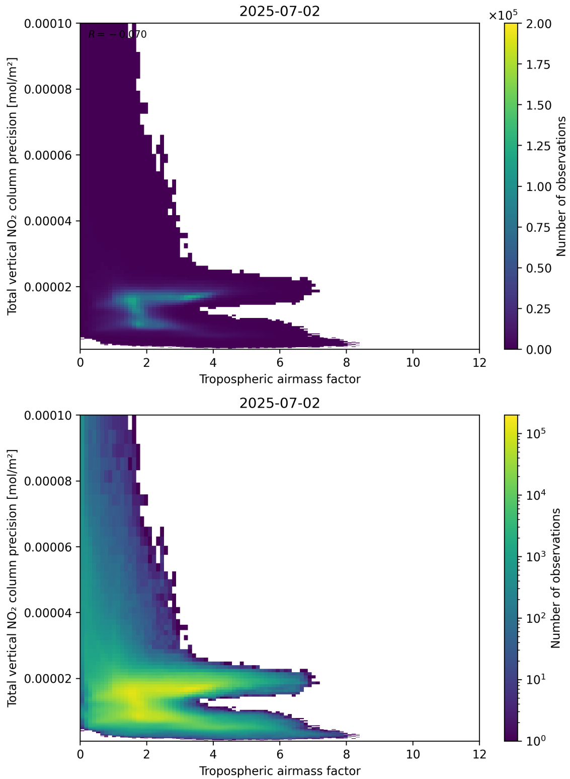
Figure 78: Scatter density plot of “Tropospheric air mass factor” against “Total vertical NO 2 column precision” for 2025-07-02 to 2025-07-03.
