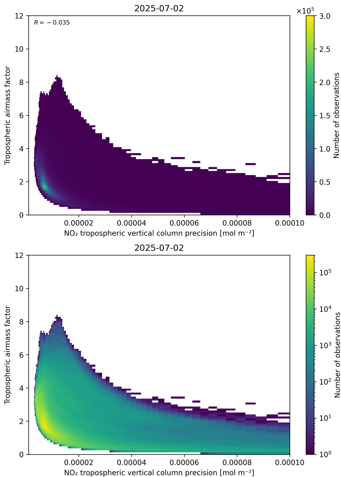
Figure 133: Scatter density plot of “NO 2 tropospheric vertical column precision” against “Tropospheric air mass factor” for 2025-07-02 to 2025-07-03.
