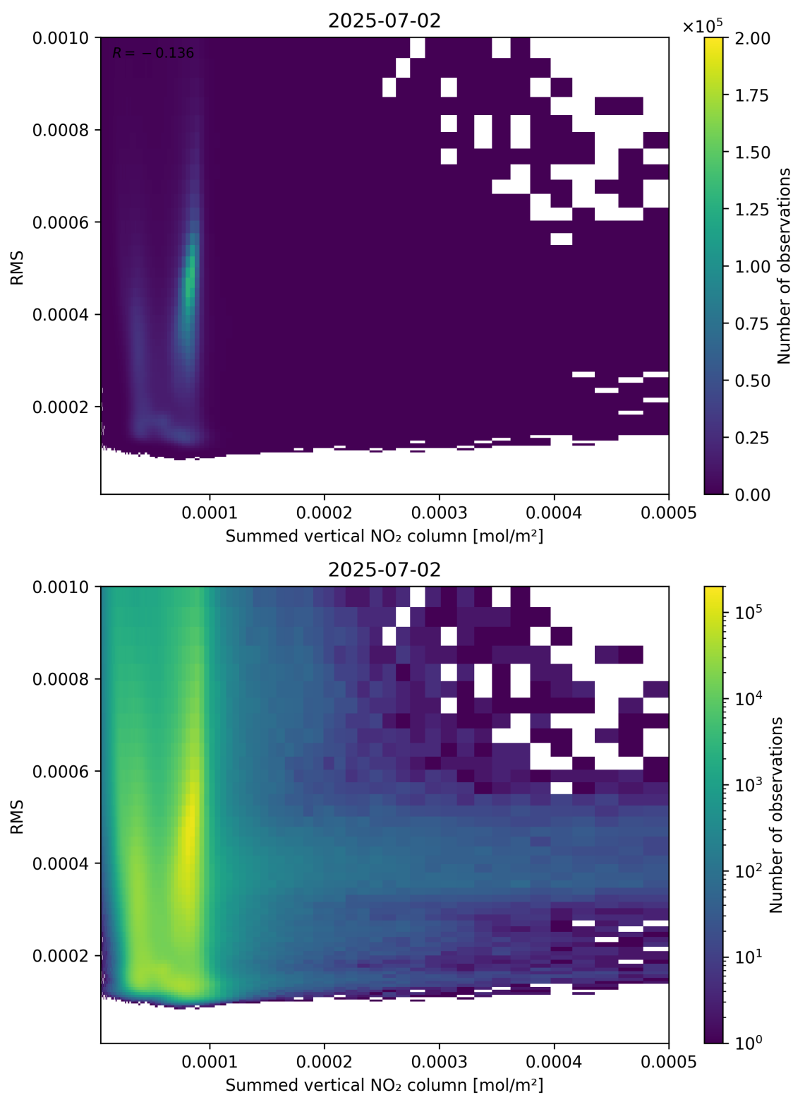
Figure 109: Scatter density plot of “Summed vertical NO 2 column” against “RMS” for 2025-07-02 to 2025-07-03.
