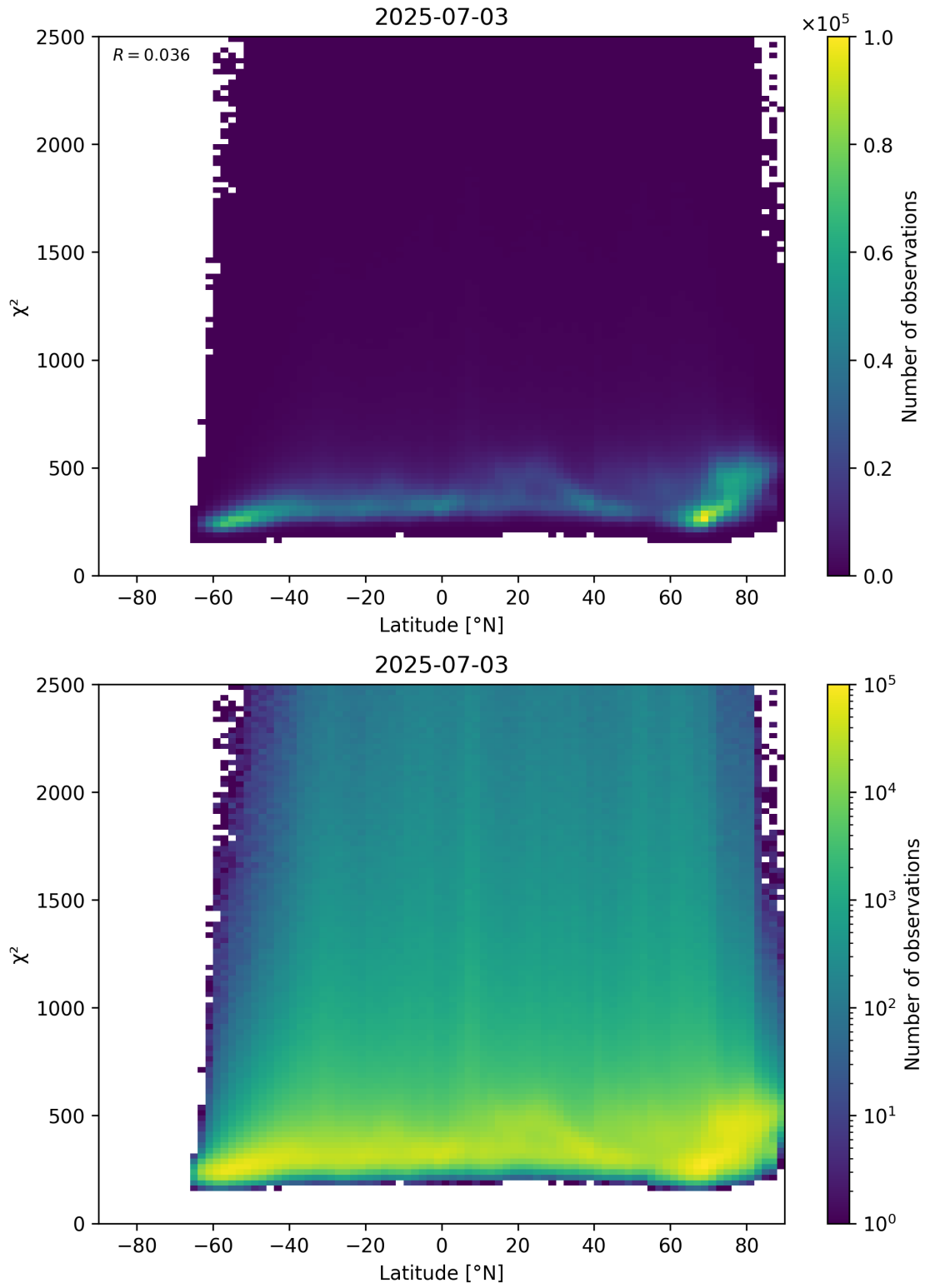
Figure 86: Scatter density plot of “Latitude” against “ \chi^2 ” for 2025-07-03 to 2025-07-04.
