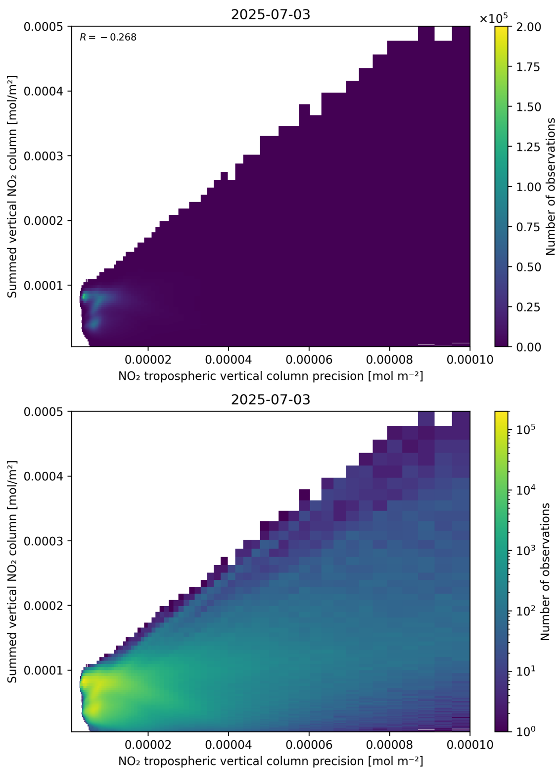
Figure 136: Scatter density plot of “NO 2 tropospheric vertical column precision” against “Summed vertical NO 2 column” for 2025-07-03 to 2025-07-04.
