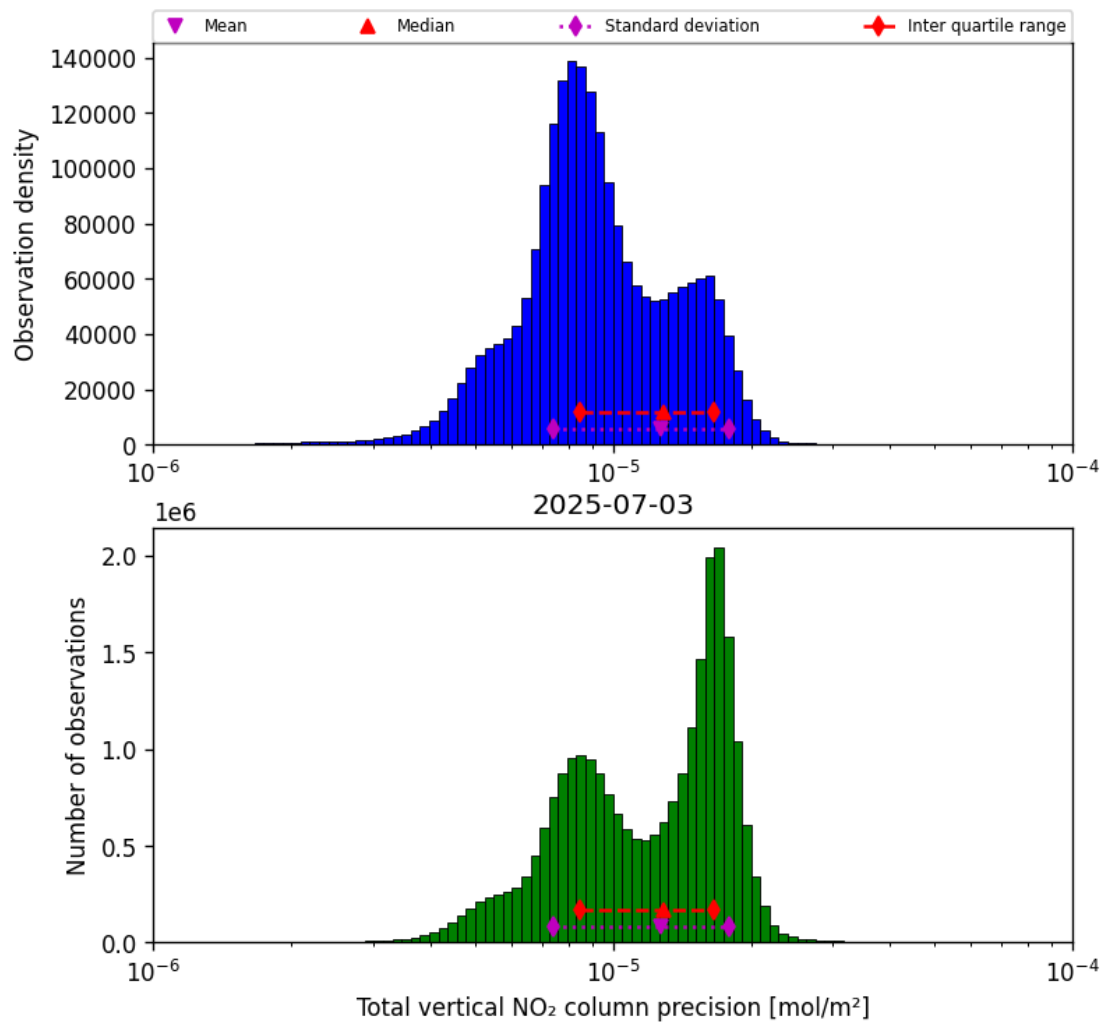
Figure 39: Histogram of “Total vertical NO 2 column precision” for 2025-07-03 to 2025-07-04
