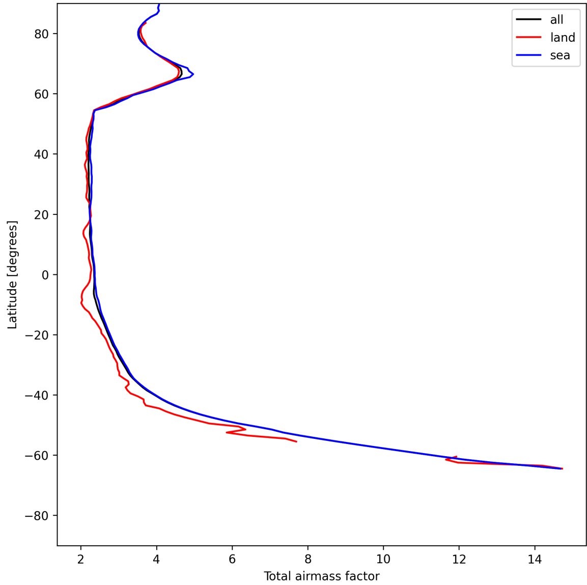
Figure 15: Zonal average of “Total airmass factor” for 2025-07-03 to 2025-07-04.
