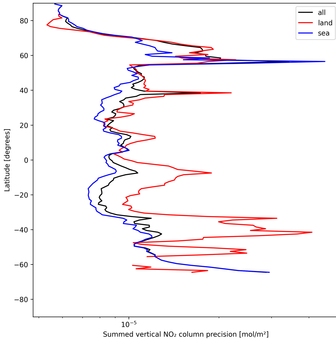
Figure 24: Zonal average of “Summed vertical NO 2 column precision” for 2025-07-03 to 2025-07-04.
