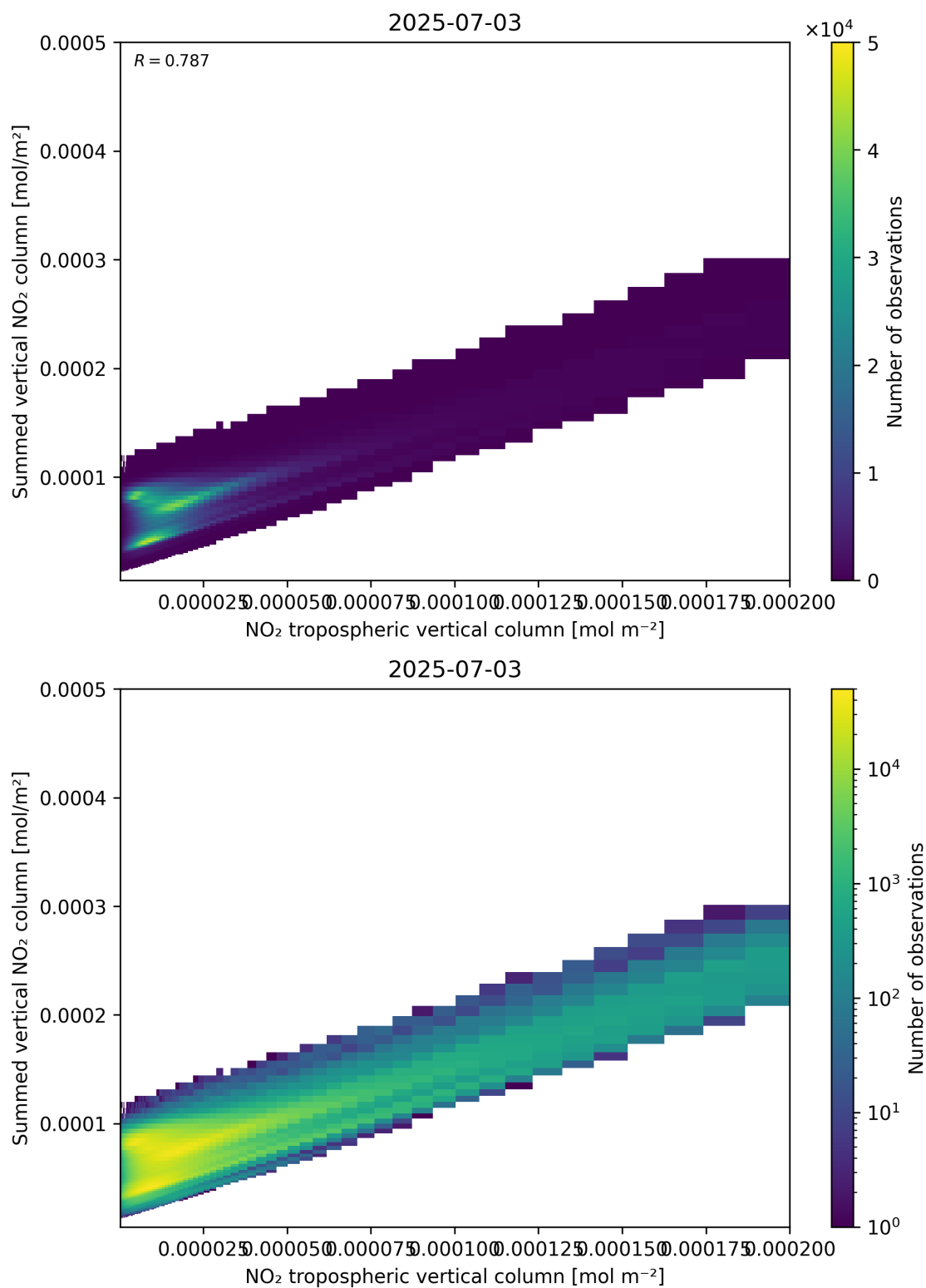
Figure 126: Scatter density plot of “NO 2 tropospheric vertical column” against “Summed vertical NO 2 column” for 2025-07-03 to 2025-07-04.
