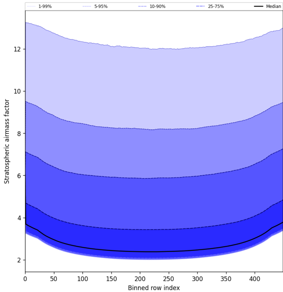
Figure 61: Along track statistics of “Stratospheric airmass factor” for 2025-07-03 to 2025-07-04
