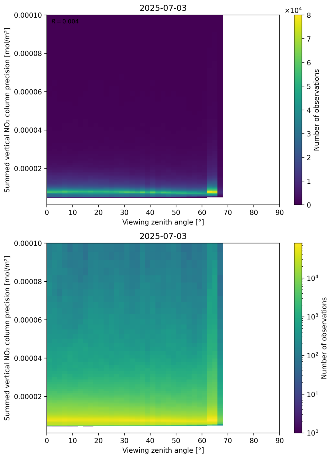
Figure 166: Scatter density plot of “Viewing zenith angle” against “Summed vertical NO 2 column precision” for 2025-07-03 to 2025-07-04.
