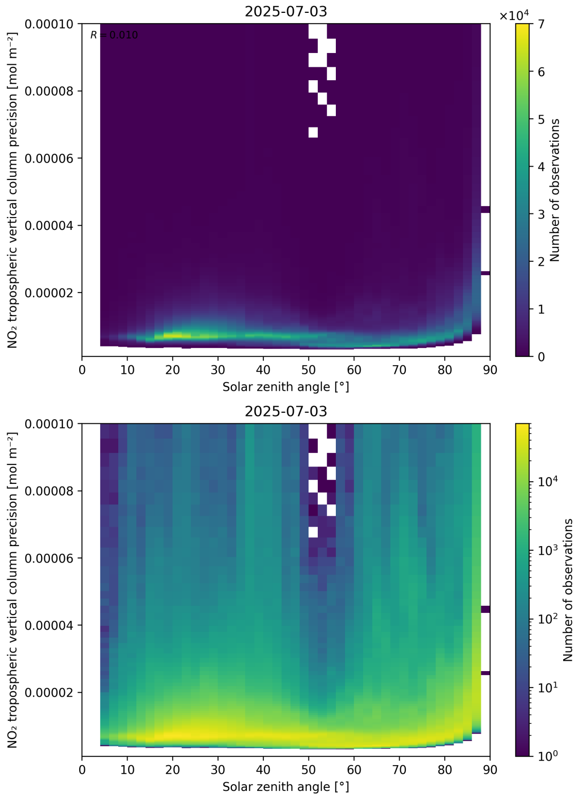
Figure 156: Scatter density plot of “Solar zenith angle” against “NO 2 tropospheric vertical column precision” for 2025-07-03 to 2025-07-04.
