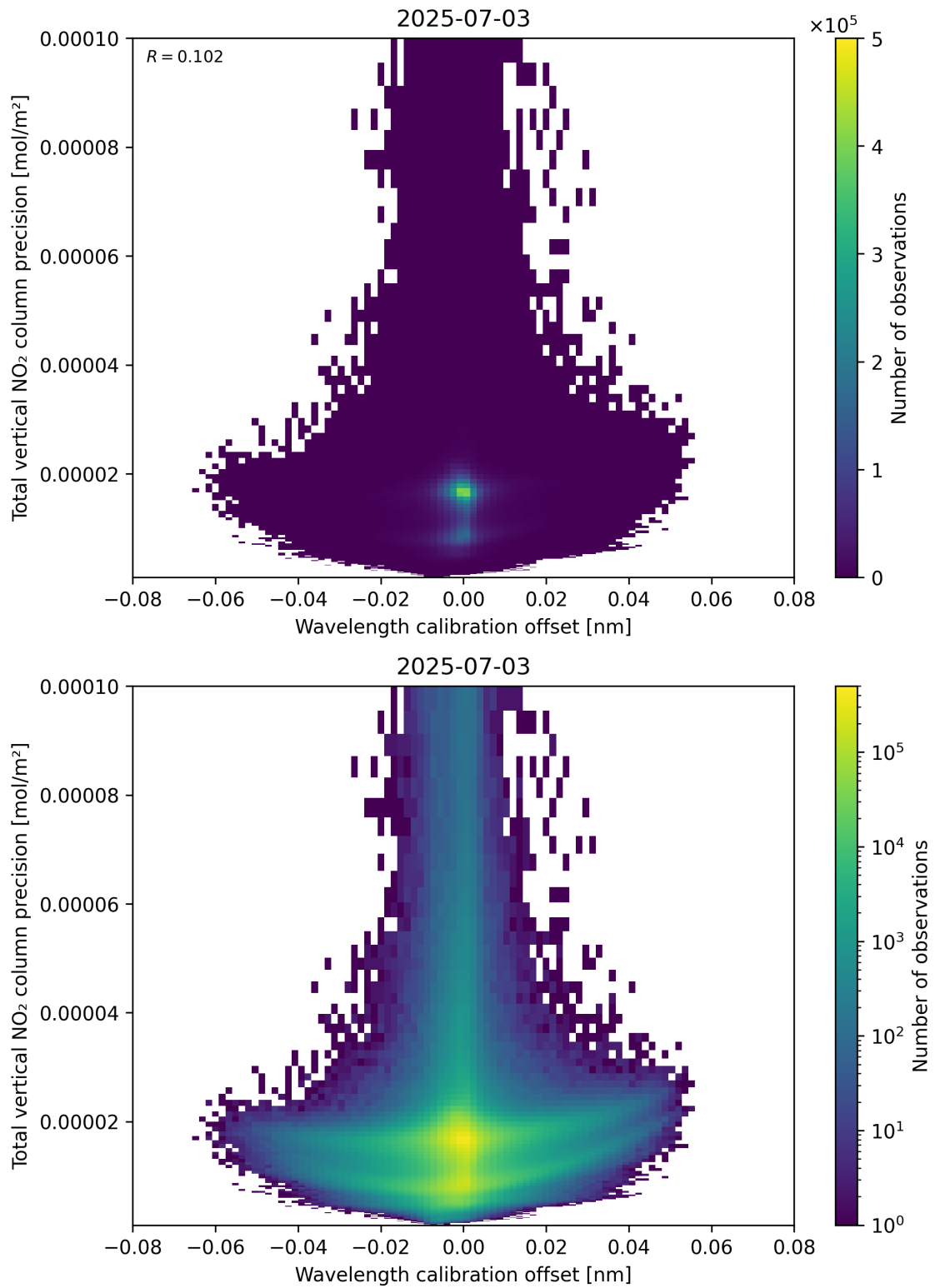
Figure 180: Scatter density plot of “Wavelength calibration offset” against “Total vertical NO 2 column precision” for 2025-07-03 to 2025-07-04.
