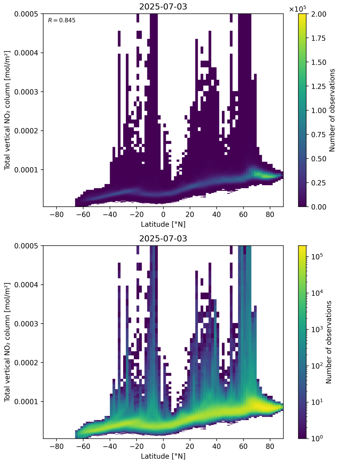
Figure 90: Scatter density plot of “Latitude” against “Total vertical NO 2 column” for 2025-07-03 to 2025-07-04.
