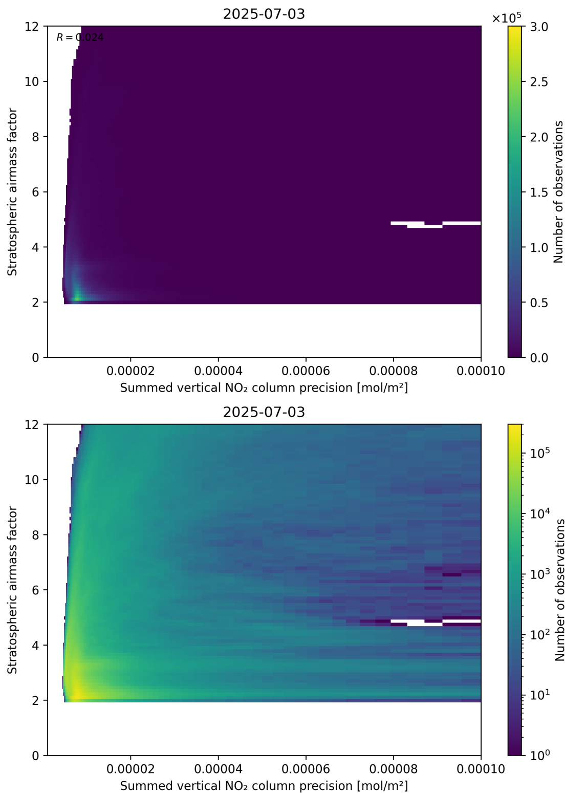
Figure 106: Scatter density plot of “Summed vertical NO 2 column precision” against “Stratospheric airmass factor” for 2025-07-03 to 2025-07-04.
