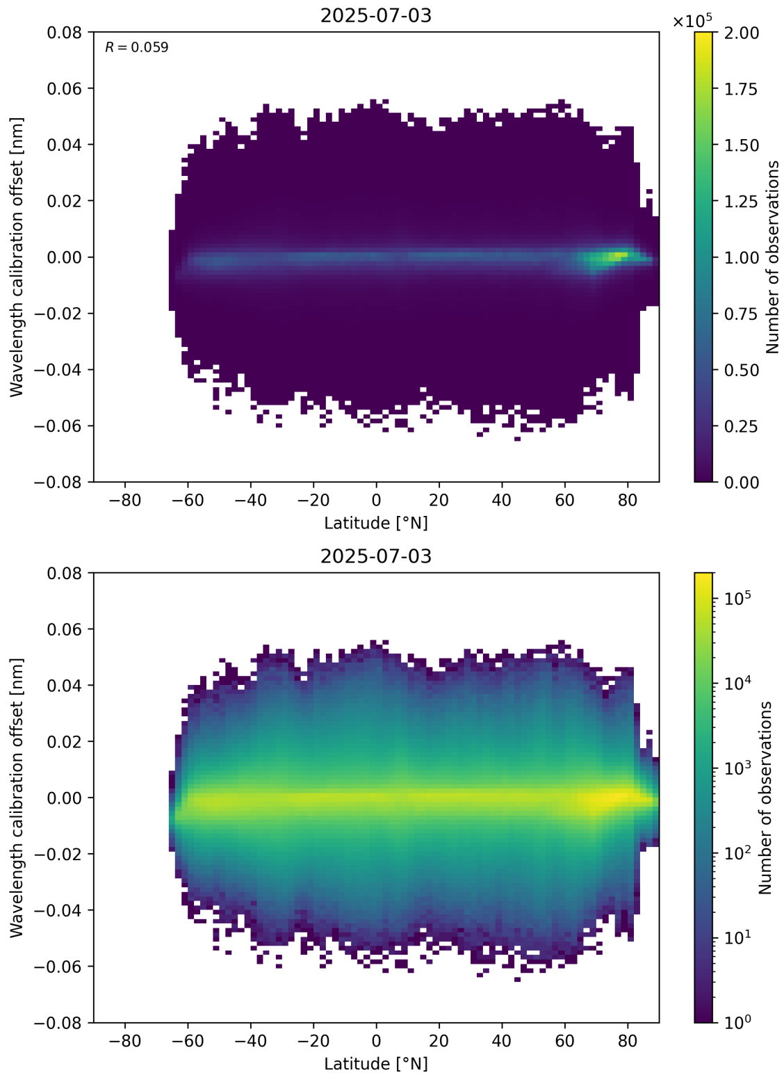
Figure 95: Scatter density plot of “Latitude” against “Wavelength calibration offset” for 2025-07-03 to 2025-07-04.
