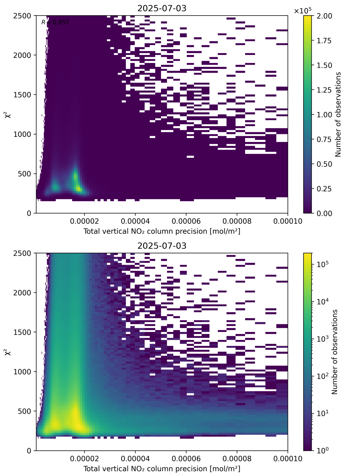
Figure 116: Scatter density plot of “Total vertical NO 2 column precision” against “ \chi^2 ” for 2025-07-03 to 2025-07-04.
