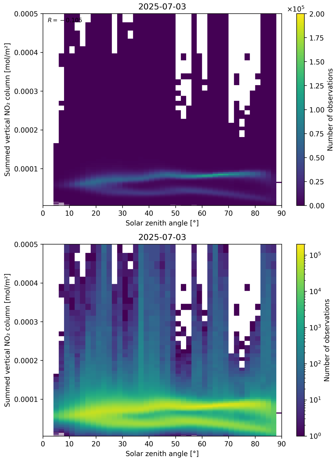
Figure 151: Scatter density plot of “Solar zenith angle” against “Summed vertical NO 2 column” for 2025-07-03 to 2025-07-04.
