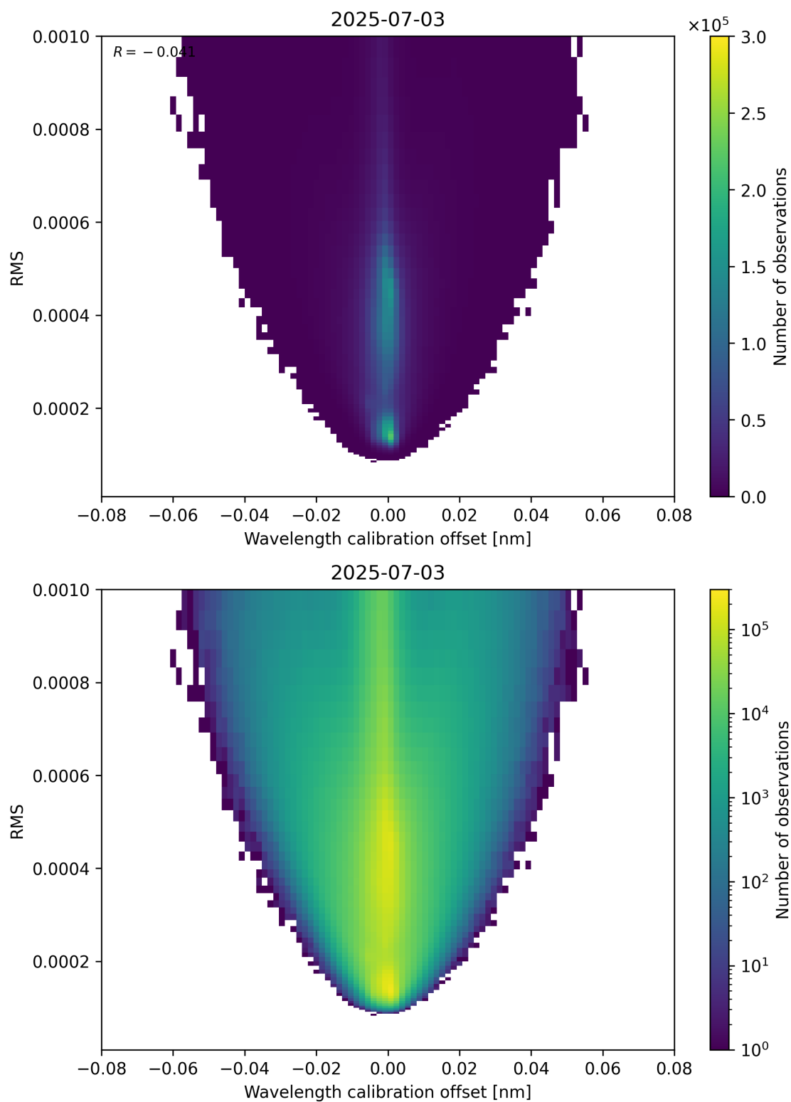
Figure 181: Scatter density plot of “Wavelength calibration offset” against “RMS” for 2025-07-03 to 2025-07-04.
