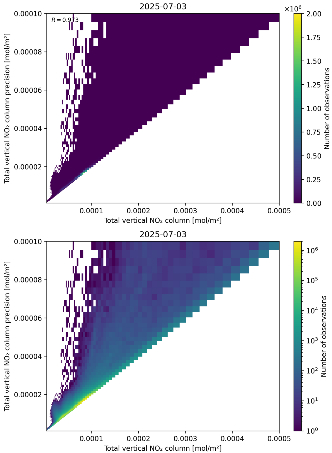
Figure 114: Scatter density plot of “Total vertical NO 2 column” against “Total vertical NO 2 column precision” for 2025-07-03 to 2025-07-04.
