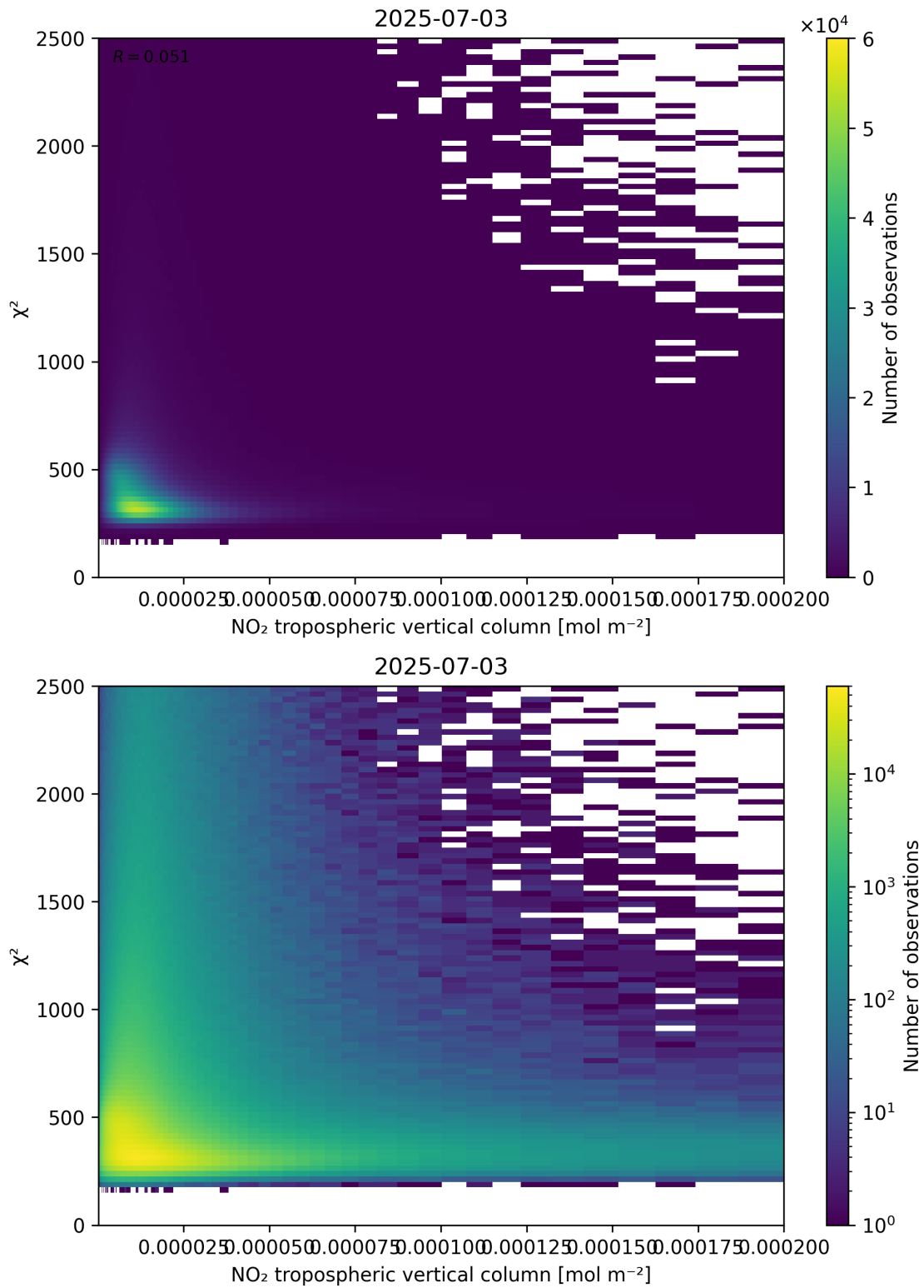
Figure 124: Scatter density plot of “NO 2 tropospheric vertical column” against “ \chi^2 ” for 2025-07-03 to 2025-07-04.
