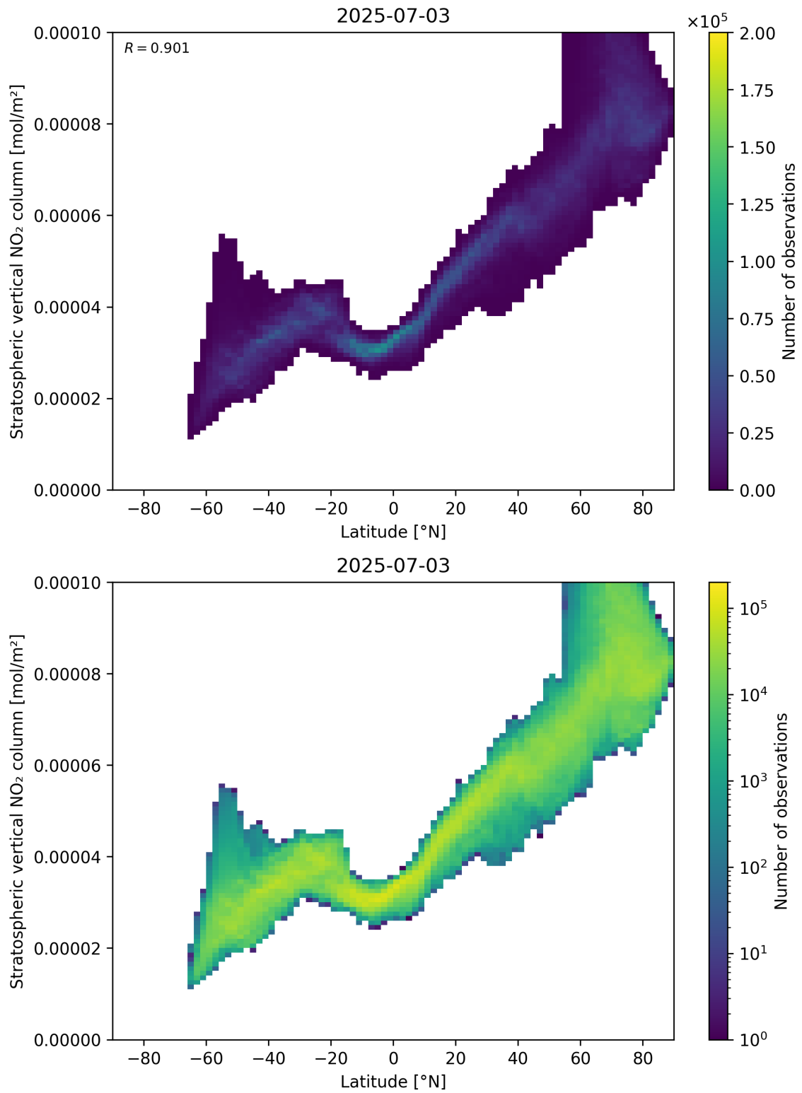
Figure 87: Scatter density plot of “Latitude” against “Stratospheric vertical \text{NO}_2 column” for 2025-07-03 to 2025-07-04.
