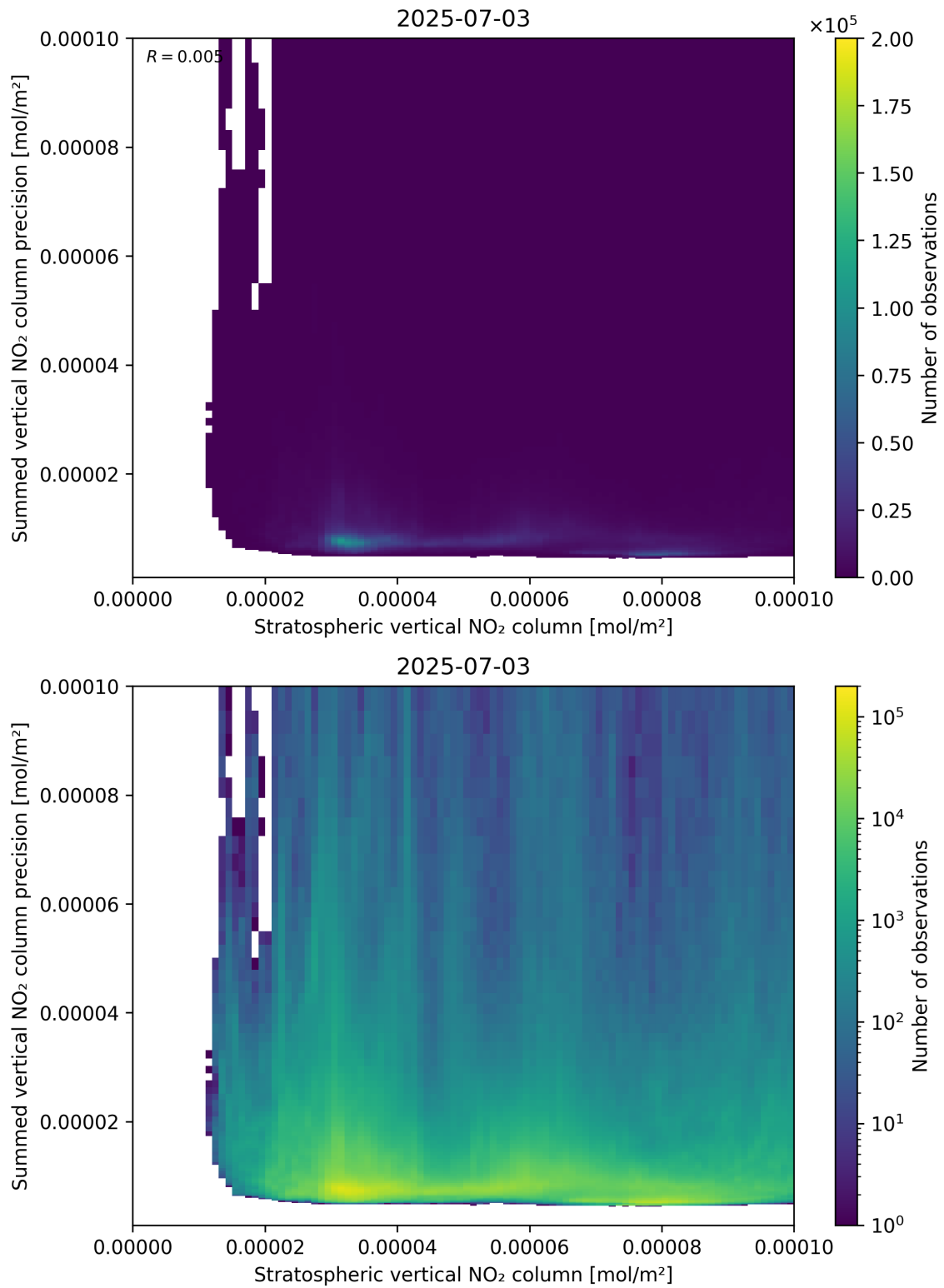
Figure 99: Scatter density plot of “Stratospheric vertical NO 2 column” against “Summed vertical NO 2 column precision” for 2025-07-03 to 2025-07-04.
