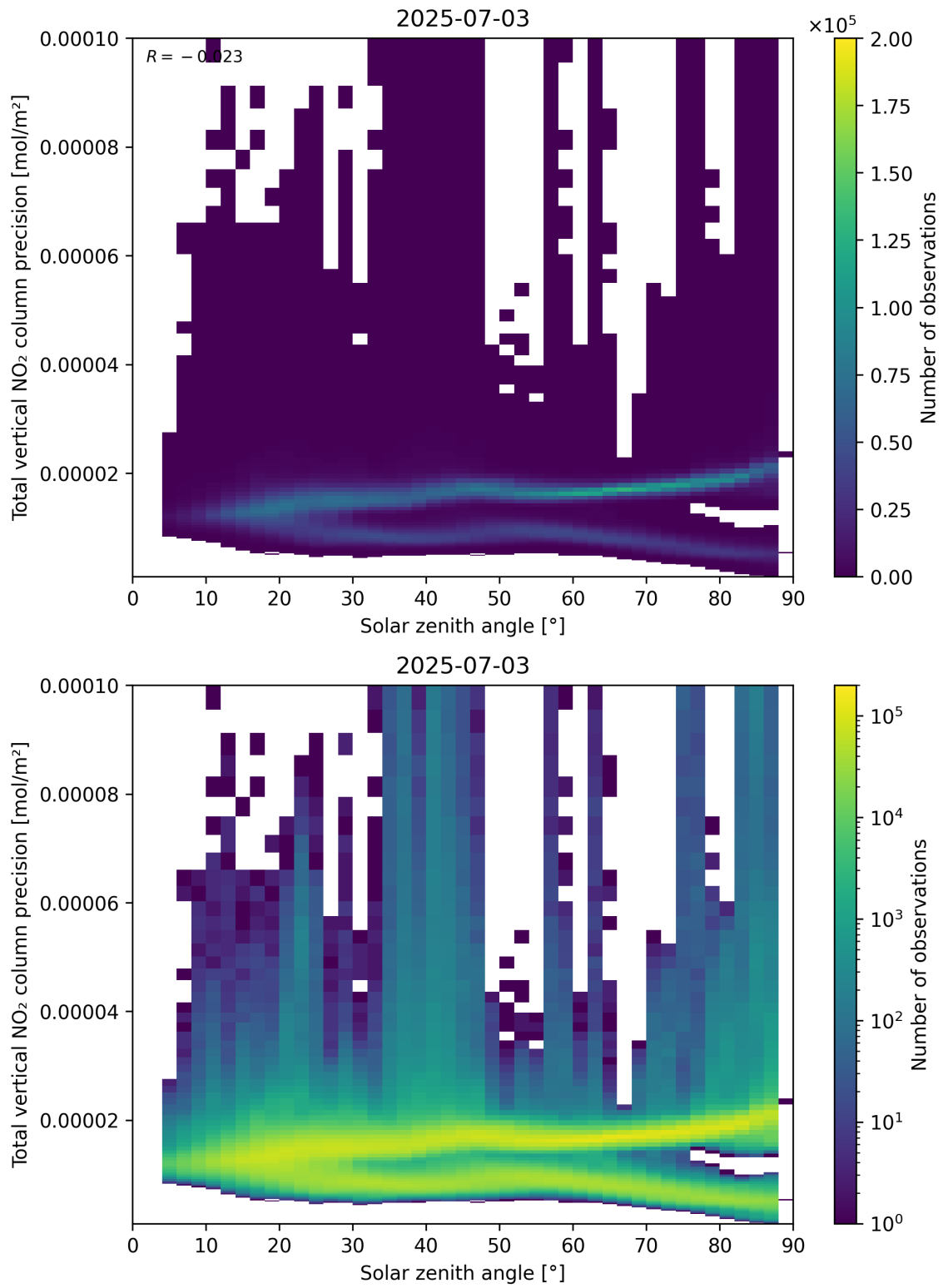
Figure 154: Scatter density plot of “Solar zenith angle” against “Total vertical NO 2 column precision” for 2025-07-03 to 2025-07-04.
