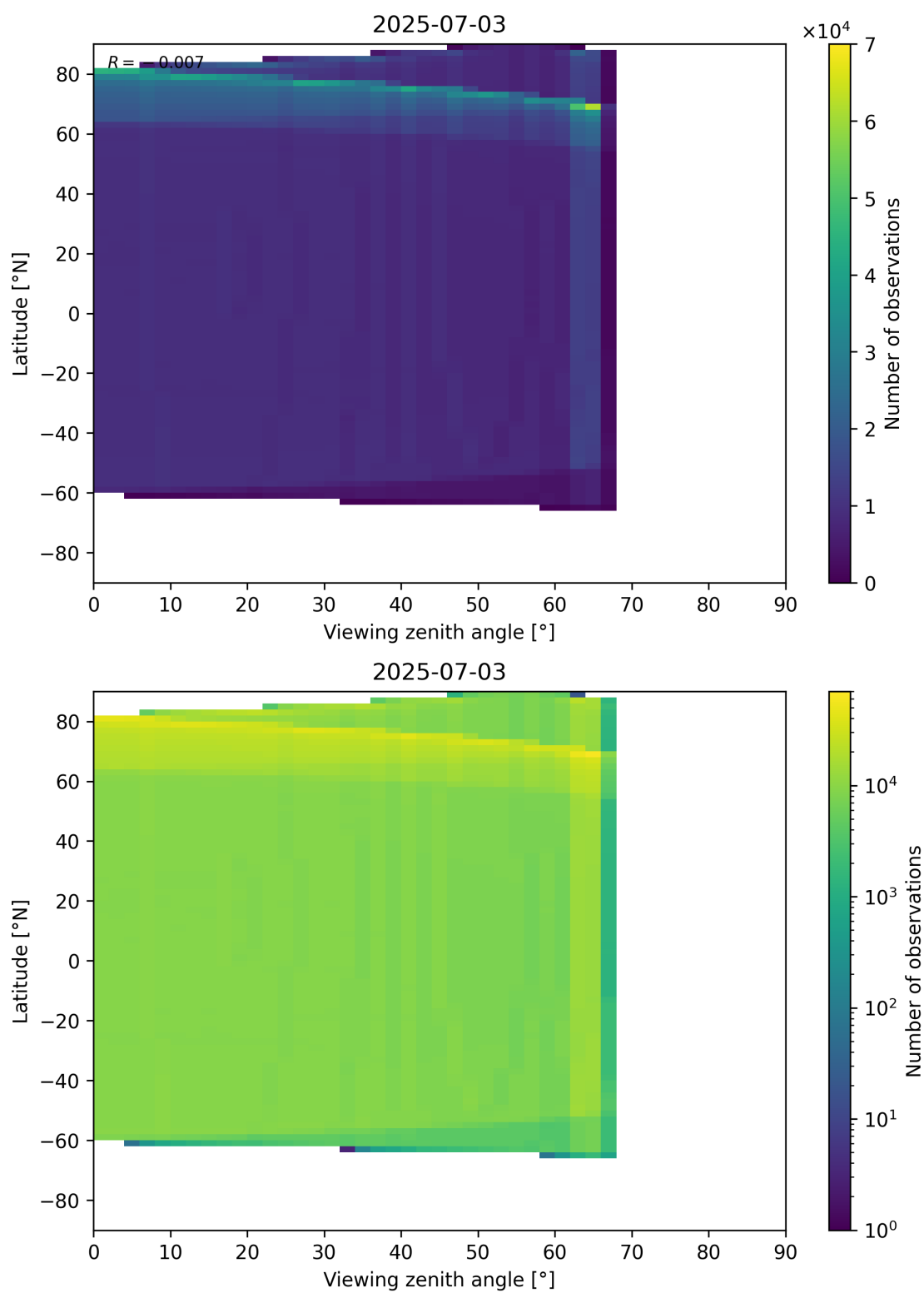
Figure 163: Scatter density plot of “Viewing zenith angle” against “Latitude” for 2025-07-03 to 2025-07-04.
