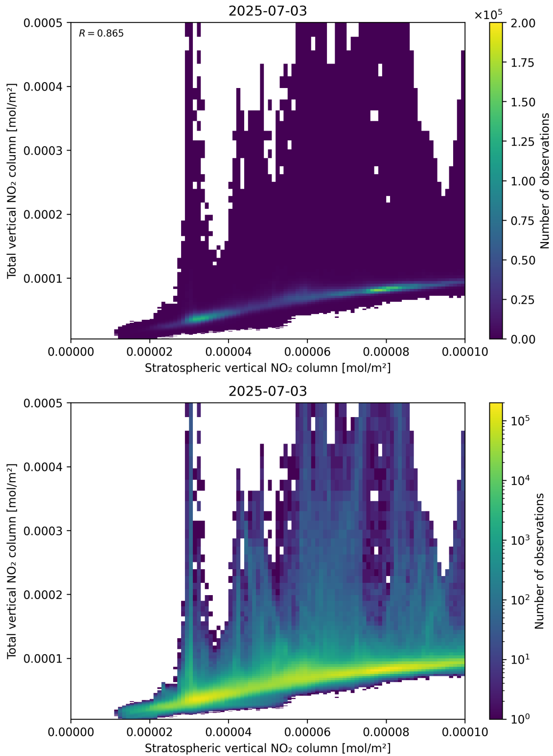
Figure 100: Scatter density plot of “Stratospheric vertical NO 2 column” against “Total vertical NO 2 column” for 2025-07-03 to 2025-07-04.
