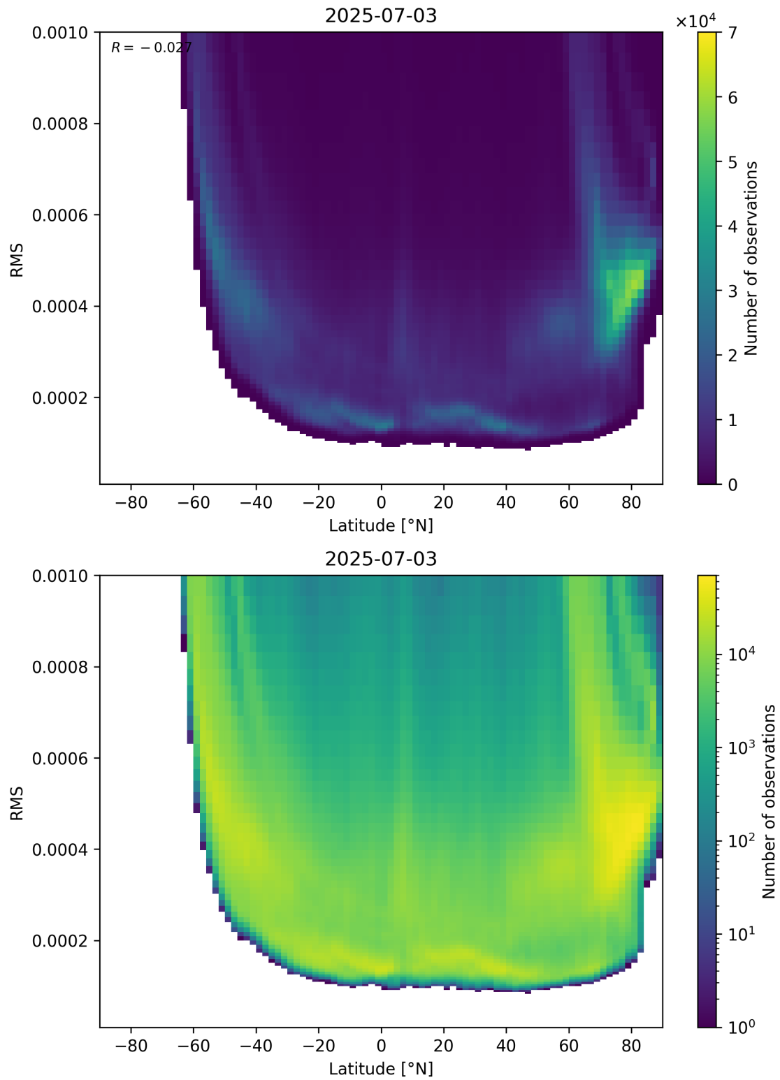
Figure 94: Scatter density plot of “Latitude” against “RMS” for 2025-07-03 to 2025-07-04.
