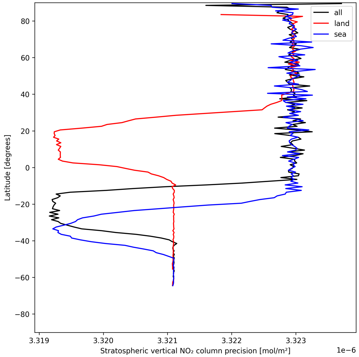
Figure 20: Zonal average of “Stratospheric vertical NO 2 column precision” for 2025-07-03 to 2025-07-04.
