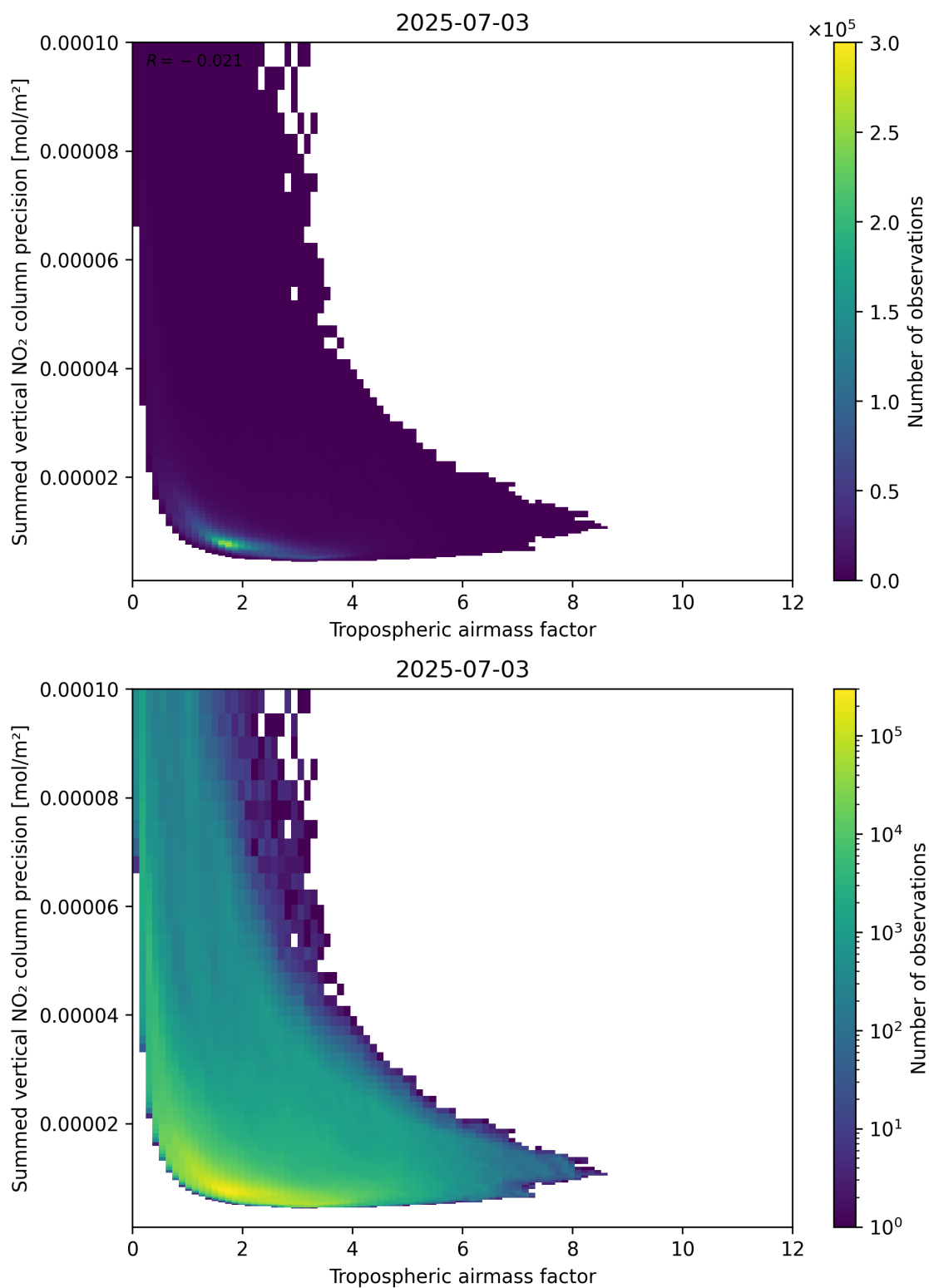
Figure 76: Scatter density plot of “Tropospheric air mass factor” against “Summed vertical NO 2 column precision” for 2025-07-03 to 2025-07-04.
