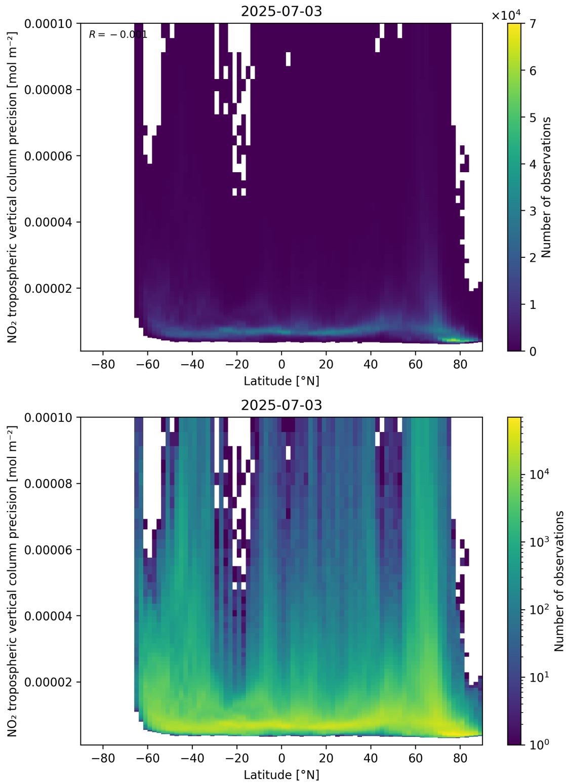
Figure 93: Scatter density plot of “Latitude” against “NO 2 tropospheric vertical column precision” for 2025-07-03 to 2025-07-04.
