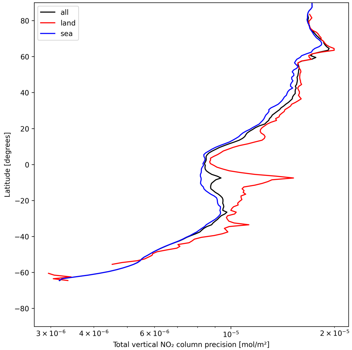
Figure 22: Zonal average of “Total vertical NO 2 column precision” for 2025-07-03 to 2025-07-04.
