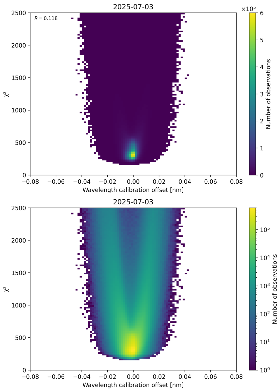
Figure 175: Scatter density plot of “Wavelength calibration offset” against “ \chi^2 ” for 2025-07-03 to 2025-07-04.
