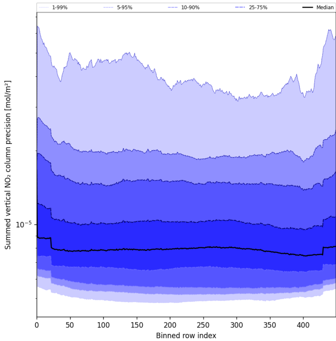
Figure 58: Along track statistics of “Summed vertical NO 2 column precision” for 2025-07-03 to 2025-07-04
