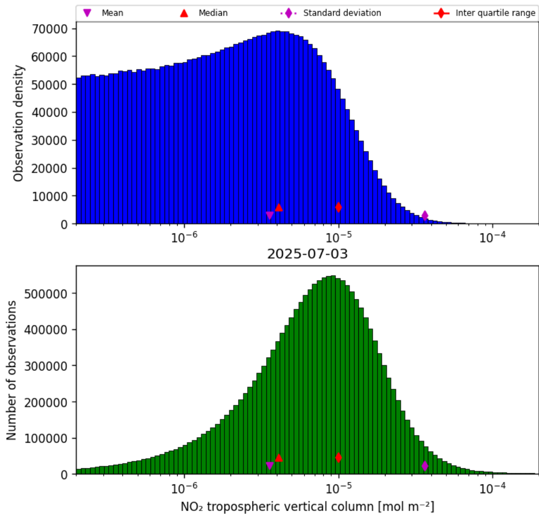
Figure 29: Histogram of “NO 2 tropospheric vertical column” for 2025-07-03 to 2025-07-04
