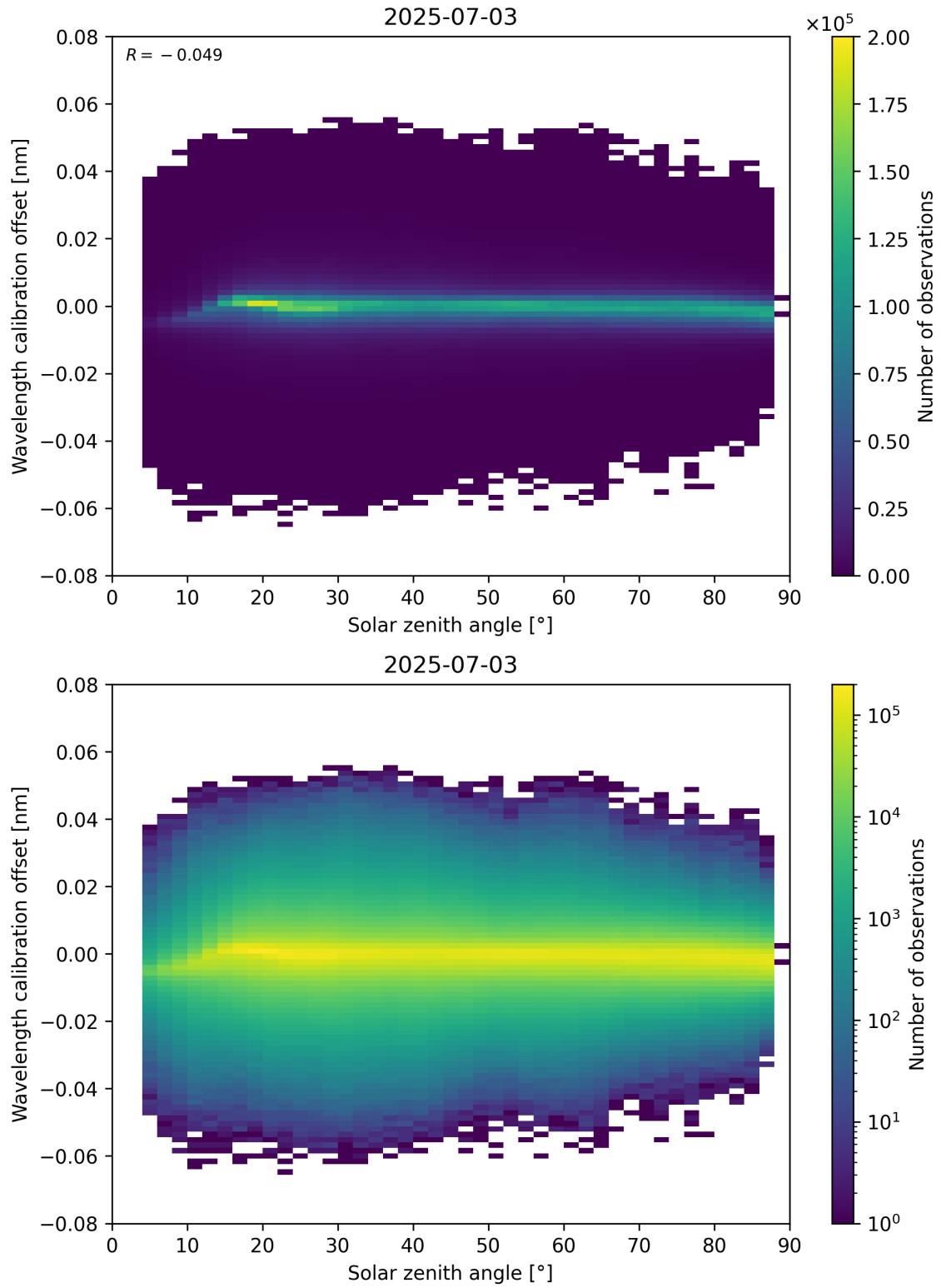
Figure 158: Scatter density plot of “Solar zenith angle” against “Wavelength calibration offset” for 2025-07-03 to 2025-07-04.
