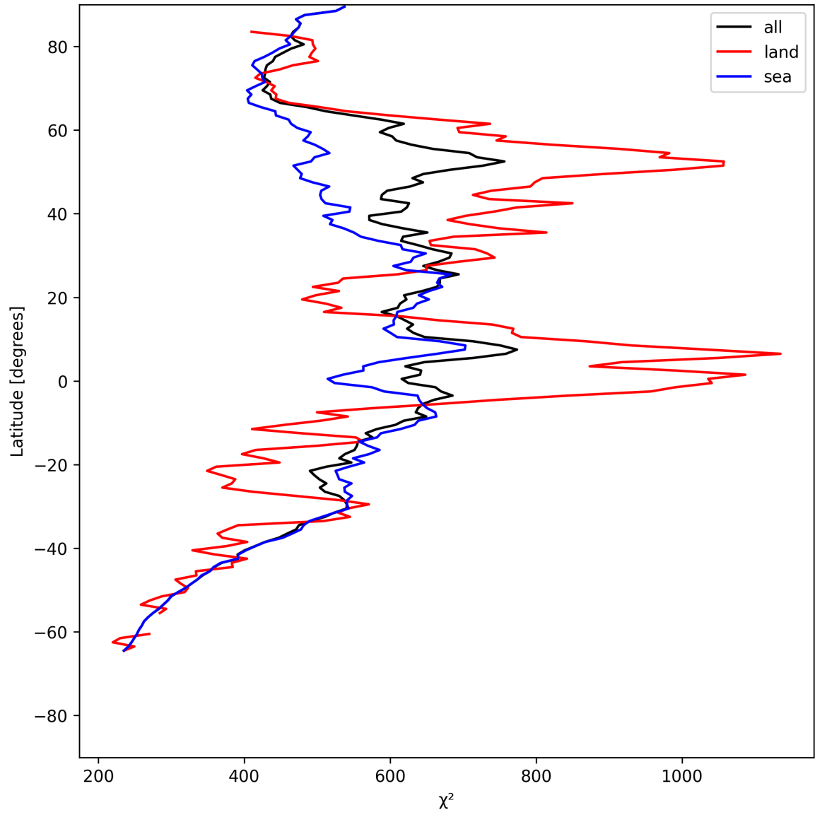
Figure 25: Zonal average of “ \chi^2 ” for 2025-07-03 to 2025-07-04.
