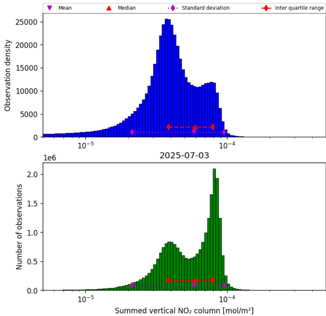
Figure 40: Histogram of “Summed vertical NO 2 column” for 2025-07-03 to 2025-07-04
