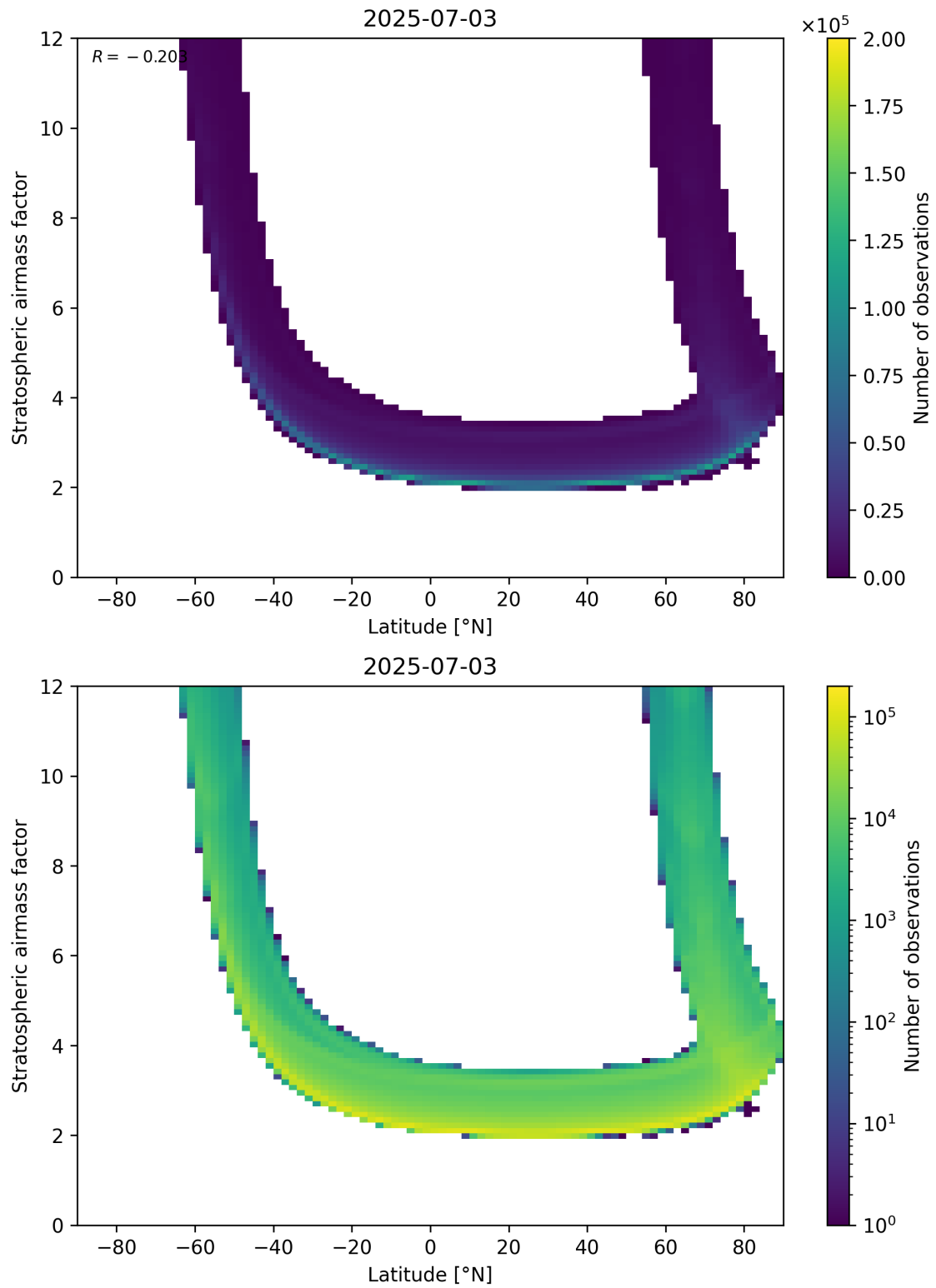
Figure 83: Scatter density plot of “Latitude” against “Stratospheric air mass factor” for 2025-07-03 to 2025-07-04.
