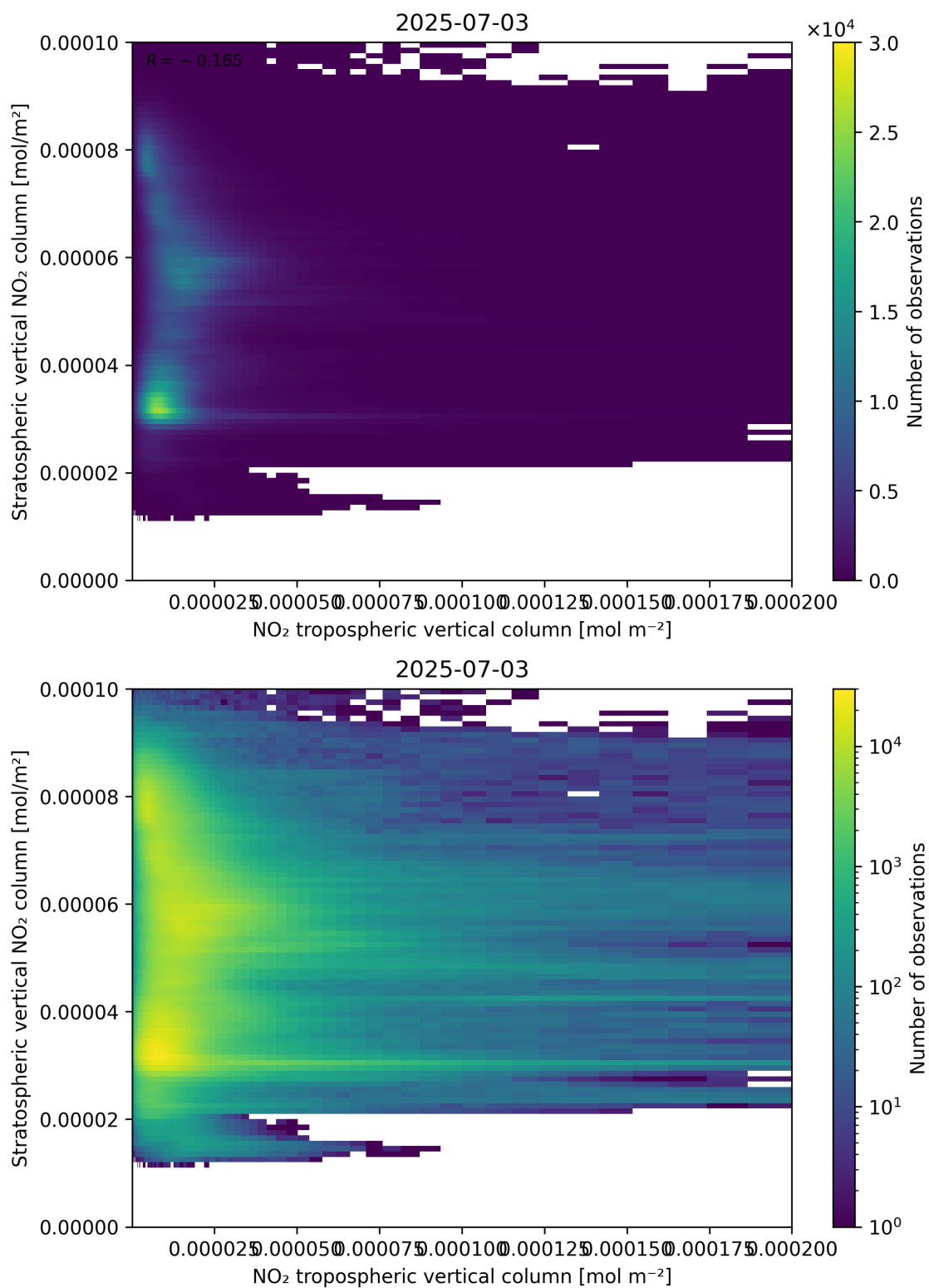
Figure 125: Scatter density plot of “NO 2 tropospheric vertical column” against “Stratospheric vertical NO 2 column” for 2025-07-03 to 2025-07-04.
