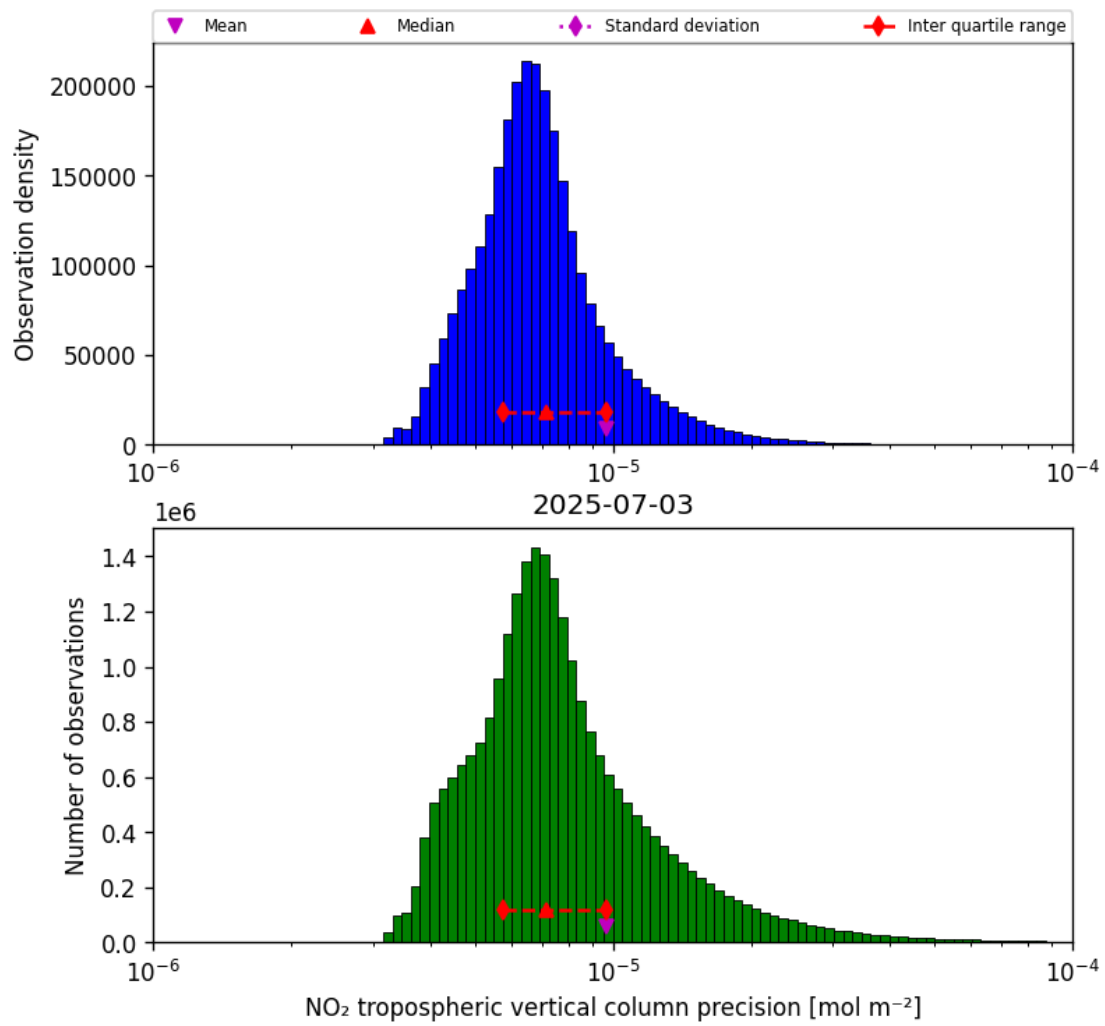
Figure 30: Histogram of “NO 2 tropospheric vertical column precision” for 2025-07-03 to 2025-07-04
