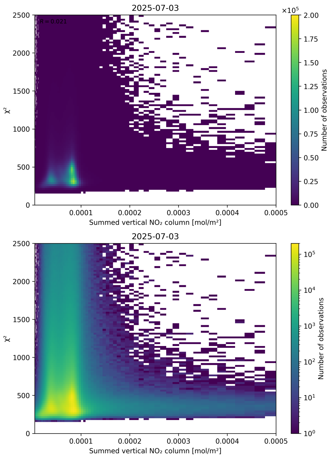
Figure 104: Scatter density plot of “Summed vertical NO 2 column” against “ \chi^2 ” for 2025-07-03 to 2025-07-04.
