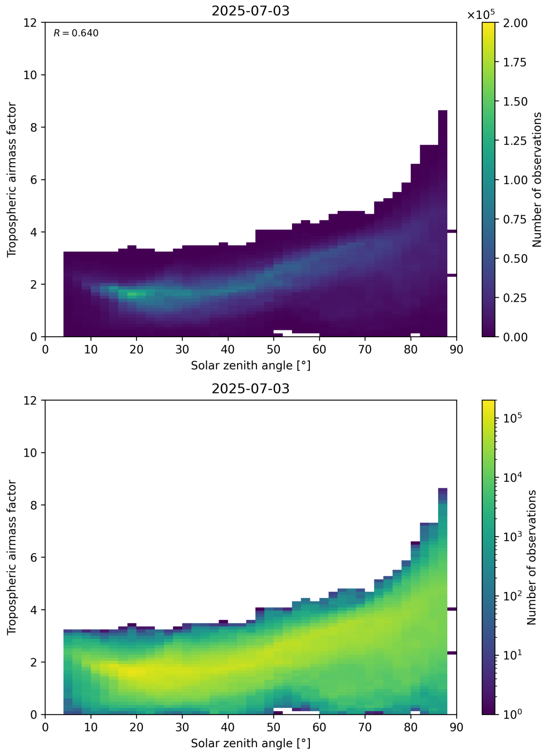
Figure 147: Scatter density plot of “Solar zenith angle” against “Tropospheric airmass factor” for 2025-07-03 to 2025-07-04.
