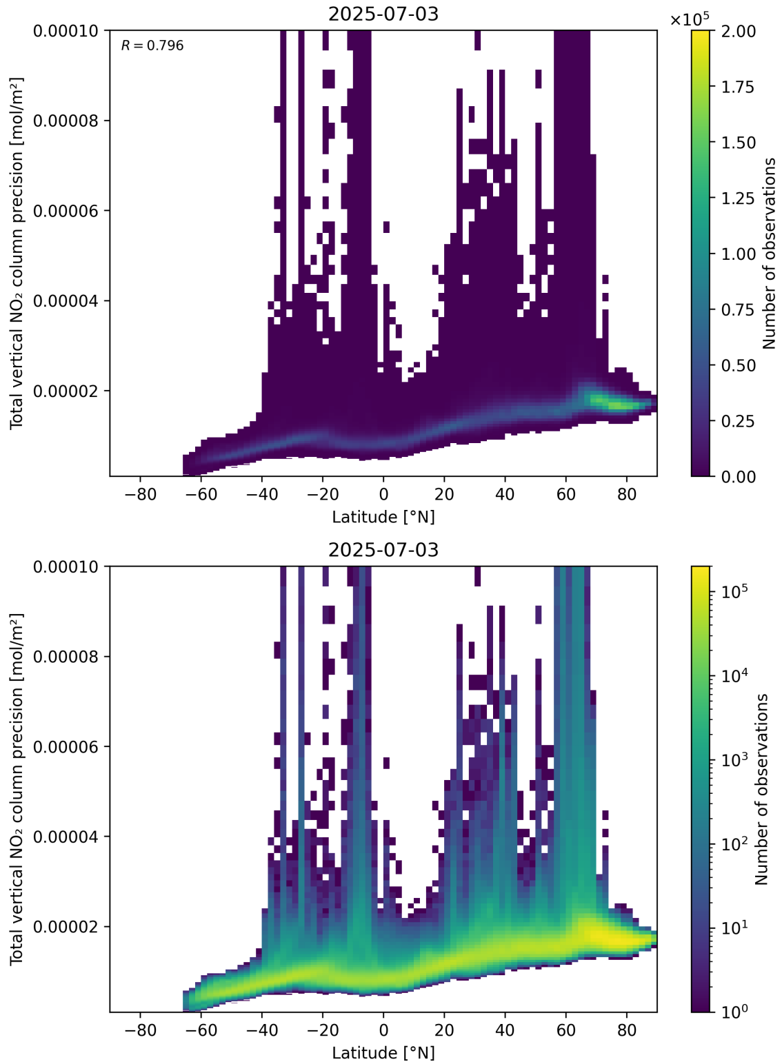
Figure 91: Scatter density plot of “Latitude” against “Total vertical NO 2 column precision” for 2025-07-03 to 2025-07-04.
