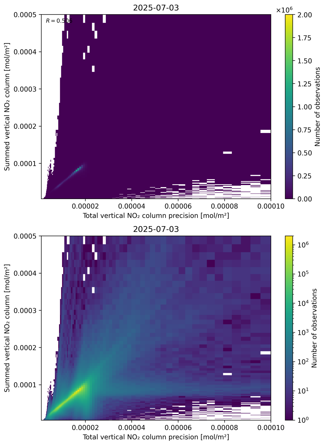
Figure 117: Scatter density plot of “Total vertical NO 2 column precision” against “Summed vertical NO 2 column” for 2025-07-03 to 2025-07-04.
