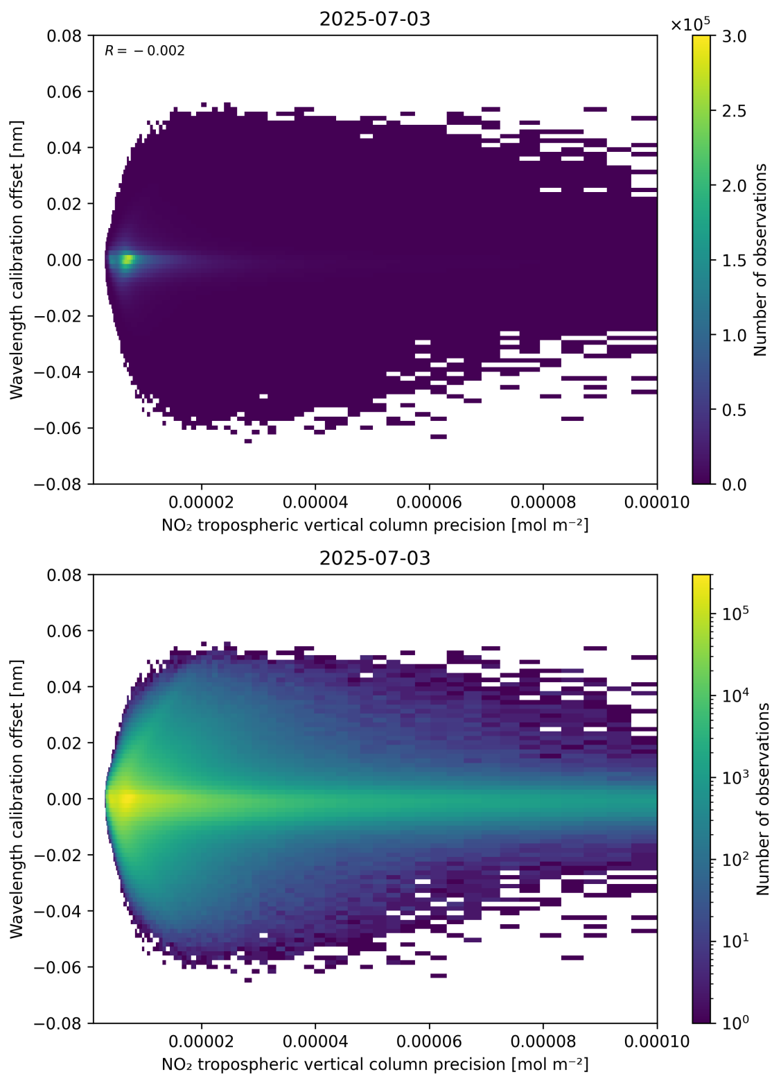
Figure 141: Scatter density plot of “NO 2 tropospheric vertical column precision” against “Wavelength calibration offset” for 2025-07-03 to 2025-07-04.
