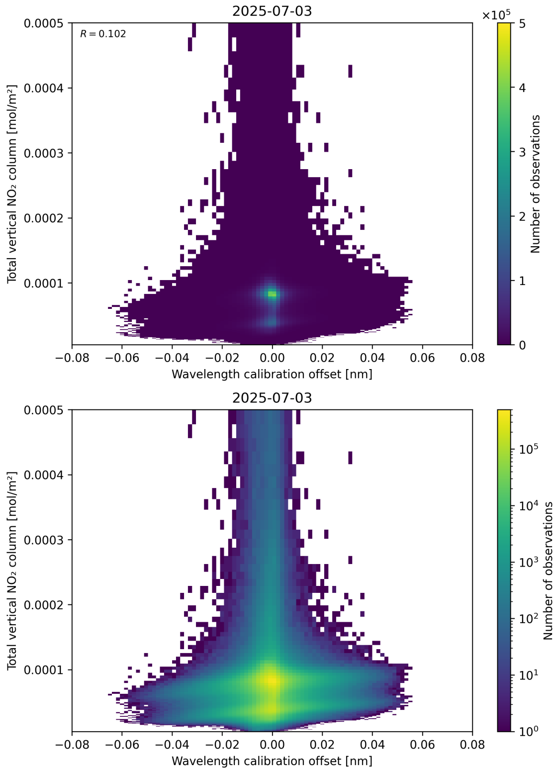
Figure 179: Scatter density plot of “Wavelength calibration offset” against “Total vertical NO 2 column” for 2025-07-03 to 2025-07-04.
