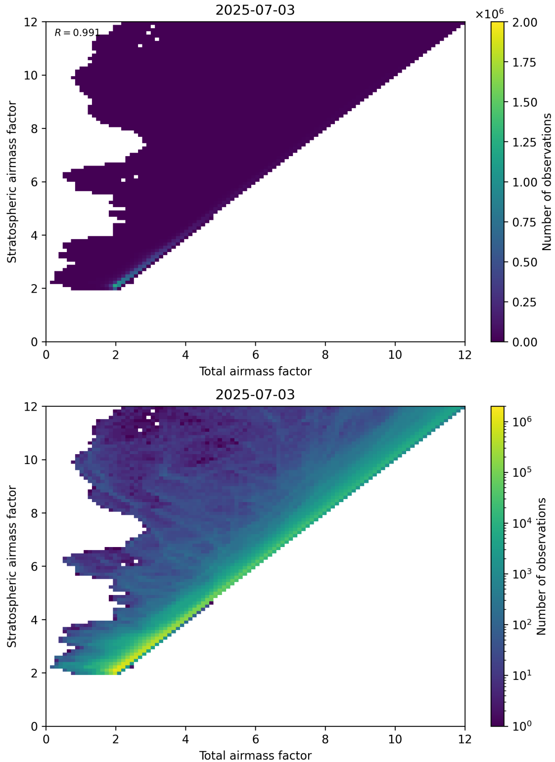
Figure 62: Scatter density plot of “Total airmass factor” against “Stratospheric airmass factor” for 2025-07-03 to 2025-07-04.
