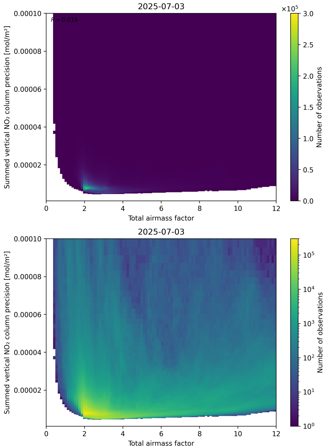
Figure 66: Scatter density plot of “Total airmass factor” against “Summed vertical NO 2 column precision” for 2025-07-03 to 2025-07-04.
