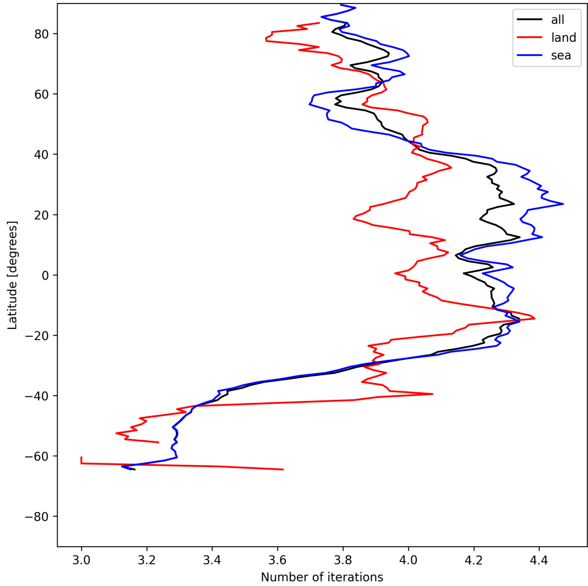
Figure 17: Zonal average of “Number of iterations” for 2025-07-03 to 2025-07-04.
