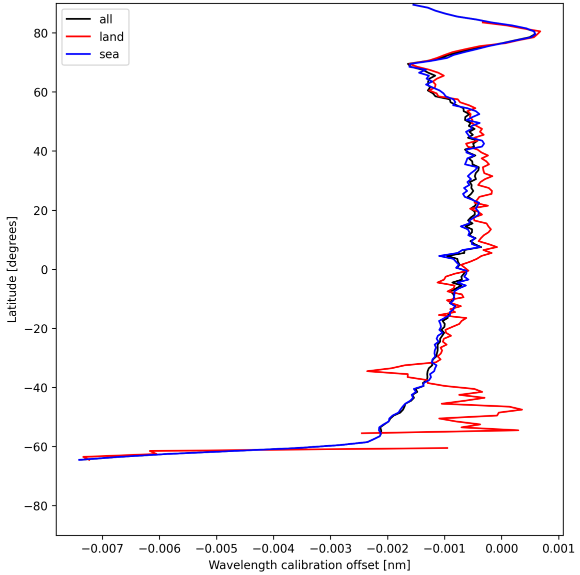
Figure 18: Zonal average of “Wavelength calibration offset” for 2025-07-03 to 2025-07-04.
