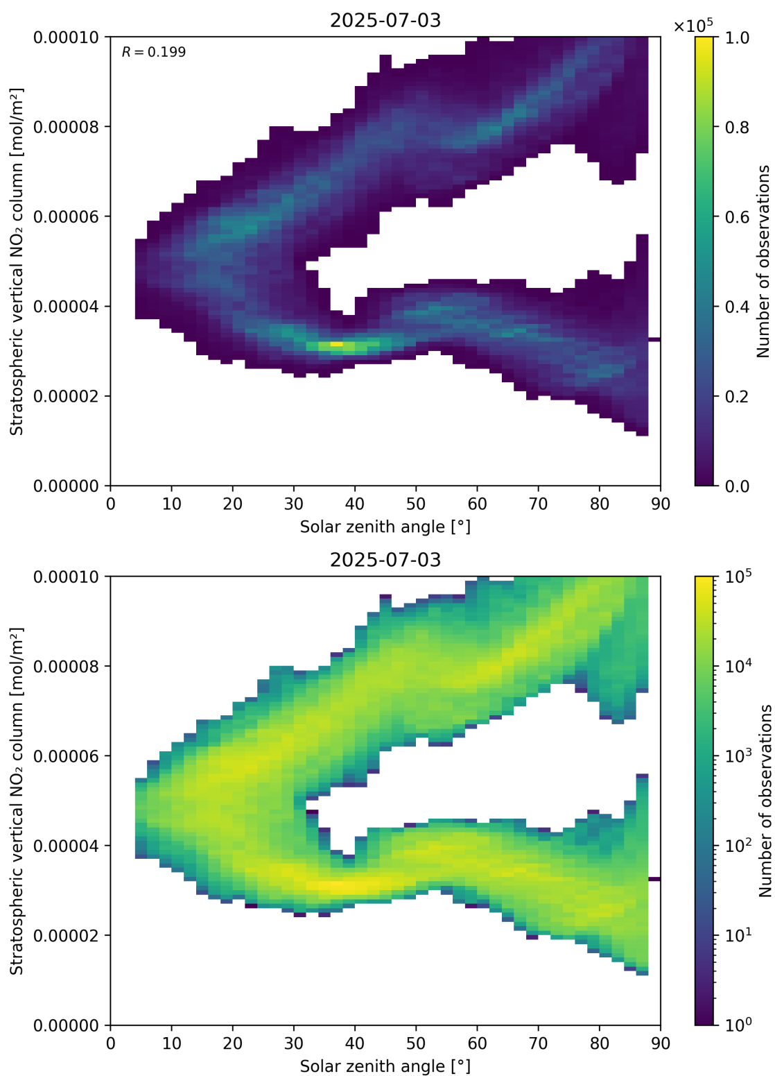
Figure 150: Scatter density plot of “Solar zenith angle” against “Stratospheric vertical NO 2 column” for 2025-07-03 to 2025-07-04.
