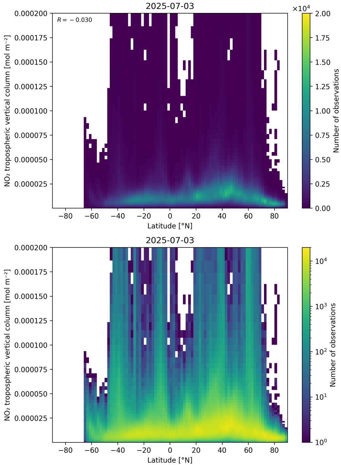
Figure 92: Scatter density plot of “Latitude” against “NO 2 tropospheric vertical column” for 2025-07-03 to 2025-07-04.
