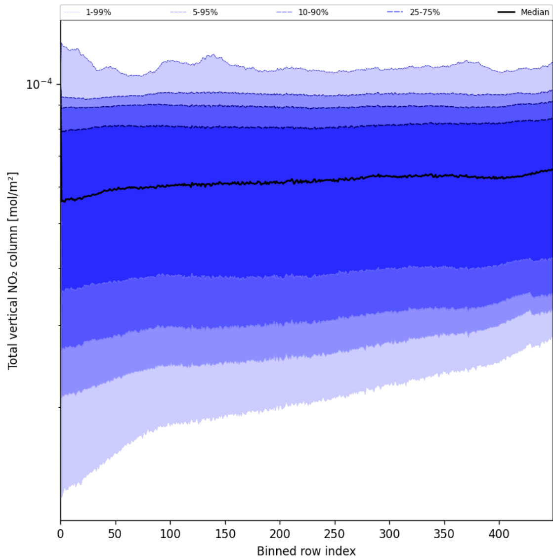
Figure 55: Along track statistics of “Total vertical NO 2 column” for 2025-07-03 to 2025-07-04
