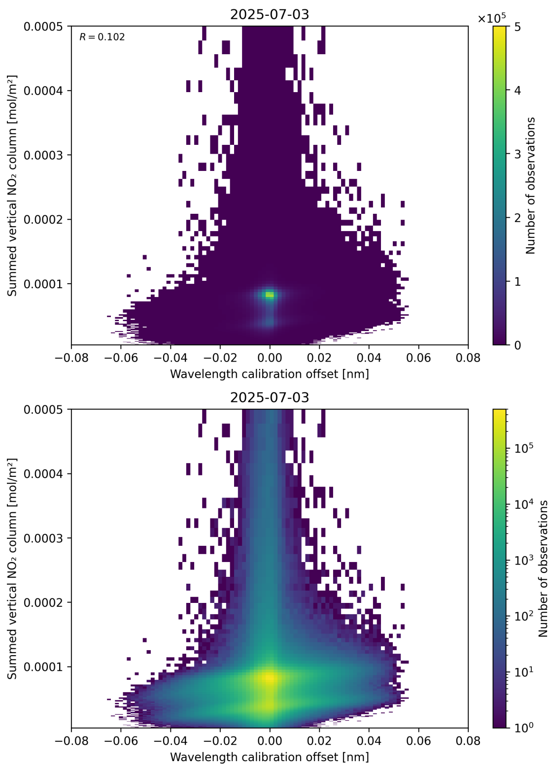
Figure 177: Scatter density plot of “Wavelength calibration offset” against “Summed vertical NO 2 column” for 2025-07-03 to 2025-07-04.
