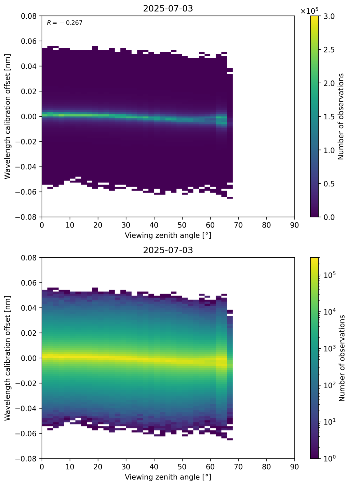
Figure 173: Scatter density plot of “Viewing zenith angle” against “Wavelength calibration offset” for 2025-07-03 to 2025-07-04.
