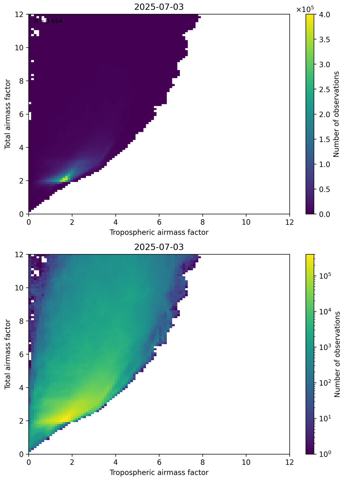
Figure 72: Scatter density plot of “Tropospheric airmass factor” against “Total airmass factor” for 2025-07-03 to 2025-07-04.
