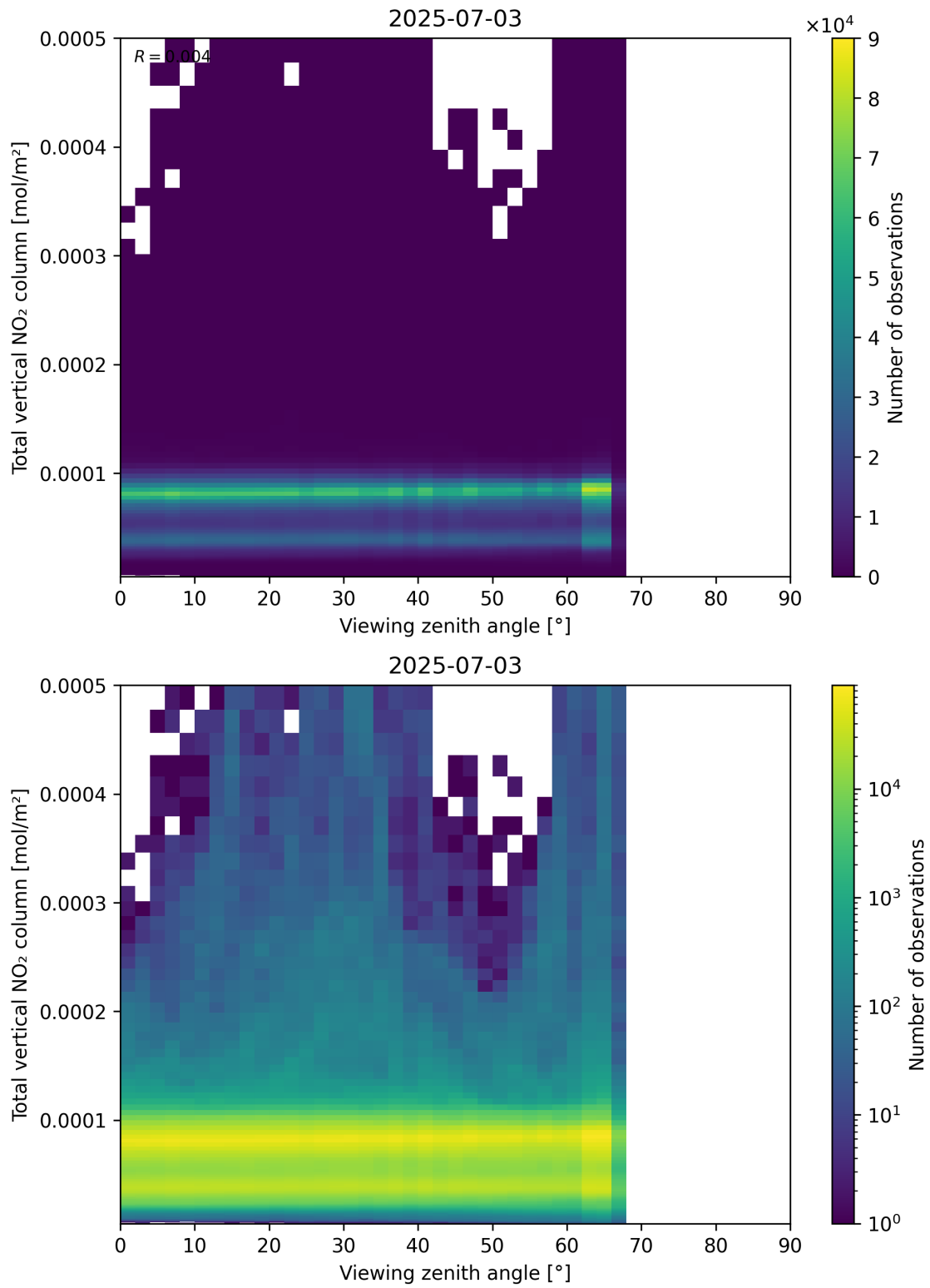
Figure 167: Scatter density plot of “Viewing zenith angle” against “Total vertical NO 2 column” for 2025-07-03 to 2025-07-04.
