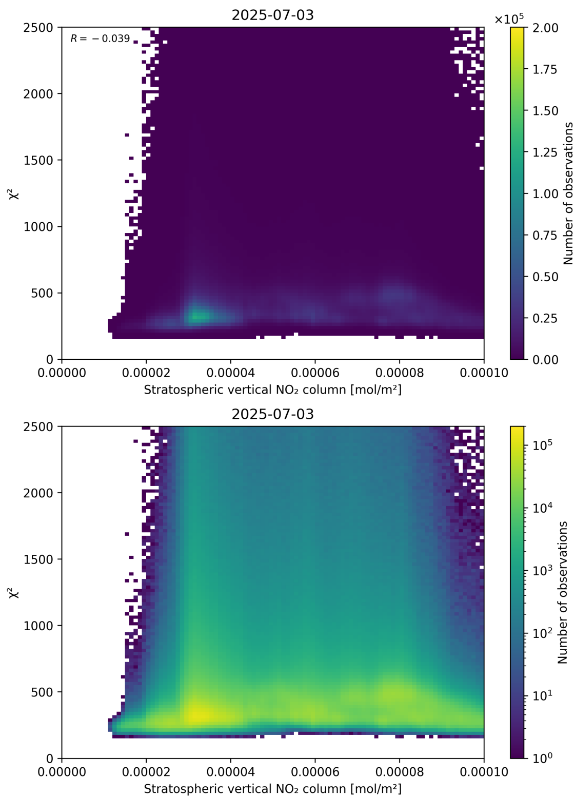
Figure 97: Scatter density plot of “Stratospheric vertical NO 2 column” against “ \chi^2 ” for 2025-07-03 to 2025-07-04.
