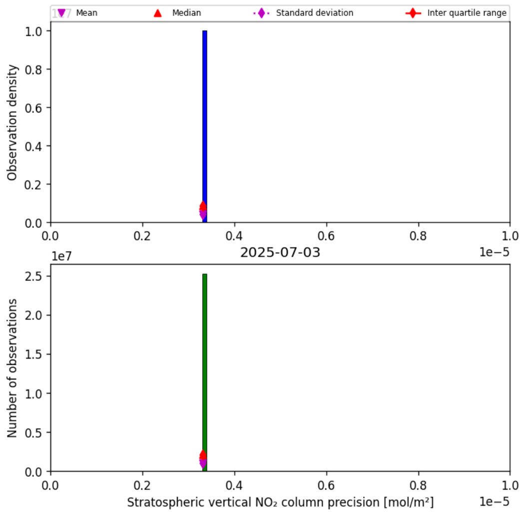
Figure 37: Histogram of “Stratospheric vertical NO 2 column precision” for 2025-07-03 to 2025-07-04
