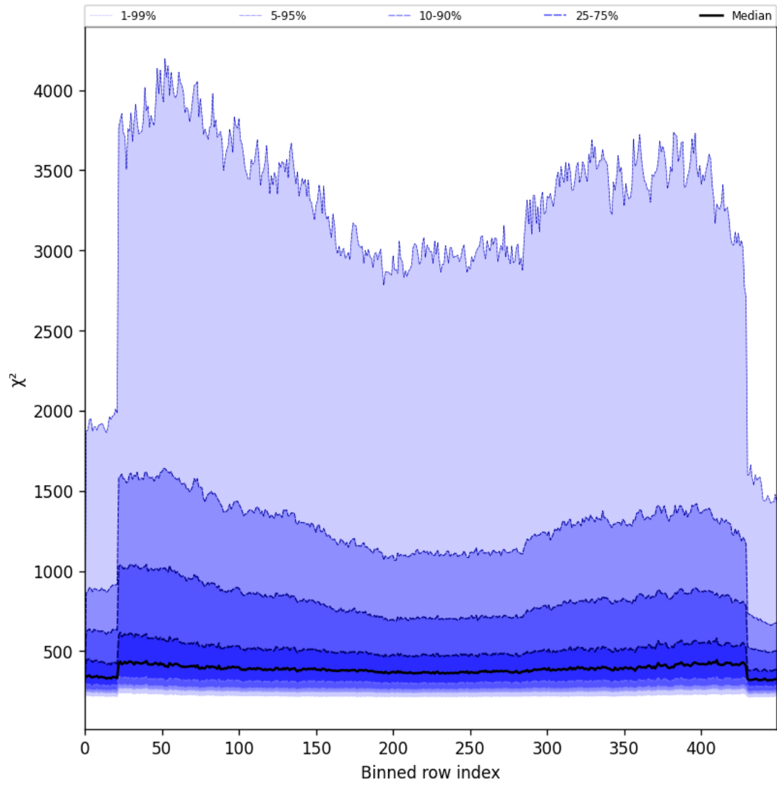
Figure 59: Along track statistics of “ \chi^2 ” for 2025-07-03 to 2025-07-04
