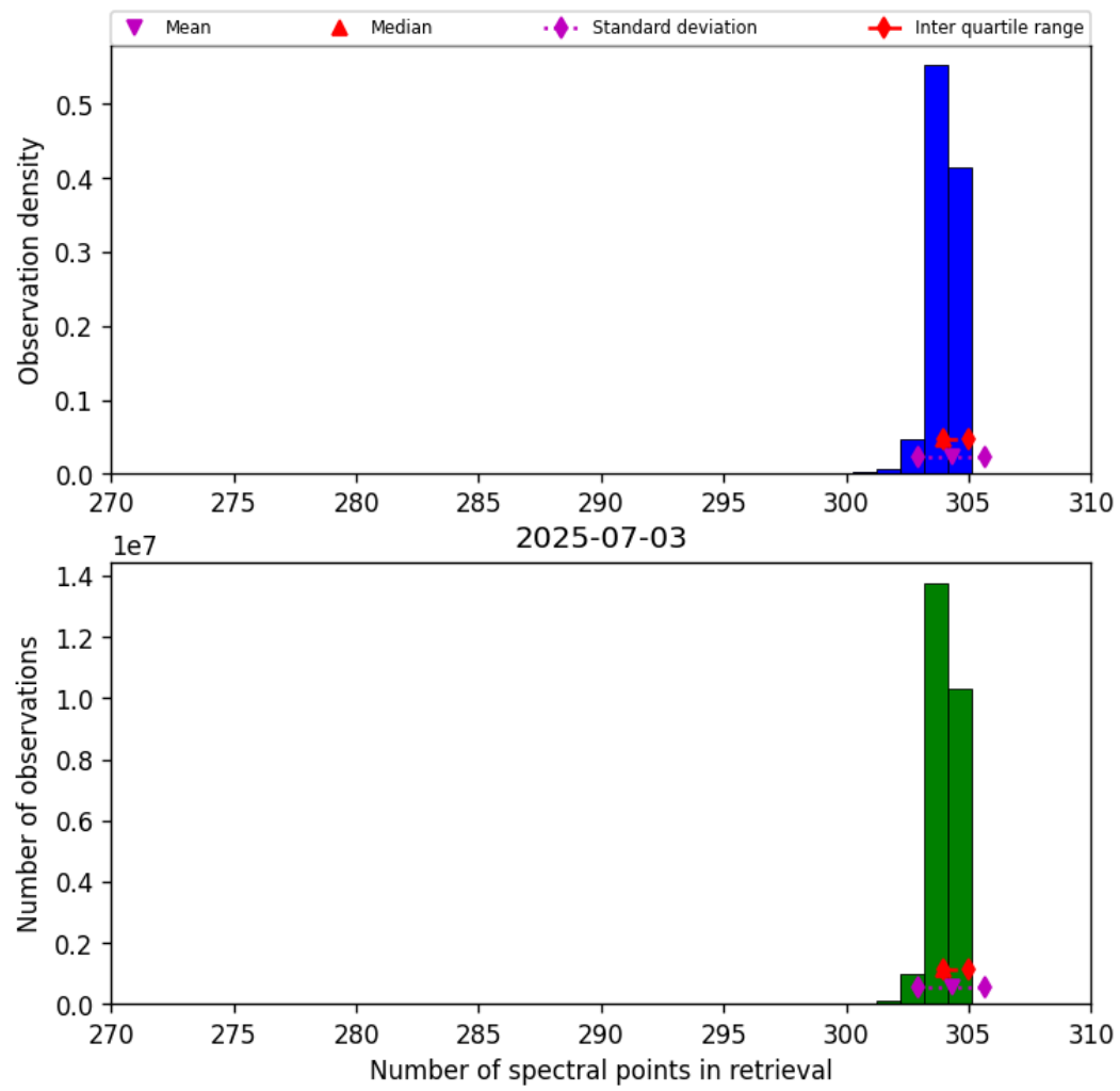
Figure 33: Histogram of “Number of spectral points in retrieval” for 2025-07-03 to 2025-07-04
