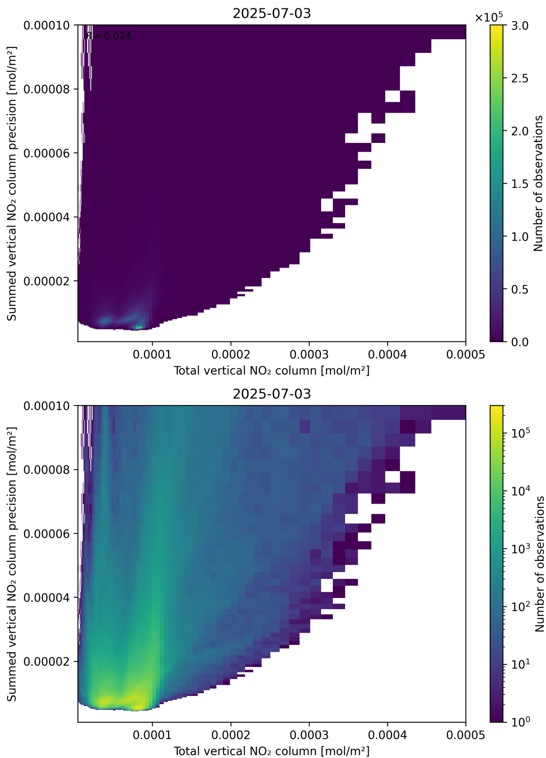
Figure 113: Scatter density plot of “Total vertical NO 2 column” against “Summed vertical NO 2 column precision” for 2025-07-03 to 2025-07-04.
