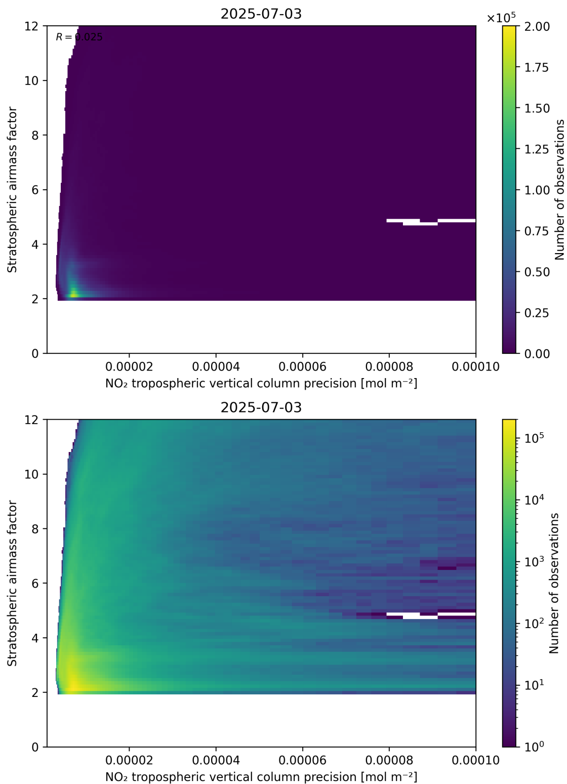
Figure 131: Scatter density plot of “NO 2 tropospheric vertical column precision” against “Stratospheric airmass factor” for 2025-07-03 to 2025-07-04.
