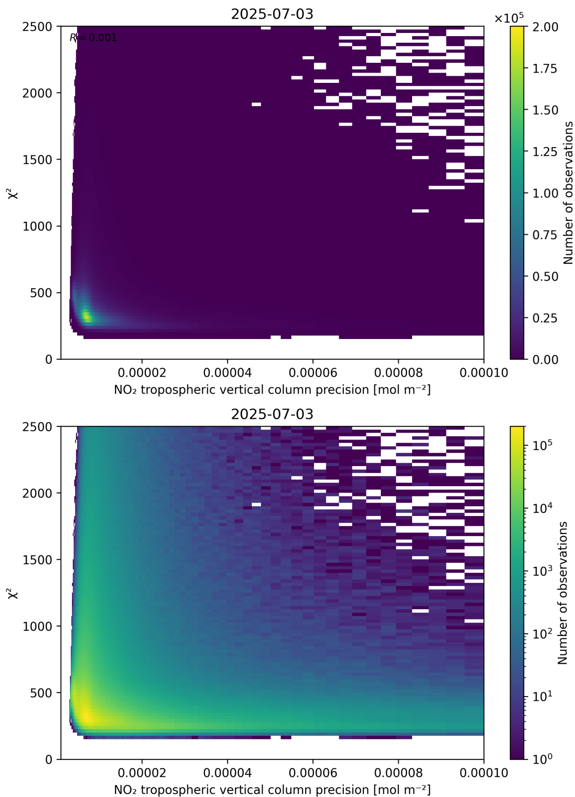
Figure 134: Scatter density plot of “NO 2 tropospheric vertical column precision” against “ \chi^2 ” for 2025-07-03 to 2025-07-04.
