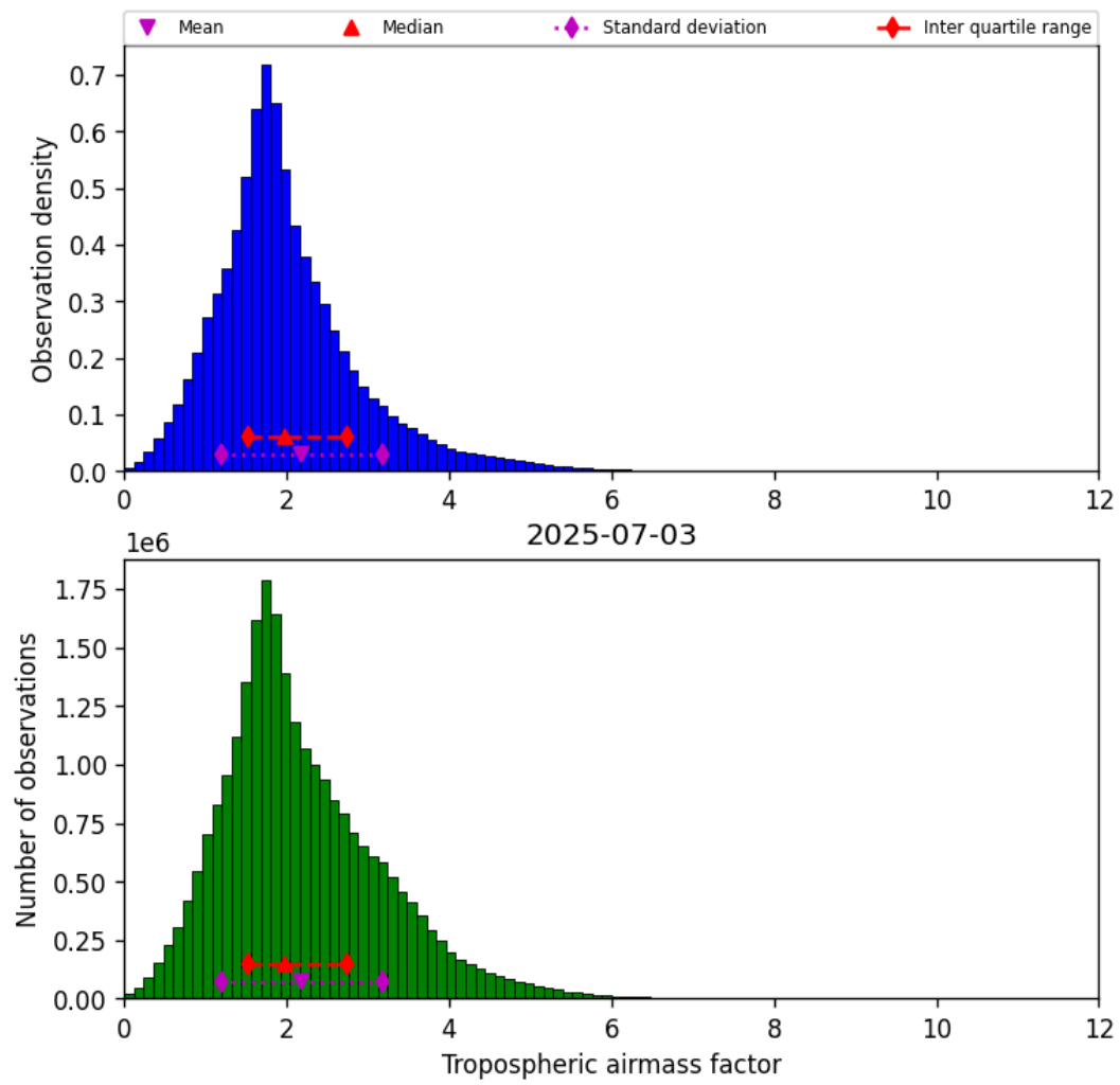
Figure 31: Histogram of “Tropospheric airmass factor” for 2025-07-03 to 2025-07-04
