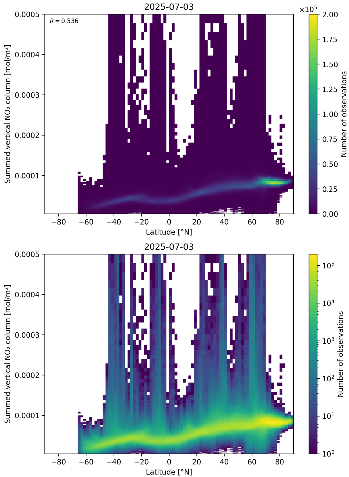
Figure 88: Scatter density plot of “Latitude” against “Summed vertical NO 2 column” for 2025-07-03 to 2025-07-04.
