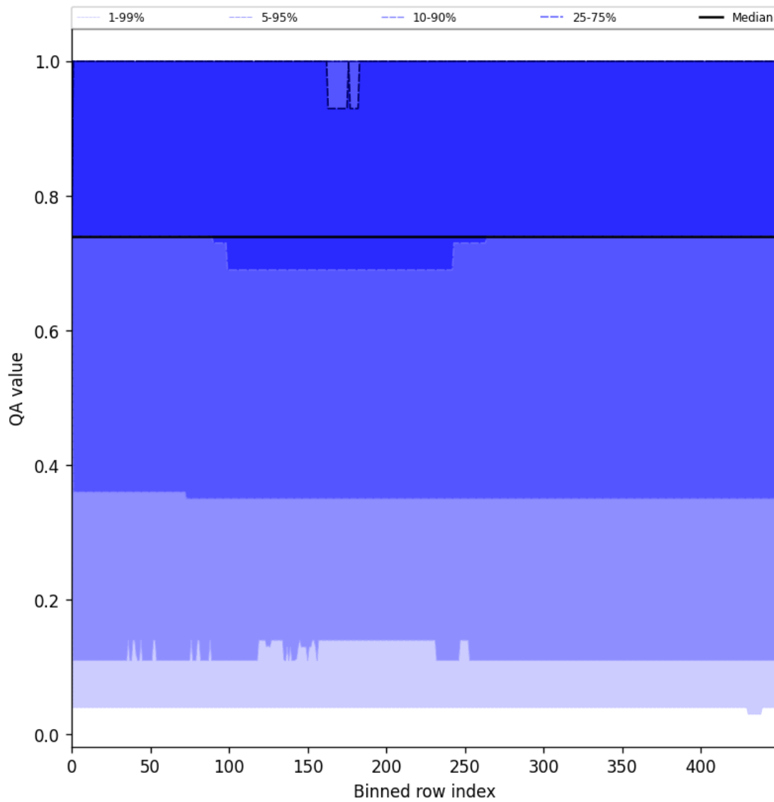
Figure 45: Along track statistics of “QA value” for 2025-07-03 to 2025-07-04
