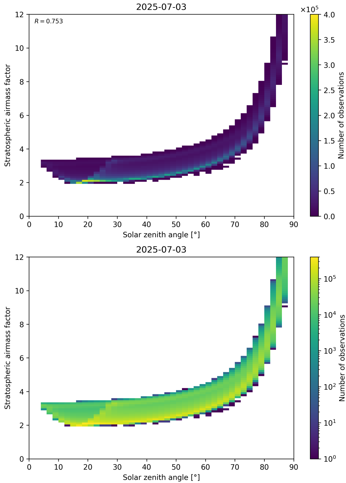
Figure 145: Scatter density plot of “Solar zenith angle” against “Stratospheric airmass factor” for 2025-07-03 to 2025-07-04.
