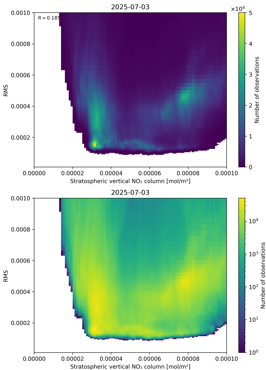
Figure 102: Scatter density plot of “Stratospheric vertical NO 2 column” against “RMS” for 2025-07-03 to 2025-07-04.
