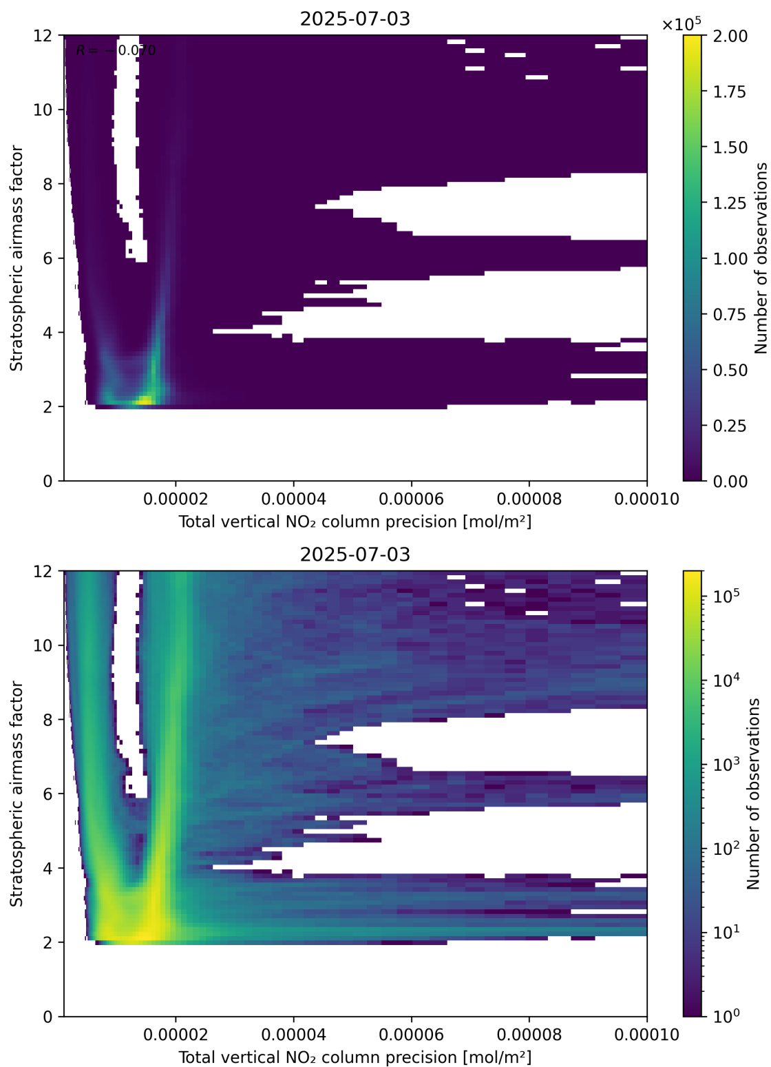
Figure 115: Scatter density plot of “Total vertical NO 2 column precision” against “Stratospheric air mass factor” for 2025-07-03 to 2025-07-04.
