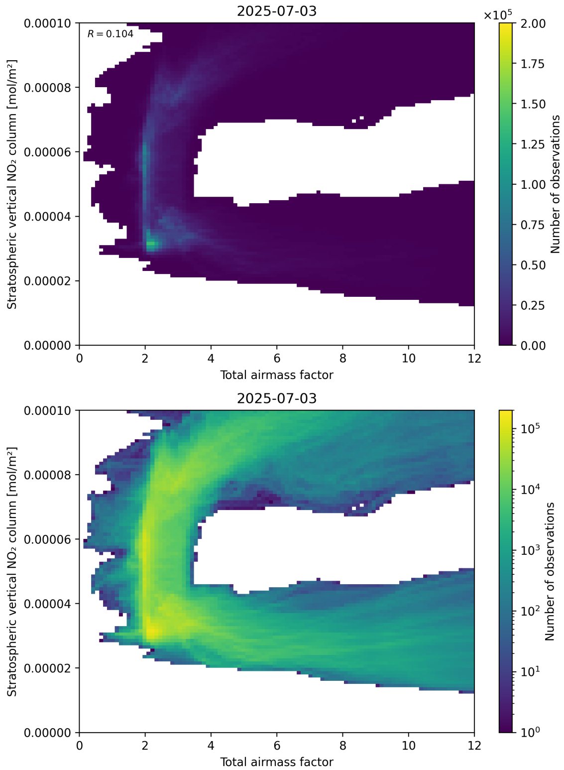
Figure 64: Scatter density plot of “Total airmass factor” against “Stratospheric vertical NO 2 column” for 2025-07-03 to 2025-07-04.
