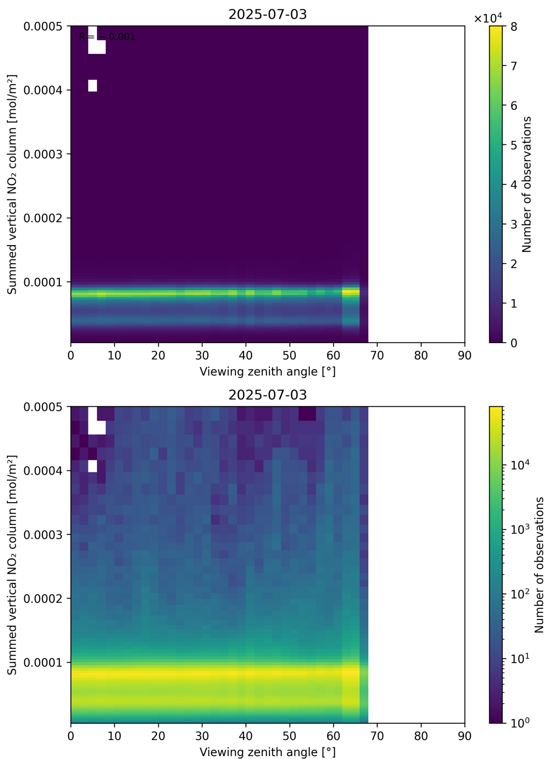
Figure 165: Scatter density plot of “Viewing zenith angle” against “Summed vertical NO 2 column” for 2025-07-03 to 2025-07-04.
