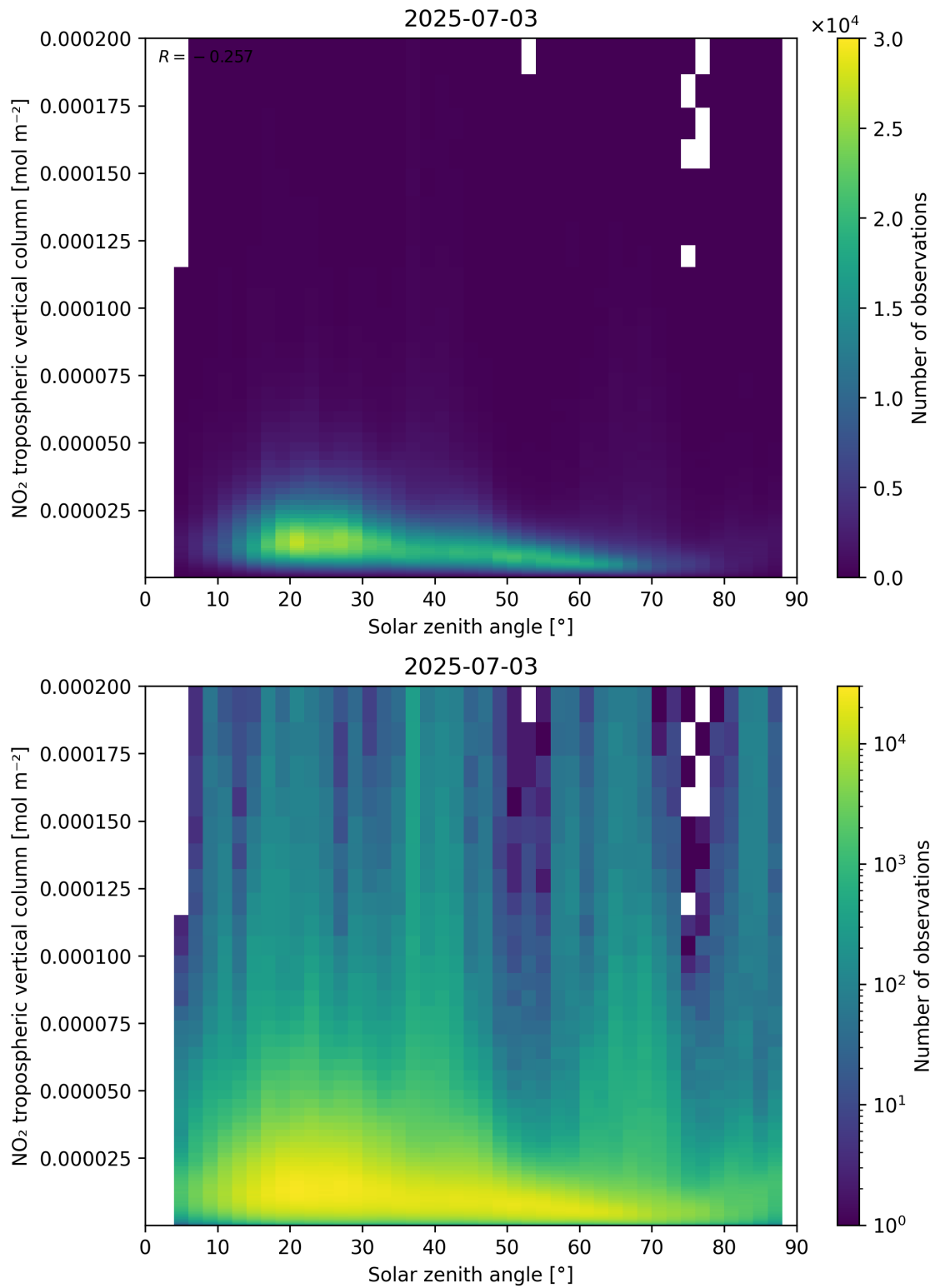
Figure 155: Scatter density plot of “Solar zenith angle” against “NO 2 tropospheric vertical column” for 2025-07-03 to 2025-07-04.
