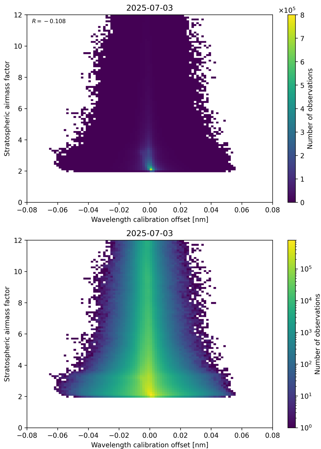
Figure 174: Scatter density plot of “Wavelength calibration offset” against “Stratospheric airmass factor” for 2025-07-03 to 2025-07-04.
