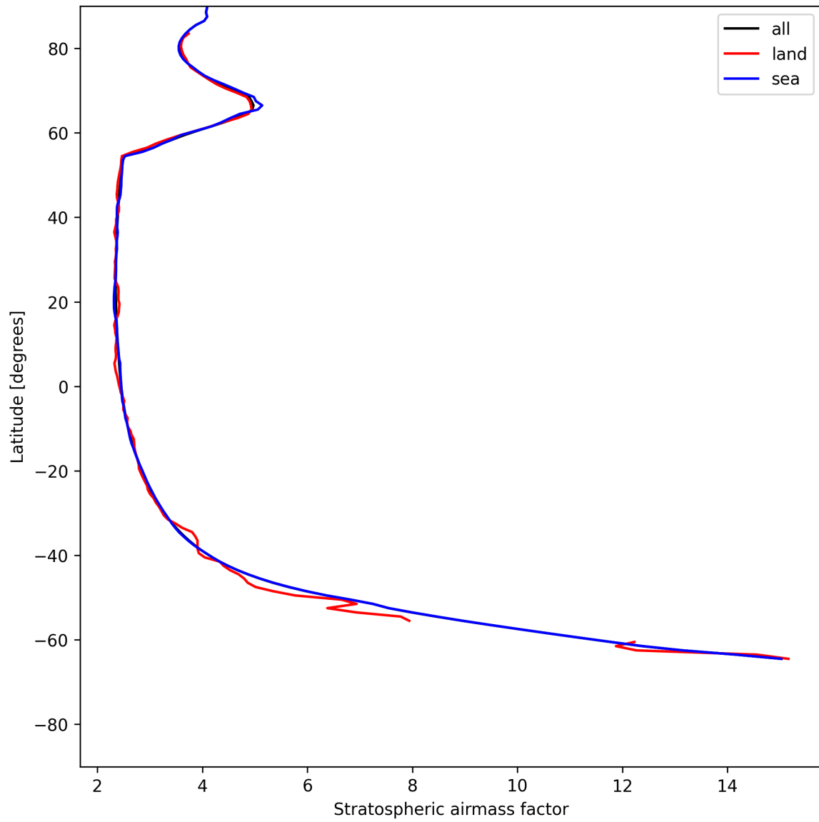
Figure 27: Zonal average of “Stratospheric air mass factor” for 2025-07-03 to 2025-07-04.
