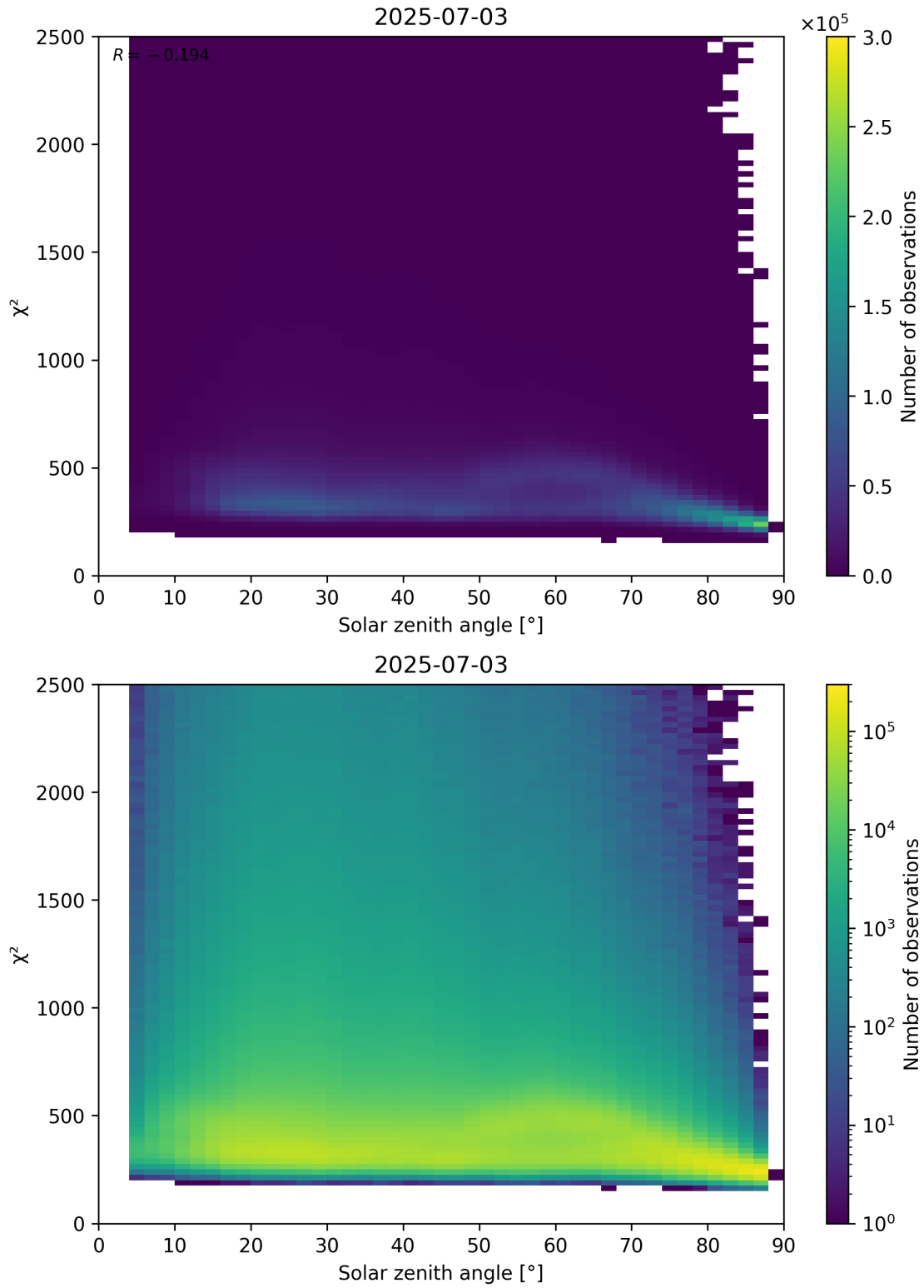
Figure 148: Scatter density plot of “Solar zenith angle” against “ \chi^2 ” for 2025-07-03 to 2025-07-04.
