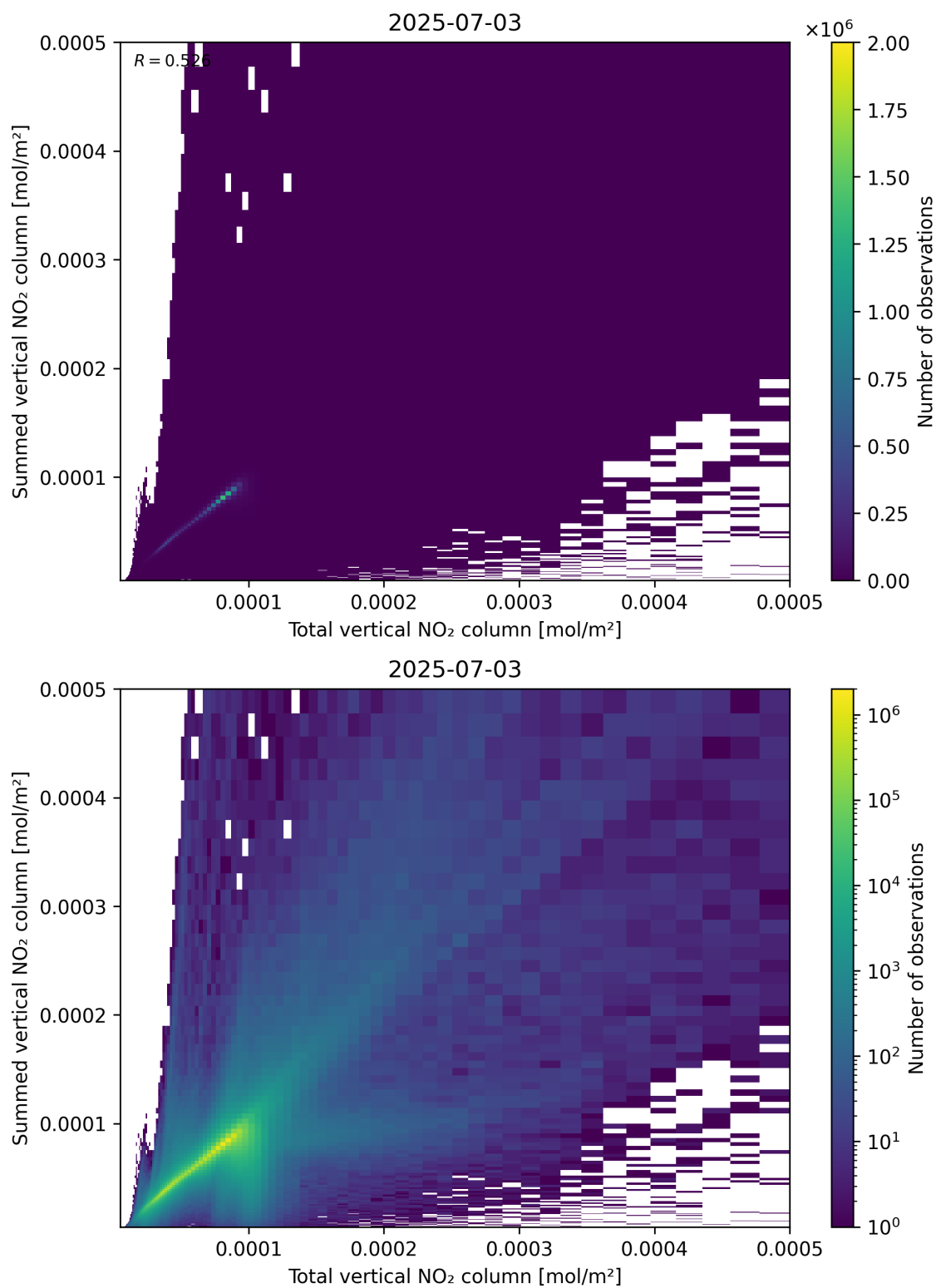
Figure 112: Scatter density plot of “Total vertical NO 2 column” against “Summed vertical NO 2 column” for 2025-07-03 to 2025-07-04.
