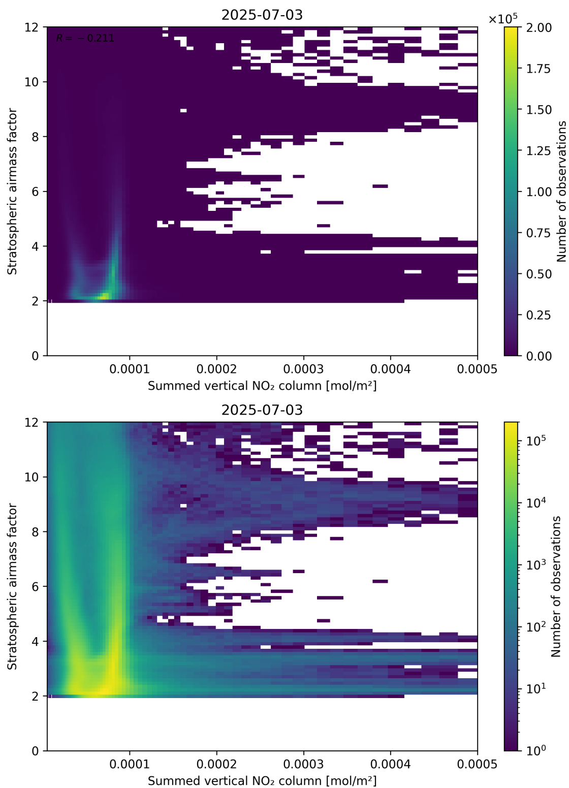
Figure 103: Scatter density plot of “Summed vertical NO 2 column” against “Stratospheric air mass factor” for 2025-07-03 to 2025-07-04.
