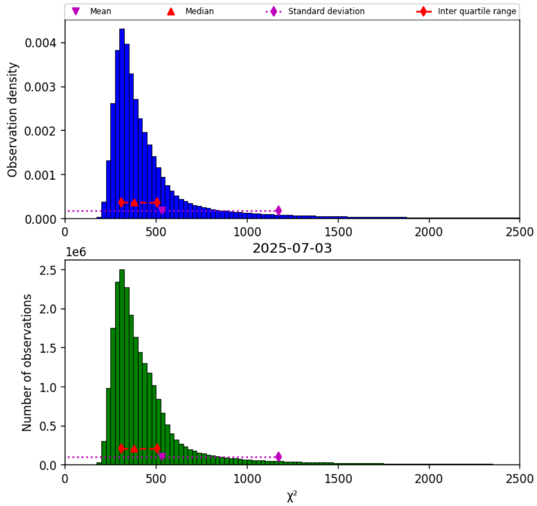
Figure 42: Histogram of “ \chi^2 ” for 2025-07-03 to 2025-07-04
