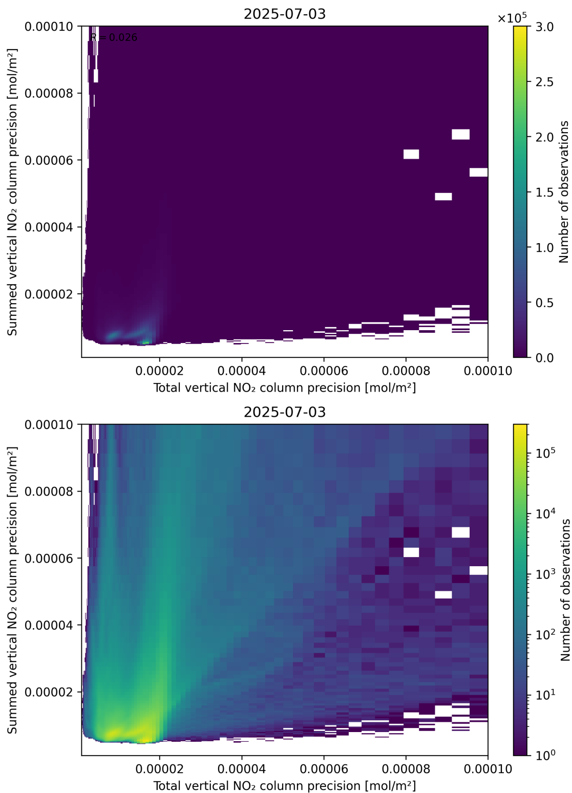
Figure 118: Scatter density plot of “Total vertical NO 2 column precision” against “Summed vertical NO 2 column precision” for 2025-07-03 to 2025-07-04.
