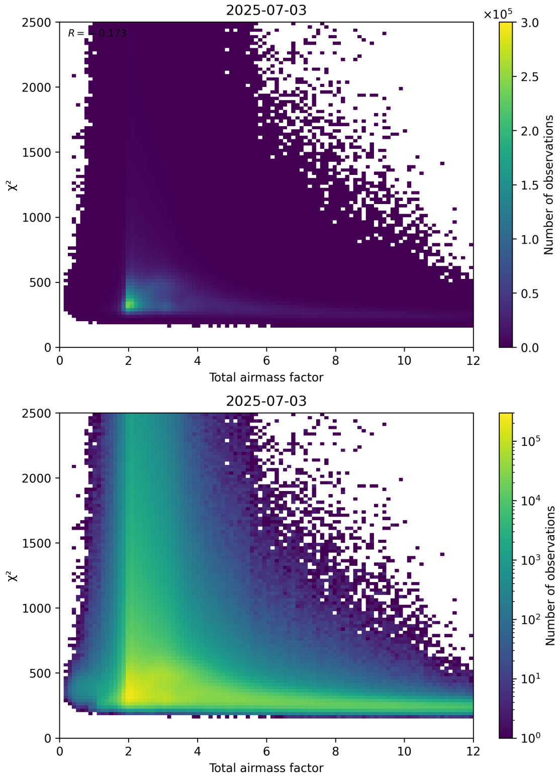
Figure 63: Scatter density plot of “Total airmass factor” against “ \chi^2 ” for 2025-07-03 to 2025-07-04.
