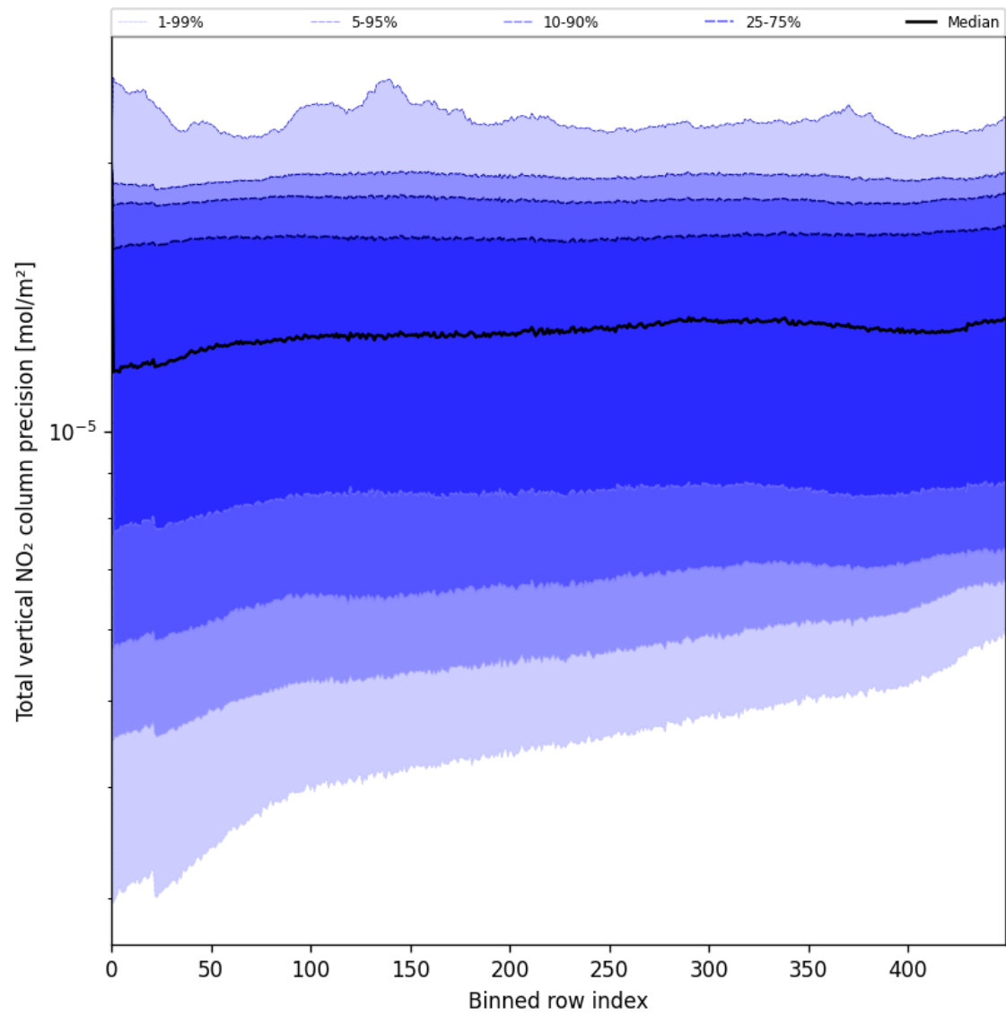
Figure 56: Along track statistics of “Total vertical NO 2 column precision” for 2025-07-03 to 2025-07-04
