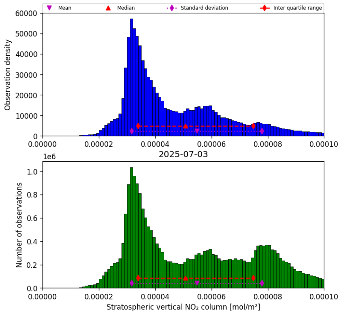
Figure 36: Histogram of “Stratospheric vertical NO 2 column” for 2025-07-03 to 2025-07-04
