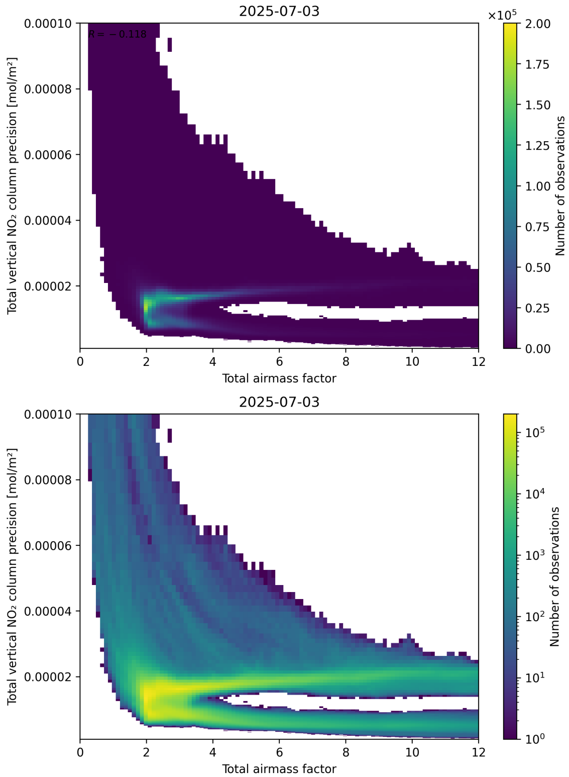
Figure 68: Scatter density plot of “Total airmass factor” against “Total vertical NO 2 column precision” for 2025-07-03 to 2025-07-04.
