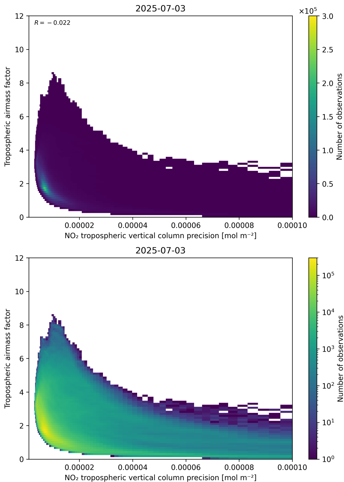
Figure 133: Scatter density plot of “NO 2 tropospheric vertical column precision” against “Tropospheric air mass factor” for 2025-07-03 to 2025-07-04.
