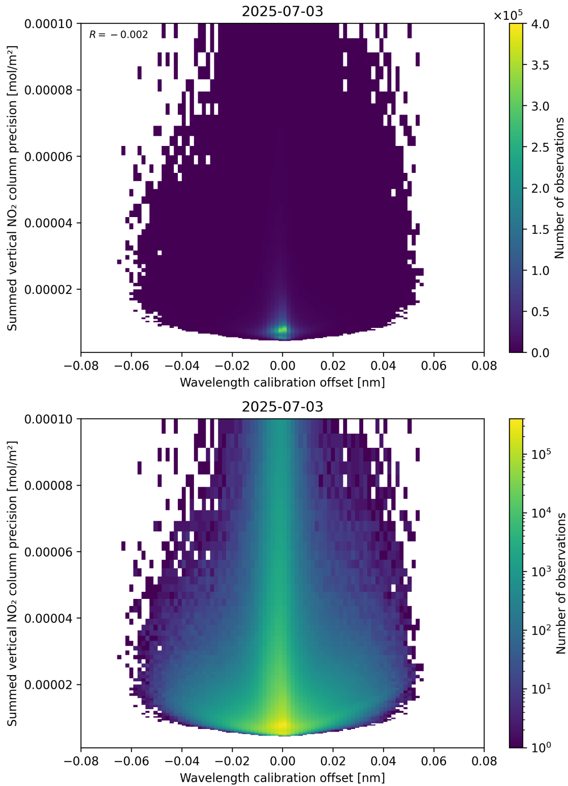
Figure 178: Scatter density plot of “Wavelength calibration offset” against “Summed vertical NO 2 column precision” for 2025-07-03 to 2025-07-04.
