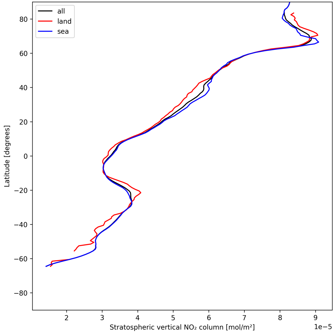
Figure 19: Zonal average of “Stratospheric vertical NO 2 column” for 2025-07-03 to 2025-07-04.
