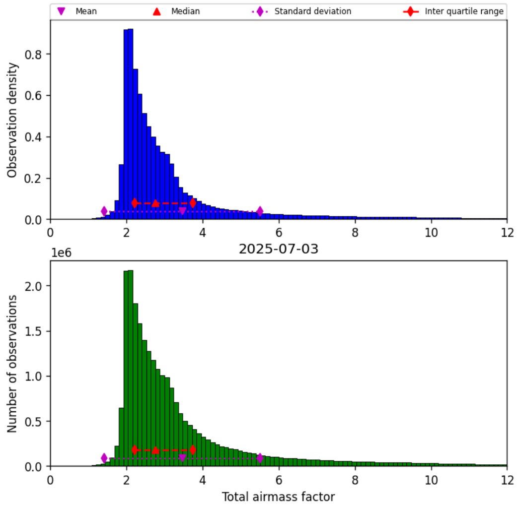
Figure 32: Histogram of “Total airmass factor” for 2025-07-03 to 2025-07-04
