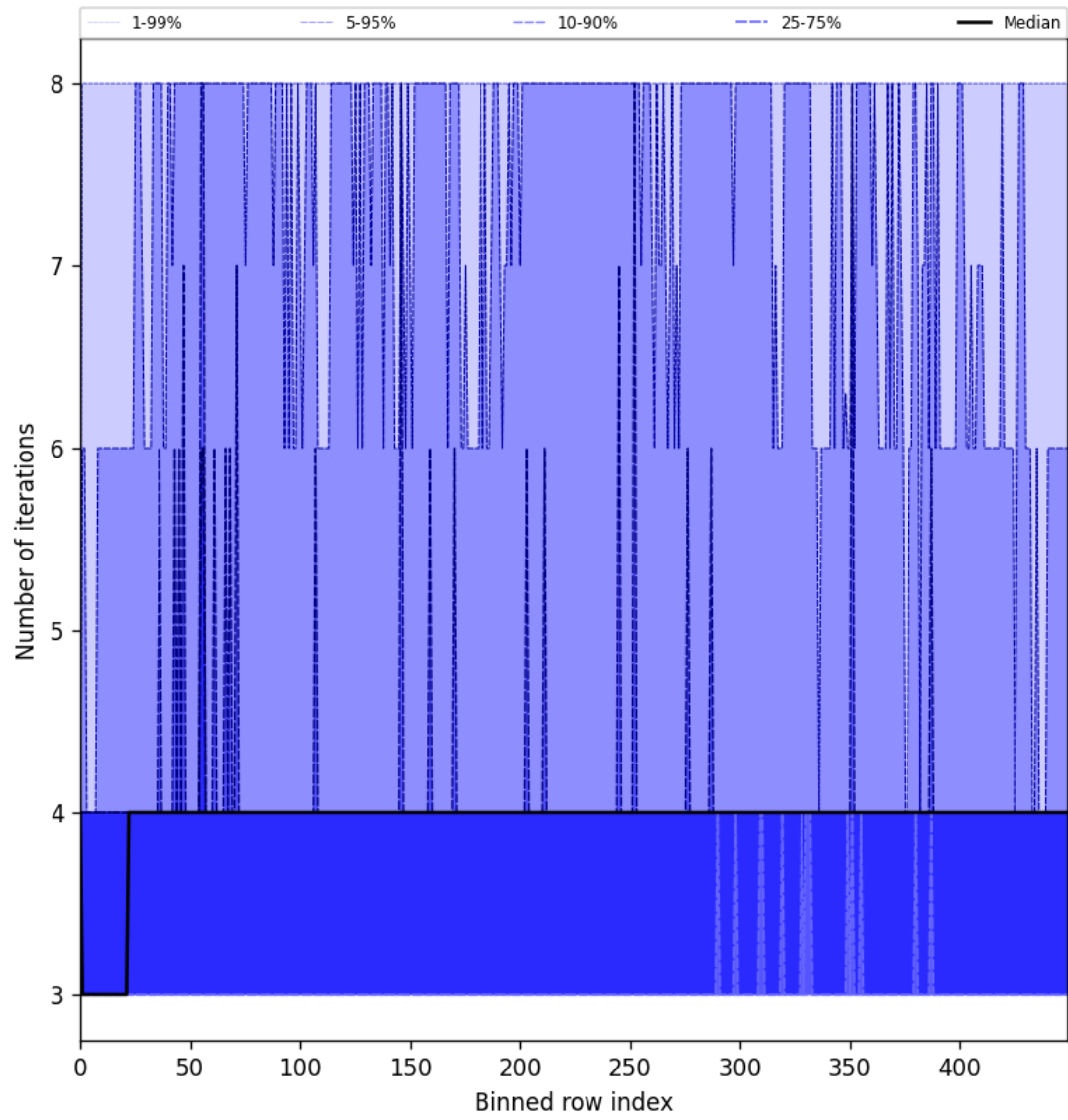
Figure 51: Along track statistics of “Number of iterations” for 2025-07-03 to 2025-07-04
