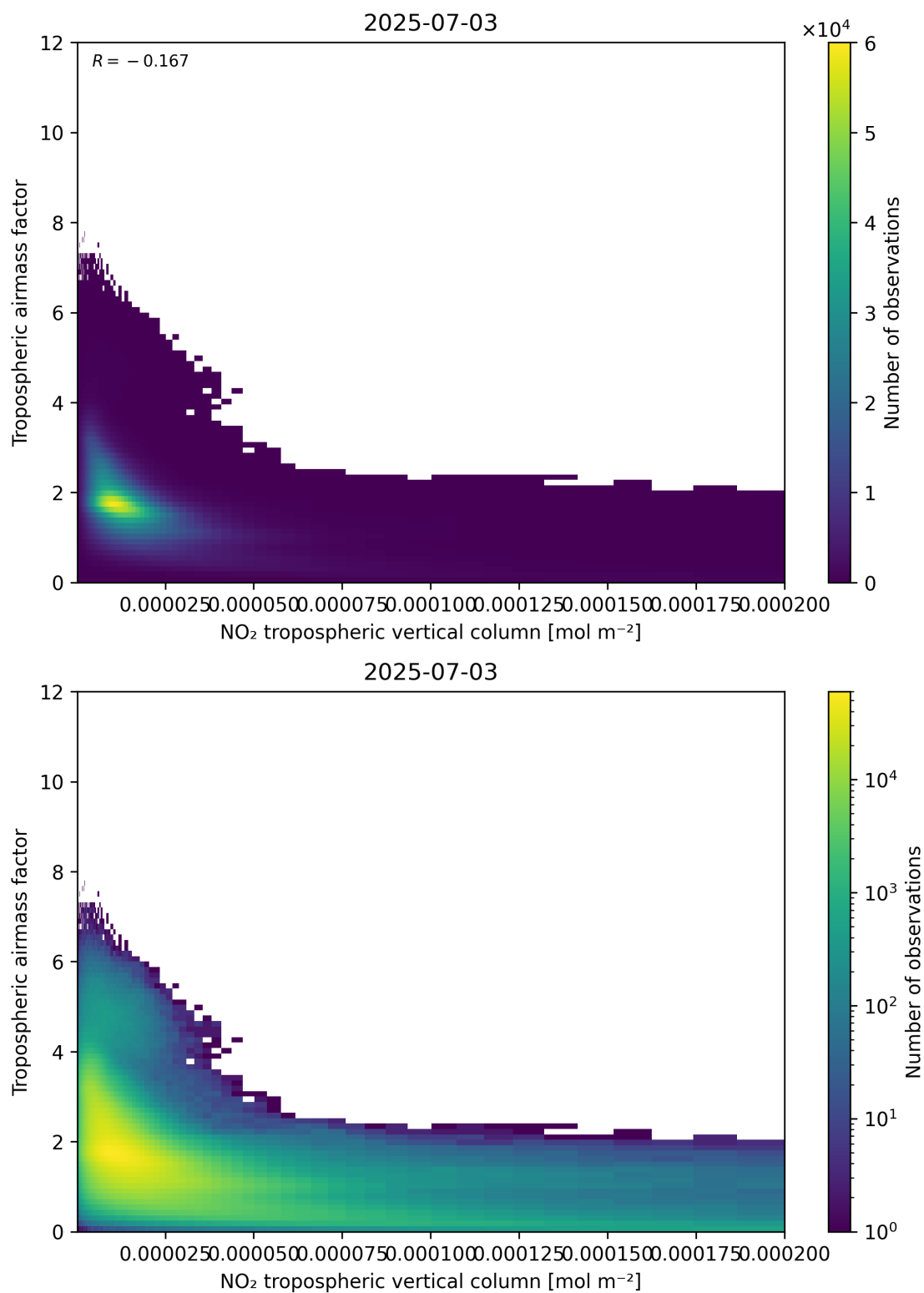
Figure 123: Scatter density plot of “NO 2 tropospheric vertical column” against “Tropospheric air mass factor” for 2025-07-03 to 2025-07-04.
