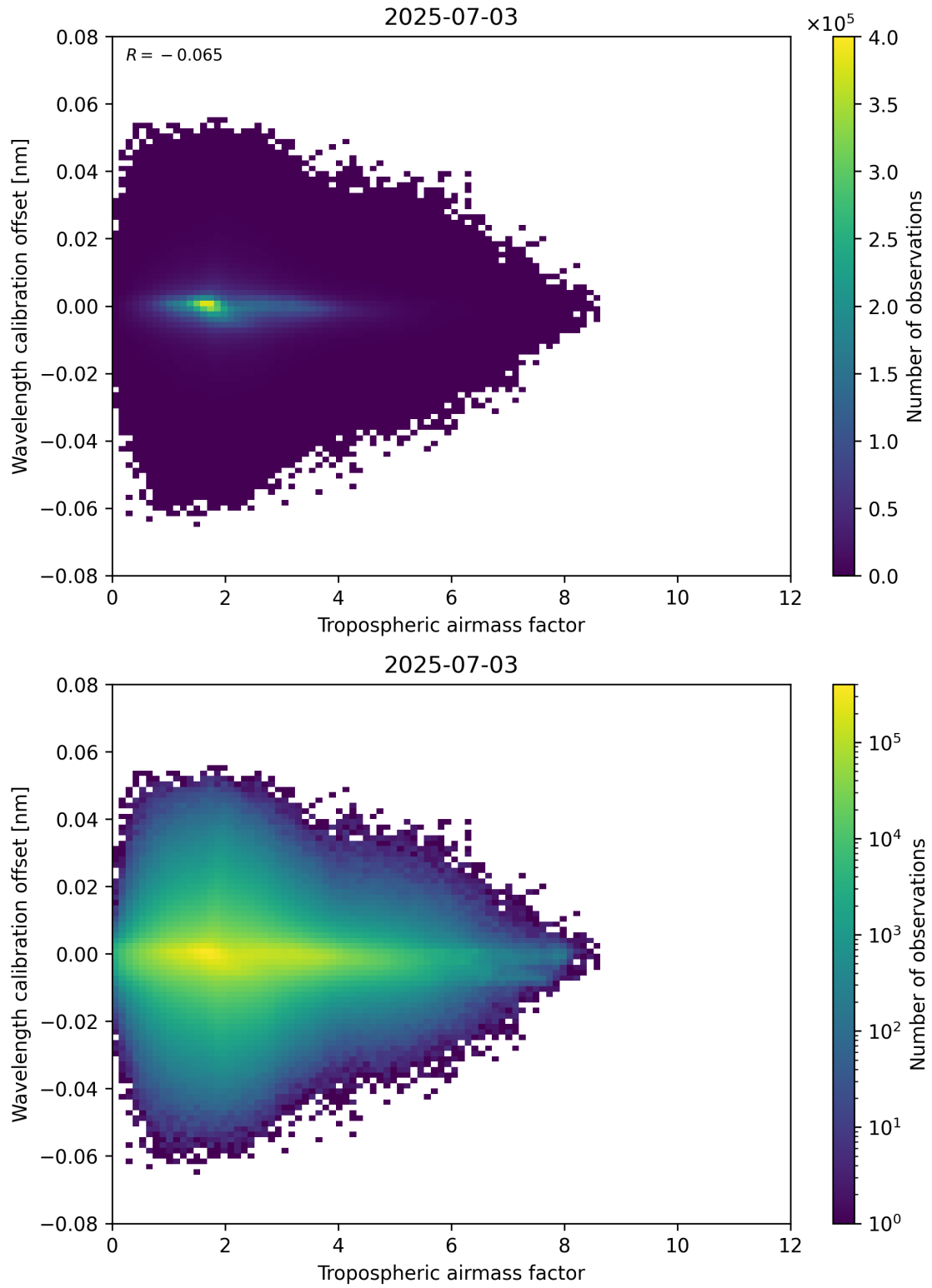
Figure 80: Scatter density plot of “Tropospheric airmass factor” against “Wavelength calibration offset” for 2025-07-03 to 2025-07-04.
