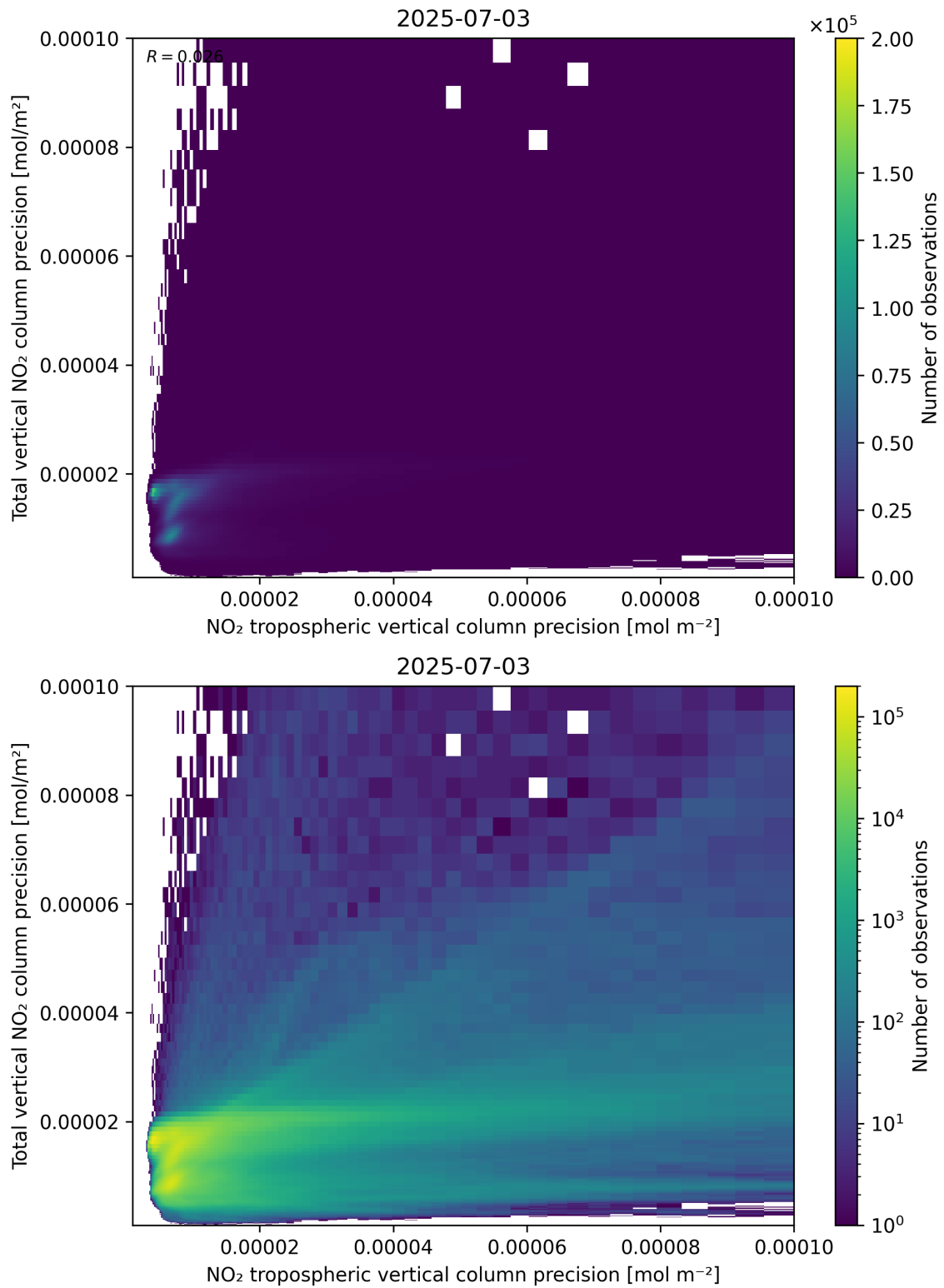
Figure 139: Scatter density plot of “NO 2 tropospheric vertical column precision” against “Total vertical NO 2 column precision” for 2025-07-03 to 2025-07-04.
