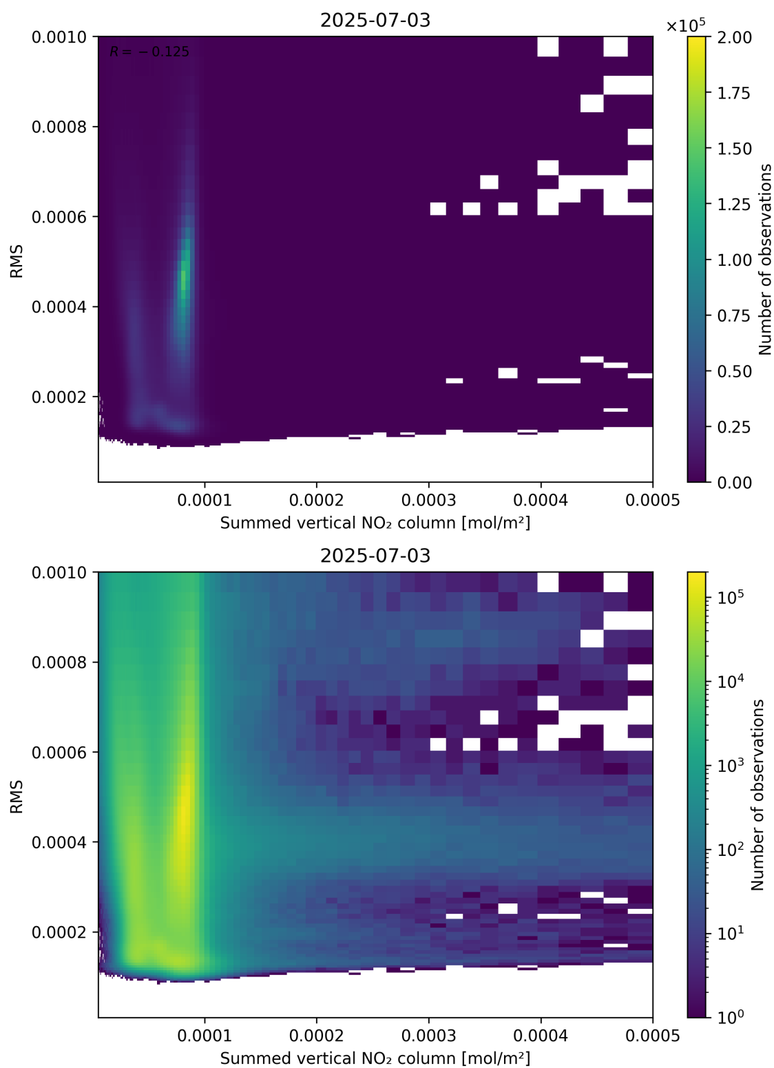
Figure 109: Scatter density plot of “Summed vertical NO 2 column” against “RMS” for 2025-07-03 to 2025-07-04.
