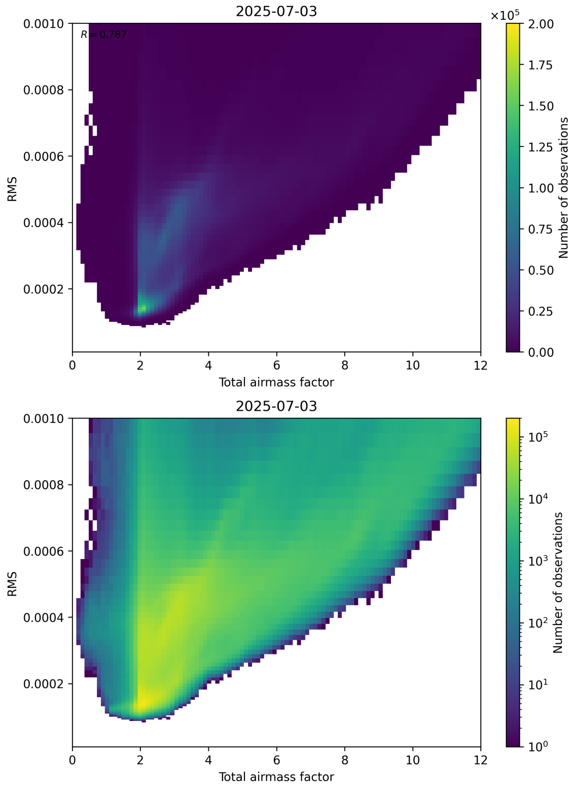
Figure 69: Scatter density plot of “Total airmass factor” against “RMS” for 2025-07-03 to 2025-07-04.
