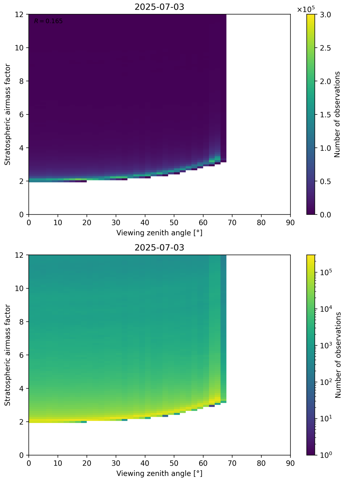
Figure 159: Scatter density plot of “Viewing zenith angle” against “Stratospheric airmass factor” for 2025-07-03 to 2025-07-04.
