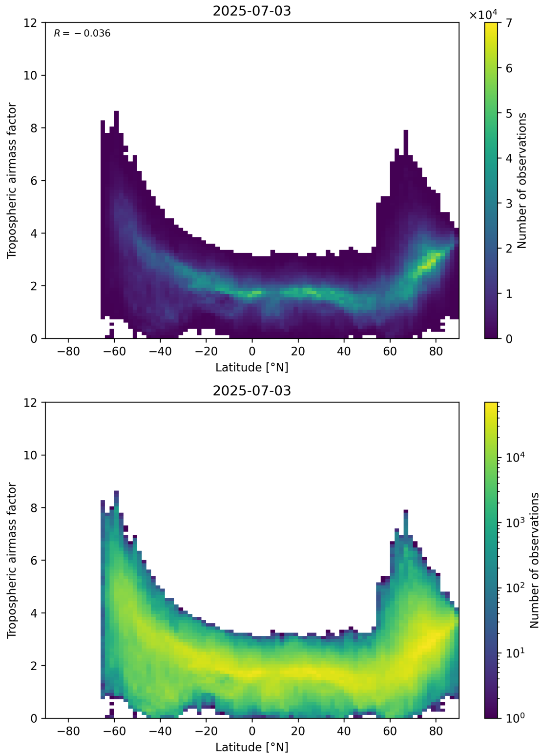
Figure 85: Scatter density plot of “Latitude” against “Tropospheric airmass factor” for 2025-07-03 to 2025-07-04.
