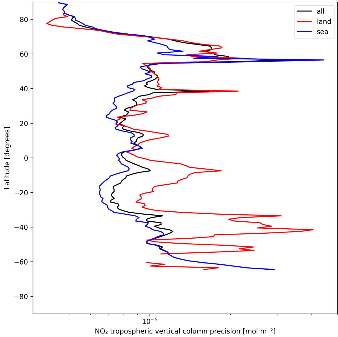
Figure 13: Zonal average of “NO 2 tropospheric vertical column precision” for 2025-07-03 to 2025-07-04.
