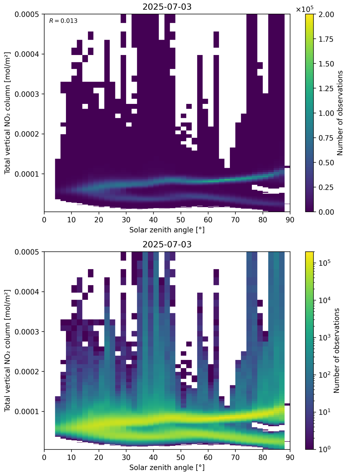
Figure 153: Scatter density plot of “Solar zenith angle” against “Total vertical NO 2 column” for 2025-07-03 to 2025-07-04.
