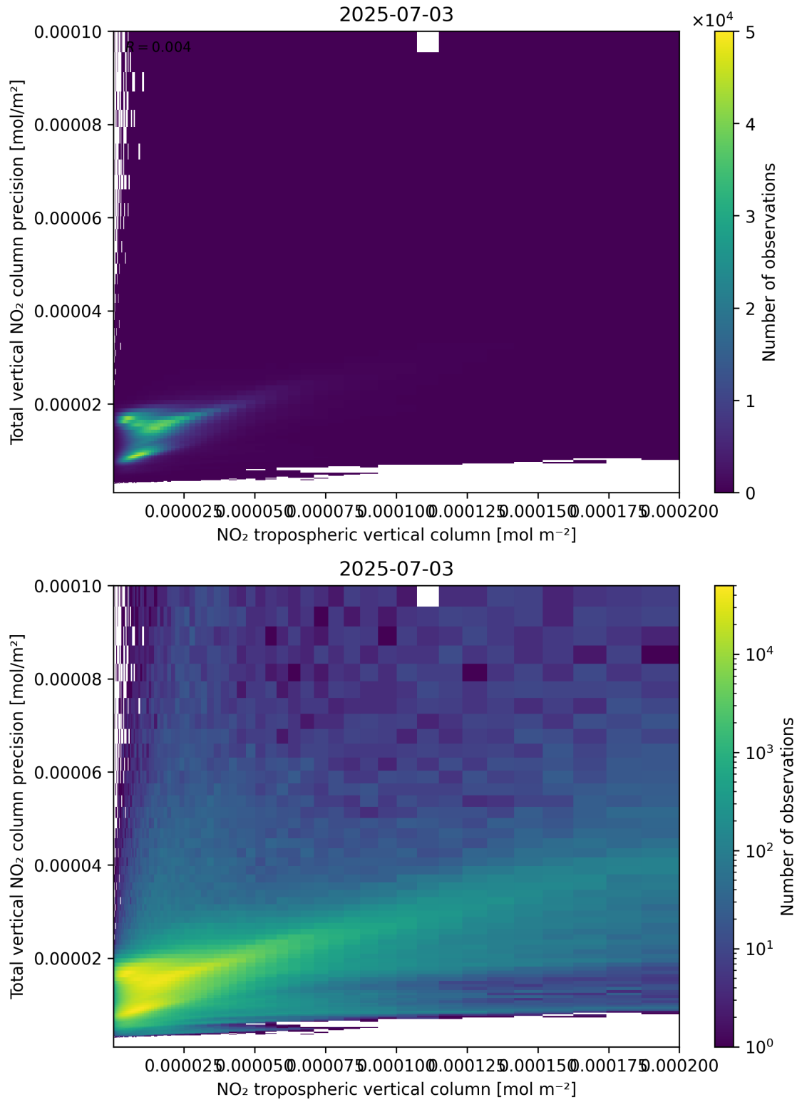
Figure 129: Scatter density plot of “NO 2 tropospheric vertical column” against “Total vertical NO 2 column precision” for 2025-07-03 to 2025-07-04.
