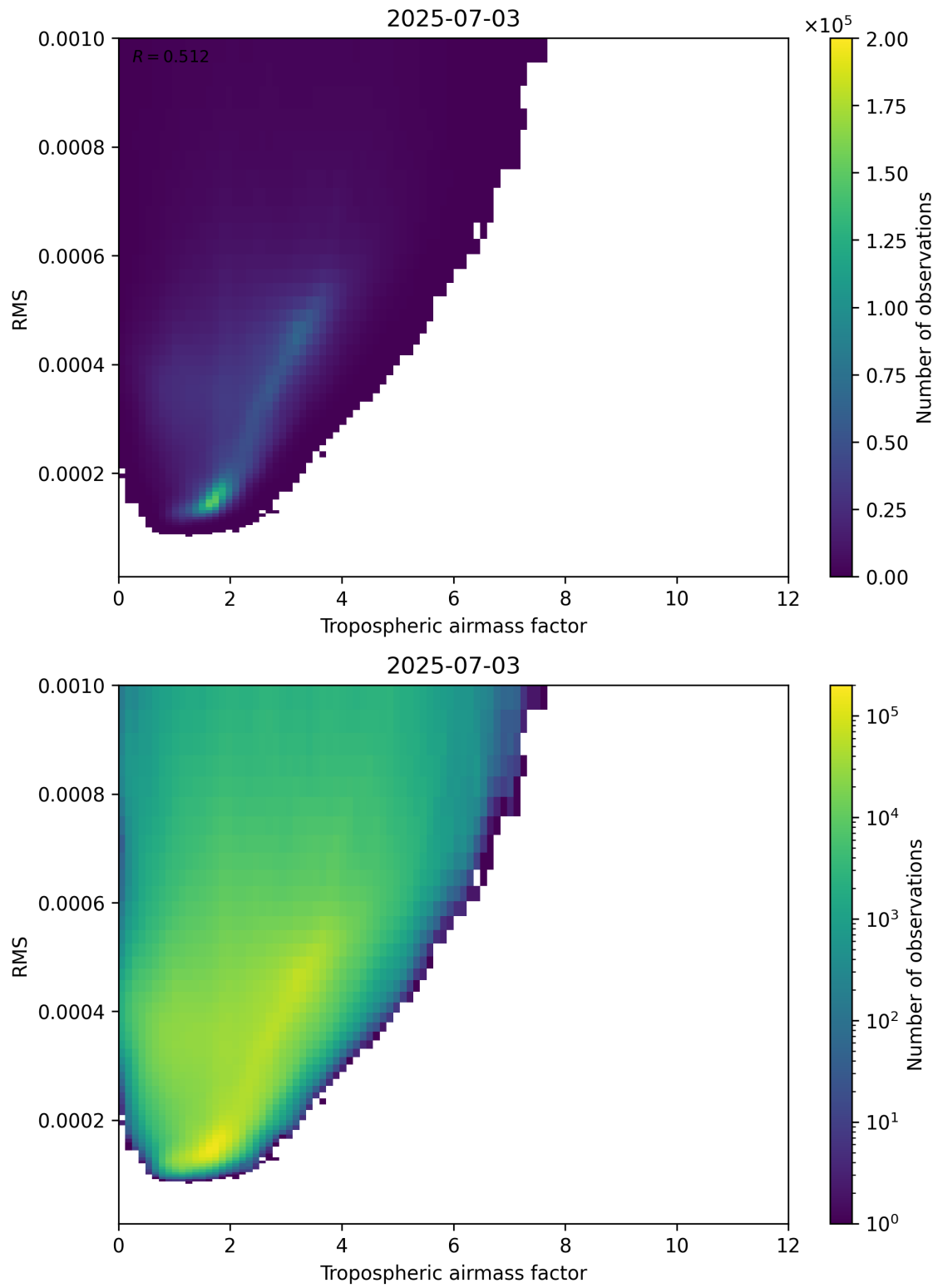
Figure 79: Scatter density plot of “Tropospheric airmass factor” against “RMS” for 2025-07-03 to 2025-07-04.
