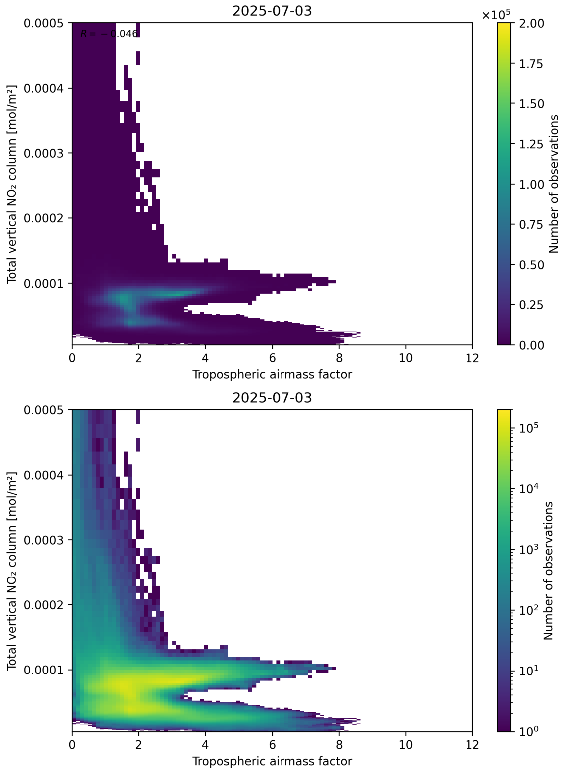
Figure 77: Scatter density plot of “Tropospheric airmass factor” against “Total vertical NO 2 column” for 2025-07-03 to 2025-07-04.
