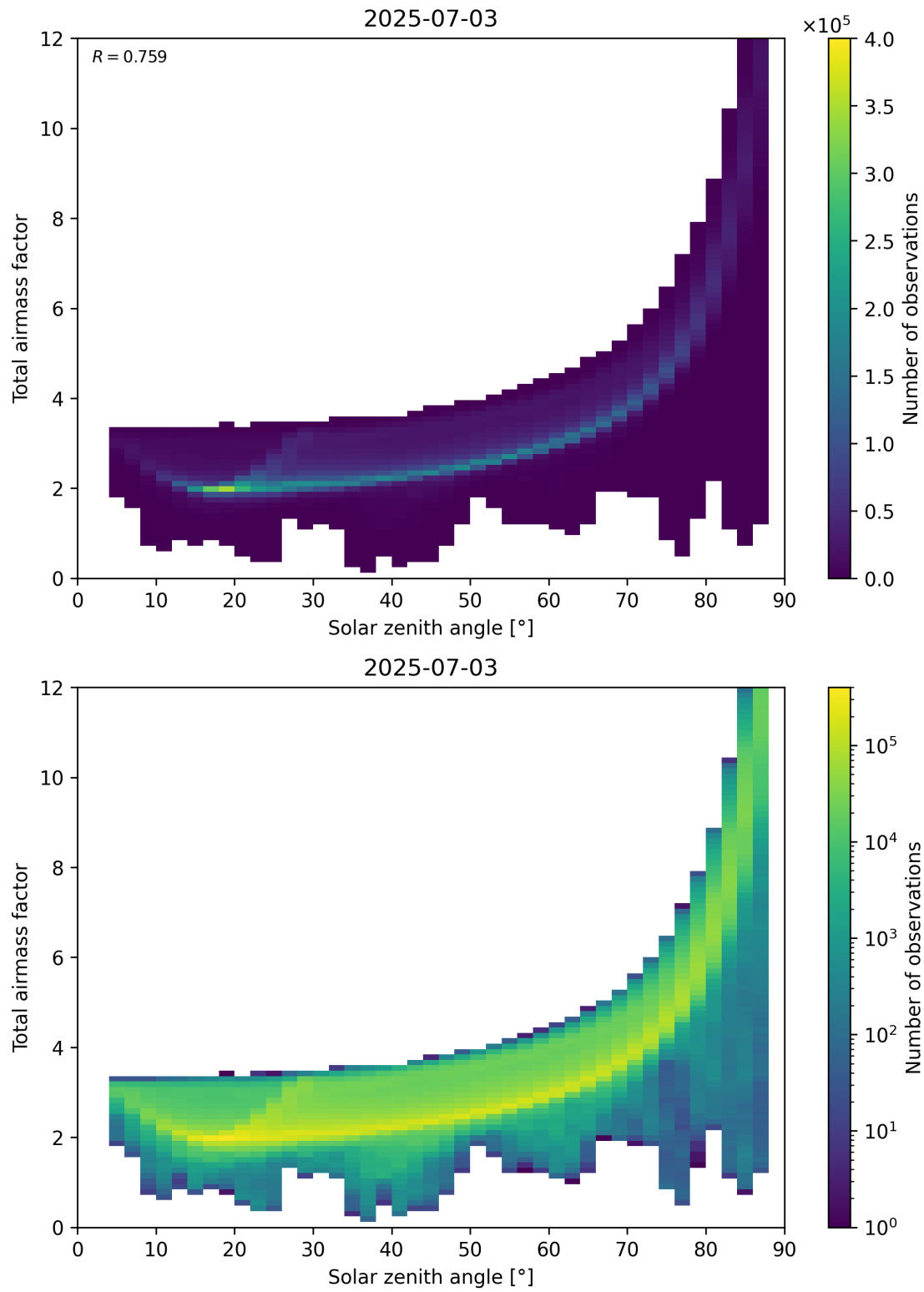
Figure 146: Scatter density plot of “Solar zenith angle” against “Total air mass factor” for 2025-07-03 to 2025-07-04.
