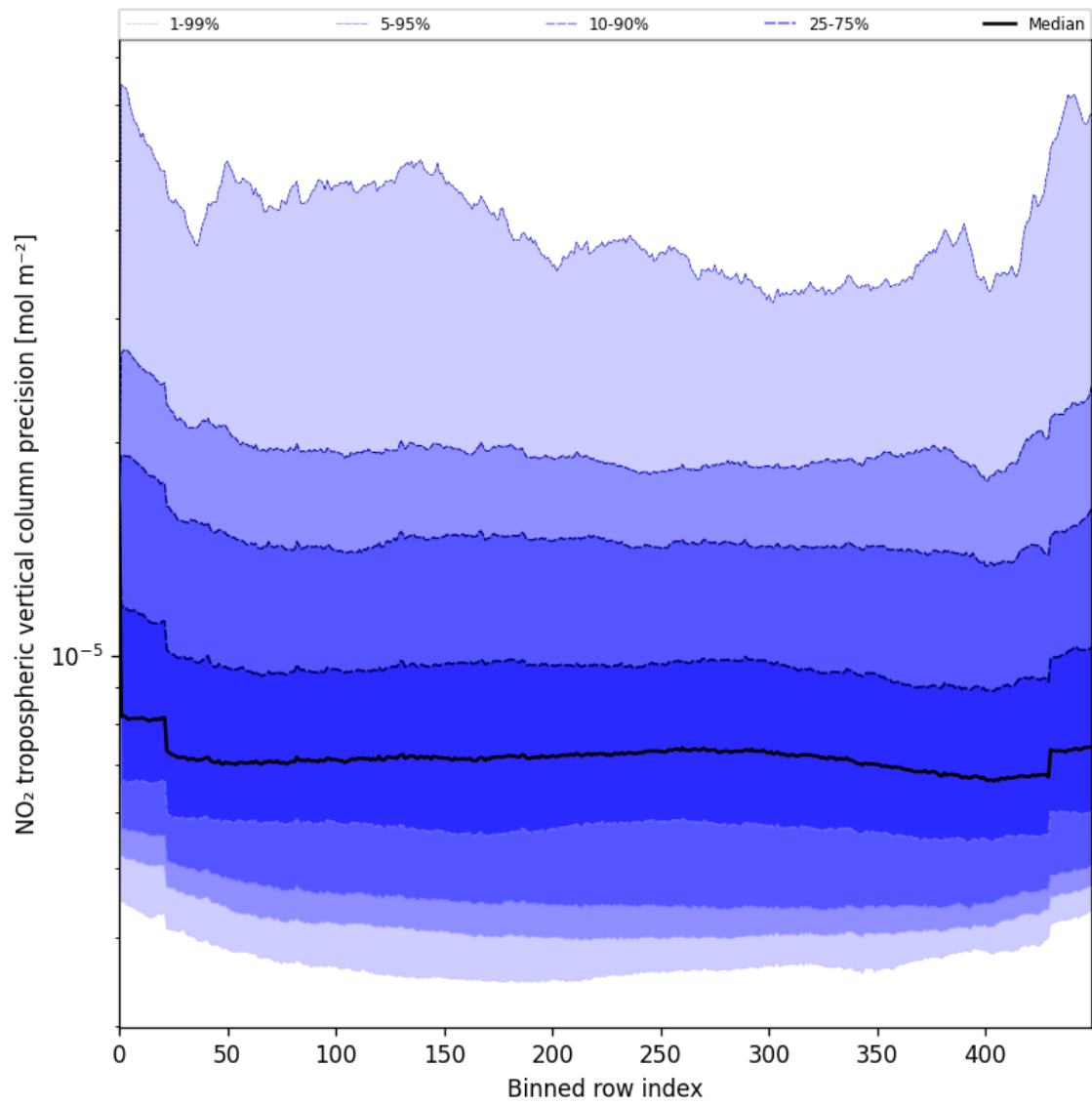
Figure 47: Along track statistics of “NO 2 tropospheric vertical column precision” for 2025-07-03 to 2025-07-04
