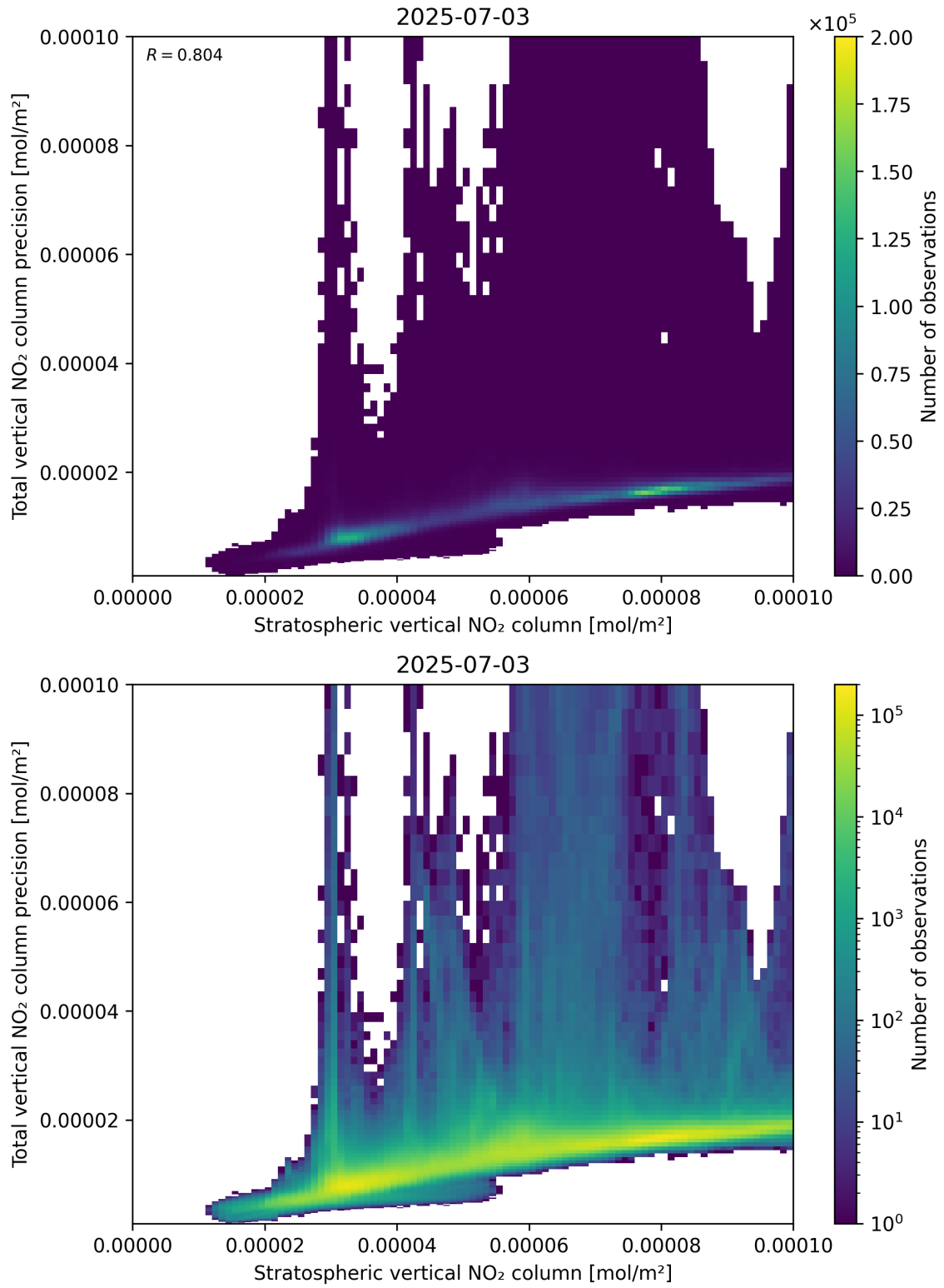
Figure 101: Scatter density plot of “Stratospheric vertical NO 2 column” against “Total vertical NO 2 column precision” for 2025-07-03 to 2025-07-04.
