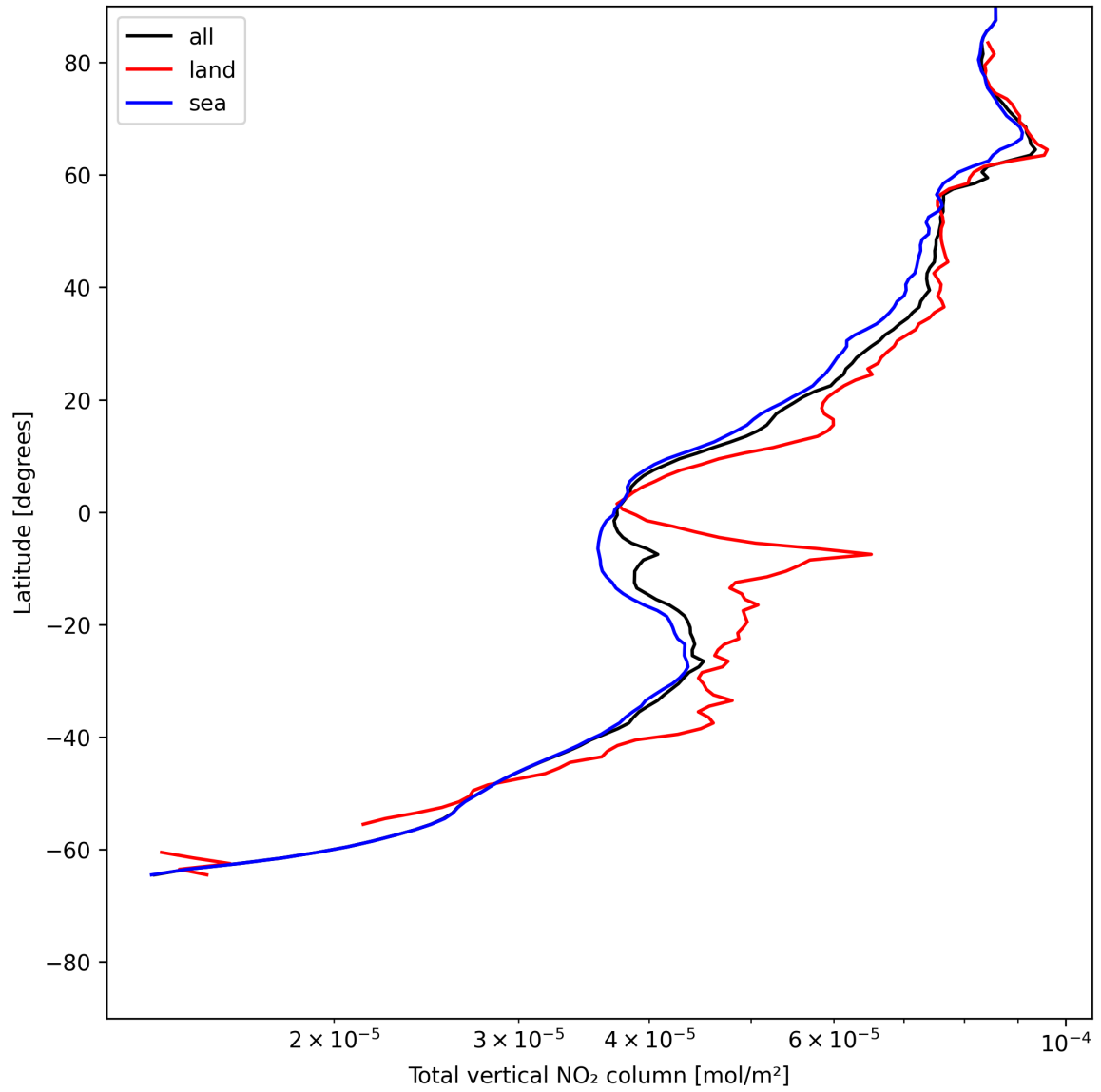
Figure 21: Zonal average of “Total vertical NO 2 column” for 2025-07-03 to 2025-07-04.
