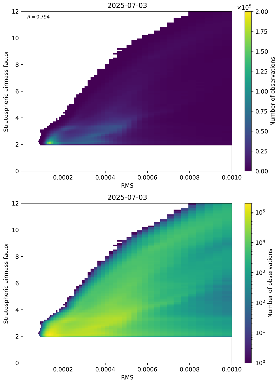
Figure 144: Scatter density plot of “RMS” against “Stratospheric airmass factor” for 2025-07-03 to 2025-07-04.
