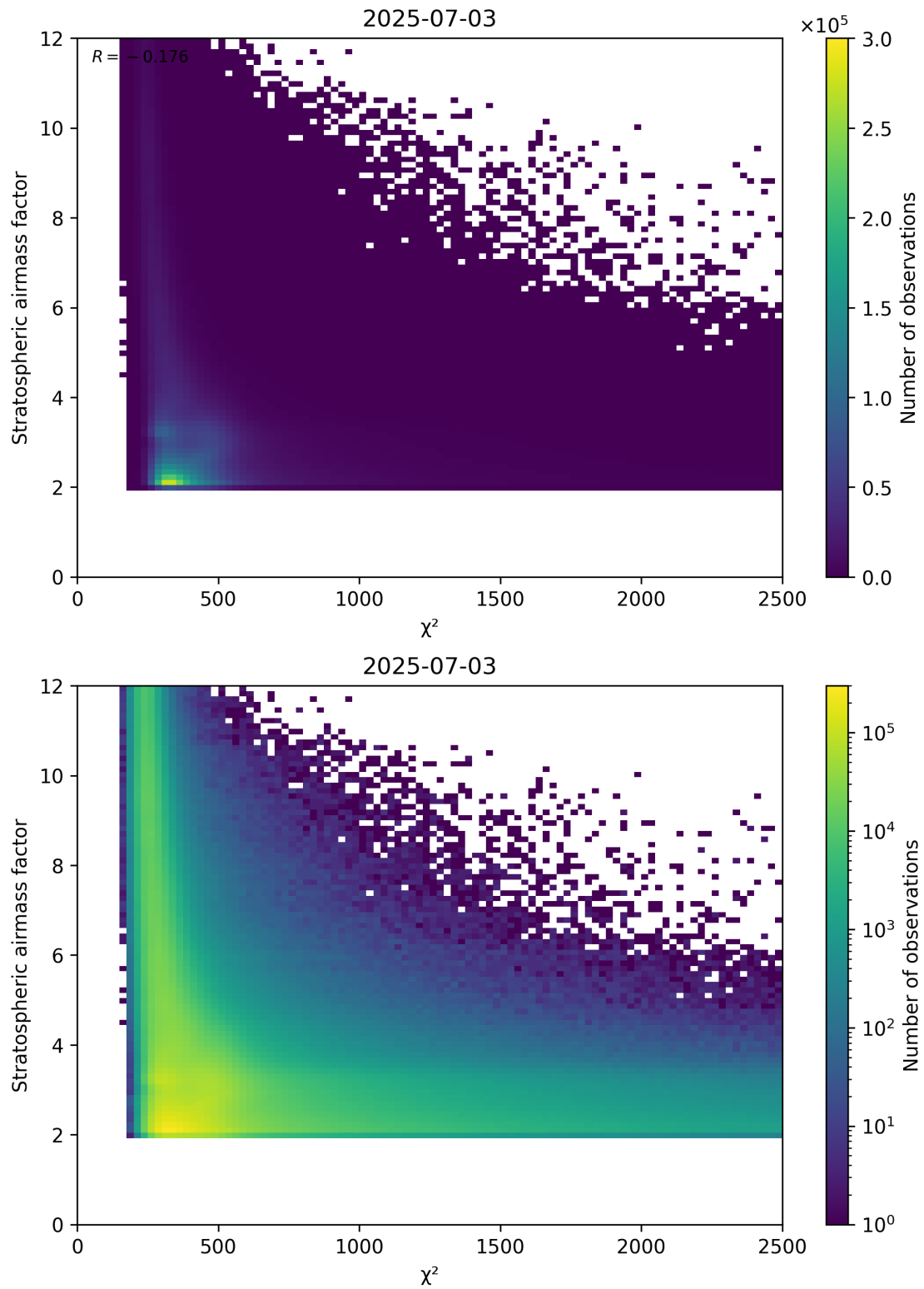
Figure 81: Scatter density plot of “ \chi^2 ” against “Stratospheric airmass factor” for 2025-07-03 to 2025-07-04.
