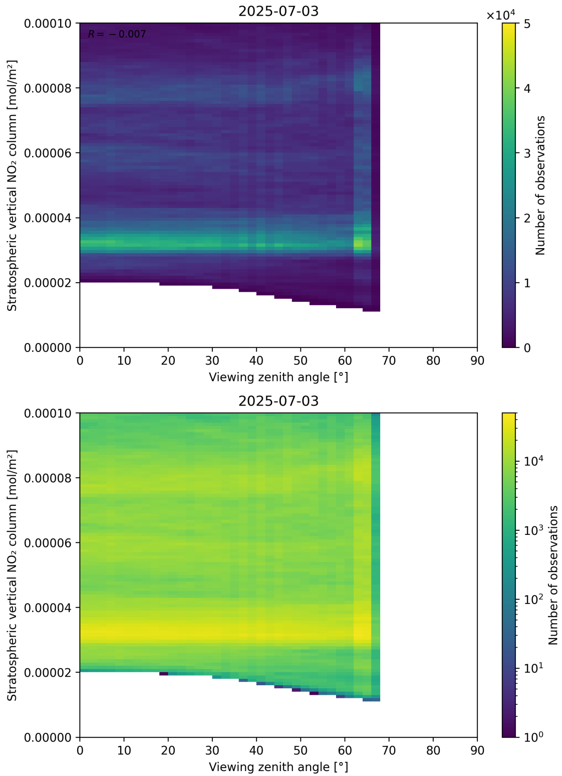
Figure 164: Scatter density plot of “Viewing zenith angle” against “Stratospheric vertical NO 2 column” for 2025-07-03 to 2025-07-04.
