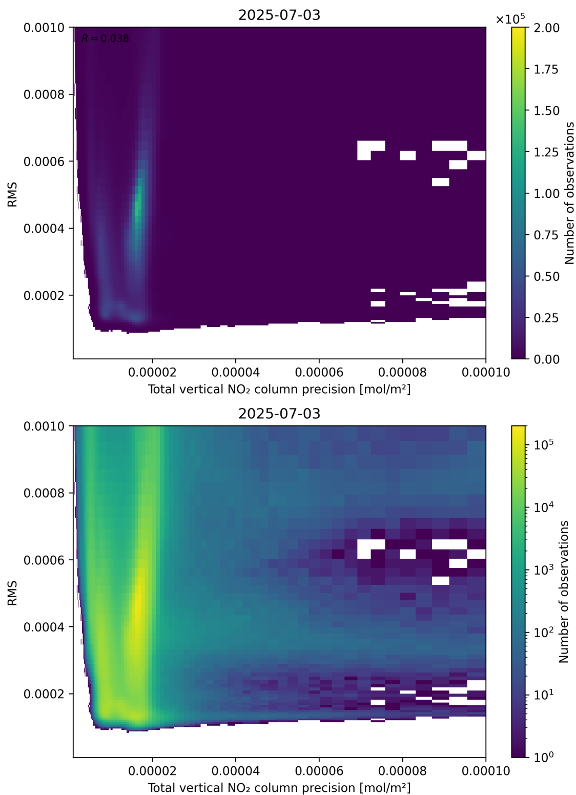
Figure 119: Scatter density plot of “Total vertical NO 2 column precision” against “RMS” for 2025-07-03 to 2025-07-04.
