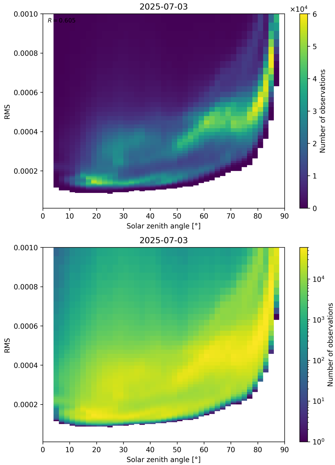
Figure 157: Scatter density plot of “Solar zenith angle” against “RMS” for 2025-07-03 to 2025-07-04.
