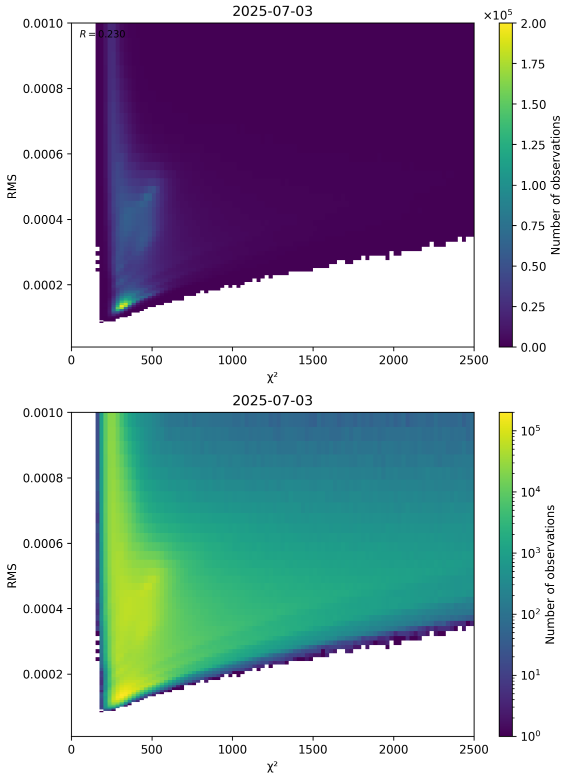
Figure 82: Scatter density plot of “ \chi^2 ” against “RMS” for 2025-07-03 to 2025-07-04.
