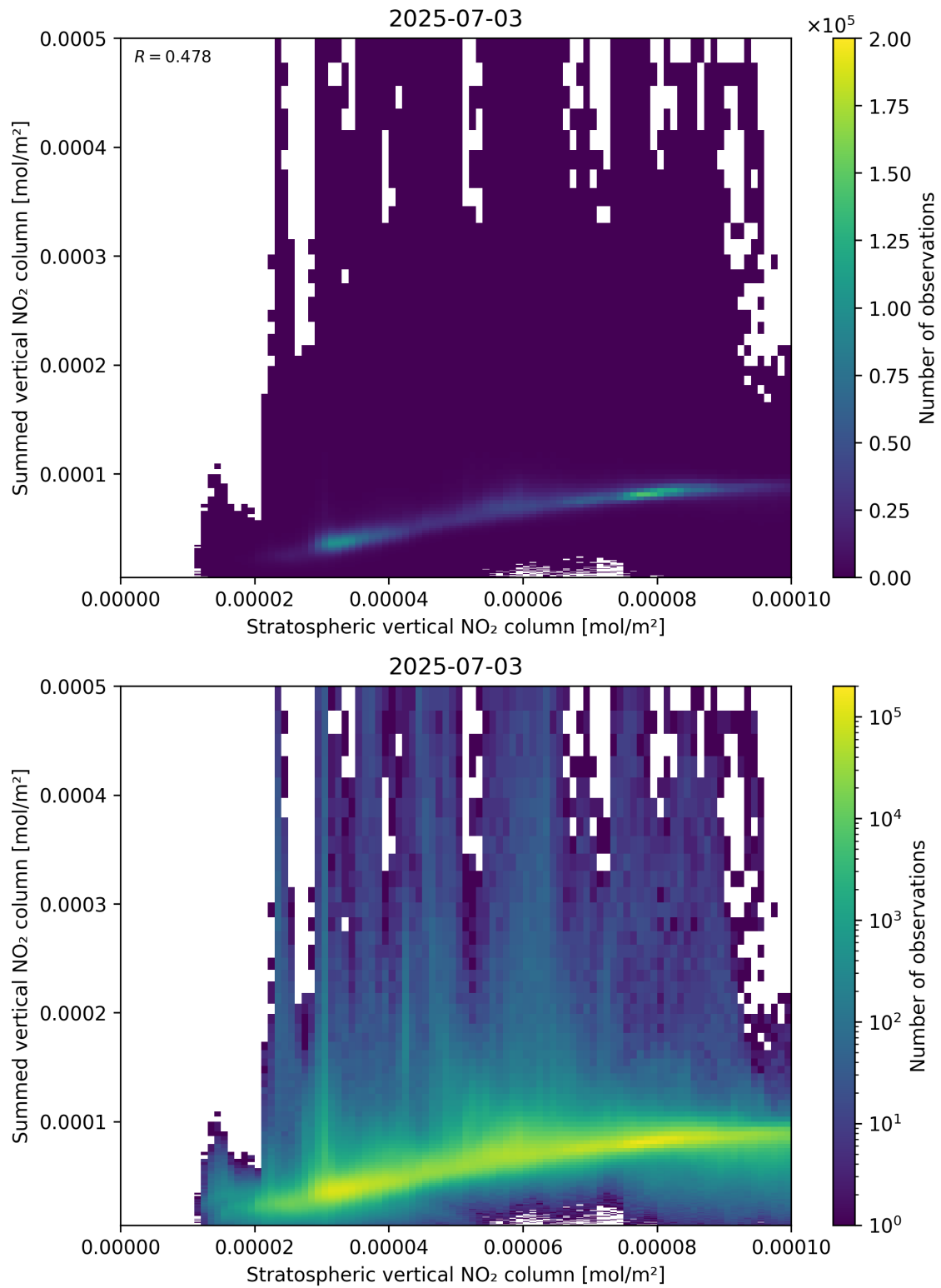
Figure 98: Scatter density plot of “Stratospheric vertical NO 2 column” against “Summed vertical NO 2 column” for 2025-07-03 to 2025-07-04.
