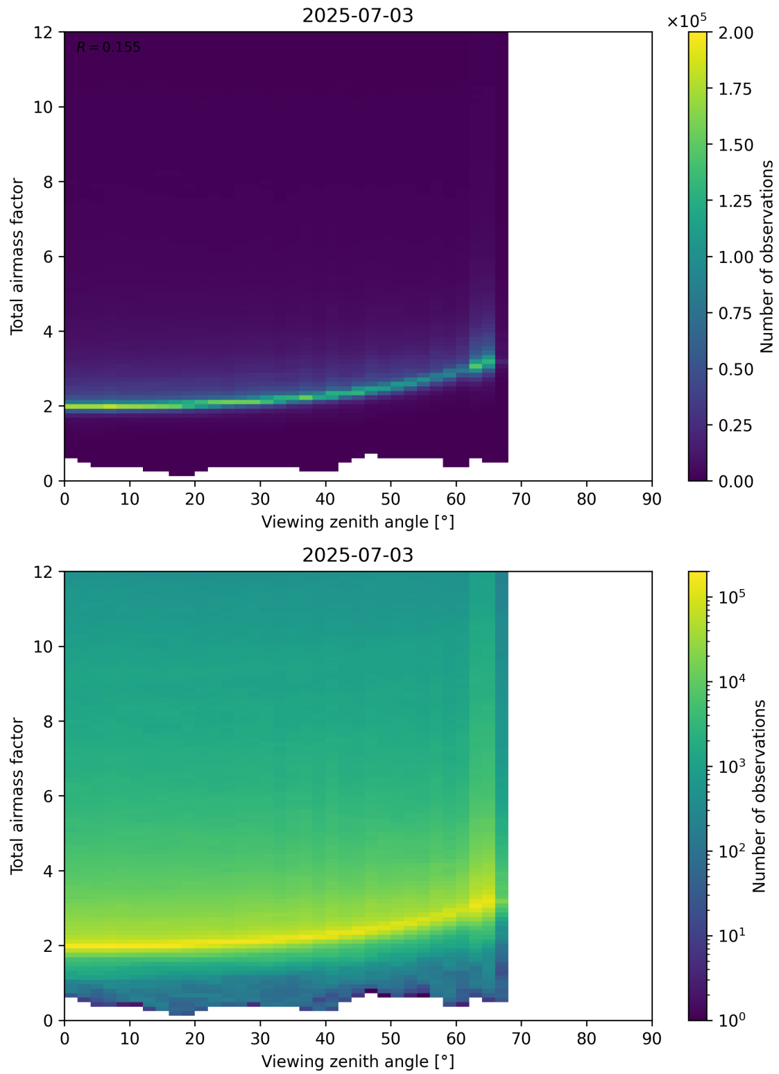
Figure 160: Scatter density plot of “Viewing zenith angle” against “Total airmass factor” for 2025-07-03 to 2025-07-04.
