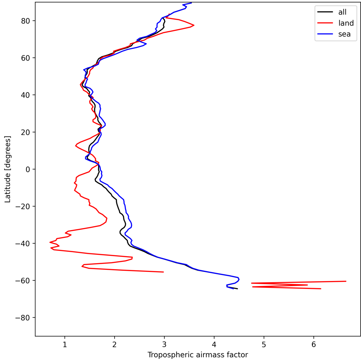
Figure 14: Zonal average of “Tropospheric airmass factor” for 2025-07-03 to 2025-07-04.
