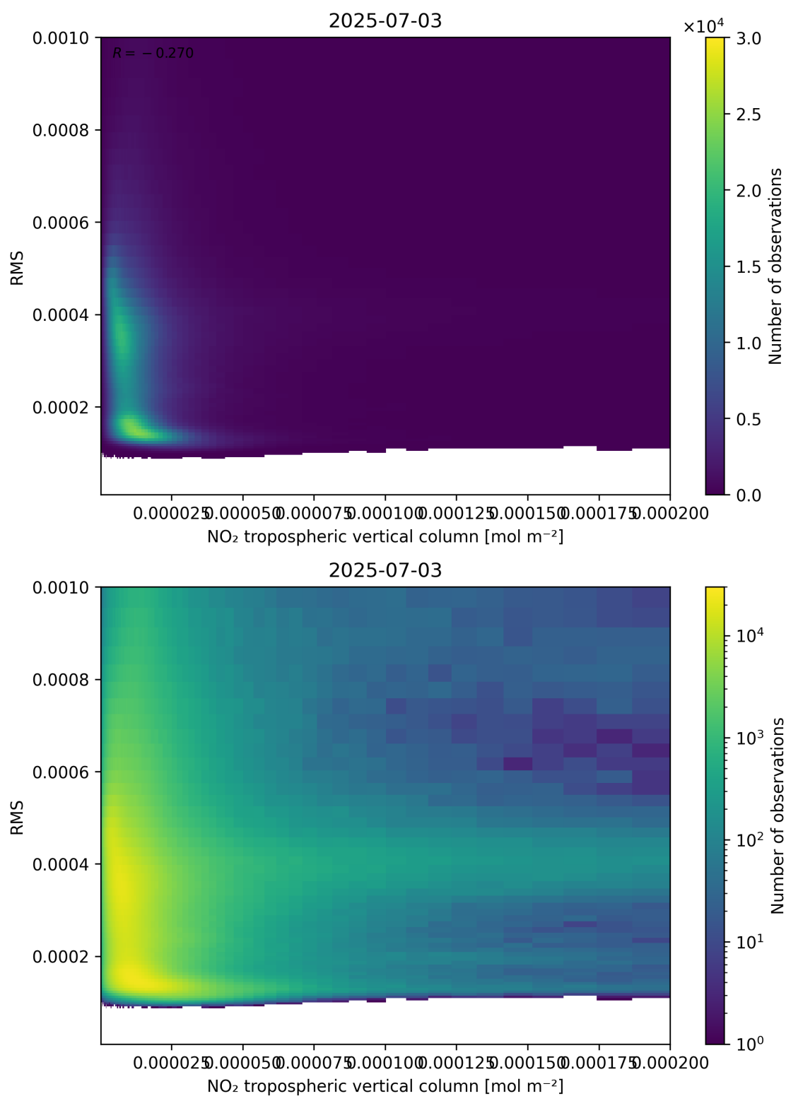
Figure 142: Scatter density plot of “NO 2 tropospheric vertical column” against “RMS” for 2025-07-03 to 2025-07-04.
