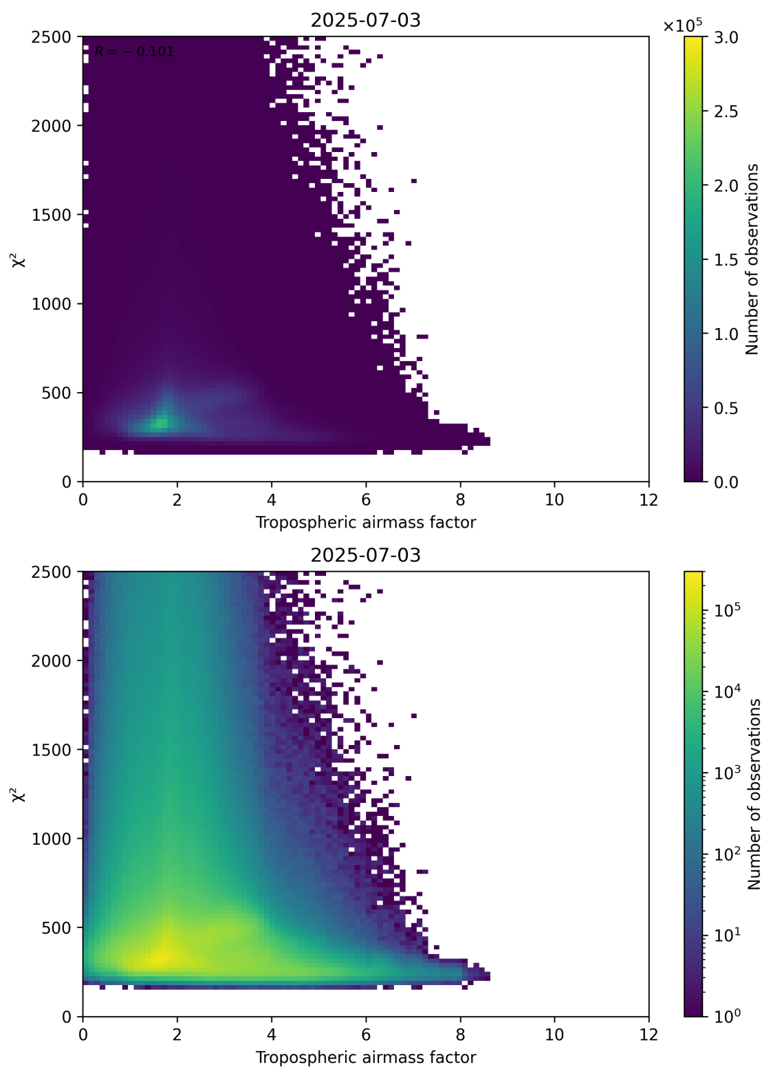
Figure 73: Scatter density plot of “Tropospheric airmass factor” against “ \chi^2 ” for 2025-07-03 to 2025-07-04.
