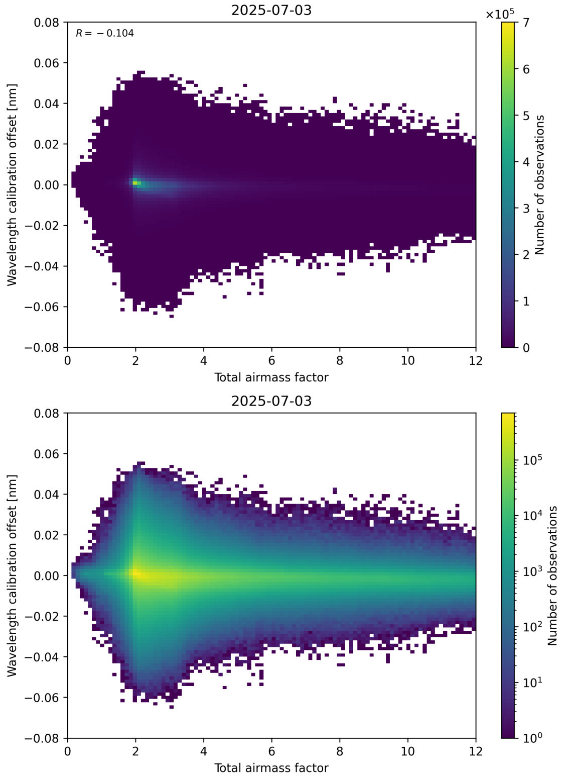
Figure 70: Scatter density plot of “Total airmass factor” against “Wavelength calibration offset” for 2025-07-03 to 2025-07-04.
