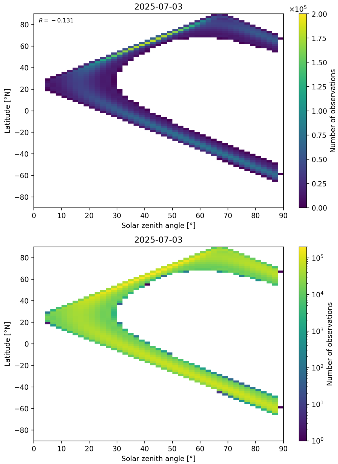
Figure 149: Scatter density plot of “Solar zenith angle” against “Latitude” for 2025-07-03 to 2025-07-04.
