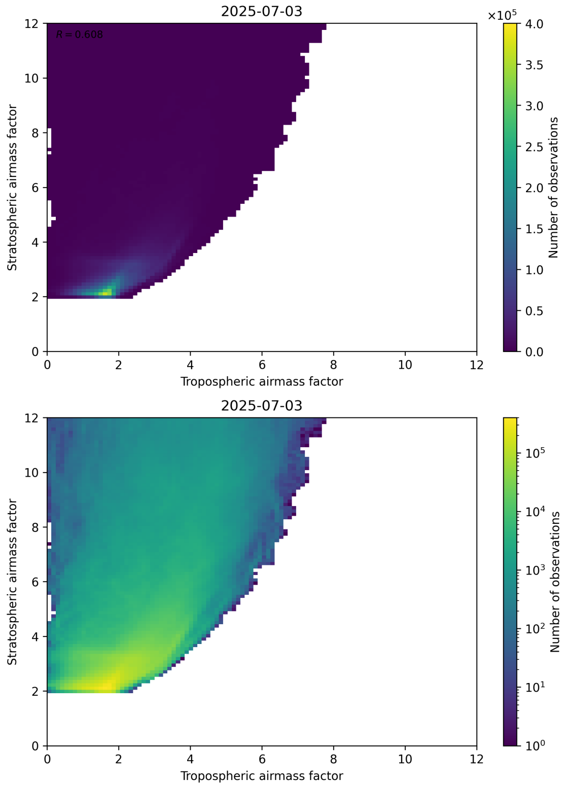
Figure 71: Scatter density plot of “Tropospheric airmass factor” against “Stratospheric airmass factor” for 2025-07-03 to 2025-07-04.
