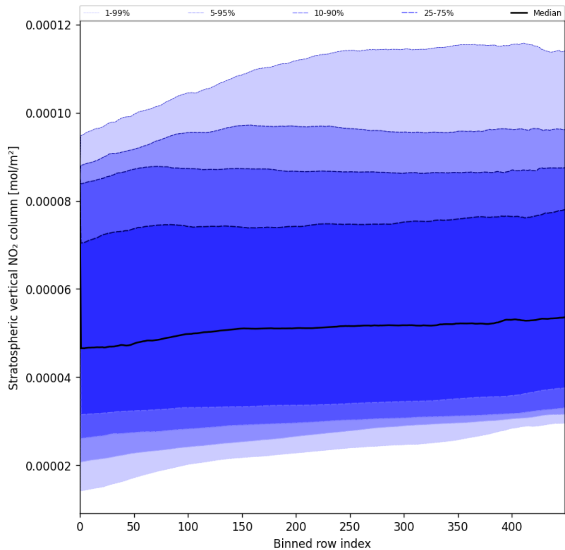
Figure 53: Along track statistics of “Stratospheric vertical NO 2 column” for 2025-07-03 to 2025-07-04
