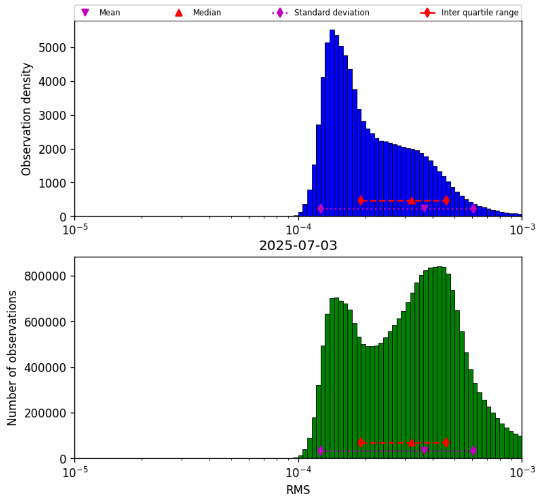
Figure 43: Histogram of “RMS” for 2025-07-03 to 2025-07-04
