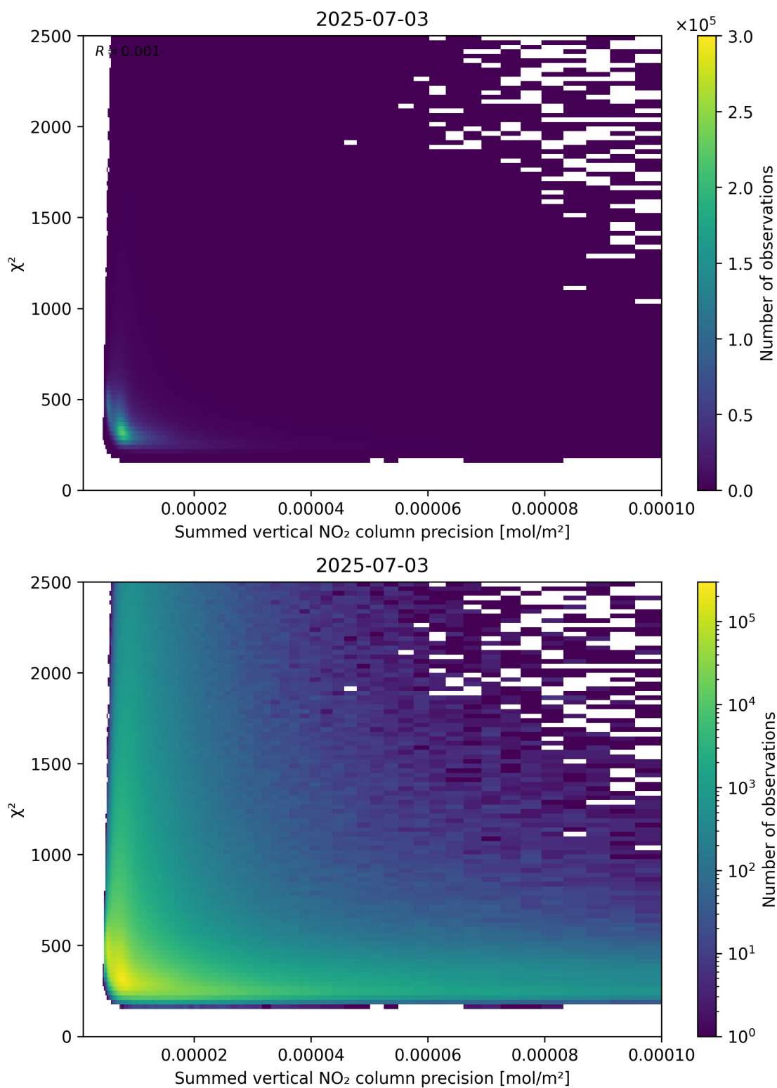
Figure 107: Scatter density plot of “Summed vertical NO 2 column precision” against “ \chi^2 ” for 2025-07-03 to 2025-07-04.
