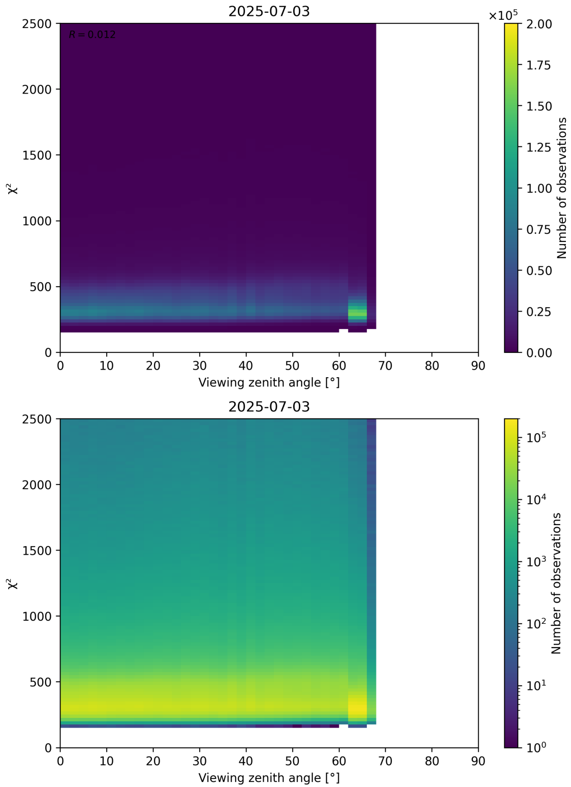
Figure 162: Scatter density plot of “Viewing zenith angle” against “ \chi^2 ” for 2025-07-03 to 2025-07-04.
