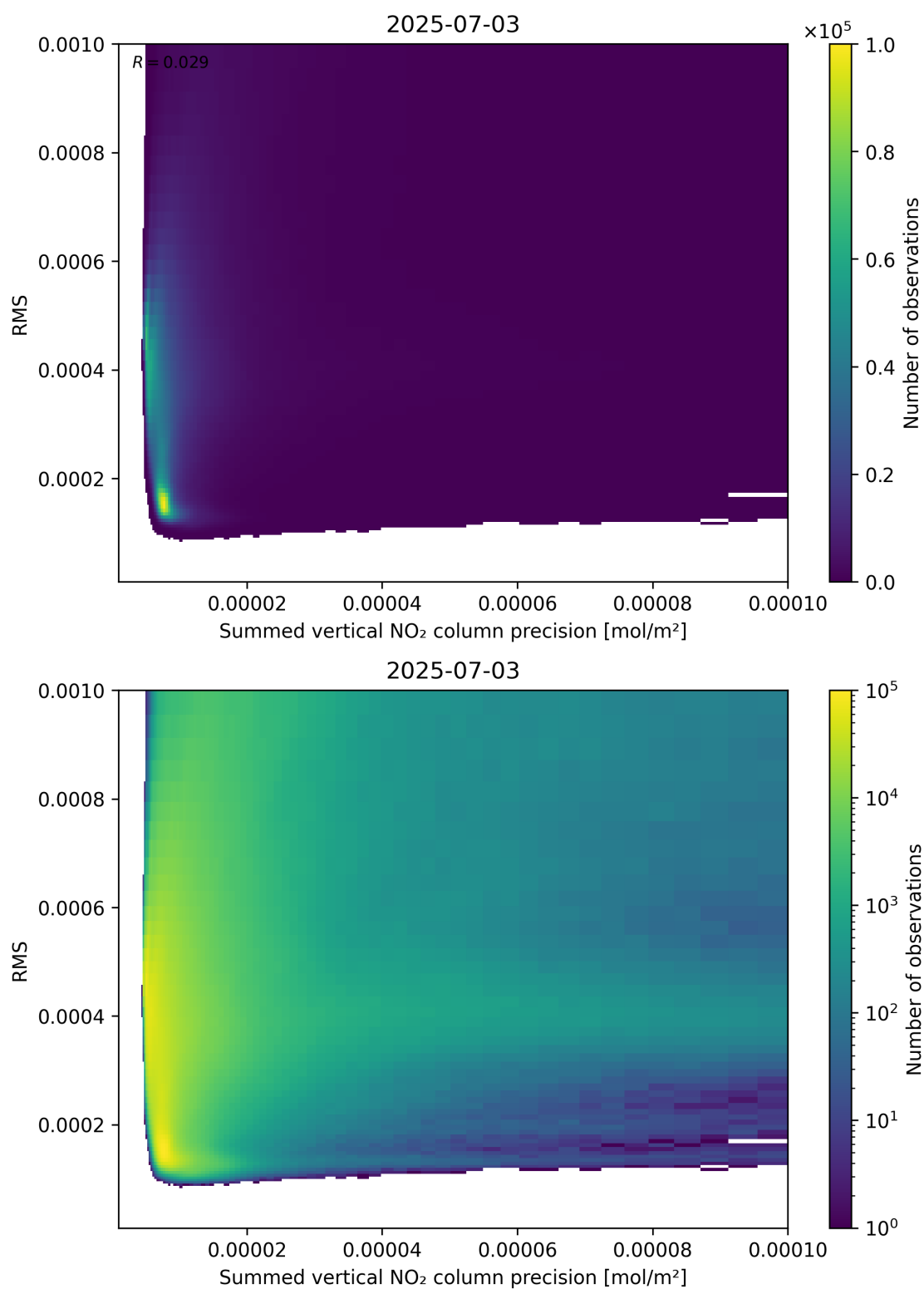
Figure 108: Scatter density plot of “Summed vertical NO 2 column precision” against “RMS” for 2025-07-03 to 2025-07-04.
