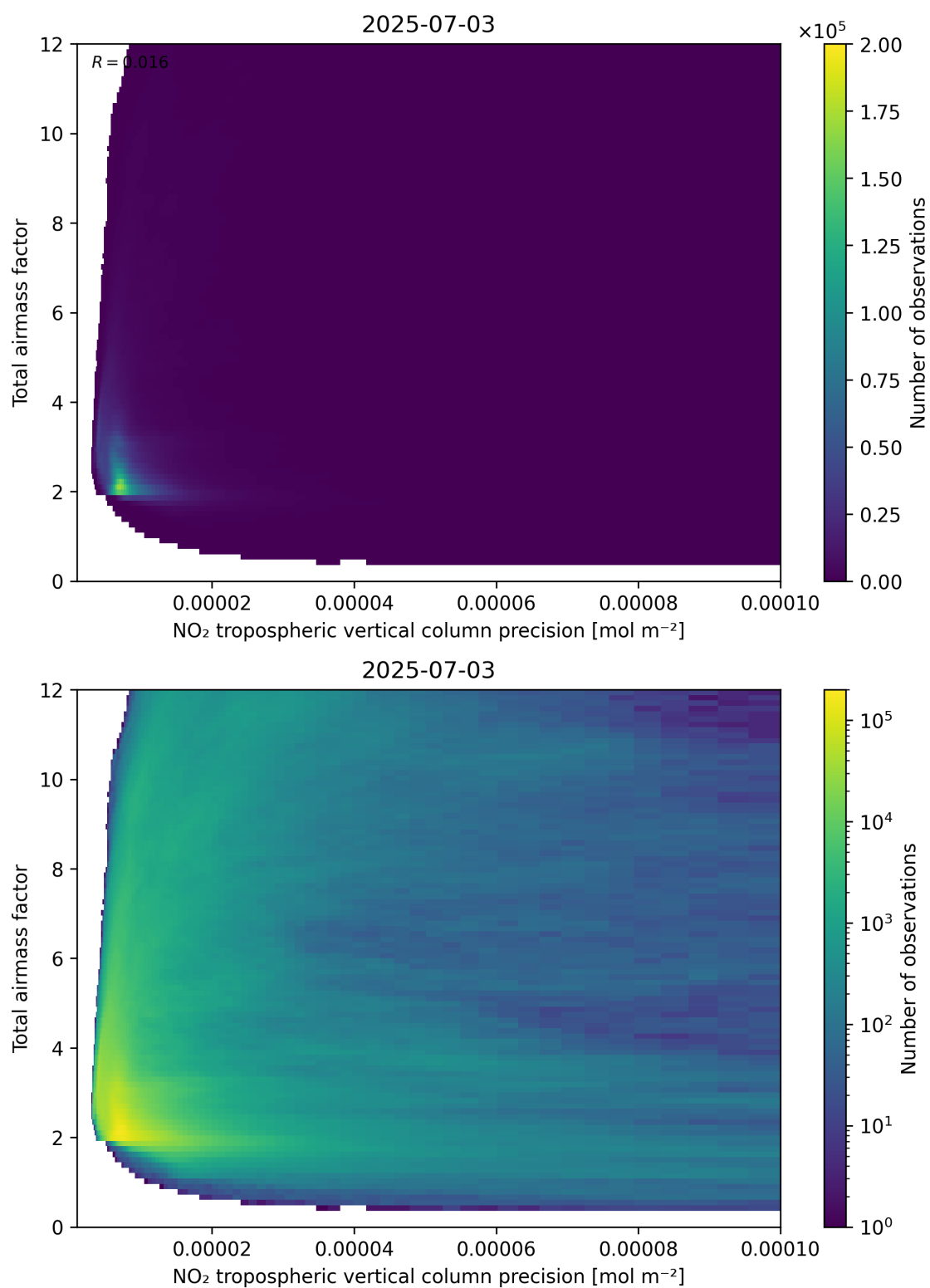
Figure 132: Scatter density plot of “NO 2 tropospheric vertical column precision” against “Total air mass factor” for 2025-07-03 to 2025-07-04.
