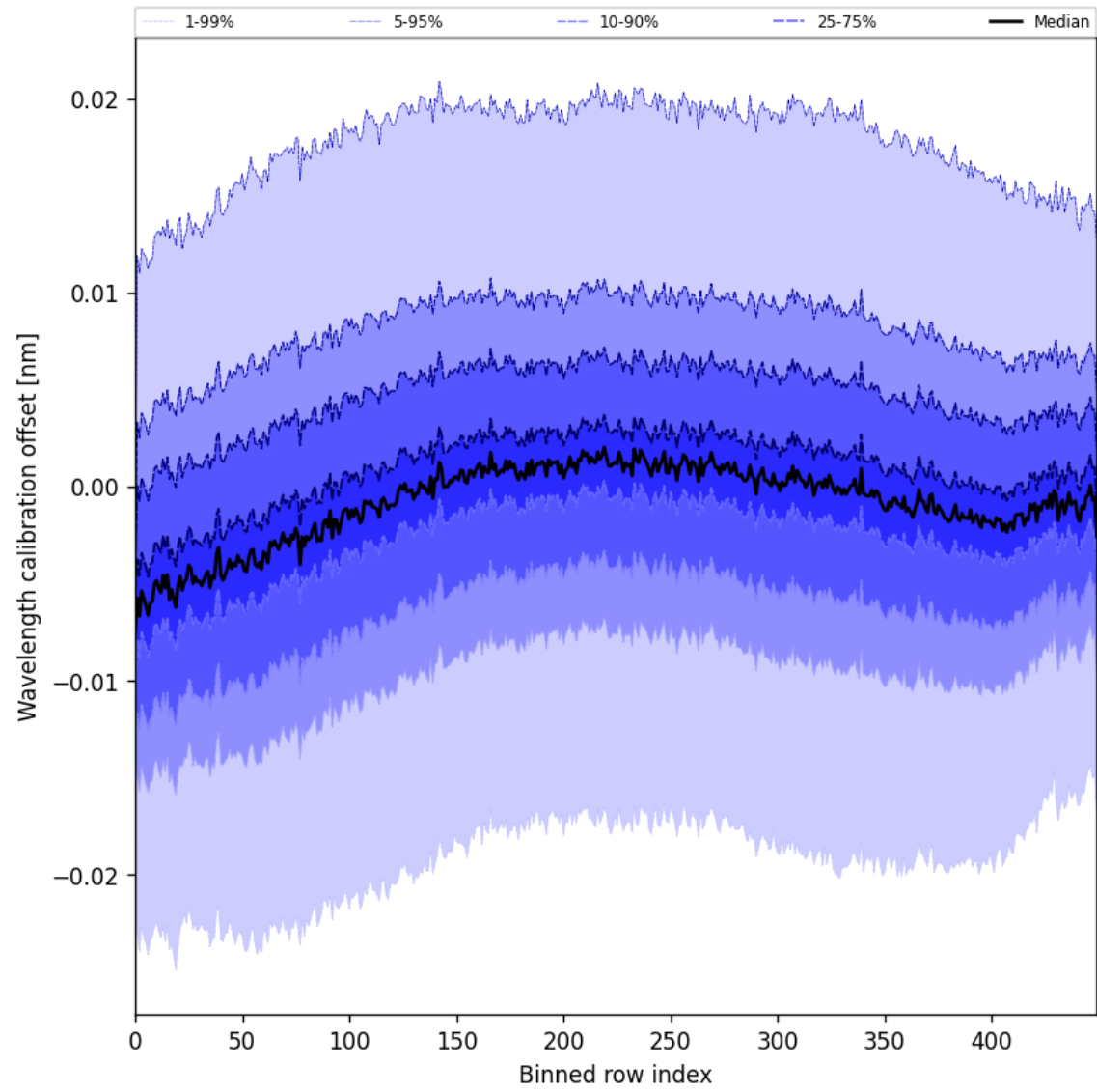
Figure 52: Along track statistics of “Wavelength calibration offset” for 2025-07-03 to 2025-07-04
