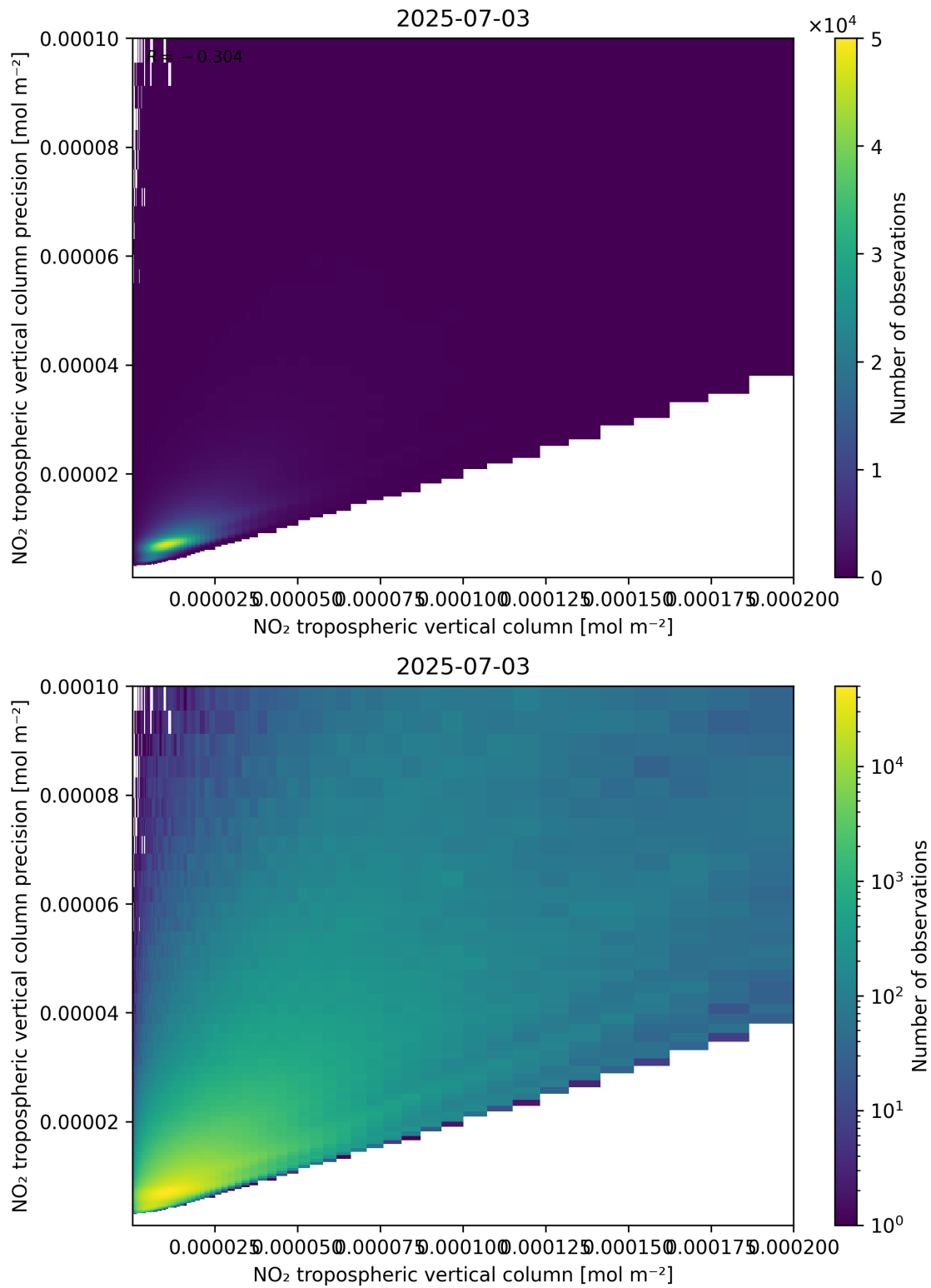
Figure 130: Scatter density plot of “NO 2 tropospheric vertical column” against “NO 2 tropospheric vertical column precision” for 2025-07-03 to 2025-07-04.
