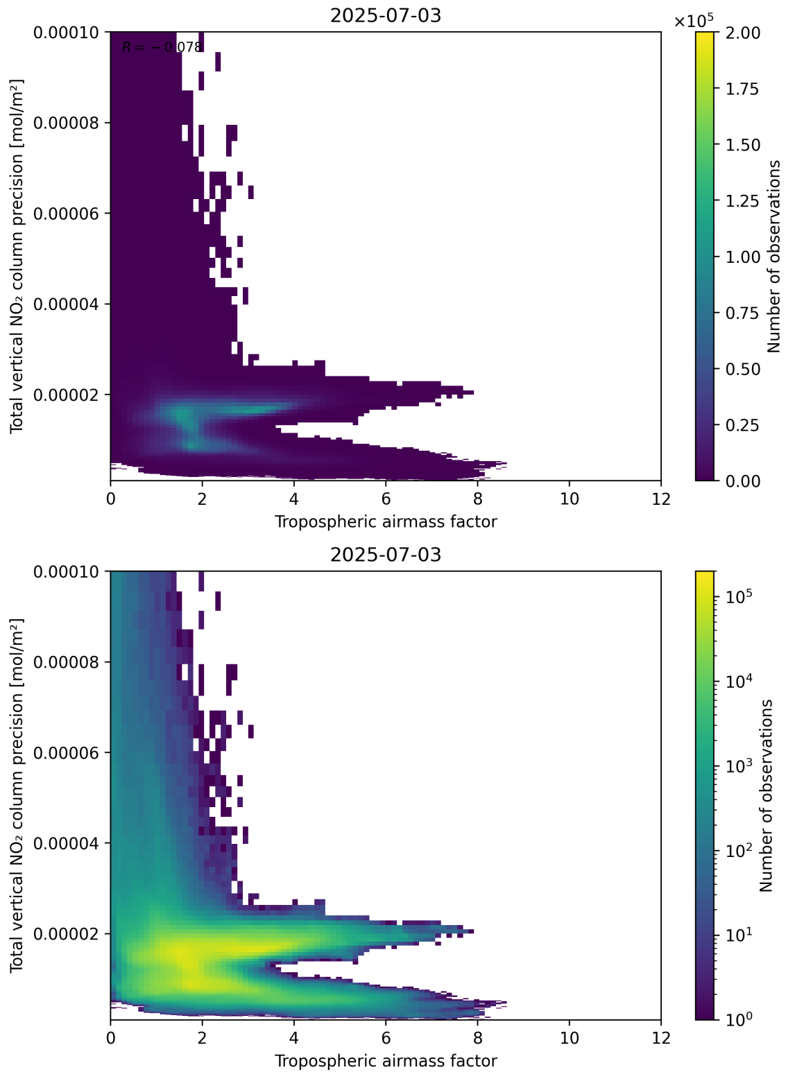
Figure 78: Scatter density plot of “Tropospheric air mass factor” against “Total vertical NO 2 column precision” for 2025-07-03 to 2025-07-04.
