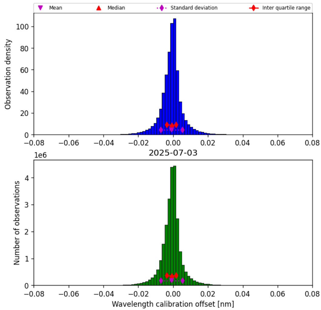
Figure 35: Histogram of “Wavelength calibration offset” for 2025-07-03 to 2025-07-04
