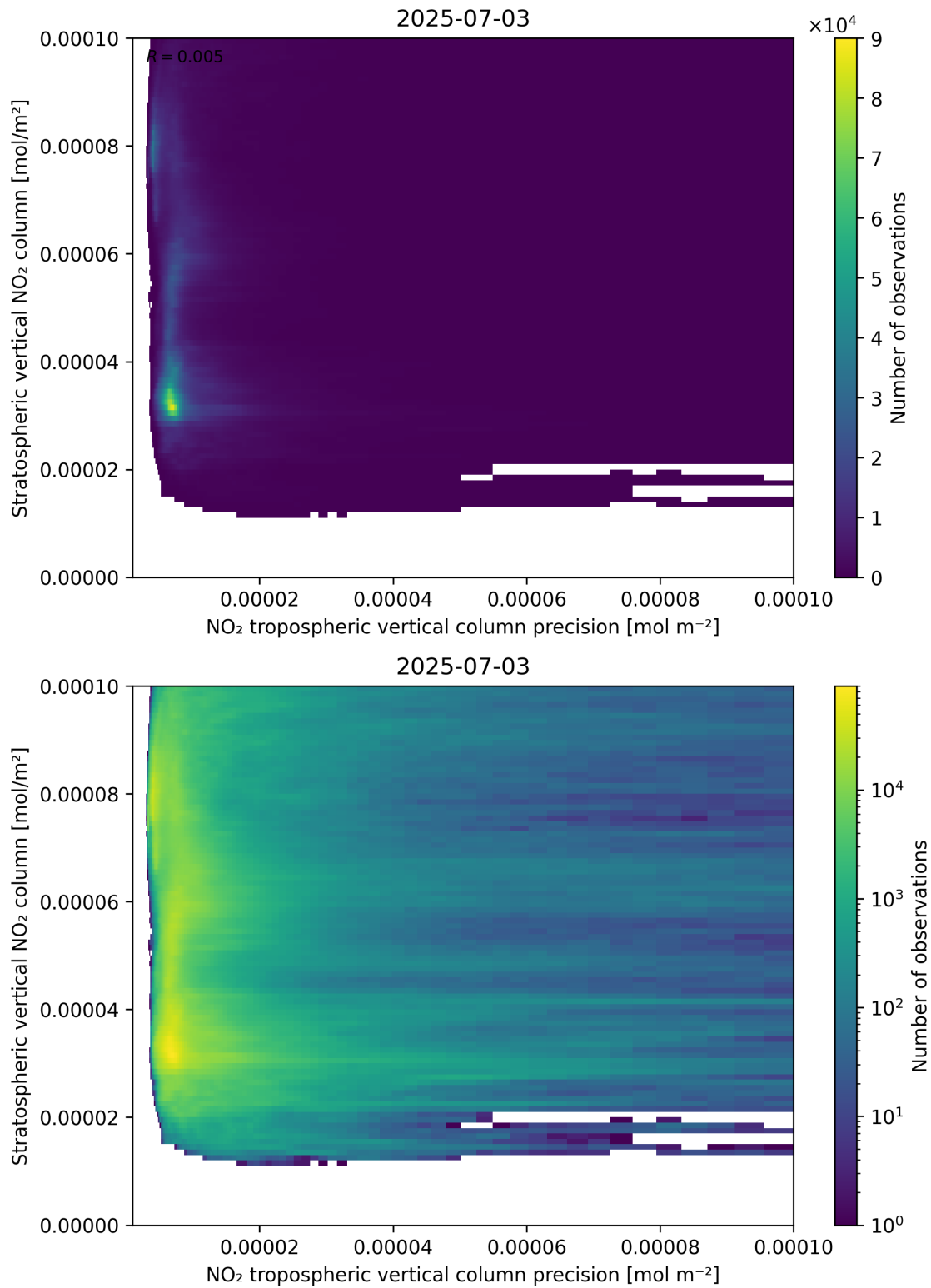
Figure 135: Scatter density plot of “NO 2 tropospheric vertical column precision” against “Stratospheric vertical NO 2 column” for 2025-07-03 to 2025-07-04.
