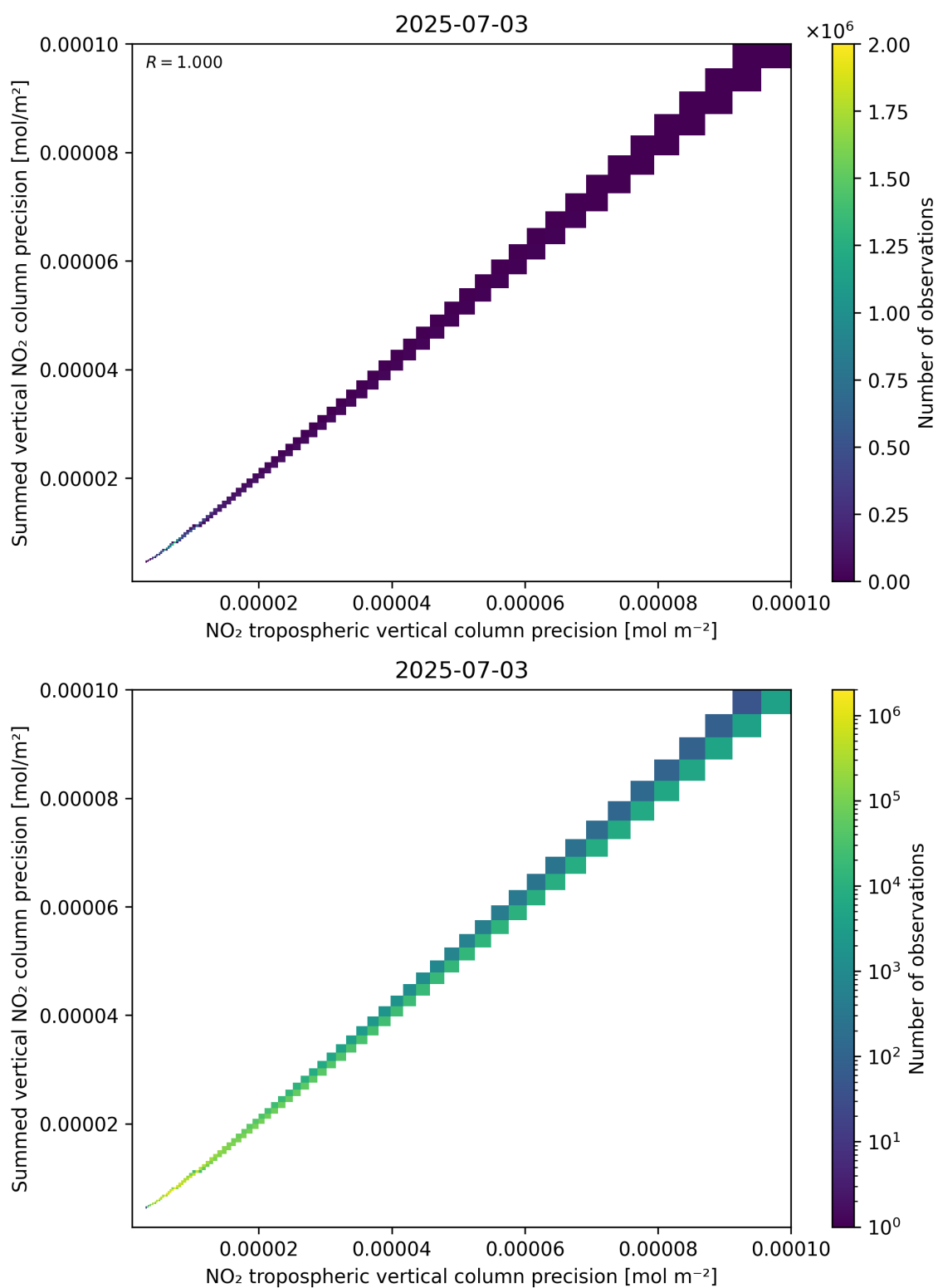
Figure 137: Scatter density plot of “NO 2 tropospheric vertical column precision” against “Summed vertical NO 2 column precision” for 2025-07-03 to 2025-07-04.
