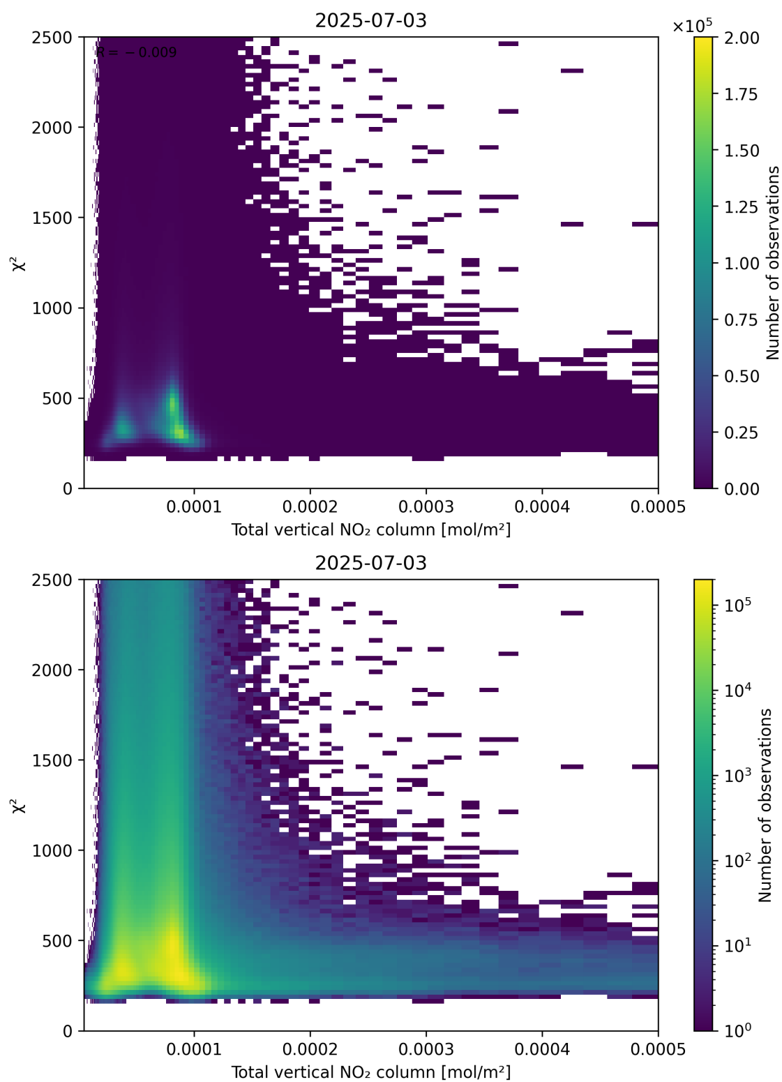
Figure 111: Scatter density plot of “Total vertical NO 2 column” against “ \chi^2 ” for 2025-07-03 to 2025-07-04.
