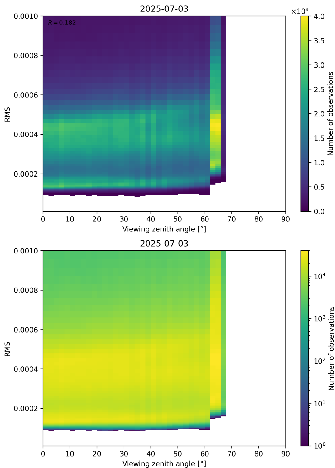
Figure 171: Scatter density plot of “Viewing zenith angle” against “RMS” for 2025-07-03 to 2025-07-04.
