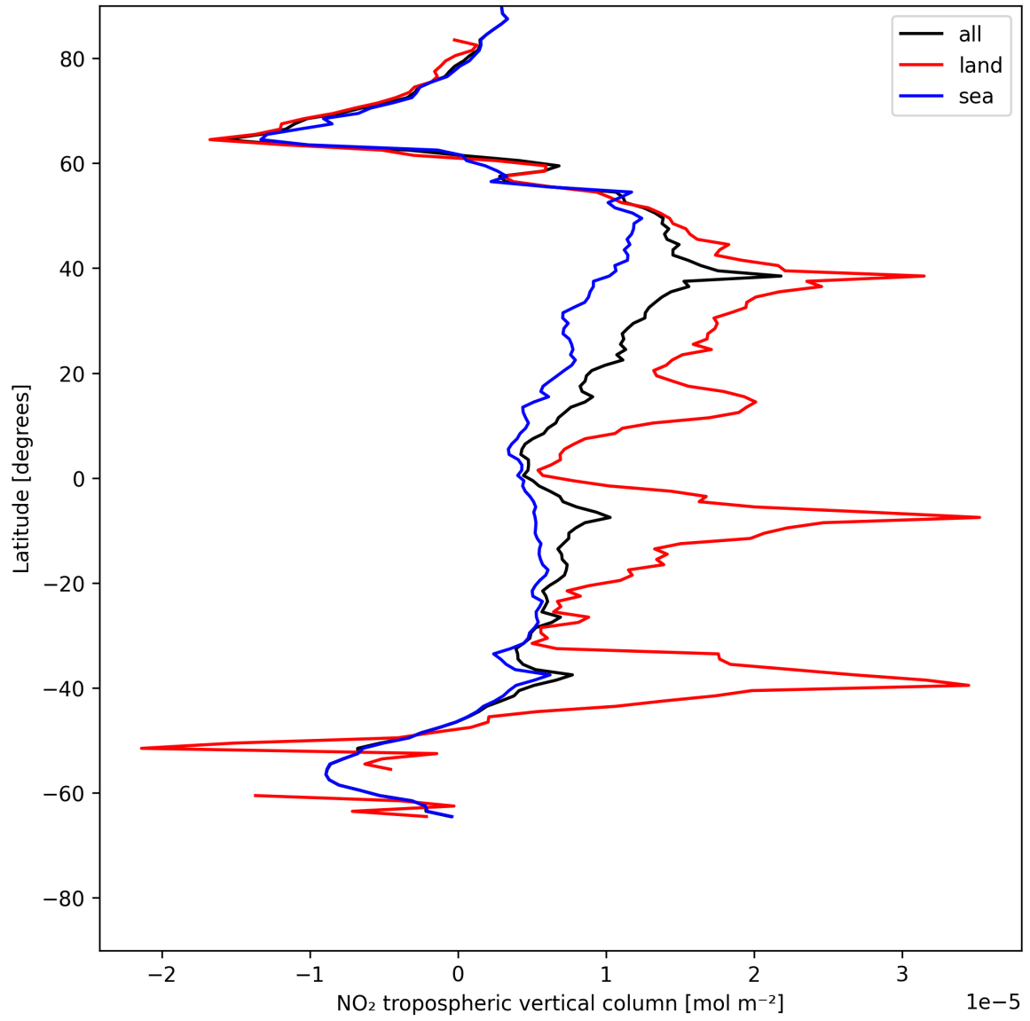
Figure 12: Zonal average of “NO 2 tropospheric vertical column” for 2025-07-03 to 2025-07-04.
