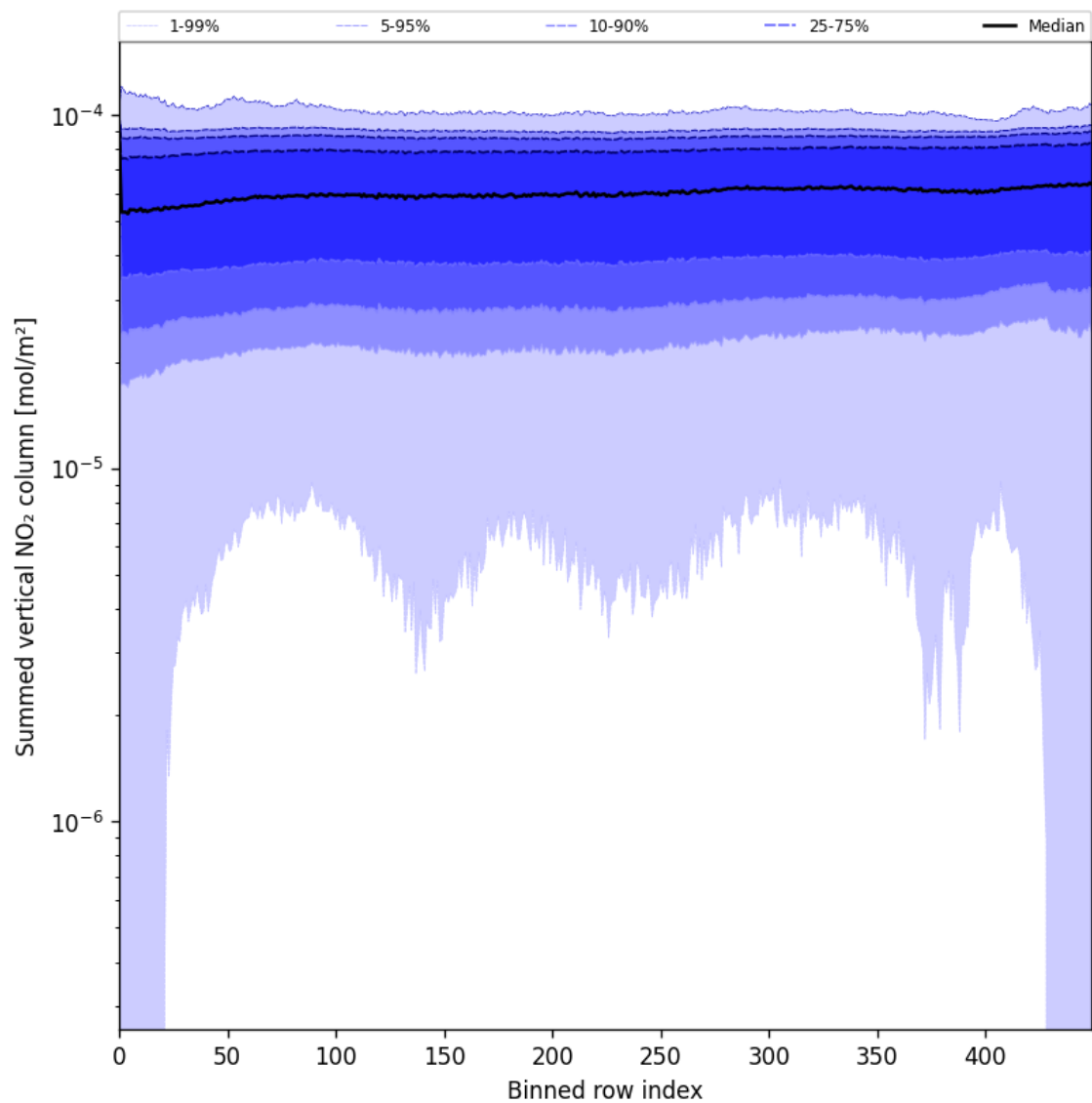
Figure 57: Along track statistics of “Summed vertical NO 2 column” for 2025-07-03 to 2025-07-04
