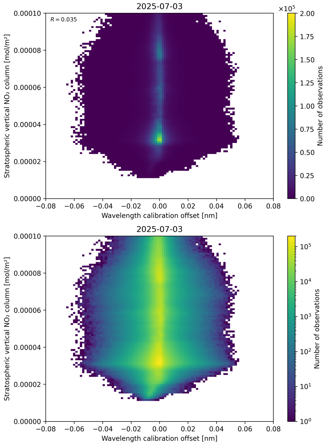
Figure 176: Scatter density plot of “Wavelength calibration offset” against “Stratospheric vertical NO 2 column” for 2025-07-03 to 2025-07-04.
