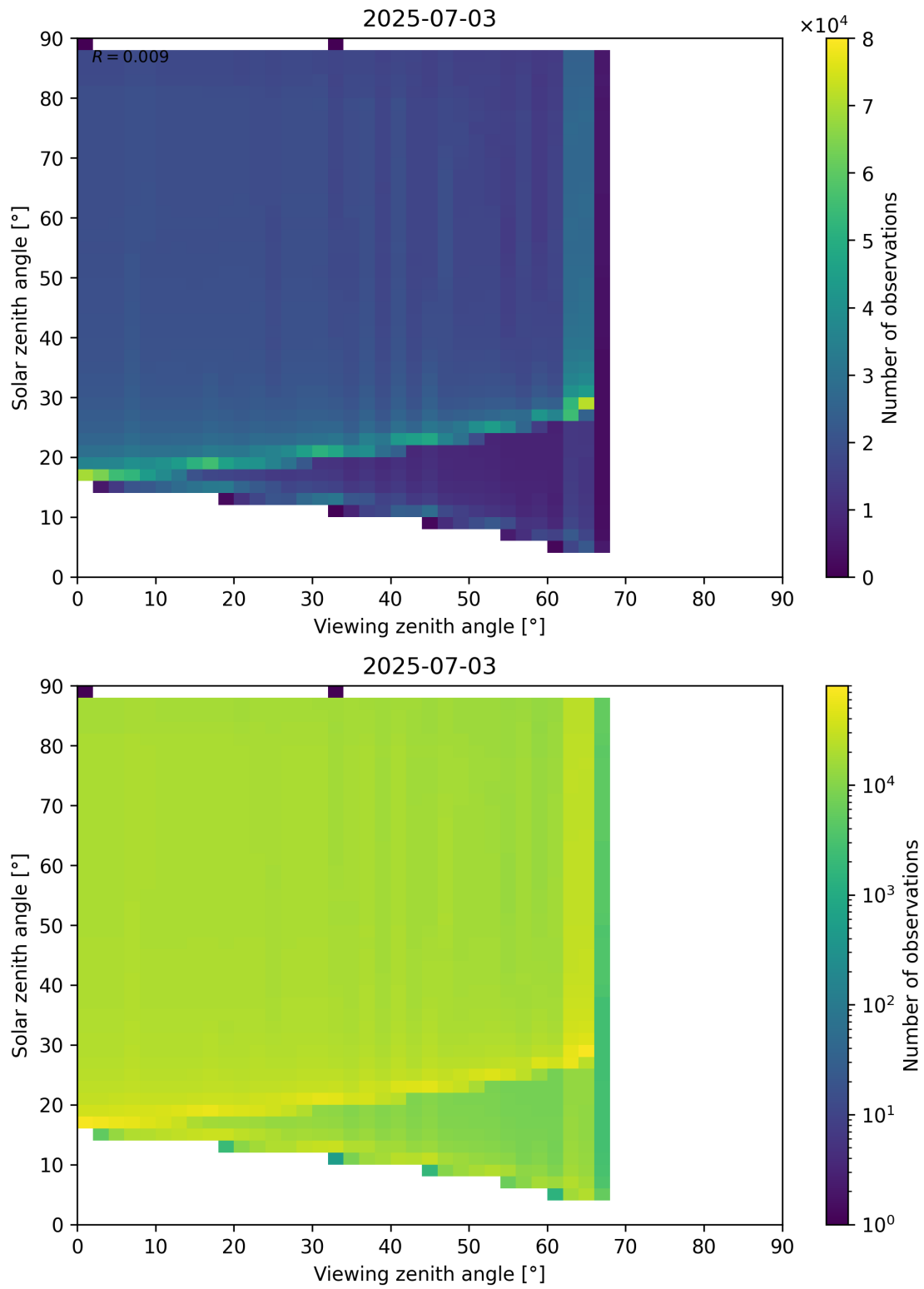
Figure 172: Scatter density plot of “Viewing zenith angle” against “Solar zenith angle” for 2025-07-03 to 2025-07-04.
