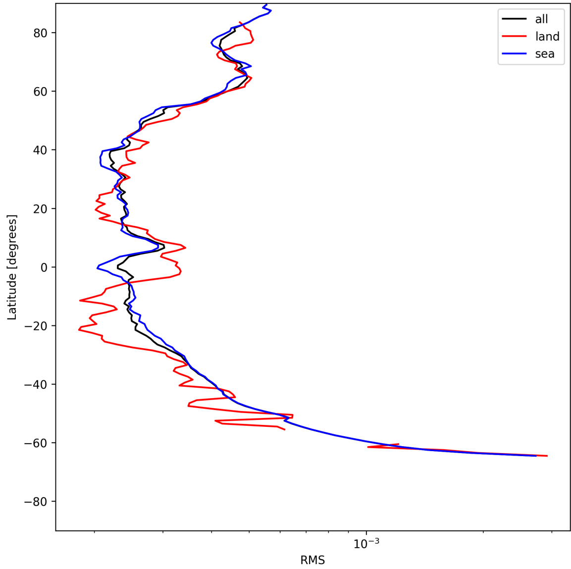
Figure 26: Zonal average of “RMS” for 2025-07-03 to 2025-07-04.
