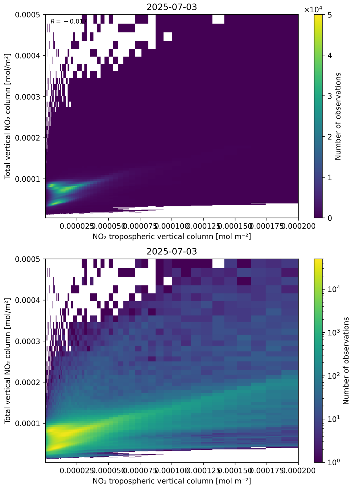
Figure 128: Scatter density plot of “NO 2 tropospheric vertical column” against “Total vertical NO 2 column” for 2025-07-03 to 2025-07-04.
