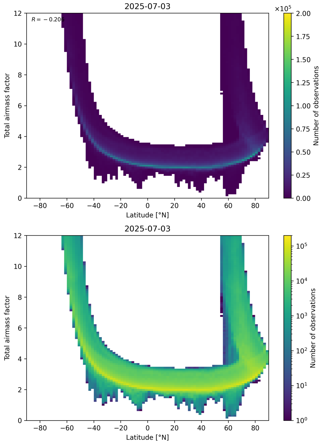
Figure 84: Scatter density plot of “Latitude” against “Total airmass factor” for 2025-07-03 to 2025-07-04.
