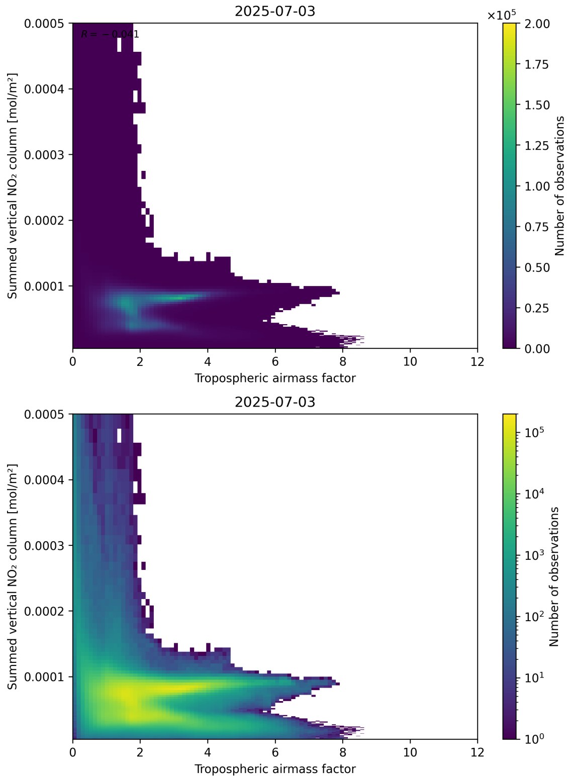
Figure 75: Scatter density plot of “Tropospheric air mass factor” against “Summed vertical NO 2 column” for 2025-07-03 to 2025-07-04.
