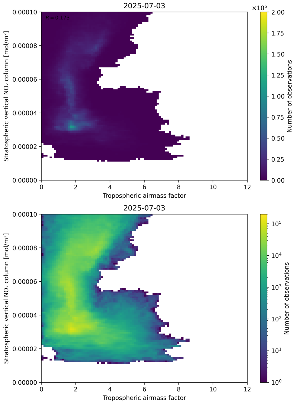
Figure 74: Scatter density plot of “Tropospheric air mass factor” against “Stratospheric vertical NO 2 column” for 2025-07-03 to 2025-07-04.
