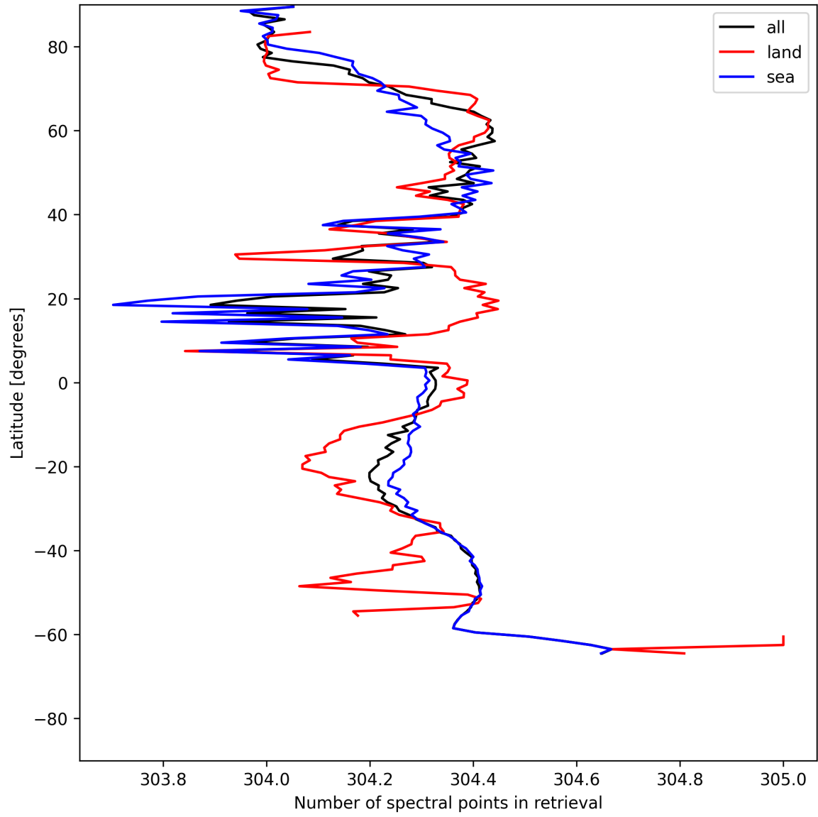
Figure 16: Zonal average of “Number of spectral points in retrieval” for 2025-07-03 to 2025-07-04.
