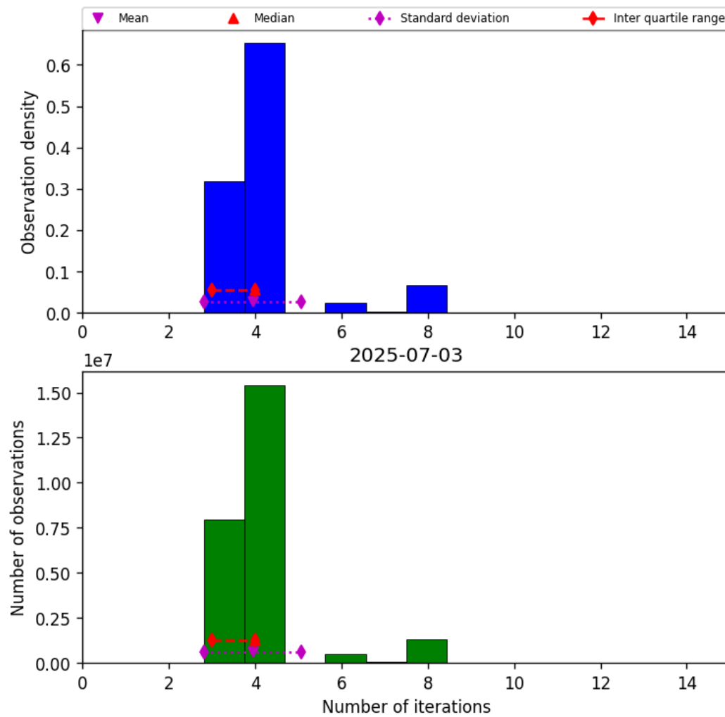
Figure 34: Histogram of “Number of iterations” for 2025-07-03 to 2025-07-04
