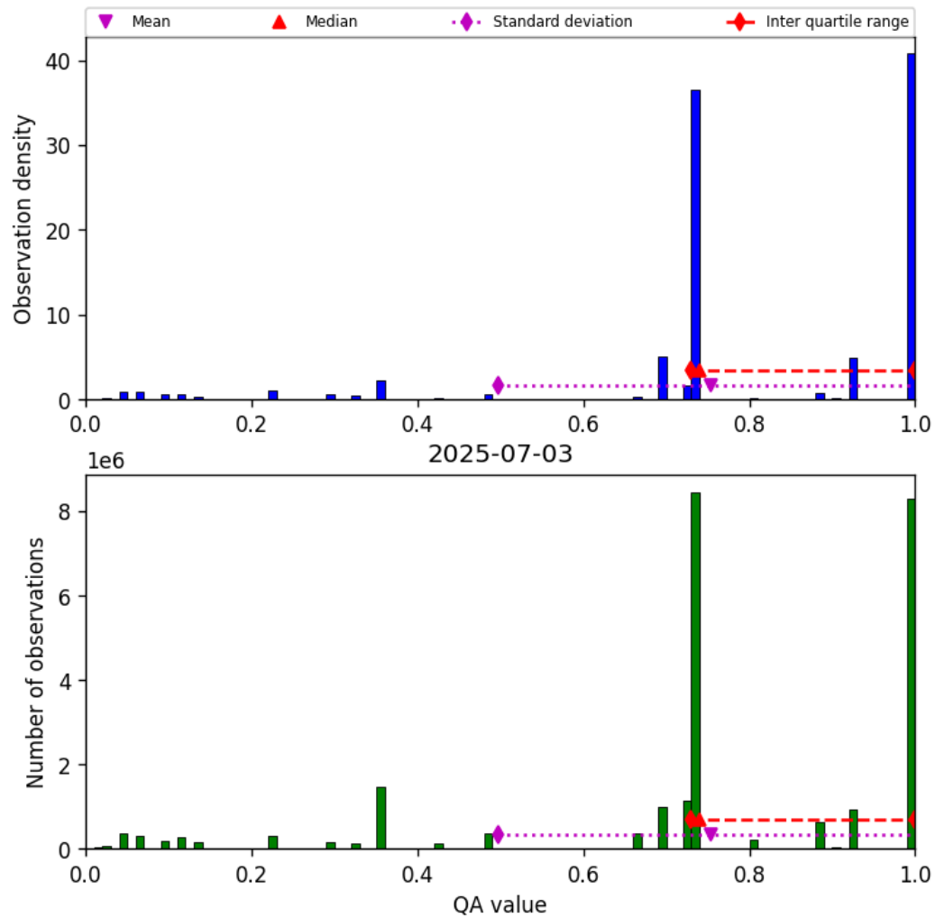
Figure 28: Histogram of “QA value” for 2025-07-03 to 2025-07-04
