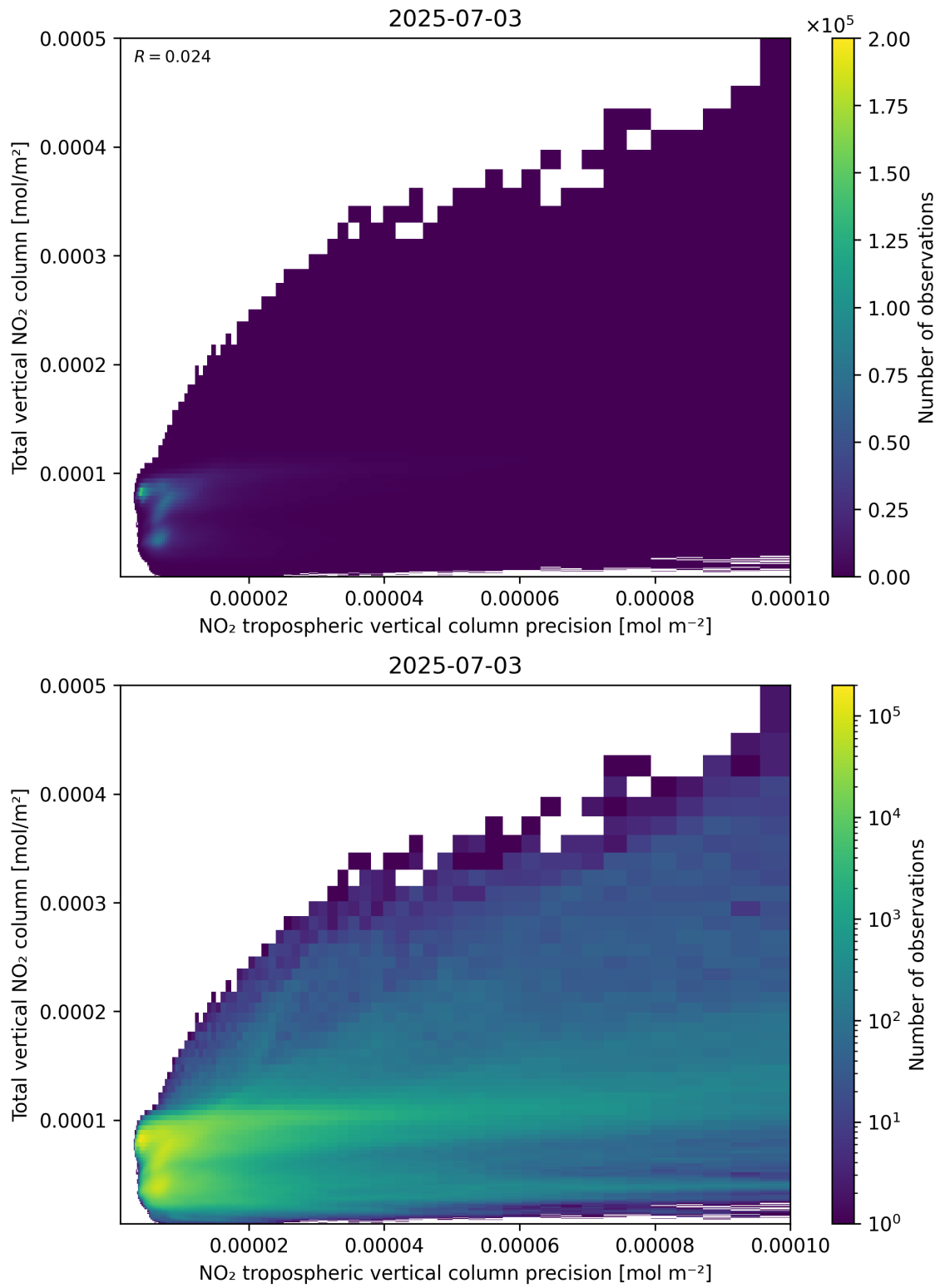
Figure 138: Scatter density plot of “NO 2 tropospheric vertical column precision” against “Total vertical NO 2 column” for 2025-07-03 to 2025-07-04.
