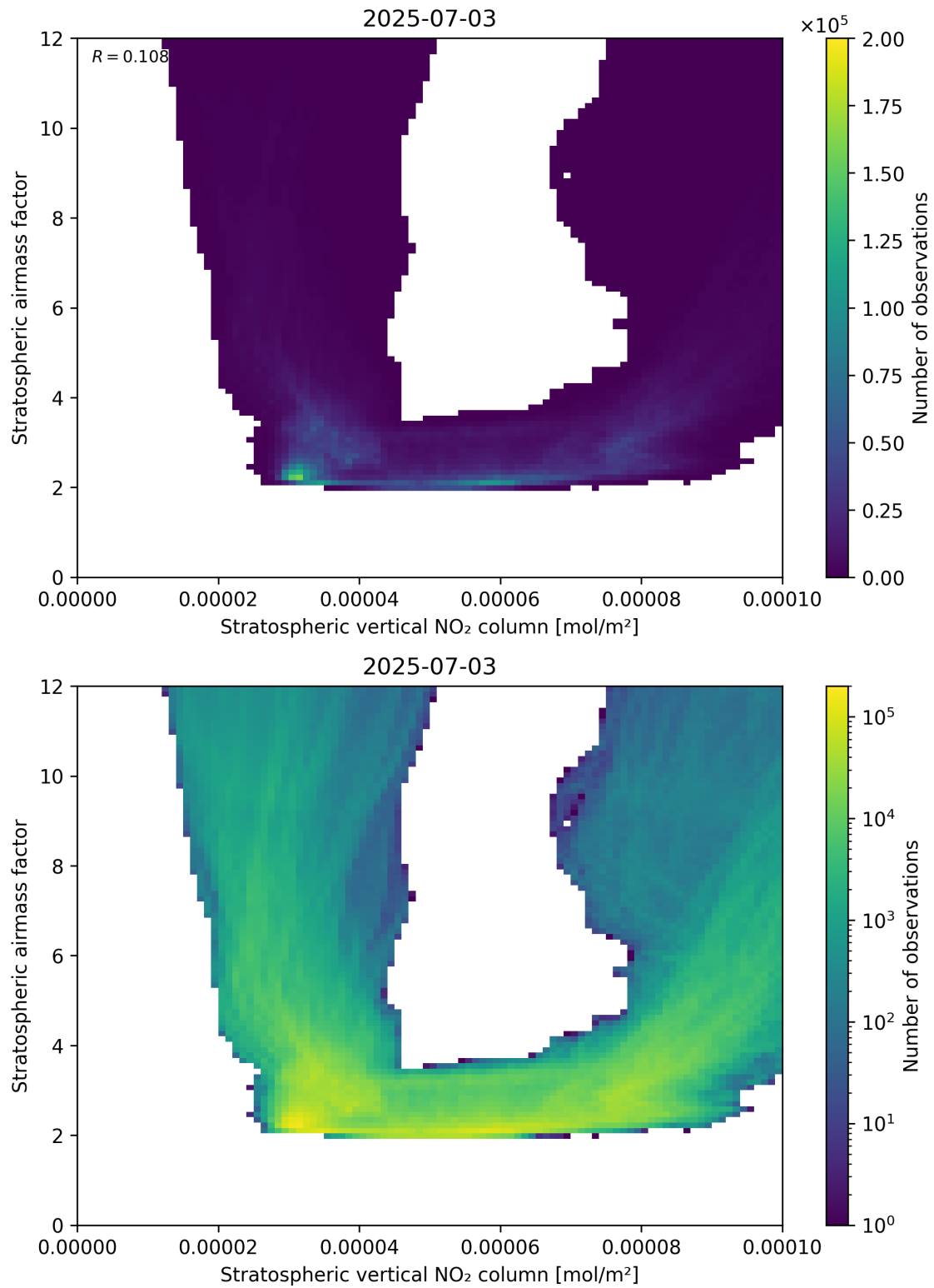
Figure 96: Scatter density plot of “Stratospheric vertical NO 2 column” against “Stratospheric airmass factor” for 2025-07-03 to 2025-07-04.
