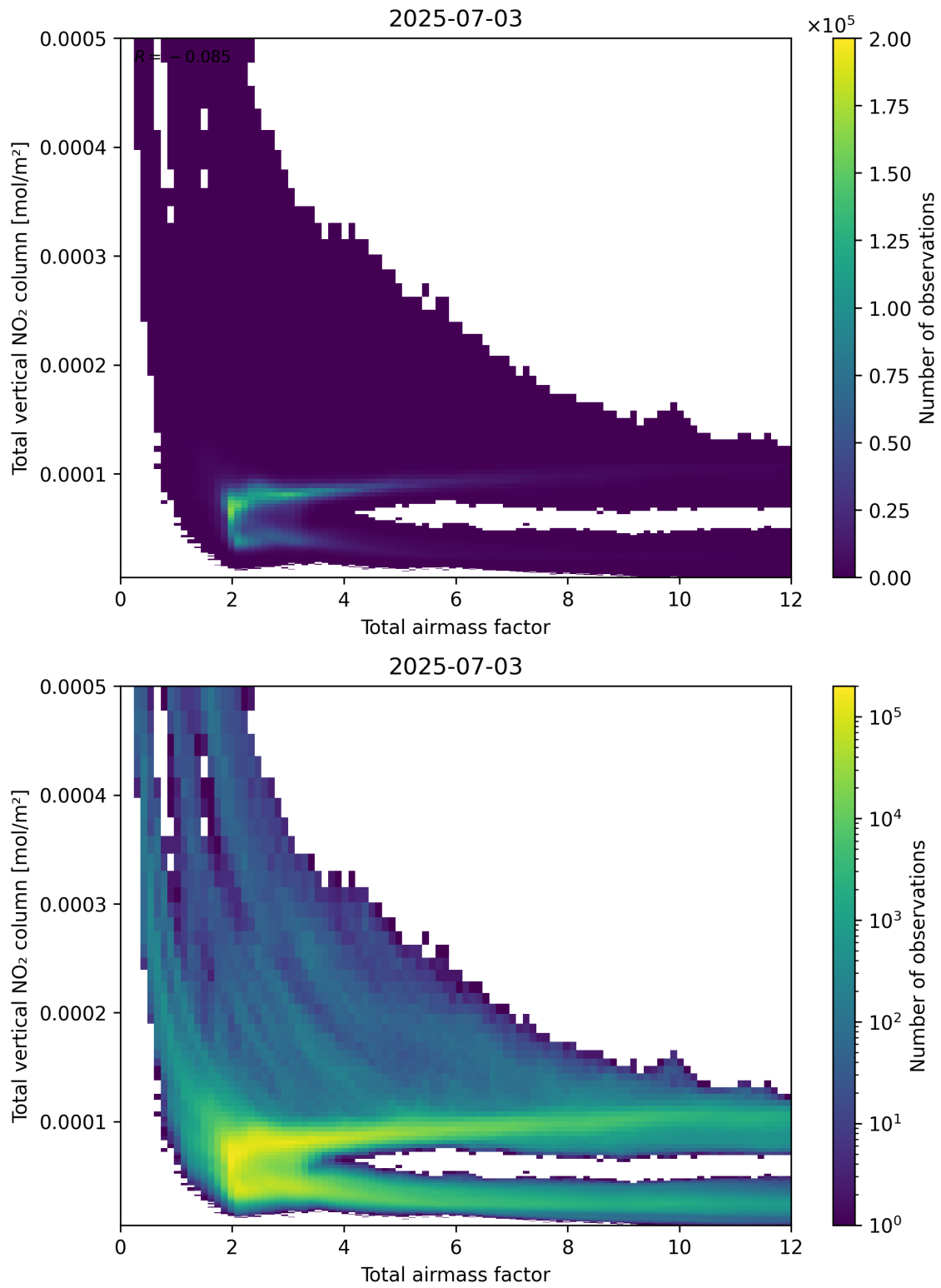
Figure 67: Scatter density plot of “Total airmass factor” against “Total vertical NO 2 column” for 2025-07-03 to 2025-07-04.
