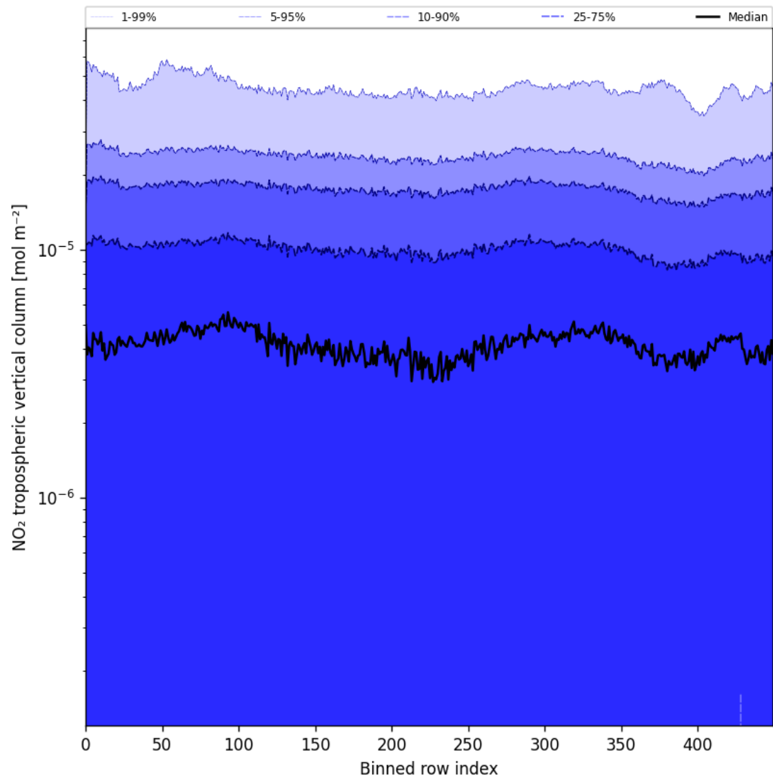
Figure 46: Along track statistics of “NO 2 tropospheric vertical column” for 2025-07-03 to 2025-07-04
