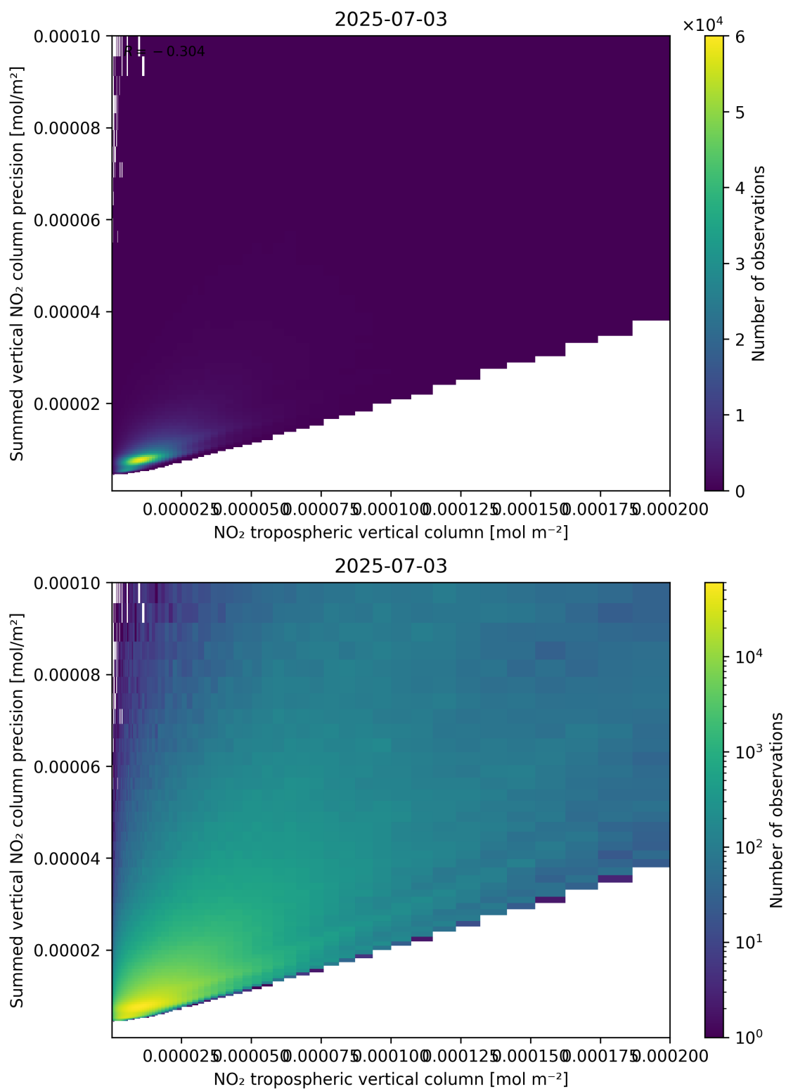
Figure 127: Scatter density plot of “NO 2 tropospheric vertical column” against “Summed vertical NO 2 column precision” for 2025-07-03 to 2025-07-04.
