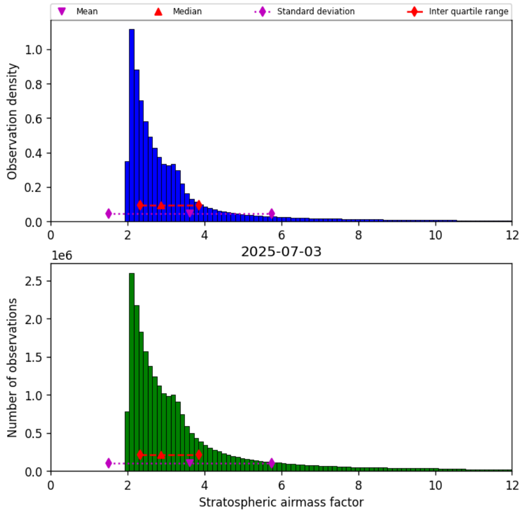
Figure 44: Histogram of “Stratospheric airmass factor” for 2025-07-03 to 2025-07-04
