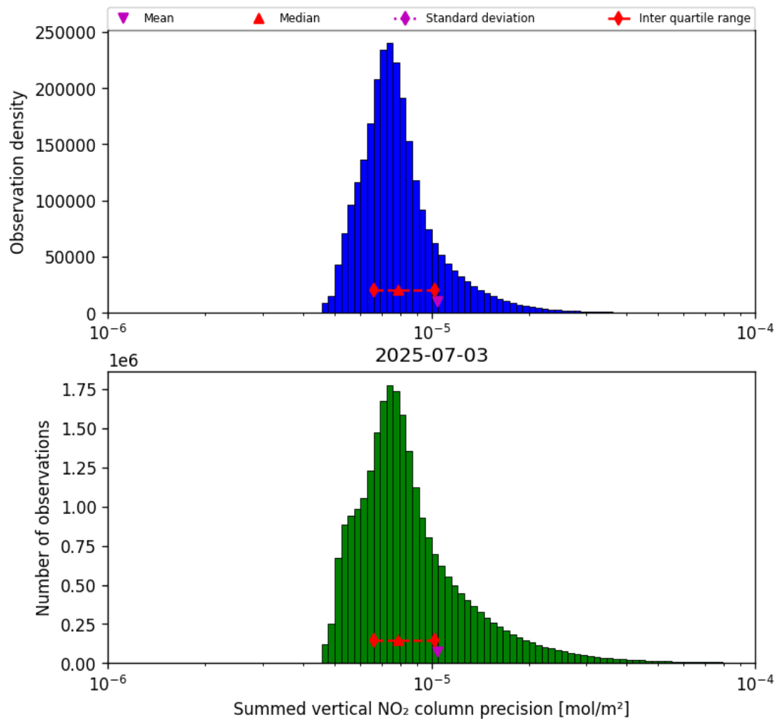
Figure 41: Histogram of "Summed vertical NO 2 column precision" for 2025-07-03 to 2025-07-04
