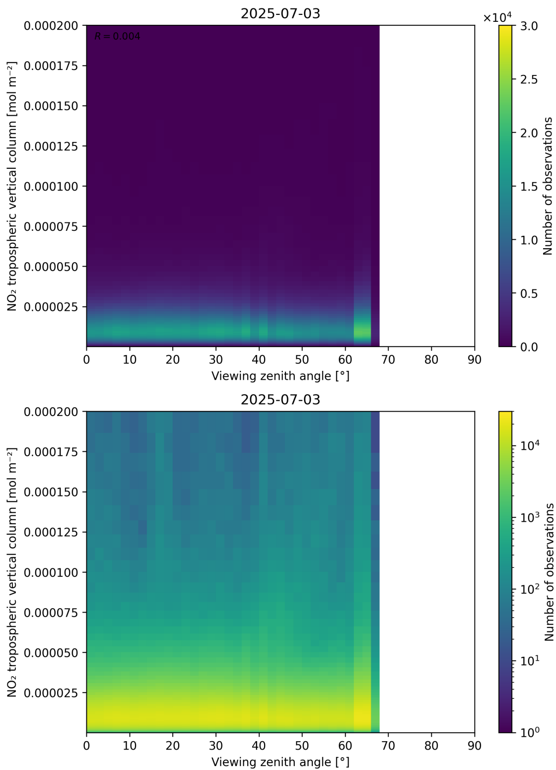
Figure 169: Scatter density plot of “Viewing zenith angle” against “NO 2 tropospheric vertical column” for 2025-07-03 to 2025-07-04.
