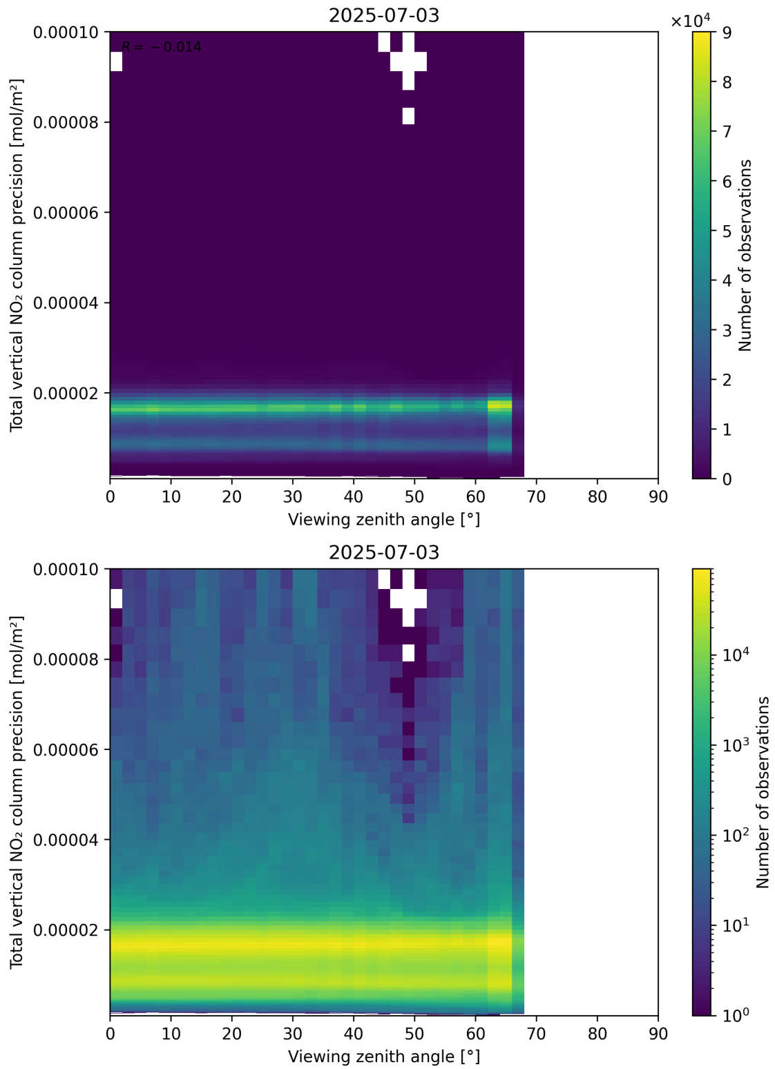
Figure 168: Scatter density plot of “Viewing zenith angle” against “Total vertical NO 2 column precision” for 2025-07-03 to 2025-07-04.
