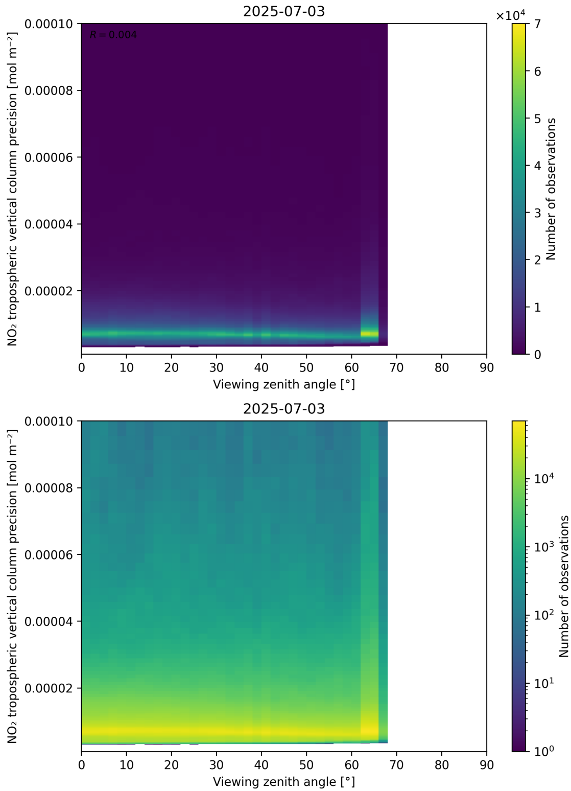
Figure 170: Scatter density plot of “Viewing zenith angle” against “NO 2 tropospheric vertical column precision” for 2025-07-03 to 2025-07-04.
