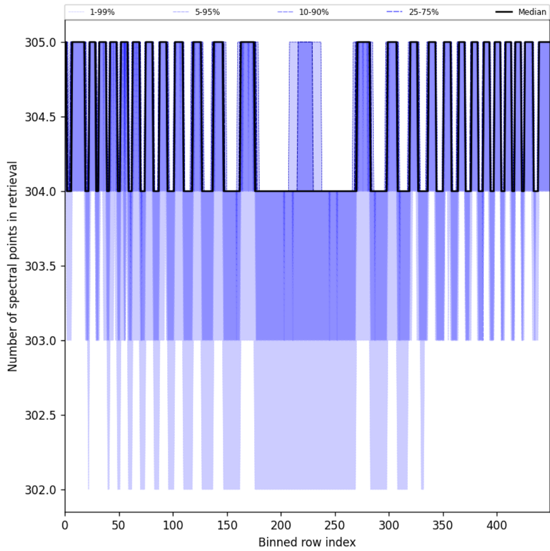
Figure 50: Along track statistics of “Number of spectral points in retrieval” for 2025-07-03 to 2025-07-04
