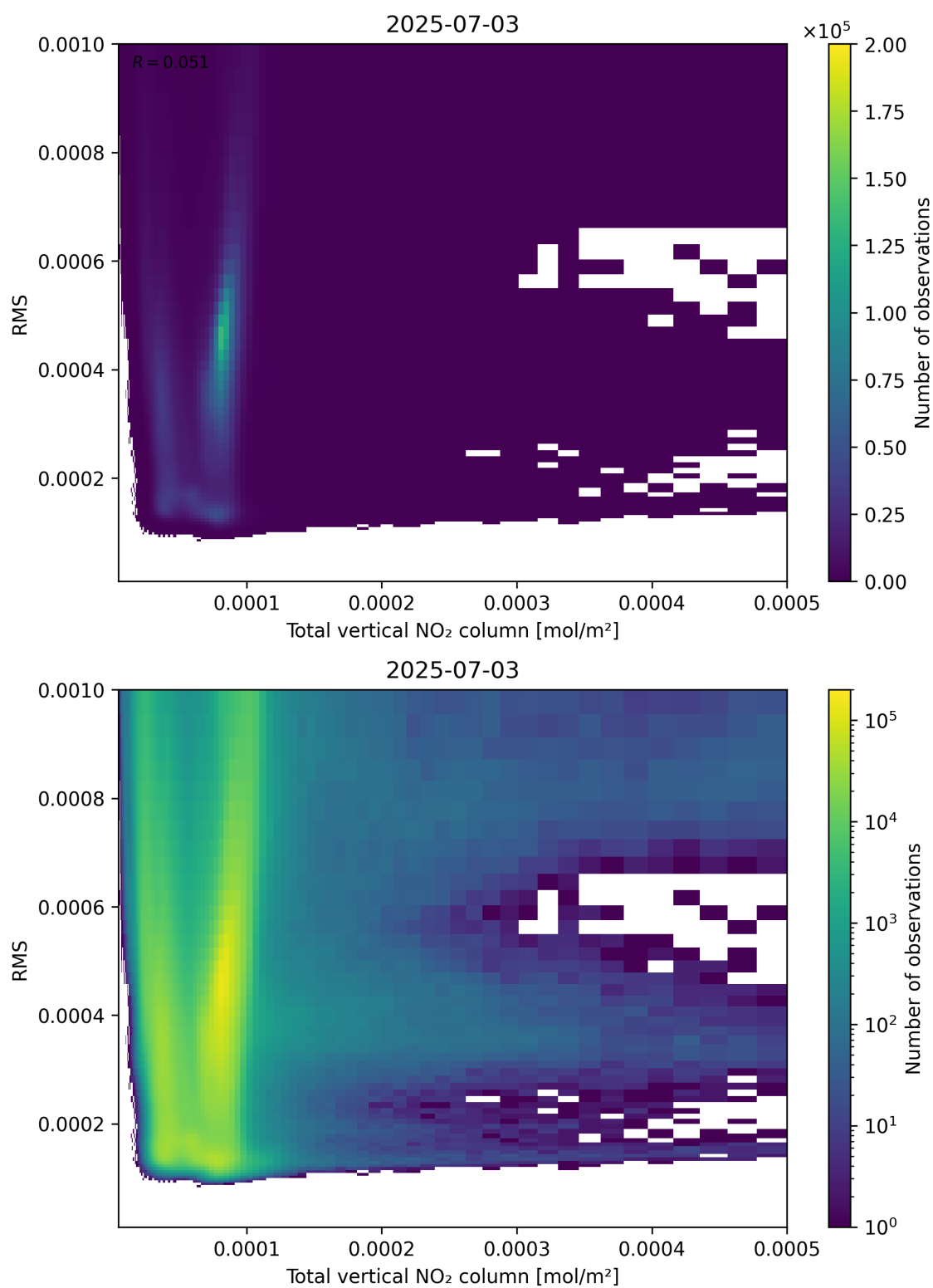
Figure 120: Scatter density plot of “Total vertical NO 2 column” against “RMS” for 2025-07-03 to 2025-07-04.
