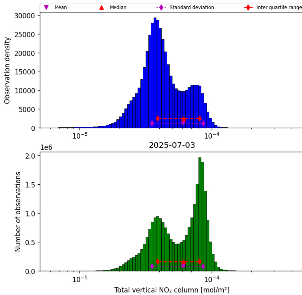
Figure 38: Histogram of “Total vertical NO 2 column” for 2025-07-03 to 2025-07-04
