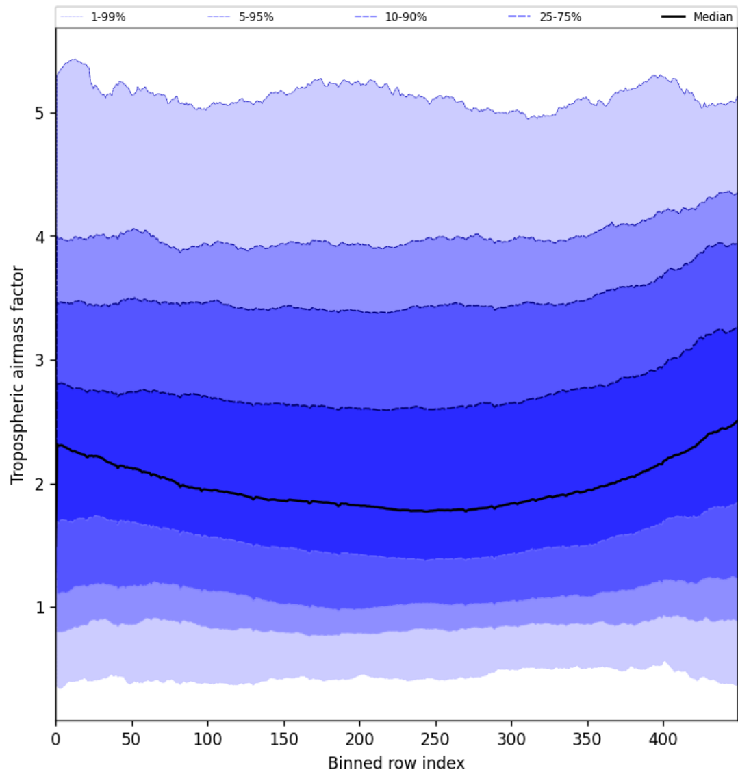
Figure 48: Along track statistics of “Tropospheric airmass factor” for 2025-07-03 to 2025-07-04
