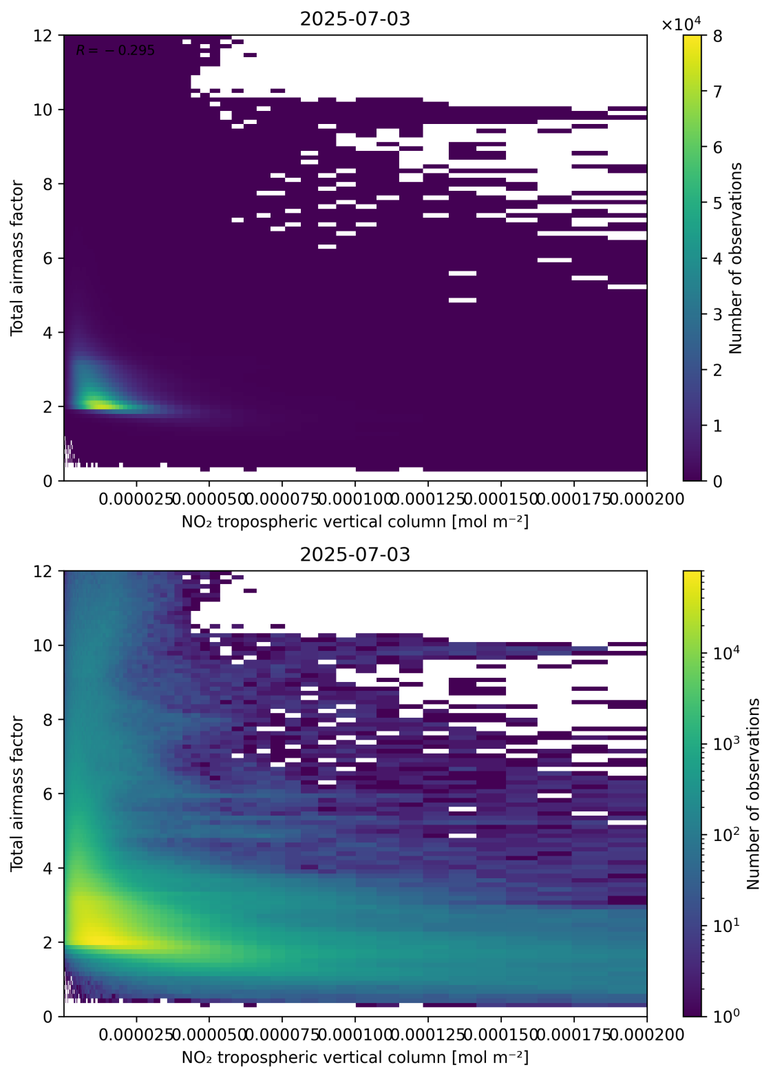
Figure 122: Scatter density plot of “NO 2 tropospheric vertical column” against “Total air mass factor” for 2025-07-03 to 2025-07-04.
