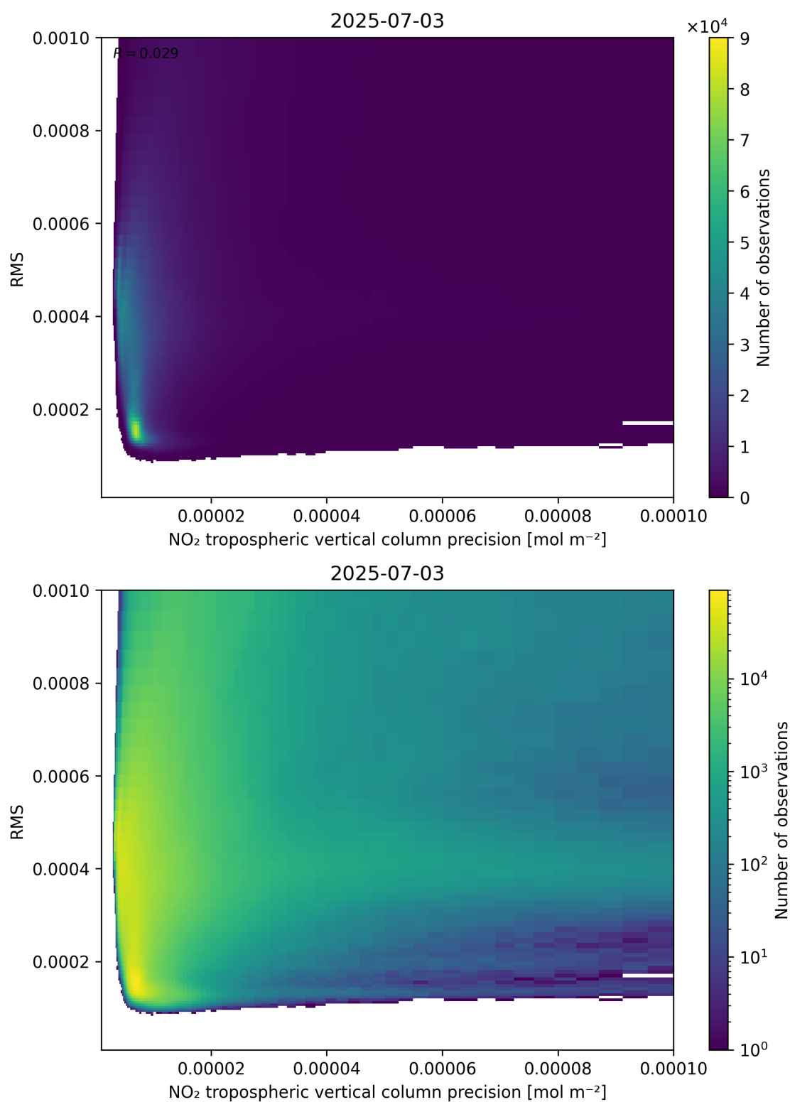
Figure 140: Scatter density plot of “NO 2 tropospheric vertical column precision” against “RMS” for 2025-07-03 to 2025-07-04.
