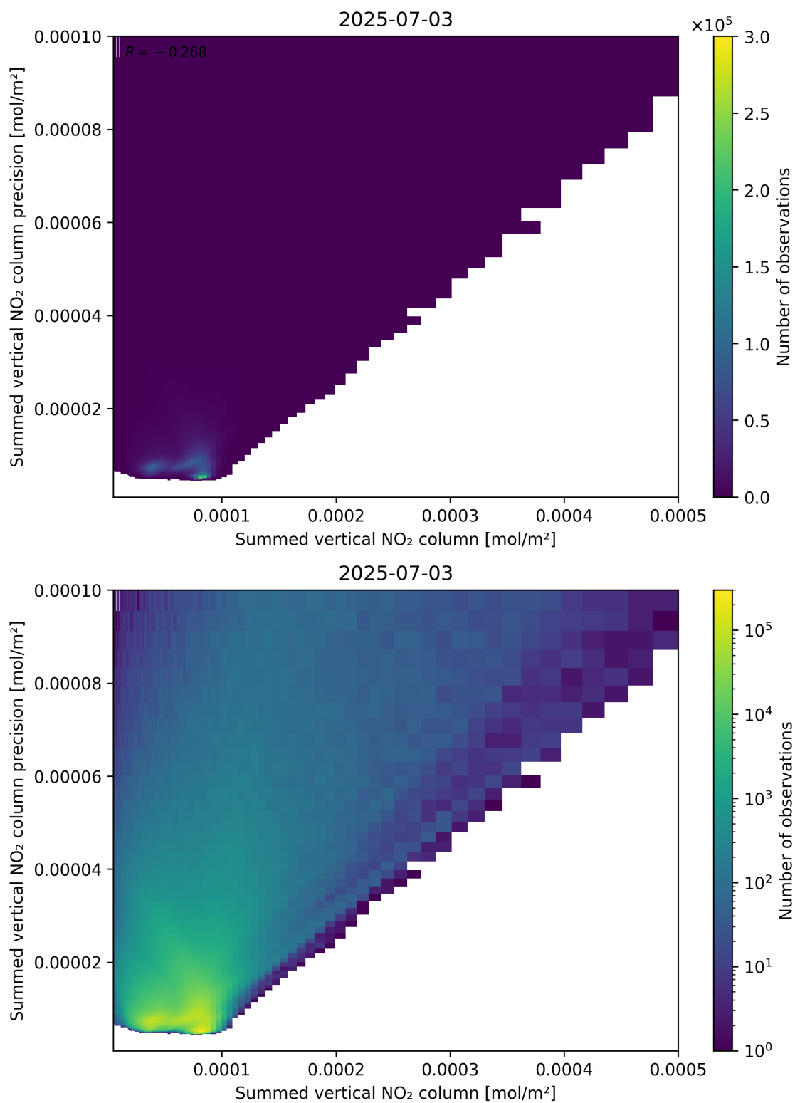
Figure 105: Scatter density plot of “Summed vertical NO 2 column” against “Summed vertical NO 2 column precision” for 2025-07-03 to 2025-07-04.
