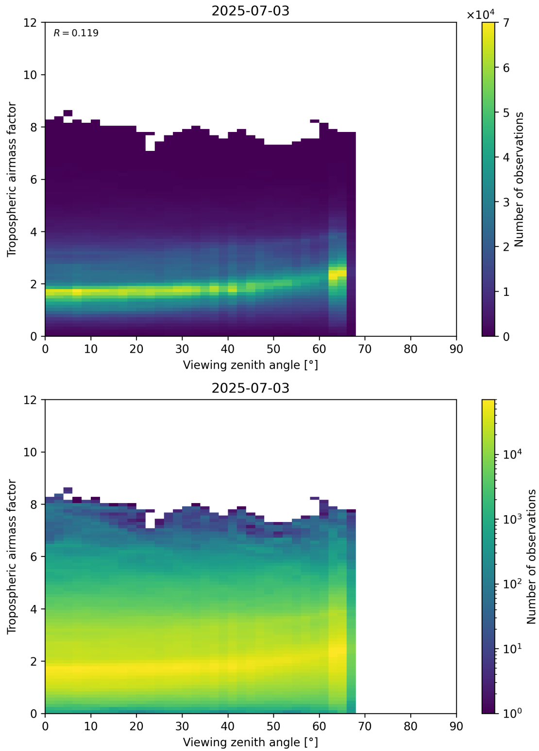
Figure 161: Scatter density plot of “Viewing zenith angle” against “Tropospheric airmass factor” for 2025-07-03 to 2025-07-04.
