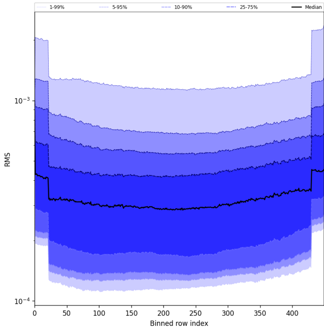
Figure 60: Along track statistics of “RMS” for 2025-07-03 to 2025-07-04
