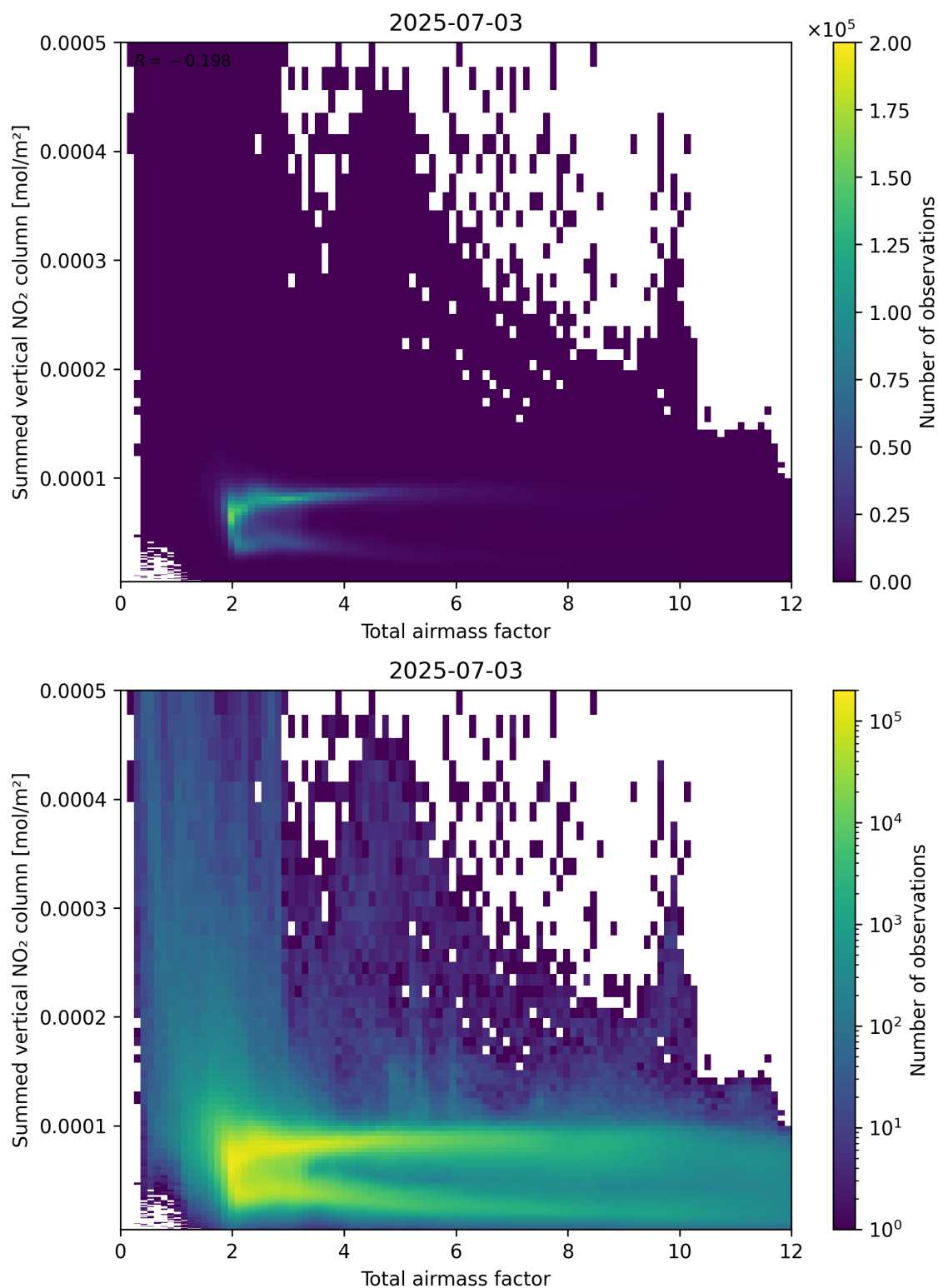
Figure 65: Scatter density plot of “Total airmass factor” against “Summed vertical NO 2 column” for 2025-07-03 to 2025-07-04.
