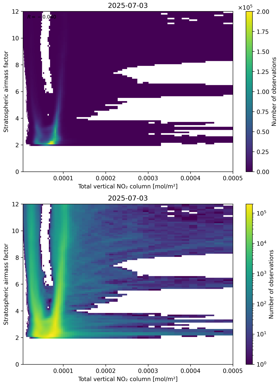
Figure 110: Scatter density plot of “Total vertical NO 2 column” against “Stratospheric airmass factor” for 2025-07-03 to 2025-07-04.
