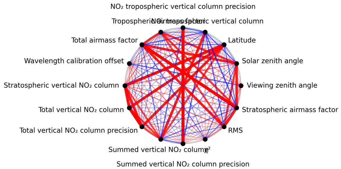
Figure 1: Map of correlation graph for 2025-07-03 to 2025-07-04.
