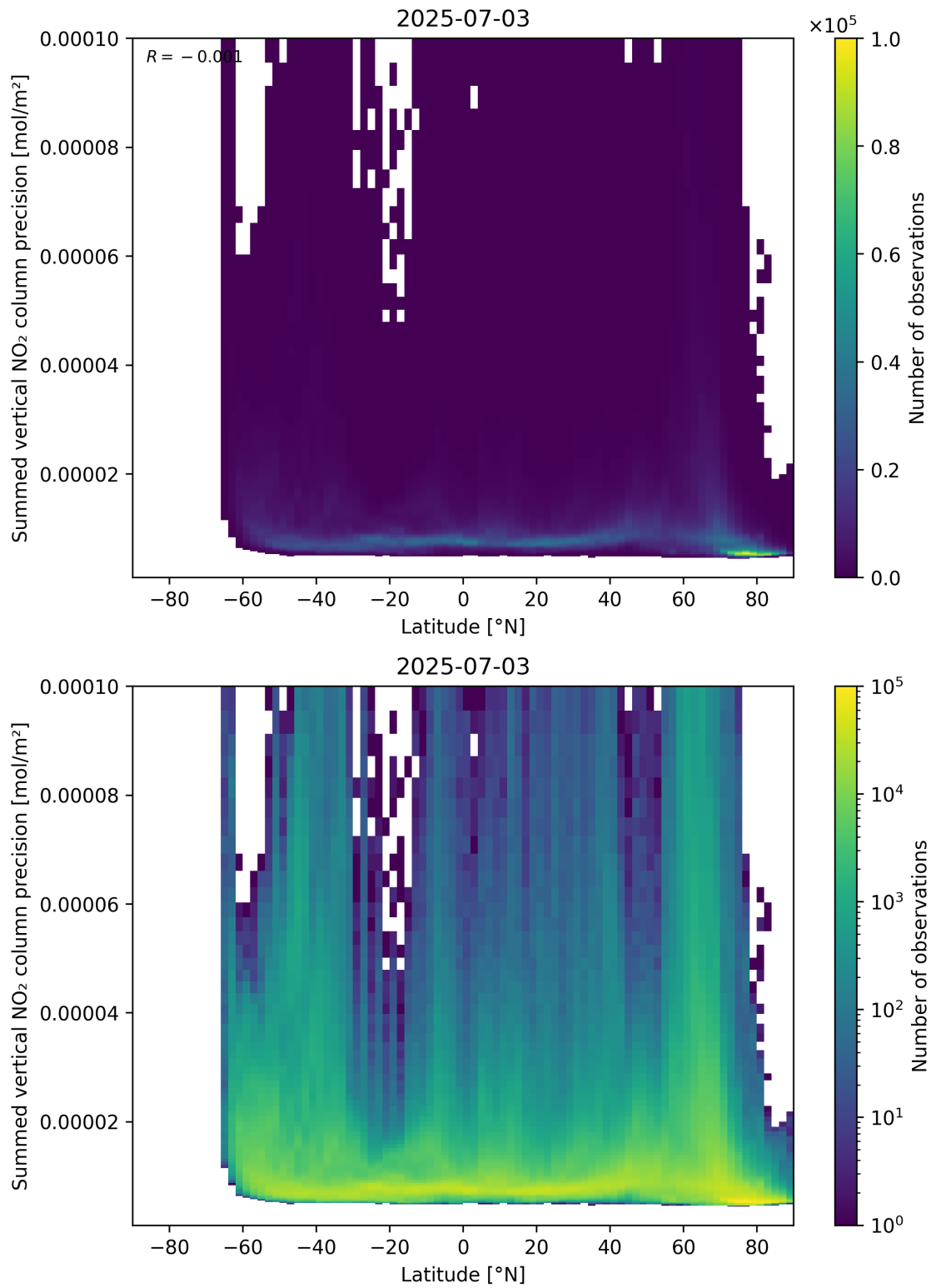
Figure 89: Scatter density plot of “Latitude” against “Summed vertical NO 2 column precision” for 2025-07-03 to 2025-07-04.
