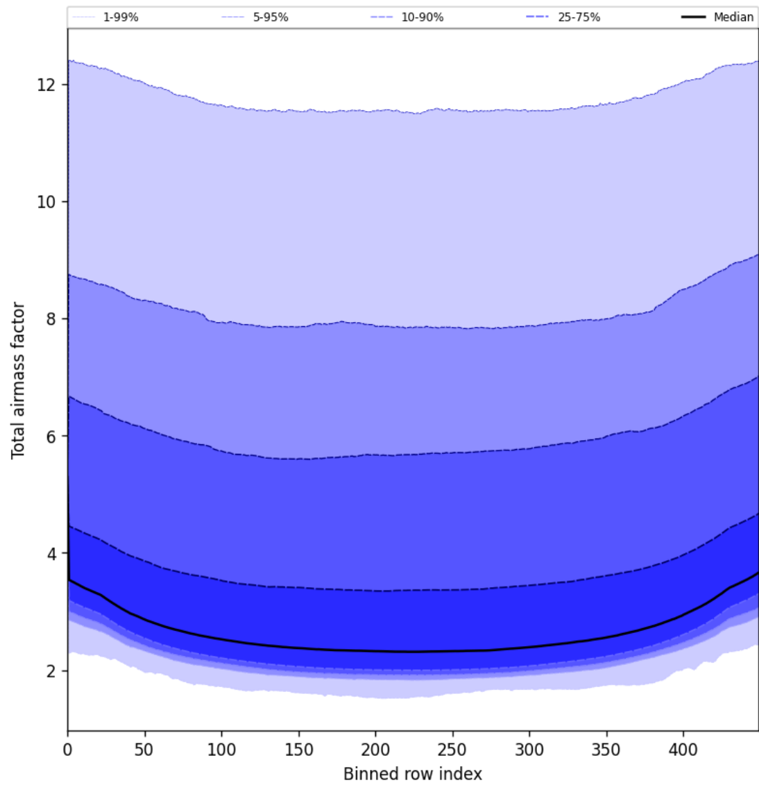
Figure 49: Along track statistics of “Total airmass factor” for 2025-07-03 to 2025-07-04
