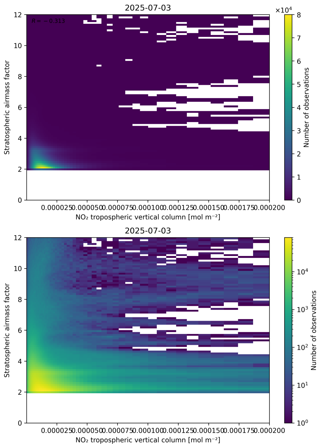
Figure 121: Scatter density plot of “NO 2 tropospheric vertical column” against “Stratospheric air mass factor” for 2025-07-03 to 2025-07-04.
