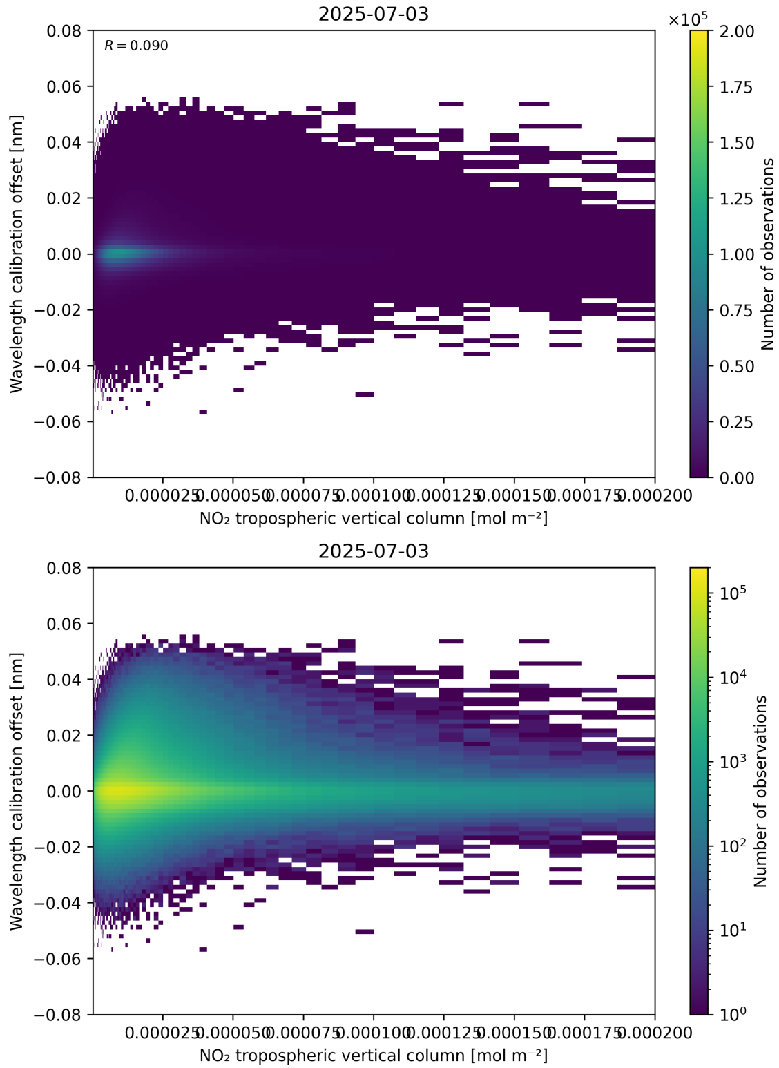
Figure 143: Scatter density plot of “NO 2 tropospheric vertical column” against “Wavelength calibration offset” for 2025-07-03 to 2025-07-04.
