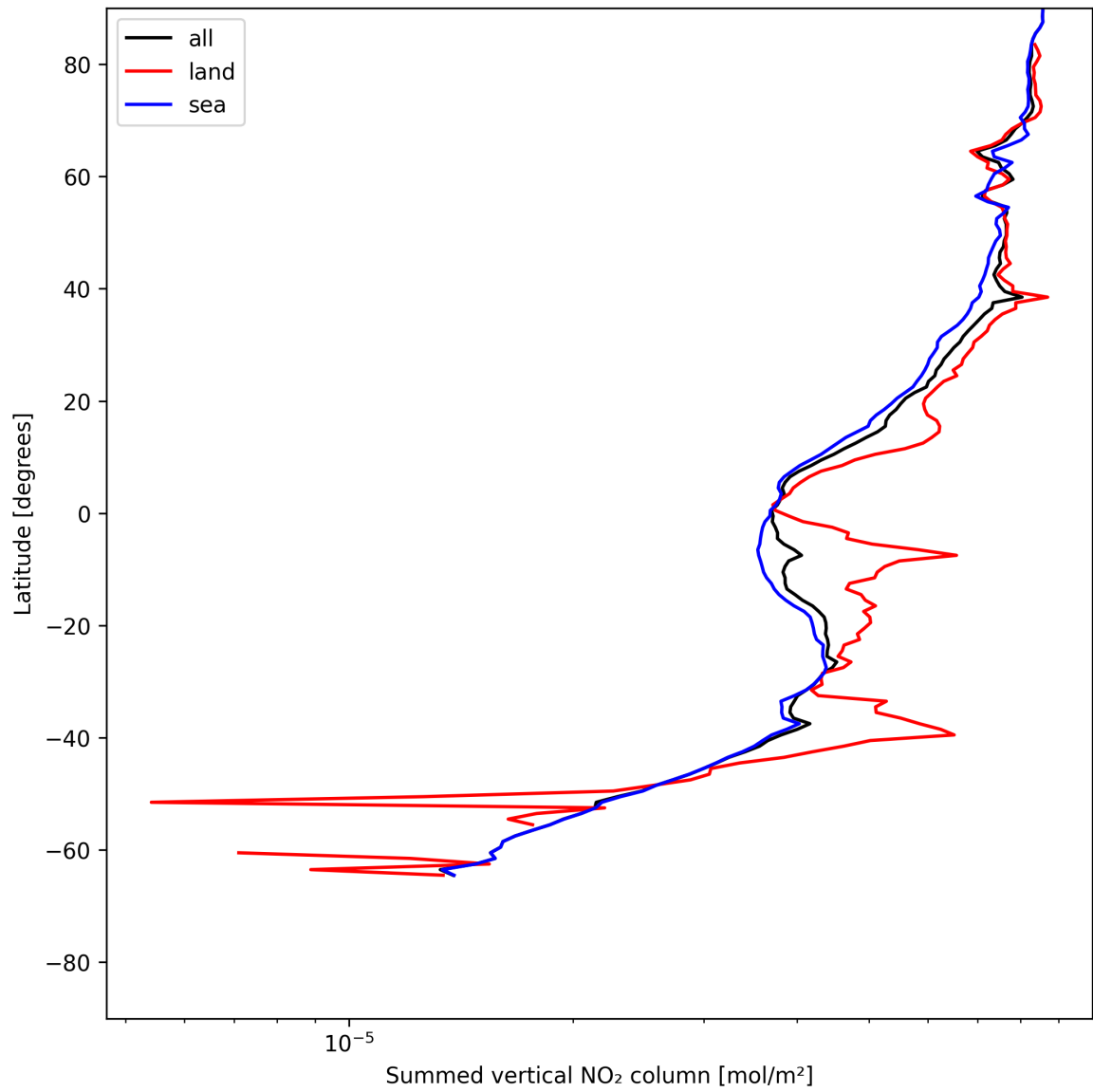
Figure 23: Zonal average of “Summed vertical NO 2 column” for 2025-07-03 to 2025-07-04.
