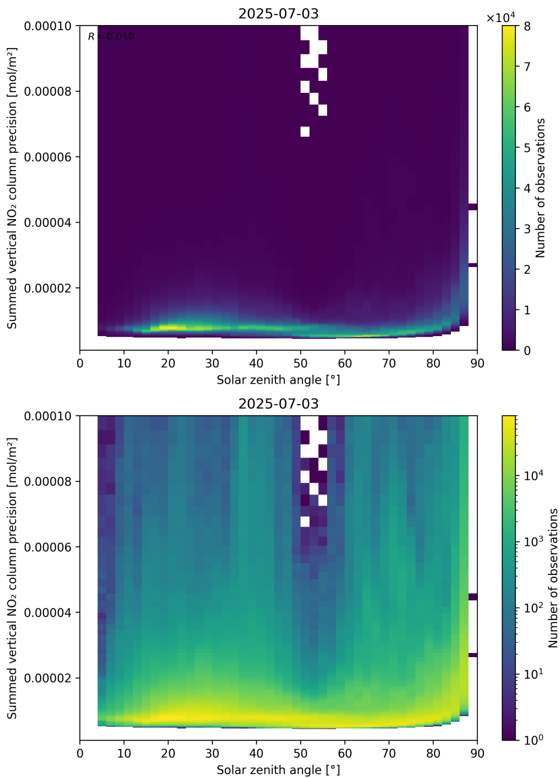
Figure 152: Scatter density plot of “Solar zenith angle” against “Summed vertical NO 2 column precision” for 2025-07-03 to 2025-07-04.
