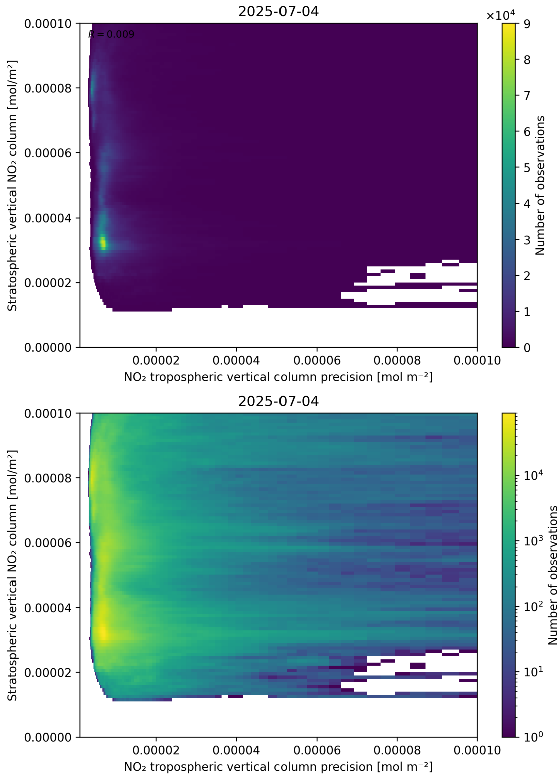
Figure 135: Scatter density plot of “NO 2 tropospheric vertical column precision” against “Stratospheric vertical NO 2 column” for 2025-07-03 to 2025-07-05.
