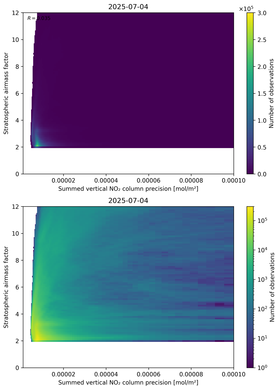
Figure 106: Scatter density plot of “Summed vertical NO 2 column precision” against “Stratospheric airmass factor” for 2025-07-03 to 2025-07-05.
