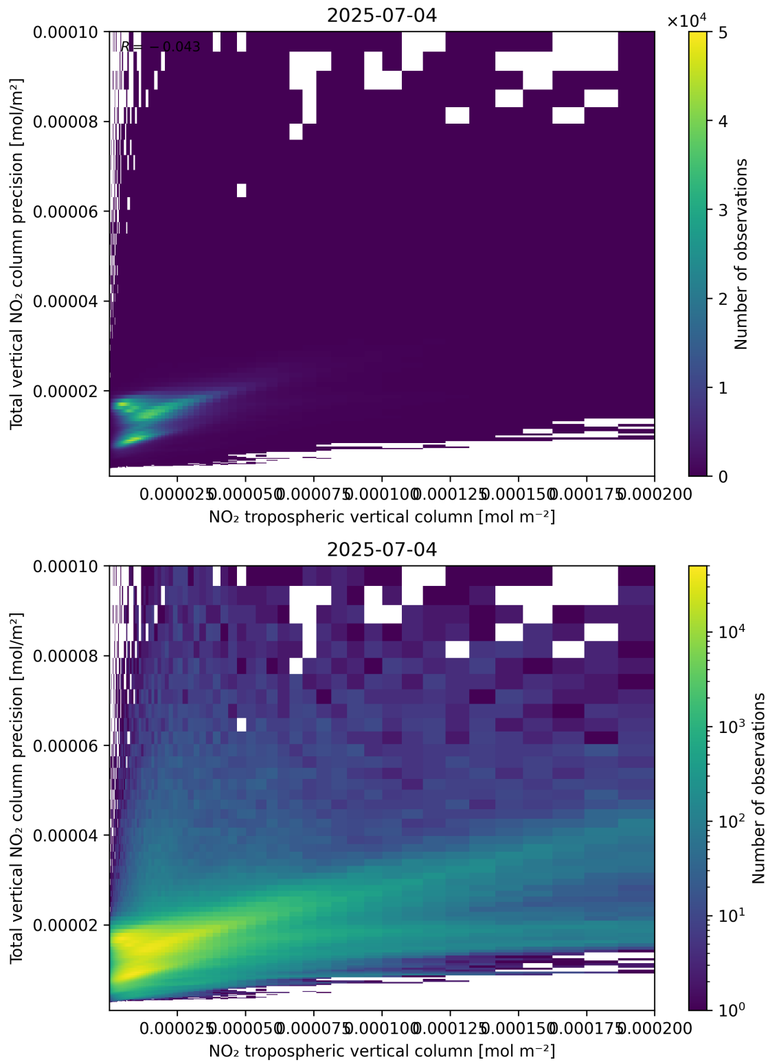
Figure 129: Scatter density plot of “NO 2 tropospheric vertical column” against “Total vertical NO 2 column precision” for 2025-07-03 to 2025-07-05.
