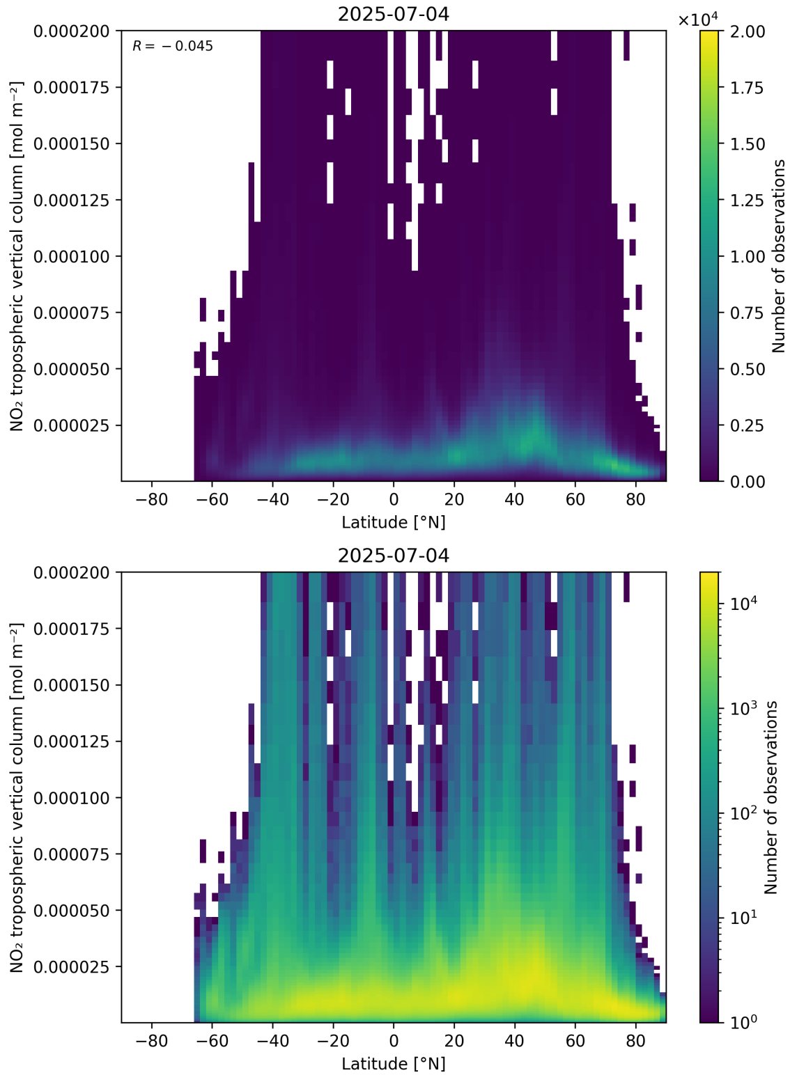
Figure 92: Scatter density plot of “Latitude” against “NO 2 tropospheric vertical column” for 2025-07-03 to 2025-07-05.
