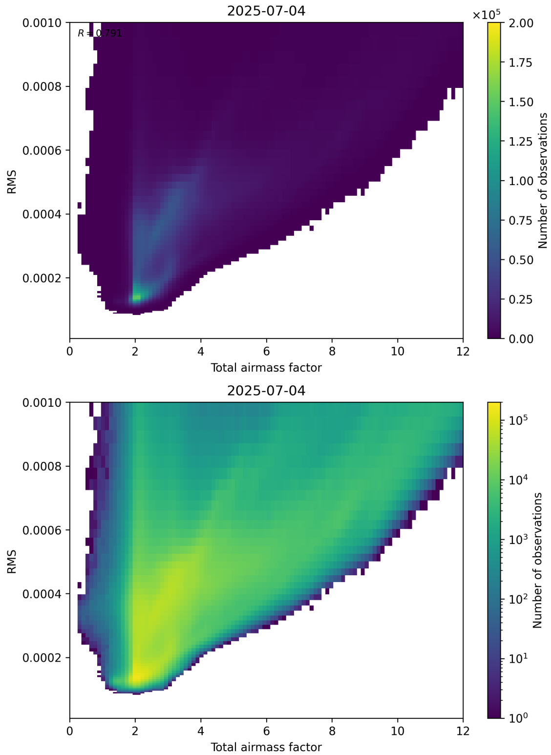
Figure 69: Scatter density plot of “Total airmass factor” against “RMS” for 2025-07-03 to 2025-07-05.
