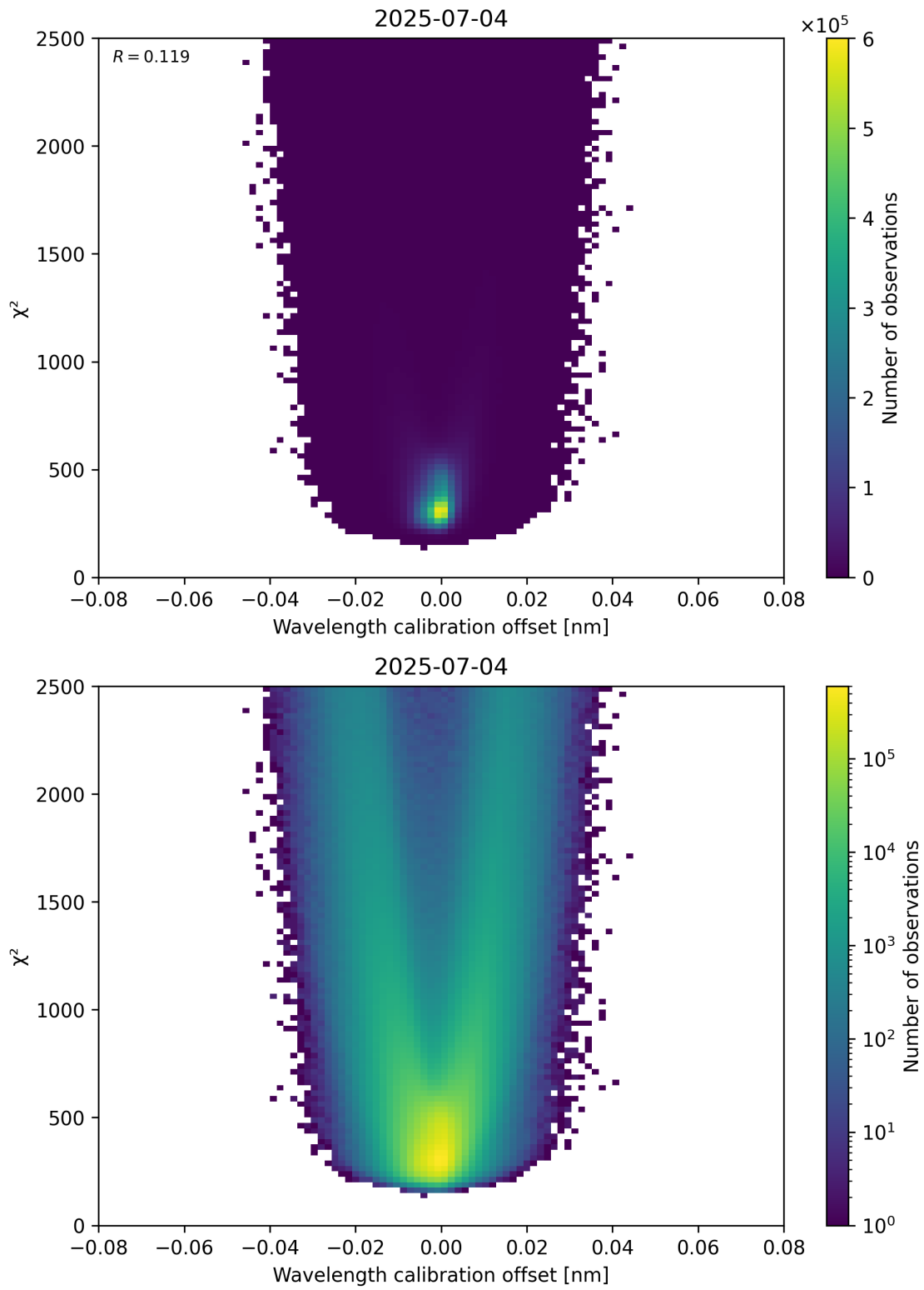
Figure 175: Scatter density plot of “Wavelength calibration offset” against “ \chi^2 ” for 2025-07-03 to 2025-07-05.
