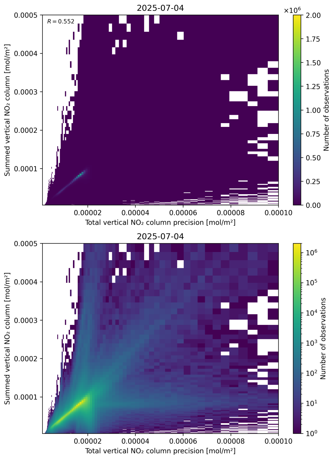
Figure 117: Scatter density plot of “Total vertical NO 2 column precision” against “Summed vertical NO 2 column” for 2025-07-03 to 2025-07-05.
