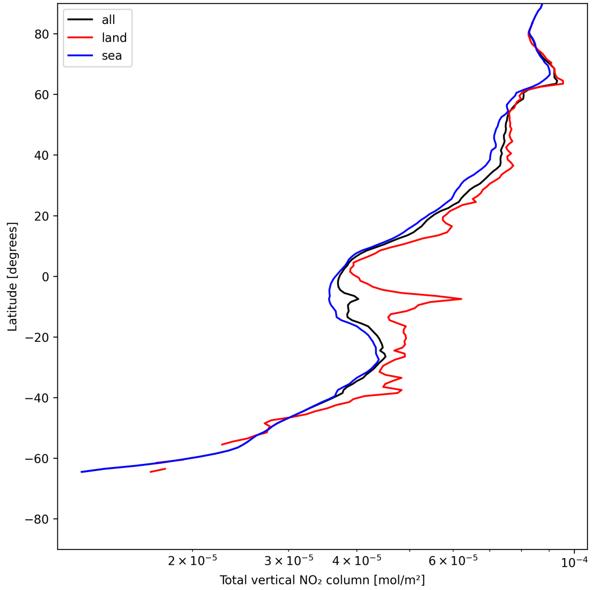
Figure 21: Zonal average of “Total vertical NO 2 column” for 2025-07-03 to 2025-07-05.
