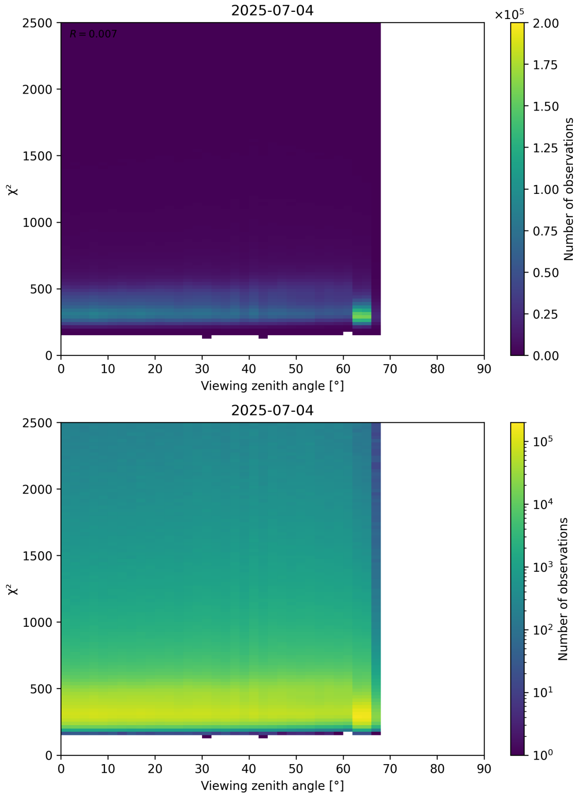
Figure 162: Scatter density plot of “Viewing zenith angle” against “ \chi^2 ” for 2025-07-03 to 2025-07-05.
