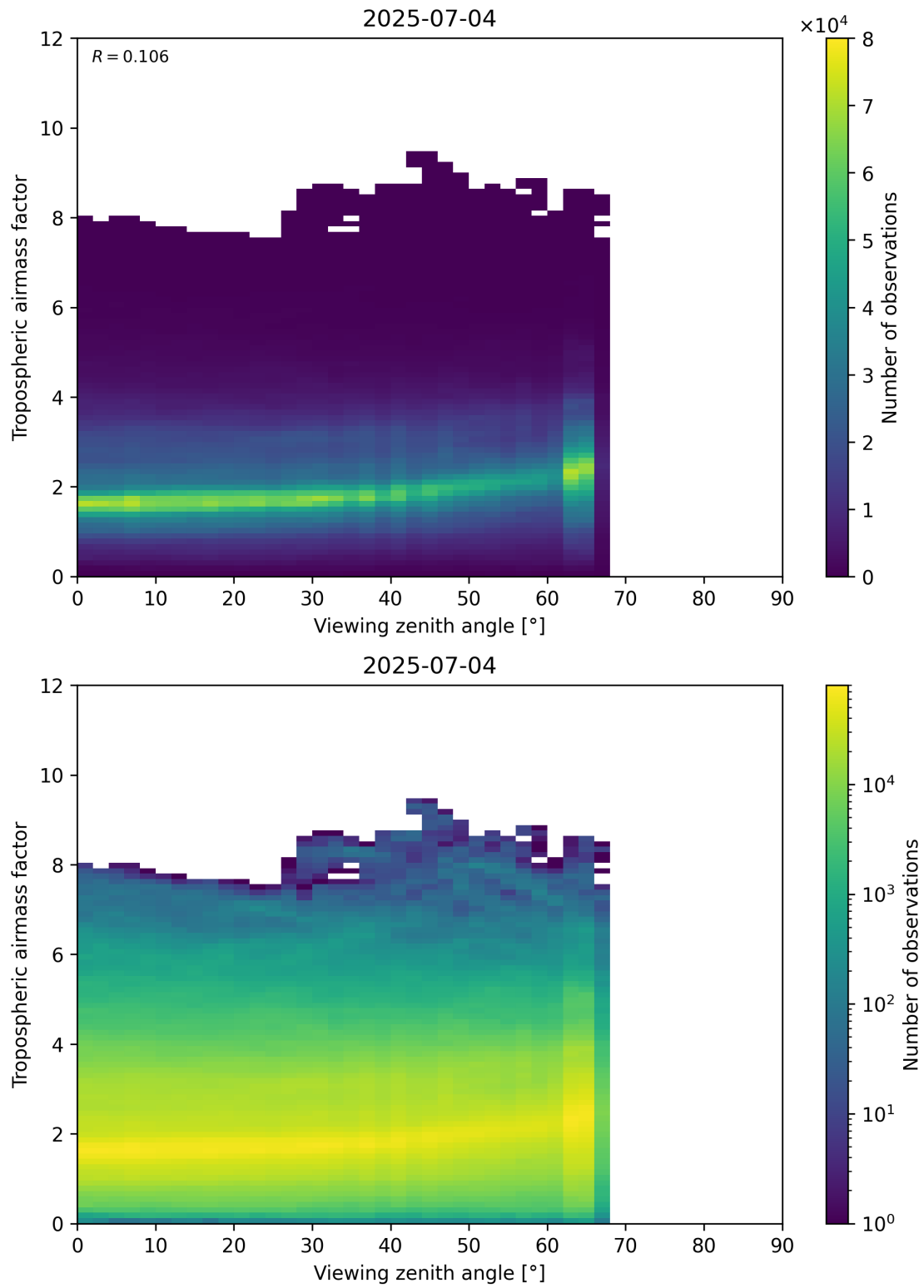
Figure 161: Scatter density plot of “Viewing zenith angle” against “Tropospheric airmass factor” for 2025-07-03 to 2025-07-05.
