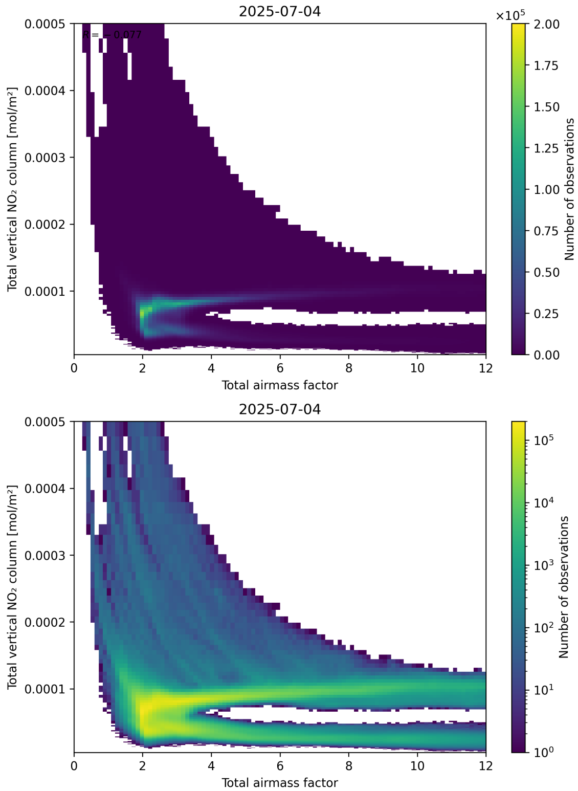
Figure 67: Scatter density plot of “Total airmass factor” against “Total vertical NO 2 column” for 2025-07-03 to 2025-07-05.
