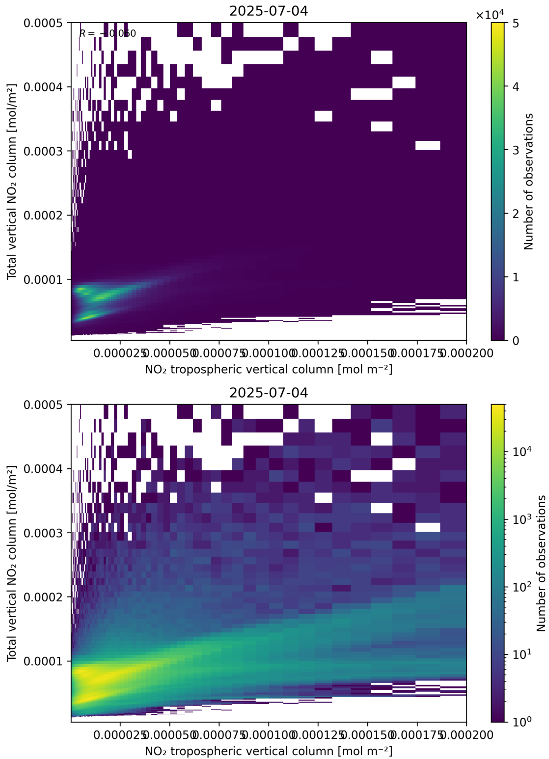
Figure 128: Scatter density plot of “NO 2 tropospheric vertical column” against “Total vertical NO 2 column” for 2025-07-03 to 2025-07-05.
