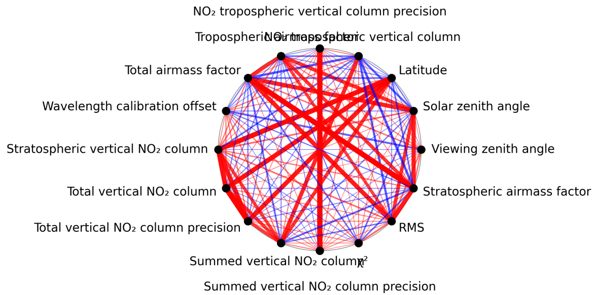
Figure 1: Map of correlation graph for 2025-07-03 to 2025-07-05.
