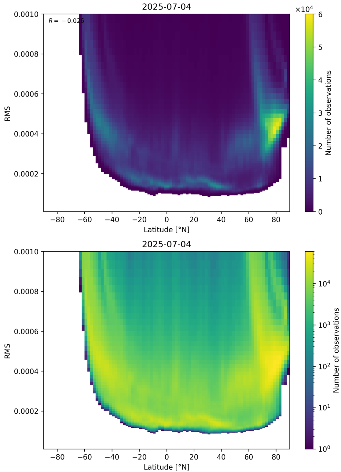
Figure 94: Scatter density plot of “Latitude” against “RMS” for 2025-07-03 to 2025-07-05.
