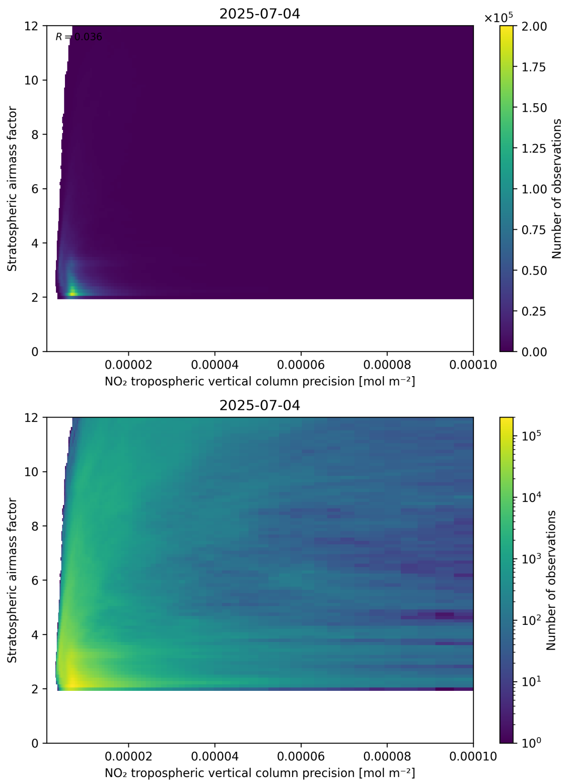
Figure 131: Scatter density plot of “NO 2 tropospheric vertical column precision” against “Stratospheric airmass factor” for 2025-07-03 to 2025-07-05.
