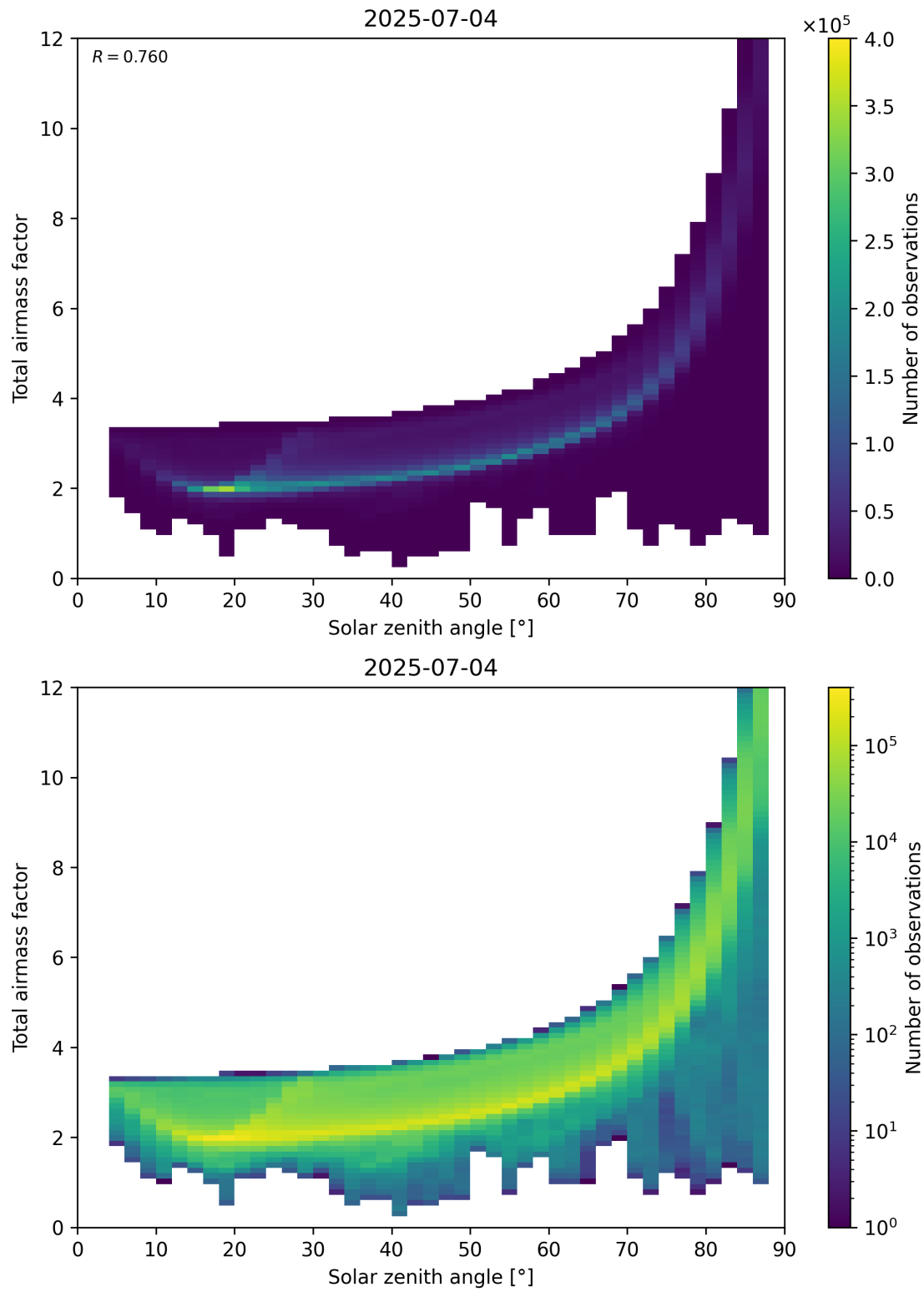
Figure 146: Scatter density plot of “Solar zenith angle” against “Total air mass factor” for 2025-07-03 to 2025-07-05.
