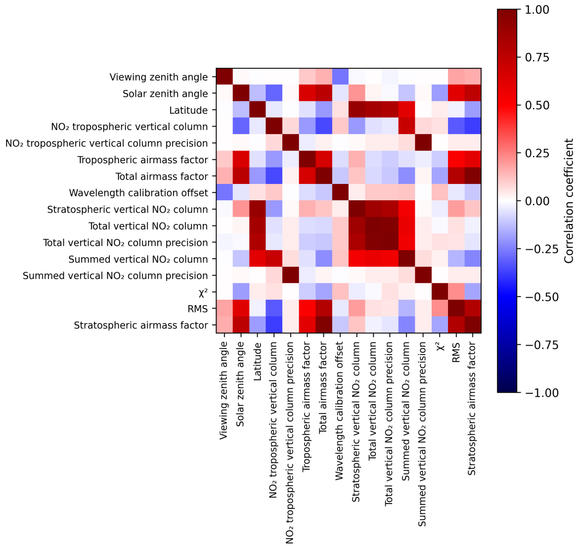
Figure 2: Map of correlation matrix for 2025-07-03 to 2025-07-05.
