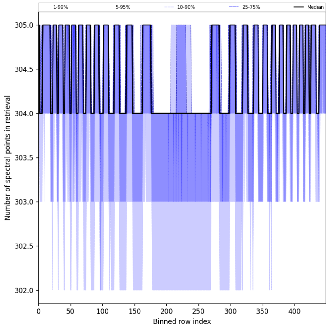
Figure 50: Along track statistics of “Number of spectral points in retrieval” for 2025-07-03 to 2025-07-05
