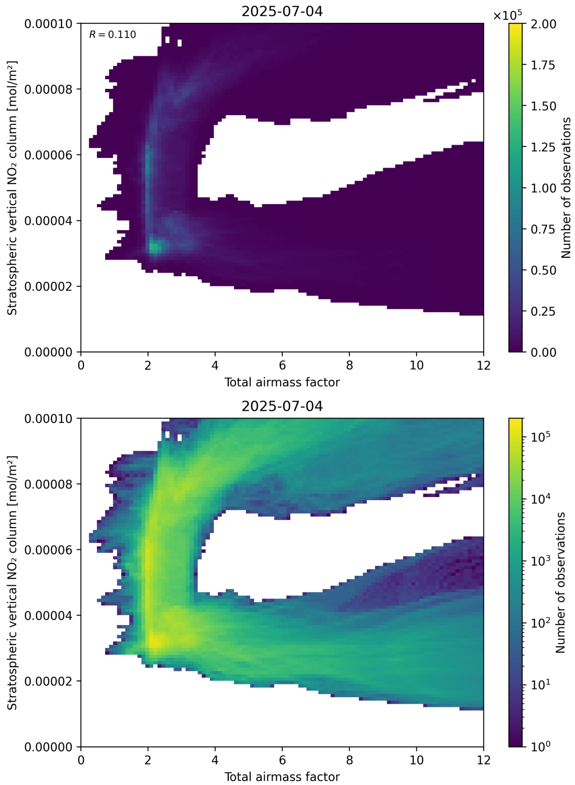
Figure 64: Scatter density plot of “Total airmass factor” against “Stratospheric vertical \text{NO}_2 column” for 2025-07-03 to 2025-07-05.
