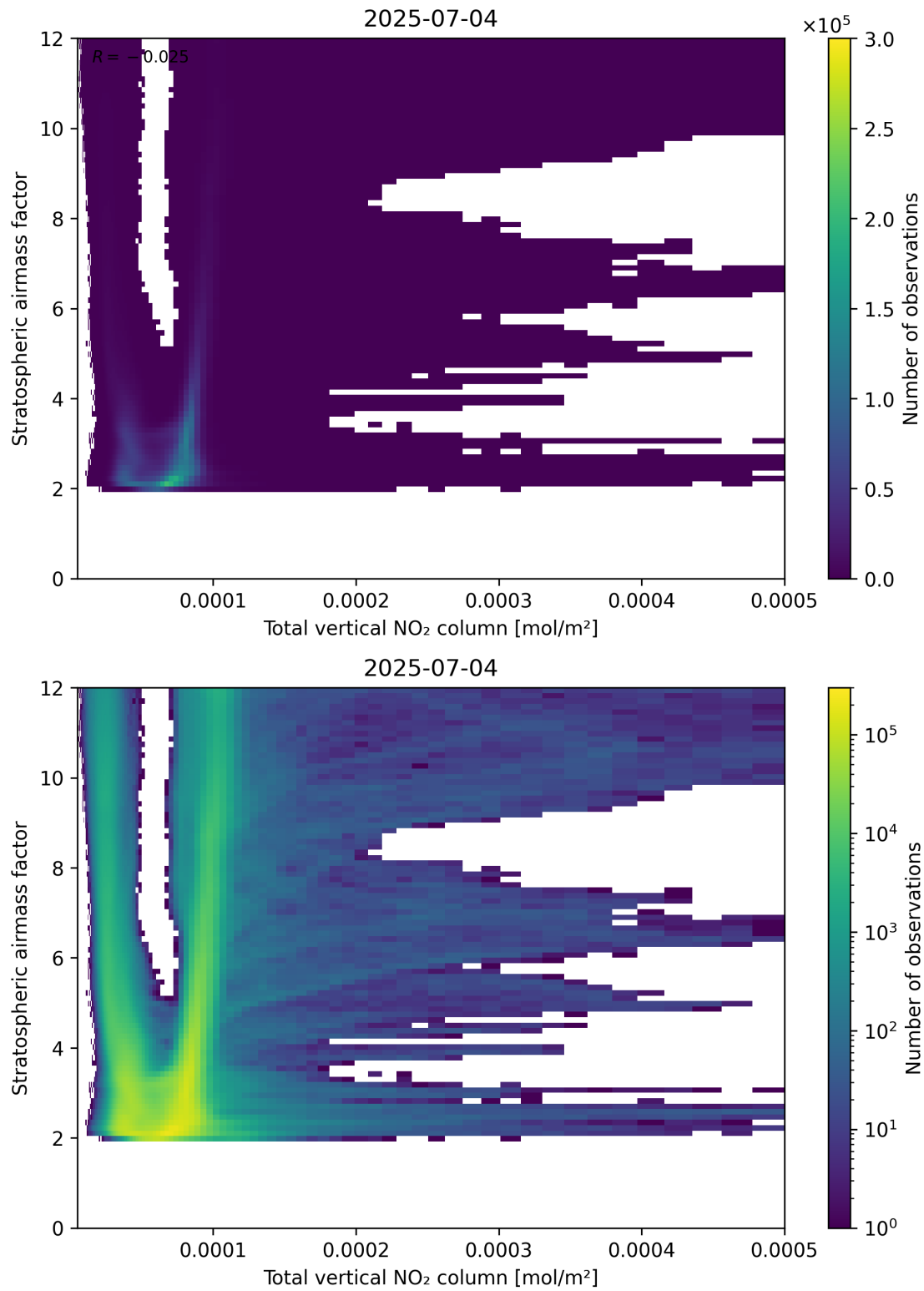
Figure 110: Scatter density plot of “Total vertical NO 2 column” against “Stratospheric airmass factor” for 2025-07-03 to 2025-07-05.
