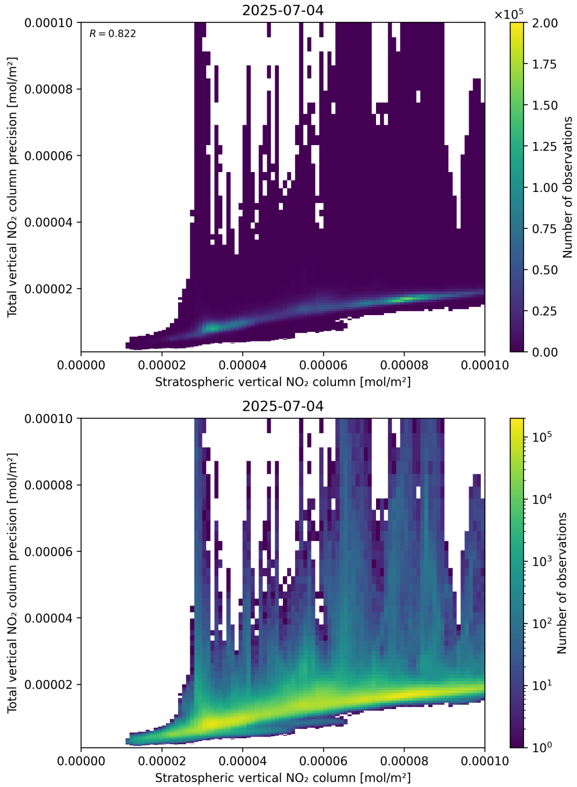
Figure 101: Scatter density plot of “Stratospheric vertical NO 2 column” against “Total vertical NO 2 column precision” for 2025-07-03 to 2025-07-05.
