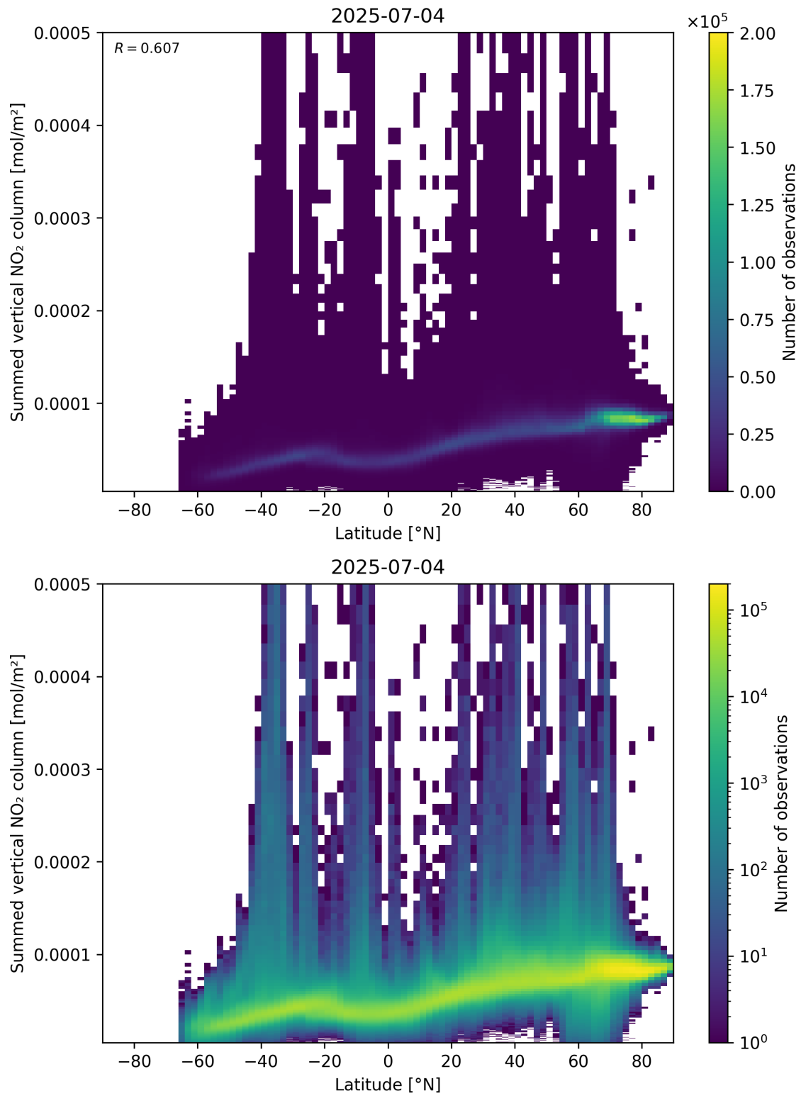
Figure 88: Scatter density plot of “Latitude” against “Summed vertical NO 2 column” for 2025-07-03 to 2025-07-05.
