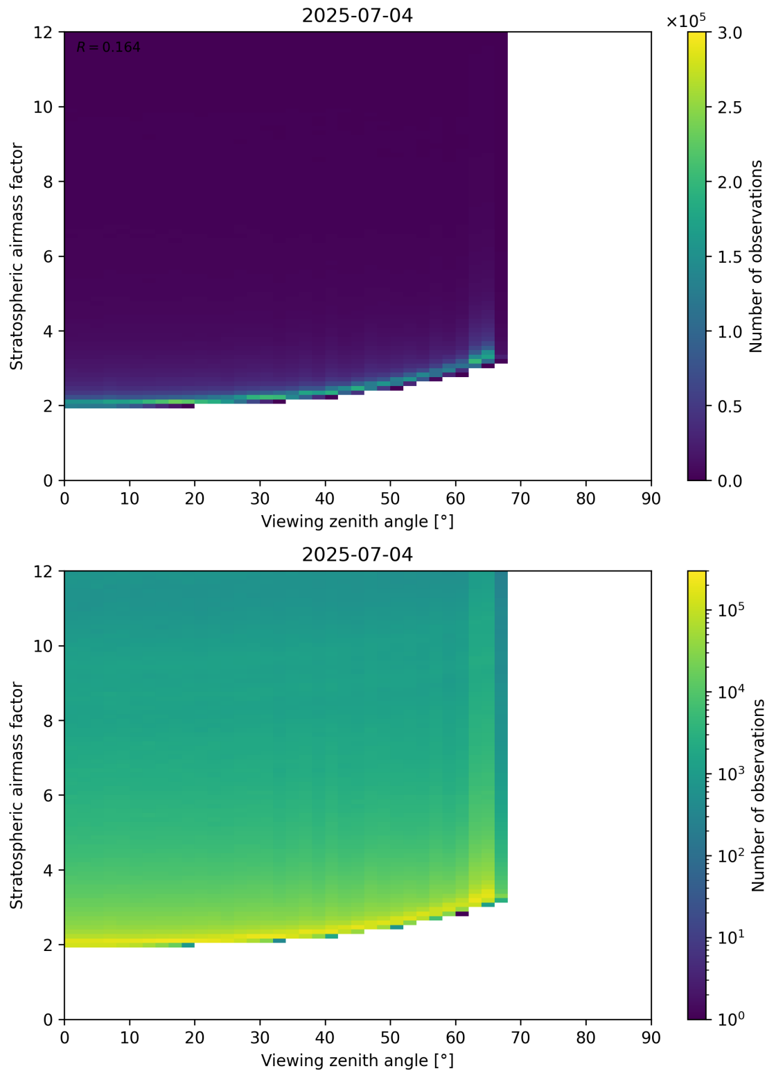
Figure 159: Scatter density plot of “Viewing zenith angle” against “Stratospheric airmass factor” for 2025-07-03 to 2025-07-05.
