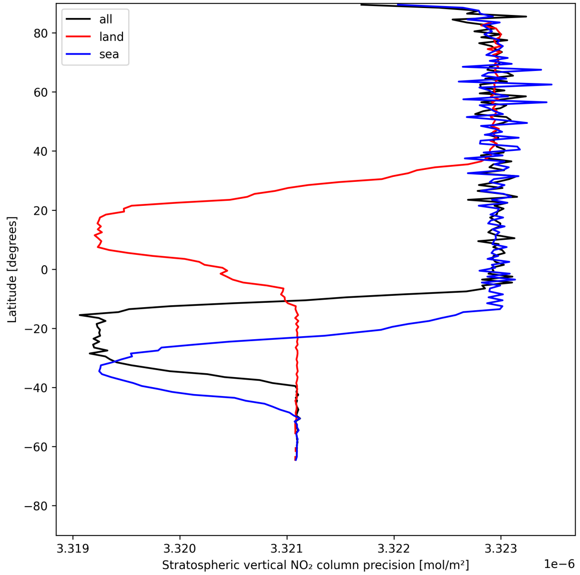
Figure 20: Zonal average of “Stratospheric vertical NO 2 column precision” for 2025-07-03 to 2025-07-05.
