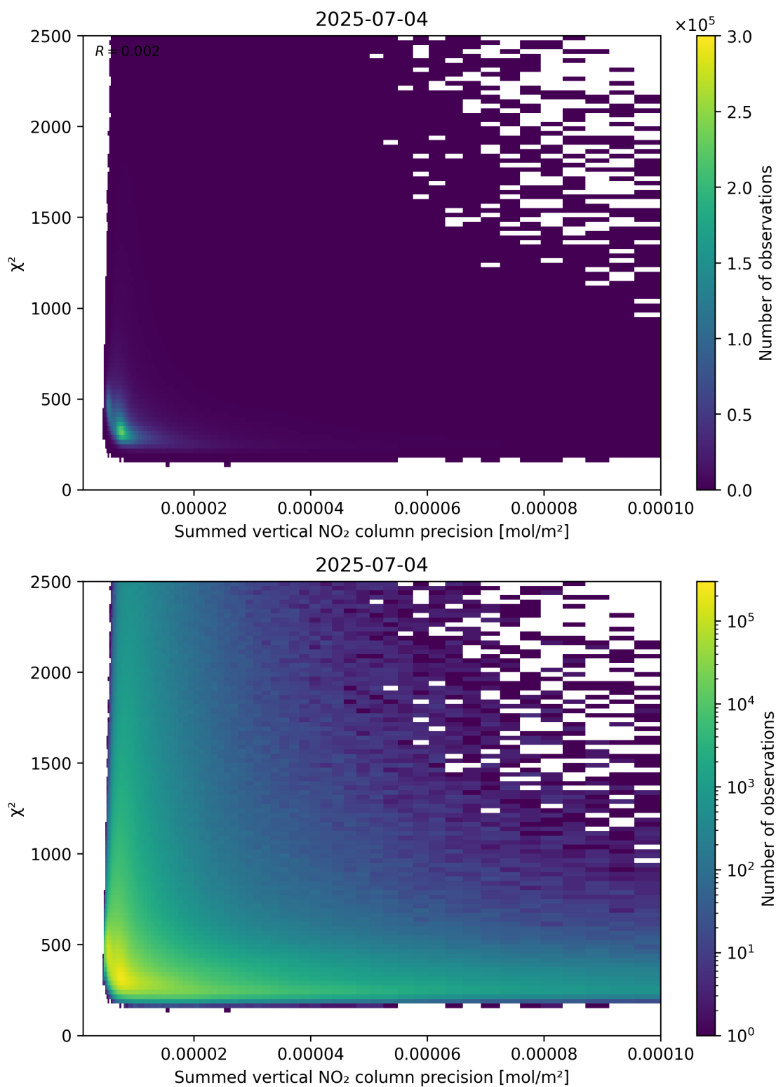
Figure 107: Scatter density plot of “Summed vertical NO 2 column precision” against “ \chi^2 ” for 2025-07-03 to 2025-07-05.
