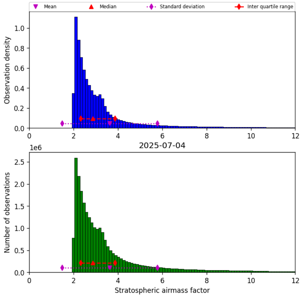
Figure 44: Histogram of “Stratospheric airmass factor” for 2025-07-03 to 2025-07-05
