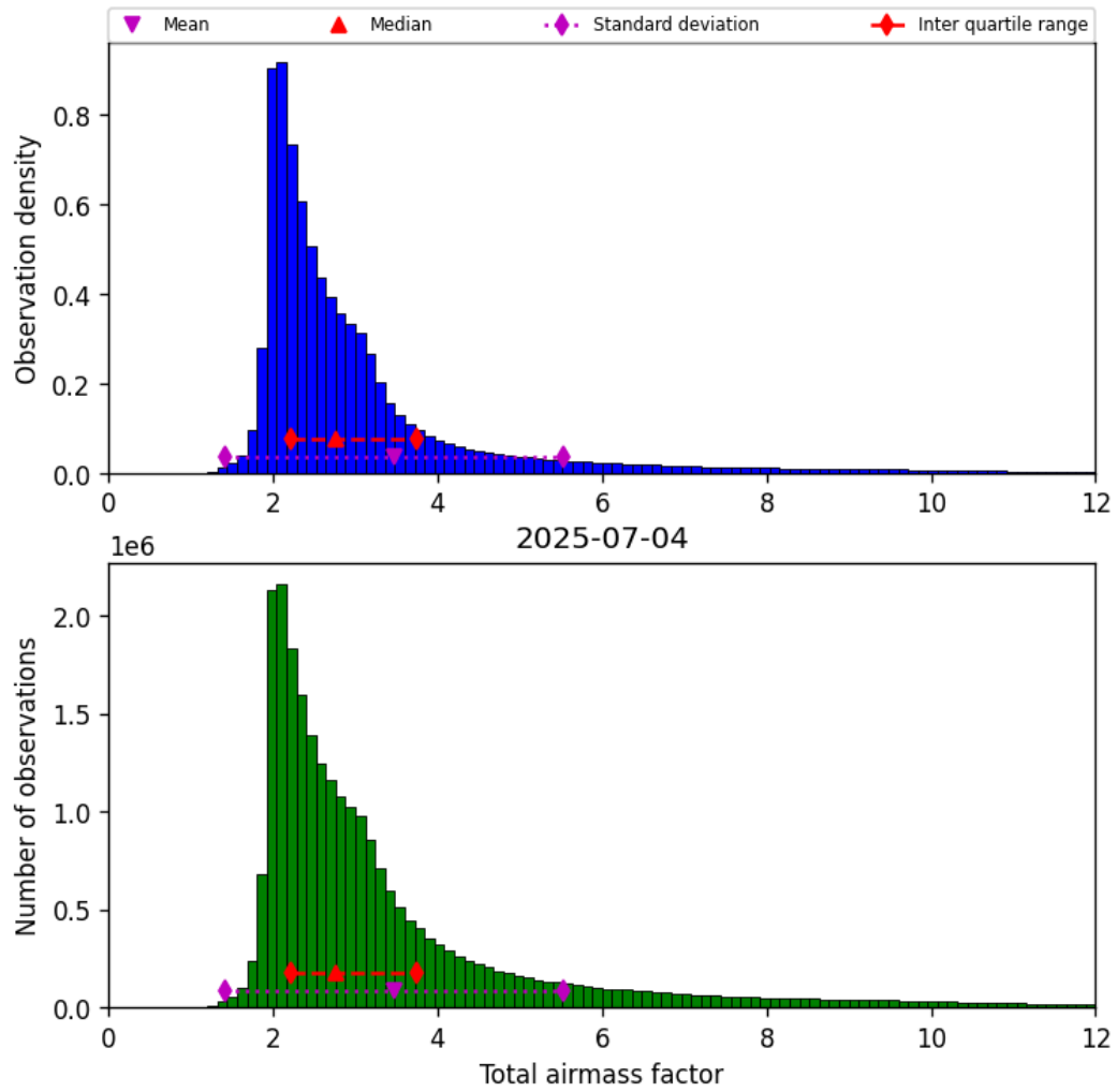
Figure 32: Histogram of “Total airmass factor” for 2025-07-03 to 2025-07-05
