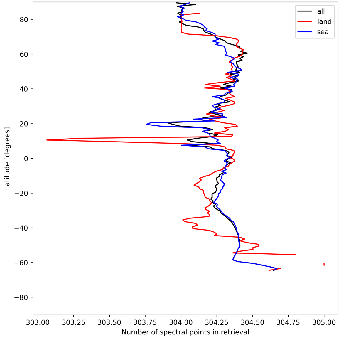
Figure 16: Zonal average of “Number of spectral points in retrieval” for 2025-07-03 to 2025-07-05.
