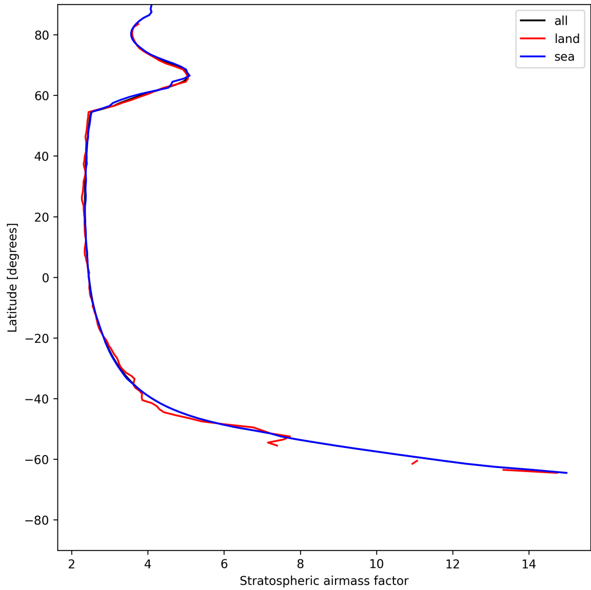
Figure 27: Zonal average of “Stratospheric airmass factor” for 2025-07-03 to 2025-07-05.
