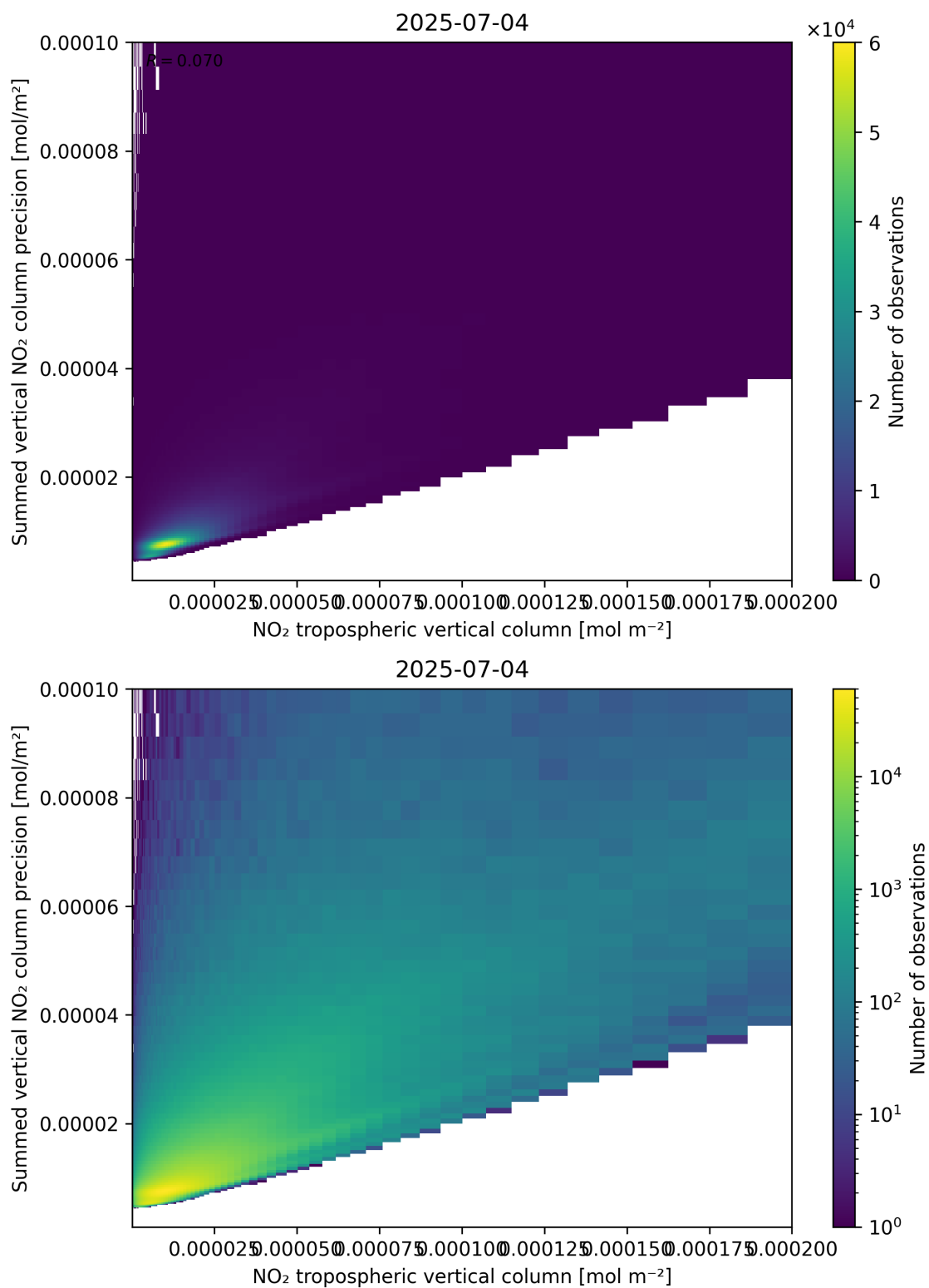
Figure 127: Scatter density plot of “NO 2 tropospheric vertical column” against “Summed vertical NO 2 column precision” for 2025-07-03 to 2025-07-05.
