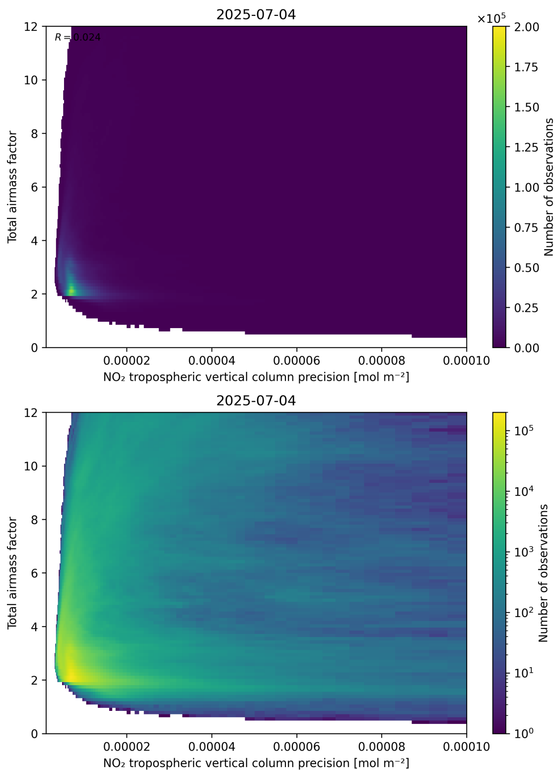
Figure 132: Scatter density plot of “NO 2 tropospheric vertical column precision” against “Total air mass factor” for 2025-07-03 to 2025-07-05.
