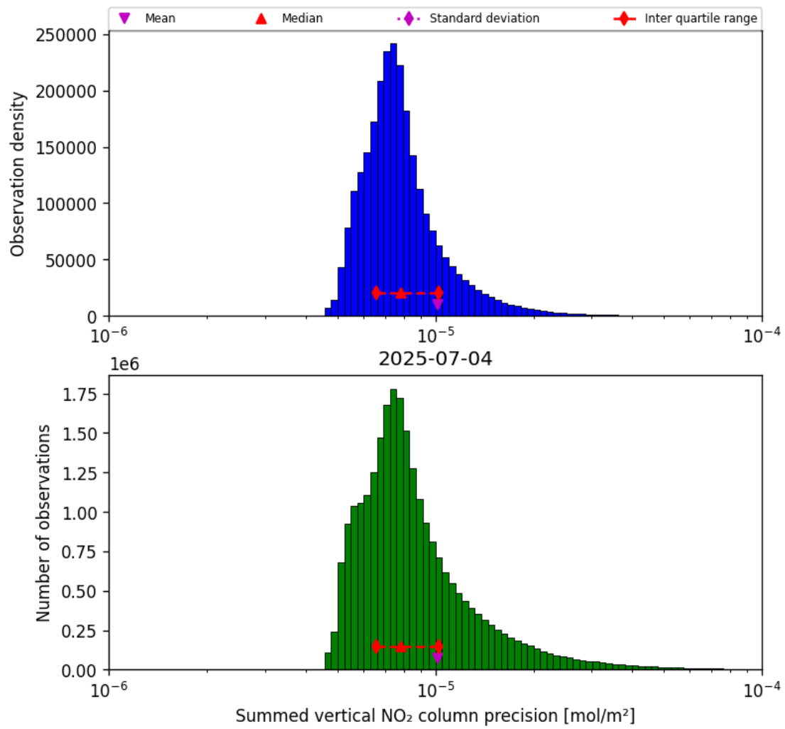
Figure 41: Histogram of "Summed vertical NO 2 column precision" for 2025-07-03 to 2025-07-05
