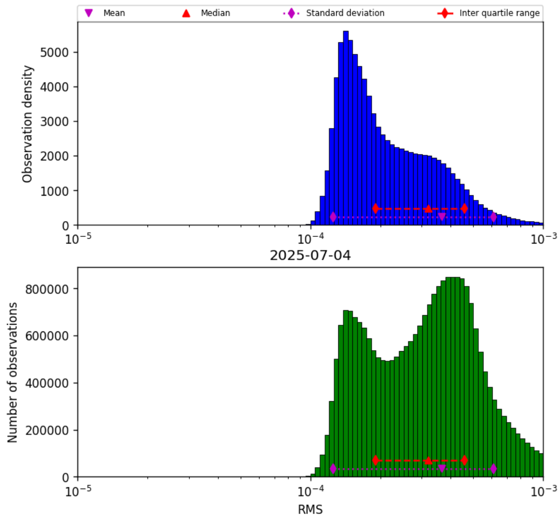
Figure 43: Histogram of “RMS” for 2025-07-03 to 2025-07-05
