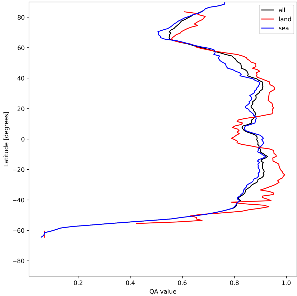
Figure 11: Zonal average of “QA value” for 2025-07-03 to 2025-07-05.
