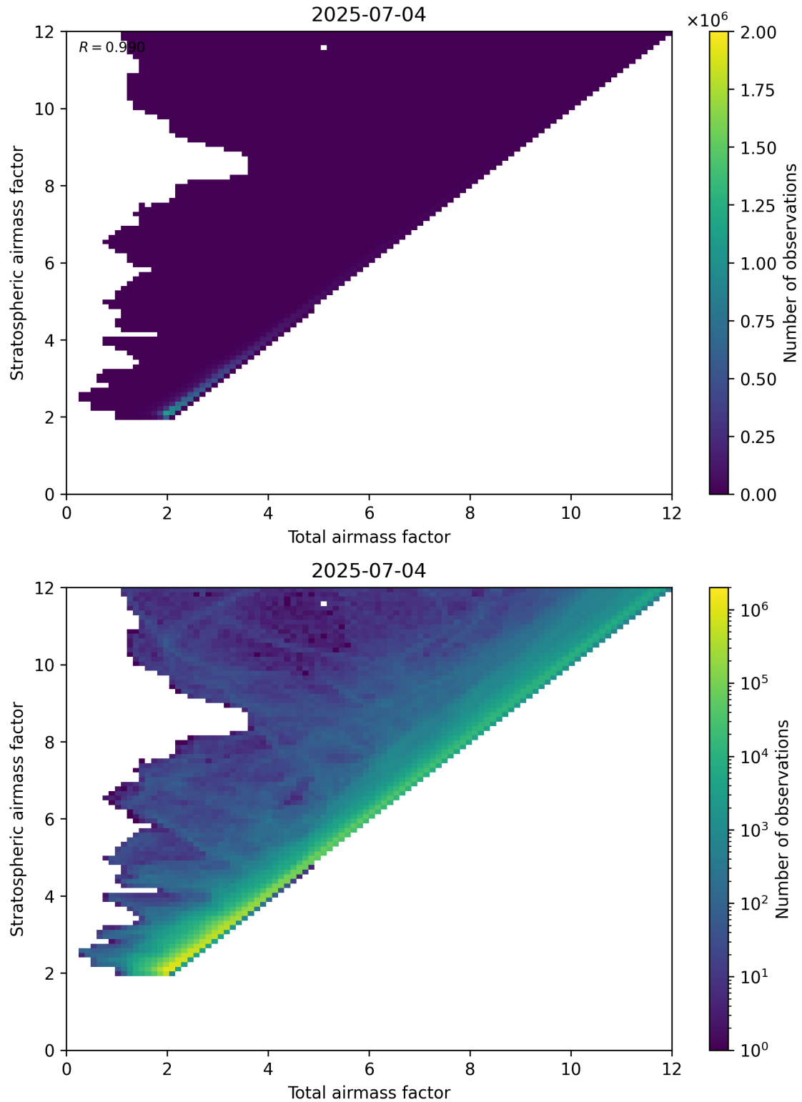
Figure 62: Scatter density plot of “Total airmass factor” against “Stratospheric airmass factor” for 2025-07-03 to 2025-07-05.
