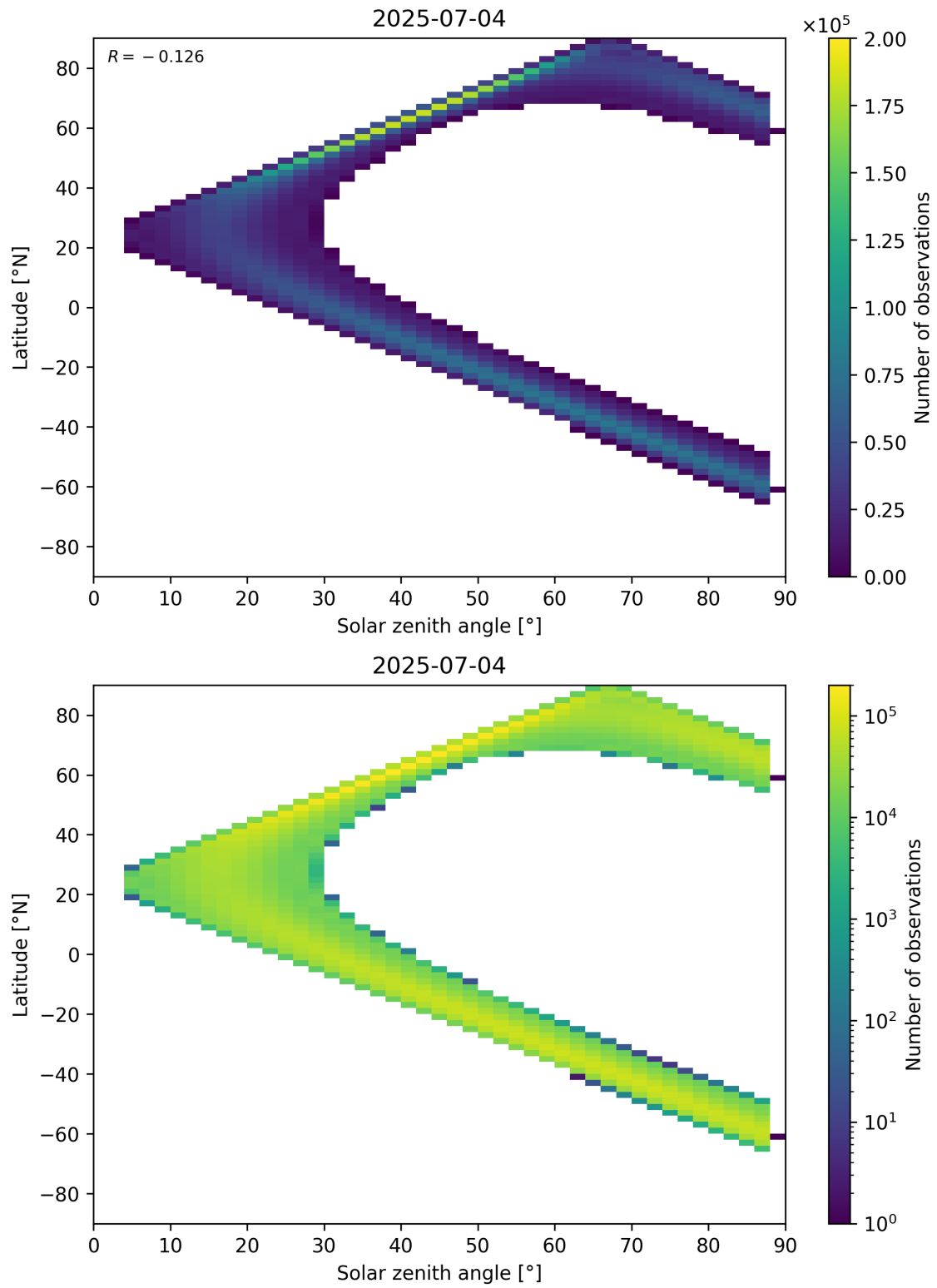
Figure 149: Scatter density plot of “Solar zenith angle” against “Latitude” for 2025-07-03 to 2025-07-05.
