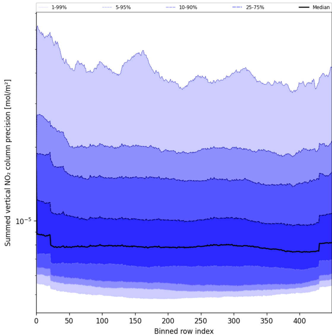
Figure 58: Along track statistics of “Summed vertical NO 2 column precision” for 2025-07-03 to 2025-07-05
