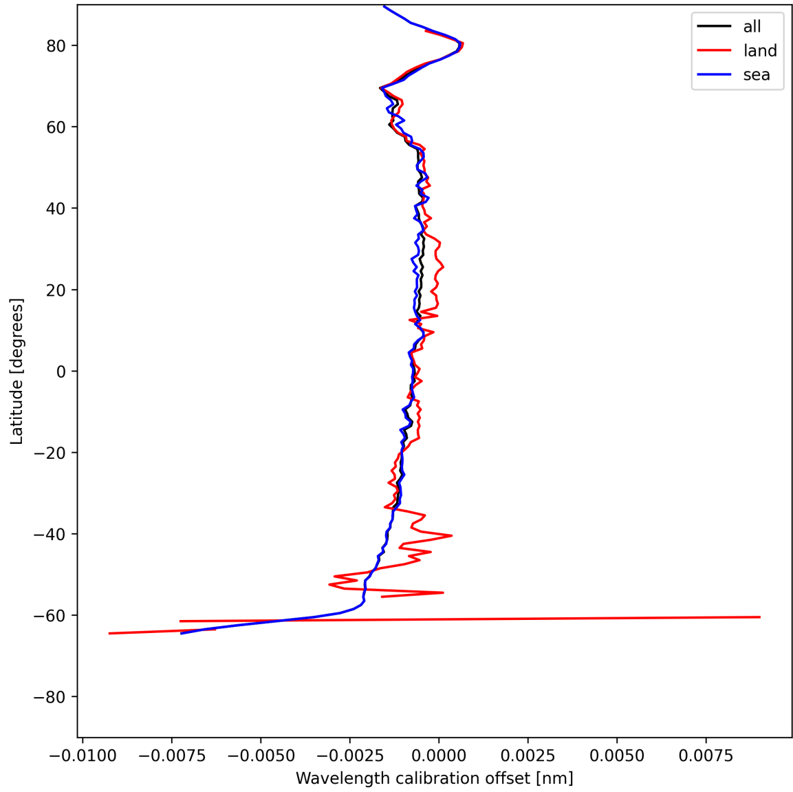
Figure 18: Zonal average of “Wavelength calibration offset” for 2025-07-03 to 2025-07-05.
