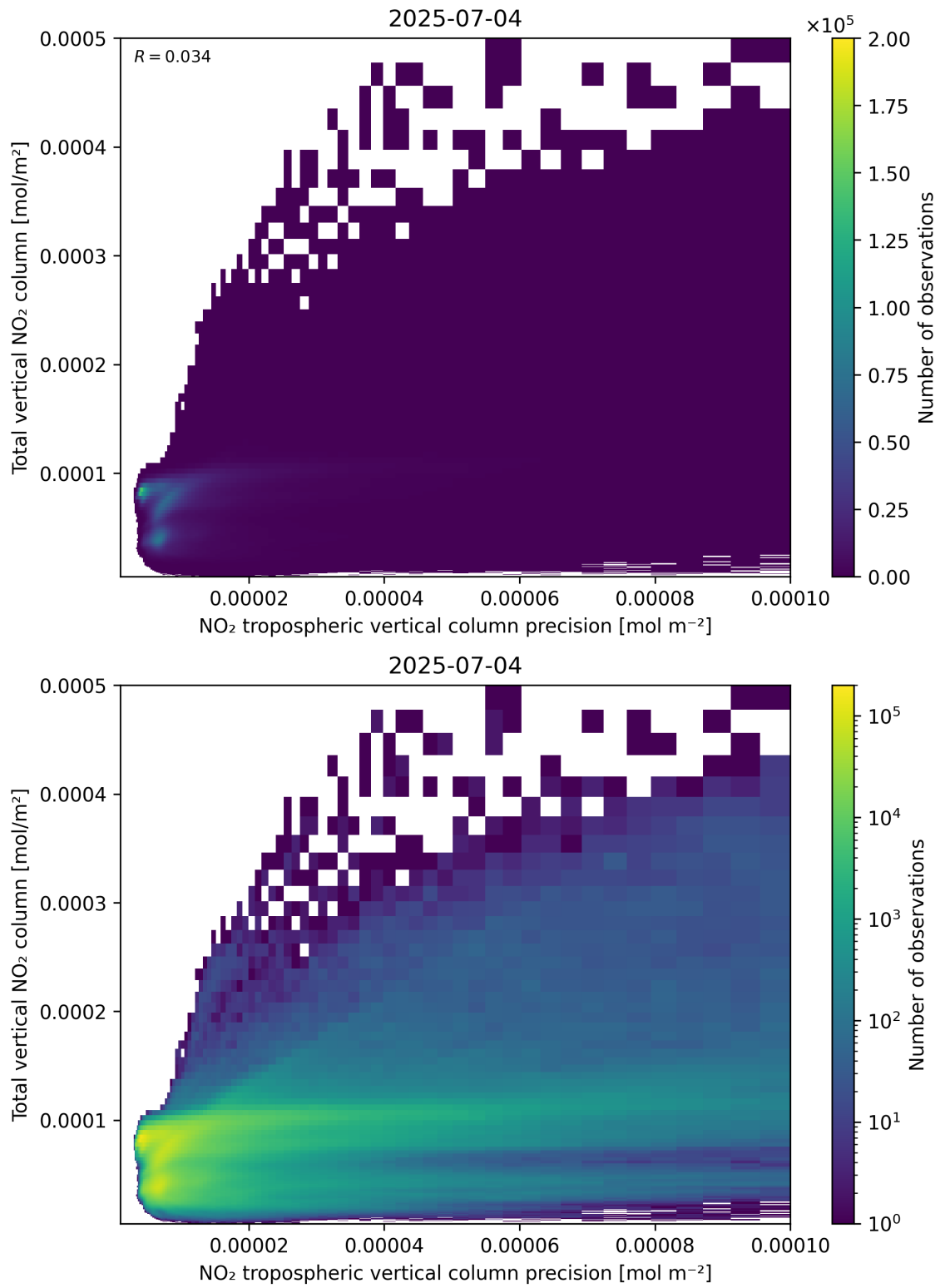
Figure 138: Scatter density plot of “NO 2 tropospheric vertical column precision” against “Total vertical NO 2 column” for 2025-07-03 to 2025-07-05.
