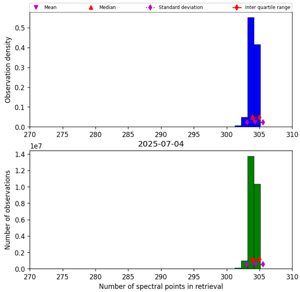
Figure 33: Histogram of “Number of spectral points in retrieval” for 2025-07-03 to 2025-07-05
