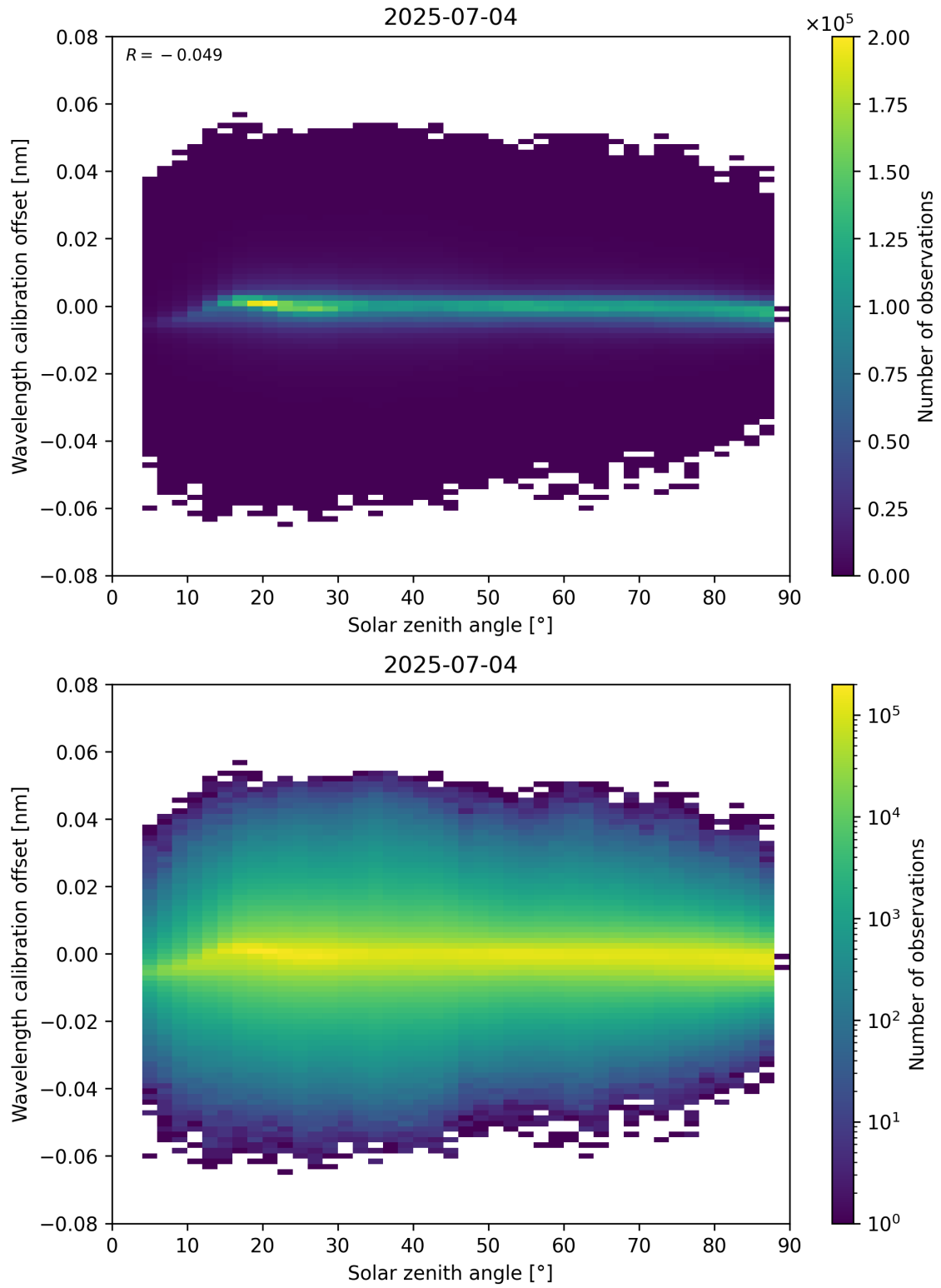
Figure 158: Scatter density plot of “Solar zenith angle” against “Wavelength calibration offset” for 2025-07-03 to 2025-07-05.
