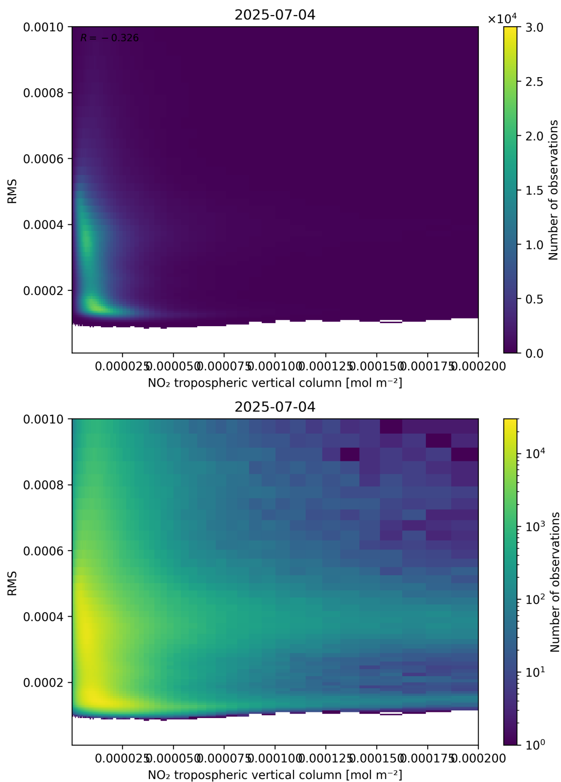
Figure 142: Scatter density plot of “NO 2 tropospheric vertical column” against “RMS” for 2025-07-03 to 2025-07-05.
