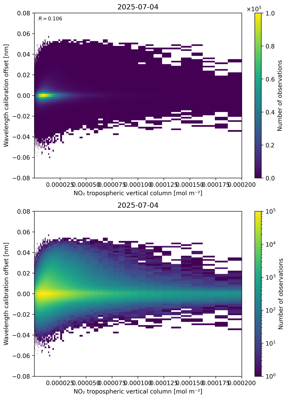
Figure 143: Scatter density plot of “NO 2 tropospheric vertical column” against “Wavelength calibration offset” for 2025-07-03 to 2025-07-05.
