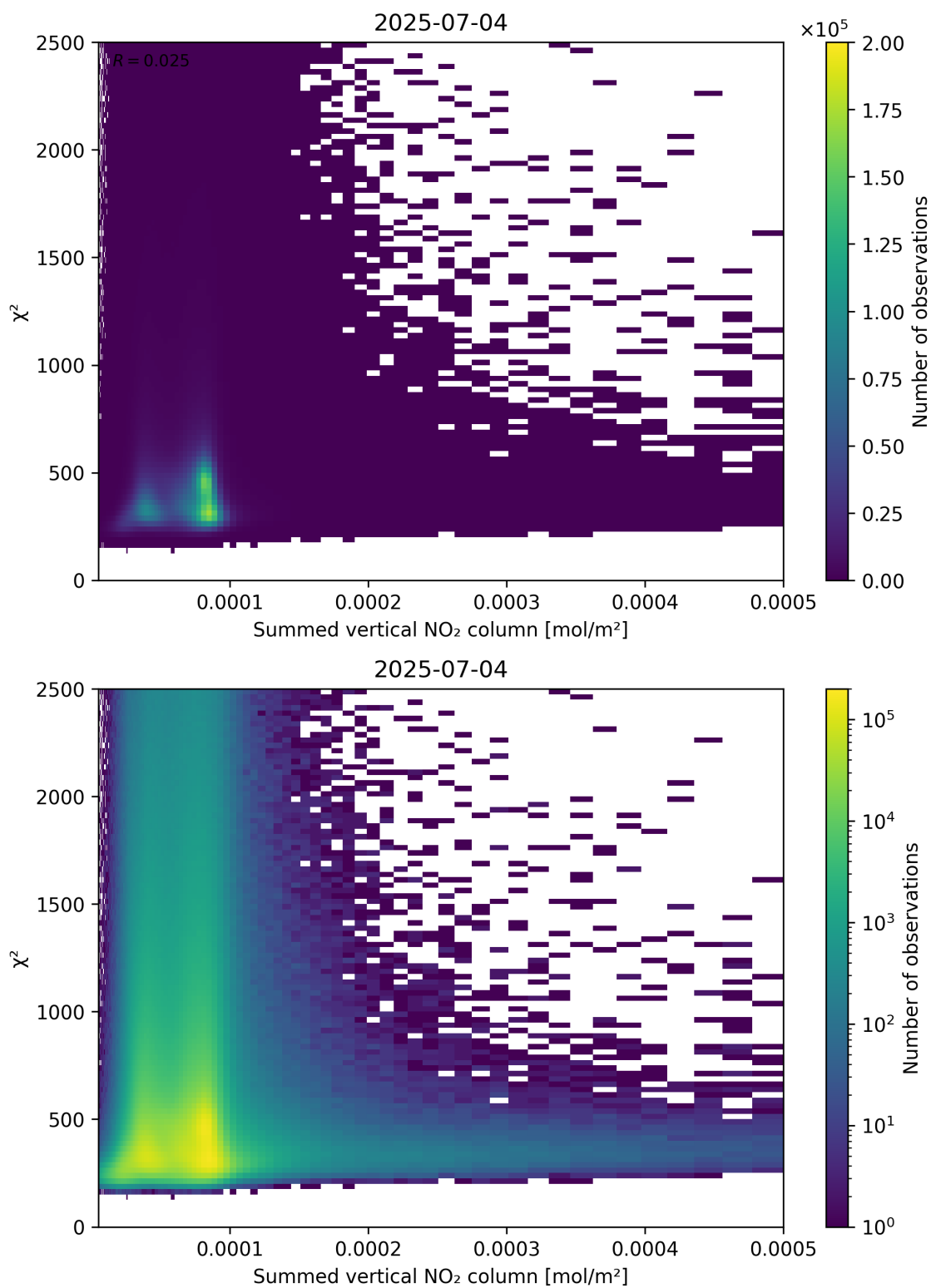
Figure 104: Scatter density plot of “Summed vertical NO 2 column” against “ \chi^2 ” for 2025-07-03 to 2025-07-05.
