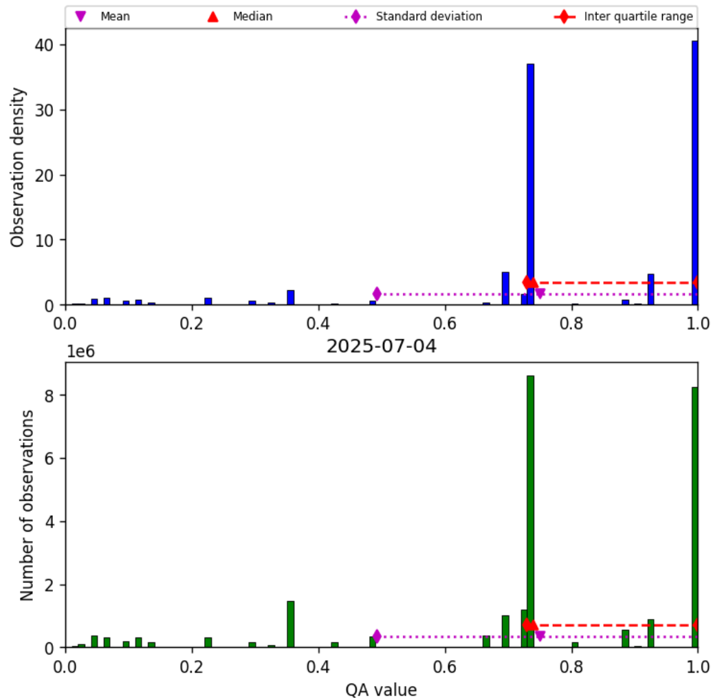
Figure 28: Histogram of “QA value” for 2025-07-03 to 2025-07-05
