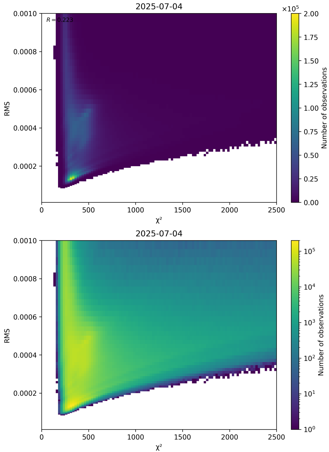
Figure 82: Scatter density plot of “ \chi^2 ” against “RMS” for 2025-07-03 to 2025-07-05.
