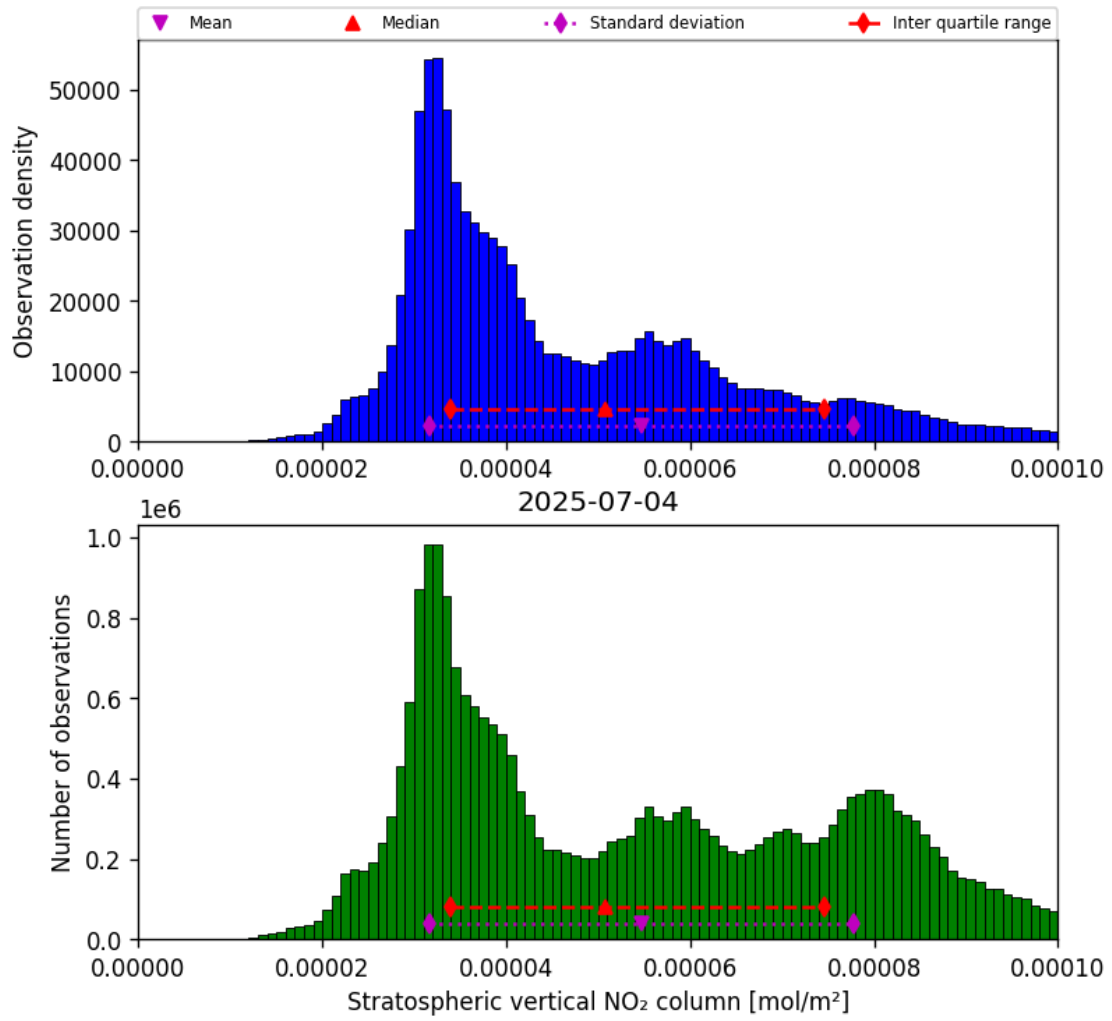
Figure 36: Histogram of “Stratospheric vertical NO 2 column” for 2025-07-03 to 2025-07-05
