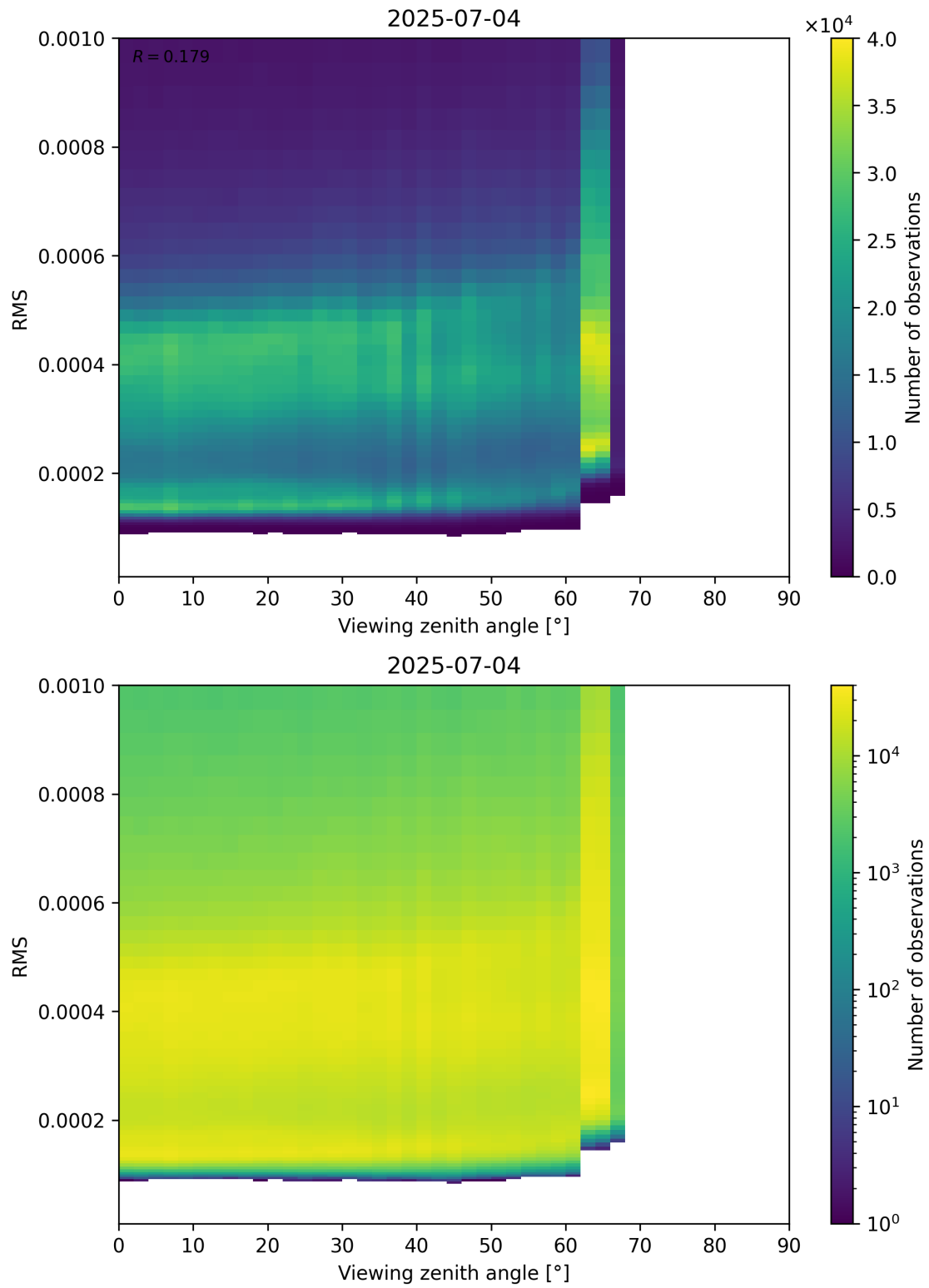
Figure 171: Scatter density plot of “Viewing zenith angle” against “RMS” for 2025-07-03 to 2025-07-05.
