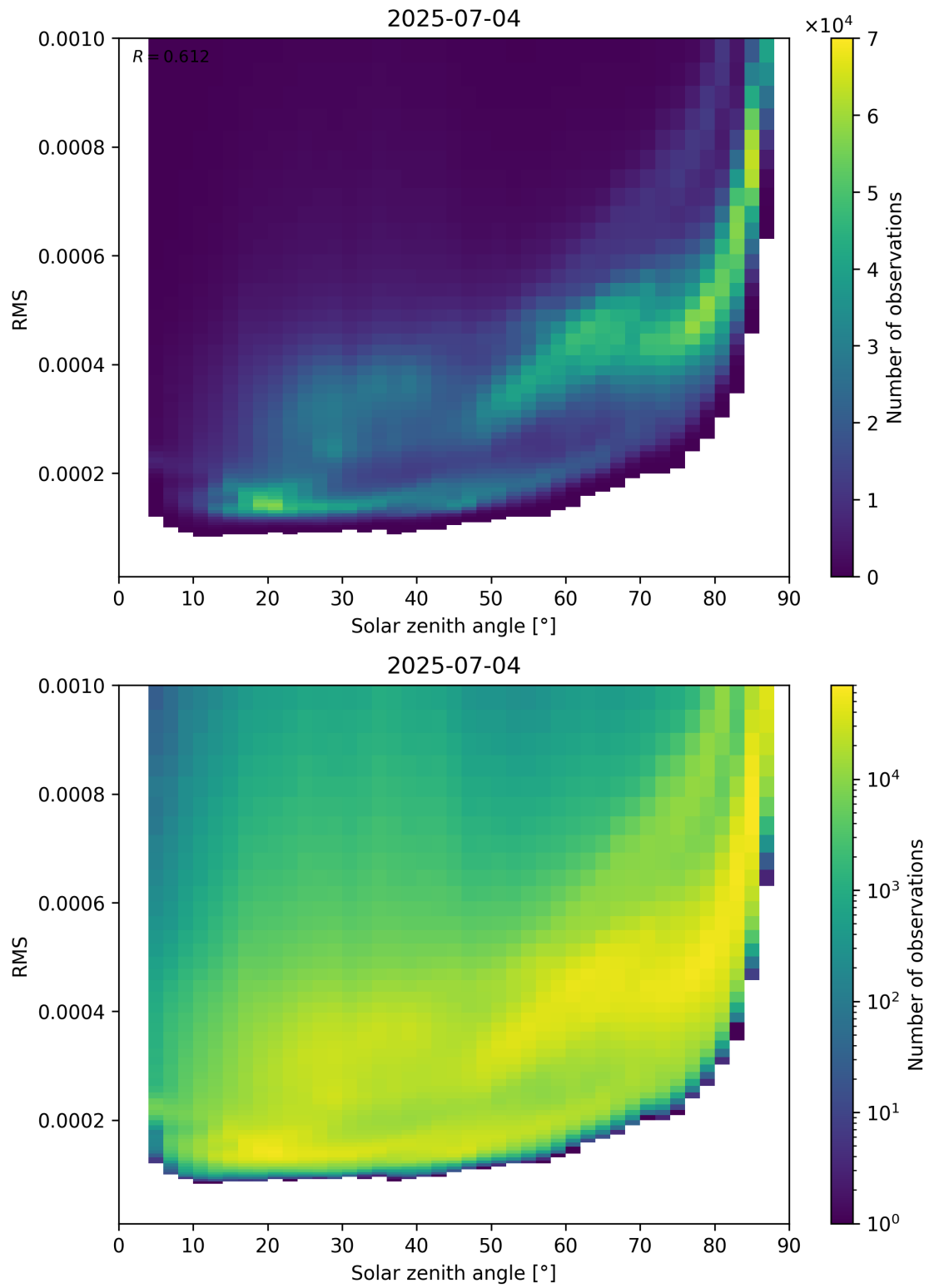
Figure 157: Scatter density plot of “Solar zenith angle” against “RMS” for 2025-07-03 to 2025-07-05.
