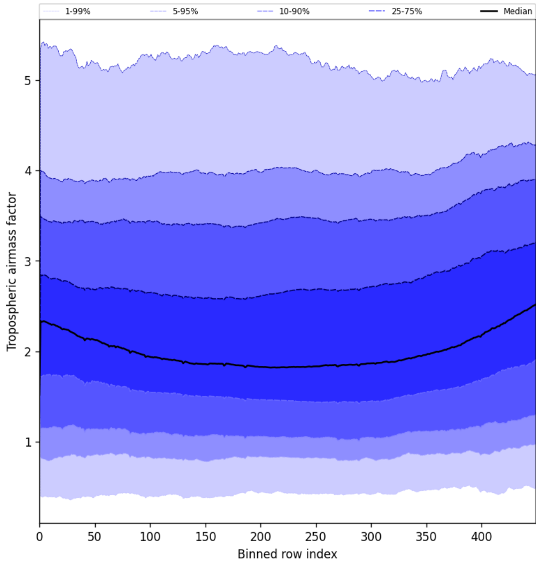
Figure 48: Along track statistics of “Tropospheric airmass factor” for 2025-07-03 to 2025-07-05
