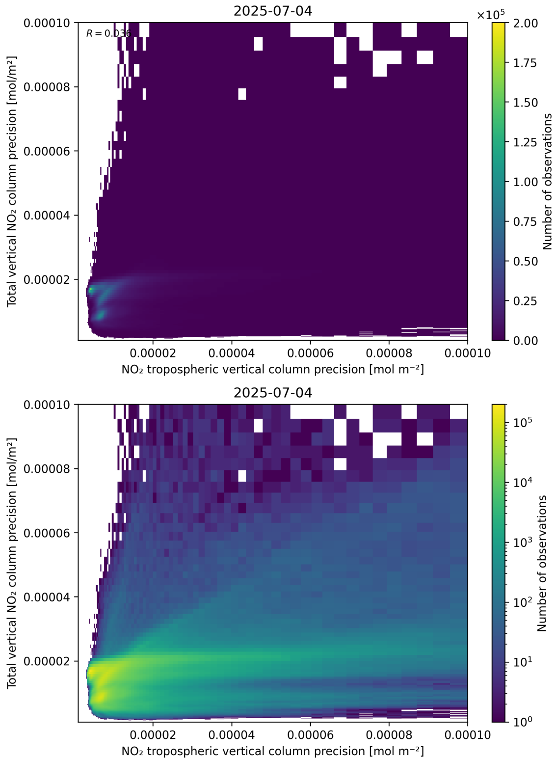
Figure 139: Scatter density plot of “NO 2 tropospheric vertical column precision” against “Total vertical NO 2 column precision” for 2025-07-03 to 2025-07-05.
