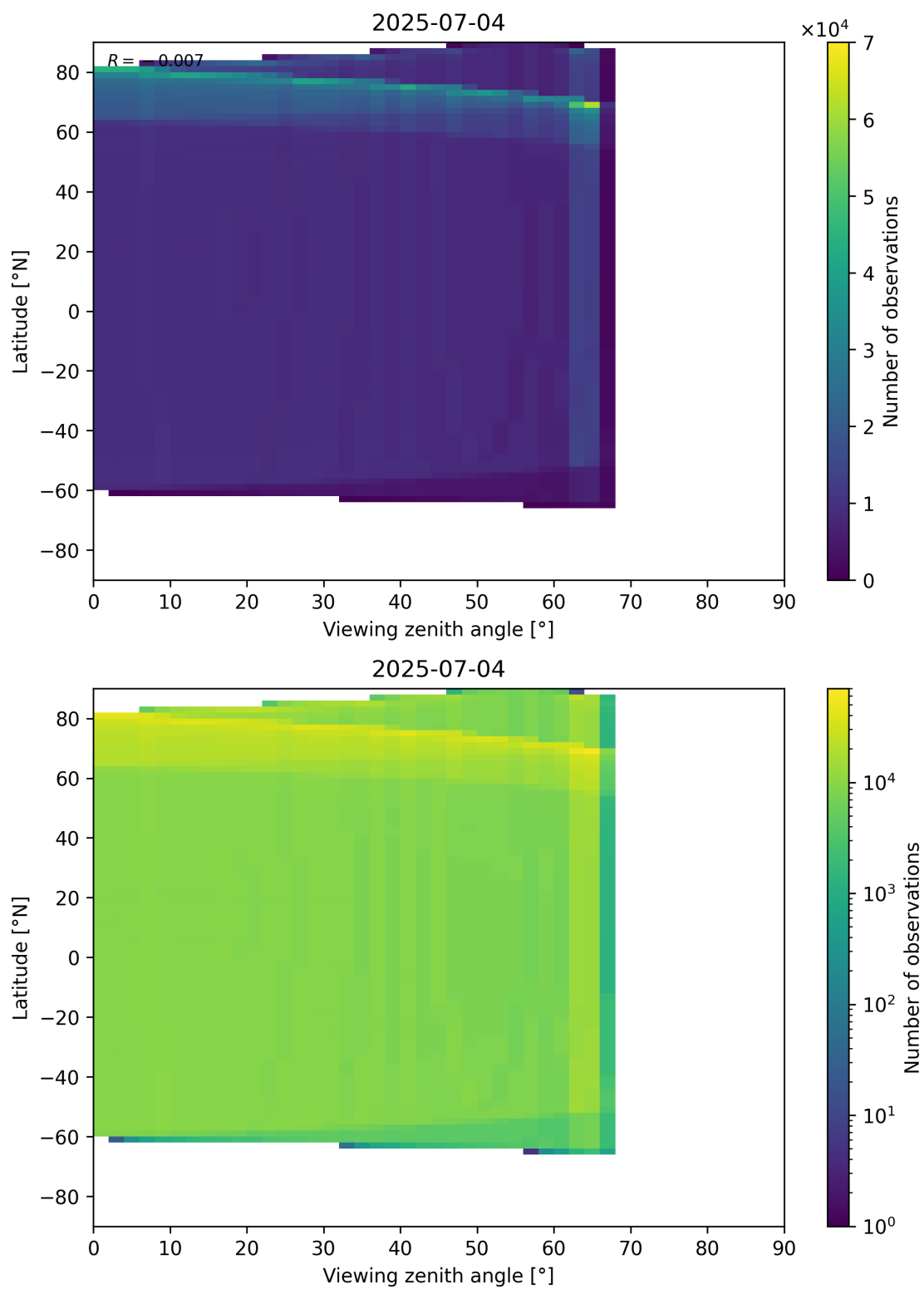
Figure 163: Scatter density plot of “Viewing zenith angle” against “Latitude” for 2025-07-03 to 2025-07-05.
