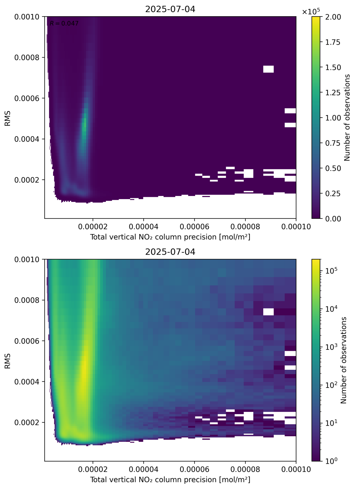
Figure 119: Scatter density plot of “Total vertical NO 2 column precision” against “RMS” for 2025-07-03 to 2025-07-05.
