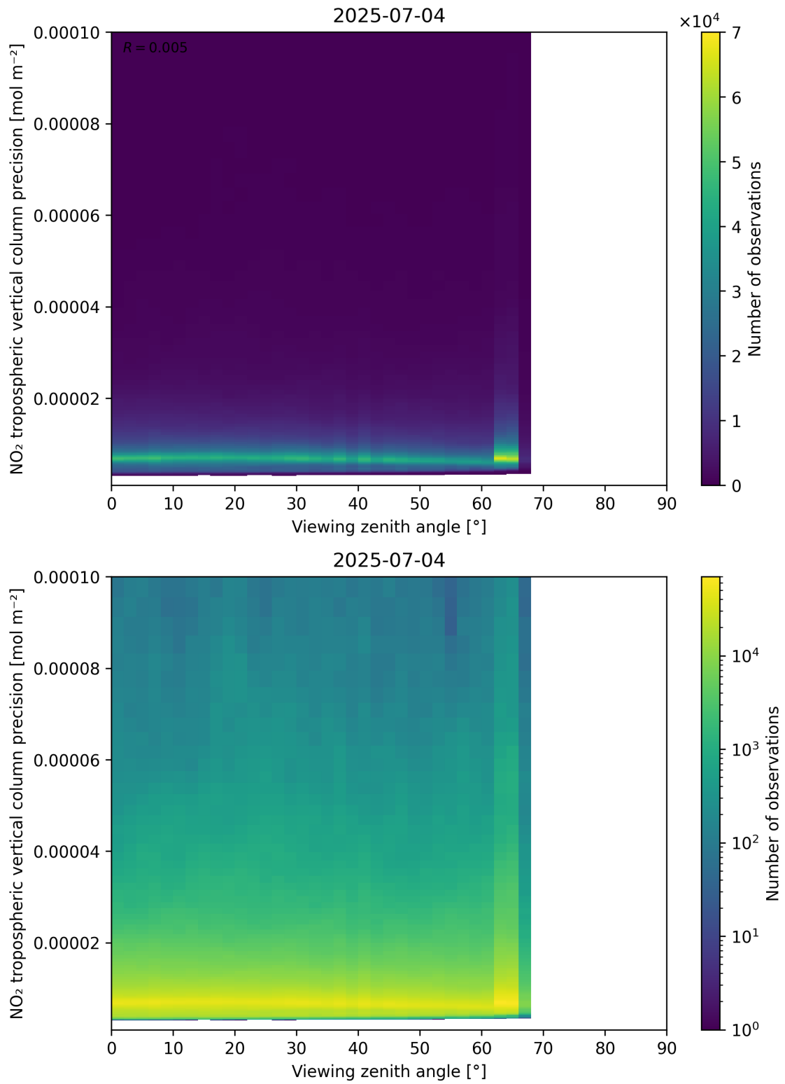
Figure 170: Scatter density plot of “Viewing zenith angle” against “NO 2 tropospheric vertical column precision” for 2025-07-03 to 2025-07-05.
