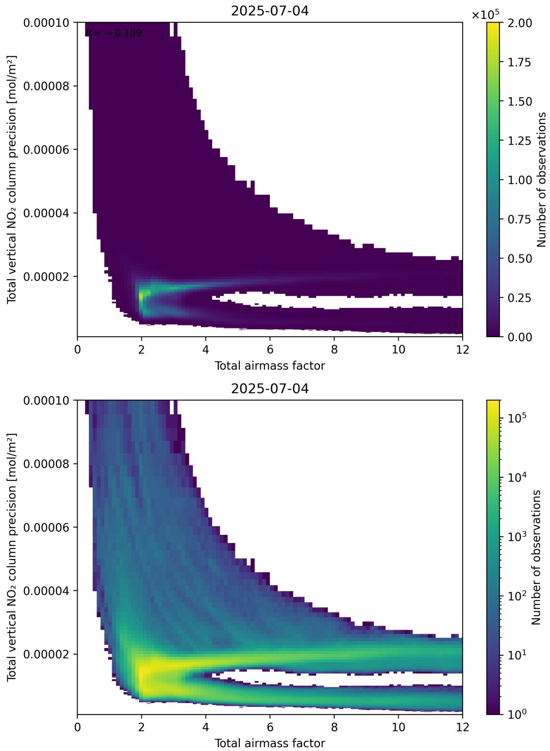
Figure 68: Scatter density plot of “Total airmass factor” against “Total vertical NO 2 column precision” for 2025-07-03 to 2025-07-05.
