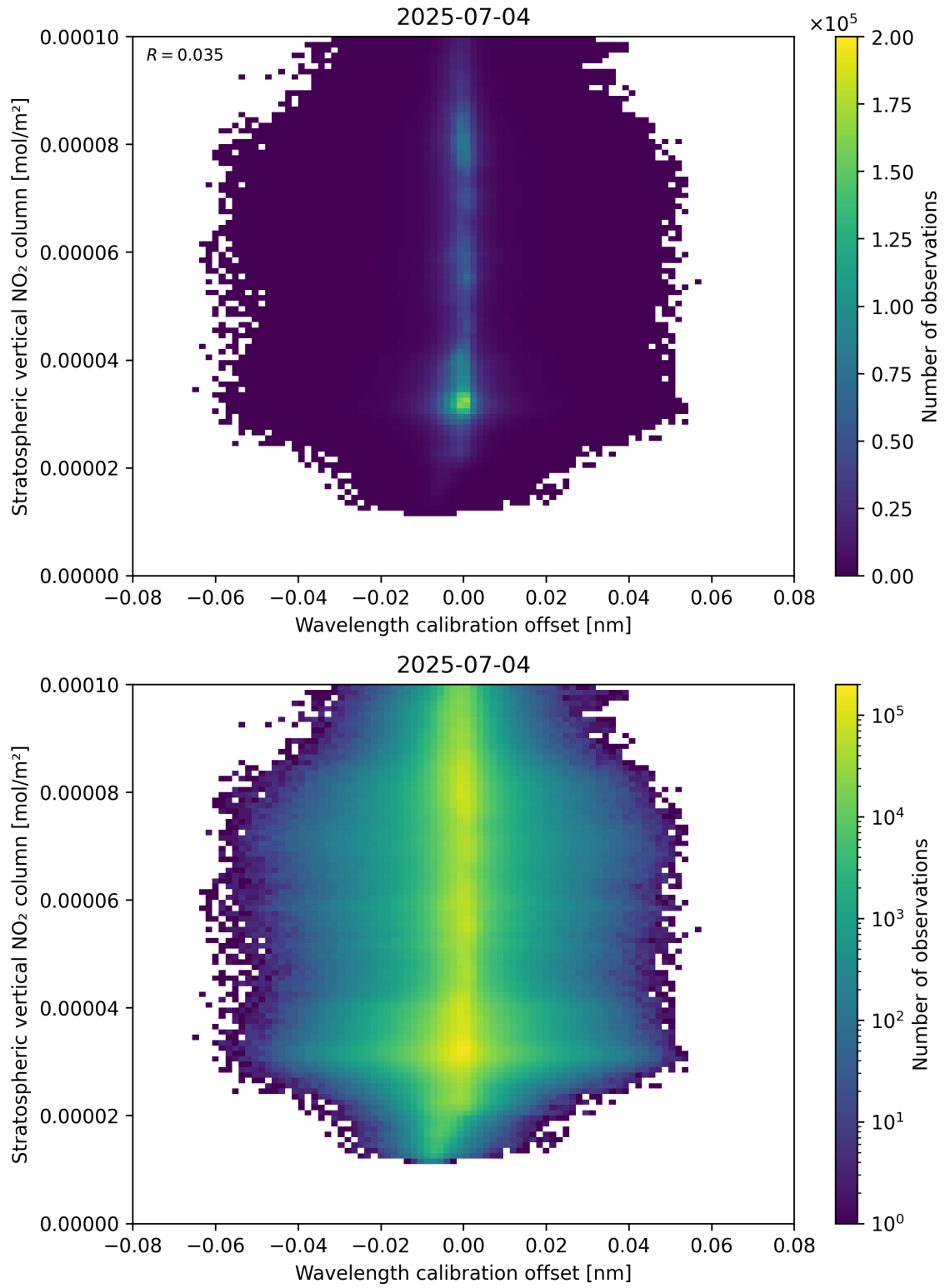
Figure 176: Scatter density plot of “Wavelength calibration offset” against “Stratospheric vertical NO 2 column” for 2025-07-03 to 2025-07-05.
