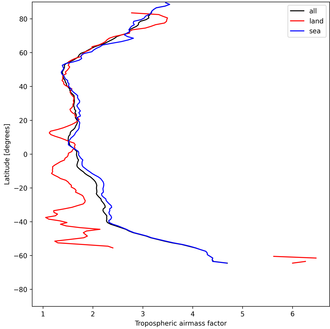
Figure 14: Zonal average of “Tropospheric airmass factor” for 2025-07-03 to 2025-07-05.
