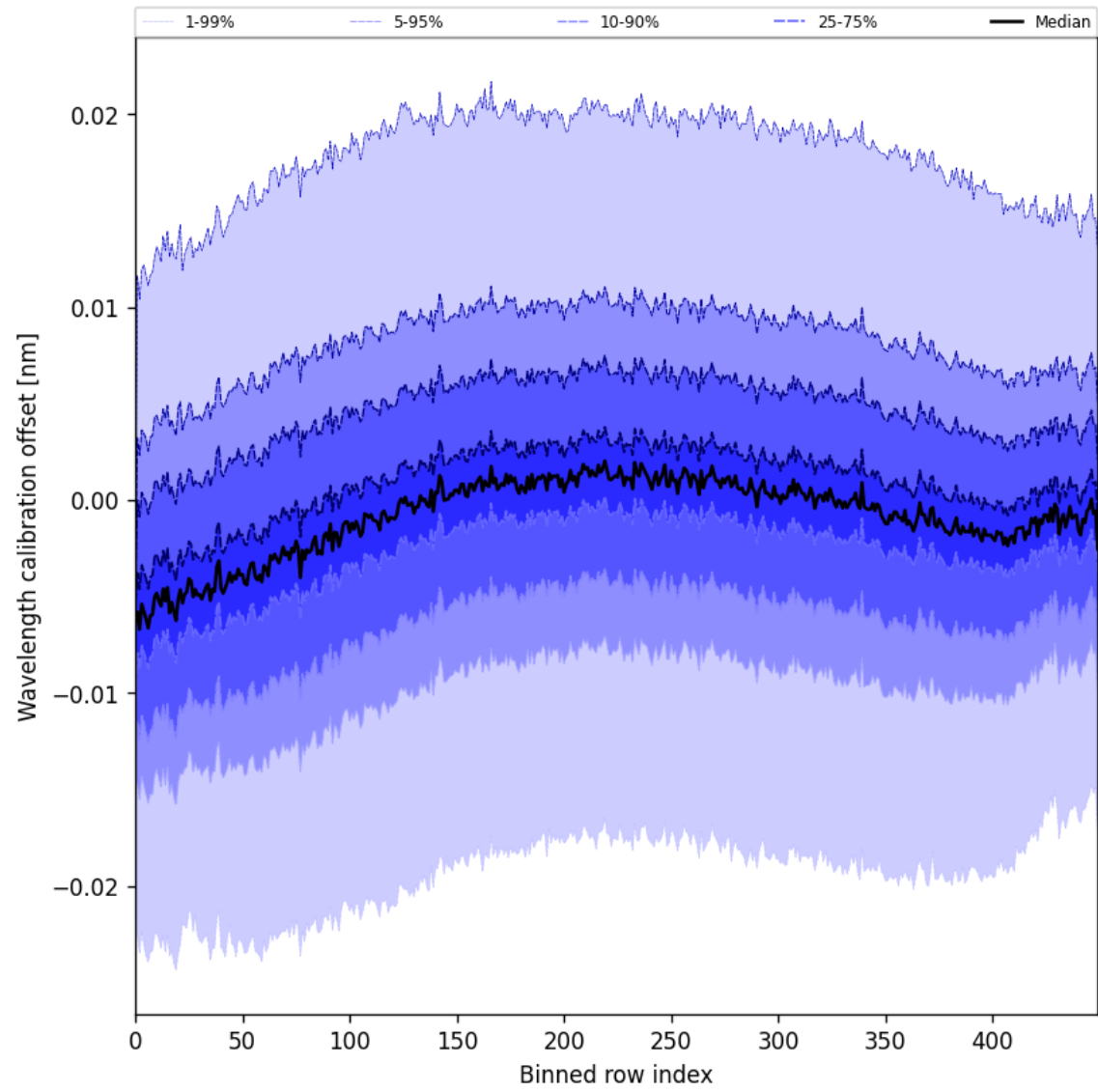
Figure 52: Along track statistics of “Wavelength calibration offset” for 2025-07-03 to 2025-07-05
