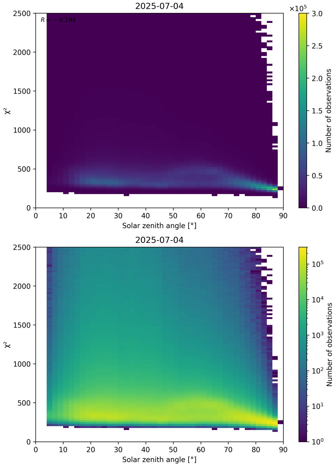
Figure 148: Scatter density plot of “Solar zenith angle” against “ \chi^2 ” for 2025-07-03 to 2025-07-05.
