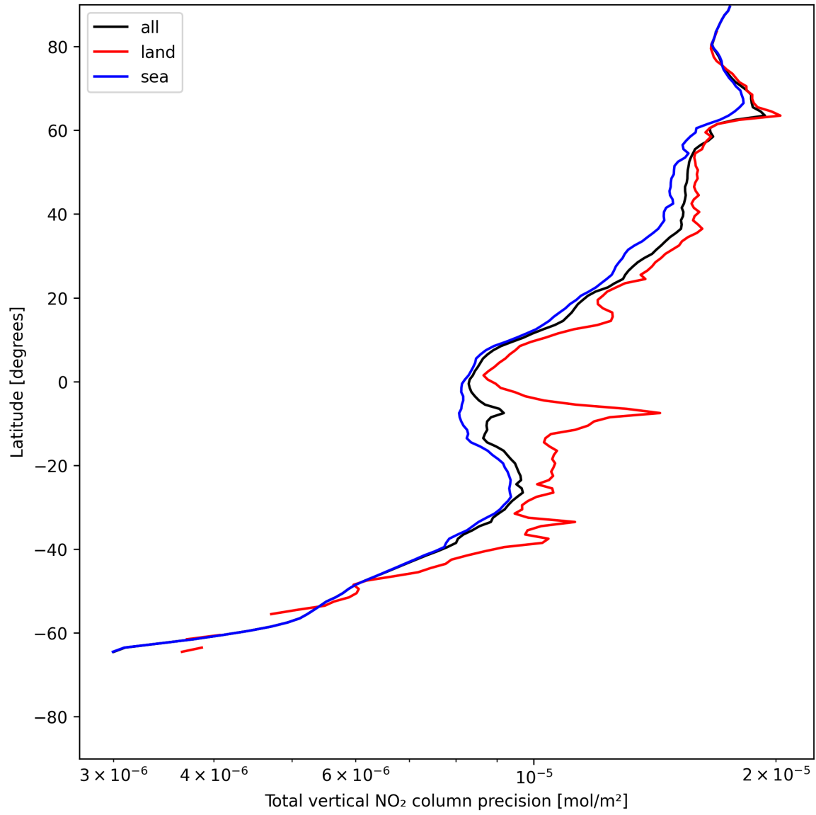
Figure 22: Zonal average of “Total vertical NO 2 column precision” for 2025-07-03 to 2025-07-05.
