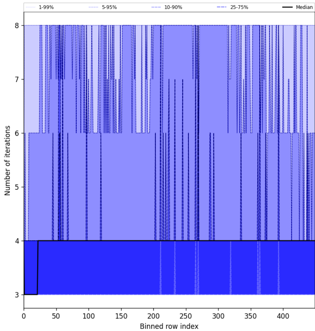
Figure 51: Along track statistics of “Number of iterations” for 2025-07-03 to 2025-07-05
