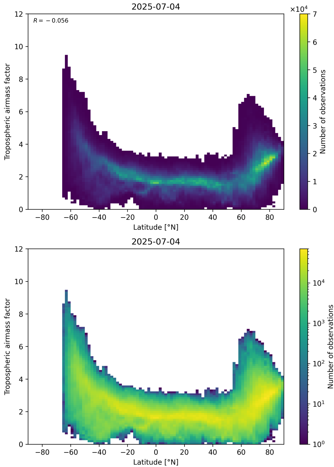
Figure 85: Scatter density plot of “Latitude” against “Tropospheric air mass factor” for 2025-07-03 to 2025-07-05.
