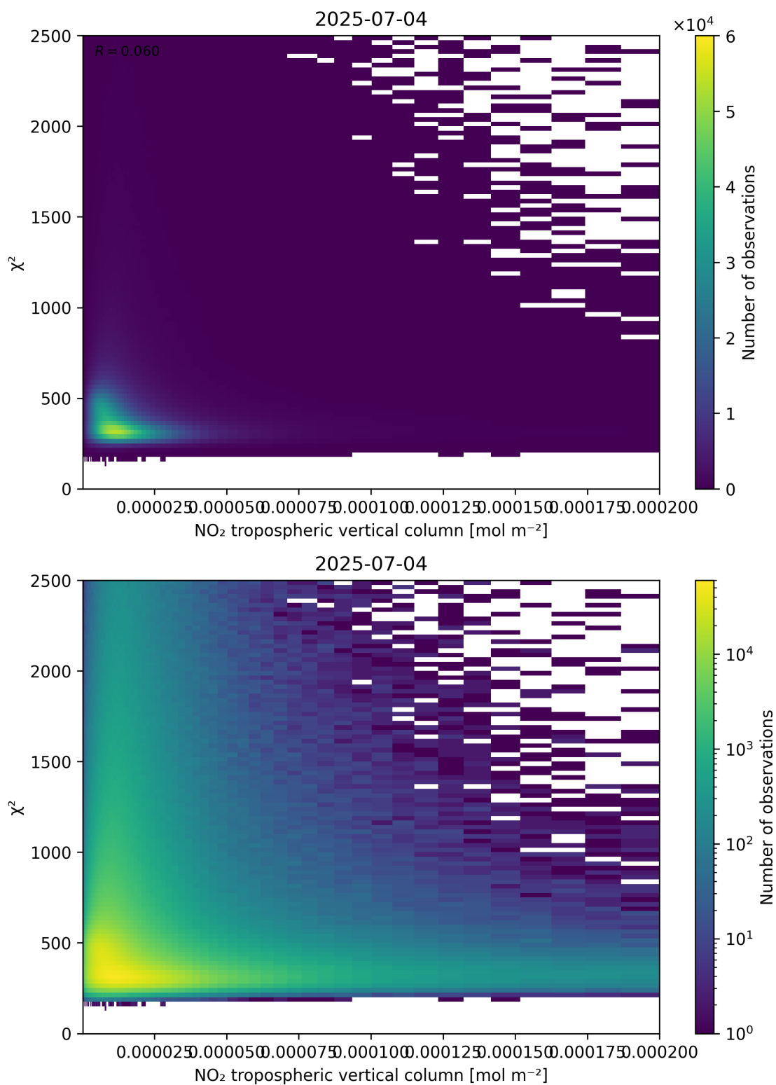
Figure 124: Scatter density plot of “NO 2 tropospheric vertical column” against “ \chi^2 ” for 2025-07-03 to 2025-07-05.
