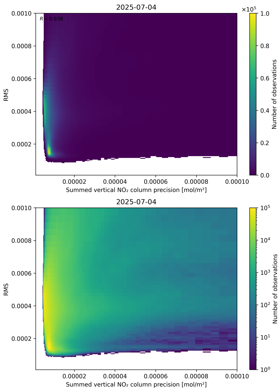
Figure 108: Scatter density plot of “Summed vertical NO 2 column precision” against “RMS” for 2025-07-03 to 2025-07-05.
