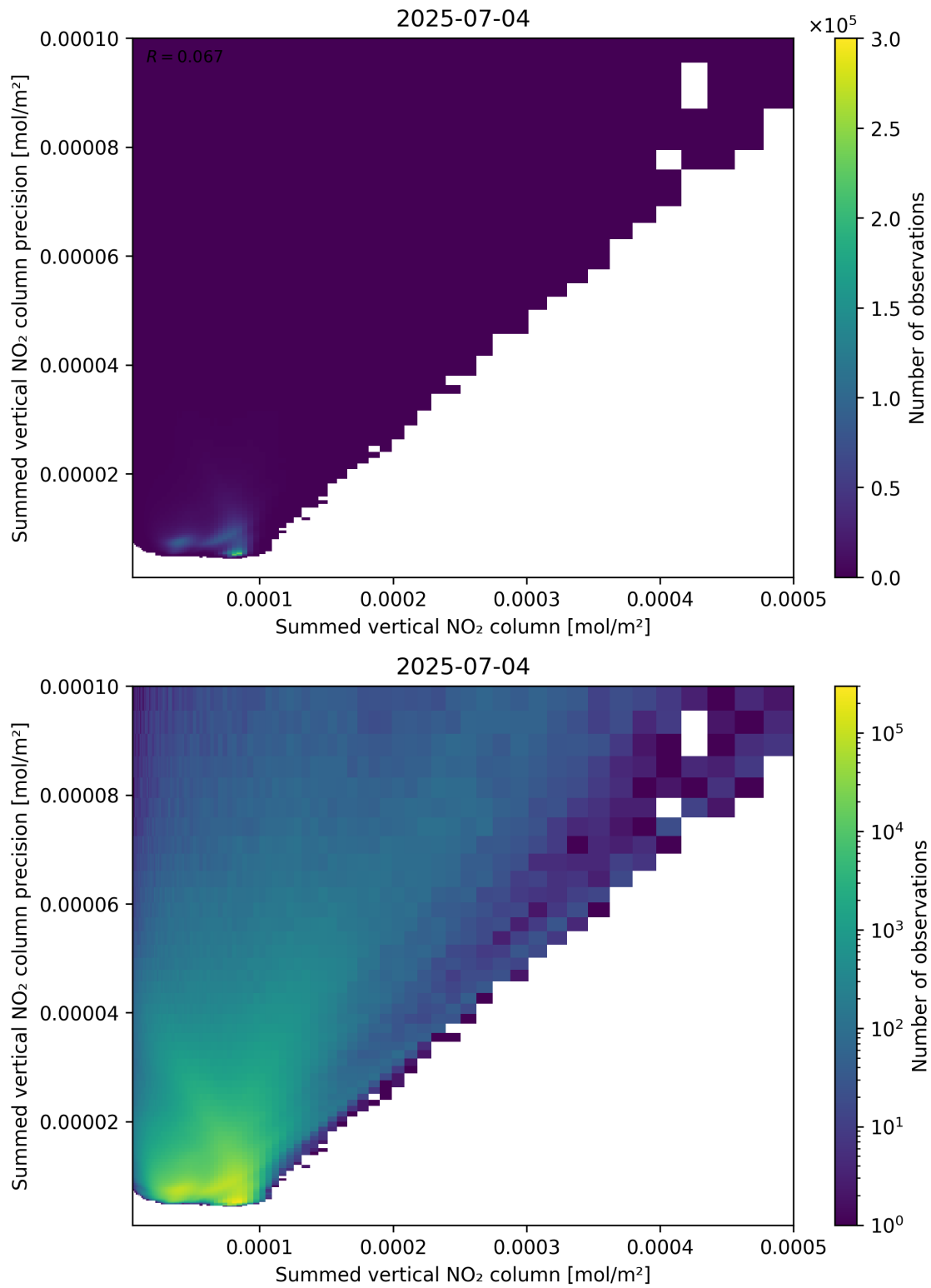
Figure 105: Scatter density plot of “Summed vertical NO 2 column” against “Summed vertical NO 2 column precision” for 2025-07-03 to 2025-07-05.
