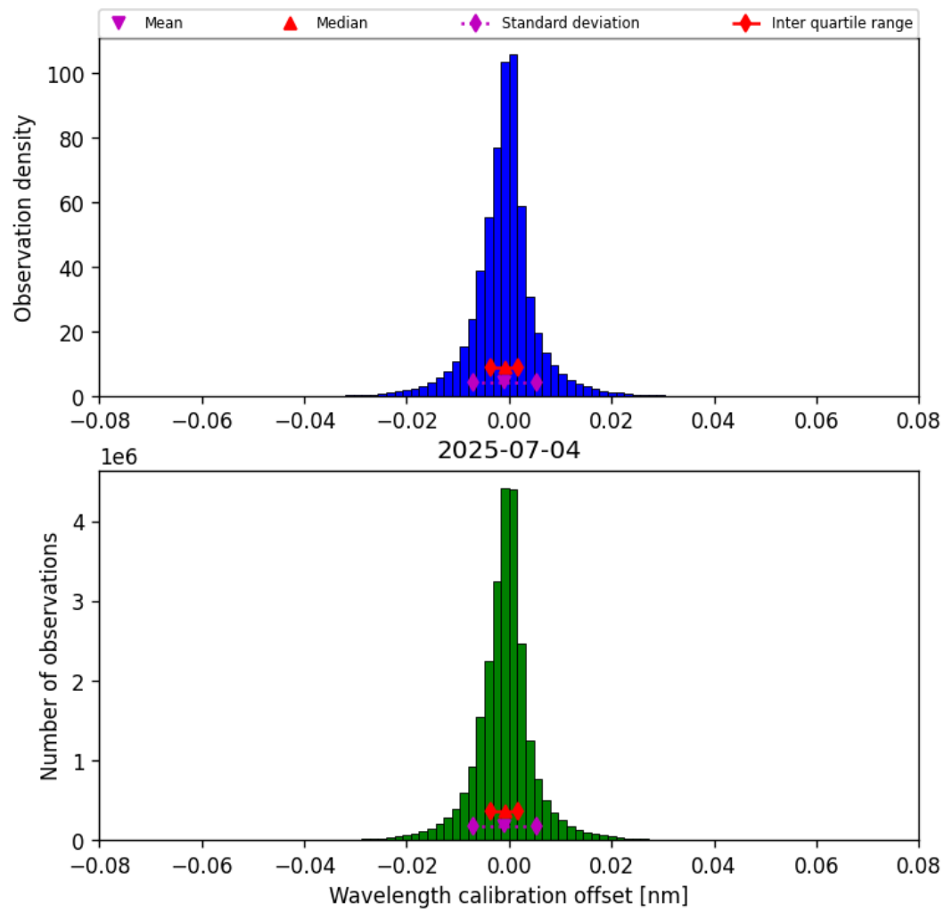
Figure 35: Histogram of “Wavelength calibration offset” for 2025-07-03 to 2025-07-05
