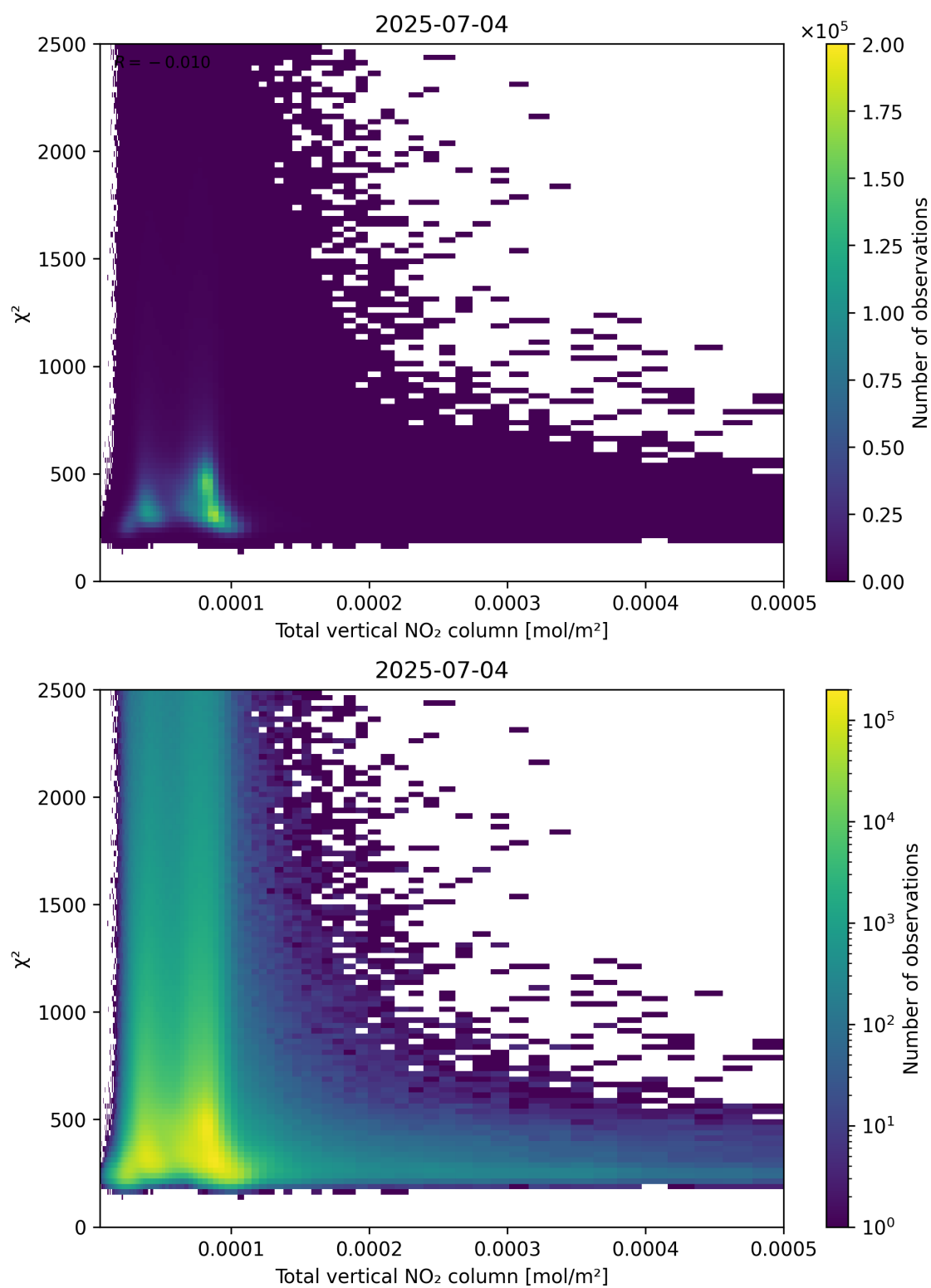
Figure 111: Scatter density plot of “Total vertical NO 2 column” against “ \chi^2 ” for 2025-07-03 to 2025-07-05.
