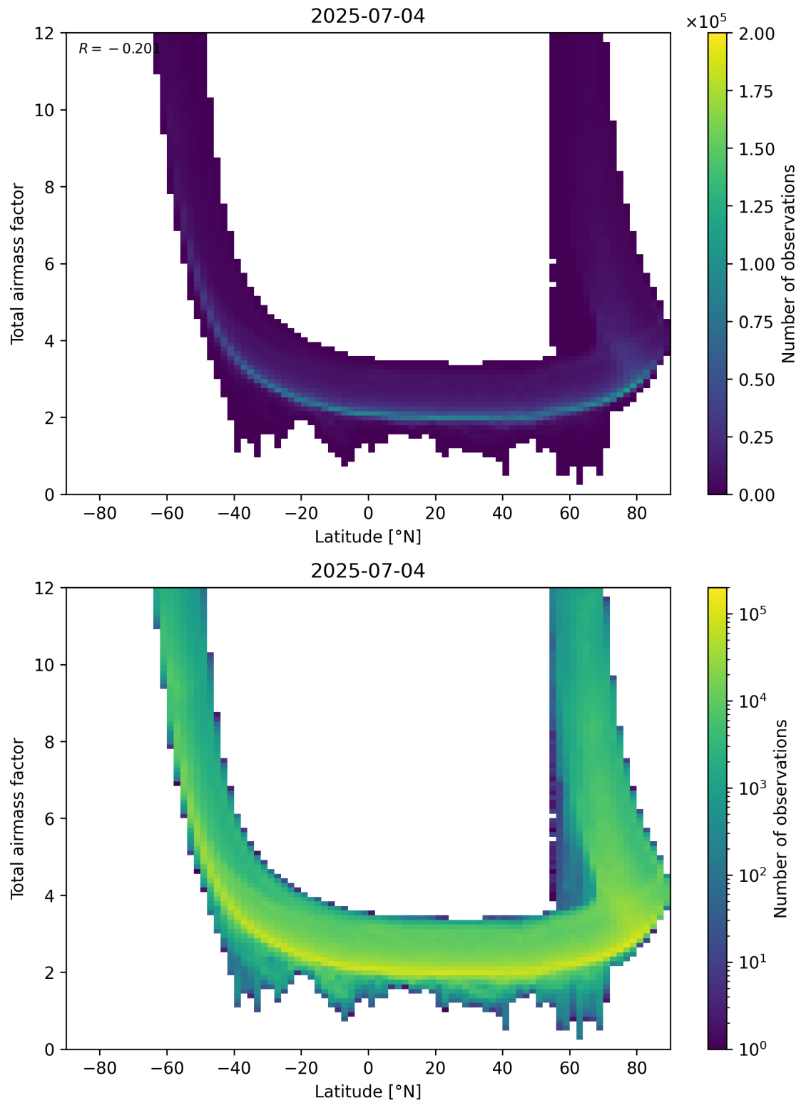
Figure 84: Scatter density plot of “Latitude” against “Total airmass factor” for 2025-07-03 to 2025-07-05.
