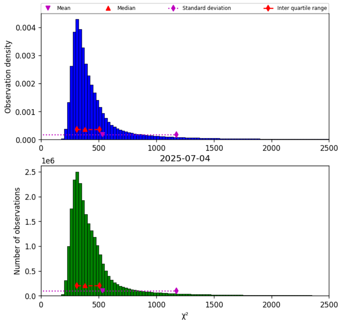
Figure 42: Histogram of “ \chi^2 ” for 2025-07-03 to 2025-07-05
