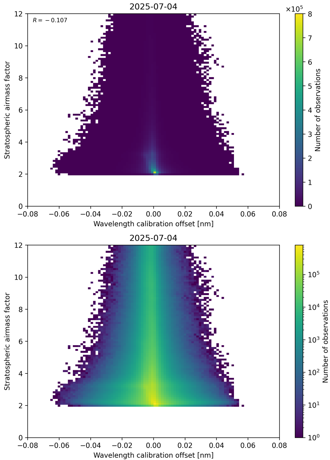
Figure 174: Scatter density plot of “Wavelength calibration offset” against “Stratospheric airmass factor” for 2025-07-03 to 2025-07-05.
