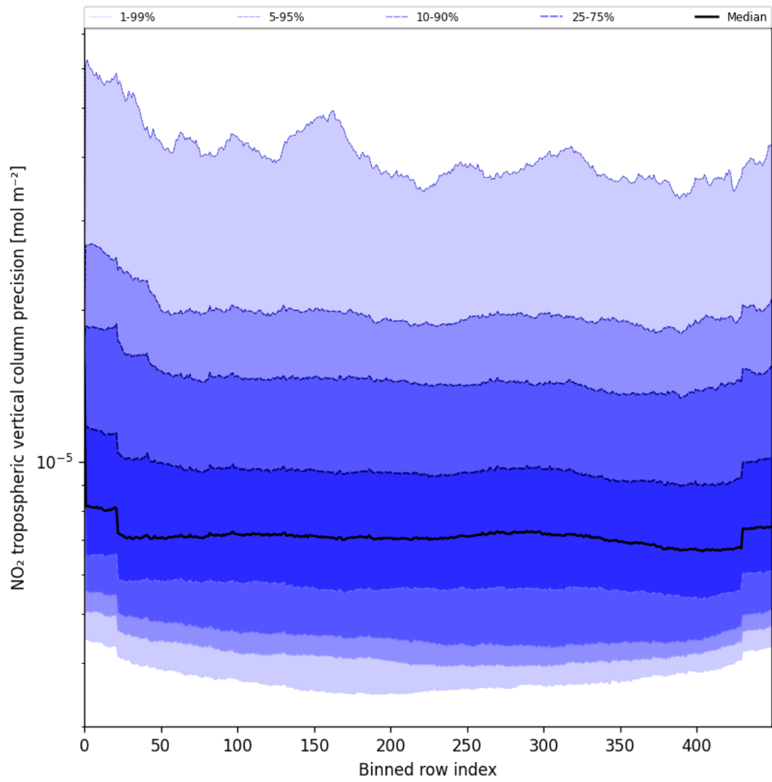
Figure 47: Along track statistics of “NO 2 tropospheric vertical column precision” for 2025-07-03 to 2025-07-05
