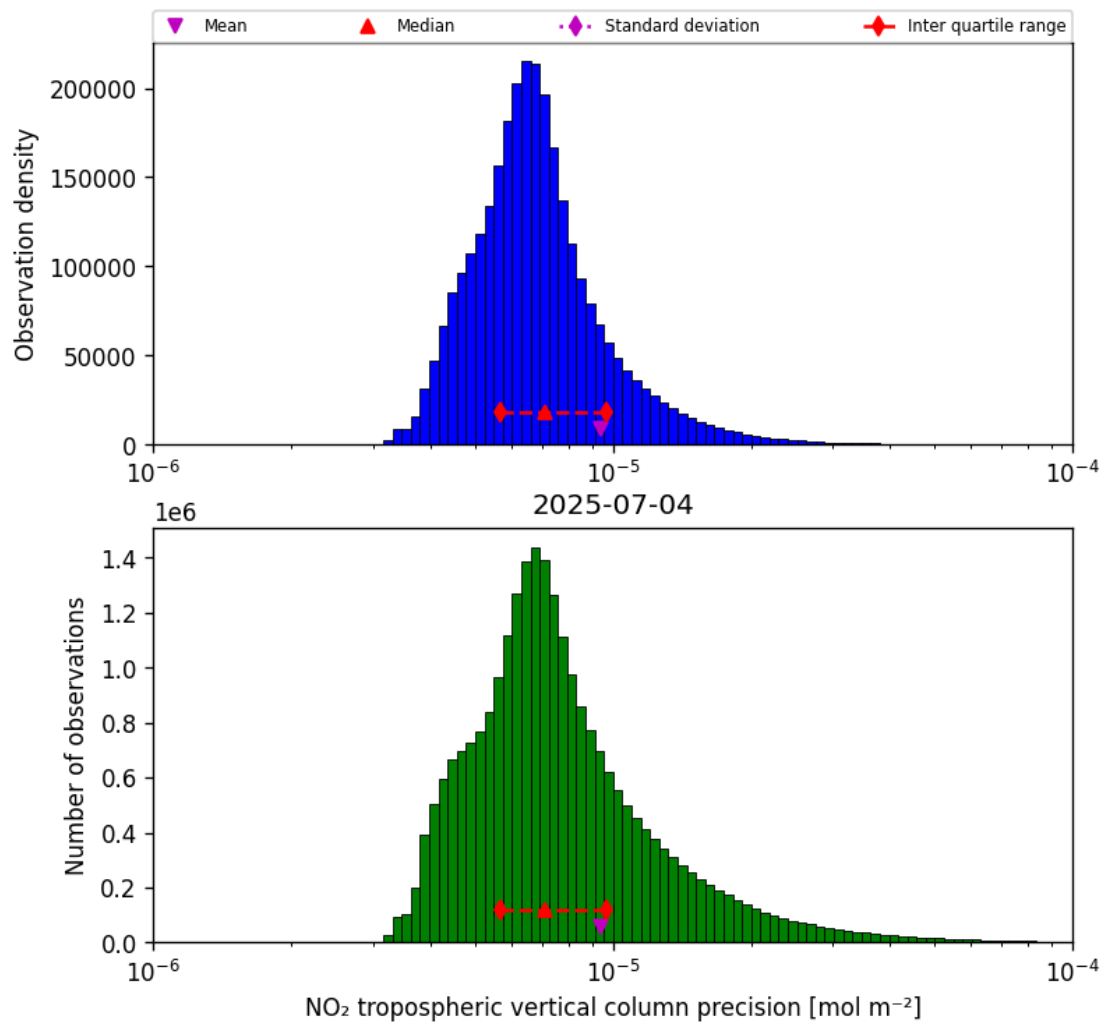
Figure 30: Histogram of “NO 2 tropospheric vertical column precision” for 2025-07-03 to 2025-07-05
