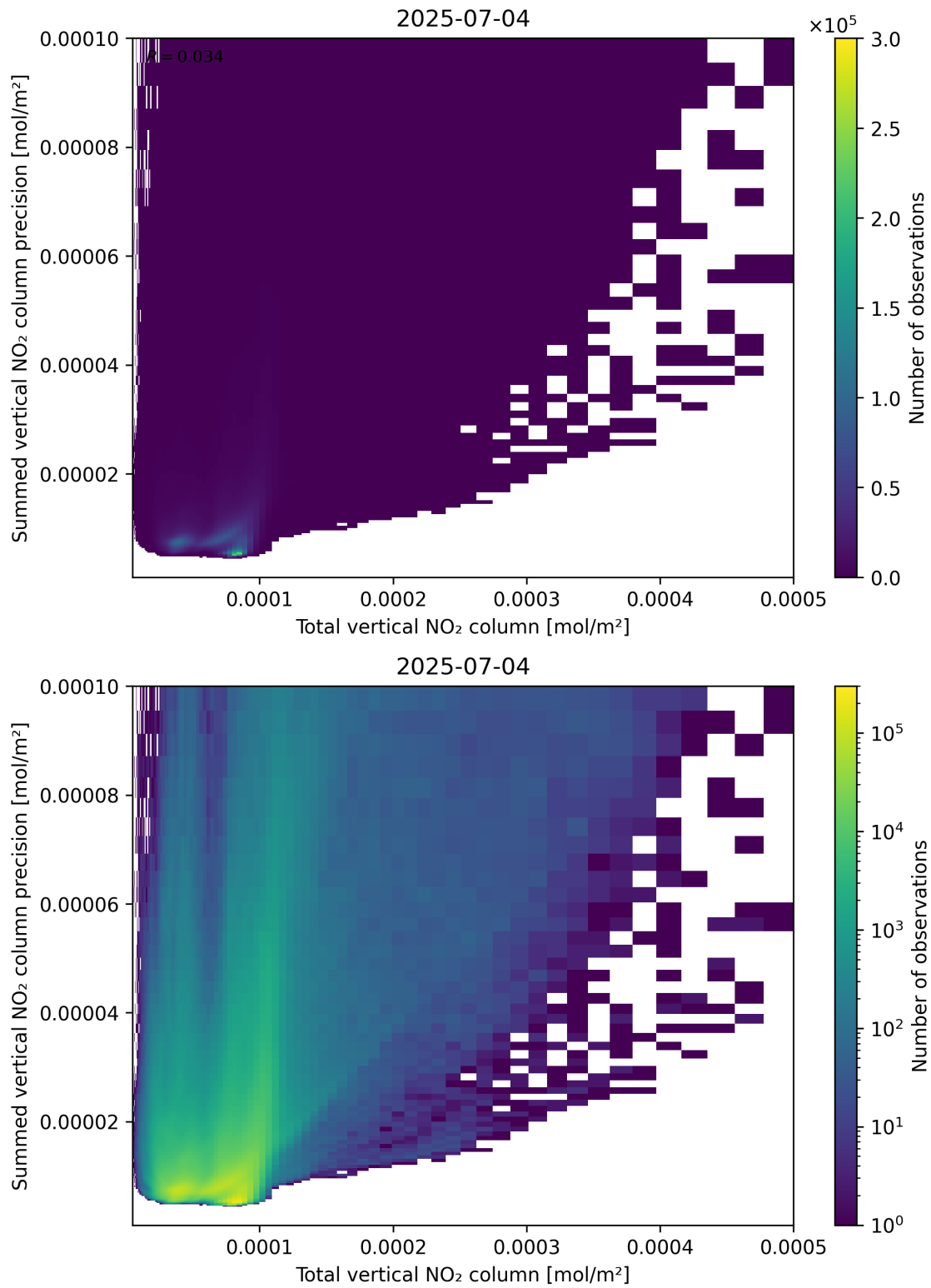
Figure 113: Scatter density plot of “Total vertical NO 2 column” against “Summed vertical NO 2 column precision” for 2025-07-03 to 2025-07-05.
