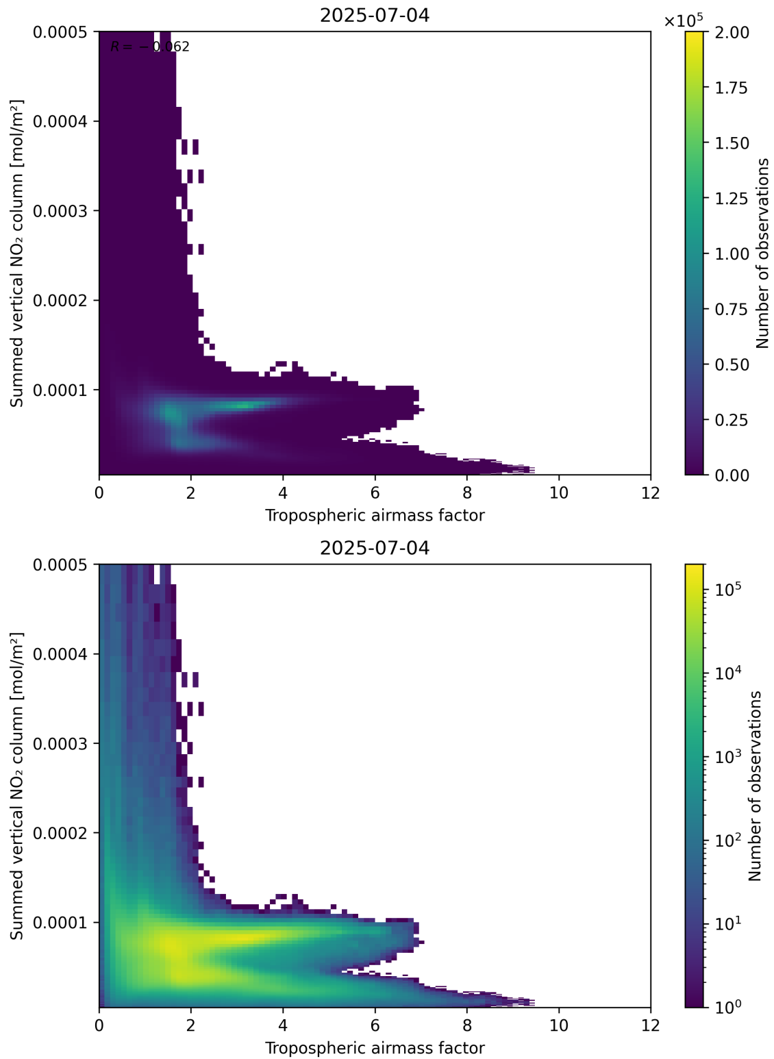
Figure 75: Scatter density plot of “Tropospheric air mass factor” against “Summed vertical NO 2 column” for 2025-07-03 to 2025-07-05.
