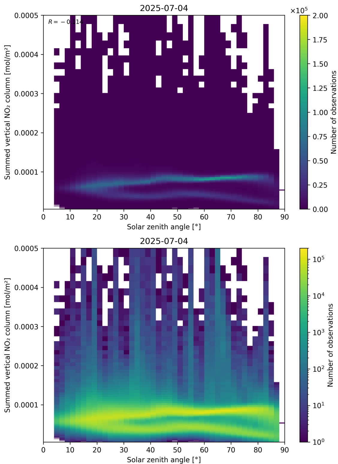
Figure 151: Scatter density plot of “Solar zenith angle” against “Summed vertical NO 2 column” for 2025-07-03 to 2025-07-05.
