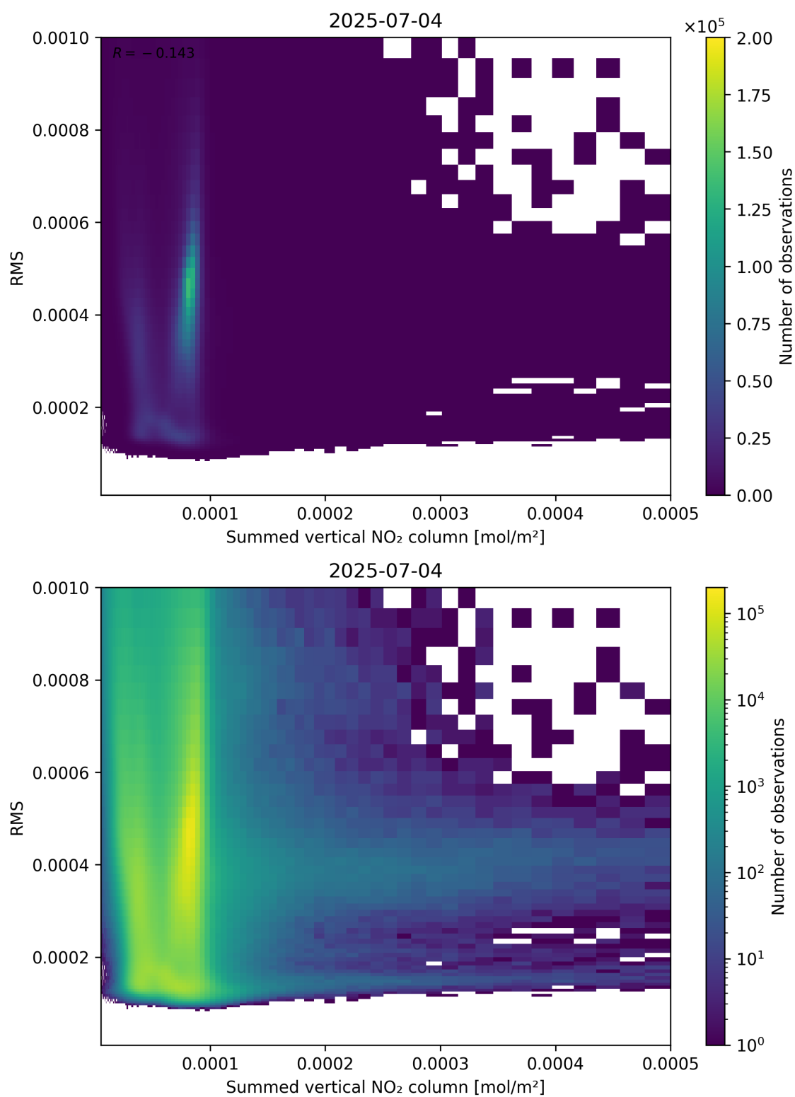
Figure 109: Scatter density plot of “Summed vertical NO 2 column” against “RMS” for 2025-07-03 to 2025-07-05.
