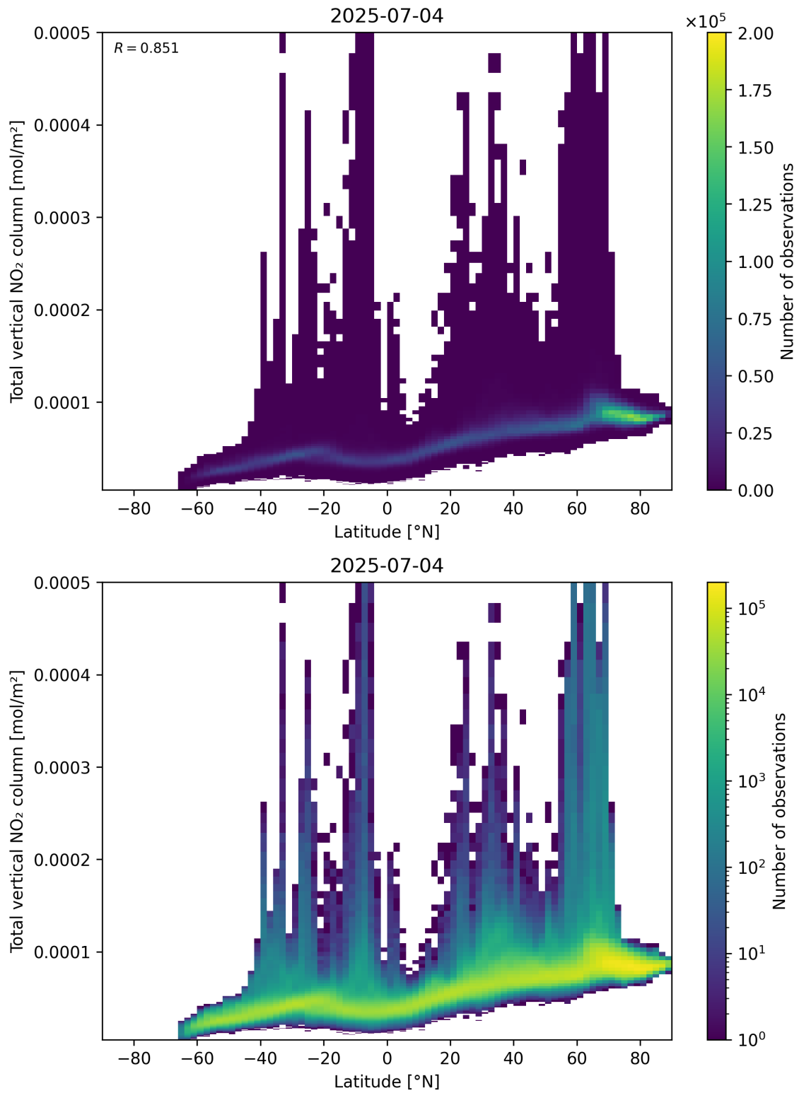
Figure 90: Scatter density plot of “Latitude” against “Total vertical NO 2 column” for 2025-07-03 to 2025-07-05.
