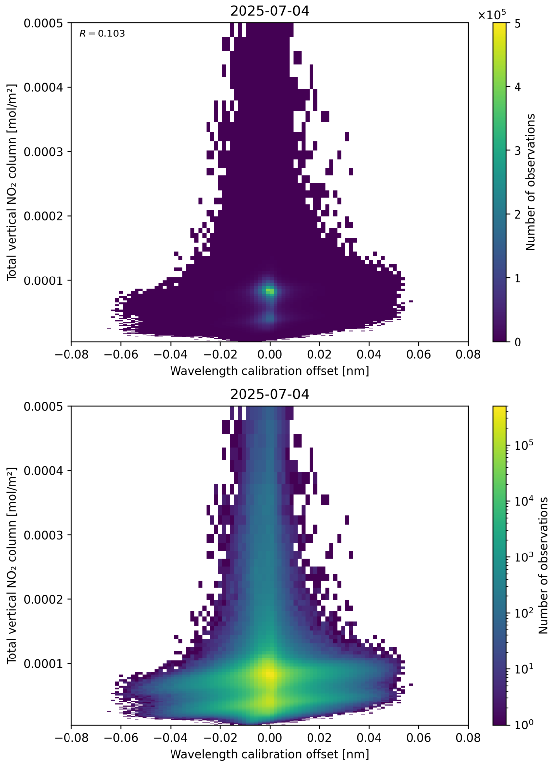
Figure 179: Scatter density plot of “Wavelength calibration offset” against “Total vertical NO 2 column” for 2025-07-03 to 2025-07-05.
