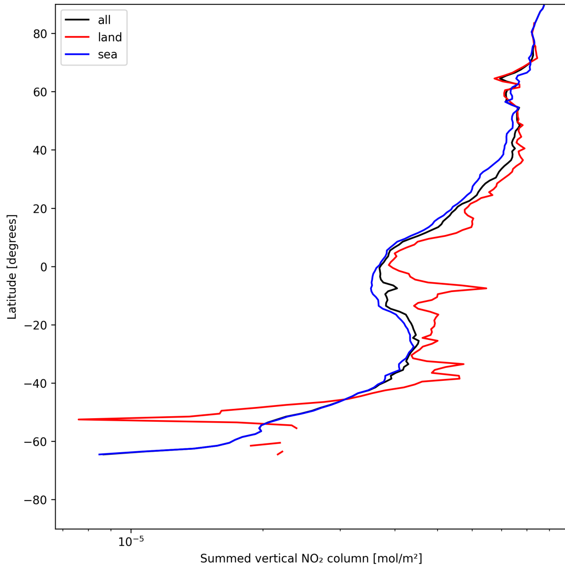
Figure 23: Zonal average of “Summed vertical NO 2 column” for 2025-07-03 to 2025-07-05.
