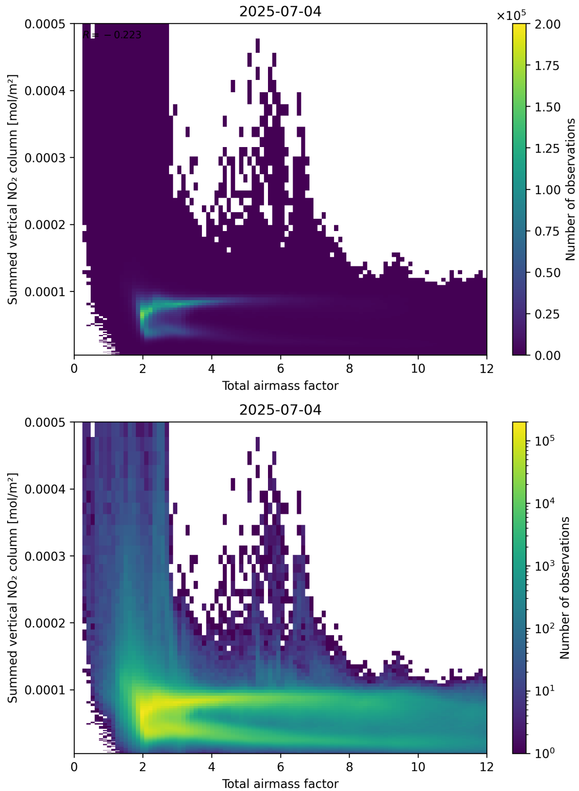
Figure 65: Scatter density plot of “Total airmass factor” against “Summed vertical NO 2 column” for 2025-07-03 to 2025-07-05.
