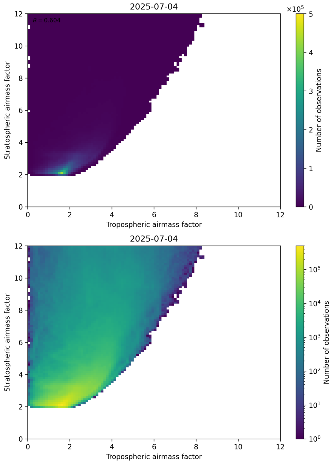
Figure 71: Scatter density plot of “Tropospheric airmass factor” against “Stratospheric airmass factor” for 2025-07-03 to 2025-07-05.
