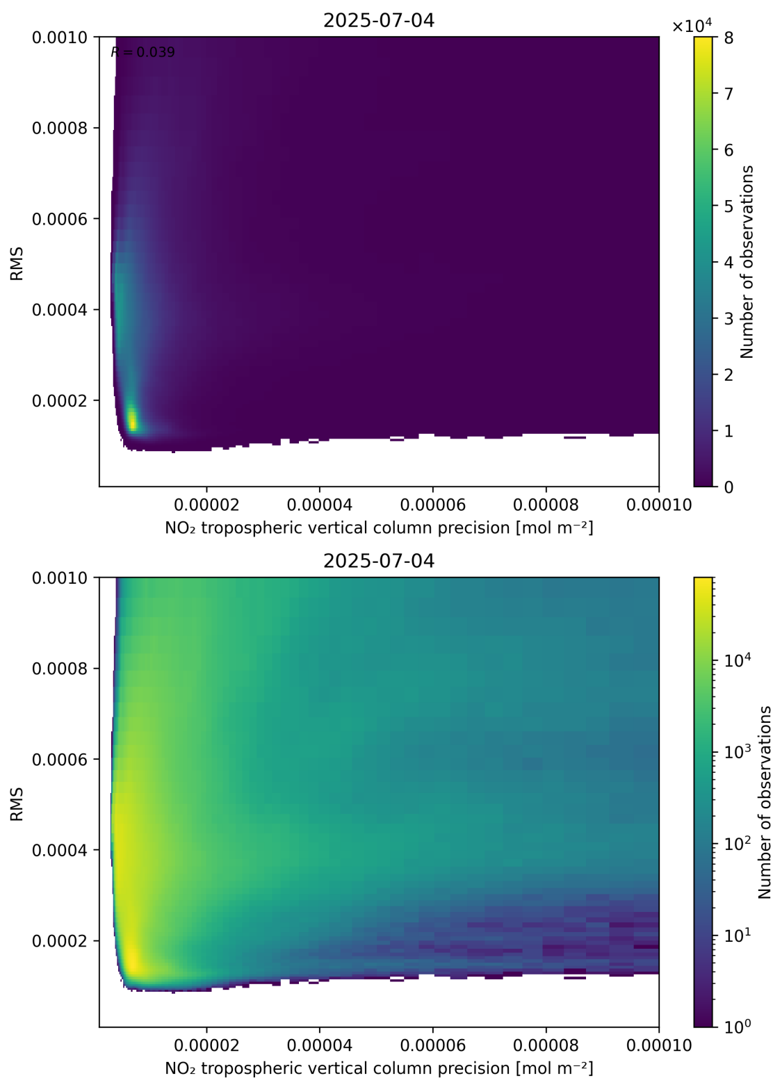
Figure 140: Scatter density plot of “NO 2 tropospheric vertical column precision” against “RMS” for 2025-07-03 to 2025-07-05.
