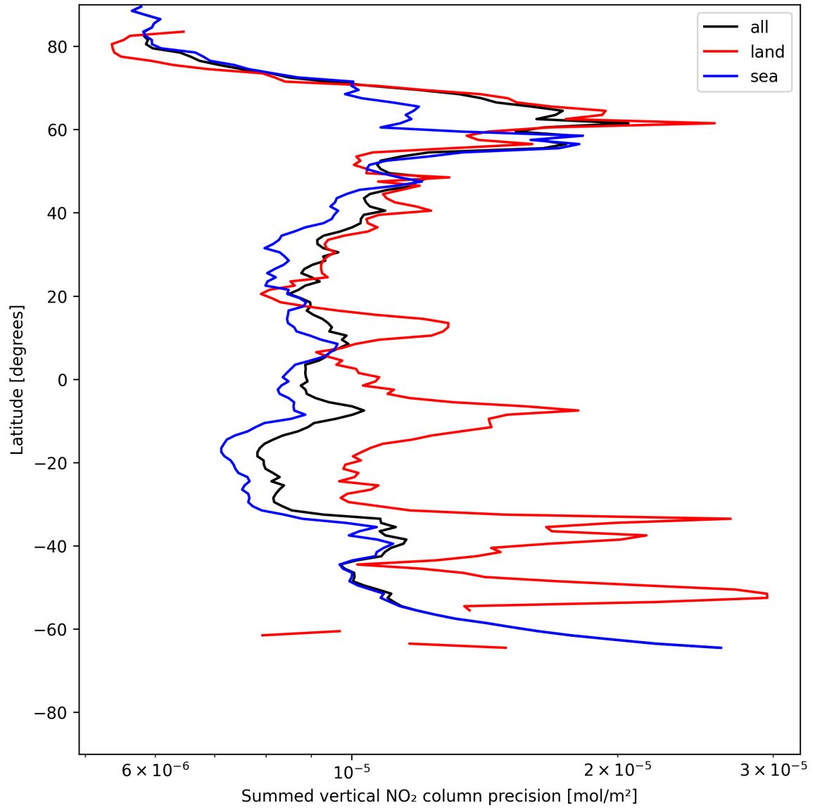
Figure 24: Zonal average of “Summed vertical NO 2 column precision” for 2025-07-03 to 2025-07-05.
