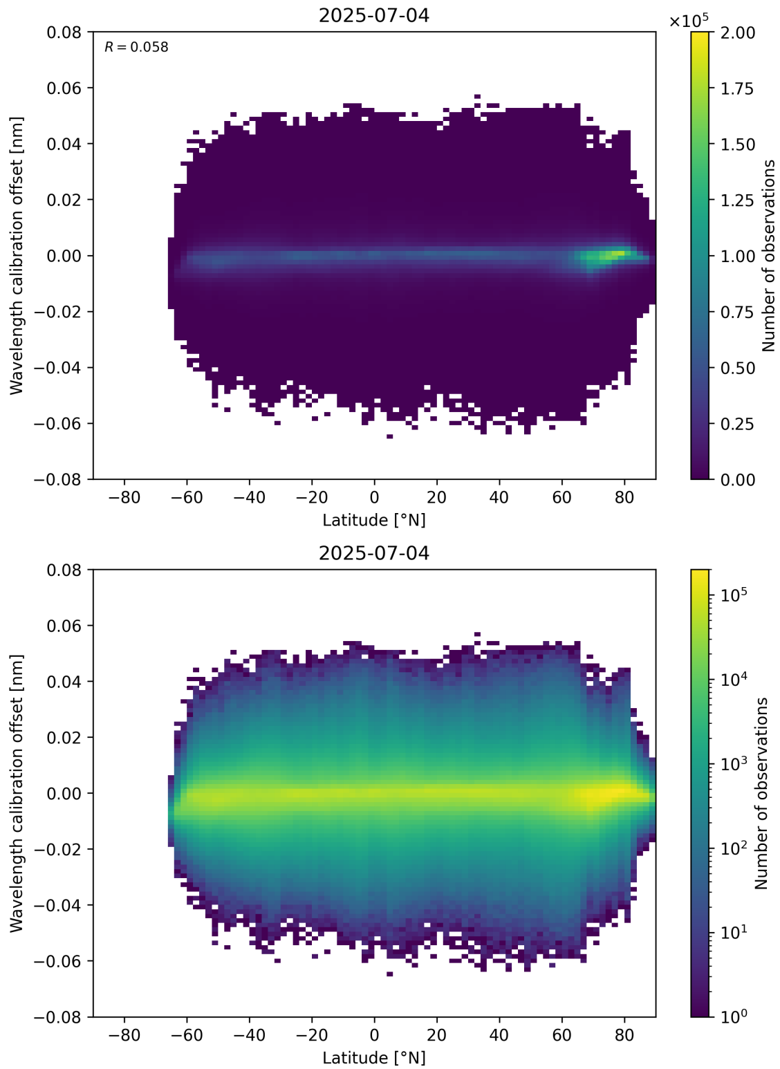
Figure 95: Scatter density plot of “Latitude” against “Wavelength calibration offset” for 2025-07-03 to 2025-07-05.
