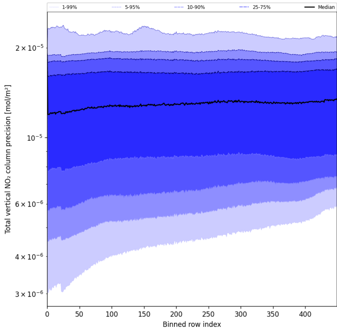
Figure 56: Along track statistics of “Total vertical NO 2 column precision” for 2025-07-03 to 2025-07-05
