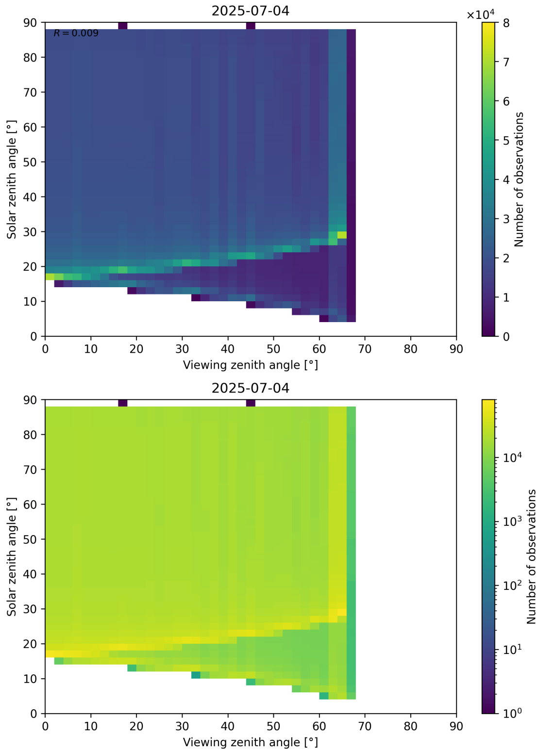
Figure 172: Scatter density plot of “Viewing zenith angle” against “Solar zenith angle” for 2025-07-03 to 2025-07-05.
