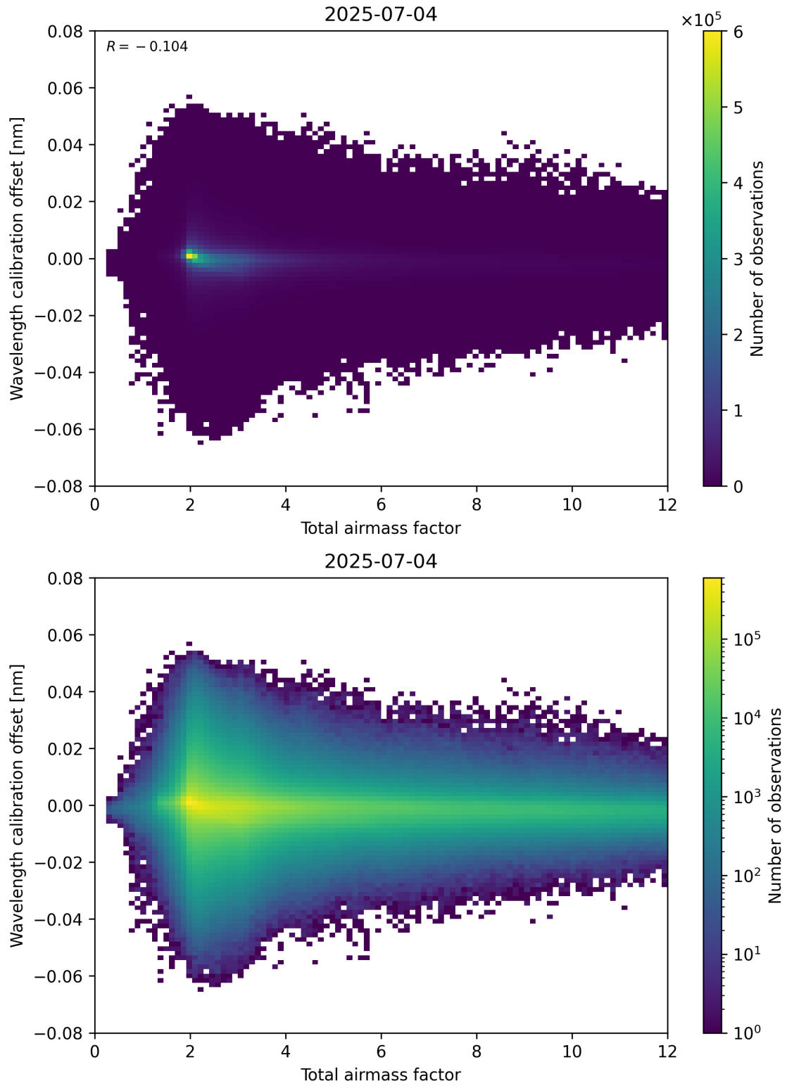
Figure 70: Scatter density plot of “Total airmass factor” against “Wavelength calibration offset” for 2025-07-03 to 2025-07-05.
