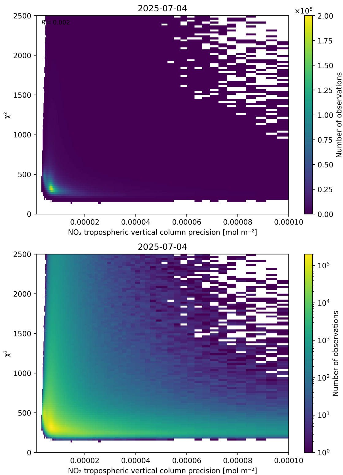
Figure 134: Scatter density plot of “NO 2 tropospheric vertical column precision” against “ \chi^2 ” for 2025-07-03 to 2025-07-05.
