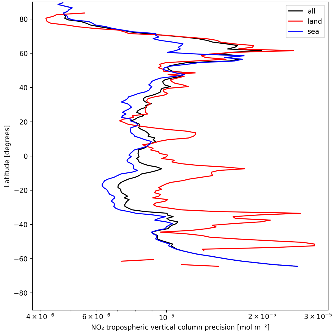
Figure 13: Zonal average of “NO 2 tropospheric vertical column precision” for 2025-07-03 to 2025-07-05.
