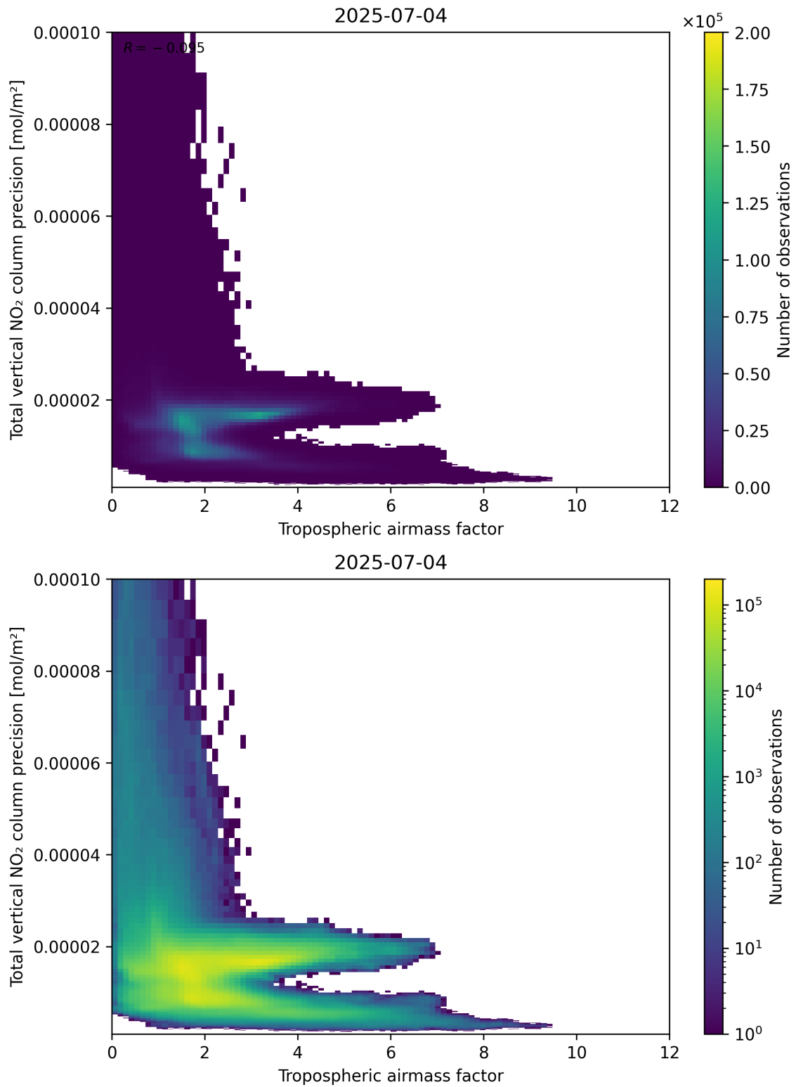
Figure 78: Scatter density plot of “Tropospheric air mass factor” against “Total vertical NO 2 column precision” for 2025-07-03 to 2025-07-05.
