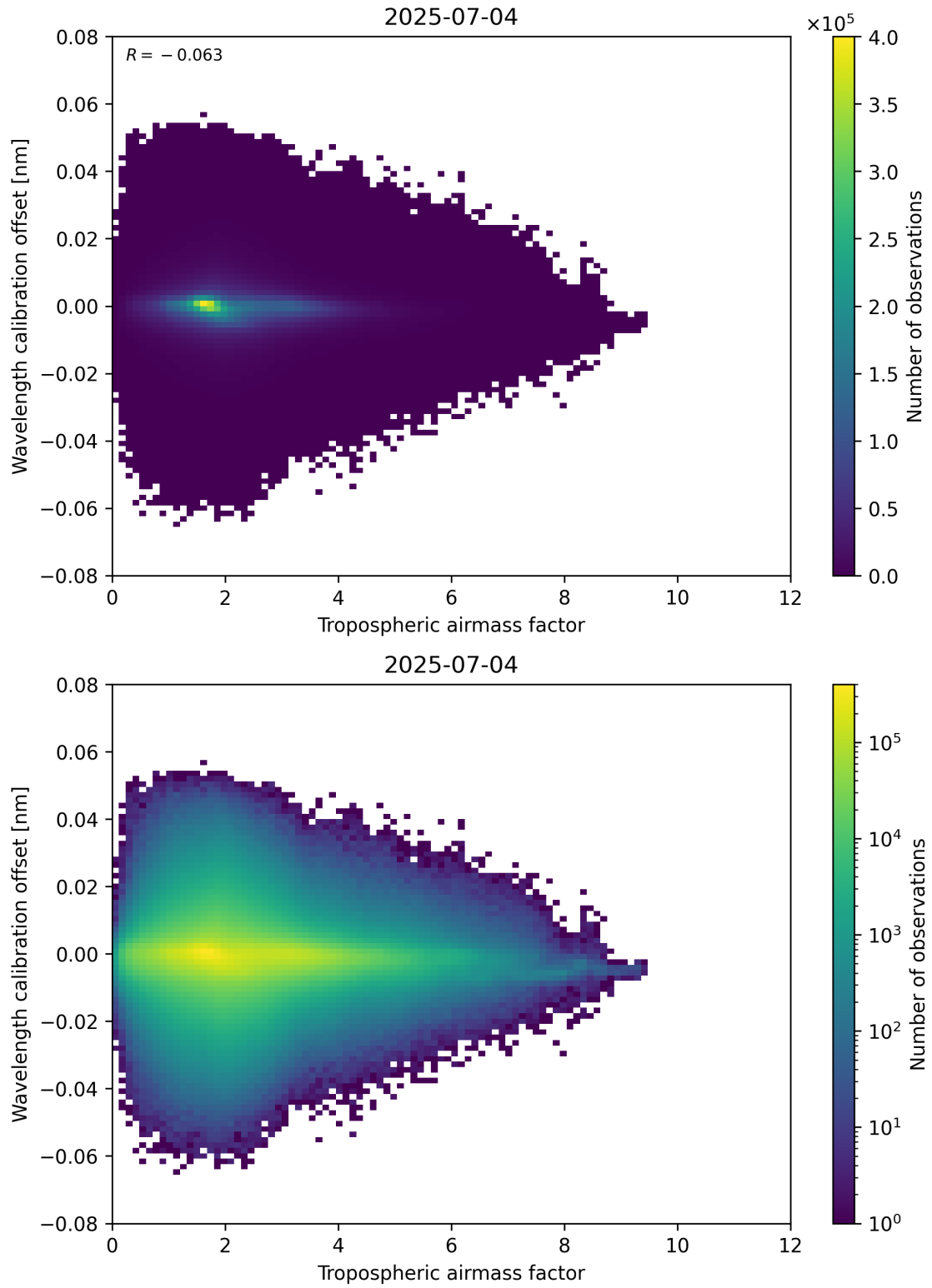
Figure 80: Scatter density plot of “Tropospheric airmass factor” against “Wavelength calibration offset” for 2025-07-03 to 2025-07-05.
