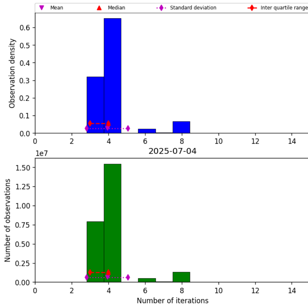
Figure 34: Histogram of “Number of iterations” for 2025-07-03 to 2025-07-05
