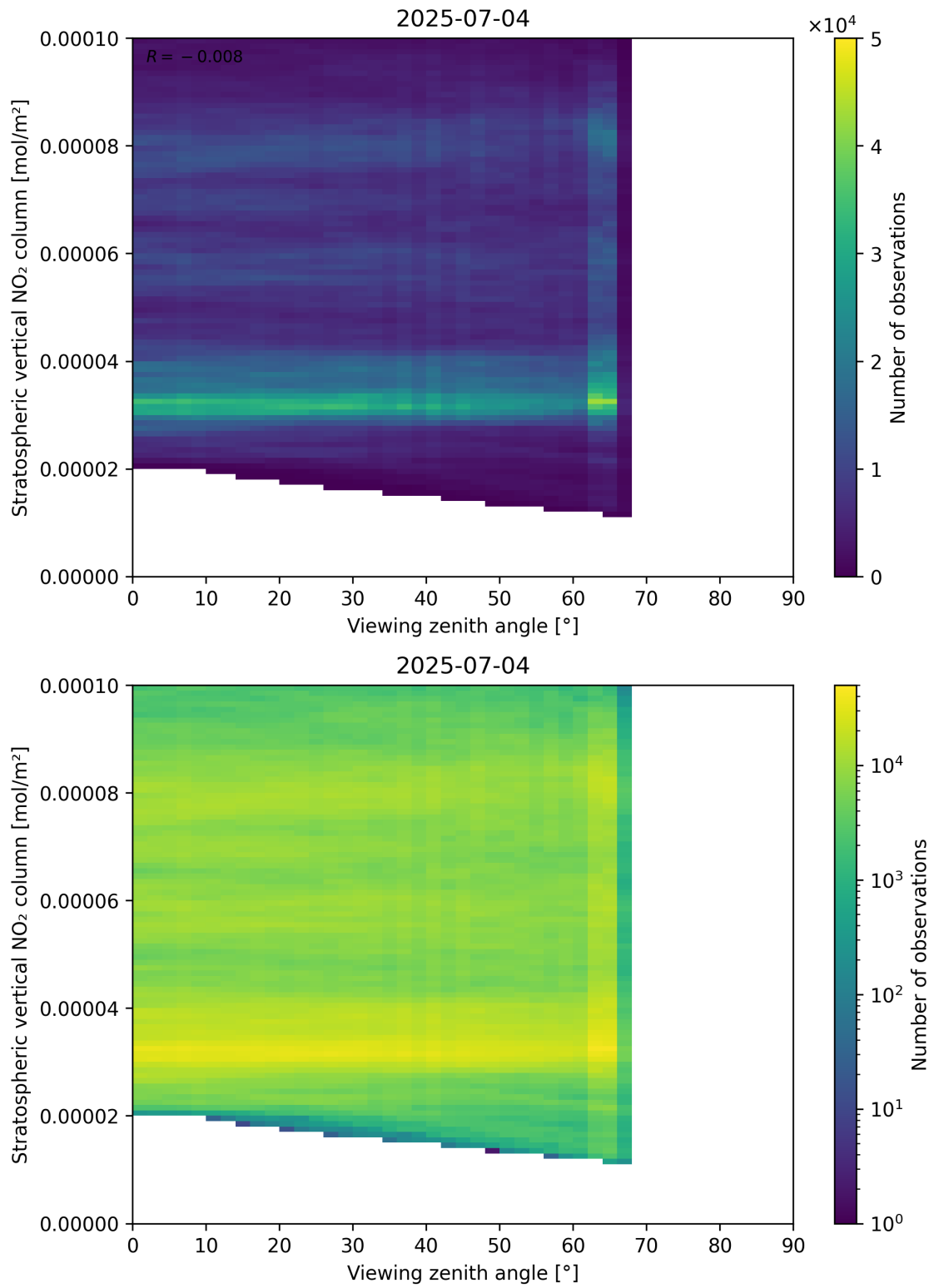
Figure 164: Scatter density plot of “Viewing zenith angle” against “Stratospheric vertical NO 2 column” for 2025-07-03 to 2025-07-05.
