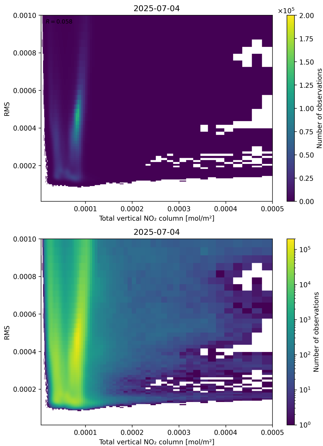
Figure 120: Scatter density plot of “Total vertical NO 2 column” against “RMS” for 2025-07-03 to 2025-07-05.
