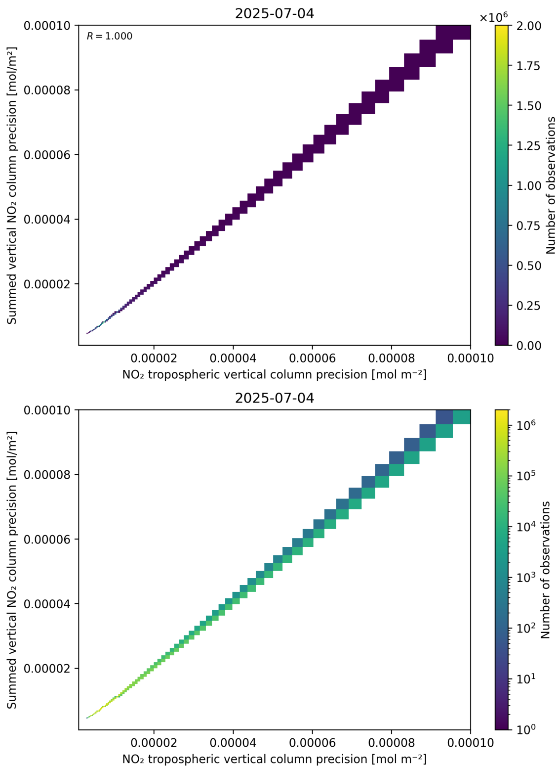
Figure 137: Scatter density plot of “NO 2 tropospheric vertical column precision” against “Summed vertical NO 2 column precision” for 2025-07-03 to 2025-07-05.
