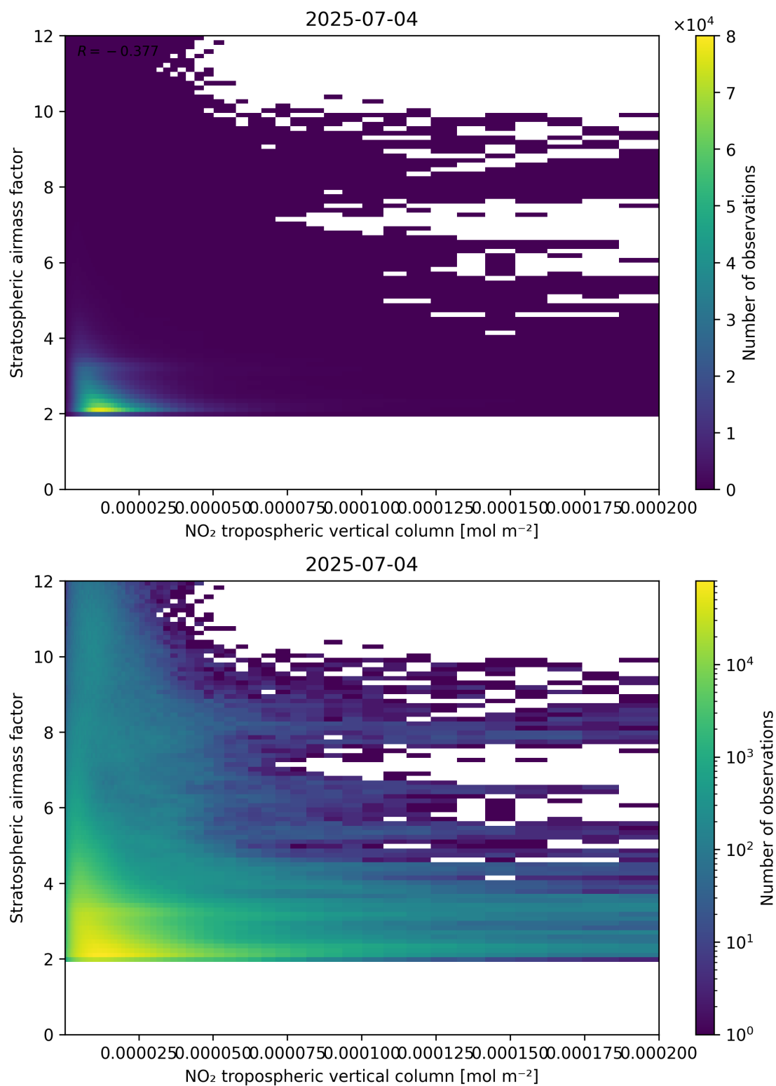
Figure 121: Scatter density plot of “NO 2 tropospheric vertical column” against “Stratospheric air mass factor” for 2025-07-03 to 2025-07-05.
