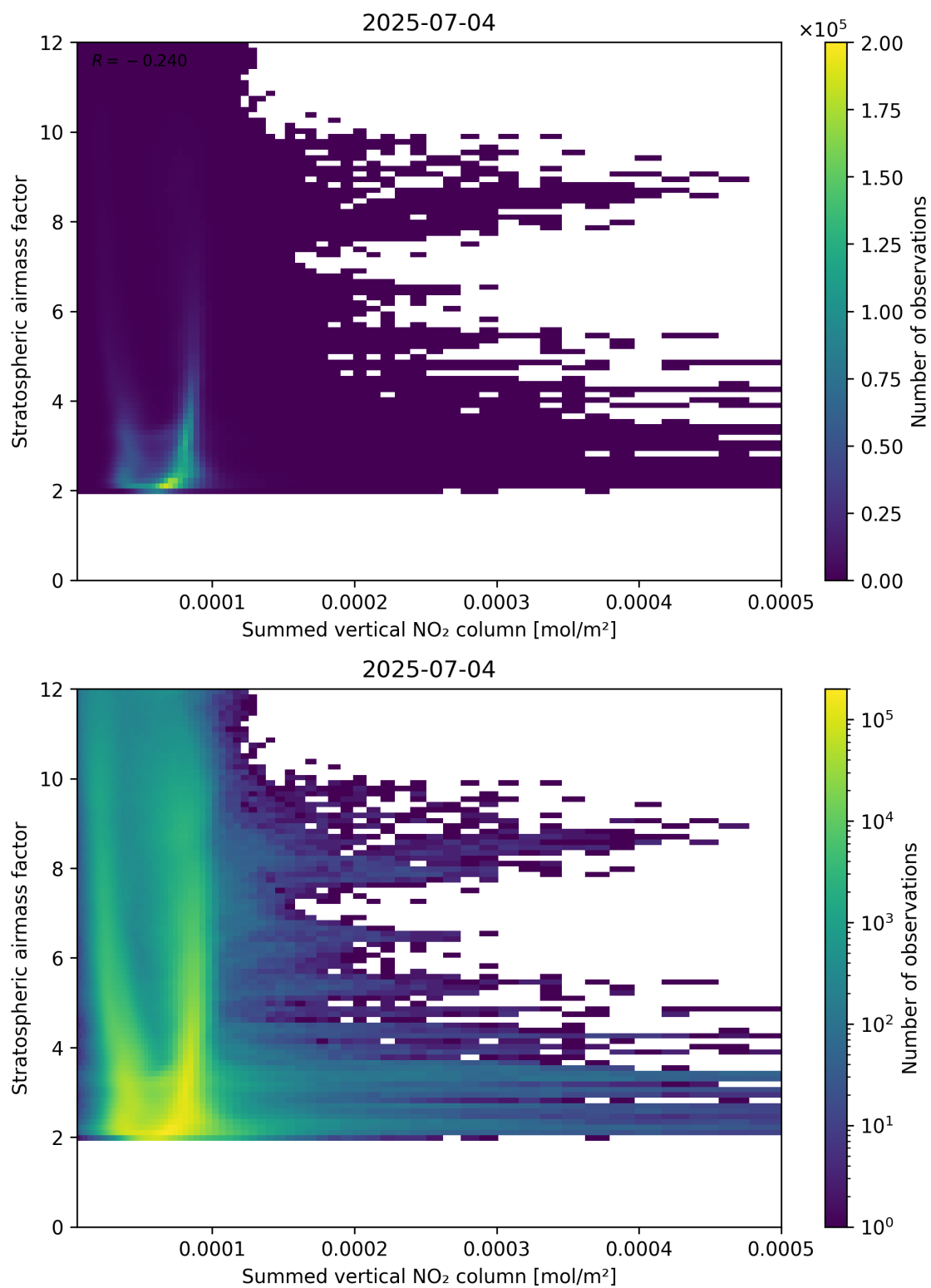
Figure 103: Scatter density plot of “Summed vertical NO 2 column” against “Stratospheric air mass factor” for 2025-07-03 to 2025-07-05.
