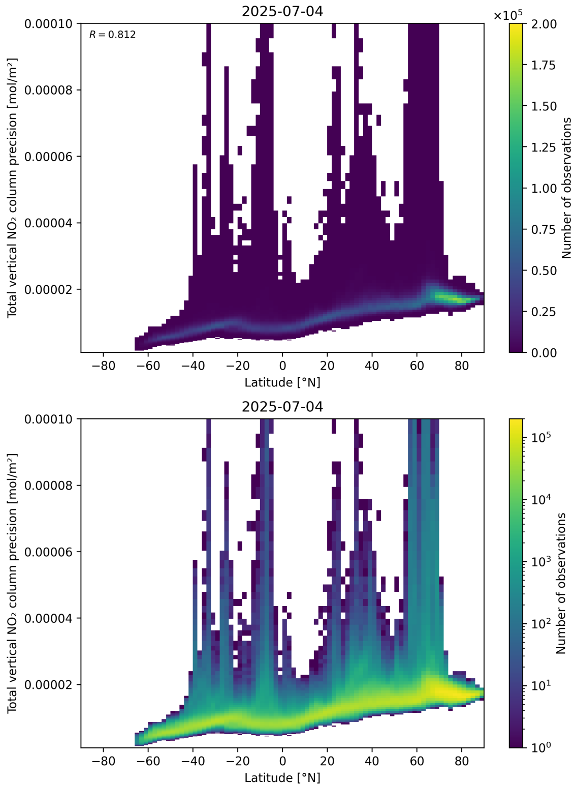
Figure 91: Scatter density plot of “Latitude” against “Total vertical NO 2 column precision” for 2025-07-03 to 2025-07-05.
