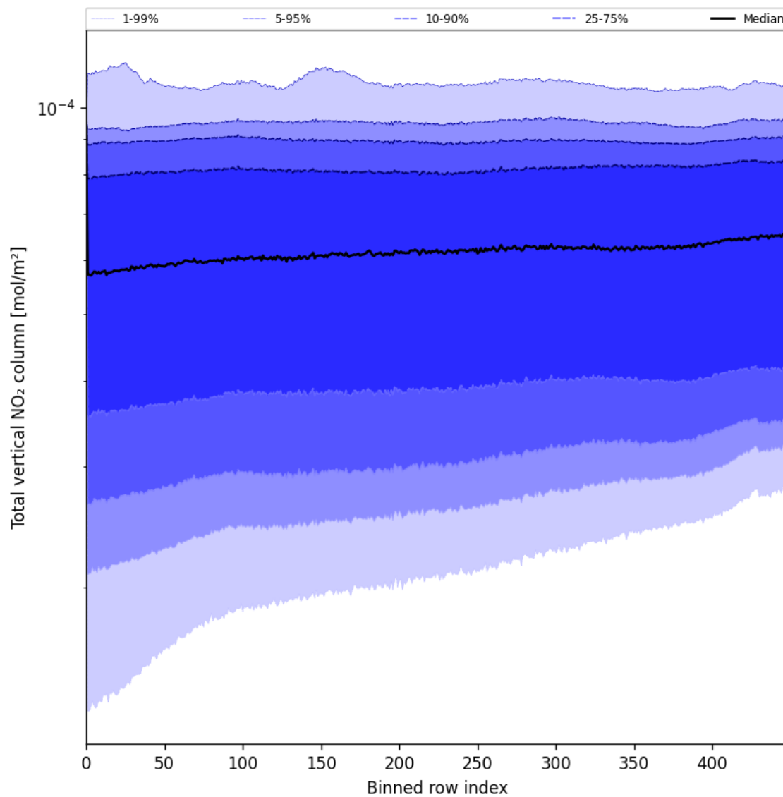
Figure 55: Along track statistics of “Total vertical NO 2 column” for 2025-07-03 to 2025-07-05
