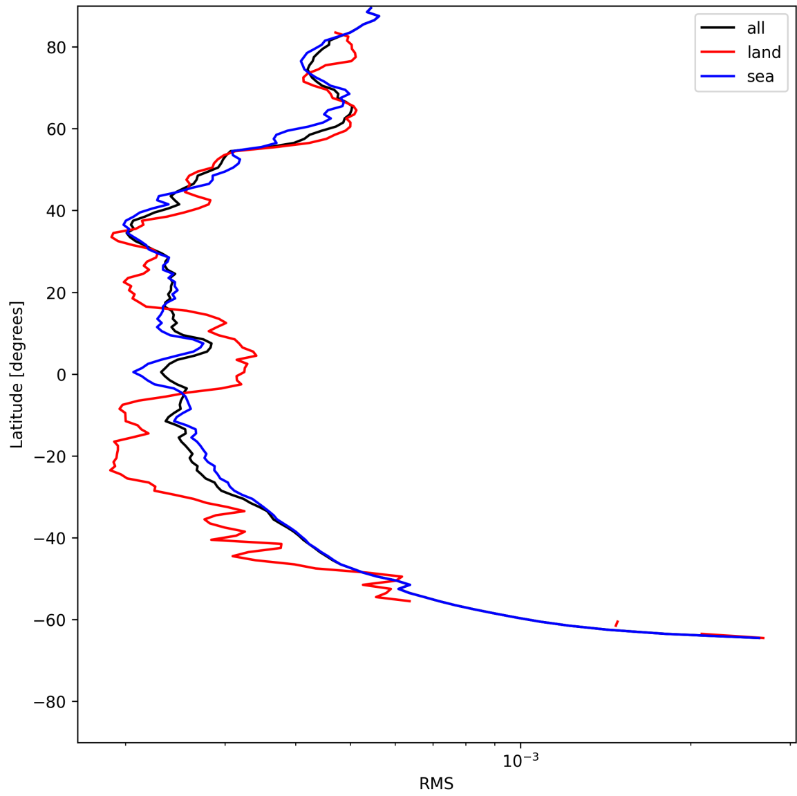
Figure 26: Zonal average of “RMS” for 2025-07-03 to 2025-07-05.
