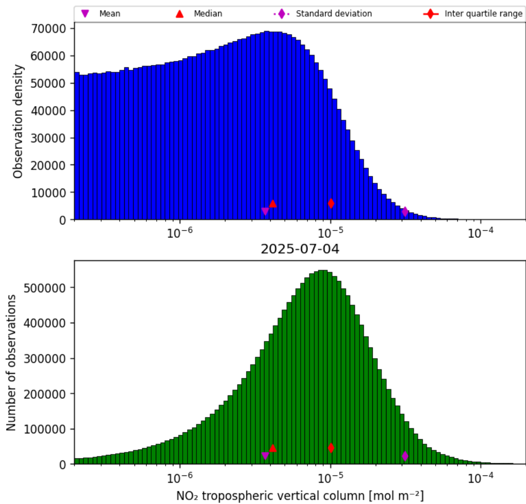
Figure 29: Histogram of “NO 2 tropospheric vertical column” for 2025-07-03 to 2025-07-05
