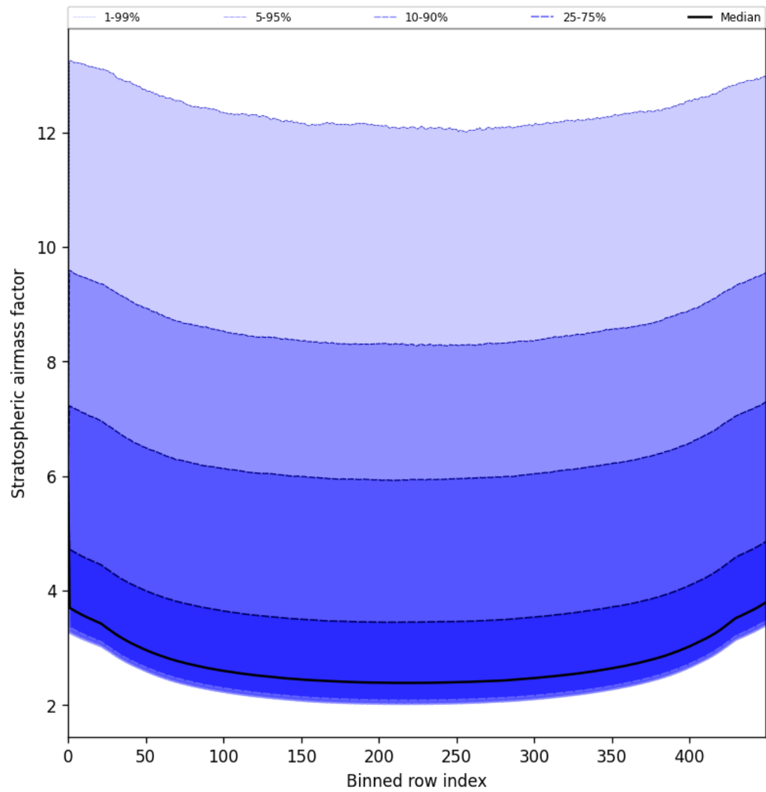
Figure 61: Along track statistics of “Stratospheric airmass factor” for 2025-07-03 to 2025-07-05
