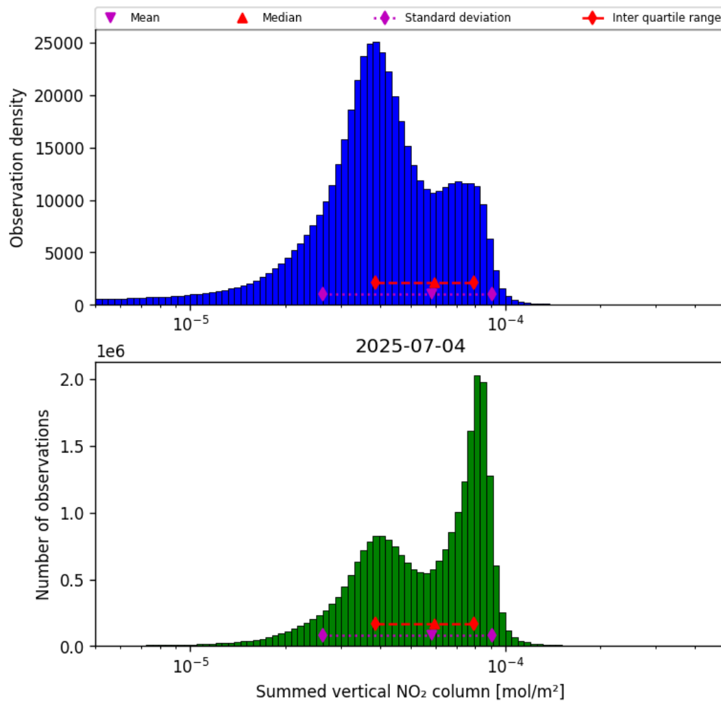
Figure 40: Histogram of “Summed vertical NO 2 column” for 2025-07-03 to 2025-07-05
