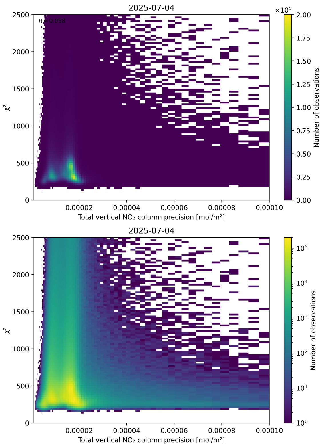
Figure 116: Scatter density plot of “Total vertical NO 2 column precision” against “ \chi^2 ” for 2025-07-03 to 2025-07-05.
