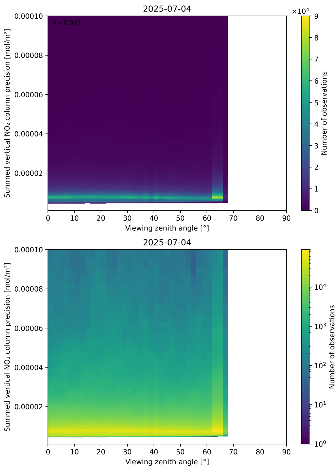
Figure 166: Scatter density plot of “Viewing zenith angle” against “Summed vertical NO 2 column precision” for 2025-07-03 to 2025-07-05.
