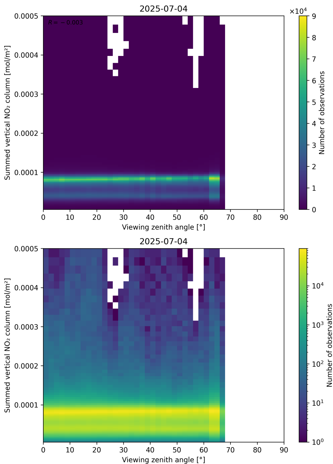
Figure 165: Scatter density plot of “Viewing zenith angle” against “Summed vertical NO 2 column” for 2025-07-03 to 2025-07-05.
