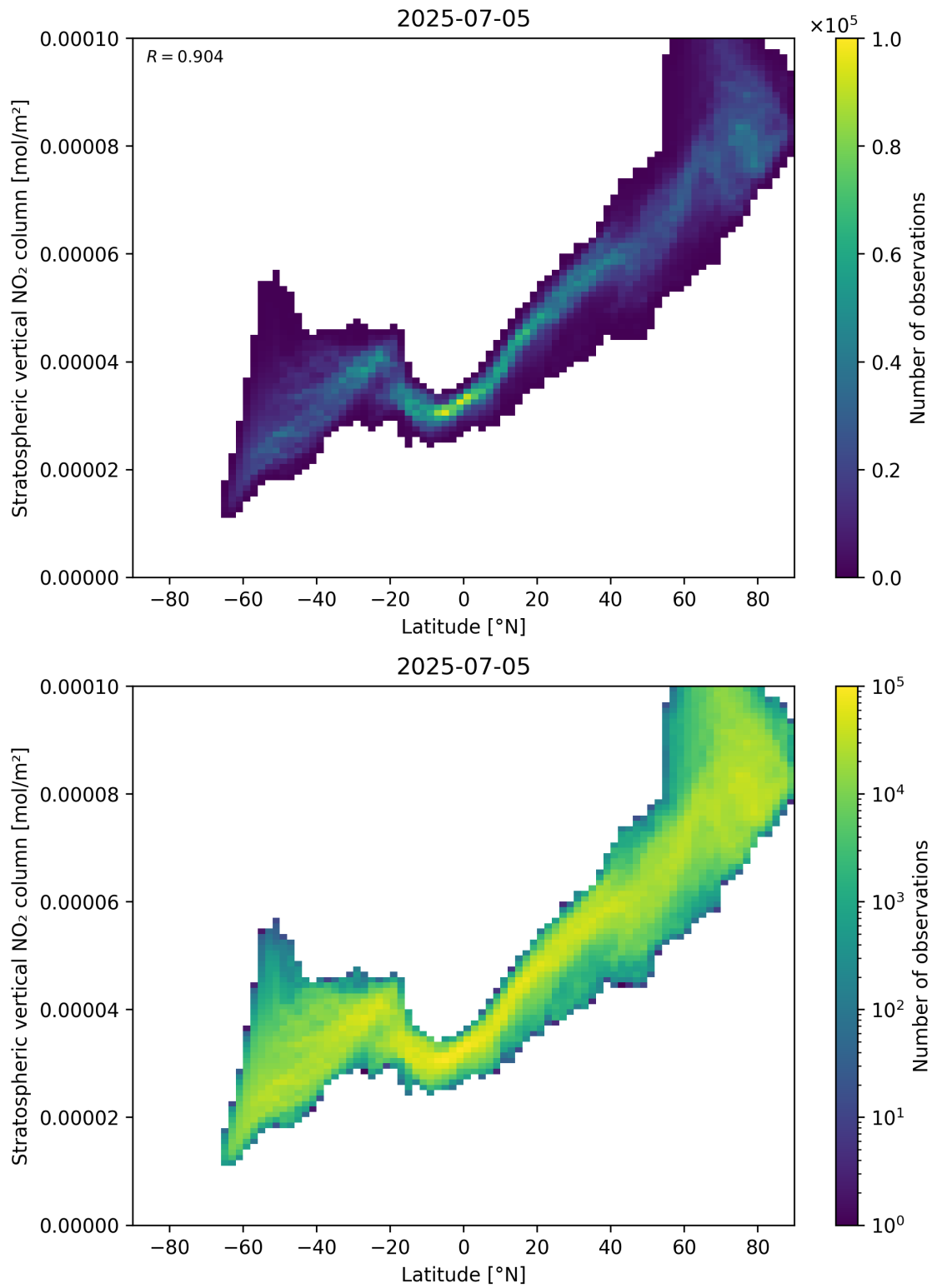
Figure 87: Scatter density plot of “Latitude” against “Stratospheric vertical NO 2 column” for 2025-07-04 to 2025-07-06.
