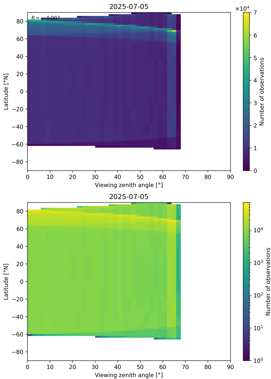
Figure 163: Scatter density plot of “Viewing zenith angle” against “Latitude” for 2025-07-04 to 2025-07-06.
