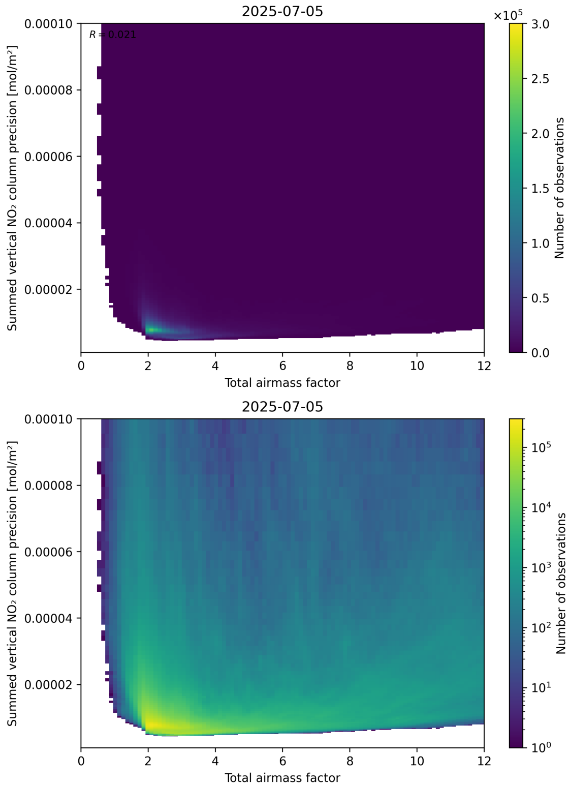
Figure 66: Scatter density plot of “Total airmass factor” against “Summed vertical NO 2 column precision” for 2025-07-04 to 2025-07-06.
