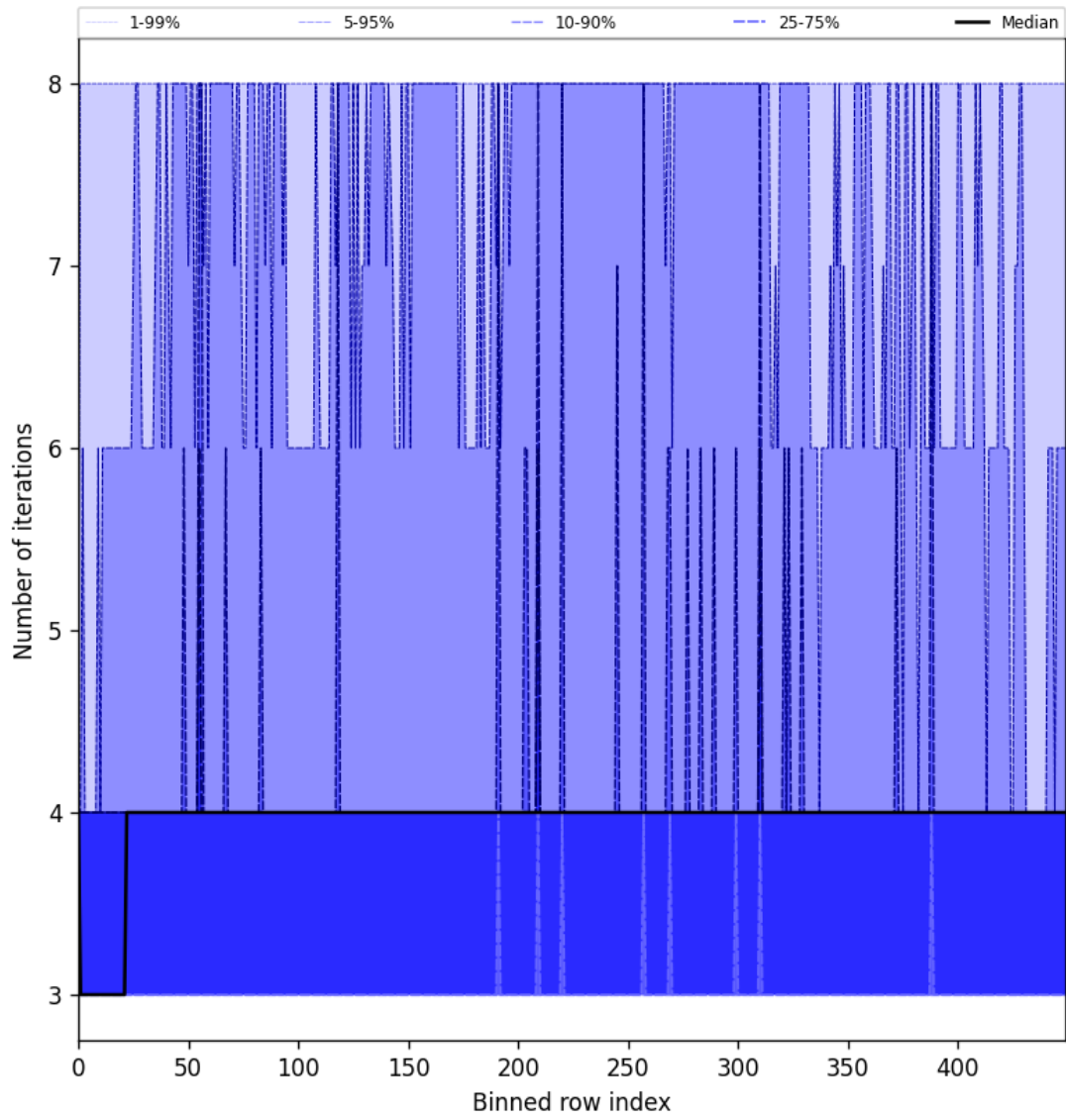
Figure 51: Along track statistics of “Number of iterations” for 2025-07-04 to 2025-07-06
