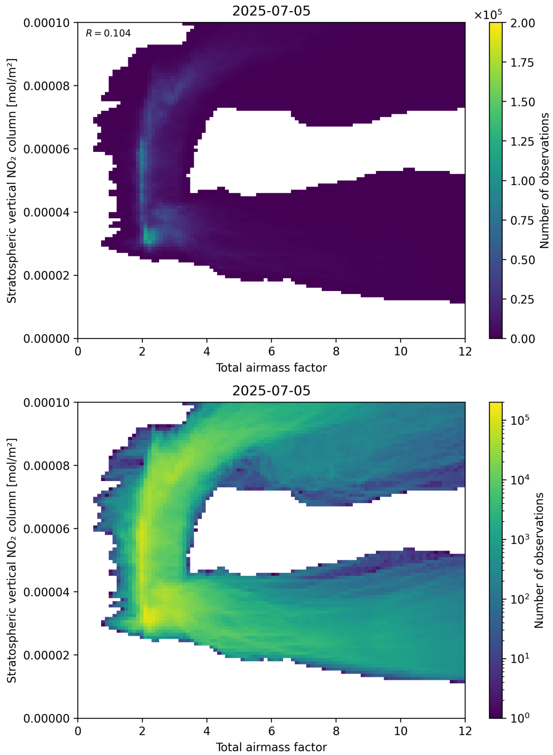
Figure 64: Scatter density plot of “Total airmass factor” against “Stratospheric vertical NO 2 column” for 2025-07-04 to 2025-07-06.
