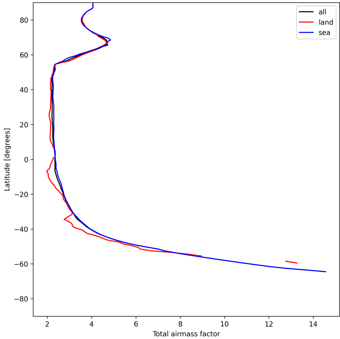
Figure 15: Zonal average of “Total airmass factor” for 2025-07-04 to 2025-07-06.
