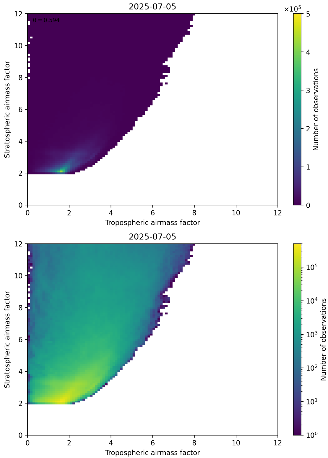
Figure 71: Scatter density plot of “Tropospheric airmass factor” against “Stratospheric airmass factor” for 2025-07-04 to 2025-07-06.
