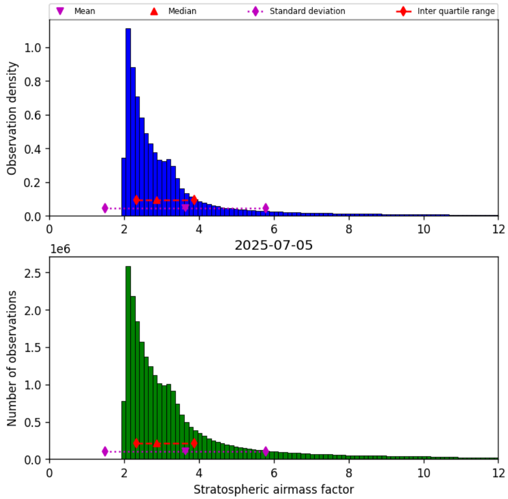
Figure 44: Histogram of “Stratospheric airmass factor” for 2025-07-04 to 2025-07-06
