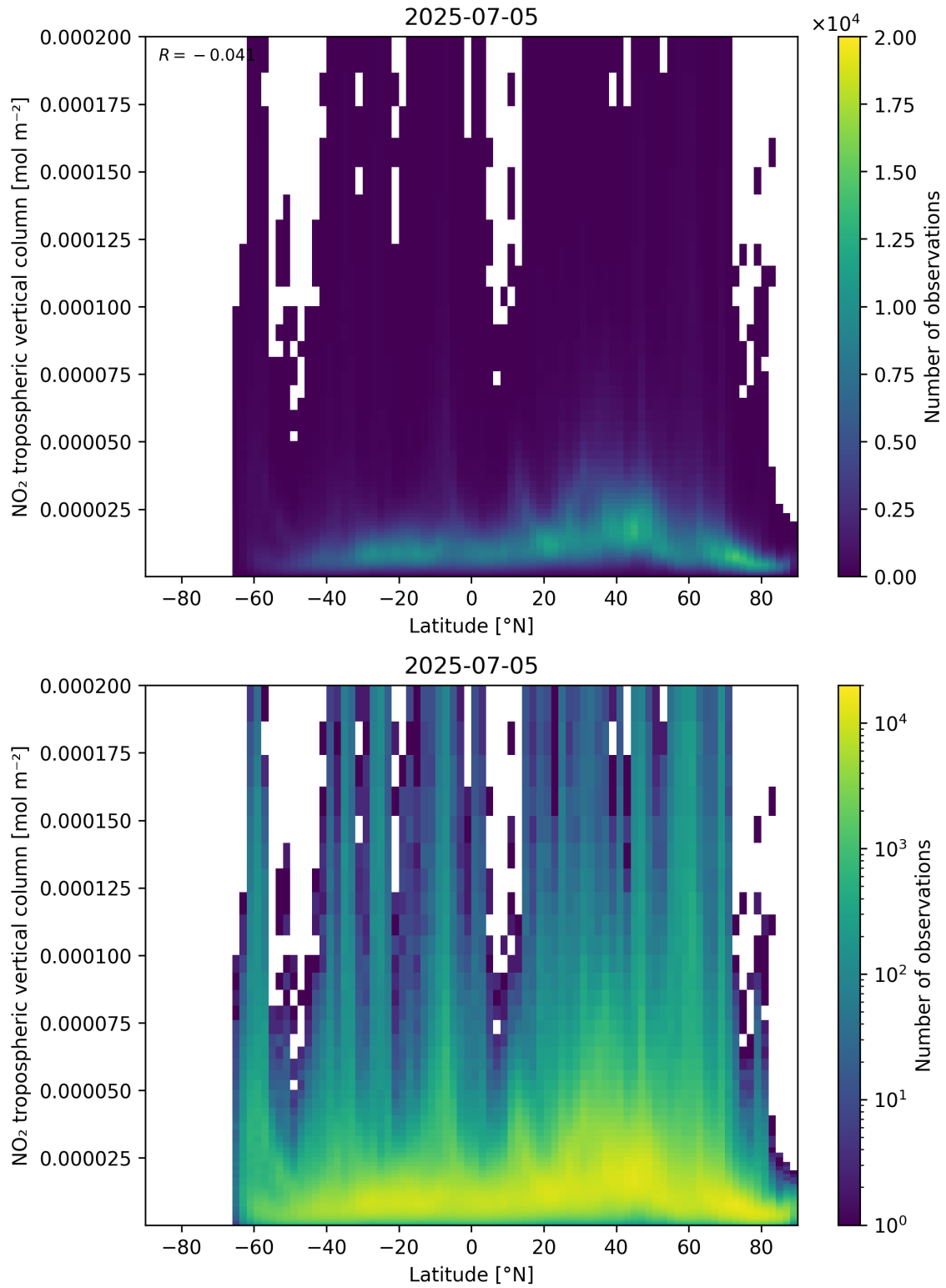
Figure 92: Scatter density plot of “Latitude” against “NO 2 tropospheric vertical column” for 2025-07-04 to 2025-07-06.
