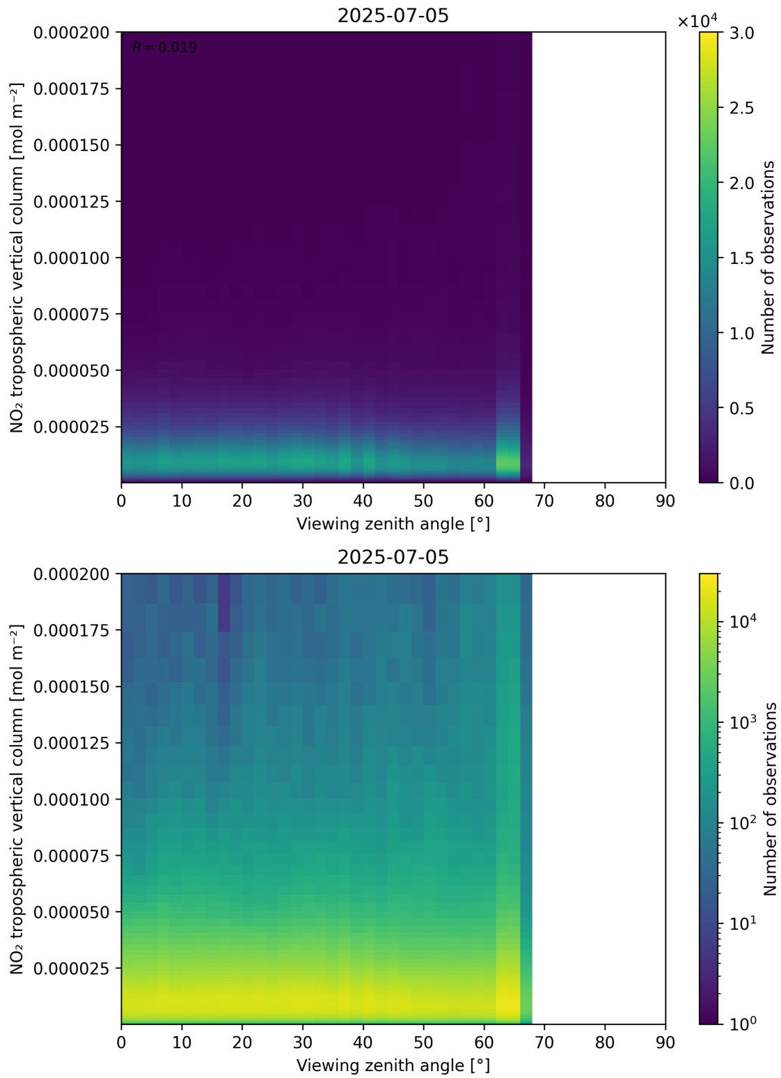
Figure 169: Scatter density plot of “Viewing zenith angle” against “NO 2 tropospheric vertical column” for 2025-07-04 to 2025-07-06.
