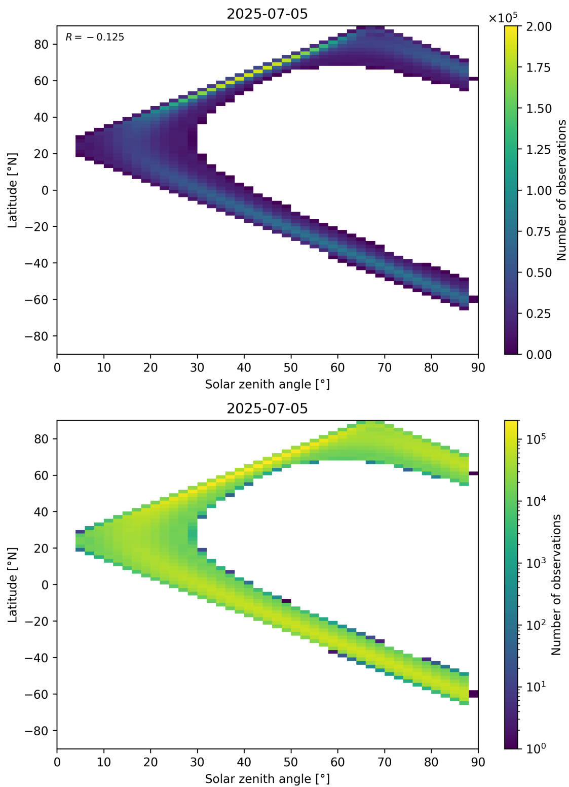
Figure 149: Scatter density plot of “Solar zenith angle” against “Latitude” for 2025-07-04 to 2025-07-06.
