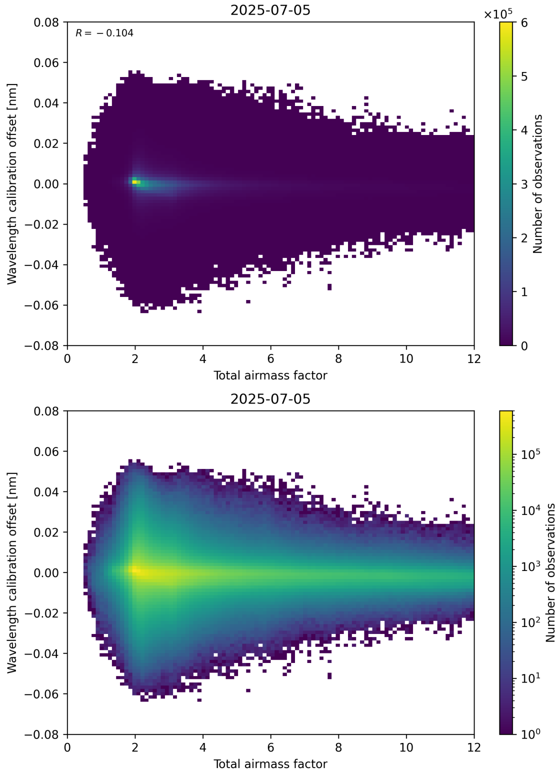
Figure 70: Scatter density plot of “Total airmass factor” against “Wavelength calibration offset” for 2025-07-04 to 2025-07-06.
