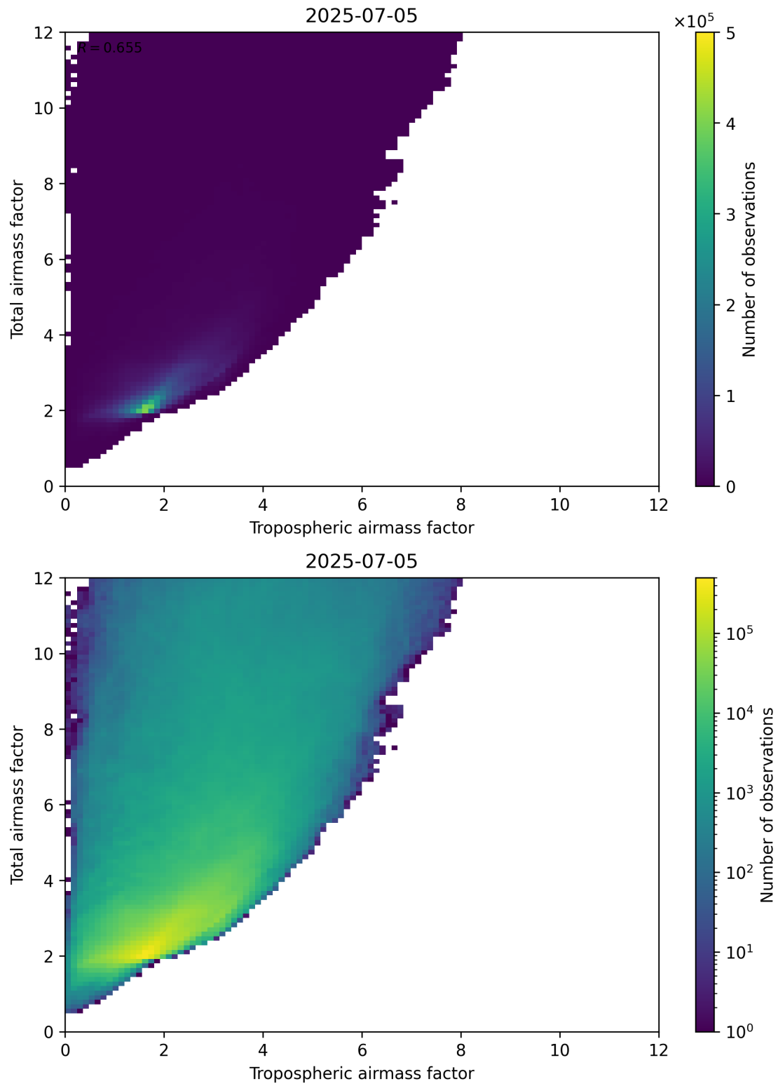
Figure 72: Scatter density plot of “Tropospheric airmass factor” against “Total airmass factor” for 2025-07-04 to 2025-07-06.
