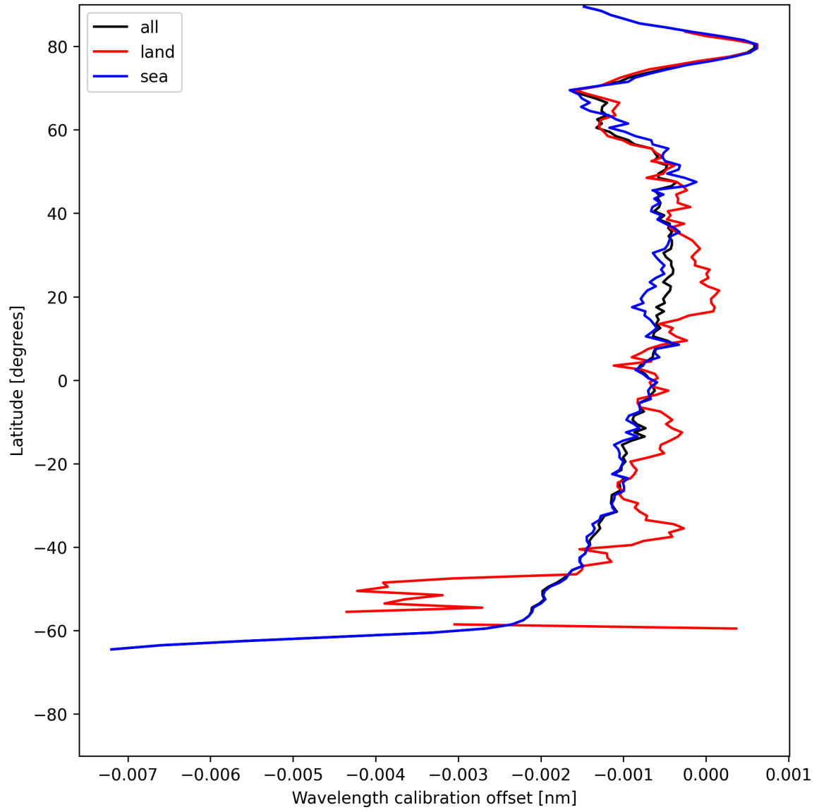
Figure 18: Zonal average of “Wavelength calibration offset” for 2025-07-04 to 2025-07-06.
