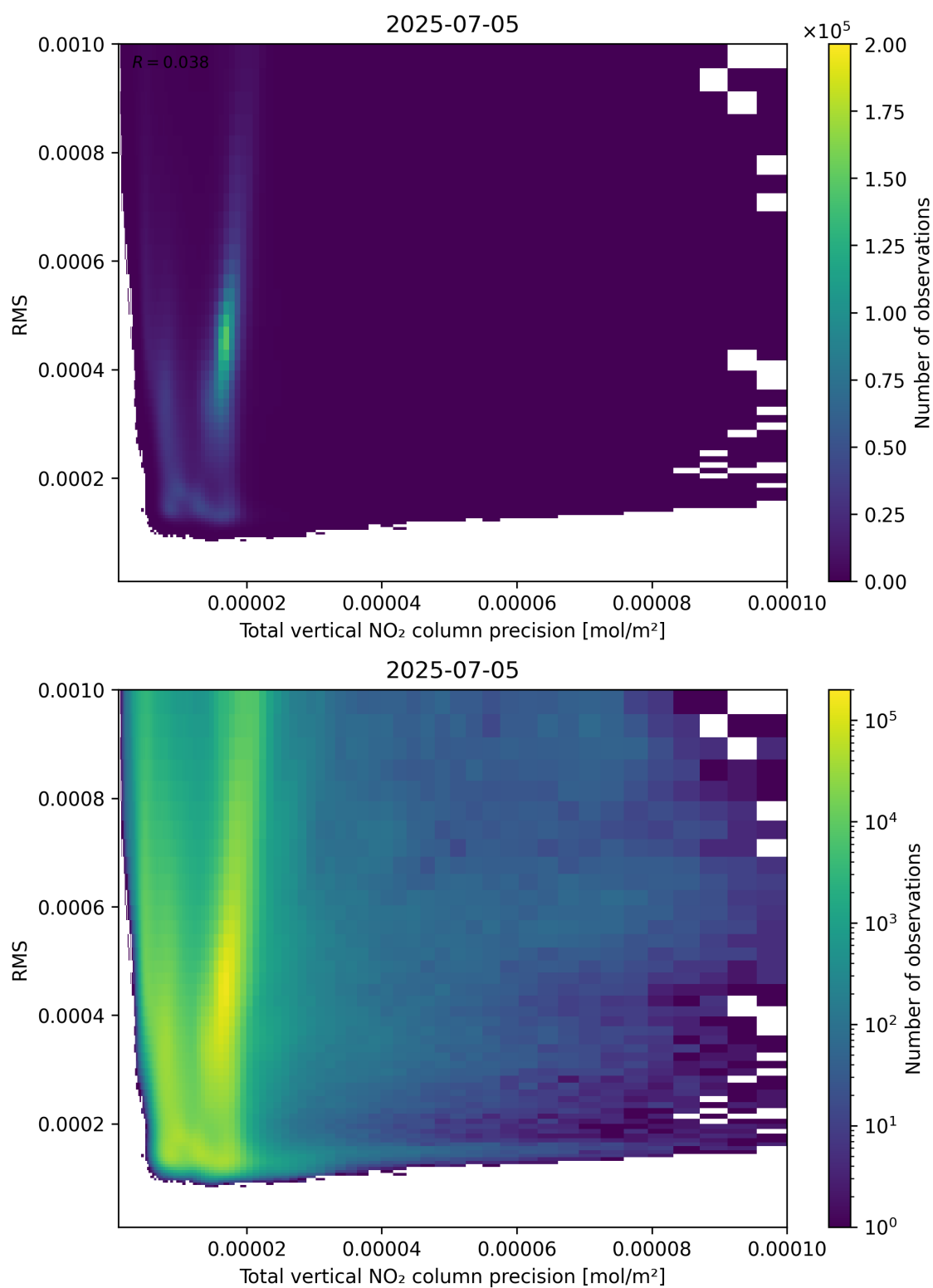
Figure 119: Scatter density plot of “Total vertical NO 2 column precision” against “RMS” for 2025-07-04 to 2025-07-06.
