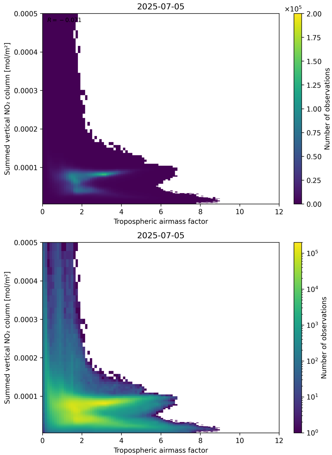
Figure 75: Scatter density plot of “Tropospheric air mass factor” against “Summed vertical NO 2 column” for 2025-07-04 to 2025-07-06.
