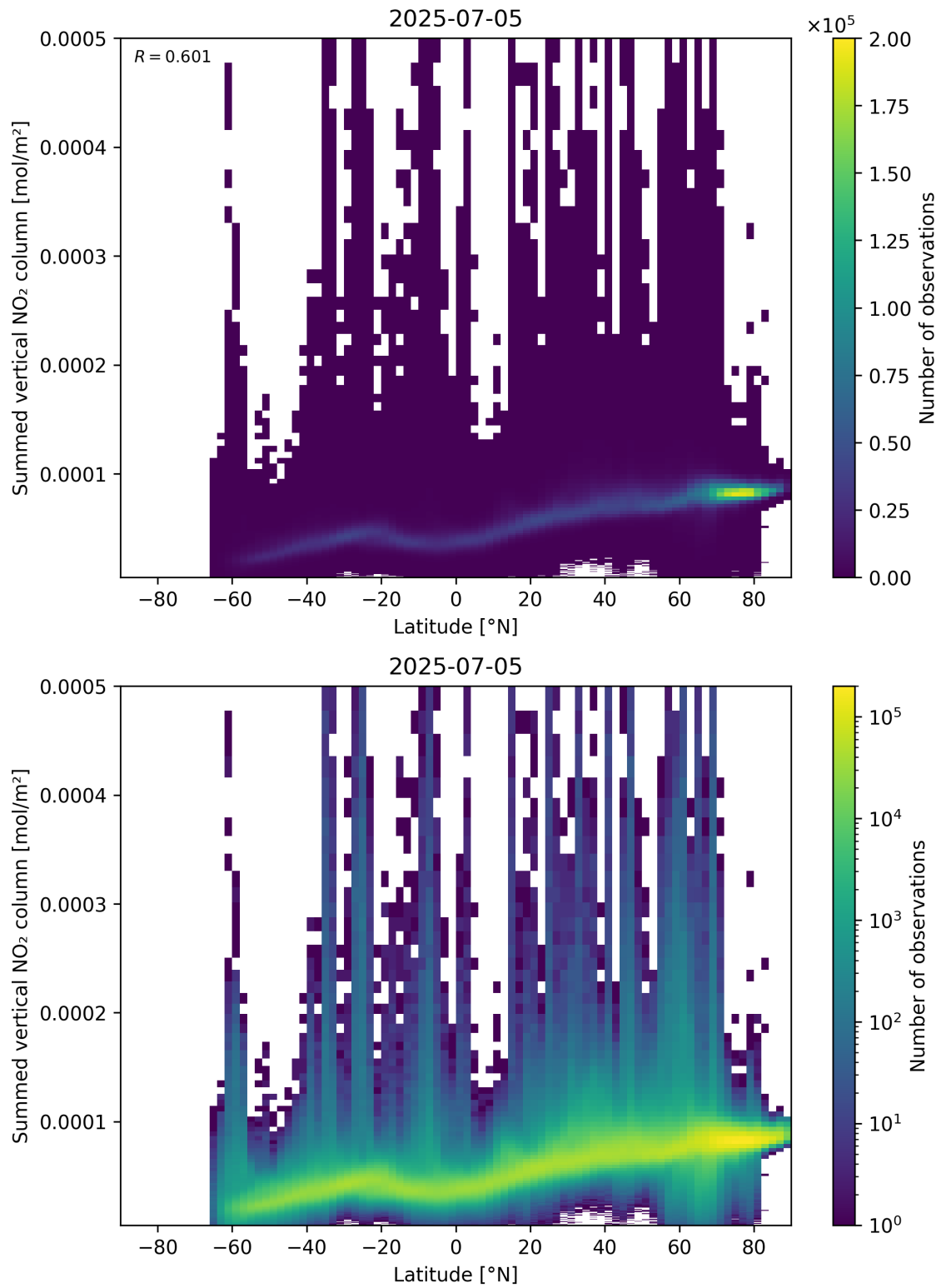
Figure 88: Scatter density plot of “Latitude” against “Summed vertical NO 2 column” for 2025-07-04 to 2025-07-06.
