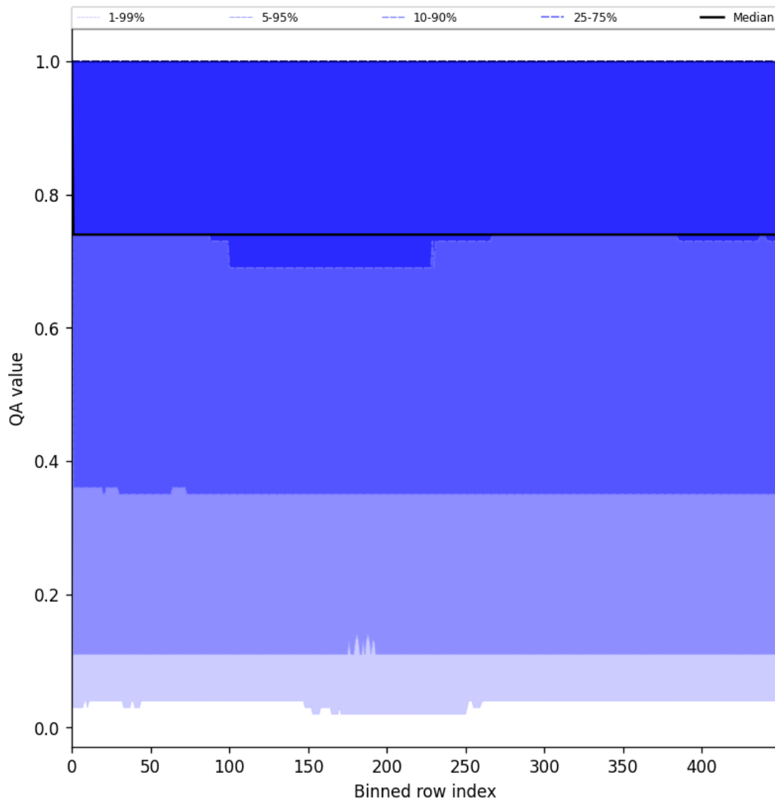
Figure 45: Along track statistics of “QA value” for 2025-07-04 to 2025-07-06
