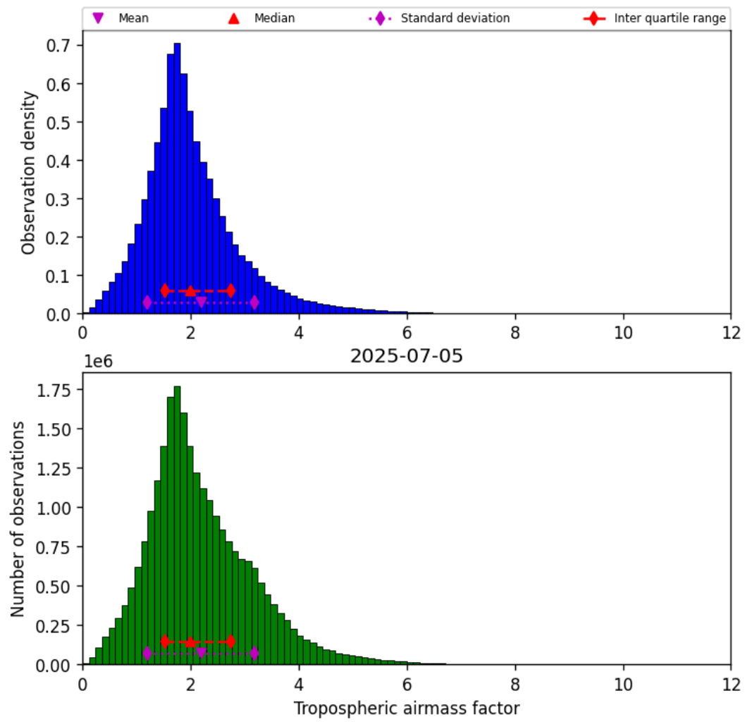
Figure 31: Histogram of “Tropospheric airmass factor” for 2025-07-04 to 2025-07-06
