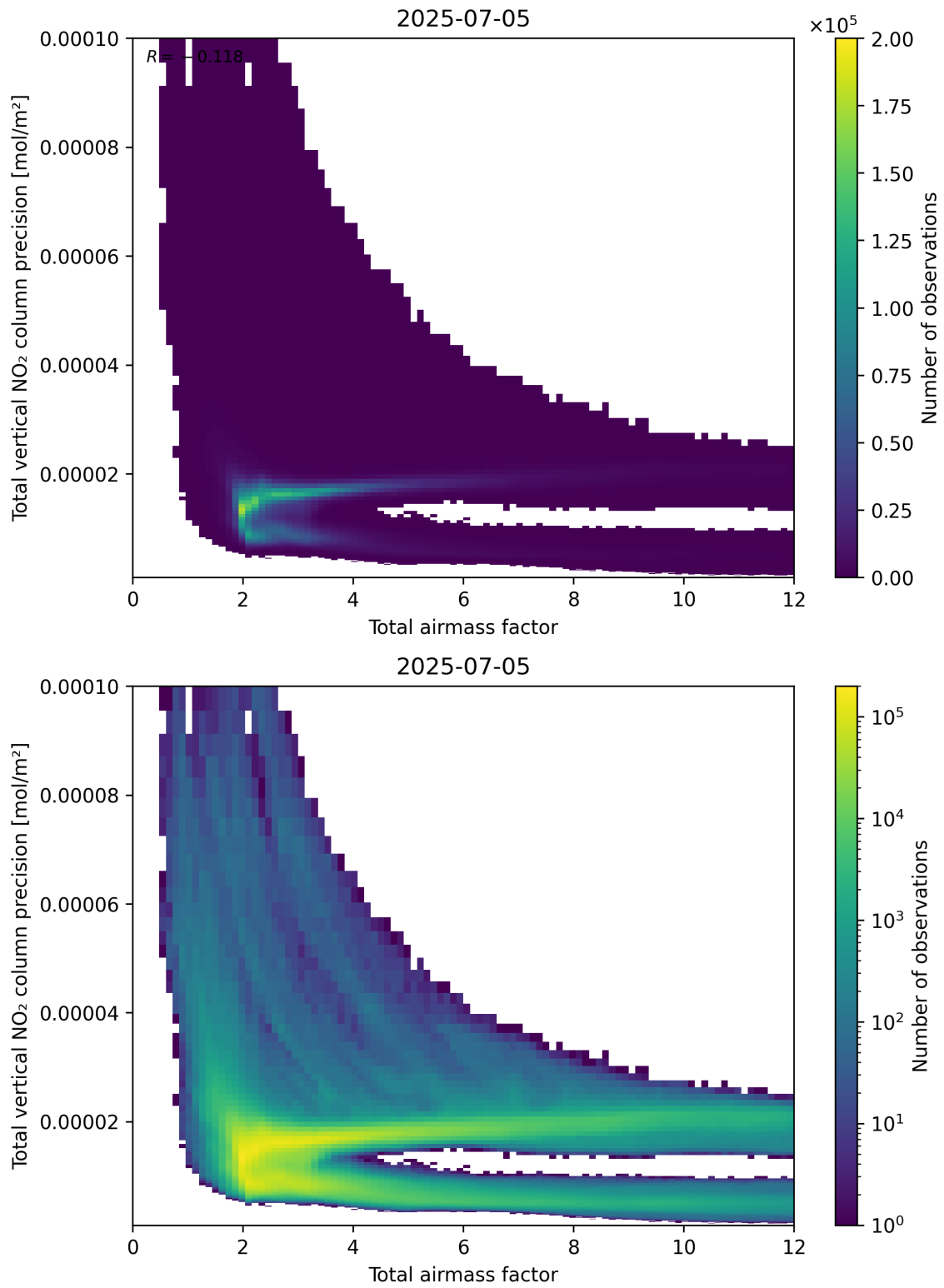
Figure 68: Scatter density plot of “Total airmass factor” against “Total vertical NO 2 column precision” for 2025-07-04 to 2025-07-06.
