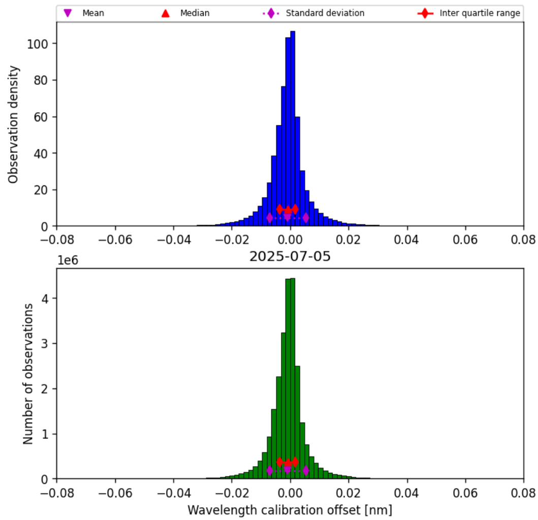
Figure 35: Histogram of “Wavelength calibration offset” for 2025-07-04 to 2025-07-06
