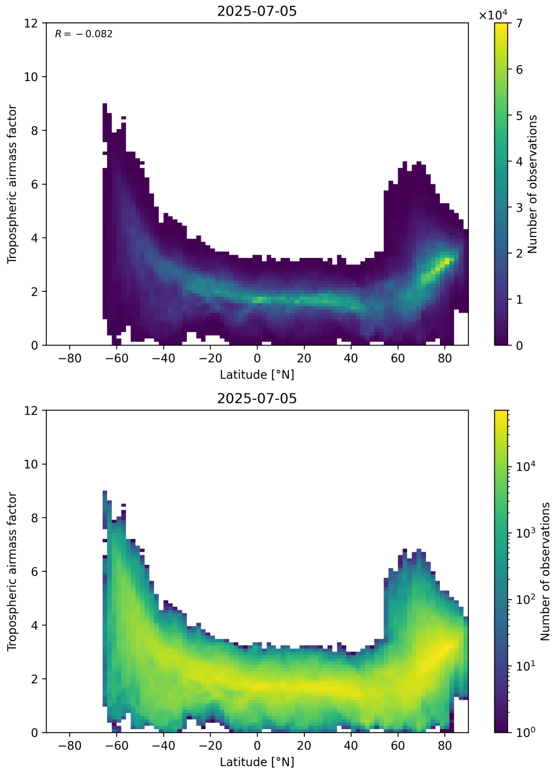
Figure 85: Scatter density plot of “Latitude” against “Tropospheric airmass factor” for 2025-07-04 to 2025-07-06.
