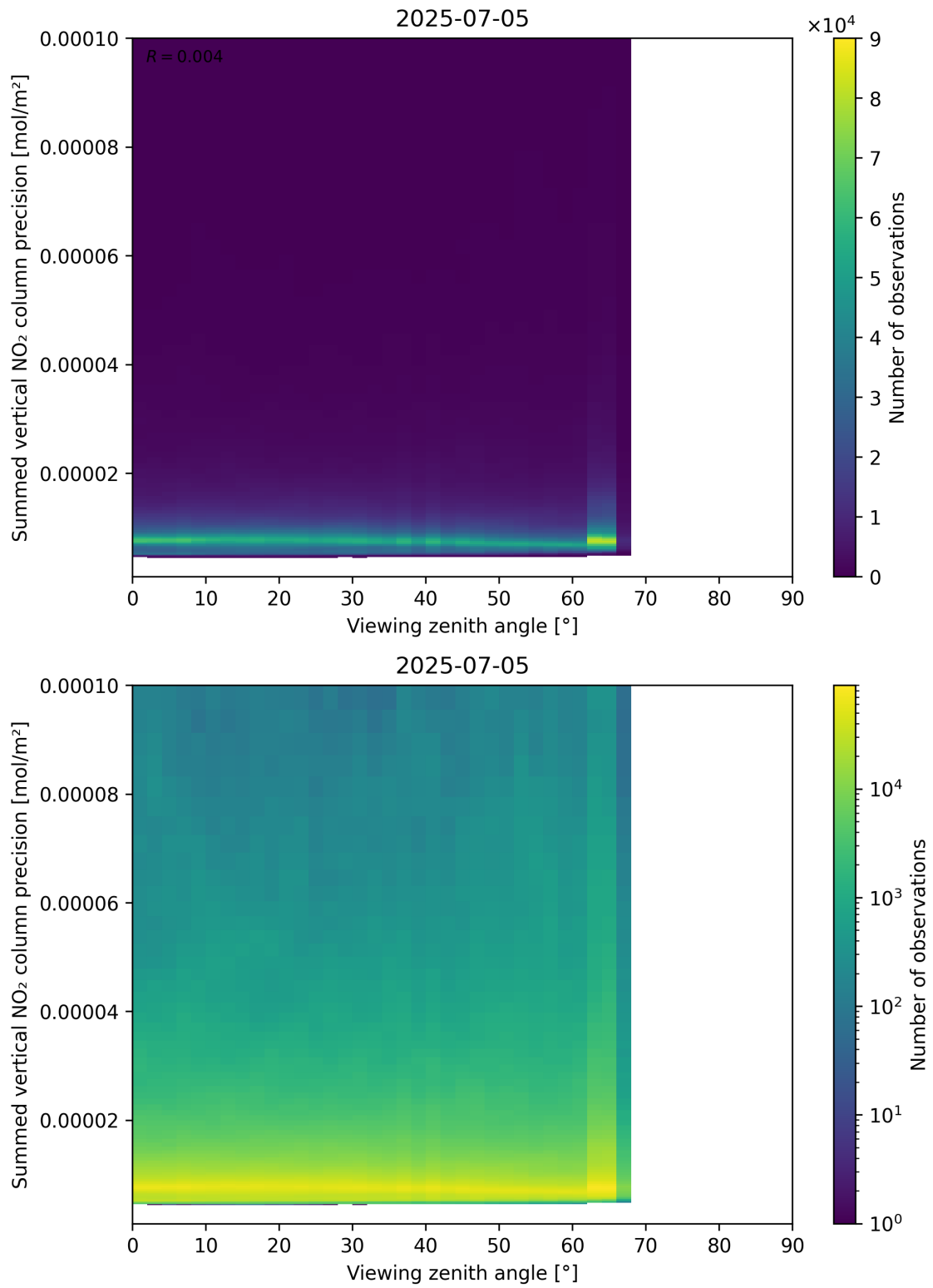
Figure 166: Scatter density plot of “Viewing zenith angle” against “Summed vertical NO 2 column precision” for 2025-07-04 to 2025-07-06.
