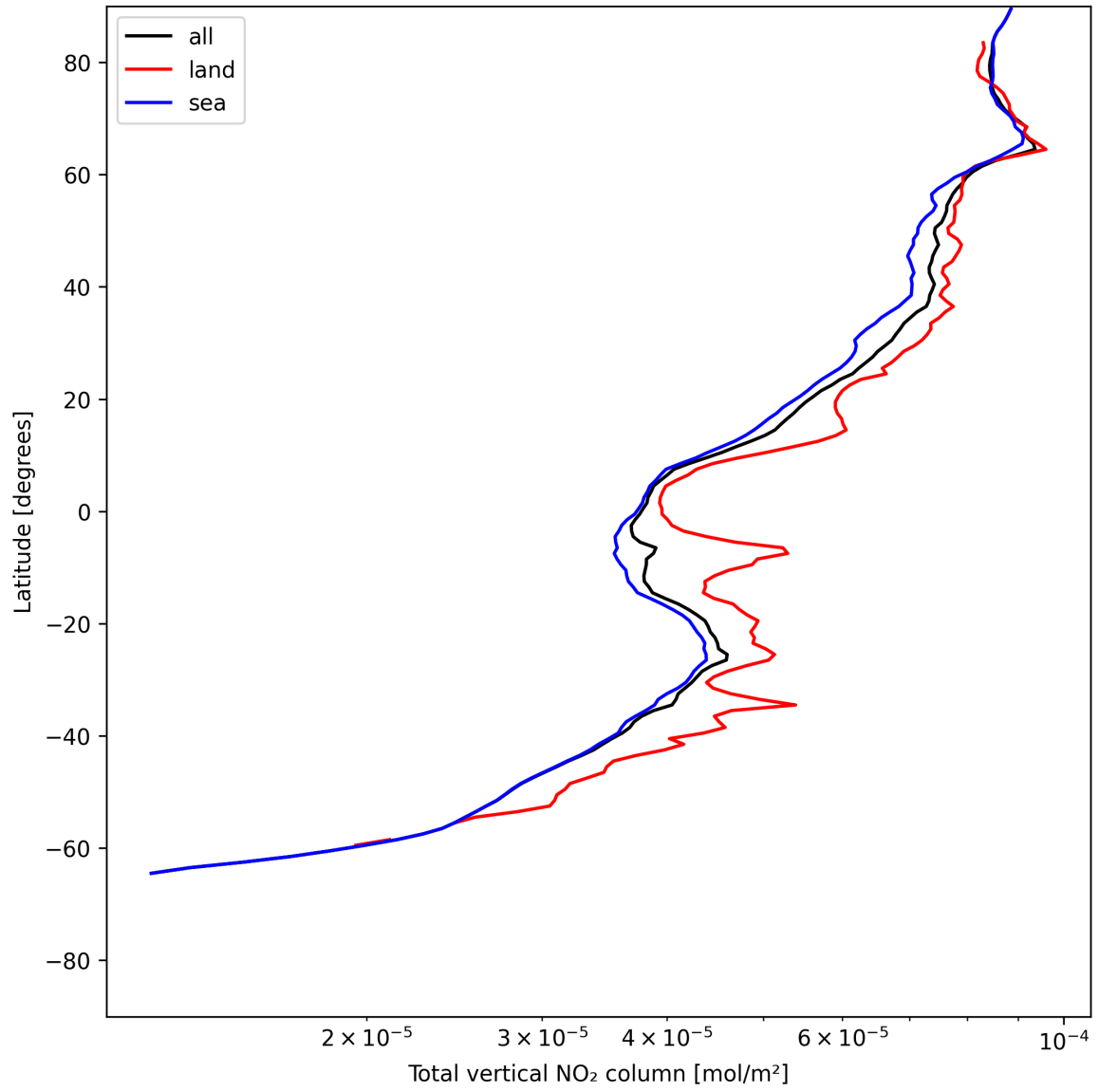
Figure 21: Zonal average of “Total vertical NO 2 column” for 2025-07-04 to 2025-07-06.
