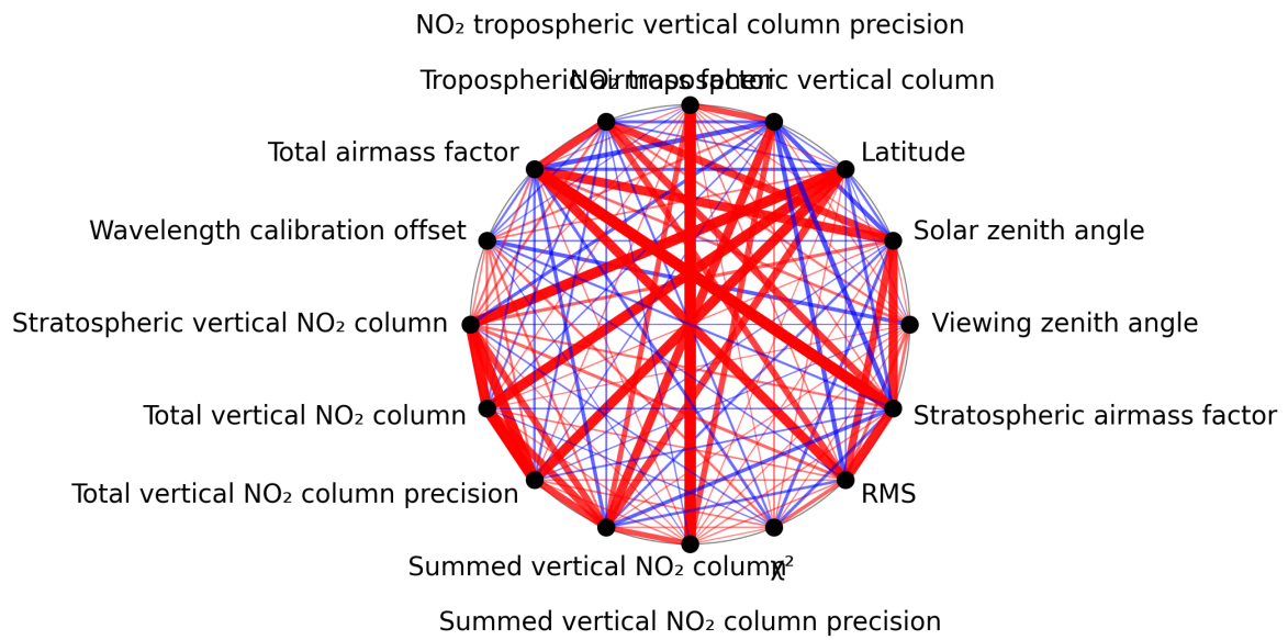
Figure 1: Map of correlation graph for 2025-07-04 to 2025-07-06.
