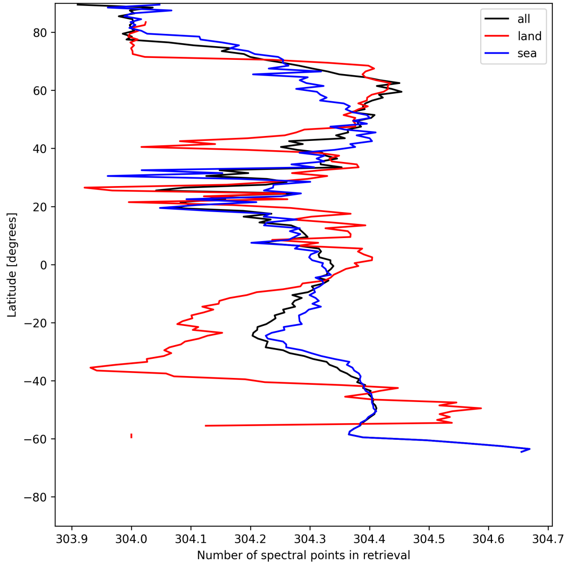
Figure 16: Zonal average of “Number of spectral points in retrieval” for 2025-07-04 to 2025-07-06.
