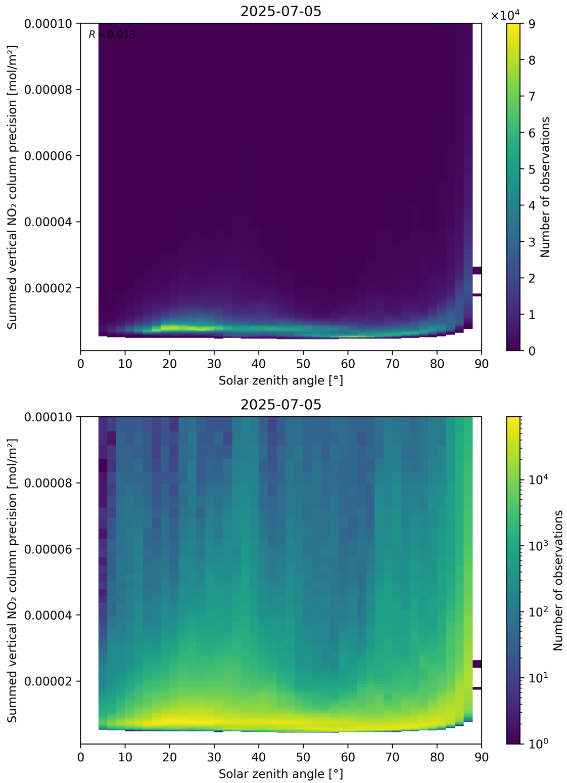
Figure 152: Scatter density plot of “Solar zenith angle” against “Summed vertical NO 2 column precision” for 2025-07-04 to 2025-07-06.
