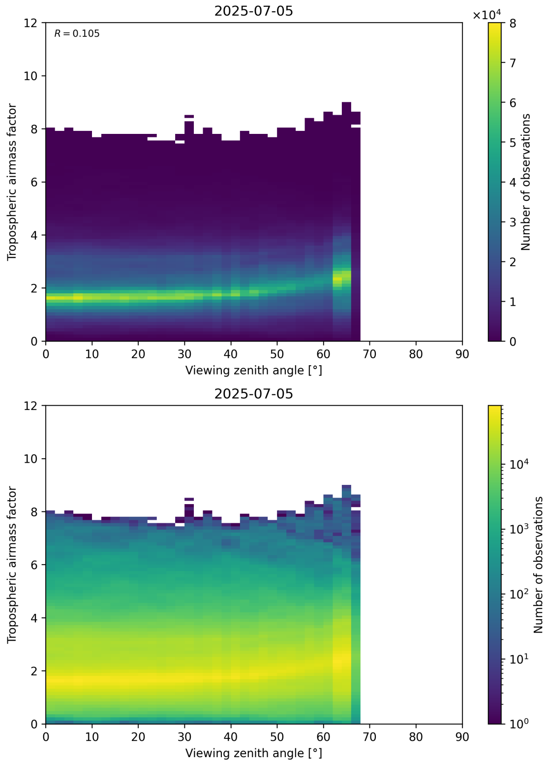
Figure 161: Scatter density plot of “Viewing zenith angle” against “Tropospheric airmass factor” for 2025-07-04 to 2025-07-06.
