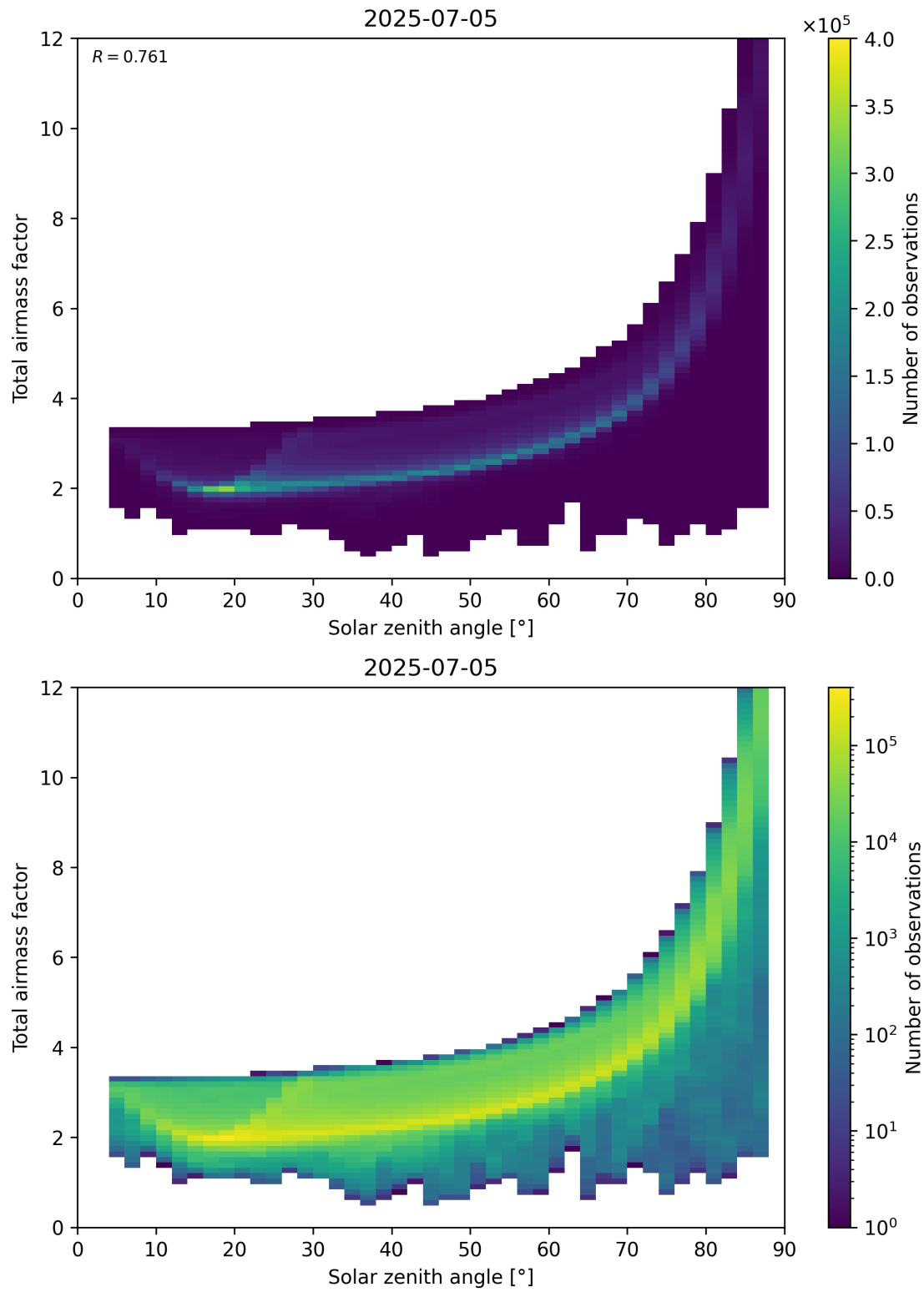
Figure 146: Scatter density plot of “Solar zenith angle” against “Total air mass factor” for 2025-07-04 to 2025-07-06.
