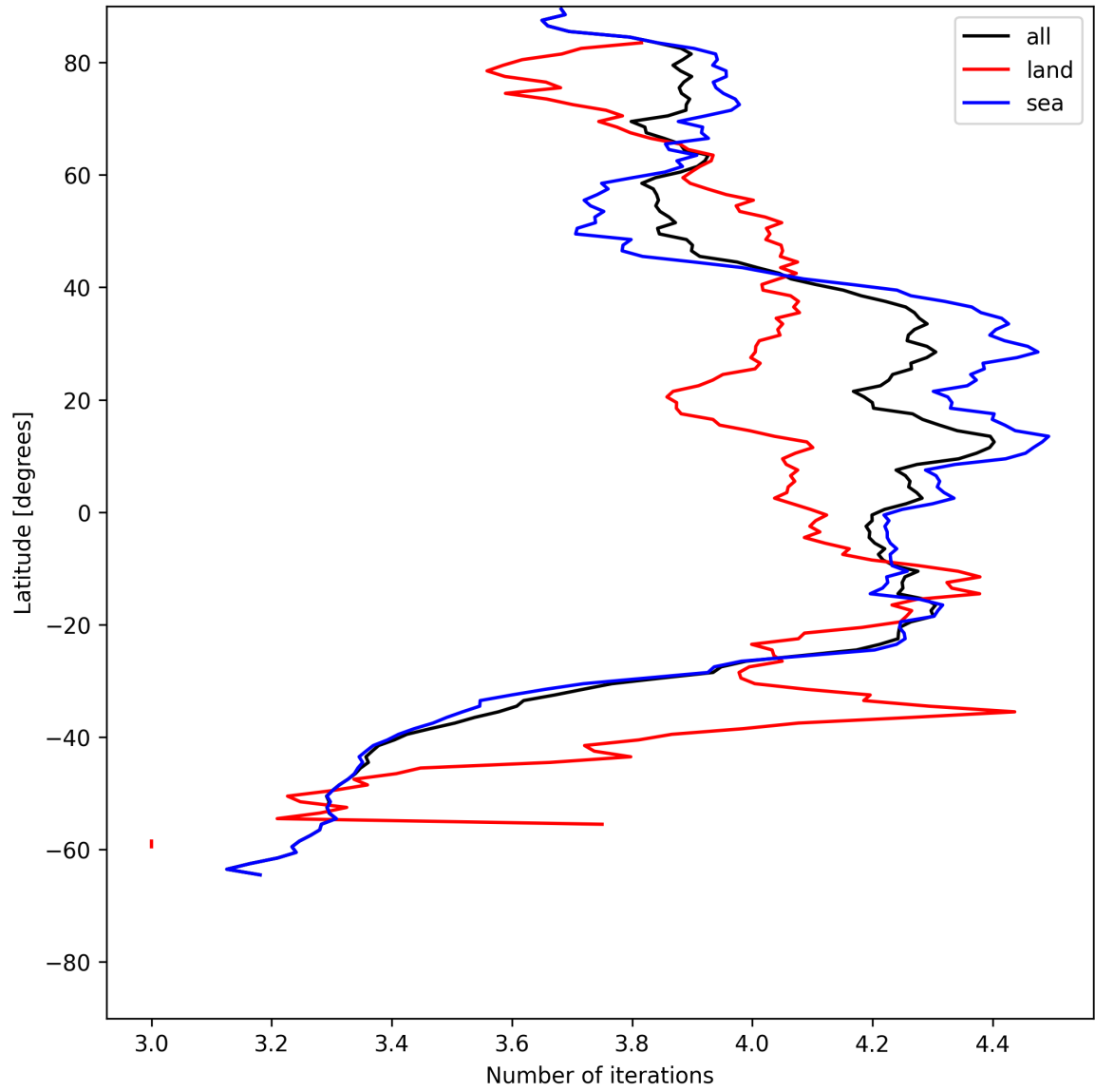
Figure 17: Zonal average of “Number of iterations” for 2025-07-04 to 2025-07-06.
