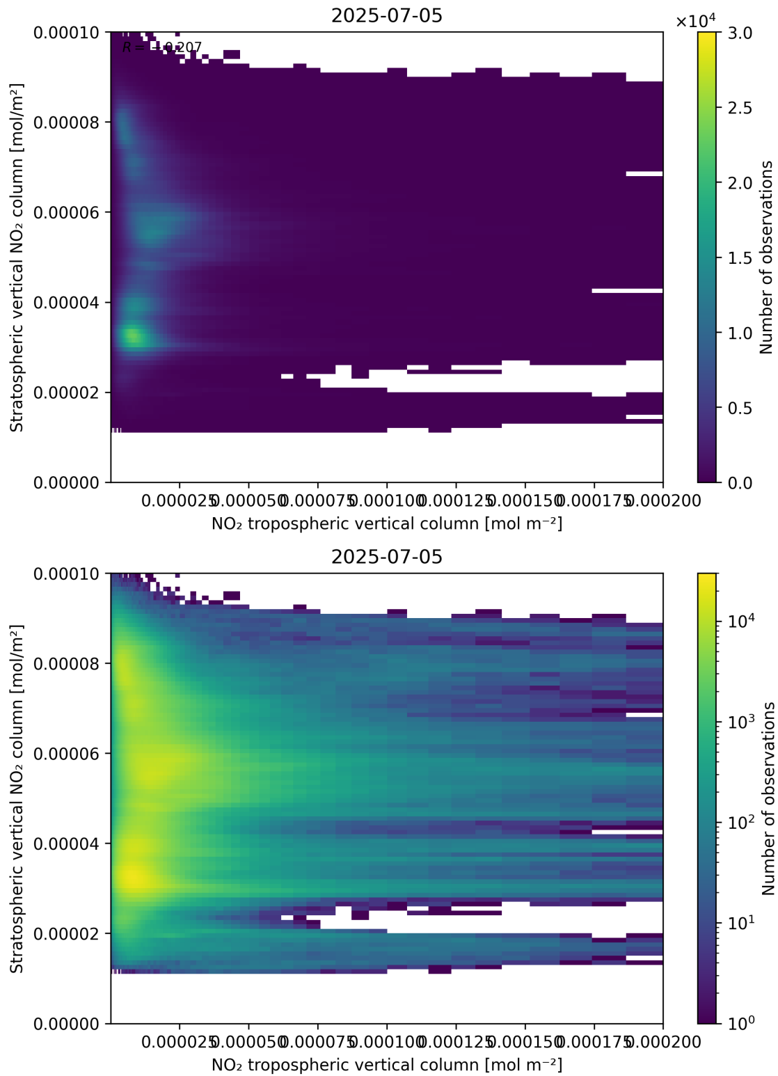
Figure 125: Scatter density plot of “NO 2 tropospheric vertical column” against “Stratospheric vertical NO 2 column” for 2025-07-04 to 2025-07-06.
