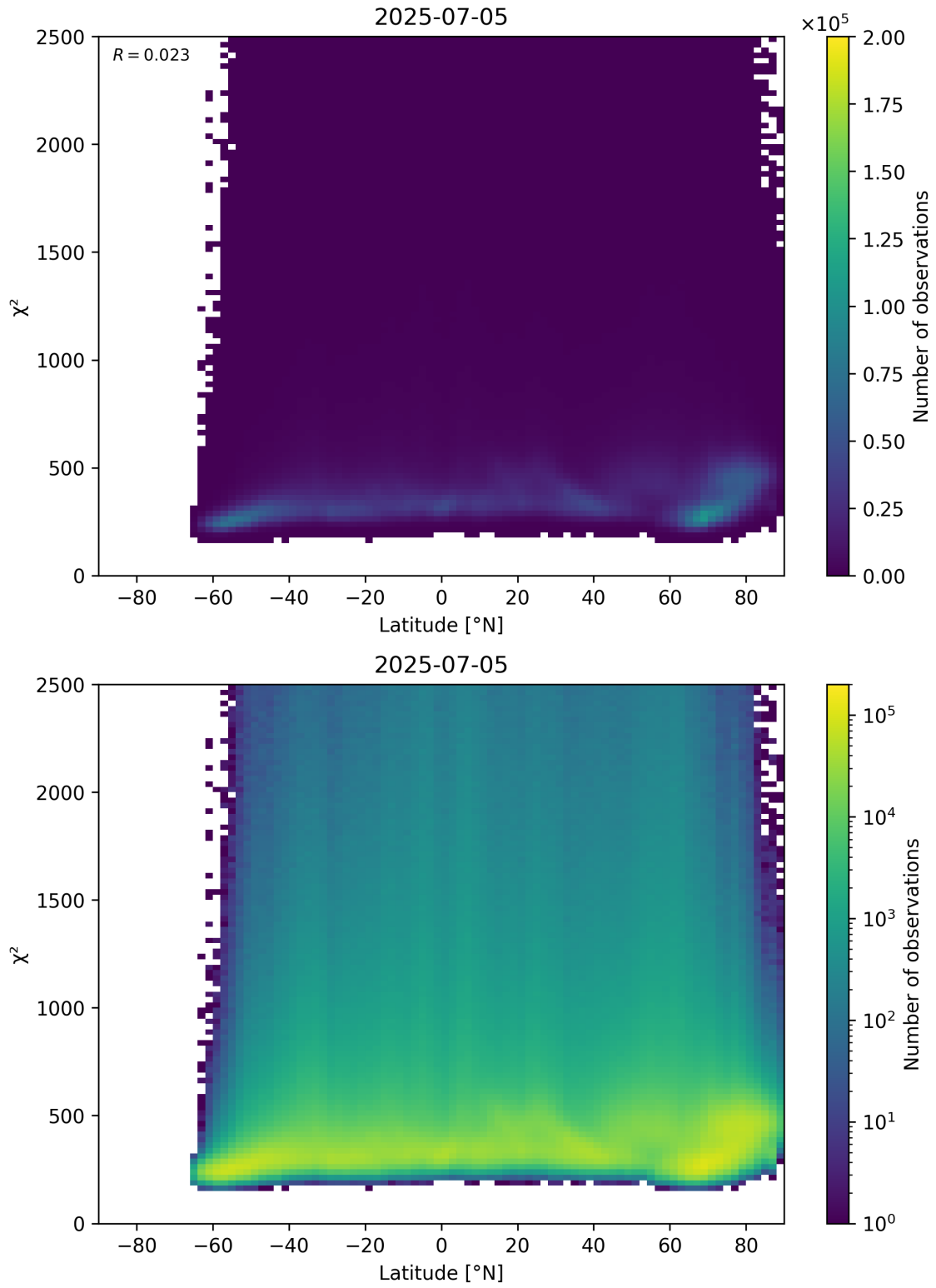
Figure 86: Scatter density plot of “Latitude” against “ \chi^2 ” for 2025-07-04 to 2025-07-06.
