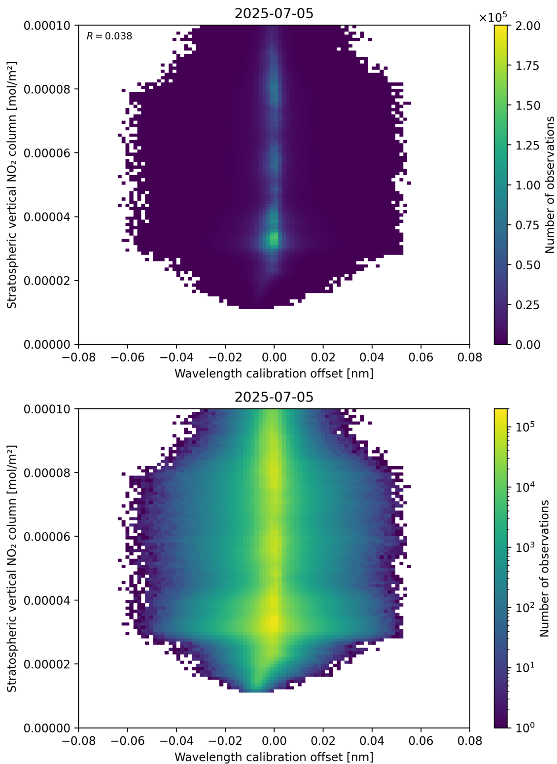
Figure 176: Scatter density plot of “Wavelength calibration offset” against “Stratospheric vertical NO 2 column” for 2025-07-04 to 2025-07-06.
