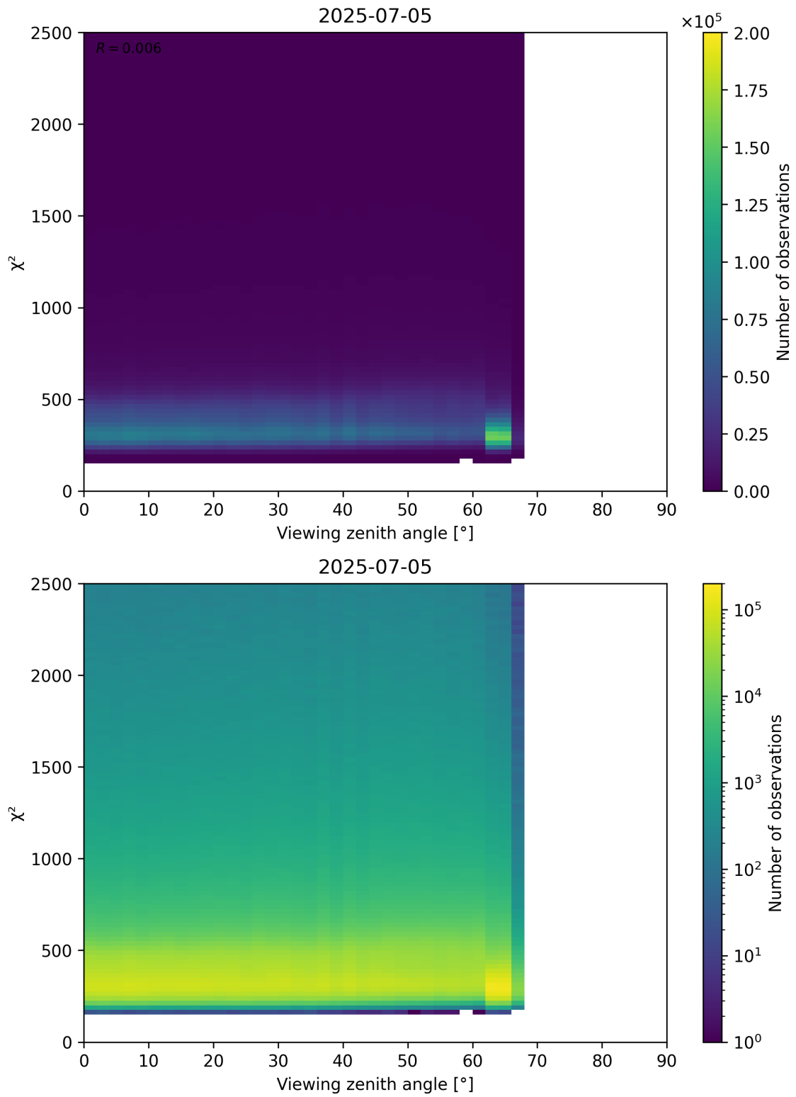
Figure 162: Scatter density plot of “Viewing zenith angle” against “ \chi^2 ” for 2025-07-04 to 2025-07-06.
