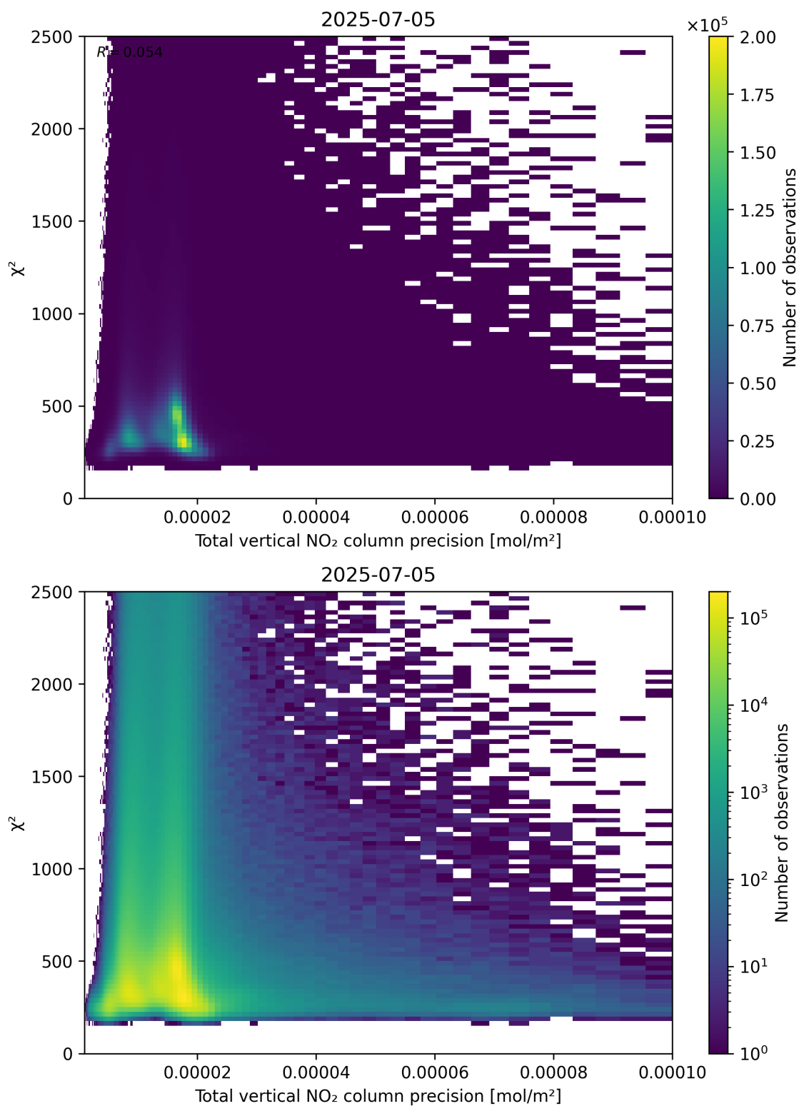
Figure 116: Scatter density plot of “Total vertical NO 2 column precision” against “ \chi^2 ” for 2025-07-04 to 2025-07-06.
