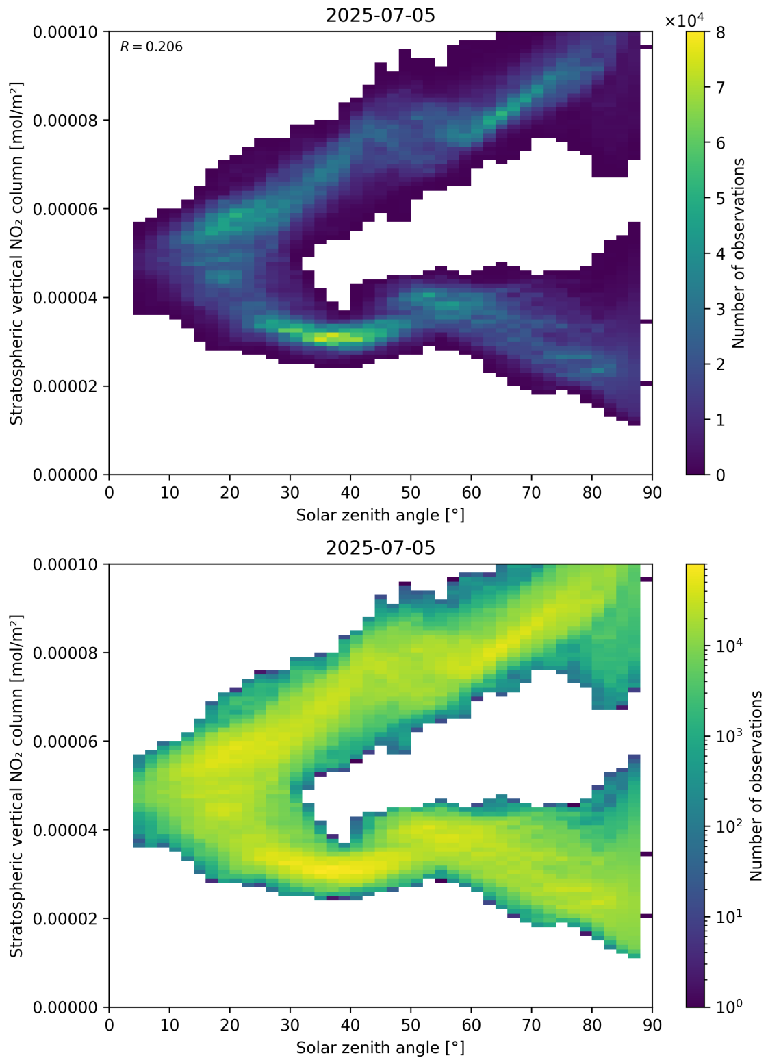
Figure 150: Scatter density plot of “Solar zenith angle” against “Stratospheric vertical NO 2 column” for 2025-07-04 to 2025-07-06.
