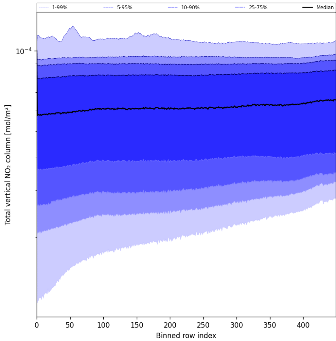
Figure 55: Along track statistics of “Total vertical NO 2 column” for 2025-07-04 to 2025-07-06
