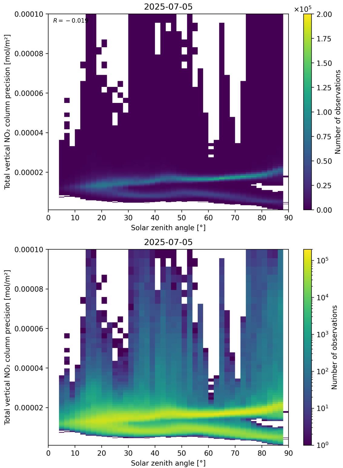
Figure 154: Scatter density plot of “Solar zenith angle” against “Total vertical NO 2 column precision” for 2025-07-04 to 2025-07-06.
