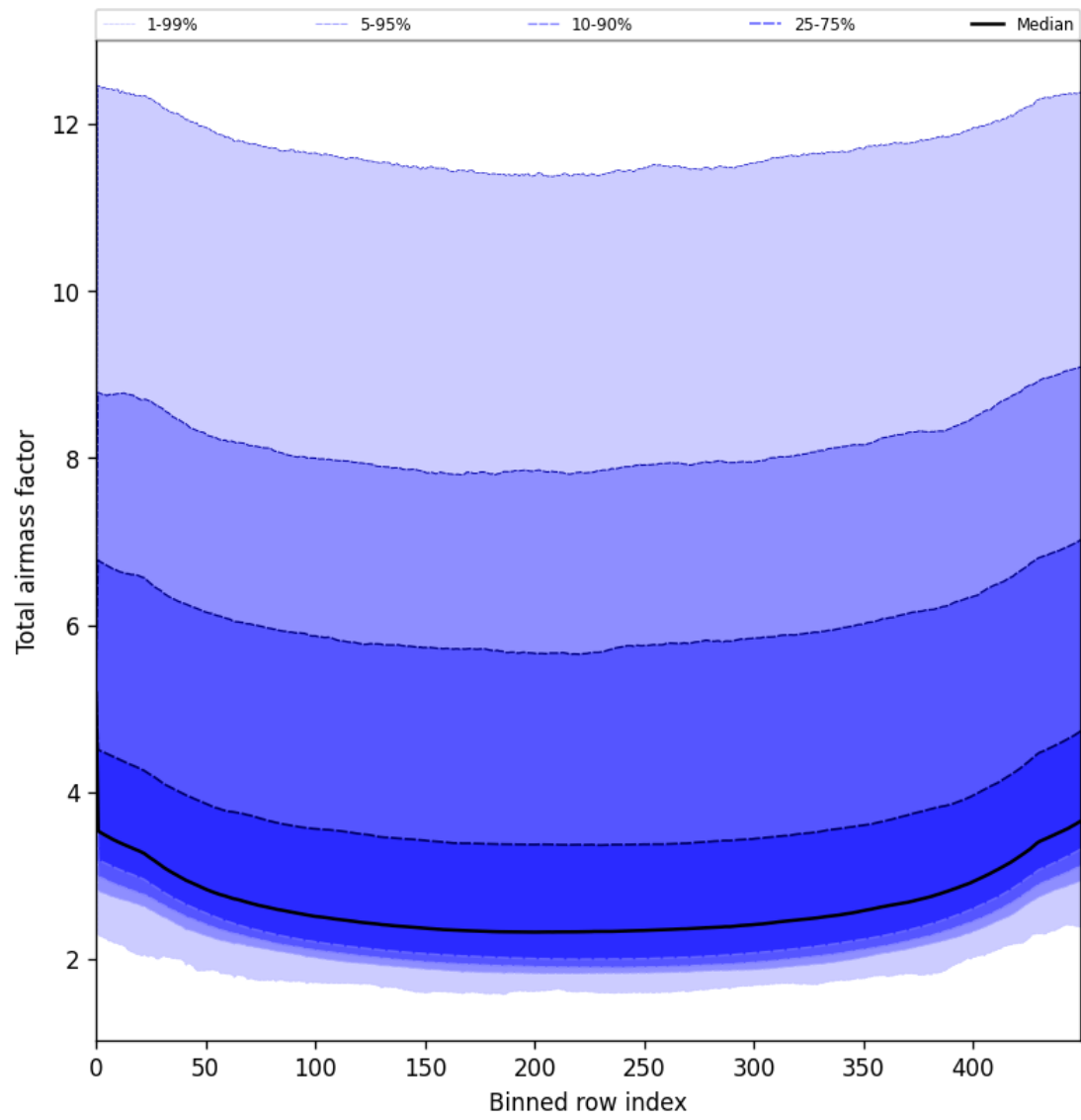
Figure 49: Along track statistics of “Total airmass factor” for 2025-07-04 to 2025-07-06
