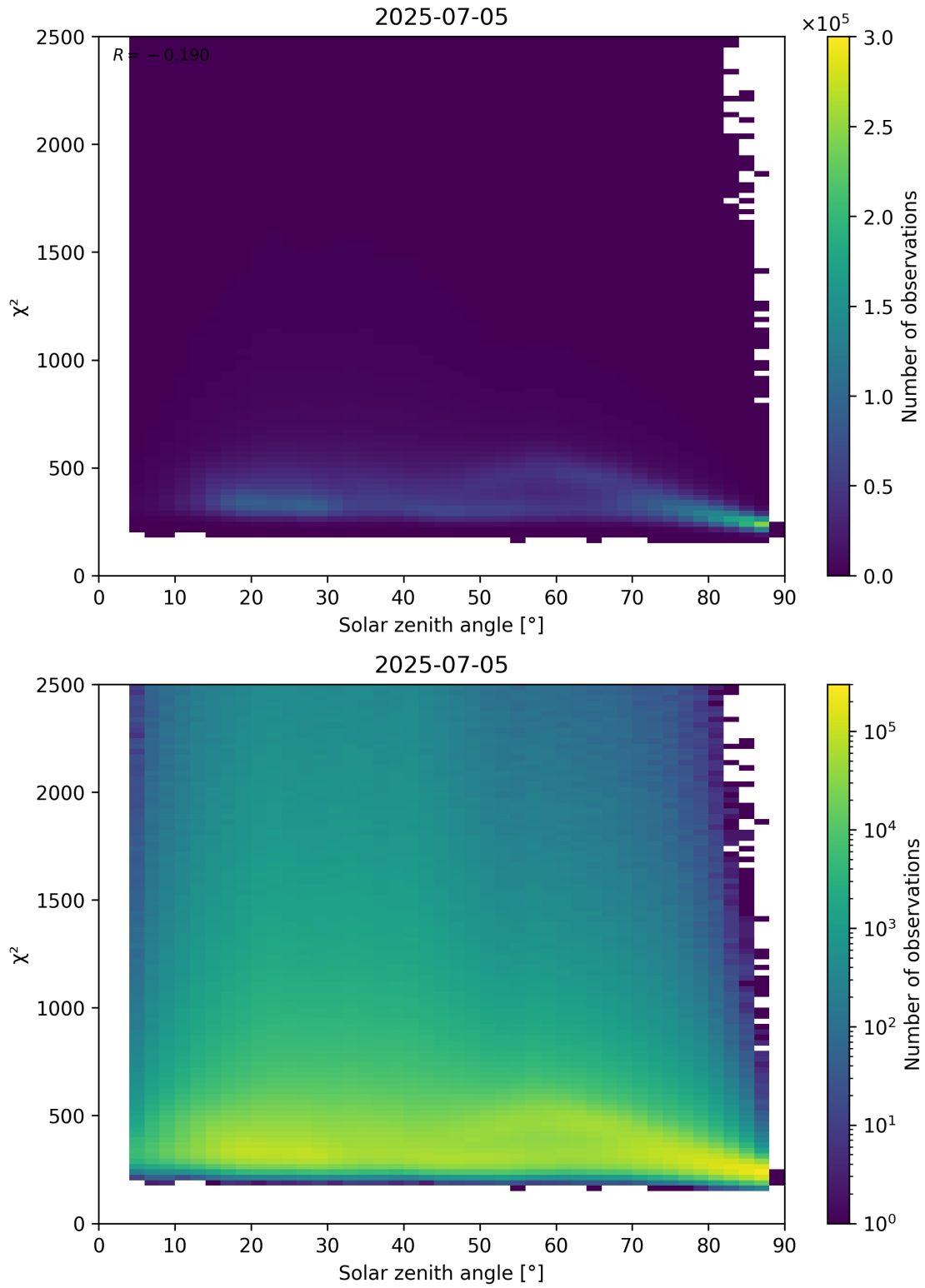
Figure 148: Scatter density plot of “Solar zenith angle” against “ \chi^2 ” for 2025-07-04 to 2025-07-06.
