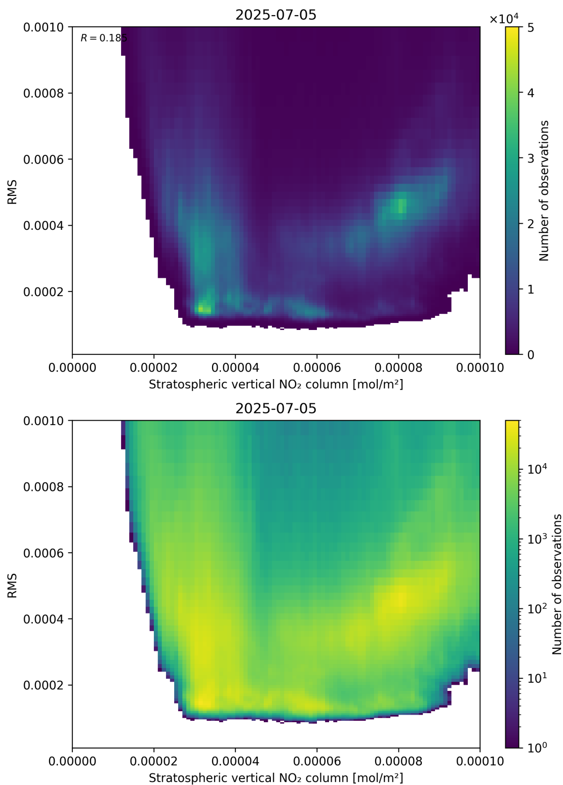
Figure 102: Scatter density plot of “Stratospheric vertical NO 2 column” against “RMS” for 2025-07-04 to 2025-07-06.
