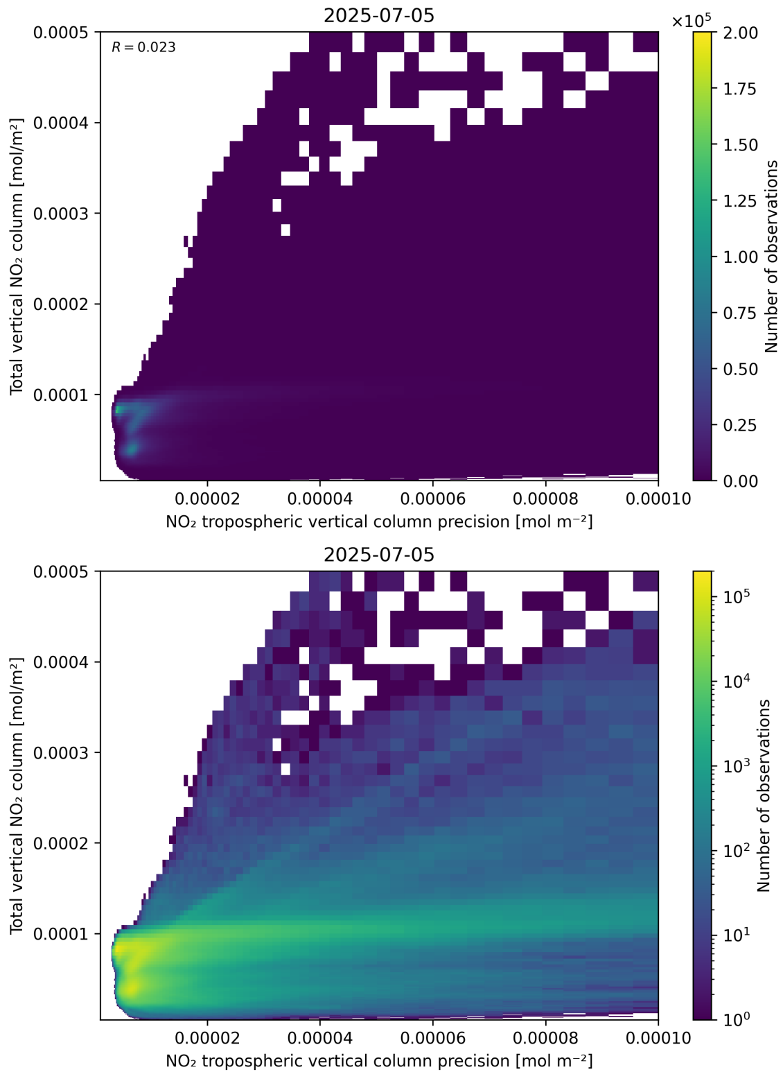
Figure 138: Scatter density plot of “NO 2 tropospheric vertical column precision” against “Total vertical NO 2 column” for 2025-07-04 to 2025-07-06.
