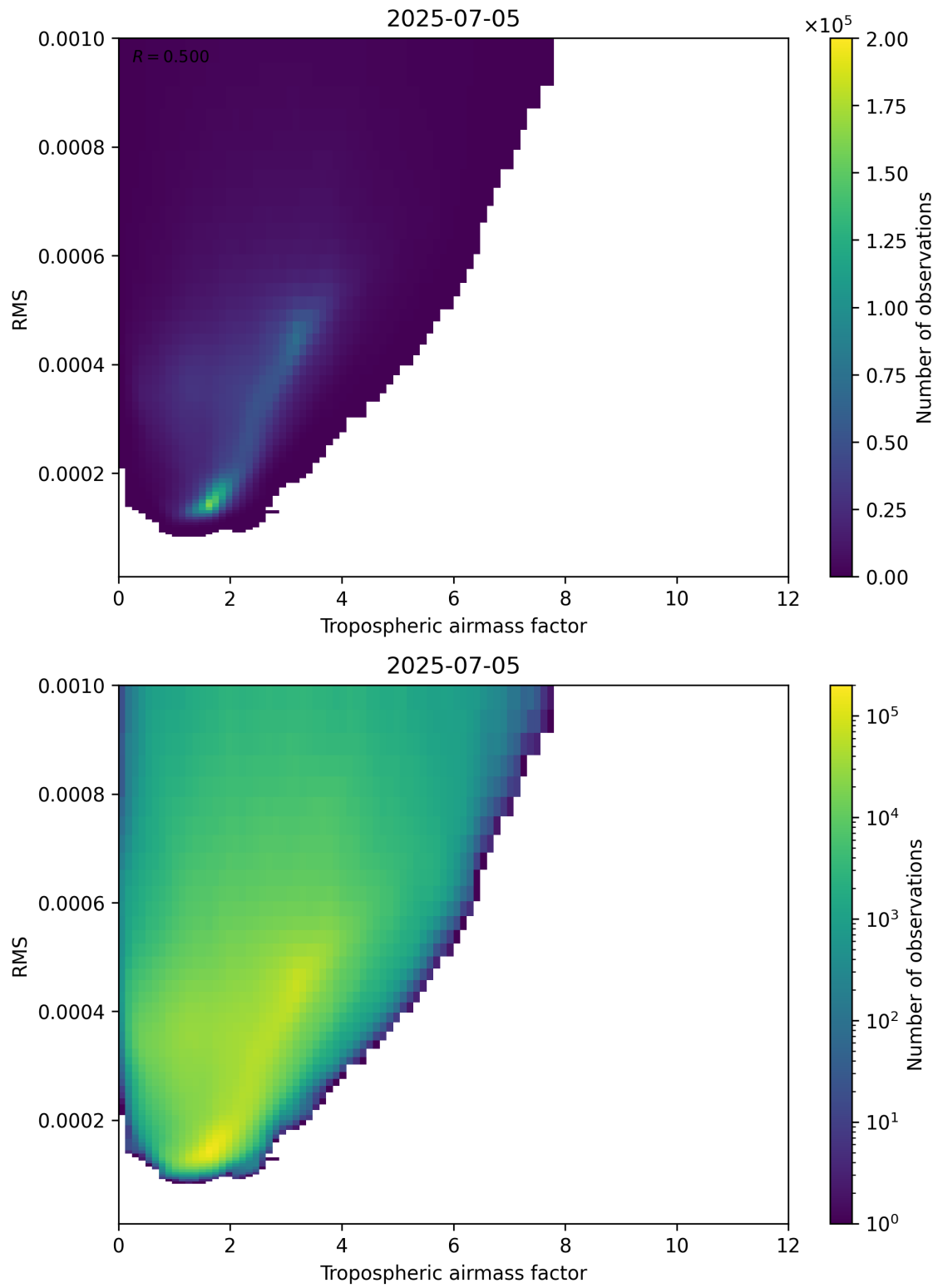
Figure 79: Scatter density plot of “Tropospheric airmass factor” against “RMS” for 2025-07-04 to 2025-07-06.
