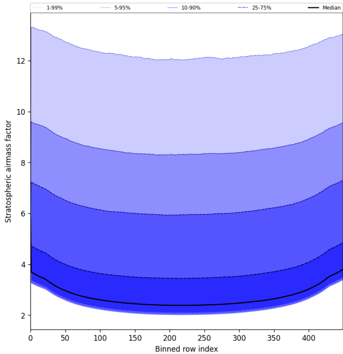
Figure 61: Along track statistics of “Stratospheric airmass factor” for 2025-07-04 to 2025-07-06
