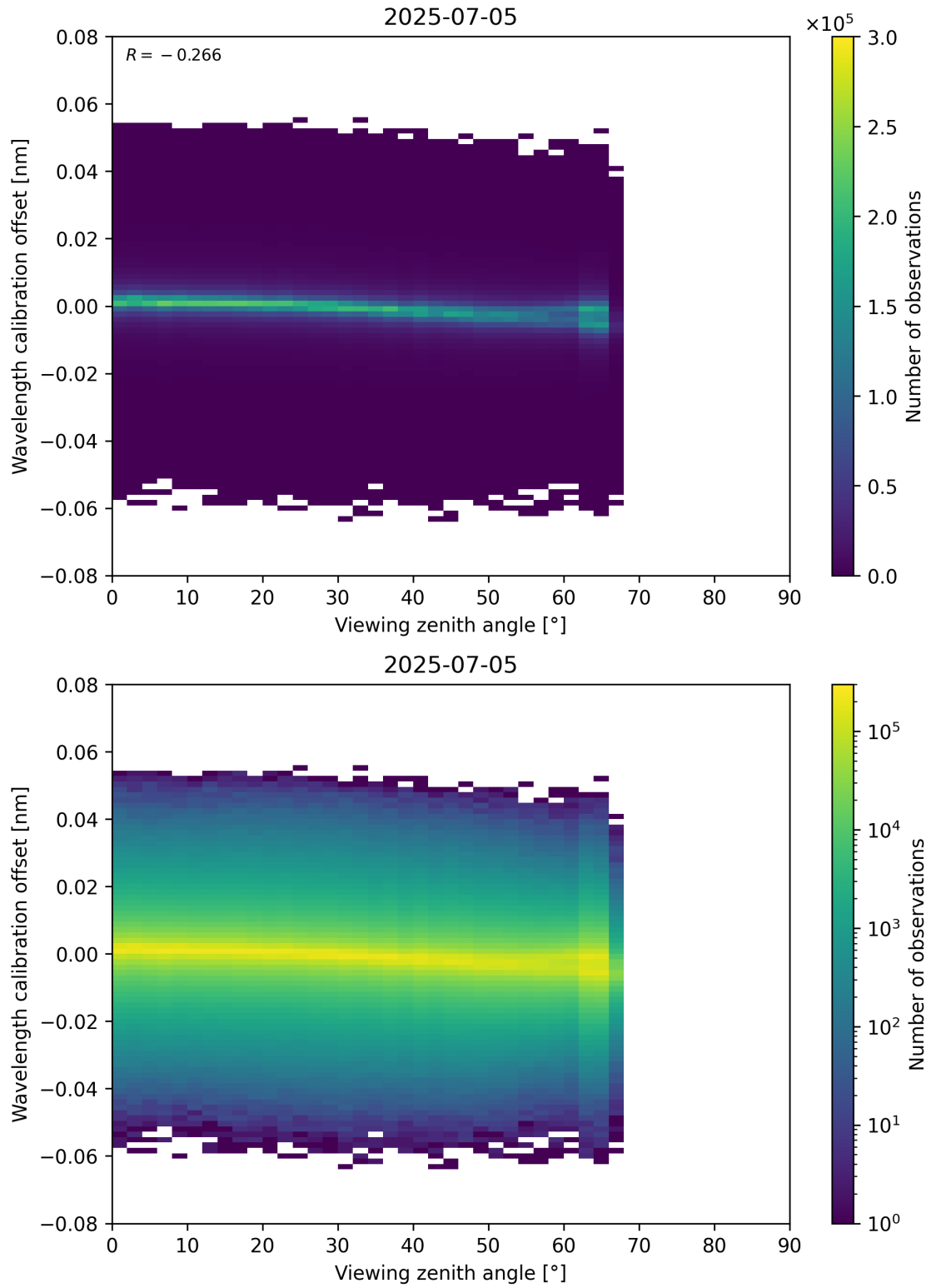
Figure 173: Scatter density plot of “Viewing zenith angle” against “Wavelength calibration offset” for 2025-07-04 to 2025-07-06.
