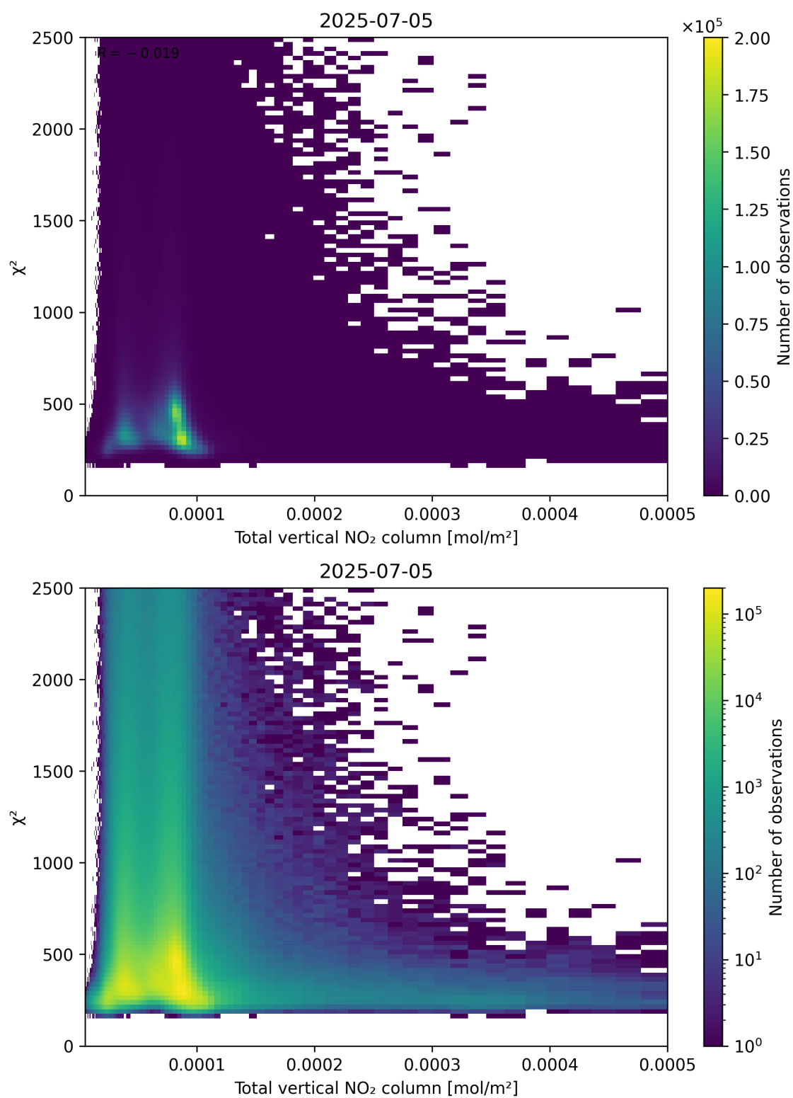
Figure 111: Scatter density plot of “Total vertical NO 2 column” against “ \chi^2 ” for 2025-07-04 to 2025-07-06.
