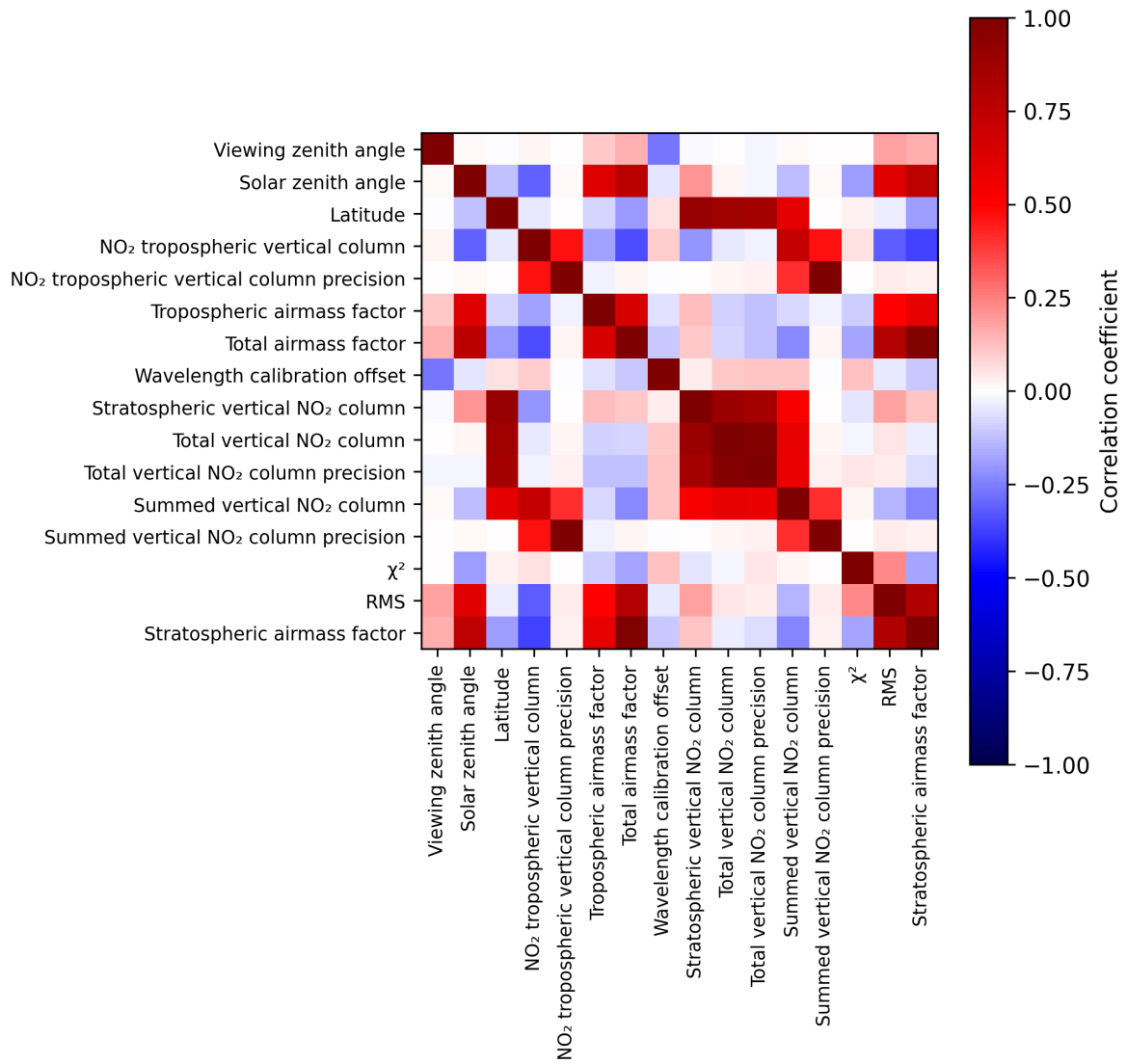
Figure 2: Map of correlation matrix for 2025-07-04 to 2025-07-06.
