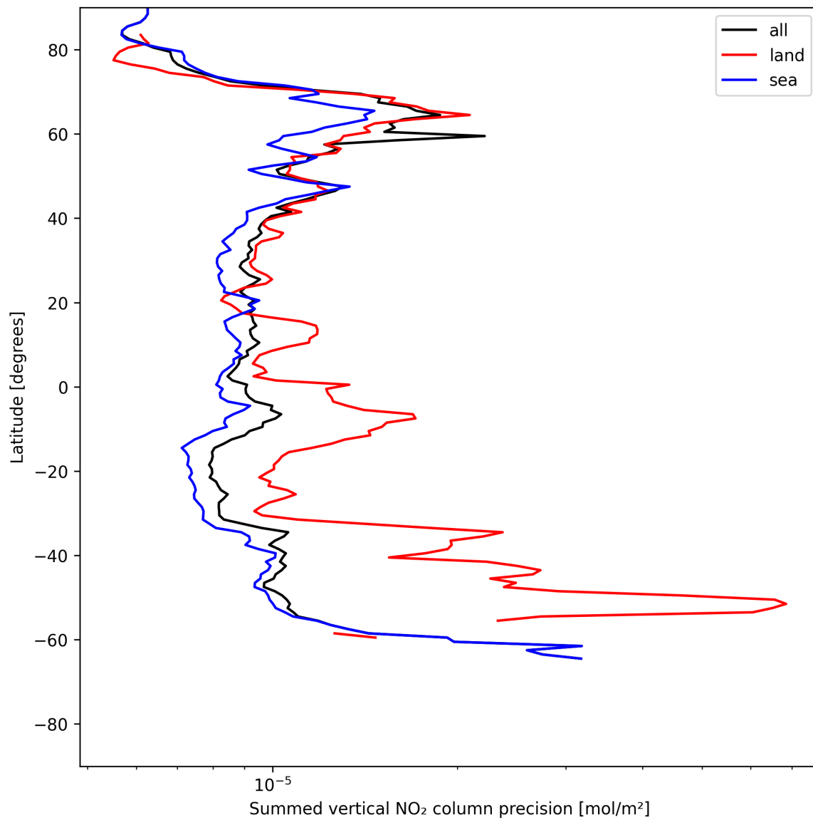
Figure 24: Zonal average of “Summed vertical NO 2 column precision” for 2025-07-04 to 2025-07-06.
