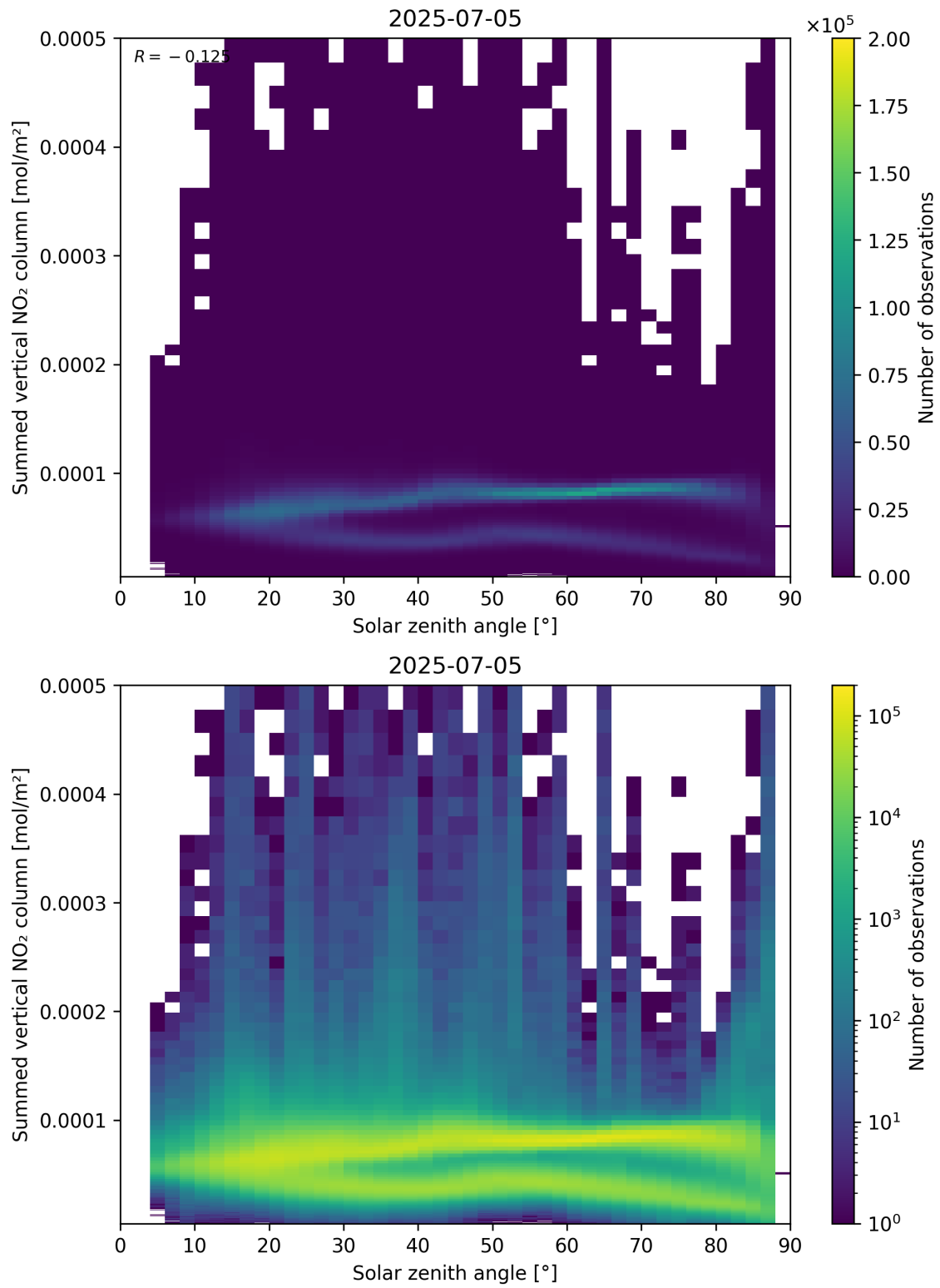
Figure 151: Scatter density plot of “Solar zenith angle” against “Summed vertical NO 2 column” for 2025-07-04 to 2025-07-06.
