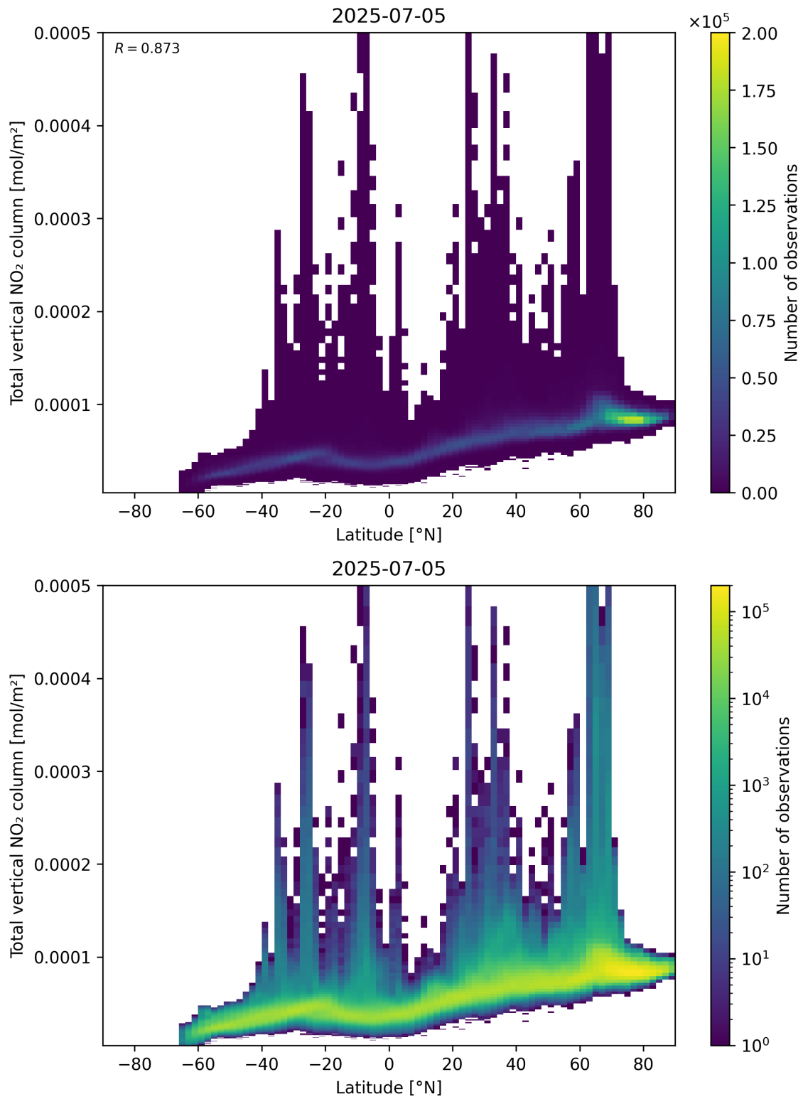
Figure 90: Scatter density plot of “Latitude” against “Total vertical NO 2 column” for 2025-07-04 to 2025-07-06.
