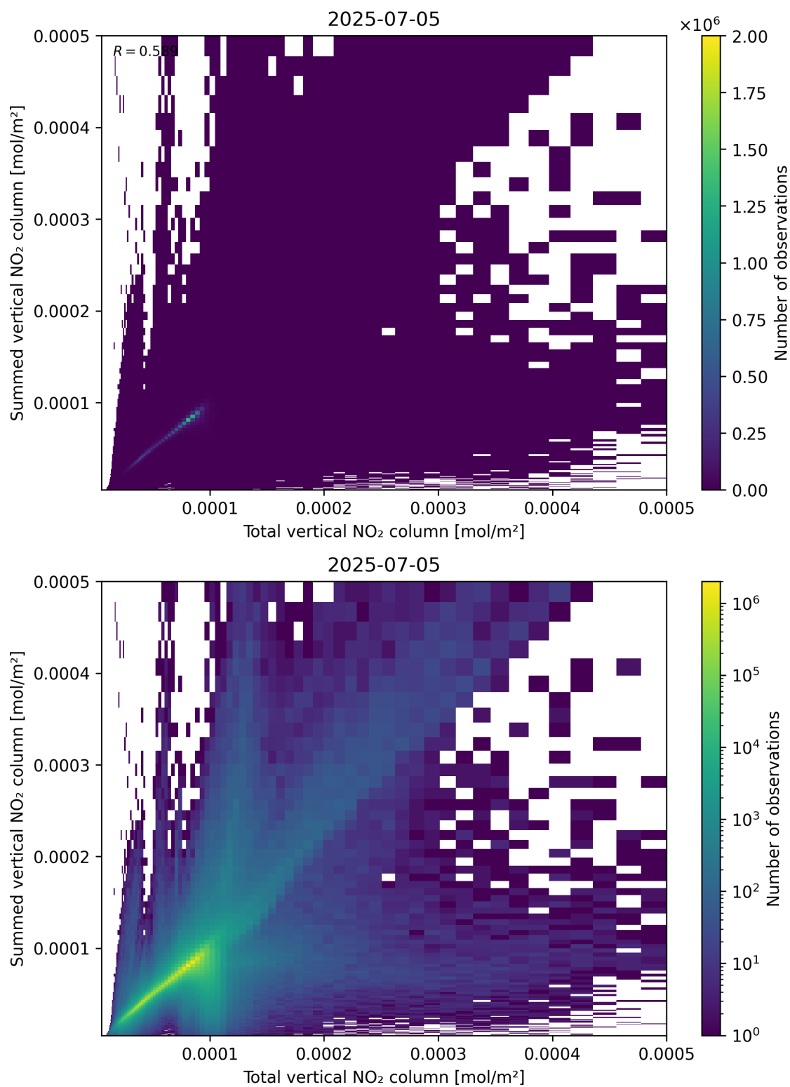
Figure 112: Scatter density plot of “Total vertical NO 2 column” against “Summed vertical NO 2 column” for 2025-07-04 to 2025-07-06.
