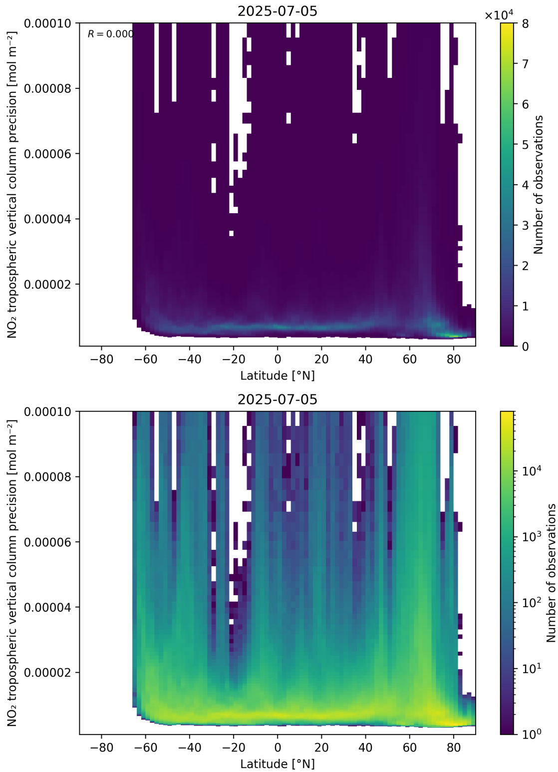
Figure 93: Scatter density plot of “Latitude” against “NO 2 tropospheric vertical column precision” for 2025-07-04 to 2025-07-06.
