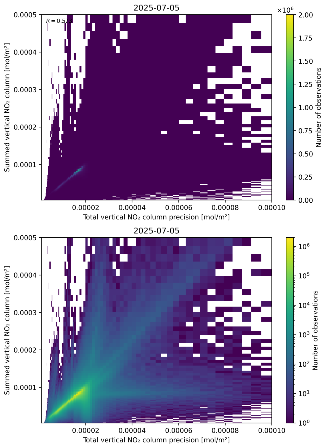
Figure 117: Scatter density plot of “Total vertical NO 2 column precision” against “Summed vertical NO 2 column” for 2025-07-04 to 2025-07-06.
