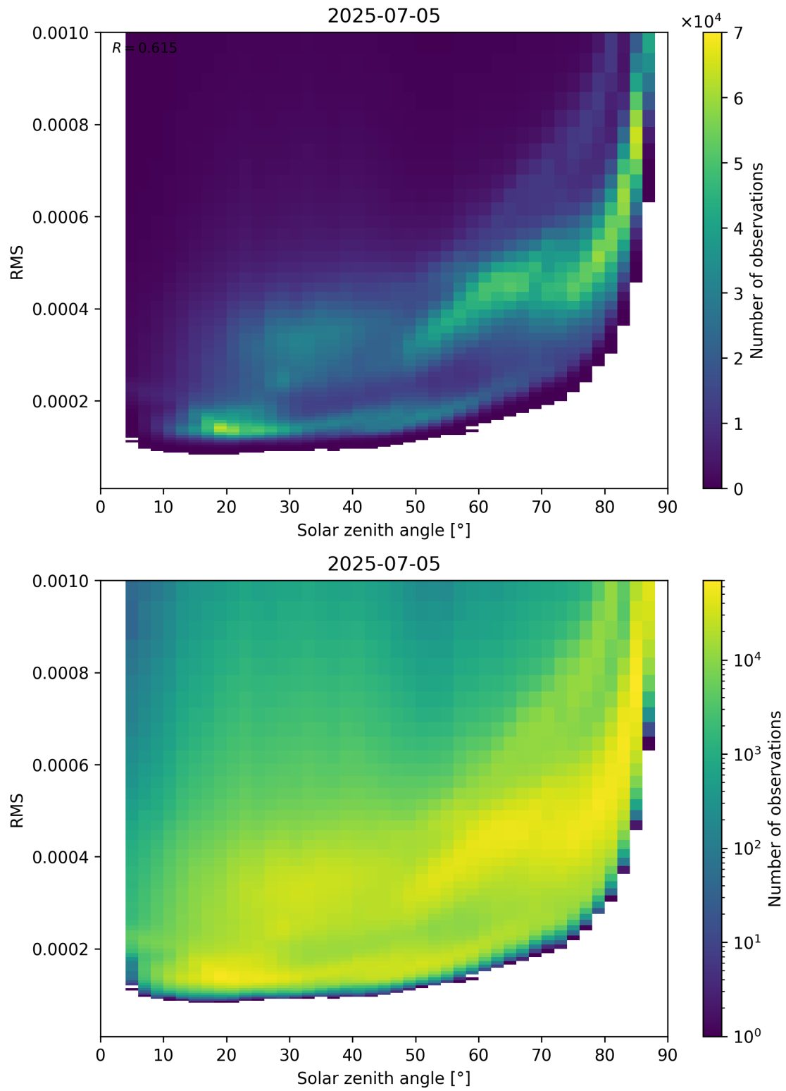
Figure 157: Scatter density plot of “Solar zenith angle” against “RMS” for 2025-07-04 to 2025-07-06.
