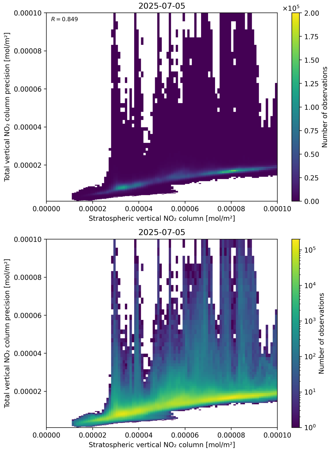
Figure 101: Scatter density plot of “Stratospheric vertical NO 2 column” against “Total vertical NO 2 column precision” for 2025-07-04 to 2025-07-06.
