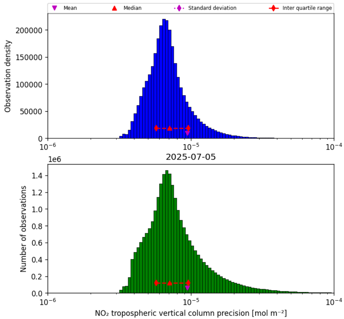
Figure 30: Histogram of “NO 2 tropospheric vertical column precision” for 2025-07-04 to 2025-07-06
