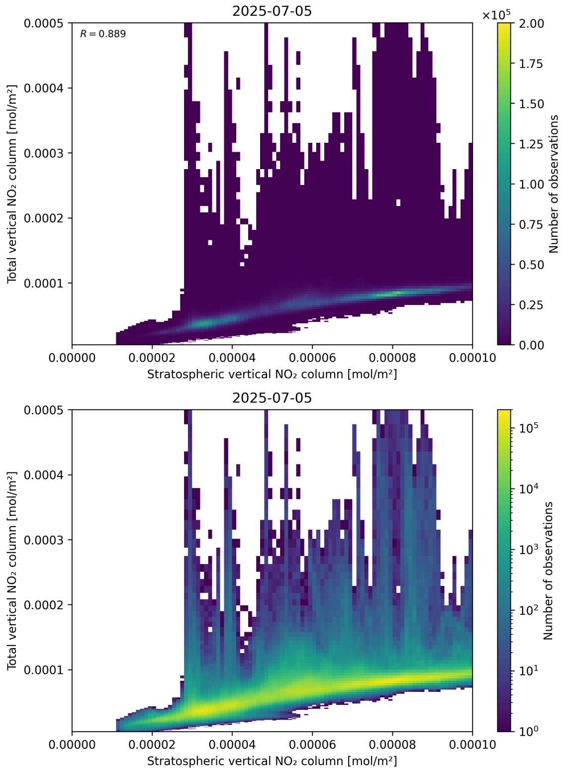
Figure 100: Scatter density plot of “Stratospheric vertical NO 2 column” against “Total vertical NO 2 column” for 2025-07-04 to 2025-07-06.
