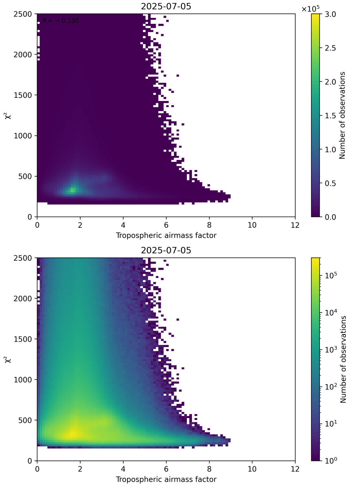
Figure 73: Scatter density plot of “Tropospheric airmass factor” against “ \chi^2 ” for 2025-07-04 to 2025-07-06.
