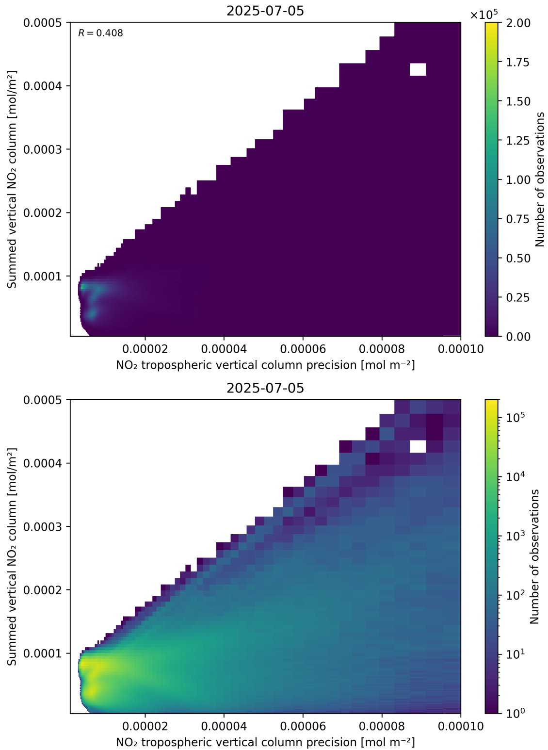
Figure 136: Scatter density plot of “NO 2 tropospheric vertical column precision” against “Summed vertical NO 2 column” for 2025-07-04 to 2025-07-06.
