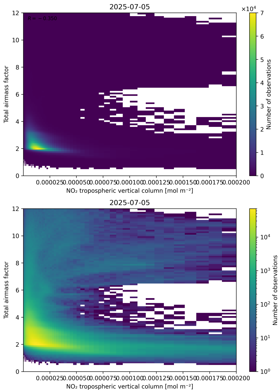
Figure 122: Scatter density plot of “NO 2 tropospheric vertical column” against “Total air mass factor” for 2025-07-04 to 2025-07-06.
