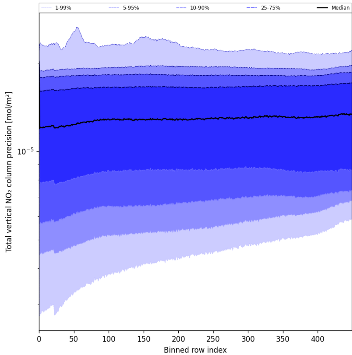
Figure 56: Along track statistics of “Total vertical NO 2 column precision” for 2025-07-04 to 2025-07-06
