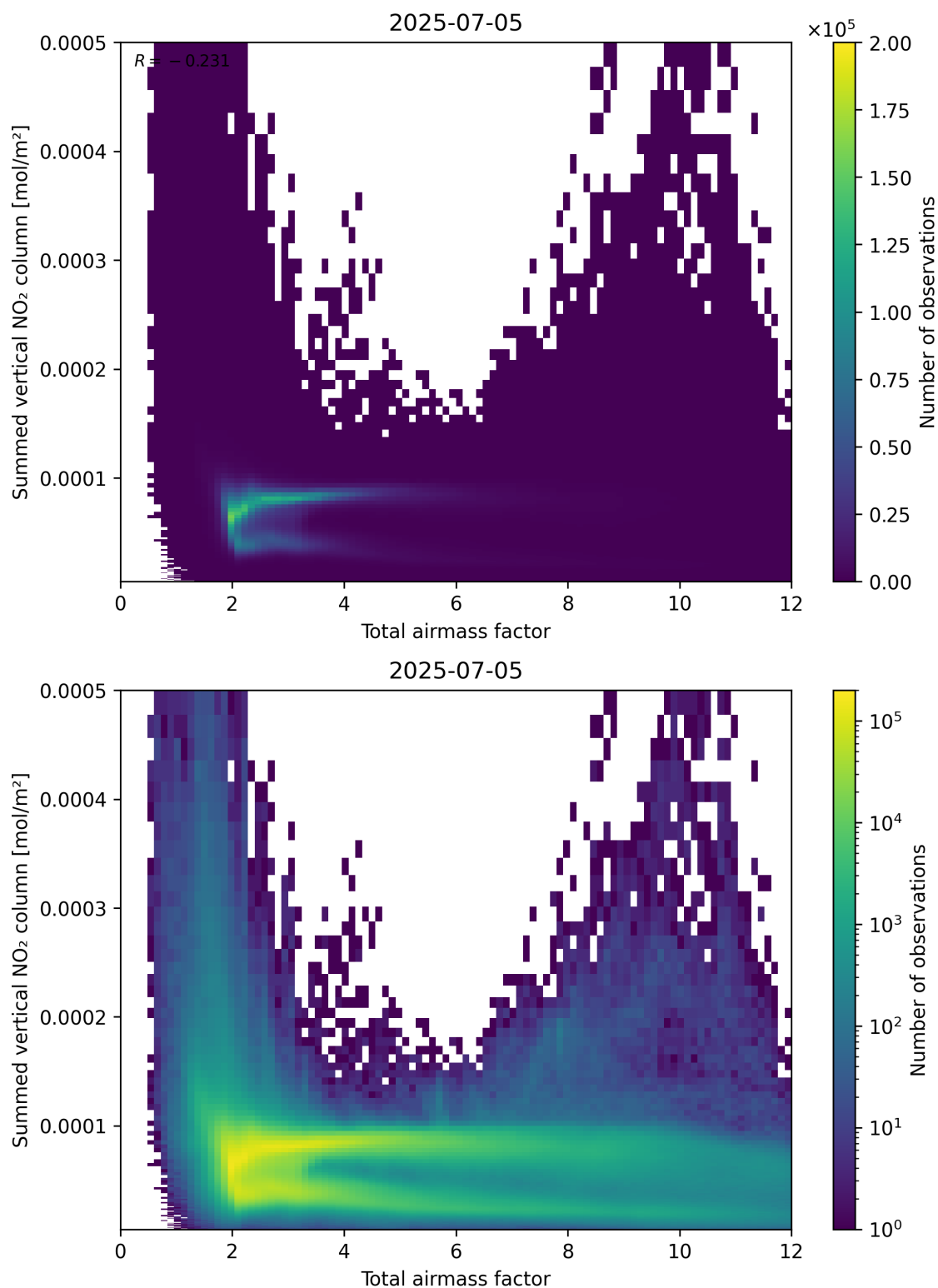
Figure 65: Scatter density plot of “Total airmass factor” against “Summed vertical NO 2 column” for 2025-07-04 to 2025-07-06.
