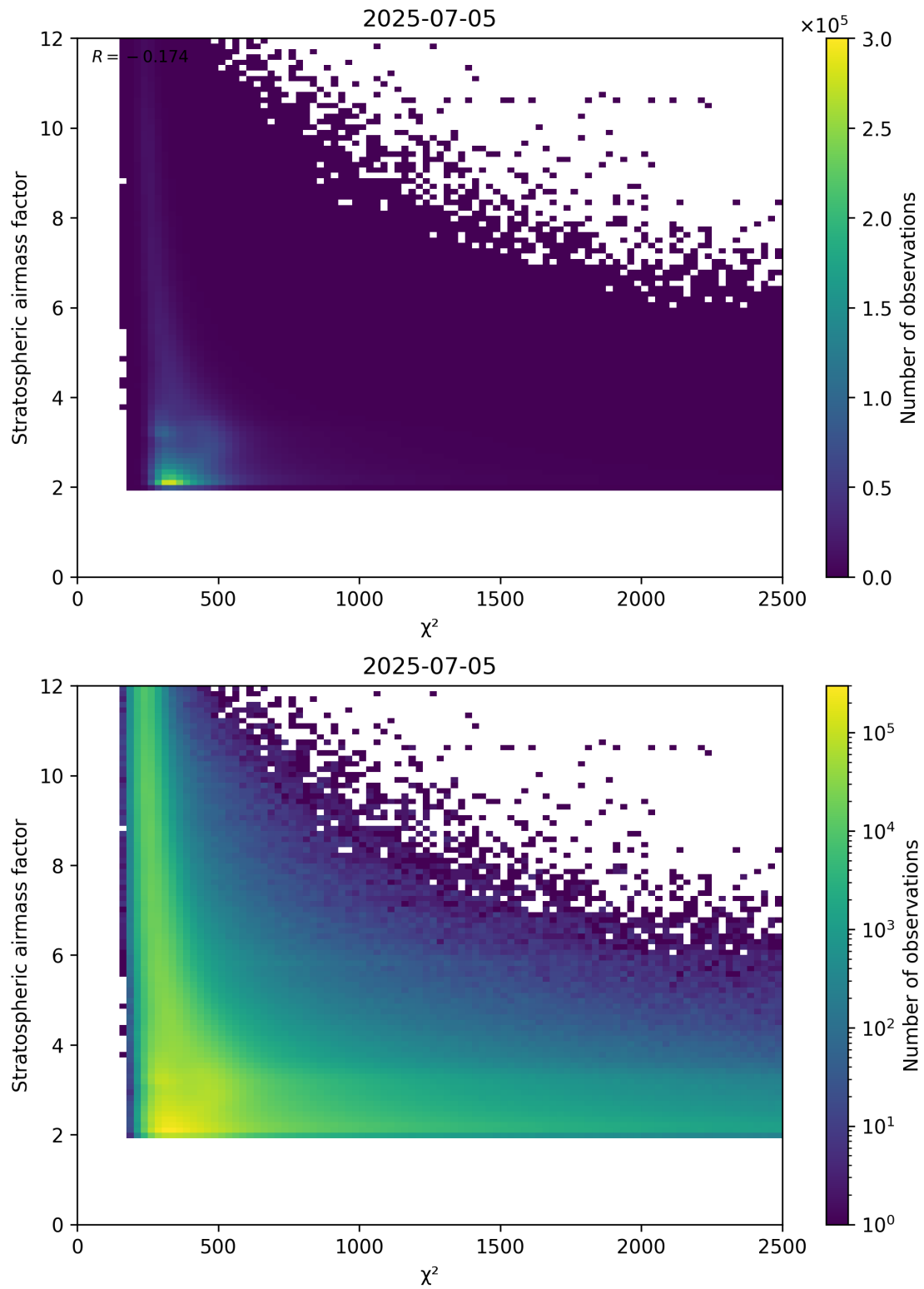
Figure 81: Scatter density plot of “ \chi^2 ” against “Stratospheric airmass factor” for 2025-07-04 to 2025-07-06.
