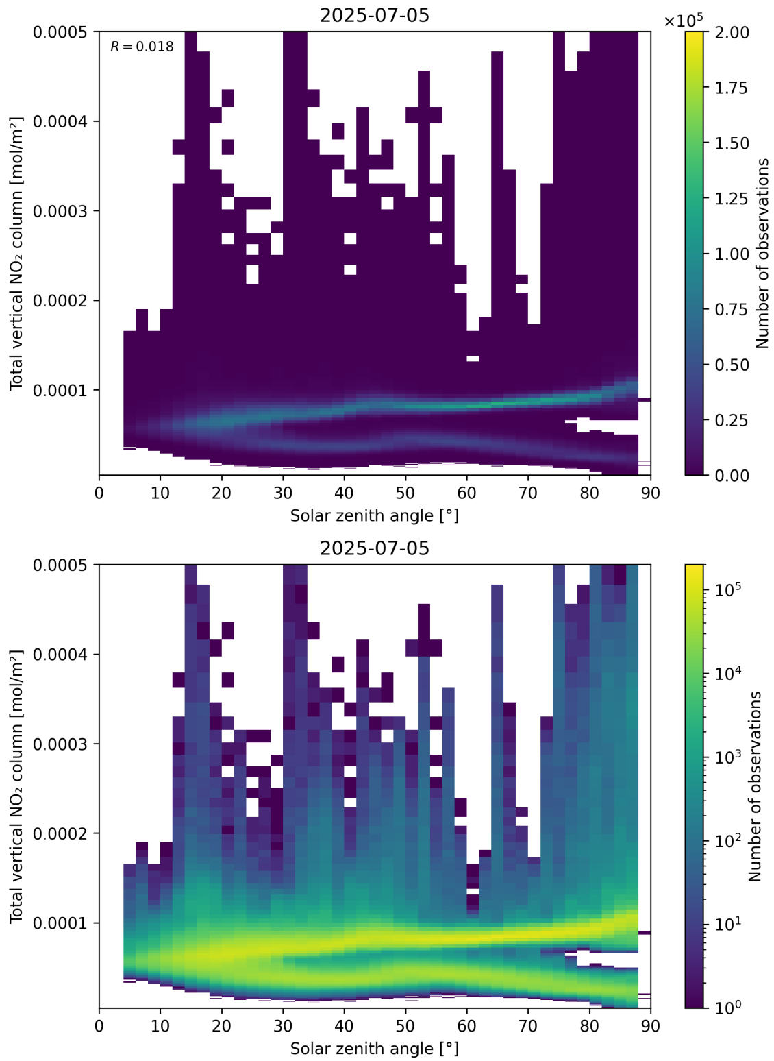
Figure 153: Scatter density plot of “Solar zenith angle” against “Total vertical NO 2 column” for 2025-07-04 to 2025-07-06.
