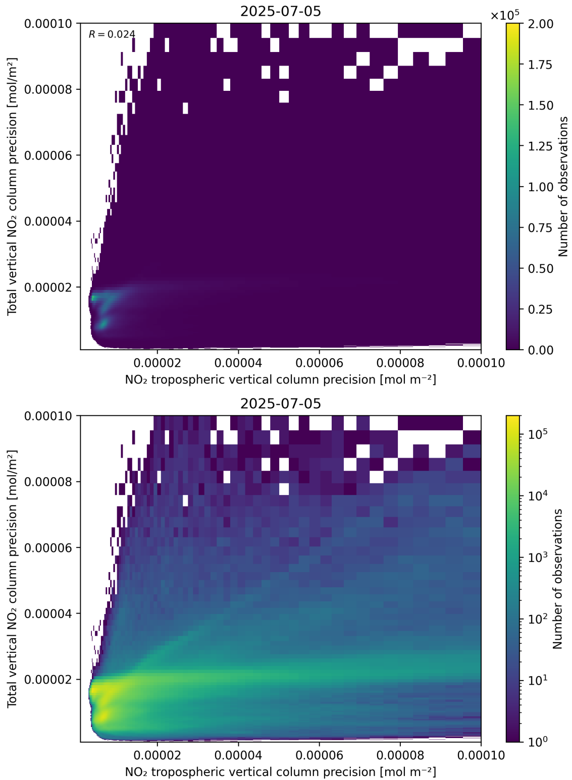
Figure 139: Scatter density plot of “NO 2 tropospheric vertical column precision” against “Total vertical NO 2 column precision” for 2025-07-04 to 2025-07-06.
