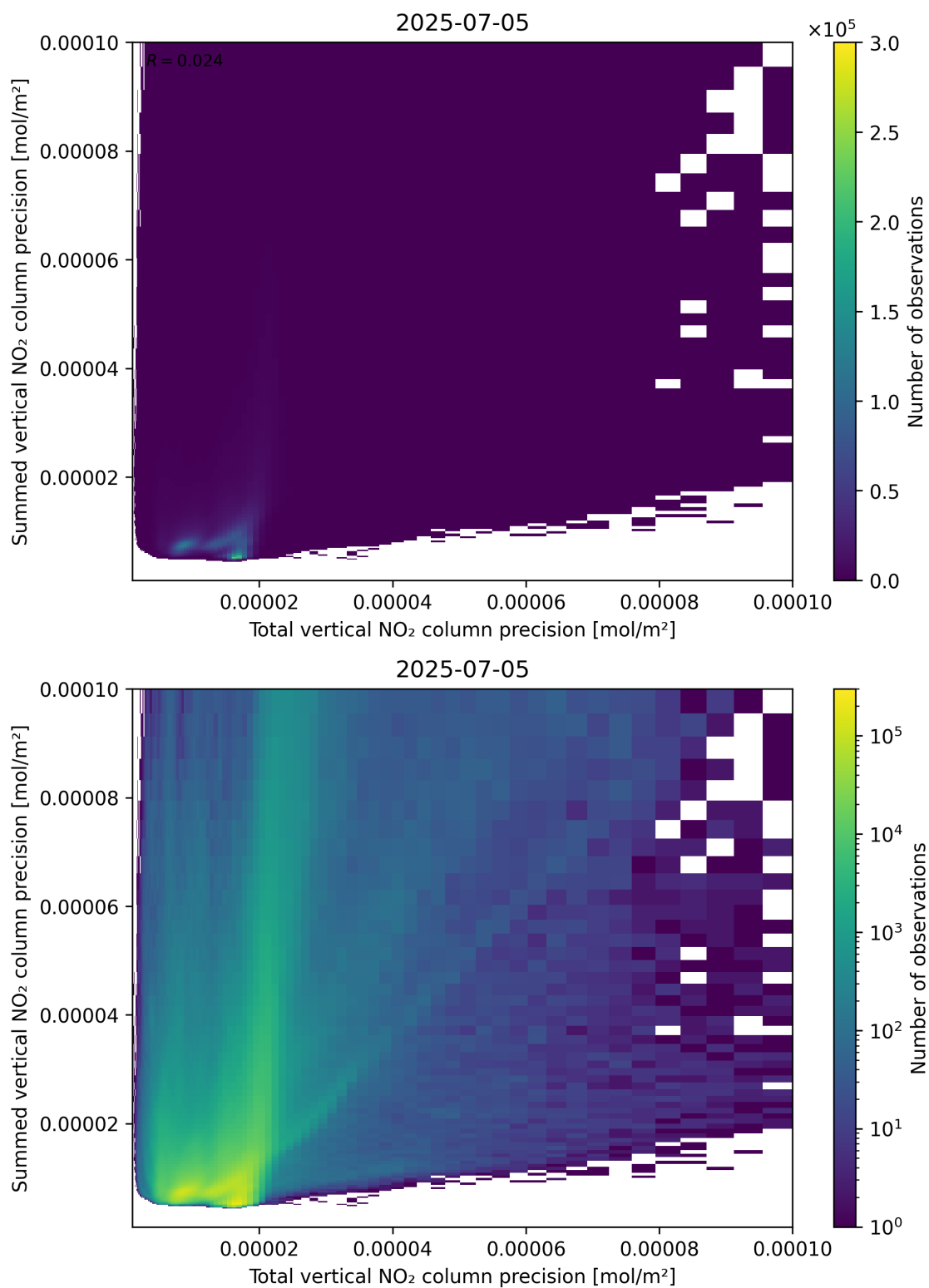
Figure 118: Scatter density plot of “Total vertical NO 2 column precision” against “Summed vertical NO 2 column precision” for 2025-07-04 to 2025-07-06.
