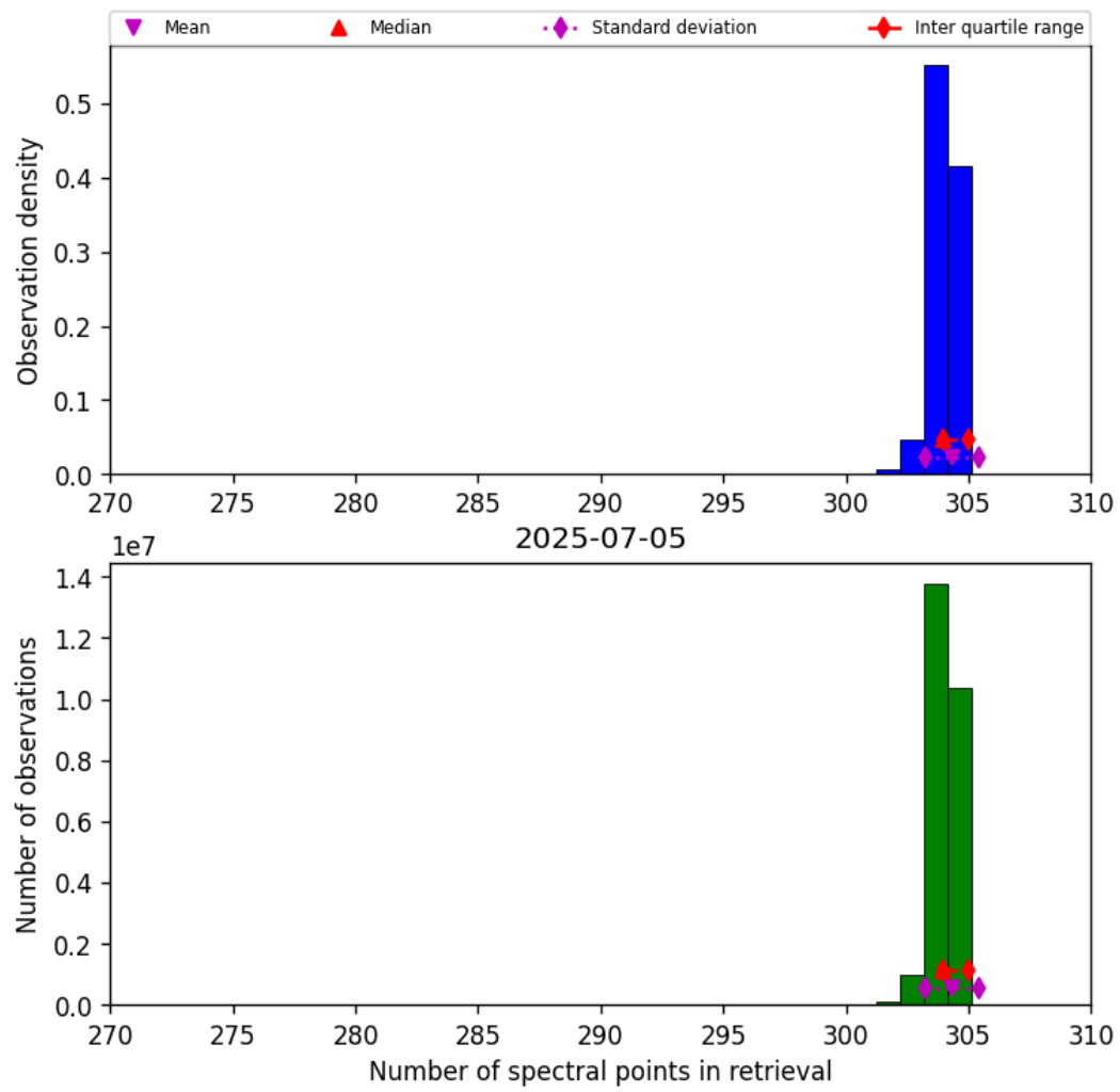
Figure 33: Histogram of “Number of spectral points in retrieval” for 2025-07-04 to 2025-07-06
