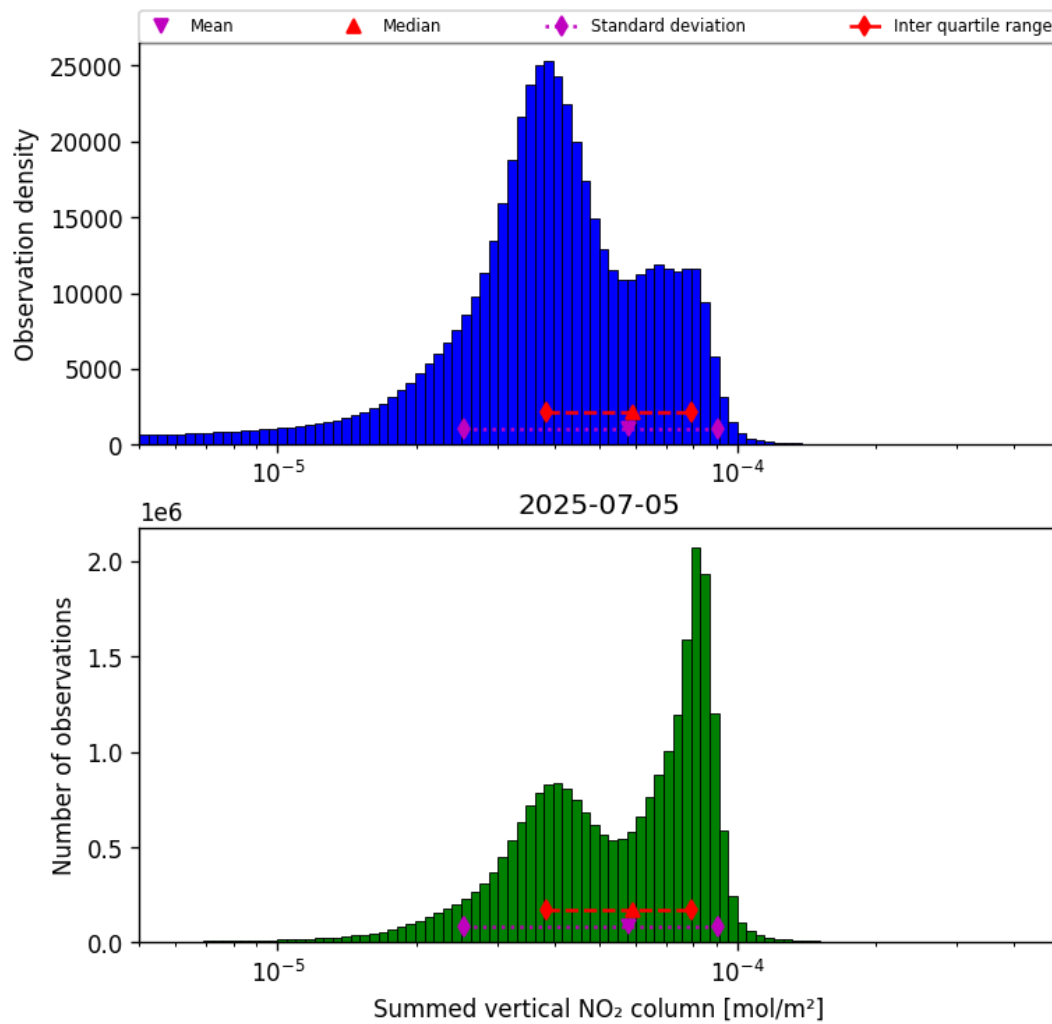
Figure 40: Histogram of “Summed vertical NO 2 column” for 2025-07-04 to 2025-07-06
