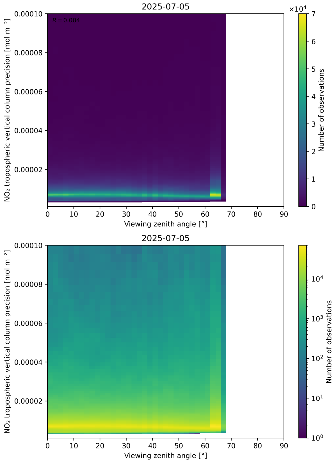
Figure 170: Scatter density plot of “Viewing zenith angle” against “NO 2 tropospheric vertical column precision” for 2025-07-04 to 2025-07-06.
