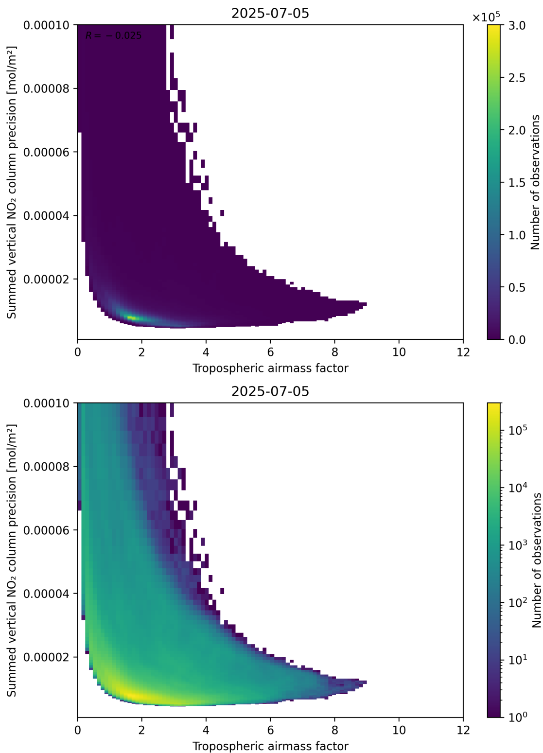
Figure 76: Scatter density plot of “Tropospheric air mass factor” against “Summed vertical NO 2 column precision” for 2025-07-04 to 2025-07-06.
