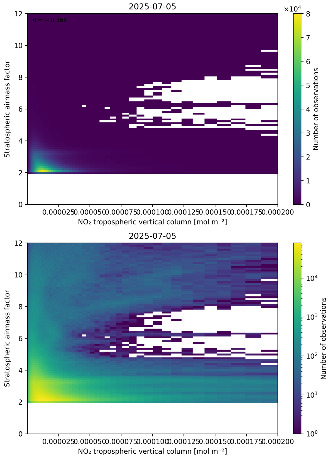
Figure 121: Scatter density plot of “NO 2 tropospheric vertical column” against “Stratospheric air mass factor” for 2025-07-04 to 2025-07-06.
