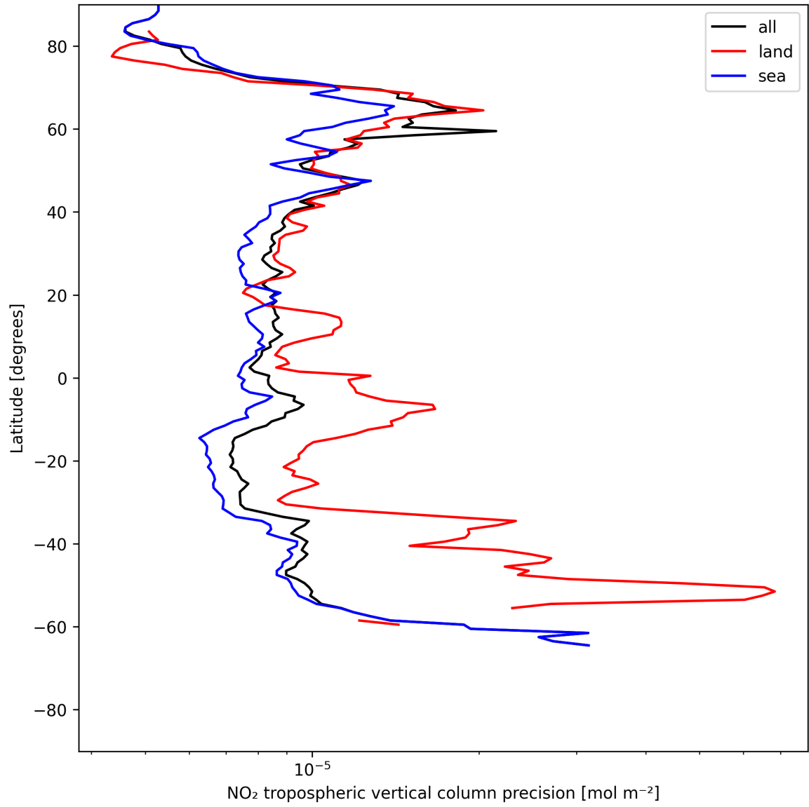
Figure 13: Zonal average of “NO 2 tropospheric vertical column precision” for 2025-07-04 to 2025-07-06.
