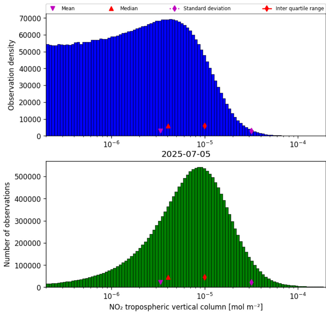
Figure 29: Histogram of “NO 2 tropospheric vertical column” for 2025-07-04 to 2025-07-06
