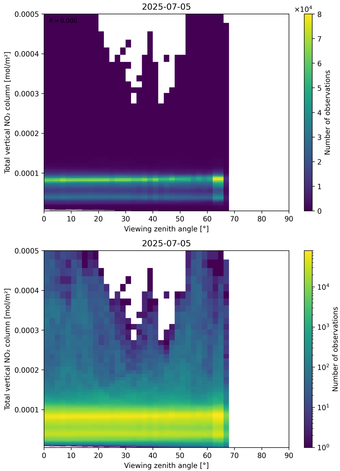
Figure 167: Scatter density plot of “Viewing zenith angle” against “Total vertical NO 2 column” for 2025-07-04 to 2025-07-06.
