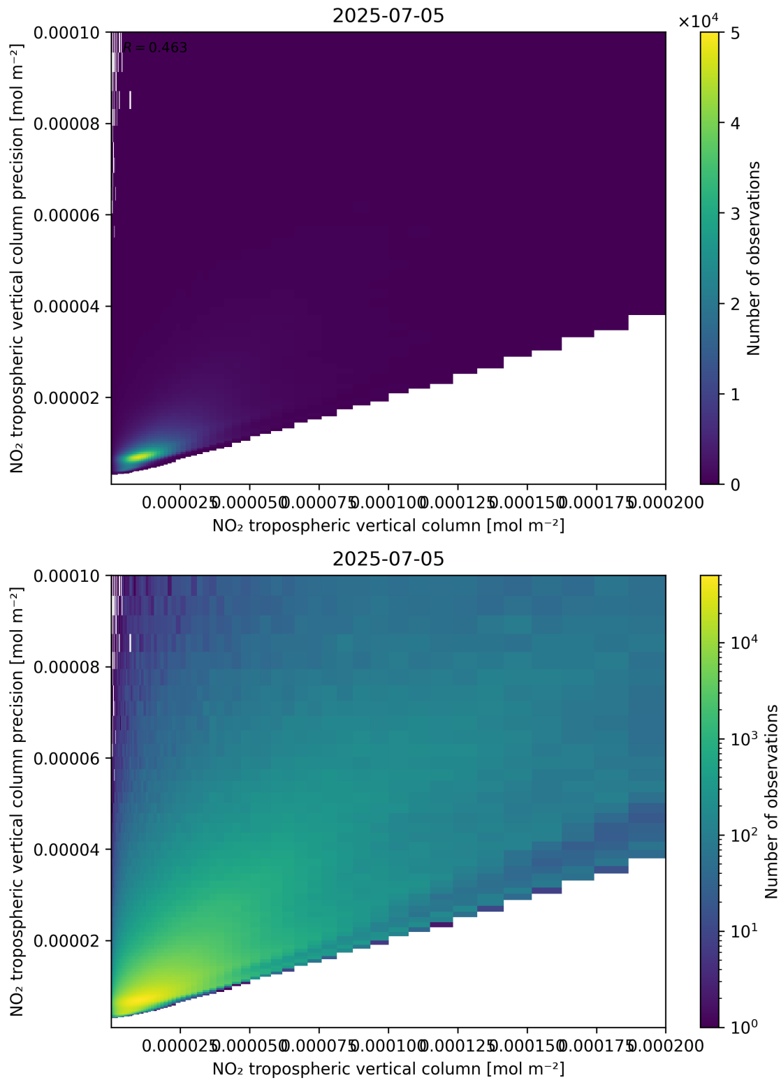
Figure 130: Scatter density plot of “NO 2 tropospheric vertical column” against “NO 2 tropospheric vertical column precision” for 2025-07-04 to 2025-07-06.
