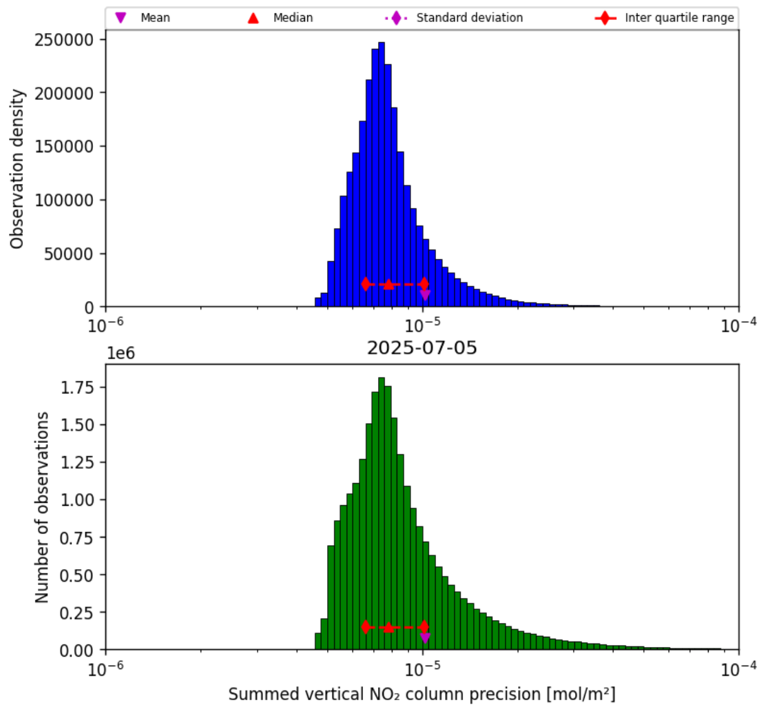
Figure 41: Histogram of "Summed vertical NO 2 column precision" for 2025-07-04 to 2025-07-06
