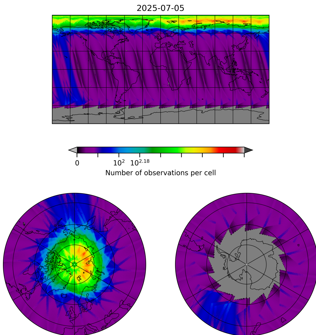
Figure 10: Map of the number of observations for 2025-07-04 to 2025-07-06
