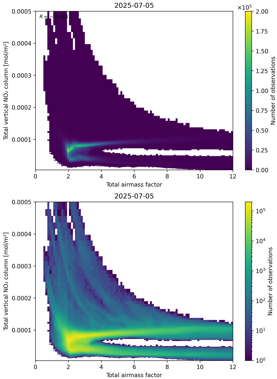
Figure 67: Scatter density plot of “Total airmass factor” against “Total vertical NO 2 column” for 2025-07-04 to 2025-07-06.
