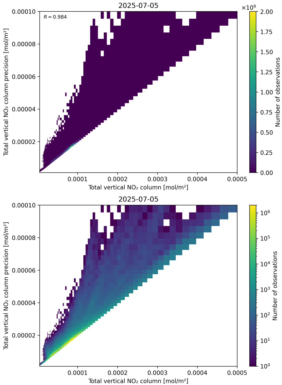
Figure 114: Scatter density plot of “Total vertical NO 2 column” against “Total vertical NO 2 column precision” for 2025-07-04 to 2025-07-06.
