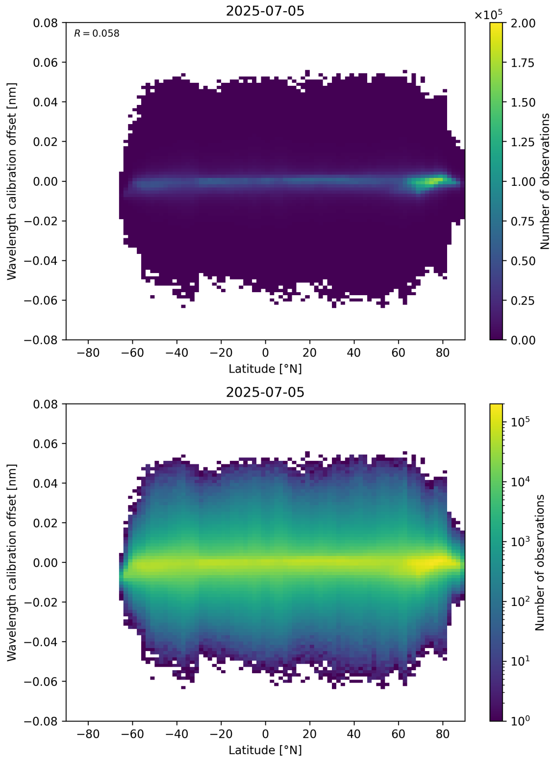
Figure 95: Scatter density plot of “Latitude” against “Wavelength calibration offset” for 2025-07-04 to 2025-07-06.
