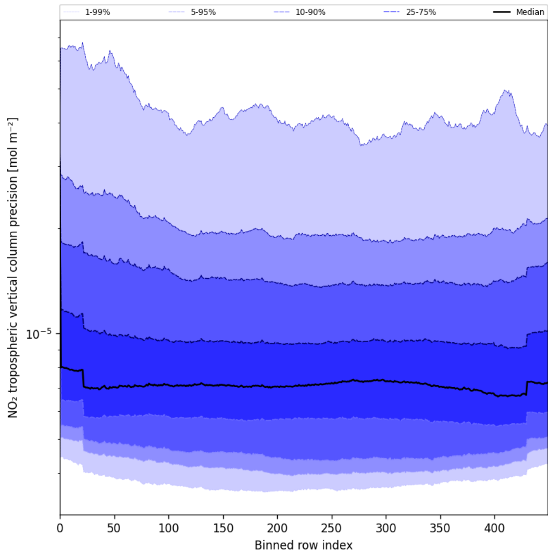
Figure 47: Along track statistics of “NO 2 tropospheric vertical column precision” for 2025-07-04 to 2025-07-06
