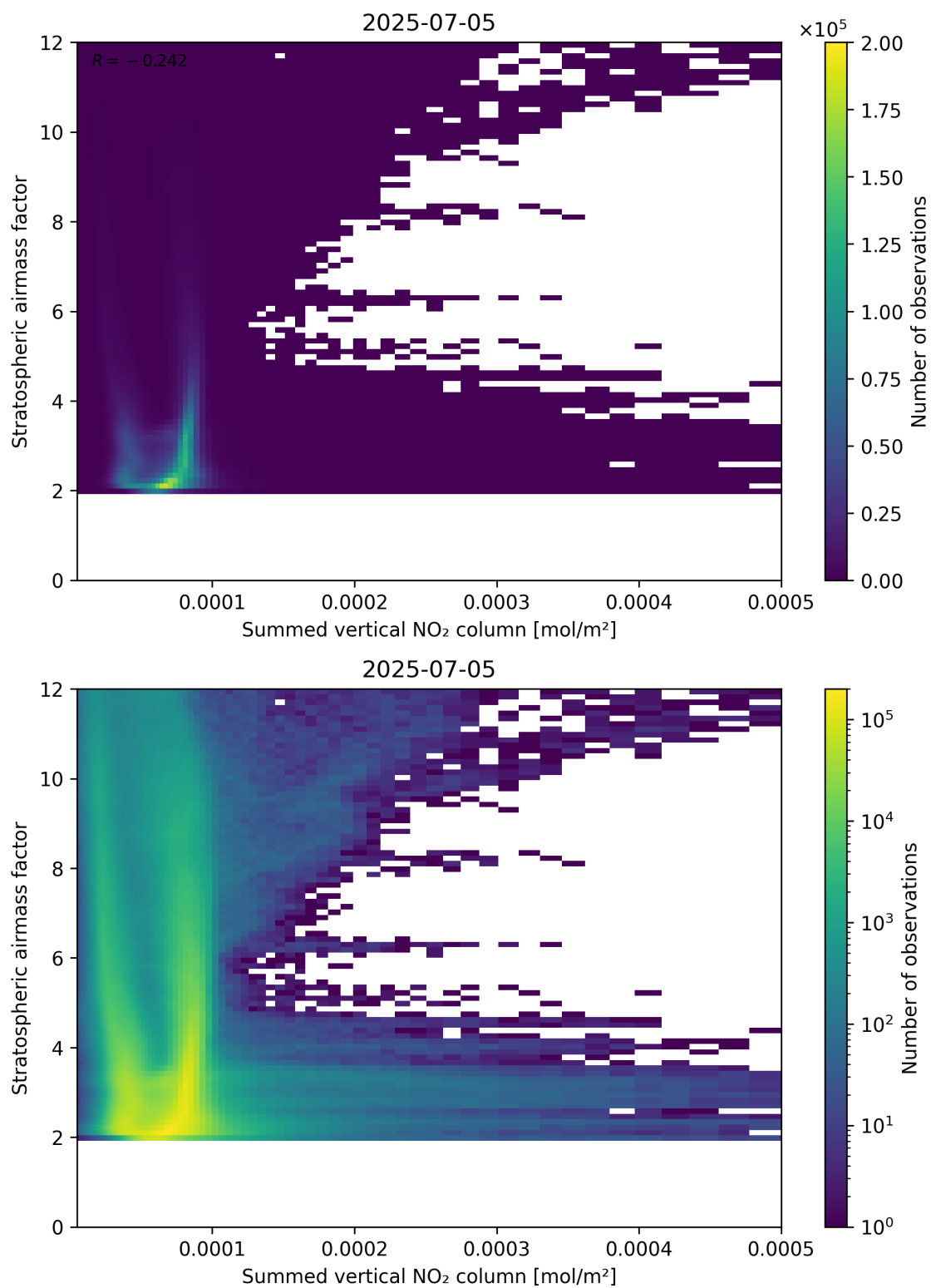
Figure 103: Scatter density plot of “Summed vertical NO 2 column” against “Stratospheric airmass factor” for 2025-07-04 to 2025-07-06.
