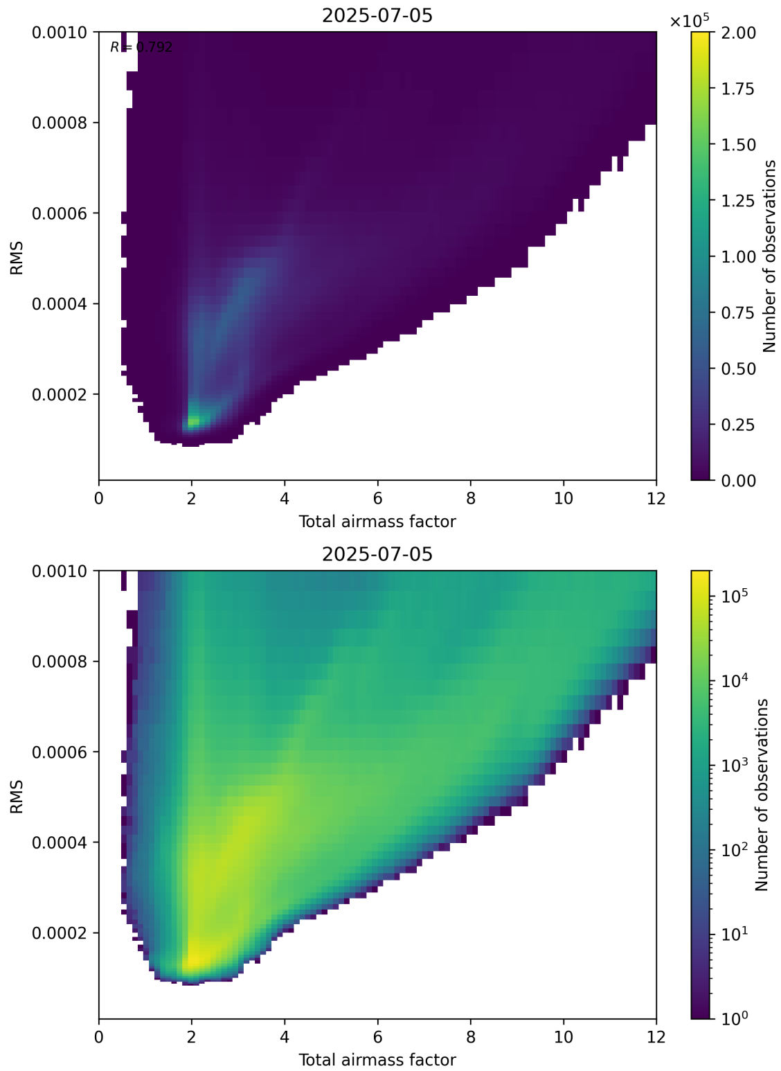
Figure 69: Scatter density plot of “Total airmass factor” against “RMS” for 2025-07-04 to 2025-07-06.
