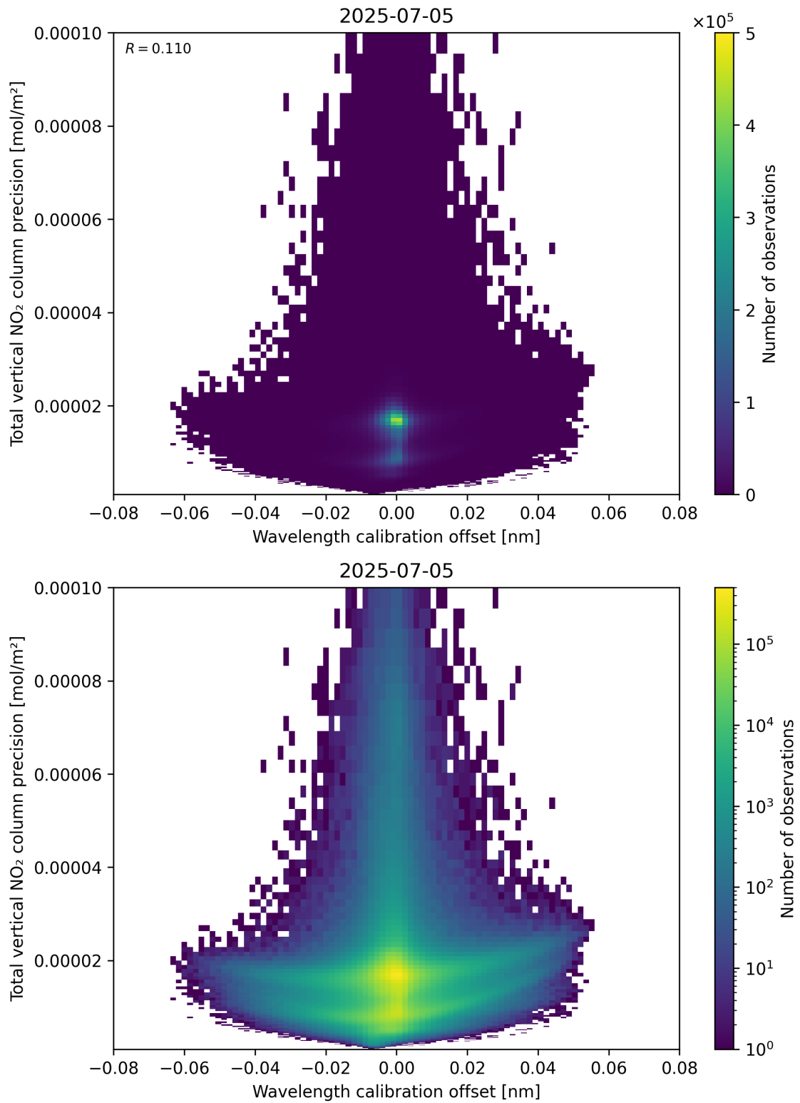
Figure 180: Scatter density plot of “Wavelength calibration offset” against “Total vertical NO 2 column precision” for 2025-07-04 to 2025-07-06.
