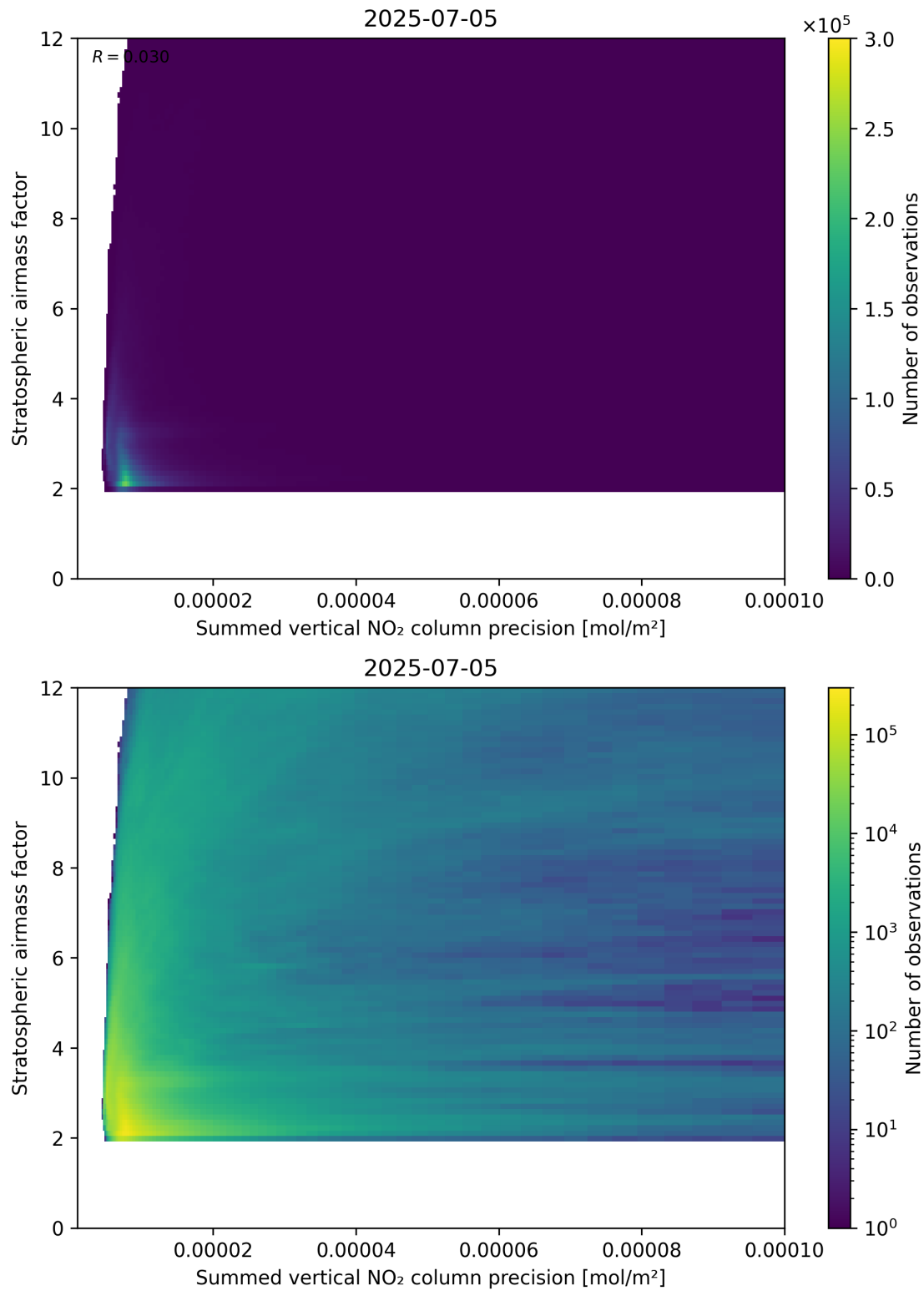
Figure 106: Scatter density plot of “Summed vertical NO 2 column precision” against “Stratospheric airmass factor” for 2025-07-04 to 2025-07-06.
