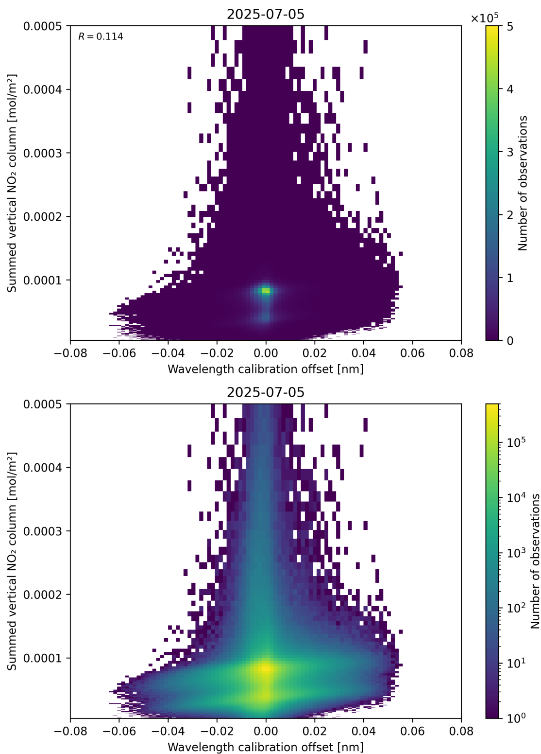
Figure 177: Scatter density plot of “Wavelength calibration offset” against “Summed vertical NO 2 column” for 2025-07-04 to 2025-07-06.
