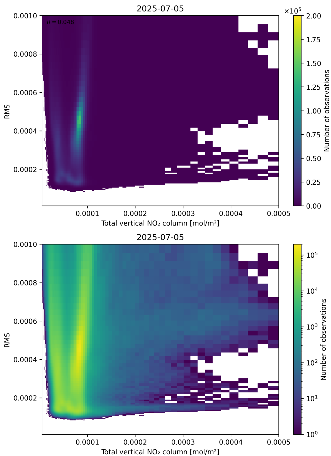
Figure 120: Scatter density plot of “Total vertical NO 2 column” against “RMS” for 2025-07-04 to 2025-07-06.
