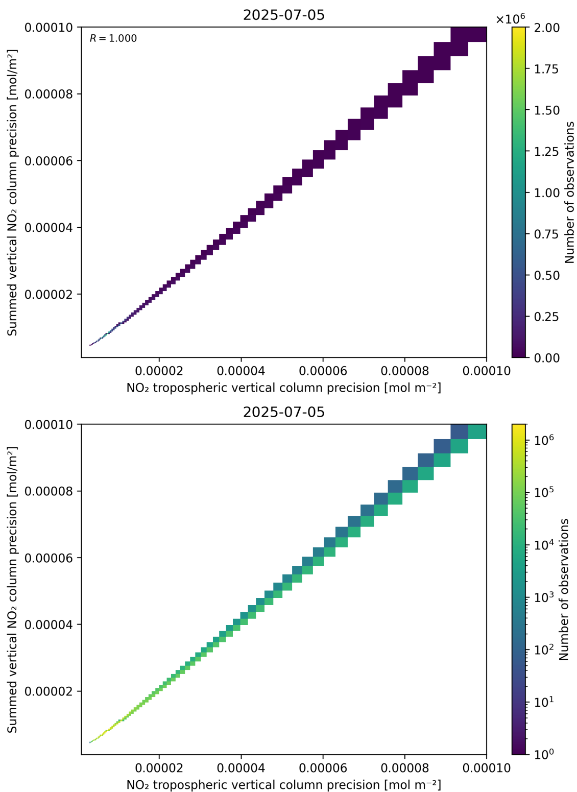
Figure 137: Scatter density plot of “NO 2 tropospheric vertical column precision” against “Summed vertical NO 2 column precision” for 2025-07-04 to 2025-07-06.
