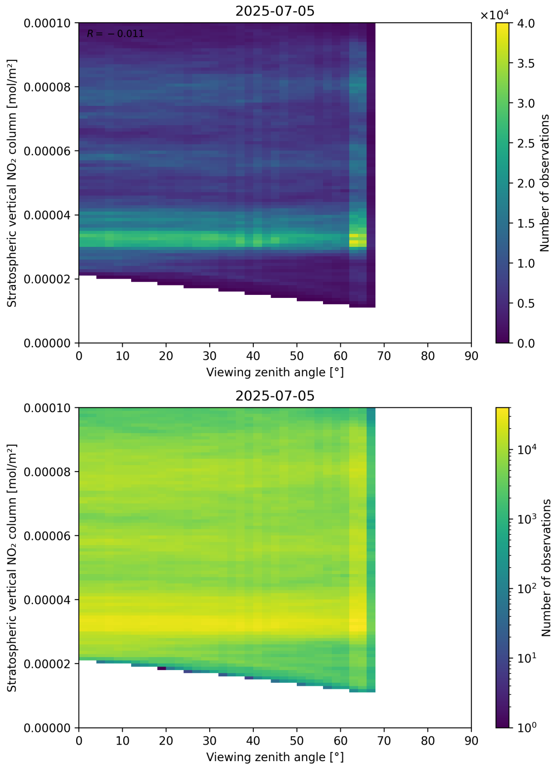
Figure 164: Scatter density plot of “Viewing zenith angle” against “Stratospheric vertical NO 2 column” for 2025-07-04 to 2025-07-06.
