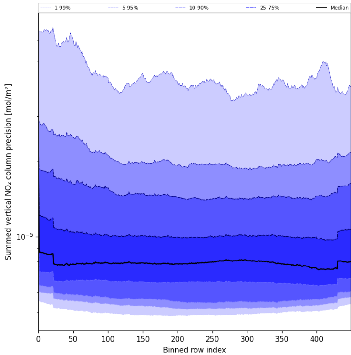
Figure 58: Along track statistics of “Summed vertical NO 2 column precision” for 2025-07-04 to 2025-07-06
