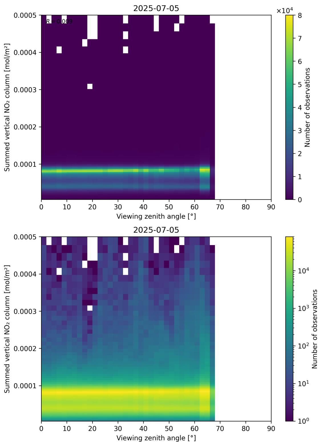
Figure 165: Scatter density plot of “Viewing zenith angle” against “Summed vertical NO 2 column” for 2025-07-04 to 2025-07-06.
