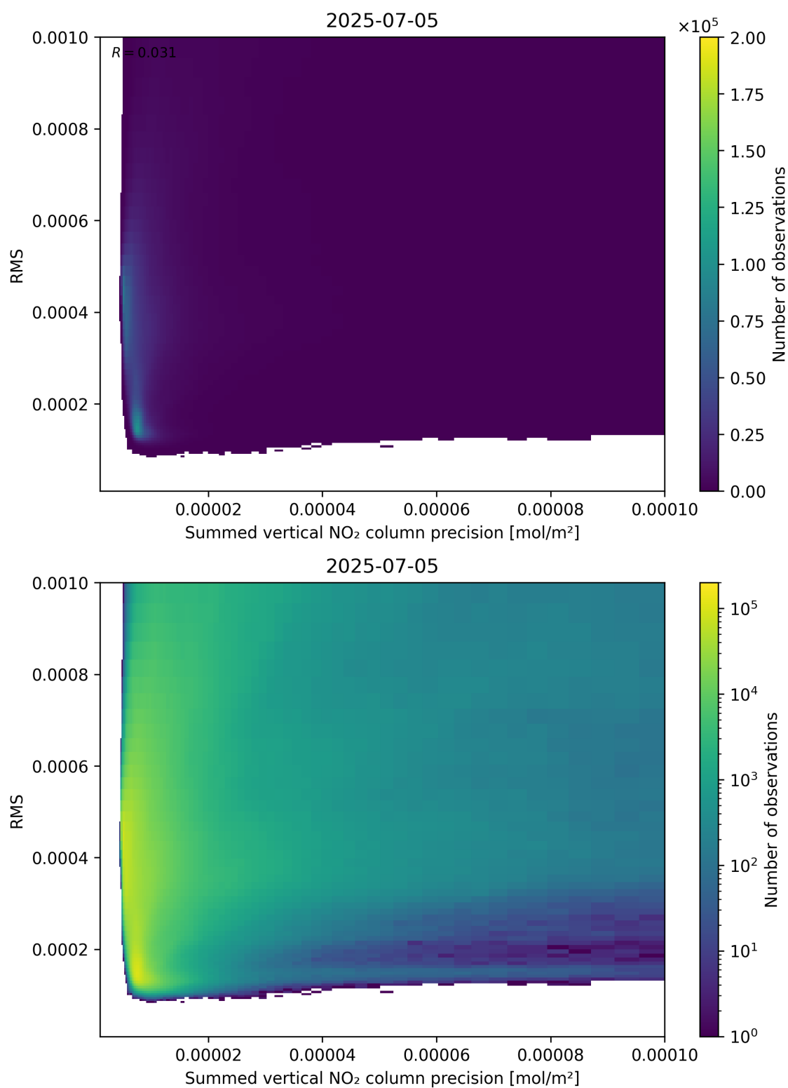
Figure 108: Scatter density plot of “Summed vertical NO 2 column precision” against “RMS” for 2025-07-04 to 2025-07-06.
