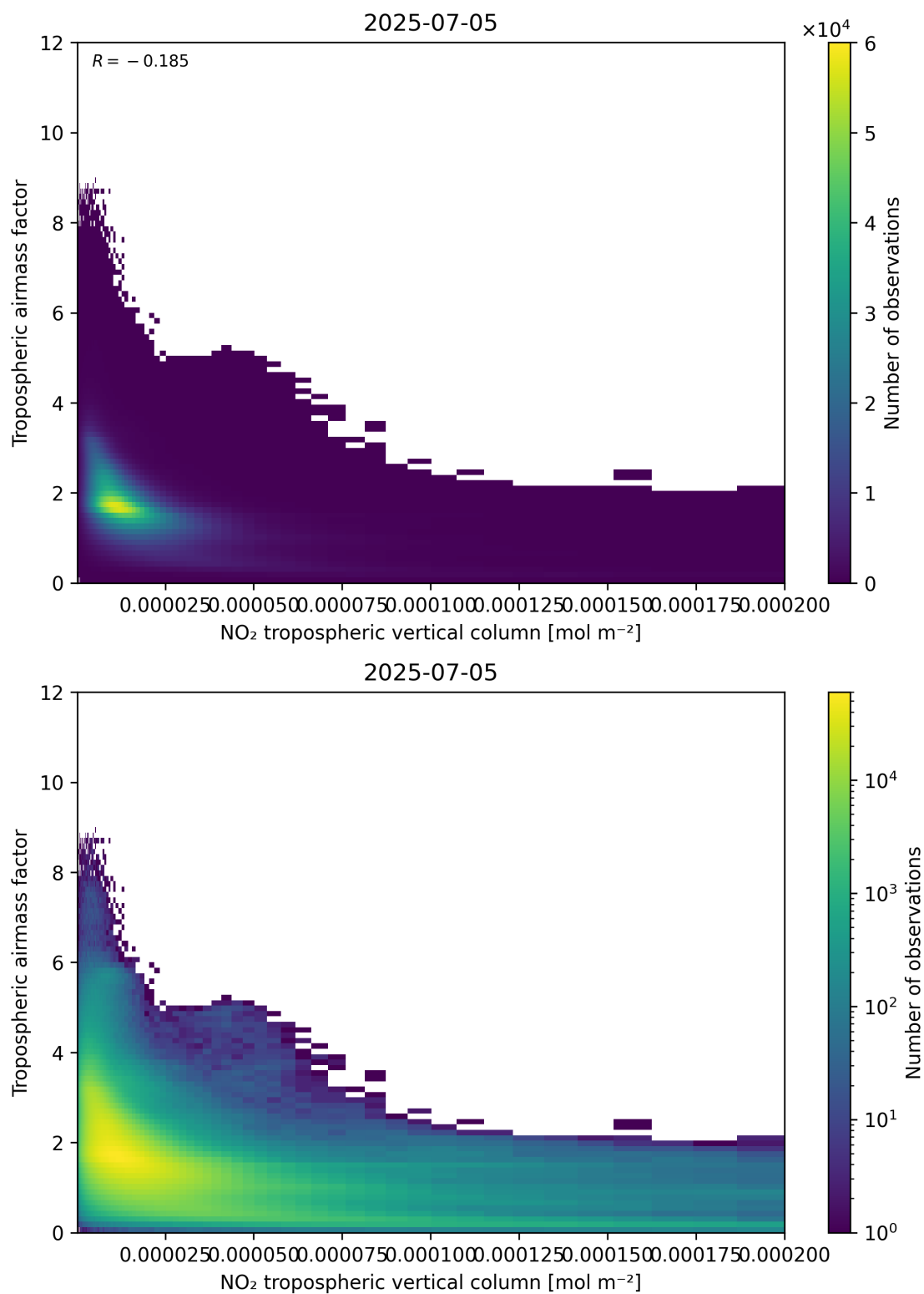
Figure 123: Scatter density plot of “NO 2 tropospheric vertical column” against “Tropospheric air mass factor” for 2025-07-04 to 2025-07-06.
