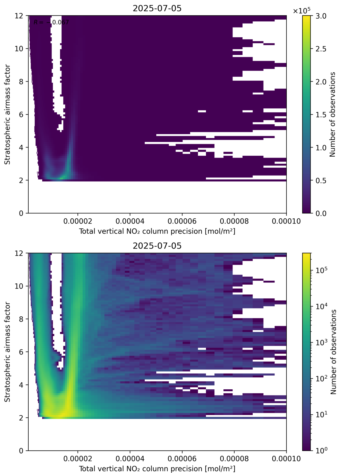
Figure 115: Scatter density plot of “Total vertical NO 2 column precision” against “Stratospheric air mass factor” for 2025-07-04 to 2025-07-06.
