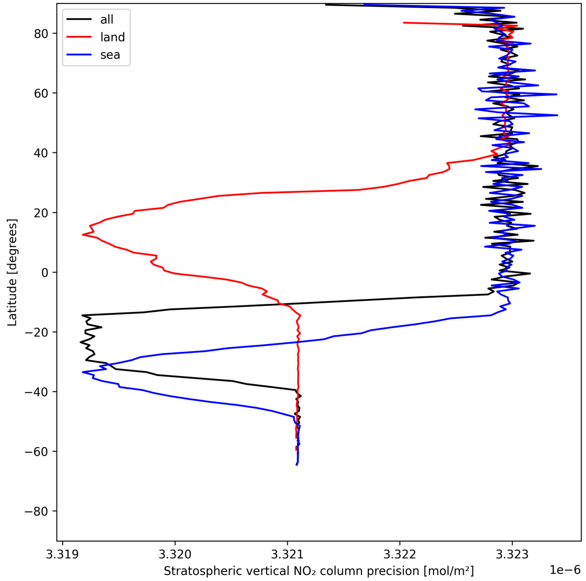
Figure 20: Zonal average of “Stratospheric vertical NO 2 column precision” for 2025-07-04 to 2025-07-06.
