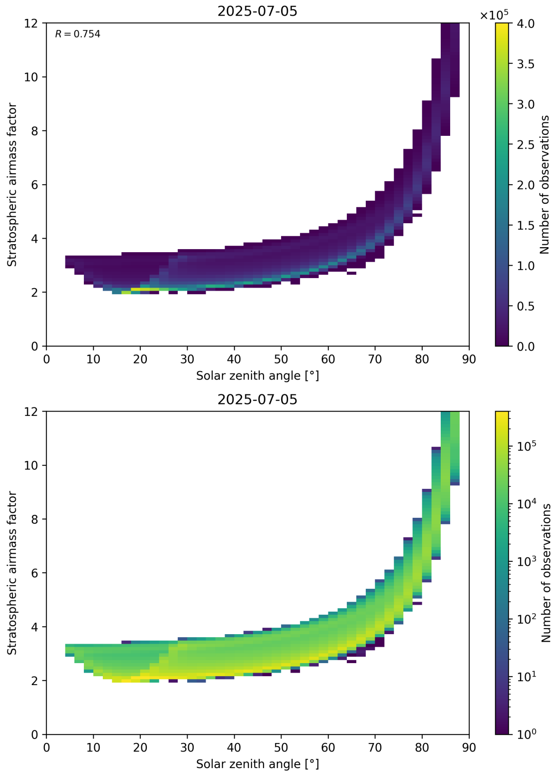
Figure 145: Scatter density plot of “Solar zenith angle” against “Stratospheric airmass factor” for 2025-07-04 to 2025-07-06.
