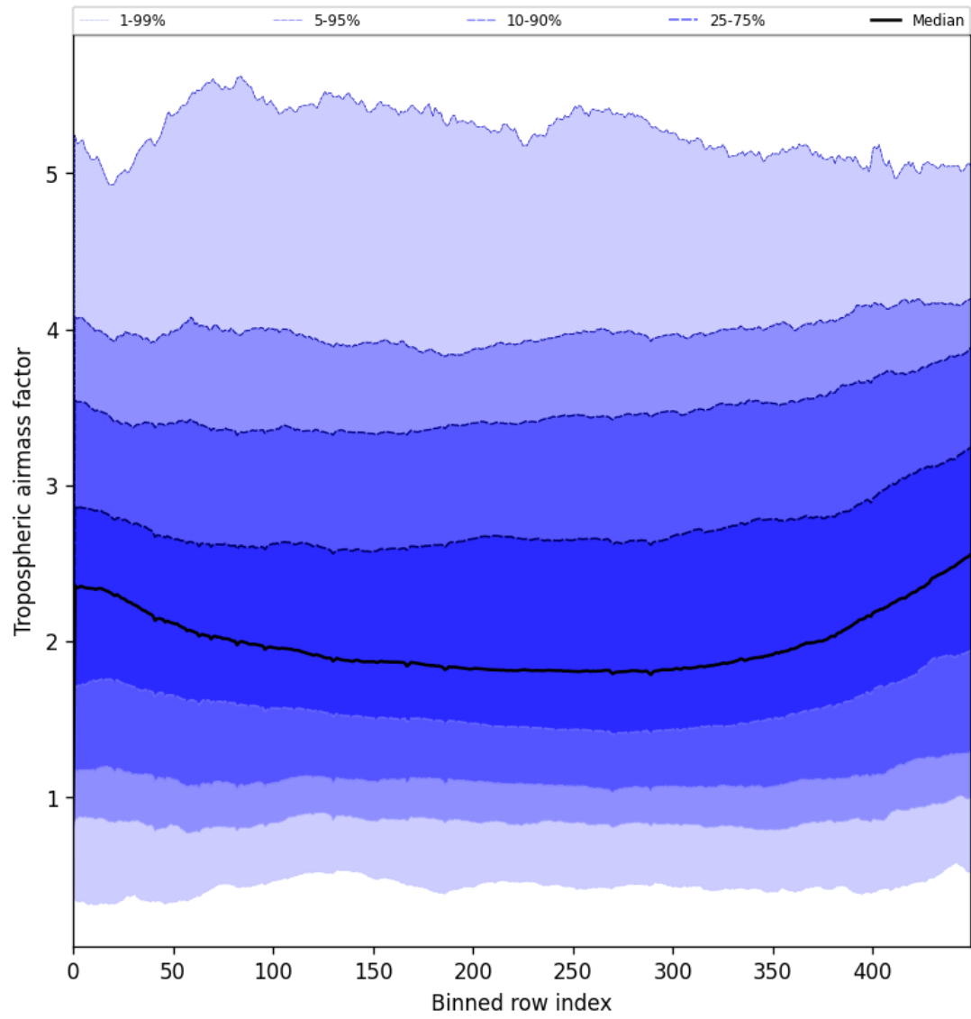
Figure 48: Along track statistics of “Tropospheric airmass factor” for 2025-07-04 to 2025-07-06
