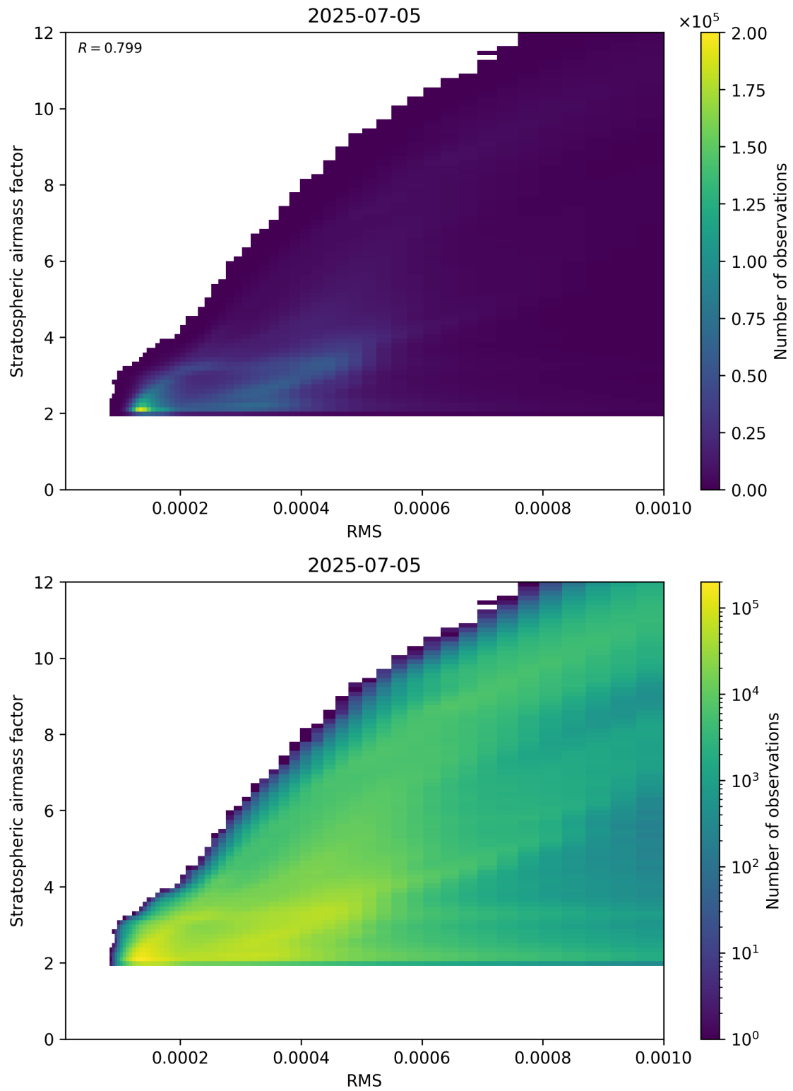
Figure 144: Scatter density plot of “RMS” against “Stratospheric airmass factor” for 2025-07-04 to 2025-07-06.
