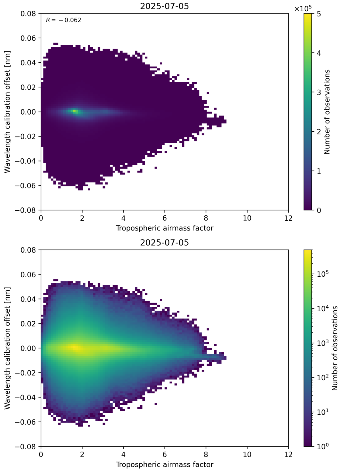
Figure 80: Scatter density plot of “Tropospheric airmass factor” against “Wavelength calibration offset” for 2025-07-04 to 2025-07-06.
