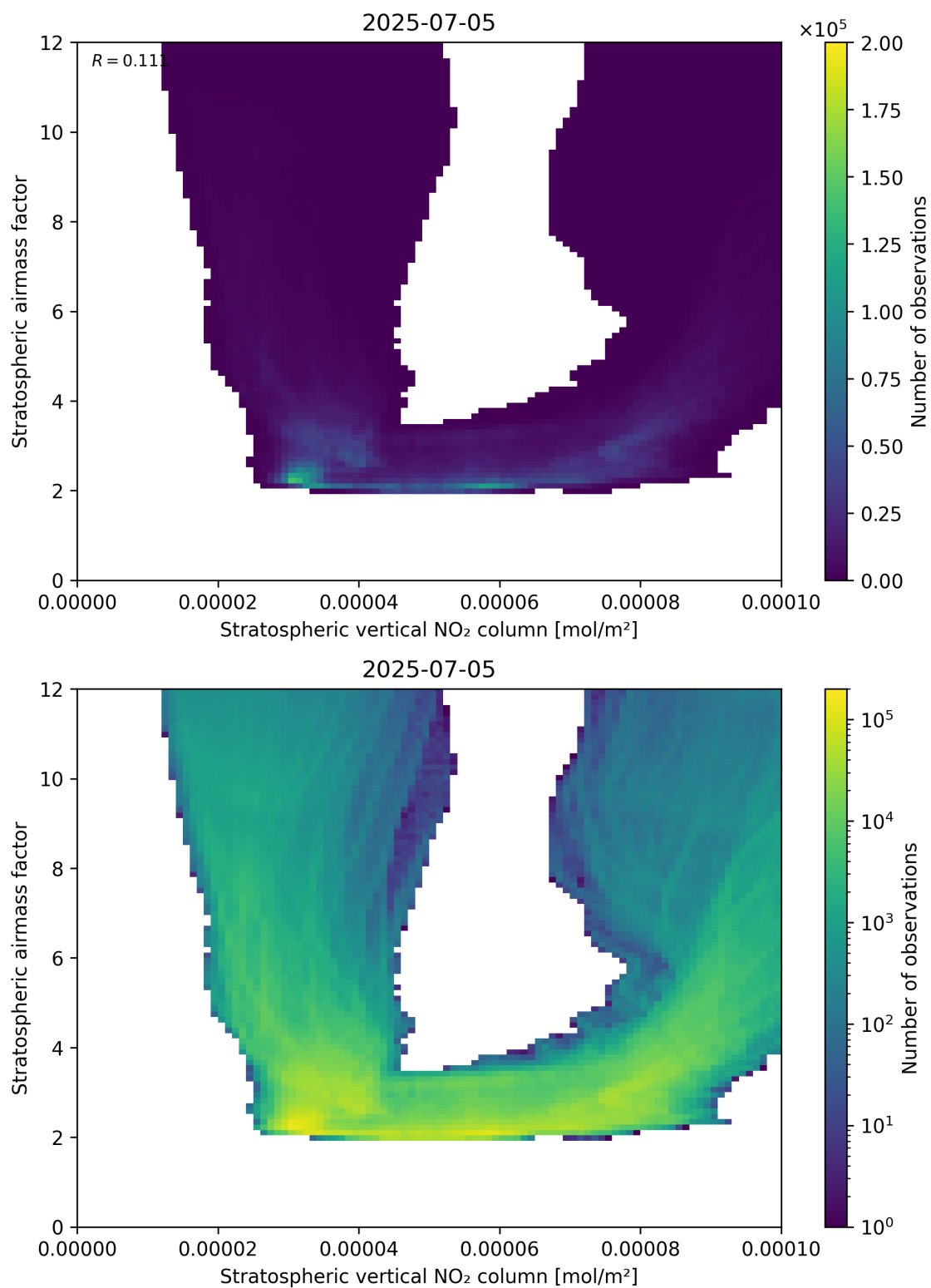
Figure 96: Scatter density plot of “Stratospheric vertical NO 2 column” against “Stratospheric airmass factor” for 2025-07-04 to 2025-07-06.
