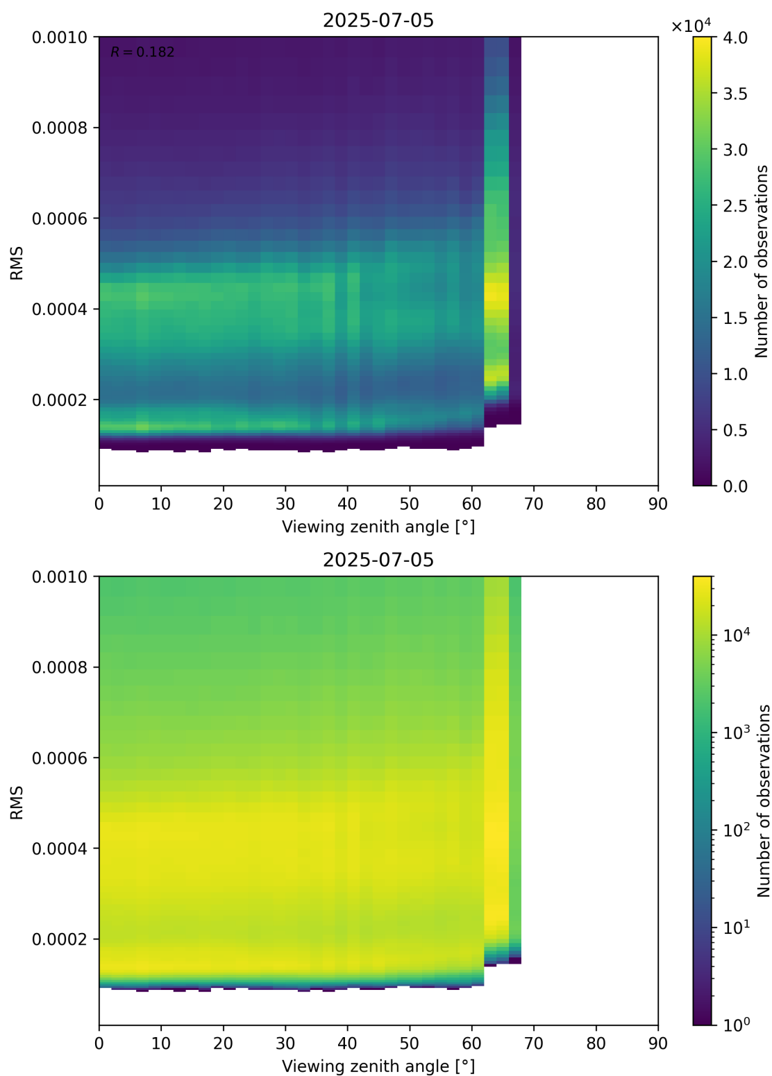
Figure 171: Scatter density plot of “Viewing zenith angle” against “RMS” for 2025-07-04 to 2025-07-06.
