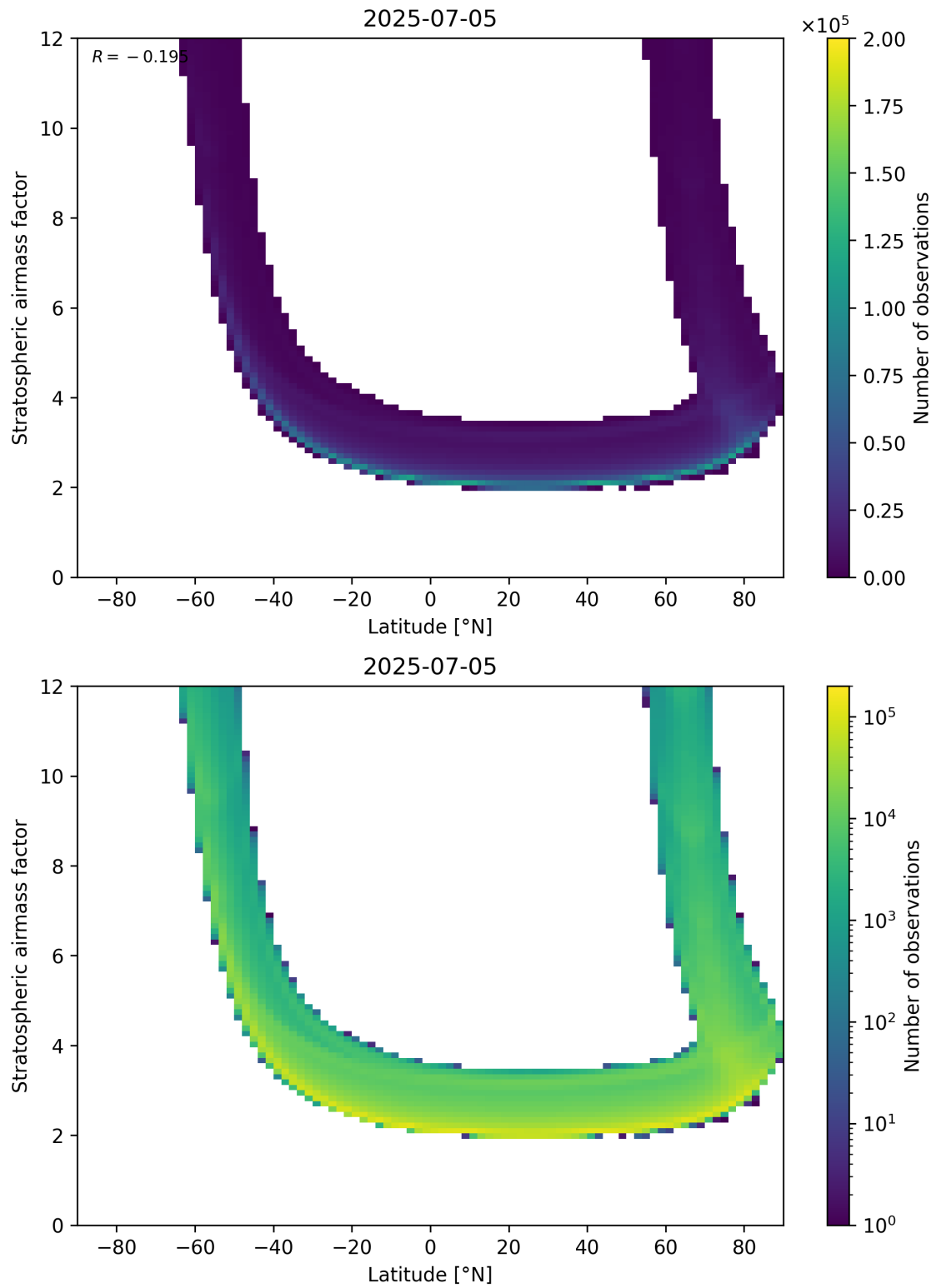
Figure 83: Scatter density plot of “Latitude” against “Stratospheric air mass factor” for 2025-07-04 to 2025-07-06.
