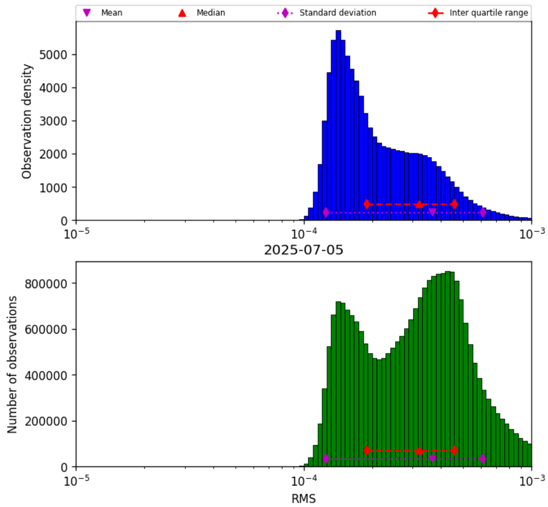
Figure 43: Histogram of “RMS” for 2025-07-04 to 2025-07-06
