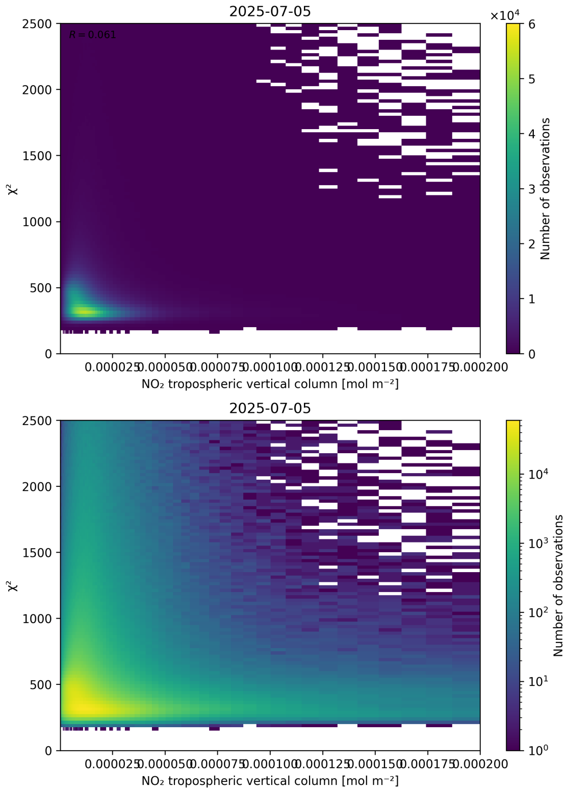
Figure 124: Scatter density plot of “NO 2 tropospheric vertical column” against “ \chi^2 ” for 2025-07-04 to 2025-07-06.
