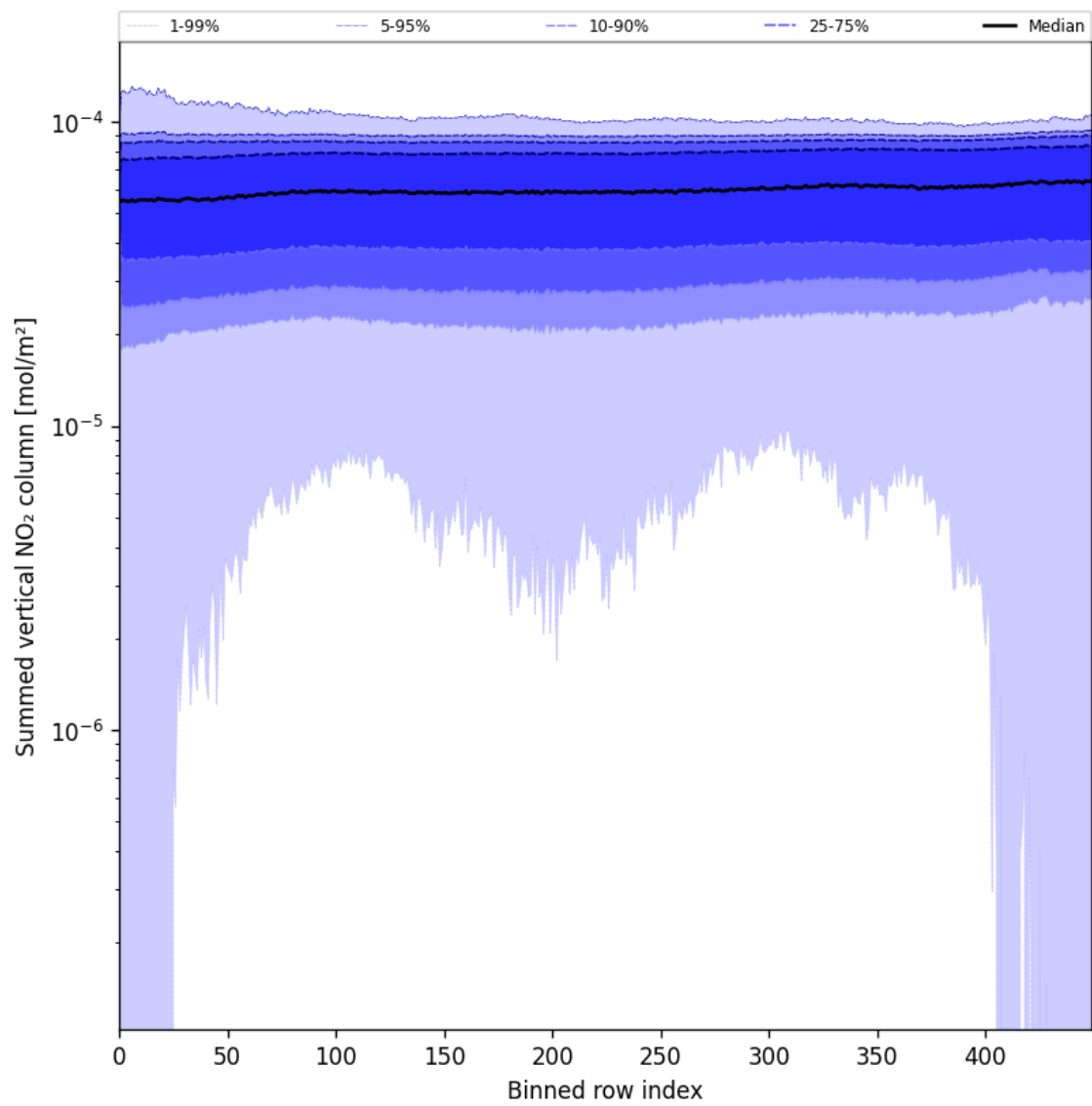
Figure 57: Along track statistics of “Summed vertical NO 2 column” for 2025-07-04 to 2025-07-06
