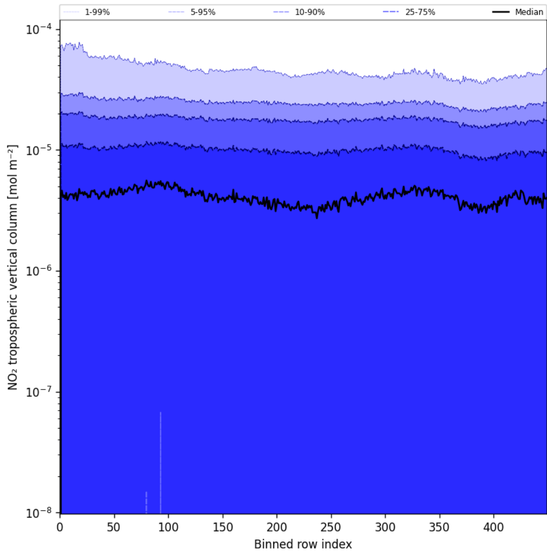
Figure 46: Along track statistics of “NO 2 tropospheric vertical column” for 2025-07-04 to 2025-07-06
