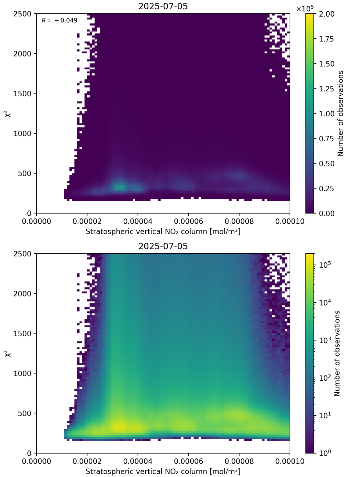
Figure 97: Scatter density plot of “Stratospheric vertical NO 2 column” against “ \chi^2 ” for 2025-07-04 to 2025-07-06.
