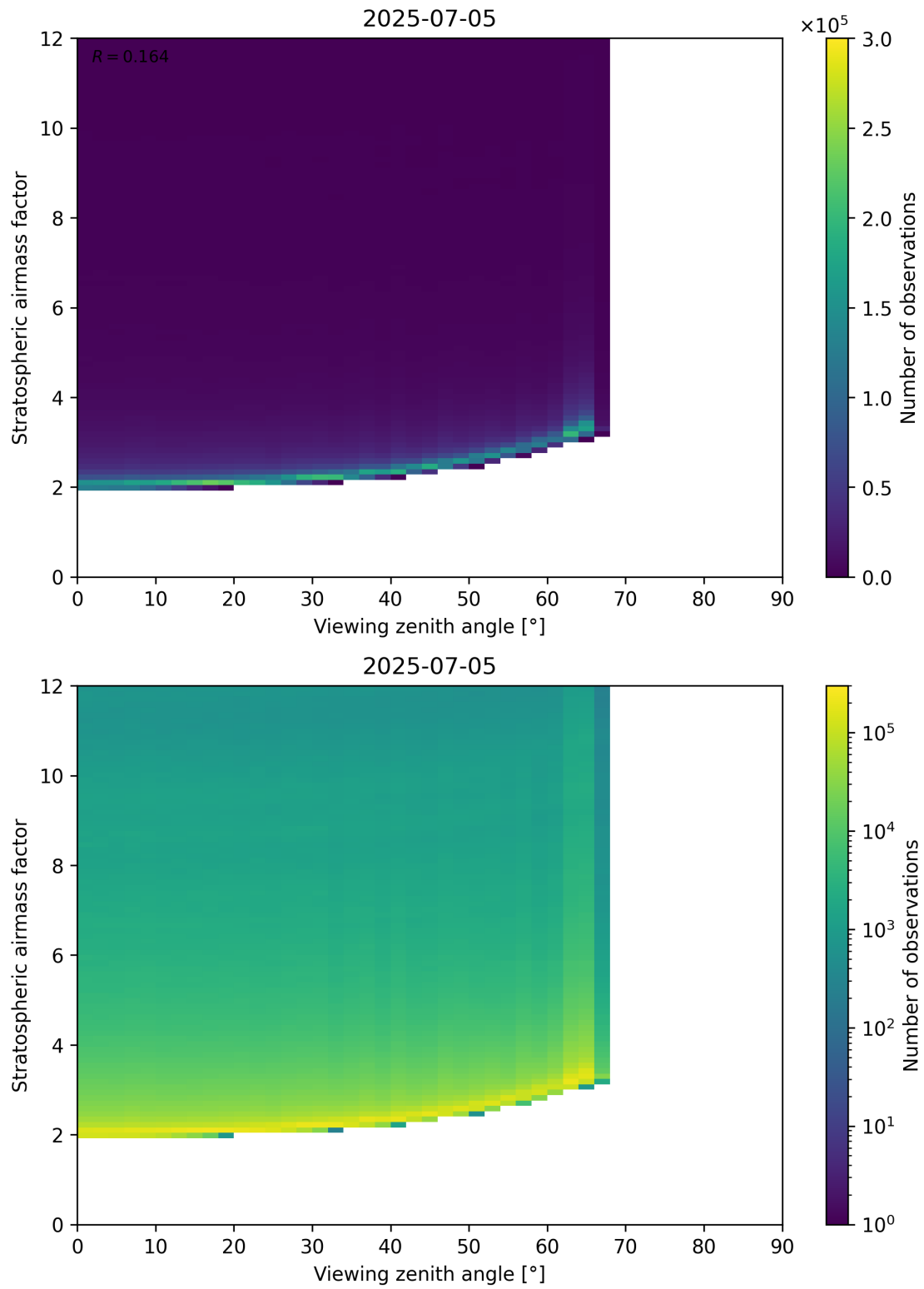
Figure 159: Scatter density plot of “Viewing zenith angle” against “Stratospheric airmass factor” for 2025-07-04 to 2025-07-06.
