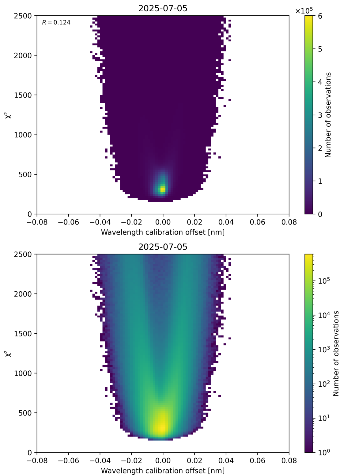
Figure 175: Scatter density plot of “Wavelength calibration offset” against “ \chi^2 ” for 2025-07-04 to 2025-07-06.
