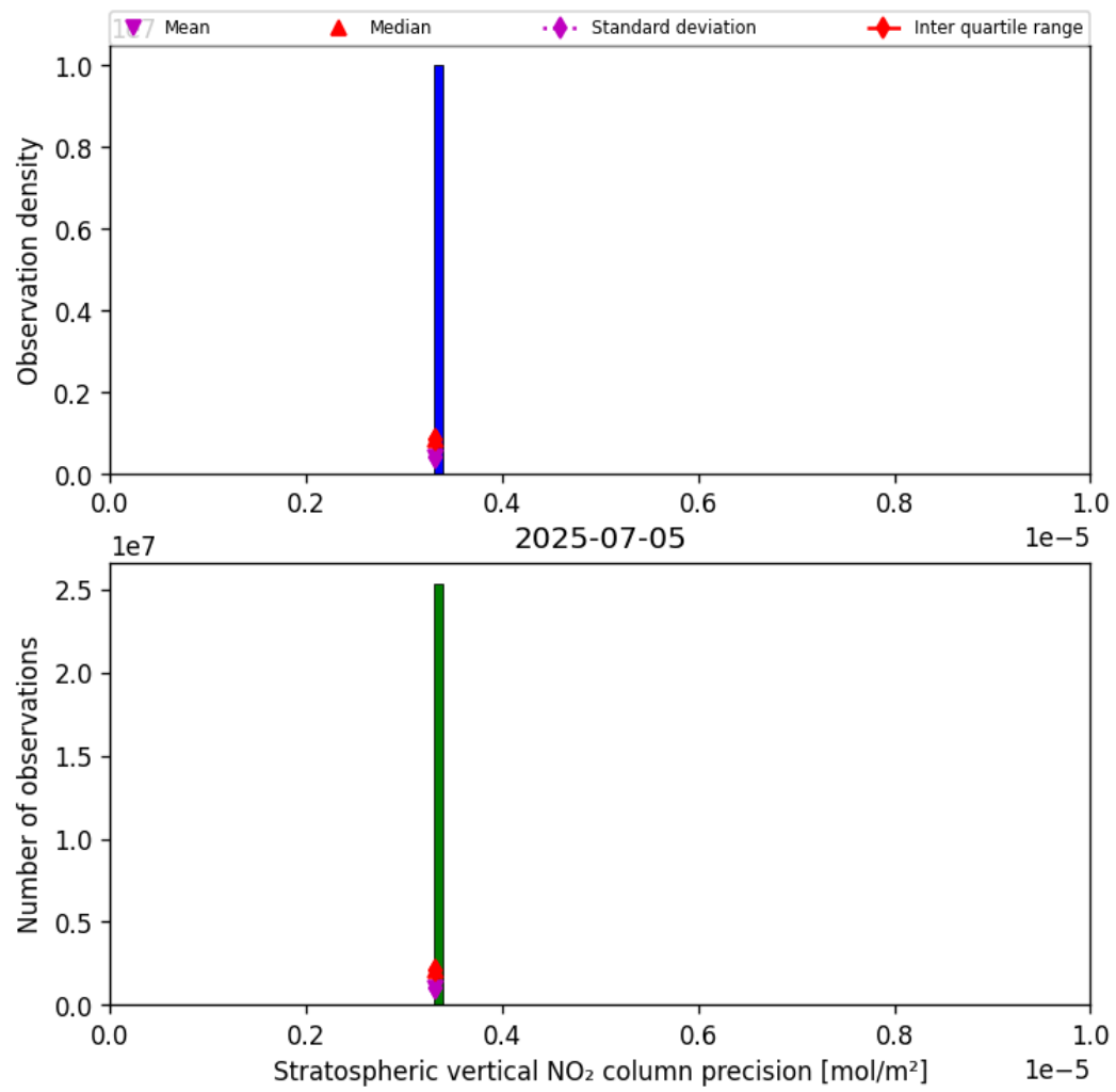
Figure 37: Histogram of “Stratospheric vertical NO 2 column precision” for 2025-07-04 to 2025-07-06
