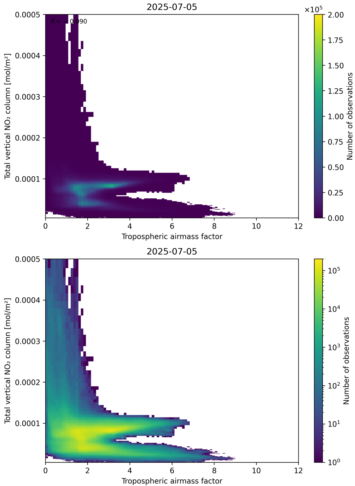
Figure 77: Scatter density plot of “Tropospheric airmass factor” against “Total vertical NO 2 column” for 2025-07-04 to 2025-07-06.
