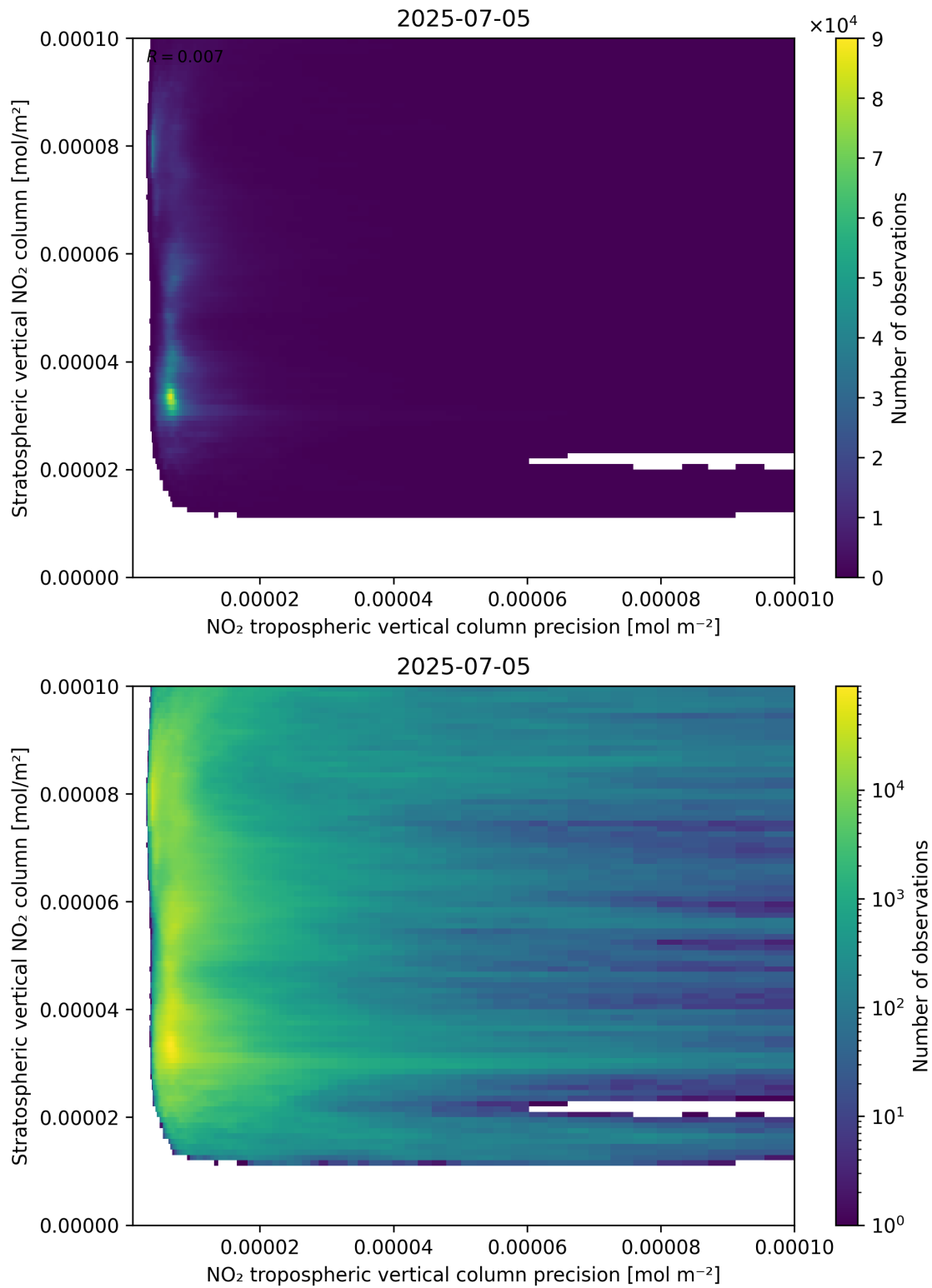
Figure 135: Scatter density plot of “NO 2 tropospheric vertical column precision” against “Stratospheric vertical NO 2 column” for 2025-07-04 to 2025-07-06.
