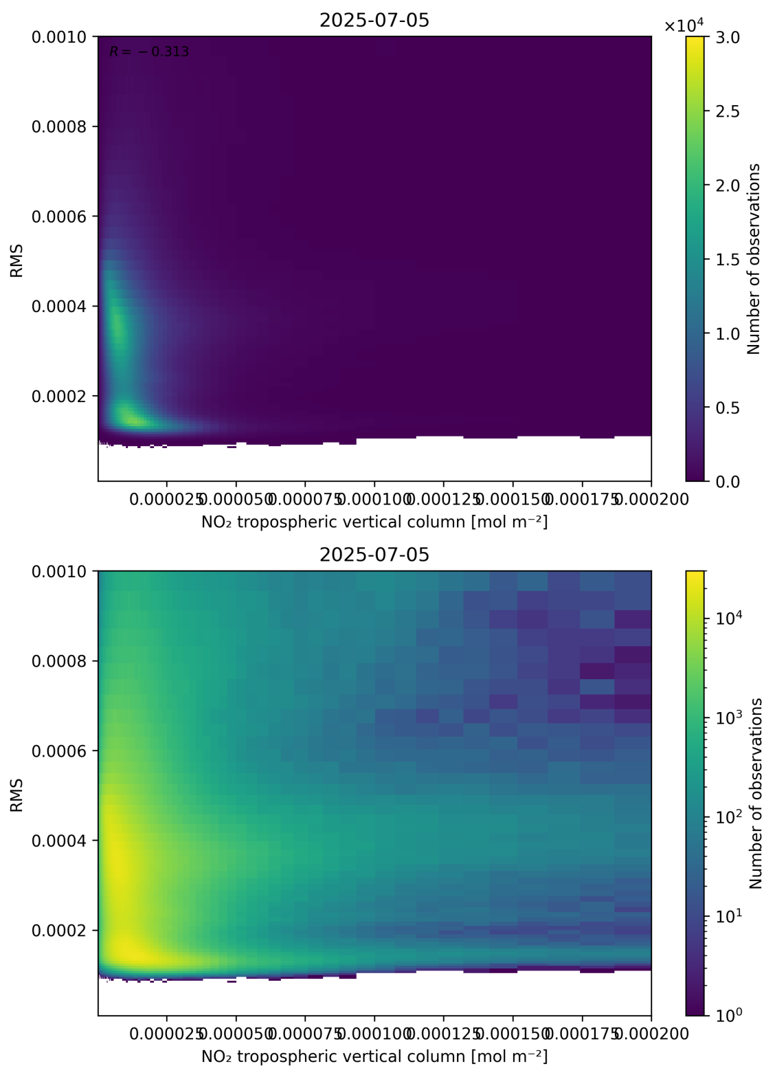
Figure 142: Scatter density plot of “NO 2 tropospheric vertical column” against “RMS” for 2025-07-04 to 2025-07-06.
