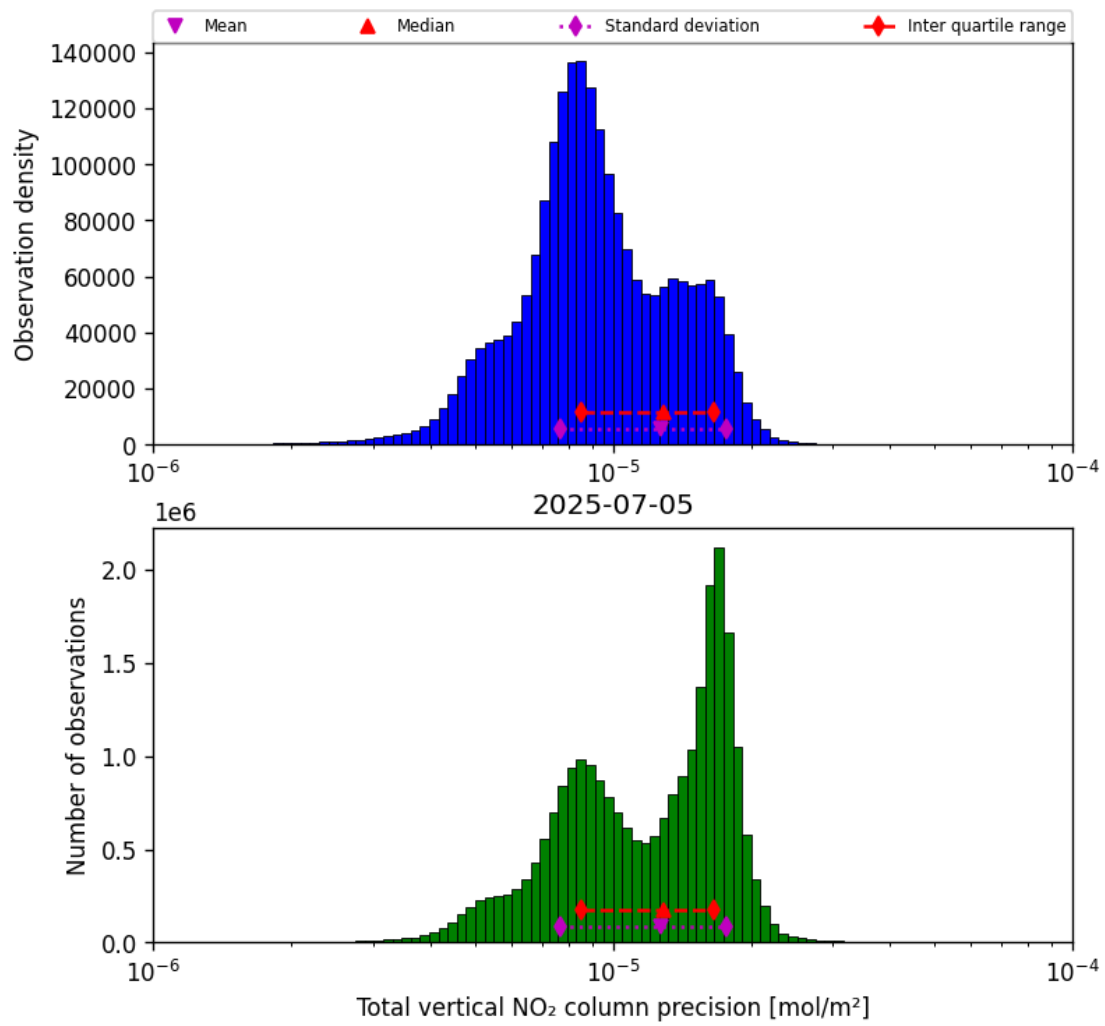
Figure 39: Histogram of “Total vertical NO 2 column precision” for 2025-07-04 to 2025-07-06
