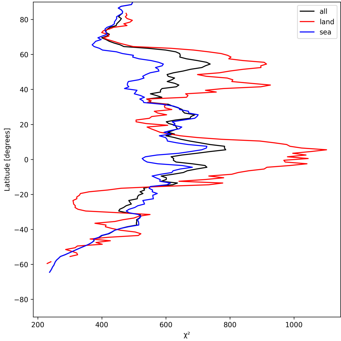
Figure 25: Zonal average of “ \chi^2 ” for 2025-07-04 to 2025-07-06.
