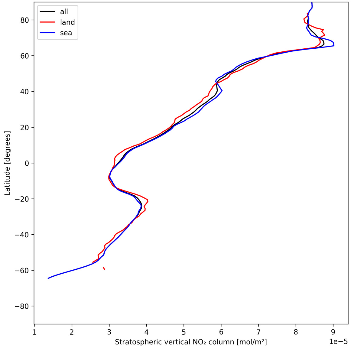
Figure 19: Zonal average of “Stratospheric vertical NO 2 column” for 2025-07-04 to 2025-07-06.
