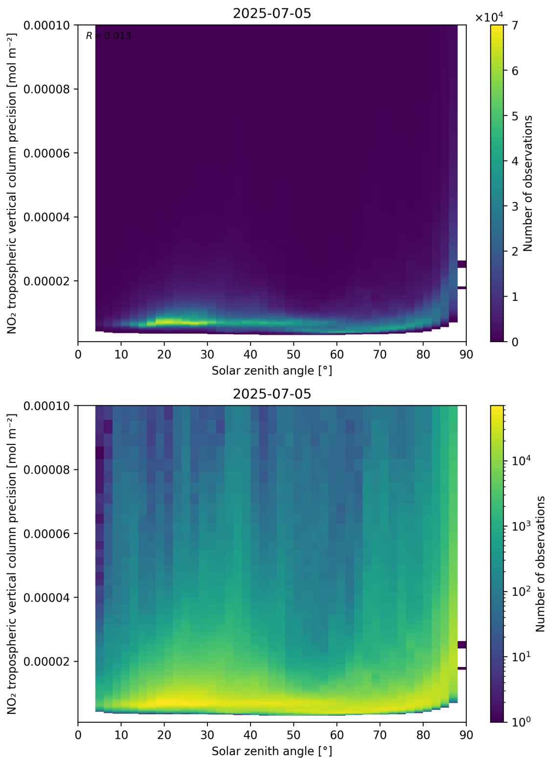
Figure 156: Scatter density plot of “Solar zenith angle” against “NO 2 tropospheric vertical column precision” for 2025-07-04 to 2025-07-06.
