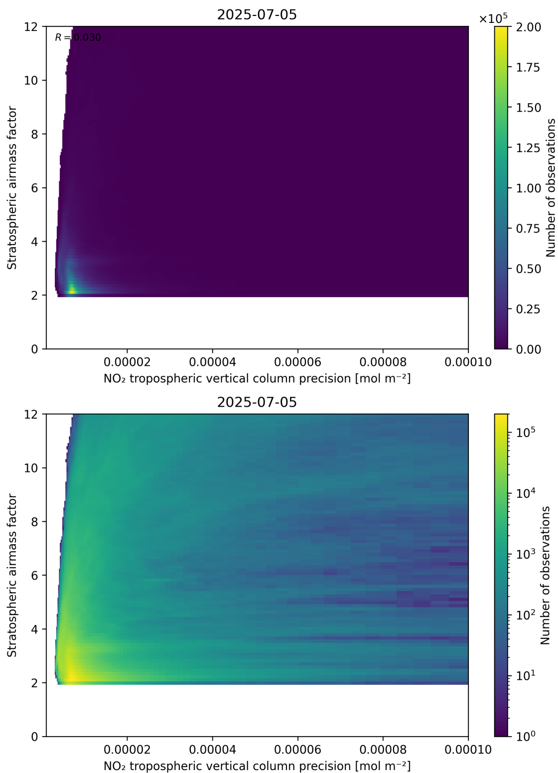
Figure 131: Scatter density plot of “NO 2 tropospheric vertical column precision” against “Stratospheric airmass factor” for 2025-07-04 to 2025-07-06.
