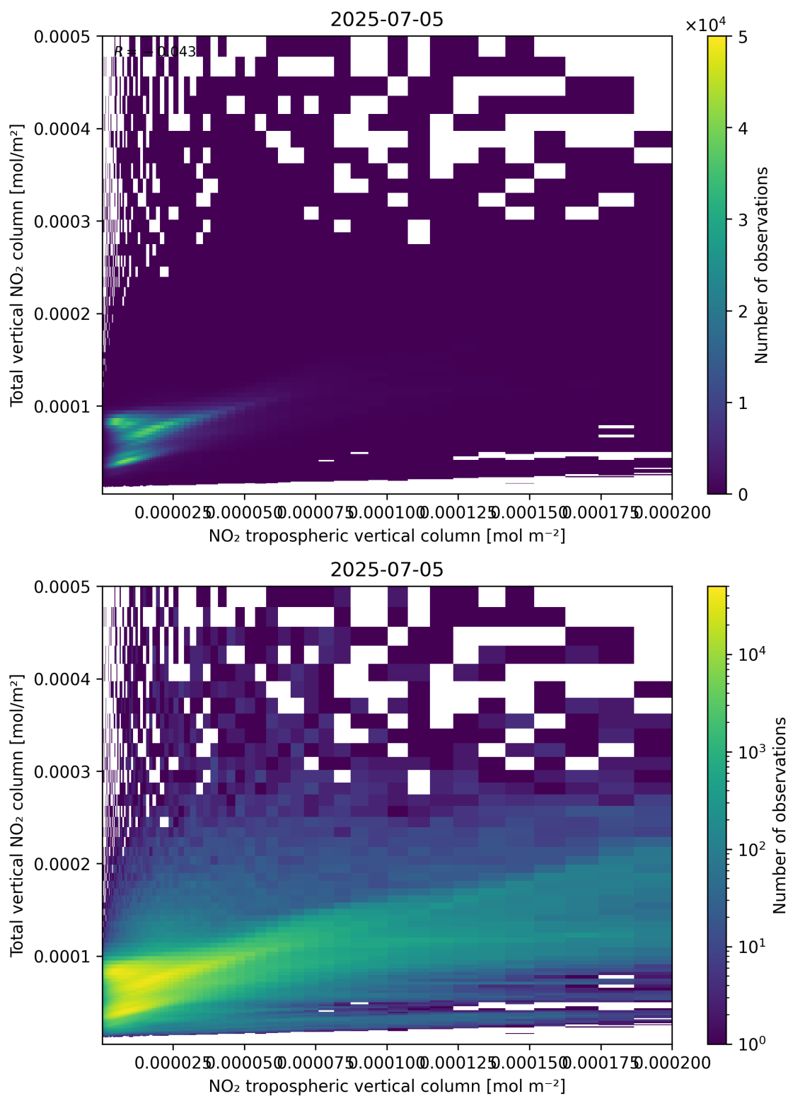
Figure 128: Scatter density plot of “NO 2 tropospheric vertical column” against “Total vertical NO 2 column” for 2025-07-04 to 2025-07-06.
