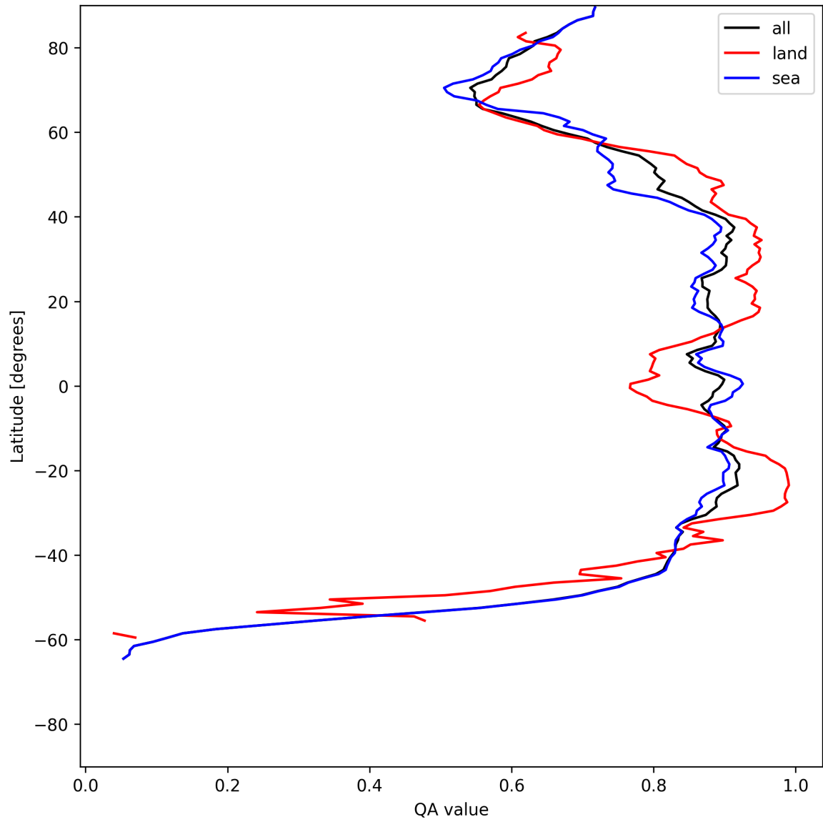
Figure 11: Zonal average of “QA value” for 2025-07-04 to 2025-07-06.
