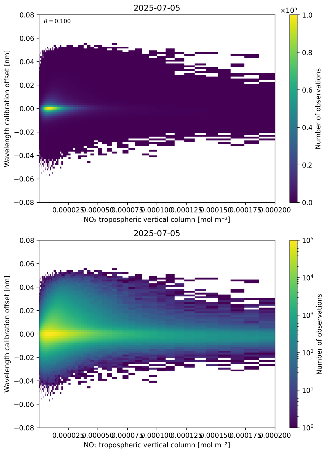
Figure 143: Scatter density plot of “NO 2 tropospheric vertical column” against “Wavelength calibration offset” for 2025-07-04 to 2025-07-06.
