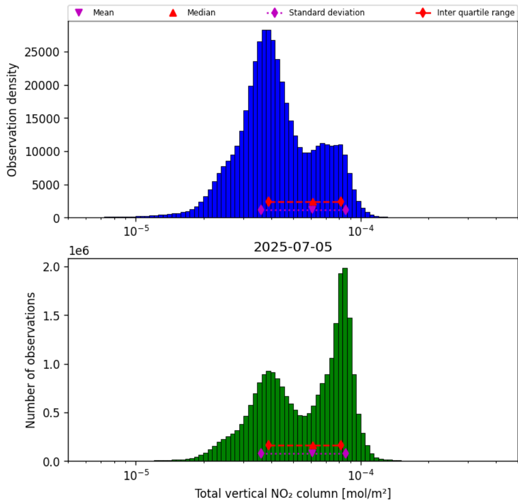
Figure 38: Histogram of “Total vertical NO 2 column” for 2025-07-04 to 2025-07-06
