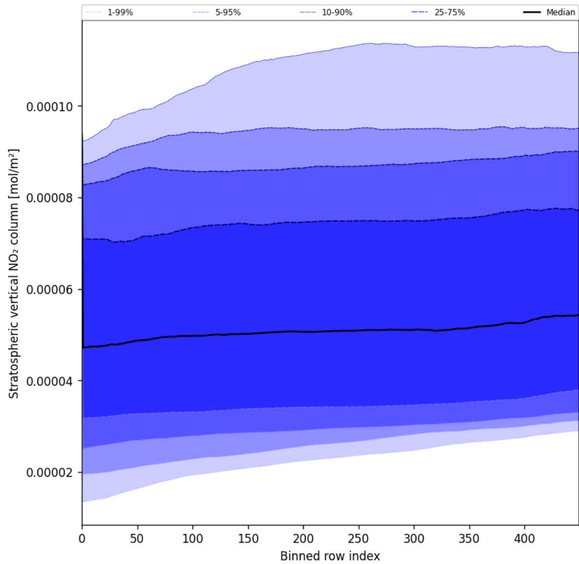
Figure 53: Along track statistics of “Stratospheric vertical NO 2 column” for 2025-07-04 to 2025-07-06
