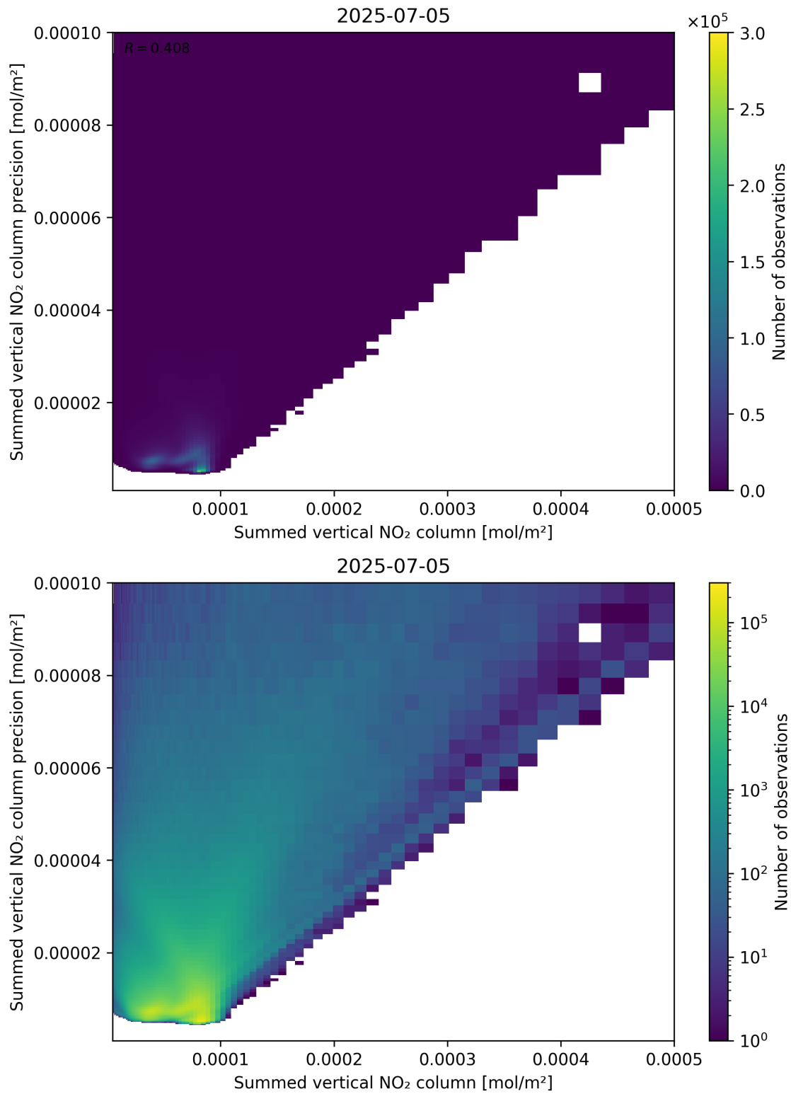
Figure 105: Scatter density plot of “Summed vertical NO 2 column” against “Summed vertical NO 2 column precision” for 2025-07-04 to 2025-07-06.
