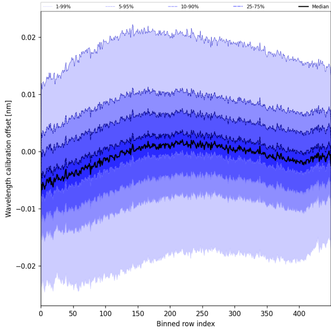
Figure 52: Along track statistics of “Wavelength calibration offset” for 2025-07-04 to 2025-07-06
