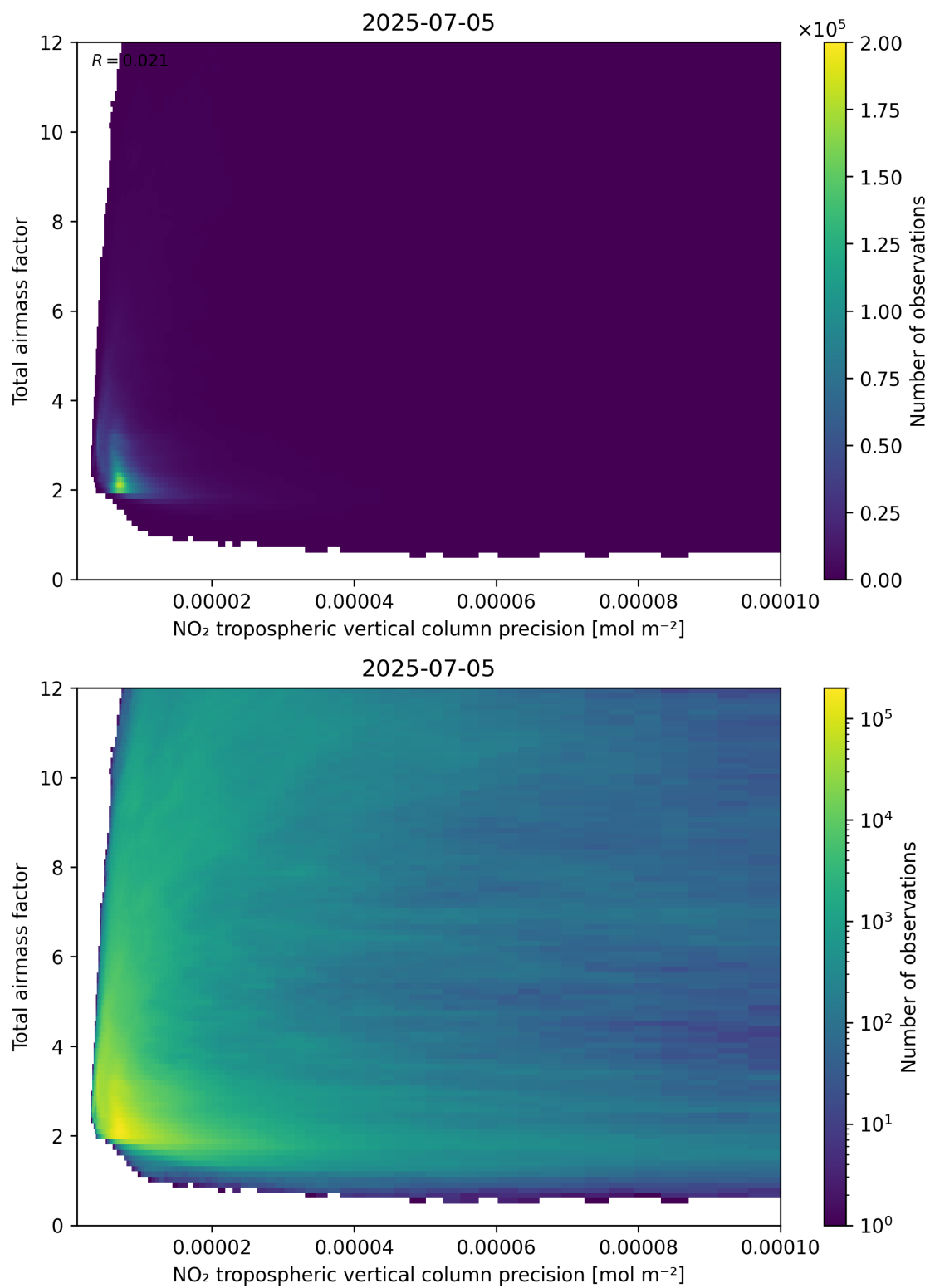
Figure 132: Scatter density plot of “NO 2 tropospheric vertical column precision” against “Total air mass factor” for 2025-07-04 to 2025-07-06.
