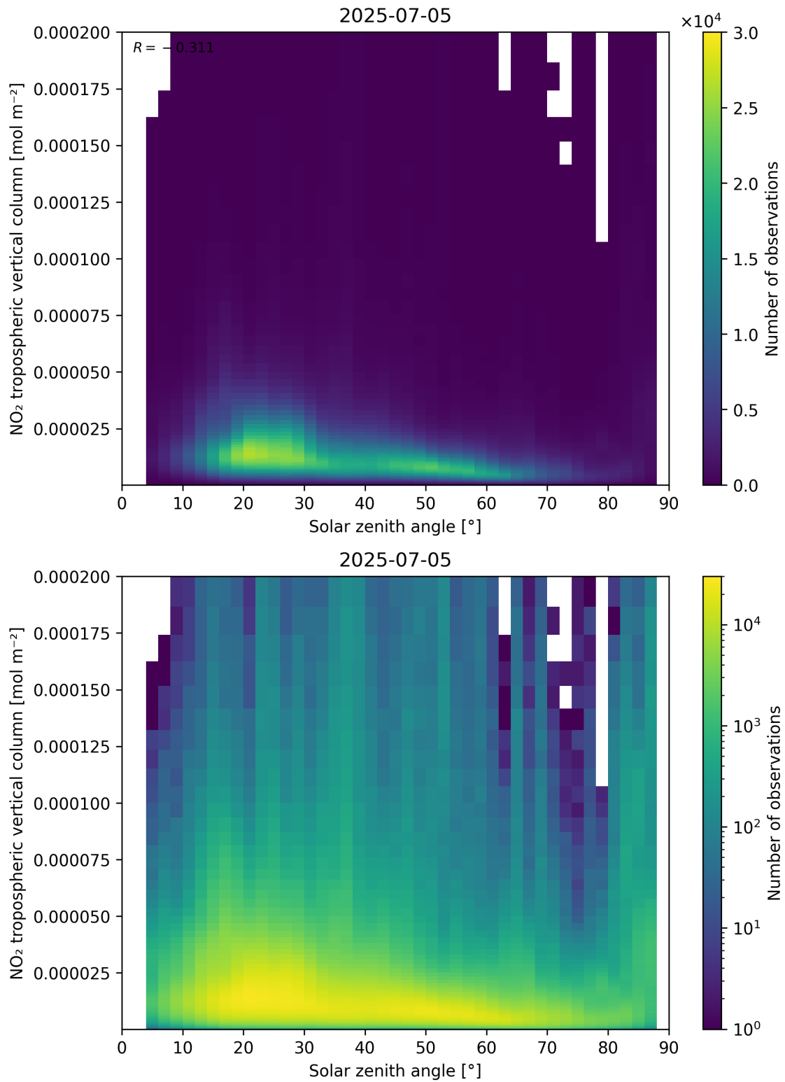
Figure 155: Scatter density plot of “Solar zenith angle” against “NO 2 tropospheric vertical column” for 2025-07-04 to 2025-07-06.
