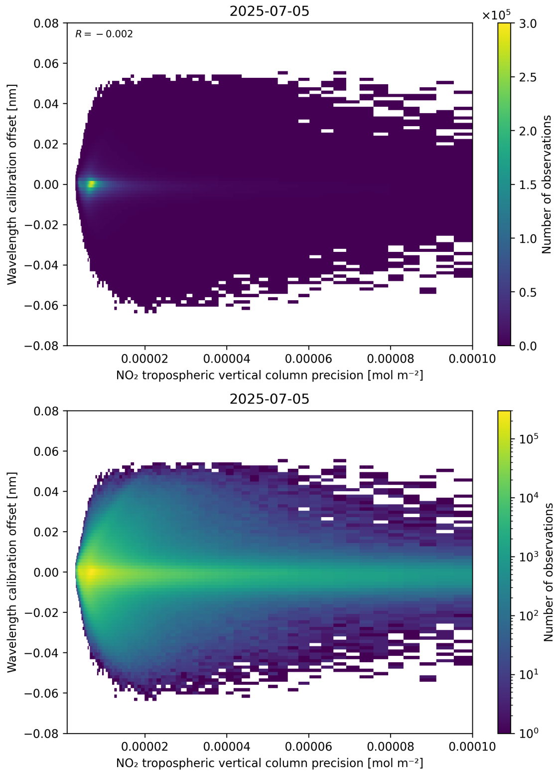
Figure 141: Scatter density plot of “NO 2 tropospheric vertical column precision” against “Wavelength calibration offset” for 2025-07-04 to 2025-07-06.
