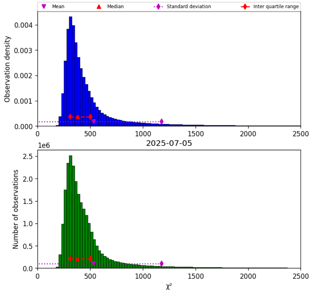
Figure 42: Histogram of “ \chi^2 ” for 2025-07-04 to 2025-07-06
