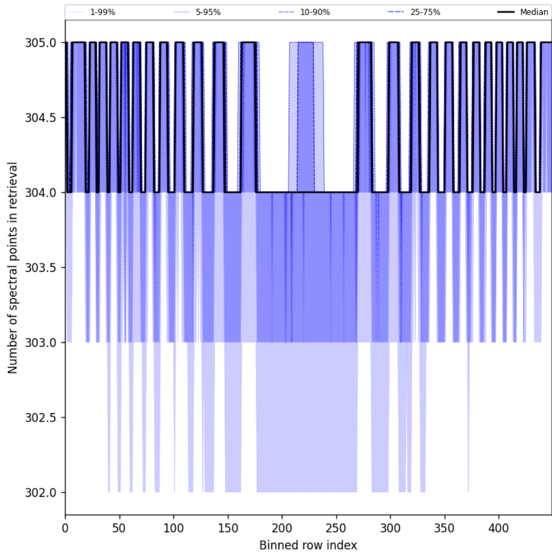
Figure 50: Along track statistics of “Number of spectral points in retrieval” for 2025-07-04 to 2025-07-06
