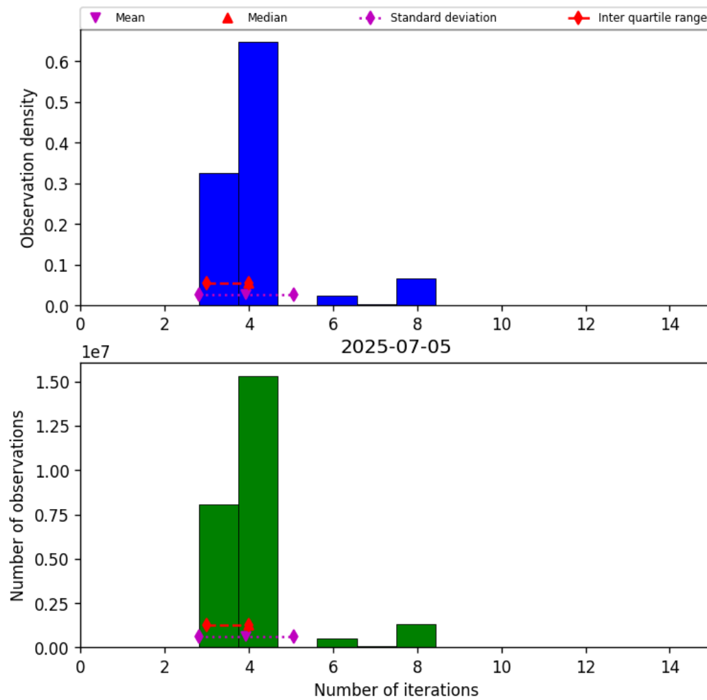
Figure 34: Histogram of “Number of iterations” for 2025-07-04 to 2025-07-06
