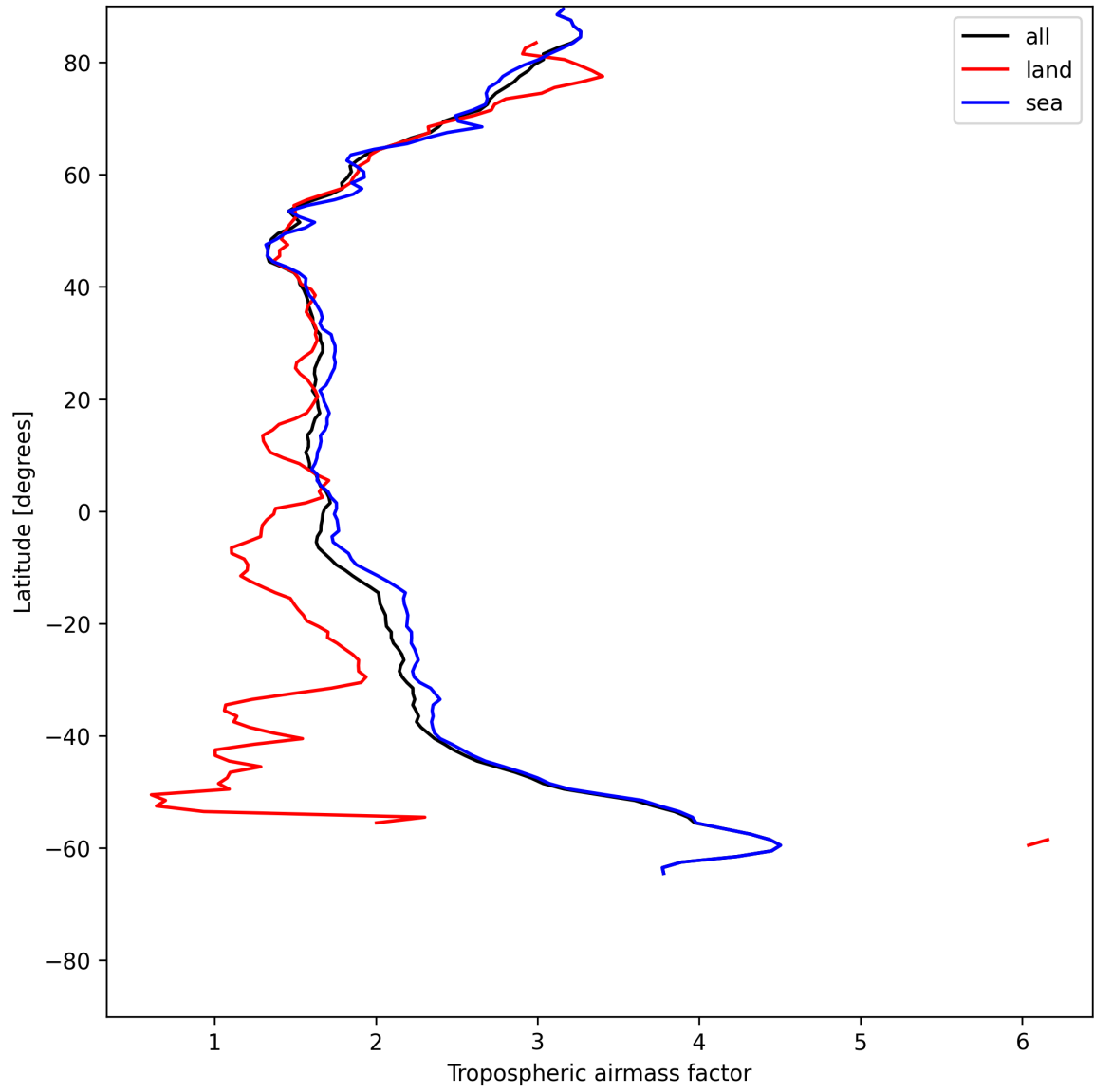
Figure 14: Zonal average of “Tropospheric airmass factor” for 2025-07-04 to 2025-07-06.
