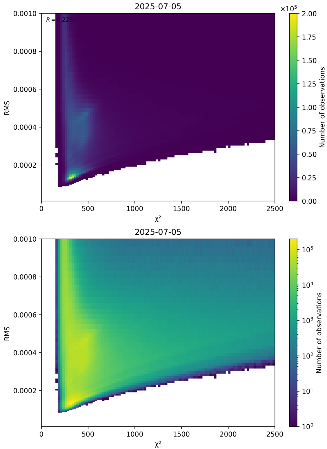
Figure 82: Scatter density plot of “ \chi^2 ” against “RMS” for 2025-07-04 to 2025-07-06.
