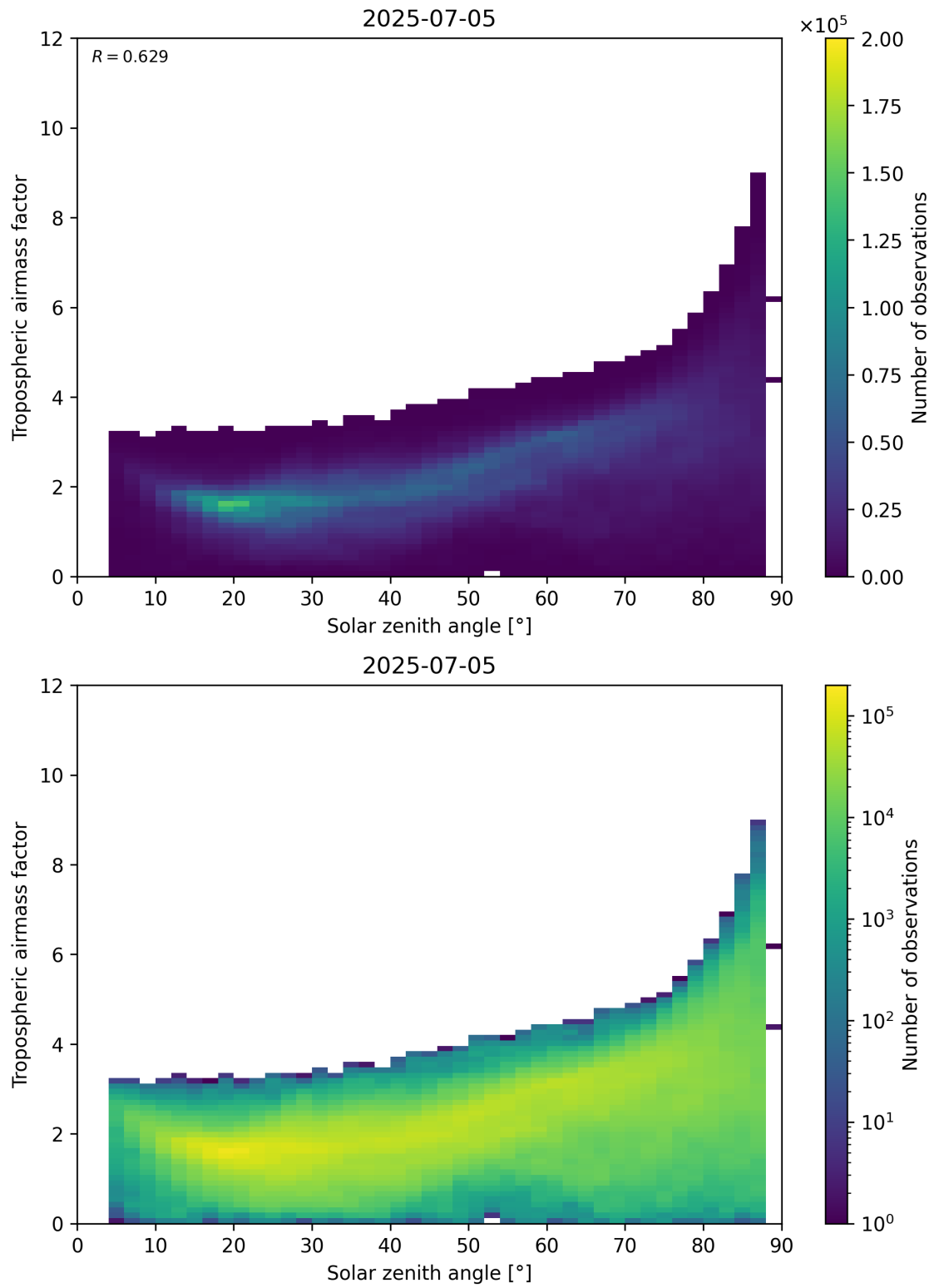
Figure 147: Scatter density plot of “Solar zenith angle” against “Tropospheric airmass factor” for 2025-07-04 to 2025-07-06.
