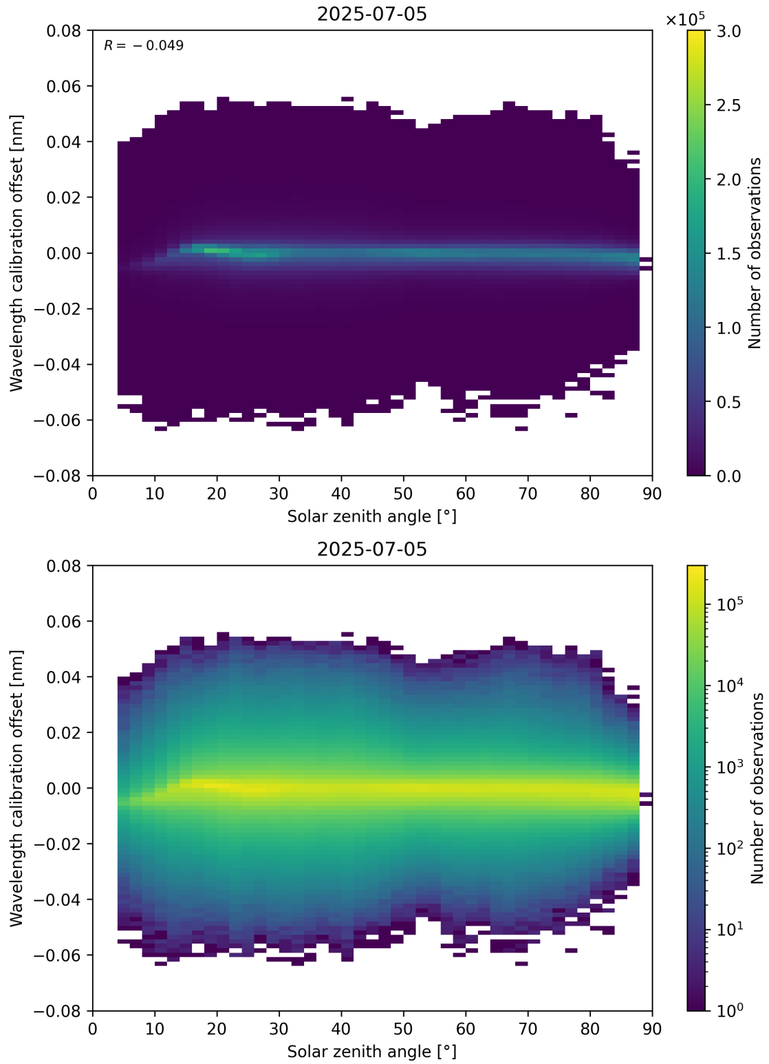
Figure 158: Scatter density plot of “Solar zenith angle” against “Wavelength calibration offset” for 2025-07-04 to 2025-07-06.
