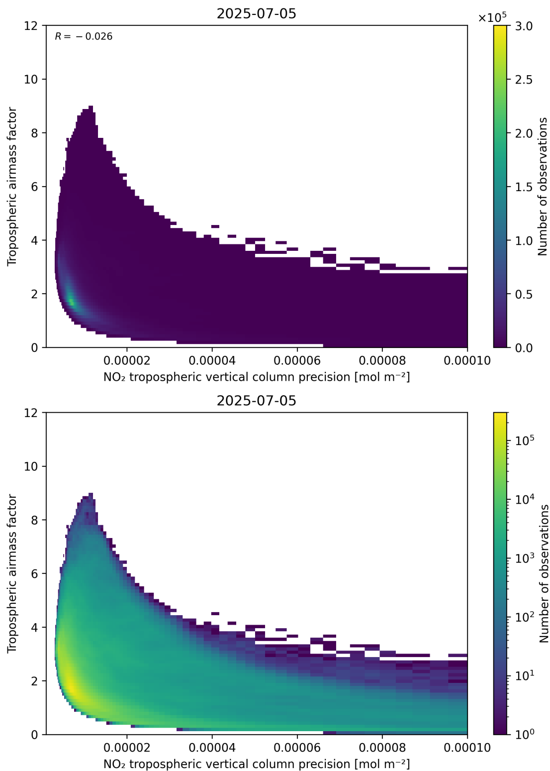
Figure 133: Scatter density plot of “NO 2 tropospheric vertical column precision” against “Tropospheric airmass factor” for 2025-07-04 to 2025-07-06.
