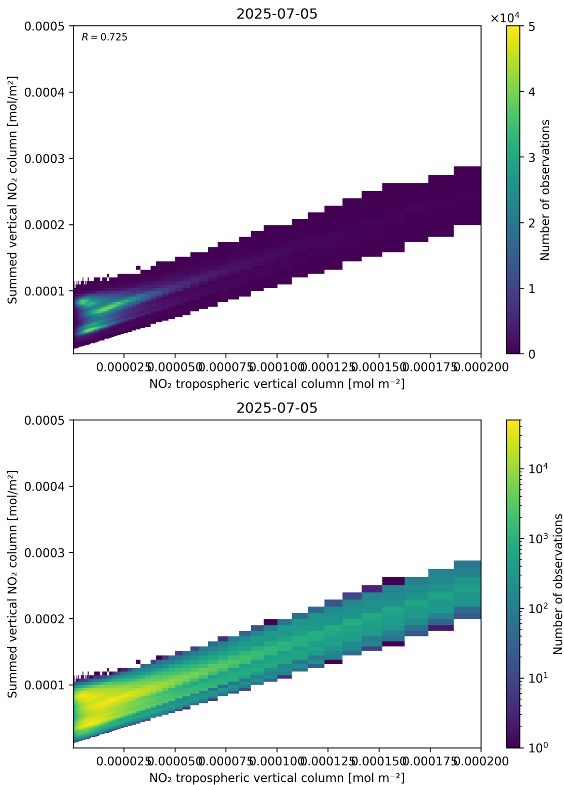
Figure 126: Scatter density plot of “NO 2 tropospheric vertical column” against “Summed vertical NO 2 column” for 2025-07-04 to 2025-07-06.
