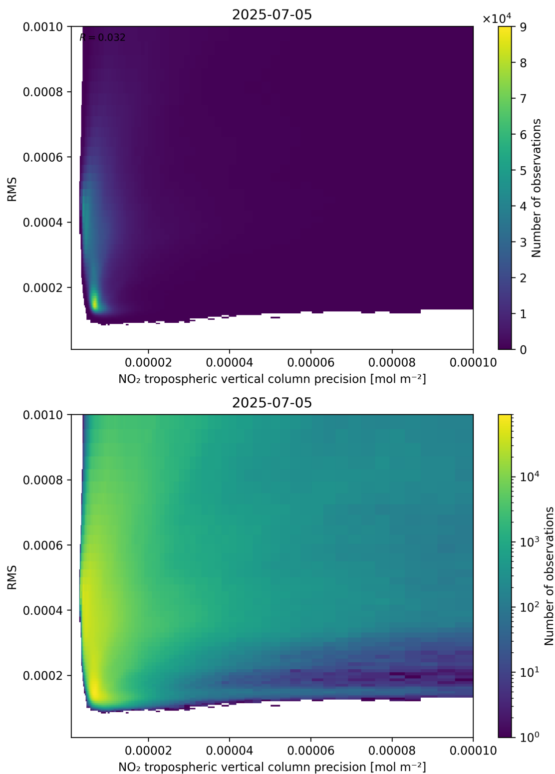
Figure 140: Scatter density plot of “NO 2 tropospheric vertical column precision” against “RMS” for 2025-07-04 to 2025-07-06.
