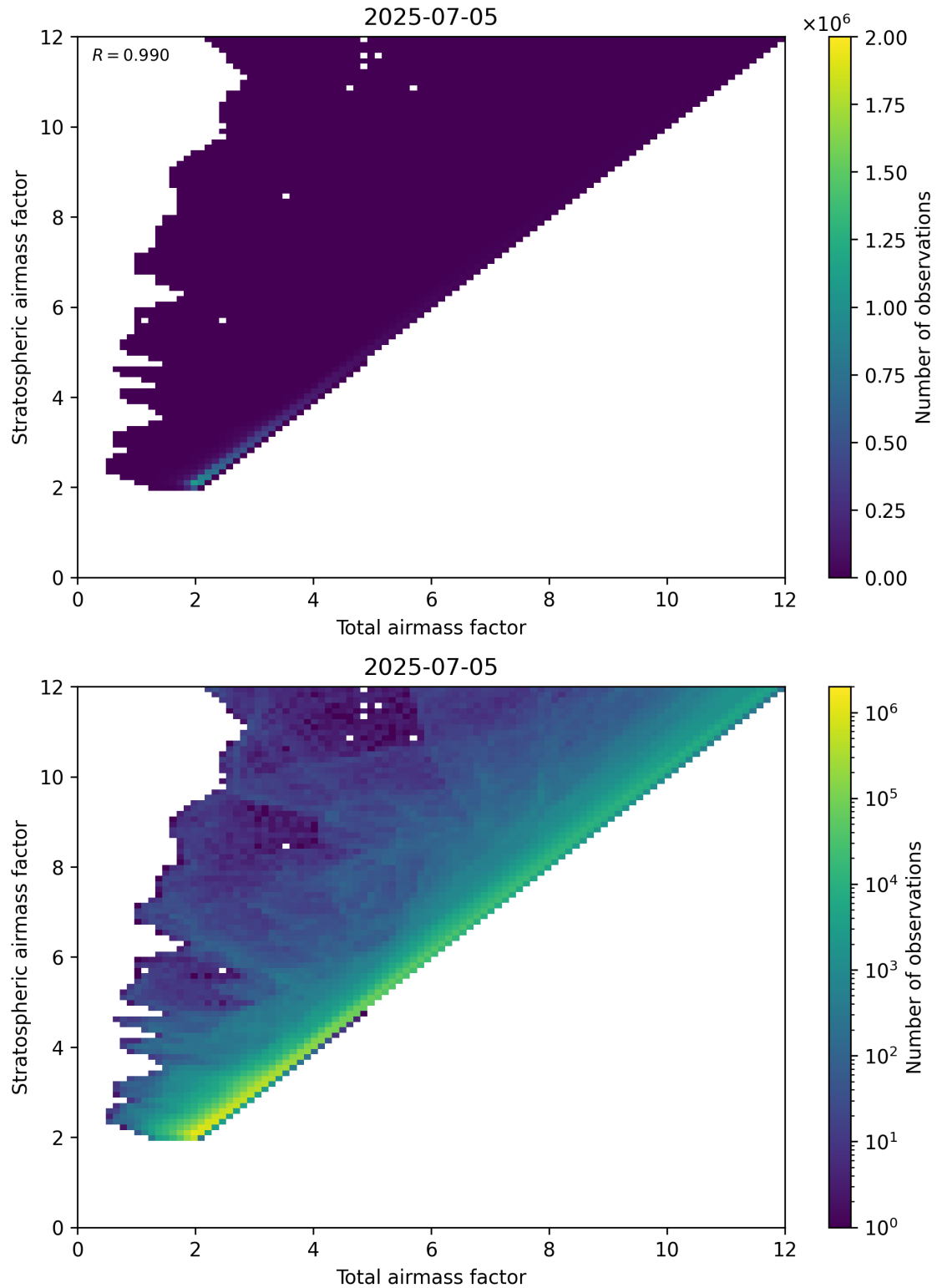
Figure 62: Scatter density plot of “Total airmass factor” against “Stratospheric airmass factor” for 2025-07-04 to 2025-07-06.
