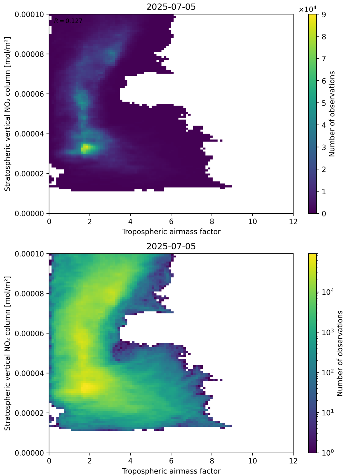
Figure 74: Scatter density plot of “Tropospheric airmass factor” against “Stratospheric vertical NO 2 column” for 2025-07-04 to 2025-07-06.
