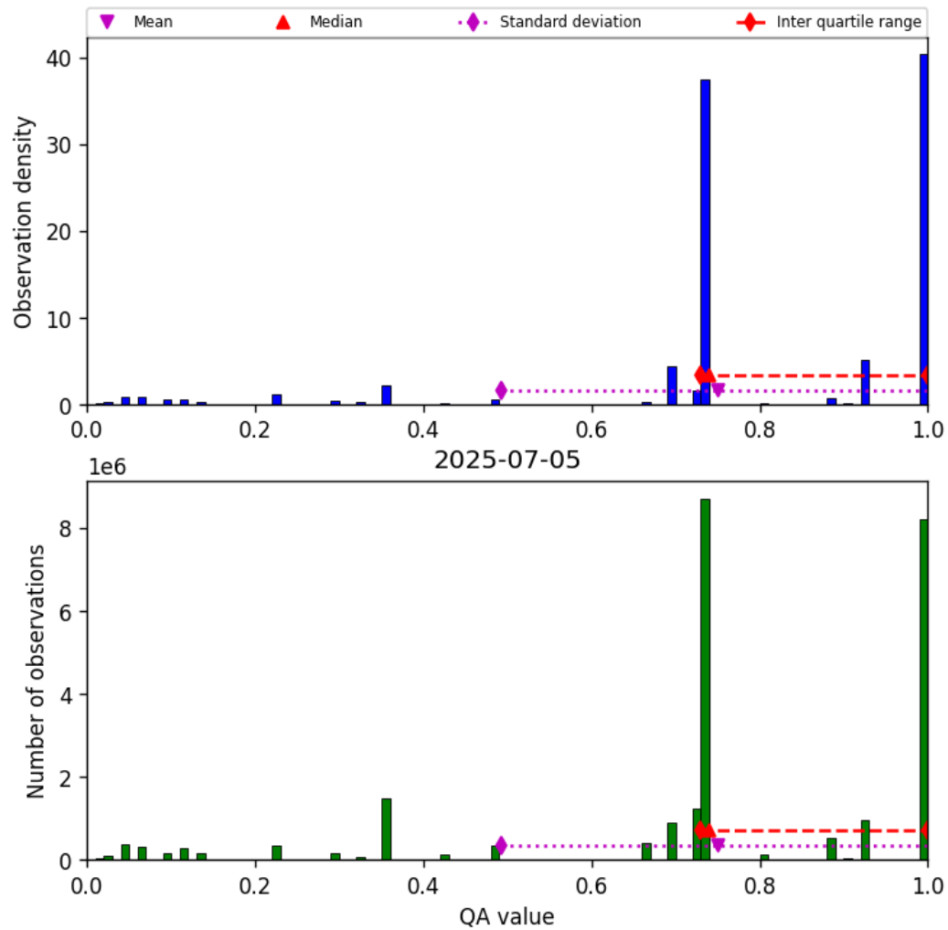
Figure 28: Histogram of “QA value” for 2025-07-04 to 2025-07-06
