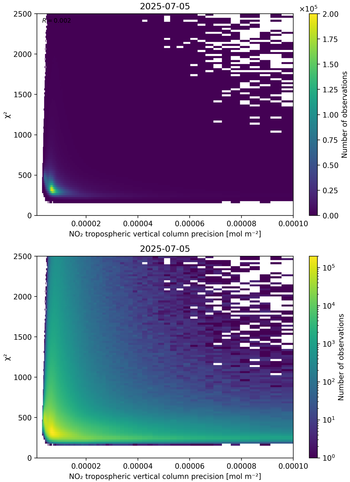
Figure 134: Scatter density plot of “NO 2 tropospheric vertical column precision” against “ \chi^2 ” for 2025-07-04 to 2025-07-06.
