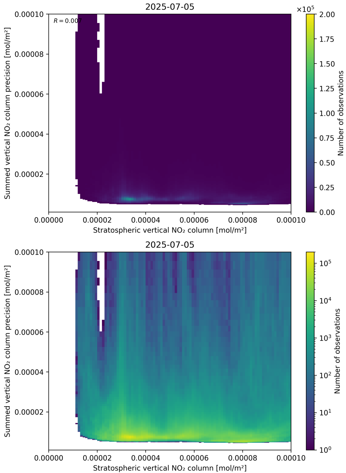
Figure 99: Scatter density plot of “Stratospheric vertical NO 2 column” against “Summed vertical NO 2 column precision” for 2025-07-04 to 2025-07-06.
