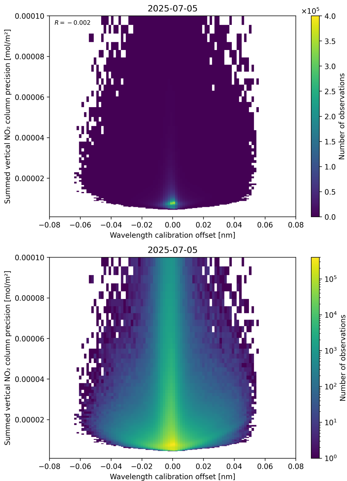
Figure 178: Scatter density plot of “Wavelength calibration offset” against “Summed vertical NO 2 column precision” for 2025-07-04 to 2025-07-06.
