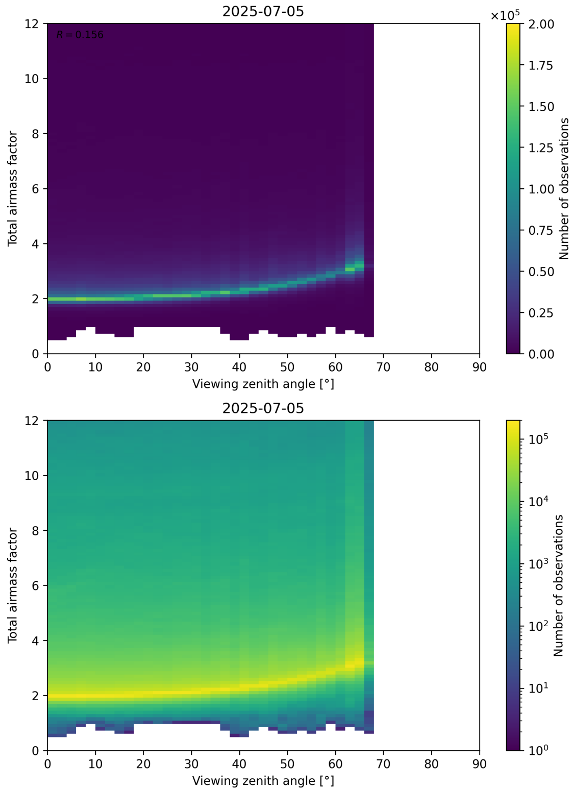
Figure 160: Scatter density plot of “Viewing zenith angle” against “Total airmass factor” for 2025-07-04 to 2025-07-06.
