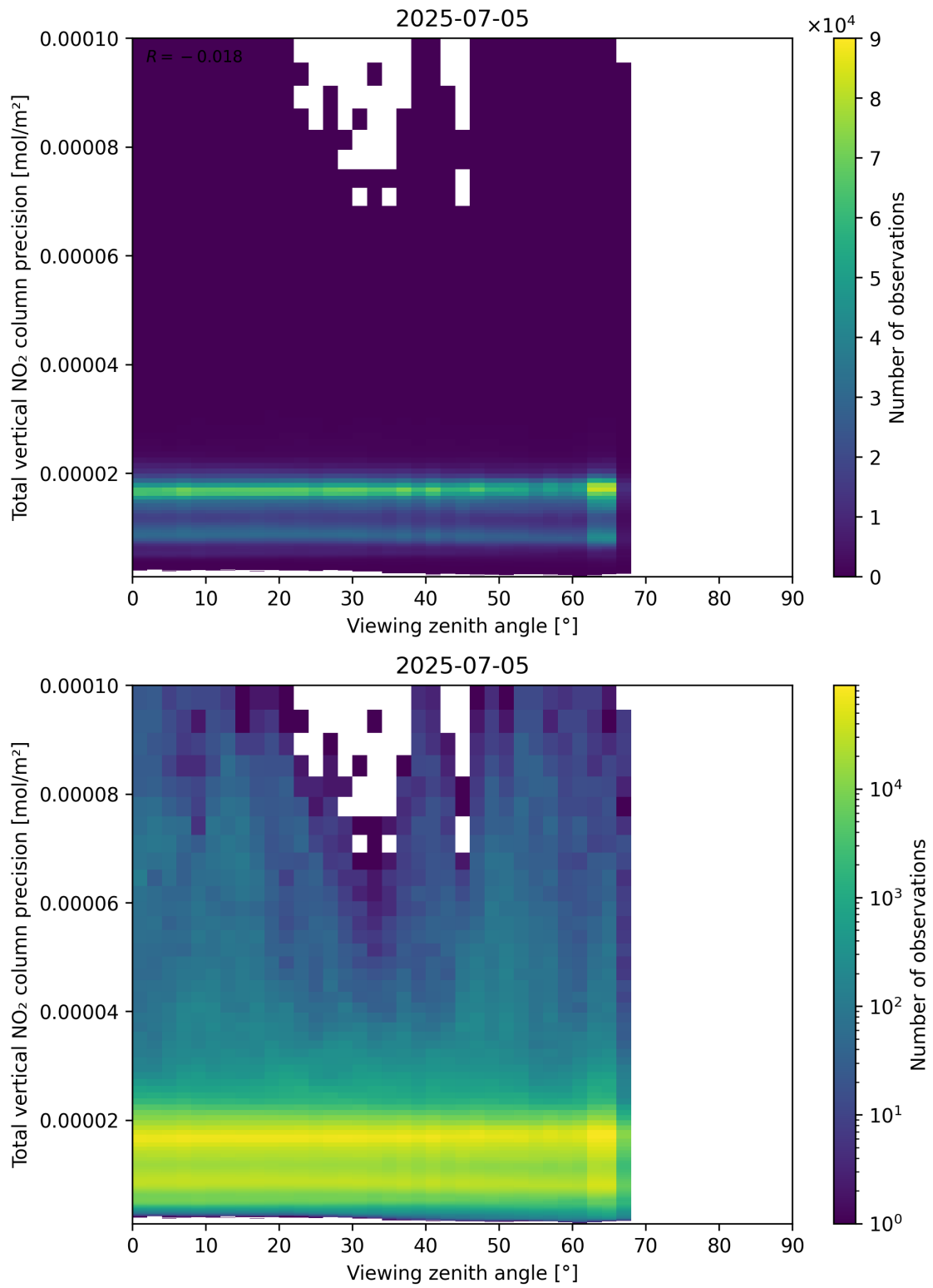
Figure 168: Scatter density plot of “Viewing zenith angle” against “Total vertical NO 2 column precision” for 2025-07-04 to 2025-07-06.
