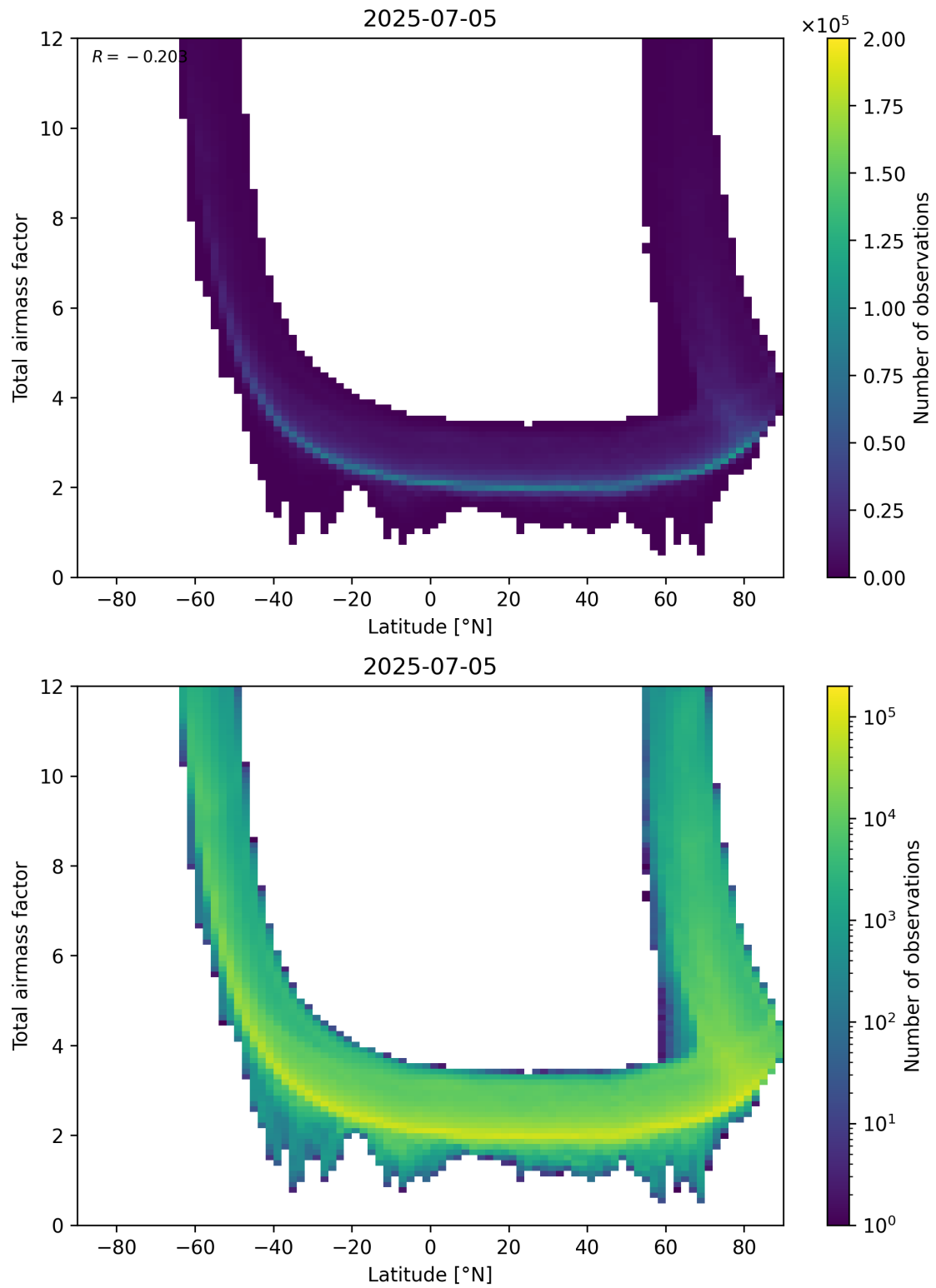
Figure 84: Scatter density plot of “Latitude” against “Total airmass factor” for 2025-07-04 to 2025-07-06.
