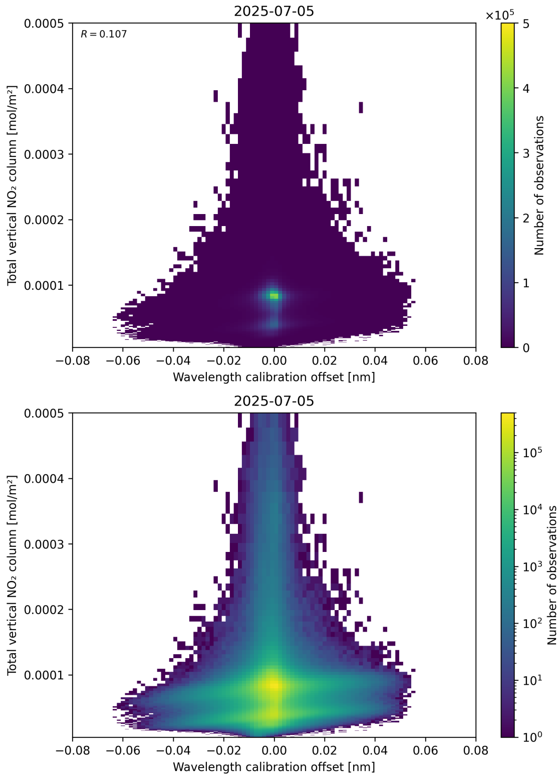
Figure 179: Scatter density plot of “Wavelength calibration offset” against “Total vertical NO 2 column” for 2025-07-04 to 2025-07-06.
