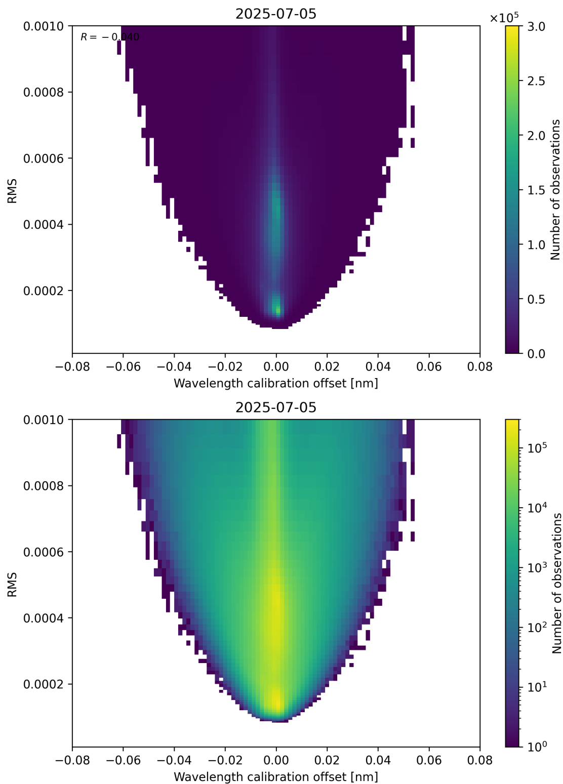
Figure 181: Scatter density plot of “Wavelength calibration offset” against “RMS” for 2025-07-04 to 2025-07-06.
