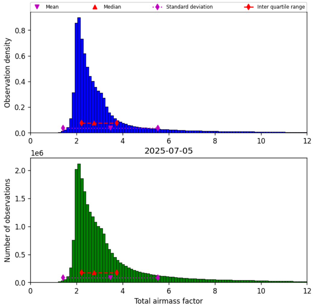
Figure 32: Histogram of “Total airmass factor” for 2025-07-04 to 2025-07-06
