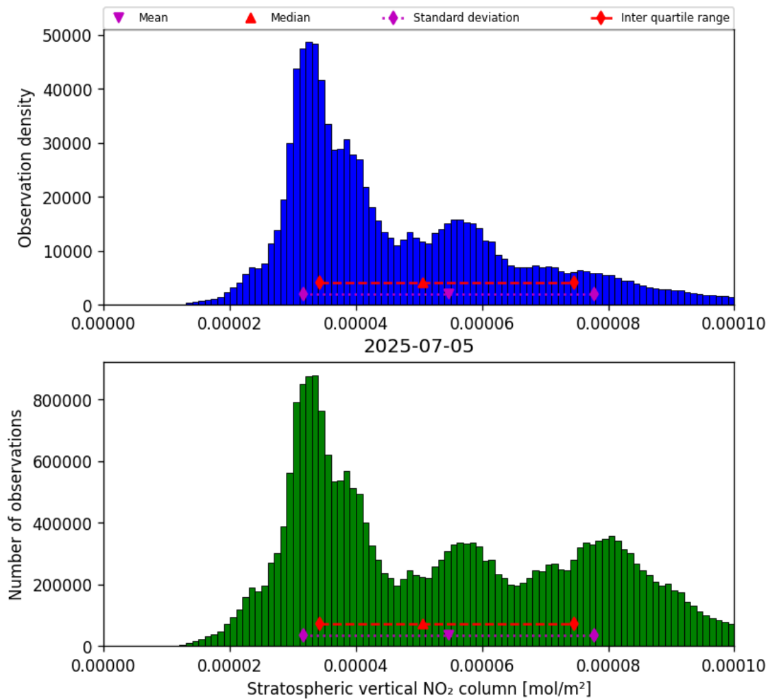
Figure 36: Histogram of “Stratospheric vertical NO 2 column” for 2025-07-04 to 2025-07-06
