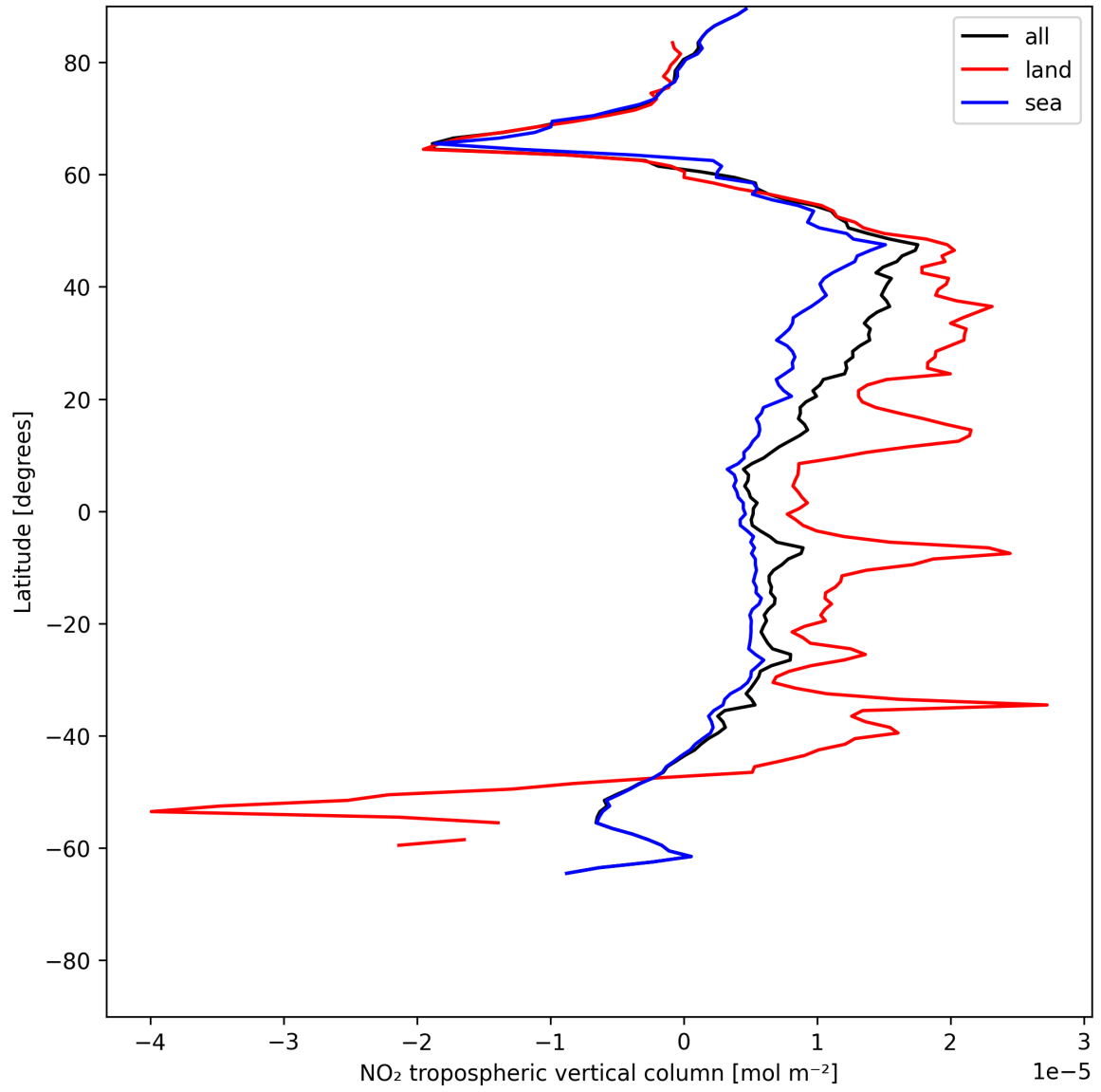
Figure 12: Zonal average of “NO 2 tropospheric vertical column” for 2025-07-04 to 2025-07-06.
