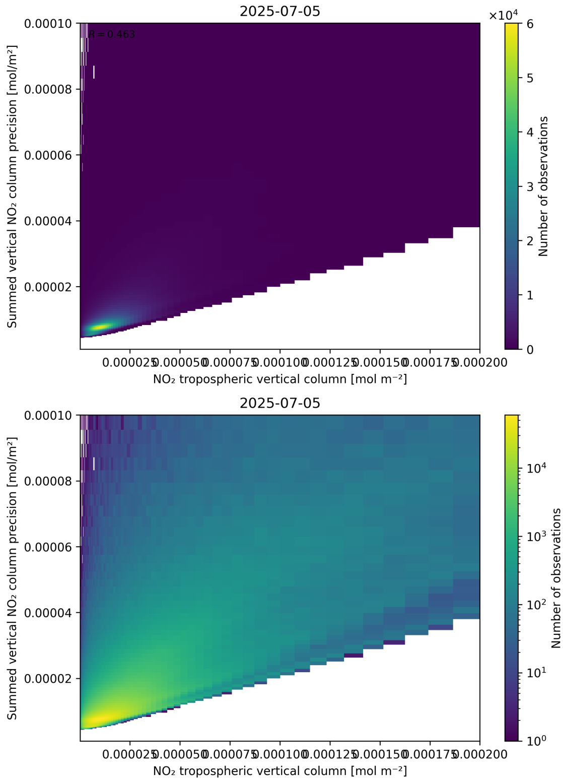
Figure 127: Scatter density plot of “NO 2 tropospheric vertical column” against “Summed vertical NO 2 column precision” for 2025-07-04 to 2025-07-06.
