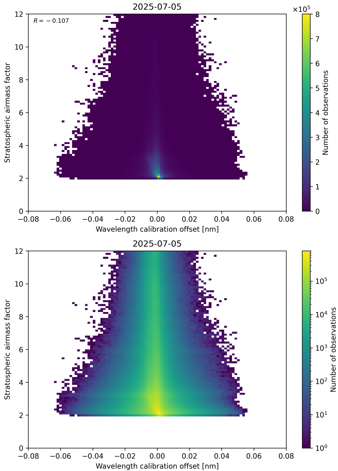
Figure 174: Scatter density plot of “Wavelength calibration offset” against “Stratospheric airmass factor” for 2025-07-04 to 2025-07-06.
