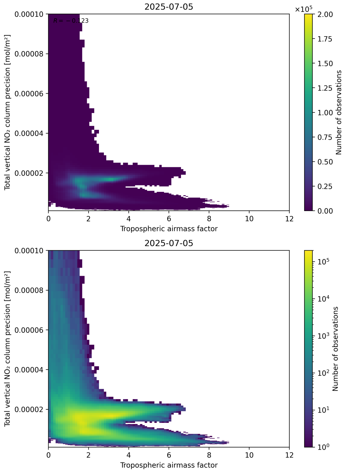
Figure 78: Scatter density plot of “Tropospheric air mass factor” against “Total vertical NO 2 column precision” for 2025-07-04 to 2025-07-06.
