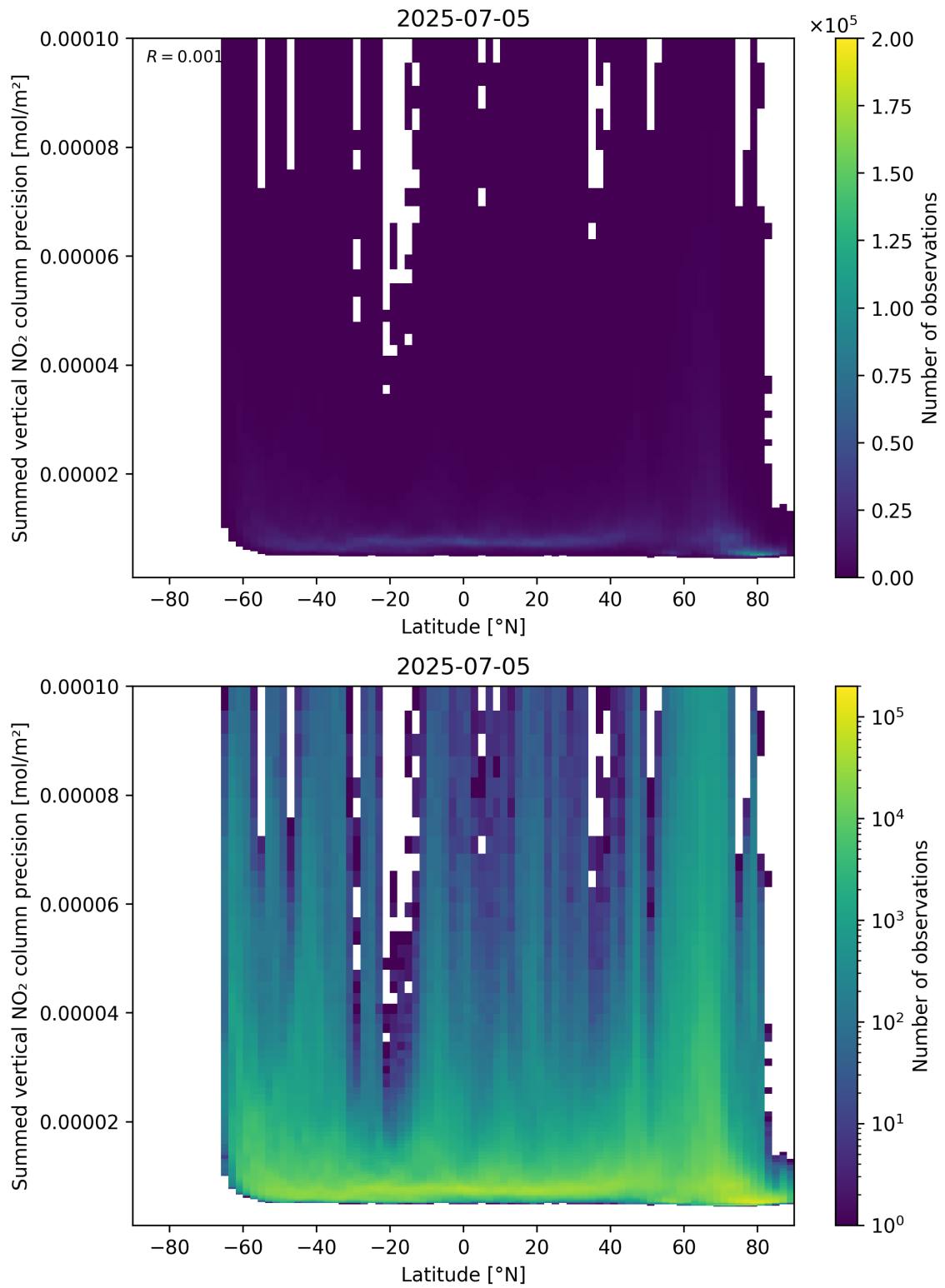
Figure 89: Scatter density plot of “Latitude” against “Summed vertical NO 2 column precision” for 2025-07-04 to 2025-07-06.
