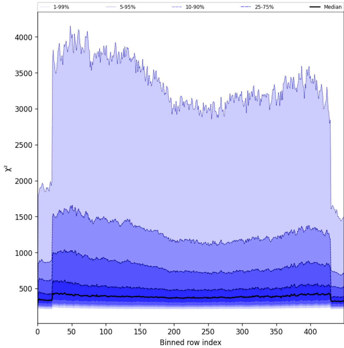
Figure 59: Along track statistics of “ \chi^2 ” for 2025-07-04 to 2025-07-06
