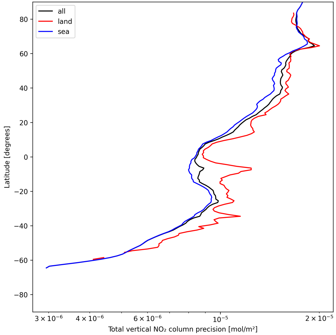
Figure 22: Zonal average of “Total vertical NO 2 column precision” for 2025-07-04 to 2025-07-06.
