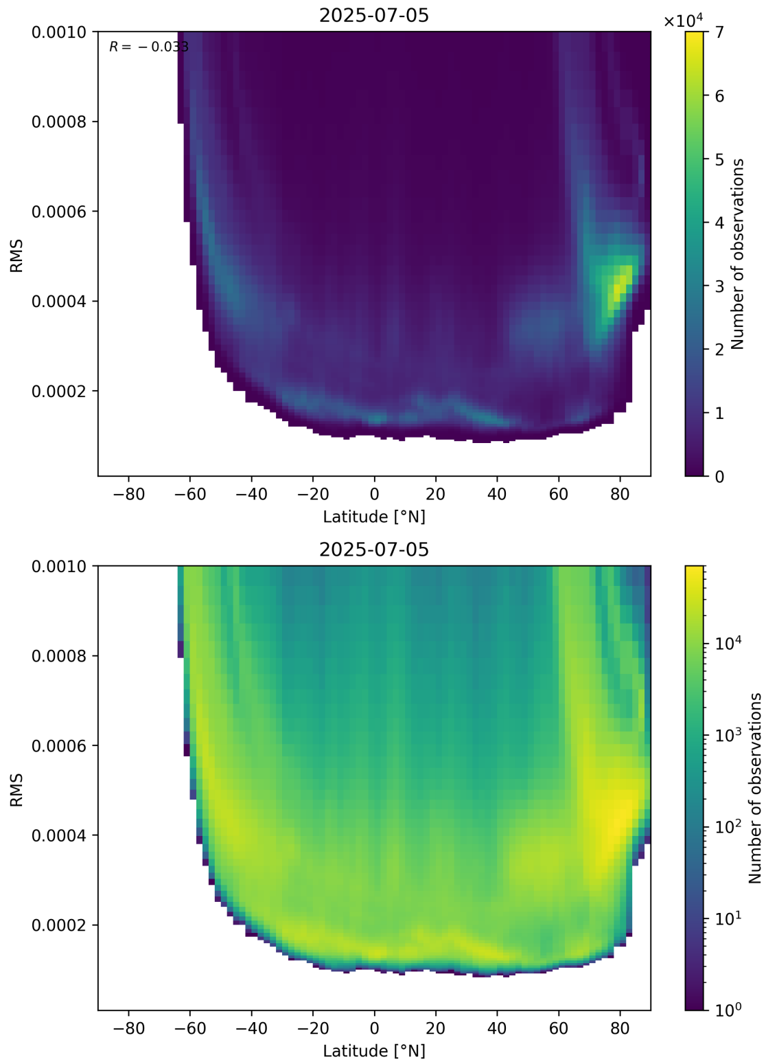
Figure 94: Scatter density plot of “Latitude” against “RMS” for 2025-07-04 to 2025-07-06.
