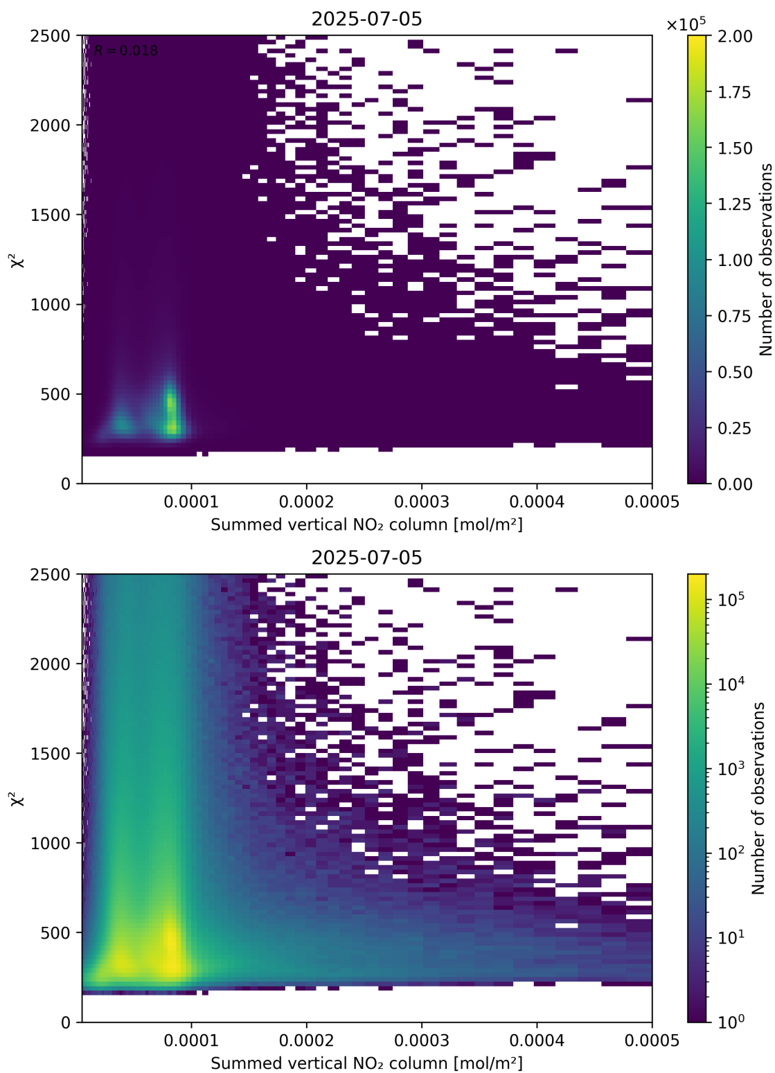
Figure 104: Scatter density plot of “Summed vertical NO 2 column” against “ \chi^2 ” for 2025-07-04 to 2025-07-06.
