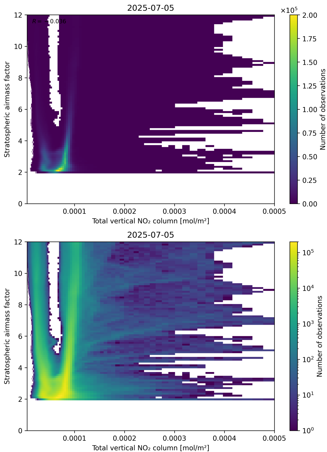
Figure 110: Scatter density plot of “Total vertical NO 2 column” against “Stratospheric airmass factor” for 2025-07-04 to 2025-07-06.
