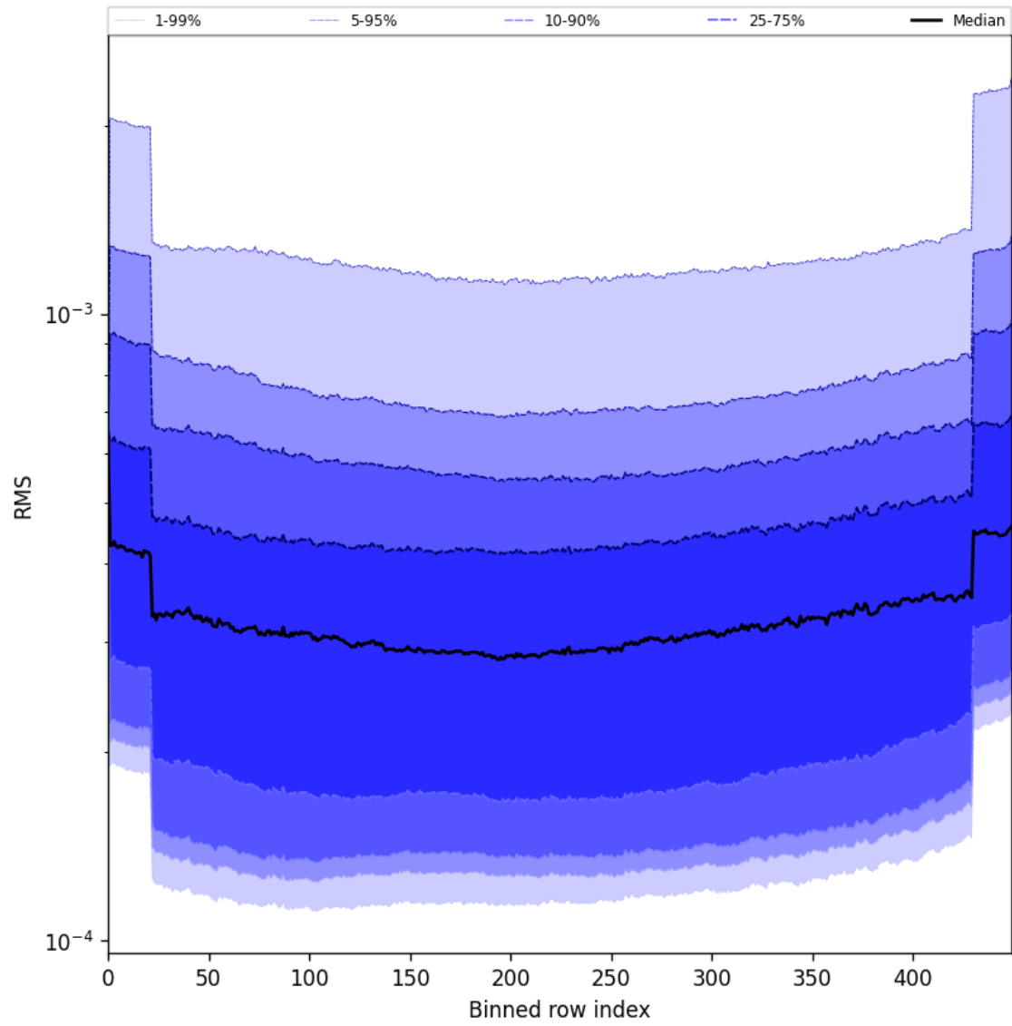
Figure 60: Along track statistics of “RMS” for 2025-07-04 to 2025-07-06
