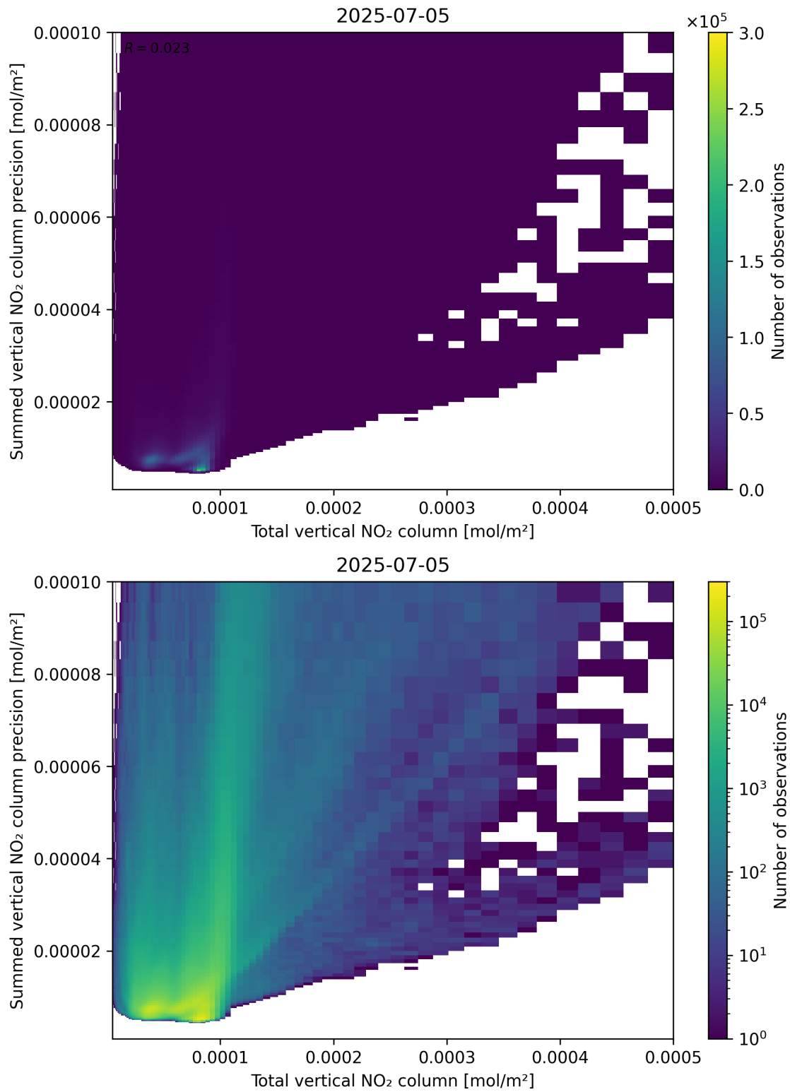
Figure 113: Scatter density plot of “Total vertical NO 2 column” against “Summed vertical NO 2 column precision” for 2025-07-04 to 2025-07-06.
