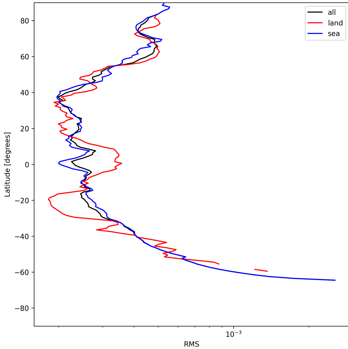
Figure 26: Zonal average of “RMS” for 2025-07-04 to 2025-07-06.
