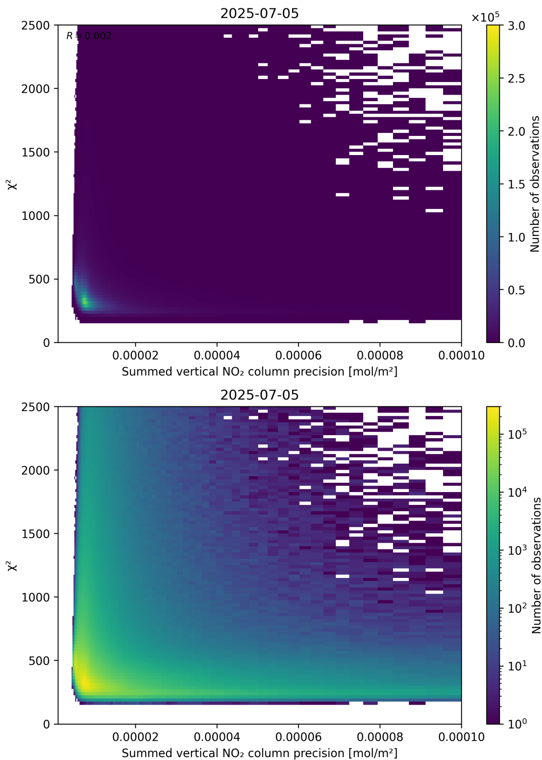
Figure 107: Scatter density plot of “Summed vertical NO 2 column precision” against “ \chi^2 ” for 2025-07-04 to 2025-07-06.
