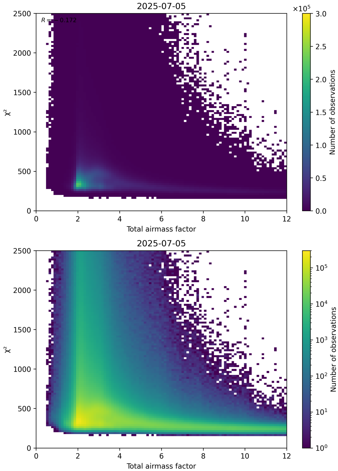
Figure 63: Scatter density plot of “Total airmass factor” against “ \chi^2 ” for 2025-07-04 to 2025-07-06.
