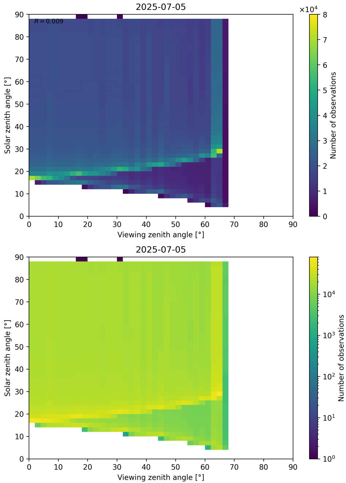
Figure 172: Scatter density plot of “Viewing zenith angle” against “Solar zenith angle” for 2025-07-04 to 2025-07-06.
