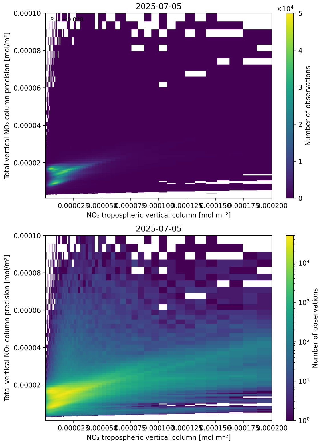
Figure 129: Scatter density plot of “NO 2 tropospheric vertical column” against “Total vertical NO 2 column precision” for 2025-07-04 to 2025-07-06.
