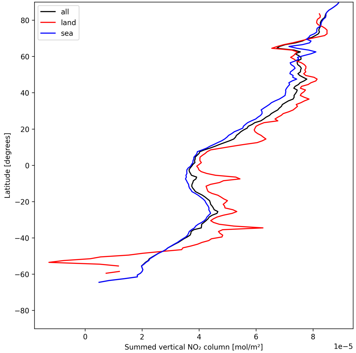
Figure 23: Zonal average of “Summed vertical NO 2 column” for 2025-07-04 to 2025-07-06.
