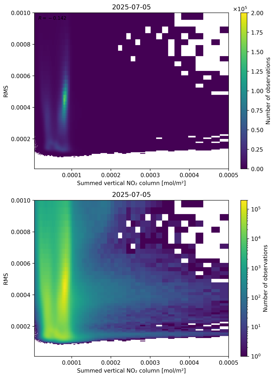
Figure 109: Scatter density plot of “Summed vertical NO 2 column” against “RMS” for 2025-07-04 to 2025-07-06.
