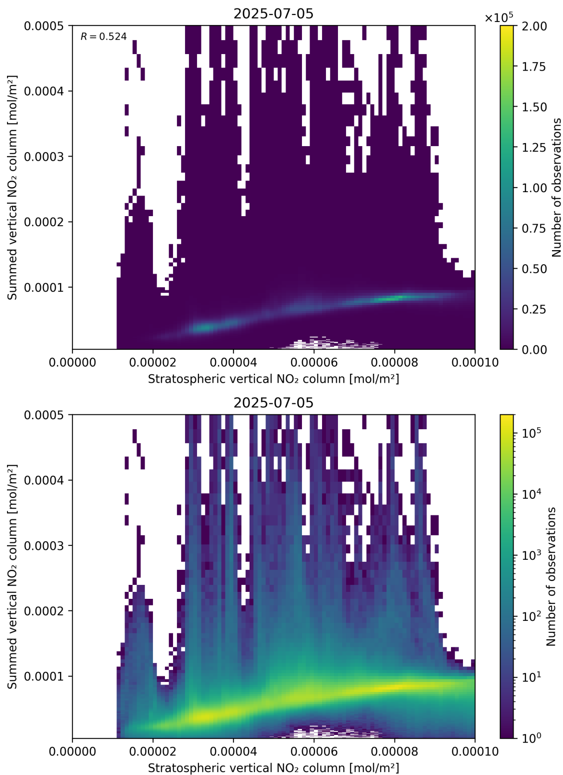
Figure 98: Scatter density plot of “Stratospheric vertical NO 2 column” against “Summed vertical NO 2 column” for 2025-07-04 to 2025-07-06.
