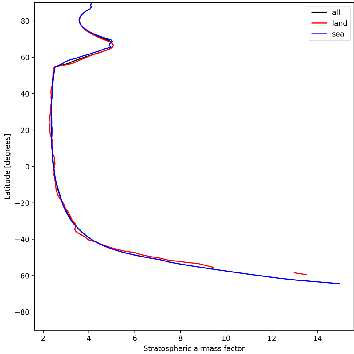
Figure 27: Zonal average of “Stratospheric airmass factor” for 2025-07-04 to 2025-07-06.
