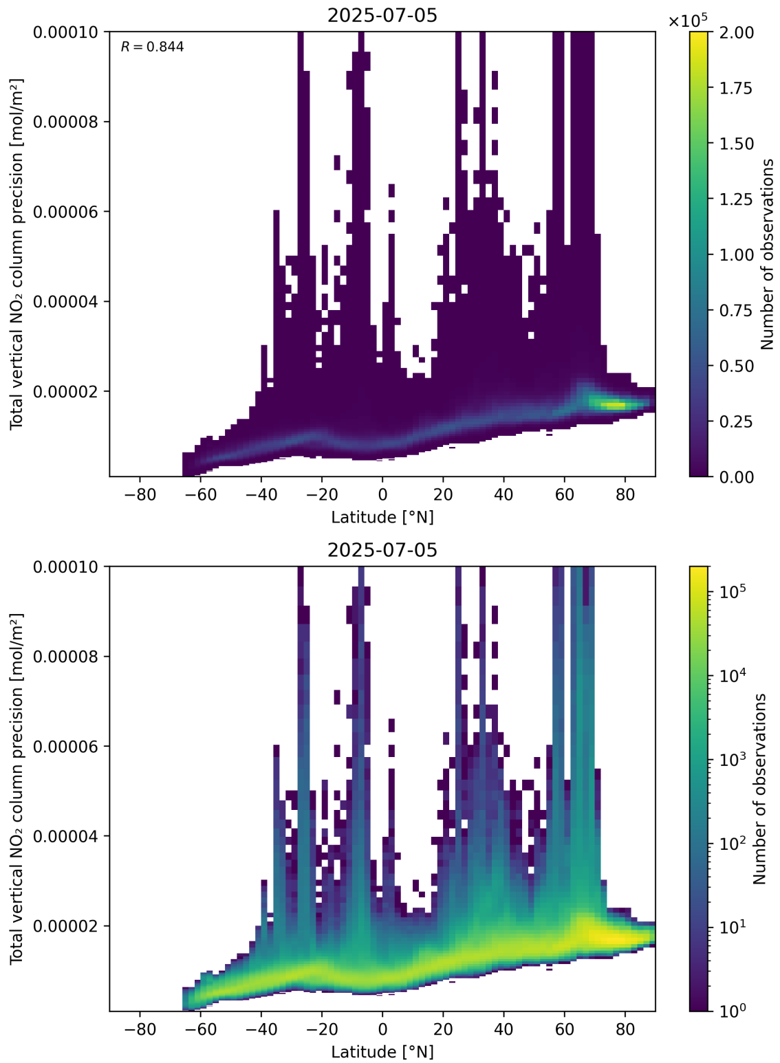
Figure 91: Scatter density plot of “Latitude” against “Total vertical NO 2 column precision” for 2025-07-04 to 2025-07-06.
