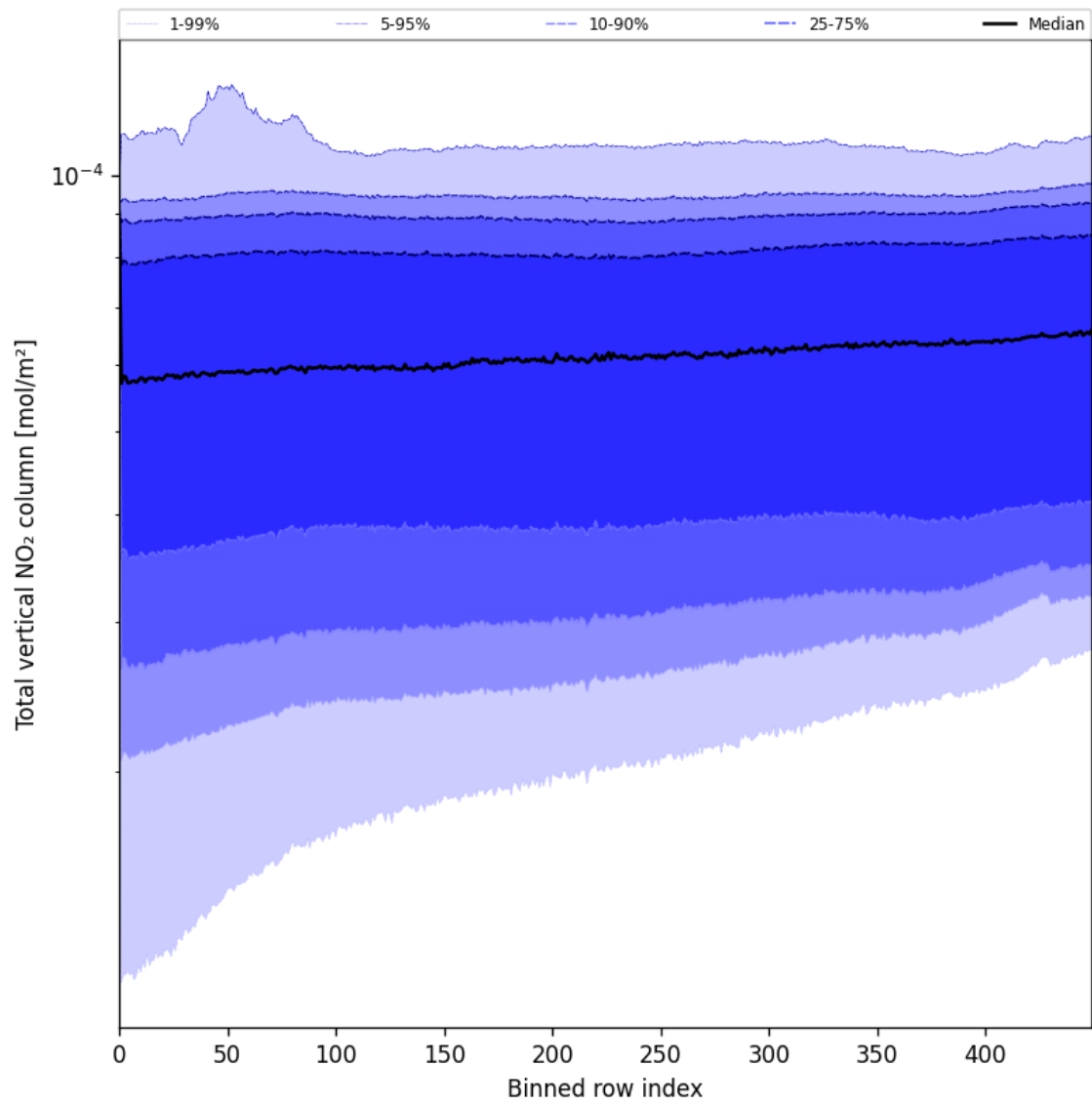
Figure 55: Along track statistics of “Total vertical NO 2 column” for 2025-07-05 to 2025-07-07
