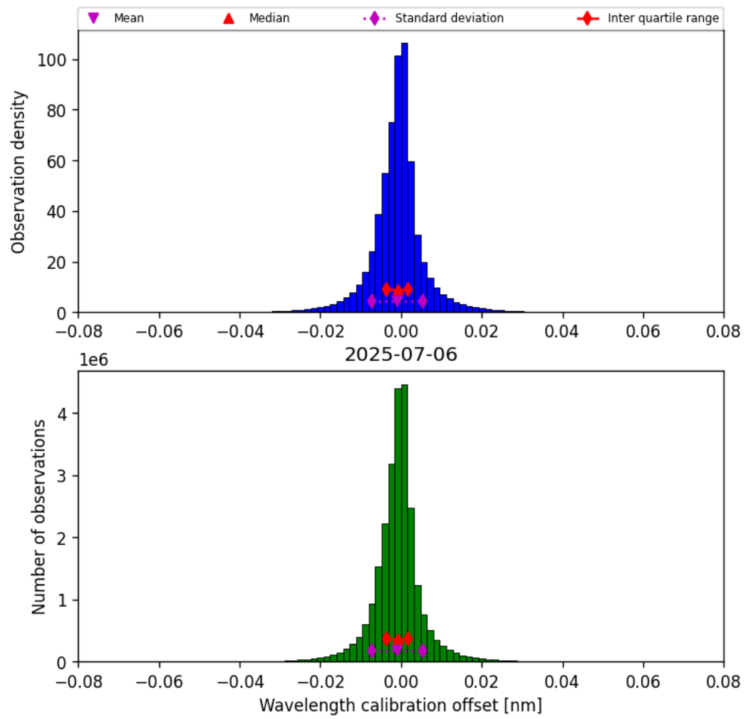
Figure 35: Histogram of “Wavelength calibration offset” for 2025-07-05 to 2025-07-07
