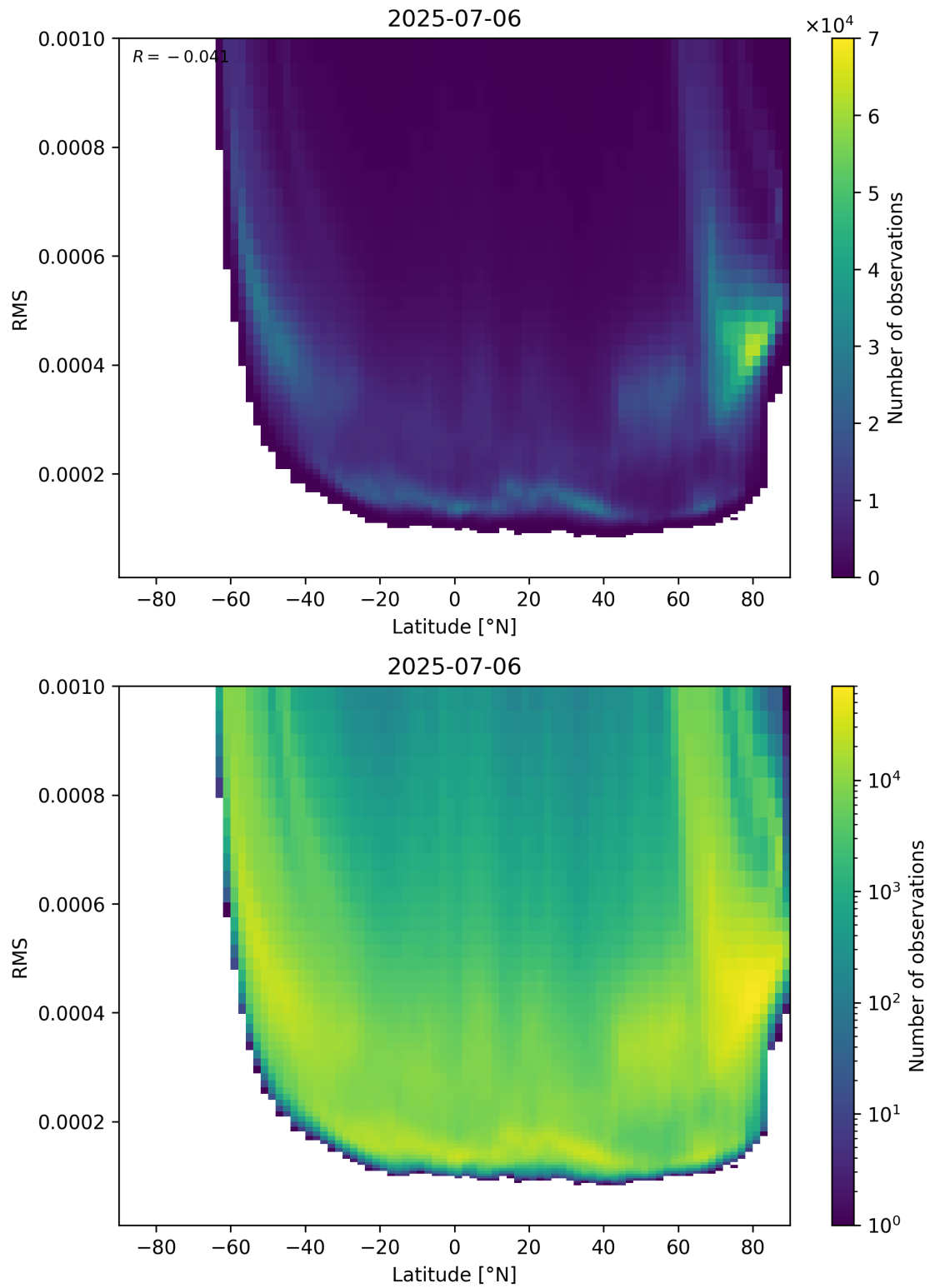
Figure 94: Scatter density plot of “Latitude” against “RMS” for 2025-07-05 to 2025-07-07.
