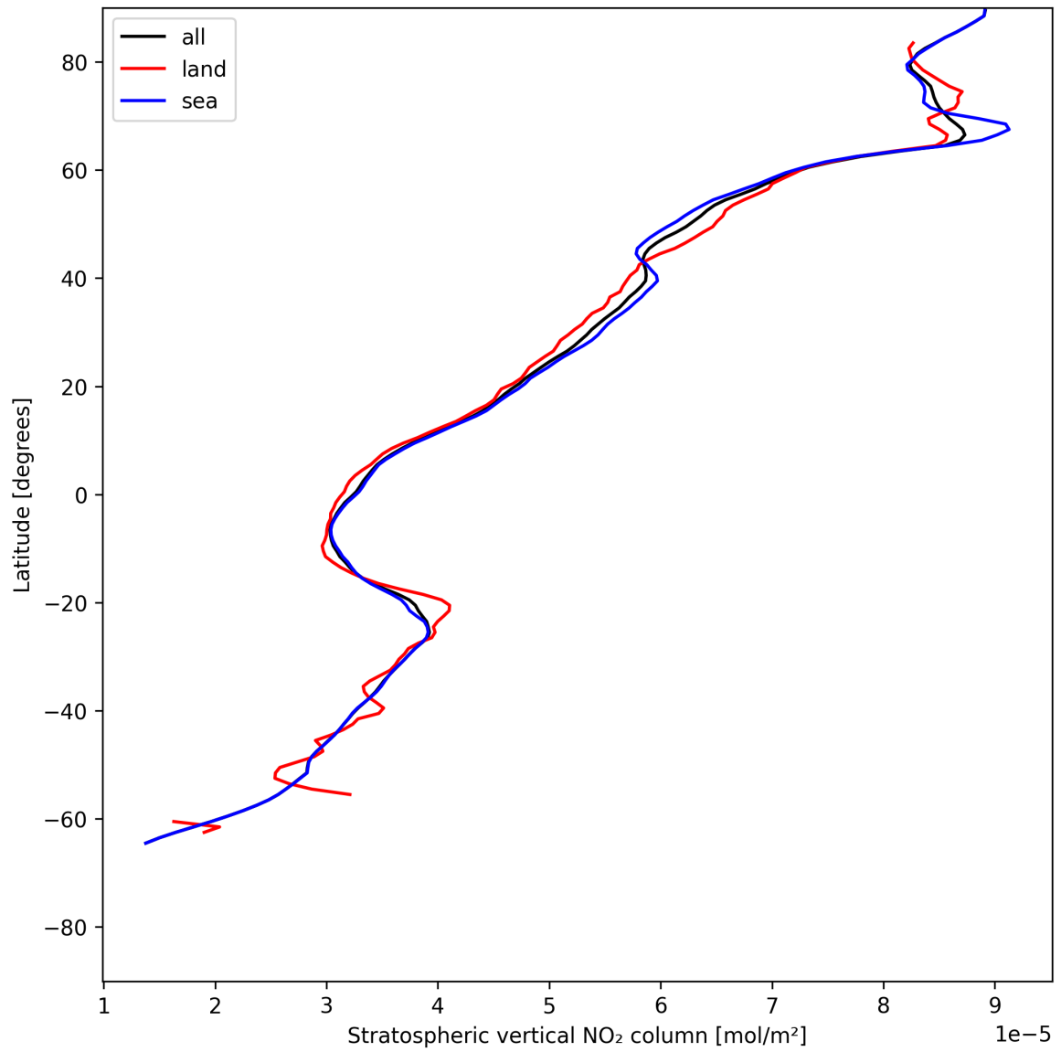
Figure 19: Zonal average of “Stratospheric vertical NO 2 column” for 2025-07-05 to 2025-07-07.
