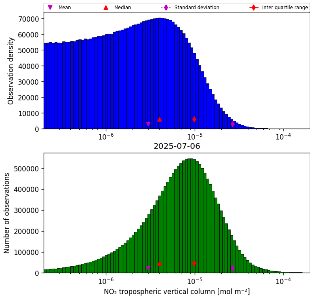
Figure 29: Histogram of “ \text{NO}_2 tropospheric vertical column” for 2025-07-05 to 2025-07-07
