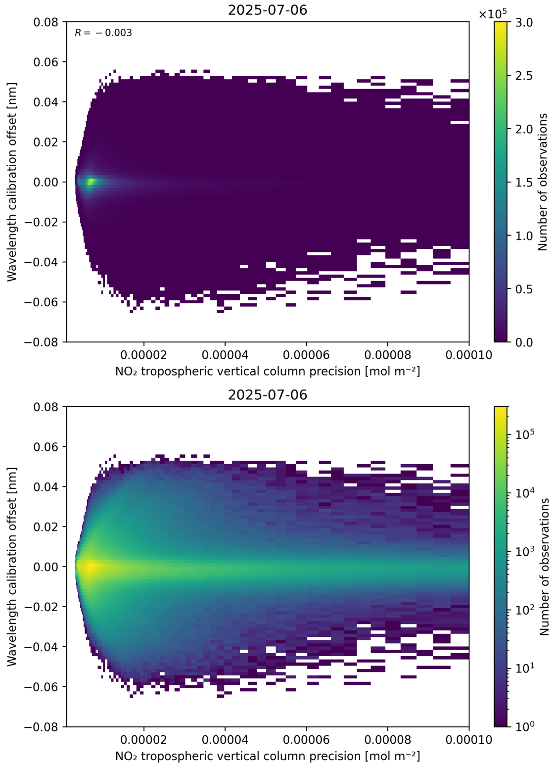
Figure 141: Scatter density plot of “NO 2 tropospheric vertical column precision” against “Wavelength calibration offset” for 2025-07-05 to 2025-07-07.
