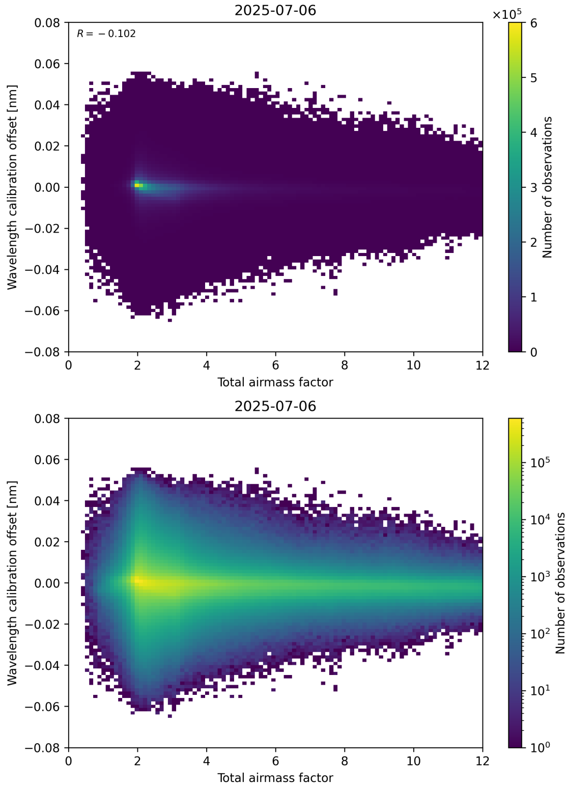
Figure 70: Scatter density plot of “Total airmass factor” against “Wavelength calibration offset” for 2025-07-05 to 2025-07-07.
