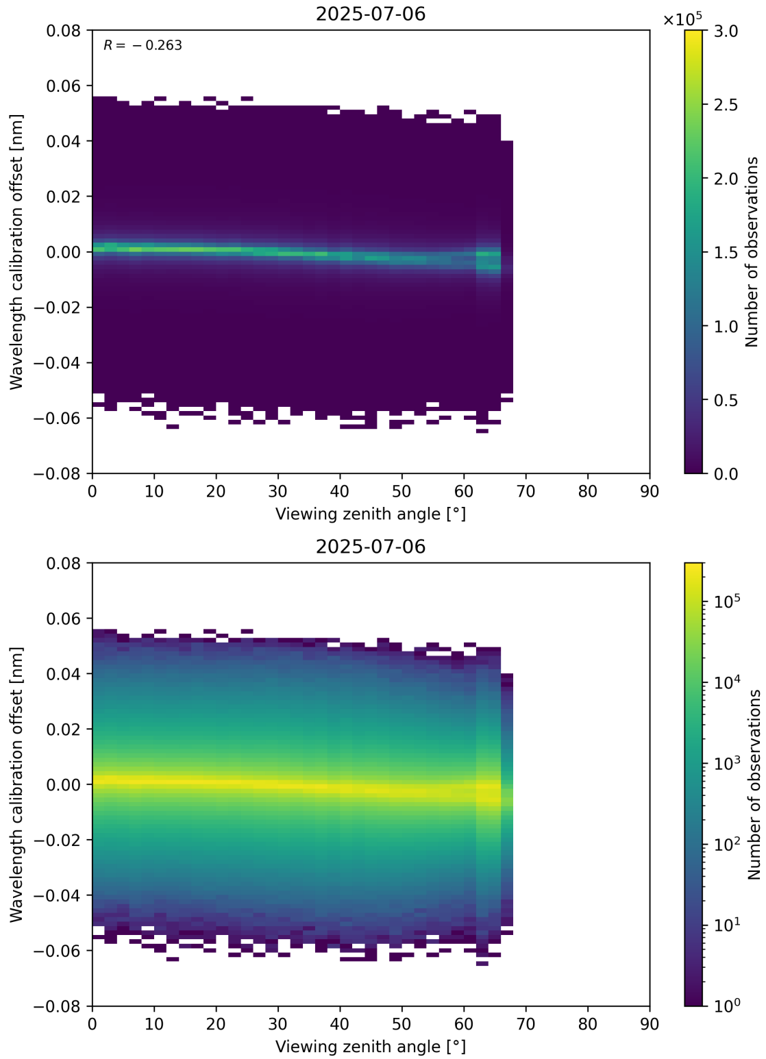
Figure 173: Scatter density plot of “Viewing zenith angle” against “Wavelength calibration offset” for 2025-07-05 to 2025-07-07.
