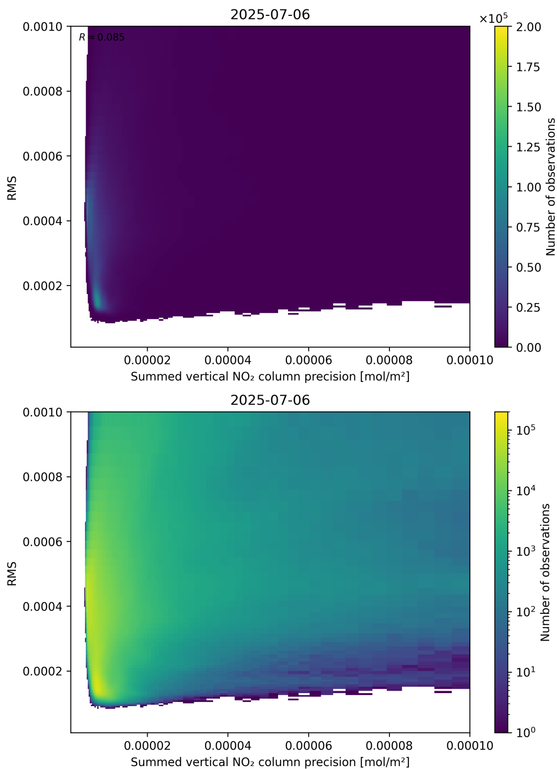
Figure 108: Scatter density plot of “Summed vertical NO 2 column precision” against “RMS” for 2025-07-05 to 2025-07-07.
