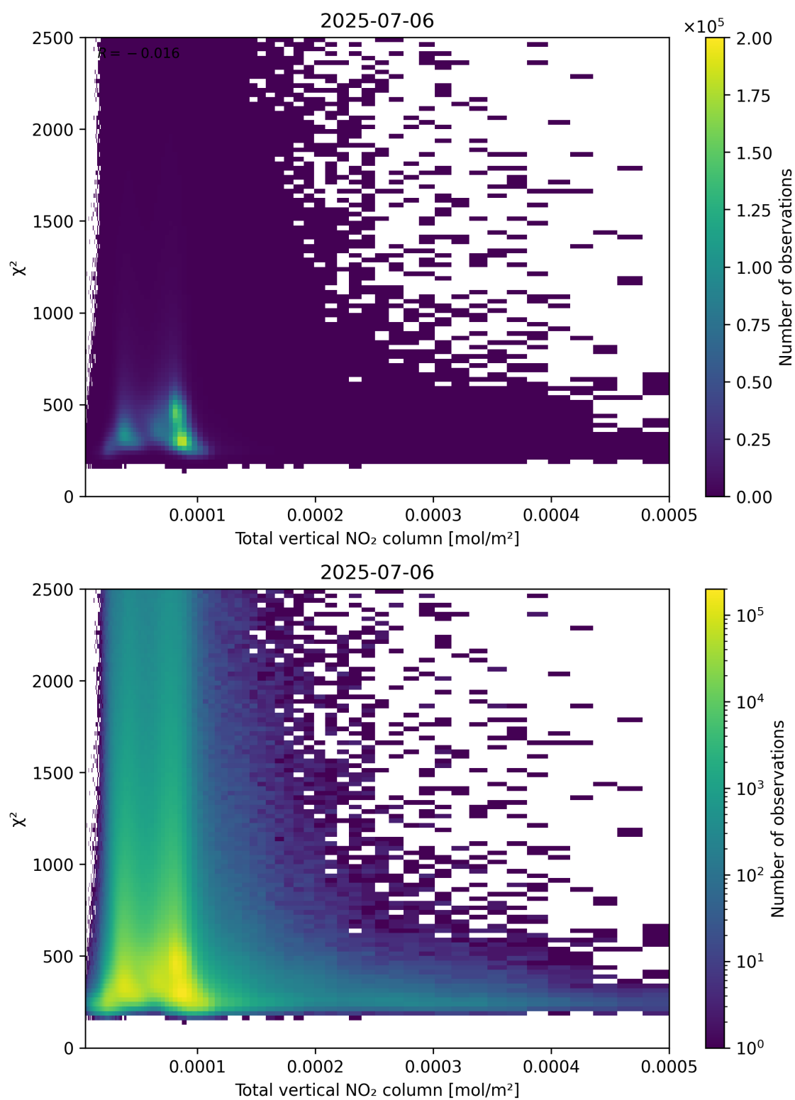
Figure 111: Scatter density plot of “Total vertical NO 2 column” against “ \chi^2 ” for 2025-07-05 to 2025-07-07.
