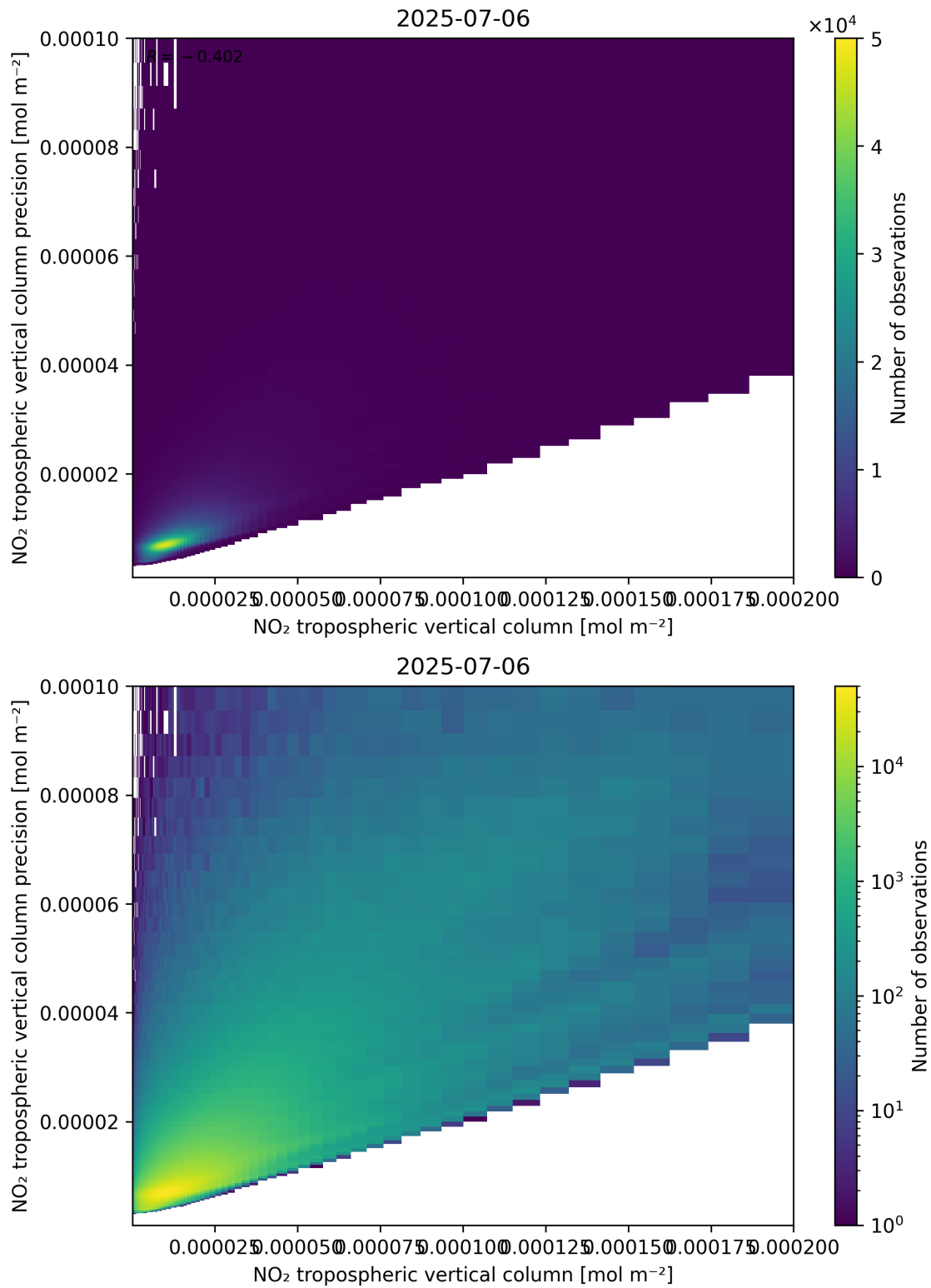
Figure 130: Scatter density plot of “NO 2 tropospheric vertical column” against “NO 2 tropospheric vertical column precision” for 2025-07-05 to 2025-07-07.
