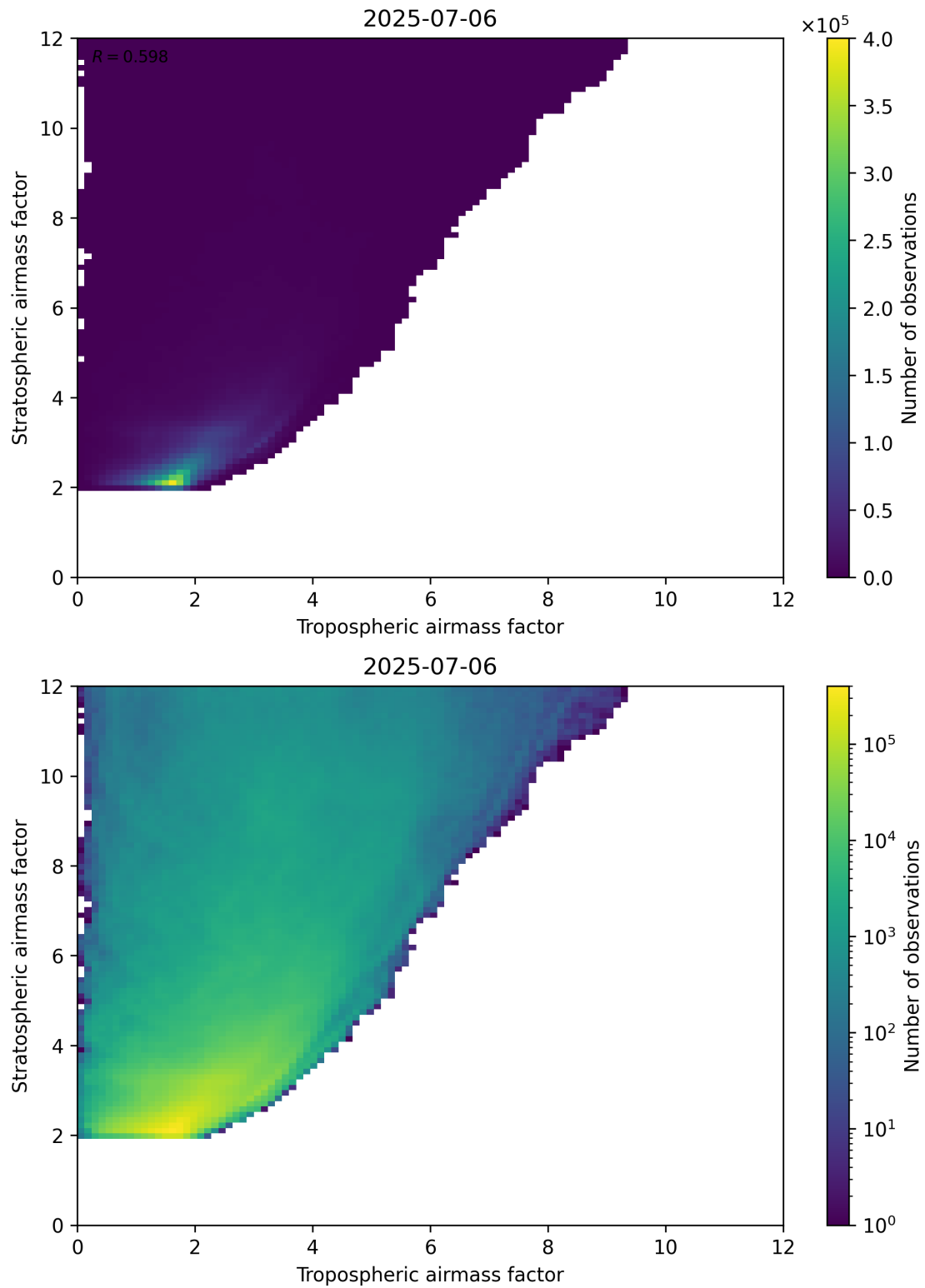
Figure 71: Scatter density plot of “Tropospheric airmass factor” against “Stratospheric airmass factor” for 2025-07-05 to 2025-07-07.
