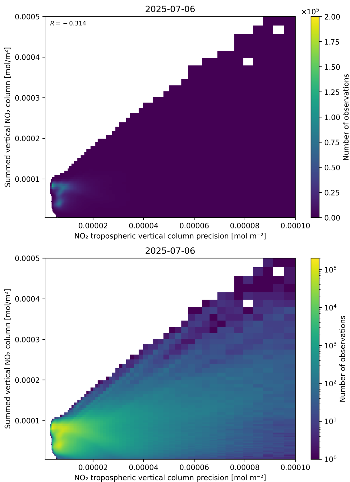
Figure 136: Scatter density plot of “NO 2 tropospheric vertical column precision” against “Summed vertical NO 2 column” for 2025-07-05 to 2025-07-07.
