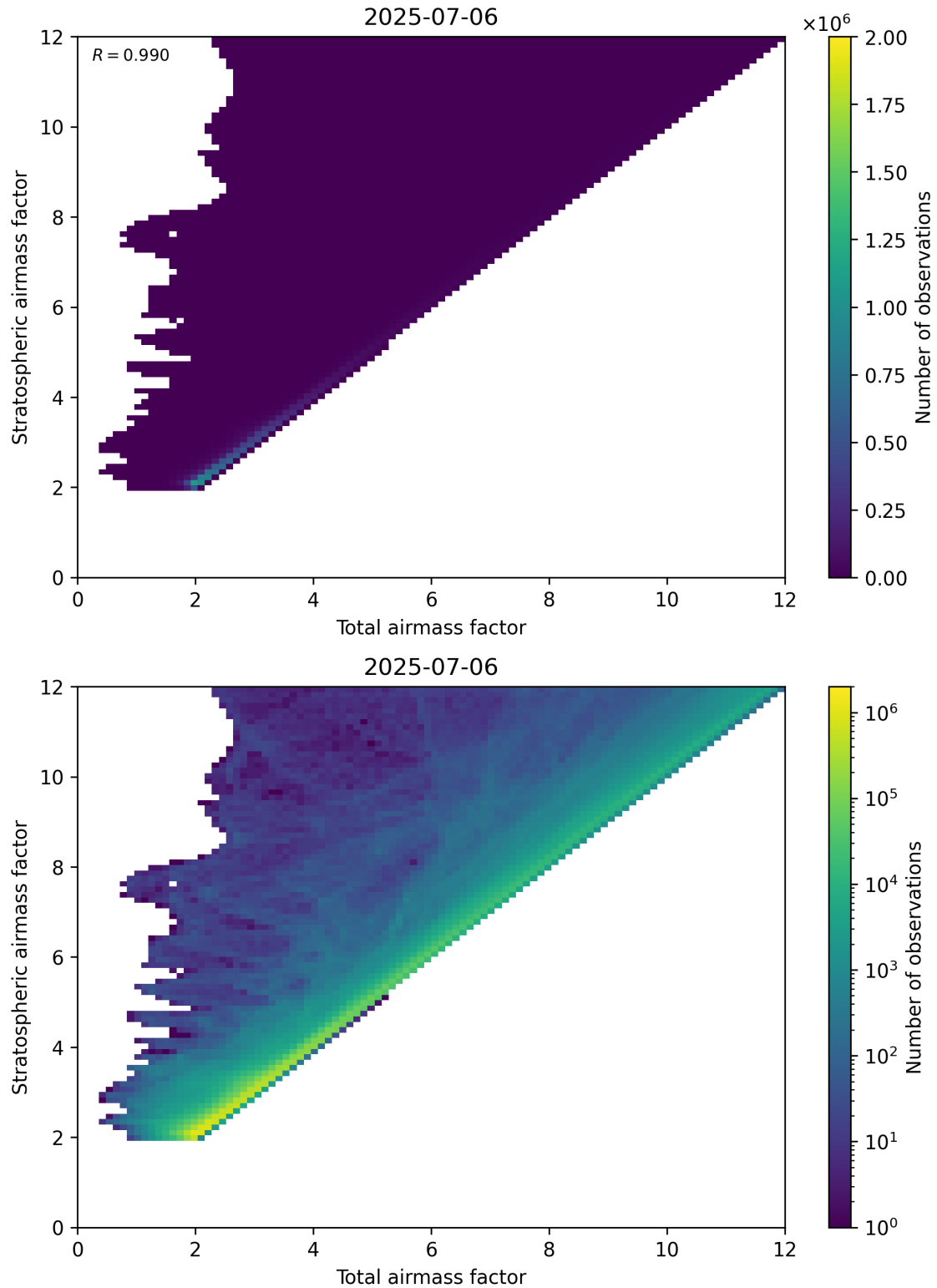
Figure 62: Scatter density plot of “Total airmass factor” against “Stratospheric airmass factor” for 2025-07-05 to 2025-07-07.
