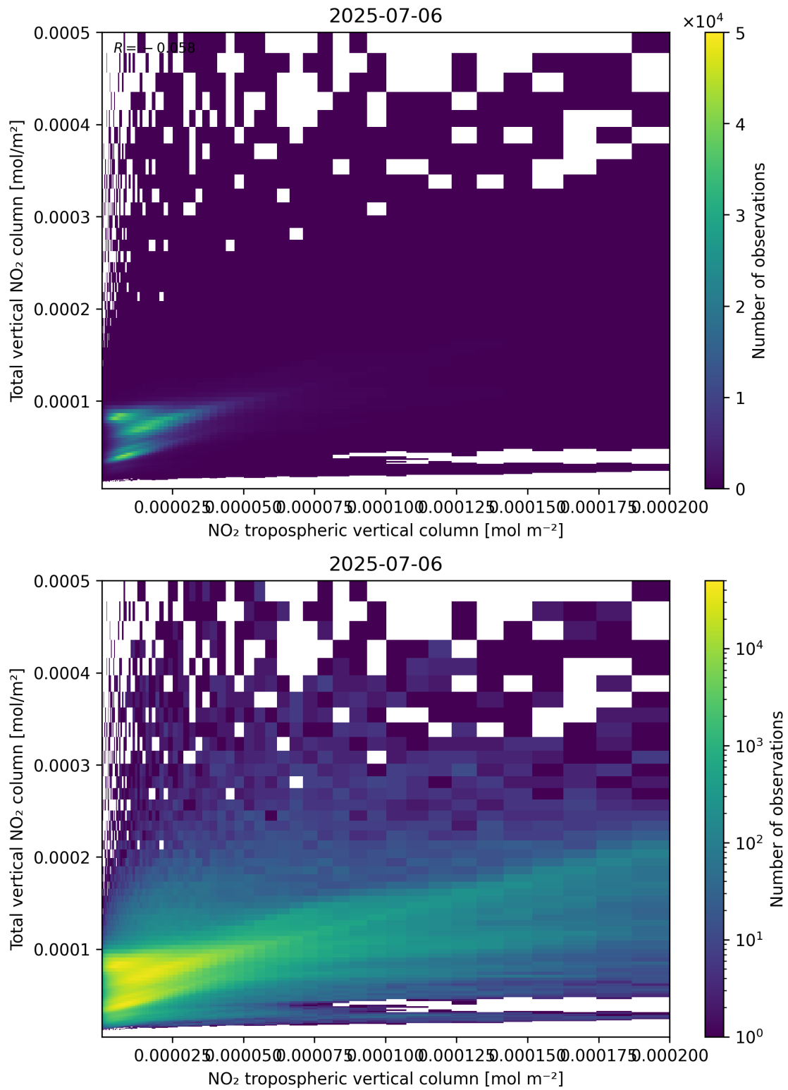
Figure 128: Scatter density plot of “NO 2 tropospheric vertical column” against “Total vertical NO 2 column” for 2025-07-05 to 2025-07-07.
