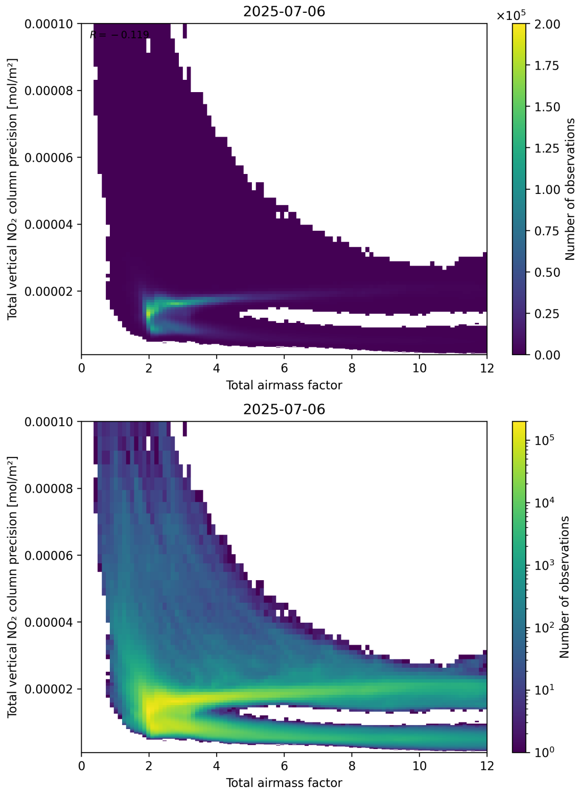
Figure 68: Scatter density plot of “Total airmass factor” against “Total vertical NO 2 column precision” for 2025-07-05 to 2025-07-07.
