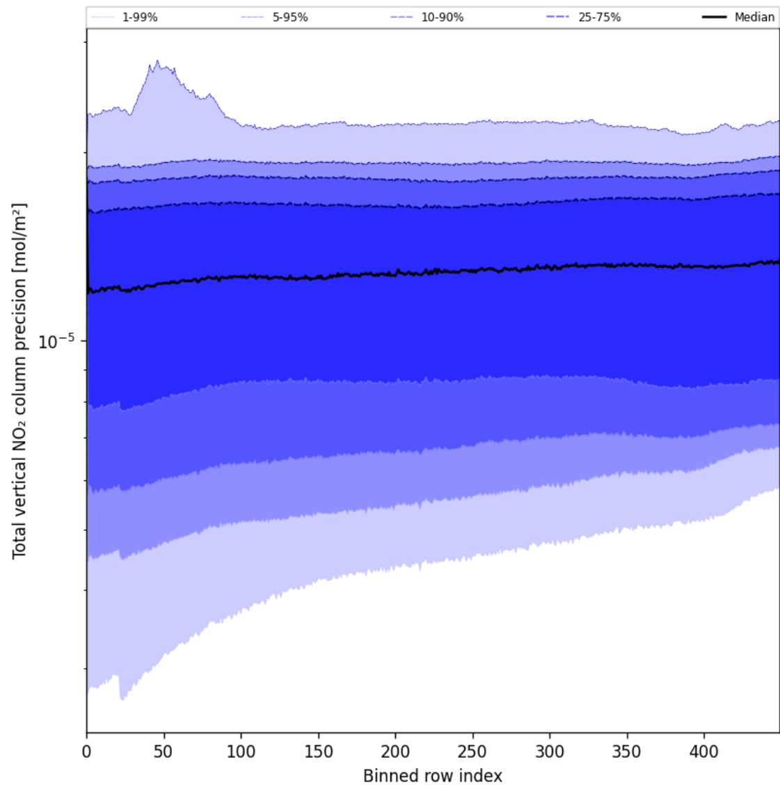
Figure 56: Along track statistics of “Total vertical NO 2 column precision” for 2025-07-05 to 2025-07-07
