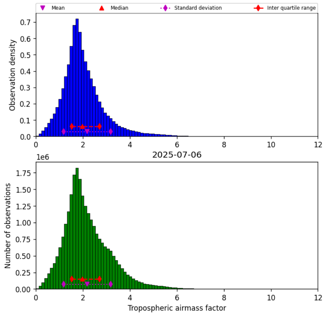
Figure 31: Histogram of “Tropospheric airmass factor” for 2025-07-05 to 2025-07-07
