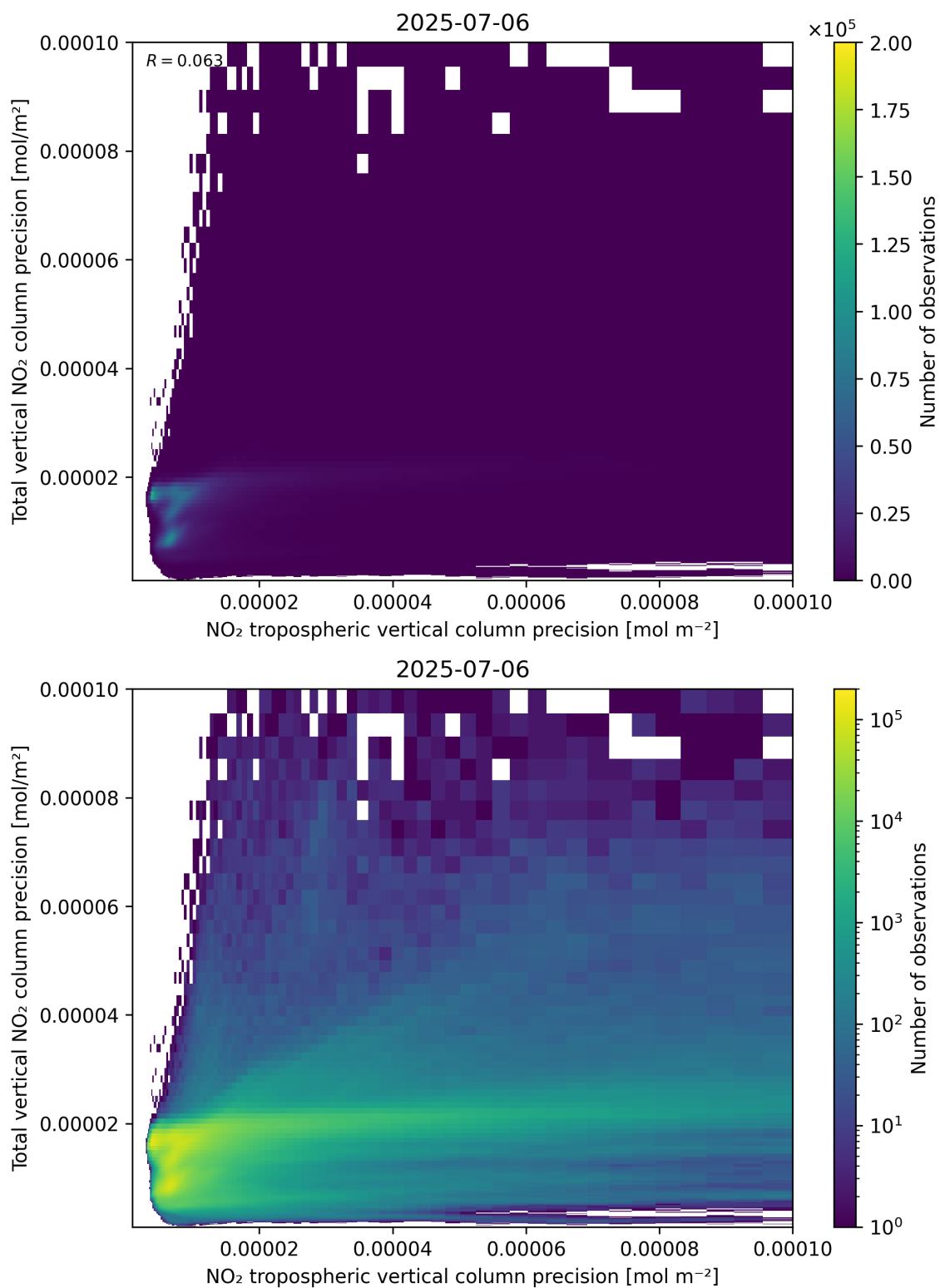
Figure 139: Scatter density plot of “NO 2 tropospheric vertical column precision” against “Total vertical NO 2 column precision” for 2025-07-05 to 2025-07-07.
