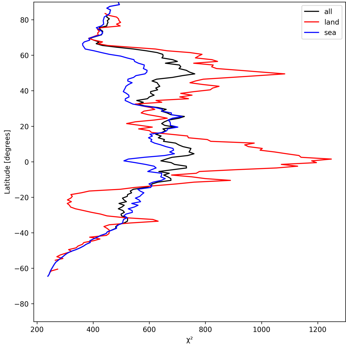
Figure 25: Zonal average of “ \chi^2 ” for 2025-07-05 to 2025-07-07.
