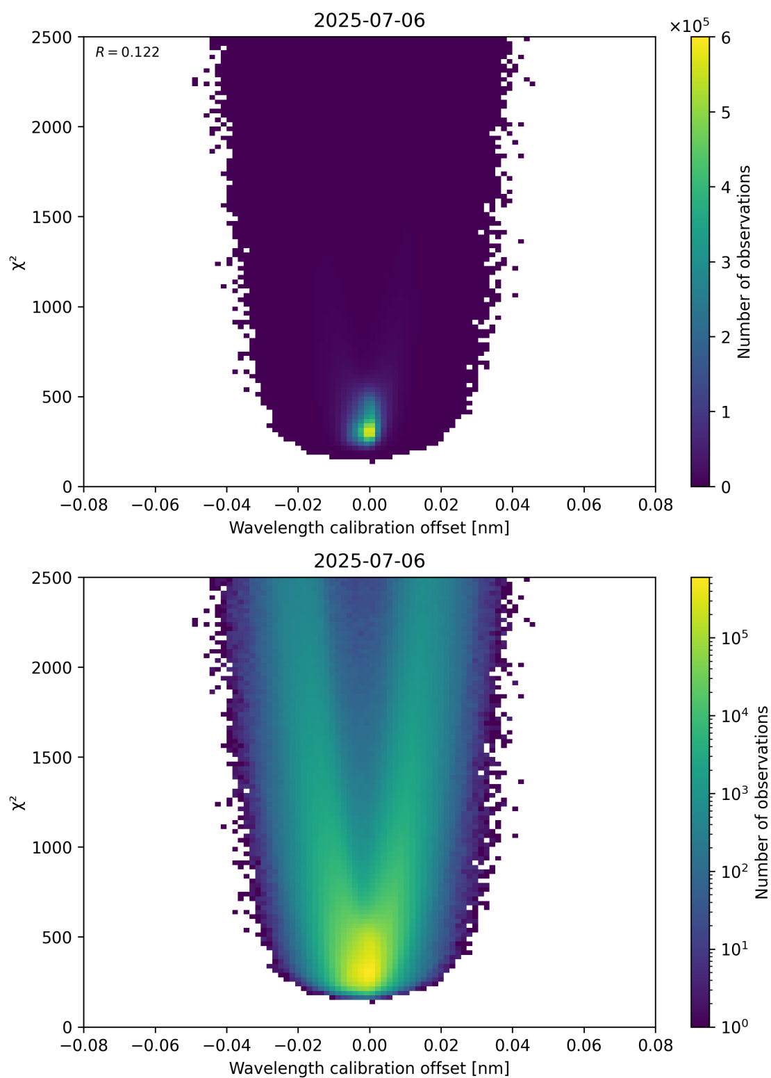
Figure 175: Scatter density plot of “Wavelength calibration offset” against “ \chi^2 ” for 2025-07-05 to 2025-07-07.
