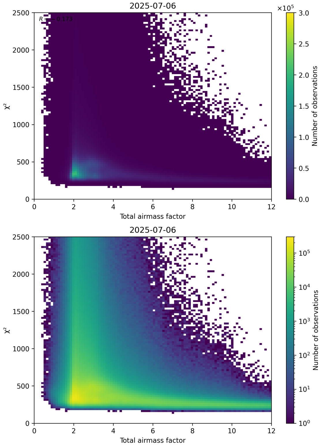
Figure 63: Scatter density plot of “Total airmass factor” against “ \chi^2 ” for 2025-07-05 to 2025-07-07.
