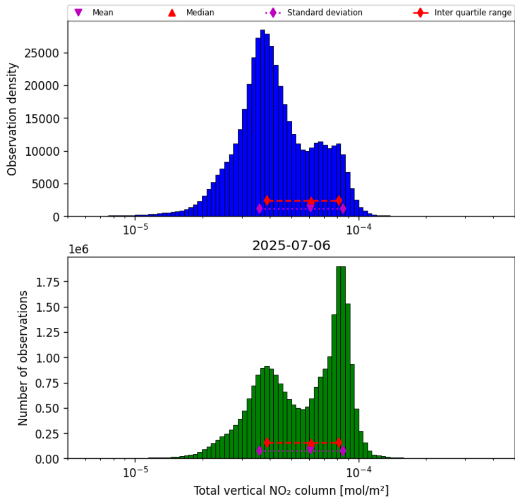
Figure 38: Histogram of “Total vertical NO 2 column” for 2025-07-05 to 2025-07-07
