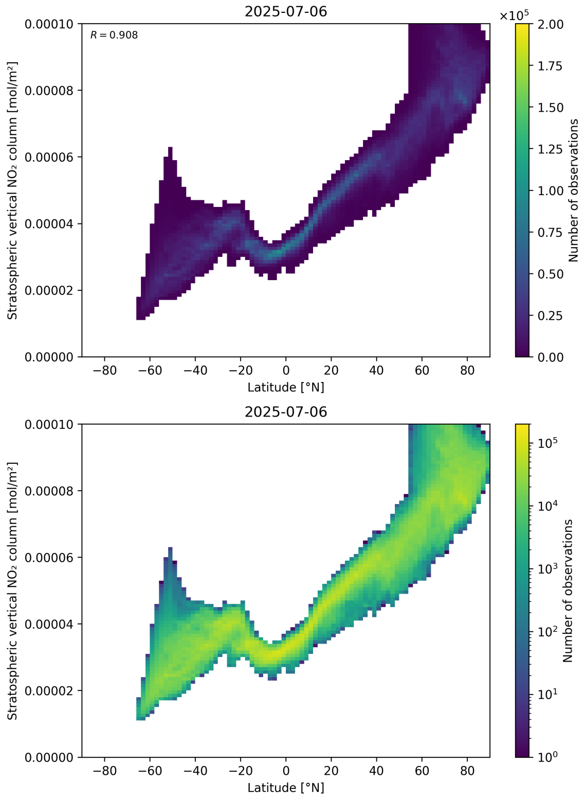
Figure 87: Scatter density plot of “Latitude” against “Stratospheric vertical NO 2 column” for 2025-07-05 to 2025-07-07.
