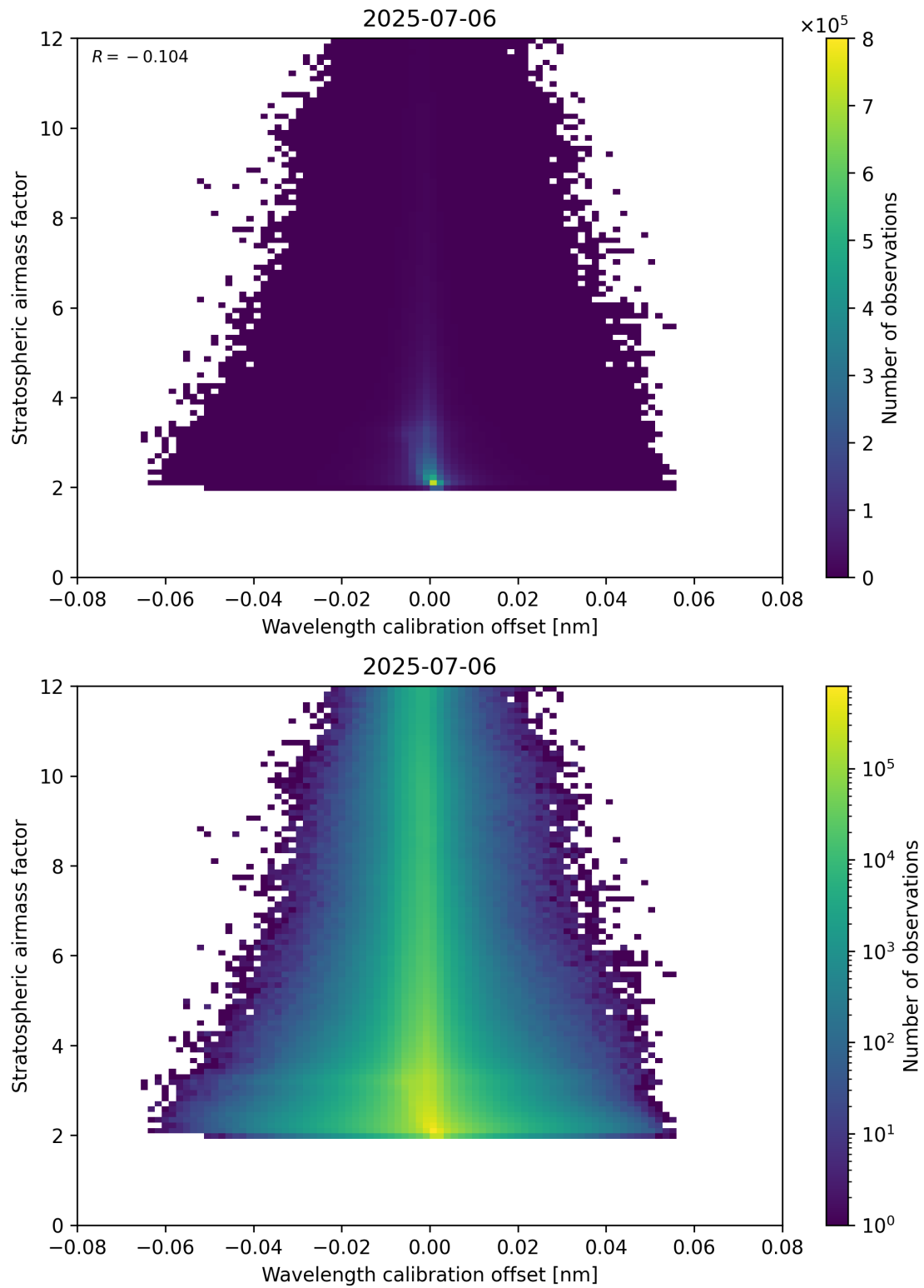
Figure 174: Scatter density plot of “Wavelength calibration offset” against “Stratospheric airmass factor” for 2025-07-05 to 2025-07-07.
