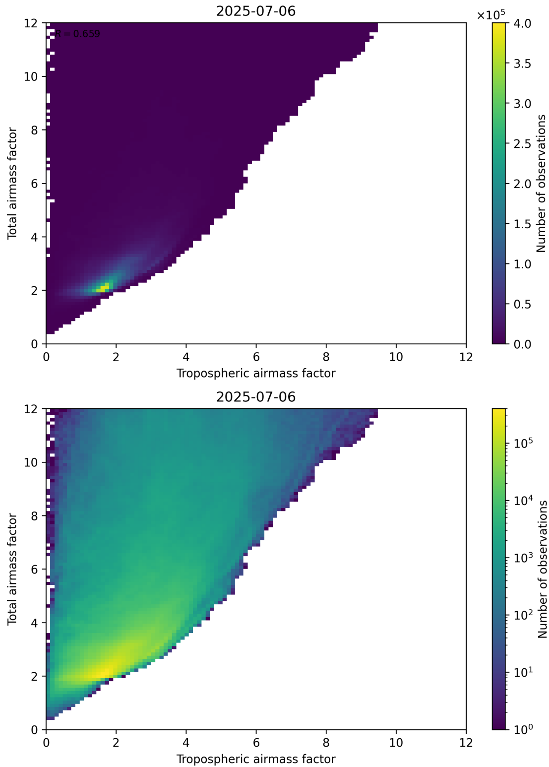
Figure 72: Scatter density plot of “Tropospheric airmass factor” against “Total airmass factor” for 2025-07-05 to 2025-07-07.
