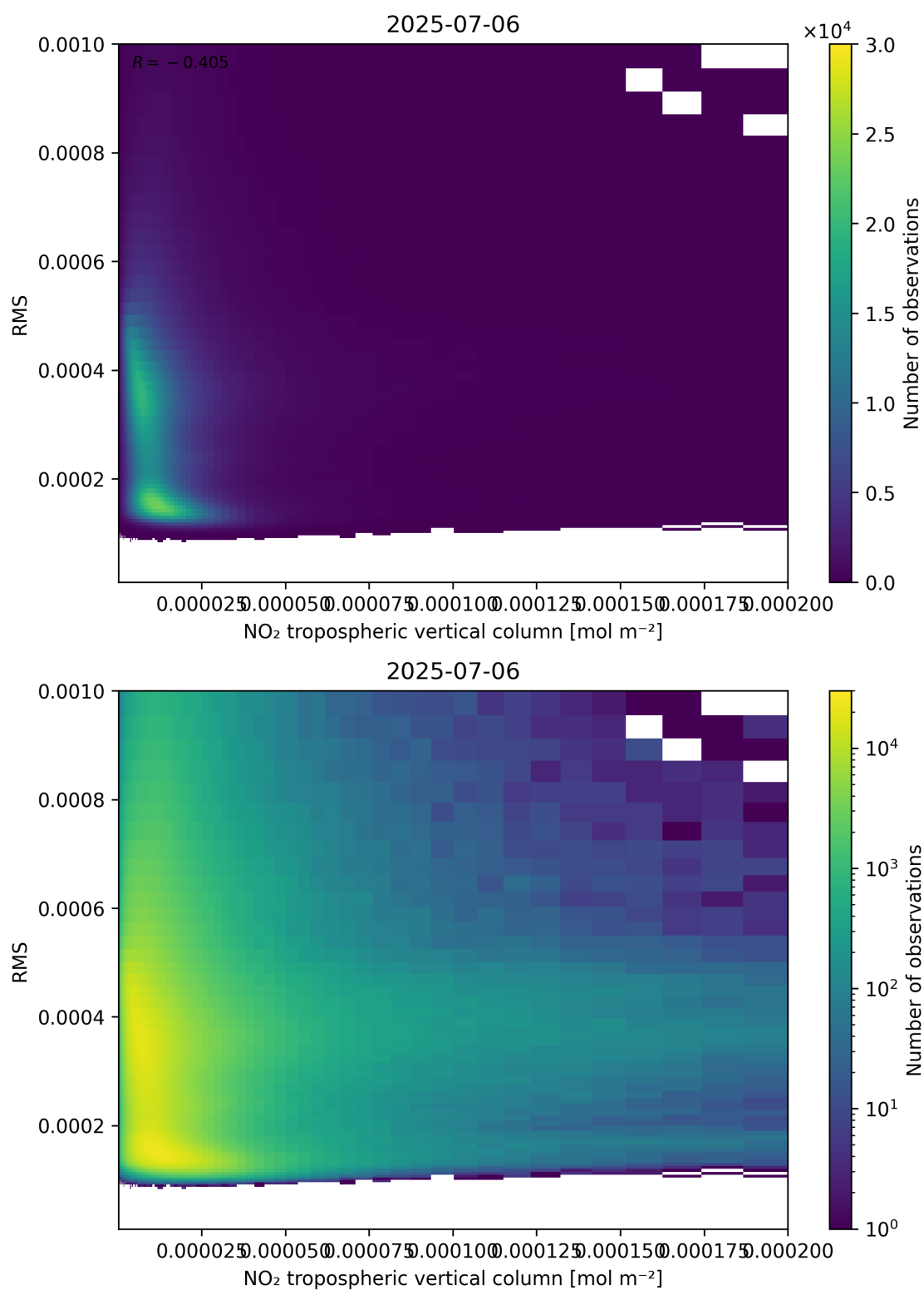
Figure 142: Scatter density plot of “NO 2 tropospheric vertical column” against “RMS” for 2025-07-05 to 2025-07-07.
