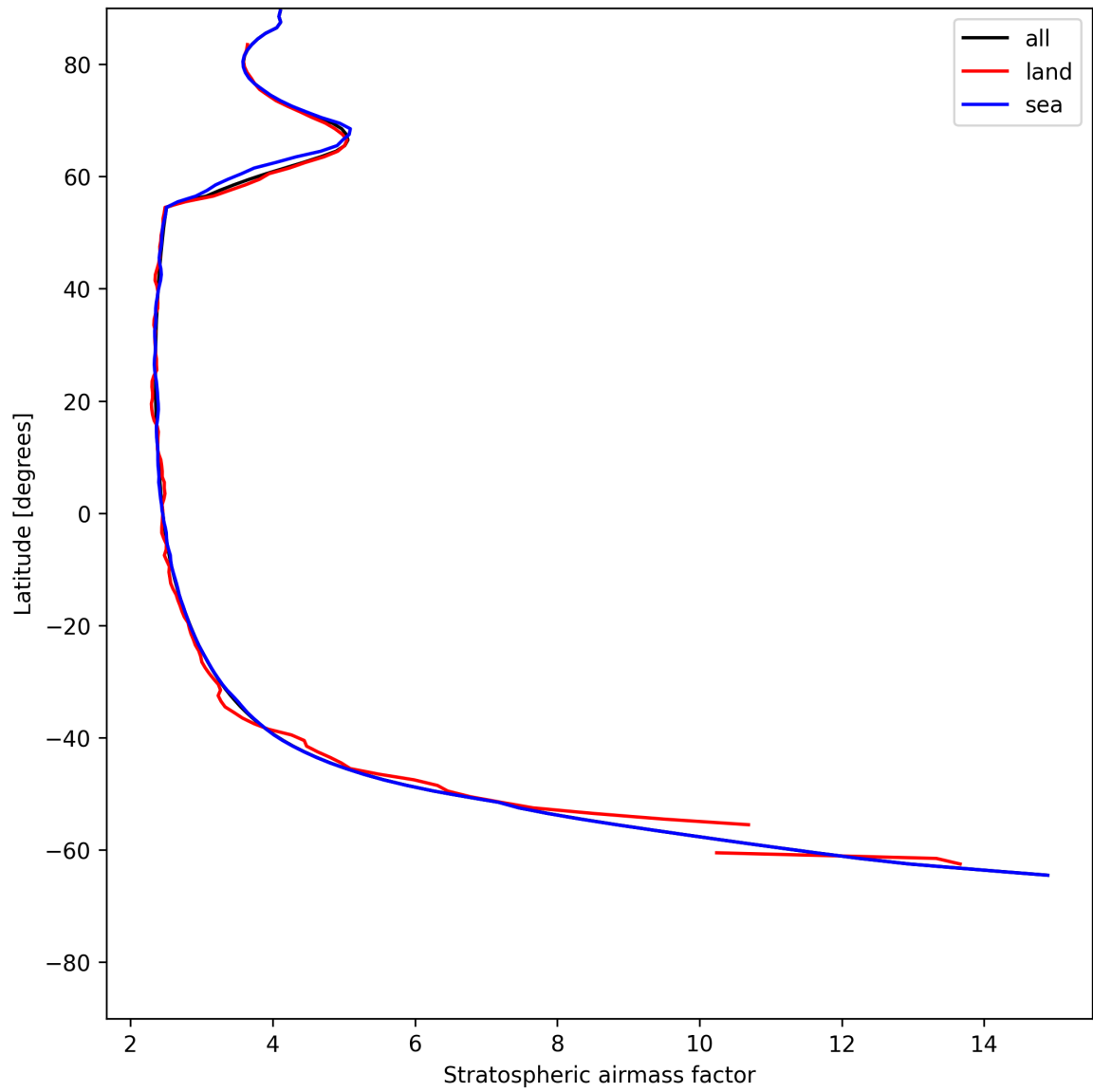
Figure 27: Zonal average of “Stratospheric airmass factor” for 2025-07-05 to 2025-07-07.
