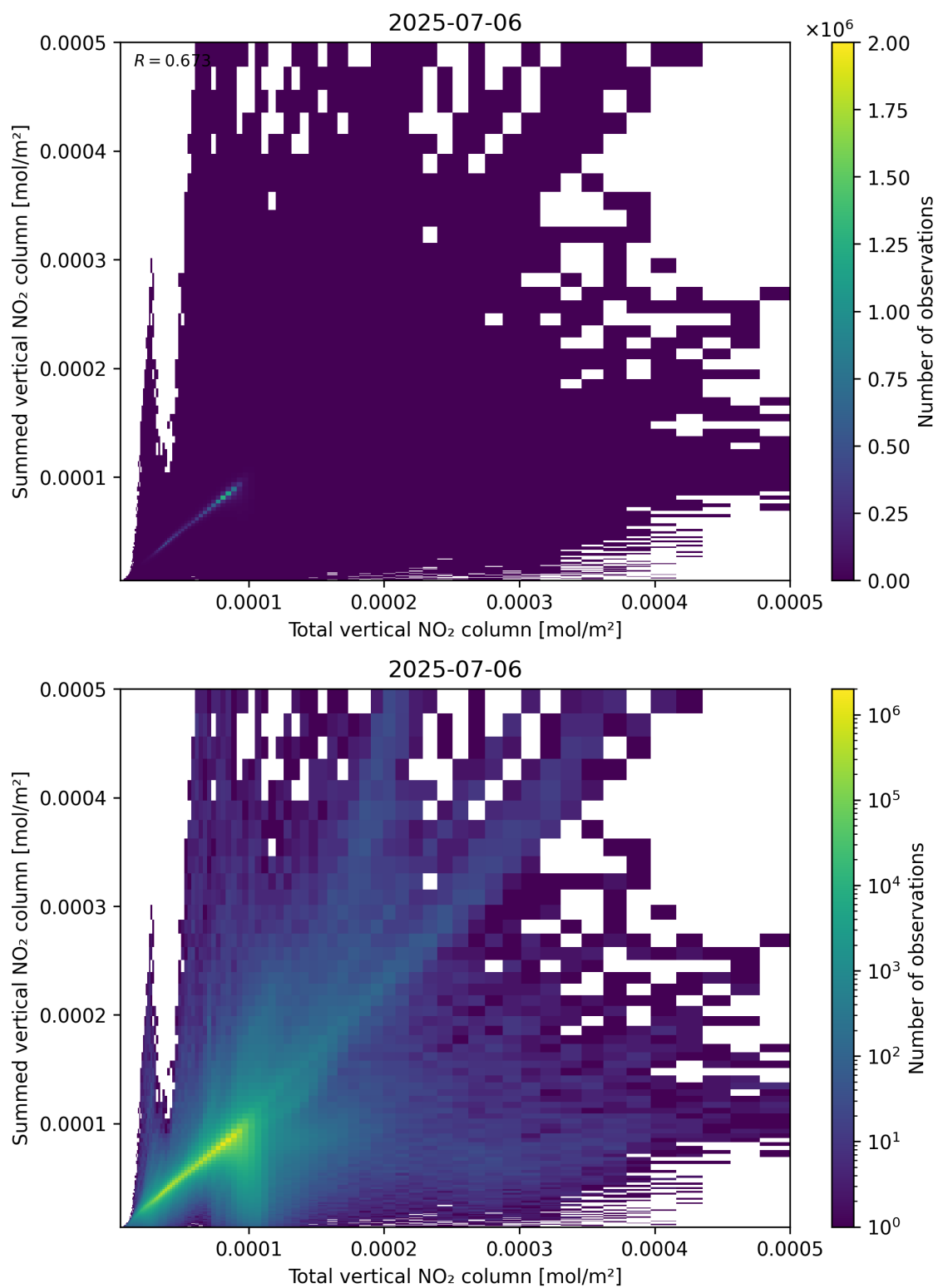
Figure 112: Scatter density plot of “Total vertical NO 2 column” against “Summed vertical NO 2 column” for 2025-07-05 to 2025-07-07.
