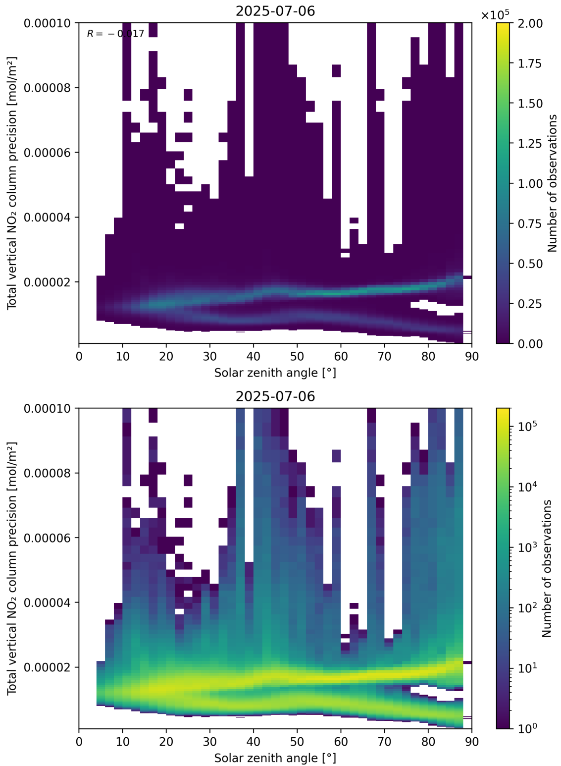
Figure 154: Scatter density plot of “Solar zenith angle” against “Total vertical NO 2 column precision” for 2025-07-05 to 2025-07-07.
