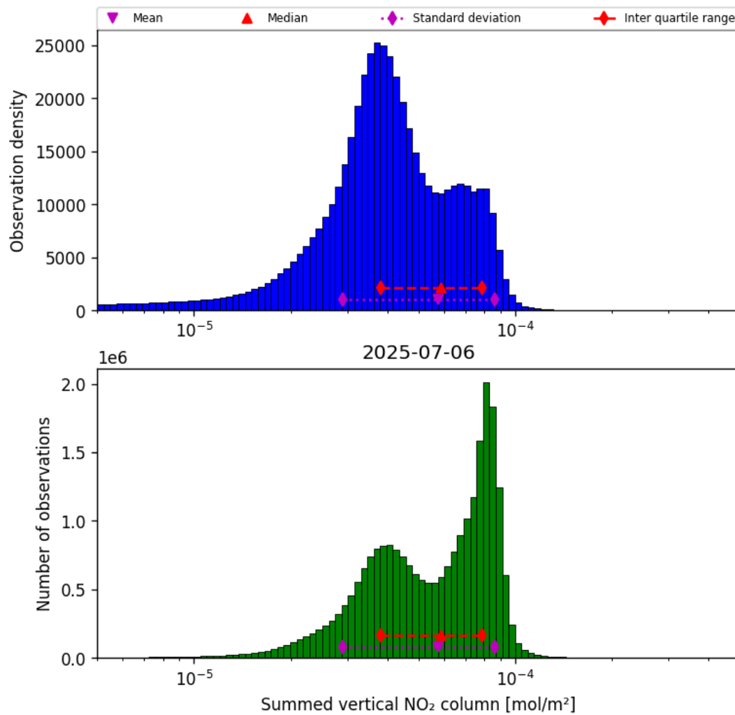
Figure 40: Histogram of “Summed vertical NO 2 column” for 2025-07-05 to 2025-07-07
