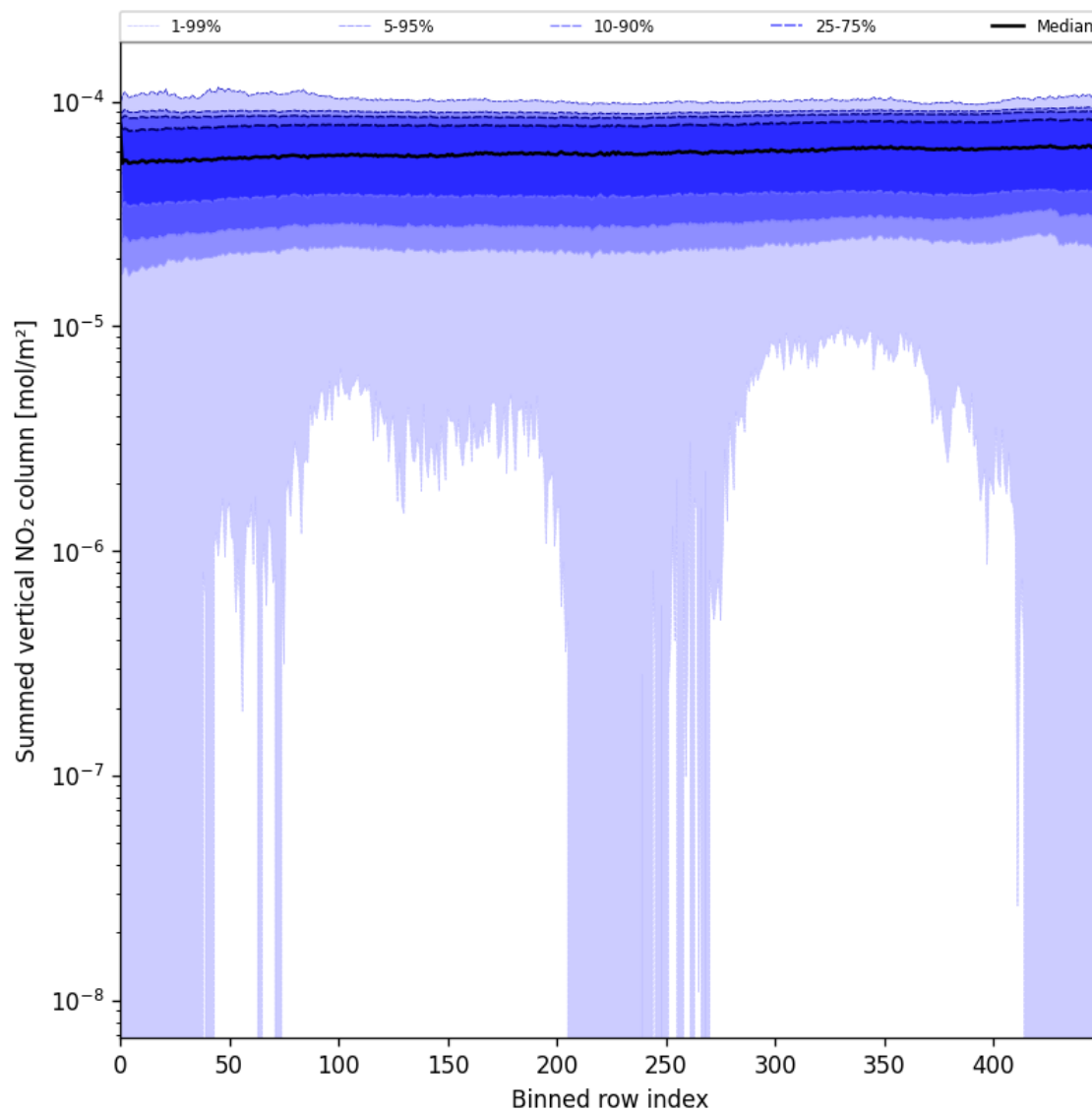
Figure 57: Along track statistics of “Summed vertical NO 2 column” for 2025-07-05 to 2025-07-07
