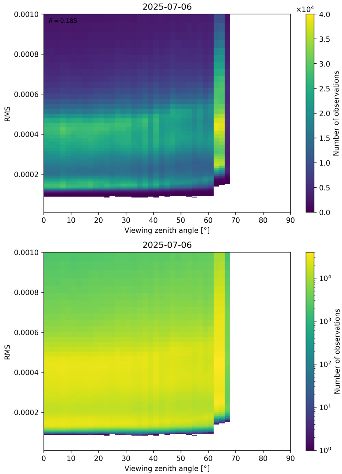
Figure 171: Scatter density plot of “Viewing zenith angle” against “RMS” for 2025-07-05 to 2025-07-07.
