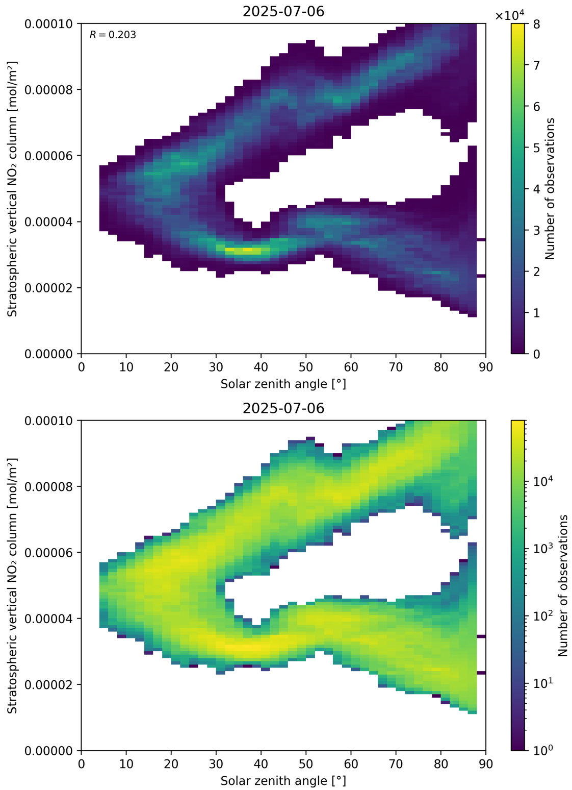
Figure 150: Scatter density plot of “Solar zenith angle” against “Stratospheric vertical NO 2 column” for 2025-07-05 to 2025-07-07.
