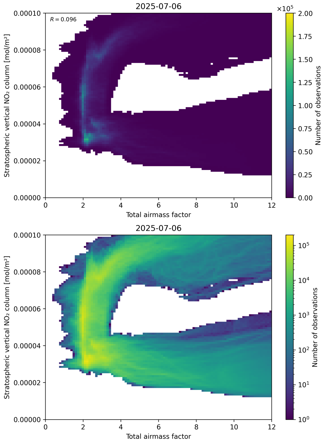
Figure 64: Scatter density plot of “Total airmass factor” against “Stratospheric vertical NO 2 column” for 2025-07-05 to 2025-07-07.
