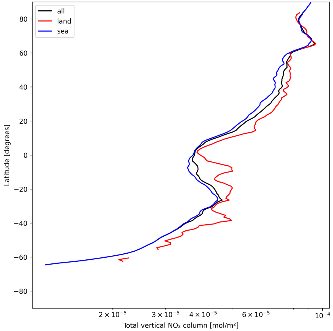
Figure 21: Zonal average of “Total vertical NO 2 column” for 2025-07-05 to 2025-07-07.
