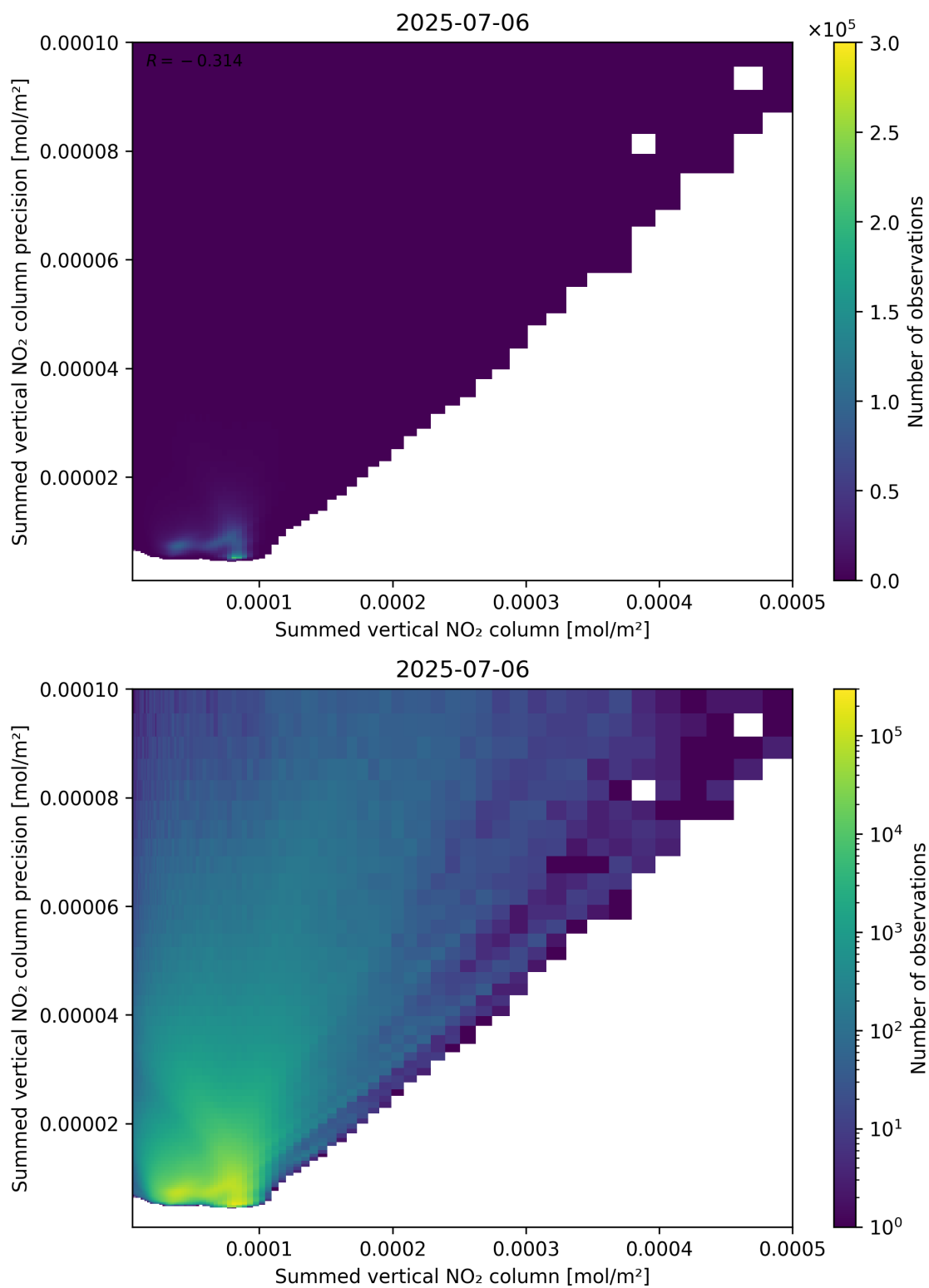
Figure 105: Scatter density plot of “Summed vertical NO 2 column” against “Summed vertical NO 2 column precision” for 2025-07-05 to 2025-07-07.
