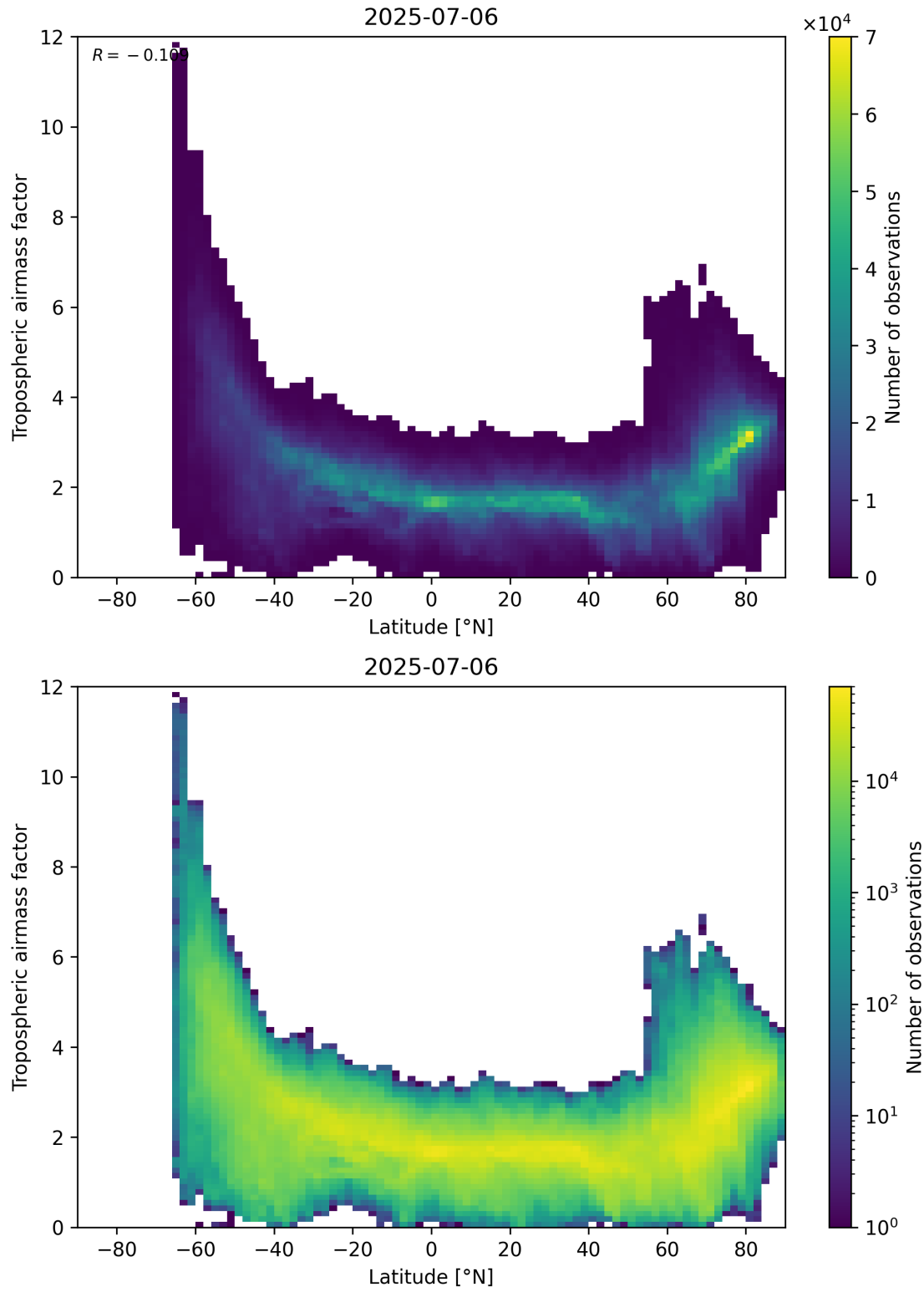
Figure 85: Scatter density plot of “Latitude” against “Tropospheric air mass factor” for 2025-07-05 to 2025-07-07.
