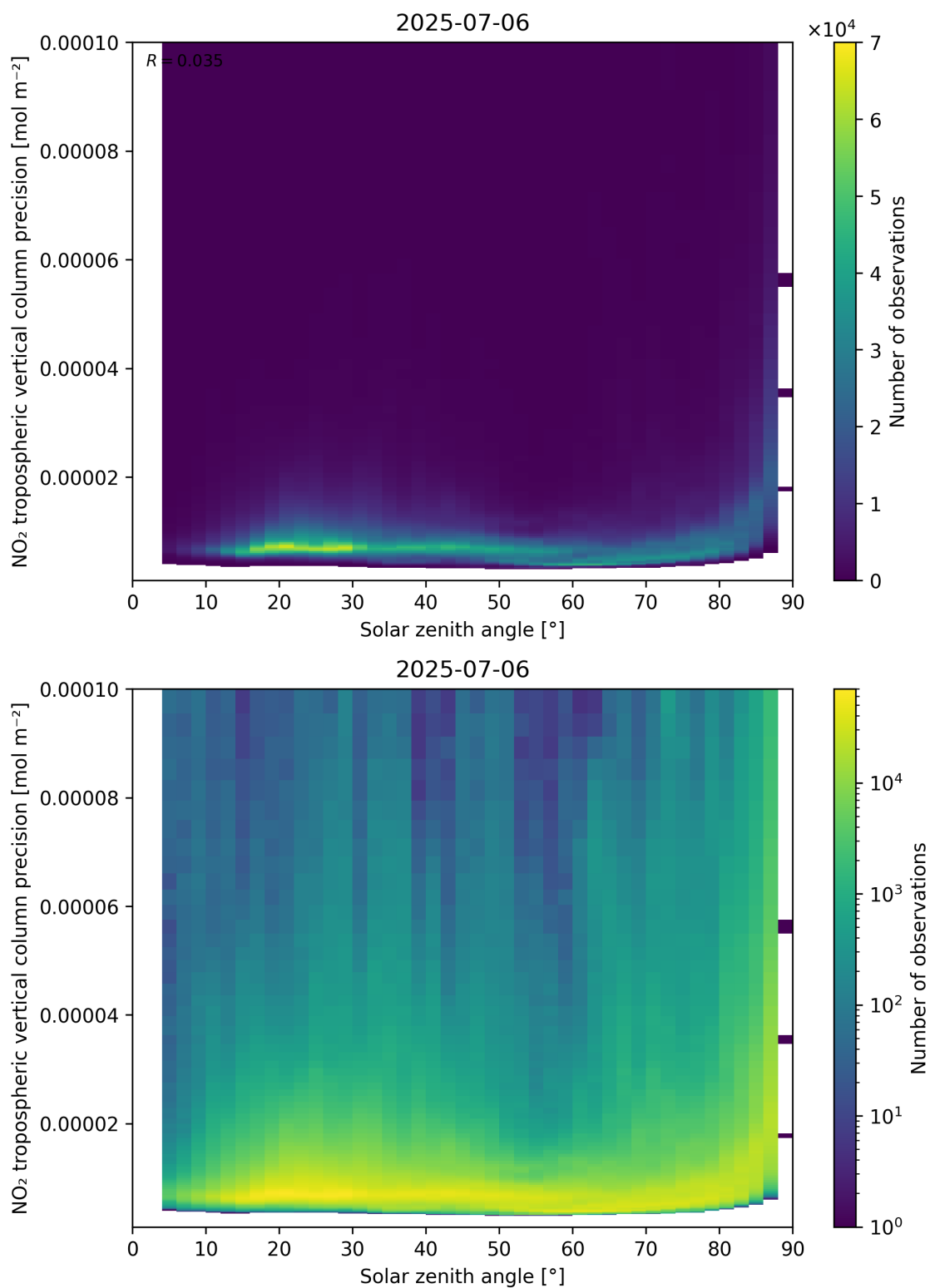
Figure 156: Scatter density plot of “Solar zenith angle” against “NO 2 tropospheric vertical column precision” for 2025-07-05 to 2025-07-07.
