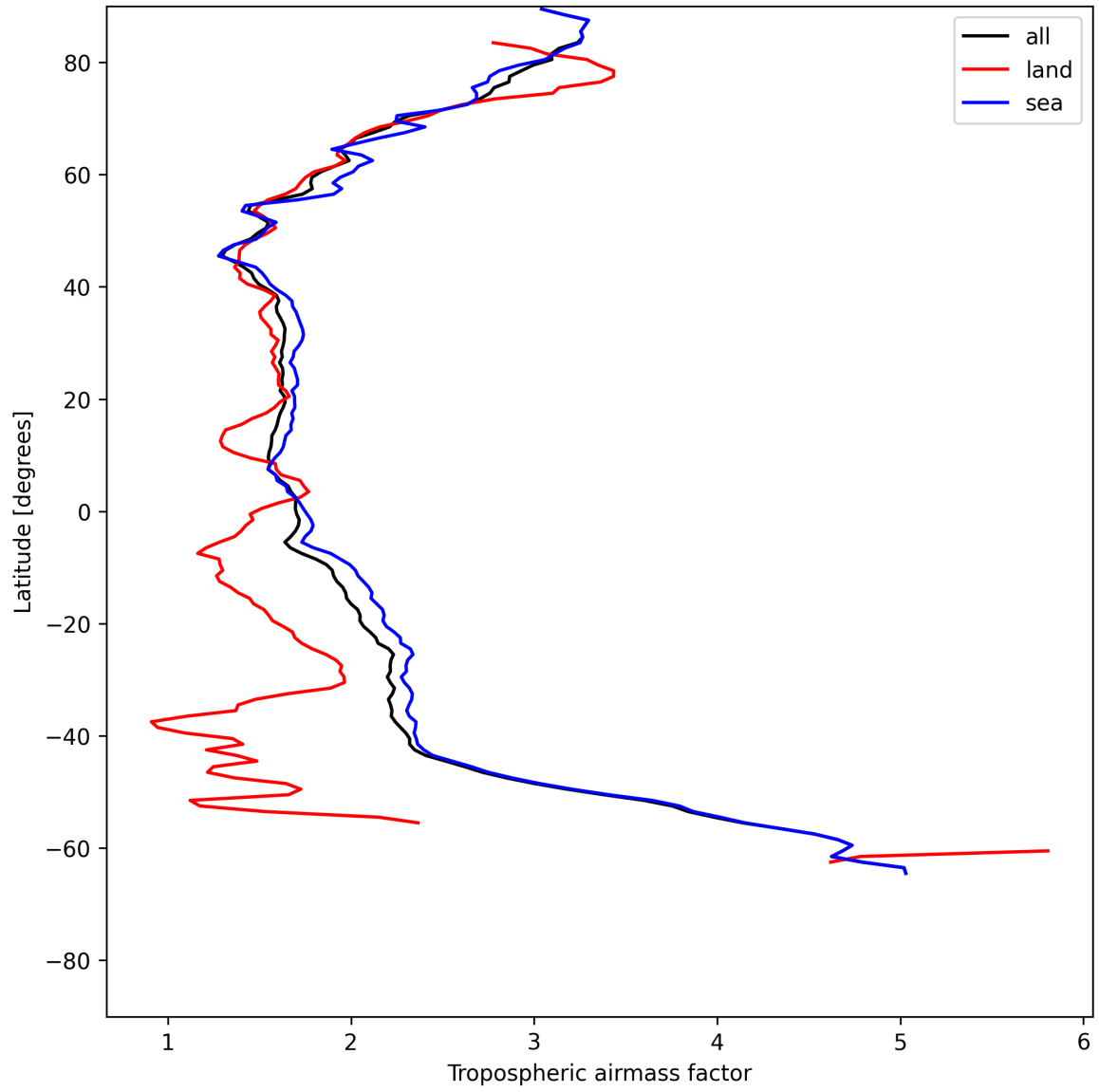
Figure 14: Zonal average of “Tropospheric airmass factor” for 2025-07-05 to 2025-07-07.
