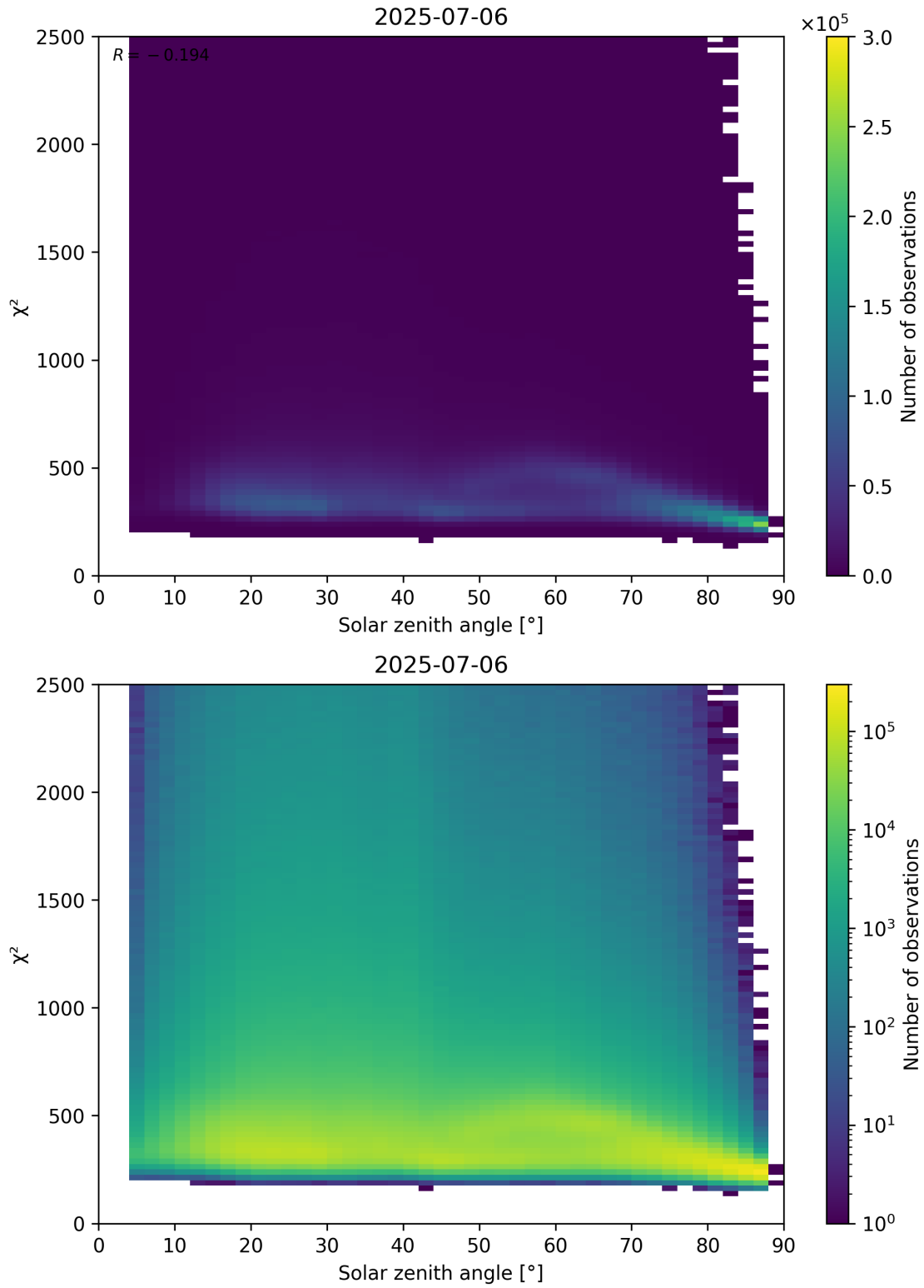
Figure 148: Scatter density plot of “Solar zenith angle” against “ \chi^2 ” for 2025-07-05 to 2025-07-07.
