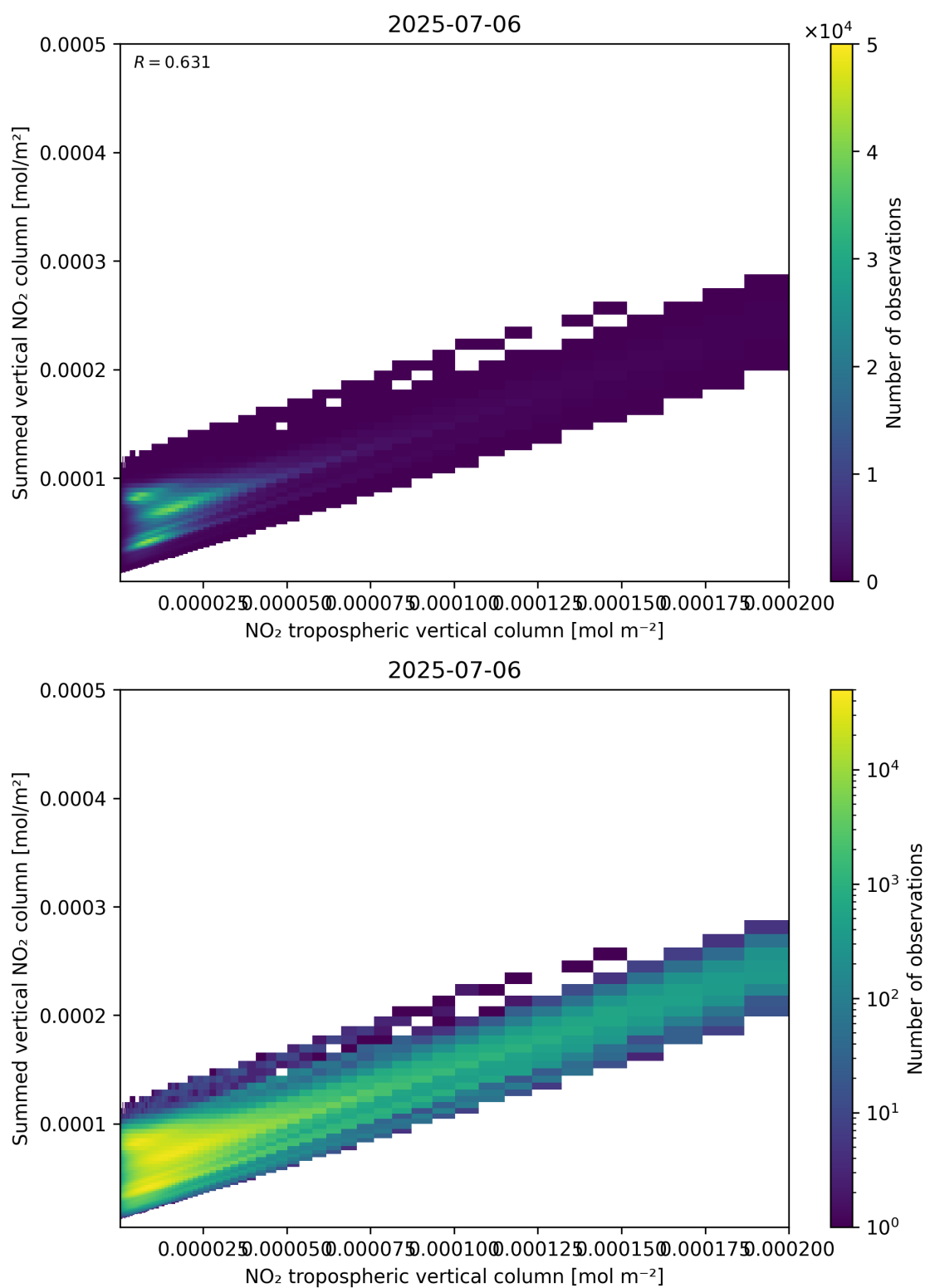
Figure 126: Scatter density plot of “NO 2 tropospheric vertical column” against “Summed vertical NO 2 column” for 2025-07-05 to 2025-07-07.
