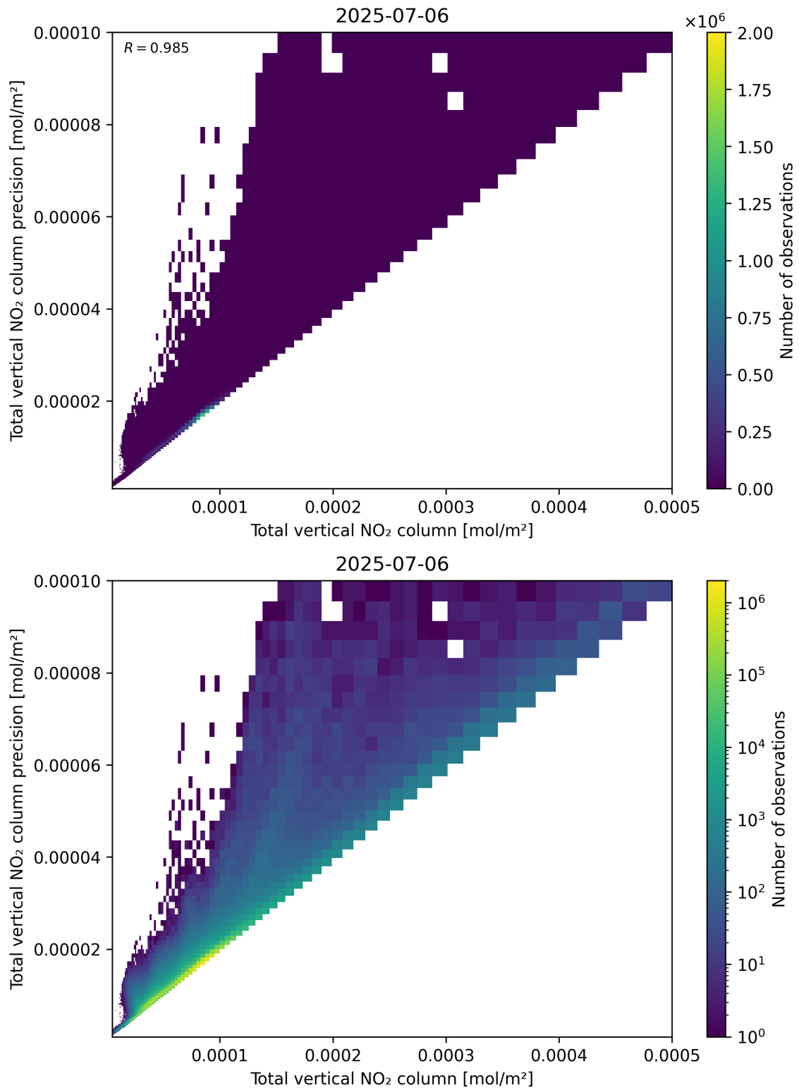
Figure 114: Scatter density plot of “Total vertical NO 2 column” against “Total vertical NO 2 column precision” for 2025-07-05 to 2025-07-07.
