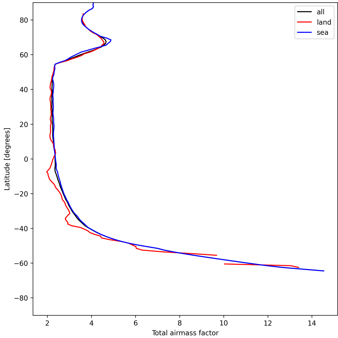
Figure 15: Zonal average of “Total airmass factor” for 2025-07-05 to 2025-07-07.
