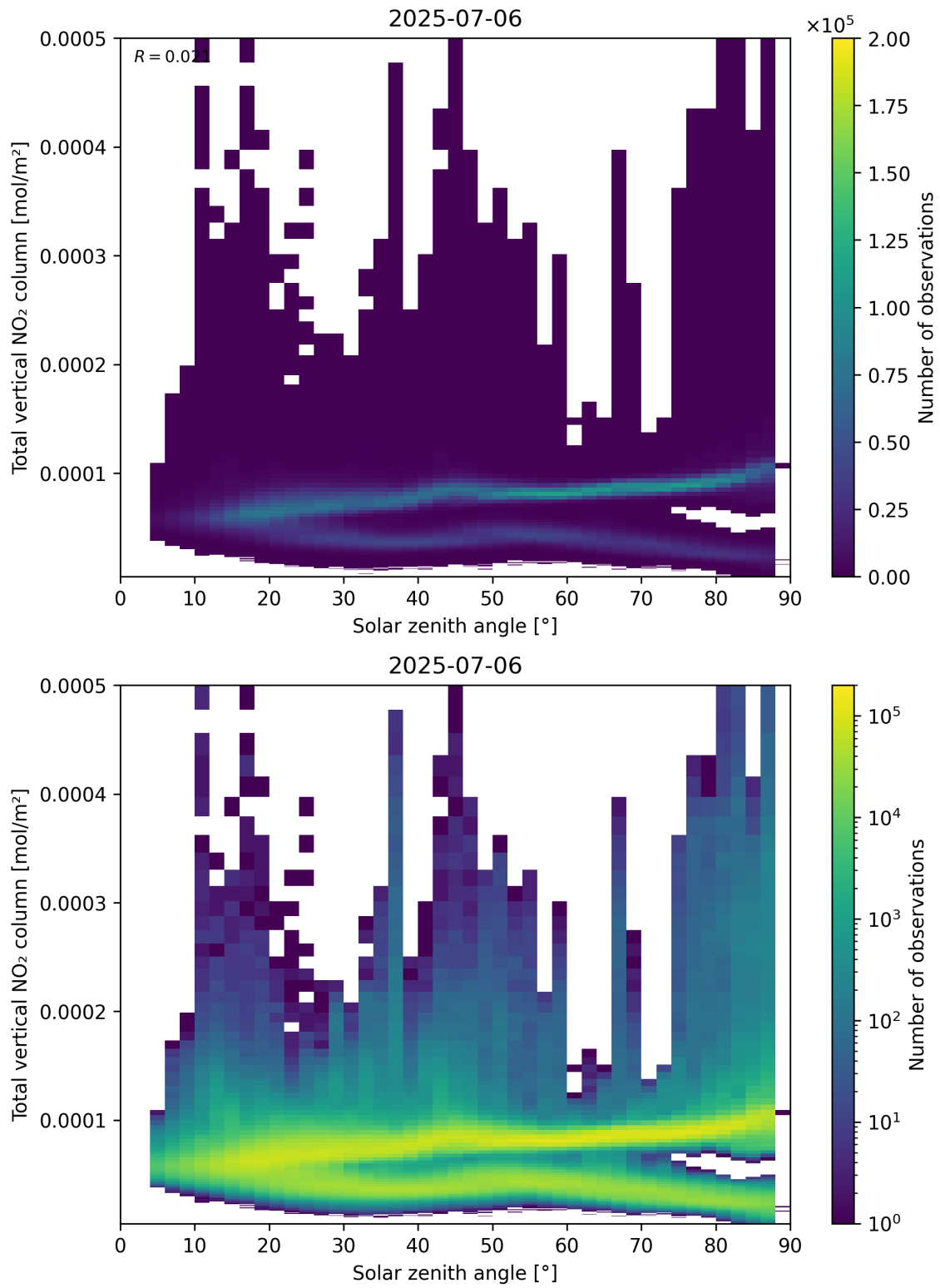
Figure 153: Scatter density plot of “Solar zenith angle” against “Total vertical NO 2 column” for 2025-07-05 to 2025-07-07.
