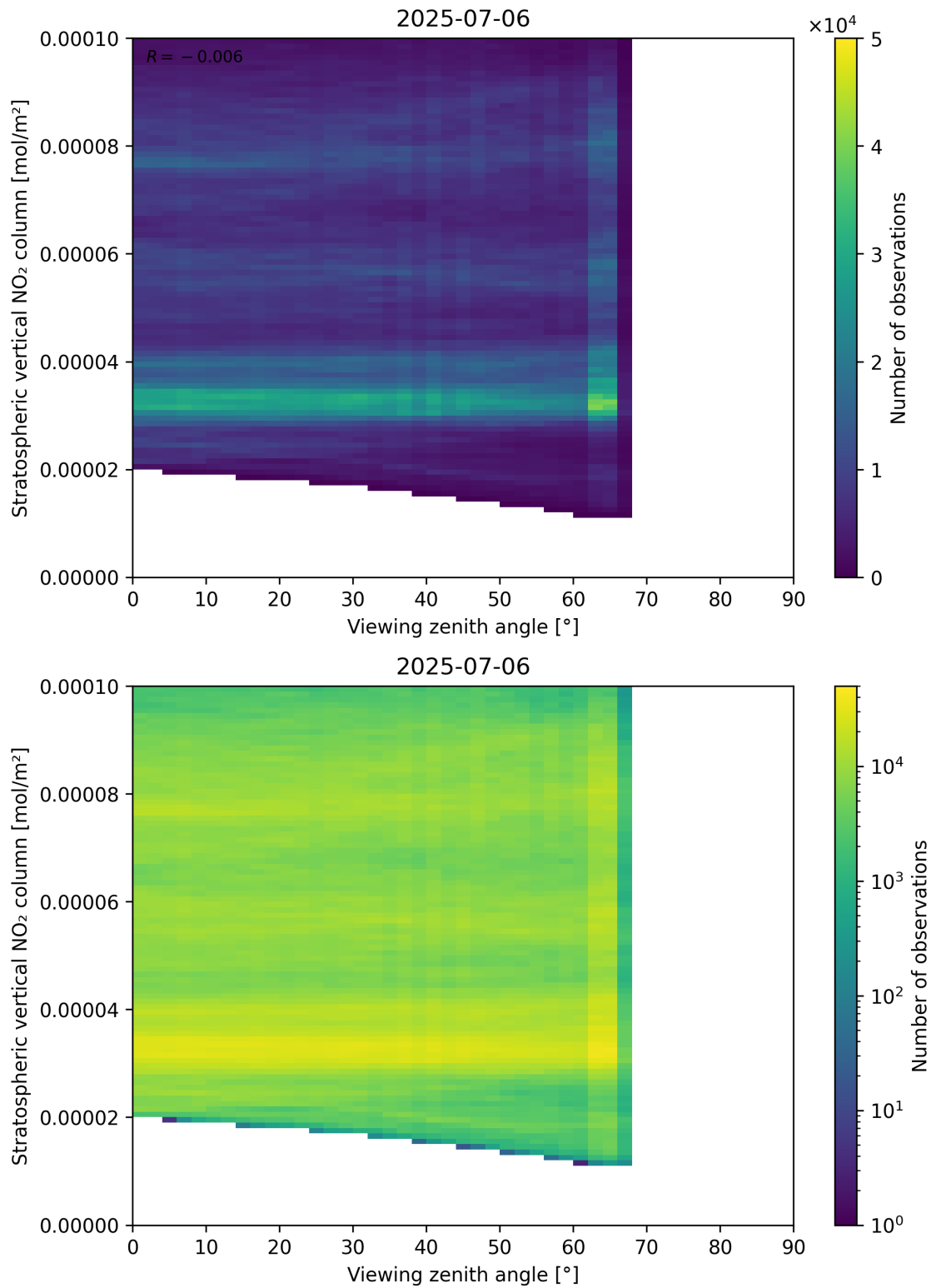
Figure 164: Scatter density plot of “Viewing zenith angle” against “Stratospheric vertical NO 2 column” for 2025-07-05 to 2025-07-07.
