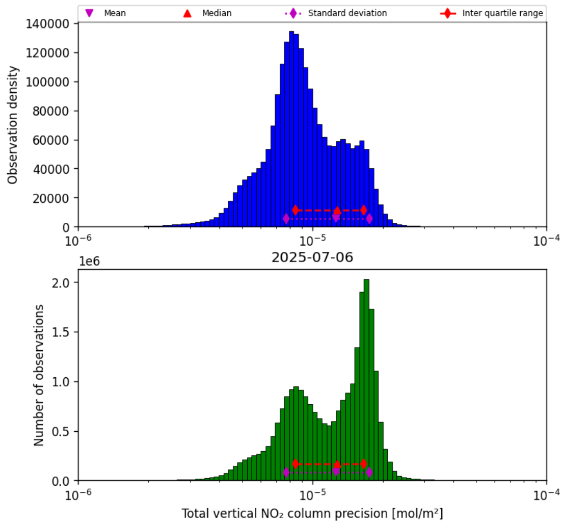
Figure 39: Histogram of “Total vertical NO 2 column precision” for 2025-07-05 to 2025-07-07
