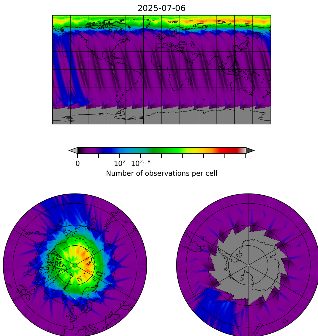
Figure 10: Map of the number of observations for 2025-07-05 to 2025-07-07
