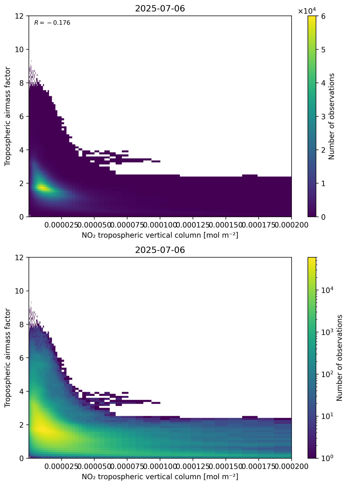
Figure 123: Scatter density plot of “NO 2 tropospheric vertical column” against “Tropospheric air mass factor” for 2025-07-05 to 2025-07-07.
