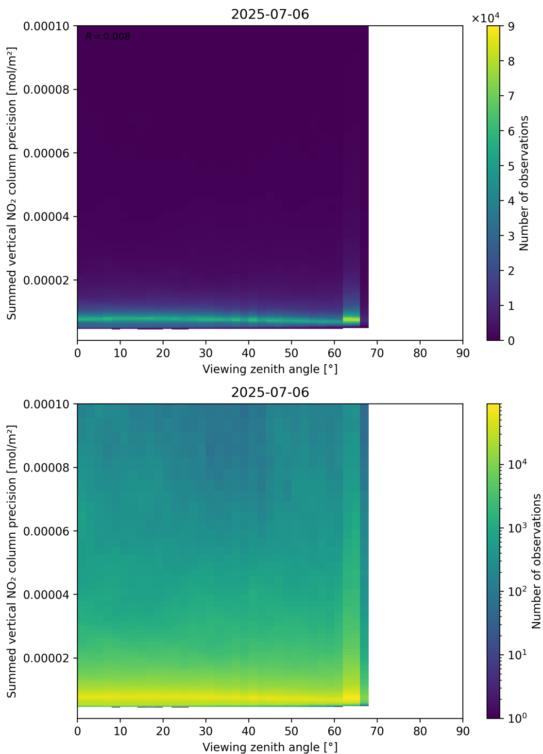
Figure 166: Scatter density plot of “Viewing zenith angle” against “Summed vertical NO 2 column precision” for 2025-07-05 to 2025-07-07.
