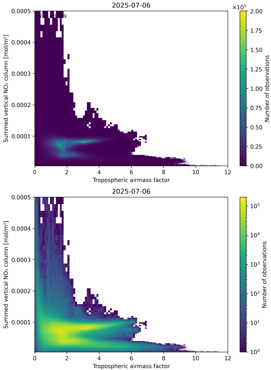
Figure 75: Scatter density plot of “Tropospheric airmass factor” against “Summed vertical NO 2 column” for 2025-07-05 to 2025-07-07.
