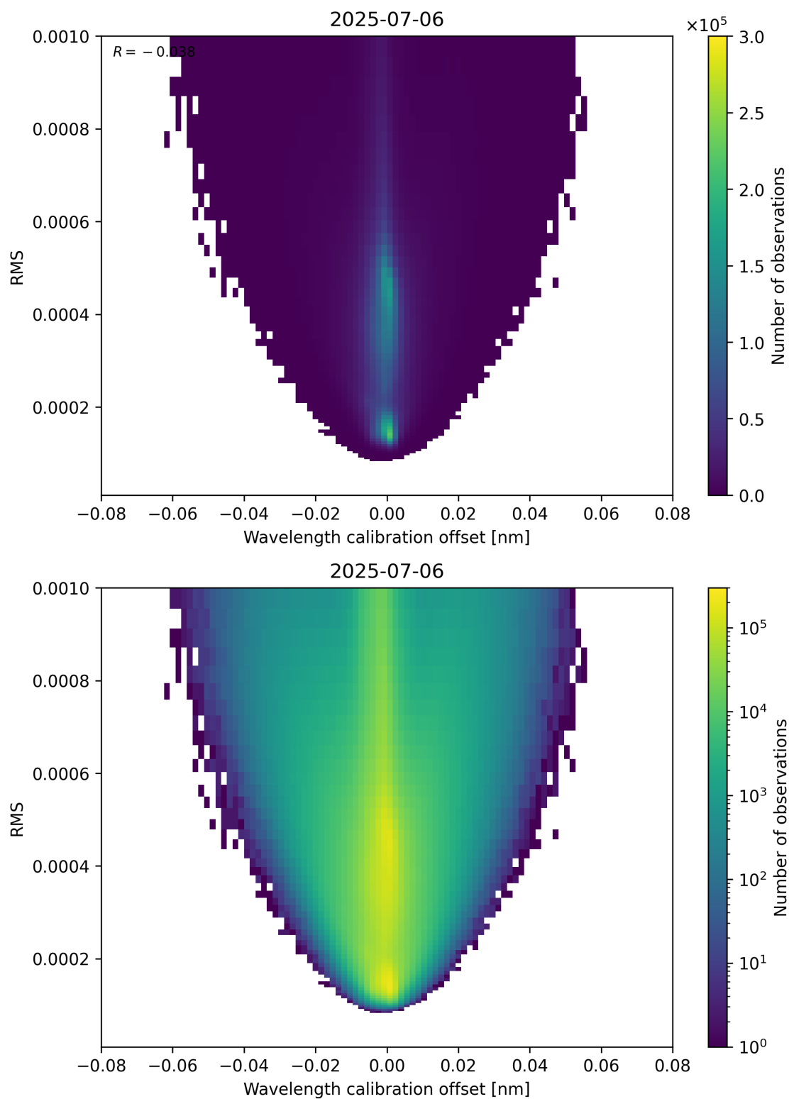
Figure 181: Scatter density plot of “Wavelength calibration offset” against “RMS” for 2025-07-05 to 2025-07-07.
