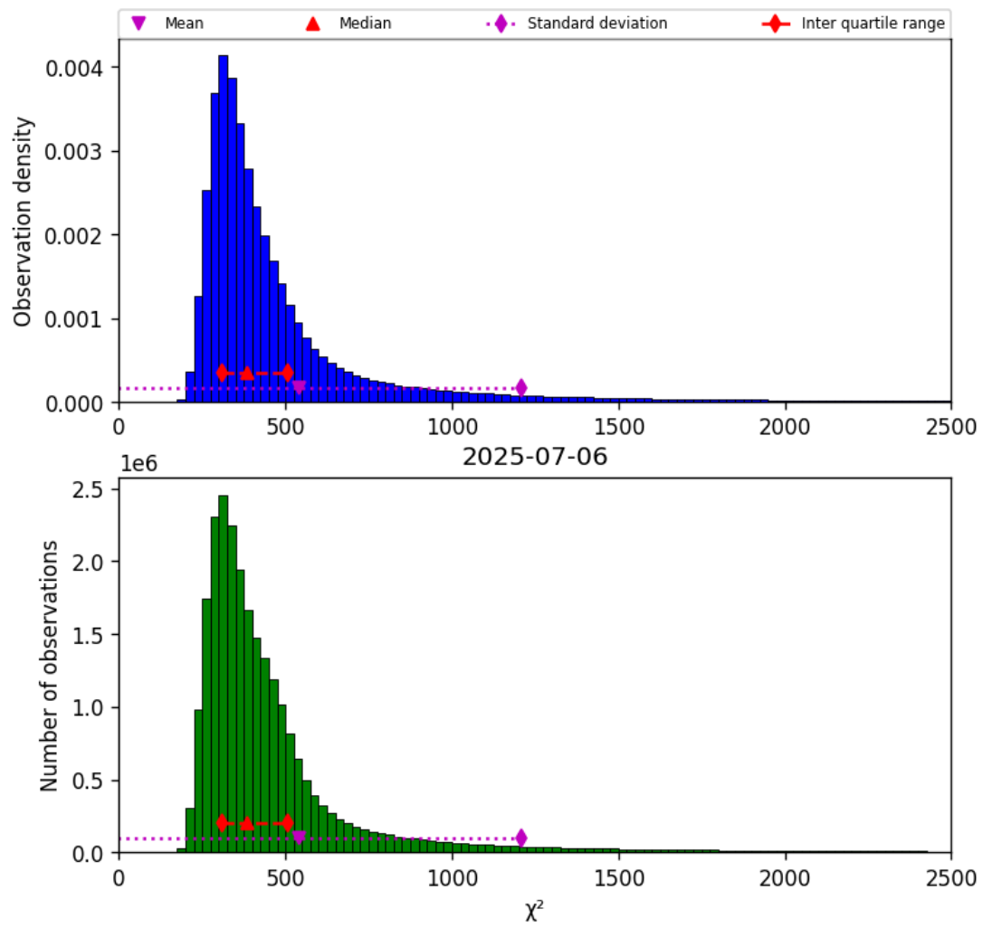
Figure 42: Histogram of “ \chi^2 ” for 2025-07-05 to 2025-07-07
