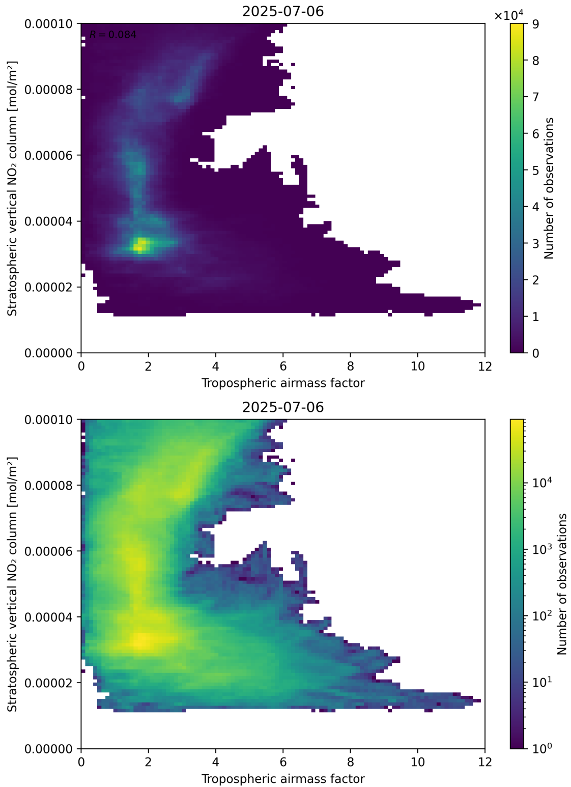
Figure 74: Scatter density plot of “Tropospheric air mass factor” against “Stratospheric vertical NO 2 column” for 2025-07-05 to 2025-07-07.
