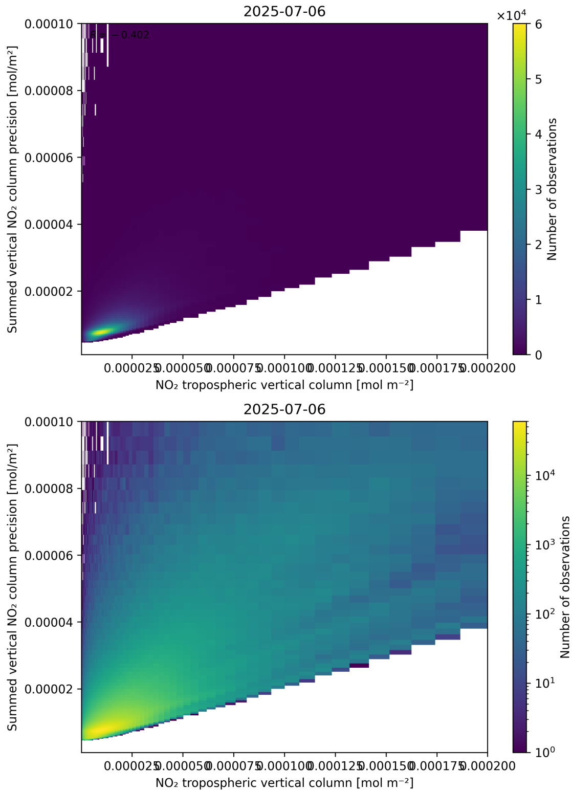
Figure 127: Scatter density plot of “NO 2 tropospheric vertical column” against “Summed vertical NO 2 column precision” for 2025-07-05 to 2025-07-07.
