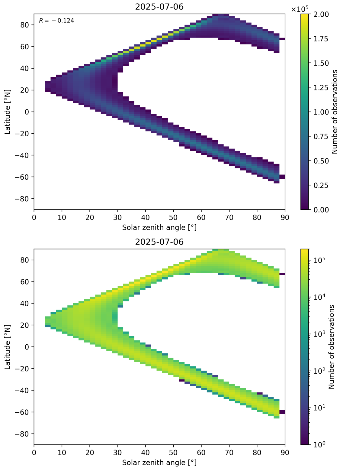
Figure 149: Scatter density plot of “Solar zenith angle” against “Latitude” for 2025-07-05 to 2025-07-07.
