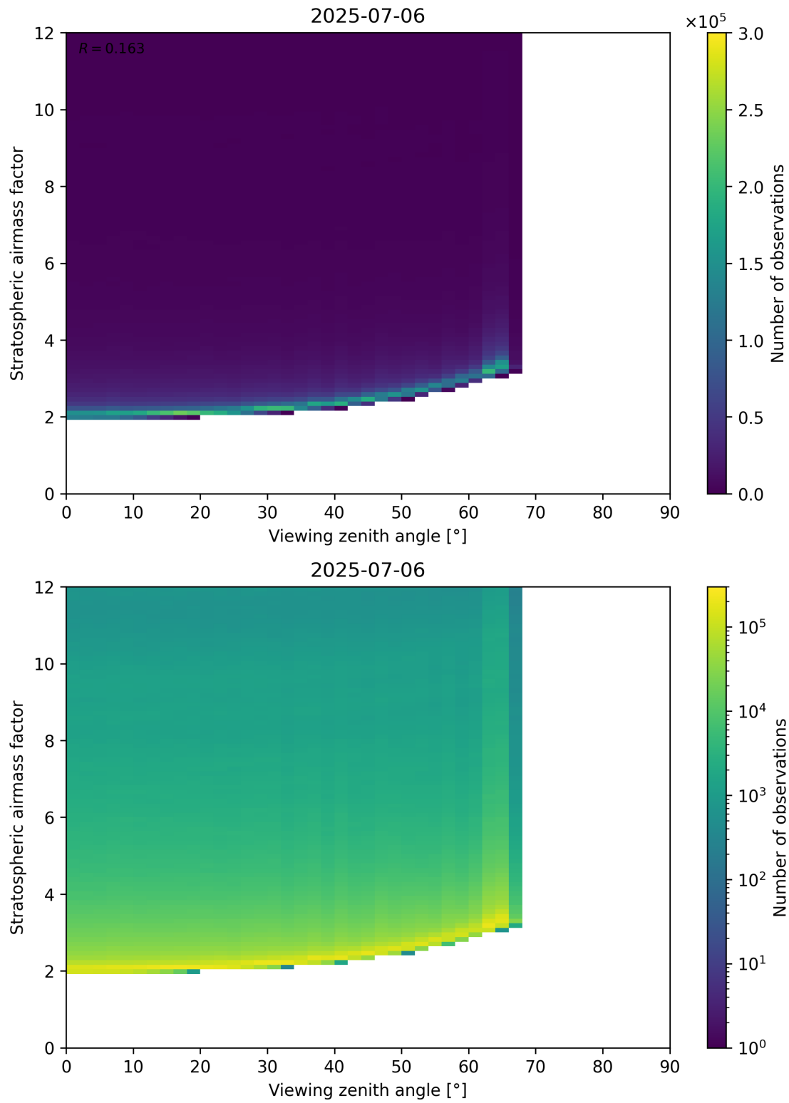
Figure 159: Scatter density plot of “Viewing zenith angle” against “Stratospheric airmass factor” for 2025-07-05 to 2025-07-07.
