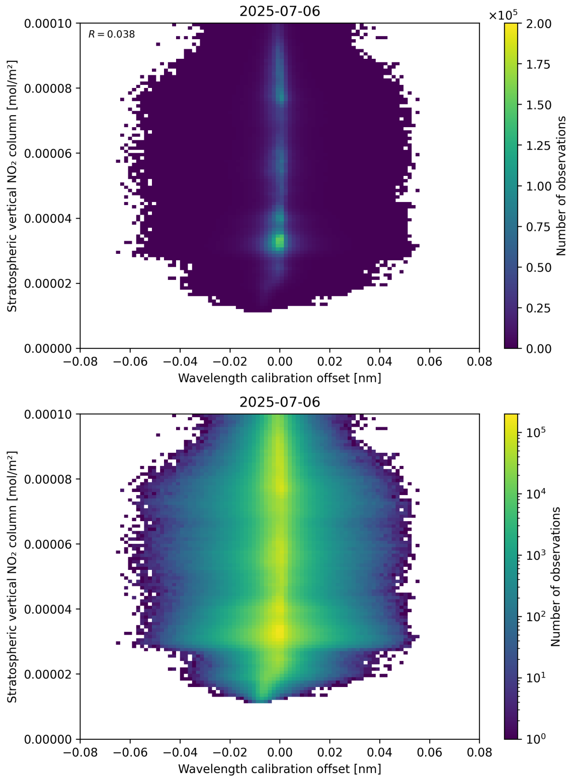
Figure 176: Scatter density plot of “Wavelength calibration offset” against “Stratospheric vertical NO 2 column” for 2025-07-05 to 2025-07-07.
