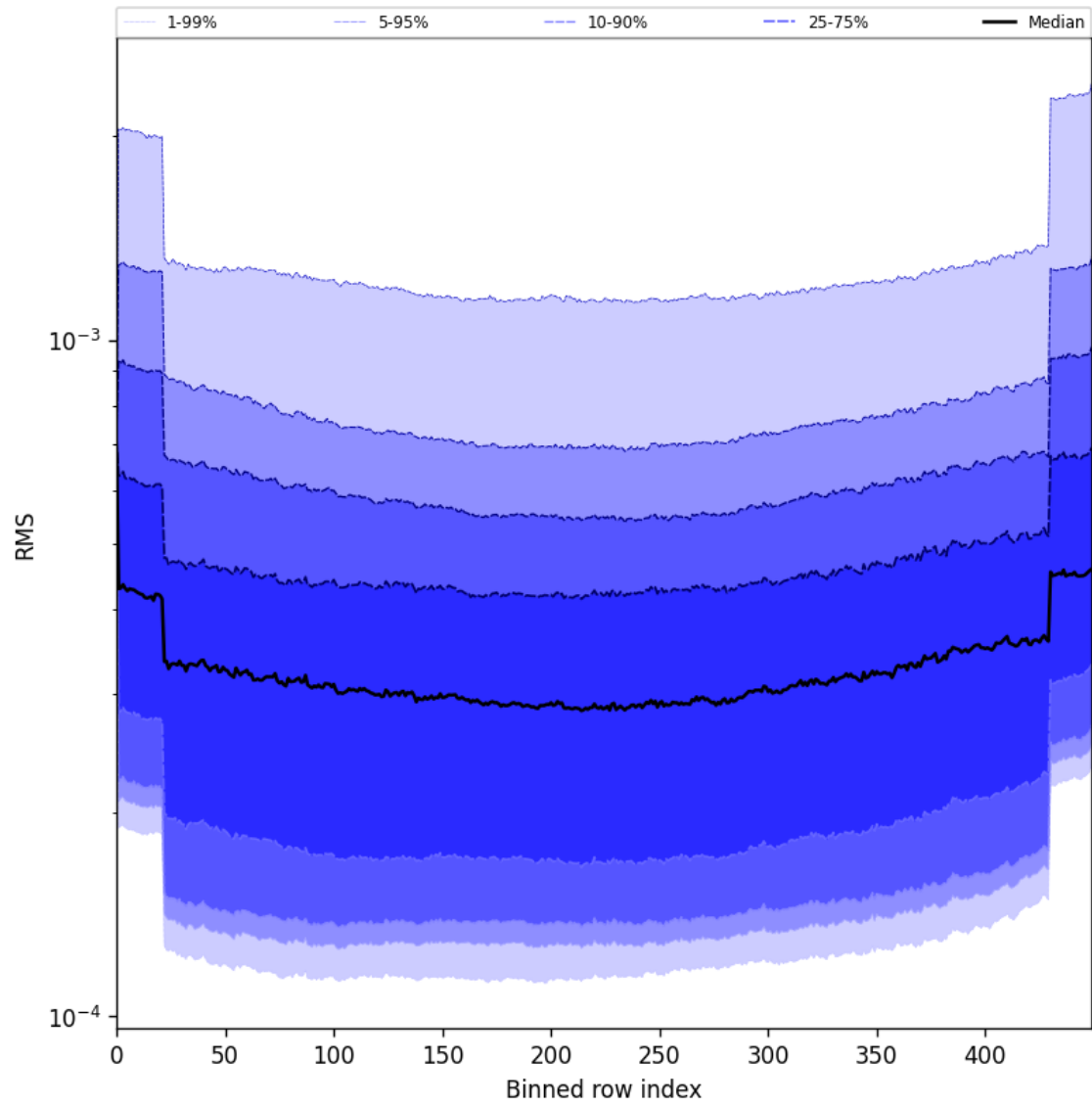
Figure 60: Along track statistics of “RMS” for 2025-07-05 to 2025-07-07
