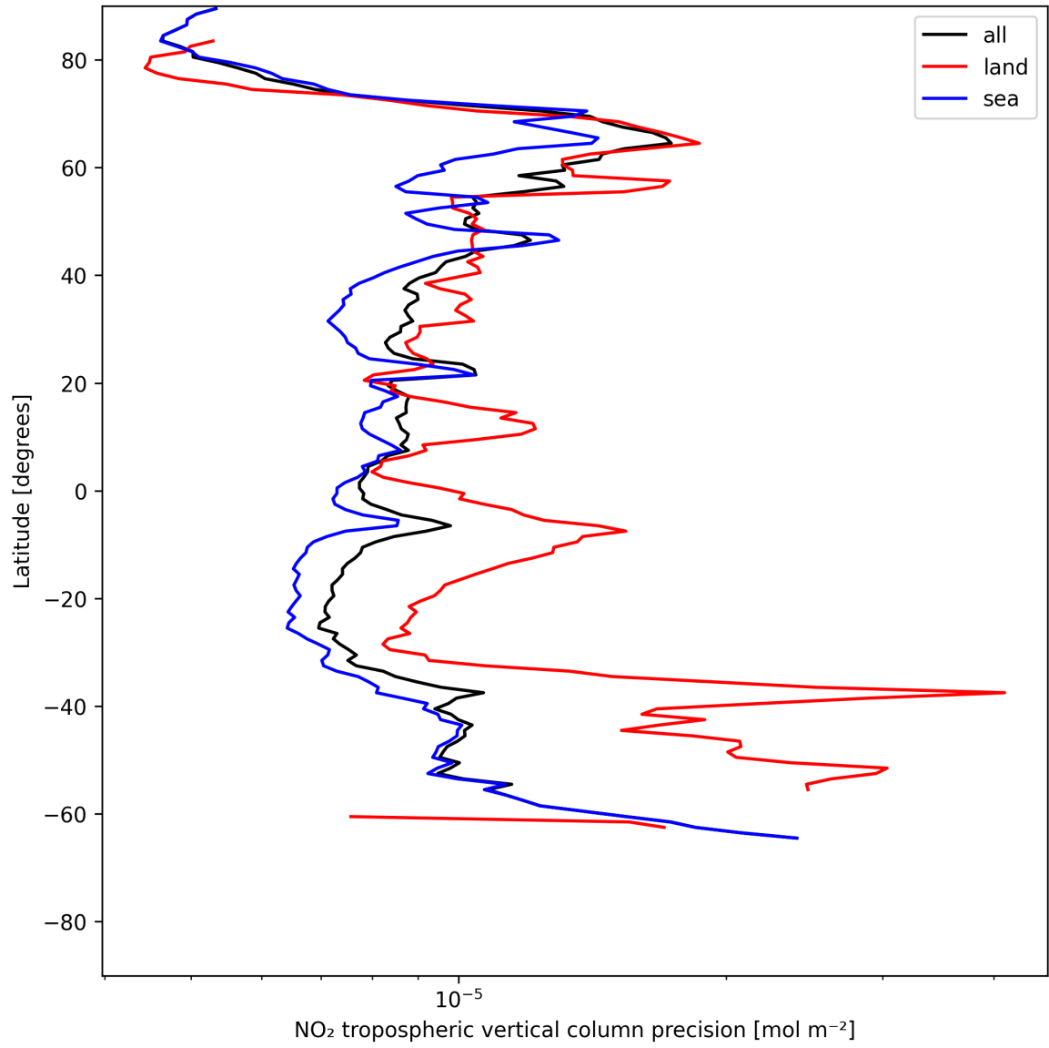
Figure 13: Zonal average of “NO 2 tropospheric vertical column precision” for 2025-07-05 to 2025-07-07.
