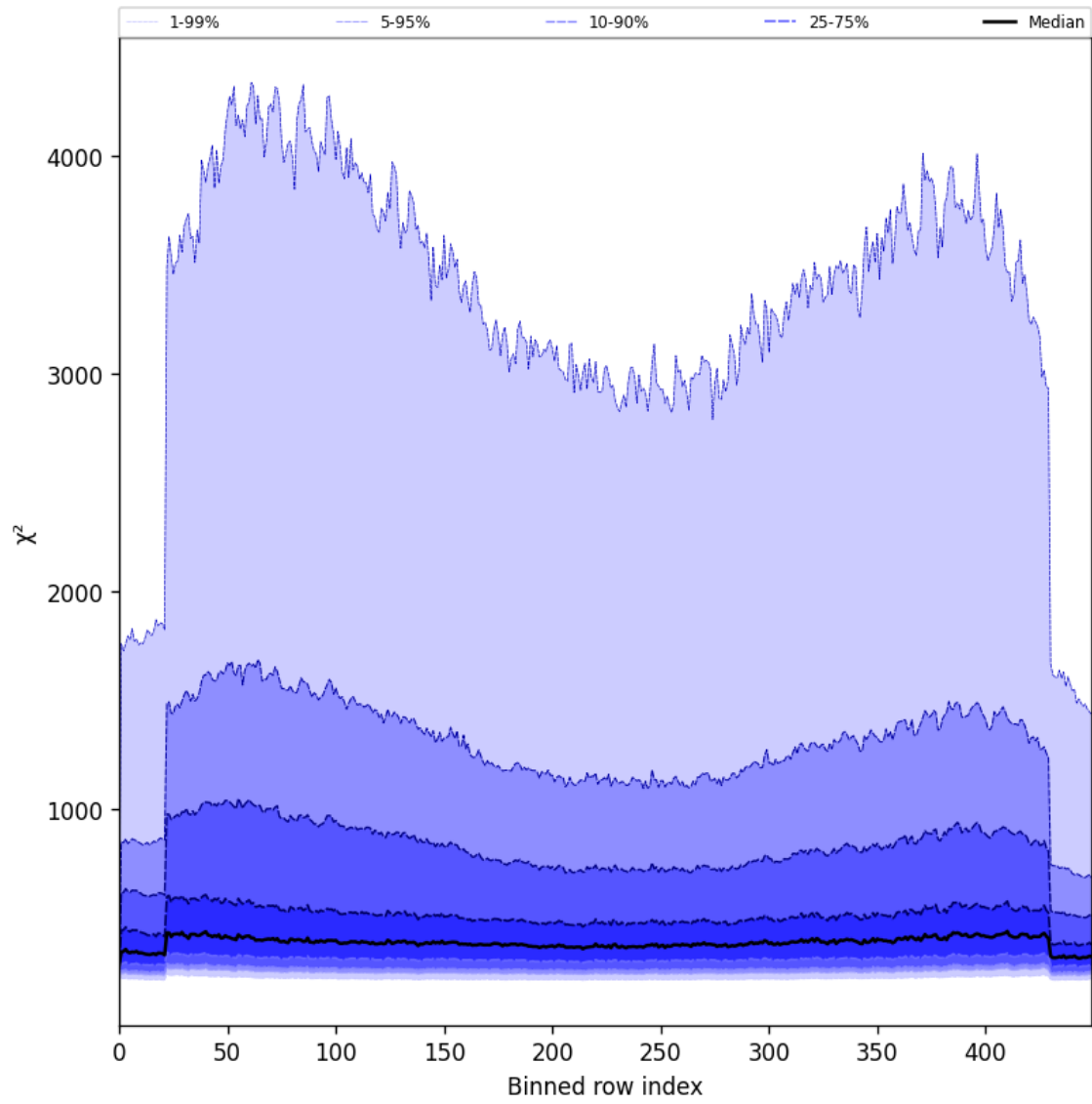
Figure 59: Along track statistics of “ \chi^2 ” for 2025-07-05 to 2025-07-07
