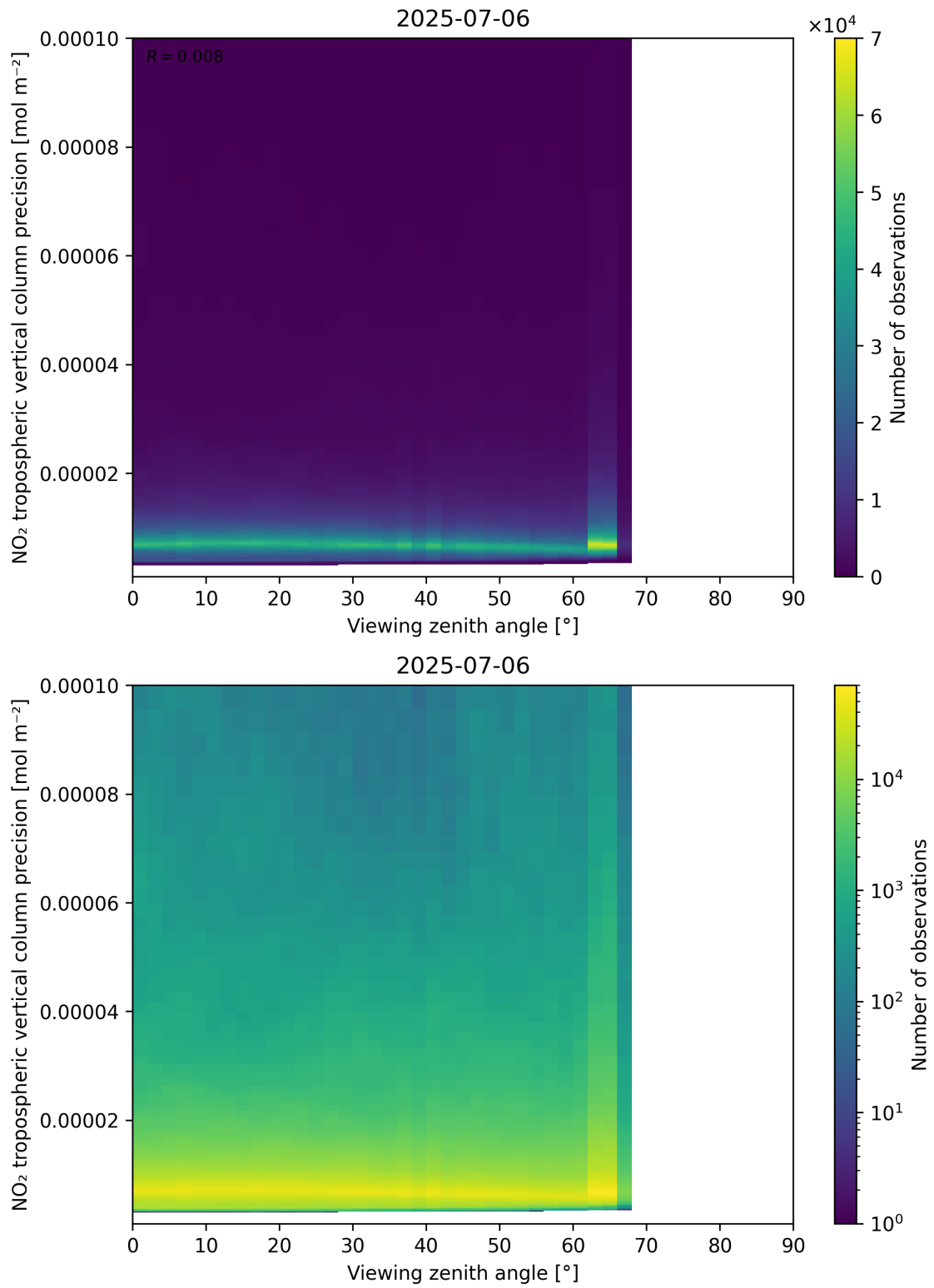
Figure 170: Scatter density plot of “Viewing zenith angle” against “NO 2 tropospheric vertical column precision” for 2025-07-05 to 2025-07-07.
