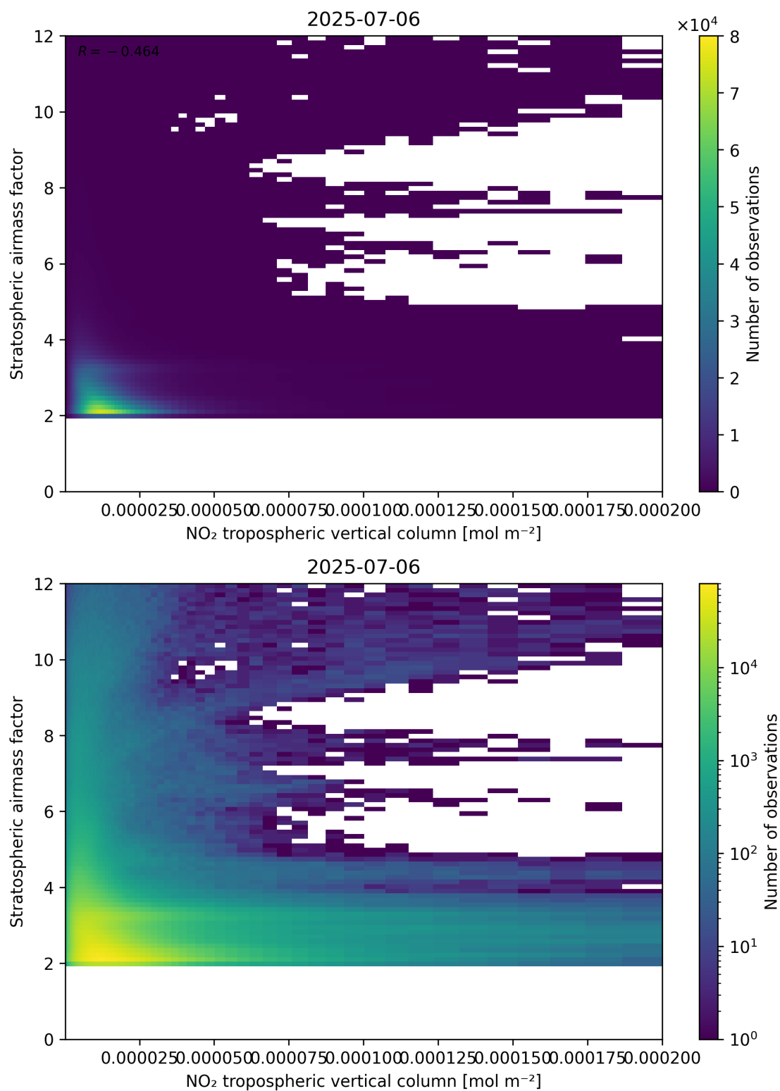
Figure 121: Scatter density plot of “NO 2 tropospheric vertical column” against “Stratospheric air mass factor” for 2025-07-05 to 2025-07-07.
