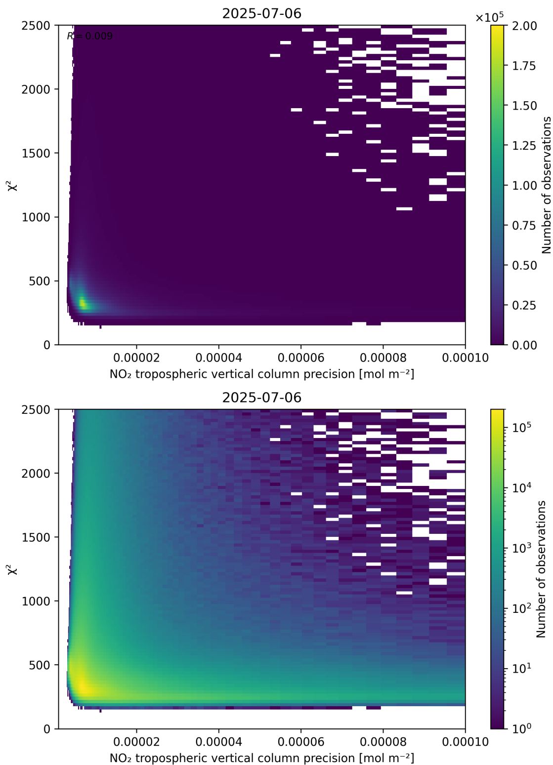
Figure 134: Scatter density plot of “NO 2 tropospheric vertical column precision” against “ \chi^2 ” for 2025-07-05 to 2025-07-07.
