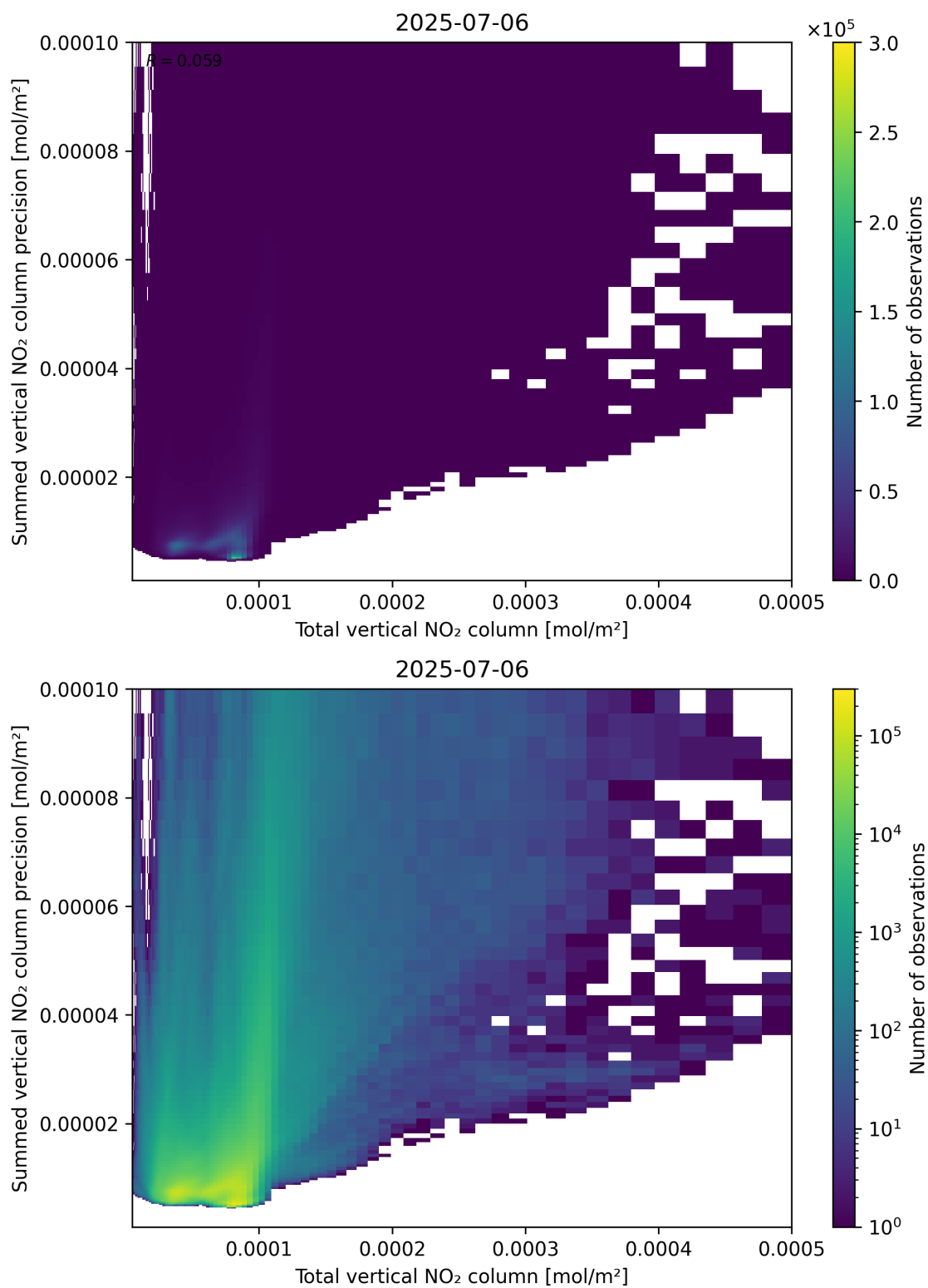
Figure 113: Scatter density plot of “Total vertical NO 2 column” against “Summed vertical NO 2 column precision” for 2025-07-05 to 2025-07-07.
