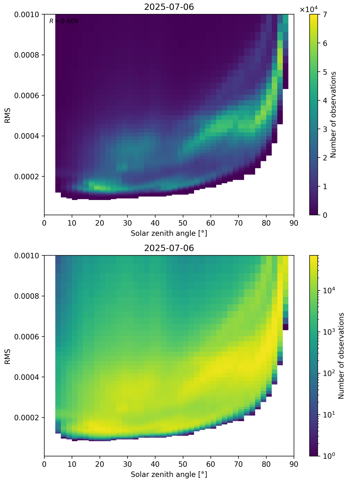
Figure 157: Scatter density plot of “Solar zenith angle” against “RMS” for 2025-07-05 to 2025-07-07.
