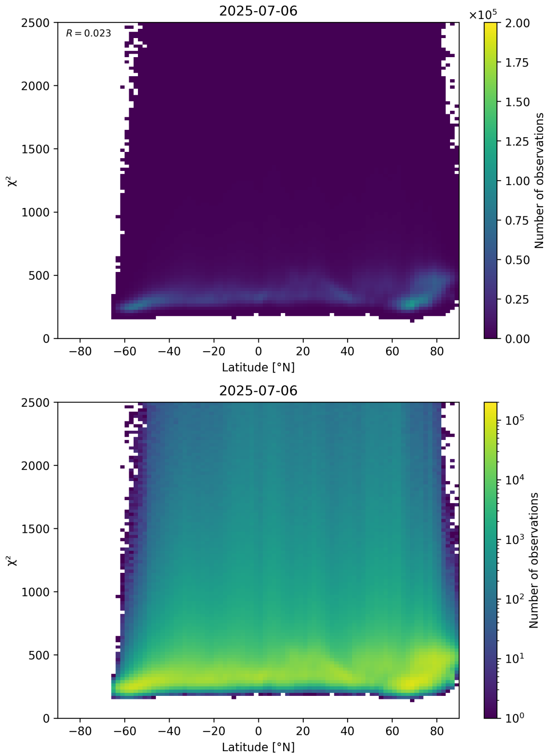
Figure 86: Scatter density plot of “Latitude” against “ \chi^2 ” for 2025-07-05 to 2025-07-07.
