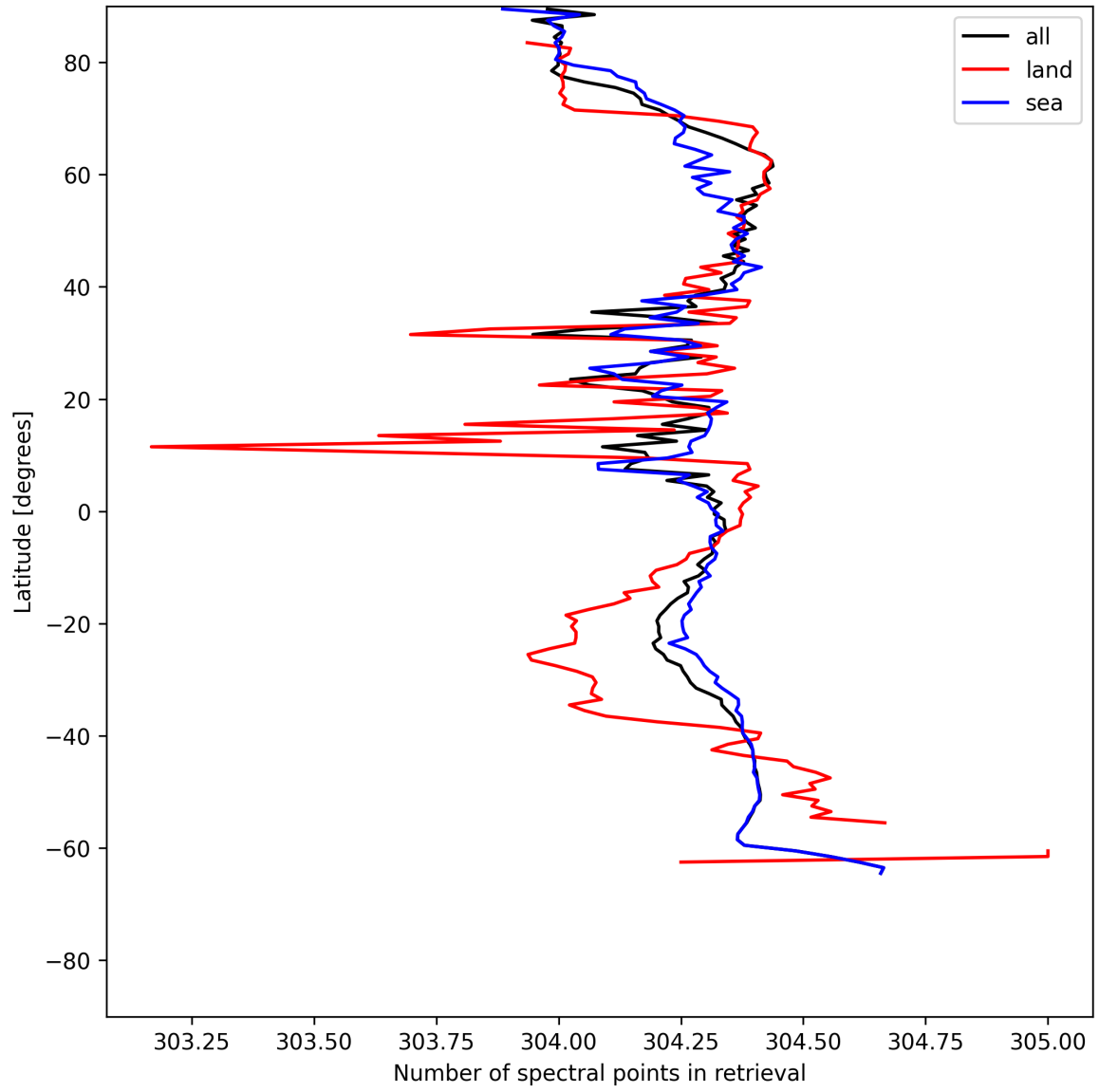
Figure 16: Zonal average of “Number of spectral points in retrieval” for 2025-07-05 to 2025-07-07.
