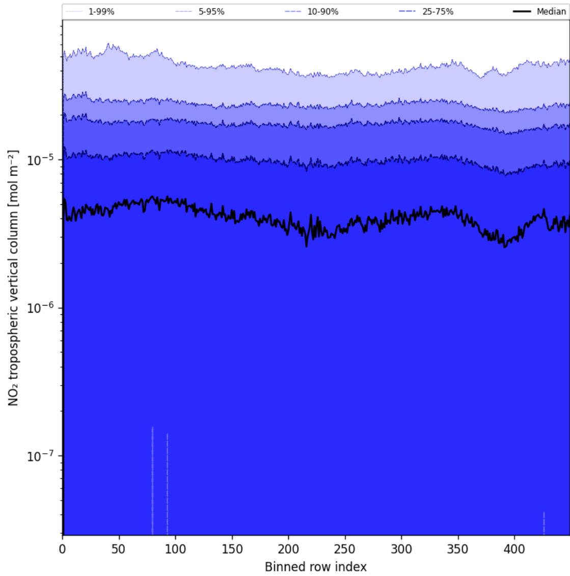
Figure 46: Along track statistics of “NO 2 tropospheric vertical column” for 2025-07-05 to 2025-07-07
