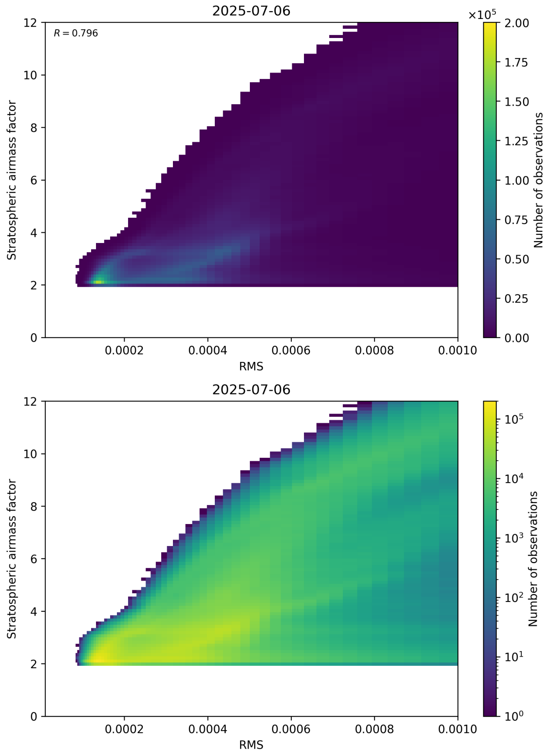
Figure 144: Scatter density plot of “RMS” against “Stratospheric airmass factor” for 2025-07-05 to 2025-07-07.
