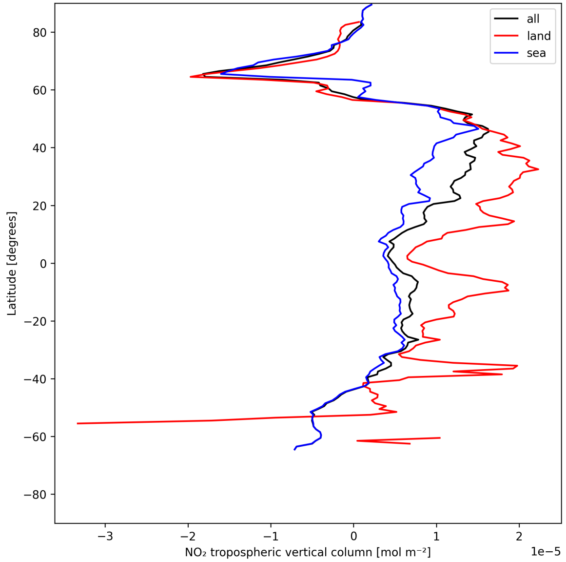
Figure 12: Zonal average of “NO 2 tropospheric vertical column” for 2025-07-05 to 2025-07-07.
