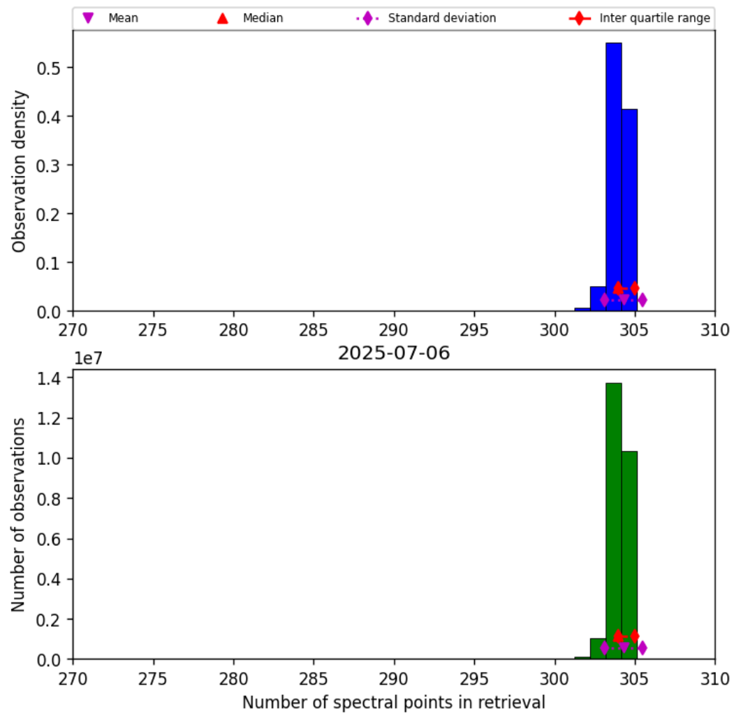
Figure 33: Histogram of “Number of spectral points in retrieval” for 2025-07-05 to 2025-07-07
