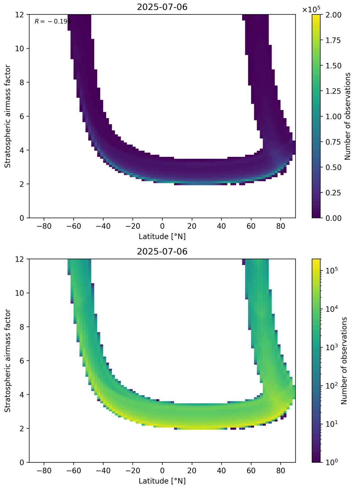
Figure 83: Scatter density plot of “Latitude” against “Stratospheric air mass factor” for 2025-07-05 to 2025-07-07.
