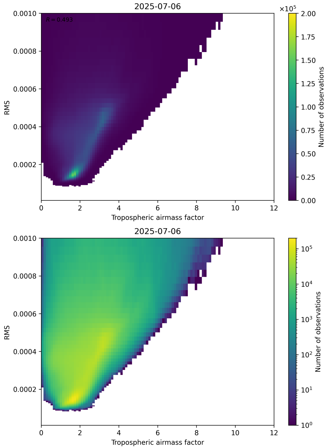
Figure 79: Scatter density plot of “Tropospheric airmass factor” against “RMS” for 2025-07-05 to 2025-07-07.
