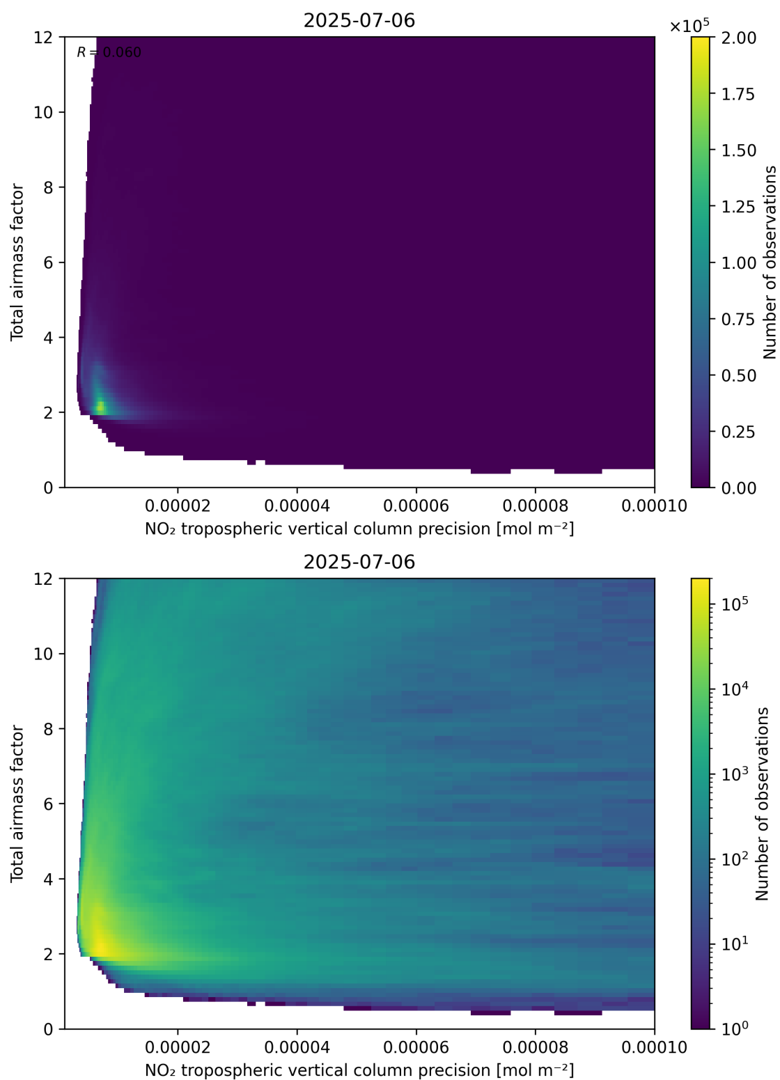
Figure 132: Scatter density plot of “NO 2 tropospheric vertical column precision” against “Total air mass factor” for 2025-07-05 to 2025-07-07.
