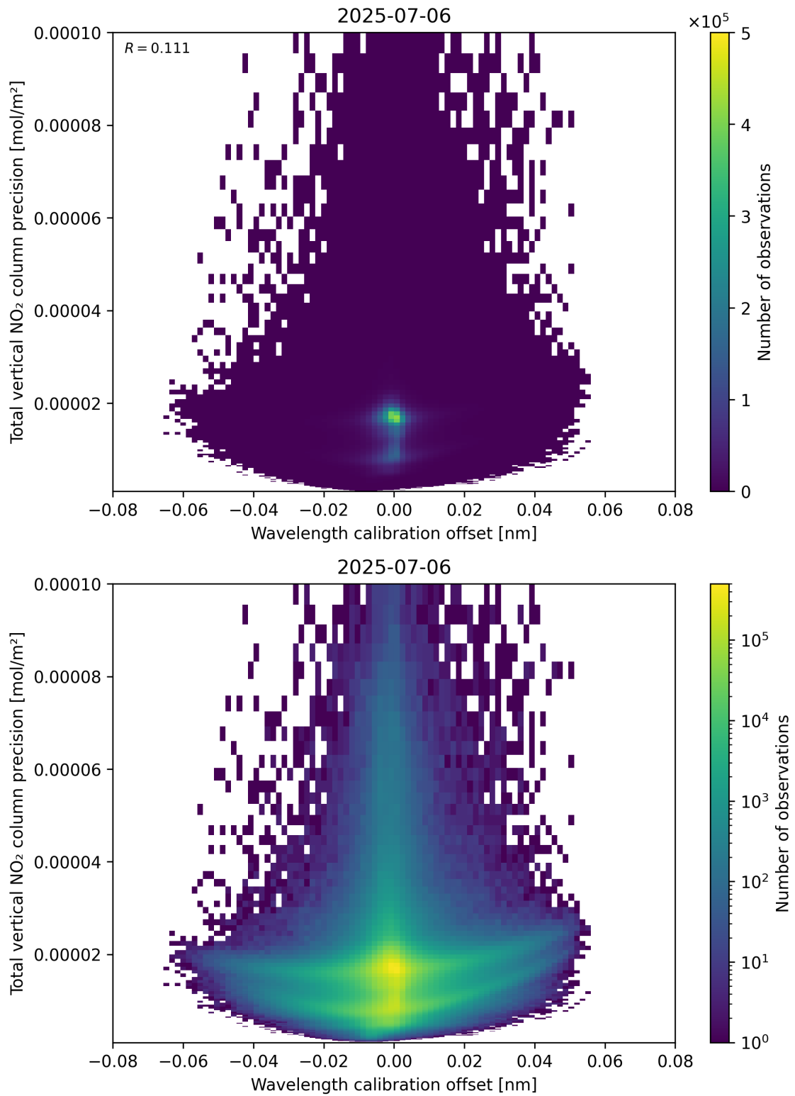
Figure 180: Scatter density plot of “Wavelength calibration offset” against “Total vertical NO 2 column precision” for 2025-07-05 to 2025-07-07.
