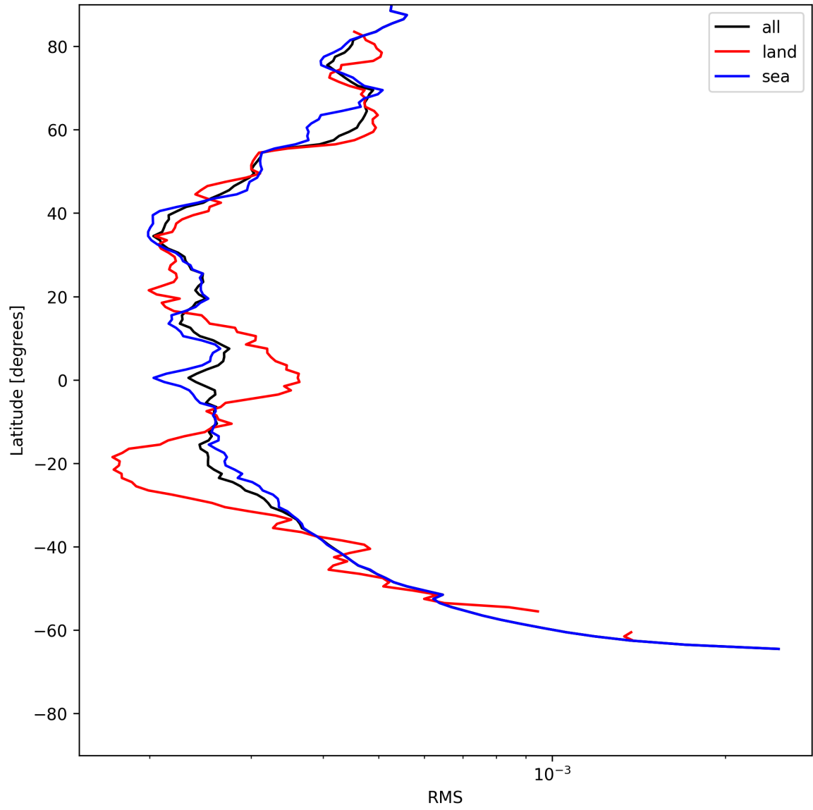
Figure 26: Zonal average of “RMS” for 2025-07-05 to 2025-07-07.
