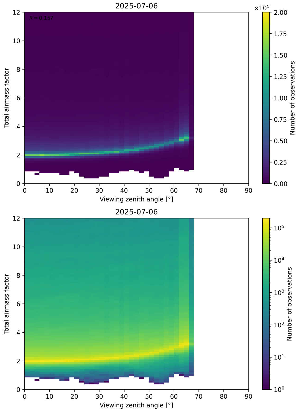
Figure 160: Scatter density plot of “Viewing zenith angle” against “Total airmass factor” for 2025-07-05 to 2025-07-07.
