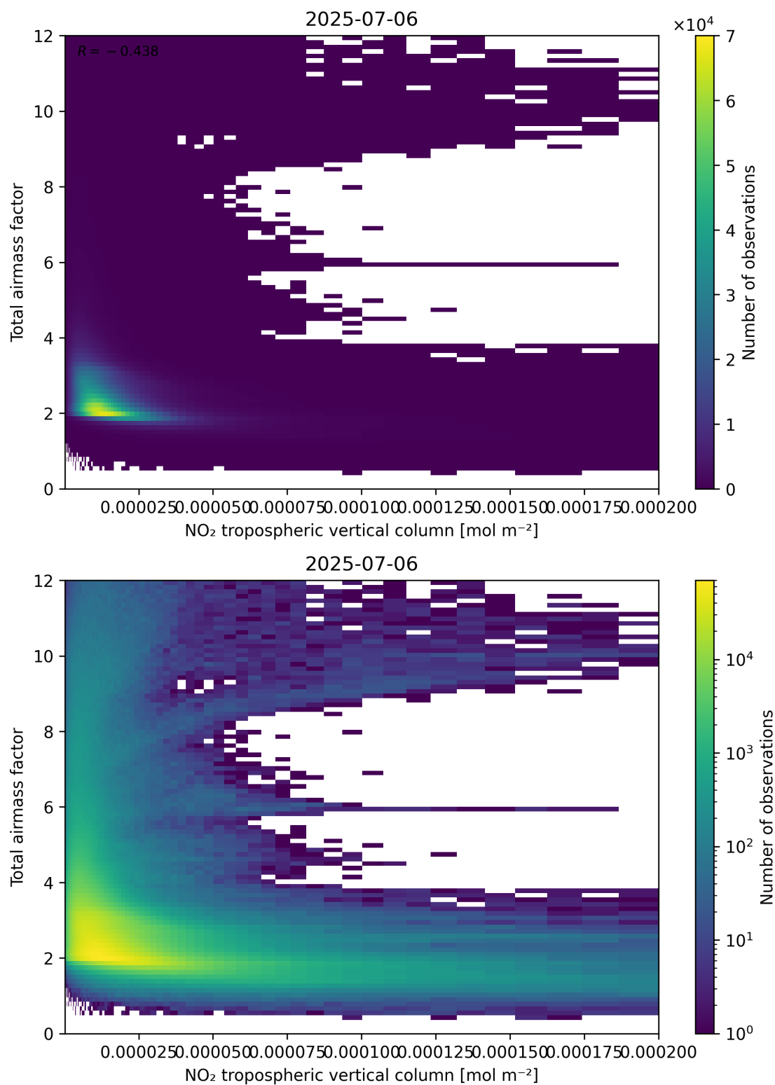
Figure 122: Scatter density plot of “NO 2 tropospheric vertical column” against “Total air mass factor” for 2025-07-05 to 2025-07-07.
