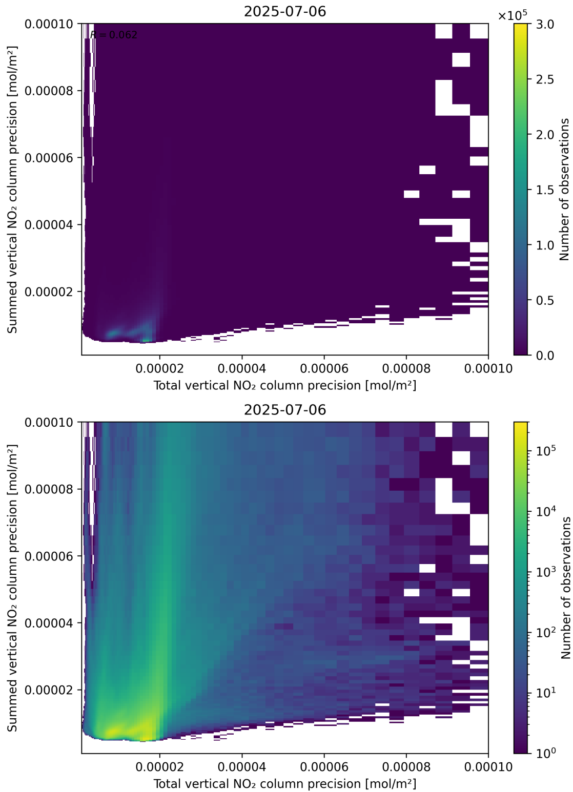
Figure 118: Scatter density plot of “Total vertical NO 2 column precision” against “Summed vertical NO 2 column precision” for 2025-07-05 to 2025-07-07.
