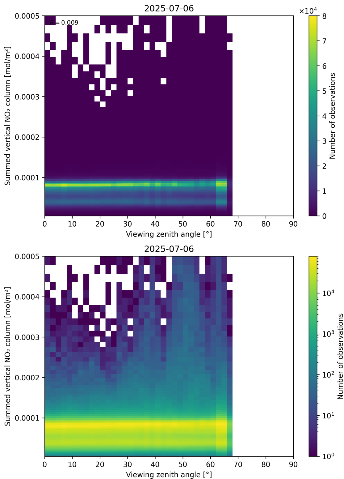
Figure 165: Scatter density plot of “Viewing zenith angle” against “Summed vertical NO 2 column” for 2025-07-05 to 2025-07-07.
