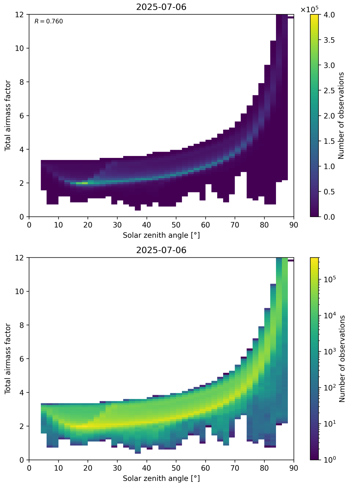
Figure 146: Scatter density plot of “Solar zenith angle” against “Total air mass factor” for 2025-07-05 to 2025-07-07.
