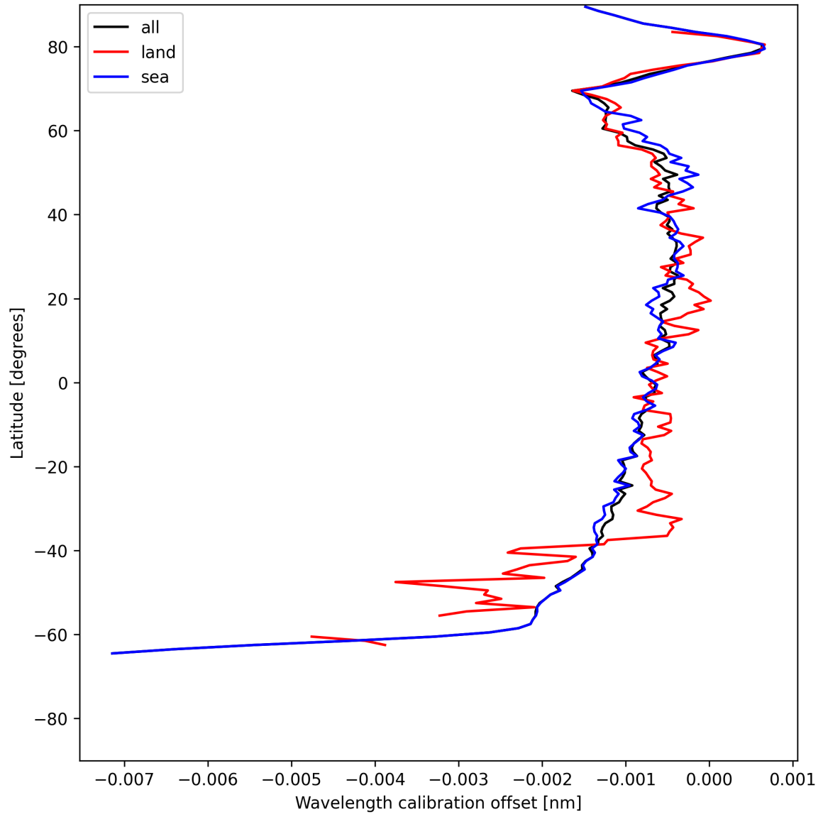
Figure 18: Zonal average of “Wavelength calibration offset” for 2025-07-05 to 2025-07-07.
