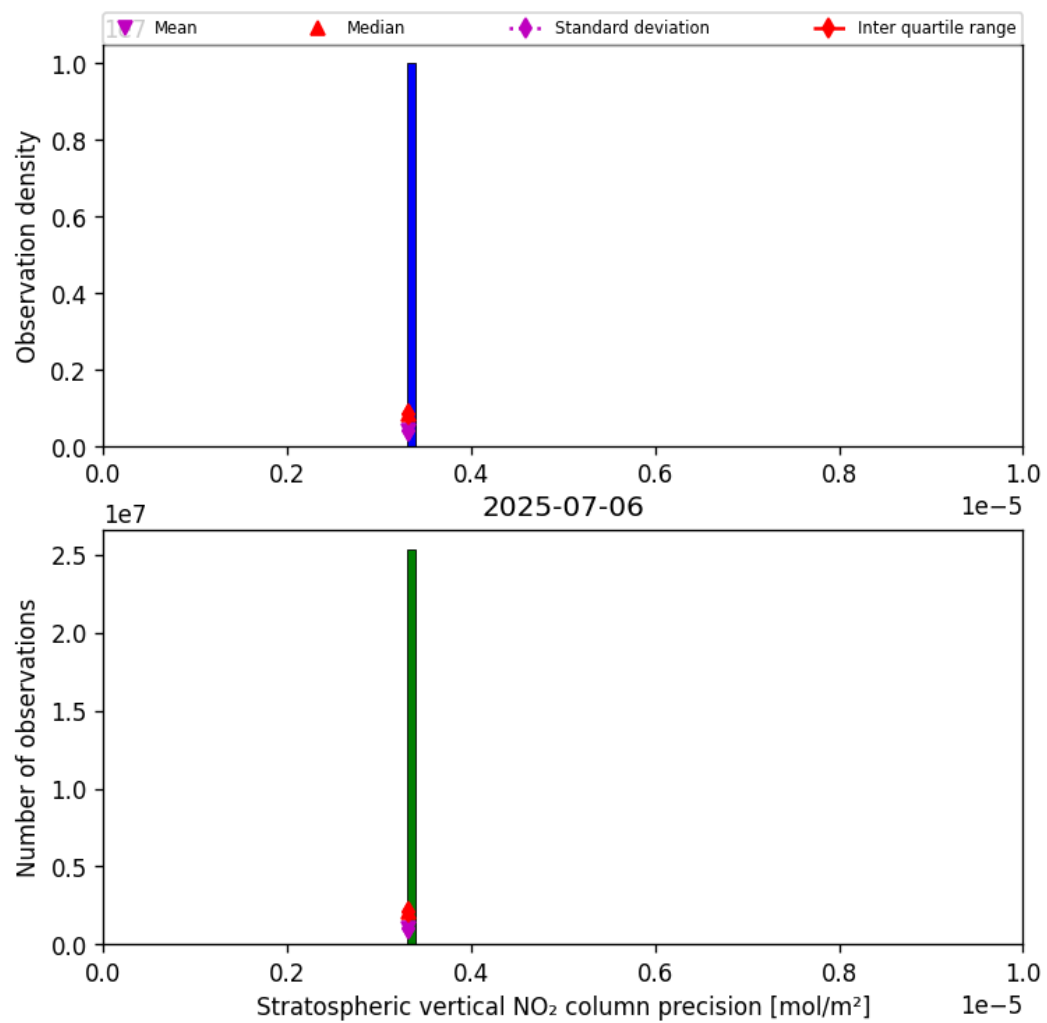
Figure 37: Histogram of “Stratospheric vertical NO 2 column precision” for 2025-07-05 to 2025-07-07
