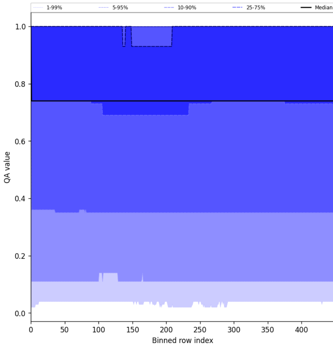
Figure 45: Along track statistics of “QA value” for 2025-07-05 to 2025-07-07
