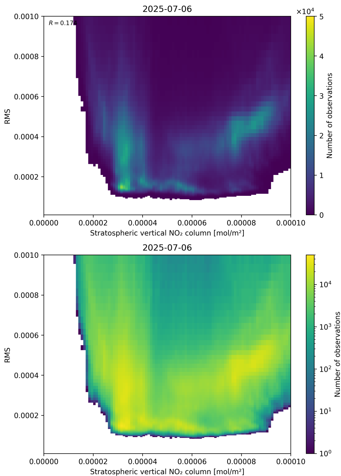
Figure 102: Scatter density plot of “Stratospheric vertical NO 2 column” against “RMS” for 2025-07-05 to 2025-07-07.
