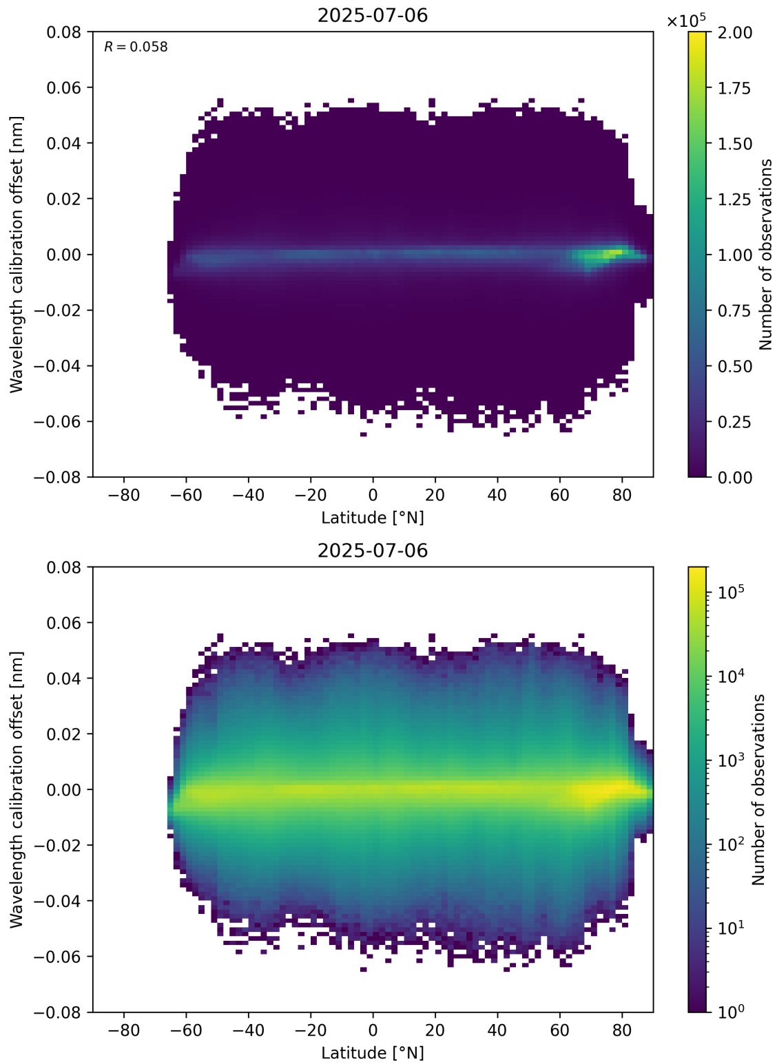
Figure 95: Scatter density plot of “Latitude” against “Wavelength calibration offset” for 2025-07-05 to 2025-07-07.
