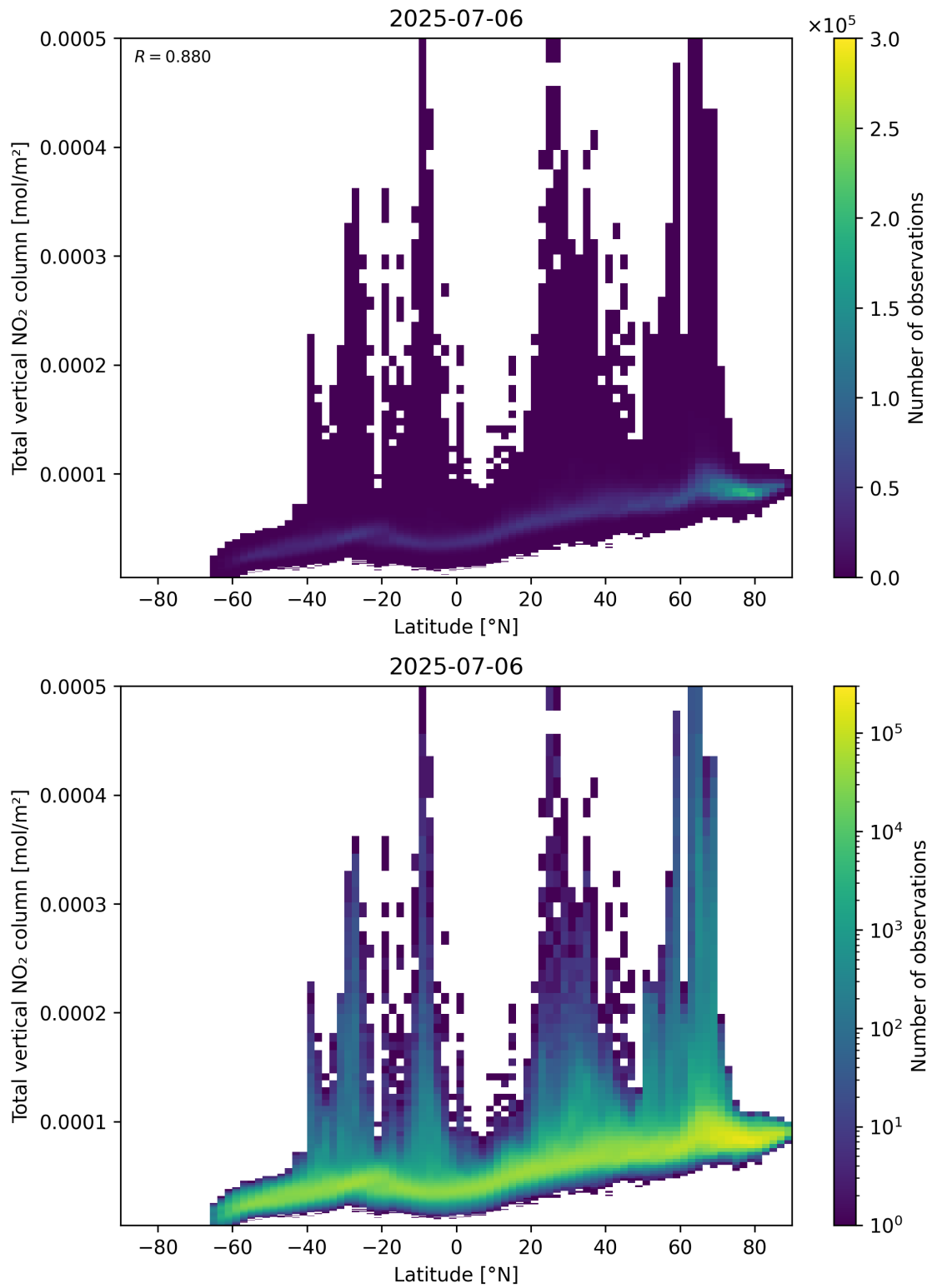
Figure 90: Scatter density plot of “Latitude” against “Total vertical NO 2 column” for 2025-07-05 to 2025-07-07.
