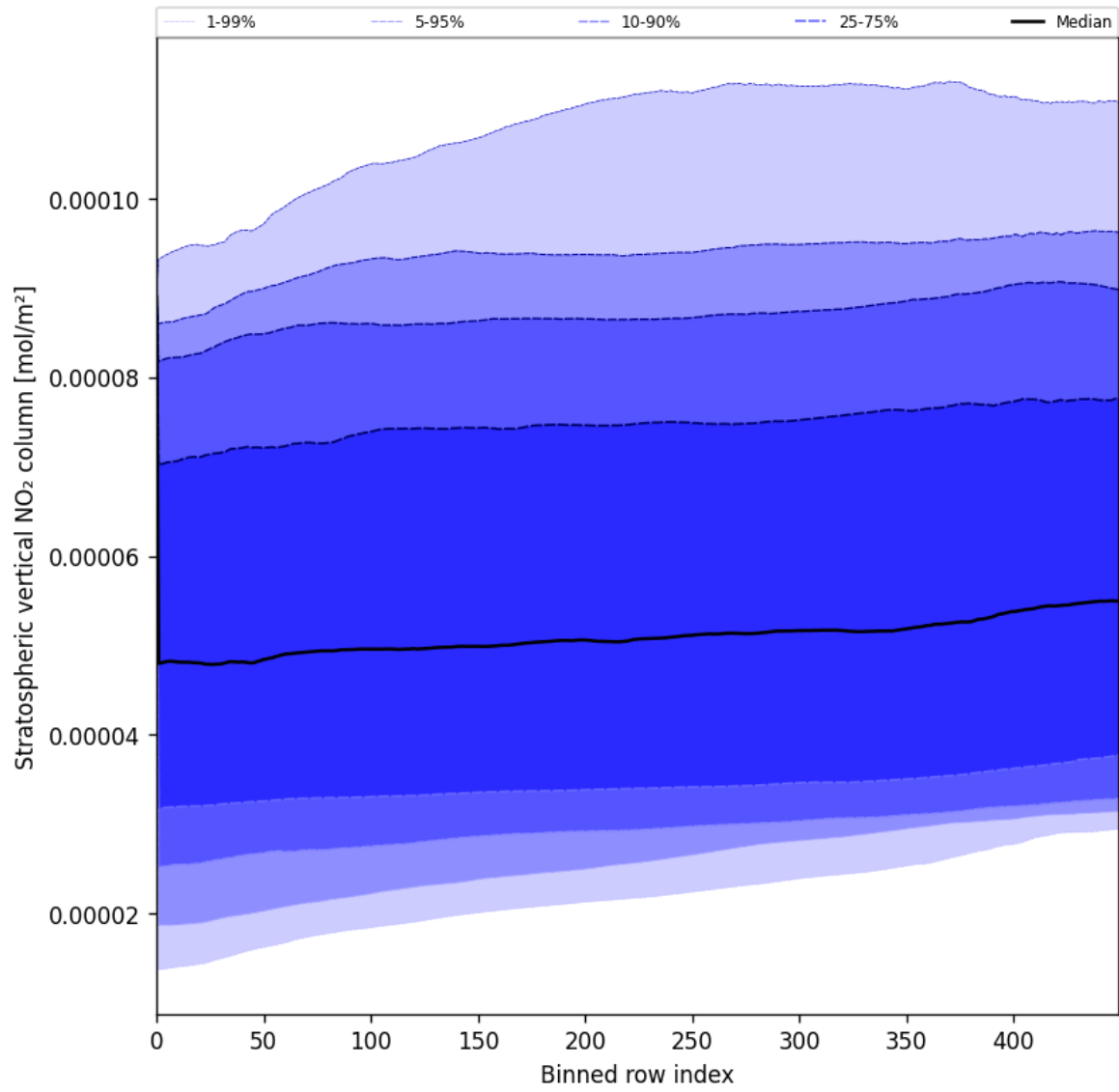
Figure 53: Along track statistics of “Stratospheric vertical NO 2 column” for 2025-07-05 to 2025-07-07
