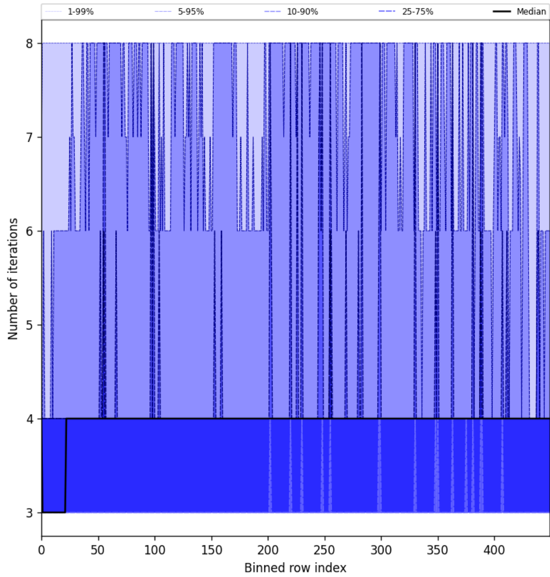
Figure 51: Along track statistics of “Number of iterations” for 2025-07-05 to 2025-07-07
