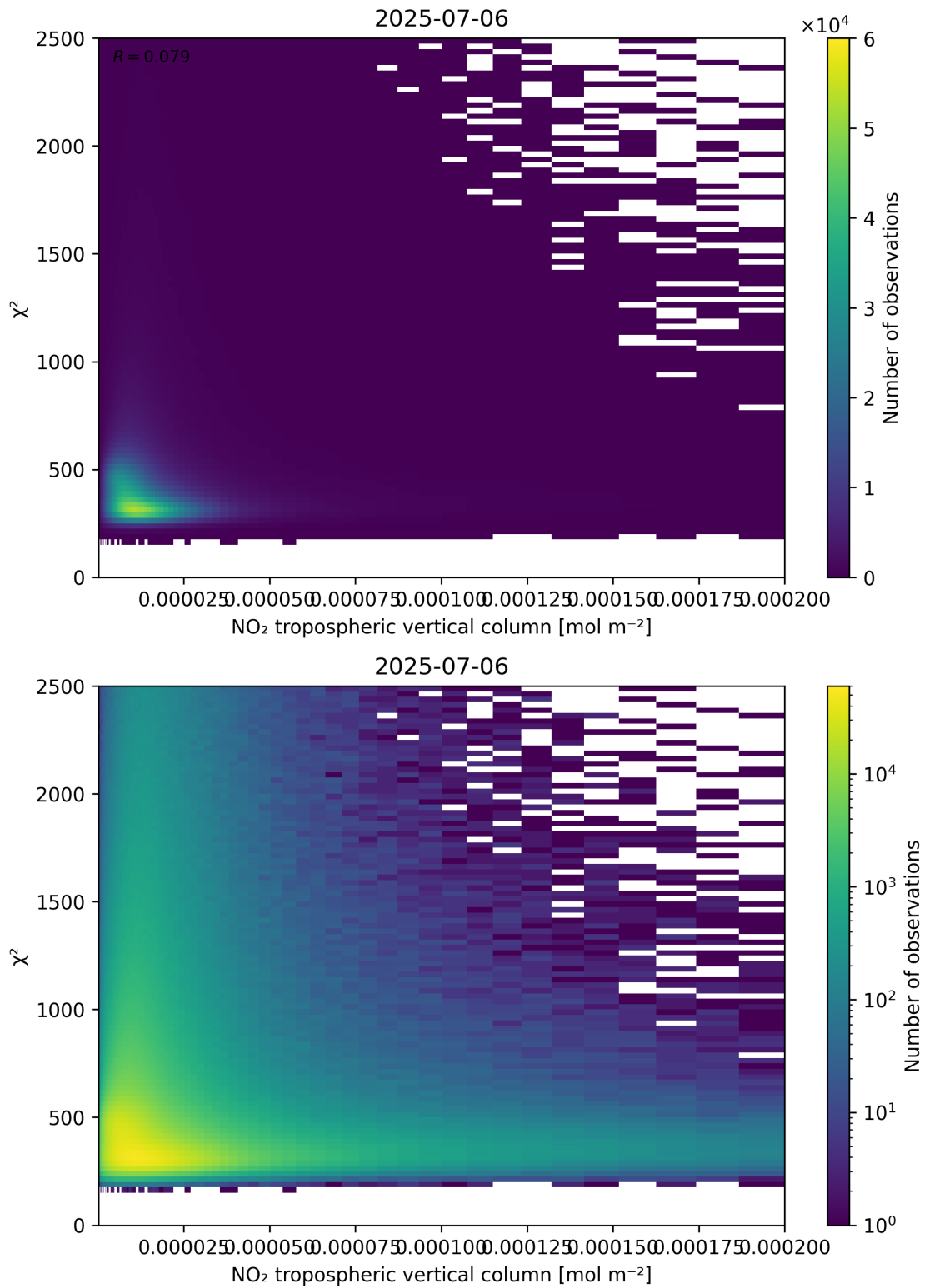
Figure 124: Scatter density plot of “NO 2 tropospheric vertical column” against “ \chi^2 ” for 2025-07-05 to 2025-07-07.
