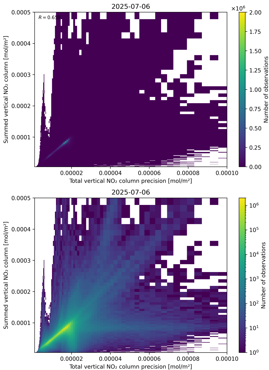
Figure 117: Scatter density plot of “Total vertical NO 2 column precision” against “Summed vertical NO 2 column” for 2025-07-05 to 2025-07-07.
