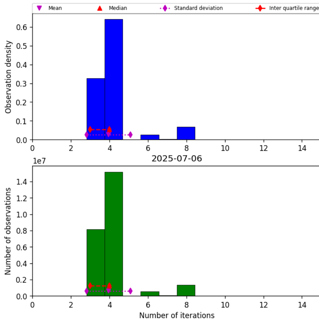
Figure 34: Histogram of “Number of iterations” for 2025-07-05 to 2025-07-07
