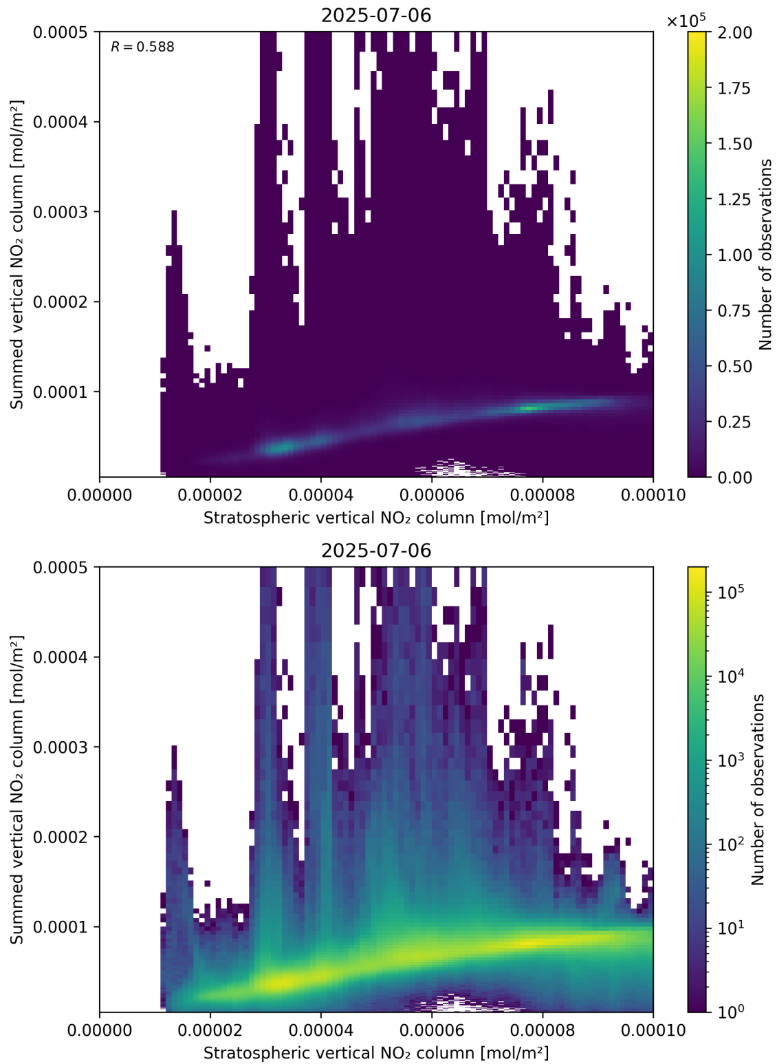
Figure 98: Scatter density plot of “Stratospheric vertical NO 2 column” against “Summed vertical NO 2 column” for 2025-07-05 to 2025-07-07.
