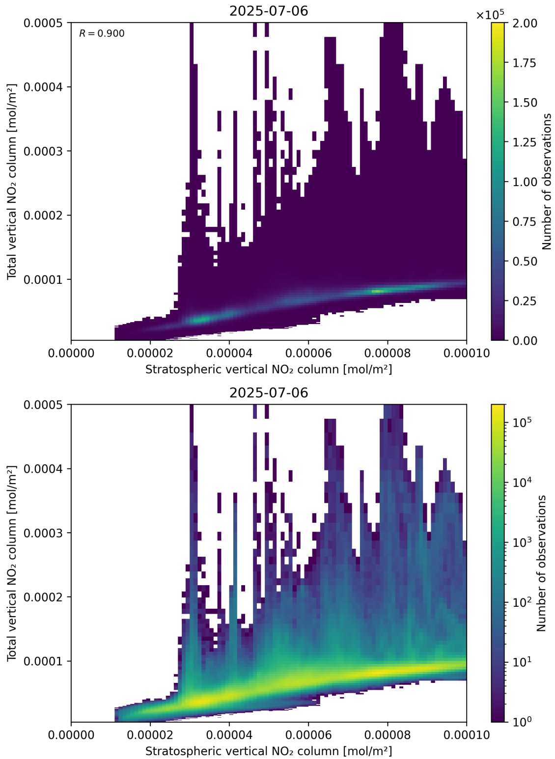
Figure 100: Scatter density plot of “Stratospheric vertical NO 2 column” against “Total vertical NO 2 column” for 2025-07-05 to 2025-07-07.
