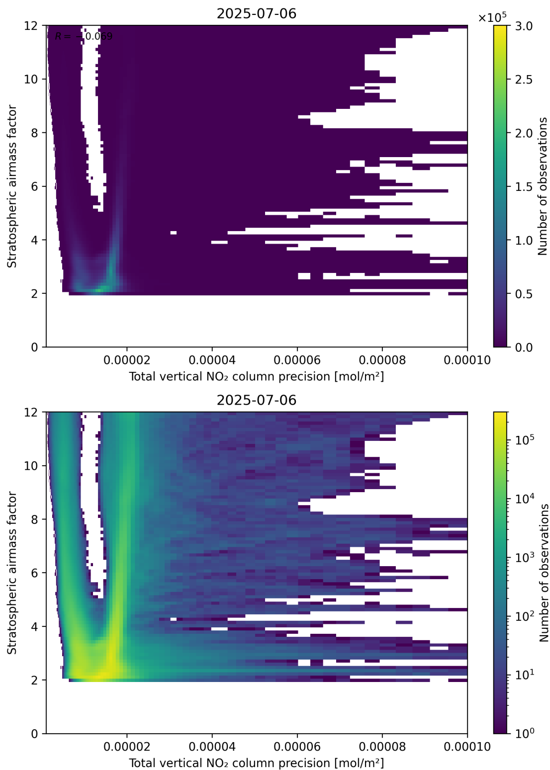
Figure 115: Scatter density plot of “Total vertical NO 2 column precision” against “Stratospheric air mass factor” for 2025-07-05 to 2025-07-07.
