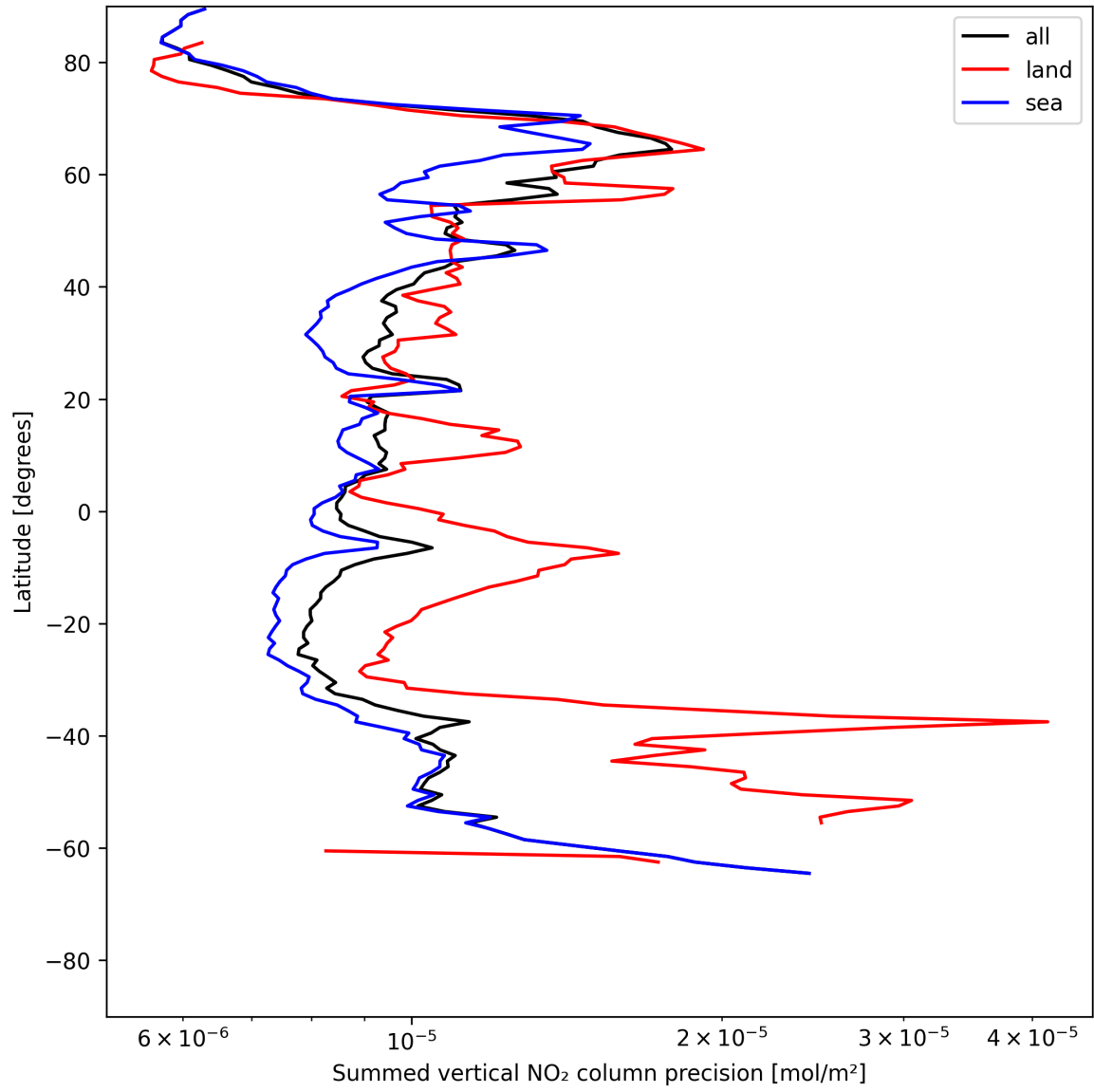
Figure 24: Zonal average of “Summed vertical NO 2 column precision” for 2025-07-05 to 2025-07-07.
