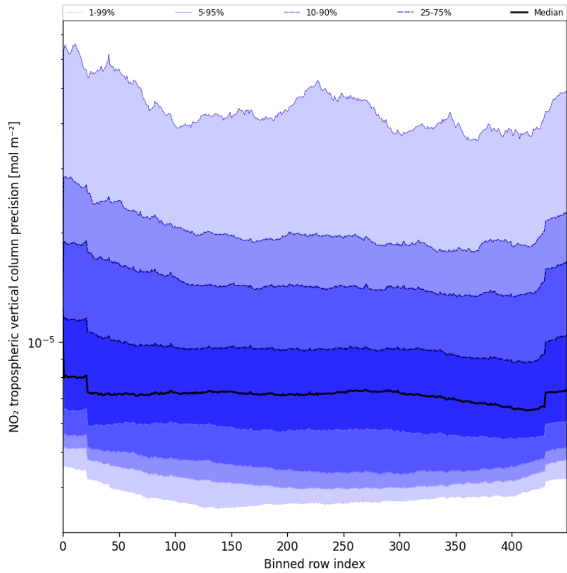
Figure 47: Along track statistics of “NO 2 tropospheric vertical column precision” for 2025-07-05 to 2025-07-07
