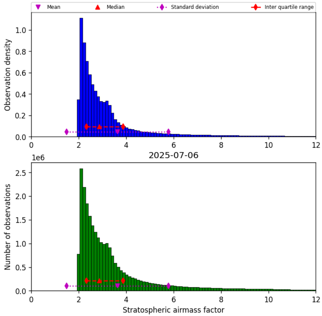
Figure 44: Histogram of “Stratospheric airmass factor” for 2025-07-05 to 2025-07-07
