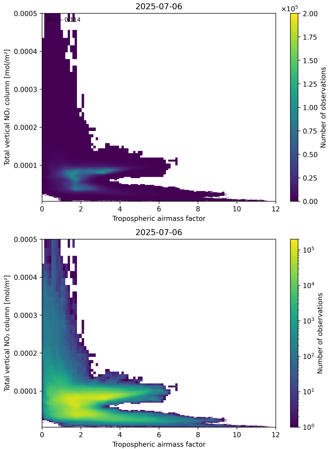
Figure 77: Scatter density plot of “Tropospheric airmass factor” against “Total vertical NO 2 column” for 2025-07-05 to 2025-07-07.
