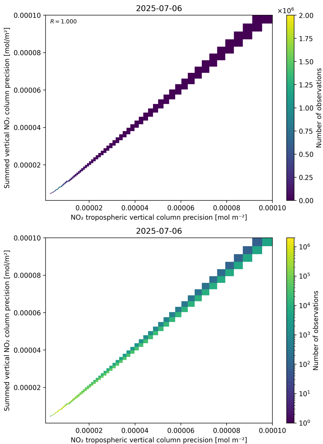
Figure 137: Scatter density plot of “NO 2 tropospheric vertical column precision” against “Summed vertical NO 2 column precision” for 2025-07-05 to 2025-07-07.
