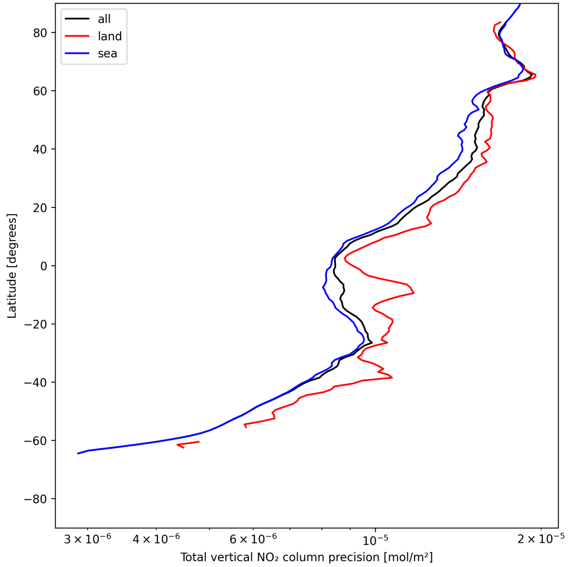
Figure 22: Zonal average of “Total vertical NO 2 column precision” for 2025-07-05 to 2025-07-07.
