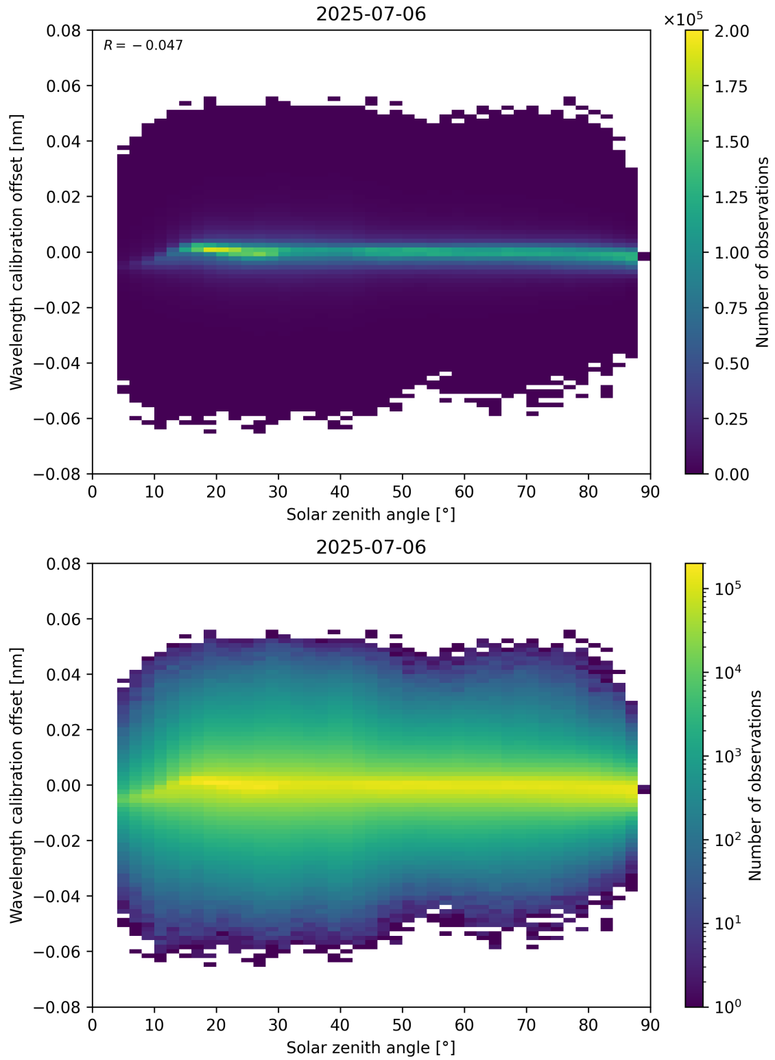
Figure 158: Scatter density plot of “Solar zenith angle” against “Wavelength calibration offset” for 2025-07-05 to 2025-07-07.
