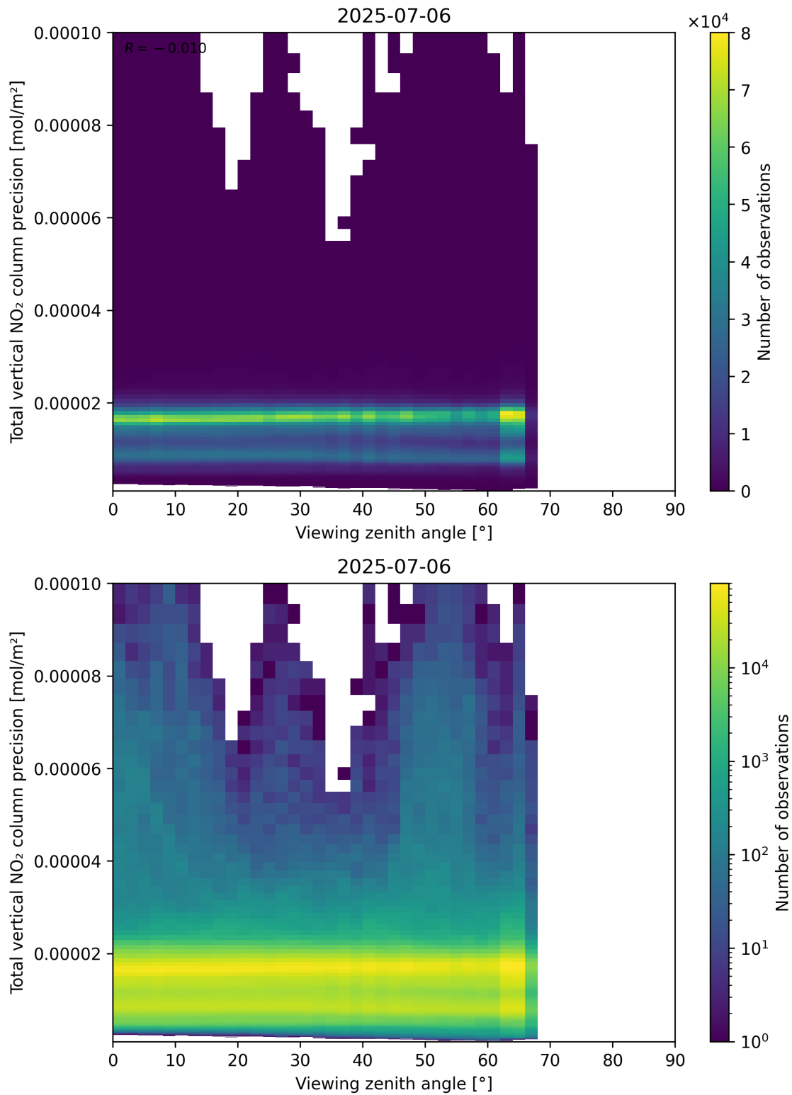
Figure 168: Scatter density plot of “Viewing zenith angle” against “Total vertical NO 2 column precision” for 2025-07-05 to 2025-07-07.
