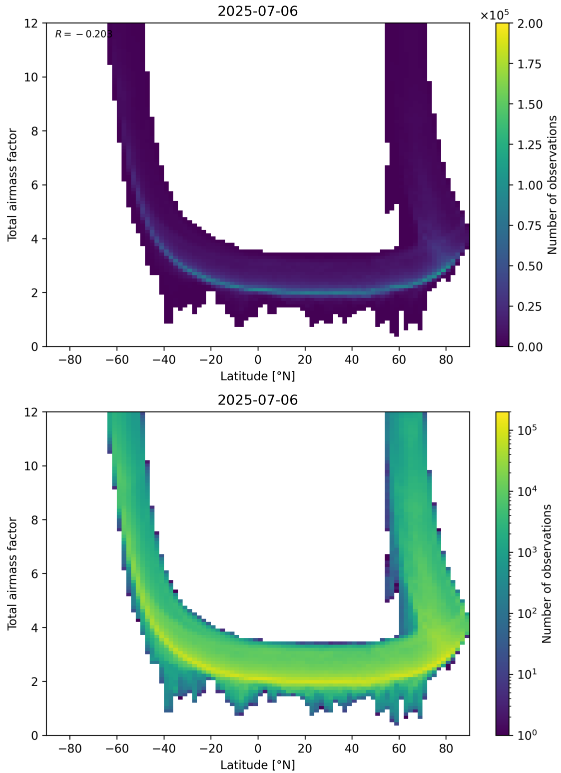
Figure 84: Scatter density plot of “Latitude” against “Total airmass factor” for 2025-07-05 to 2025-07-07.
