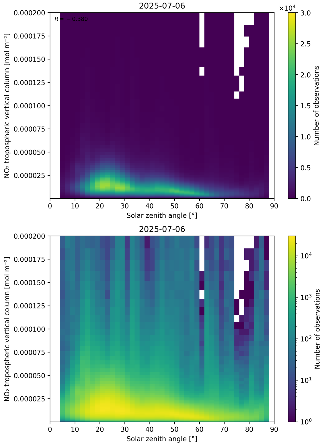
Figure 155: Scatter density plot of “Solar zenith angle” against “NO 2 tropospheric vertical column” for 2025-07-05 to 2025-07-07.
