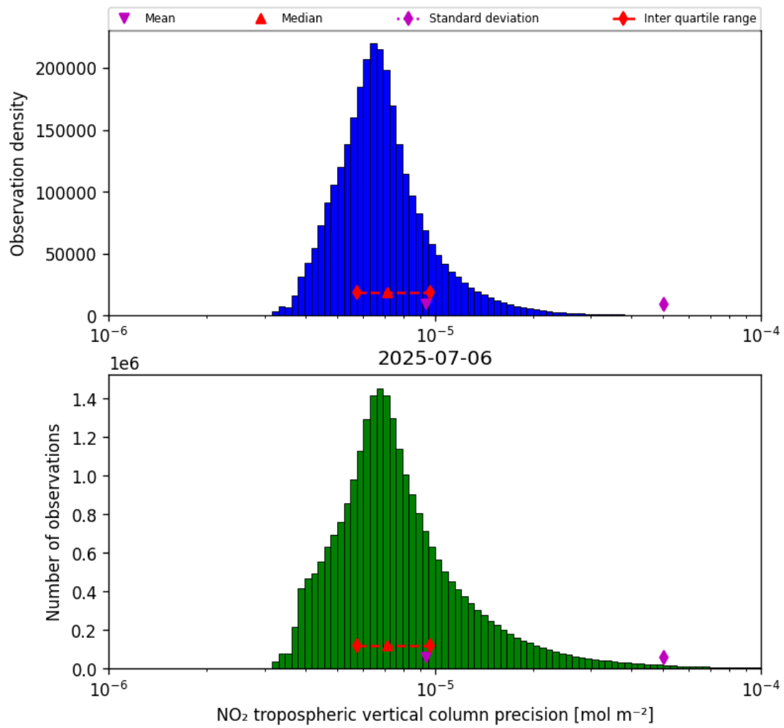
Figure 30: Histogram of “NO 2 tropospheric vertical column precision” for 2025-07-05 to 2025-07-07
