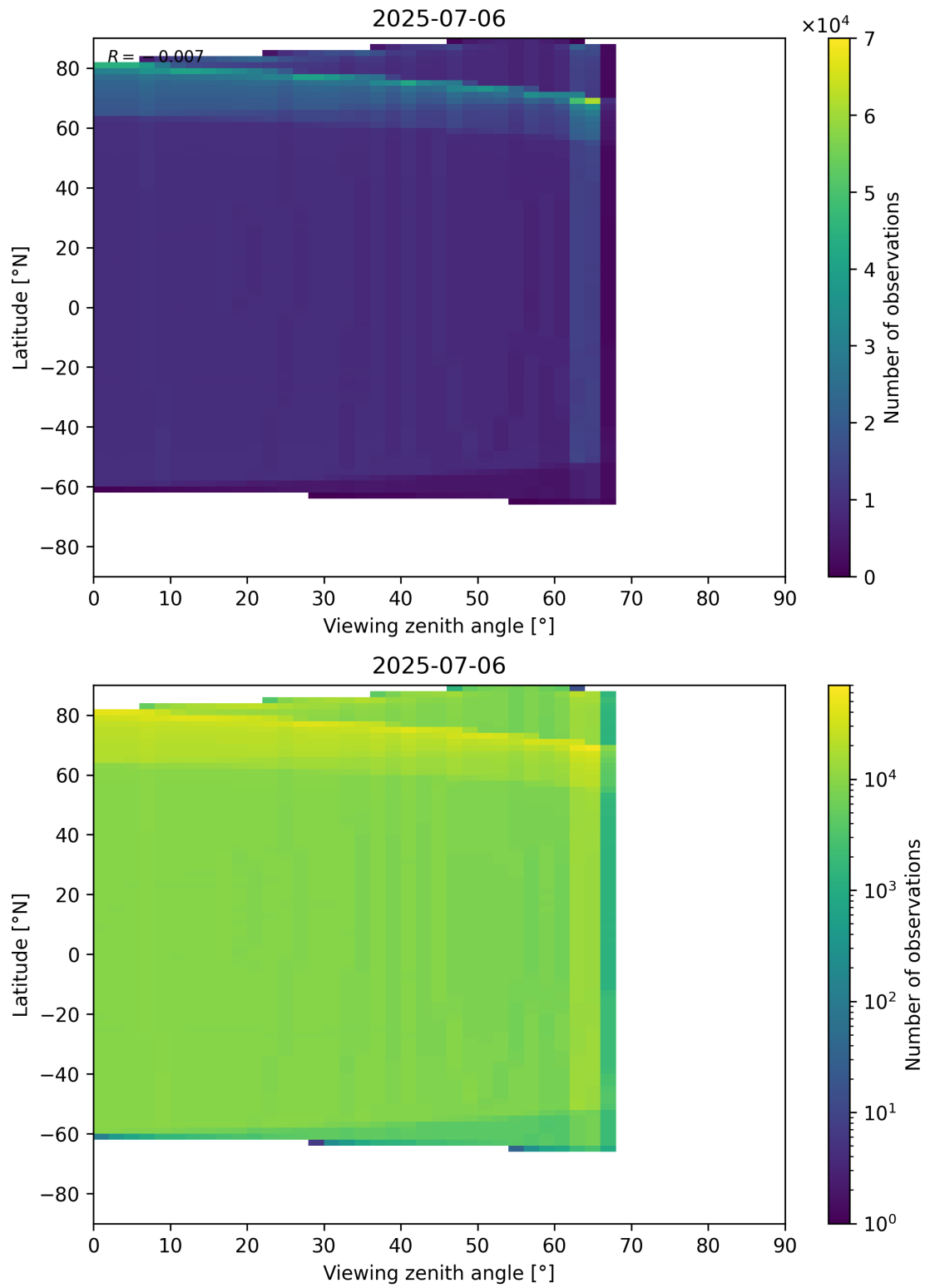
Figure 163: Scatter density plot of “Viewing zenith angle” against “Latitude” for 2025-07-05 to 2025-07-07.
