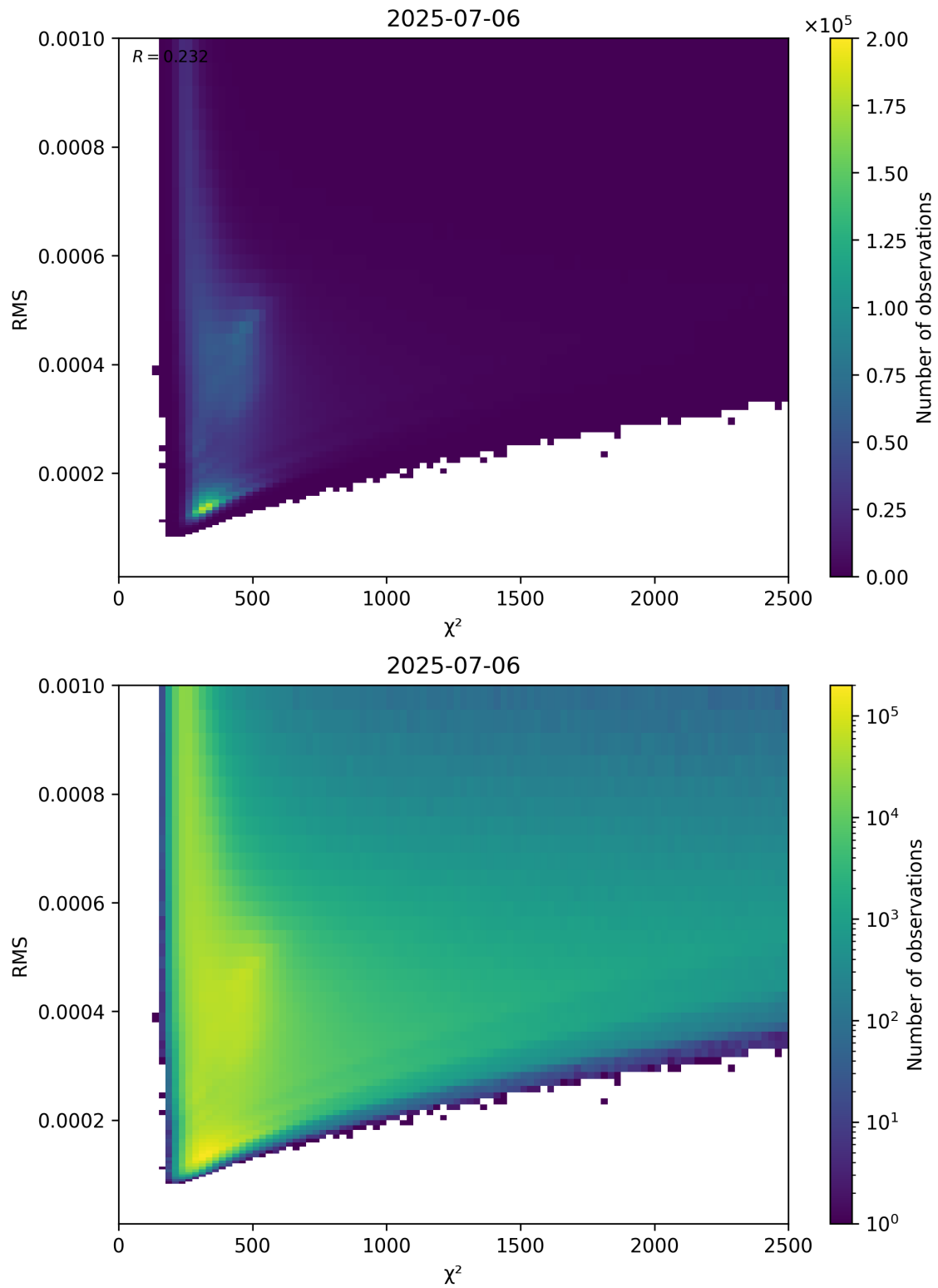
Figure 82: Scatter density plot of “ \chi^2 ” against “RMS” for 2025-07-05 to 2025-07-07.
