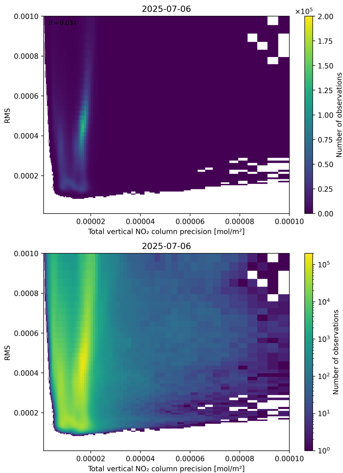
Figure 119: Scatter density plot of “Total vertical NO 2 column precision” against “RMS” for 2025-07-05 to 2025-07-07.
