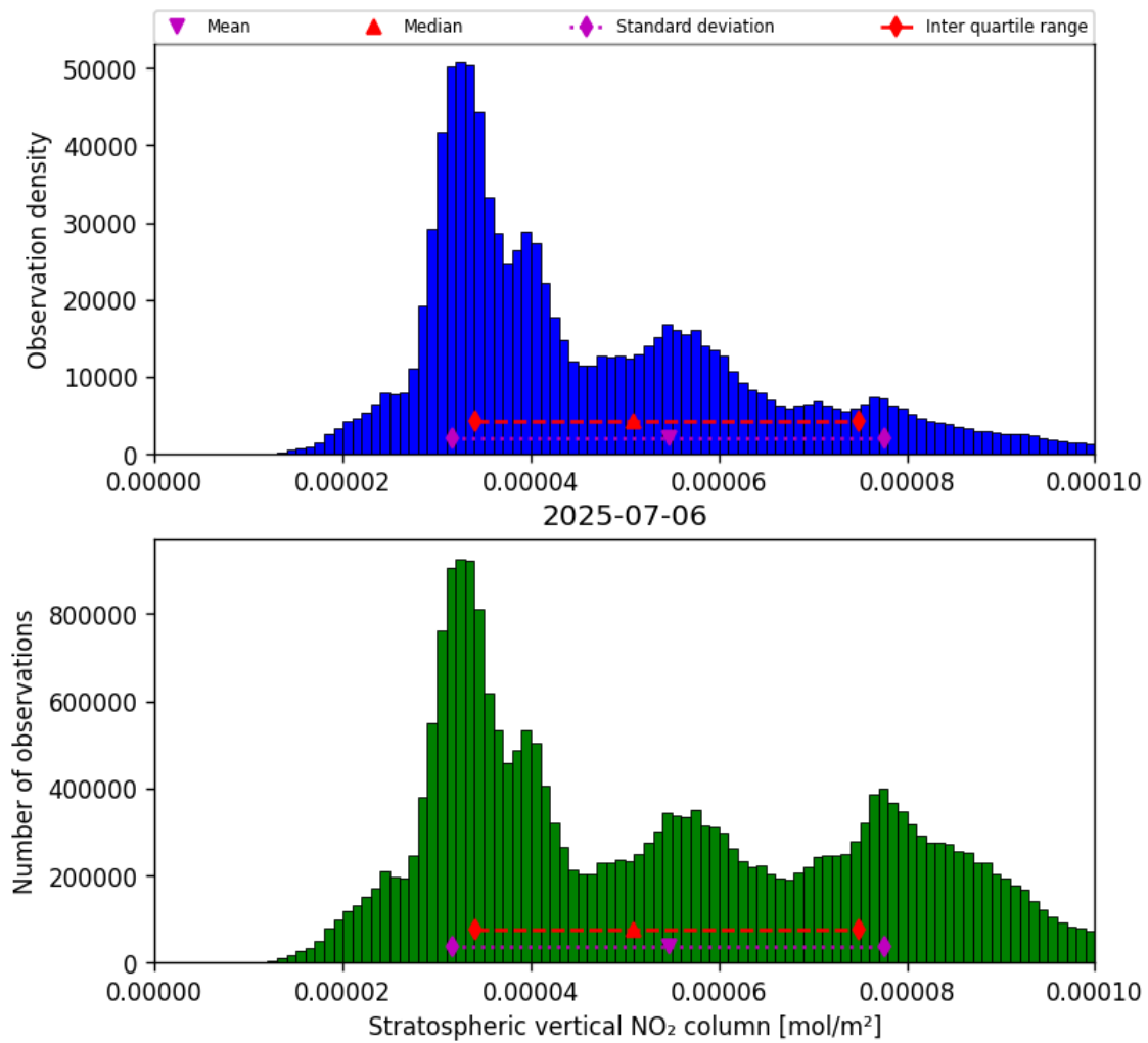
Figure 36: Histogram of “Stratospheric vertical NO 2 column” for 2025-07-05 to 2025-07-07
