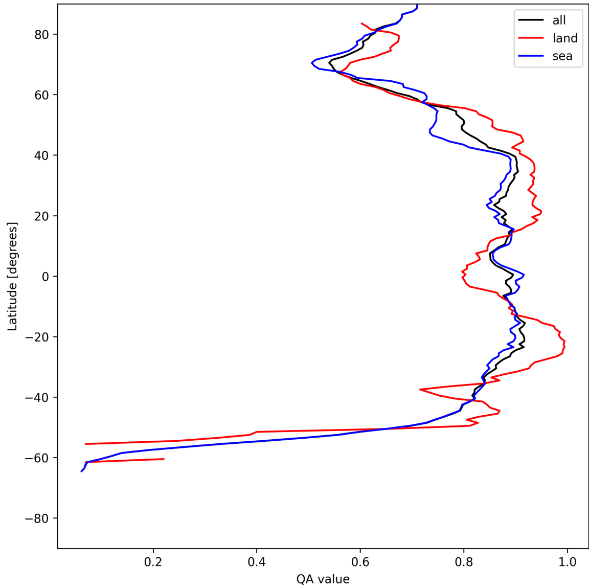
Figure 11: Zonal average of “QA value” for 2025-07-05 to 2025-07-07.
