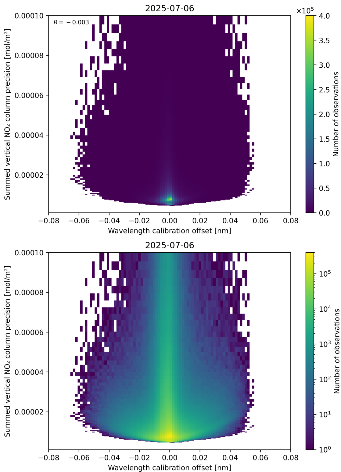
Figure 178: Scatter density plot of “Wavelength calibration offset” against “Summed vertical NO 2 column precision” for 2025-07-05 to 2025-07-07.
