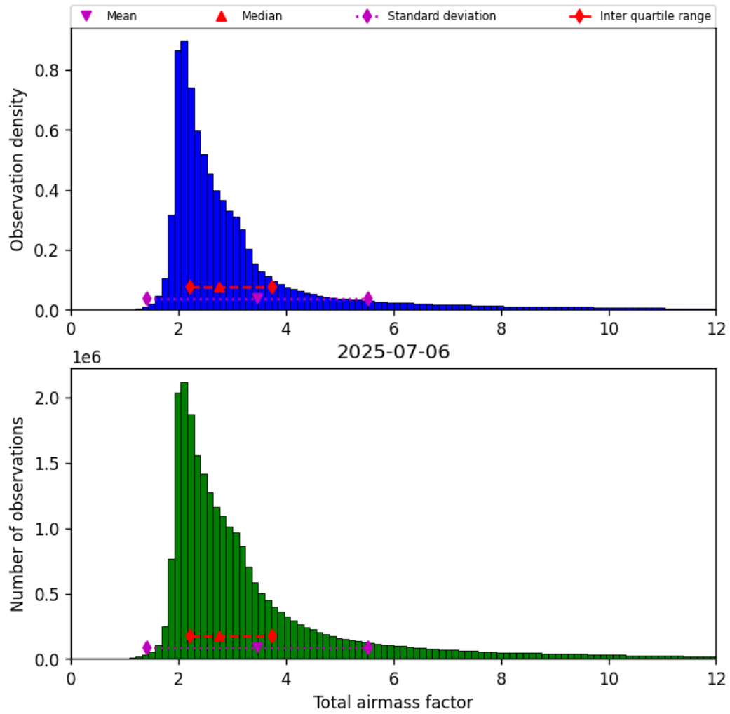
Figure 32: Histogram of “Total airmass factor” for 2025-07-05 to 2025-07-07
