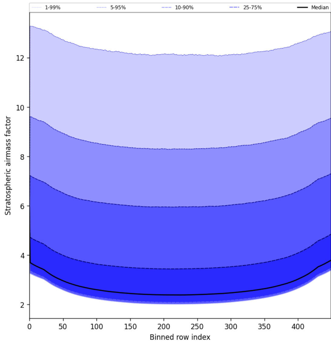
Figure 61: Along track statistics of “Stratospheric airmass factor” for 2025-07-05 to 2025-07-07
