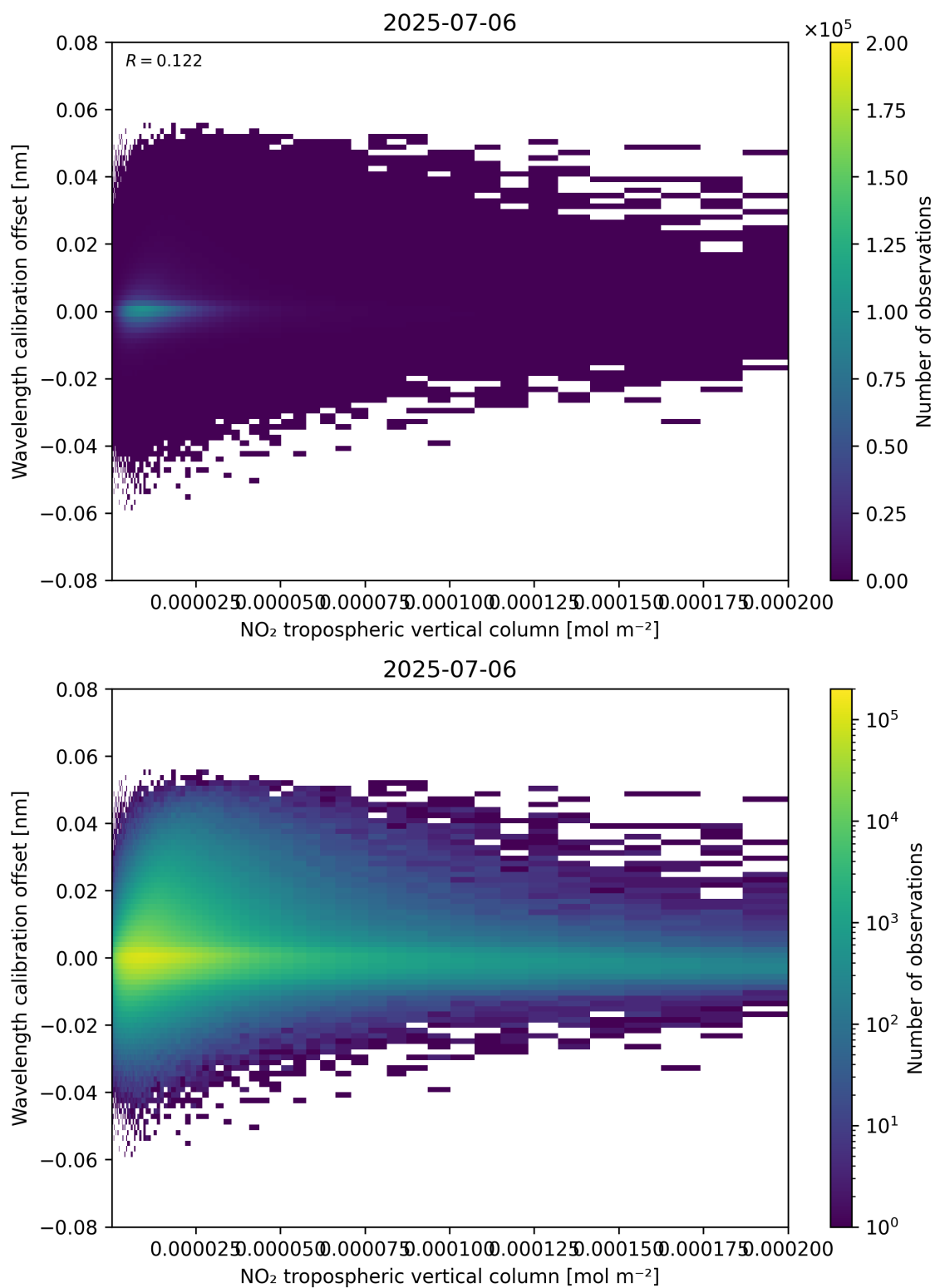
Figure 143: Scatter density plot of “NO 2 tropospheric vertical column” against “Wavelength calibration offset” for 2025-07-05 to 2025-07-07.
