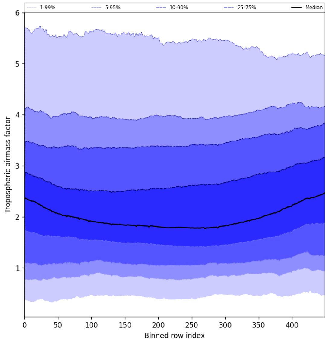
Figure 48: Along track statistics of “Tropospheric airmass factor” for 2025-07-05 to 2025-07-07
