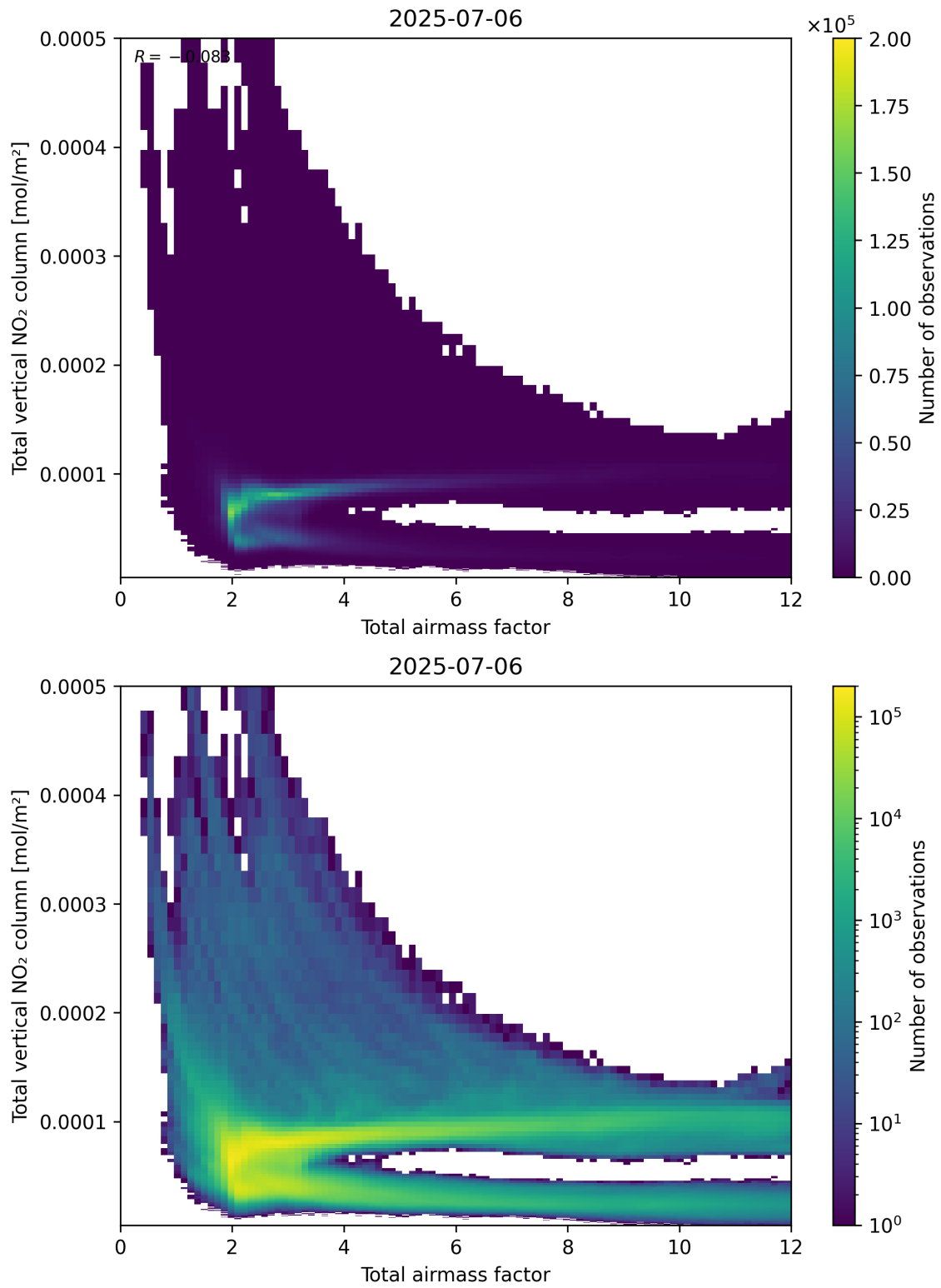
Figure 67: Scatter density plot of “Total airmass factor” against “Total vertical NO 2 column” for 2025-07-05 to 2025-07-07.
