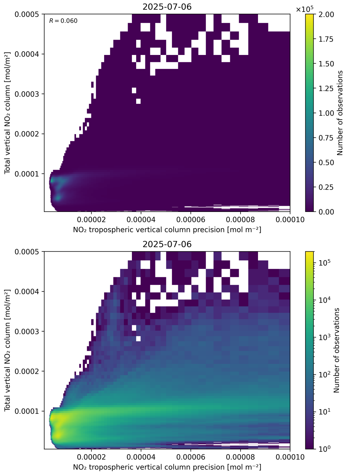
Figure 138: Scatter density plot of “NO 2 tropospheric vertical column precision” against “Total vertical NO 2 column” for 2025-07-05 to 2025-07-07.
