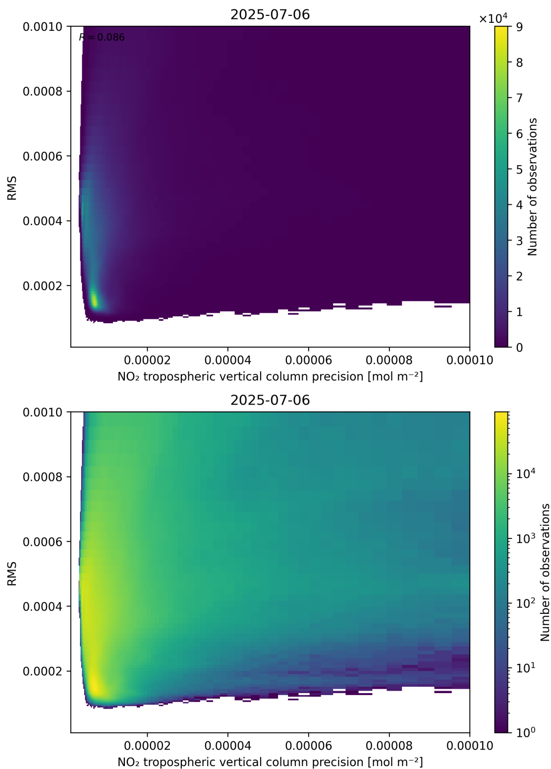
Figure 140: Scatter density plot of “NO 2 tropospheric vertical column precision” against “RMS” for 2025-07-05 to 2025-07-07.
