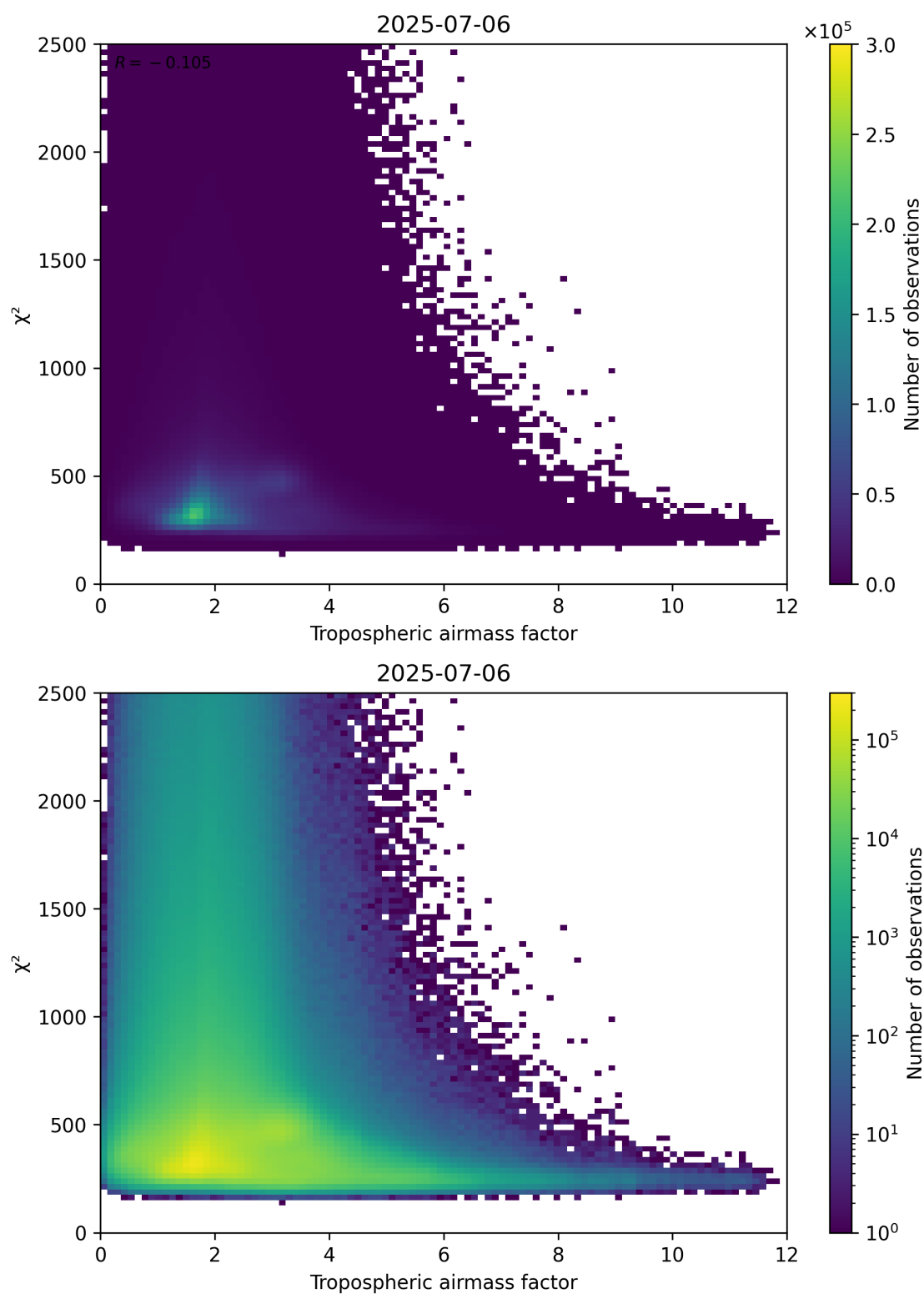
Figure 73: Scatter density plot of “Tropospheric airmass factor” against “ \chi^2 ” for 2025-07-05 to 2025-07-07.
