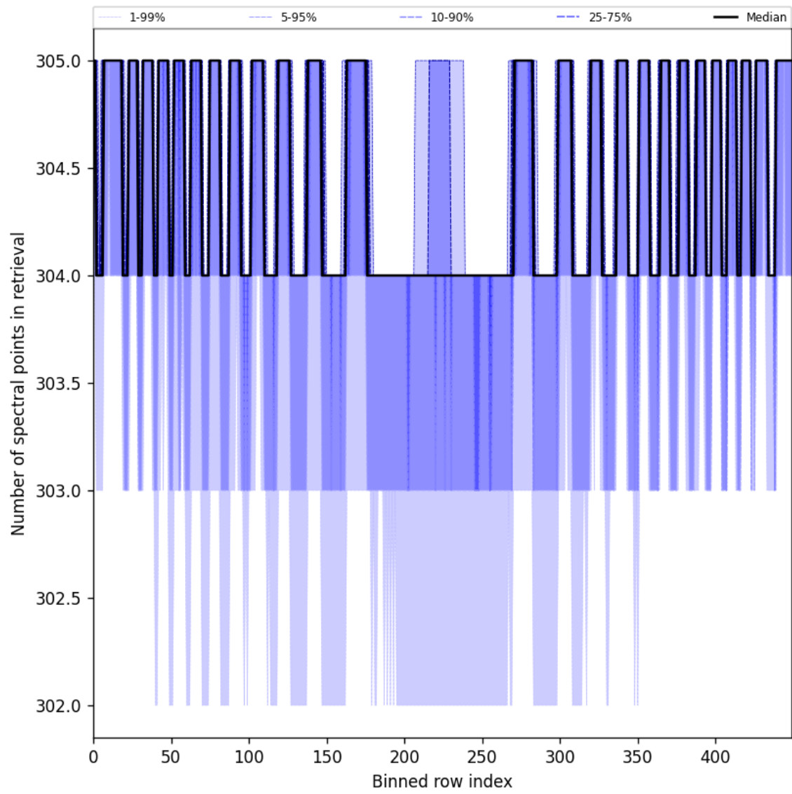
Figure 50: Along track statistics of “Number of spectral points in retrieval” for 2025-07-05 to 2025-07-07
