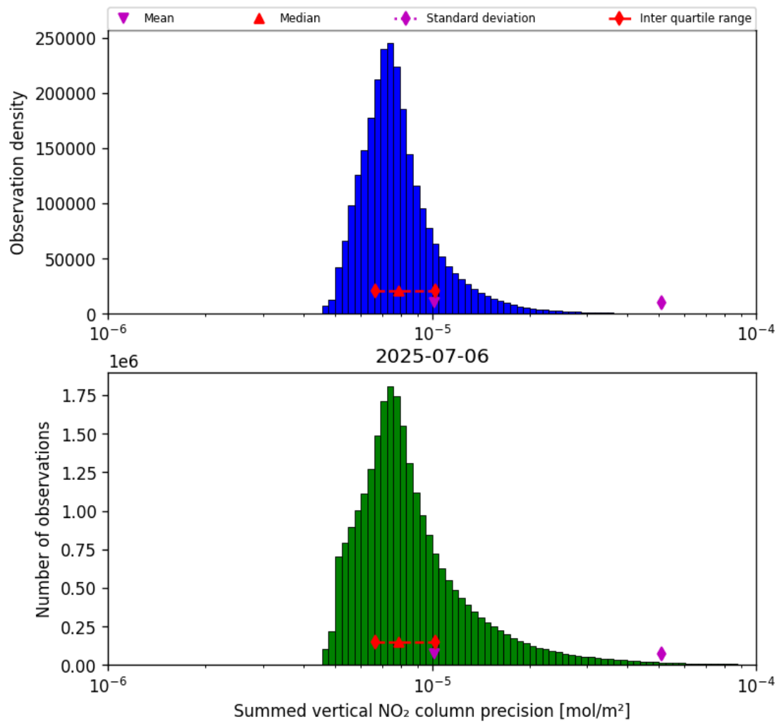
Figure 41: Histogram of "Summed vertical NO 2 column precision" for 2025-07-05 to 2025-07-07
