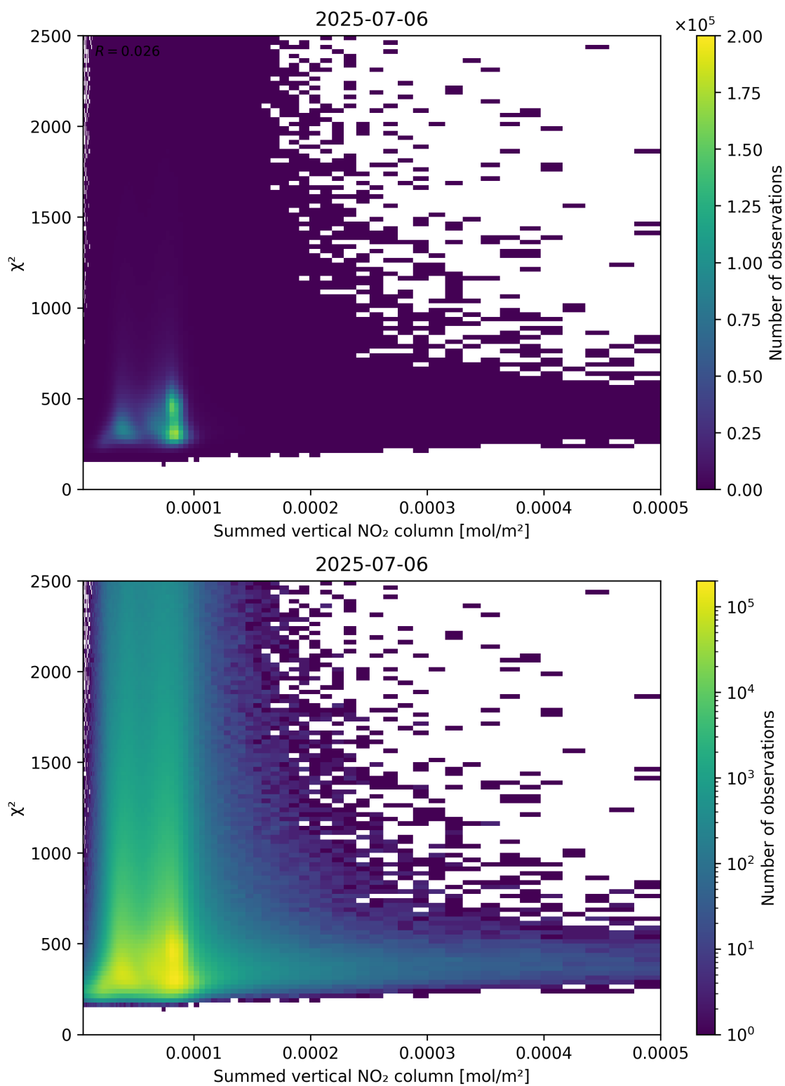
Figure 104: Scatter density plot of “Summed vertical NO 2 column” against “ \chi^2 ” for 2025-07-05 to 2025-07-07.
