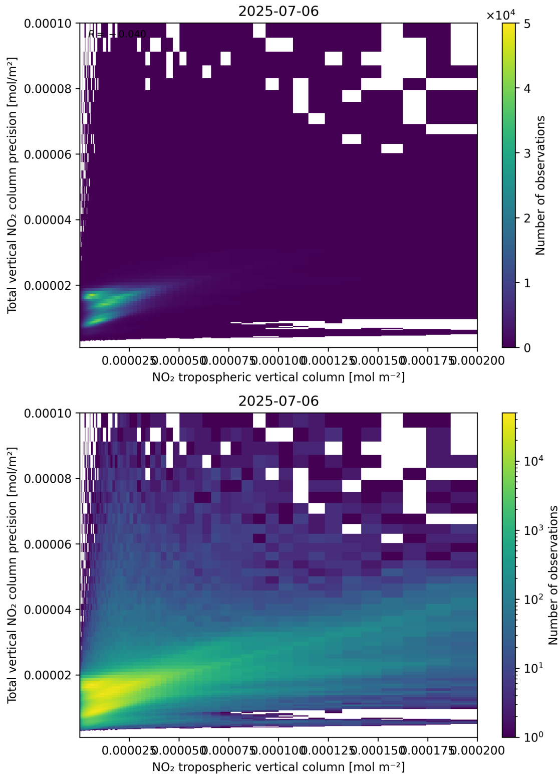
Figure 129: Scatter density plot of “NO 2 tropospheric vertical column” against “Total vertical NO 2 column precision” for 2025-07-05 to 2025-07-07.
