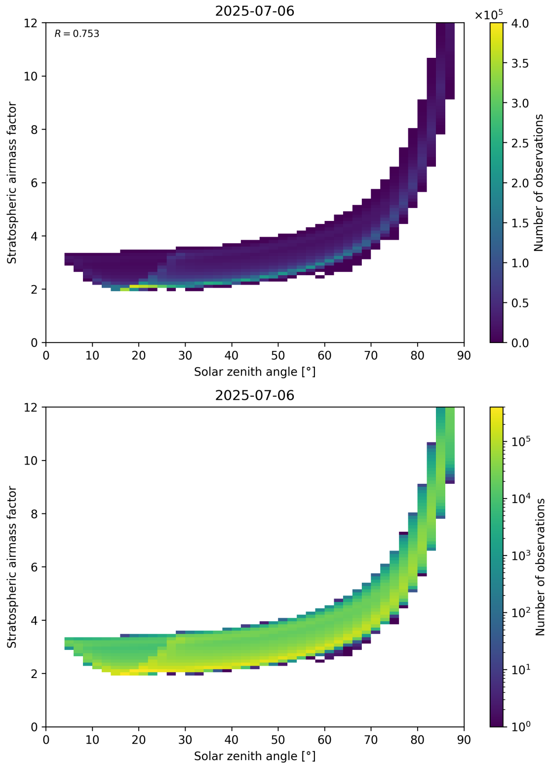
Figure 145: Scatter density plot of “Solar zenith angle” against “Stratospheric airmass factor” for 2025-07-05 to 2025-07-07.
