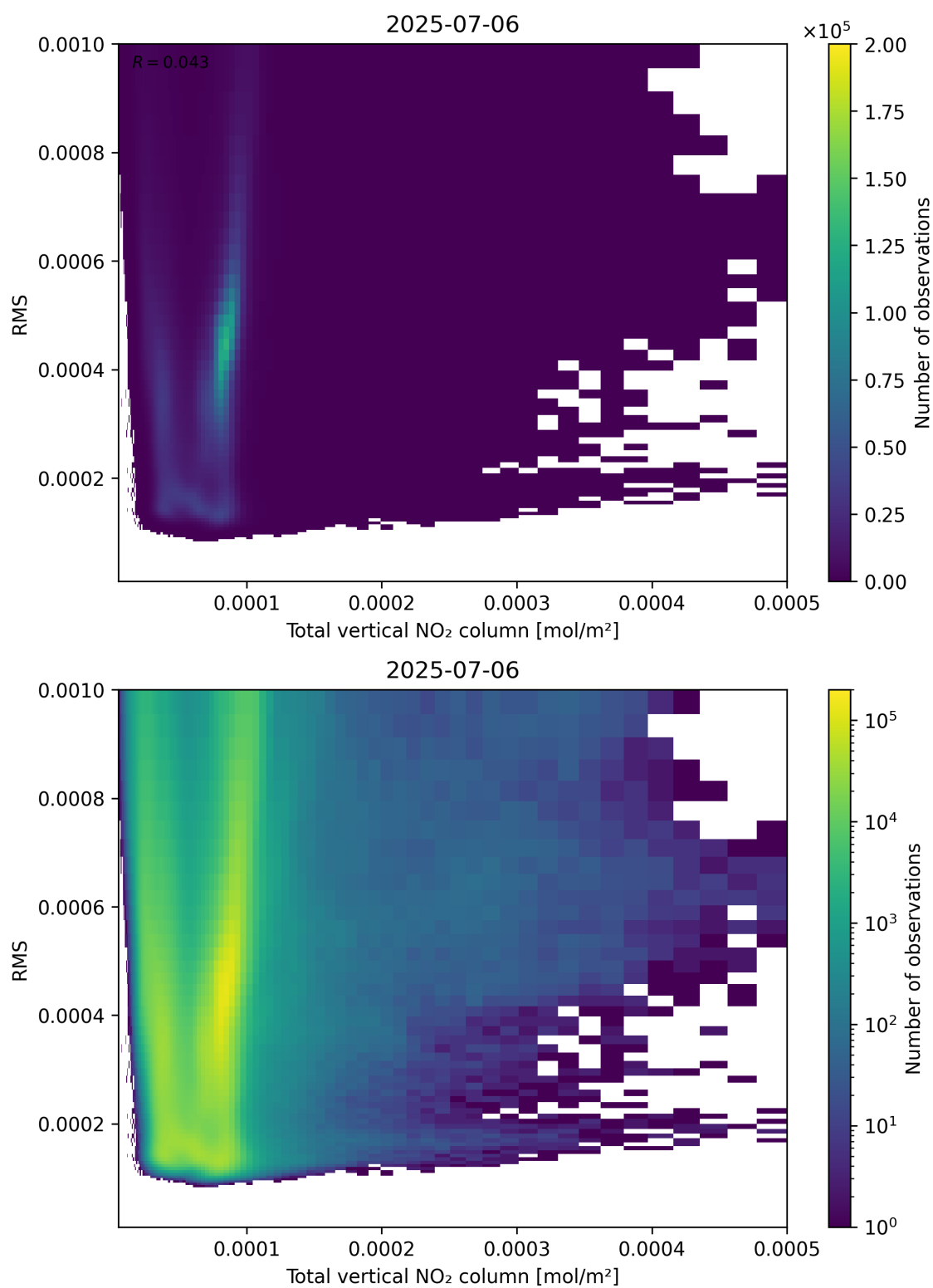
Figure 120: Scatter density plot of “Total vertical NO 2 column” against “RMS” for 2025-07-05 to 2025-07-07.
