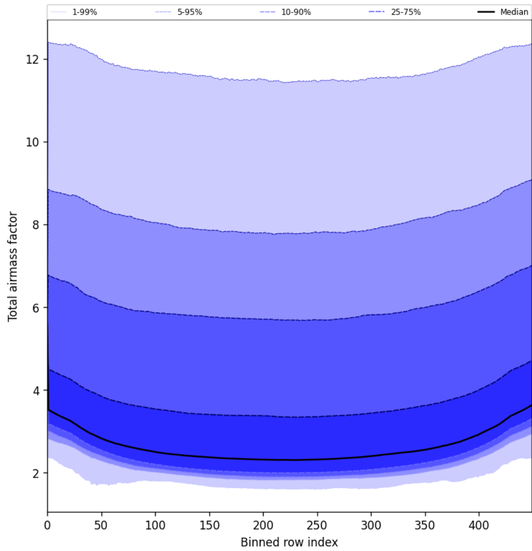
Figure 49: Along track statistics of “Total airmass factor” for 2025-07-05 to 2025-07-07
