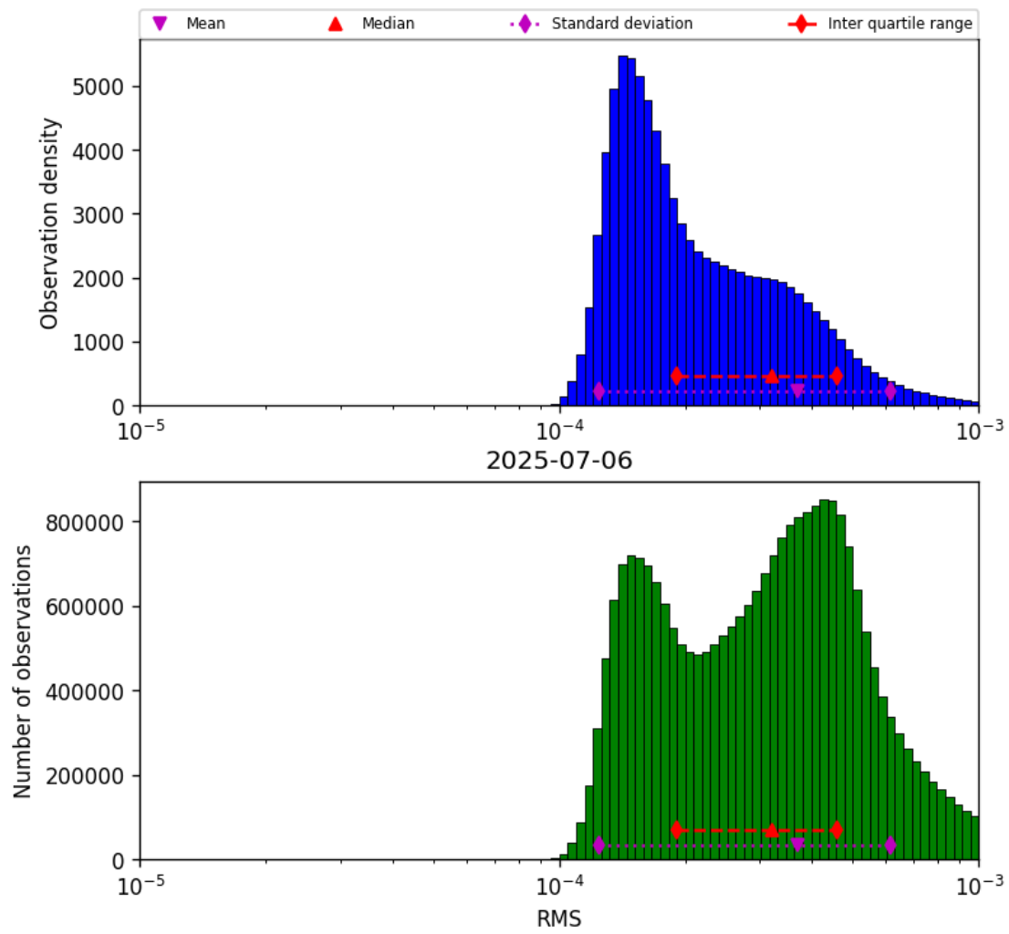
Figure 43: Histogram of “RMS” for 2025-07-05 to 2025-07-07
