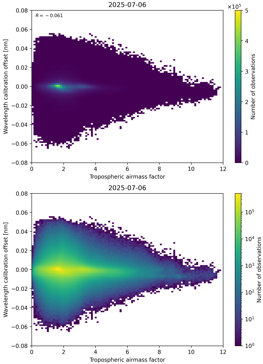
Figure 80: Scatter density plot of “Tropospheric airmass factor” against “Wavelength calibration offset” for 2025-07-05 to 2025-07-07.
