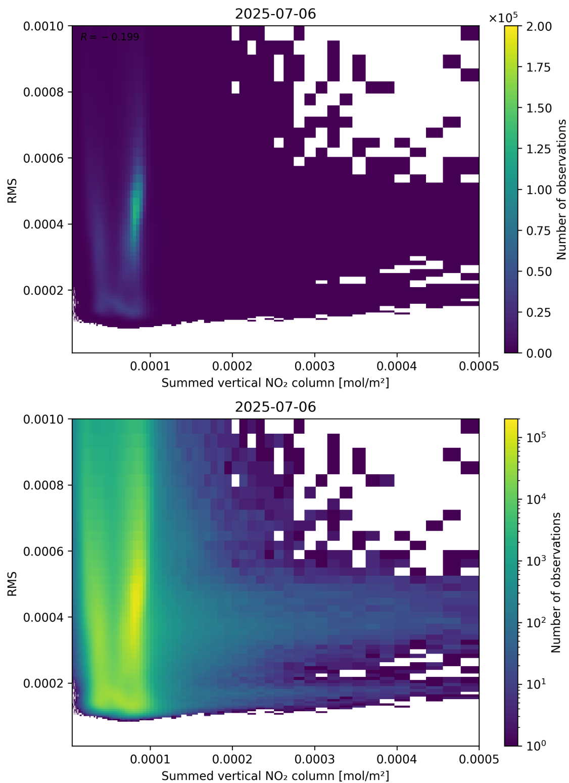
Figure 109: Scatter density plot of “Summed vertical NO 2 column” against “RMS” for 2025-07-05 to 2025-07-07.
