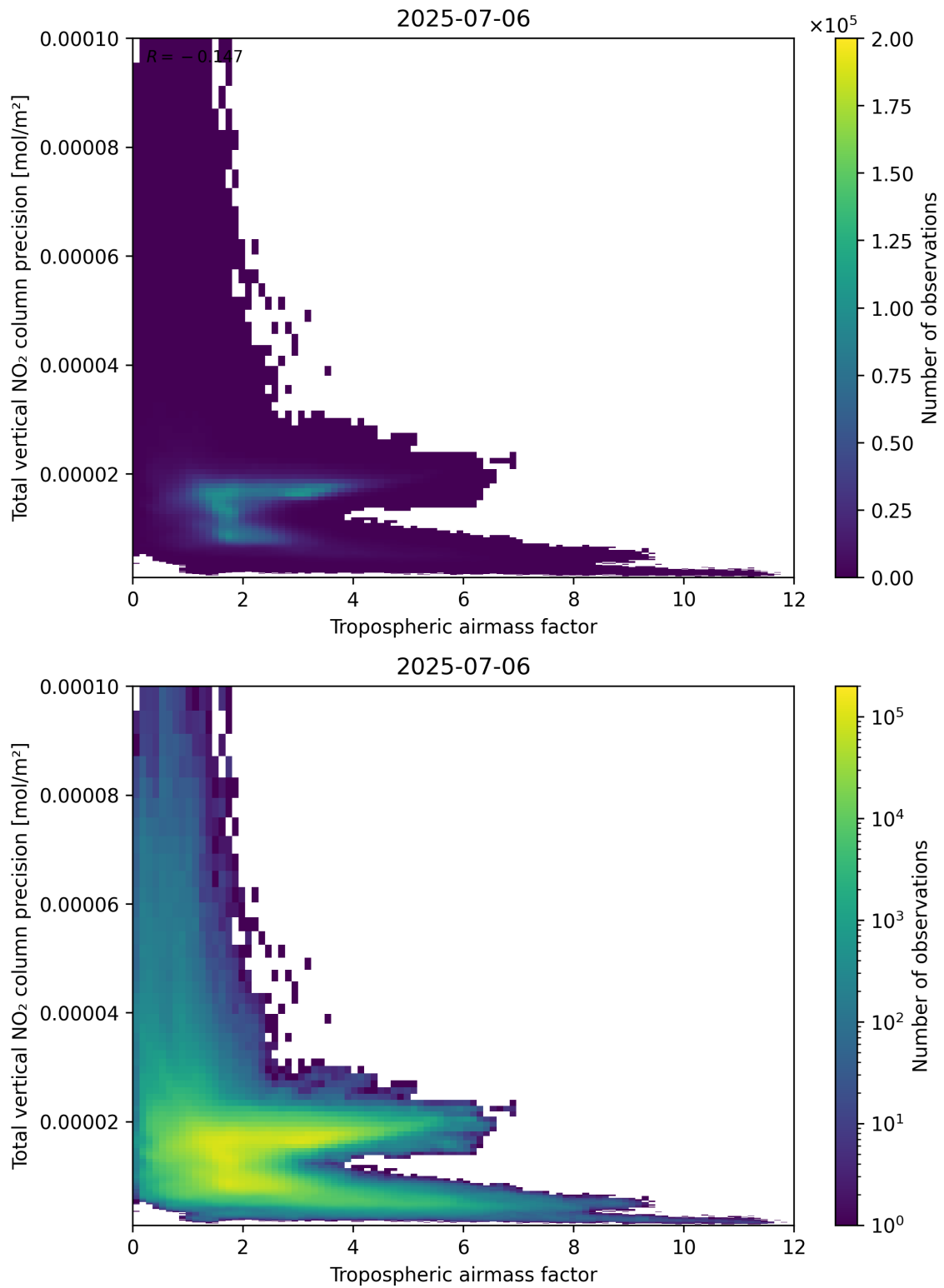
Figure 78: Scatter density plot of “Tropospheric airmass factor” against “Total vertical NO 2 column precision” for 2025-07-05 to 2025-07-07.
