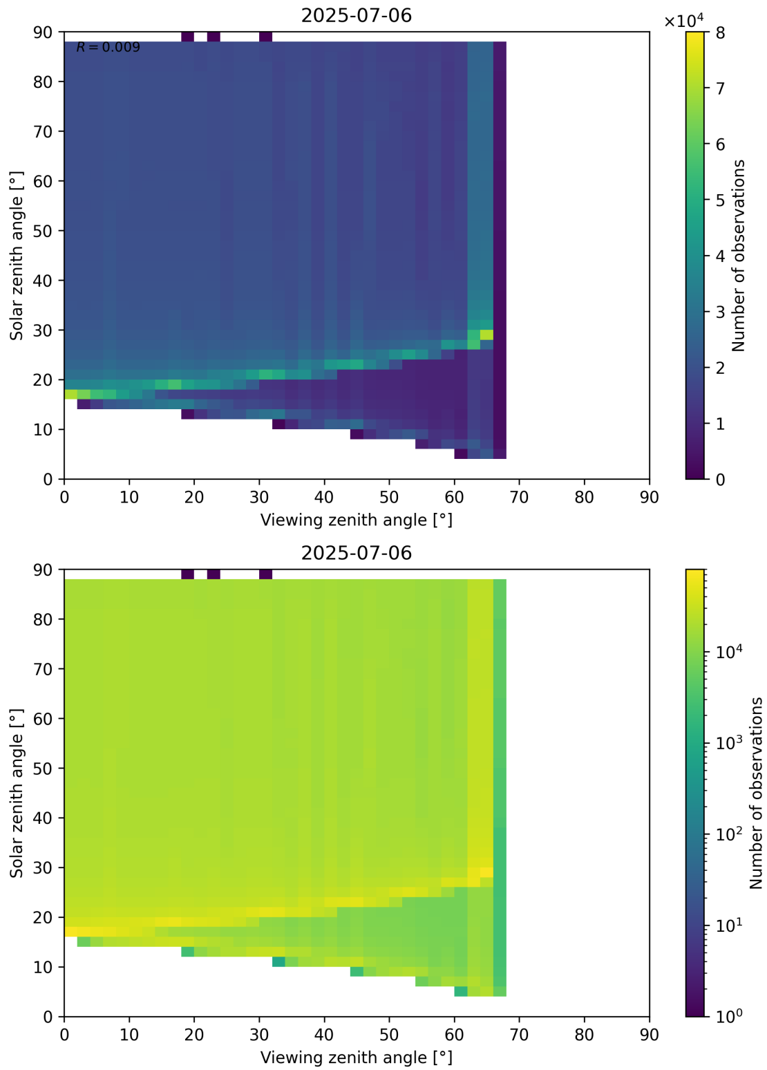
Figure 172: Scatter density plot of “Viewing zenith angle” against “Solar zenith angle” for 2025-07-05 to 2025-07-07.
