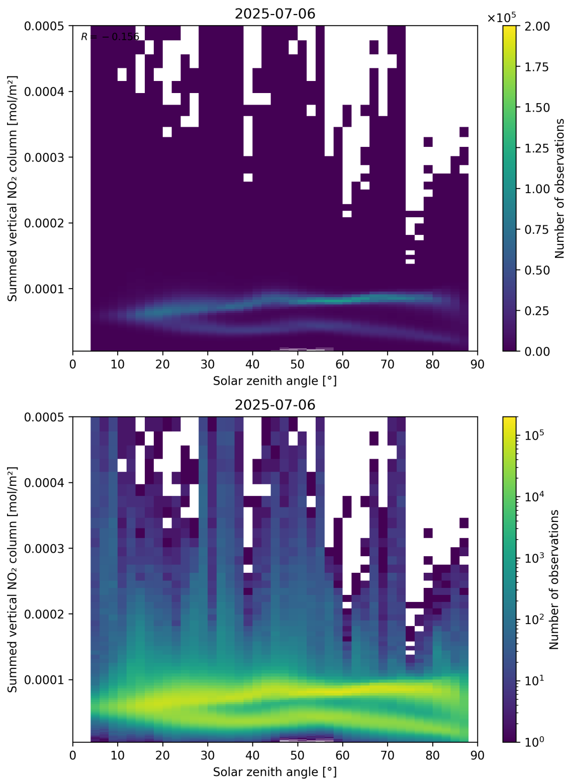
Figure 151: Scatter density plot of “Solar zenith angle” against “Summed vertical NO 2 column” for 2025-07-05 to 2025-07-07.
