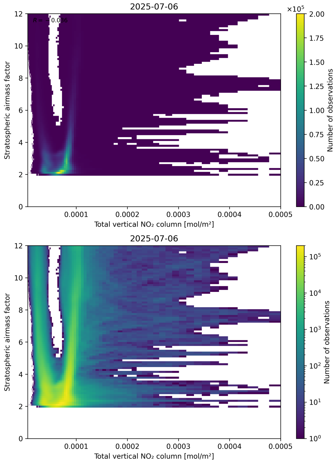
Figure 110: Scatter density plot of “Total vertical NO 2 column” against “Stratospheric airmass factor” for 2025-07-05 to 2025-07-07.
