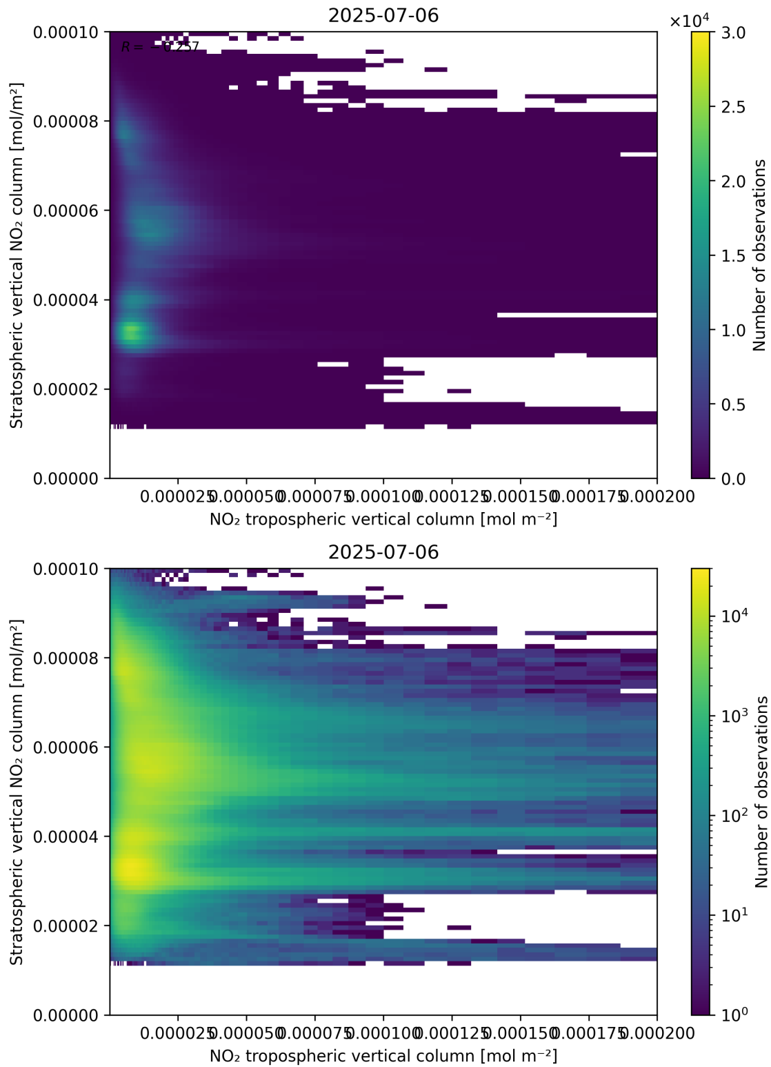
Figure 125: Scatter density plot of “NO 2 tropospheric vertical column” against “Stratospheric vertical NO 2 column” for 2025-07-05 to 2025-07-07.
