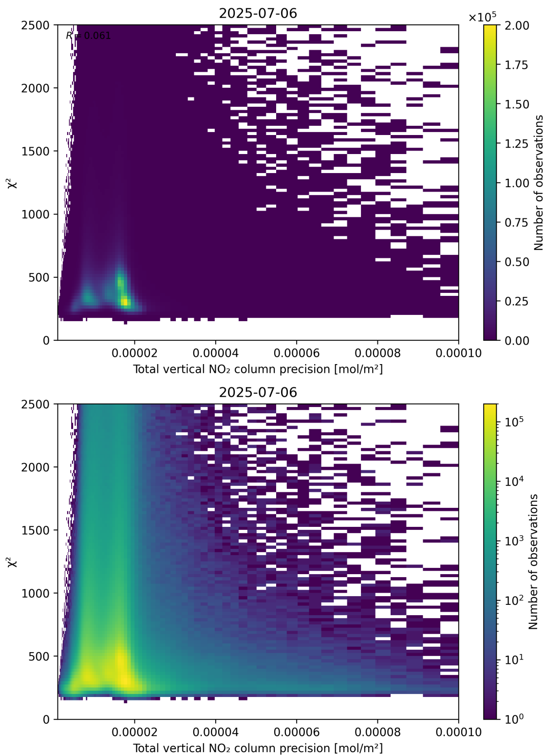
Figure 116: Scatter density plot of “Total vertical NO 2 column precision” against “ \chi^2 ” for 2025-07-05 to 2025-07-07.
