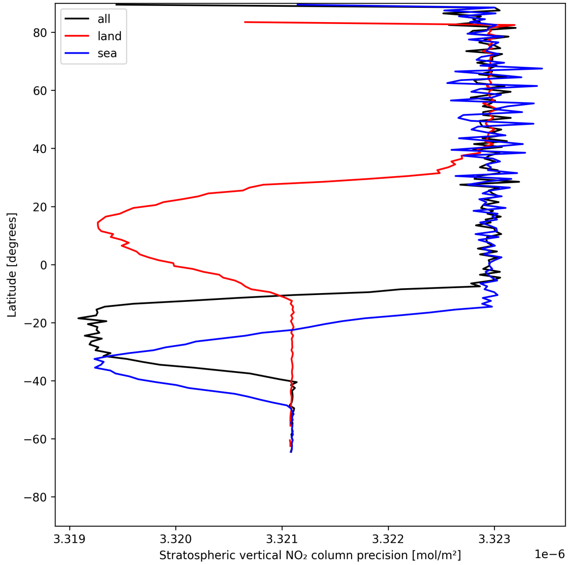
Figure 20: Zonal average of “Stratospheric vertical NO 2 column precision” for 2025-07-05 to 2025-07-07.
