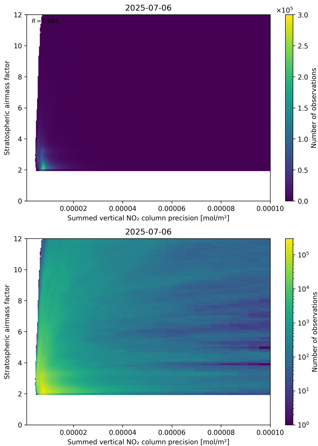
Figure 106: Scatter density plot of “Summed vertical NO 2 column precision” against “Stratospheric airmass factor” for 2025-07-05 to 2025-07-07.
