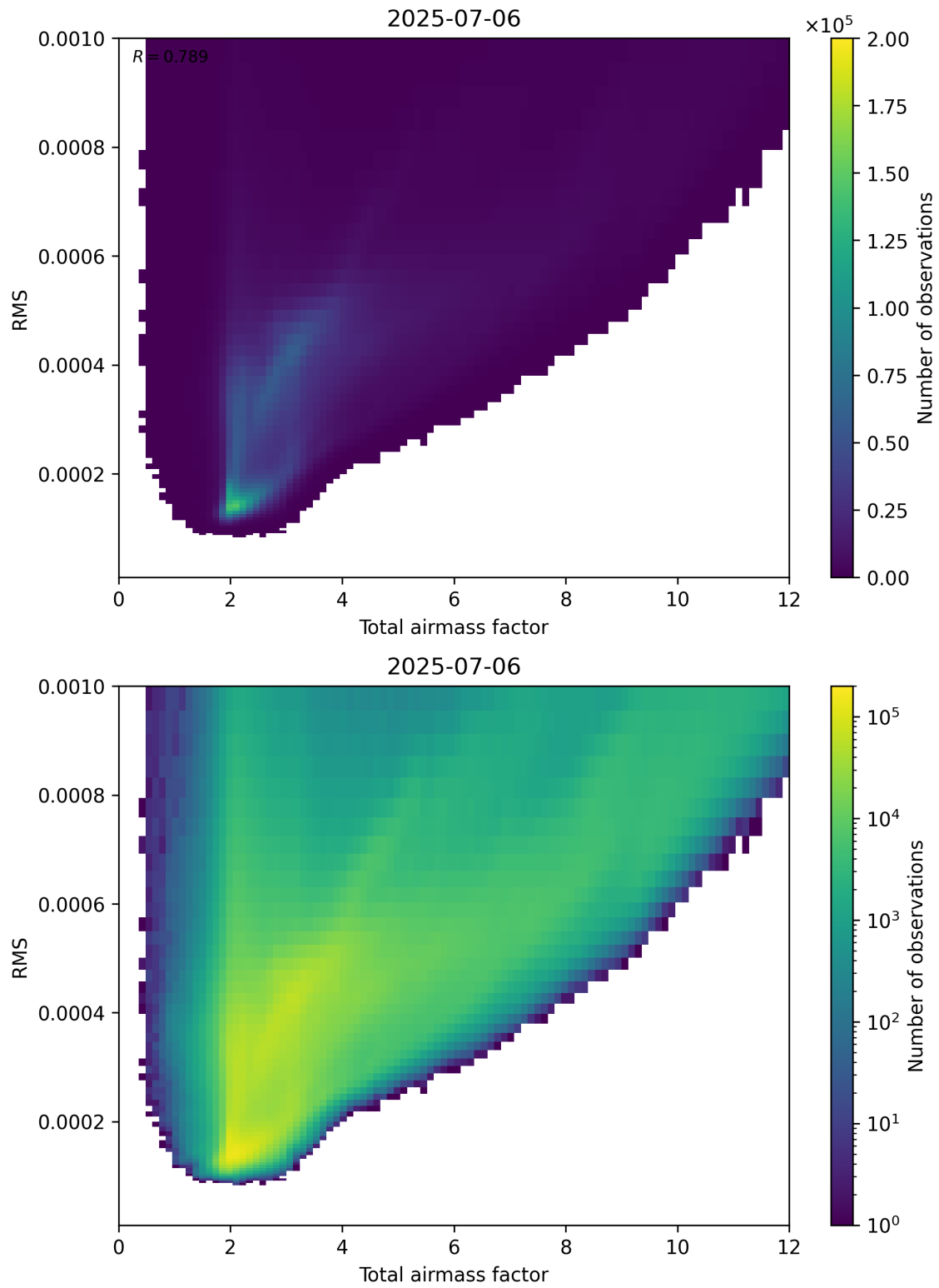
Figure 69: Scatter density plot of “Total airmass factor” against “RMS” for 2025-07-05 to 2025-07-07.
