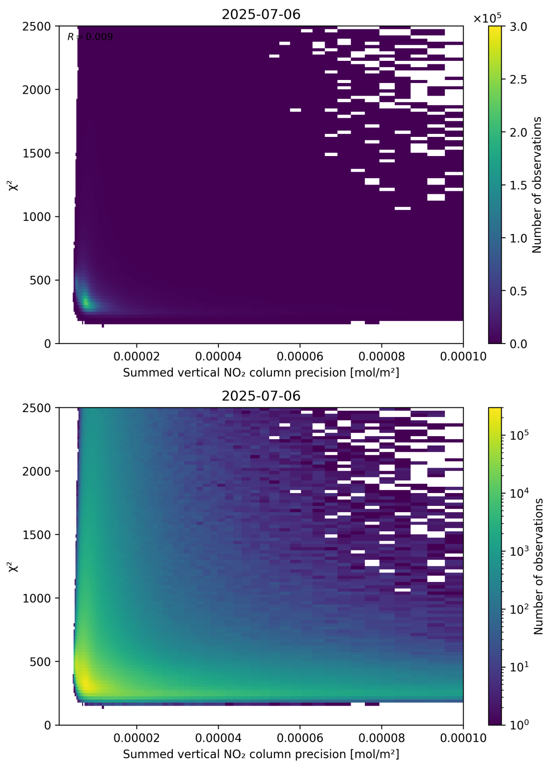
Figure 107: Scatter density plot of “Summed vertical NO 2 column precision” against “ \chi^2 ” for 2025-07-05 to 2025-07-07.
