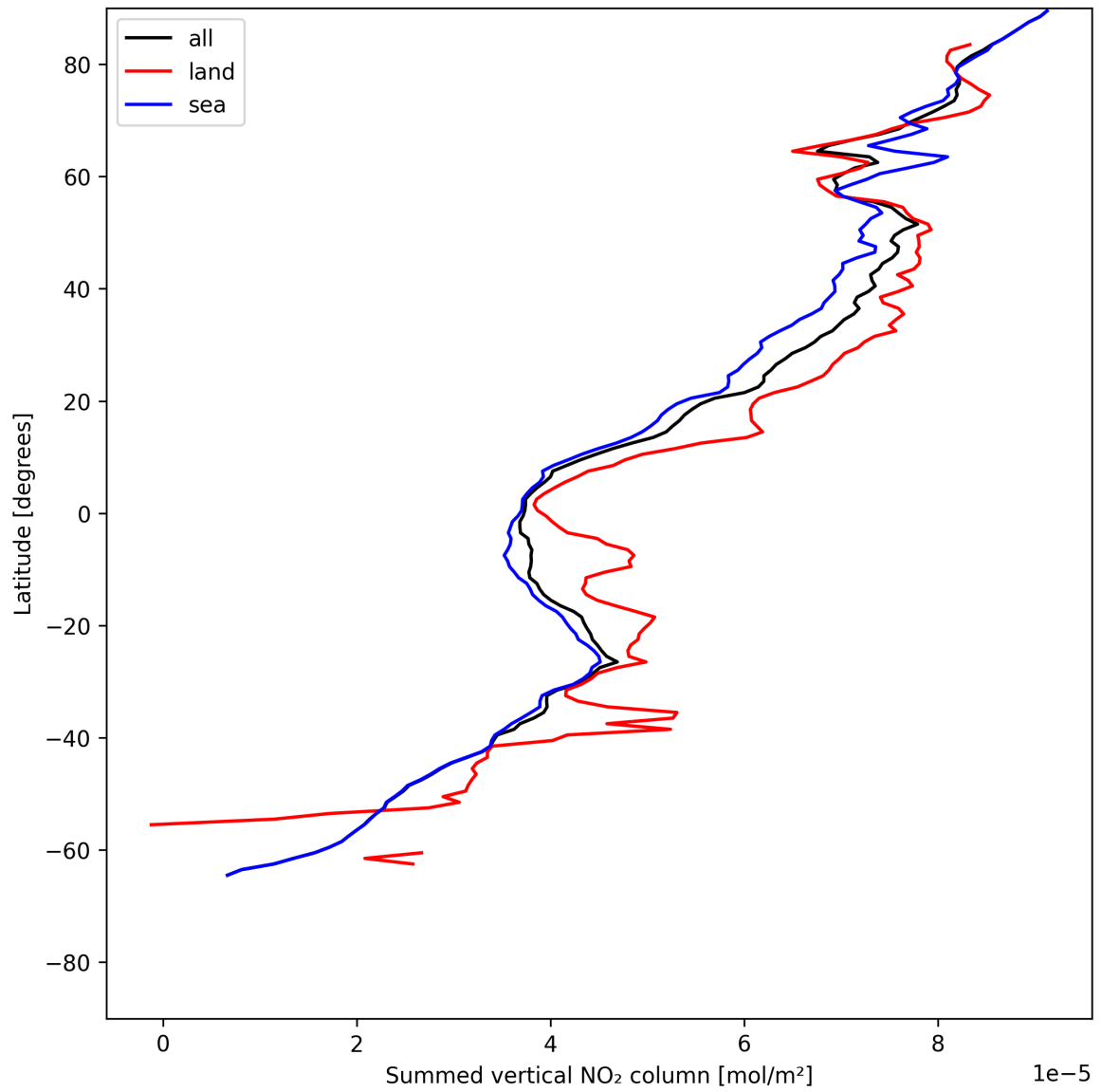
Figure 23: Zonal average of “Summed vertical NO 2 column” for 2025-07-05 to 2025-07-07.
