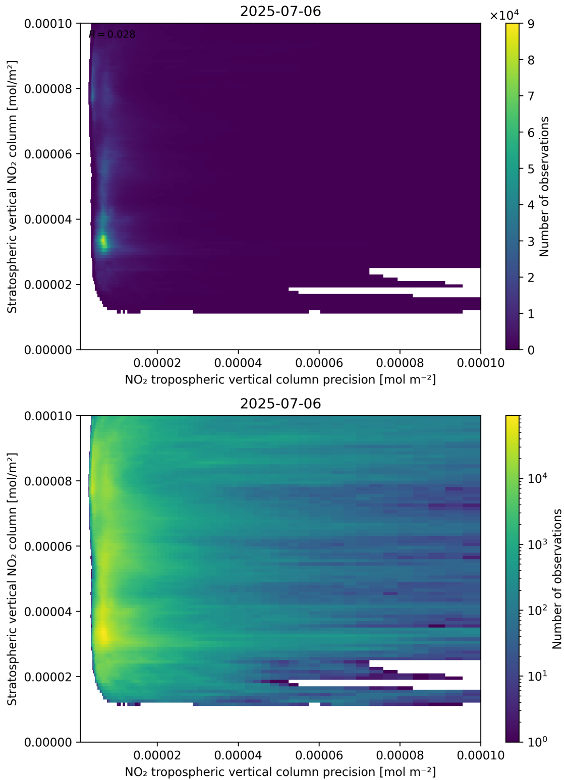
Figure 135: Scatter density plot of “NO 2 tropospheric vertical column precision” against “Stratospheric vertical NO 2 column” for 2025-07-05 to 2025-07-07.
