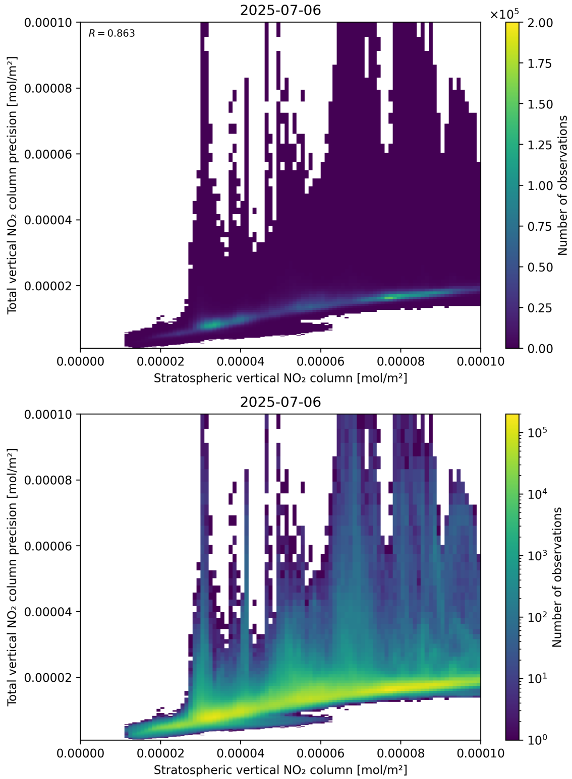
Figure 101: Scatter density plot of “Stratospheric vertical NO 2 column” against “Total vertical NO 2 column precision” for 2025-07-05 to 2025-07-07.
