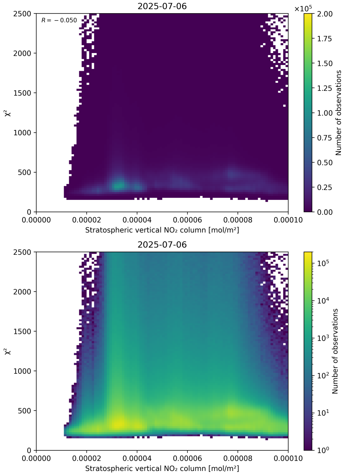
Figure 97: Scatter density plot of “Stratospheric vertical NO 2 column” against “ \chi^2 ” for 2025-07-05 to 2025-07-07.
