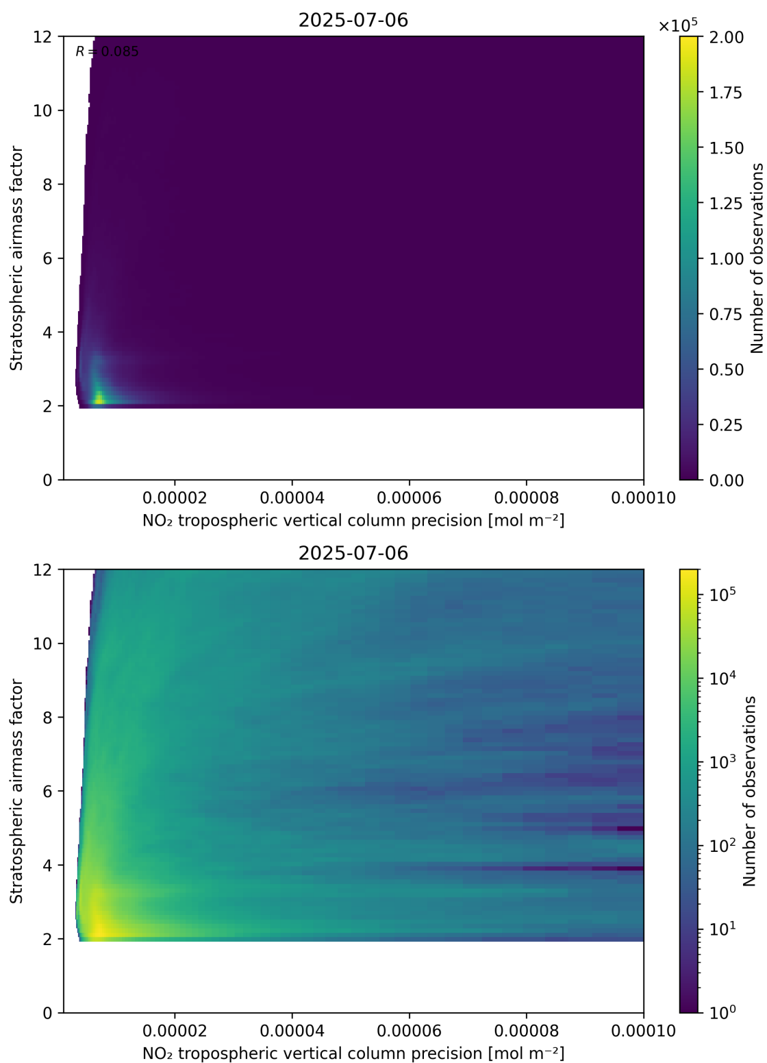
Figure 131: Scatter density plot of “NO 2 tropospheric vertical column precision” against “Stratospheric airmass factor” for 2025-07-05 to 2025-07-07.
