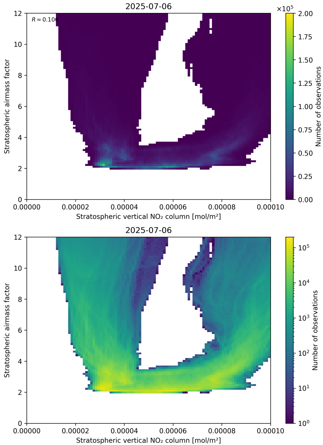
Figure 96: Scatter density plot of “Stratospheric vertical NO 2 column” against “Stratospheric airmass factor” for 2025-07-05 to 2025-07-07.
