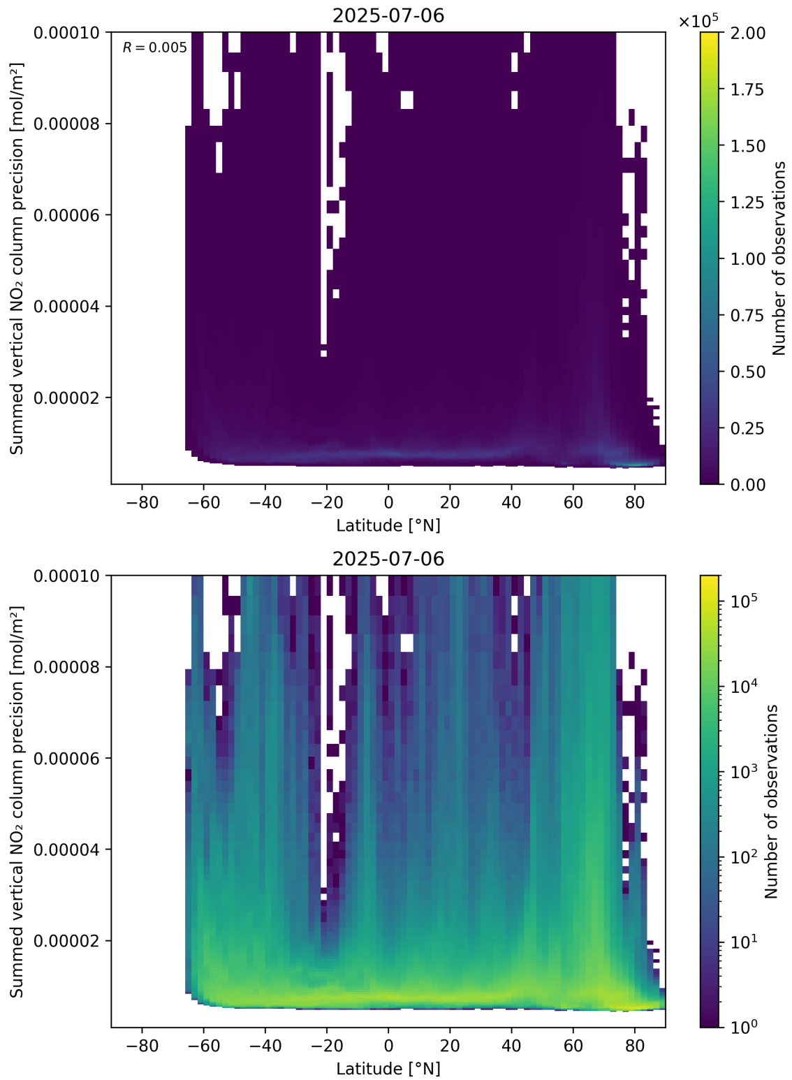
Figure 89: Scatter density plot of “Latitude” against “Summed vertical NO 2 column precision” for 2025-07-05 to 2025-07-07.
