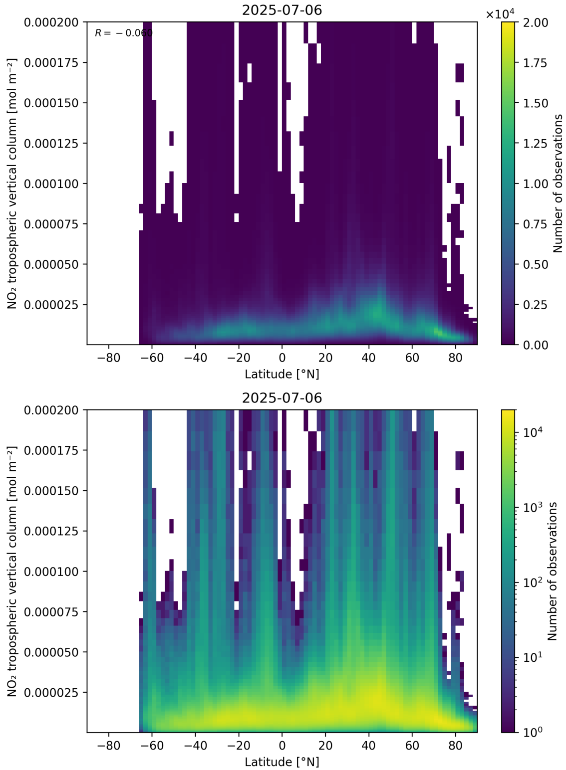
Figure 92: Scatter density plot of “Latitude” against “NO 2 tropospheric vertical column” for 2025-07-05 to 2025-07-07.
