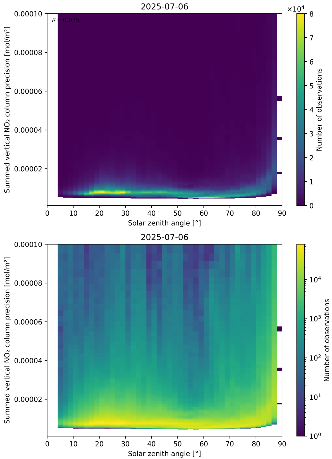
Figure 152: Scatter density plot of “Solar zenith angle” against “Summed vertical NO 2 column precision” for 2025-07-05 to 2025-07-07.
