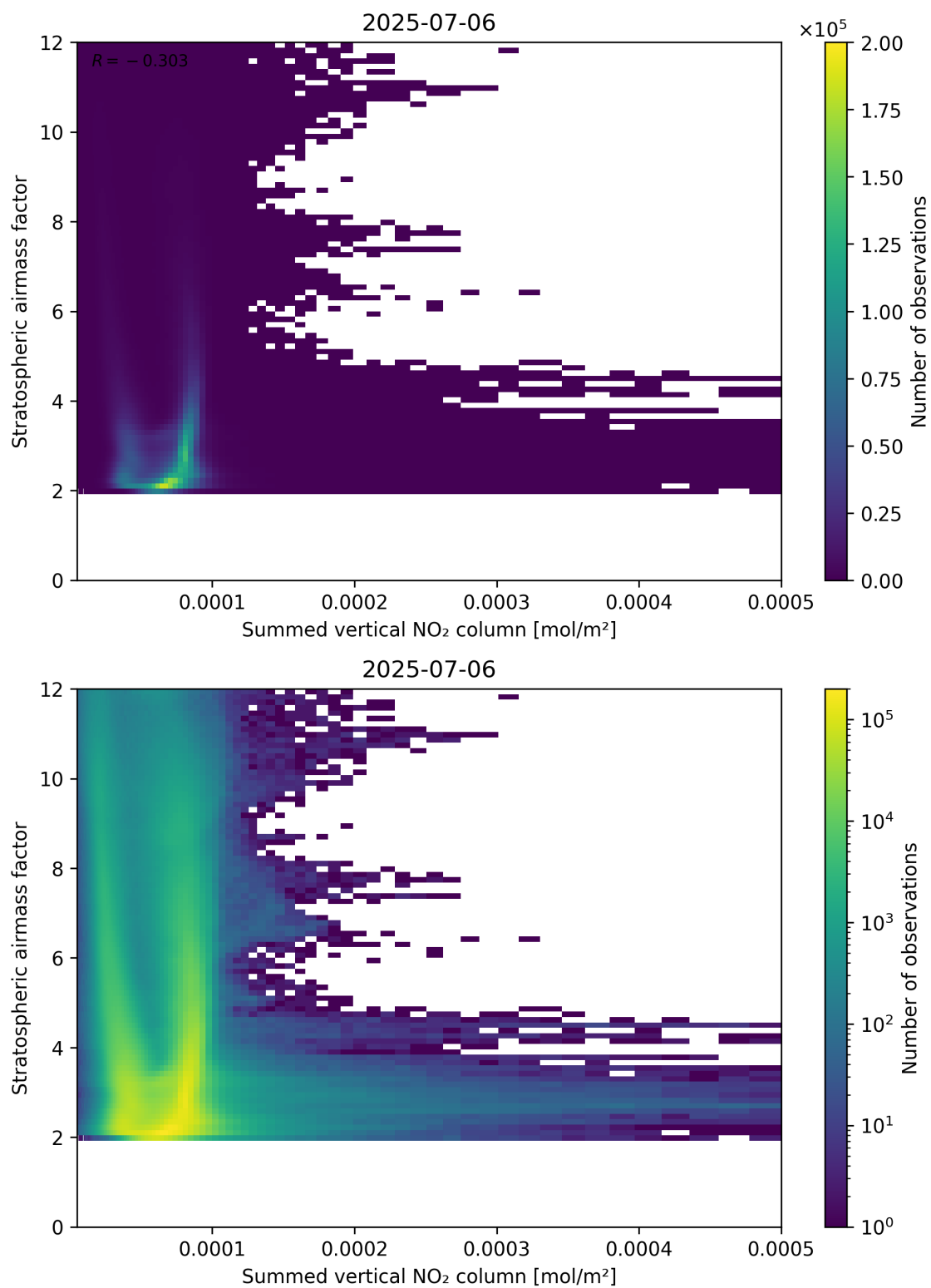
Figure 103: Scatter density plot of “Summed vertical NO 2 column” against “Stratospheric air mass factor” for 2025-07-05 to 2025-07-07.
