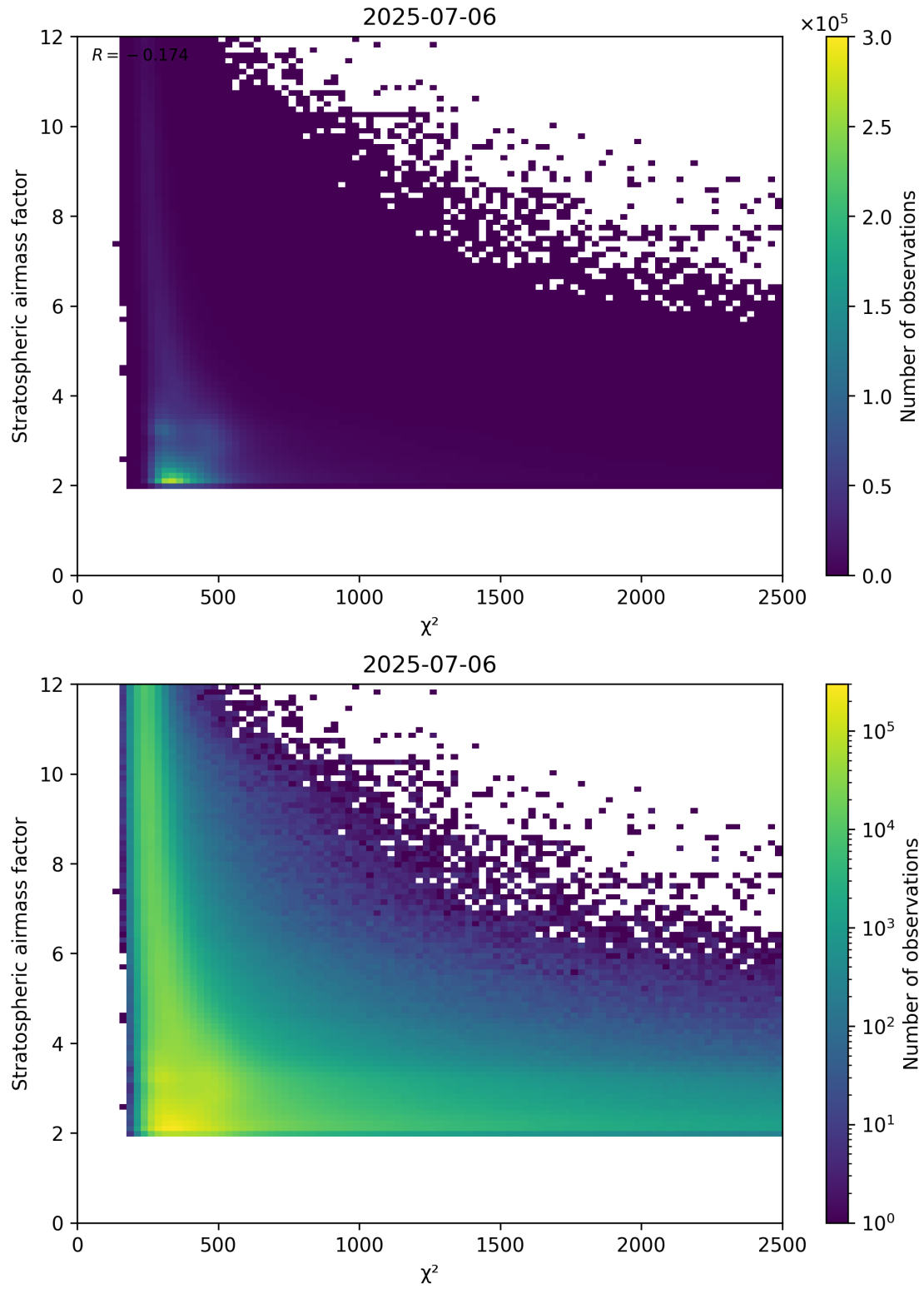
Figure 81: Scatter density plot of “ \chi^2 ” against “Stratospheric airmass factor” for 2025-07-05 to 2025-07-07.
