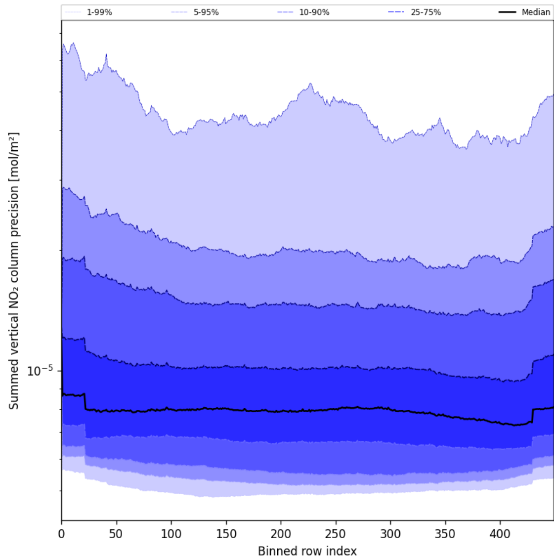
Figure 58: Along track statistics of “Summed vertical NO 2 column precision” for 2025-07-05 to 2025-07-07
