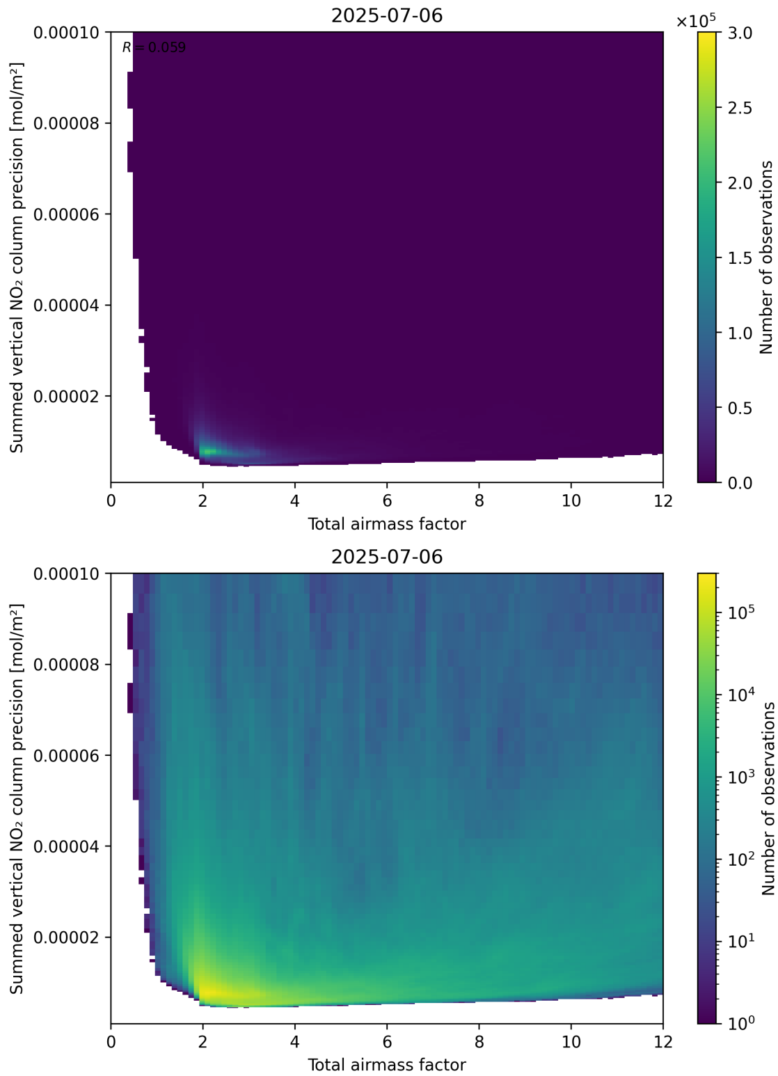
Figure 66: Scatter density plot of “Total airmass factor” against “Summed vertical NO 2 column precision” for 2025-07-05 to 2025-07-07.
