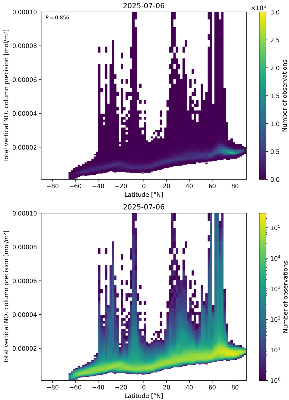
Figure 91: Scatter density plot of “Latitude” against “Total vertical NO 2 column precision” for 2025-07-05 to 2025-07-07.
