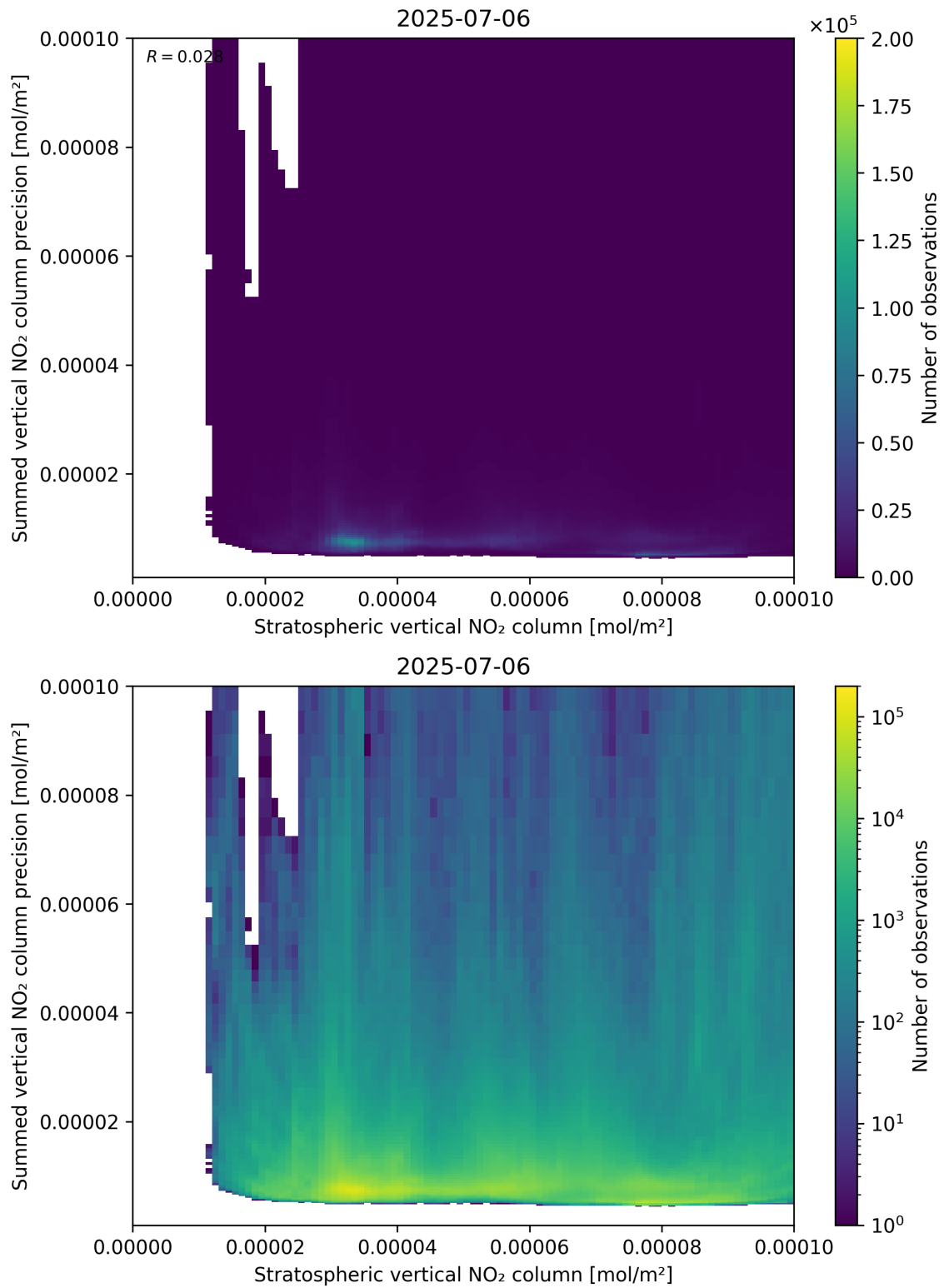
Figure 99: Scatter density plot of “Stratospheric vertical NO 2 column” against “Summed vertical NO 2 column precision” for 2025-07-05 to 2025-07-07.
