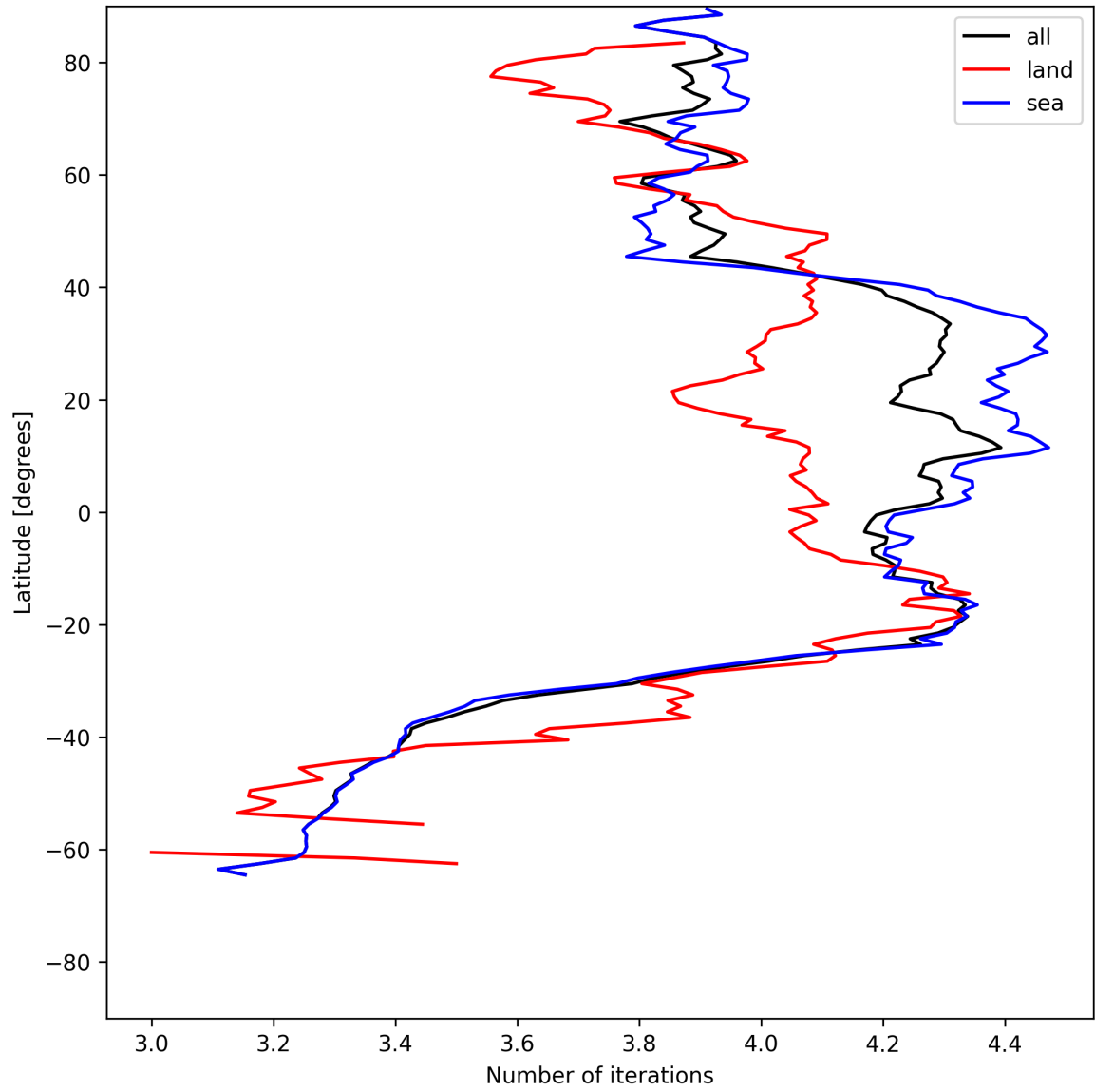
Figure 17: Zonal average of “Number of iterations” for 2025-07-05 to 2025-07-07.
