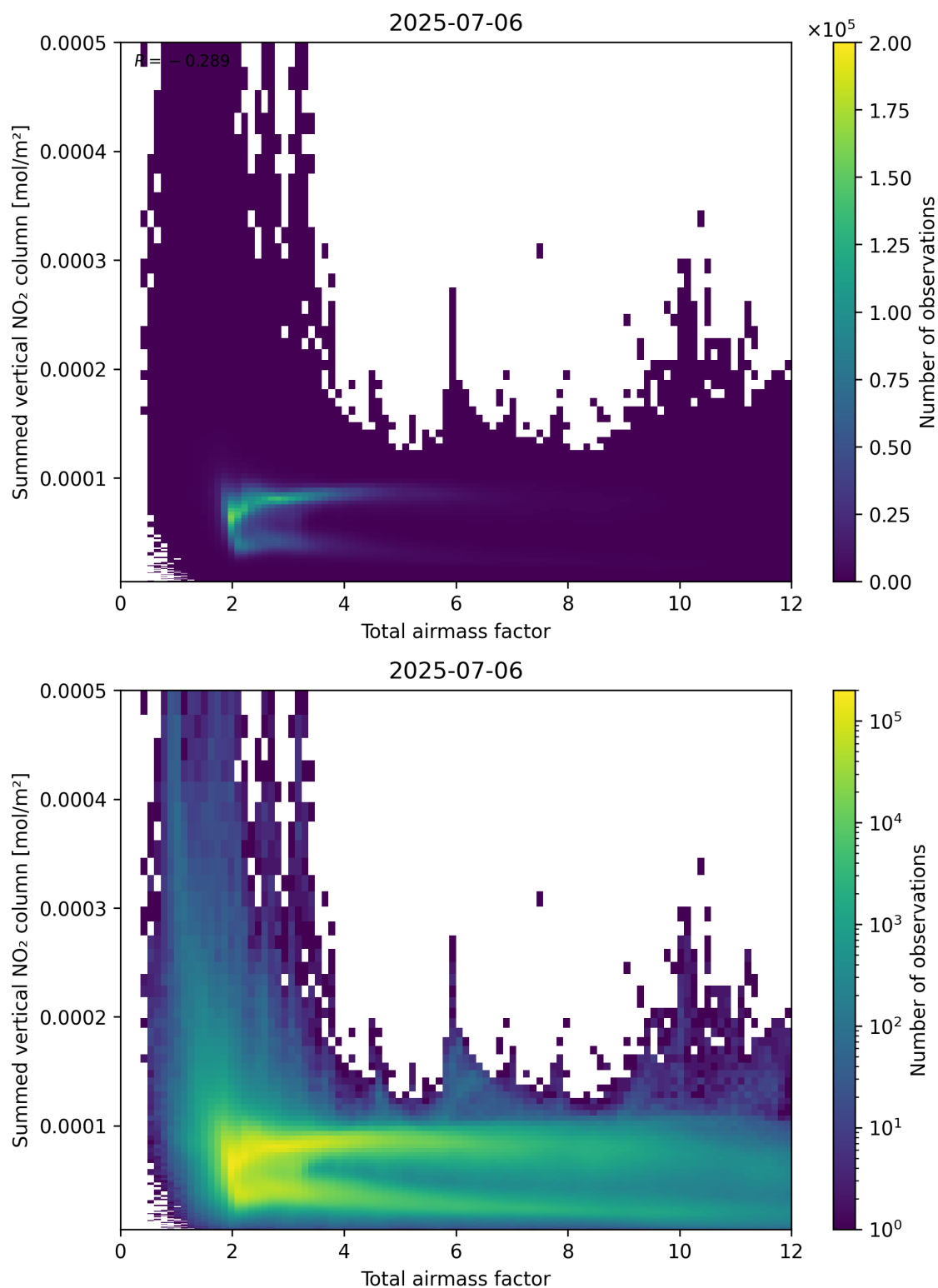
Figure 65: Scatter density plot of “Total airmass factor” against “Summed vertical NO 2 column” for 2025-07-05 to 2025-07-07.
