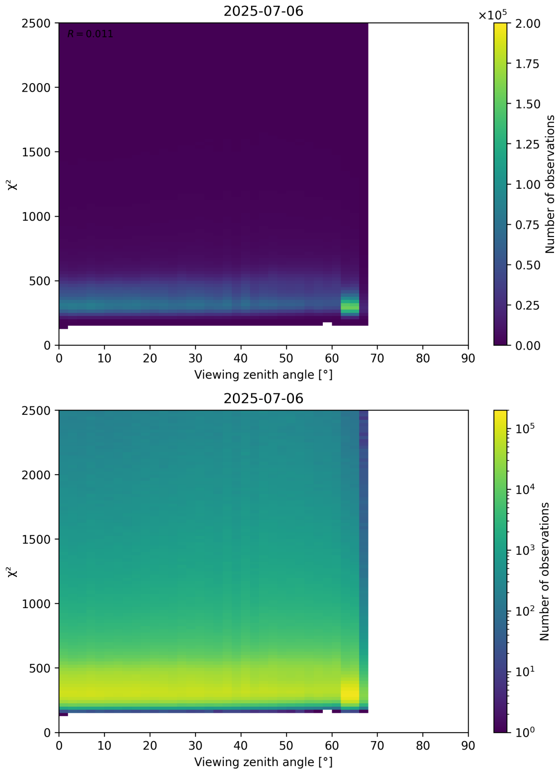
Figure 162: Scatter density plot of “Viewing zenith angle” against “ \chi^2 ” for 2025-07-05 to 2025-07-07.
