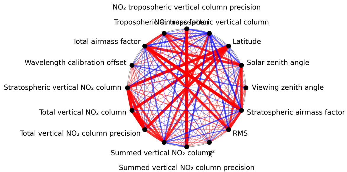
Figure 1: Map of correlation graph for 2025-07-05 to 2025-07-07.
