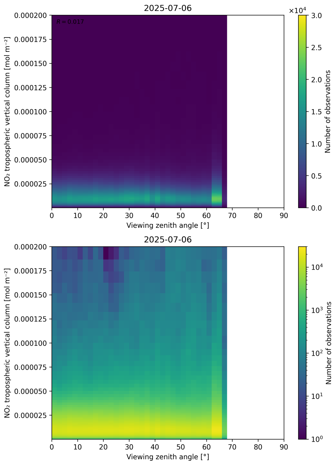
Figure 169: Scatter density plot of “Viewing zenith angle” against “NO 2 tropospheric vertical column” for 2025-07-05 to 2025-07-07.
