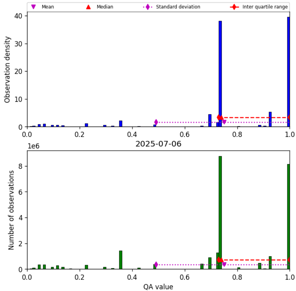
Figure 28: Histogram of “QA value” for 2025-07-05 to 2025-07-07
