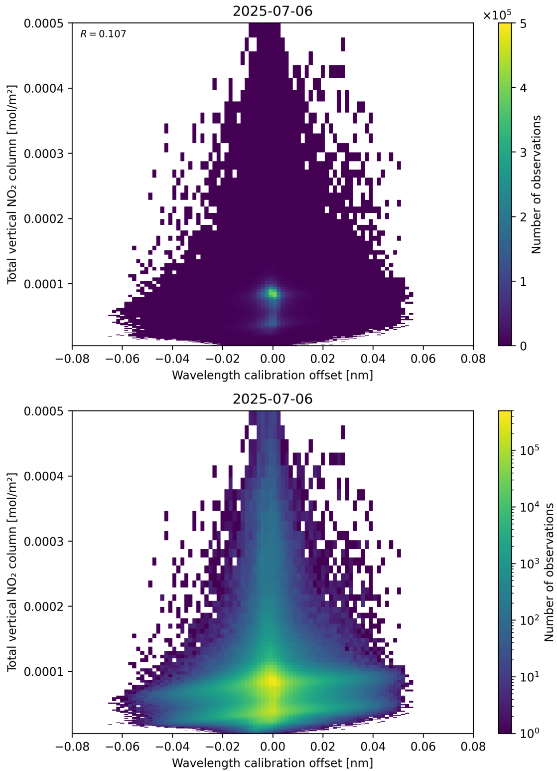
Figure 179: Scatter density plot of “Wavelength calibration offset” against “Total vertical NO 2 column” for 2025-07-05 to 2025-07-07.
