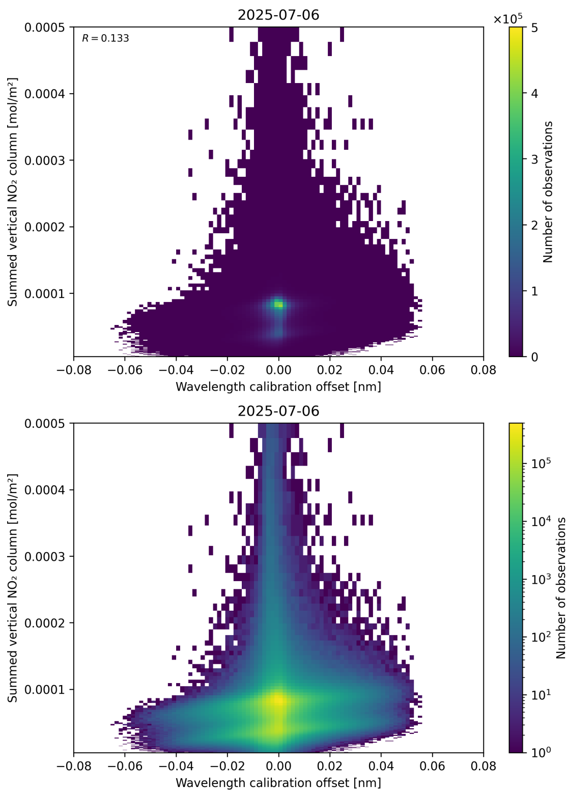
Figure 177: Scatter density plot of “Wavelength calibration offset” against “Summed vertical NO 2 column” for 2025-07-05 to 2025-07-07.
