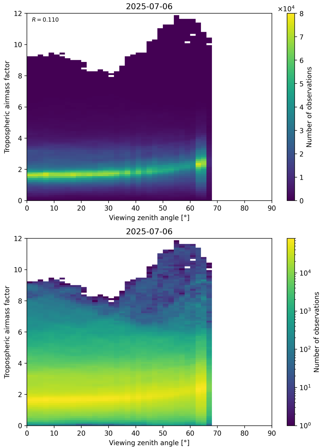
Figure 161: Scatter density plot of “Viewing zenith angle” against “Tropospheric airmass factor” for 2025-07-05 to 2025-07-07.
