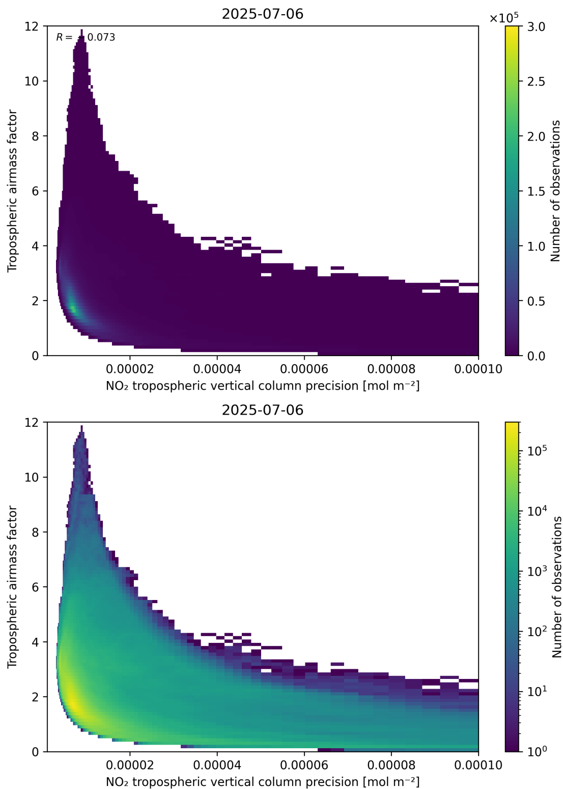
Figure 133: Scatter density plot of “NO 2 tropospheric vertical column precision” against “Tropospheric air mass factor” for 2025-07-05 to 2025-07-07.
