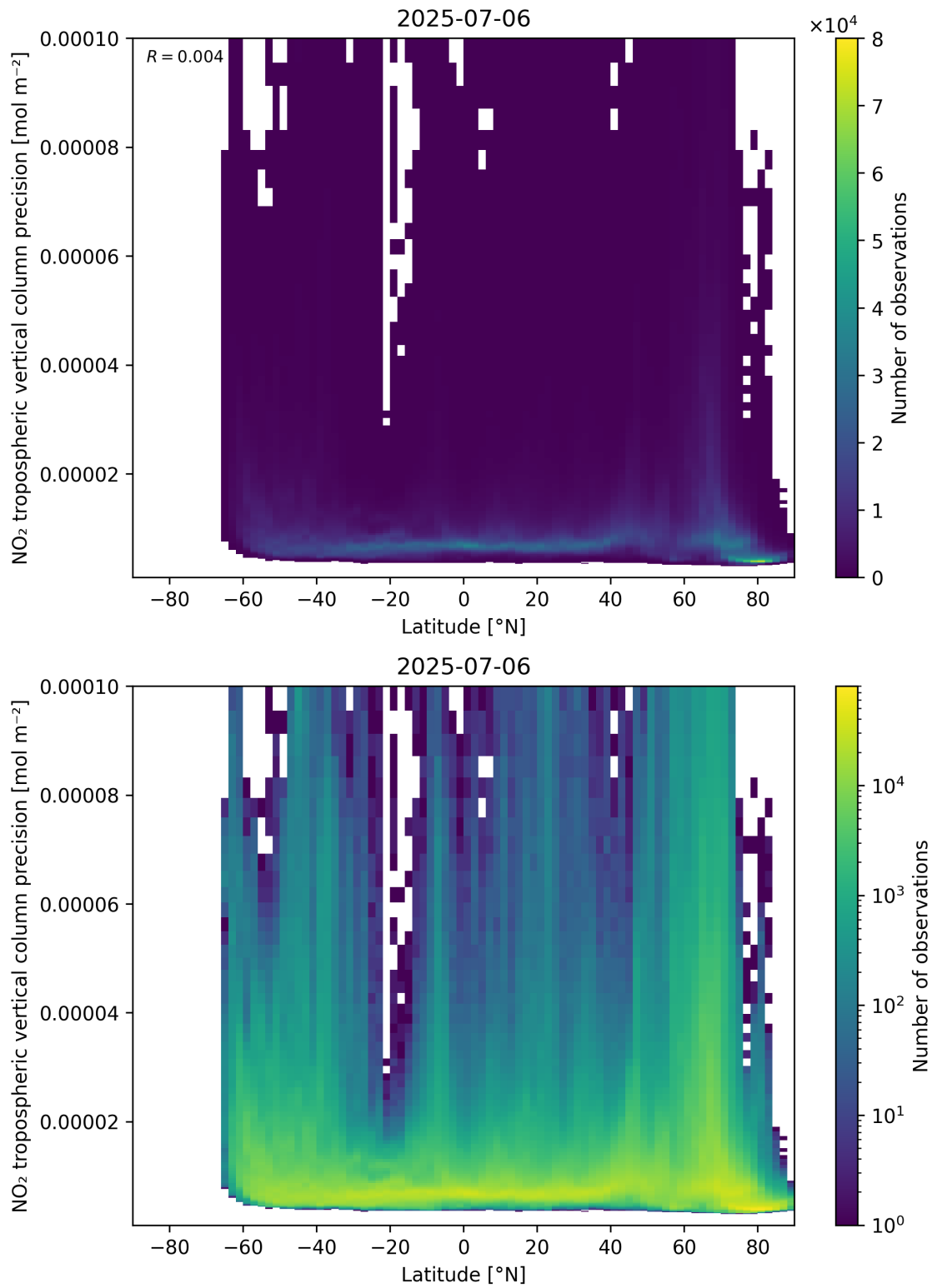
Figure 93: Scatter density plot of “Latitude” against “NO 2 tropospheric vertical column precision” for 2025-07-05 to 2025-07-07.
