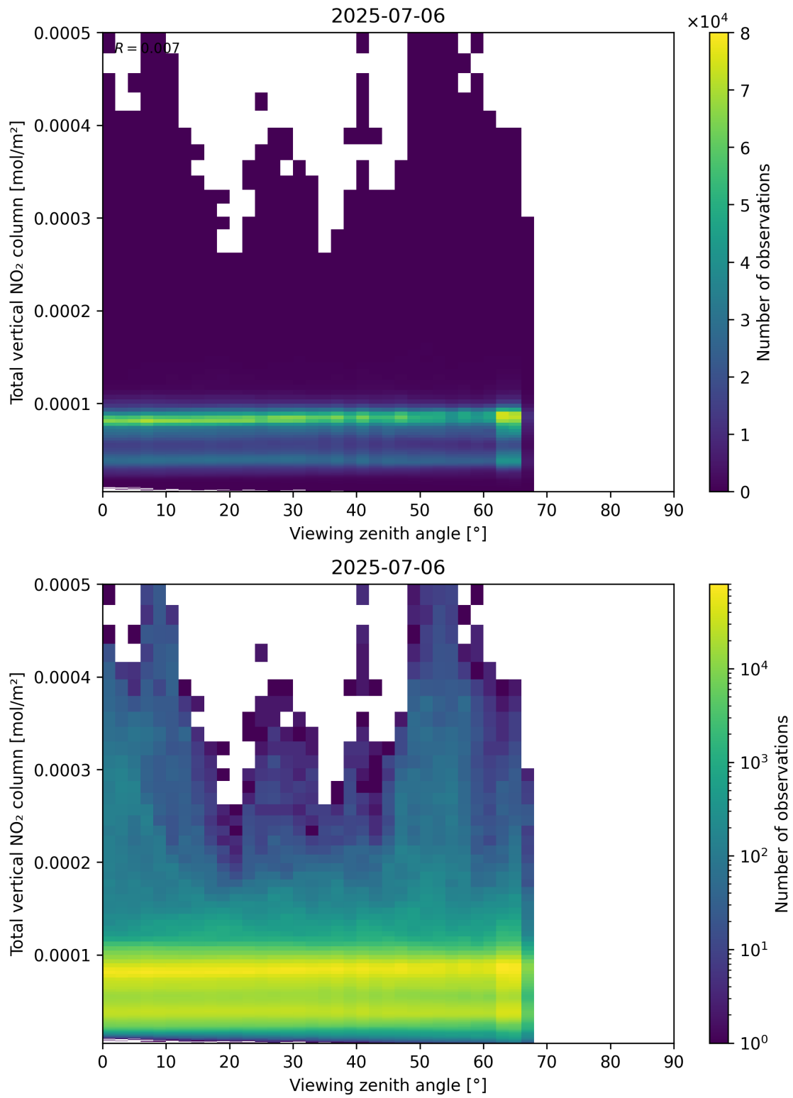
Figure 167: Scatter density plot of “Viewing zenith angle” against “Total vertical NO 2 column” for 2025-07-05 to 2025-07-07.
