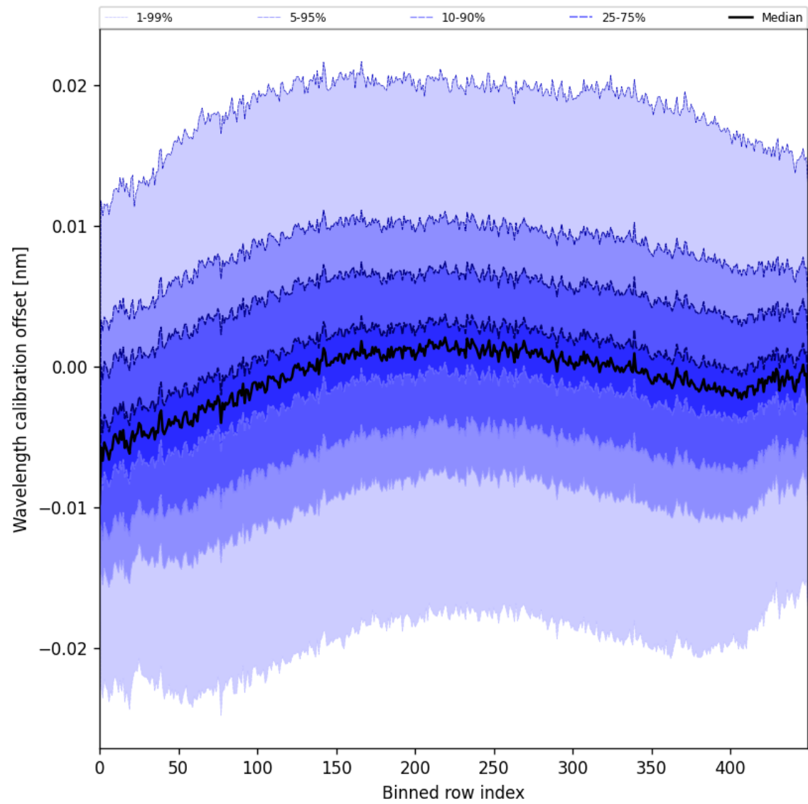
Figure 52: Along track statistics of “Wavelength calibration offset” for 2025-07-05 to 2025-07-07
