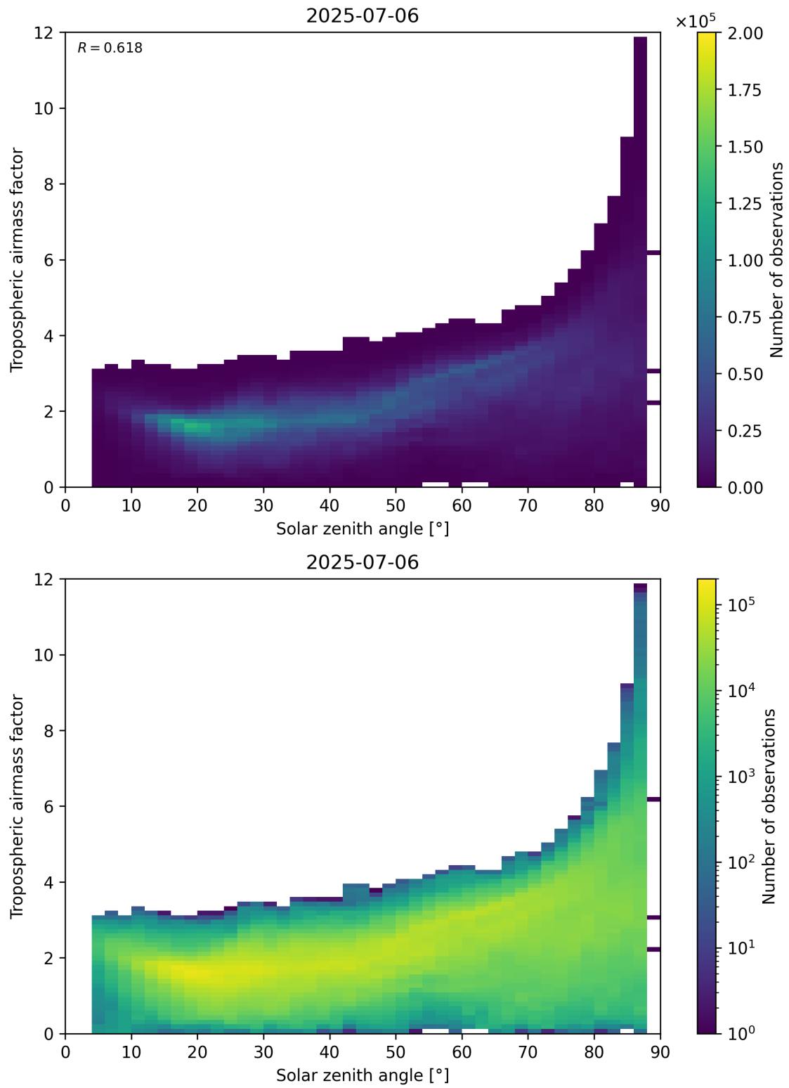
Figure 147: Scatter density plot of “Solar zenith angle” against “Tropospheric airmass factor” for 2025-07-05 to 2025-07-07.
