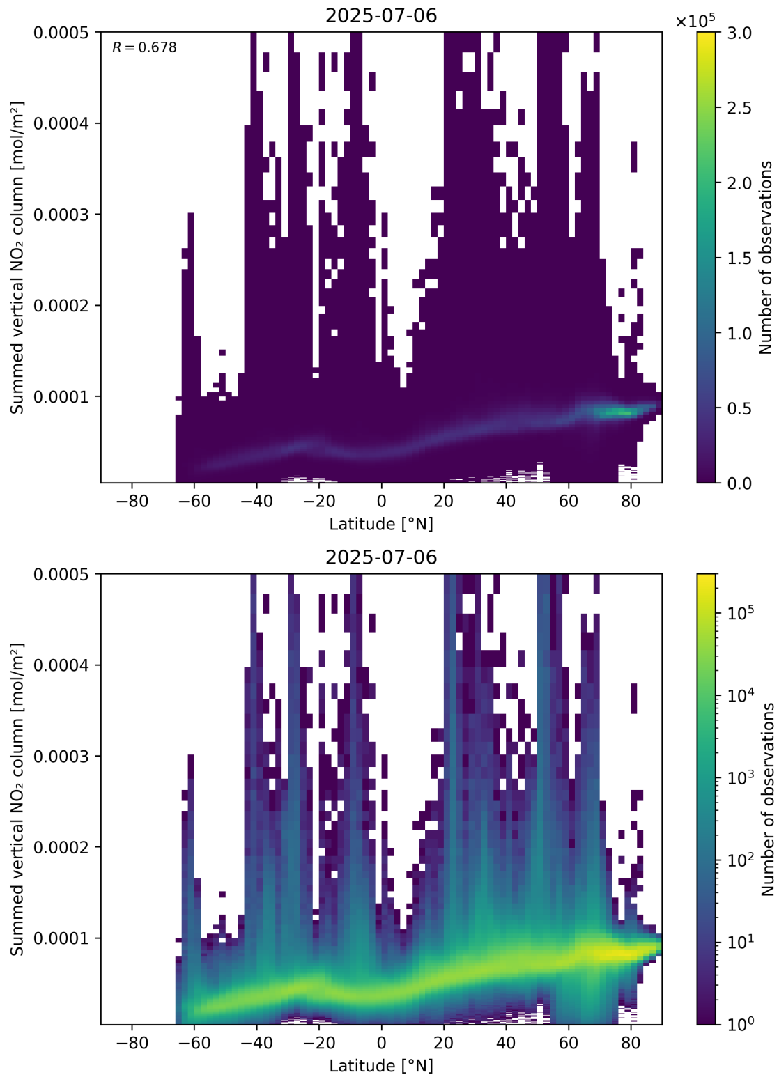
Figure 88: Scatter density plot of “Latitude” against “Summed vertical NO 2 column” for 2025-07-05 to 2025-07-07.
