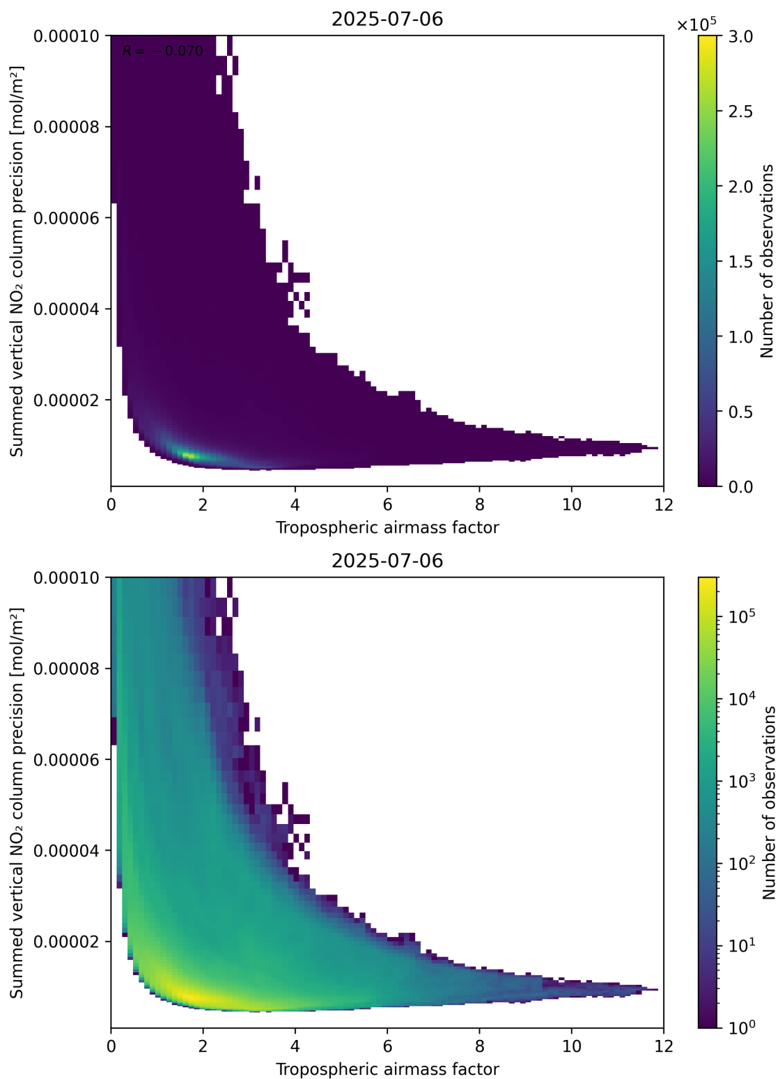
Figure 76: Scatter density plot of “Tropospheric air mass factor” against “Summed vertical NO 2 column precision” for 2025-07-05 to 2025-07-07.
