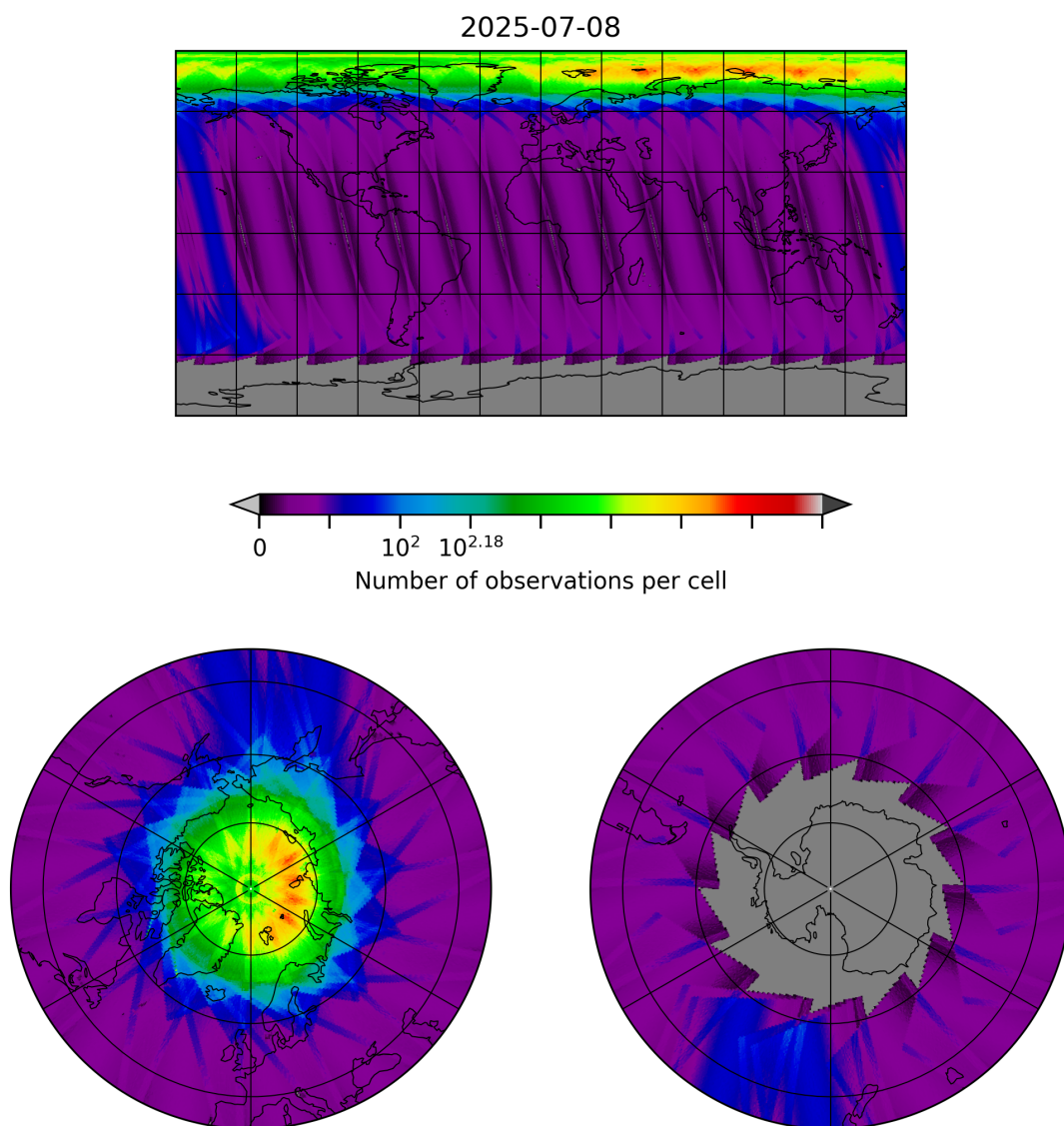
Figure 10: Map of the number of observations for 2025-07-08 to 2025-07-09
