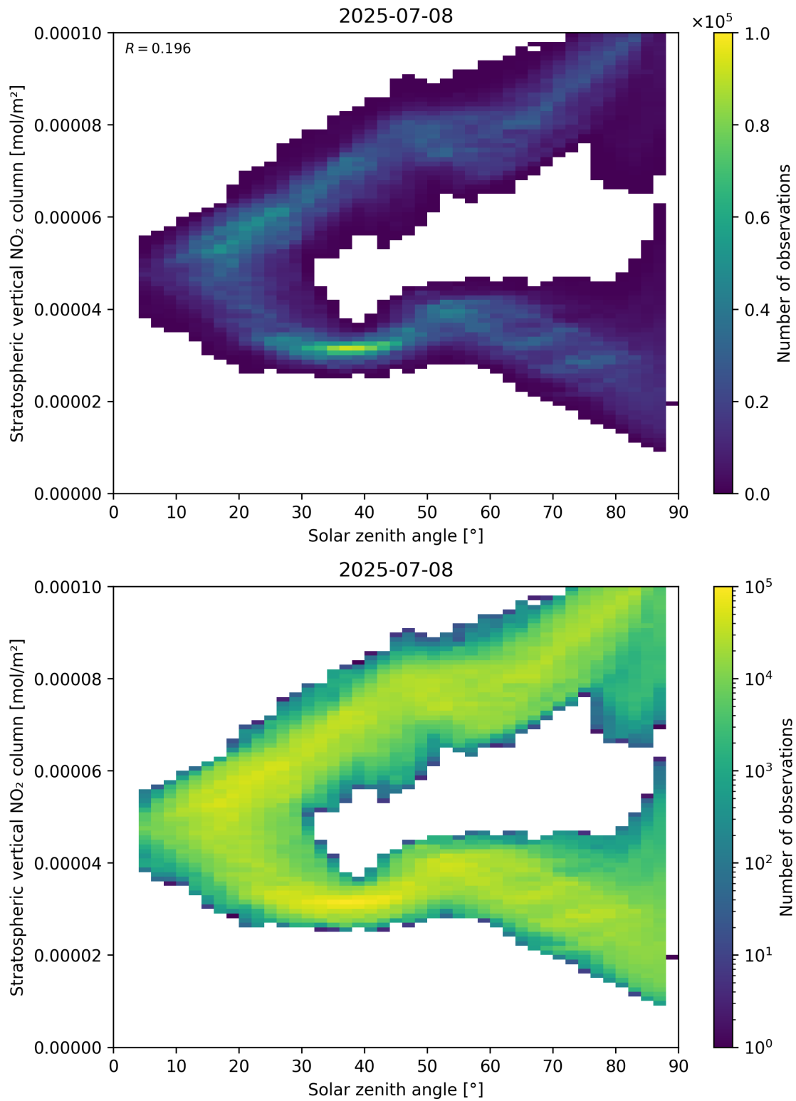
Figure 150: Scatter density plot of “Solar zenith angle” against “Stratospheric vertical NO 2 column” for 2025-07-08 to 2025-07-09.
