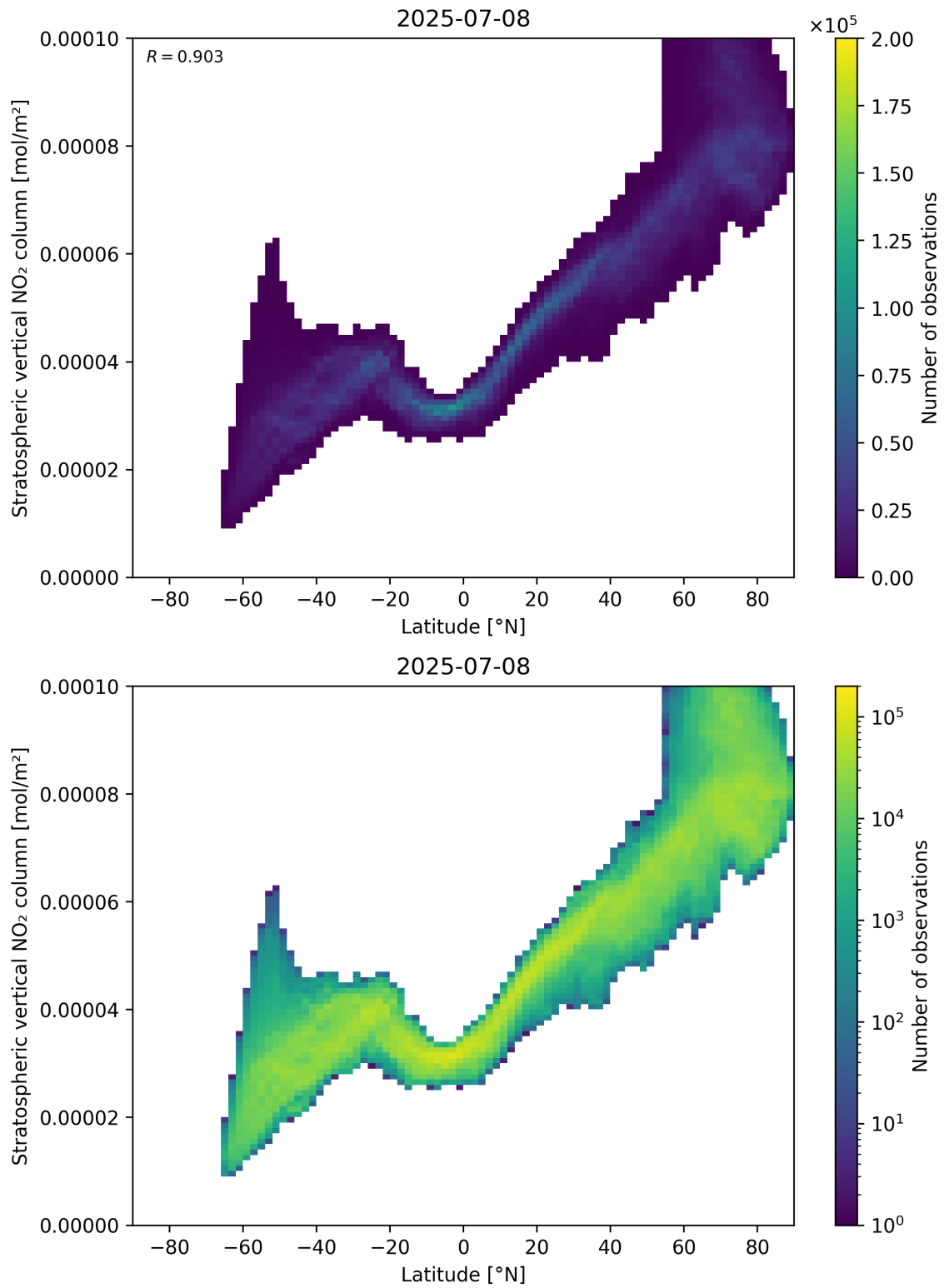
Figure 87: Scatter density plot of “Latitude” against “Stratospheric vertical \text{NO}_2 column” for 2025-07-08 to 2025-07-09.
