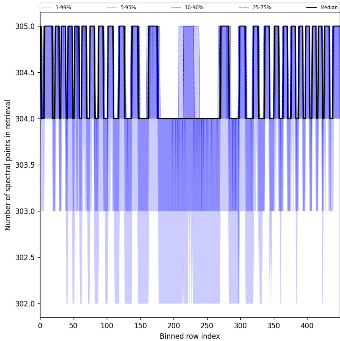
Figure 50: Along track statistics of “Number of spectral points in retrieval” for 2025-07-08 to 2025-07-09
