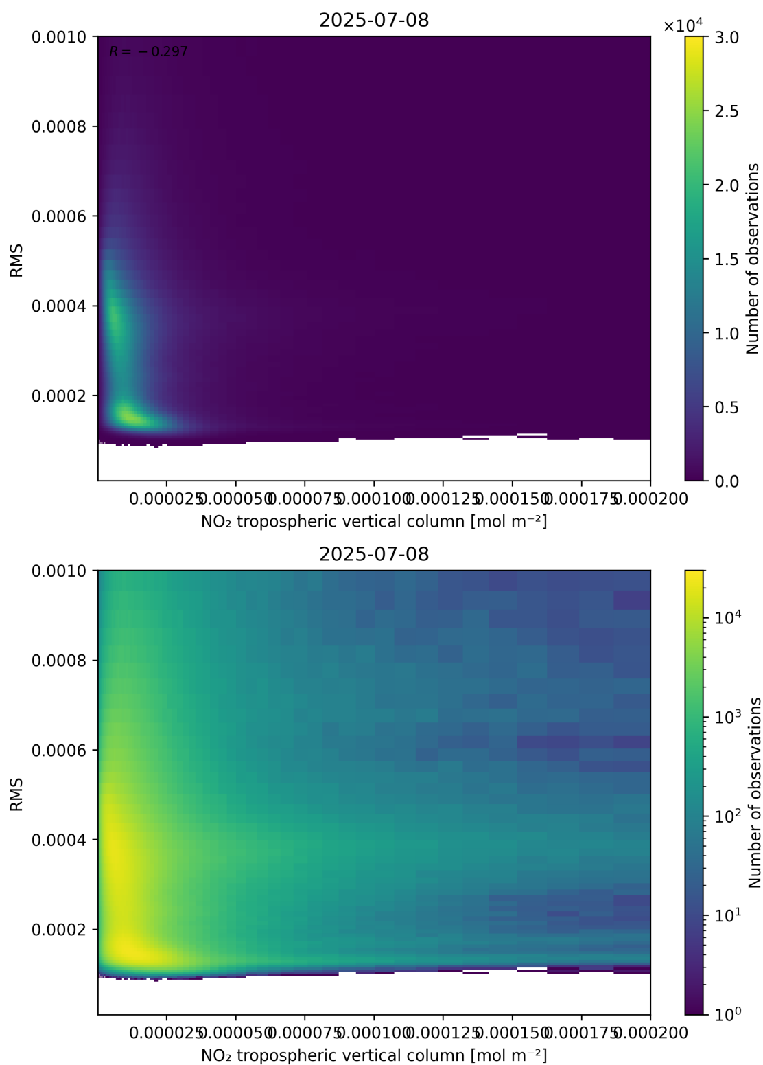
Figure 142: Scatter density plot of “NO 2 tropospheric vertical column” against “RMS” for 2025-07-08 to 2025-07-09.
