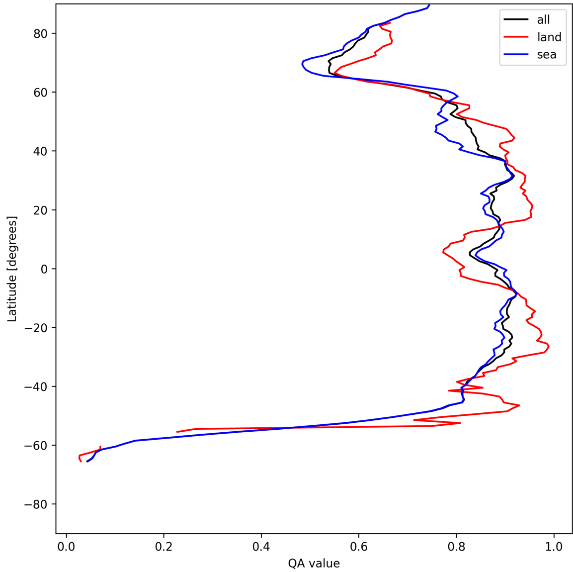
Figure 11: Zonal average of “QA value” for 2025-07-08 to 2025-07-09.
