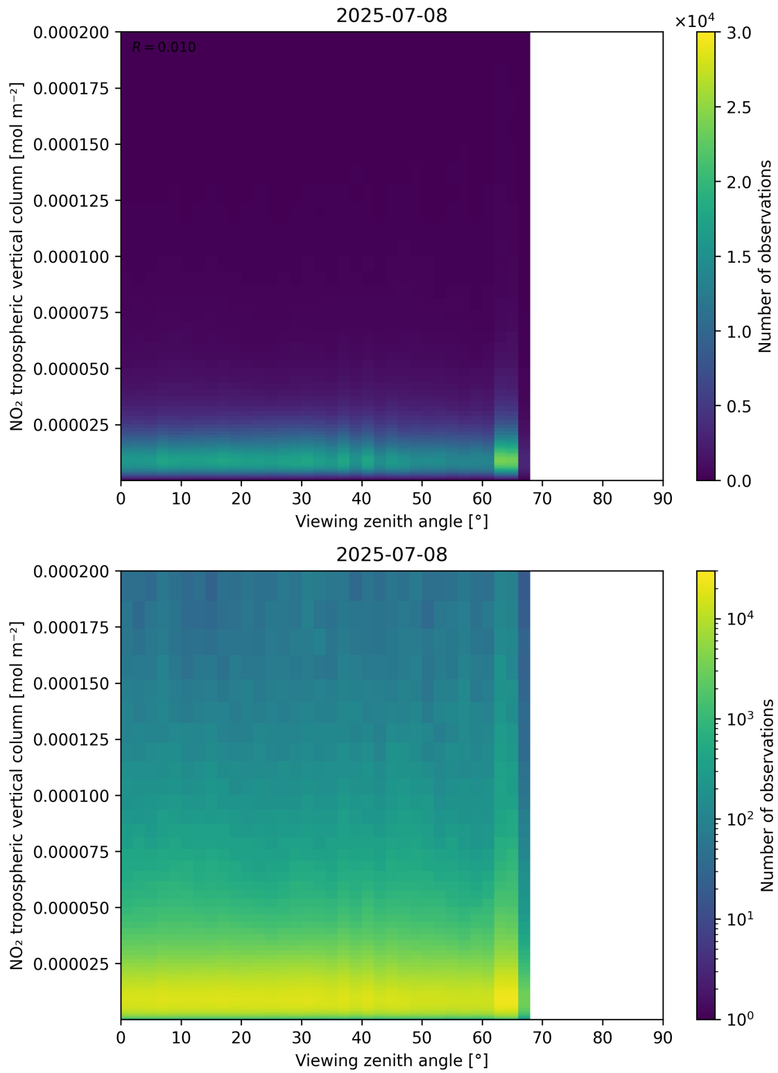
Figure 169: Scatter density plot of “Viewing zenith angle” against “NO 2 tropospheric vertical column” for 2025-07-08 to 2025-07-09.
