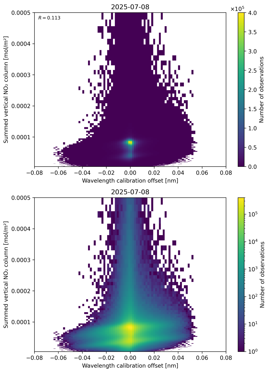
Figure 177: Scatter density plot of “Wavelength calibration offset” against “Summed vertical NO 2 column” for 2025-07-08 to 2025-07-09.
