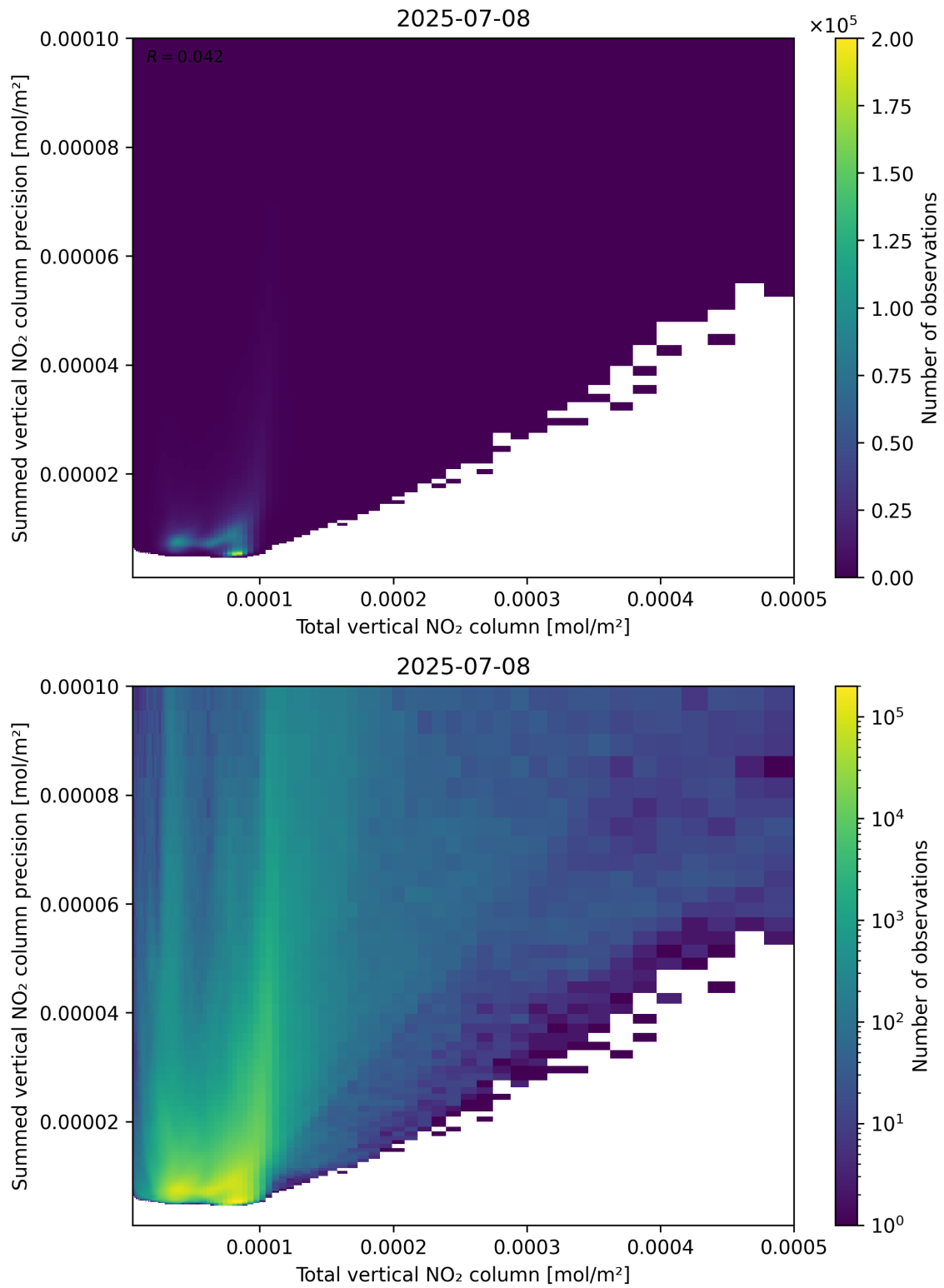
Figure 113: Scatter density plot of “Total vertical NO 2 column” against “Summed vertical NO 2 column precision” for 2025-07-08 to 2025-07-09.
