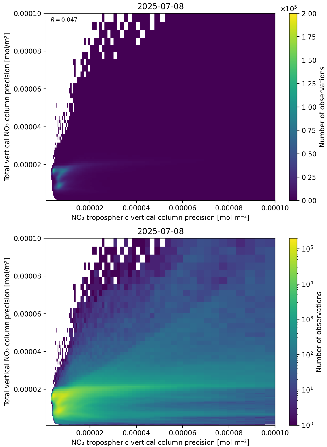
Figure 139: Scatter density plot of “NO 2 tropospheric vertical column precision” against “Total vertical NO 2 column precision” for 2025-07-08 to 2025-07-09.
