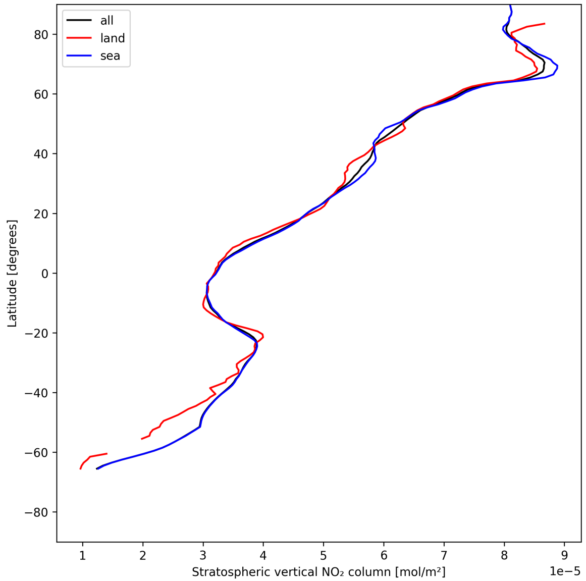
Figure 19: Zonal average of “Stratospheric vertical NO 2 column” for 2025-07-08 to 2025-07-09.
