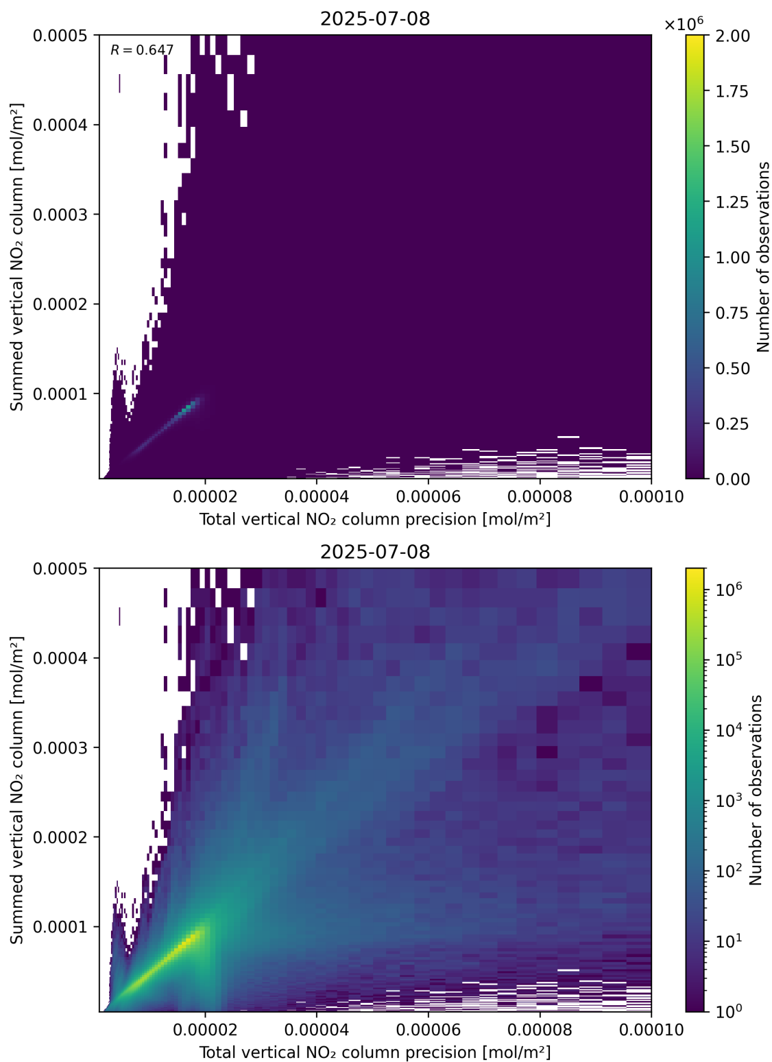
Figure 117: Scatter density plot of “Total vertical NO 2 column precision” against “Summed vertical NO 2 column” for 2025-07-08 to 2025-07-09.
