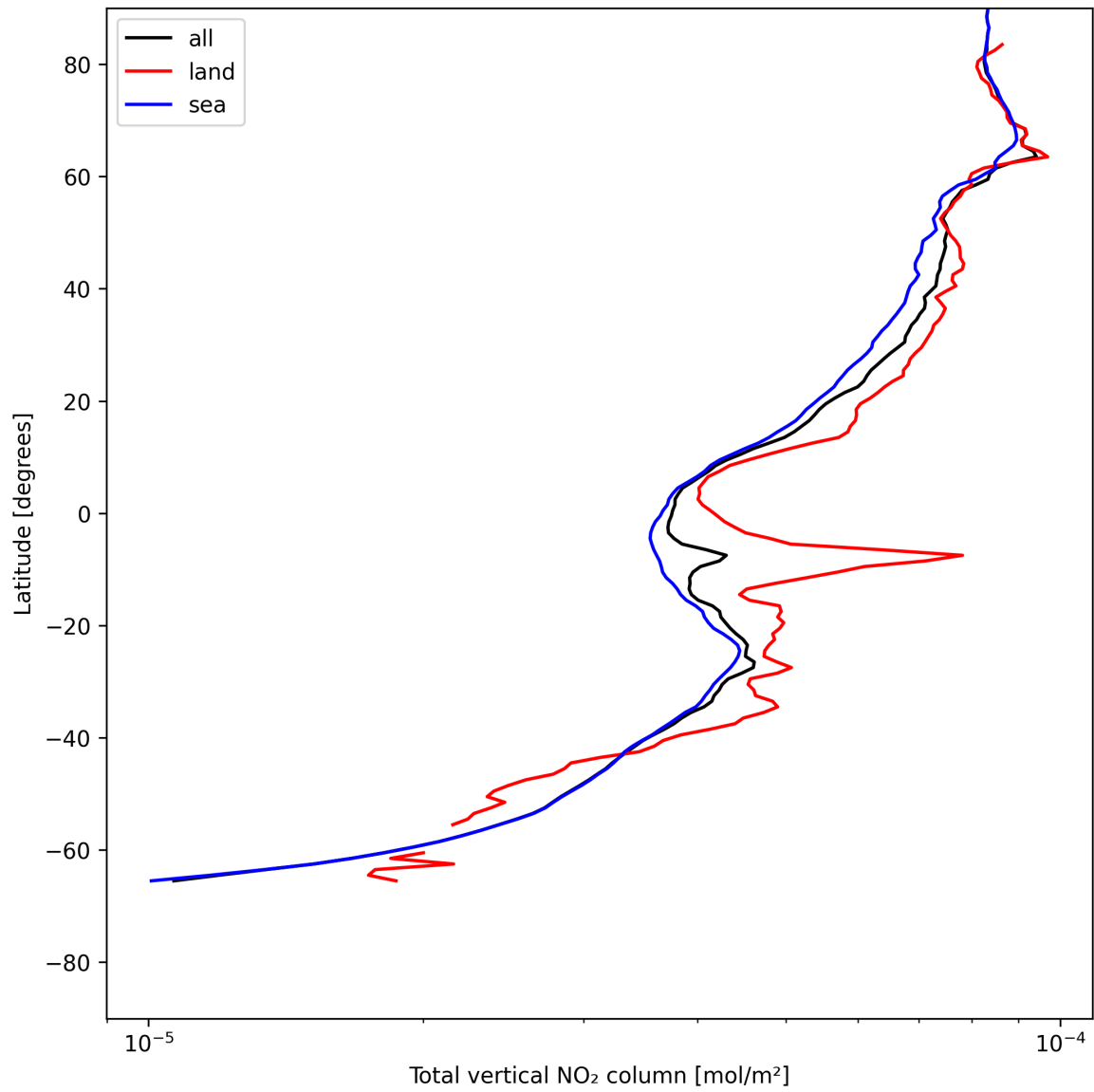
Figure 21: Zonal average of “Total vertical NO 2 column” for 2025-07-08 to 2025-07-09.
