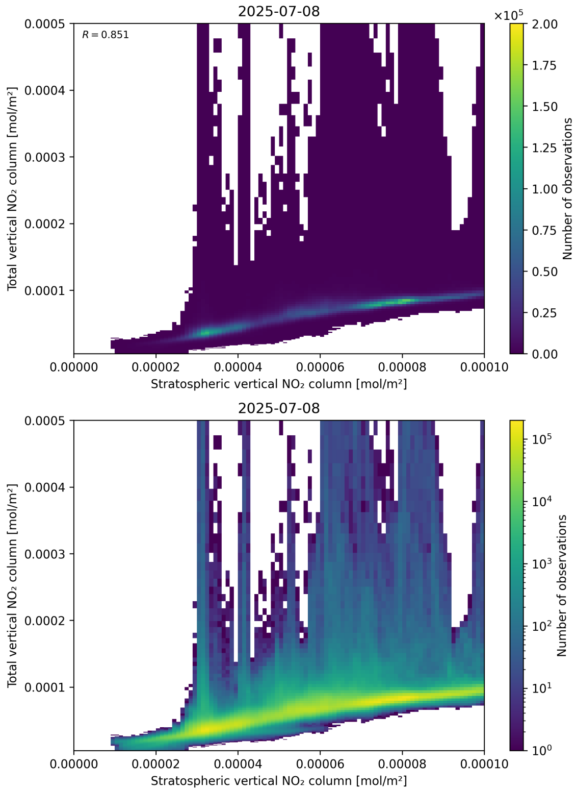
Figure 100: Scatter density plot of “Stratospheric vertical NO 2 column” against “Total vertical NO 2 column” for 2025-07-08 to 2025-07-09.
