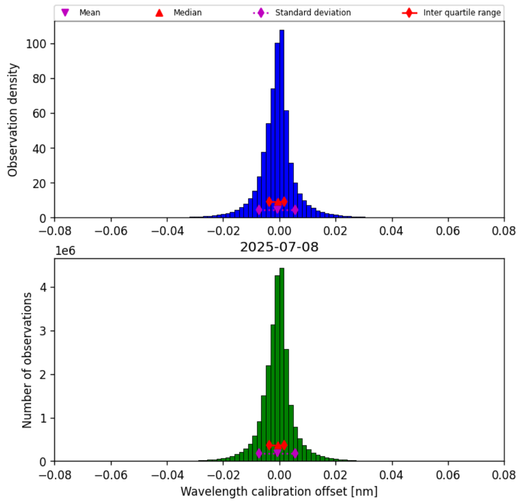
Figure 35: Histogram of “Wavelength calibration offset” for 2025-07-08 to 2025-07-09
