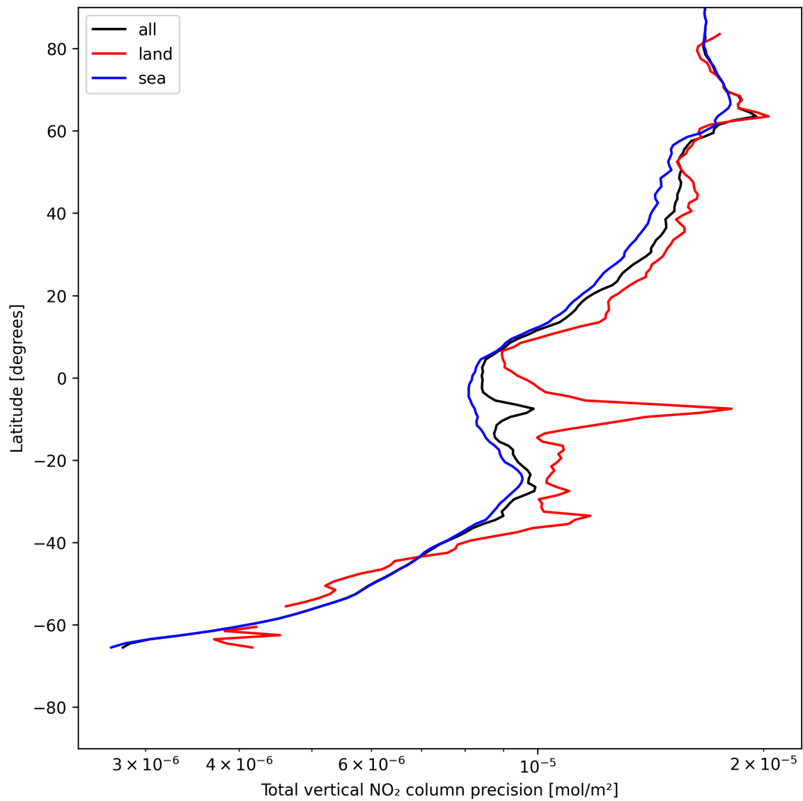
Figure 22: Zonal average of “Total vertical NO 2 column precision” for 2025-07-08 to 2025-07-09.
