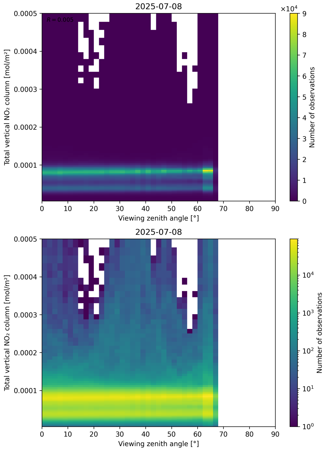
Figure 167: Scatter density plot of “Viewing zenith angle” against “Total vertical NO 2 column” for 2025-07-08 to 2025-07-09.
