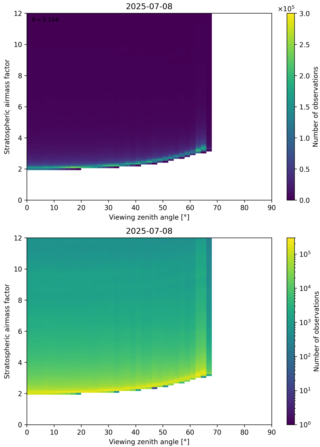
Figure 159: Scatter density plot of “Viewing zenith angle” against “Stratospheric airmass factor” for 2025-07-08 to 2025-07-09.
