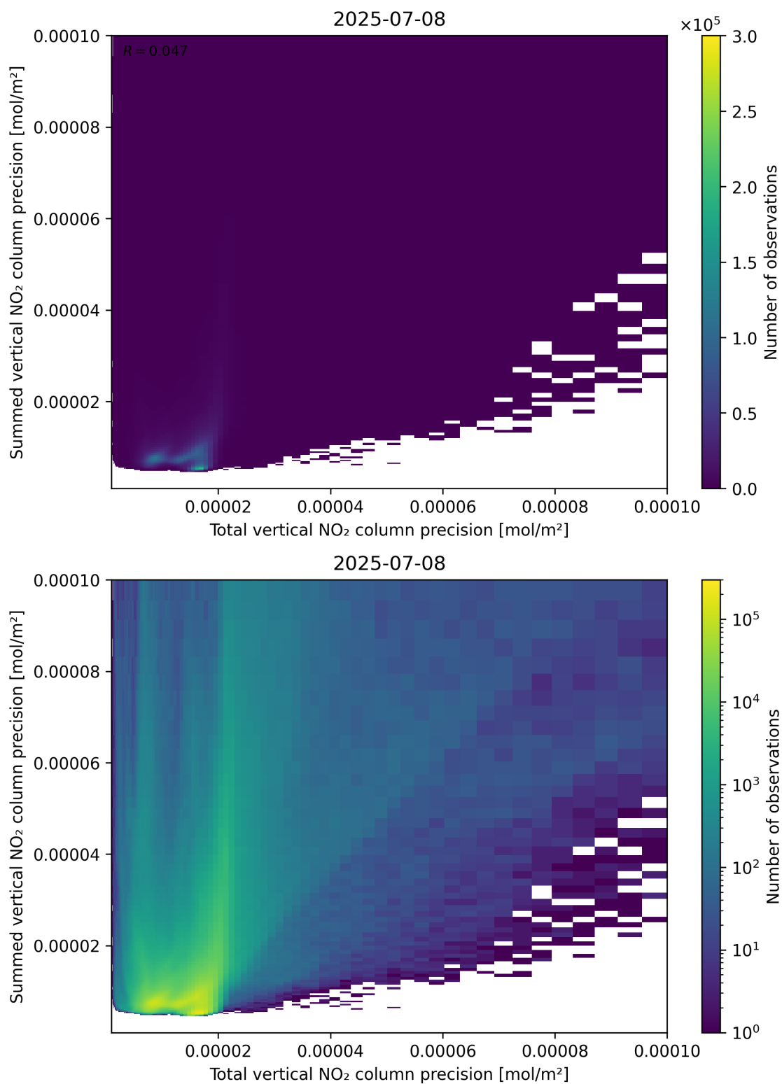
Figure 118: Scatter density plot of “Total vertical NO 2 column precision” against “Summed vertical NO 2 column precision” for 2025-07-08 to 2025-07-09.
