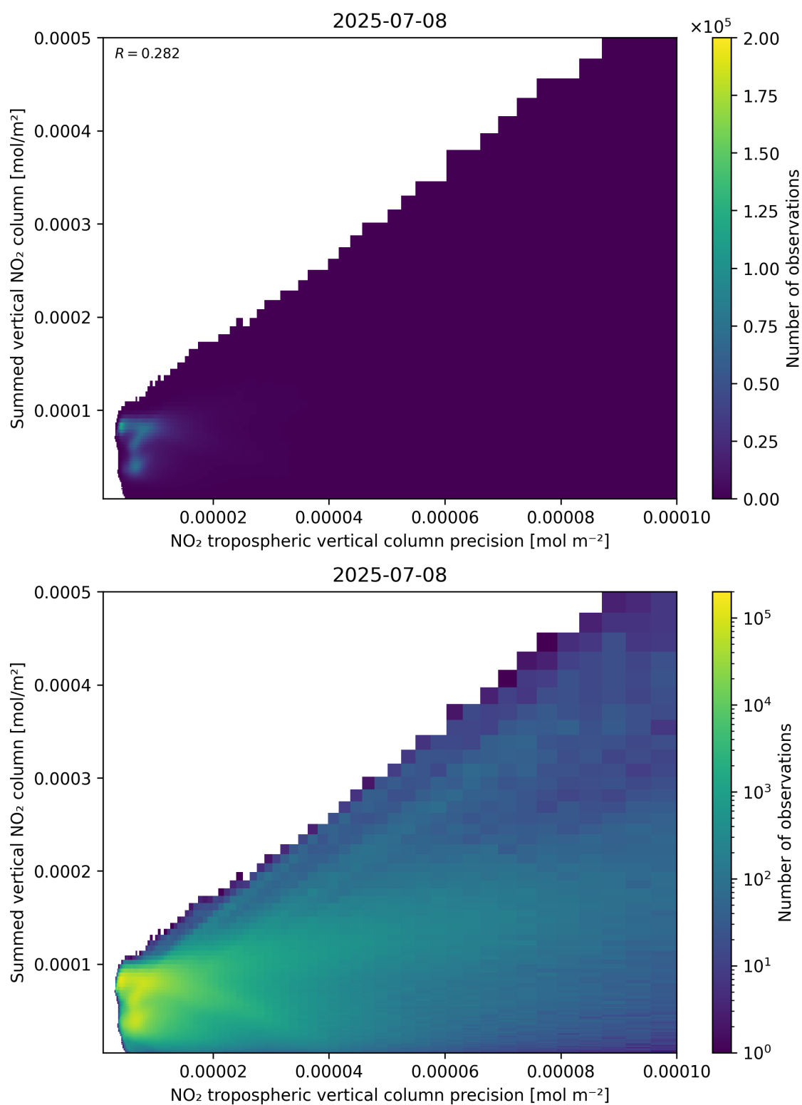
Figure 136: Scatter density plot of “NO 2 tropospheric vertical column precision” against “Summed vertical NO 2 column” for 2025-07-08 to 2025-07-09.
