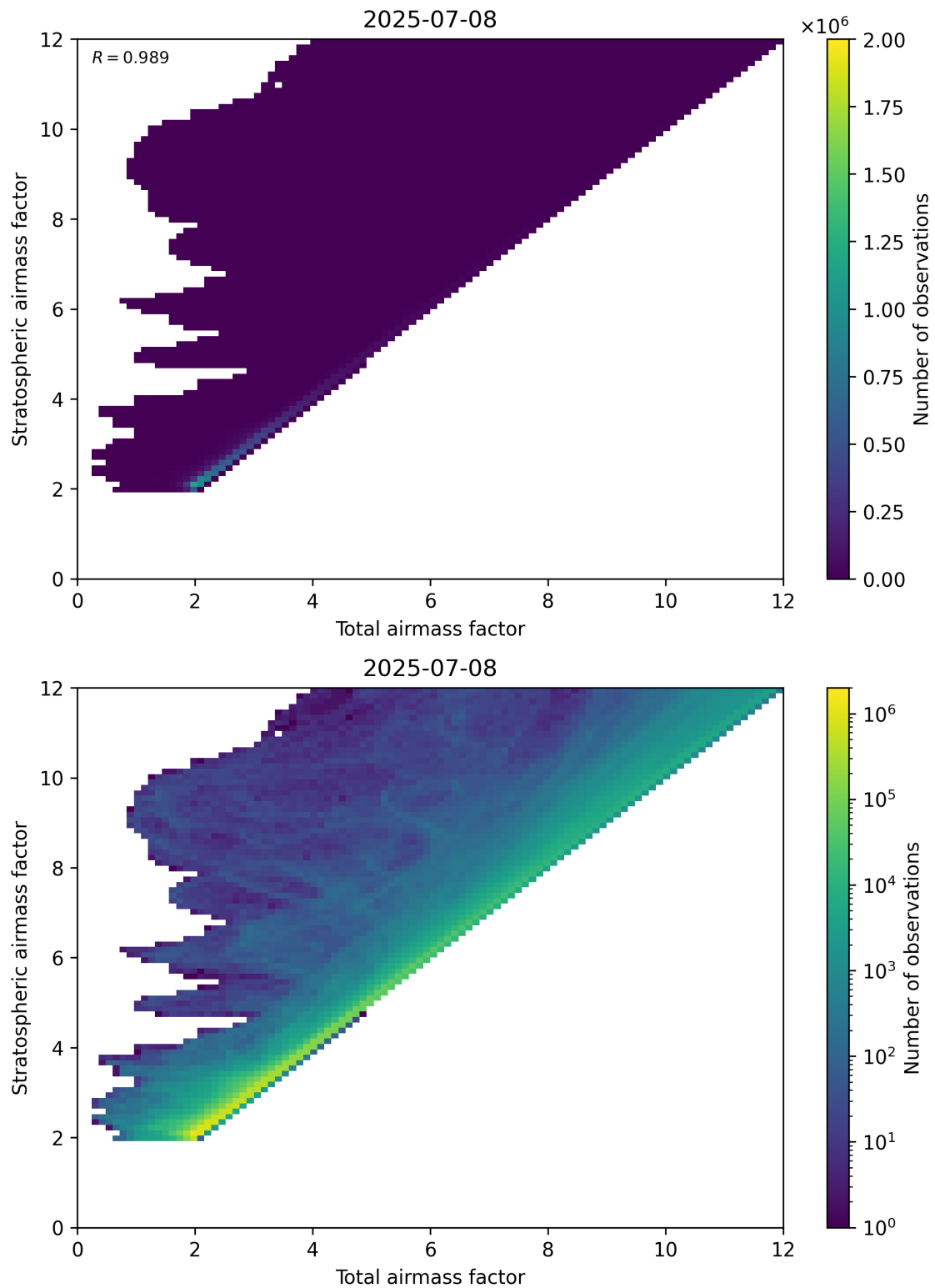
Figure 62: Scatter density plot of “Total airmass factor” against “Stratospheric airmass factor” for 2025-07-08 to 2025-07-09.
