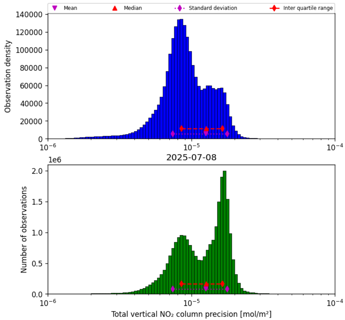
Figure 39: Histogram of “Total vertical NO 2 column precision” for 2025-07-08 to 2025-07-09
