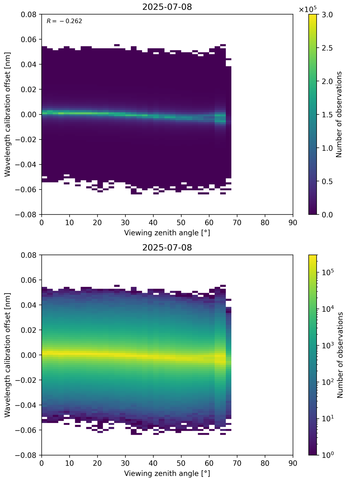
Figure 173: Scatter density plot of “Viewing zenith angle” against “Wavelength calibration offset” for 2025-07-08 to 2025-07-09.
