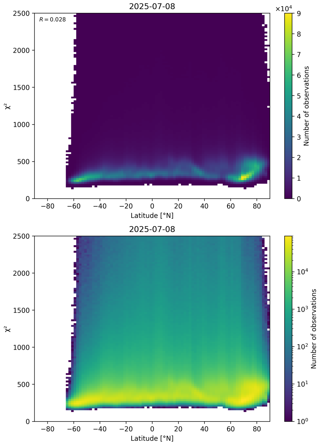
Figure 86: Scatter density plot of “Latitude” against “ \chi^2 ” for 2025-07-08 to 2025-07-09.
