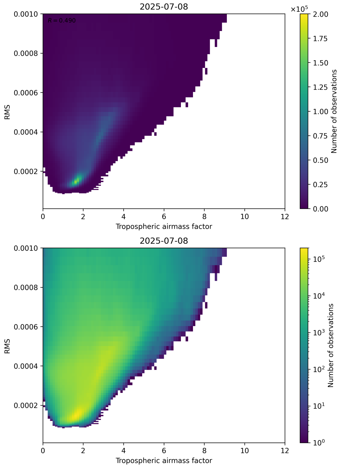
Figure 79: Scatter density plot of “Tropospheric airmass factor” against “RMS” for 2025-07-08 to 2025-07-09.
