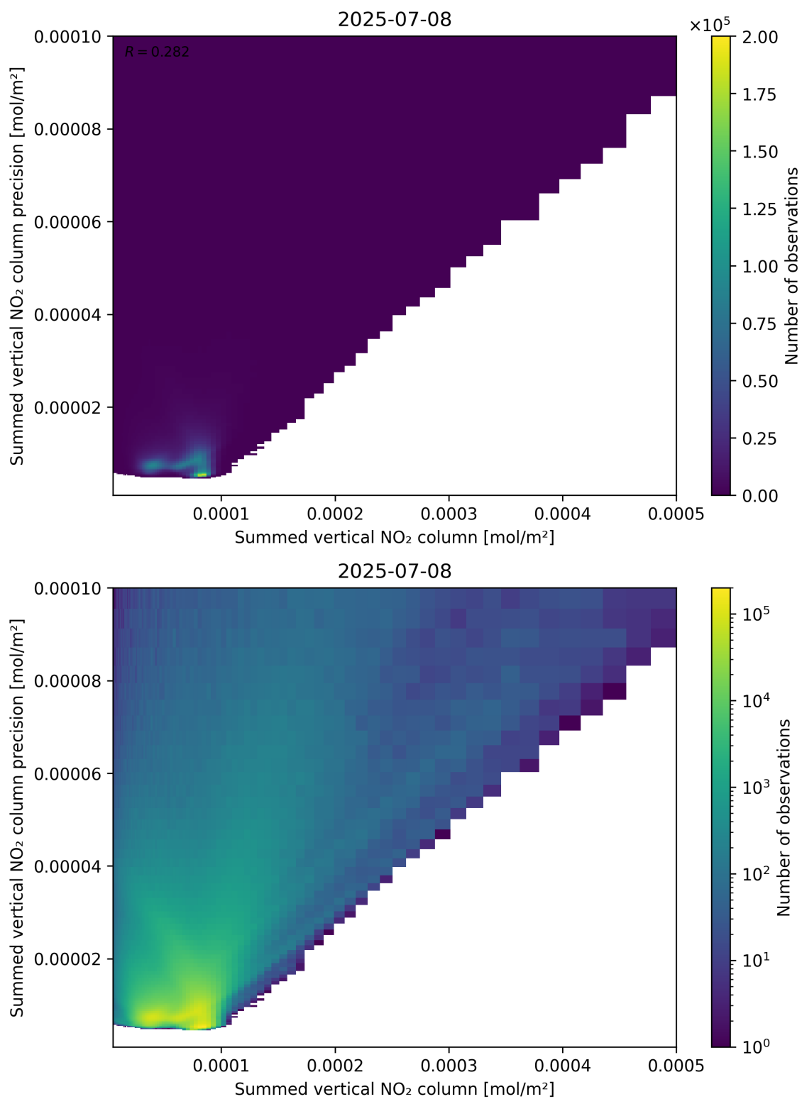
Figure 105: Scatter density plot of “Summed vertical NO 2 column” against “Summed vertical NO 2 column precision” for 2025-07-08 to 2025-07-09.
