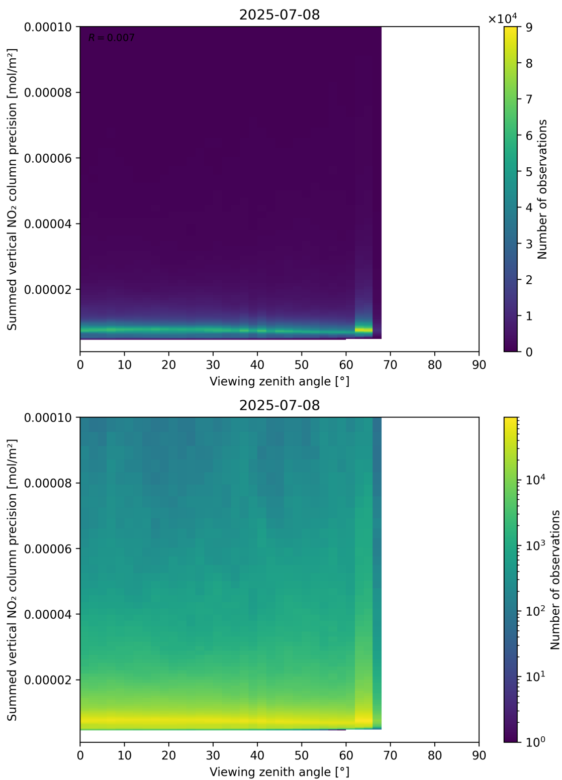
Figure 166: Scatter density plot of “Viewing zenith angle” against “Summed vertical NO 2 column precision” for 2025-07-08 to 2025-07-09.
