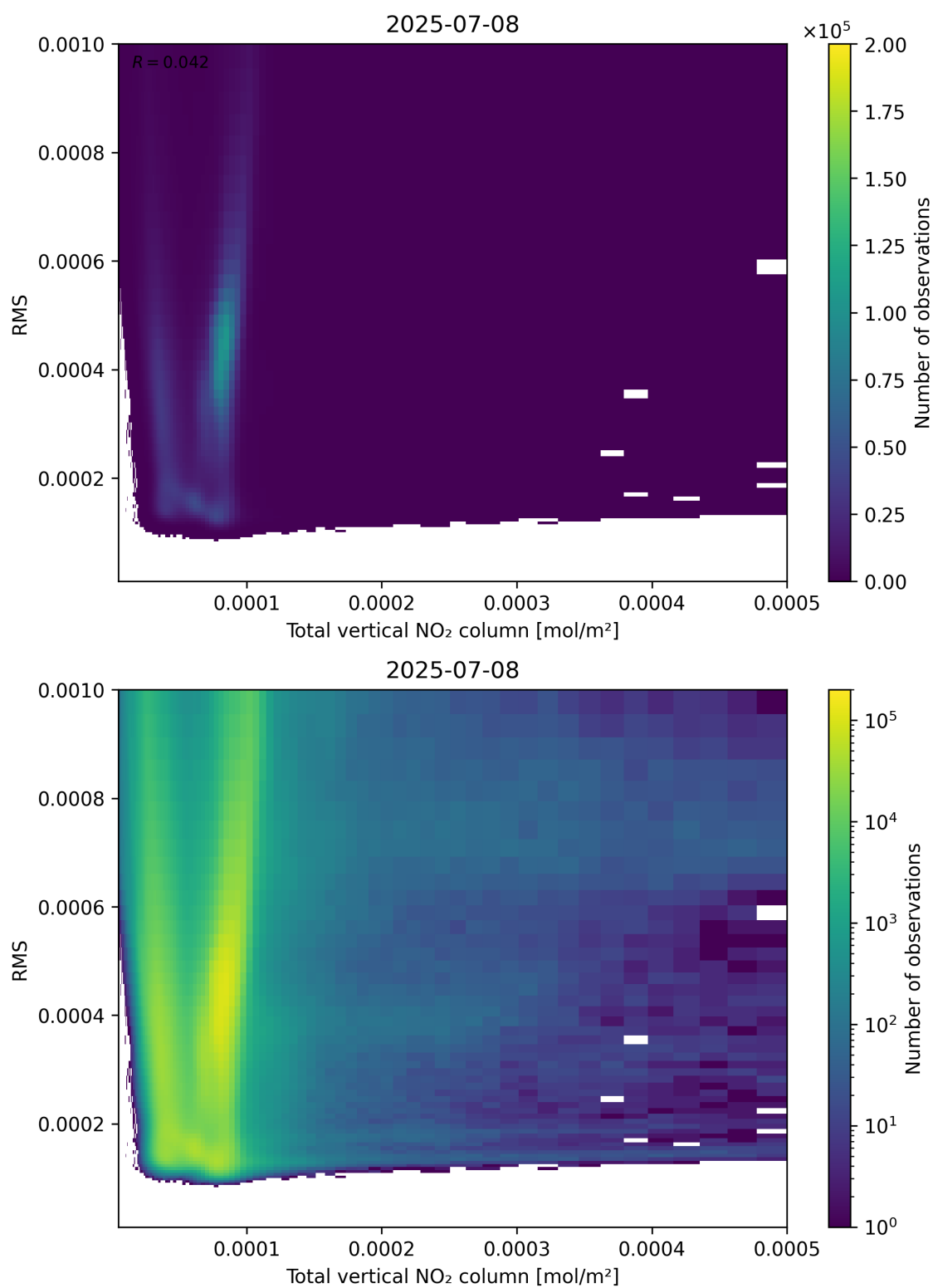
Figure 120: Scatter density plot of “Total vertical NO 2 column” against “RMS” for 2025-07-08 to 2025-07-09.
