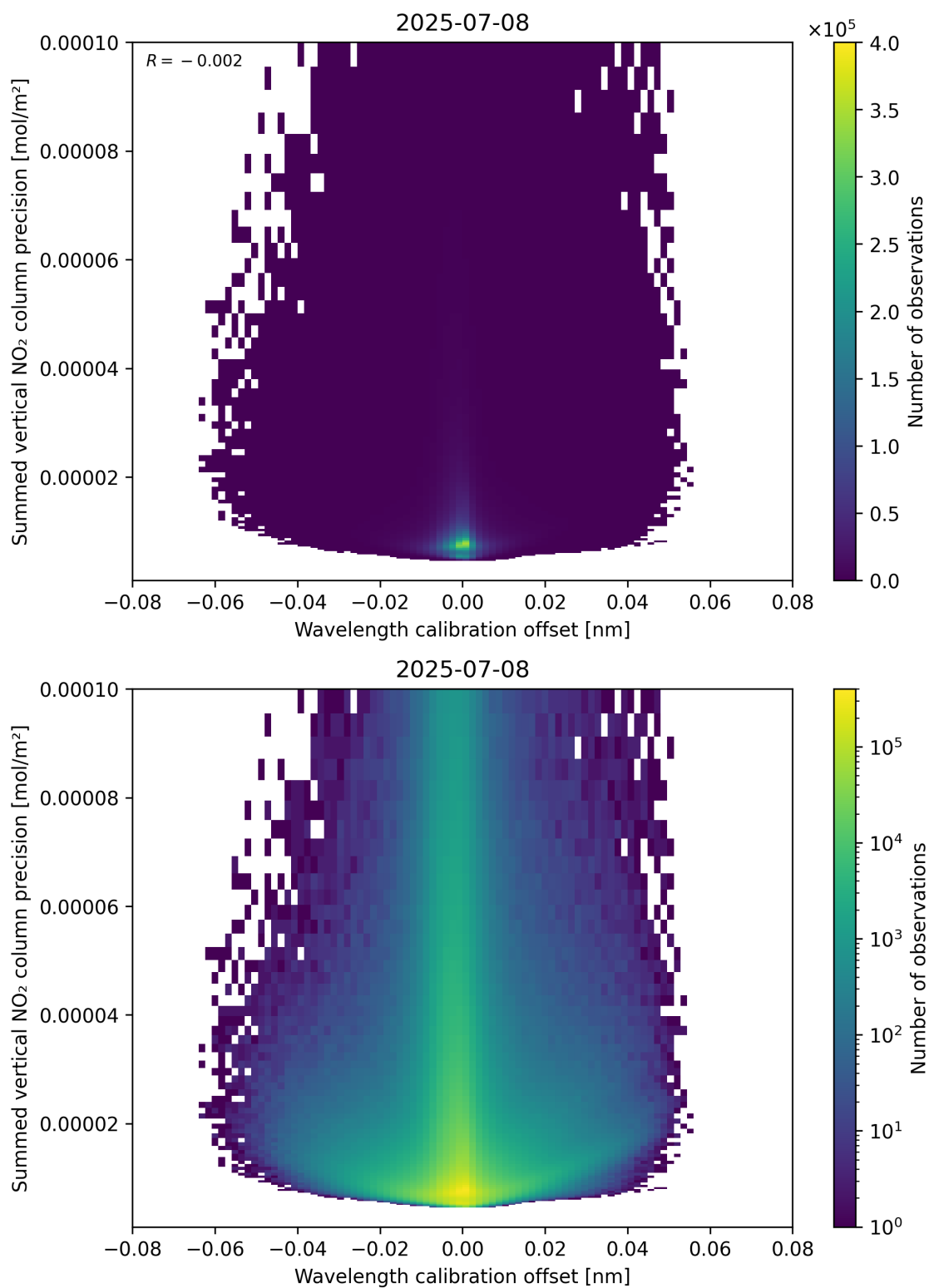
Figure 178: Scatter density plot of “Wavelength calibration offset” against “Summed vertical NO 2 column precision” for 2025-07-08 to 2025-07-09.
