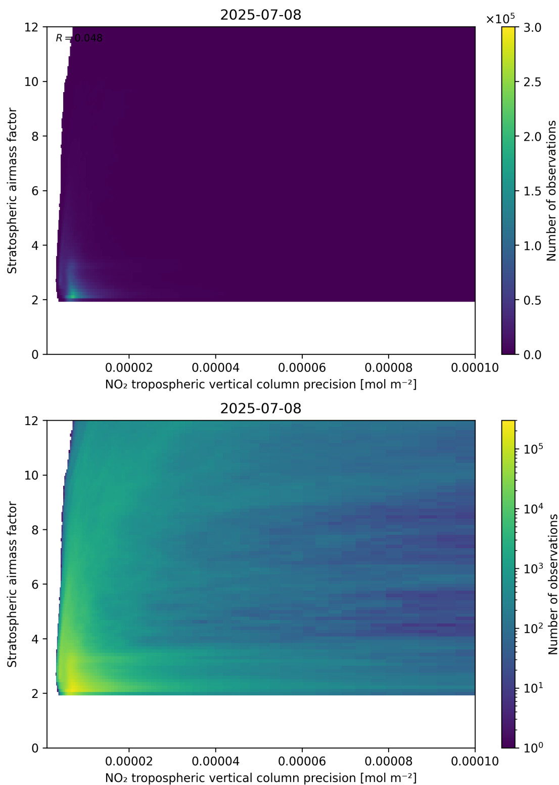
Figure 131: Scatter density plot of “NO 2 tropospheric vertical column precision” against “Stratospheric airmass factor” for 2025-07-08 to 2025-07-09.
