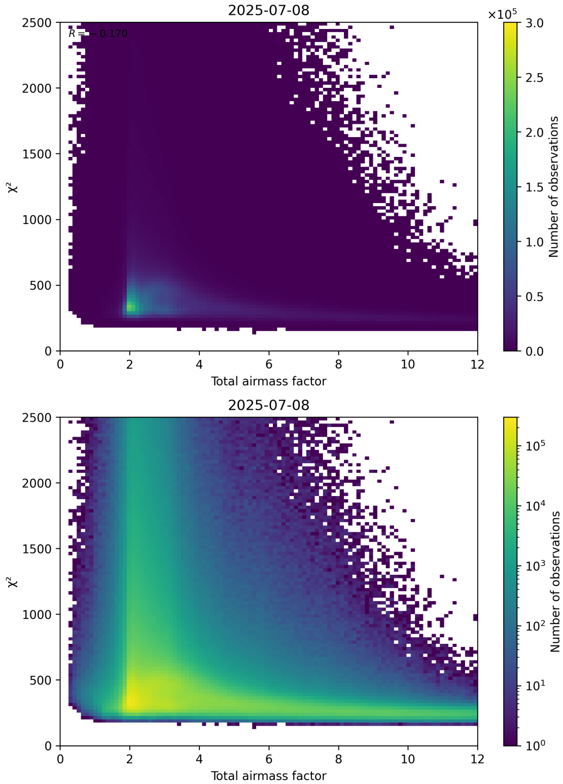
Figure 63: Scatter density plot of “Total airmass factor” against “ \chi^2 ” for 2025-07-08 to 2025-07-09.
