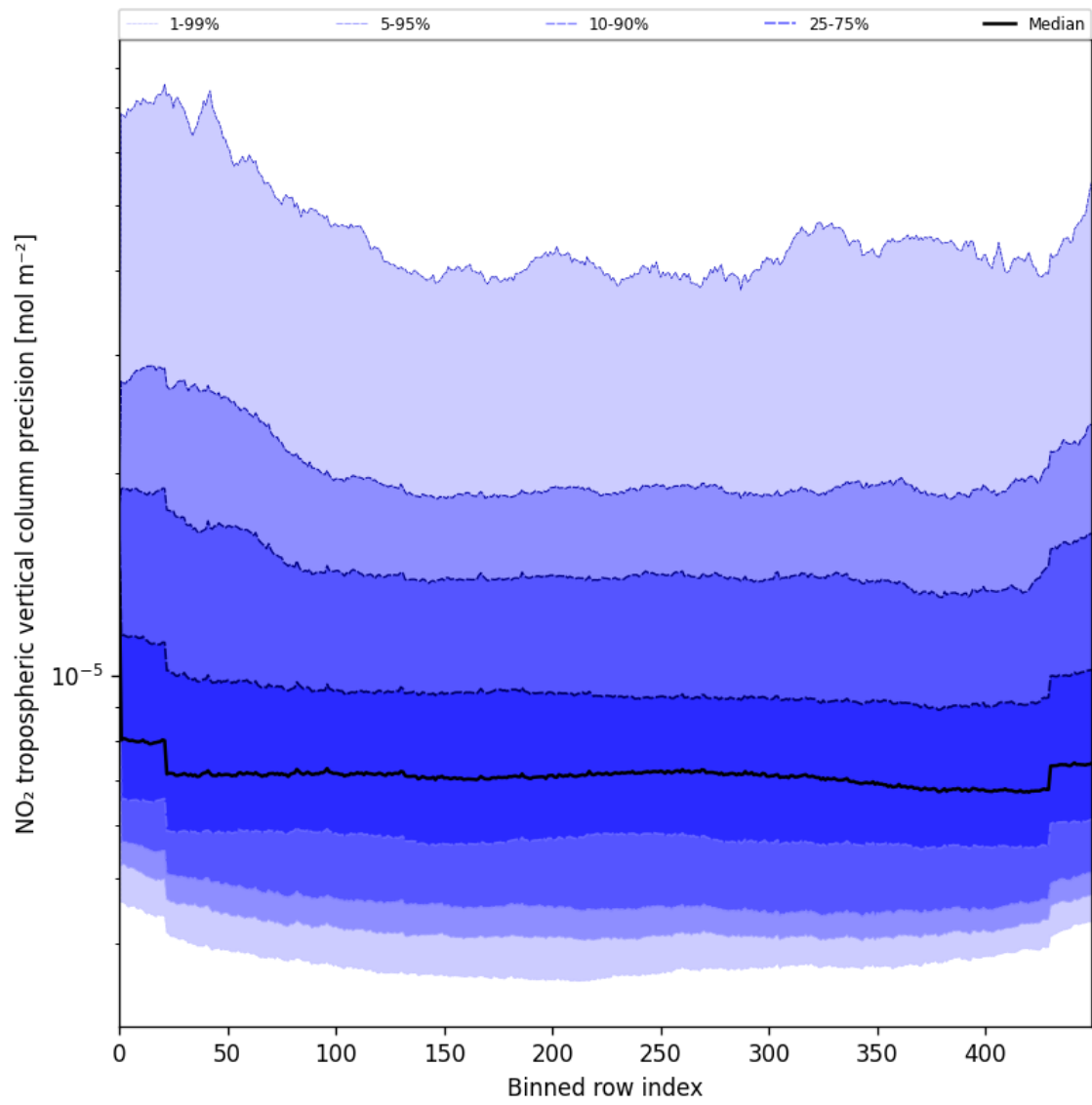
Figure 47: Along track statistics of “NO 2 tropospheric vertical column precision” for 2025-07-08 to 2025-07-09
