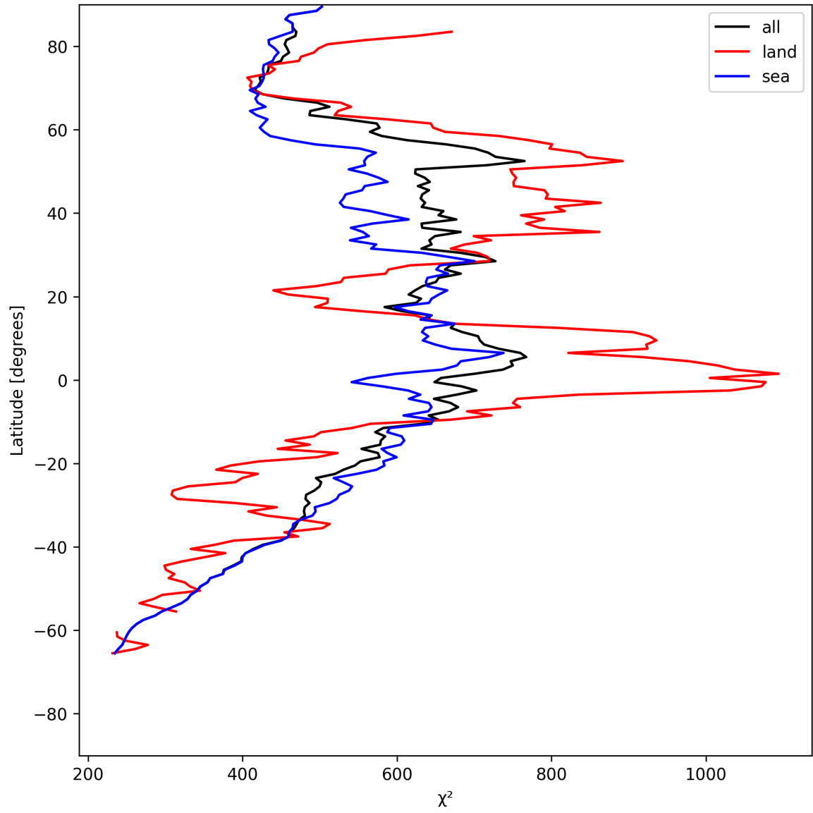
Figure 25: Zonal average of “ \chi^2 ” for 2025-07-08 to 2025-07-09.
