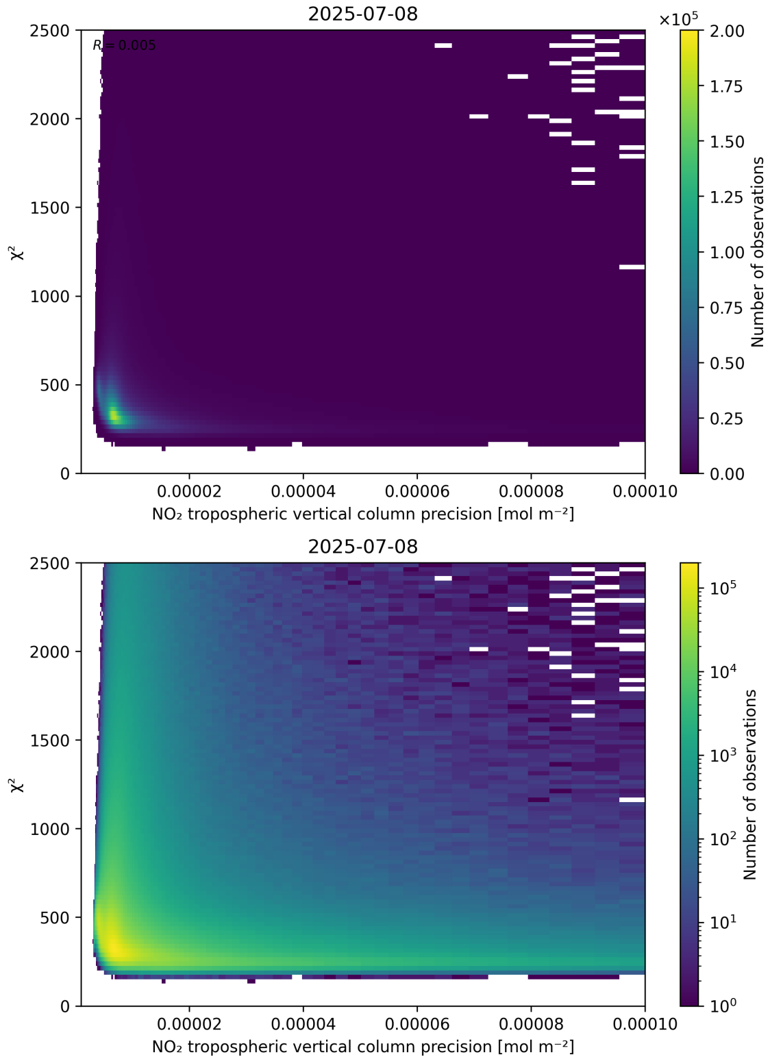
Figure 134: Scatter density plot of “NO 2 tropospheric vertical column precision” against “ \chi^2 ” for 2025-07-08 to 2025-07-09.
