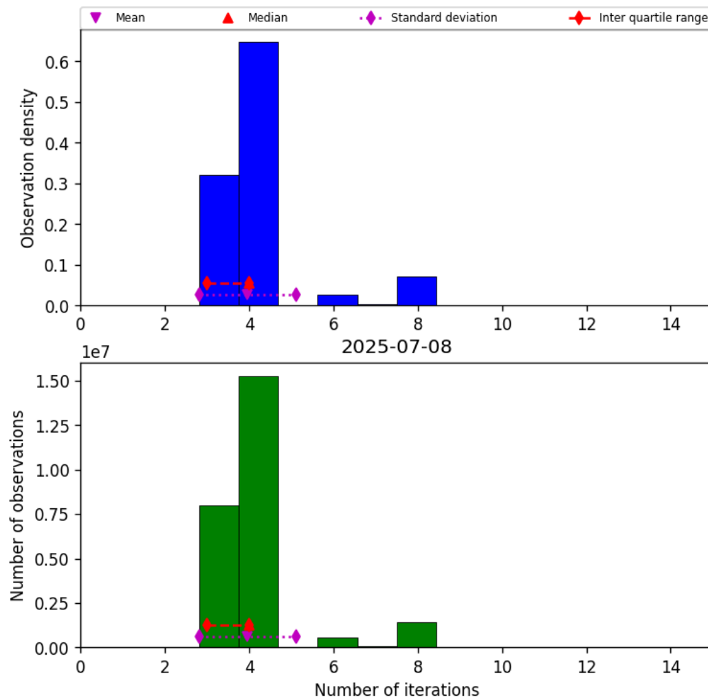
Figure 34: Histogram of “Number of iterations” for 2025-07-08 to 2025-07-09
