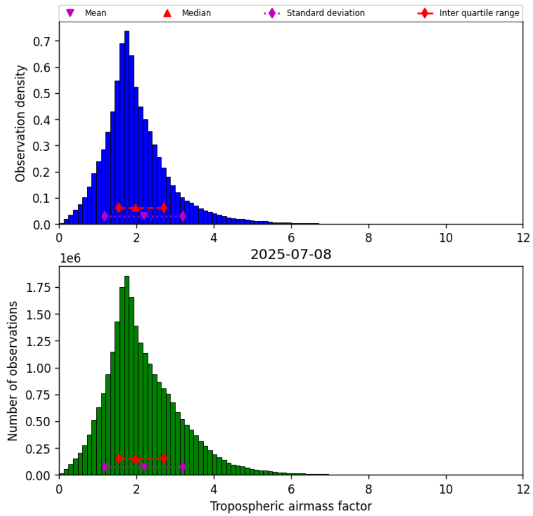
Figure 31: Histogram of “Tropospheric airmass factor” for 2025-07-08 to 2025-07-09
