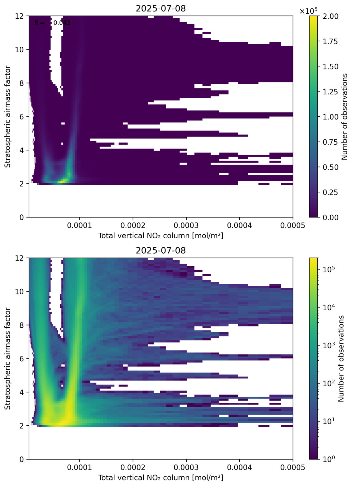
Figure 110: Scatter density plot of “Total vertical NO 2 column” against “Stratospheric air mass factor” for 2025-07-08 to 2025-07-09.
