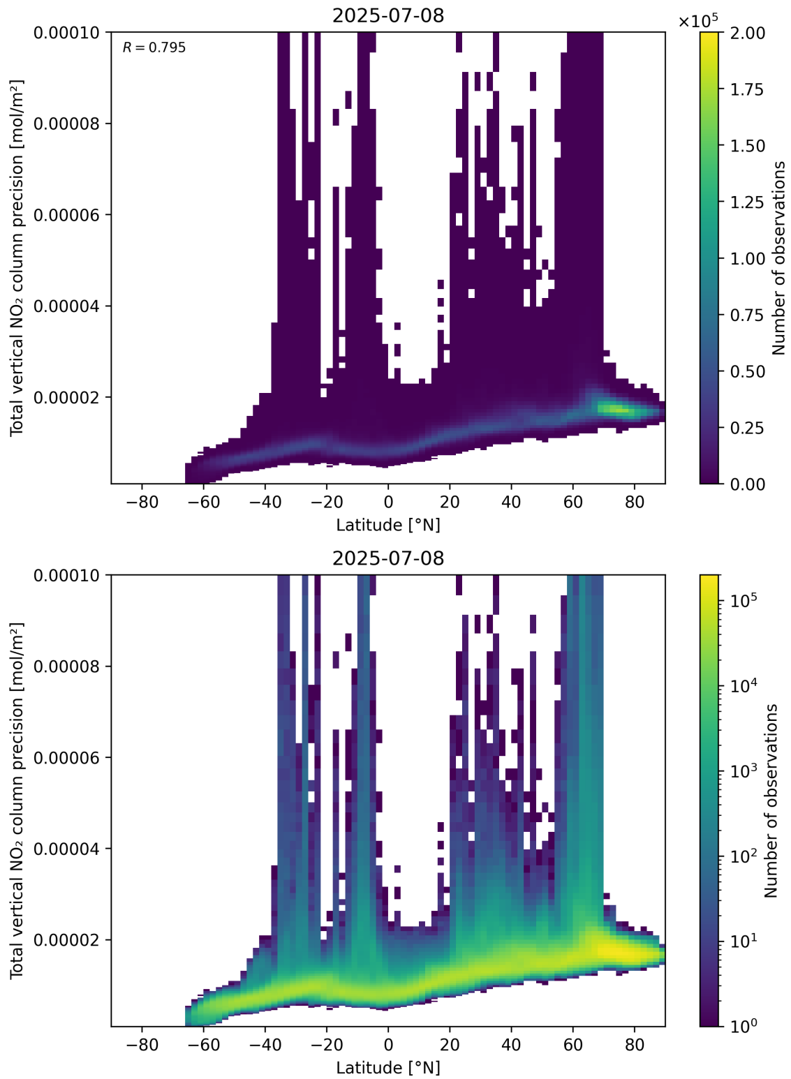
Figure 91: Scatter density plot of “Latitude” against “Total vertical NO 2 column precision” for 2025-07-08 to 2025-07-09.
