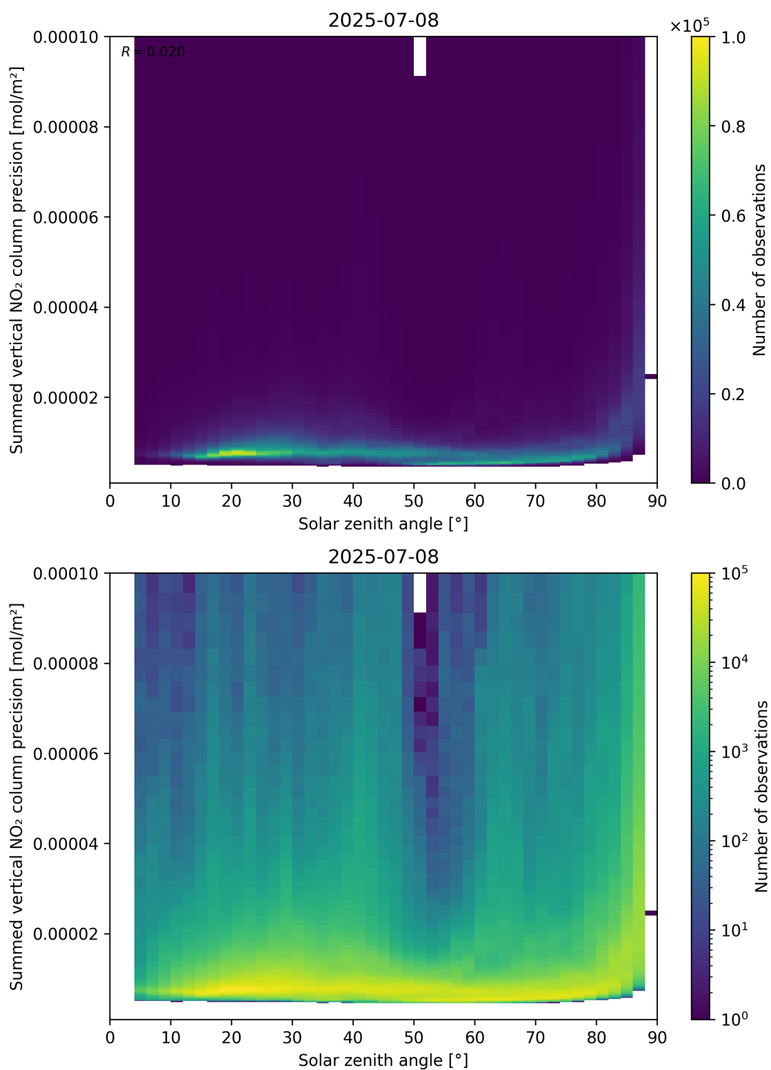
Figure 152: Scatter density plot of “Solar zenith angle” against “Summed vertical NO 2 column precision” for 2025-07-08 to 2025-07-09.
