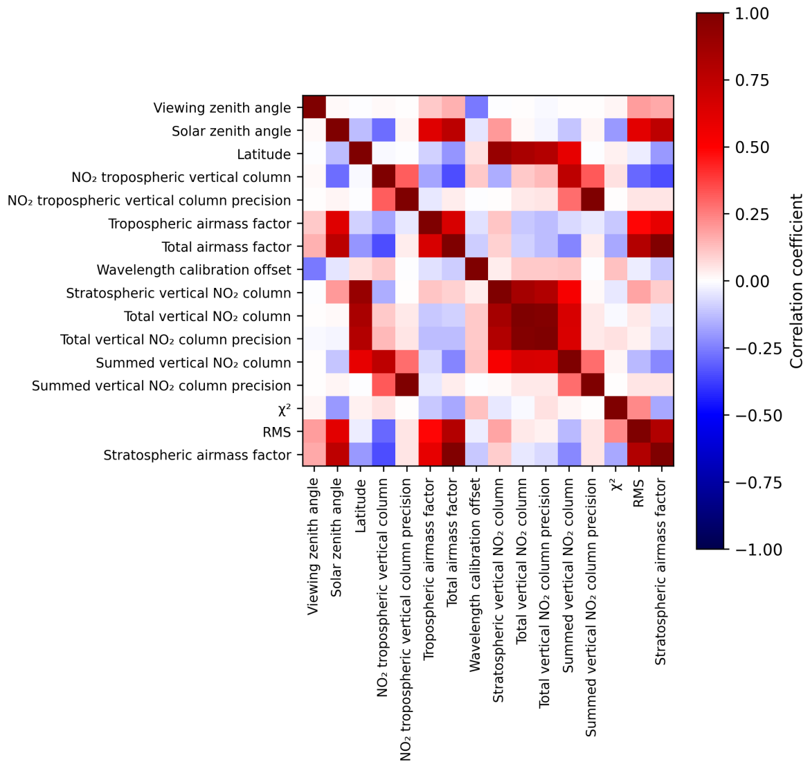
Figure 2: Map of correlation matrix for 2025-07-08 to 2025-07-09.
