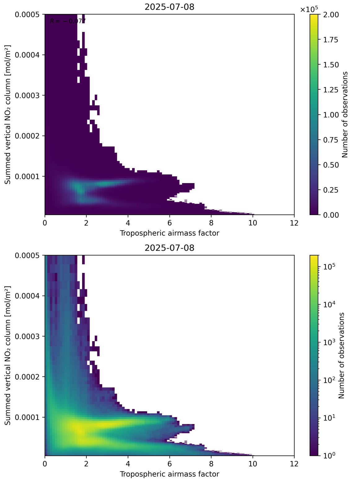
Figure 75: Scatter density plot of “Tropospheric air mass factor” against “Summed vertical NO 2 column” for 2025-07-08 to 2025-07-09.
