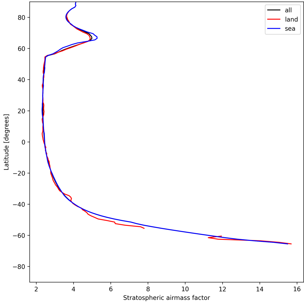
Figure 27: Zonal average of “Stratospheric airmass factor” for 2025-07-08 to 2025-07-09.
