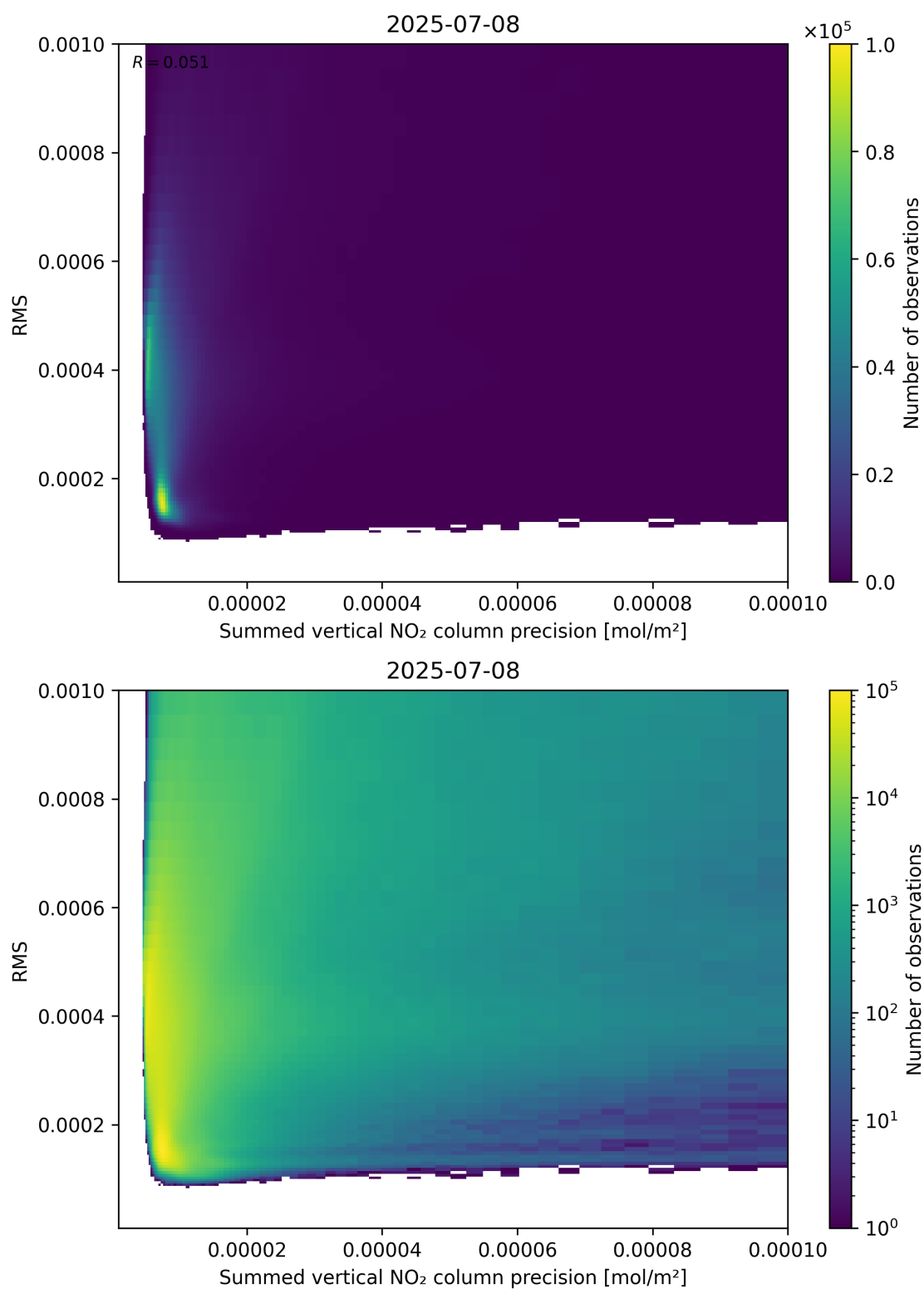
Figure 108: Scatter density plot of “Summed vertical NO 2 column precision” against “RMS” for 2025-07-08 to 2025-07-09.
