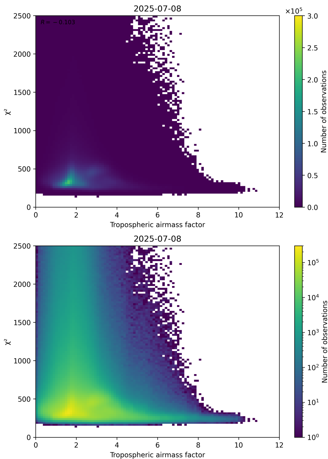
Figure 73: Scatter density plot of “Tropospheric airmass factor” against “ \chi^2 ” for 2025-07-08 to 2025-07-09.
