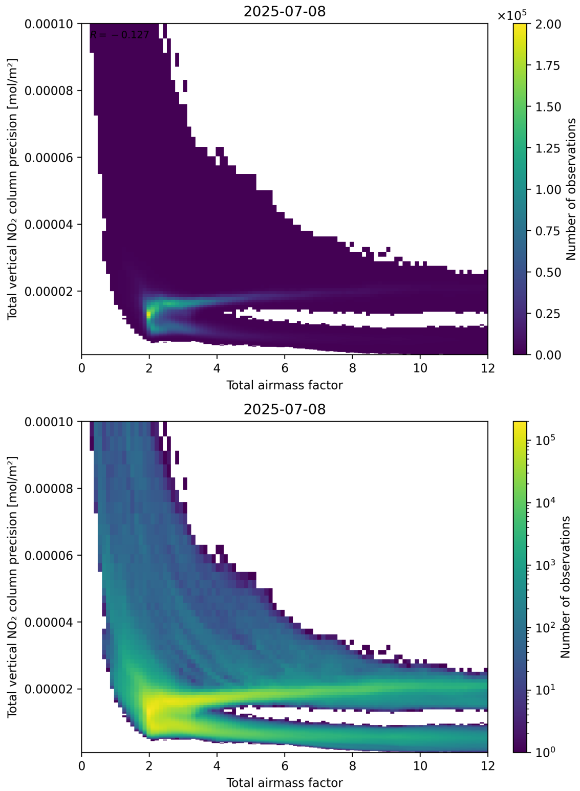
Figure 68: Scatter density plot of “Total airmass factor” against “Total vertical NO 2 column precision” for 2025-07-08 to 2025-07-09.
