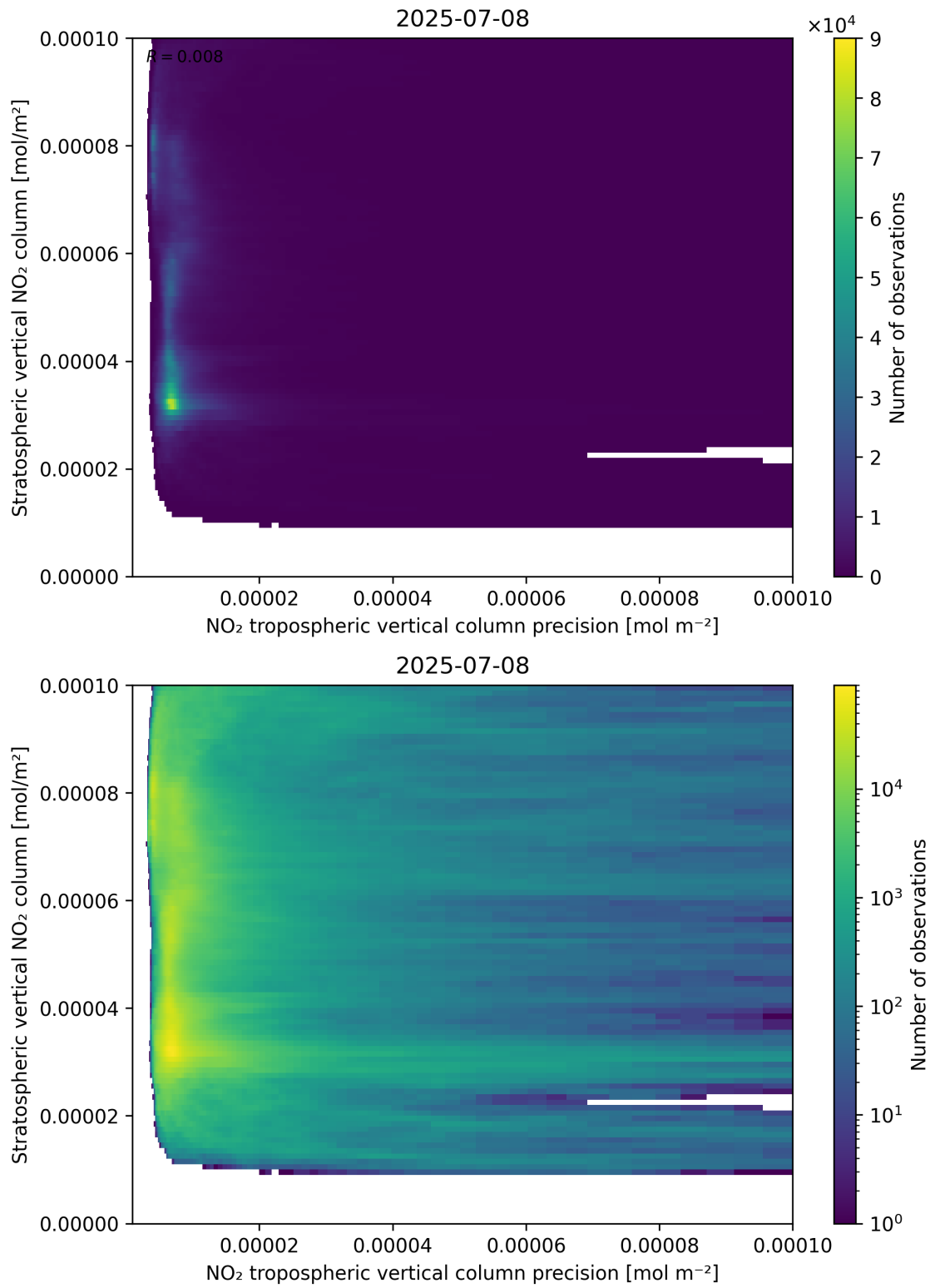
Figure 135: Scatter density plot of “NO 2 tropospheric vertical column precision” against “Stratospheric vertical NO 2 column” for 2025-07-08 to 2025-07-09.
