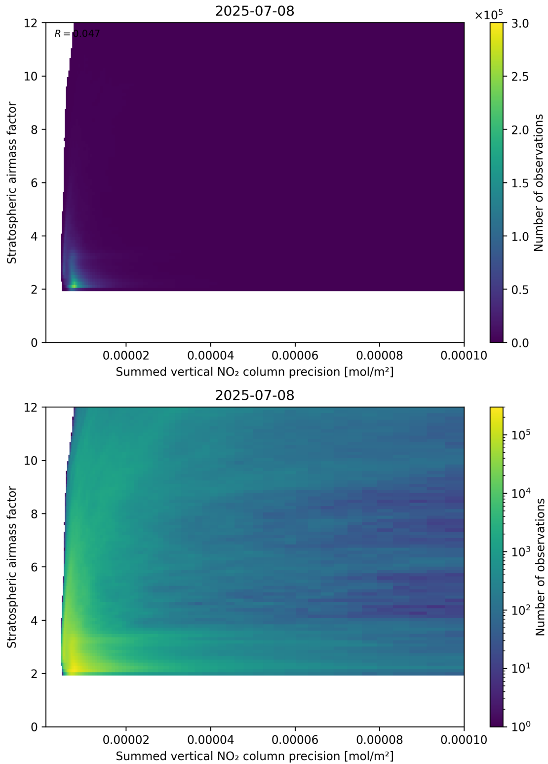
Figure 106: Scatter density plot of “Summed vertical NO 2 column precision” against “Stratospheric airmass factor” for 2025-07-08 to 2025-07-09.
