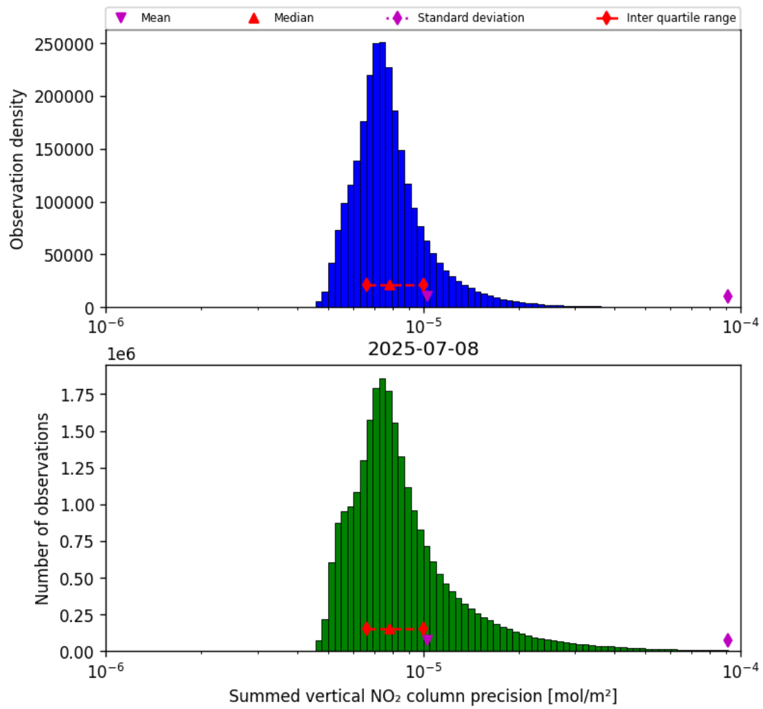
Figure 41: Histogram of “Summed vertical NO 2 column precision” for 2025-07-08 to 2025-07-09
