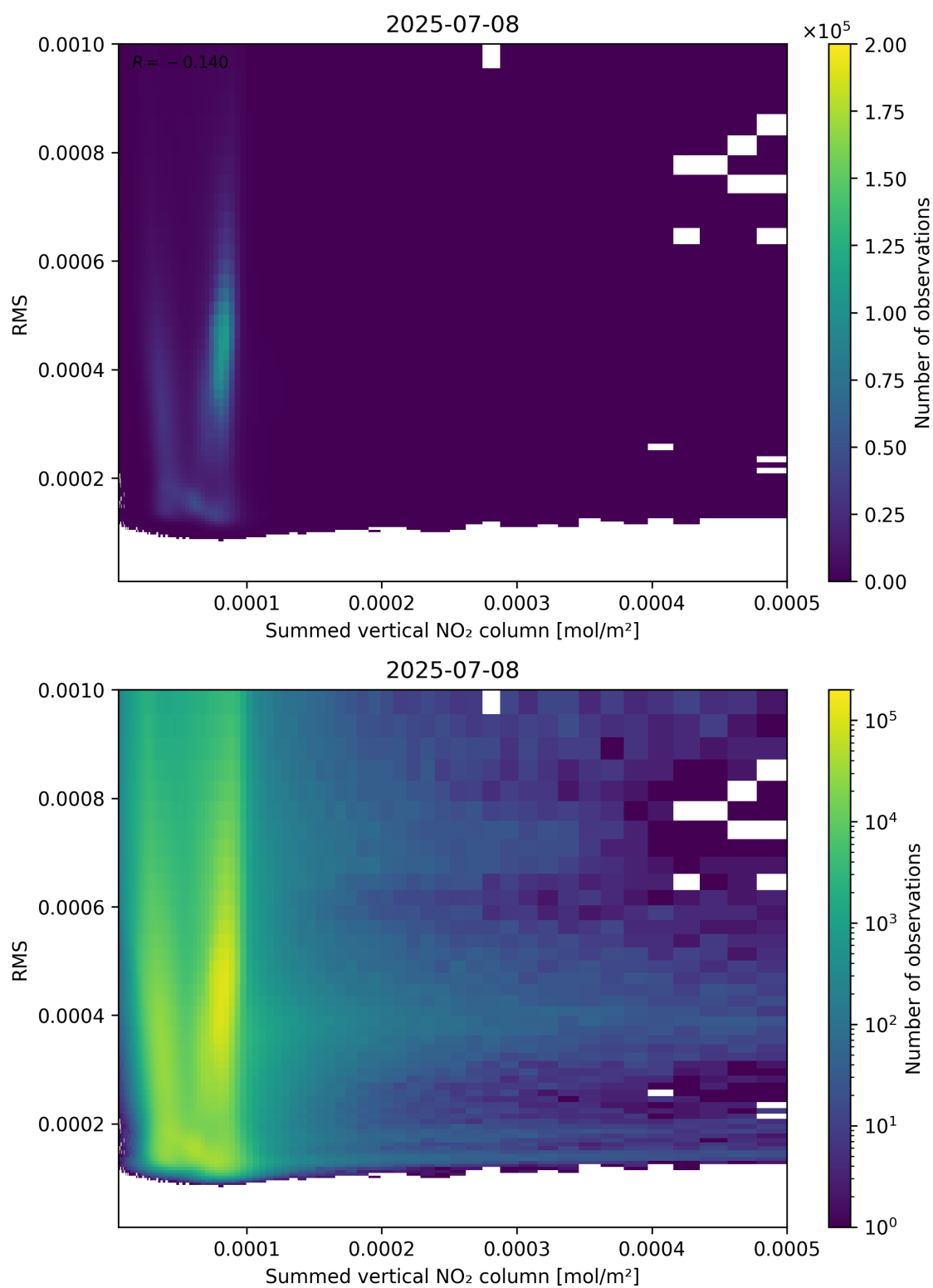
Figure 109: Scatter density plot of “Summed vertical NO 2 column” against “RMS” for 2025-07-08 to 2025-07-09.
