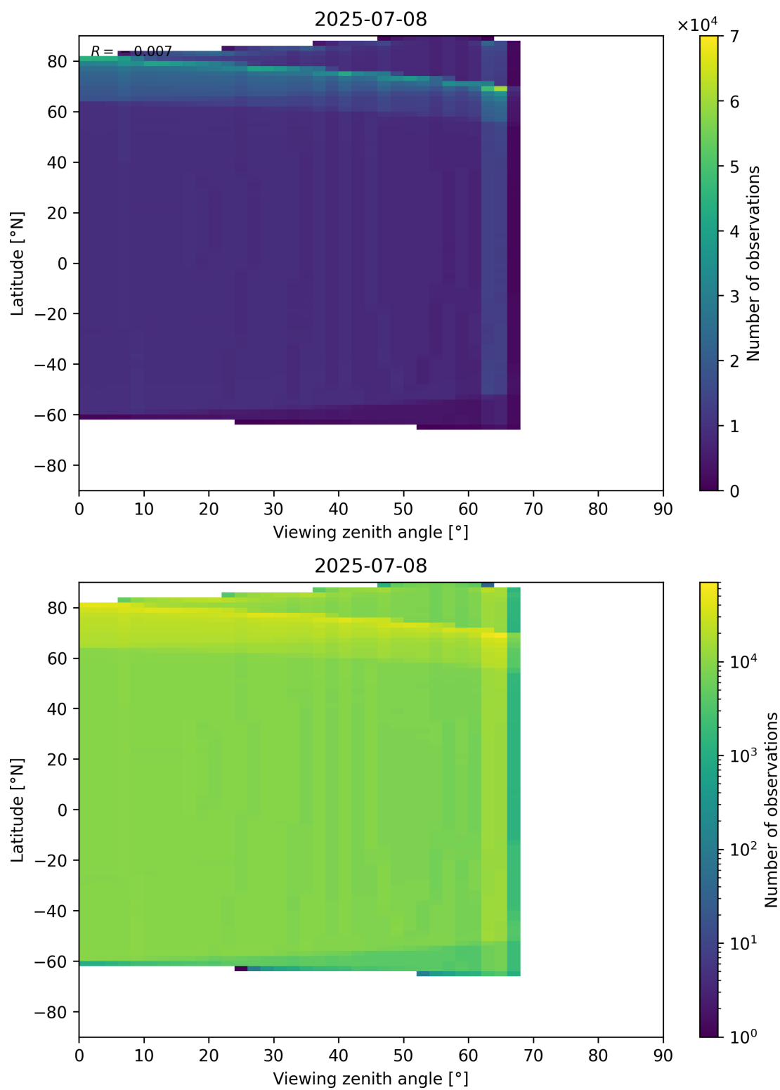
Figure 163: Scatter density plot of “Viewing zenith angle” against “Latitude” for 2025-07-08 to 2025-07-09.
