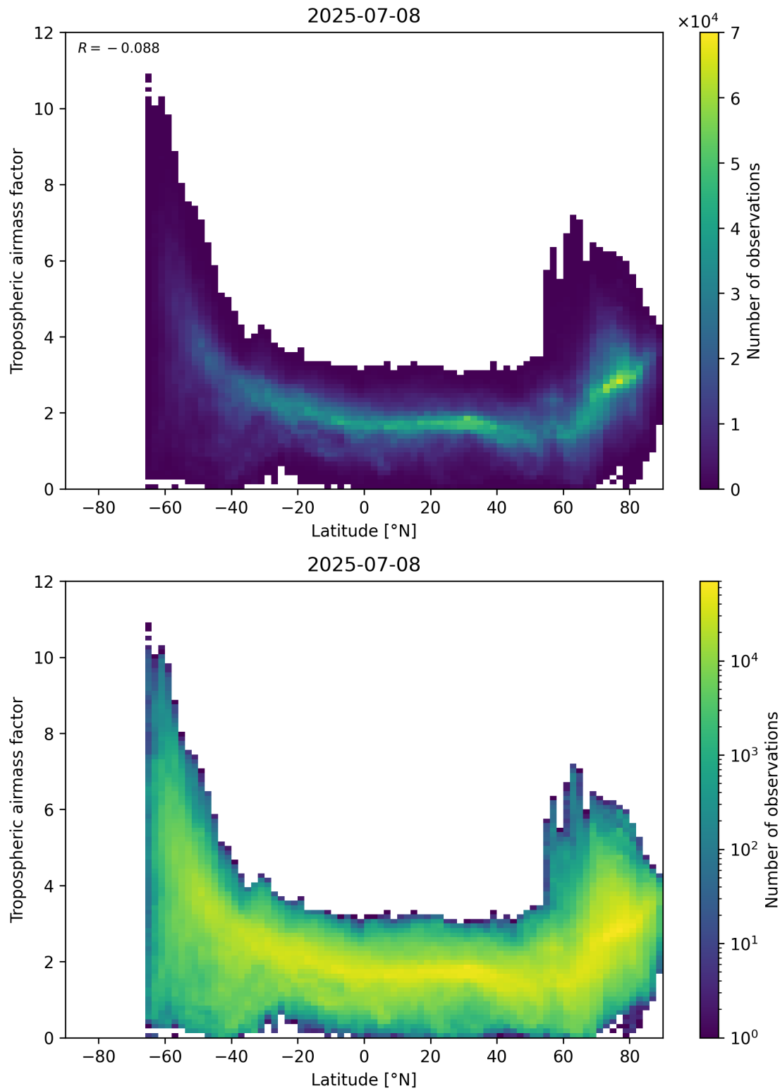
Figure 85: Scatter density plot of “Latitude” against “Tropospheric air mass factor” for 2025-07-08 to 2025-07-09.
