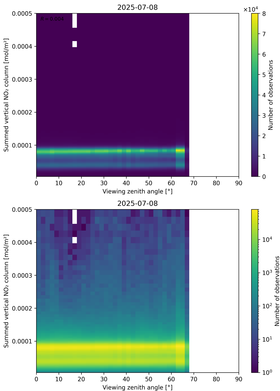
Figure 165: Scatter density plot of “Viewing zenith angle” against “Summed vertical NO 2 column” for 2025-07-08 to 2025-07-09.
