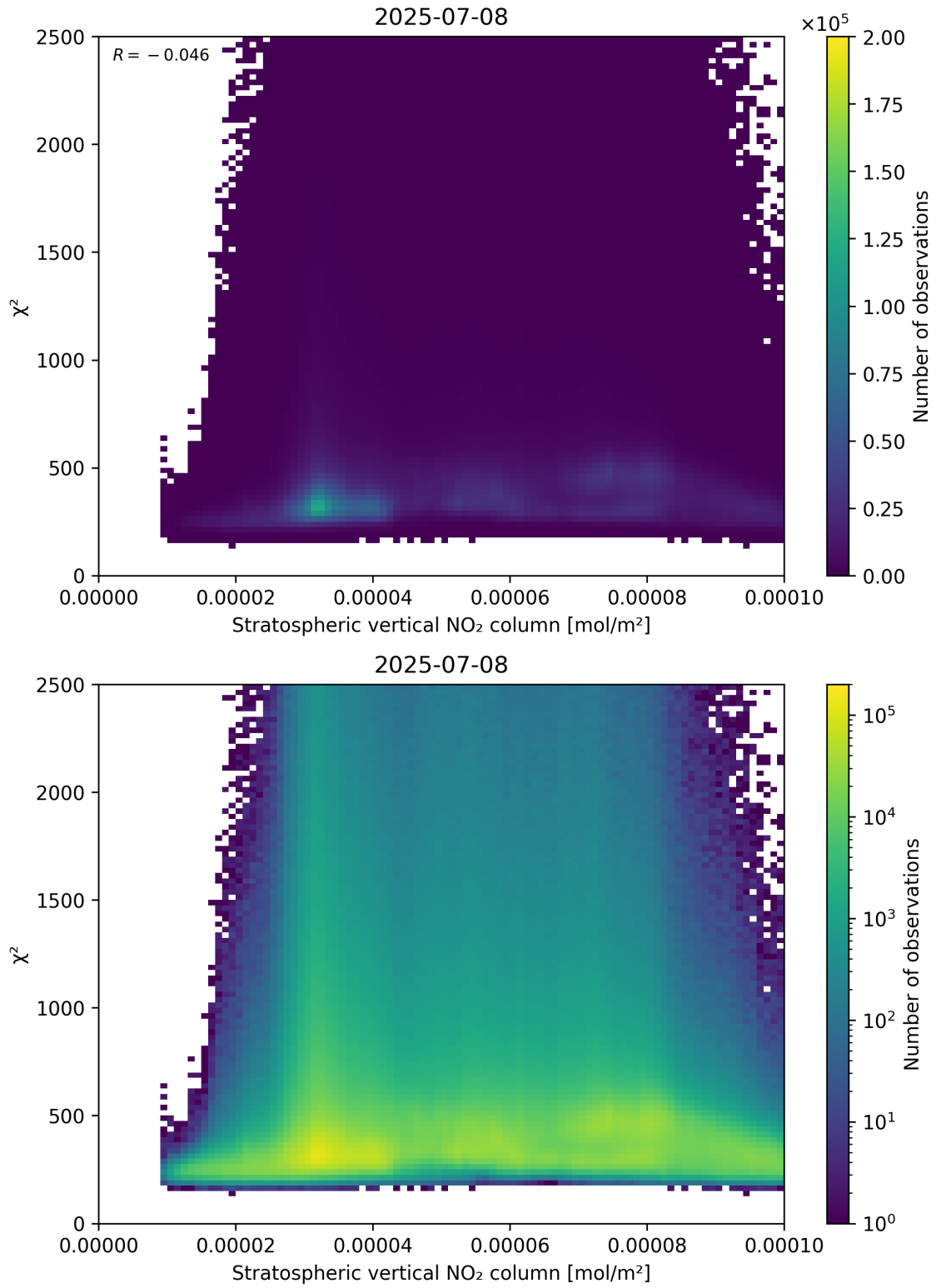
Figure 97: Scatter density plot of “Stratospheric vertical NO 2 column” against “ \chi^2 ” for 2025-07-08 to 2025-07-09.
