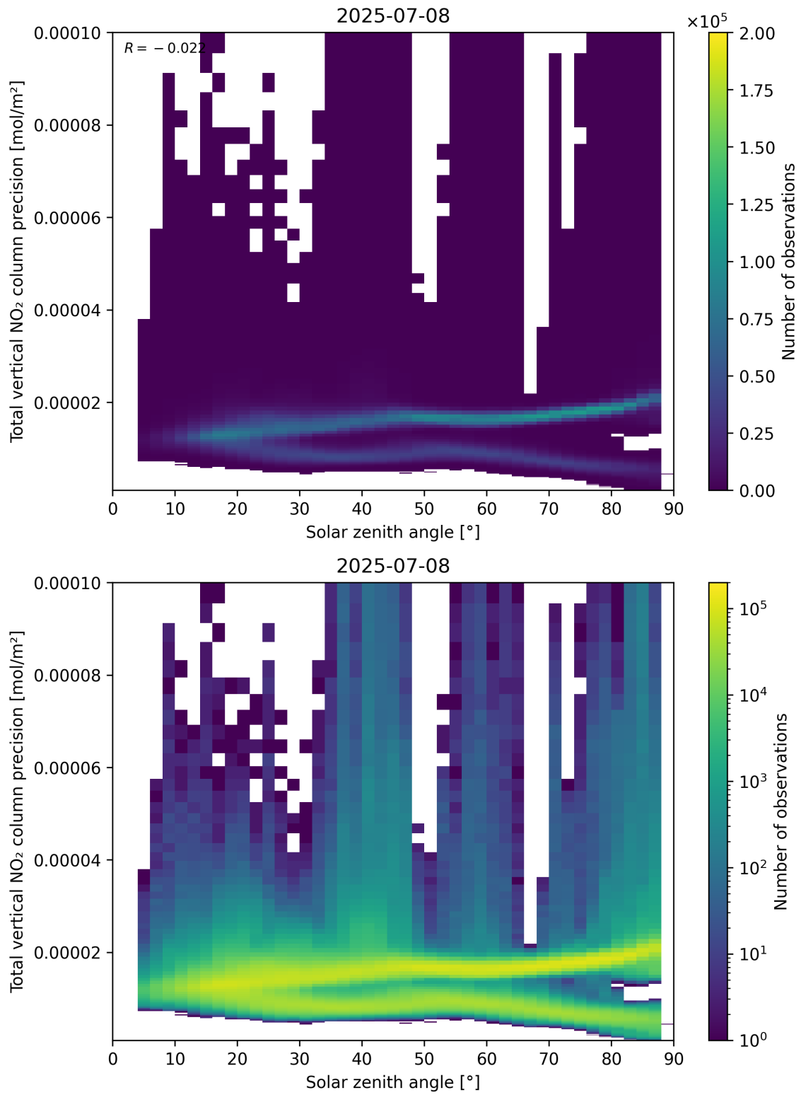
Figure 154: Scatter density plot of “Solar zenith angle” against “Total vertical NO 2 column precision” for 2025-07-08 to 2025-07-09.
