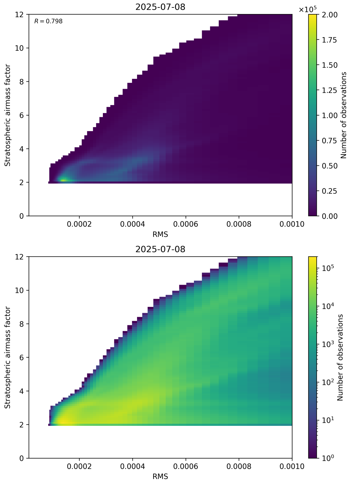
Figure 144: Scatter density plot of “RMS” against “Stratospheric airmass factor” for 2025-07-08 to 2025-07-09.
