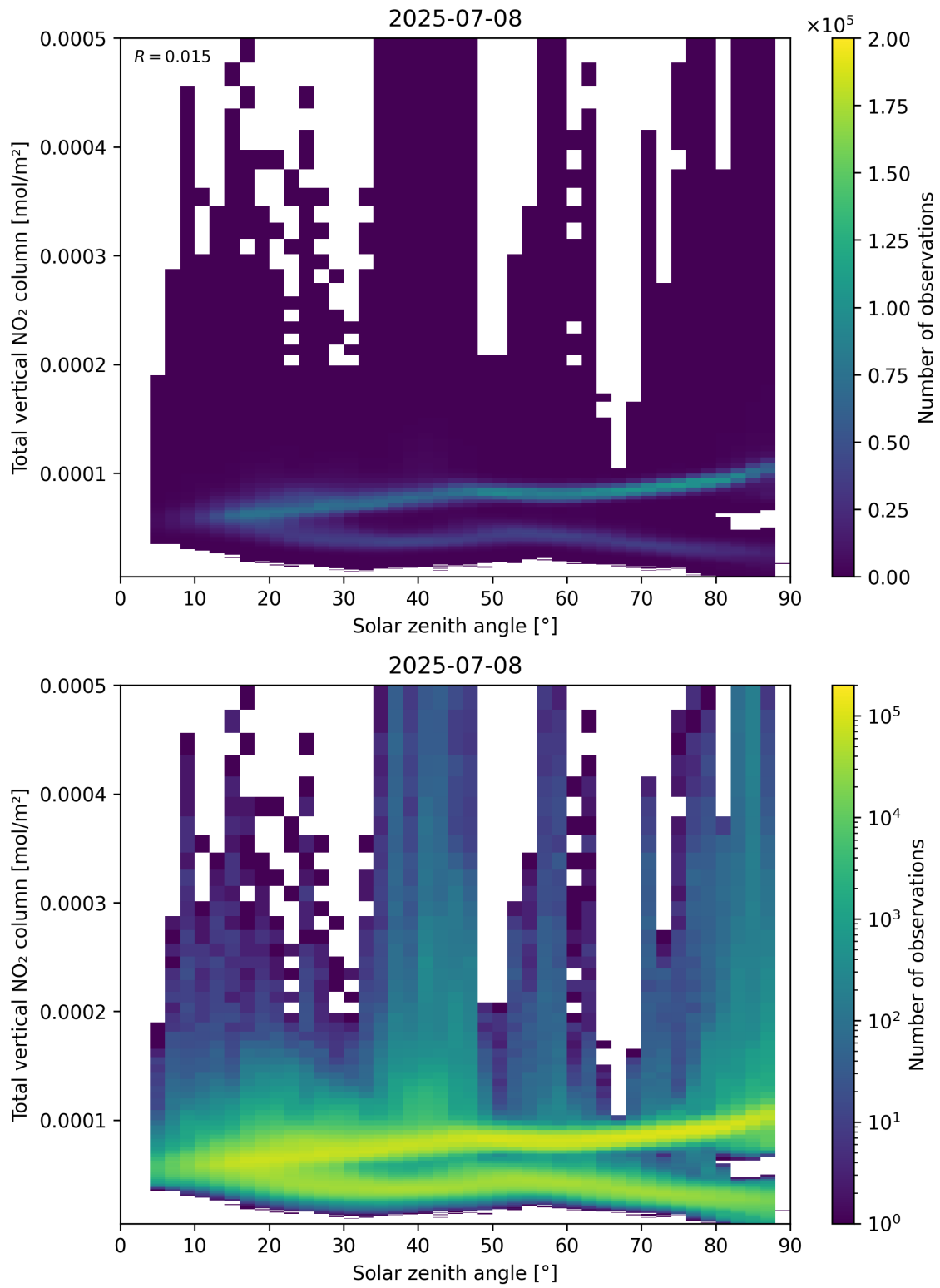
Figure 153: Scatter density plot of “Solar zenith angle” against “Total vertical NO 2 column” for 2025-07-08 to 2025-07-09.
