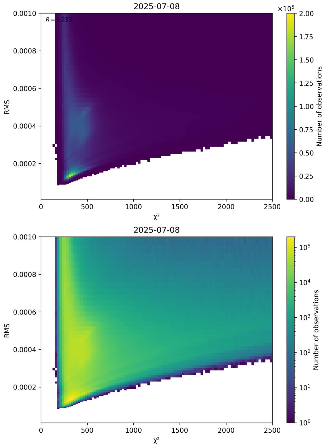
Figure 82: Scatter density plot of “ \chi^2 ” against “RMS” for 2025-07-08 to 2025-07-09.
