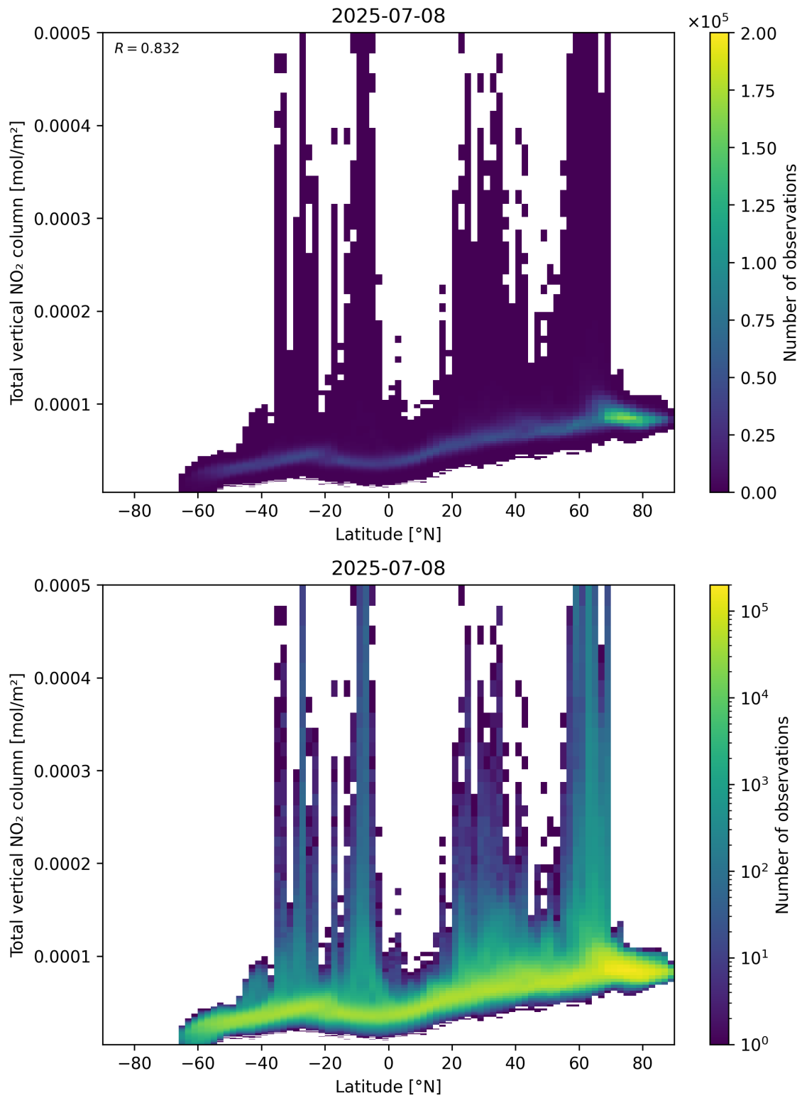
Figure 90: Scatter density plot of “Latitude” against “Total vertical NO 2 column” for 2025-07-08 to 2025-07-09.
