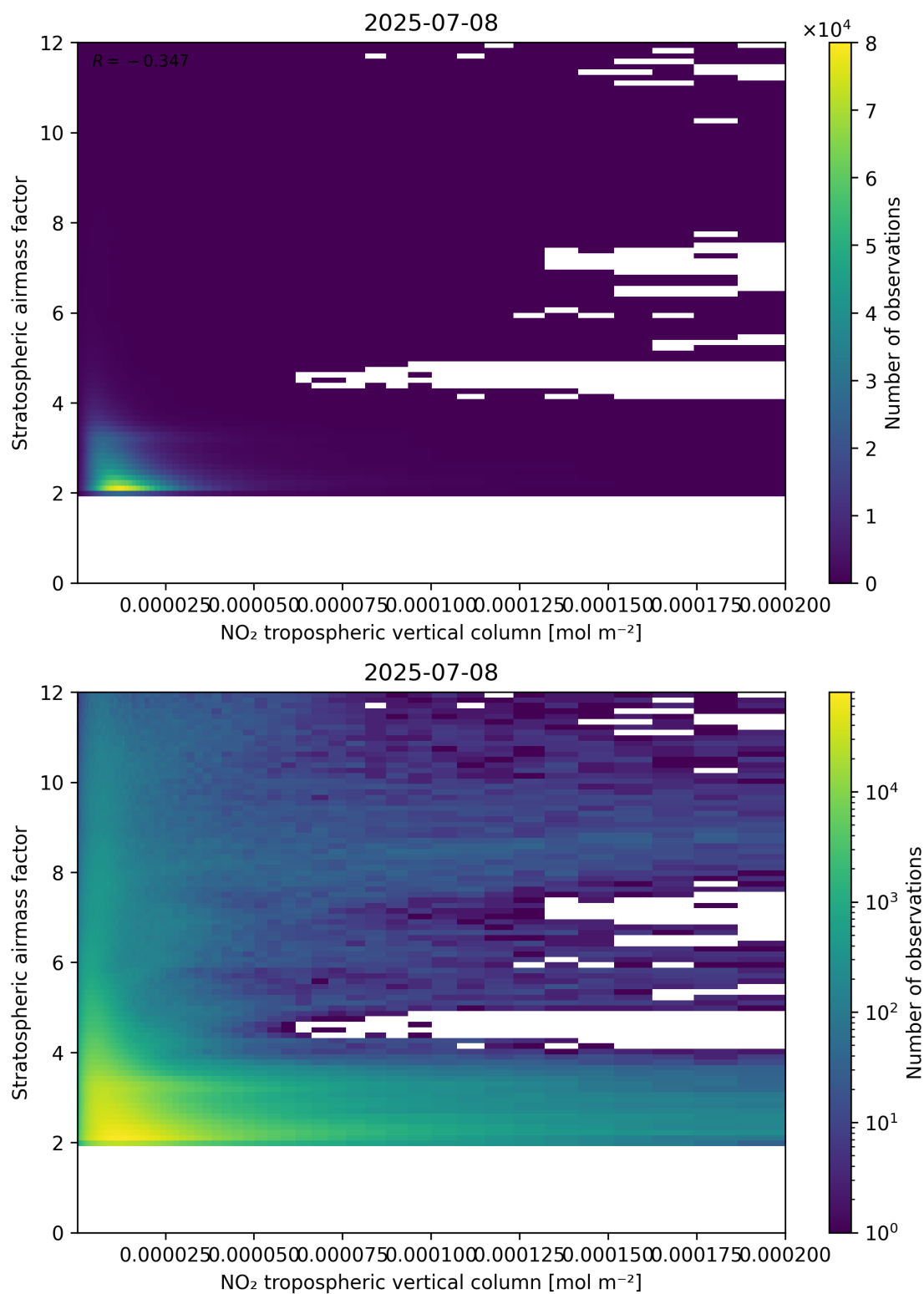
Figure 121: Scatter density plot of “NO 2 tropospheric vertical column” against “Stratospheric air mass factor” for 2025-07-08 to 2025-07-09.
