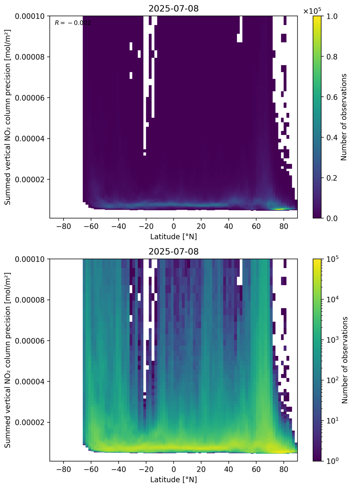
Figure 89: Scatter density plot of “Latitude” against “Summed vertical NO 2 column precision” for 2025-07-08 to 2025-07-09.
