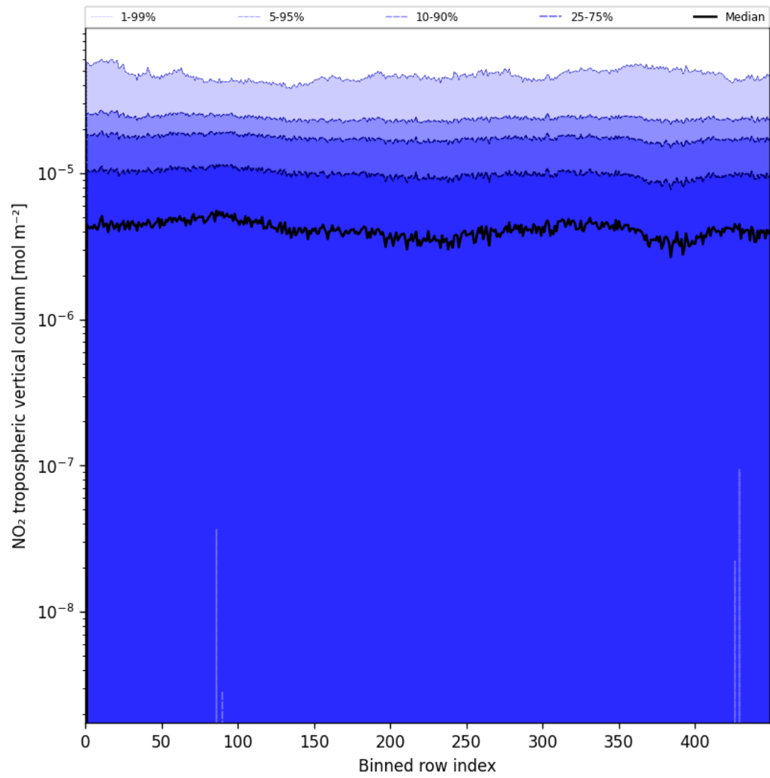
Figure 46: Along track statistics of “NO 2 tropospheric vertical column” for 2025-07-08 to 2025-07-09
