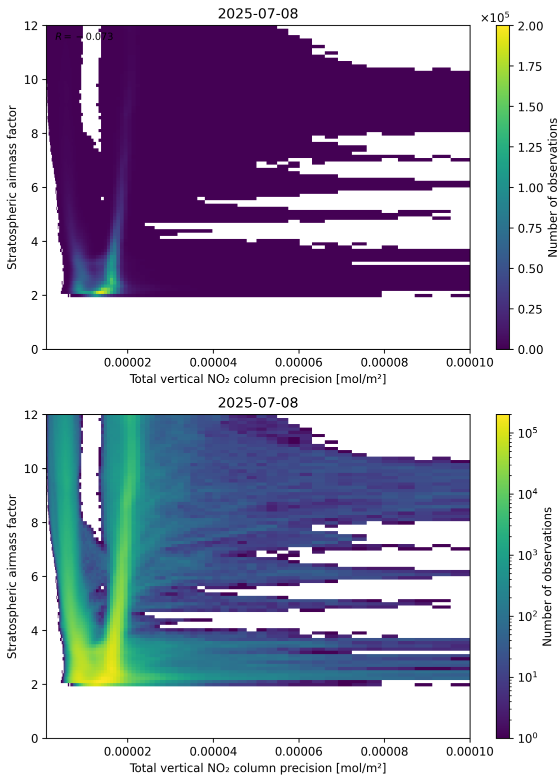
Figure 115: Scatter density plot of “Total vertical NO 2 column precision” against “Stratospheric air mass factor” for 2025-07-08 to 2025-07-09.
