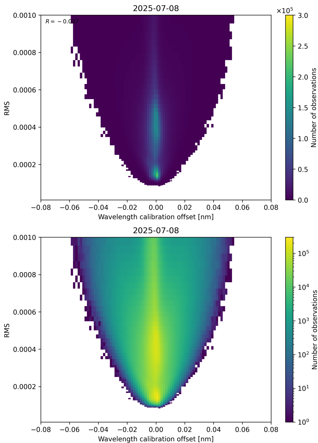
Figure 181: Scatter density plot of “Wavelength calibration offset” against “RMS” for 2025-07-08 to 2025-07-09.
