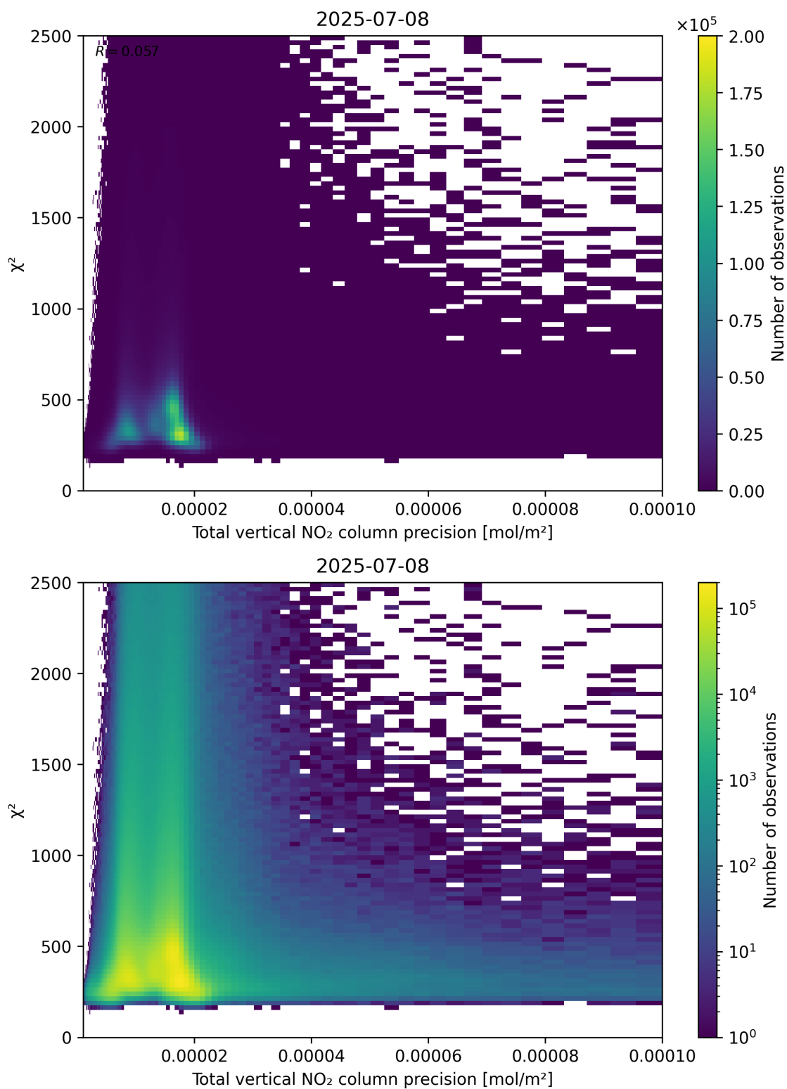
Figure 116: Scatter density plot of “Total vertical NO 2 column precision” against “ \chi^2 ” for 2025-07-08 to 2025-07-09.
