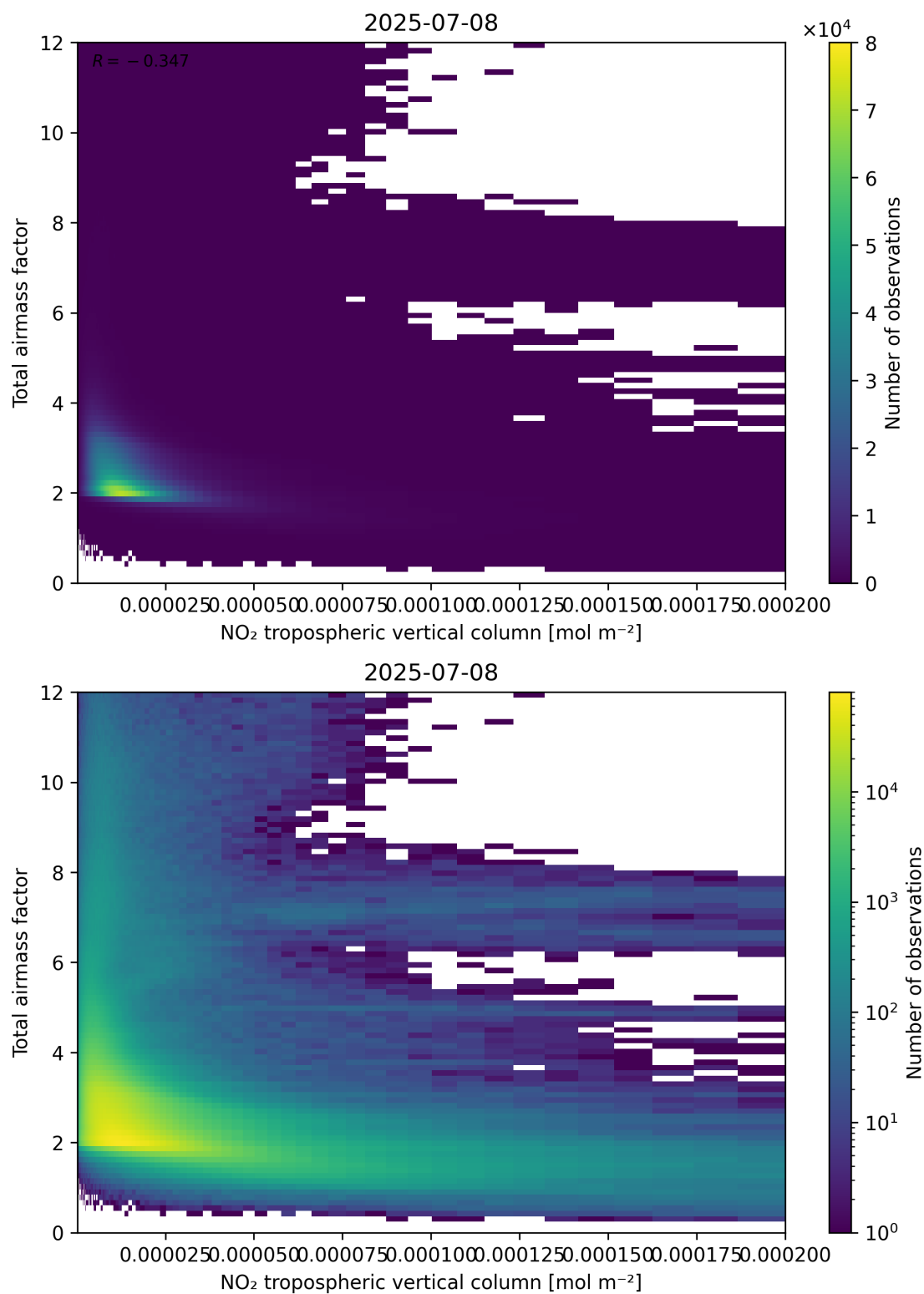
Figure 122: Scatter density plot of “NO 2 tropospheric vertical column” against “Total air mass factor” for 2025-07-08 to 2025-07-09.
