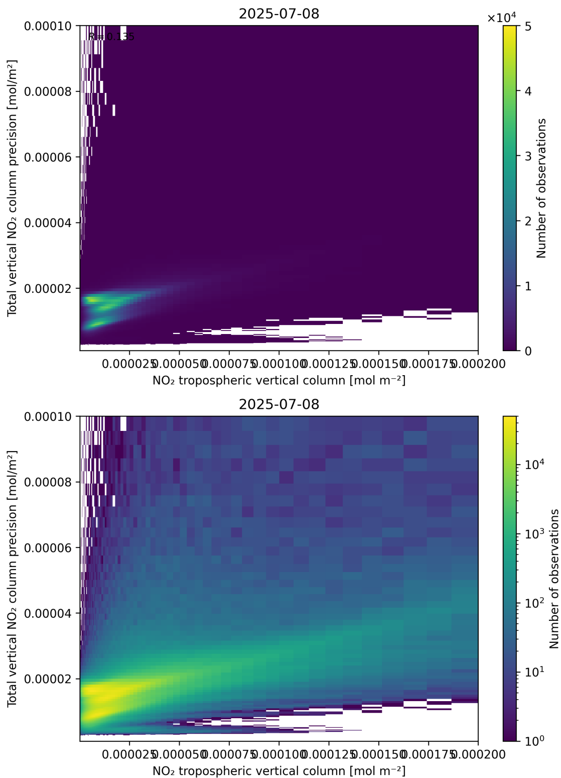
Figure 129: Scatter density plot of “NO 2 tropospheric vertical column” against “Total vertical NO 2 column precision” for 2025-07-08 to 2025-07-09.
