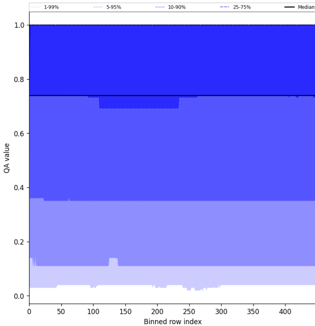
Figure 45: Along track statistics of “QA value” for 2025-07-08 to 2025-07-09
