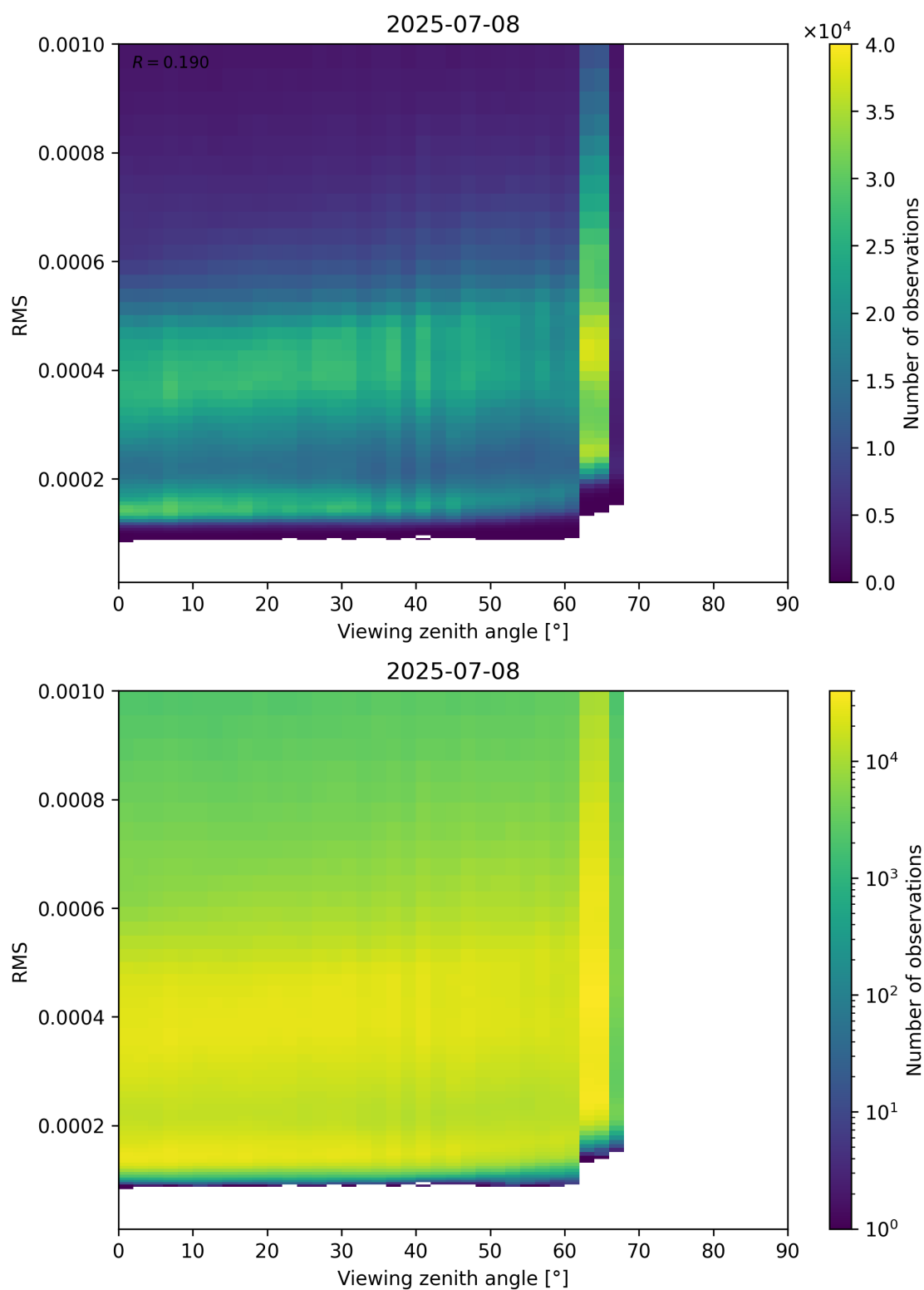
Figure 171: Scatter density plot of “Viewing zenith angle” against “RMS” for 2025-07-08 to 2025-07-09.
