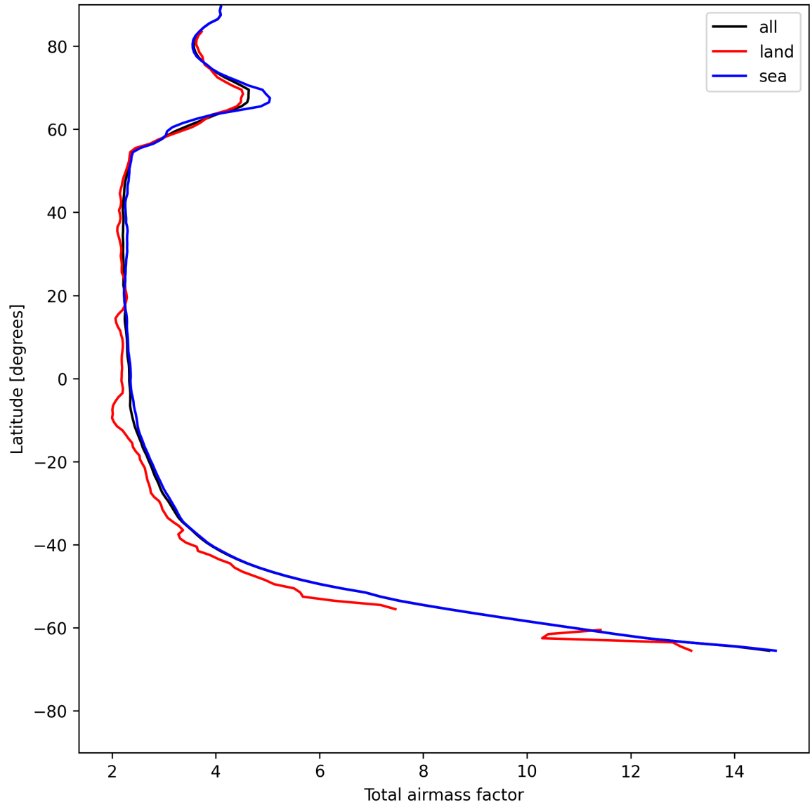
Figure 15: Zonal average of “Total airmass factor” for 2025-07-08 to 2025-07-09.
