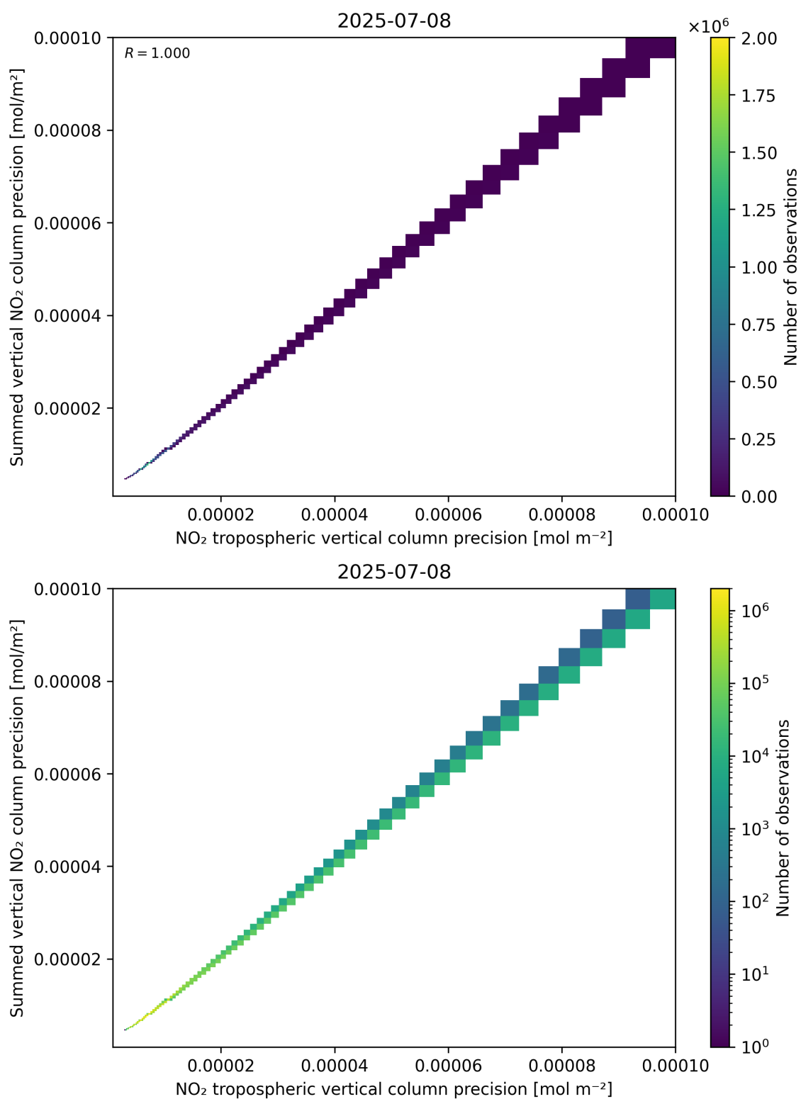
Figure 137: Scatter density plot of “NO 2 tropospheric vertical column precision” against “Summed vertical NO 2 column precision” for 2025-07-08 to 2025-07-09.
