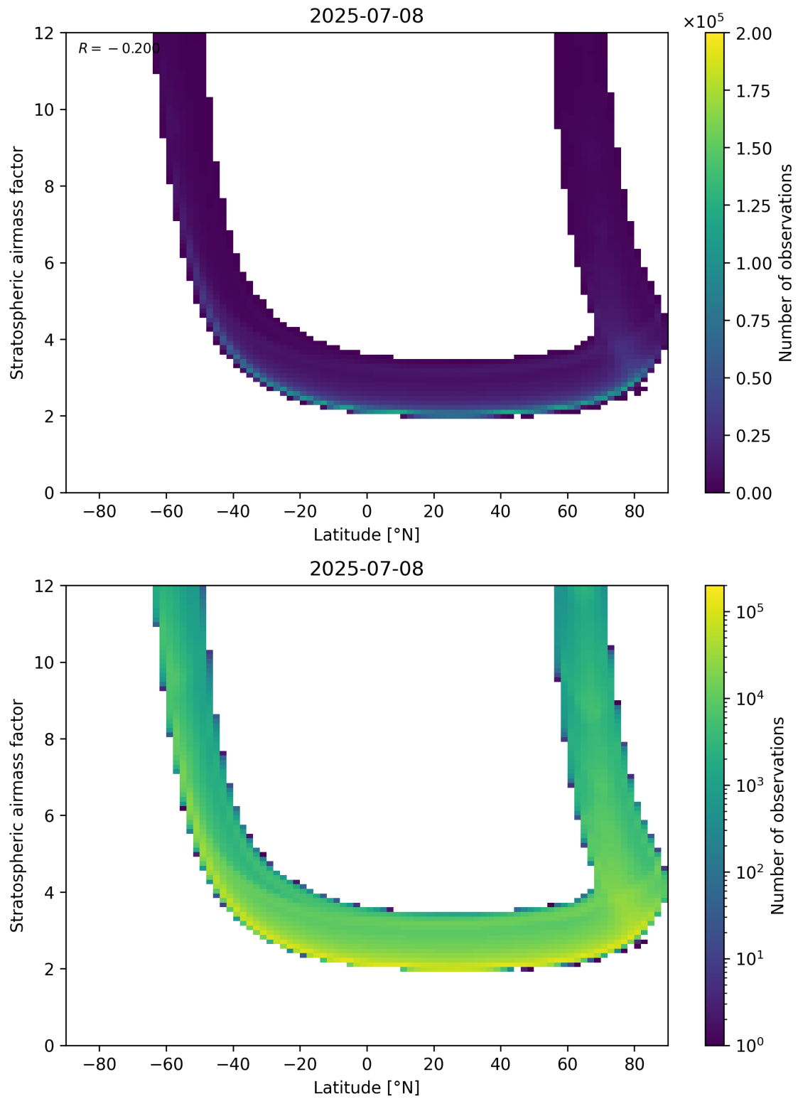
Figure 83: Scatter density plot of “Latitude” against “Stratospheric air mass factor” for 2025-07-08 to 2025-07-09.
