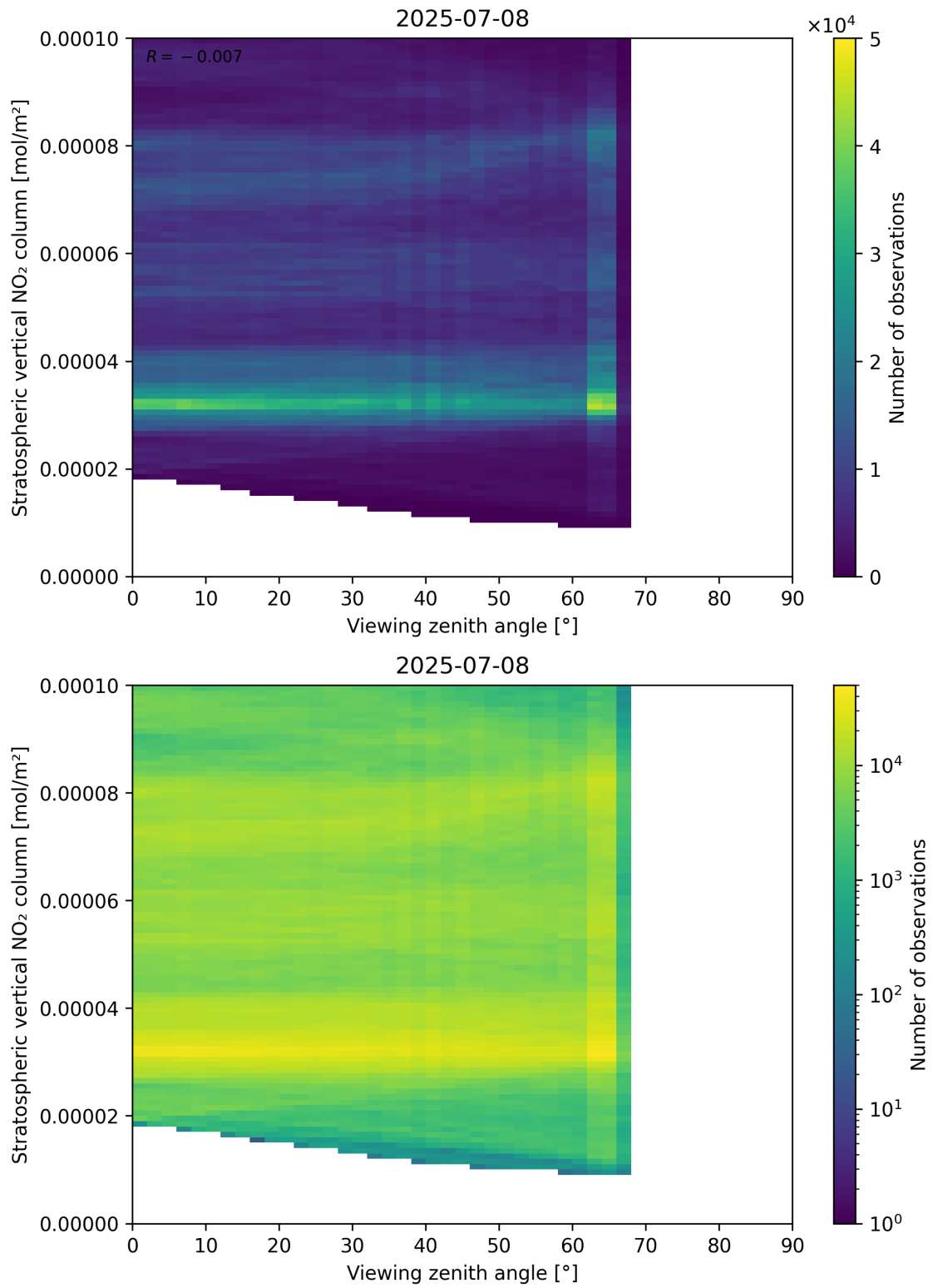
Figure 164: Scatter density plot of “Viewing zenith angle” against “Stratospheric vertical NO 2 column” for 2025-07-08 to 2025-07-09.
