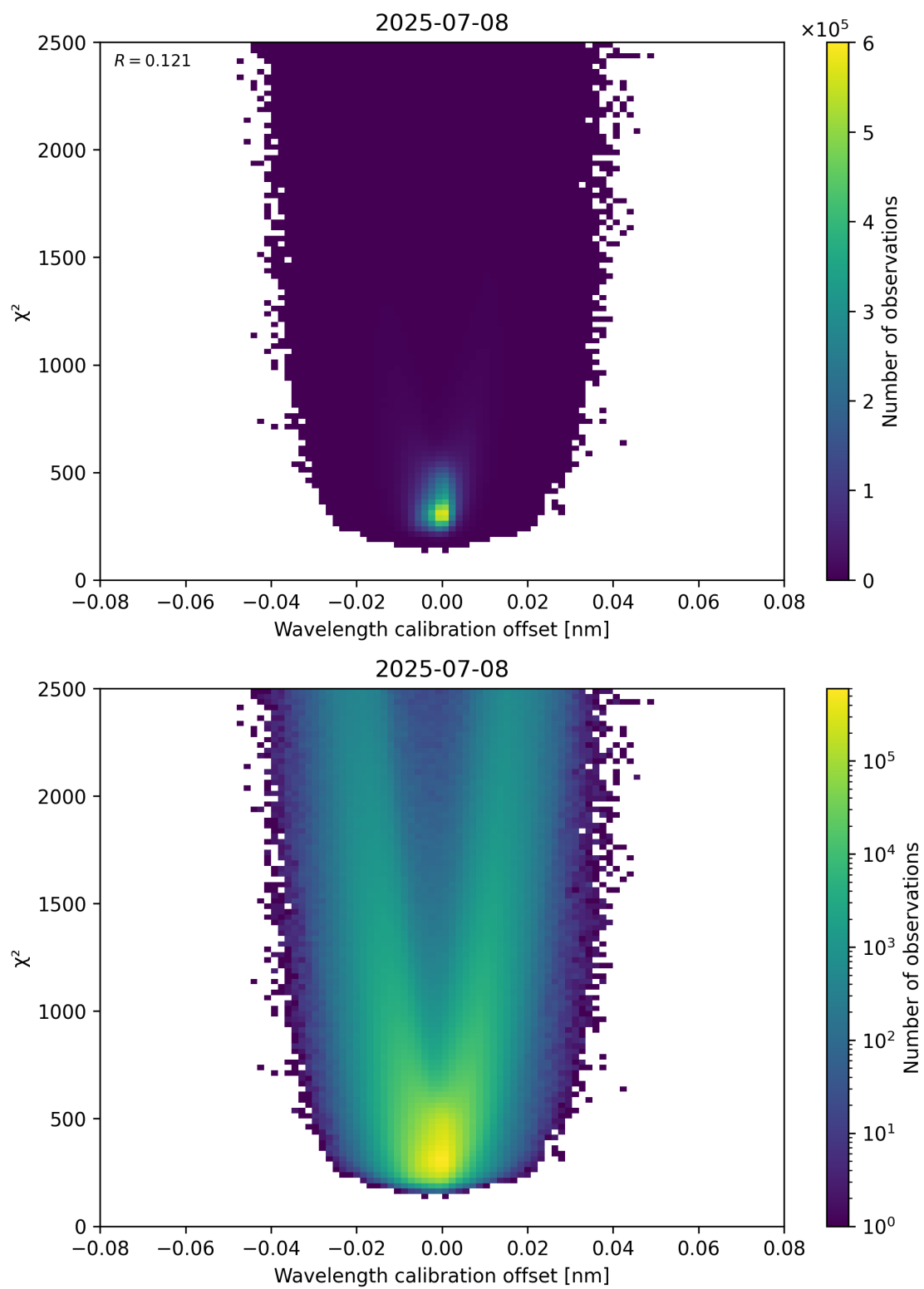
Figure 175: Scatter density plot of “Wavelength calibration offset” against “ \chi^2 ” for 2025-07-08 to 2025-07-09.
