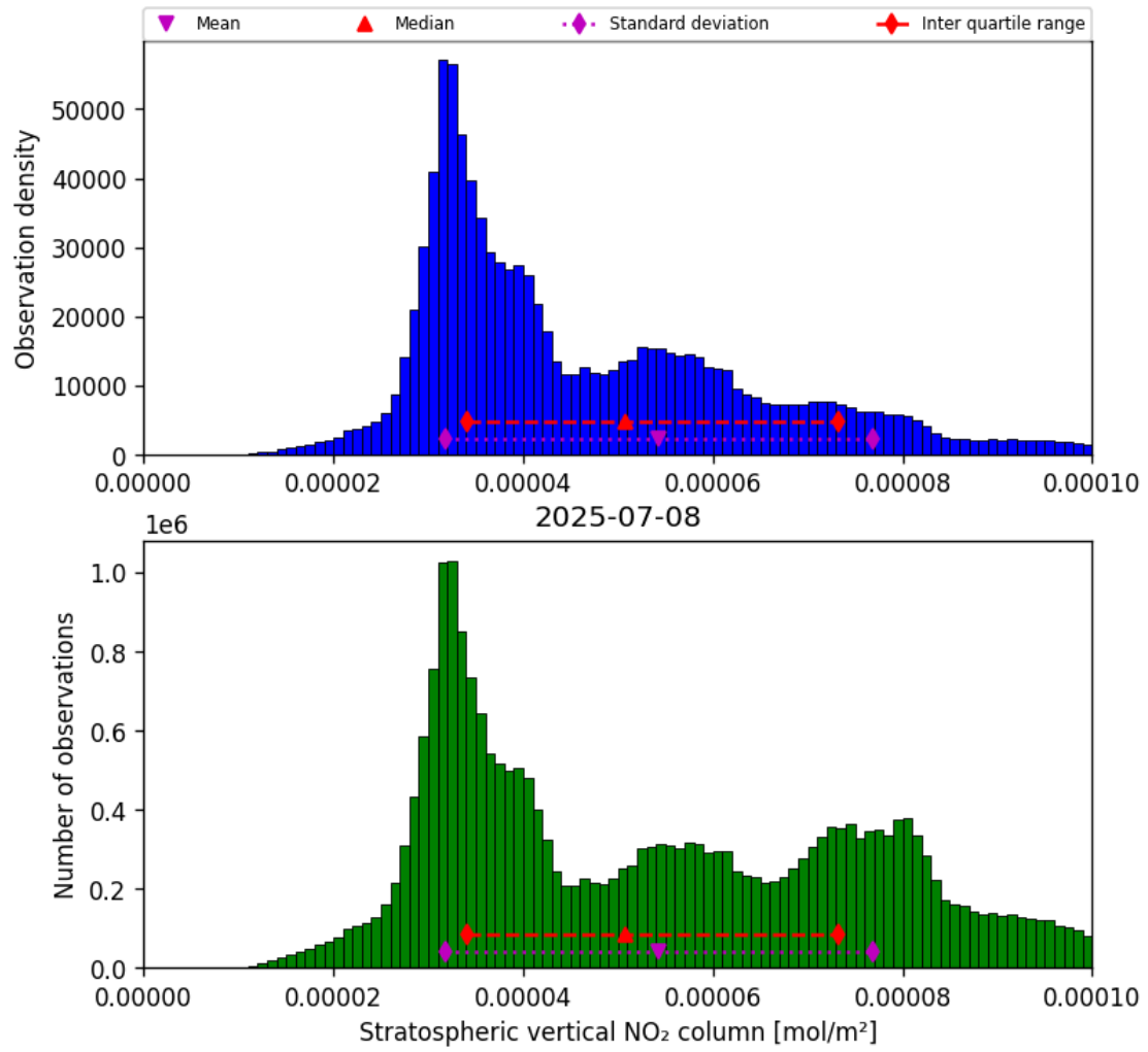
Figure 36: Histogram of “Stratospheric vertical NO 2 column” for 2025-07-08 to 2025-07-09
