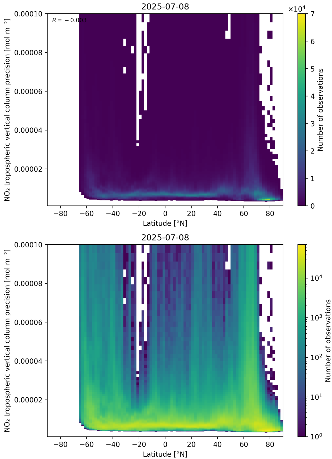
Figure 93: Scatter density plot of “Latitude” against “NO 2 tropospheric vertical column precision” for 2025-07-08 to 2025-07-09.
