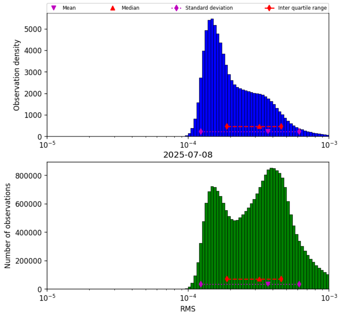
Figure 43: Histogram of “RMS” for 2025-07-08 to 2025-07-09
