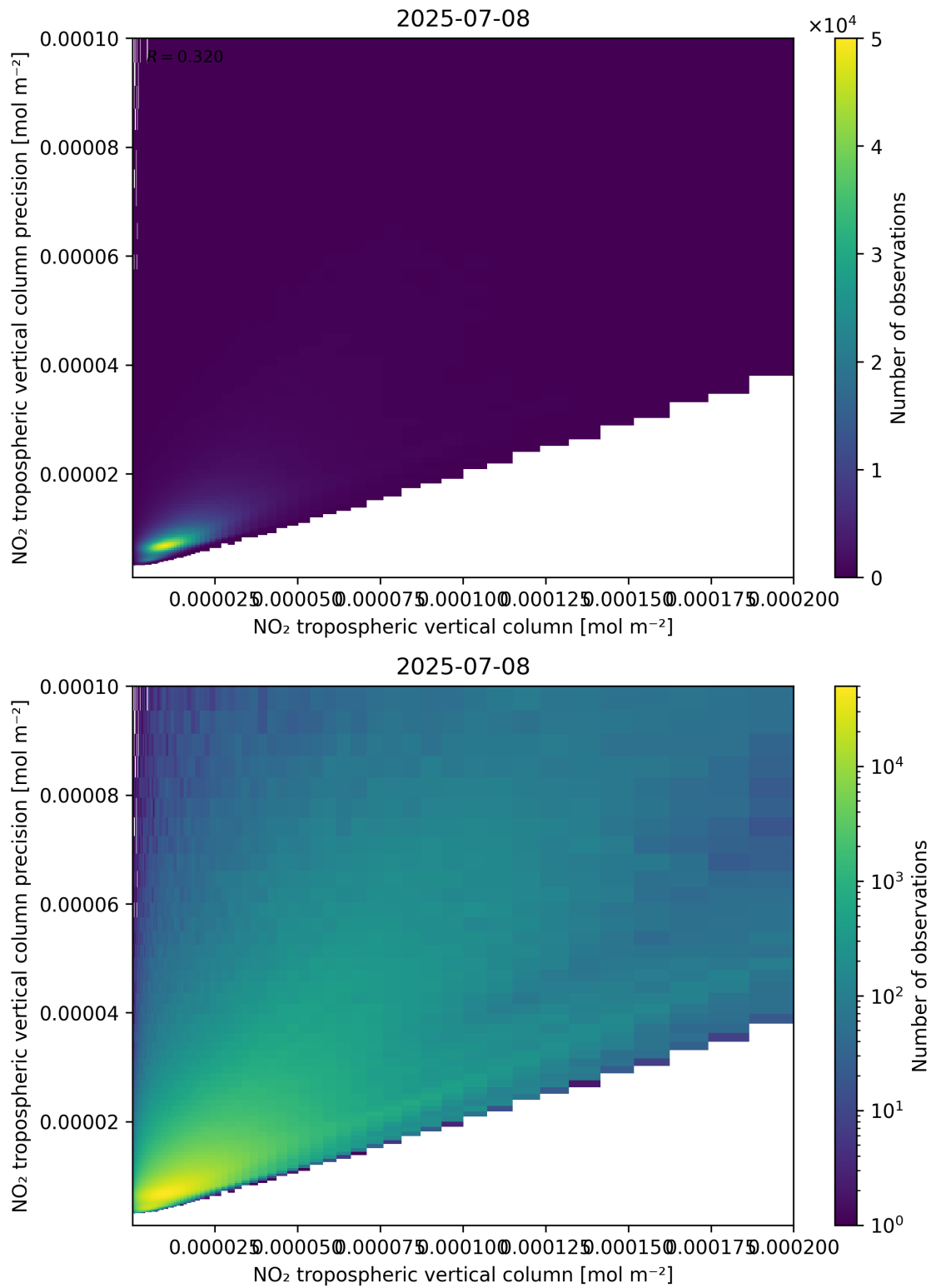
Figure 130: Scatter density plot of “NO 2 tropospheric vertical column” against “NO 2 tropospheric vertical column precision” for 2025-07-08 to 2025-07-09.
