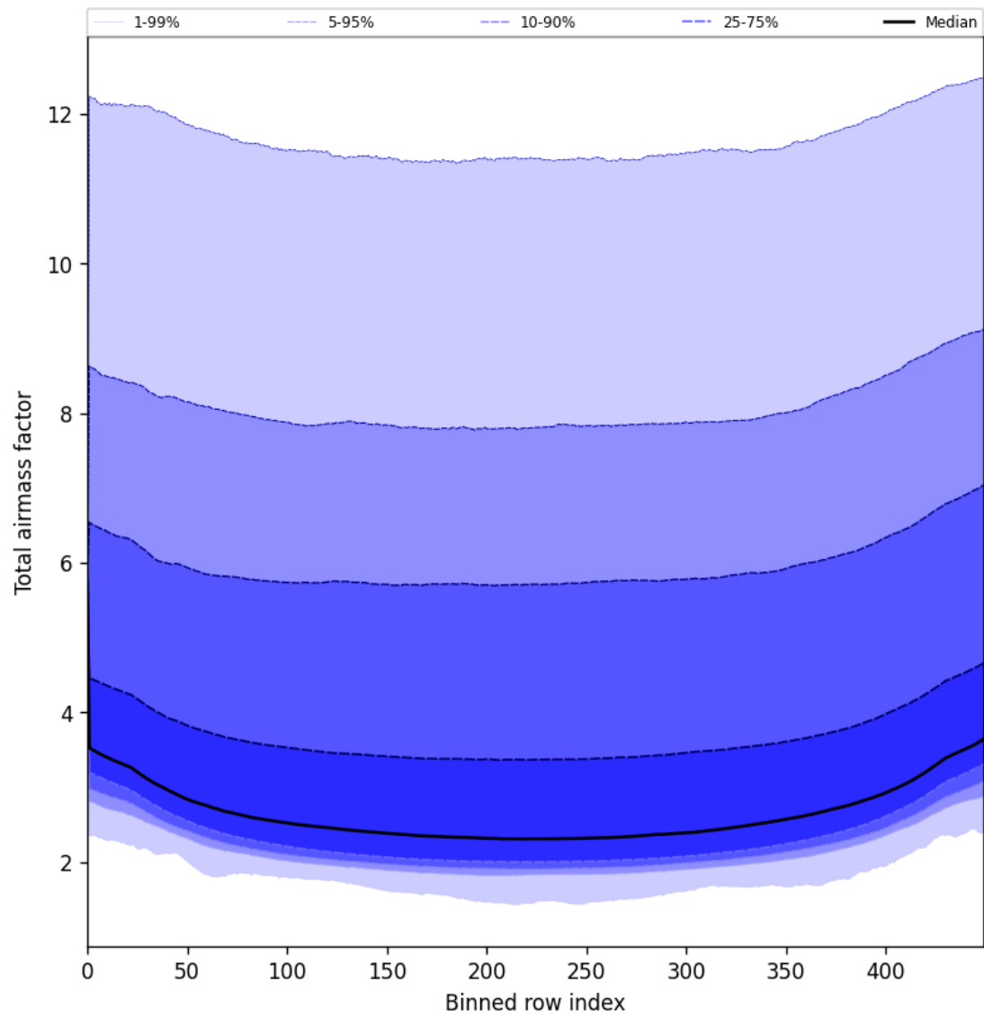
Figure 49: Along track statistics of “Total airmass factor” for 2025-07-08 to 2025-07-09
