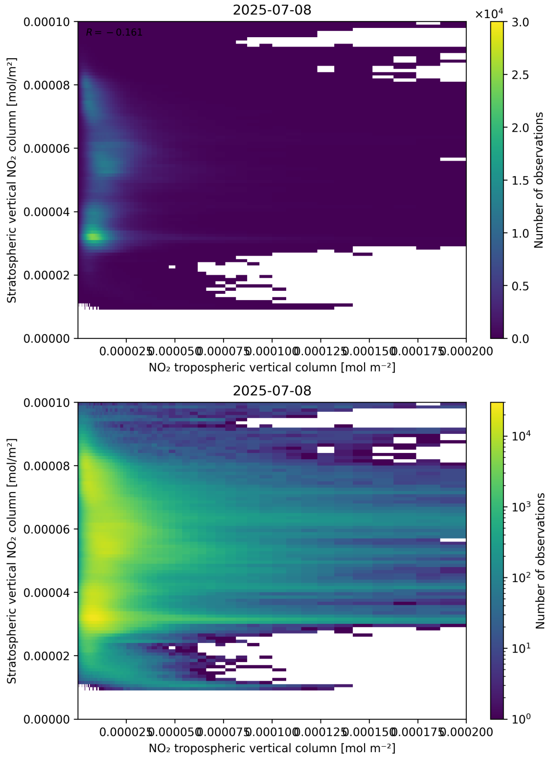
Figure 125: Scatter density plot of “NO 2 tropospheric vertical column” against “Stratospheric vertical NO 2 column” for 2025-07-08 to 2025-07-09.
