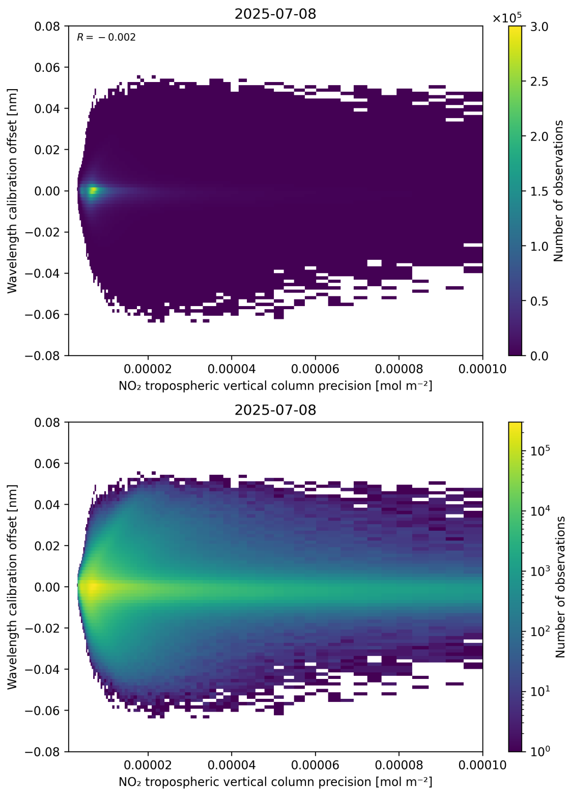
Figure 141: Scatter density plot of “NO 2 tropospheric vertical column precision” against “Wavelength calibration offset” for 2025-07-08 to 2025-07-09.
