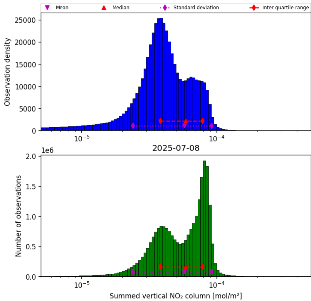
Figure 40: Histogram of “Summed vertical NO 2 column” for 2025-07-08 to 2025-07-09
