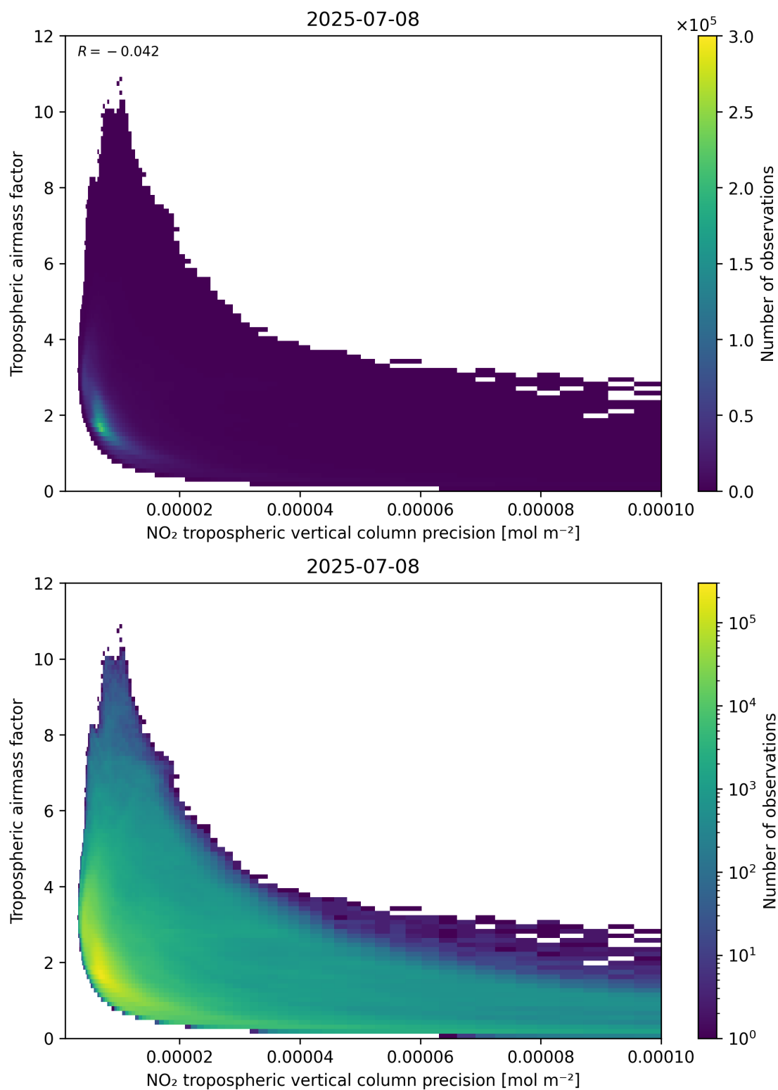
Figure 133: Scatter density plot of “NO 2 tropospheric vertical column precision” against “Tropospheric air mass factor” for 2025-07-08 to 2025-07-09.
