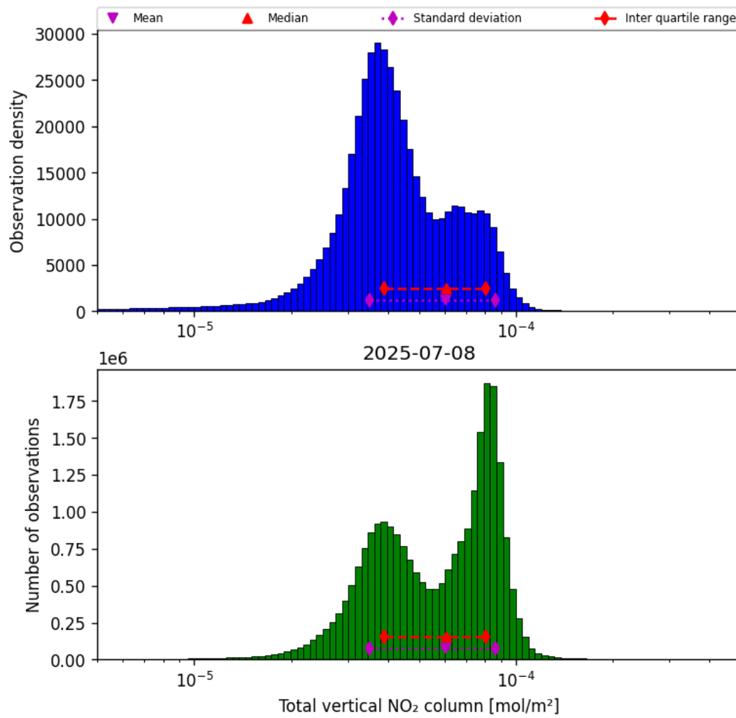
Figure 38: Histogram of “Total vertical NO 2 column” for 2025-07-08 to 2025-07-09
