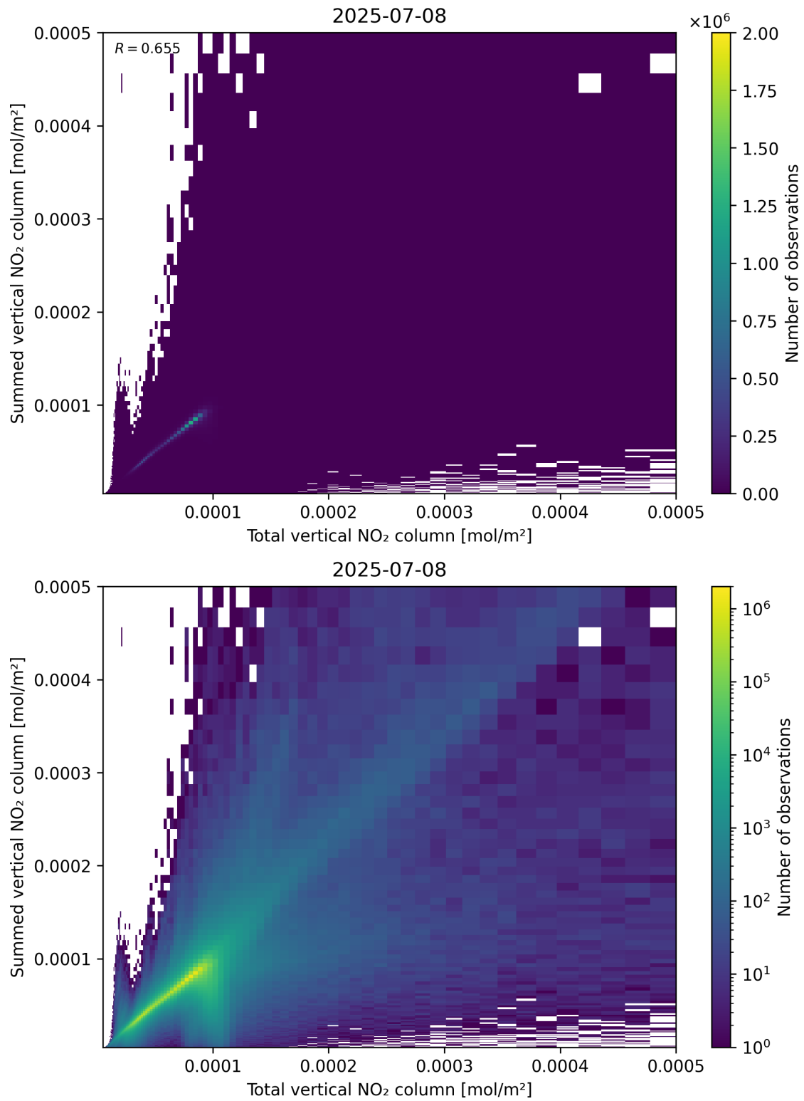
Figure 112: Scatter density plot of “Total vertical NO 2 column” against “Summed vertical NO 2 column” for 2025-07-08 to 2025-07-09.
