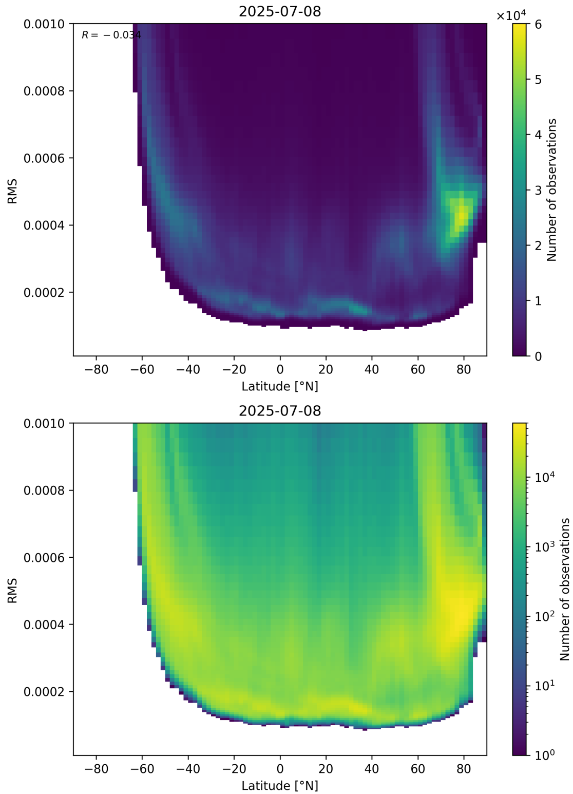
Figure 94: Scatter density plot of “Latitude” against “RMS” for 2025-07-08 to 2025-07-09.
