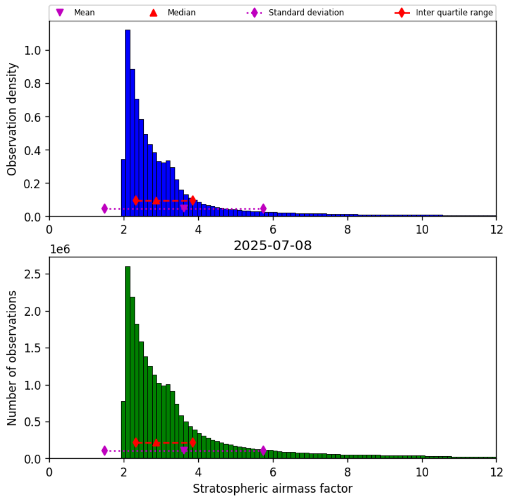
Figure 44: Histogram of “Stratospheric airmass factor” for 2025-07-08 to 2025-07-09
