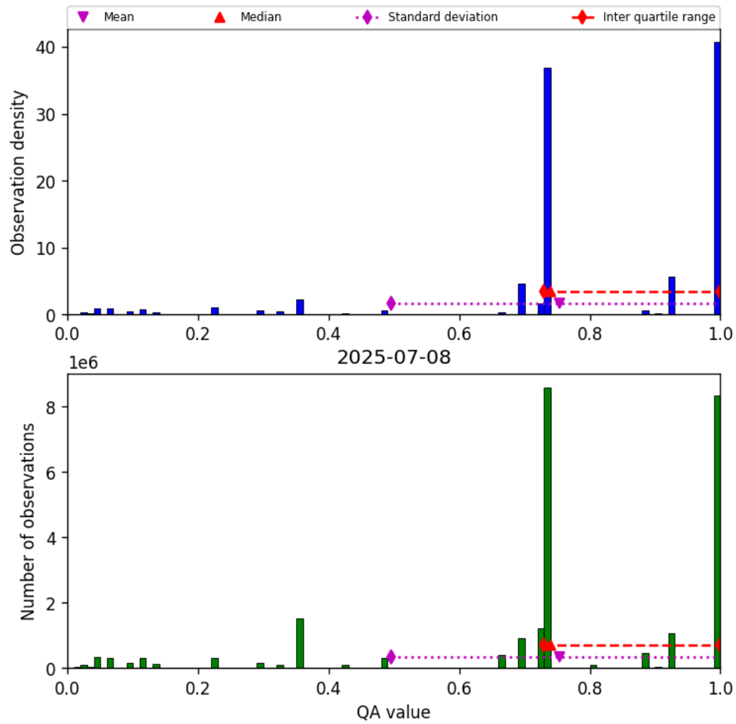
Figure 28: Histogram of “QA value” for 2025-07-08 to 2025-07-09
