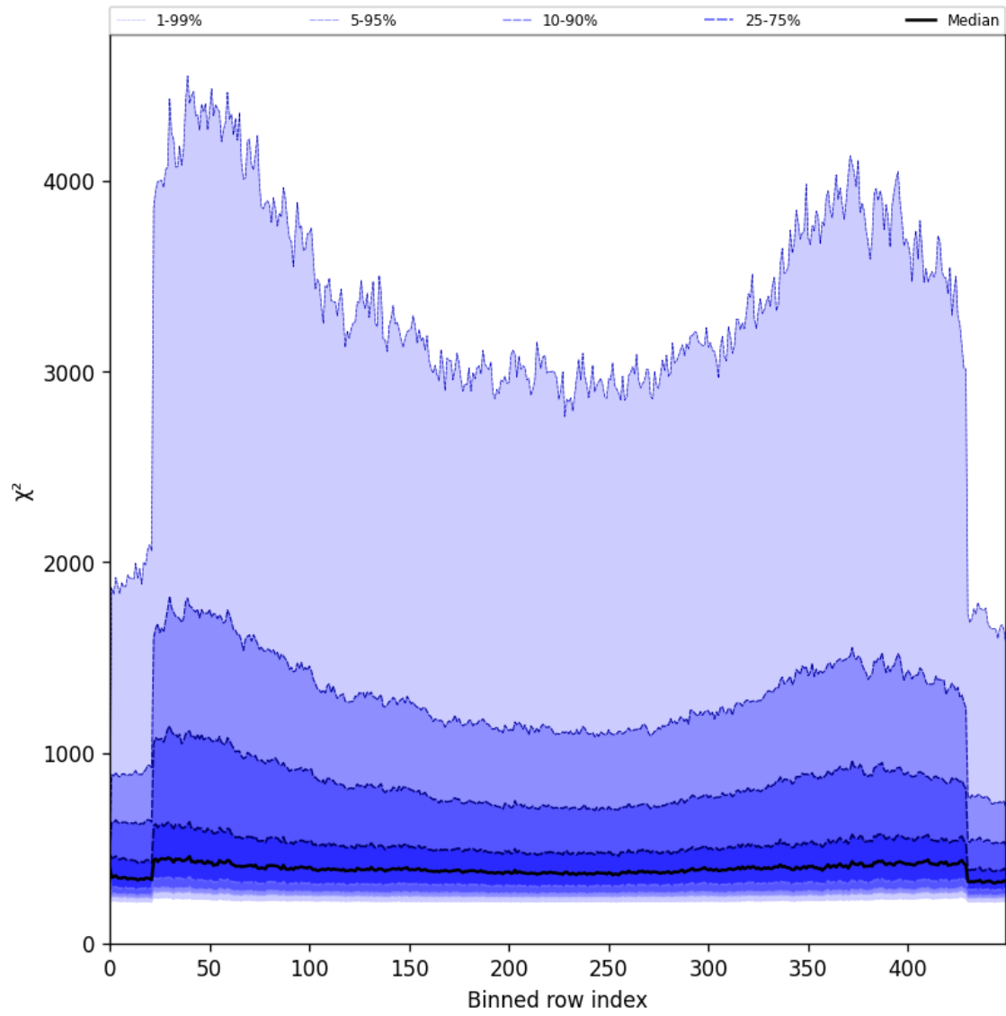
Figure 59: Along track statistics of “ \chi^2 ” for 2025-07-08 to 2025-07-09
