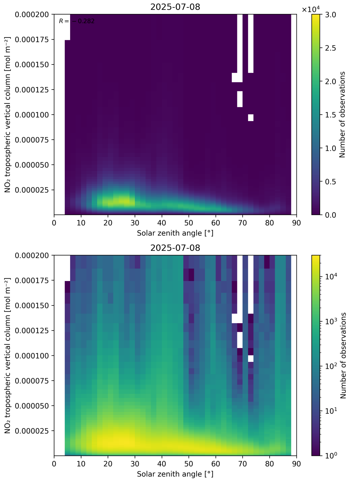
Figure 155: Scatter density plot of “Solar zenith angle” against “NO 2 tropospheric vertical column” for 2025-07-08 to 2025-07-09.
