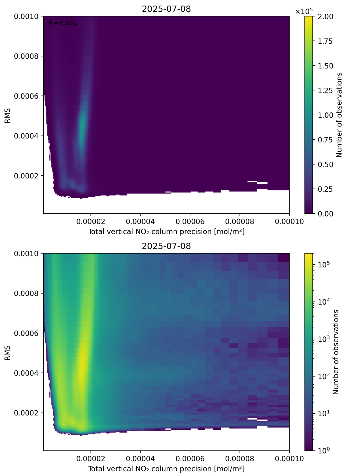
Figure 119: Scatter density plot of “Total vertical NO 2 column precision” against “RMS” for 2025-07-08 to 2025-07-09.
