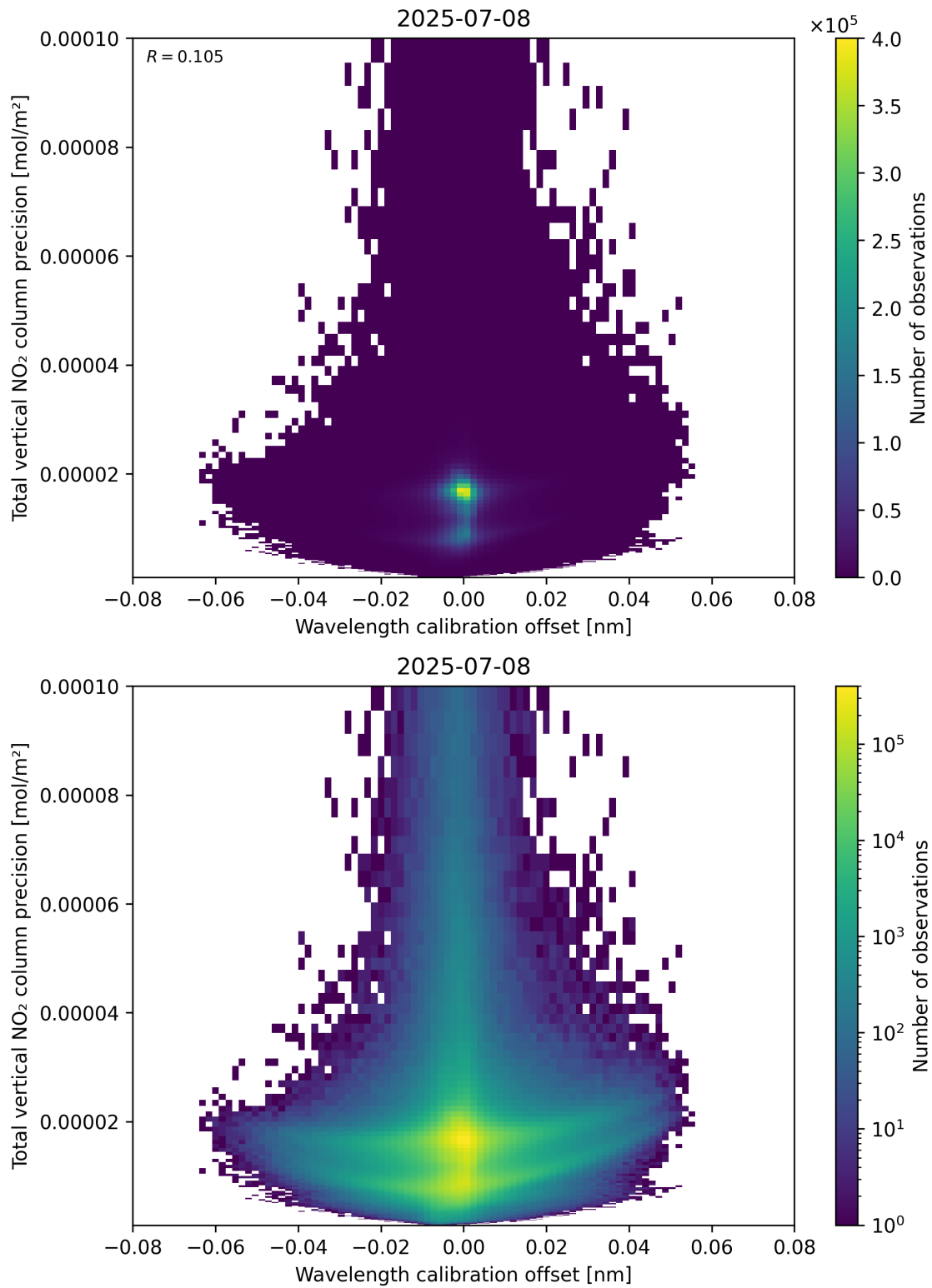
Figure 180: Scatter density plot of “Wavelength calibration offset” against “Total vertical NO 2 column precision” for 2025-07-08 to 2025-07-09.
