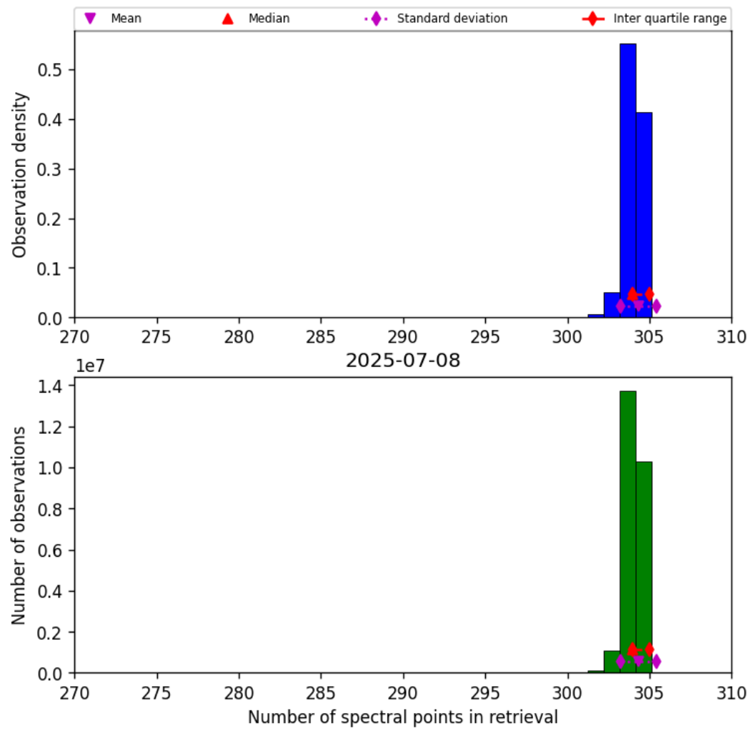
Figure 33: Histogram of “Number of spectral points in retrieval” for 2025-07-08 to 2025-07-09
