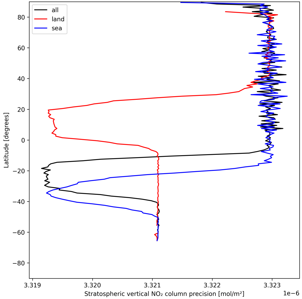
Figure 20: Zonal average of “Stratospheric vertical NO 2 column precision” for 2025-07-08 to 2025-07-09.
