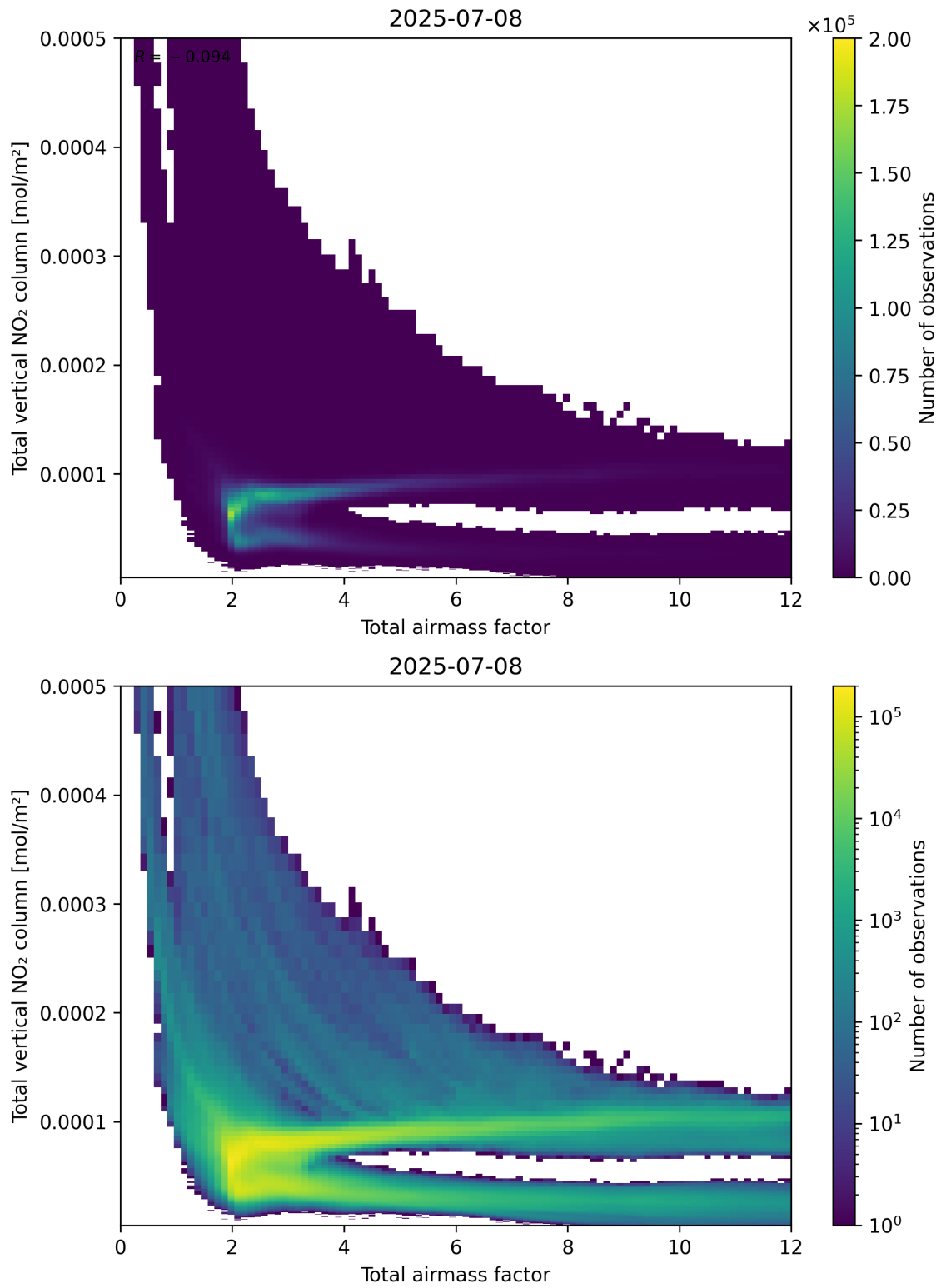
Figure 67: Scatter density plot of “Total airmass factor” against “Total vertical NO 2 column” for 2025-07-08 to 2025-07-09.
