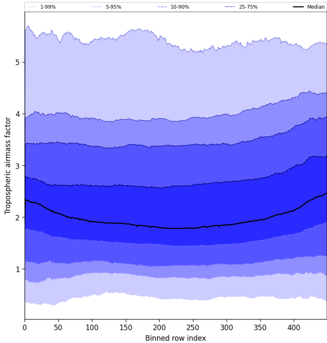
Figure 48: Along track statistics of “Tropospheric airmass factor” for 2025-07-08 to 2025-07-09
