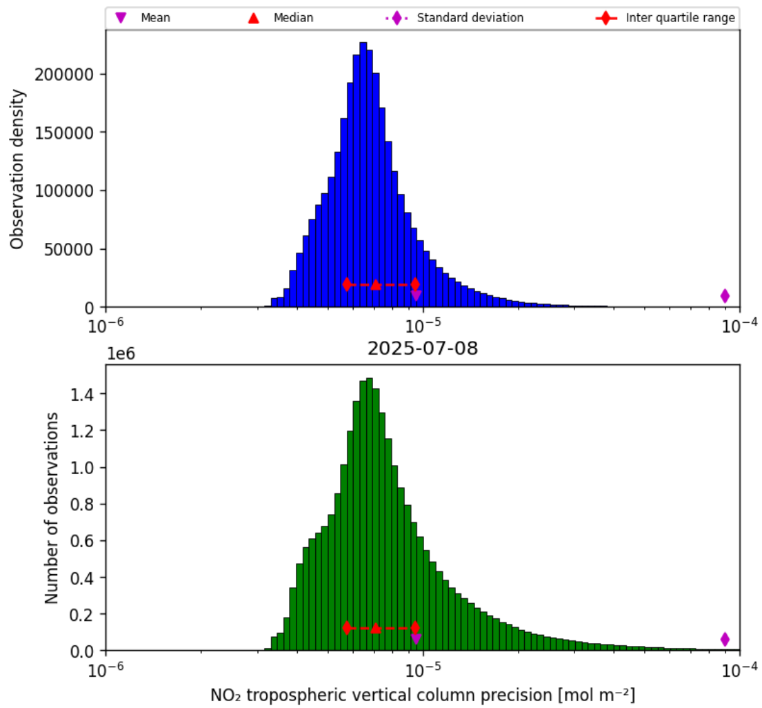
Figure 30: Histogram of “NO 2 tropospheric vertical column precision” for 2025-07-08 to 2025-07-09
