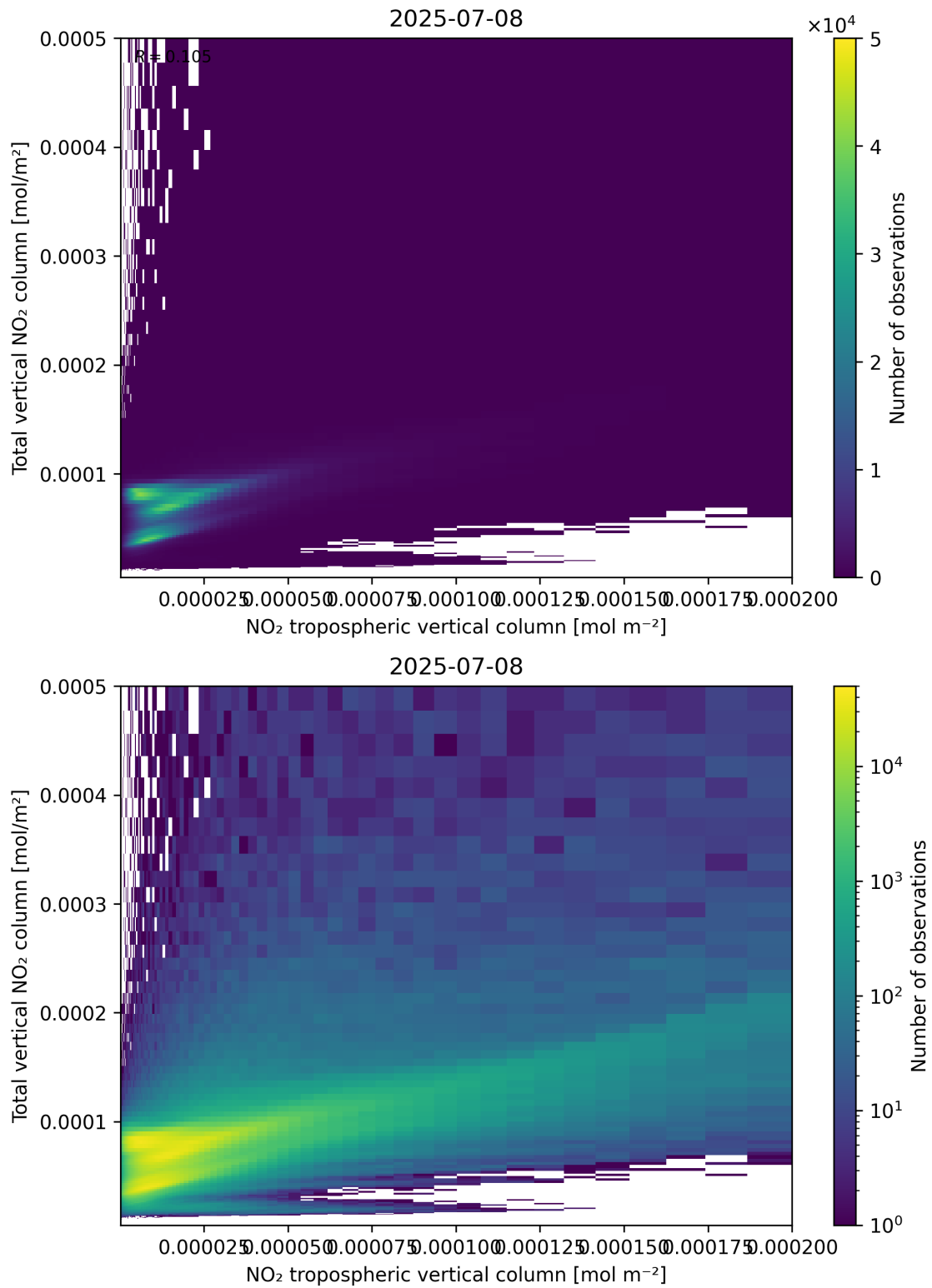
Figure 128: Scatter density plot of “NO 2 tropospheric vertical column” against “Total vertical NO 2 column” for 2025-07-08 to 2025-07-09.
