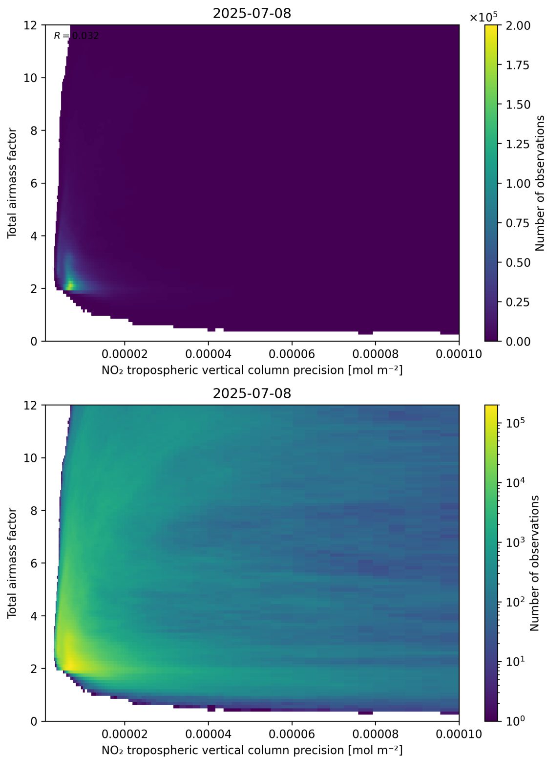
Figure 132: Scatter density plot of “NO 2 tropospheric vertical column precision” against “Total air mass factor” for 2025-07-08 to 2025-07-09.
