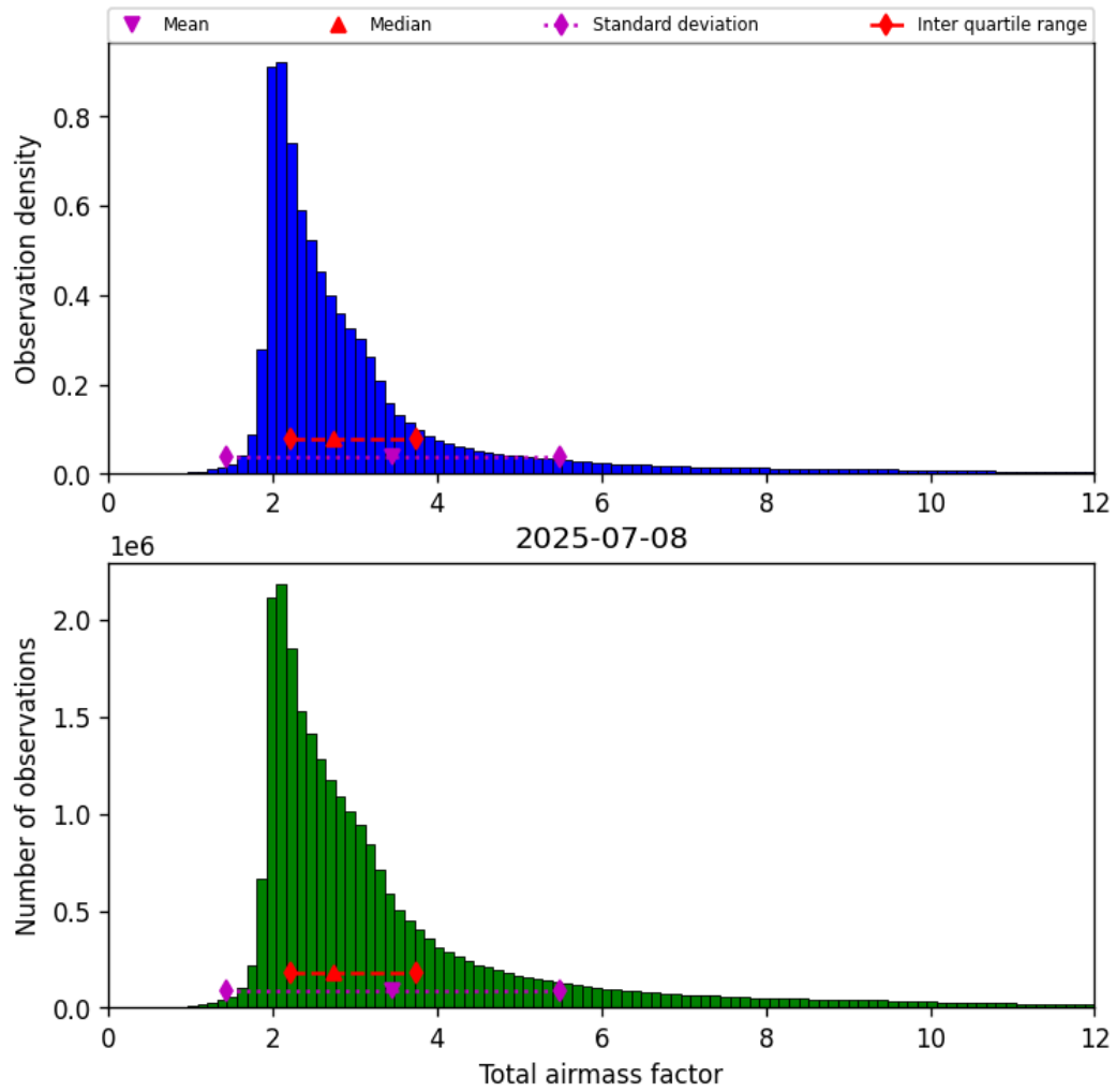
Figure 32: Histogram of “Total airmass factor” for 2025-07-08 to 2025-07-09
