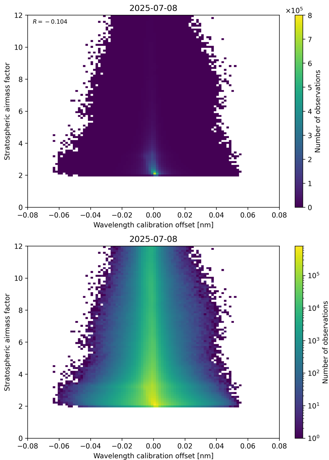
Figure 174: Scatter density plot of “Wavelength calibration offset” against “Stratospheric airmass factor” for 2025-07-08 to 2025-07-09.
