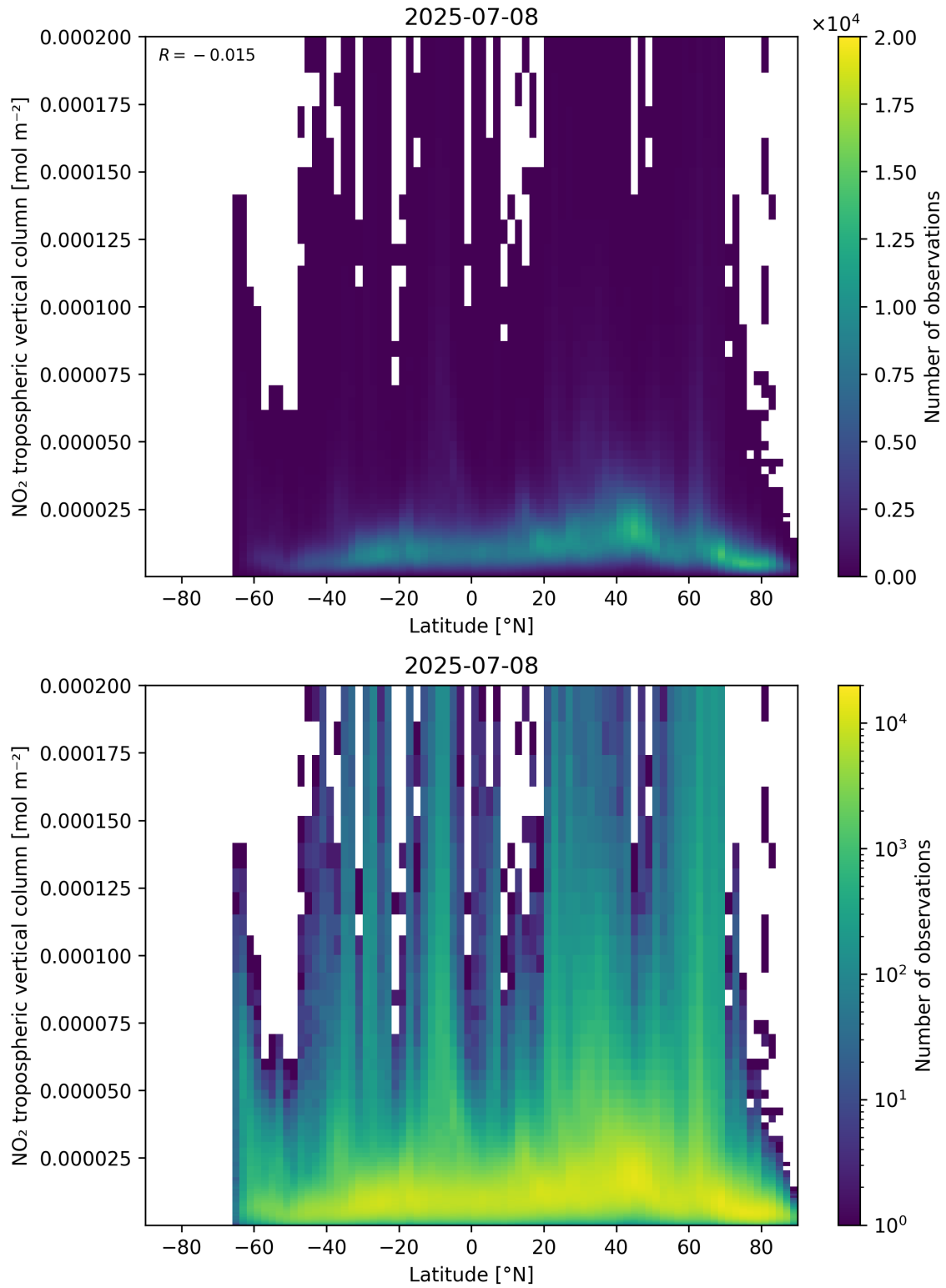
Figure 92: Scatter density plot of “Latitude” against “NO 2 tropospheric vertical column” for 2025-07-08 to 2025-07-09.
