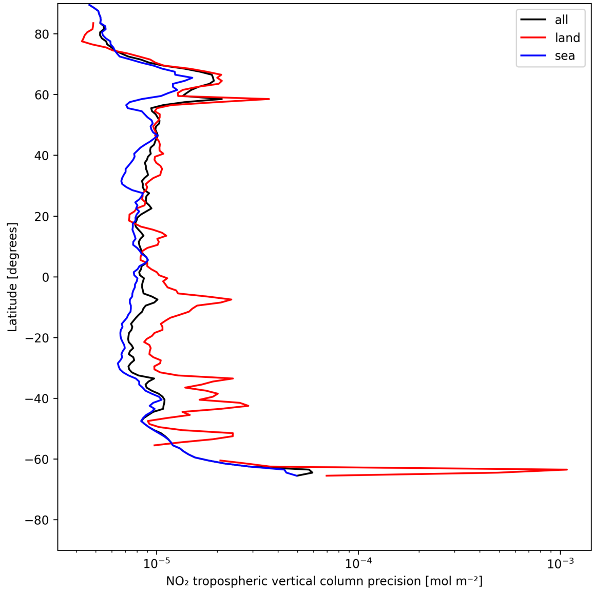
Figure 13: Zonal average of “NO 2 tropospheric vertical column precision” for 2025-07-08 to 2025-07-09.
