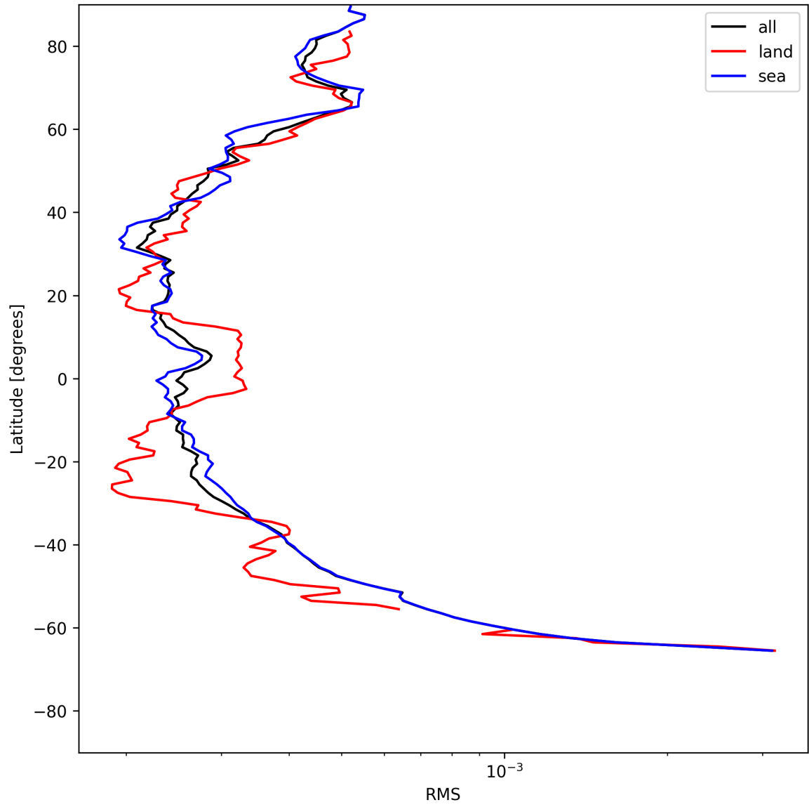
Figure 26: Zonal average of “RMS” for 2025-07-08 to 2025-07-09.
