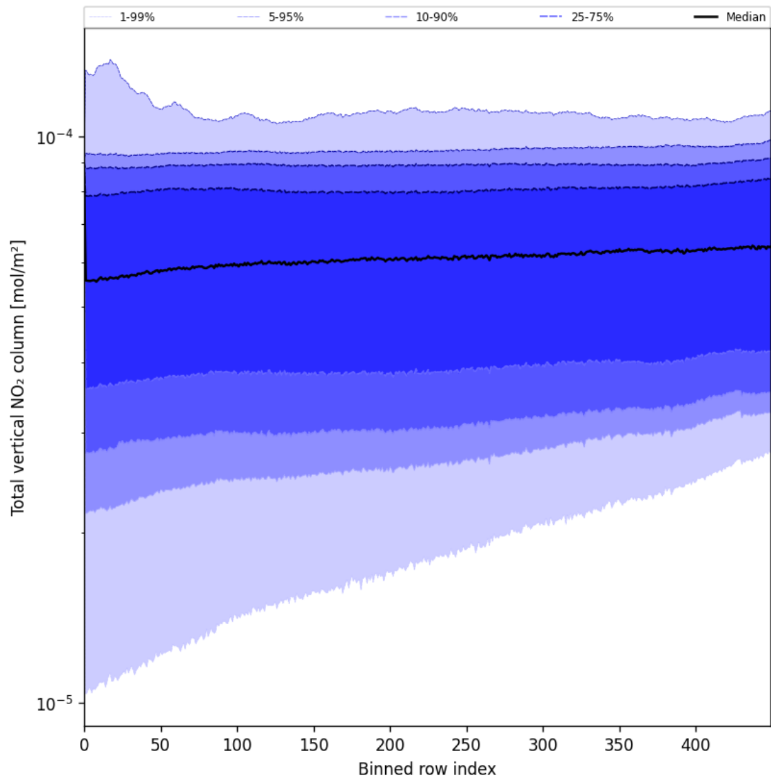
Figure 55: Along track statistics of “Total vertical NO 2 column” for 2025-07-08 to 2025-07-09
