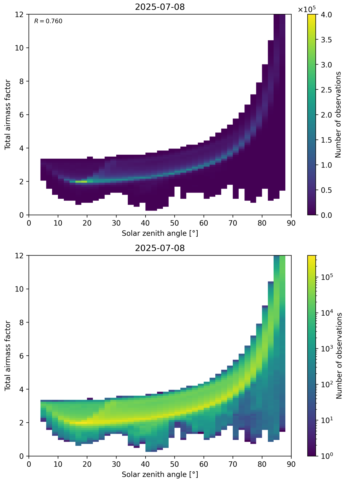
Figure 146: Scatter density plot of “Solar zenith angle” against “Total air mass factor” for 2025-07-08 to 2025-07-09.
