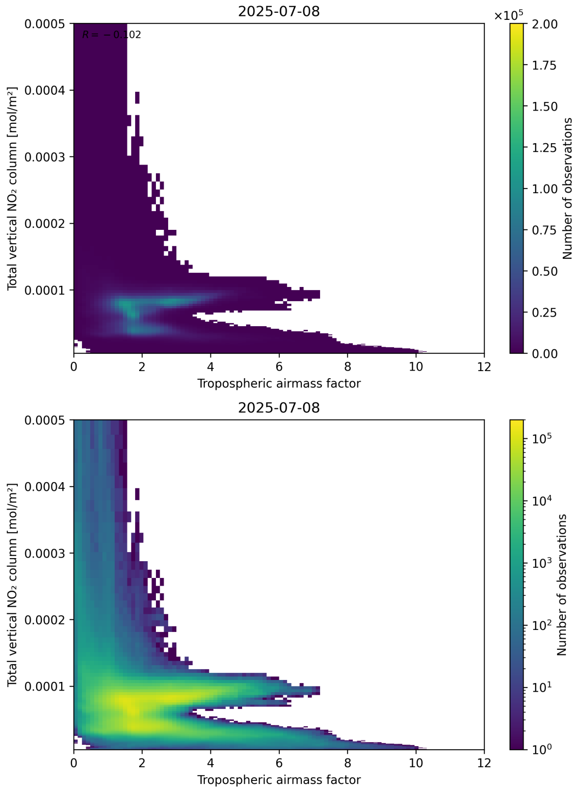
Figure 77: Scatter density plot of “Tropospheric airmass factor” against “Total vertical NO 2 column” for 2025-07-08 to 2025-07-09.
