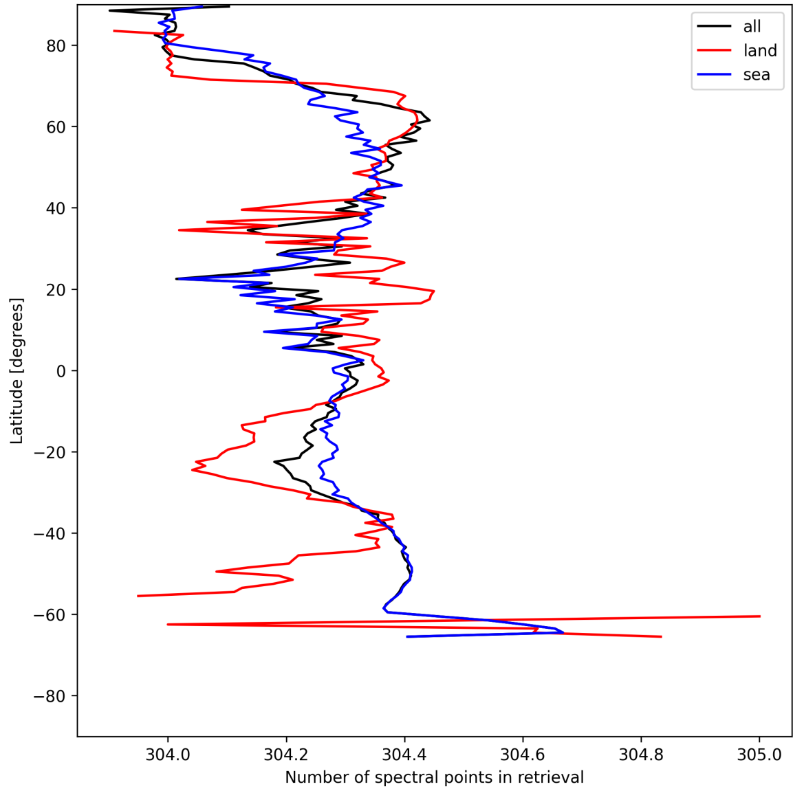
Figure 16: Zonal average of “Number of spectral points in retrieval” for 2025-07-08 to 2025-07-09.
