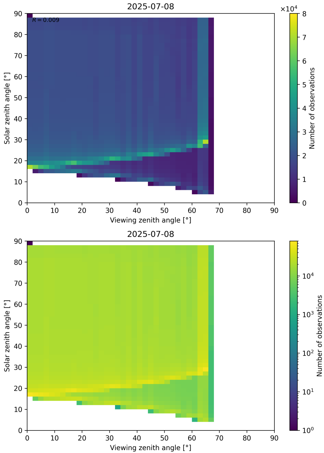
Figure 172: Scatter density plot of “Viewing zenith angle” against “Solar zenith angle” for 2025-07-08 to 2025-07-09.
