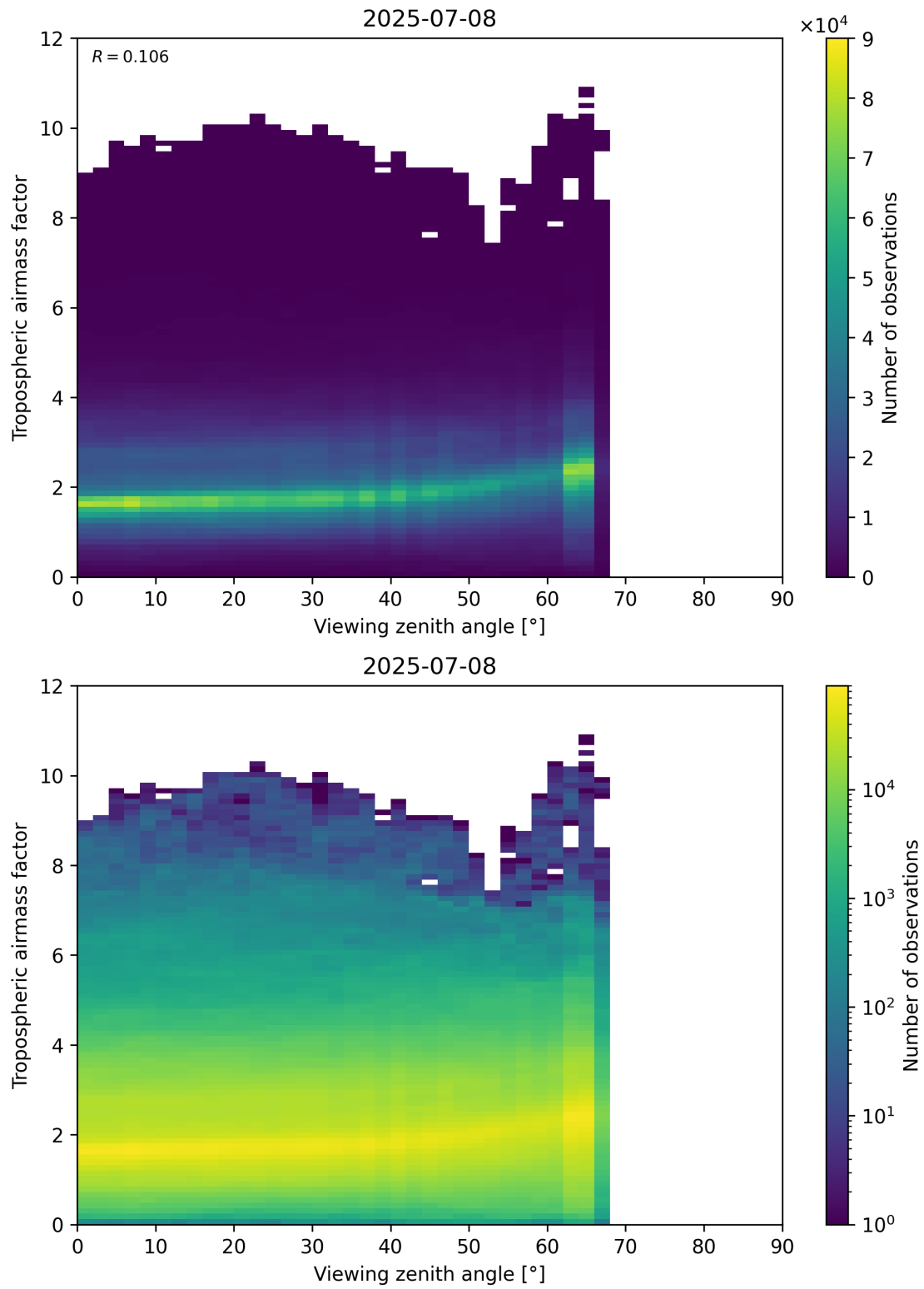
Figure 161: Scatter density plot of “Viewing zenith angle” against “Tropospheric airmass factor” for 2025-07-08 to 2025-07-09.
