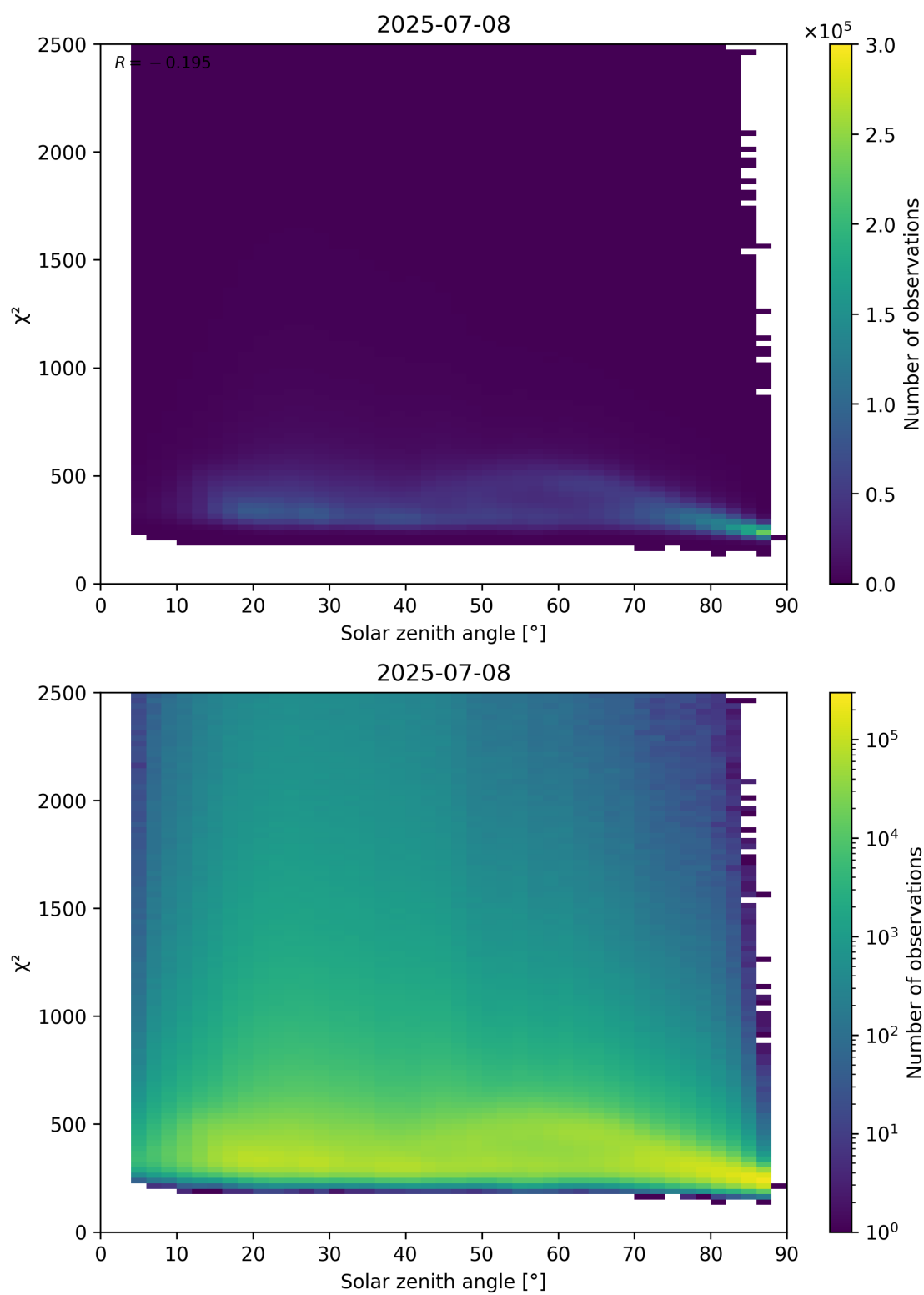
Figure 148: Scatter density plot of “Solar zenith angle” against “ \chi^2 ” for 2025-07-08 to 2025-07-09.
