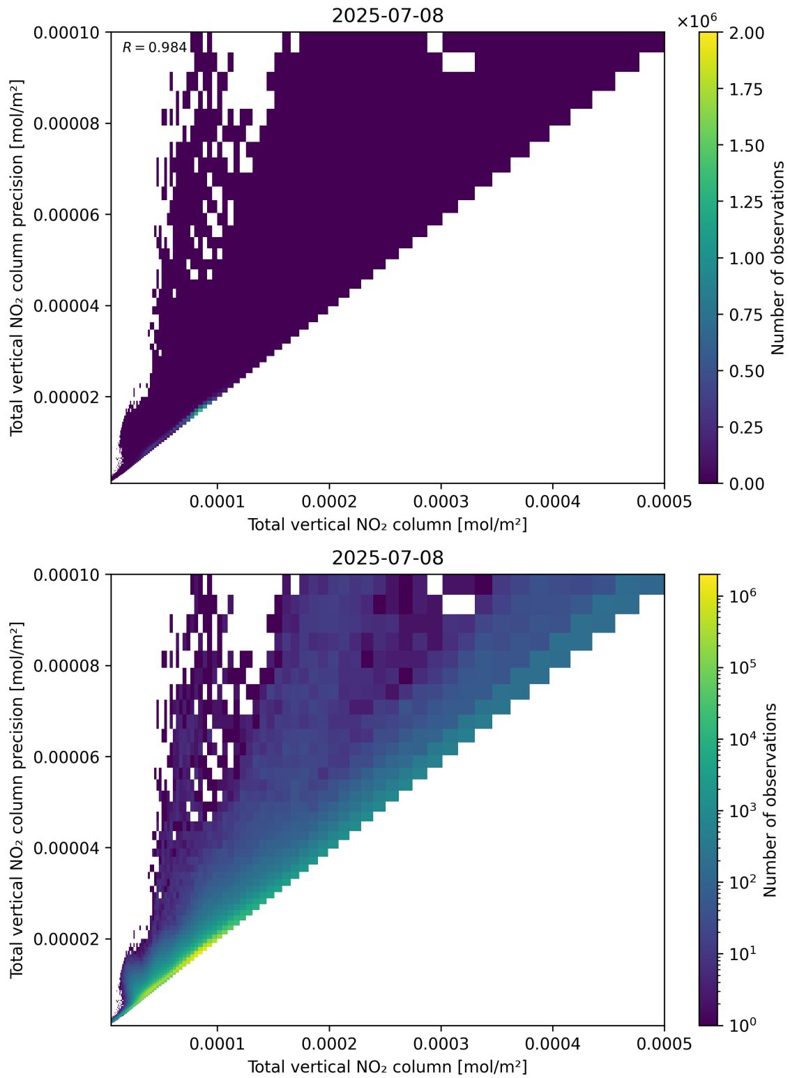
Figure 114: Scatter density plot of “Total vertical NO 2 column” against “Total vertical NO 2 column precision” for 2025-07-08 to 2025-07-09.
