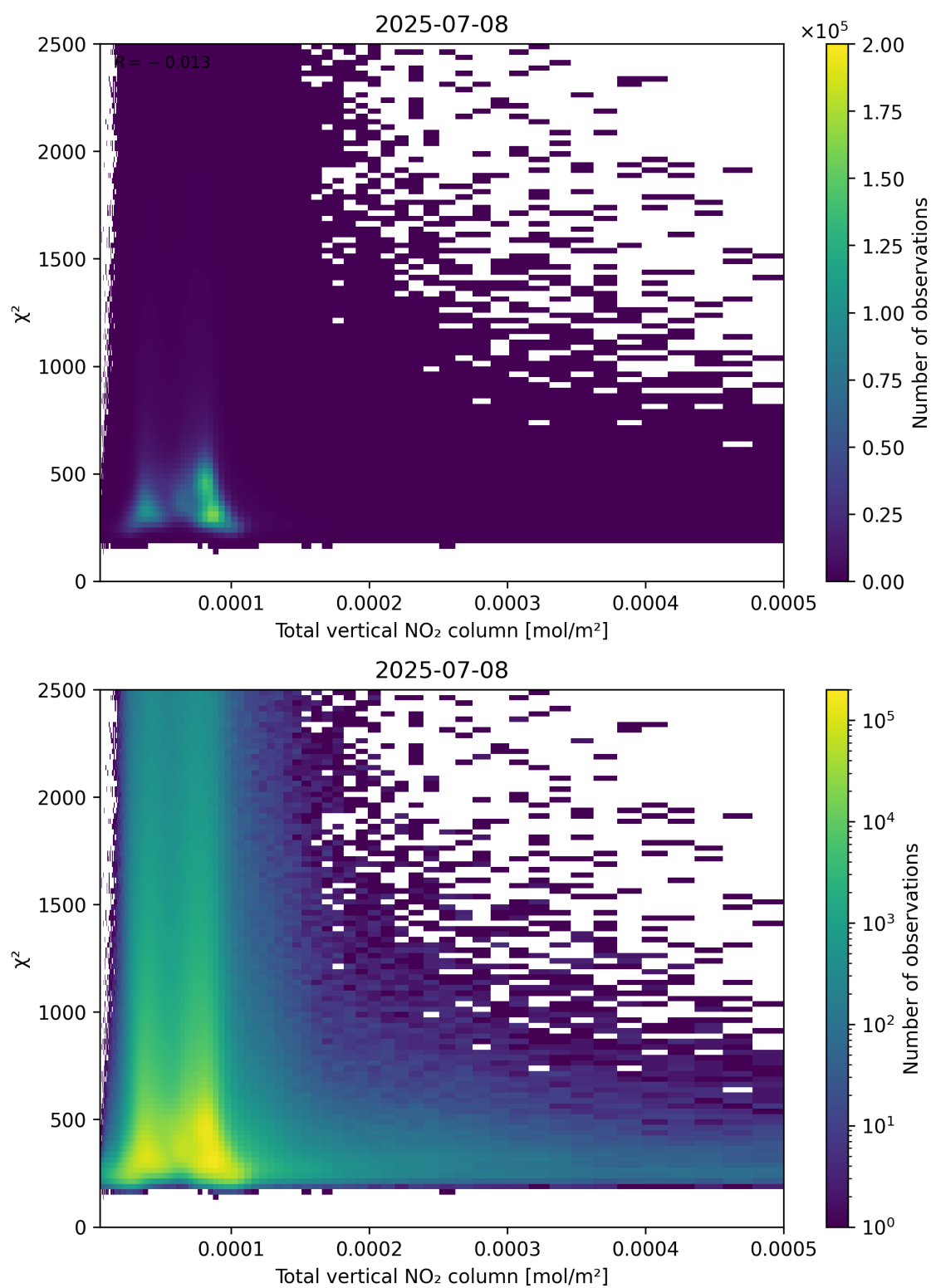
Figure 111: Scatter density plot of “Total vertical NO 2 column” against “ \chi^2 ” for 2025-07-08 to 2025-07-09.
