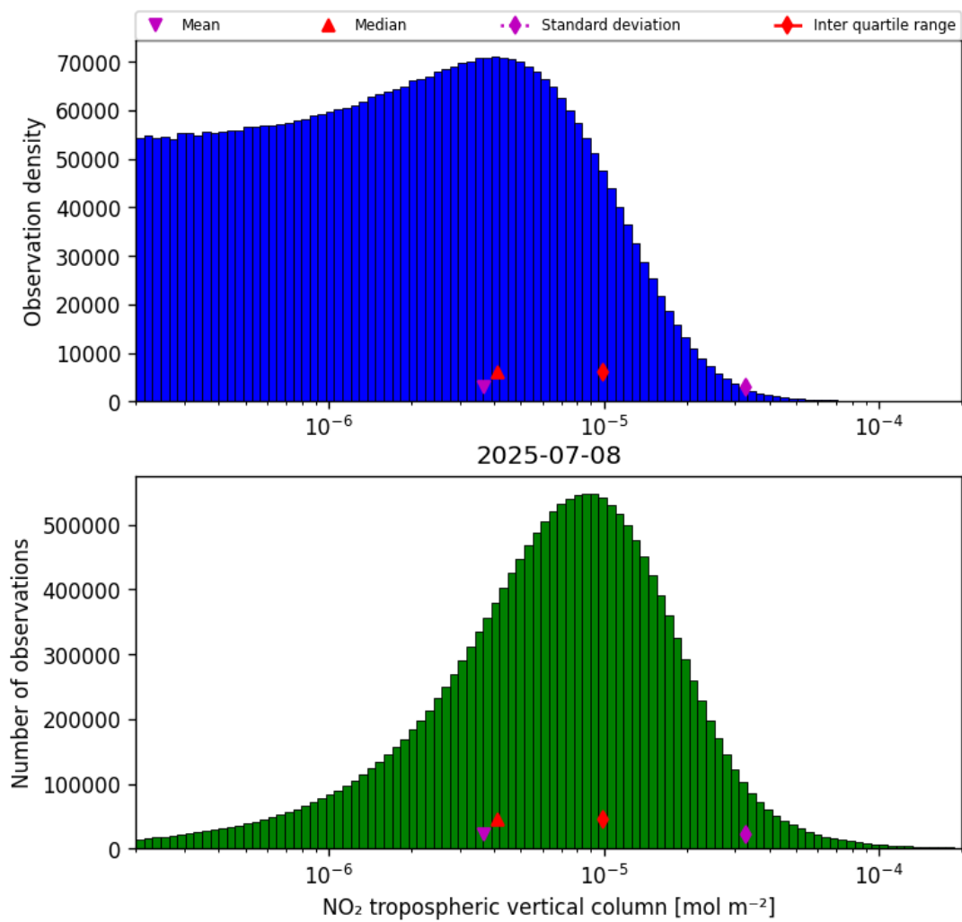
Figure 29: Histogram of “NO 2 tropospheric vertical column” for 2025-07-08 to 2025-07-09
