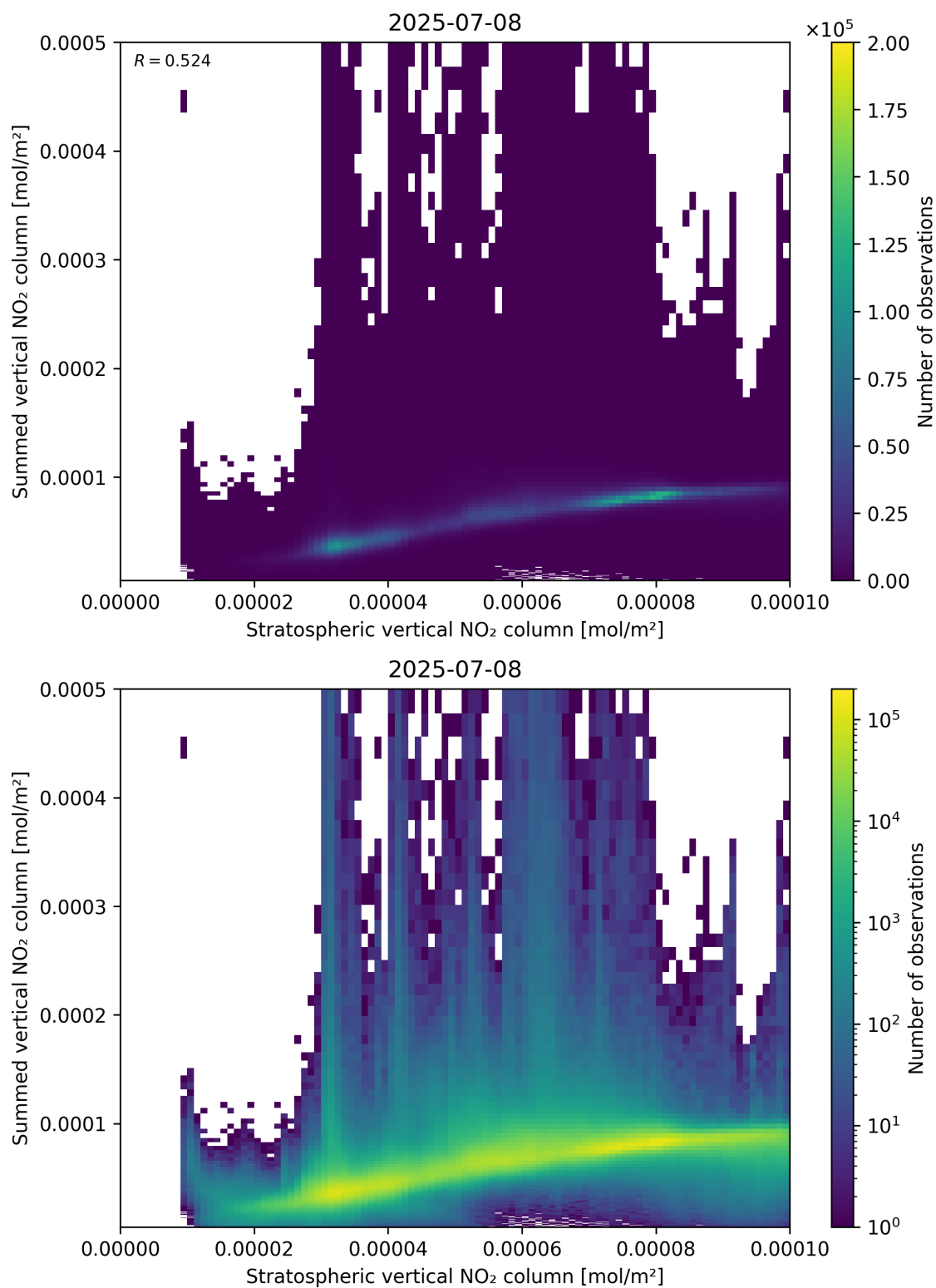
Figure 98: Scatter density plot of “Stratospheric vertical NO 2 column” against “Summed vertical NO 2 column” for 2025-07-08 to 2025-07-09.
