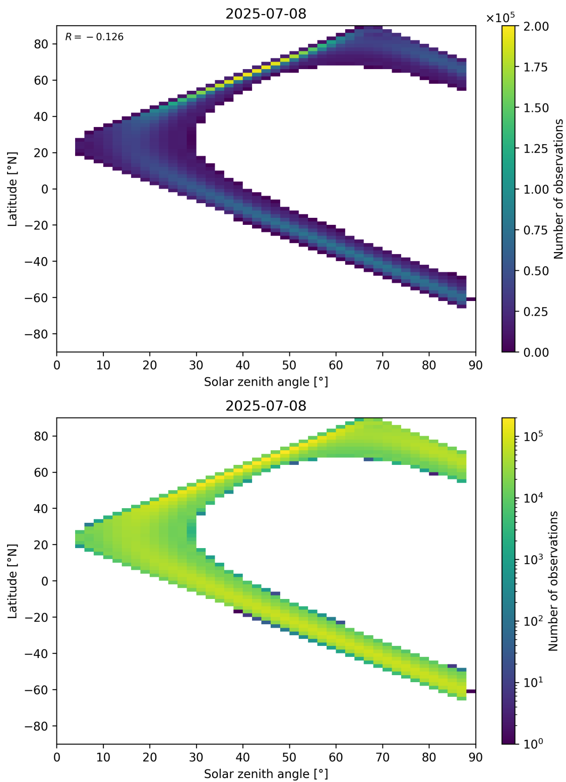
Figure 149: Scatter density plot of “Solar zenith angle” against “Latitude” for 2025-07-08 to 2025-07-09.
