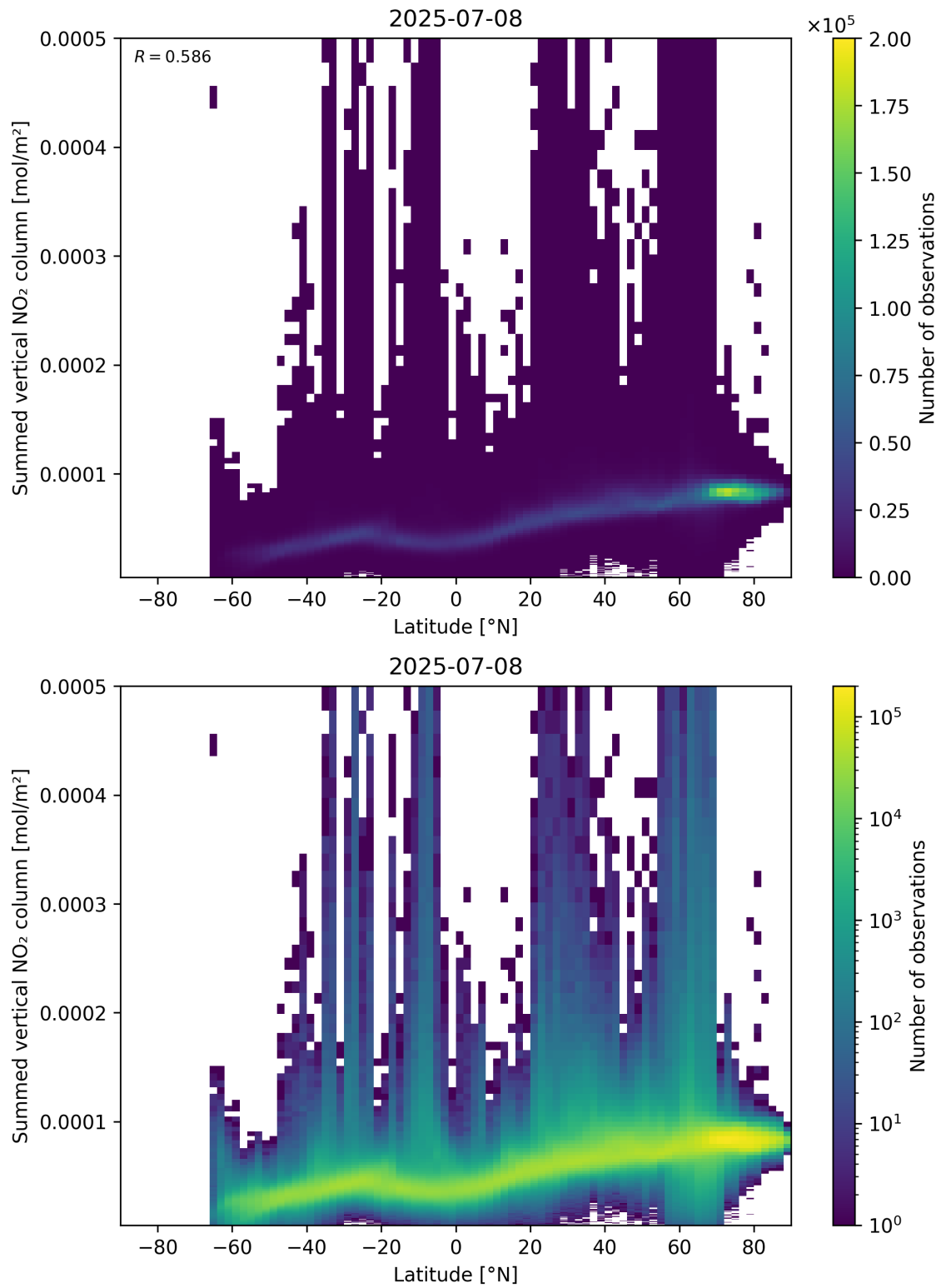
Figure 88: Scatter density plot of “Latitude” against “Summed vertical NO 2 column” for 2025-07-08 to 2025-07-09.
