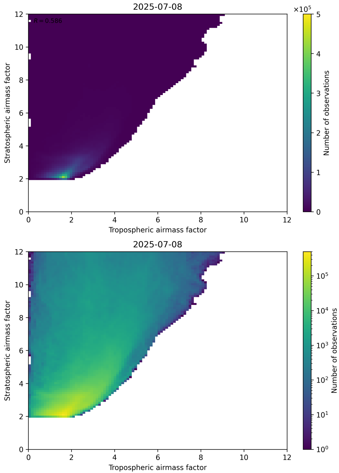
Figure 71: Scatter density plot of “Tropospheric airmass factor” against “Stratospheric airmass factor” for 2025-07-08 to 2025-07-09.
