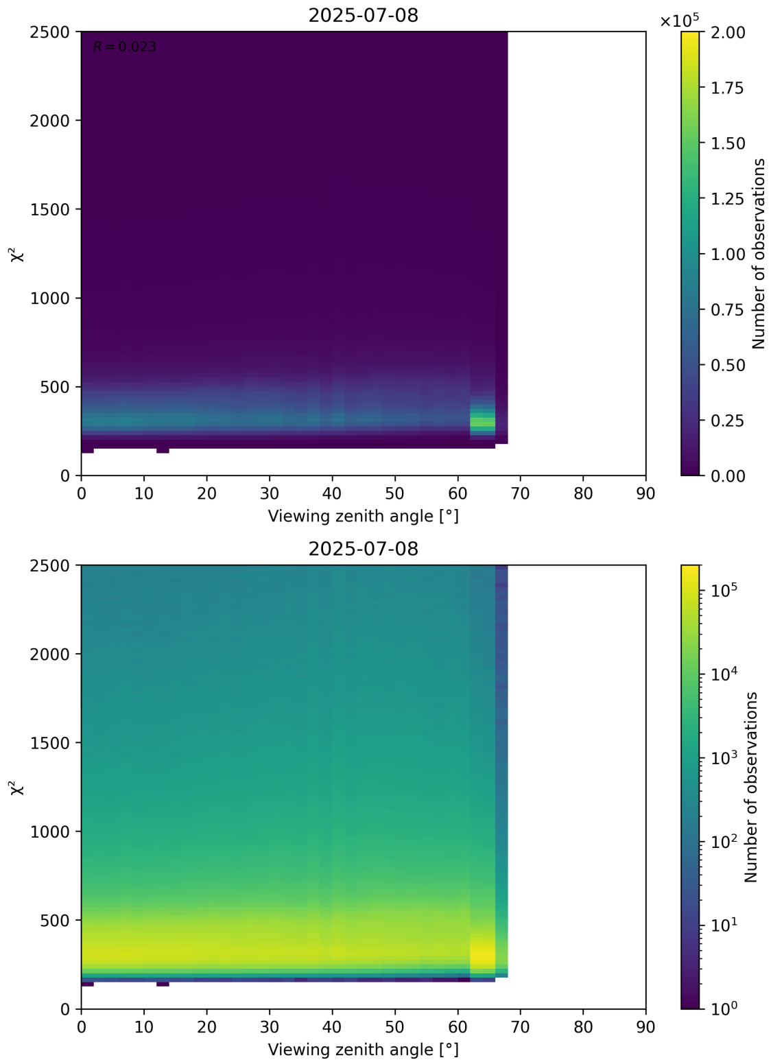
Figure 162: Scatter density plot of “Viewing zenith angle” against “ \chi^2 ” for 2025-07-08 to 2025-07-09.
