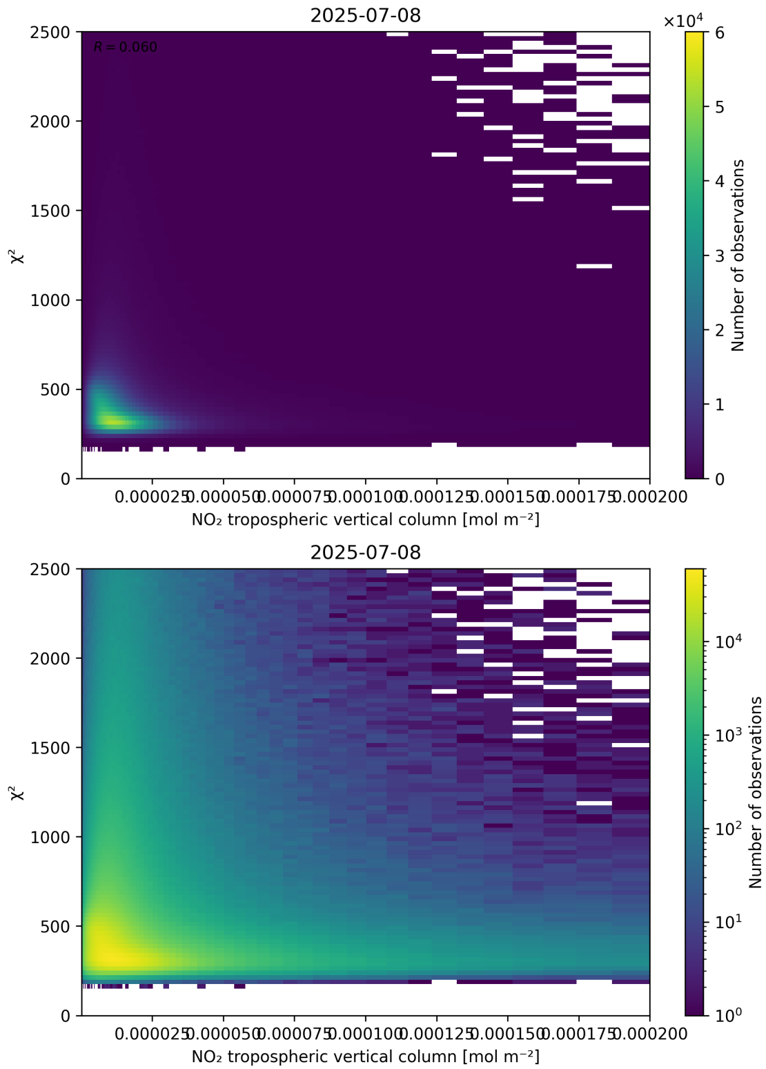
Figure 124: Scatter density plot of “NO 2 tropospheric vertical column” against “ \chi^2 ” for 2025-07-08 to 2025-07-09.
