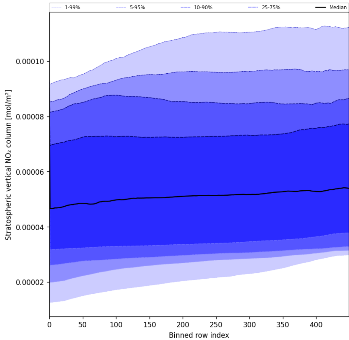
Figure 53: Along track statistics of “Stratospheric vertical NO 2 column” for 2025-07-08 to 2025-07-09
