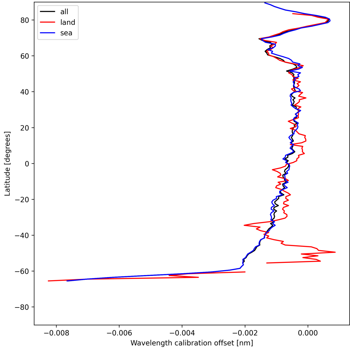
Figure 18: Zonal average of “Wavelength calibration offset” for 2025-07-08 to 2025-07-09.
