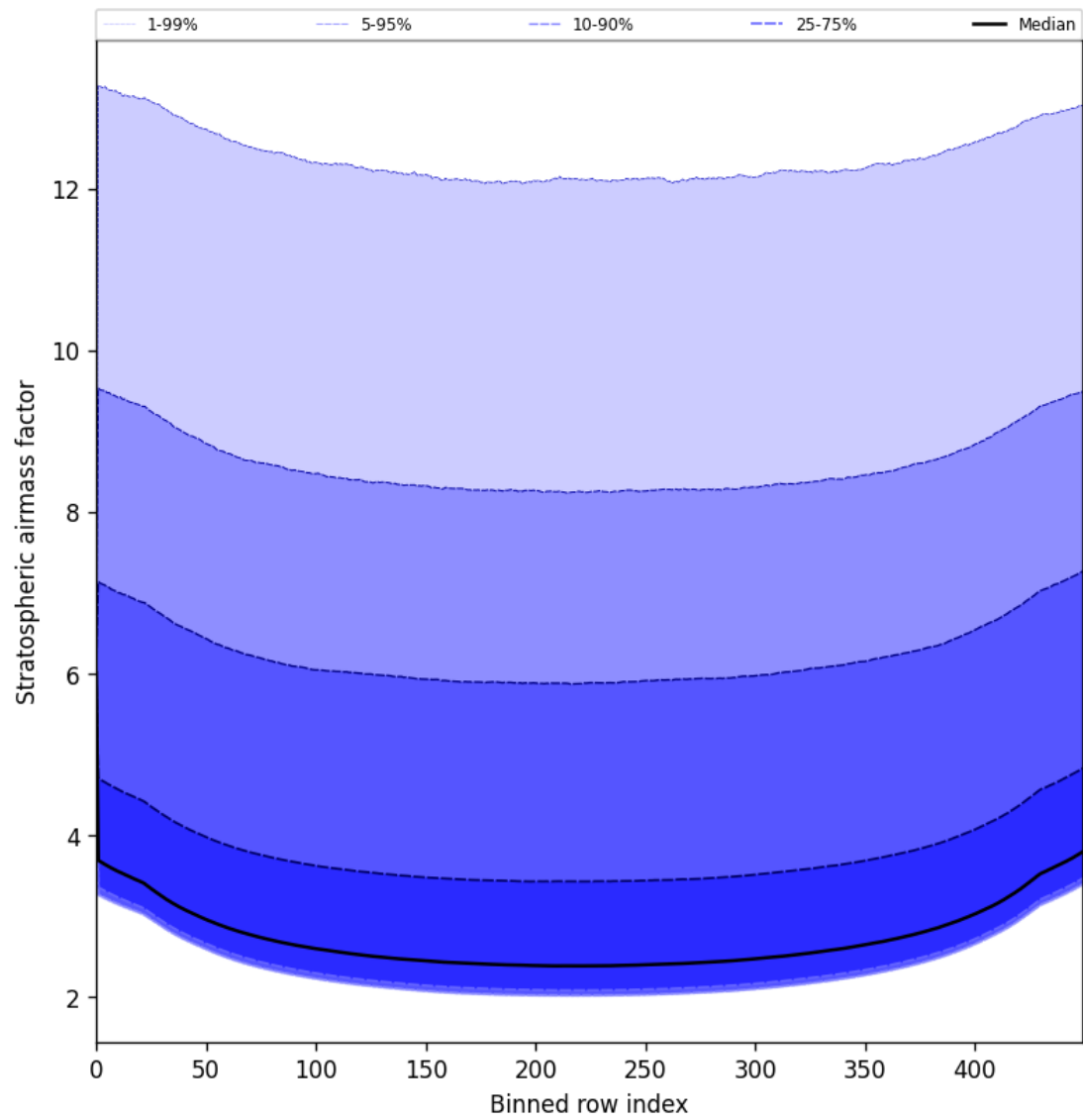
Figure 61: Along track statistics of “Stratospheric airmass factor” for 2025-07-08 to 2025-07-09
