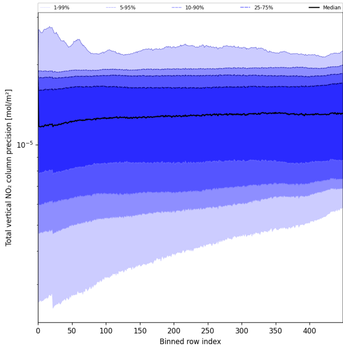
Figure 56: Along track statistics of “Total vertical NO 2 column precision” for 2025-07-08 to 2025-07-09
