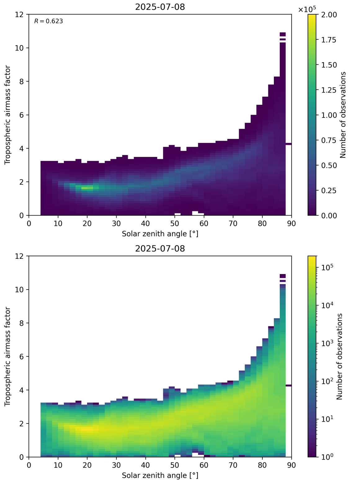
Figure 147: Scatter density plot of “Solar zenith angle” against “Tropospheric airmass factor” for 2025-07-08 to 2025-07-09.
