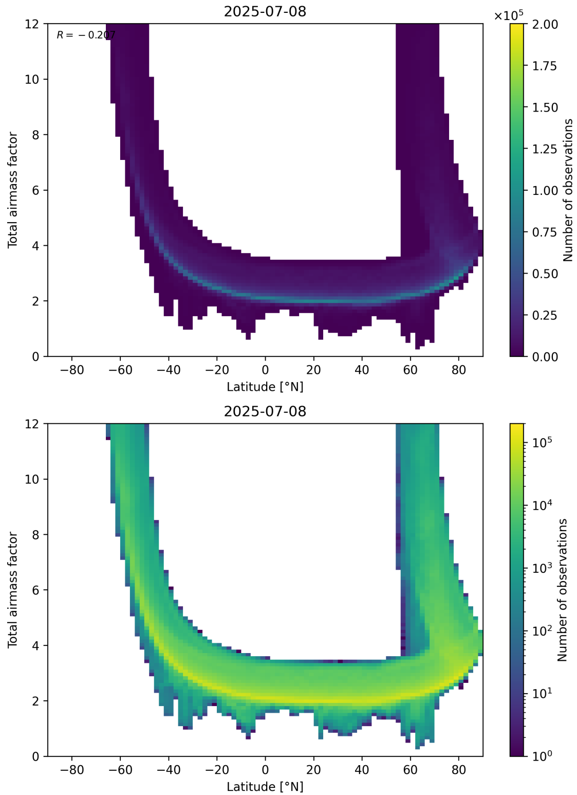
Figure 84: Scatter density plot of “Latitude” against “Total airmass factor” for 2025-07-08 to 2025-07-09.
