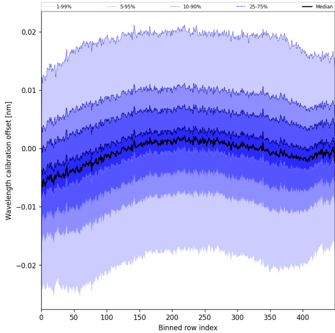
Figure 52: Along track statistics of “Wavelength calibration offset” for 2025-07-08 to 2025-07-09
