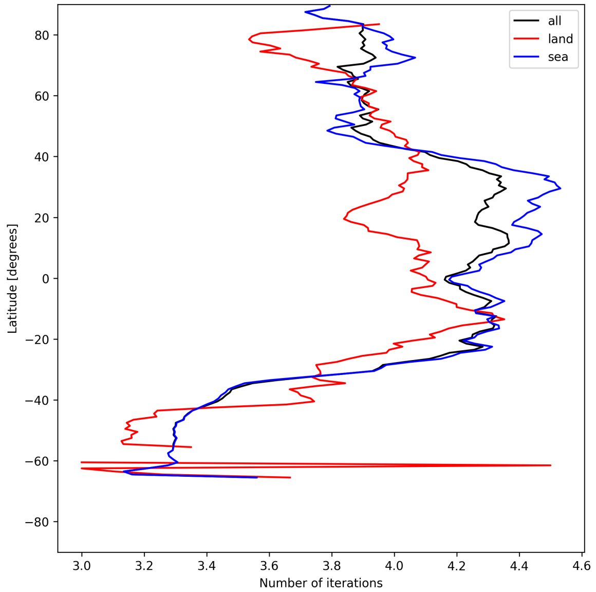
Figure 17: Zonal average of “Number of iterations” for 2025-07-08 to 2025-07-09.
