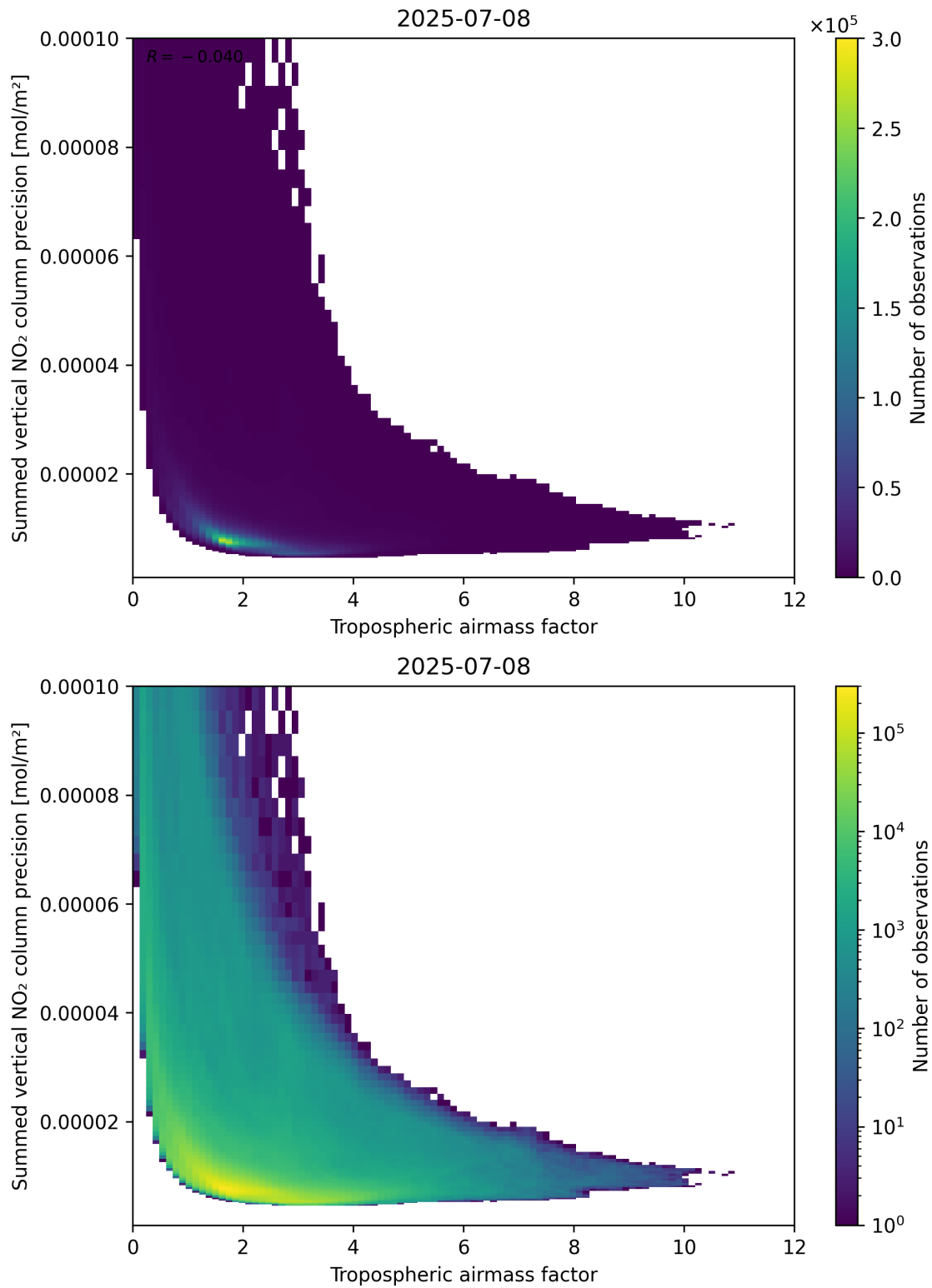
Figure 76: Scatter density plot of “Tropospheric air mass factor” against “Summed vertical NO 2 column precision” for 2025-07-08 to 2025-07-09.
