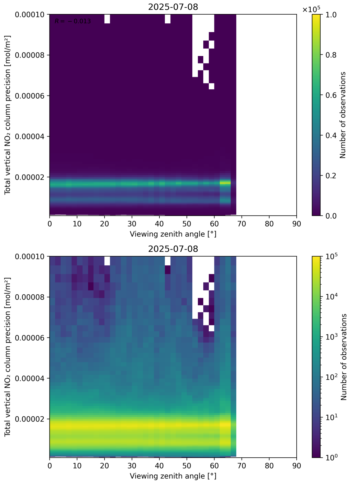
Figure 168: Scatter density plot of “Viewing zenith angle” against “Total vertical NO 2 column precision” for 2025-07-08 to 2025-07-09.
