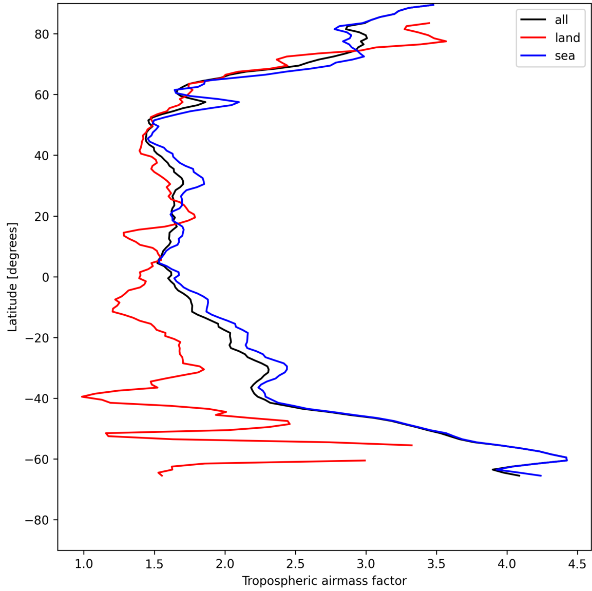
Figure 14: Zonal average of “Tropospheric airmass factor” for 2025-07-08 to 2025-07-09.
