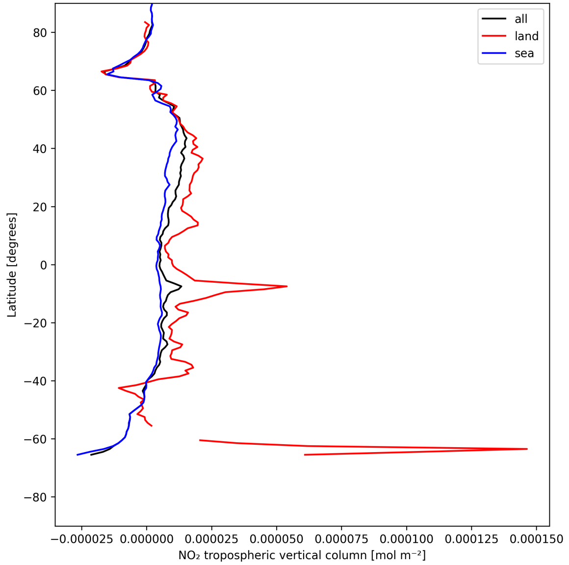
Figure 12: Zonal average of “NO 2 tropospheric vertical column” for 2025-07-08 to 2025-07-09.
