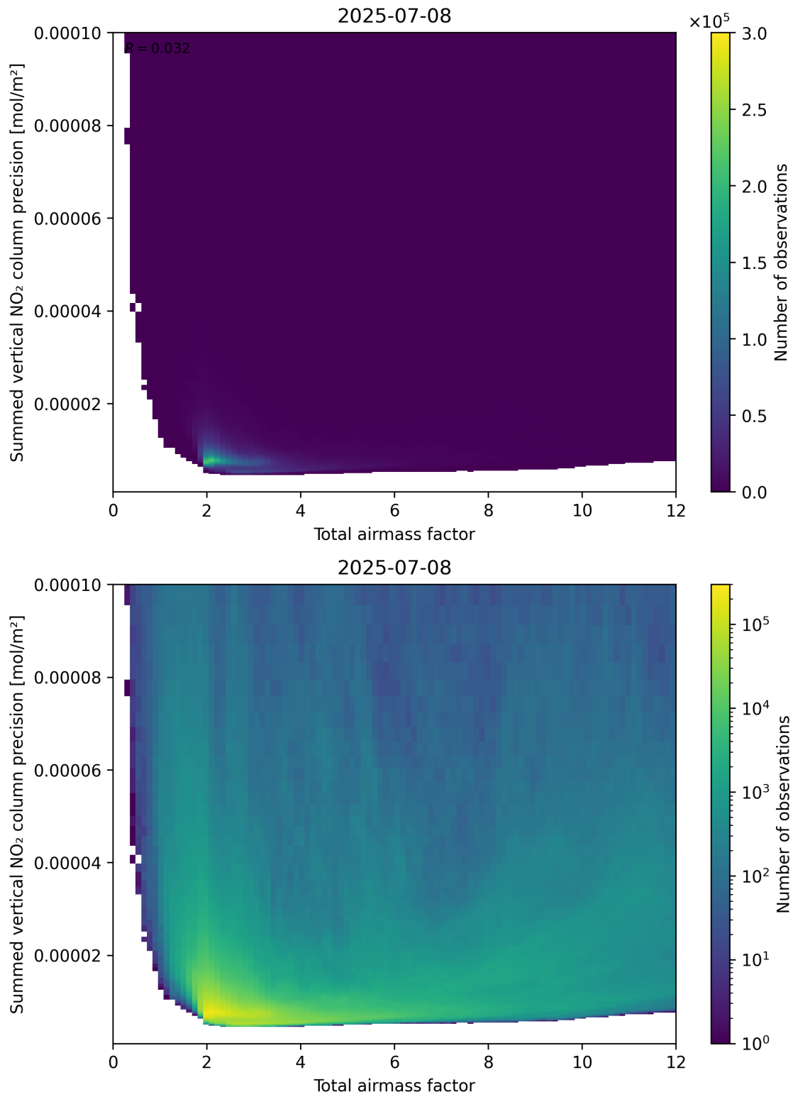
Figure 66: Scatter density plot of “Total airmass factor” against “Summed vertical NO 2 column precision” for 2025-07-08 to 2025-07-09.
