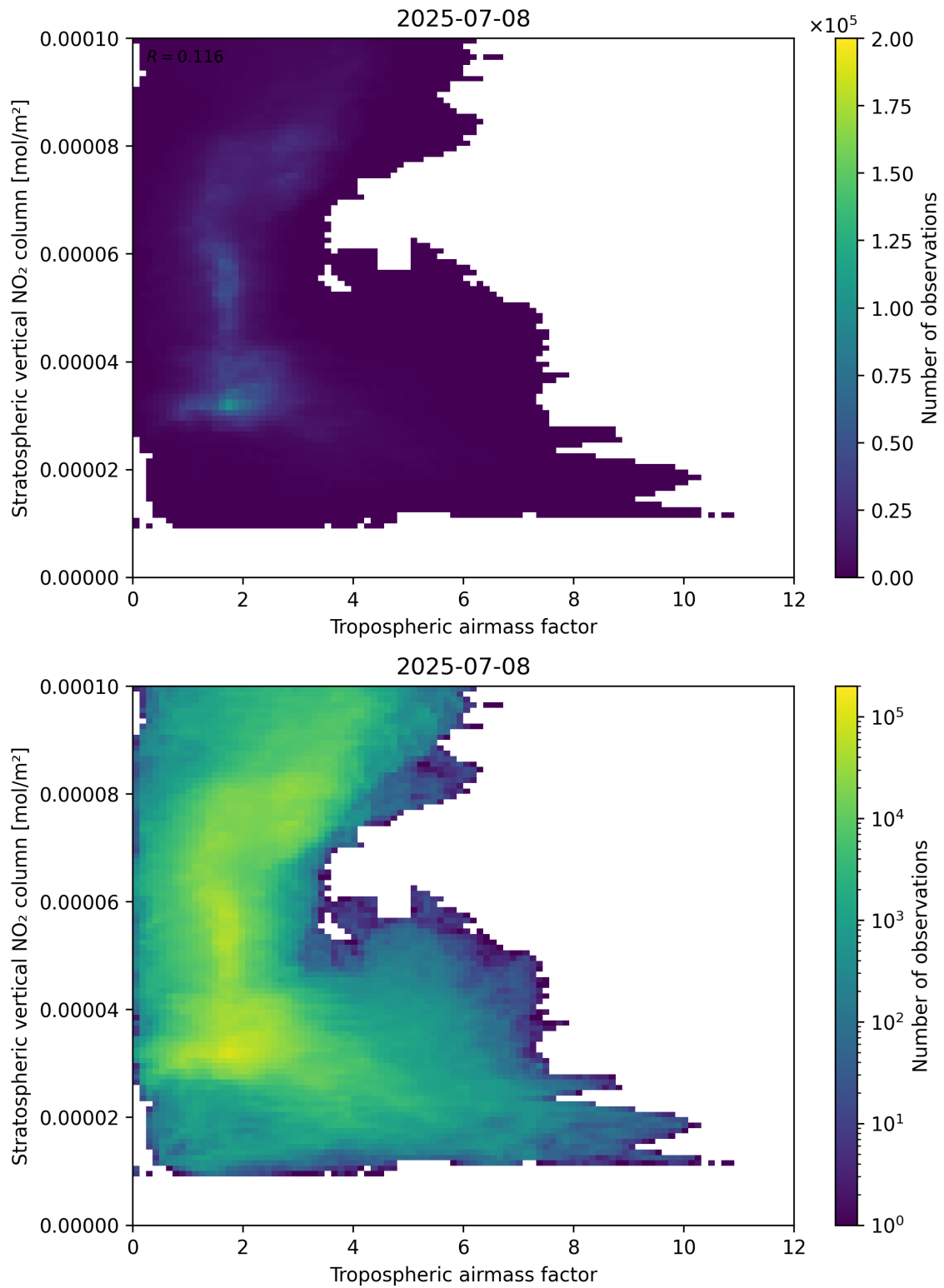
Figure 74: Scatter density plot of “Tropospheric air mass factor” against “Stratospheric vertical NO 2 column” for 2025-07-08 to 2025-07-09.
