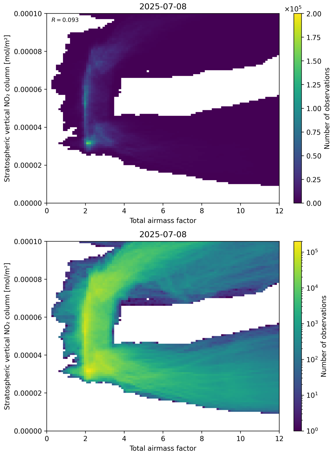
Figure 64: Scatter density plot of “Total airmass factor” against “Stratospheric vertical \text{NO}_2 column” for 2025-07-08 to 2025-07-09.
