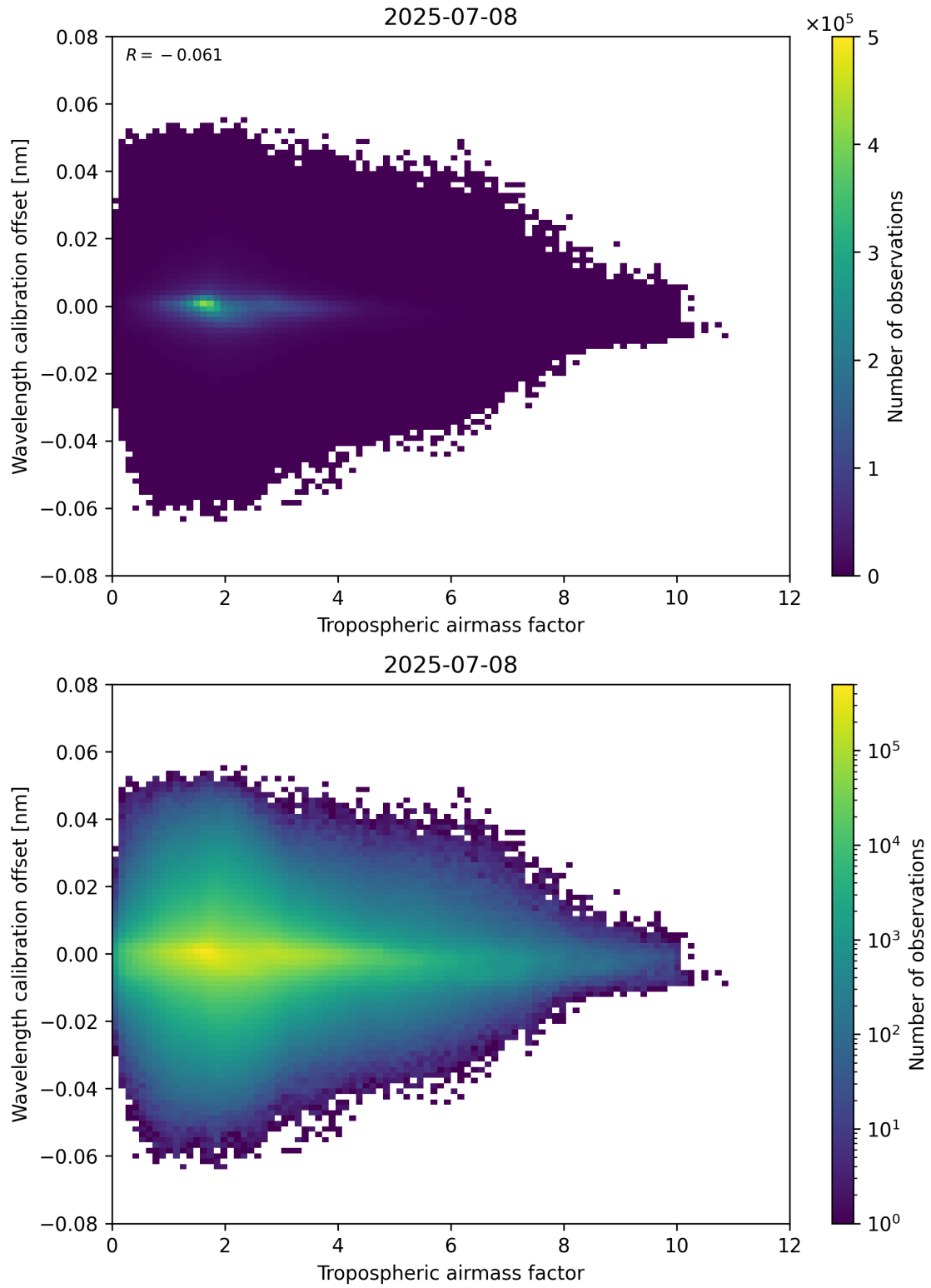
Figure 80: Scatter density plot of “Tropospheric air mass factor” against “Wavelength calibration offset” for 2025-07-08 to 2025-07-09.
