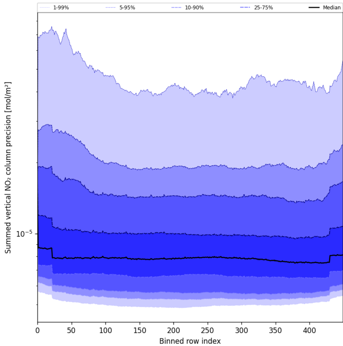
Figure 58: Along track statistics of “Summed vertical NO 2 column precision” for 2025-07-08 to 2025-07-09
