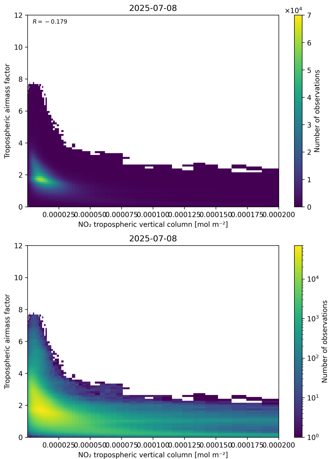
Figure 123: Scatter density plot of “NO 2 tropospheric vertical column” against “Tropospheric air mass factor” for 2025-07-08 to 2025-07-09.
