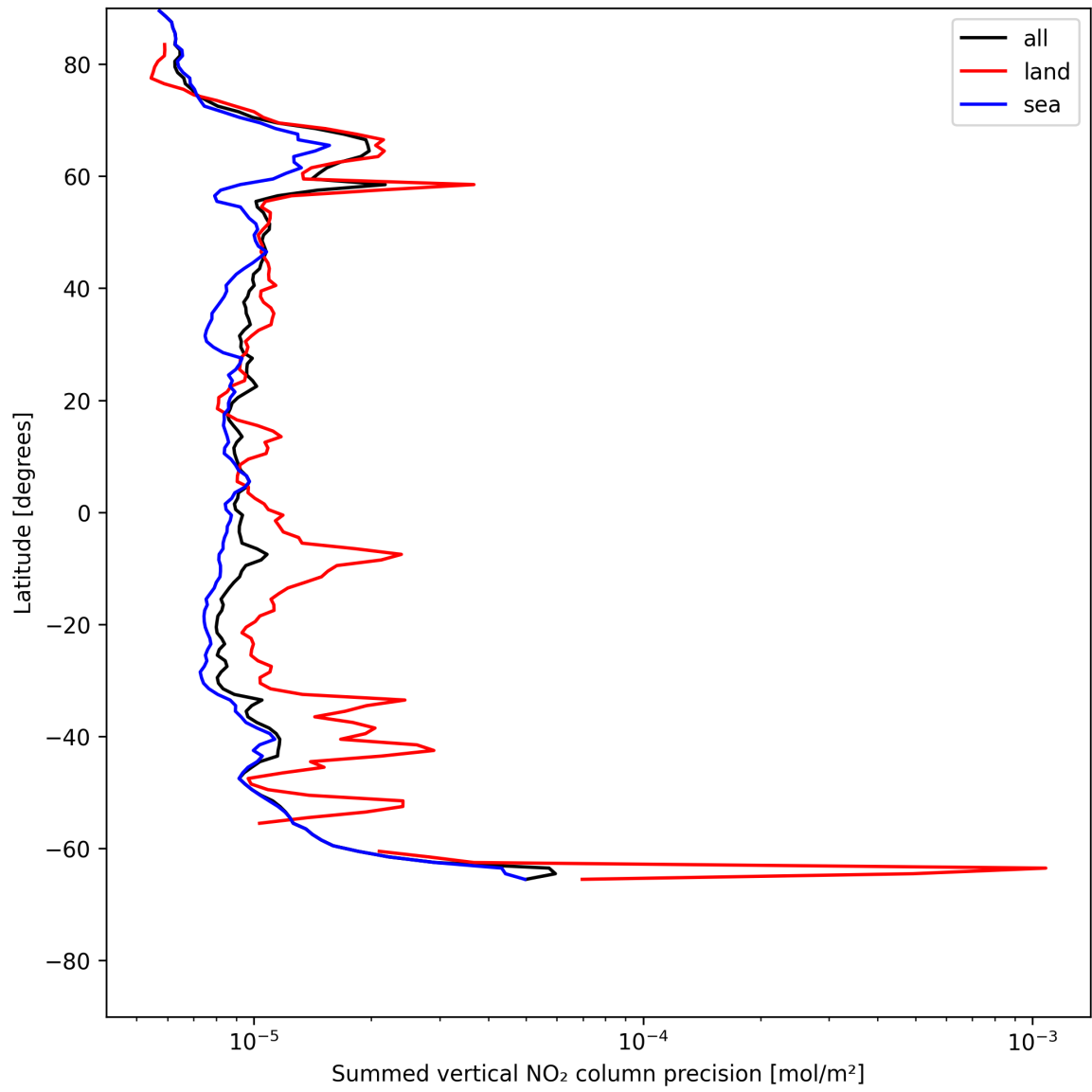
Figure 24: Zonal average of “Summed vertical NO 2 column precision” for 2025-07-08 to 2025-07-09.
