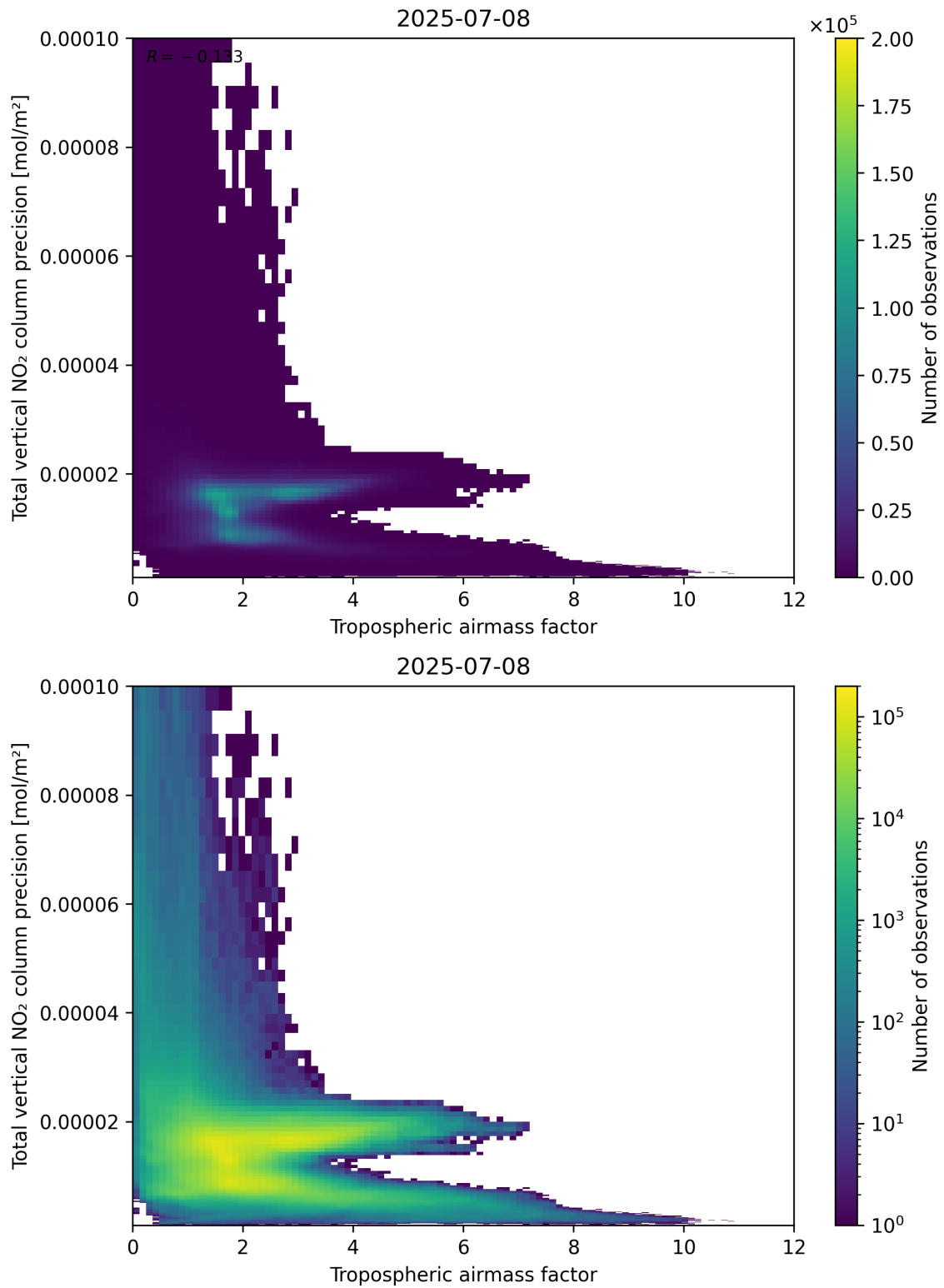
Figure 78: Scatter density plot of “Tropospheric air mass factor” against “Total vertical NO 2 column precision” for 2025-07-08 to 2025-07-09.
