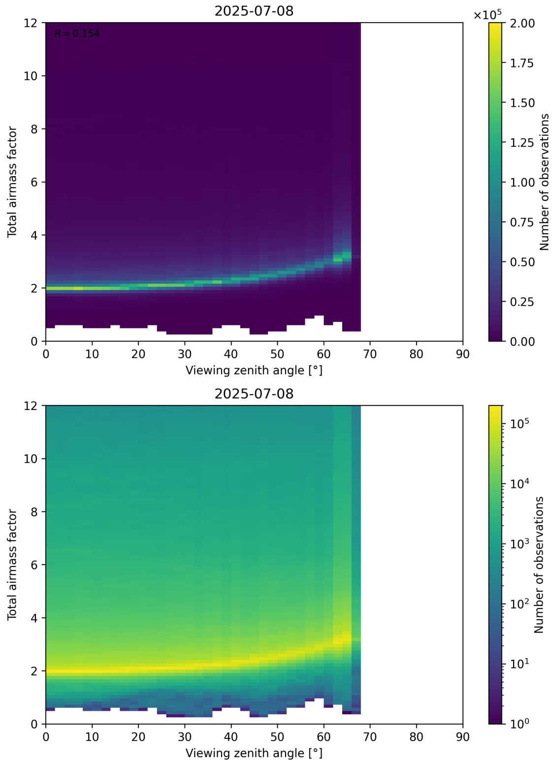
Figure 160: Scatter density plot of “Viewing zenith angle” against “Total airmass factor” for 2025-07-08 to 2025-07-09.
