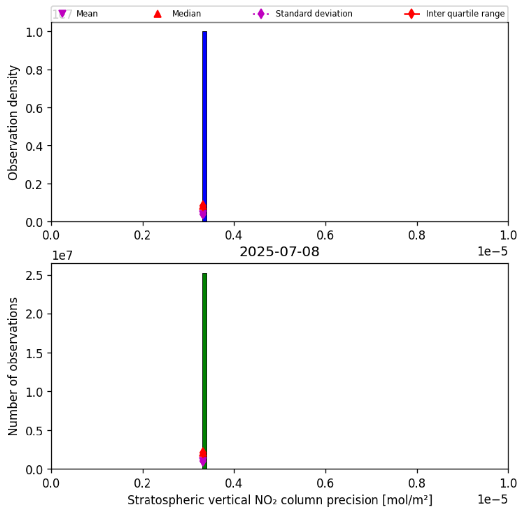
Figure 37: Histogram of “Stratospheric vertical NO 2 column precision” for 2025-07-08 to 2025-07-09
