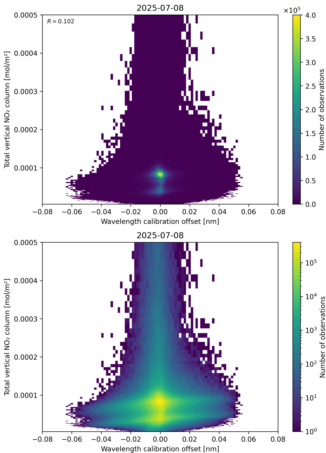
Figure 179: Scatter density plot of “Wavelength calibration offset” against “Total vertical NO 2 column” for 2025-07-08 to 2025-07-09.
