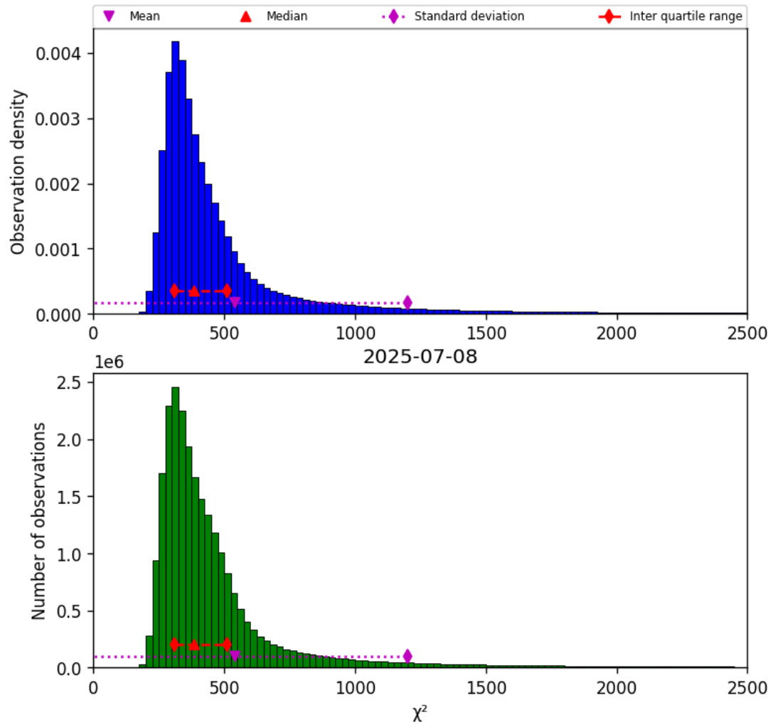
Figure 42: Histogram of " \chi^2 " for 2025-07-08 to 2025-07-09
