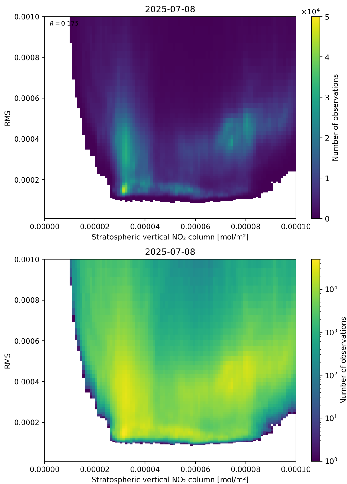
Figure 102: Scatter density plot of “Stratospheric vertical NO 2 column” against “RMS” for 2025-07-08 to 2025-07-09.
