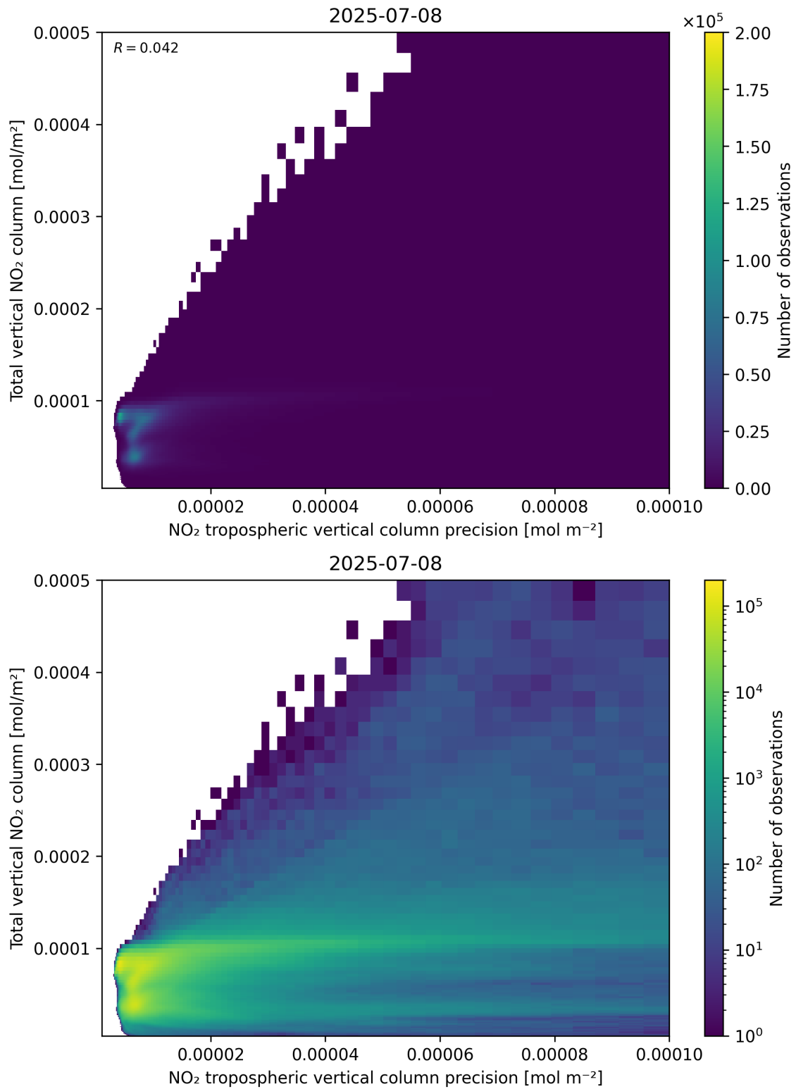
Figure 138: Scatter density plot of “NO 2 tropospheric vertical column precision” against “Total vertical NO 2 column” for 2025-07-08 to 2025-07-09.
