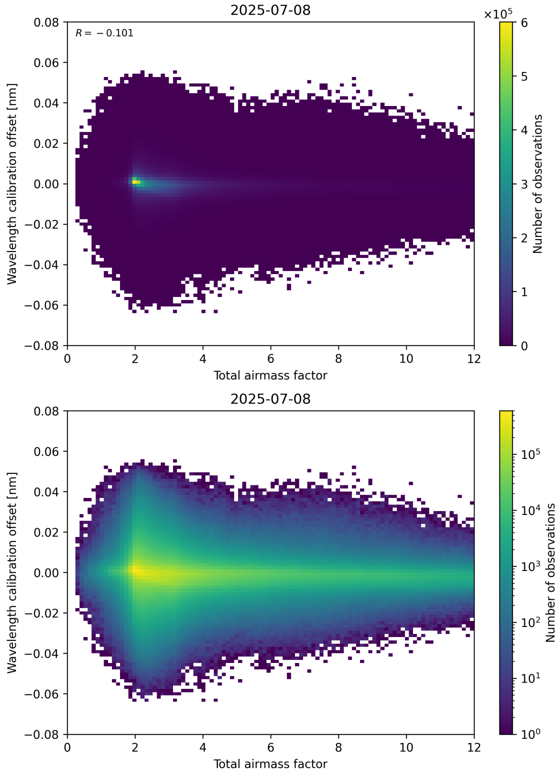
Figure 70: Scatter density plot of “Total airmass factor” against “Wavelength calibration offset” for 2025-07-08 to 2025-07-09.
