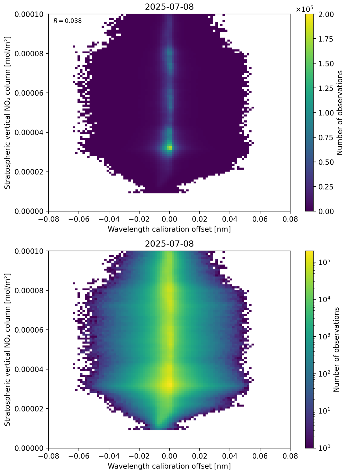
Figure 176: Scatter density plot of “Wavelength calibration offset” against “Stratospheric vertical NO 2 column” for 2025-07-08 to 2025-07-09.
