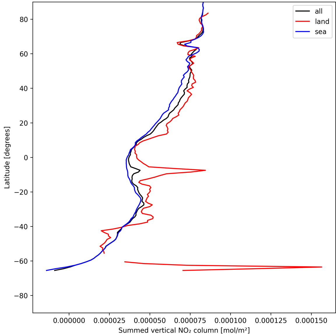
Figure 23: Zonal average of “Summed vertical NO 2 column” for 2025-07-08 to 2025-07-09.
