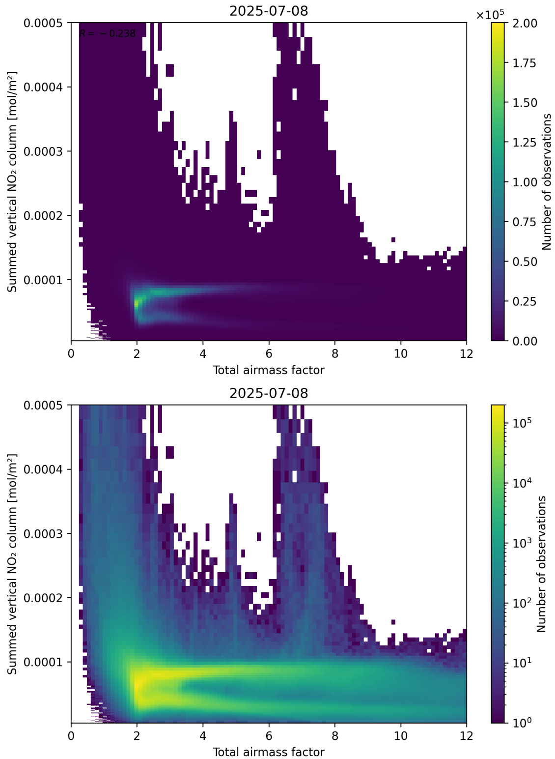
Figure 65: Scatter density plot of “Total airmass factor” against “Summed vertical NO 2 column” for 2025-07-08 to 2025-07-09.
