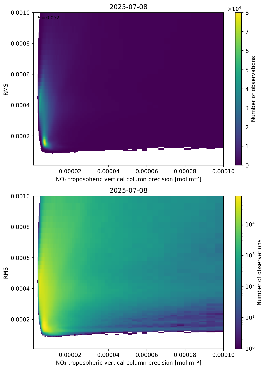
Figure 140: Scatter density plot of “NO 2 tropospheric vertical column precision” against “RMS” for 2025-07-08 to 2025-07-09.
