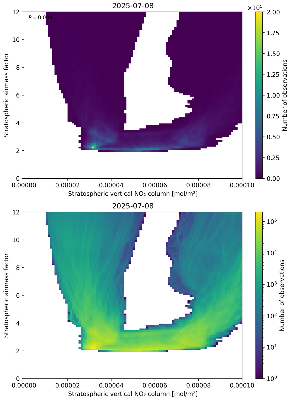
Figure 96: Scatter density plot of “Stratospheric vertical NO 2 column” against “Stratospheric airmass factor” for 2025-07-08 to 2025-07-09.
