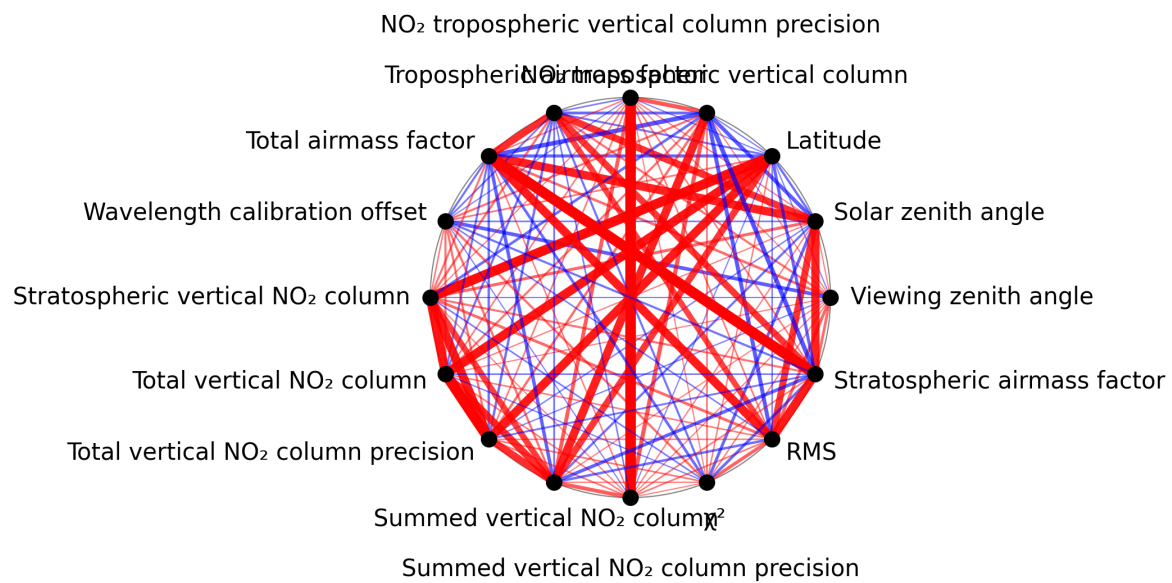
Figure 1: Map of correlation graph for 2025-07-08 to 2025-07-09.
