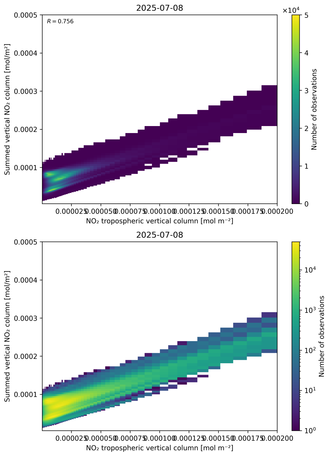
Figure 126: Scatter density plot of “NO 2 tropospheric vertical column” against “Summed vertical NO 2 column” for 2025-07-08 to 2025-07-09.
