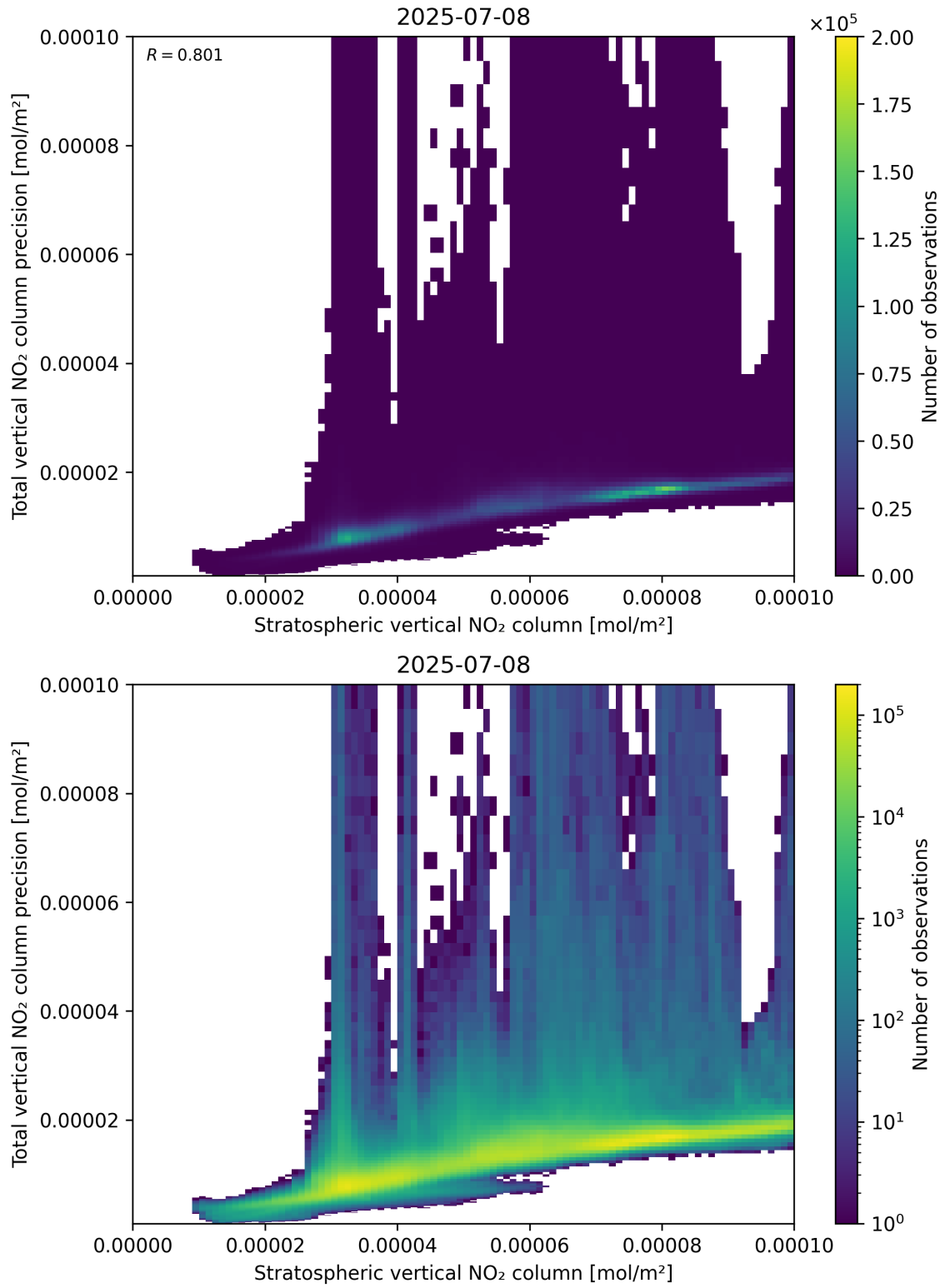
Figure 101: Scatter density plot of “Stratospheric vertical NO 2 column” against “Total vertical NO 2 column precision” for 2025-07-08 to 2025-07-09.
