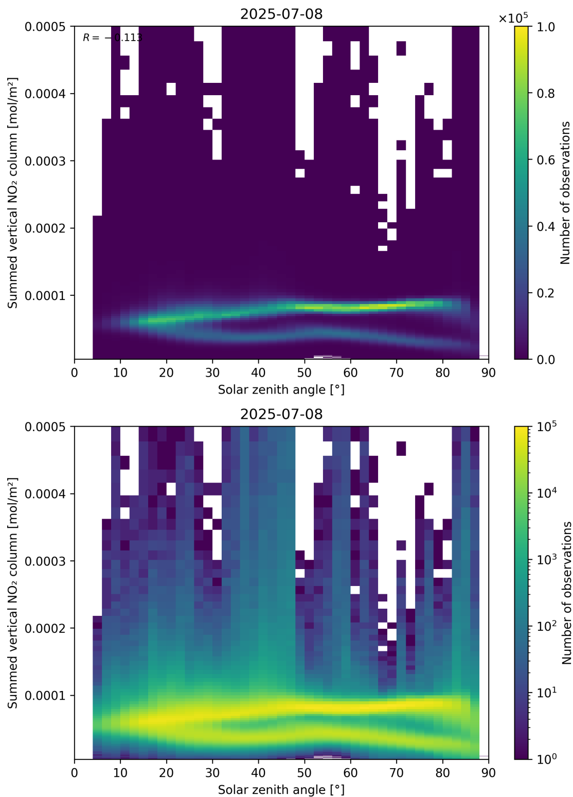
Figure 151: Scatter density plot of “Solar zenith angle” against “Summed vertical NO 2 column” for 2025-07-08 to 2025-07-09.
