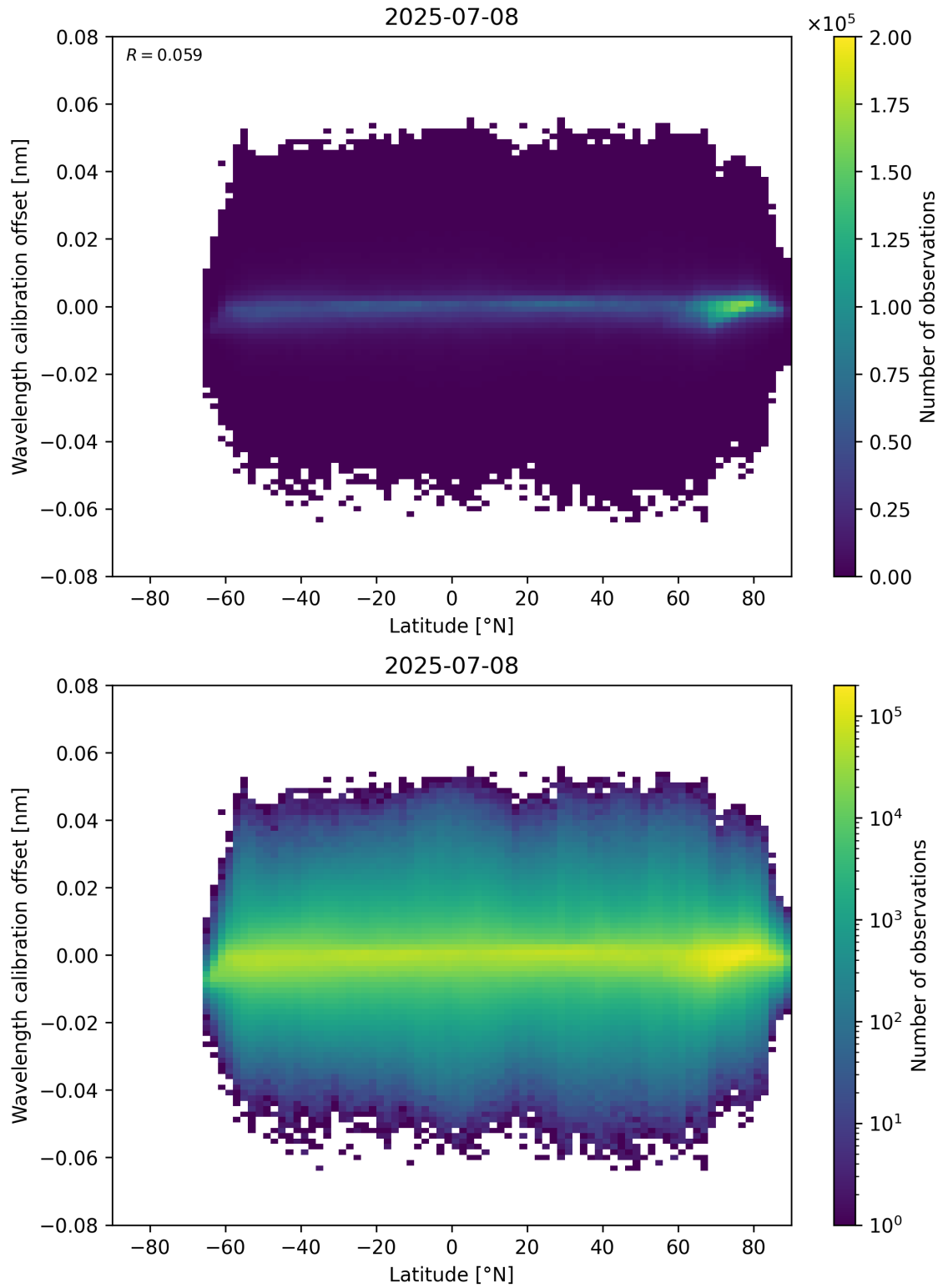
Figure 95: Scatter density plot of “Latitude” against “Wavelength calibration offset” for 2025-07-08 to 2025-07-09.
