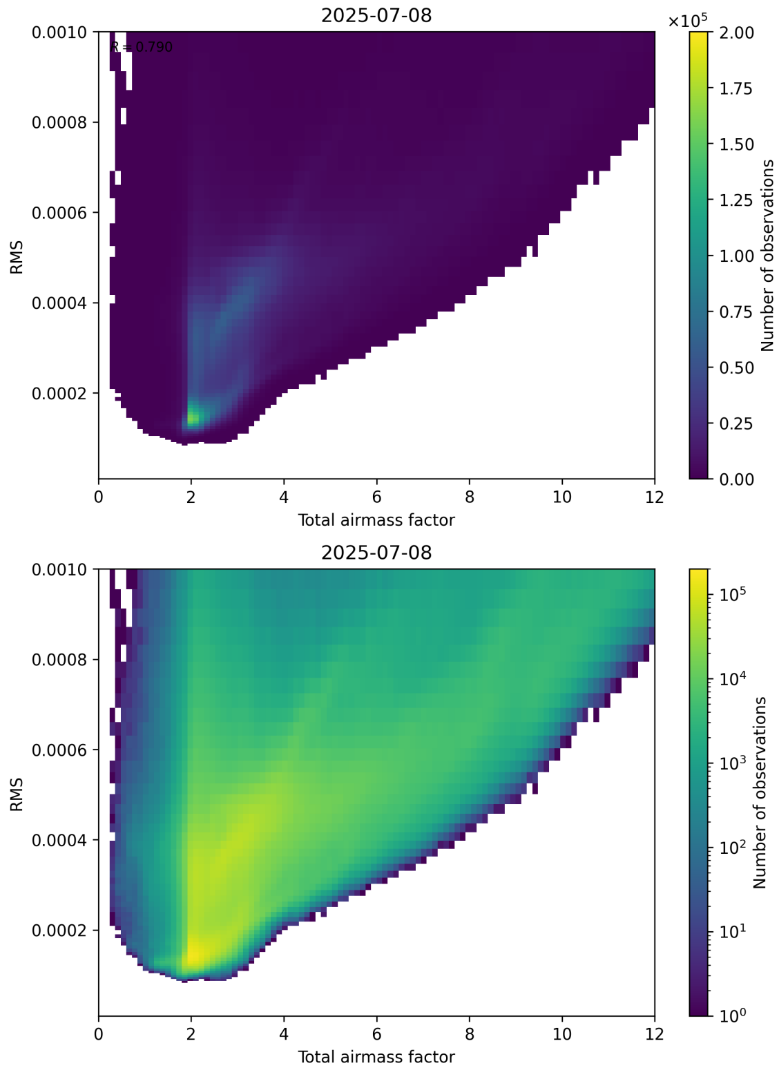
Figure 69: Scatter density plot of “Total airmass factor” against “RMS” for 2025-07-08 to 2025-07-09.
