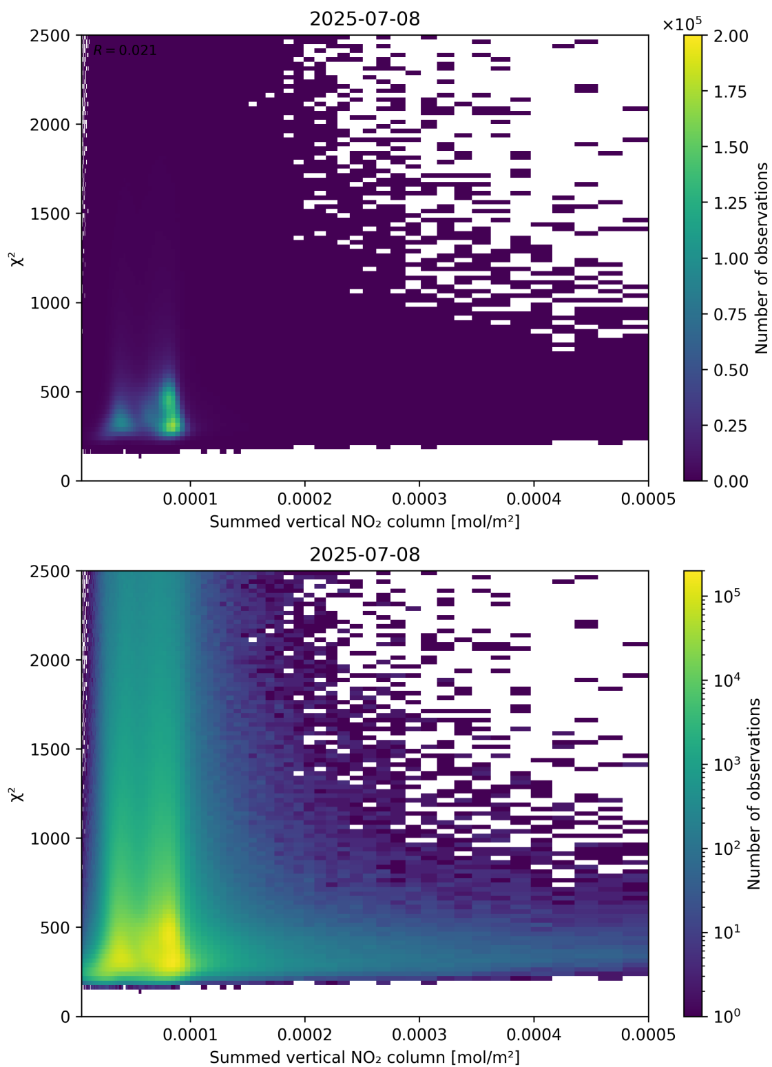
Figure 104: Scatter density plot of “Summed vertical NO 2 column” against “ \chi^2 ” for 2025-07-08 to 2025-07-09.
