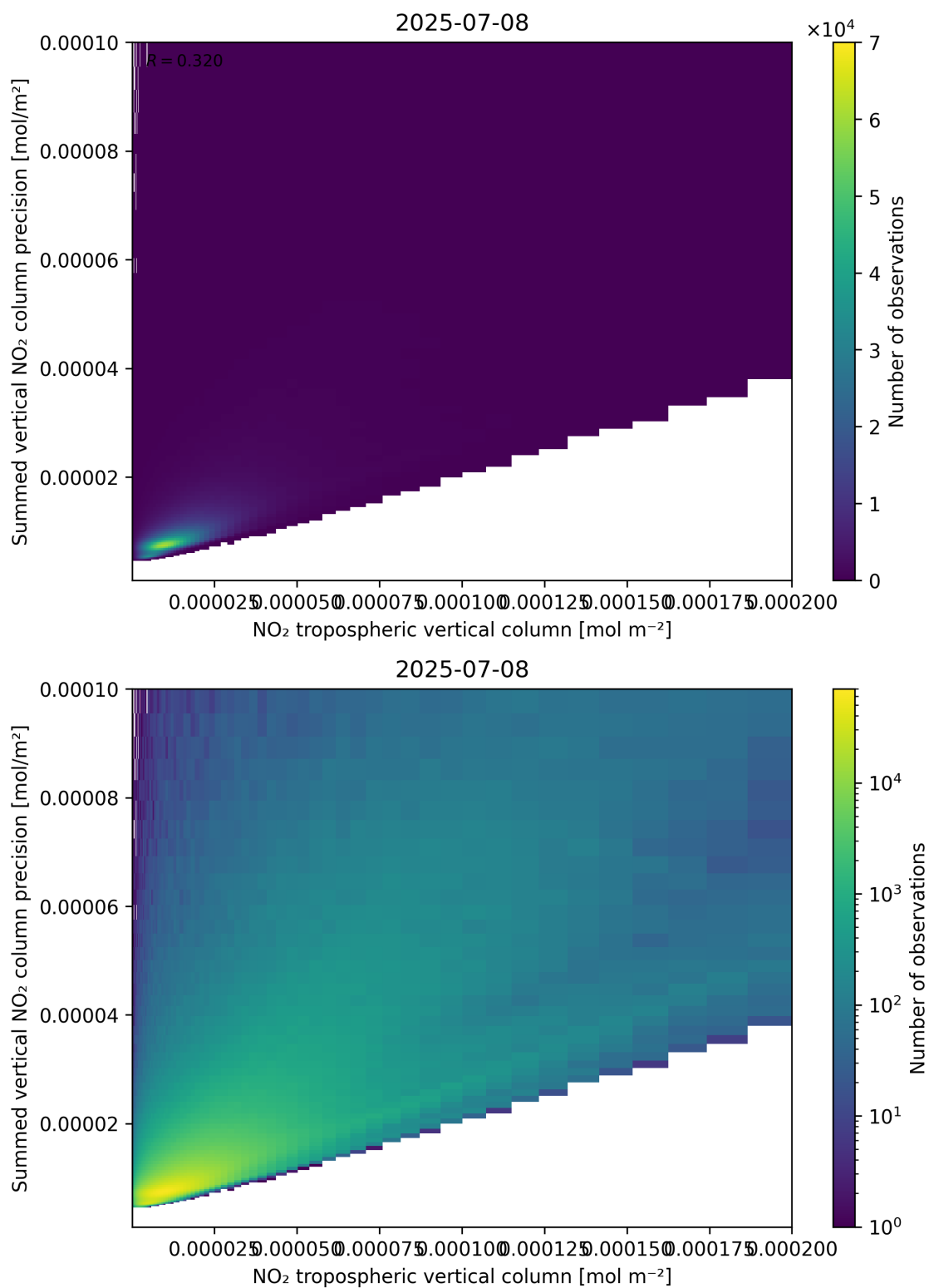
Figure 127: Scatter density plot of “NO 2 tropospheric vertical column” against “Summed vertical NO 2 column precision” for 2025-07-08 to 2025-07-09.
