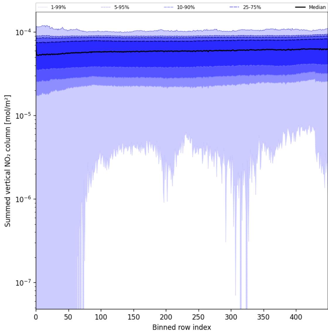
Figure 57: Along track statistics of “Summed vertical NO 2 column” for 2025-07-08 to 2025-07-09
