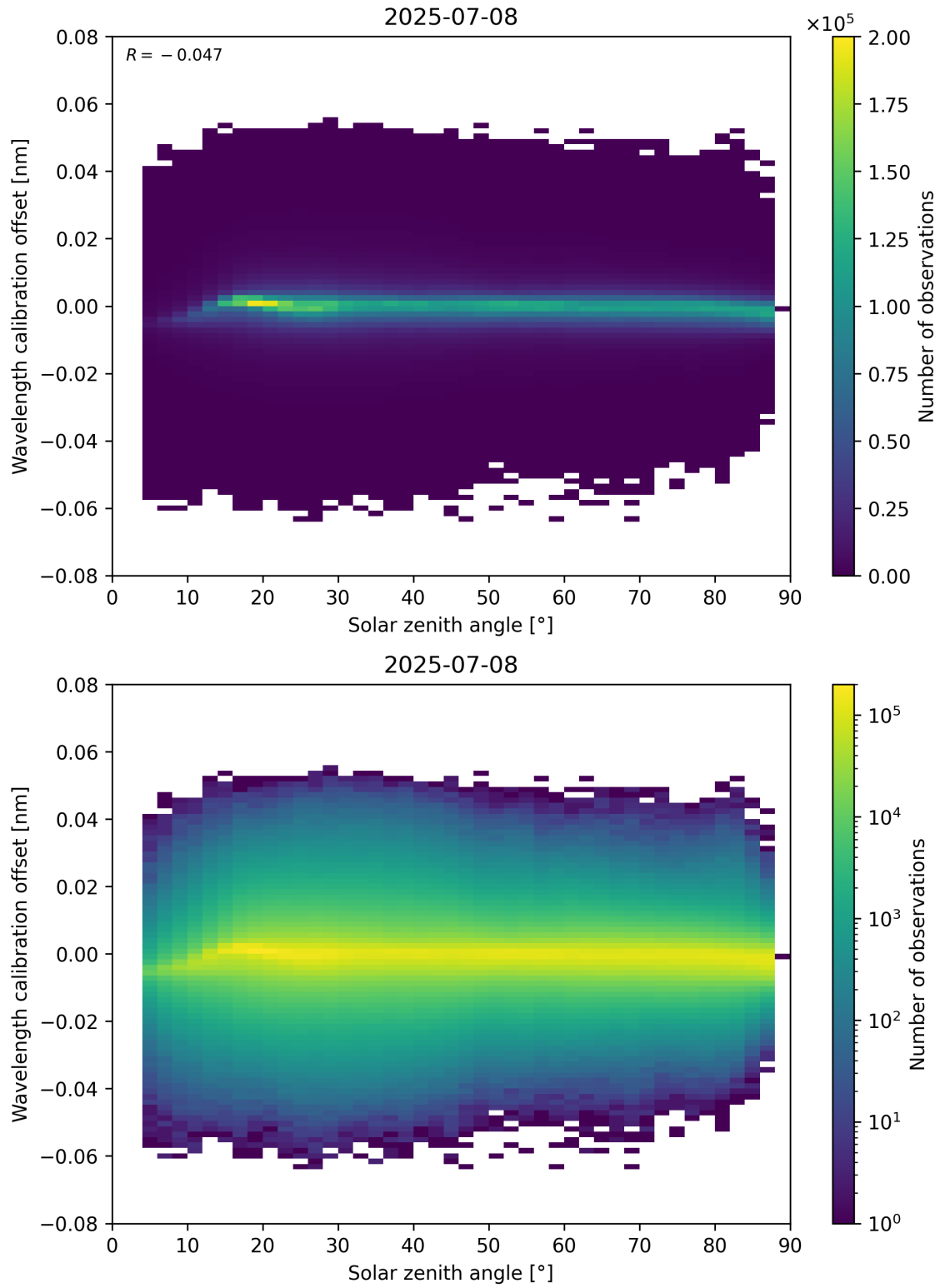
Figure 158: Scatter density plot of “Solar zenith angle” against “Wavelength calibration offset” for 2025-07-08 to 2025-07-09.
