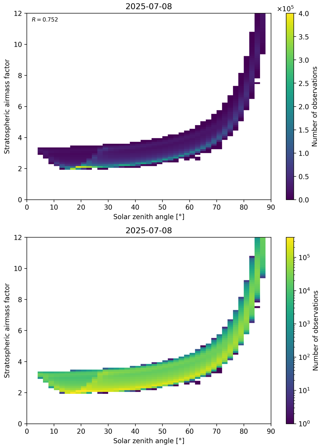
Figure 145: Scatter density plot of “Solar zenith angle” against “Stratospheric airmass factor” for 2025-07-08 to 2025-07-09.
