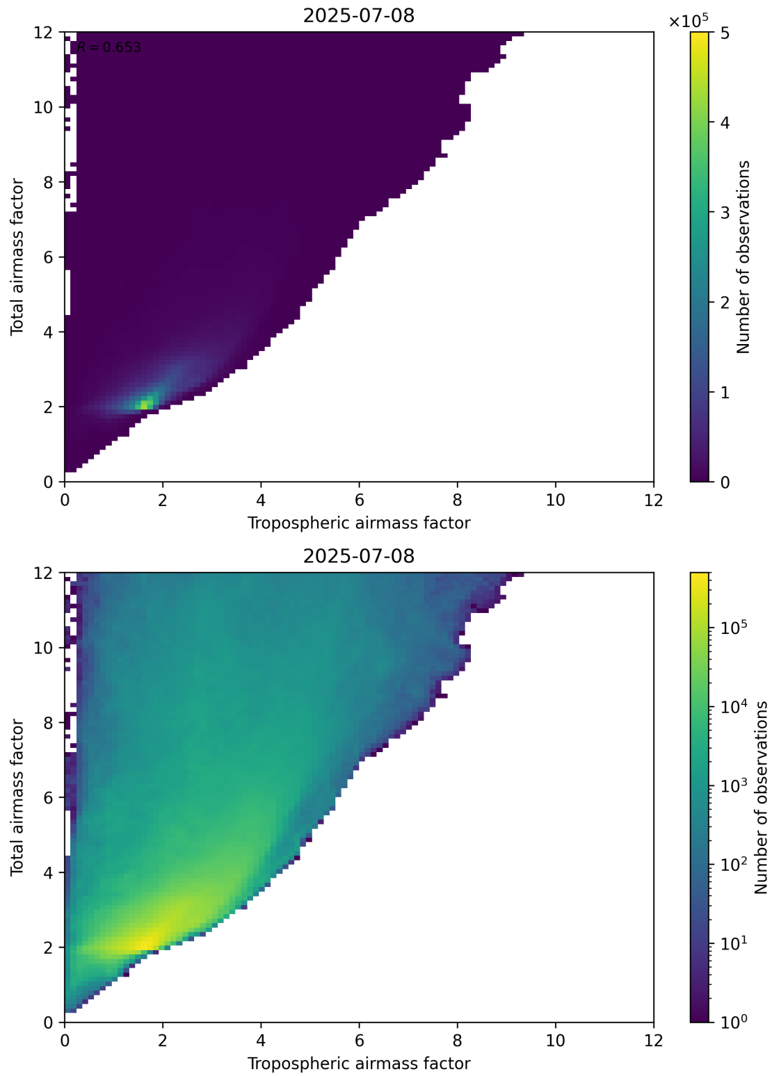
Figure 72: Scatter density plot of “Tropospheric airmass factor” against “Total airmass factor” for 2025-07-08 to 2025-07-09.
