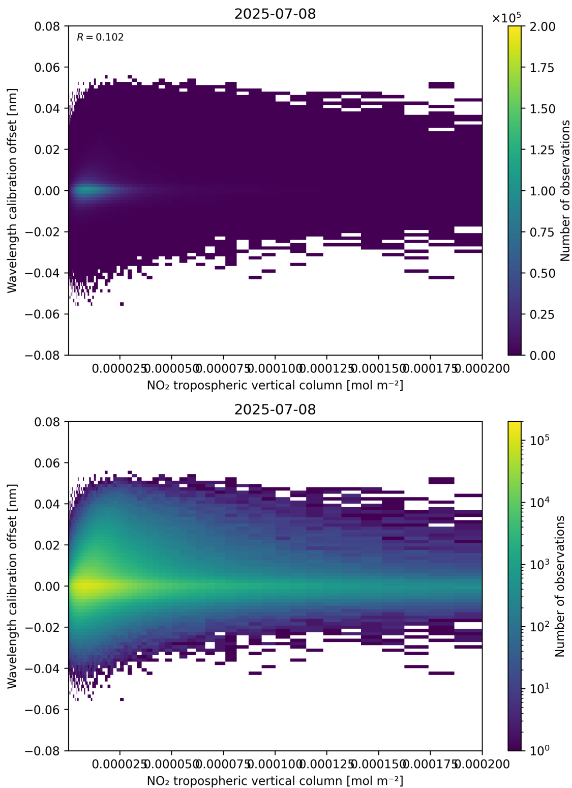
Figure 143: Scatter density plot of “NO 2 tropospheric vertical column” against “Wavelength calibration offset” for 2025-07-08 to 2025-07-09.
