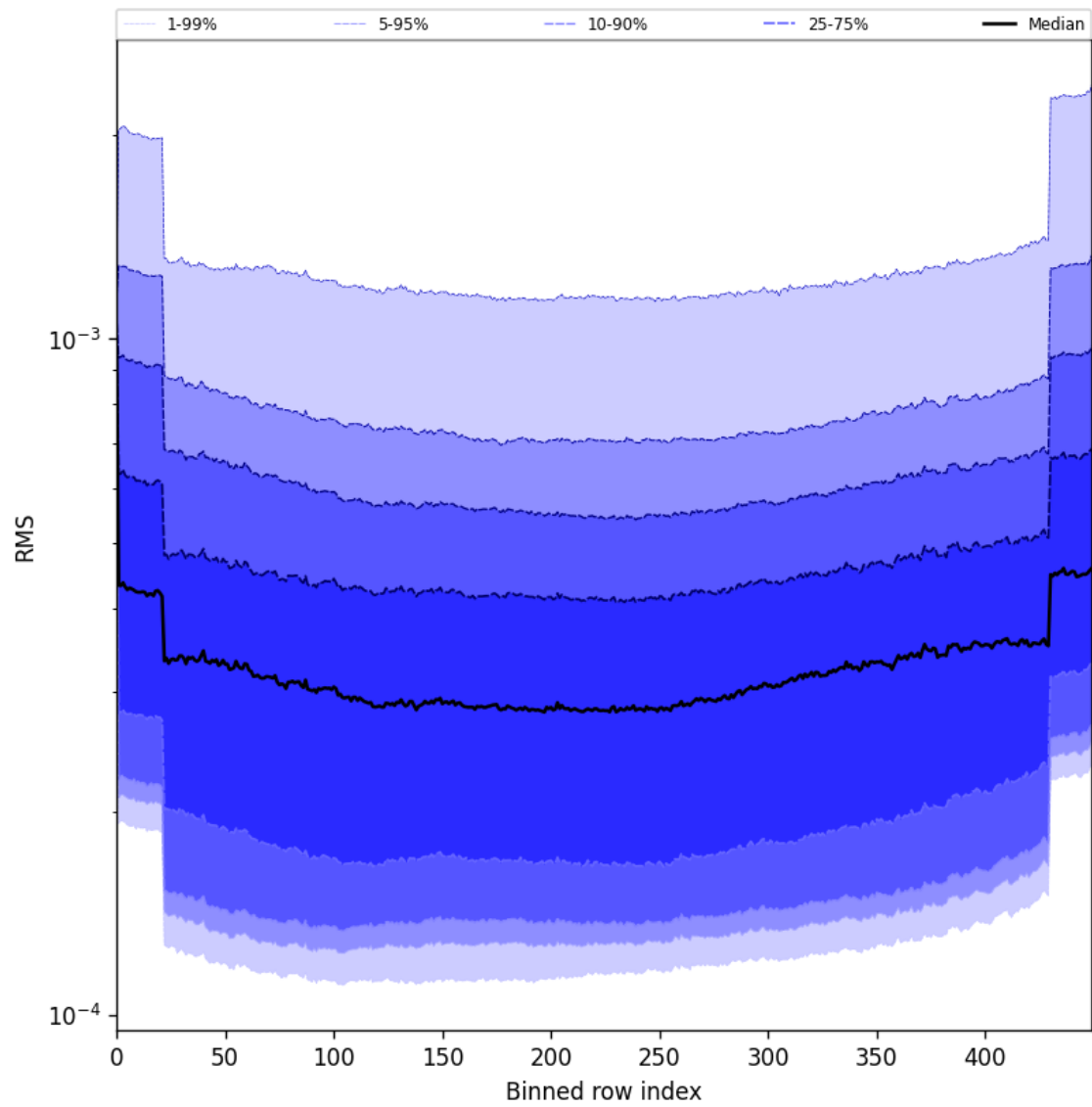
Figure 60: Along track statistics of “RMS” for 2025-07-08 to 2025-07-09
