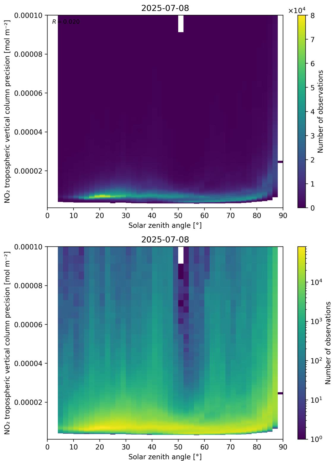
Figure 156: Scatter density plot of “Solar zenith angle” against “NO 2 tropospheric vertical column precision” for 2025-07-08 to 2025-07-09.
