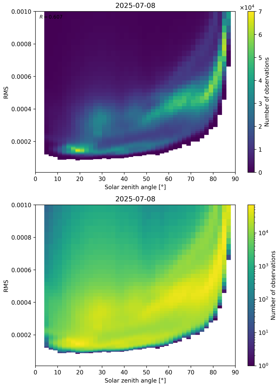
Figure 157: Scatter density plot of “Solar zenith angle” against “RMS” for 2025-07-08 to 2025-07-09.
