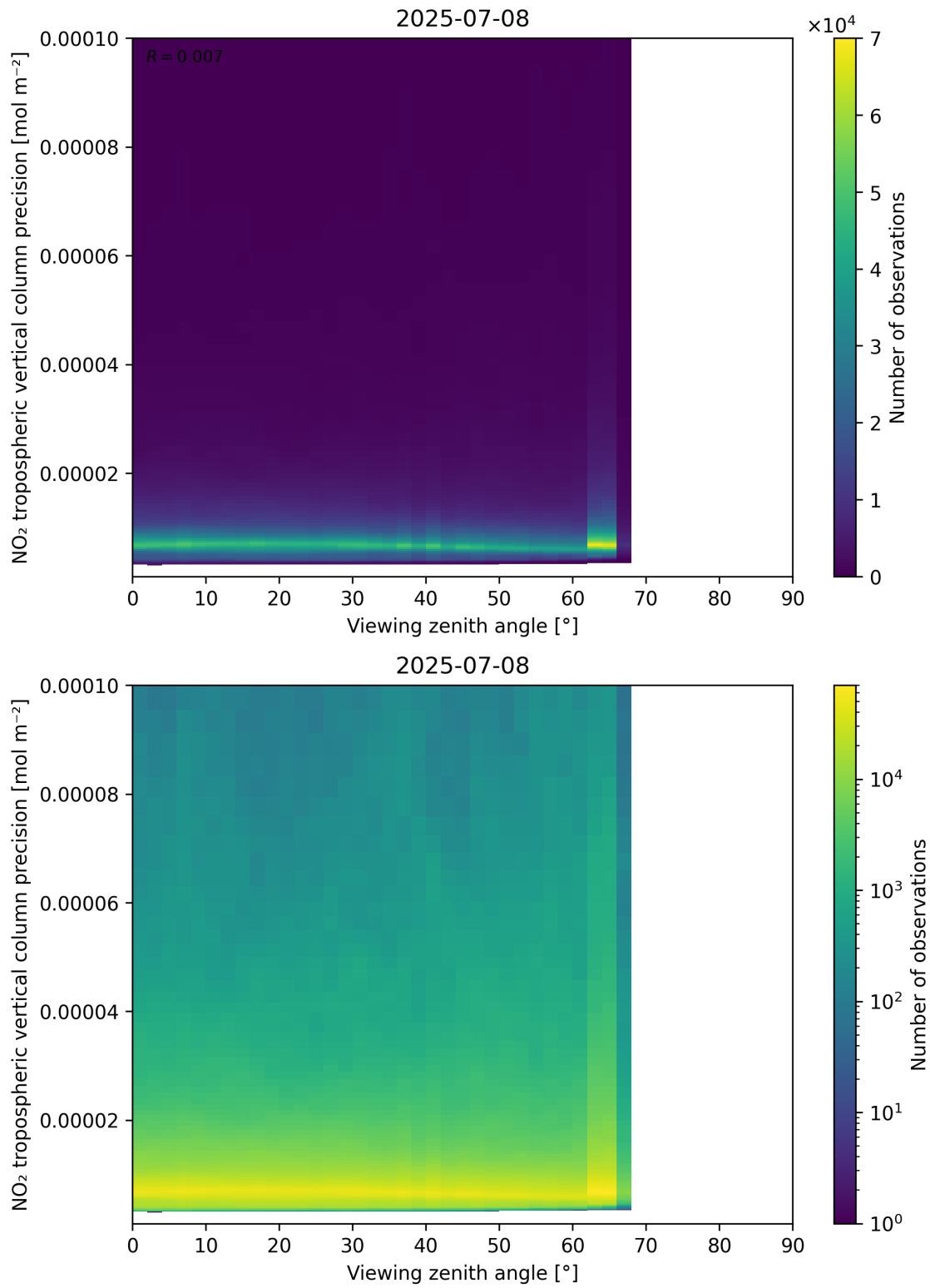
Figure 170: Scatter density plot of “Viewing zenith angle” against “NO 2 tropospheric vertical column precision” for 2025-07-08 to 2025-07-09.
