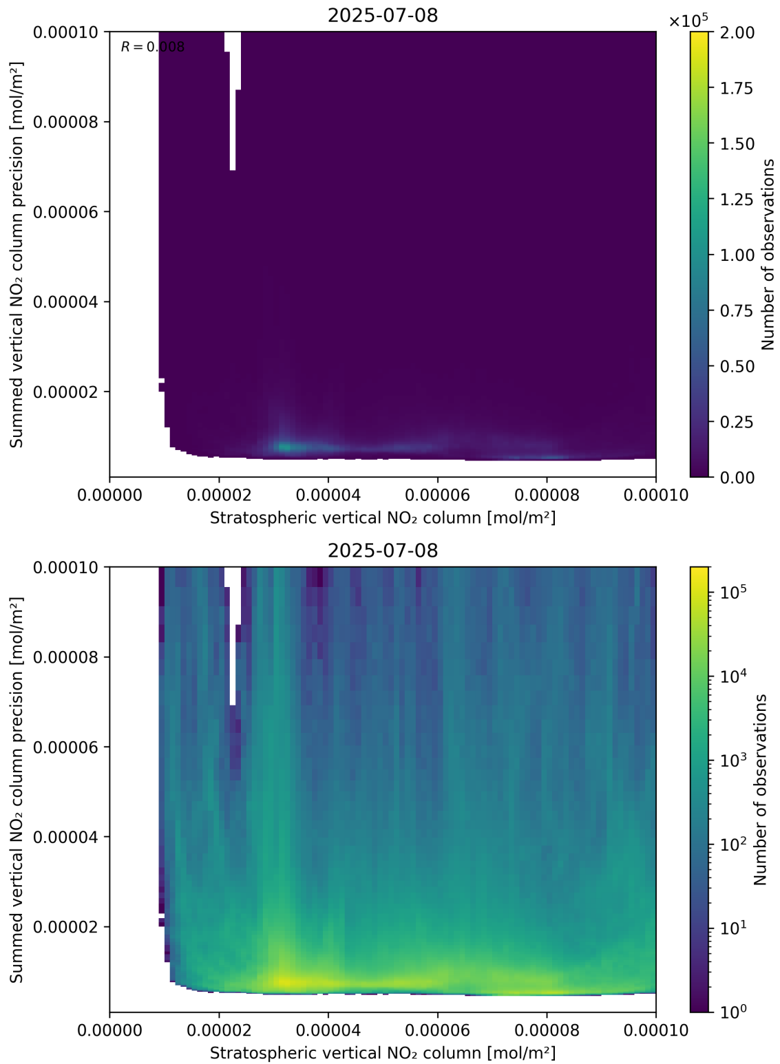
Figure 99: Scatter density plot of “Stratospheric vertical NO 2 column” against “Summed vertical NO 2 column precision” for 2025-07-08 to 2025-07-09.
