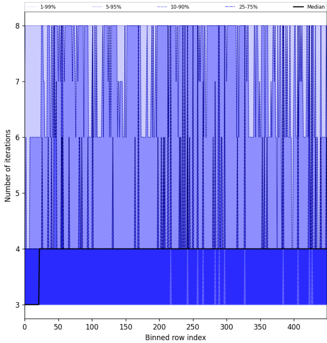
Figure 51: Along track statistics of “Number of iterations” for 2025-07-08 to 2025-07-09
