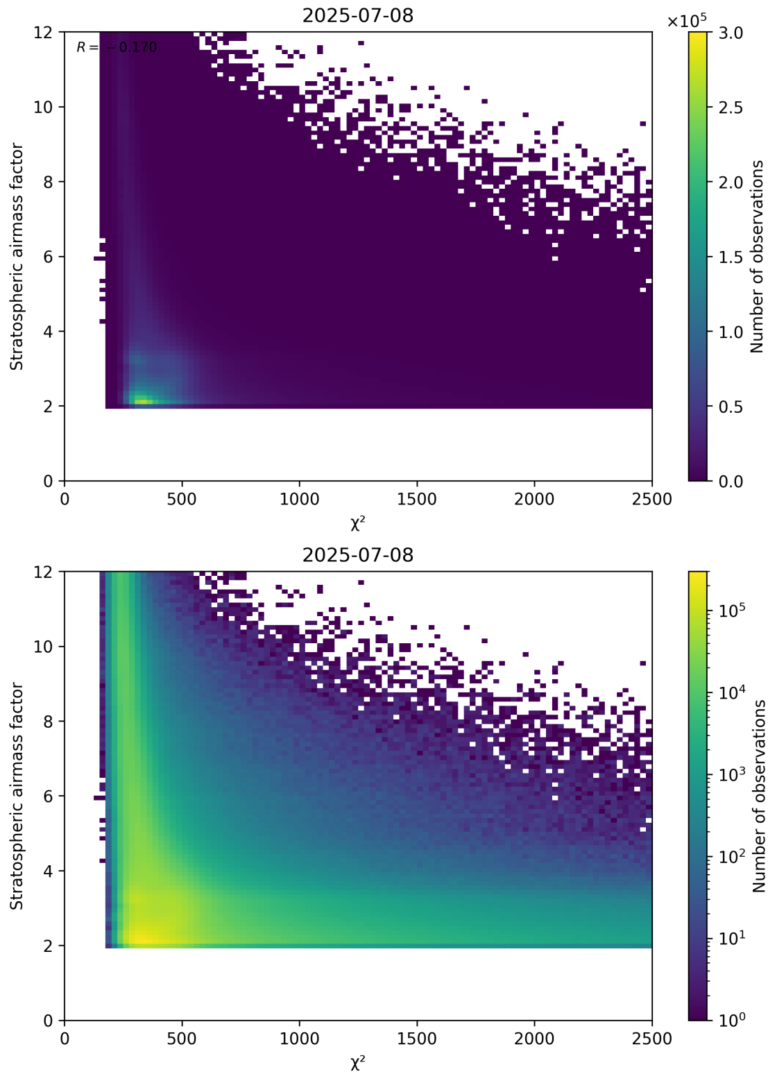
Figure 81: Scatter density plot of “ \chi^2 ” against “Stratospheric airmass factor” for 2025-07-08 to 2025-07-09.
