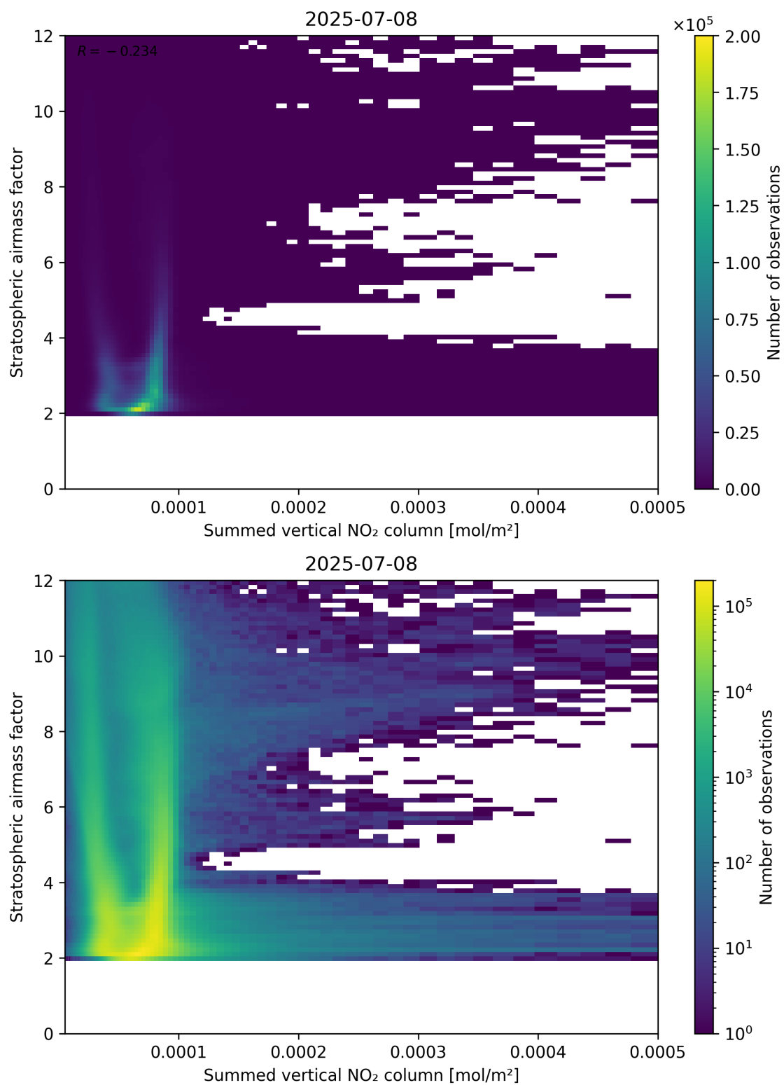
Figure 103: Scatter density plot of “Summed vertical NO 2 column” against “Stratospheric airmass factor” for 2025-07-08 to 2025-07-09.
