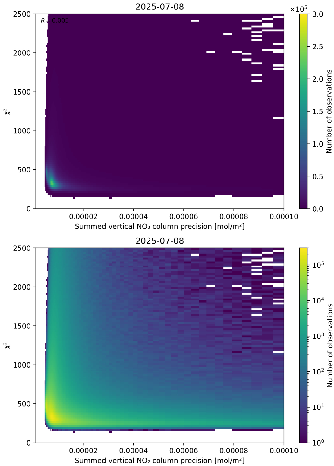
Figure 107: Scatter density plot of “Summed vertical NO 2 column precision” against “ \chi^2 ” for 2025-07-08 to 2025-07-09.
