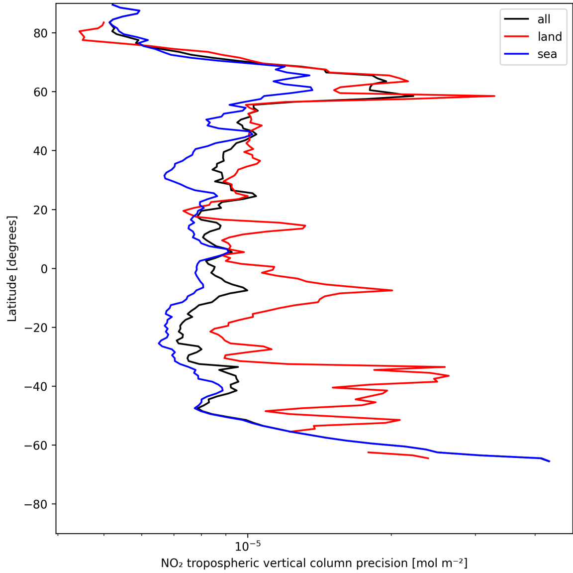
Figure 13: Zonal average of “NO 2 tropospheric vertical column precision” for 2025-07-08 to 2025-07-10.
