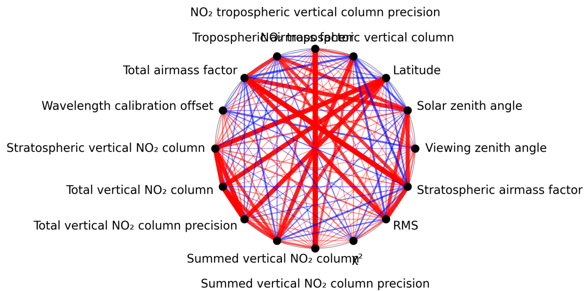
Figure 1: Map of correlation graph for 2025-07-08 to 2025-07-10.
