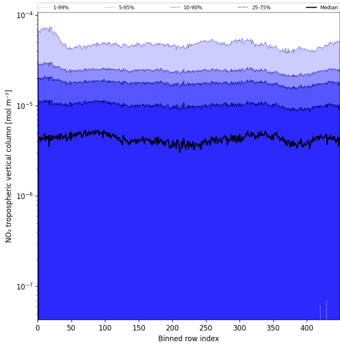
Figure 46: Along track statistics of “NO 2 tropospheric vertical column” for 2025-07-08 to 2025-07-10
