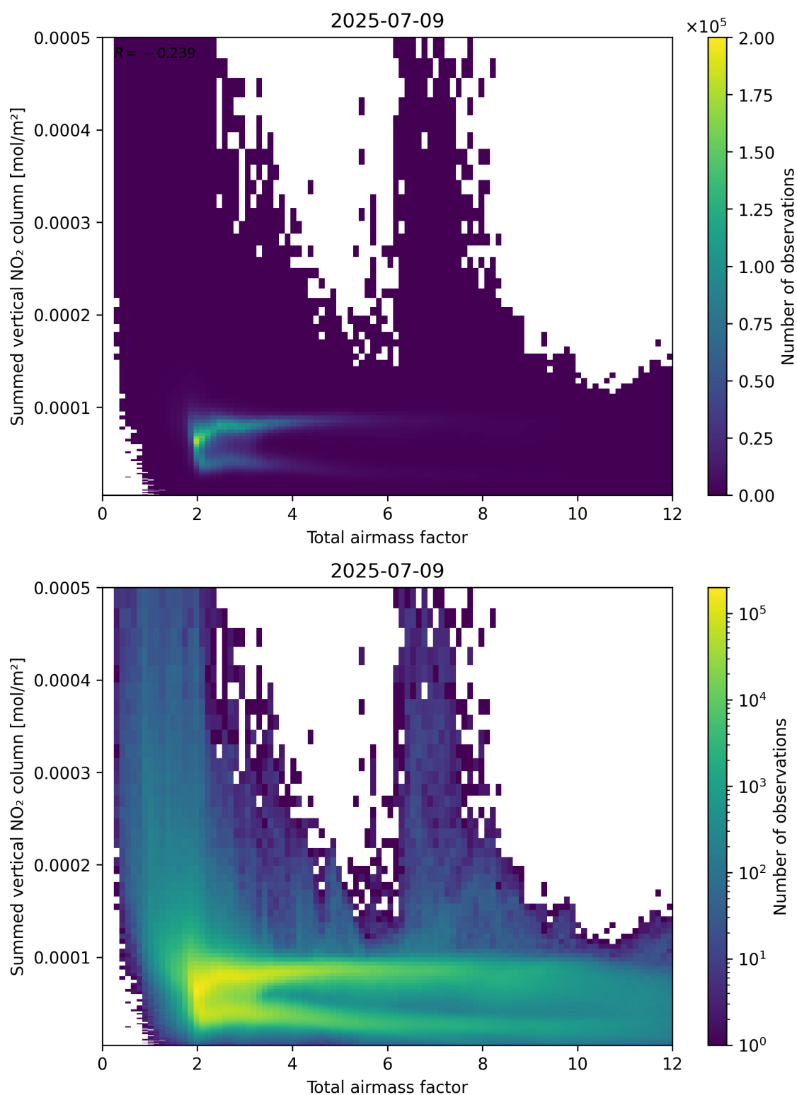
Figure 65: Scatter density plot of “Total airmass factor” against “Summed vertical NO 2 column” for 2025-07-08 to 2025-07-10.
