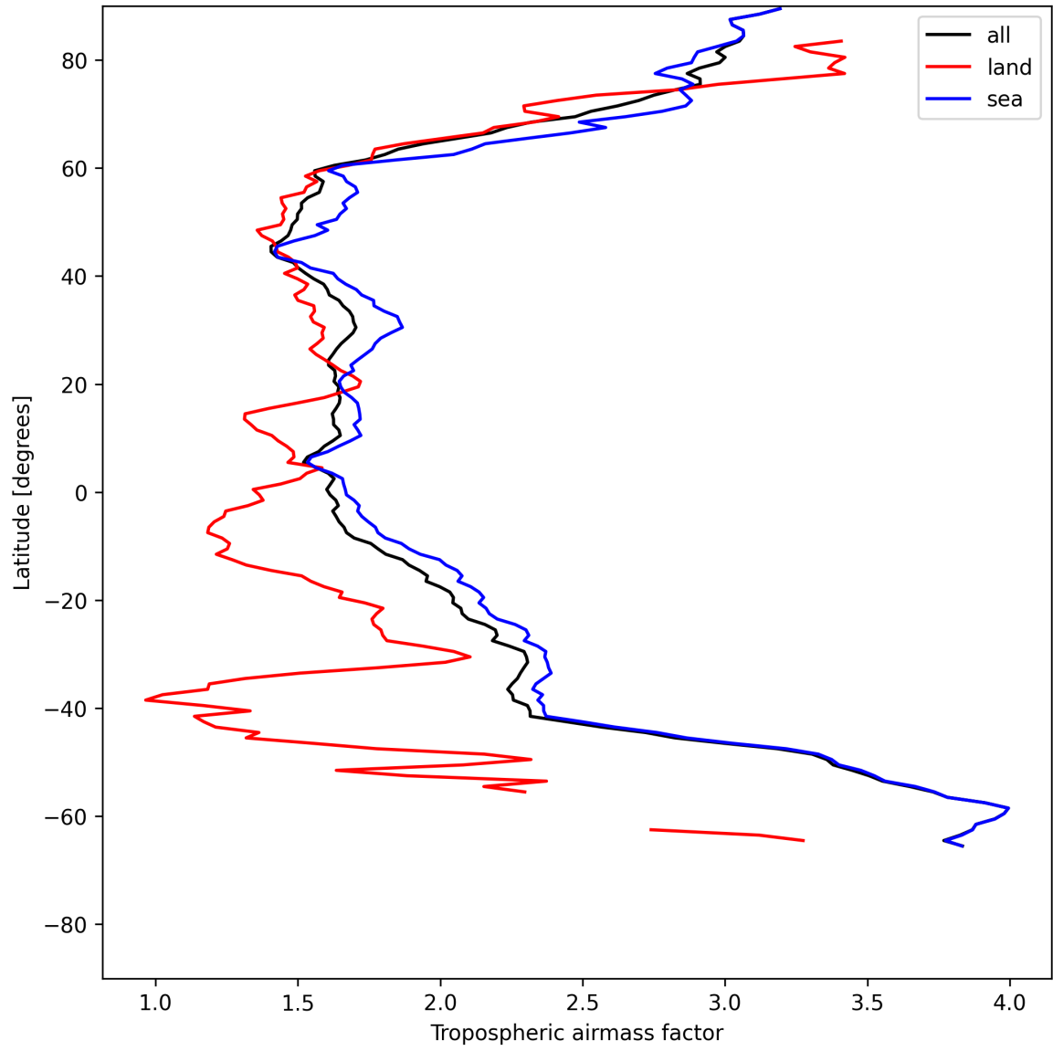
Figure 14: Zonal average of “Tropospheric air mass factor” for 2025-07-08 to 2025-07-10.
