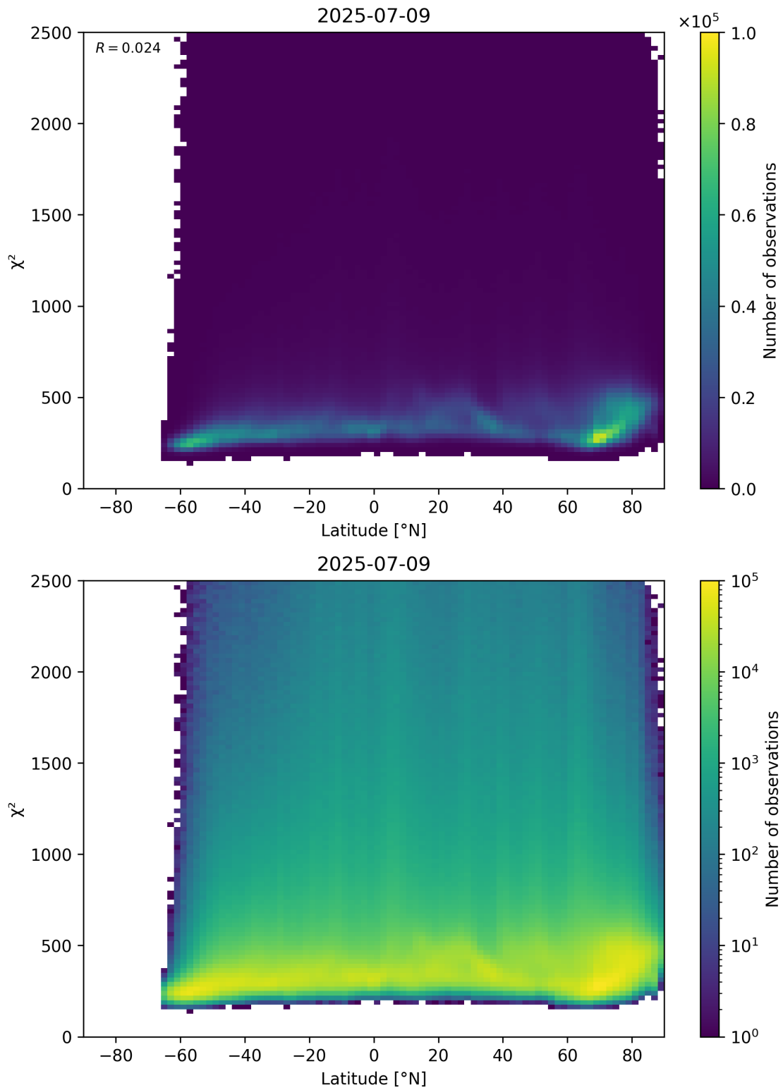
Figure 86: Scatter density plot of “Latitude” against “ \chi^2 ” for 2025-07-08 to 2025-07-10.
