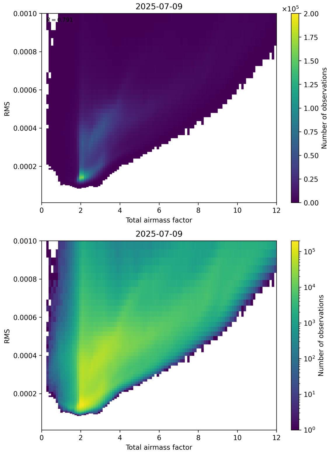
Figure 69: Scatter density plot of “Total airmass factor” against “RMS” for 2025-07-08 to 2025-07-10.
