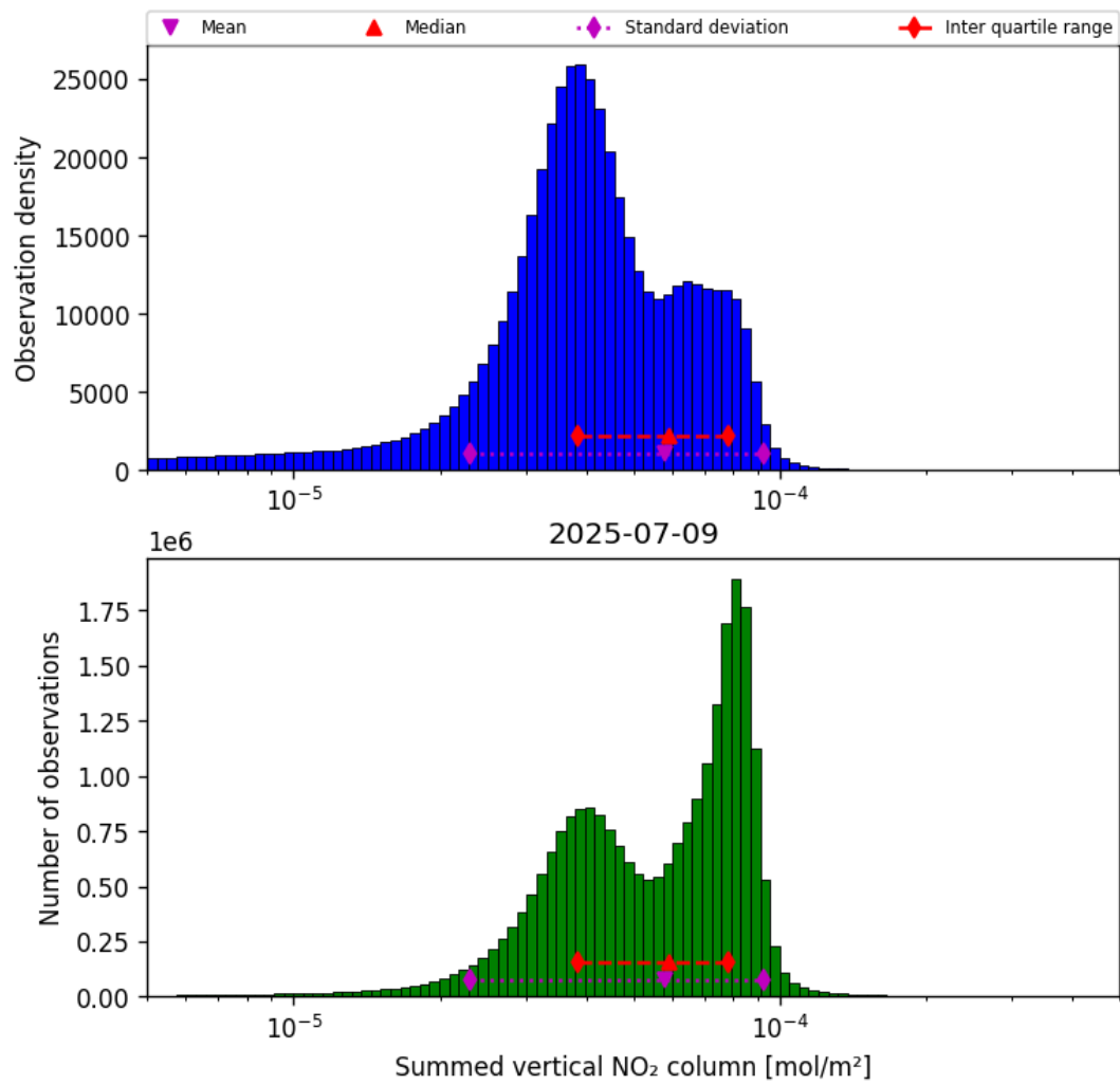
Figure 40: Histogram of “Summed vertical NO 2 column” for 2025-07-08 to 2025-07-10
