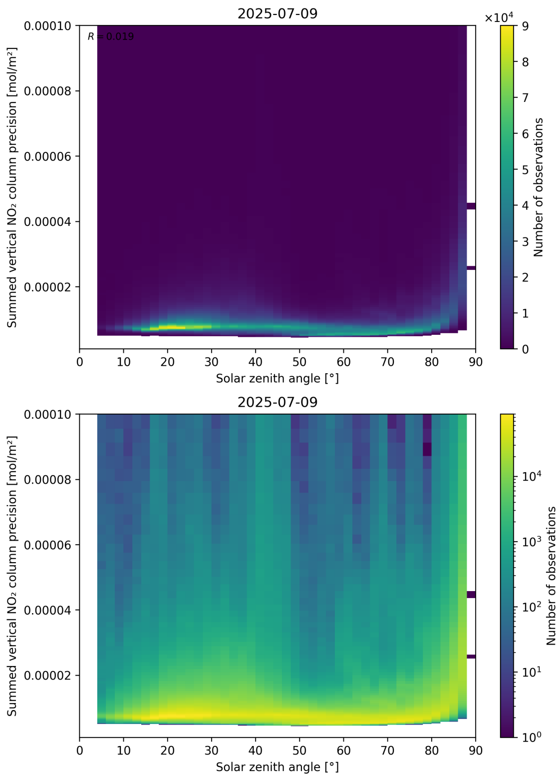
Figure 152: Scatter density plot of “Solar zenith angle” against “Summed vertical NO 2 column precision” for 2025-07-08 to 2025-07-10.
