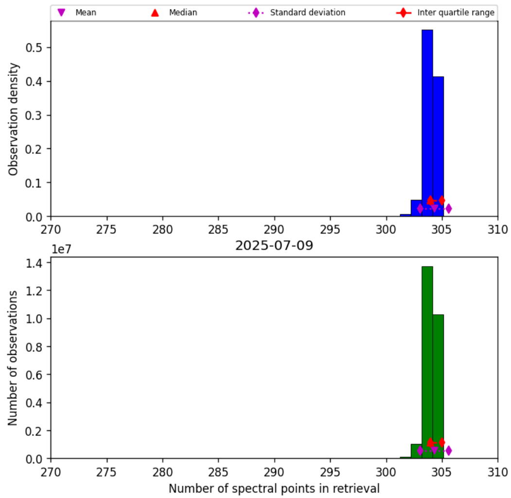
Figure 33: Histogram of “Number of spectral points in retrieval” for 2025-07-08 to 2025-07-10
