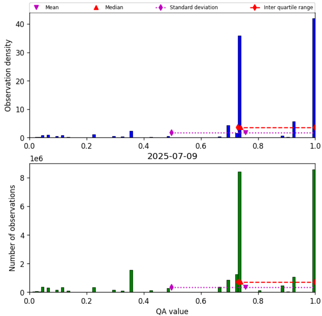
Figure 28: Histogram of “QA value” for 2025-07-08 to 2025-07-10
