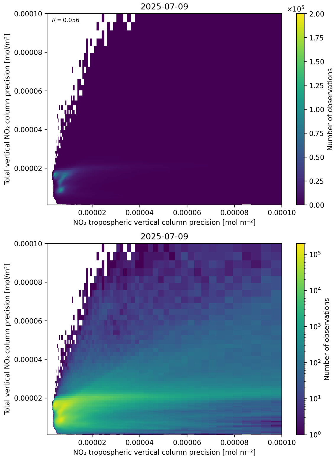
Figure 139: Scatter density plot of “NO 2 tropospheric vertical column precision” against “Total vertical NO 2 column precision” for 2025-07-08 to 2025-07-10.
