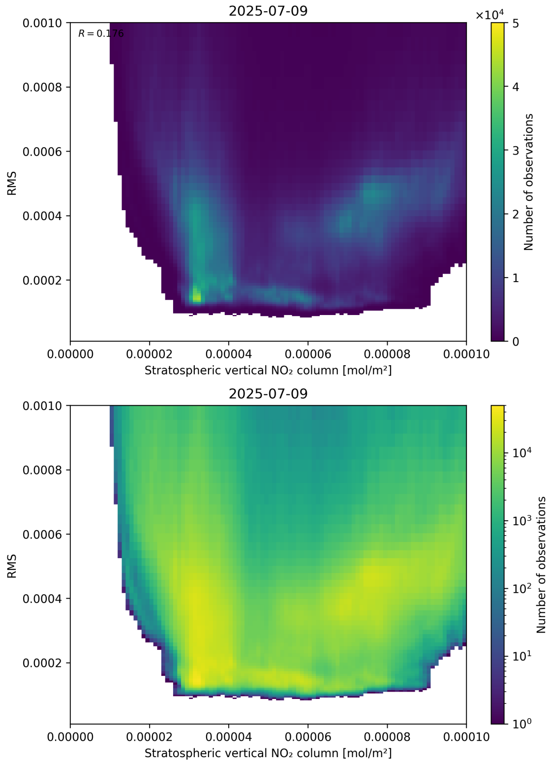
Figure 102: Scatter density plot of “Stratospheric vertical NO 2 column” against “RMS” for 2025-07-08 to 2025-07-10.
