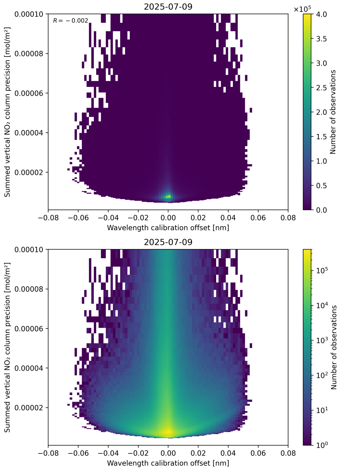
Figure 178: Scatter density plot of “Wavelength calibration offset” against “Summed vertical NO 2 column precision” for 2025-07-08 to 2025-07-10.
