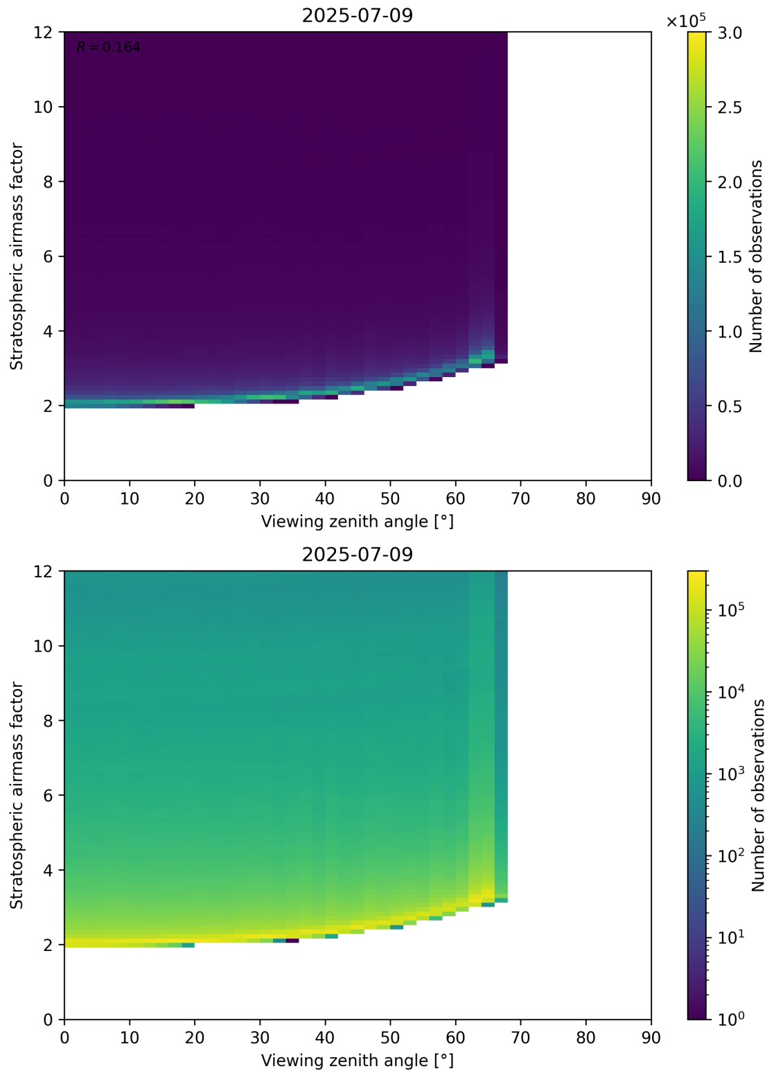
Figure 159: Scatter density plot of “Viewing zenith angle” against “Stratospheric airmass factor” for 2025-07-08 to 2025-07-10.
