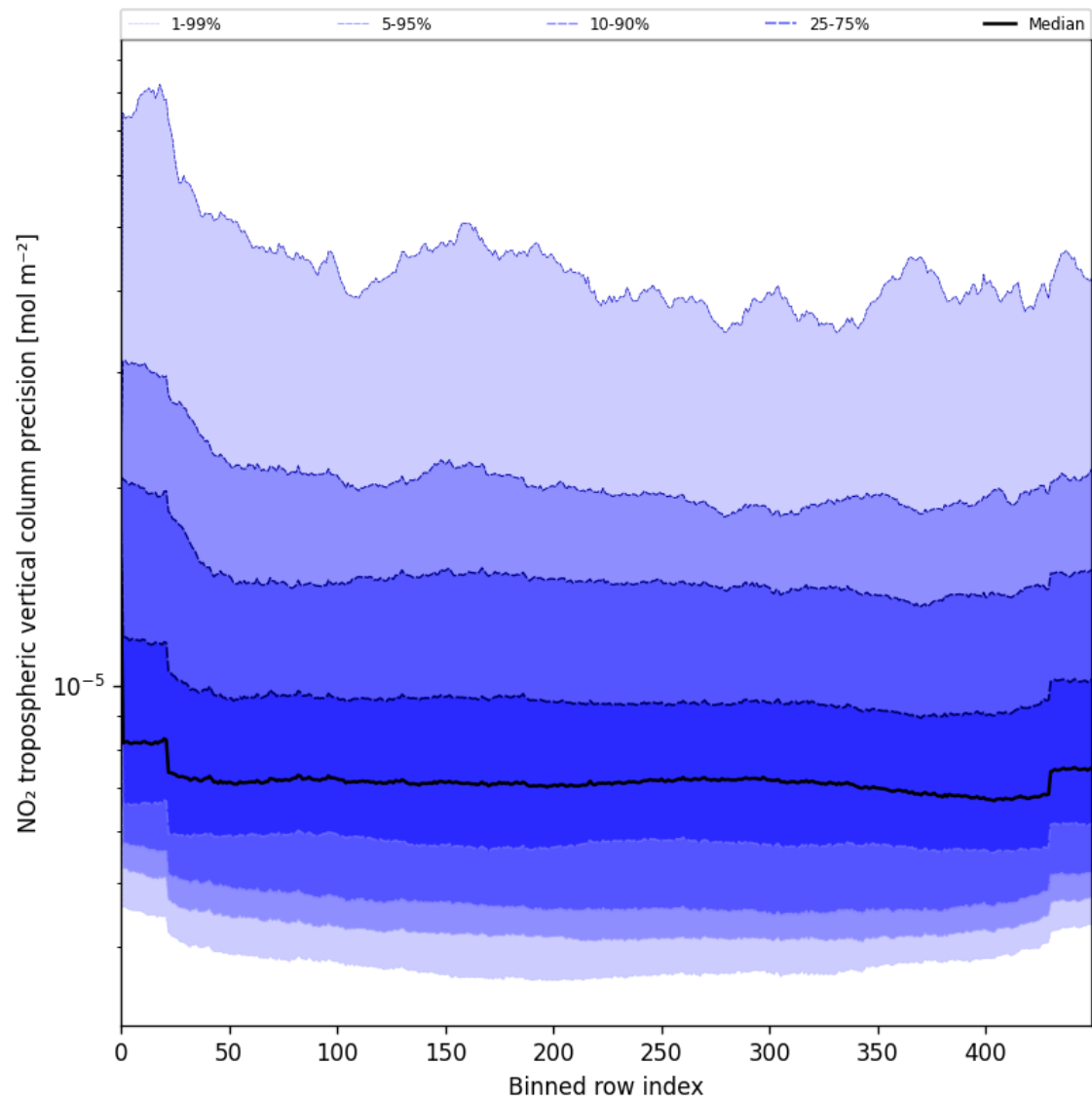
Figure 47: Along track statistics of “NO 2 tropospheric vertical column precision” for 2025-07-08 to 2025-07-10
