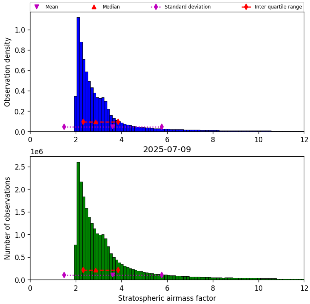
Figure 44: Histogram of “Stratospheric airmass factor” for 2025-07-08 to 2025-07-10
