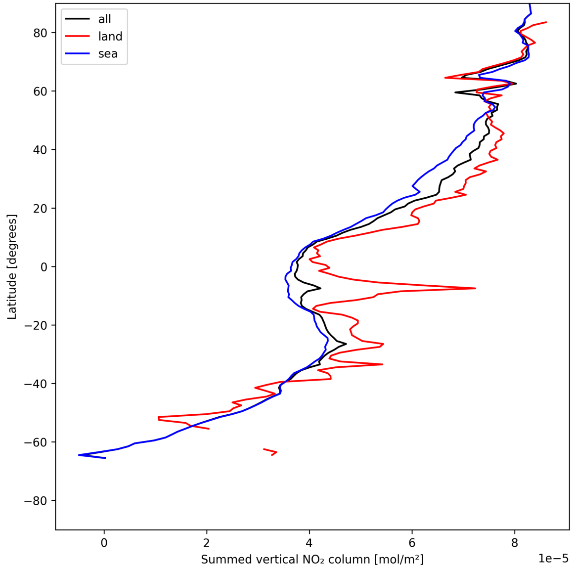
Figure 23: Zonal average of “Summed vertical NO 2 column” for 2025-07-08 to 2025-07-10.
