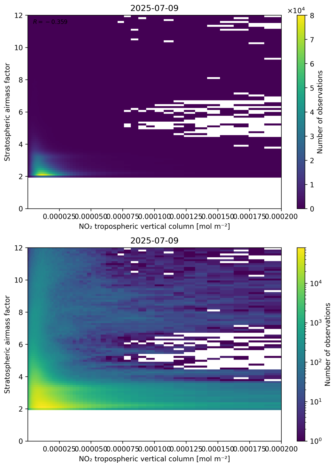
Figure 121: Scatter density plot of “NO 2 tropospheric vertical column” against “Stratospheric air mass factor” for 2025-07-08 to 2025-07-10.
