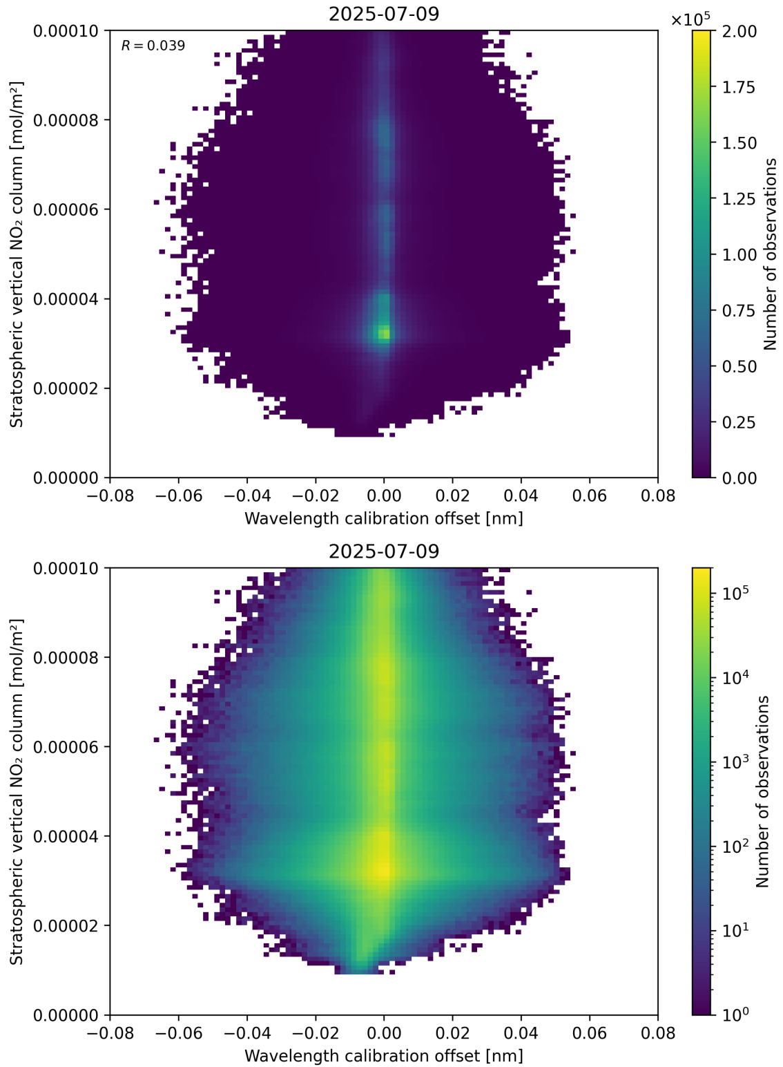
Figure 176: Scatter density plot of “Wavelength calibration offset” against “Stratospheric vertical NO 2 column” for 2025-07-08 to 2025-07-10.
