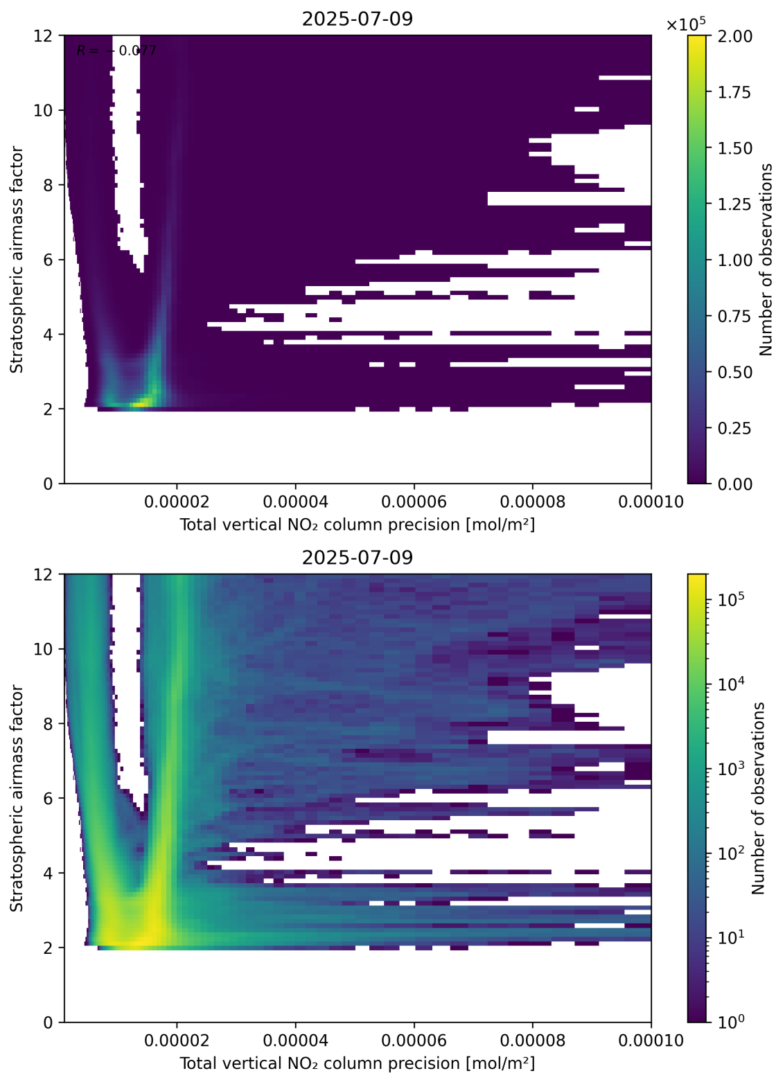
Figure 115: Scatter density plot of “Total vertical NO 2 column precision” against “Stratospheric air mass factor” for 2025-07-08 to 2025-07-10.
