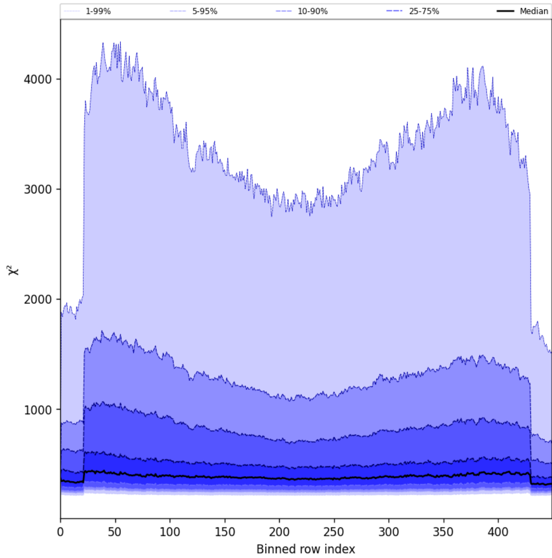
Figure 59: Along track statistics of “ \chi^2 ” for 2025-07-08 to 2025-07-10
