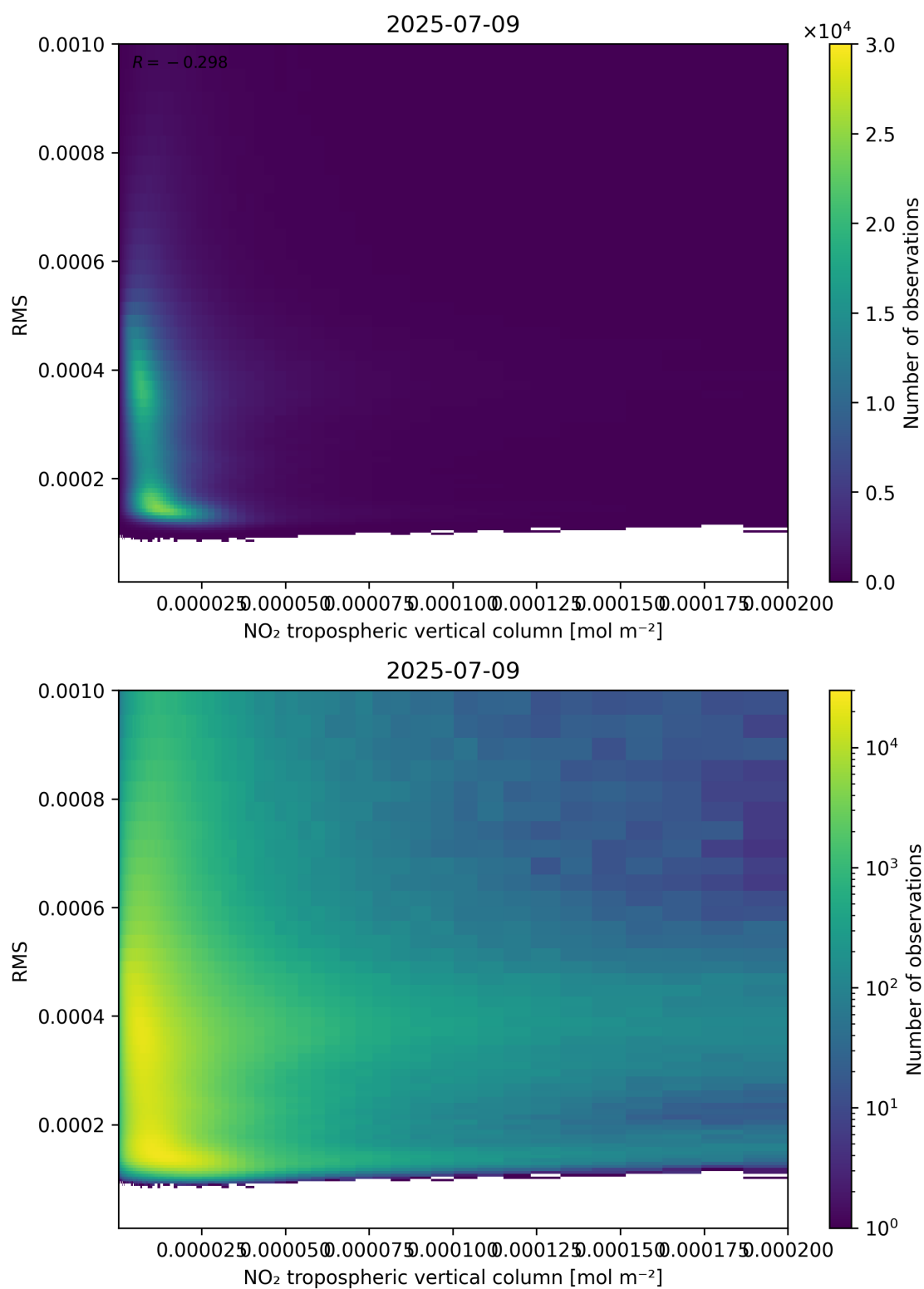
Figure 142: Scatter density plot of “NO 2 tropospheric vertical column” against “RMS” for 2025-07-08 to 2025-07-10.
