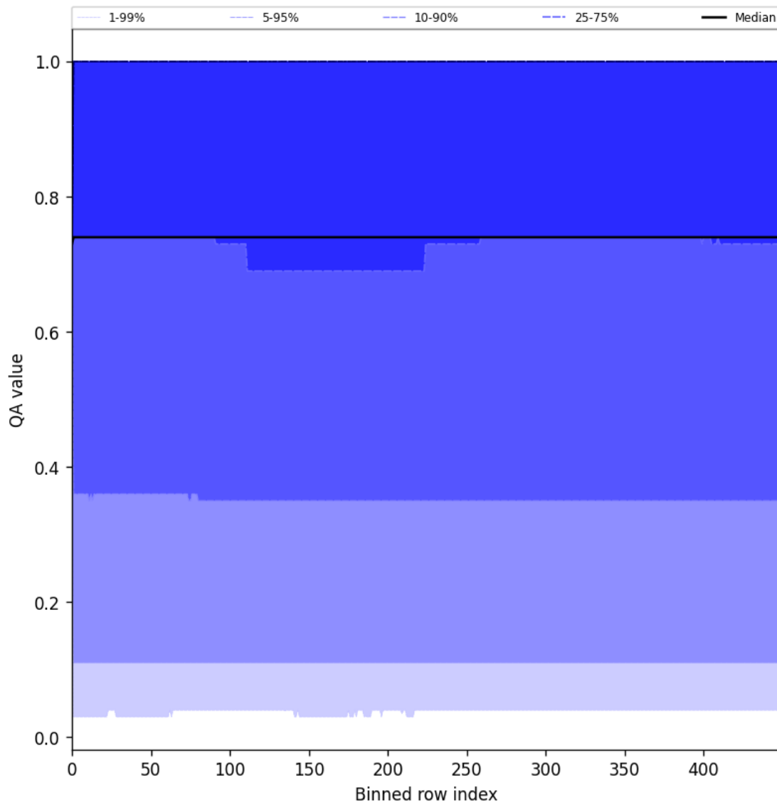
Figure 45: Along track statistics of “QA value” for 2025-07-08 to 2025-07-10
