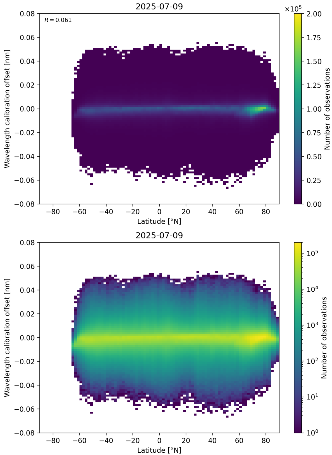
Figure 95: Scatter density plot of “Latitude” against “Wavelength calibration offset” for 2025-07-08 to 2025-07-10.
