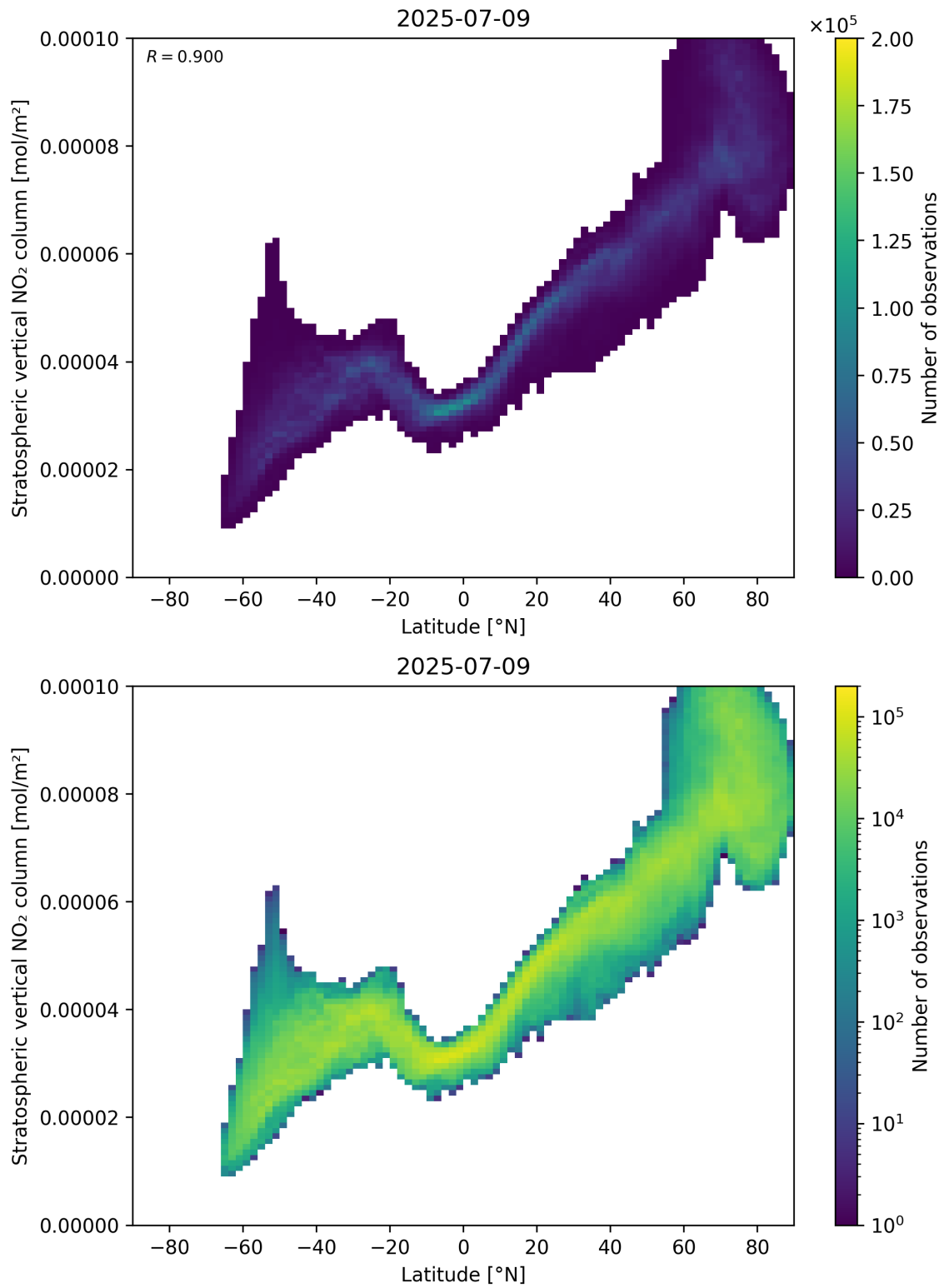
Figure 87: Scatter density plot of “Latitude” against “Stratospheric vertical \text{NO}_2 column” for 2025-07-08 to 2025-07-10.
