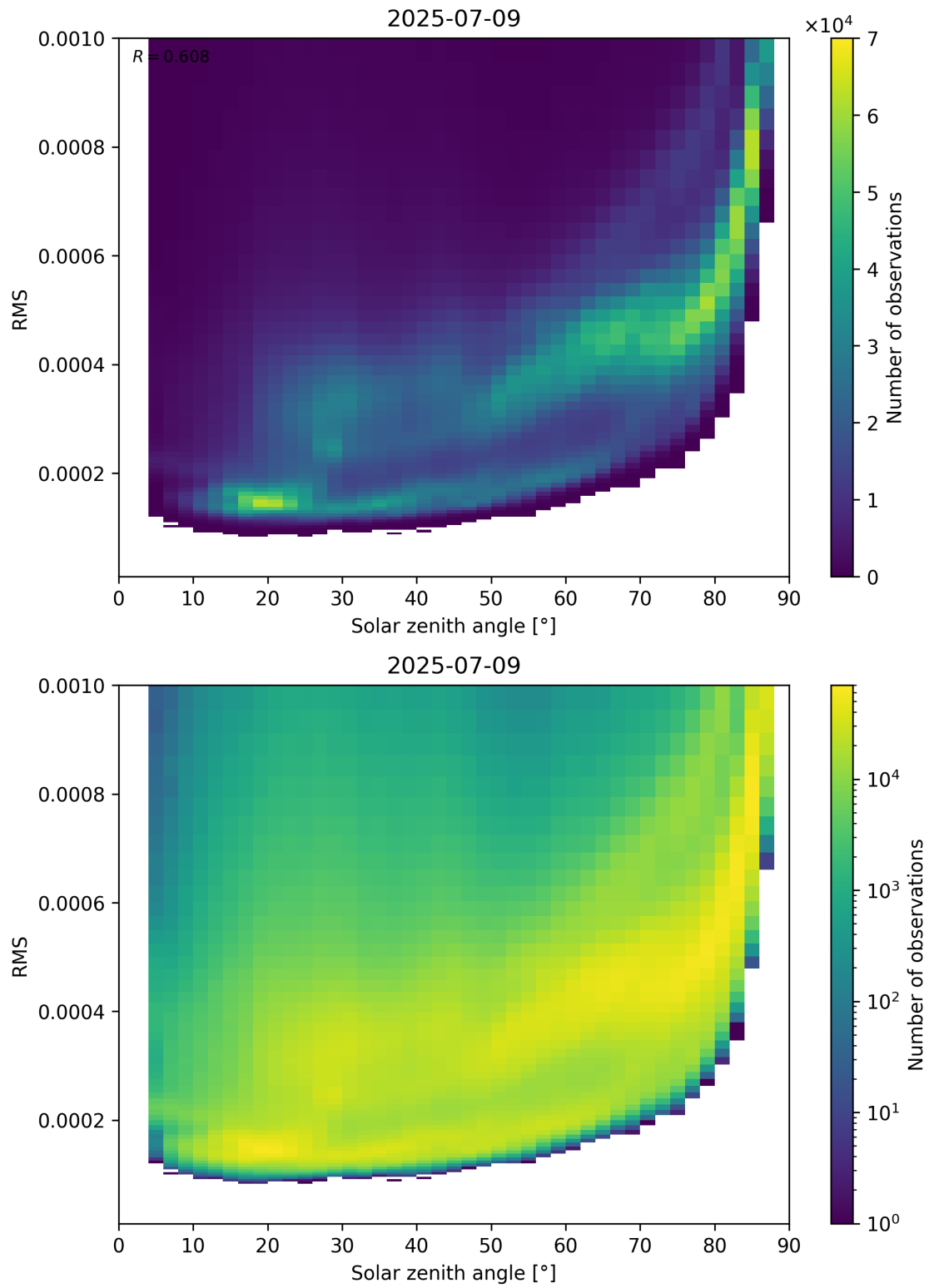
Figure 157: Scatter density plot of “Solar zenith angle” against “RMS” for 2025-07-08 to 2025-07-10.
