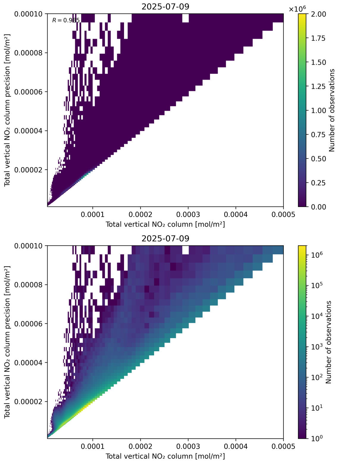
Figure 114: Scatter density plot of “Total vertical NO 2 column” against “Total vertical NO 2 column precision” for 2025-07-08 to 2025-07-10.
