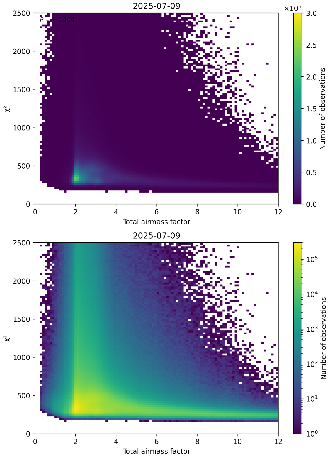
Figure 63: Scatter density plot of “Total airmass factor” against “ \chi^2 ” for 2025-07-08 to 2025-07-10.
