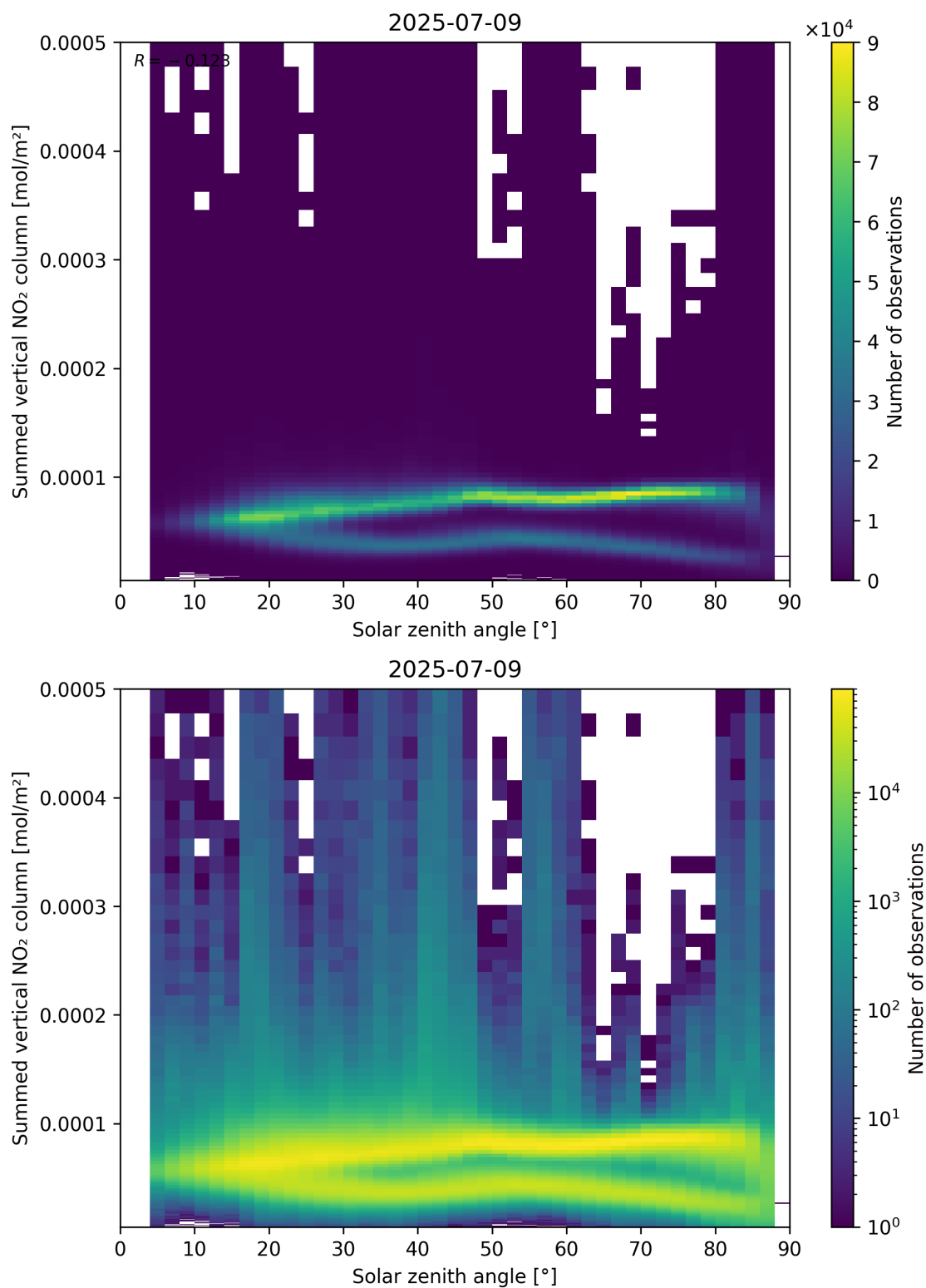
Figure 151: Scatter density plot of “Solar zenith angle” against “Summed vertical NO 2 column” for 2025-07-08 to 2025-07-10.
