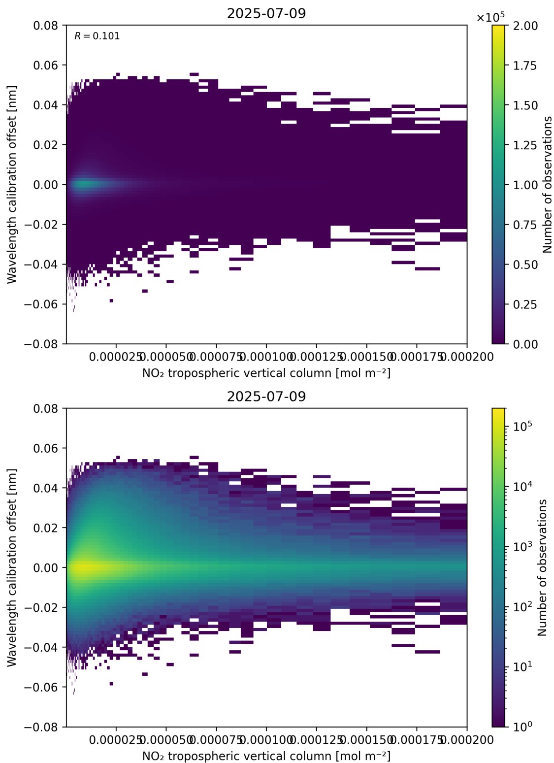
Figure 143: Scatter density plot of “NO 2 tropospheric vertical column” against “Wavelength calibration offset” for 2025-07-08 to 2025-07-10.
