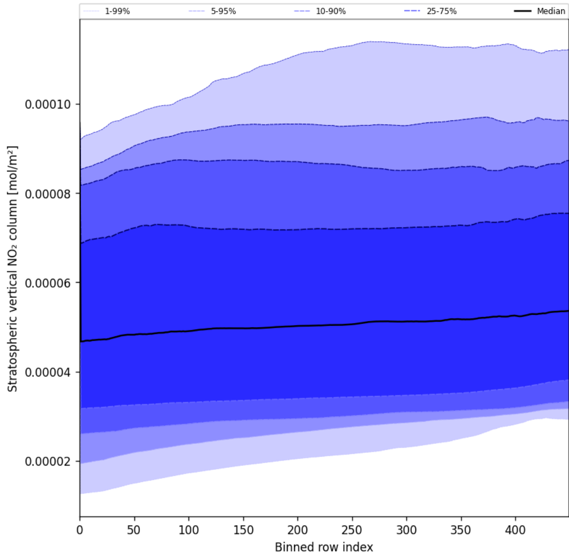
Figure 53: Along track statistics of “Stratospheric vertical NO 2 column” for 2025-07-08 to 2025-07-10
