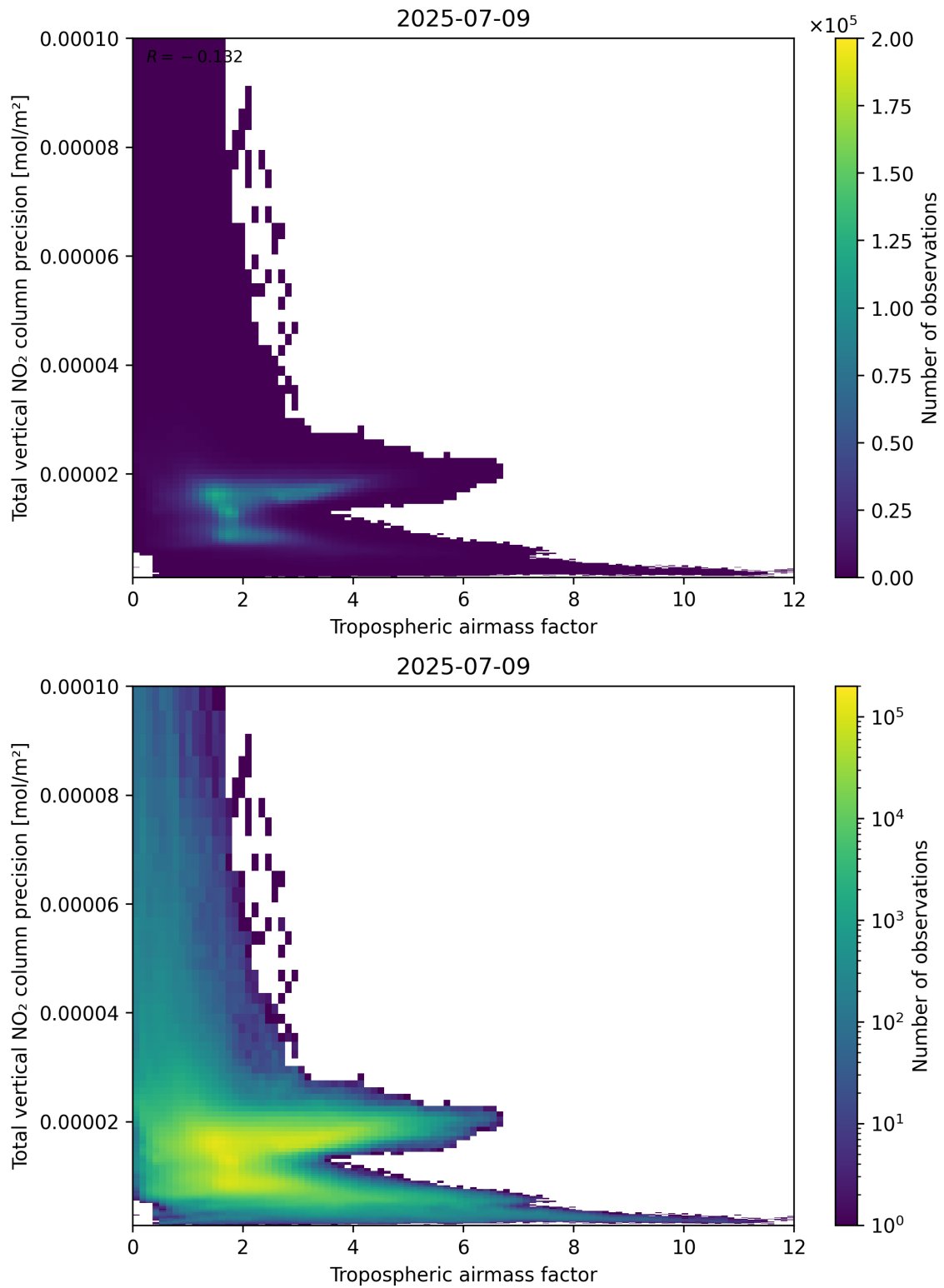
Figure 78: Scatter density plot of “Tropospheric air mass factor” against “Total vertical NO 2 column precision” for 2025-07-08 to 2025-07-10.
