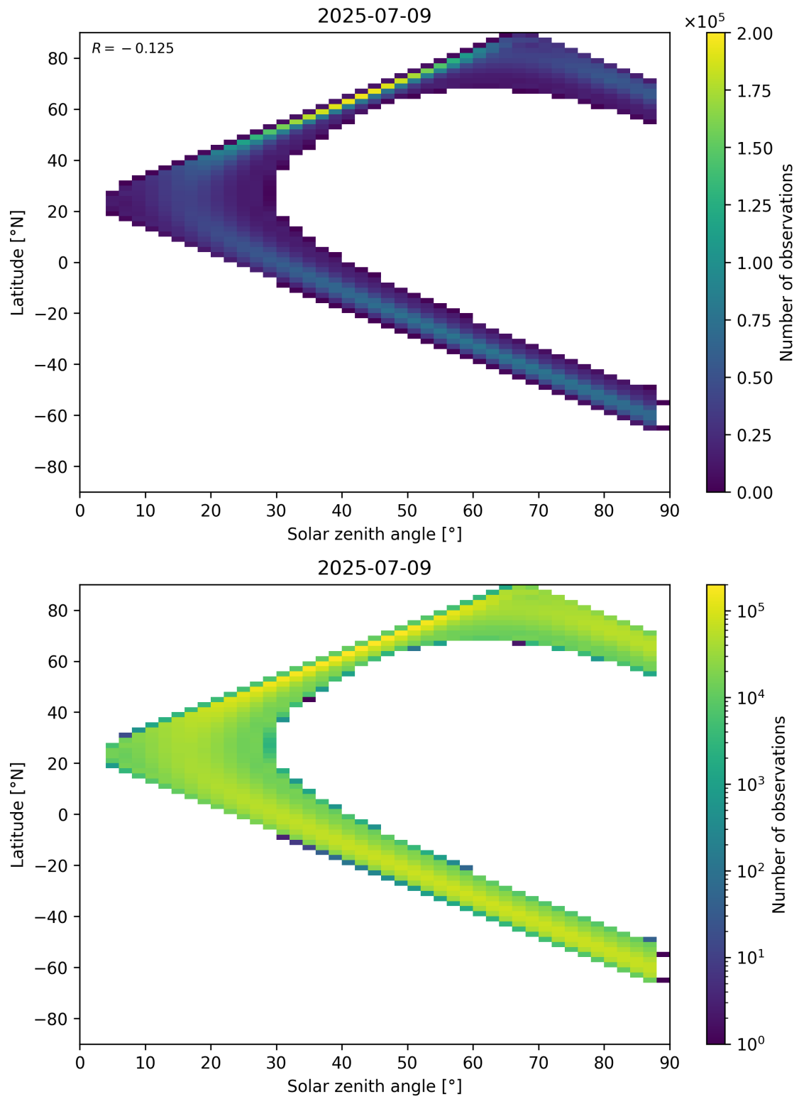
Figure 149: Scatter density plot of “Solar zenith angle” against “Latitude” for 2025-07-08 to 2025-07-10.
