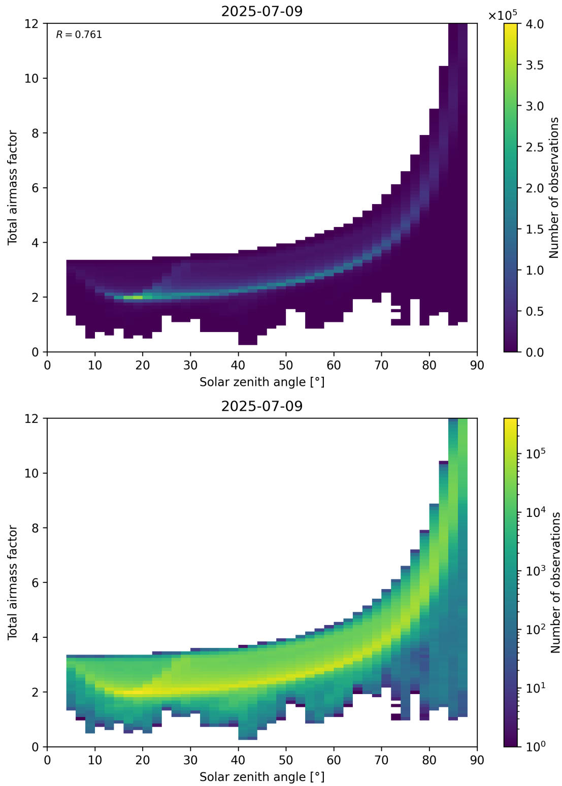
Figure 146: Scatter density plot of “Solar zenith angle” against “Total air mass factor” for 2025-07-08 to 2025-07-10.
