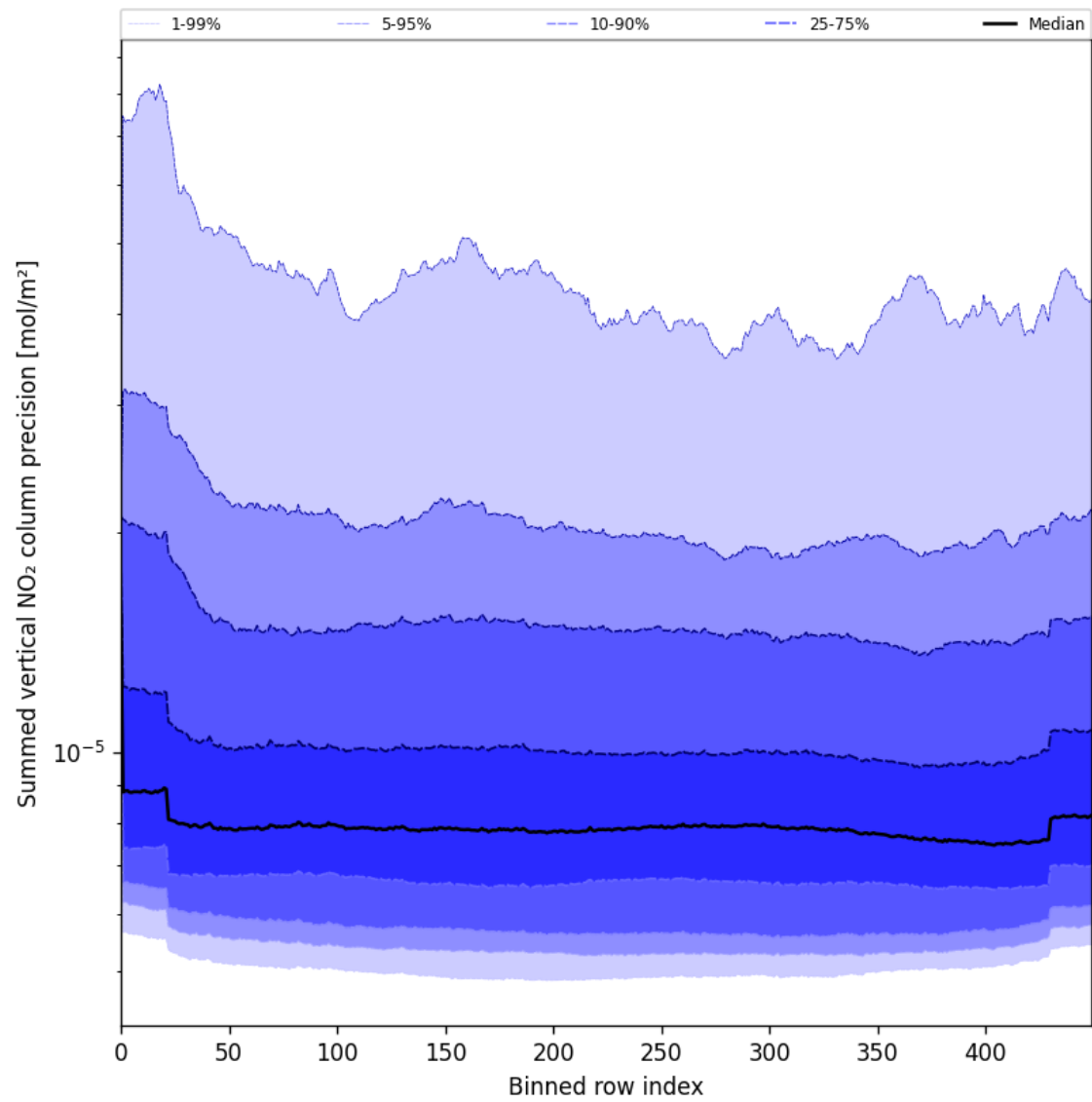
Figure 58: Along track statistics of “Summed vertical NO 2 column precision” for 2025-07-08 to 2025-07-10
