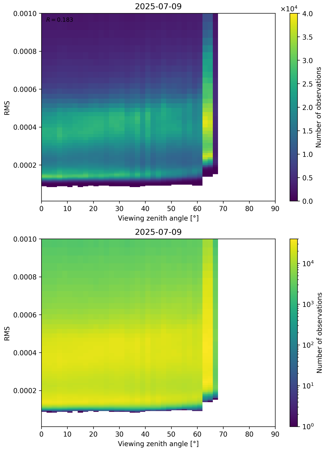
Figure 171: Scatter density plot of “Viewing zenith angle” against “RMS” for 2025-07-08 to 2025-07-10.
