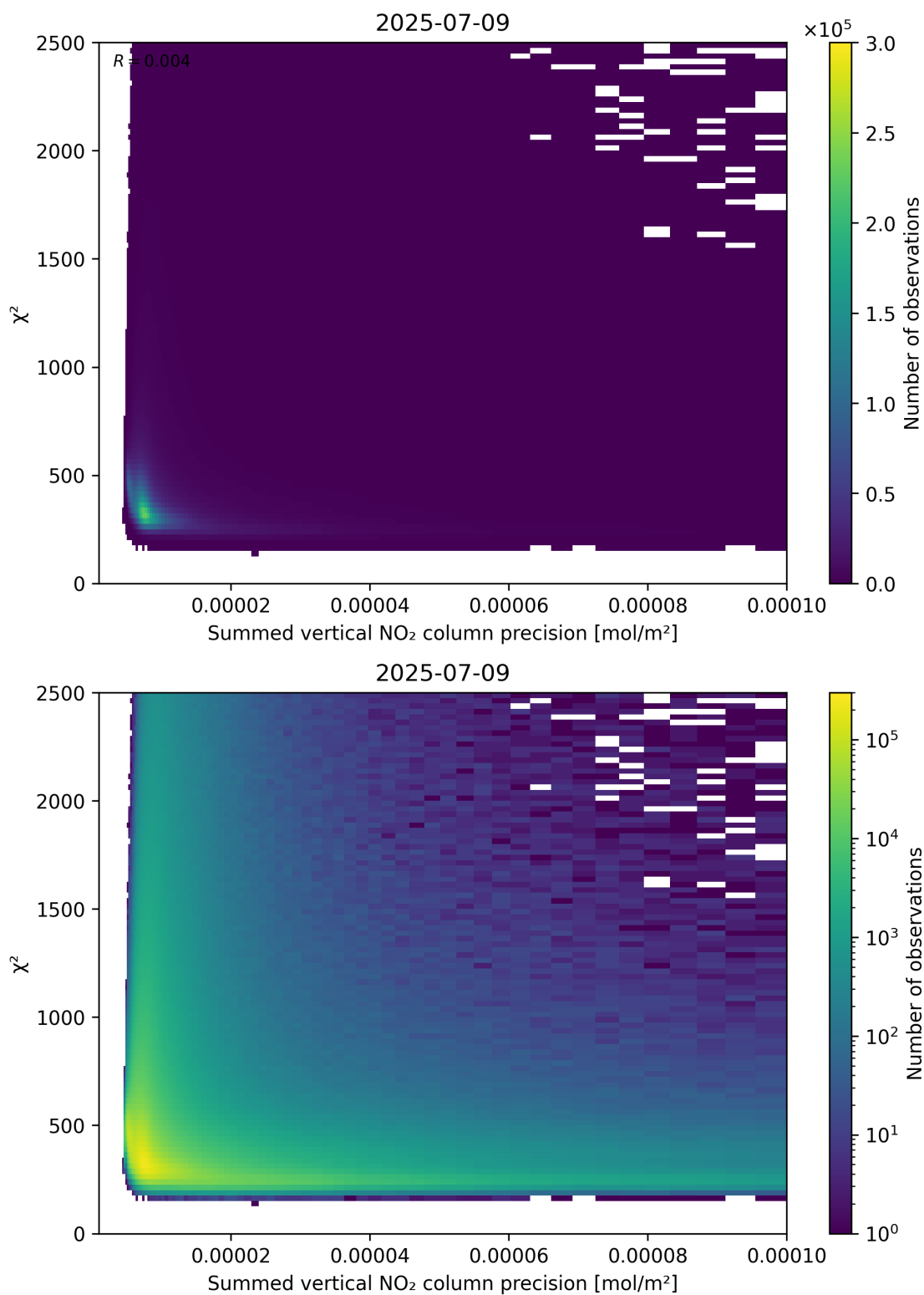
Figure 107: Scatter density plot of “Summed vertical NO 2 column precision” against “ \chi^2 ” for 2025-07-08 to 2025-07-10.
