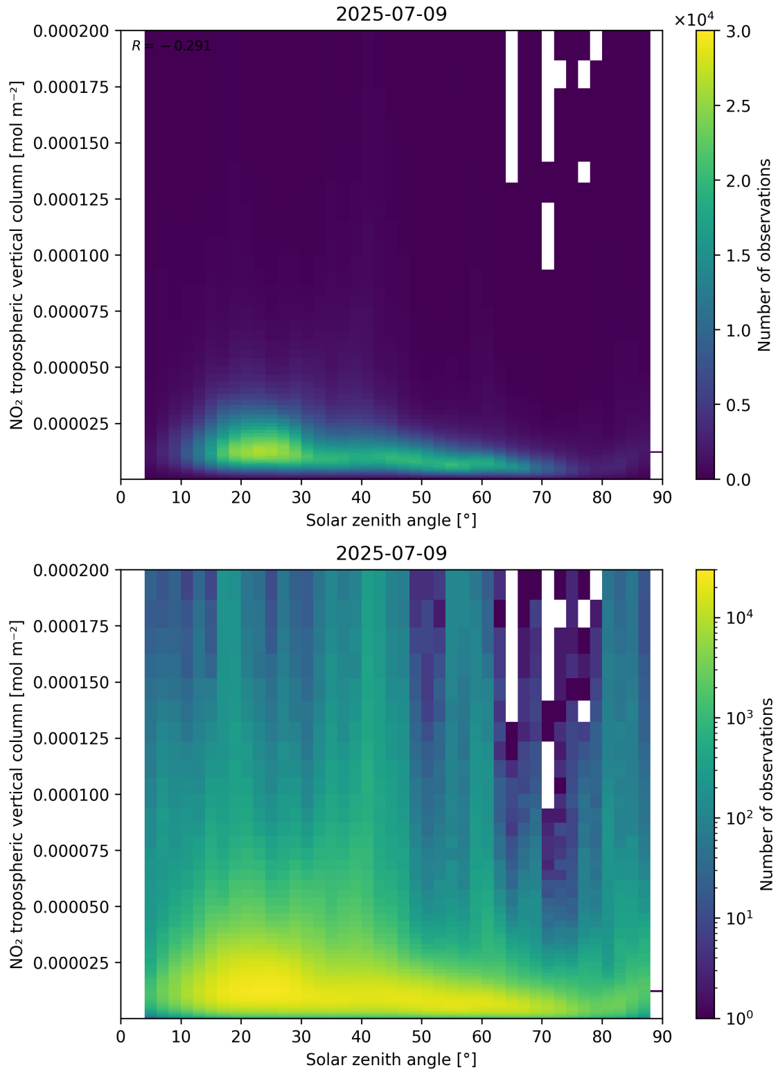
Figure 155: Scatter density plot of “Solar zenith angle” against “NO 2 tropospheric vertical column” for 2025-07-08 to 2025-07-10.
