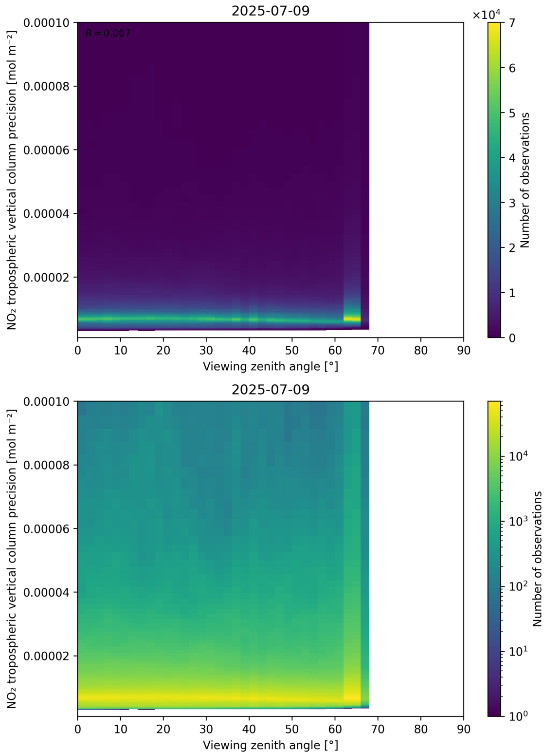
Figure 170: Scatter density plot of “Viewing zenith angle” against “NO 2 tropospheric vertical column precision” for 2025-07-08 to 2025-07-10.
