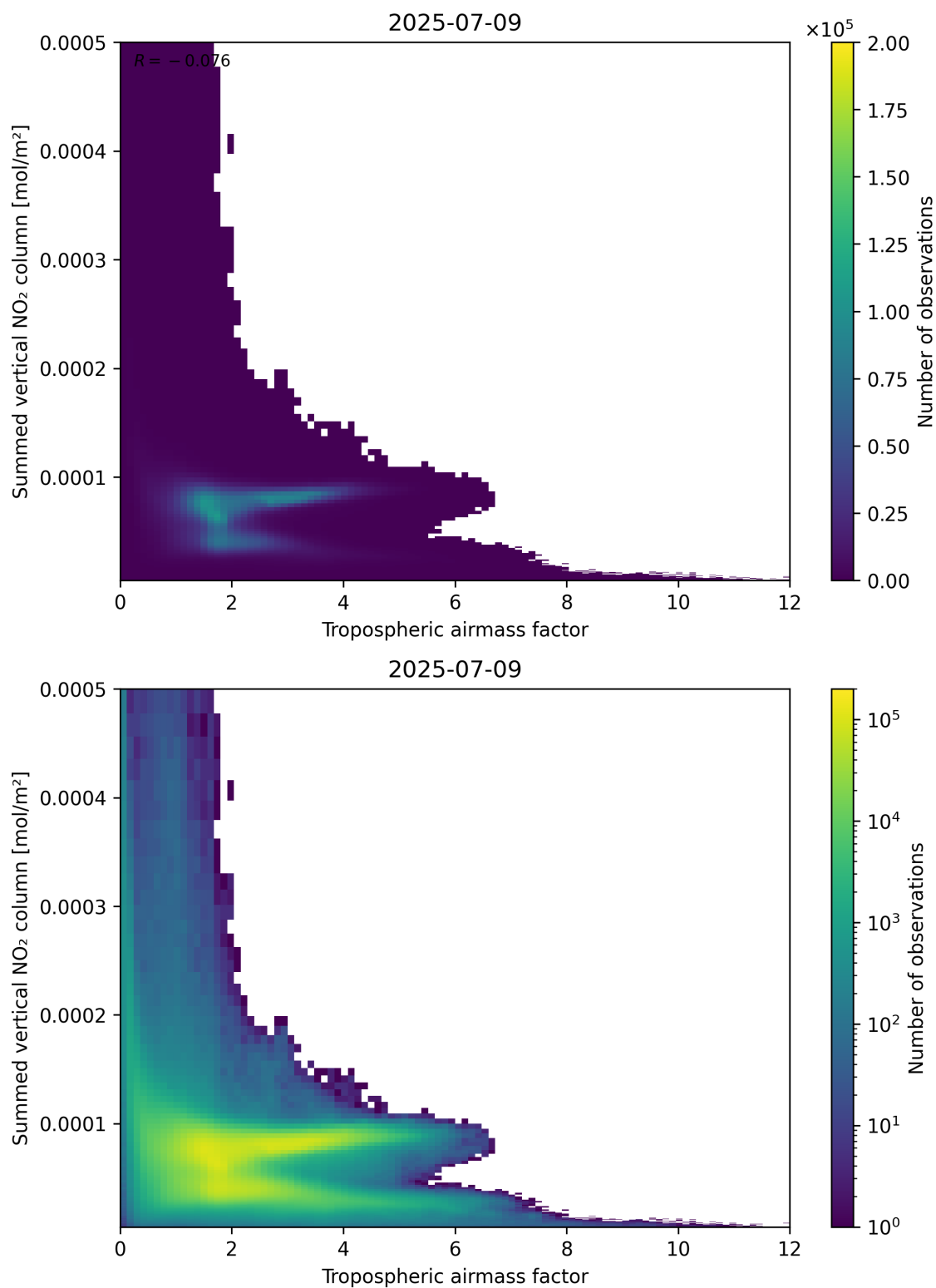
Figure 75: Scatter density plot of “Tropospheric airmass factor” against “Summed vertical NO 2 column” for 2025-07-08 to 2025-07-10.
