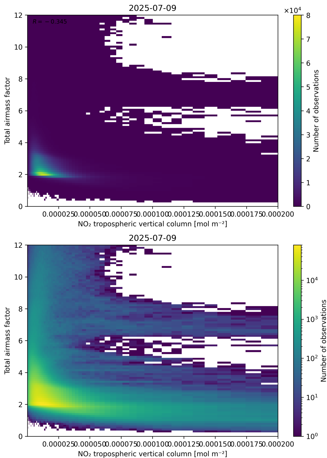
Figure 122: Scatter density plot of “NO 2 tropospheric vertical column” against “Total air mass factor” for 2025-07-08 to 2025-07-10.
