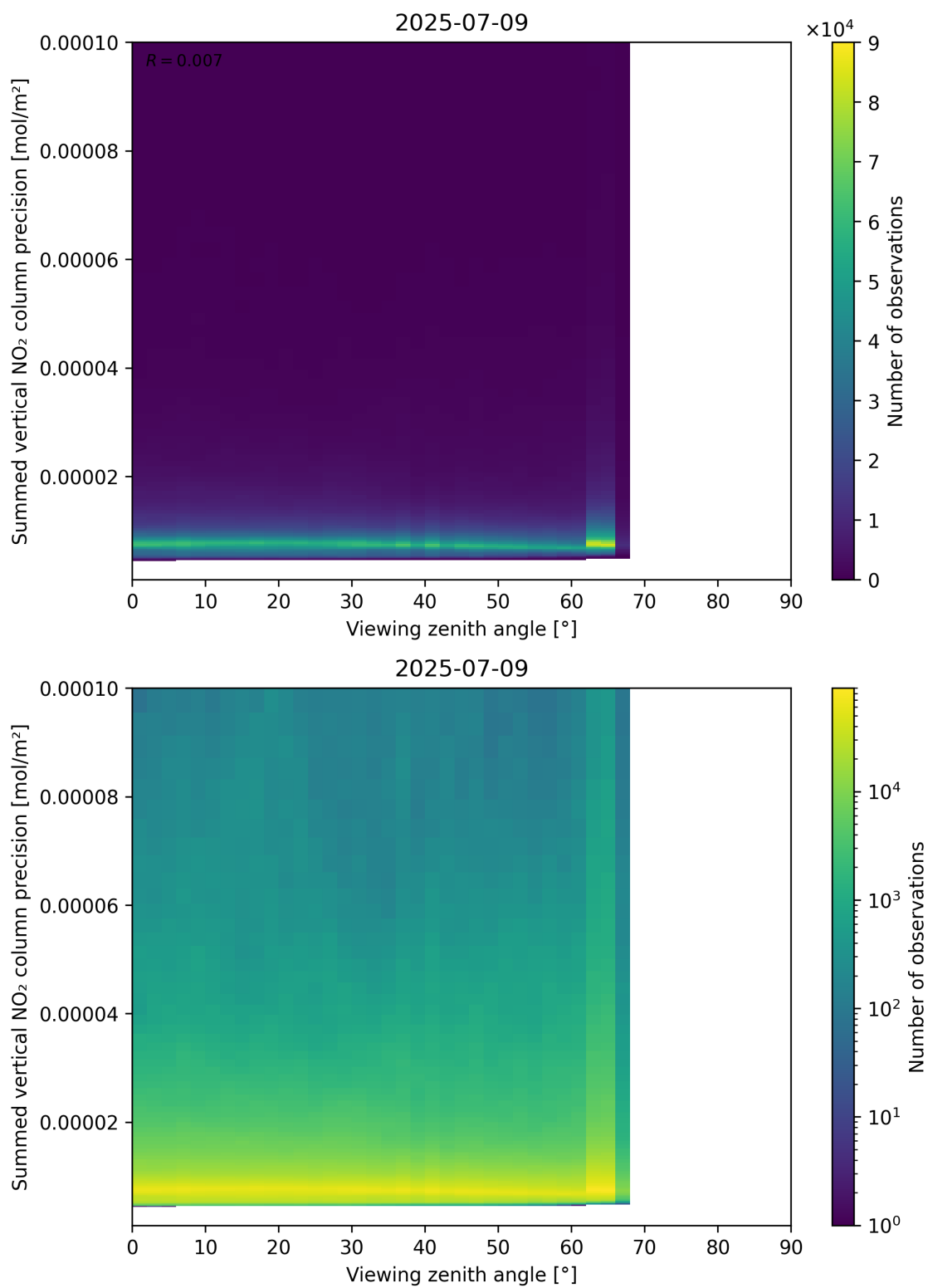
Figure 166: Scatter density plot of “Viewing zenith angle” against “Summed vertical NO 2 column precision” for 2025-07-08 to 2025-07-10.
