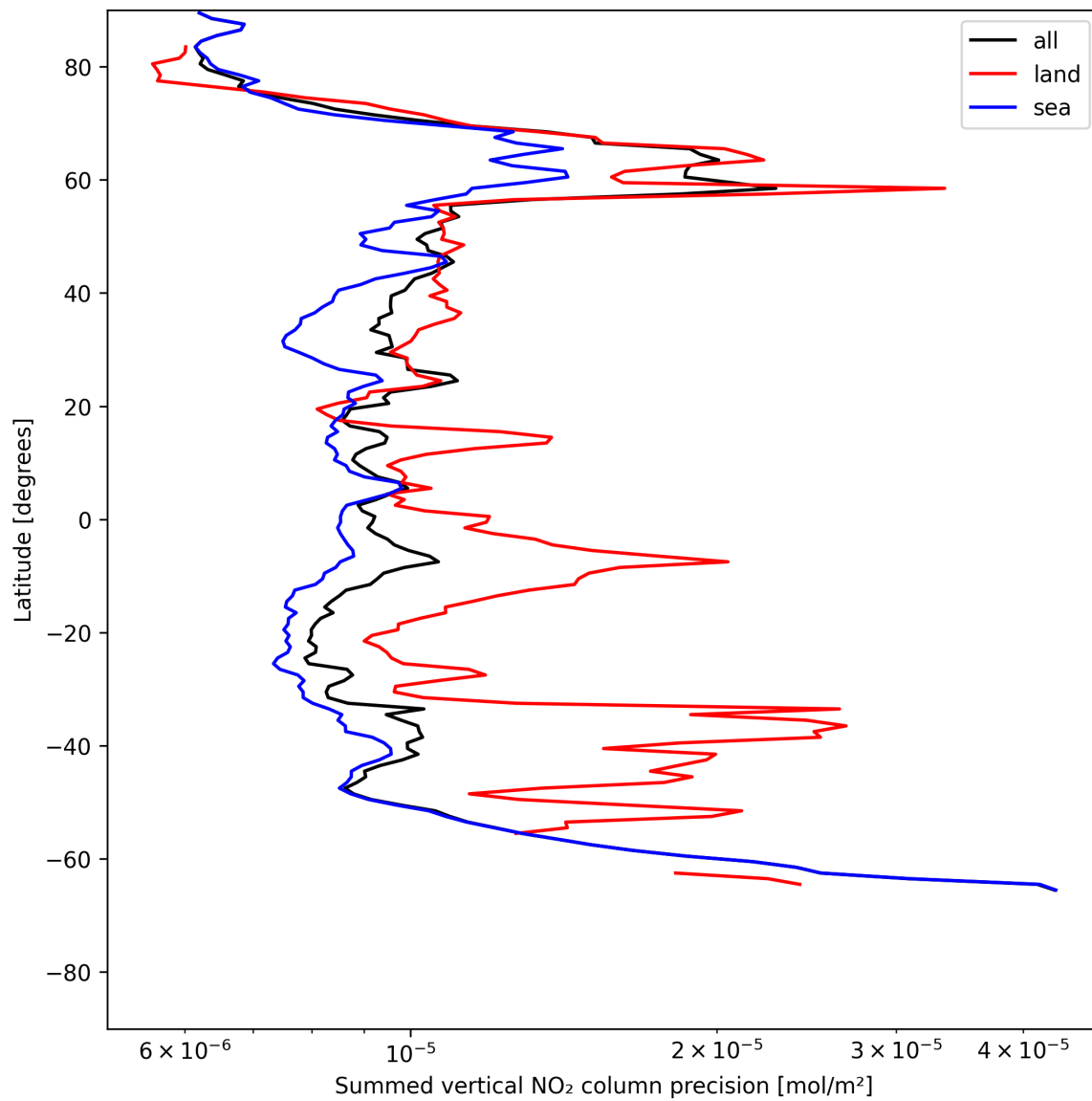
Figure 24: Zonal average of “Summed vertical NO 2 column precision” for 2025-07-08 to 2025-07-10.
