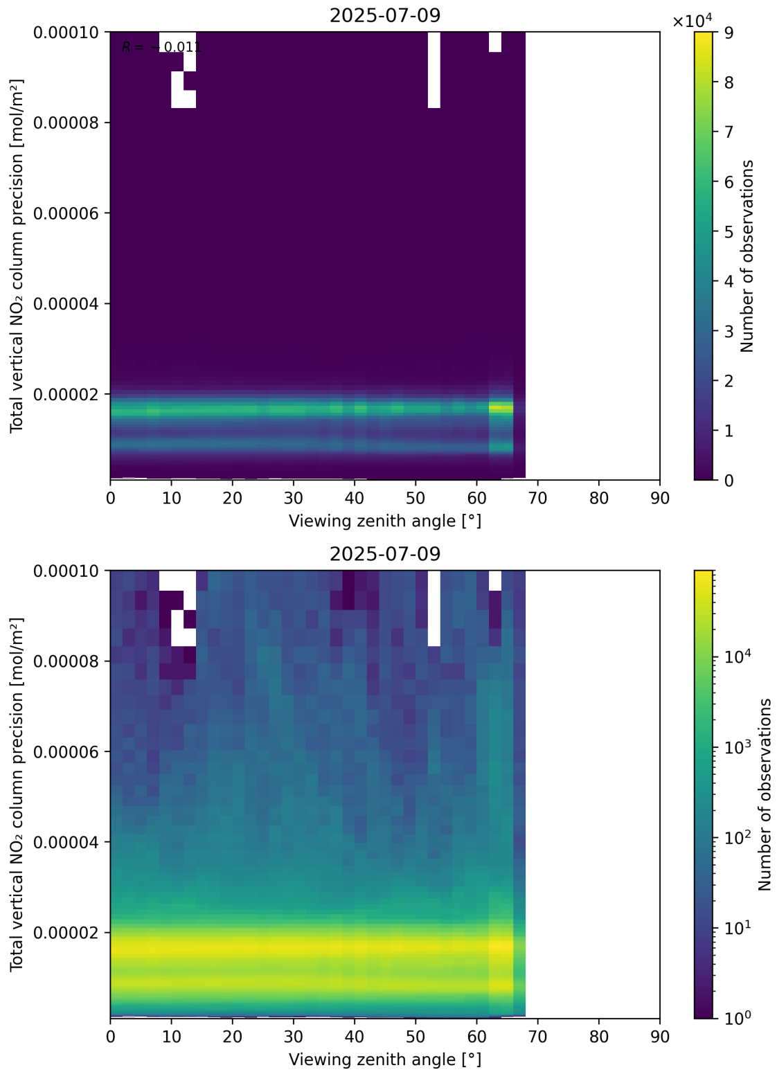
Figure 168: Scatter density plot of “Viewing zenith angle” against “Total vertical NO 2 column precision” for 2025-07-08 to 2025-07-10.
