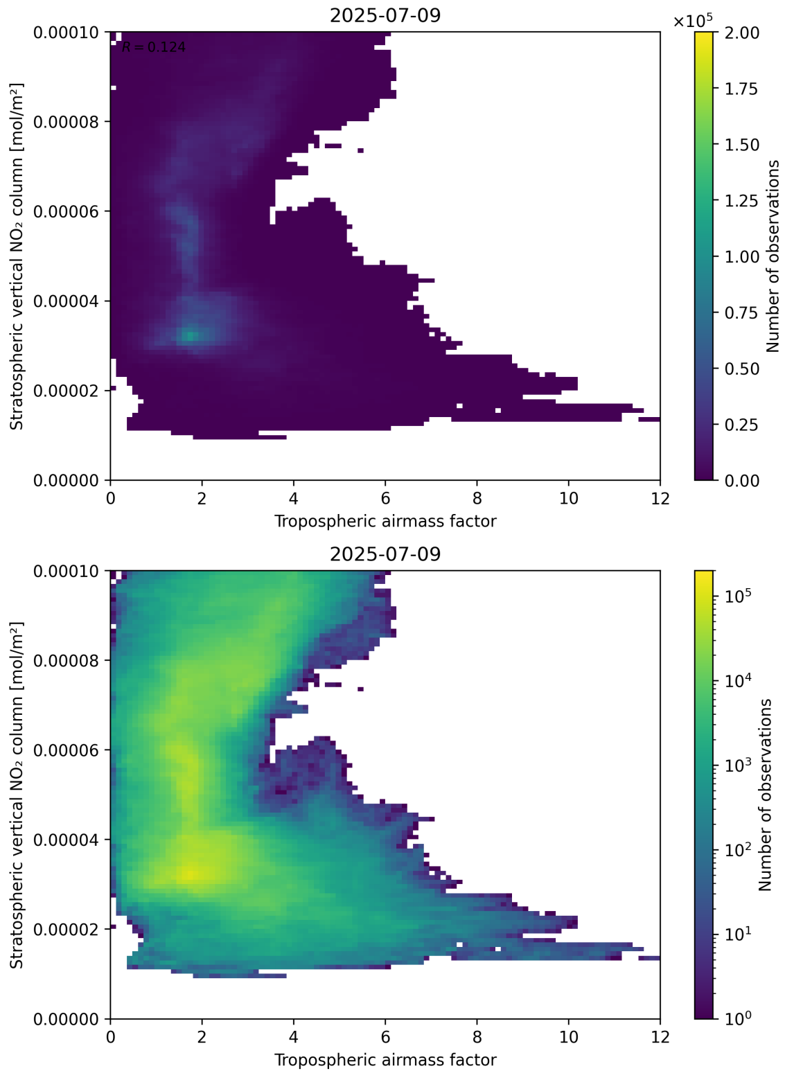
Figure 74: Scatter density plot of “Tropospheric air mass factor” against “Stratospheric vertical NO 2 column” for 2025-07-08 to 2025-07-10.
