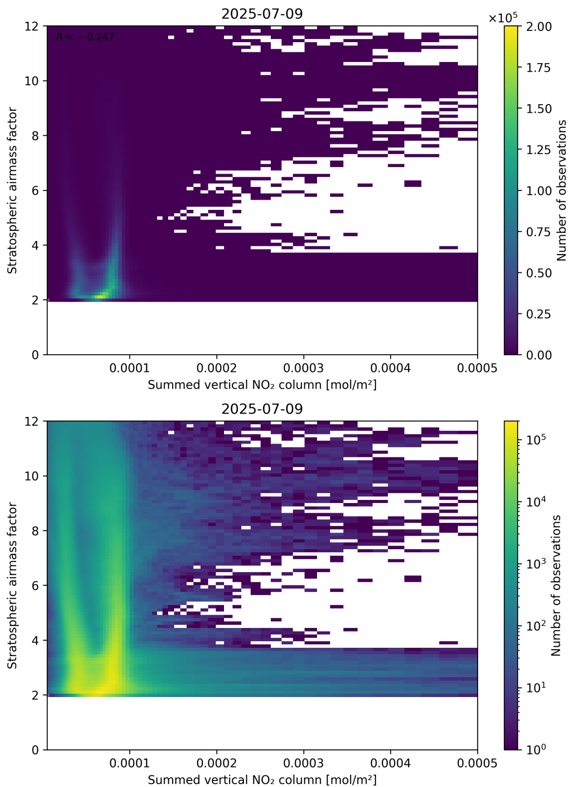
Figure 103: Scatter density plot of “Summed vertical NO 2 column” against “Stratospheric air mass factor” for 2025-07-08 to 2025-07-10.
