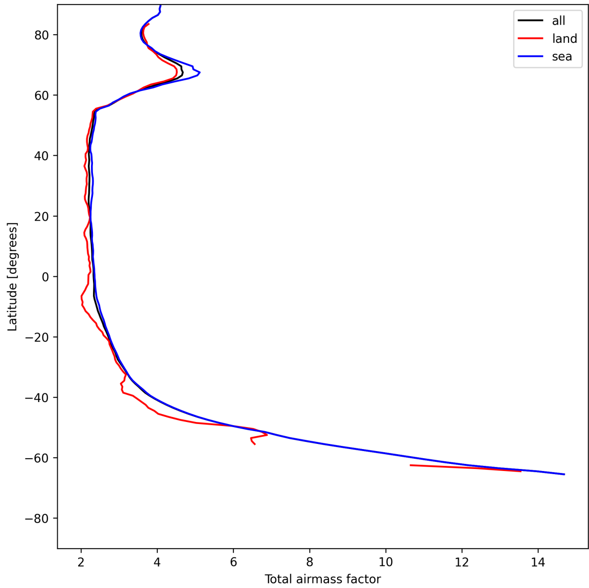
Figure 15: Zonal average of “Total airmass factor” for 2025-07-08 to 2025-07-10.
