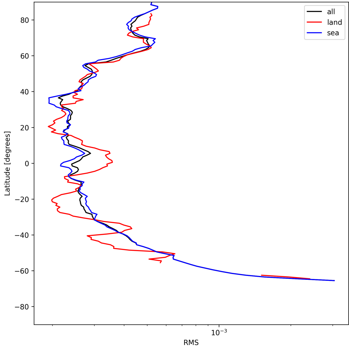
Figure 26: Zonal average of “RMS” for 2025-07-08 to 2025-07-10.
