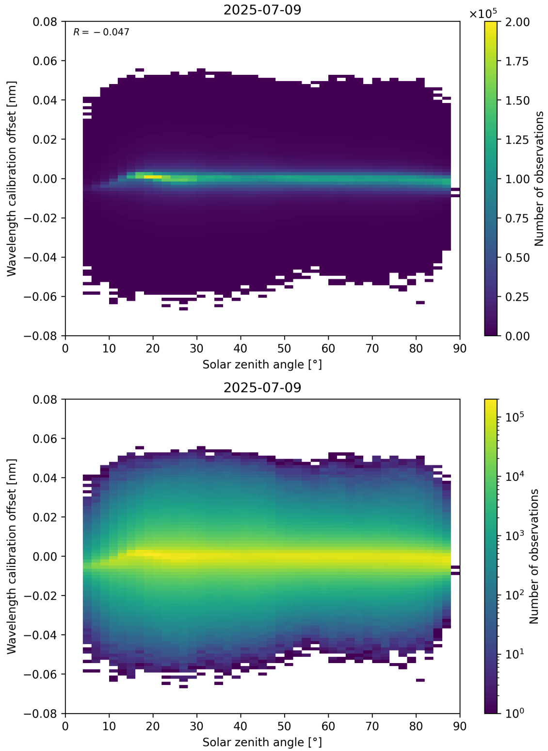
Figure 158: Scatter density plot of “Solar zenith angle” against “Wavelength calibration offset” for 2025-07-08 to 2025-07-10.
