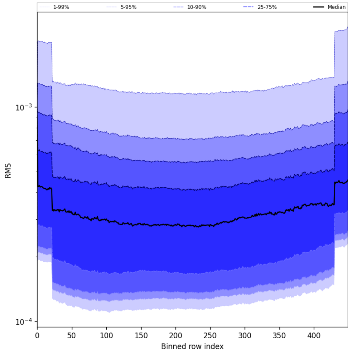
Figure 60: Along track statistics of “RMS” for 2025-07-08 to 2025-07-10
