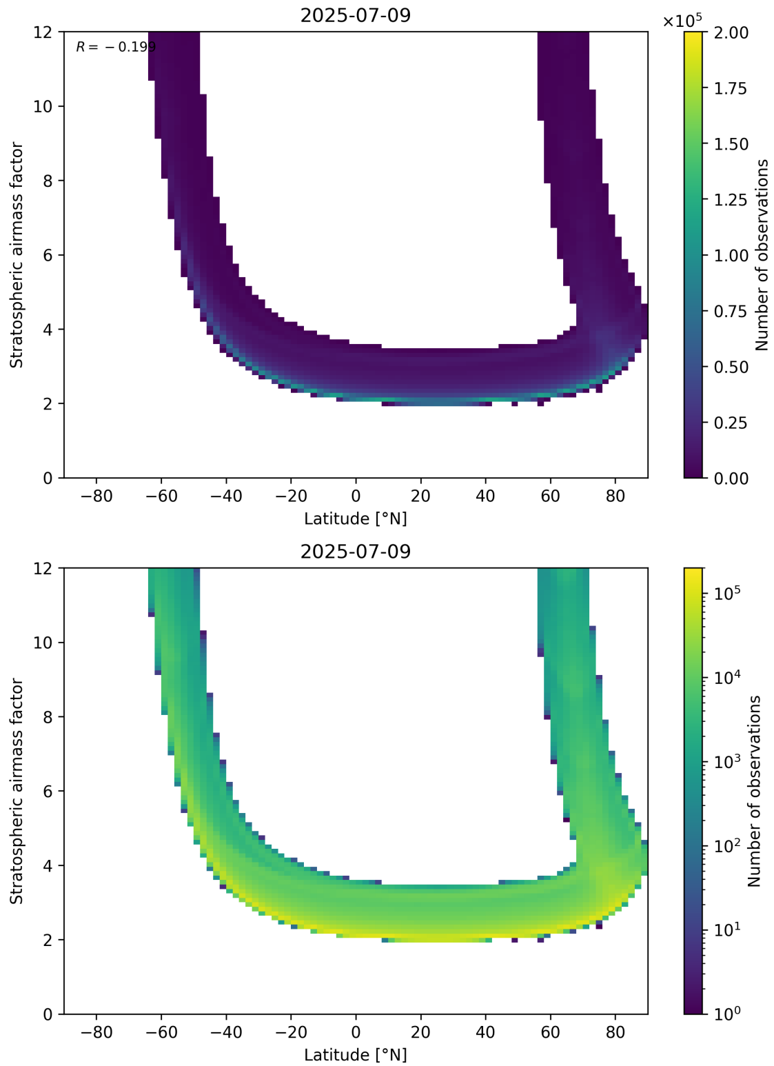
Figure 83: Scatter density plot of “Latitude” against “Stratospheric air mass factor” for 2025-07-08 to 2025-07-10.
