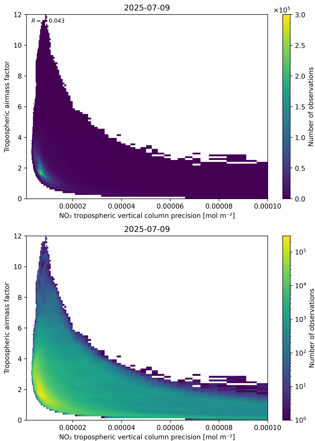
Figure 133: Scatter density plot of “NO 2 tropospheric vertical column precision” against “Tropospheric airmass factor” for 2025-07-08 to 2025-07-10.
