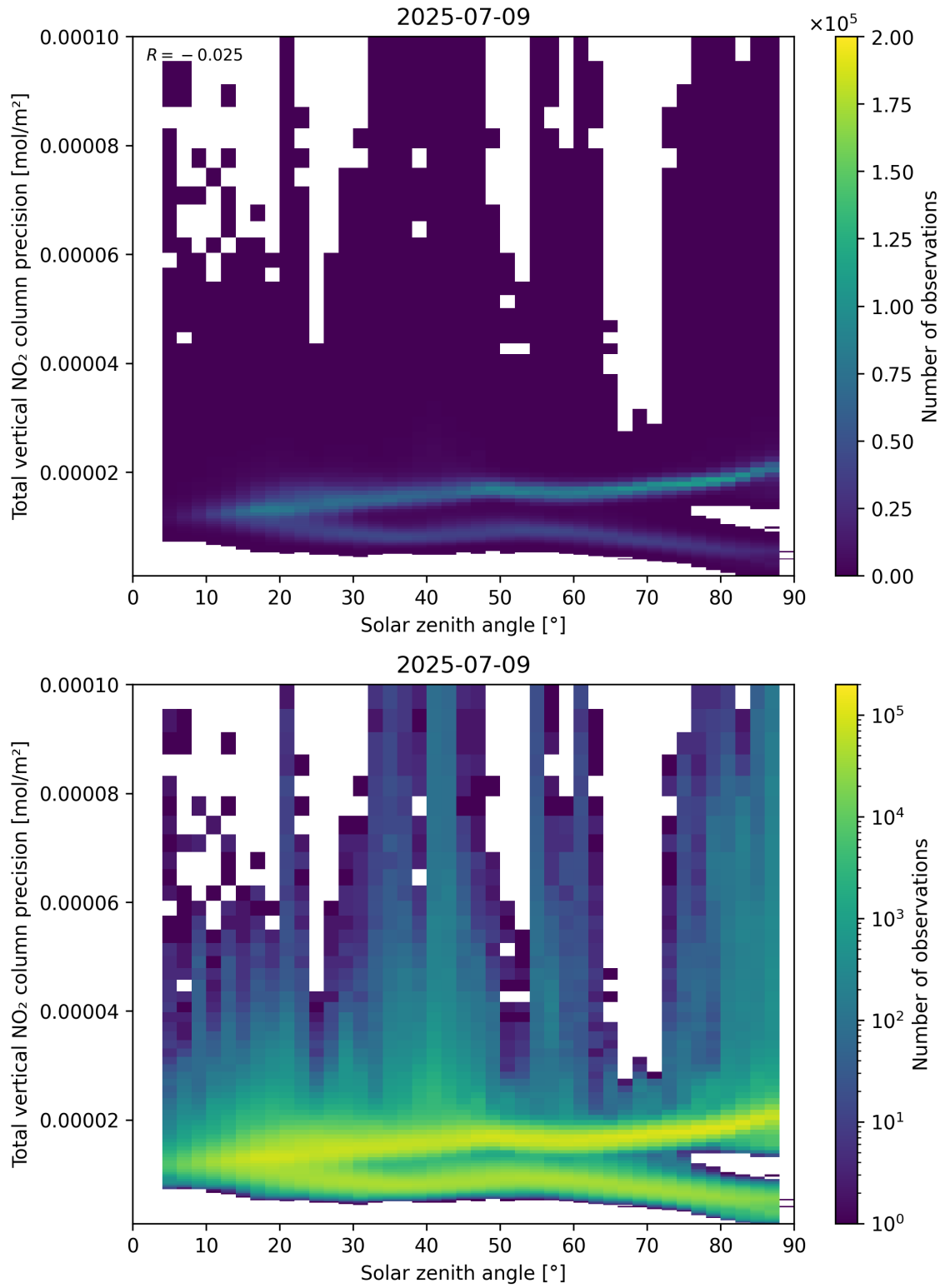
Figure 154: Scatter density plot of “Solar zenith angle” against “Total vertical NO 2 column precision” for 2025-07-08 to 2025-07-10.
