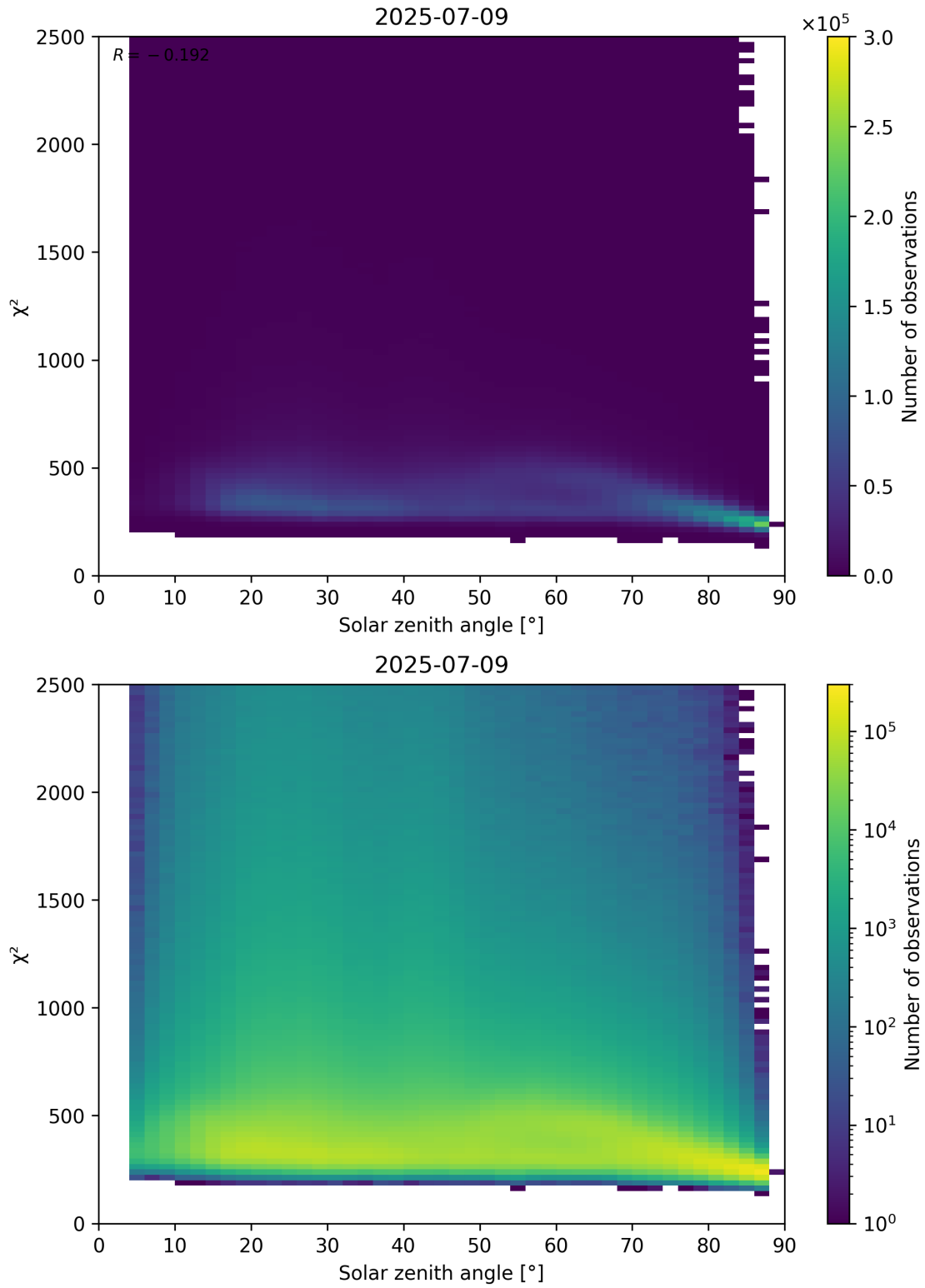
Figure 148: Scatter density plot of “Solar zenith angle” against “ \chi^2 ” for 2025-07-08 to 2025-07-10.
