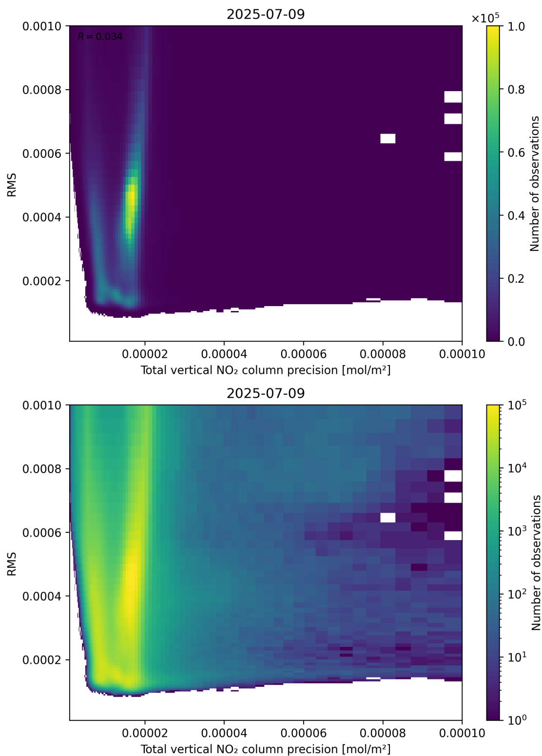
Figure 119: Scatter density plot of “Total vertical NO 2 column precision” against “RMS” for 2025-07-08 to 2025-07-10.
