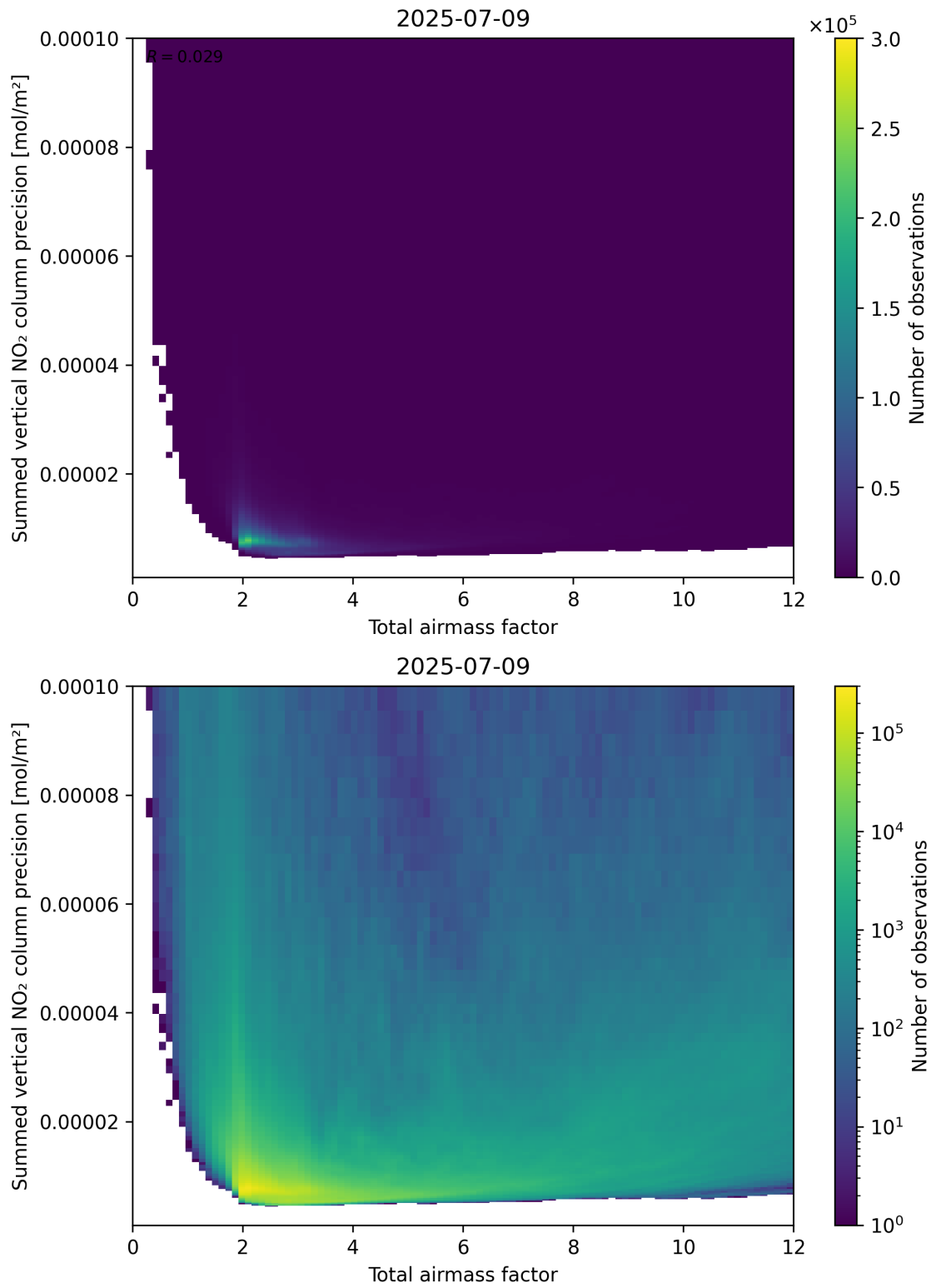
Figure 66: Scatter density plot of “Total airmass factor” against “Summed vertical NO 2 column precision” for 2025-07-08 to 2025-07-10.
