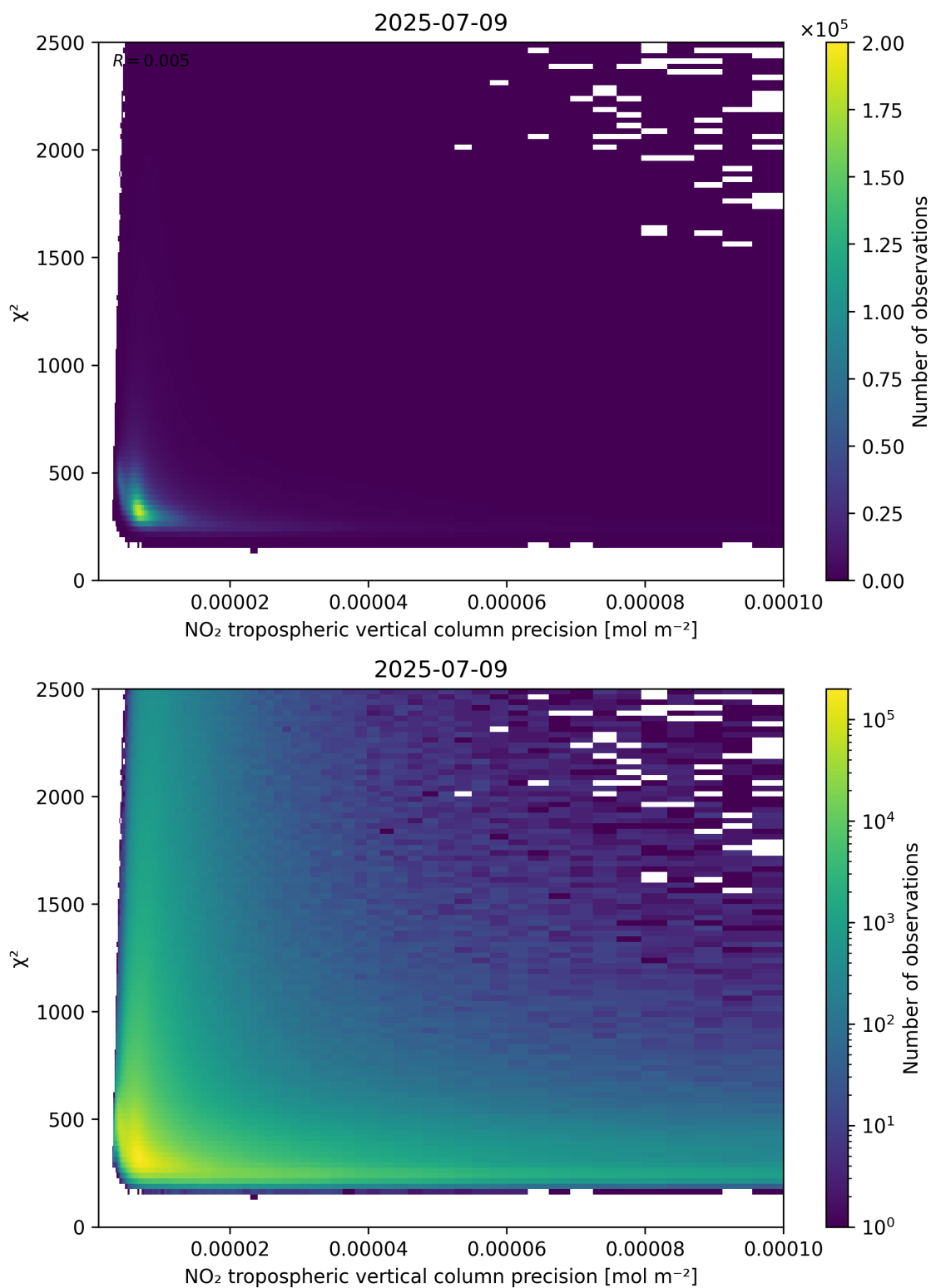
Figure 134: Scatter density plot of “NO 2 tropospheric vertical column precision” against “ \chi^2 ” for 2025-07-08 to 2025-07-10.
