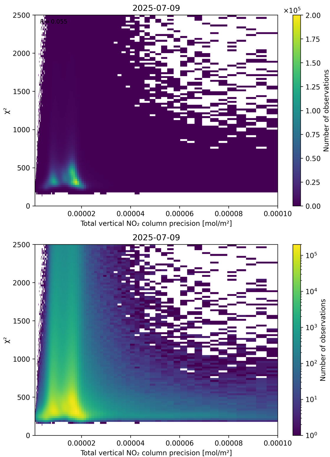
Figure 116: Scatter density plot of “Total vertical NO 2 column precision” against “ \chi^2 ” for 2025-07-08 to 2025-07-10.
