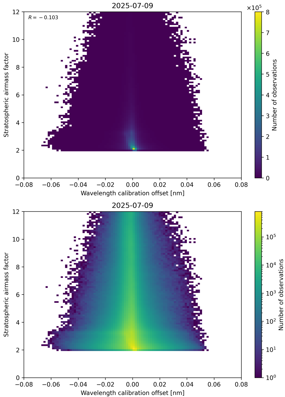
Figure 174: Scatter density plot of “Wavelength calibration offset” against “Stratospheric airmass factor” for 2025-07-08 to 2025-07-10.
