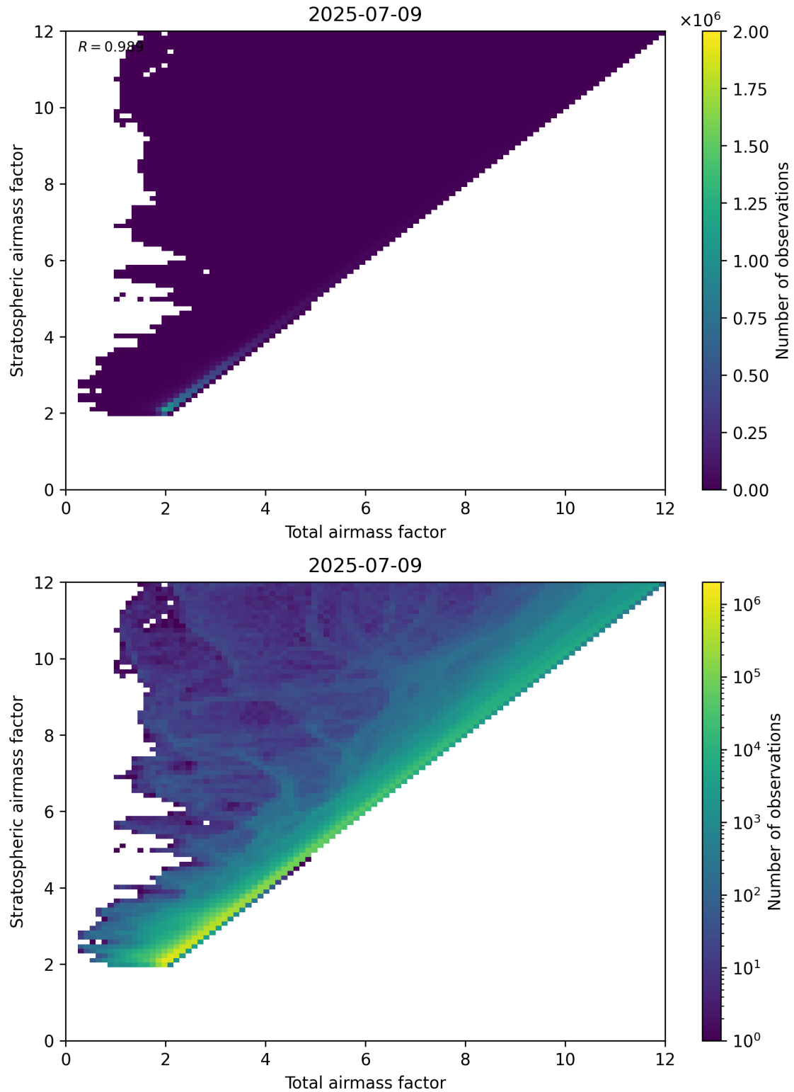
Figure 62: Scatter density plot of “Total airmass factor” against “Stratospheric airmass factor” for 2025-07-08 to 2025-07-10.
