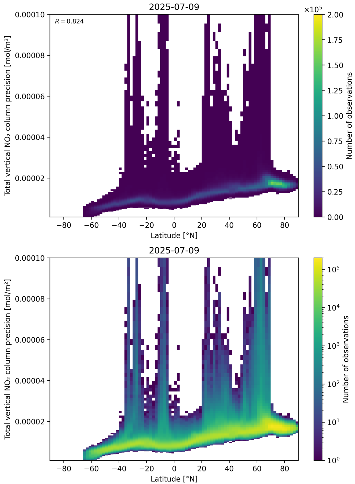
Figure 91: Scatter density plot of “Latitude” against “Total vertical NO 2 column precision” for 2025-07-08 to 2025-07-10.
