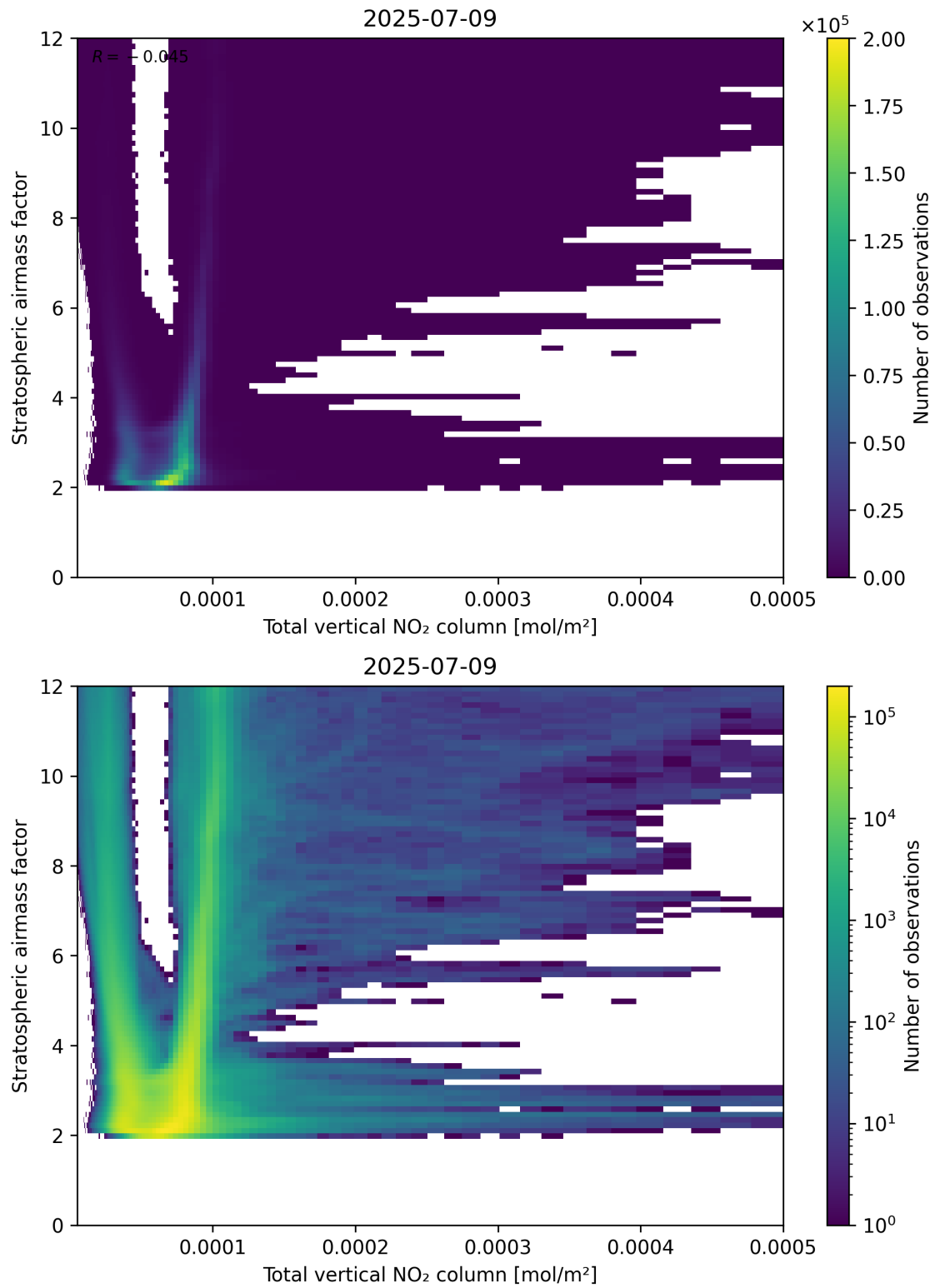
Figure 110: Scatter density plot of “Total vertical NO 2 column” against “Stratospheric airmass factor” for 2025-07-08 to 2025-07-10.
