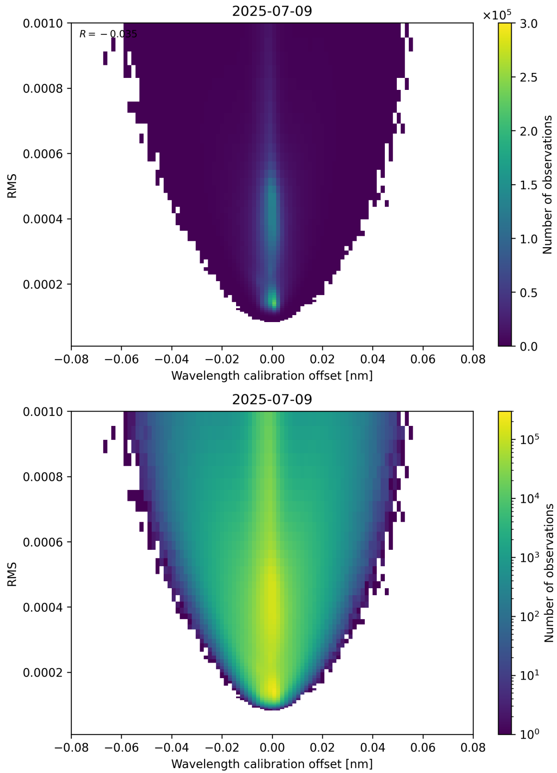
Figure 181: Scatter density plot of “Wavelength calibration offset” against “RMS” for 2025-07-08 to 2025-07-10.
