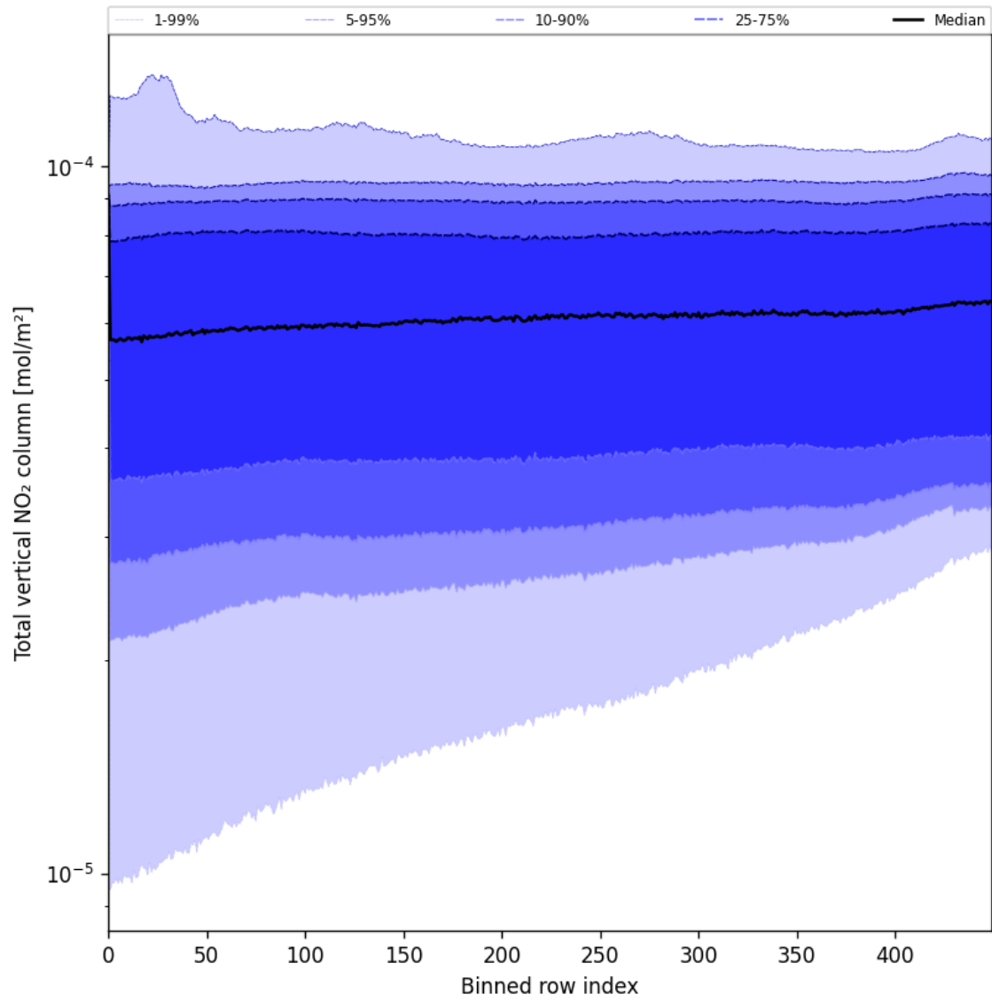
Figure 55: Along track statistics of “Total vertical NO 2 column” for 2025-07-08 to 2025-07-10
