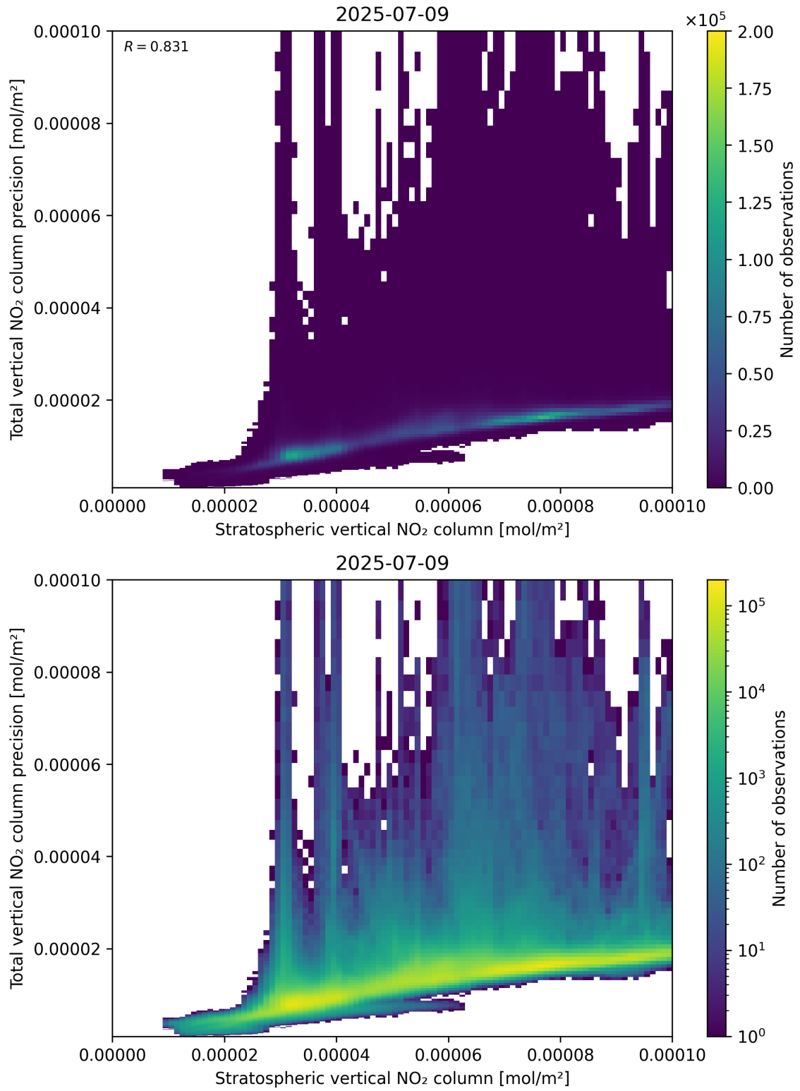
Figure 101: Scatter density plot of “Stratospheric vertical NO 2 column” against “Total vertical NO 2 column precision” for 2025-07-08 to 2025-07-10.
