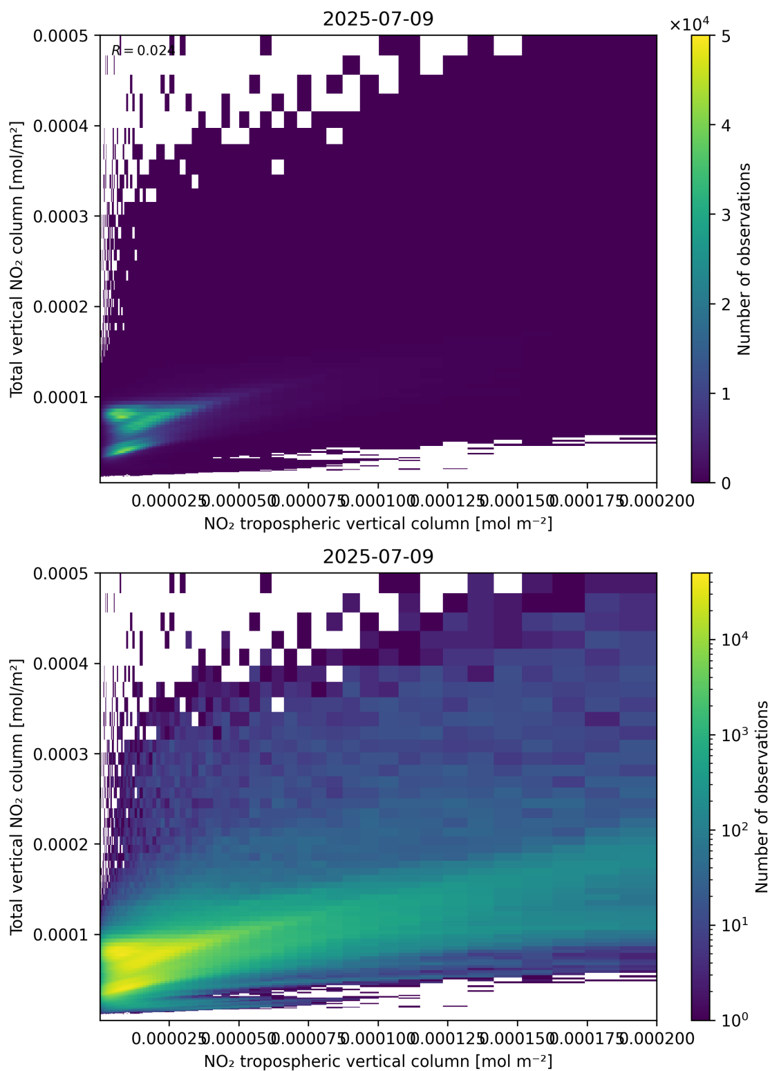
Figure 128: Scatter density plot of “NO 2 tropospheric vertical column” against “Total vertical NO 2 column” for 2025-07-08 to 2025-07-10.
