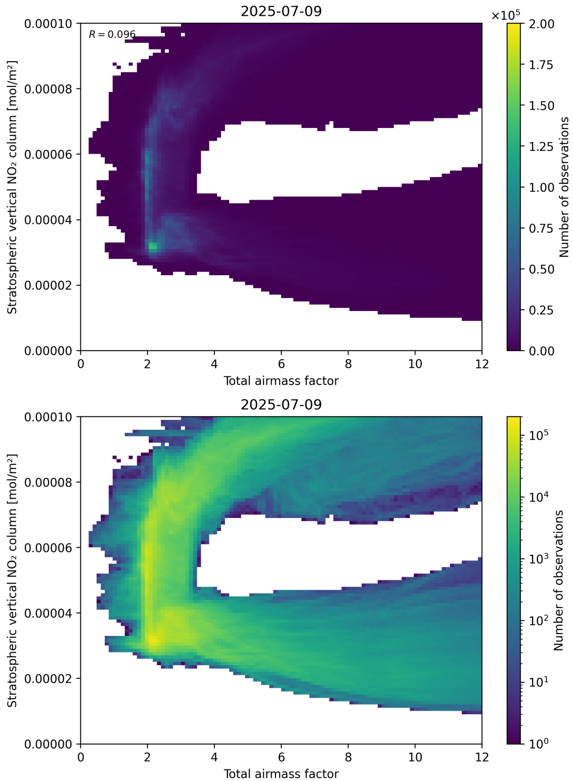
Figure 64: Scatter density plot of “Total airmass factor” against “Stratospheric vertical NO 2 column” for 2025-07-08 to 2025-07-10.
