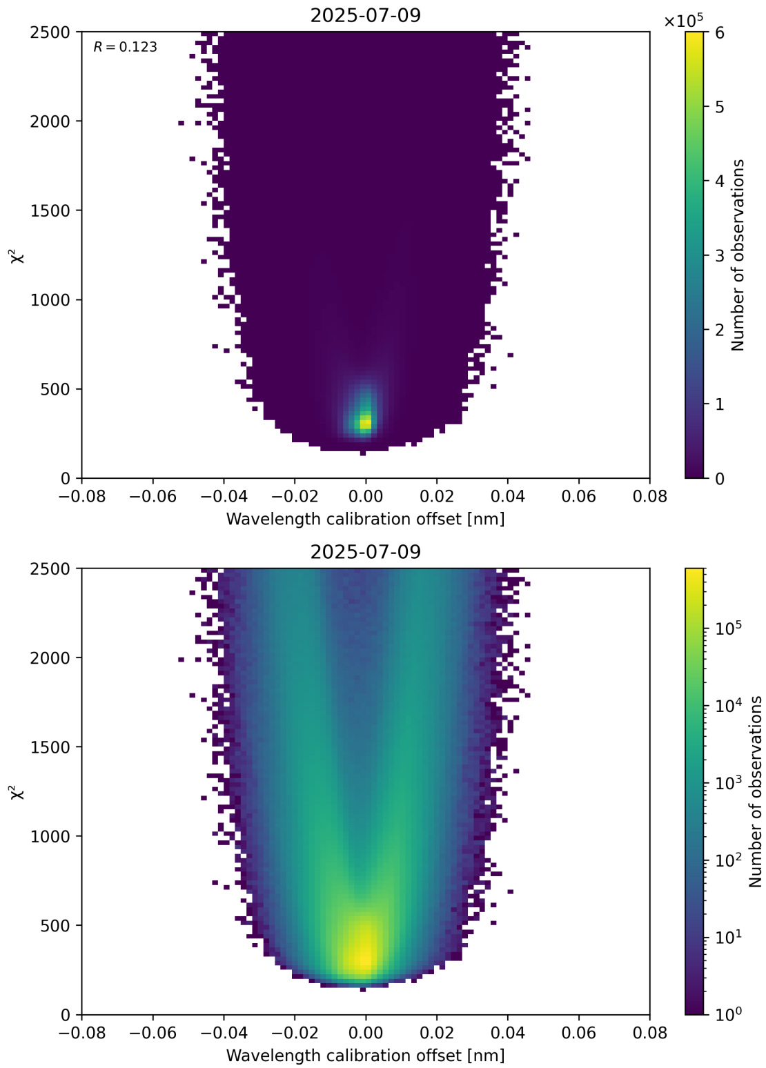
Figure 175: Scatter density plot of “Wavelength calibration offset” against “ \chi^2 ” for 2025-07-08 to 2025-07-10.
