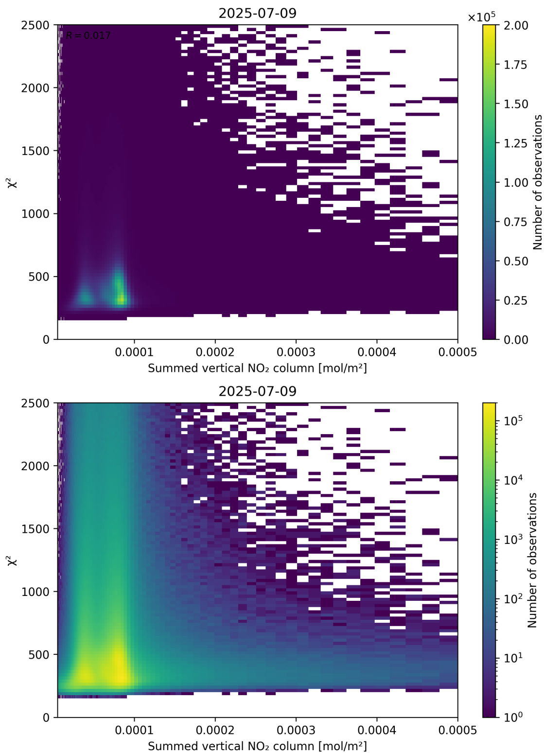
Figure 104: Scatter density plot of “Summed vertical NO 2 column” against “ \chi^2 ” for 2025-07-08 to 2025-07-10.
