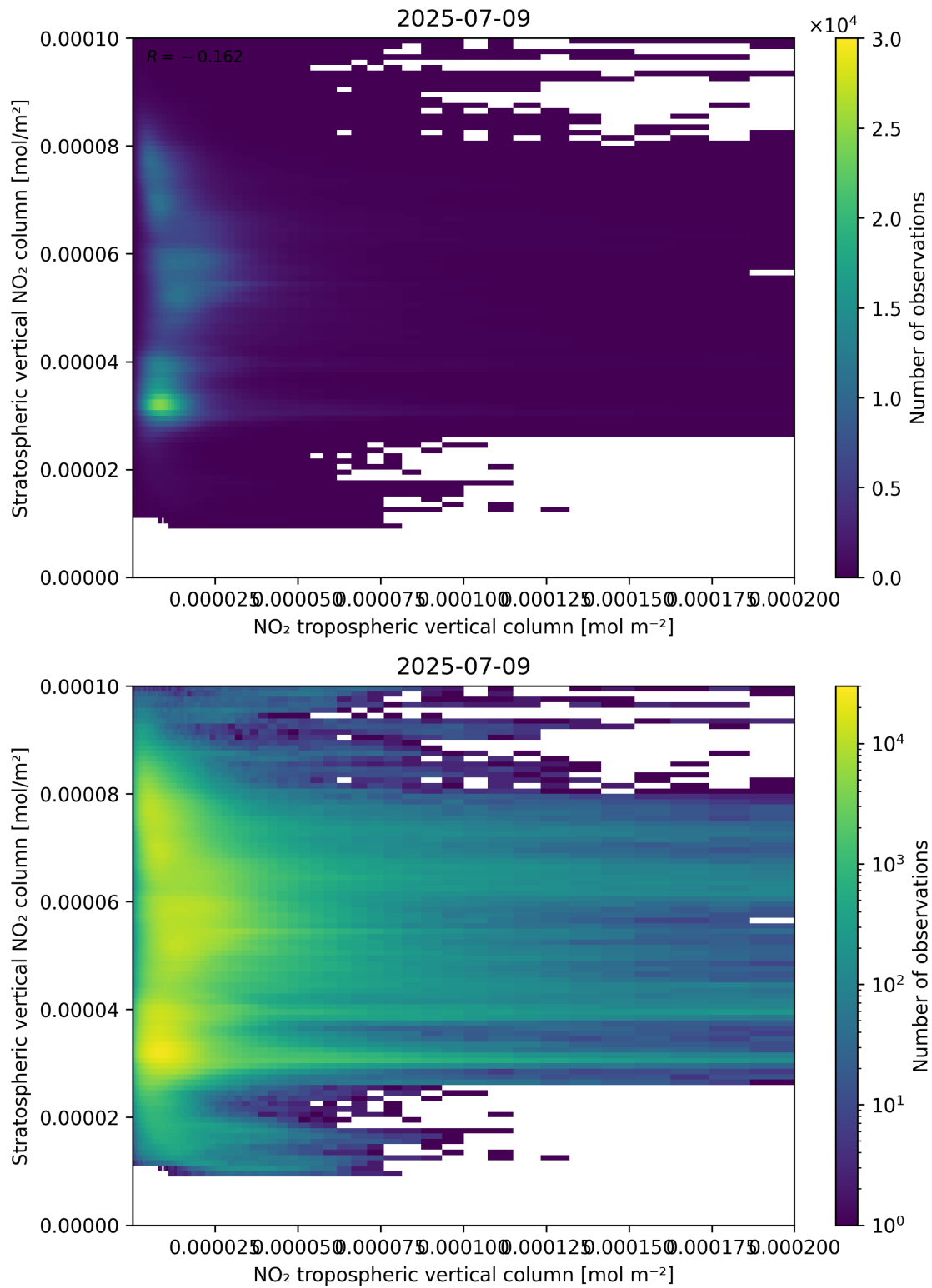
Figure 125: Scatter density plot of “NO 2 tropospheric vertical column” against “Stratospheric vertical NO 2 column” for 2025-07-08 to 2025-07-10.
