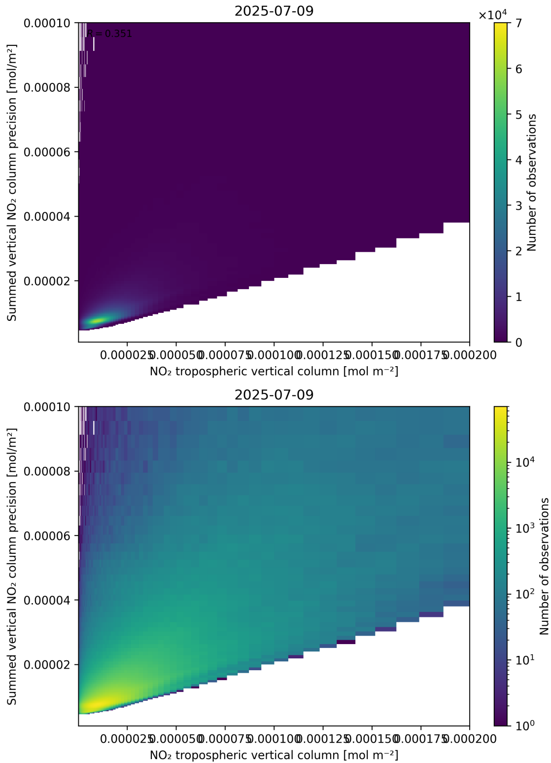
Figure 127: Scatter density plot of “NO 2 tropospheric vertical column” against “Summed vertical NO 2 column precision” for 2025-07-08 to 2025-07-10.
