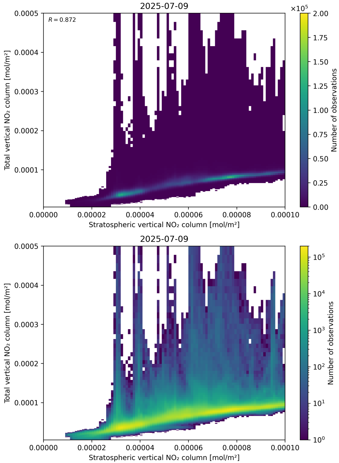
Figure 100: Scatter density plot of “Stratospheric vertical NO 2 column” against “Total vertical NO 2 column” for 2025-07-08 to 2025-07-10.
