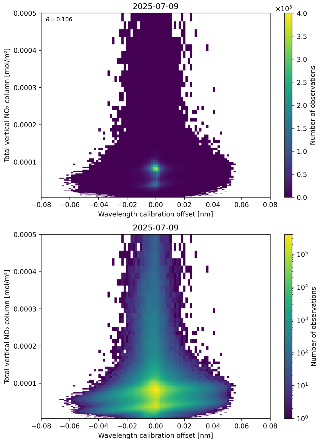
Figure 179: Scatter density plot of “Wavelength calibration offset” against “Total vertical NO 2 column” for 2025-07-08 to 2025-07-10.
