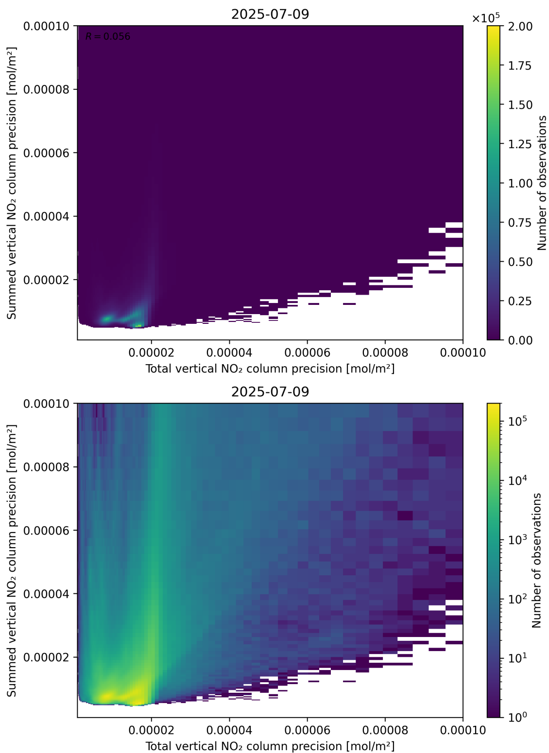
Figure 118: Scatter density plot of “Total vertical NO 2 column precision” against “Summed vertical NO 2 column precision” for 2025-07-08 to 2025-07-10.
