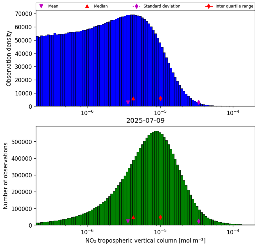
Figure 29: Histogram of “NO 2 tropospheric vertical column” for 2025-07-08 to 2025-07-10
