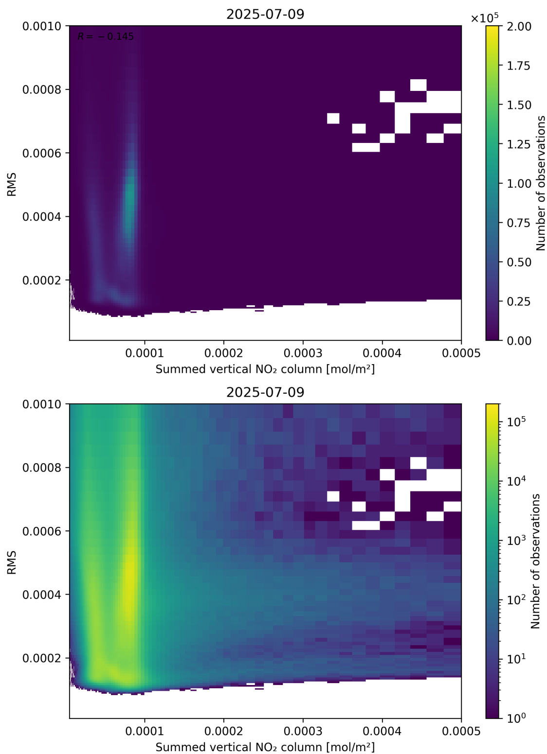
Figure 109: Scatter density plot of “Summed vertical NO 2 column” against “RMS” for 2025-07-08 to 2025-07-10.
