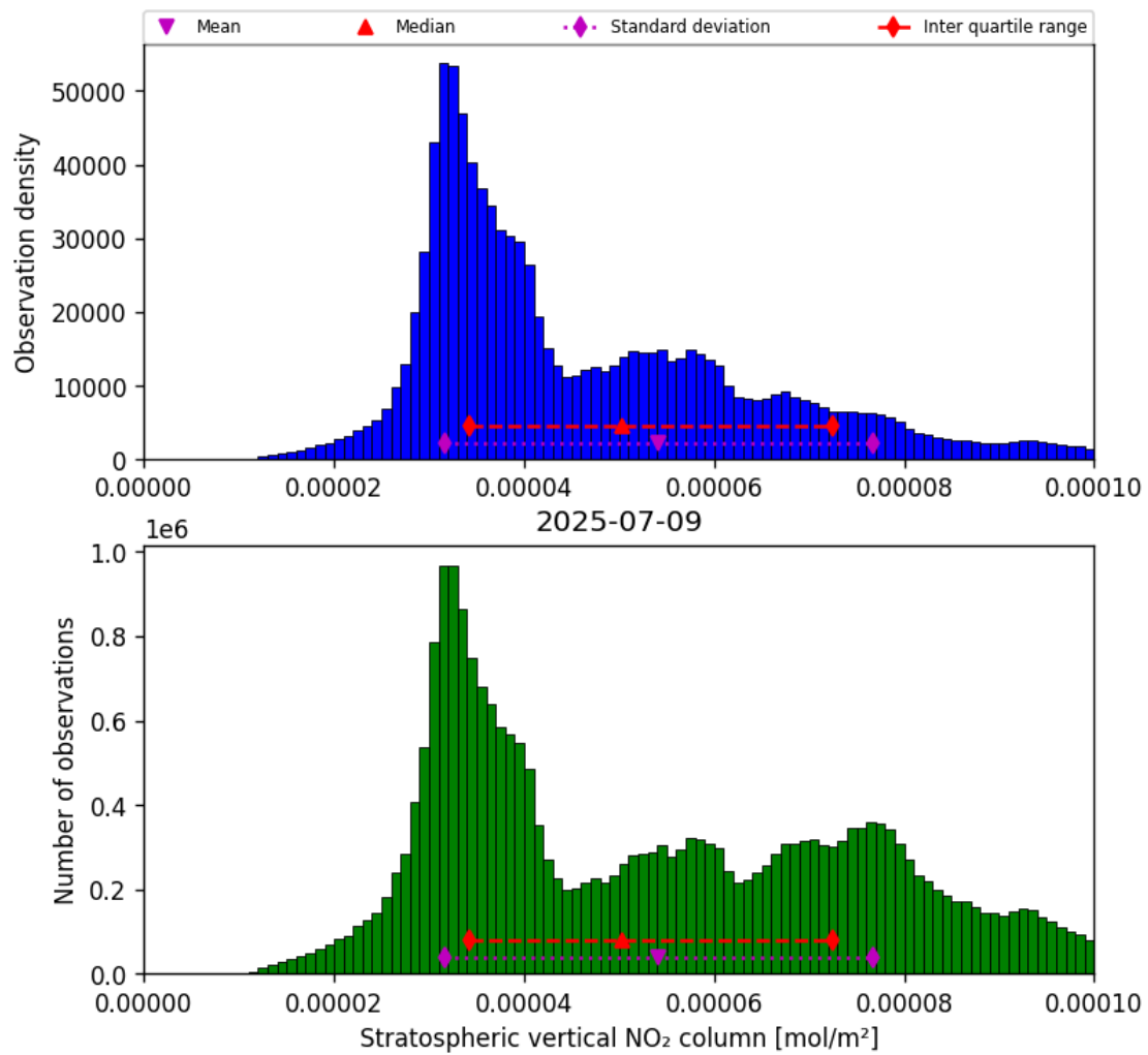
Figure 36: Histogram of “Stratospheric vertical NO 2 column” for 2025-07-08 to 2025-07-10
