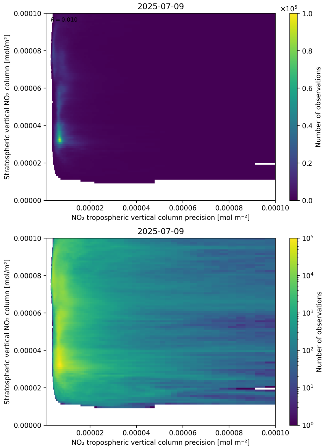
Figure 135: Scatter density plot of “NO 2 tropospheric vertical column precision” against “Stratospheric vertical NO 2 column” for 2025-07-08 to 2025-07-10.
