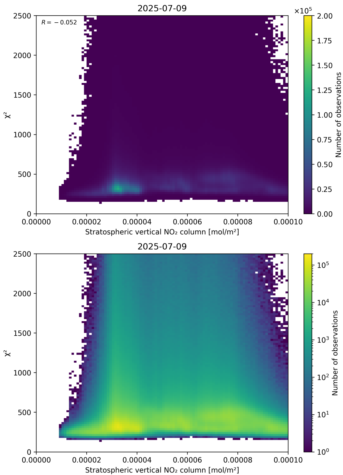
Figure 97: Scatter density plot of “Stratospheric vertical NO 2 column” against “ \chi^2 ” for 2025-07-08 to 2025-07-10.
