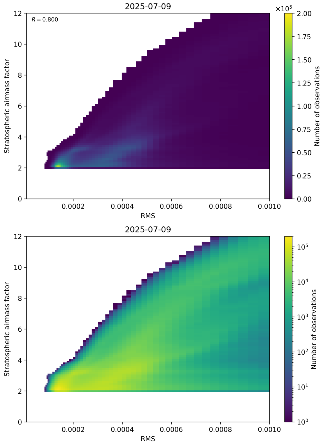
Figure 144: Scatter density plot of “RMS” against “Stratospheric airmass factor” for 2025-07-08 to 2025-07-10.
