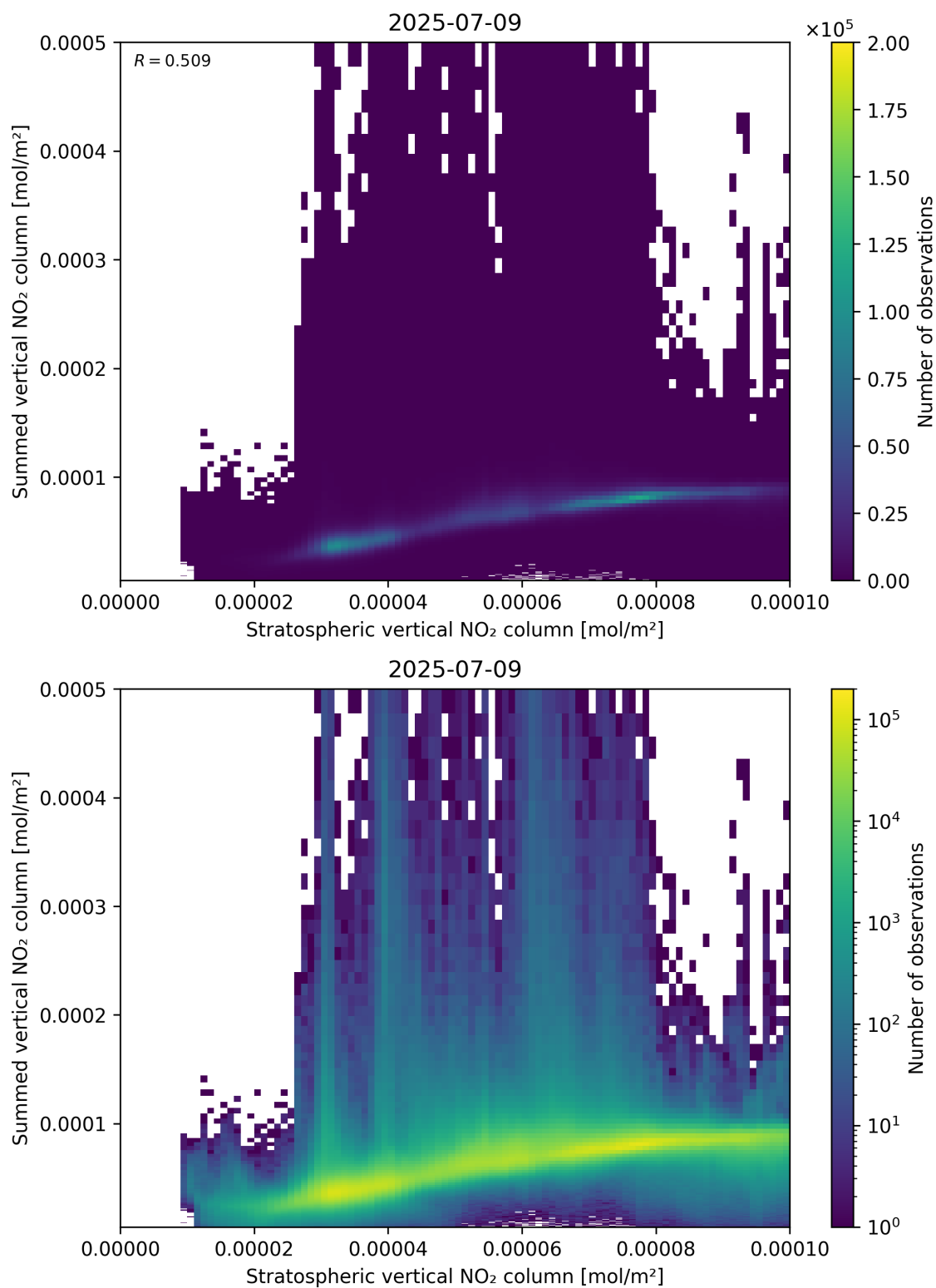
Figure 98: Scatter density plot of “Stratospheric vertical NO 2 column” against “Summed vertical NO 2 column” for 2025-07-08 to 2025-07-10.
