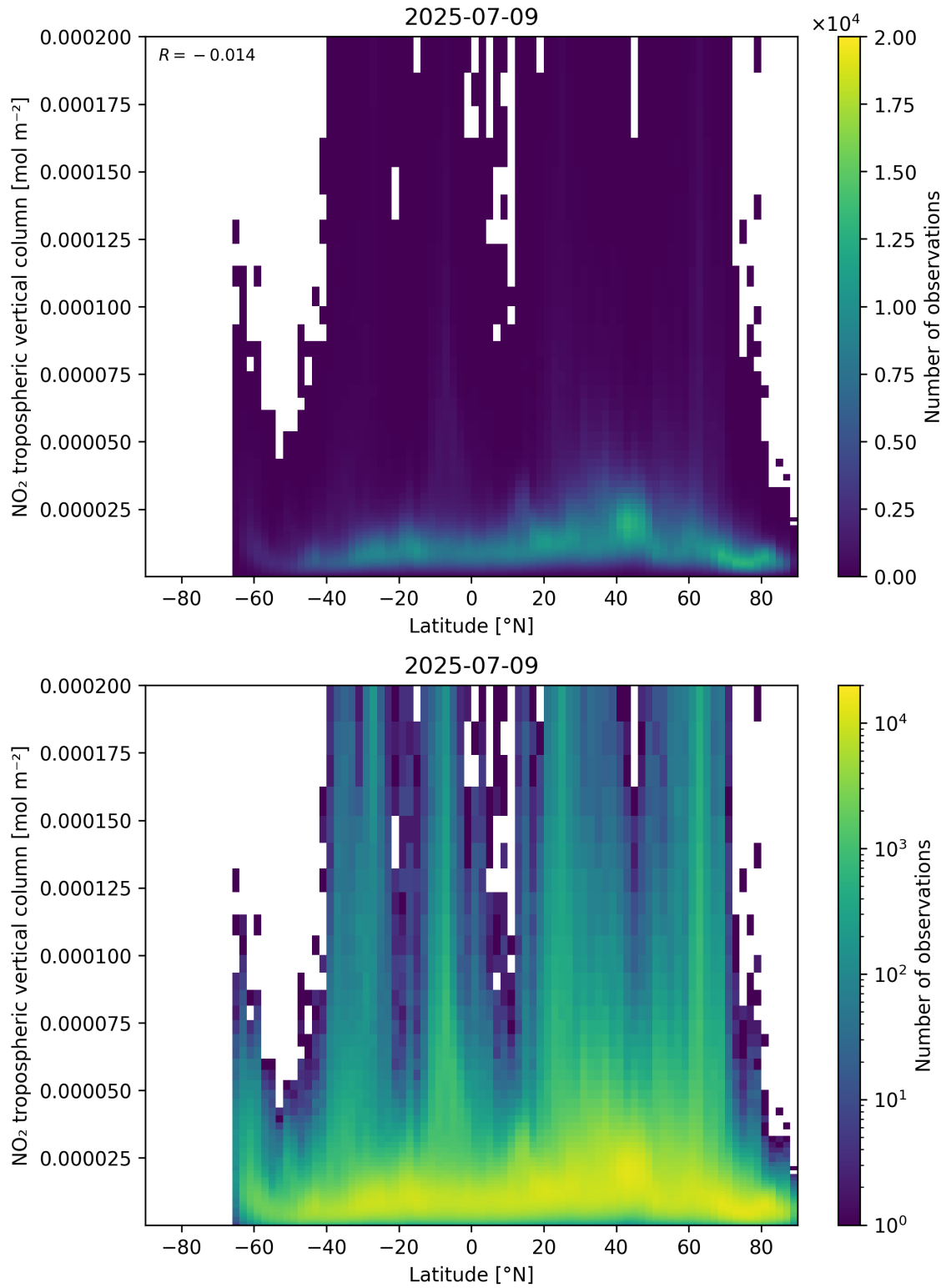
Figure 92: Scatter density plot of “Latitude” against “NO 2 tropospheric vertical column” for 2025-07-08 to 2025-07-10.
