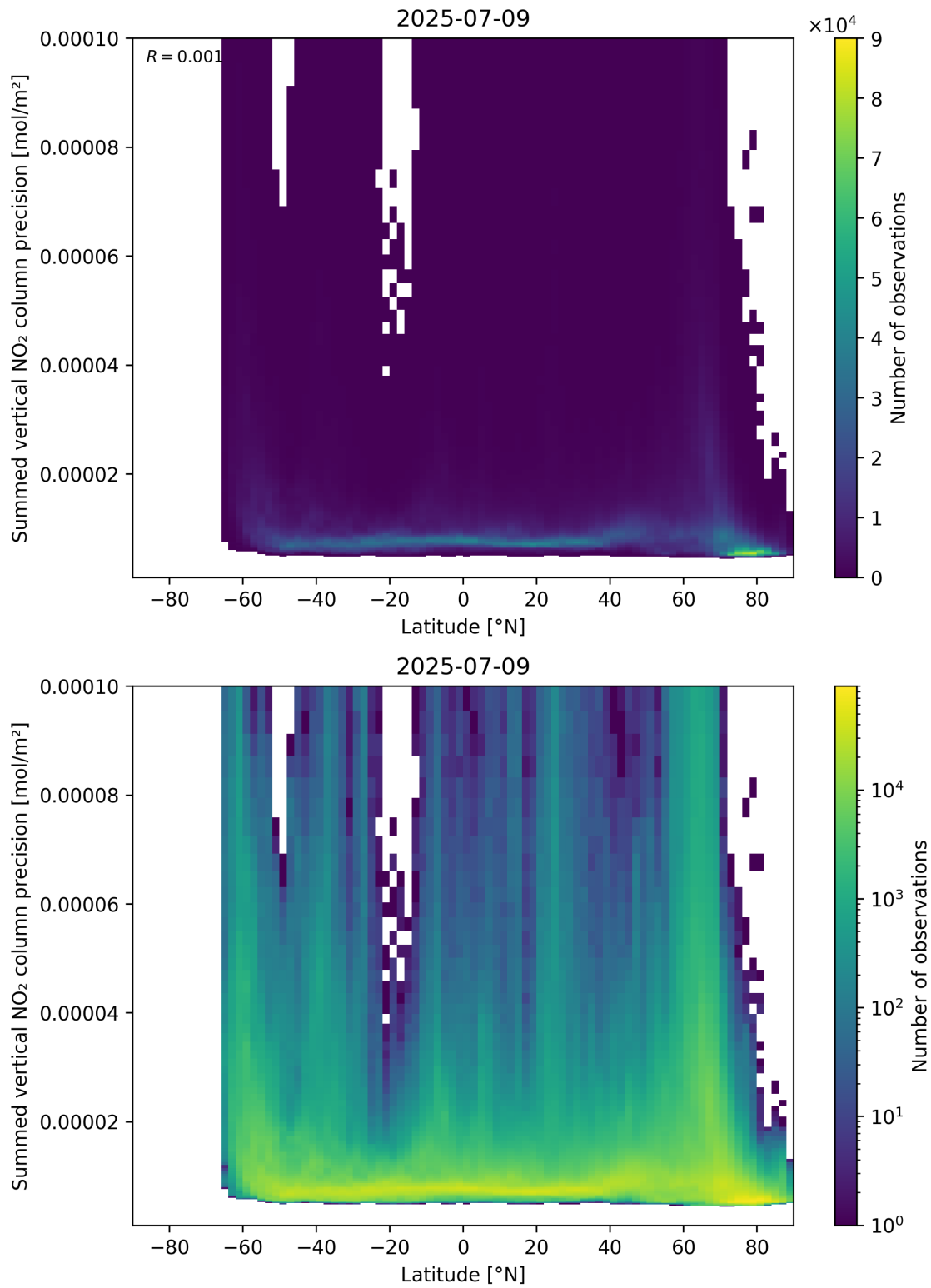
Figure 89: Scatter density plot of “Latitude” against “Summed vertical NO 2 column precision” for 2025-07-08 to 2025-07-10.
