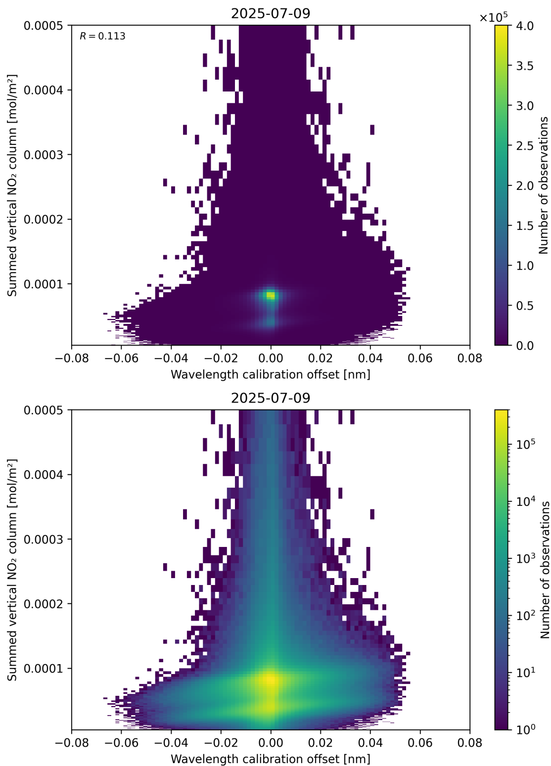
Figure 177: Scatter density plot of “Wavelength calibration offset” against “Summed vertical NO 2 column” for 2025-07-08 to 2025-07-10.
