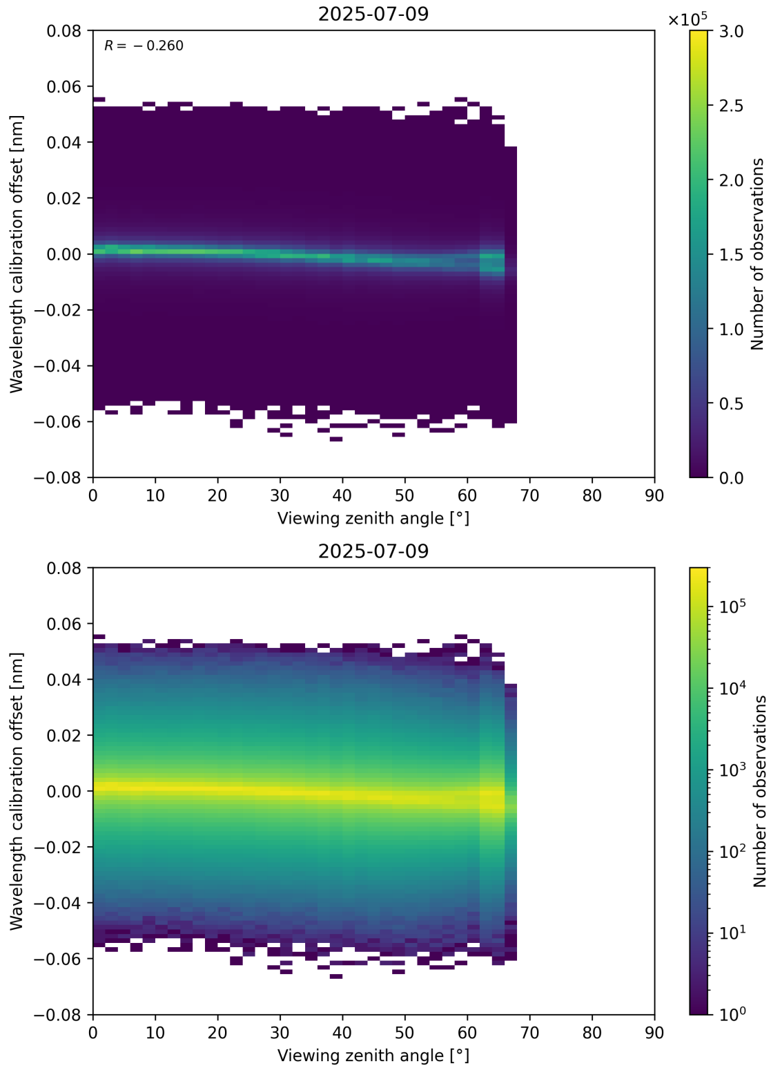
Figure 173: Scatter density plot of “Viewing zenith angle” against “Wavelength calibration offset” for 2025-07-08 to 2025-07-10.
