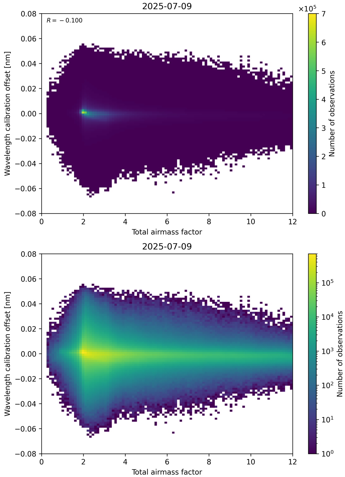
Figure 70: Scatter density plot of “Total airmass factor” against “Wavelength calibration offset” for 2025-07-08 to 2025-07-10.
