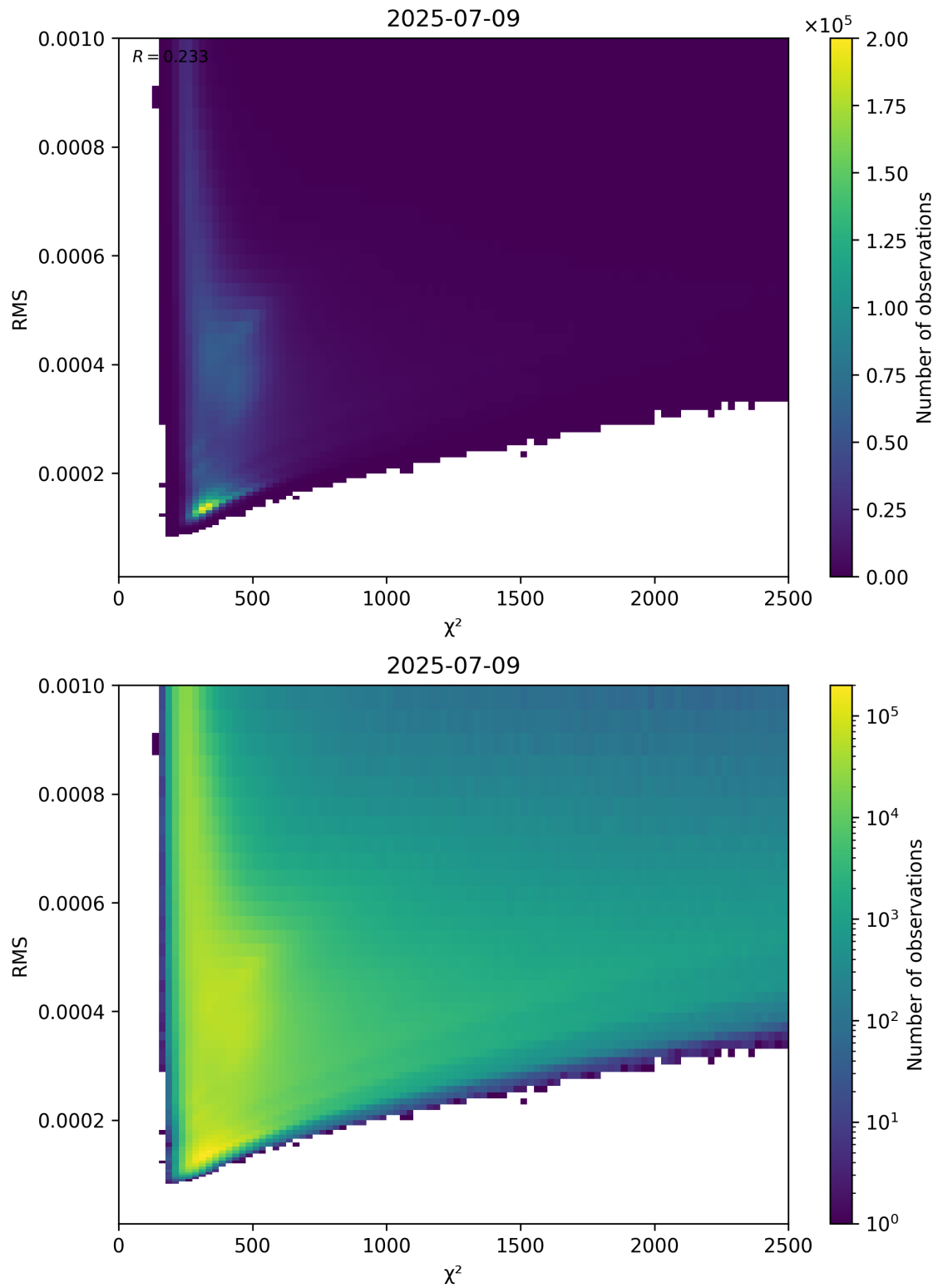
Figure 82: Scatter density plot of “ \chi^2 ” against “RMS” for 2025-07-08 to 2025-07-10.
