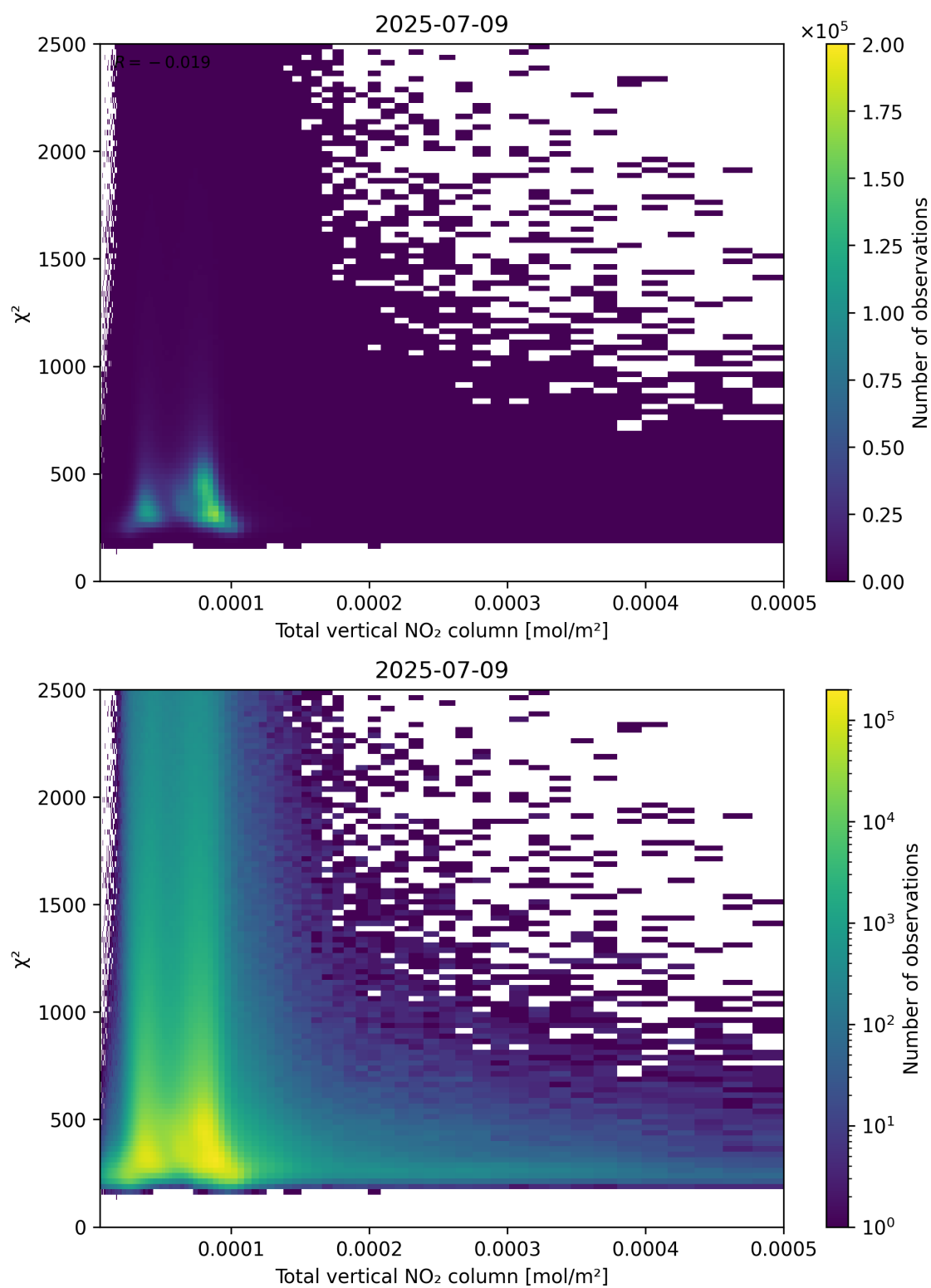
Figure 111: Scatter density plot of “Total vertical NO 2 column” against “ \chi^2 ” for 2025-07-08 to 2025-07-10.
