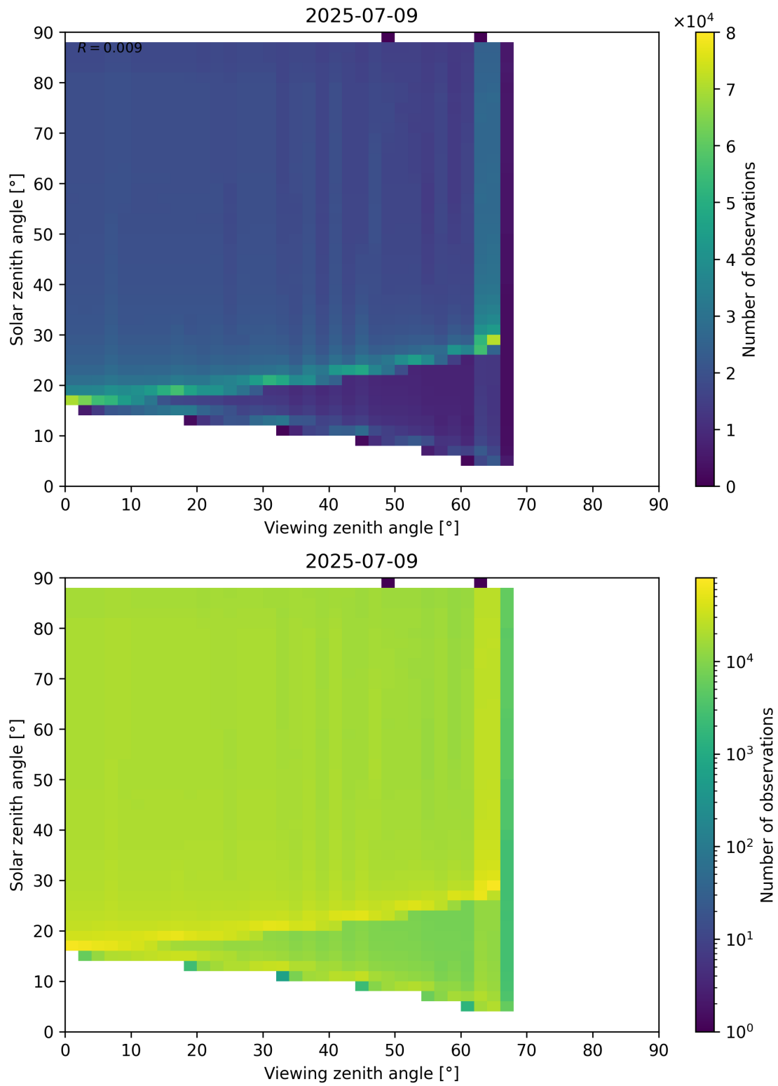
Figure 172: Scatter density plot of “Viewing zenith angle” against “Solar zenith angle” for 2025-07-08 to 2025-07-10.
