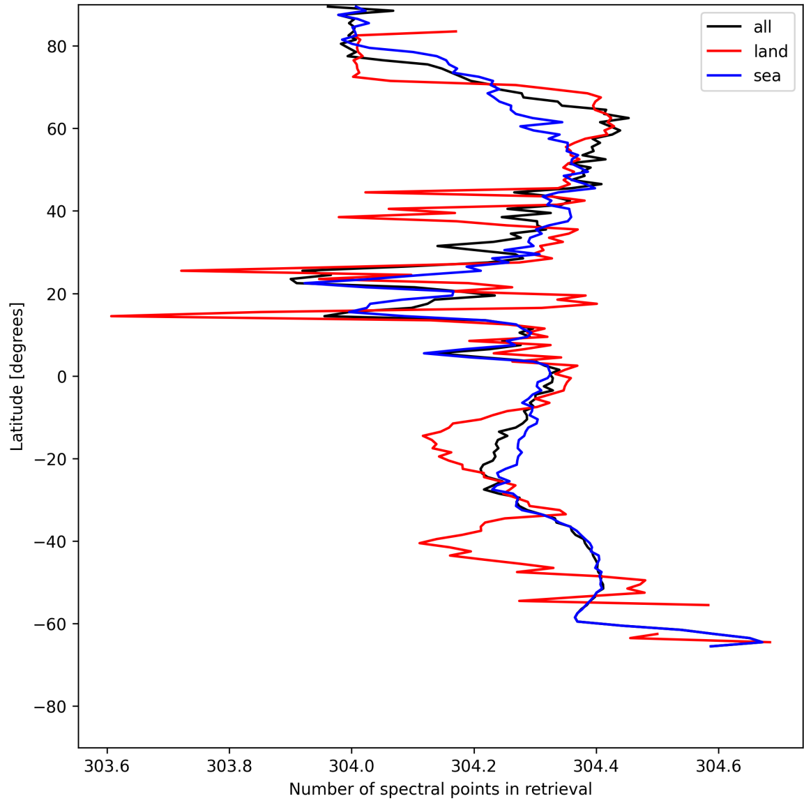
Figure 16: Zonal average of “Number of spectral points in retrieval” for 2025-07-08 to 2025-07-10.
