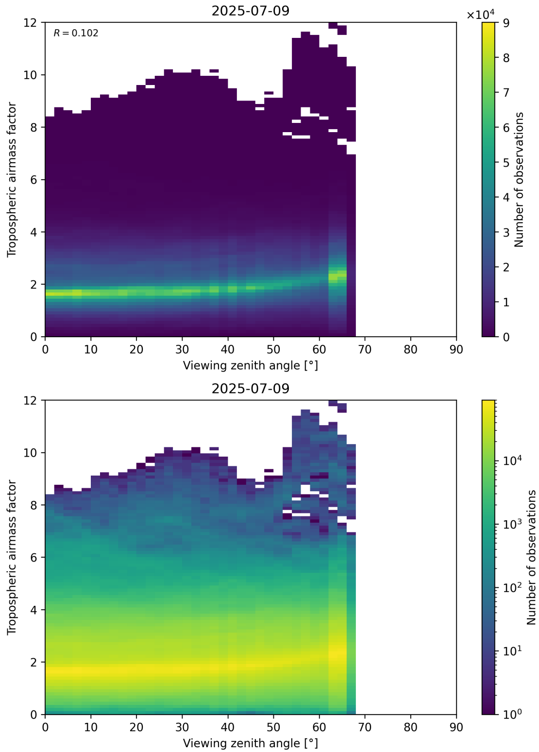
Figure 161: Scatter density plot of “Viewing zenith angle” against “Tropospheric airmass factor” for 2025-07-08 to 2025-07-10.
