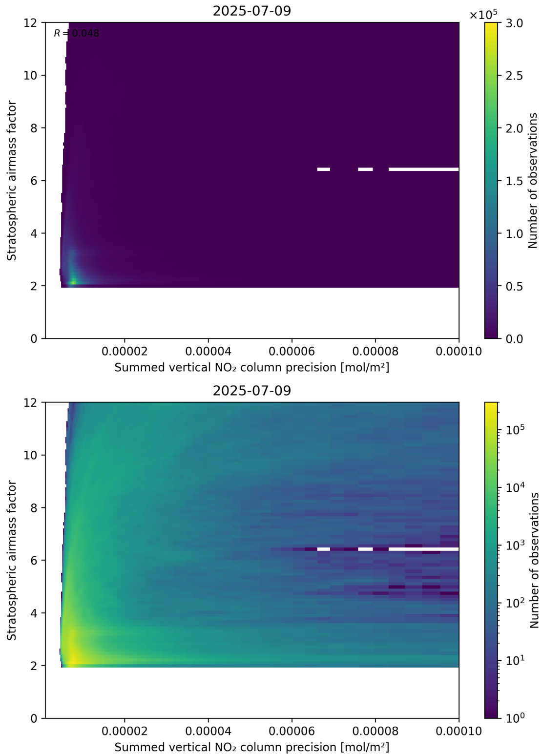
Figure 106: Scatter density plot of “Summed vertical NO 2 column precision” against “Stratospheric airmass factor” for 2025-07-08 to 2025-07-10.
