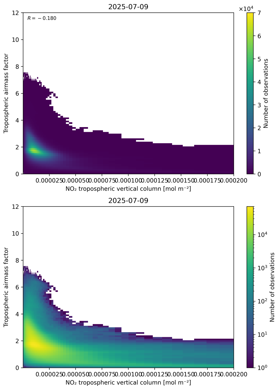
Figure 123: Scatter density plot of “NO 2 tropospheric vertical column” against “Tropospheric air mass factor” for 2025-07-08 to 2025-07-10.
