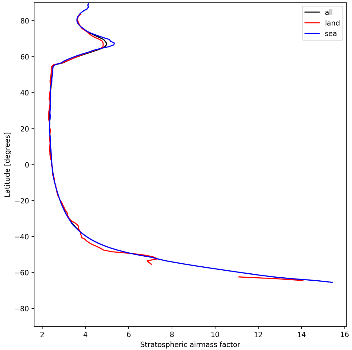
Figure 27: Zonal average of “Stratospheric airmass factor” for 2025-07-08 to 2025-07-10.
