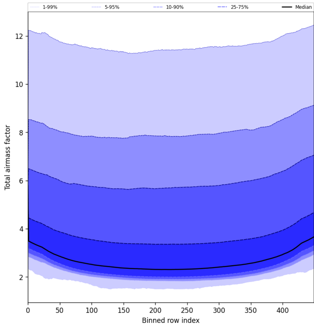
Figure 49: Along track statistics of “Total airmass factor” for 2025-07-08 to 2025-07-10
