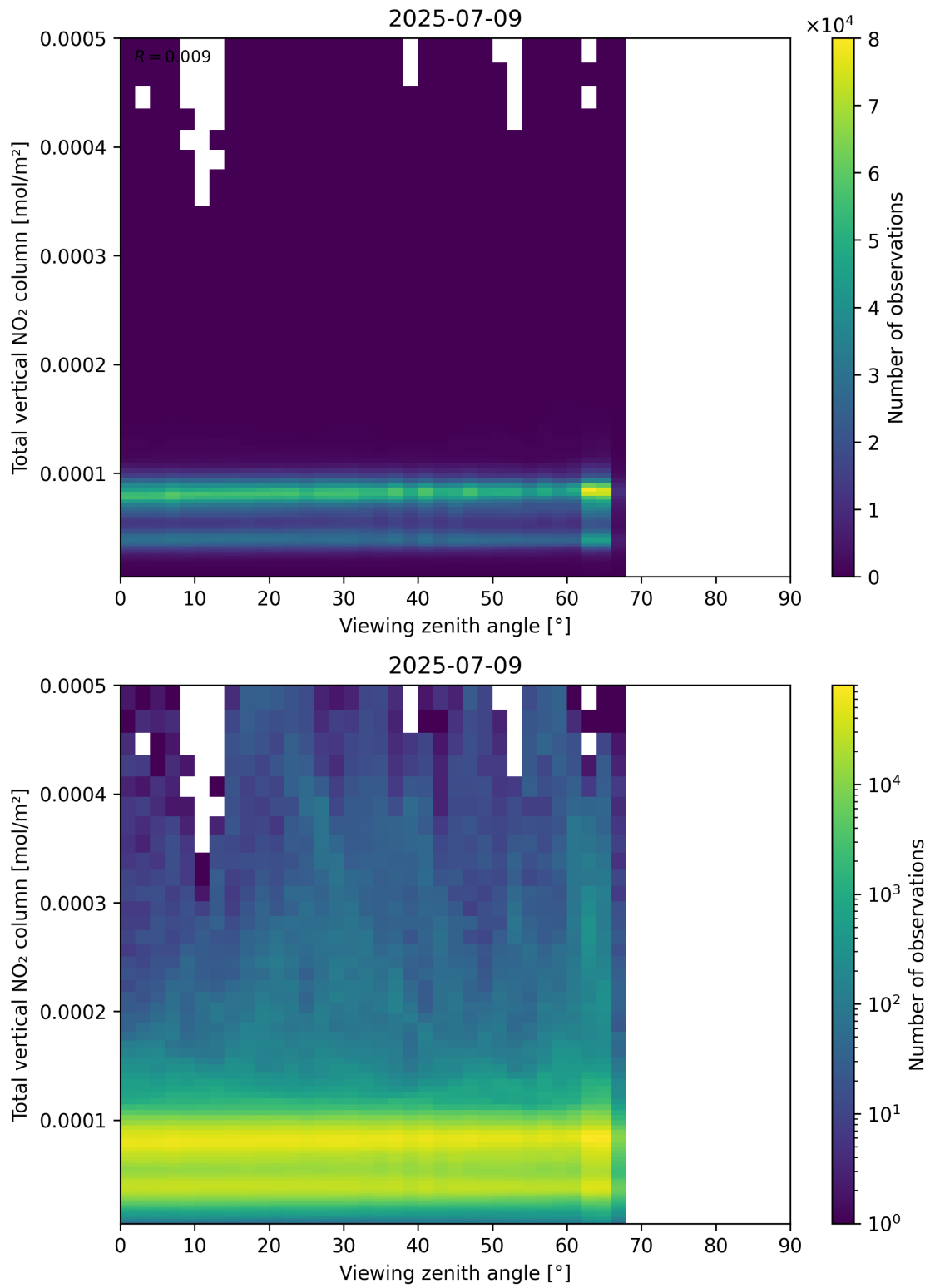
Figure 167: Scatter density plot of “Viewing zenith angle” against “Total vertical NO 2 column” for 2025-07-08 to 2025-07-10.
