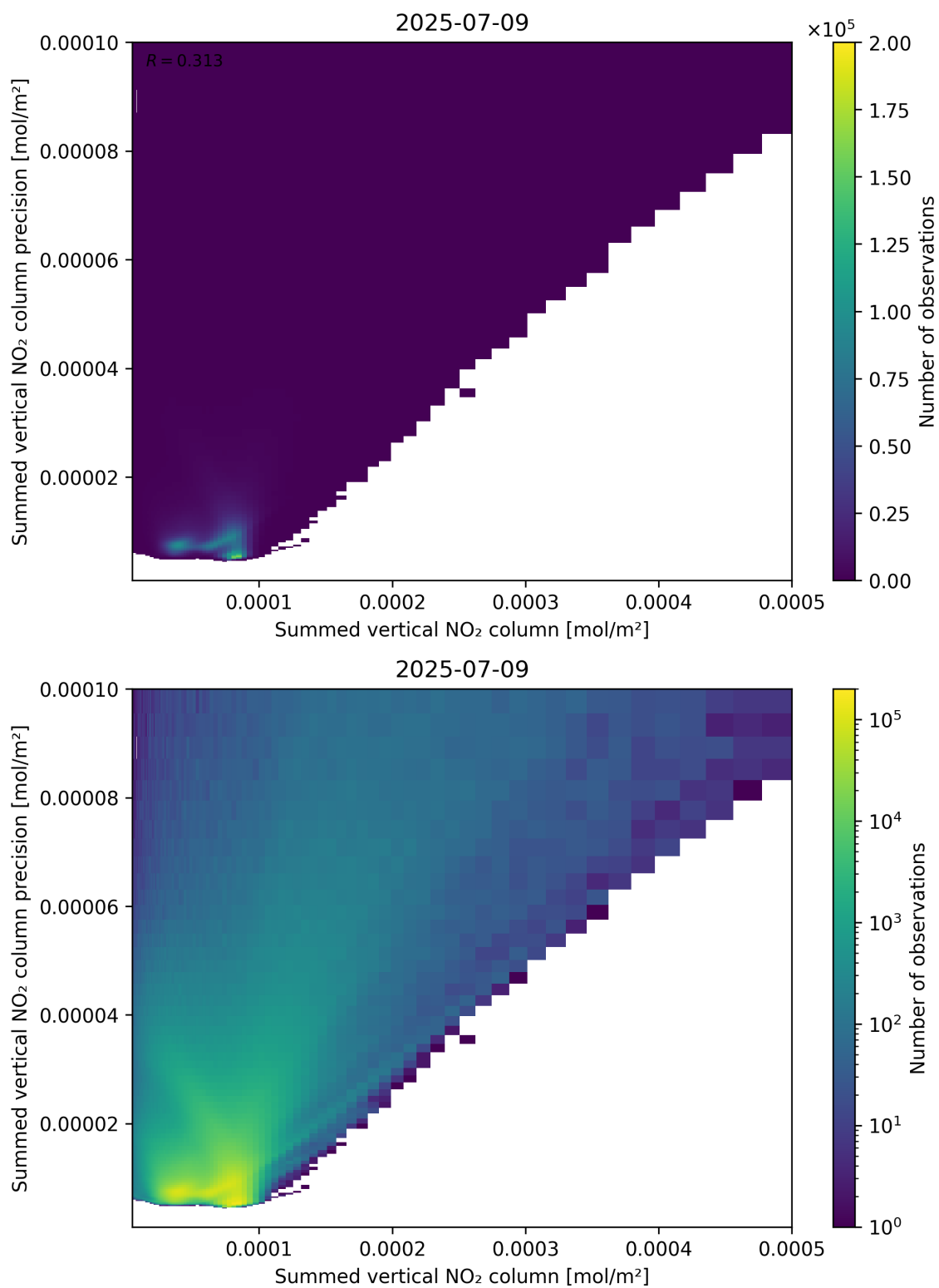
Figure 105: Scatter density plot of “Summed vertical NO 2 column” against “Summed vertical NO 2 column precision” for 2025-07-08 to 2025-07-10.
