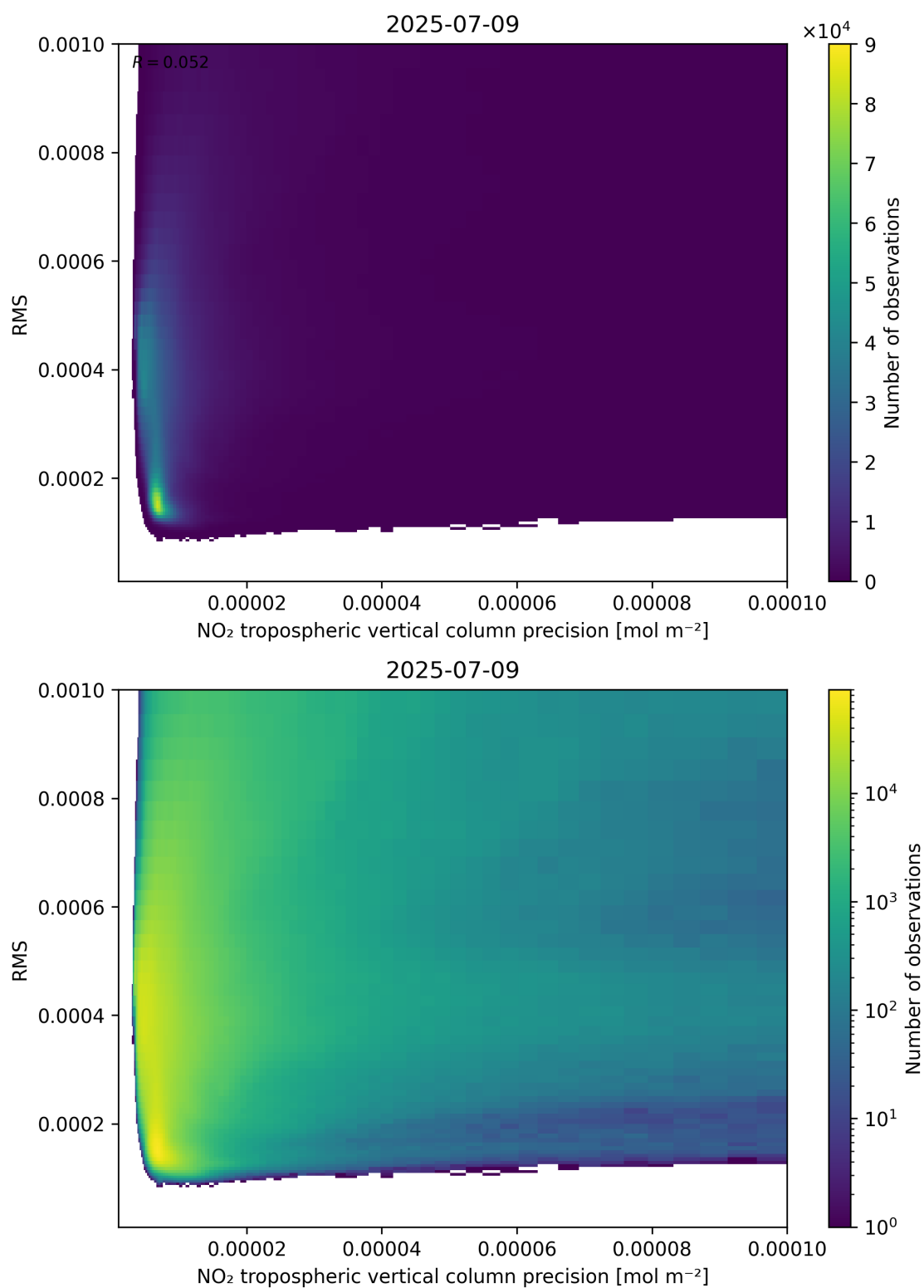
Figure 140: Scatter density plot of “NO 2 tropospheric vertical column precision” against “RMS” for 2025-07-08 to 2025-07-10.
