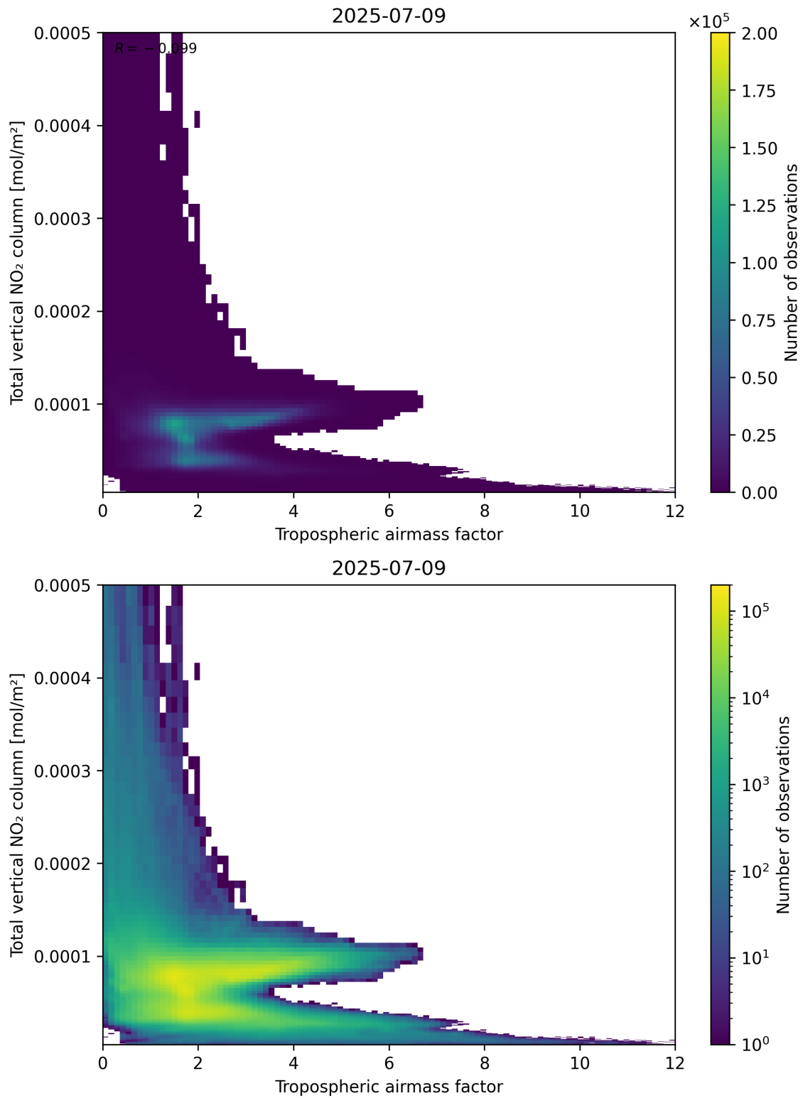
Figure 77: Scatter density plot of “Tropospheric airmass factor” against “Total vertical NO 2 column” for 2025-07-08 to 2025-07-10.
