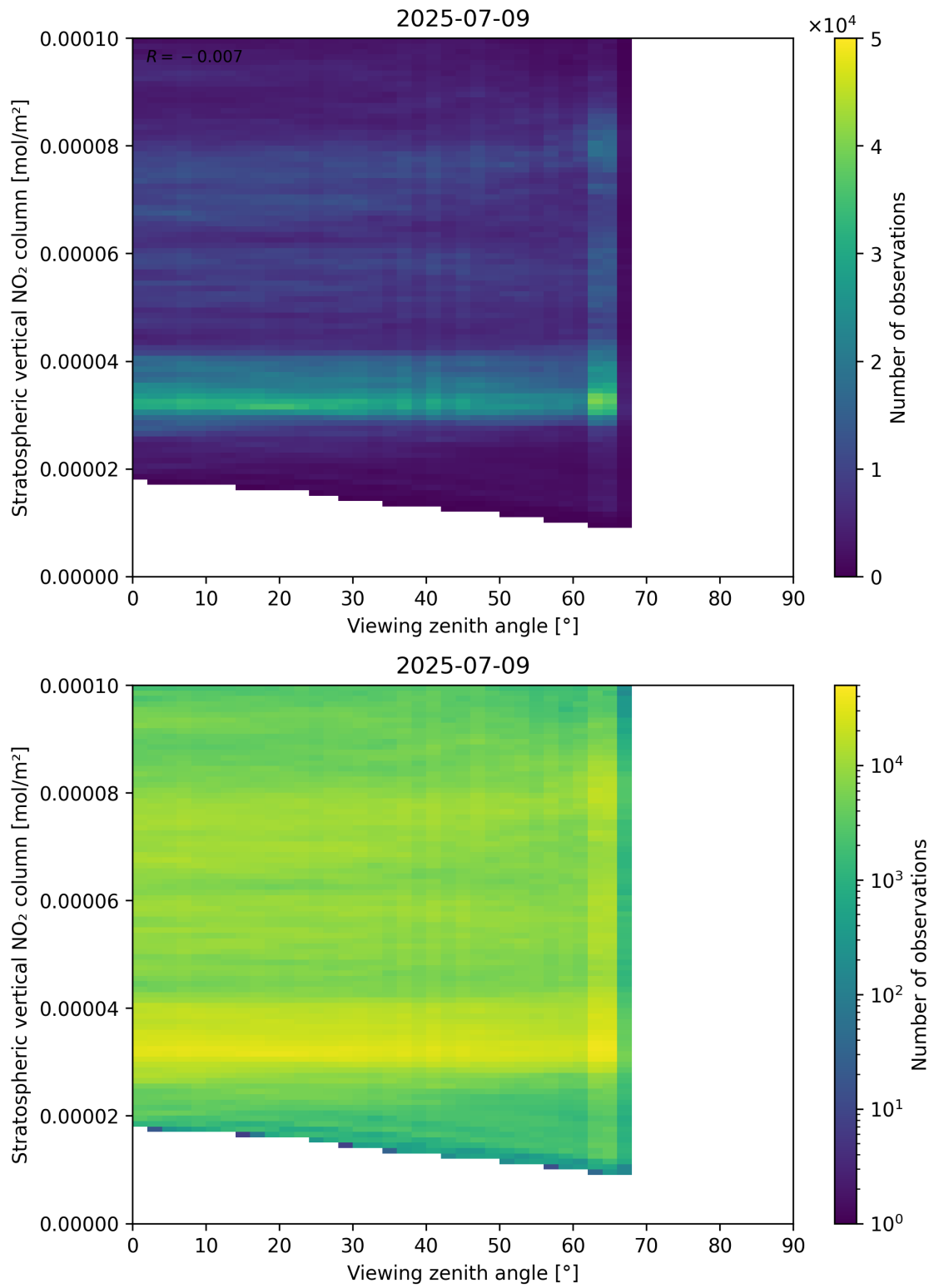
Figure 164: Scatter density plot of “Viewing zenith angle” against “Stratospheric vertical NO 2 column” for 2025-07-08 to 2025-07-10.
