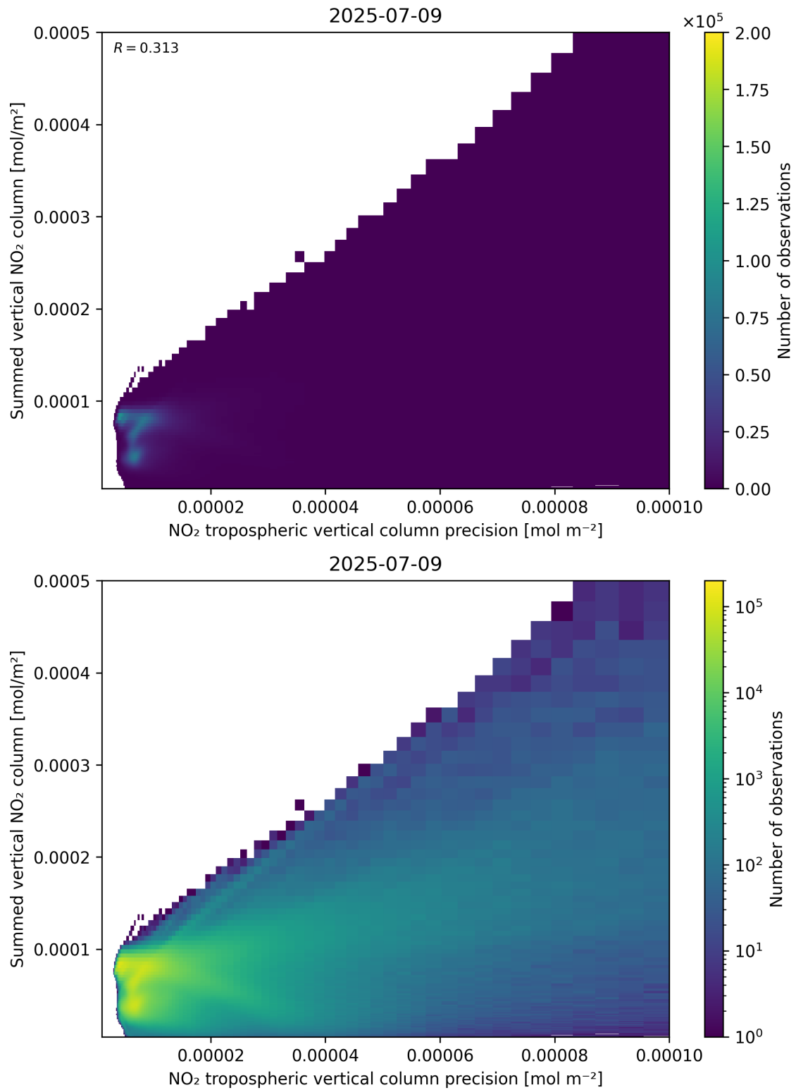
Figure 136: Scatter density plot of “NO 2 tropospheric vertical column precision” against “Summed vertical NO 2 column” for 2025-07-08 to 2025-07-10.
