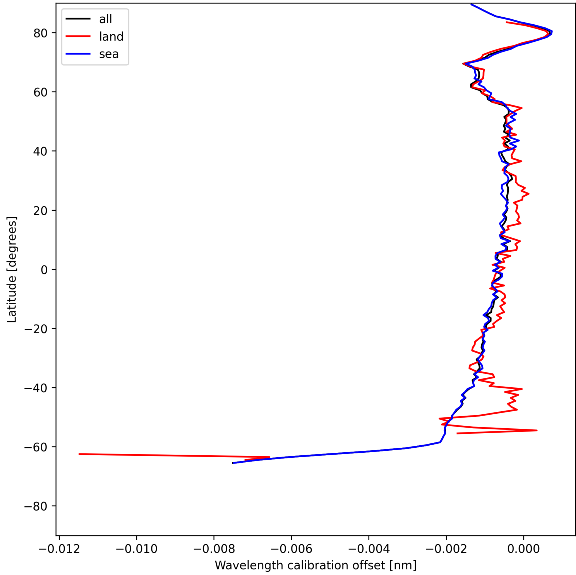
Figure 18: Zonal average of “Wavelength calibration offset” for 2025-07-08 to 2025-07-10.
