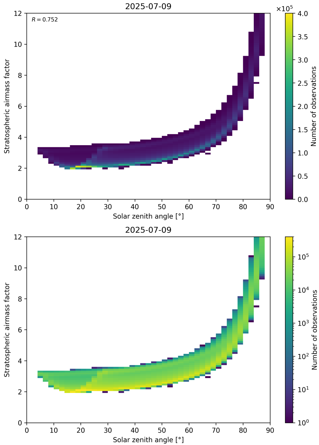
Figure 145: Scatter density plot of “Solar zenith angle” against “Stratospheric airmass factor” for 2025-07-08 to 2025-07-10.
