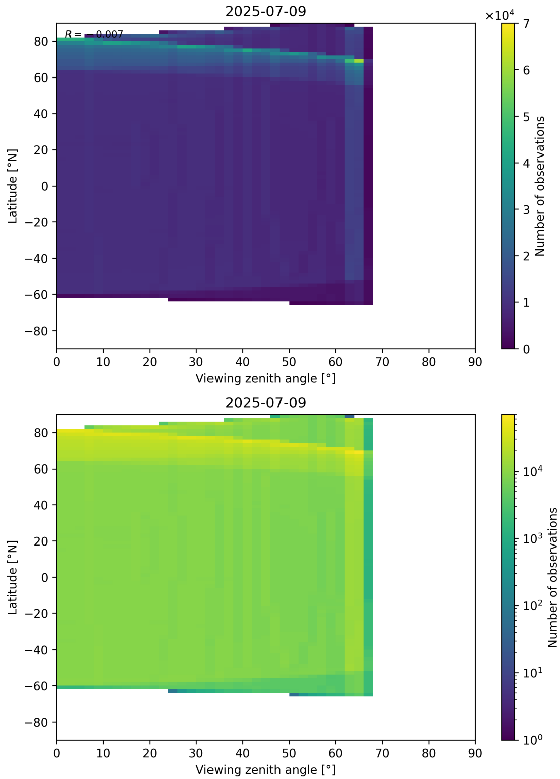
Figure 163: Scatter density plot of “Viewing zenith angle” against “Latitude” for 2025-07-08 to 2025-07-10.
