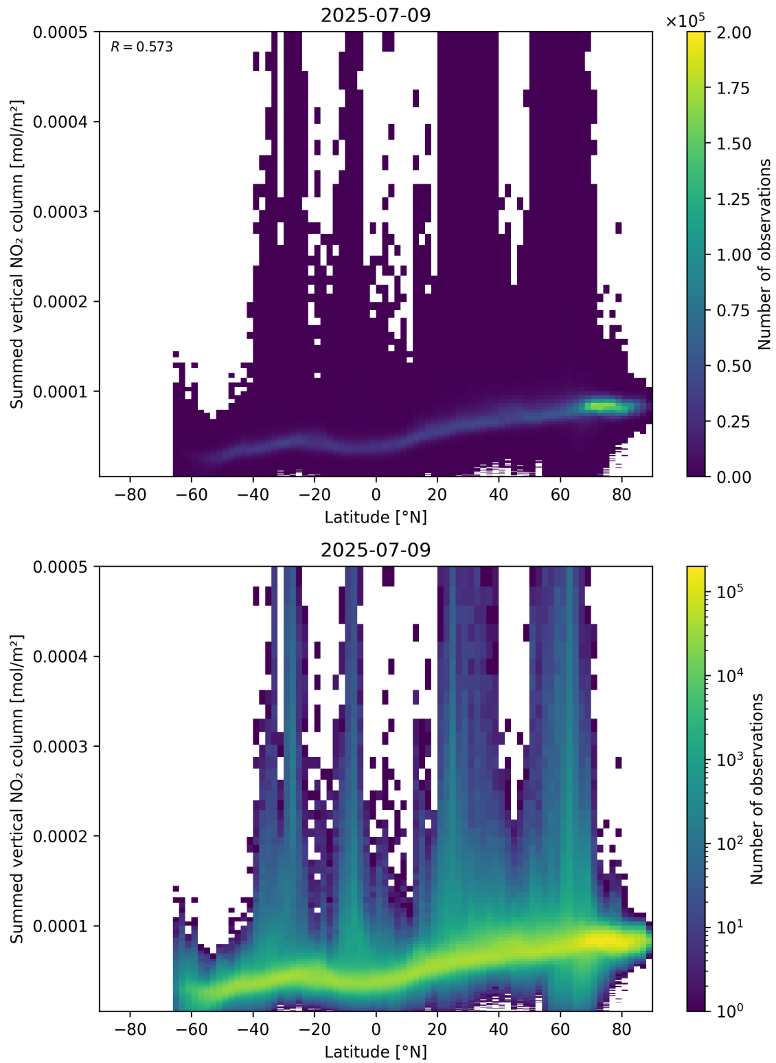
Figure 88: Scatter density plot of “Latitude” against “Summed vertical NO 2 column” for 2025-07-08 to 2025-07-10.
