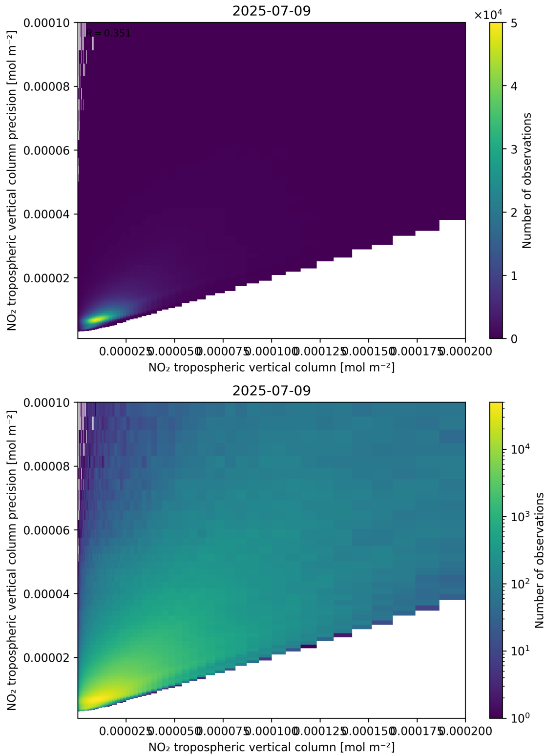
Figure 130: Scatter density plot of “NO 2 tropospheric vertical column” against “NO 2 tropospheric vertical column precision” for 2025-07-08 to 2025-07-10.
