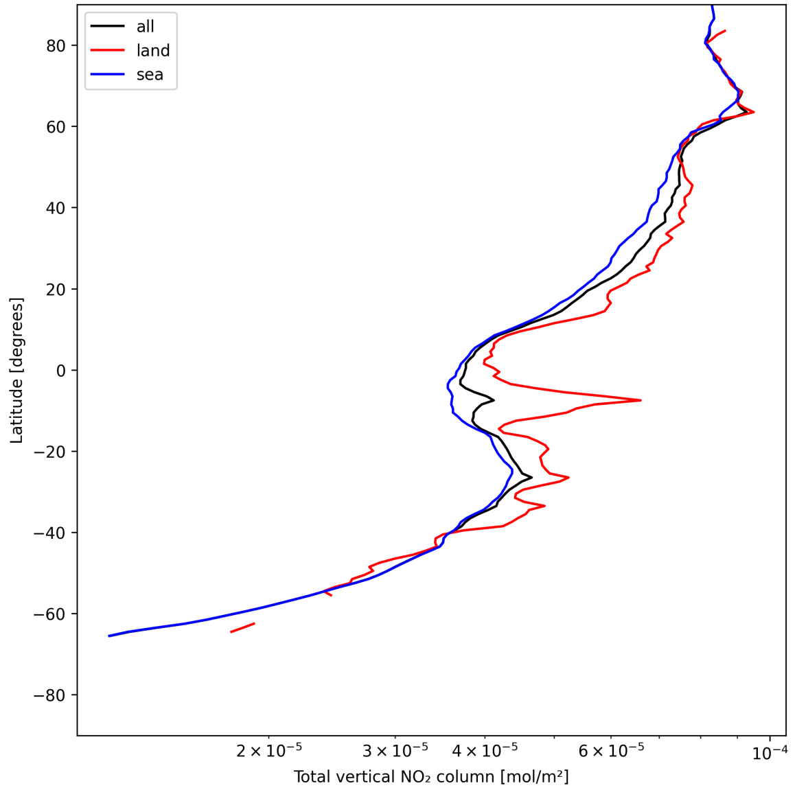
Figure 21: Zonal average of “Total vertical NO 2 column” for 2025-07-08 to 2025-07-10.
