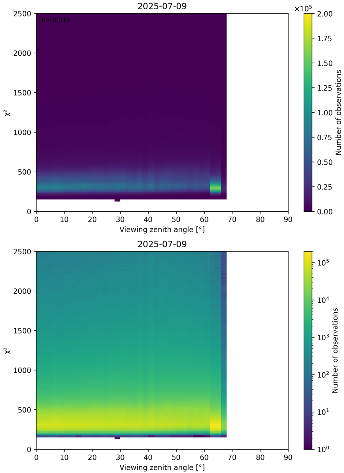
Figure 162: Scatter density plot of “Viewing zenith angle” against “ \chi^2 ” for 2025-07-08 to 2025-07-10.
