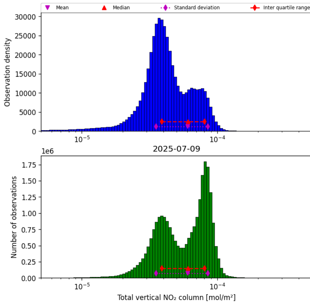
Figure 38: Histogram of “Total vertical NO 2 column” for 2025-07-08 to 2025-07-10
