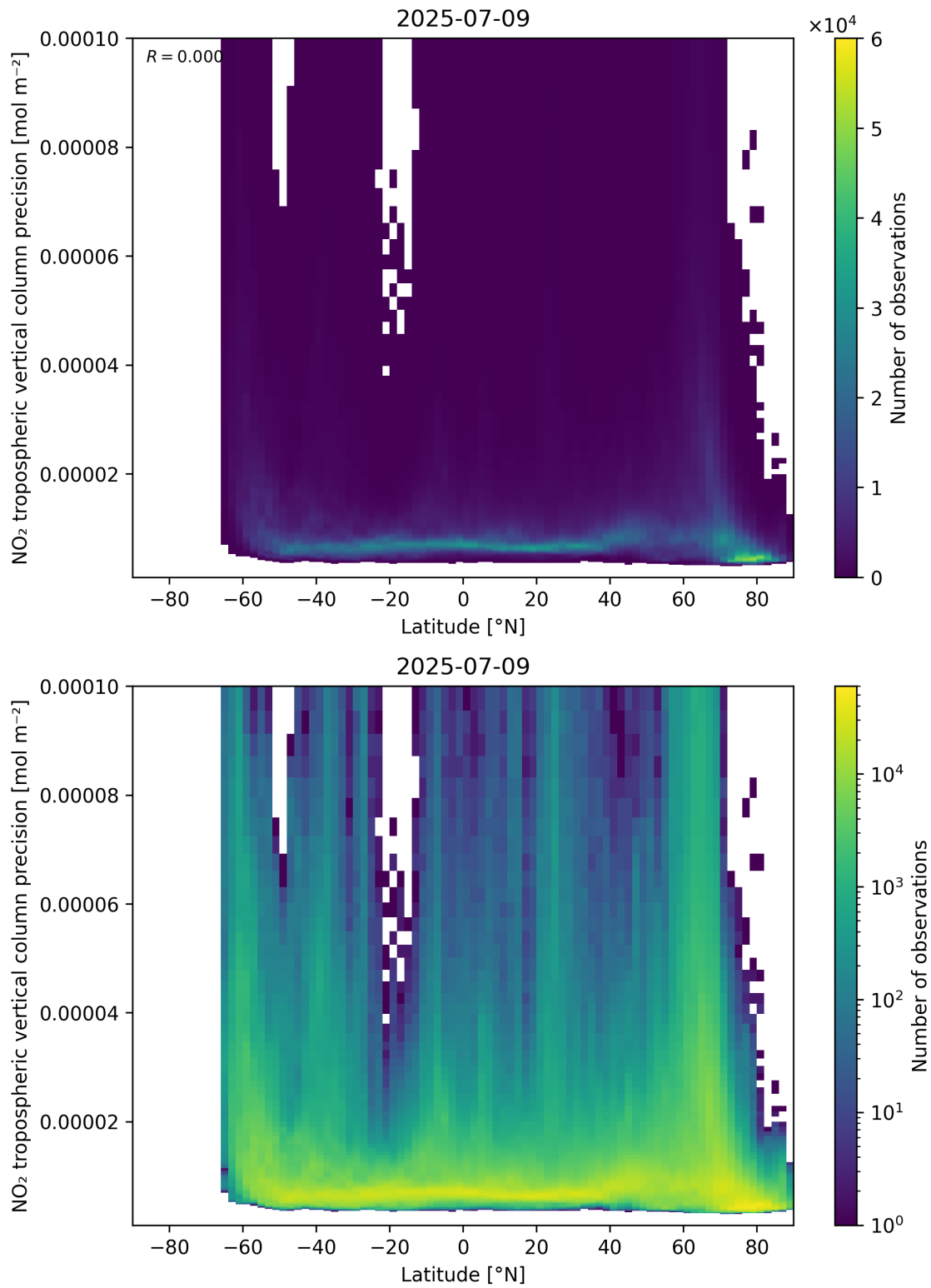
Figure 93: Scatter density plot of “Latitude” against “NO 2 tropospheric vertical column precision” for 2025-07-08 to 2025-07-10.
