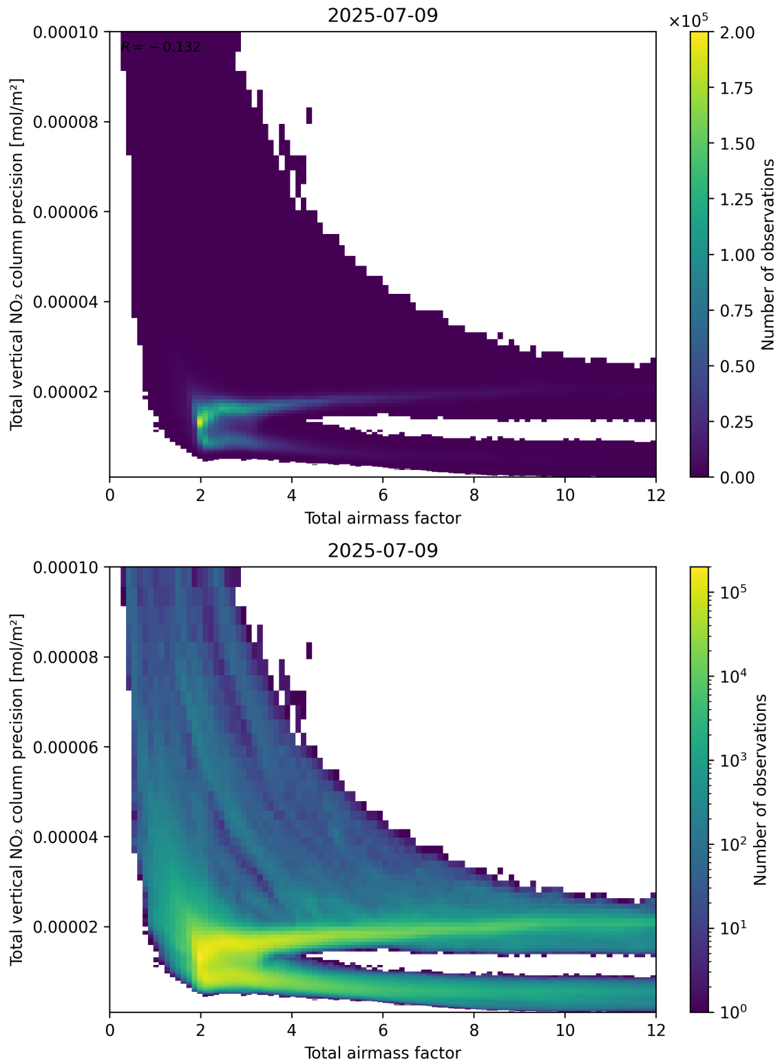
Figure 68: Scatter density plot of “Total airmass factor” against “Total vertical NO 2 column precision” for 2025-07-08 to 2025-07-10.
