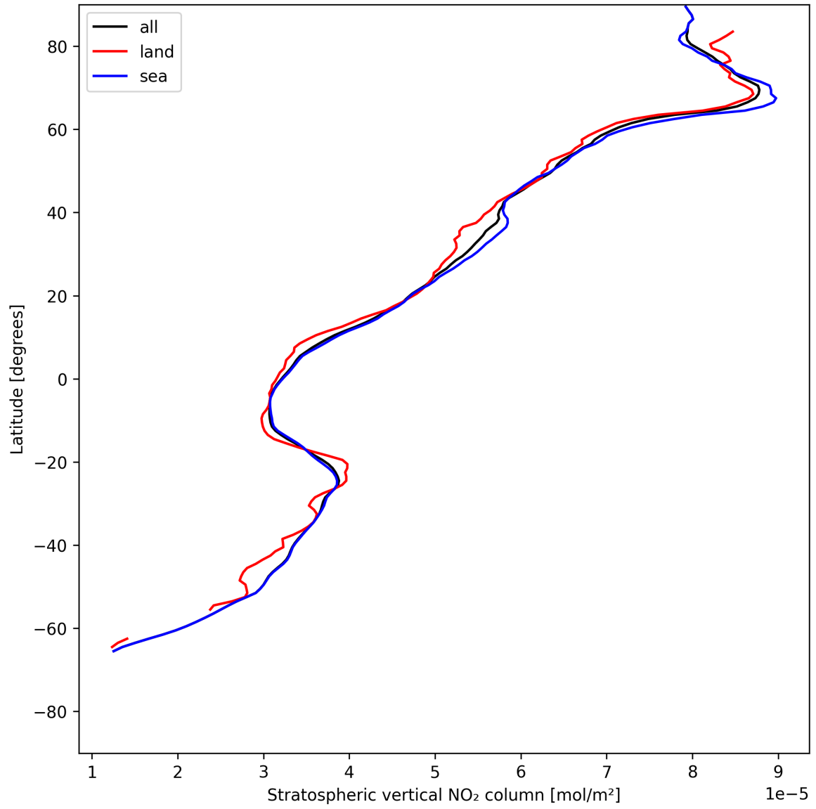
Figure 19: Zonal average of “Stratospheric vertical NO 2 column” for 2025-07-08 to 2025-07-10.
