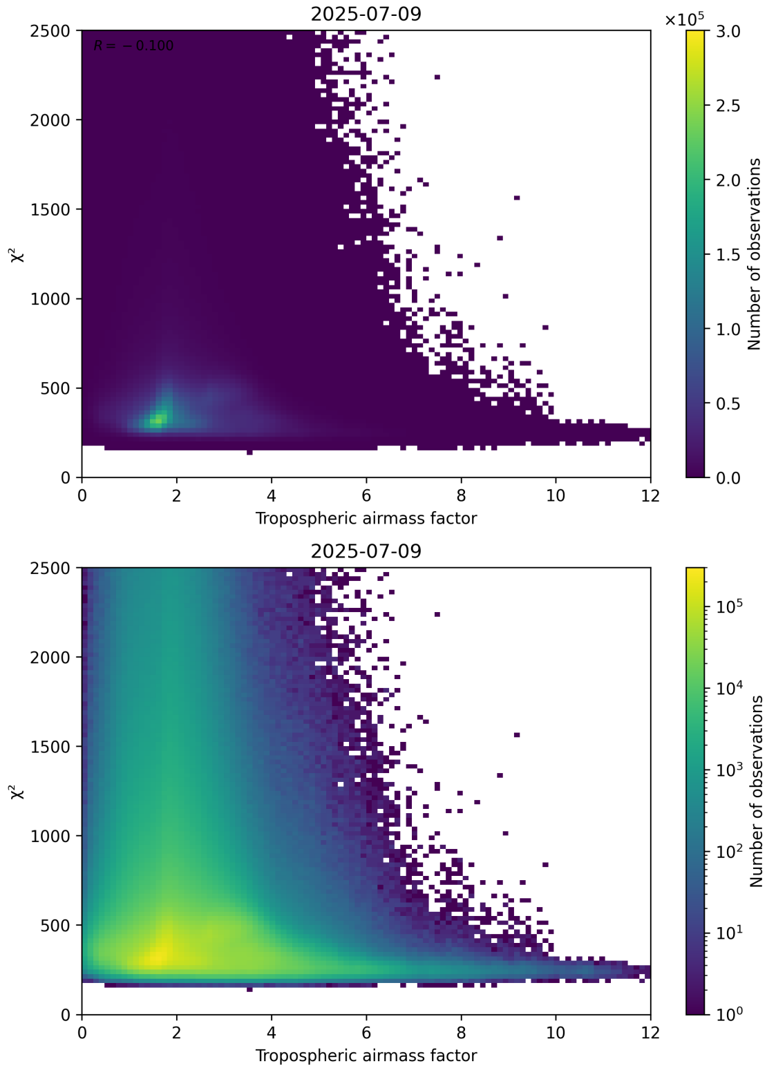
Figure 73: Scatter density plot of “Tropospheric airmass factor” against “ \chi^2 ” for 2025-07-08 to 2025-07-10.
