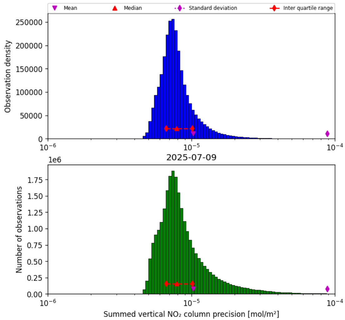
Figure 41: Histogram of “Summed vertical NO 2 column precision” for 2025-07-08 to 2025-07-10
