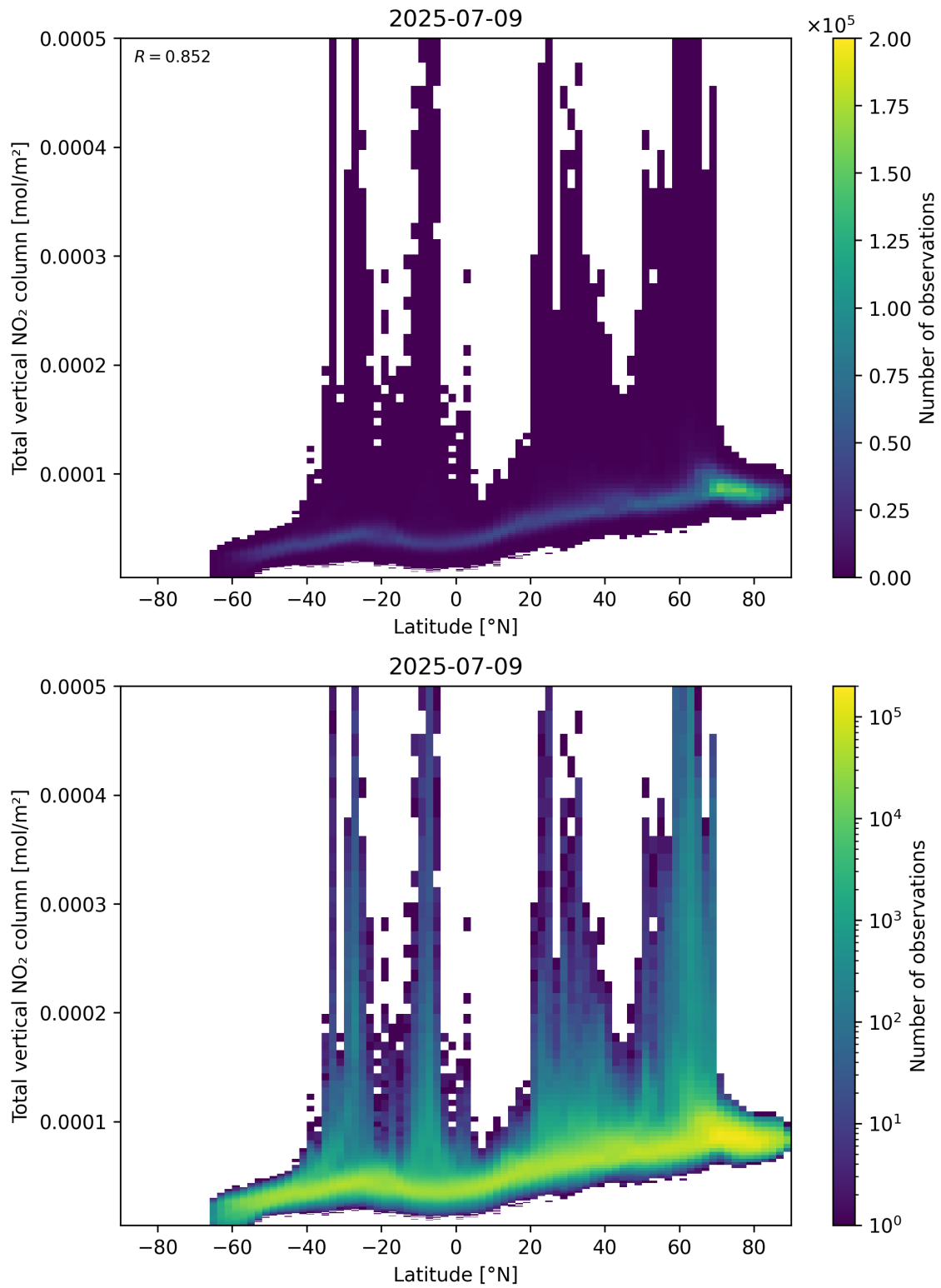
Figure 90: Scatter density plot of “Latitude” against “Total vertical \text{NO}_2 column” for 2025-07-08 to 2025-07-10.
