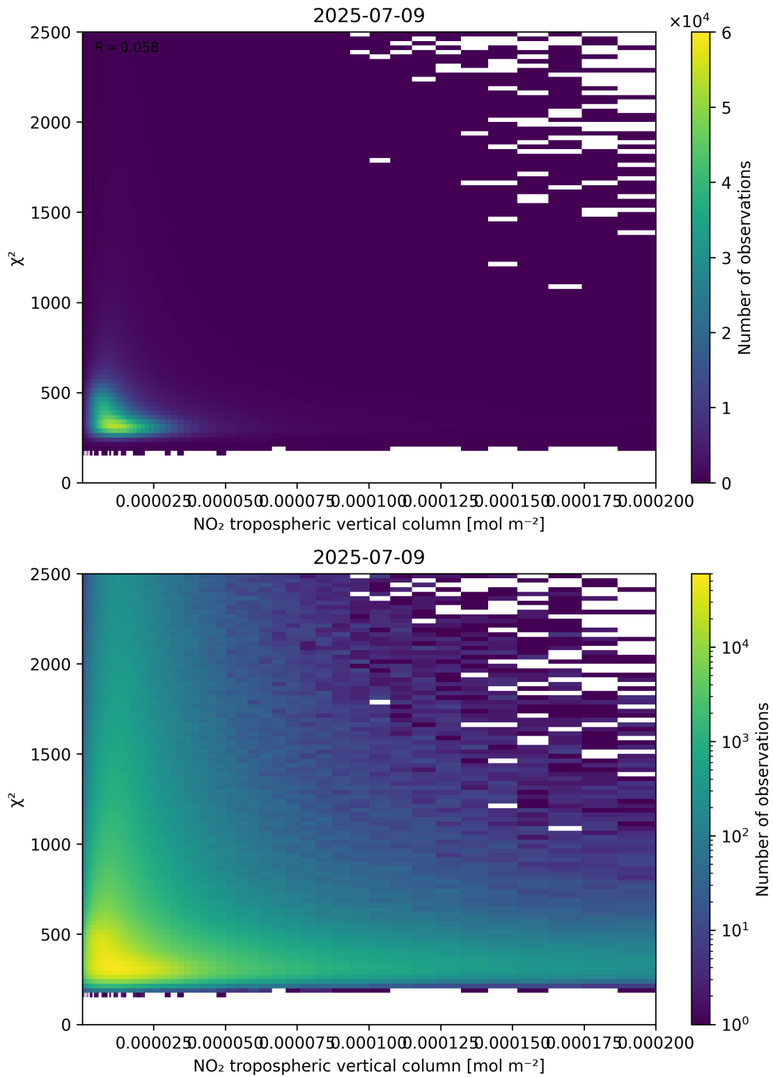
Figure 124: Scatter density plot of “NO 2 tropospheric vertical column” against “ \chi^2 ” for 2025-07-08 to 2025-07-10.
