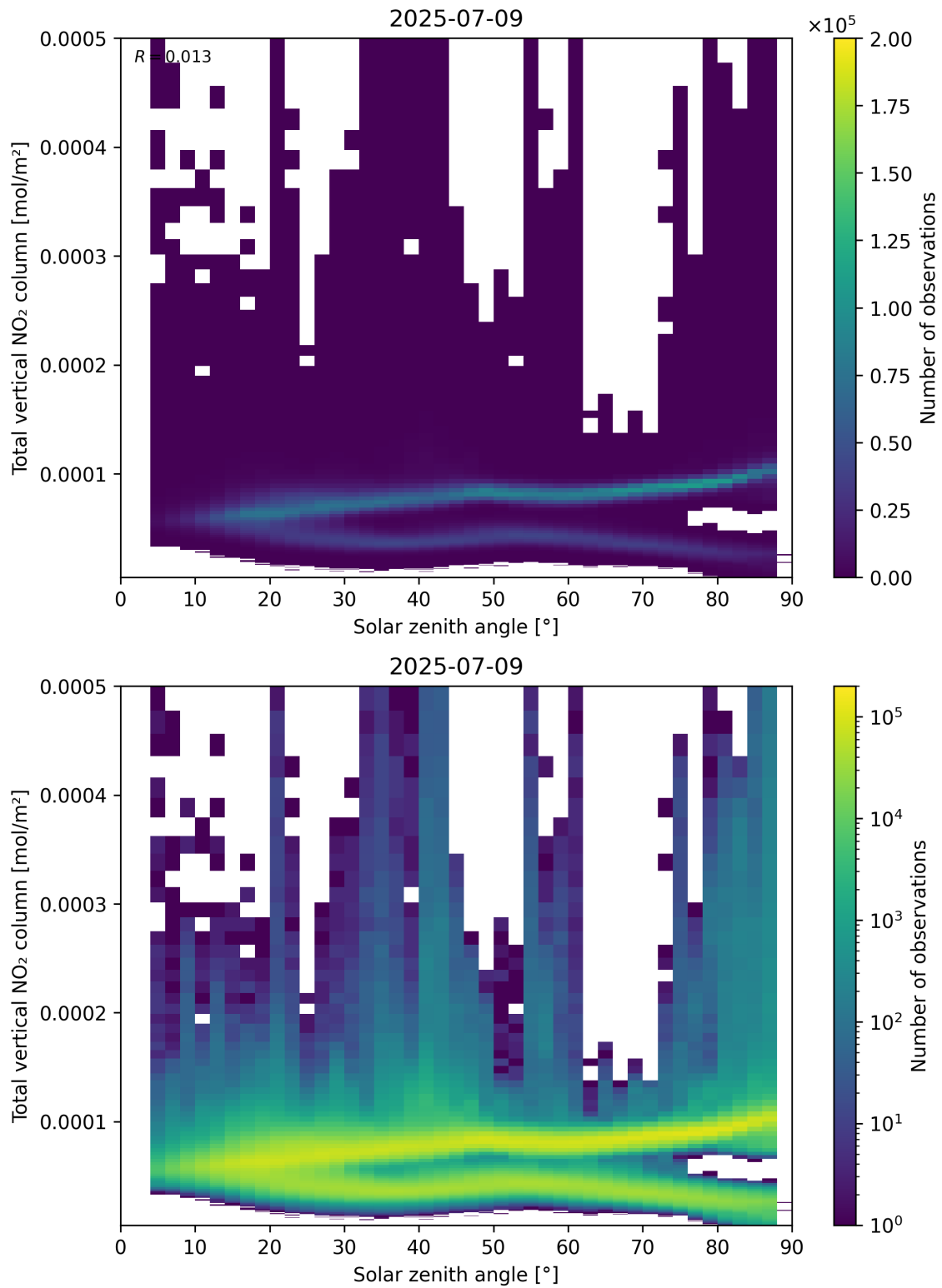
Figure 153: Scatter density plot of “Solar zenith angle” against “Total vertical NO 2 column” for 2025-07-08 to 2025-07-10.
