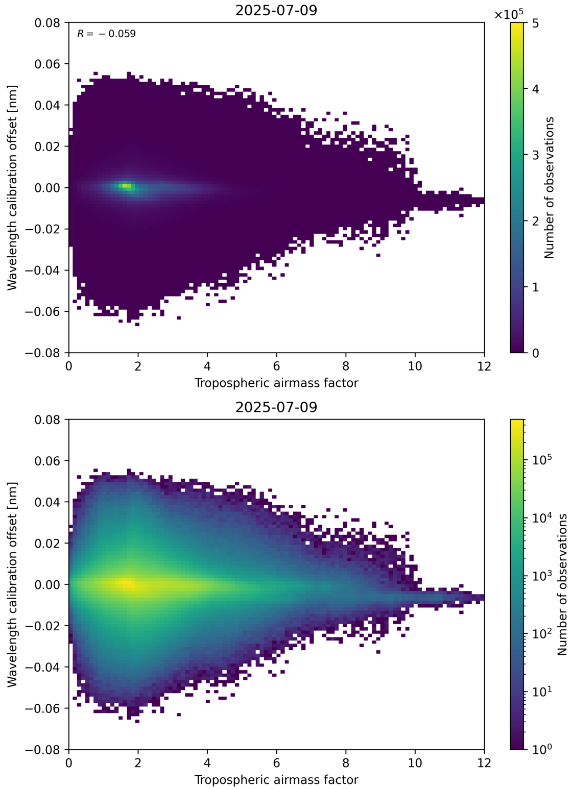
Figure 80: Scatter density plot of “Tropospheric air mass factor” against “Wavelength calibration offset” for 2025-07-08 to 2025-07-10.
