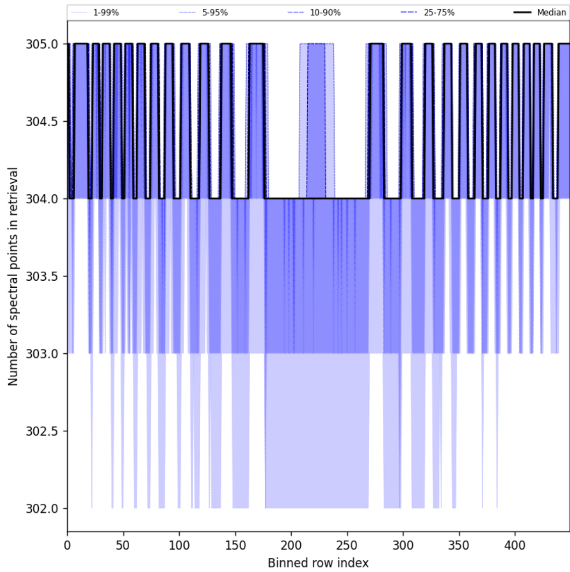
Figure 50: Along track statistics of “Number of spectral points in retrieval” for 2025-07-08 to 2025-07-10
