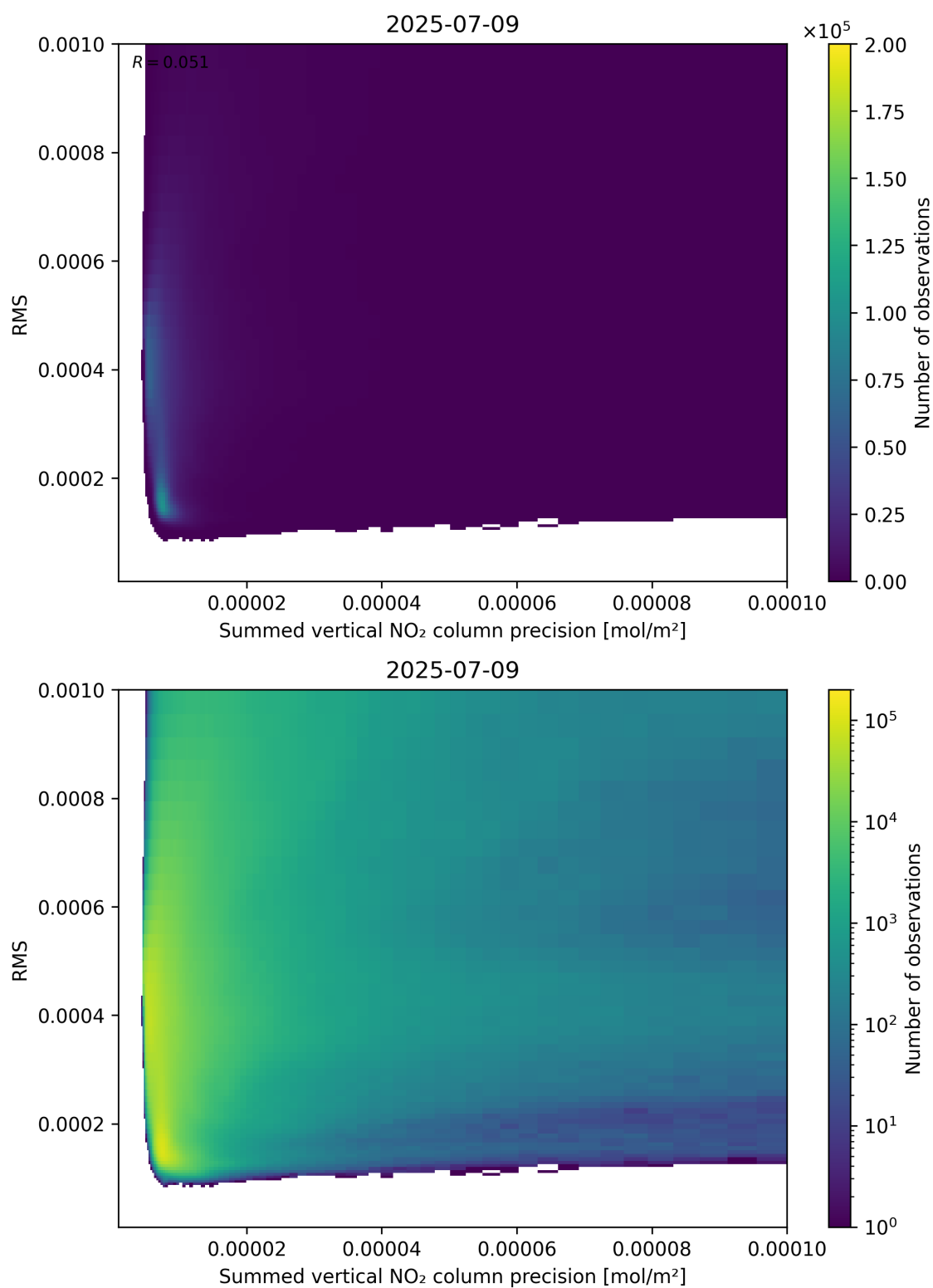
Figure 108: Scatter density plot of “Summed vertical NO 2 column precision” against “RMS” for 2025-07-08 to 2025-07-10.
