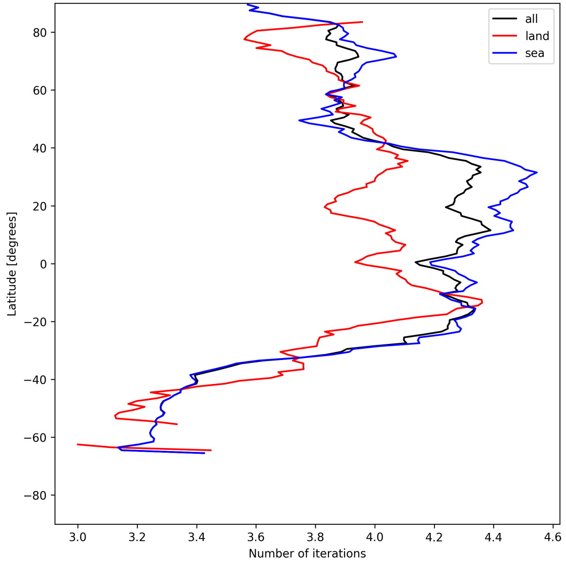
Figure 17: Zonal average of “Number of iterations” for 2025-07-08 to 2025-07-10.
