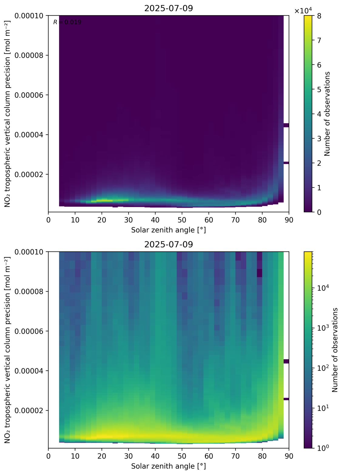
Figure 156: Scatter density plot of “Solar zenith angle” against “NO 2 tropospheric vertical column precision” for 2025-07-08 to 2025-07-10.
