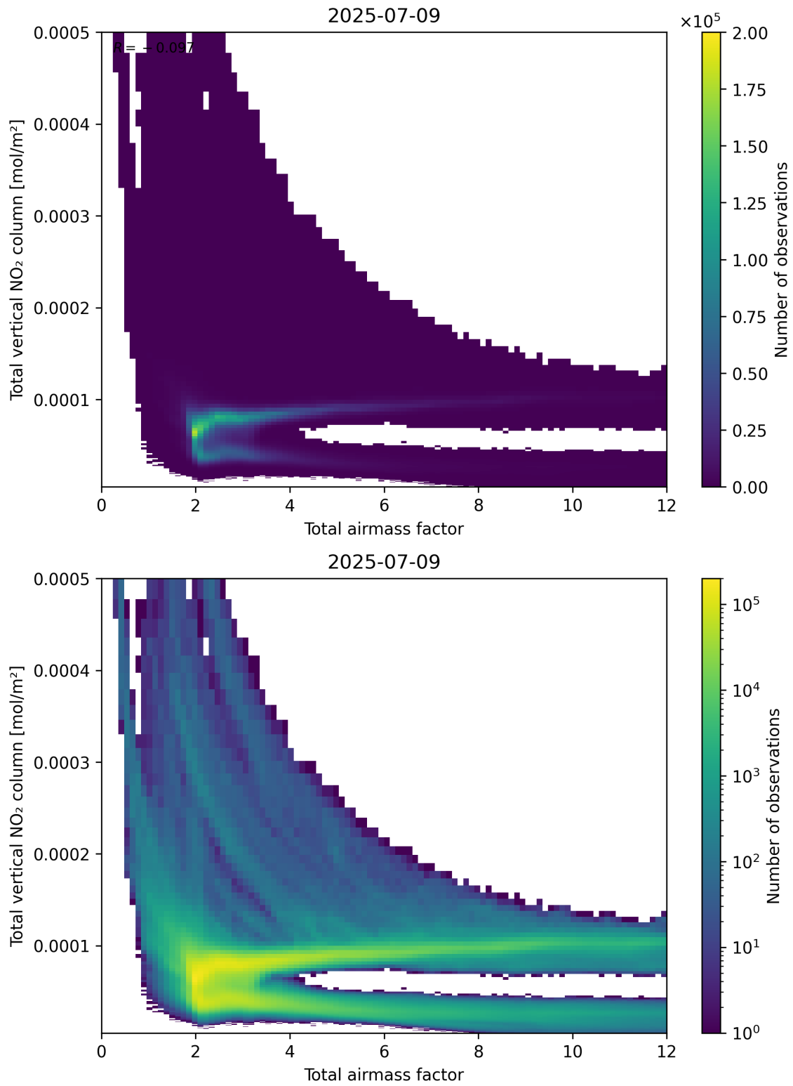
Figure 67: Scatter density plot of “Total airmass factor” against “Total vertical NO 2 column” for 2025-07-08 to 2025-07-10.
