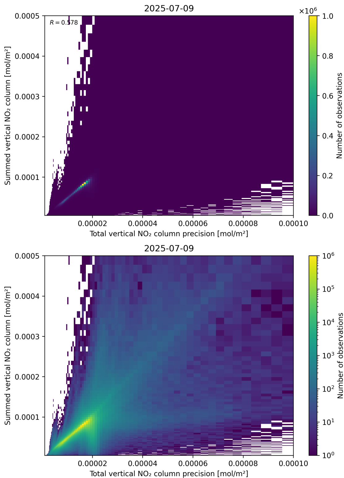
Figure 117: Scatter density plot of “Total vertical NO 2 column precision” against “Summed vertical NO 2 column” for 2025-07-08 to 2025-07-10.
