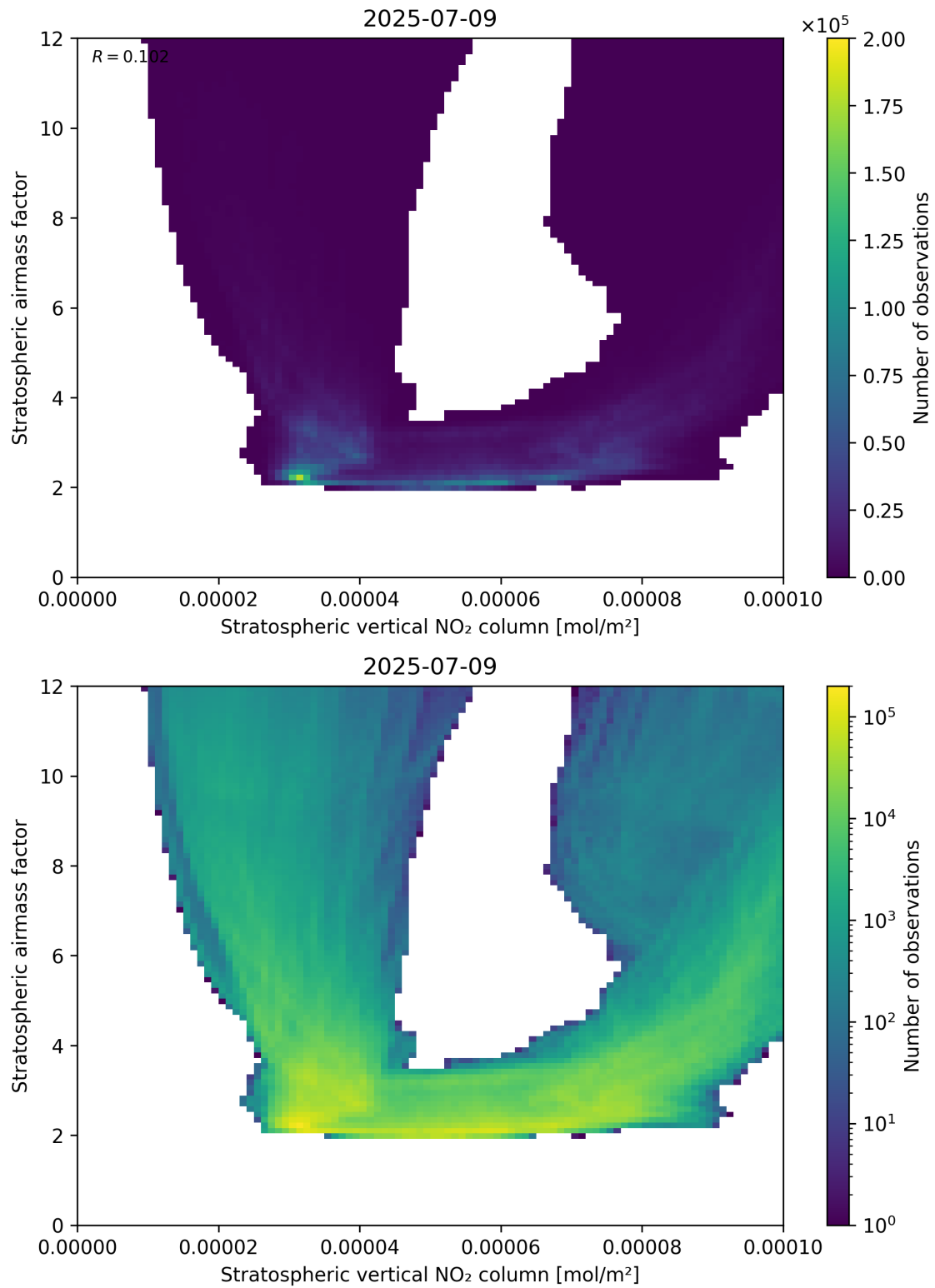
Figure 96: Scatter density plot of “Stratospheric vertical NO 2 column” against “Stratospheric airmass factor” for 2025-07-08 to 2025-07-10.
