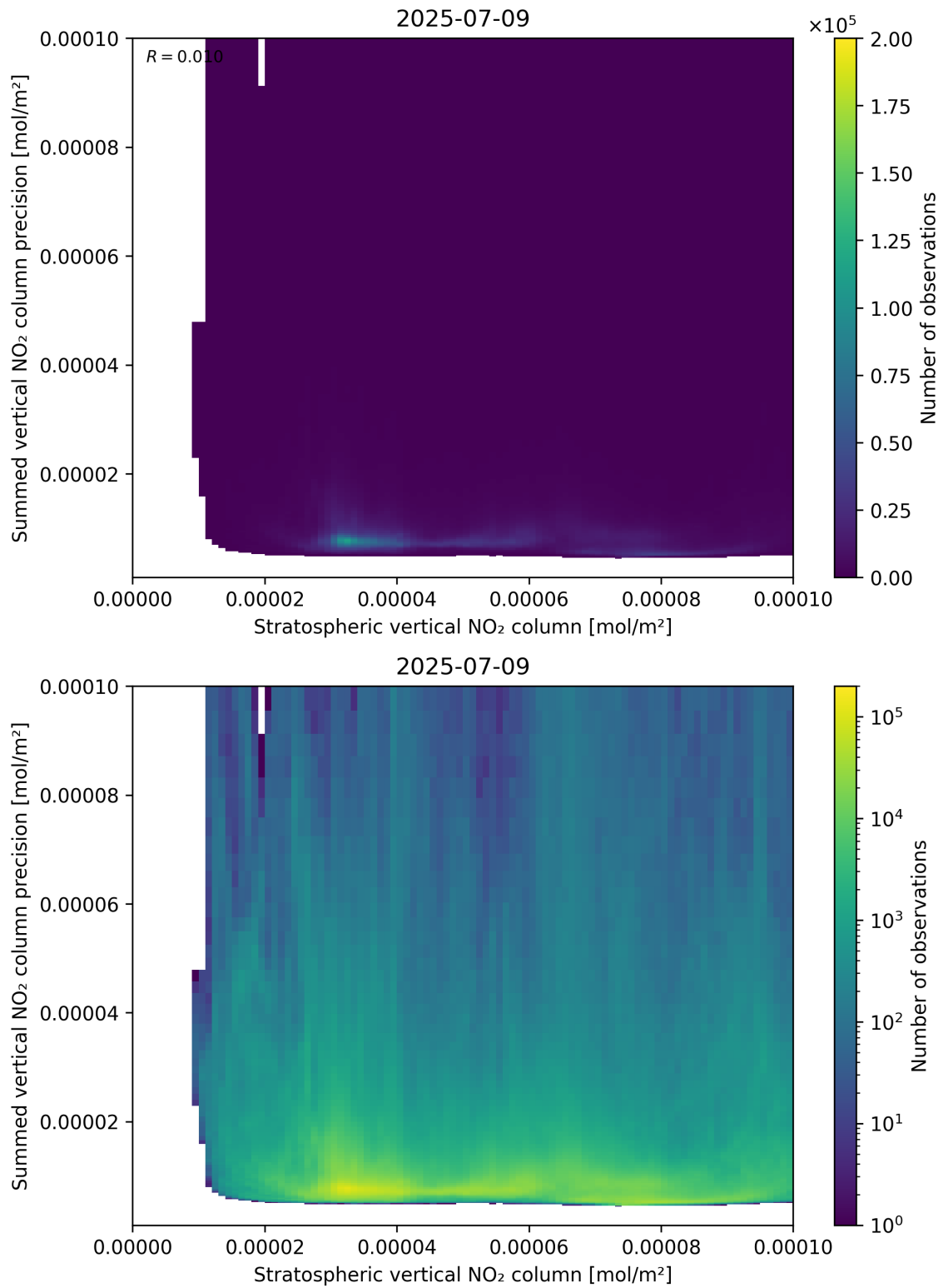
Figure 99: Scatter density plot of “Stratospheric vertical NO 2 column” against “Summed vertical NO 2 column precision” for 2025-07-08 to 2025-07-10.
