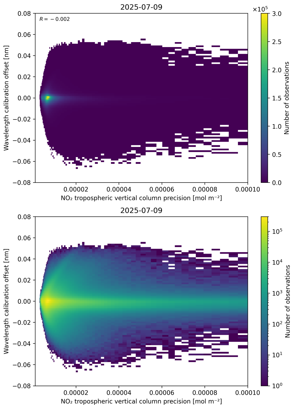
Figure 141: Scatter density plot of “NO 2 tropospheric vertical column precision” against “Wavelength calibration offset” for 2025-07-08 to 2025-07-10.
