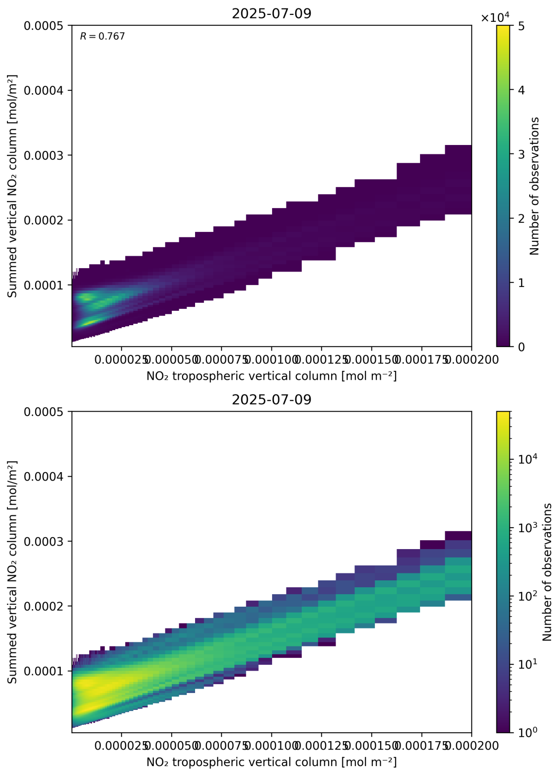
Figure 126: Scatter density plot of “NO 2 tropospheric vertical column” against “Summed vertical NO 2 column” for 2025-07-08 to 2025-07-10.
