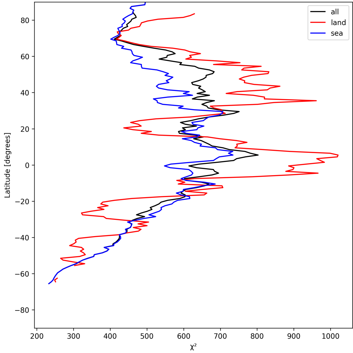
Figure 25: Zonal average of " \chi^2 " for 2025-07-08 to 2025-07-10.
