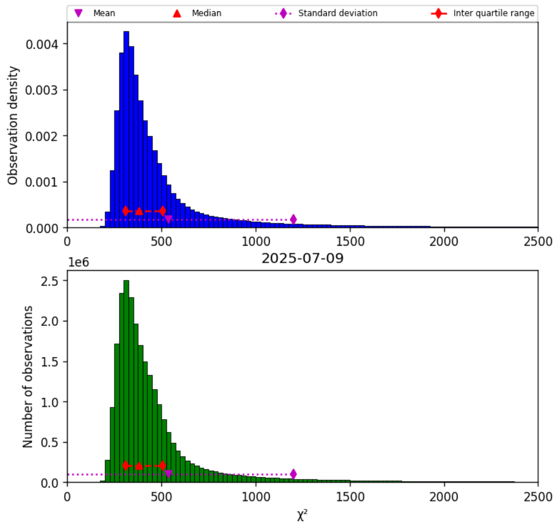
Figure 42: Histogram of “ \chi^2 ” for 2025-07-08 to 2025-07-10
