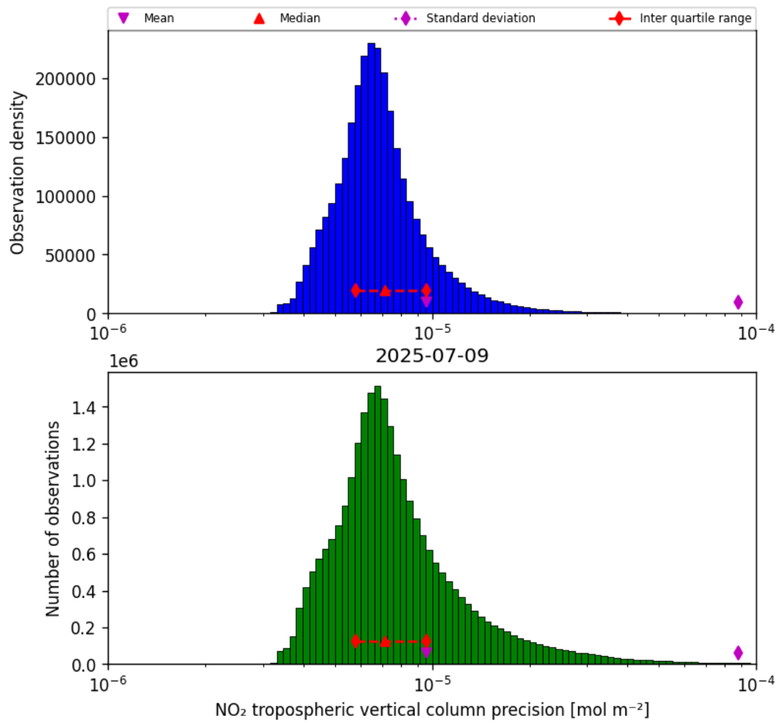
Figure 30: Histogram of “NO 2 tropospheric vertical column precision” for 2025-07-08 to 2025-07-10
