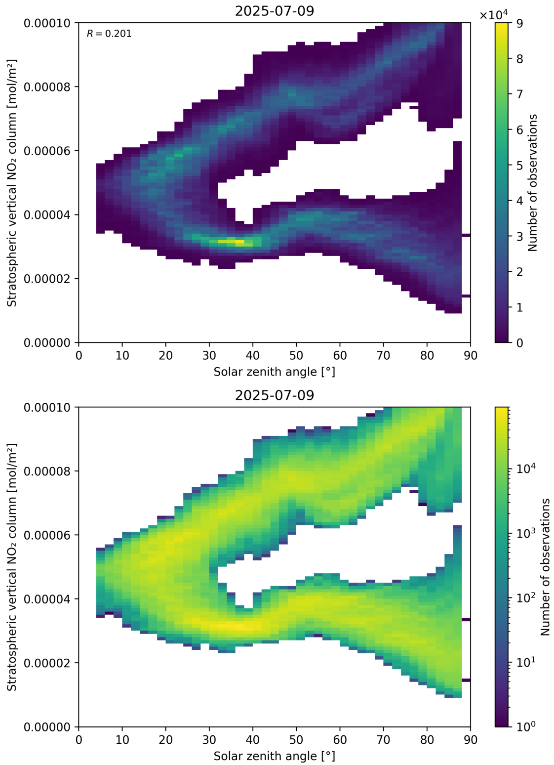
Figure 150: Scatter density plot of “Solar zenith angle” against “Stratospheric vertical NO 2 column” for 2025-07-08 to 2025-07-10.
