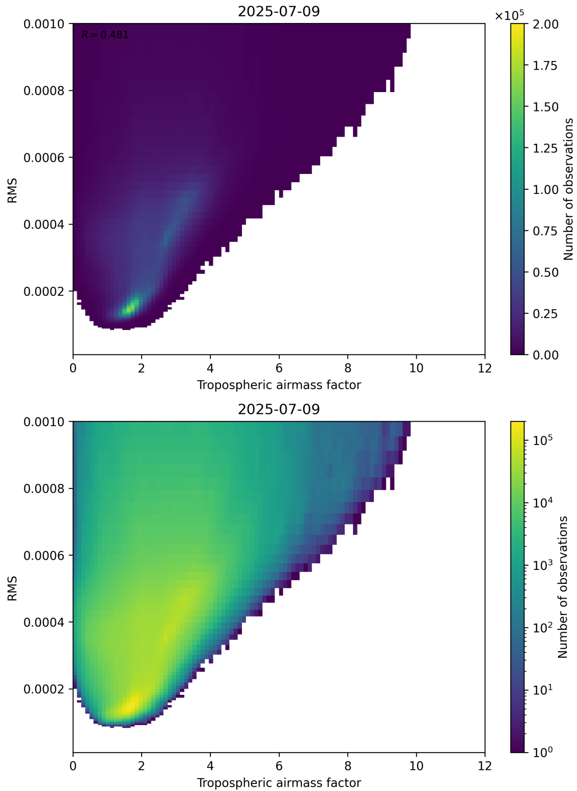
Figure 79: Scatter density plot of “Tropospheric airmass factor” against “RMS” for 2025-07-08 to 2025-07-10.
