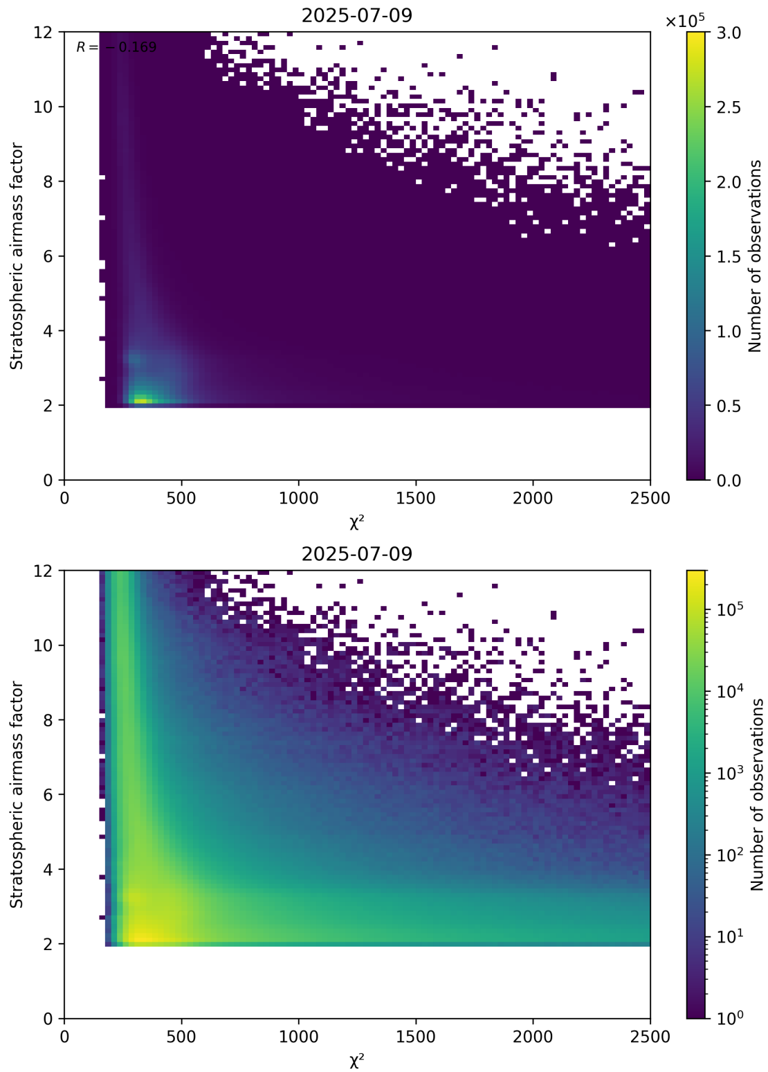
Figure 81: Scatter density plot of “ \chi^2 ” against “Stratospheric airmass factor” for 2025-07-08 to 2025-07-10.
