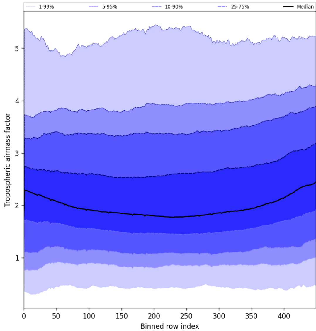
Figure 48: Along track statistics of “Tropospheric airmass factor” for 2025-07-08 to 2025-07-10
