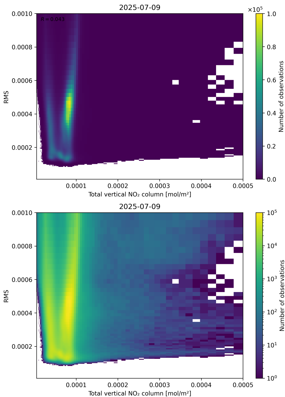
Figure 120: Scatter density plot of “Total vertical NO 2 column” against “RMS” for 2025-07-08 to 2025-07-10.
