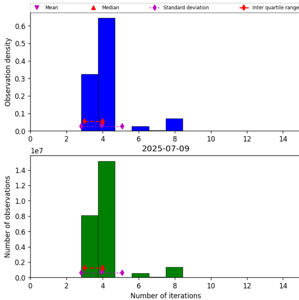
Figure 34: Histogram of “Number of iterations” for 2025-07-08 to 2025-07-10
