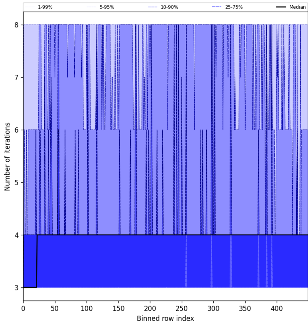
Figure 51: Along track statistics of “Number of iterations” for 2025-07-08 to 2025-07-10
