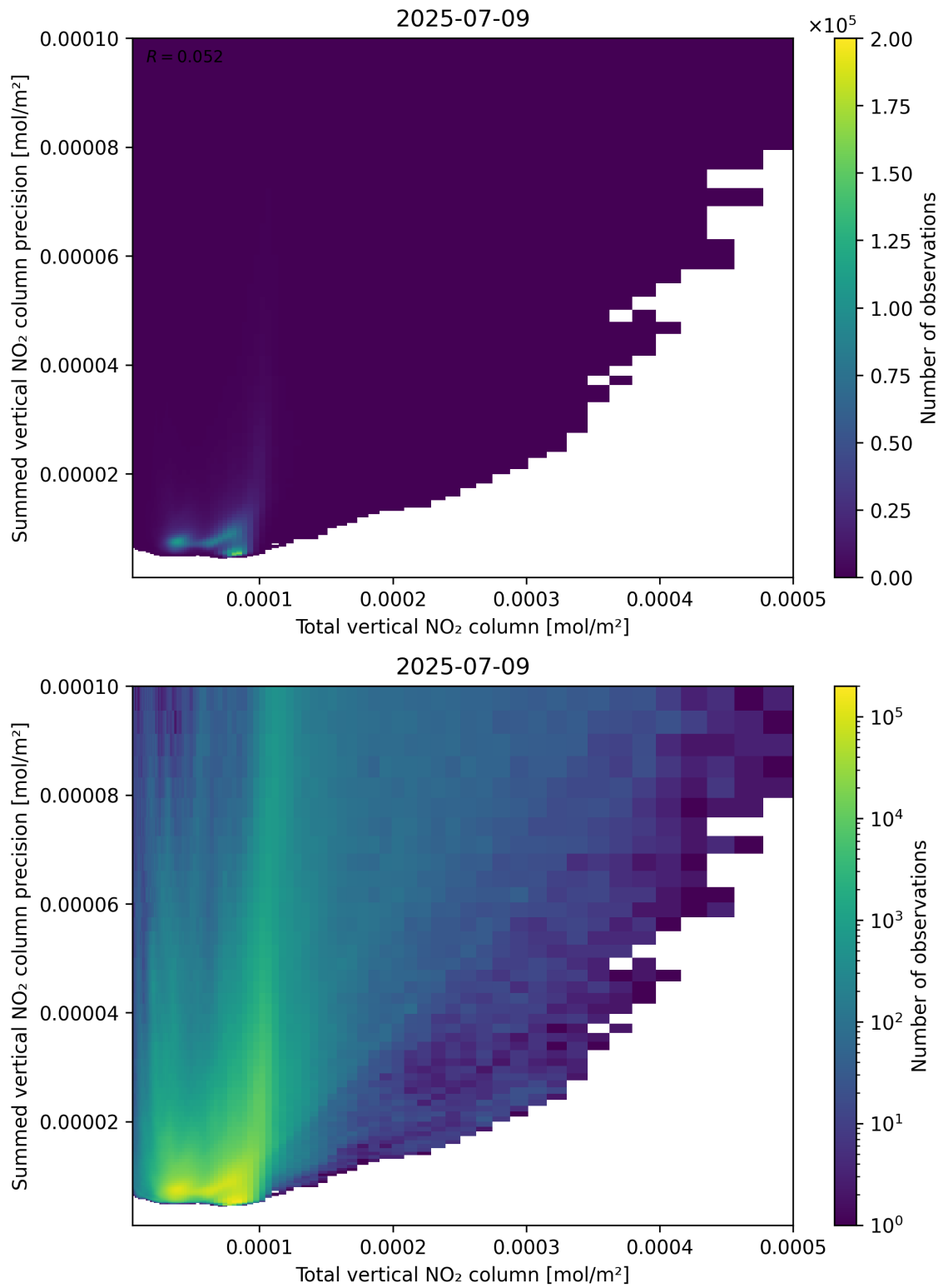
Figure 113: Scatter density plot of “Total vertical NO 2 column” against “Summed vertical NO 2 column precision” for 2025-07-08 to 2025-07-10.
