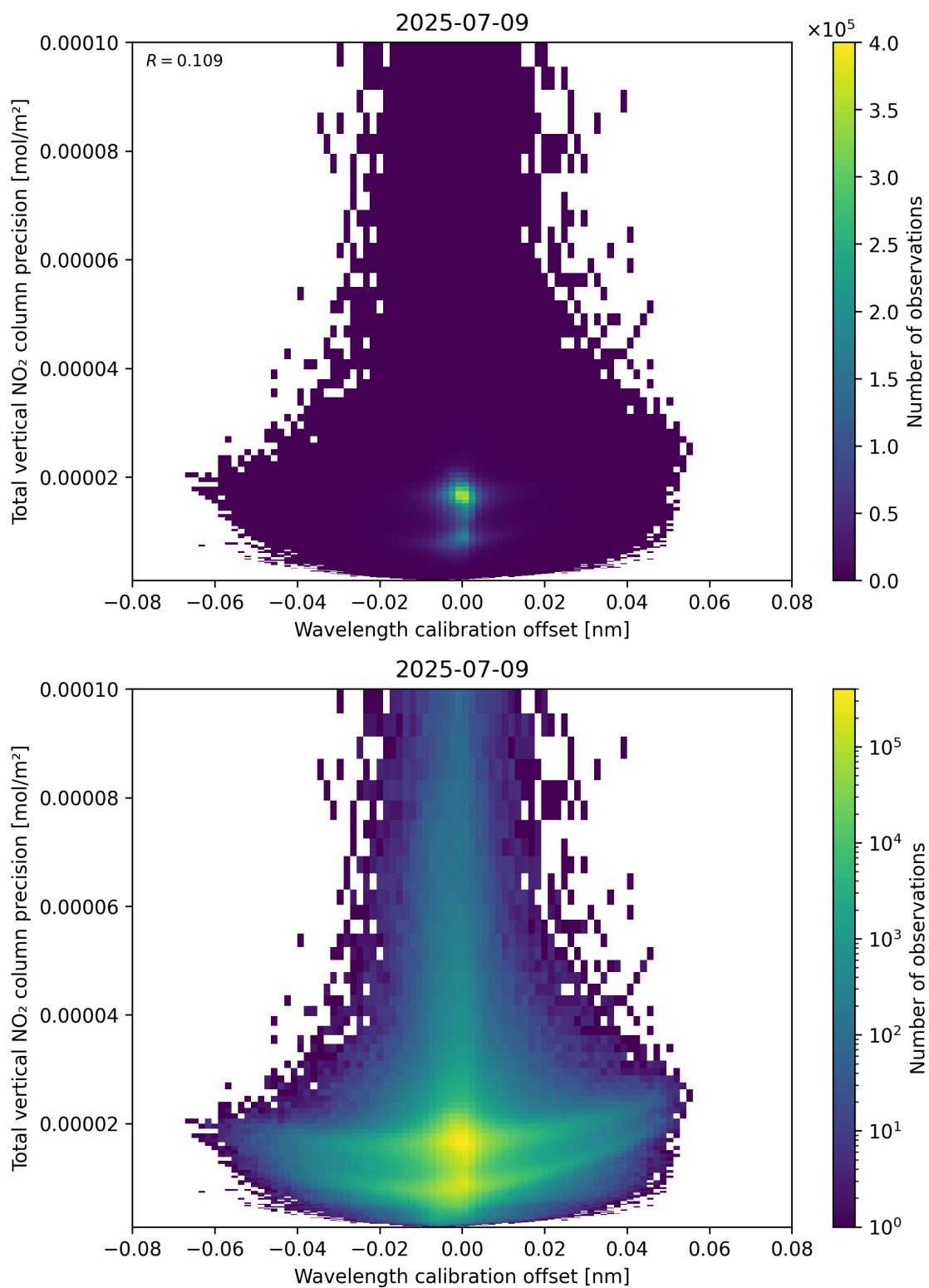
Figure 180: Scatter density plot of “Wavelength calibration offset” against “Total vertical NO 2 column precision” for 2025-07-08 to 2025-07-10.
