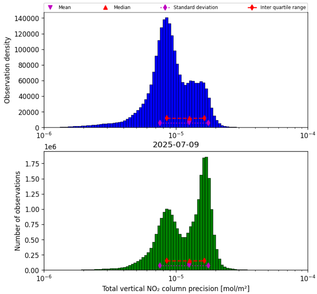
Figure 39: Histogram of “Total vertical NO 2 column precision” for 2025-07-08 to 2025-07-10
