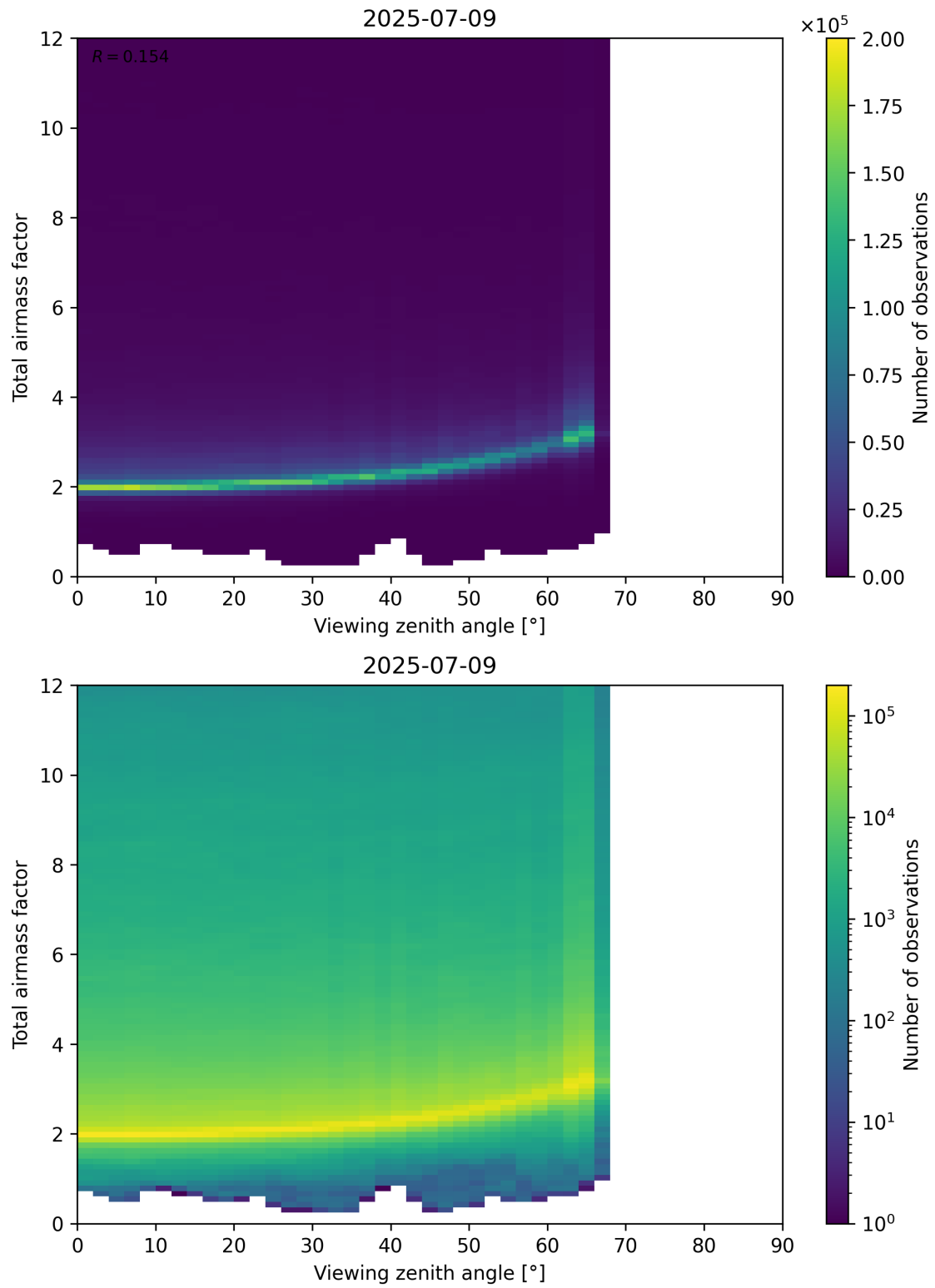
Figure 160: Scatter density plot of “Viewing zenith angle” against “Total airmass factor” for 2025-07-08 to 2025-07-10.
