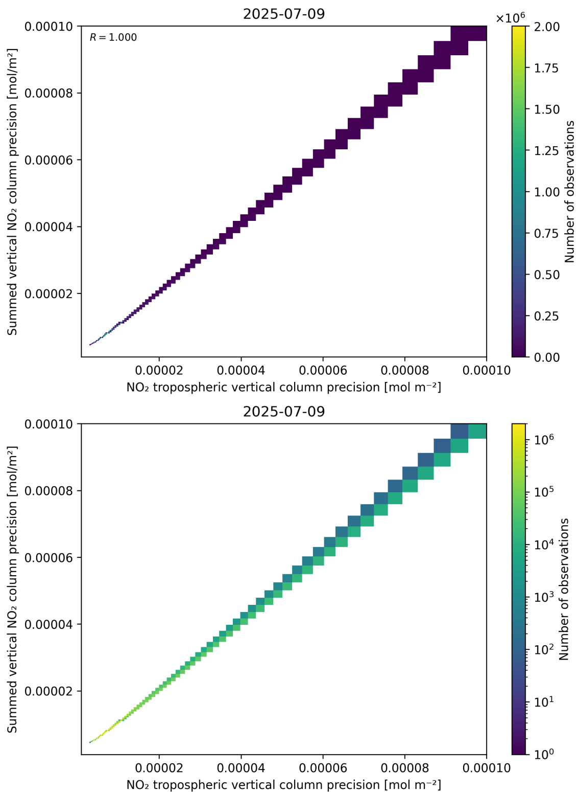
Figure 137: Scatter density plot of “NO 2 tropospheric vertical column precision” against “Summed vertical NO 2 column precision” for 2025-07-08 to 2025-07-10.
