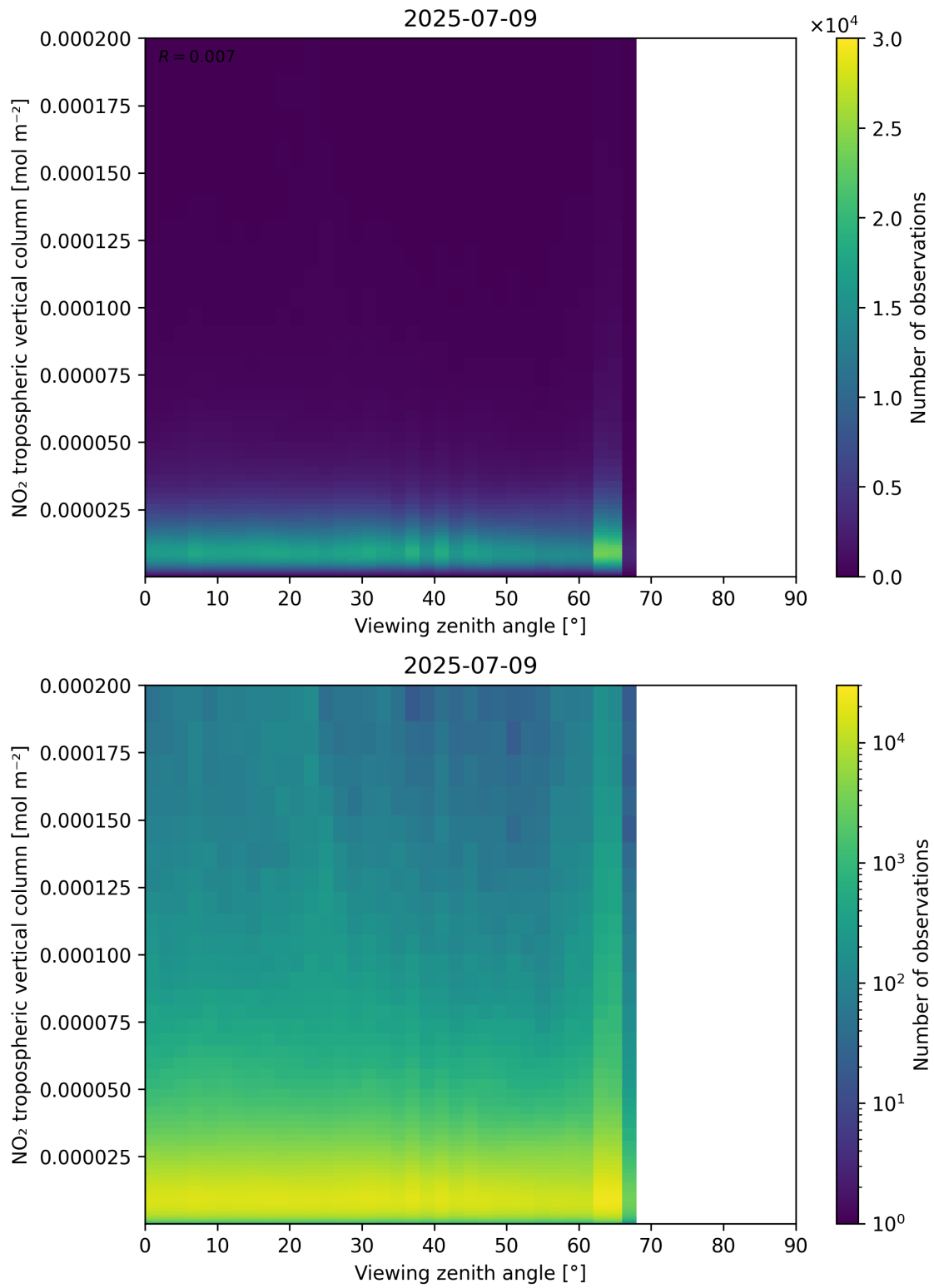
Figure 169: Scatter density plot of “Viewing zenith angle” against “NO 2 tropospheric vertical column” for 2025-07-08 to 2025-07-10.
