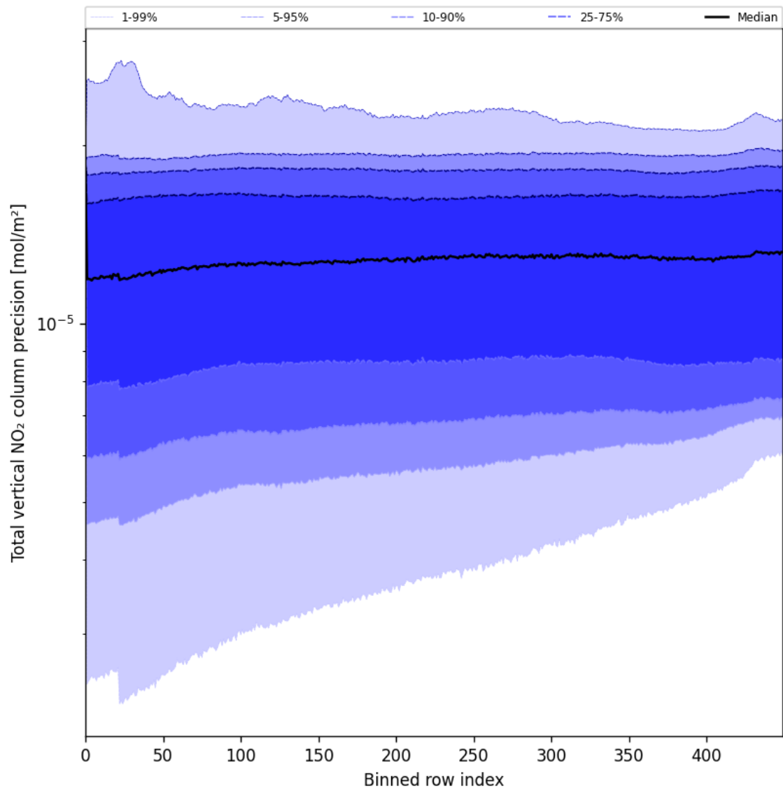
Figure 56: Along track statistics of “Total vertical NO 2 column precision” for 2025-07-08 to 2025-07-10
