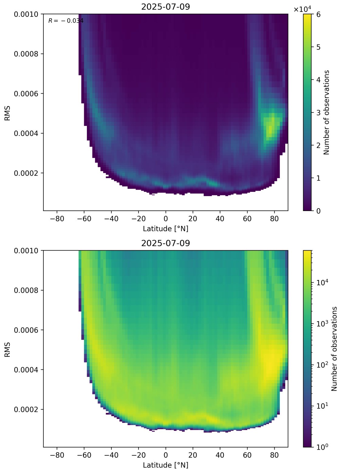
Figure 94: Scatter density plot of “Latitude” against “RMS” for 2025-07-08 to 2025-07-10.
