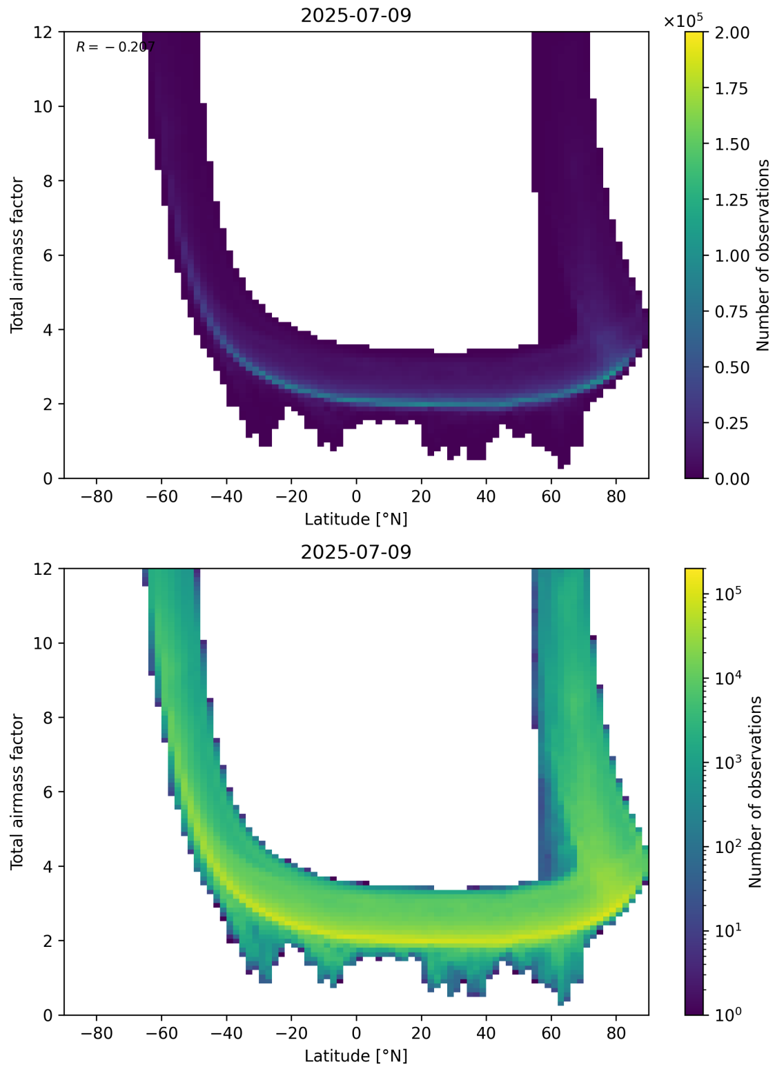
Figure 84: Scatter density plot of “Latitude” against “Total airmass factor” for 2025-07-08 to 2025-07-10.
