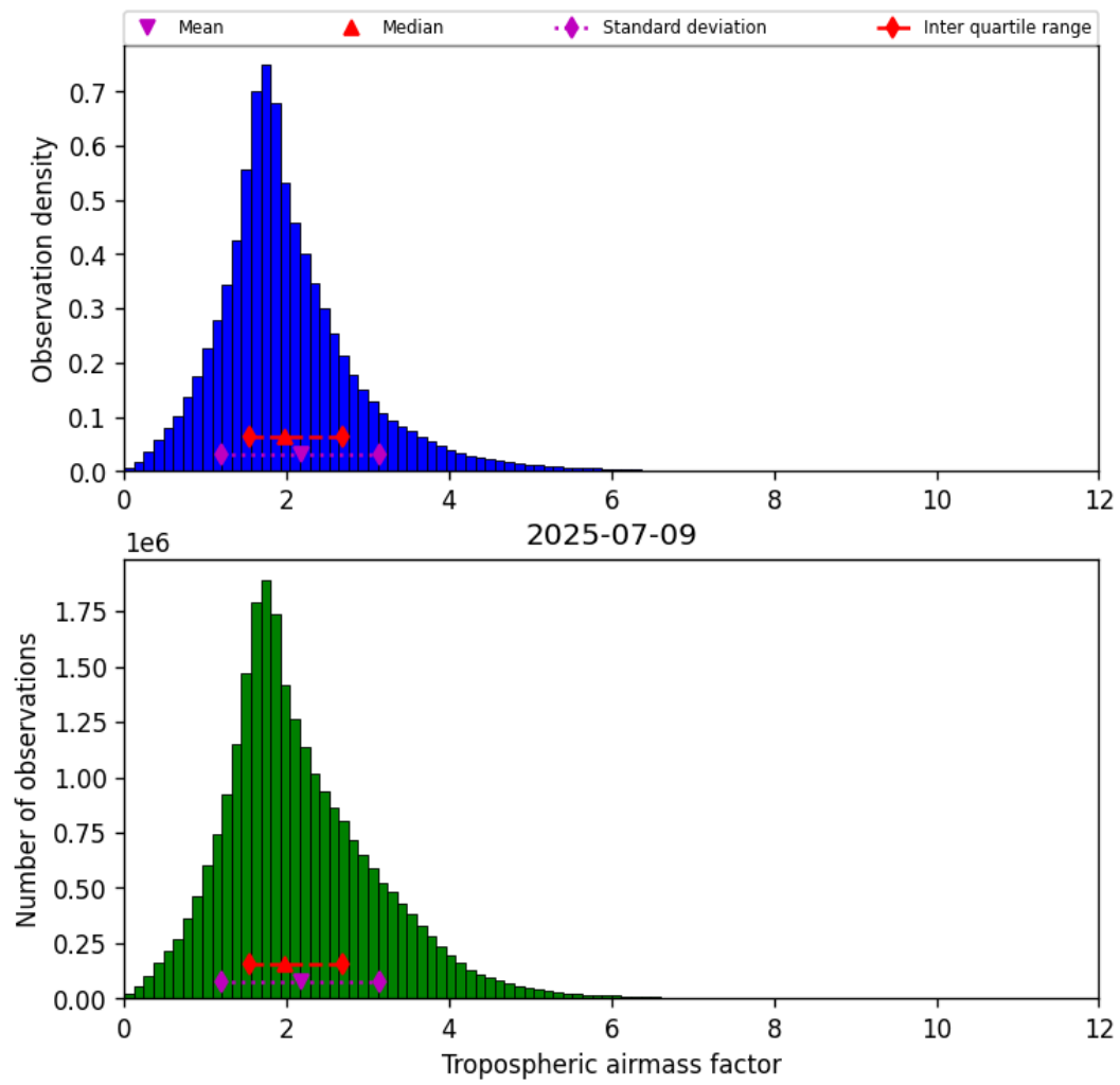
Figure 31: Histogram of “Tropospheric airmass factor” for 2025-07-08 to 2025-07-10
