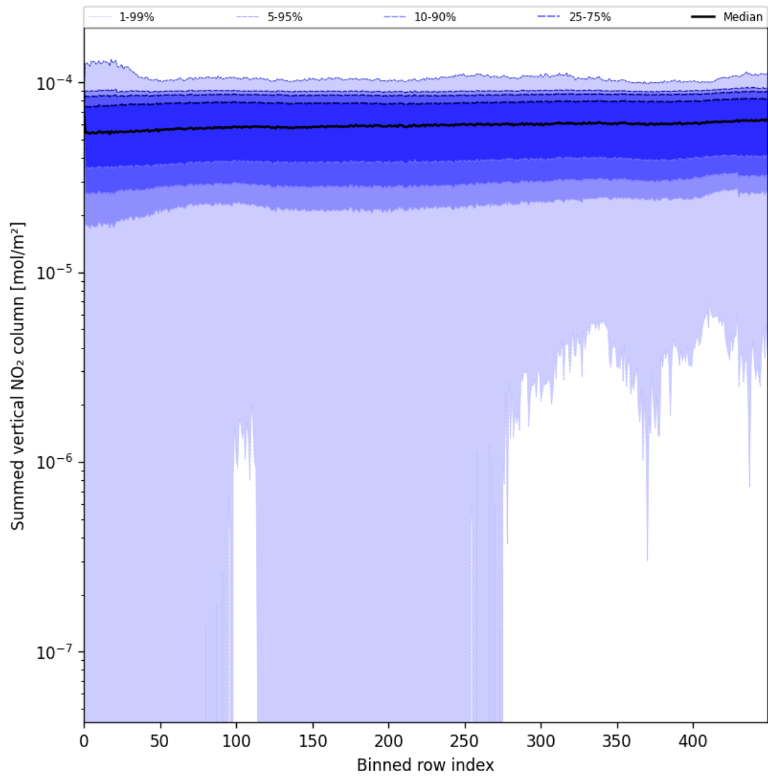
Figure 57: Along track statistics of “Summed vertical NO 2 column” for 2025-07-08 to 2025-07-10
