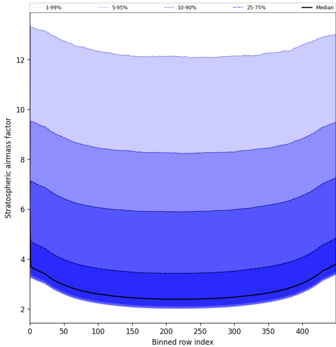
Figure 61: Along track statistics of “Stratospheric airmass factor” for 2025-07-08 to 2025-07-10
