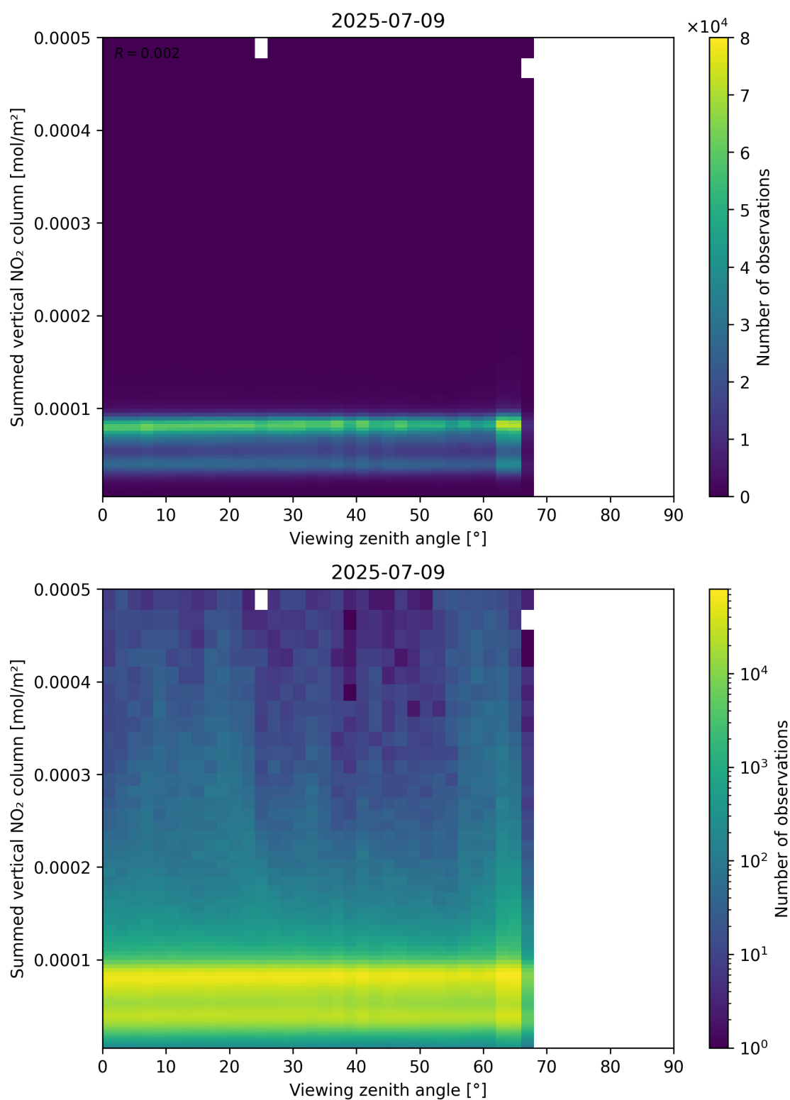
Figure 165: Scatter density plot of “Viewing zenith angle” against “Summed vertical NO 2 column” for 2025-07-08 to 2025-07-10.
