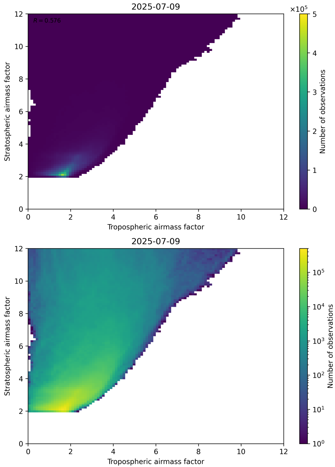
Figure 71: Scatter density plot of “Tropospheric airmass factor” against “Stratospheric airmass factor” for 2025-07-08 to 2025-07-10.
