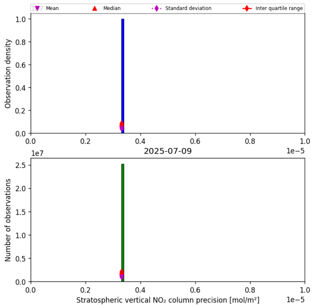
Figure 37: Histogram of “Stratospheric vertical NO 2 column precision” for 2025-07-08 to 2025-07-10
