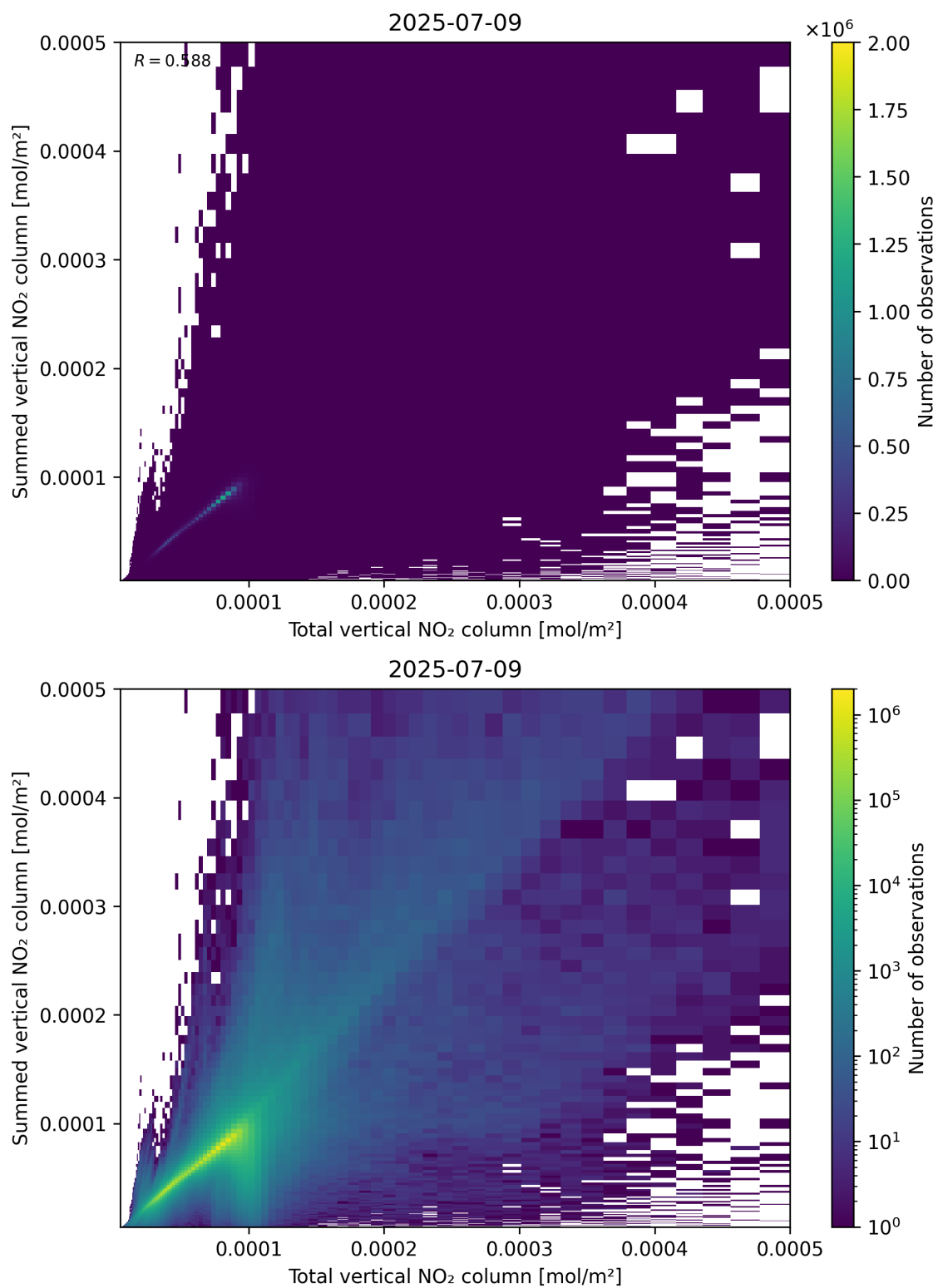
Figure 112: Scatter density plot of “Total vertical NO 2 column” against “Summed vertical NO 2 column” for 2025-07-08 to 2025-07-10.
