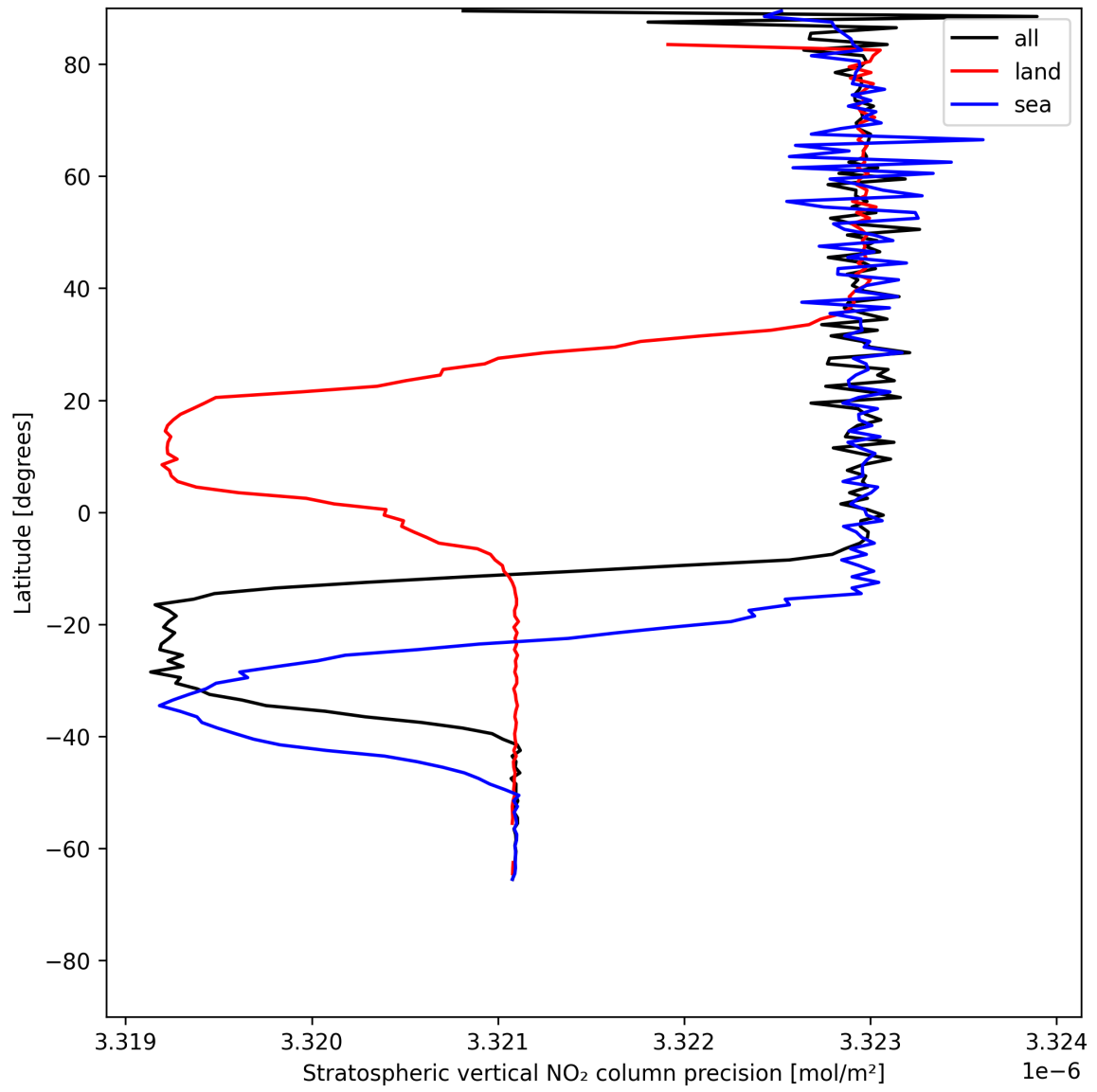
Figure 20: Zonal average of “Stratospheric vertical NO 2 column precision” for 2025-07-08 to 2025-07-10.
