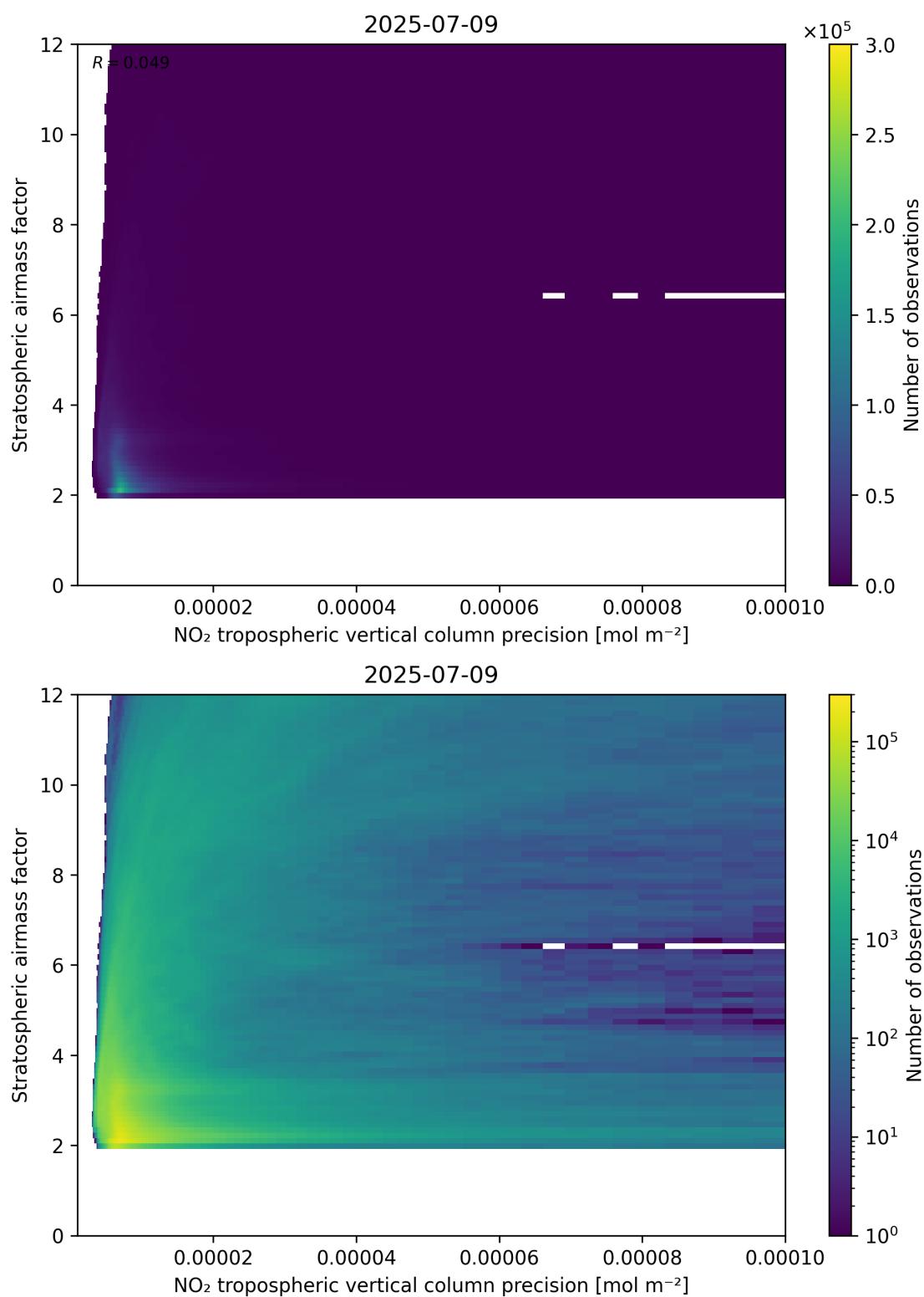
Figure 131: Scatter density plot of “NO 2 tropospheric vertical column precision” against “Stratospheric airmass factor” for 2025-07-08 to 2025-07-10.
