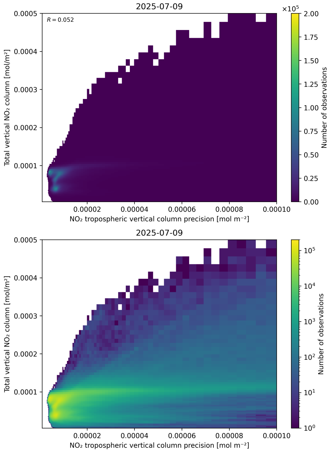
Figure 138: Scatter density plot of “NO 2 tropospheric vertical column precision” against “Total vertical NO 2 column” for 2025-07-08 to 2025-07-10.
