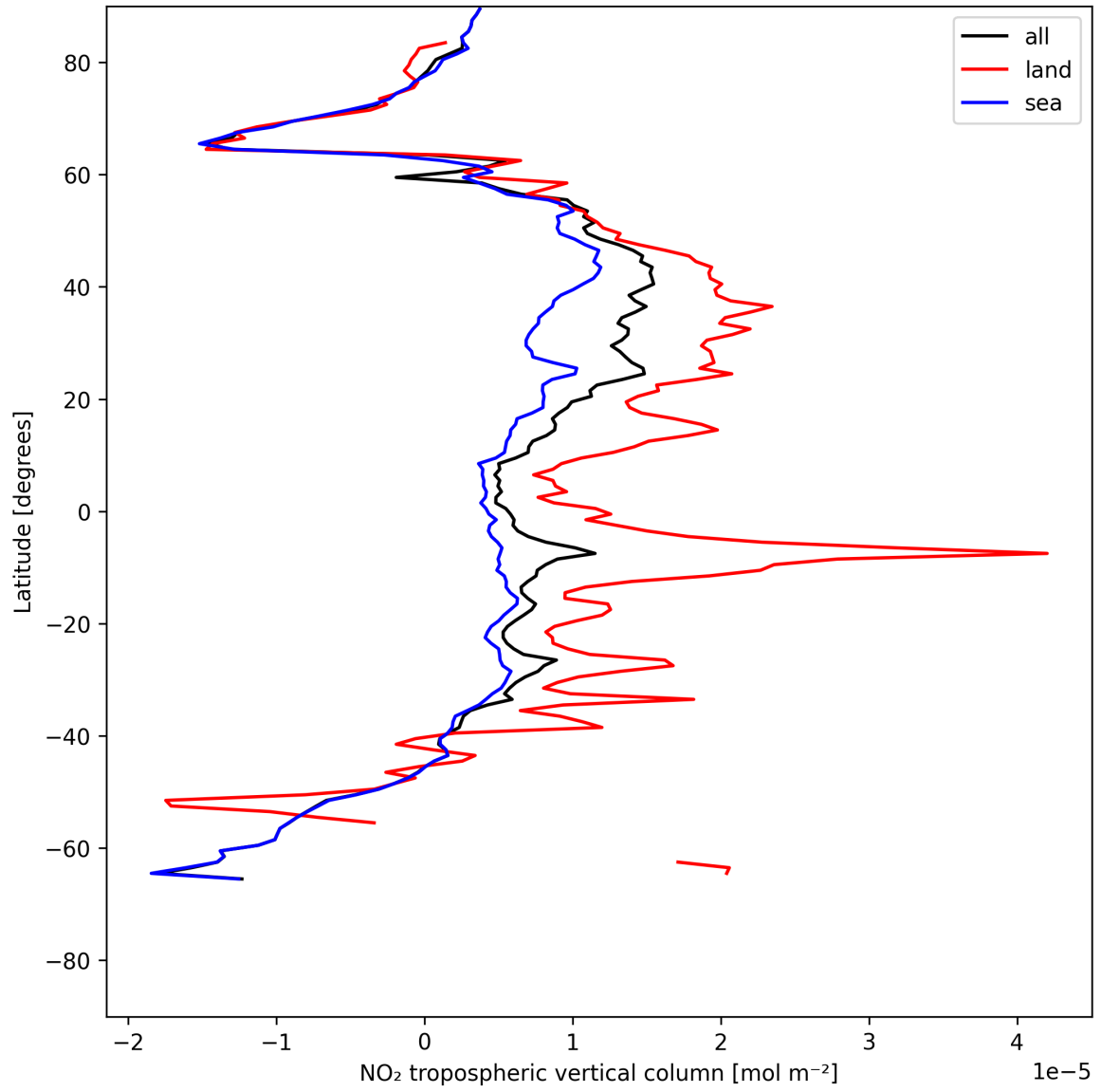
Figure 12: Zonal average of “NO 2 tropospheric vertical column” for 2025-07-08 to 2025-07-10.
