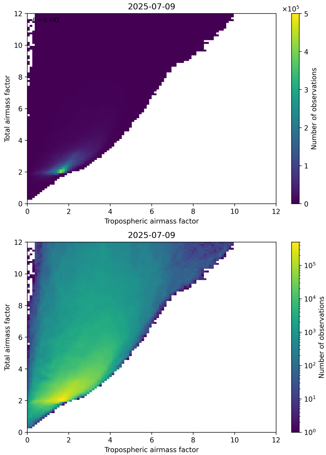
Figure 72: Scatter density plot of “Tropospheric airmass factor” against “Total airmass factor” for 2025-07-08 to 2025-07-10.
