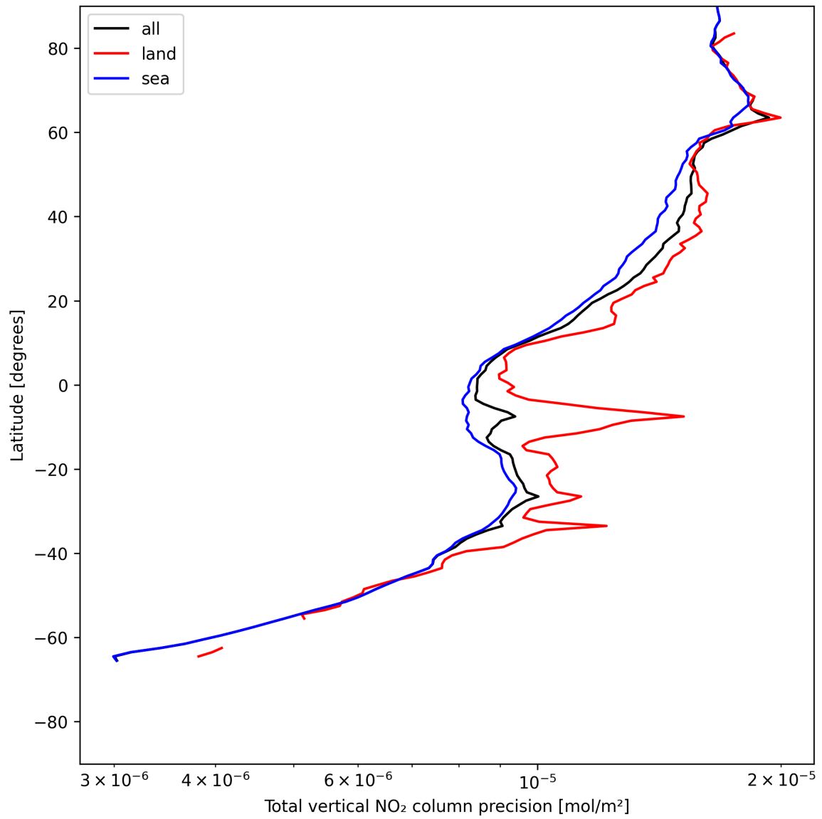
Figure 22: Zonal average of “Total vertical NO 2 column precision” for 2025-07-08 to 2025-07-10.
