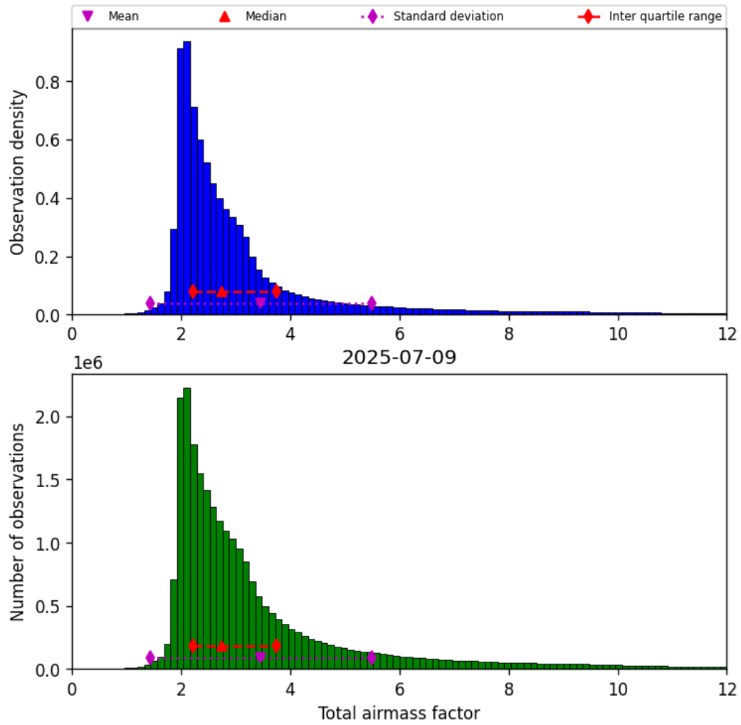
Figure 32: Histogram of “Total airmass factor” for 2025-07-08 to 2025-07-10
