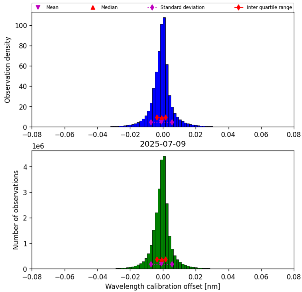
Figure 35: Histogram of “Wavelength calibration offset” for 2025-07-08 to 2025-07-10
