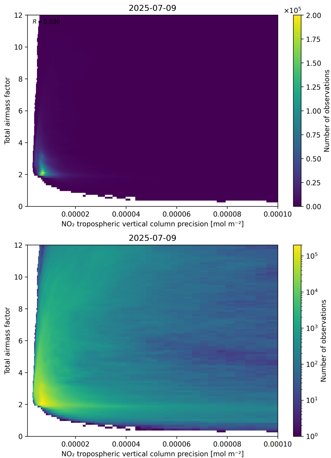
Figure 132: Scatter density plot of “NO 2 tropospheric vertical column precision” against “Total air mass factor” for 2025-07-08 to 2025-07-10.
