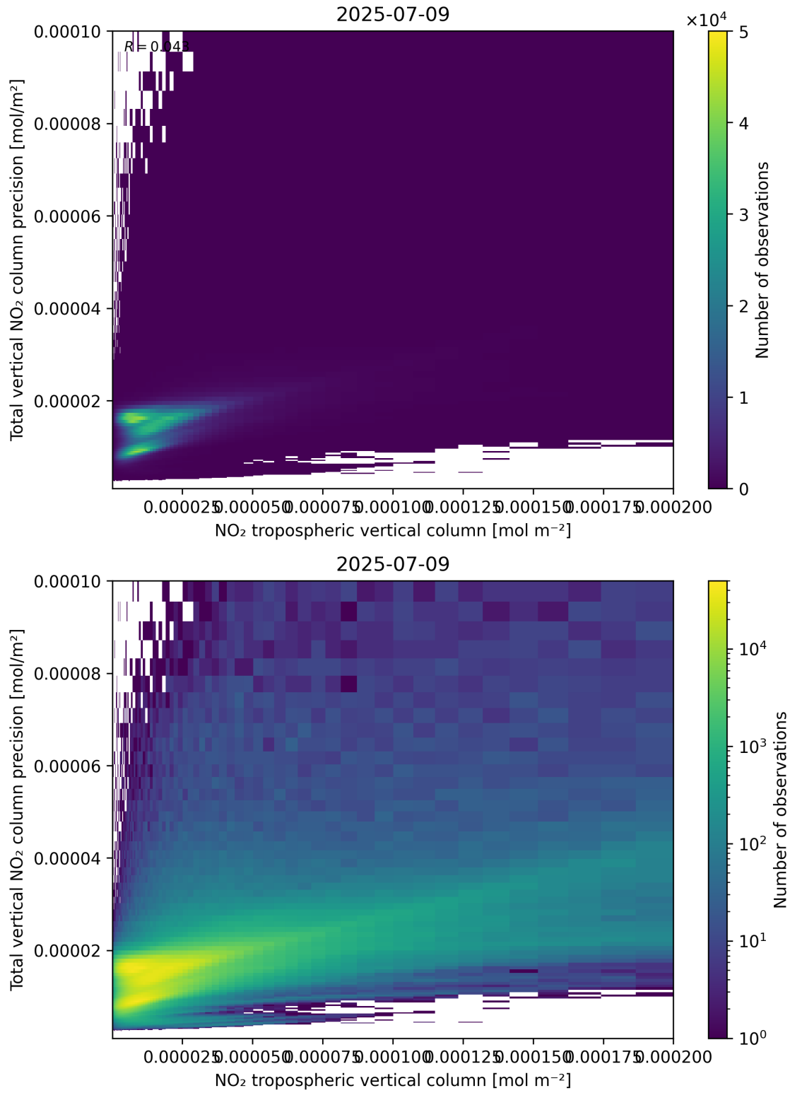
Figure 129: Scatter density plot of “NO 2 tropospheric vertical column” against “Total vertical NO 2 column precision” for 2025-07-08 to 2025-07-10.
