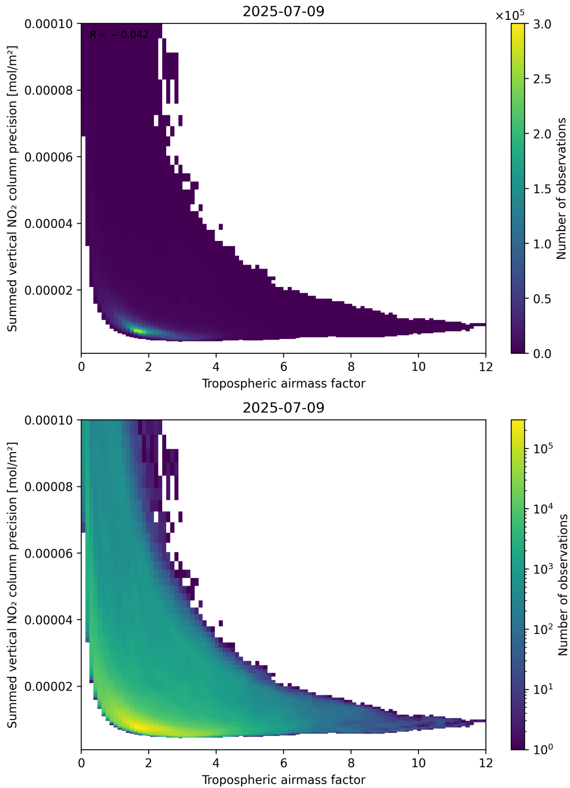
Figure 76: Scatter density plot of “Tropospheric air mass factor” against “Summed vertical NO 2 column precision” for 2025-07-08 to 2025-07-10.
