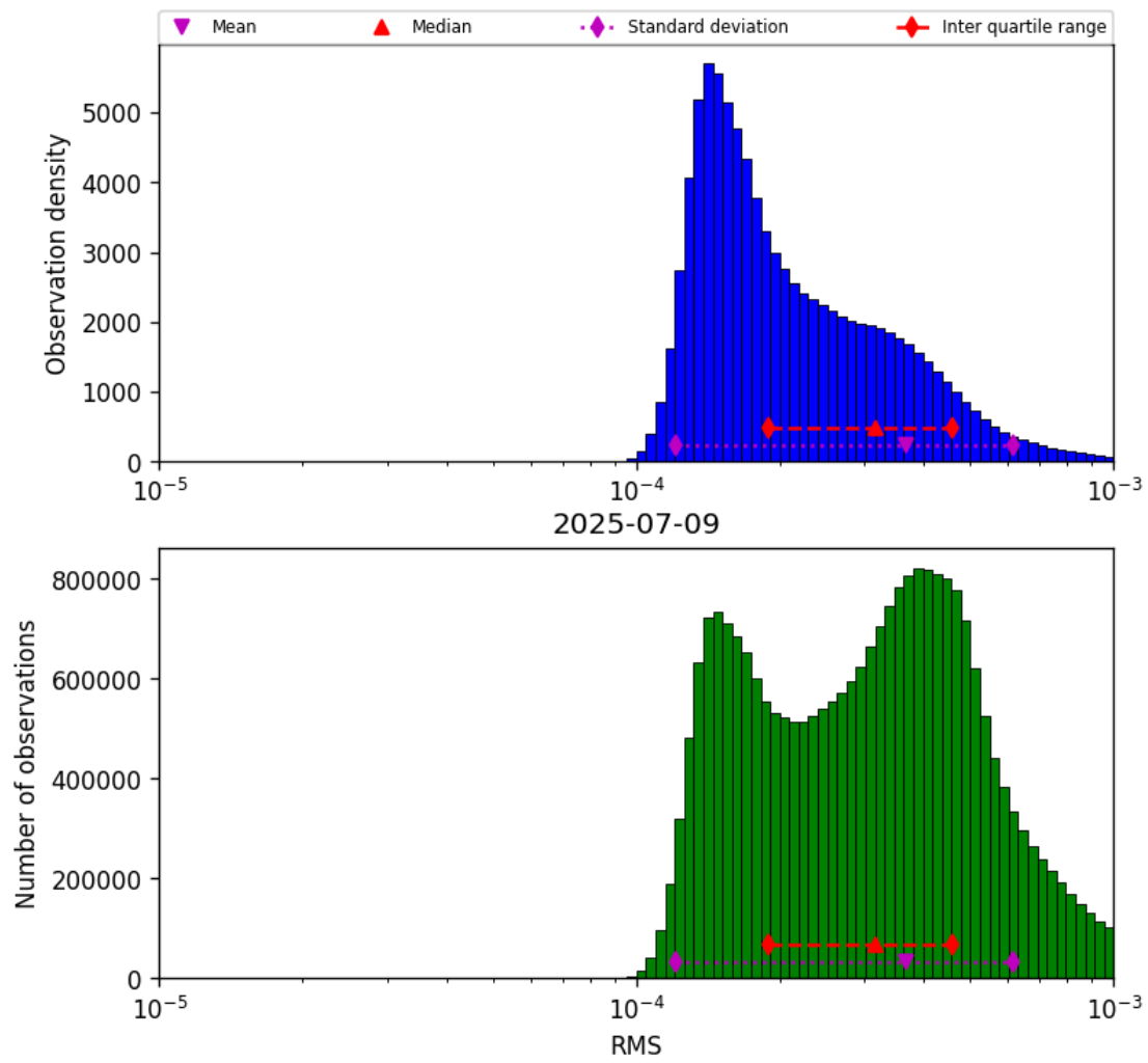
Figure 43: Histogram of “RMS” for 2025-07-08 to 2025-07-10
