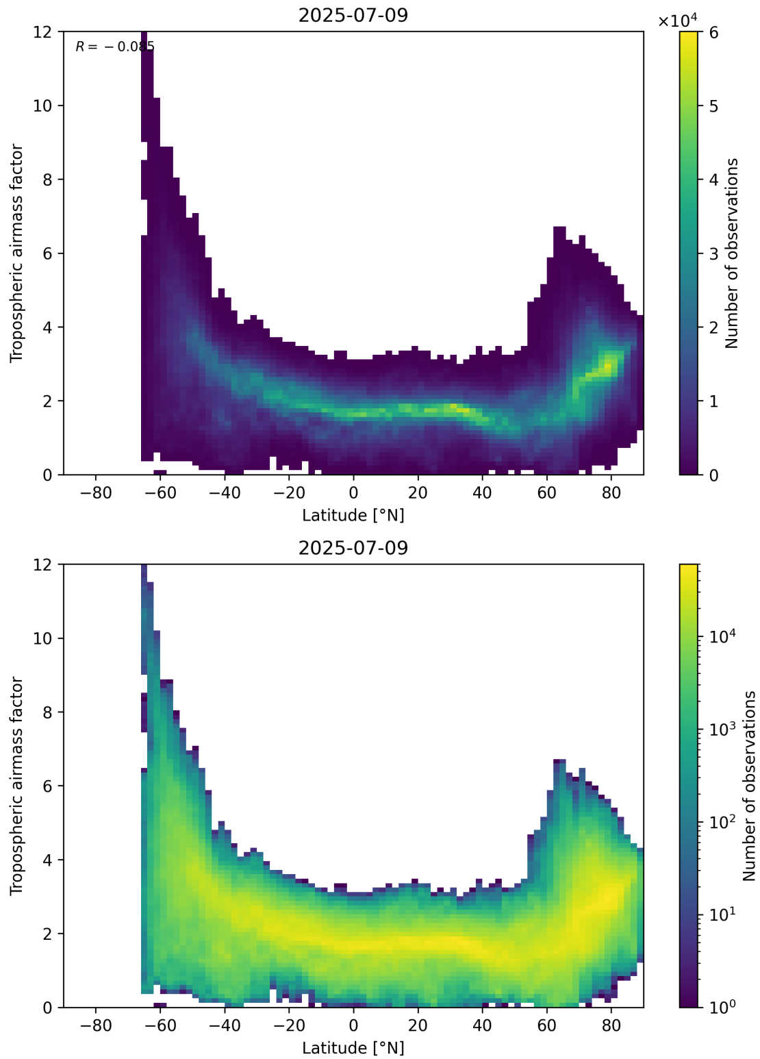
Figure 85: Scatter density plot of “Latitude” against “Tropospheric air mass factor” for 2025-07-08 to 2025-07-10.
