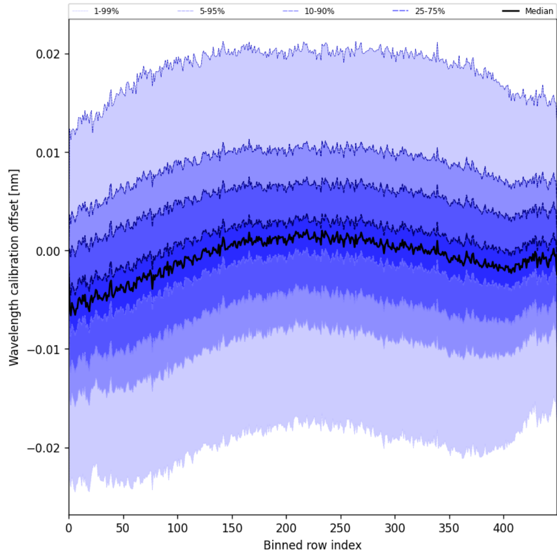
Figure 52: Along track statistics of “Wavelength calibration offset” for 2025-07-08 to 2025-07-10
