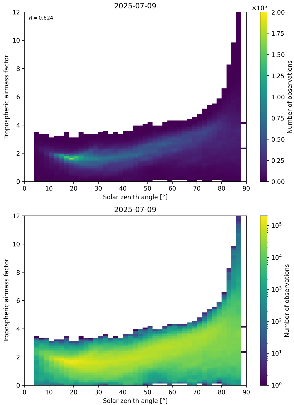
Figure 147: Scatter density plot of “Solar zenith angle” against “Tropospheric airmass factor” for 2025-07-08 to 2025-07-10.
