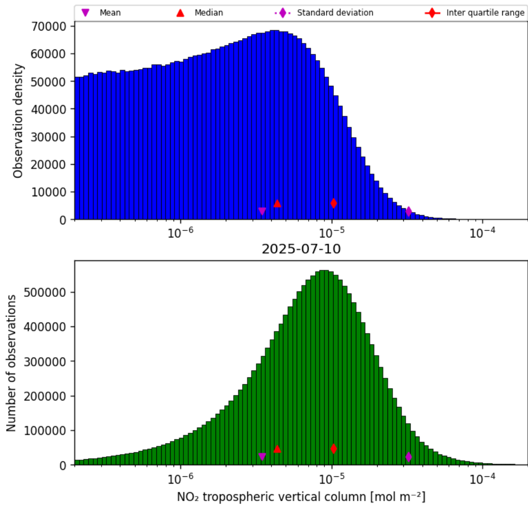
Figure 29: Histogram of “NO 2 tropospheric vertical column” for 2025-07-09 to 2025-07-11
