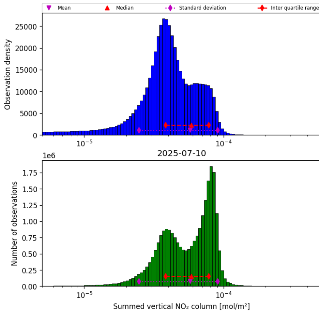
Figure 40: Histogram of “Summed vertical NO 2 column” for 2025-07-09 to 2025-07-11
