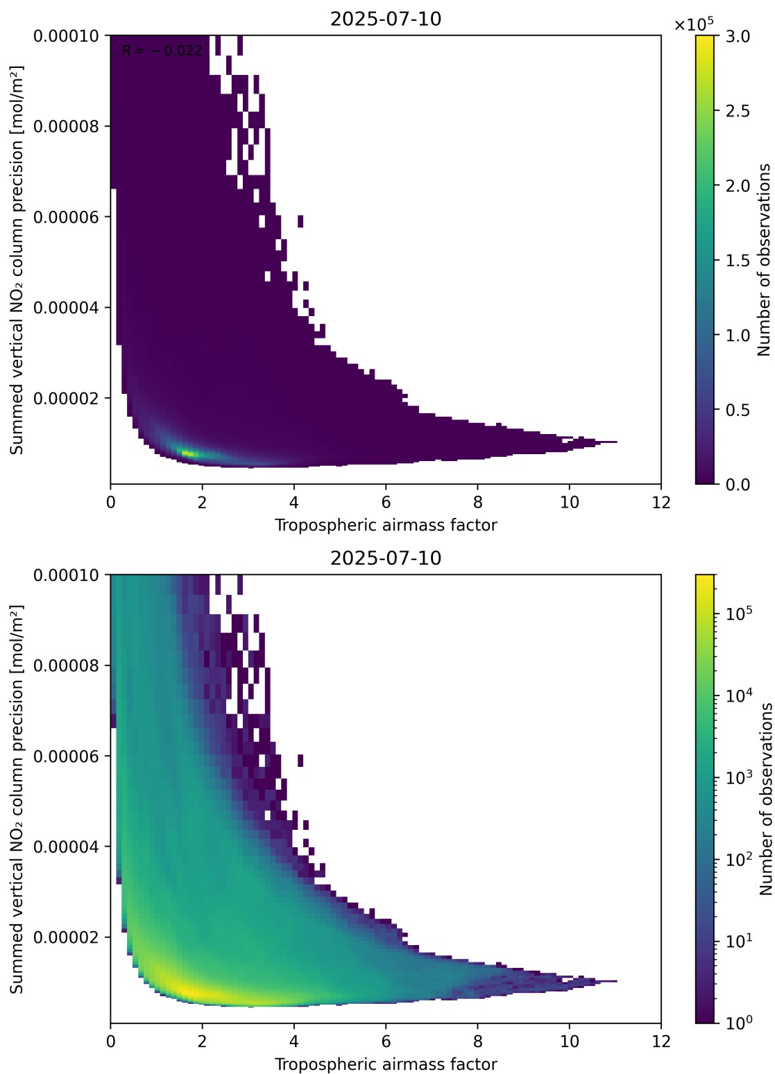
Figure 76: Scatter density plot of “Tropospheric air mass factor” against “Summed vertical NO 2 column precision” for 2025-07-09 to 2025-07-11.
