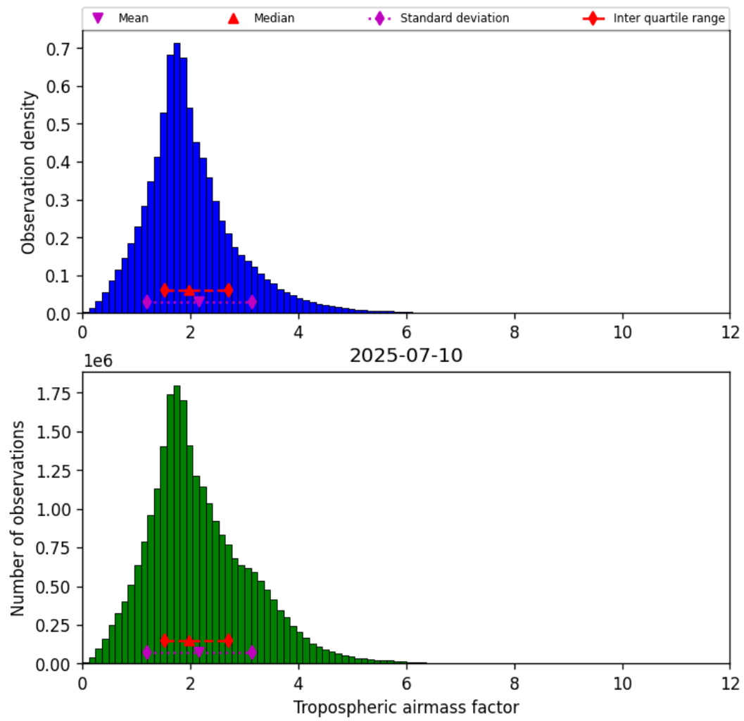
Figure 31: Histogram of “Tropospheric airmass factor” for 2025-07-09 to 2025-07-11
