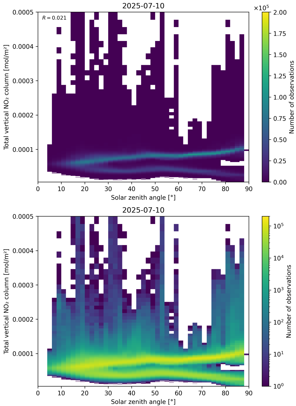
Figure 153: Scatter density plot of “Solar zenith angle” against “Total vertical NO 2 column” for 2025-07-09 to 2025-07-11.
