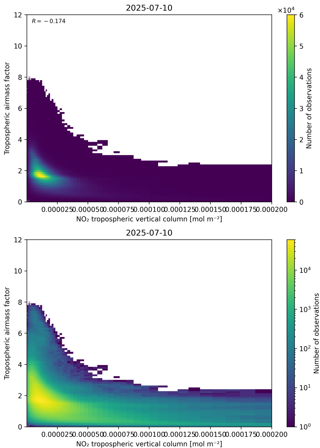
Figure 123: Scatter density plot of “NO 2 tropospheric vertical column” against “Tropospheric airmass factor” for 2025-07-09 to 2025-07-11.
