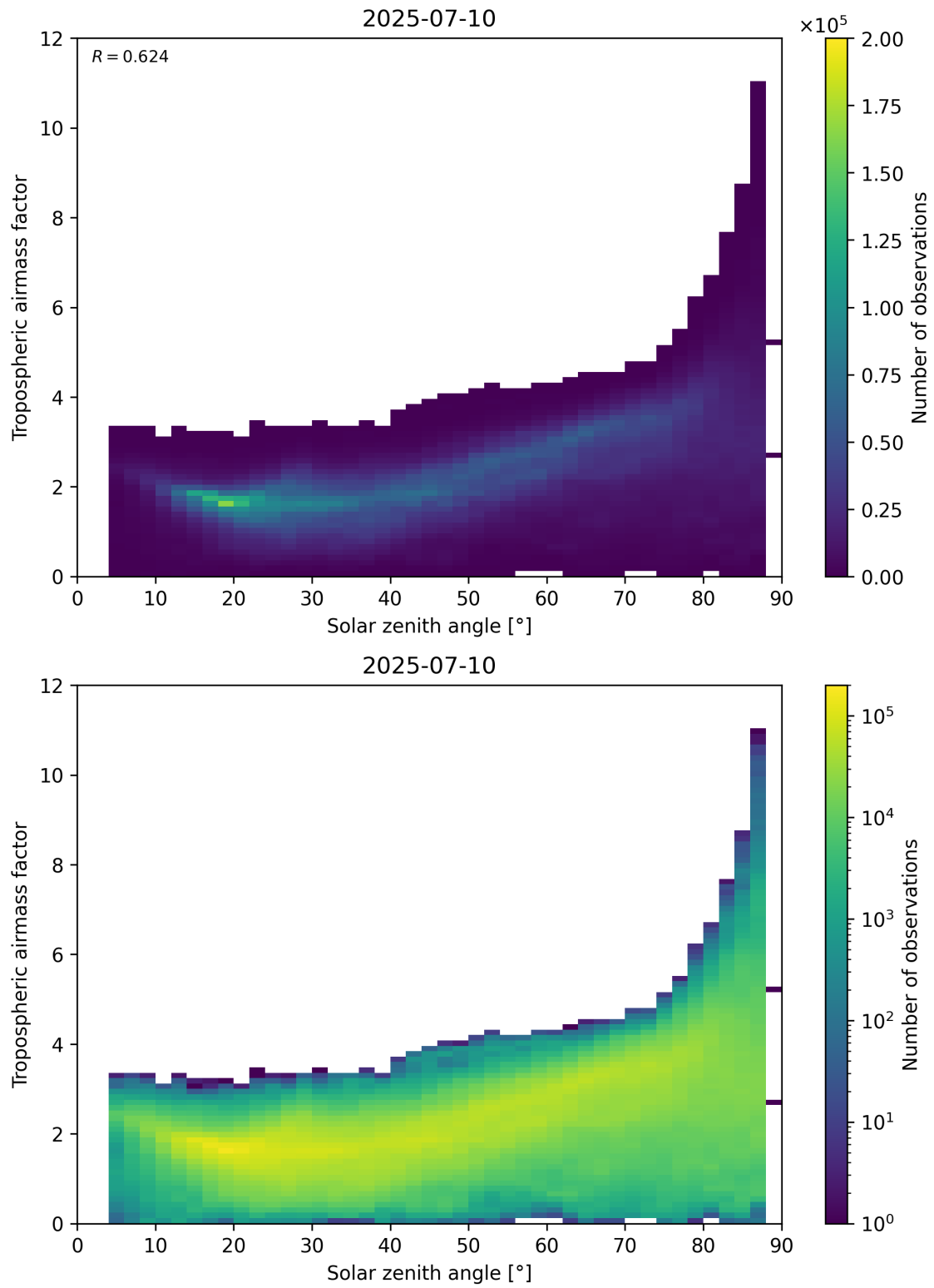
Figure 147: Scatter density plot of “Solar zenith angle” against “Tropospheric airmass factor” for 2025-07-09 to 2025-07-11.
