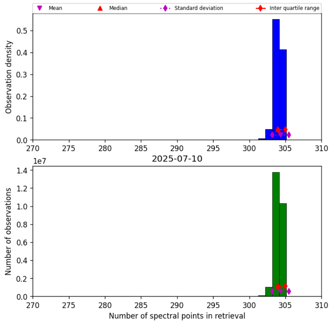
Figure 33: Histogram of “Number of spectral points in retrieval” for 2025-07-09 to 2025-07-11
