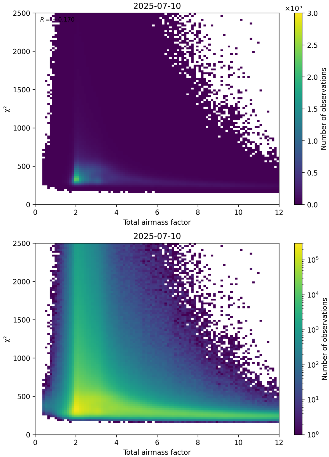
Figure 63: Scatter density plot of “Total airmass factor” against “ \chi^2 ” for 2025-07-09 to 2025-07-11.
