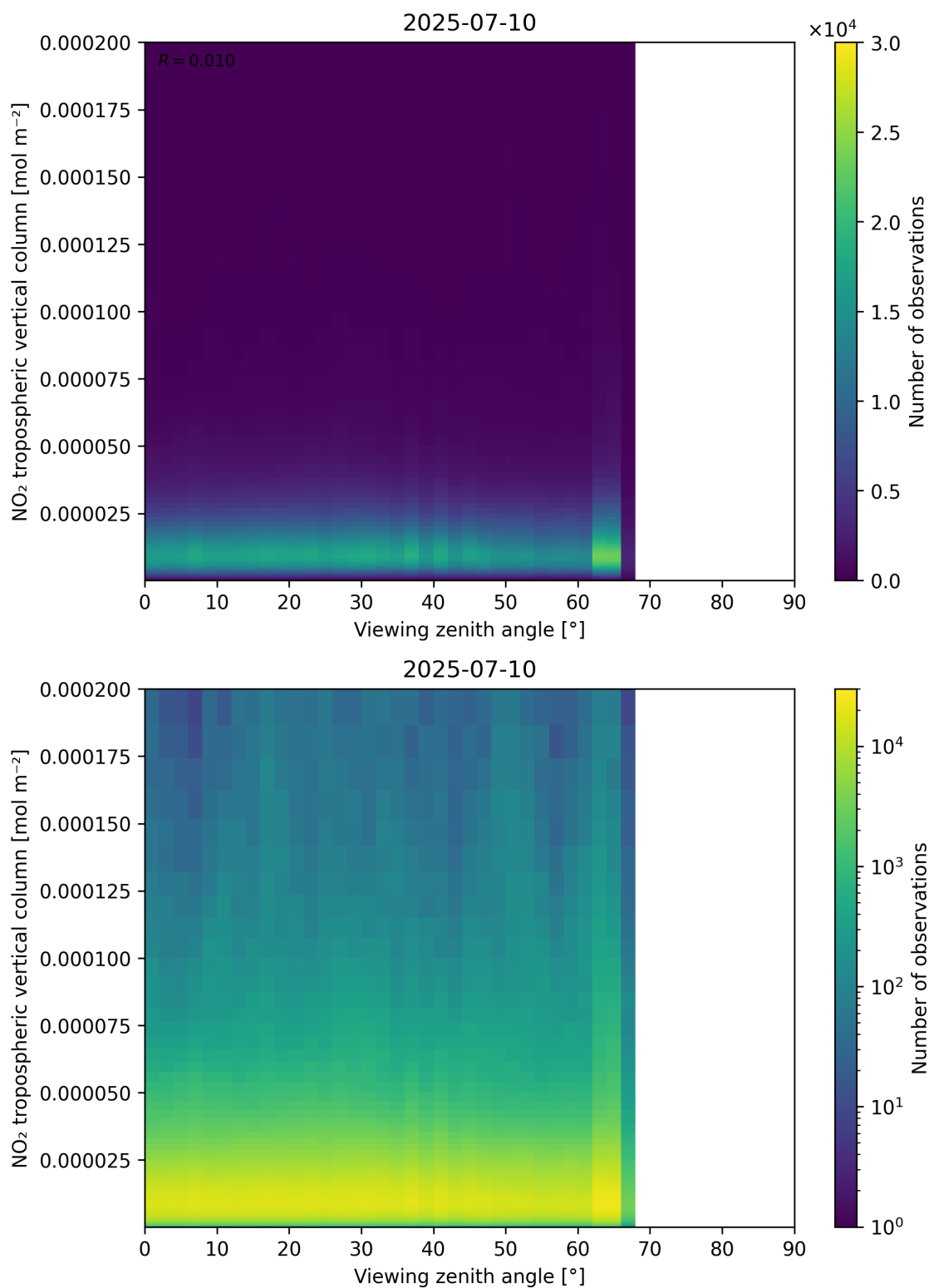
Figure 169: Scatter density plot of “Viewing zenith angle” against “NO 2 tropospheric vertical column” for 2025-07-09 to 2025-07-11.
