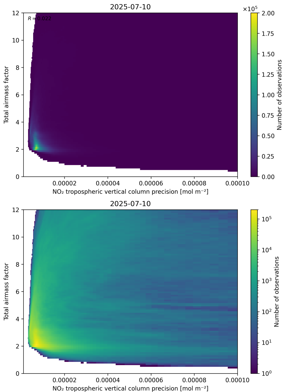
Figure 132: Scatter density plot of “NO 2 tropospheric vertical column precision” against “Total air mass factor” for 2025-07-09 to 2025-07-11.
