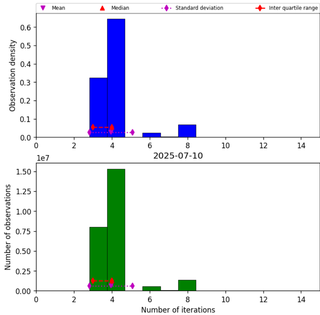
Figure 34: Histogram of “Number of iterations” for 2025-07-09 to 2025-07-11
