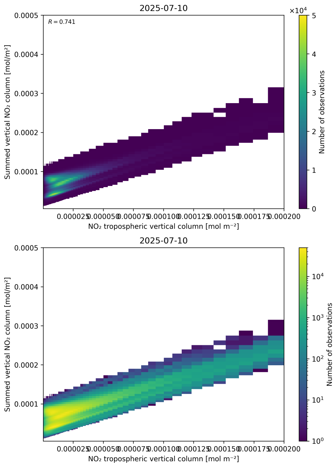
Figure 126: Scatter density plot of “NO 2 tropospheric vertical column” against “Summed vertical NO 2 column” for 2025-07-09 to 2025-07-11.
