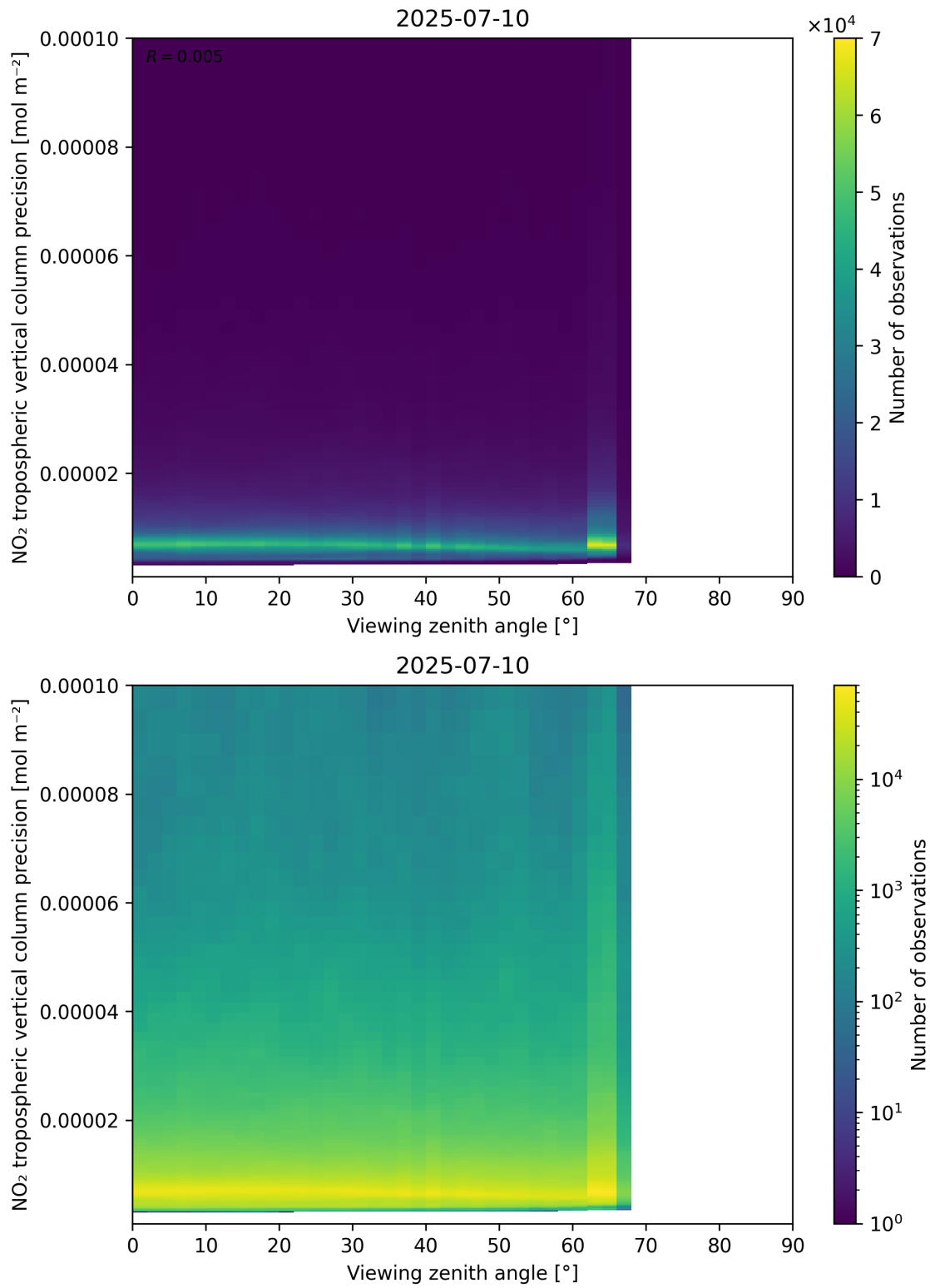
Figure 170: Scatter density plot of “Viewing zenith angle” against “NO 2 tropospheric vertical column precision” for 2025-07-09 to 2025-07-11.
