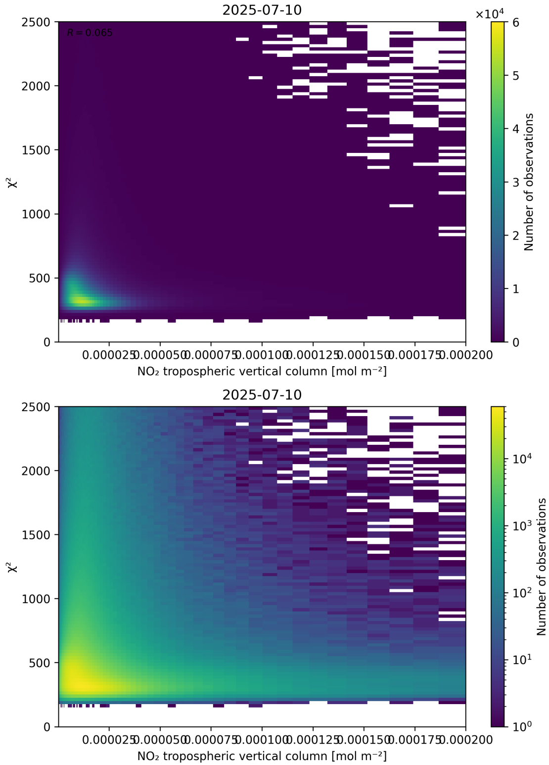
Figure 124: Scatter density plot of “NO 2 tropospheric vertical column” against “ \chi^2 ” for 2025-07-09 to 2025-07-11.
