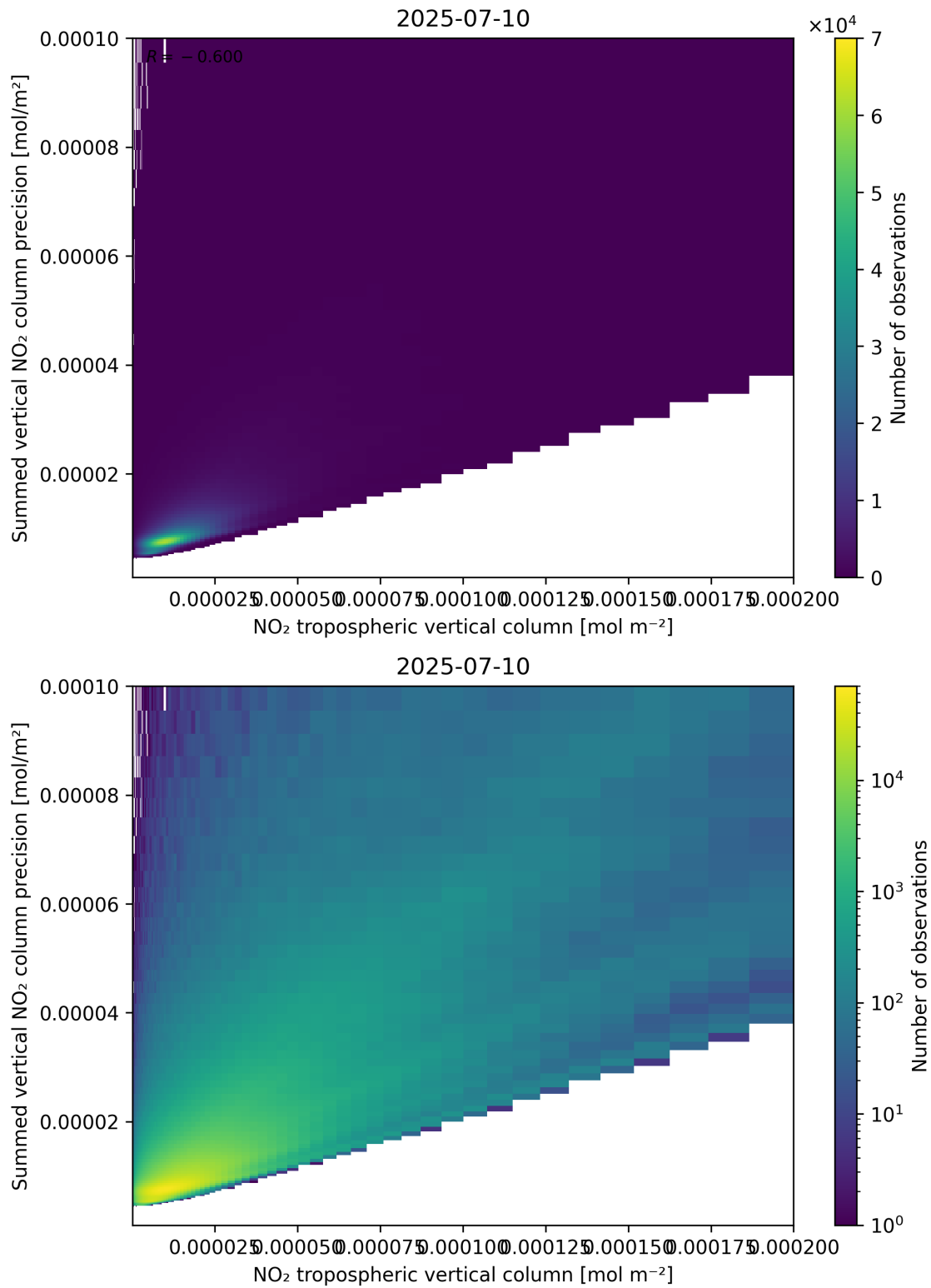
Figure 127: Scatter density plot of “NO 2 tropospheric vertical column” against “Summed vertical NO 2 column precision” for 2025-07-09 to 2025-07-11.
