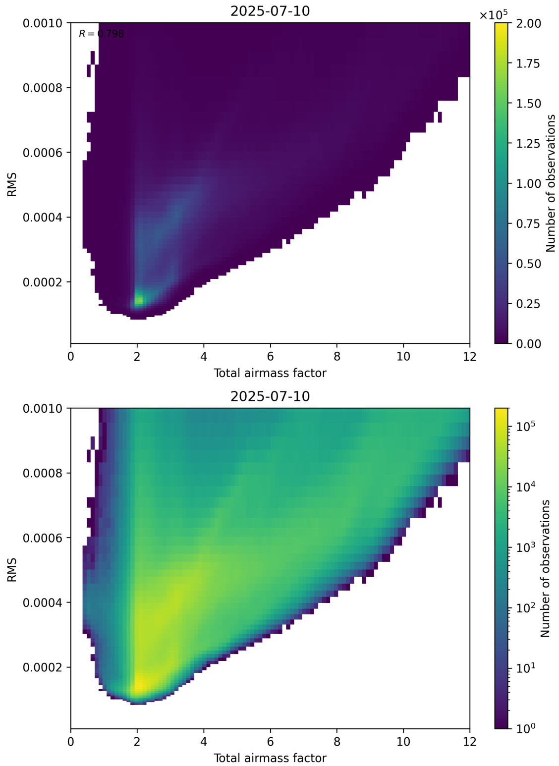
Figure 69: Scatter density plot of “Total airmass factor” against “RMS” for 2025-07-09 to 2025-07-11.
