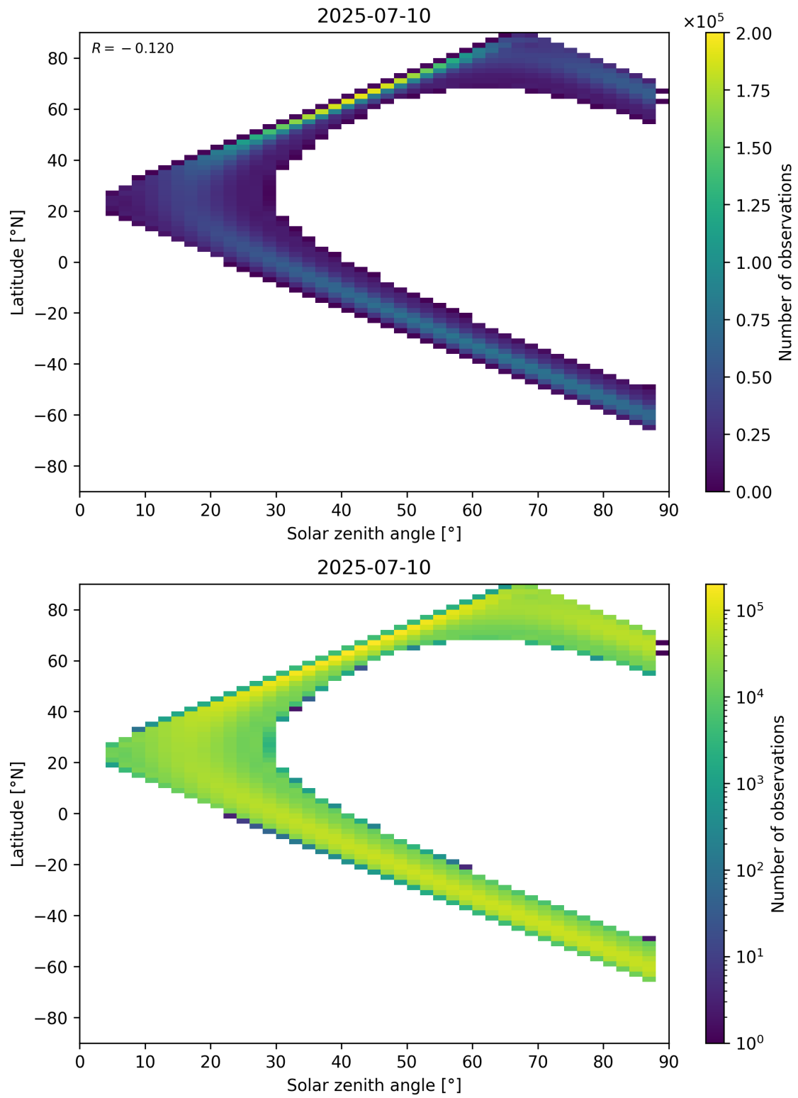
Figure 149: Scatter density plot of “Solar zenith angle” against “Latitude” for 2025-07-09 to 2025-07-11.
