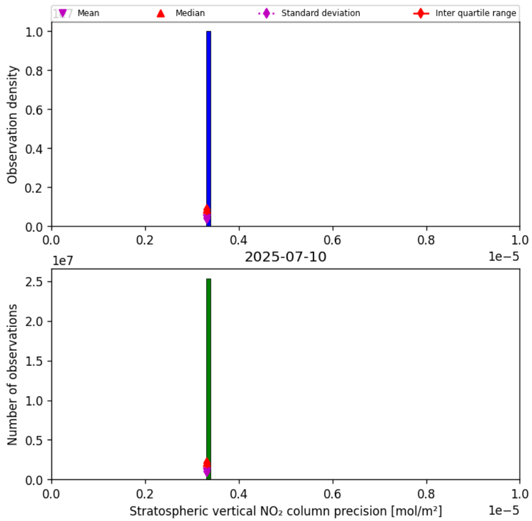
Figure 37: Histogram of “Stratospheric vertical NO 2 column precision” for 2025-07-09 to 2025-07-11
