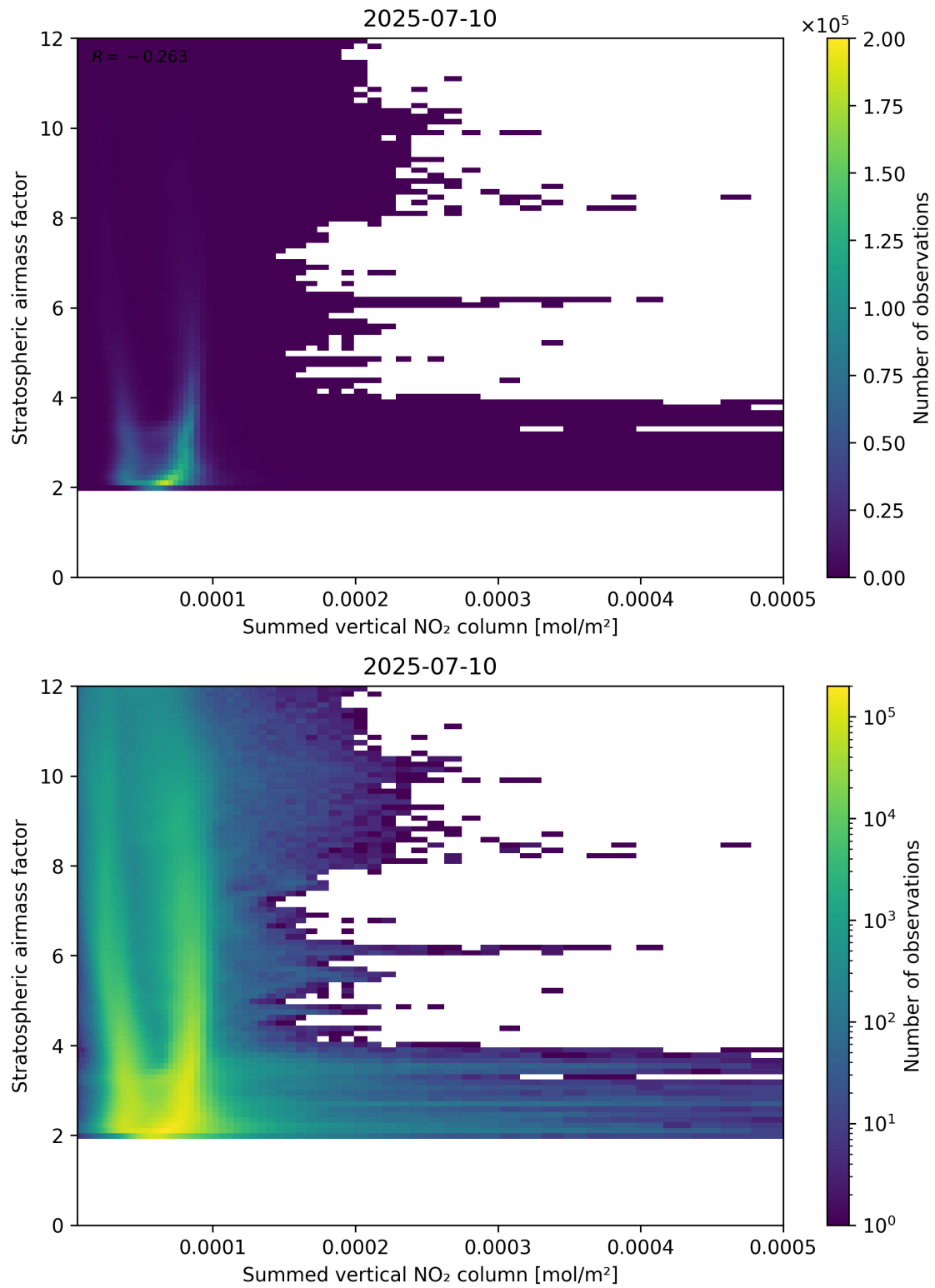
Figure 103: Scatter density plot of “Summed vertical NO 2 column” against “Stratospheric airmass factor” for 2025-07-09 to 2025-07-11.
