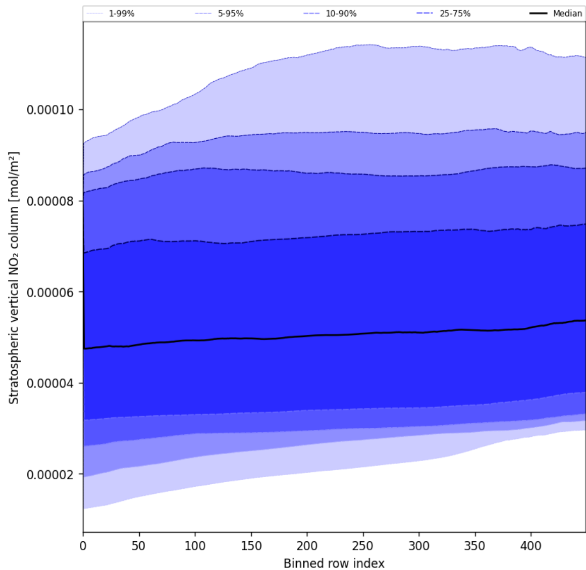
Figure 53: Along track statistics of “Stratospheric vertical NO 2 column” for 2025-07-09 to 2025-07-11
