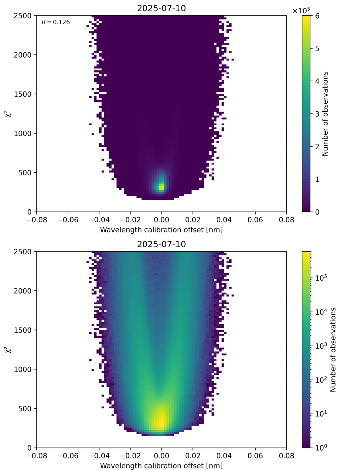
Figure 175: Scatter density plot of “Wavelength calibration offset” against “ \chi^2 ” for 2025-07-09 to 2025-07-11.
