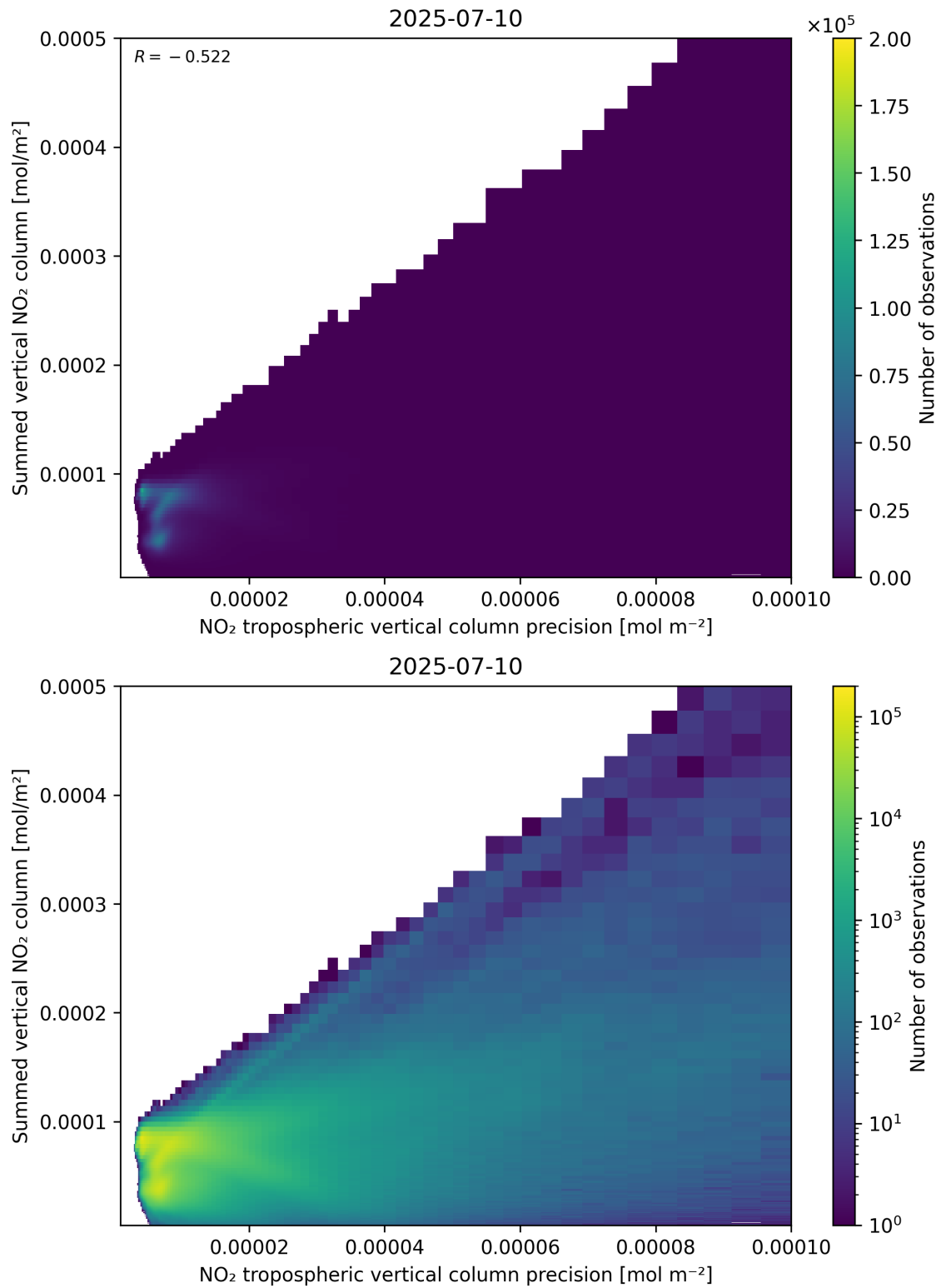
Figure 136: Scatter density plot of “NO 2 tropospheric vertical column precision” against “Summed vertical NO 2 column” for 2025-07-09 to 2025-07-11.
