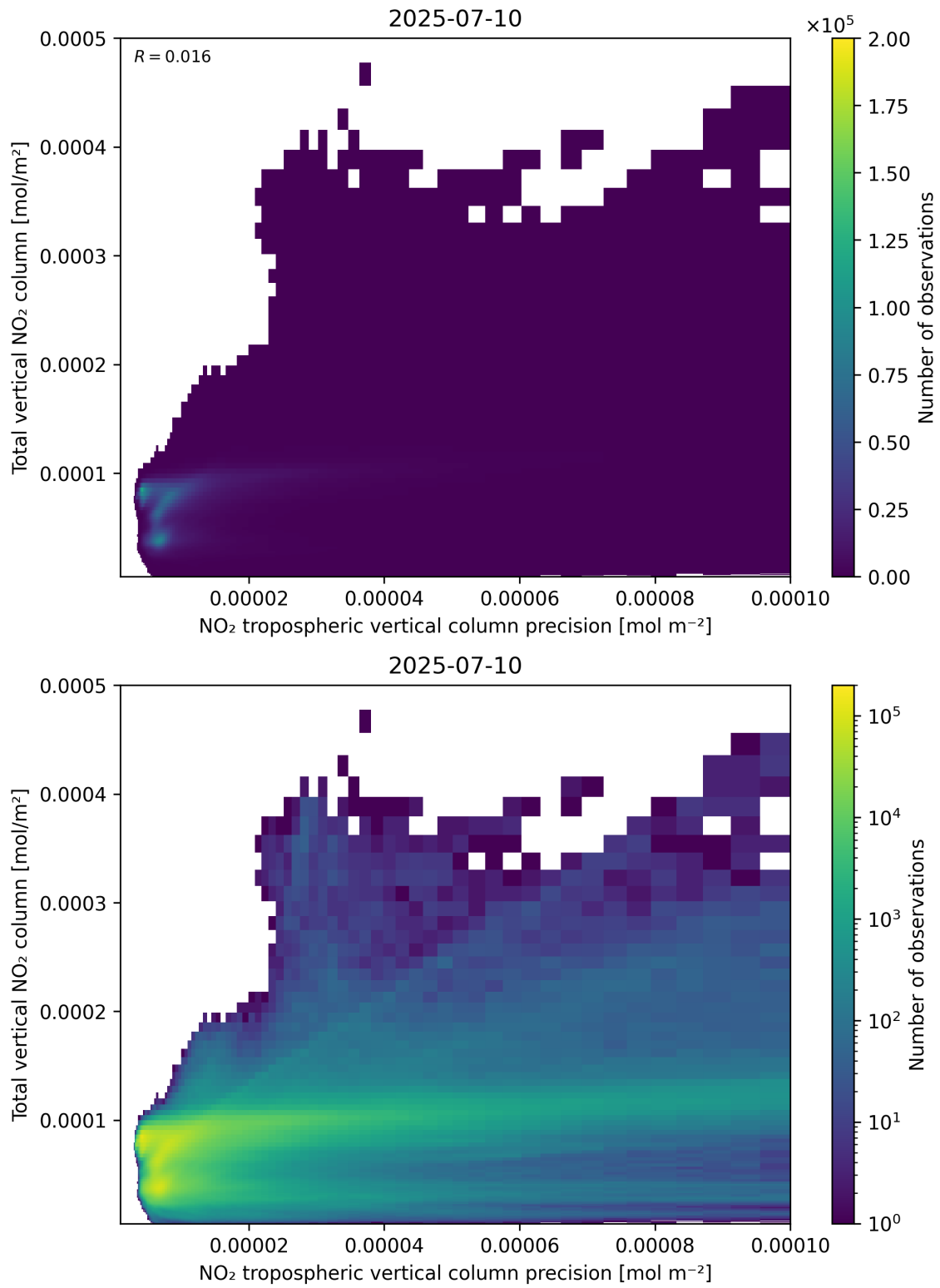
Figure 138: Scatter density plot of “NO 2 tropospheric vertical column precision” against “Total vertical NO 2 column” for 2025-07-09 to 2025-07-11.
