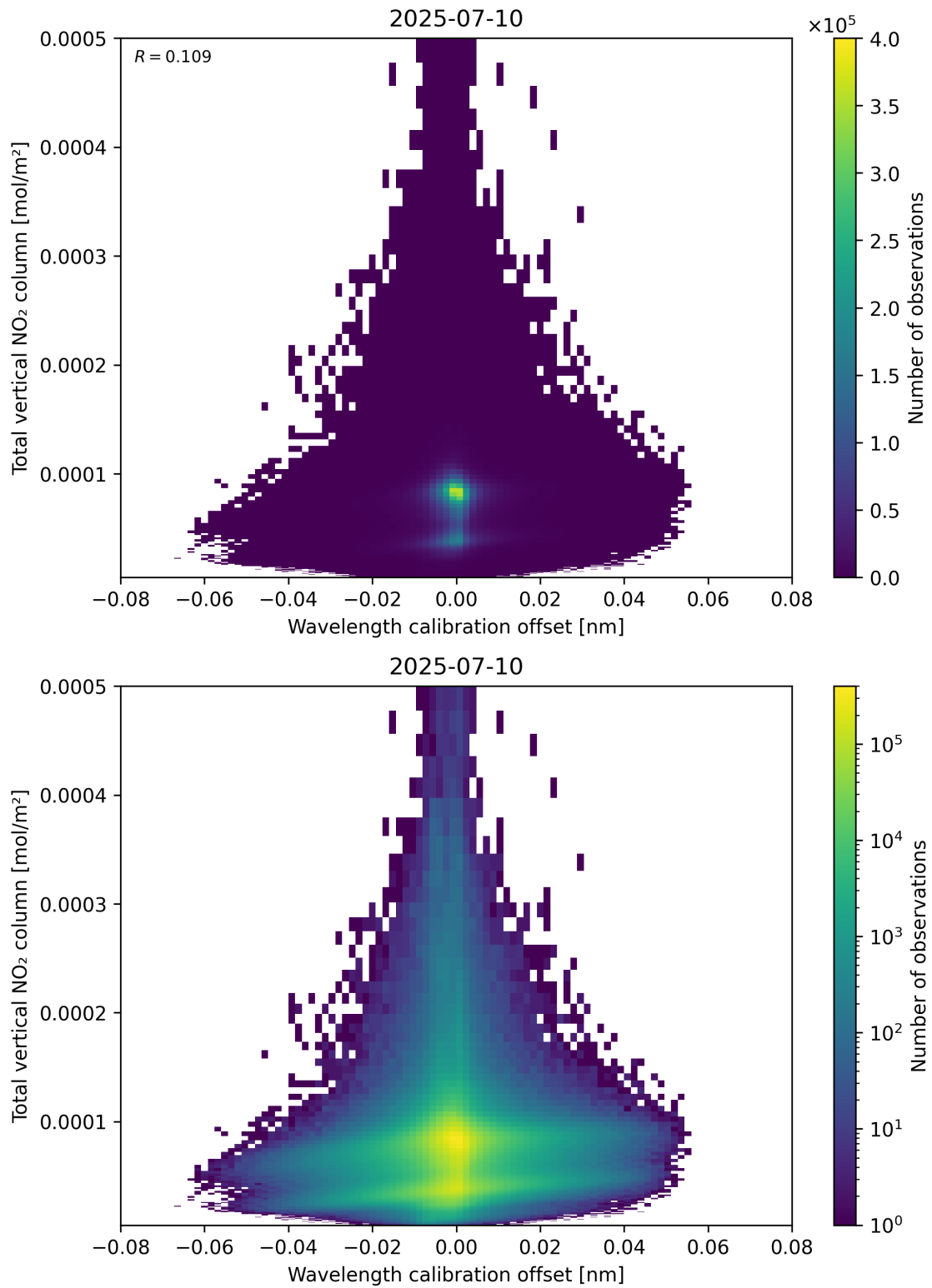
Figure 179: Scatter density plot of “Wavelength calibration offset” against “Total vertical NO 2 column” for 2025-07-09 to 2025-07-11.
