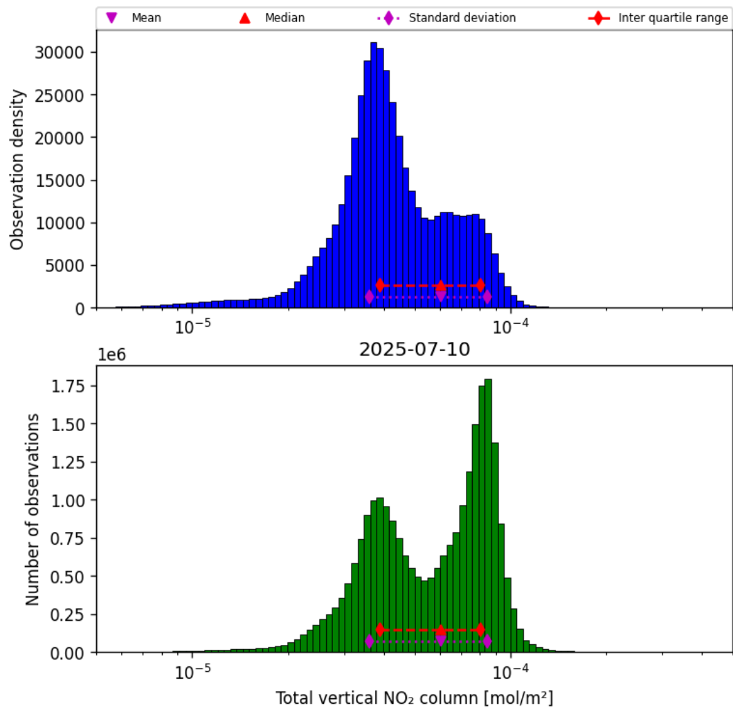
Figure 38: Histogram of “Total vertical NO 2 column” for 2025-07-09 to 2025-07-11
