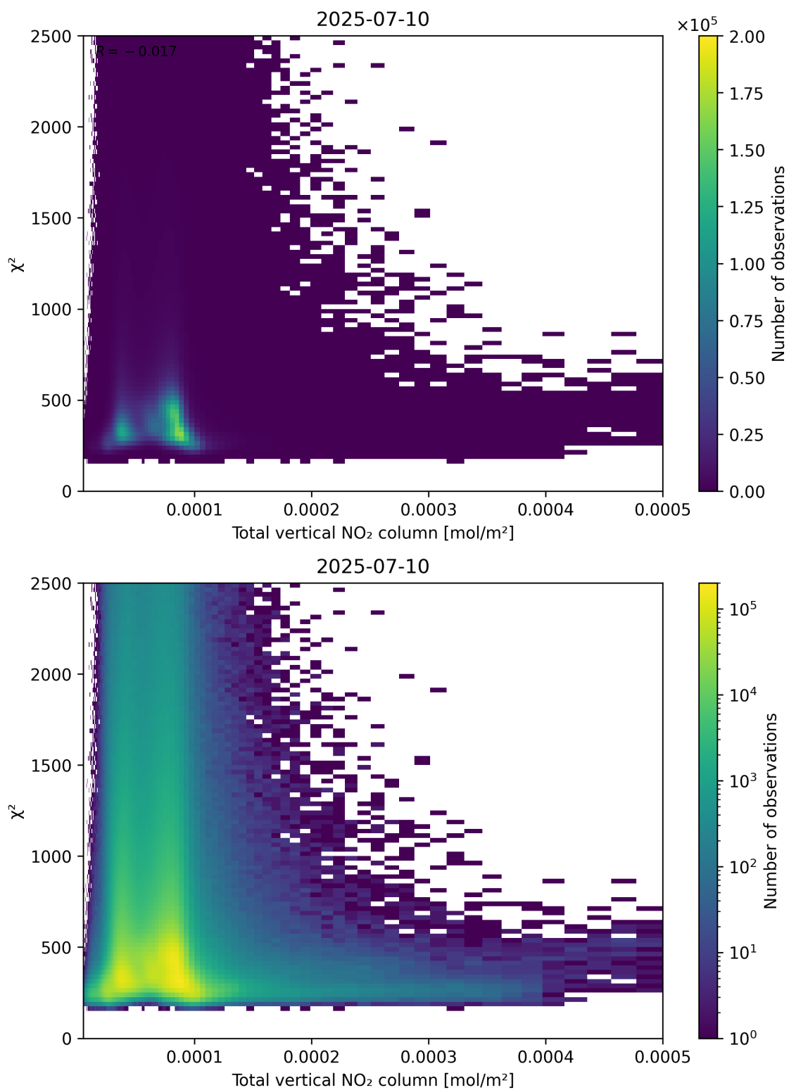
Figure 111: Scatter density plot of “Total vertical NO 2 column” against “ \chi^2 ” for 2025-07-09 to 2025-07-11.
