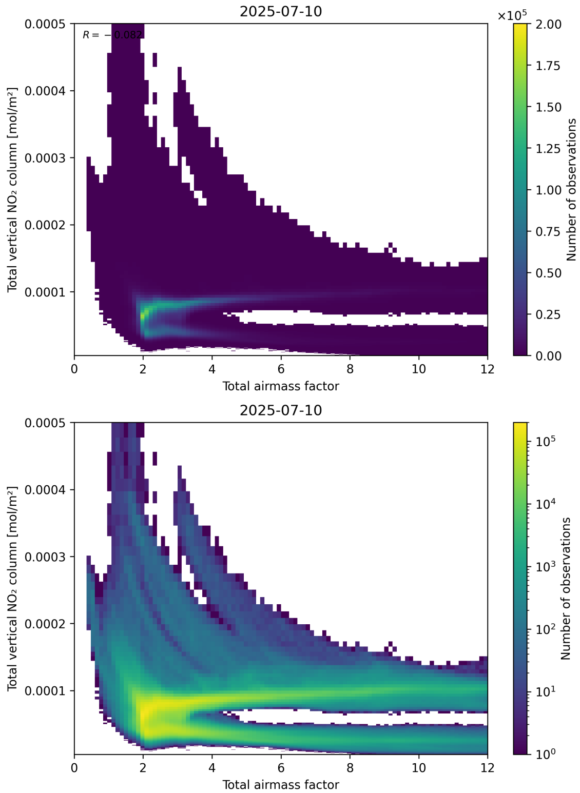
Figure 67: Scatter density plot of “Total airmass factor” against “Total vertical NO 2 column” for 2025-07-09 to 2025-07-11.
