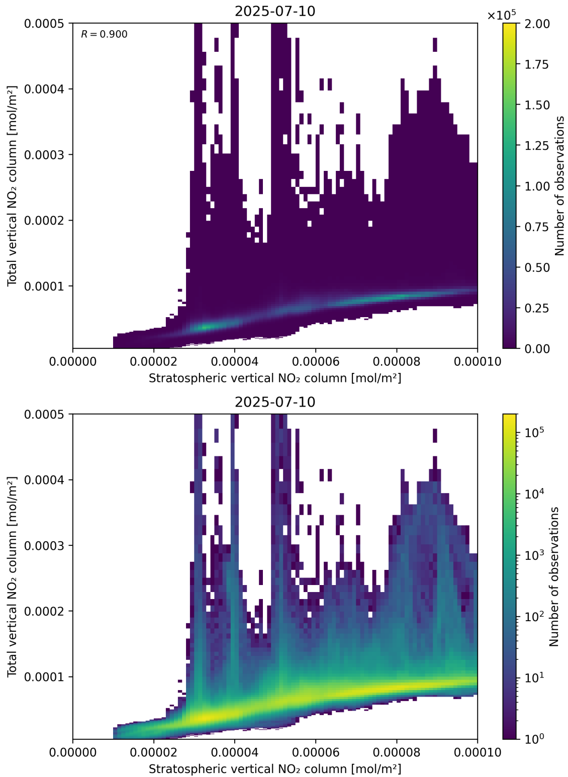
Figure 100: Scatter density plot of “Stratospheric vertical NO 2 column” against “Total vertical NO 2 column” for 2025-07-09 to 2025-07-11.
