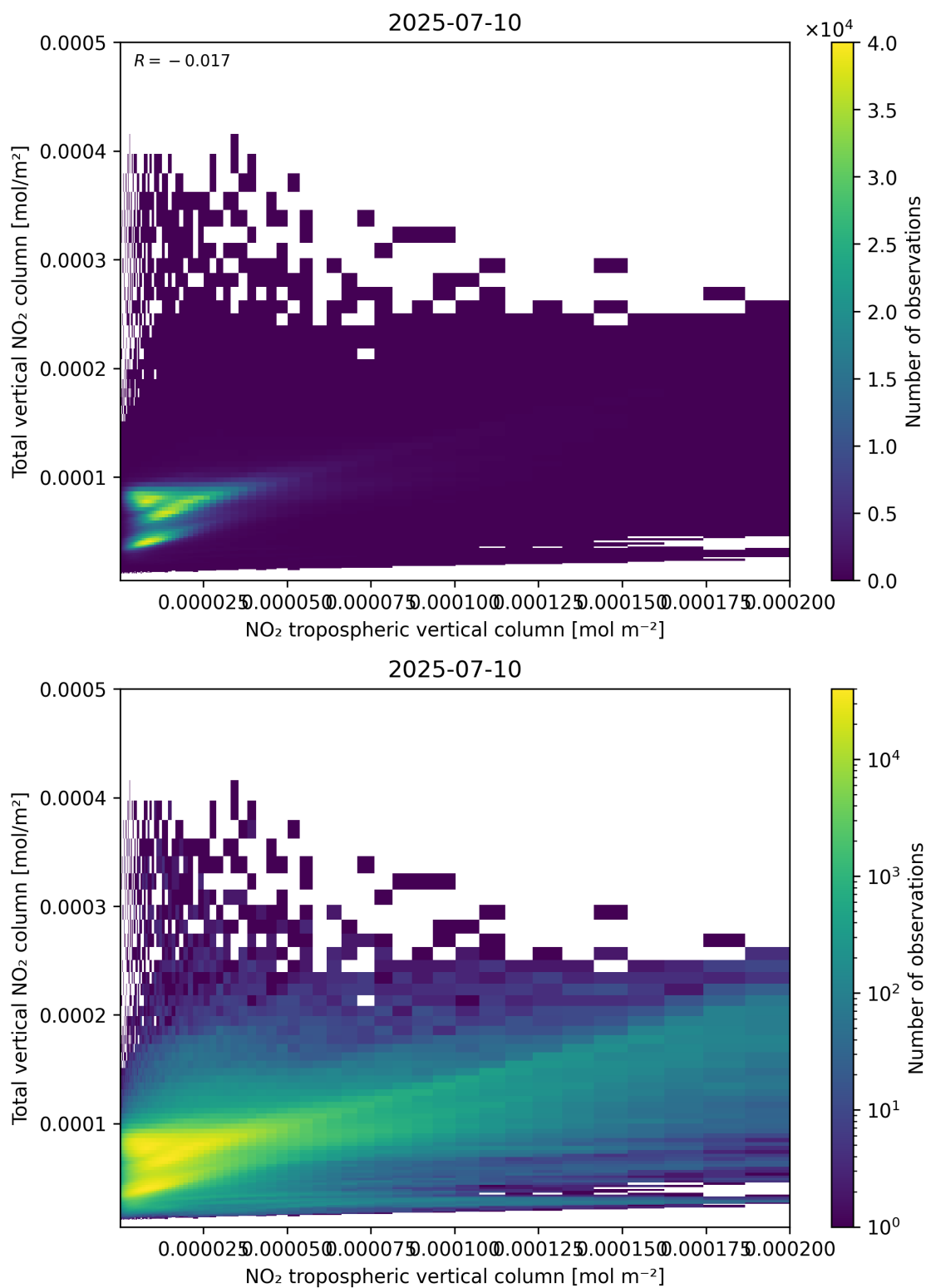
Figure 128: Scatter density plot of “NO 2 tropospheric vertical column” against “Total vertical NO 2 column” for 2025-07-09 to 2025-07-11.
