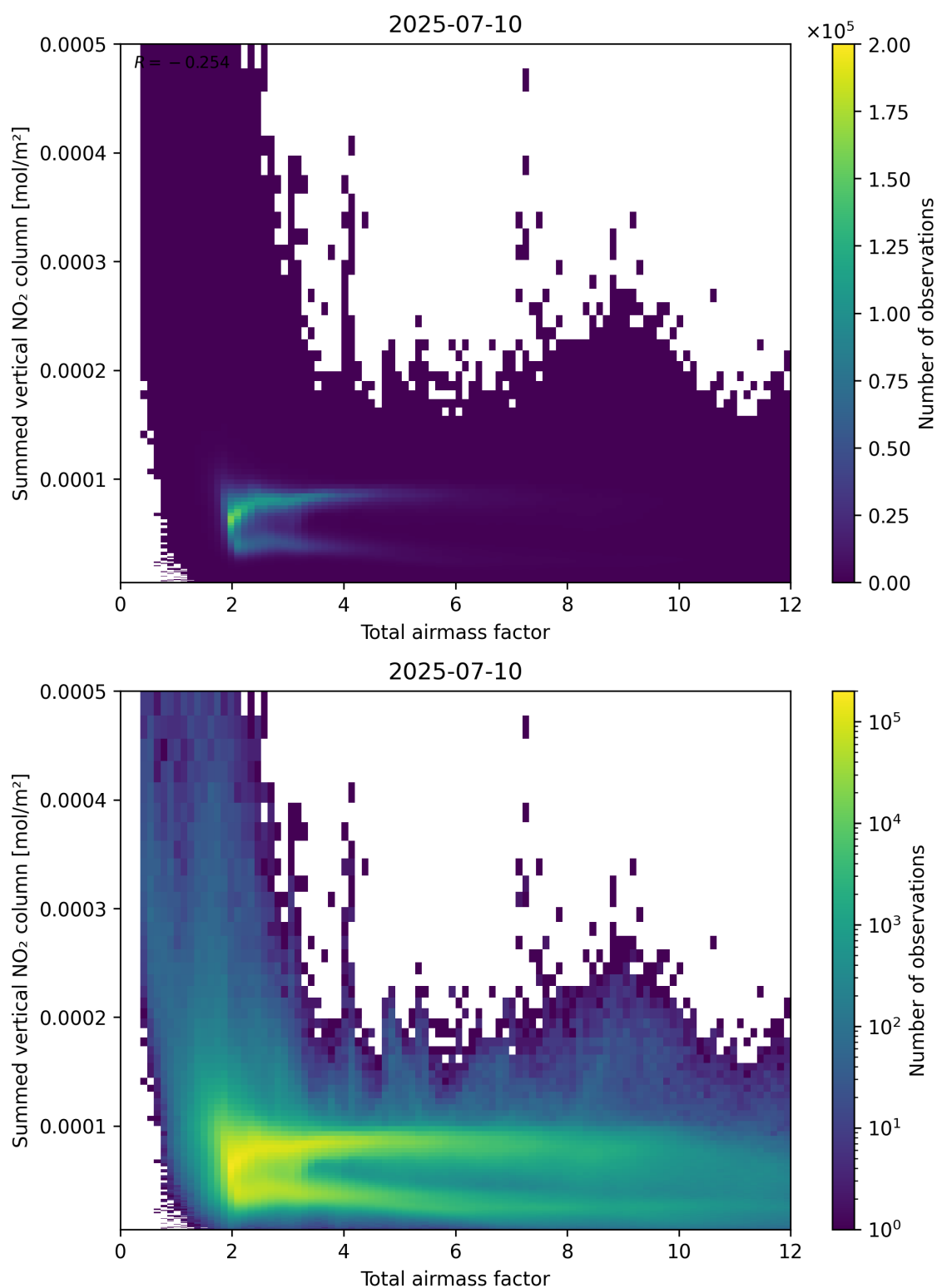
Figure 65: Scatter density plot of “Total airmass factor” against “Summed vertical NO 2 column” for 2025-07-09 to 2025-07-11.
