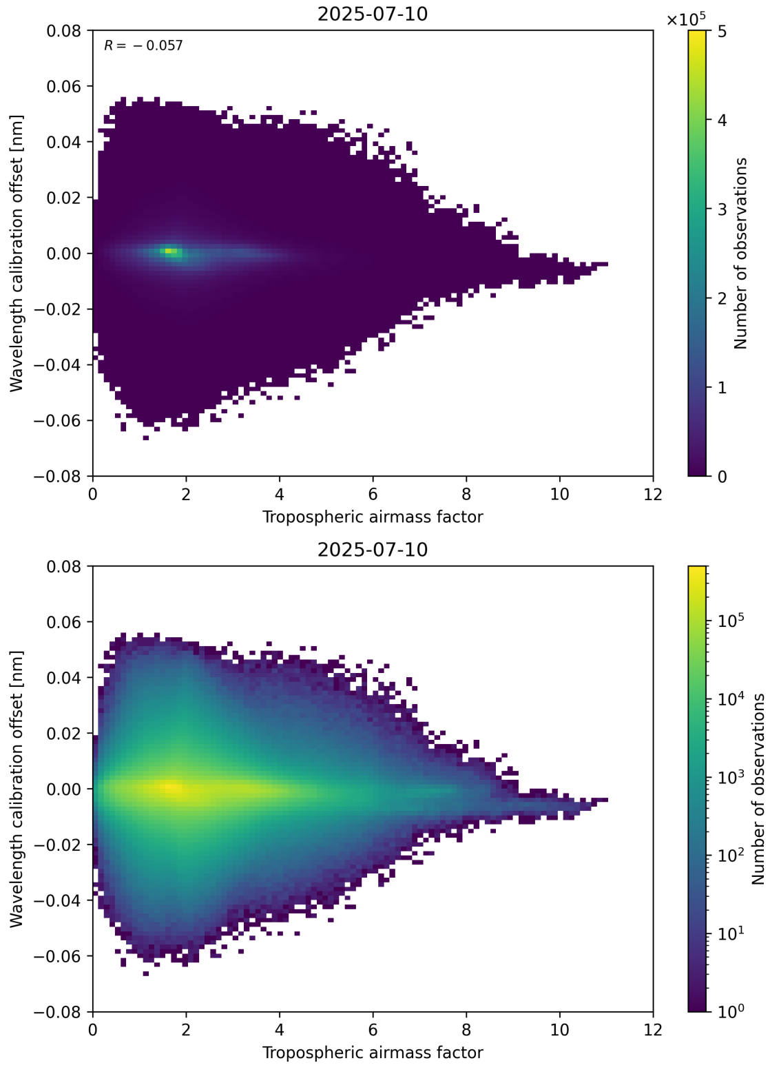
Figure 80: Scatter density plot of “Tropospheric airmass factor” against “Wavelength calibration offset” for 2025-07-09 to 2025-07-11.
