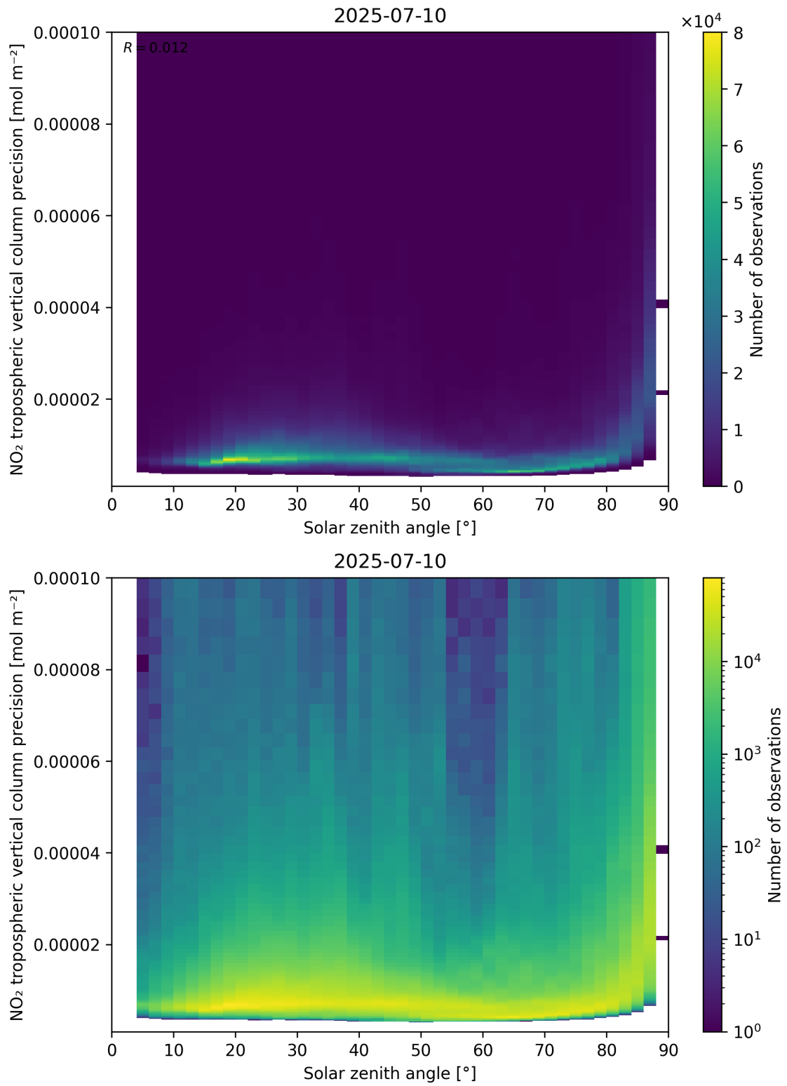
Figure 156: Scatter density plot of “Solar zenith angle” against “NO 2 tropospheric vertical column precision” for 2025-07-09 to 2025-07-11.
