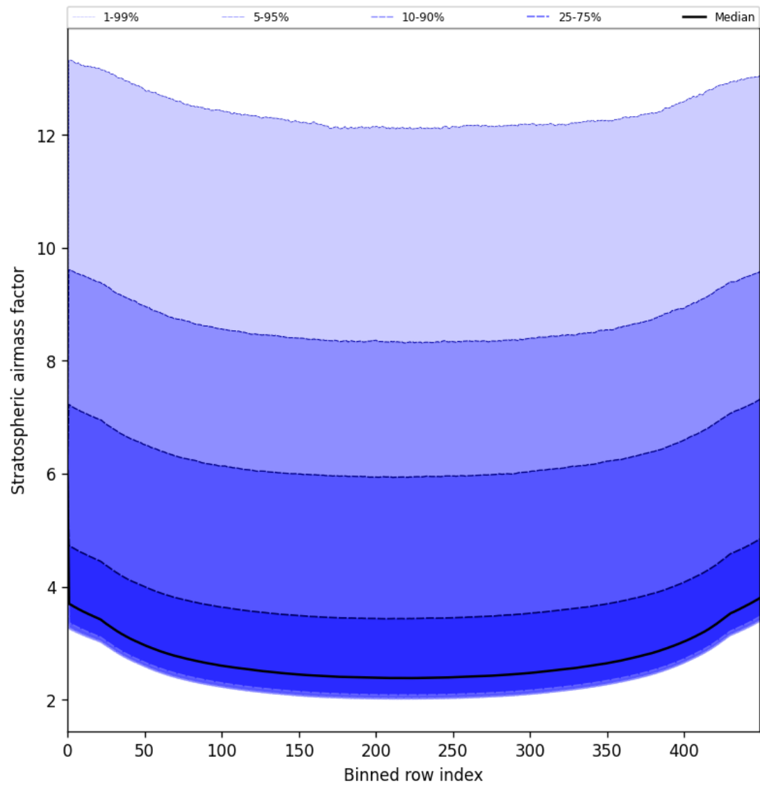
Figure 61: Along track statistics of “Stratospheric airmass factor” for 2025-07-09 to 2025-07-11
