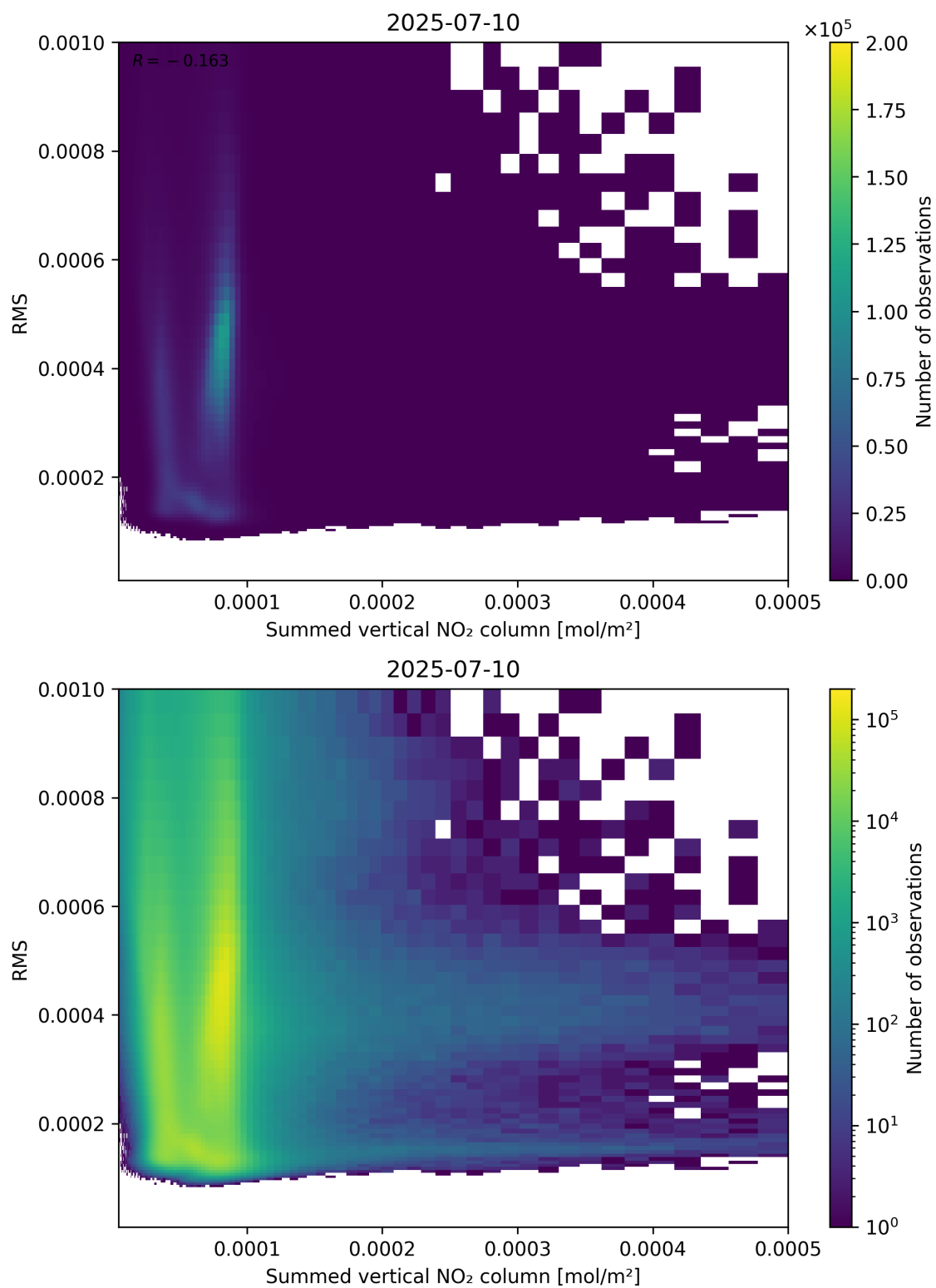
Figure 109: Scatter density plot of “Summed vertical NO 2 column” against “RMS” for 2025-07-09 to 2025-07-11.
