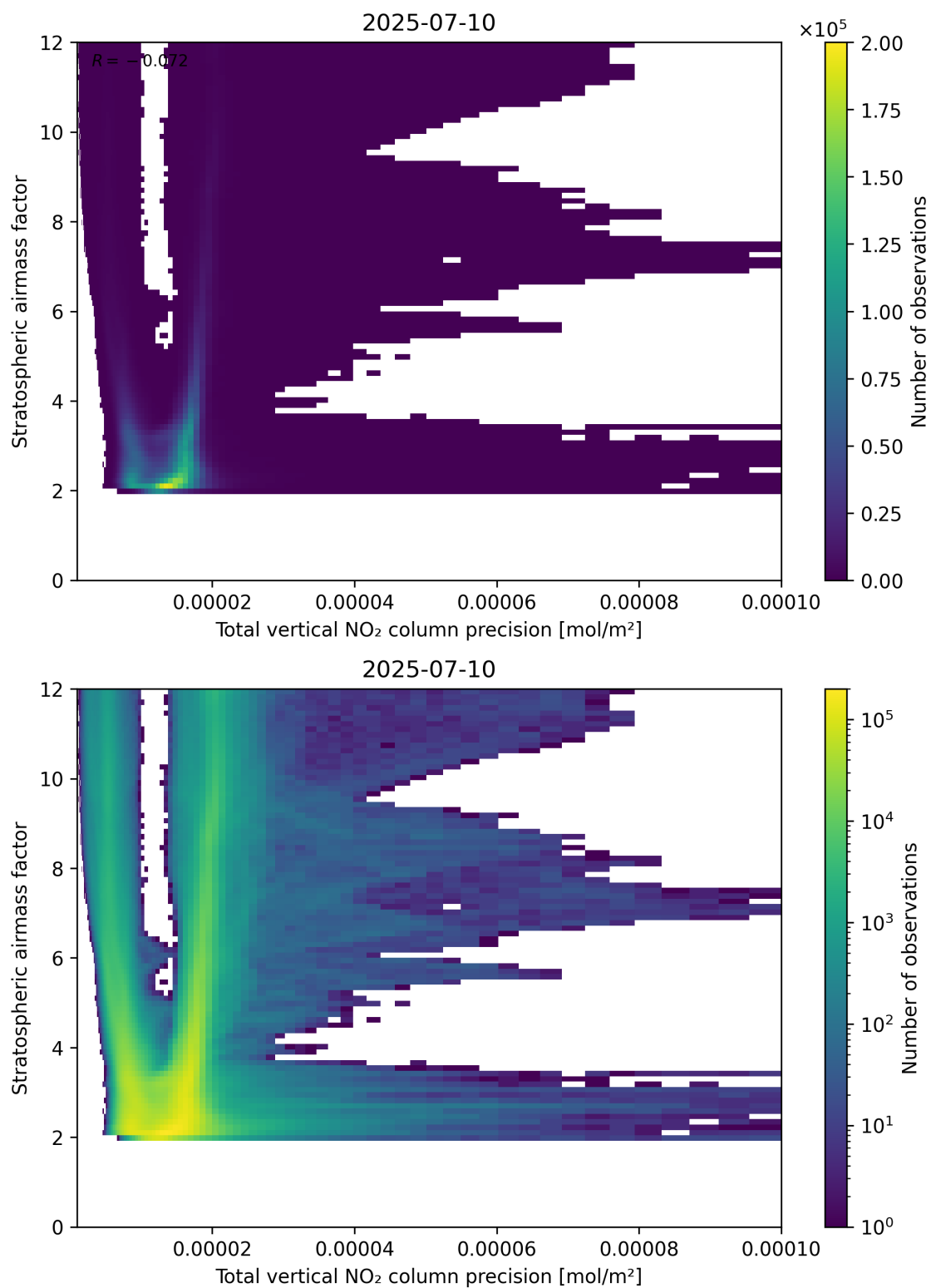
Figure 115: Scatter density plot of “Total vertical NO 2 column precision” against “Stratospheric airmass factor” for 2025-07-09 to 2025-07-11.
