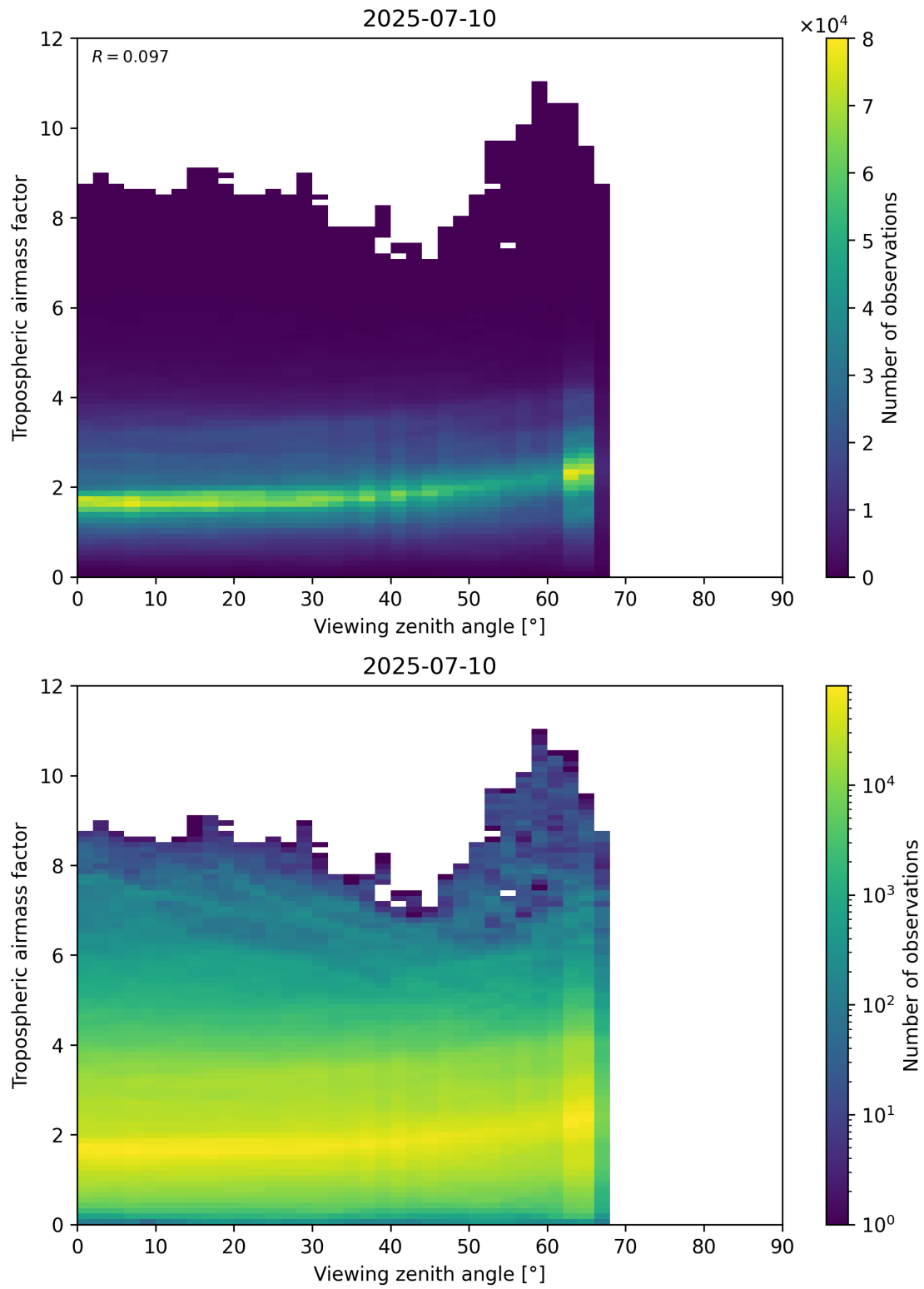
Figure 161: Scatter density plot of “Viewing zenith angle” against “Tropospheric airmass factor” for 2025-07-09 to 2025-07-11.
