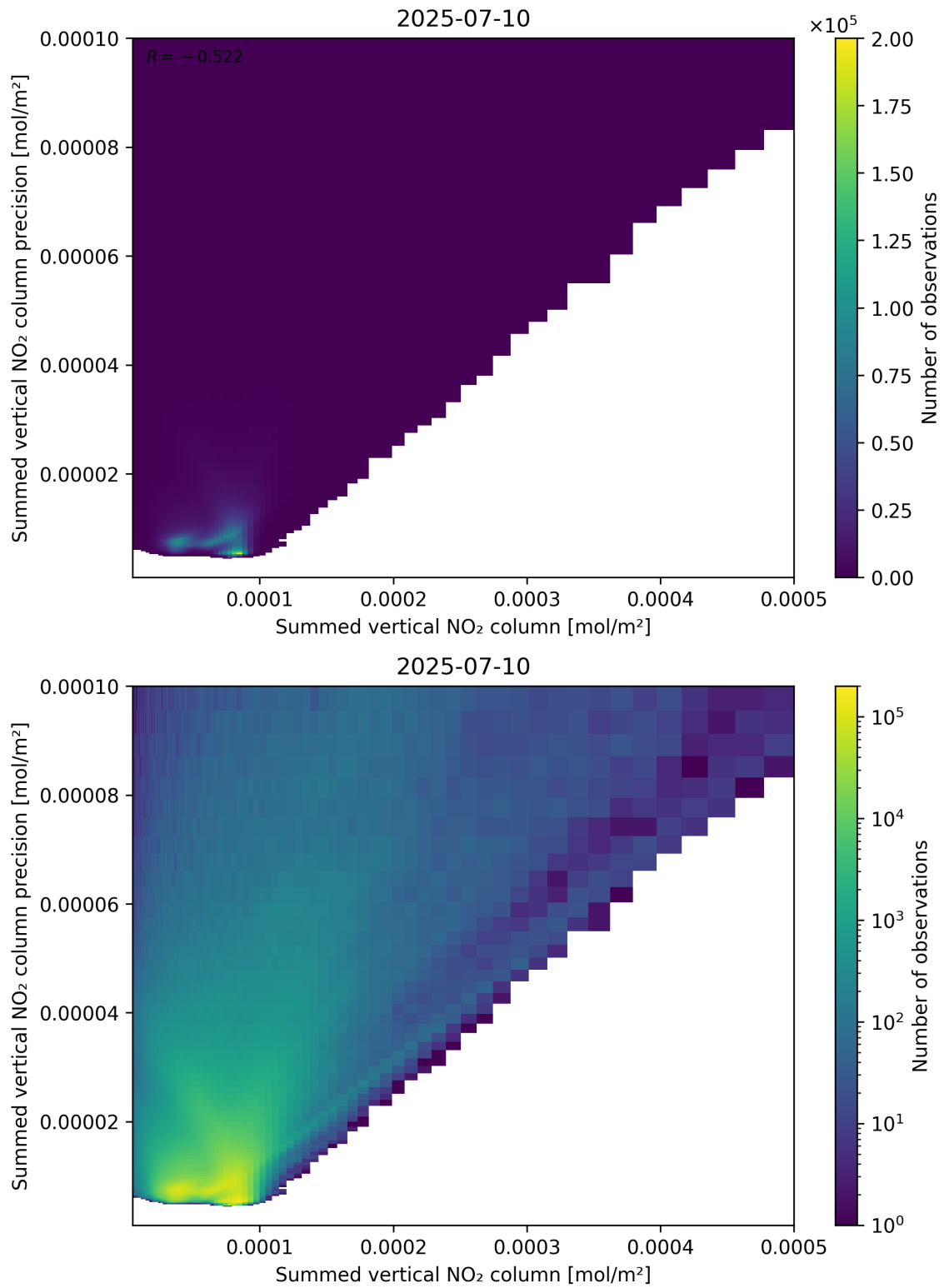
Figure 105: Scatter density plot of “Summed vertical NO 2 column” against “Summed vertical NO 2 column precision” for 2025-07-09 to 2025-07-11.
