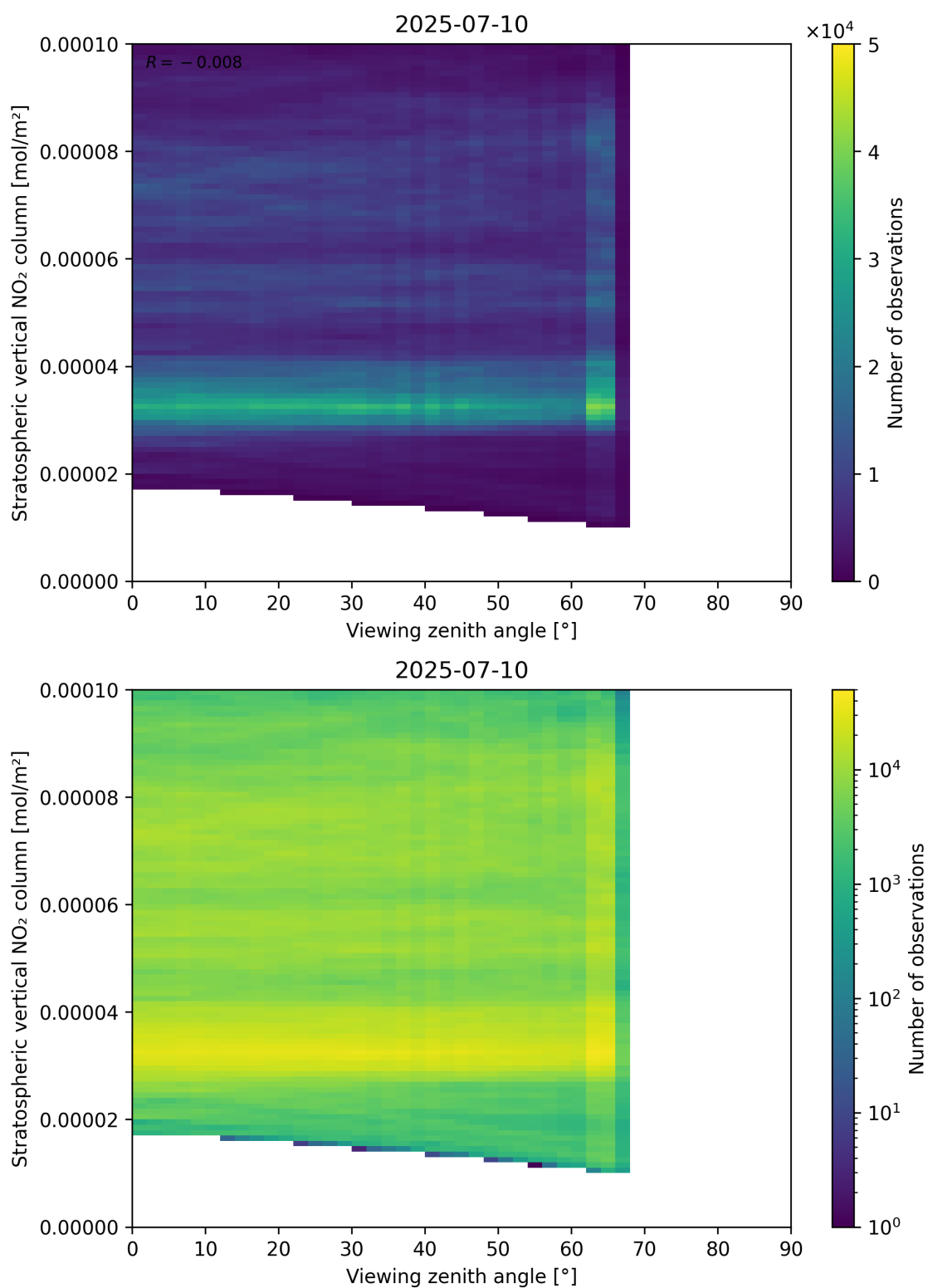
Figure 164: Scatter density plot of “Viewing zenith angle” against “Stratospheric vertical NO 2 column” for 2025-07-09 to 2025-07-11.
