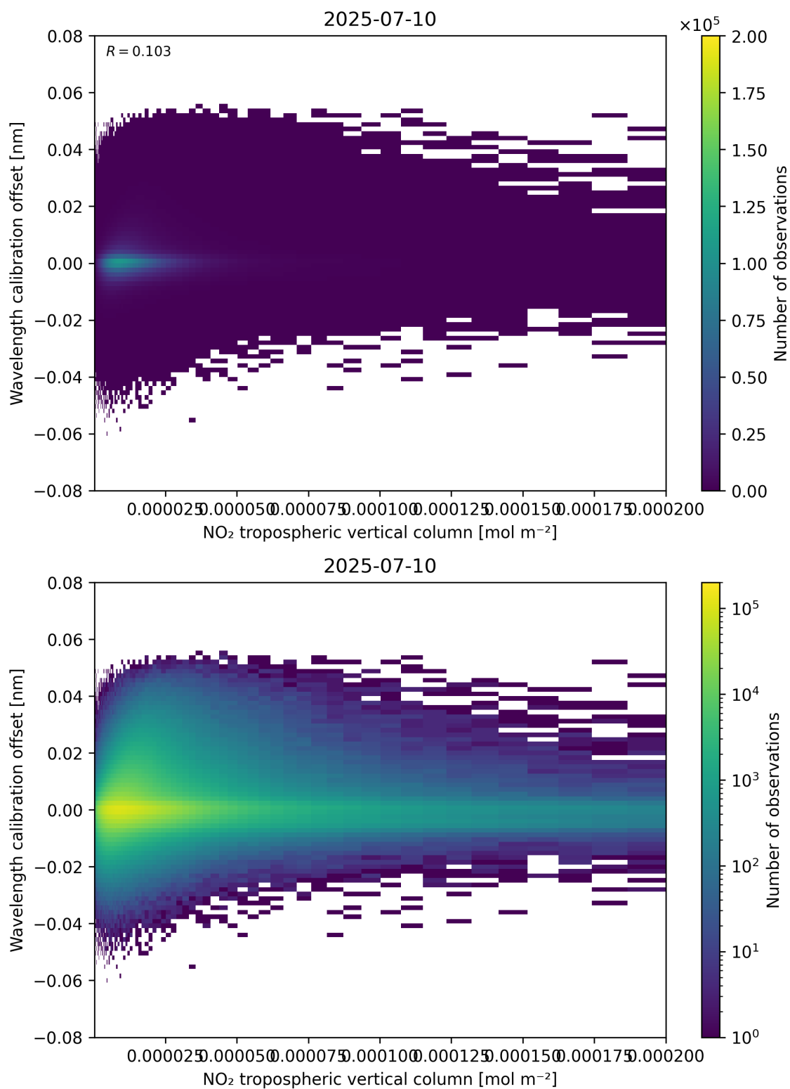
Figure 143: Scatter density plot of “NO 2 tropospheric vertical column” against “Wavelength calibration offset” for 2025-07-09 to 2025-07-11.
