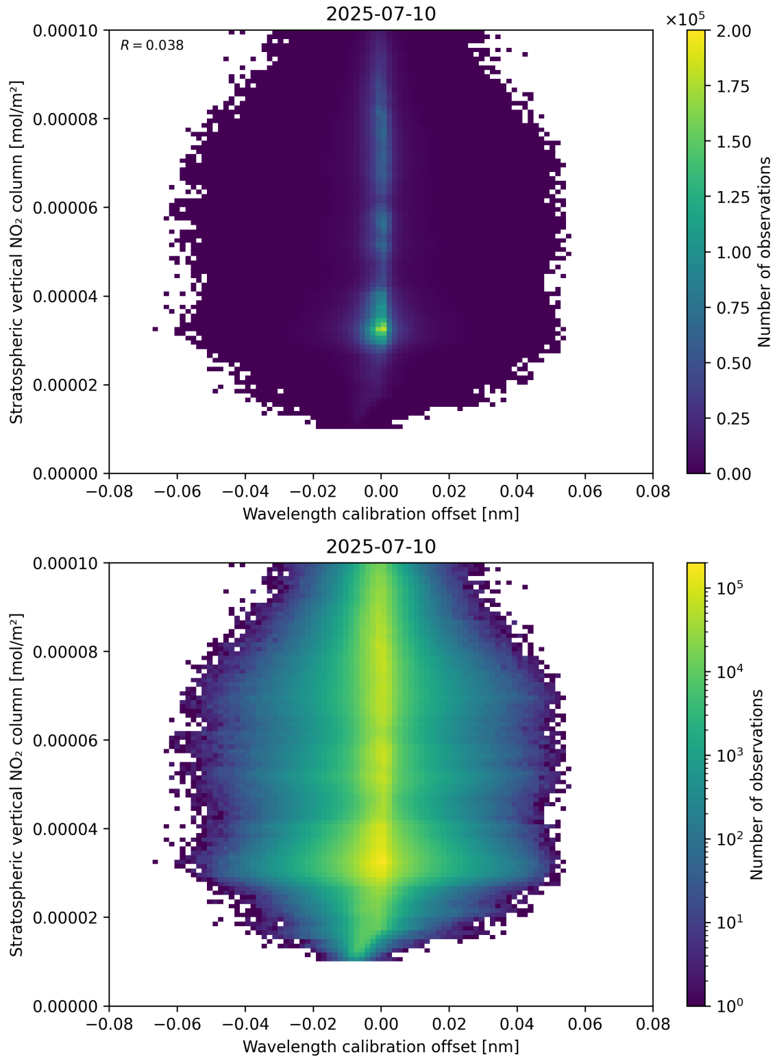
Figure 176: Scatter density plot of “Wavelength calibration offset” against “Stratospheric vertical NO 2 column” for 2025-07-09 to 2025-07-11.
