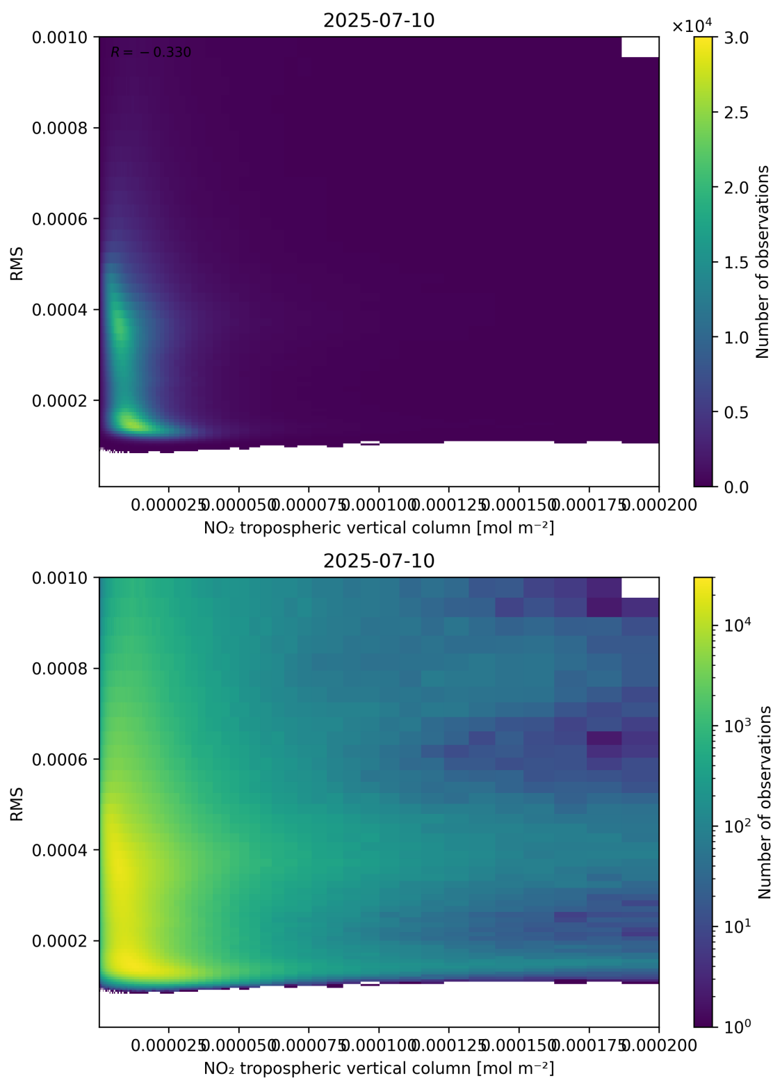
Figure 142: Scatter density plot of “NO 2 tropospheric vertical column” against “RMS” for 2025-07-09 to 2025-07-11.
