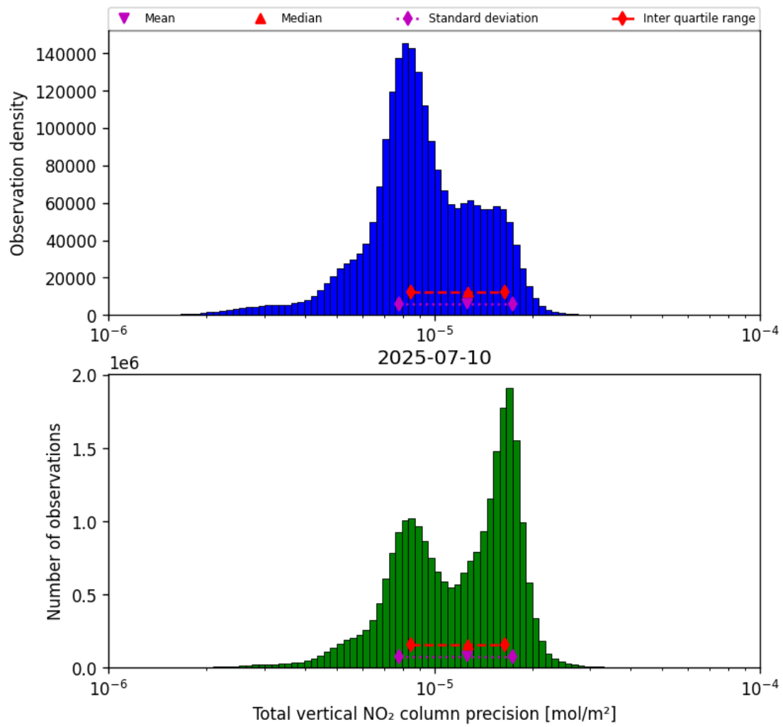
Figure 39: Histogram of “Total vertical NO 2 column precision” for 2025-07-09 to 2025-07-11
