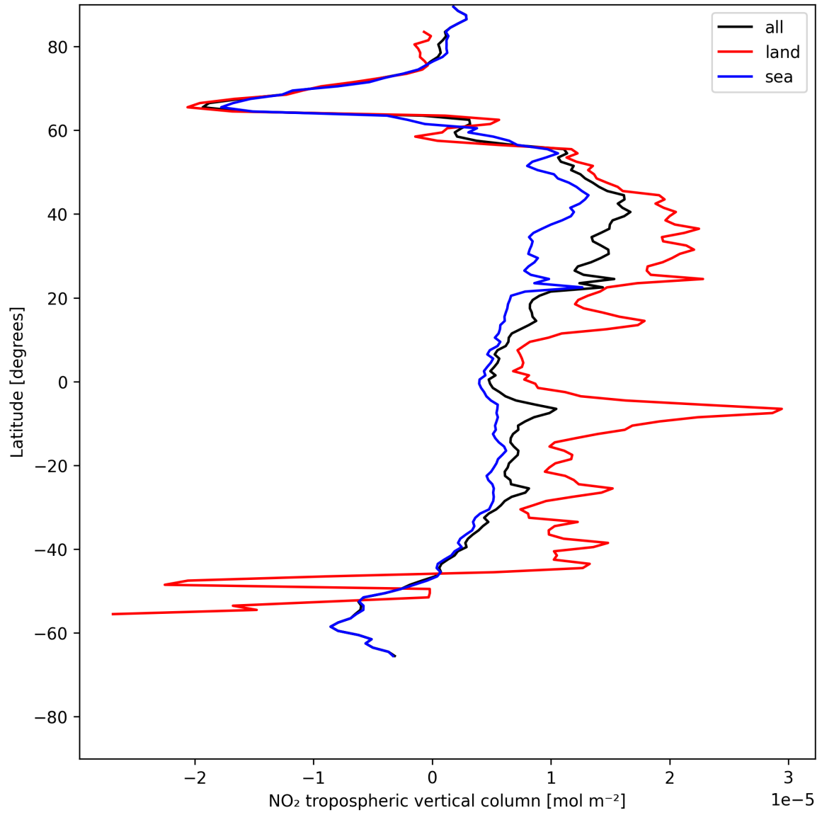
Figure 12: Zonal average of “NO 2 tropospheric vertical column” for 2025-07-09 to 2025-07-11.
