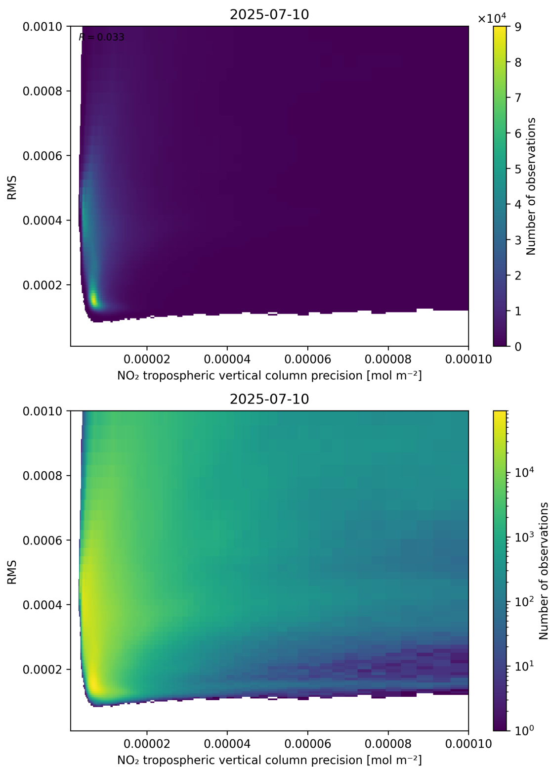
Figure 140: Scatter density plot of “NO 2 tropospheric vertical column precision” against “RMS” for 2025-07-09 to 2025-07-11.
