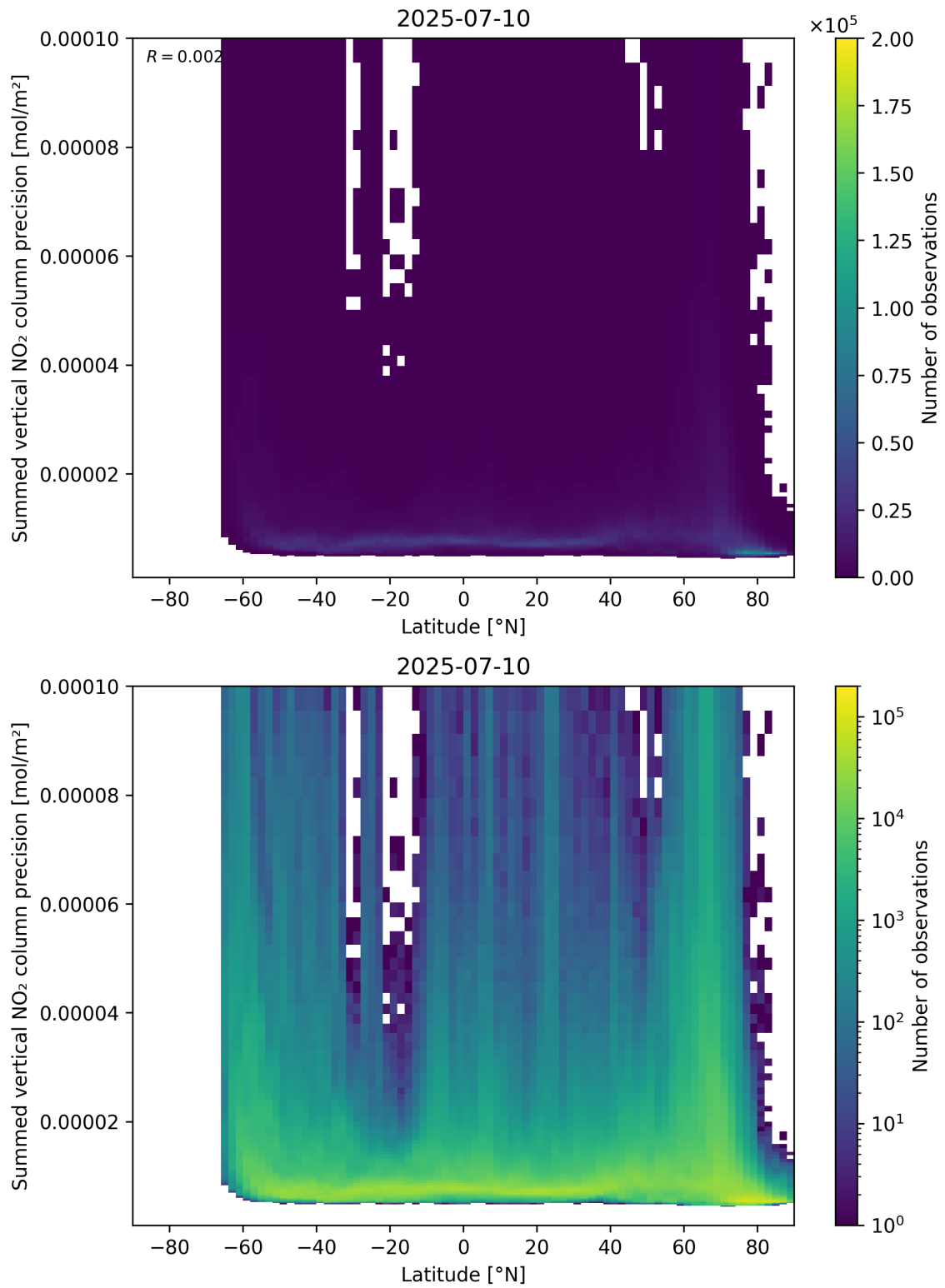
Figure 89: Scatter density plot of “Latitude” against “Summed vertical NO 2 column precision” for 2025-07-09 to 2025-07-11.
