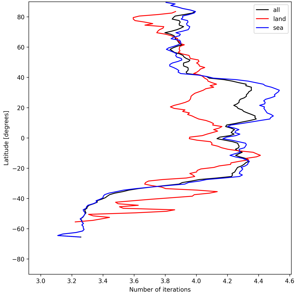
Figure 17: Zonal average of “Number of iterations” for 2025-07-09 to 2025-07-11.
