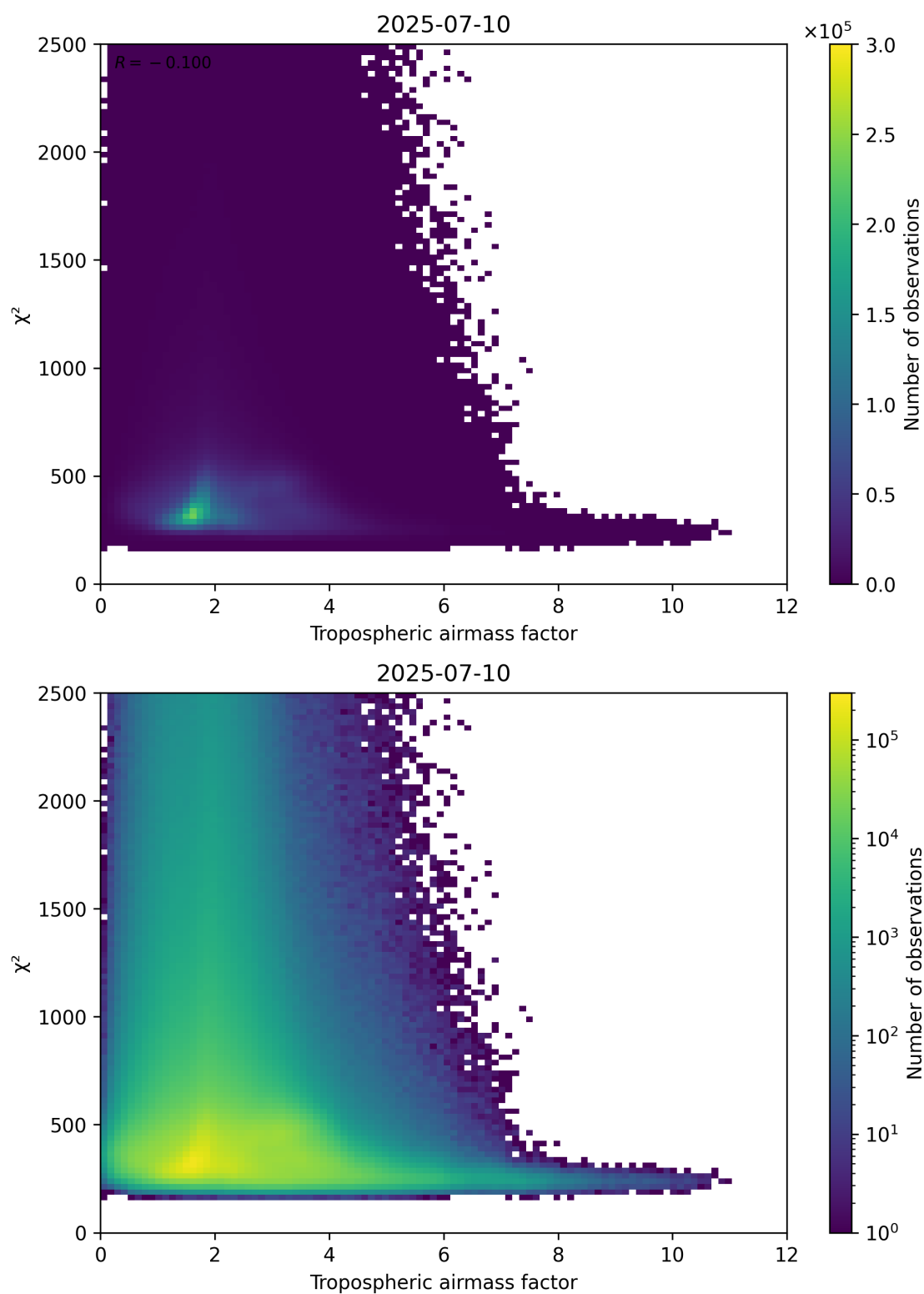
Figure 73: Scatter density plot of “Tropospheric airmass factor” against “ \chi^2 ” for 2025-07-09 to 2025-07-11.
