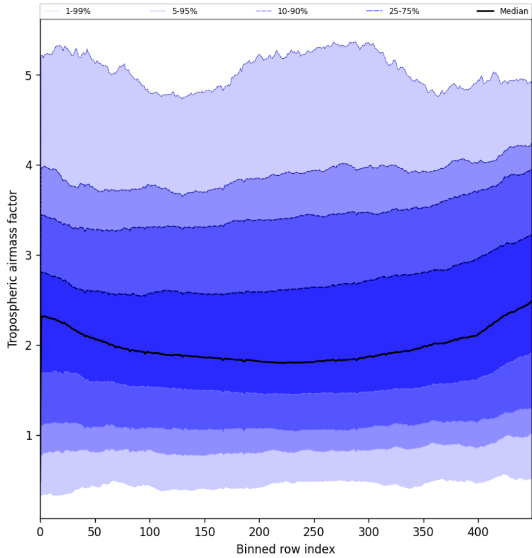
Figure 48: Along track statistics of “Tropospheric airmass factor” for 2025-07-09 to 2025-07-11
