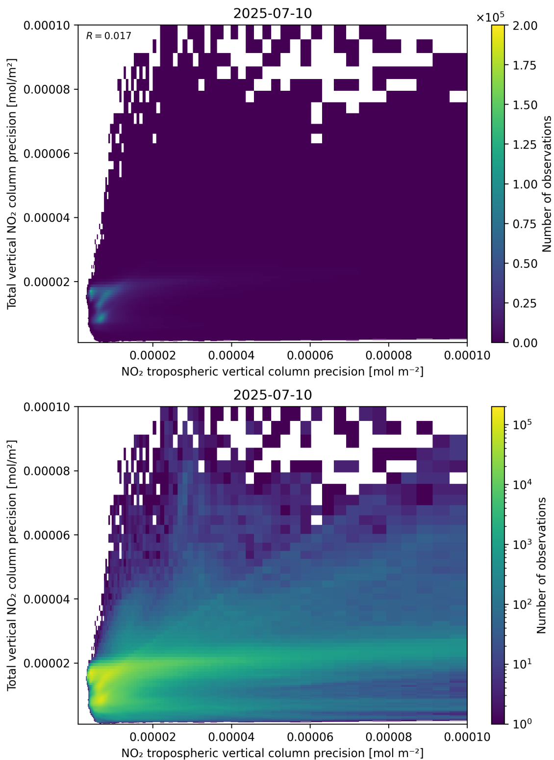
Figure 139: Scatter density plot of “NO 2 tropospheric vertical column precision” against “Total vertical NO 2 column precision” for 2025-07-09 to 2025-07-11.
