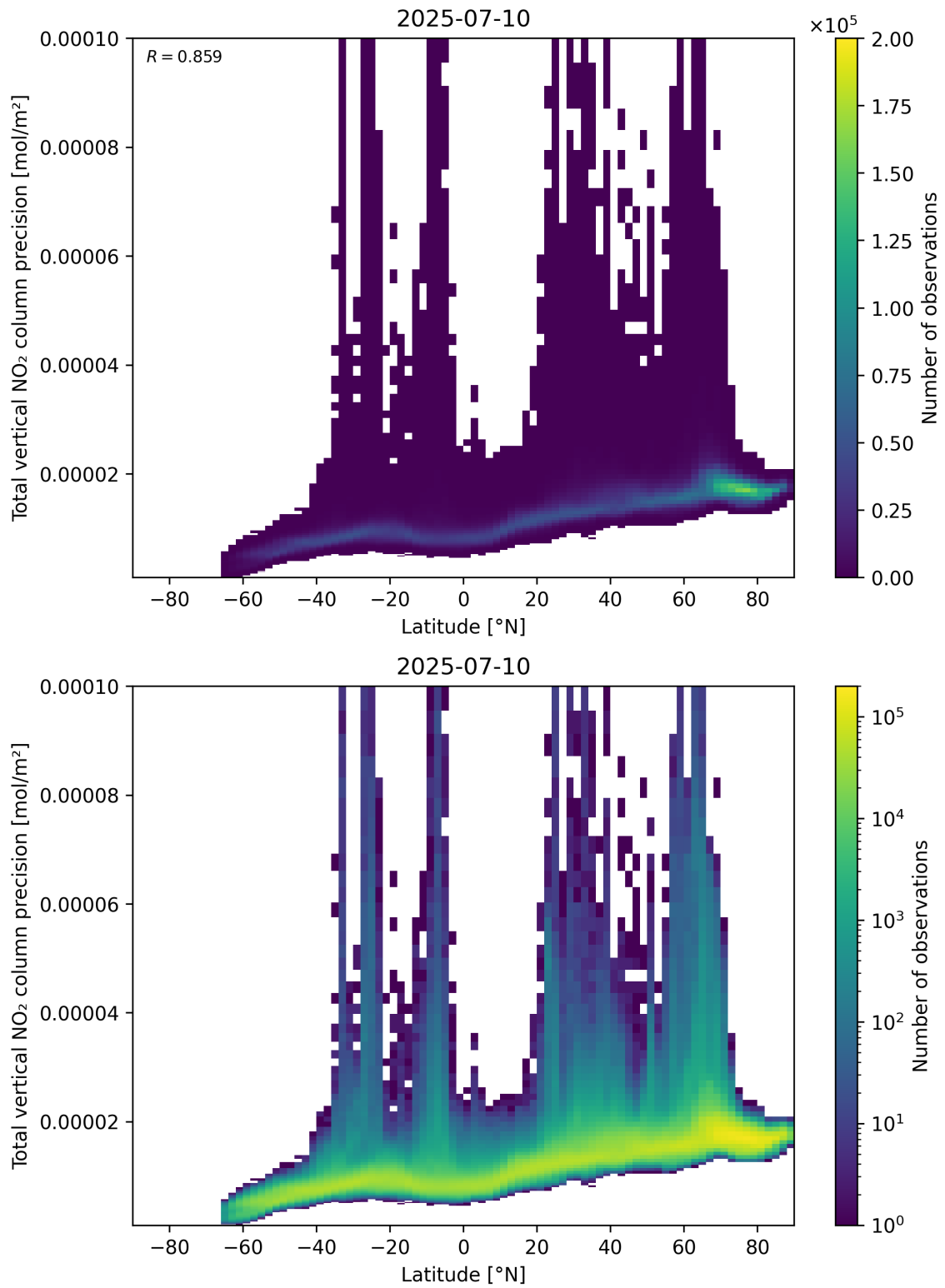
Figure 91: Scatter density plot of “Latitude” against “Total vertical NO 2 column precision” for 2025-07-09 to 2025-07-11.
