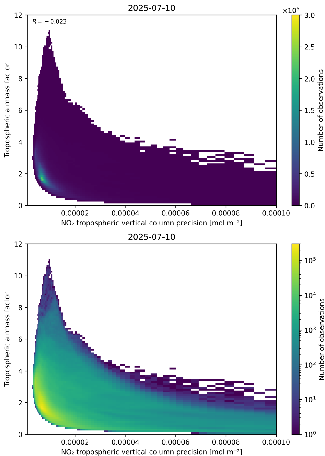
Figure 133: Scatter density plot of “NO 2 tropospheric vertical column precision” against “Tropospheric air mass factor” for 2025-07-09 to 2025-07-11.
