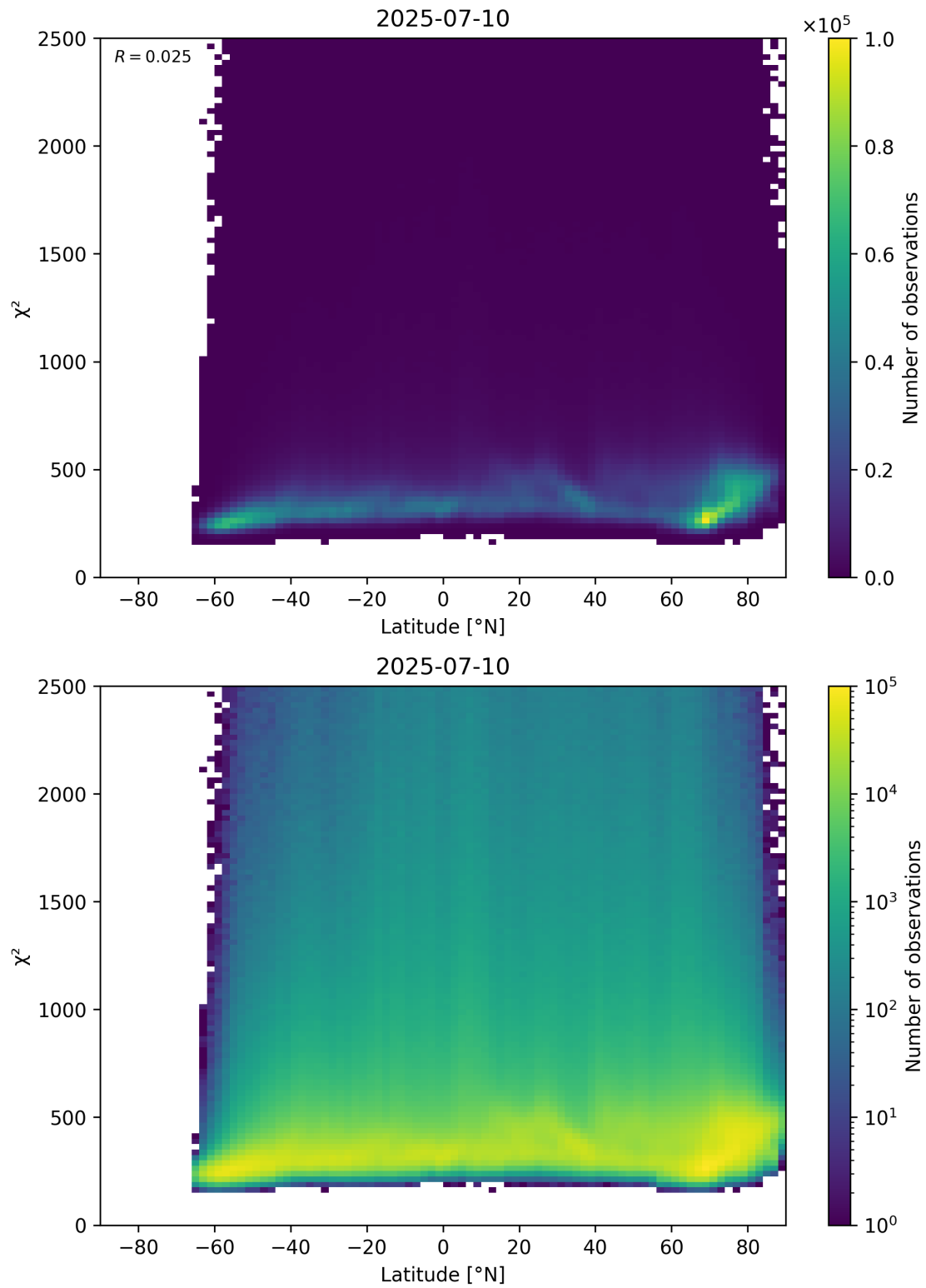
Figure 86: Scatter density plot of “Latitude” against “ \chi^2 ” for 2025-07-09 to 2025-07-11.
