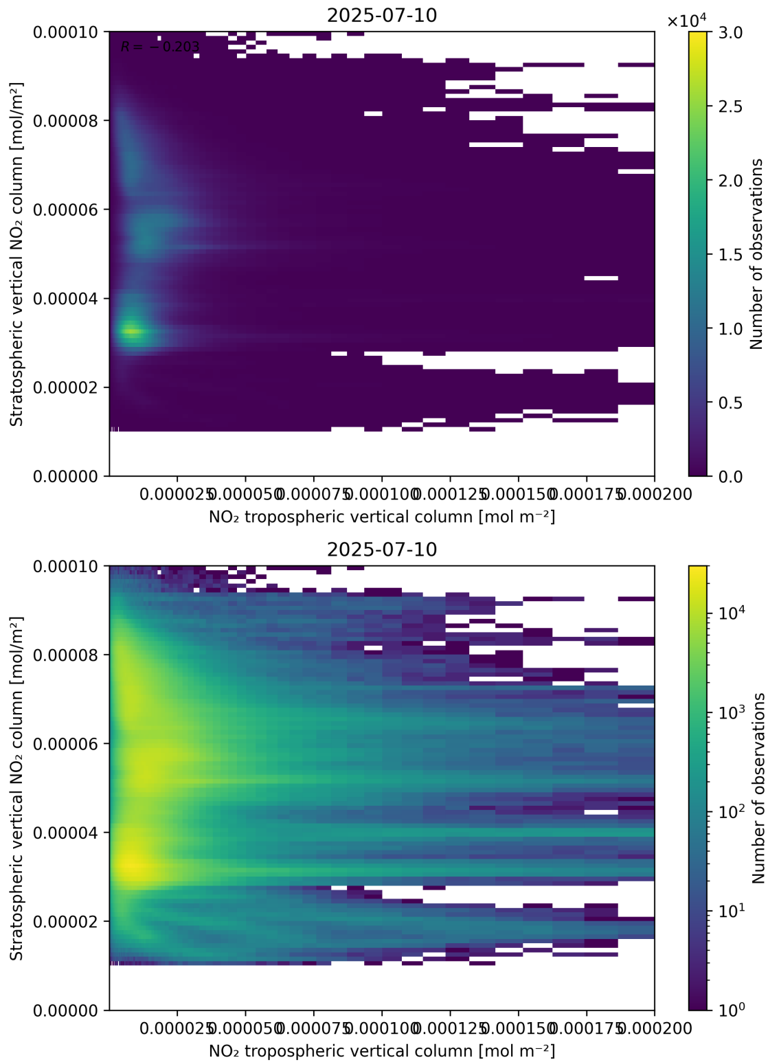
Figure 125: Scatter density plot of “NO 2 tropospheric vertical column” against “Stratospheric vertical NO 2 column” for 2025-07-09 to 2025-07-11.
