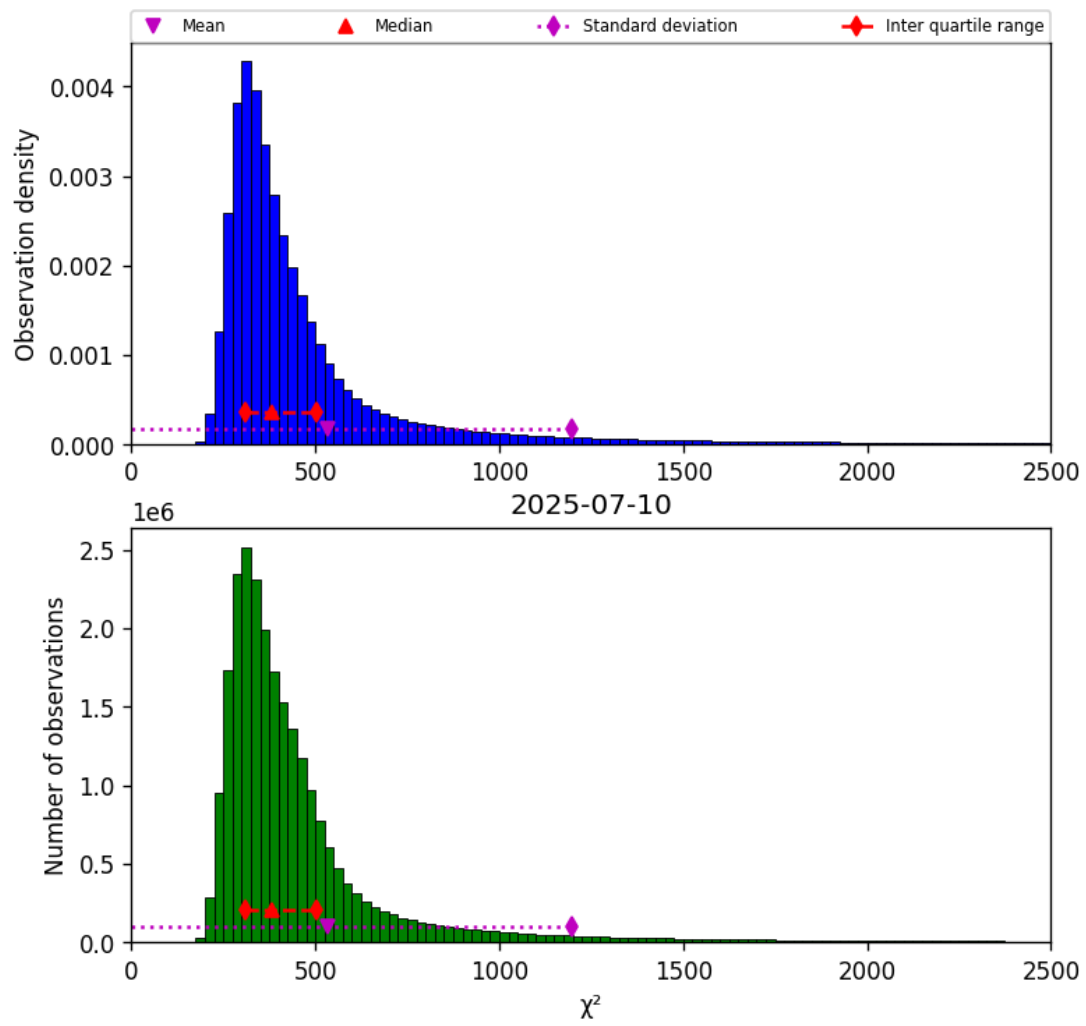
Figure 42: Histogram of “ \chi^2 ” for 2025-07-09 to 2025-07-11
