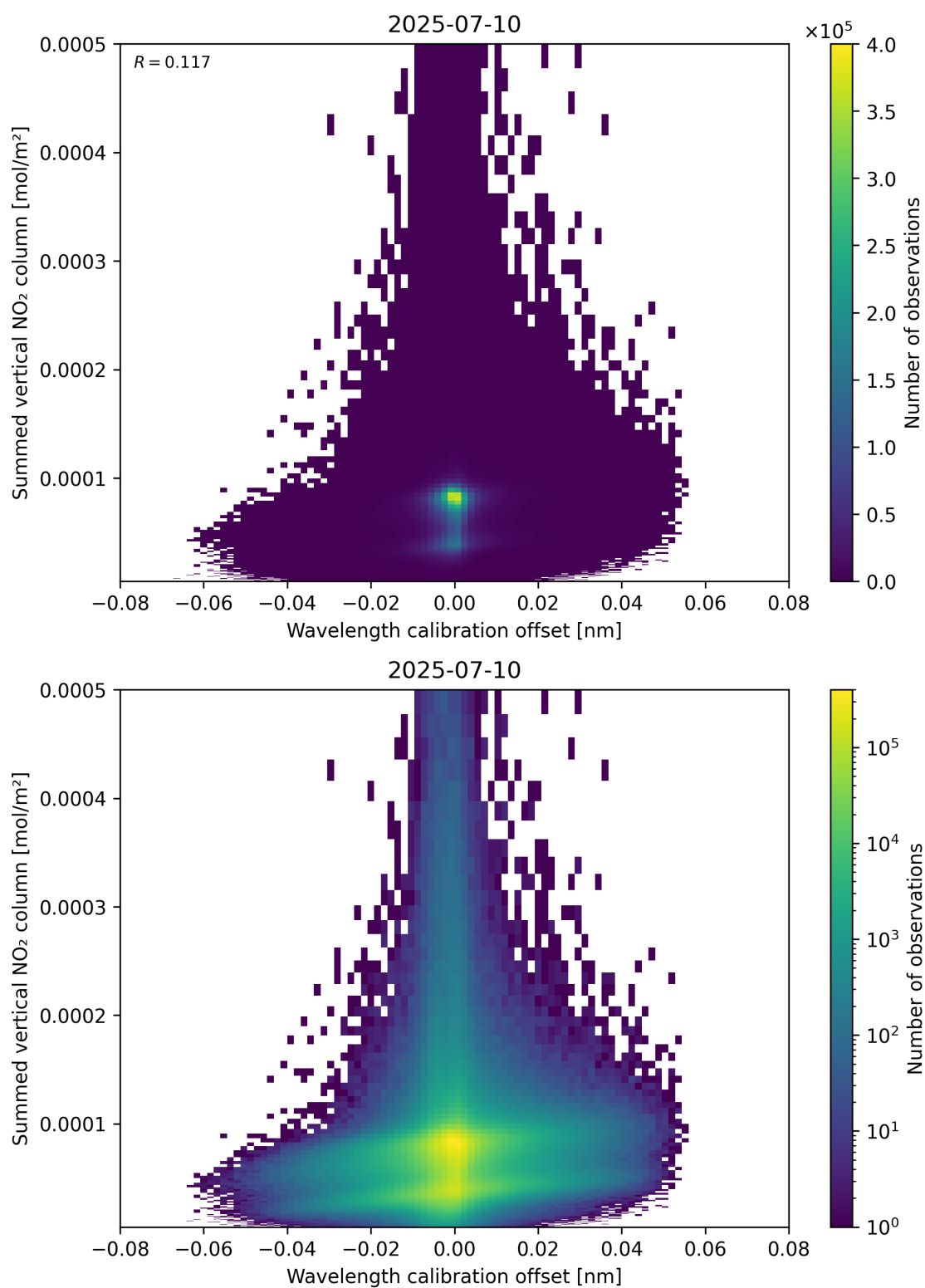
Figure 177: Scatter density plot of “Wavelength calibration offset” against “Summed vertical NO 2 column” for 2025-07-09 to 2025-07-11.
