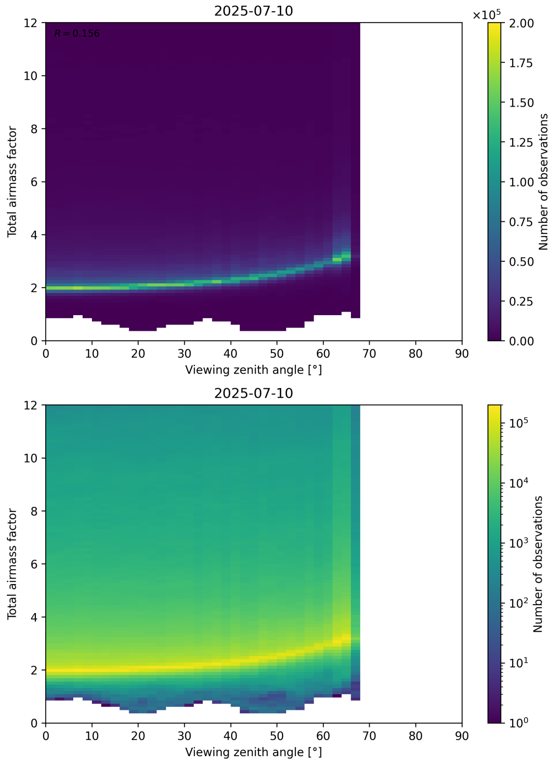
Figure 160: Scatter density plot of “Viewing zenith angle” against “Total airmass factor” for 2025-07-09 to 2025-07-11.
