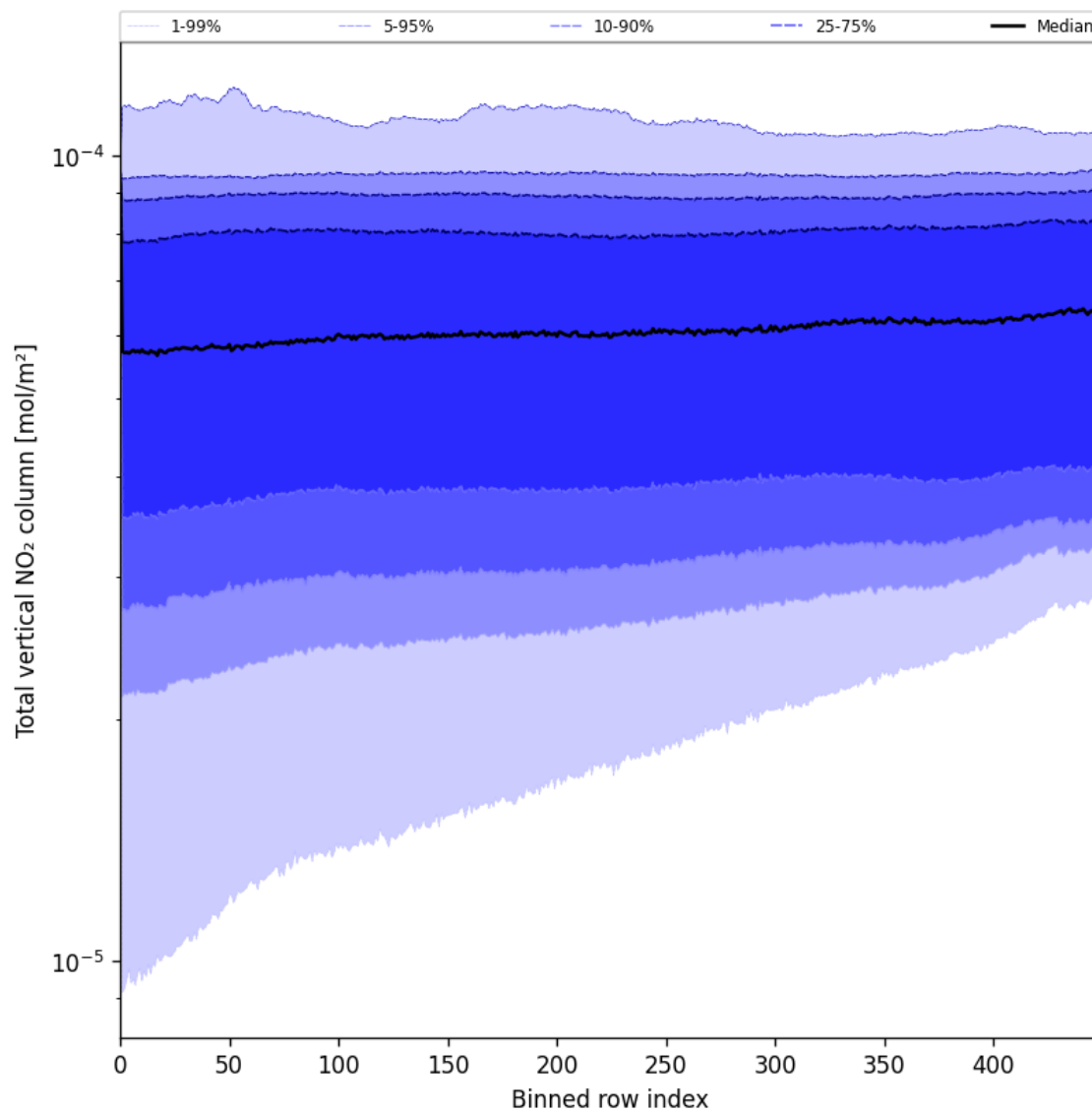
Figure 55: Along track statistics of “Total vertical NO 2 column” for 2025-07-09 to 2025-07-11
