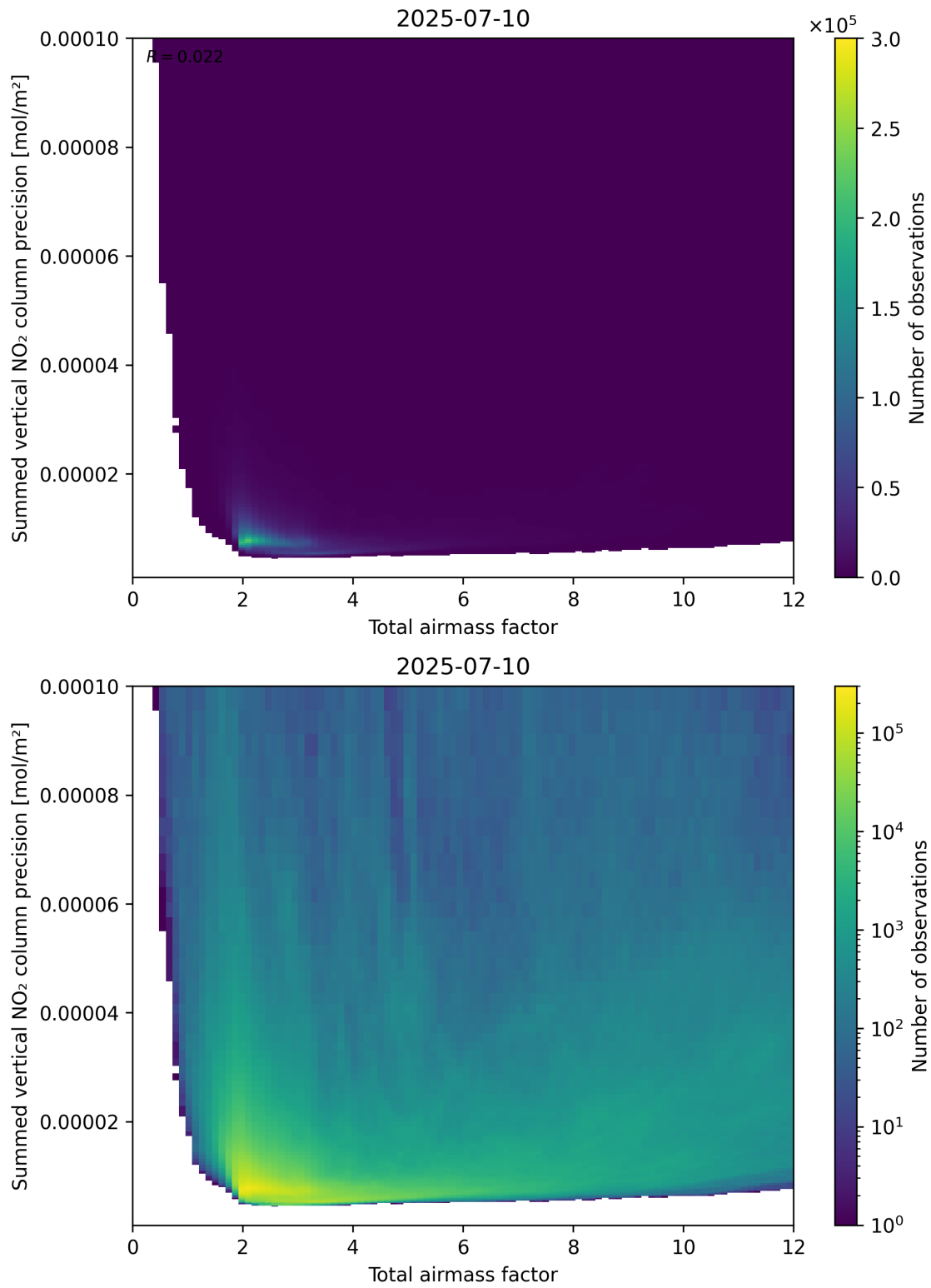
Figure 66: Scatter density plot of “Total airmass factor” against “Summed vertical NO 2 column precision” for 2025-07-09 to 2025-07-11.
