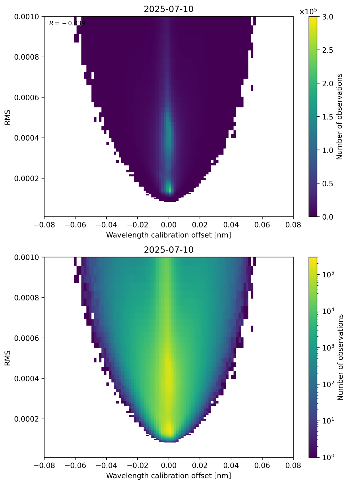
Figure 181: Scatter density plot of “Wavelength calibration offset” against “RMS” for 2025-07-09 to 2025-07-11.
