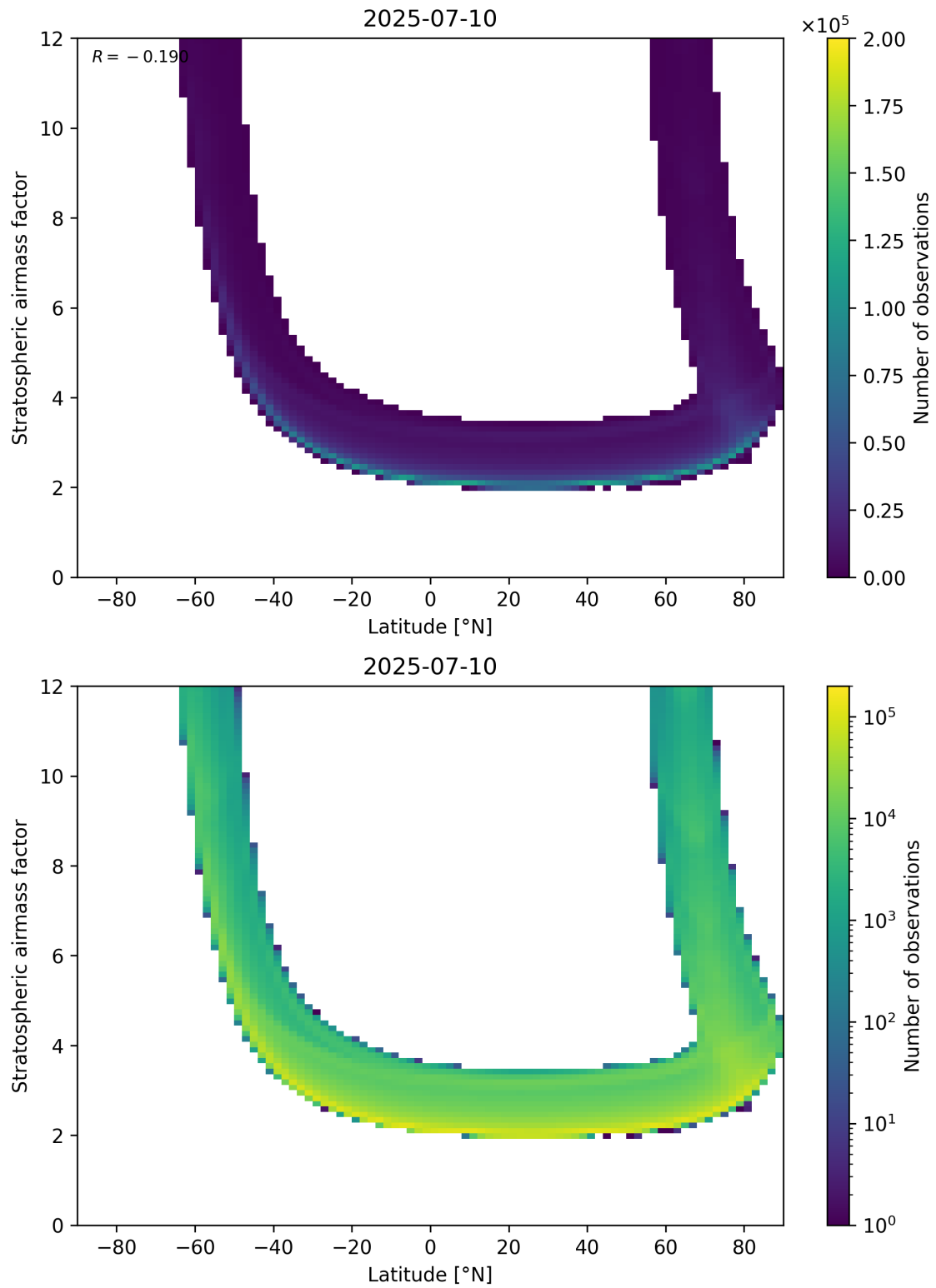
Figure 83: Scatter density plot of “Latitude” against “Stratospheric air mass factor” for 2025-07-09 to 2025-07-11.
