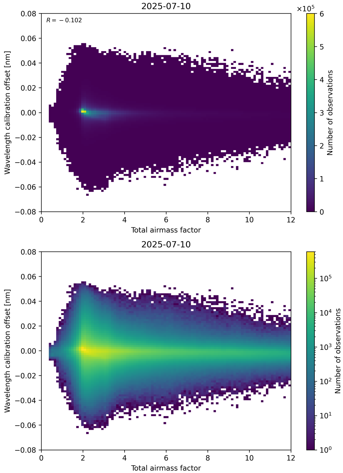
Figure 70: Scatter density plot of “Total airmass factor” against “Wavelength calibration offset” for 2025-07-09 to 2025-07-11.
