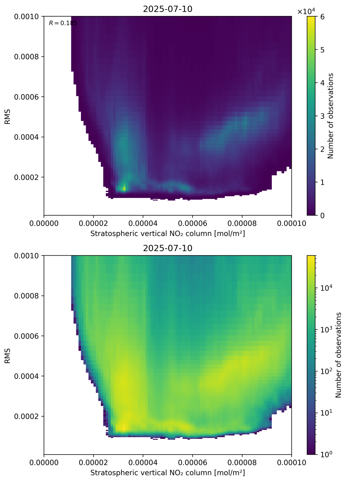
Figure 102: Scatter density plot of “Stratospheric vertical NO 2 column” against “RMS” for 2025-07-09 to 2025-07-11.
