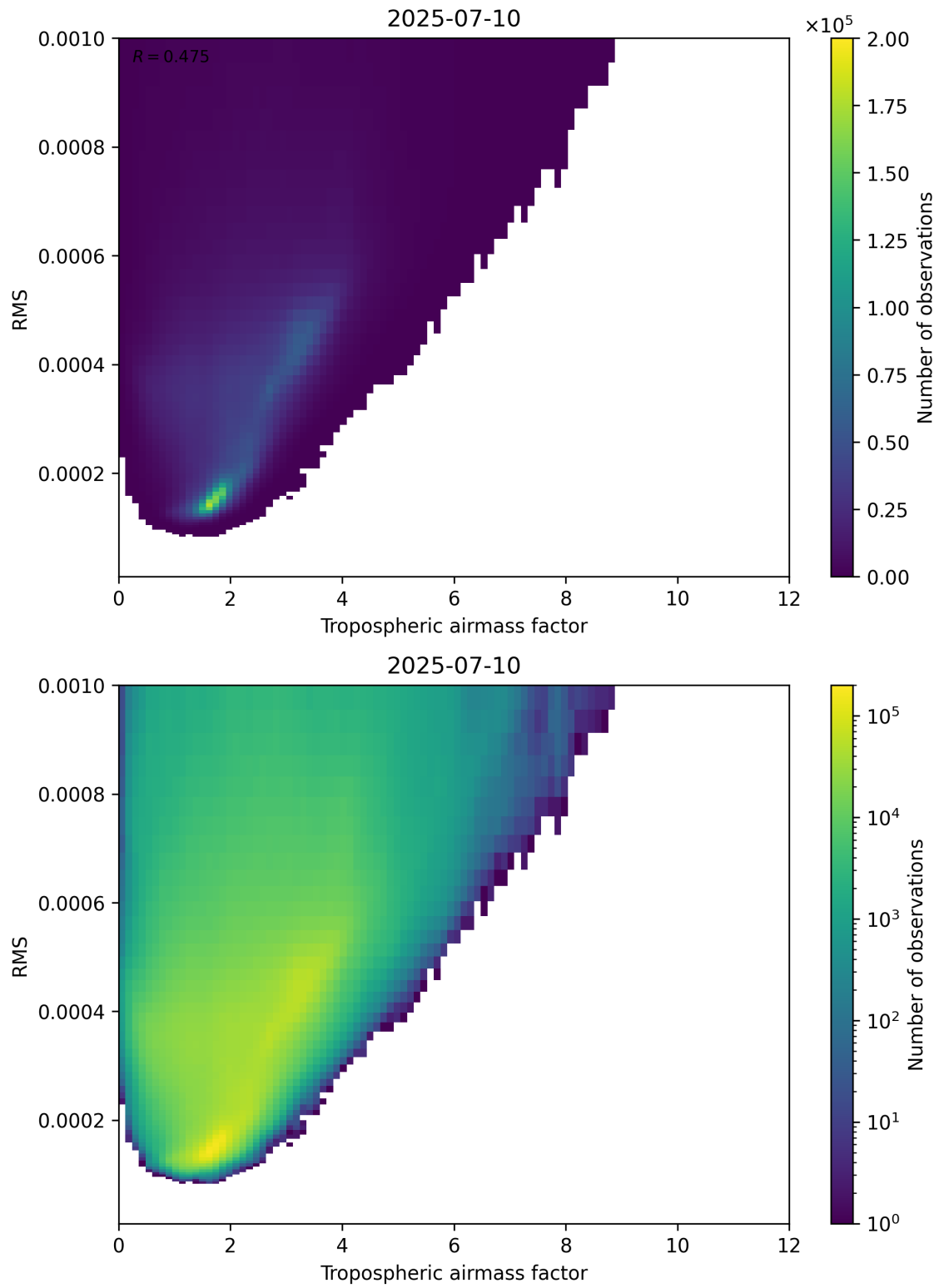
Figure 79: Scatter density plot of “Tropospheric airmass factor” against “RMS” for 2025-07-09 to 2025-07-11.
