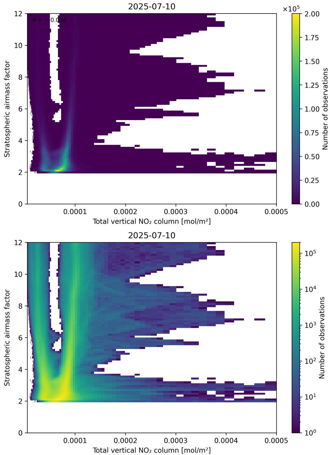
Figure 110: Scatter density plot of “Total vertical NO 2 column” against “Stratospheric air mass factor” for 2025-07-09 to 2025-07-11.
