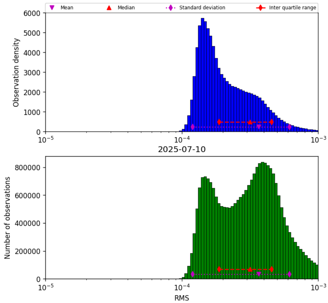
Figure 43: Histogram of “RMS” for 2025-07-09 to 2025-07-11
