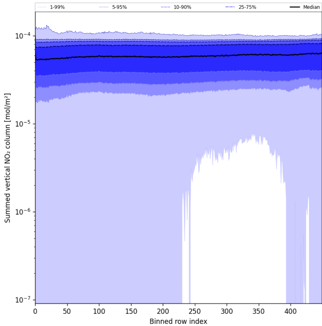
Figure 57: Along track statistics of “Summed vertical NO 2 column” for 2025-07-09 to 2025-07-11
