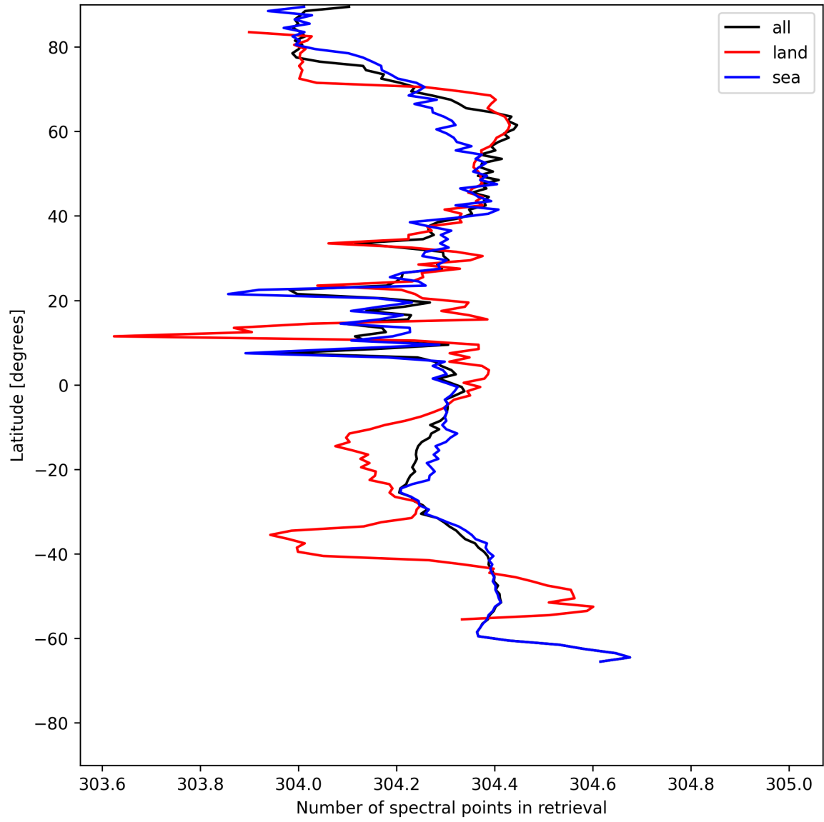
Figure 16: Zonal average of “Number of spectral points in retrieval” for 2025-07-09 to 2025-07-11.
