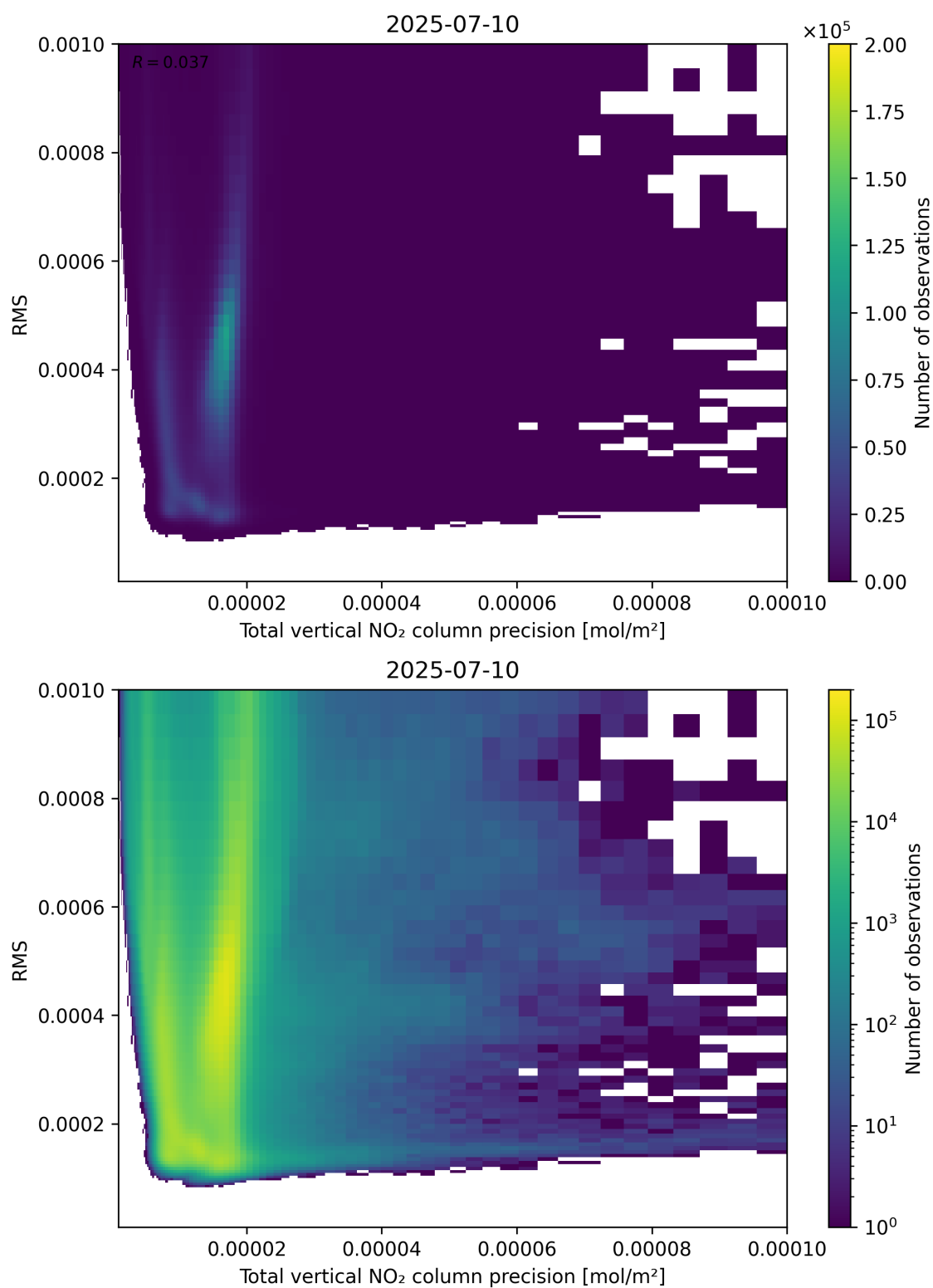
Figure 119: Scatter density plot of “Total vertical NO 2 column precision” against “RMS” for 2025-07-09 to 2025-07-11.
