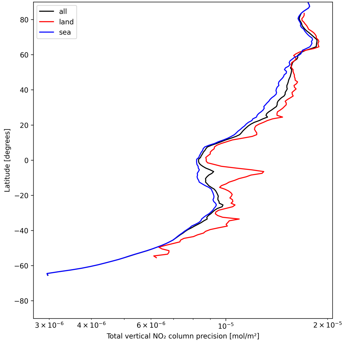
Figure 22: Zonal average of “Total vertical NO 2 column precision” for 2025-07-09 to 2025-07-11.
