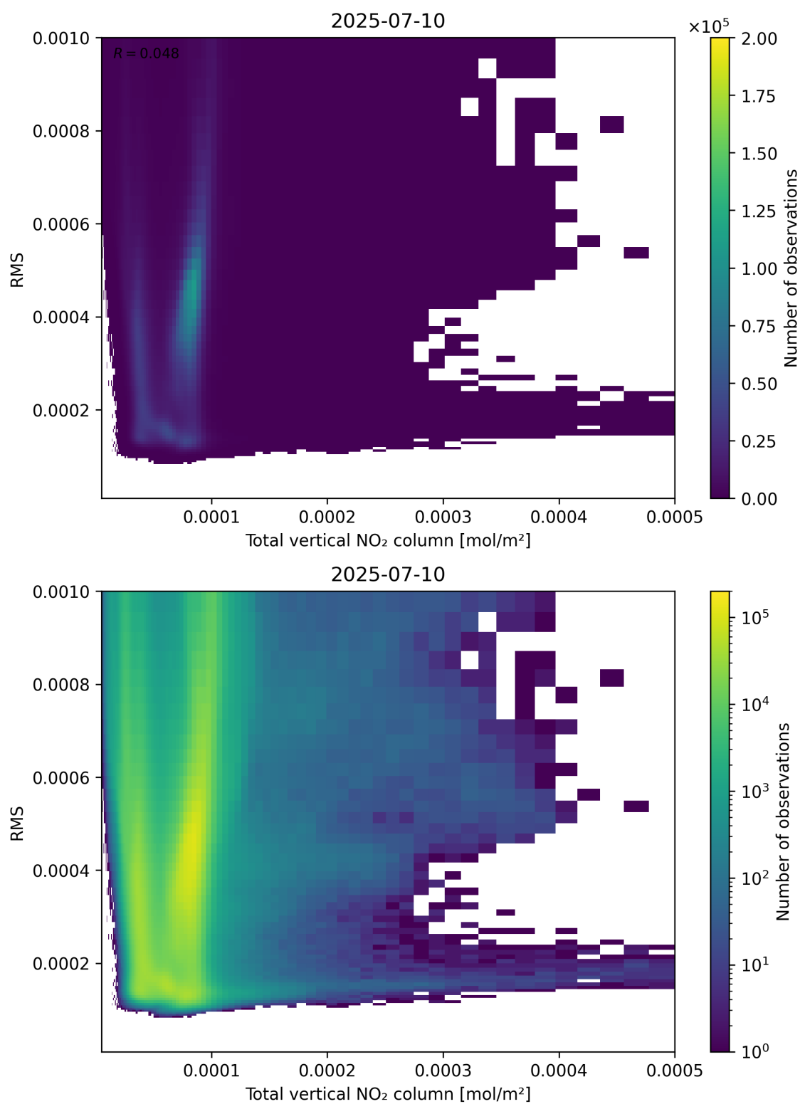
Figure 120: Scatter density plot of “Total vertical NO 2 column” against “RMS” for 2025-07-09 to 2025-07-11.
