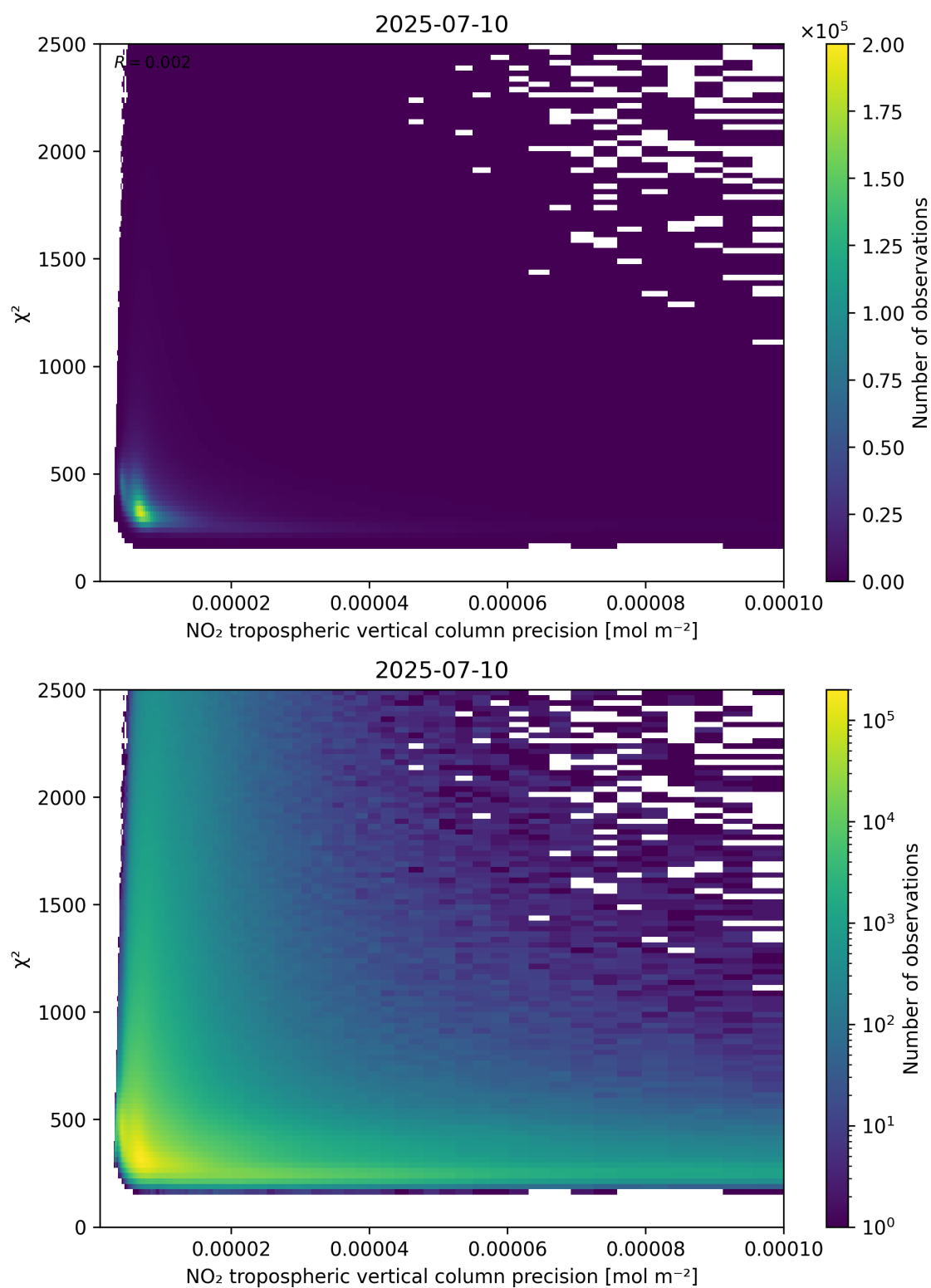
Figure 134: Scatter density plot of “NO 2 tropospheric vertical column precision” against “ \chi^2 ” for 2025-07-09 to 2025-07-11.
