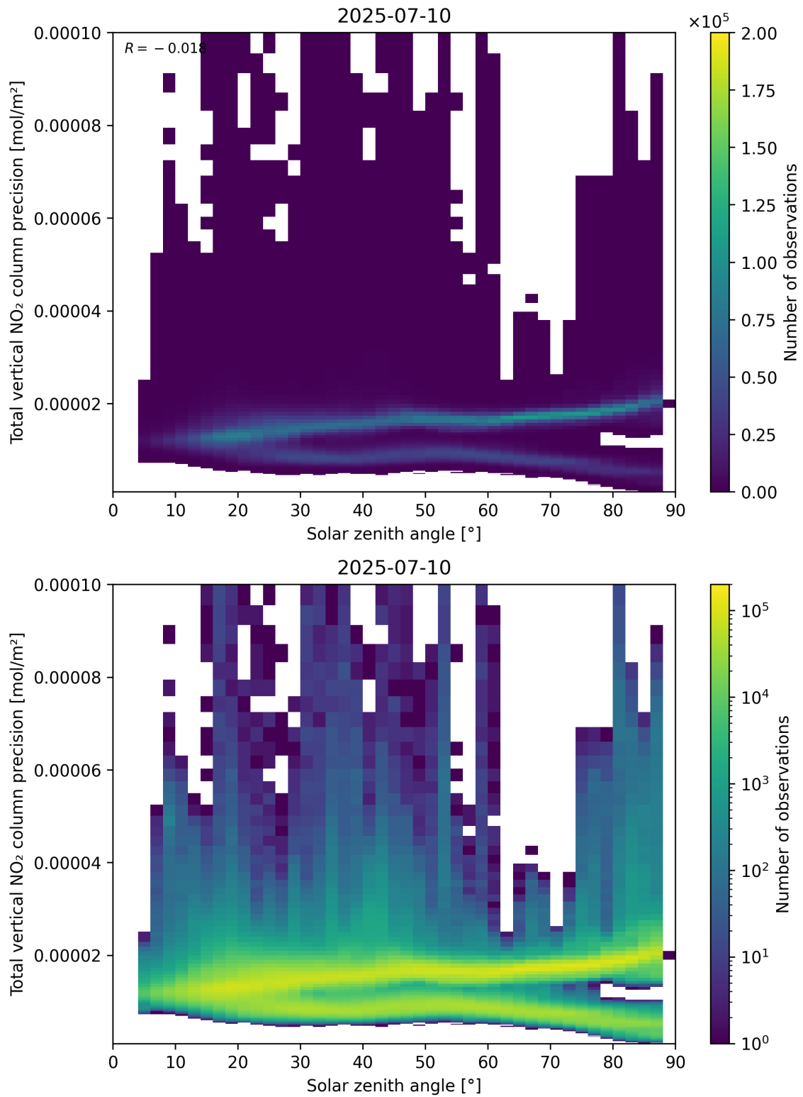
Figure 154: Scatter density plot of “Solar zenith angle” against “Total vertical NO 2 column precision” for 2025-07-09 to 2025-07-11.
