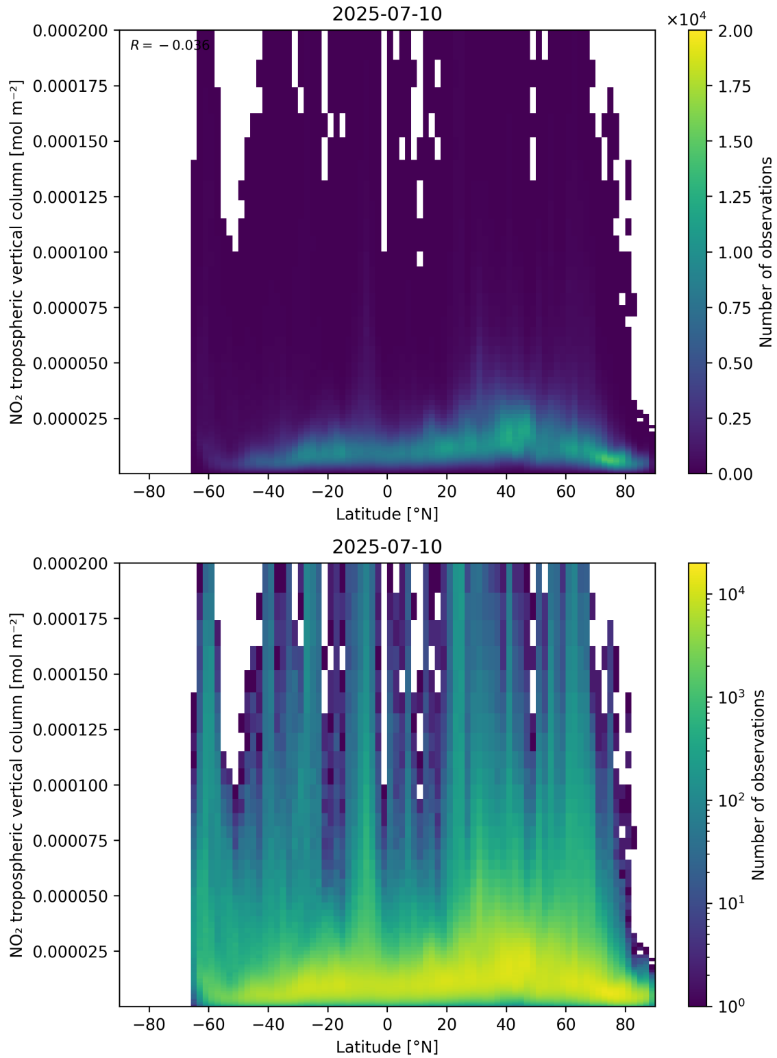
Figure 92: Scatter density plot of “Latitude” against “NO 2 tropospheric vertical column” for 2025-07-09 to 2025-07-11.
