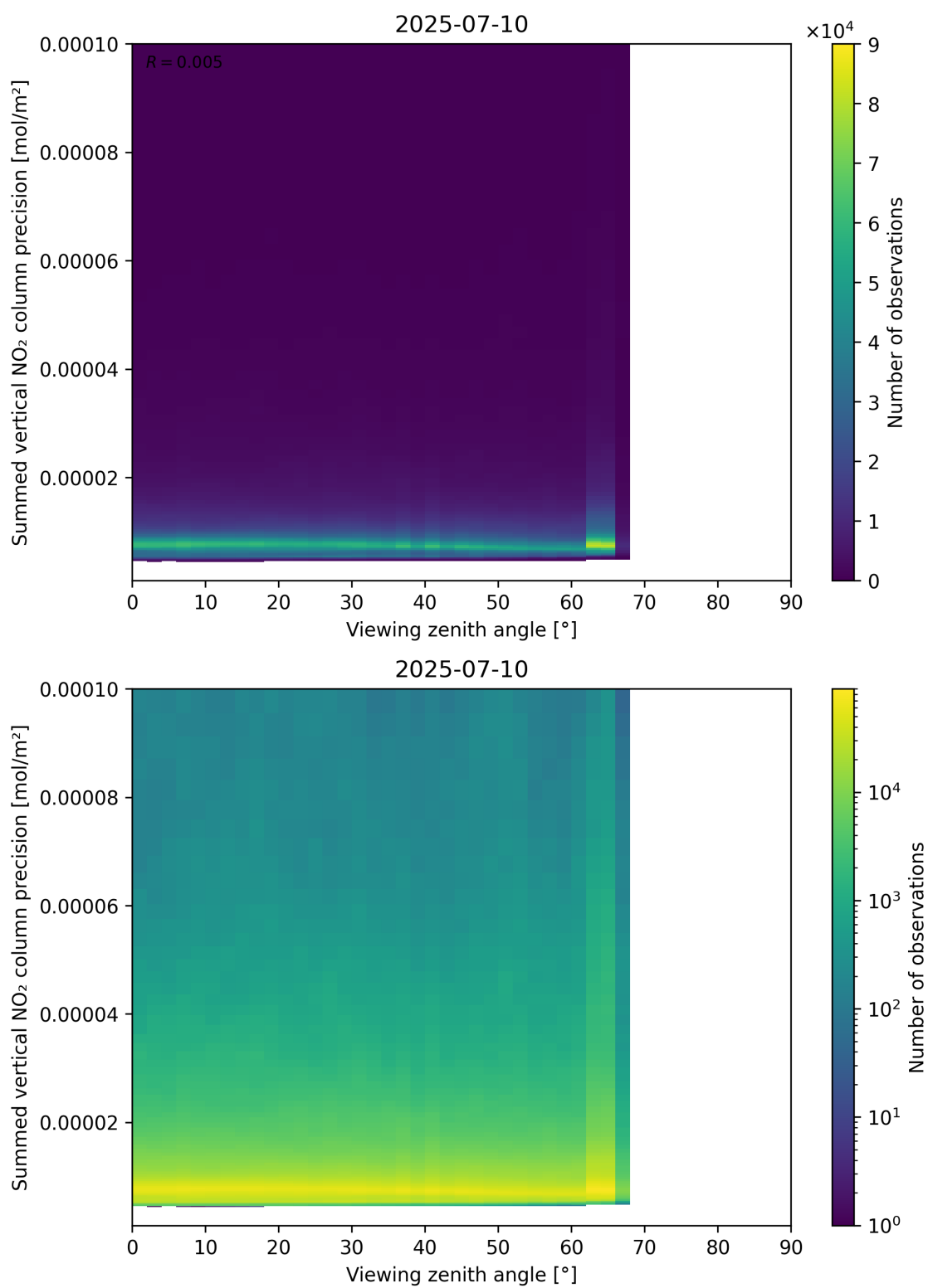
Figure 166: Scatter density plot of “Viewing zenith angle” against “Summed vertical NO 2 column precision” for 2025-07-09 to 2025-07-11.
