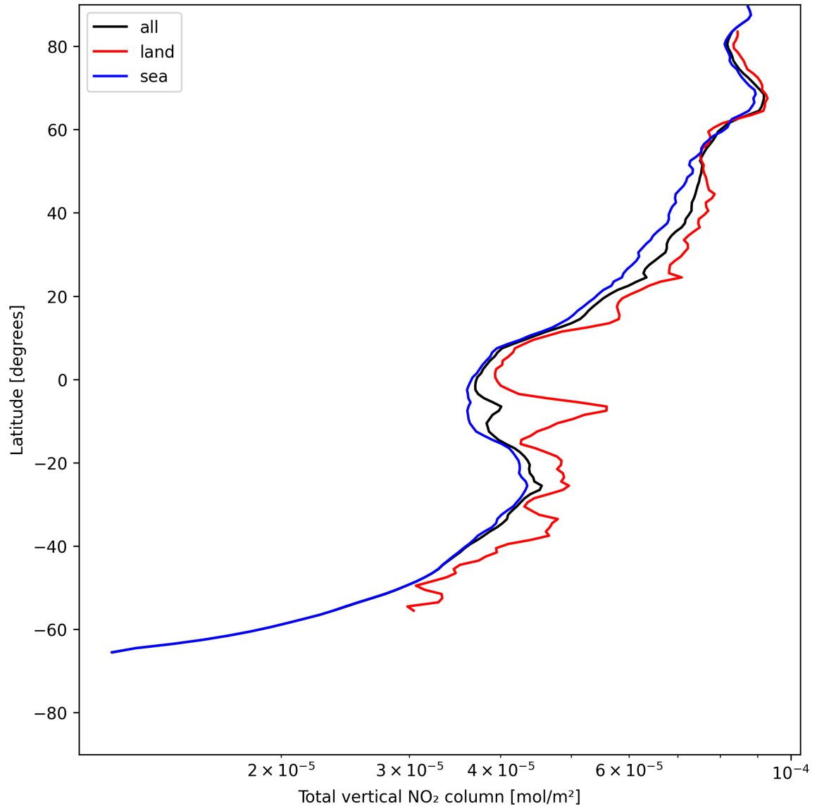
Figure 21: Zonal average of “Total vertical NO 2 column” for 2025-07-09 to 2025-07-11.
