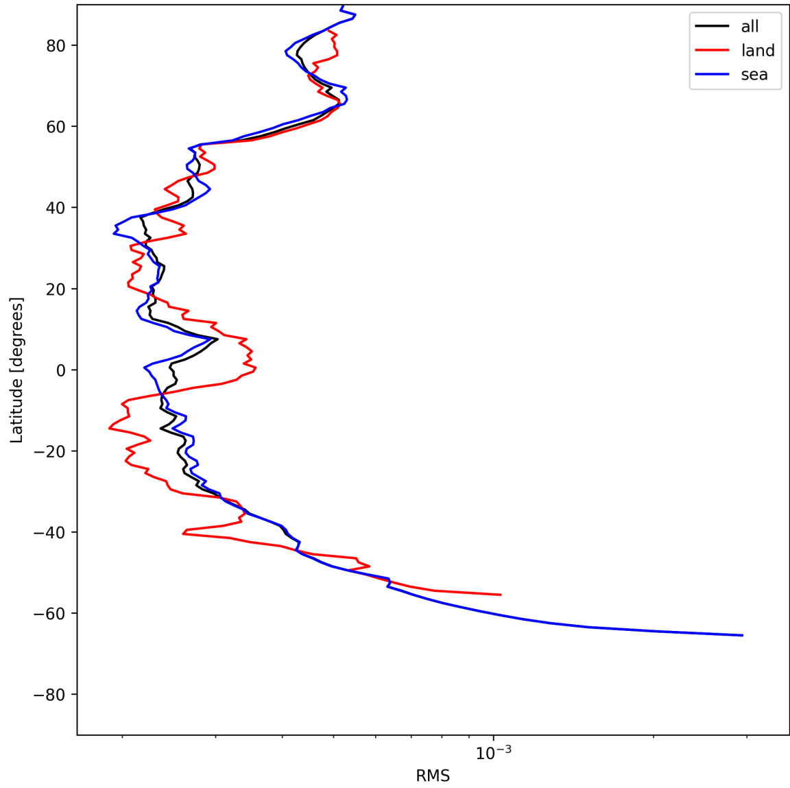
Figure 26: Zonal average of “RMS” for 2025-07-09 to 2025-07-11.
