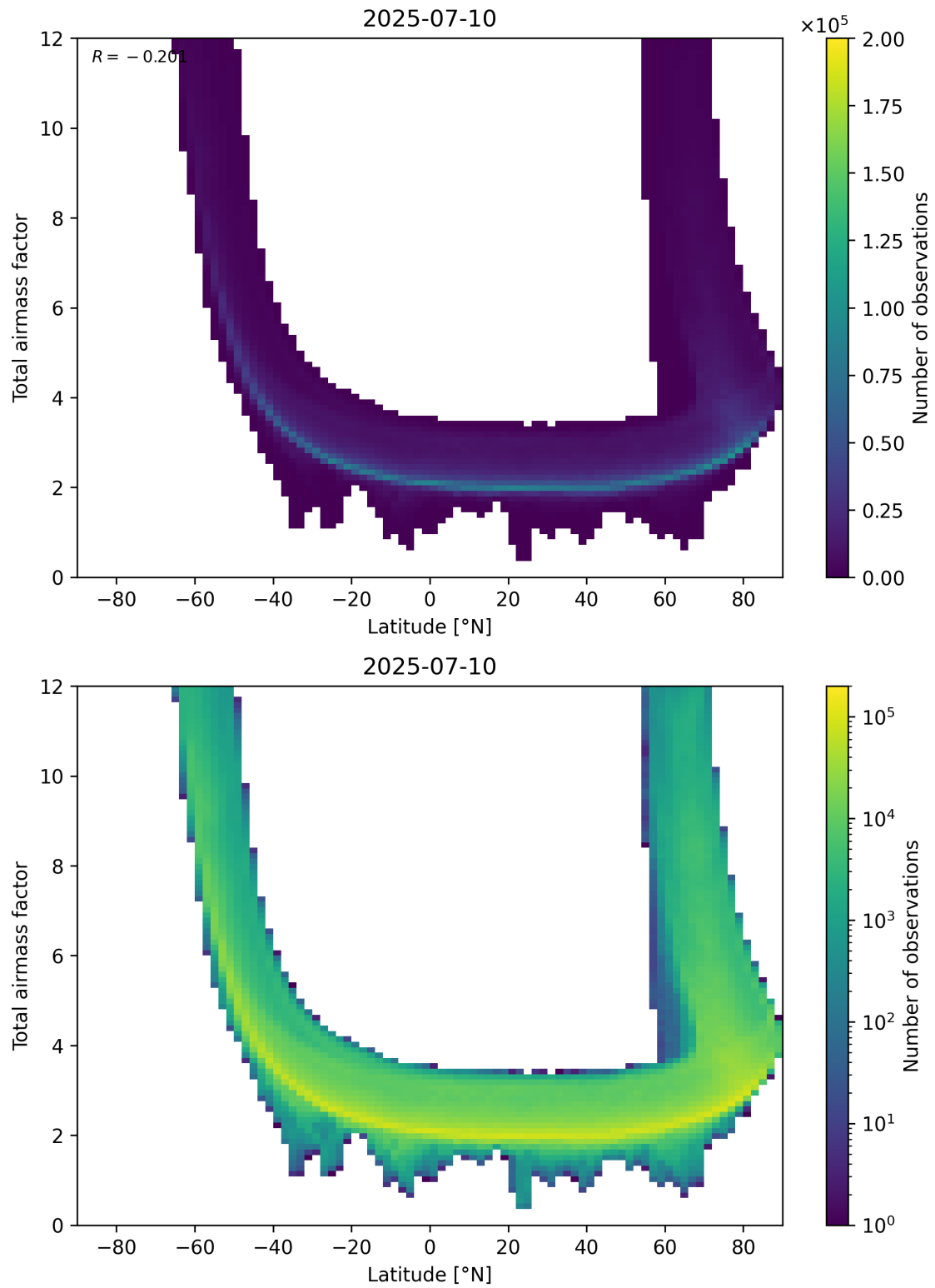
Figure 84: Scatter density plot of “Latitude” against “Total airmass factor” for 2025-07-09 to 2025-07-11.
