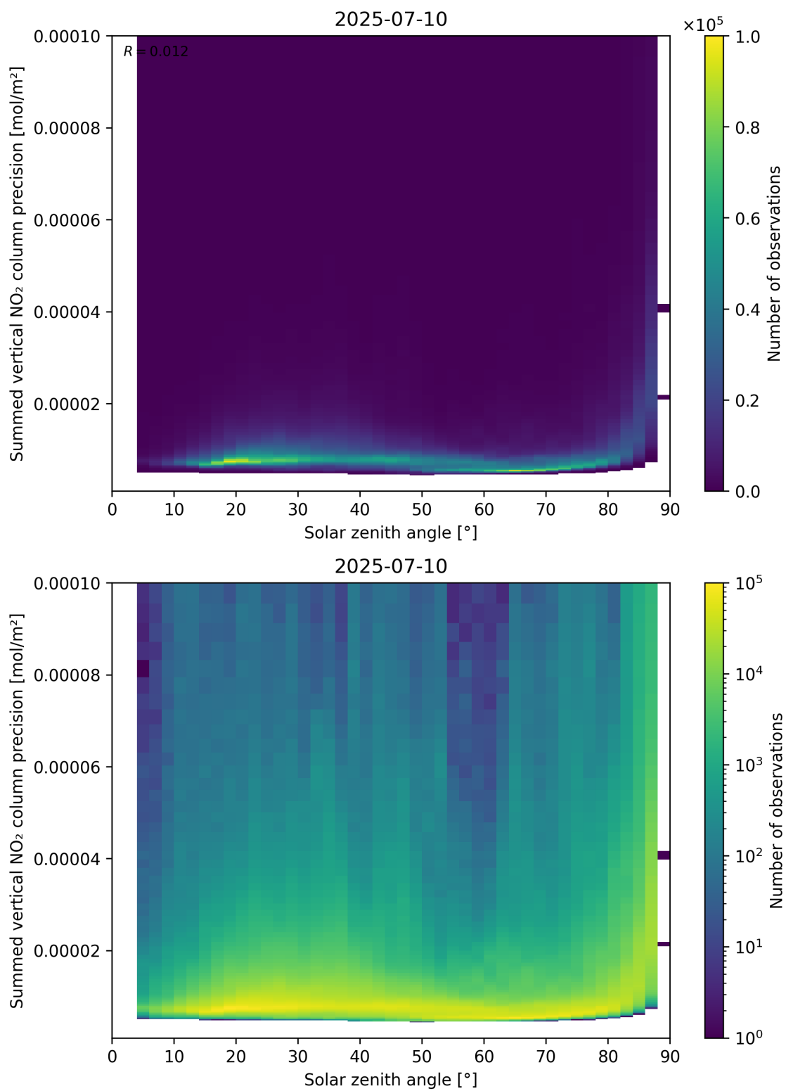
Figure 152: Scatter density plot of “Solar zenith angle” against “Summed vertical NO 2 column precision” for 2025-07-09 to 2025-07-11.
