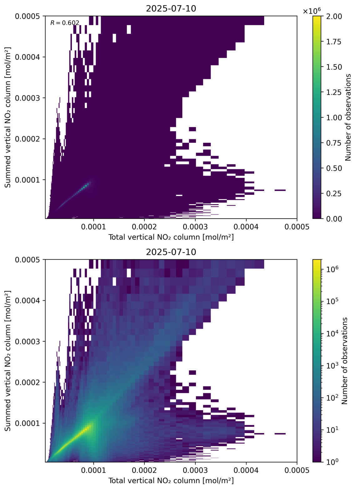
Figure 112: Scatter density plot of “Total vertical NO 2 column” against “Summed vertical NO 2 column” for 2025-07-09 to 2025-07-11.
