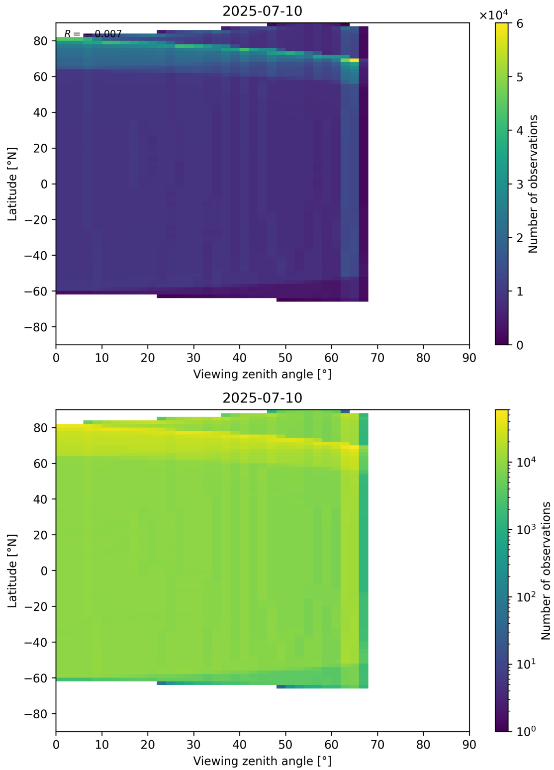
Figure 163: Scatter density plot of “Viewing zenith angle” against “Latitude” for 2025-07-09 to 2025-07-11.
