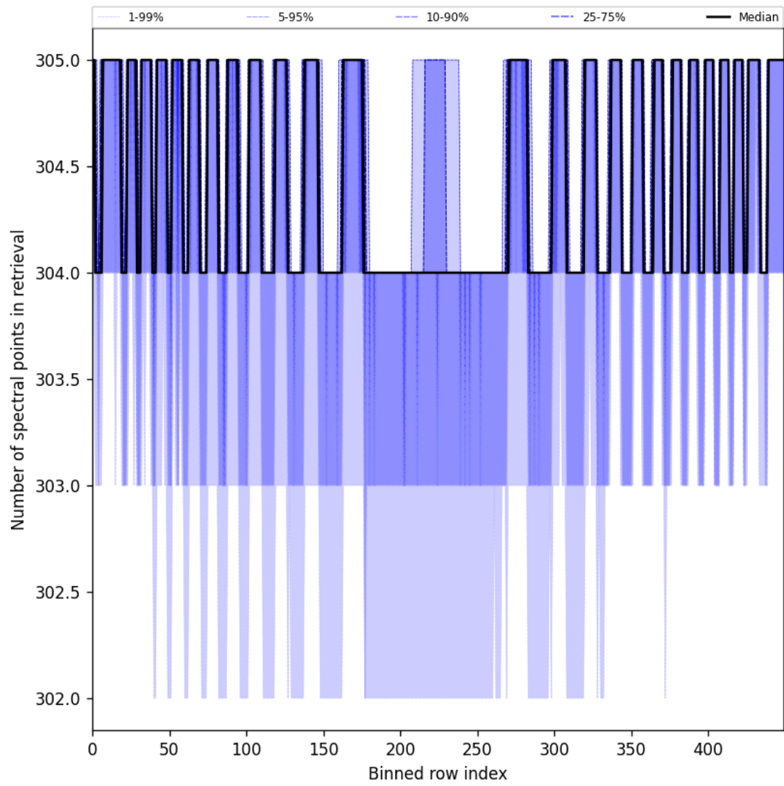
Figure 50: Along track statistics of “Number of spectral points in retrieval” for 2025-07-09 to 2025-07-11
