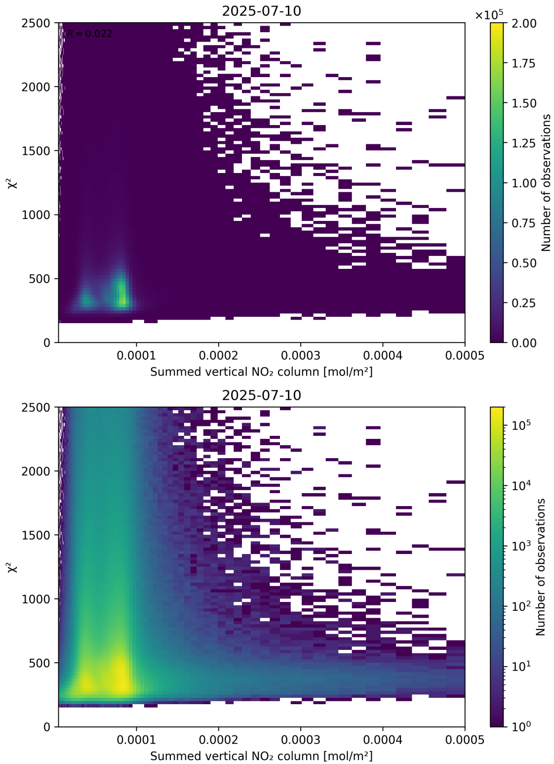
Figure 104: Scatter density plot of “Summed vertical NO 2 column” against “ \chi^2 ” for 2025-07-09 to 2025-07-11.
