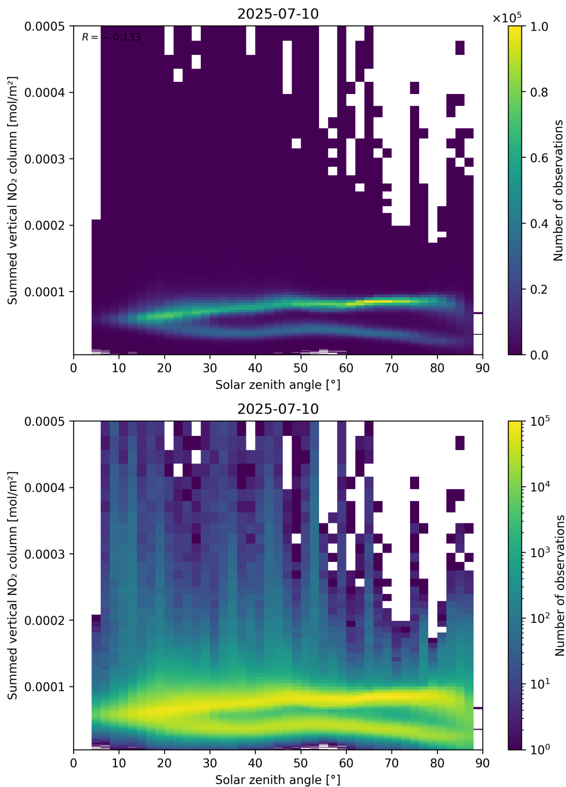
Figure 151: Scatter density plot of “Solar zenith angle” against “Summed vertical NO 2 column” for 2025-07-09 to 2025-07-11.
