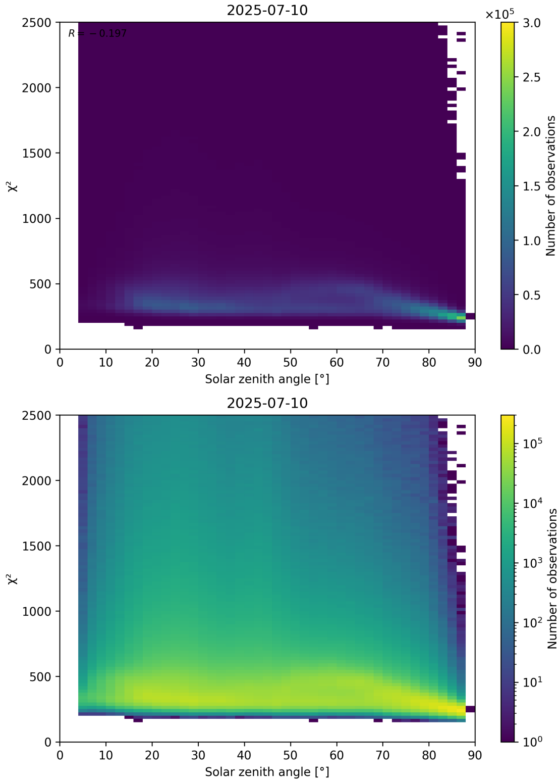
Figure 148: Scatter density plot of “Solar zenith angle” against “ \chi^2 ” for 2025-07-09 to 2025-07-11.
