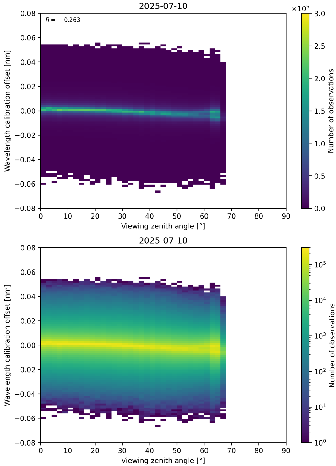
Figure 173: Scatter density plot of “Viewing zenith angle” against “Wavelength calibration offset” for 2025-07-09 to 2025-07-11.
