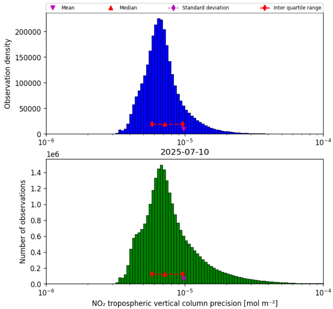
Figure 30: Histogram of “NO 2 tropospheric vertical column precision” for 2025-07-09 to 2025-07-11
