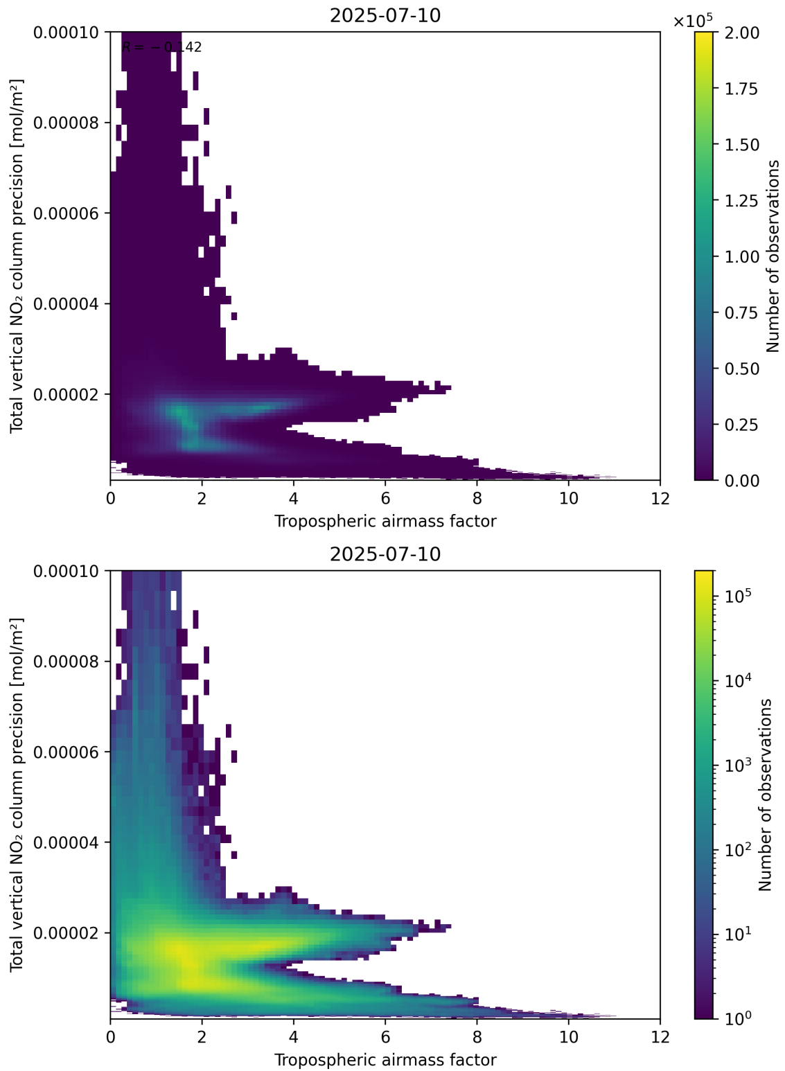
Figure 78: Scatter density plot of “Tropospheric air mass factor” against “Total vertical NO 2 column precision” for 2025-07-09 to 2025-07-11.
