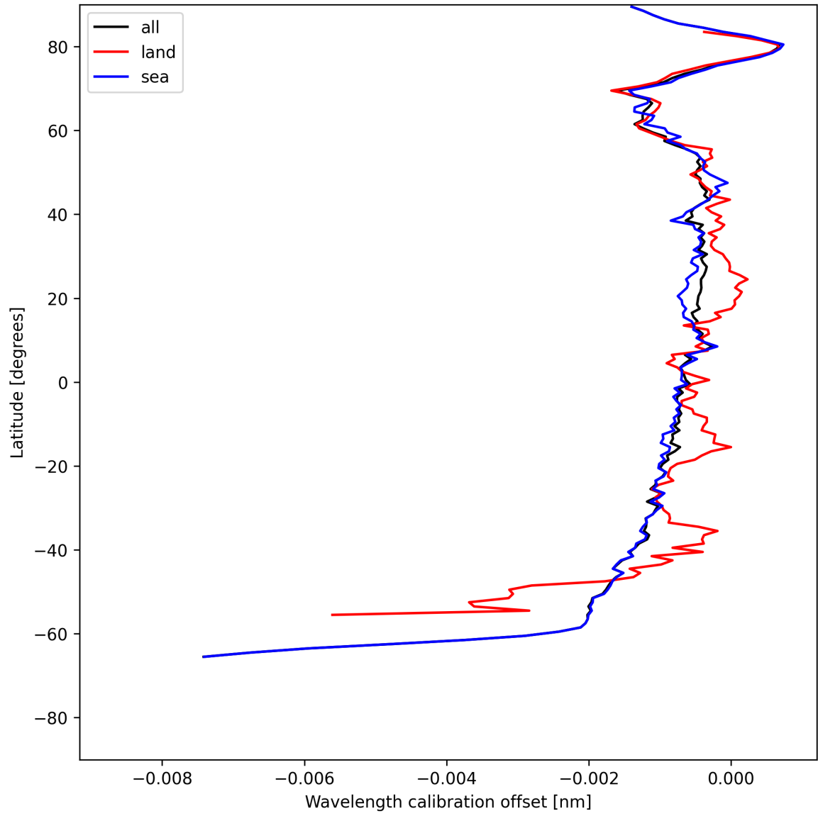
Figure 18: Zonal average of “Wavelength calibration offset” for 2025-07-09 to 2025-07-11.
