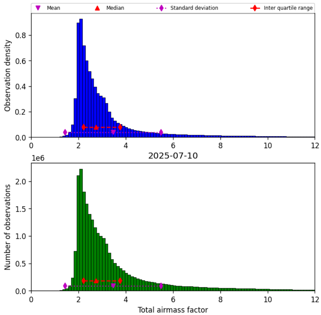
Figure 32: Histogram of “Total airmass factor” for 2025-07-09 to 2025-07-11
