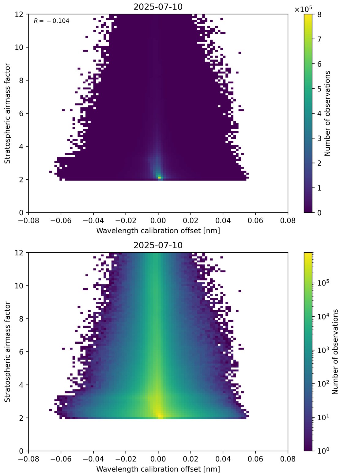
Figure 174: Scatter density plot of “Wavelength calibration offset” against “Stratospheric airmass factor” for 2025-07-09 to 2025-07-11.
