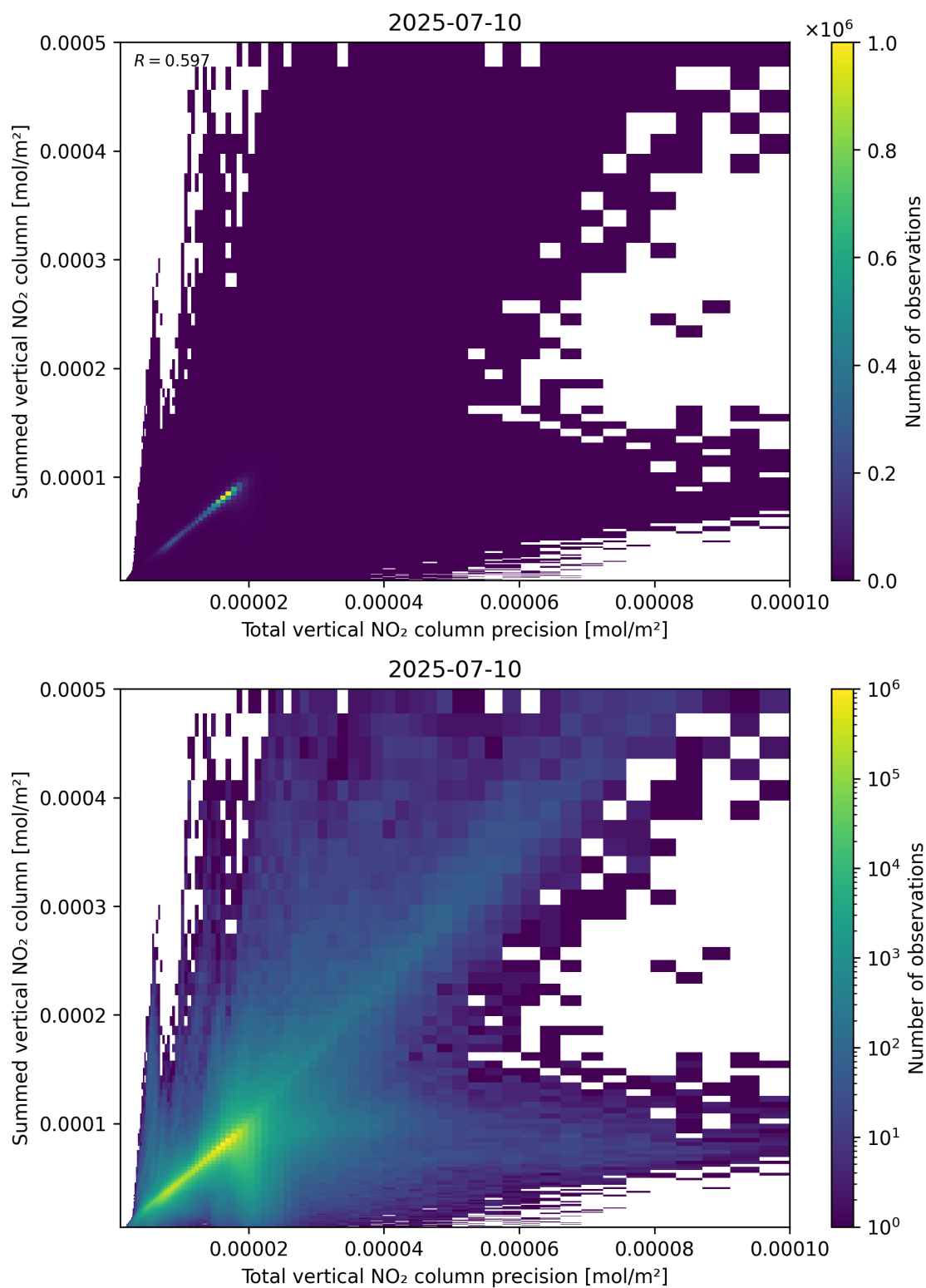
Figure 117: Scatter density plot of “Total vertical NO 2 column precision” against “Summed vertical NO 2 column” for 2025-07-09 to 2025-07-11.
