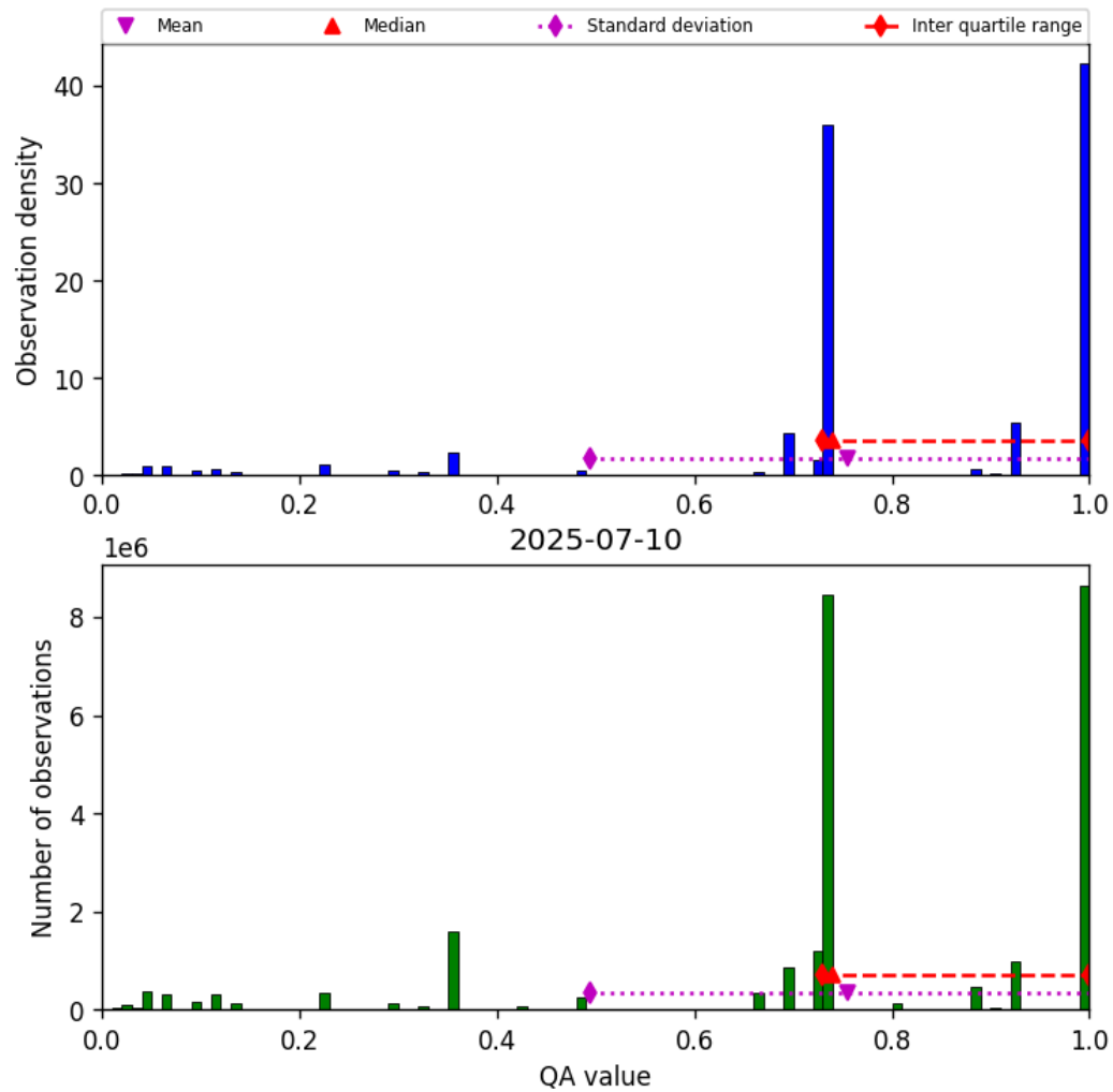
Figure 28: Histogram of “QA value” for 2025-07-09 to 2025-07-11
