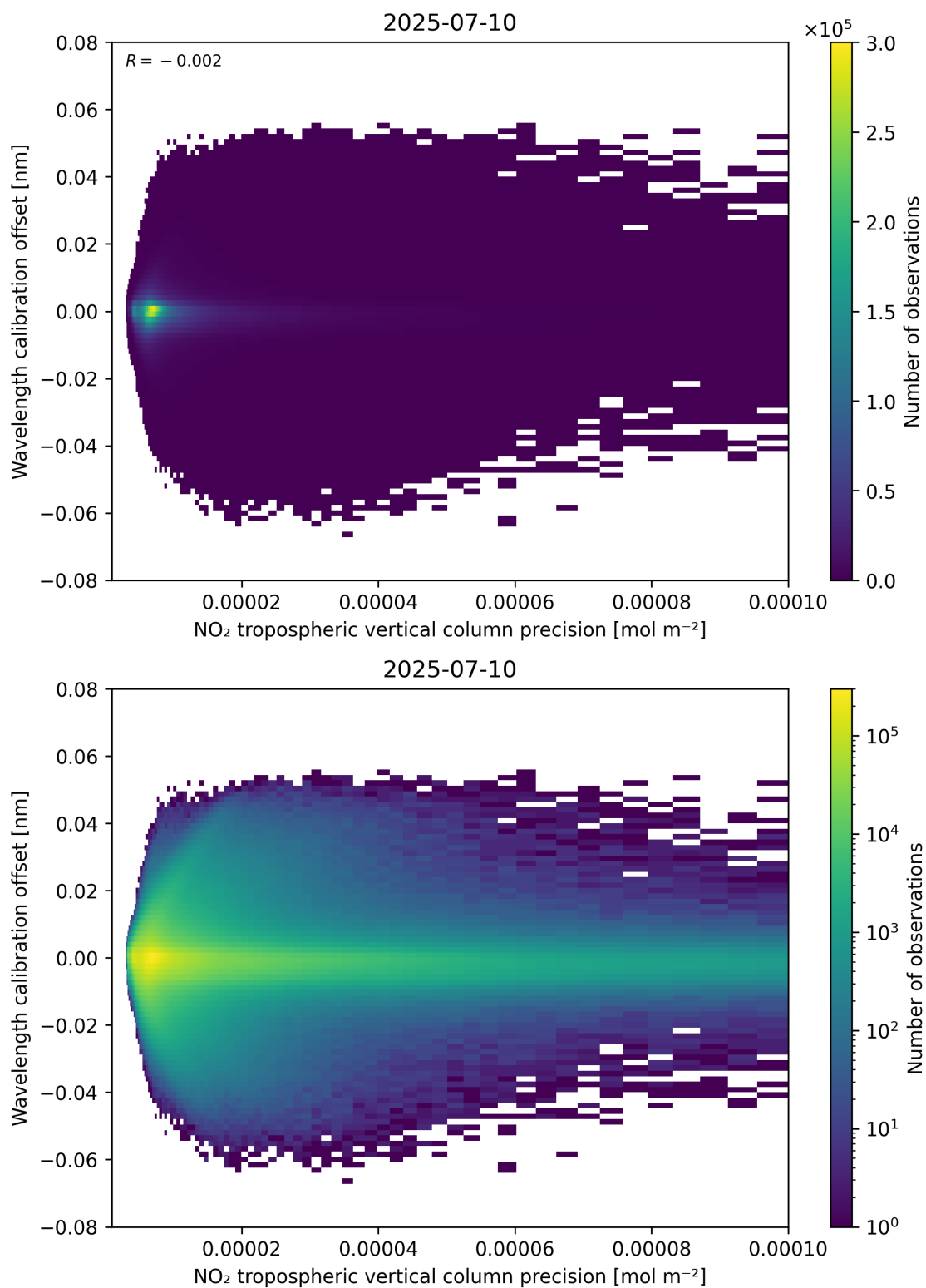
Figure 141: Scatter density plot of “NO 2 tropospheric vertical column precision” against “Wavelength calibration offset” for 2025-07-09 to 2025-07-11.
