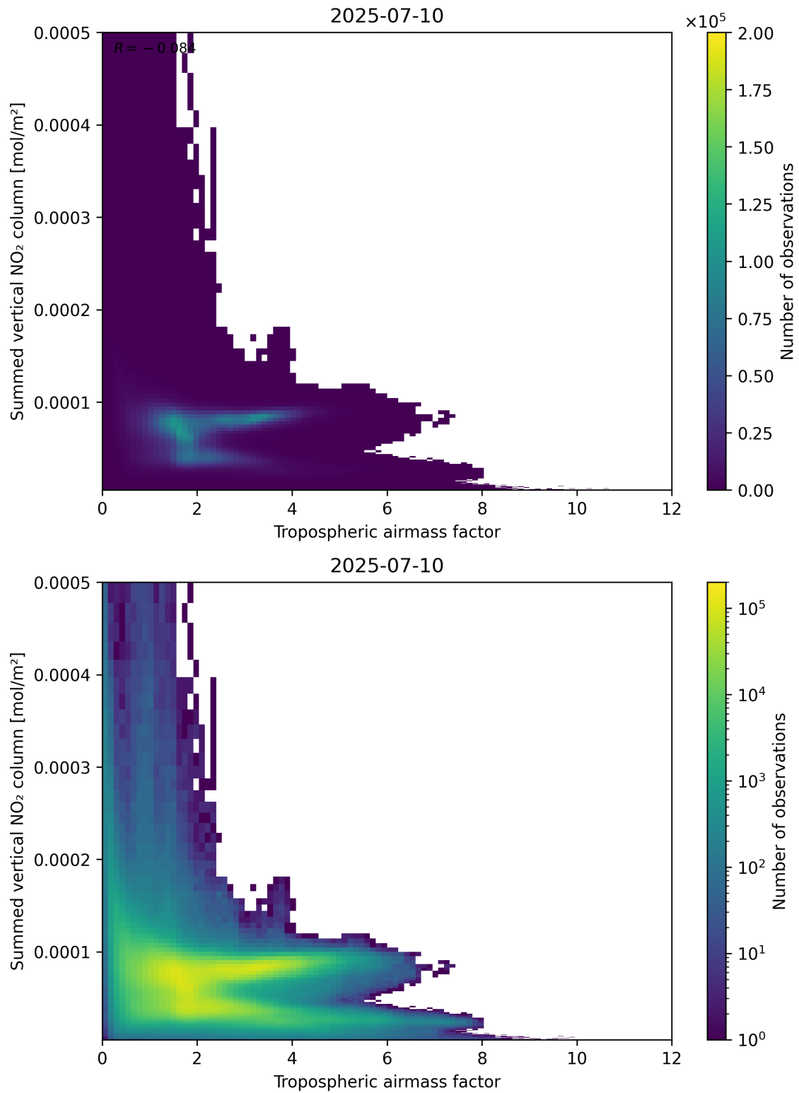
Figure 75: Scatter density plot of “Tropospheric airmass factor” against “Summed vertical NO 2 column” for 2025-07-09 to 2025-07-11.
