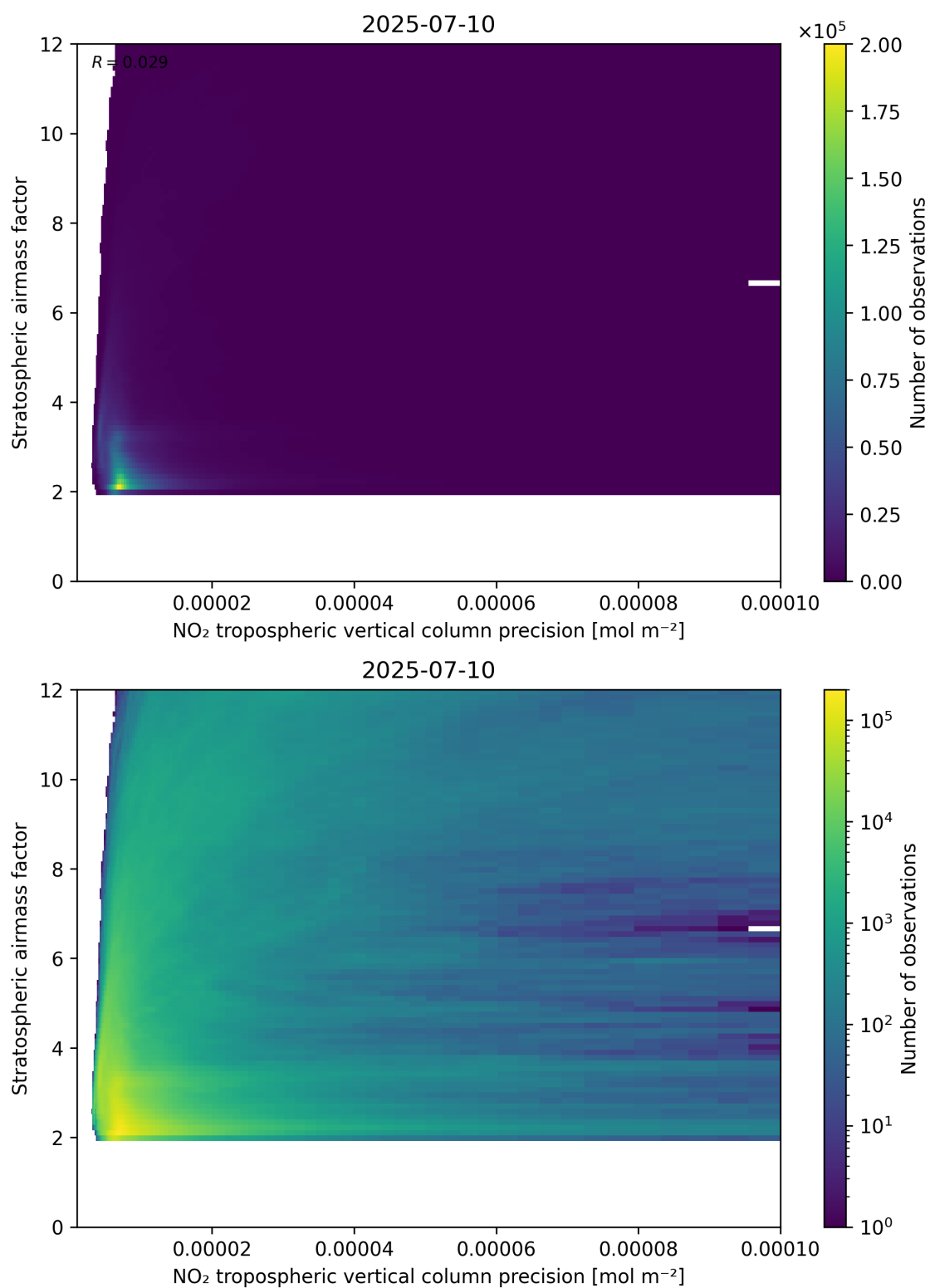
Figure 131: Scatter density plot of “NO 2 tropospheric vertical column precision” against “Stratospheric airmass factor” for 2025-07-09 to 2025-07-11.
