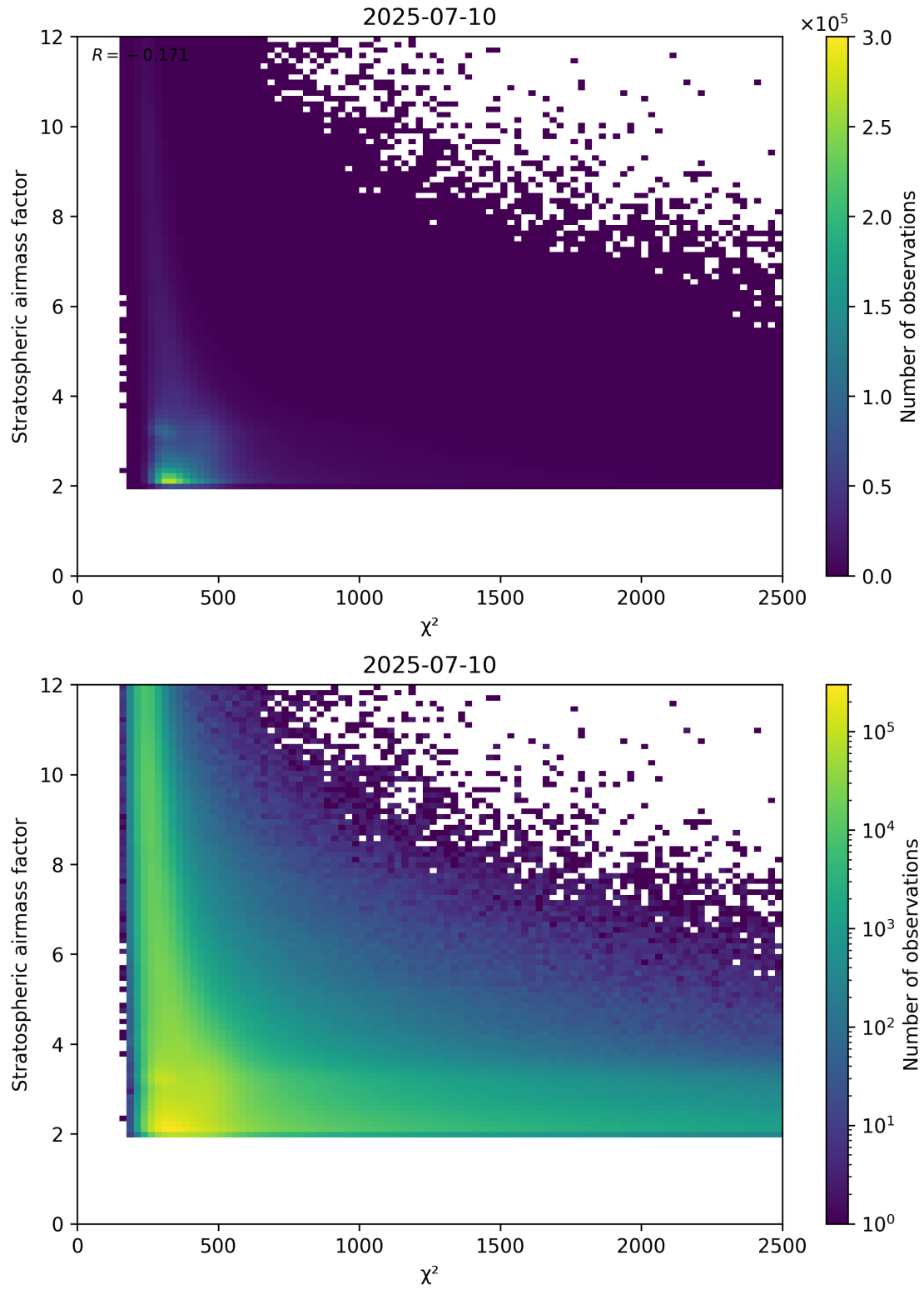
Figure 81: Scatter density plot of “ \chi^2 ” against “Stratospheric airmass factor” for 2025-07-09 to 2025-07-11.
