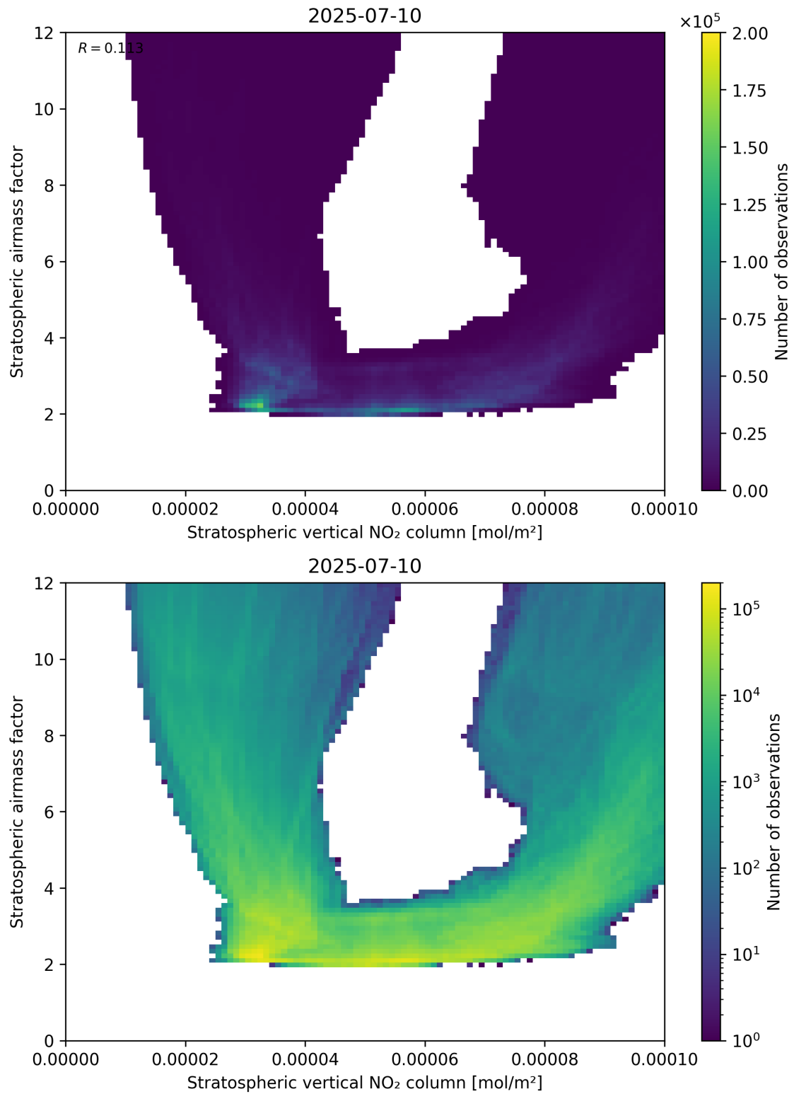
Figure 96: Scatter density plot of “Stratospheric vertical NO 2 column” against “Stratospheric airmass factor” for 2025-07-09 to 2025-07-11.
