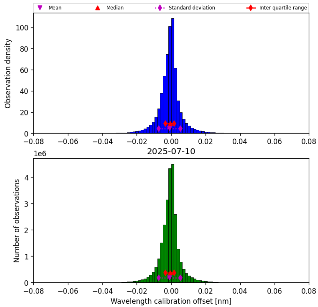
Figure 35: Histogram of “Wavelength calibration offset” for 2025-07-09 to 2025-07-11
