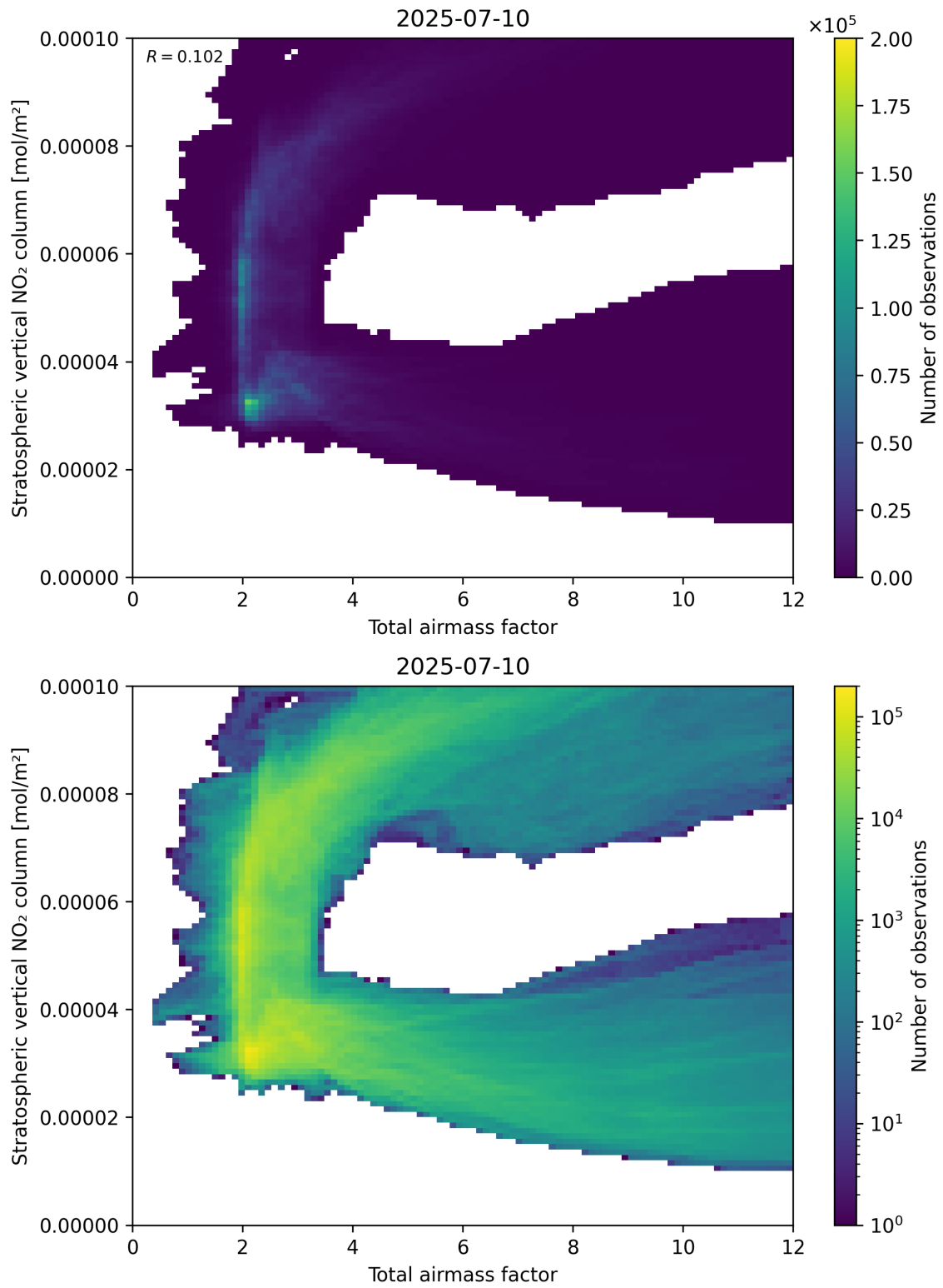
Figure 64: Scatter density plot of “Total airmass factor” against “Stratospheric vertical NO 2 column” for 2025-07-09 to 2025-07-11.
