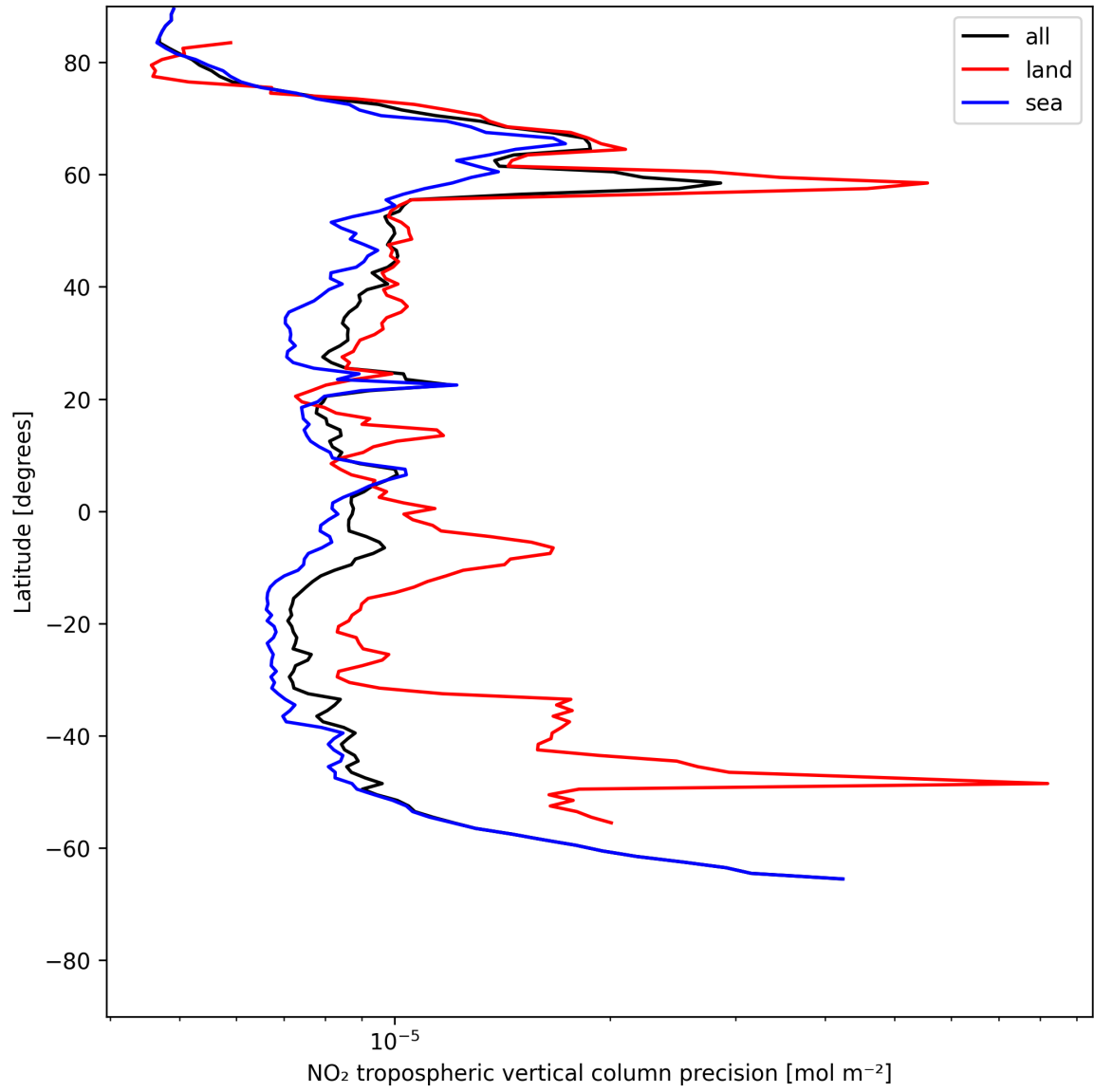
Figure 13: Zonal average of “NO 2 tropospheric vertical column precision” for 2025-07-09 to 2025-07-11.
