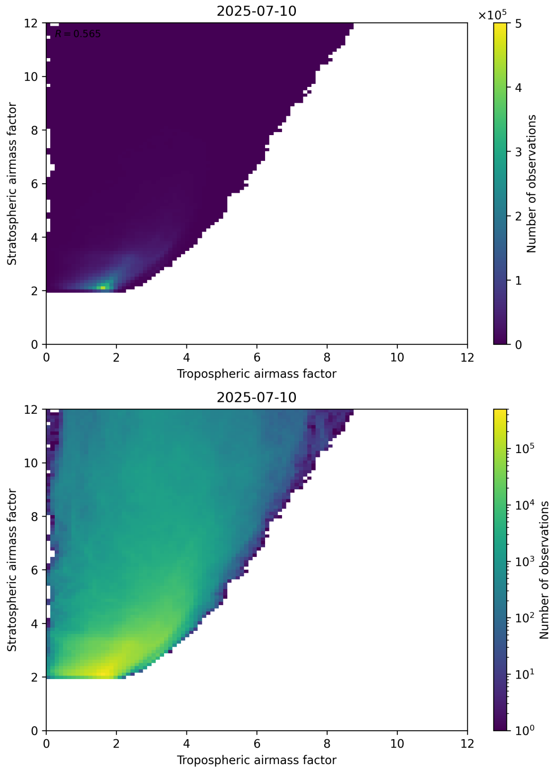
Figure 71: Scatter density plot of “Tropospheric airmass factor” against “Stratospheric airmass factor” for 2025-07-09 to 2025-07-11.
