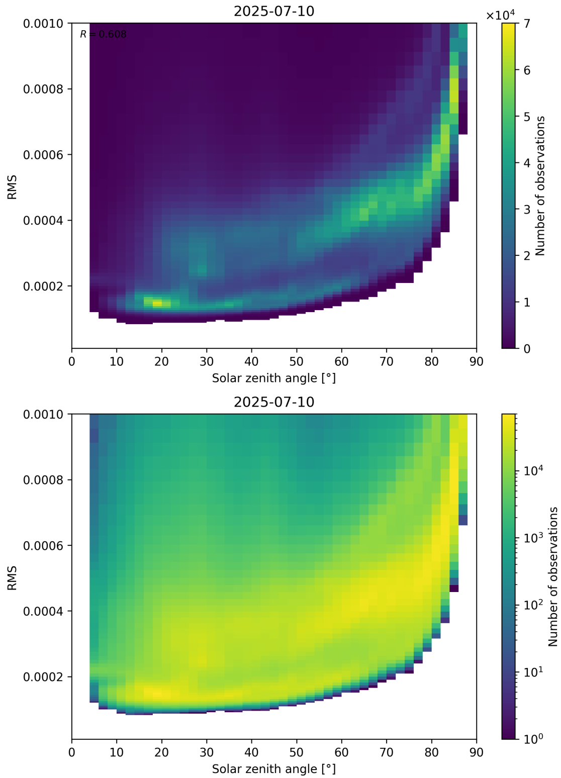
Figure 157: Scatter density plot of “Solar zenith angle” against “RMS” for 2025-07-09 to 2025-07-11.
