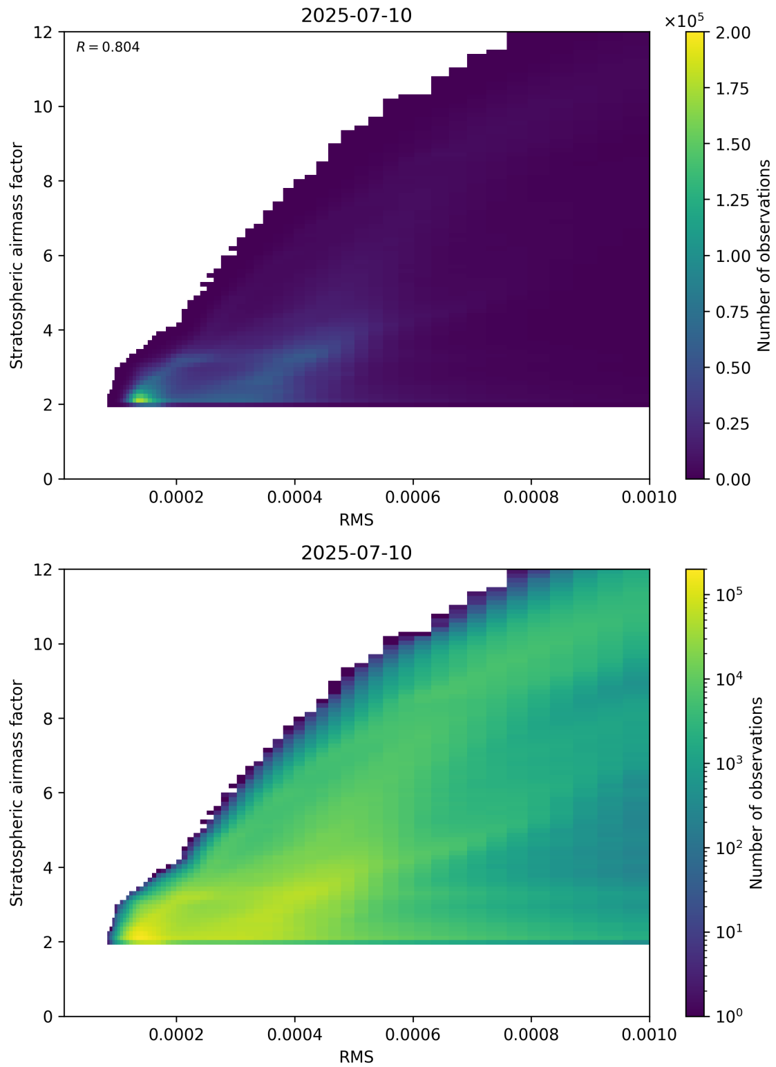
Figure 144: Scatter density plot of “RMS” against “Stratospheric airmass factor” for 2025-07-09 to 2025-07-11.
