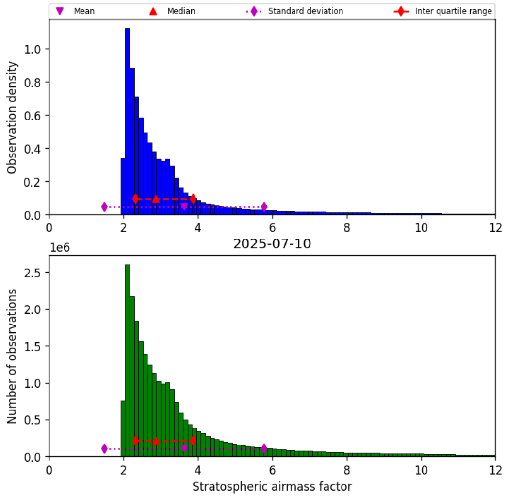
Figure 44: Histogram of “Stratospheric airmass factor” for 2025-07-09 to 2025-07-11
