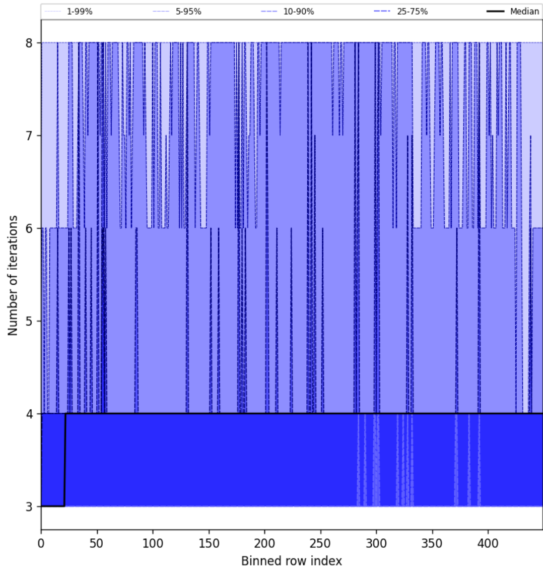
Figure 51: Along track statistics of “Number of iterations” for 2025-07-09 to 2025-07-11
