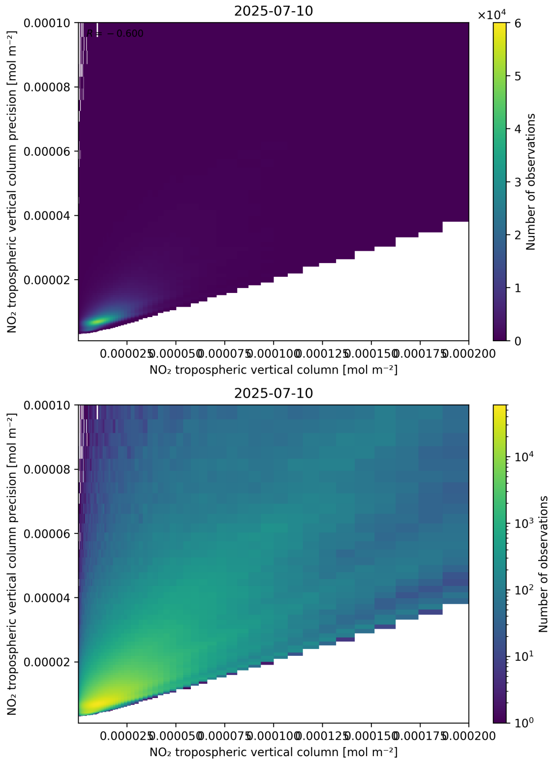
Figure 130: Scatter density plot of “NO 2 tropospheric vertical column” against “NO 2 tropospheric vertical column precision” for 2025-07-09 to 2025-07-11.
