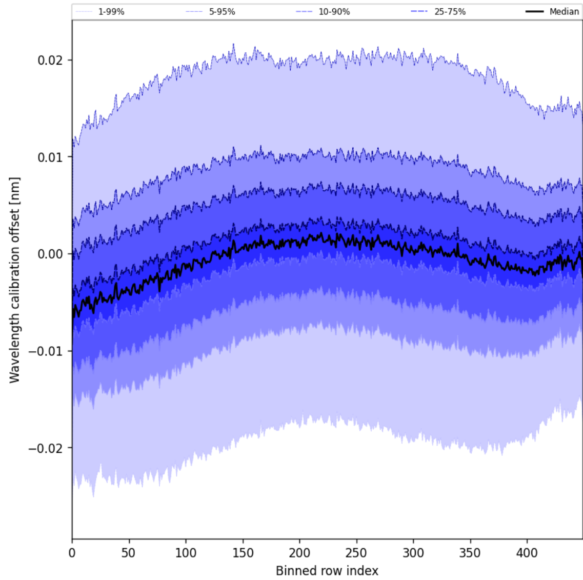
Figure 52: Along track statistics of “Wavelength calibration offset” for 2025-07-09 to 2025-07-11
