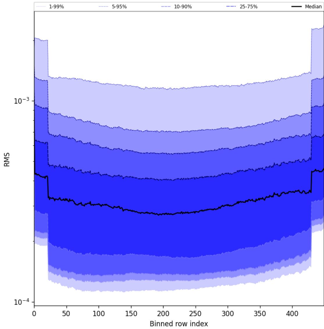
Figure 60: Along track statistics of “RMS” for 2025-07-09 to 2025-07-11
