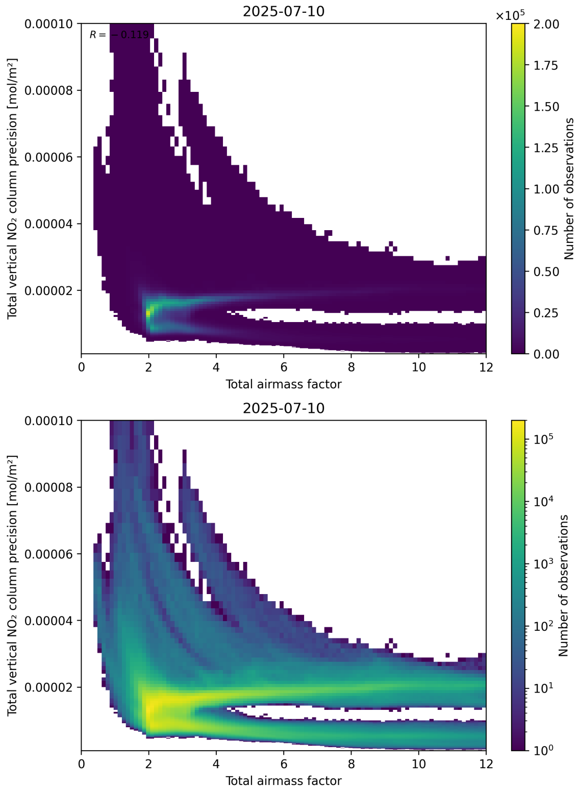
Figure 68: Scatter density plot of “Total airmass factor” against “Total vertical NO 2 column precision” for 2025-07-09 to 2025-07-11.
