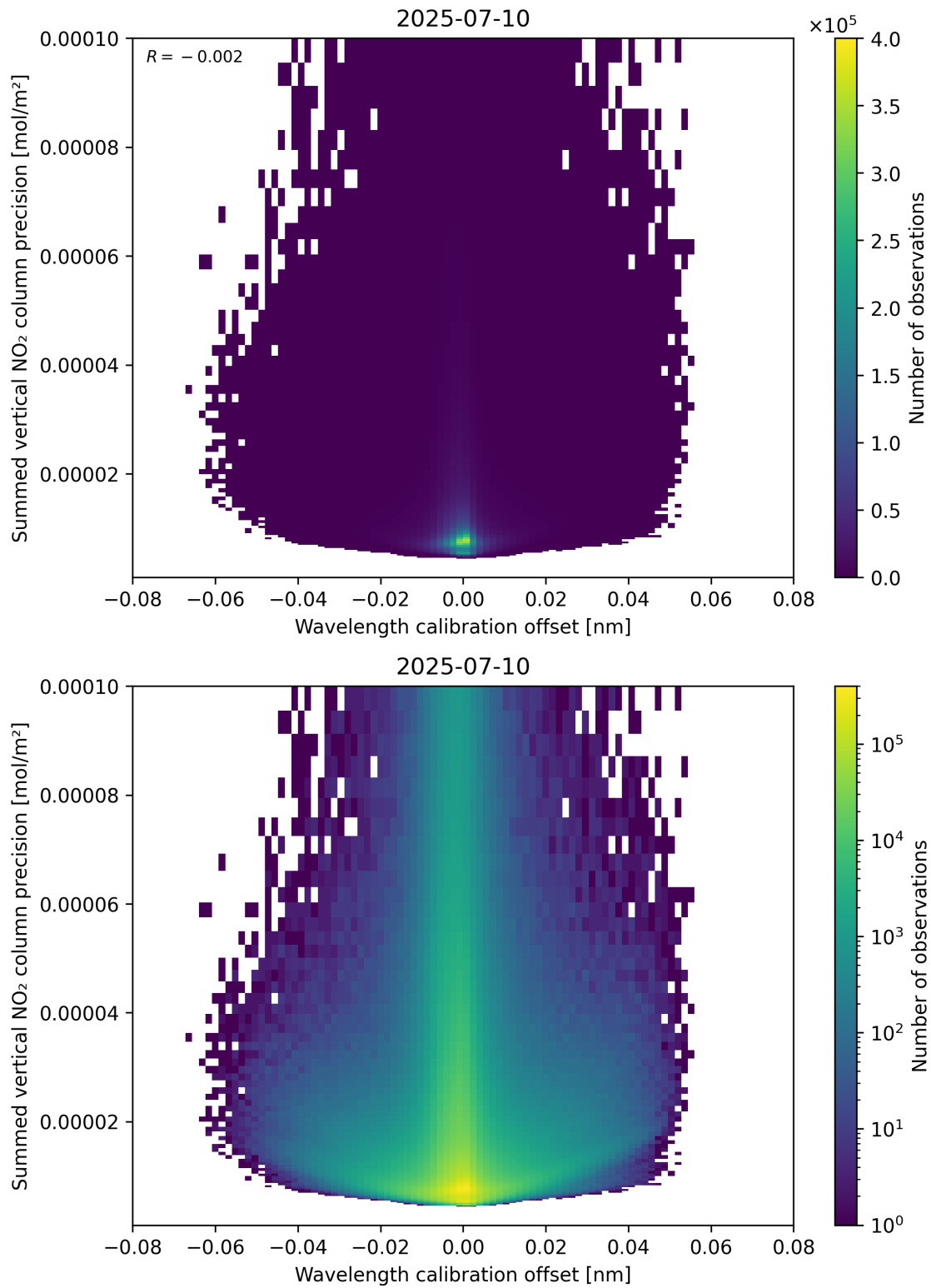
Figure 178: Scatter density plot of “Wavelength calibration offset” against “Summed vertical NO 2 column precision” for 2025-07-09 to 2025-07-11.
