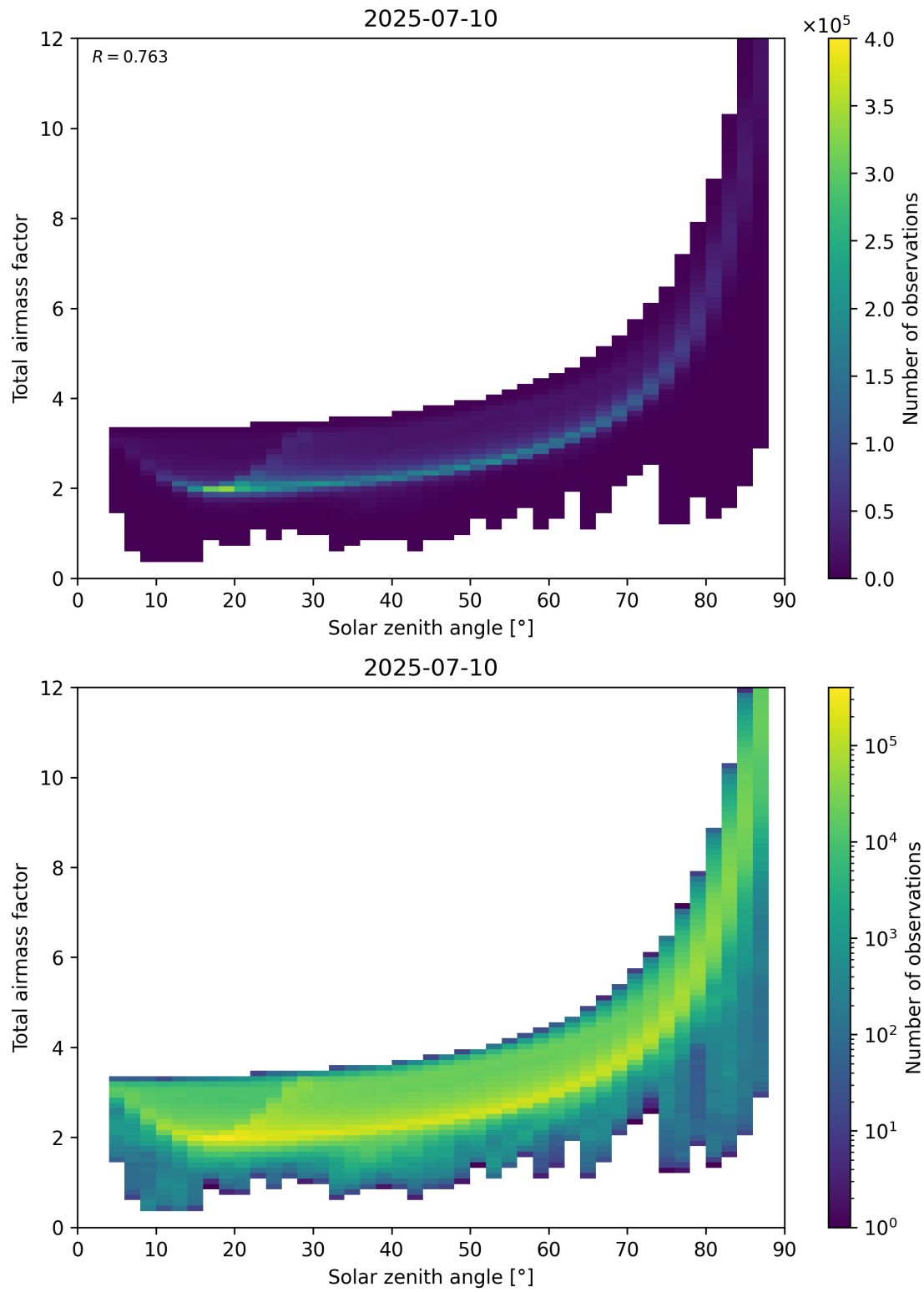
Figure 146: Scatter density plot of “Solar zenith angle” against “Total air mass factor” for 2025-07-09 to 2025-07-11.
