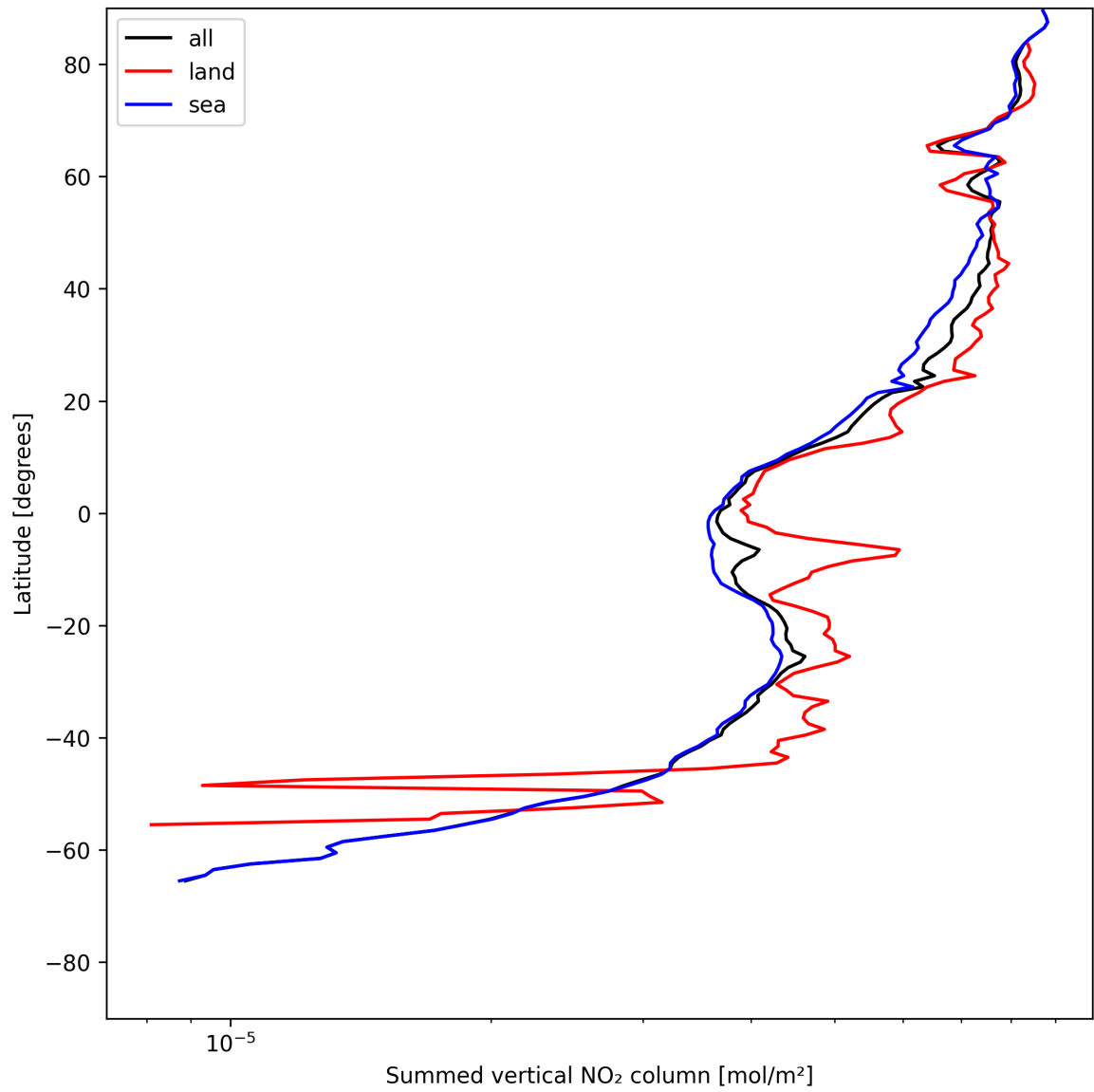
Figure 23: Zonal average of “Summed vertical NO 2 column” for 2025-07-09 to 2025-07-11.
