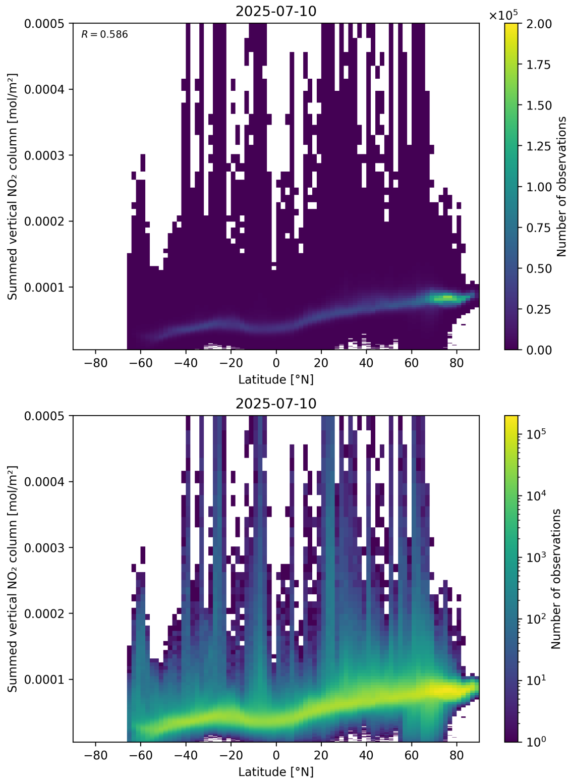
Figure 88: Scatter density plot of “Latitude” against “Summed vertical NO 2 column” for 2025-07-09 to 2025-07-11.
