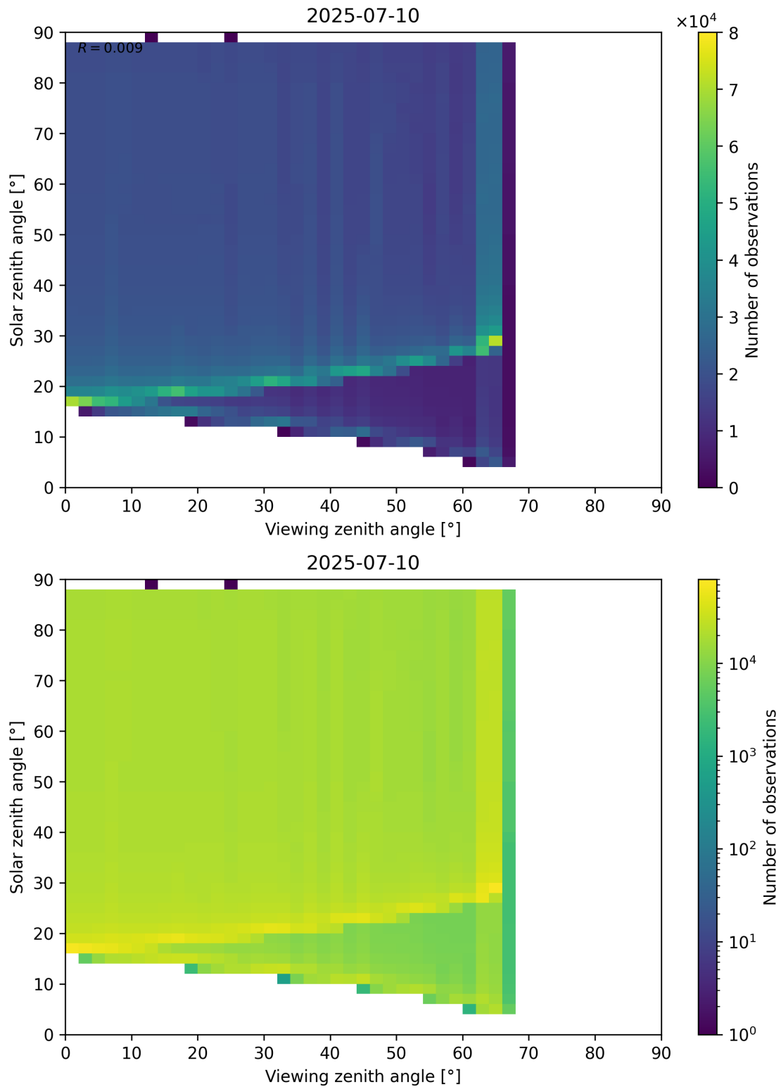
Figure 172: Scatter density plot of “Viewing zenith angle” against “Solar zenith angle” for 2025-07-09 to 2025-07-11.
