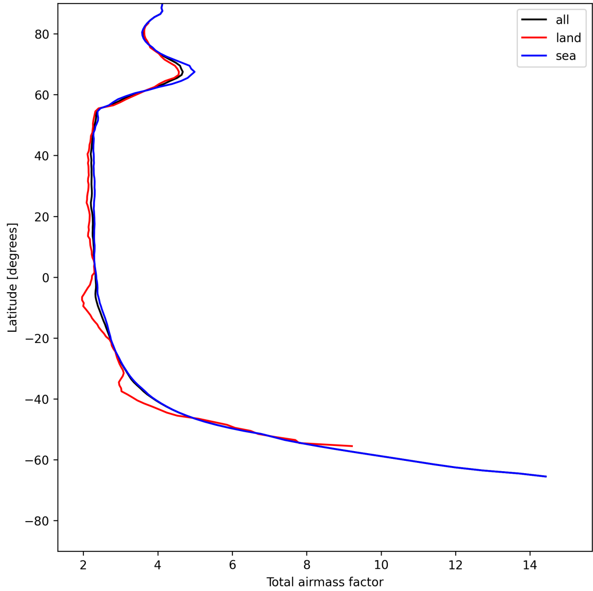
Figure 15: Zonal average of “Total airmass factor” for 2025-07-09 to 2025-07-11.
