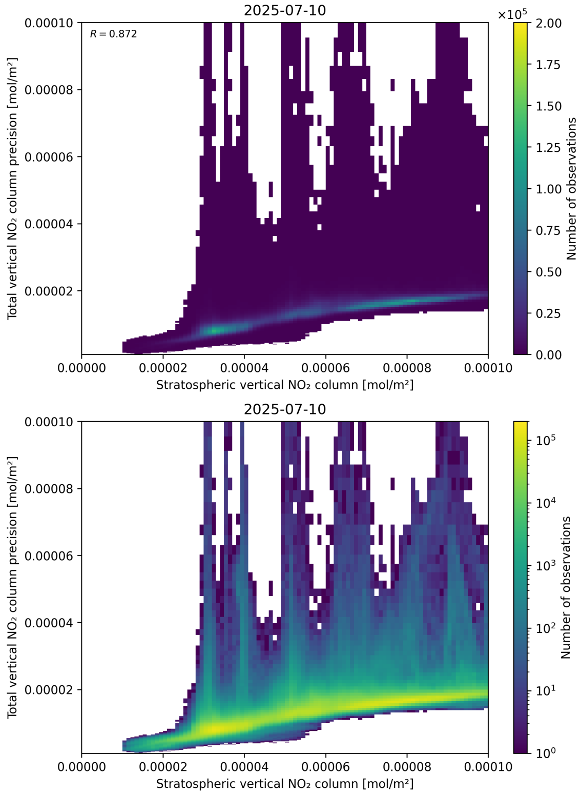
Figure 101: Scatter density plot of “Stratospheric vertical NO 2 column” against “Total vertical NO 2 column precision” for 2025-07-09 to 2025-07-11.
