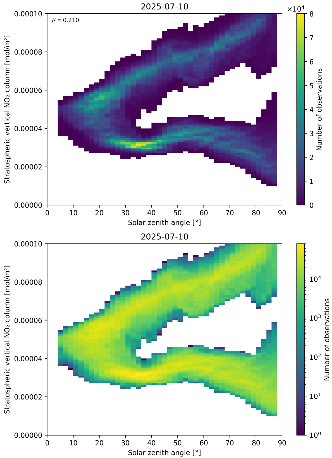
Figure 150: Scatter density plot of “Solar zenith angle” against “Stratospheric vertical NO 2 column” for 2025-07-09 to 2025-07-11.
