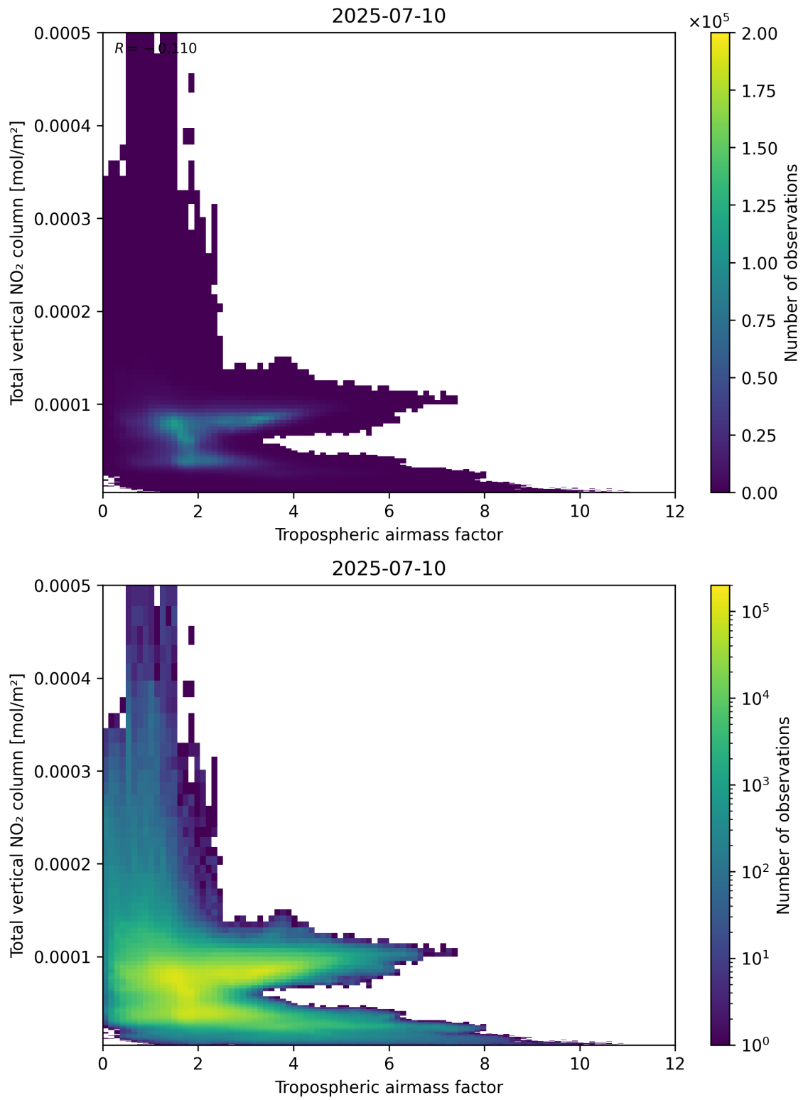
Figure 77: Scatter density plot of “Tropospheric airmass factor” against “Total vertical NO 2 column” for 2025-07-09 to 2025-07-11.
