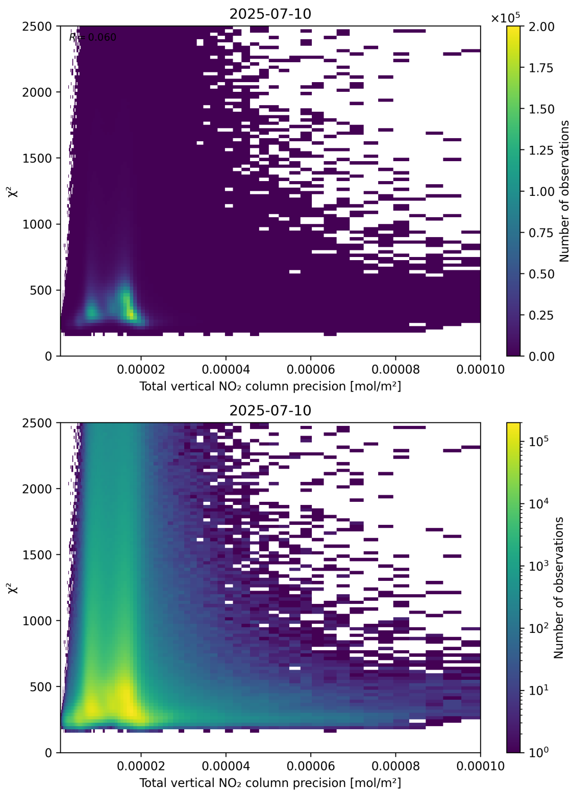
Figure 116: Scatter density plot of “Total vertical NO 2 column precision” against “ \chi^2 ” for 2025-07-09 to 2025-07-11.
