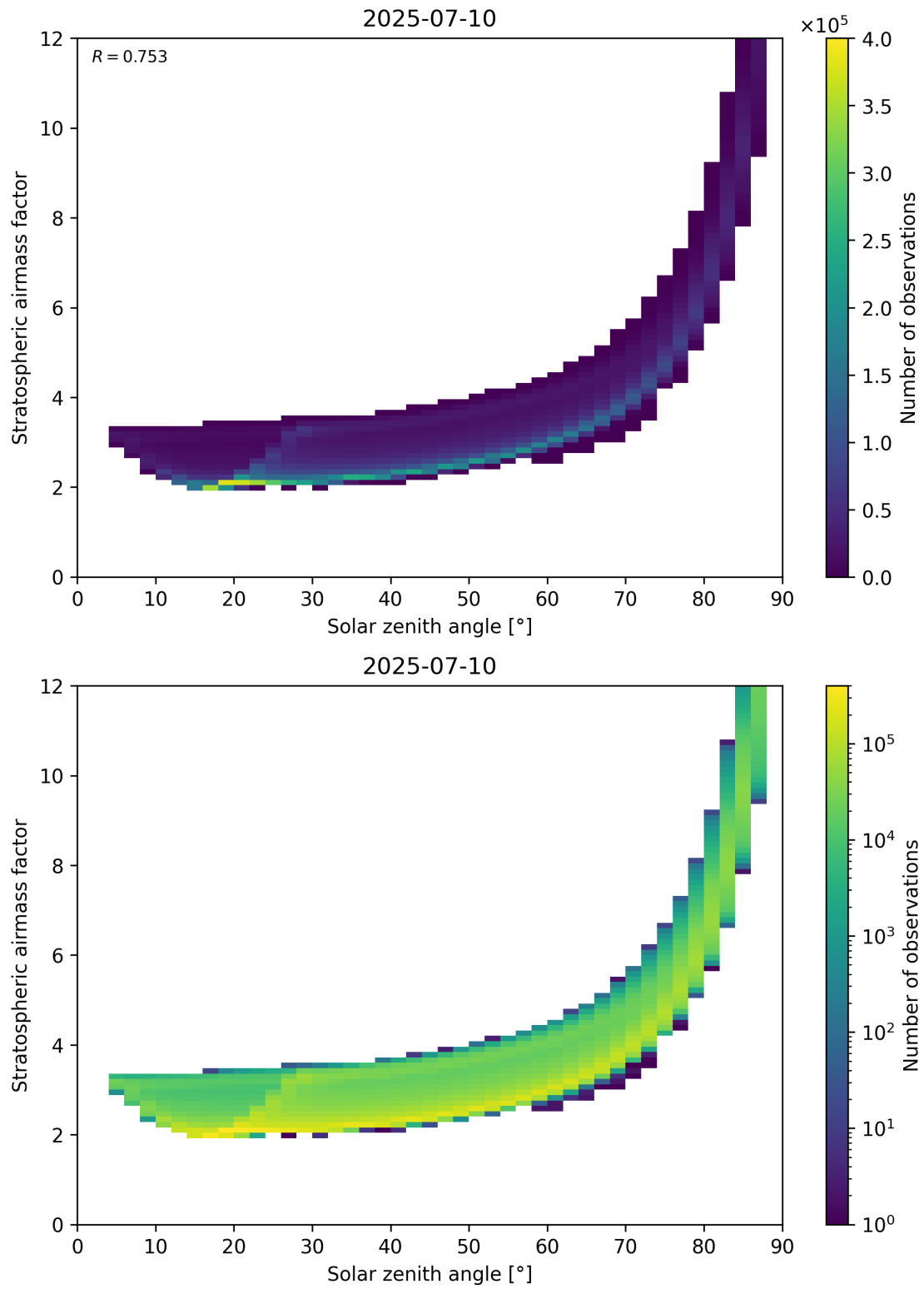
Figure 145: Scatter density plot of “Solar zenith angle” against “Stratospheric airmass factor” for 2025-07-09 to 2025-07-11.
