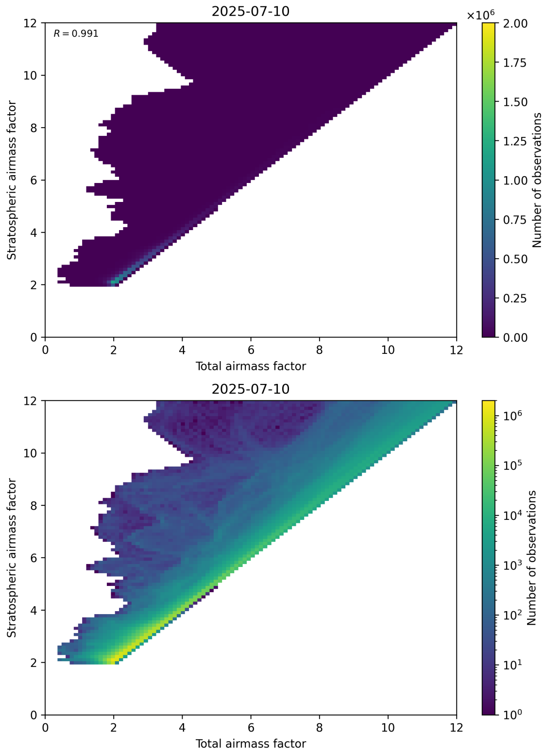
Figure 62: Scatter density plot of “Total airmass factor” against “Stratospheric airmass factor” for 2025-07-09 to 2025-07-11.
