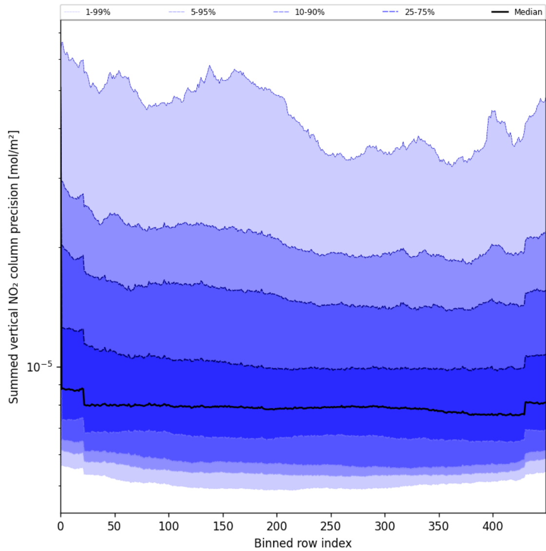
Figure 58: Along track statistics of “Summed vertical NO 2 column precision” for 2025-07-09 to 2025-07-11
