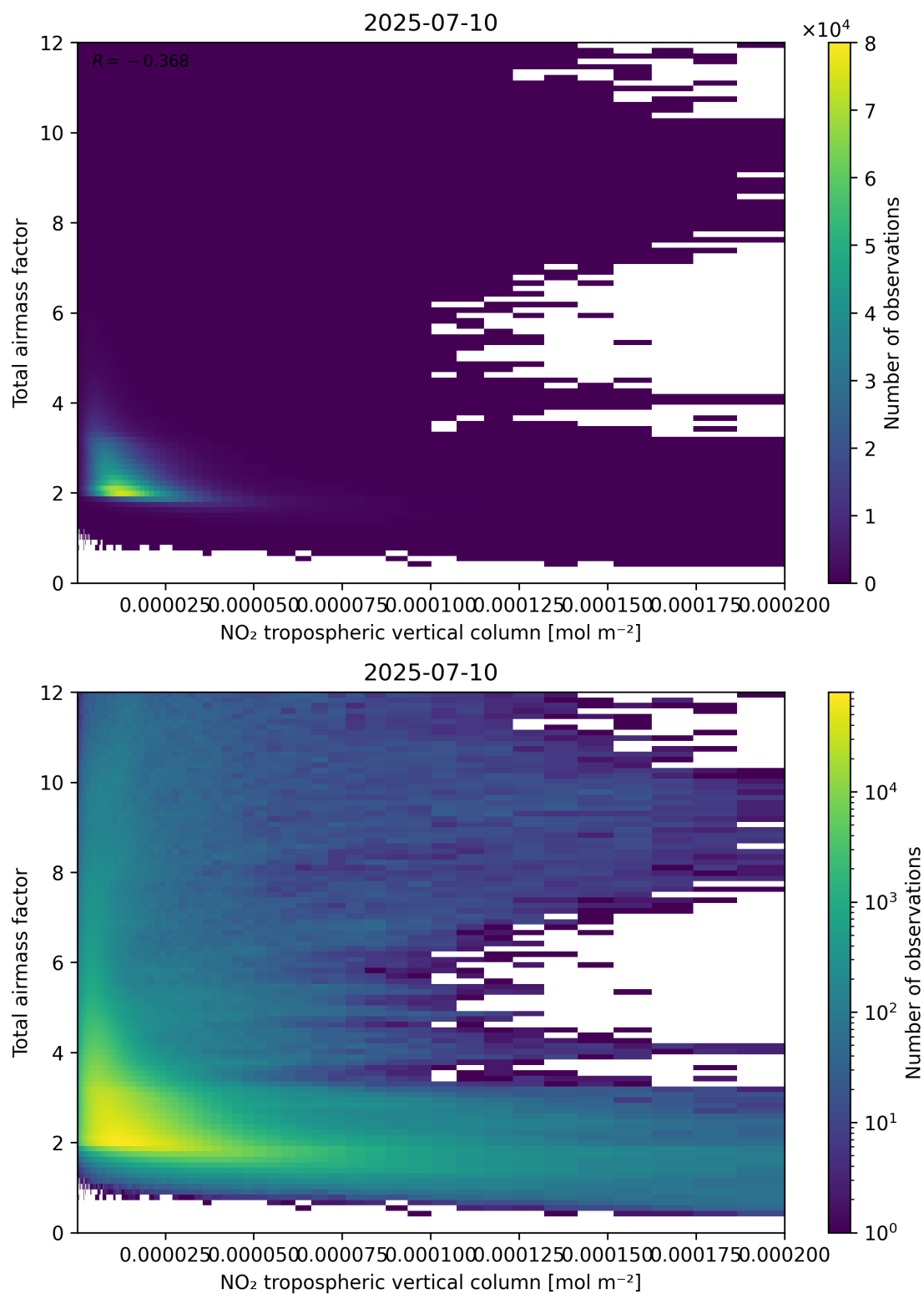
Figure 122: Scatter density plot of “NO 2 tropospheric vertical column” against “Total air mass factor” for 2025-07-09 to 2025-07-11.
