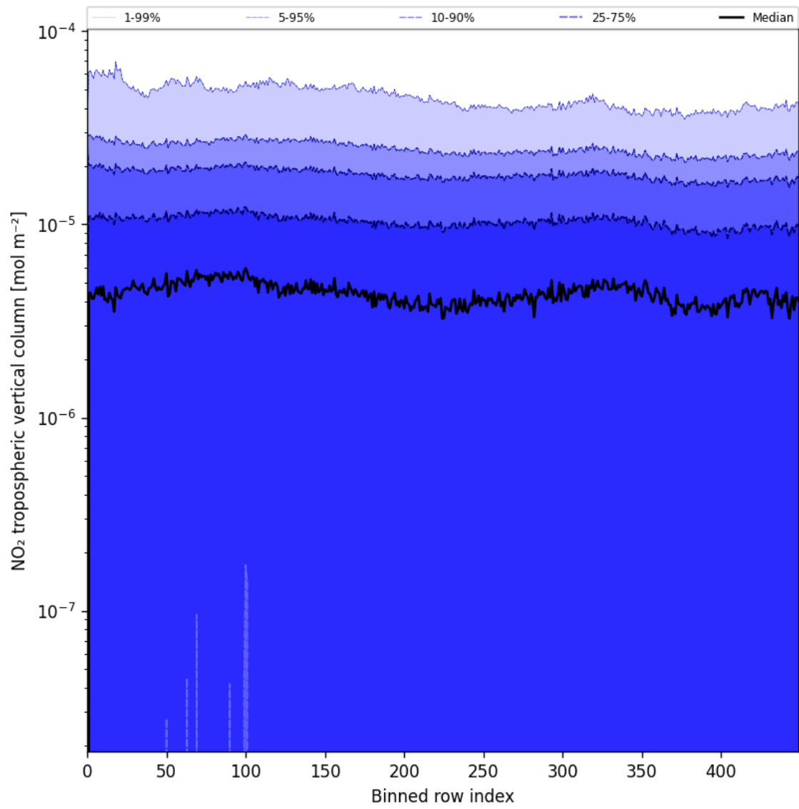
Figure 46: Along track statistics of “NO 2 tropospheric vertical column” for 2025-07-09 to 2025-07-11
