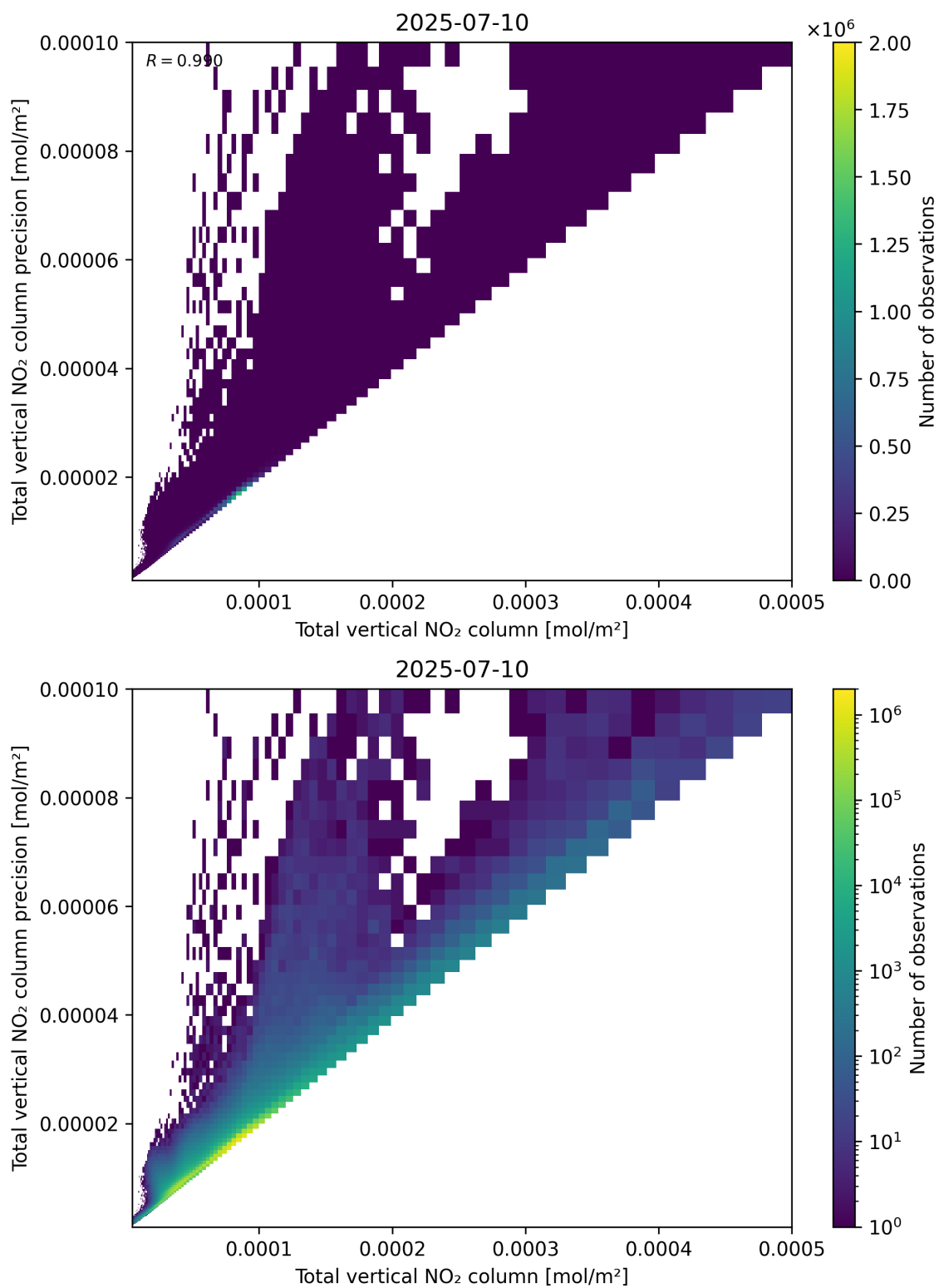
Figure 114: Scatter density plot of “Total vertical NO 2 column” against “Total vertical NO 2 column precision” for 2025-07-09 to 2025-07-11.
