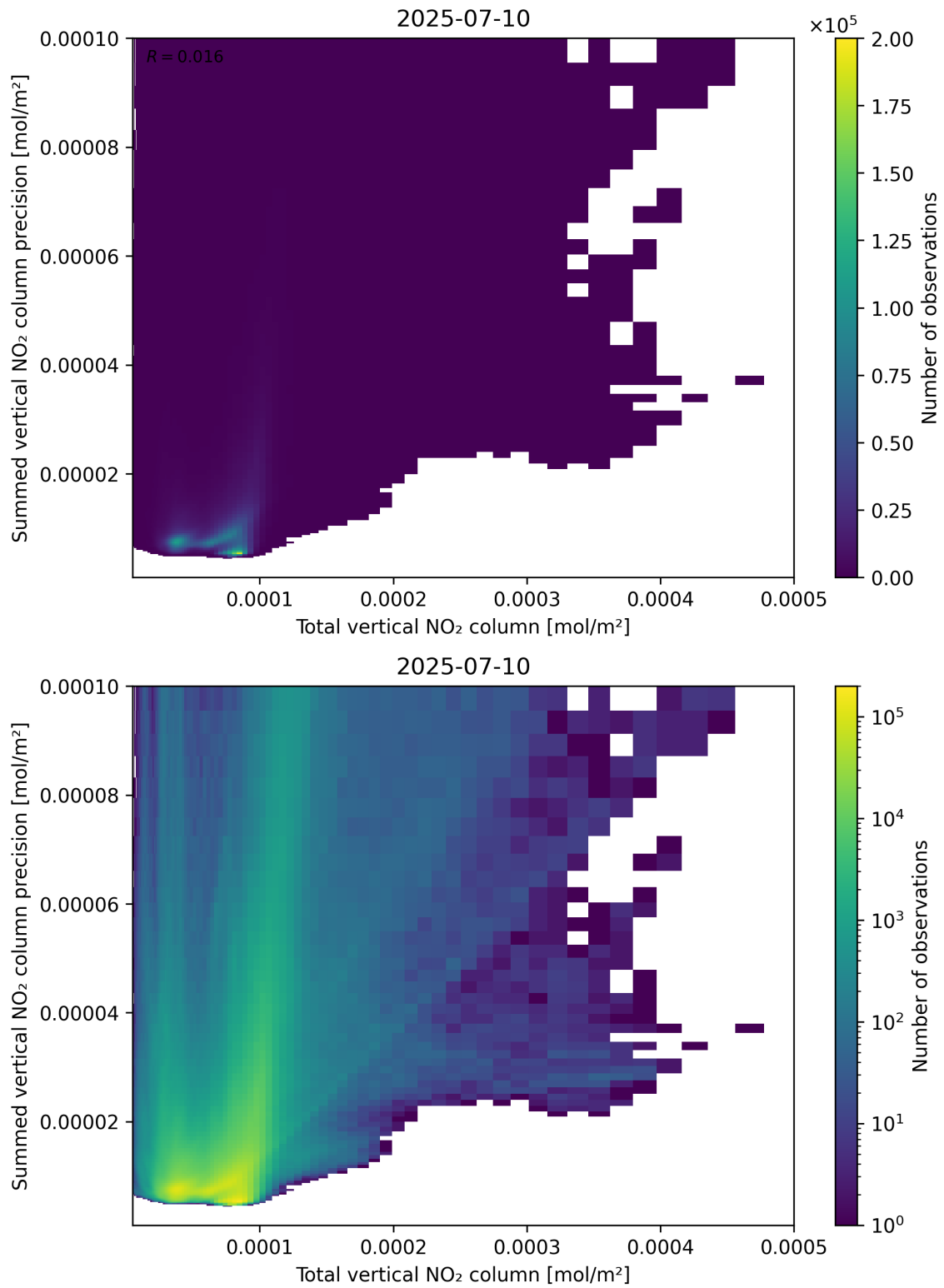
Figure 113: Scatter density plot of “Total vertical NO 2 column” against “Summed vertical NO 2 column precision” for 2025-07-09 to 2025-07-11.
