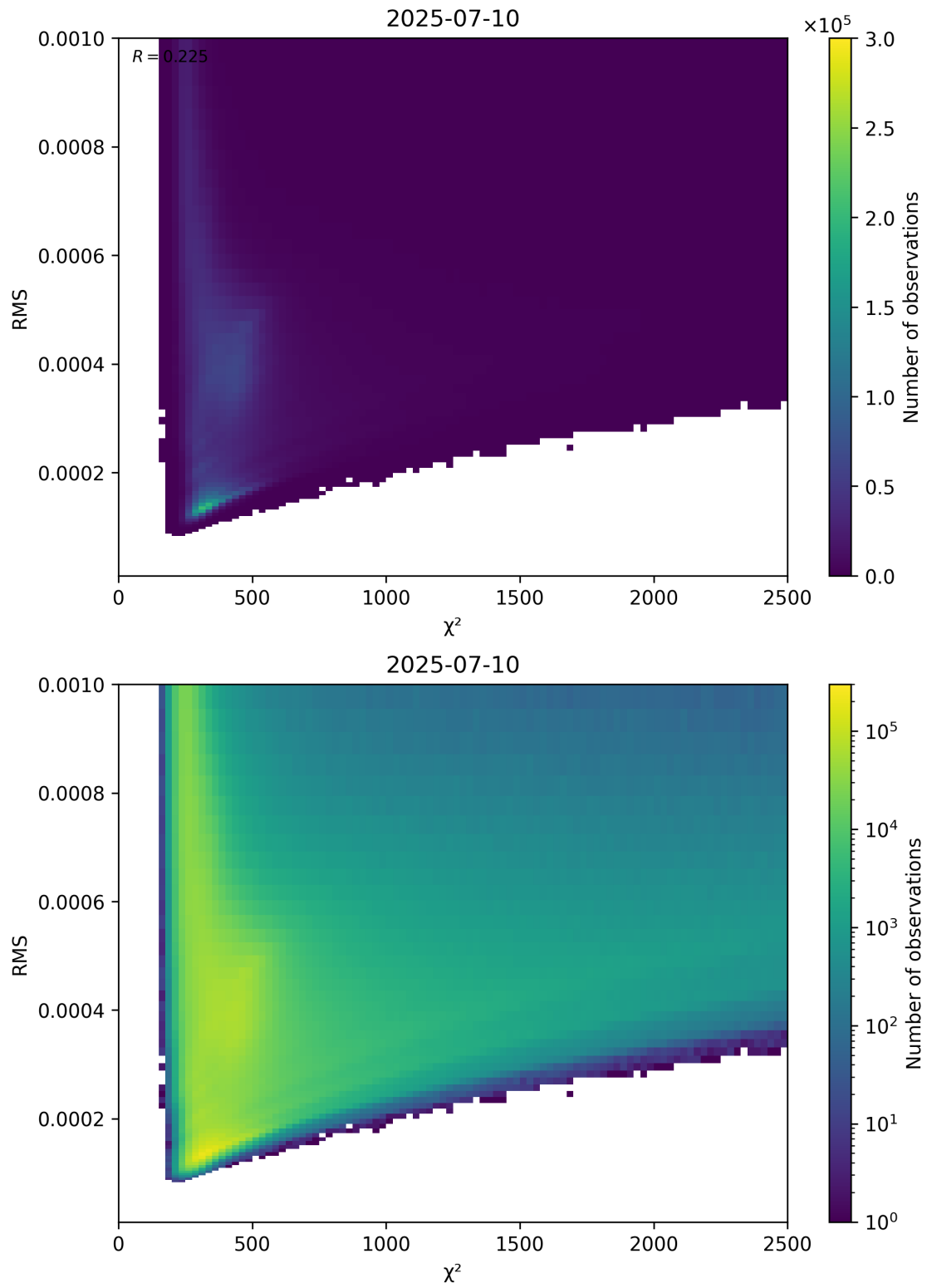
Figure 82: Scatter density plot of “ \chi^2 ” against “RMS” for 2025-07-09 to 2025-07-11.
