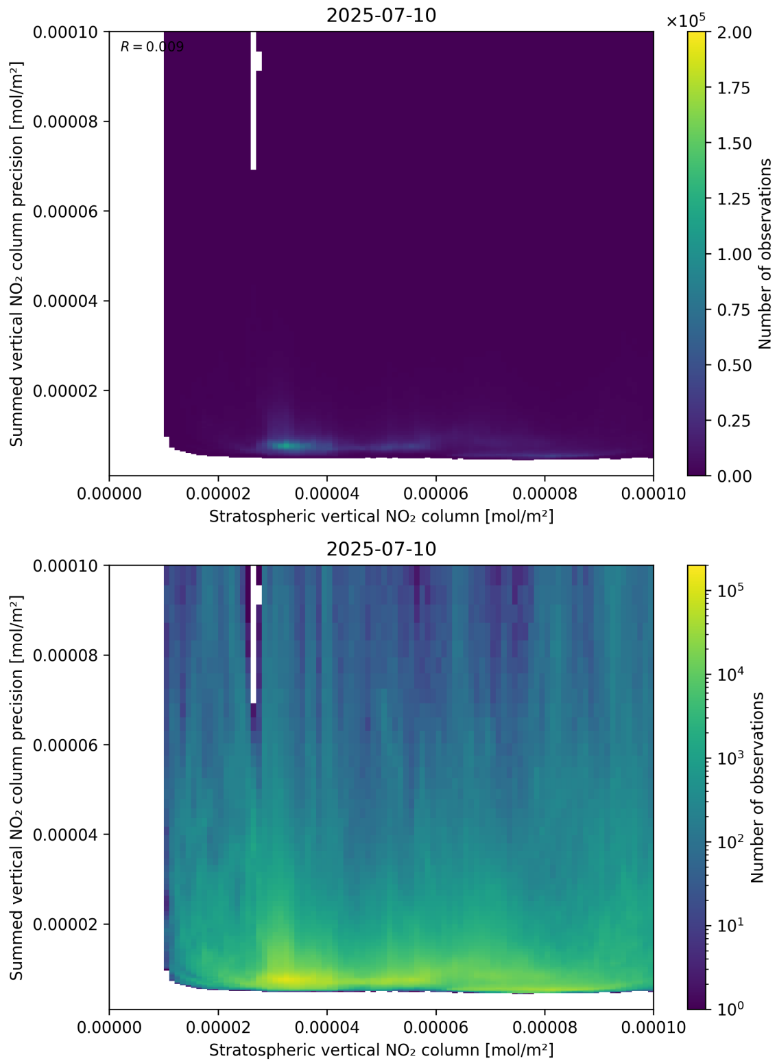
Figure 99: Scatter density plot of “Stratospheric vertical NO 2 column” against “Summed vertical NO 2 column precision” for 2025-07-09 to 2025-07-11.
