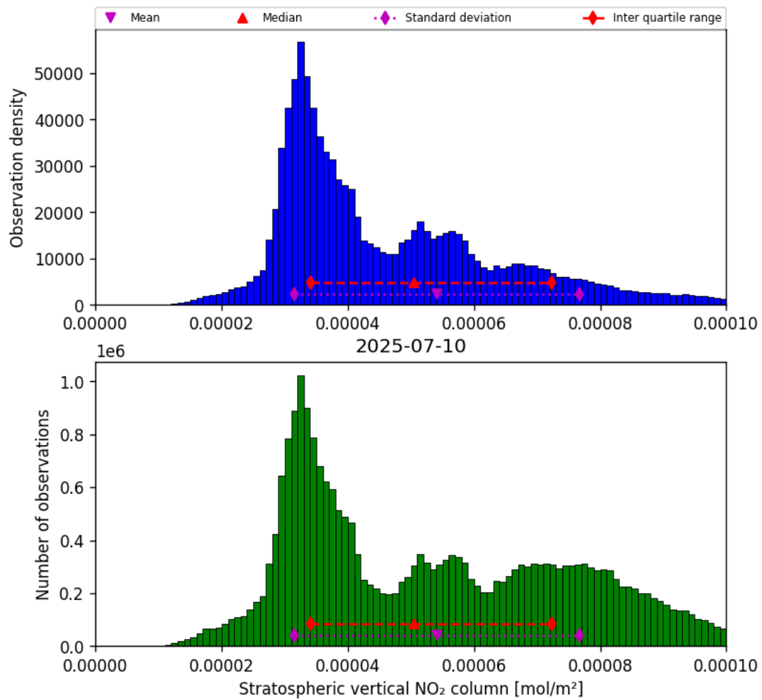
Figure 36: Histogram of “Stratospheric vertical NO 2 column” for 2025-07-09 to 2025-07-11
