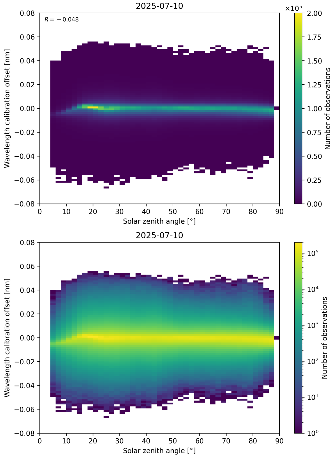
Figure 158: Scatter density plot of “Solar zenith angle” against “Wavelength calibration offset” for 2025-07-09 to 2025-07-11.
