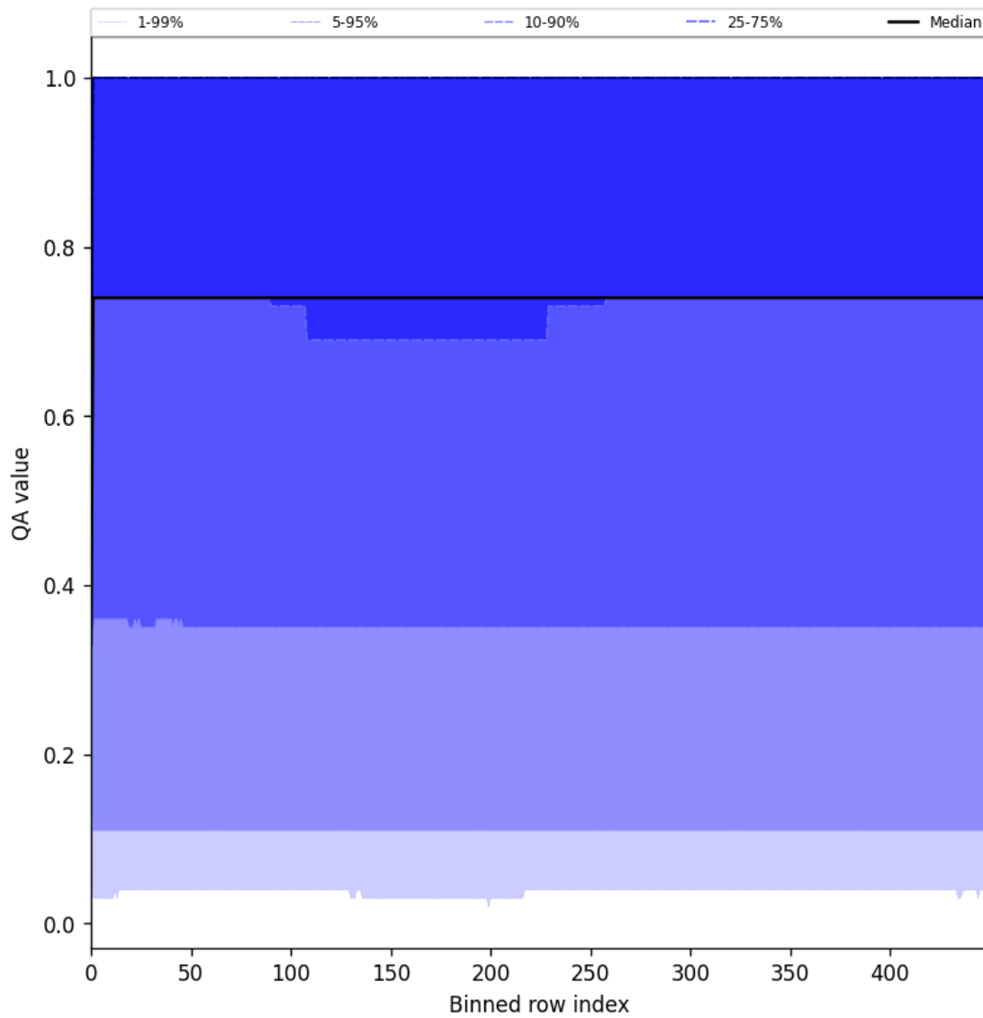
Figure 45: Along track statistics of “QA value” for 2025-07-09 to 2025-07-11
