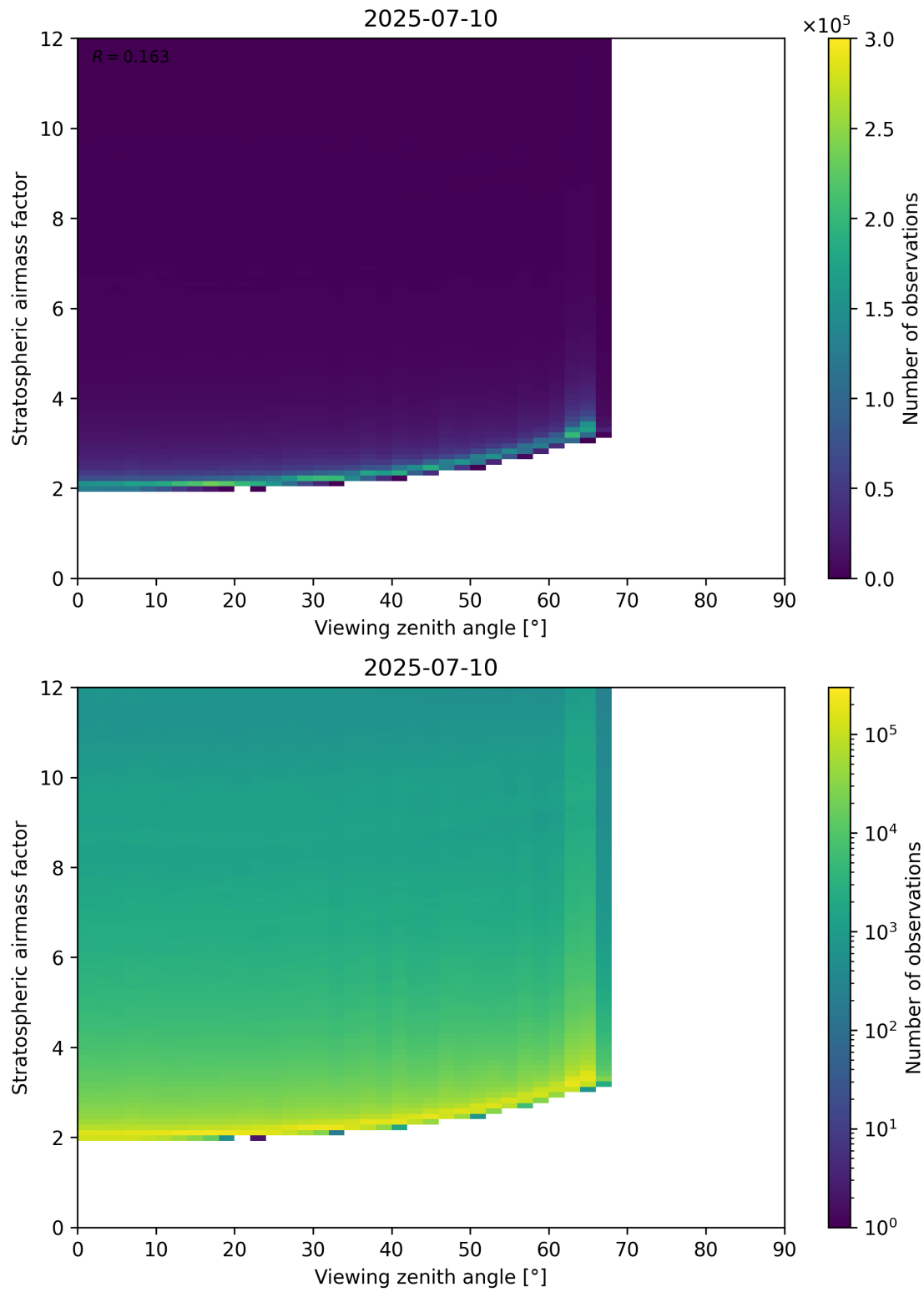
Figure 159: Scatter density plot of “Viewing zenith angle” against “Stratospheric airmass factor” for 2025-07-09 to 2025-07-11.
