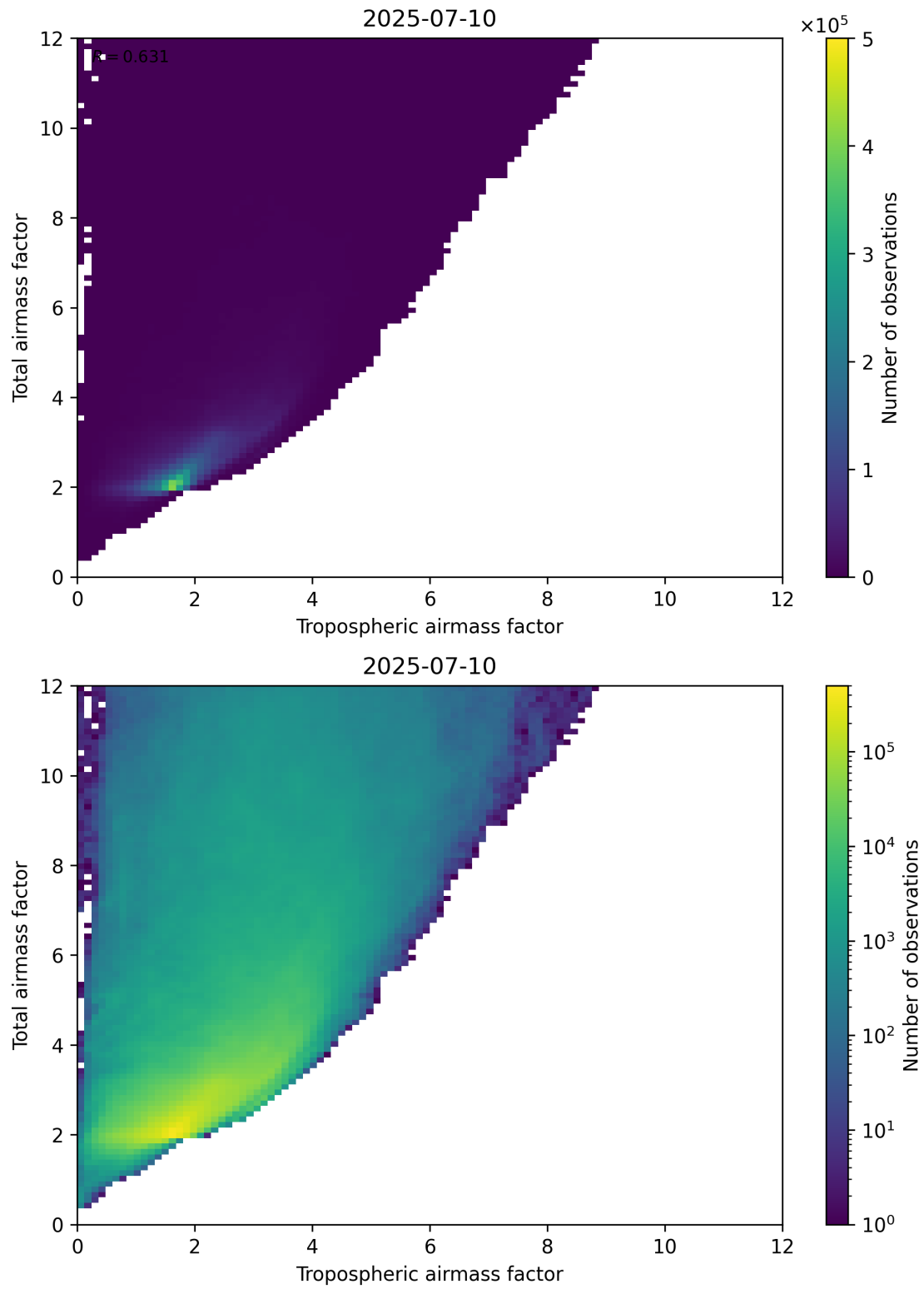
Figure 72: Scatter density plot of “Tropospheric airmass factor” against “Total airmass factor” for 2025-07-09 to 2025-07-11.
