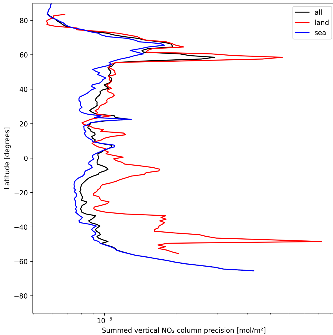
Figure 24: Zonal average of “Summed vertical NO 2 column precision” for 2025-07-09 to 2025-07-11.
