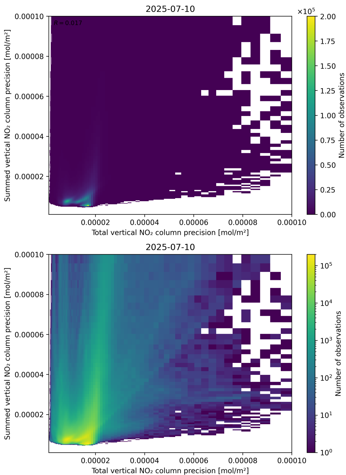
Figure 118: Scatter density plot of “Total vertical NO 2 column precision” against “Summed vertical NO 2 column precision” for 2025-07-09 to 2025-07-11.
