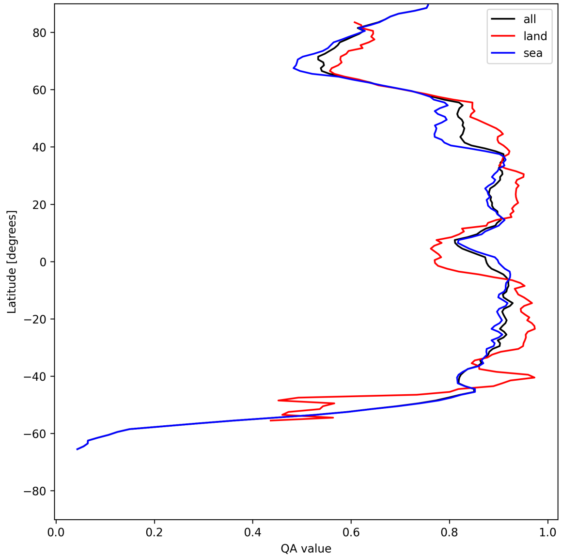
Figure 11: Zonal average of “QA value” for 2025-07-09 to 2025-07-11.
