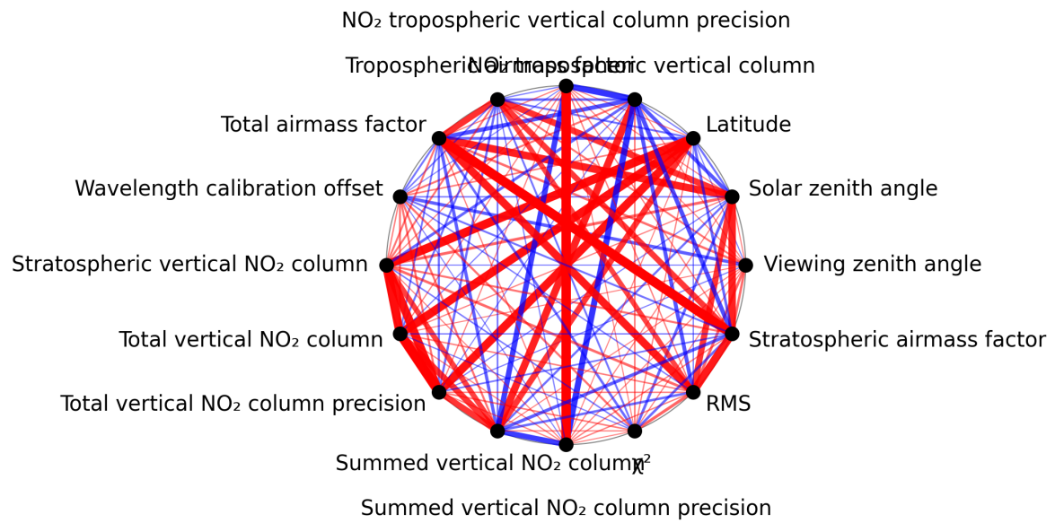
Figure 1: Map of correlation graph for 2025-07-09 to 2025-07-11.
