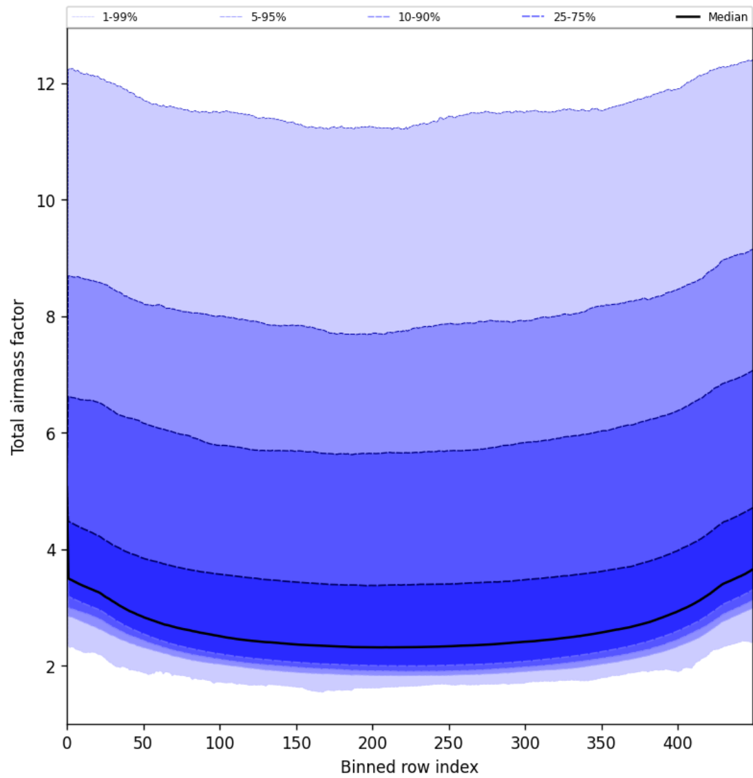
Figure 49: Along track statistics of “Total airmass factor” for 2025-07-09 to 2025-07-11
