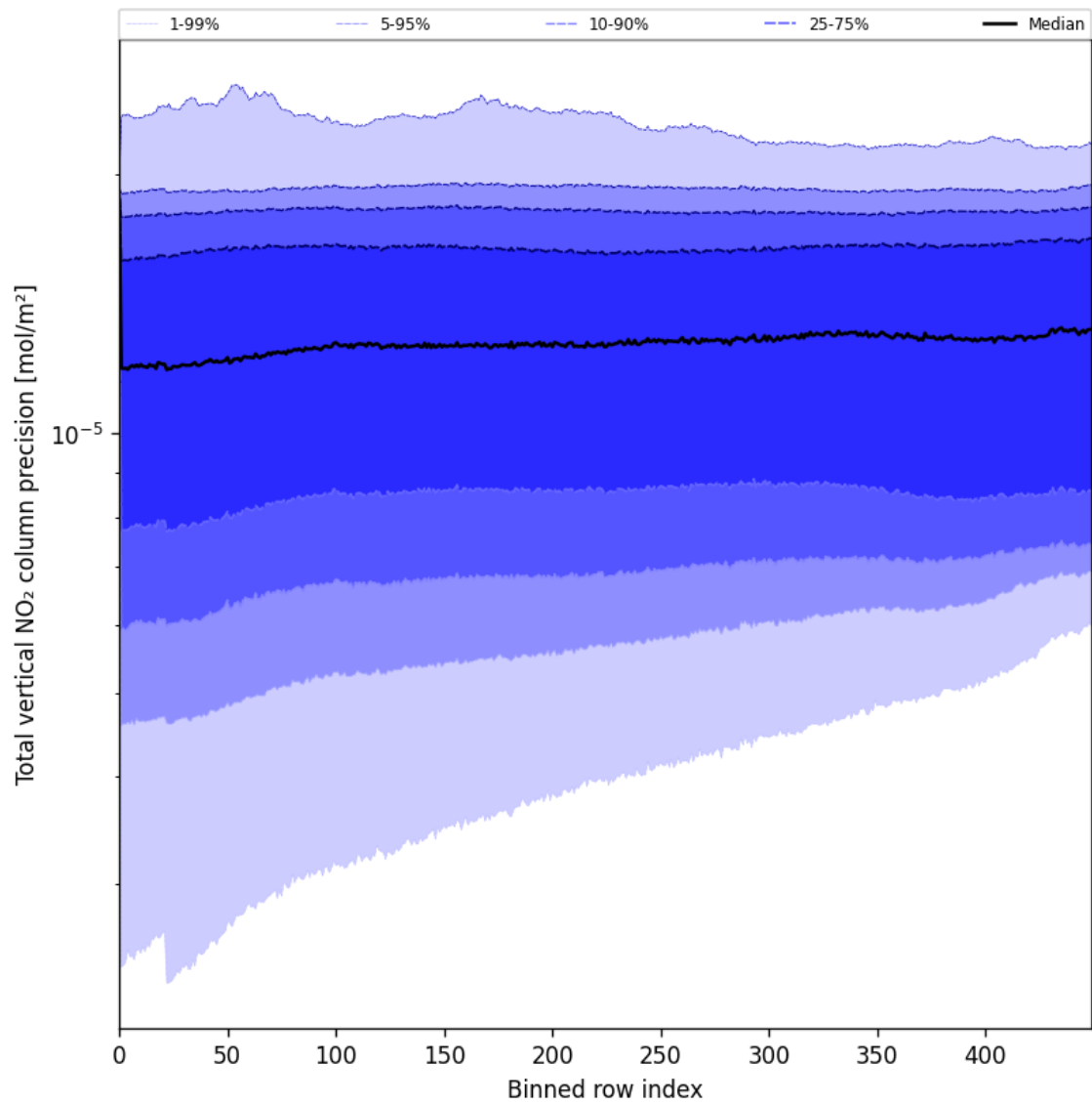
Figure 56: Along track statistics of “Total vertical NO 2 column precision” for 2025-07-09 to 2025-07-11
