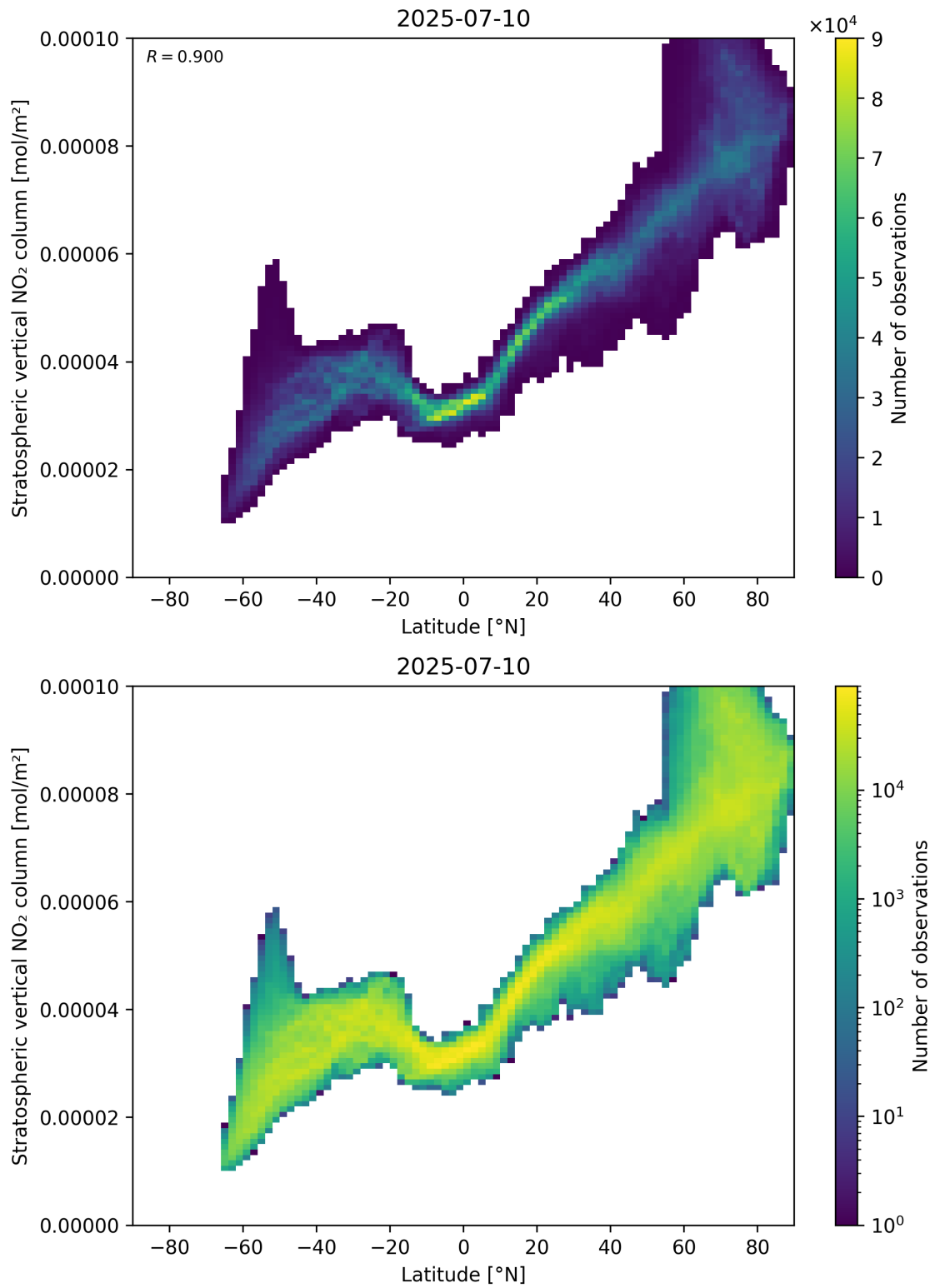
Figure 87: Scatter density plot of “Latitude” against “Stratospheric vertical NO 2 column” for 2025-07-09 to 2025-07-11.
