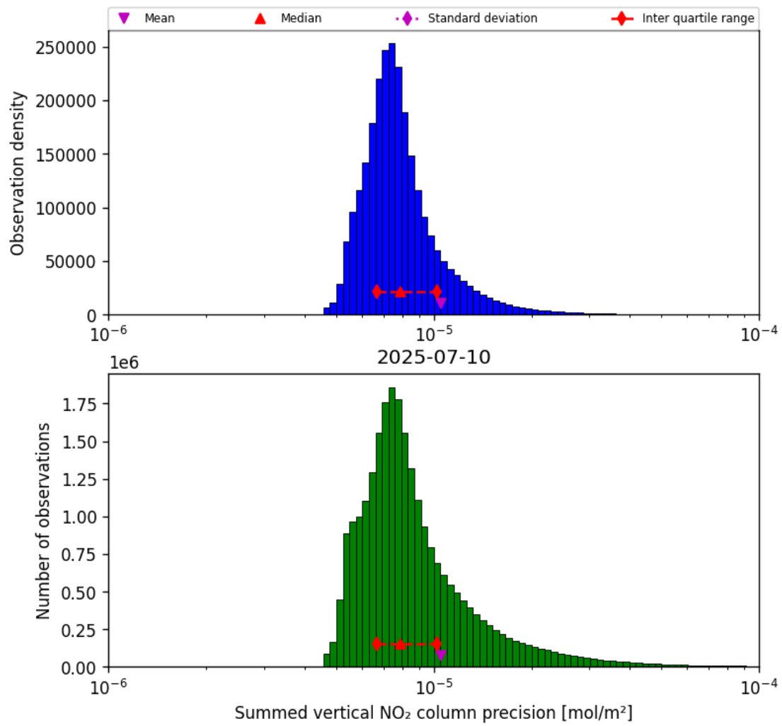
Figure 41: Histogram of "Summed vertical NO 2 column precision" for 2025-07-09 to 2025-07-11
