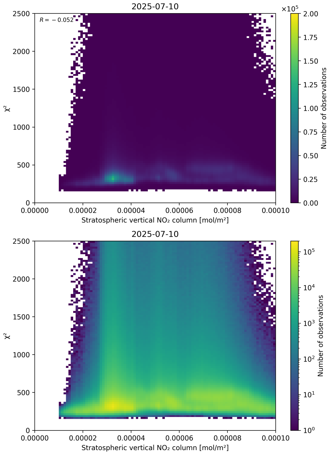
Figure 97: Scatter density plot of “Stratospheric vertical NO 2 column” against “ \chi^2 ” for 2025-07-09 to 2025-07-11.
