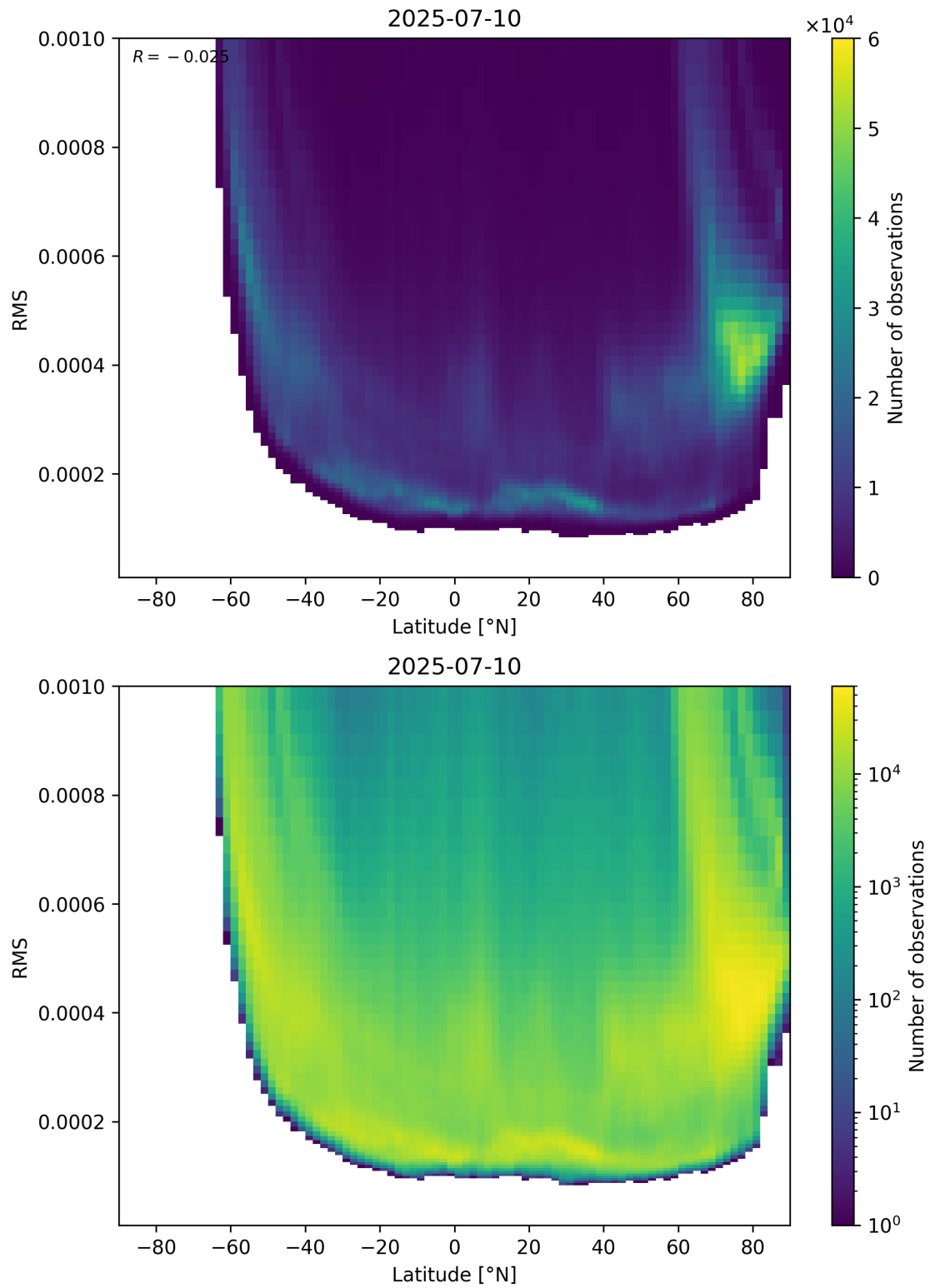
Figure 94: Scatter density plot of “Latitude” against “RMS” for 2025-07-09 to 2025-07-11.
