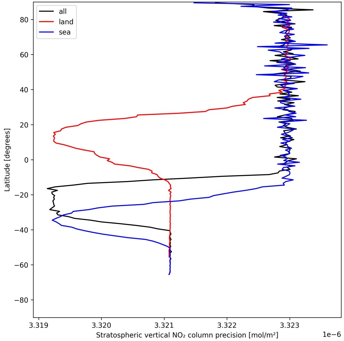
Figure 20: Zonal average of “Stratospheric vertical NO 2 column precision” for 2025-07-09 to 2025-07-11.
