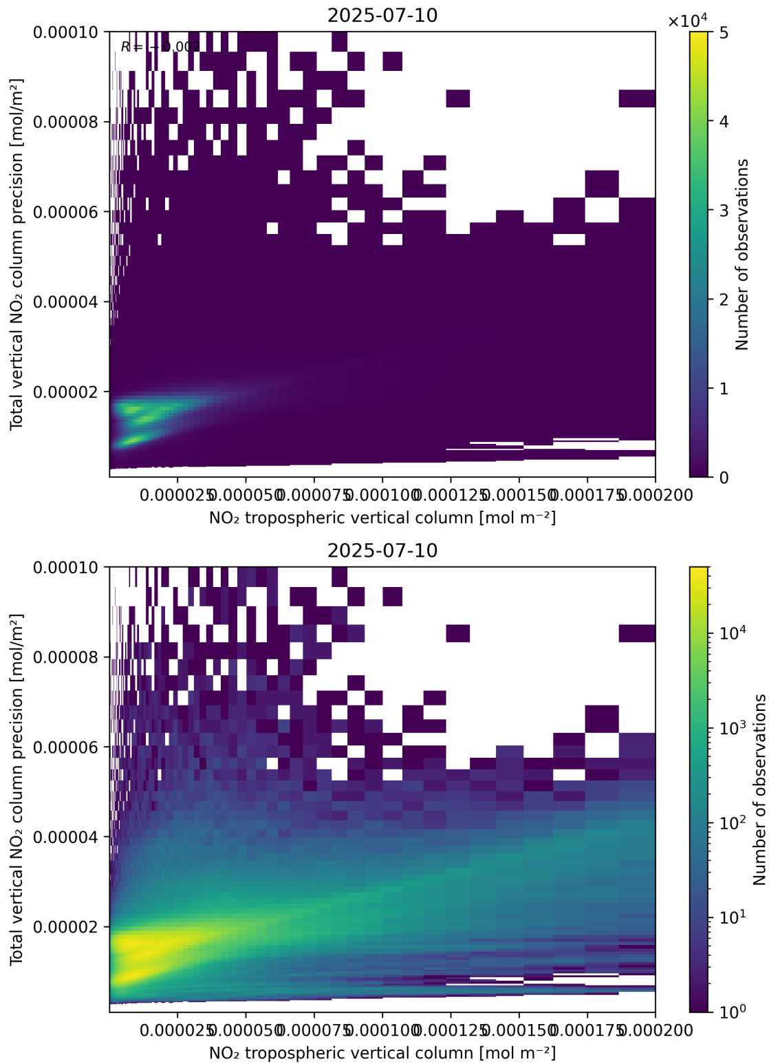
Figure 129: Scatter density plot of “NO 2 tropospheric vertical column” against “Total vertical NO 2 column precision” for 2025-07-09 to 2025-07-11.
