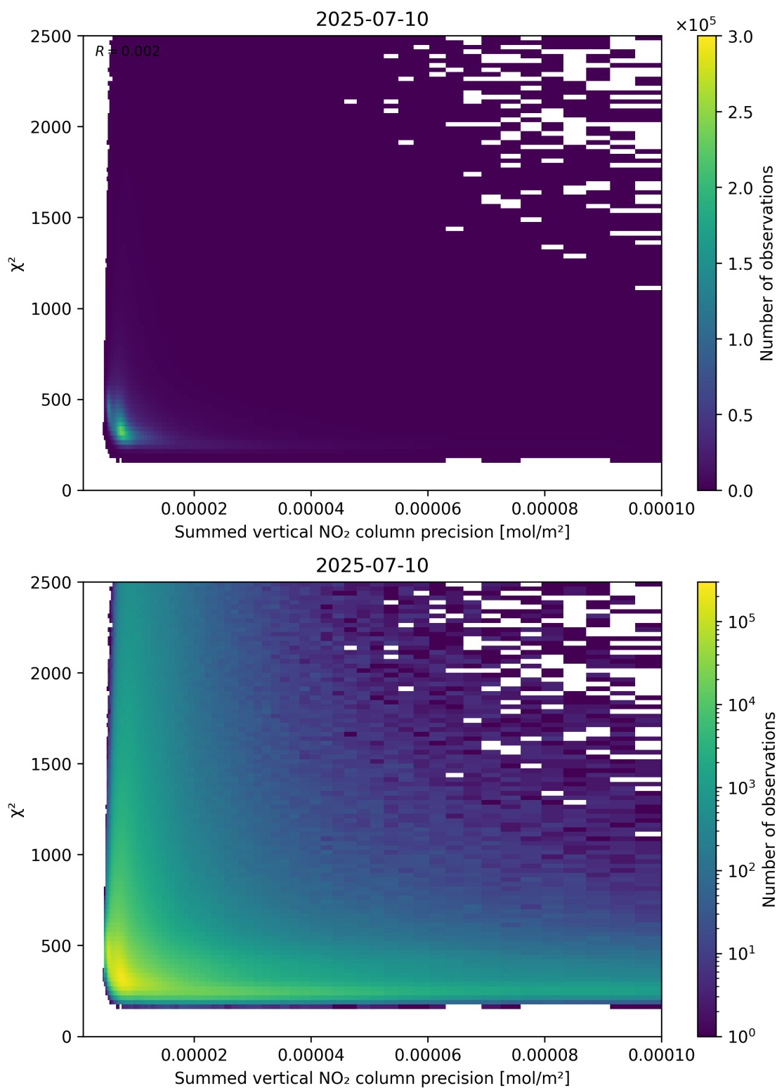
Figure 107: Scatter density plot of “Summed vertical NO 2 column precision” against “ \chi^2 ” for 2025-07-09 to 2025-07-11.
