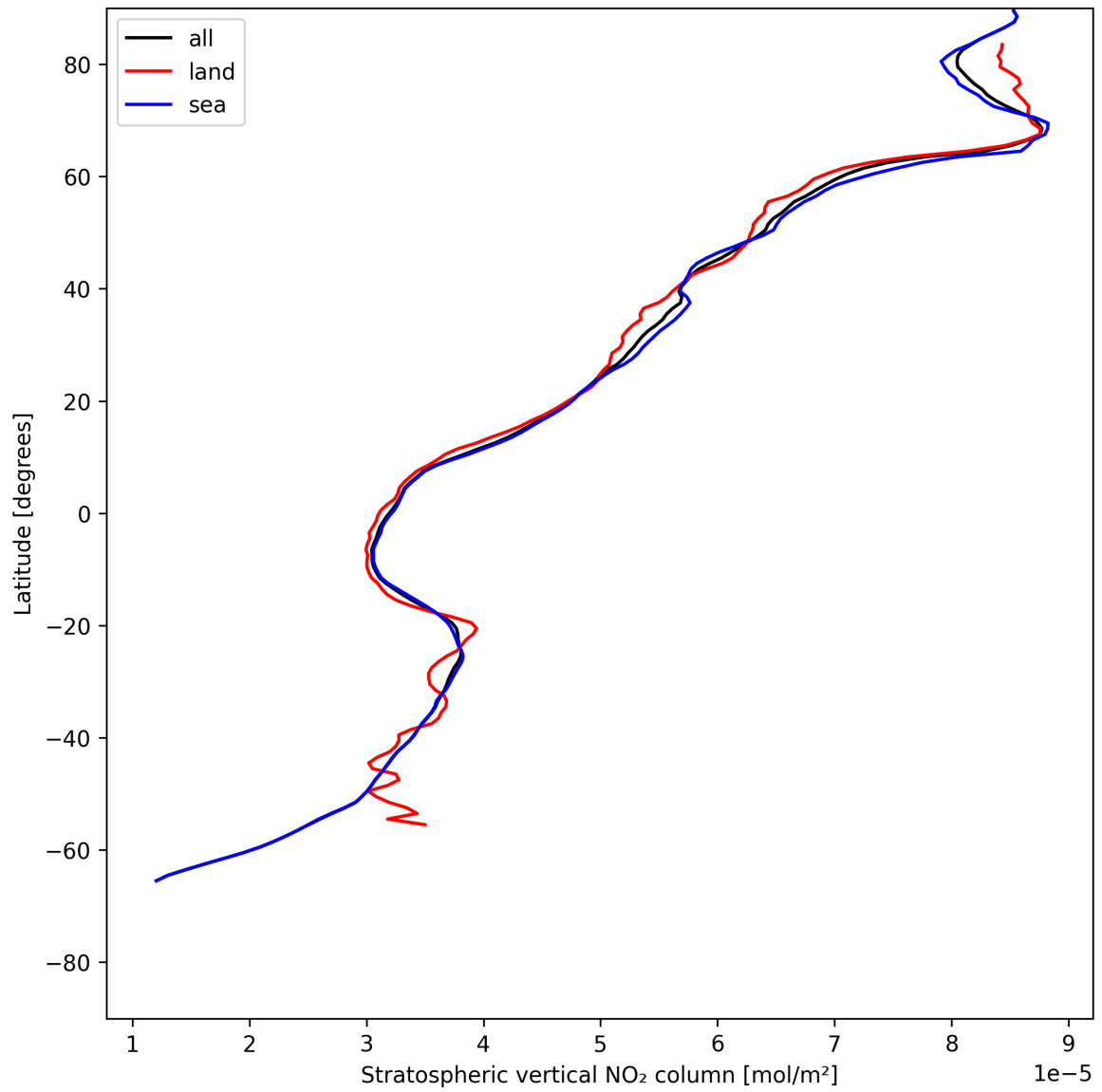
Figure 19: Zonal average of “Stratospheric vertical NO 2 column” for 2025-07-09 to 2025-07-11.
