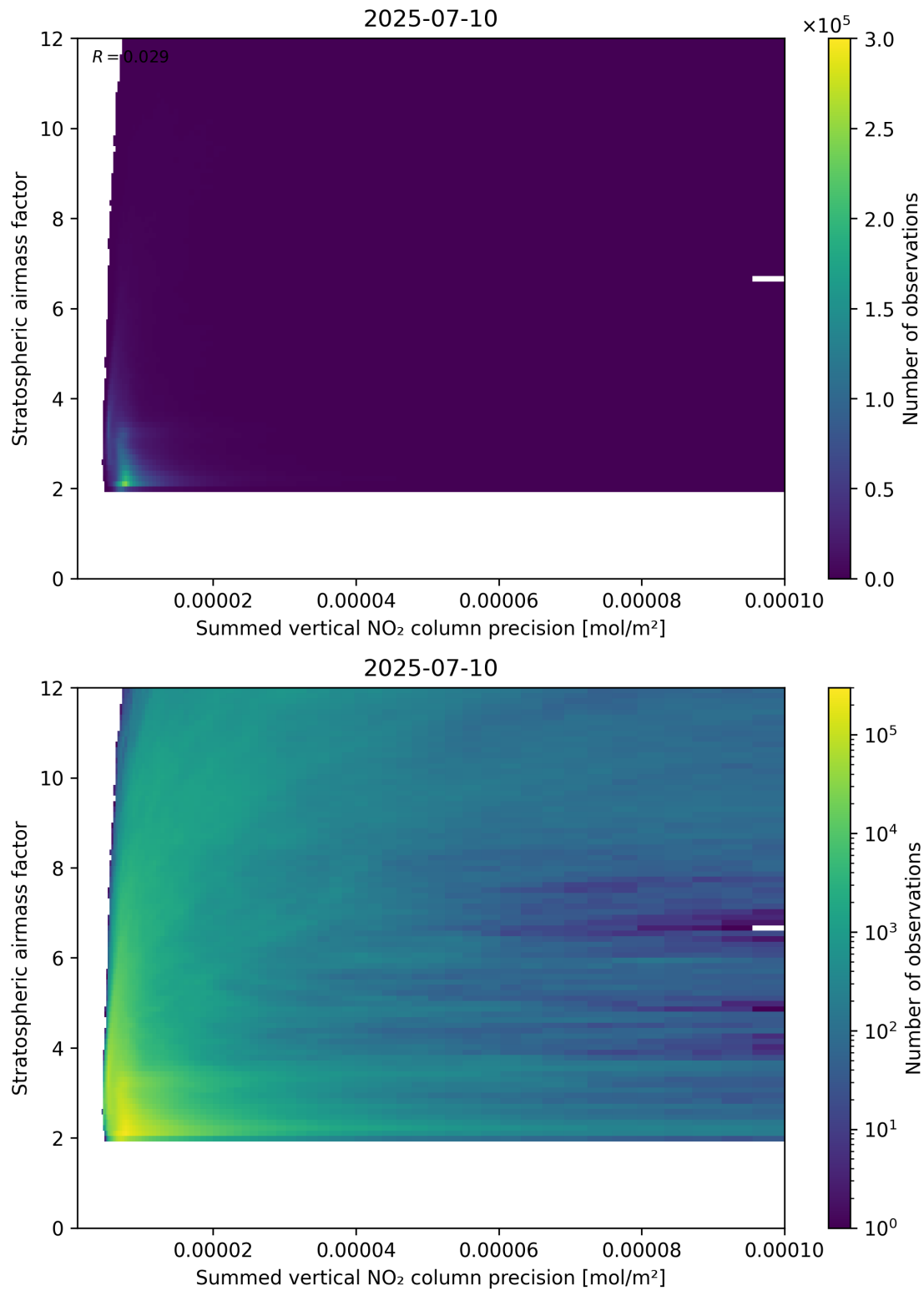
Figure 106: Scatter density plot of “Summed vertical NO 2 column precision” against “Stratospheric airmass factor” for 2025-07-09 to 2025-07-11.
