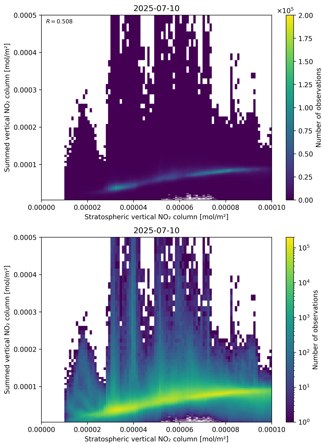
Figure 98: Scatter density plot of “Stratospheric vertical NO 2 column” against “Summed vertical NO 2 column” for 2025-07-09 to 2025-07-11.
