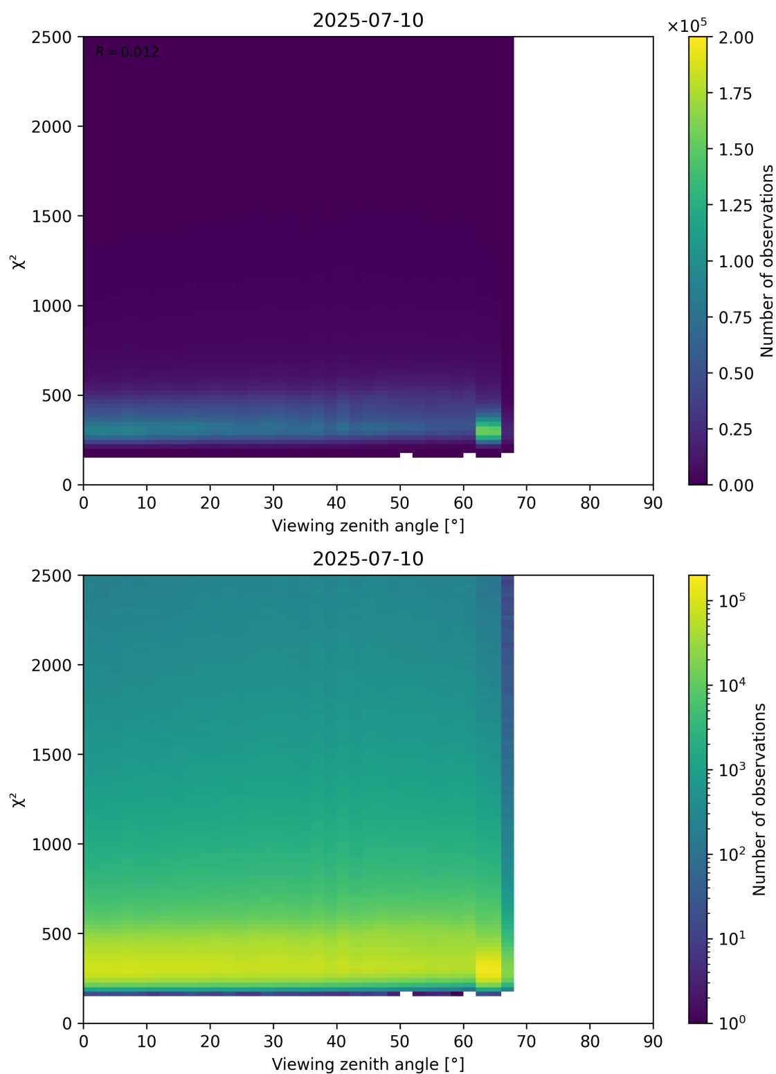
Figure 162: Scatter density plot of “Viewing zenith angle” against “ \chi^2 ” for 2025-07-09 to 2025-07-11.
