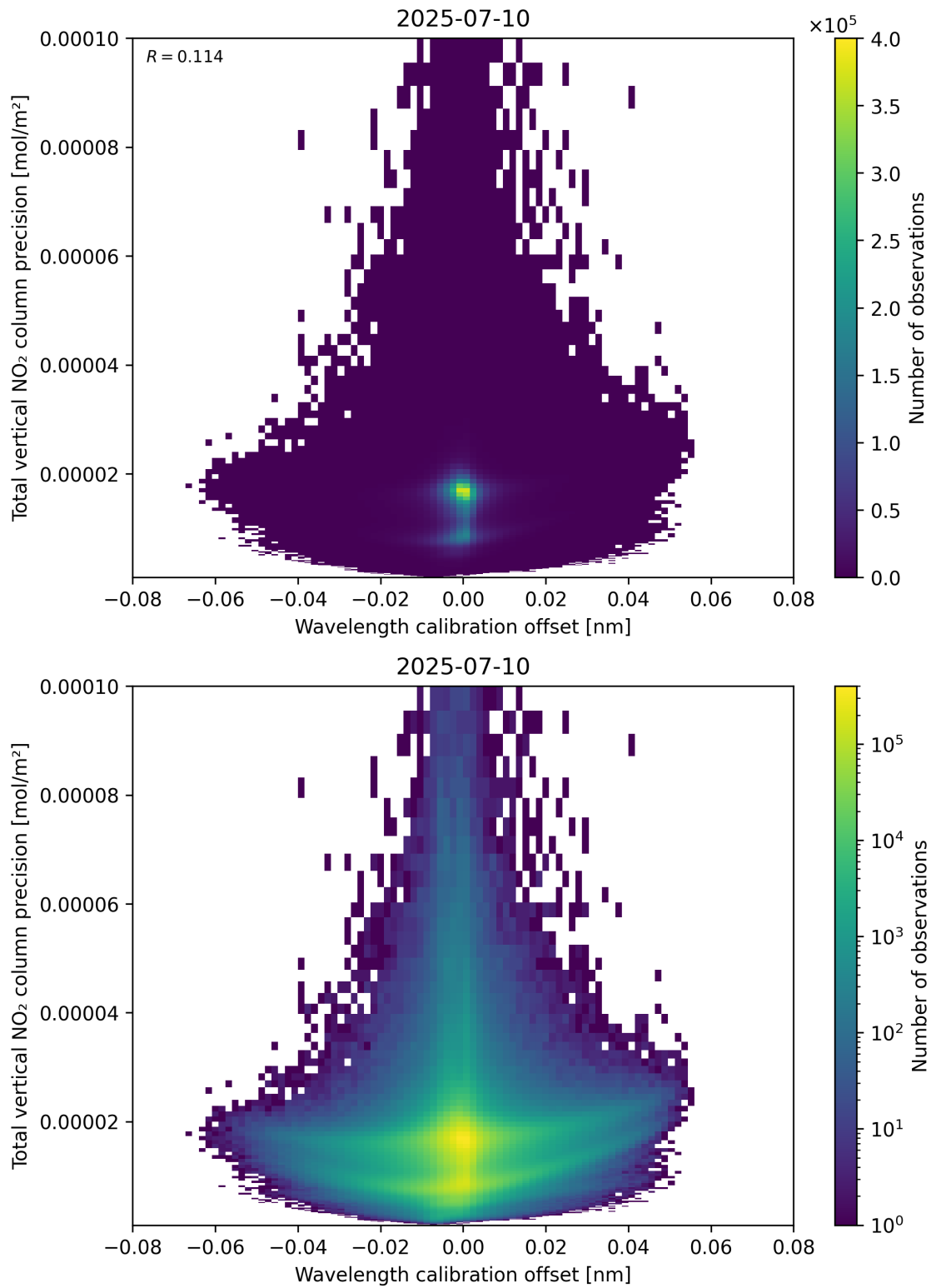
Figure 180: Scatter density plot of “Wavelength calibration offset” against “Total vertical NO 2 column precision” for 2025-07-09 to 2025-07-11.
