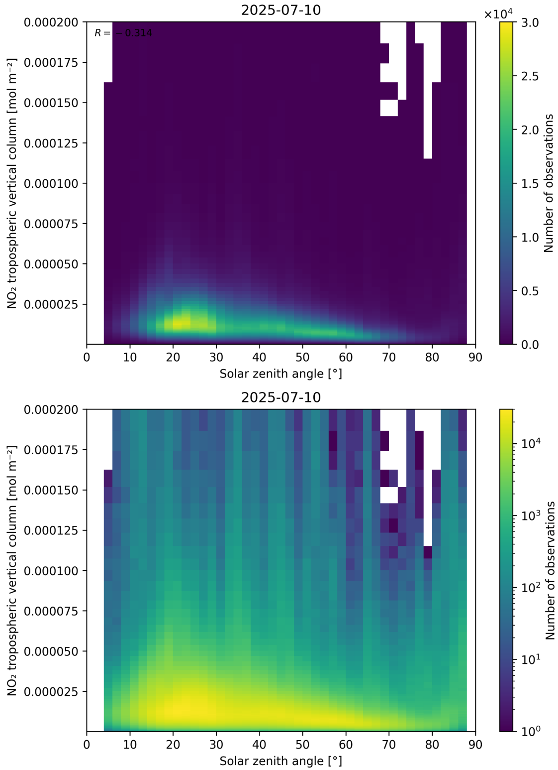
Figure 155: Scatter density plot of “Solar zenith angle” against “NO 2 tropospheric vertical column” for 2025-07-09 to 2025-07-11.
