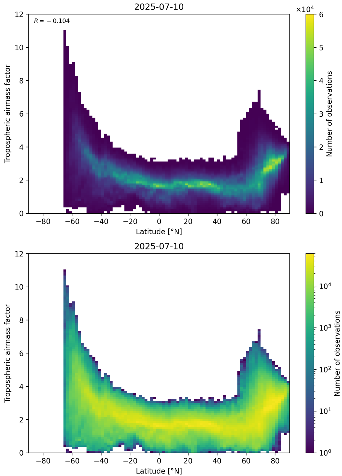
Figure 85: Scatter density plot of “Latitude” against “Tropospheric air mass factor” for 2025-07-09 to 2025-07-11.
