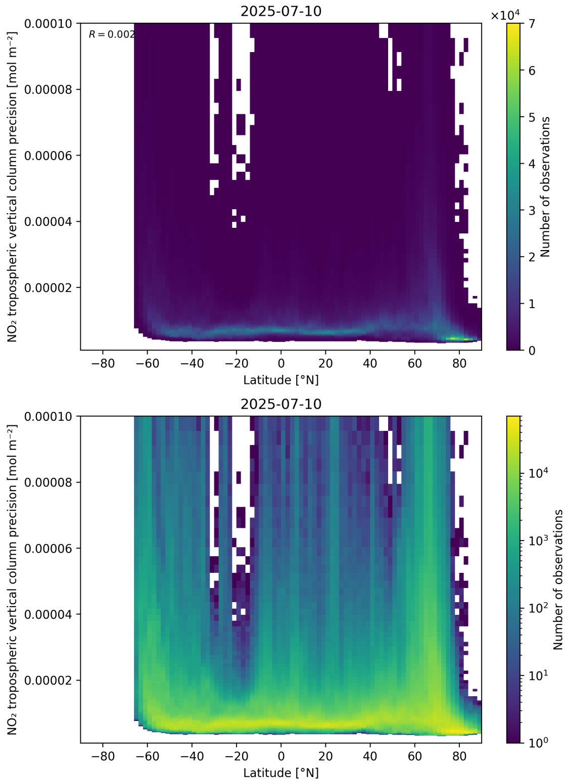
Figure 93: Scatter density plot of “Latitude” against “NO 2 tropospheric vertical column precision” for 2025-07-09 to 2025-07-11.
