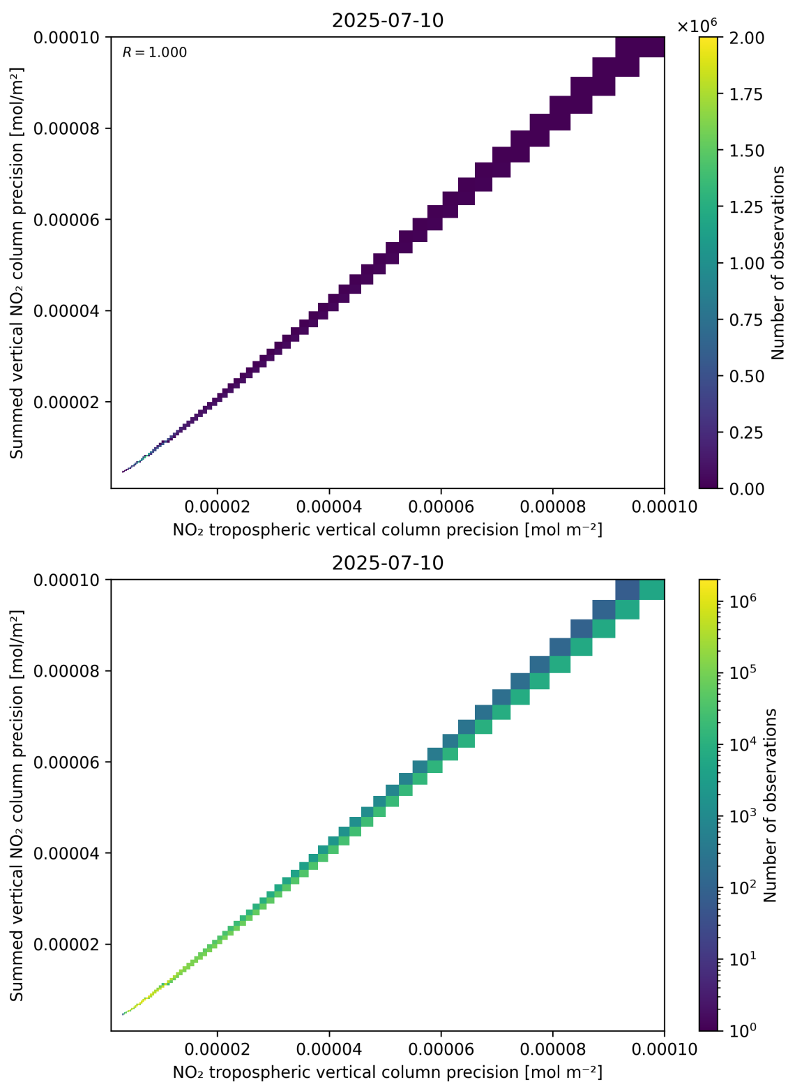
Figure 137: Scatter density plot of “NO 2 tropospheric vertical column precision” against “Summed vertical NO 2 column precision” for 2025-07-09 to 2025-07-11.
