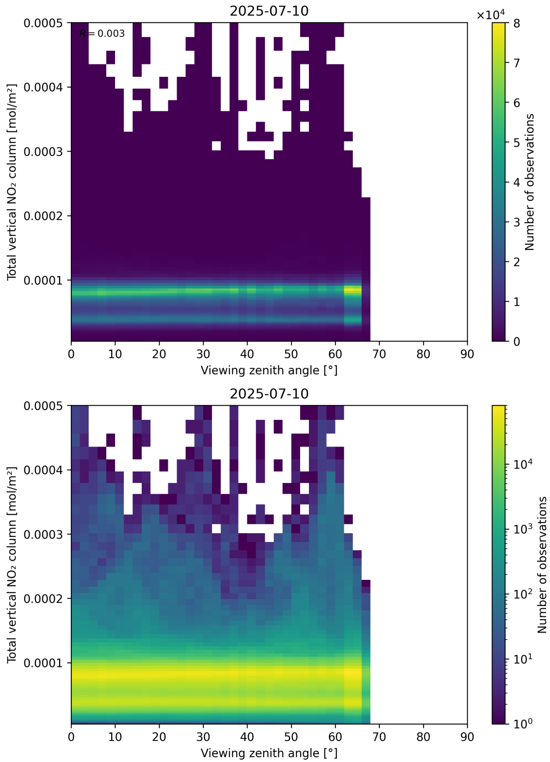
Figure 167: Scatter density plot of “Viewing zenith angle” against “Total vertical NO 2 column” for 2025-07-09 to 2025-07-11.
