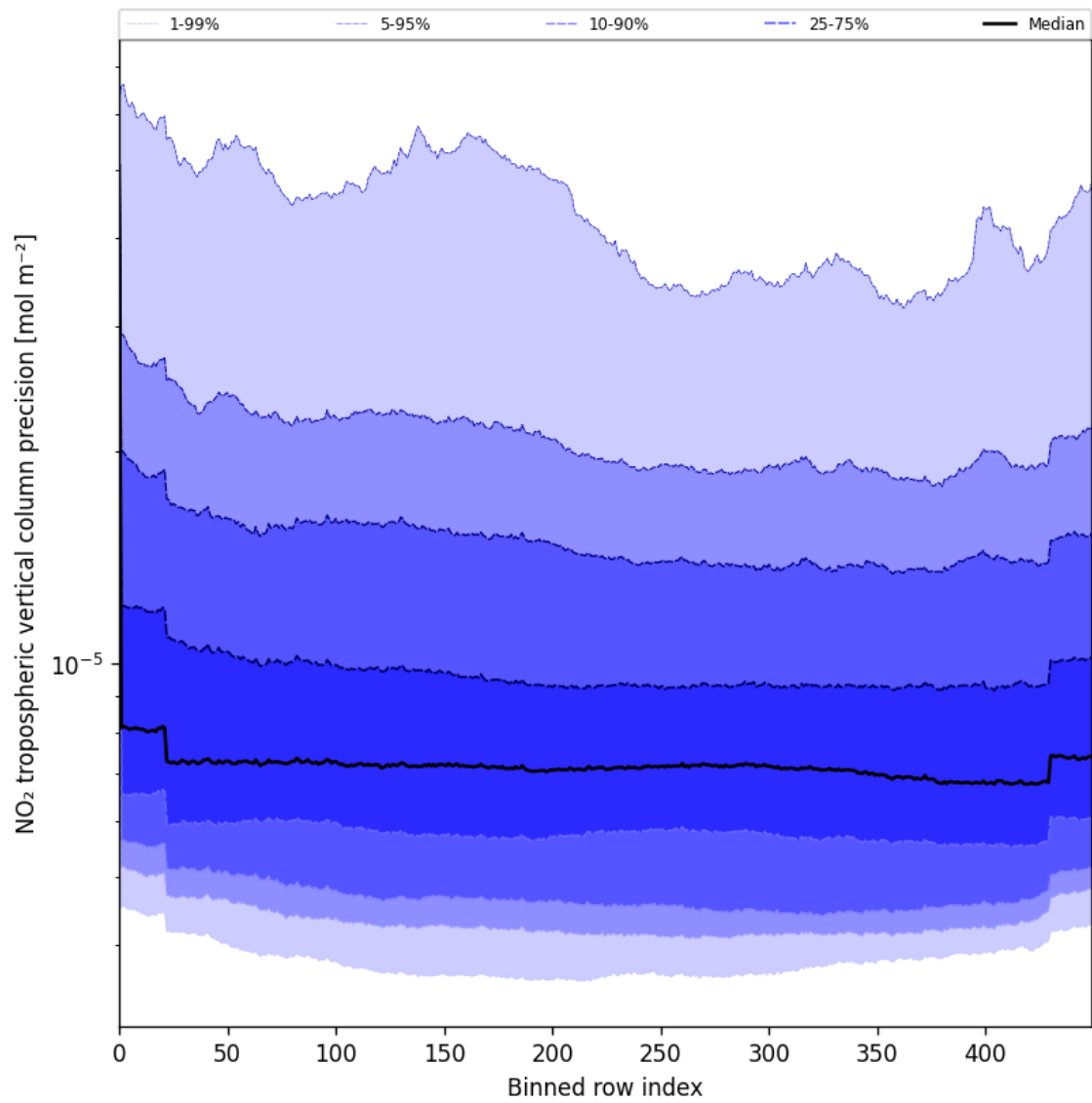
Figure 47: Along track statistics of “NO 2 tropospheric vertical column precision” for 2025-07-09 to 2025-07-11
