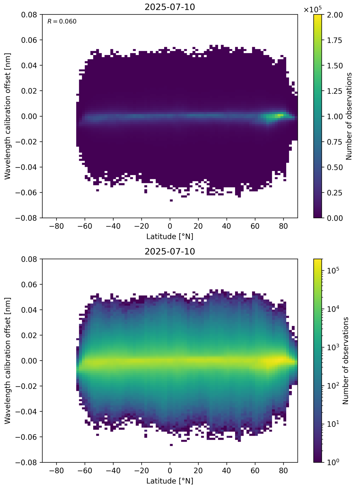
Figure 95: Scatter density plot of “Latitude” against “Wavelength calibration offset” for 2025-07-09 to 2025-07-11.
