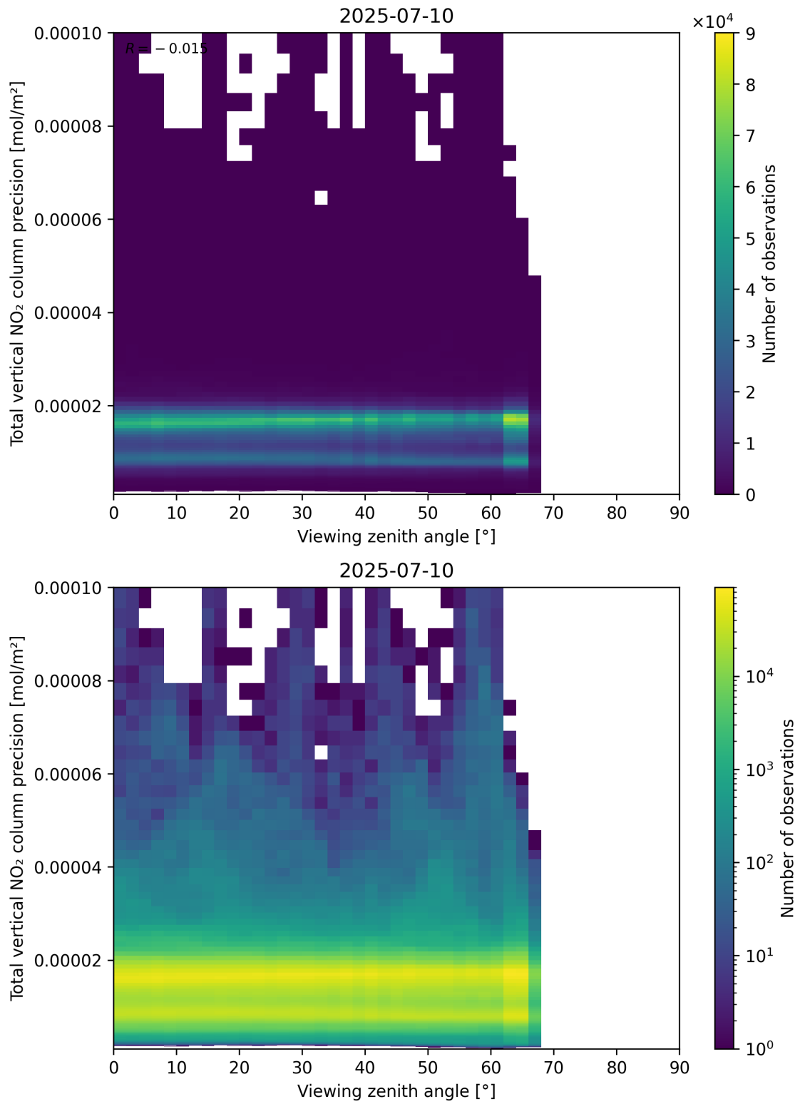
Figure 168: Scatter density plot of “Viewing zenith angle” against “Total vertical NO 2 column precision” for 2025-07-09 to 2025-07-11.
