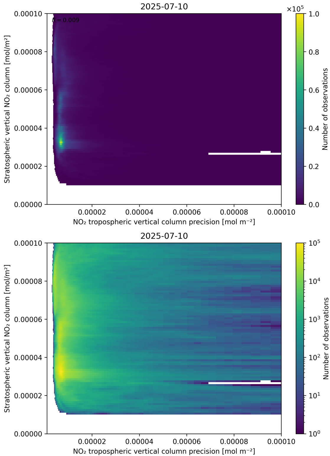
Figure 135: Scatter density plot of “NO 2 tropospheric vertical column precision” against “Stratospheric vertical NO 2 column” for 2025-07-09 to 2025-07-11.
