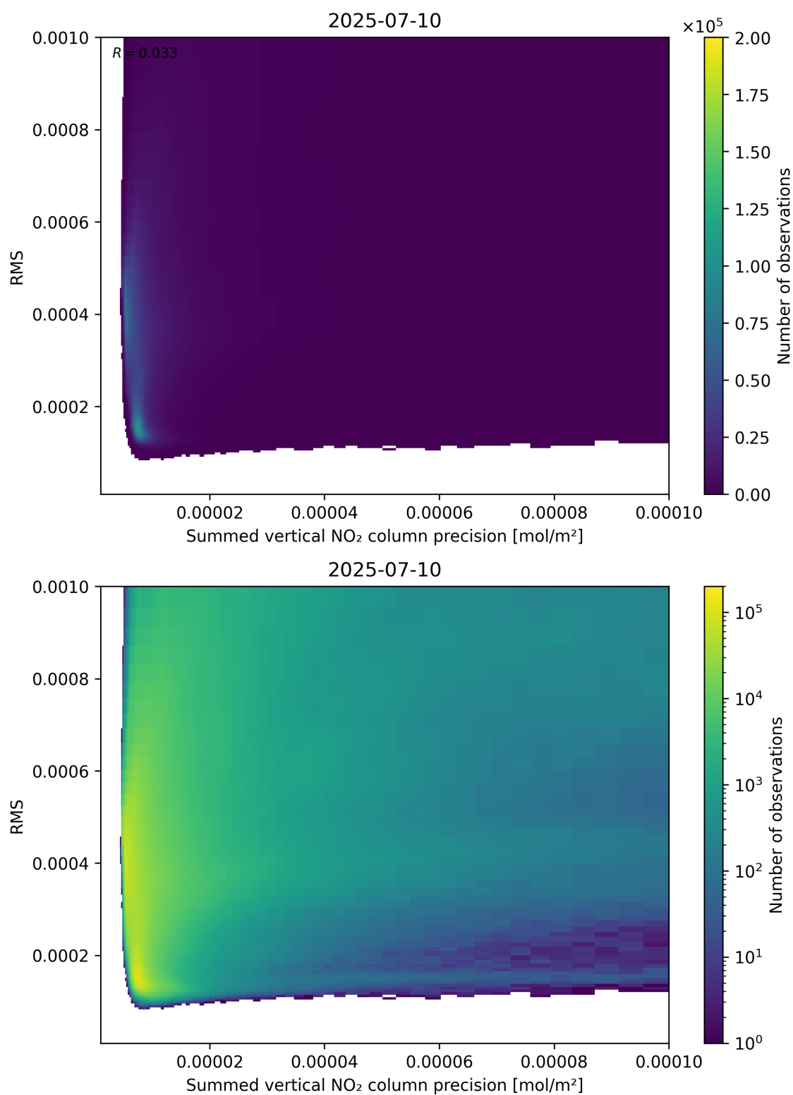
Figure 108: Scatter density plot of “Summed vertical NO 2 column precision” against “RMS” for 2025-07-09 to 2025-07-11.
