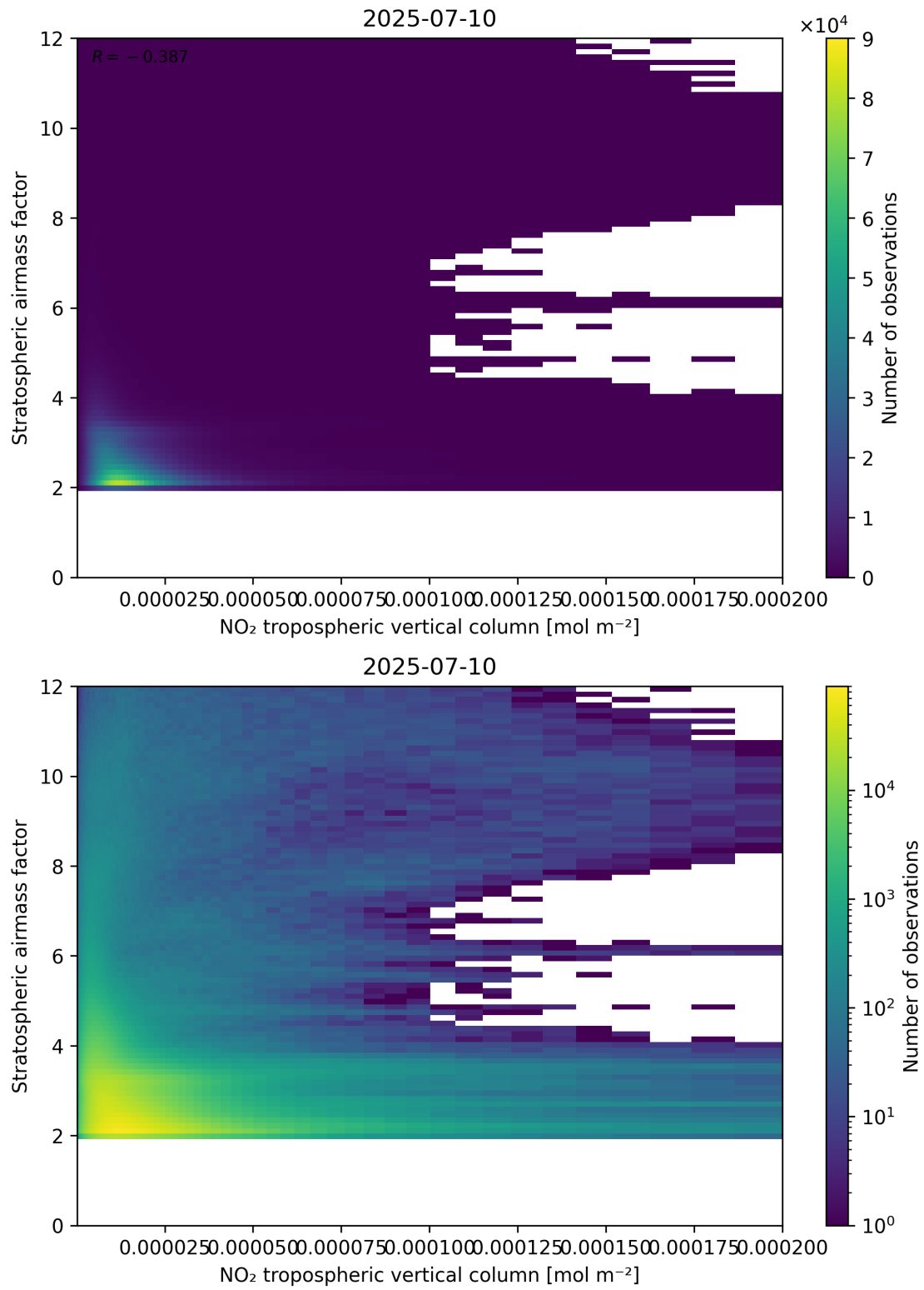
Figure 121: Scatter density plot of “NO 2 tropospheric vertical column” against “Stratospheric air mass factor” for 2025-07-09 to 2025-07-11.
