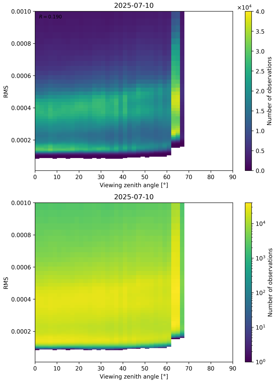
Figure 171: Scatter density plot of “Viewing zenith angle” against “RMS” for 2025-07-09 to 2025-07-11.
