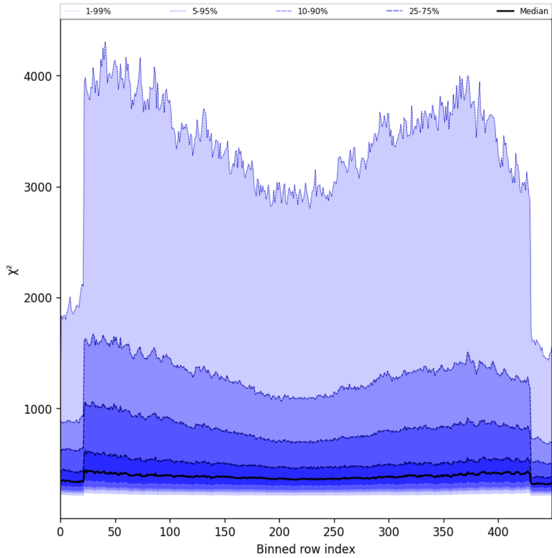
Figure 59: Along track statistics of “ \chi^2 ” for 2025-07-09 to 2025-07-11
