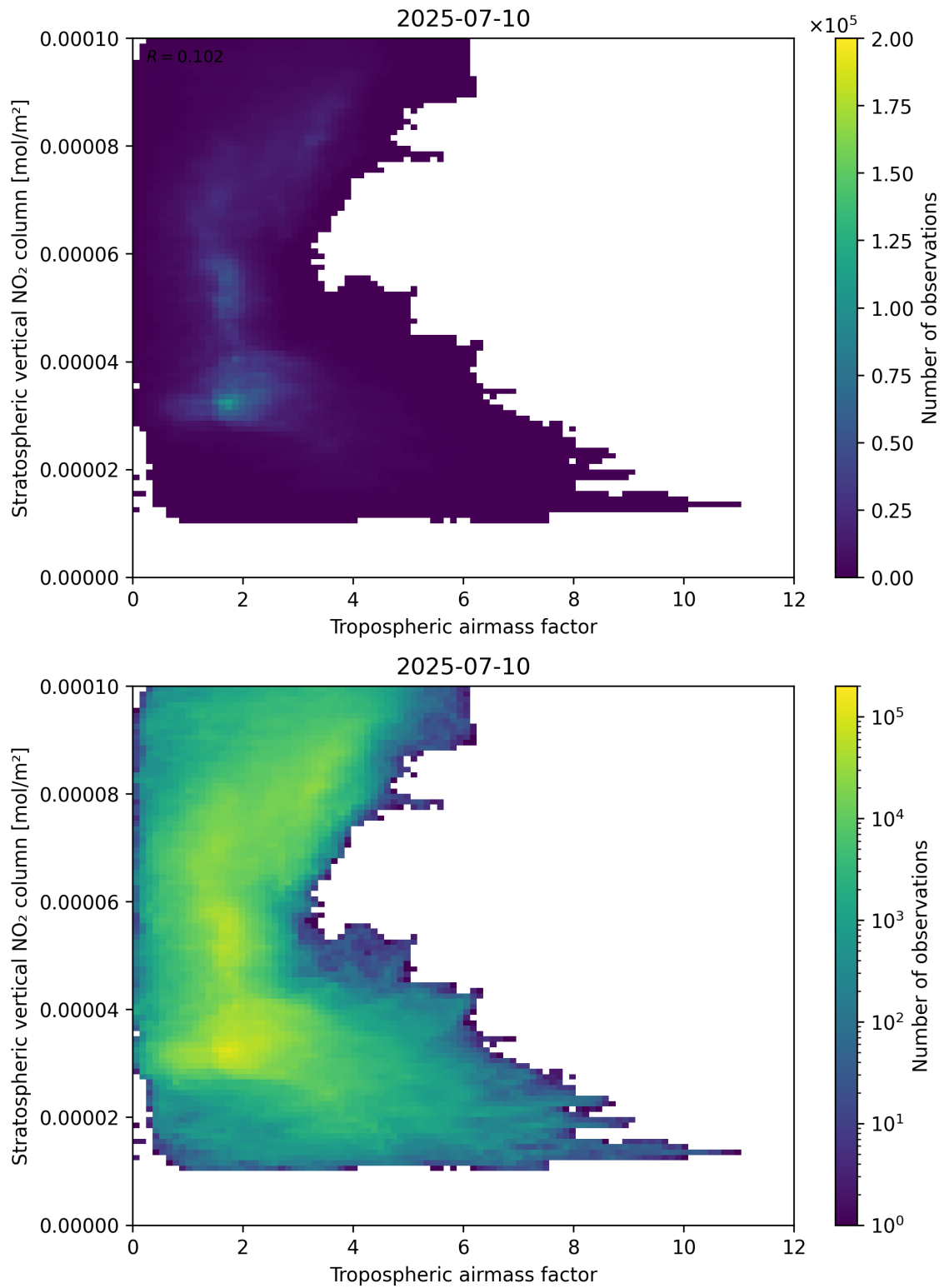
Figure 74: Scatter density plot of “Tropospheric airmass factor” against “Stratospheric vertical NO 2 column” for 2025-07-09 to 2025-07-11.
