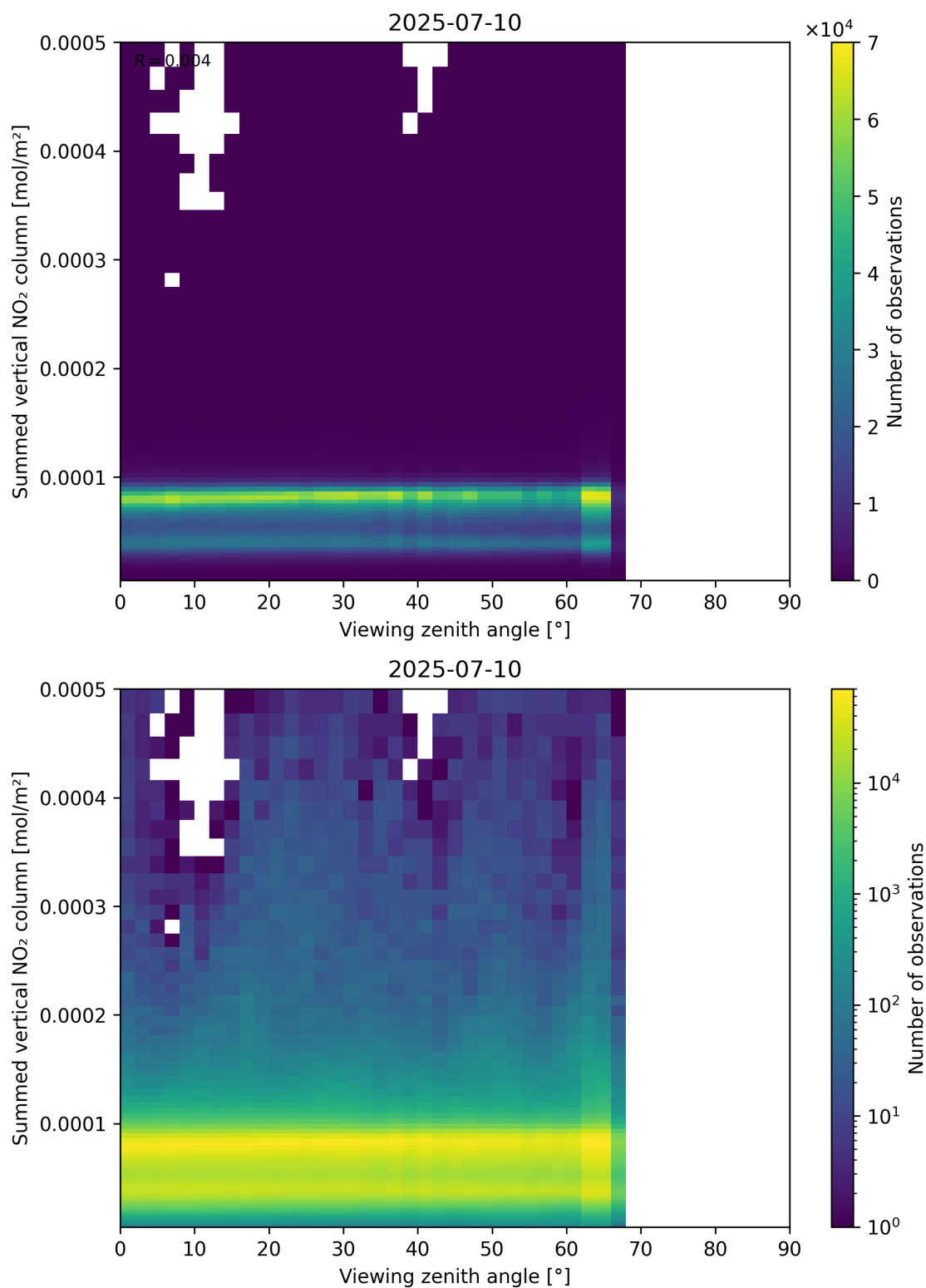
Figure 165: Scatter density plot of “Viewing zenith angle” against “Summed vertical NO 2 column” for 2025-07-09 to 2025-07-11.
