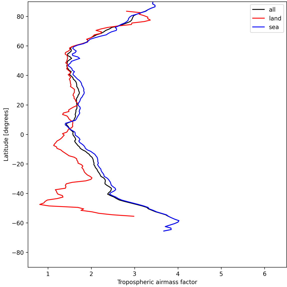
Figure 14: Zonal average of “Tropospheric airmass factor” for 2025-07-09 to 2025-07-11.
