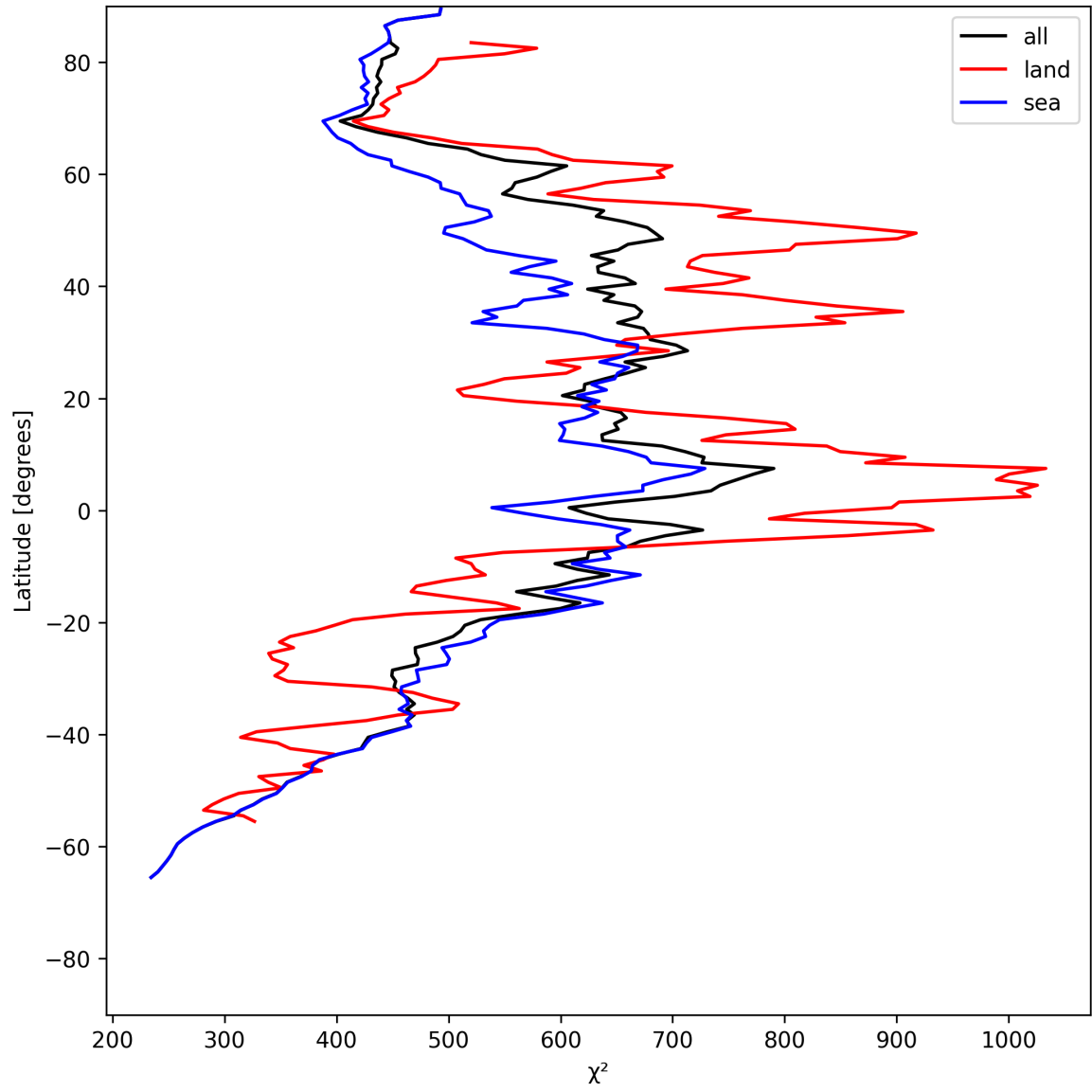
Figure 25: Zonal average of “ \chi^2 ” for 2025-07-09 to 2025-07-11.
