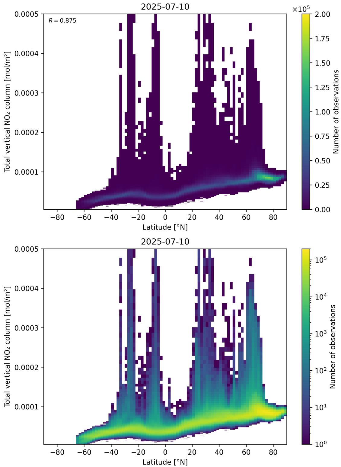
Figure 90: Scatter density plot of “Latitude” against “Total vertical NO 2 column” for 2025-07-09 to 2025-07-11.
