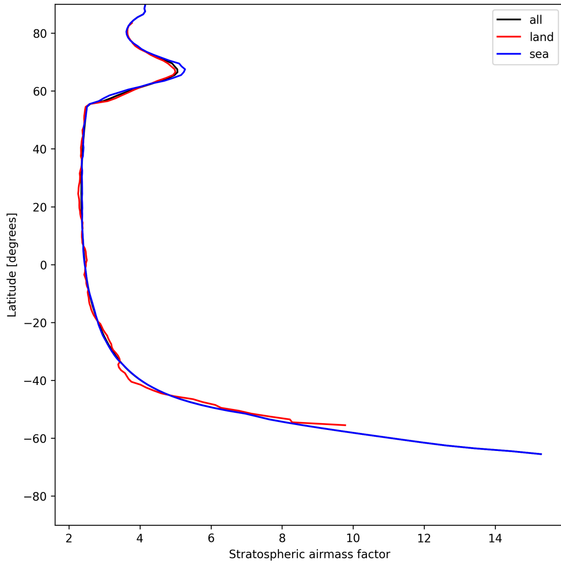
Figure 27: Zonal average of “Stratospheric air mass factor” for 2025-07-09 to 2025-07-11.
