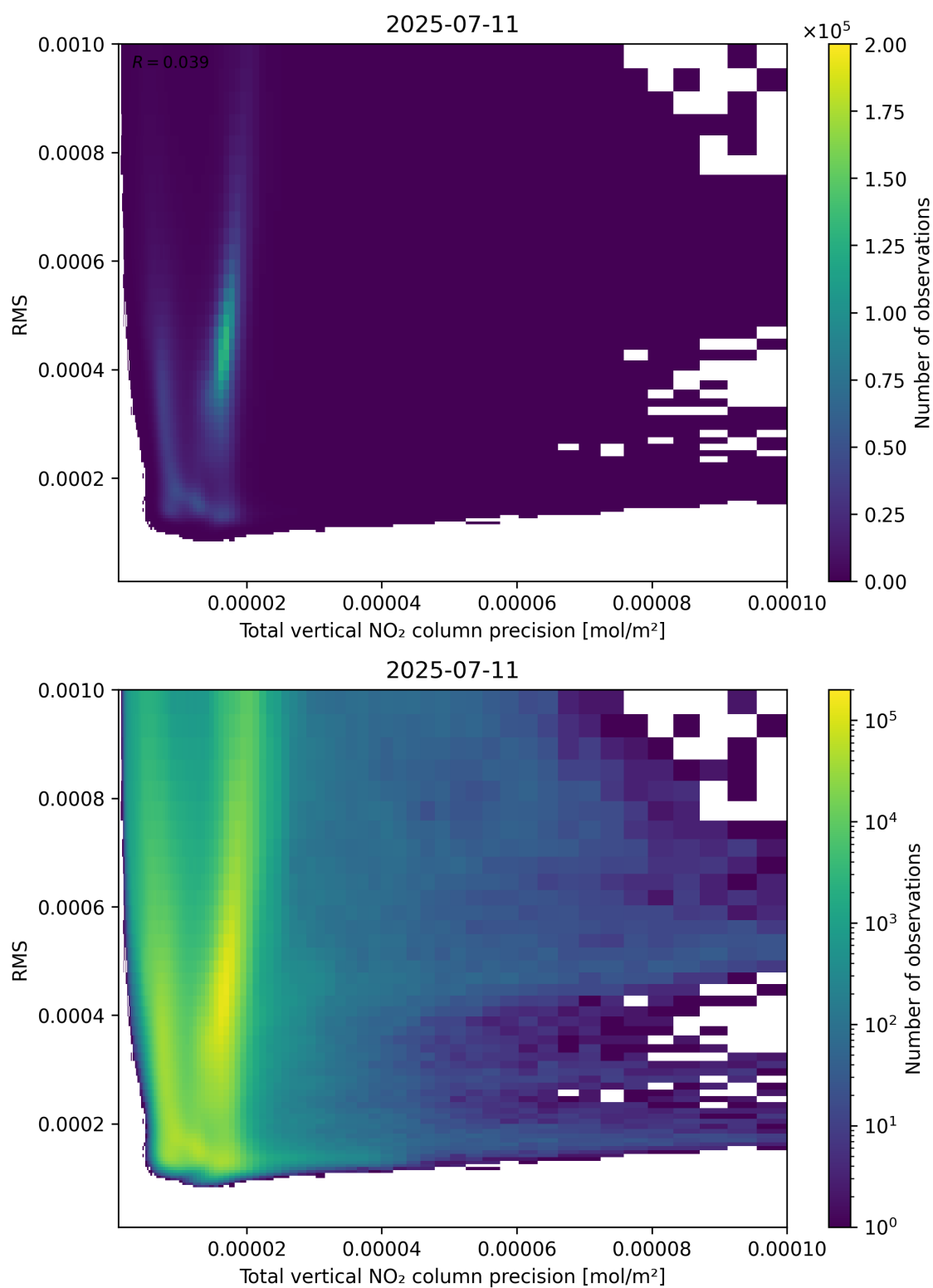
Figure 119: Scatter density plot of “Total vertical NO 2 column precision” against “RMS” for 2025-07-10 to 2025-07-12.
