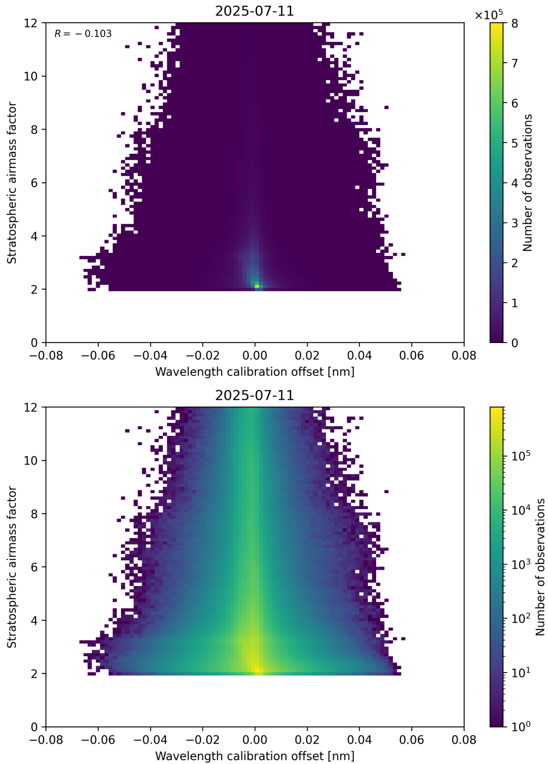
Figure 174: Scatter density plot of “Wavelength calibration offset” against “Stratospheric airmass factor” for 2025-07-10 to 2025-07-12.
