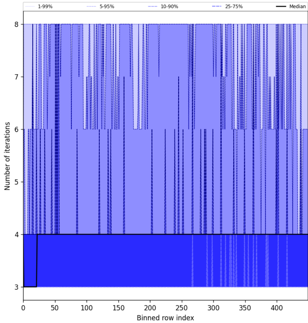
Figure 51: Along track statistics of “Number of iterations” for 2025-07-10 to 2025-07-12
