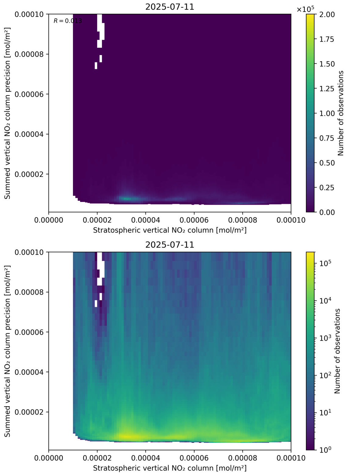
Figure 99: Scatter density plot of “Stratospheric vertical NO 2 column” against “Summed vertical NO 2 column precision” for 2025-07-10 to 2025-07-12.
