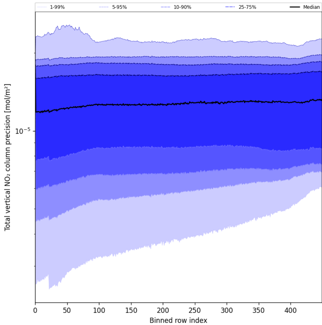
Figure 56: Along track statistics of “Total vertical NO 2 column precision” for 2025-07-10 to 2025-07-12
