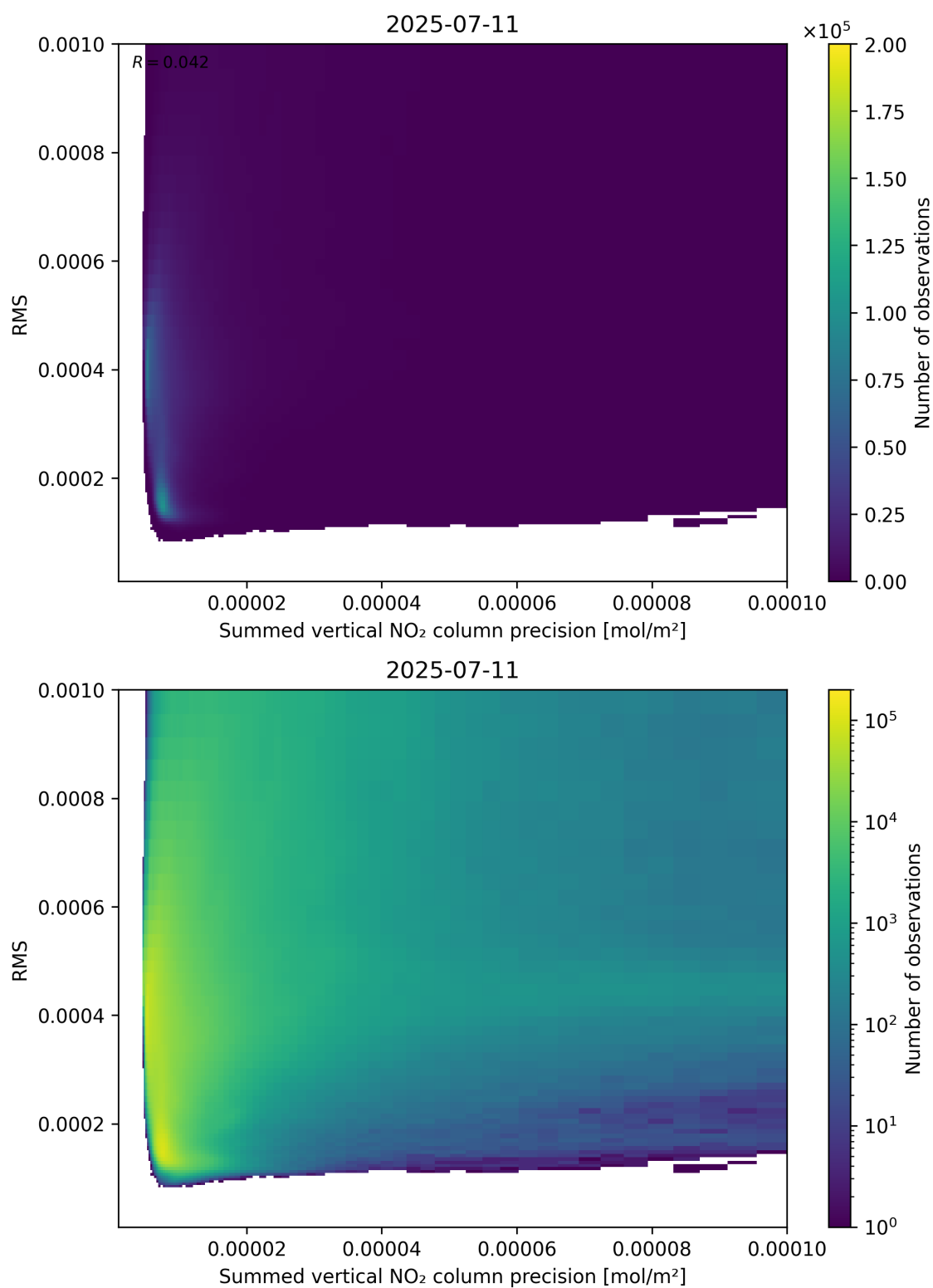
Figure 108: Scatter density plot of “Summed vertical NO 2 column precision” against “RMS” for 2025-07-10 to 2025-07-12.
