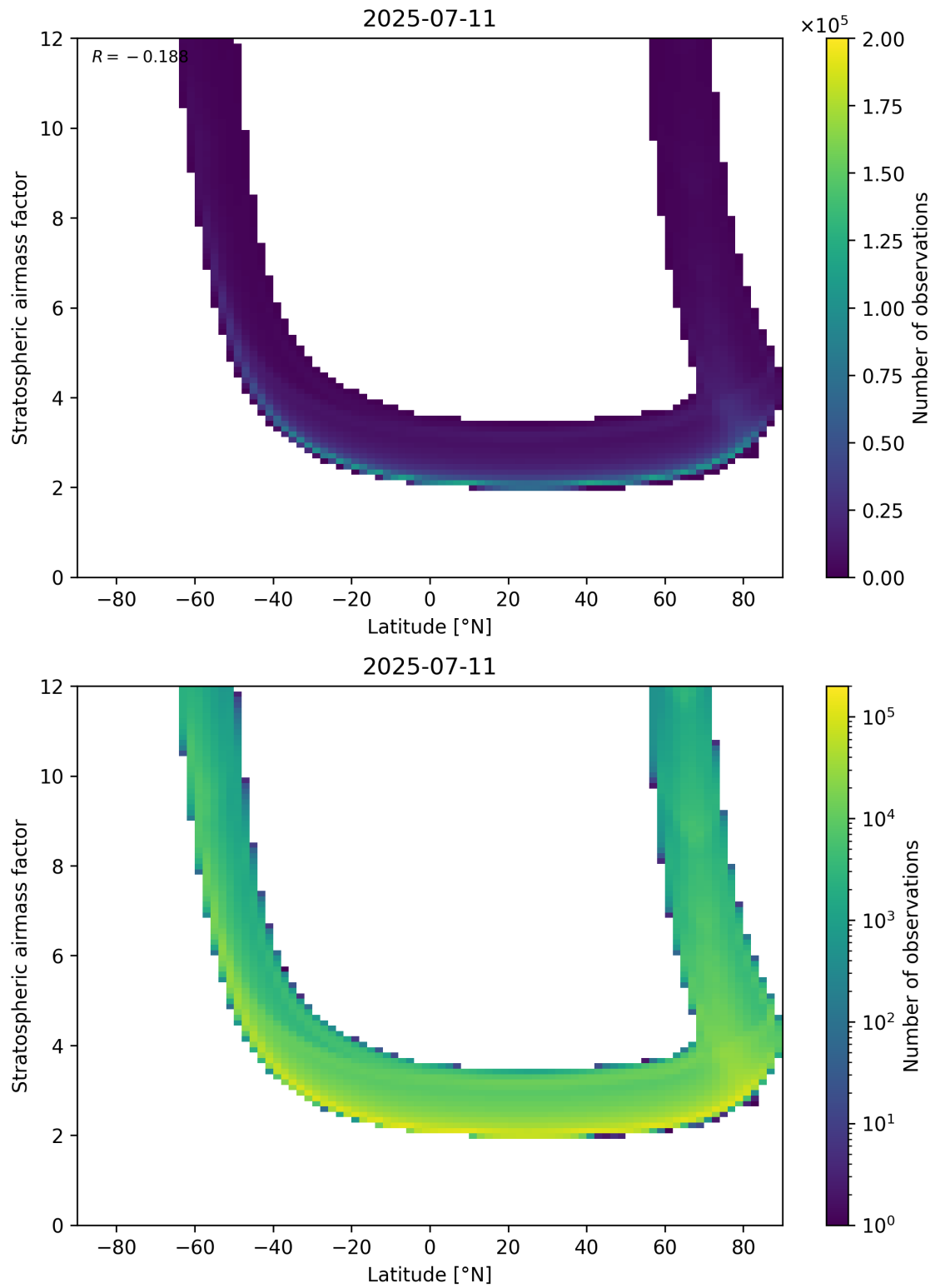
Figure 83: Scatter density plot of “Latitude” against “Stratospheric air mass factor” for 2025-07-10 to 2025-07-12.
