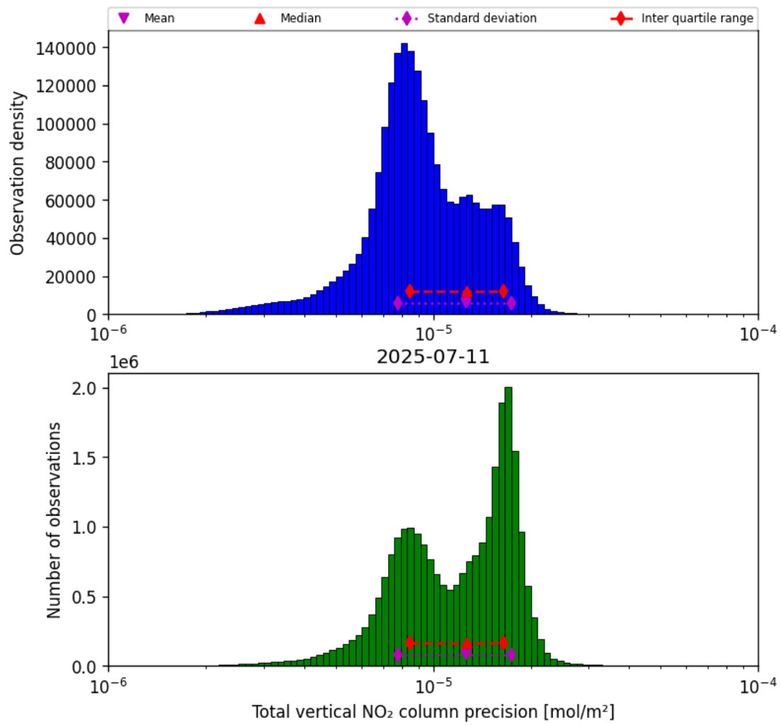
Figure 39: Histogram of “Total vertical NO 2 column precision” for 2025-07-10 to 2025-07-12
