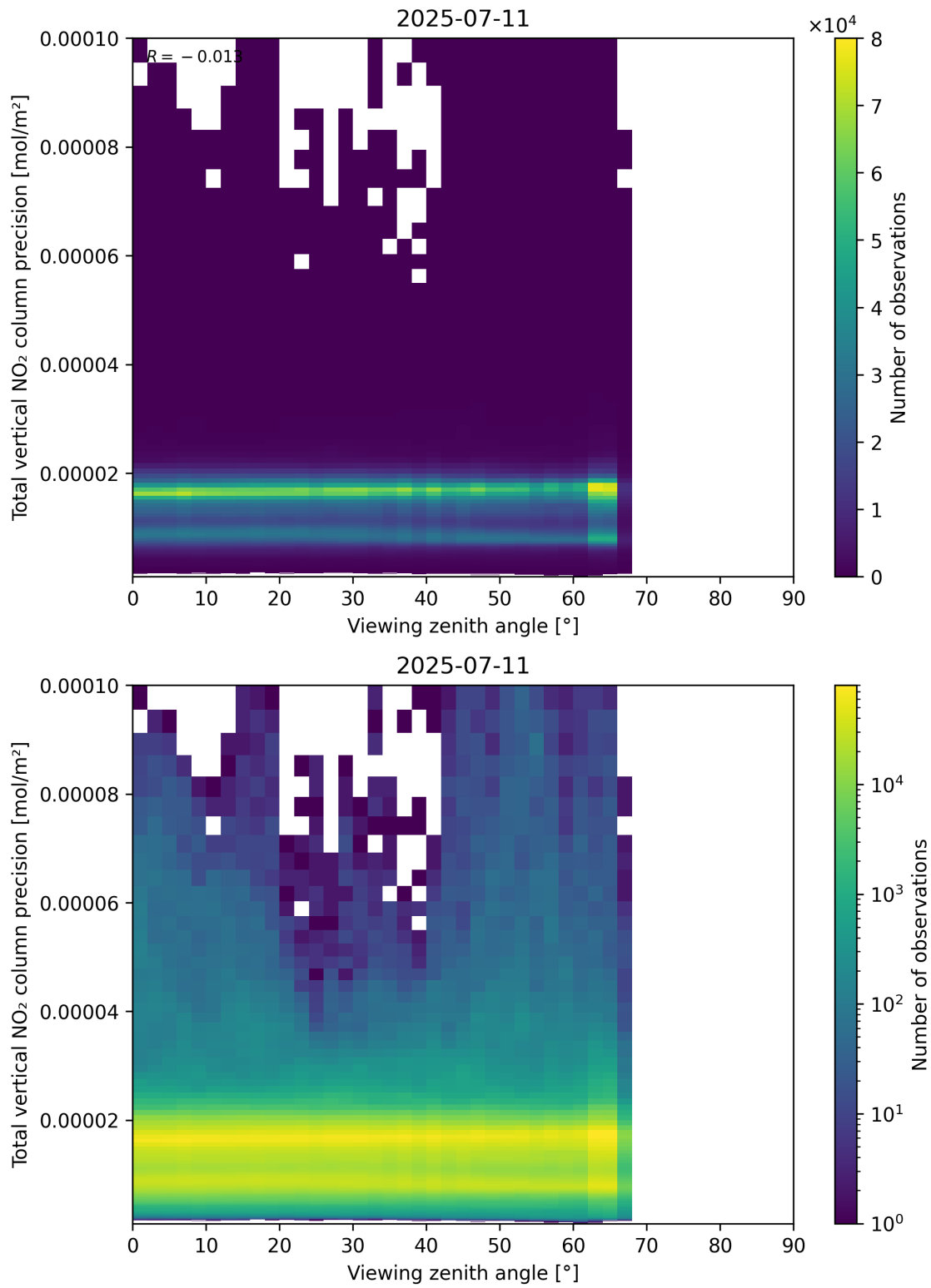
Figure 168: Scatter density plot of “Viewing zenith angle” against “Total vertical NO 2 column precision” for 2025-07-10 to 2025-07-12.
