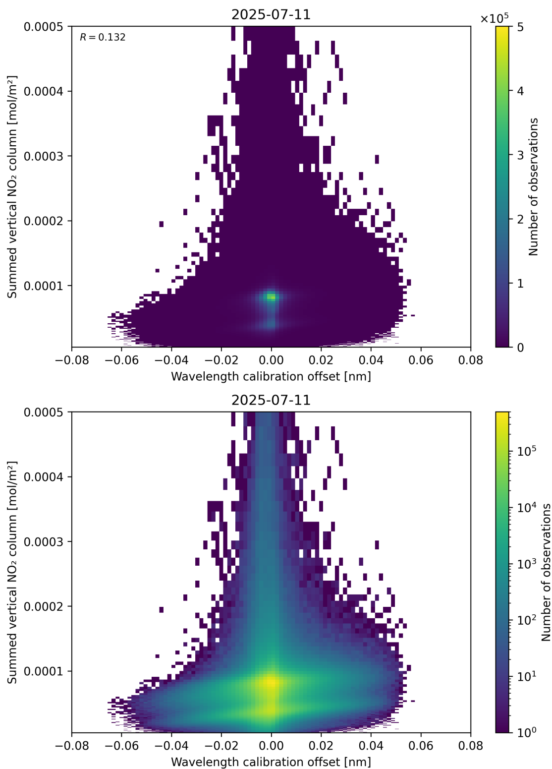
Figure 177: Scatter density plot of “Wavelength calibration offset” against “Summed vertical NO 2 column” for 2025-07-10 to 2025-07-12.
