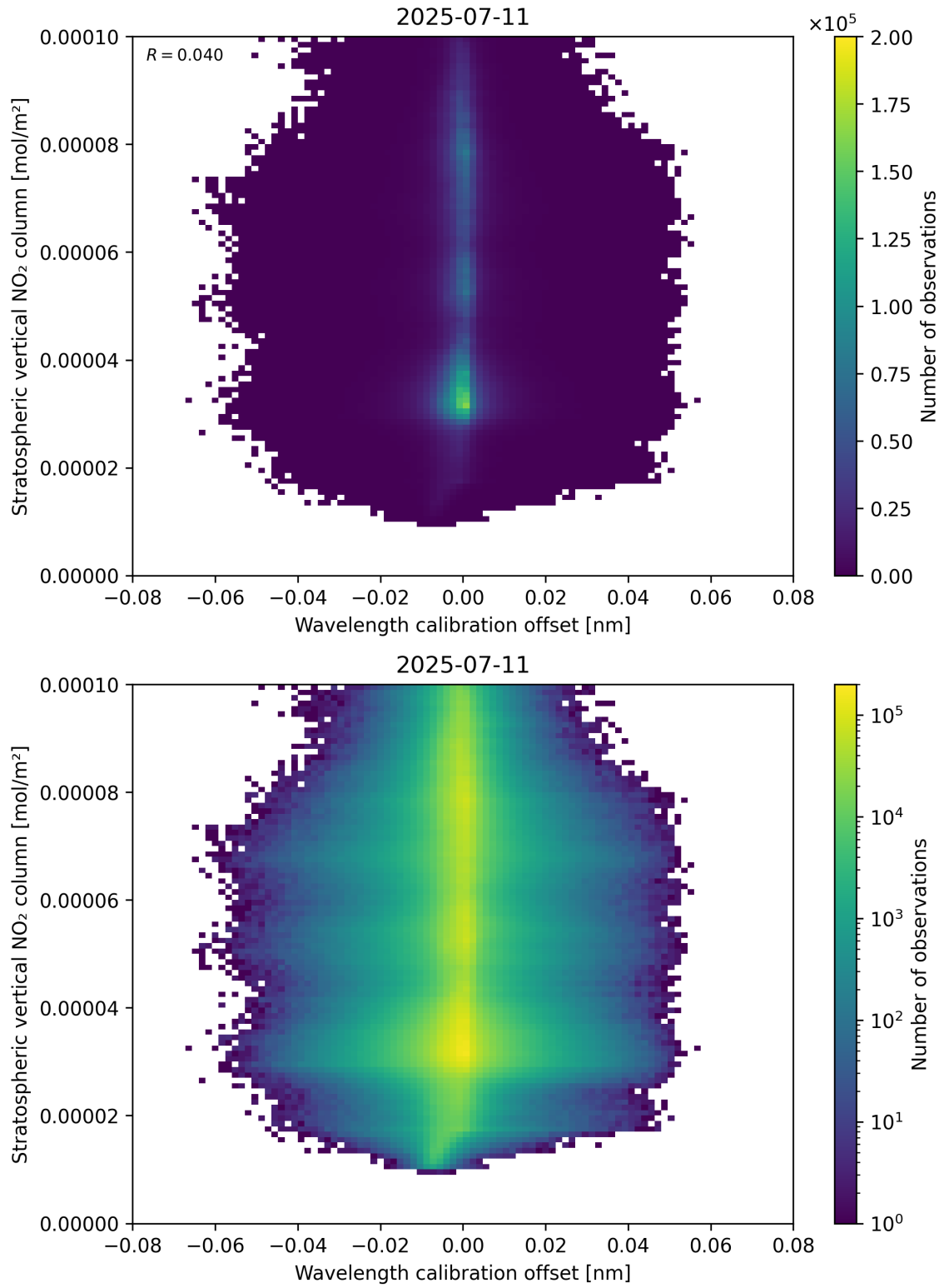
Figure 176: Scatter density plot of “Wavelength calibration offset” against “Stratospheric vertical NO 2 column” for 2025-07-10 to 2025-07-12.
