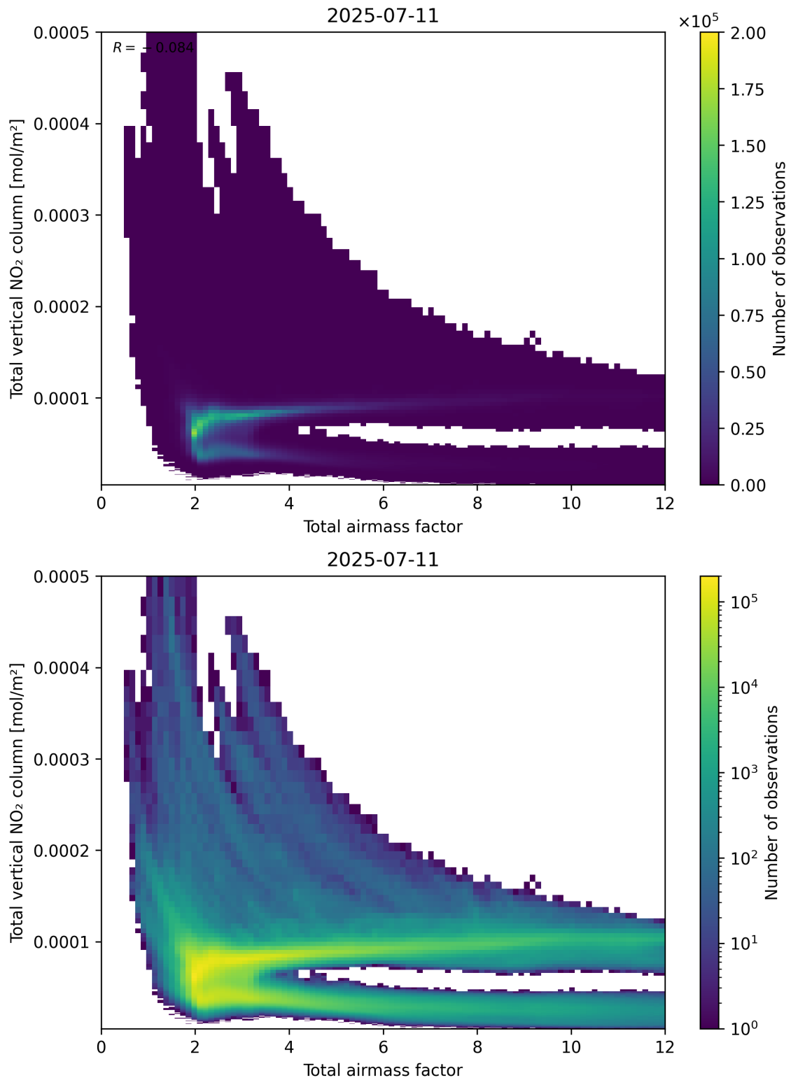
Figure 67: Scatter density plot of “Total airmass factor” against “Total vertical NO 2 column” for 2025-07-10 to 2025-07-12.
