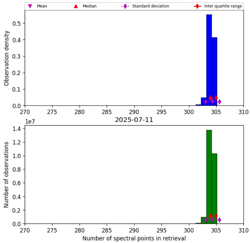
Figure 33: Histogram of “Number of spectral points in retrieval” for 2025-07-10 to 2025-07-12
