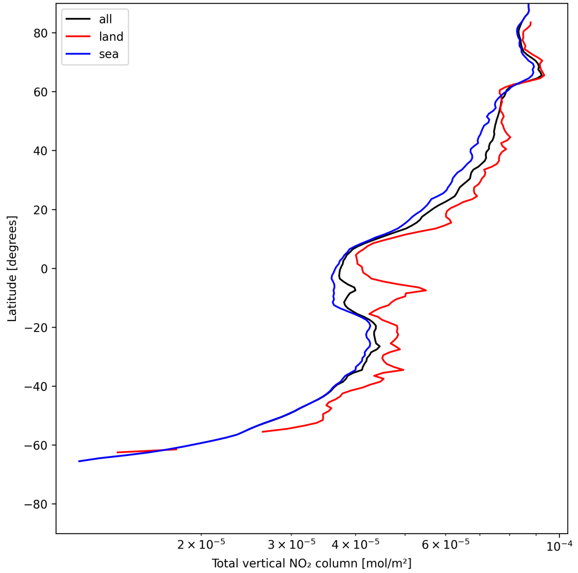
Figure 21: Zonal average of “Total vertical NO 2 column” for 2025-07-10 to 2025-07-12.
