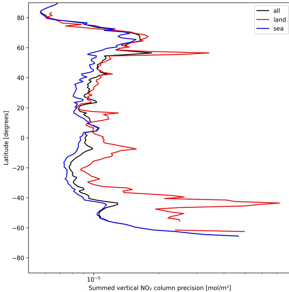
Figure 24: Zonal average of “Summed vertical NO 2 column precision” for 2025-07-10 to 2025-07-12.
