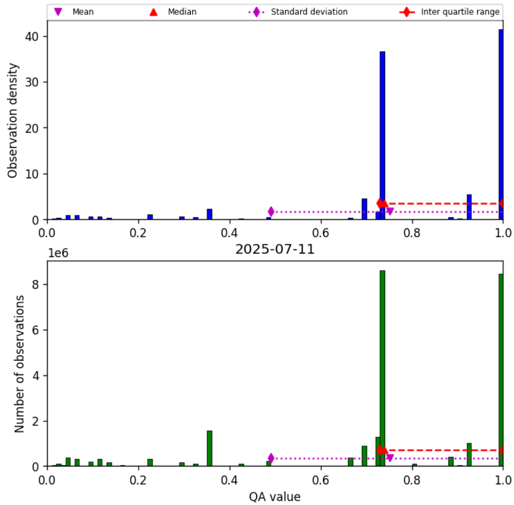
Figure 28: Histogram of “QA value” for 2025-07-10 to 2025-07-12
