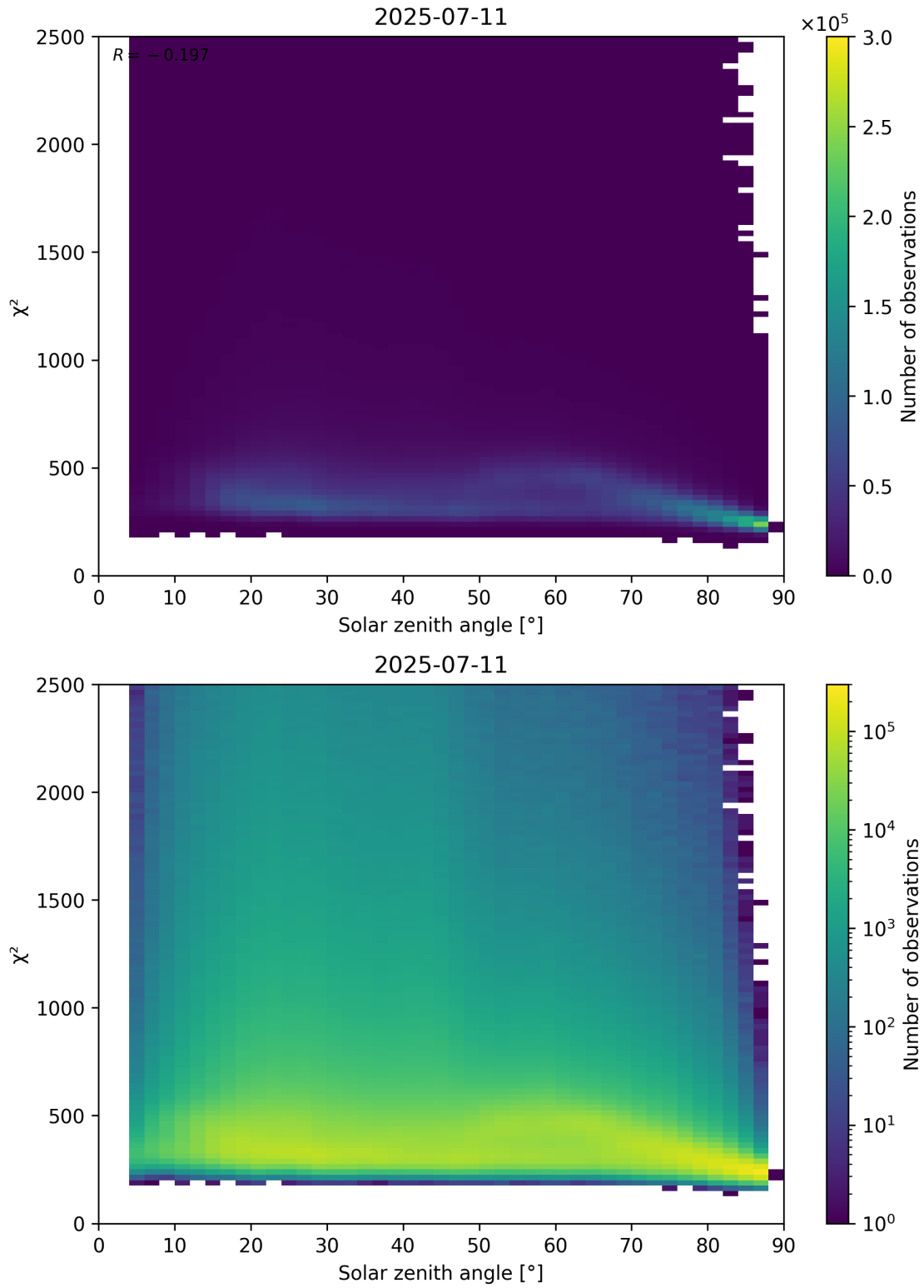
Figure 148: Scatter density plot of “Solar zenith angle” against “ \chi^2 ” for 2025-07-10 to 2025-07-12.
