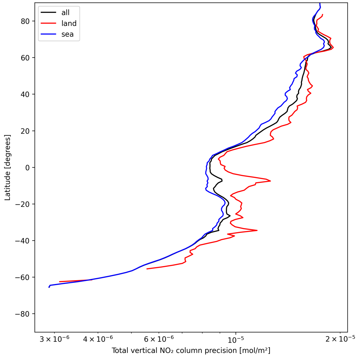
Figure 22: Zonal average of “Total vertical NO 2 column precision” for 2025-07-10 to 2025-07-12.
