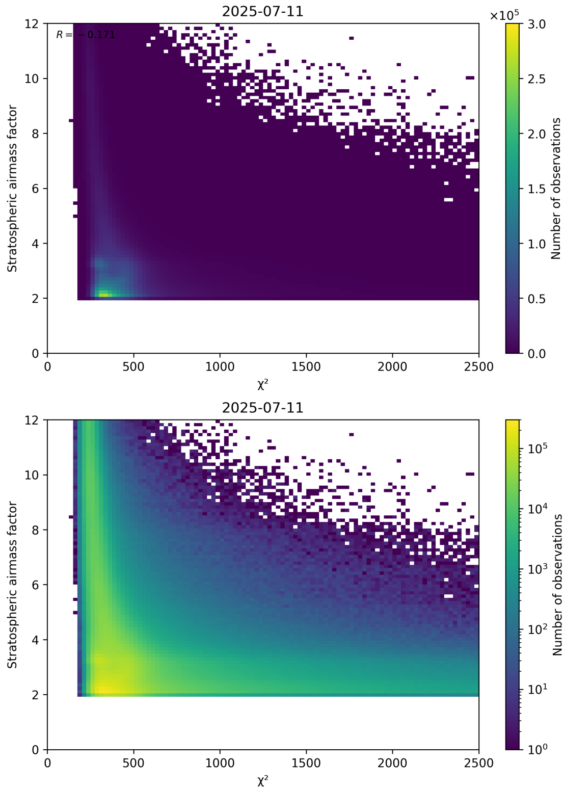
Figure 81: Scatter density plot of “ \chi^2 ” against “Stratospheric airmass factor” for 2025-07-10 to 2025-07-12.
