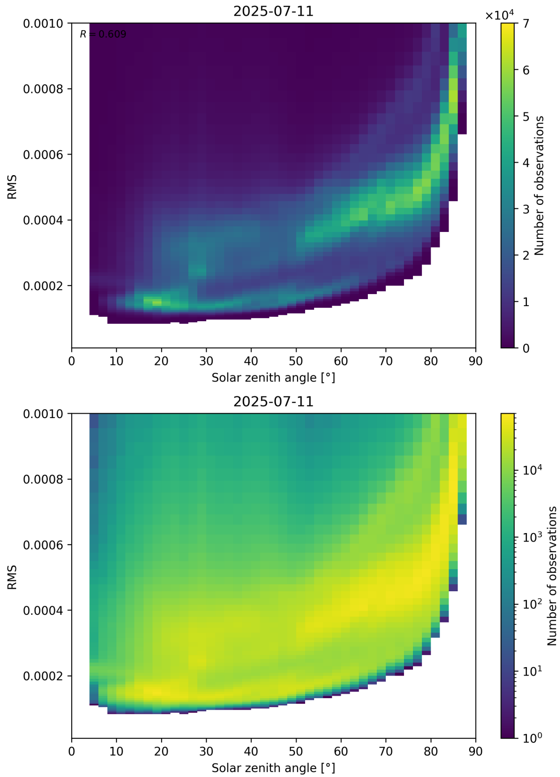
Figure 157: Scatter density plot of “Solar zenith angle” against “RMS” for 2025-07-10 to 2025-07-12.
