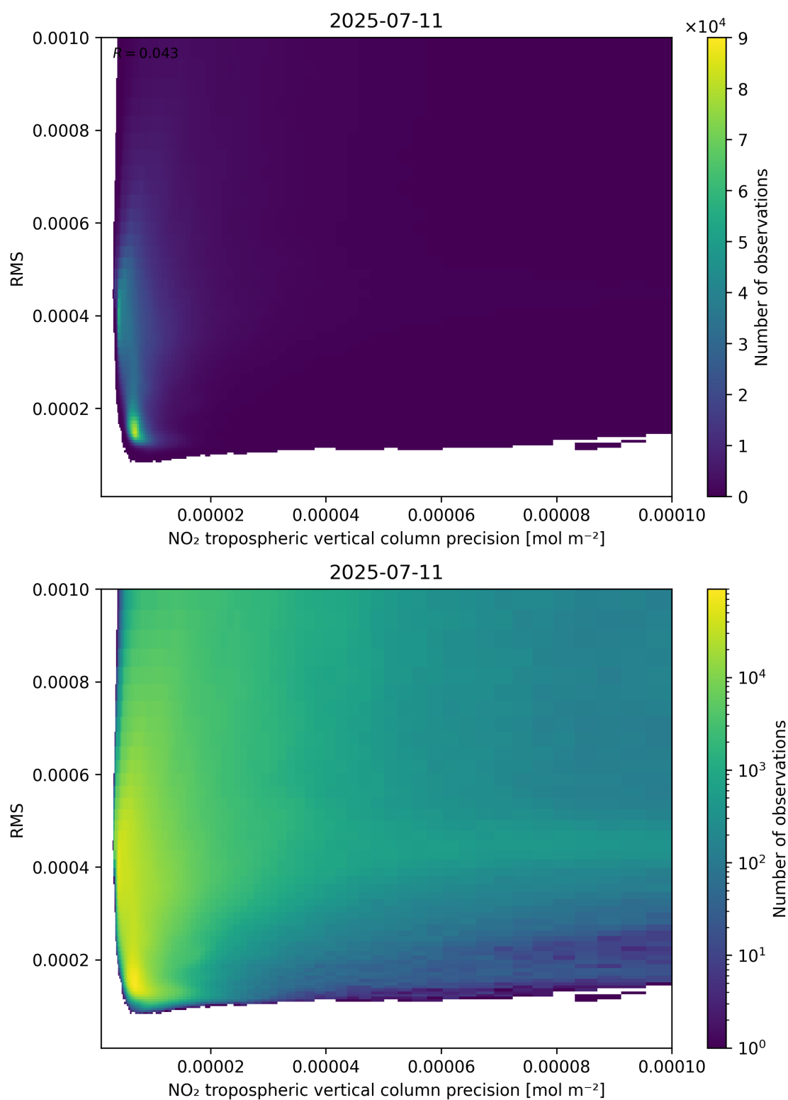
Figure 140: Scatter density plot of “NO 2 tropospheric vertical column precision” against “RMS” for 2025-07-10 to 2025-07-12.
