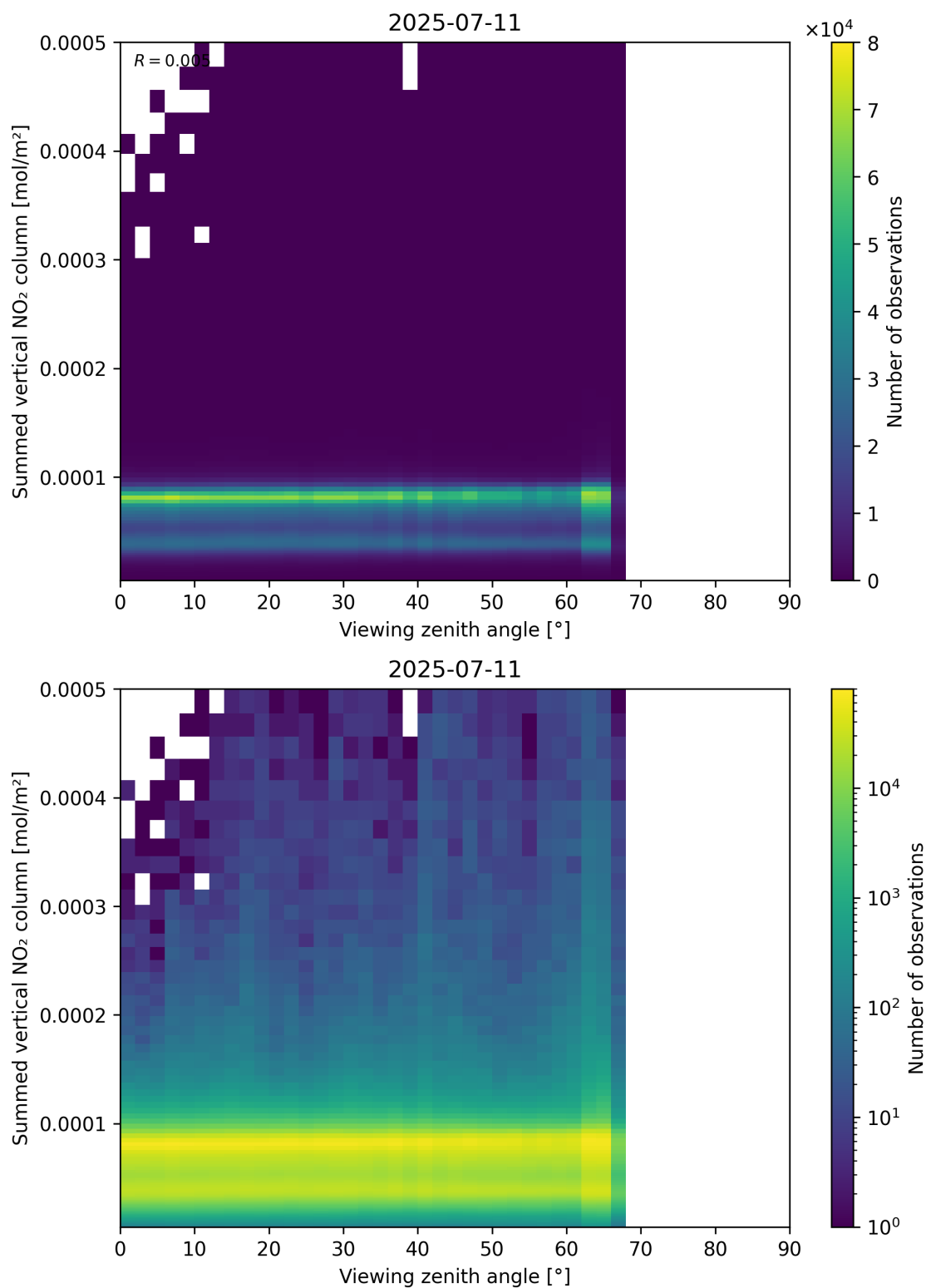
Figure 165: Scatter density plot of “Viewing zenith angle” against “Summed vertical NO 2 column” for 2025-07-10 to 2025-07-12.
