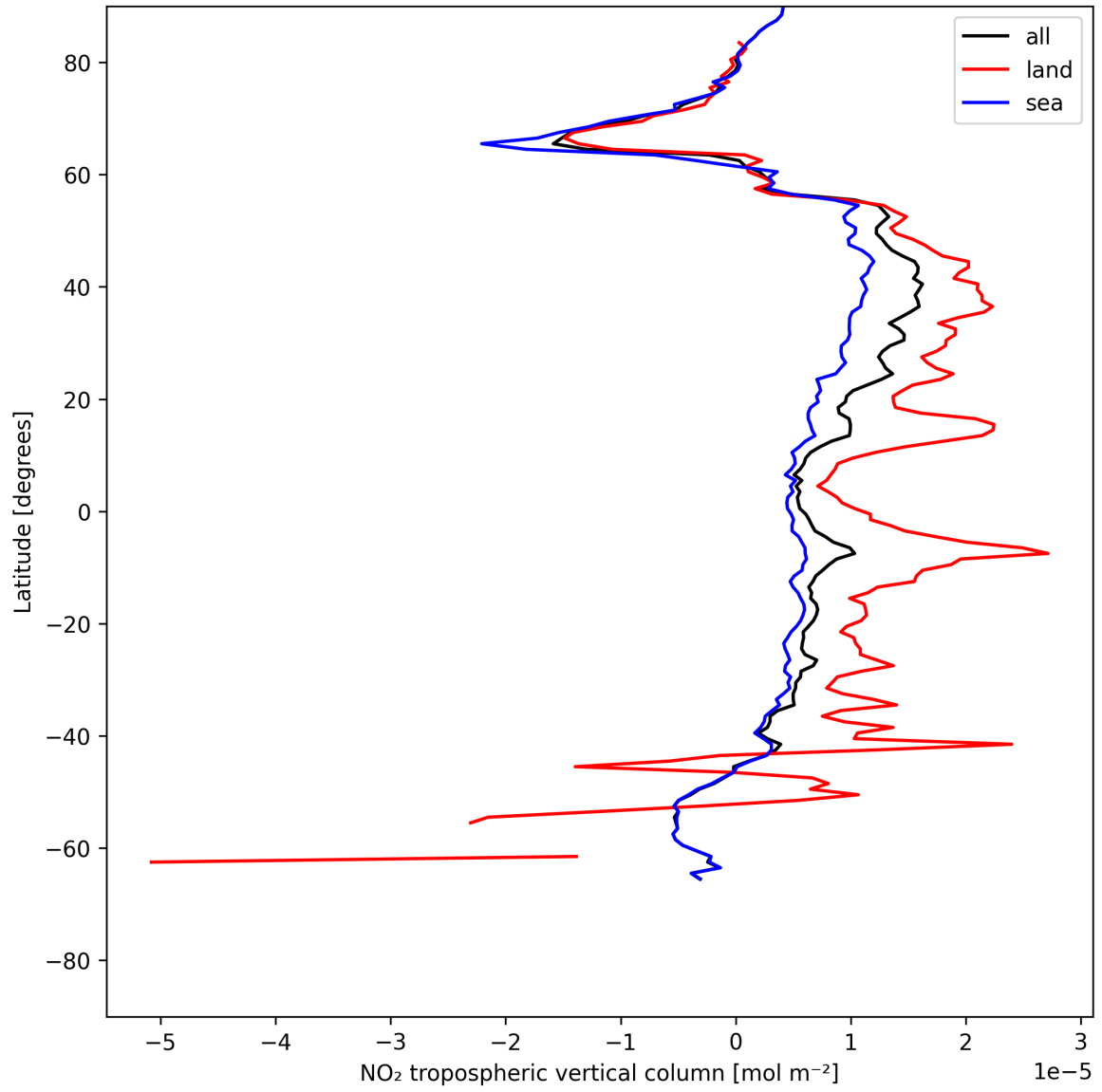
Figure 12: Zonal average of “NO 2 tropospheric vertical column” for 2025-07-10 to 2025-07-12.
