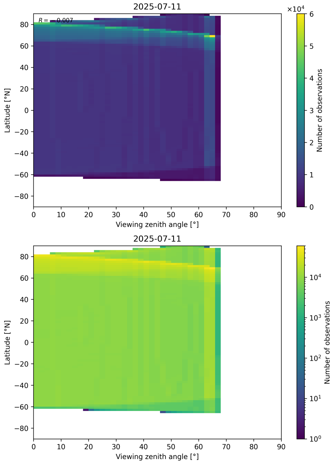
Figure 163: Scatter density plot of “Viewing zenith angle” against “Latitude” for 2025-07-10 to 2025-07-12.
