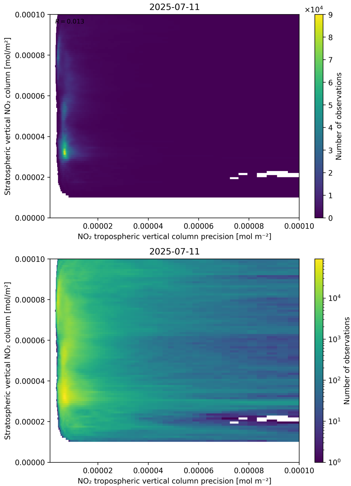
Figure 135: Scatter density plot of “NO 2 tropospheric vertical column precision” against “Stratospheric vertical NO 2 column” for 2025-07-10 to 2025-07-12.
