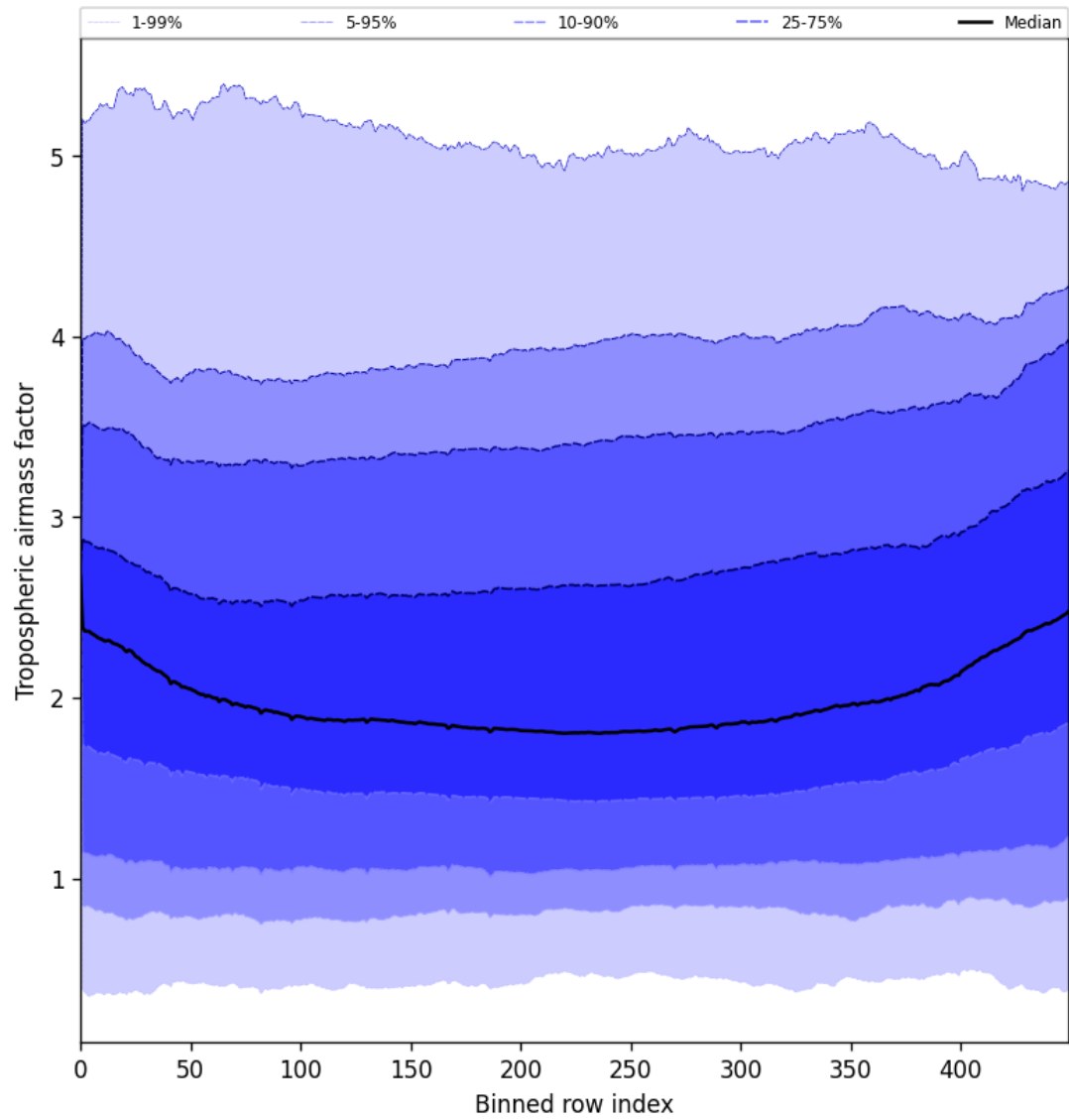
Figure 48: Along track statistics of “Tropospheric airmass factor” for 2025-07-10 to 2025-07-12
