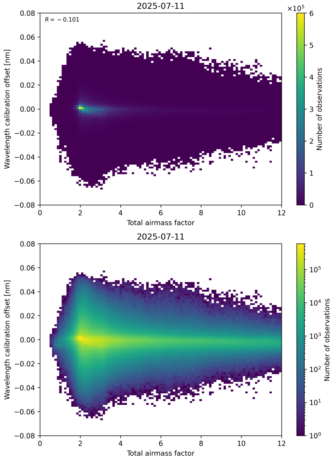
Figure 70: Scatter density plot of “Total airmass factor” against “Wavelength calibration offset” for 2025-07-10 to 2025-07-12.
