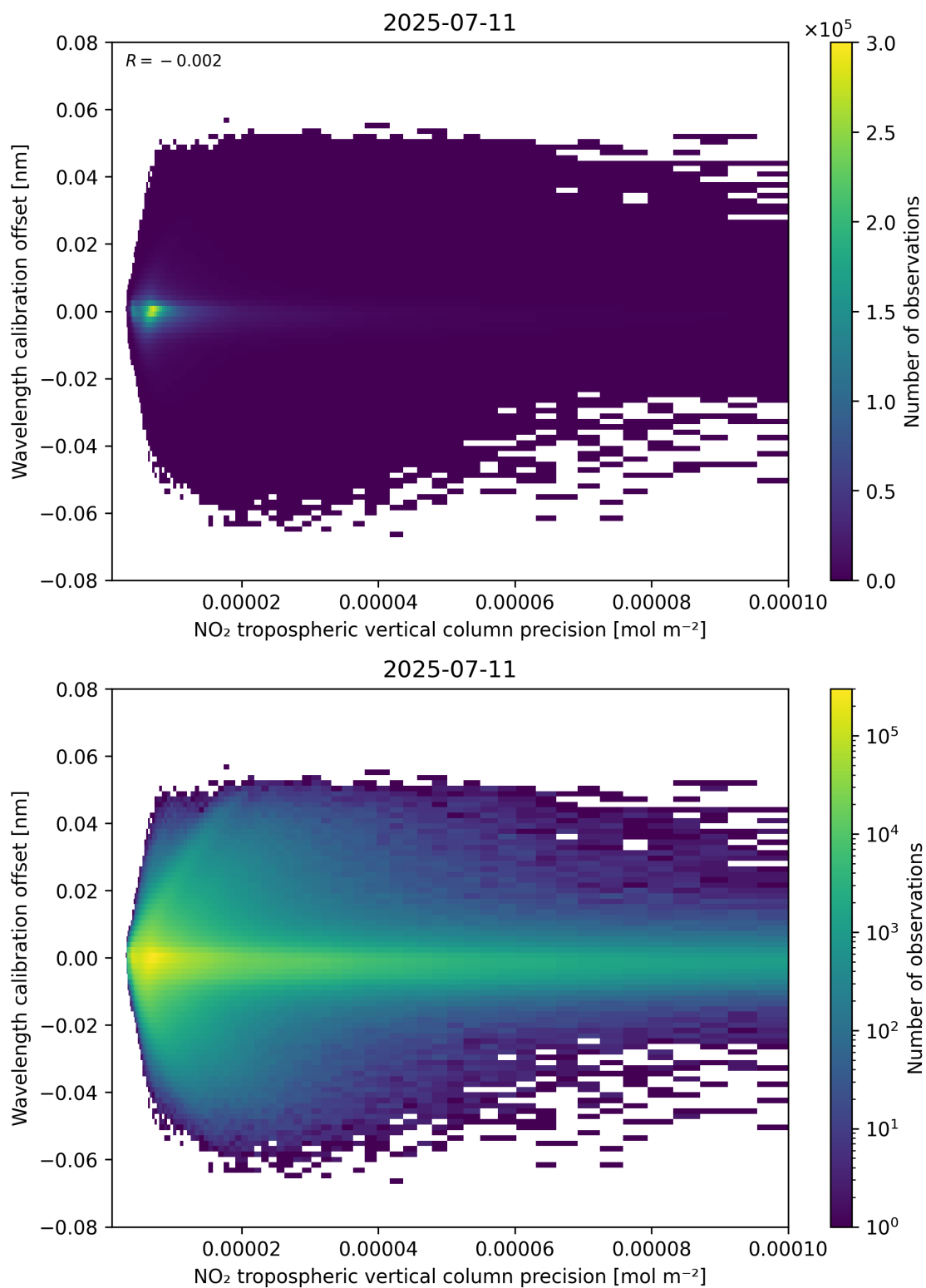
Figure 141: Scatter density plot of “NO 2 tropospheric vertical column precision” against “Wavelength calibration offset” for 2025-07-10 to 2025-07-12.
