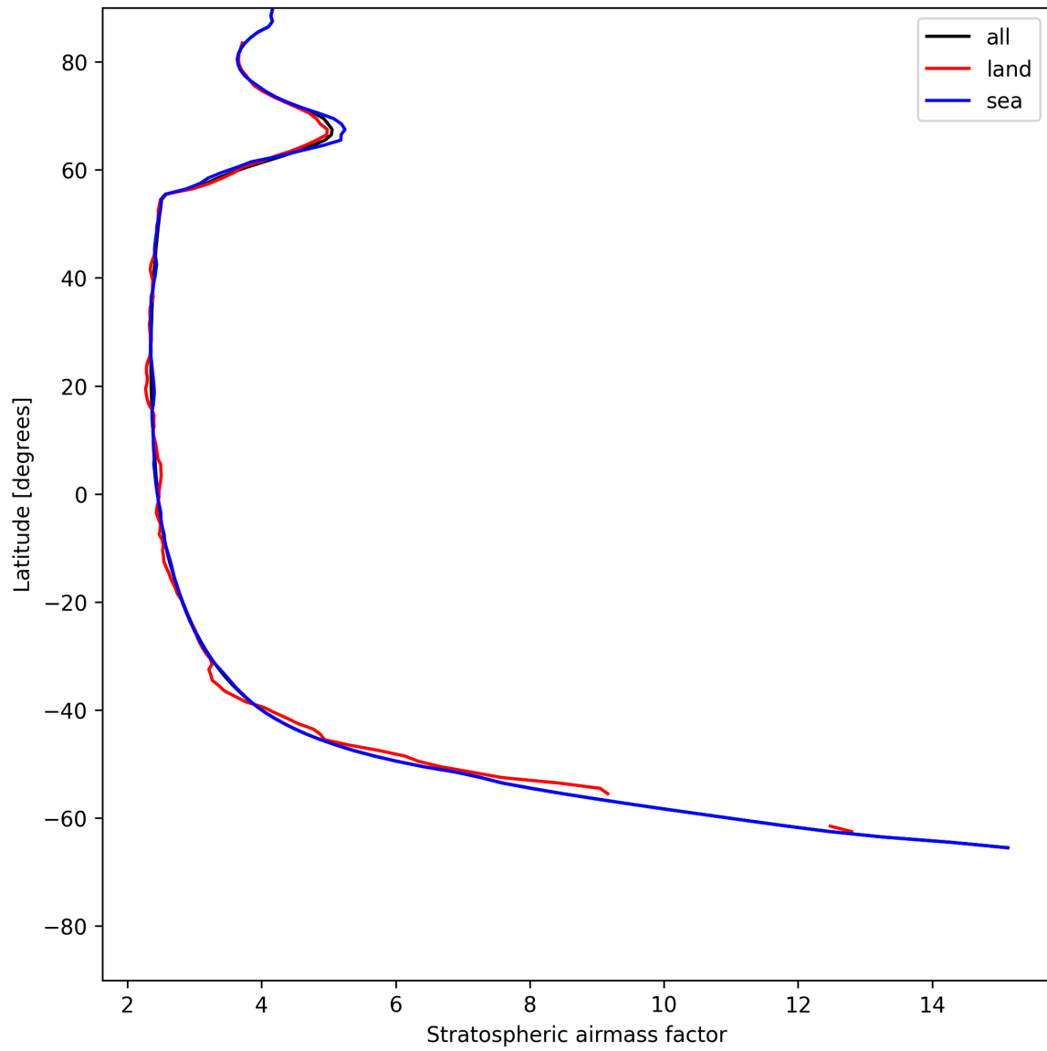
Figure 27: Zonal average of “Stratospheric air mass factor” for 2025-07-10 to 2025-07-12.
