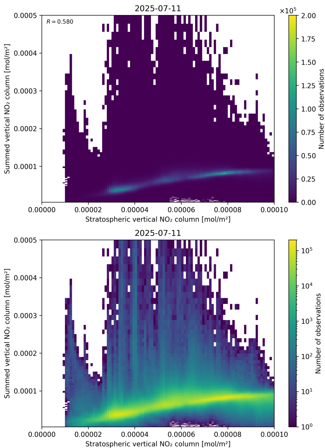
Figure 98: Scatter density plot of “Stratospheric vertical NO 2 column” against “Summed vertical NO 2 column” for 2025-07-10 to 2025-07-12.
