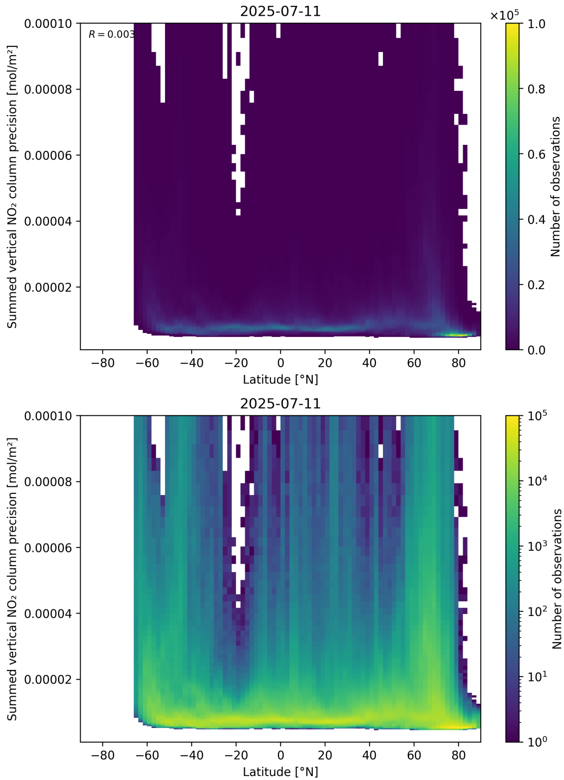
Figure 89: Scatter density plot of “Latitude” against “Summed vertical NO 2 column precision” for 2025-07-10 to 2025-07-12.
