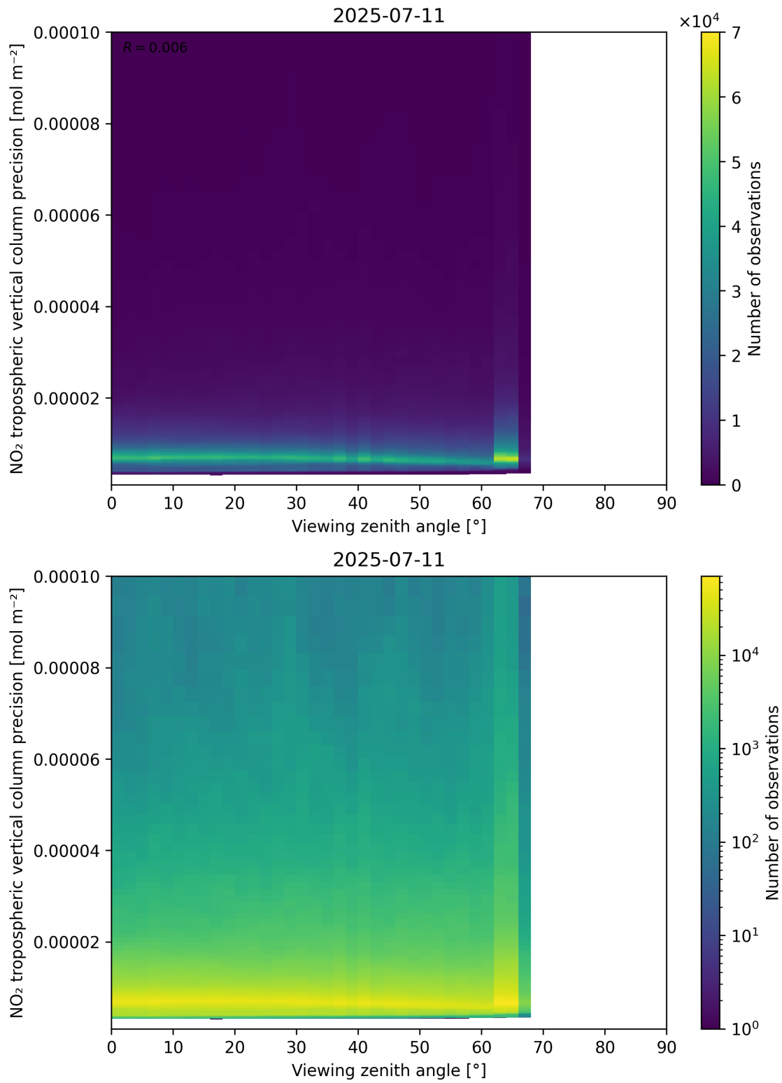
Figure 170: Scatter density plot of “Viewing zenith angle” against “NO 2 tropospheric vertical column precision” for 2025-07-10 to 2025-07-12.
