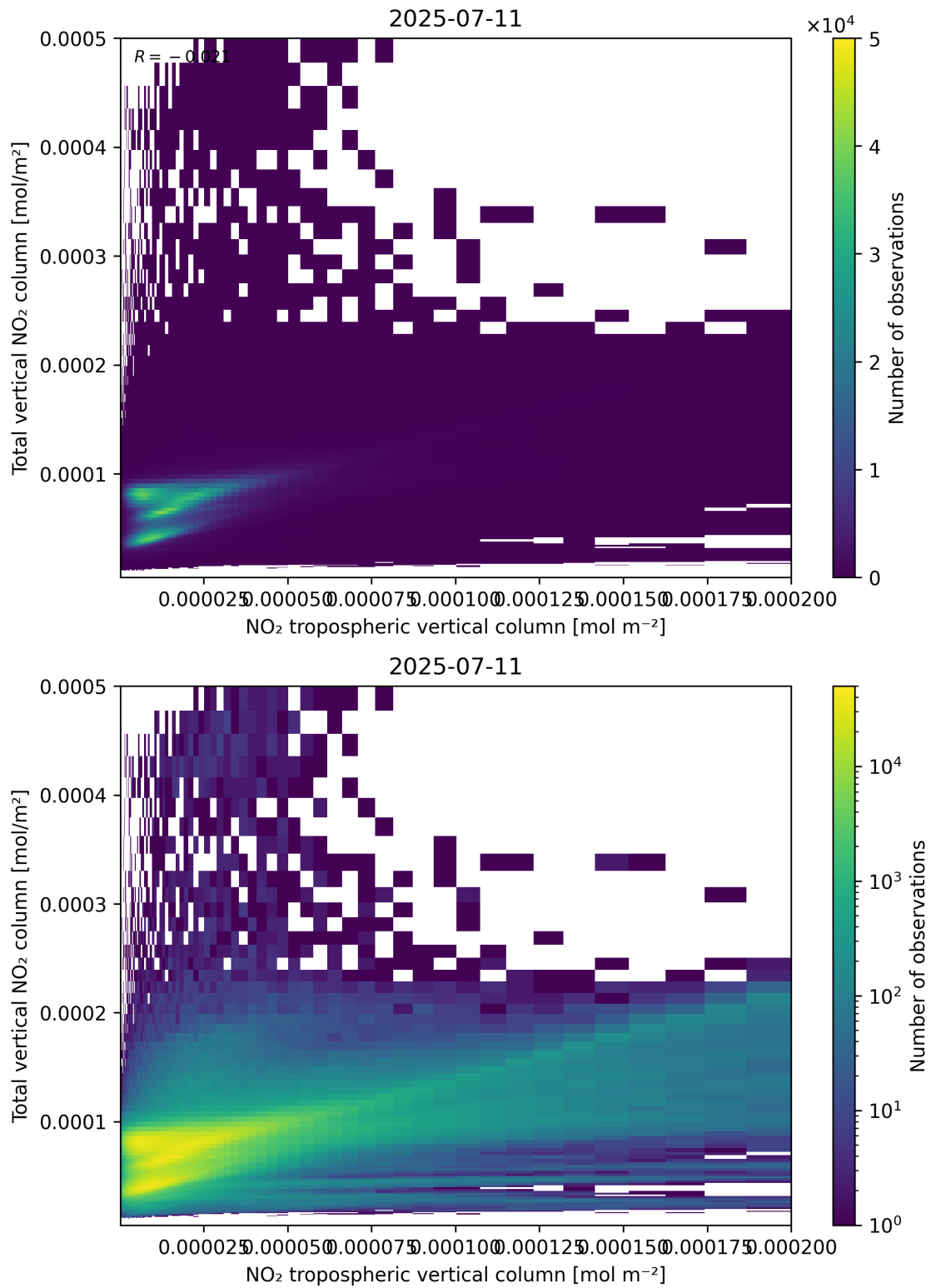
Figure 128: Scatter density plot of “NO 2 tropospheric vertical column” against “Total vertical NO 2 column” for 2025-07-10 to 2025-07-12.
