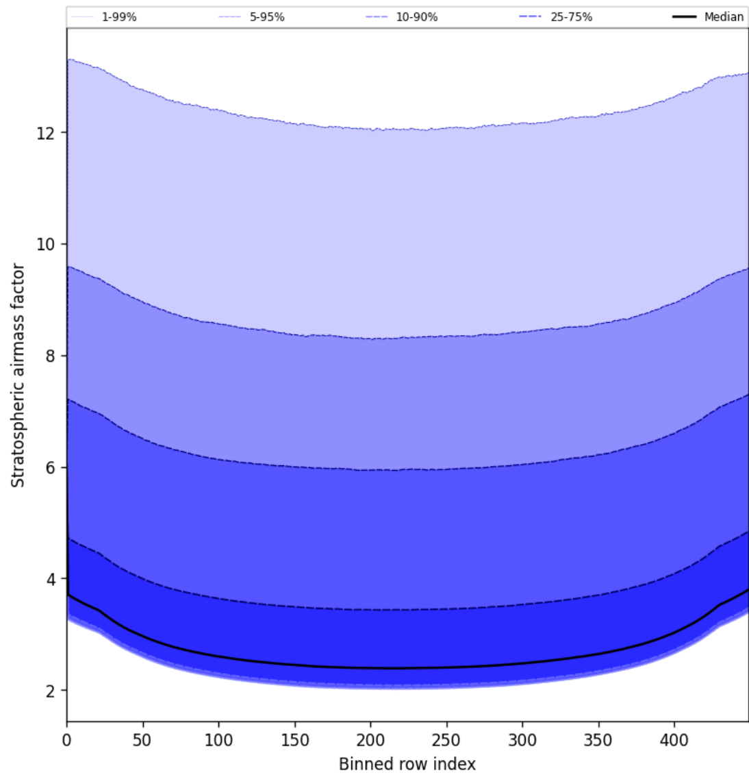
Figure 61: Along track statistics of “Stratospheric airmass factor” for 2025-07-10 to 2025-07-12
