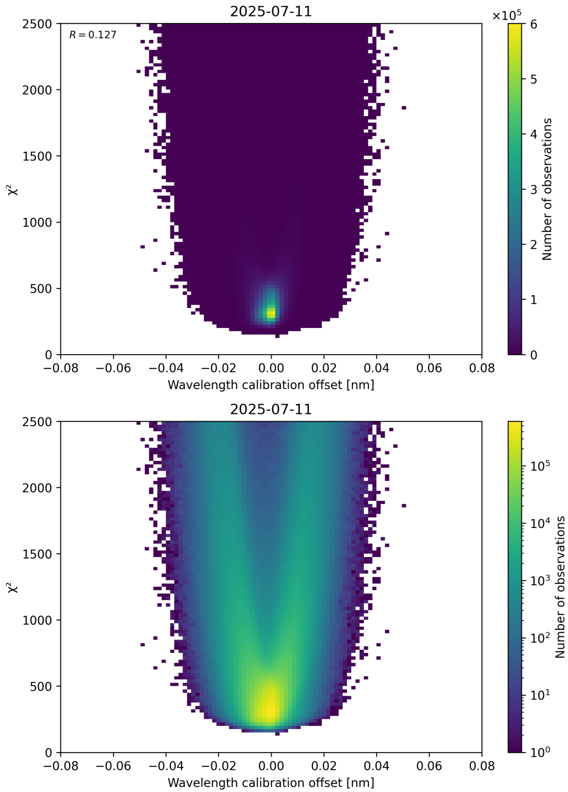
Figure 175: Scatter density plot of “Wavelength calibration offset” against “ \chi^2 ” for 2025-07-10 to 2025-07-12.
