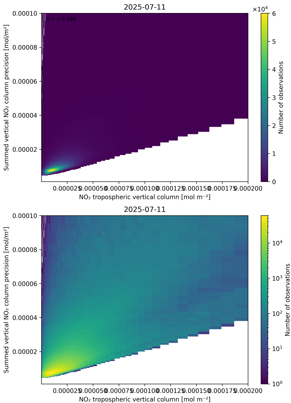
Figure 127: Scatter density plot of “NO 2 tropospheric vertical column” against “Summed vertical NO 2 column precision” for 2025-07-10 to 2025-07-12.
