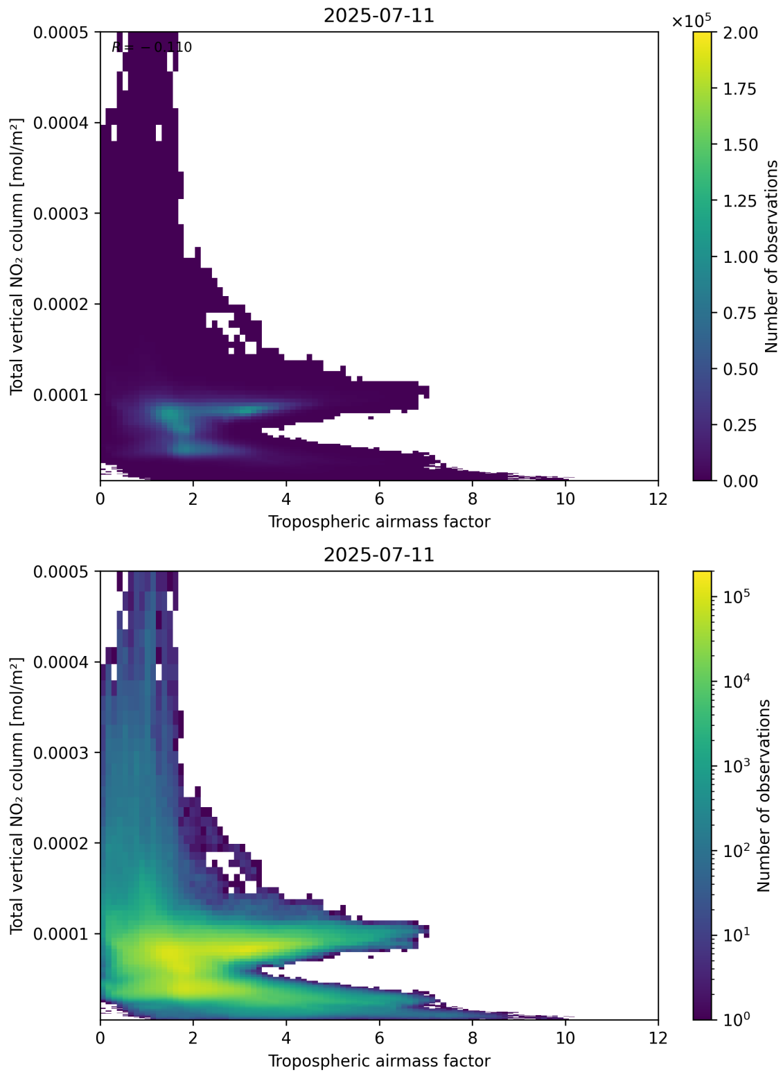
Figure 77: Scatter density plot of “Tropospheric airmass factor” against “Total vertical NO 2 column” for 2025-07-10 to 2025-07-12.
