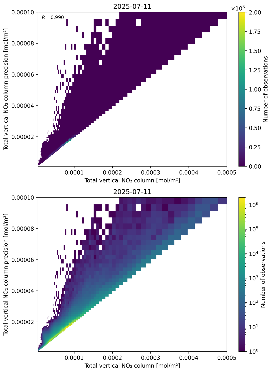
Figure 114: Scatter density plot of “Total vertical NO 2 column” against “Total vertical NO 2 column precision” for 2025-07-10 to 2025-07-12.
