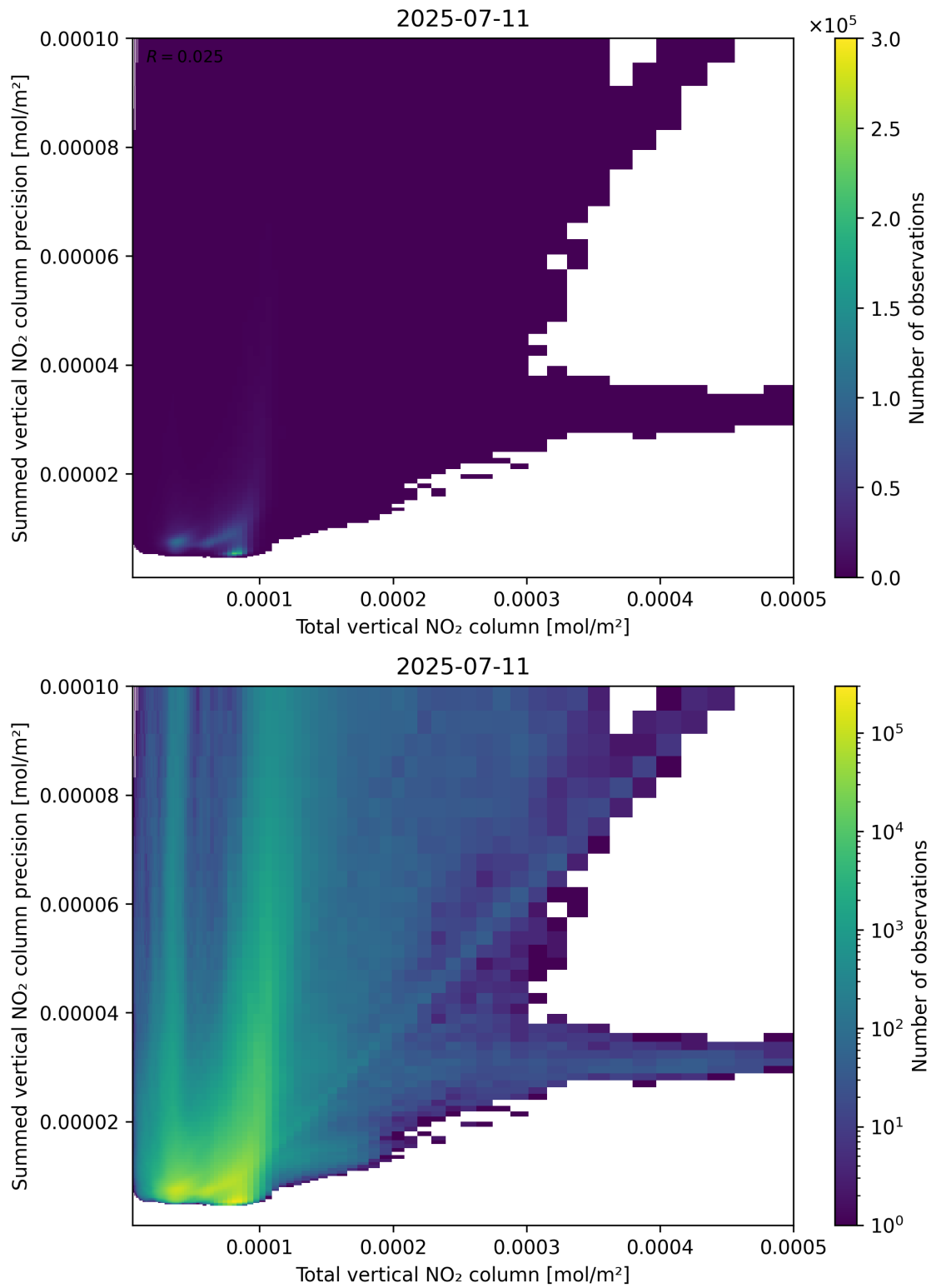
Figure 113: Scatter density plot of “Total vertical NO 2 column” against “Summed vertical NO 2 column precision” for 2025-07-10 to 2025-07-12.
