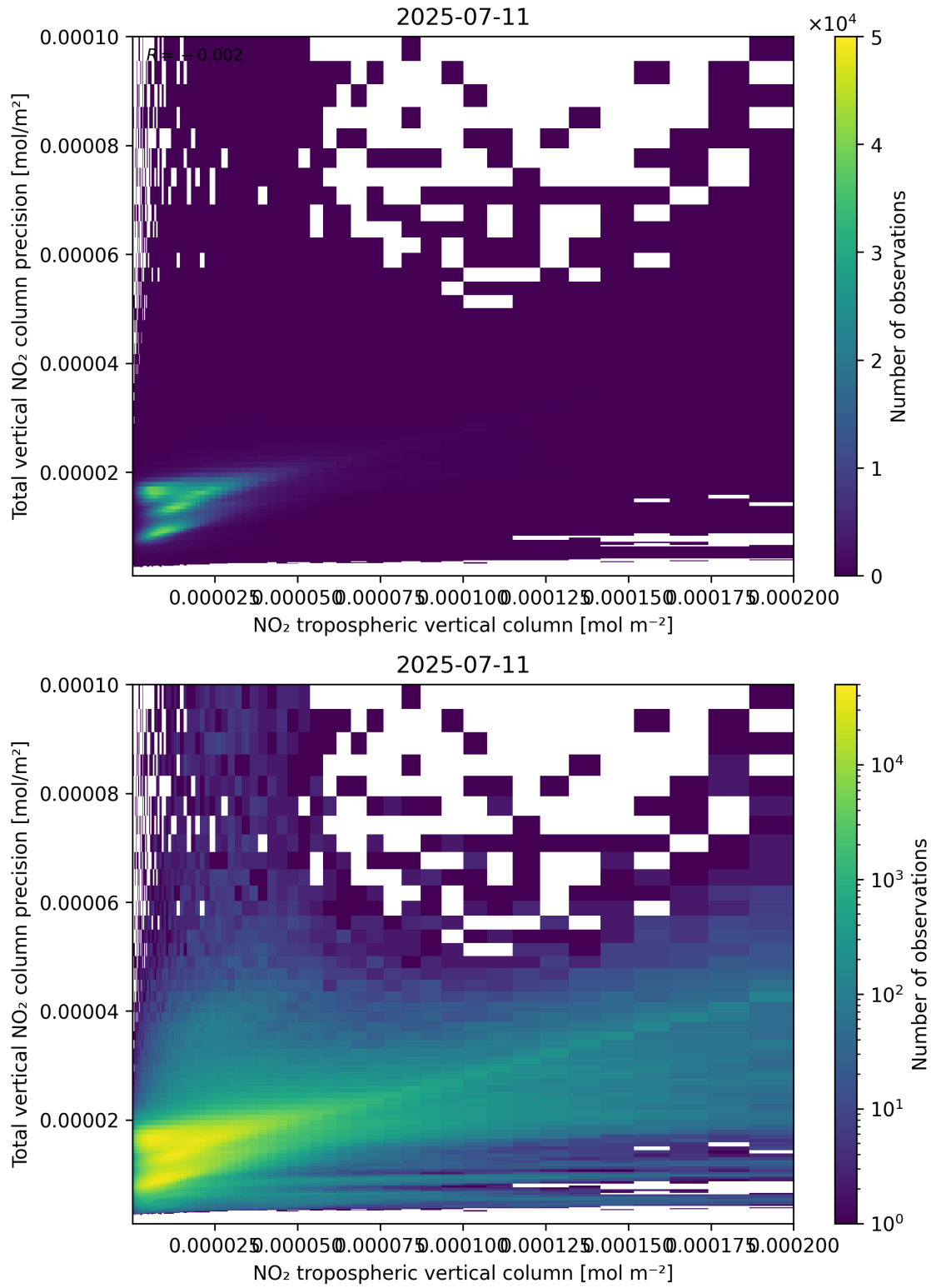
Figure 129: Scatter density plot of “NO 2 tropospheric vertical column” against “Total vertical NO 2 column precision” for 2025-07-10 to 2025-07-12.
