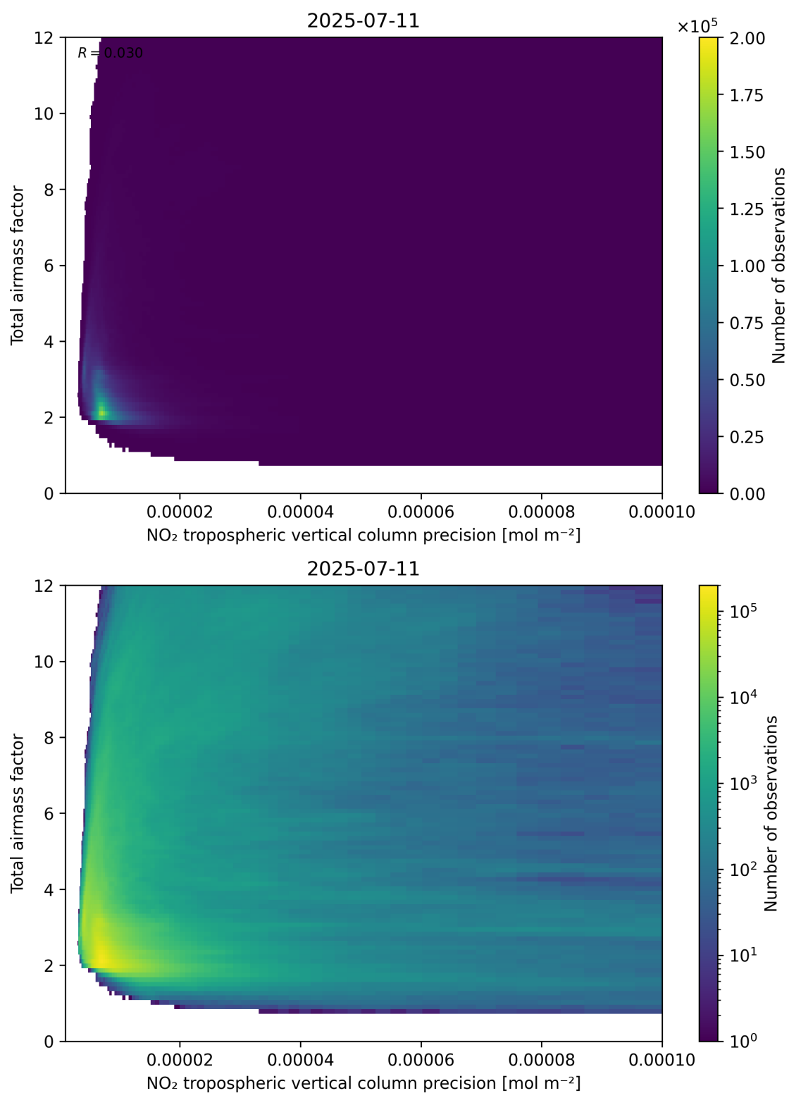
Figure 132: Scatter density plot of “NO 2 tropospheric vertical column precision” against “Total air mass factor” for 2025-07-10 to 2025-07-12.
