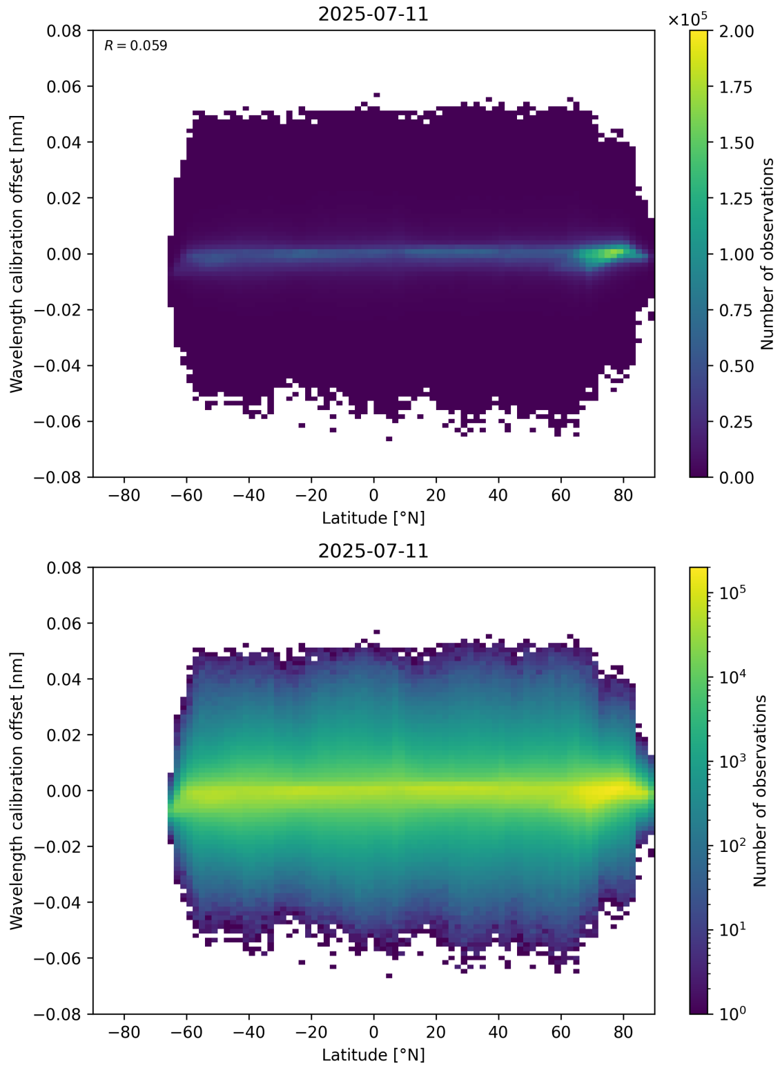
Figure 95: Scatter density plot of “Latitude” against “Wavelength calibration offset” for 2025-07-10 to 2025-07-12.
