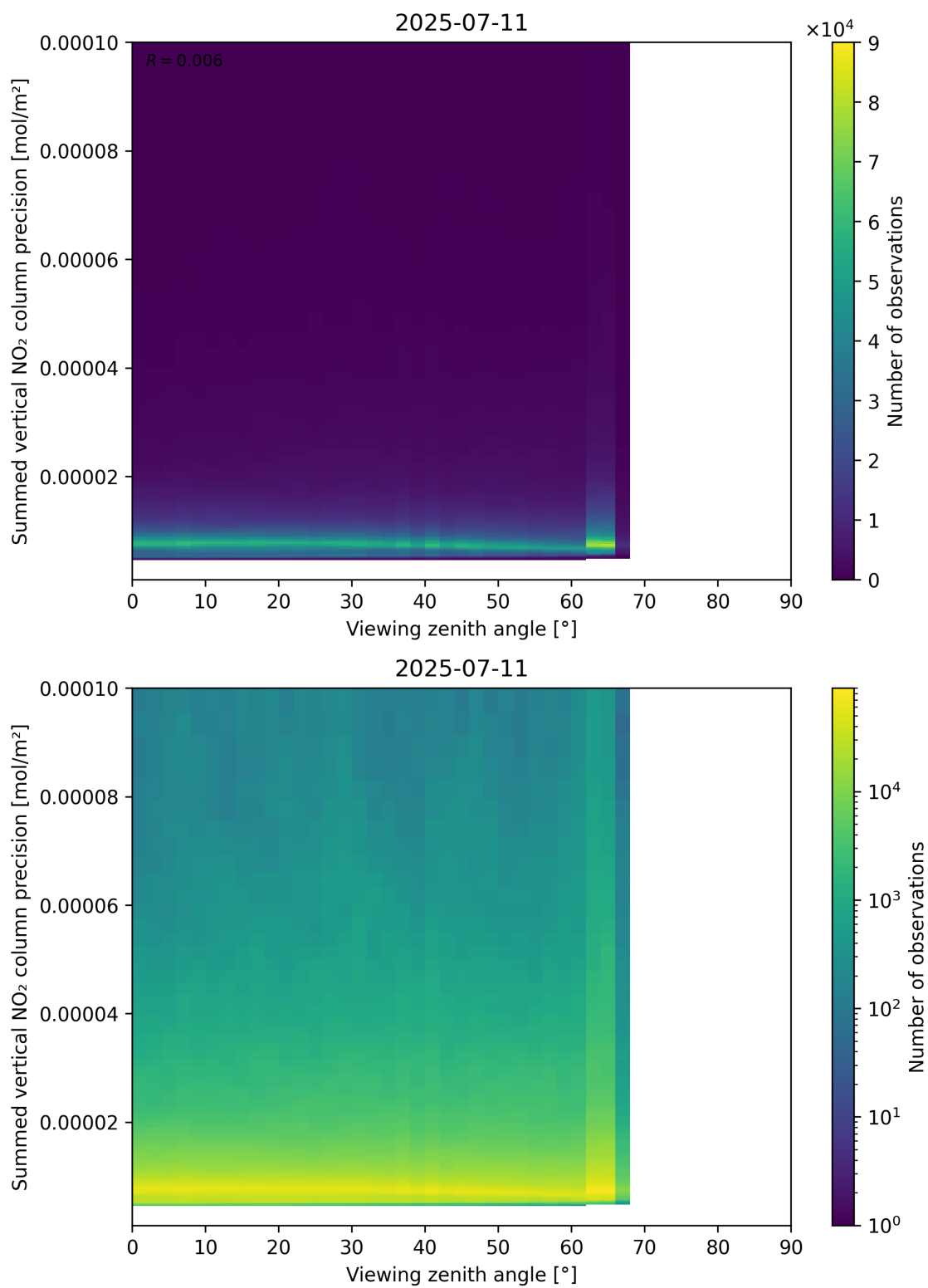
Figure 166: Scatter density plot of “Viewing zenith angle” against “Summed vertical NO 2 column precision” for 2025-07-10 to 2025-07-12.
