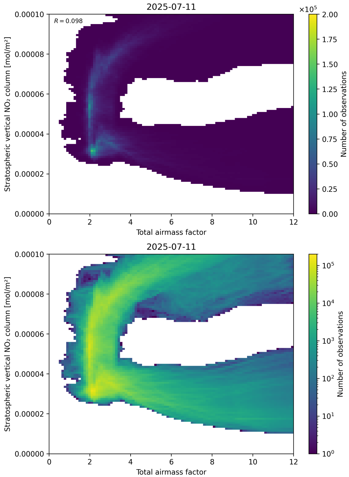
Figure 64: Scatter density plot of “Total airmass factor” against “Stratospheric vertical \text{NO}_2 column” for 2025-07-10 to 2025-07-12.
