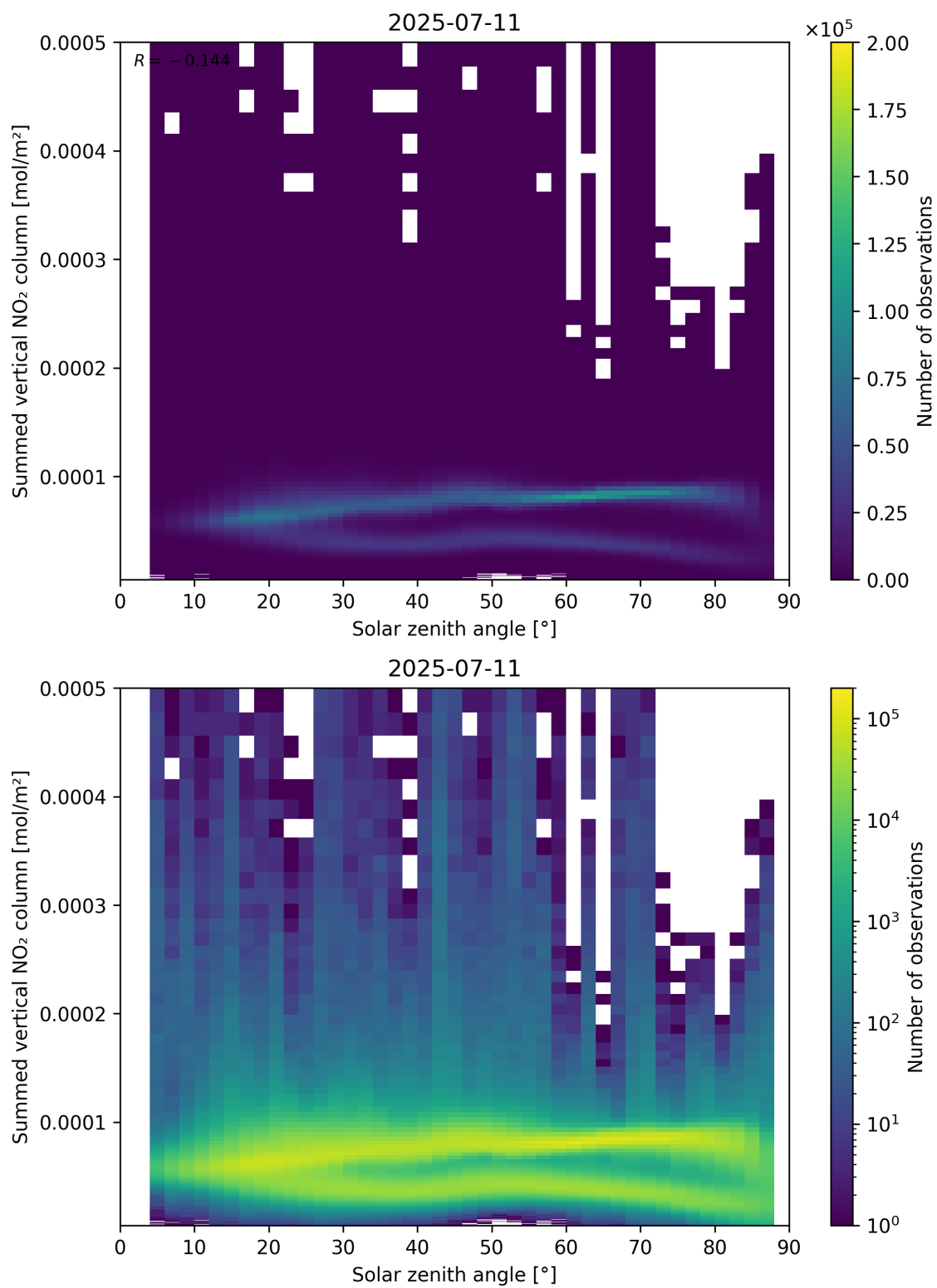
Figure 151: Scatter density plot of “Solar zenith angle” against “Summed vertical NO 2 column” for 2025-07-10 to 2025-07-12.
