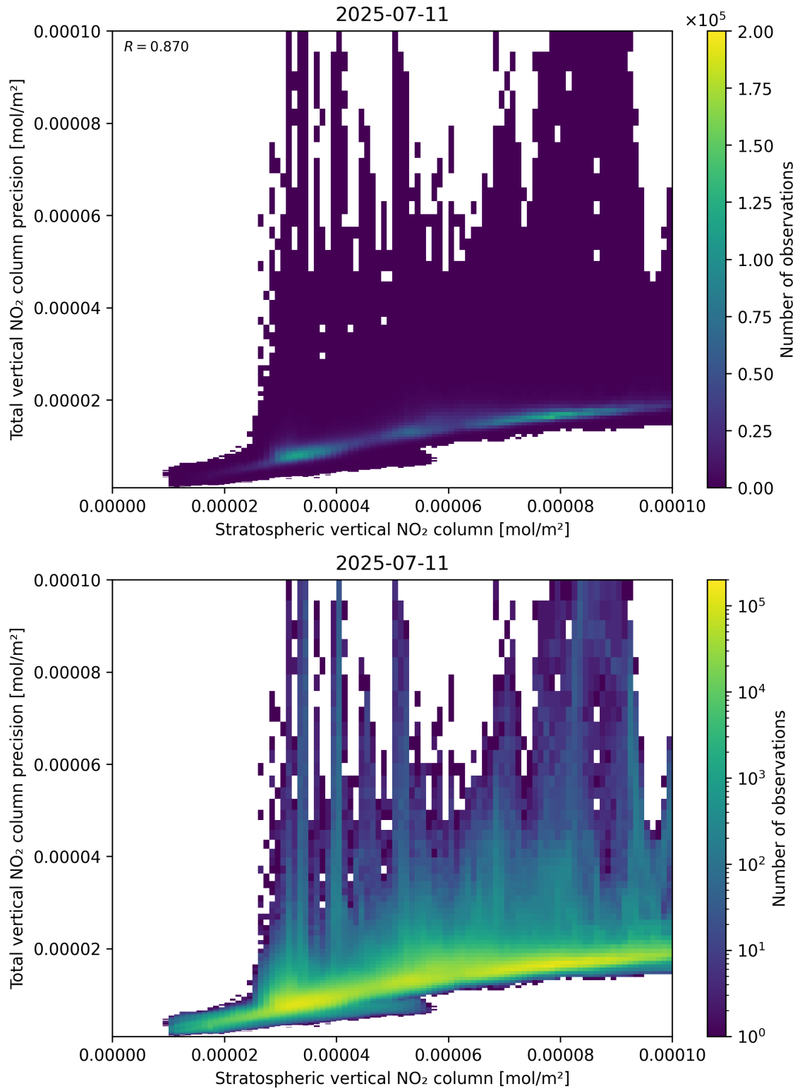
Figure 101: Scatter density plot of “Stratospheric vertical NO 2 column” against “Total vertical NO 2 column precision” for 2025-07-10 to 2025-07-12.
