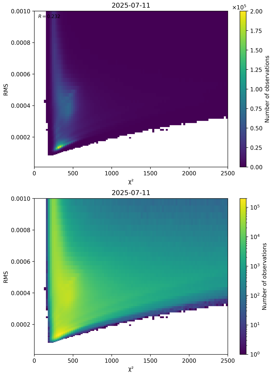
Figure 82: Scatter density plot of “ \chi^2 ” against “RMS” for 2025-07-10 to 2025-07-12.
