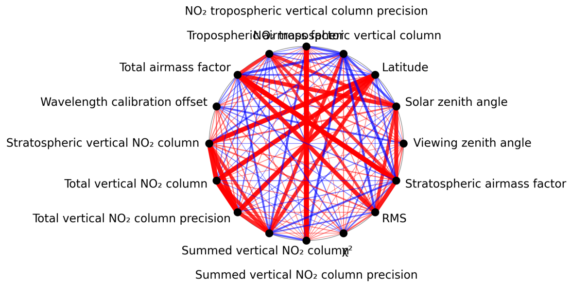
Figure 1: Map of correlation graph for 2025-07-10 to 2025-07-12.
