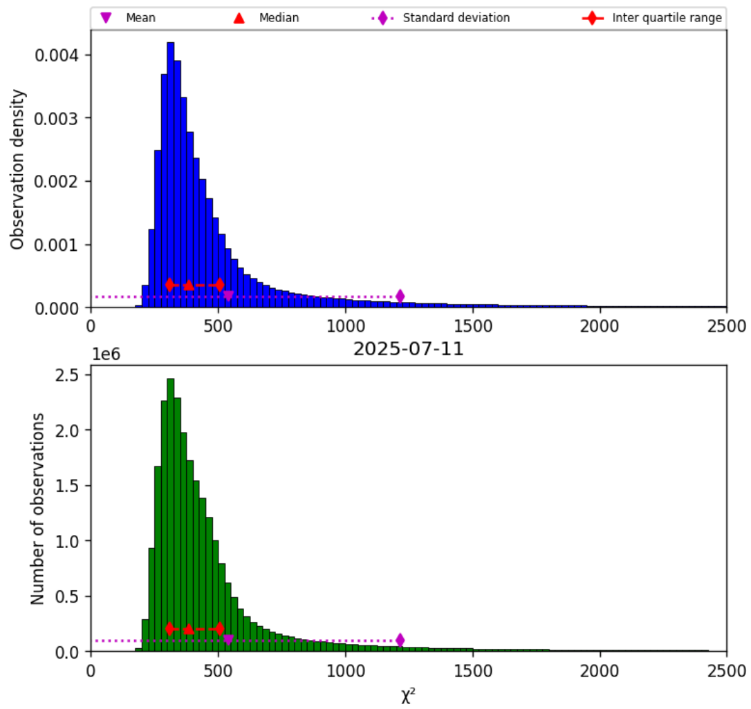
Figure 42: Histogram of “ \chi^2 ” for 2025-07-10 to 2025-07-12
