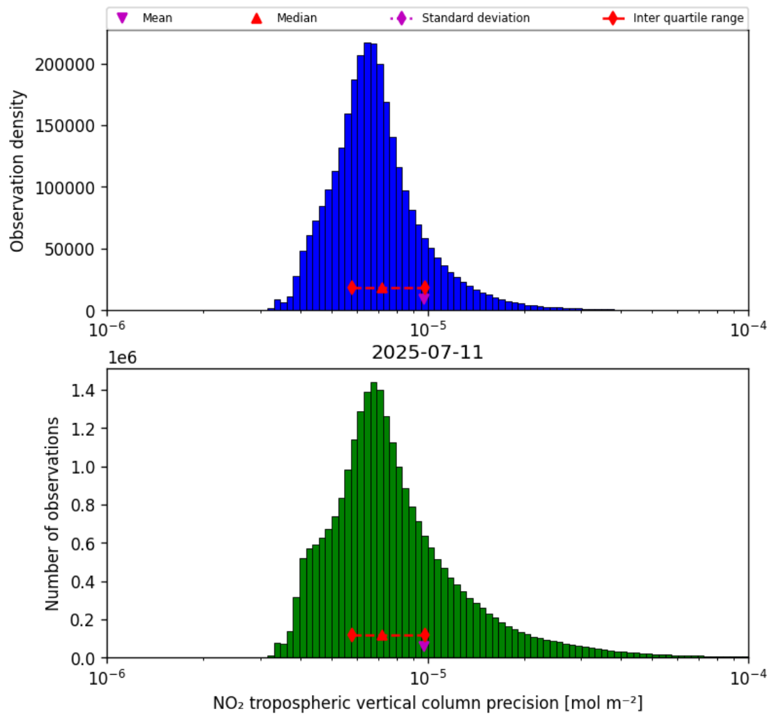
Figure 30: Histogram of “NO 2 tropospheric vertical column precision” for 2025-07-10 to 2025-07-12
