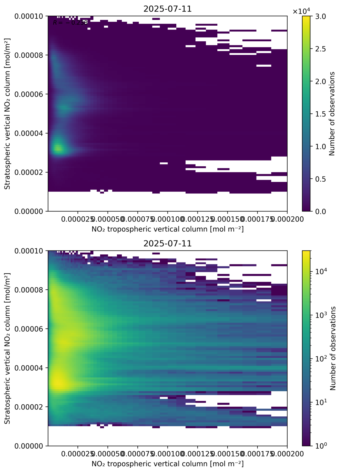
Figure 125: Scatter density plot of “NO 2 tropospheric vertical column” against “Stratospheric vertical NO 2 column” for 2025-07-10 to 2025-07-12.
