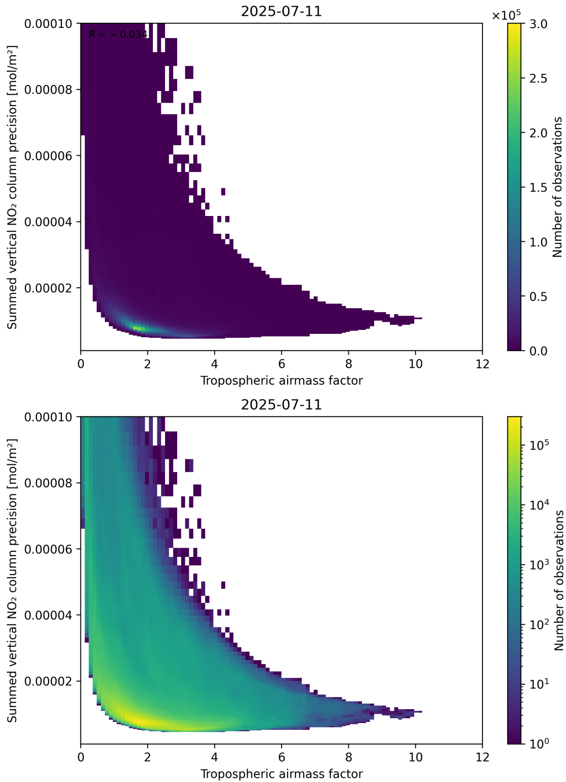
Figure 76: Scatter density plot of “Tropospheric air mass factor” against “Summed vertical NO 2 column precision” for 2025-07-10 to 2025-07-12.
