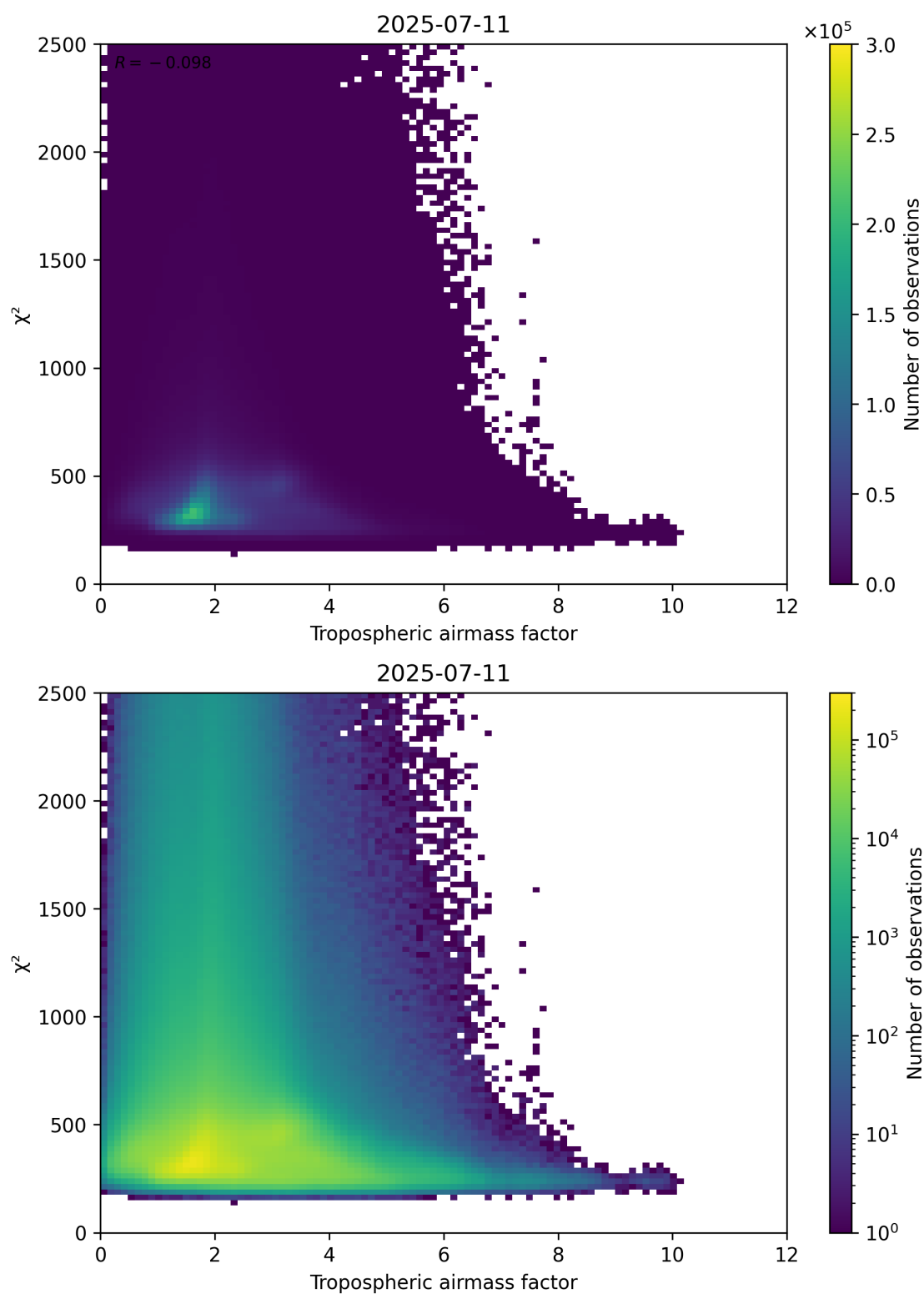
Figure 73: Scatter density plot of “Tropospheric airmass factor” against “ \chi^2 ” for 2025-07-10 to 2025-07-12.
