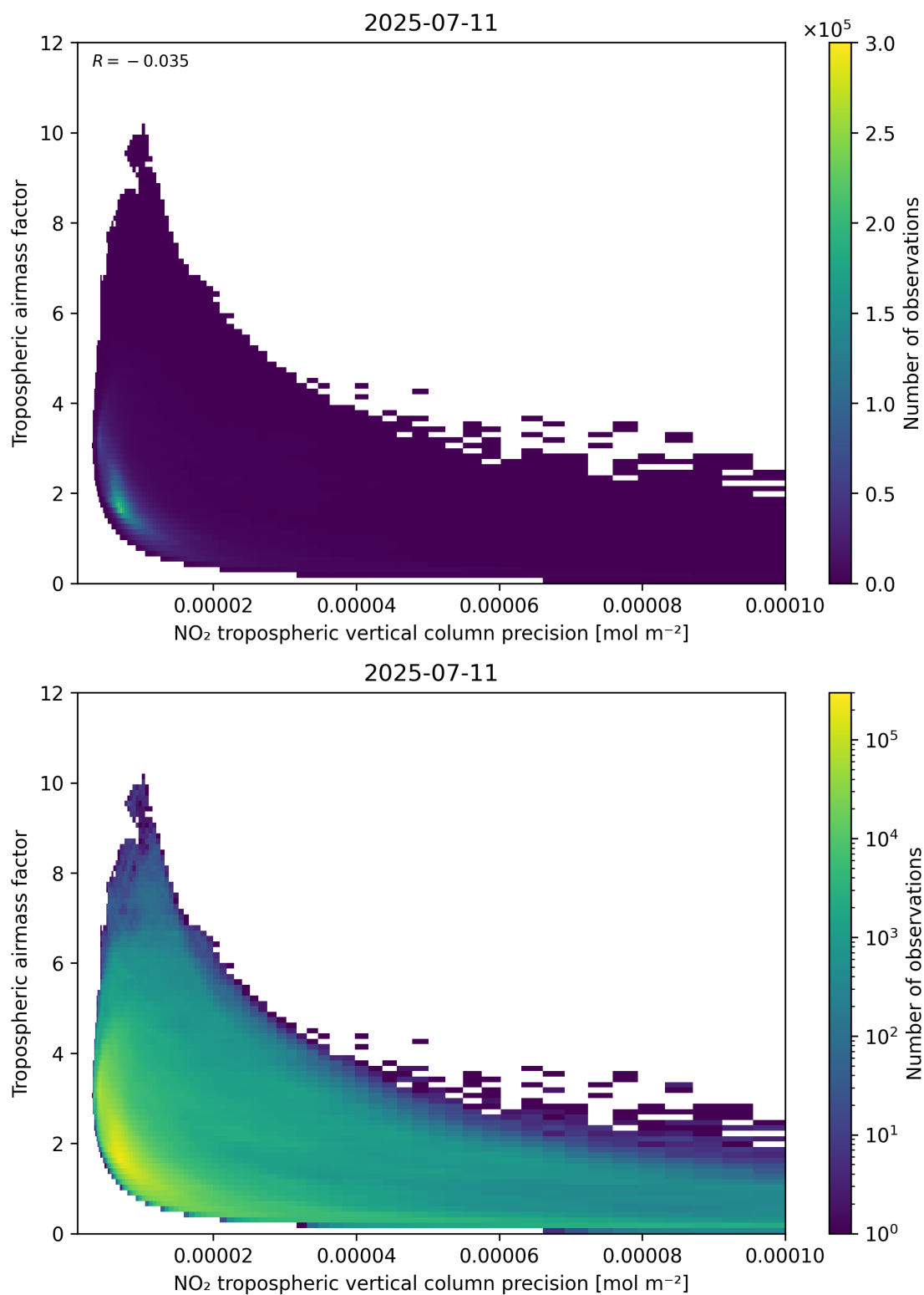
Figure 133: Scatter density plot of “NO 2 tropospheric vertical column precision” against “Tropospheric airmass factor” for 2025-07-10 to 2025-07-12.
