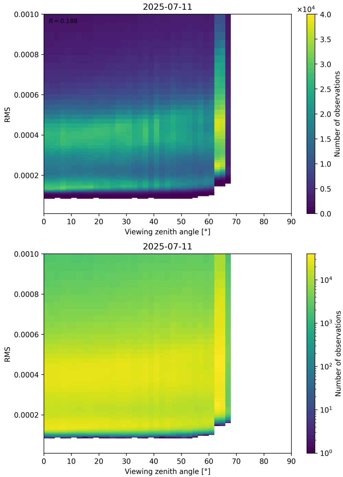
Figure 171: Scatter density plot of “Viewing zenith angle” against “RMS” for 2025-07-10 to 2025-07-12.
