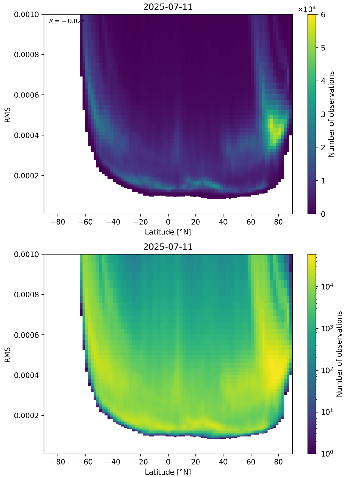
Figure 94: Scatter density plot of “Latitude” against “RMS” for 2025-07-10 to 2025-07-12.
