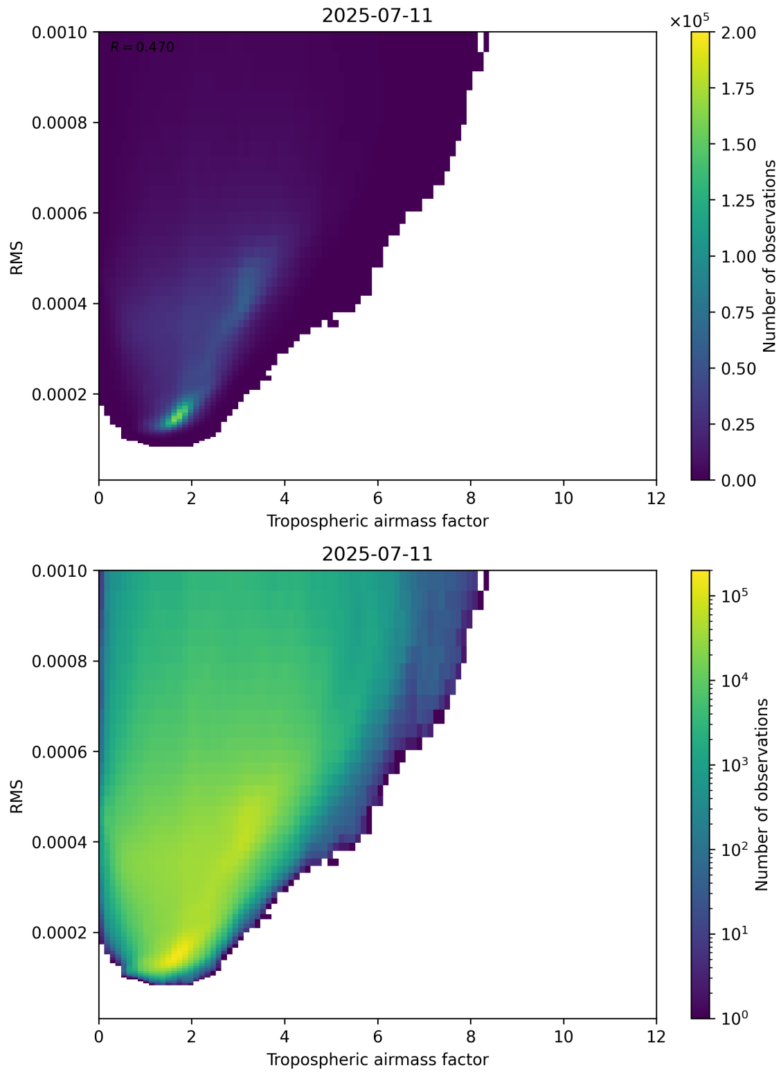
Figure 79: Scatter density plot of “Tropospheric airmass factor” against “RMS” for 2025-07-10 to 2025-07-12.
