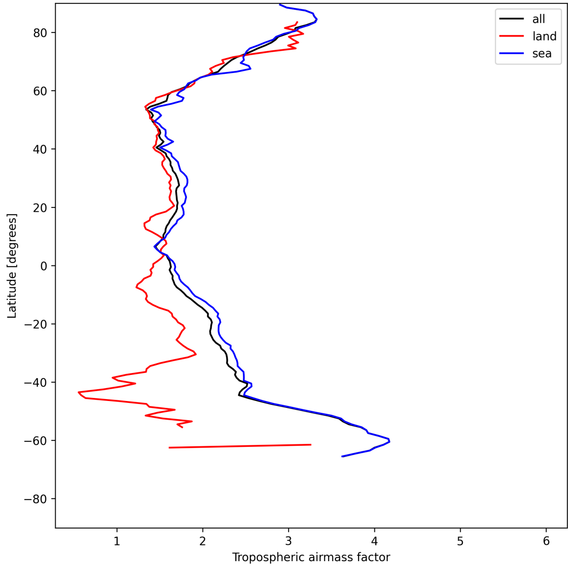
Figure 14: Zonal average of “Tropospheric air mass factor” for 2025-07-10 to 2025-07-12.
