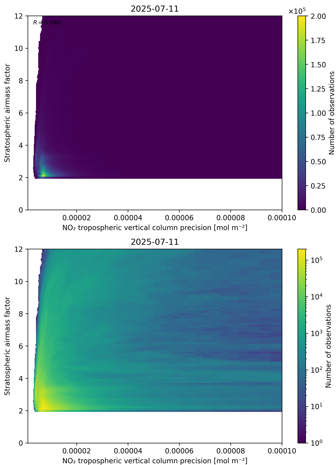
Figure 131: Scatter density plot of “NO 2 tropospheric vertical column precision” against “Stratospheric airmass factor” for 2025-07-10 to 2025-07-12.
