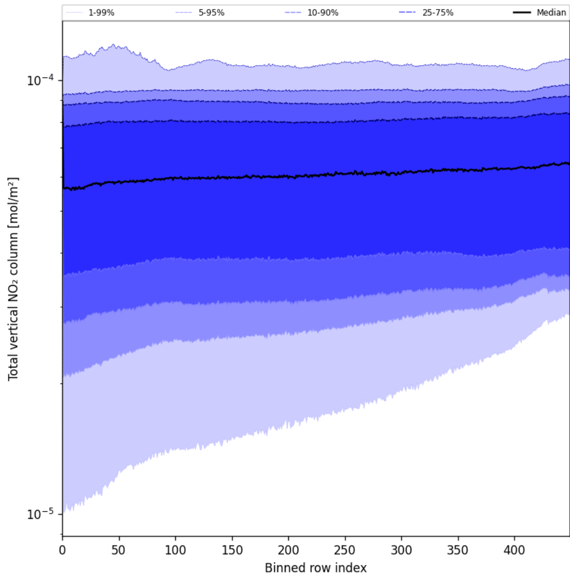
Figure 55: Along track statistics of “Total vertical NO 2 column” for 2025-07-10 to 2025-07-12
