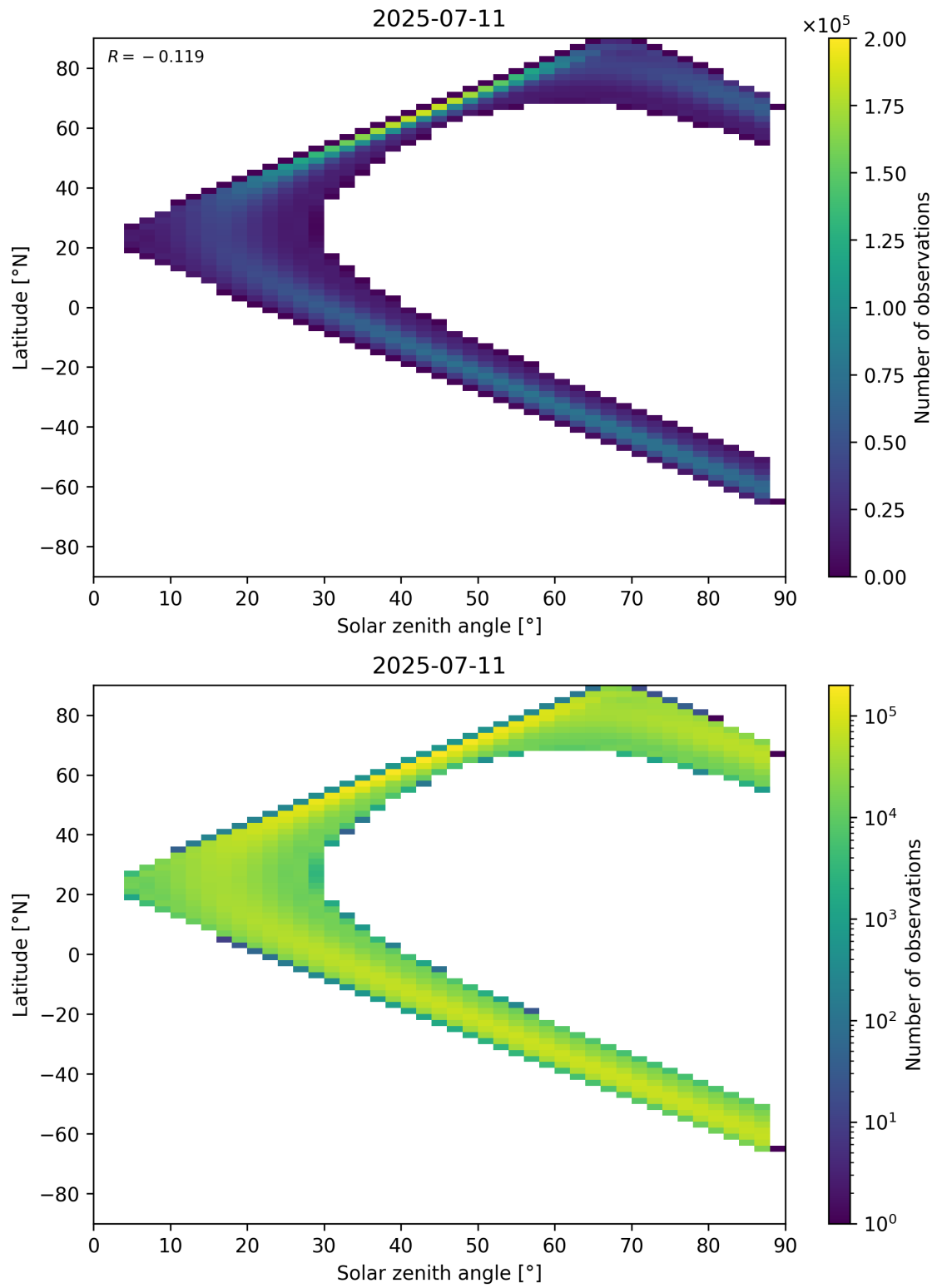
Figure 149: Scatter density plot of “Solar zenith angle” against “Latitude” for 2025-07-10 to 2025-07-12.
