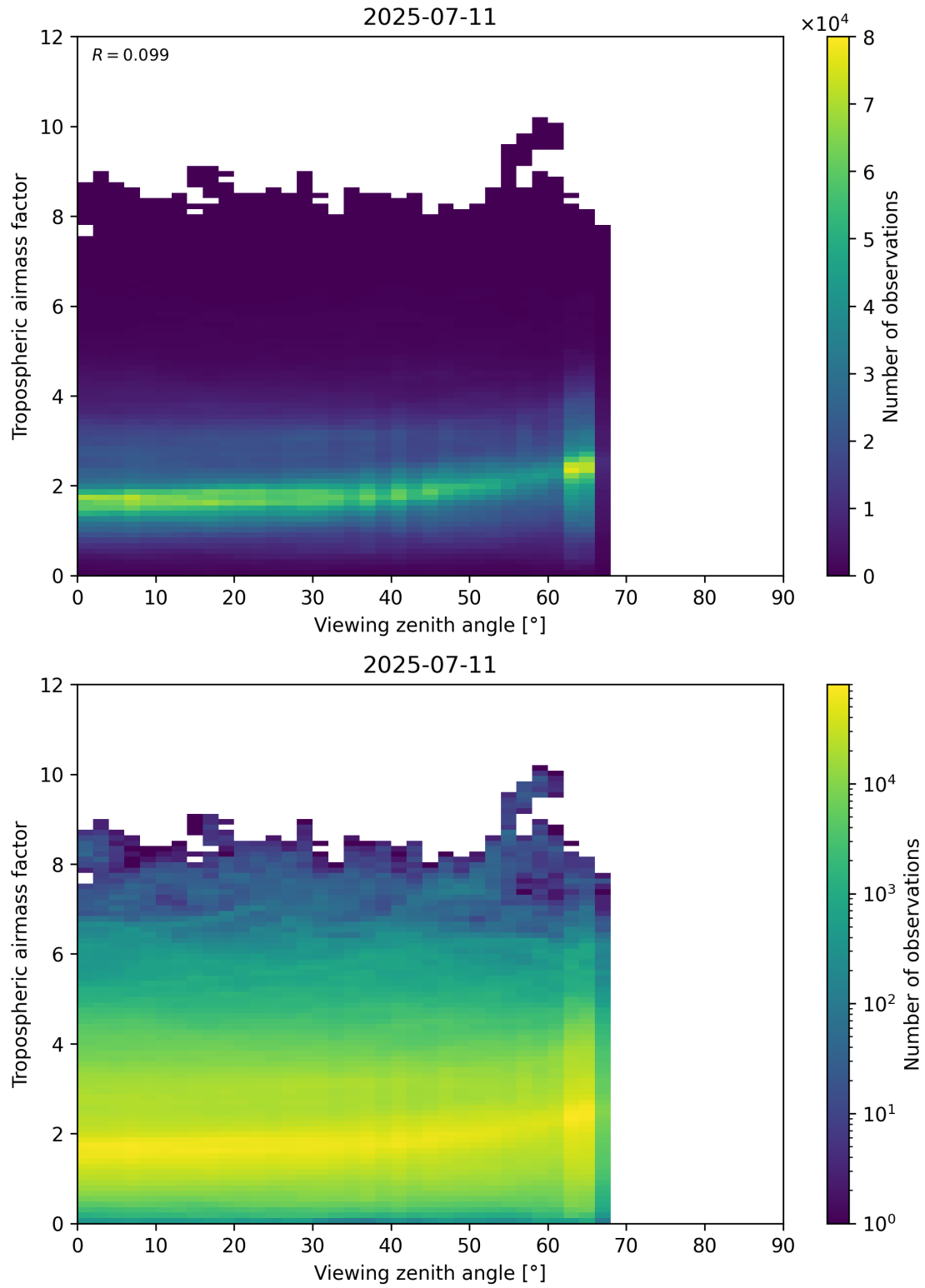
Figure 161: Scatter density plot of “Viewing zenith angle” against “Tropospheric airmass factor” for 2025-07-10 to 2025-07-12.
