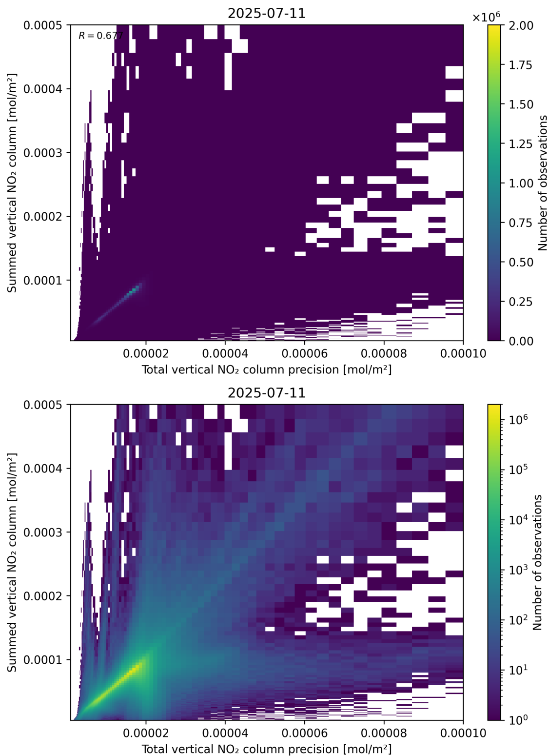
Figure 117: Scatter density plot of “Total vertical NO 2 column precision” against “Summed vertical NO 2 column” for 2025-07-10 to 2025-07-12.
