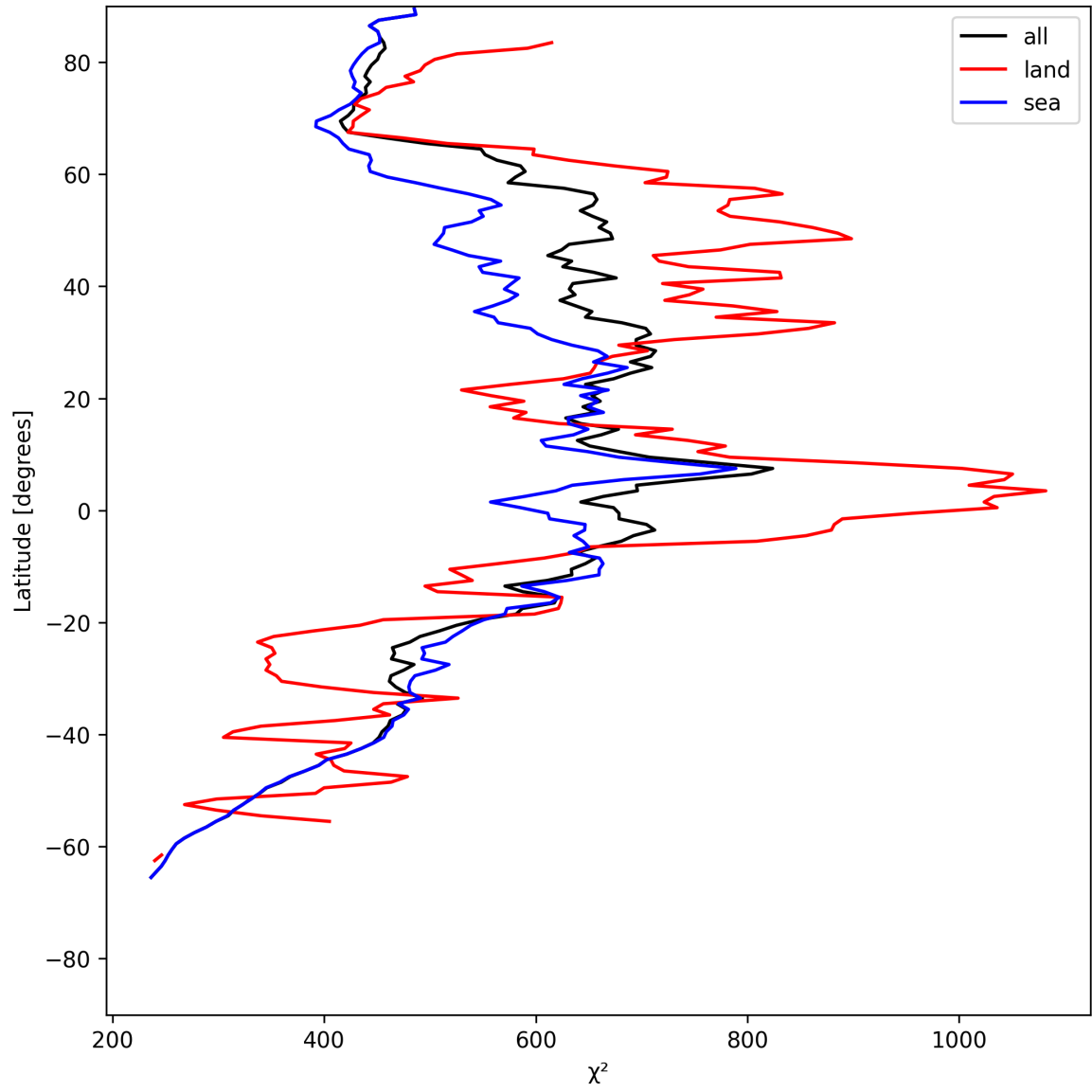
Figure 25: Zonal average of “ \chi^2 ” for 2025-07-10 to 2025-07-12.
