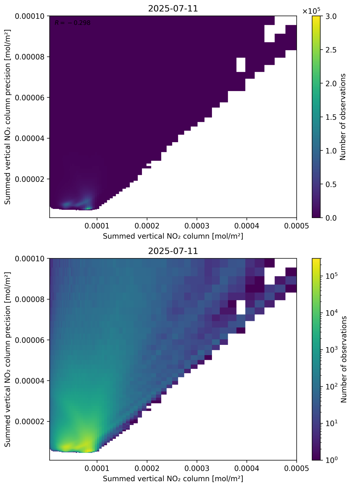
Figure 105: Scatter density plot of “Summed vertical NO 2 column” against “Summed vertical NO 2 column precision” for 2025-07-10 to 2025-07-12.
