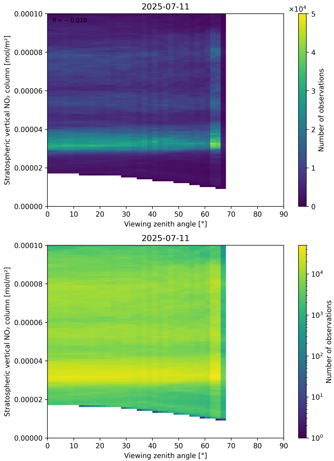
Figure 164: Scatter density plot of “Viewing zenith angle” against “Stratospheric vertical NO 2 column” for 2025-07-10 to 2025-07-12.
