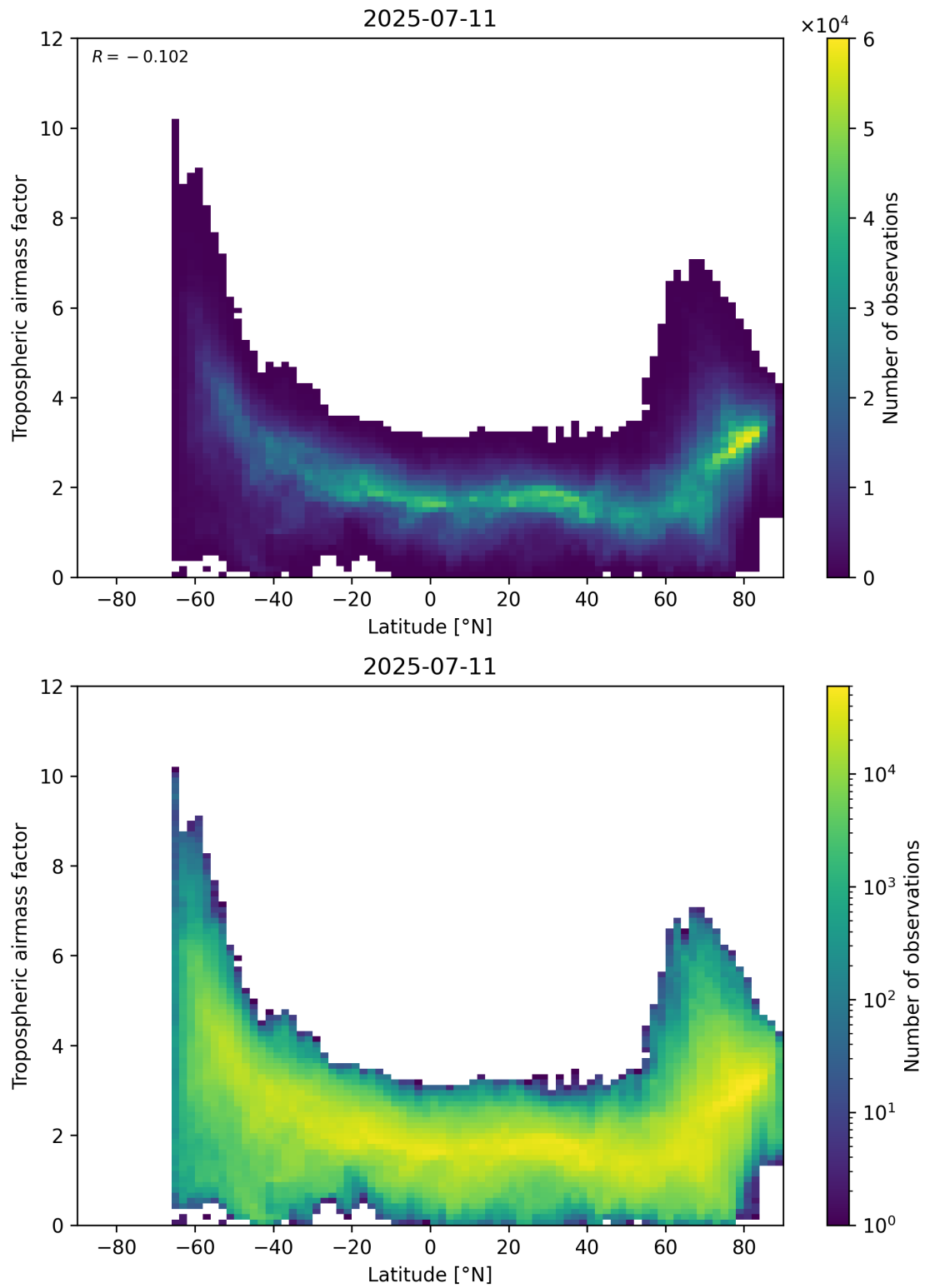
Figure 85: Scatter density plot of “Latitude” against “Tropospheric air mass factor” for 2025-07-10 to 2025-07-12.
