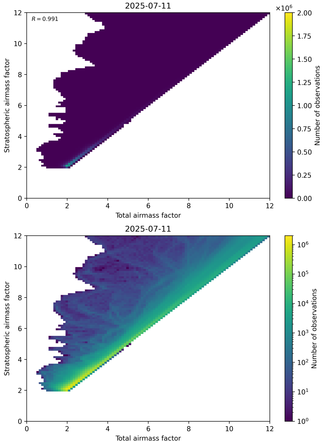
Figure 62: Scatter density plot of “Total airmass factor” against “Stratospheric airmass factor” for 2025-07-10 to 2025-07-12.
