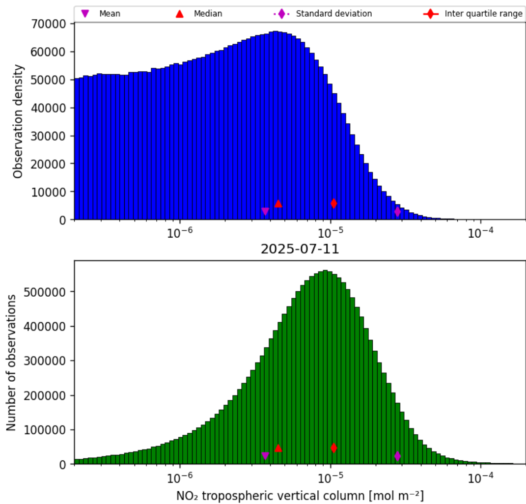
Figure 29: Histogram of “NO 2 tropospheric vertical column” for 2025-07-10 to 2025-07-12
