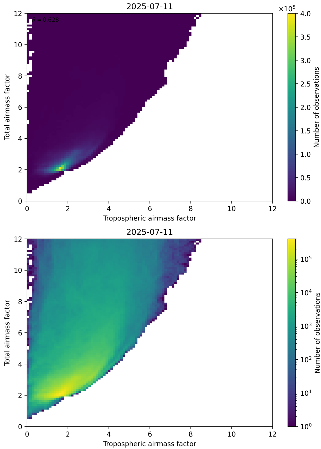
Figure 72: Scatter density plot of “Tropospheric airmass factor” against “Total airmass factor” for 2025-07-10 to 2025-07-12.
