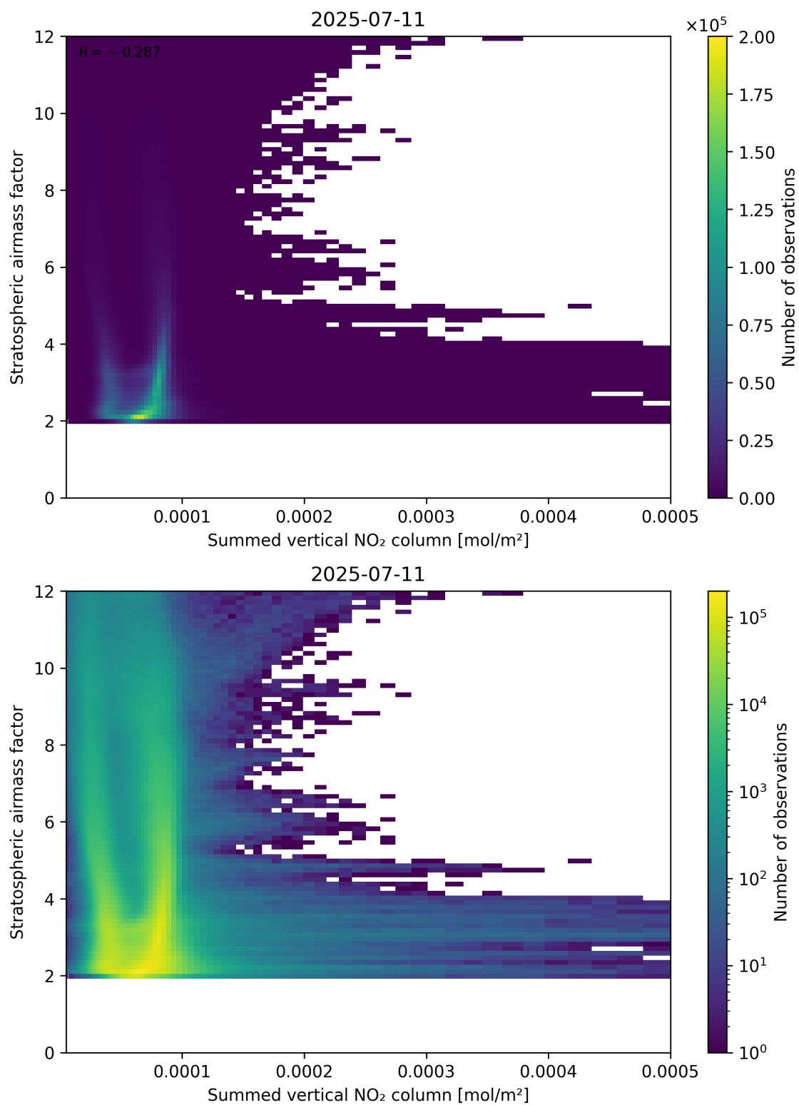
Figure 103: Scatter density plot of “Summed vertical NO 2 column” against “Stratospheric air mass factor” for 2025-07-10 to 2025-07-12.
