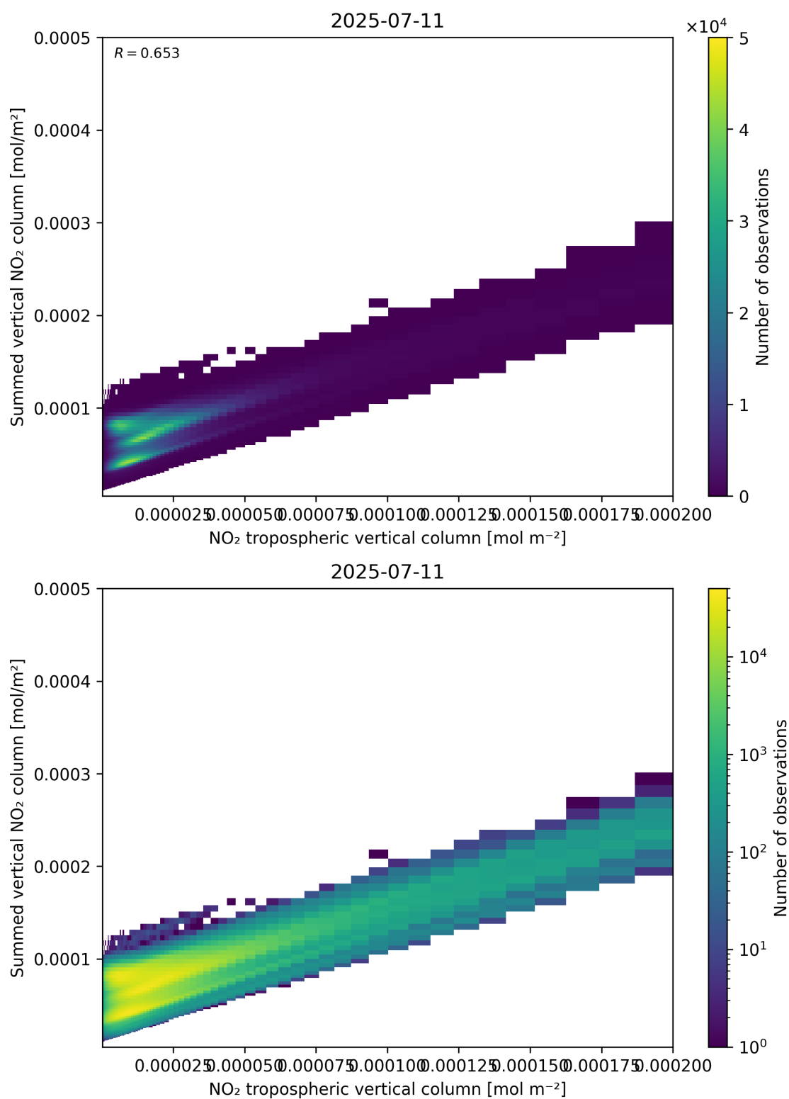
Figure 126: Scatter density plot of “NO 2 tropospheric vertical column” against “Summed vertical NO 2 column” for 2025-07-10 to 2025-07-12.
