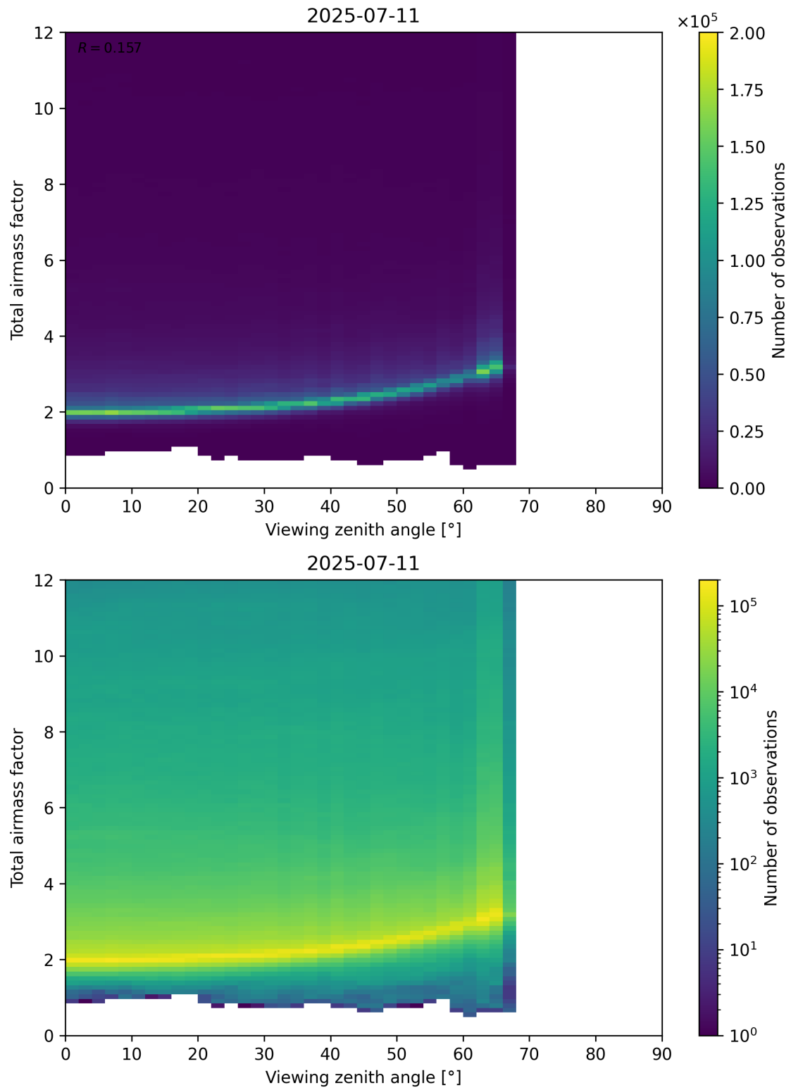
Figure 160: Scatter density plot of “Viewing zenith angle” against “Total airmass factor” for 2025-07-10 to 2025-07-12.
