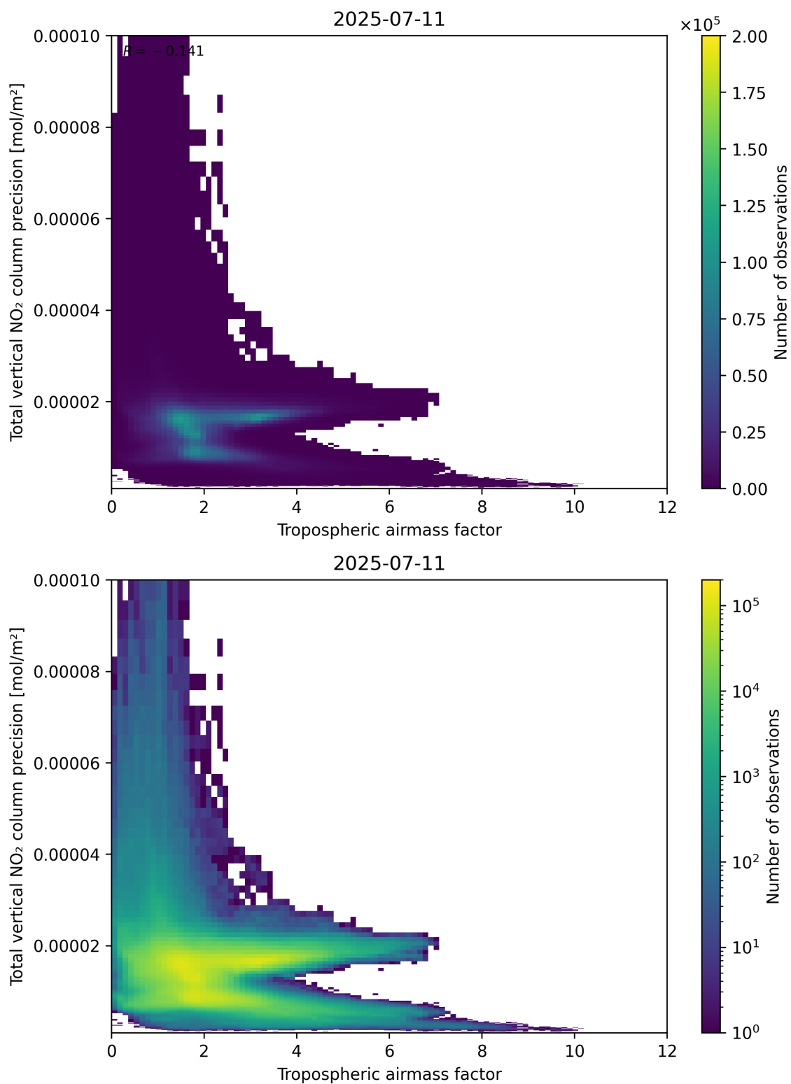
Figure 78: Scatter density plot of “Tropospheric airmass factor” against “Total vertical NO 2 column precision” for 2025-07-10 to 2025-07-12.
