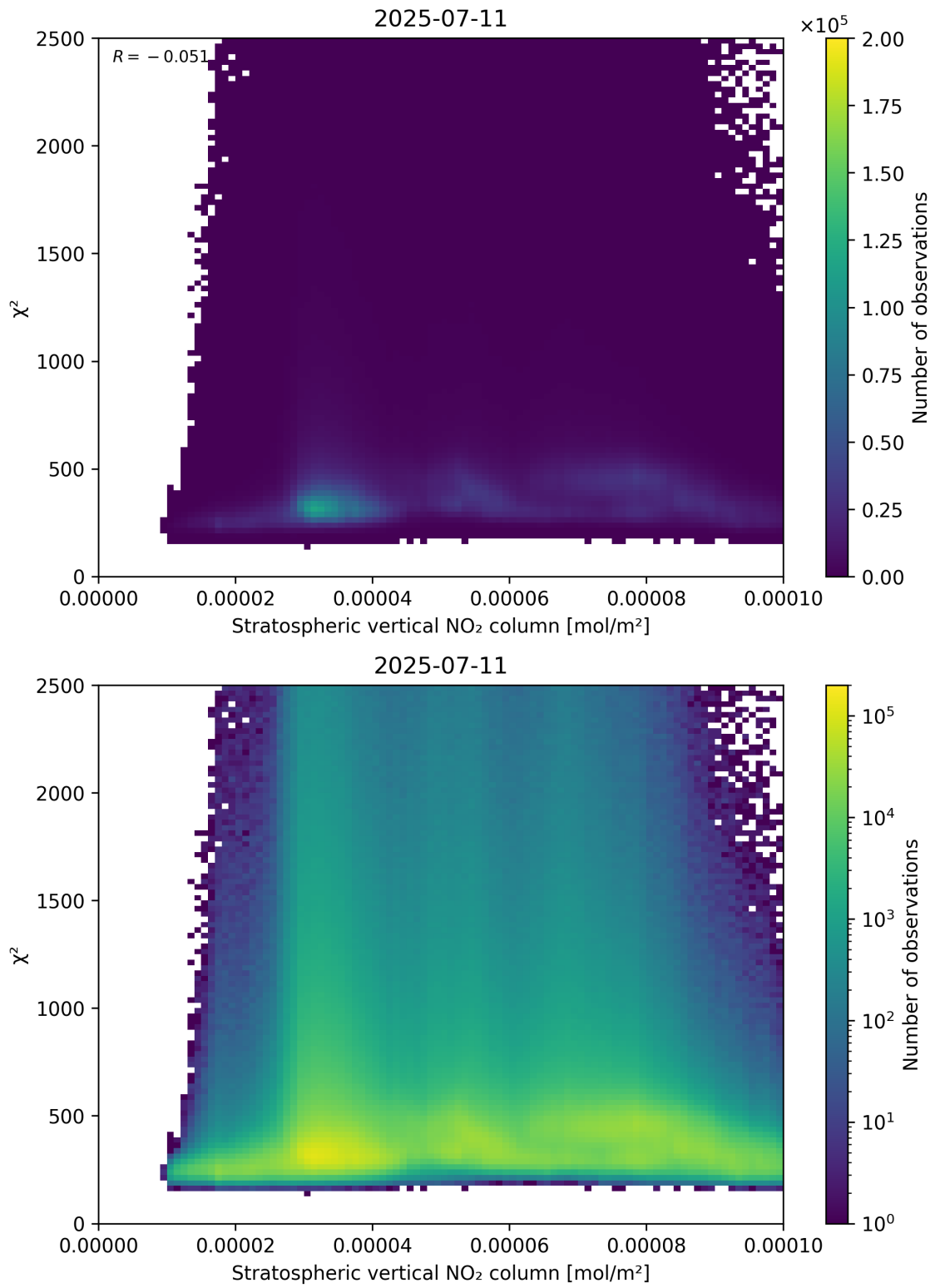
Figure 97: Scatter density plot of “Stratospheric vertical NO 2 column” against “ \chi^2 ” for 2025-07-10 to 2025-07-12.
