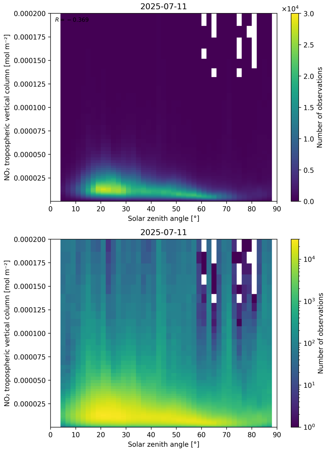
Figure 155: Scatter density plot of “Solar zenith angle” against “NO 2 tropospheric vertical column” for 2025-07-10 to 2025-07-12.
