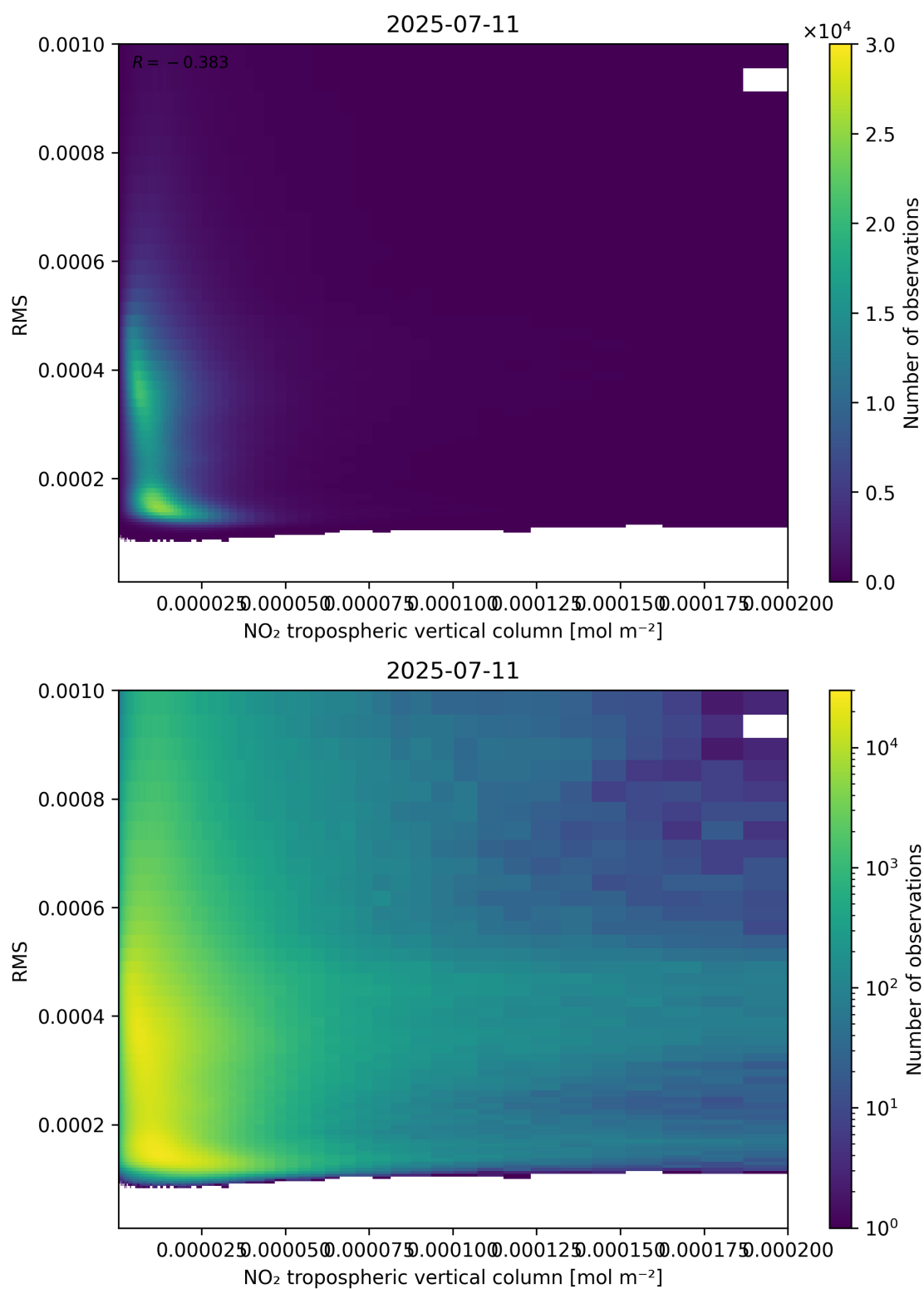
Figure 142: Scatter density plot of “NO 2 tropospheric vertical column” against “RMS” for 2025-07-10 to 2025-07-12.
