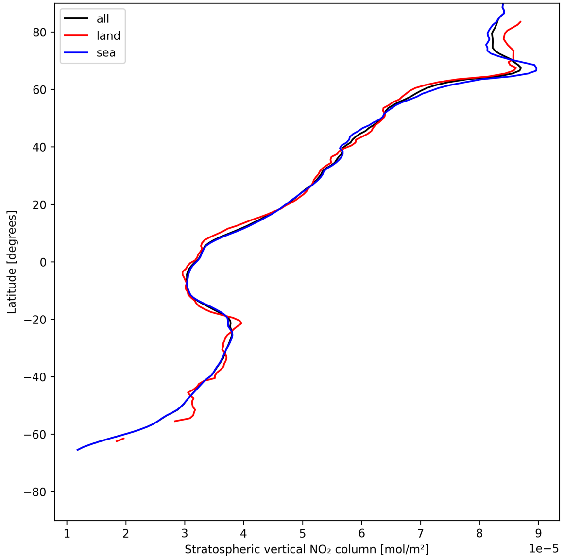
Figure 19: Zonal average of “Stratospheric vertical NO 2 column” for 2025-07-10 to 2025-07-12.
