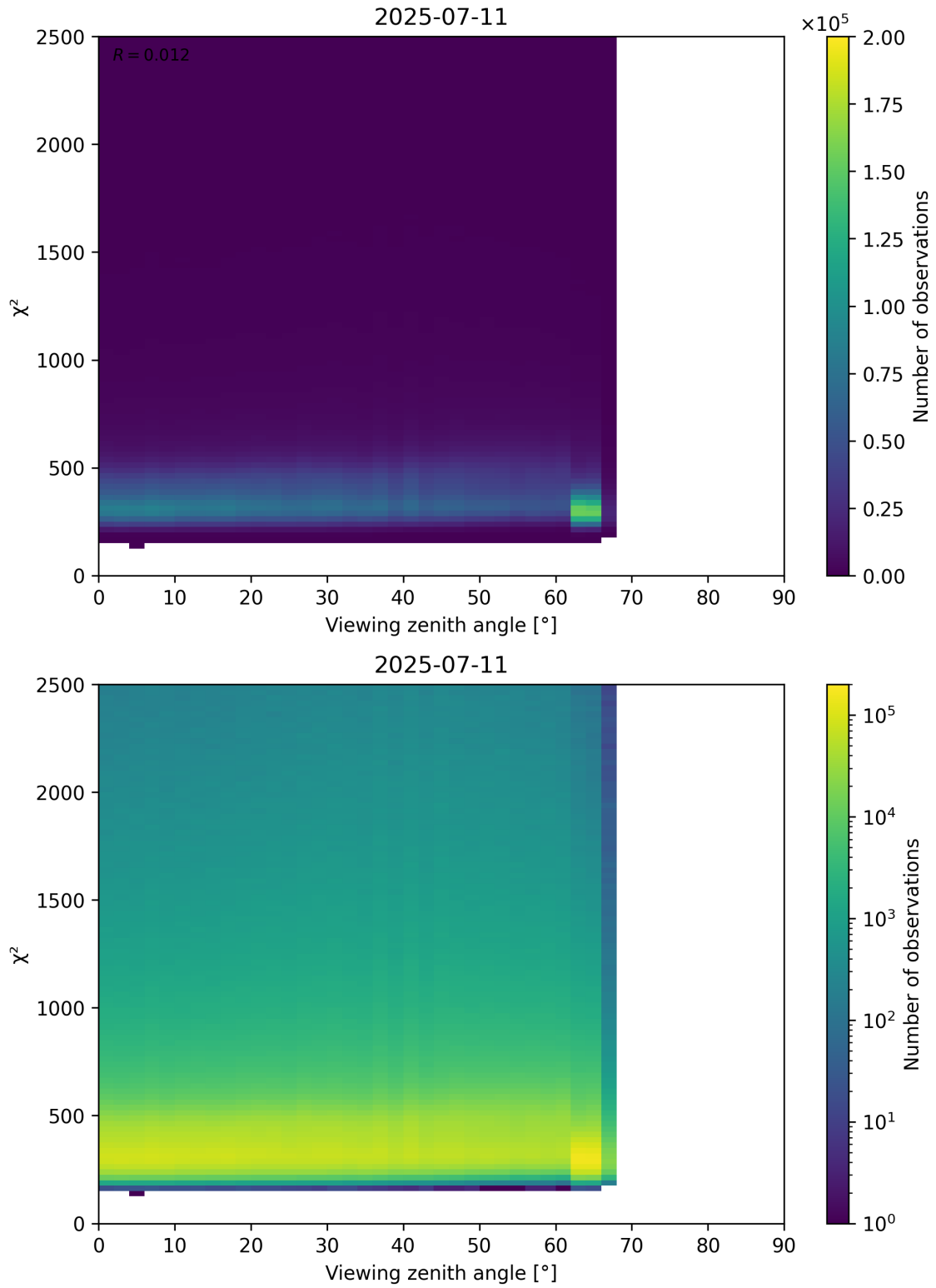
Figure 162: Scatter density plot of “Viewing zenith angle” against “ \chi^2 ” for 2025-07-10 to 2025-07-12.
