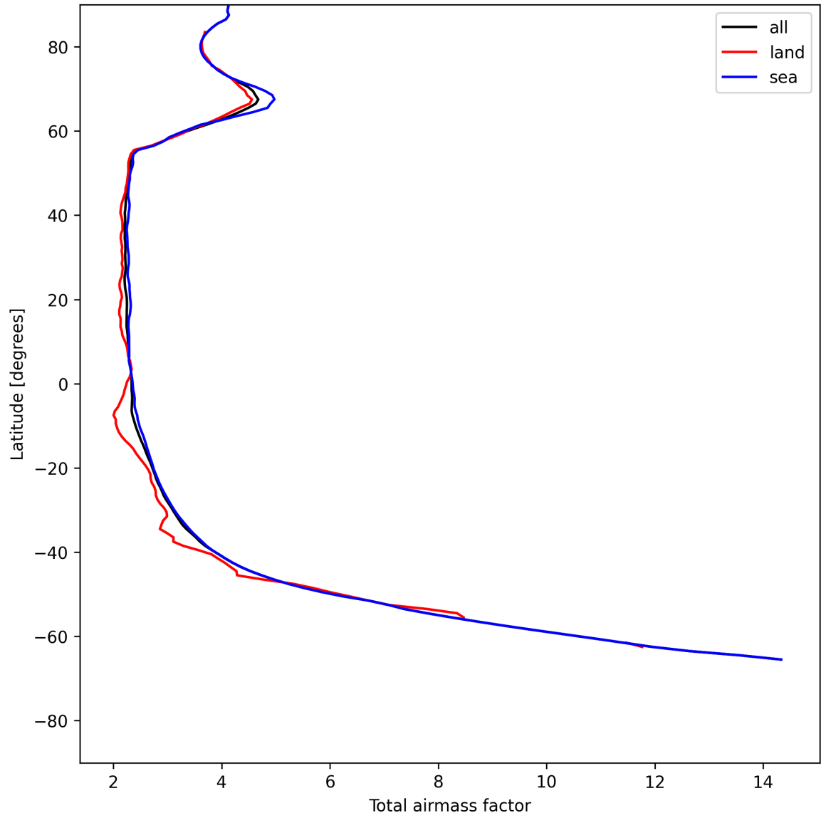
Figure 15: Zonal average of “Total airmass factor” for 2025-07-10 to 2025-07-12.
