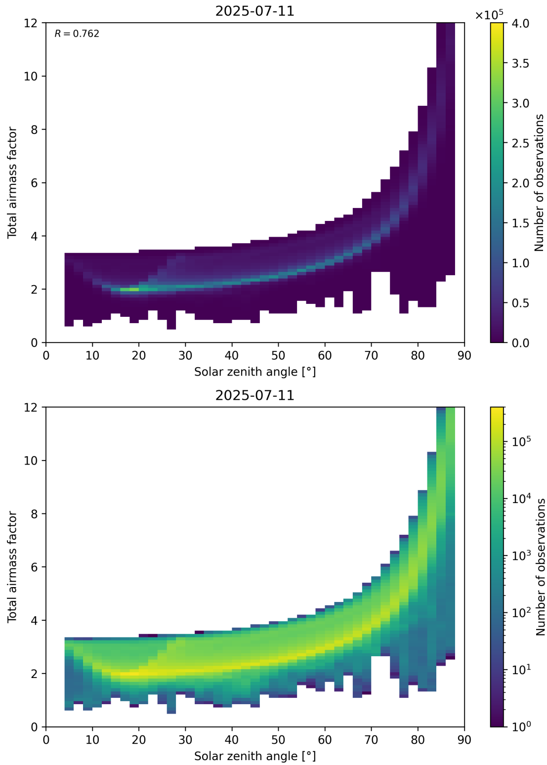
Figure 146: Scatter density plot of “Solar zenith angle” against “Total air mass factor” for 2025-07-10 to 2025-07-12.
