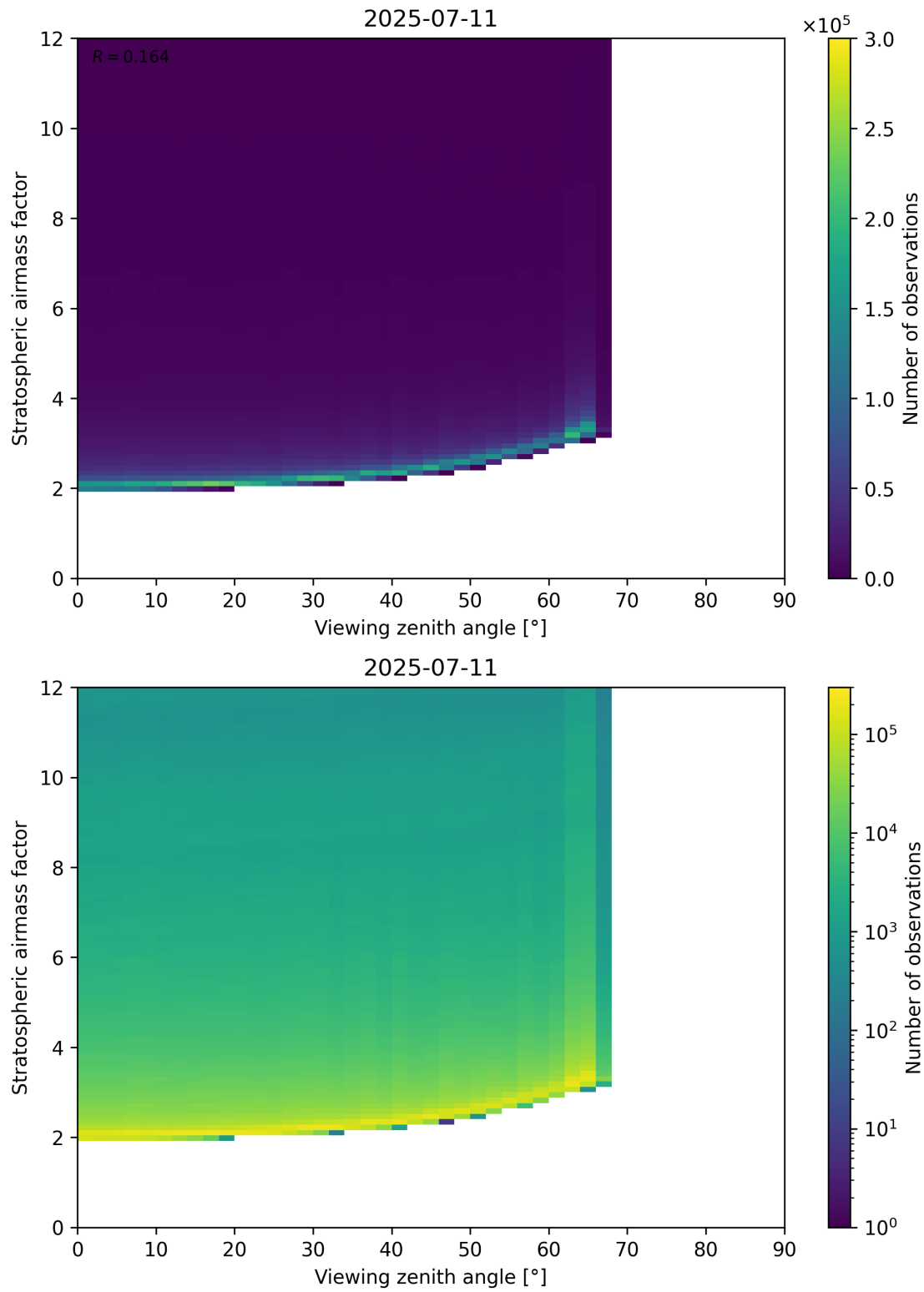
Figure 159: Scatter density plot of “Viewing zenith angle” against “Stratospheric airmass factor” for 2025-07-10 to 2025-07-12.
