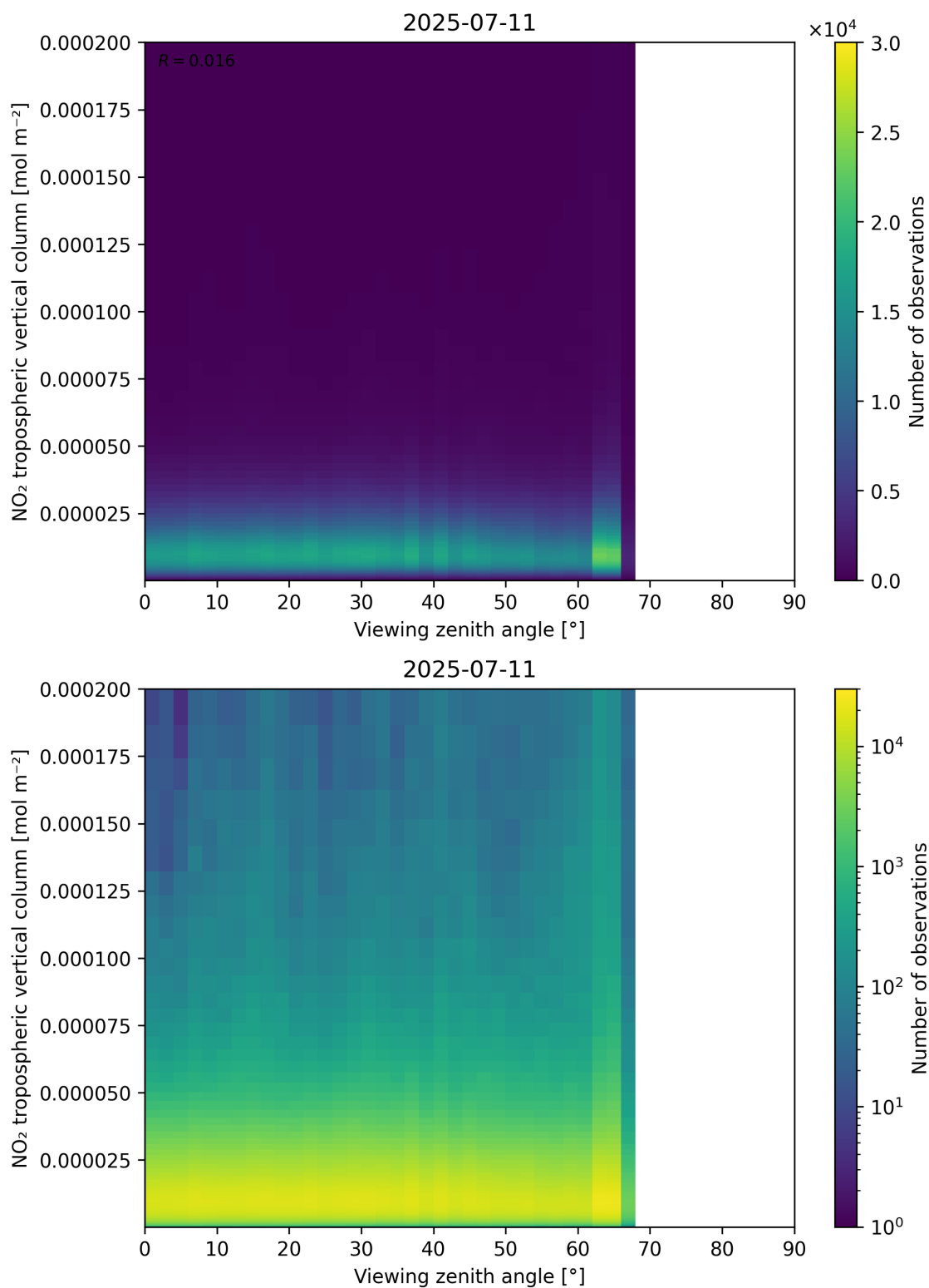
Figure 169: Scatter density plot of “Viewing zenith angle” against “NO 2 tropospheric vertical column” for 2025-07-10 to 2025-07-12.
