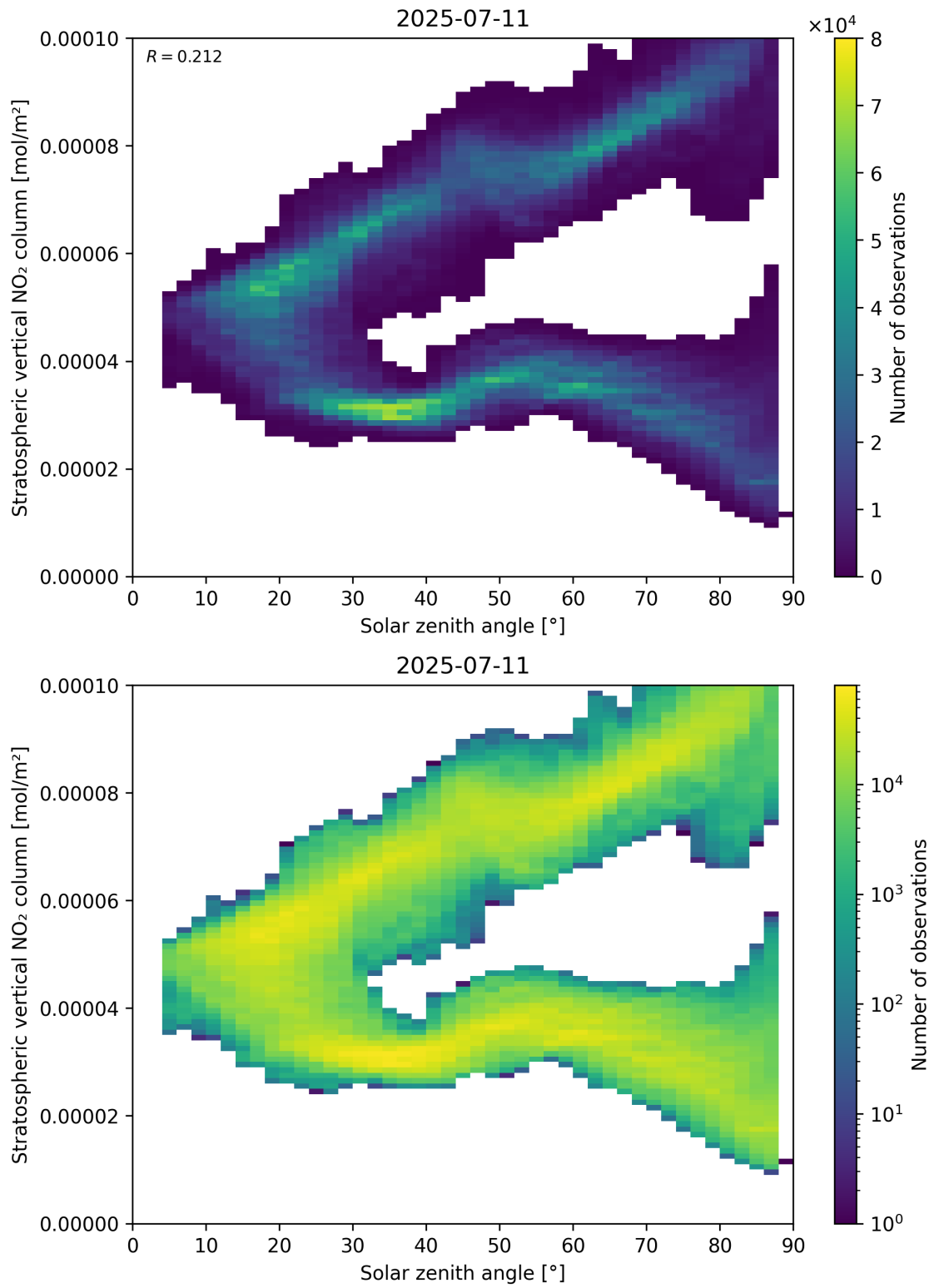
Figure 150: Scatter density plot of “Solar zenith angle” against “Stratospheric vertical NO 2 column” for 2025-07-10 to 2025-07-12.
