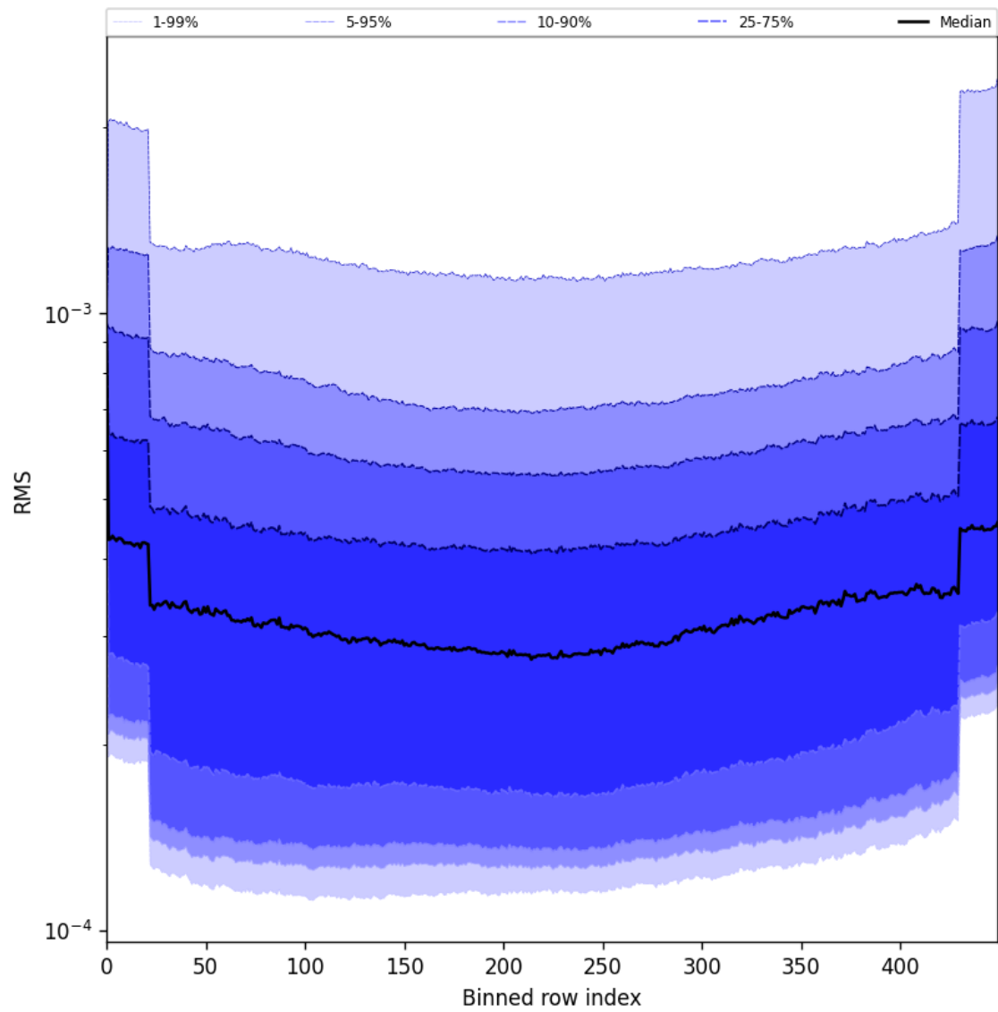
Figure 60: Along track statistics of “RMS” for 2025-07-10 to 2025-07-12
