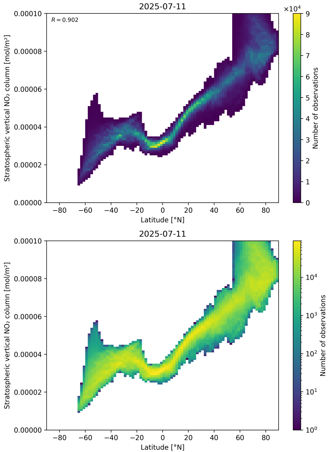
Figure 87: Scatter density plot of “Latitude” against “Stratospheric vertical NO 2 column” for 2025-07-10 to 2025-07-12.
