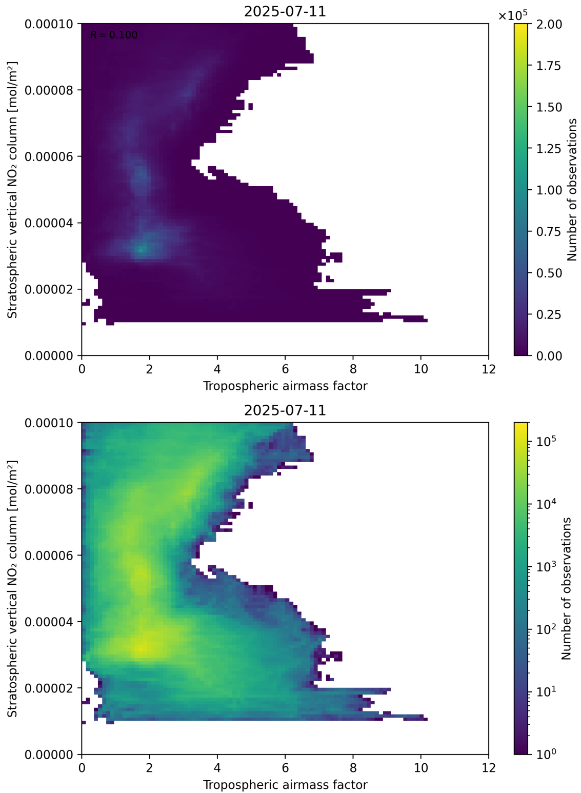
Figure 74: Scatter density plot of “Tropospheric airmass factor” against “Stratospheric vertical NO 2 column” for 2025-07-10 to 2025-07-12.
