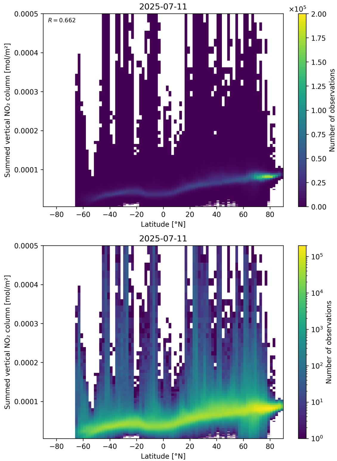
Figure 88: Scatter density plot of “Latitude” against “Summed vertical NO 2 column” for 2025-07-10 to 2025-07-12.
