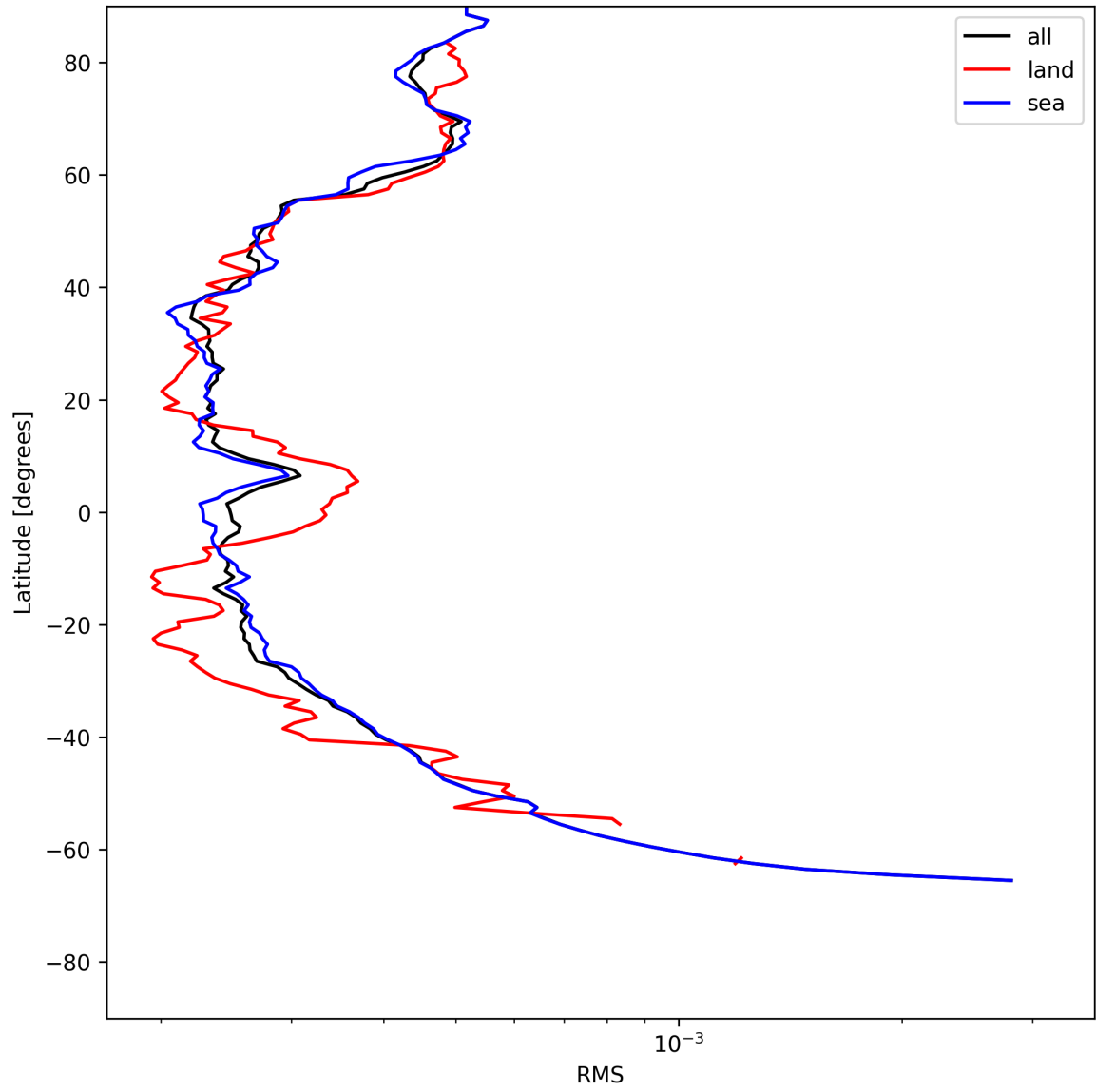
Figure 26: Zonal average of “RMS” for 2025-07-10 to 2025-07-12.
