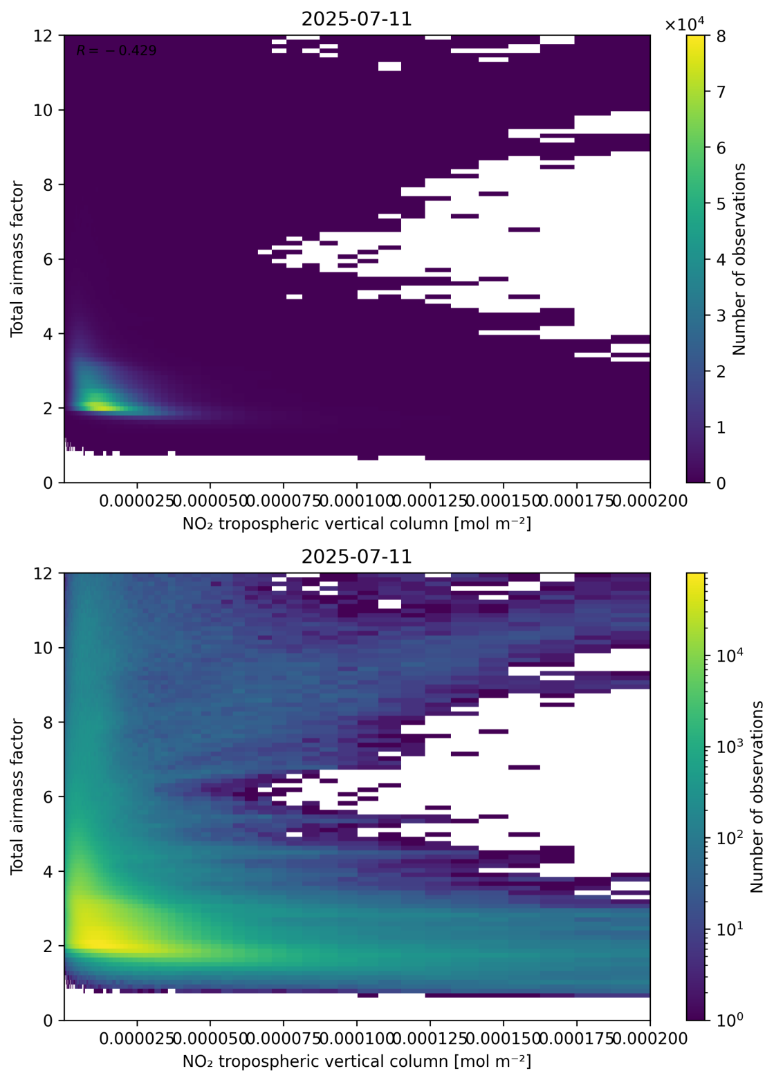
Figure 122: Scatter density plot of “NO 2 tropospheric vertical column” against “Total air mass factor” for 2025-07-10 to 2025-07-12.
