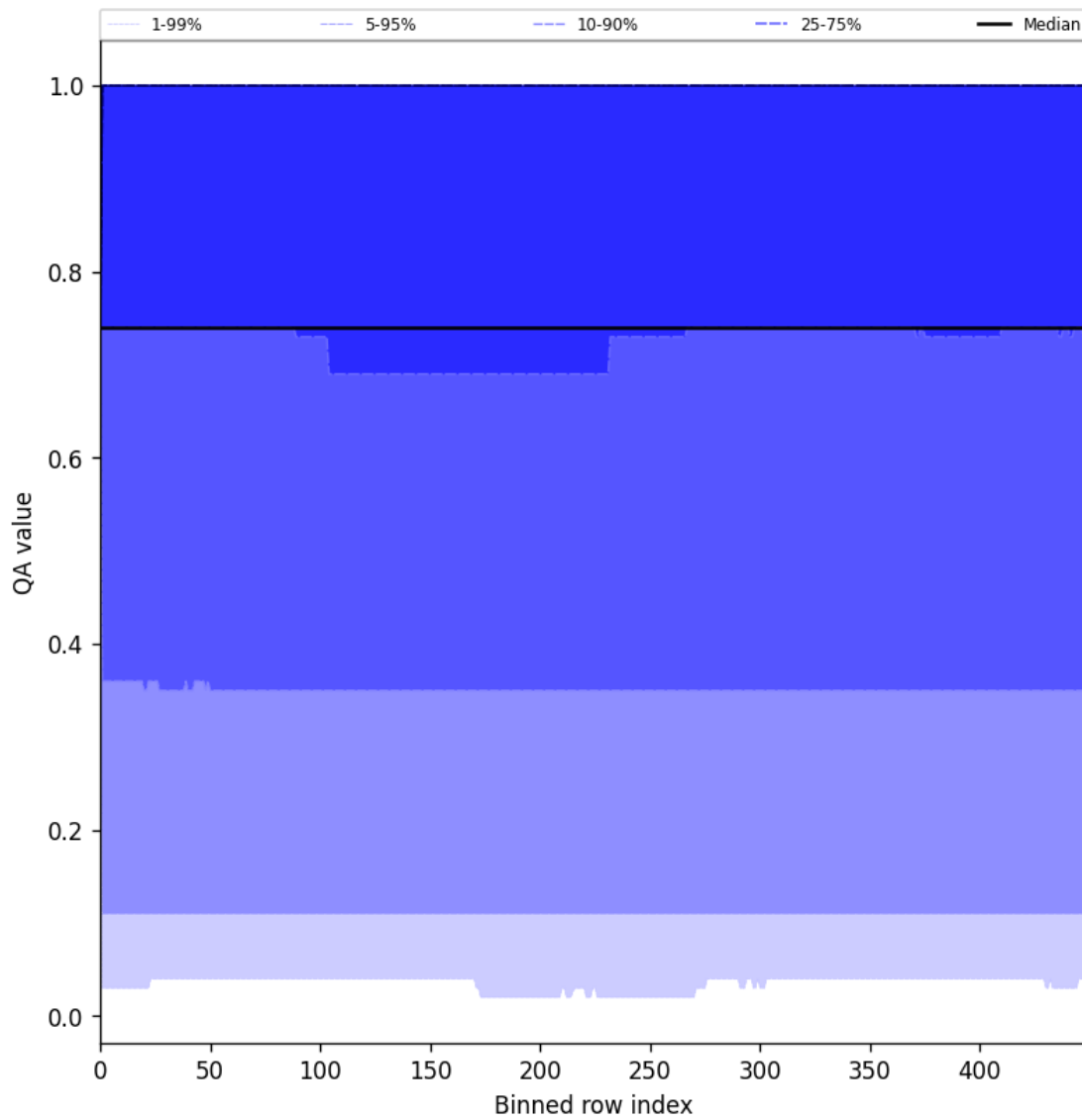
Figure 45: Along track statistics of “QA value” for 2025-07-10 to 2025-07-12
