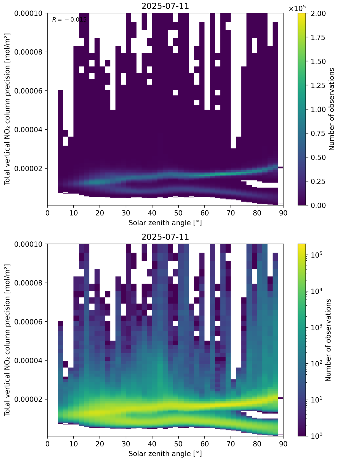
Figure 154: Scatter density plot of “Solar zenith angle” against “Total vertical NO 2 column precision” for 2025-07-10 to 2025-07-12.
