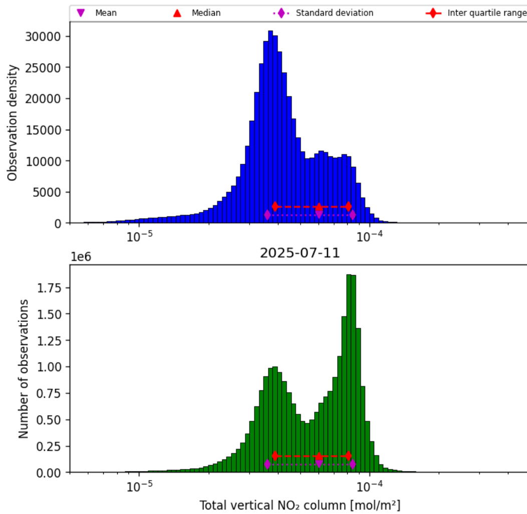
Figure 38: Histogram of “Total vertical NO 2 column” for 2025-07-10 to 2025-07-12
