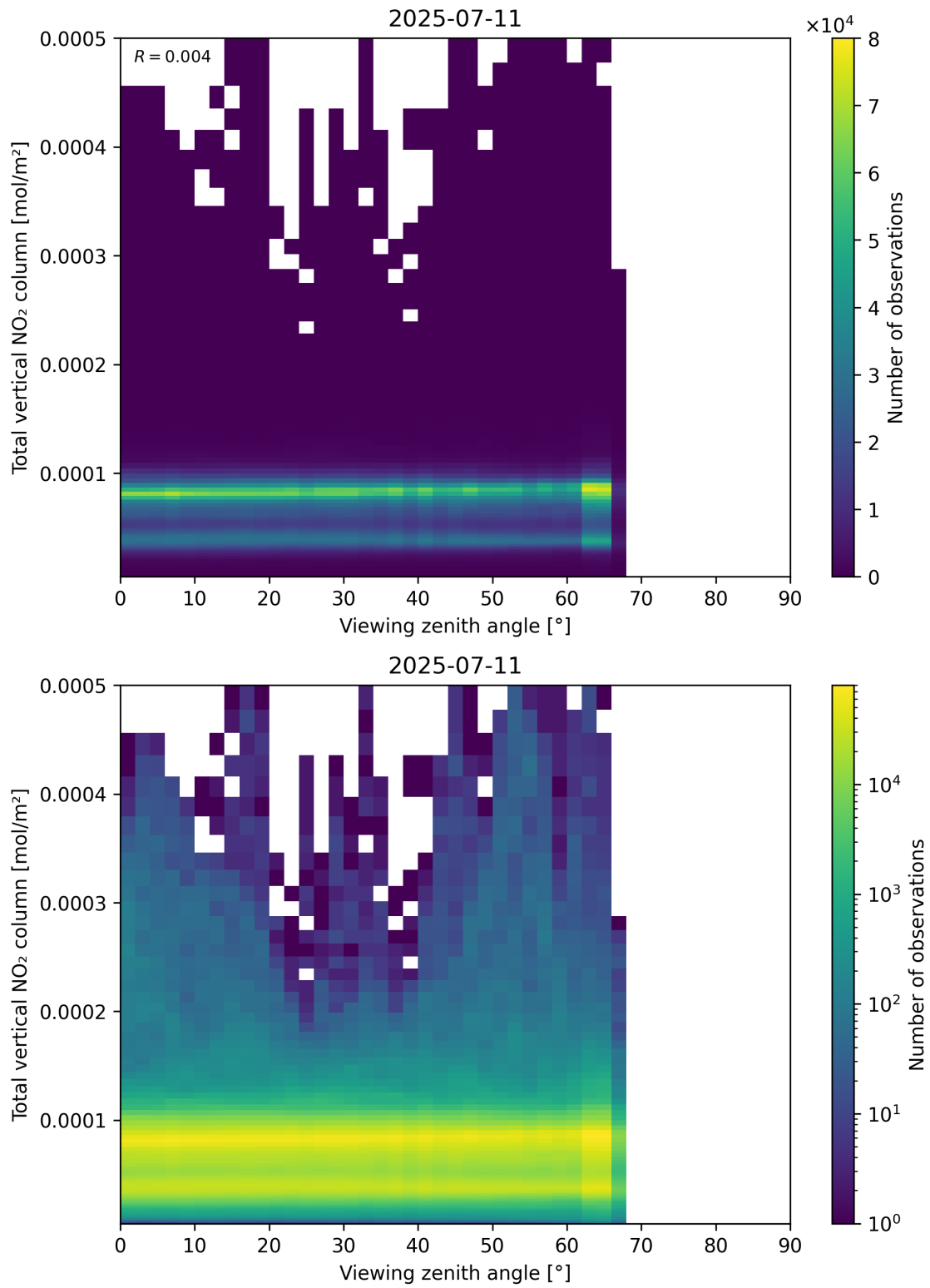
Figure 167: Scatter density plot of “Viewing zenith angle” against “Total vertical NO 2 column” for 2025-07-10 to 2025-07-12.
