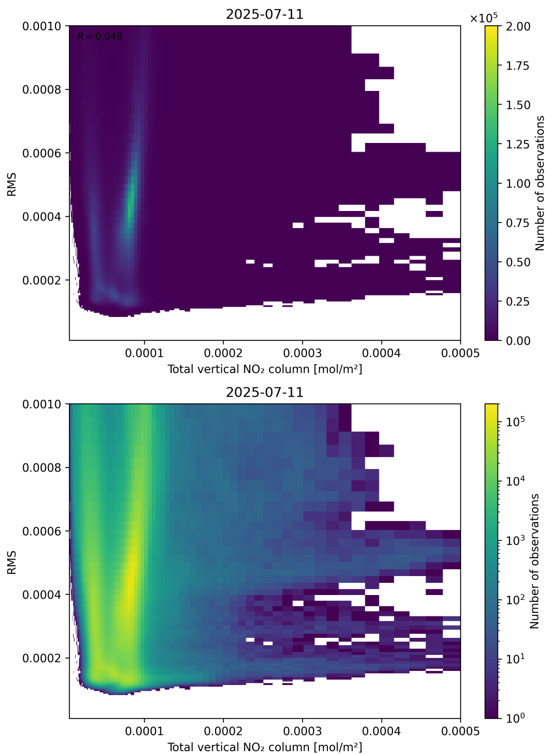
Figure 120: Scatter density plot of “Total vertical NO 2 column” against “RMS” for 2025-07-10 to 2025-07-12.
