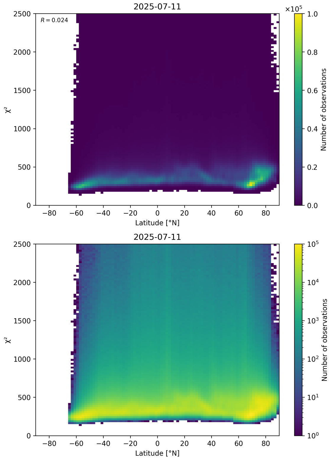
Figure 86: Scatter density plot of “Latitude” against “ \chi^2 ” for 2025-07-10 to 2025-07-12.
