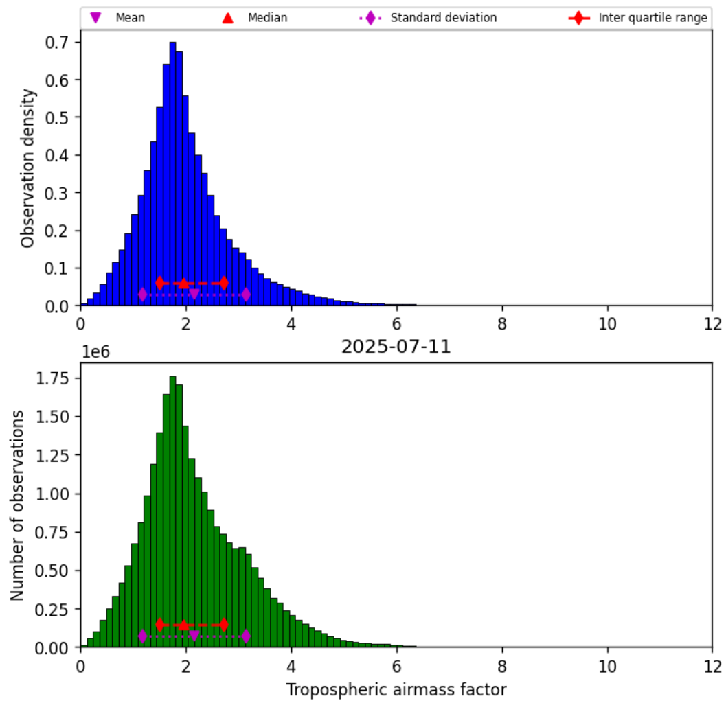
Figure 31: Histogram of “Tropospheric airmass factor” for 2025-07-10 to 2025-07-12
