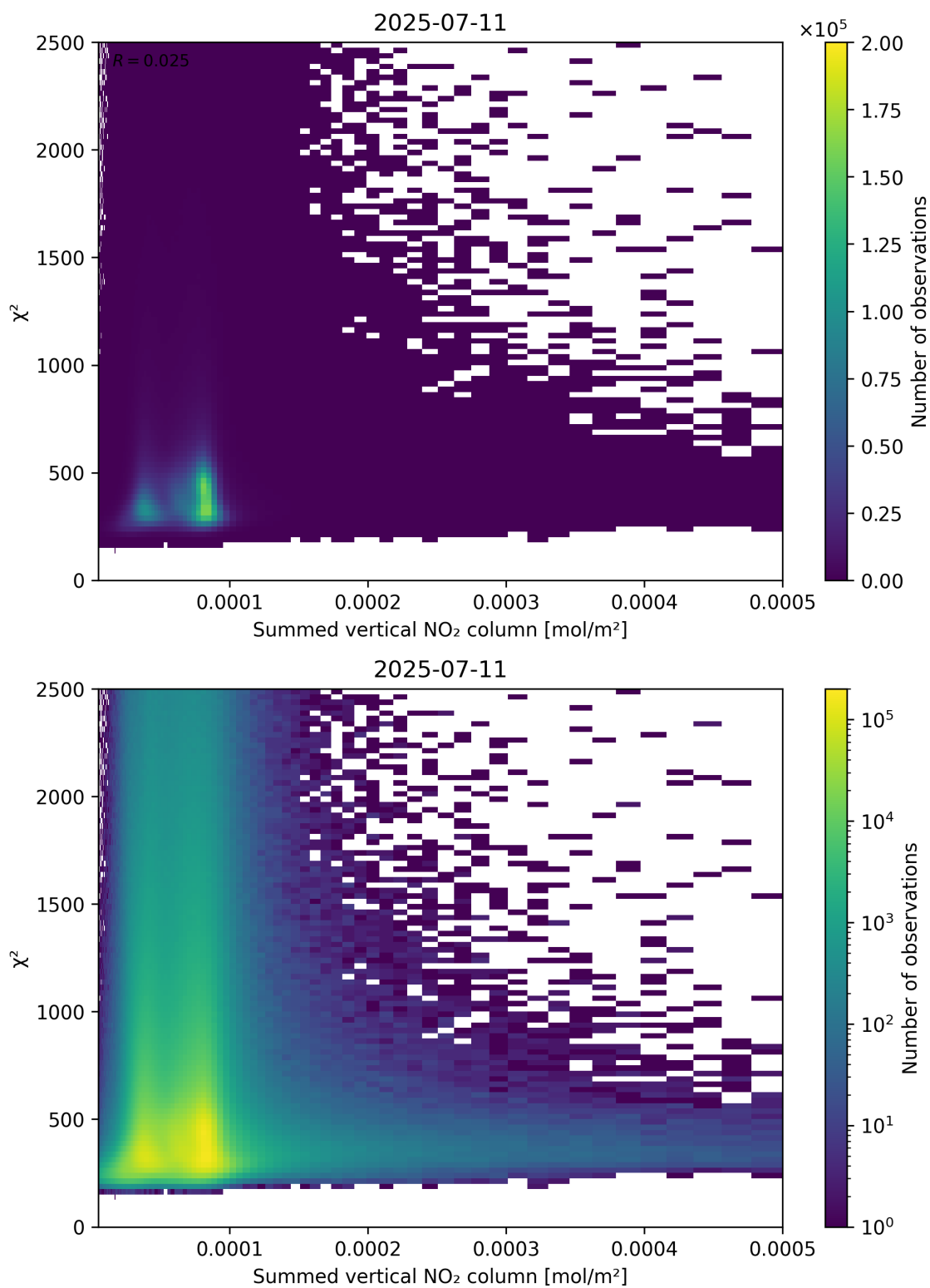
Figure 104: Scatter density plot of “Summed vertical NO 2 column” against “ \chi^2 ” for 2025-07-10 to 2025-07-12.
