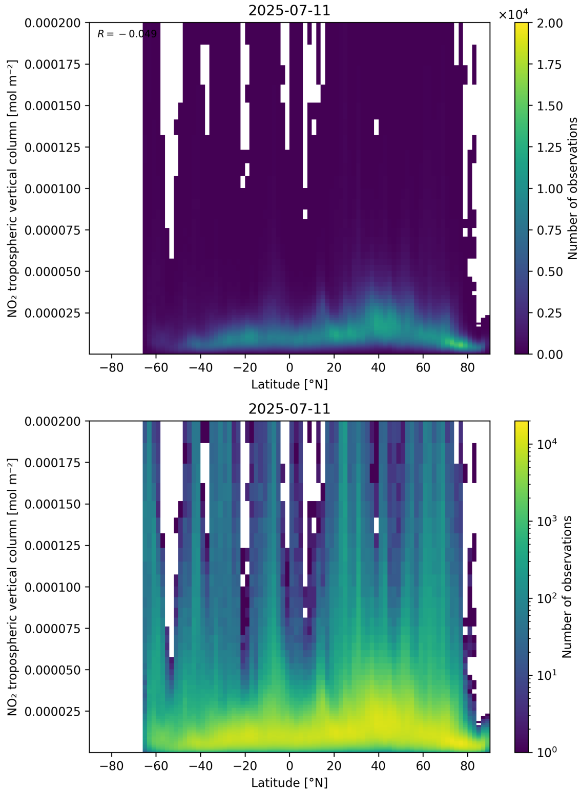
Figure 92: Scatter density plot of “Latitude” against “NO 2 tropospheric vertical column” for 2025-07-10 to 2025-07-12.
