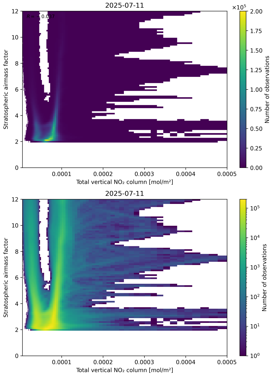
Figure 110: Scatter density plot of “Total vertical NO 2 column” against “Stratospheric airmass factor” for 2025-07-10 to 2025-07-12.
