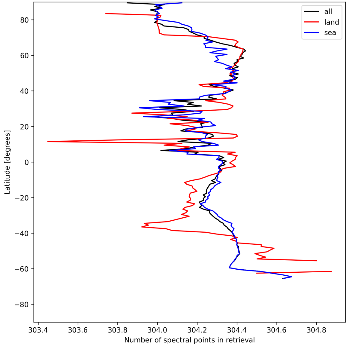
Figure 16: Zonal average of “Number of spectral points in retrieval” for 2025-07-10 to 2025-07-12.
