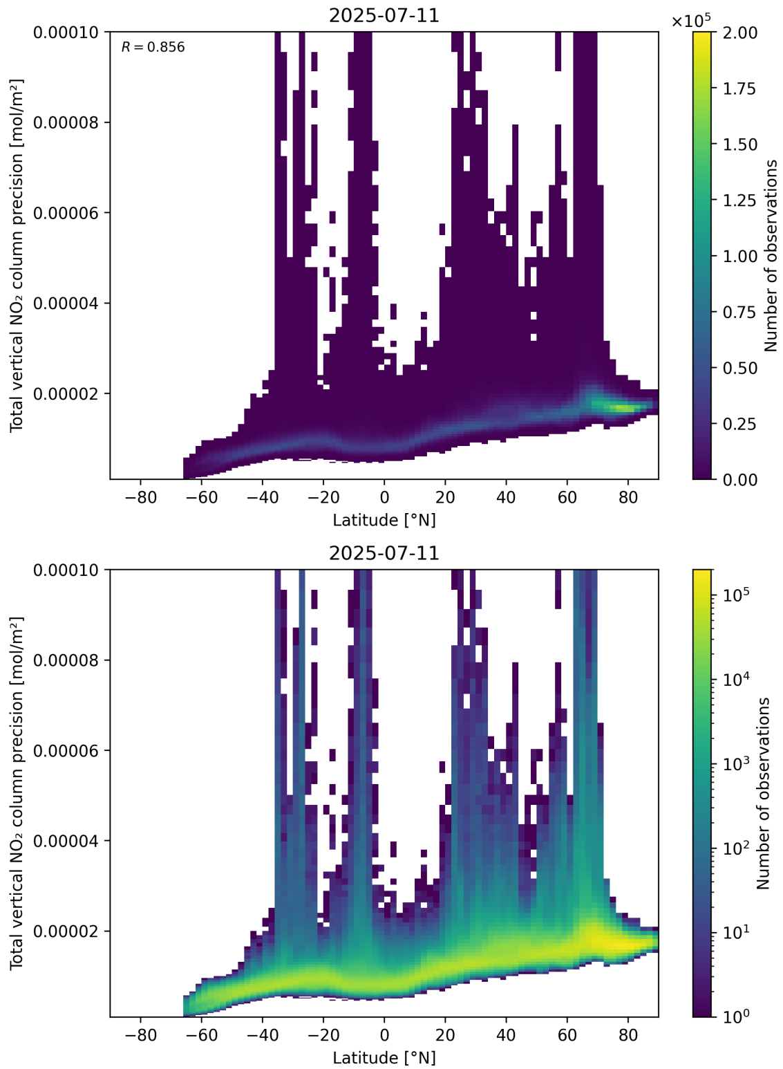
Figure 91: Scatter density plot of “Latitude” against “Total vertical NO 2 column precision” for 2025-07-10 to 2025-07-12.
