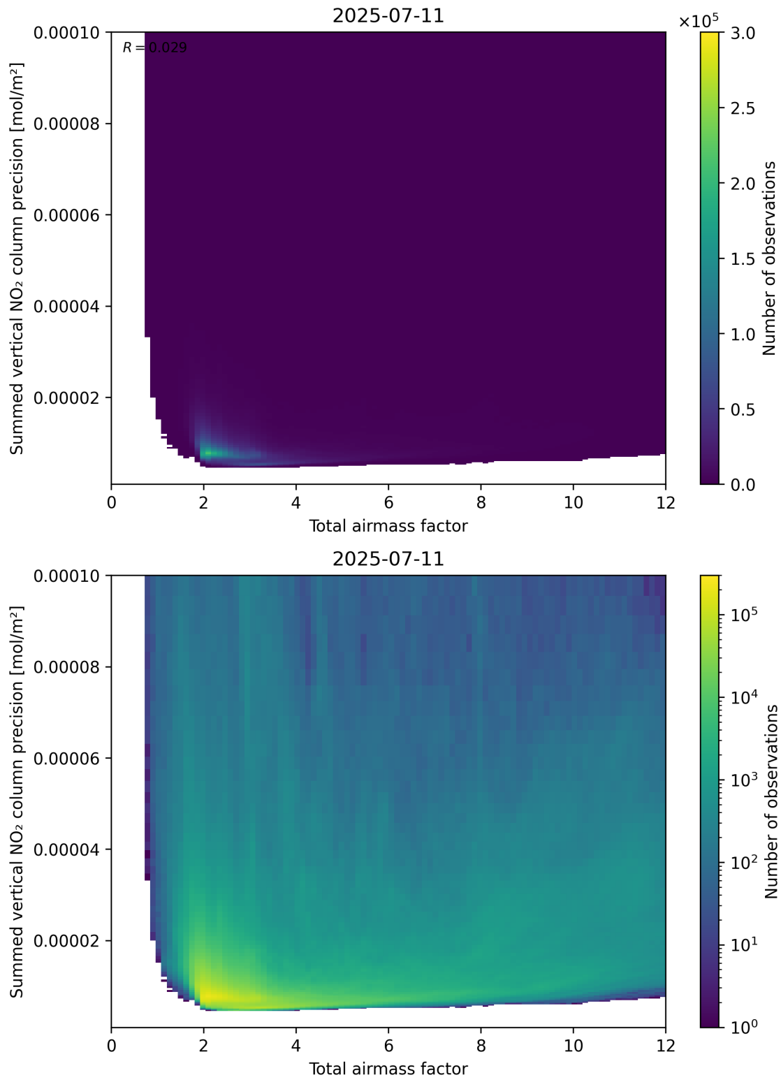
Figure 66: Scatter density plot of “Total airmass factor” against “Summed vertical NO 2 column precision” for 2025-07-10 to 2025-07-12.
