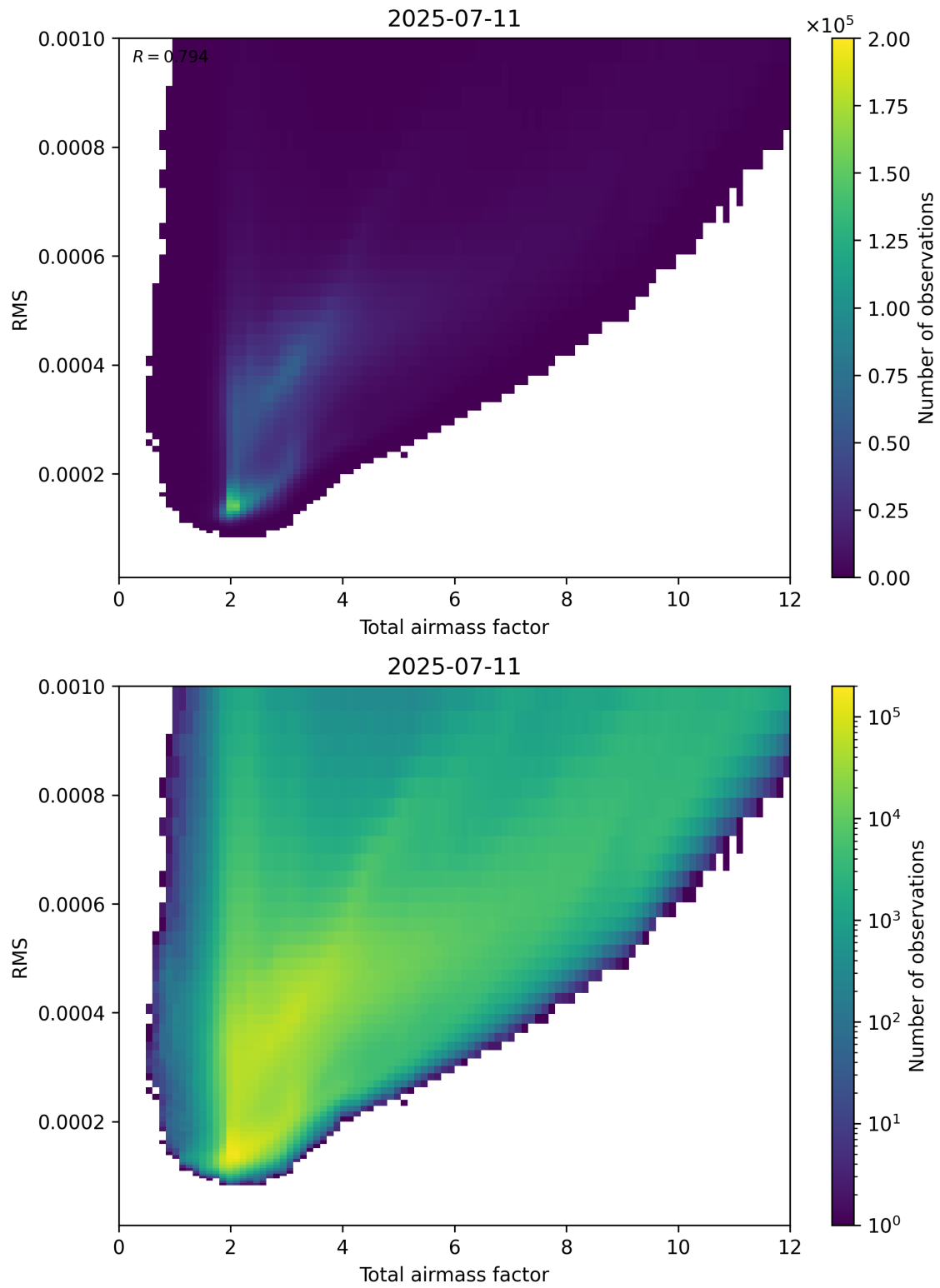
Figure 69: Scatter density plot of “Total airmass factor” against “RMS” for 2025-07-10 to 2025-07-12.
