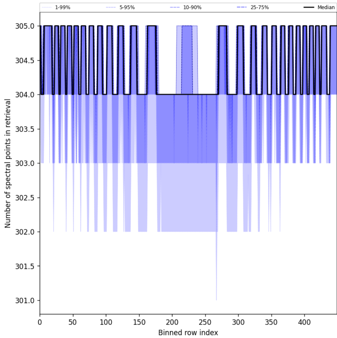
Figure 50: Along track statistics of “Number of spectral points in retrieval” for 2025-07-10 to 2025-07-12
