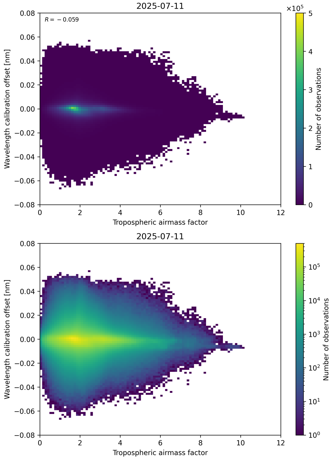
Figure 80: Scatter density plot of “Tropospheric airmass factor” against “Wavelength calibration offset” for 2025-07-10 to 2025-07-12.
