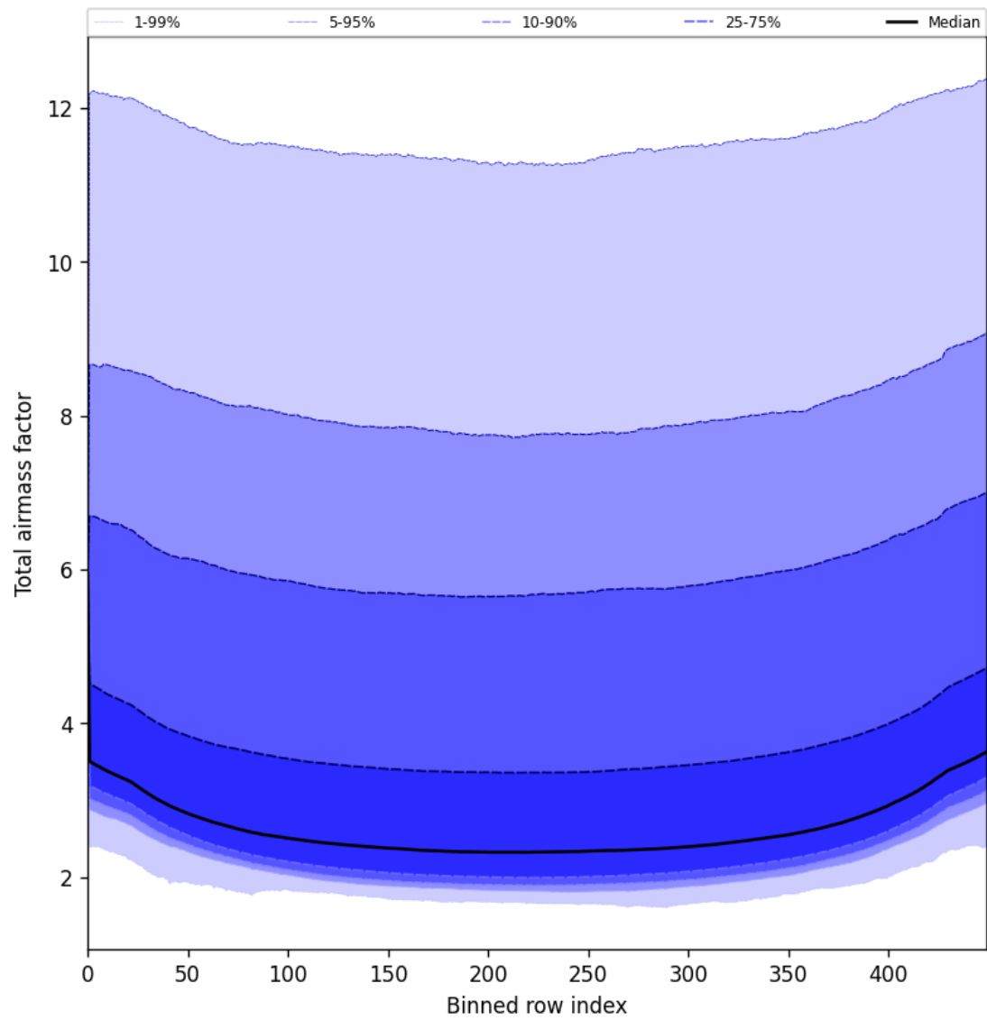
Figure 49: Along track statistics of “Total airmass factor” for 2025-07-10 to 2025-07-12
