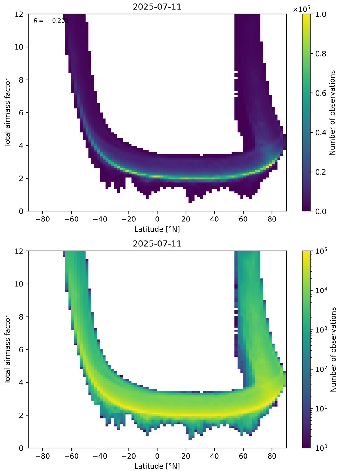
Figure 84: Scatter density plot of “Latitude” against “Total airmass factor” for 2025-07-10 to 2025-07-12.
