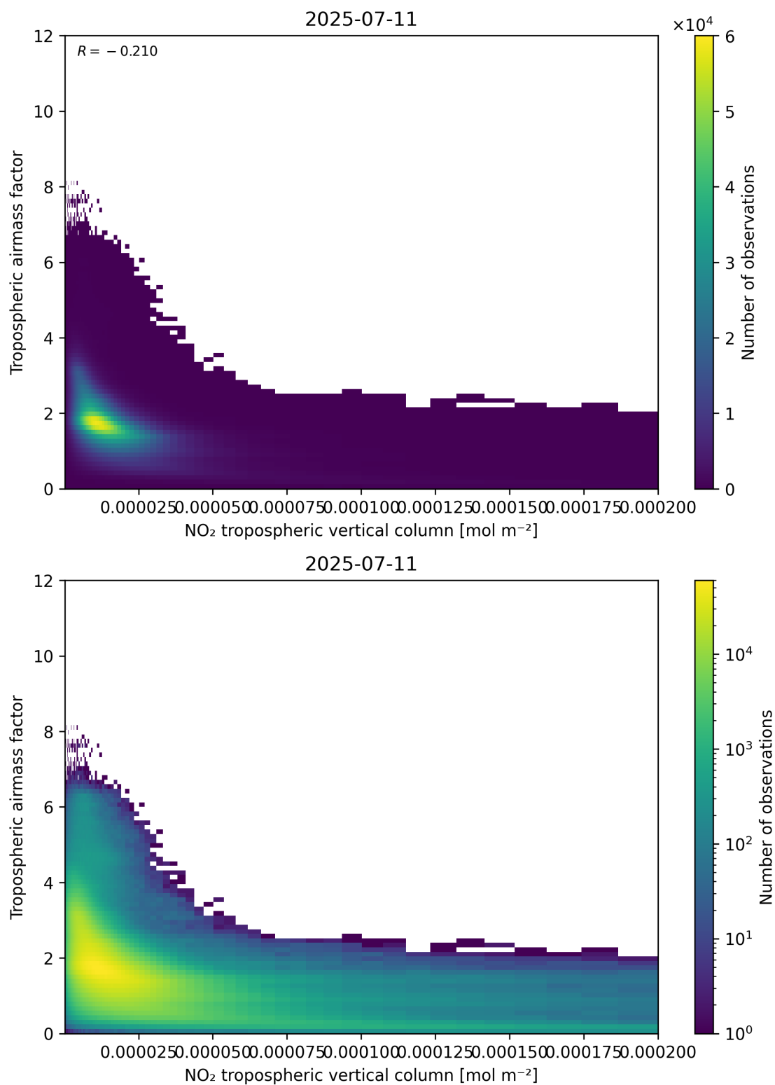
Figure 123: Scatter density plot of “NO 2 tropospheric vertical column” against “Tropospheric air mass factor” for 2025-07-10 to 2025-07-12.
