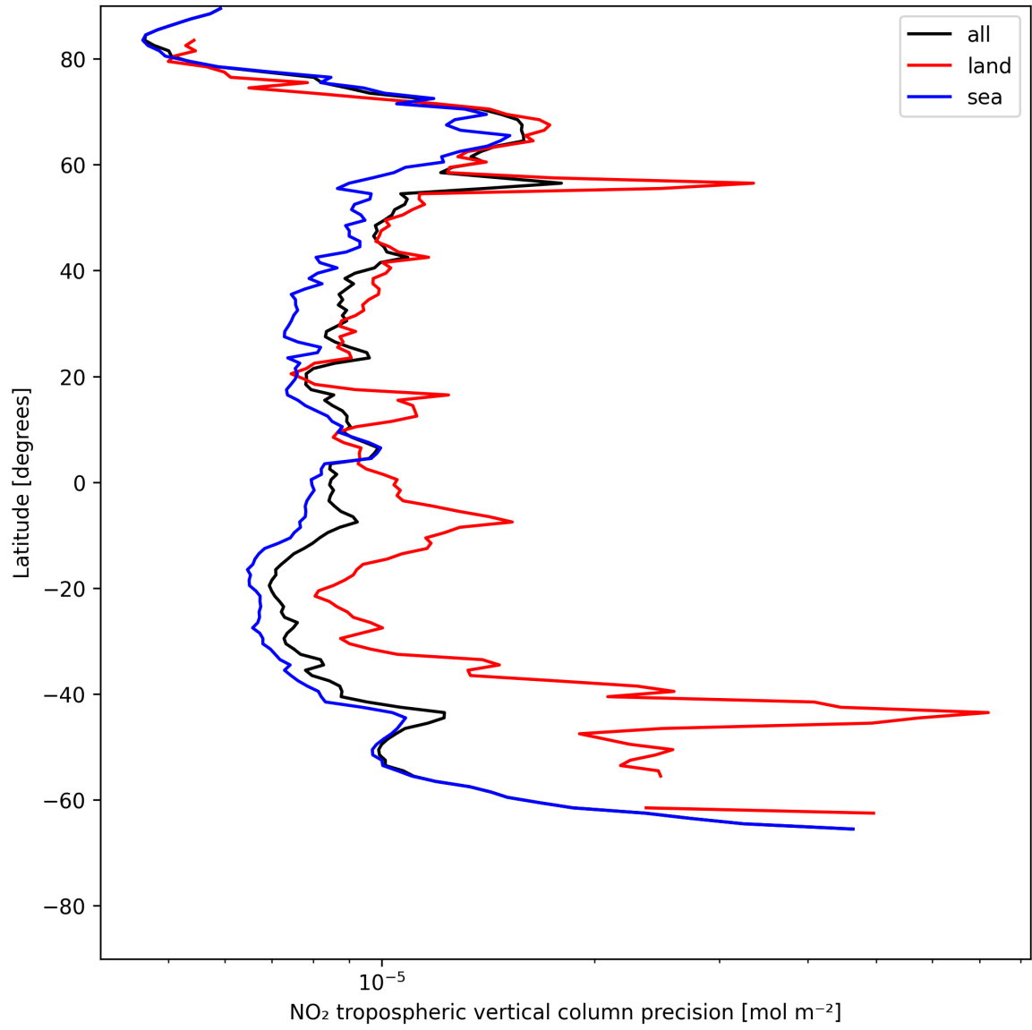
Figure 13: Zonal average of "NO 2 tropospheric vertical column precision" for 2025-07-10 to 2025-07-12.
