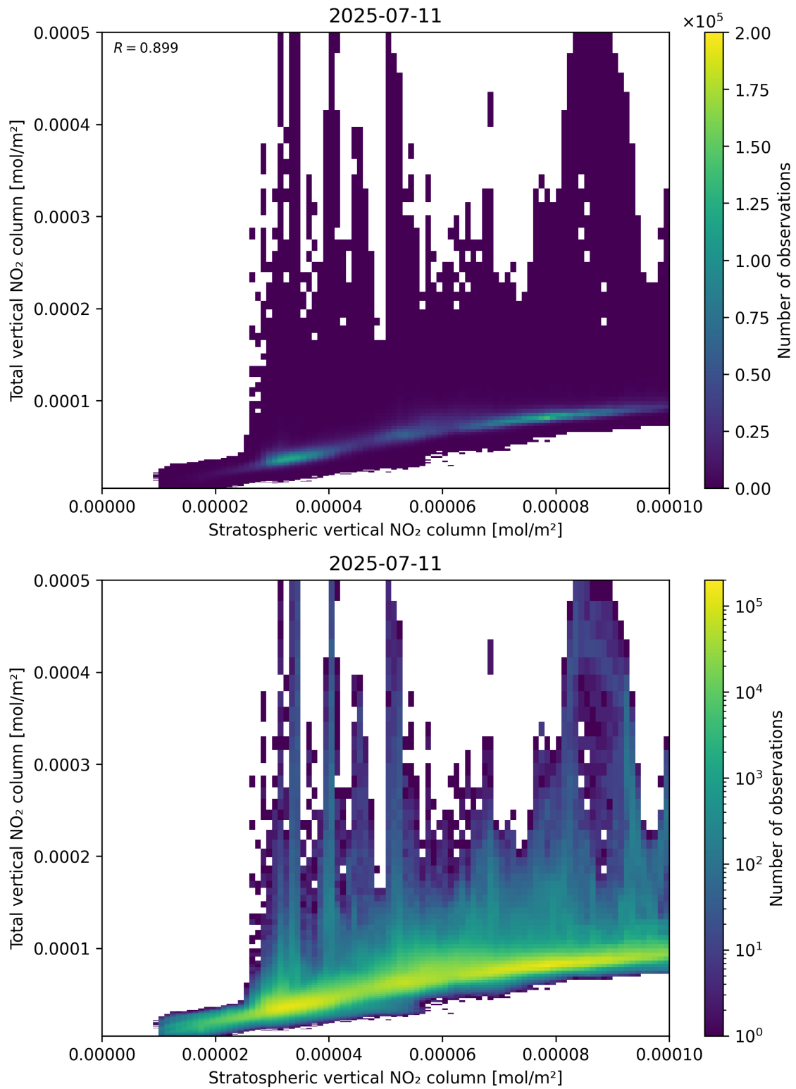
Figure 100: Scatter density plot of “Stratospheric vertical NO 2 column” against “Total vertical NO 2 column” for 2025-07-10 to 2025-07-12.
