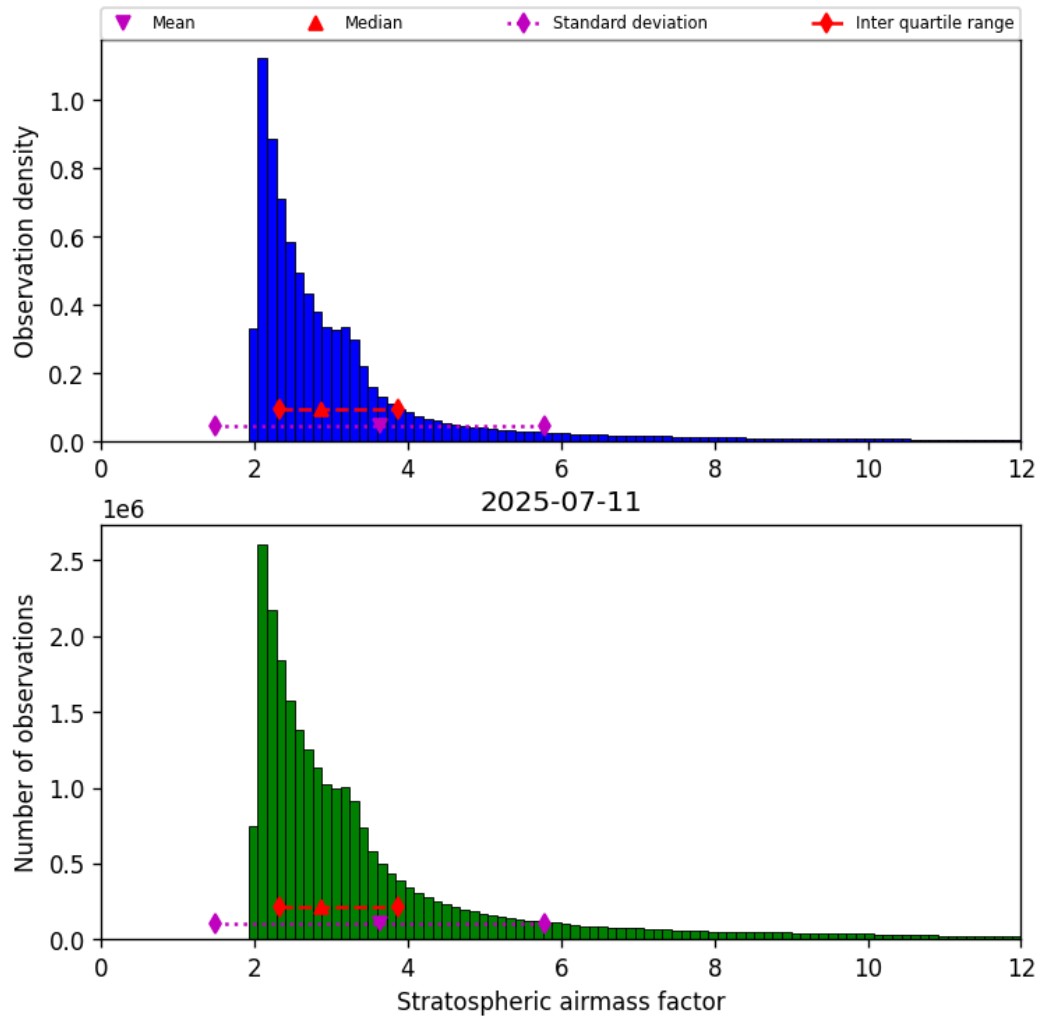
Figure 44: Histogram of “Stratospheric airmass factor” for 2025-07-10 to 2025-07-12
