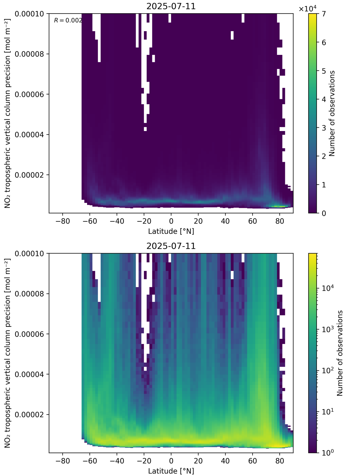
Figure 93: Scatter density plot of “Latitude” against “NO 2 tropospheric vertical column precision” for 2025-07-10 to 2025-07-12.
