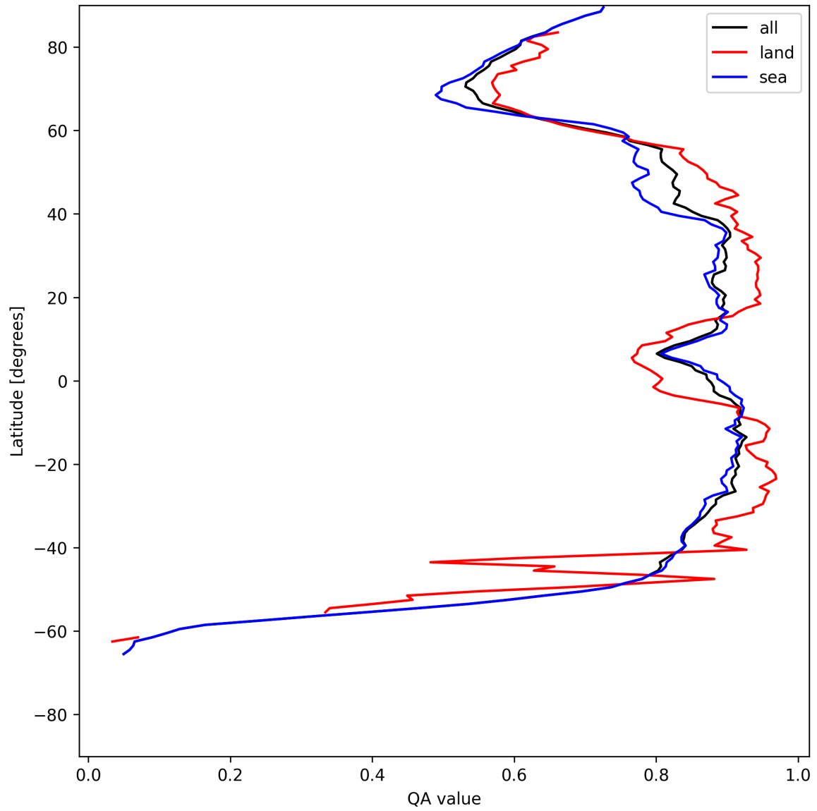
Figure 11: Zonal average of “QA value” for 2025-07-10 to 2025-07-12.
