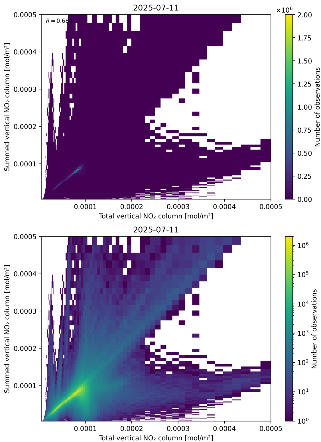
Figure 112: Scatter density plot of “Total vertical NO 2 column” against “Summed vertical NO 2 column” for 2025-07-10 to 2025-07-12.
