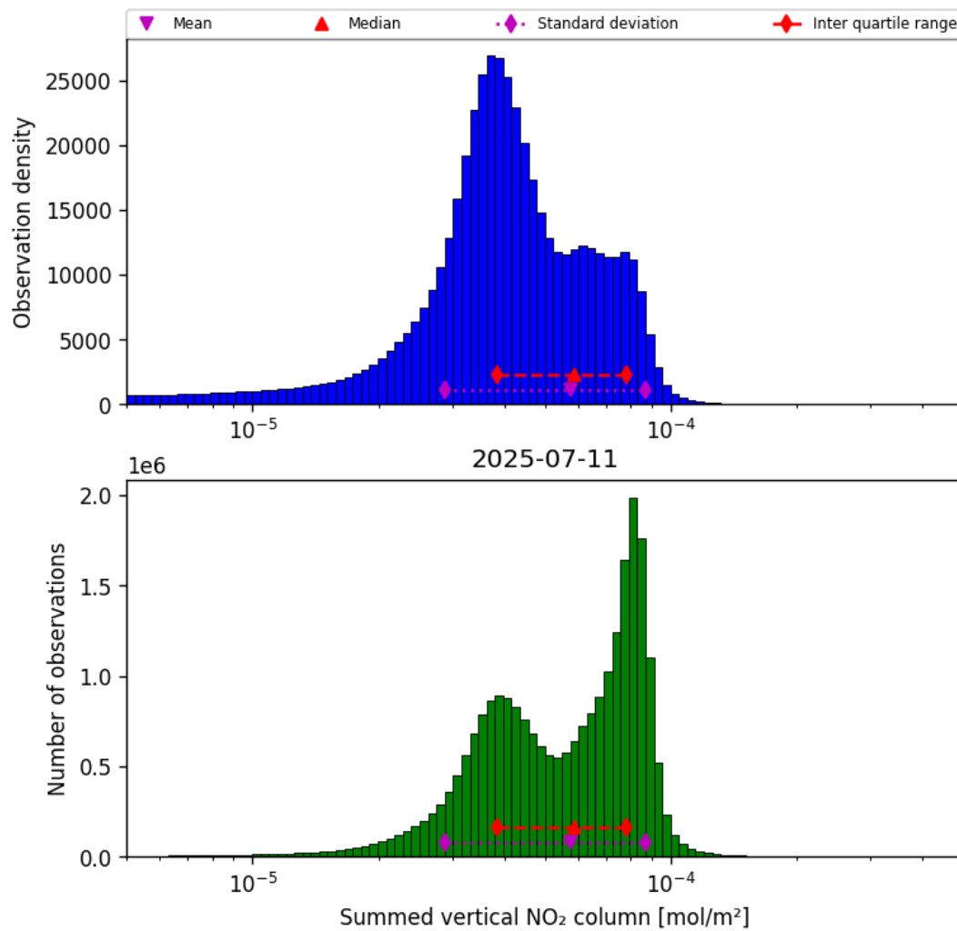
Figure 40: Histogram of “Summed vertical NO 2 column” for 2025-07-10 to 2025-07-12
