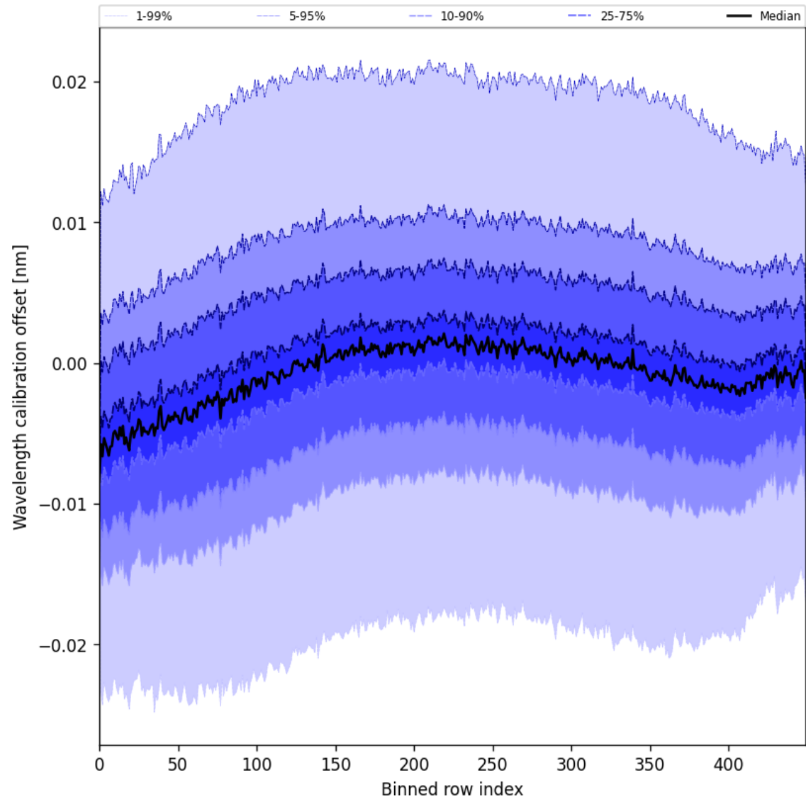
Figure 52: Along track statistics of “Wavelength calibration offset” for 2025-07-10 to 2025-07-12
