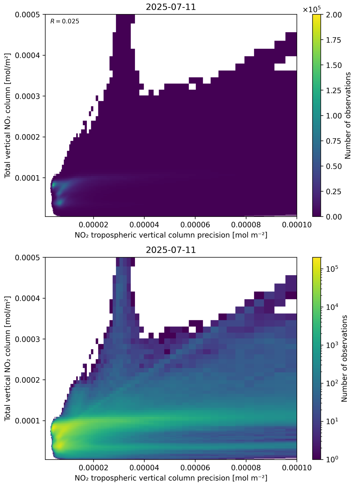
Figure 138: Scatter density plot of “NO 2 tropospheric vertical column precision” against “Total vertical NO 2 column” for 2025-07-10 to 2025-07-12.
