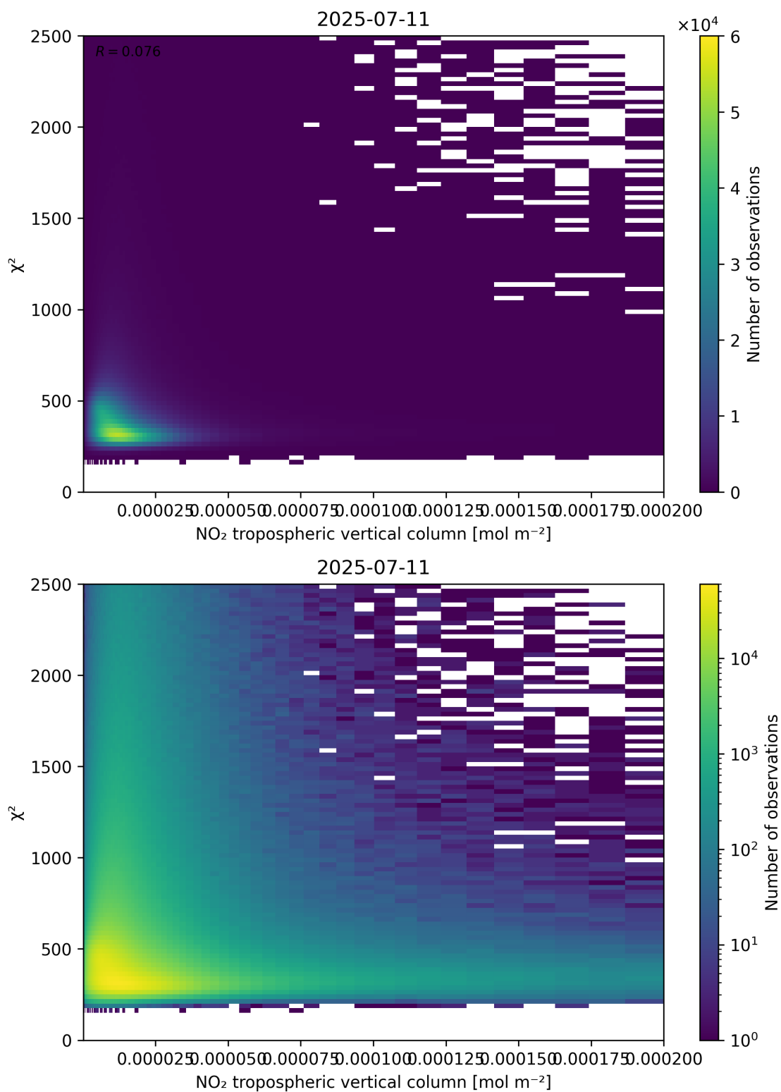
Figure 124: Scatter density plot of “NO 2 tropospheric vertical column” against “ \chi^2 ” for 2025-07-10 to 2025-07-12.
