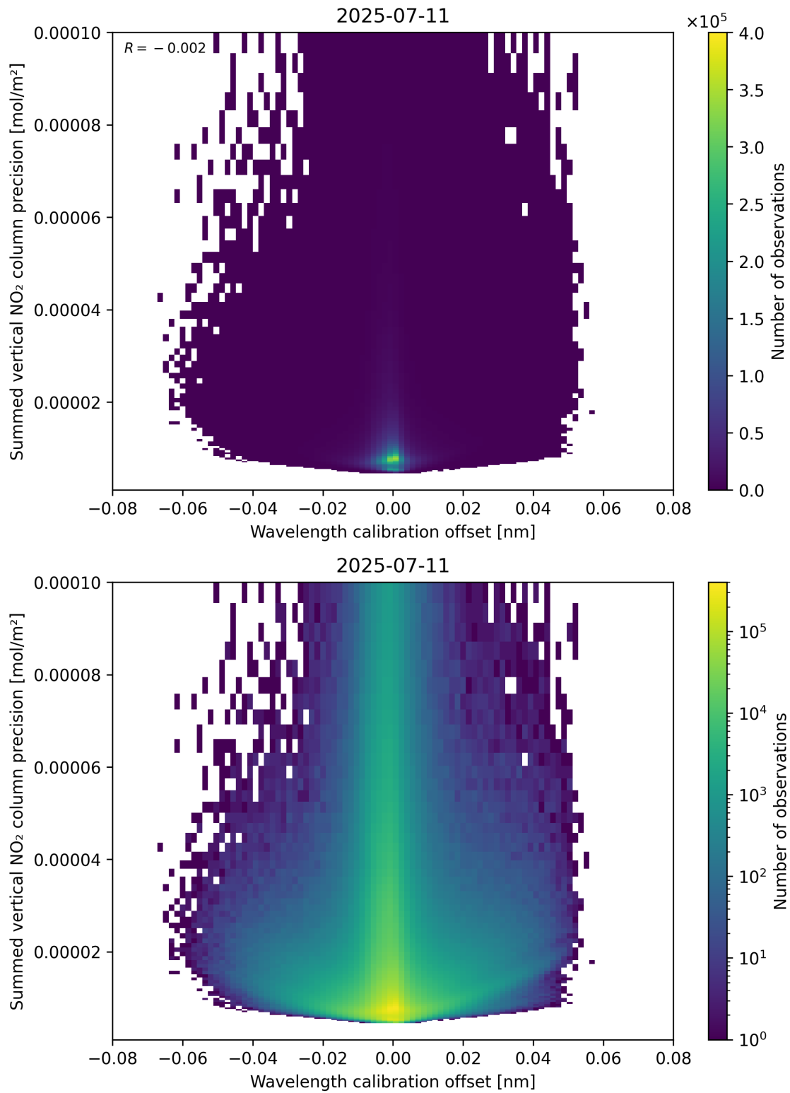
Figure 178: Scatter density plot of “Wavelength calibration offset” against “Summed vertical NO 2 column precision” for 2025-07-10 to 2025-07-12.
