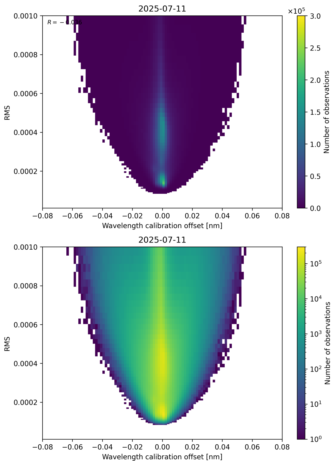
Figure 181: Scatter density plot of “Wavelength calibration offset” against “RMS” for 2025-07-10 to 2025-07-12.
