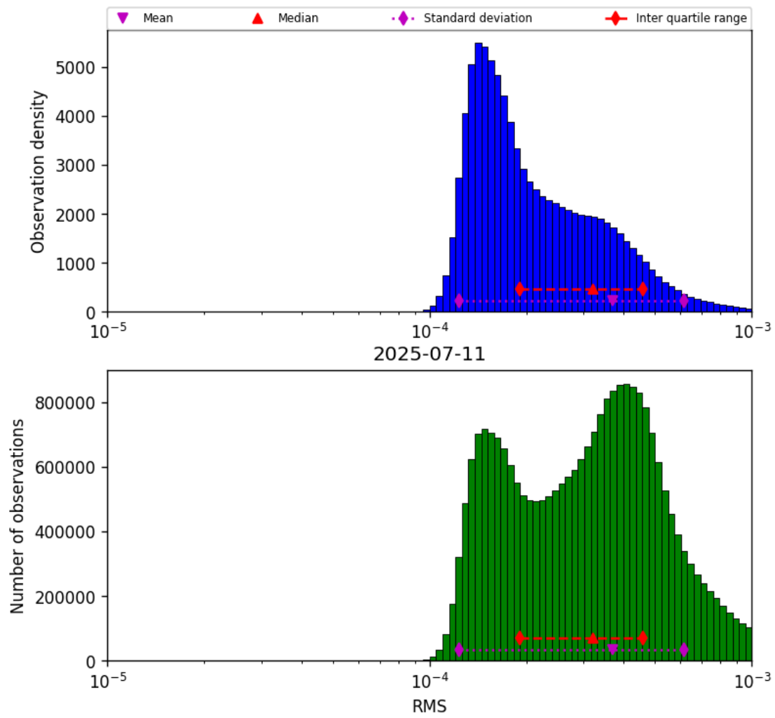
Figure 43: Histogram of “RMS” for 2025-07-10 to 2025-07-12
