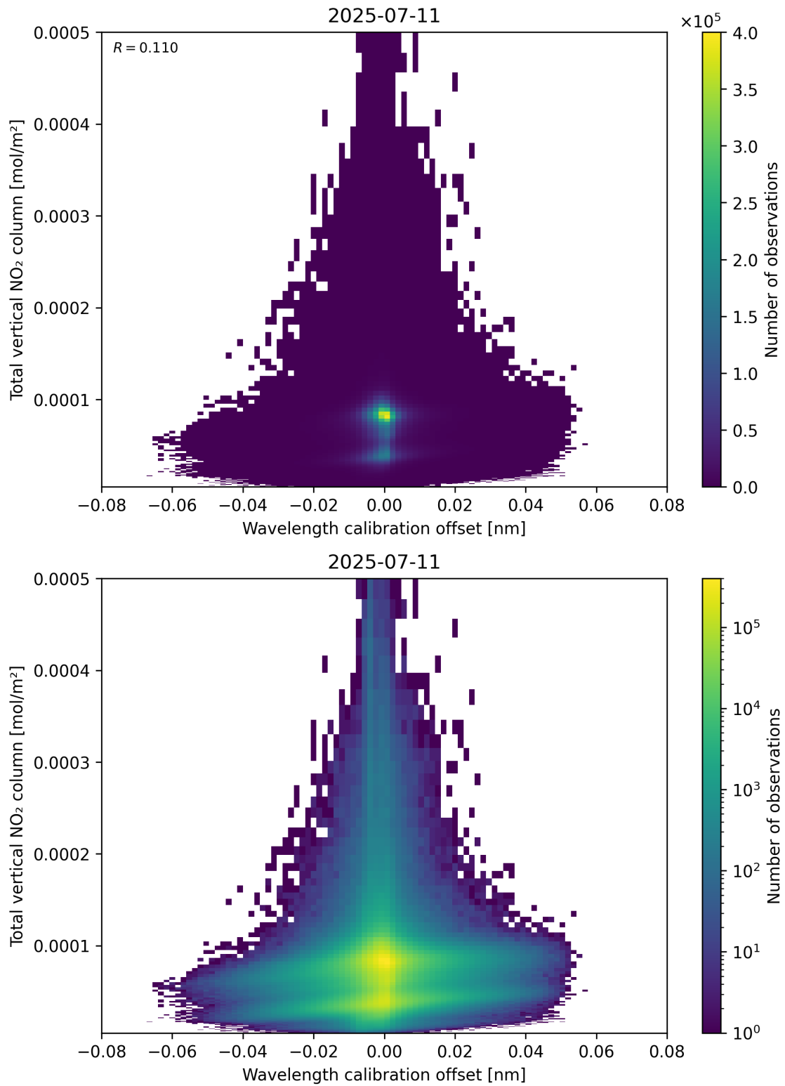
Figure 179: Scatter density plot of “Wavelength calibration offset” against “Total vertical NO 2 column” for 2025-07-10 to 2025-07-12.
