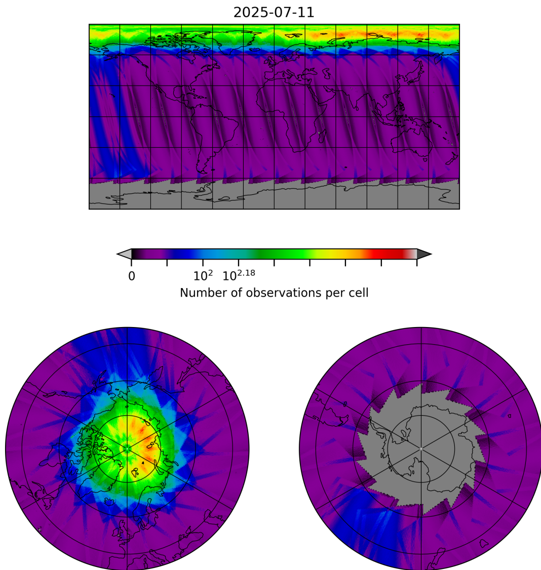
Figure 10: Map of the number of observations for 2025-07-10 to 2025-07-12
