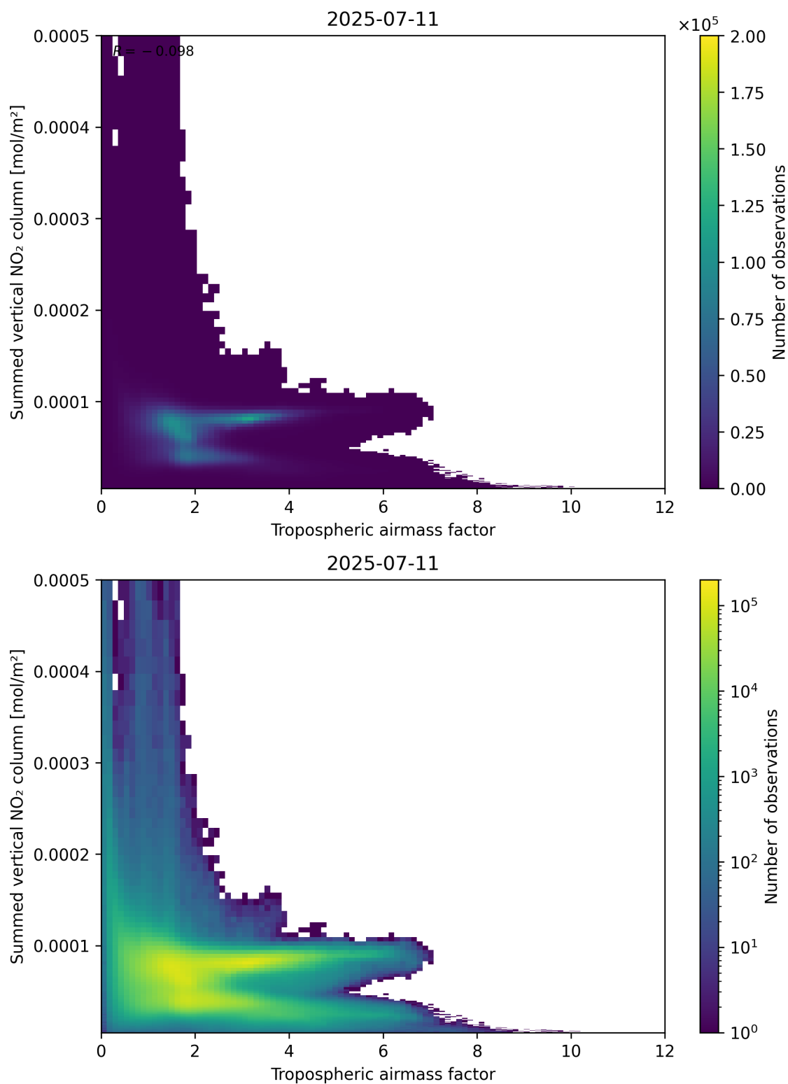
Figure 75: Scatter density plot of “Tropospheric air mass factor” against “Summed vertical NO 2 column” for 2025-07-10 to 2025-07-12.
