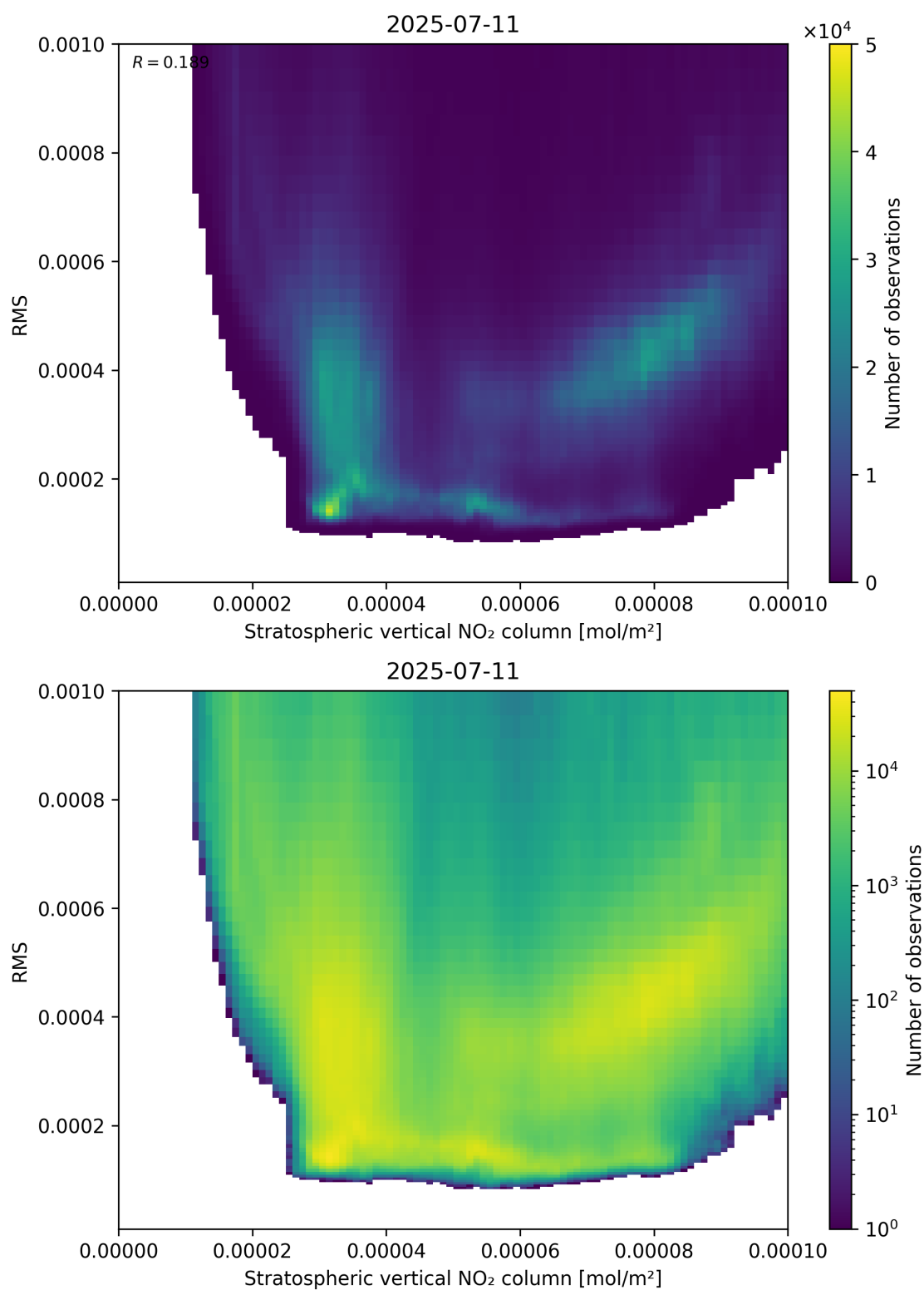
Figure 102: Scatter density plot of “Stratospheric vertical NO 2 column” against “RMS” for 2025-07-10 to 2025-07-12.
