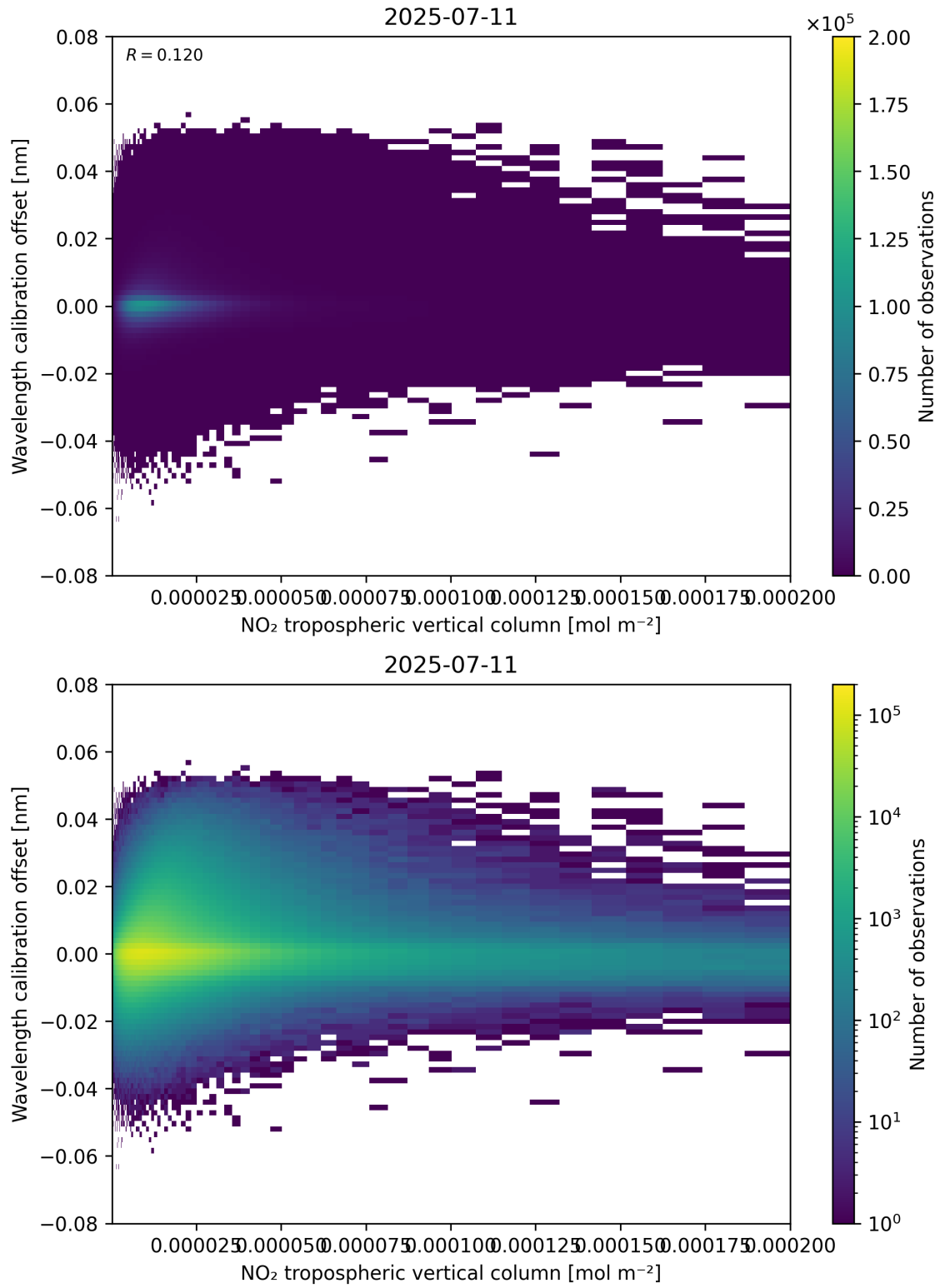
Figure 143: Scatter density plot of “NO 2 tropospheric vertical column” against “Wavelength calibration offset” for 2025-07-10 to 2025-07-12.
