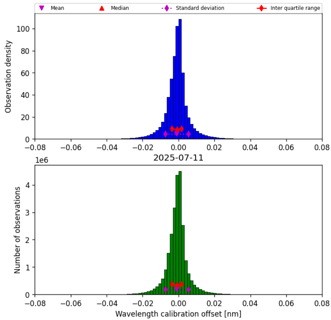
Figure 35: Histogram of “Wavelength calibration offset” for 2025-07-10 to 2025-07-12
