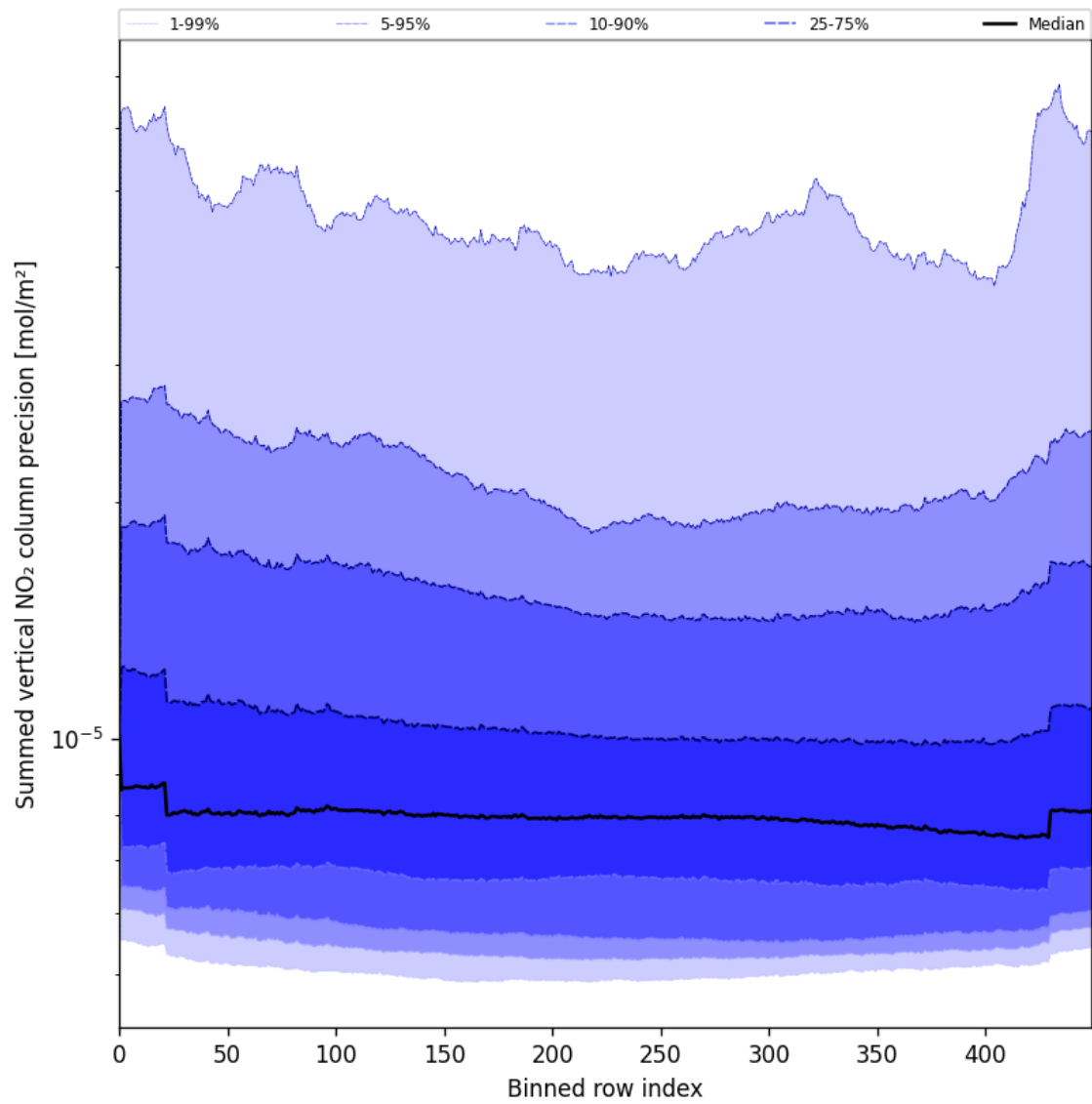
Figure 58: Along track statistics of “Summed vertical NO 2 column precision” for 2025-07-10 to 2025-07-12
