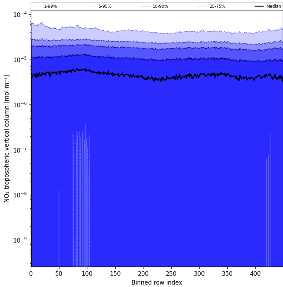
Figure 46: Along track statistics of “NO 2 tropospheric vertical column” for 2025-07-10 to 2025-07-12
