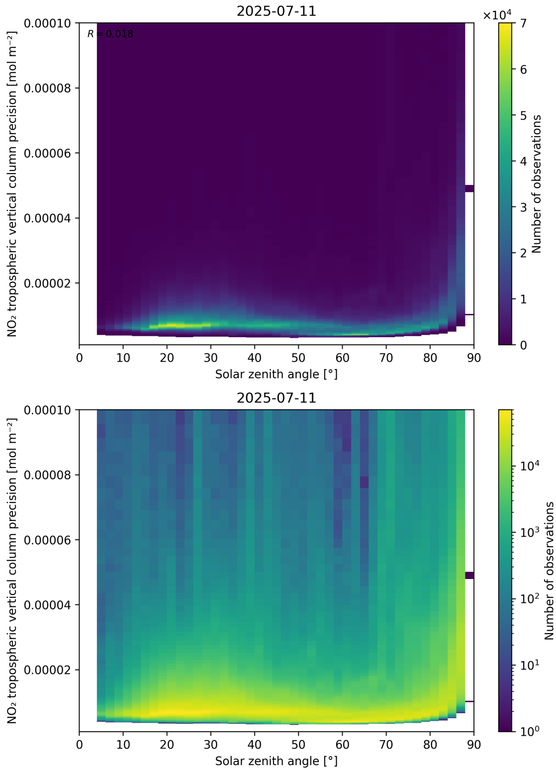
Figure 156: Scatter density plot of “Solar zenith angle” against “NO 2 tropospheric vertical column precision” for 2025-07-10 to 2025-07-12.
