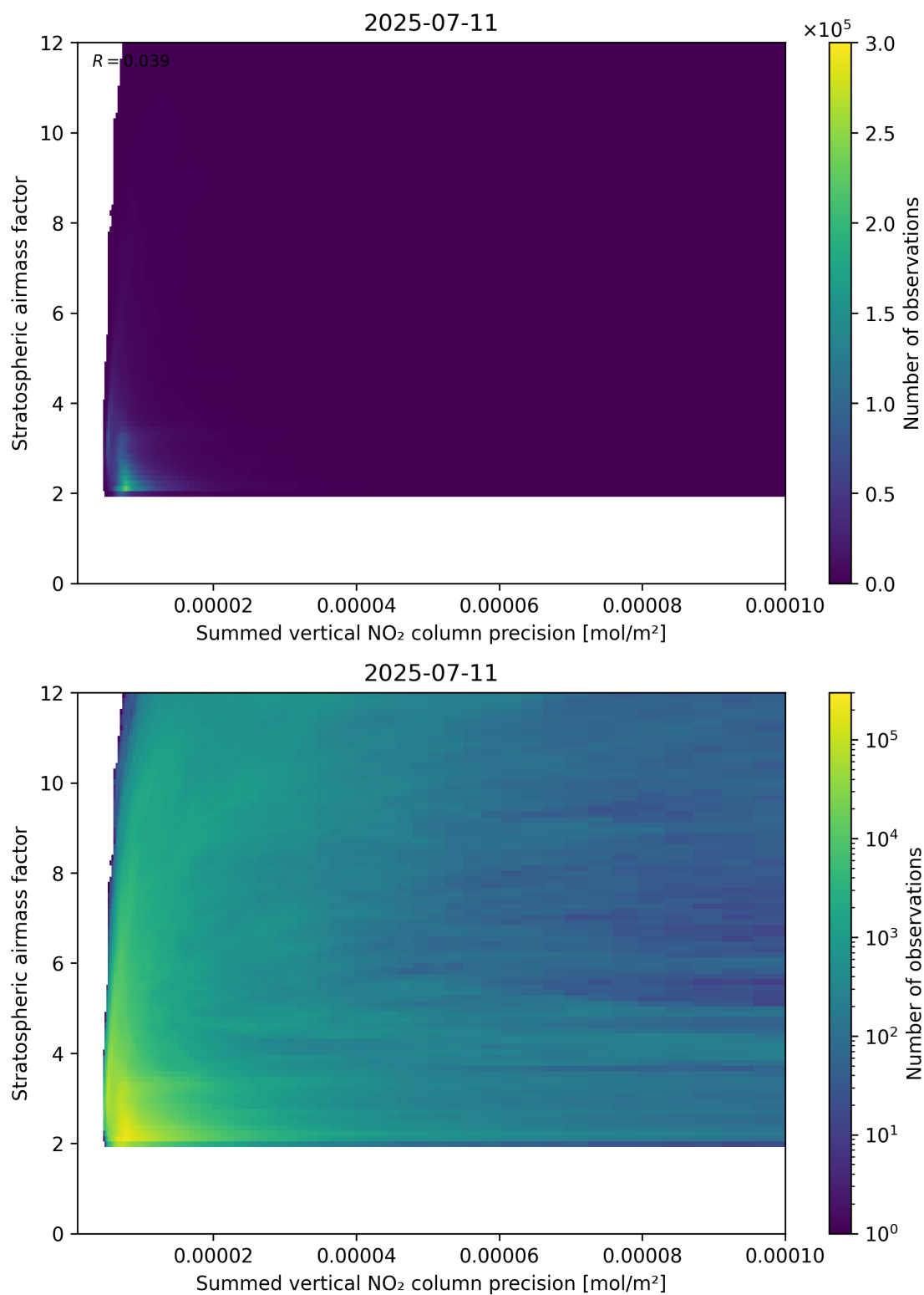
Figure 106: Scatter density plot of “Summed vertical NO 2 column precision” against “Stratospheric airmass factor” for 2025-07-10 to 2025-07-12.
