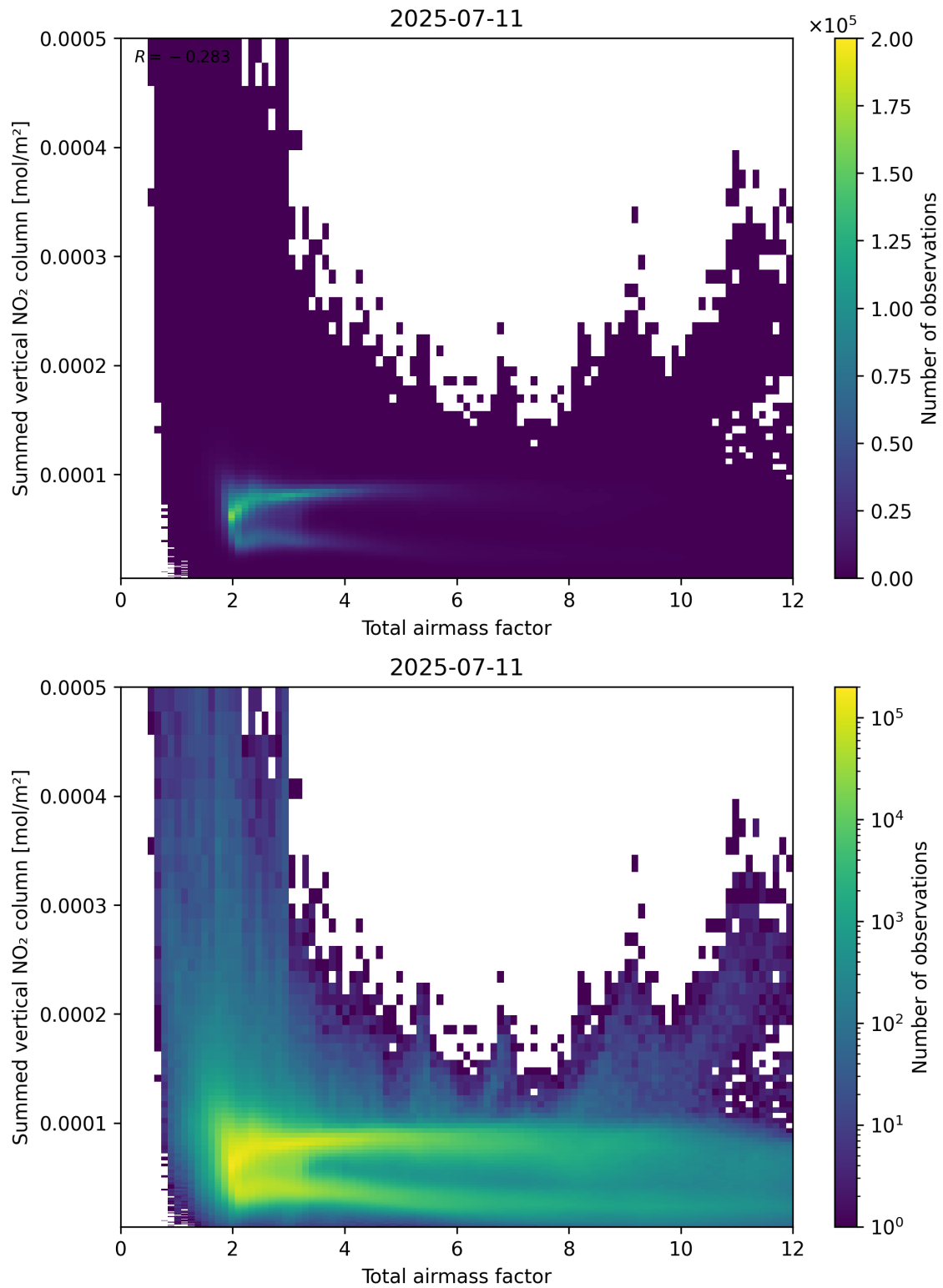
Figure 65: Scatter density plot of “Total airmass factor” against “Summed vertical NO 2 column” for 2025-07-10 to 2025-07-12.
