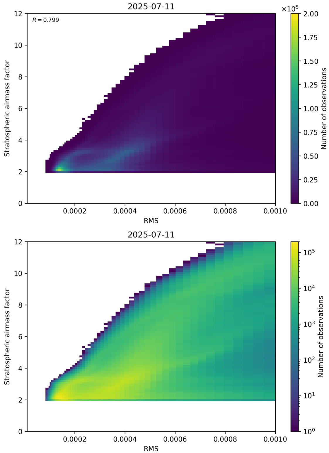
Figure 144: Scatter density plot of “RMS” against “Stratospheric airmass factor” for 2025-07-10 to 2025-07-12.
