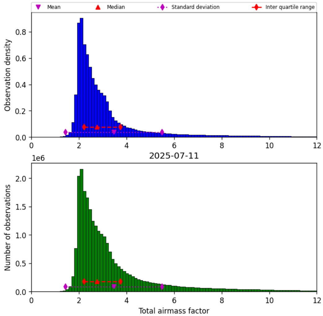
Figure 32: Histogram of “Total airmass factor” for 2025-07-10 to 2025-07-12
