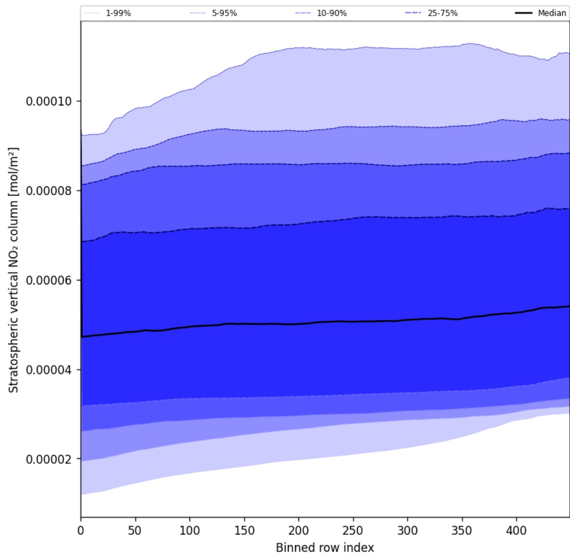
Figure 53: Along track statistics of “Stratospheric vertical NO 2 column” for 2025-07-10 to 2025-07-12
