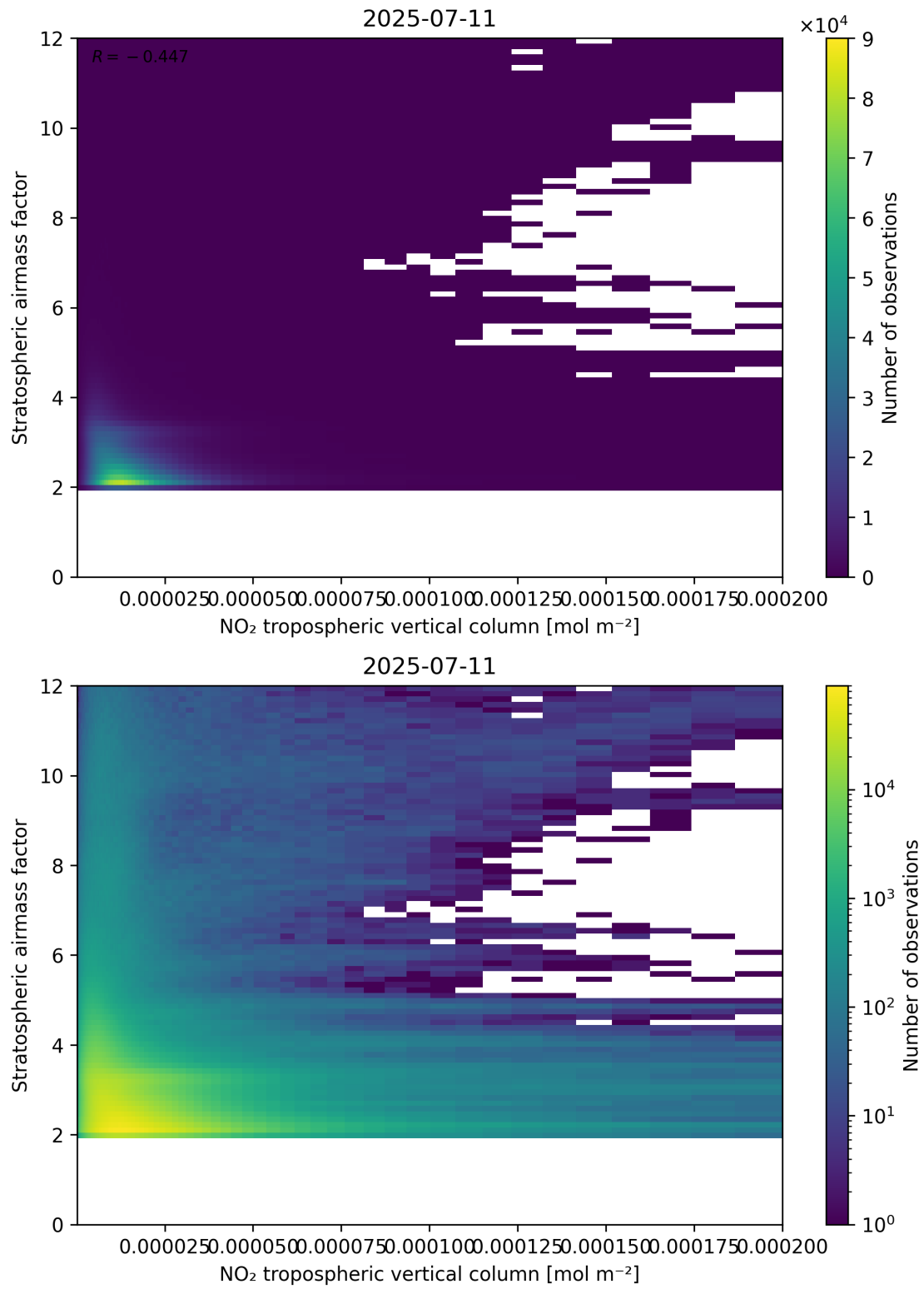
Figure 121: Scatter density plot of “NO 2 tropospheric vertical column” against “Stratospheric air mass factor” for 2025-07-10 to 2025-07-12.
