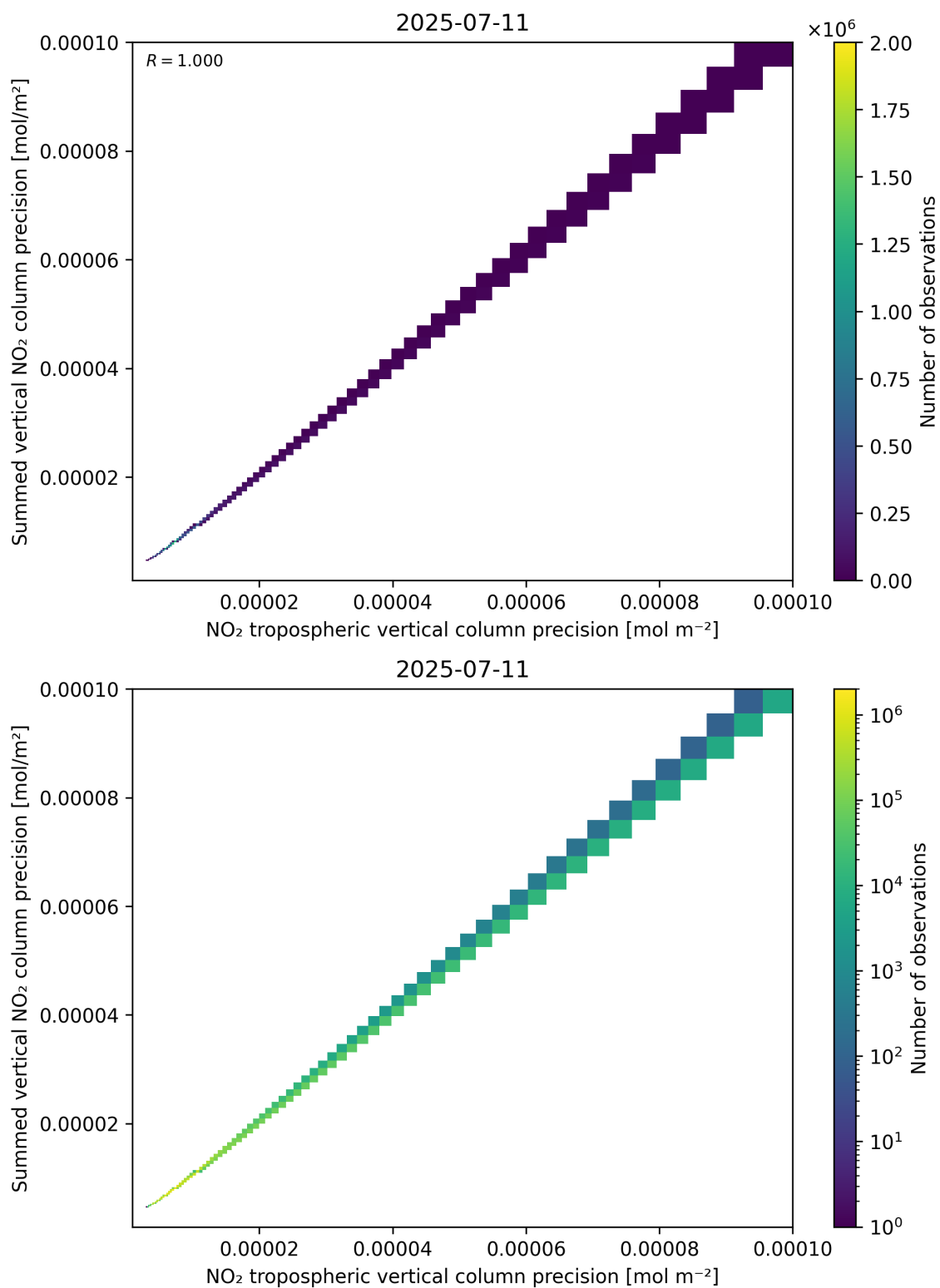
Figure 137: Scatter density plot of “NO 2 tropospheric vertical column precision” against “Summed vertical NO 2 column precision” for 2025-07-10 to 2025-07-12.
