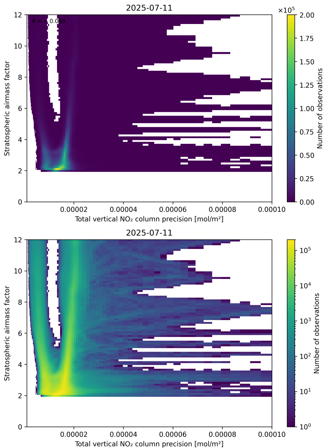
Figure 115: Scatter density plot of “Total vertical NO 2 column precision” against “Stratospheric air mass factor” for 2025-07-10 to 2025-07-12.
