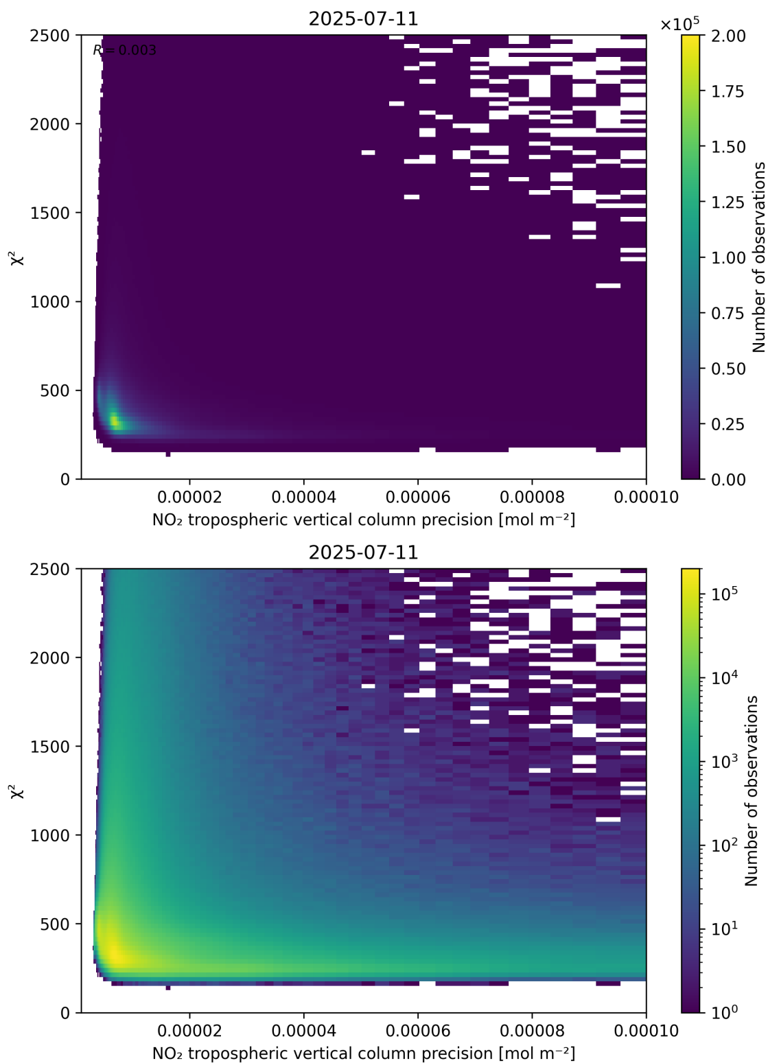
Figure 134: Scatter density plot of “NO 2 tropospheric vertical column precision” against “ \chi^2 ” for 2025-07-10 to 2025-07-12.
