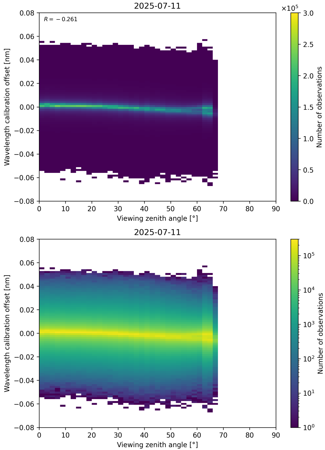
Figure 173: Scatter density plot of “Viewing zenith angle” against “Wavelength calibration offset” for 2025-07-10 to 2025-07-12.
