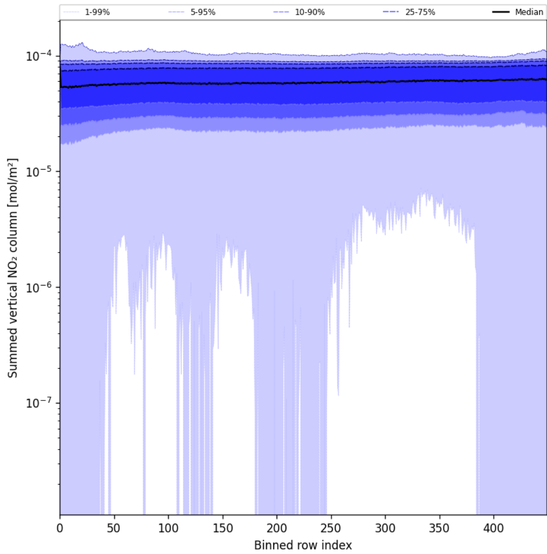
Figure 57: Along track statistics of “Summed vertical NO 2 column” for 2025-07-10 to 2025-07-12
