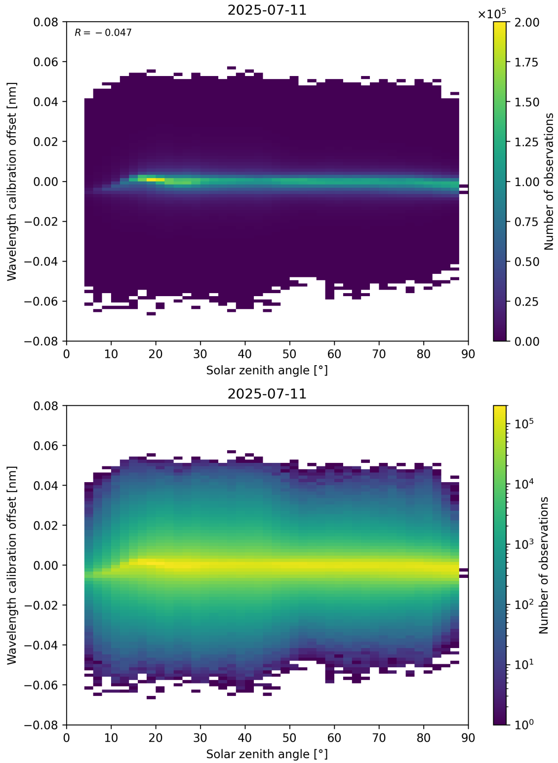
Figure 158: Scatter density plot of “Solar zenith angle” against “Wavelength calibration offset” for 2025-07-10 to 2025-07-12.
