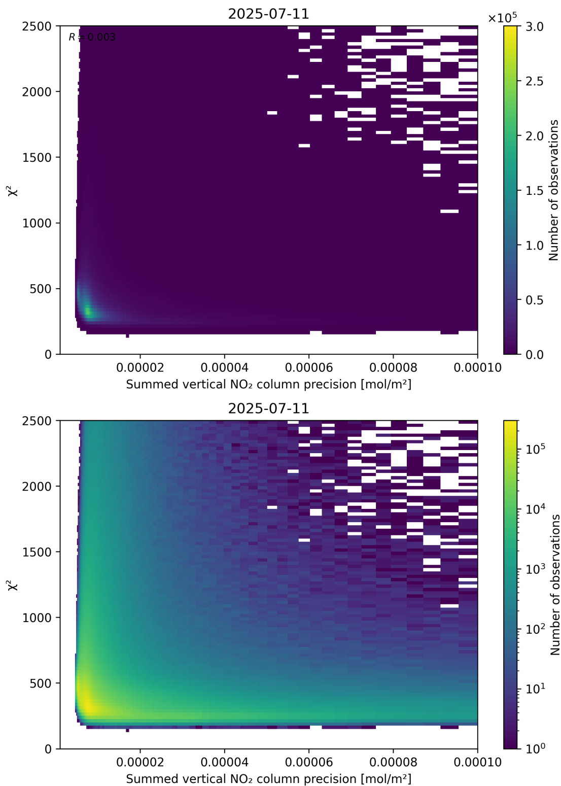
Figure 107: Scatter density plot of “Summed vertical NO 2 column precision” against “ \chi^2 ” for 2025-07-10 to 2025-07-12.
