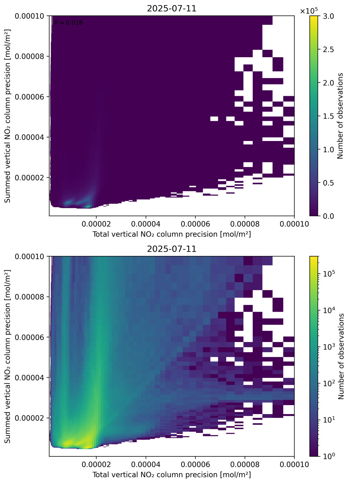
Figure 118: Scatter density plot of “Total vertical NO 2 column precision” against “Summed vertical NO 2 column precision” for 2025-07-10 to 2025-07-12.
