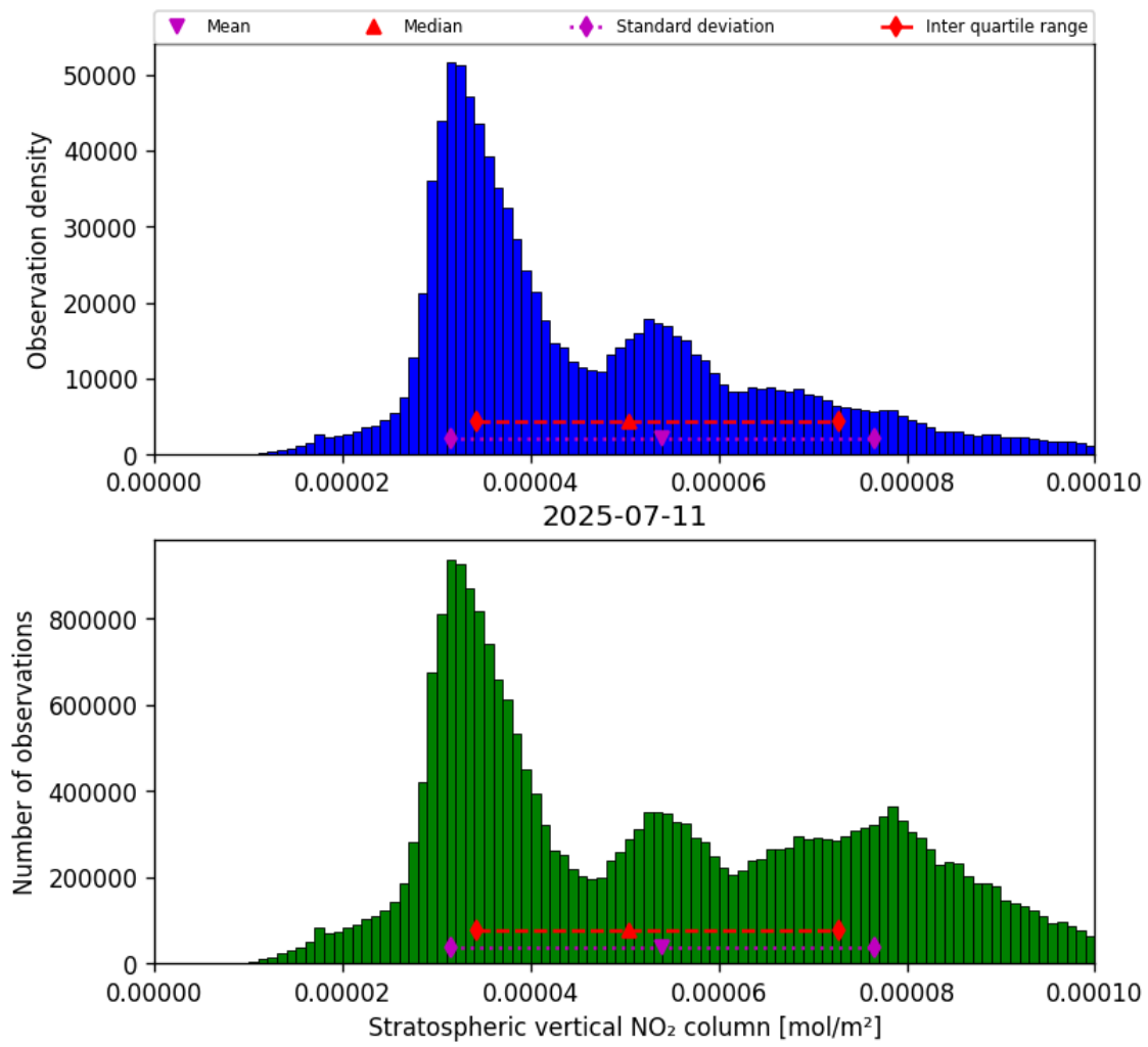
Figure 36: Histogram of “Stratospheric vertical NO 2 column” for 2025-07-10 to 2025-07-12
