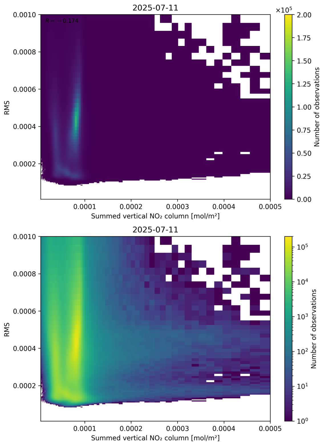
Figure 109: Scatter density plot of “Summed vertical NO 2 column” against “RMS” for 2025-07-10 to 2025-07-12.
