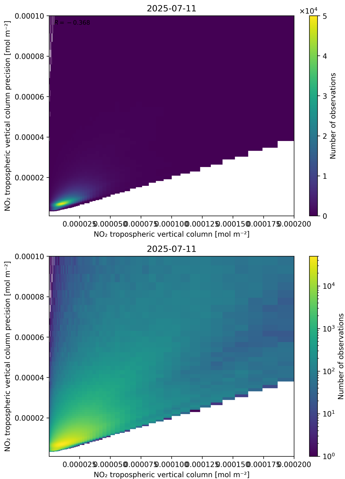
Figure 130: Scatter density plot of “NO 2 tropospheric vertical column” against “NO 2 tropospheric vertical column precision” for 2025-07-10 to 2025-07-12.
