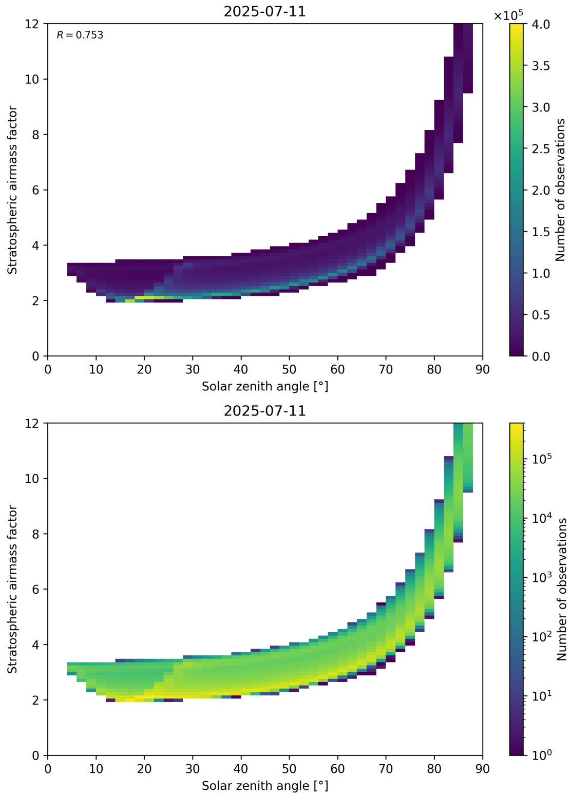
Figure 145: Scatter density plot of “Solar zenith angle” against “Stratospheric airmass factor” for 2025-07-10 to 2025-07-12.
