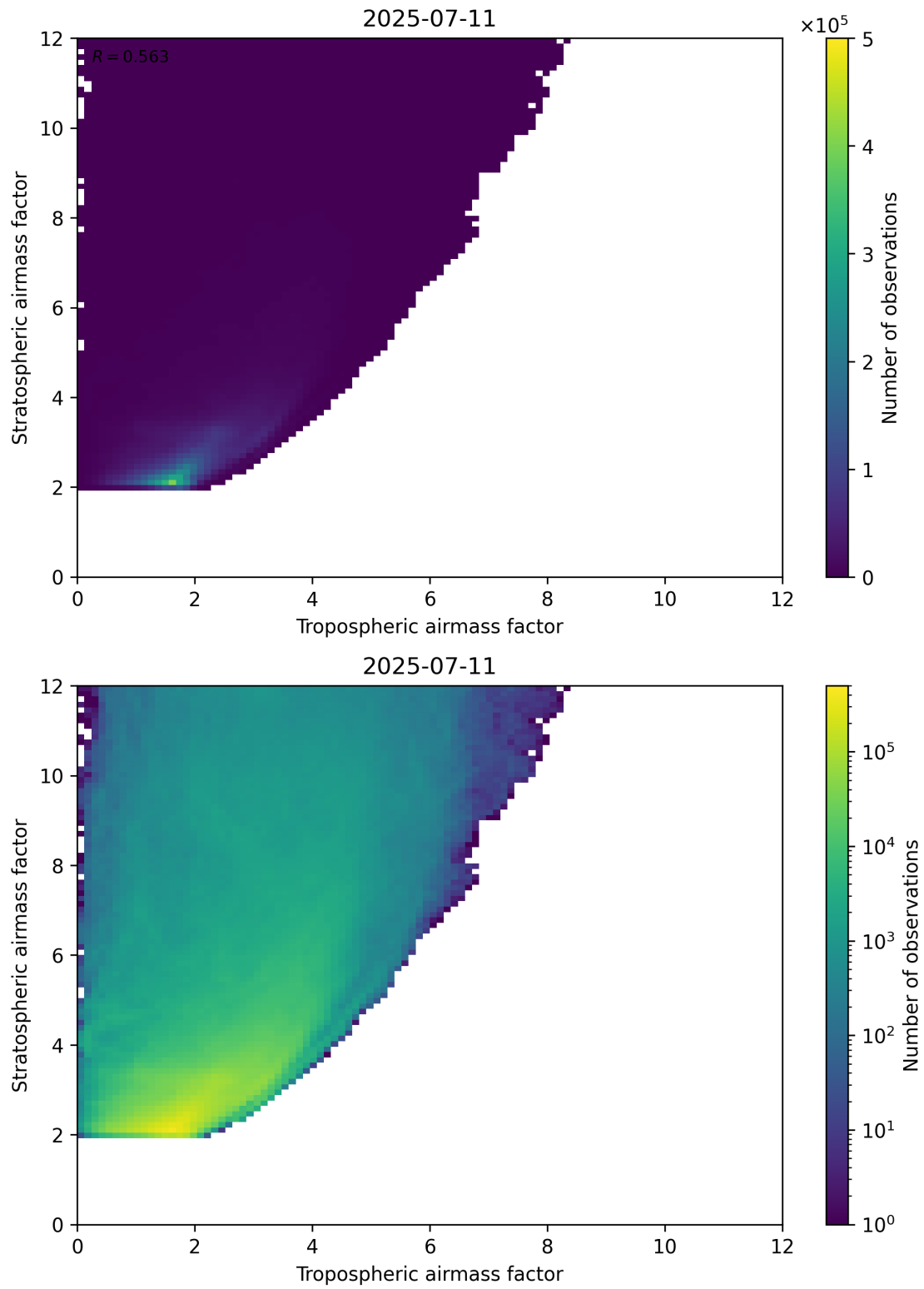
Figure 71: Scatter density plot of “Tropospheric airmass factor” against “Stratospheric airmass factor” for 2025-07-10 to 2025-07-12.
