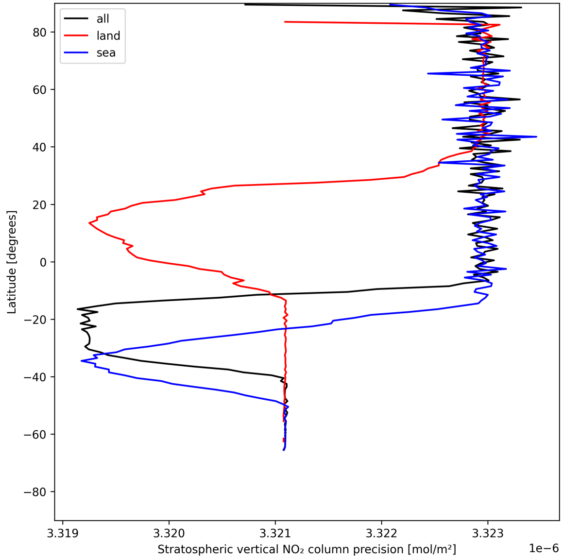
Figure 20: Zonal average of “Stratospheric vertical NO 2 column precision” for 2025-07-10 to 2025-07-12.
