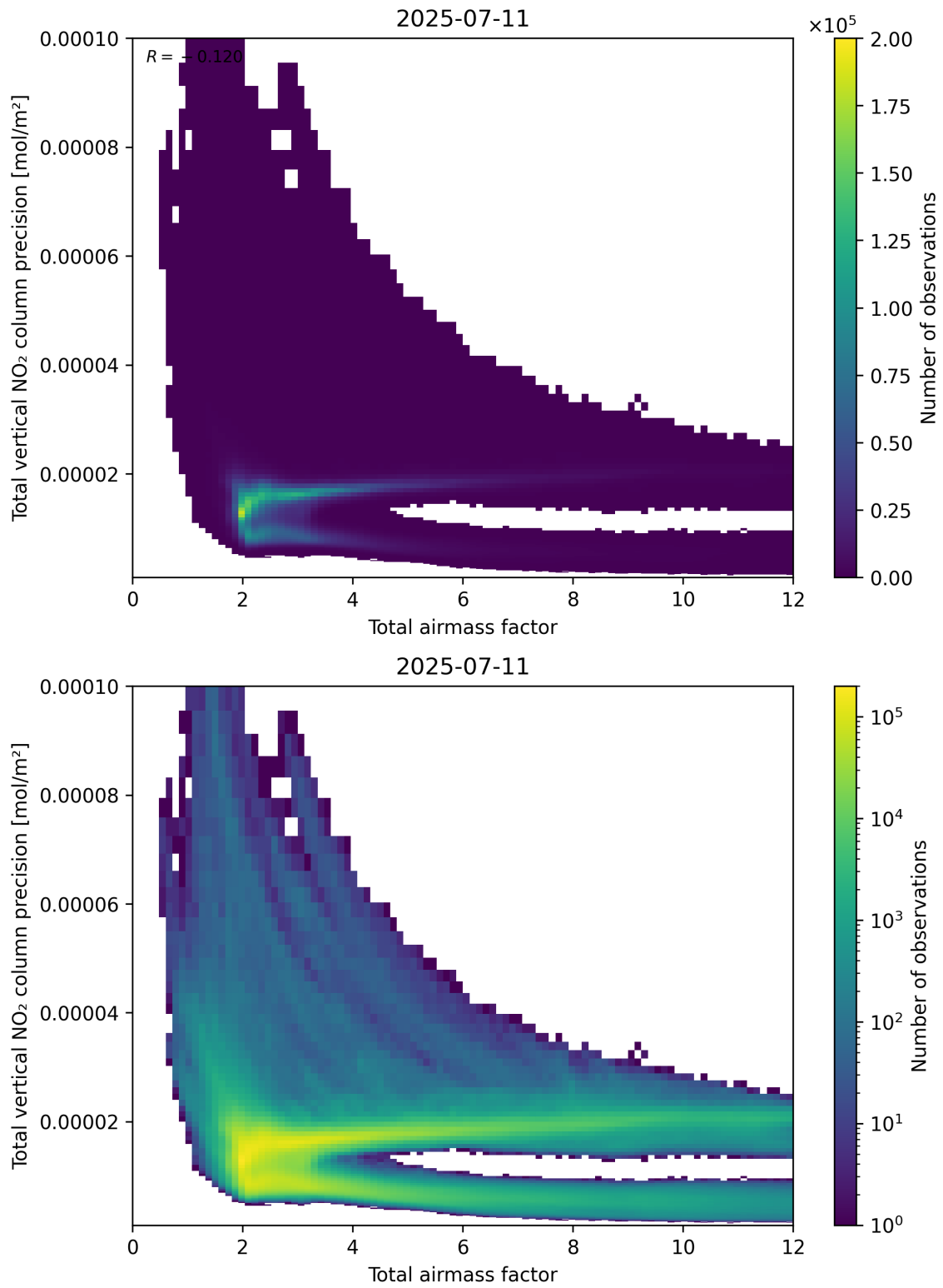
Figure 68: Scatter density plot of “Total airmass factor” against “Total vertical NO 2 column precision” for 2025-07-10 to 2025-07-12.
