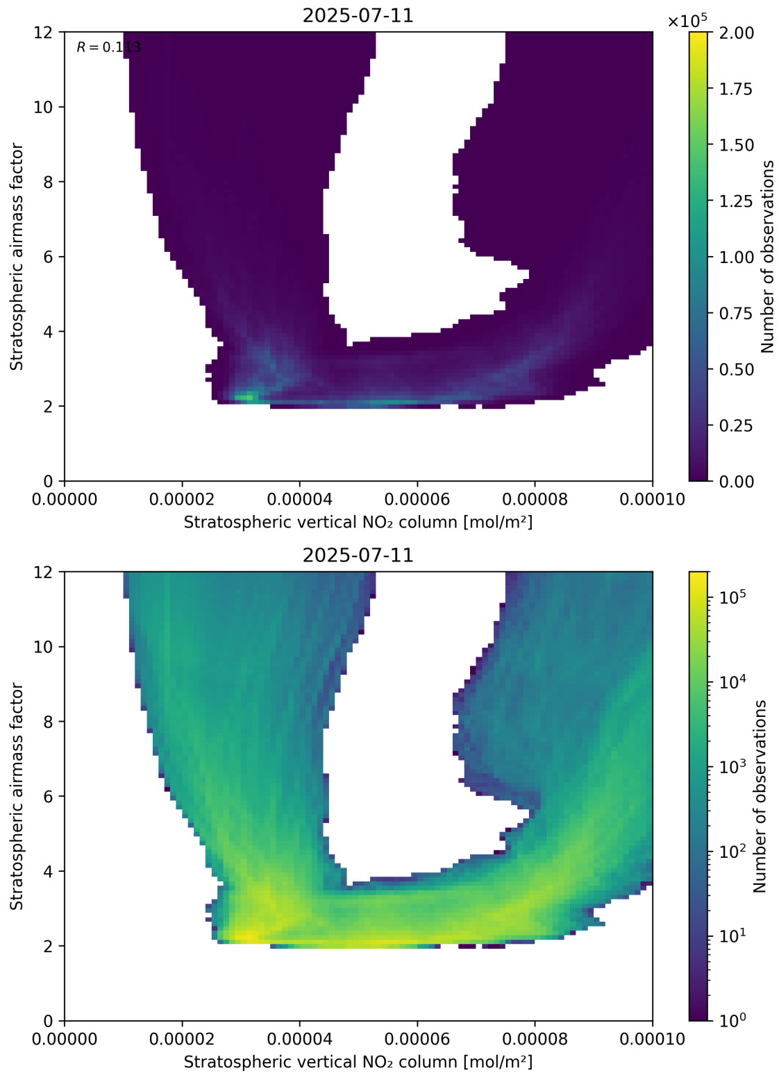
Figure 96: Scatter density plot of “Stratospheric vertical NO 2 column” against “Stratospheric airmass factor” for 2025-07-10 to 2025-07-12.
