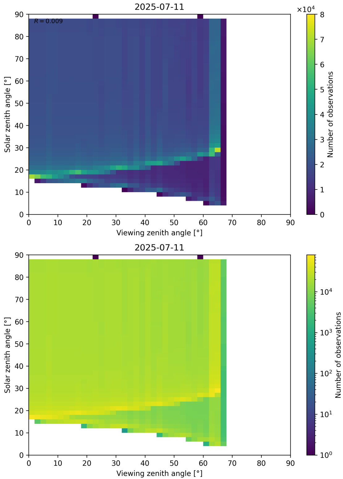
Figure 172: Scatter density plot of “Viewing zenith angle” against “Solar zenith angle” for 2025-07-10 to 2025-07-12.
