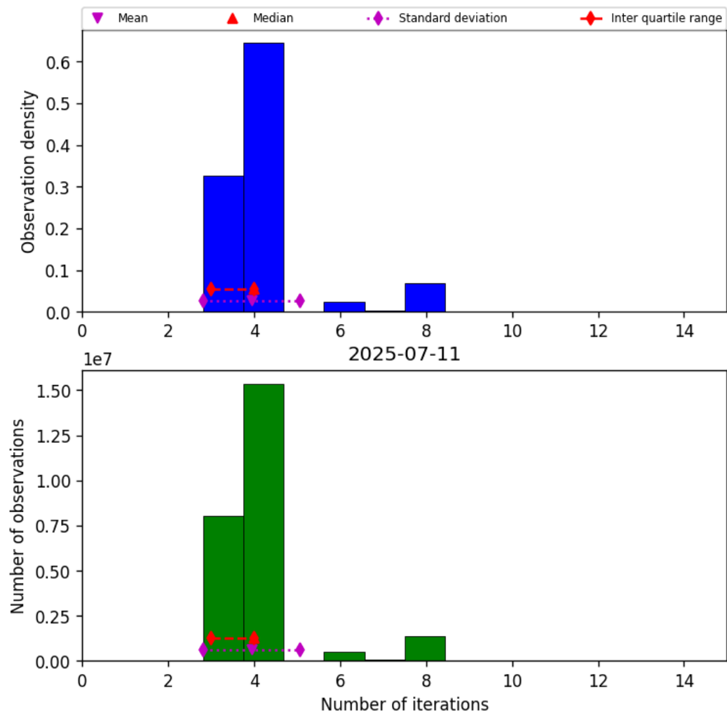
Figure 34: Histogram of “Number of iterations” for 2025-07-10 to 2025-07-12
