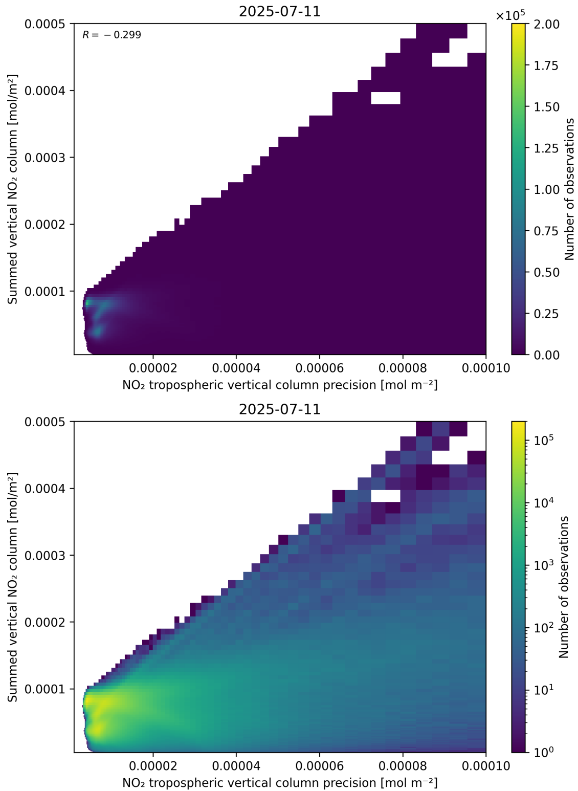
Figure 136: Scatter density plot of “NO 2 tropospheric vertical column precision” against “Summed vertical NO 2 column” for 2025-07-10 to 2025-07-12.
