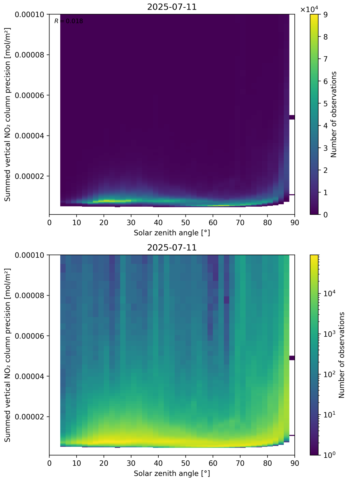
Figure 152: Scatter density plot of “Solar zenith angle” against “Summed vertical NO 2 column precision” for 2025-07-10 to 2025-07-12.
