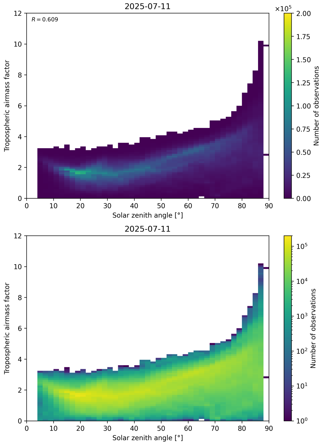
Figure 147: Scatter density plot of “Solar zenith angle” against “Tropospheric airmass factor” for 2025-07-10 to 2025-07-12.
