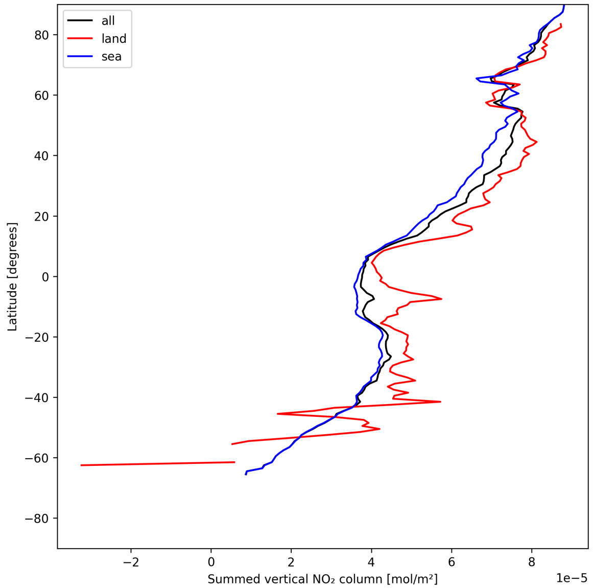
Figure 23: Zonal average of “Summed vertical NO 2 column” for 2025-07-10 to 2025-07-12.
