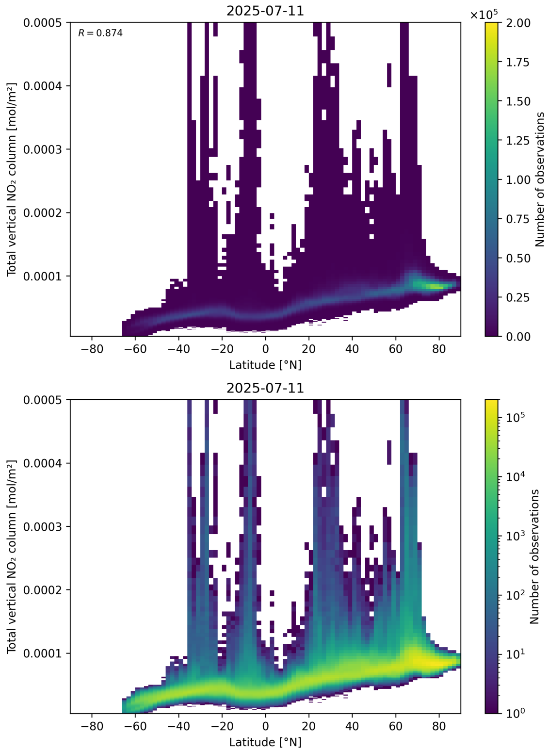
Figure 90: Scatter density plot of “Latitude” against “Total vertical NO 2 column” for 2025-07-10 to 2025-07-12.
