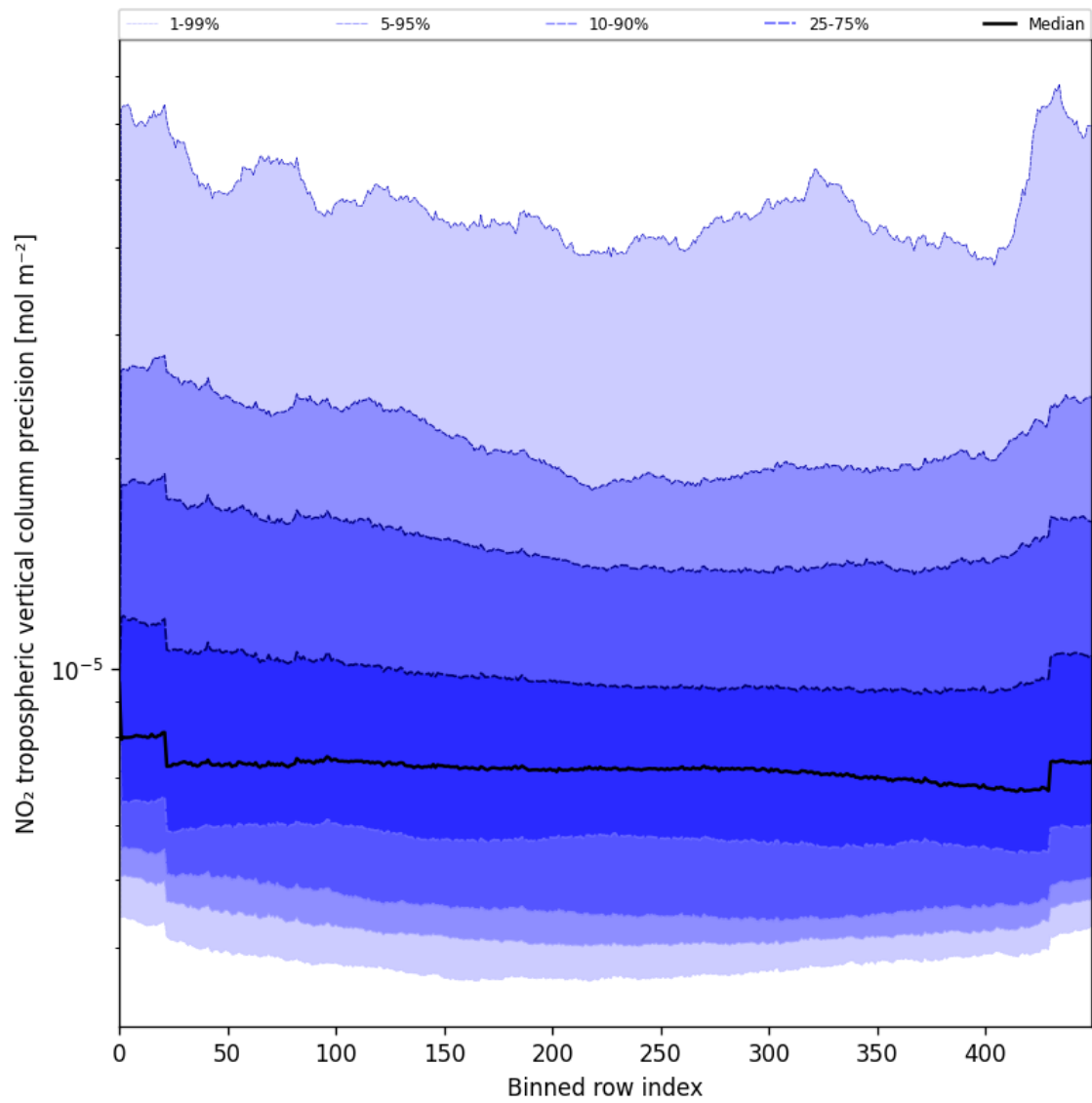
Figure 47: Along track statistics of “NO 2 tropospheric vertical column precision” for 2025-07-10 to 2025-07-12
