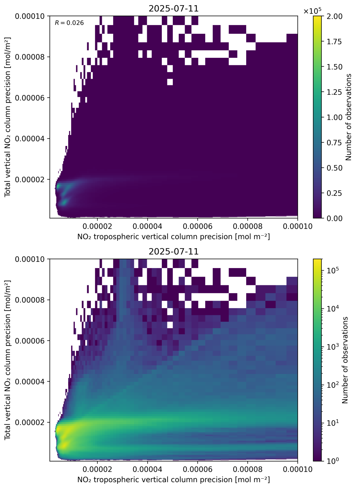
Figure 139: Scatter density plot of “NO 2 tropospheric vertical column precision” against “Total vertical NO 2 column precision” for 2025-07-10 to 2025-07-12.
