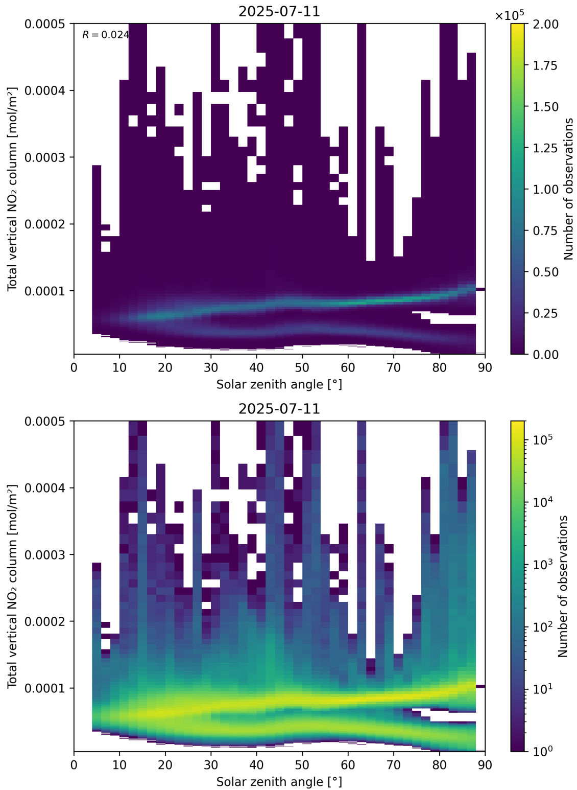
Figure 153: Scatter density plot of “Solar zenith angle” against “Total vertical NO 2 column” for 2025-07-10 to 2025-07-12.
