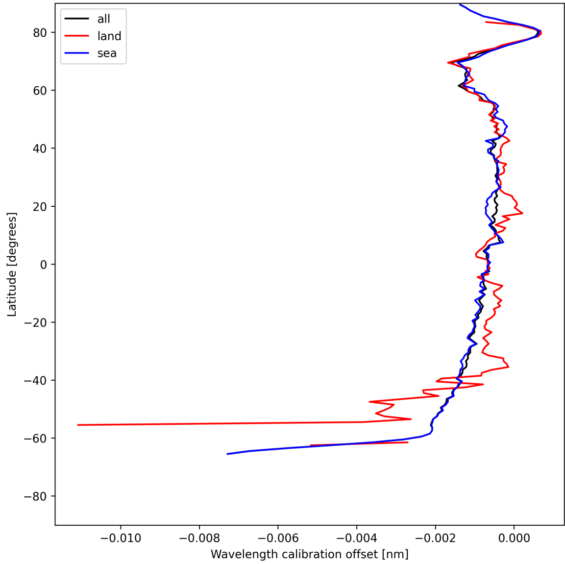
Figure 18: Zonal average of “Wavelength calibration offset” for 2025-07-10 to 2025-07-12.
