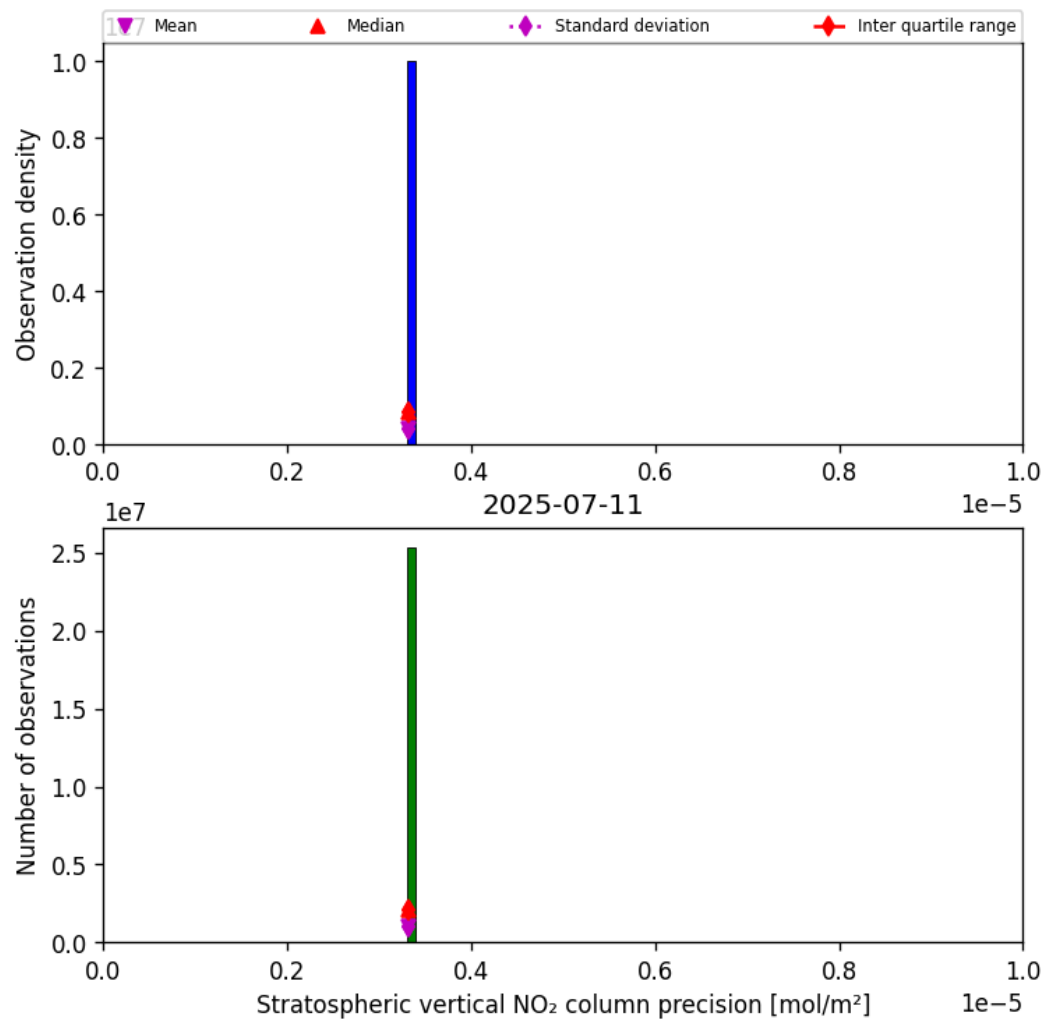
Figure 37: Histogram of “Stratospheric vertical NO 2 column precision” for 2025-07-10 to 2025-07-12
