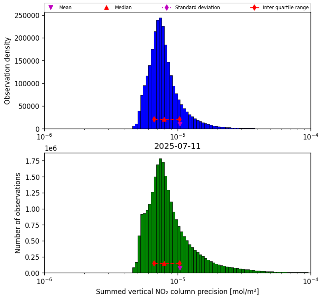
Figure 41: Histogram of "Summed vertical NO 2 column precision" for 2025-07-10 to 2025-07-12
