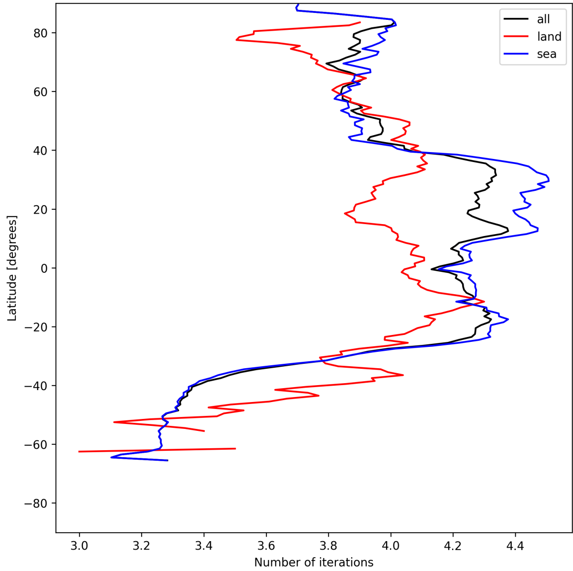
Figure 17: Zonal average of “Number of iterations” for 2025-07-10 to 2025-07-12.
