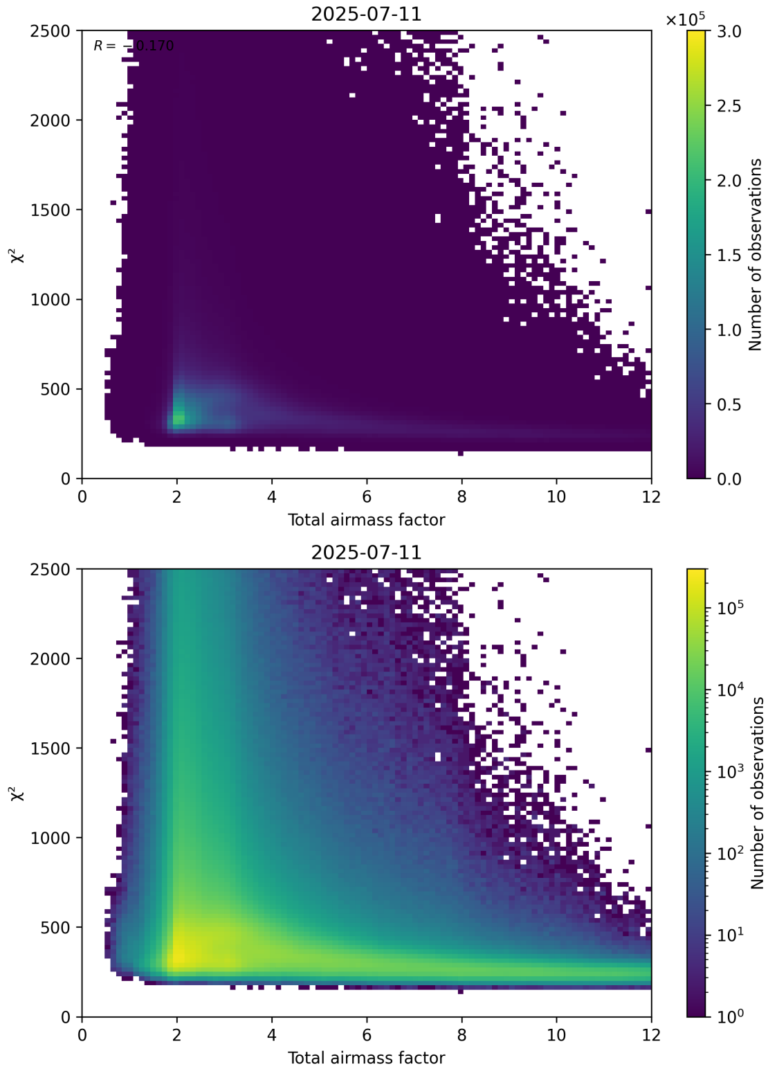
Figure 63: Scatter density plot of “Total airmass factor” against “ \chi^2 ” for 2025-07-10 to 2025-07-12.
