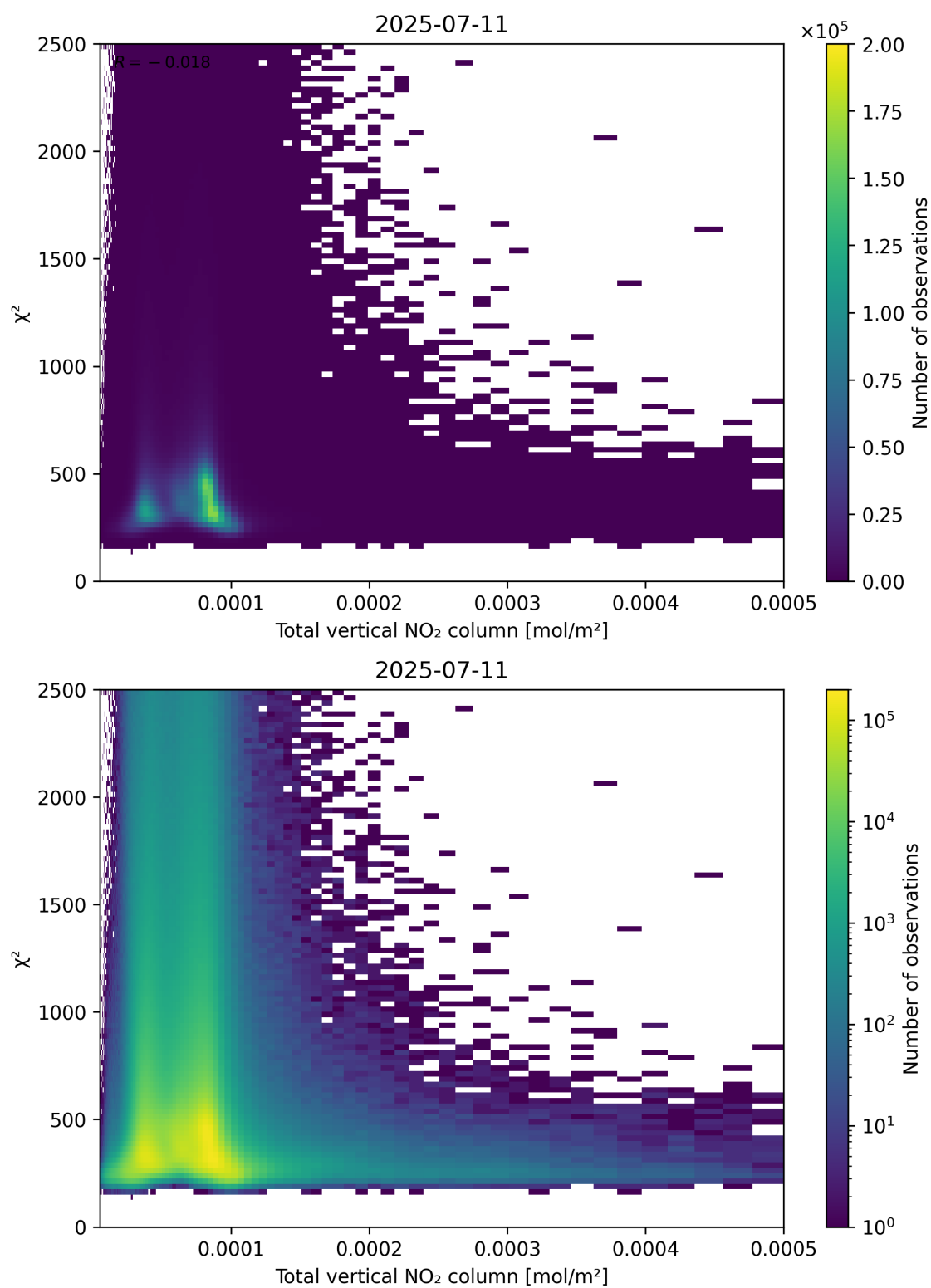
Figure 111: Scatter density plot of “Total vertical NO 2 column” against “ \chi^2 ” for 2025-07-10 to 2025-07-12.
