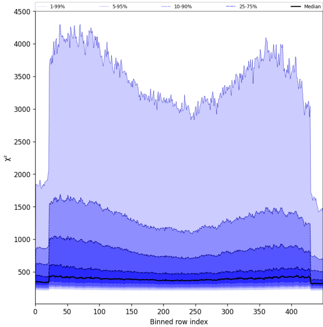
Figure 59: Along track statistics of “ \chi^2 ” for 2025-07-10 to 2025-07-12
