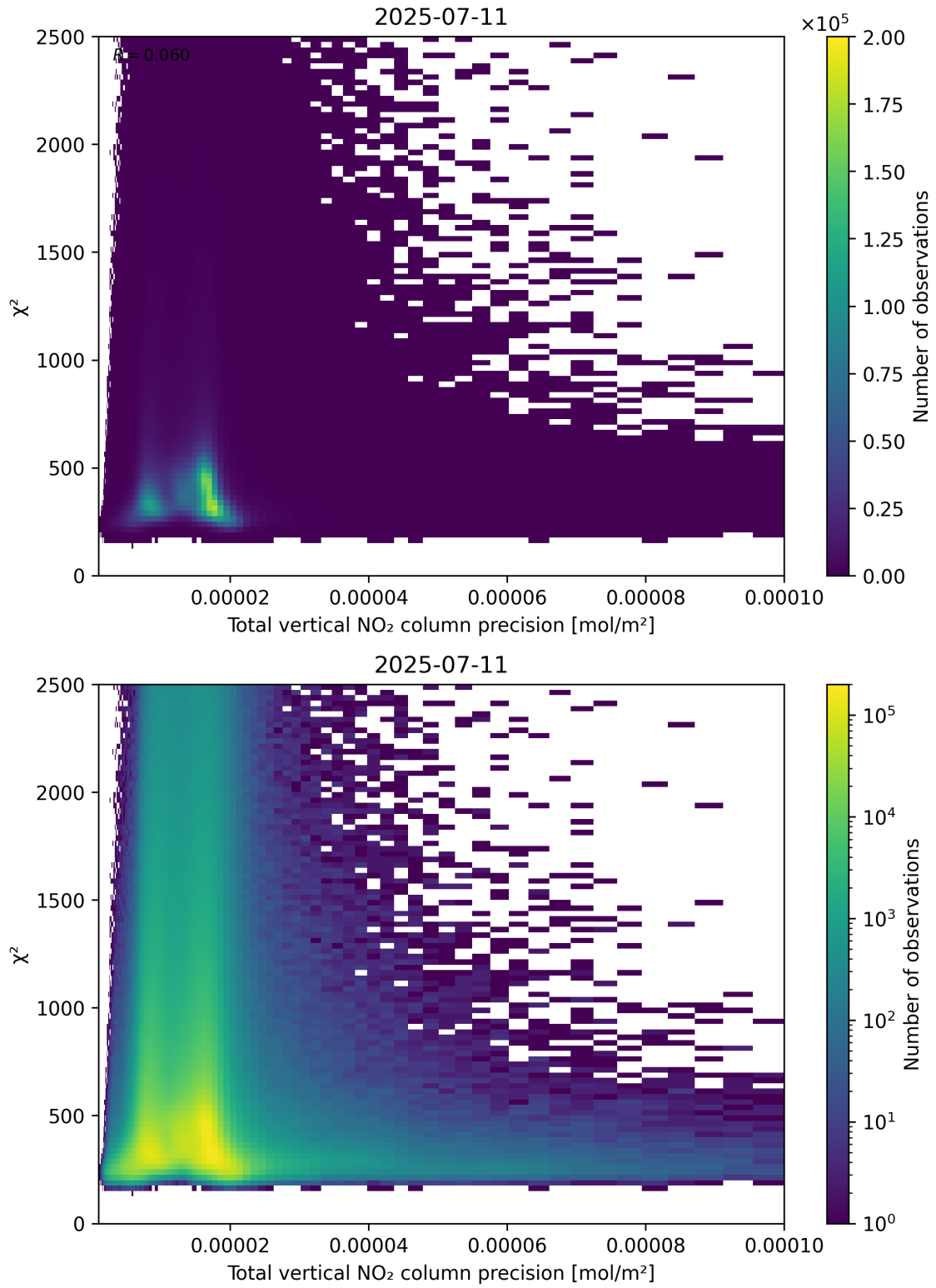
Figure 116: Scatter density plot of “Total vertical NO 2 column precision” against “ \chi^2 ” for 2025-07-10 to 2025-07-12.
