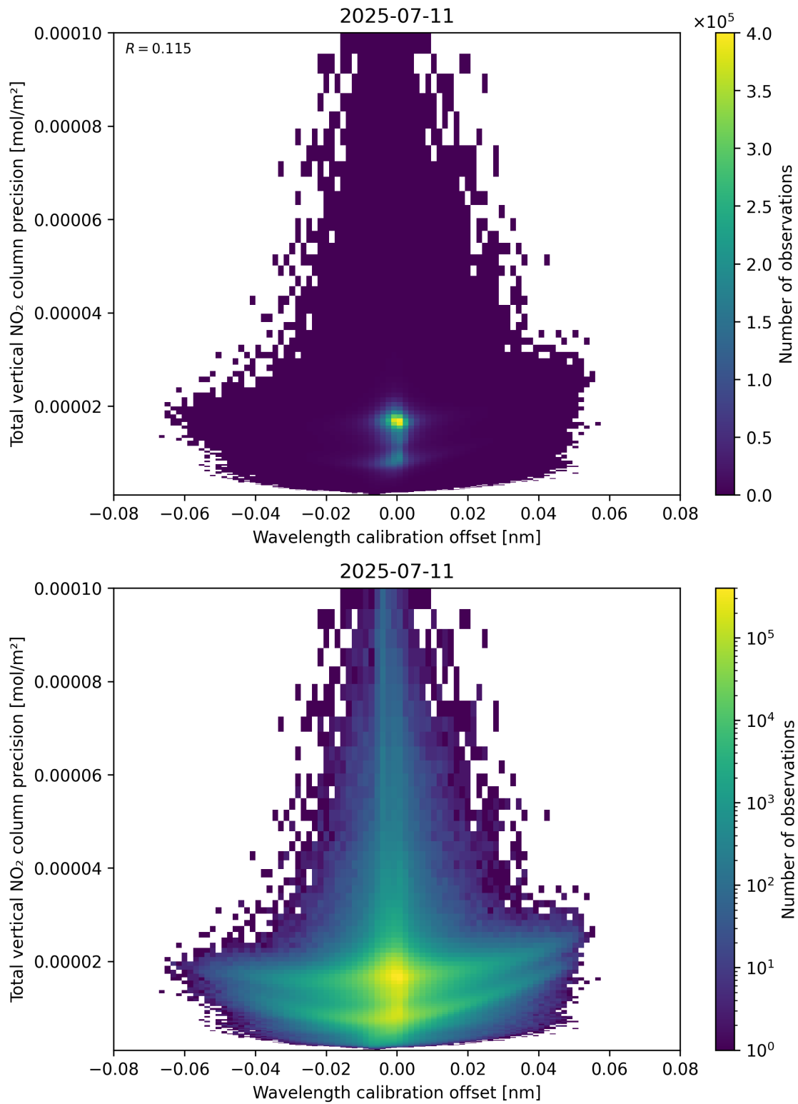
Figure 180: Scatter density plot of “Wavelength calibration offset” against “Total vertical NO 2 column precision” for 2025-07-10 to 2025-07-12.
