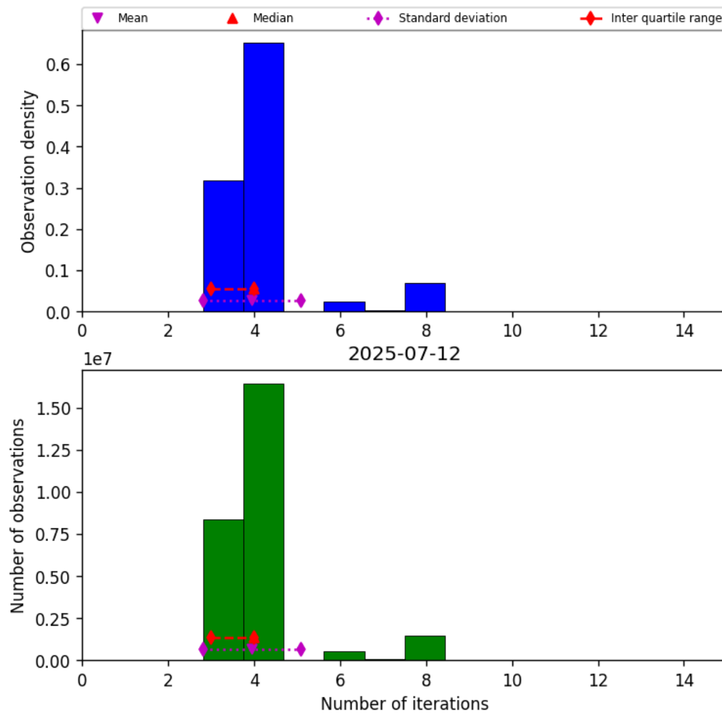
Figure 34: Histogram of “Number of iterations” for 2025-07-11 to 2025-07-13
