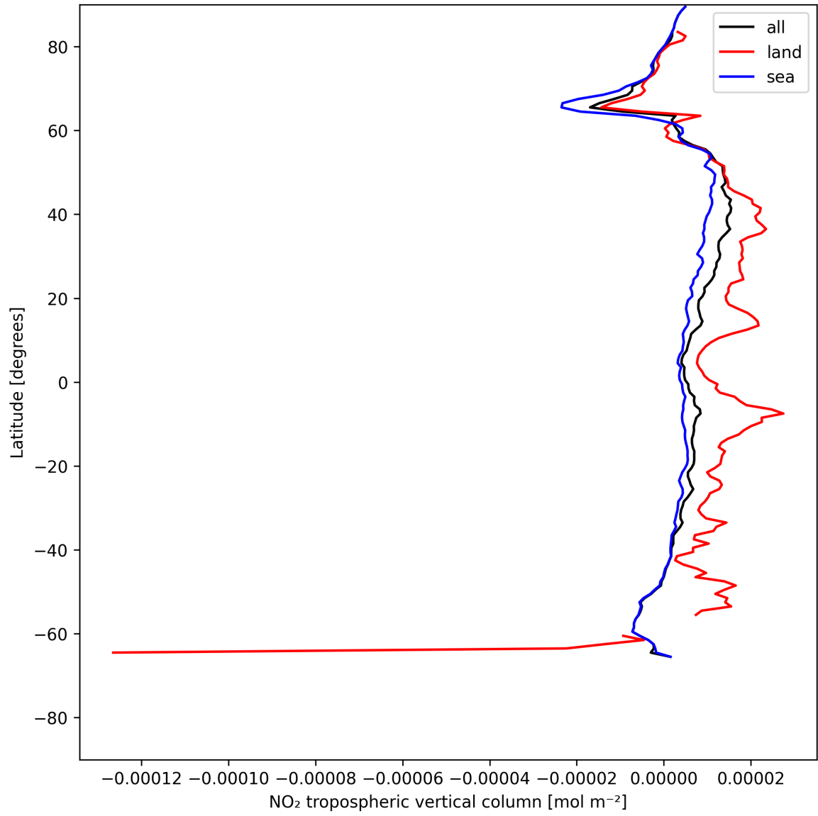
Figure 12: Zonal average of “NO 2 tropospheric vertical column” for 2025-07-11 to 2025-07-13.
