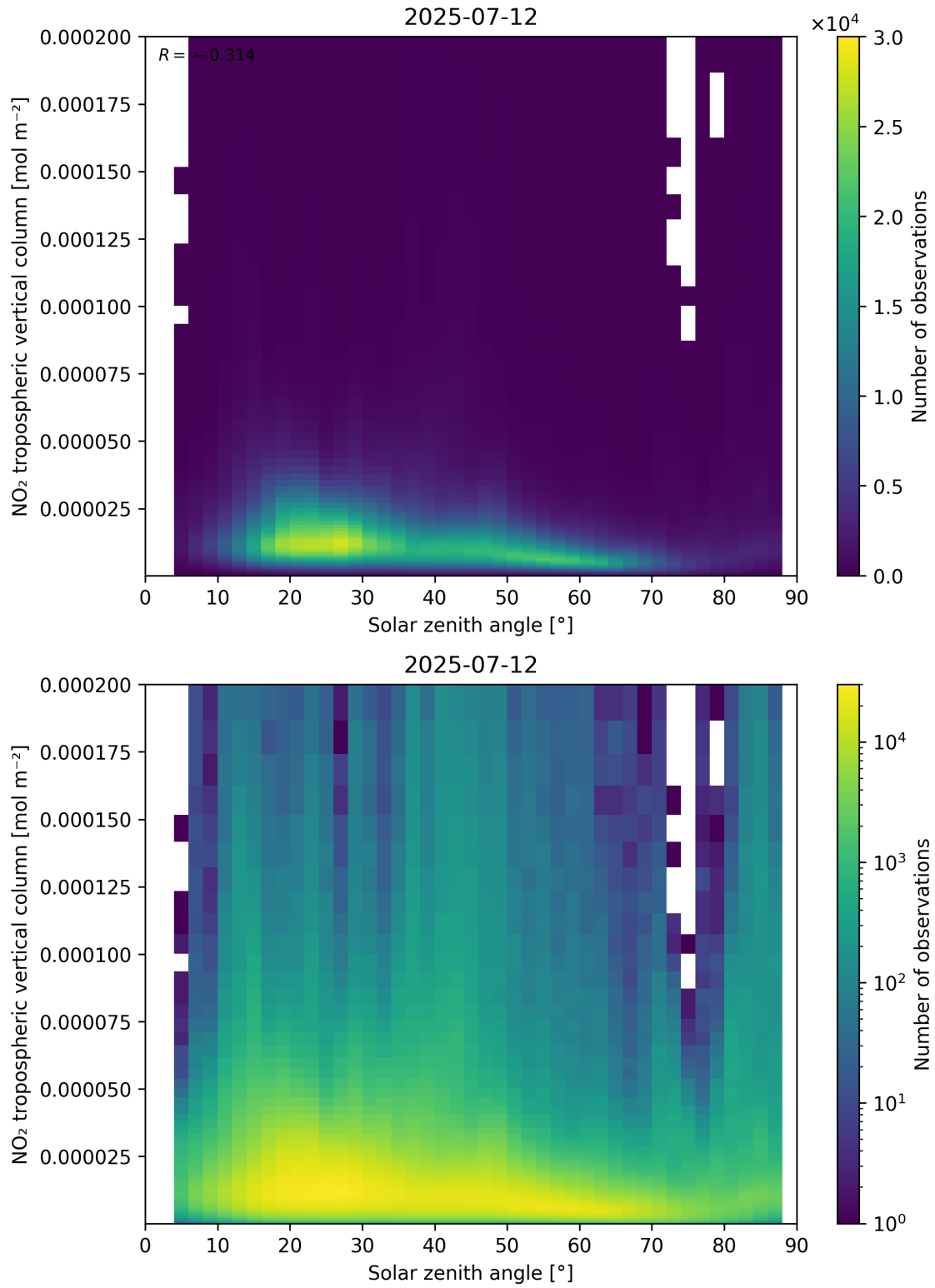
Figure 155: Scatter density plot of “Solar zenith angle” against “NO 2 tropospheric vertical column” for 2025-07-11 to 2025-07-13.
