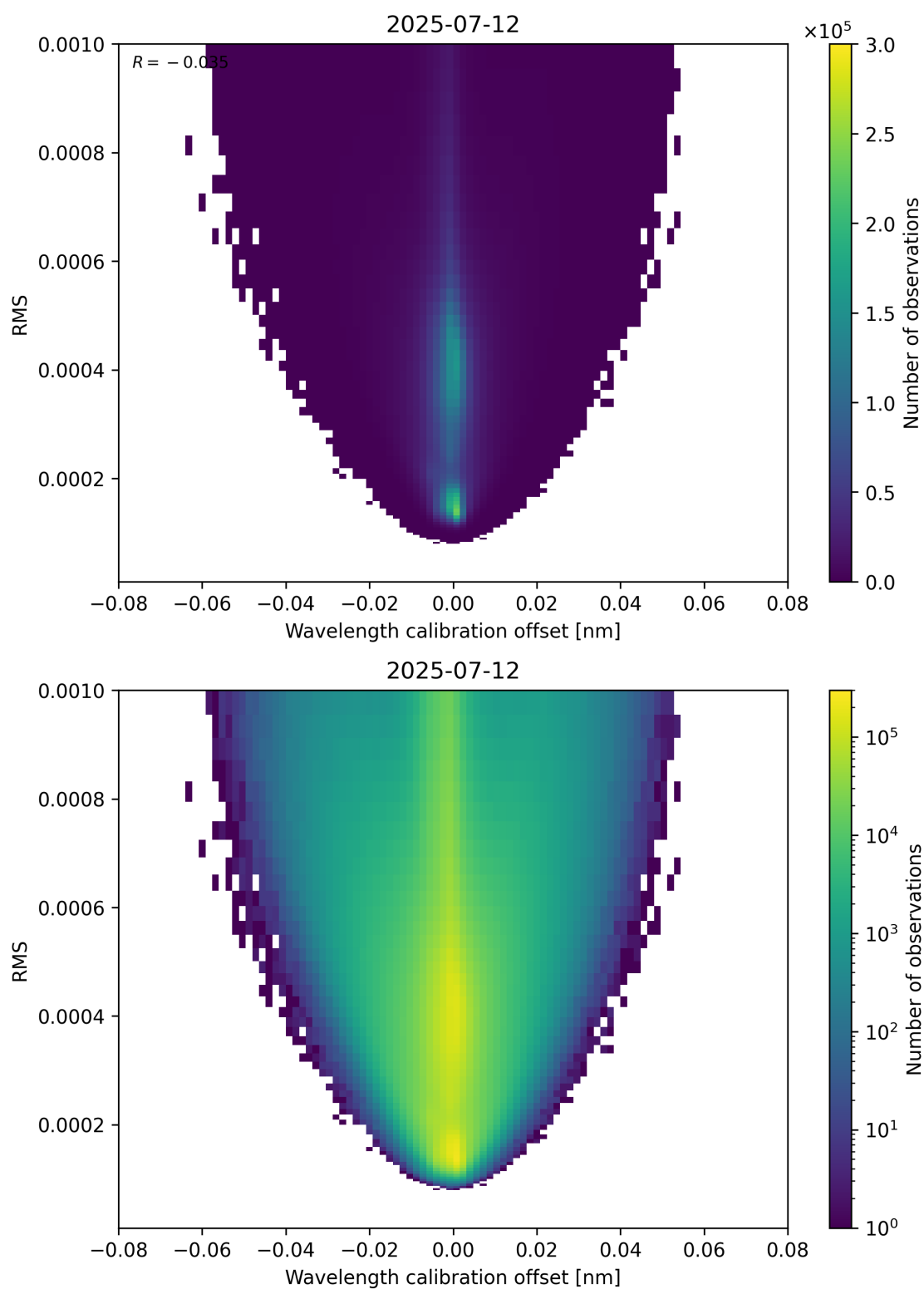
Figure 181: Scatter density plot of “Wavelength calibration offset” against “RMS” for 2025-07-11 to 2025-07-13.
