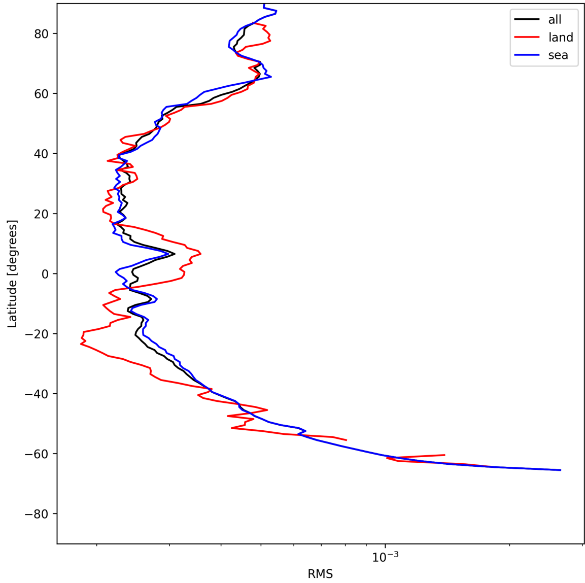
Figure 26: Zonal average of “RMS” for 2025-07-11 to 2025-07-13.
