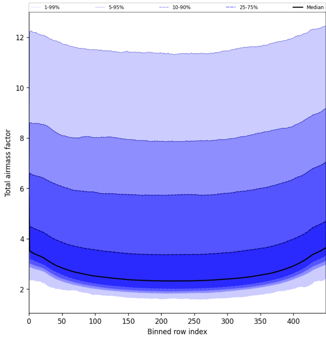
Figure 49: Along track statistics of “Total airmass factor” for 2025-07-11 to 2025-07-13
