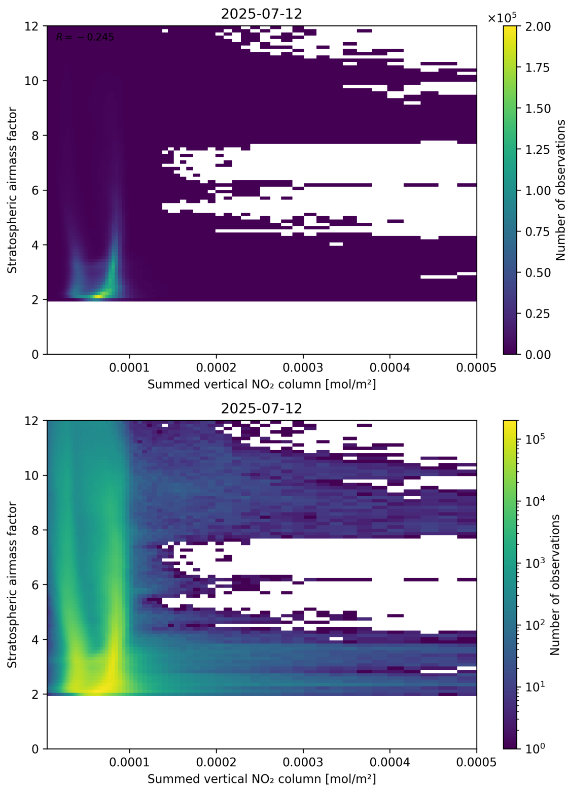
Figure 103: Scatter density plot of “Summed vertical NO 2 column” against “Stratospheric air mass factor” for 2025-07-11 to 2025-07-13.
