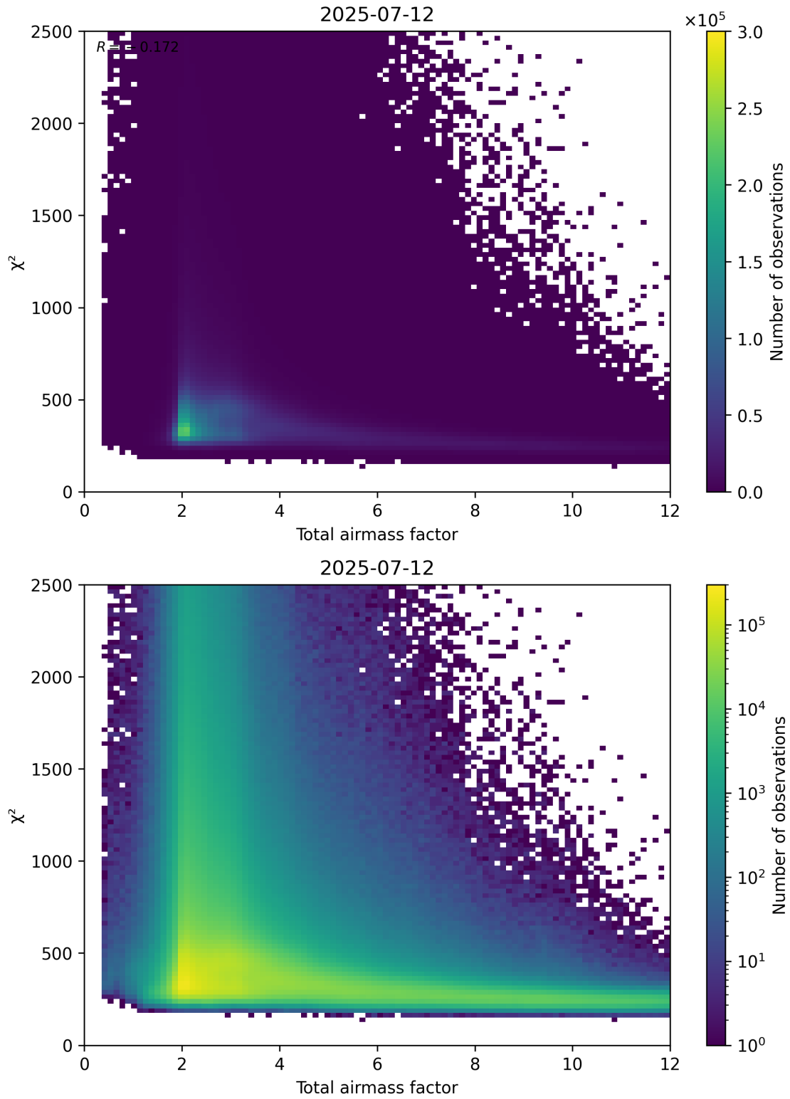
Figure 63: Scatter density plot of “Total airmass factor” against “ \chi^2 ” for 2025-07-11 to 2025-07-13.
