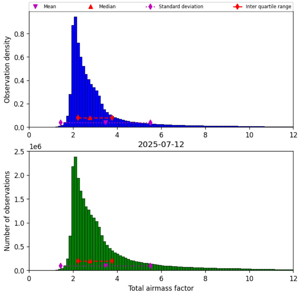
Figure 32: Histogram of “Total airmass factor” for 2025-07-11 to 2025-07-13
