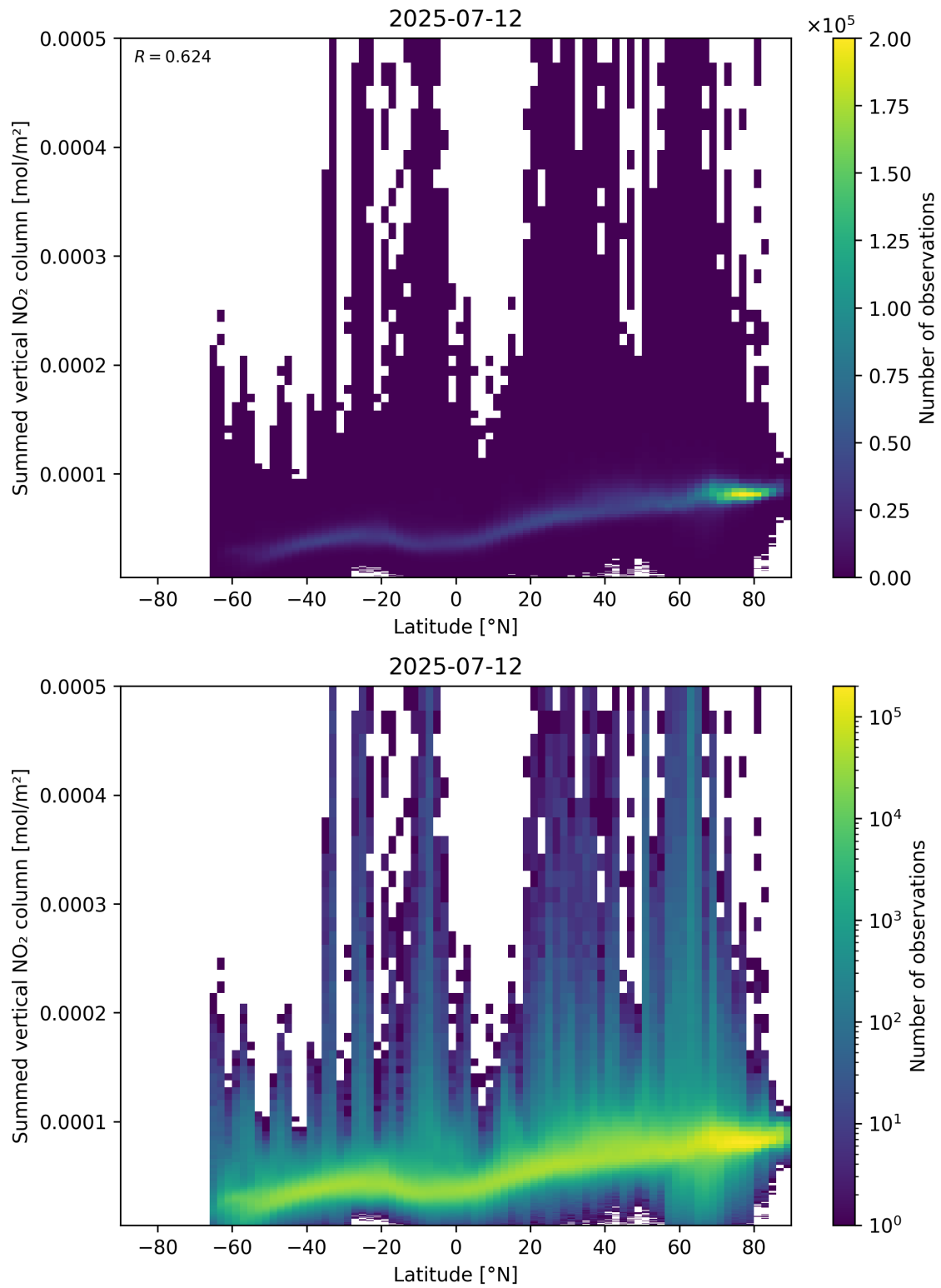
Figure 88: Scatter density plot of “Latitude” against “Summed vertical NO 2 column” for 2025-07-11 to 2025-07-13.
