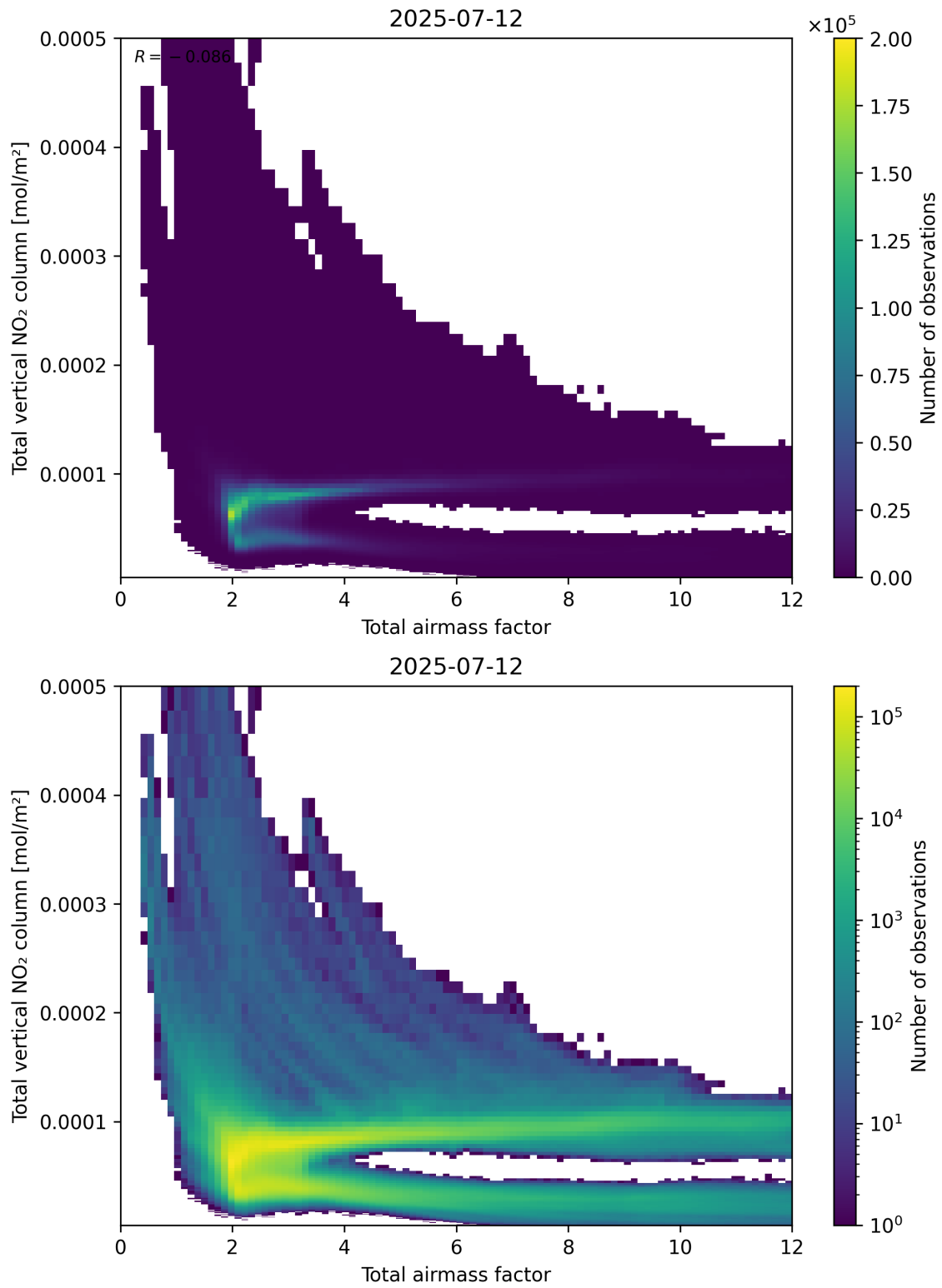
Figure 67: Scatter density plot of “Total airmass factor” against “Total vertical NO 2 column” for 2025-07-11 to 2025-07-13.
