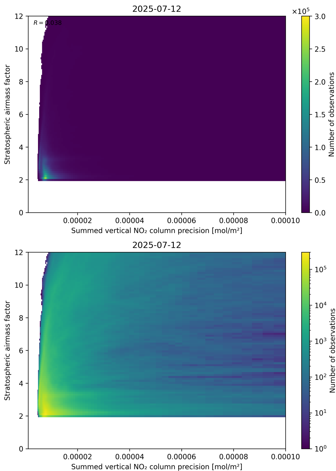
Figure 106: Scatter density plot of “Summed vertical NO 2 column precision” against “Stratospheric airmass factor” for 2025-07-11 to 2025-07-13.
