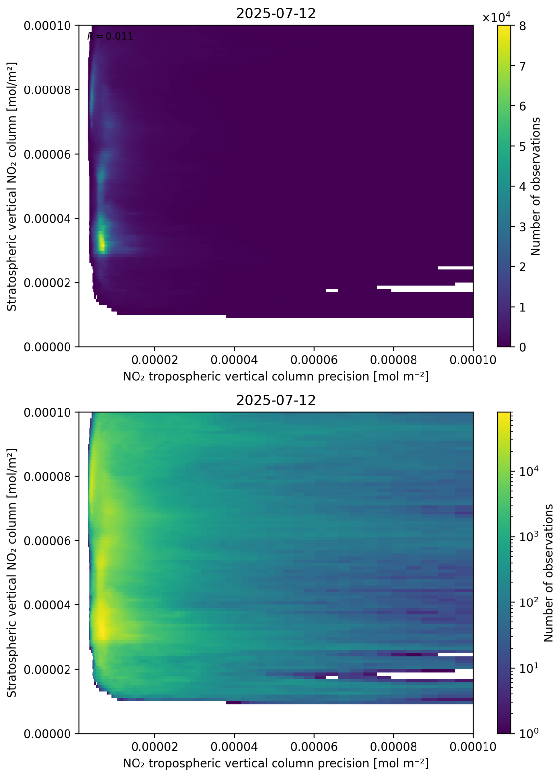
Figure 135: Scatter density plot of “NO 2 tropospheric vertical column precision” against “Stratospheric vertical NO 2 column” for 2025-07-11 to 2025-07-13.
