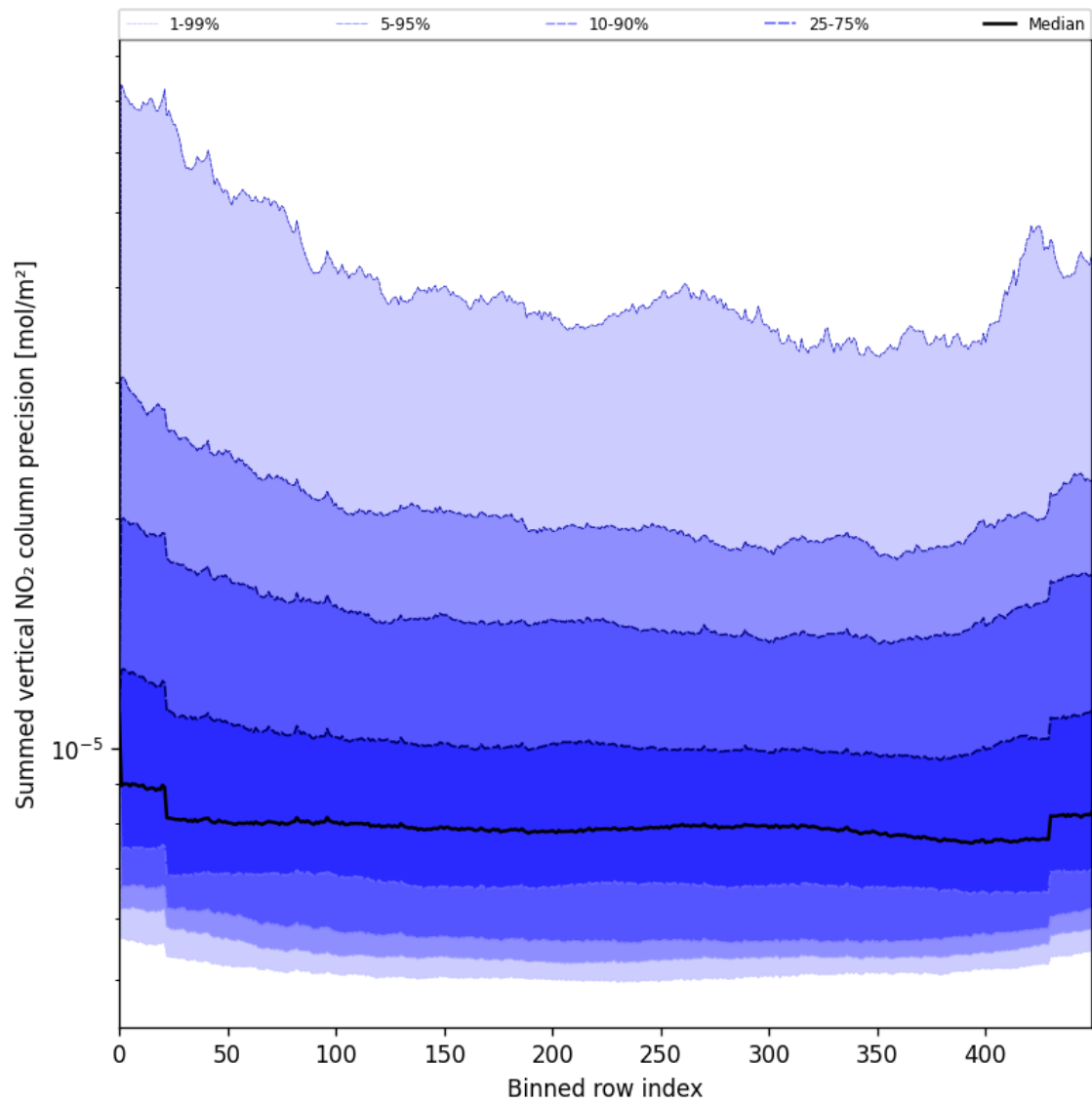
Figure 58: Along track statistics of “Summed vertical NO 2 column precision” for 2025-07-11 to 2025-07-13
