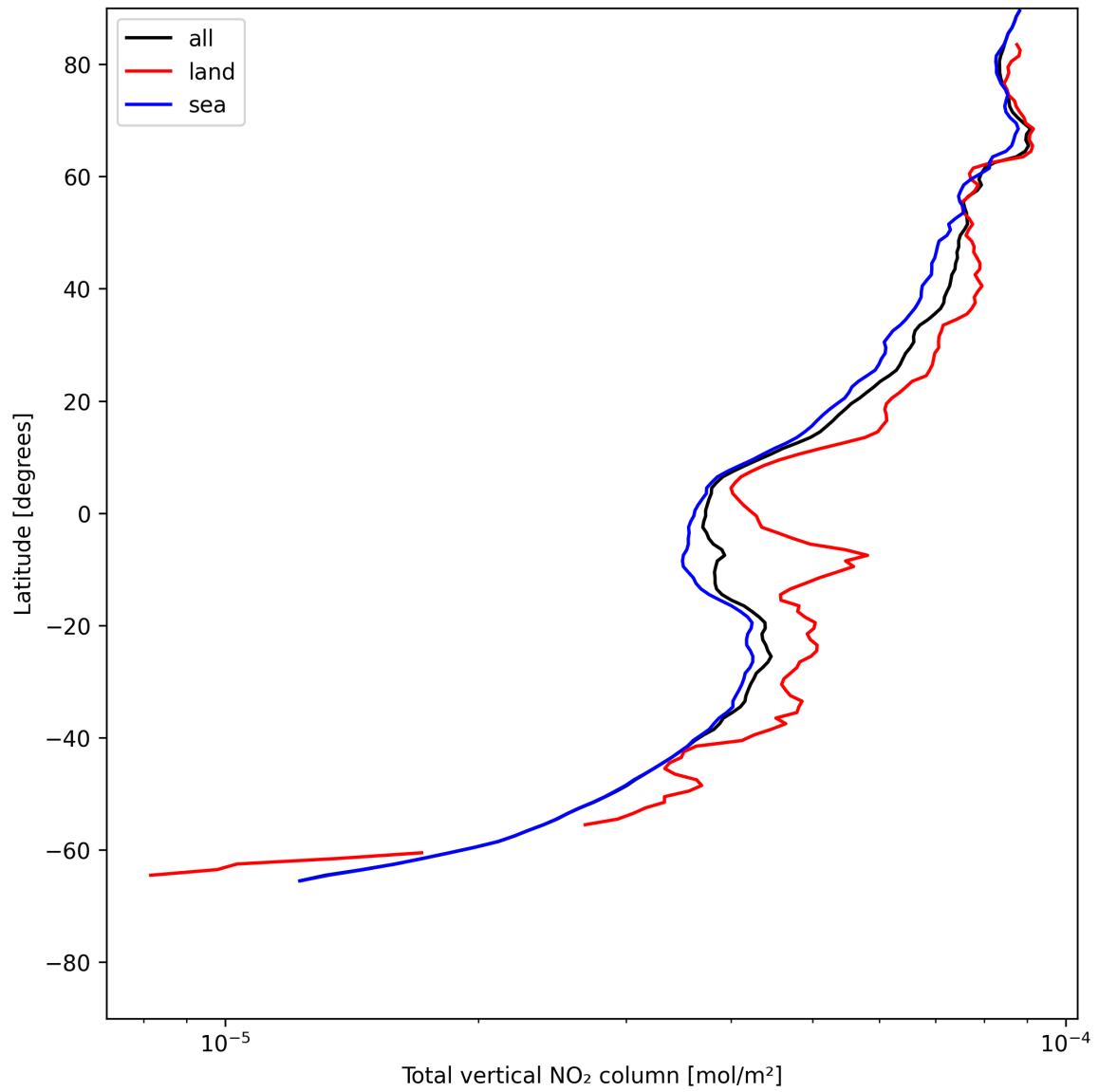
Figure 21: Zonal average of “Total vertical NO 2 column” for 2025-07-11 to 2025-07-13.
