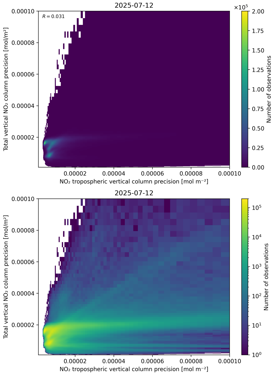
Figure 139: Scatter density plot of “NO 2 tropospheric vertical column precision” against “Total vertical NO 2 column precision” for 2025-07-11 to 2025-07-13.
