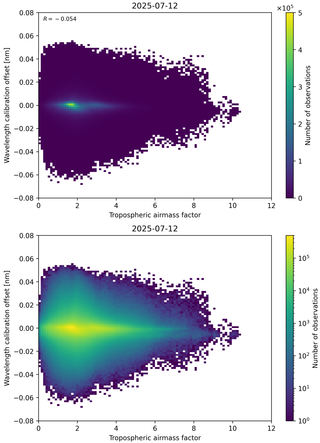
Figure 80: Scatter density plot of “Tropospheric airmass factor” against “Wavelength calibration offset” for 2025-07-11 to 2025-07-13.
