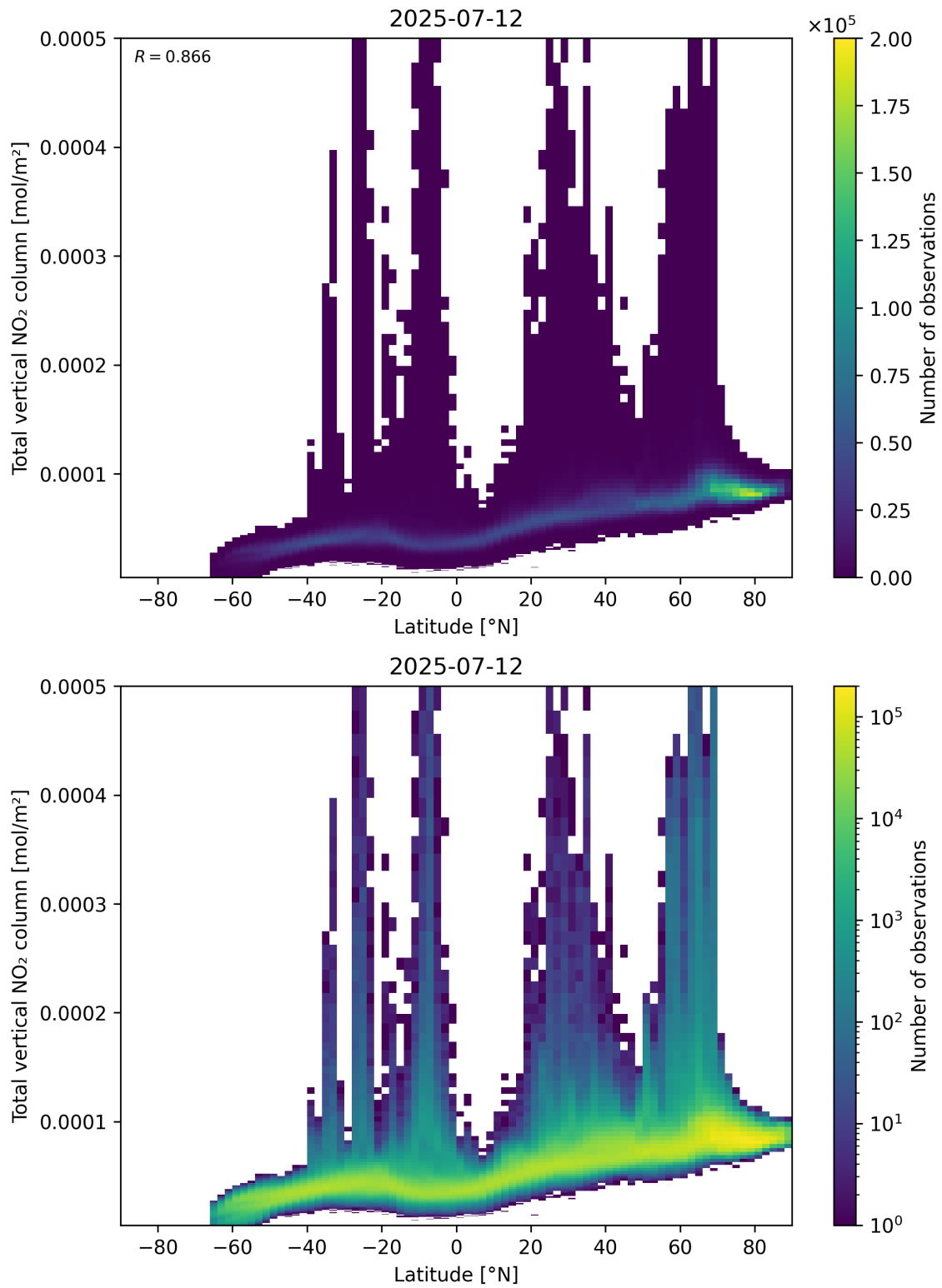
Figure 90: Scatter density plot of “Latitude” against “Total vertical NO 2 column” for 2025-07-11 to 2025-07-13.
