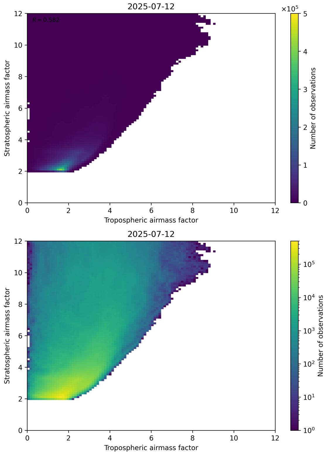
Figure 71: Scatter density plot of “Tropospheric airmass factor” against “Stratospheric airmass factor” for 2025-07-11 to 2025-07-13.
