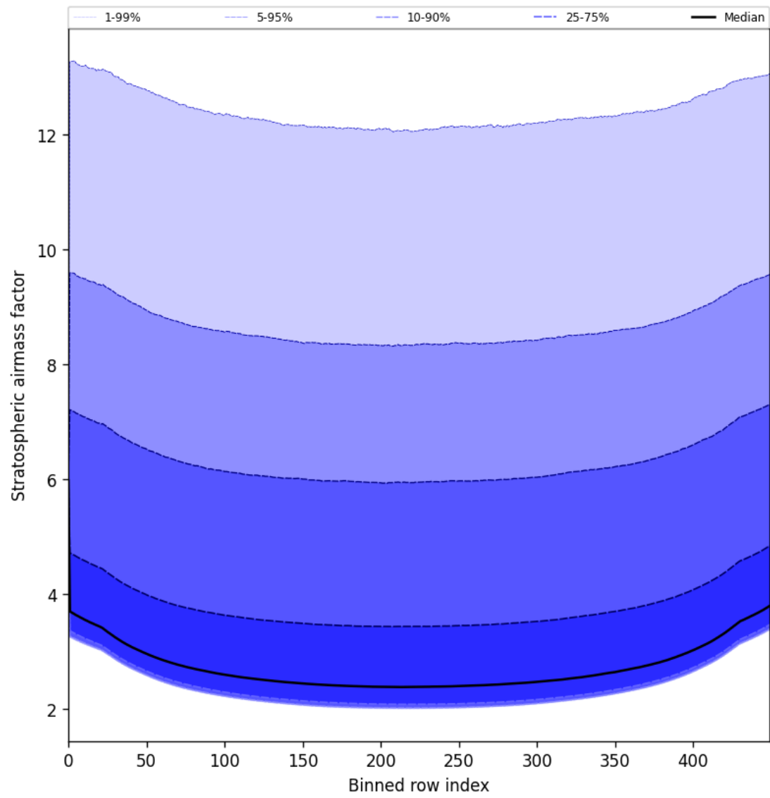
Figure 61: Along track statistics of “Stratospheric airmass factor” for 2025-07-11 to 2025-07-13
