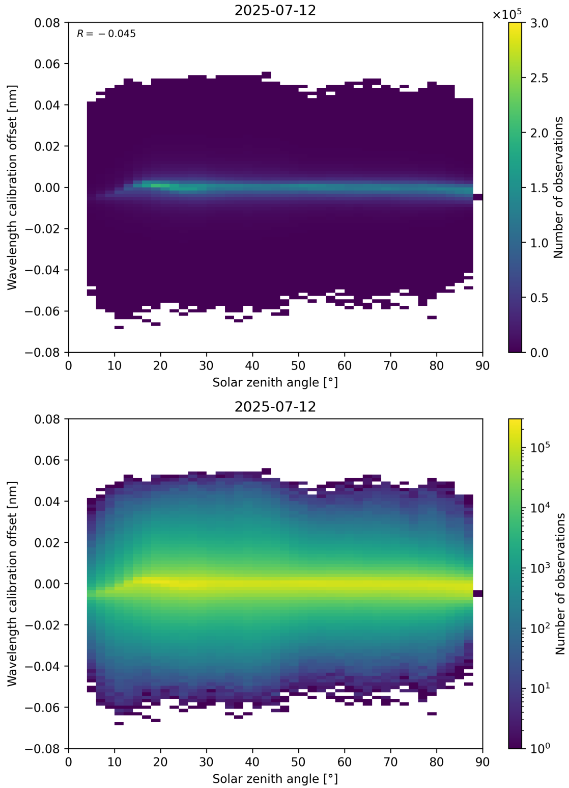
Figure 158: Scatter density plot of “Solar zenith angle” against “Wavelength calibration offset” for 2025-07-11 to 2025-07-13.
