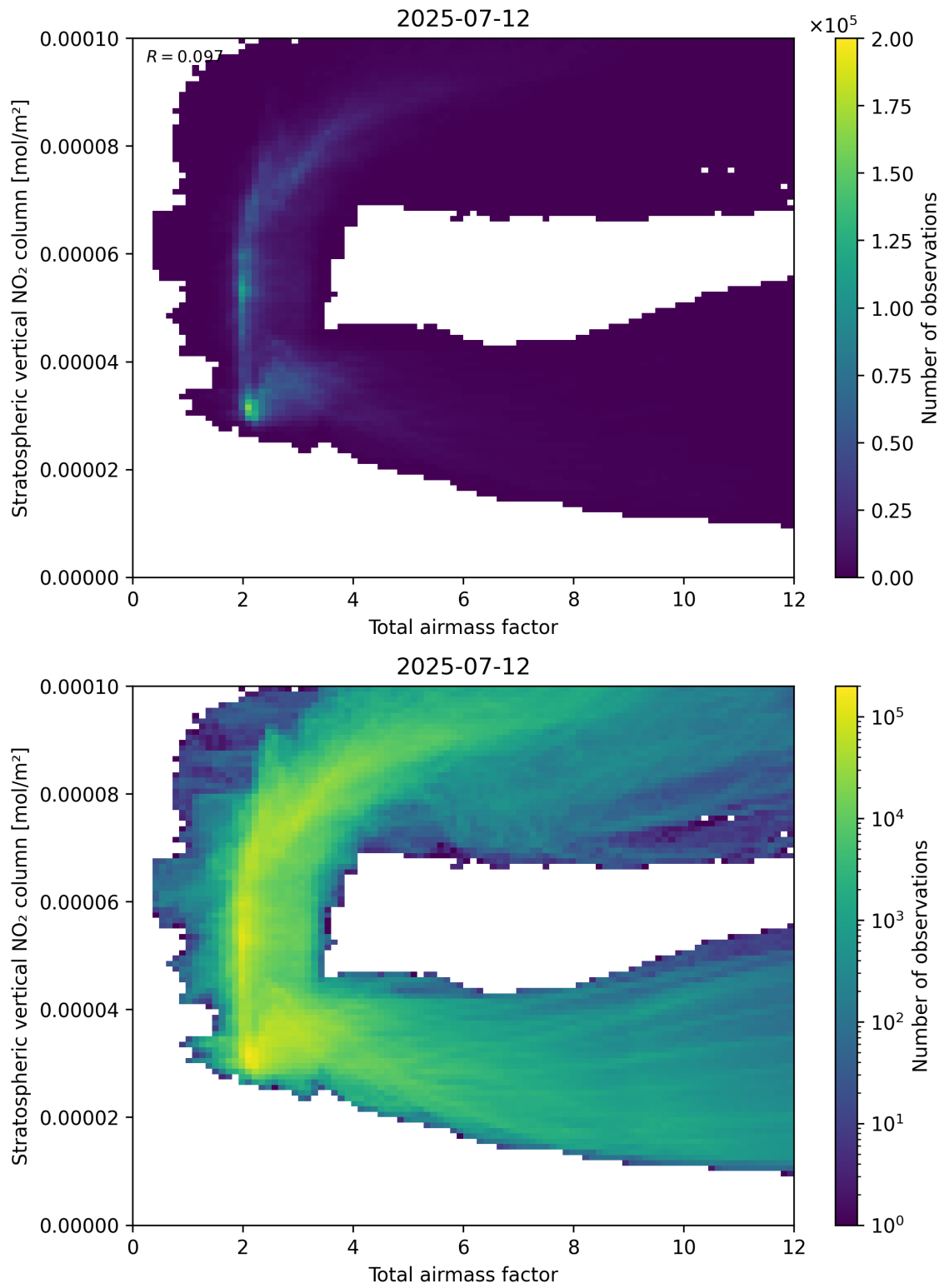
Figure 64: Scatter density plot of “Total airmass factor” against “Stratospheric vertical NO 2 column” for 2025-07-11 to 2025-07-13.
