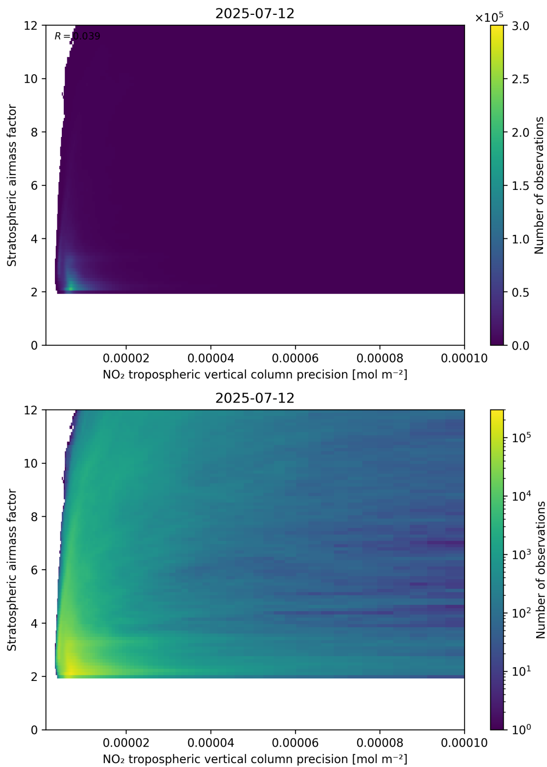
Figure 131: Scatter density plot of “NO 2 tropospheric vertical column precision” against “Stratospheric airmass factor” for 2025-07-11 to 2025-07-13.
