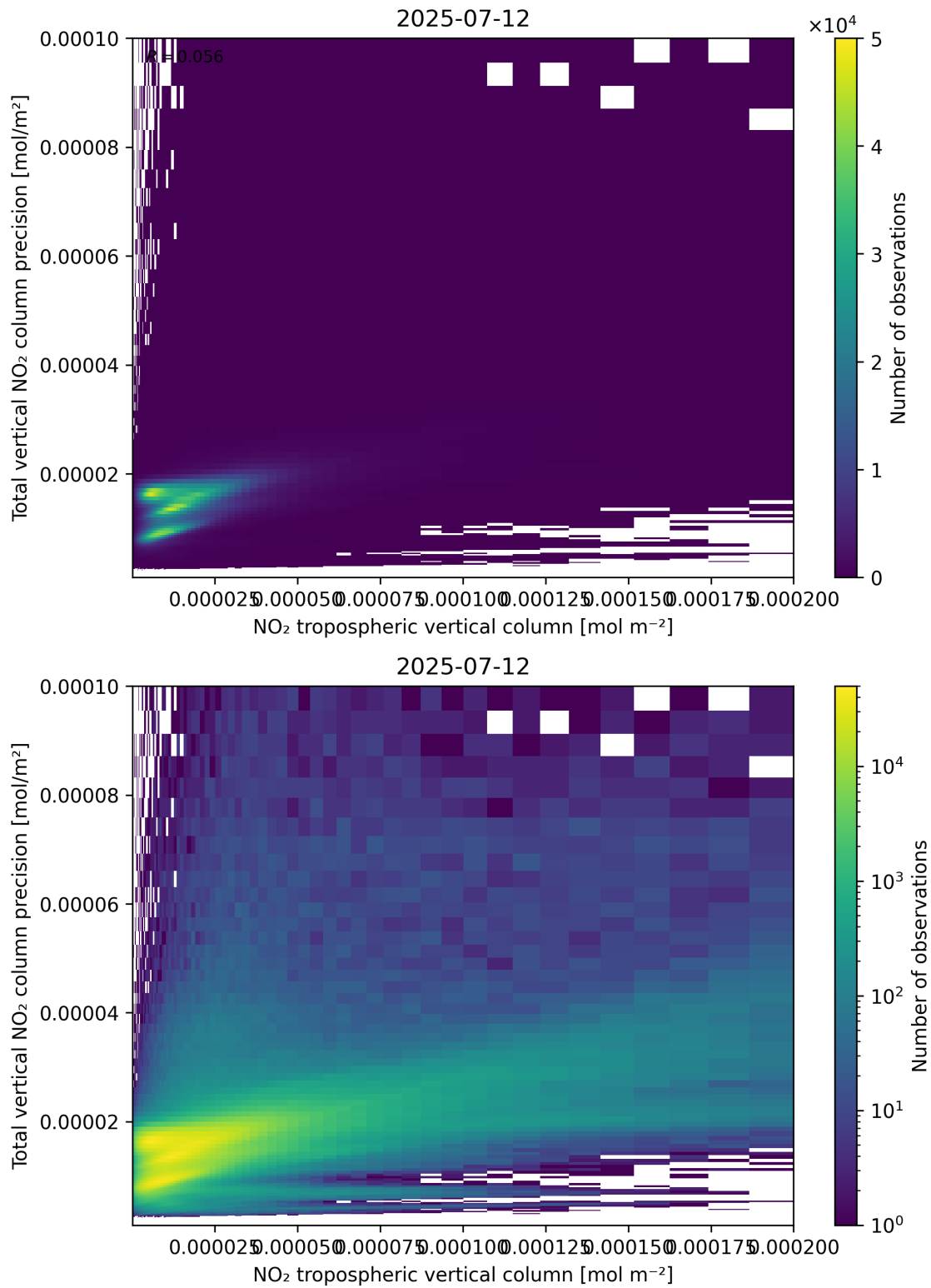
Figure 129: Scatter density plot of “NO 2 tropospheric vertical column” against “Total vertical NO 2 column precision” for 2025-07-11 to 2025-07-13.
