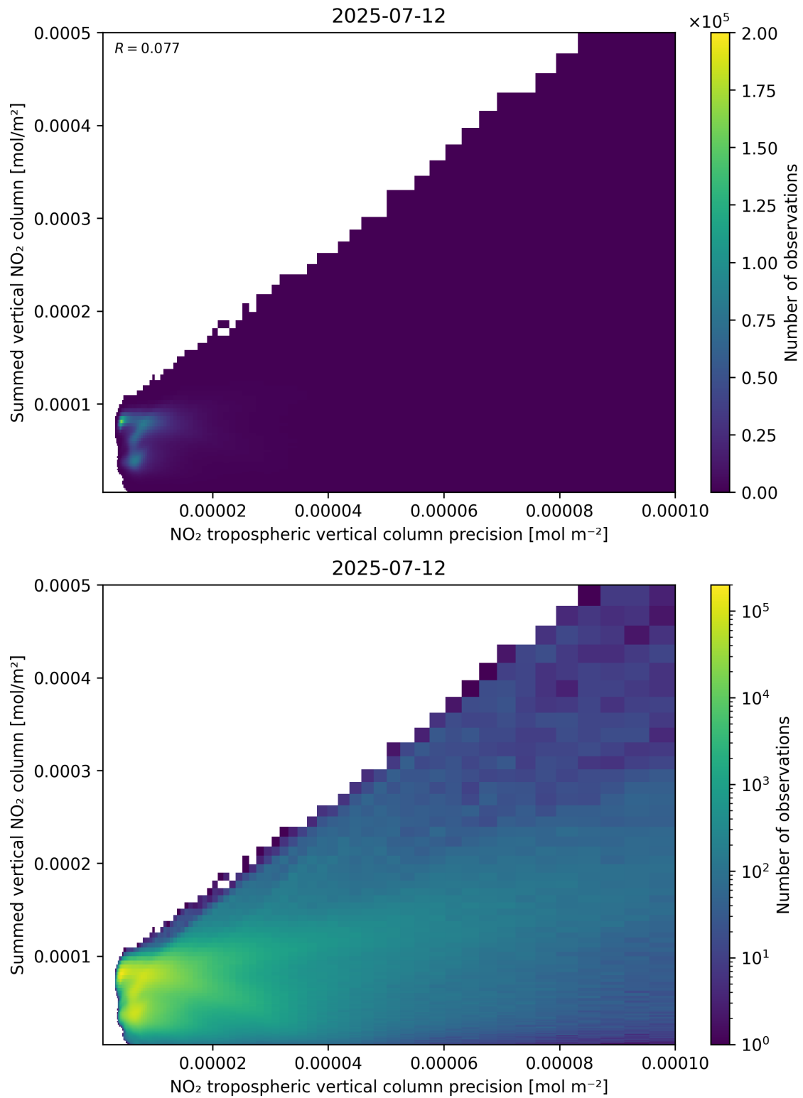
Figure 136: Scatter density plot of “NO 2 tropospheric vertical column precision” against “Summed vertical NO 2 column” for 2025-07-11 to 2025-07-13.
