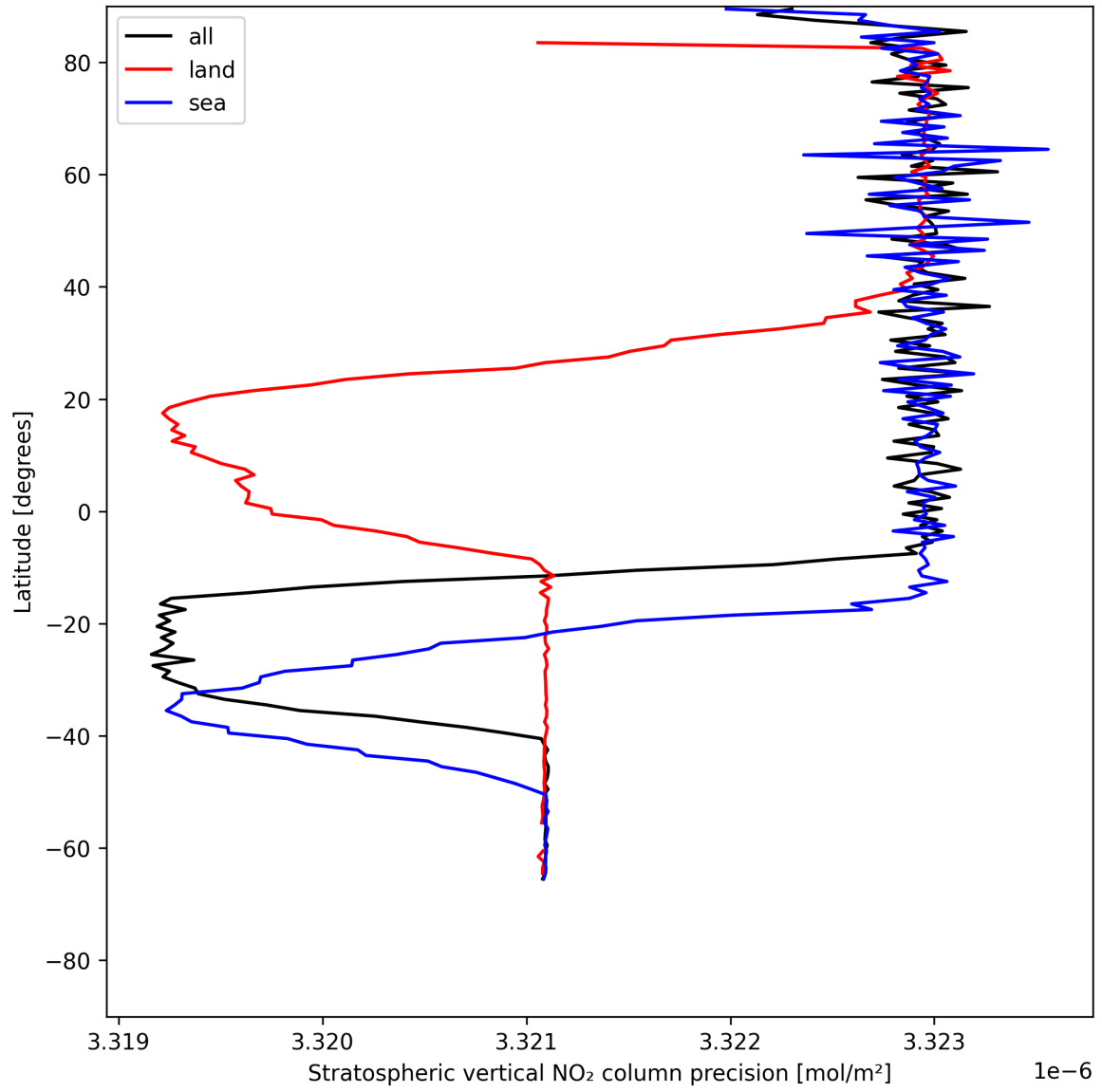
Figure 20: Zonal average of “Stratospheric vertical NO 2 column precision” for 2025-07-11 to 2025-07-13.
