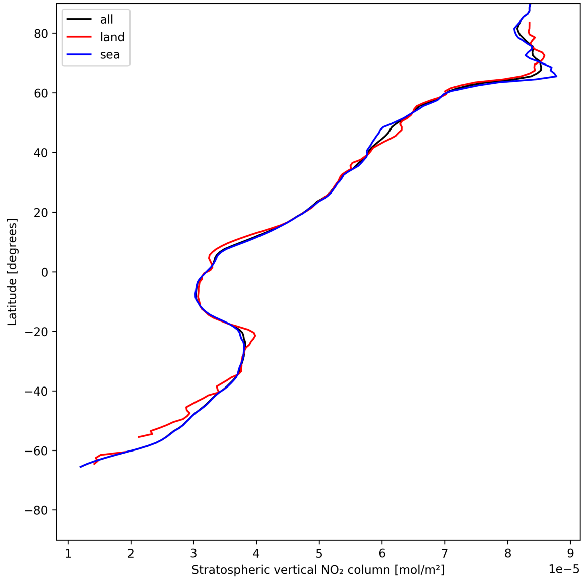
Figure 19: Zonal average of “Stratospheric vertical NO 2 column” for 2025-07-11 to 2025-07-13.
