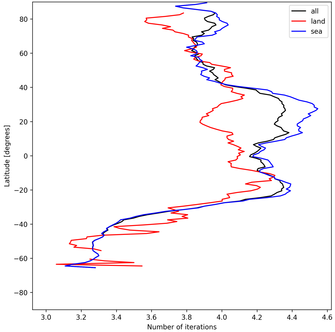
Figure 17: Zonal average of “Number of iterations” for 2025-07-11 to 2025-07-13.
