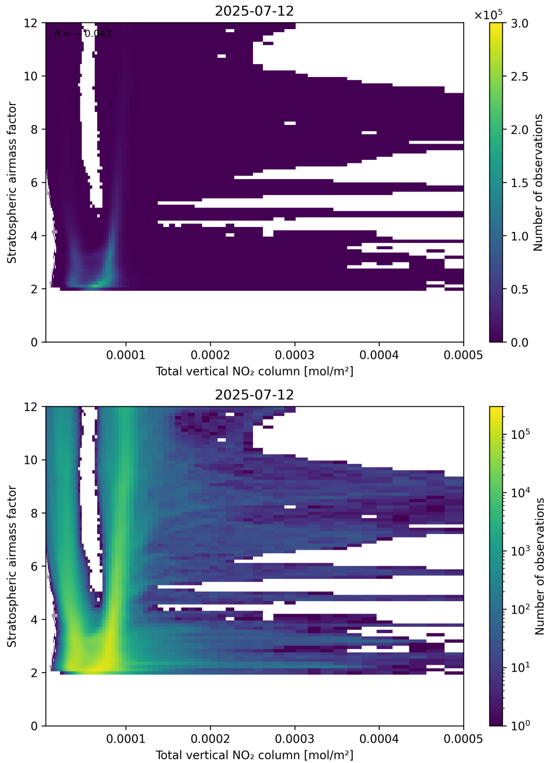
Figure 110: Scatter density plot of “Total vertical NO 2 column” against “Stratospheric air mass factor” for 2025-07-11 to 2025-07-13.
