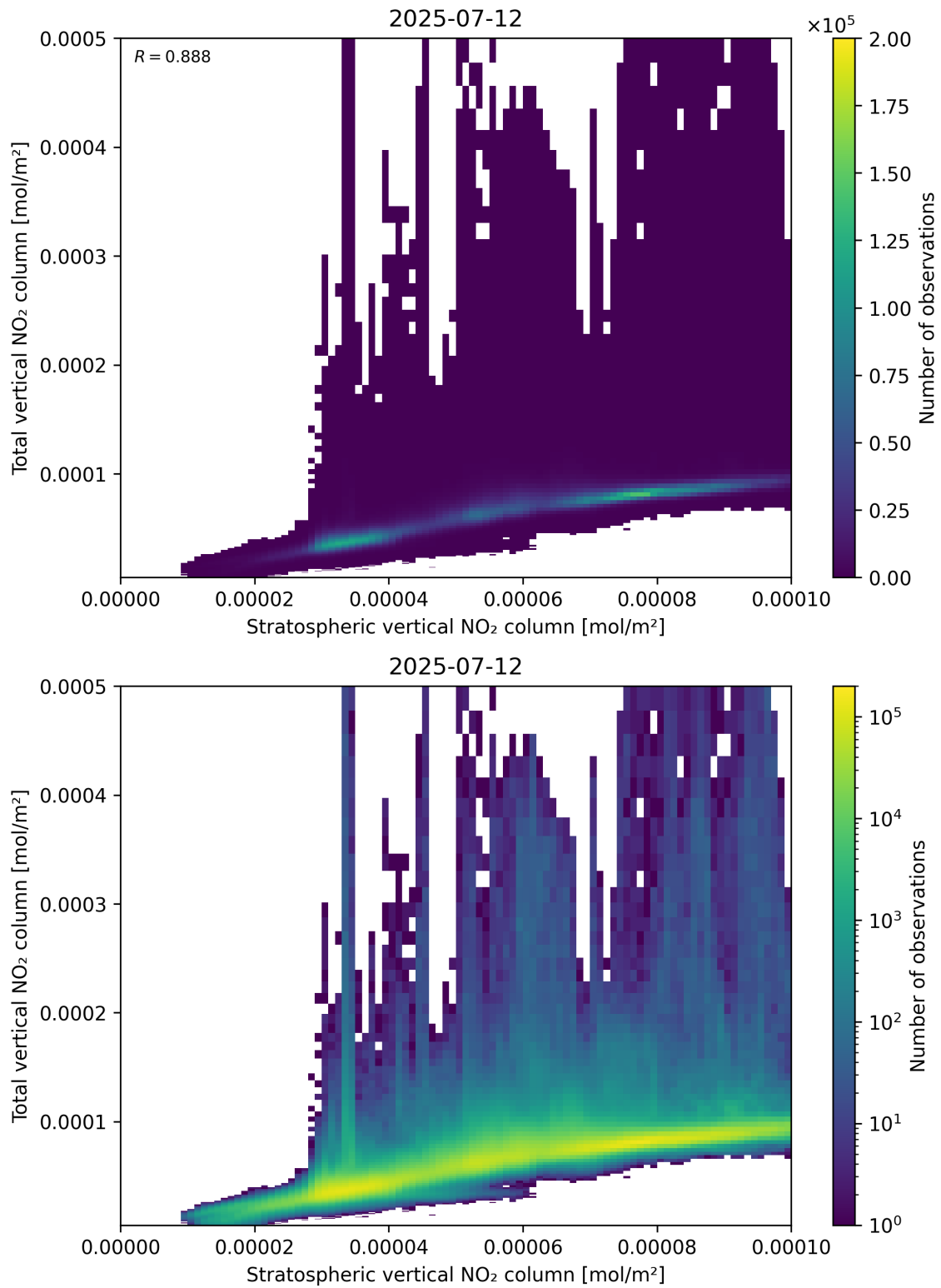
Figure 100: Scatter density plot of “Stratospheric vertical NO 2 column” against “Total vertical NO 2 column” for 2025-07-11 to 2025-07-13.
