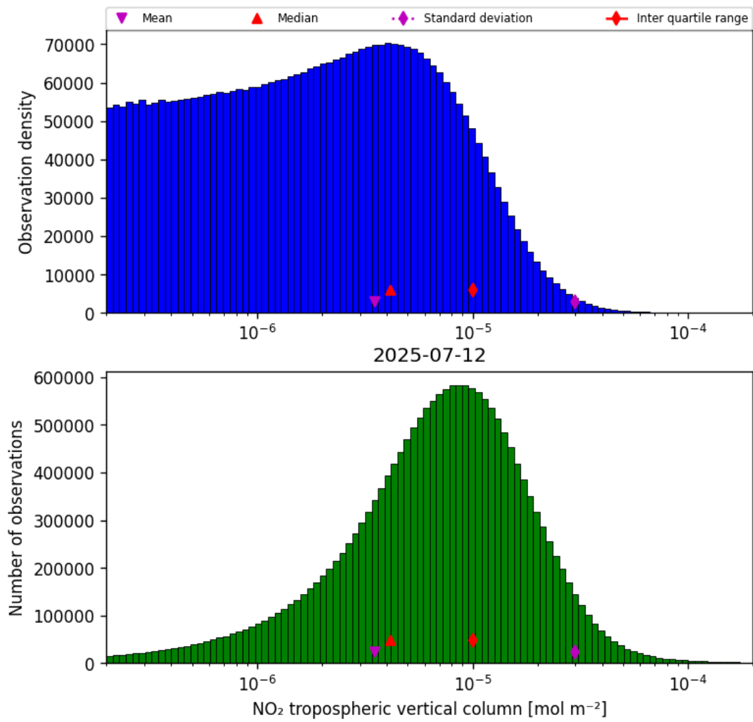
Figure 29: Histogram of “NO 2 tropospheric vertical column” for 2025-07-11 to 2025-07-13
