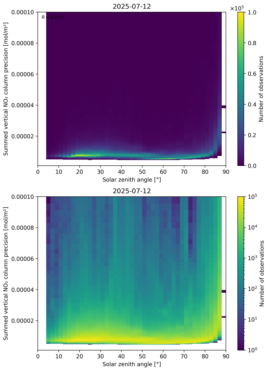
Figure 152: Scatter density plot of “Solar zenith angle” against “Summed vertical NO 2 column precision” for 2025-07-11 to 2025-07-13.
