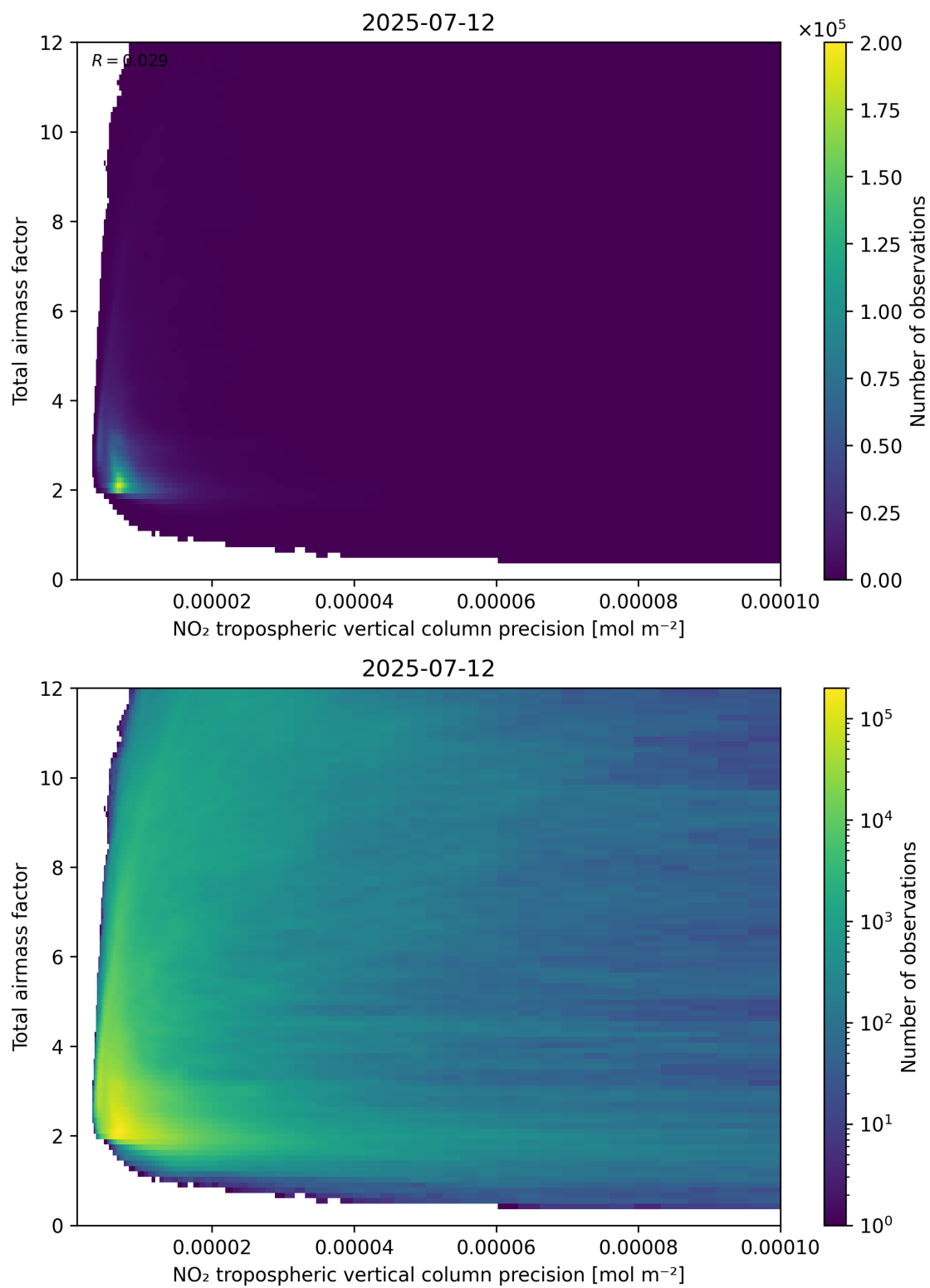
Figure 132: Scatter density plot of “NO 2 tropospheric vertical column precision” against “Total air mass factor” for 2025-07-11 to 2025-07-13.
