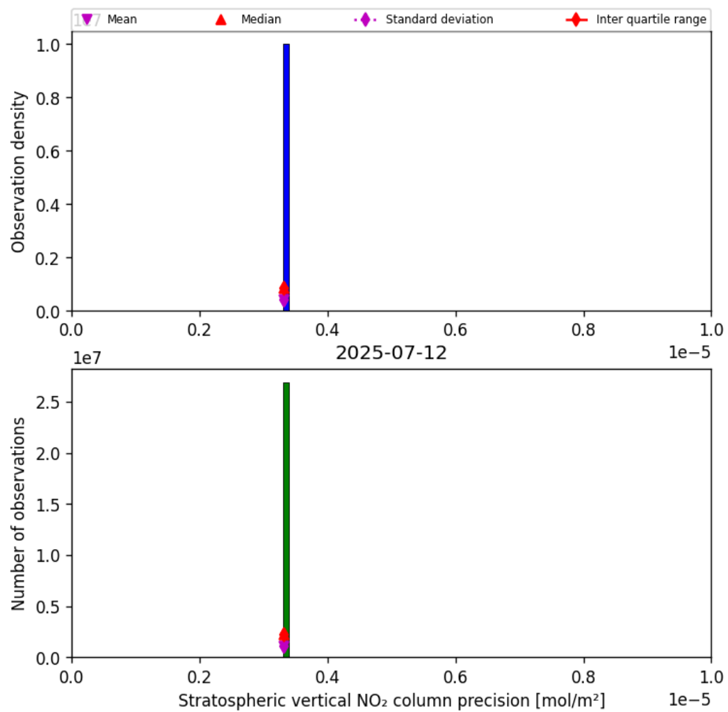
Figure 37: Histogram of “Stratospheric vertical NO 2 column precision” for 2025-07-11 to 2025-07-13
