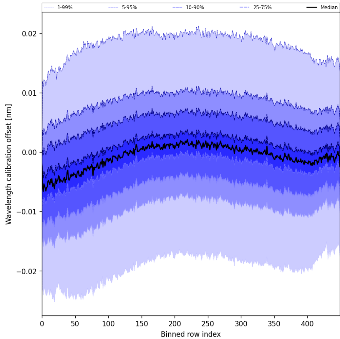
Figure 52: Along track statistics of “Wavelength calibration offset” for 2025-07-11 to 2025-07-13
