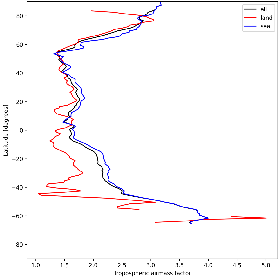
Figure 14: Zonal average of “Tropospheric airmass factor” for 2025-07-11 to 2025-07-13.
