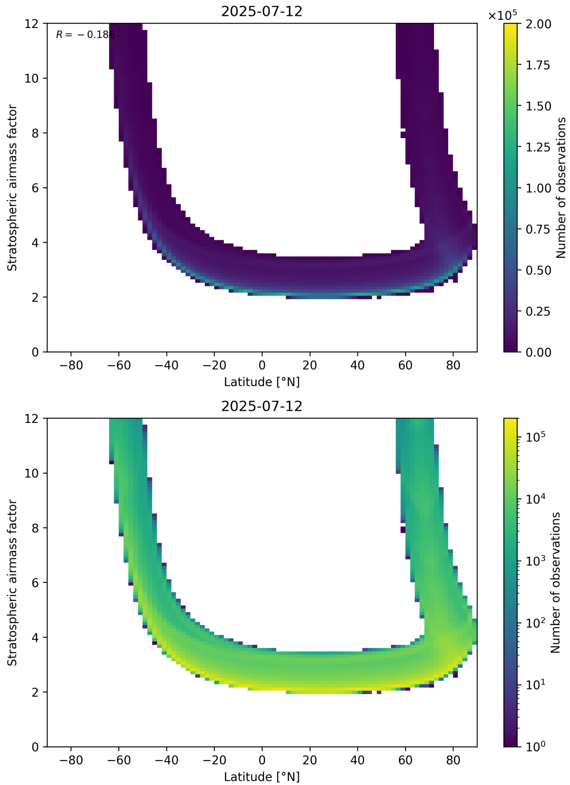
Figure 83: Scatter density plot of “Latitude” against “Stratospheric air mass factor” for 2025-07-11 to 2025-07-13.
