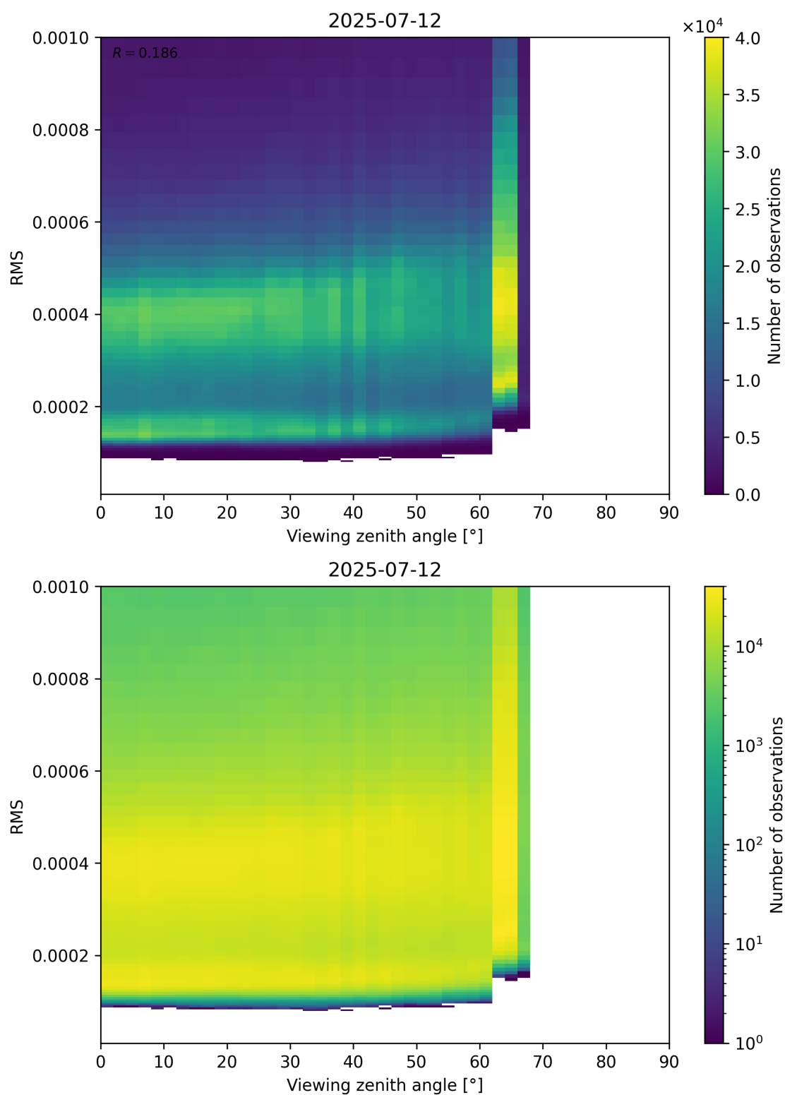
Figure 171: Scatter density plot of “Viewing zenith angle” against “RMS” for 2025-07-11 to 2025-07-13.
