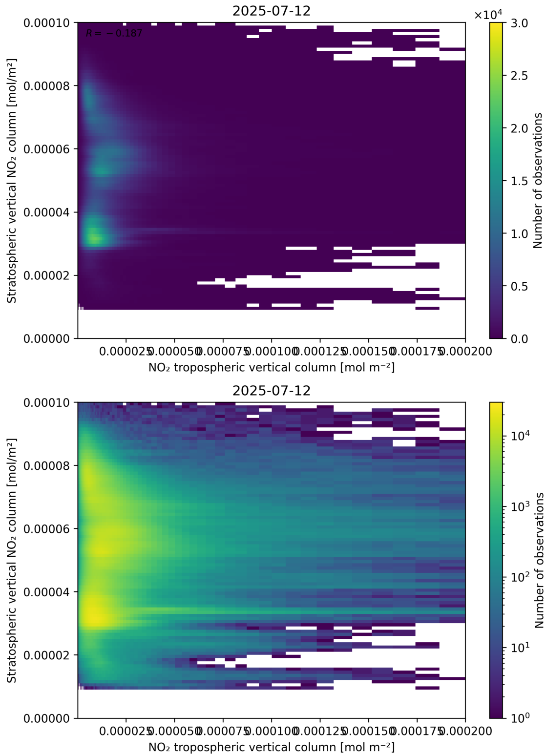
Figure 125: Scatter density plot of “NO 2 tropospheric vertical column” against “Stratospheric vertical NO 2 column” for 2025-07-11 to 2025-07-13.
