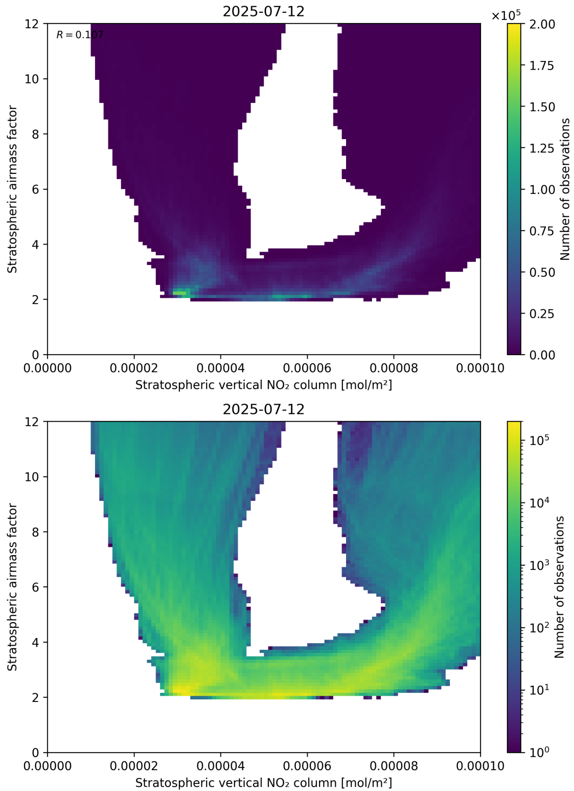
Figure 96: Scatter density plot of “Stratospheric vertical NO 2 column” against “Stratospheric airmass factor” for 2025-07-11 to 2025-07-13.
