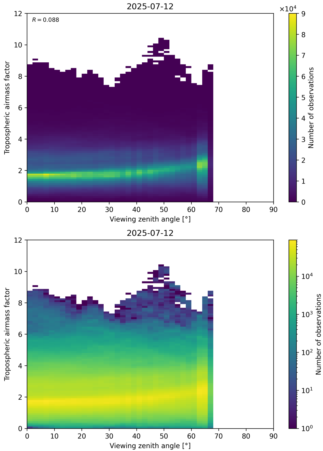
Figure 161: Scatter density plot of “Viewing zenith angle” against “Tropospheric airmass factor” for 2025-07-11 to 2025-07-13.
