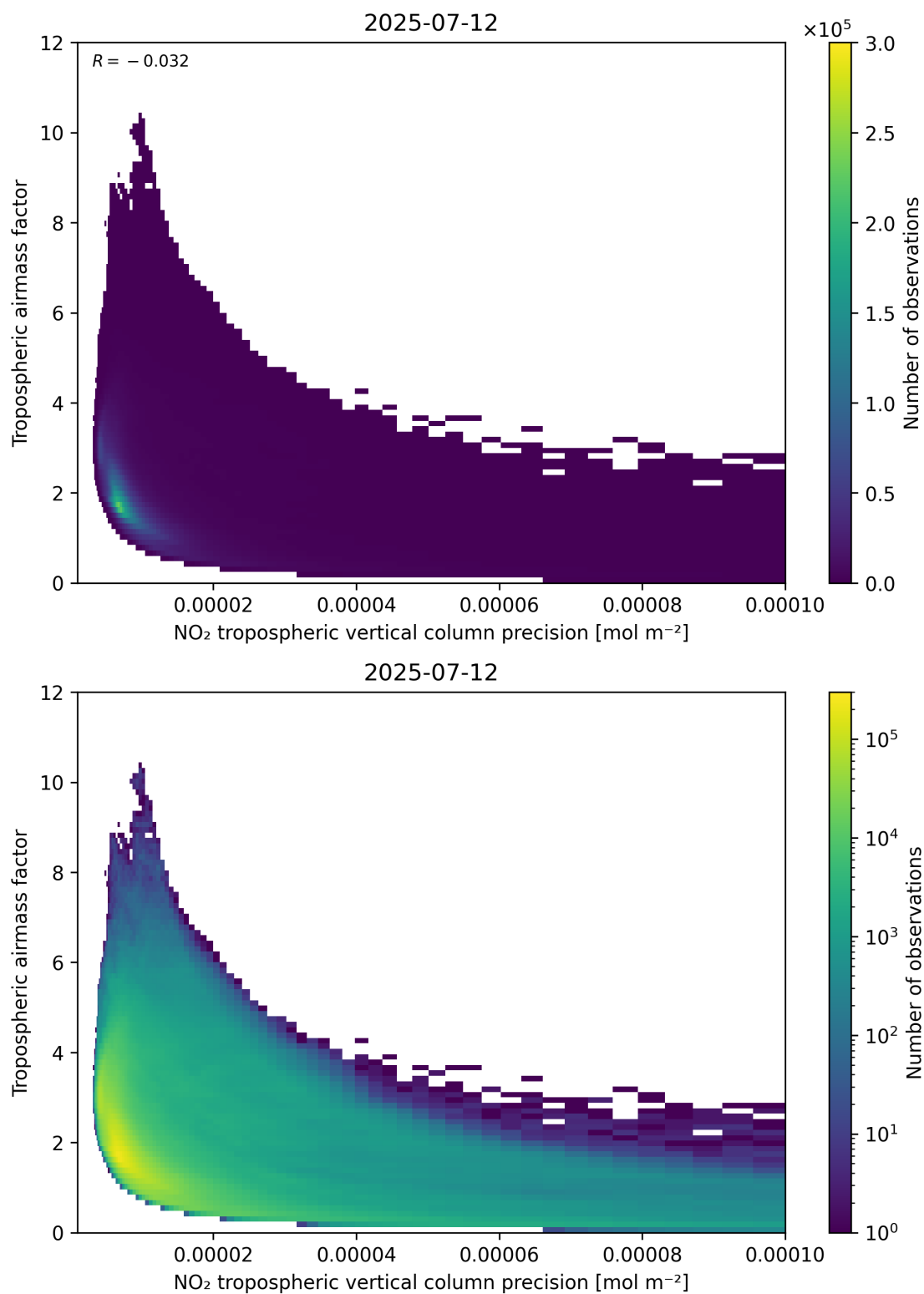
Figure 133: Scatter density plot of “NO 2 tropospheric vertical column precision” against “Tropospheric airmass factor” for 2025-07-11 to 2025-07-13.
