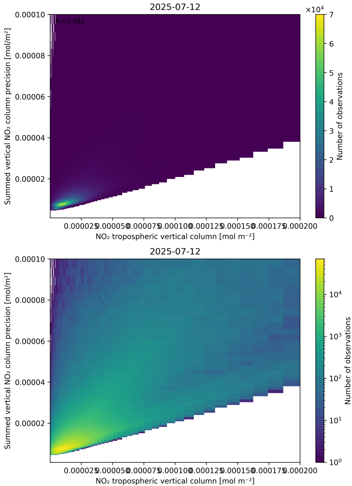
Figure 127: Scatter density plot of “NO 2 tropospheric vertical column” against “Summed vertical NO 2 column precision” for 2025-07-11 to 2025-07-13.
