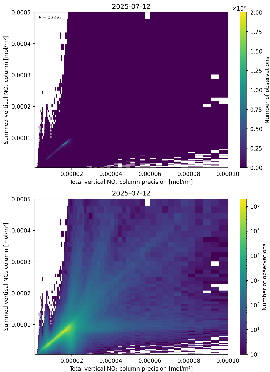
Figure 117: Scatter density plot of “Total vertical NO 2 column precision” against “Summed vertical NO 2 column” for 2025-07-11 to 2025-07-13.
