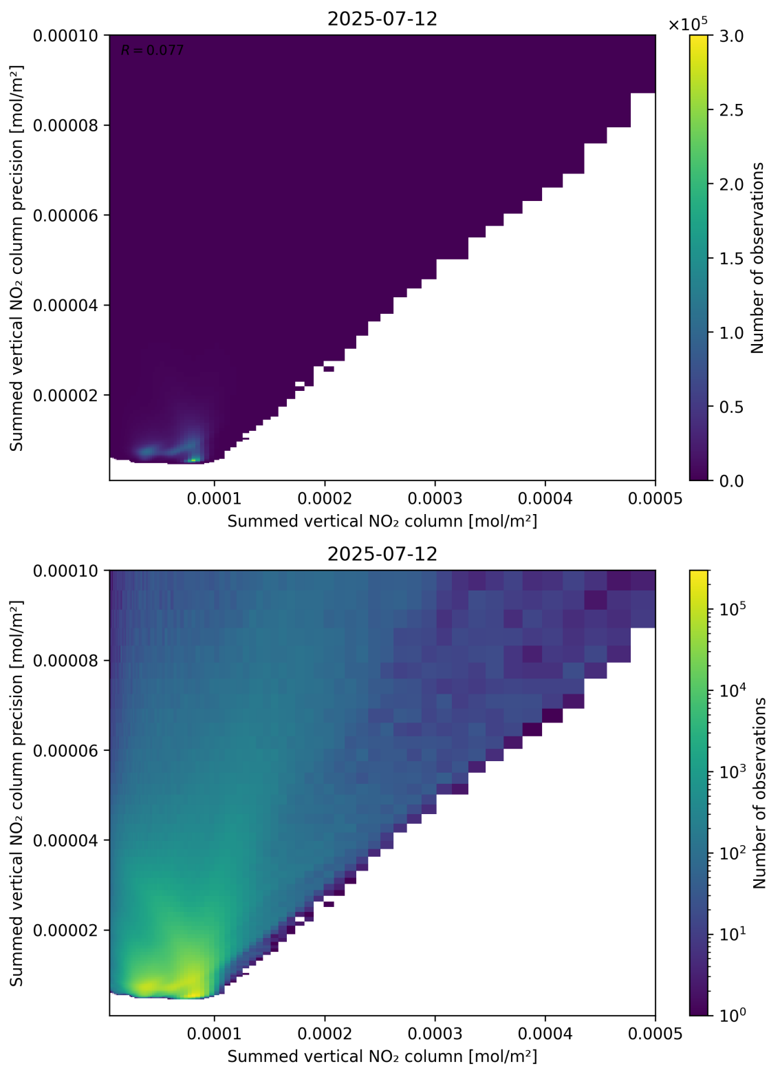
Figure 105: Scatter density plot of “Summed vertical NO 2 column” against “Summed vertical NO 2 column precision” for 2025-07-11 to 2025-07-13.
