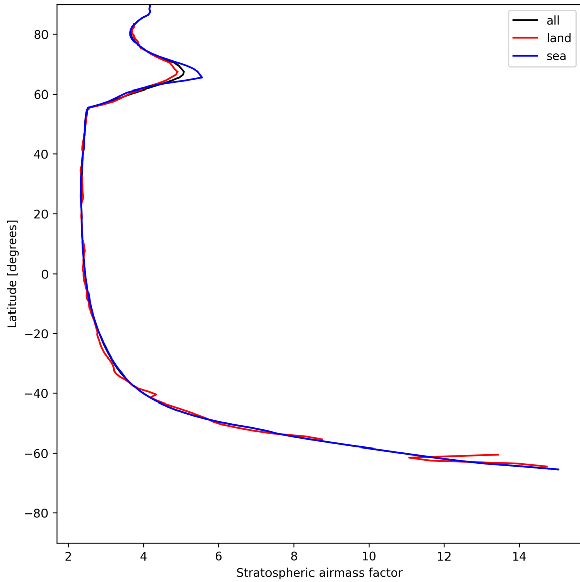
Figure 27: Zonal average of “Stratospheric air mass factor” for 2025-07-11 to 2025-07-13.
