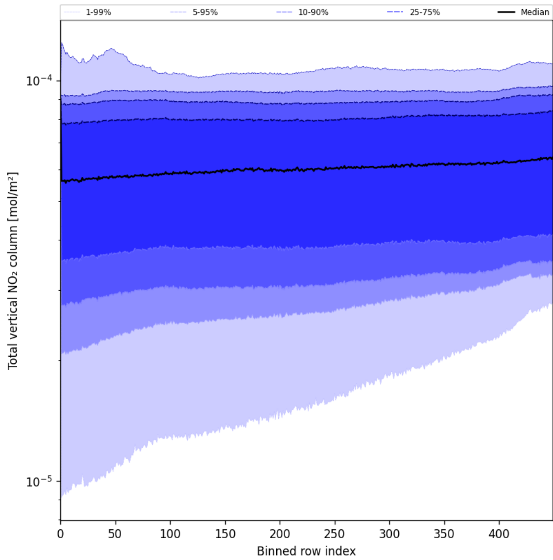
Figure 55: Along track statistics of “Total vertical NO 2 column” for 2025-07-11 to 2025-07-13
