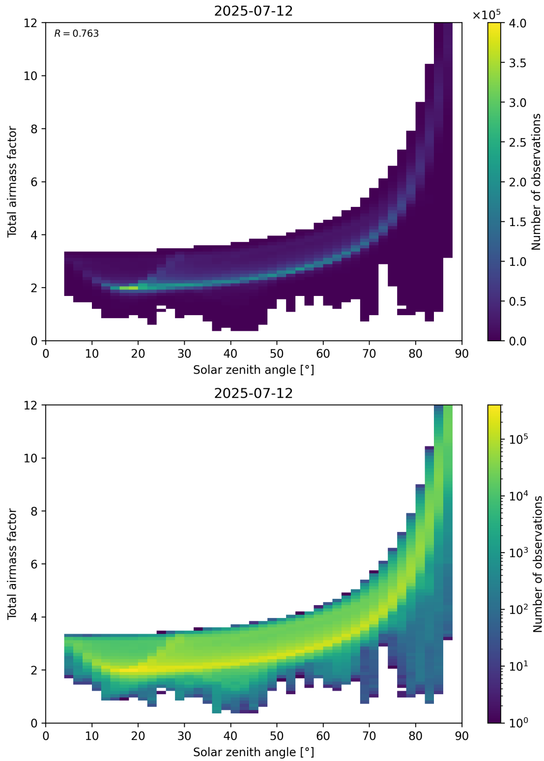
Figure 146: Scatter density plot of “Solar zenith angle” against “Total air mass factor” for 2025-07-11 to 2025-07-13.
