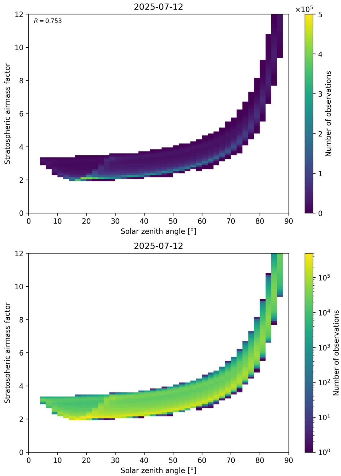
Figure 145: Scatter density plot of “Solar zenith angle” against “Stratospheric airmass factor” for 2025-07-11 to 2025-07-13.
