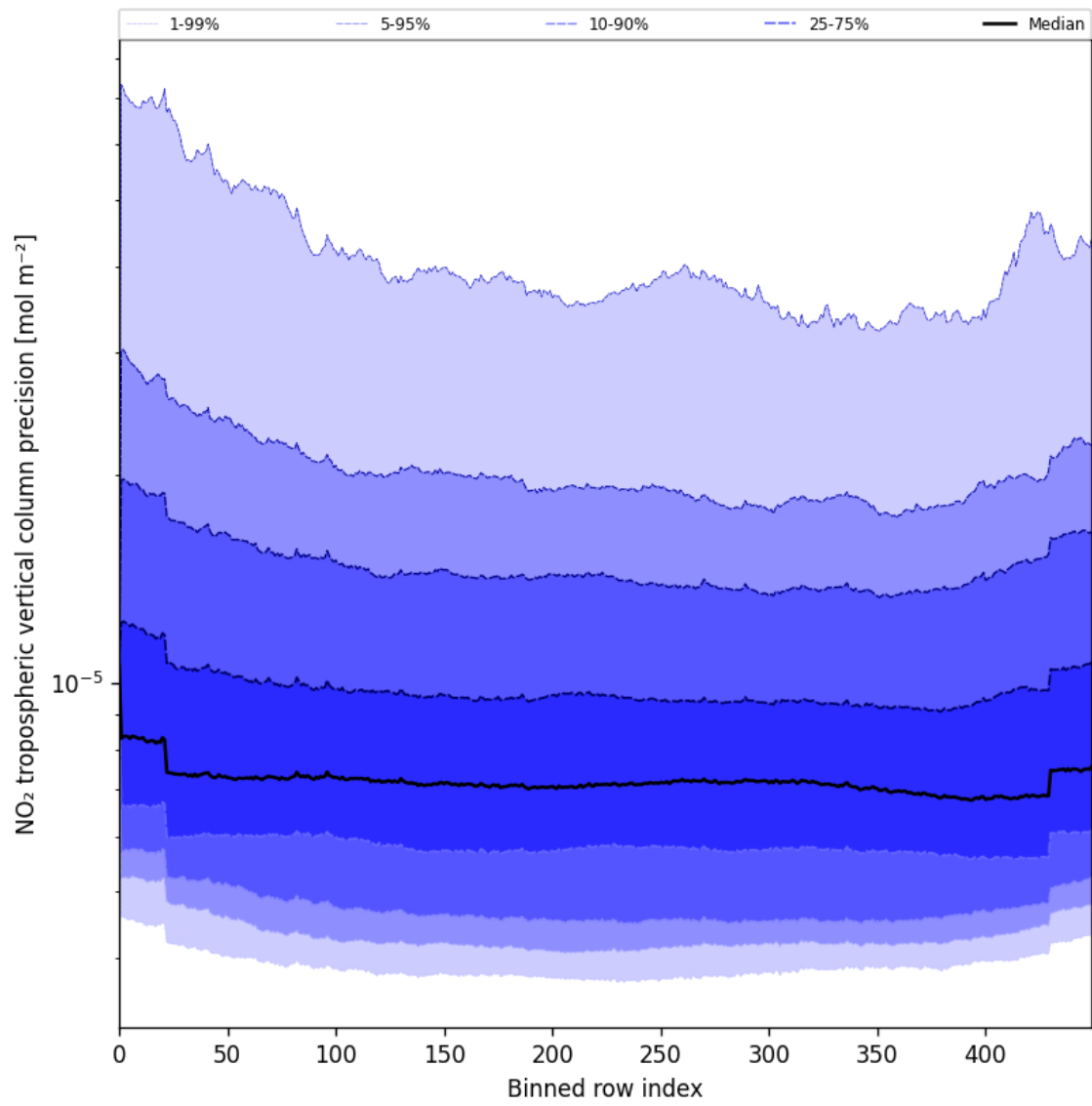
Figure 47: Along track statistics of “NO 2 tropospheric vertical column precision” for 2025-07-11 to 2025-07-13
