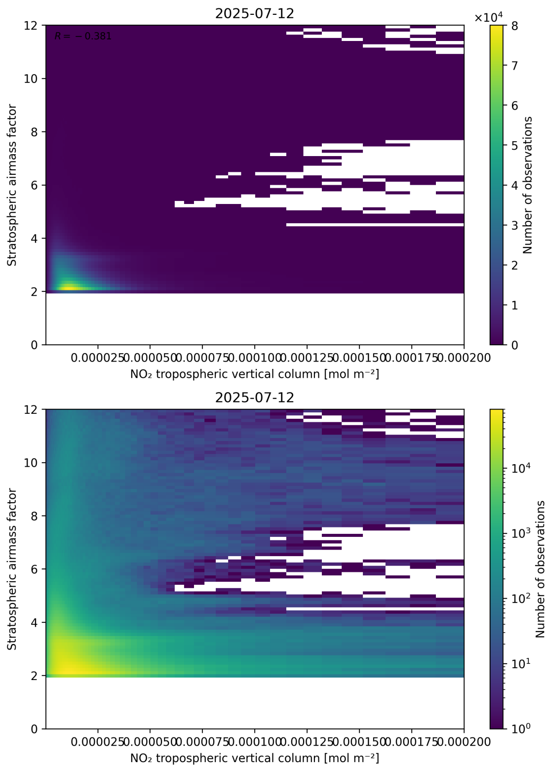
Figure 121: Scatter density plot of “NO 2 tropospheric vertical column” against “Stratospheric air mass factor” for 2025-07-11 to 2025-07-13.
