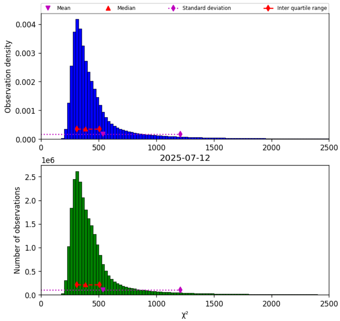
Figure 42: Histogram of “ \chi^2 ” for 2025-07-11 to 2025-07-13
