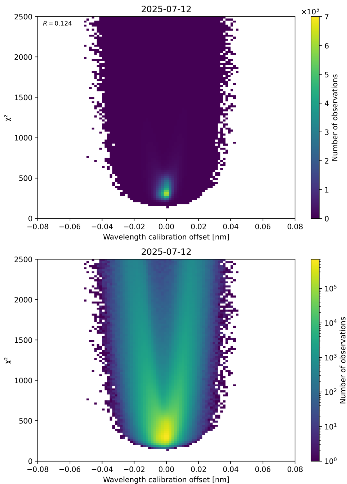
Figure 175: Scatter density plot of “Wavelength calibration offset” against “ \chi^2 ” for 2025-07-11 to 2025-07-13.
