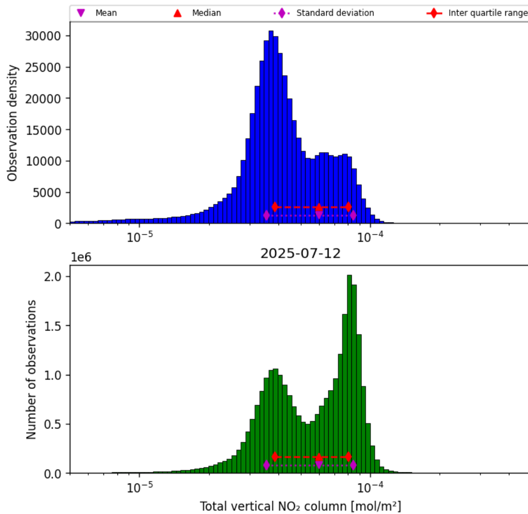
Figure 38: Histogram of “Total vertical NO 2 column” for 2025-07-11 to 2025-07-13
