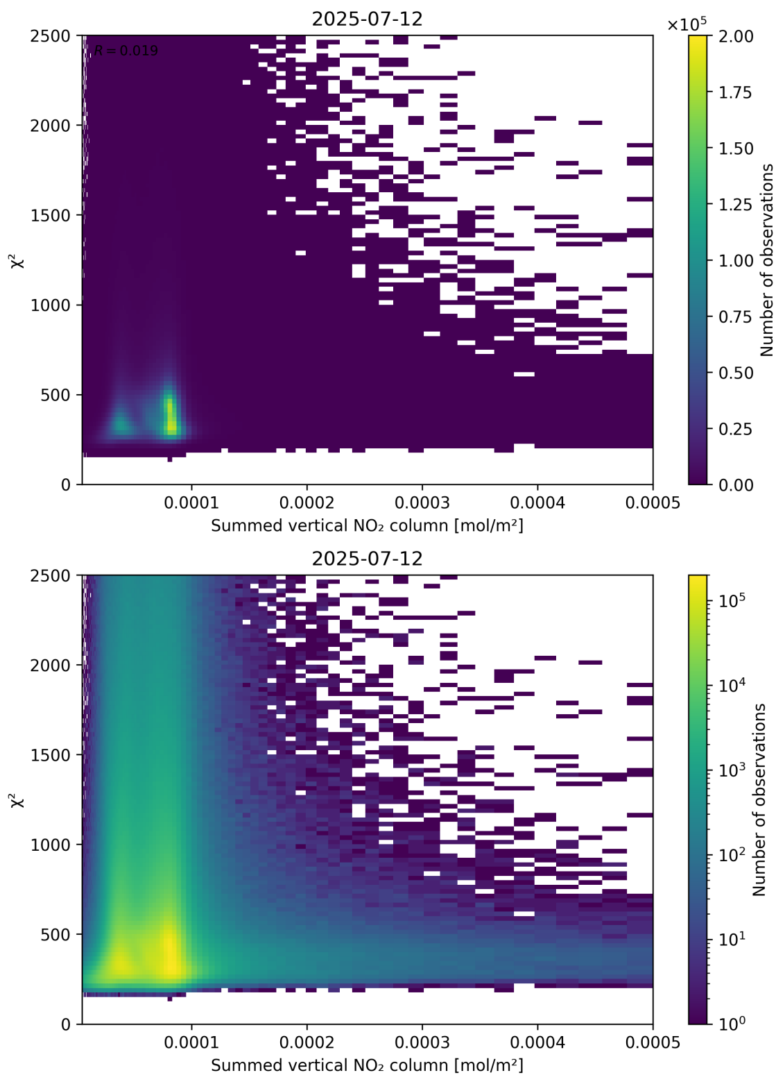
Figure 104: Scatter density plot of “Summed vertical NO 2 column” against “ \chi^2 ” for 2025-07-11 to 2025-07-13.
