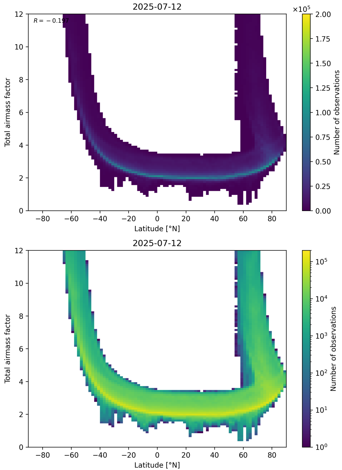
Figure 84: Scatter density plot of “Latitude” against “Total airmass factor” for 2025-07-11 to 2025-07-13.
