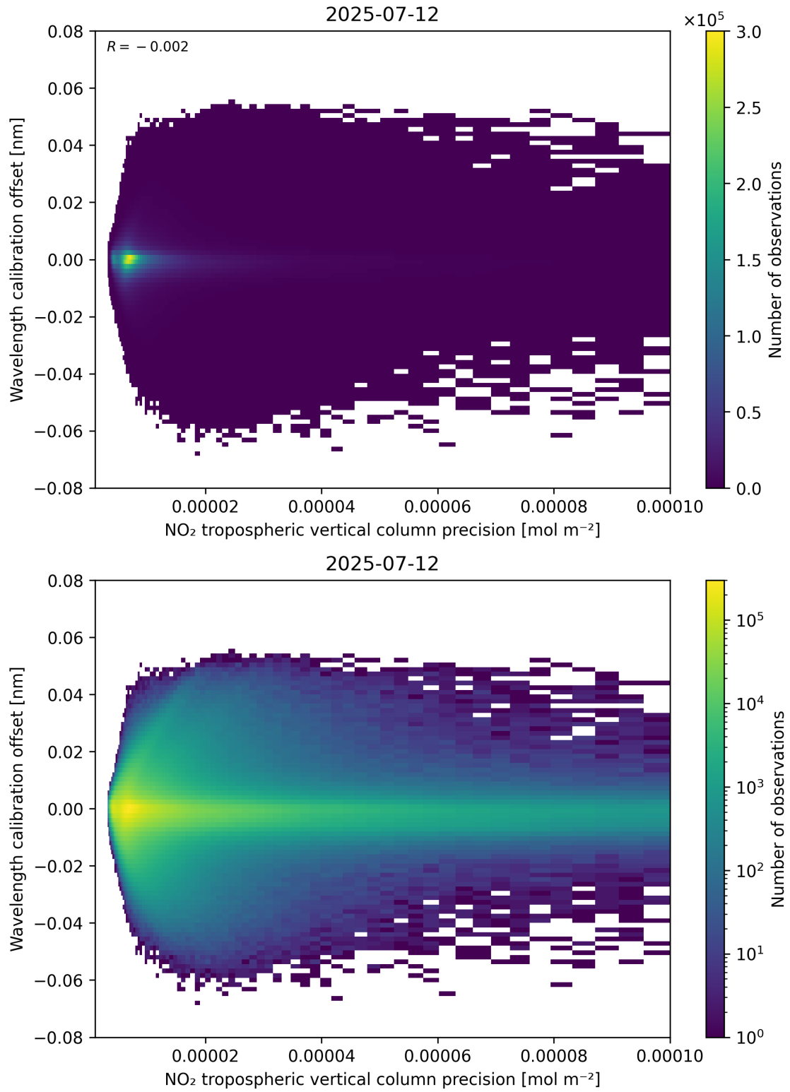
Figure 141: Scatter density plot of “NO 2 tropospheric vertical column precision” against “Wavelength calibration offset” for 2025-07-11 to 2025-07-13.
