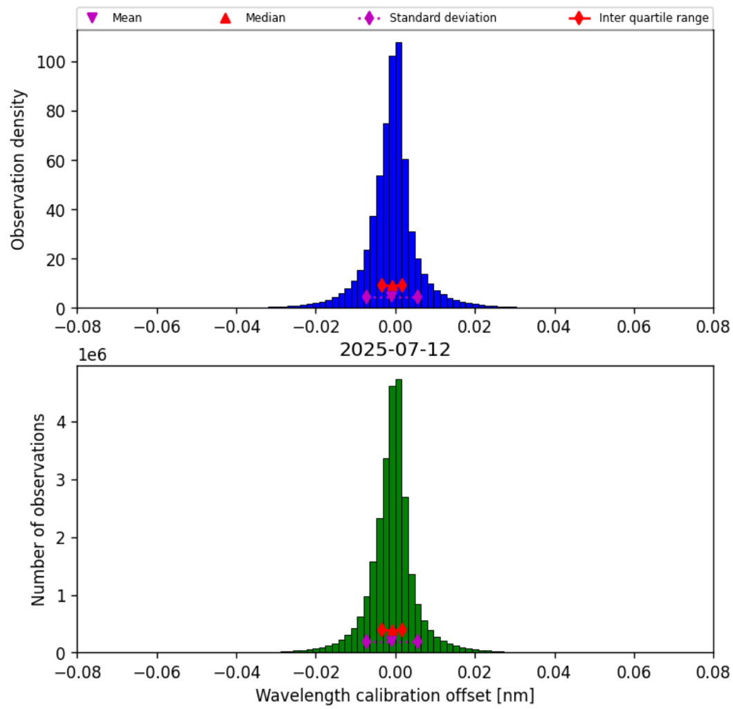
Figure 35: Histogram of “Wavelength calibration offset” for 2025-07-11 to 2025-07-13
