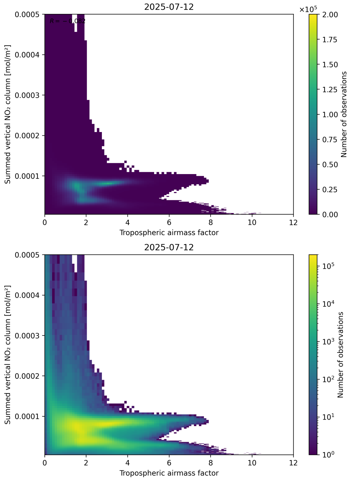
Figure 75: Scatter density plot of “Tropospheric air mass factor” against “Summed vertical NO 2 column” for 2025-07-11 to 2025-07-13.
