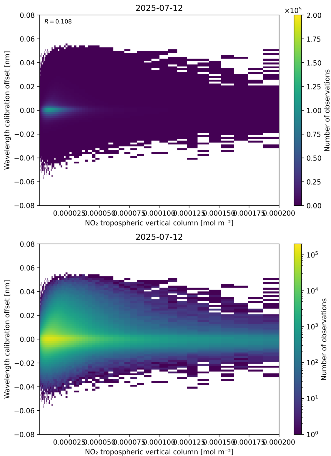
Figure 143: Scatter density plot of “NO 2 tropospheric vertical column” against “Wavelength calibration offset” for 2025-07-11 to 2025-07-13.
