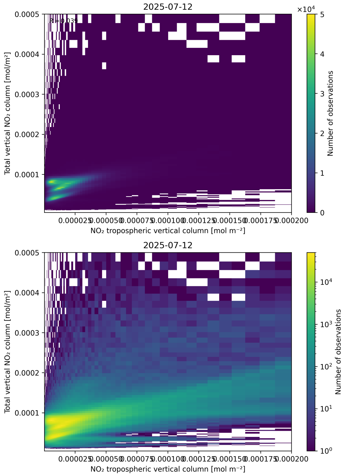
Figure 128: Scatter density plot of “NO 2 tropospheric vertical column” against “Total vertical NO 2 column” for 2025-07-11 to 2025-07-13.
