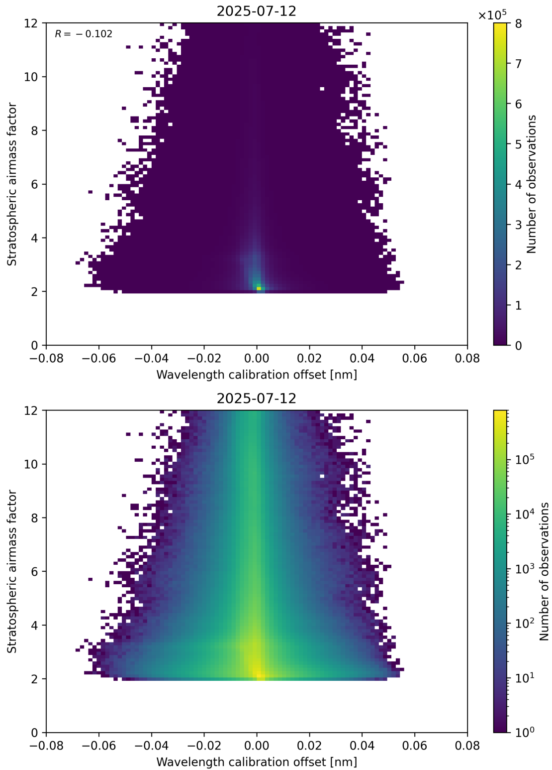
Figure 174: Scatter density plot of “Wavelength calibration offset” against “Stratospheric airmass factor” for 2025-07-11 to 2025-07-13.
