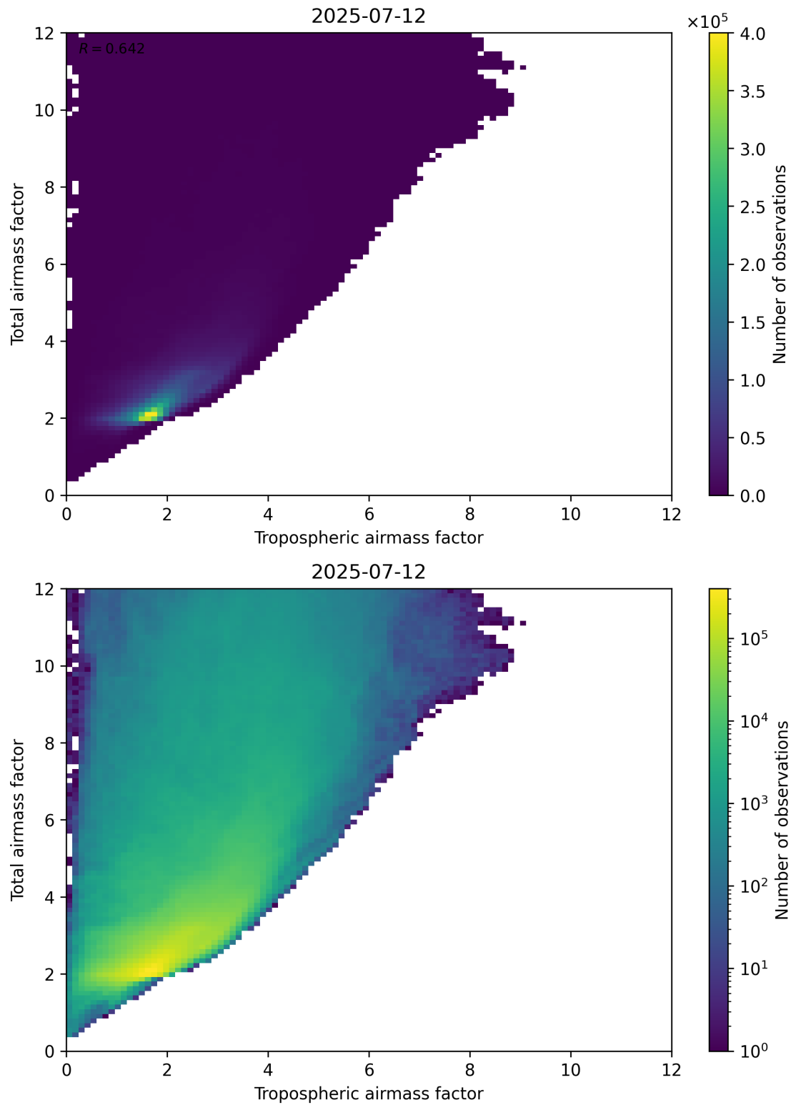
Figure 72: Scatter density plot of “Tropospheric airmass factor” against “Total airmass factor” for 2025-07-11 to 2025-07-13.
