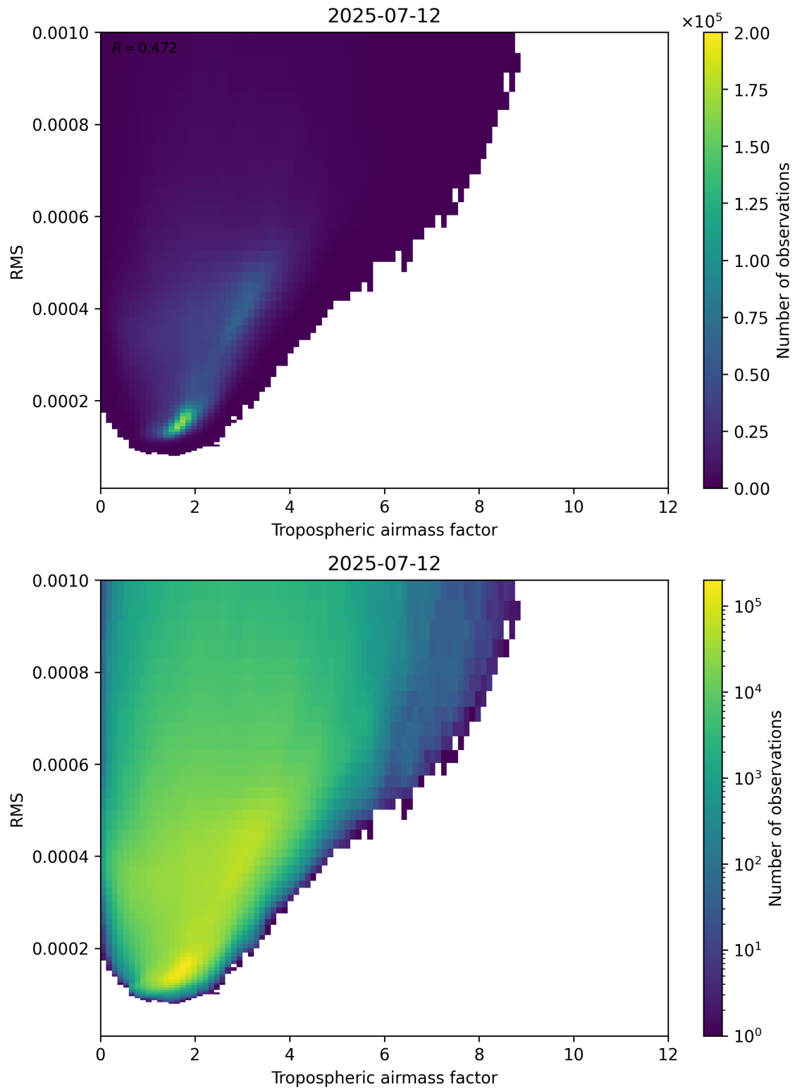
Figure 79: Scatter density plot of “Tropospheric airmass factor” against “RMS” for 2025-07-11 to 2025-07-13.
