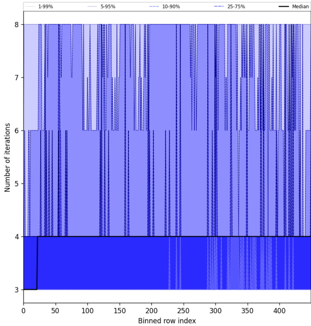
Figure 51: Along track statistics of “Number of iterations” for 2025-07-11 to 2025-07-13
