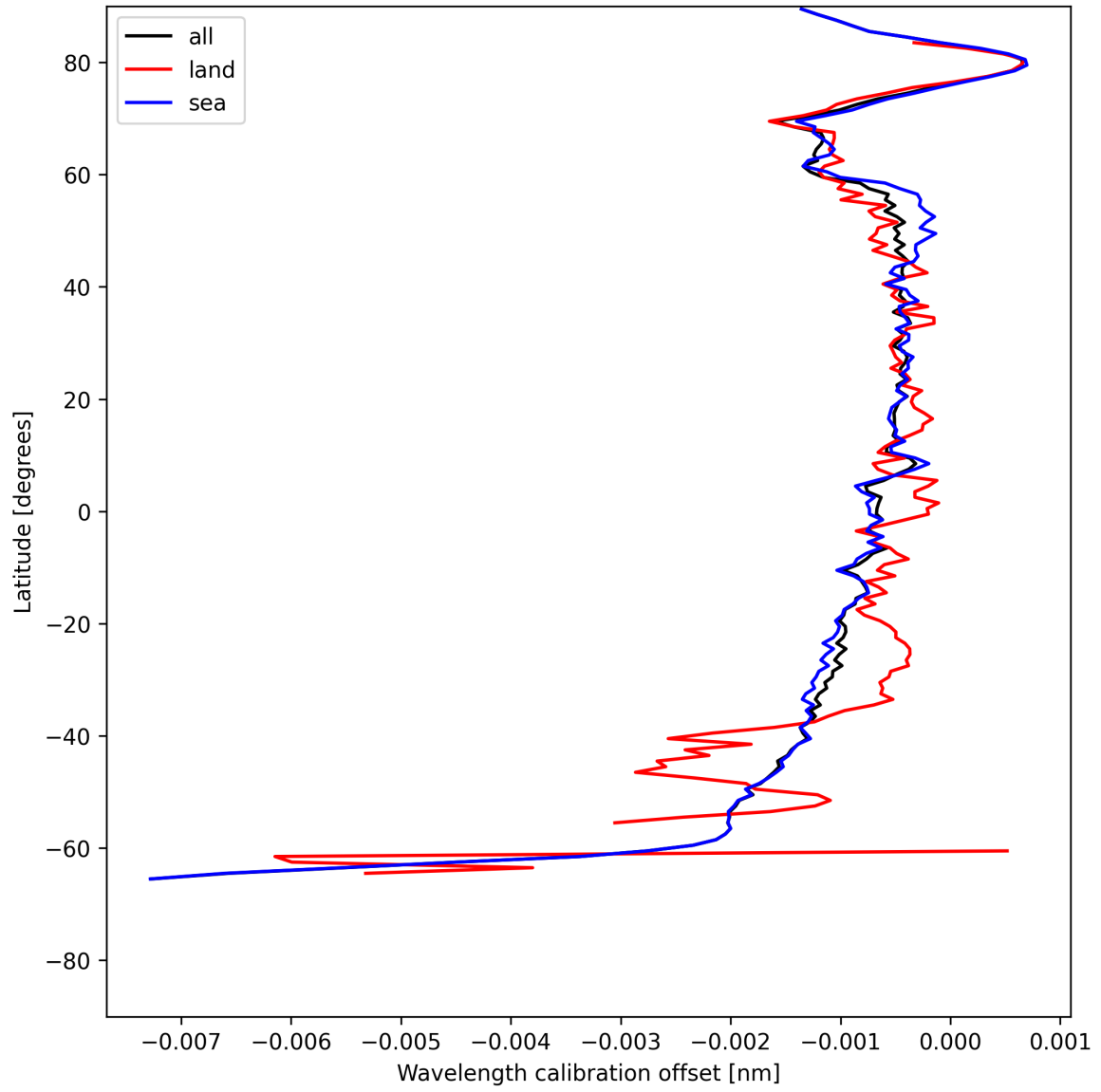
Figure 18: Zonal average of “Wavelength calibration offset” for 2025-07-11 to 2025-07-13.
