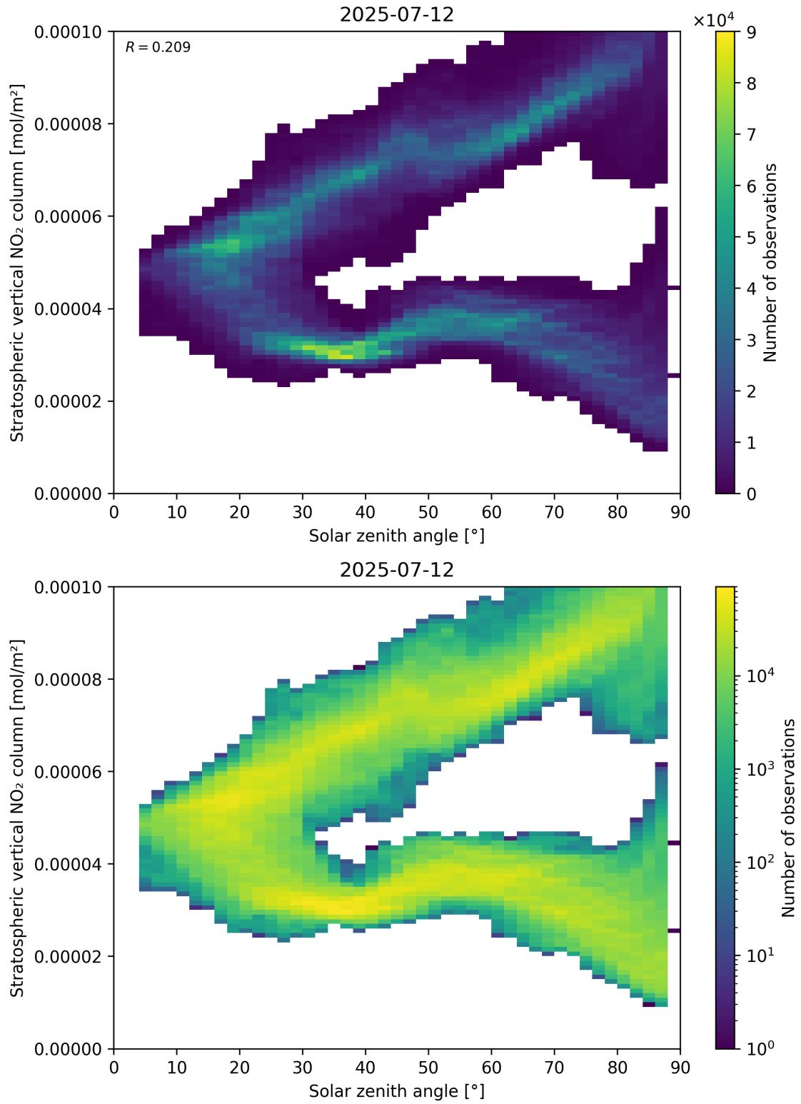
Figure 150: Scatter density plot of “Solar zenith angle” against “Stratospheric vertical NO 2 column” for 2025-07-11 to 2025-07-13.
