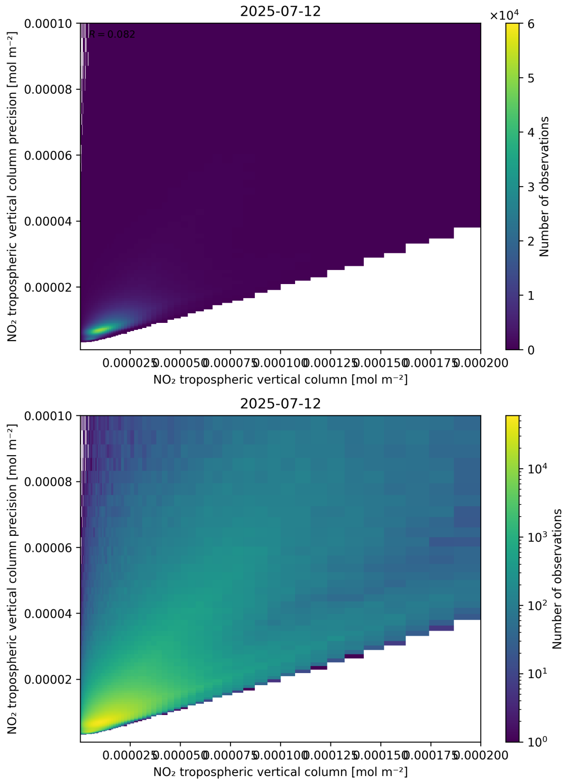
Figure 130: Scatter density plot of “NO 2 tropospheric vertical column” against “NO 2 tropospheric vertical column precision” for 2025-07-11 to 2025-07-13.
