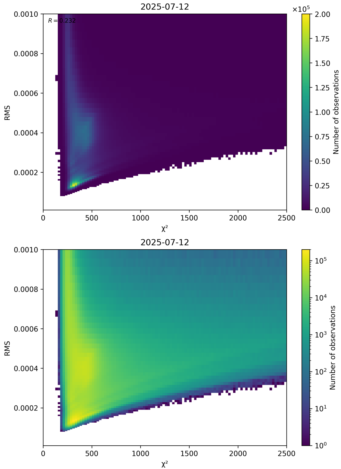
Figure 82: Scatter density plot of “ \chi^2 ” against “RMS” for 2025-07-11 to 2025-07-13.
