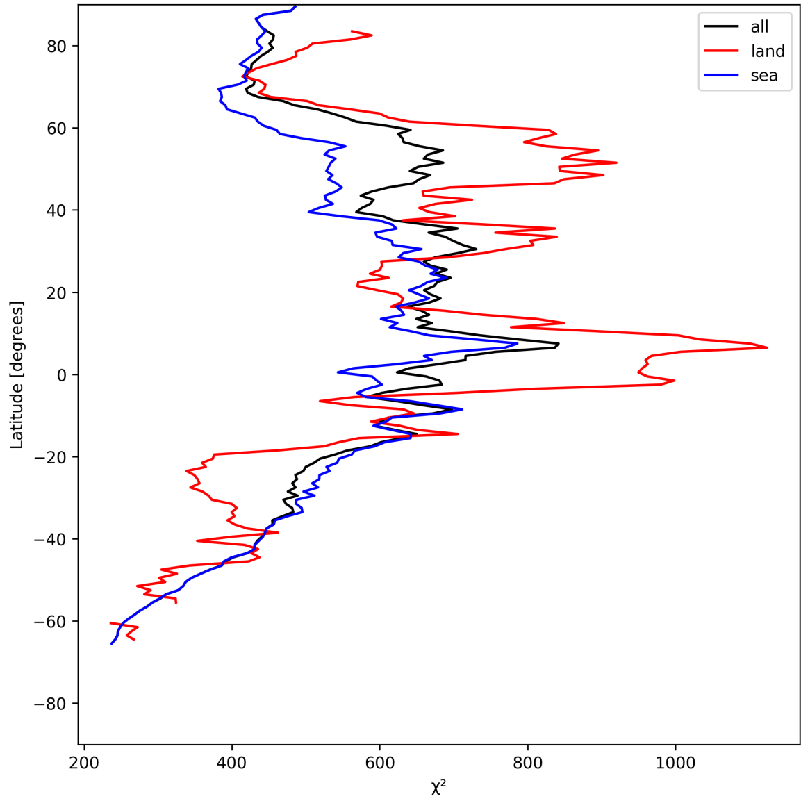
Figure 25: Zonal average of “ \chi^2 ” for 2025-07-11 to 2025-07-13.
