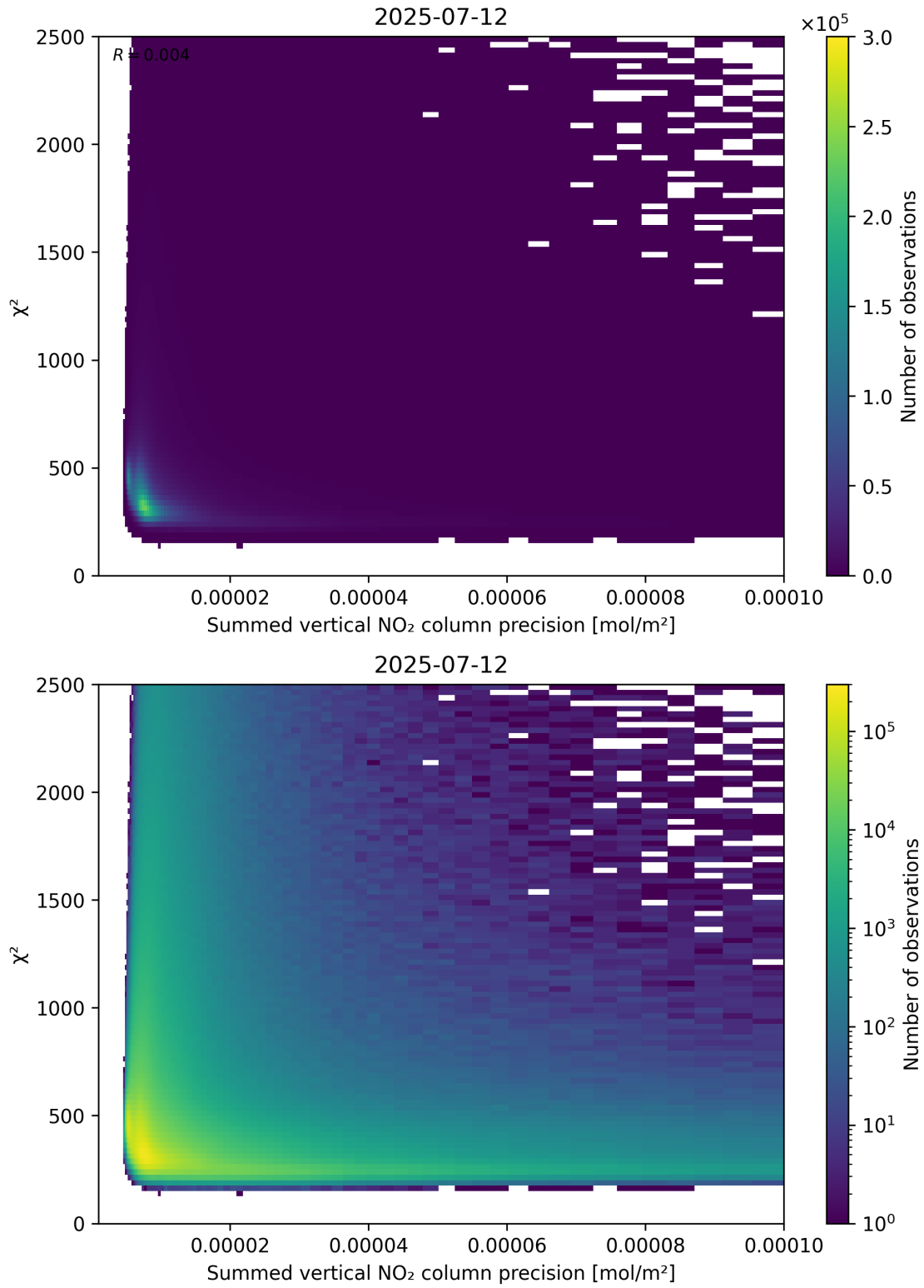
Figure 107: Scatter density plot of “Summed vertical NO 2 column precision” against “ \chi^2 ” for 2025-07-11 to 2025-07-13.
