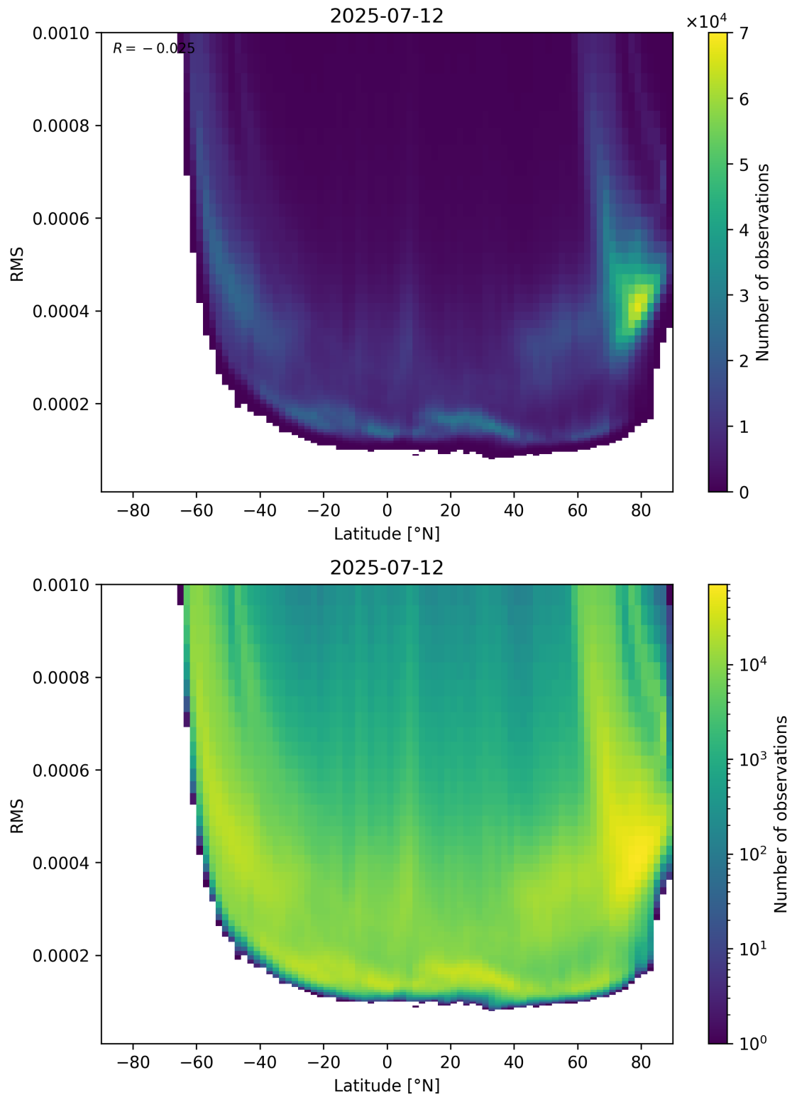
Figure 94: Scatter density plot of “Latitude” against “RMS” for 2025-07-11 to 2025-07-13.
