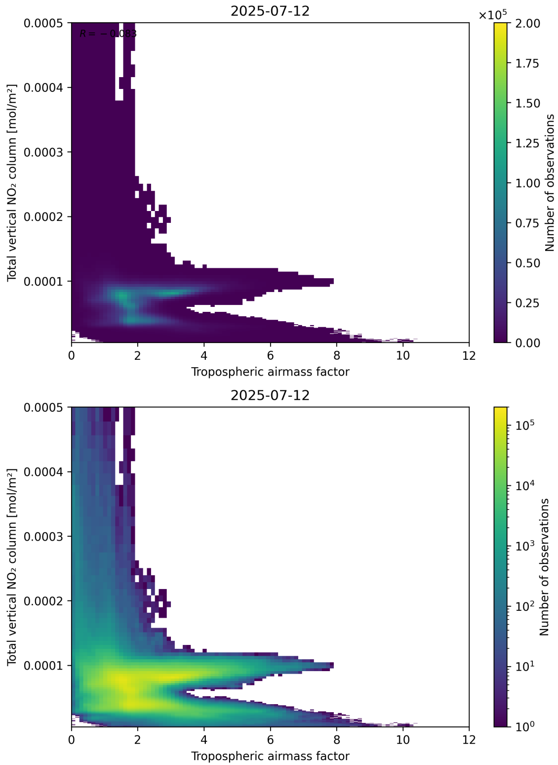
Figure 77: Scatter density plot of “Tropospheric airmass factor” against “Total vertical NO 2 column” for 2025-07-11 to 2025-07-13.
