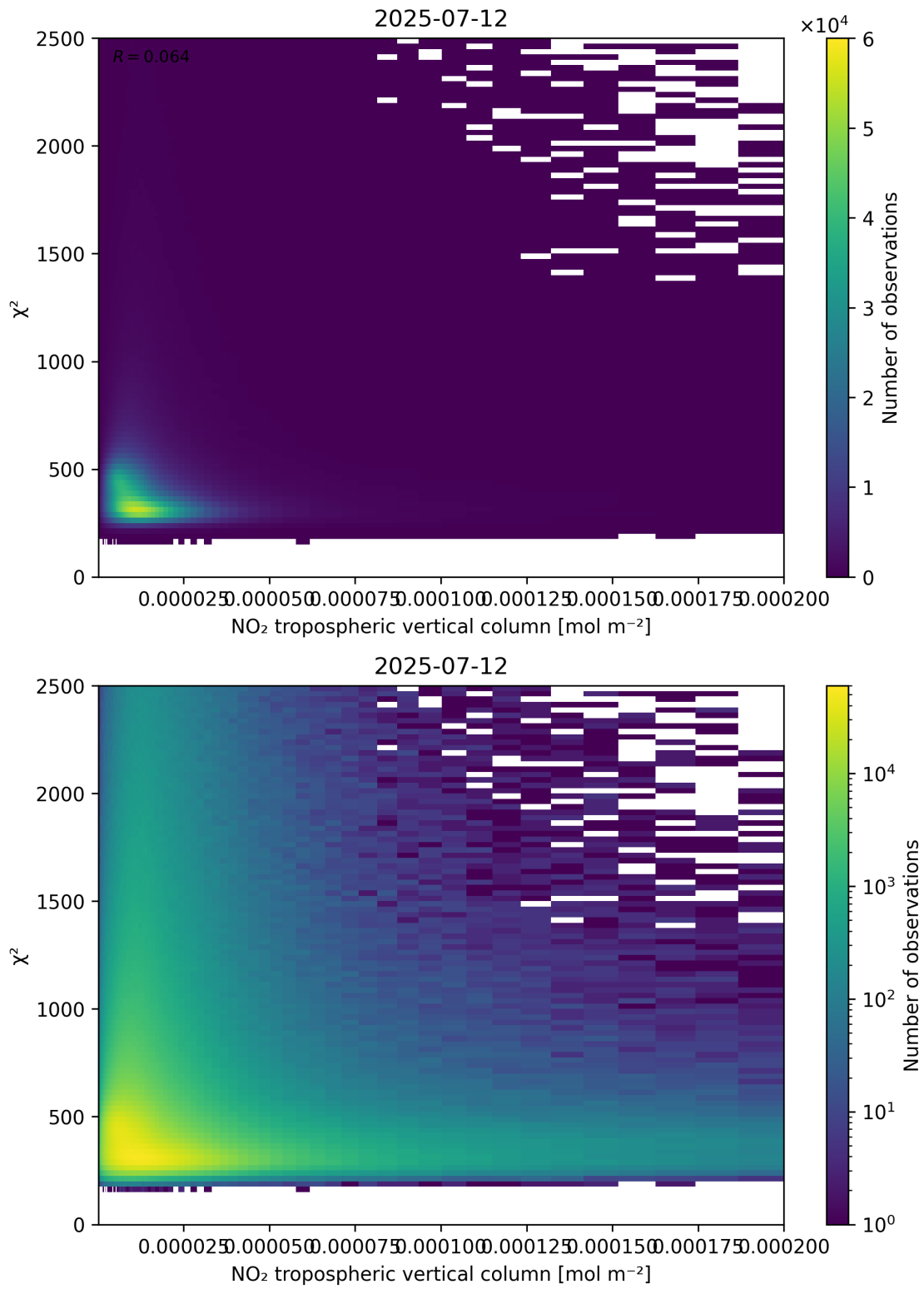
Figure 124: Scatter density plot of “NO 2 tropospheric vertical column” against “ \chi^2 ” for 2025-07-11 to 2025-07-13.
