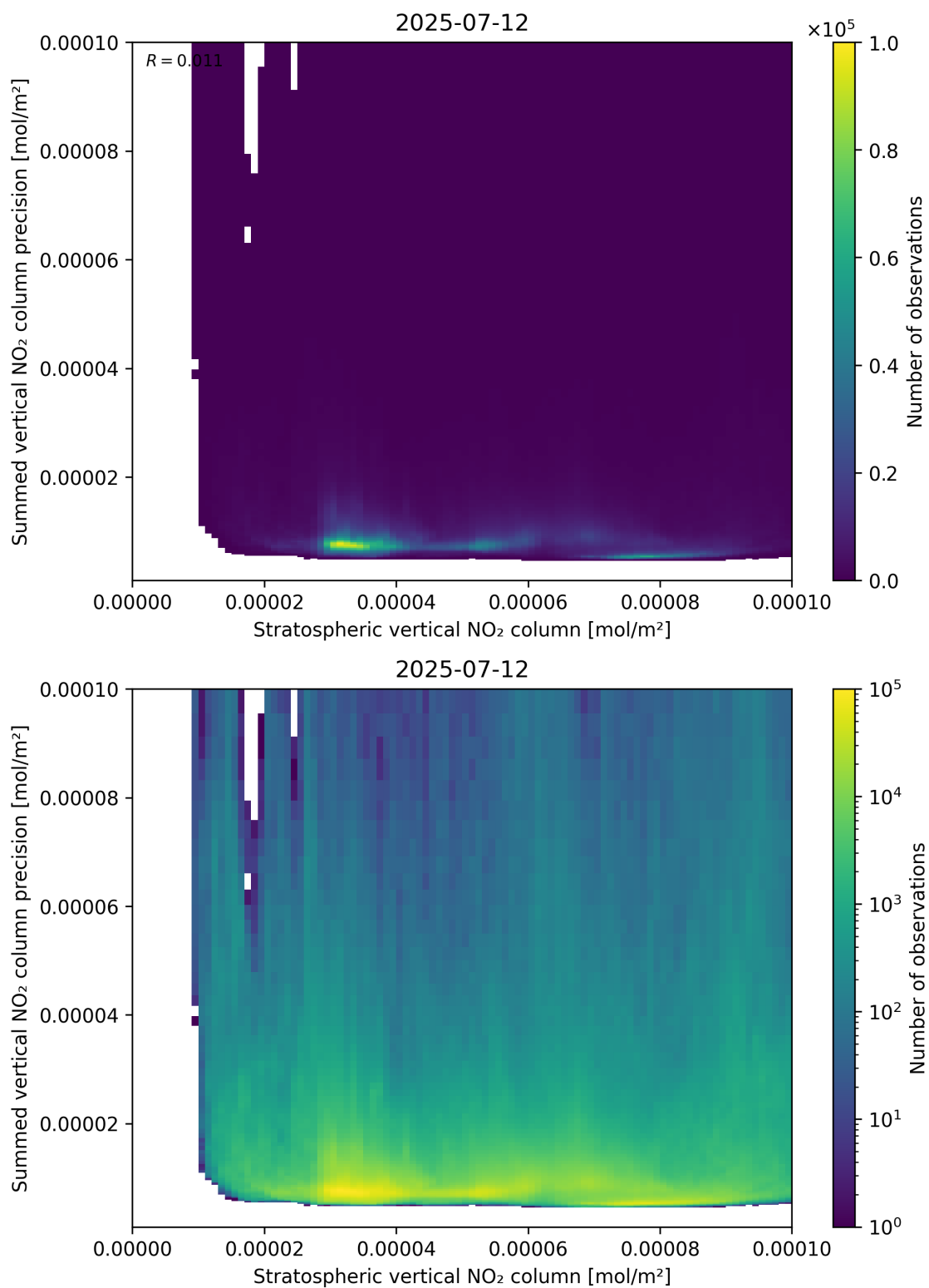
Figure 99: Scatter density plot of “Stratospheric vertical NO 2 column” against “Summed vertical NO 2 column precision” for 2025-07-11 to 2025-07-13.
