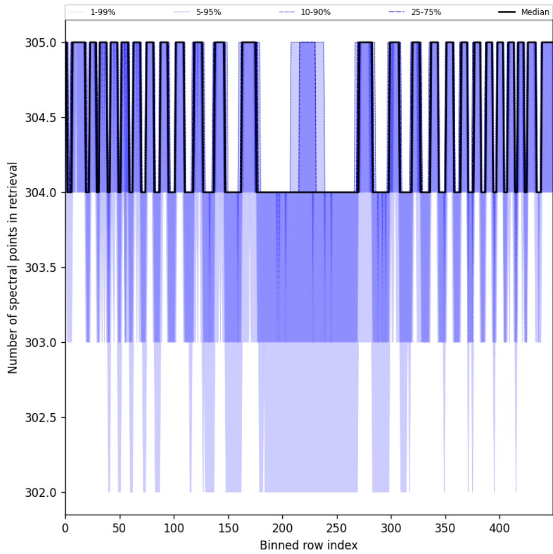
Figure 50: Along track statistics of “Number of spectral points in retrieval” for 2025-07-11 to 2025-07-13
