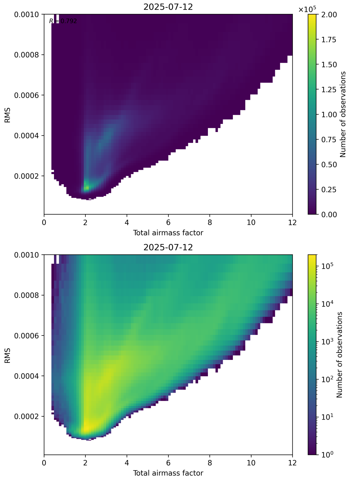
Figure 69: Scatter density plot of “Total airmass factor” against “RMS” for 2025-07-11 to 2025-07-13.
