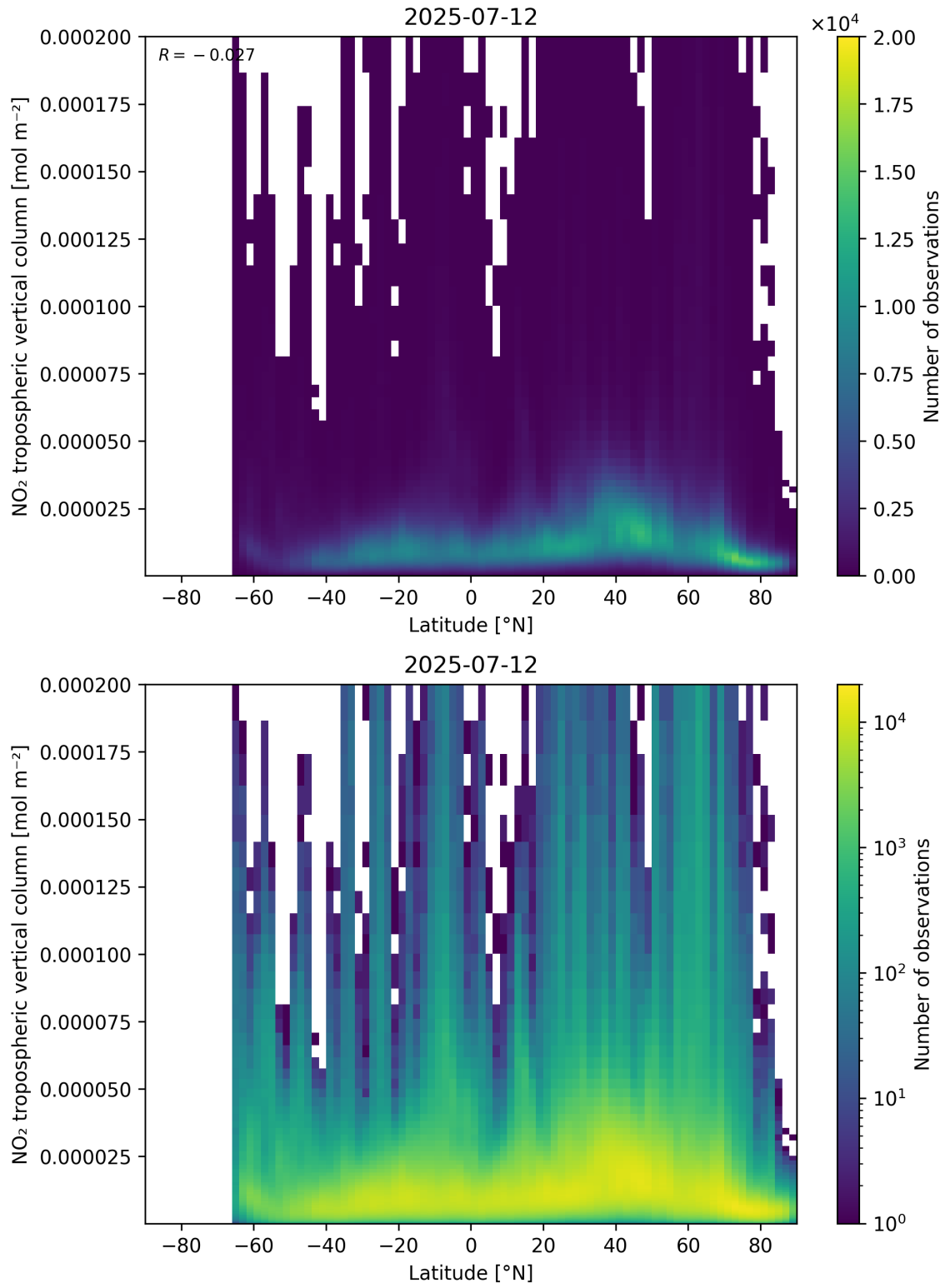
Figure 92: Scatter density plot of “Latitude” against “NO 2 tropospheric vertical column” for 2025-07-11 to 2025-07-13.
