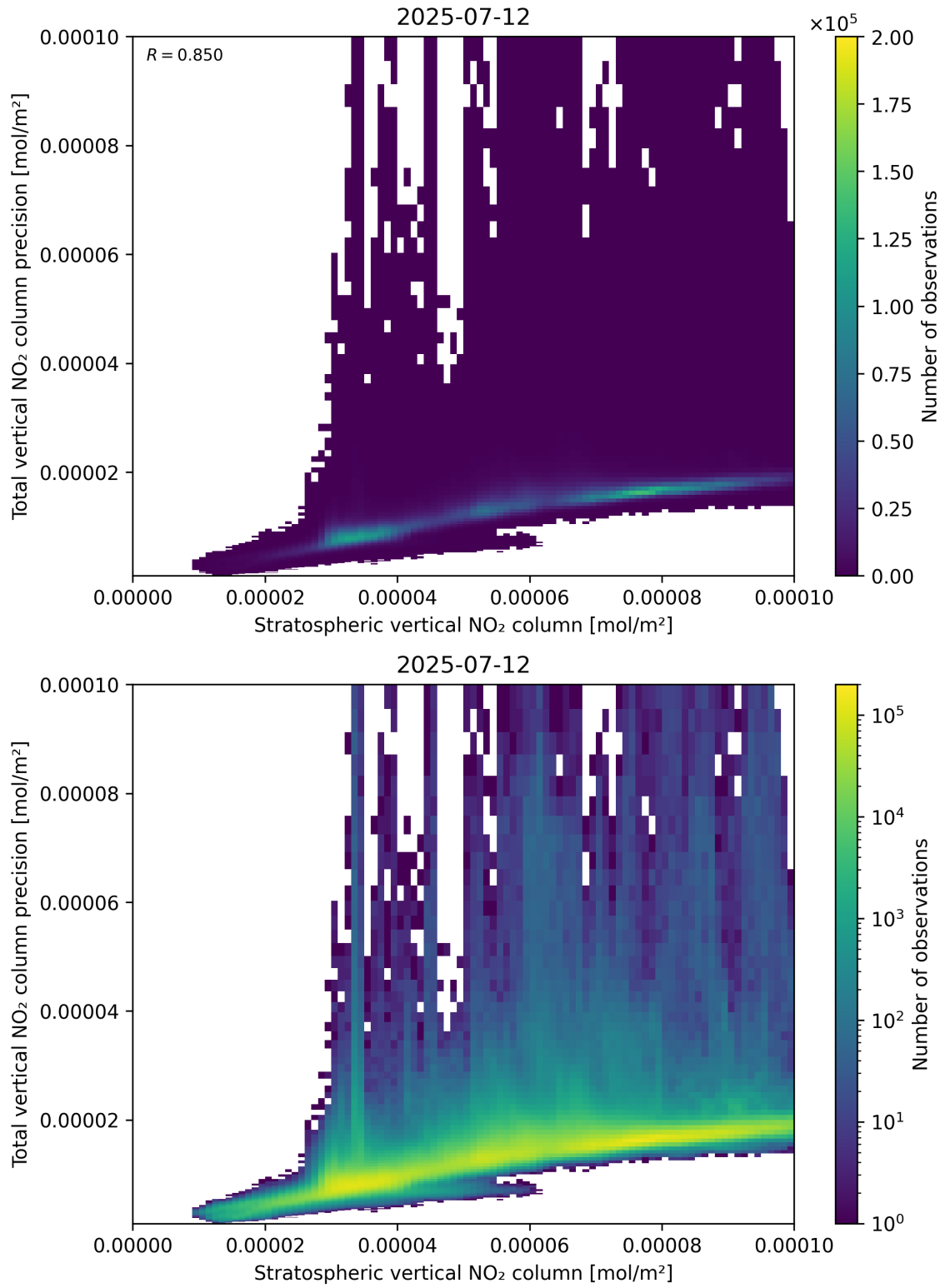
Figure 101: Scatter density plot of “Stratospheric vertical NO 2 column” against “Total vertical NO 2 column precision” for 2025-07-11 to 2025-07-13.
