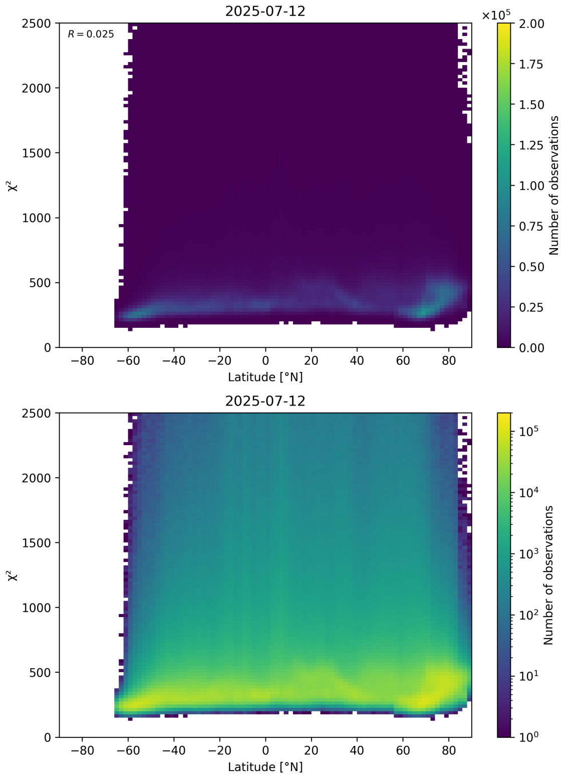
Figure 86: Scatter density plot of “Latitude” against “ \chi^2 ” for 2025-07-11 to 2025-07-13.
