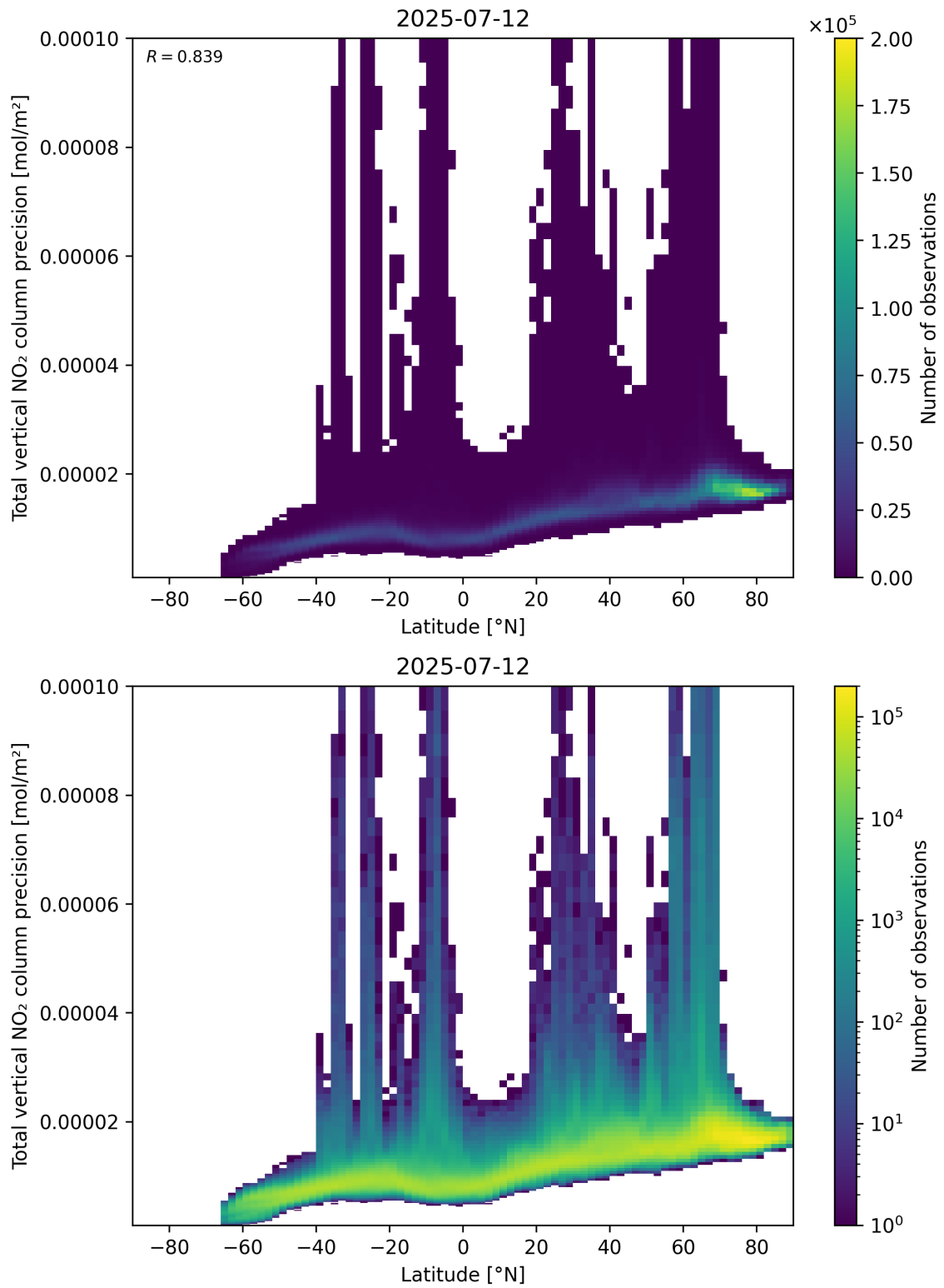
Figure 91: Scatter density plot of “Latitude” against “Total vertical NO 2 column precision” for 2025-07-11 to 2025-07-13.
