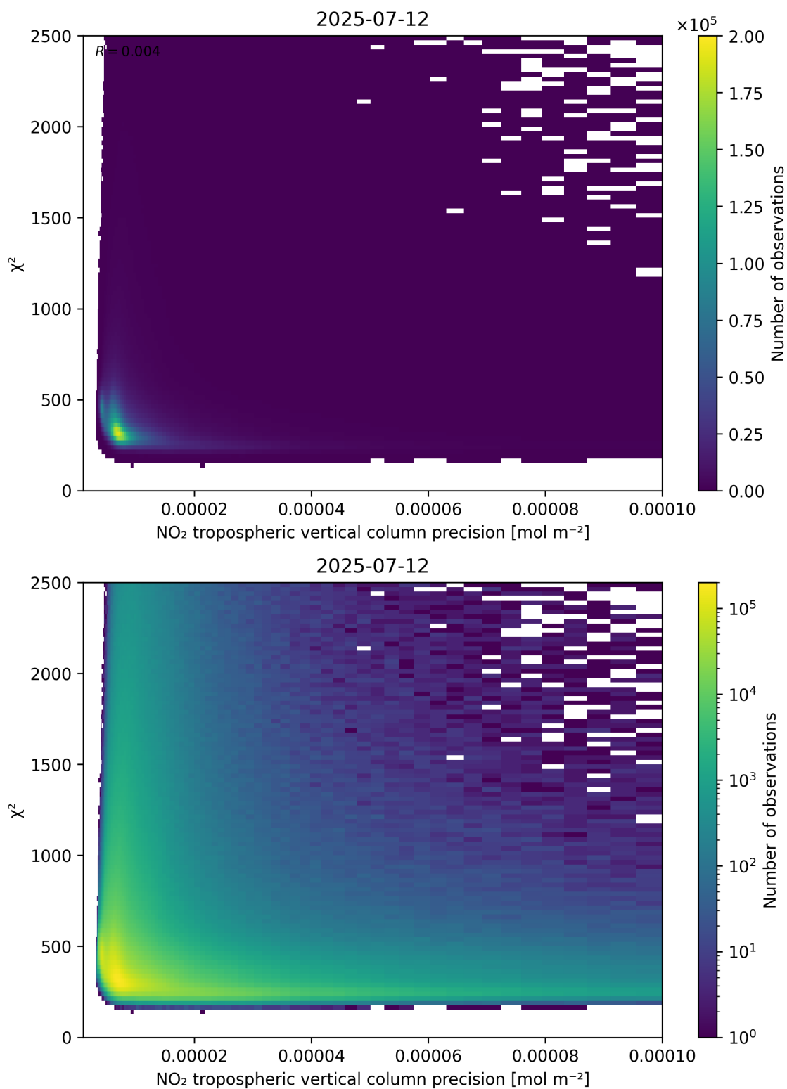
Figure 134: Scatter density plot of “NO 2 tropospheric vertical column precision” against “ \chi^2 ” for 2025-07-11 to 2025-07-13.
