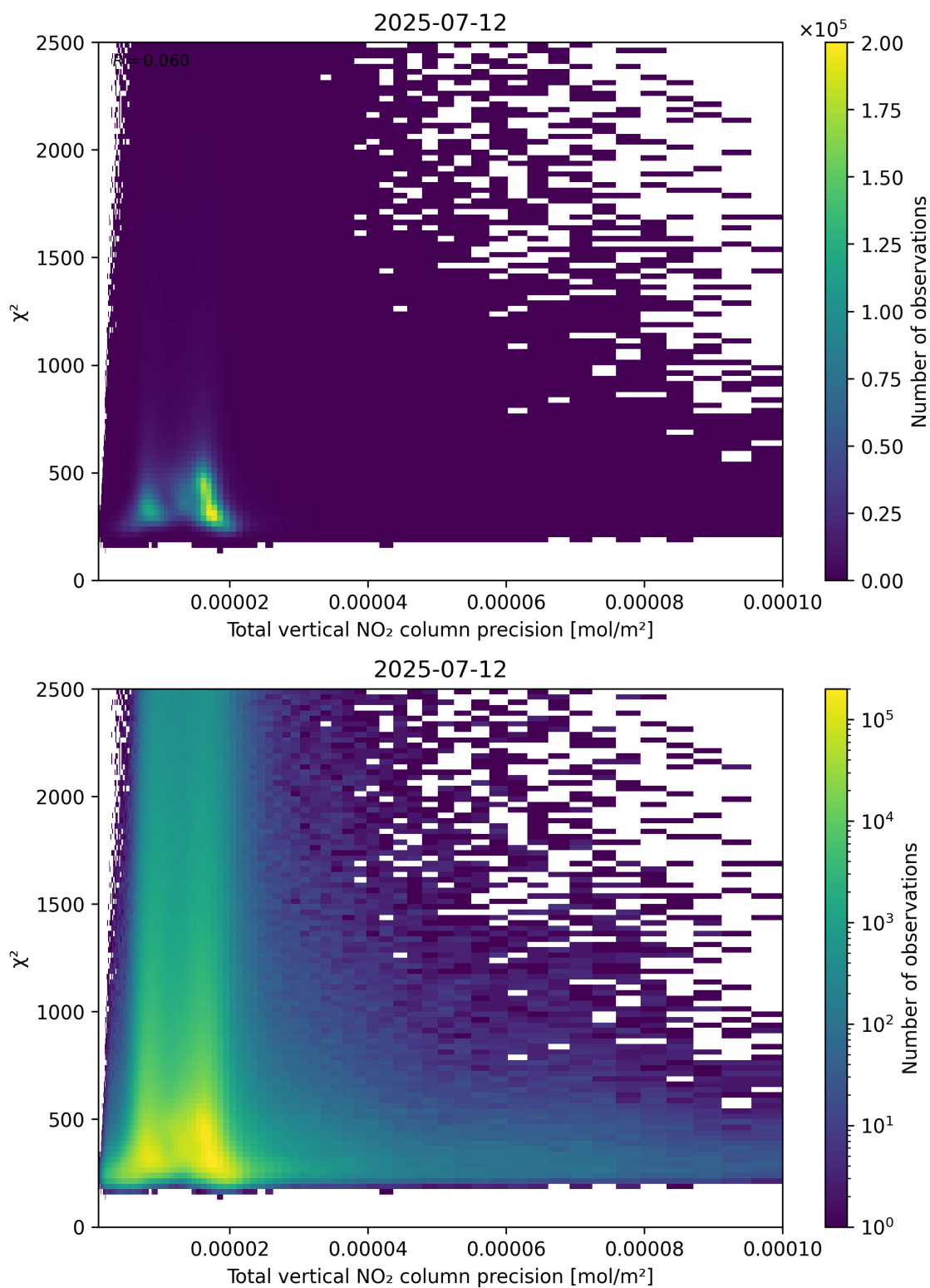
Figure 116: Scatter density plot of “Total vertical NO 2 column precision” against “ \chi^2 ” for 2025-07-11 to 2025-07-13.
