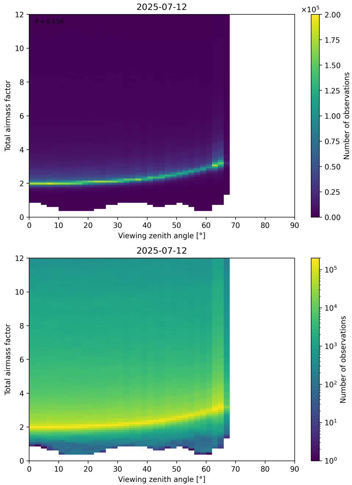
Figure 160: Scatter density plot of “Viewing zenith angle” against “Total airmass factor” for 2025-07-11 to 2025-07-13.
