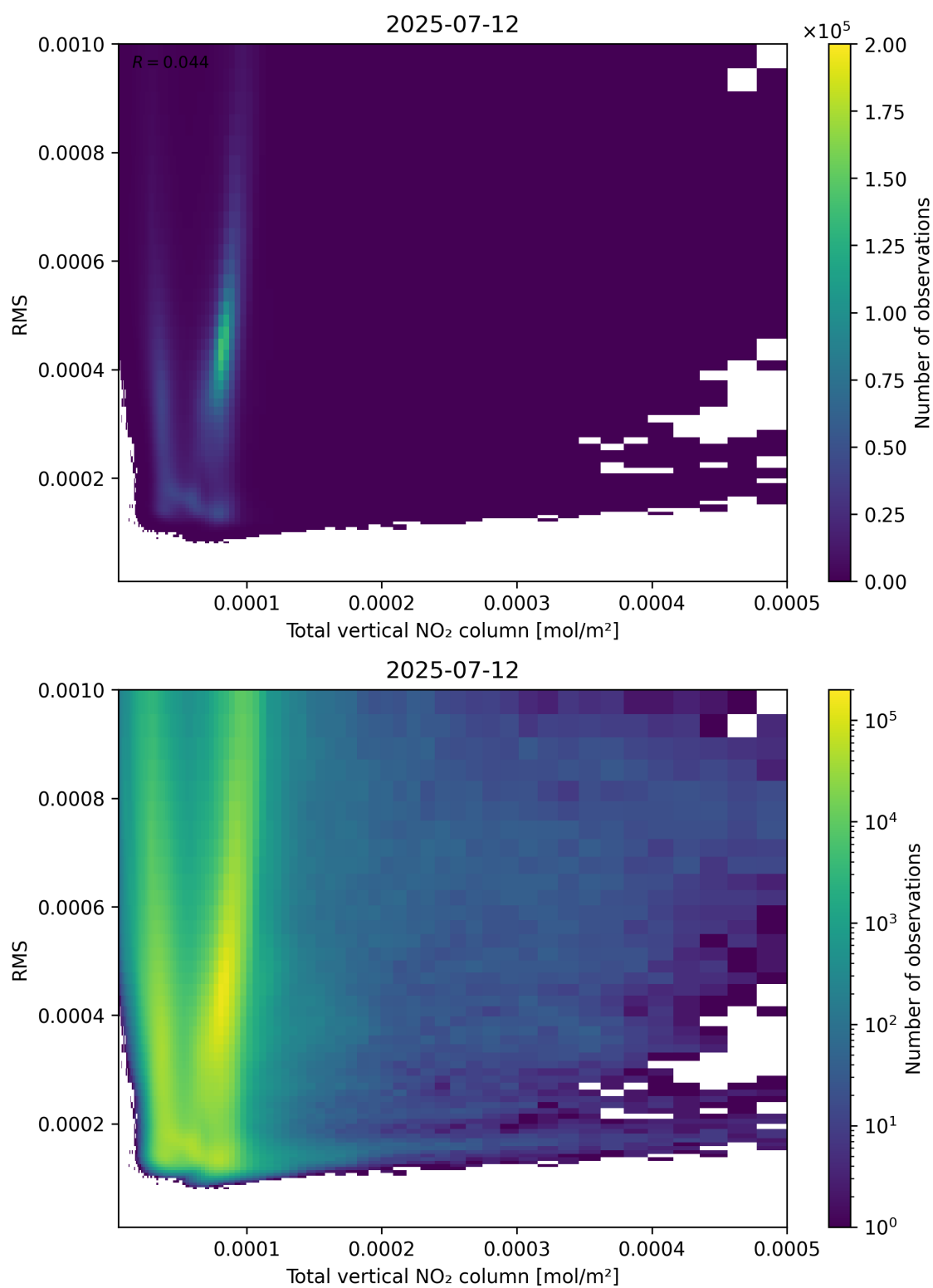
Figure 120: Scatter density plot of “Total vertical NO 2 column” against “RMS” for 2025-07-11 to 2025-07-13.
