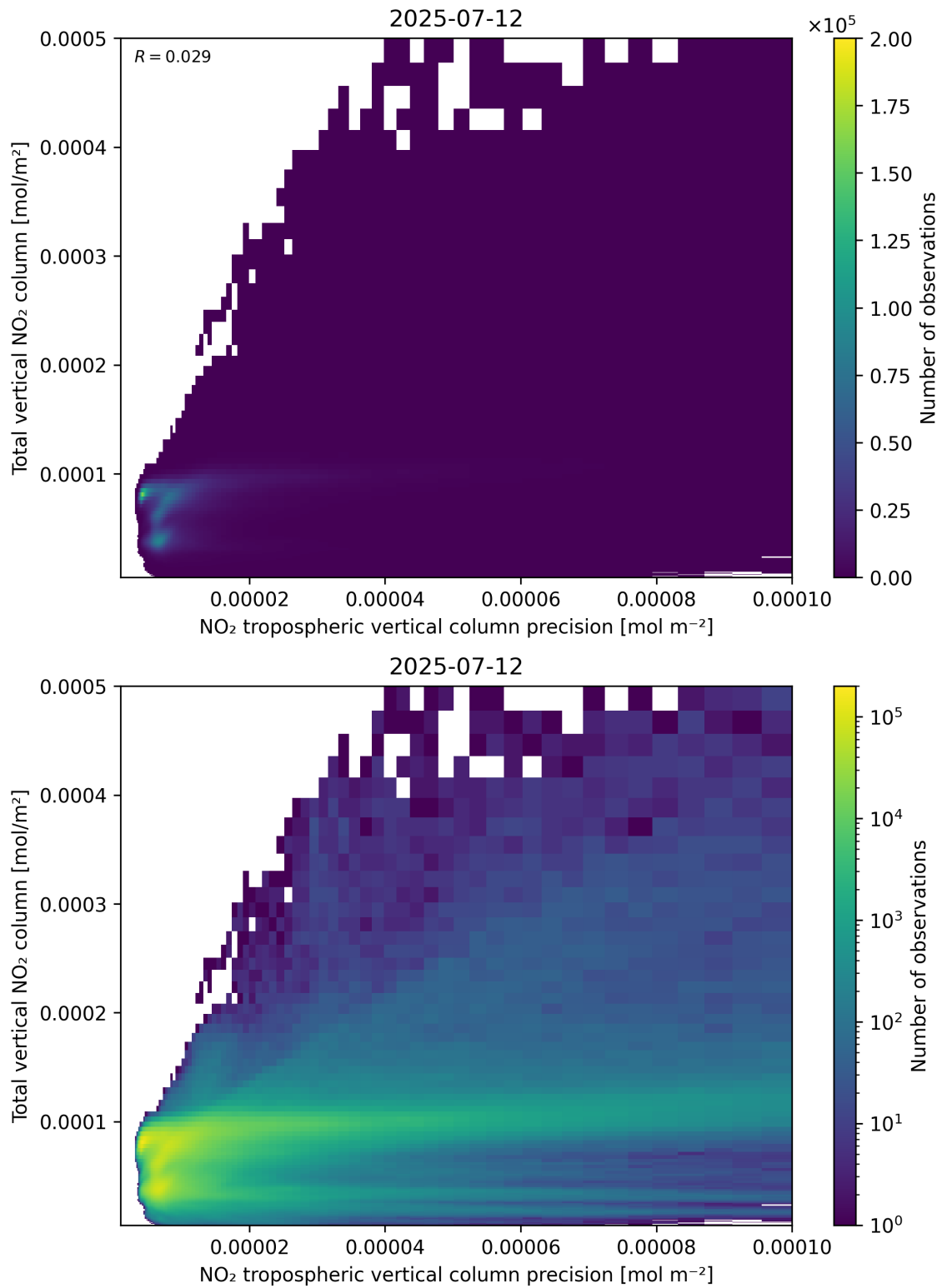
Figure 138: Scatter density plot of “NO 2 tropospheric vertical column precision” against “Total vertical NO 2 column” for 2025-07-11 to 2025-07-13.
