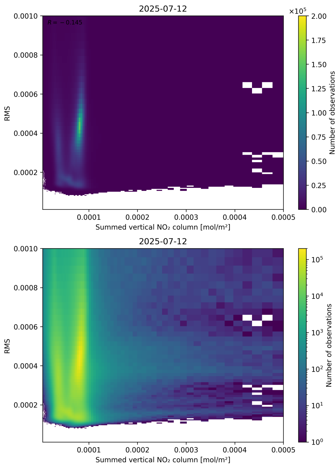
Figure 109: Scatter density plot of “Summed vertical NO 2 column” against “RMS” for 2025-07-11 to 2025-07-13.
