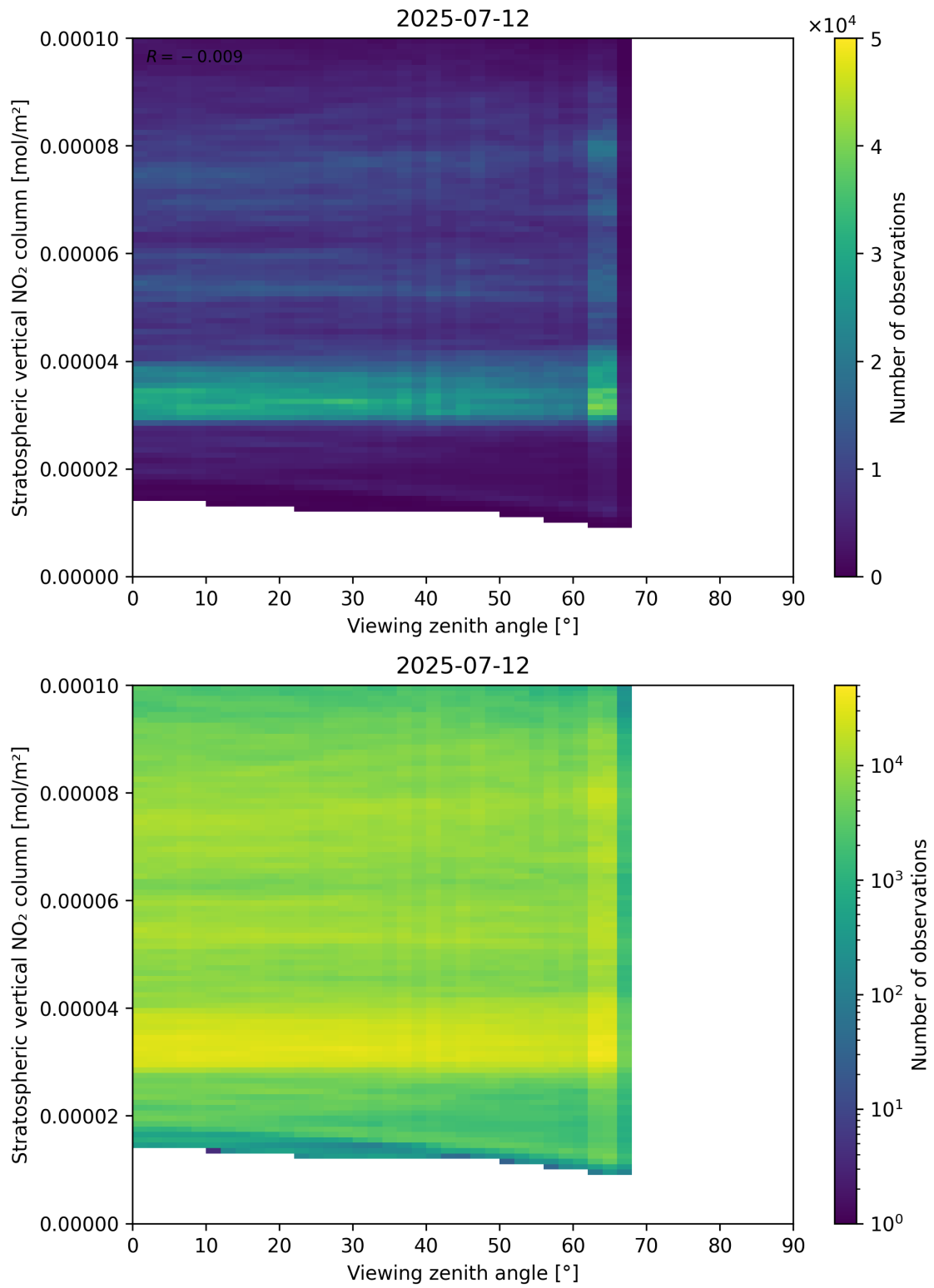
Figure 164: Scatter density plot of “Viewing zenith angle” against “Stratospheric vertical NO 2 column” for 2025-07-11 to 2025-07-13.
