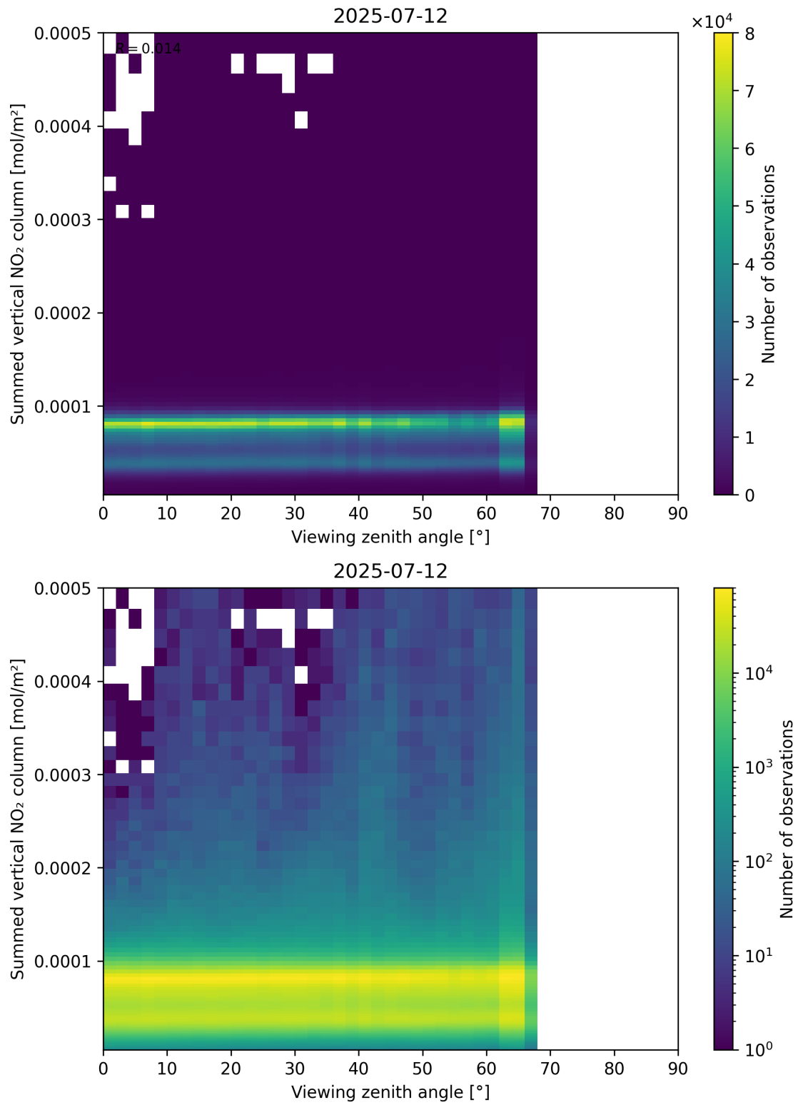
Figure 165: Scatter density plot of “Viewing zenith angle” against “Summed vertical NO 2 column” for 2025-07-11 to 2025-07-13.
