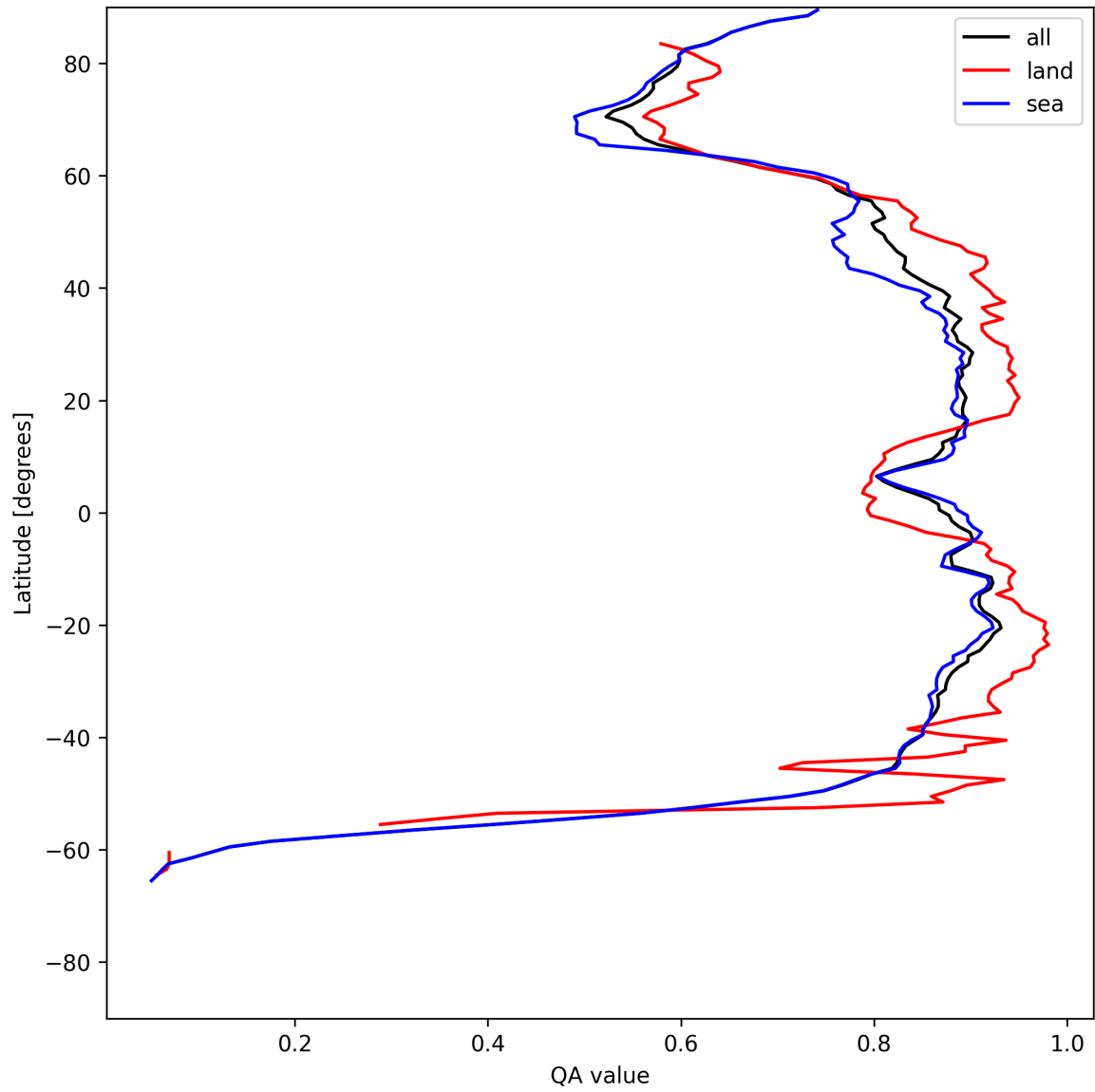
Figure 11: Zonal average of “QA value” for 2025-07-11 to 2025-07-13.
