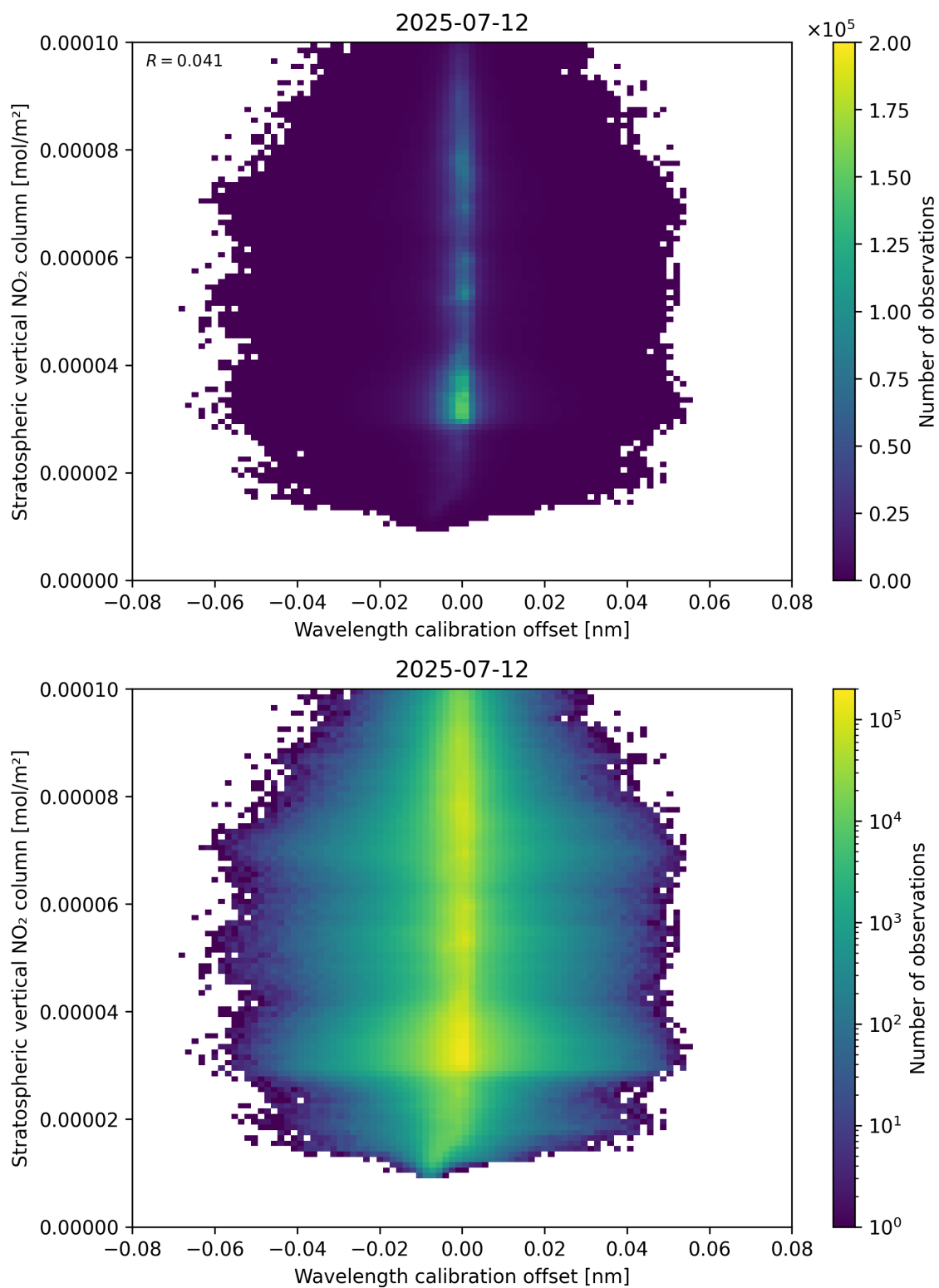
Figure 176: Scatter density plot of “Wavelength calibration offset” against “Stratospheric vertical NO 2 column” for 2025-07-11 to 2025-07-13.
