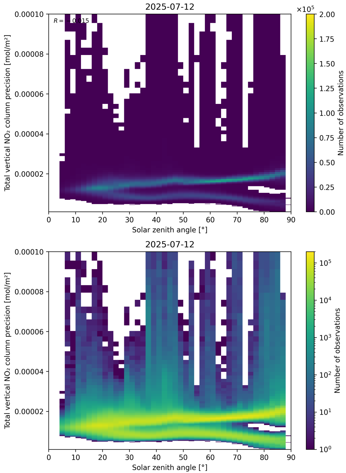
Figure 154: Scatter density plot of “Solar zenith angle” against “Total vertical NO 2 column precision” for 2025-07-11 to 2025-07-13.
