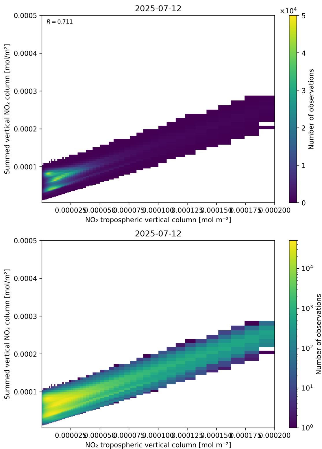
Figure 126: Scatter density plot of “NO 2 tropospheric vertical column” against “Summed vertical NO 2 column” for 2025-07-11 to 2025-07-13.
