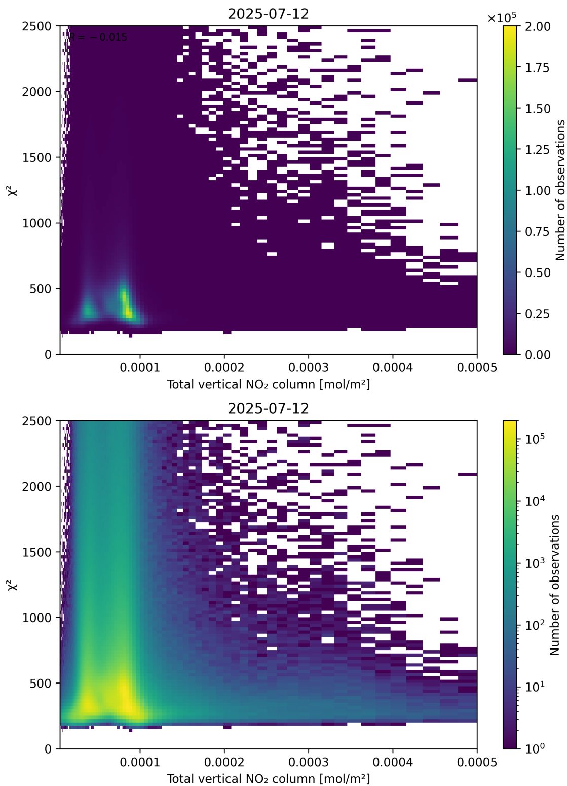
Figure 111: Scatter density plot of “Total vertical NO 2 column” against “ \chi^2 ” for 2025-07-11 to 2025-07-13.
