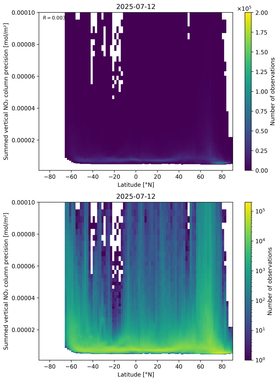
Figure 89: Scatter density plot of “Latitude” against “Summed vertical NO 2 column precision” for 2025-07-11 to 2025-07-13.
