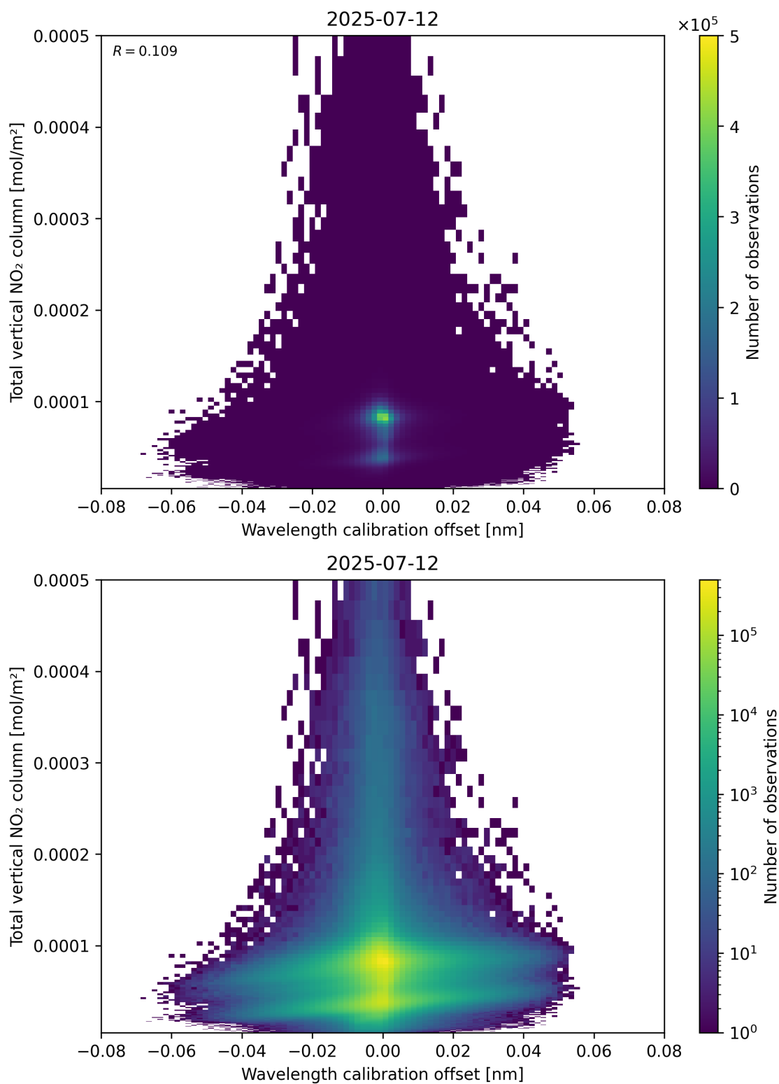
Figure 179: Scatter density plot of “Wavelength calibration offset” against “Total vertical NO 2 column” for 2025-07-11 to 2025-07-13.
