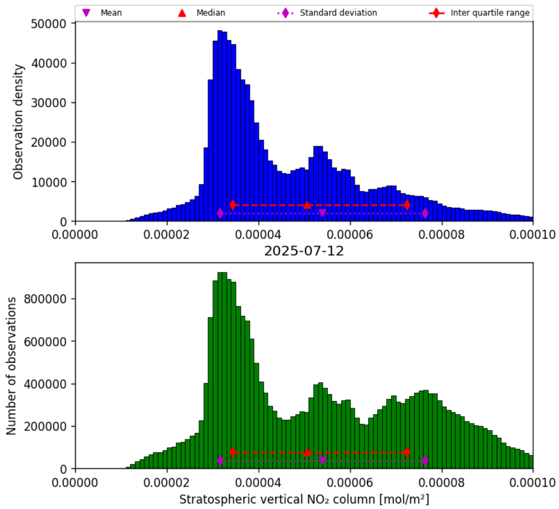
Figure 36: Histogram of “Stratospheric vertical NO 2 column” for 2025-07-11 to 2025-07-13
