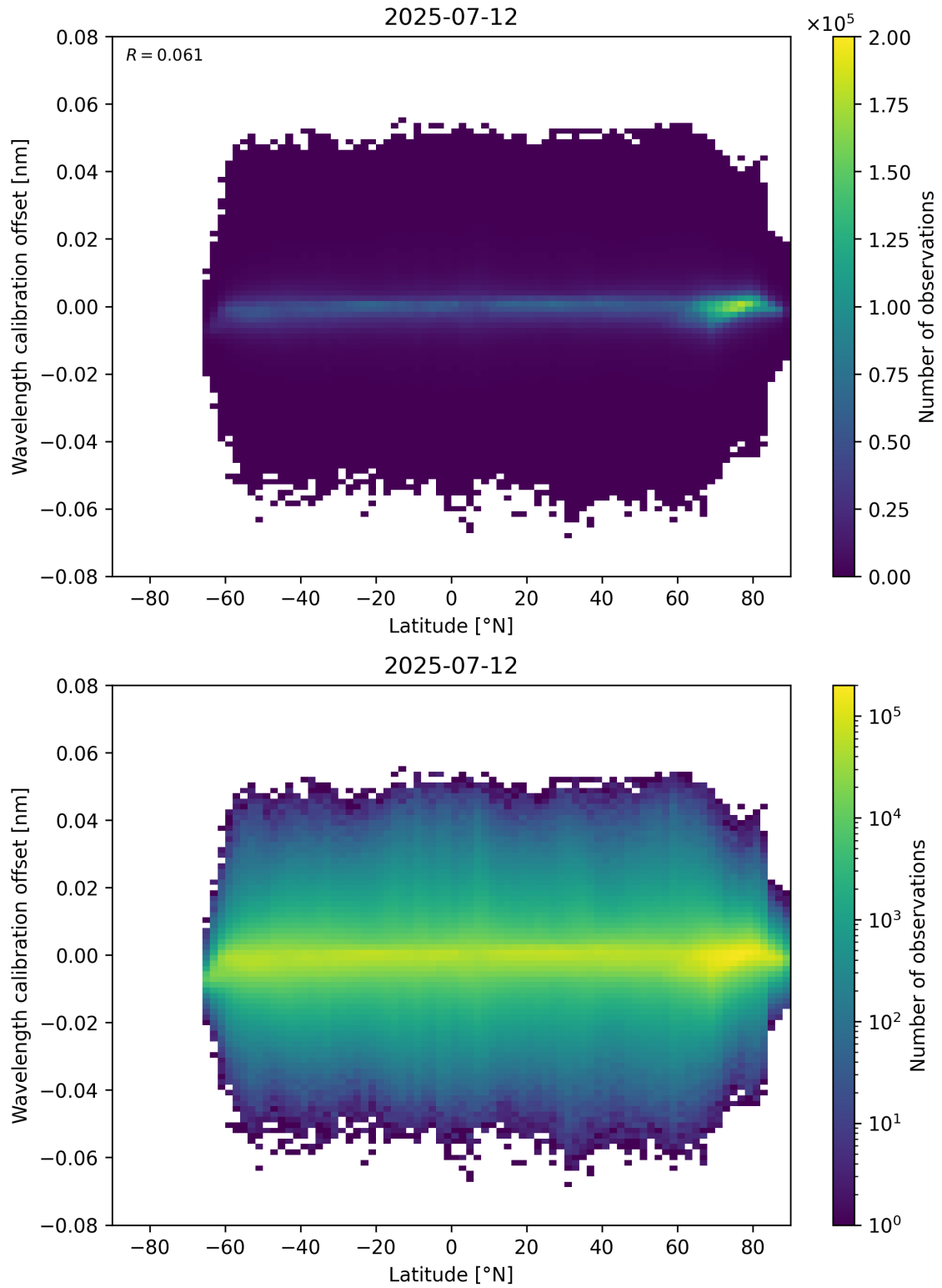
Figure 95: Scatter density plot of “Latitude” against “Wavelength calibration offset” for 2025-07-11 to 2025-07-13.
