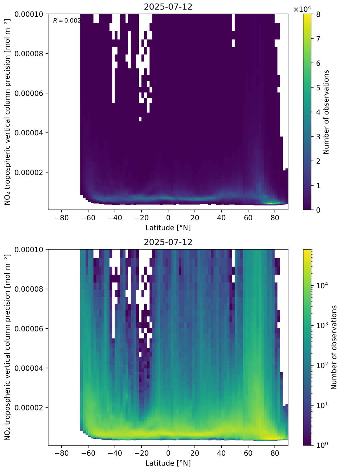
Figure 93: Scatter density plot of “Latitude” against “NO 2 tropospheric vertical column precision” for 2025-07-11 to 2025-07-13.
