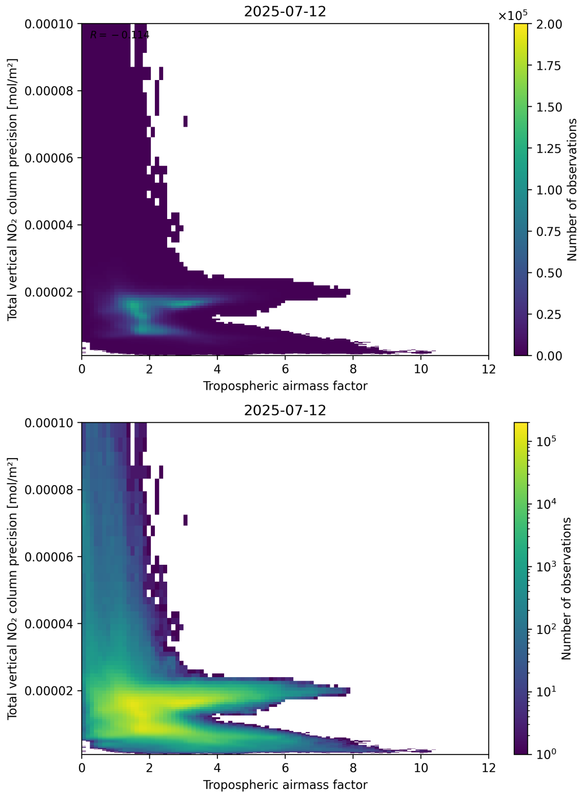
Figure 78: Scatter density plot of “Tropospheric air mass factor” against “Total vertical NO 2 column precision” for 2025-07-11 to 2025-07-13.
