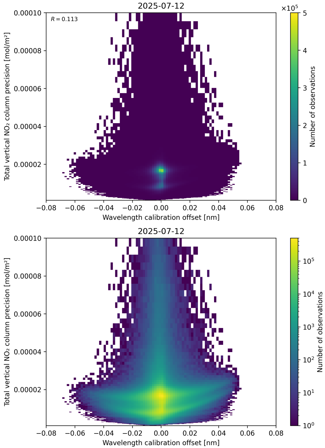
Figure 180: Scatter density plot of “Wavelength calibration offset” against “Total vertical NO 2 column precision” for 2025-07-11 to 2025-07-13.
