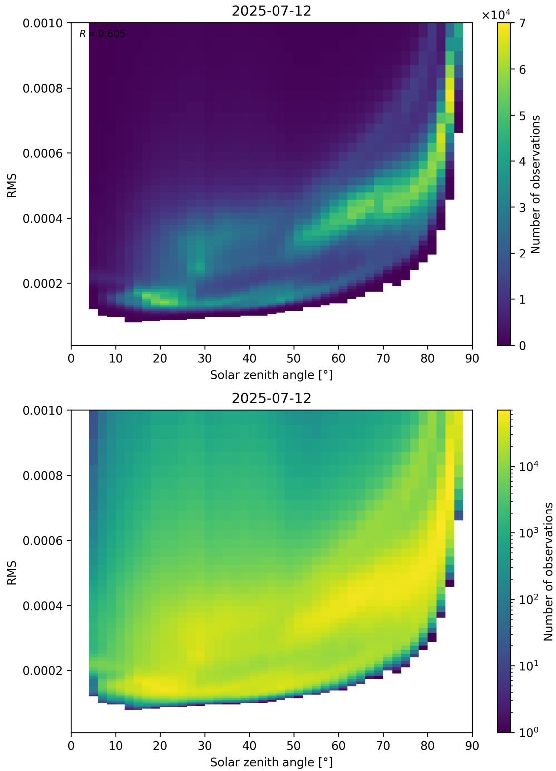
Figure 157: Scatter density plot of “Solar zenith angle” against “RMS” for 2025-07-11 to 2025-07-13.
