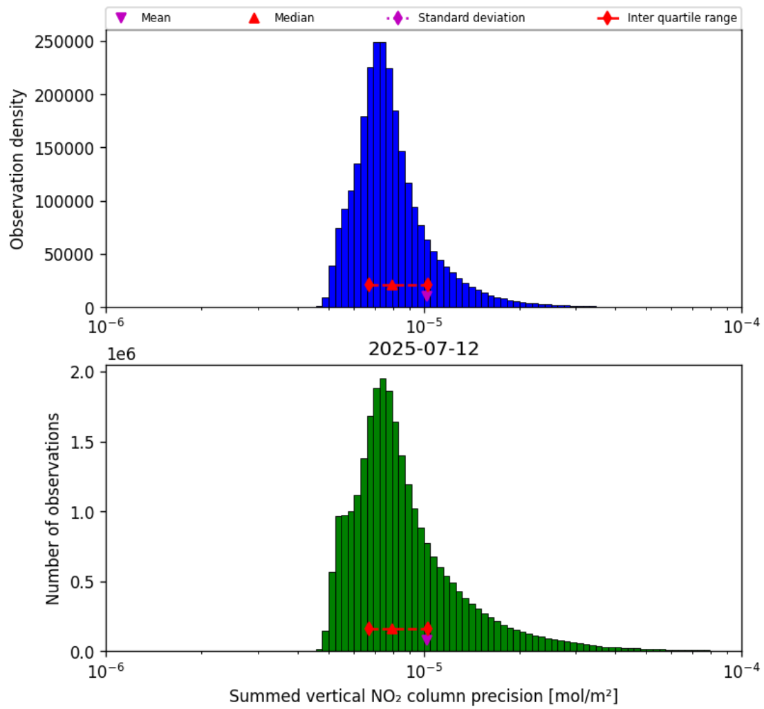
Figure 41: Histogram of "Summed vertical NO 2 column precision" for 2025-07-11 to 2025-07-13
