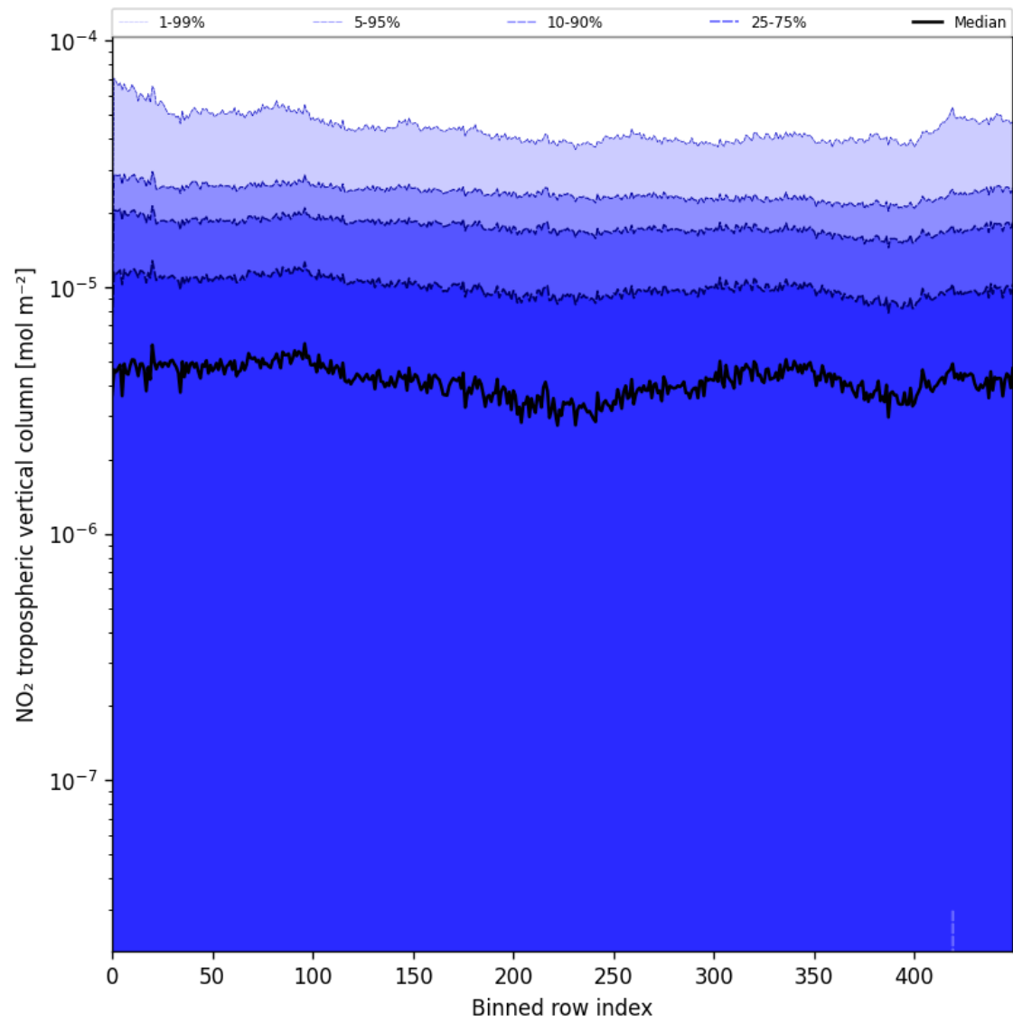
Figure 46: Along track statistics of “NO 2 tropospheric vertical column” for 2025-07-11 to 2025-07-13
