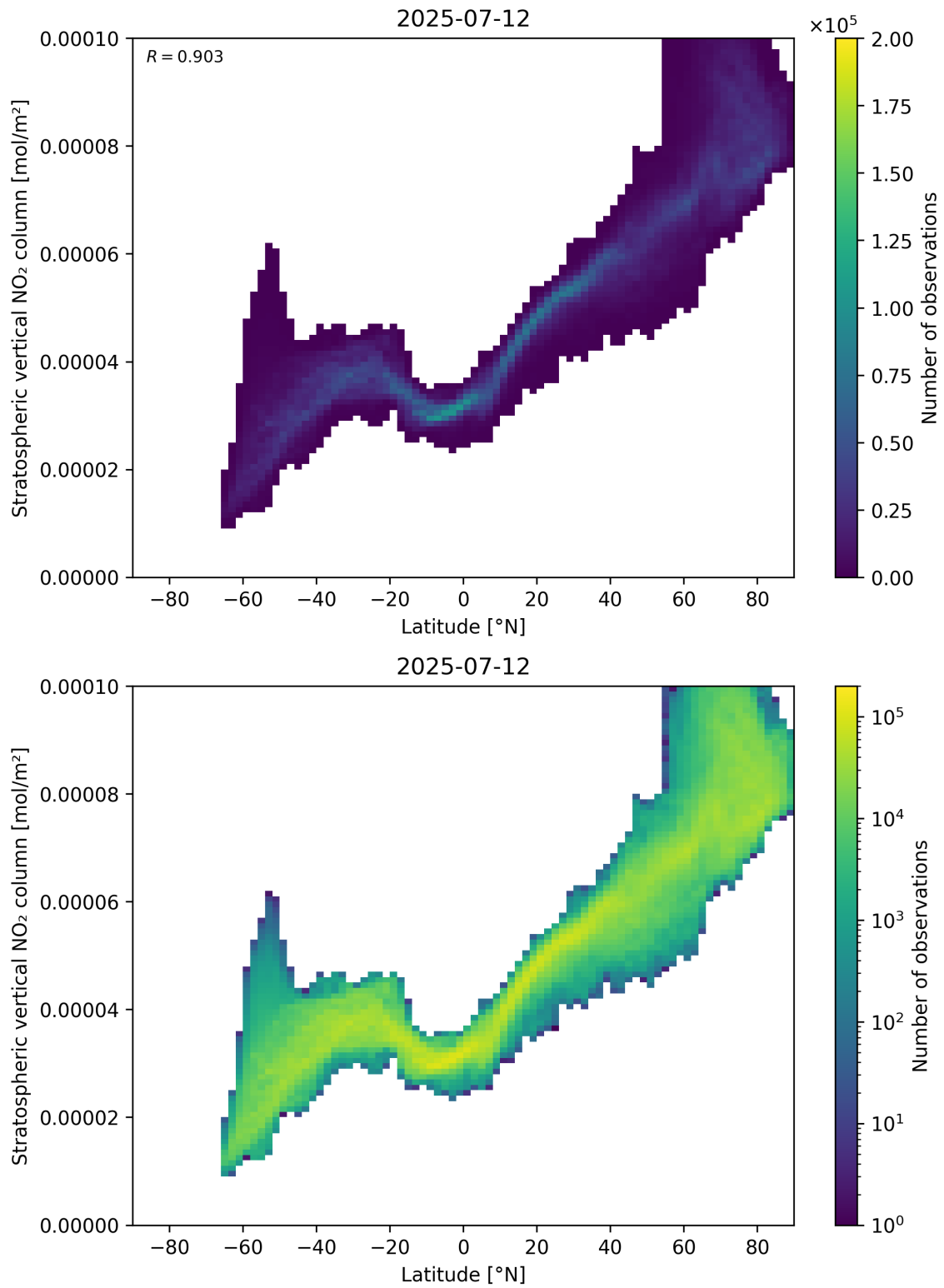
Figure 87: Scatter density plot of “Latitude” against “Stratospheric vertical \text{NO}_2 column” for 2025-07-11 to 2025-07-13.
