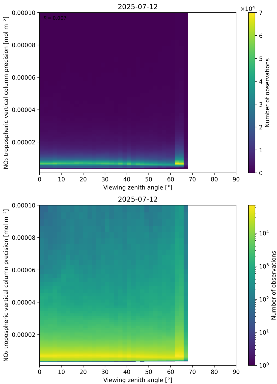
Figure 170: Scatter density plot of “Viewing zenith angle” against “NO 2 tropospheric vertical column precision” for 2025-07-11 to 2025-07-13.
