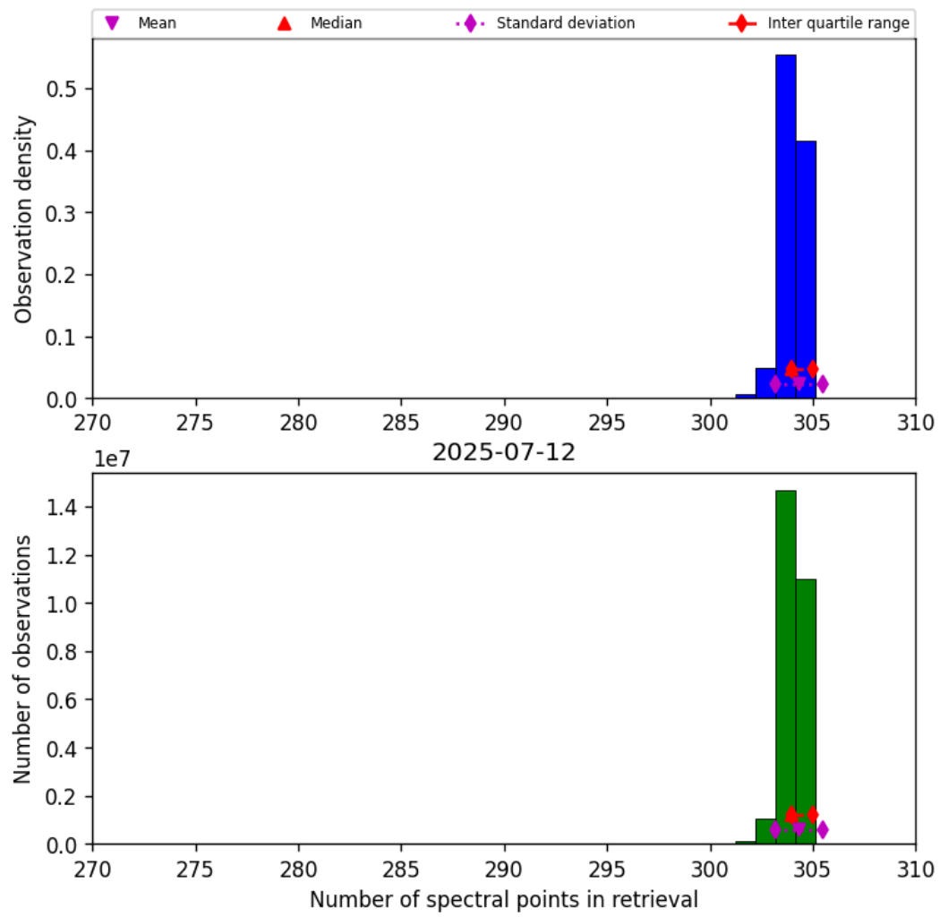
Figure 33: Histogram of “Number of spectral points in retrieval” for 2025-07-11 to 2025-07-13
