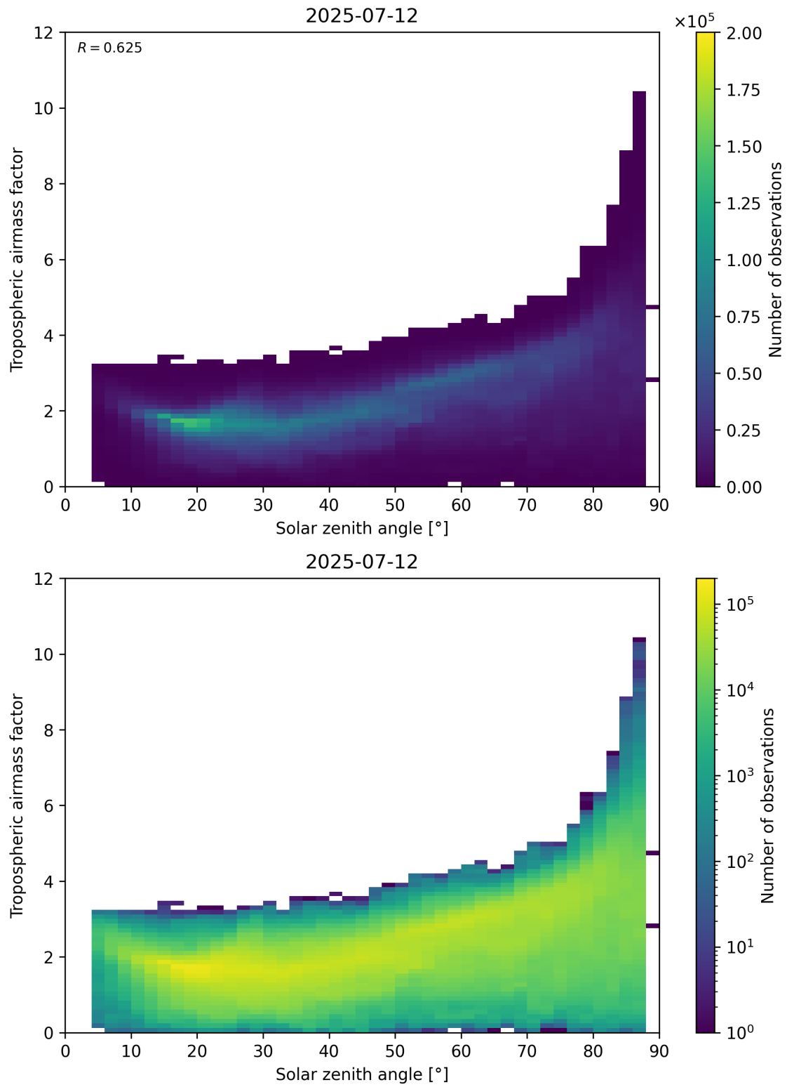
Figure 147: Scatter density plot of “Solar zenith angle” against “Tropospheric airmass factor” for 2025-07-11 to 2025-07-13.
