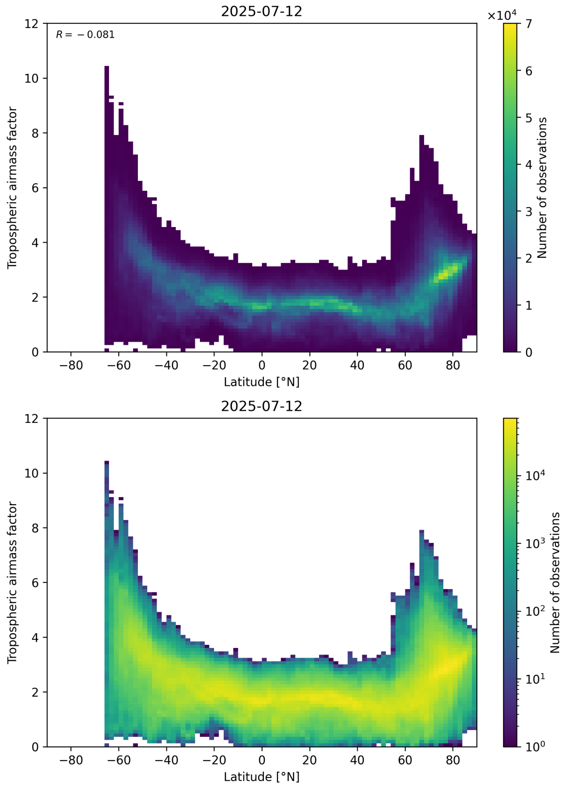
Figure 85: Scatter density plot of “Latitude” against “Tropospheric air mass factor” for 2025-07-11 to 2025-07-13.
