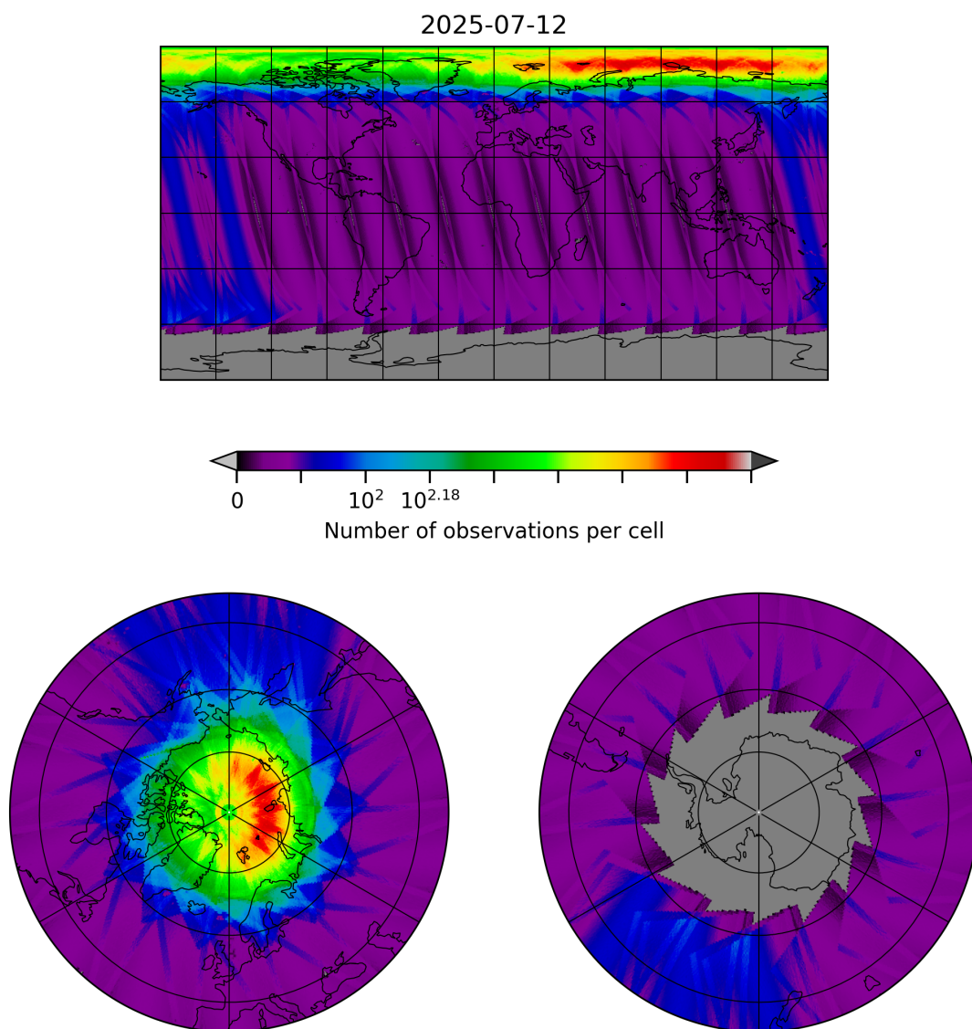
Figure 10: Map of the number of observations for 2025-07-11 to 2025-07-13
