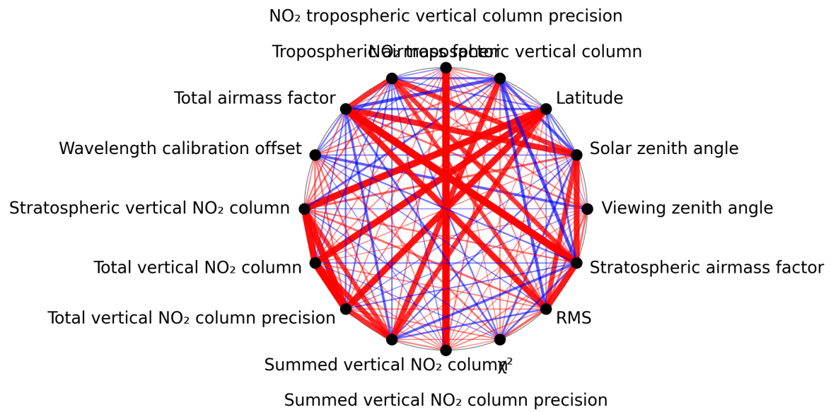
Figure 1: Map of correlation graph for 2025-07-11 to 2025-07-13.
