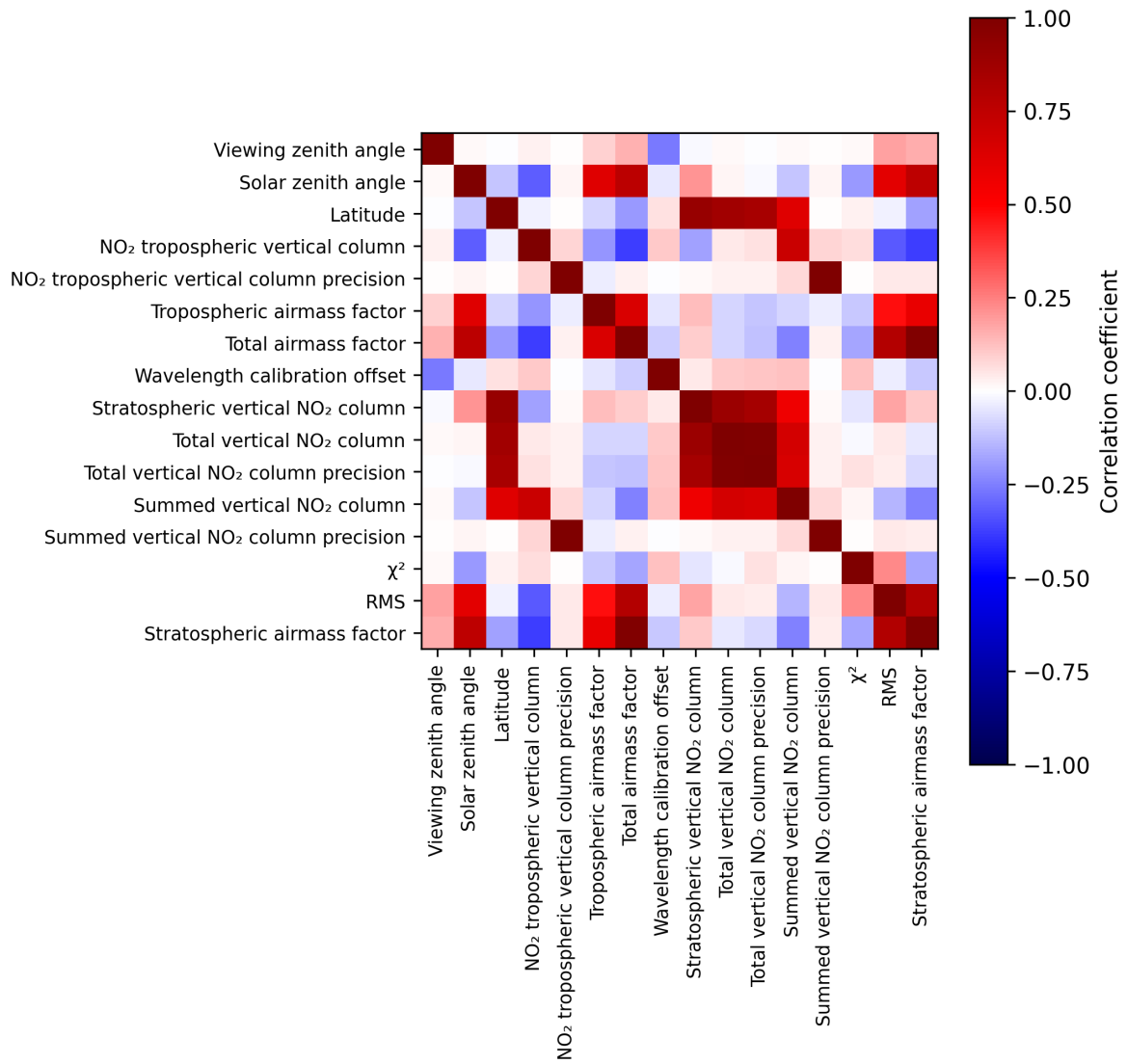
Figure 2: Map of correlation matrix for 2025-07-11 to 2025-07-13.
