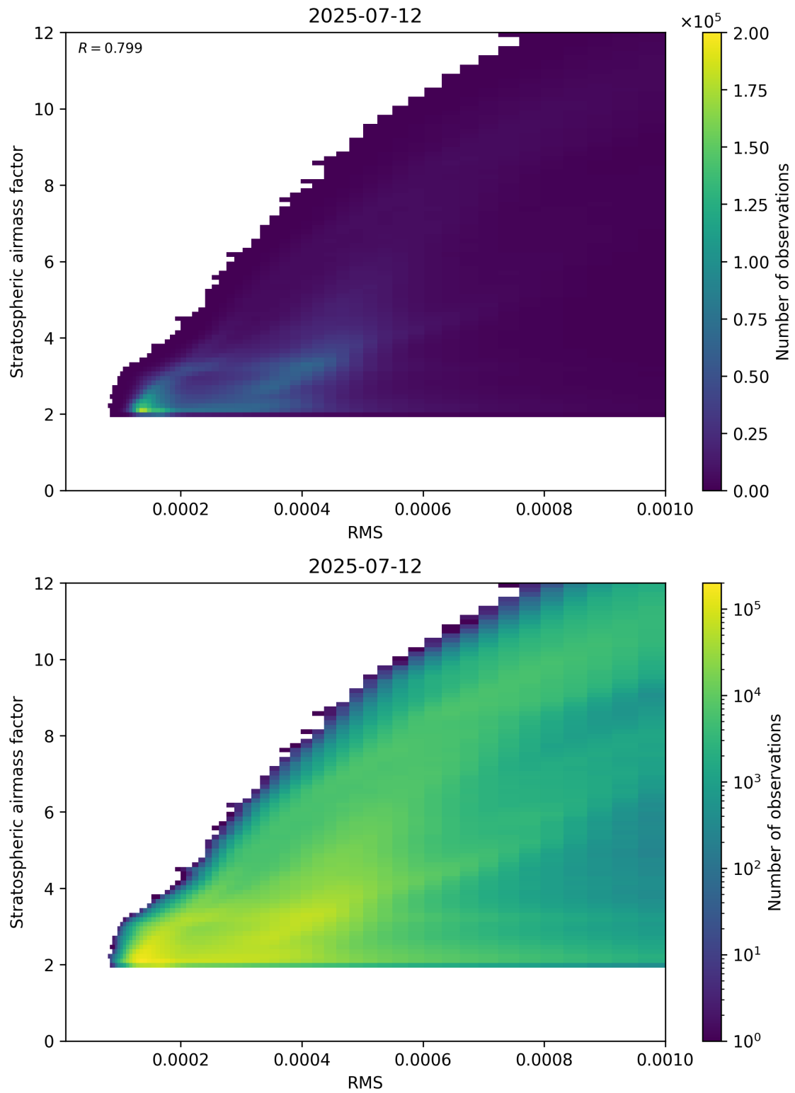
Figure 144: Scatter density plot of “RMS” against “Stratospheric airmass factor” for 2025-07-11 to 2025-07-13.
