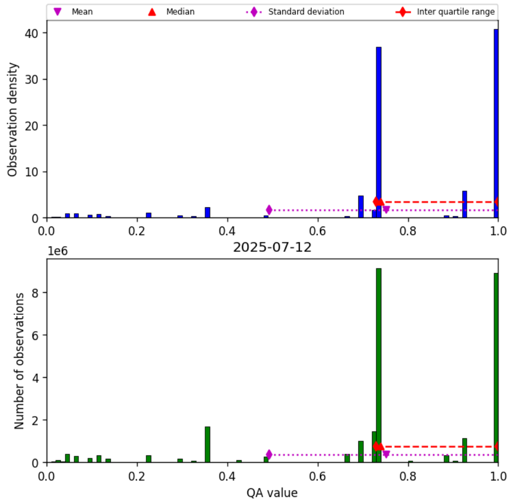
Figure 28: Histogram of “QA value” for 2025-07-11 to 2025-07-13
