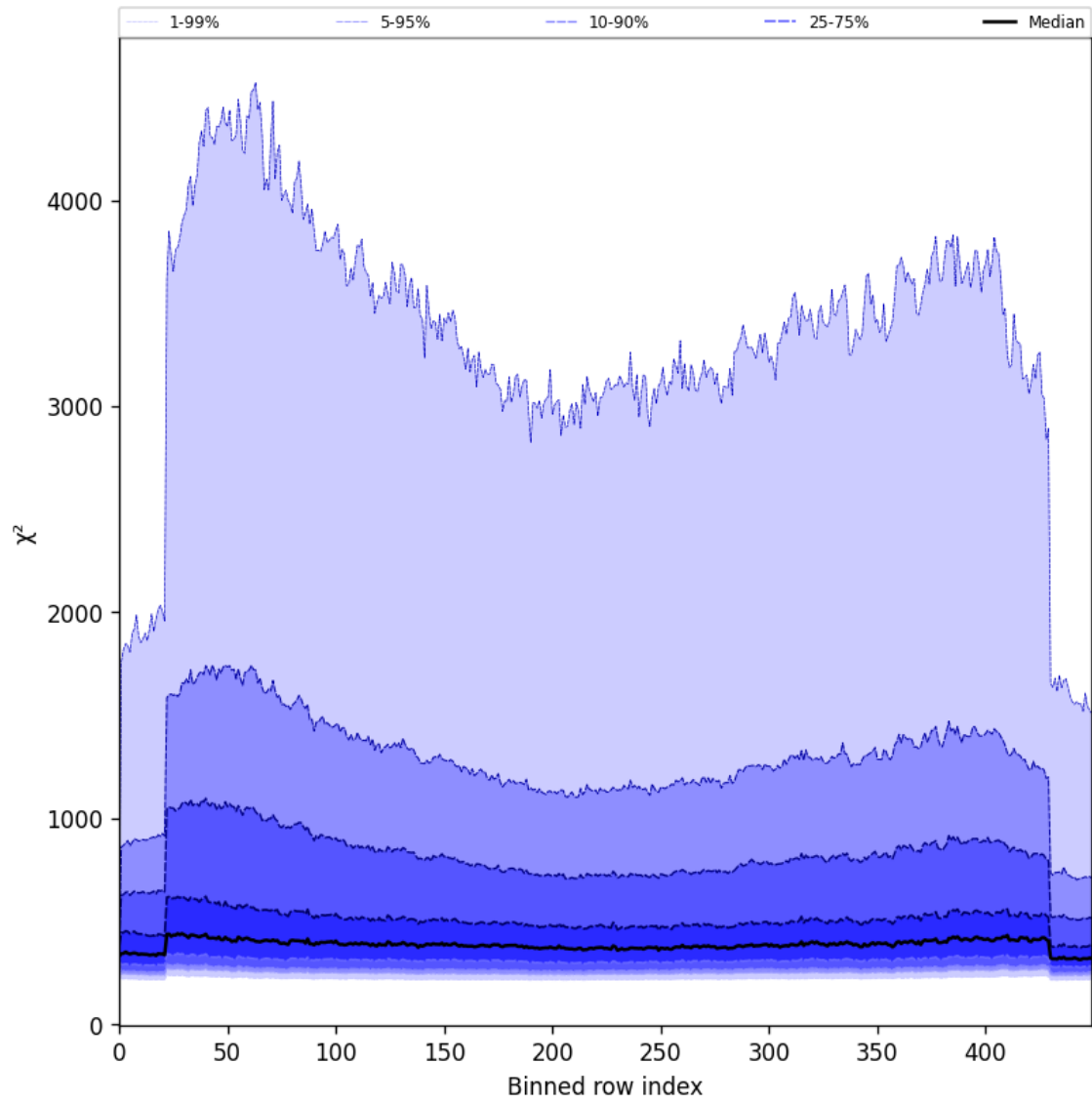
Figure 59: Along track statistics of “ \chi^2 ” for 2025-07-11 to 2025-07-13
