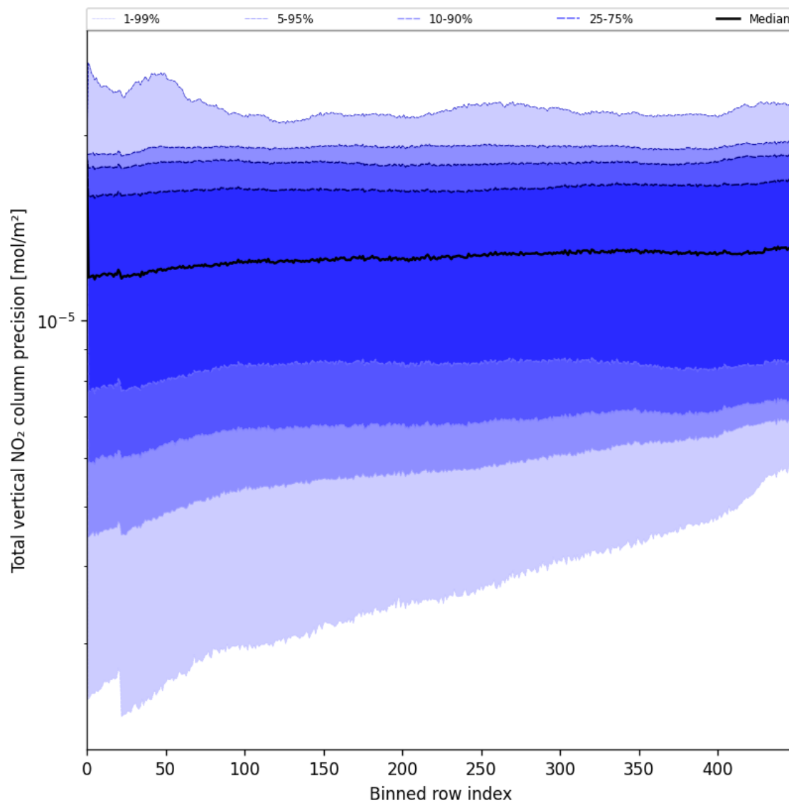
Figure 56: Along track statistics of “Total vertical NO 2 column precision” for 2025-07-11 to 2025-07-13
