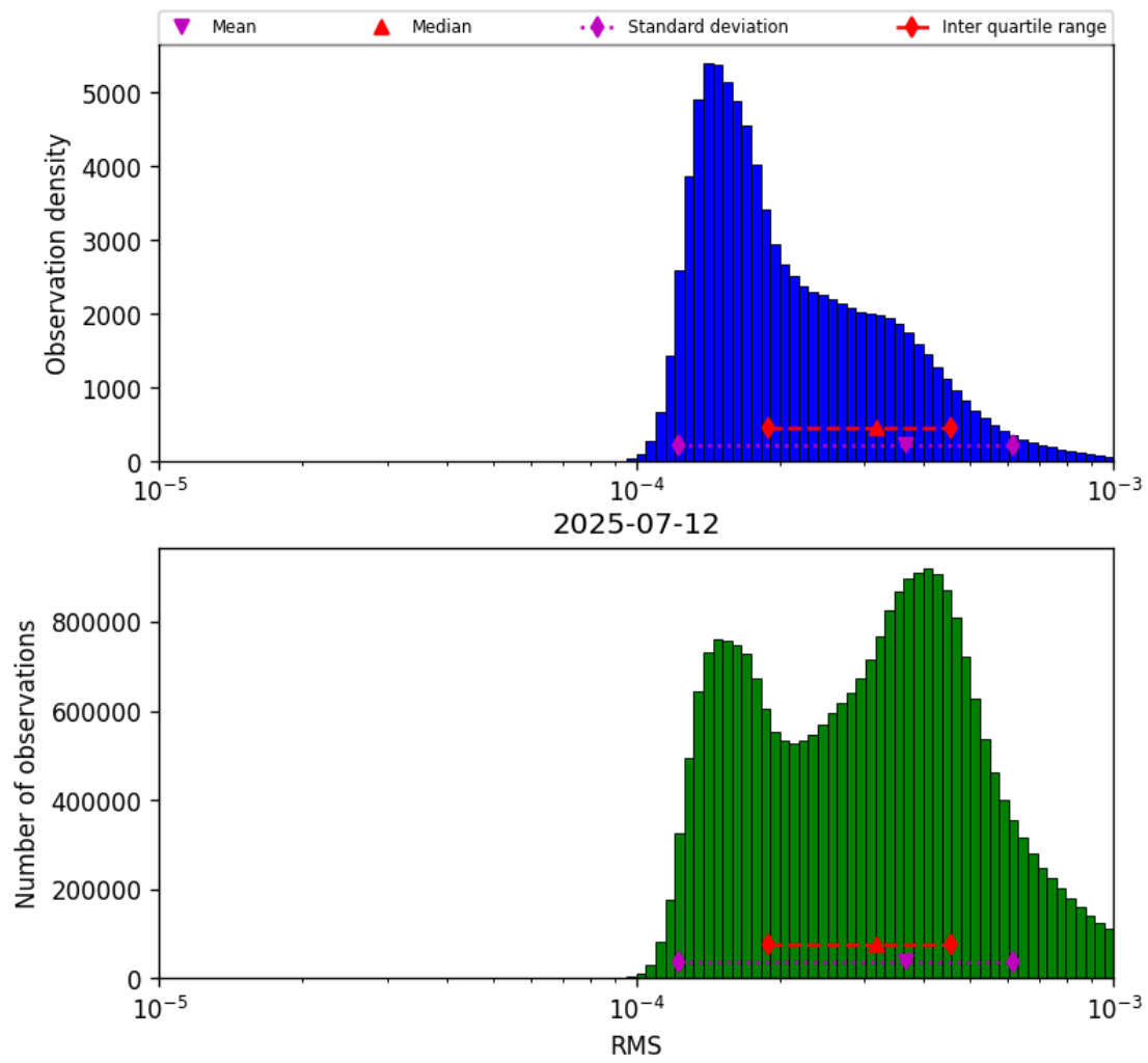
Figure 43: Histogram of “RMS” for 2025-07-11 to 2025-07-13
