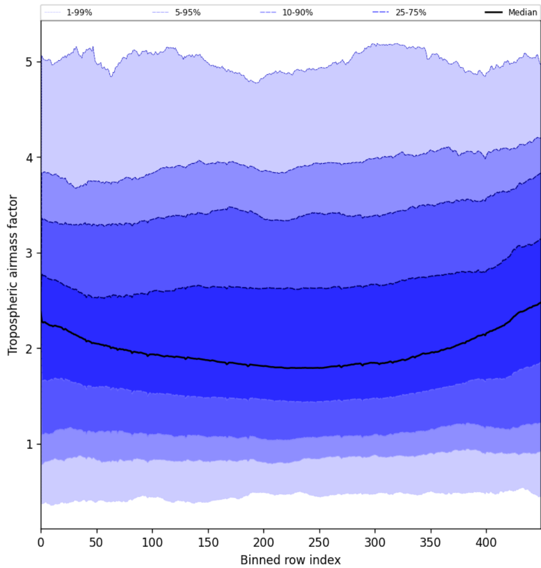
Figure 48: Along track statistics of “Tropospheric airmass factor” for 2025-07-11 to 2025-07-13
