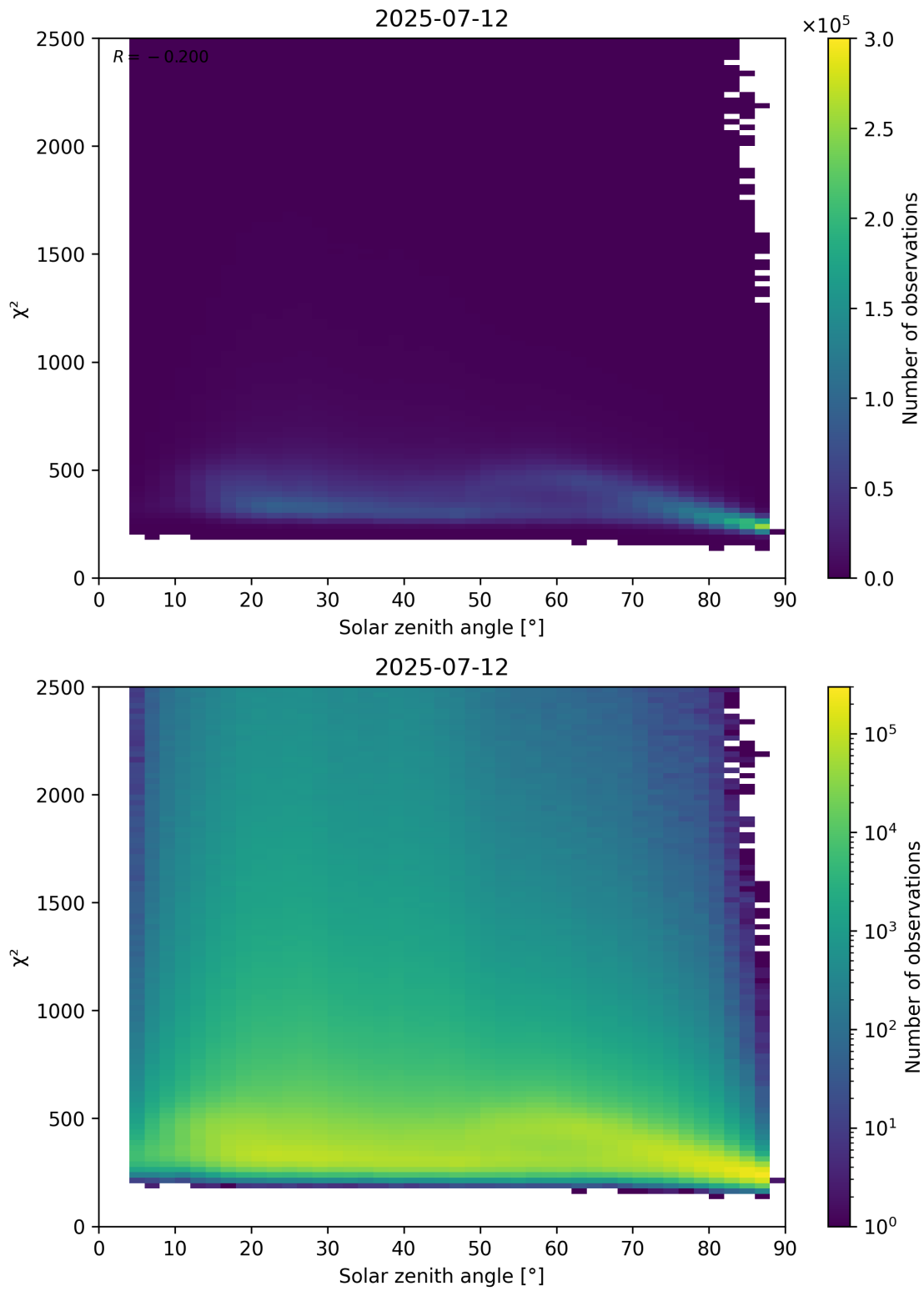
Figure 148: Scatter density plot of “Solar zenith angle” against “ \chi^2 ” for 2025-07-11 to 2025-07-13.
