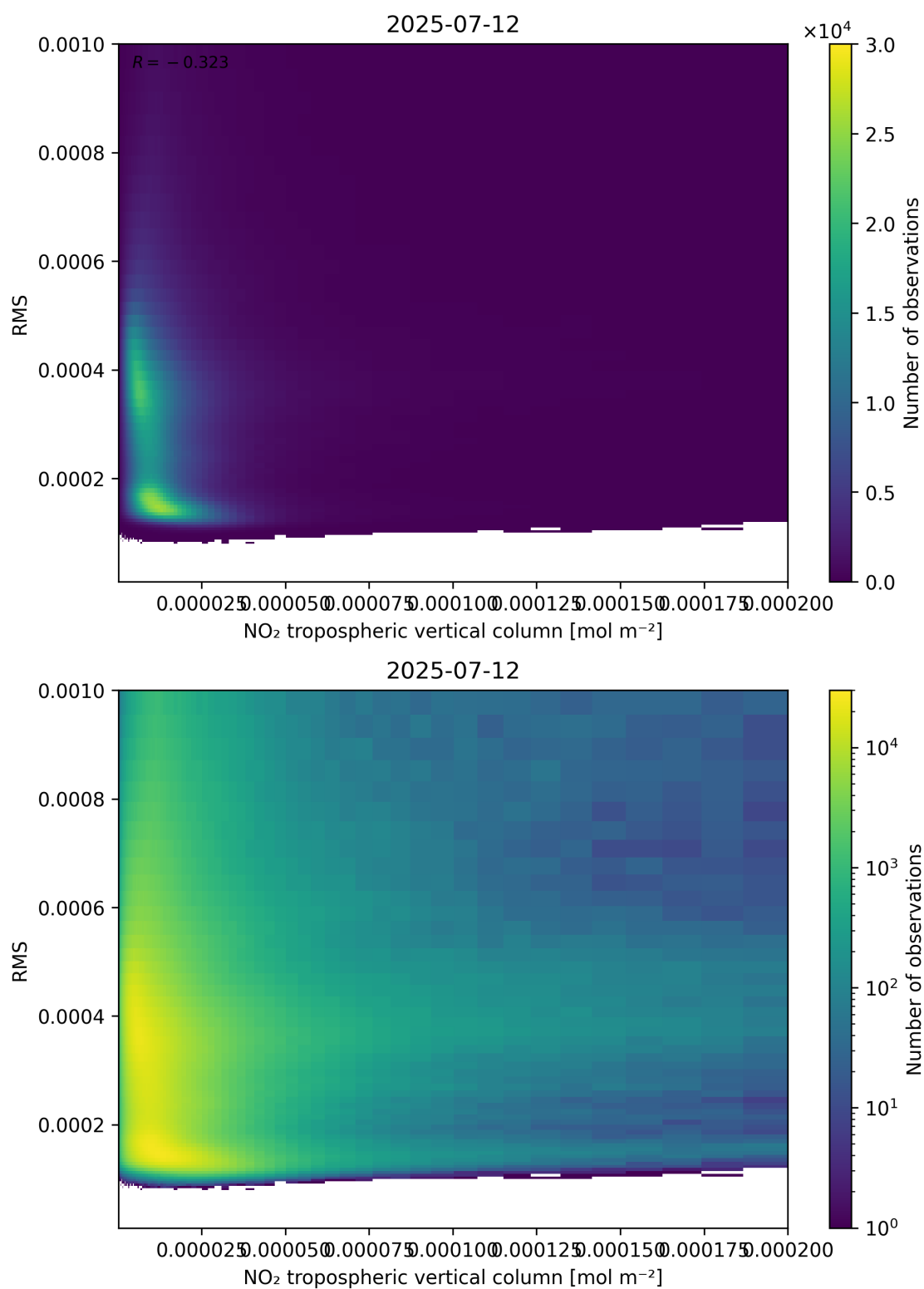
Figure 142: Scatter density plot of “NO 2 tropospheric vertical column” against “RMS” for 2025-07-11 to 2025-07-13.
