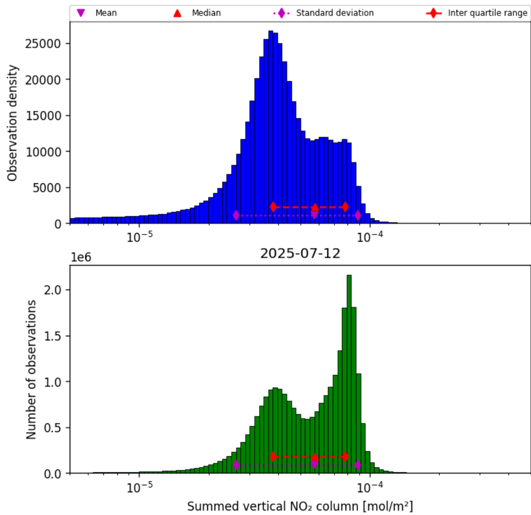
Figure 40: Histogram of “Summed vertical NO 2 column” for 2025-07-11 to 2025-07-13
