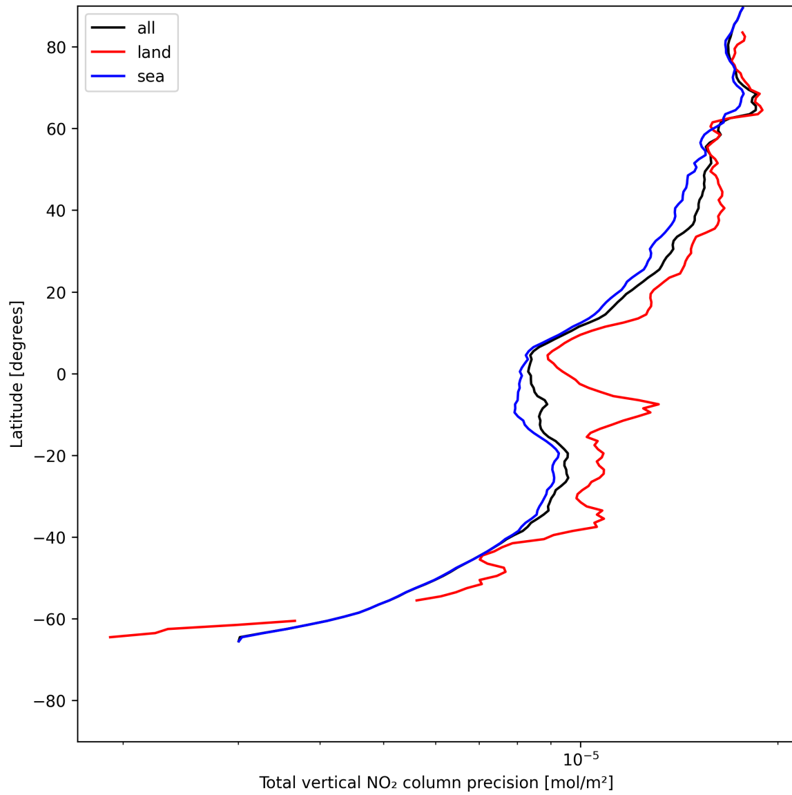
Figure 22: Zonal average of “Total vertical NO 2 column precision” for 2025-07-11 to 2025-07-13.
