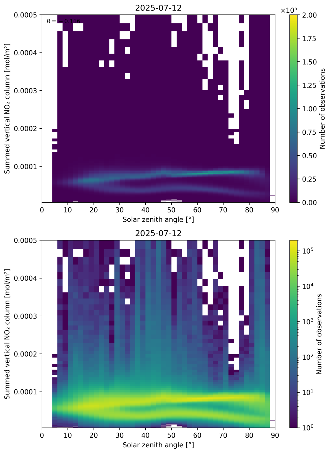
Figure 151: Scatter density plot of “Solar zenith angle” against “Summed vertical NO 2 column” for 2025-07-11 to 2025-07-13.
