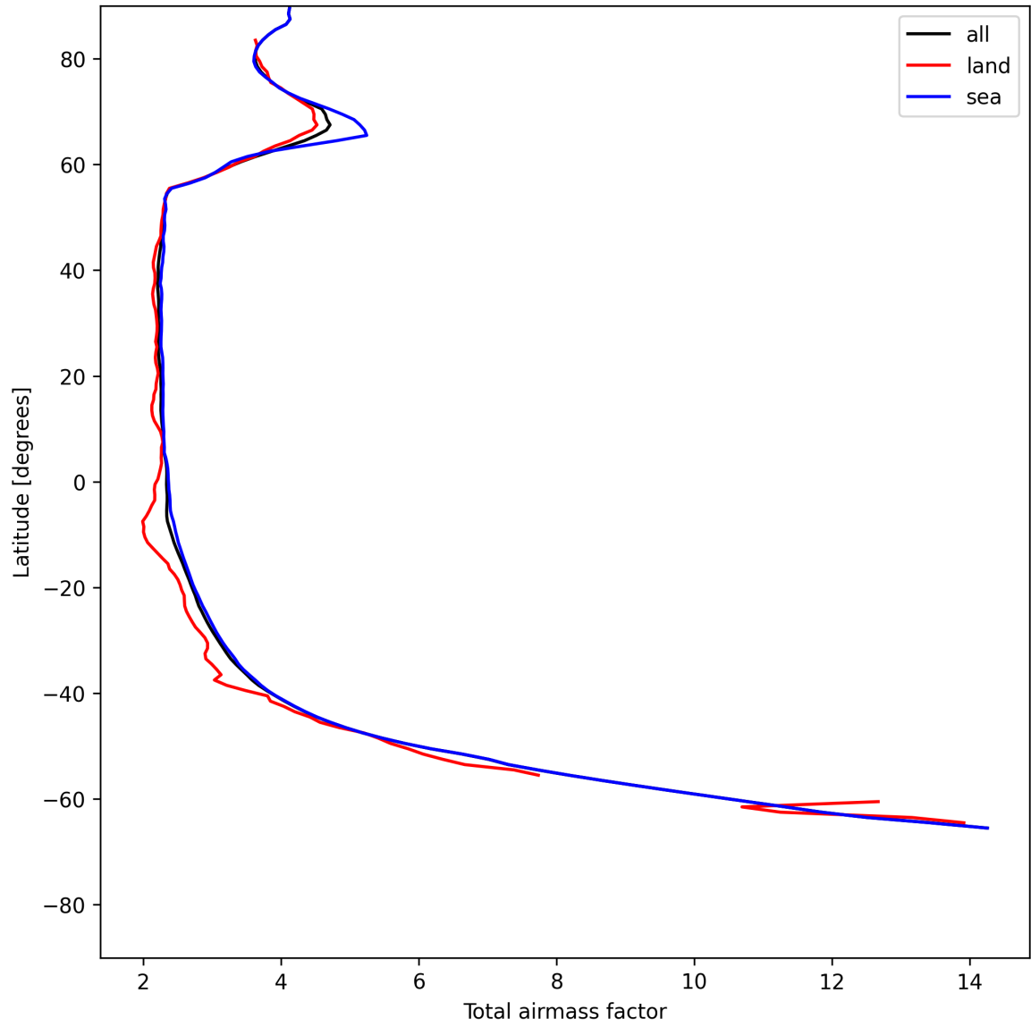
Figure 15: Zonal average of “Total airmass factor” for 2025-07-11 to 2025-07-13.
