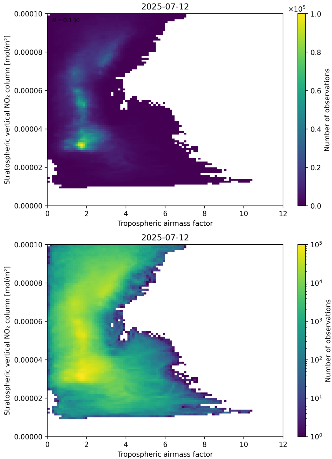
Figure 74: Scatter density plot of “Tropospheric air mass factor” against “Stratospheric vertical NO 2 column” for 2025-07-11 to 2025-07-13.
