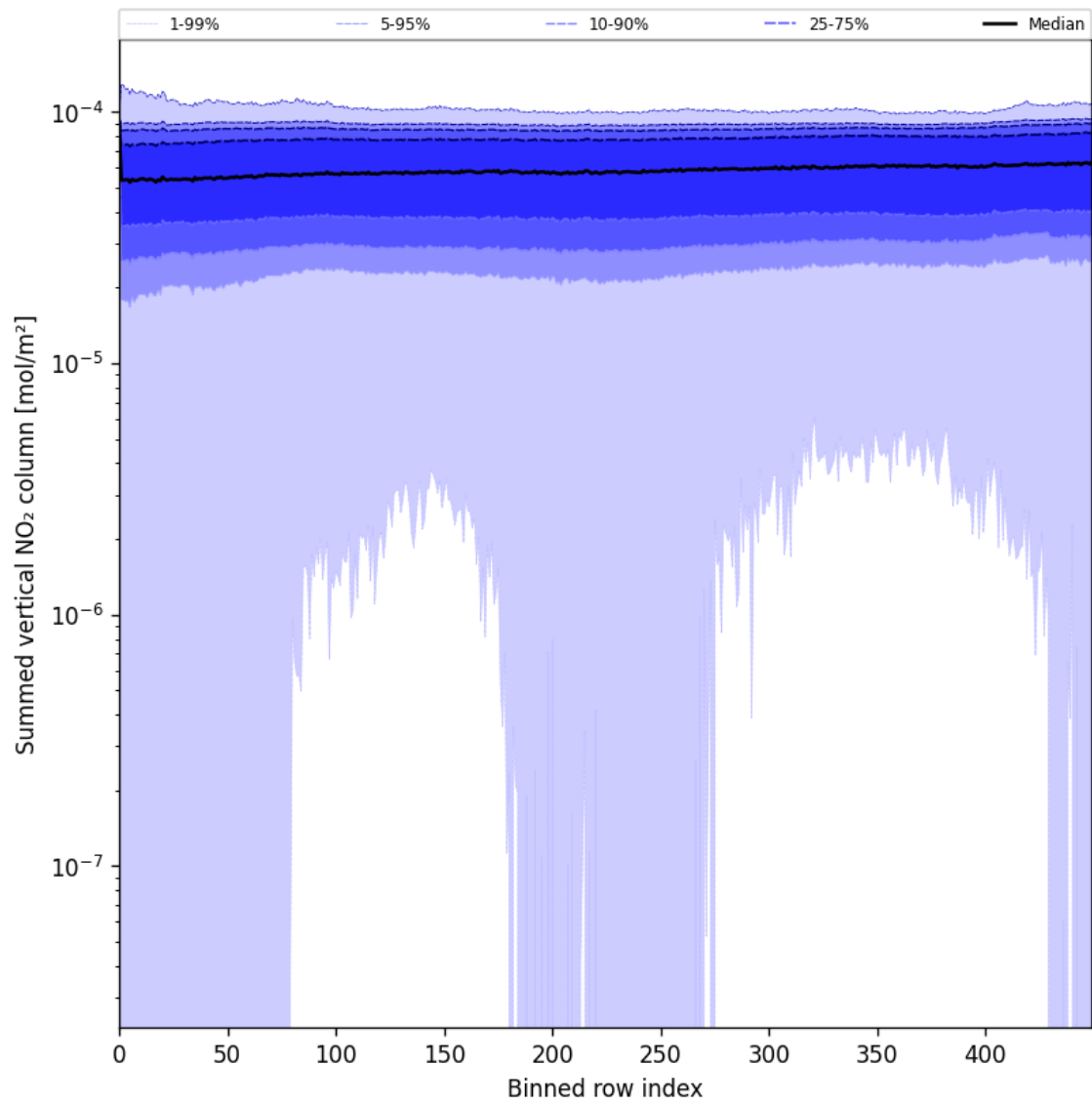
Figure 57: Along track statistics of “Summed vertical NO 2 column” for 2025-07-11 to 2025-07-13
