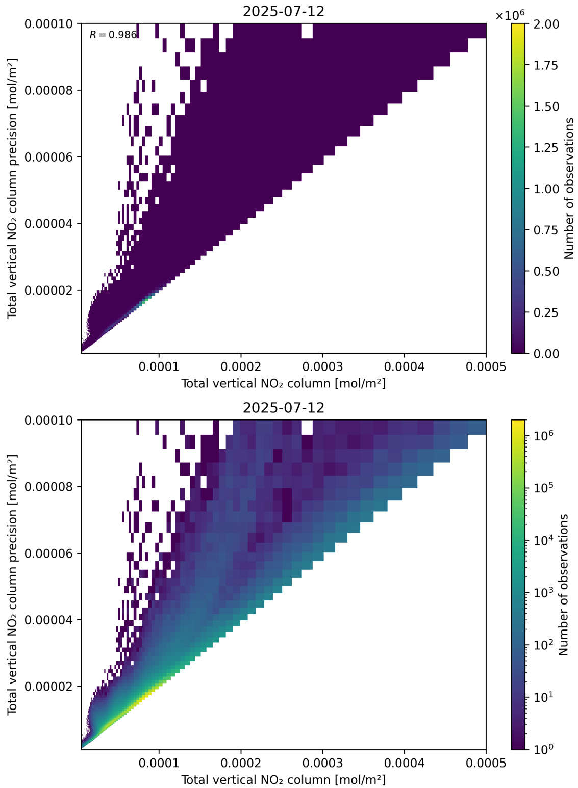
Figure 114: Scatter density plot of “Total vertical NO 2 column” against “Total vertical NO 2 column precision” for 2025-07-11 to 2025-07-13.
