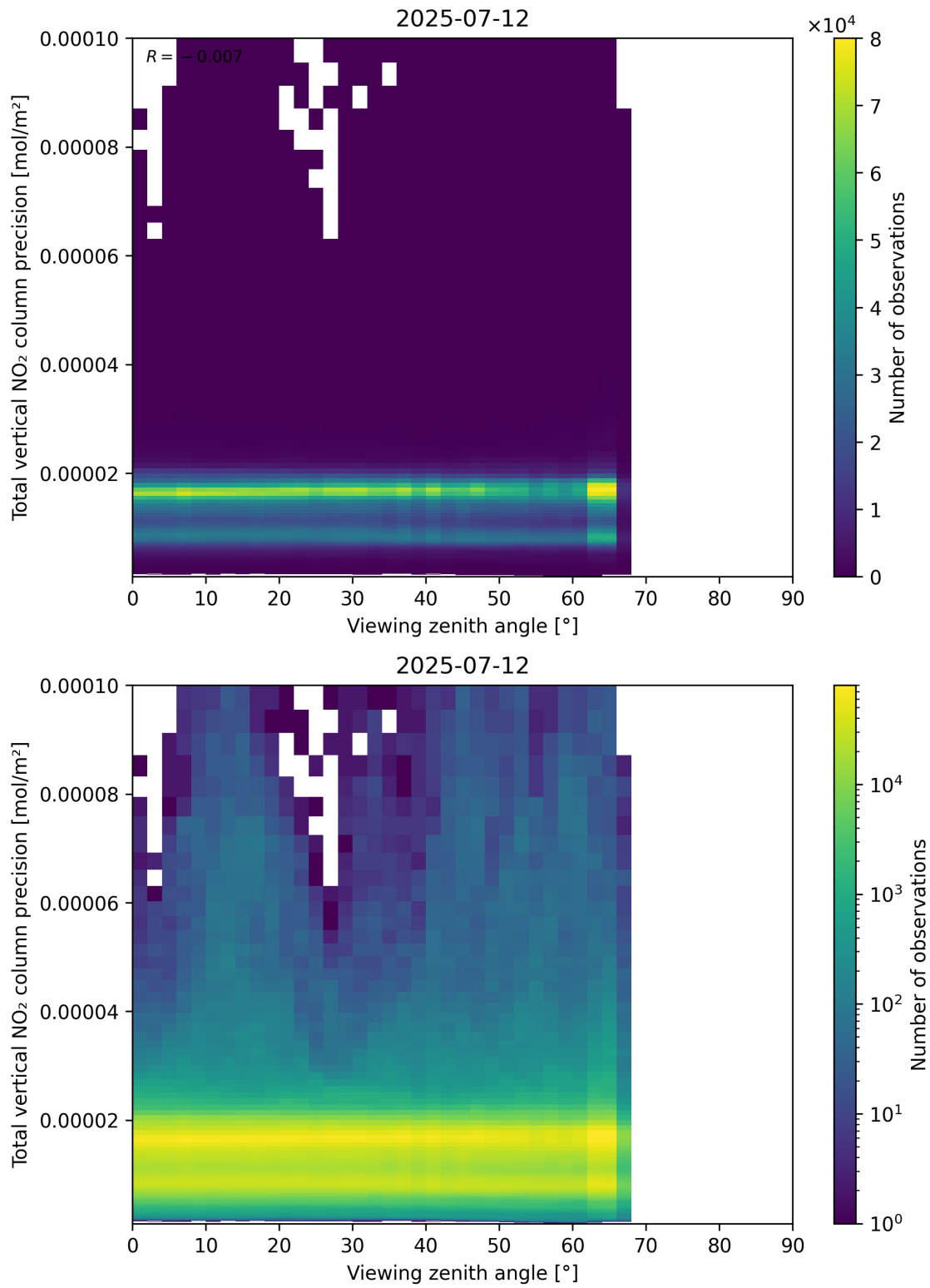
Figure 168: Scatter density plot of “Viewing zenith angle” against “Total vertical NO 2 column precision” for 2025-07-11 to 2025-07-13.
