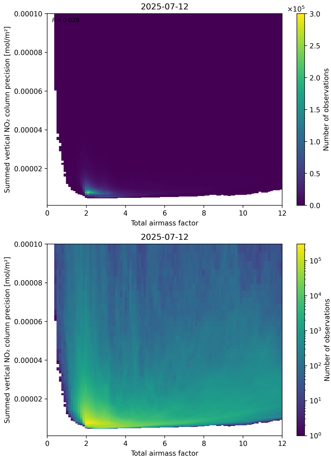
Figure 66: Scatter density plot of “Total airmass factor” against “Summed vertical NO 2 column precision” for 2025-07-11 to 2025-07-13.
