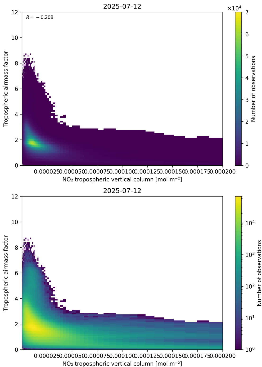
Figure 123: Scatter density plot of “NO 2 tropospheric vertical column” against “Tropospheric air mass factor” for 2025-07-11 to 2025-07-13.
