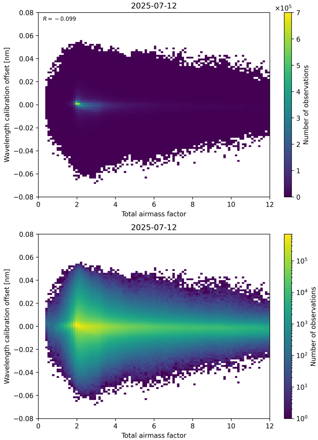
Figure 70: Scatter density plot of “Total airmass factor” against “Wavelength calibration offset” for 2025-07-11 to 2025-07-13.
