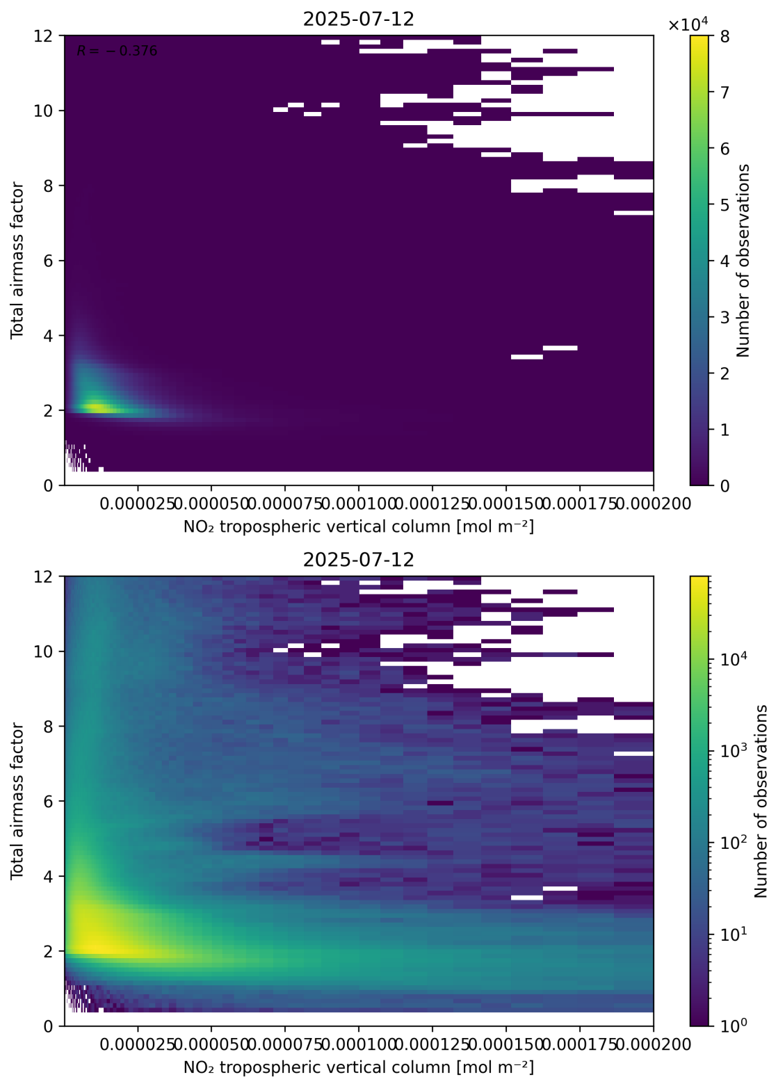
Figure 122: Scatter density plot of “NO 2 tropospheric vertical column” against “Total air mass factor” for 2025-07-11 to 2025-07-13.
