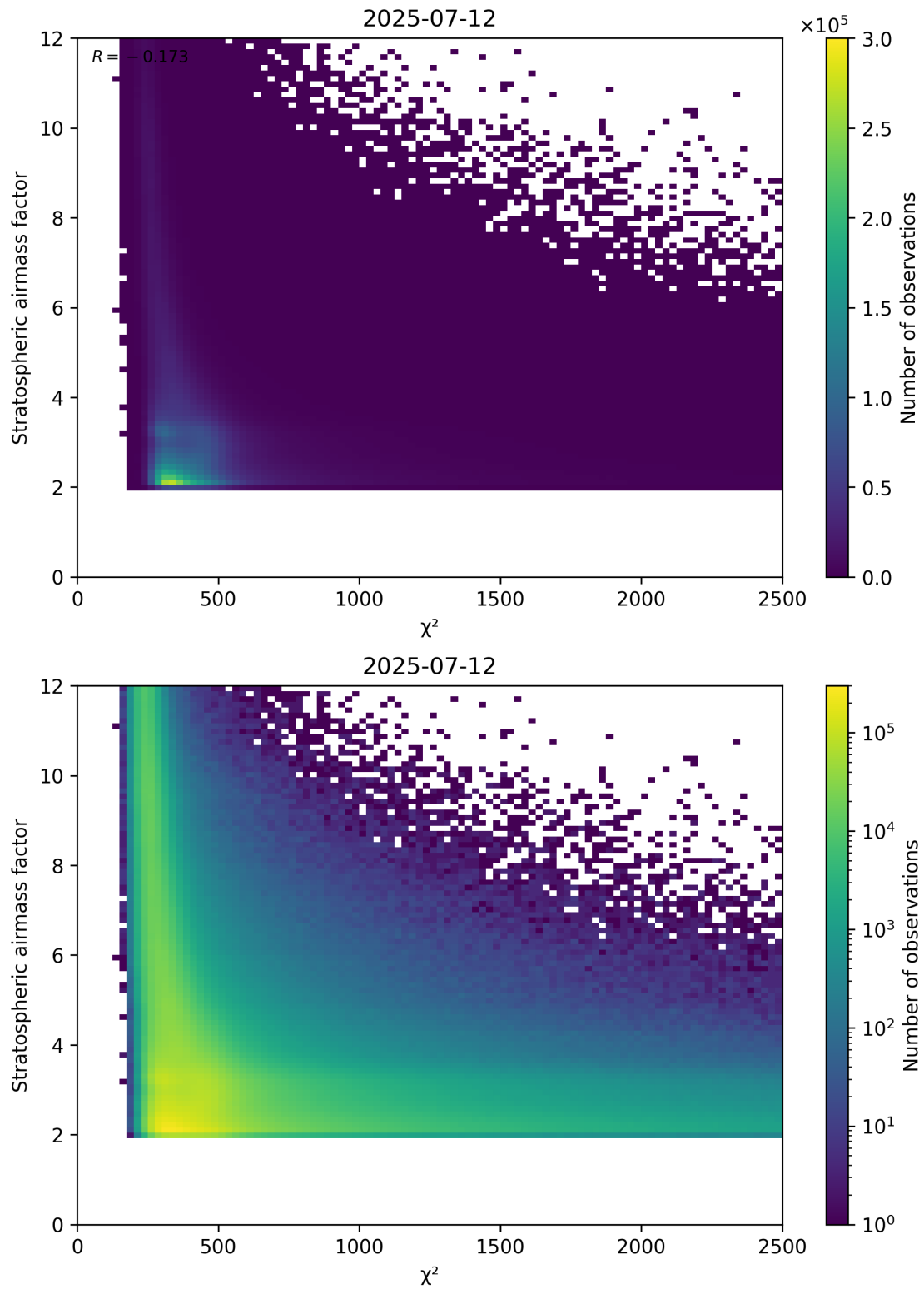
Figure 81: Scatter density plot of “ \chi^2 ” against “Stratospheric airmass factor” for 2025-07-11 to 2025-07-13.
