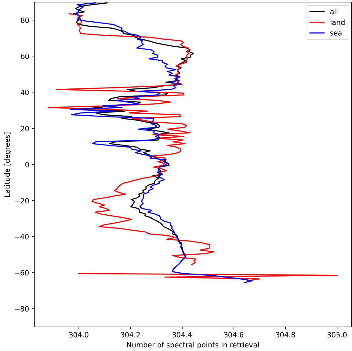
Figure 16: Zonal average of “Number of spectral points in retrieval” for 2025-07-11 to 2025-07-13.
