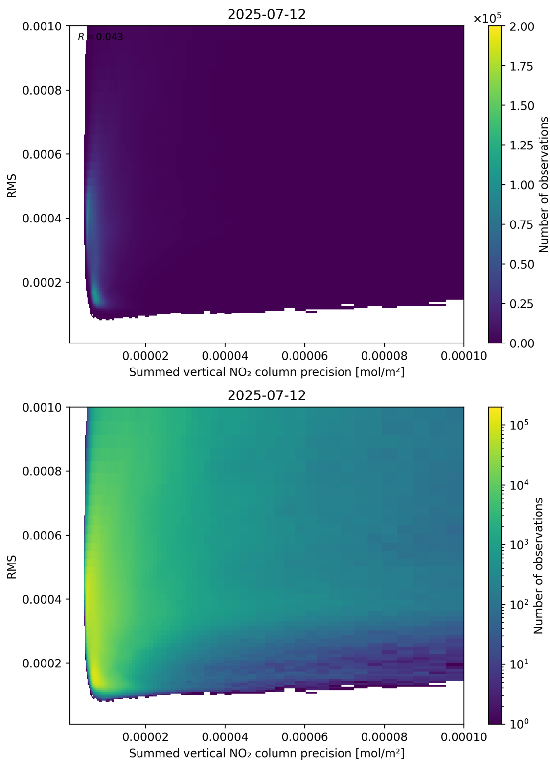
Figure 108: Scatter density plot of “Summed vertical NO 2 column precision” against “RMS” for 2025-07-11 to 2025-07-13.
