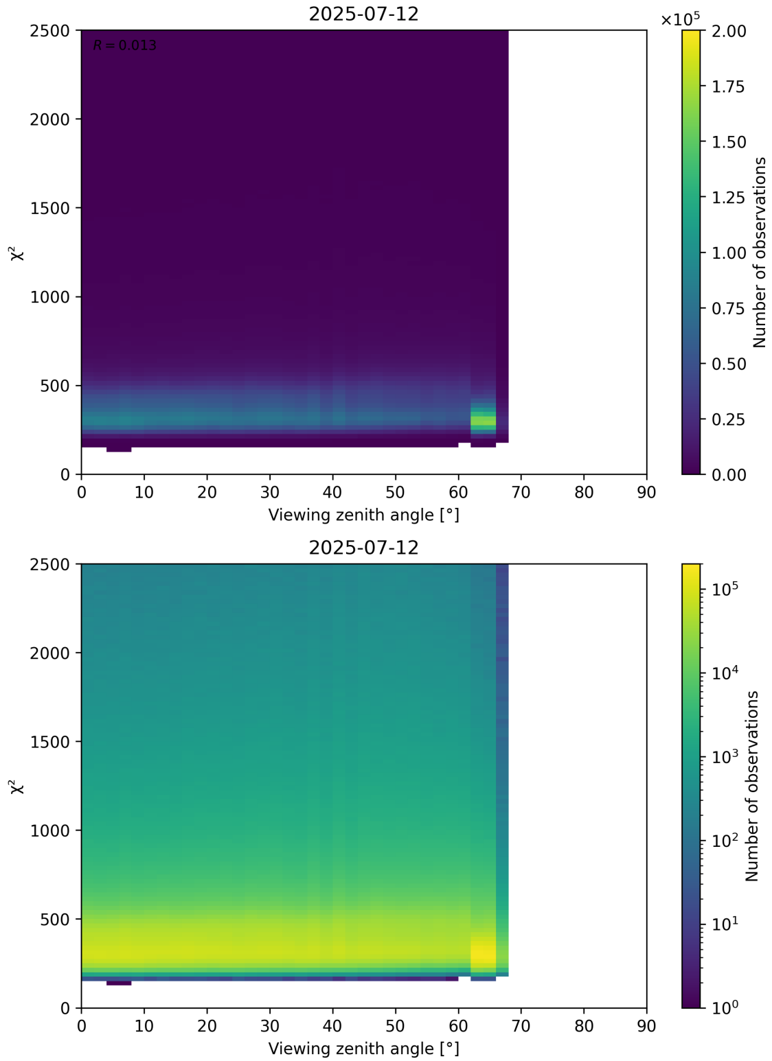
Figure 162: Scatter density plot of “Viewing zenith angle” against “ \chi^2 ” for 2025-07-11 to 2025-07-13.
