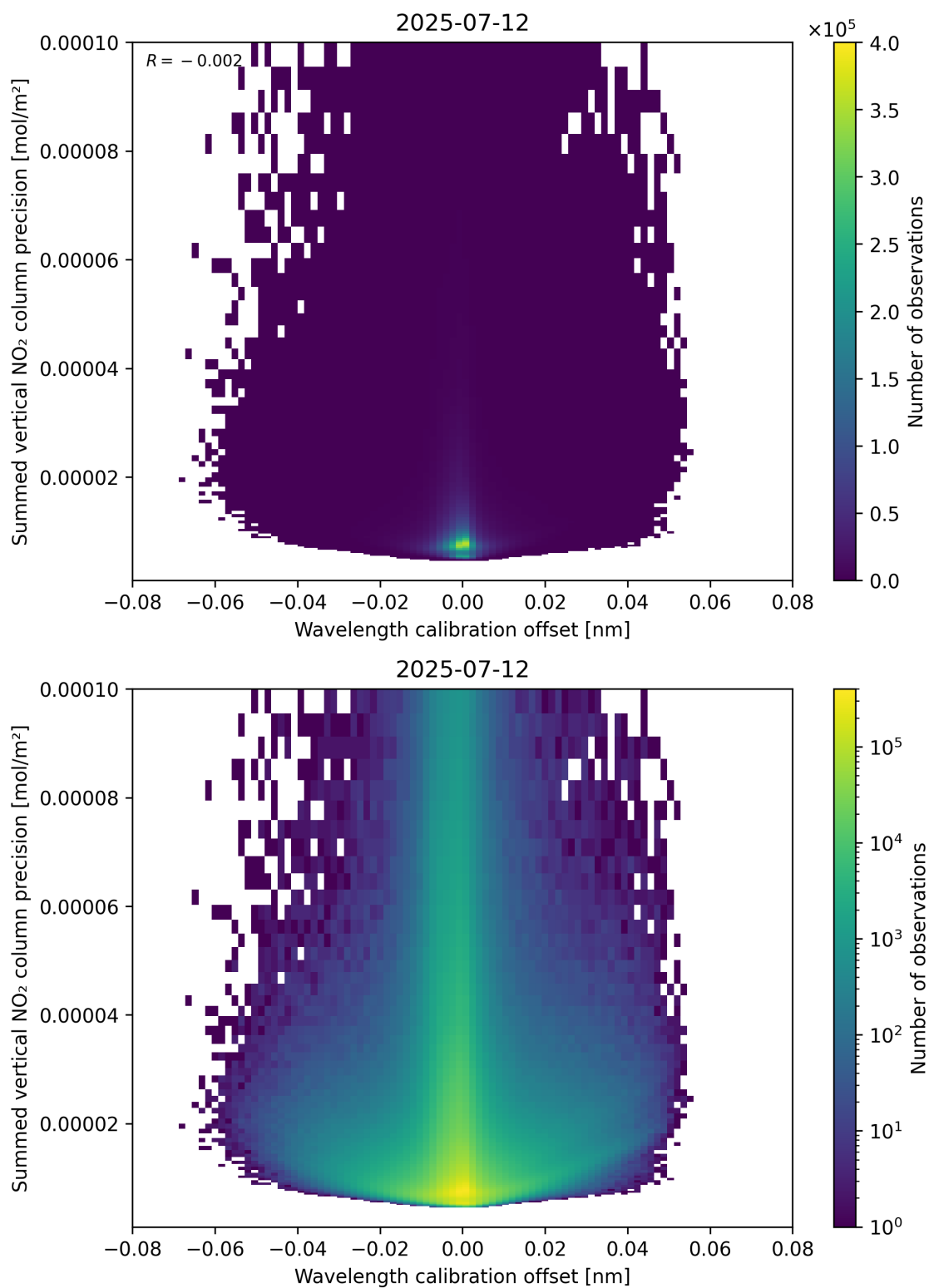
Figure 178: Scatter density plot of “Wavelength calibration offset” against “Summed vertical NO 2 column precision” for 2025-07-11 to 2025-07-13.
