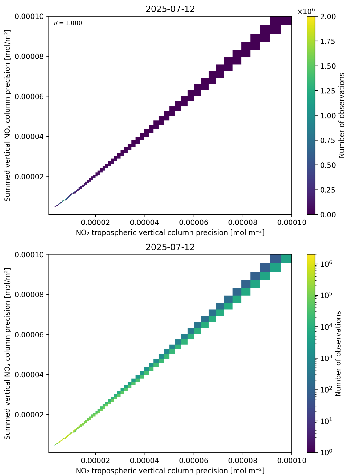
Figure 137: Scatter density plot of “NO 2 tropospheric vertical column precision” against “Summed vertical NO 2 column precision” for 2025-07-11 to 2025-07-13.
