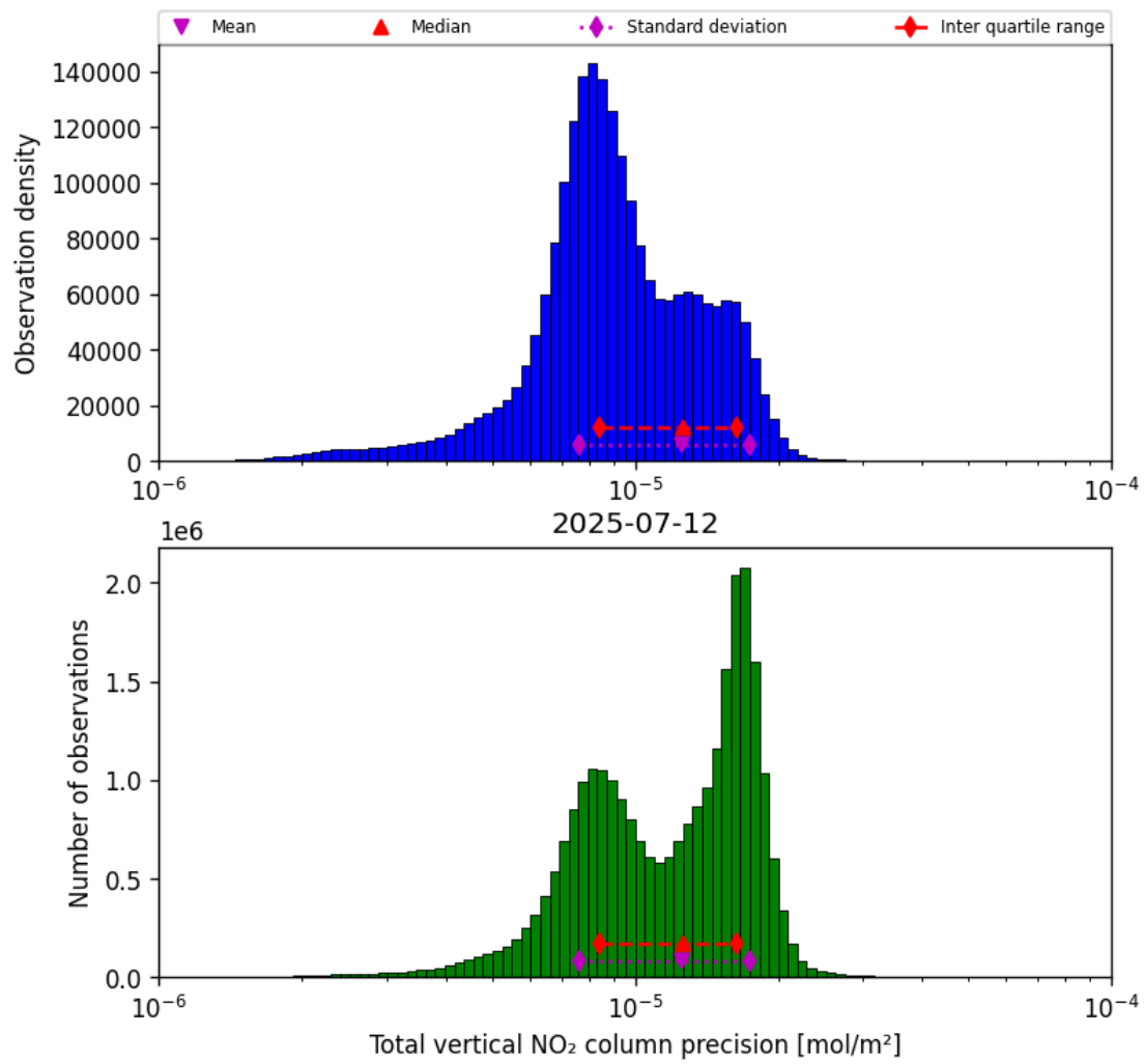
Figure 39: Histogram of “Total vertical NO 2 column precision” for 2025-07-11 to 2025-07-13
