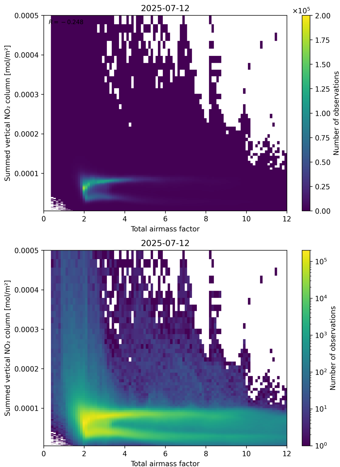
Figure 65: Scatter density plot of “Total airmass factor” against “Summed vertical NO 2 column” for 2025-07-11 to 2025-07-13.
