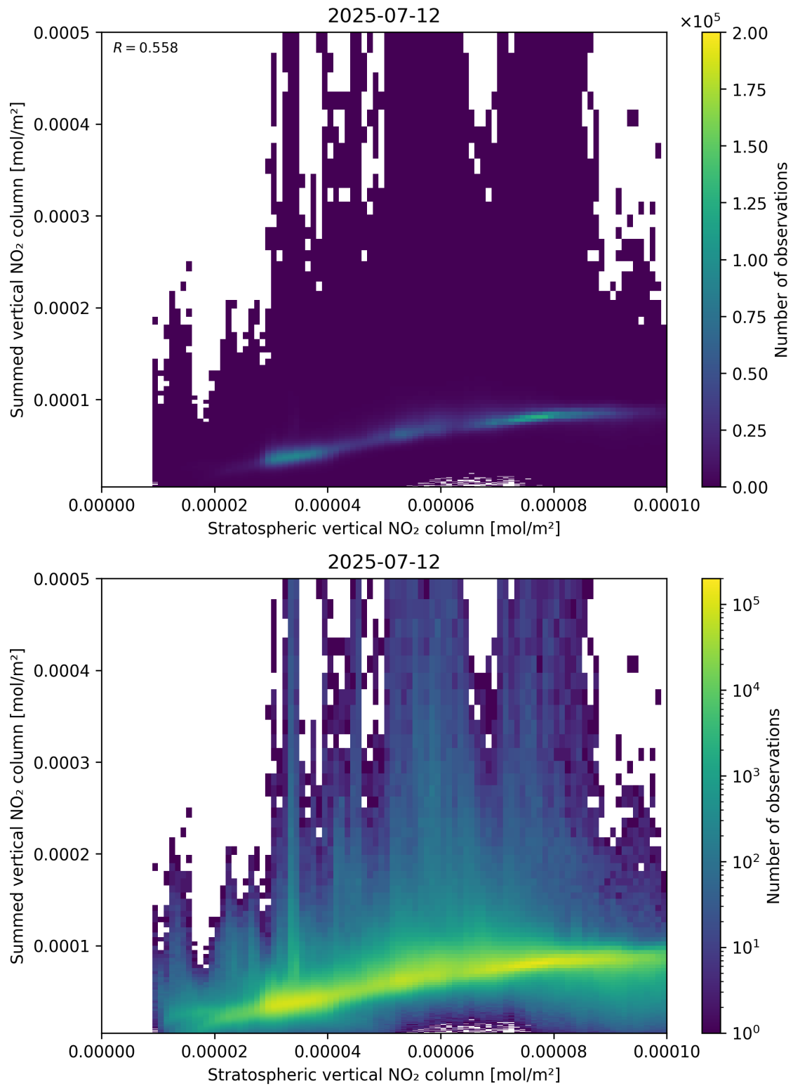
Figure 98: Scatter density plot of “Stratospheric vertical NO 2 column” against “Summed vertical NO 2 column” for 2025-07-11 to 2025-07-13.
