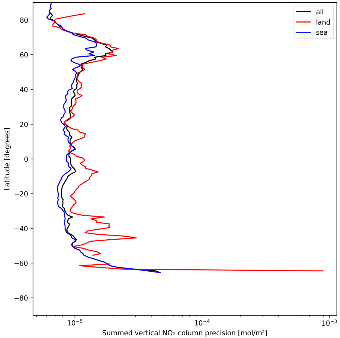
Figure 24: Zonal average of “Summed vertical NO 2 column precision” for 2025-07-11 to 2025-07-13.
