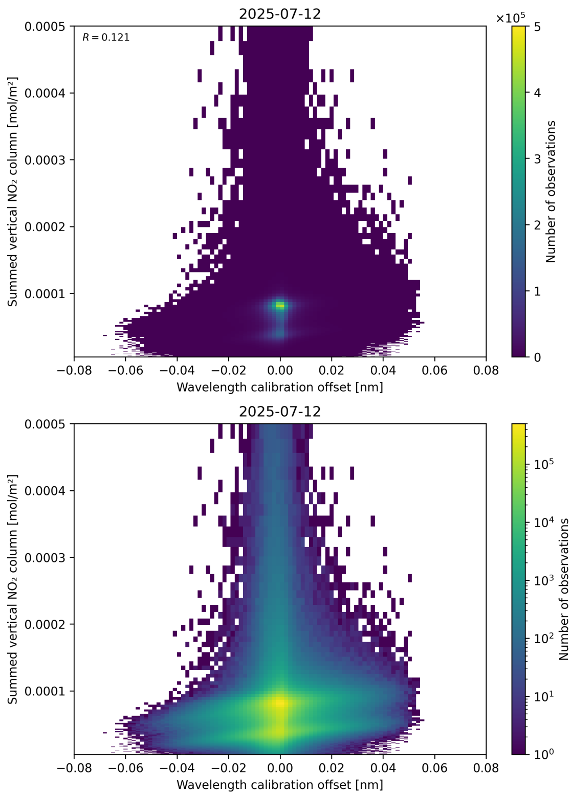
Figure 177: Scatter density plot of “Wavelength calibration offset” against “Summed vertical NO 2 column” for 2025-07-11 to 2025-07-13.
