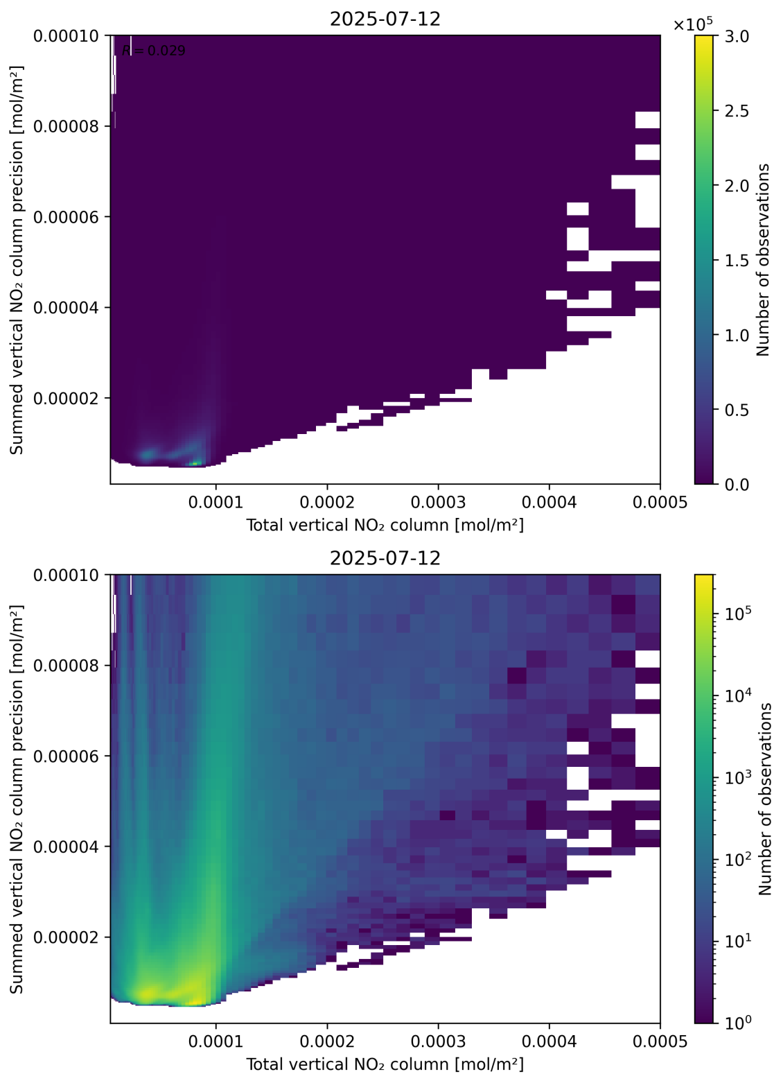
Figure 113: Scatter density plot of “Total vertical NO 2 column” against “Summed vertical NO 2 column precision” for 2025-07-11 to 2025-07-13.
