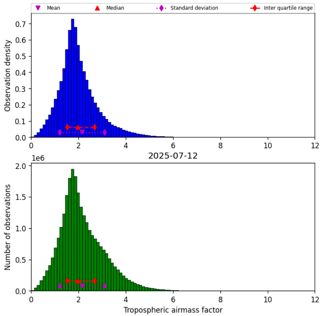
Figure 31: Histogram of “Tropospheric airmass factor” for 2025-07-11 to 2025-07-13
