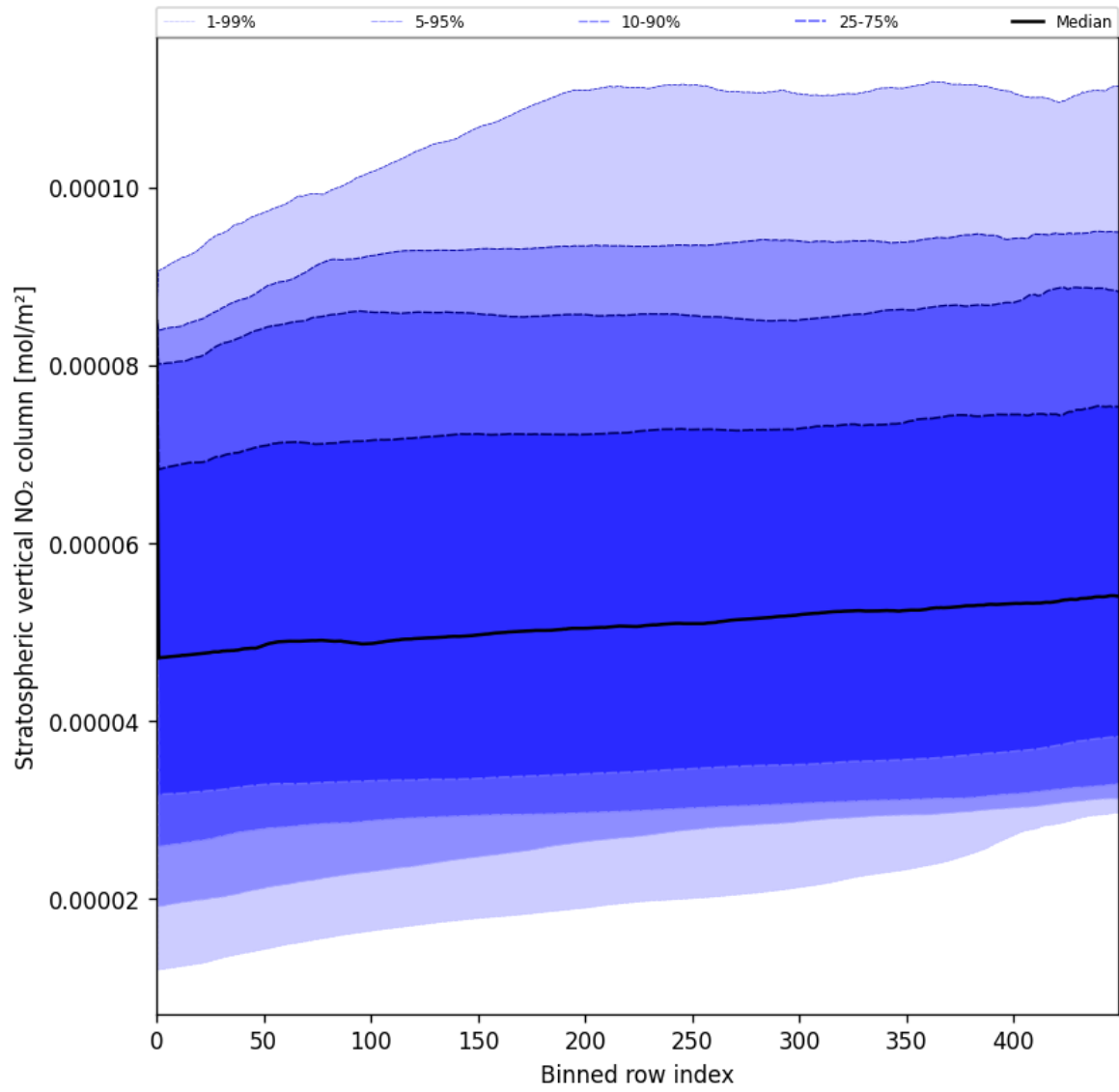
Figure 53: Along track statistics of “Stratospheric vertical NO 2 column” for 2025-07-11 to 2025-07-13
