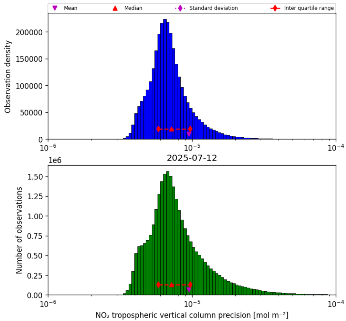
Figure 30: Histogram of "NO 2 tropospheric vertical column precision" for 2025-07-11 to 2025-07-13
