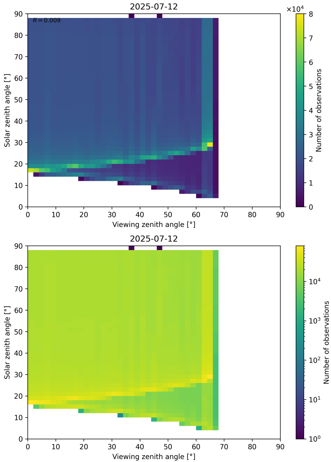
Figure 172: Scatter density plot of “Viewing zenith angle” against “Solar zenith angle” for 2025-07-11 to 2025-07-13.
