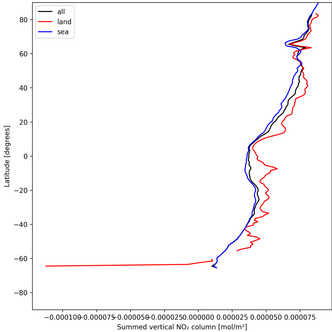
Figure 23: Zonal average of “Summed vertical NO 2 column” for 2025-07-11 to 2025-07-13.
