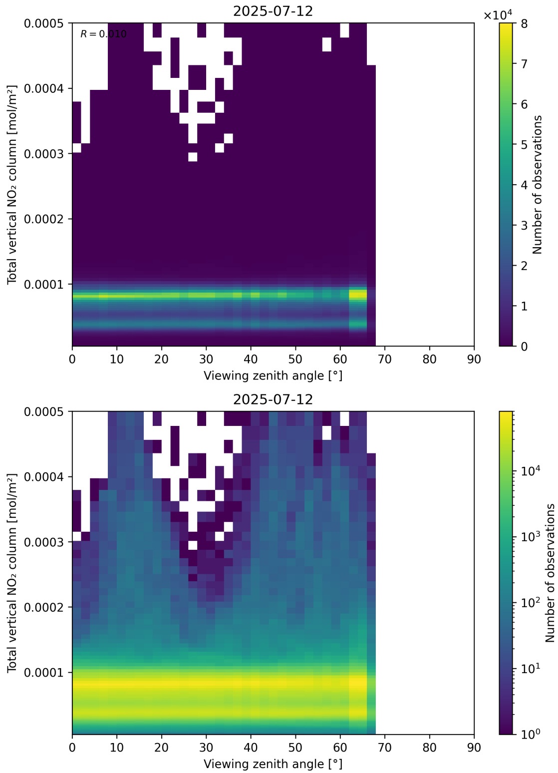
Figure 167: Scatter density plot of “Viewing zenith angle” against “Total vertical NO 2 column” for 2025-07-11 to 2025-07-13.
