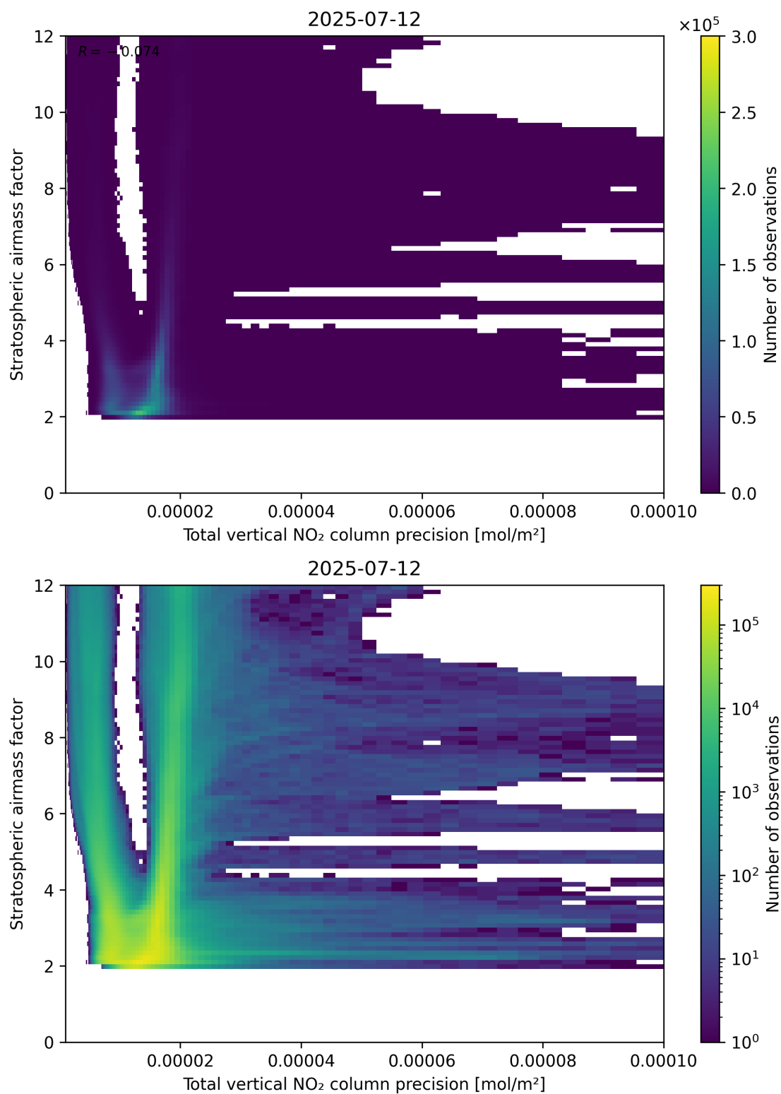
Figure 115: Scatter density plot of “Total vertical NO 2 column precision” against “Stratospheric air mass factor” for 2025-07-11 to 2025-07-13.
