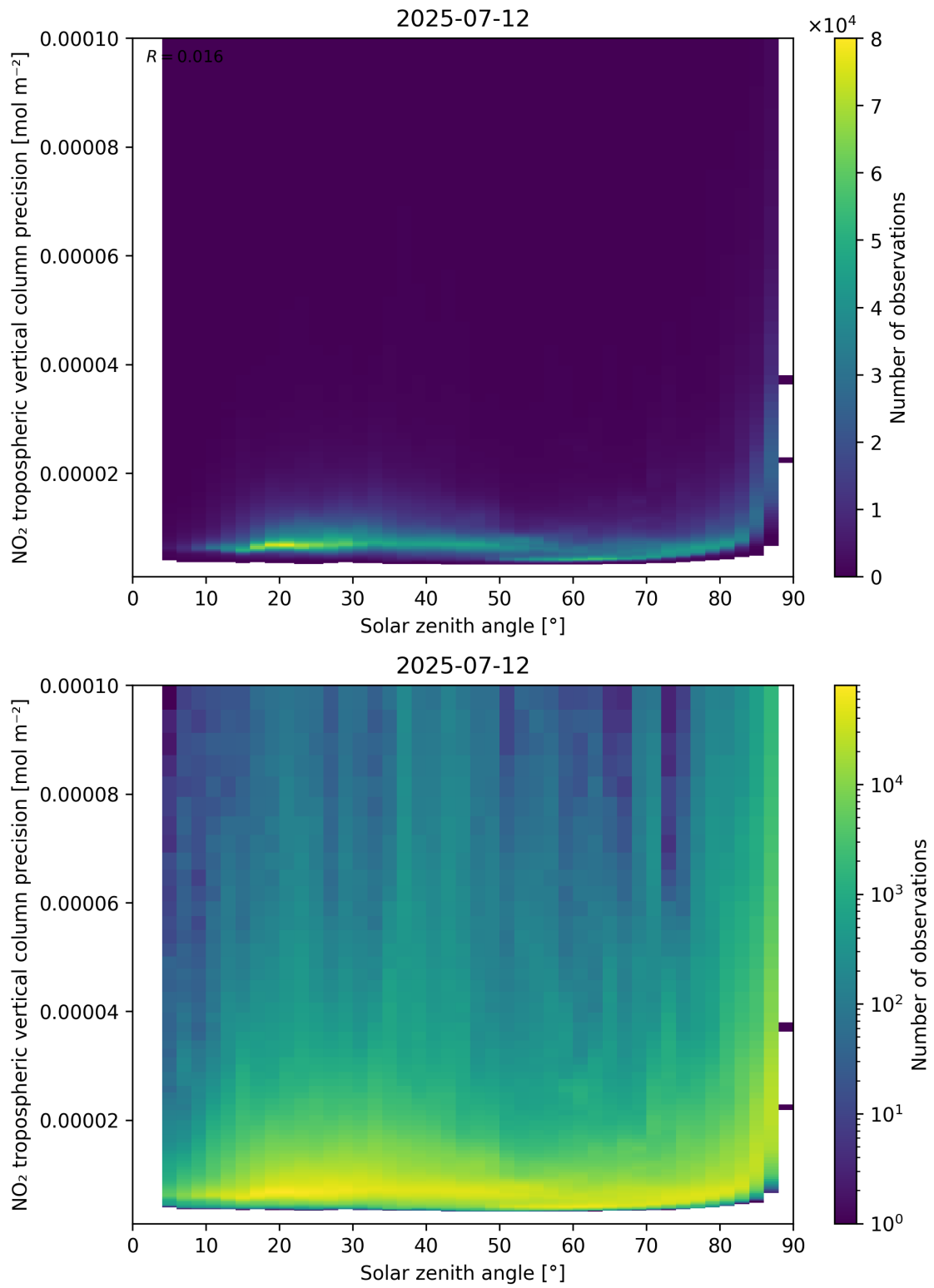
Figure 156: Scatter density plot of “Solar zenith angle” against “NO 2 tropospheric vertical column precision” for 2025-07-11 to 2025-07-13.
