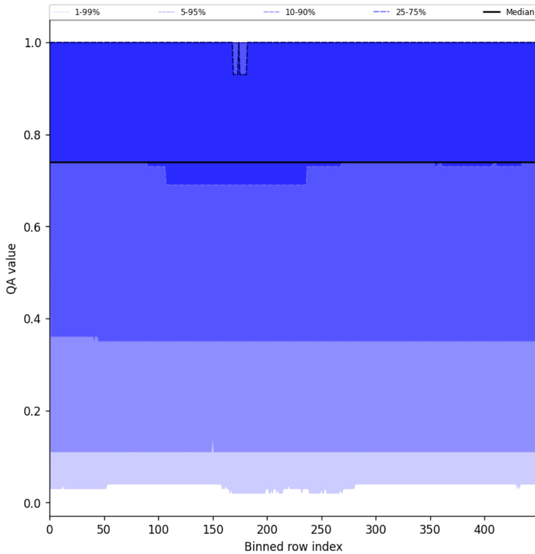
Figure 45: Along track statistics of “QA value” for 2025-07-11 to 2025-07-13
