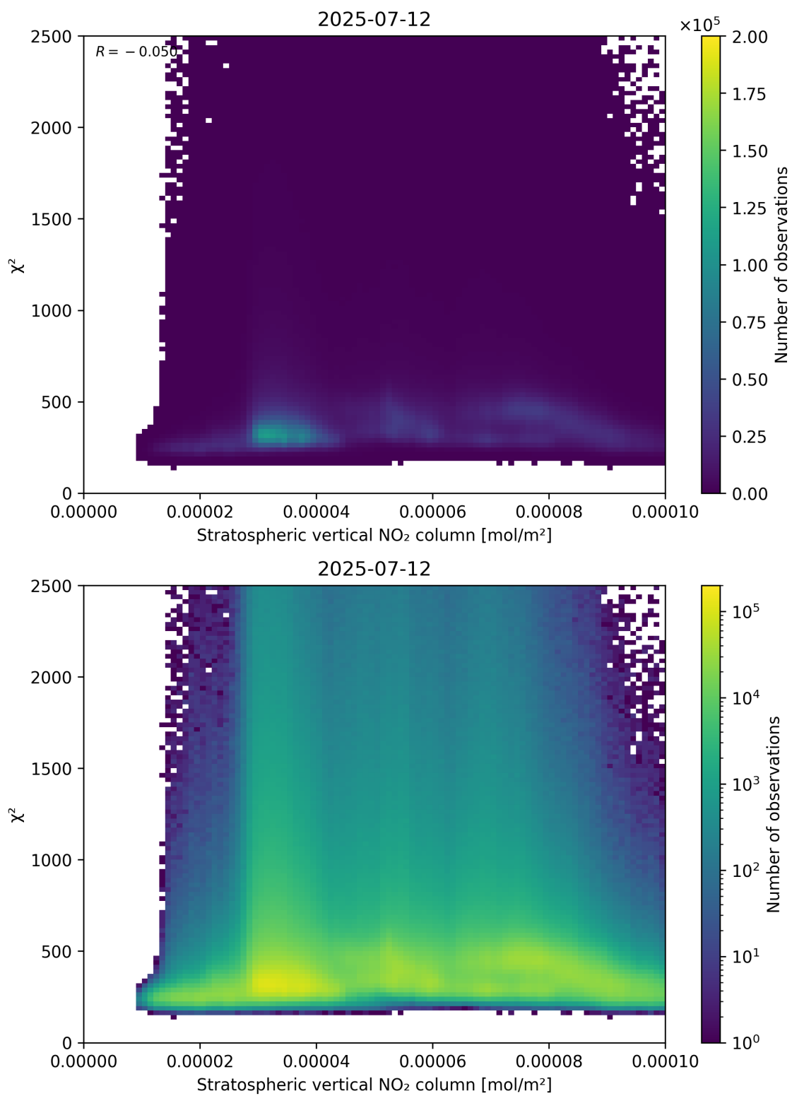
Figure 97: Scatter density plot of “Stratospheric vertical NO 2 column” against “ \chi^2 ” for 2025-07-11 to 2025-07-13.
