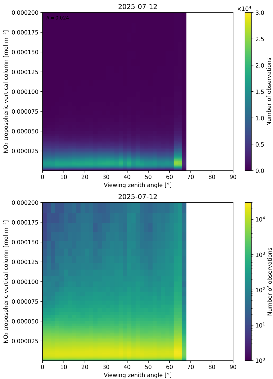
Figure 169: Scatter density plot of “Viewing zenith angle” against “NO 2 tropospheric vertical column” for 2025-07-11 to 2025-07-13.
