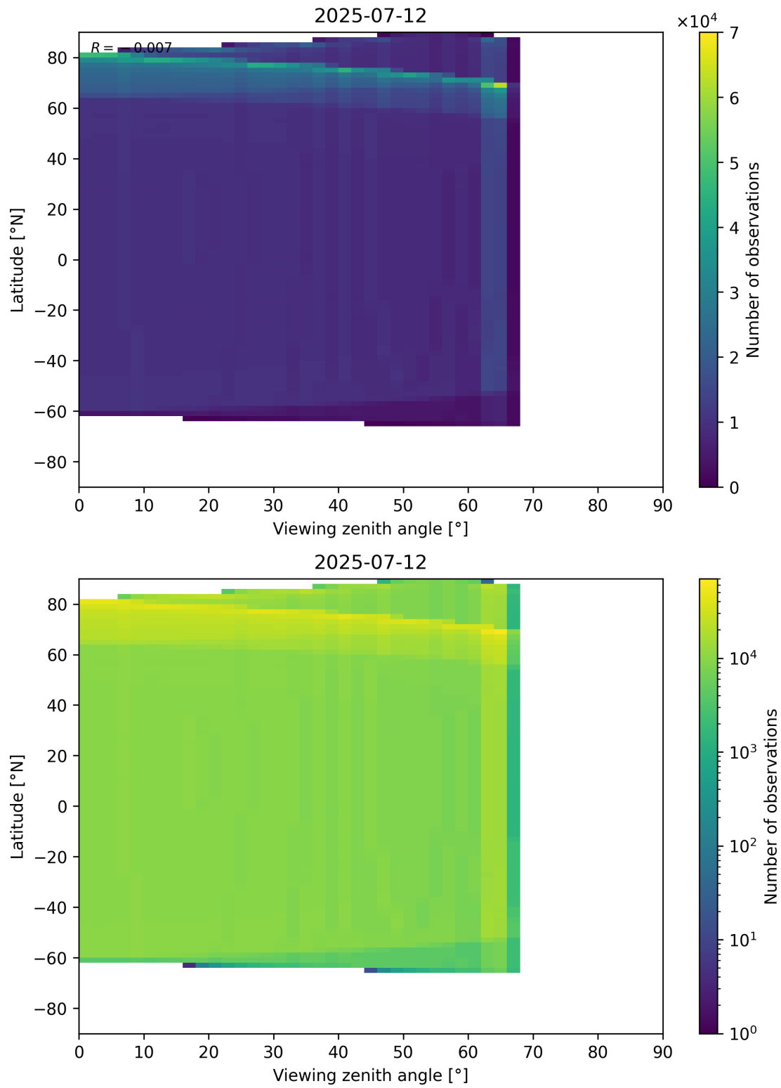
Figure 163: Scatter density plot of “Viewing zenith angle” against “Latitude” for 2025-07-11 to 2025-07-13.
