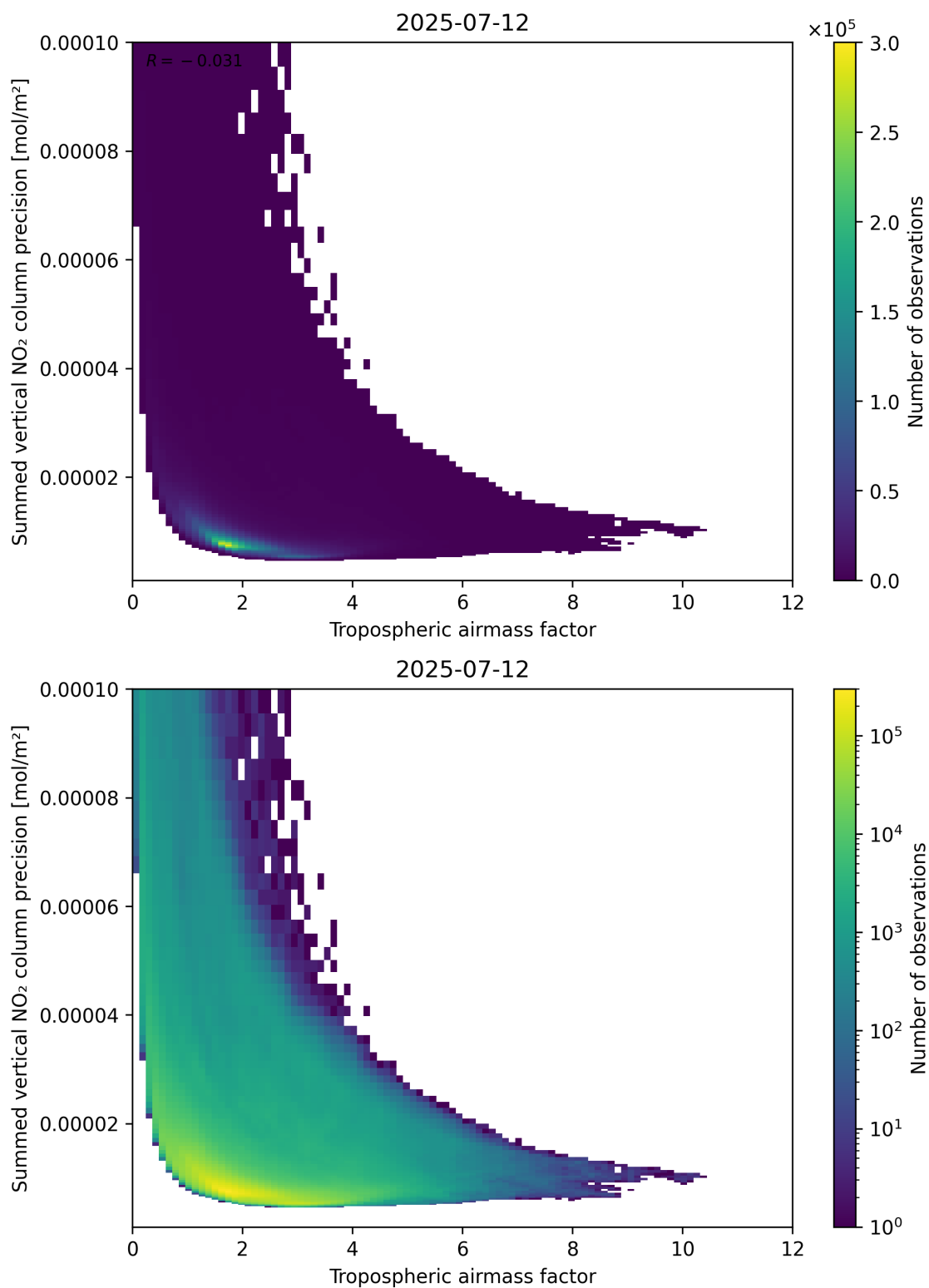
Figure 76: Scatter density plot of “Tropospheric airmass factor” against “Summed vertical NO 2 column precision” for 2025-07-11 to 2025-07-13.
