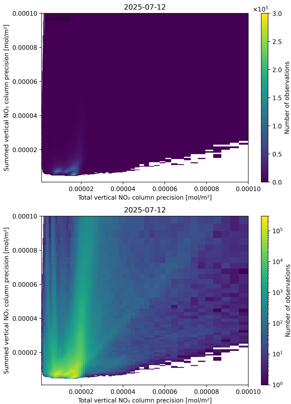
Figure 118: Scatter density plot of “Total vertical NO 2 column precision” against “Summed vertical NO 2 column precision” for 2025-07-11 to 2025-07-13.
