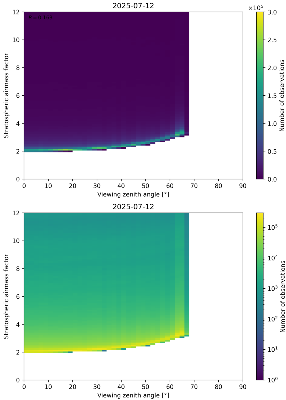
Figure 159: Scatter density plot of “Viewing zenith angle” against “Stratospheric airmass factor” for 2025-07-11 to 2025-07-13.
