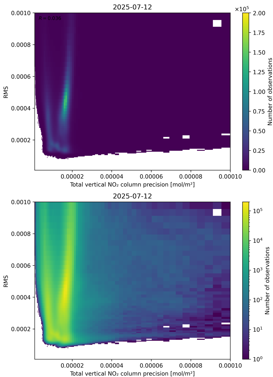
Figure 119: Scatter density plot of “Total vertical NO 2 column precision” against “RMS” for 2025-07-11 to 2025-07-13.
