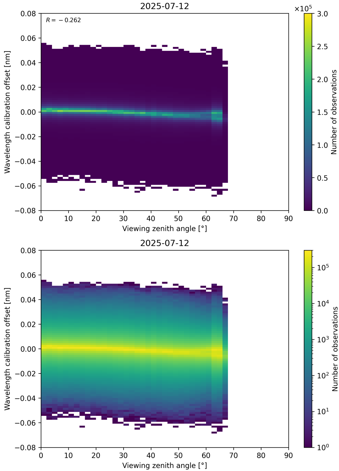
Figure 173: Scatter density plot of “Viewing zenith angle” against “Wavelength calibration offset” for 2025-07-11 to 2025-07-13.
