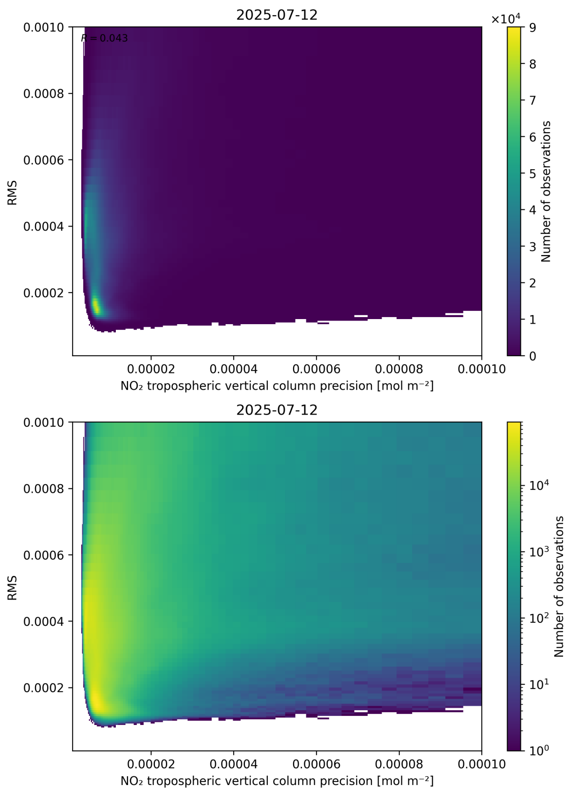
Figure 140: Scatter density plot of “NO 2 tropospheric vertical column precision” against “RMS” for 2025-07-11 to 2025-07-13.
