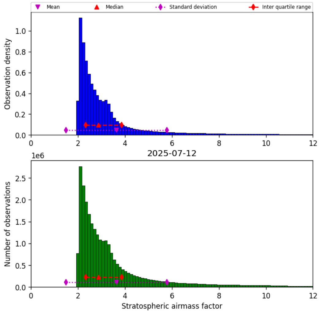
Figure 44: Histogram of “Stratospheric airmass factor” for 2025-07-11 to 2025-07-13
