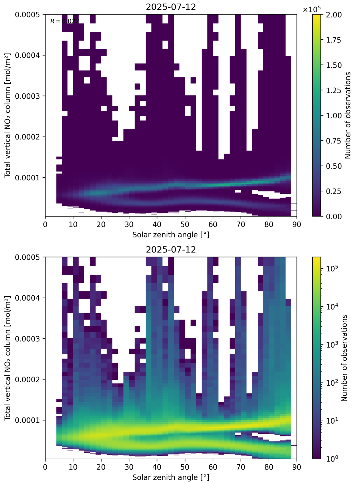
Figure 153: Scatter density plot of “Solar zenith angle” against “Total vertical NO 2 column” for 2025-07-11 to 2025-07-13.
