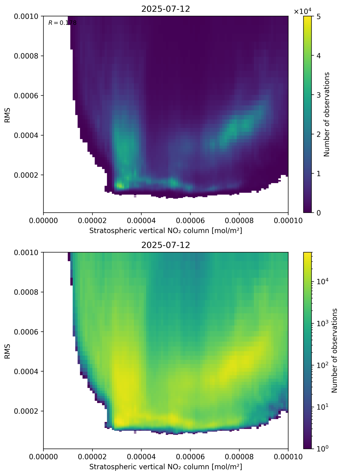
Figure 102: Scatter density plot of “Stratospheric vertical NO 2 column” against “RMS” for 2025-07-11 to 2025-07-13.
