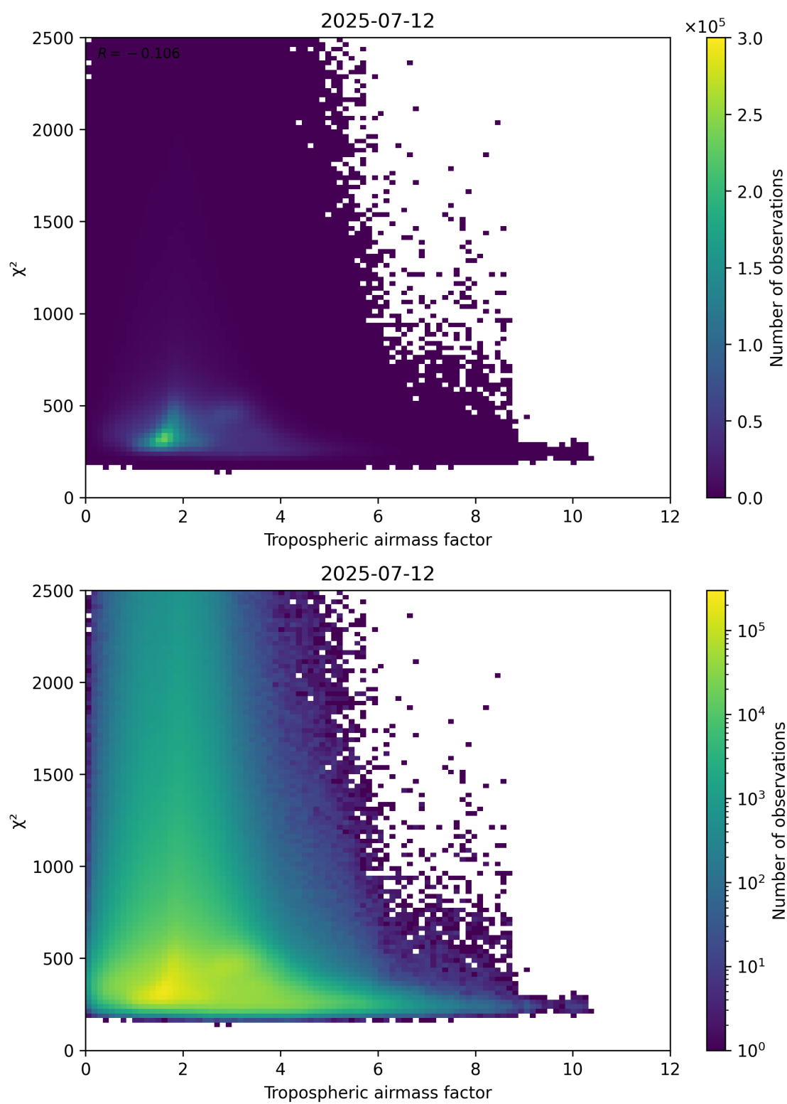
Figure 73: Scatter density plot of “Tropospheric airmass factor” against “ \chi^2 ” for 2025-07-11 to 2025-07-13.
