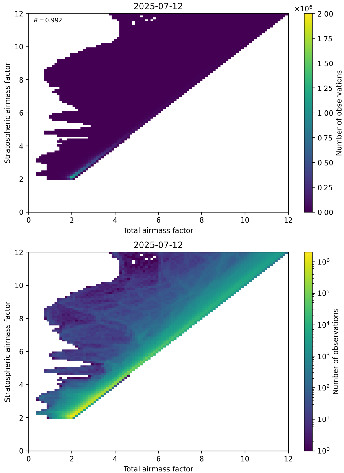
Figure 62: Scatter density plot of “Total airmass factor” against “Stratospheric airmass factor” for 2025-07-11 to 2025-07-13.
