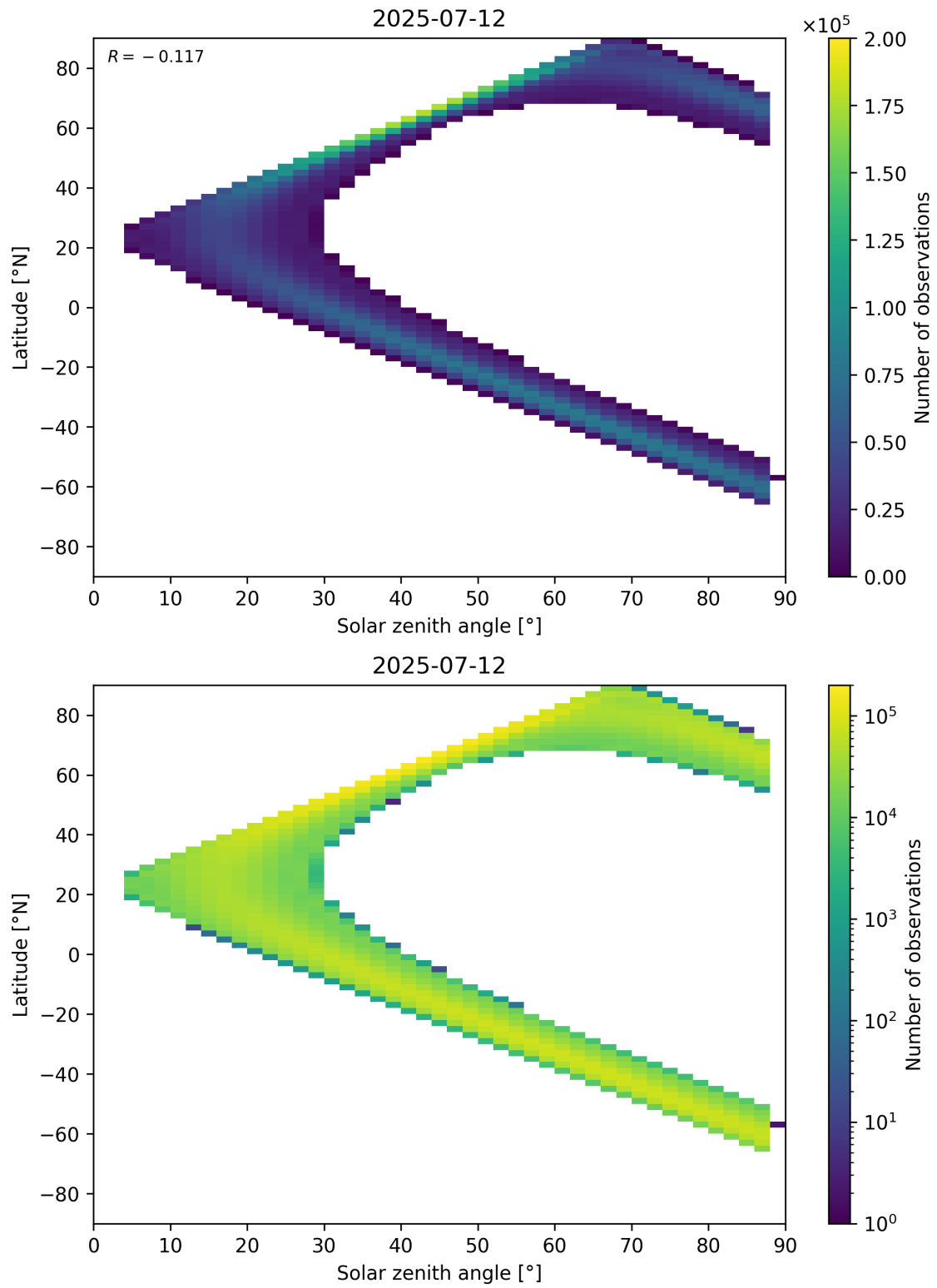
Figure 149: Scatter density plot of “Solar zenith angle” against “Latitude” for 2025-07-11 to 2025-07-13.
