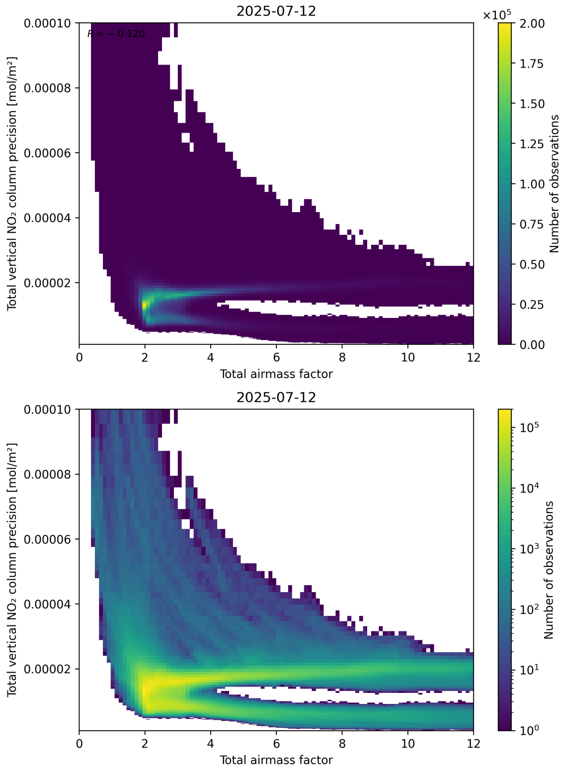
Figure 68: Scatter density plot of “Total airmass factor” against “Total vertical NO 2 column precision” for 2025-07-11 to 2025-07-13.
