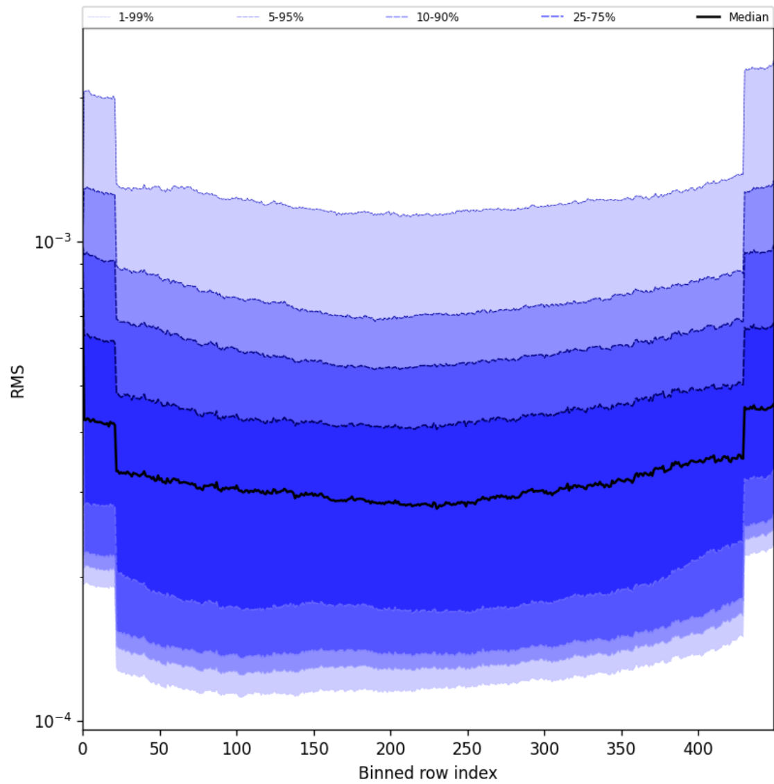
Figure 60: Along track statistics of “RMS” for 2025-07-11 to 2025-07-13
