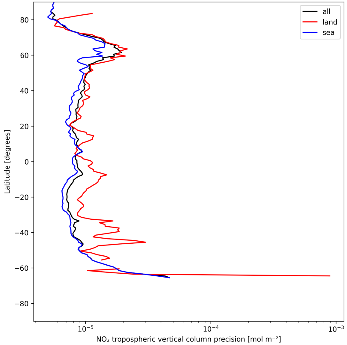
Figure 13: Zonal average of “NO 2 tropospheric vertical column precision” for 2025-07-11 to 2025-07-13.
