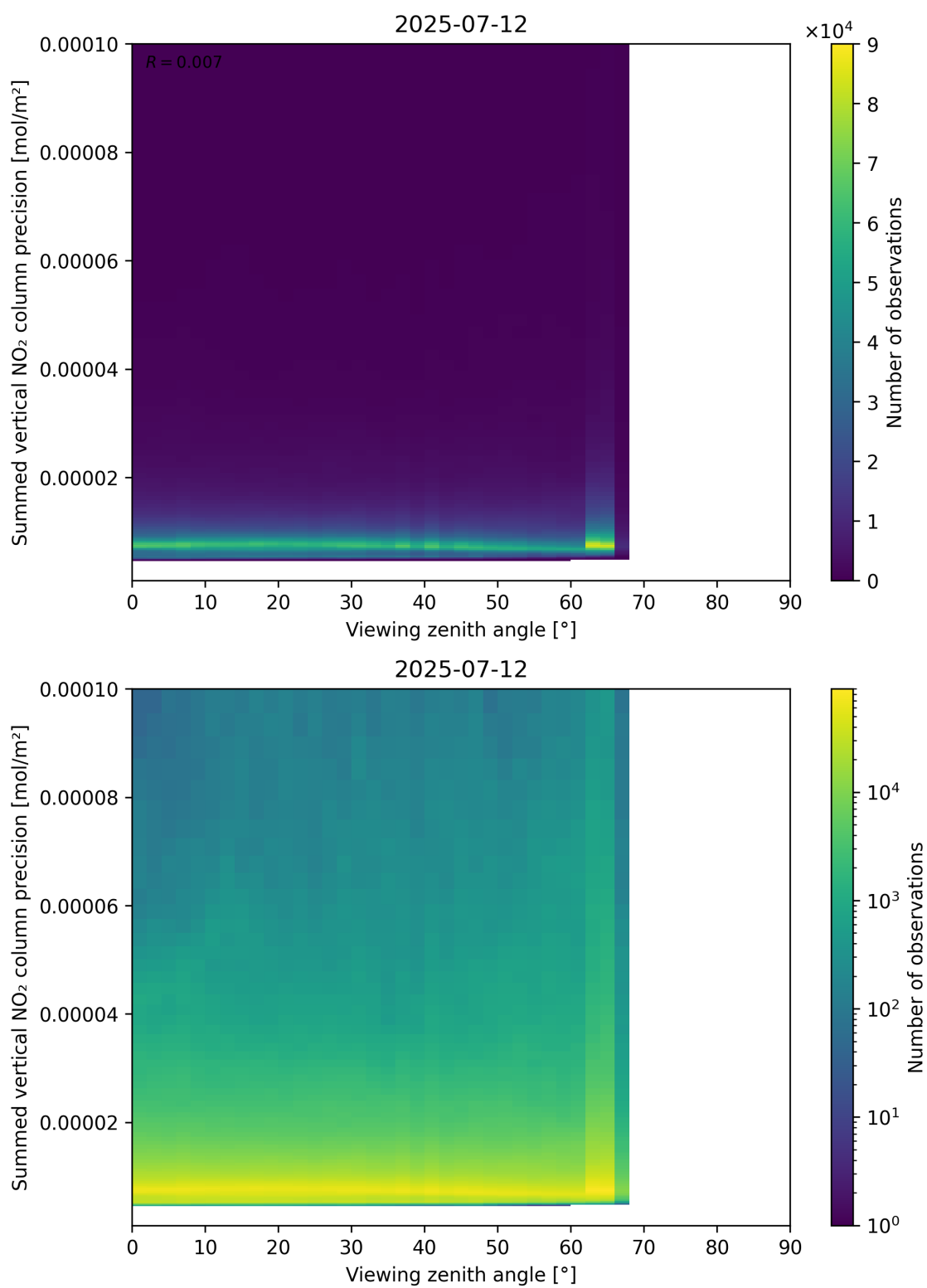
Figure 166: Scatter density plot of “Viewing zenith angle” against “Summed vertical NO 2 column precision” for 2025-07-11 to 2025-07-13.
