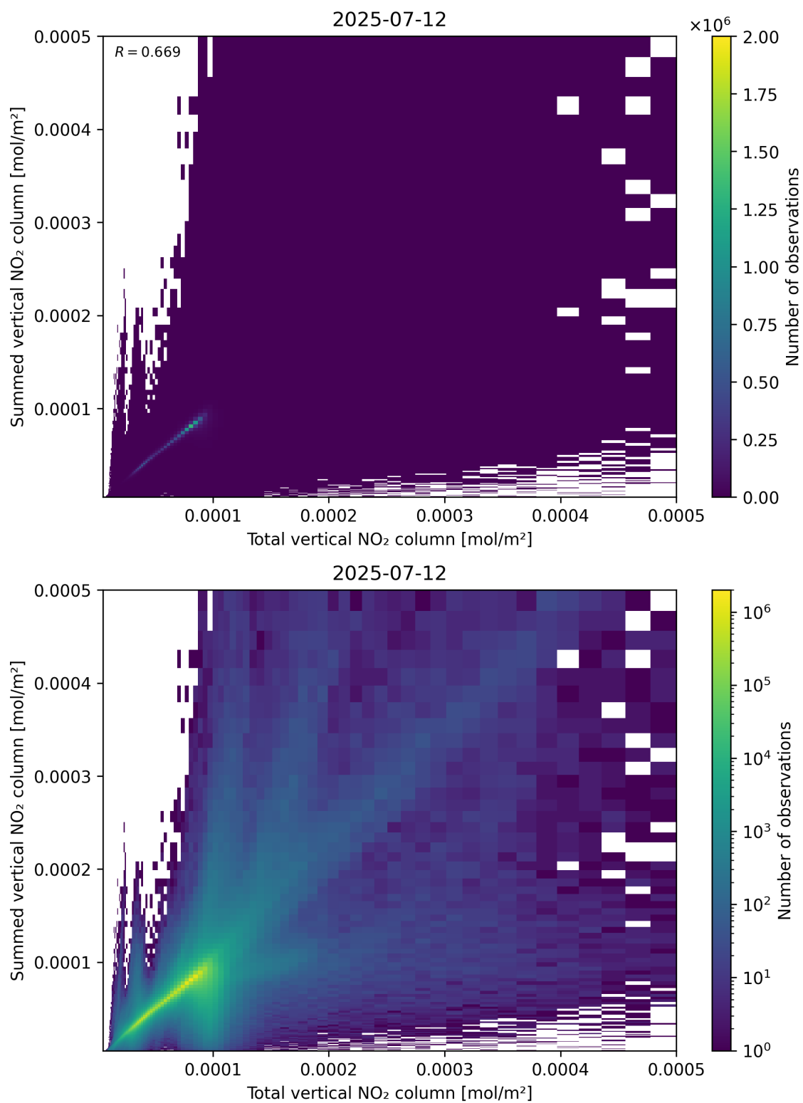
Figure 112: Scatter density plot of “Total vertical NO 2 column” against “Summed vertical NO 2 column” for 2025-07-11 to 2025-07-13.
