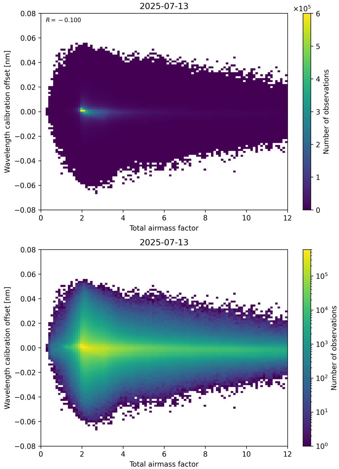
Figure 70: Scatter density plot of “Total airmass factor” against “Wavelength calibration offset” for 2025-07-13 to 2025-07-14.
