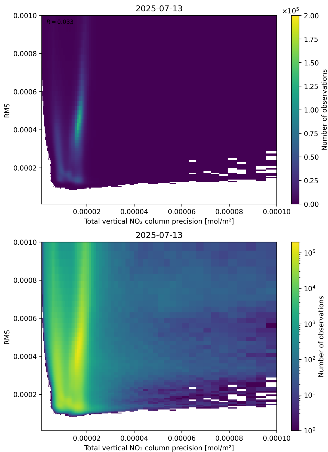
Figure 119: Scatter density plot of “Total vertical NO 2 column precision” against “RMS” for 2025-07-13 to 2025-07-14.
