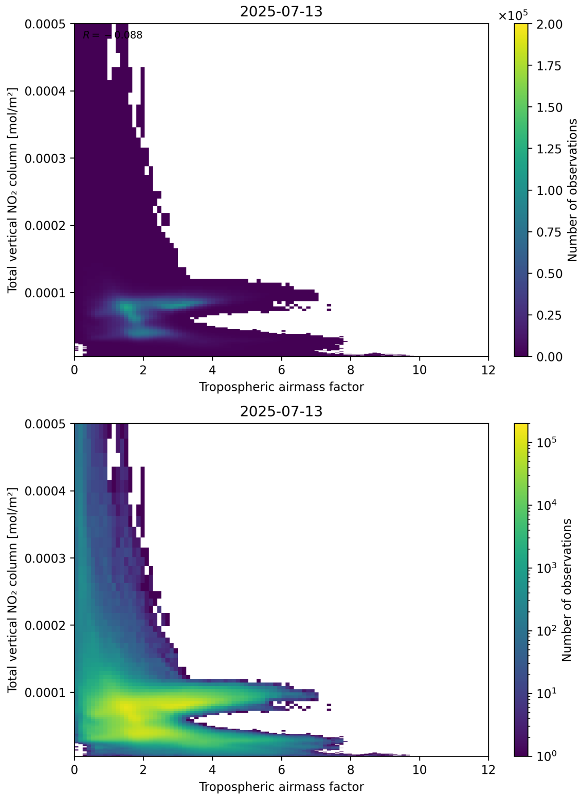
Figure 77: Scatter density plot of “Tropospheric airmass factor” against “Total vertical \text{NO}_2 column” for 2025-07-13 to 2025-07-14.
