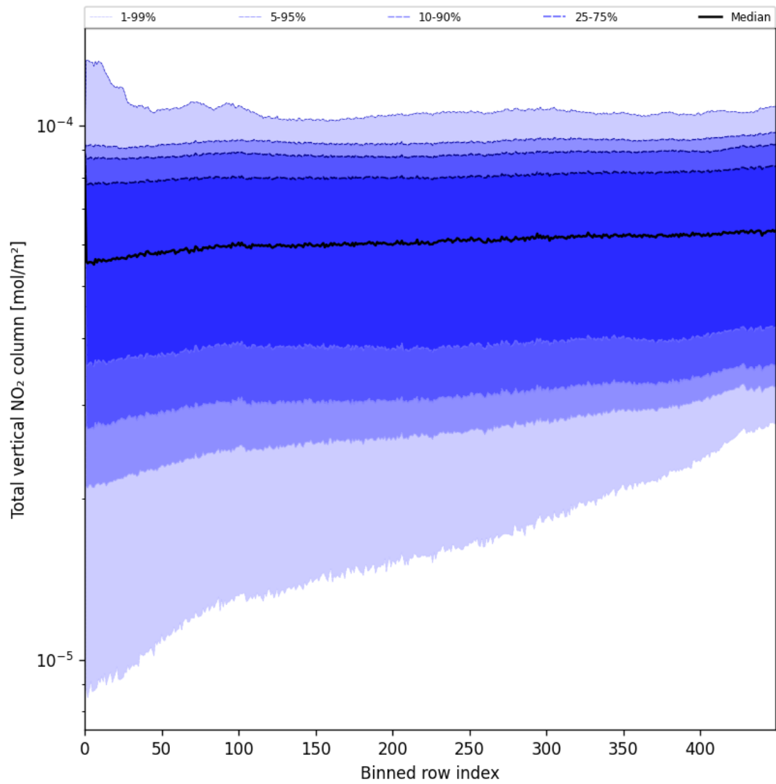
Figure 55: Along track statistics of “Total vertical NO 2 column” for 2025-07-13 to 2025-07-14
