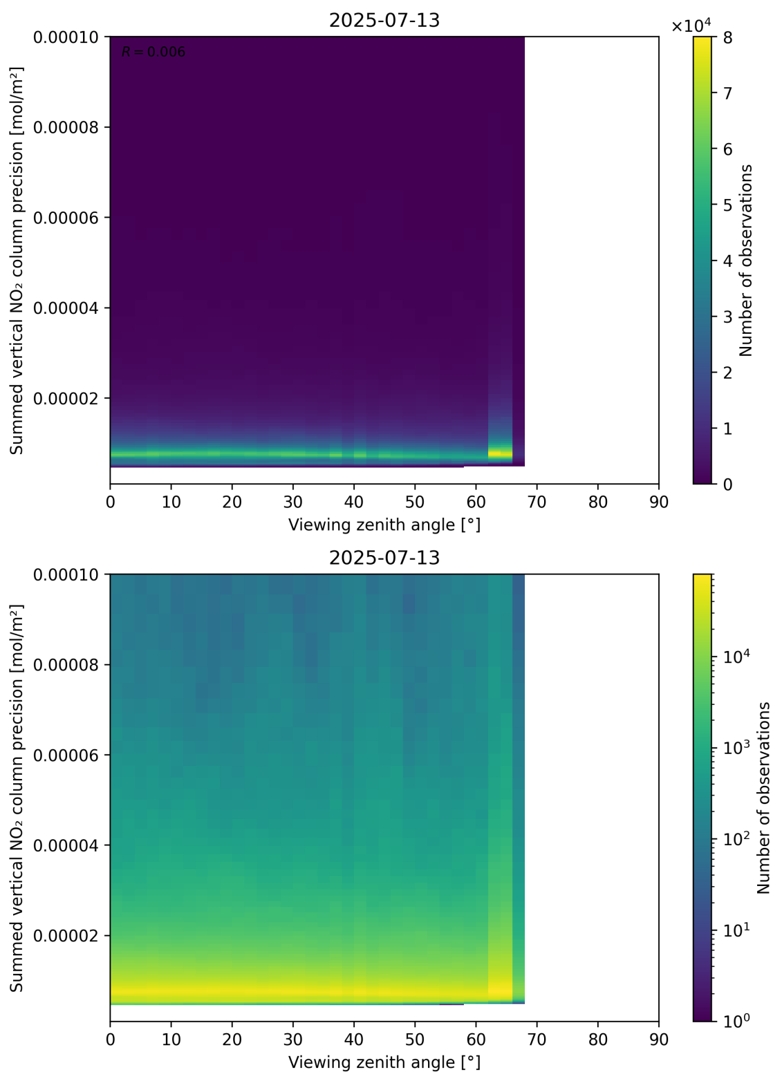
Figure 166: Scatter density plot of “Viewing zenith angle” against “Summed vertical NO 2 column precision” for 2025-07-13 to 2025-07-14.
