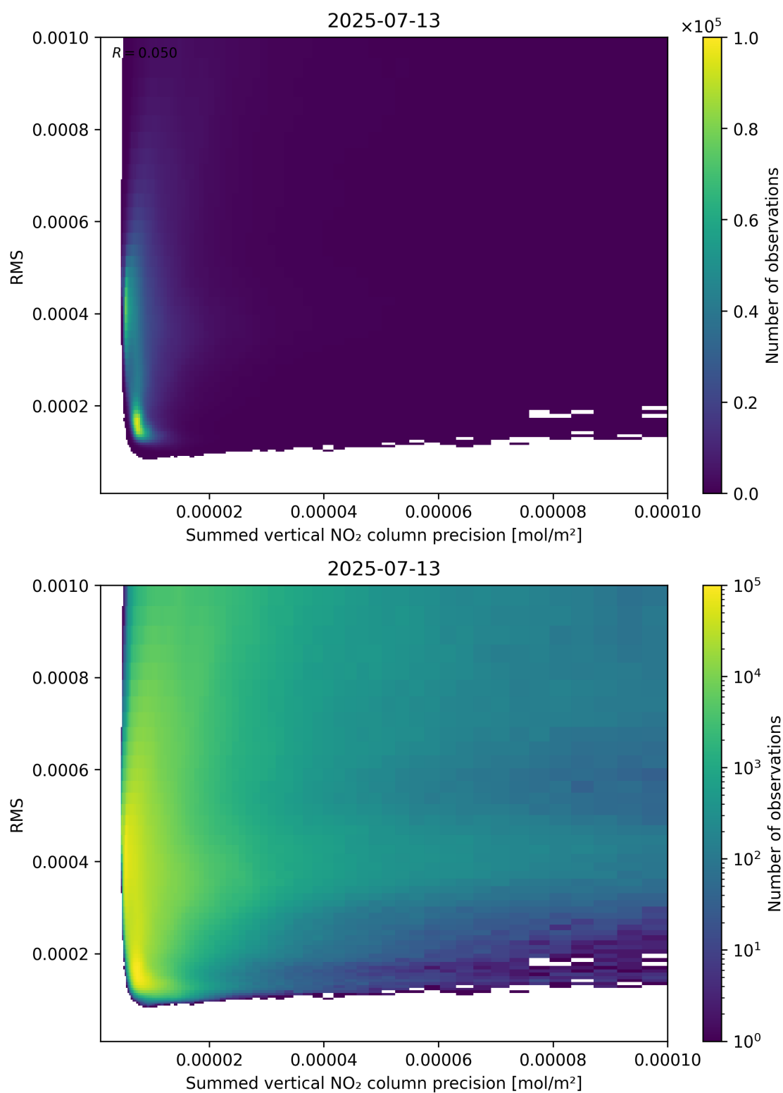
Figure 108: Scatter density plot of “Summed vertical NO 2 column precision” against “RMS” for 2025-07-13 to 2025-07-14.
