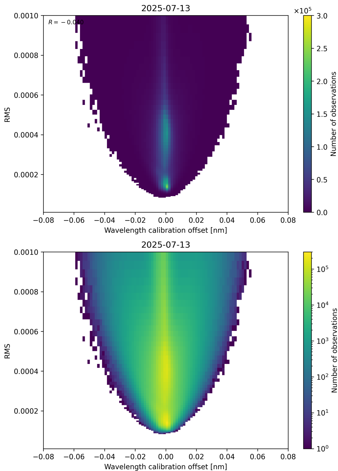
Figure 181: Scatter density plot of “Wavelength calibration offset” against “RMS” for 2025-07-13 to 2025-07-14.
