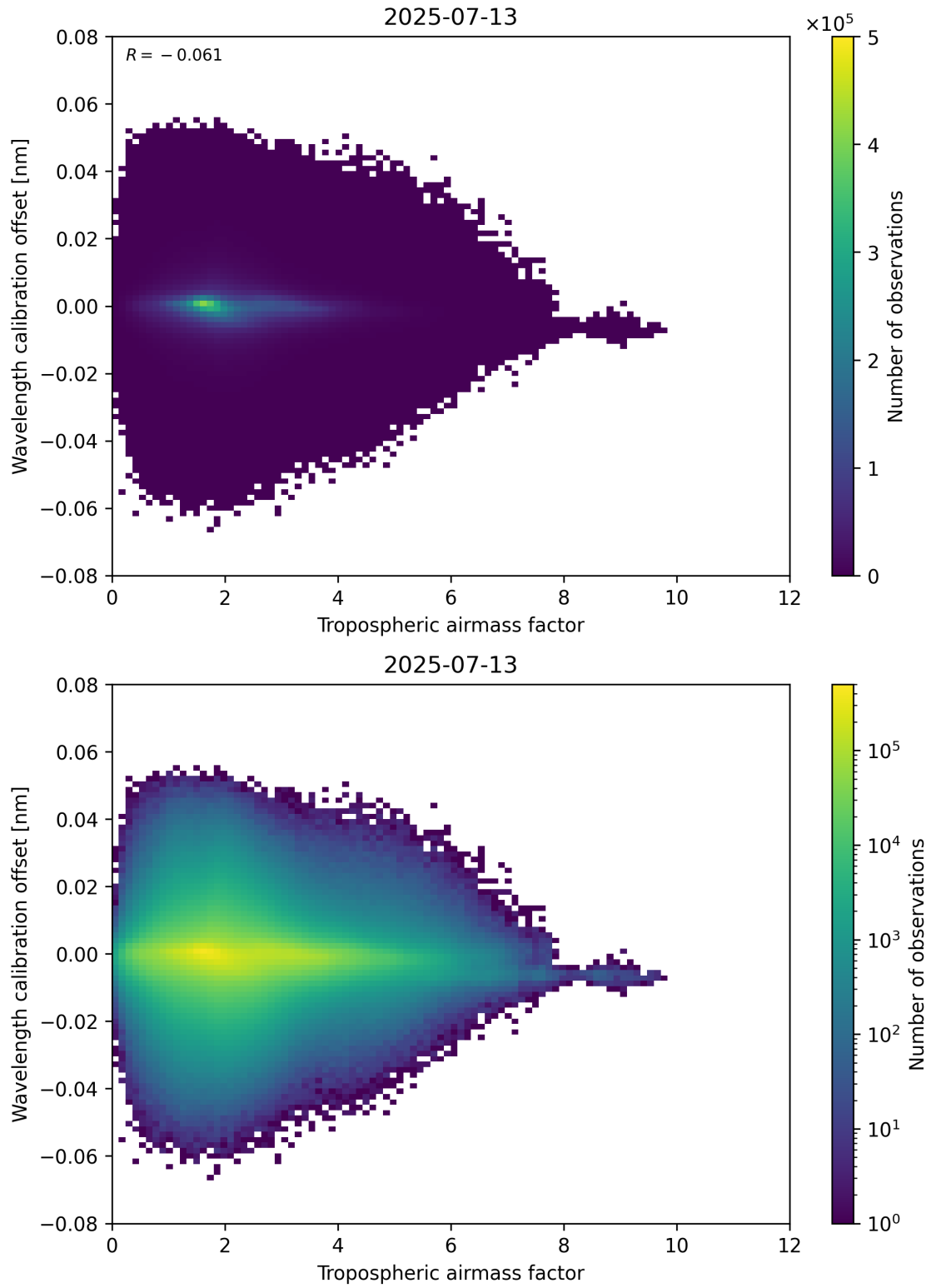
Figure 80: Scatter density plot of “Tropospheric airmass factor” against “Wavelength calibration offset” for 2025-07-13 to 2025-07-14.
