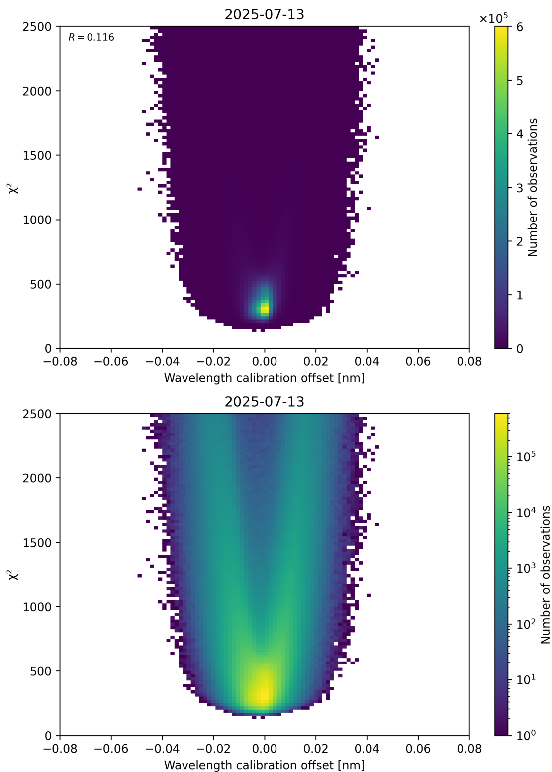
Figure 175: Scatter density plot of “Wavelength calibration offset” against “ \chi^2 ” for 2025-07-13 to 2025-07-14.
