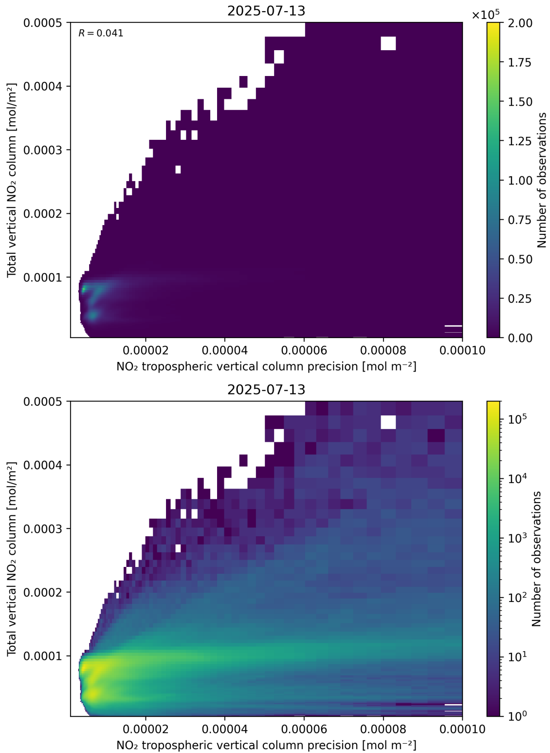
Figure 138: Scatter density plot of “NO 2 tropospheric vertical column precision” against “Total vertical NO 2 column” for 2025-07-13 to 2025-07-14.
