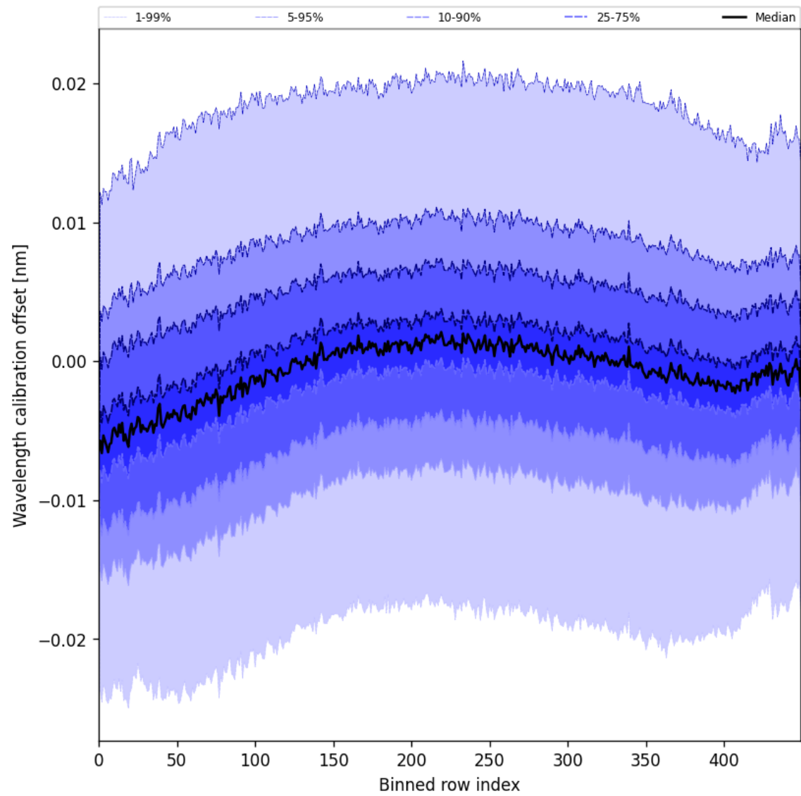
Figure 52: Along track statistics of “Wavelength calibration offset” for 2025-07-13 to 2025-07-14
