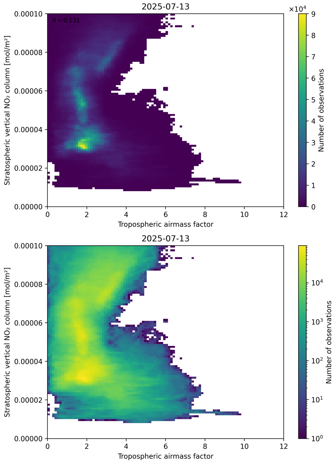
Figure 74: Scatter density plot of “Tropospheric airmass factor” against “Stratospheric vertical NO 2 column” for 2025-07-13 to 2025-07-14.
