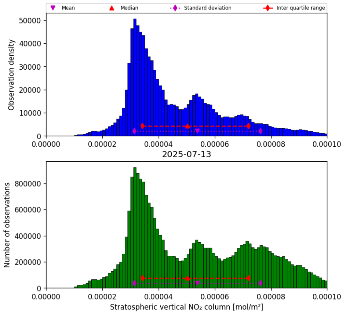
Figure 36: Histogram of “Stratospheric vertical NO 2 column” for 2025-07-13 to 2025-07-14
