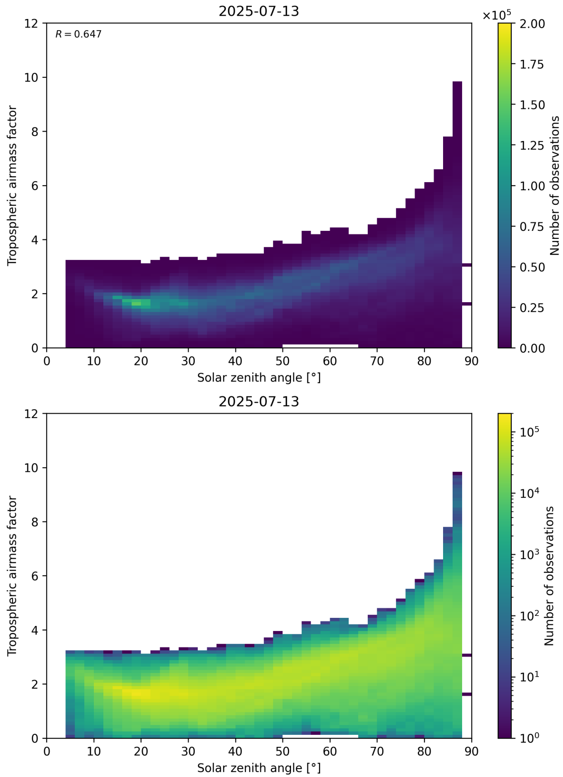
Figure 147: Scatter density plot of “Solar zenith angle” against “Tropospheric airmass factor” for 2025-07-13 to 2025-07-14.
