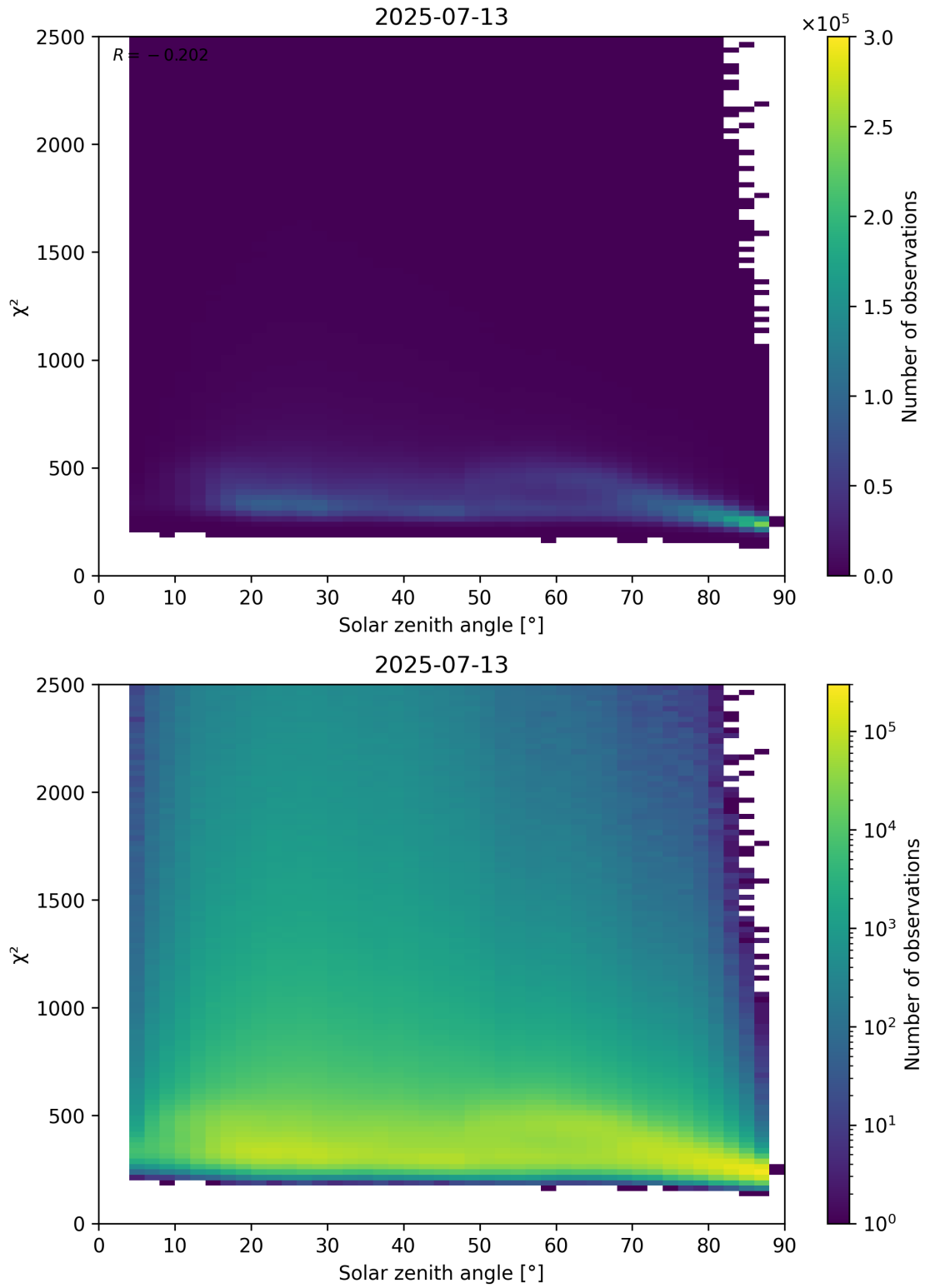
Figure 148: Scatter density plot of “Solar zenith angle” against “ \chi^2 ” for 2025-07-13 to 2025-07-14.
