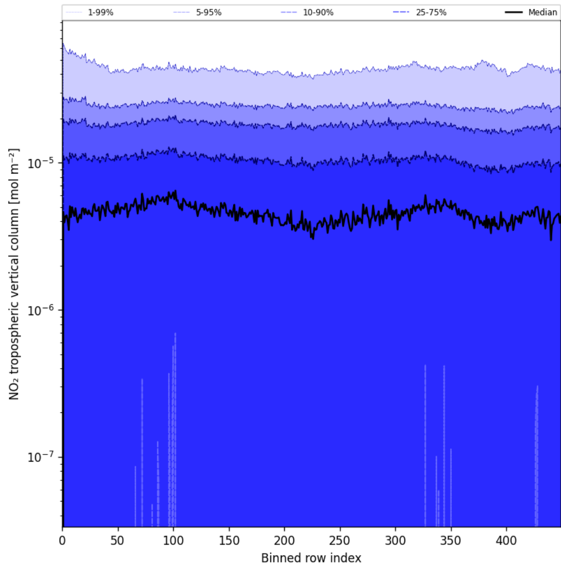
Figure 46: Along track statistics of “NO 2 tropospheric vertical column” for 2025-07-13 to 2025-07-14
