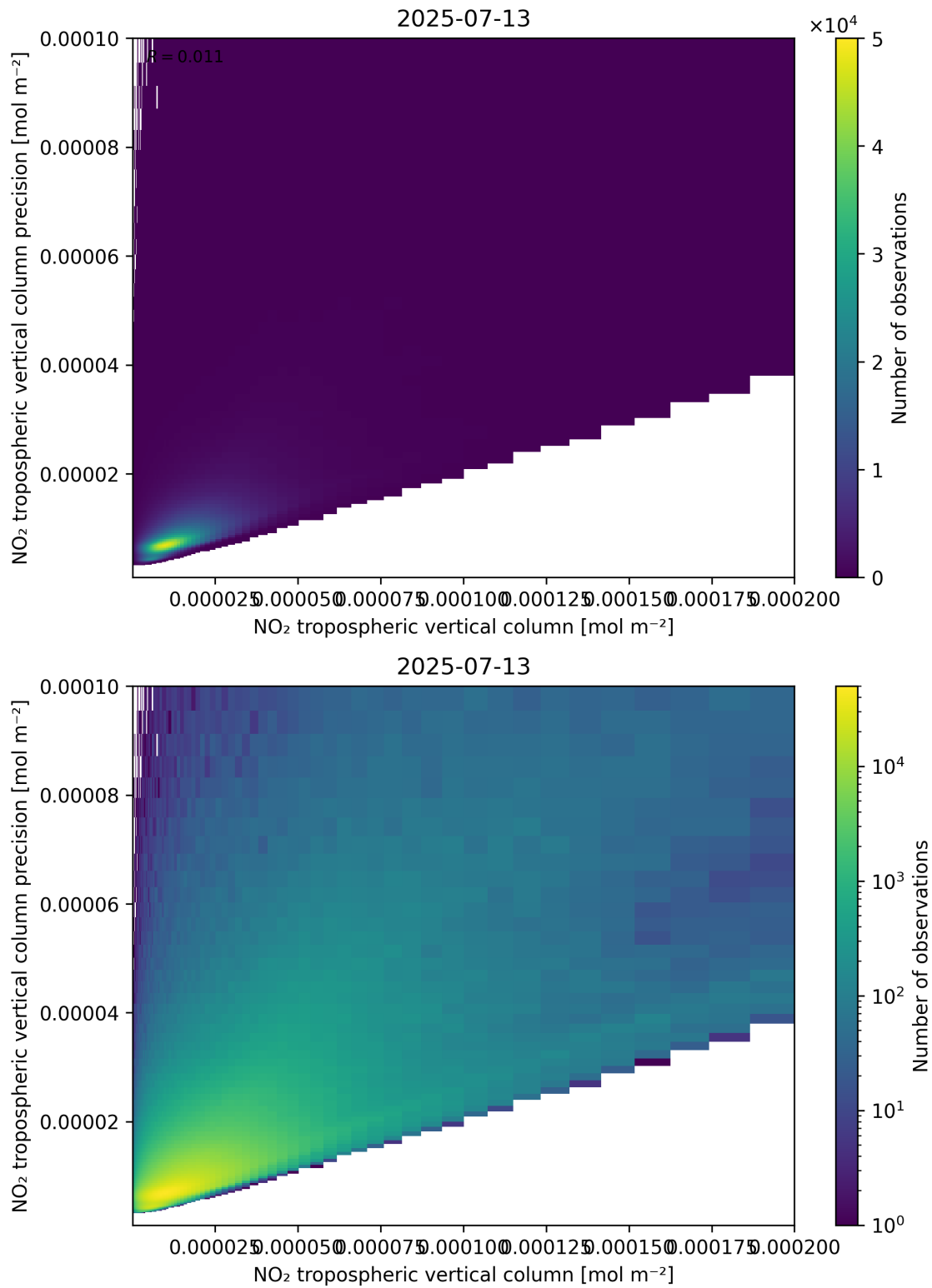
Figure 130: Scatter density plot of “NO 2 tropospheric vertical column” against “NO 2 tropospheric vertical column precision” for 2025-07-13 to 2025-07-14.
