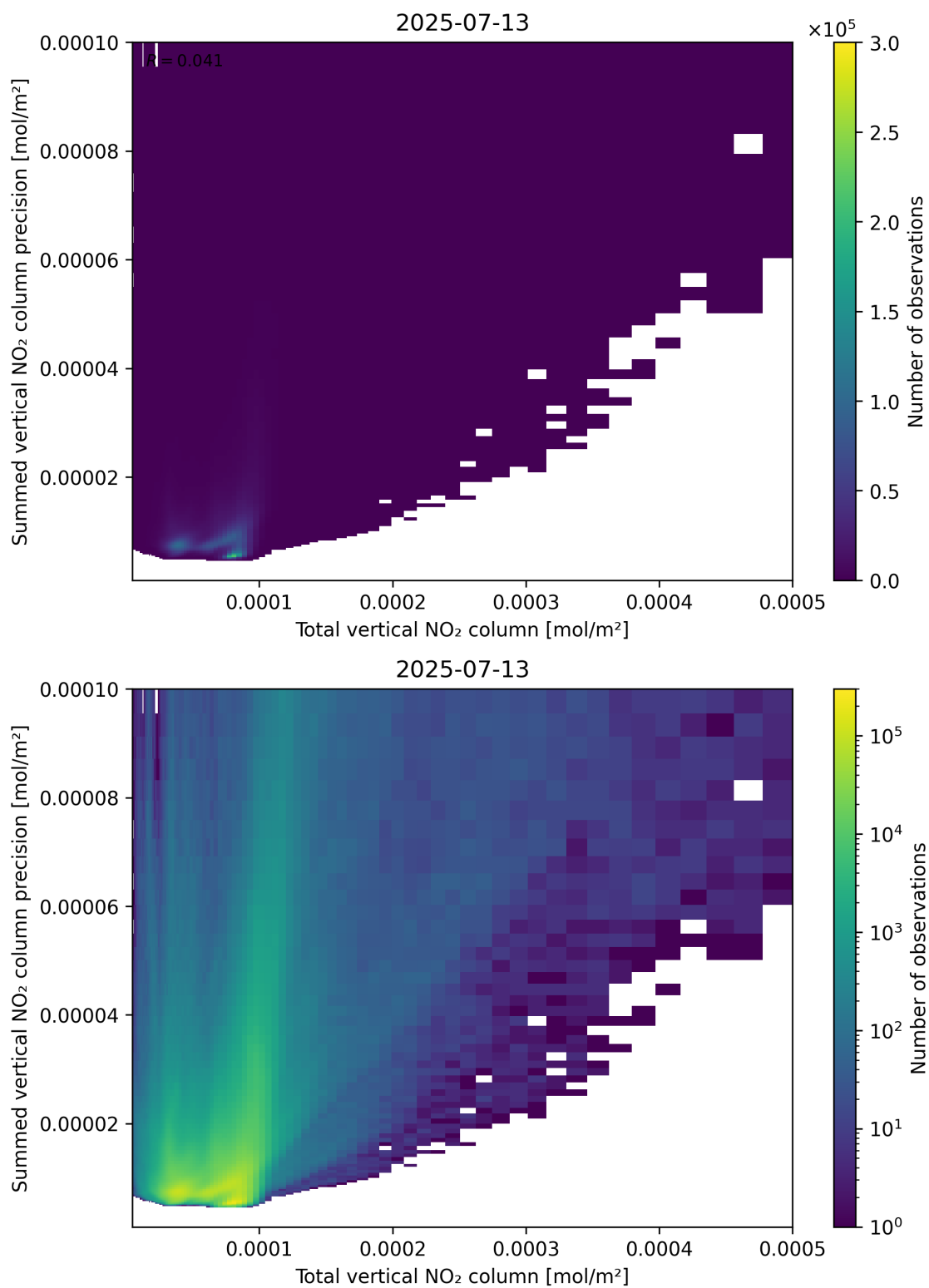
Figure 113: Scatter density plot of “Total vertical NO 2 column” against “Summed vertical NO 2 column precision” for 2025-07-13 to 2025-07-14.
