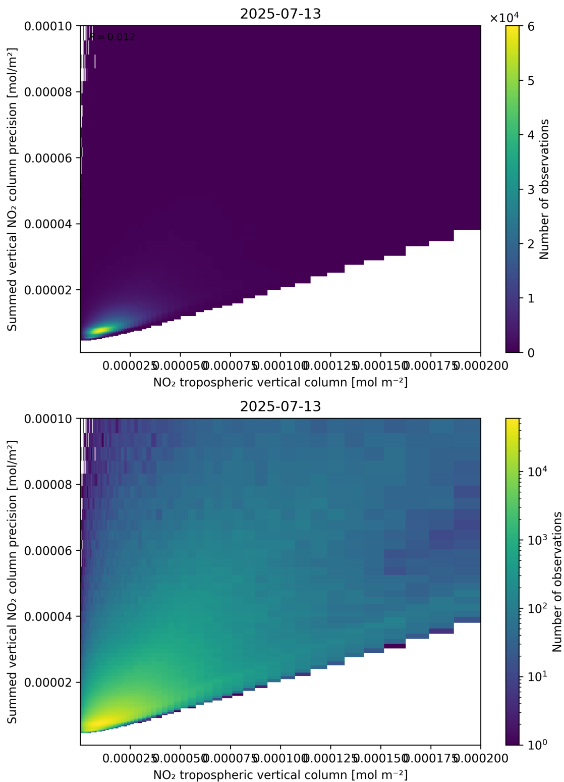
Figure 127: Scatter density plot of “NO 2 tropospheric vertical column” against “Summed vertical NO 2 column precision” for 2025-07-13 to 2025-07-14.
