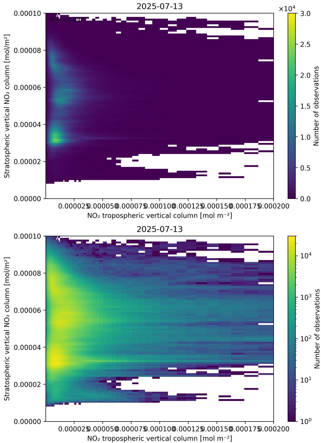
Figure 125: Scatter density plot of “NO 2 tropospheric vertical column” against “Stratospheric vertical NO 2 column” for 2025-07-13 to 2025-07-14.
