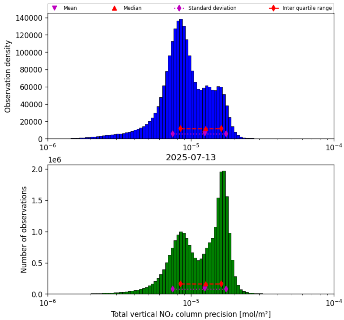
Figure 39: Histogram of “Total vertical NO 2 column precision” for 2025-07-13 to 2025-07-14
