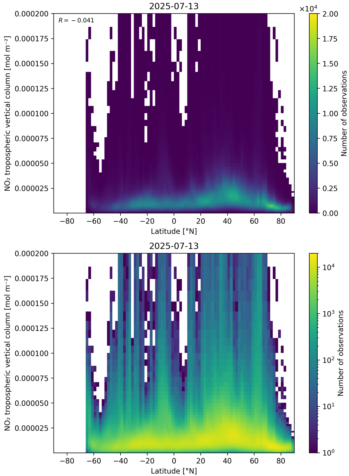
Figure 92: Scatter density plot of “Latitude” against “NO 2 tropospheric vertical column” for 2025-07-13 to 2025-07-14.
