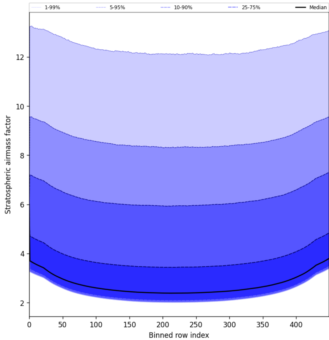
Figure 61: Along track statistics of “Stratospheric airmass factor” for 2025-07-13 to 2025-07-14
