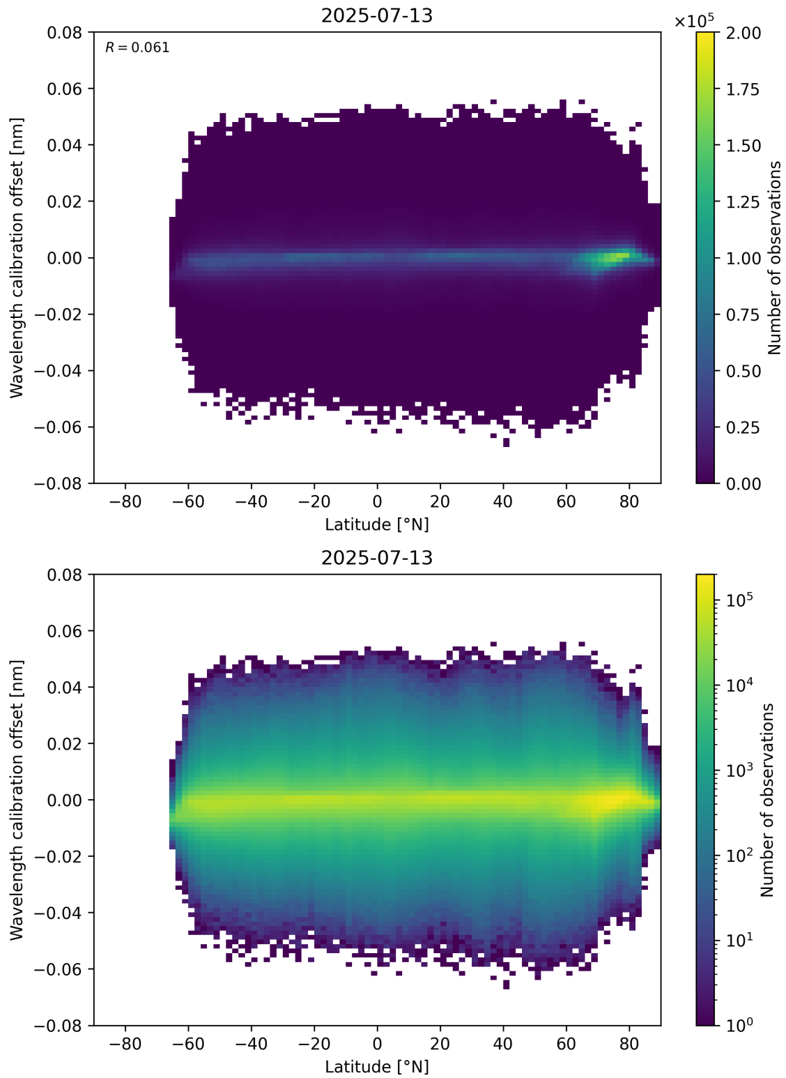
Figure 95: Scatter density plot of “Latitude” against “Wavelength calibration offset” for 2025-07-13 to 2025-07-14.
