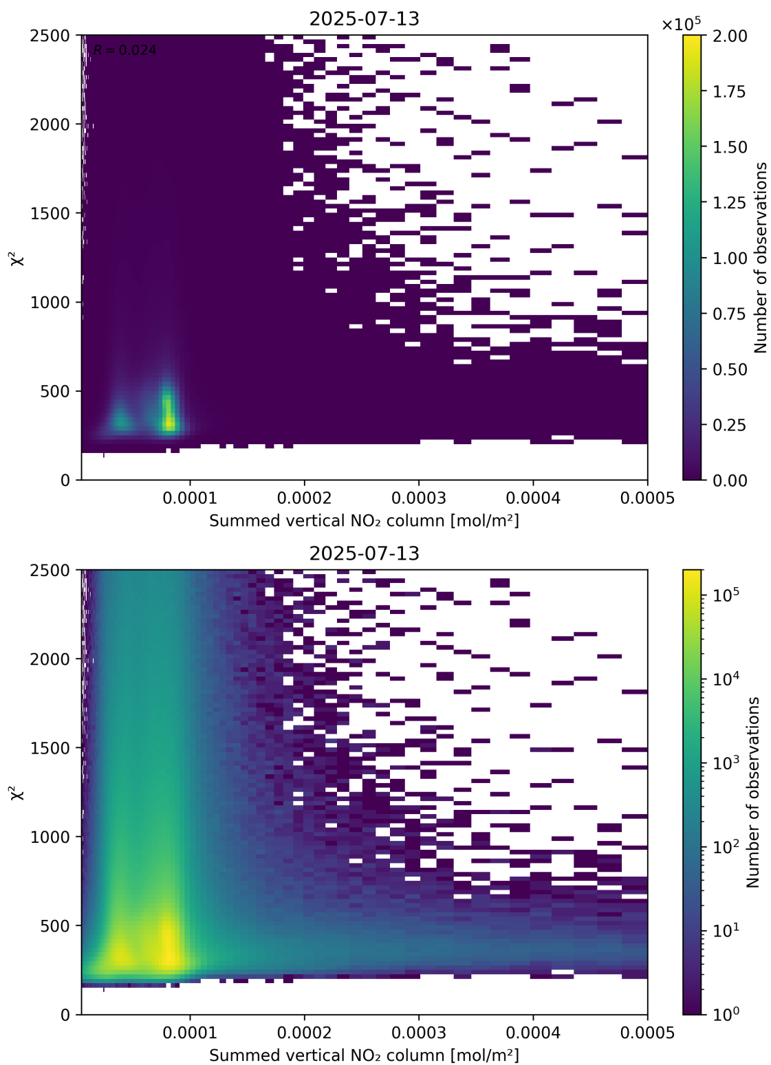
Figure 104: Scatter density plot of “Summed vertical NO 2 column” against “ \chi^2 ” for 2025-07-13 to 2025-07-14.
