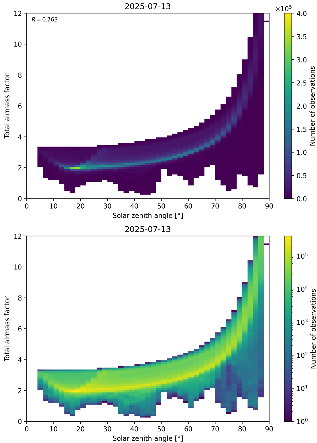
Figure 146: Scatter density plot of “Solar zenith angle” against “Total air mass factor” for 2025-07-13 to 2025-07-14.
