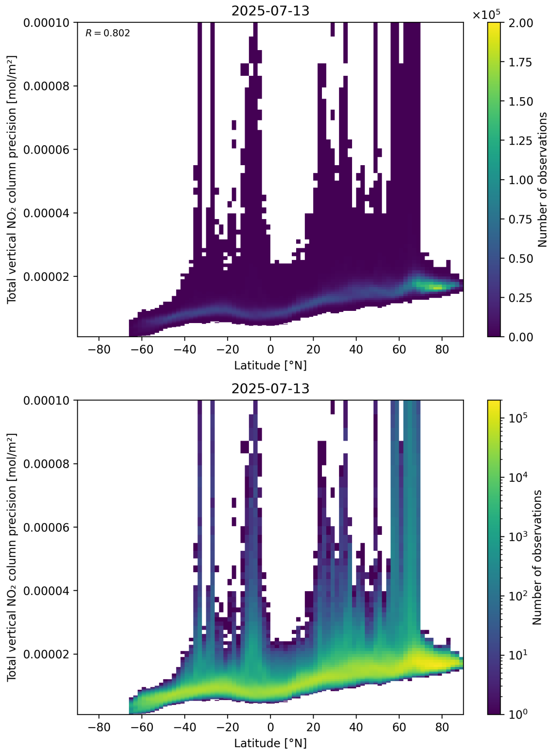
Figure 91: Scatter density plot of “Latitude” against “Total vertical NO 2 column precision” for 2025-07-13 to 2025-07-14.
