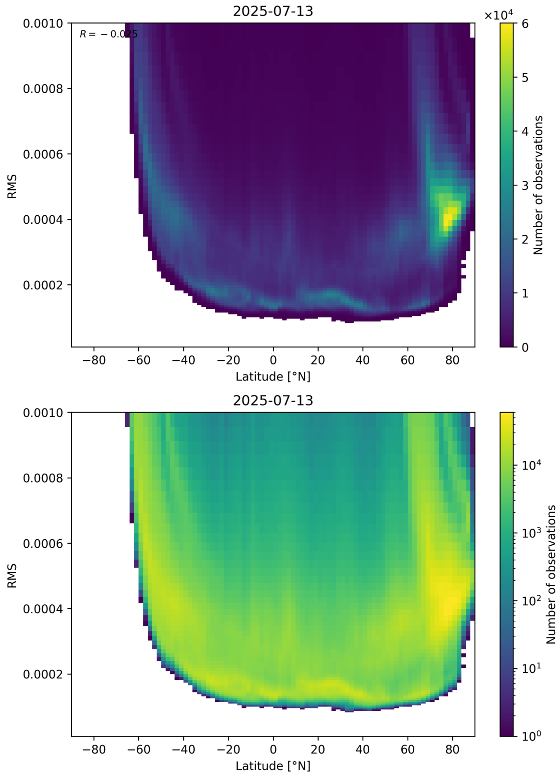
Figure 94: Scatter density plot of “Latitude” against “RMS” for 2025-07-13 to 2025-07-14.
