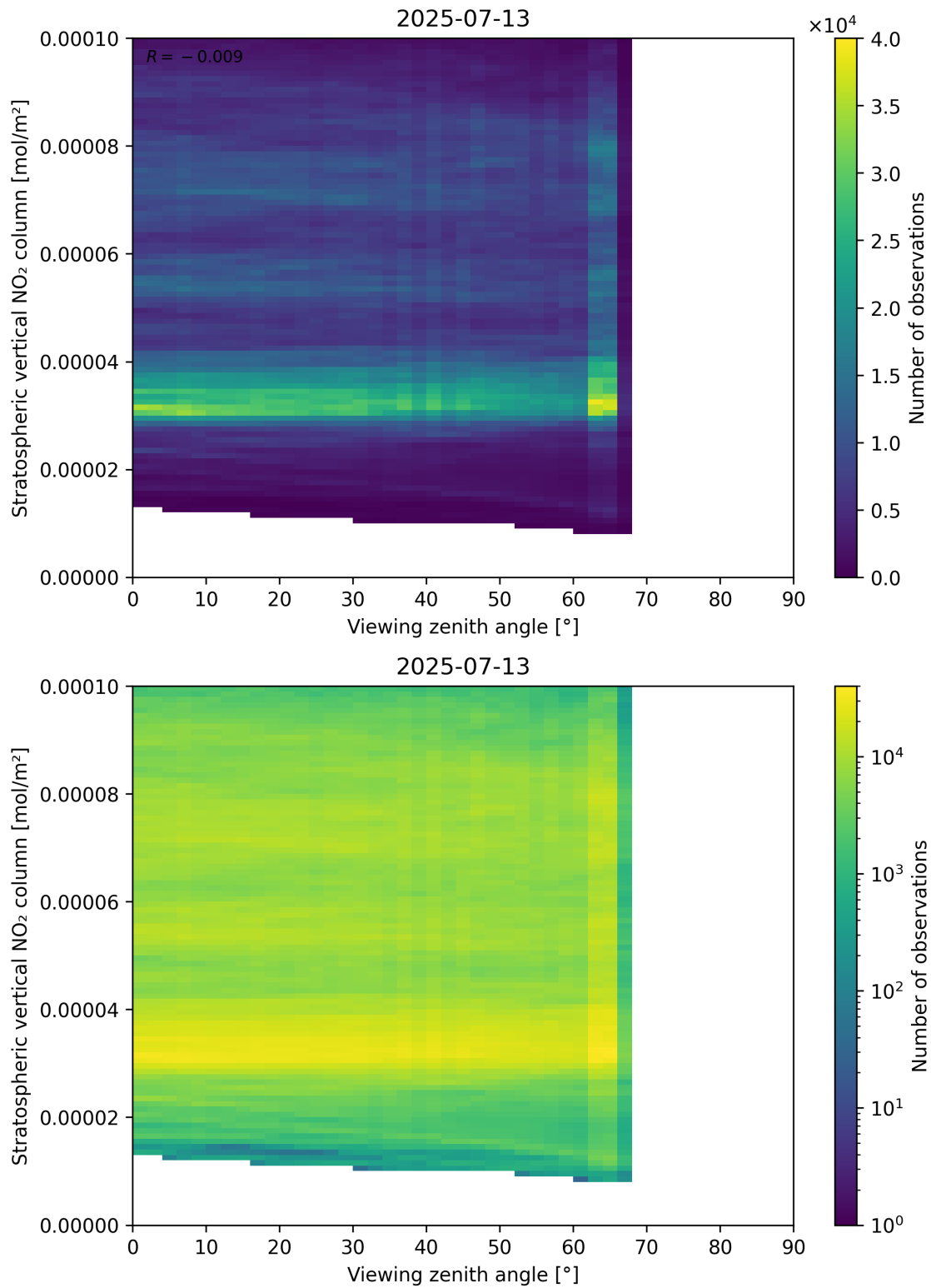
Figure 164: Scatter density plot of “Viewing zenith angle” against “Stratospheric vertical NO 2 column” for 2025-07-13 to 2025-07-14.
