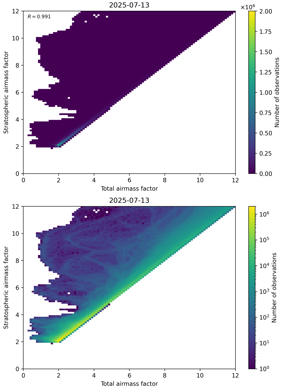
Figure 62: Scatter density plot of “Total airmass factor” against “Stratospheric airmass factor” for 2025-07-13 to 2025-07-14.
