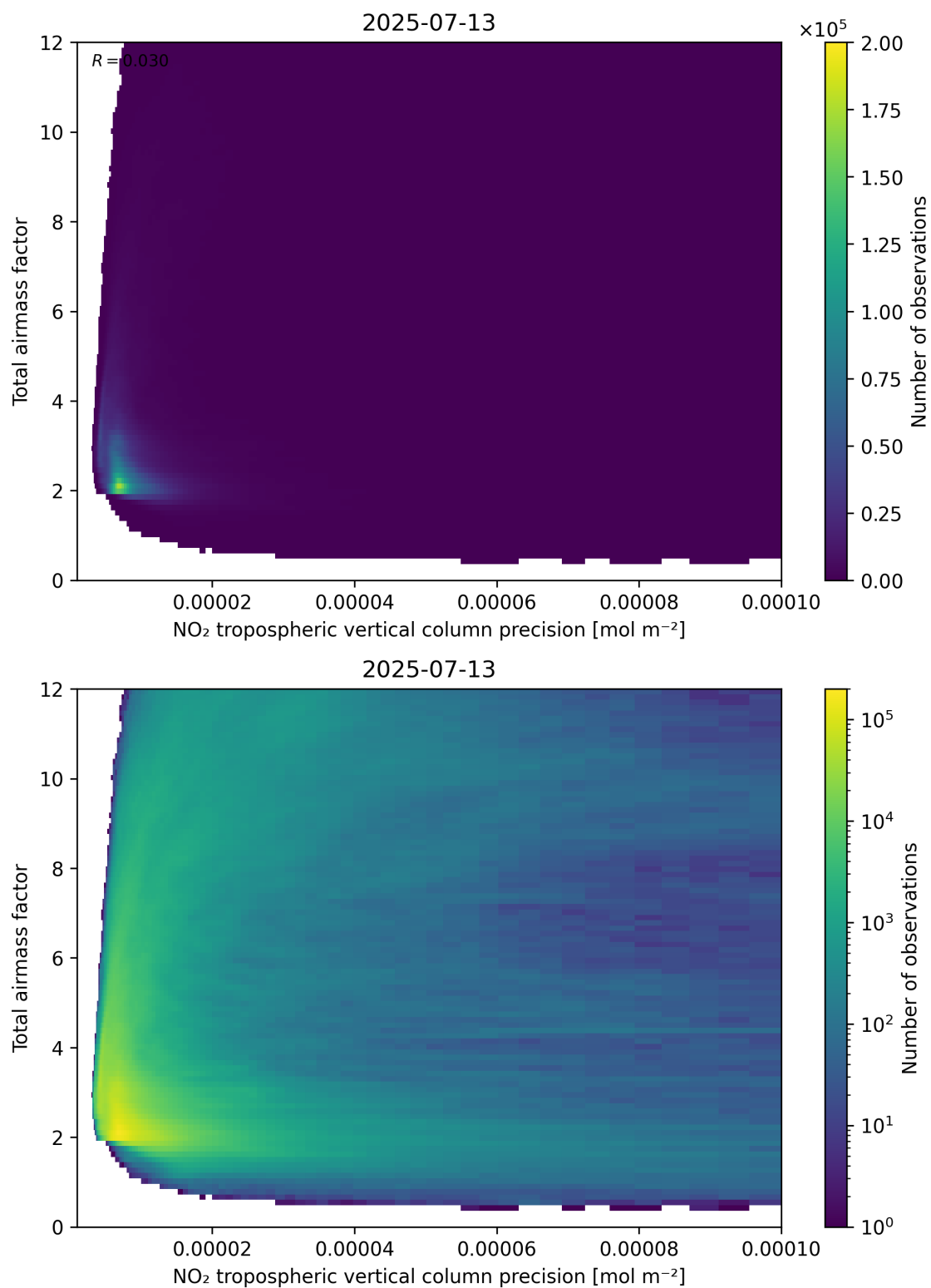
Figure 132: Scatter density plot of “NO 2 tropospheric vertical column precision” against “Total air mass factor” for 2025-07-13 to 2025-07-14.
