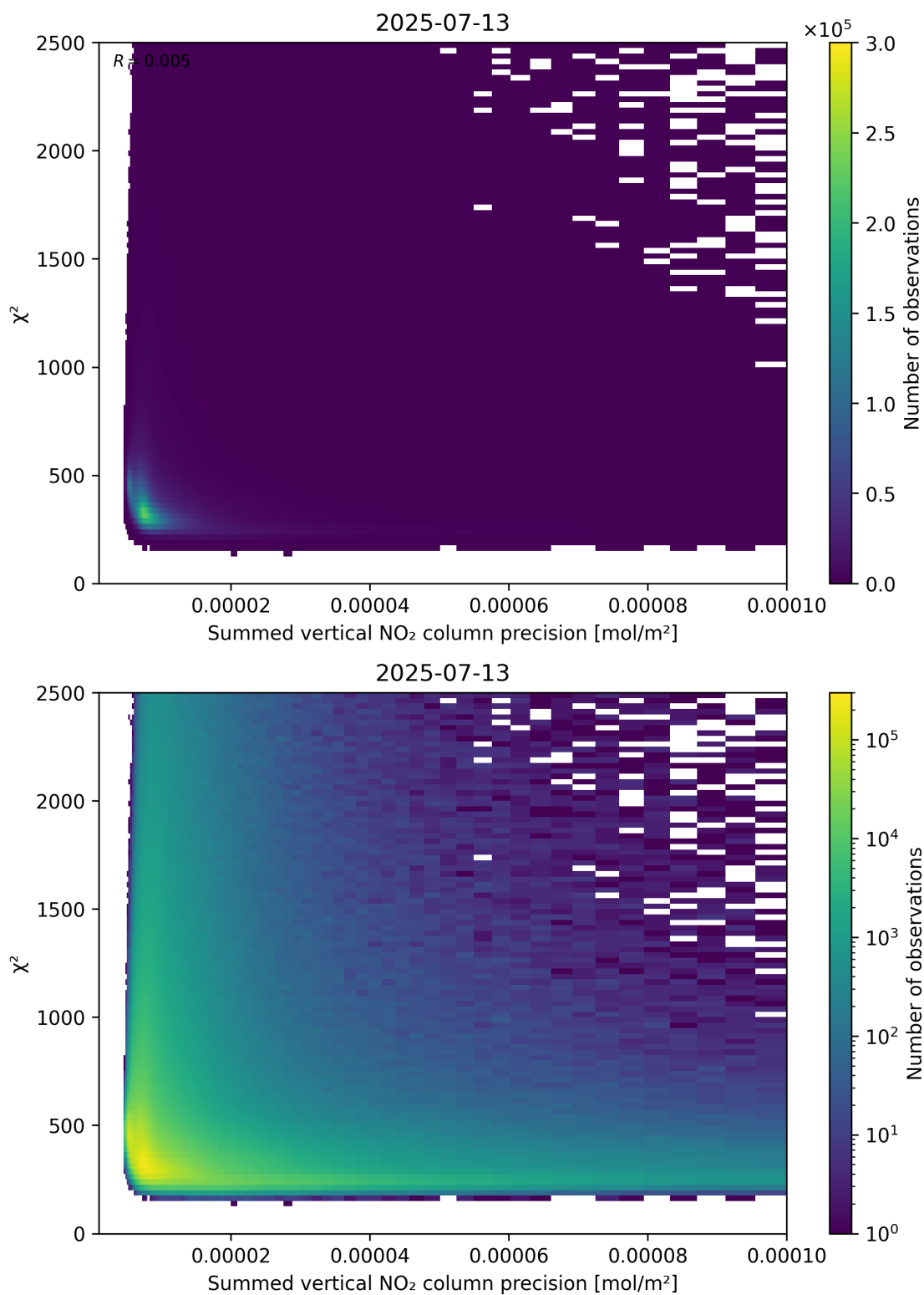
Figure 107: Scatter density plot of “Summed vertical NO 2 column precision” against “ \chi^2 ” for 2025-07-13 to 2025-07-14.
