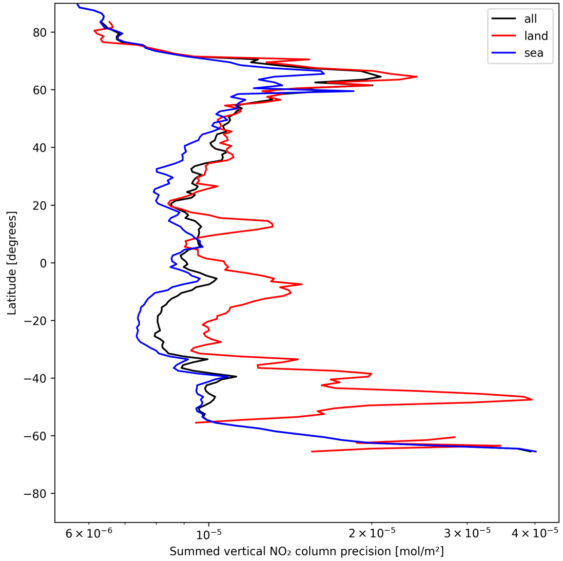
Figure 24: Zonal average of “Summed vertical NO 2 column precision” for 2025-07-13 to 2025-07-14.
