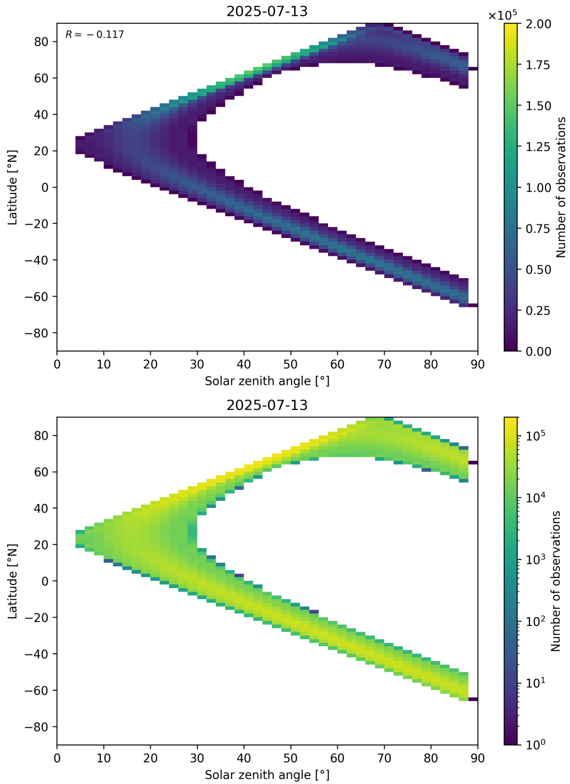
Figure 149: Scatter density plot of “Solar zenith angle” against “Latitude” for 2025-07-13 to 2025-07-14.
