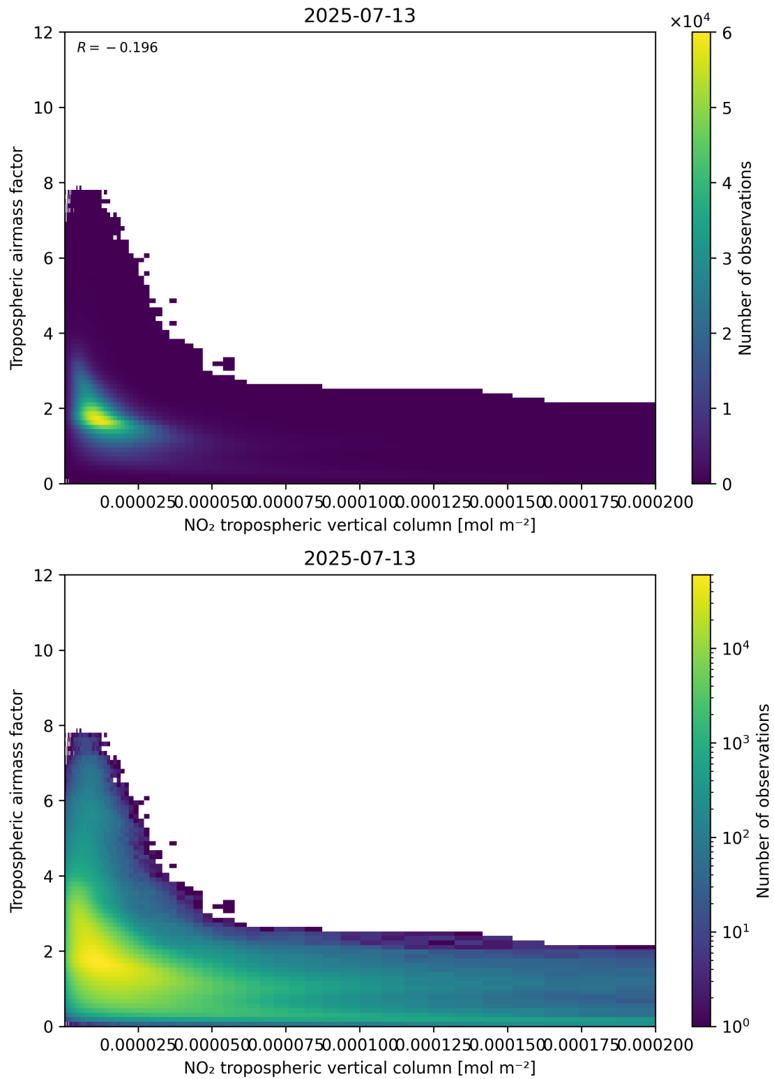
Figure 123: Scatter density plot of “NO 2 tropospheric vertical column” against “Tropospheric airmass factor” for 2025-07-13 to 2025-07-14.
