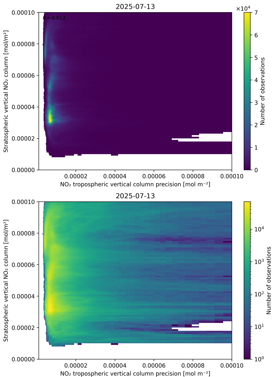
Figure 135: Scatter density plot of “NO 2 tropospheric vertical column precision” against “Stratospheric vertical NO 2 column” for 2025-07-13 to 2025-07-14.
