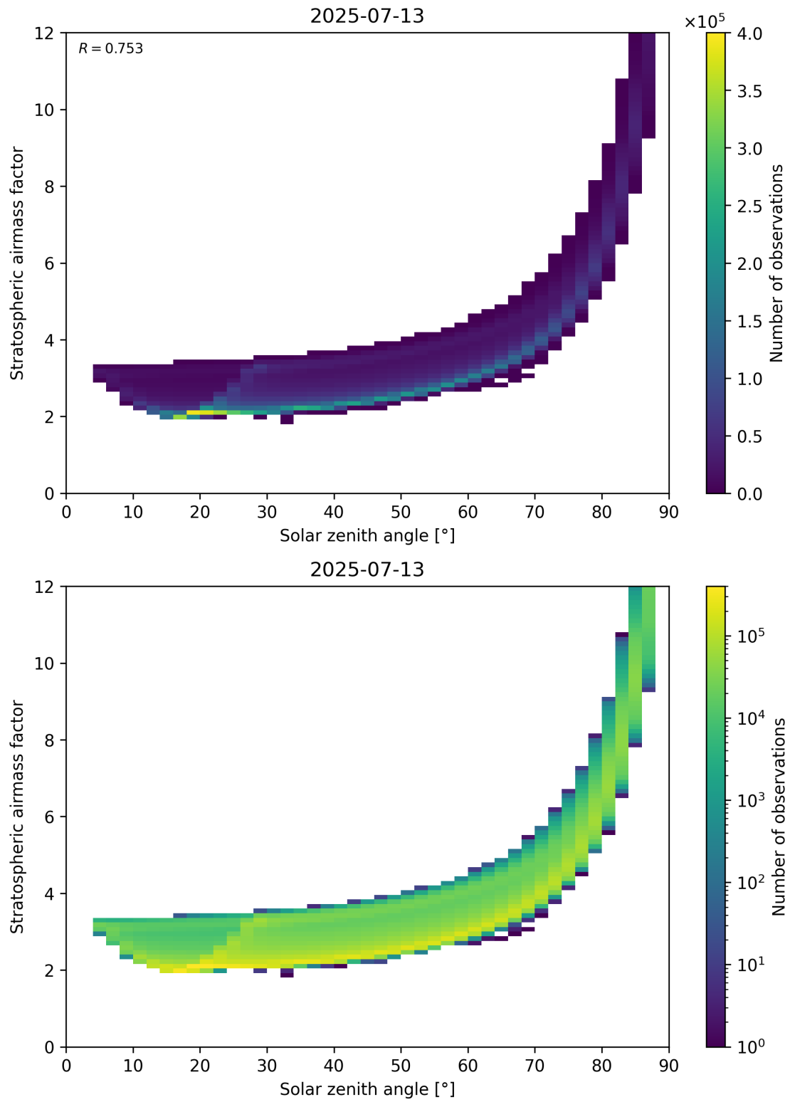
Figure 145: Scatter density plot of “Solar zenith angle” against “Stratospheric airmass factor” for 2025-07-13 to 2025-07-14.
