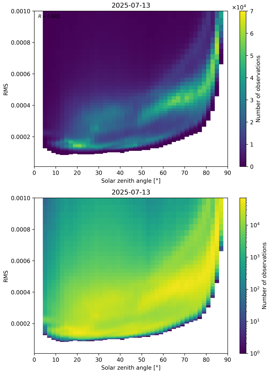
Figure 157: Scatter density plot of “Solar zenith angle” against “RMS” for 2025-07-13 to 2025-07-14.
