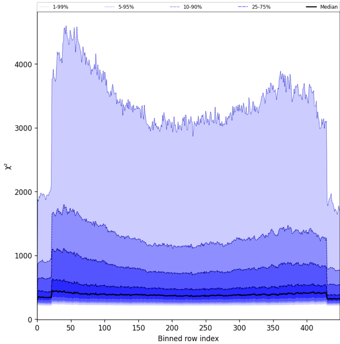
Figure 59: Along track statistics of “ \chi^2 ” for 2025-07-13 to 2025-07-14
