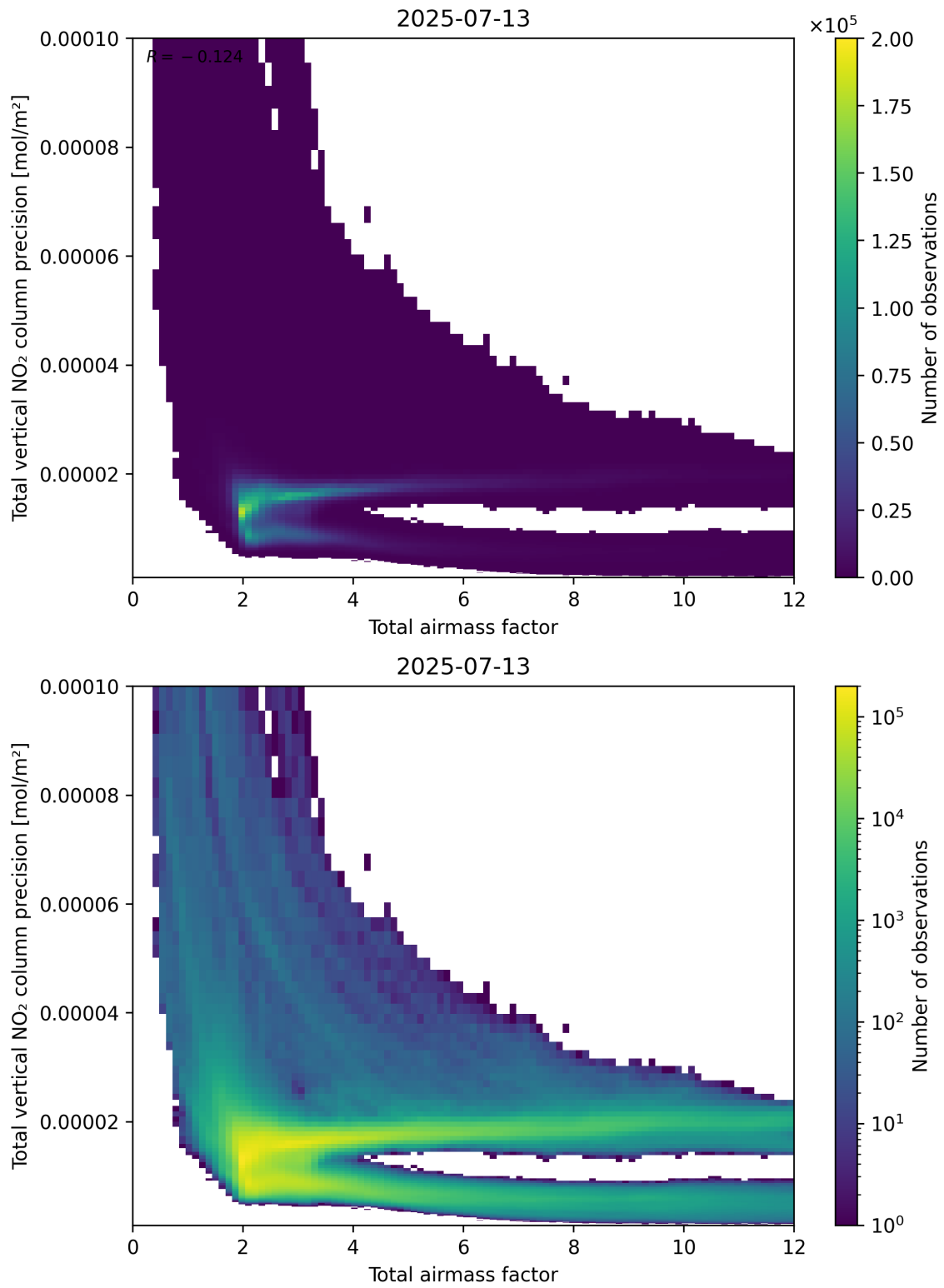
Figure 68: Scatter density plot of “Total airmass factor” against “Total vertical NO 2 column precision” for 2025-07-13 to 2025-07-14.
