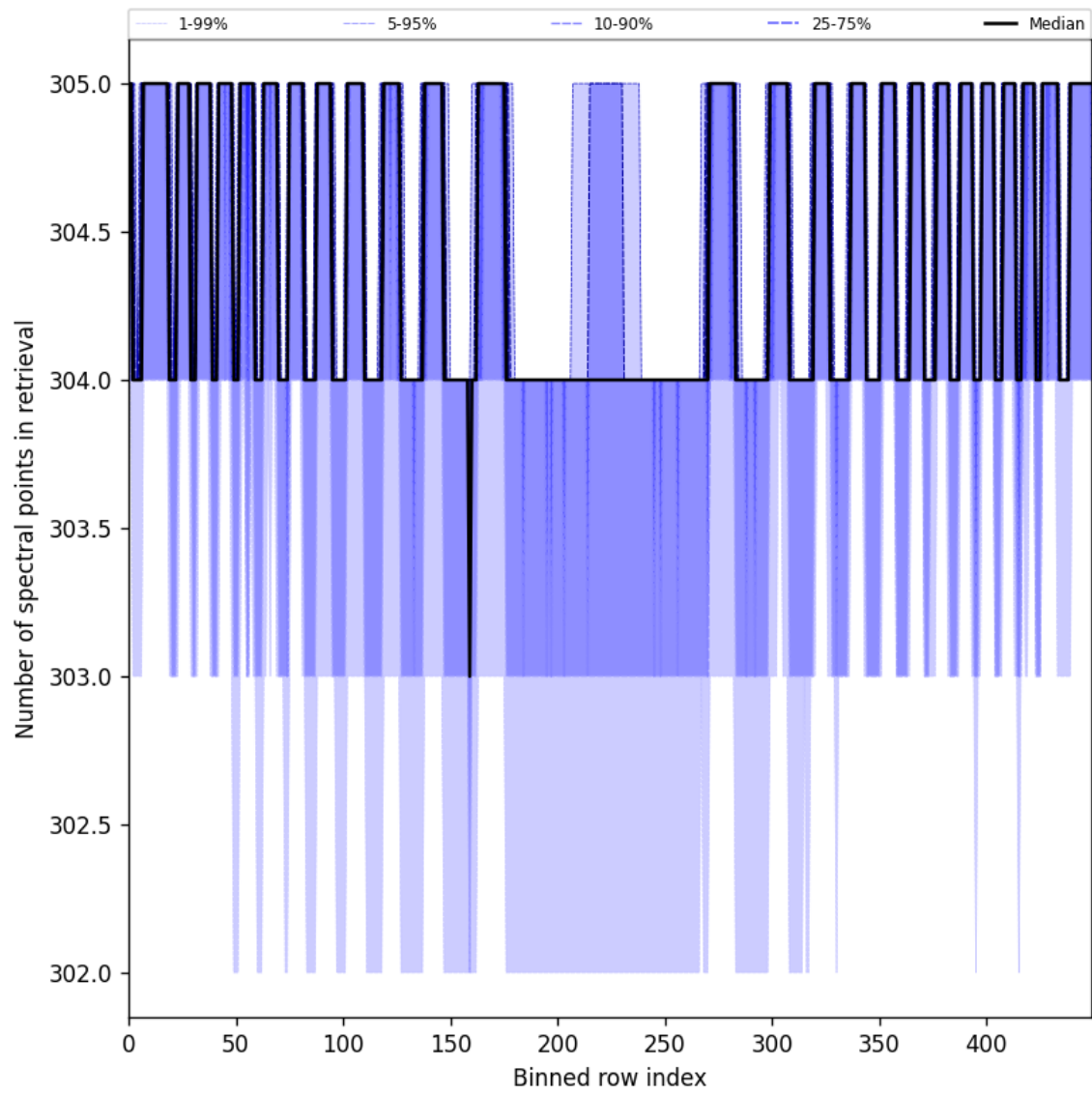
Figure 50: Along track statistics of “Number of spectral points in retrieval” for 2025-07-13 to 2025-07-14
