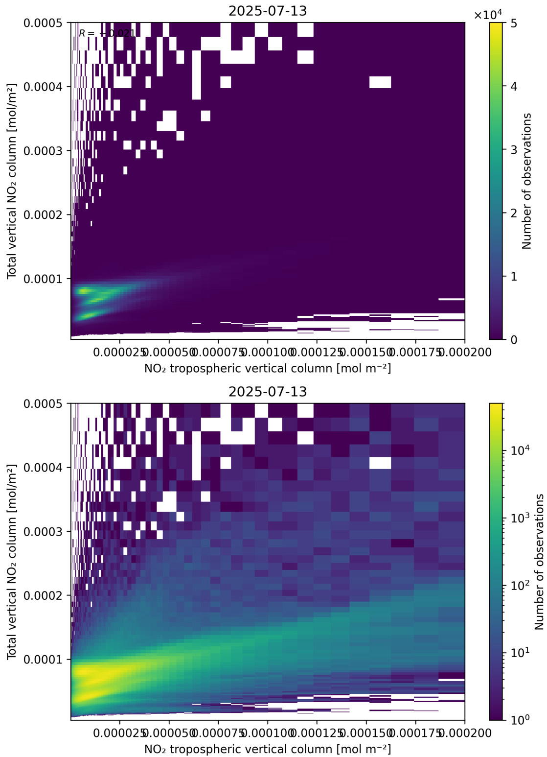
Figure 128: Scatter density plot of “NO 2 tropospheric vertical column” against “Total vertical NO 2 column” for 2025-07-13 to 2025-07-14.
