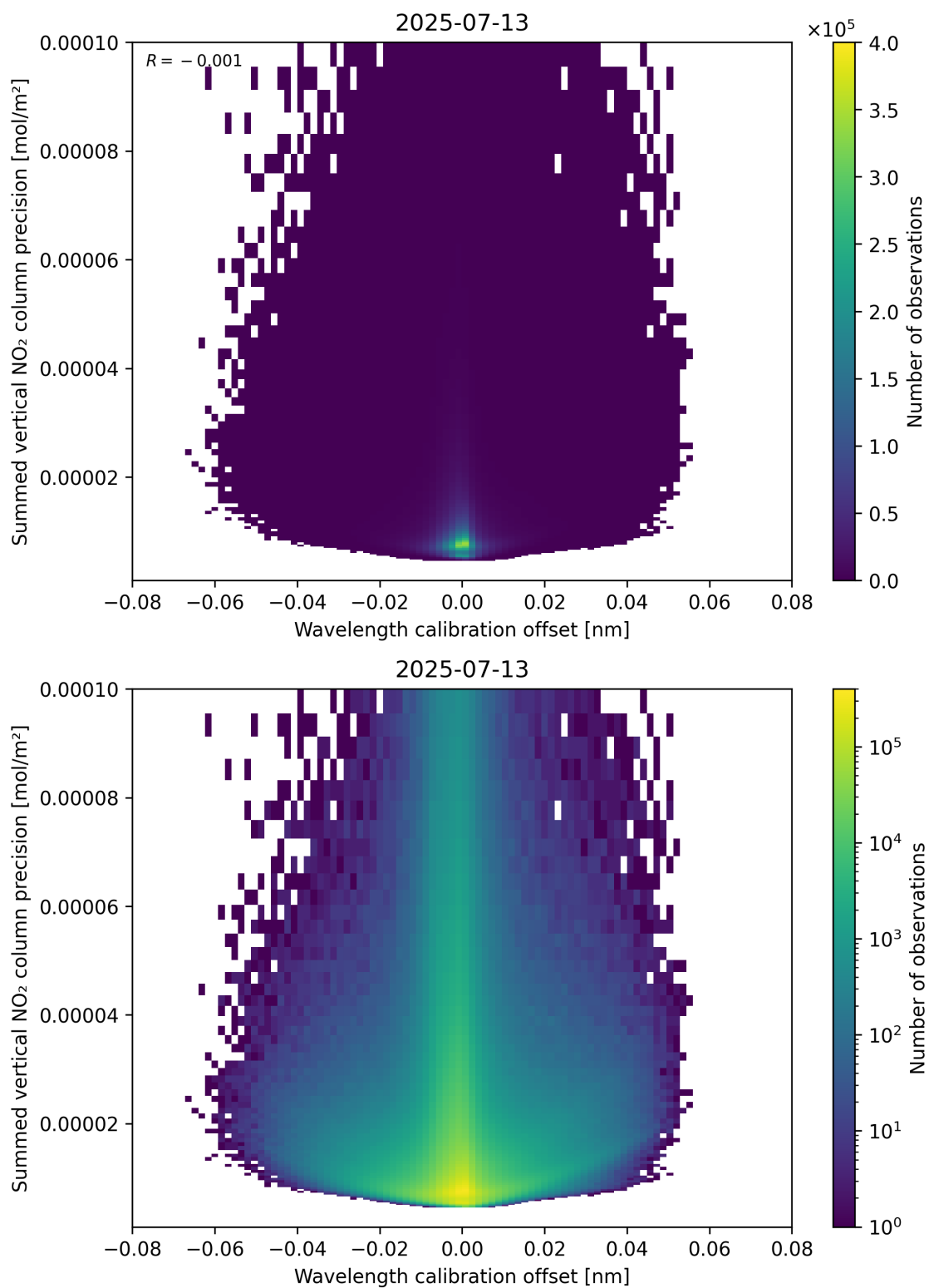
Figure 178: Scatter density plot of “Wavelength calibration offset” against “Summed vertical NO 2 column precision” for 2025-07-13 to 2025-07-14.
