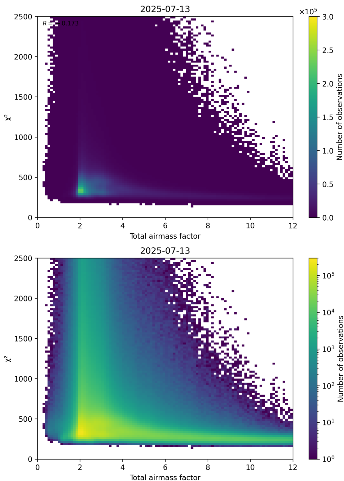
Figure 63: Scatter density plot of “Total airmass factor” against “ \chi^2 ” for 2025-07-13 to 2025-07-14.
