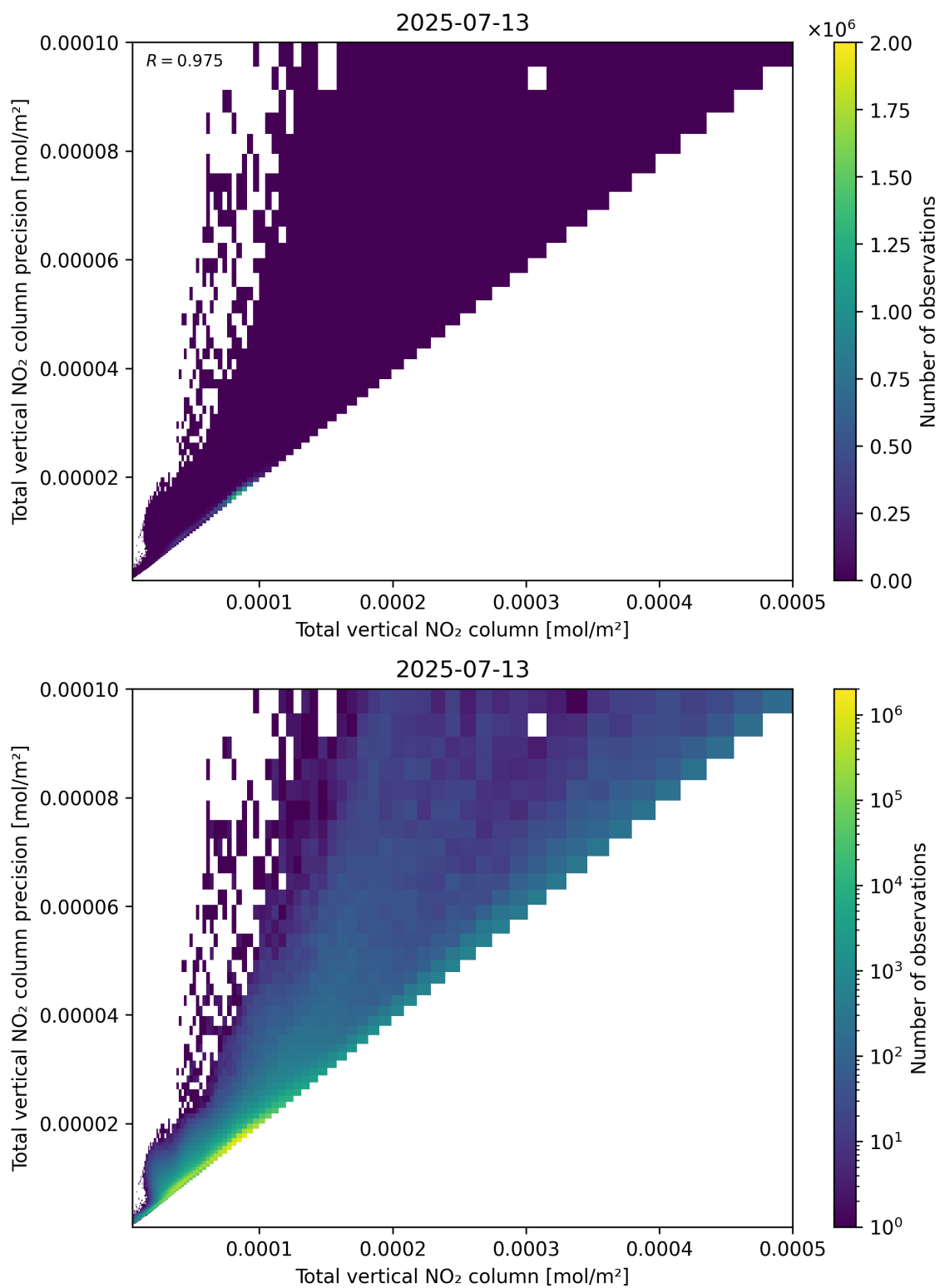
Figure 114: Scatter density plot of “Total vertical NO 2 column” against “Total vertical NO 2 column precision” for 2025-07-13 to 2025-07-14.
