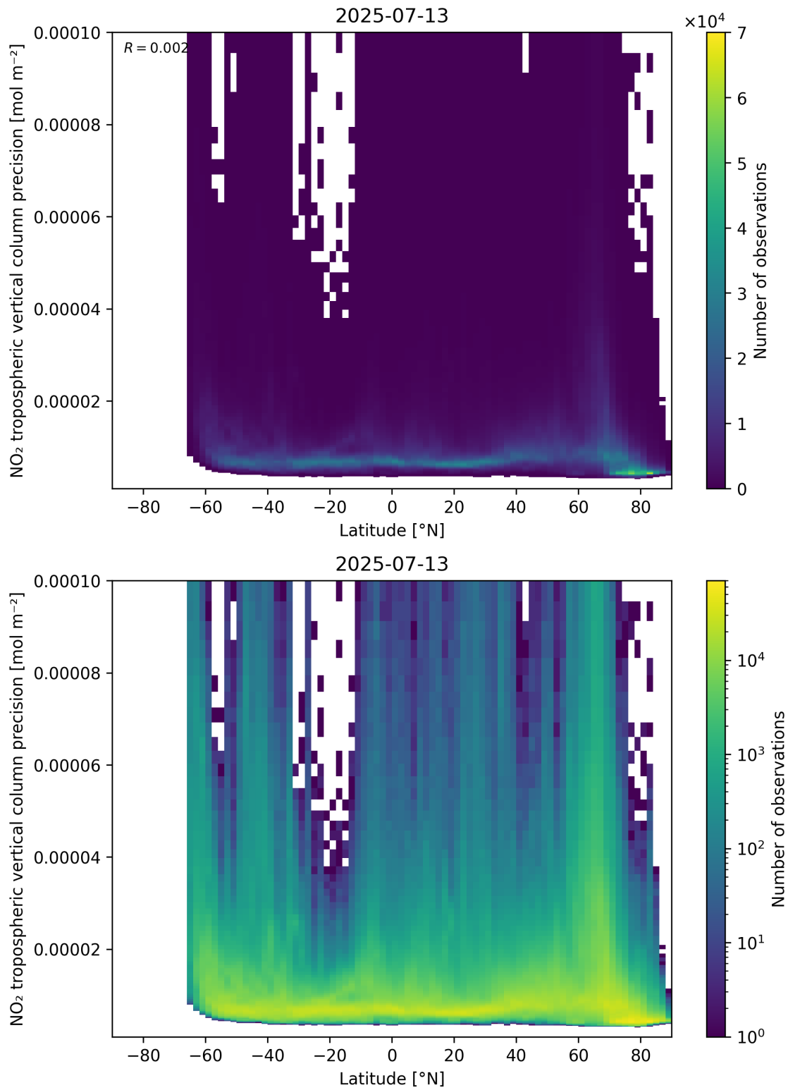
Figure 93: Scatter density plot of “Latitude” against “NO 2 tropospheric vertical column precision” for 2025-07-13 to 2025-07-14.
