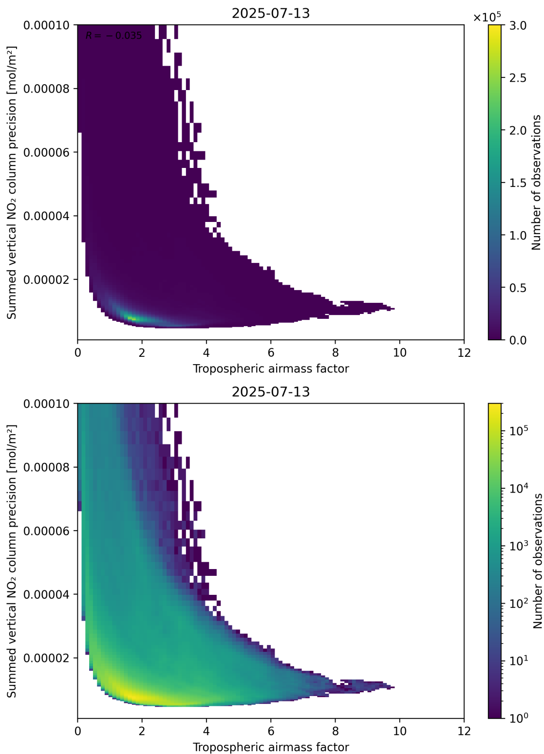
Figure 76: Scatter density plot of “Tropospheric air mass factor” against “Summed vertical NO 2 column precision” for 2025-07-13 to 2025-07-14.
