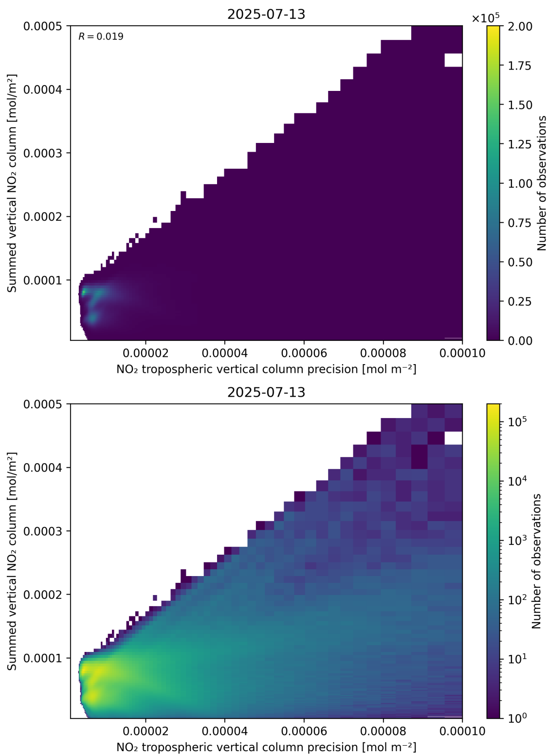
Figure 136: Scatter density plot of “NO 2 tropospheric vertical column precision” against “Summed vertical NO 2 column” for 2025-07-13 to 2025-07-14.
