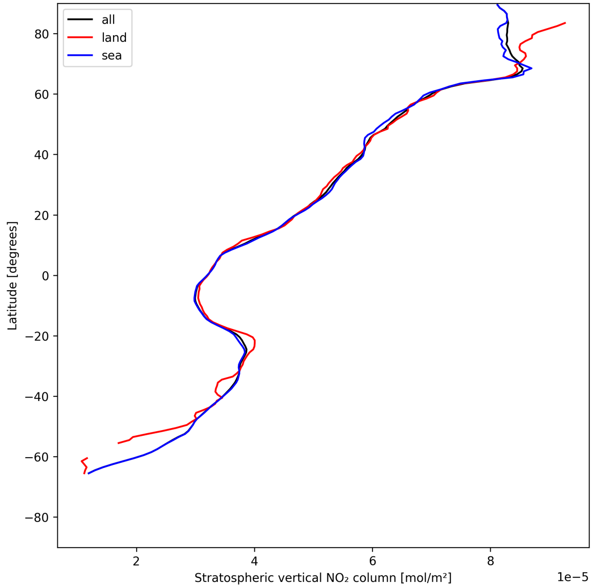
Figure 19: Zonal average of “Stratospheric vertical NO 2 column” for 2025-07-13 to 2025-07-14.
