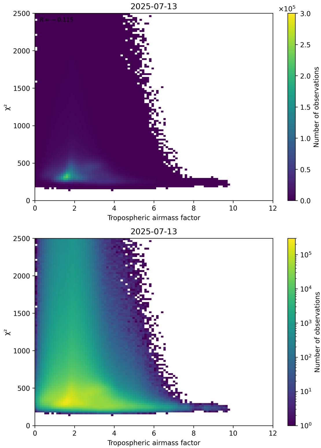
Figure 73: Scatter density plot of “Tropospheric airmass factor” against “ \chi^2 ” for 2025-07-13 to 2025-07-14.
