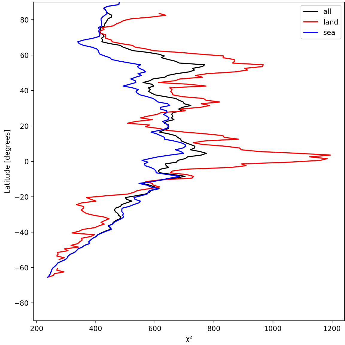
Figure 25: Zonal average of “ \chi^2 ” for 2025-07-13 to 2025-07-14.
