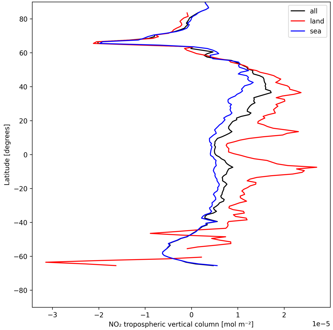
Figure 12: Zonal average of “NO 2 tropospheric vertical column” for 2025-07-13 to 2025-07-14.
