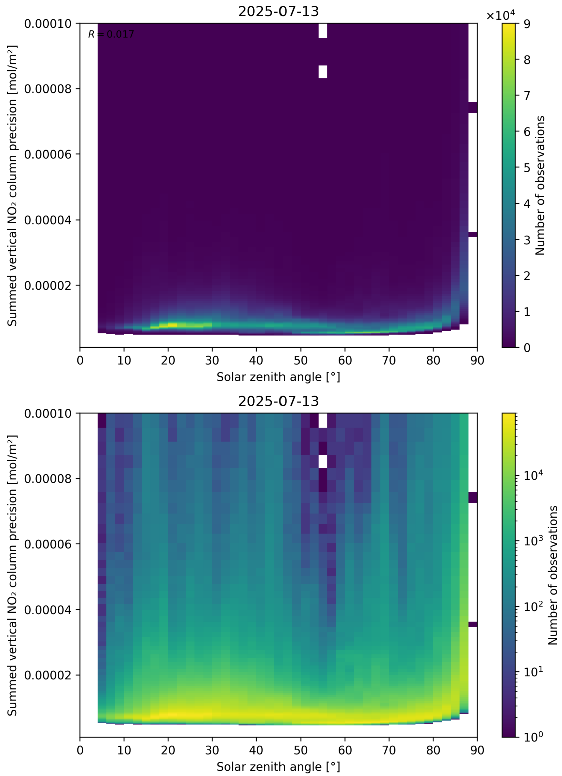
Figure 152: Scatter density plot of “Solar zenith angle” against “Summed vertical NO 2 column precision” for 2025-07-13 to 2025-07-14.
