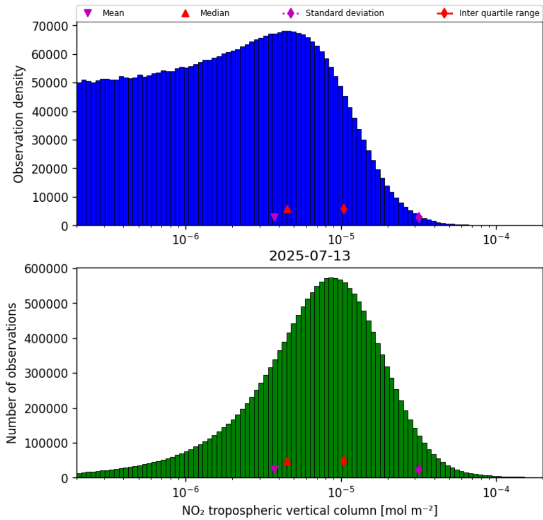
Figure 29: Histogram of “NO 2 tropospheric vertical column” for 2025-07-13 to 2025-07-14
