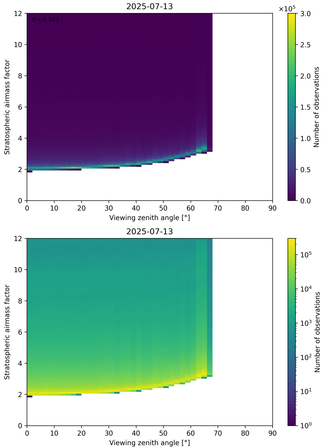
Figure 159: Scatter density plot of “Viewing zenith angle” against “Stratospheric airmass factor” for 2025-07-13 to 2025-07-14.
