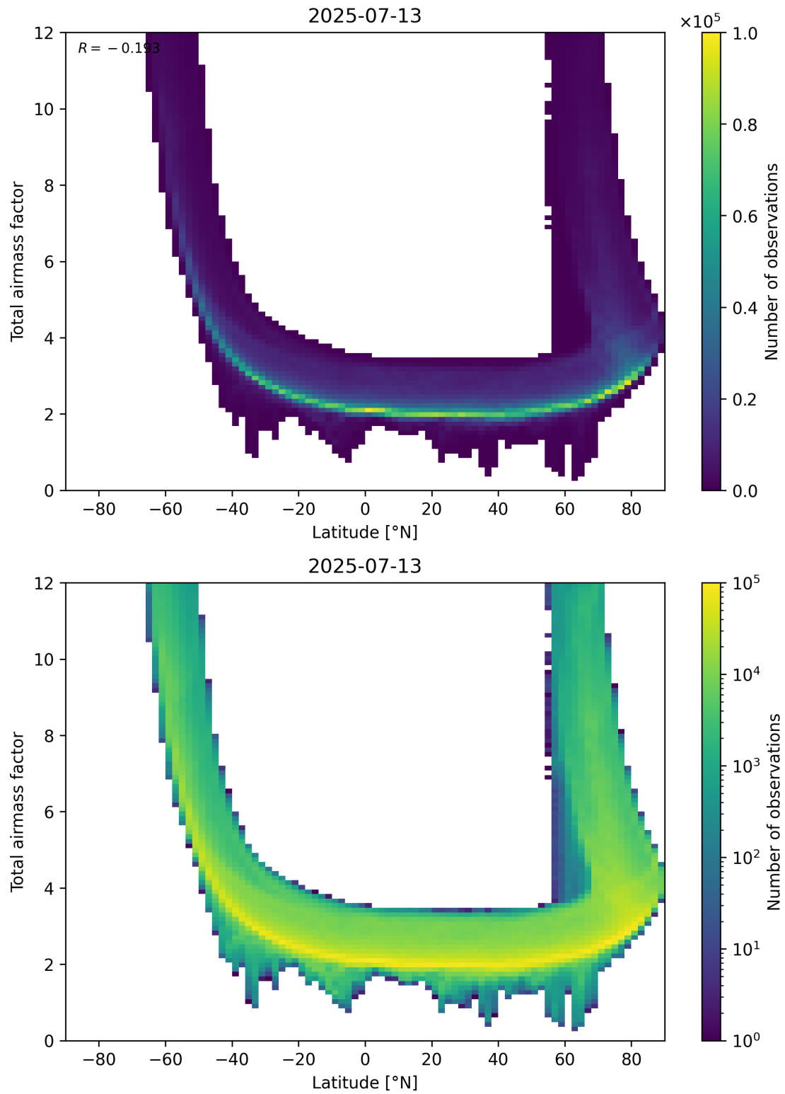
Figure 84: Scatter density plot of “Latitude” against “Total airmass factor” for 2025-07-13 to 2025-07-14.
