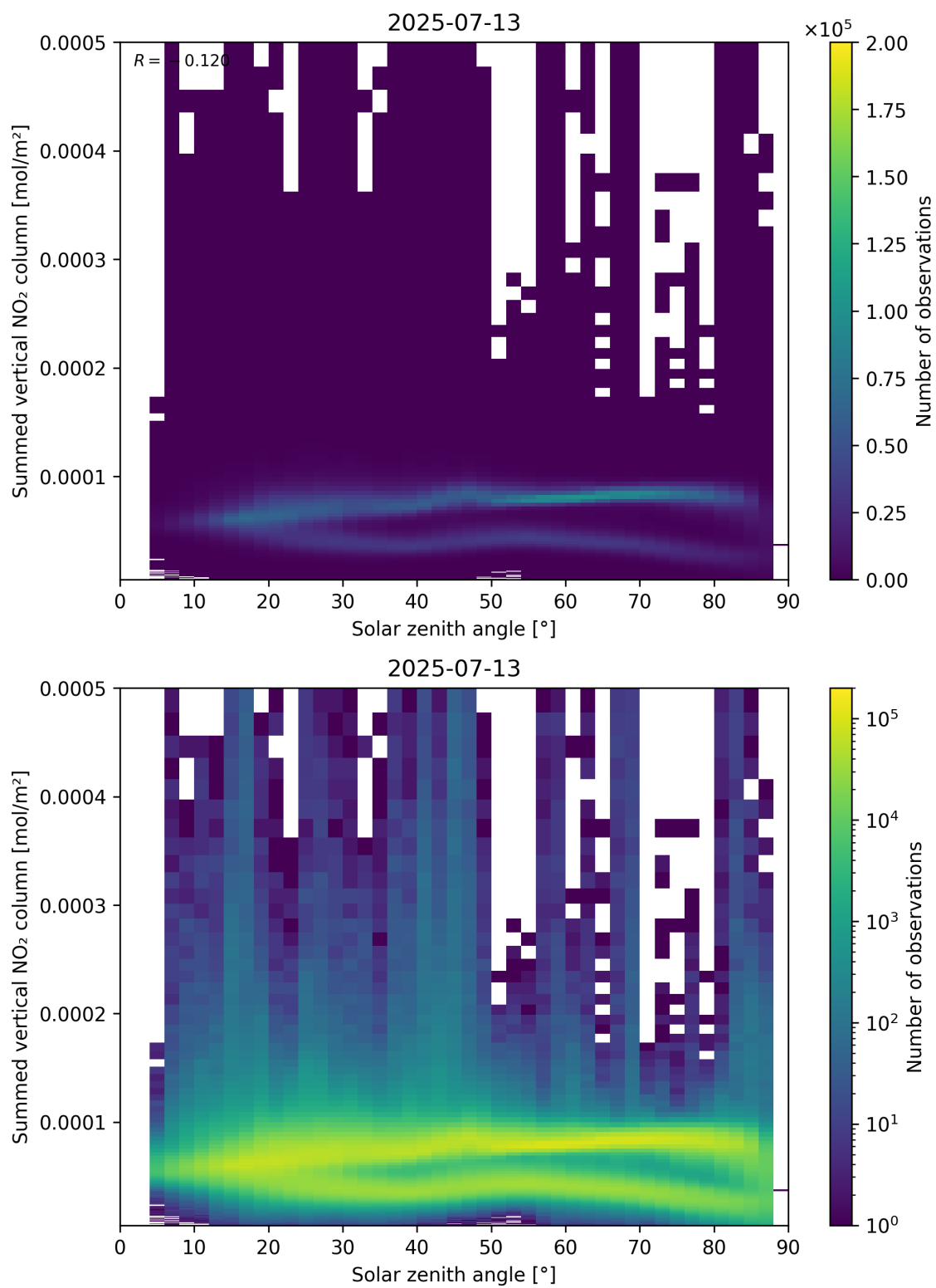
Figure 151: Scatter density plot of “Solar zenith angle” against “Summed vertical NO 2 column” for 2025-07-13 to 2025-07-14.
