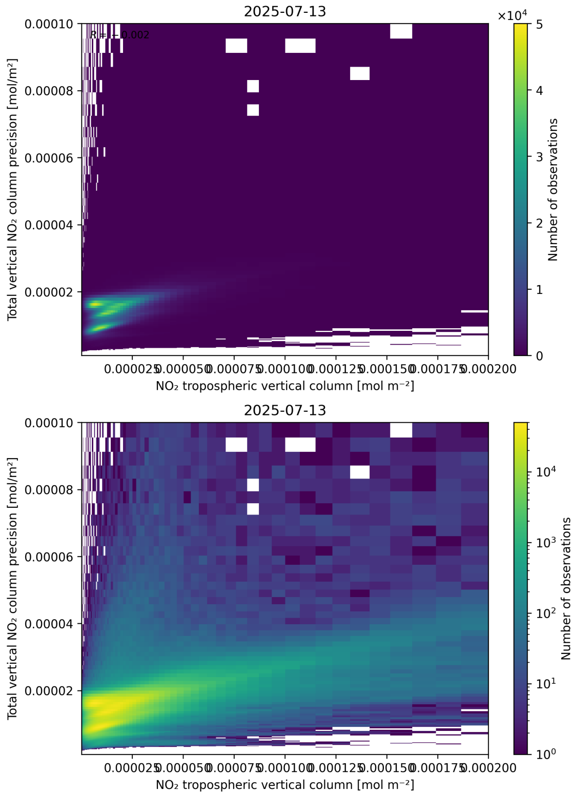
Figure 129: Scatter density plot of “NO 2 tropospheric vertical column” against “Total vertical NO 2 column precision” for 2025-07-13 to 2025-07-14.
