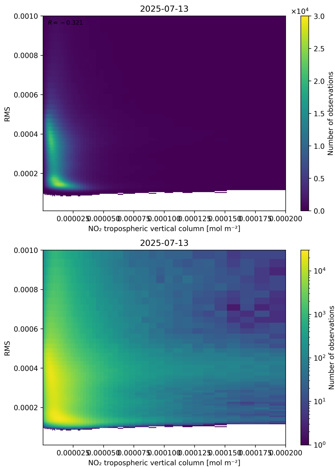
Figure 142: Scatter density plot of “NO 2 tropospheric vertical column” against “RMS” for 2025-07-13 to 2025-07-14.
