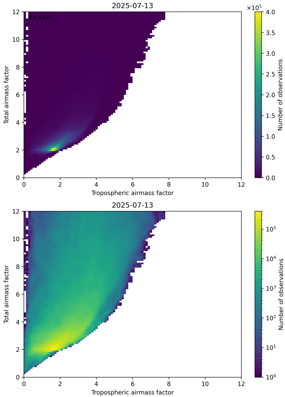
Figure 72: Scatter density plot of “Tropospheric airmass factor” against “Total airmass factor” for 2025-07-13 to 2025-07-14.
