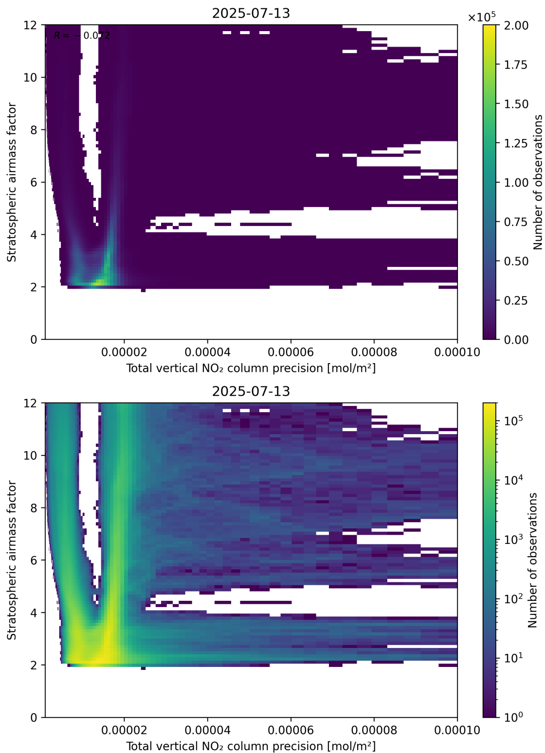
Figure 115: Scatter density plot of “Total vertical NO 2 column precision” against “Stratospheric airmass factor” for 2025-07-13 to 2025-07-14.
