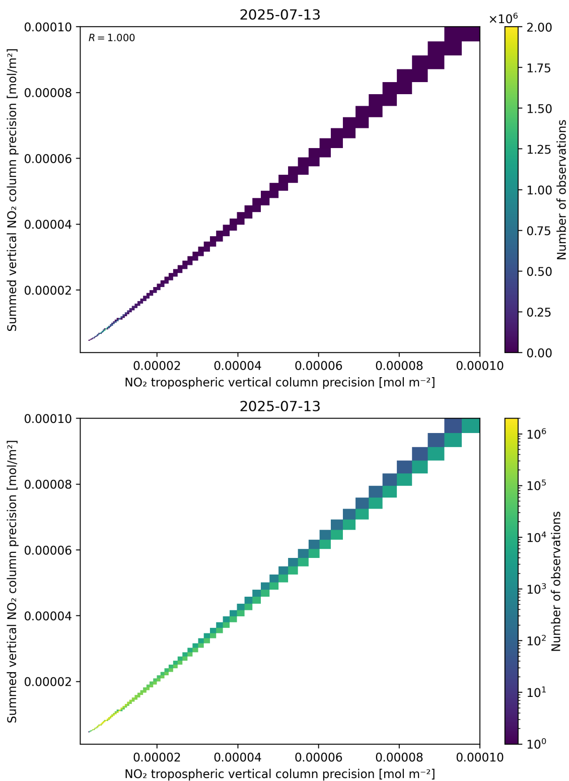
Figure 137: Scatter density plot of “NO 2 tropospheric vertical column precision” against “Summed vertical NO 2 column precision” for 2025-07-13 to 2025-07-14.
