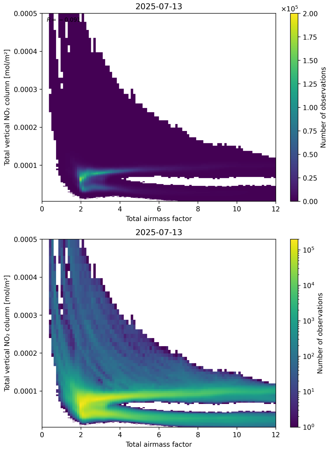
Figure 67: Scatter density plot of “Total airmass factor” against “Total vertical NO 2 column” for 2025-07-13 to 2025-07-14.
