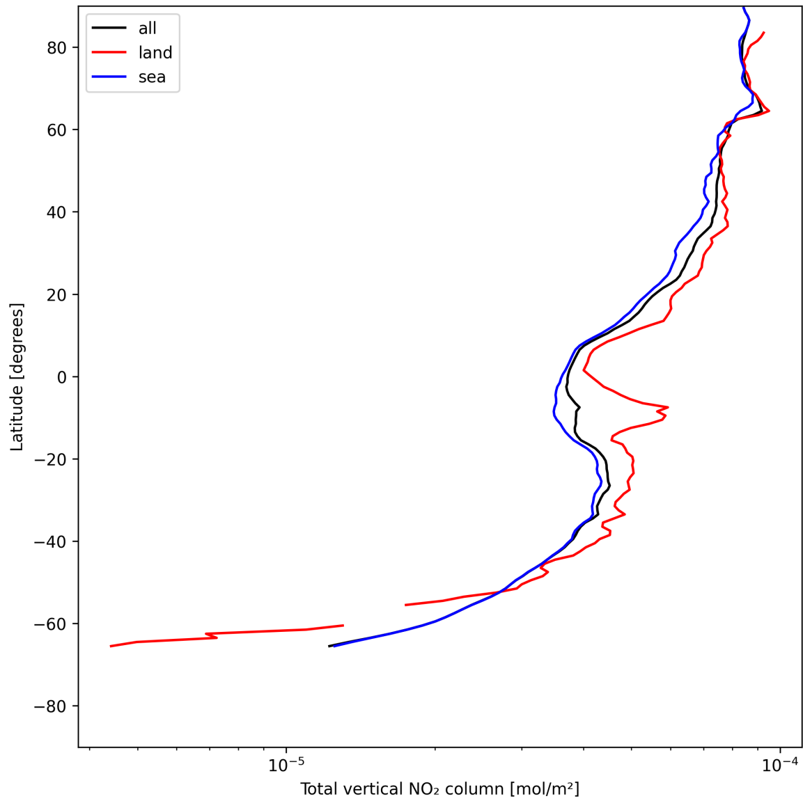
Figure 21: Zonal average of “Total vertical NO 2 column” for 2025-07-13 to 2025-07-14.
