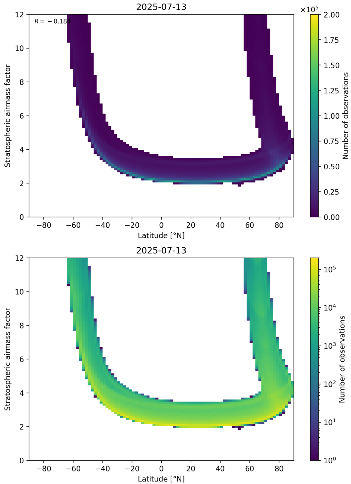
Figure 83: Scatter density plot of “Latitude” against “Stratospheric air mass factor” for 2025-07-13 to 2025-07-14.
