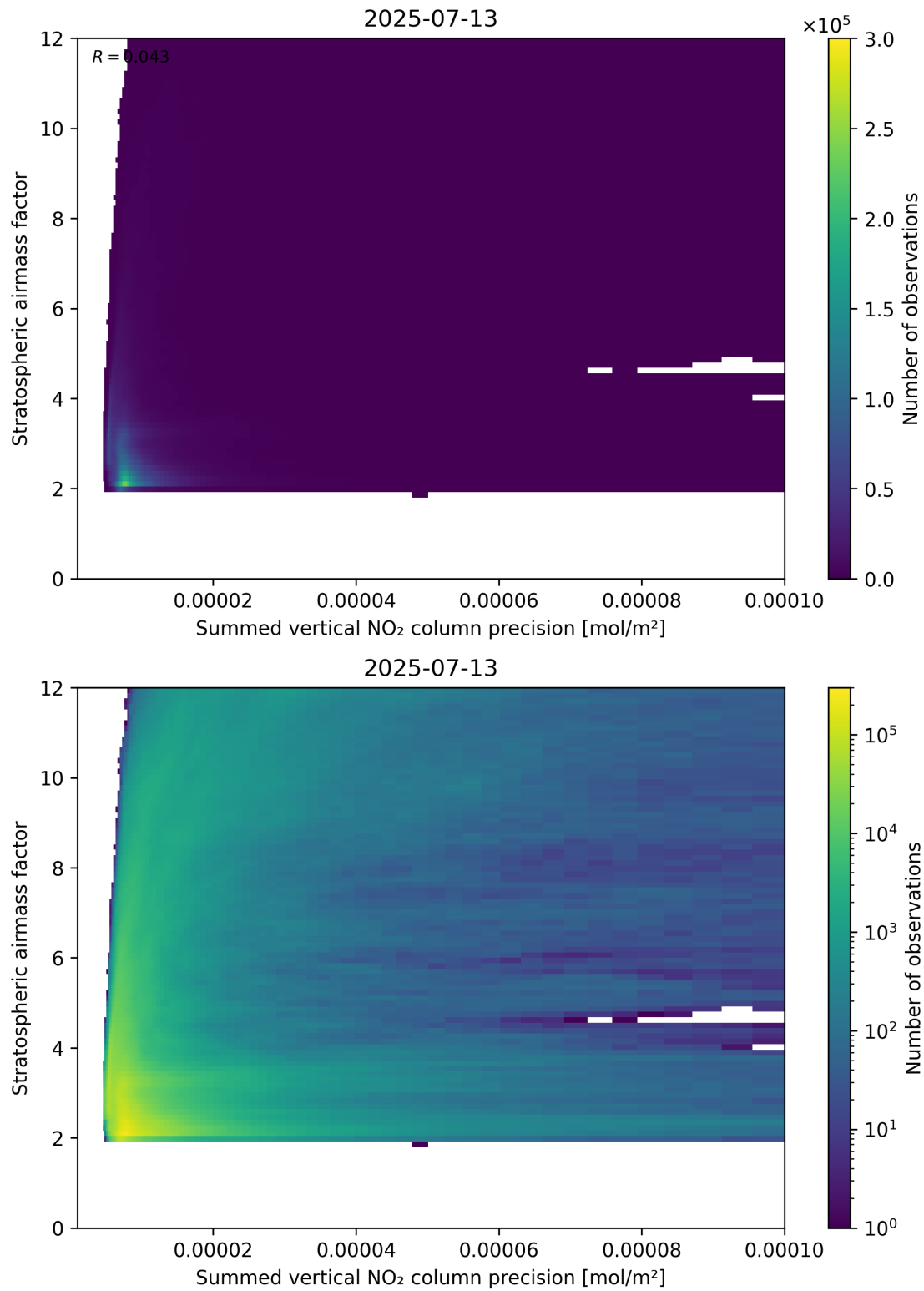
Figure 106: Scatter density plot of “Summed vertical NO 2 column precision” against “Stratospheric airmass factor” for 2025-07-13 to 2025-07-14.
