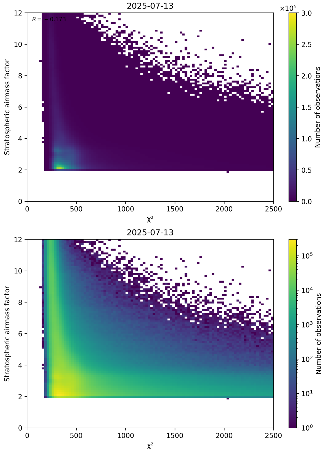
Figure 81: Scatter density plot of “ \chi^2 ” against “Stratospheric airmass factor” for 2025-07-13 to 2025-07-14.
