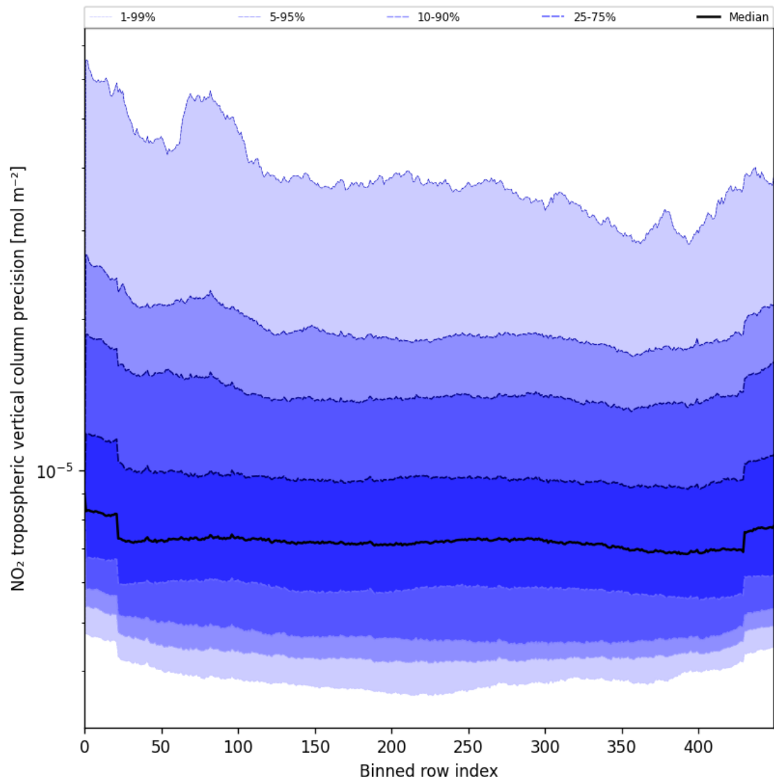
Figure 47: Along track statistics of “NO 2 tropospheric vertical column precision” for 2025-07-13 to 2025-07-14
