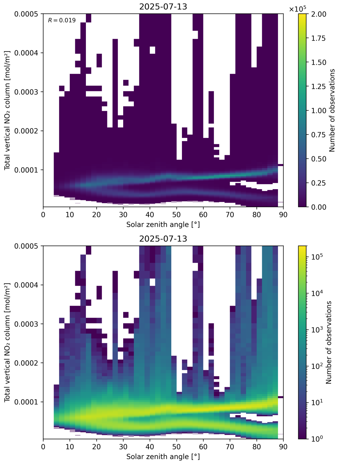
Figure 153: Scatter density plot of “Solar zenith angle” against “Total vertical \text{NO}_2 column” for 2025-07-13 to 2025-07-14.
