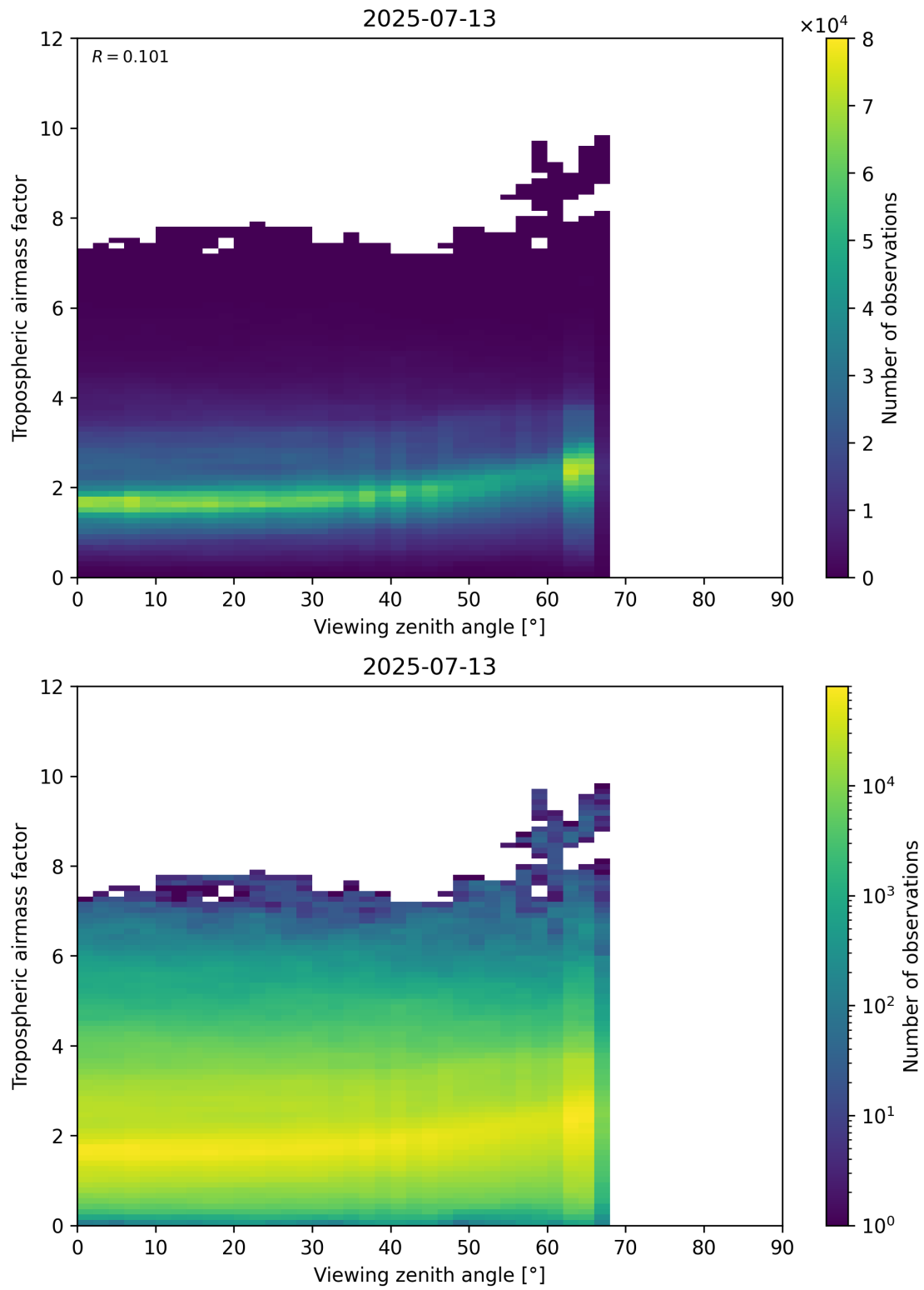
Figure 161: Scatter density plot of “Viewing zenith angle” against “Tropospheric airmass factor” for 2025-07-13 to 2025-07-14.
