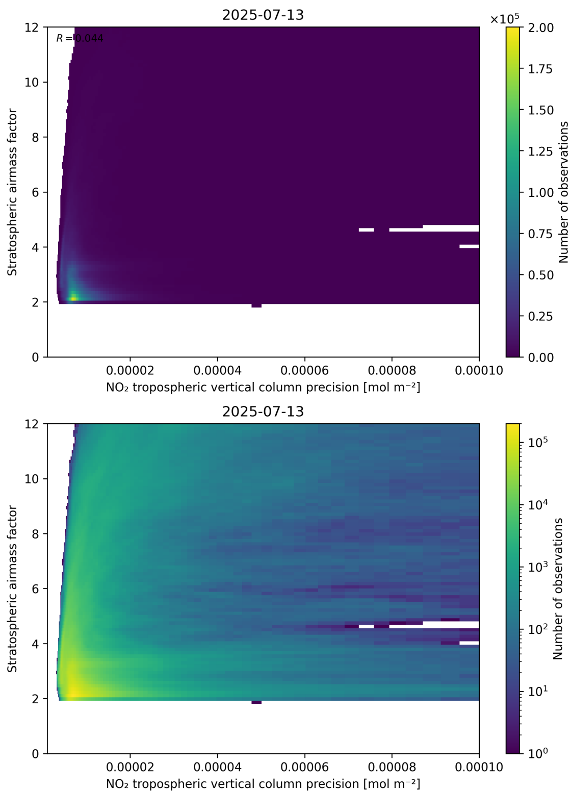
Figure 131: Scatter density plot of “NO 2 tropospheric vertical column precision” against “Stratospheric airmass factor” for 2025-07-13 to 2025-07-14.
