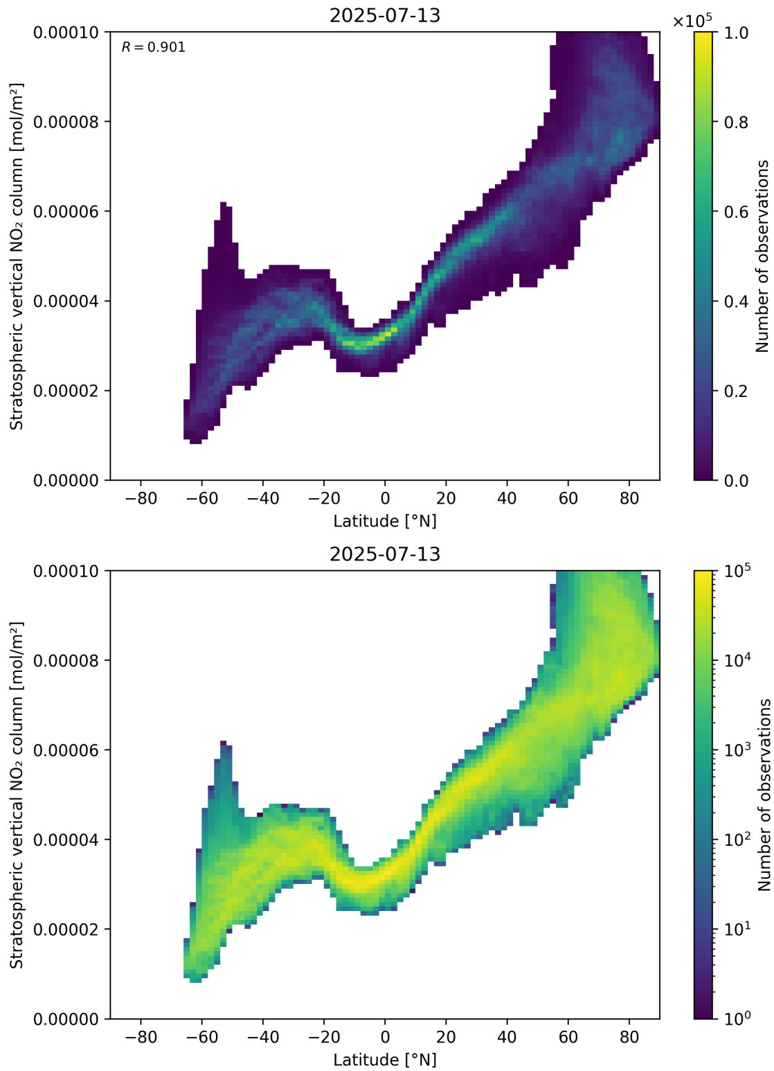
Figure 87: Scatter density plot of “Latitude” against “Stratospheric vertical NO 2 column” for 2025-07-13 to 2025-07-14.
