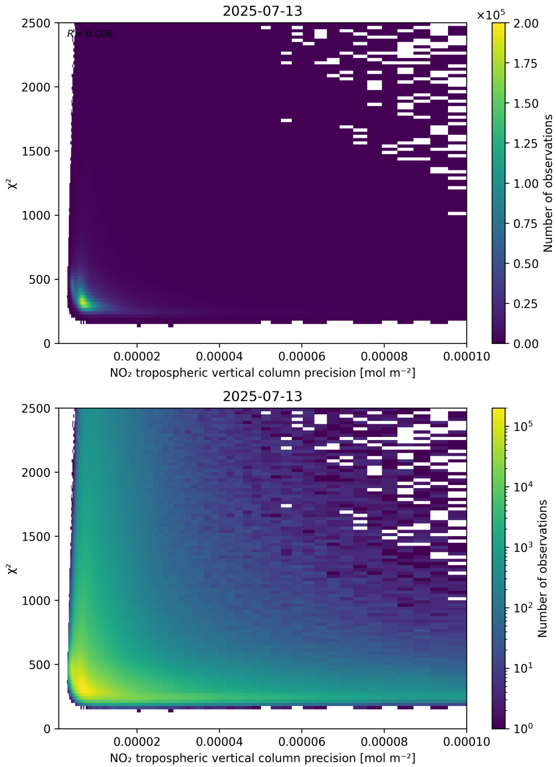
Figure 134: Scatter density plot of “NO 2 tropospheric vertical column precision” against “ \chi^2 ” for 2025-07-13 to 2025-07-14.
