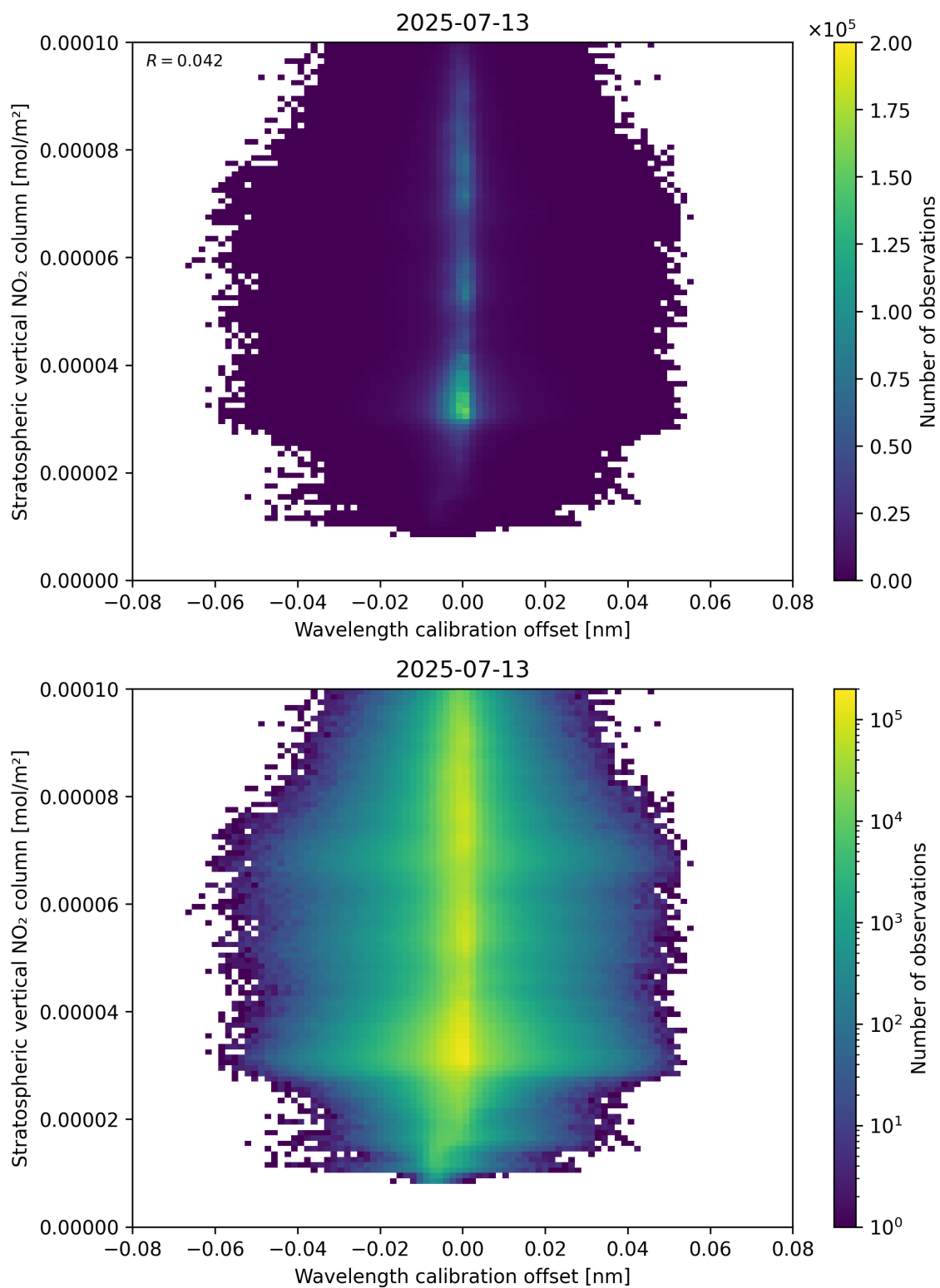
Figure 176: Scatter density plot of “Wavelength calibration offset” against “Stratospheric vertical NO 2 column” for 2025-07-13 to 2025-07-14.
