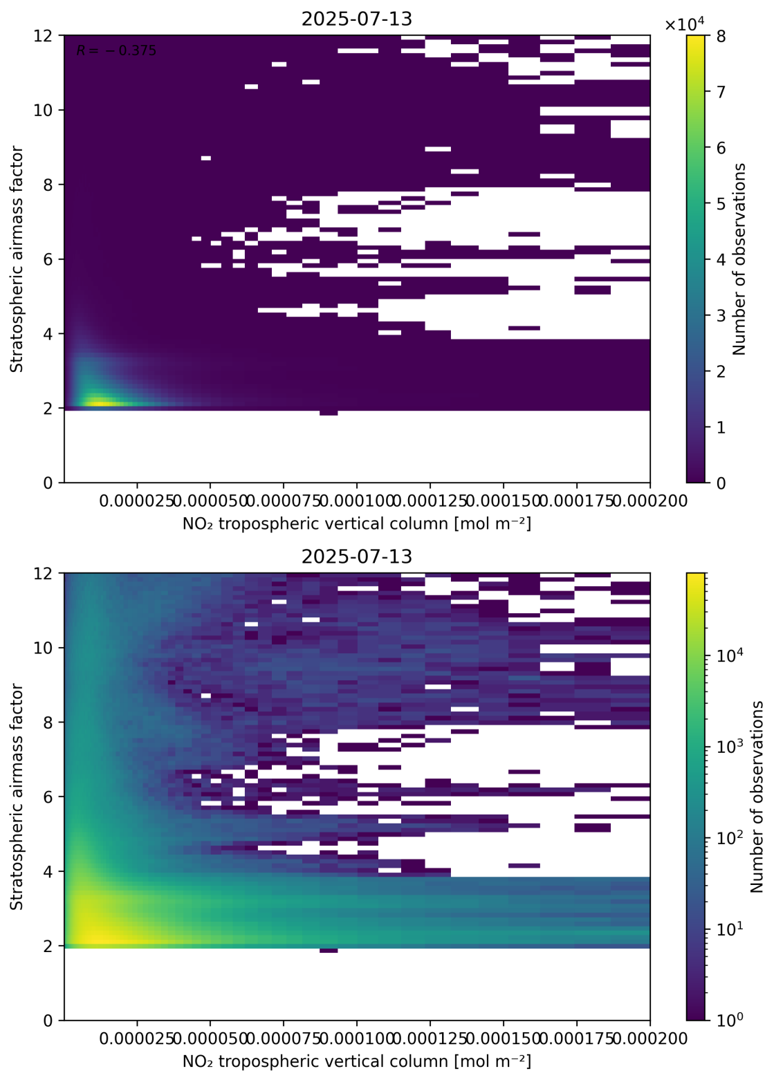
Figure 121: Scatter density plot of “NO 2 tropospheric vertical column” against “Stratospheric air mass factor” for 2025-07-13 to 2025-07-14.
