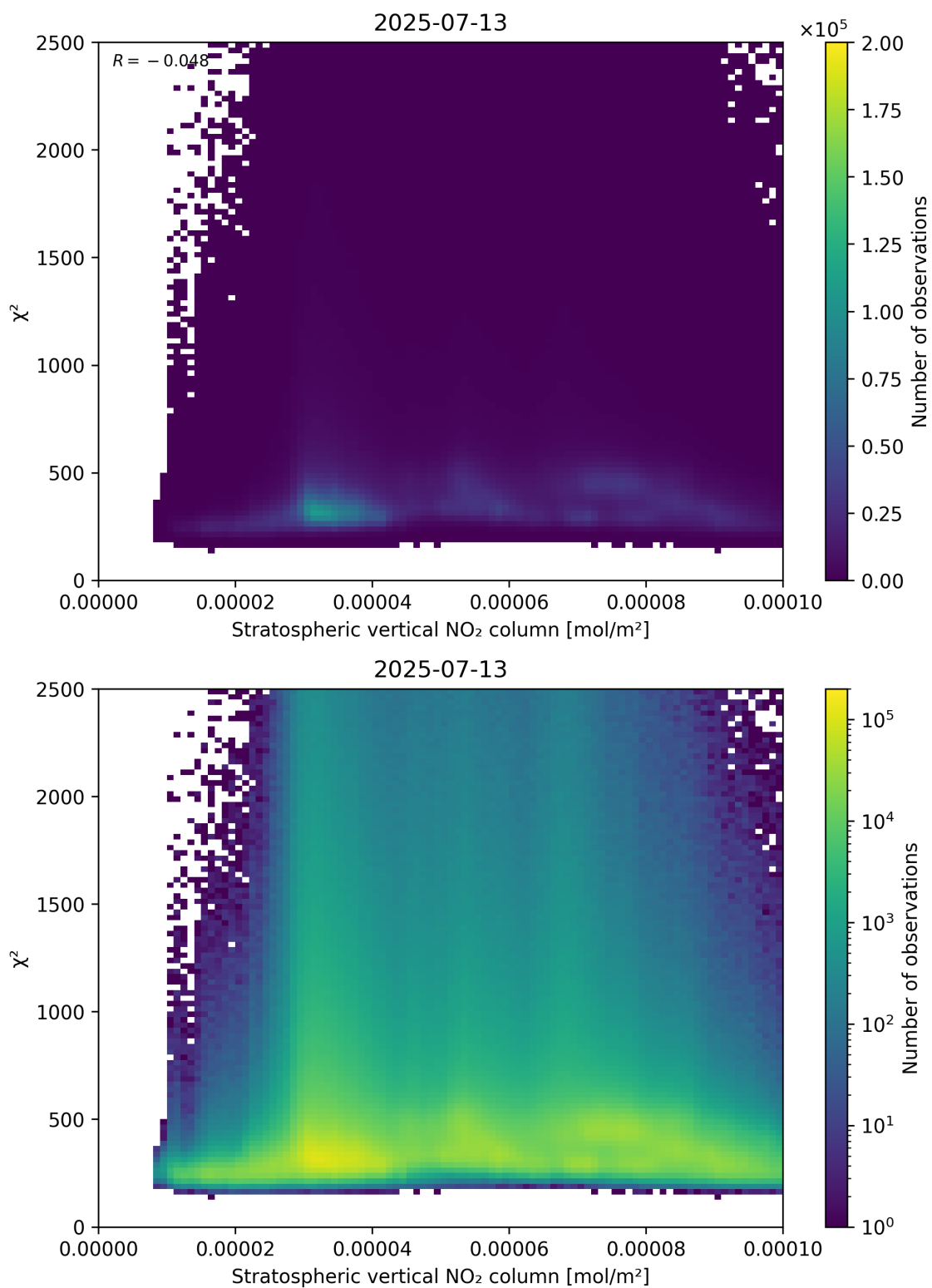
Figure 97: Scatter density plot of “Stratospheric vertical NO 2 column” against “ \chi^2 ” for 2025-07-13 to 2025-07-14.
