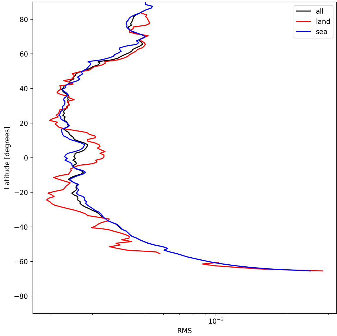
Figure 26: Zonal average of “RMS” for 2025-07-13 to 2025-07-14.
