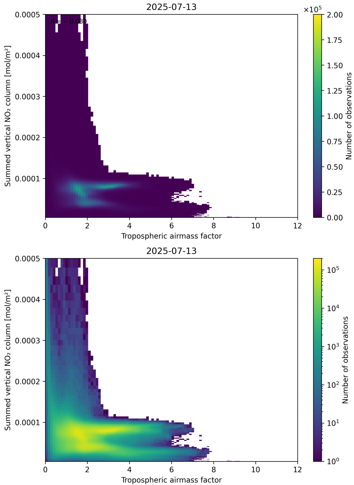
Figure 75: Scatter density plot of “Tropospheric air mass factor” against “Summed vertical NO 2 column” for 2025-07-13 to 2025-07-14.
