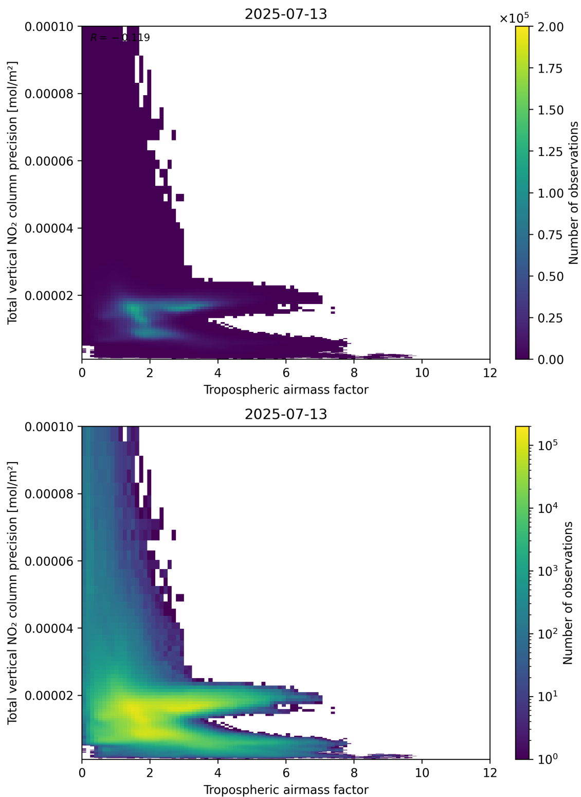
Figure 78: Scatter density plot of “Tropospheric air mass factor” against “Total vertical NO 2 column precision” for 2025-07-13 to 2025-07-14.
