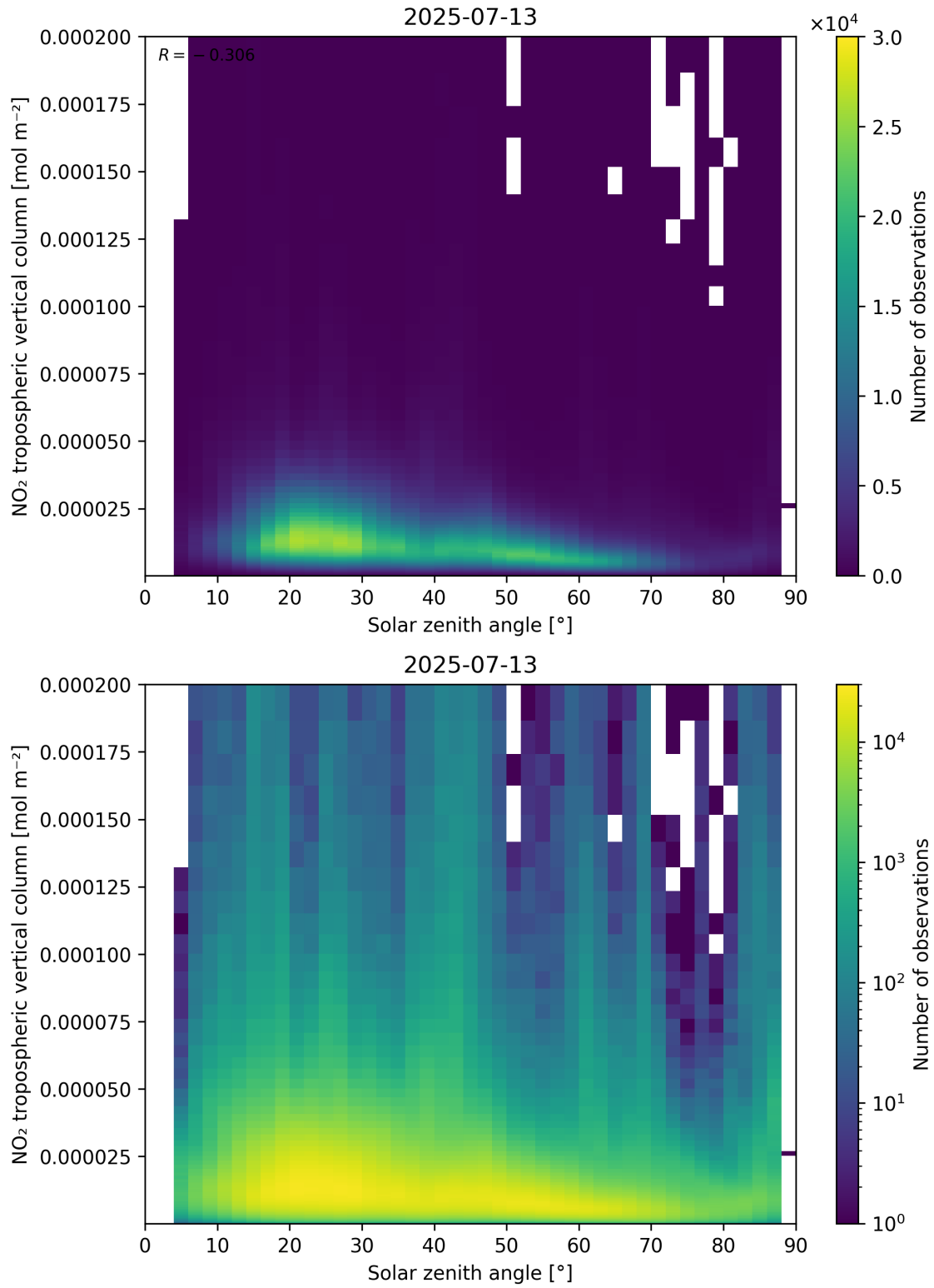
Figure 155: Scatter density plot of “Solar zenith angle” against “NO 2 tropospheric vertical column” for 2025-07-13 to 2025-07-14.
