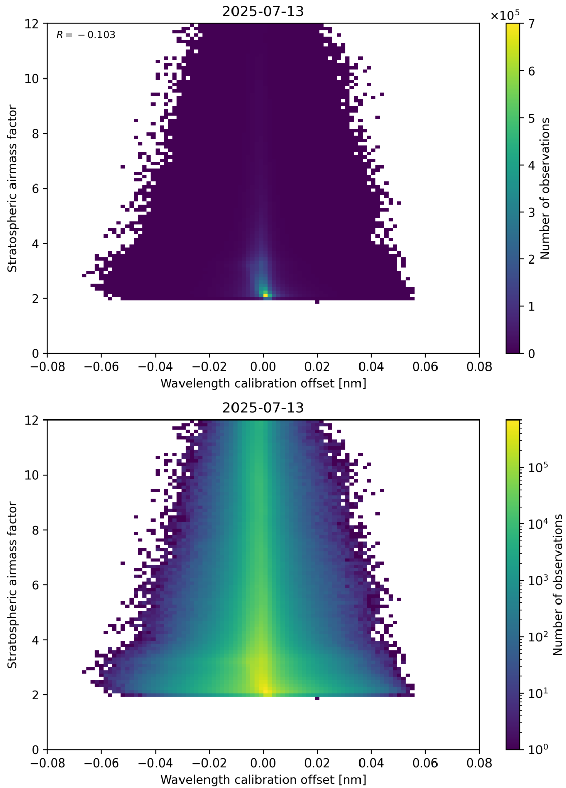
Figure 174: Scatter density plot of “Wavelength calibration offset” against “Stratospheric airmass factor” for 2025-07-13 to 2025-07-14.
