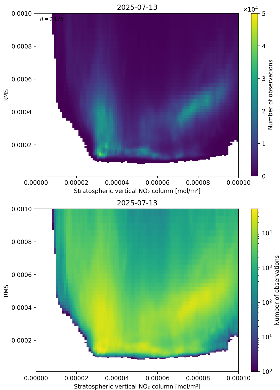
Figure 102: Scatter density plot of “Stratospheric vertical NO 2 column” against “RMS” for 2025-07-13 to 2025-07-14.
