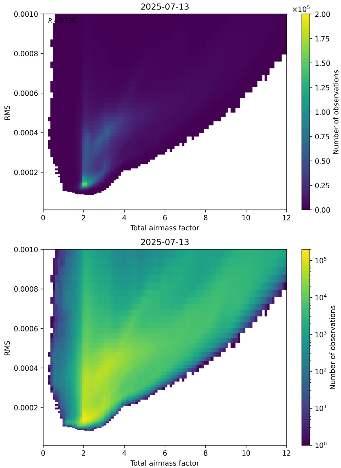
Figure 69: Scatter density plot of “Total airmass factor” against “RMS” for 2025-07-13 to 2025-07-14.
