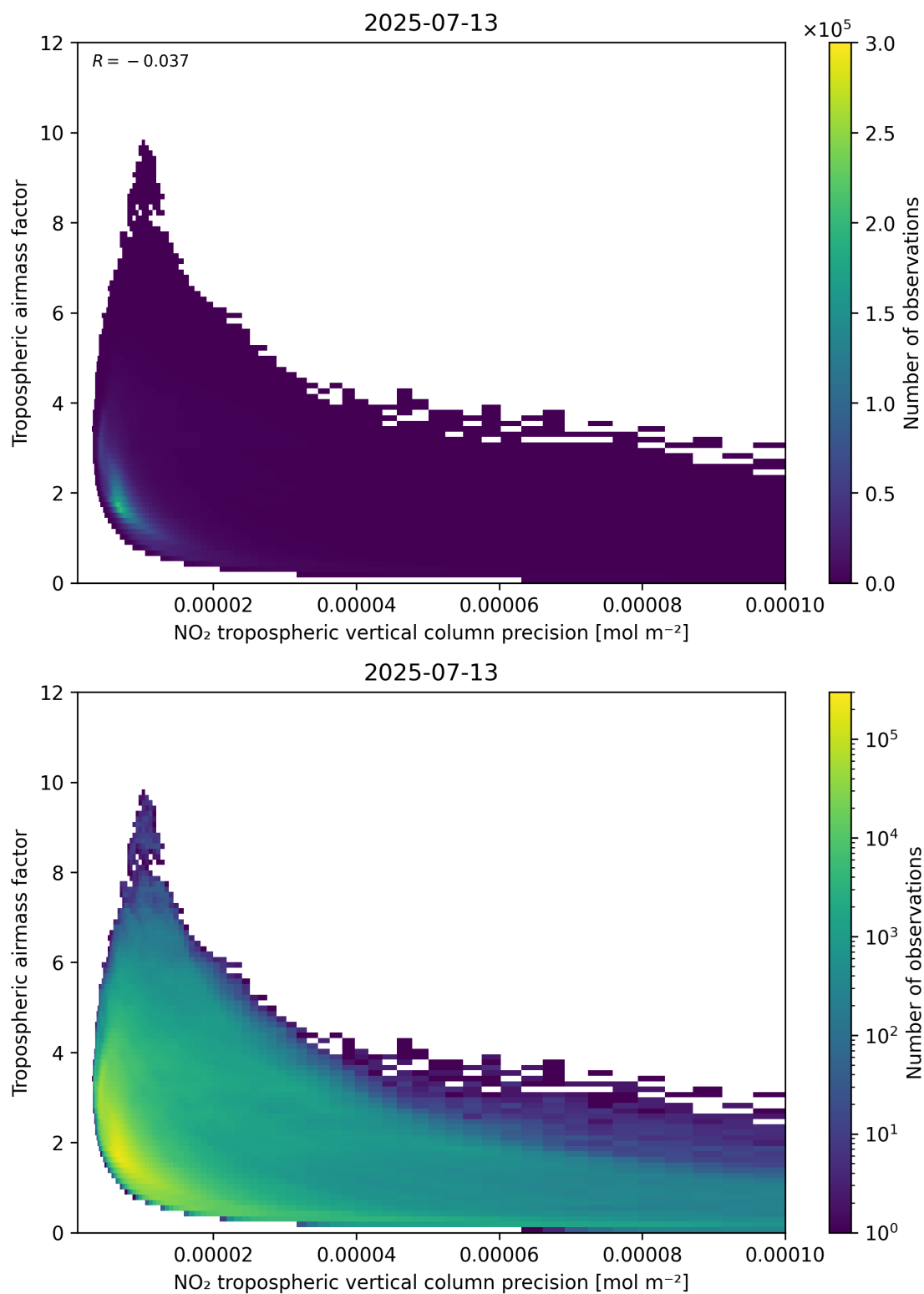
Figure 133: Scatter density plot of “NO 2 tropospheric vertical column precision” against “Tropospheric air mass factor” for 2025-07-13 to 2025-07-14.
