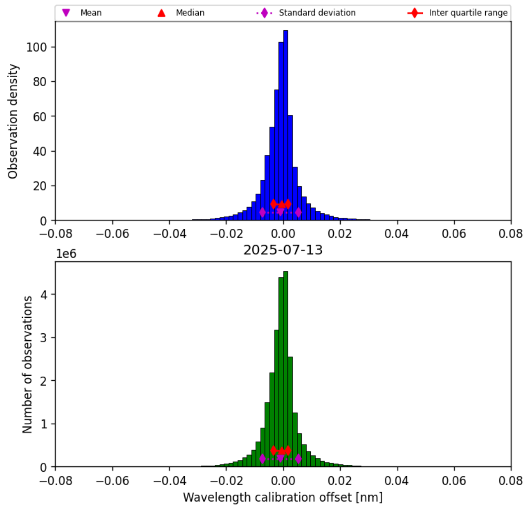
Figure 35: Histogram of “Wavelength calibration offset” for 2025-07-13 to 2025-07-14
