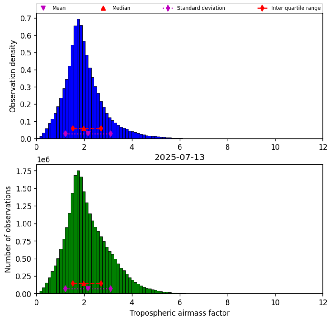
Figure 31: Histogram of “Tropospheric airmass factor” for 2025-07-13 to 2025-07-14
