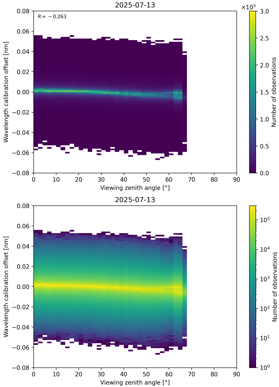
Figure 173: Scatter density plot of “Viewing zenith angle” against “Wavelength calibration offset” for 2025-07-13 to 2025-07-14.
