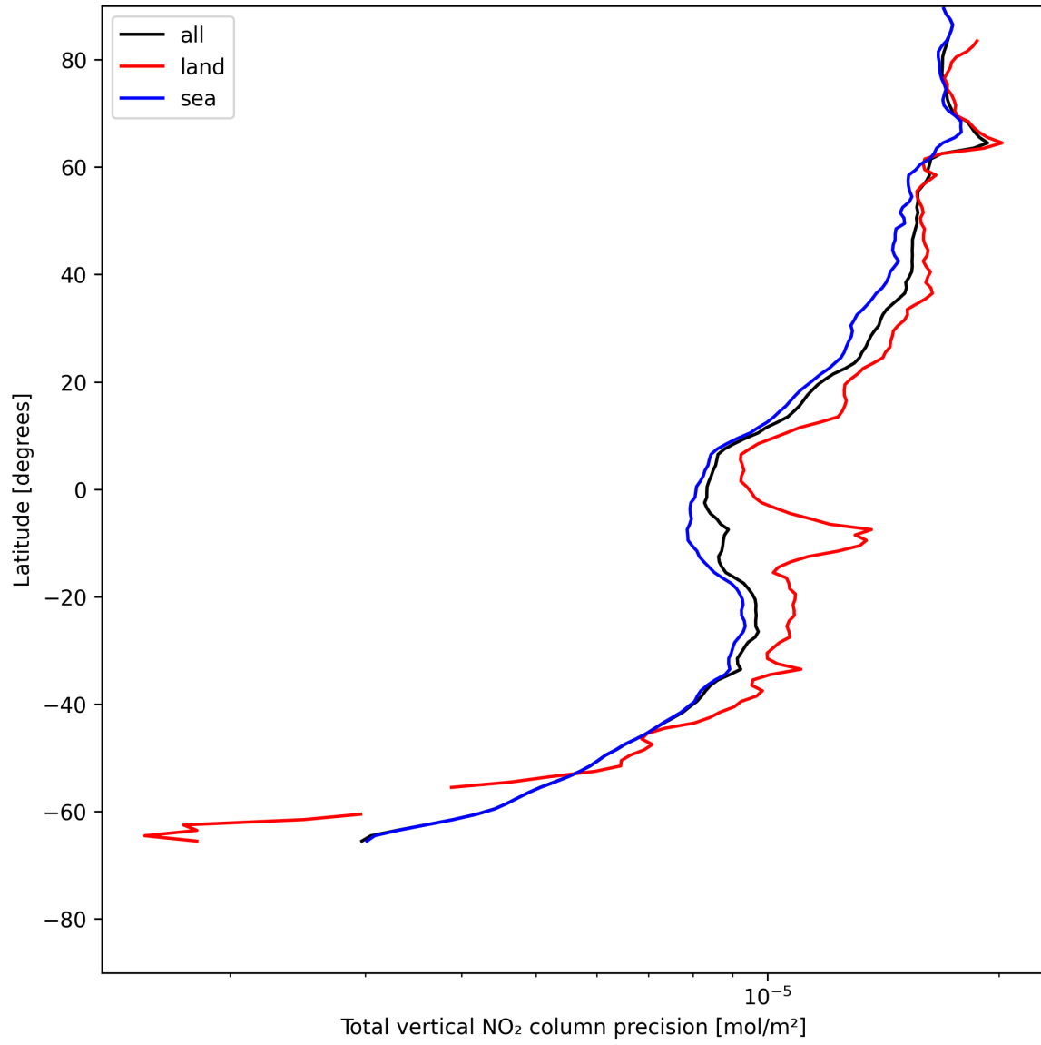
Figure 22: Zonal average of “Total vertical NO 2 column precision” for 2025-07-13 to 2025-07-14.
