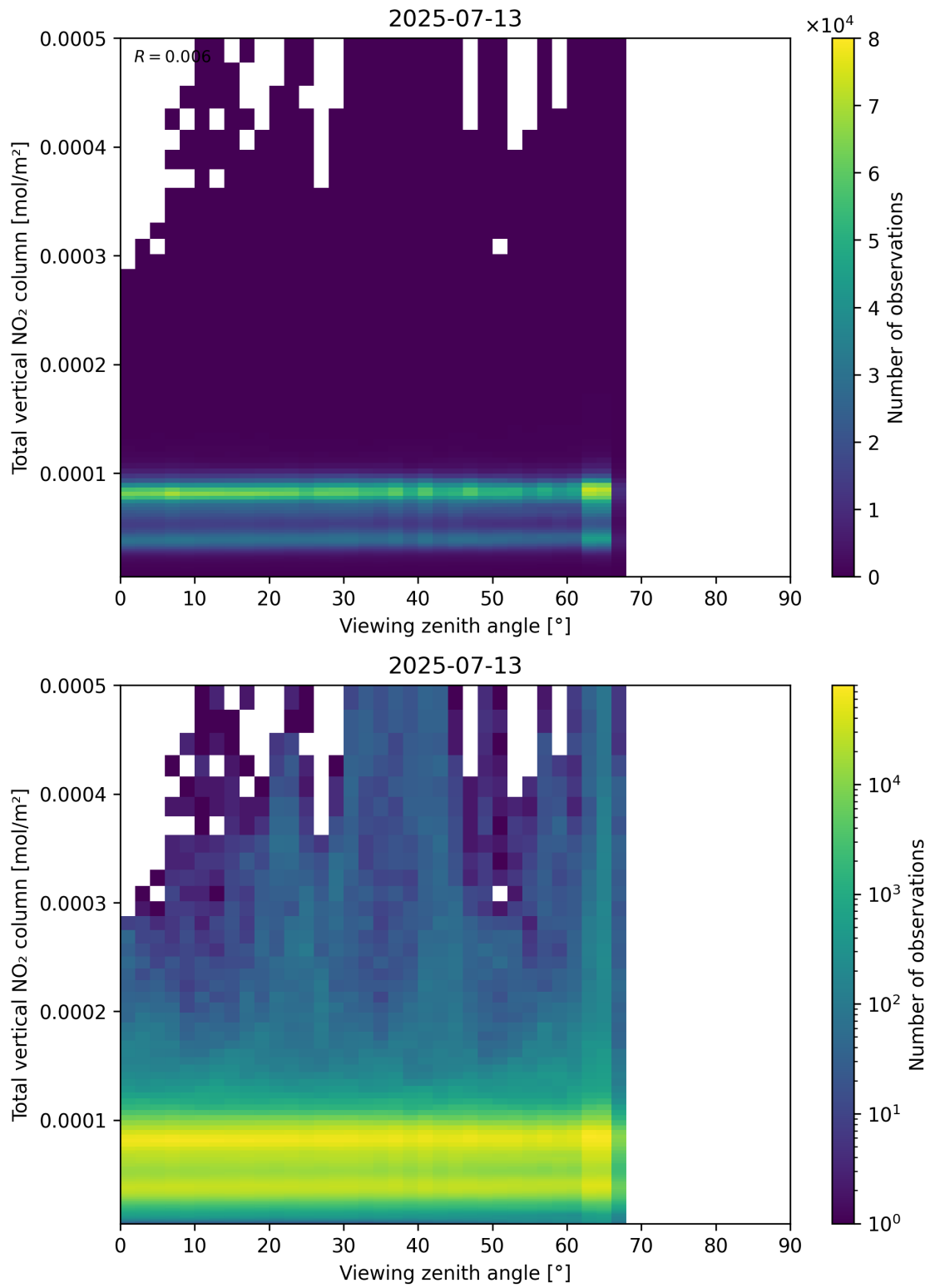
Figure 167: Scatter density plot of “Viewing zenith angle” against “Total vertical NO 2 column” for 2025-07-13 to 2025-07-14.
