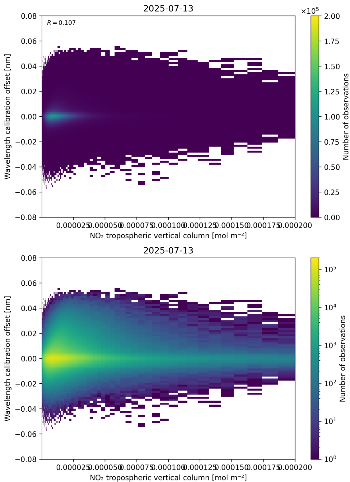
Figure 143: Scatter density plot of “NO 2 tropospheric vertical column” against “Wavelength calibration offset” for 2025-07-13 to 2025-07-14.
