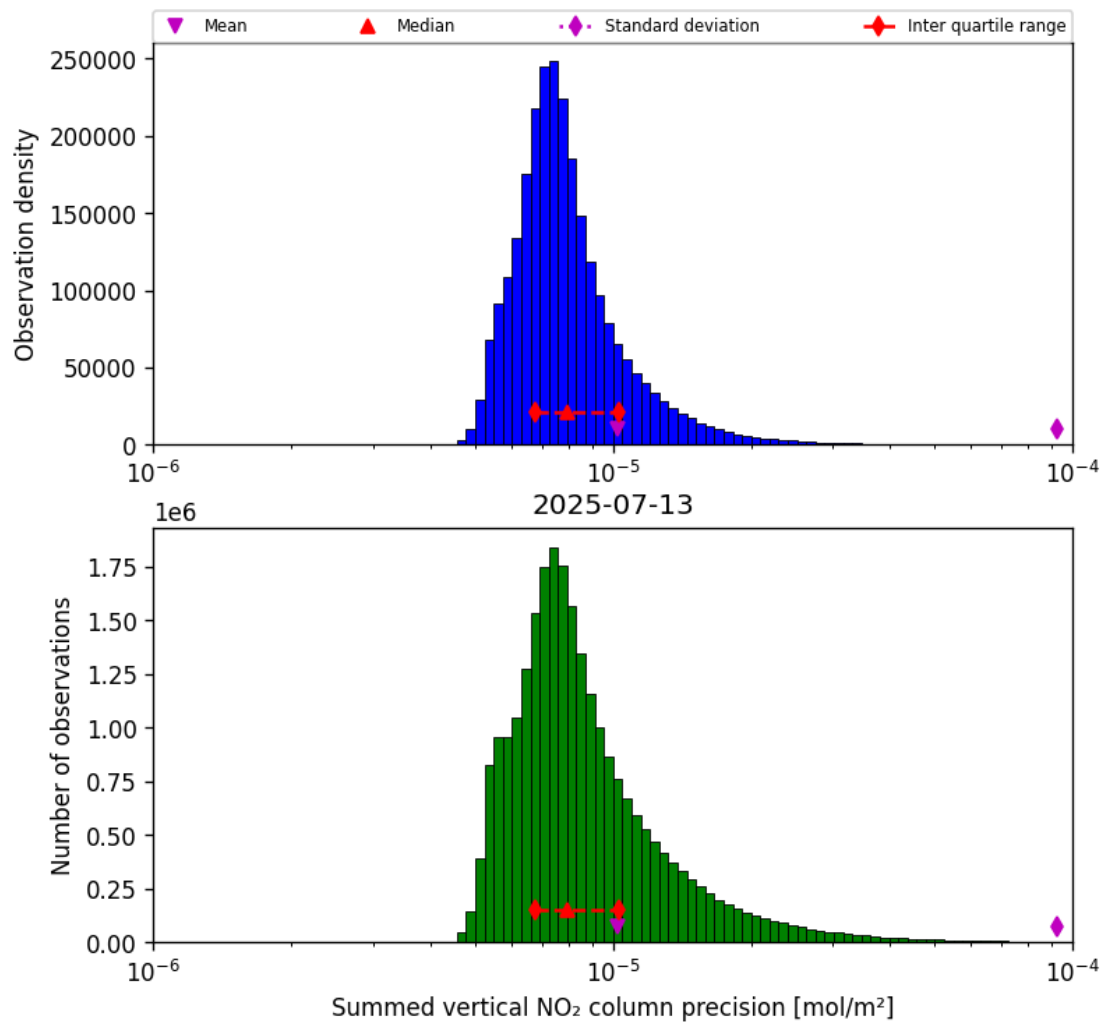
Figure 41: Histogram of "Summed vertical NO 2 column precision" for 2025-07-13 to 2025-07-14
