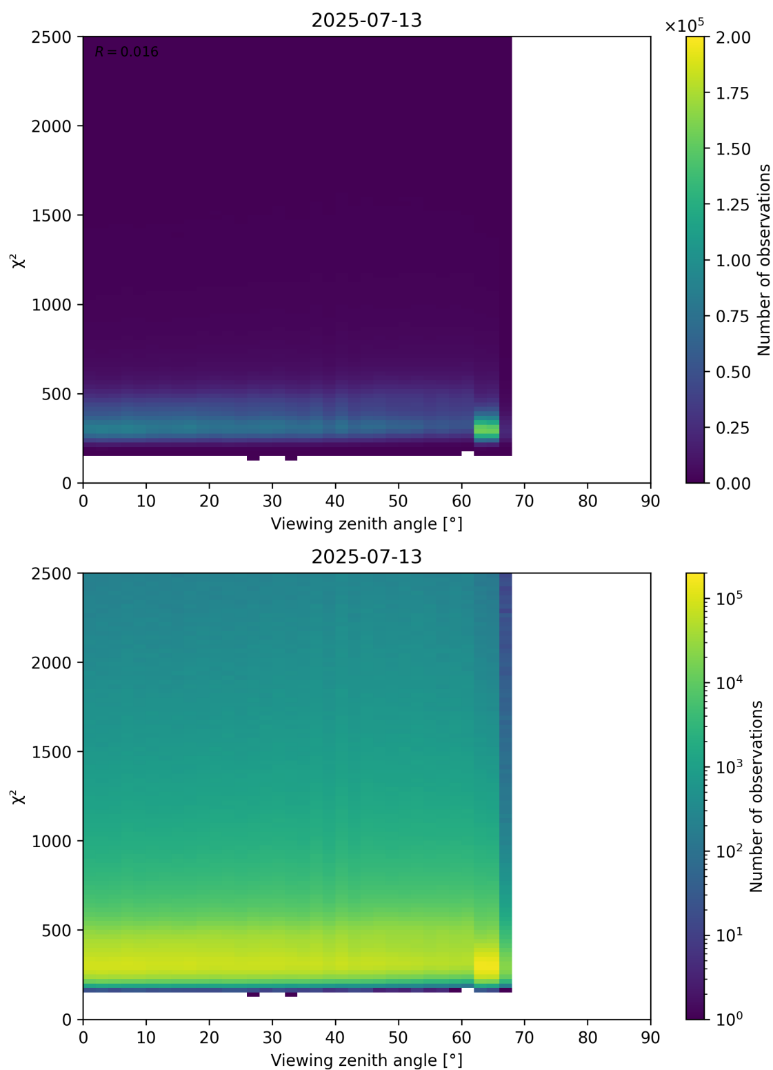
Figure 162: Scatter density plot of “Viewing zenith angle” against “ \chi^2 ” for 2025-07-13 to 2025-07-14.
