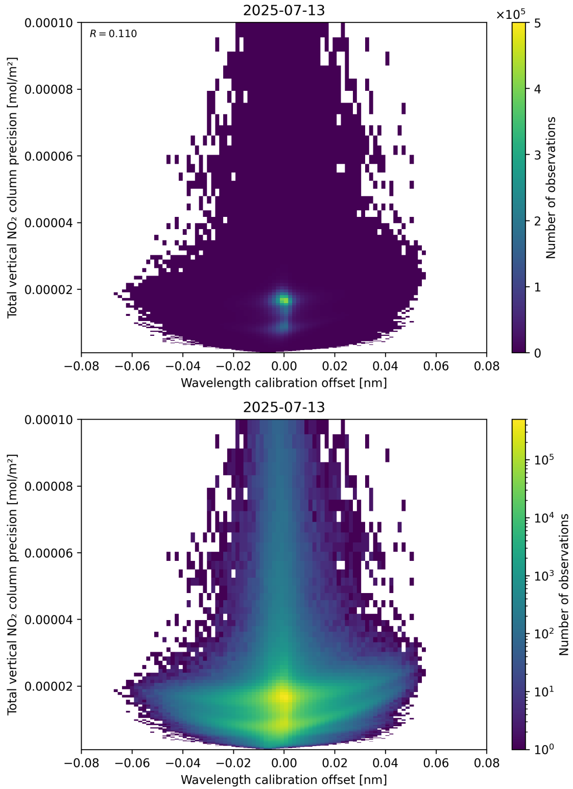
Figure 180: Scatter density plot of “Wavelength calibration offset” against “Total vertical NO 2 column precision” for 2025-07-13 to 2025-07-14.
