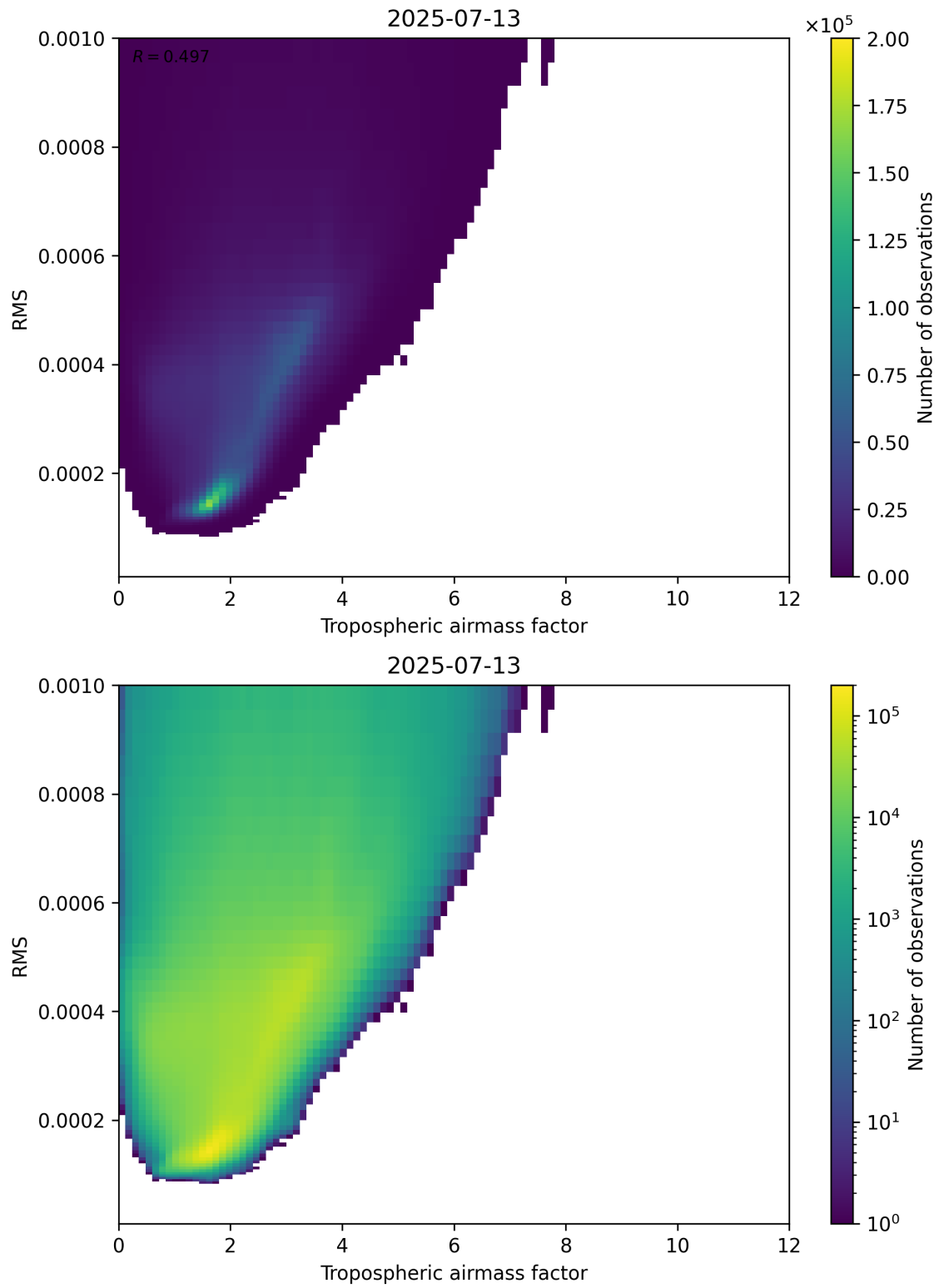
Figure 79: Scatter density plot of “Tropospheric airmass factor” against “RMS” for 2025-07-13 to 2025-07-14.
