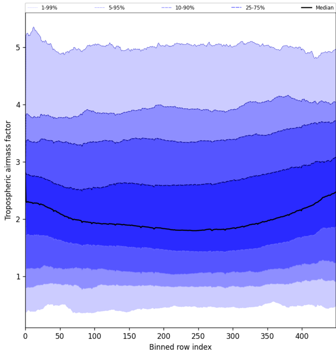
Figure 48: Along track statistics of “Tropospheric airmass factor” for 2025-07-13 to 2025-07-14
