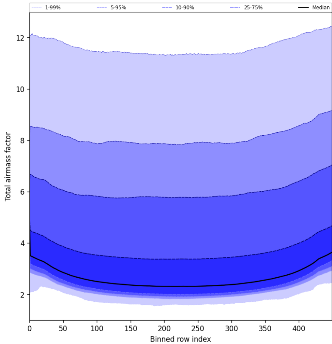
Figure 49: Along track statistics of “Total airmass factor” for 2025-07-13 to 2025-07-14
