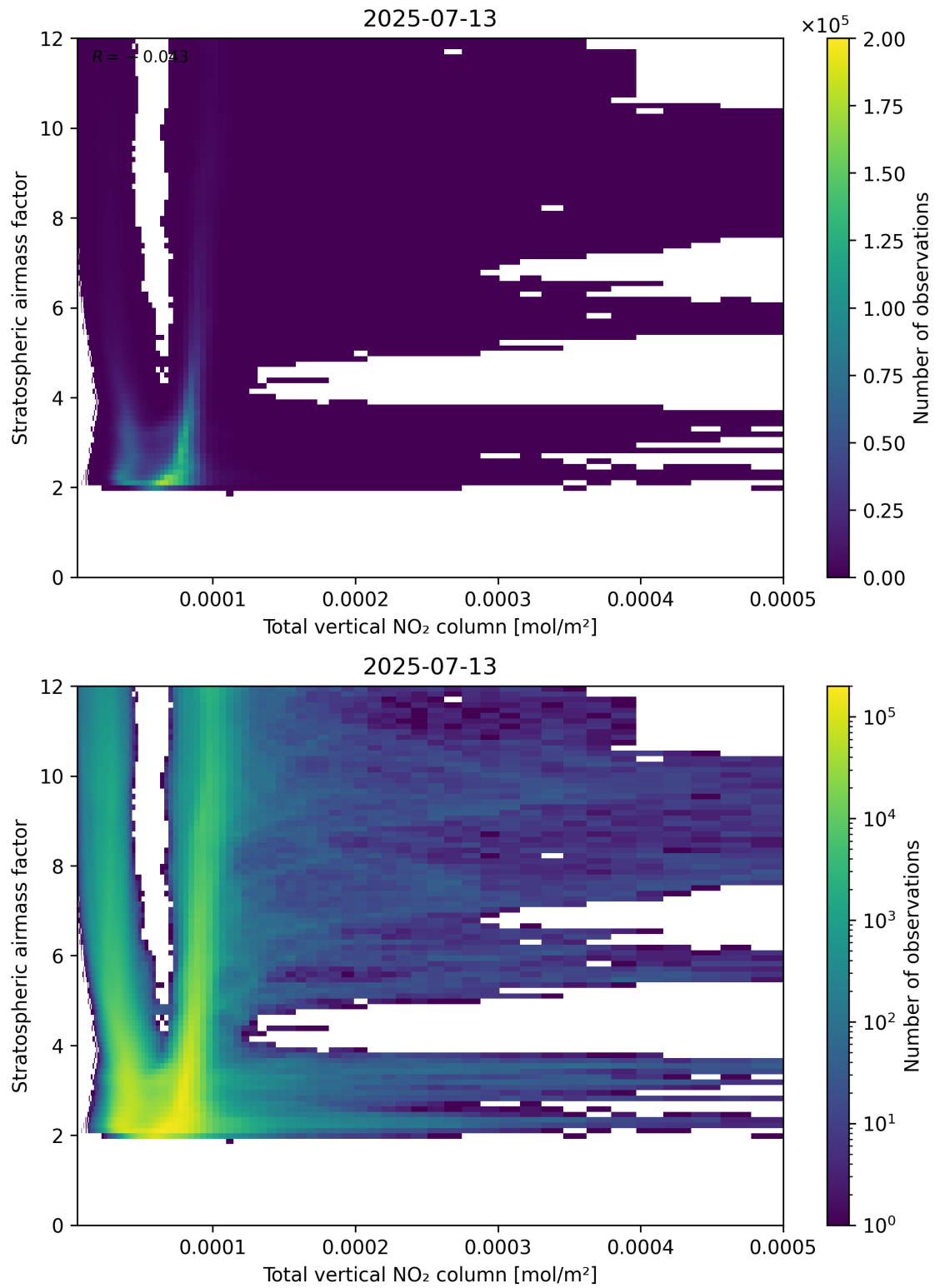
Figure 110: Scatter density plot of “Total vertical NO 2 column” against “Stratospheric airmass factor” for 2025-07-13 to 2025-07-14.
