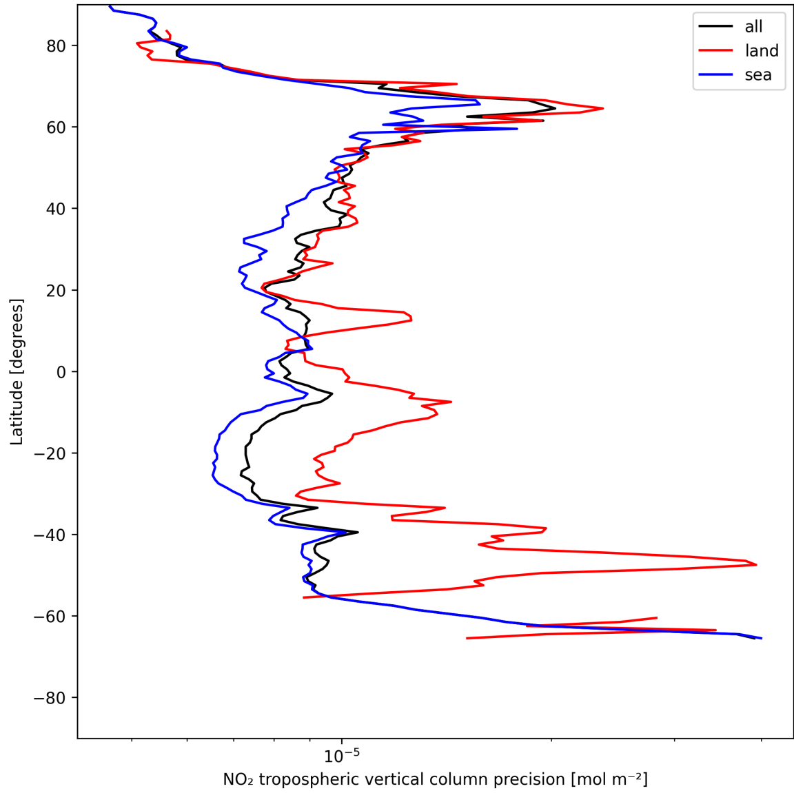
Figure 13: Zonal average of “NO 2 tropospheric vertical column precision” for 2025-07-13 to 2025-07-14.
