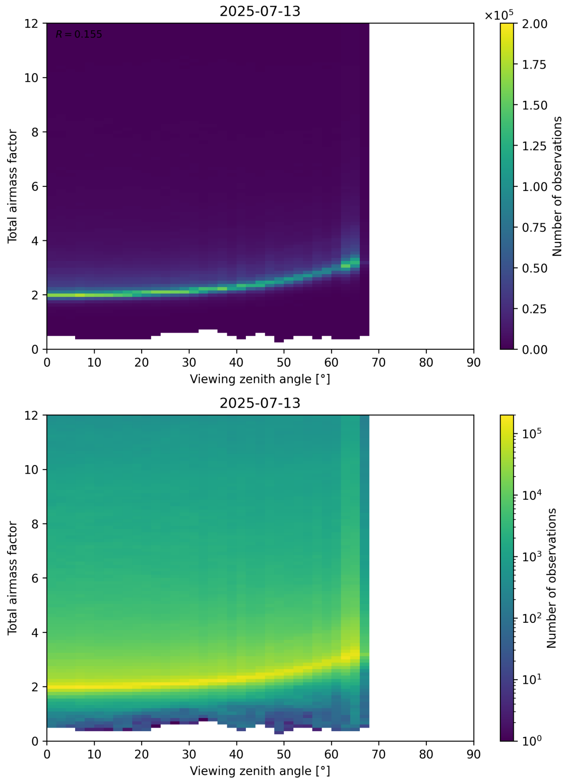
Figure 160: Scatter density plot of “Viewing zenith angle” against “Total airmass factor” for 2025-07-13 to 2025-07-14.
