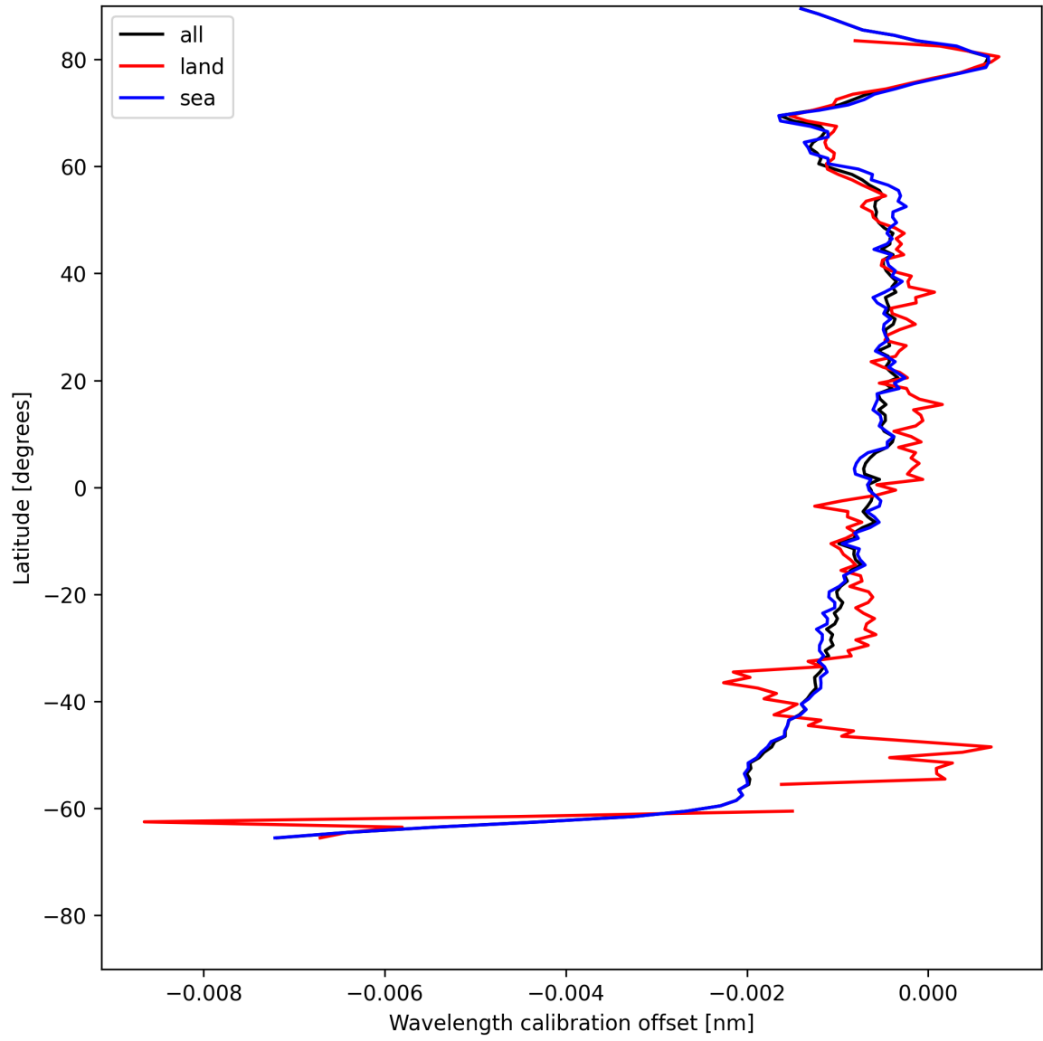
Figure 18: Zonal average of “Wavelength calibration offset” for 2025-07-13 to 2025-07-14.
