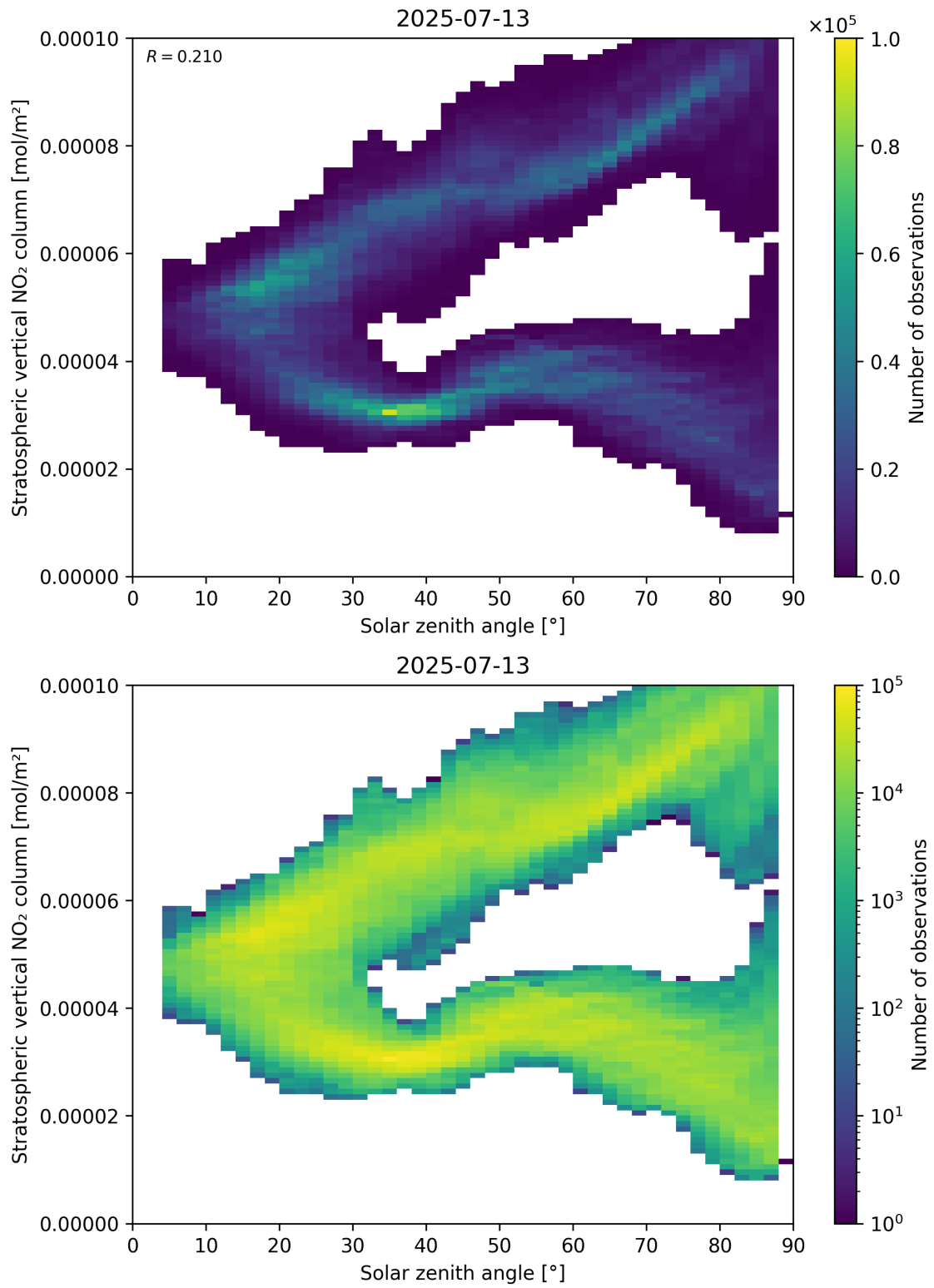
Figure 150: Scatter density plot of “Solar zenith angle” against “Stratospheric vertical NO 2 column” for 2025-07-13 to 2025-07-14.
