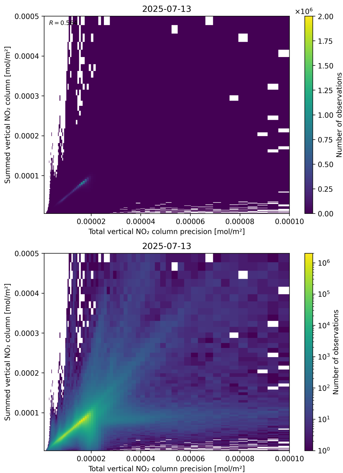
Figure 117: Scatter density plot of “Total vertical NO 2 column precision” against “Summed vertical NO 2 column” for 2025-07-13 to 2025-07-14.
