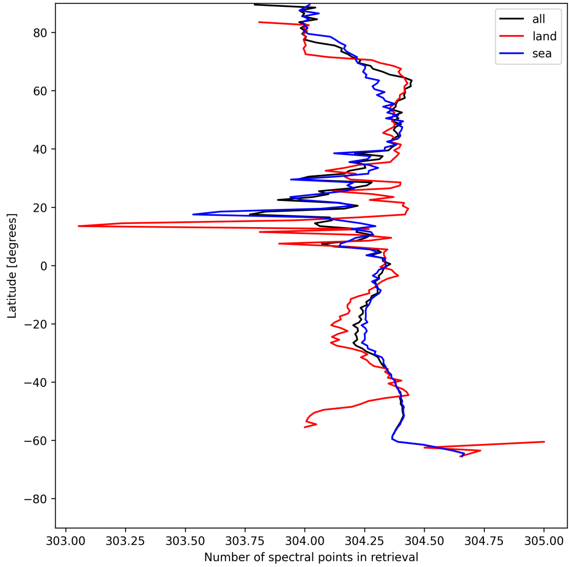
Figure 16: Zonal average of “Number of spectral points in retrieval” for 2025-07-13 to 2025-07-14.
