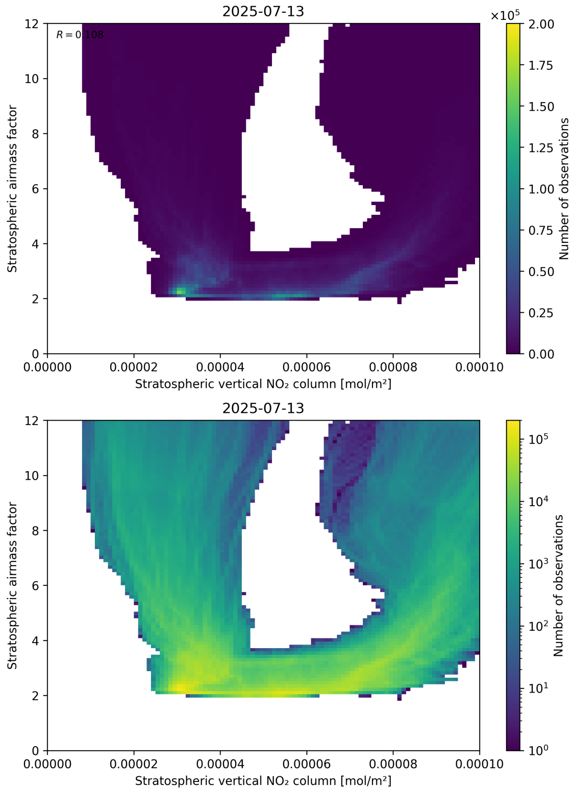
Figure 96: Scatter density plot of “Stratospheric vertical NO 2 column” against “Stratospheric airmass factor” for 2025-07-13 to 2025-07-14.
