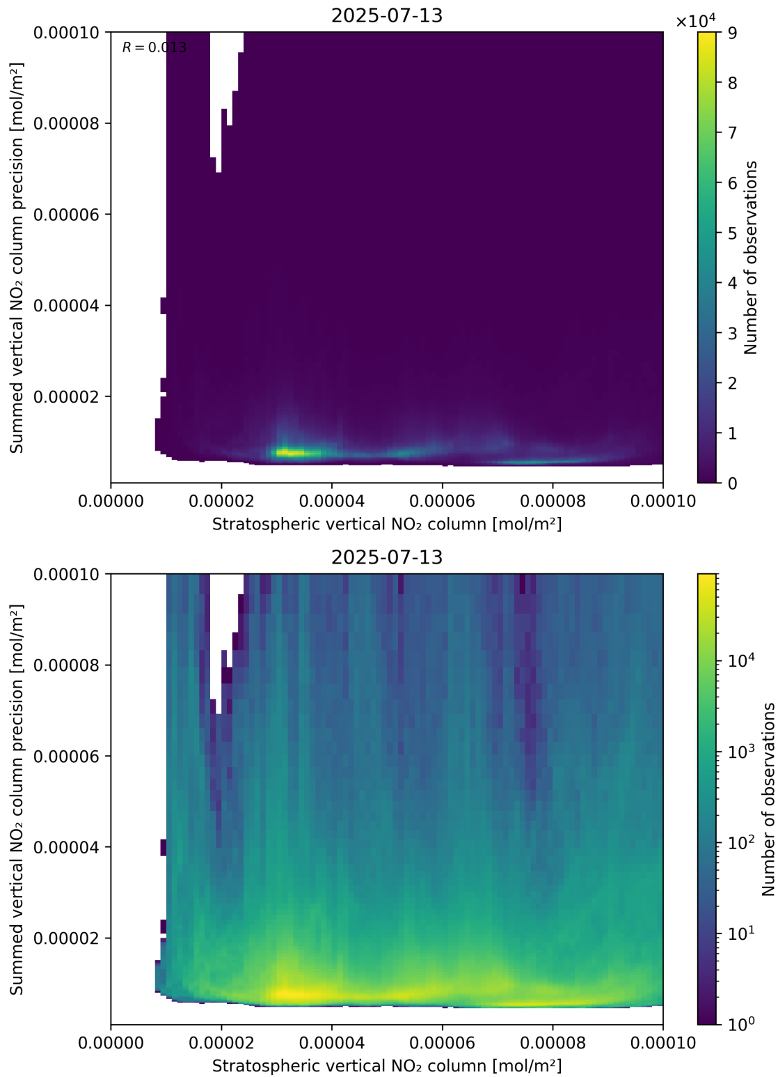
Figure 99: Scatter density plot of “Stratospheric vertical NO 2 column” against “Summed vertical NO 2 column precision” for 2025-07-13 to 2025-07-14.
