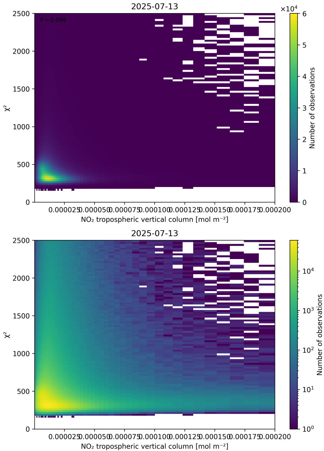
Figure 124: Scatter density plot of “NO 2 tropospheric vertical column” against “ \chi^2 ” for 2025-07-13 to 2025-07-14.
