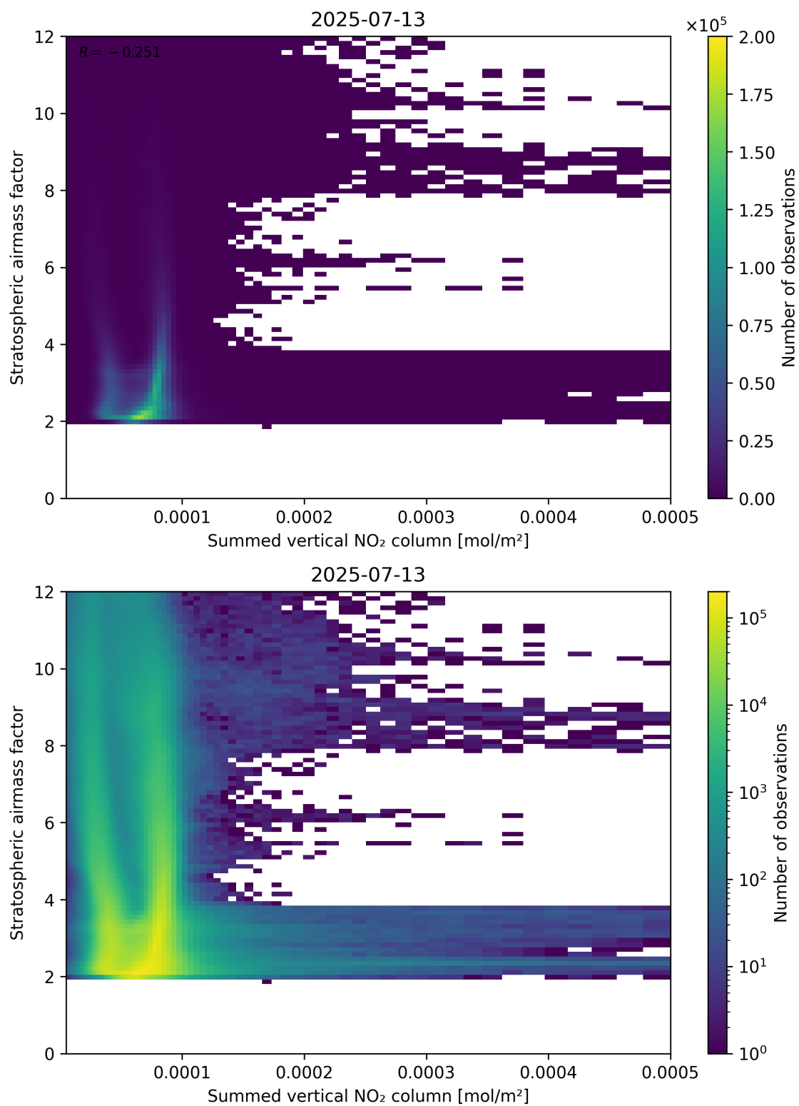
Figure 103: Scatter density plot of “Summed vertical NO 2 column” against “Stratospheric airmass factor” for 2025-07-13 to 2025-07-14.
