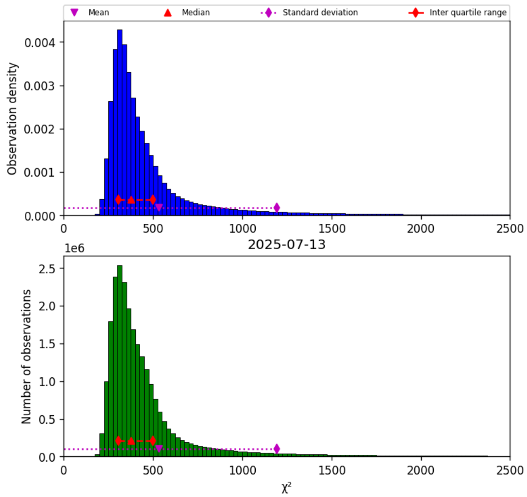
Figure 42: Histogram of “ \chi^2 ” for 2025-07-13 to 2025-07-14
