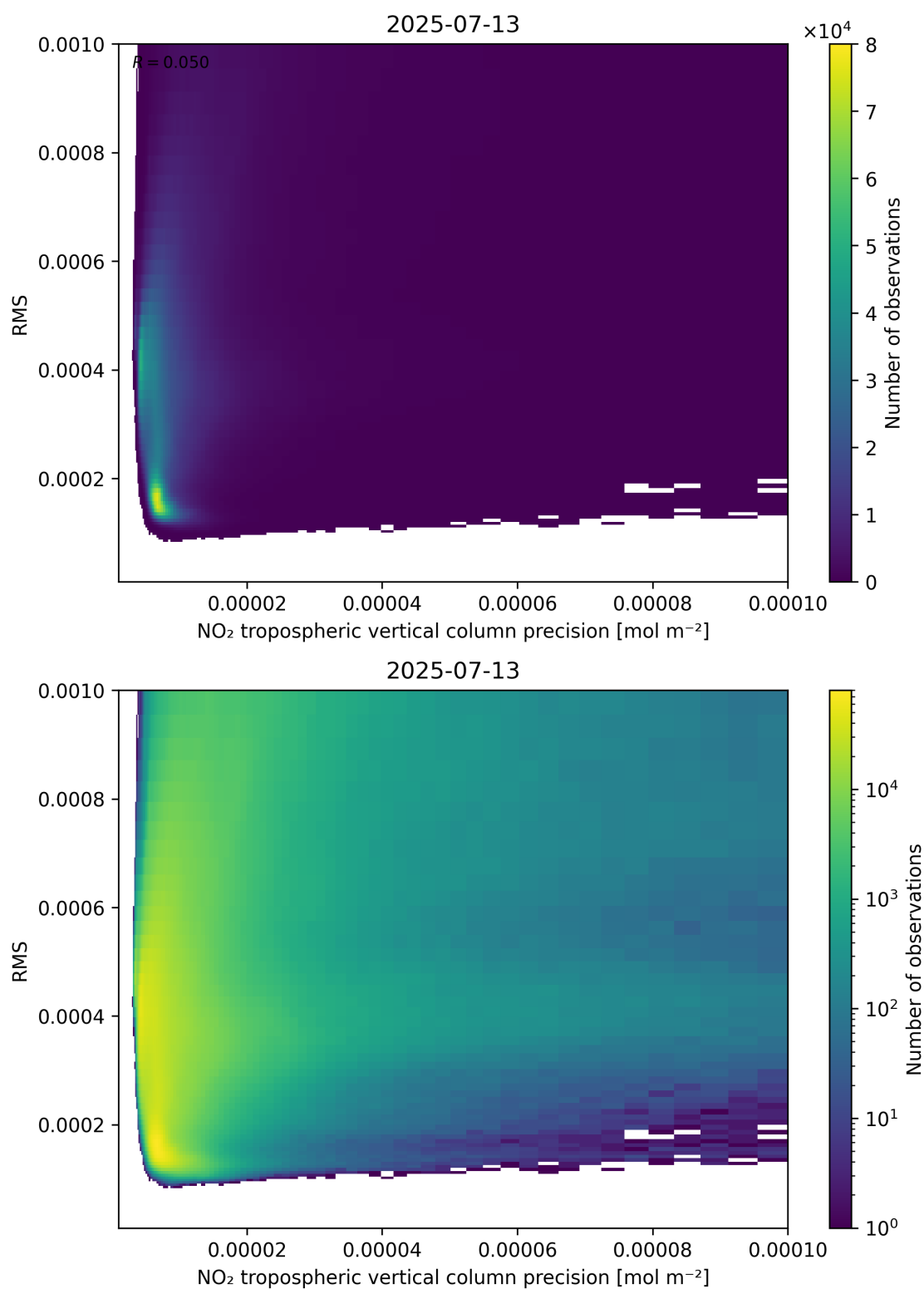
Figure 140: Scatter density plot of “NO 2 tropospheric vertical column precision” against “RMS” for 2025-07-13 to 2025-07-14.
