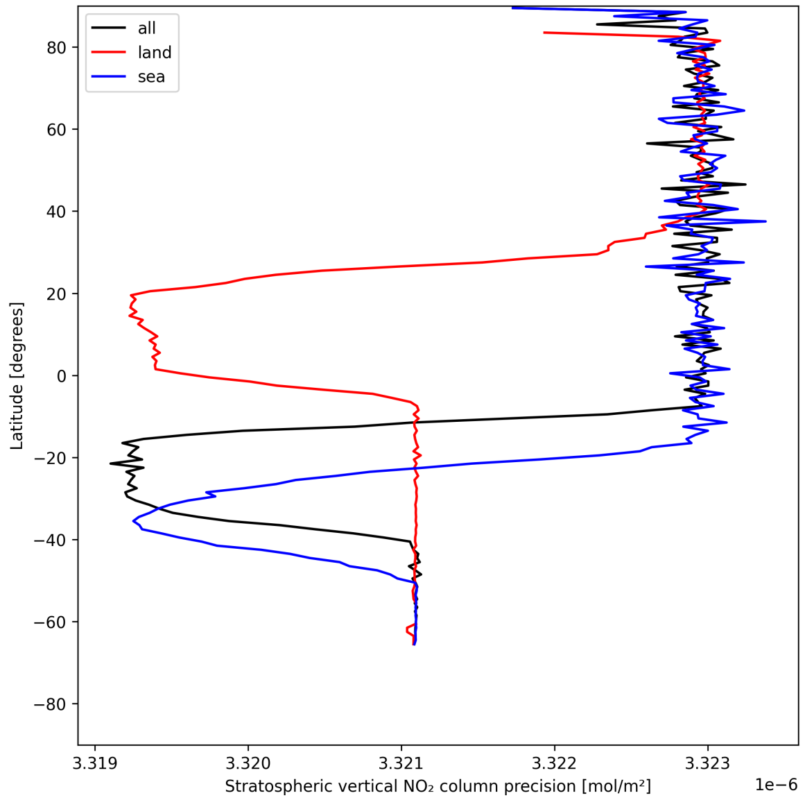
Figure 20: Zonal average of “Stratospheric vertical NO 2 column precision” for 2025-07-13 to 2025-07-14.
