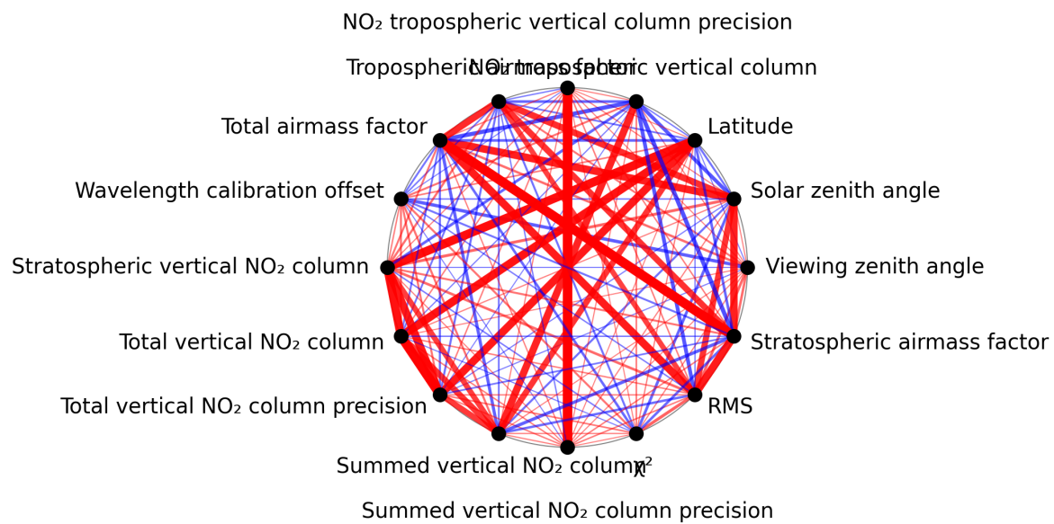
Figure 1: Map of correlation graph for 2025-07-13 to 2025-07-14.
