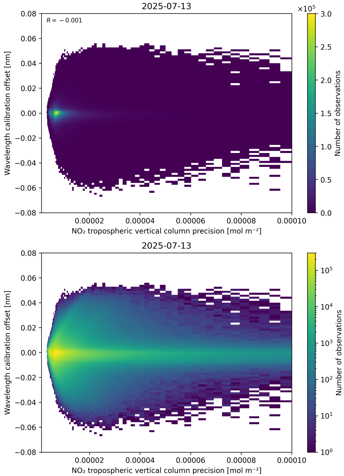
Figure 141: Scatter density plot of “NO 2 tropospheric vertical column precision” against “Wavelength calibration offset” for 2025-07-13 to 2025-07-14.
