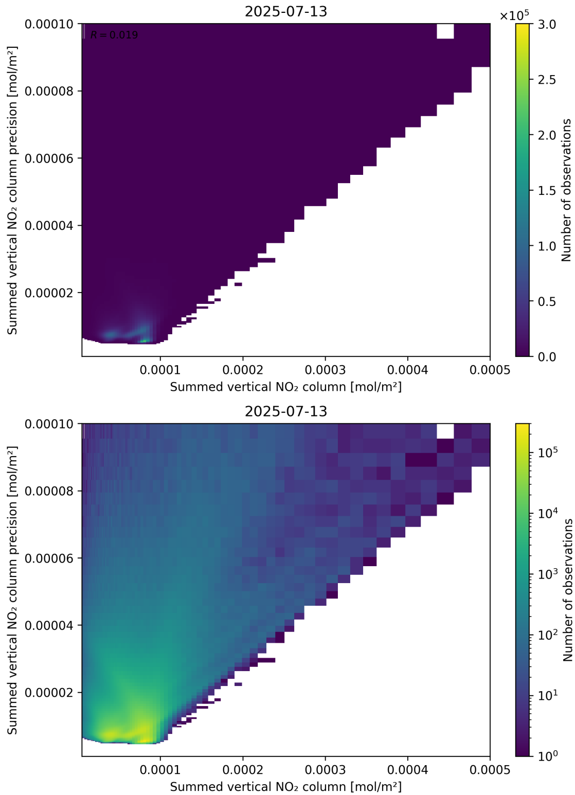
Figure 105: Scatter density plot of “Summed vertical NO 2 column” against “Summed vertical NO 2 column precision” for 2025-07-13 to 2025-07-14.
