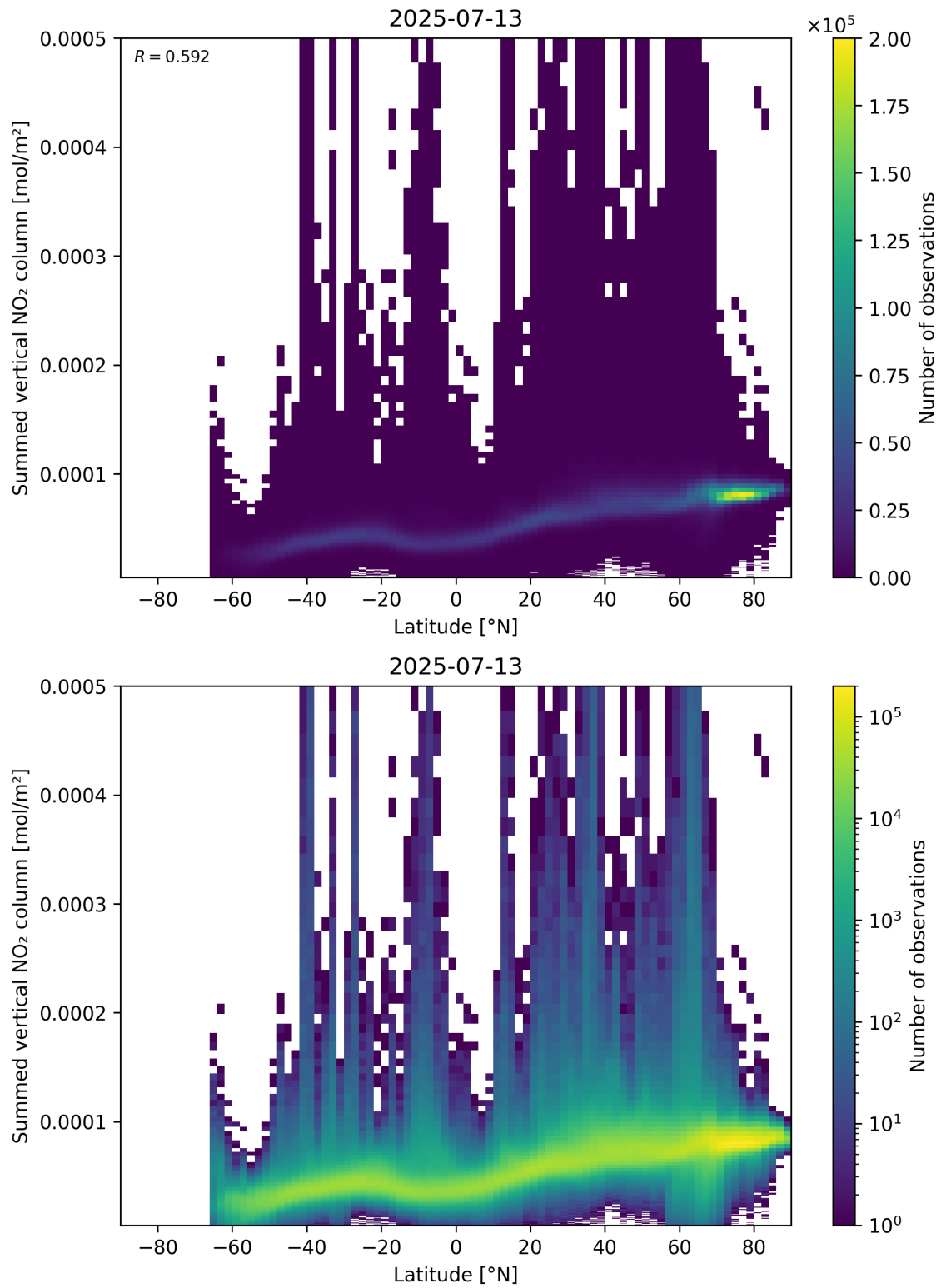
Figure 88: Scatter density plot of “Latitude” against “Summed vertical NO 2 column” for 2025-07-13 to 2025-07-14.
