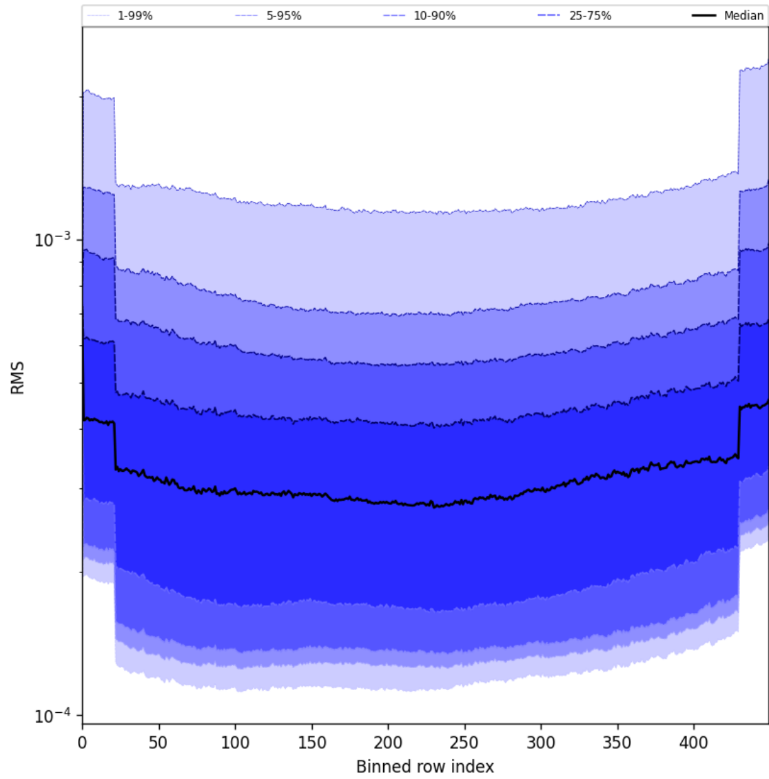
Figure 60: Along track statistics of “RMS” for 2025-07-13 to 2025-07-14
