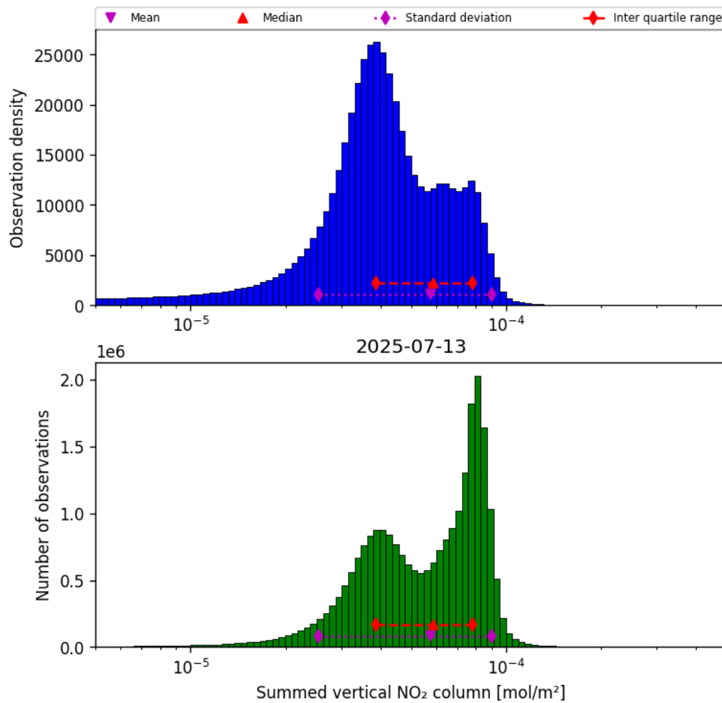
Figure 40: Histogram of “Summed vertical NO 2 column” for 2025-07-13 to 2025-07-14
