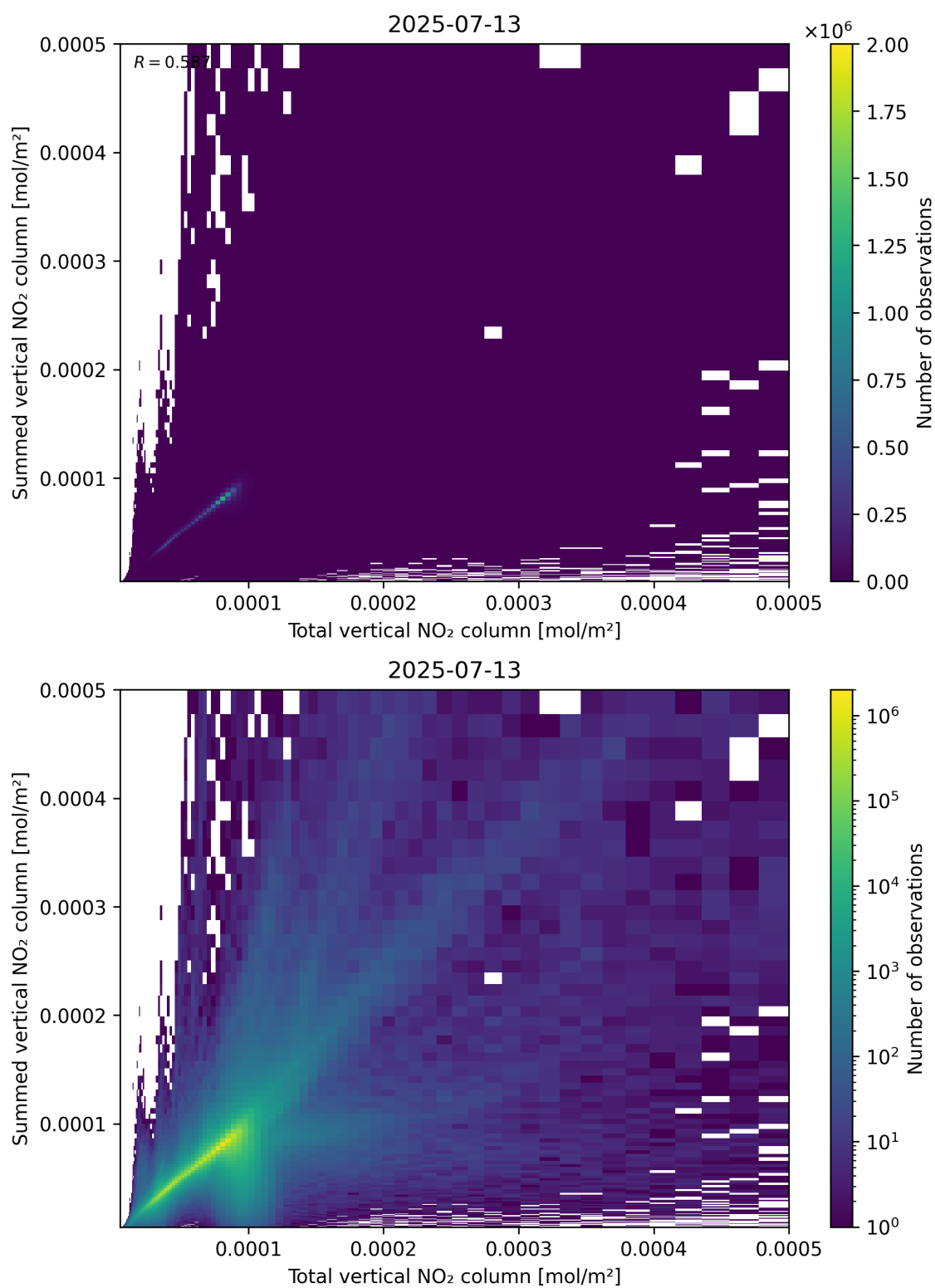
Figure 112: Scatter density plot of “Total vertical NO 2 column” against “Summed vertical NO 2 column” for 2025-07-13 to 2025-07-14.
