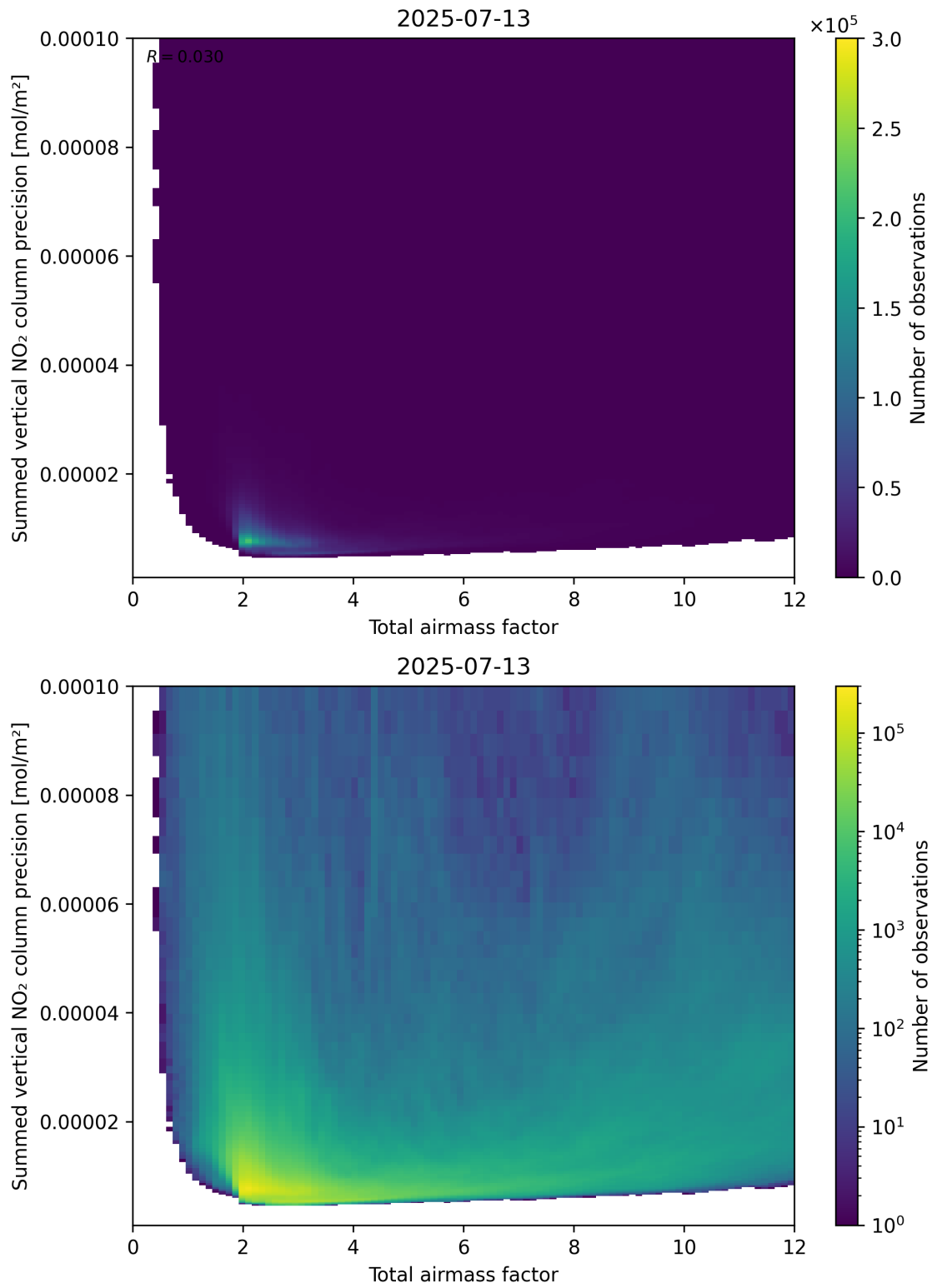
Figure 66: Scatter density plot of “Total airmass factor” against “Summed vertical NO 2 column precision” for 2025-07-13 to 2025-07-14.
