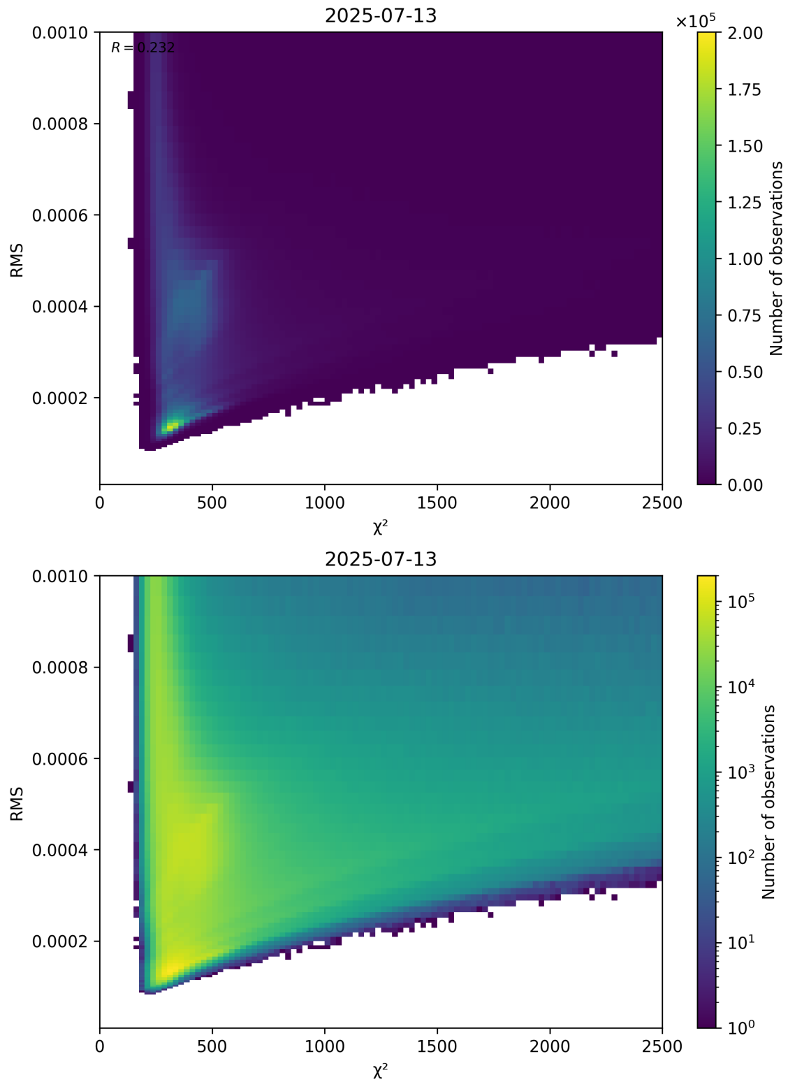
Figure 82: Scatter density plot of “ \chi^2 ” against “RMS” for 2025-07-13 to 2025-07-14.
