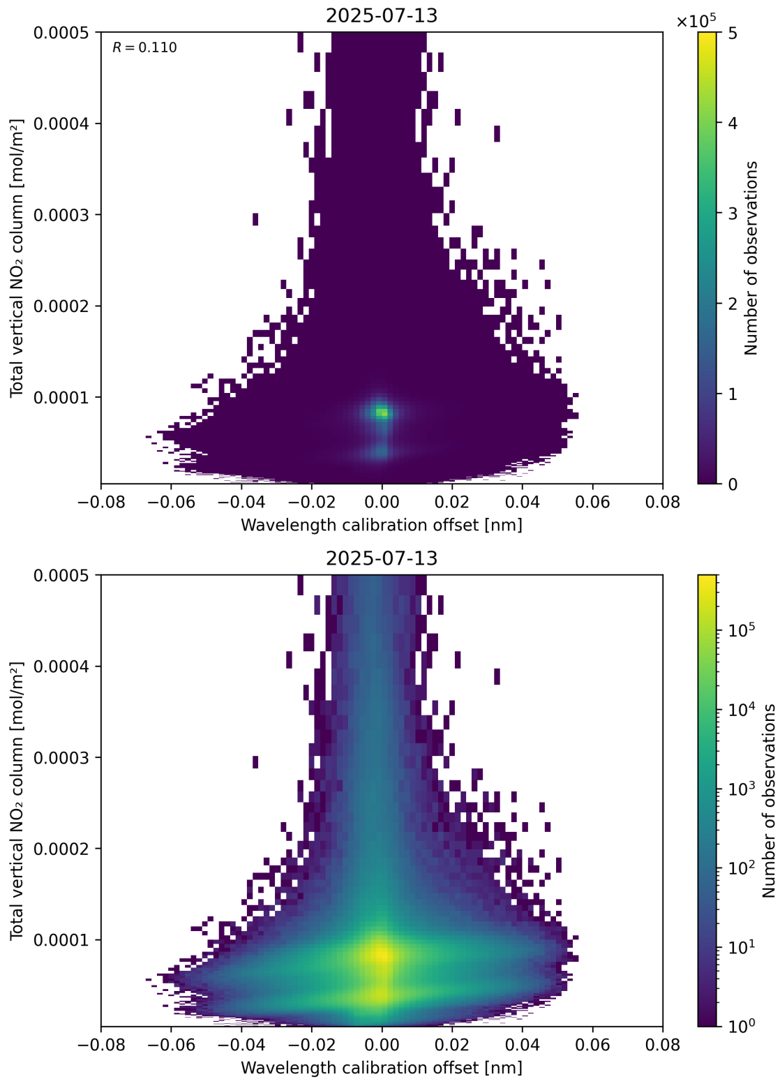
Figure 179: Scatter density plot of “Wavelength calibration offset” against “Total vertical NO 2 column” for 2025-07-13 to 2025-07-14.
