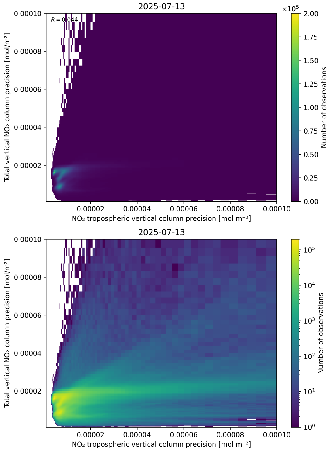
Figure 139: Scatter density plot of “NO 2 tropospheric vertical column precision” against “Total vertical NO 2 column precision” for 2025-07-13 to 2025-07-14.
