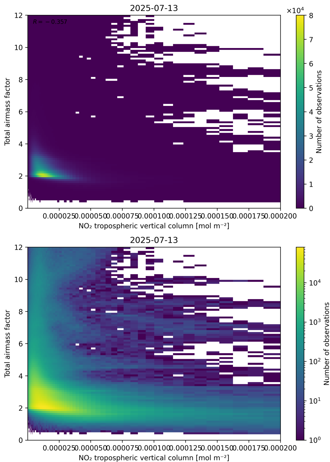
Figure 122: Scatter density plot of “NO 2 tropospheric vertical column” against “Total air mass factor” for 2025-07-13 to 2025-07-14.
