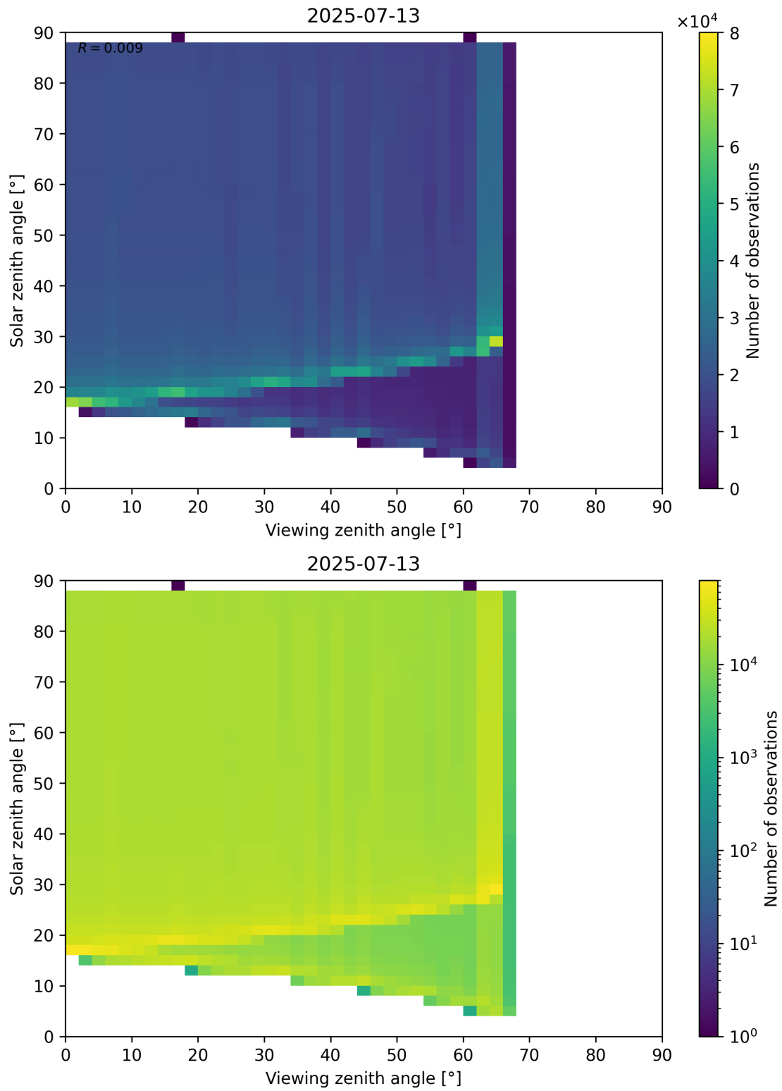
Figure 172: Scatter density plot of “Viewing zenith angle” against “Solar zenith angle” for 2025-07-13 to 2025-07-14.
