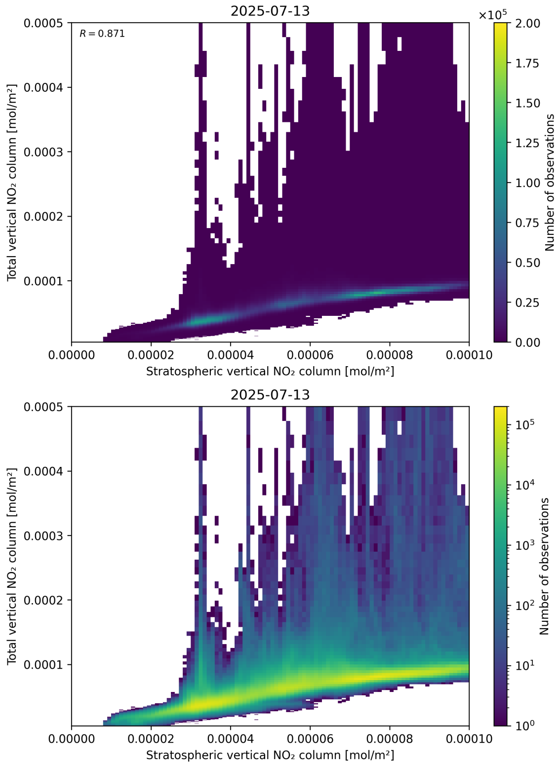
Figure 100: Scatter density plot of “Stratospheric vertical NO 2 column” against “Total vertical NO 2 column” for 2025-07-13 to 2025-07-14.
