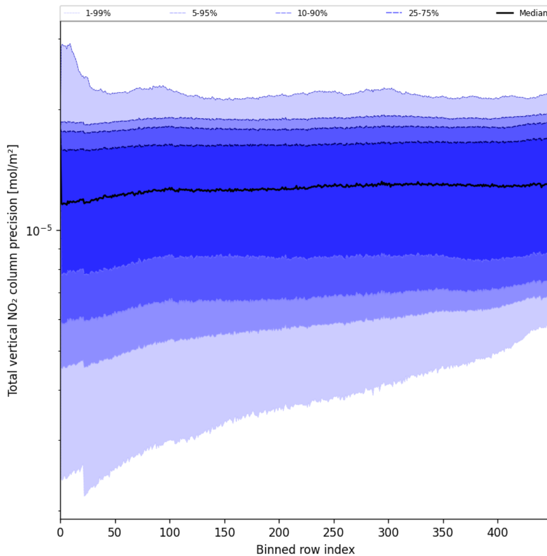
Figure 56: Along track statistics of “Total vertical NO 2 column precision” for 2025-07-13 to 2025-07-14
