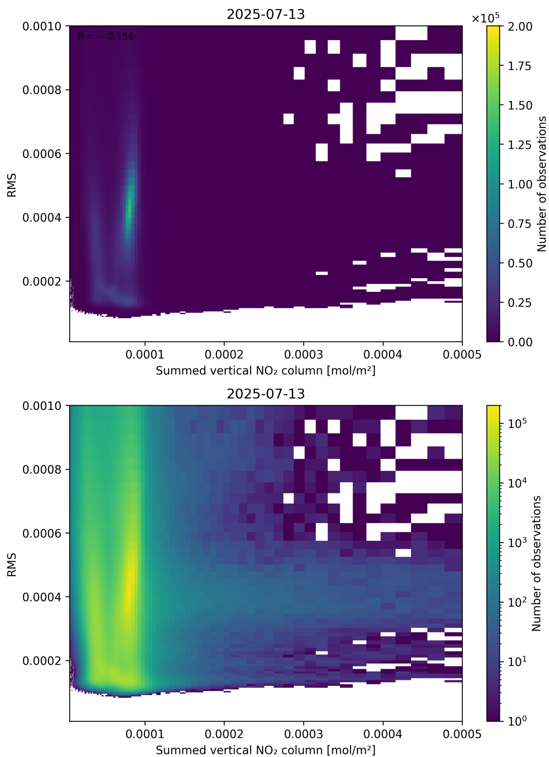
Figure 109: Scatter density plot of “Summed vertical NO 2 column” against “RMS” for 2025-07-13 to 2025-07-14.
