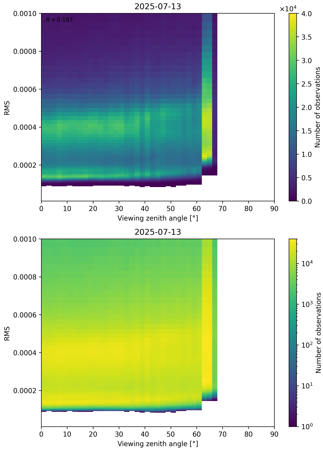
Figure 171: Scatter density plot of “Viewing zenith angle” against “RMS” for 2025-07-13 to 2025-07-14.
