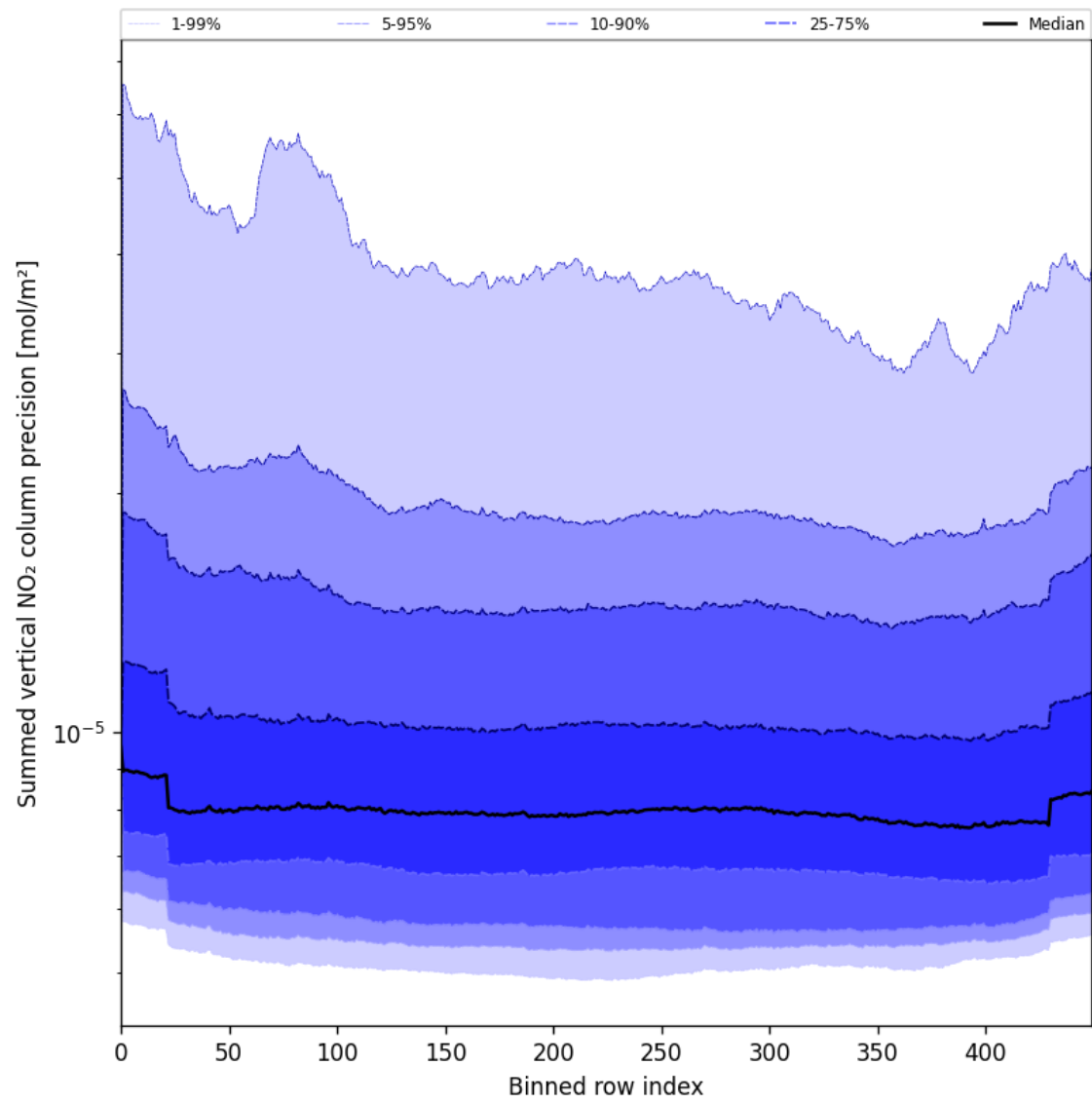
Figure 58: Along track statistics of “Summed vertical NO 2 column precision” for 2025-07-13 to 2025-07-14
