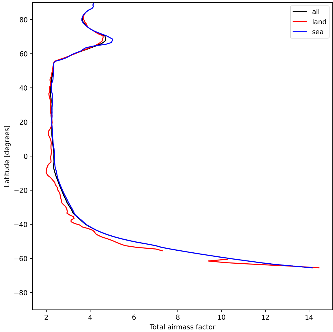
Figure 15: Zonal average of “Total airmass factor” for 2025-07-13 to 2025-07-14.
