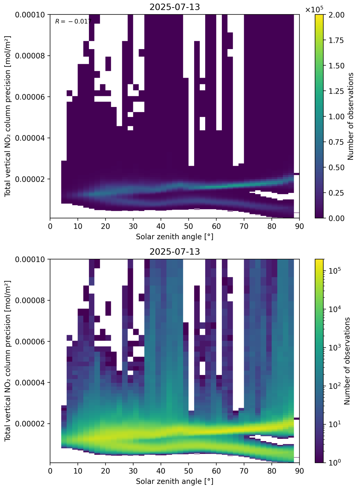
Figure 154: Scatter density plot of “Solar zenith angle” against “Total vertical NO 2 column precision” for 2025-07-13 to 2025-07-14.
