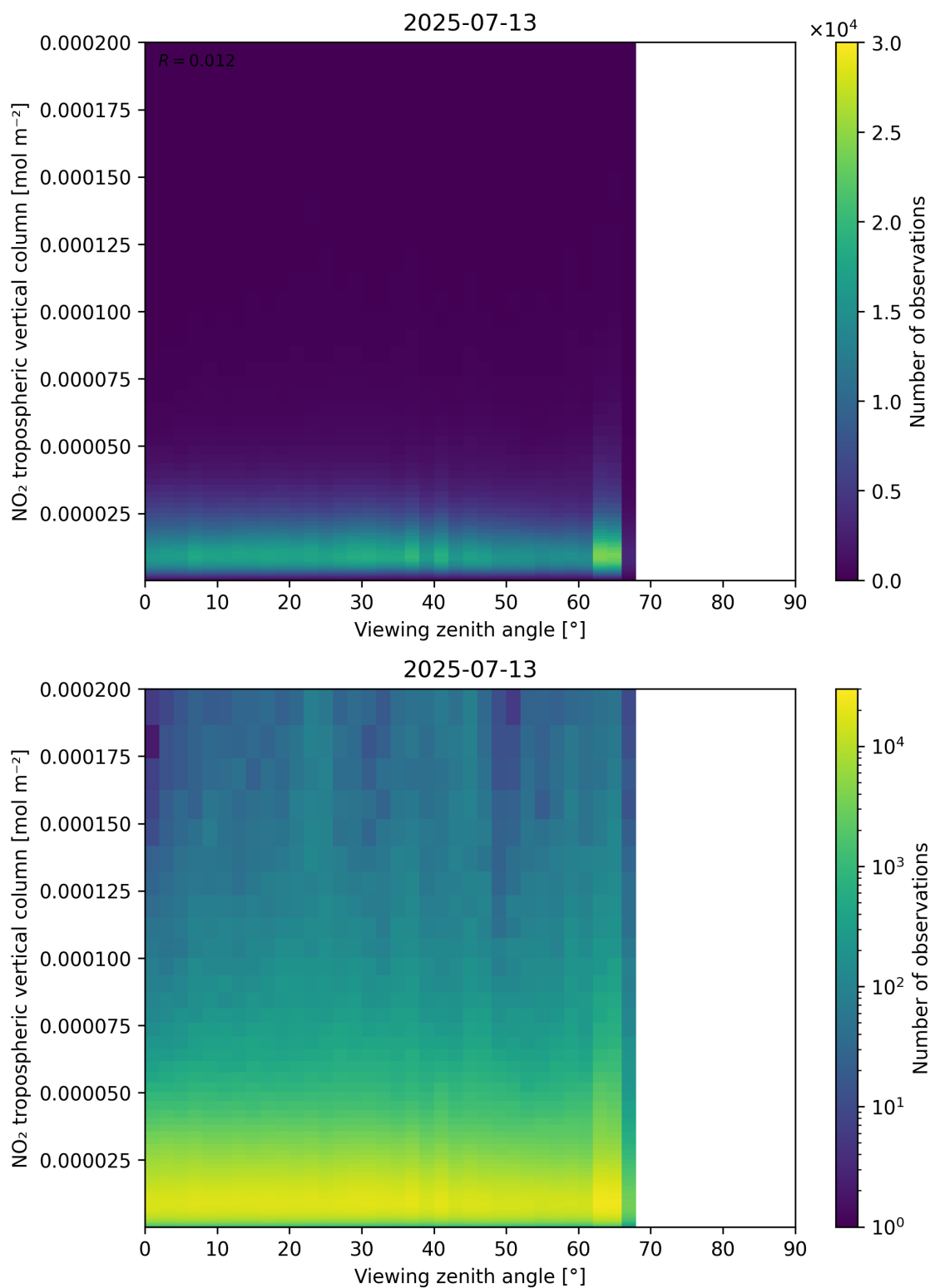
Figure 169: Scatter density plot of “Viewing zenith angle” against “NO 2 tropospheric vertical column” for 2025-07-13 to 2025-07-14.
