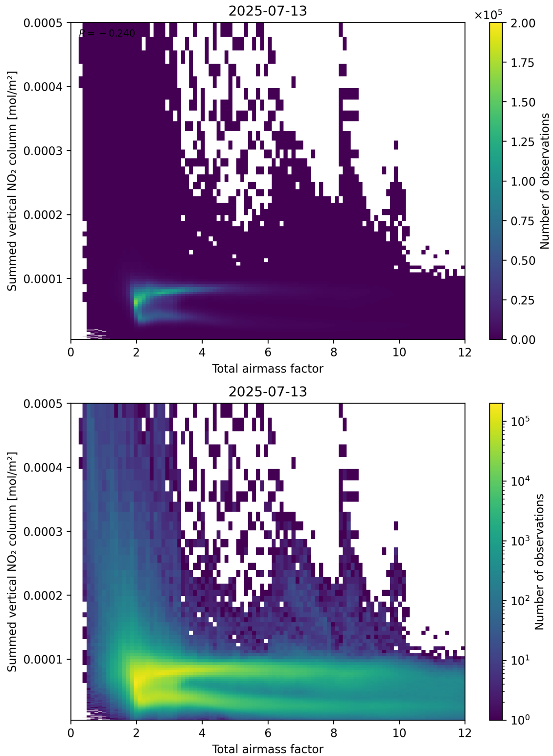
Figure 65: Scatter density plot of “Total airmass factor” against “Summed vertical NO 2 column” for 2025-07-13 to 2025-07-14.
