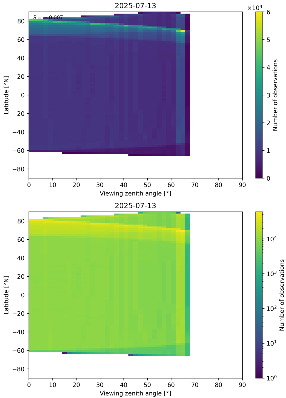
Figure 163: Scatter density plot of “Viewing zenith angle” against “Latitude” for 2025-07-13 to 2025-07-14.
