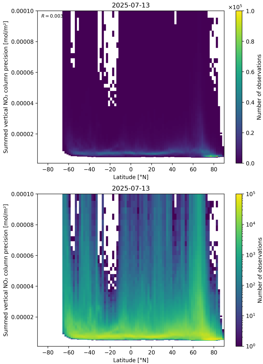
Figure 89: Scatter density plot of “Latitude” against “Summed vertical NO 2 column precision” for 2025-07-13 to 2025-07-14.
