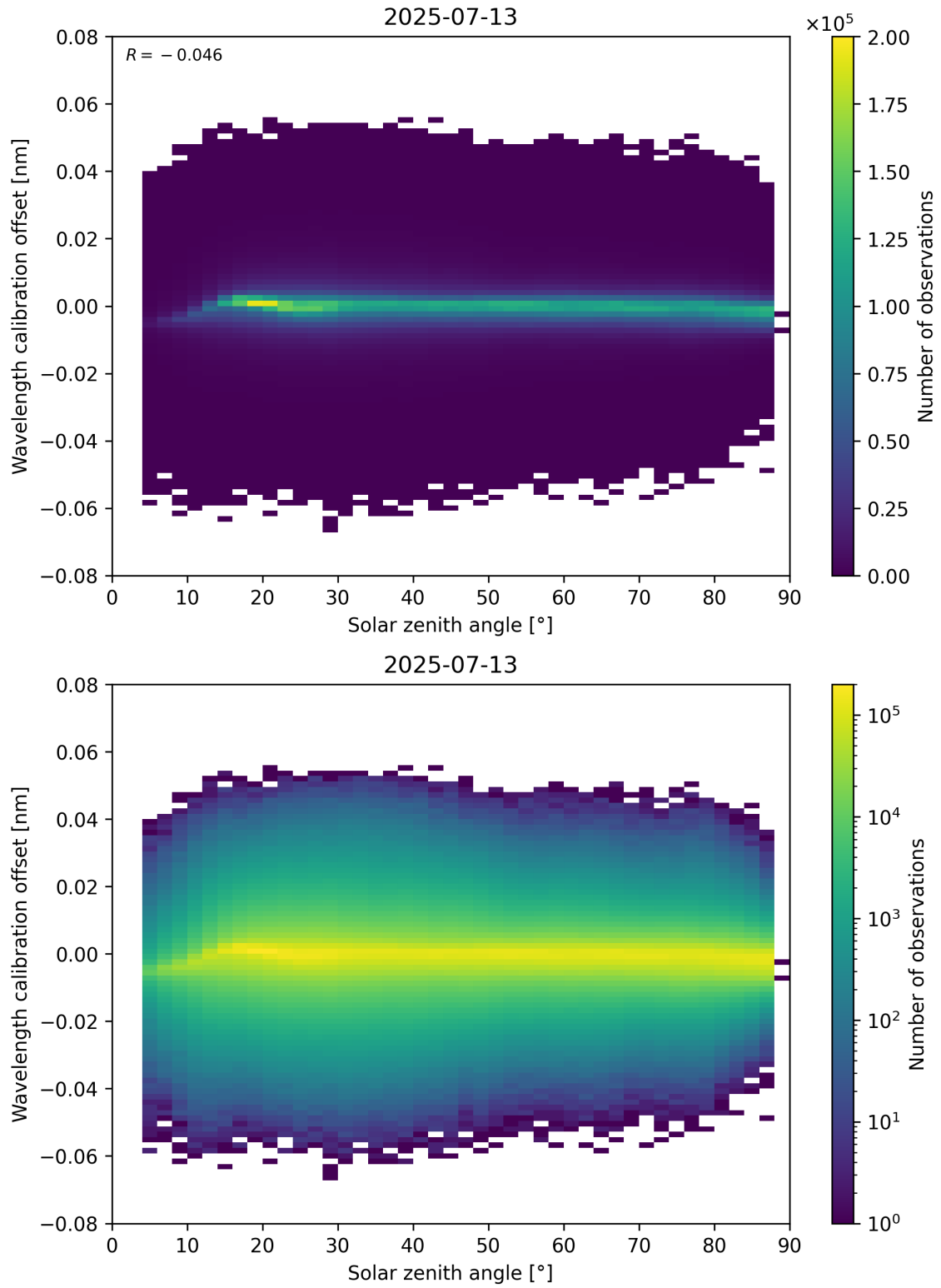
Figure 158: Scatter density plot of “Solar zenith angle” against “Wavelength calibration offset” for 2025-07-13 to 2025-07-14.
