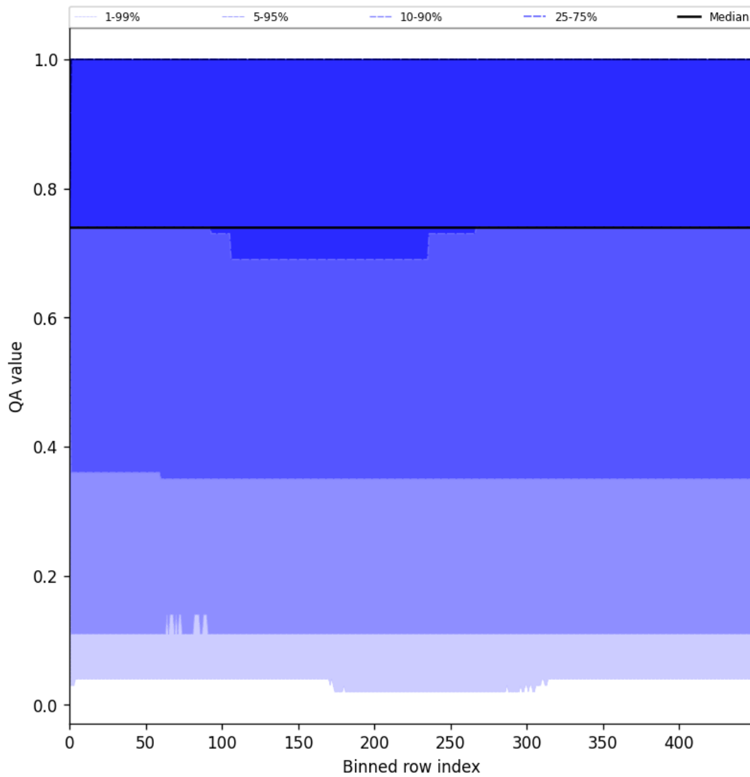
Figure 45: Along track statistics of “QA value” for 2025-07-13 to 2025-07-14
