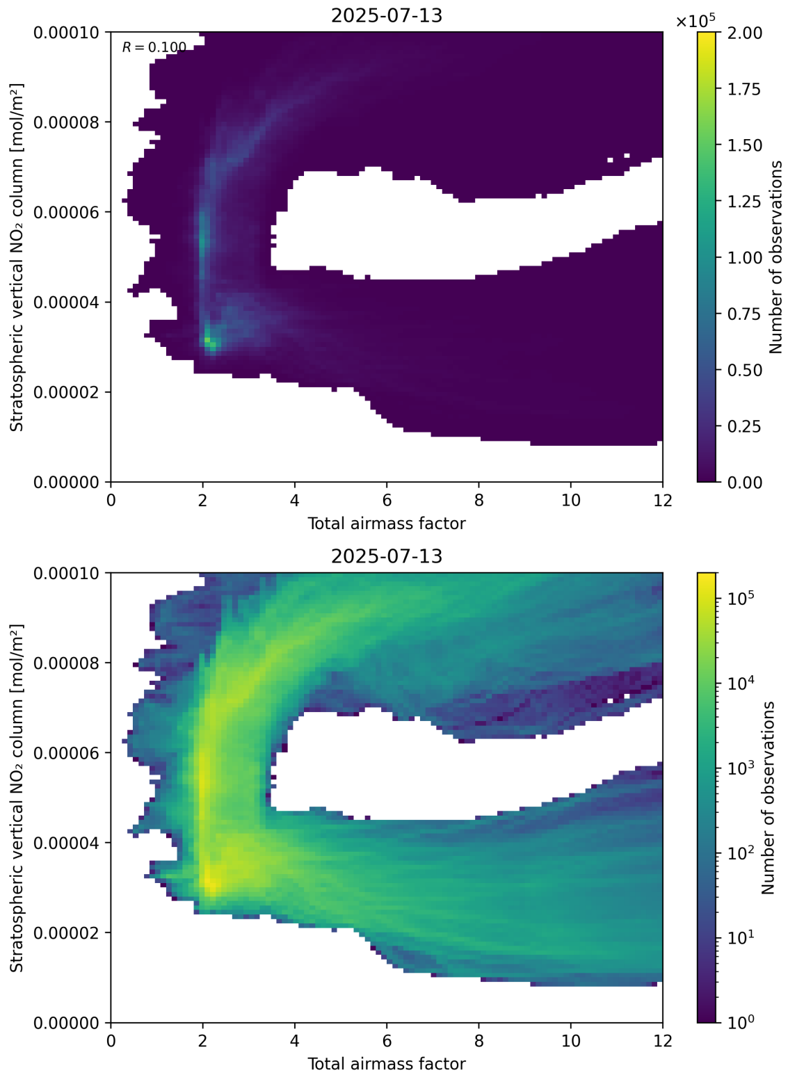
Figure 64: Scatter density plot of “Total airmass factor” against “Stratospheric vertical NO 2 column” for 2025-07-13 to 2025-07-14.
