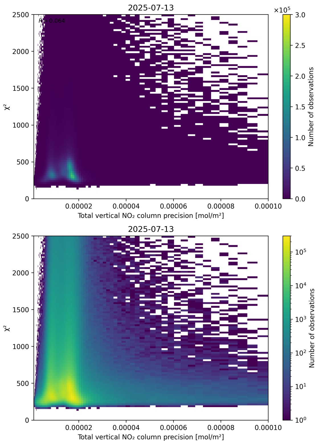
Figure 116: Scatter density plot of “Total vertical NO 2 column precision” against “ \chi^2 ” for 2025-07-13 to 2025-07-14.
