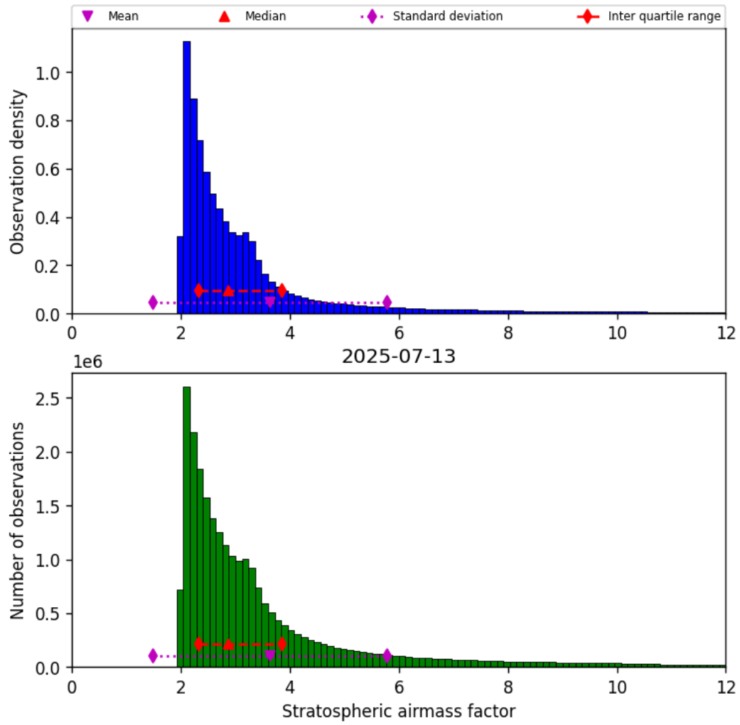
Figure 44: Histogram of “Stratospheric airmass factor” for 2025-07-13 to 2025-07-14
