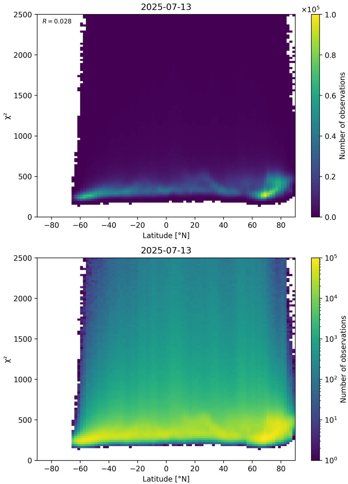
Figure 86: Scatter density plot of “Latitude” against “ \chi^2 ” for 2025-07-13 to 2025-07-14.
