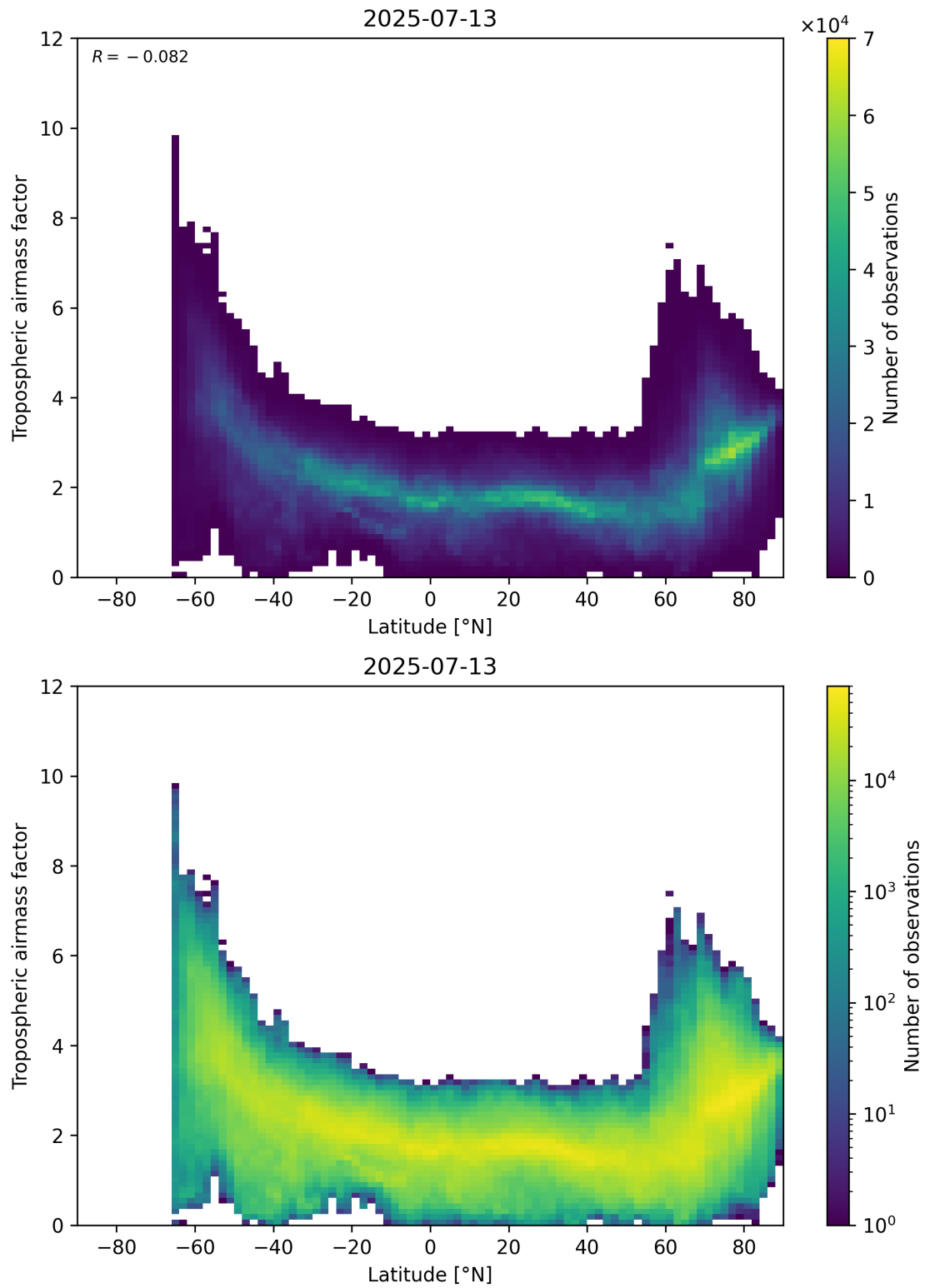
Figure 85: Scatter density plot of “Latitude” against “Tropospheric air mass factor” for 2025-07-13 to 2025-07-14.
