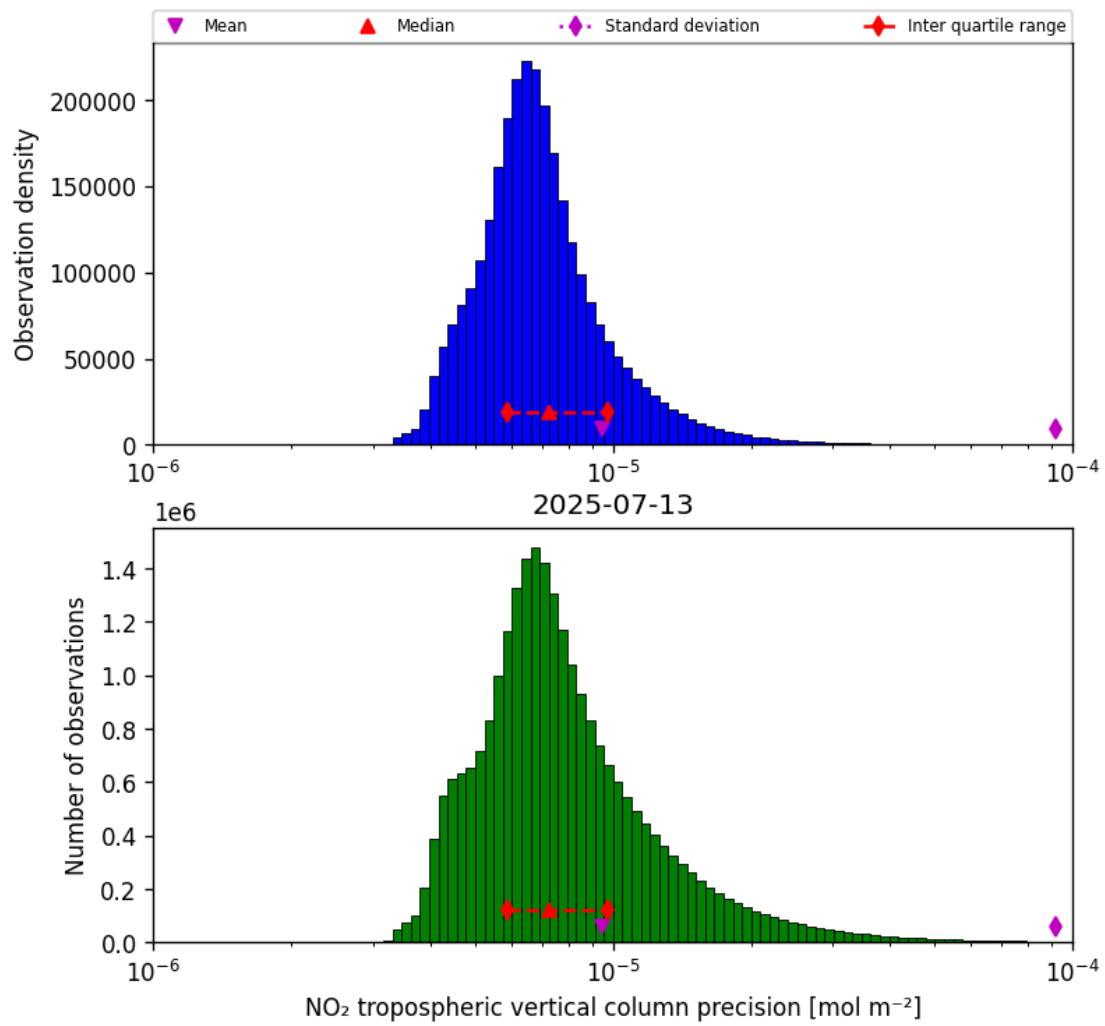
Figure 30: Histogram of “NO 2 tropospheric vertical column precision” for 2025-07-13 to 2025-07-14
