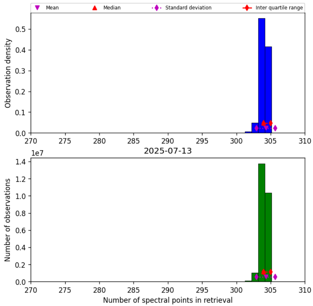
Figure 33: Histogram of “Number of spectral points in retrieval” for 2025-07-13 to 2025-07-14
