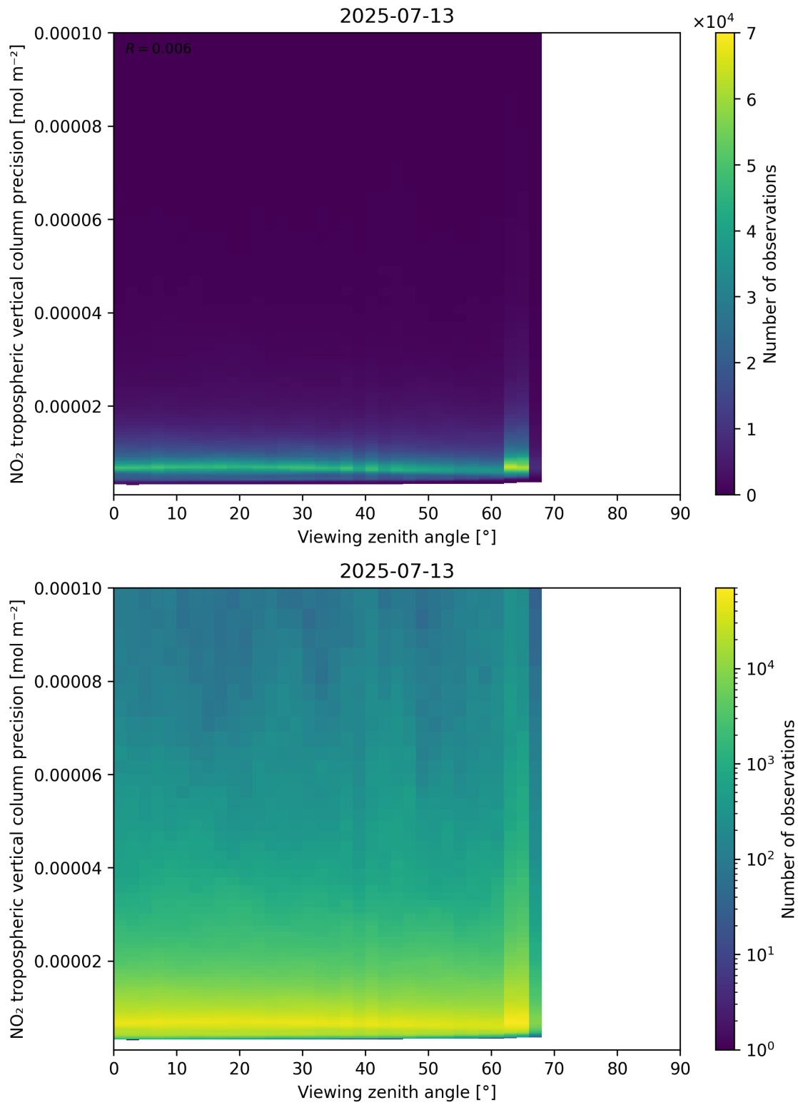
Figure 170: Scatter density plot of “Viewing zenith angle” against “NO 2 tropospheric vertical column precision” for 2025-07-13 to 2025-07-14.
