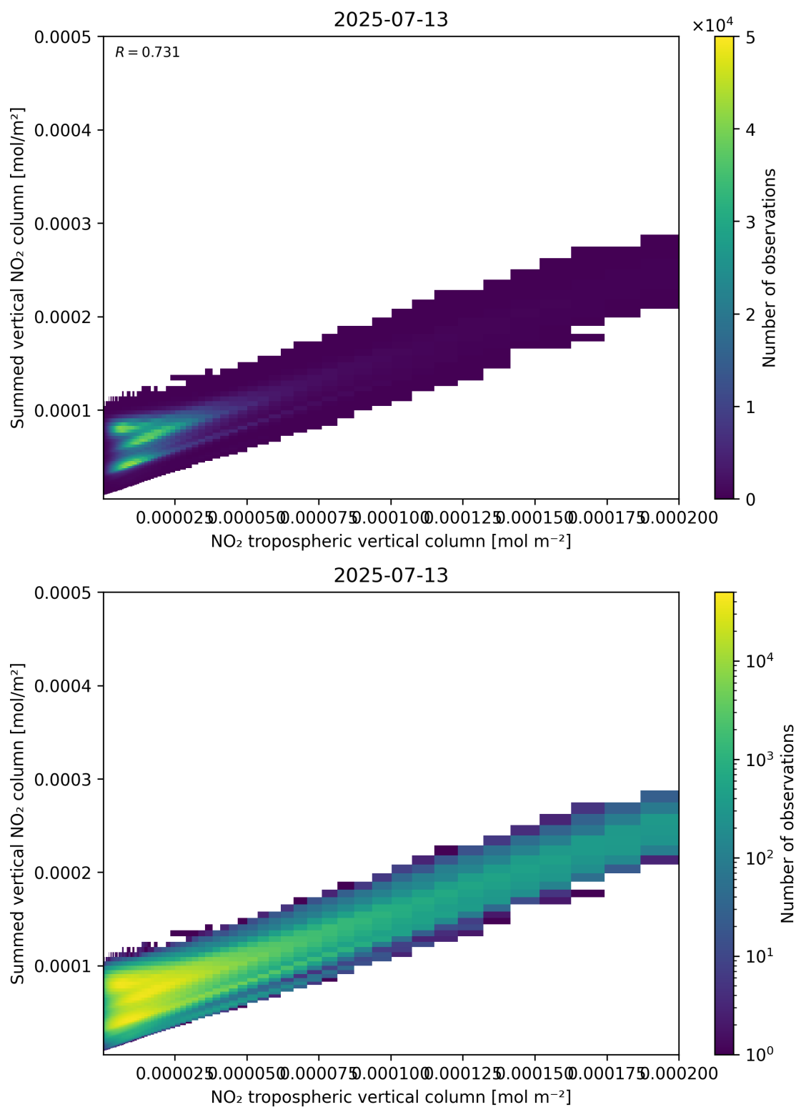
Figure 126: Scatter density plot of “NO 2 tropospheric vertical column” against “Summed vertical NO 2 column” for 2025-07-13 to 2025-07-14.
