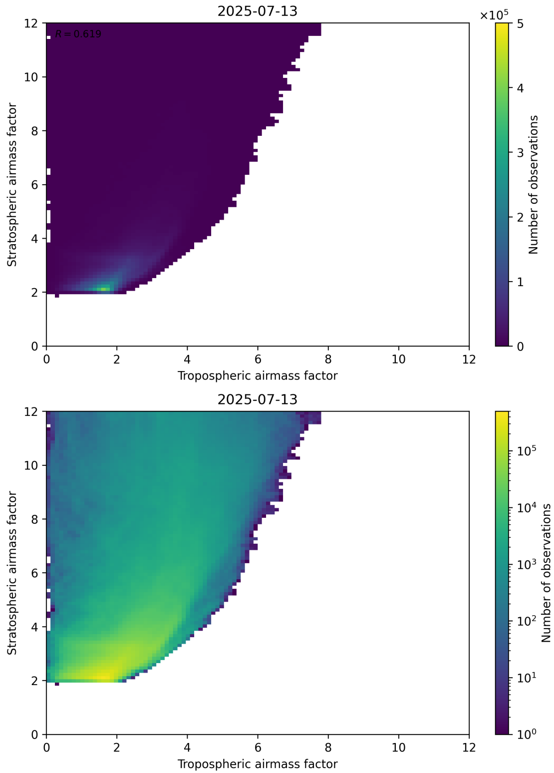
Figure 71: Scatter density plot of “Tropospheric airmass factor” against “Stratospheric airmass factor” for 2025-07-13 to 2025-07-14.
