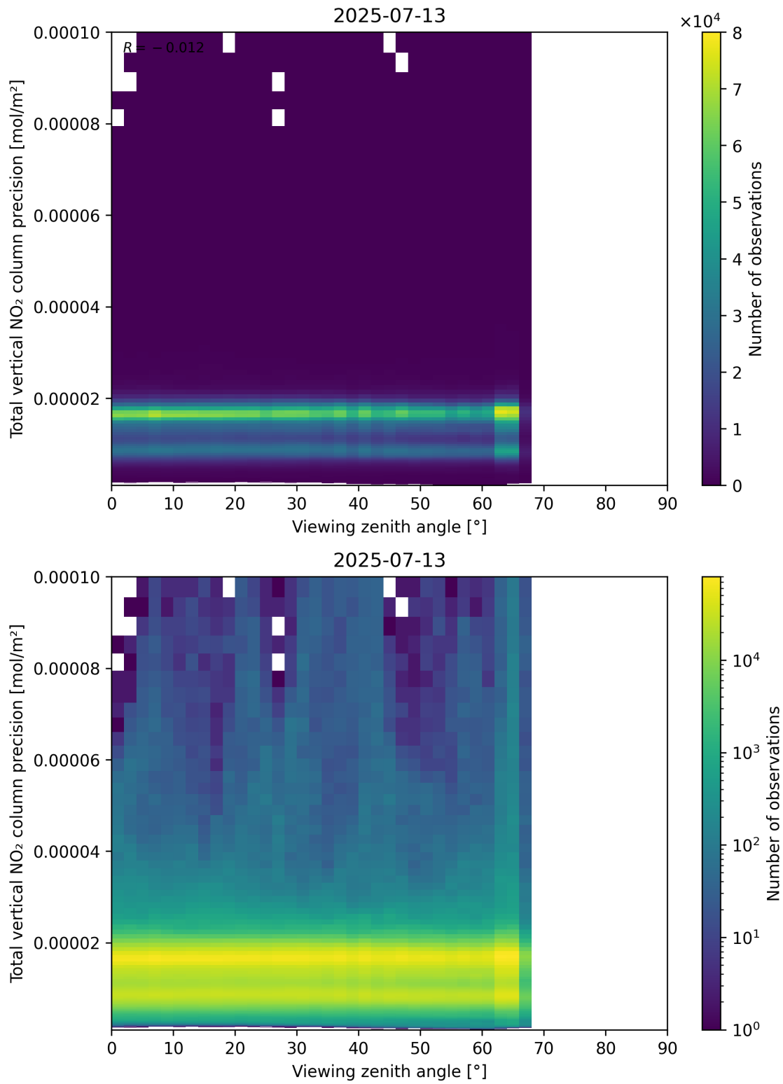
Figure 168: Scatter density plot of “Viewing zenith angle” against “Total vertical NO 2 column precision” for 2025-07-13 to 2025-07-14.
