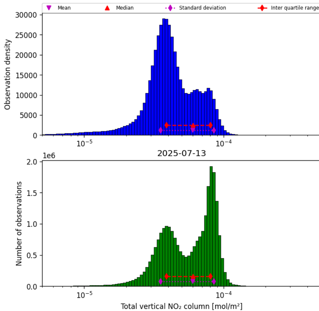
Figure 38: Histogram of "Total vertical NO 2 column" for 2025-07-13 to 2025-07-14
