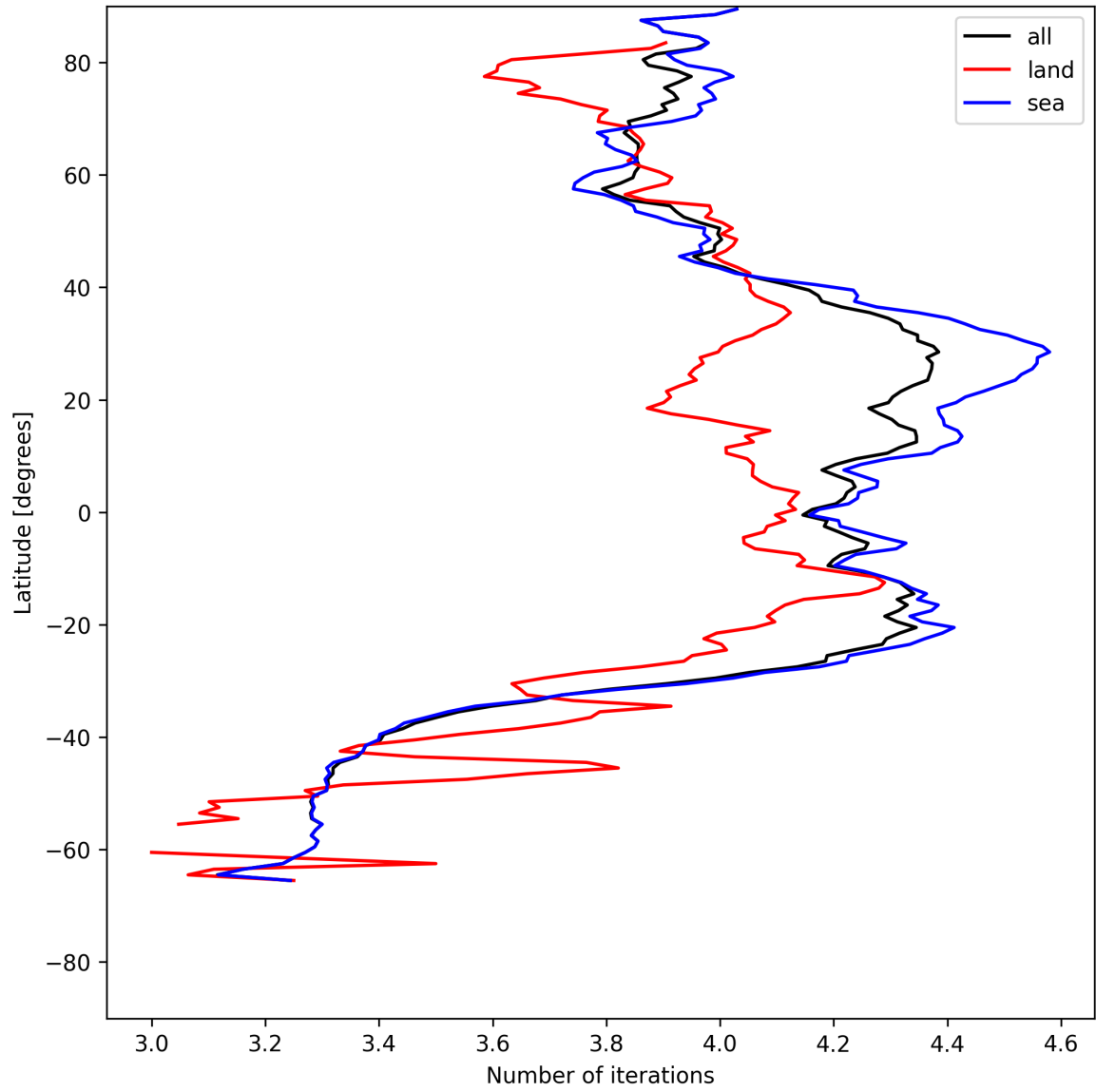
Figure 17: Zonal average of “Number of iterations” for 2025-07-13 to 2025-07-14.
