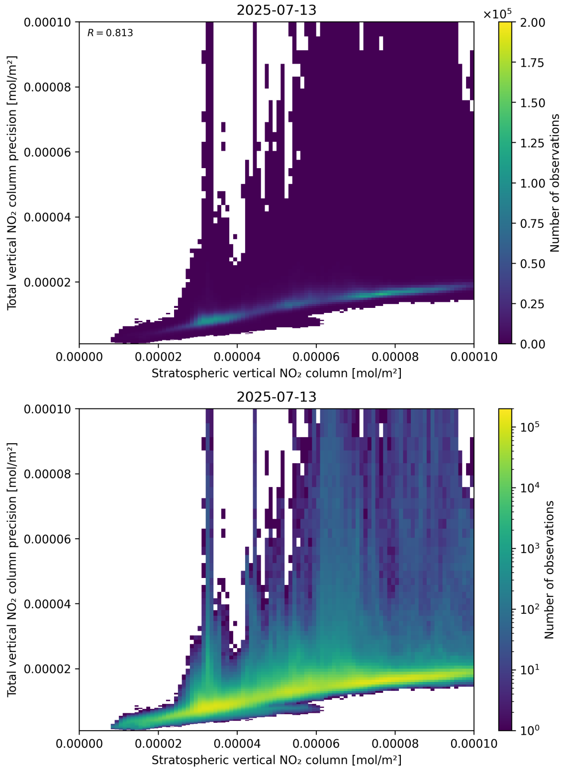
Figure 101: Scatter density plot of “Stratospheric vertical NO 2 column” against “Total vertical NO 2 column precision” for 2025-07-13 to 2025-07-14.
