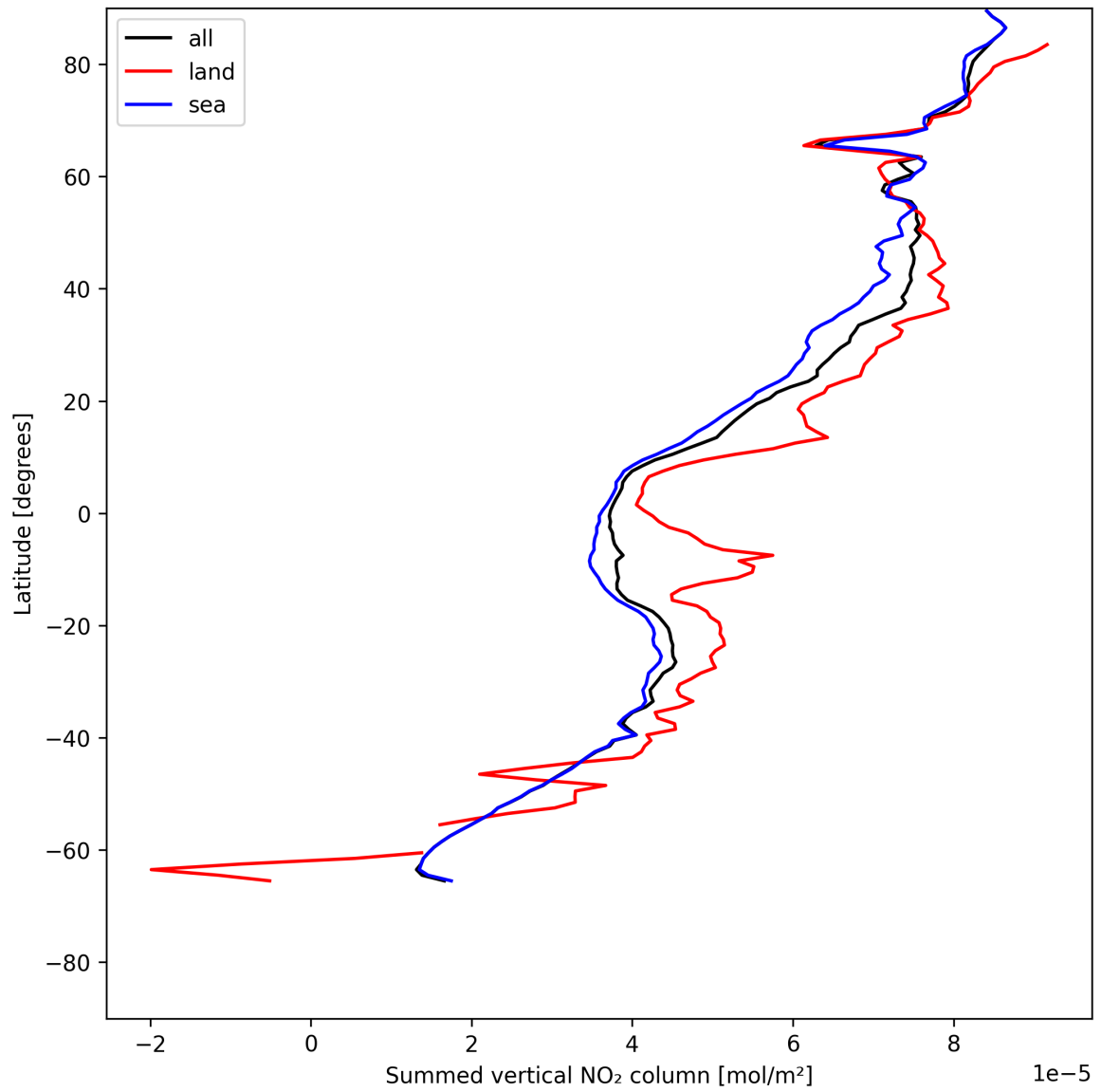
Figure 23: Zonal average of “Summed vertical NO 2 column” for 2025-07-13 to 2025-07-14.
