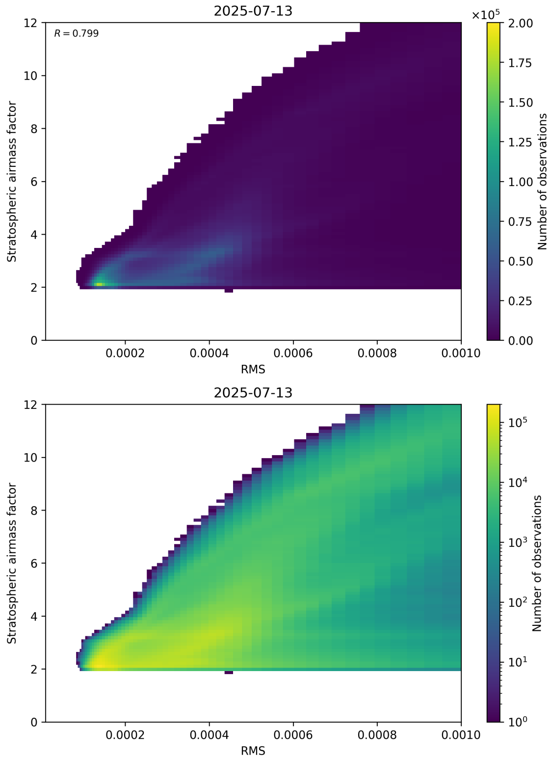
Figure 144: Scatter density plot of “RMS” against “Stratospheric airmass factor” for 2025-07-13 to 2025-07-14.
