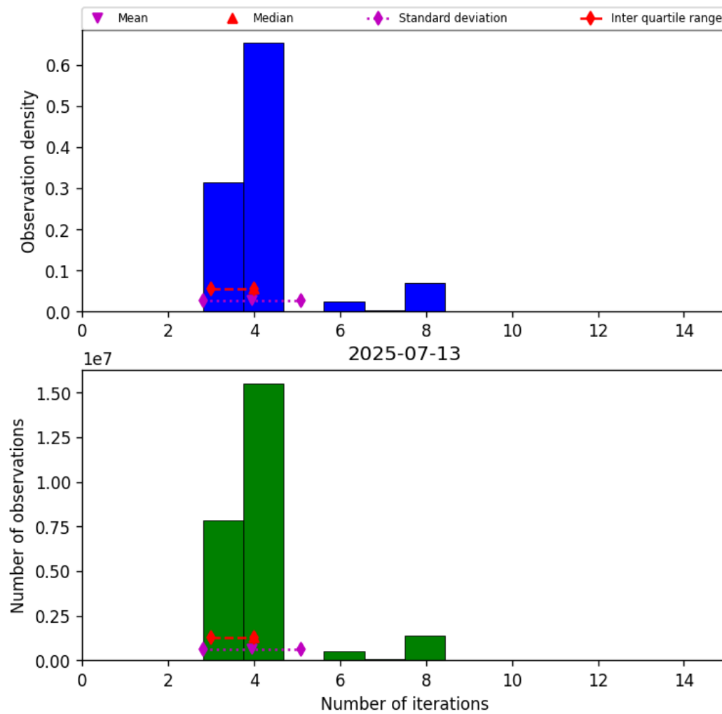
Figure 34: Histogram of “Number of iterations” for 2025-07-13 to 2025-07-14
