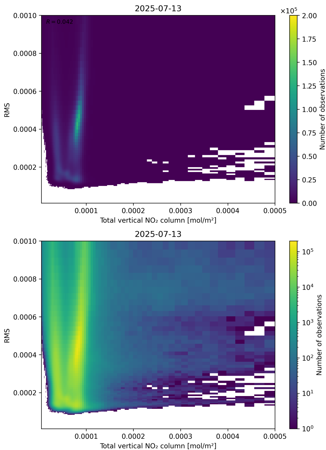
Figure 120: Scatter density plot of “Total vertical NO 2 column” against “RMS” for 2025-07-13 to 2025-07-14.
