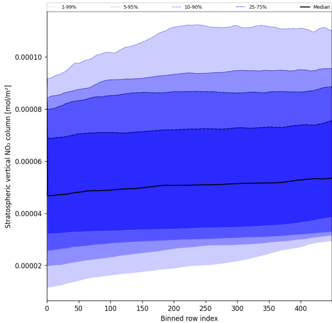
Figure 53: Along track statistics of “Stratospheric vertical NO 2 column” for 2025-07-13 to 2025-07-14
