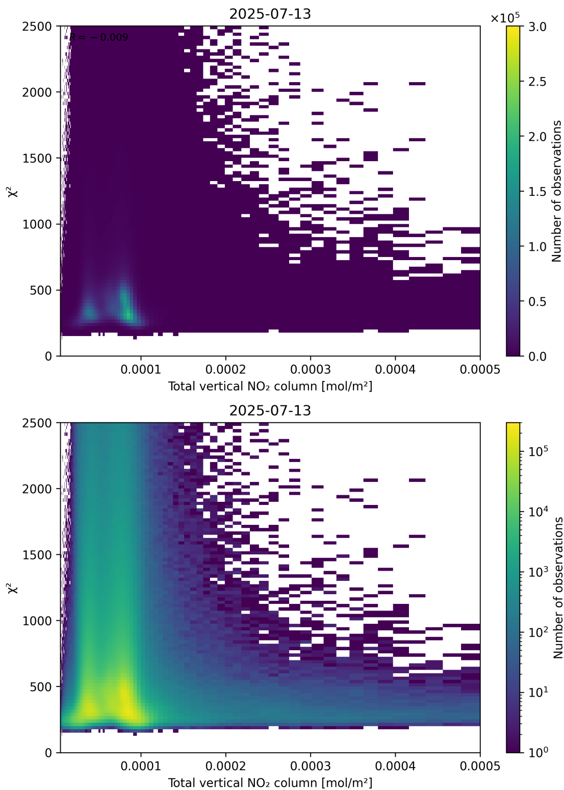
Figure 111: Scatter density plot of “Total vertical NO 2 column” against “ \chi^2 ” for 2025-07-13 to 2025-07-14.
