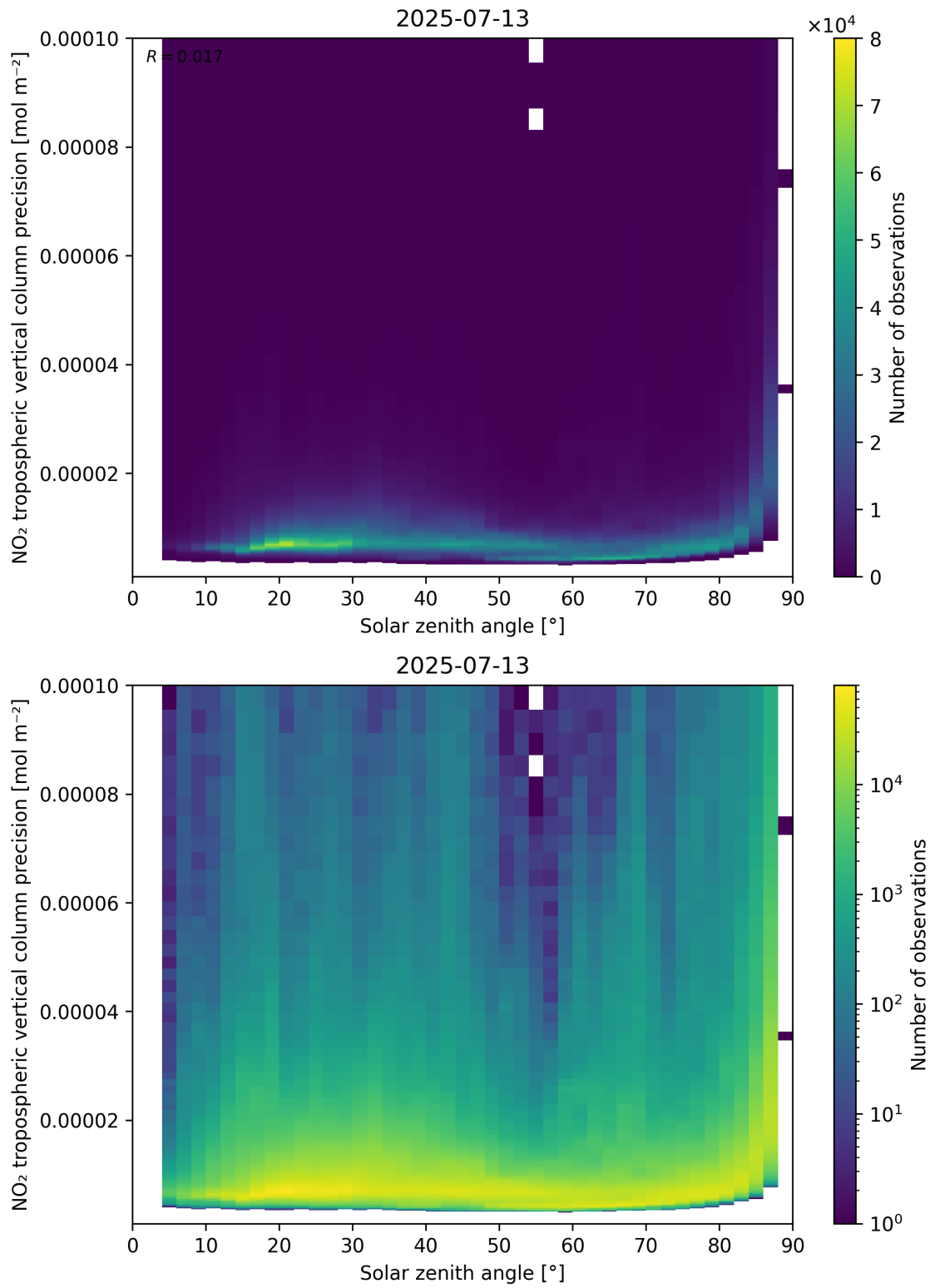
Figure 156: Scatter density plot of “Solar zenith angle” against “NO 2 tropospheric vertical column precision” for 2025-07-13 to 2025-07-14.
