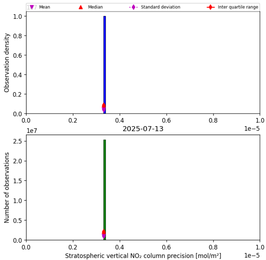
Figure 37: Histogram of “Stratospheric vertical NO 2 column precision” for 2025-07-13 to 2025-07-14
