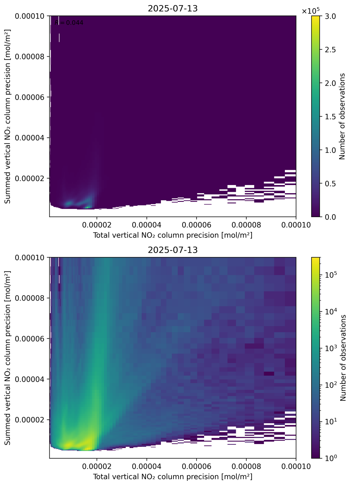
Figure 118: Scatter density plot of “Total vertical NO 2 column precision” against “Summed vertical NO 2 column precision” for 2025-07-13 to 2025-07-14.
