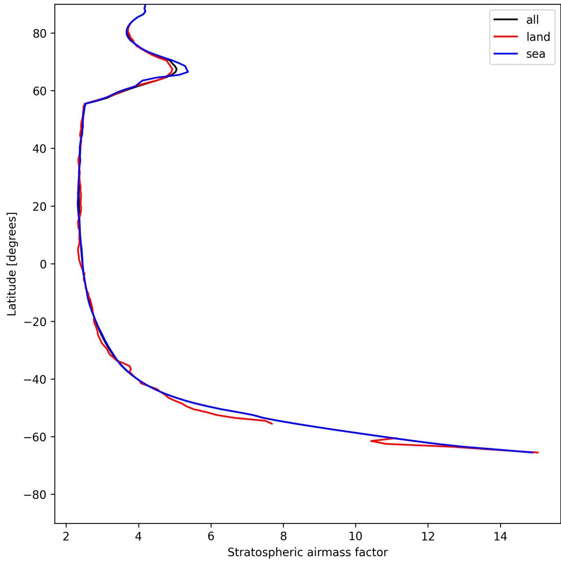
Figure 27: Zonal average of “Stratospheric air mass factor” for 2025-07-13 to 2025-07-14.
