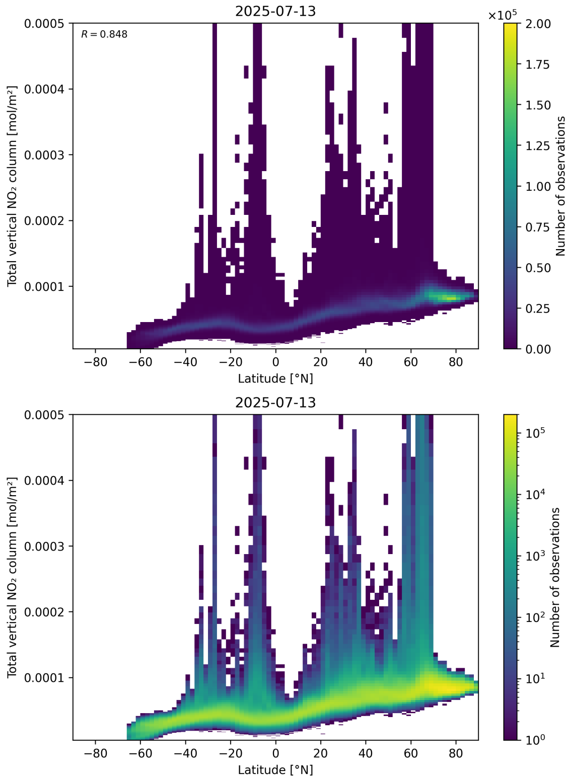
Figure 90: Scatter density plot of “Latitude” against “Total vertical NO 2 column” for 2025-07-13 to 2025-07-14.
