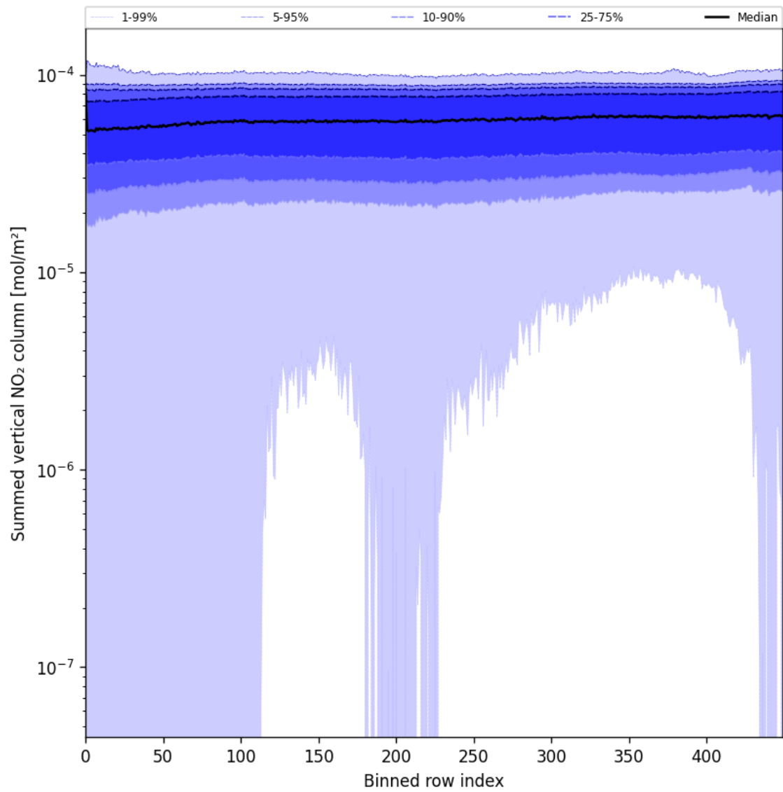
Figure 57: Along track statistics of “Summed vertical NO 2 column” for 2025-07-13 to 2025-07-14
