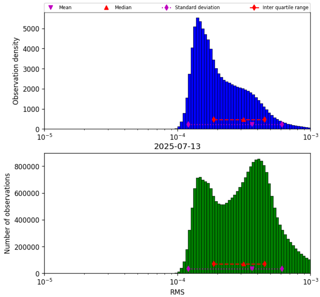
Figure 43: Histogram of “RMS” for 2025-07-13 to 2025-07-14
