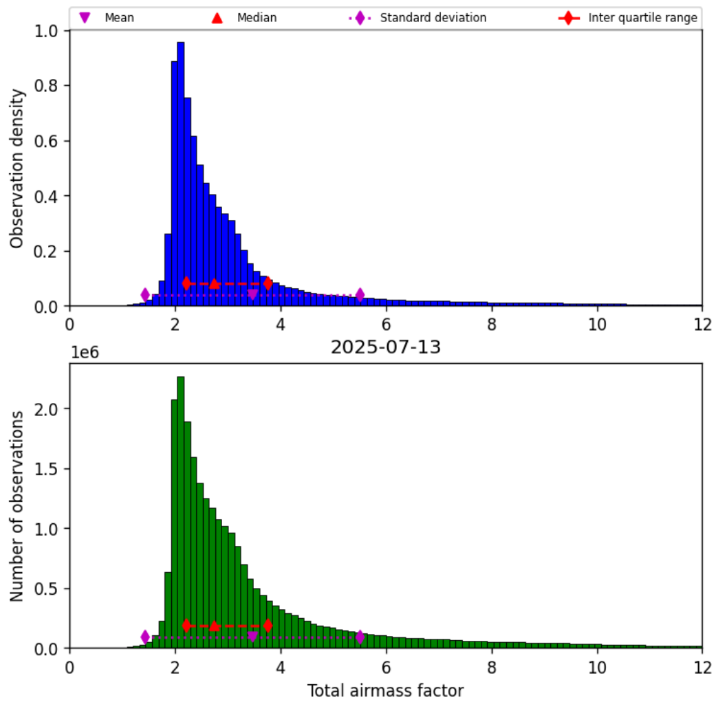
Figure 32: Histogram of “Total airmass factor” for 2025-07-13 to 2025-07-14
