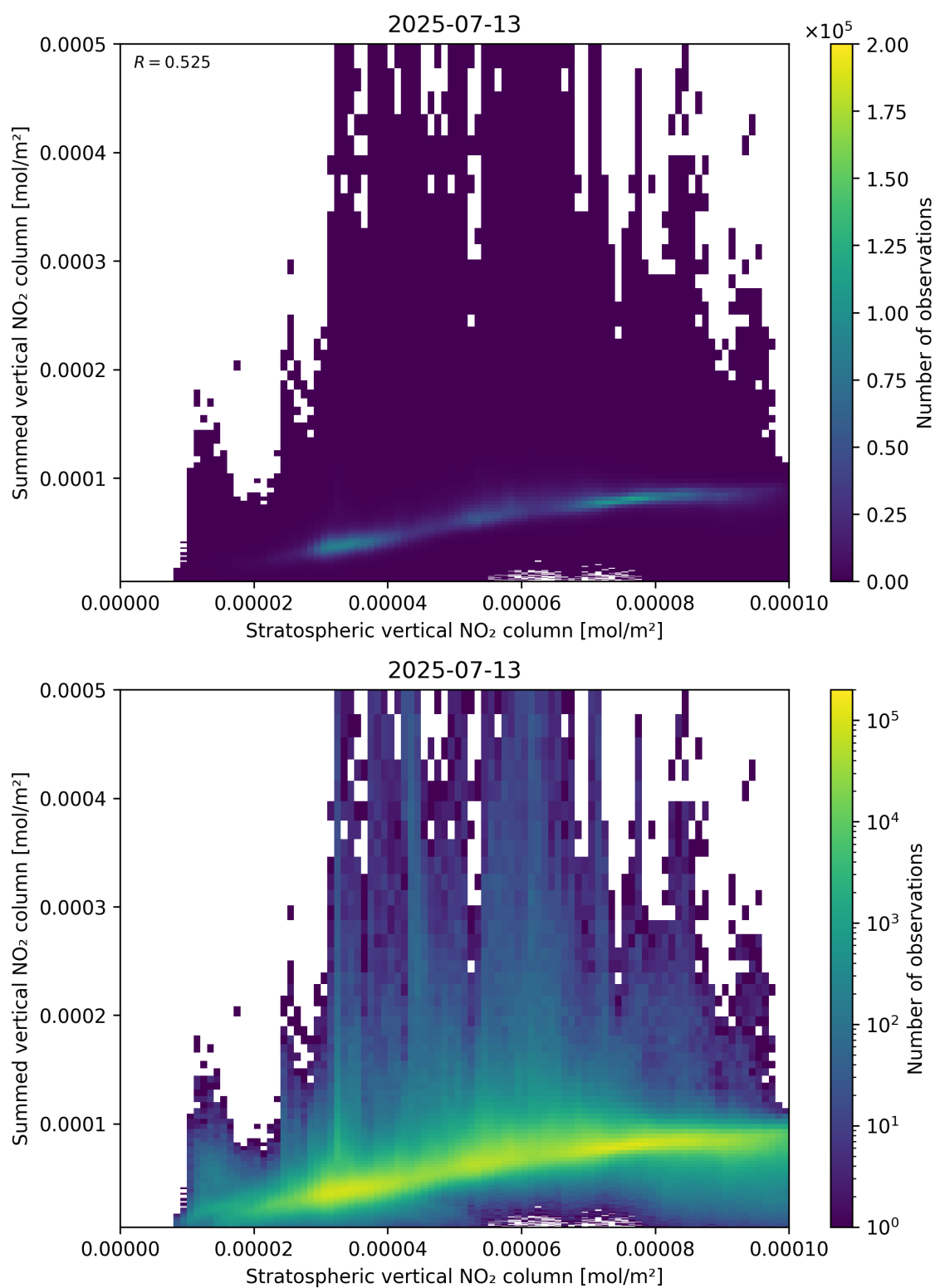
Figure 98: Scatter density plot of “Stratospheric vertical NO 2 column” against “Summed vertical NO 2 column” for 2025-07-13 to 2025-07-14.
