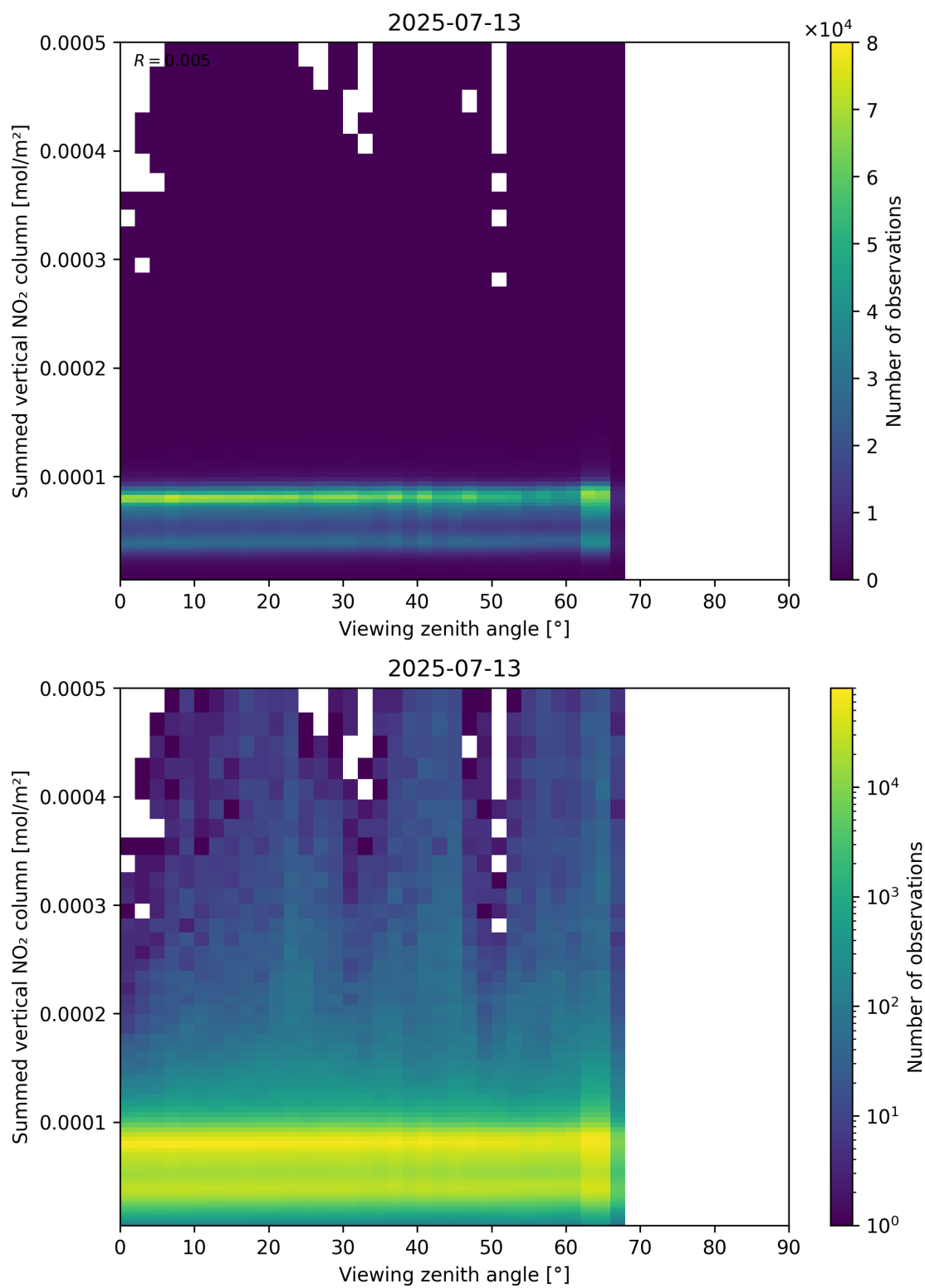
Figure 165: Scatter density plot of “Viewing zenith angle” against “Summed vertical NO 2 column” for 2025-07-13 to 2025-07-14.
