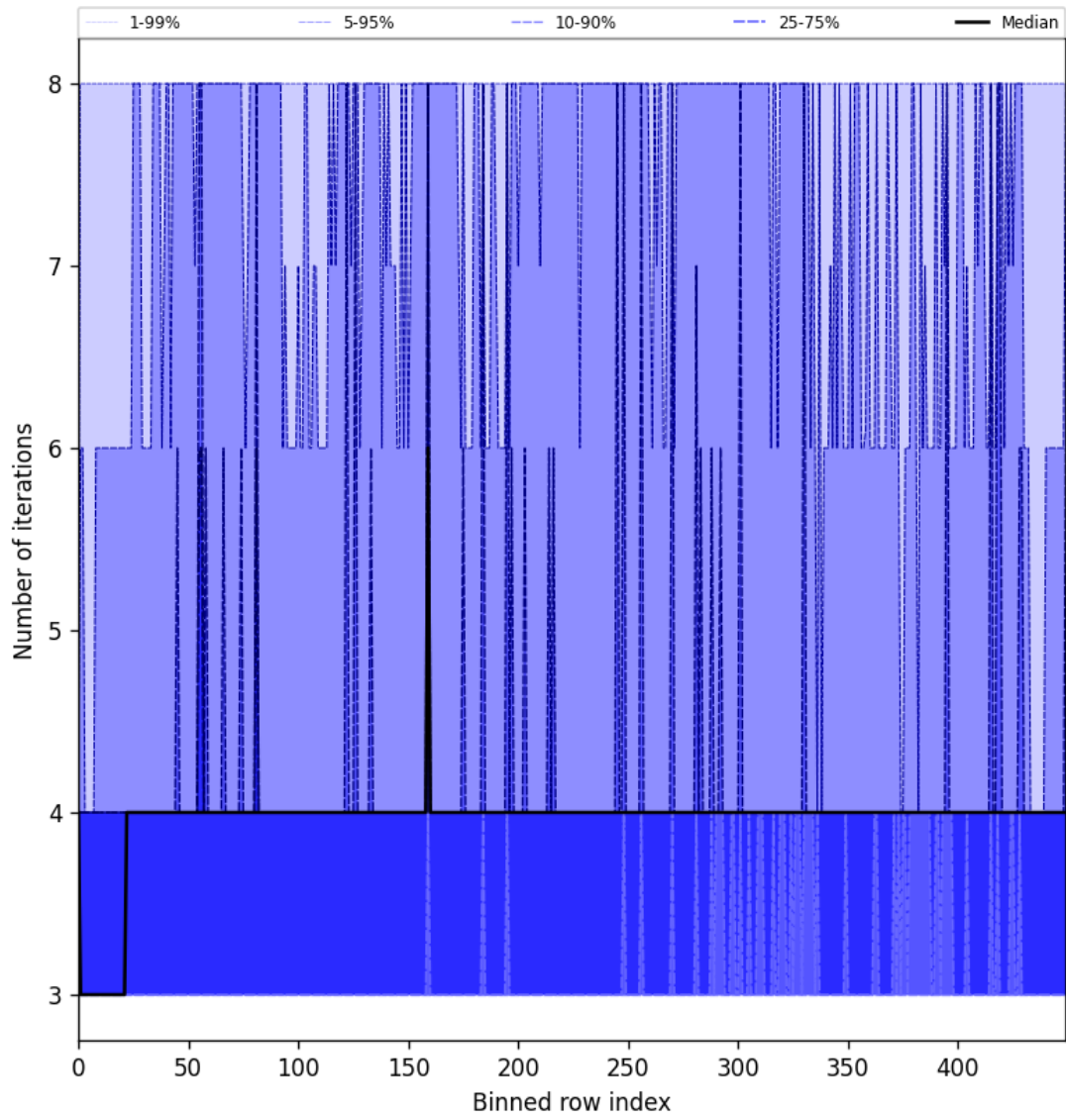
Figure 51: Along track statistics of “Number of iterations” for 2025-07-13 to 2025-07-14
