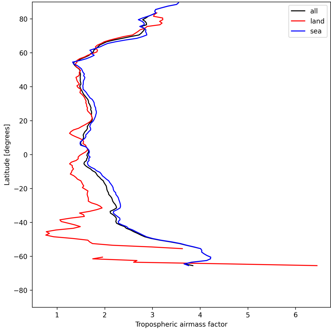
Figure 14: Zonal average of “Tropospheric airmass factor” for 2025-07-13 to 2025-07-14.
