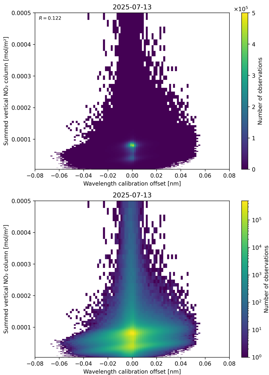
Figure 177: Scatter density plot of “Wavelength calibration offset” against “Summed vertical NO 2 column” for 2025-07-13 to 2025-07-14.
