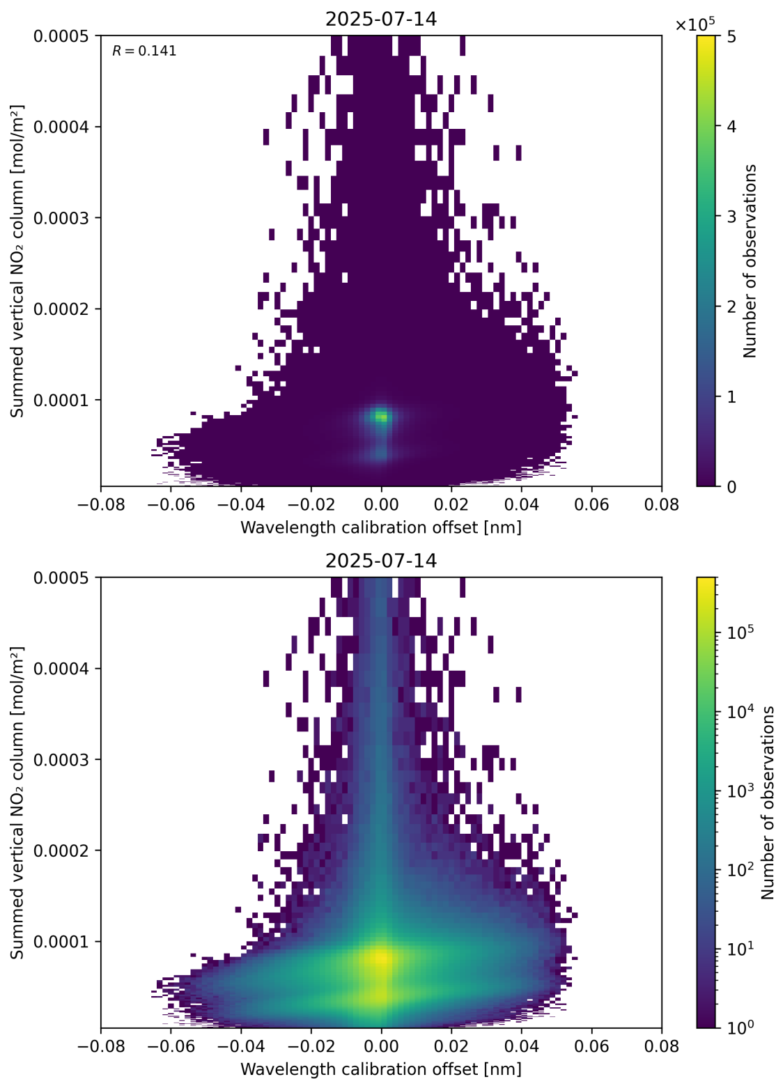
Figure 177: Scatter density plot of “Wavelength calibration offset” against “Summed vertical NO 2 column” for 2025-07-13 to 2025-07-15.
