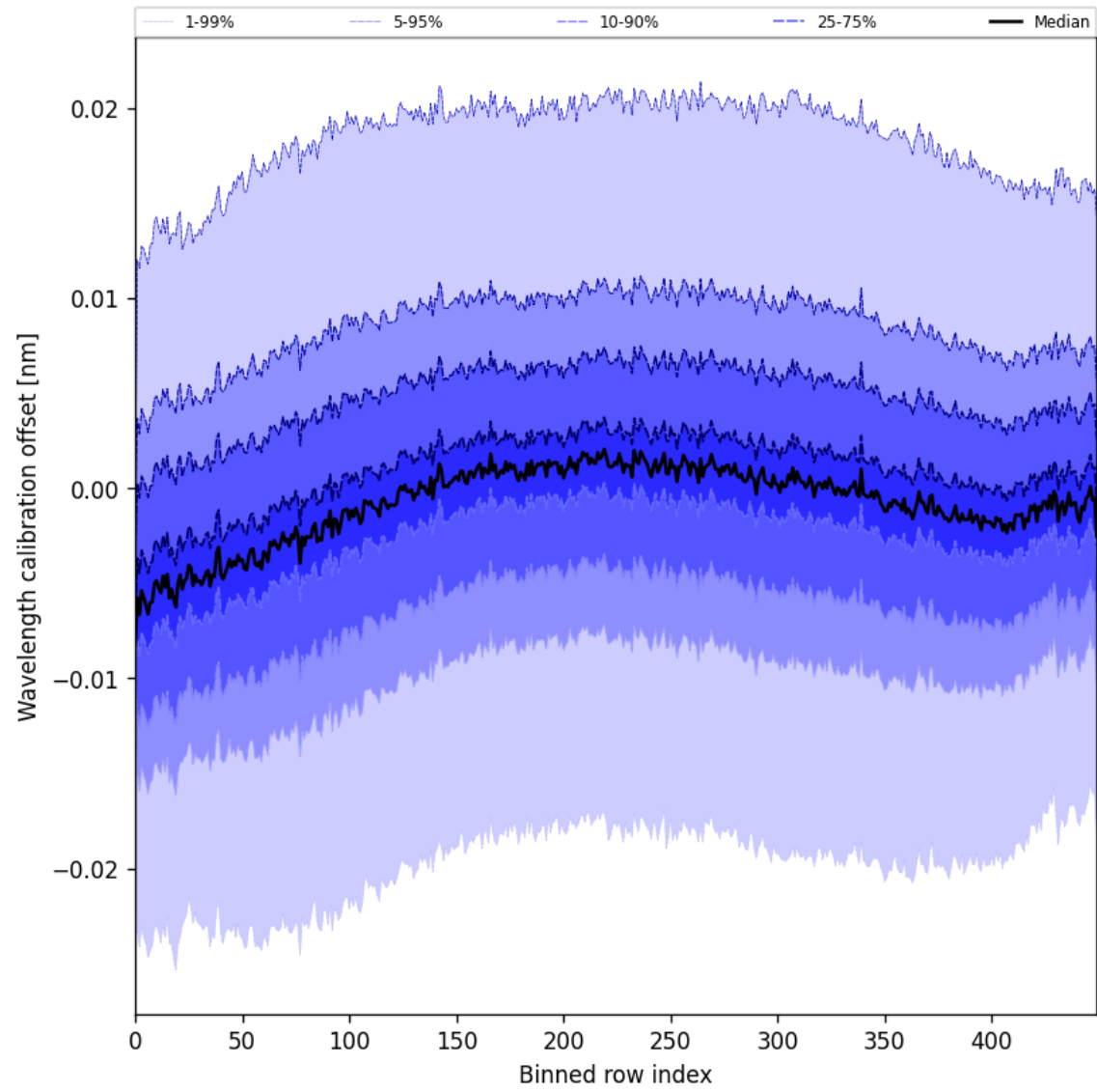
Figure 52: Along track statistics of “Wavelength calibration offset” for 2025-07-13 to 2025-07-15
