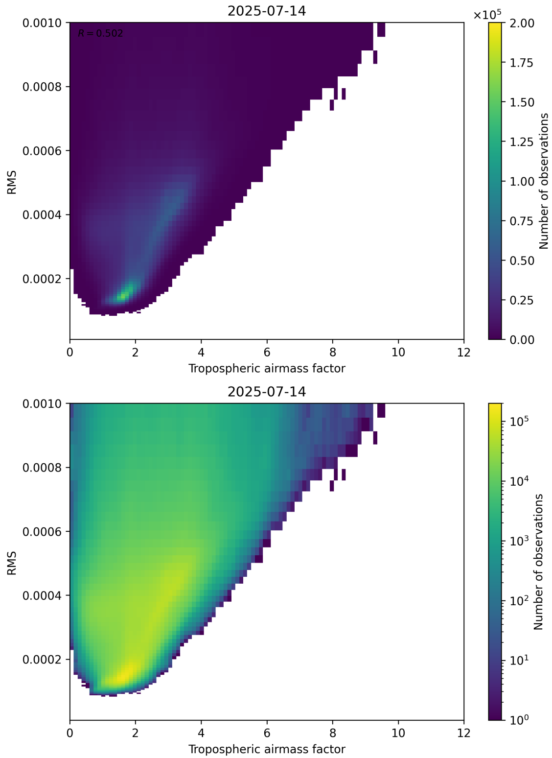
Figure 79: Scatter density plot of “Tropospheric airmass factor” against “RMS” for 2025-07-13 to 2025-07-15.
