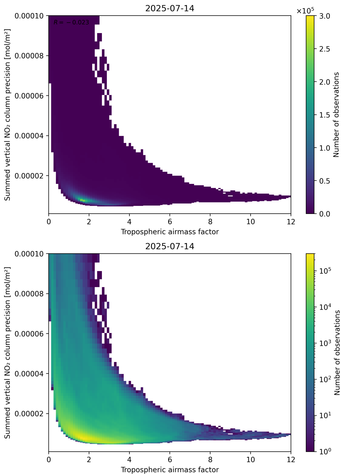
Figure 76: Scatter density plot of “Tropospheric air mass factor” against “Summed vertical NO 2 column precision” for 2025-07-13 to 2025-07-15.
