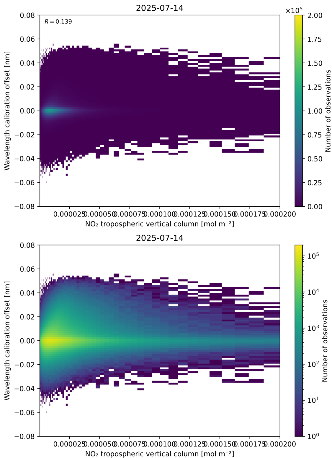
Figure 143: Scatter density plot of “NO 2 tropospheric vertical column” against “Wavelength calibration offset” for 2025-07-13 to 2025-07-15.
