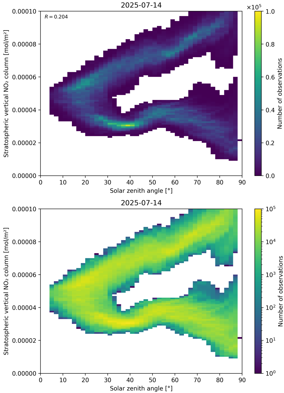
Figure 150: Scatter density plot of “Solar zenith angle” against “Stratospheric vertical NO 2 column” for 2025-07-13 to 2025-07-15.
