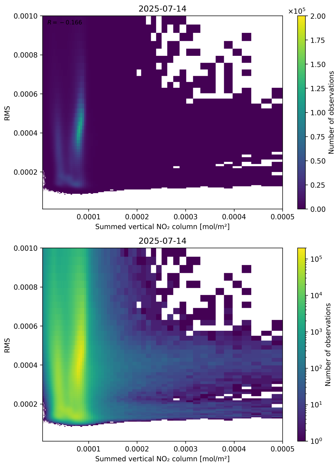
Figure 109: Scatter density plot of “Summed vertical NO 2 column” against “RMS” for 2025-07-13 to 2025-07-15.
