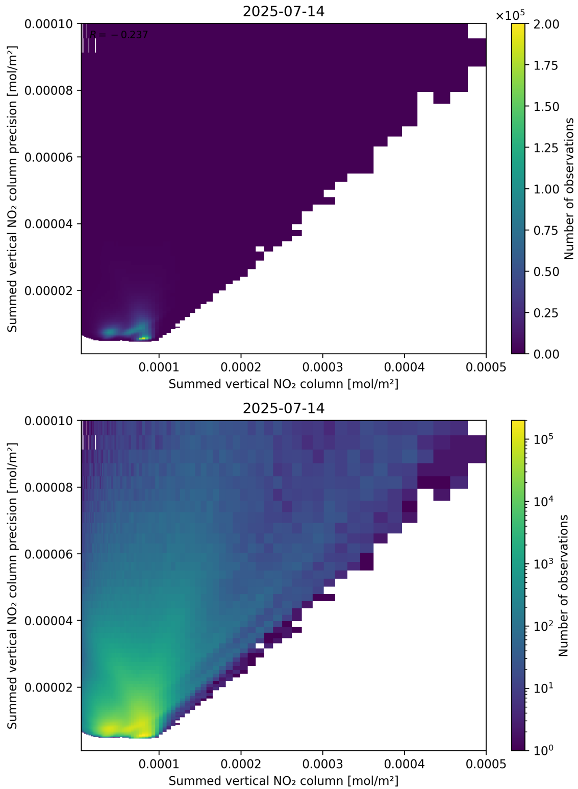
Figure 105: Scatter density plot of “Summed vertical NO 2 column” against “Summed vertical NO 2 column precision” for 2025-07-13 to 2025-07-15.
