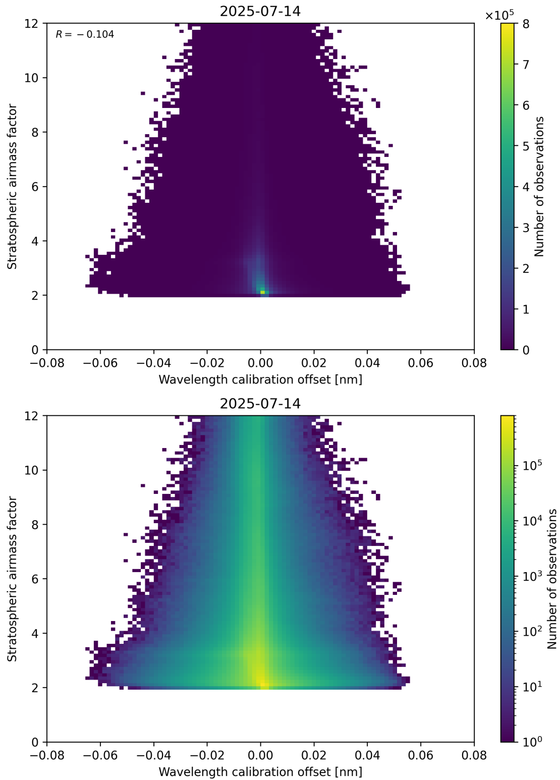
Figure 174: Scatter density plot of “Wavelength calibration offset” against “Stratospheric airmass factor” for 2025-07-13 to 2025-07-15.
