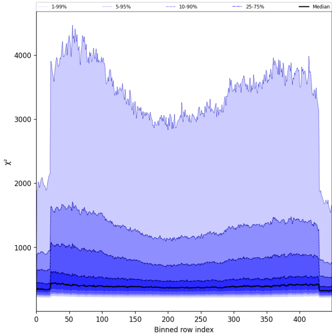
Figure 59: Along track statistics of “ \chi^2 ” for 2025-07-13 to 2025-07-15
