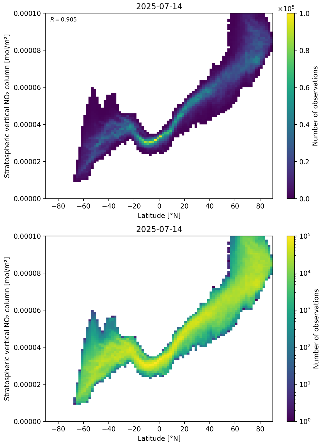
Figure 87: Scatter density plot of “Latitude” against “Stratospheric vertical \text{NO}_2 column” for 2025-07-13 to 2025-07-15.
