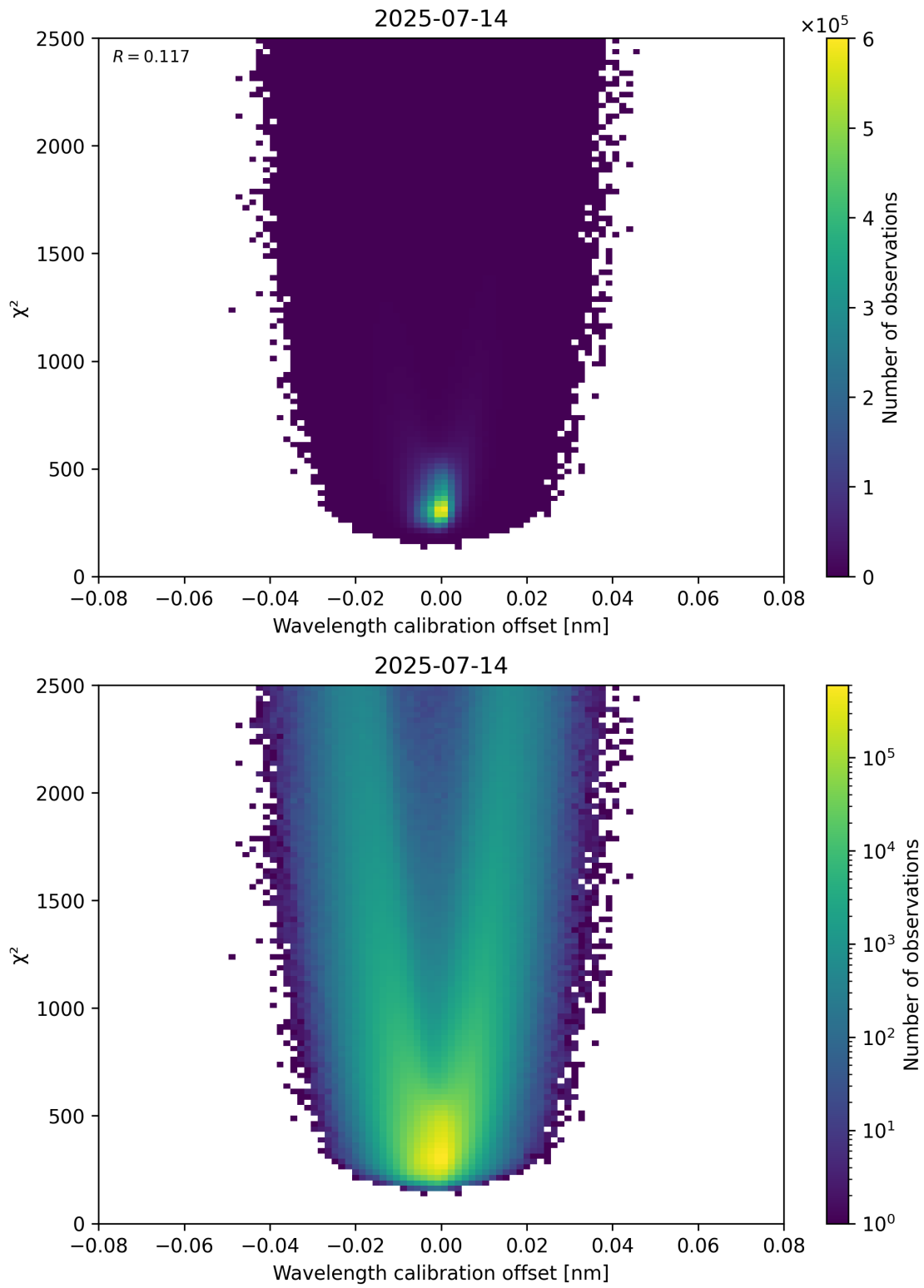
Figure 175: Scatter density plot of “Wavelength calibration offset” against “ \chi^2 ” for 2025-07-13 to 2025-07-15.
