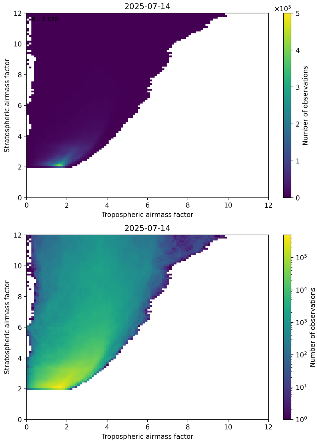
Figure 71: Scatter density plot of “Tropospheric airmass factor” against “Stratospheric airmass factor” for 2025-07-13 to 2025-07-15.
