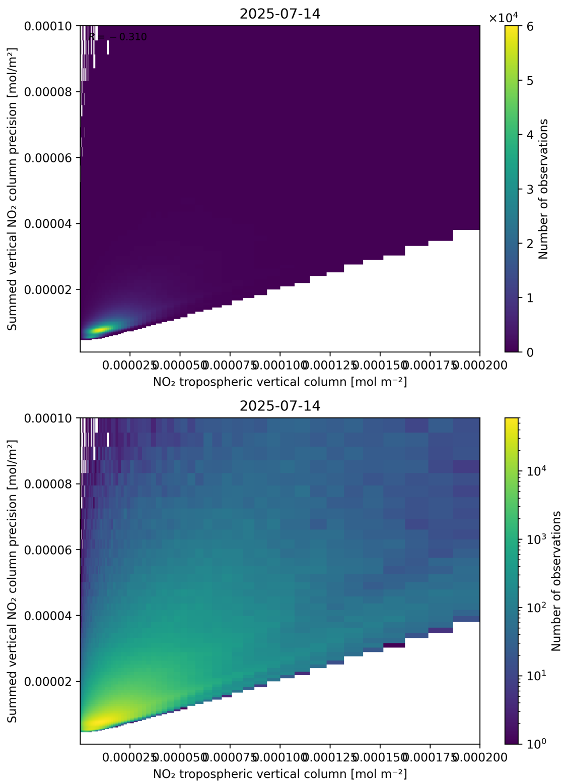
Figure 127: Scatter density plot of “NO 2 tropospheric vertical column” against “Summed vertical NO 2 column precision” for 2025-07-13 to 2025-07-15.
