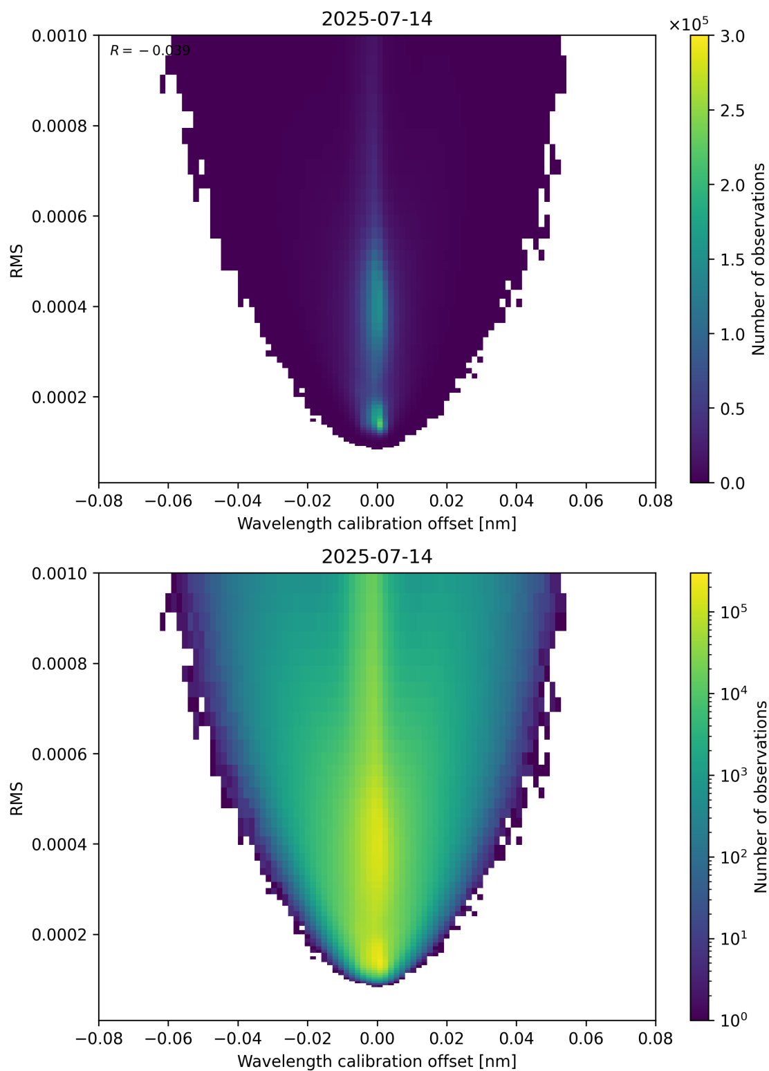
Figure 181: Scatter density plot of “Wavelength calibration offset” against “RMS” for 2025-07-13 to 2025-07-15.
