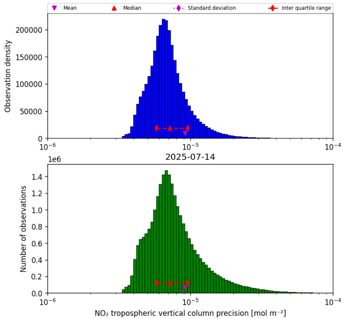
Figure 30: Histogram of “NO 2 tropospheric vertical column precision” for 2025-07-13 to 2025-07-15
