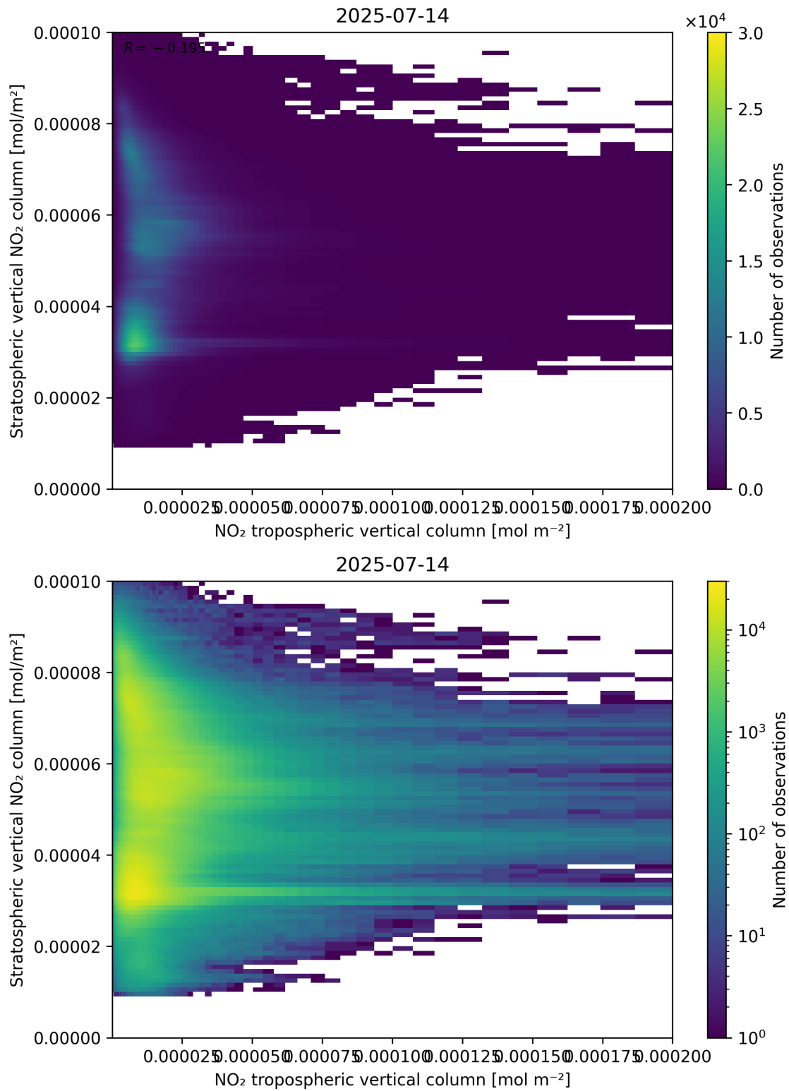
Figure 125: Scatter density plot of “NO 2 tropospheric vertical column” against “Stratospheric vertical NO 2 column” for 2025-07-13 to 2025-07-15.
