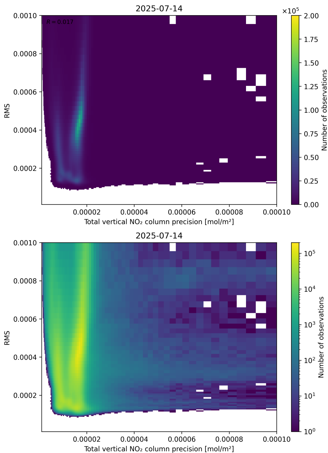
Figure 119: Scatter density plot of “Total vertical NO 2 column precision” against “RMS” for 2025-07-13 to 2025-07-15.
