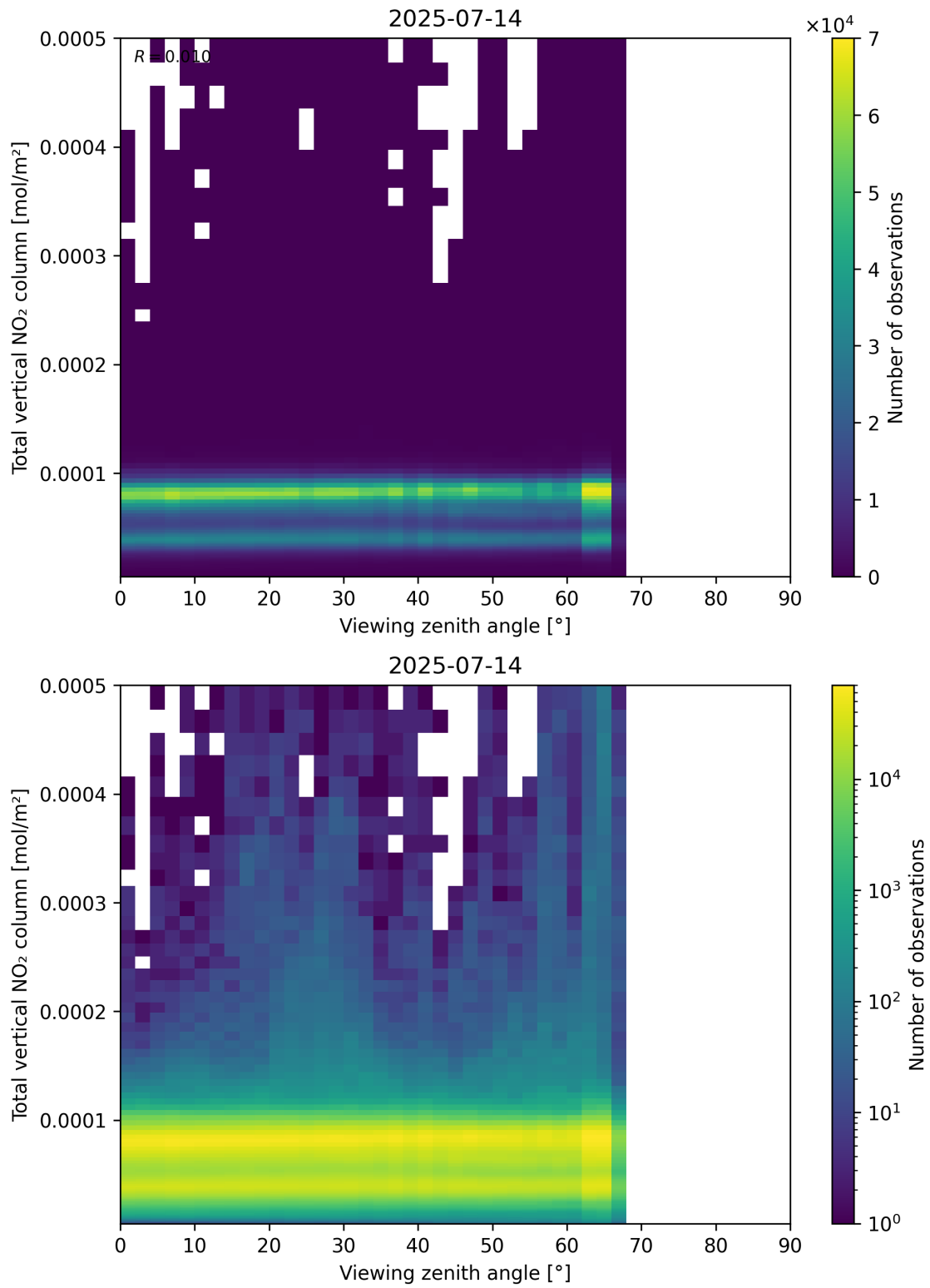
Figure 167: Scatter density plot of “Viewing zenith angle” against “Total vertical NO 2 column” for 2025-07-13 to 2025-07-15.
