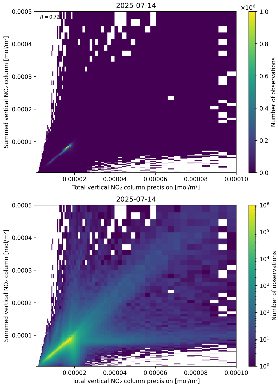
Figure 117: Scatter density plot of “Total vertical NO 2 column precision” against “Summed vertical NO 2 column” for 2025-07-13 to 2025-07-15.
