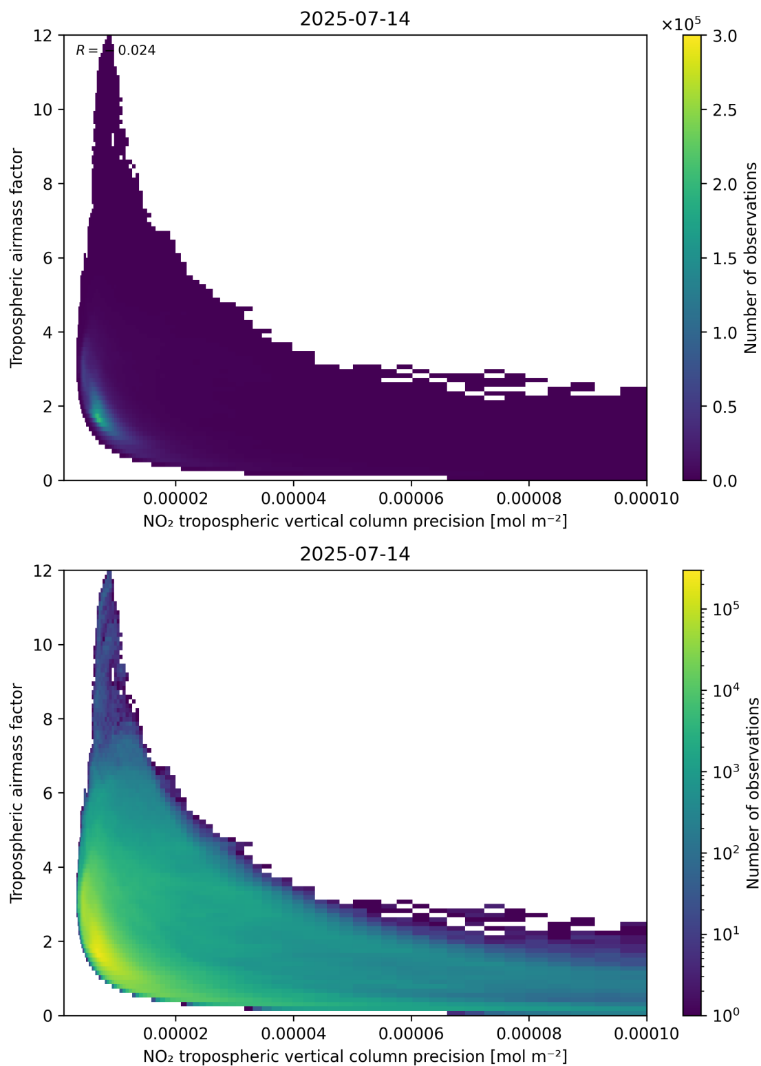
Figure 133: Scatter density plot of “NO 2 tropospheric vertical column precision” against “Tropospheric airmass factor” for 2025-07-13 to 2025-07-15.
