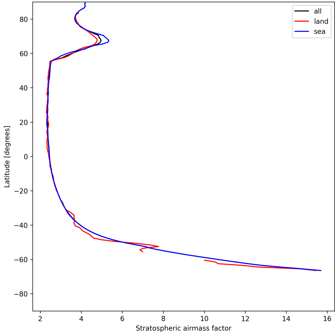
Figure 27: Zonal average of “Stratospheric airmass factor” for 2025-07-13 to 2025-07-15.
