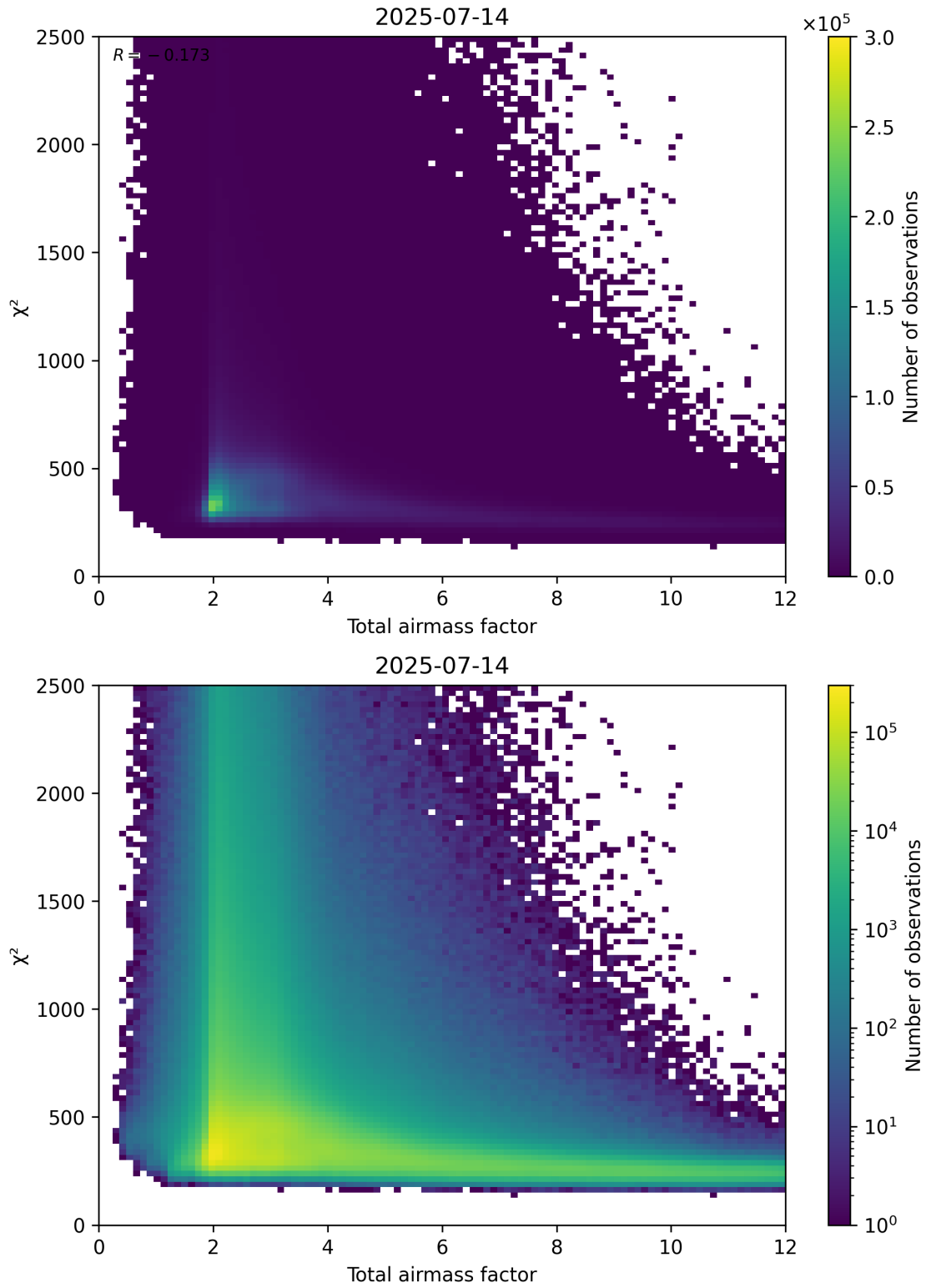
Figure 63: Scatter density plot of “Total airmass factor” against “ \chi^2 ” for 2025-07-13 to 2025-07-15.
