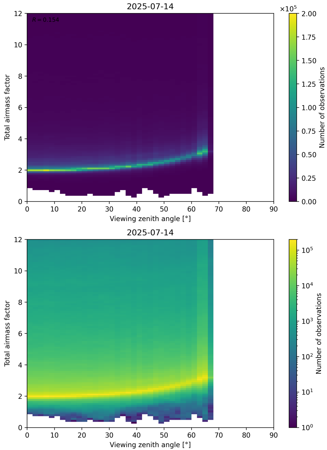
Figure 160: Scatter density plot of “Viewing zenith angle” against “Total airmass factor” for 2025-07-13 to 2025-07-15.
