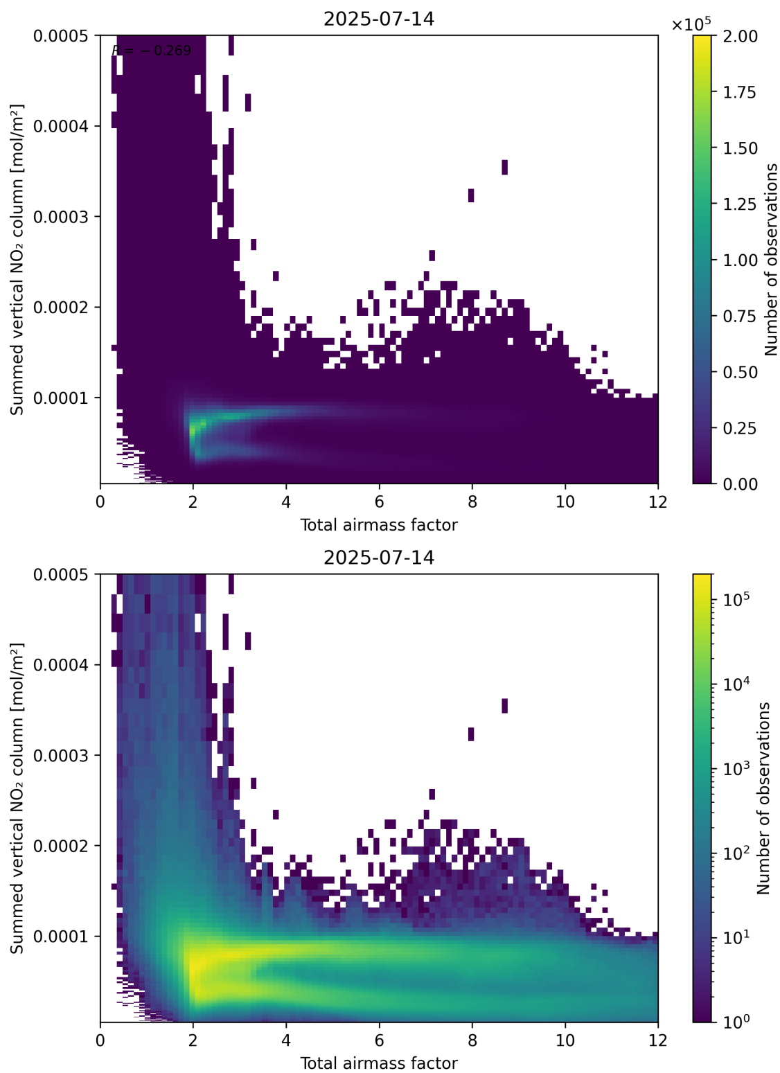
Figure 65: Scatter density plot of “Total airmass factor” against “Summed vertical NO 2 column” for 2025-07-13 to 2025-07-15.
