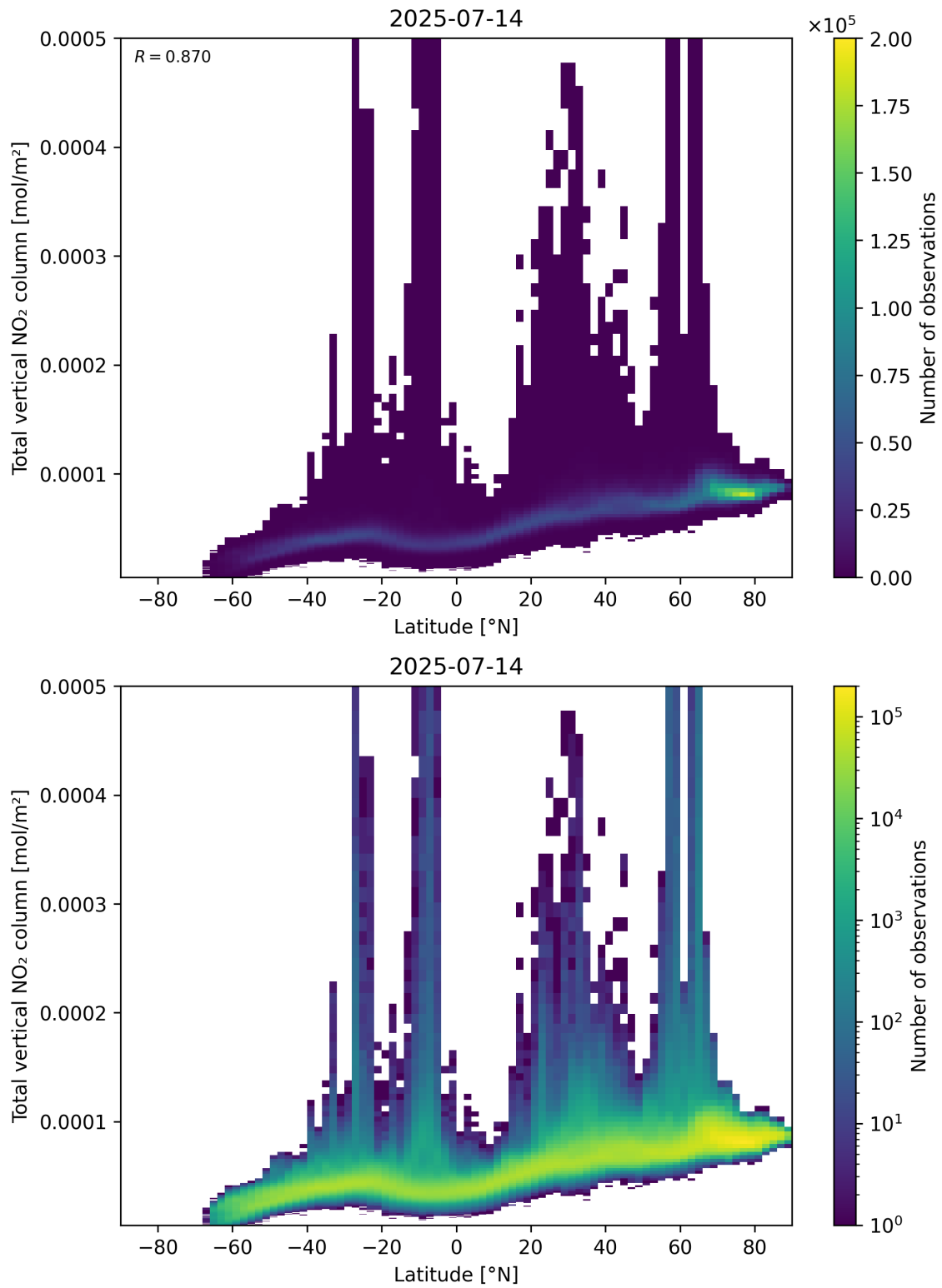
Figure 90: Scatter density plot of “Latitude” against “Total vertical NO 2 column” for 2025-07-13 to 2025-07-15.
