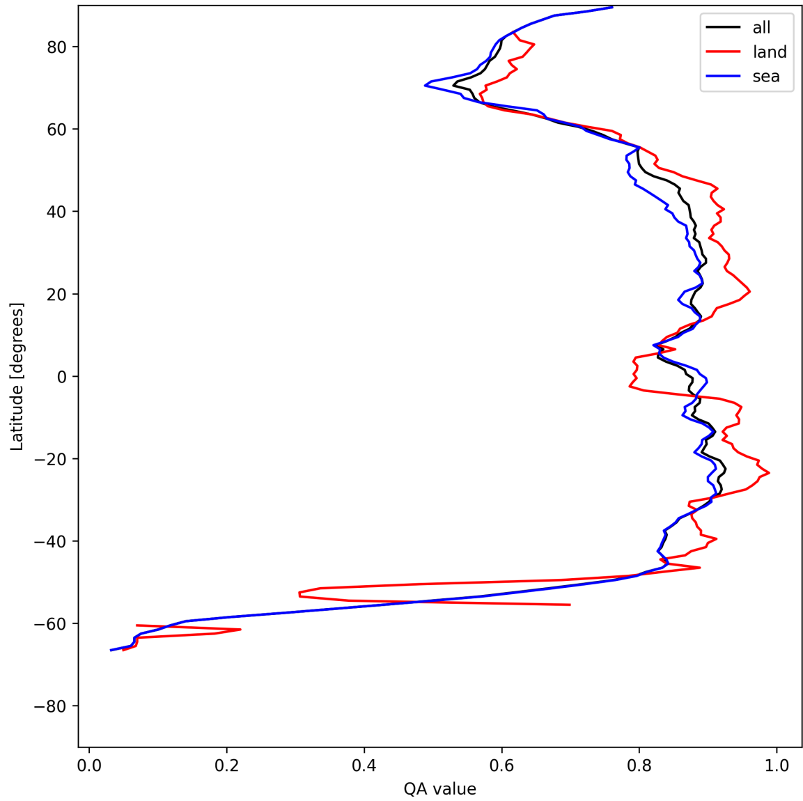
Figure 11: Zonal average of “QA value” for 2025-07-13 to 2025-07-15.
