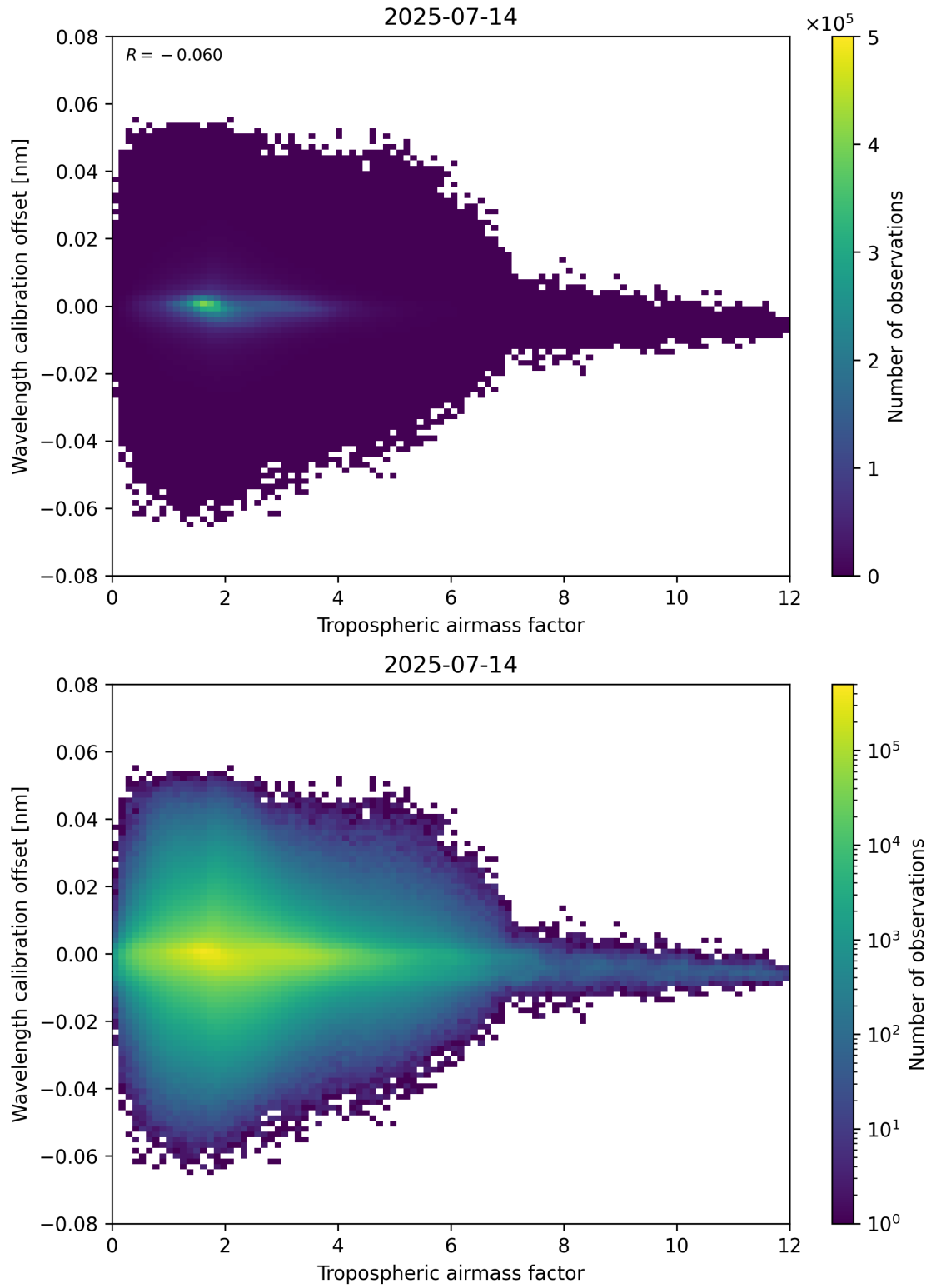
Figure 80: Scatter density plot of “Tropospheric airmass factor” against “Wavelength calibration offset” for 2025-07-13 to 2025-07-15.
