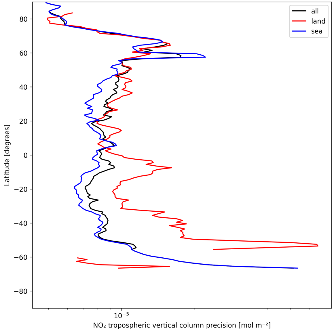
Figure 13: Zonal average of “NO 2 tropospheric vertical column precision” for 2025-07-13 to 2025-07-15.
