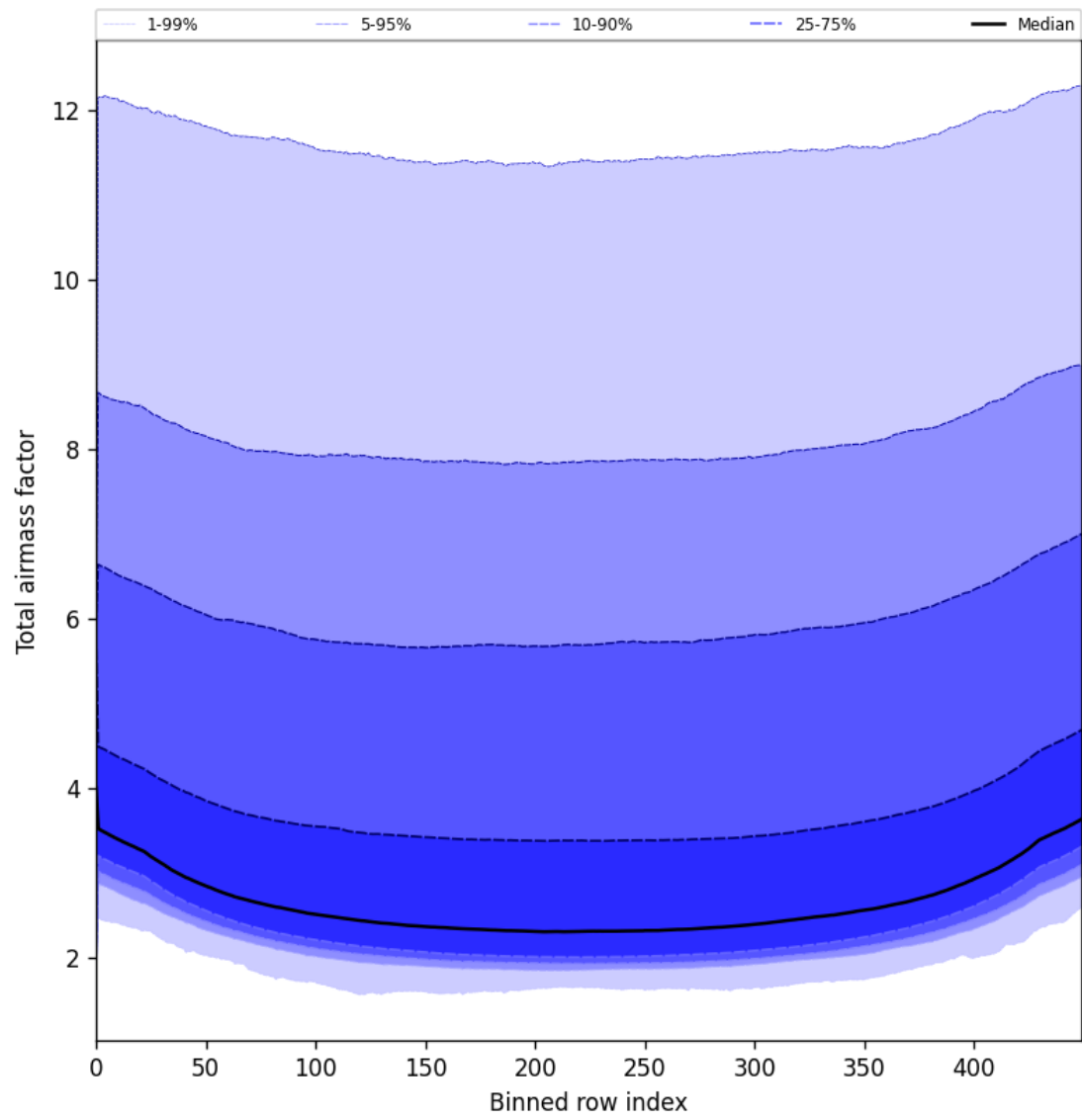
Figure 49: Along track statistics of “Total airmass factor” for 2025-07-13 to 2025-07-15
