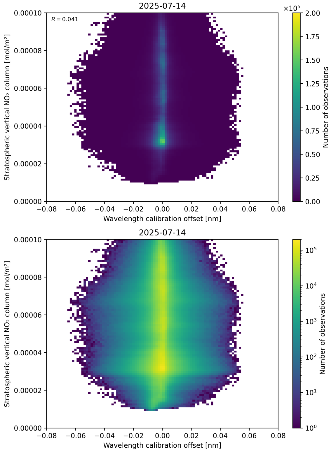
Figure 176: Scatter density plot of “Wavelength calibration offset” against “Stratospheric vertical NO 2 column” for 2025-07-13 to 2025-07-15.
