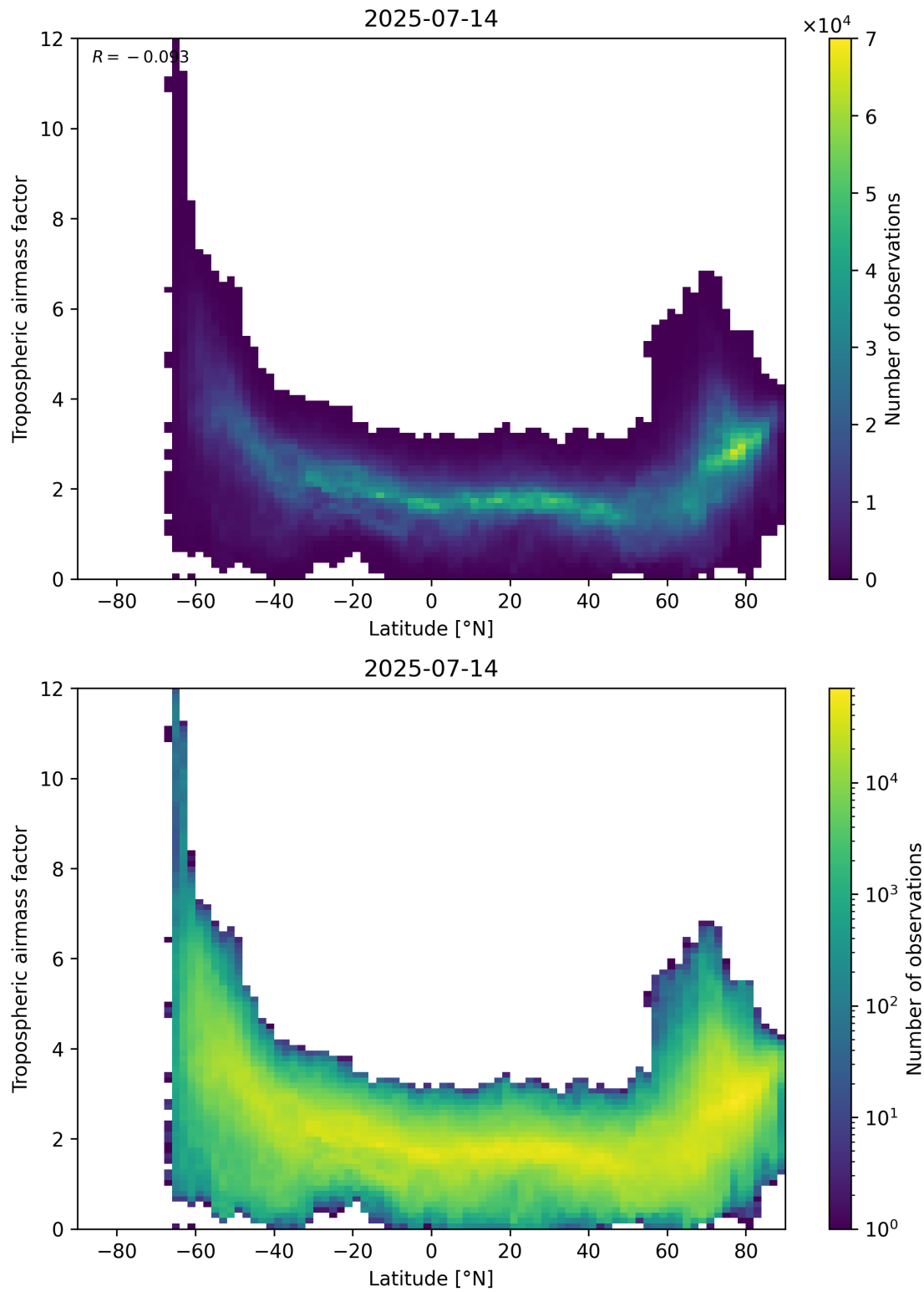
Figure 85: Scatter density plot of “Latitude” against “Tropospheric air mass factor” for 2025-07-13 to 2025-07-15.
