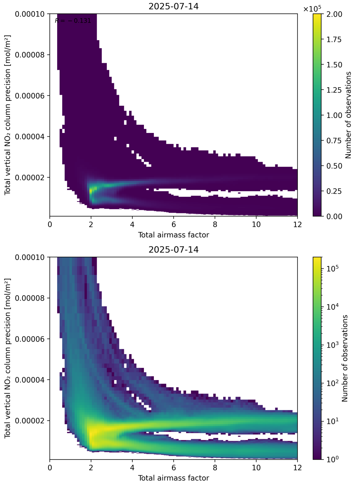
Figure 68: Scatter density plot of “Total airmass factor” against “Total vertical NO 2 column precision” for 2025-07-13 to 2025-07-15.
