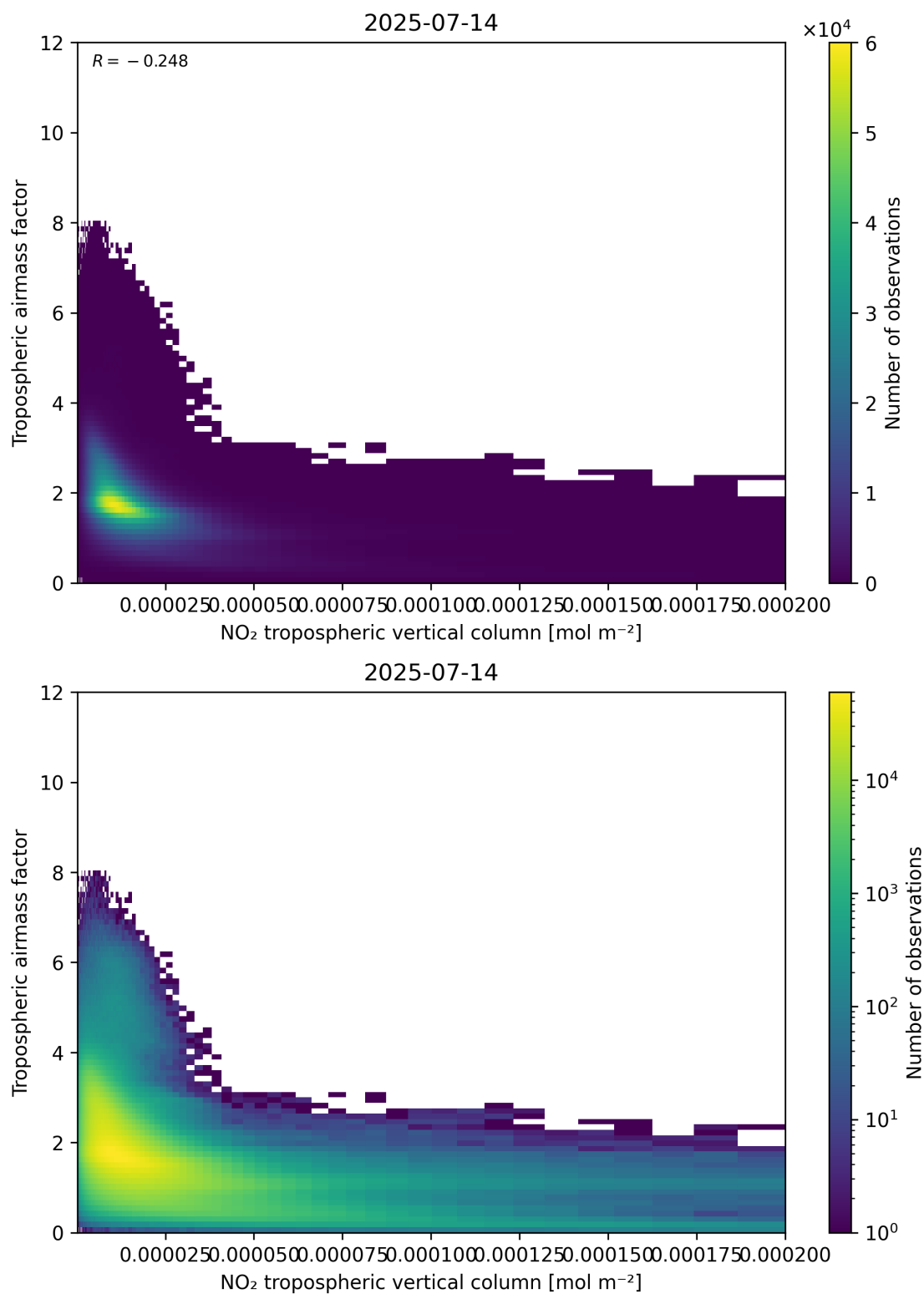
Figure 123: Scatter density plot of “NO 2 tropospheric vertical column” against “Tropospheric air mass factor” for 2025-07-13 to 2025-07-15.
