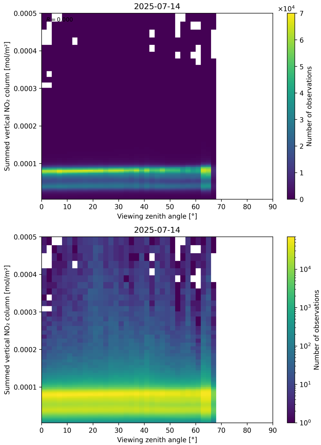
Figure 165: Scatter density plot of “Viewing zenith angle” against “Summed vertical NO 2 column” for 2025-07-13 to 2025-07-15.
