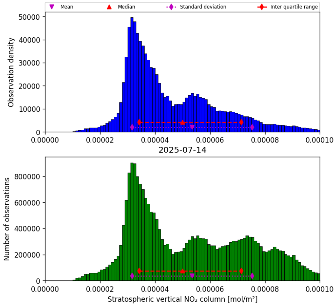
Figure 36: Histogram of “Stratospheric vertical NO 2 column” for 2025-07-13 to 2025-07-15
