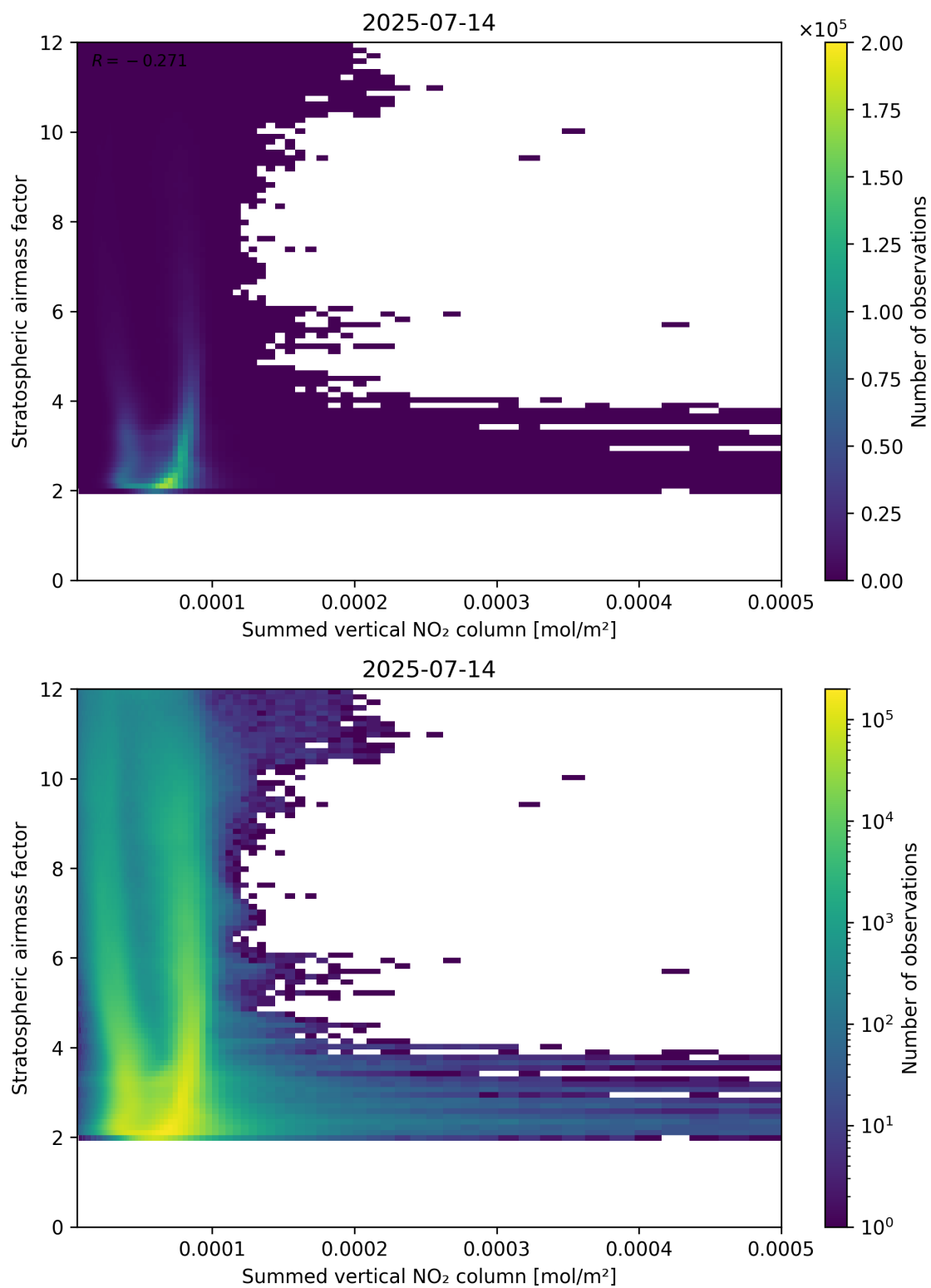
Figure 103: Scatter density plot of “Summed vertical NO 2 column” against “Stratospheric airmass factor” for 2025-07-13 to 2025-07-15.
