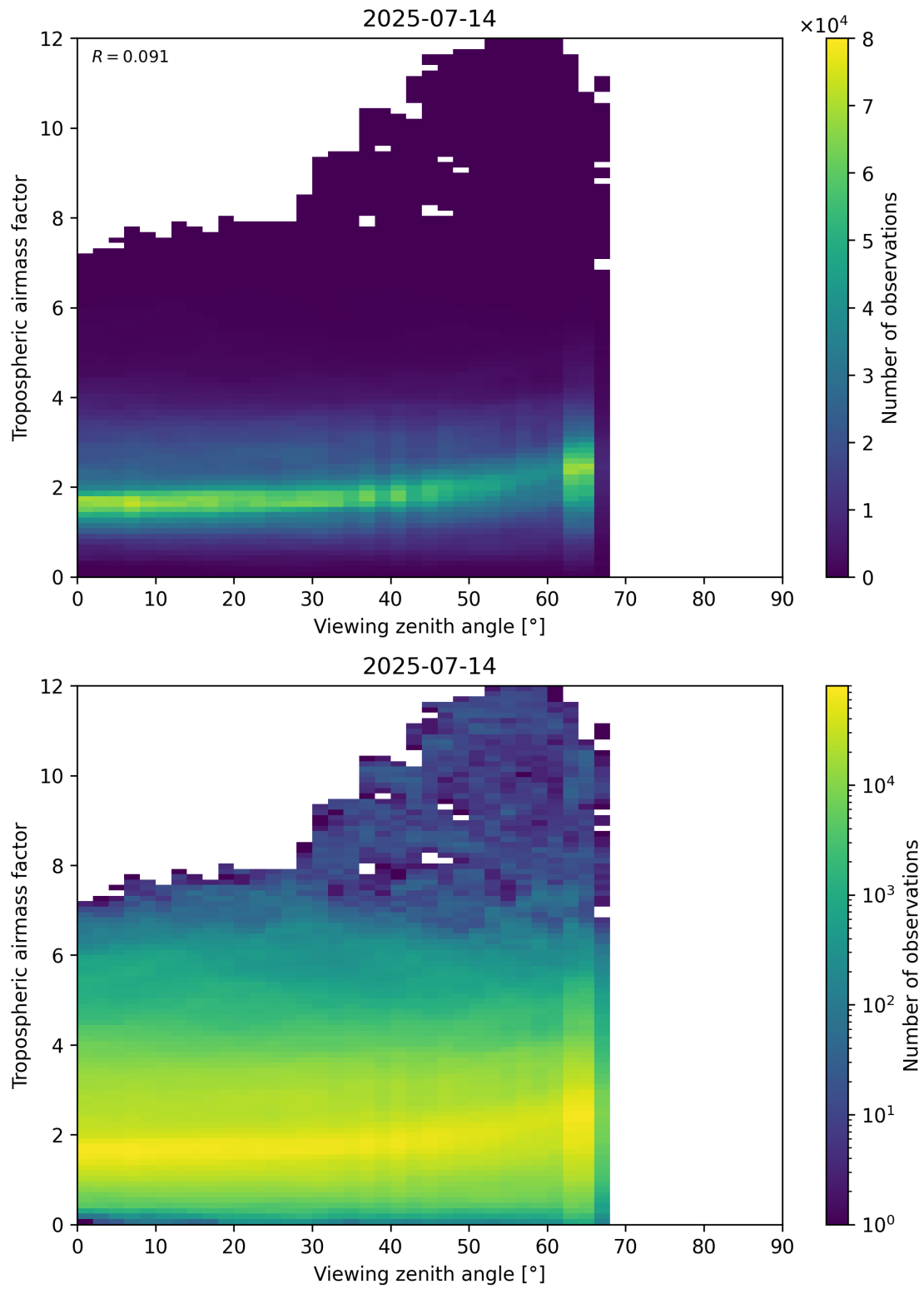
Figure 161: Scatter density plot of “Viewing zenith angle” against “Tropospheric airmass factor” for 2025-07-13 to 2025-07-15.
