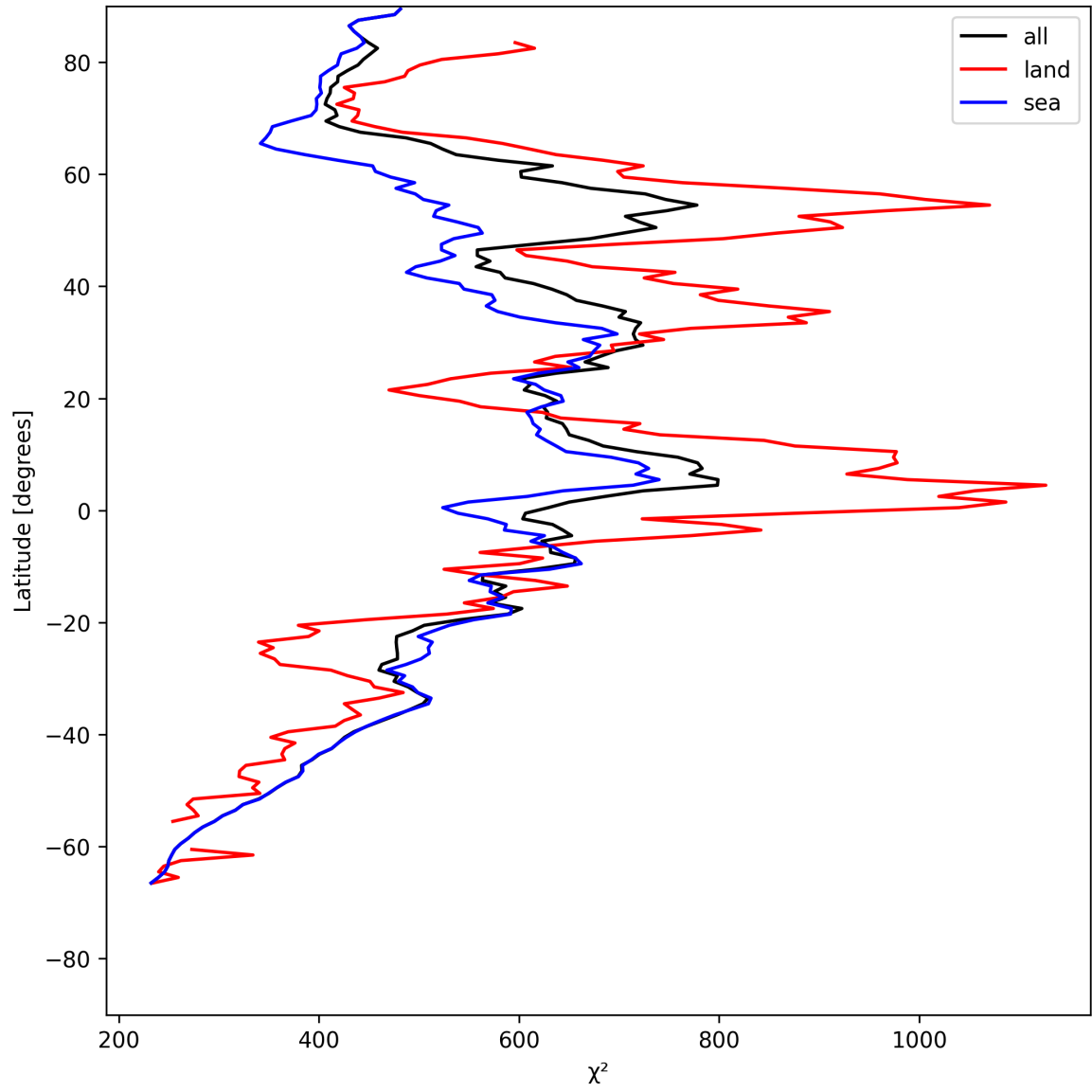
Figure 25: Zonal average of “ \chi^2 ” for 2025-07-13 to 2025-07-15.
