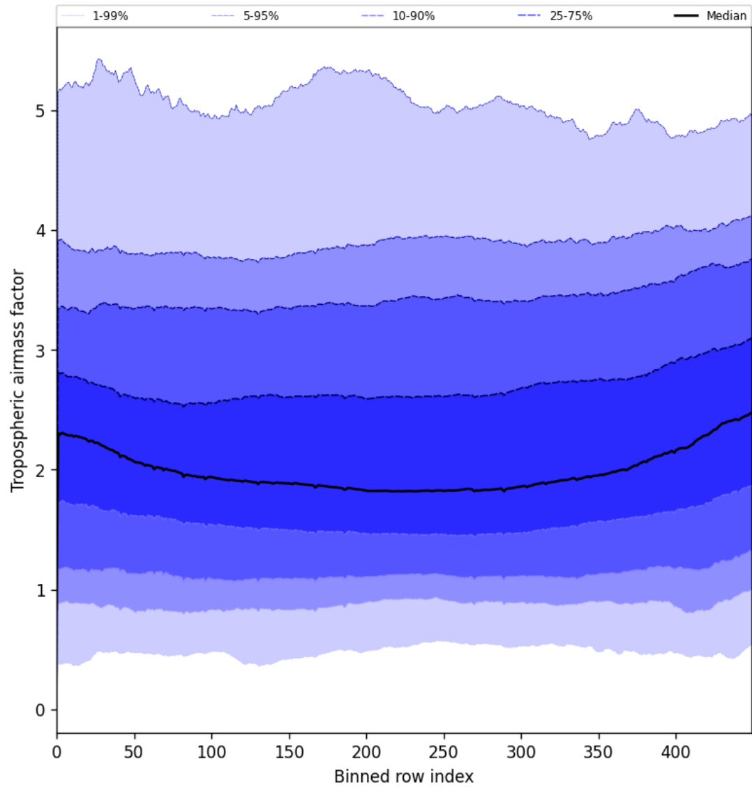
Figure 48: Along track statistics of “Tropospheric airmass factor” for 2025-07-13 to 2025-07-15
