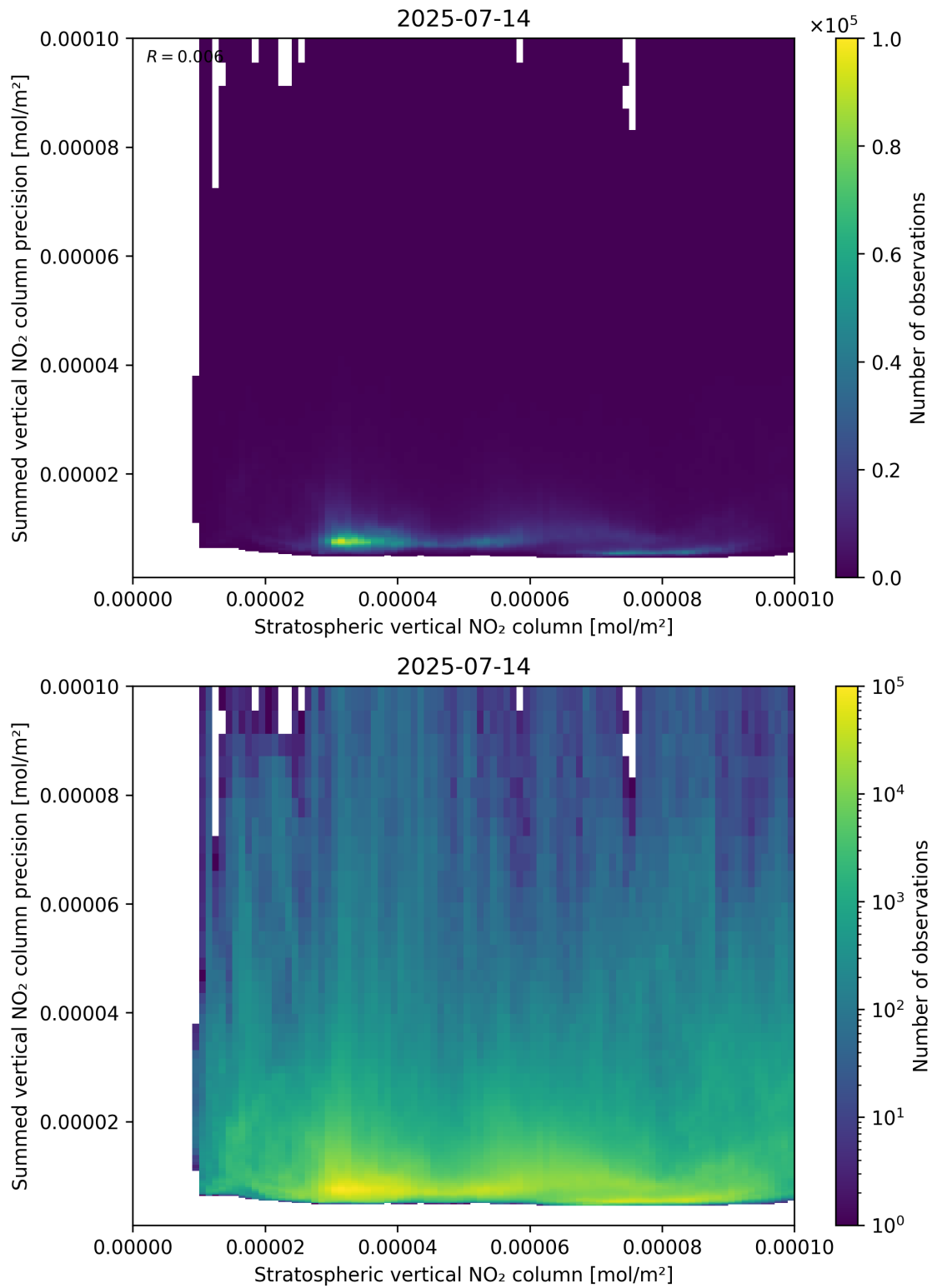
Figure 99: Scatter density plot of “Stratospheric vertical NO 2 column” against “Summed vertical NO 2 column precision” for 2025-07-13 to 2025-07-15.
