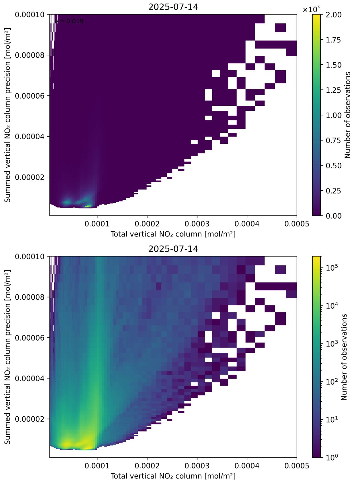
Figure 113: Scatter density plot of “Total vertical NO 2 column” against “Summed vertical NO 2 column precision” for 2025-07-13 to 2025-07-15.
