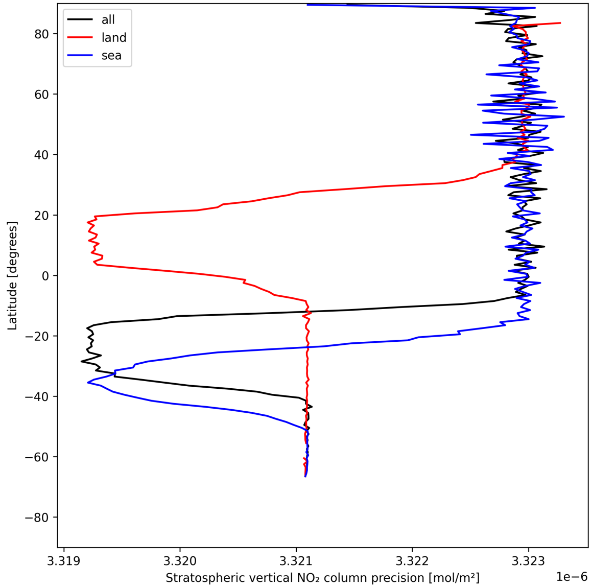
Figure 20: Zonal average of “Stratospheric vertical NO 2 column precision” for 2025-07-13 to 2025-07-15.
