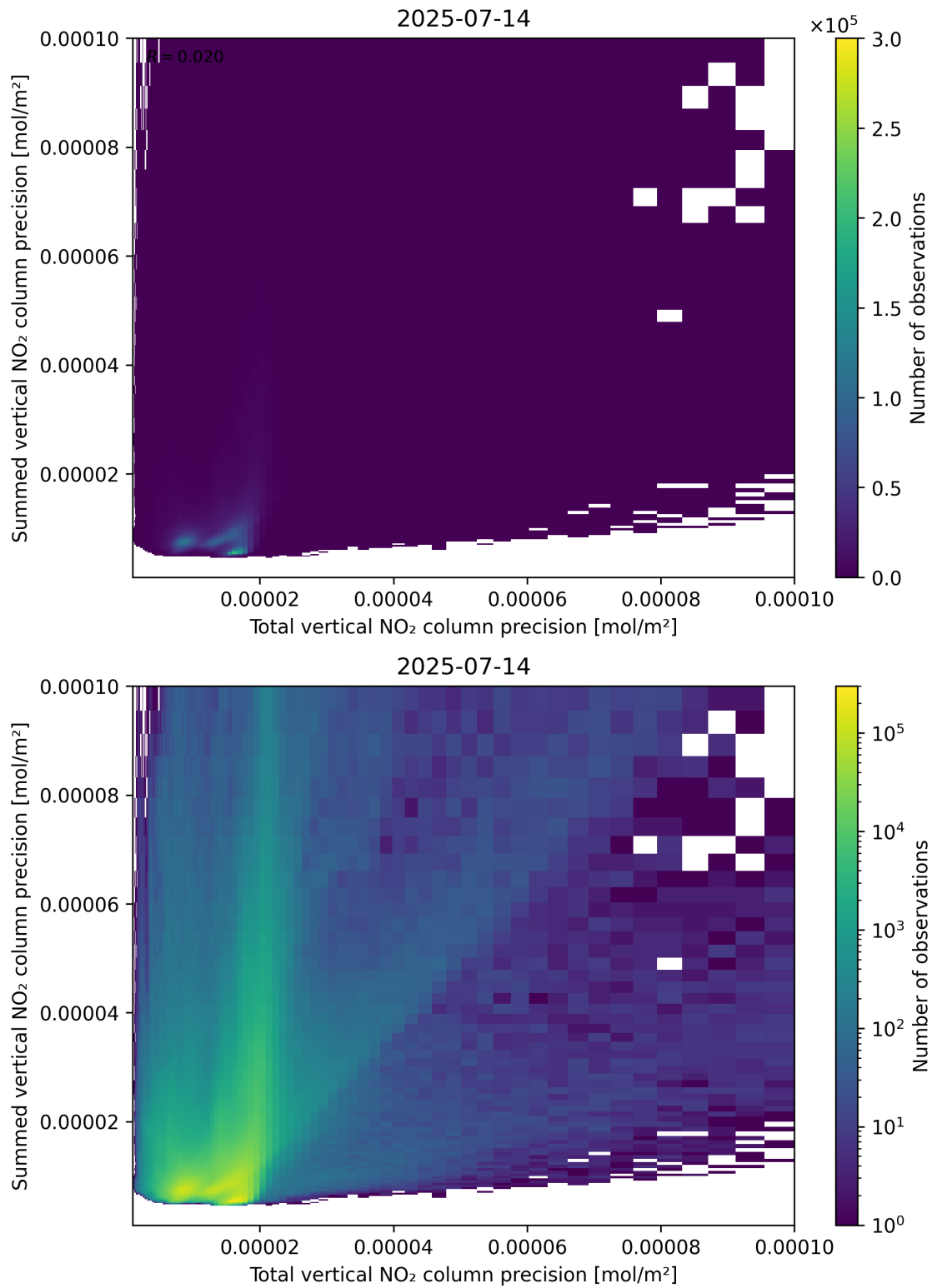
Figure 118: Scatter density plot of “Total vertical NO 2 column precision” against “Summed vertical NO 2 column precision” for 2025-07-13 to 2025-07-15.
