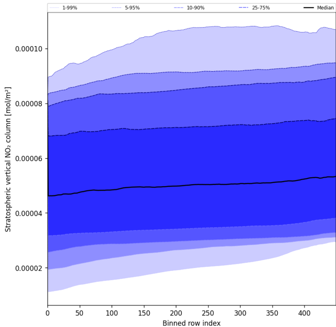
Figure 53: Along track statistics of “Stratospheric vertical NO 2 column” for 2025-07-13 to 2025-07-15
