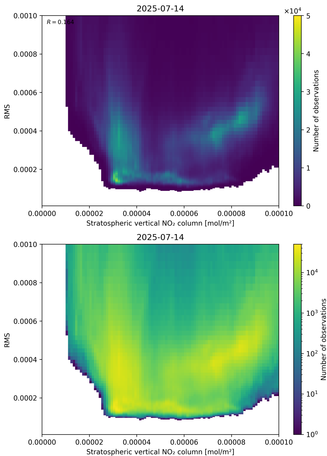
Figure 102: Scatter density plot of “Stratospheric vertical NO 2 column” against “RMS” for 2025-07-13 to 2025-07-15.
