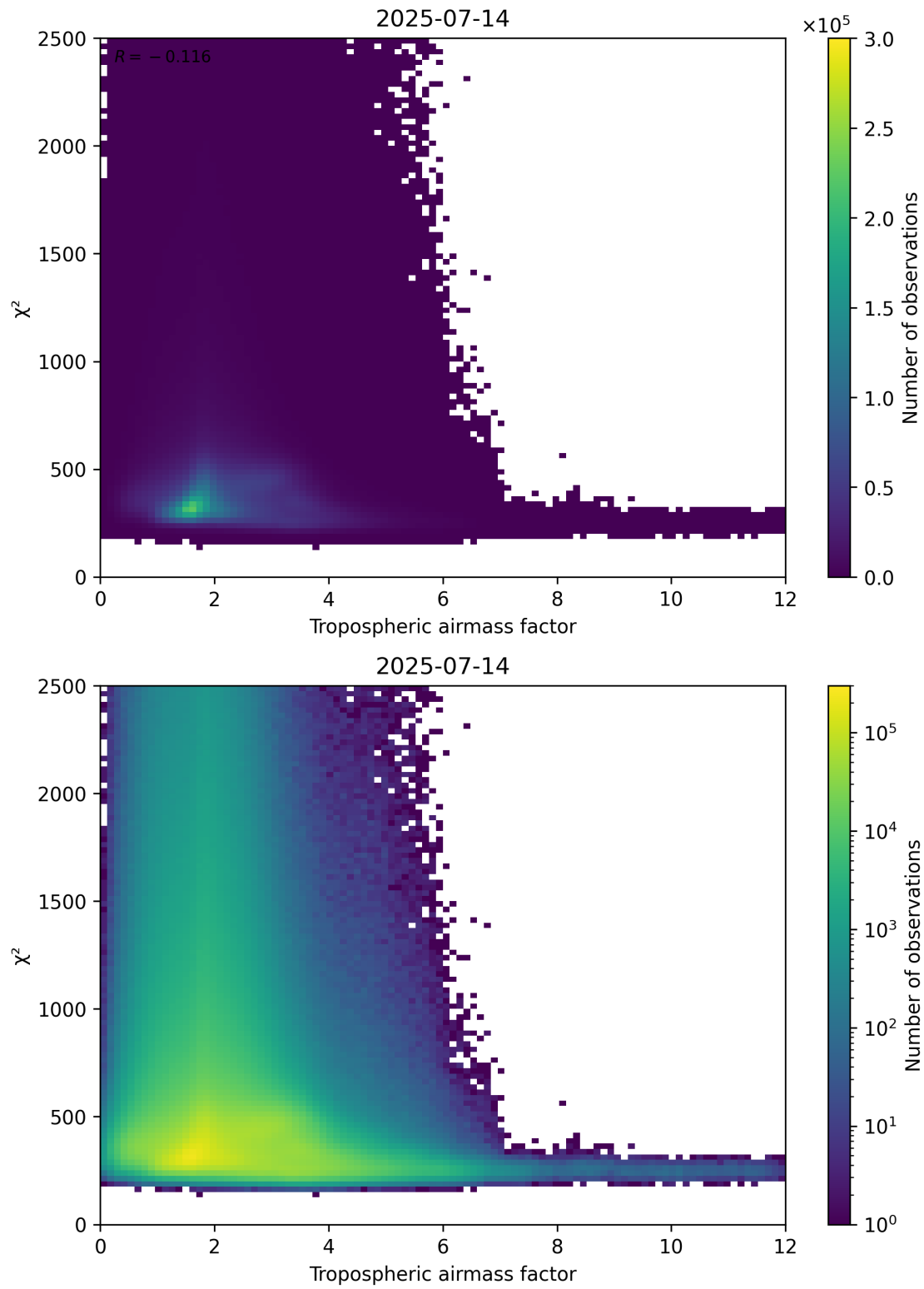
Figure 73: Scatter density plot of “Tropospheric airmass factor” against “ \chi^2 ” for 2025-07-13 to 2025-07-15.
