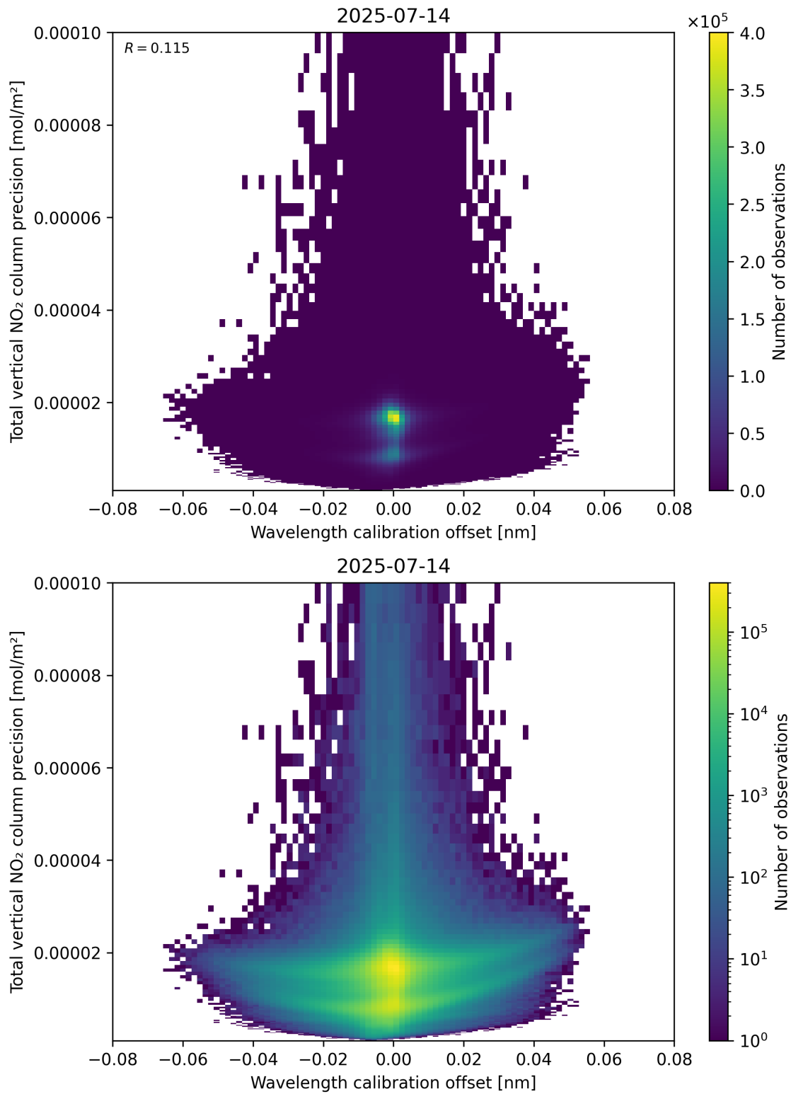
Figure 180: Scatter density plot of “Wavelength calibration offset” against “Total vertical NO 2 column precision” for 2025-07-13 to 2025-07-15.
