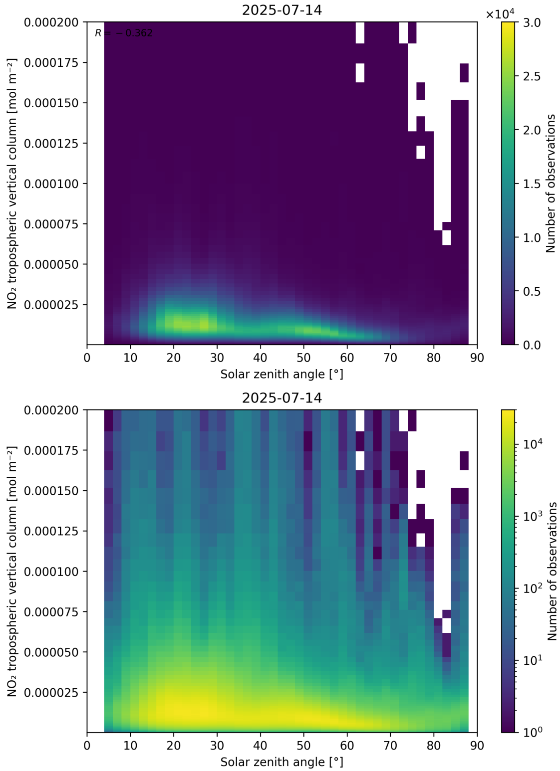
Figure 155: Scatter density plot of “Solar zenith angle” against “NO 2 tropospheric vertical column” for 2025-07-13 to 2025-07-15.
