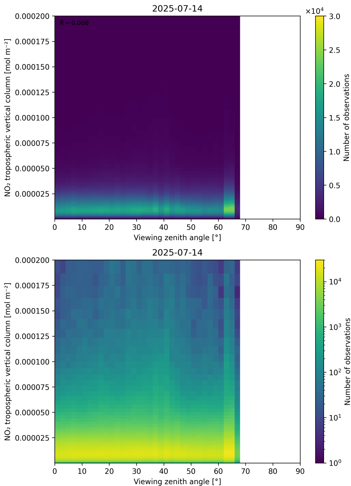
Figure 169: Scatter density plot of “Viewing zenith angle” against “NO 2 tropospheric vertical column” for 2025-07-13 to 2025-07-15.
