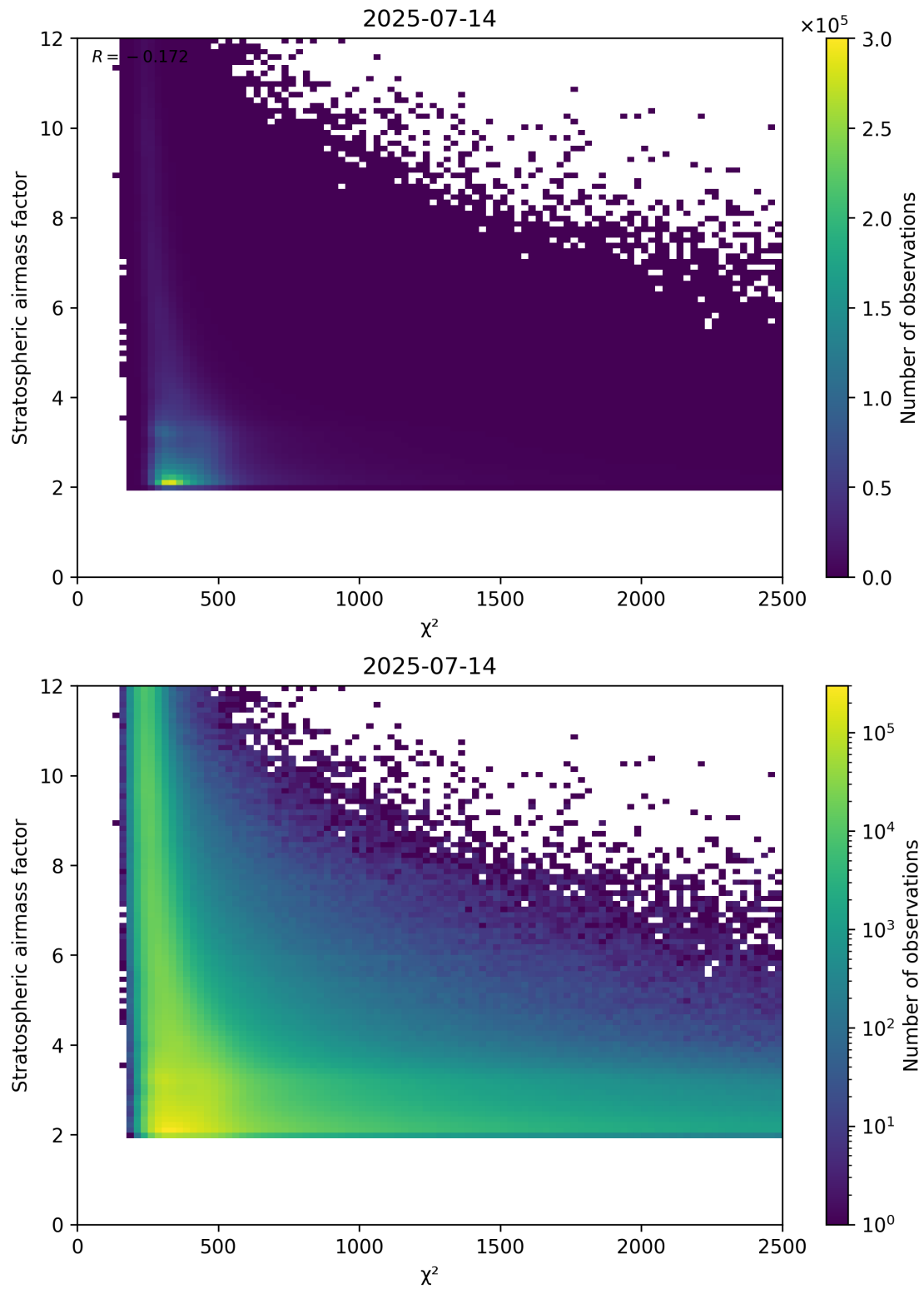
Figure 81: Scatter density plot of “ \chi^2 ” against “Stratospheric airmass factor” for 2025-07-13 to 2025-07-15.
