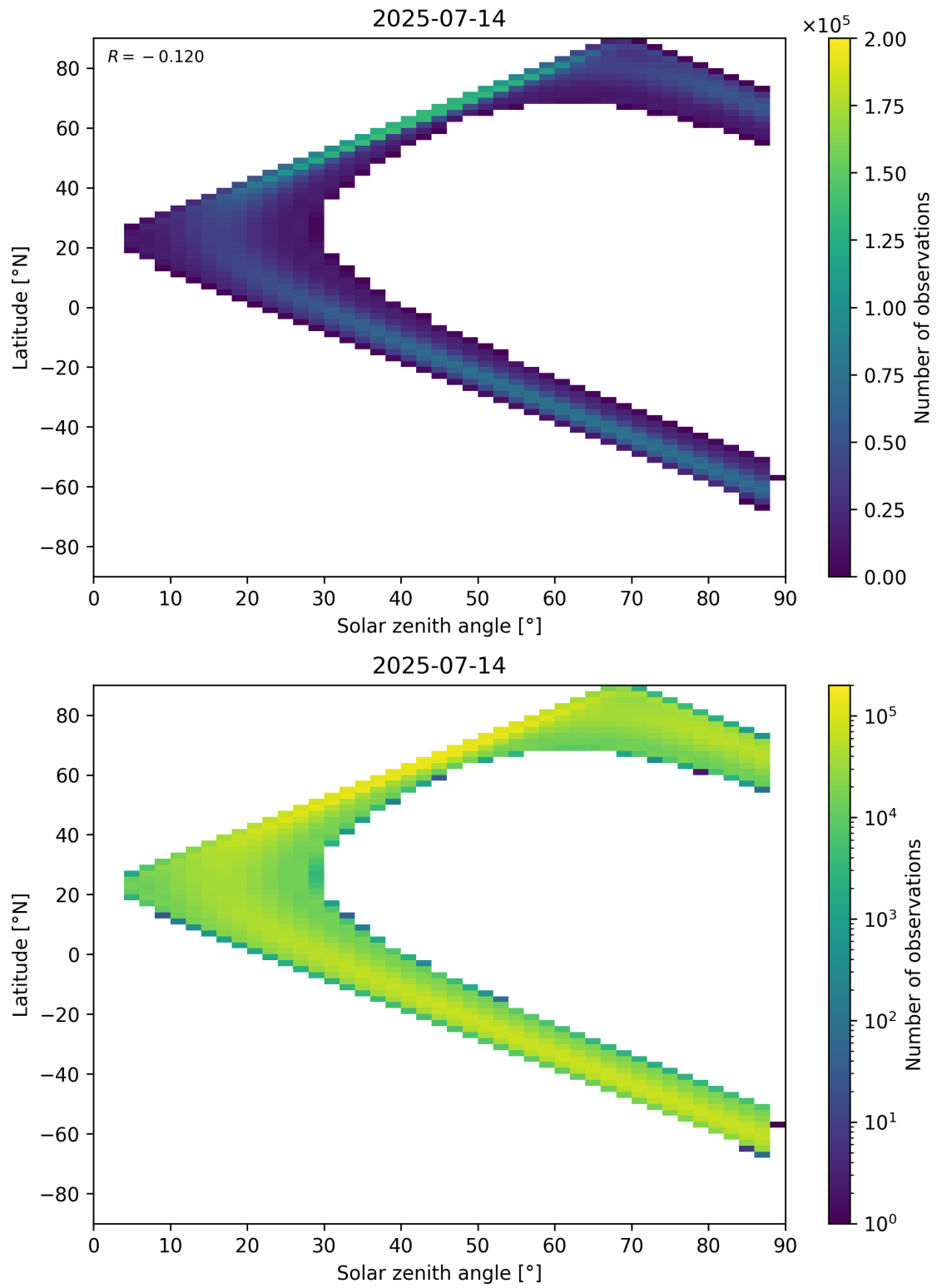
Figure 149: Scatter density plot of “Solar zenith angle” against “Latitude” for 2025-07-13 to 2025-07-15.
