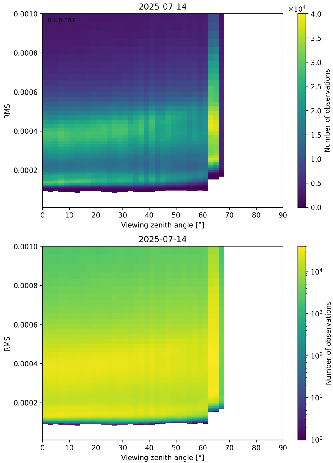
Figure 171: Scatter density plot of “Viewing zenith angle” against “RMS” for 2025-07-13 to 2025-07-15.
