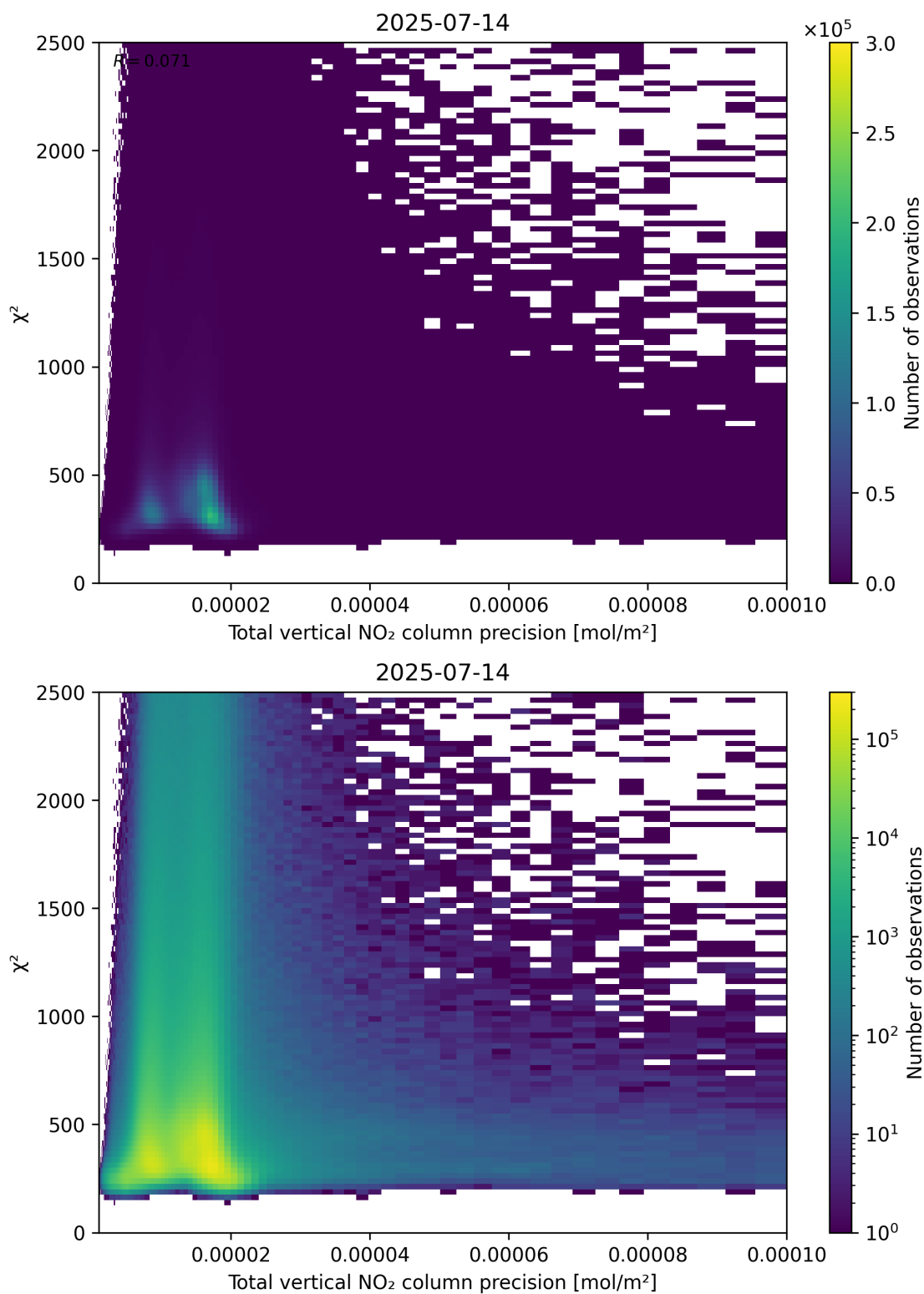
Figure 116: Scatter density plot of “Total vertical NO 2 column precision” against “ \chi^2 ” for 2025-07-13 to 2025-07-15.
