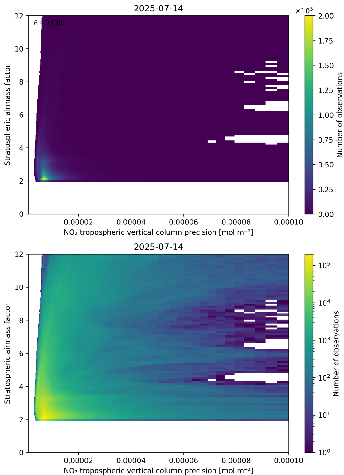
Figure 131: Scatter density plot of “NO 2 tropospheric vertical column precision” against “Stratospheric airmass factor” for 2025-07-13 to 2025-07-15.
