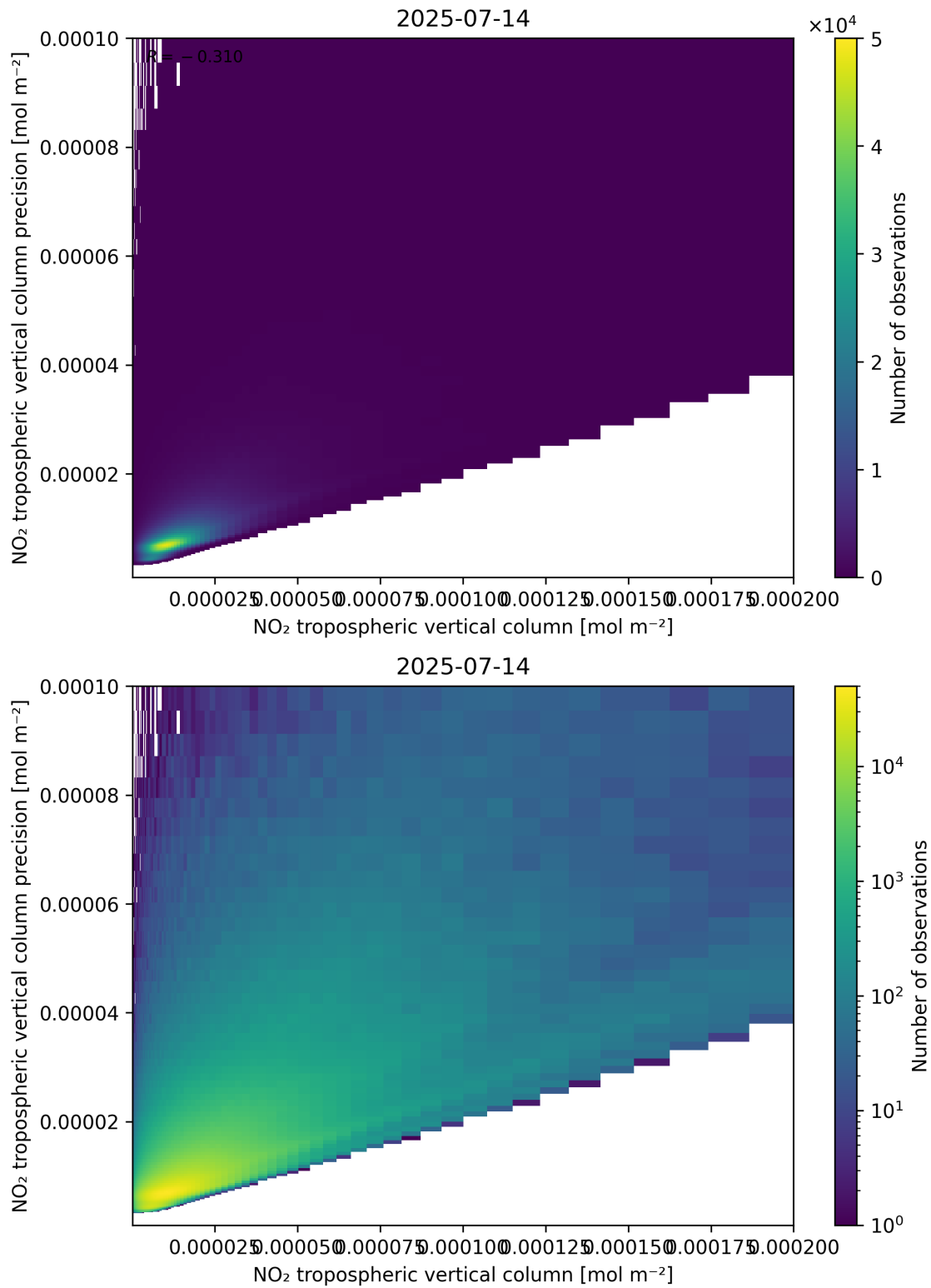
Figure 130: Scatter density plot of “NO 2 tropospheric vertical column” against “NO 2 tropospheric vertical column precision” for 2025-07-13 to 2025-07-15.
