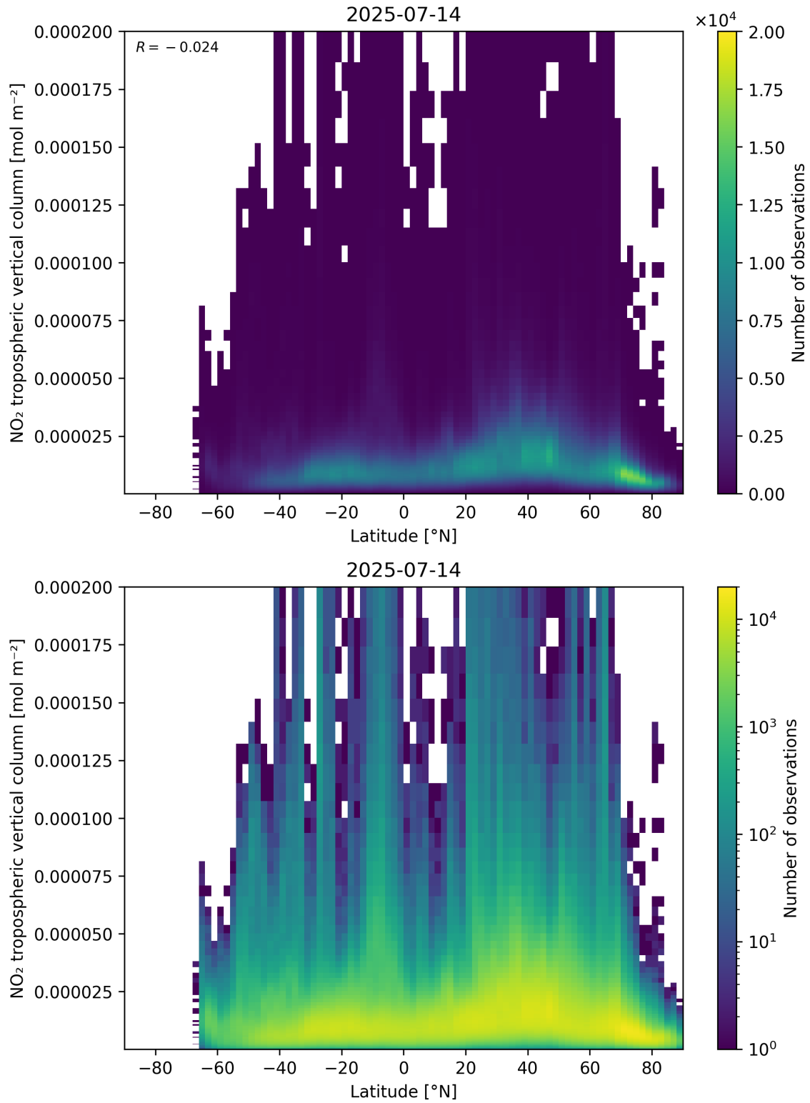
Figure 92: Scatter density plot of “Latitude” against “NO 2 tropospheric vertical column” for 2025-07-13 to 2025-07-15.
