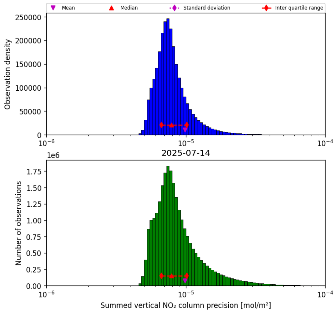
Figure 41: Histogram of "Summed vertical NO 2 column precision" for 2025-07-13 to 2025-07-15
