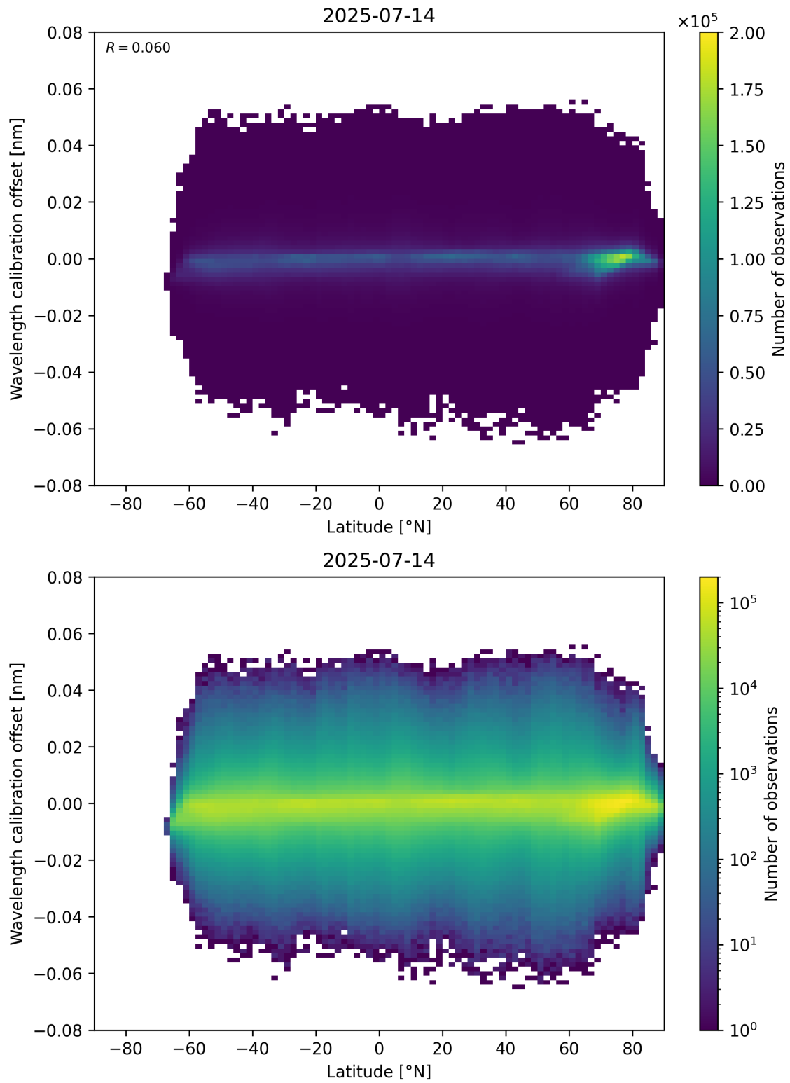
Figure 95: Scatter density plot of “Latitude” against “Wavelength calibration offset” for 2025-07-13 to 2025-07-15.
