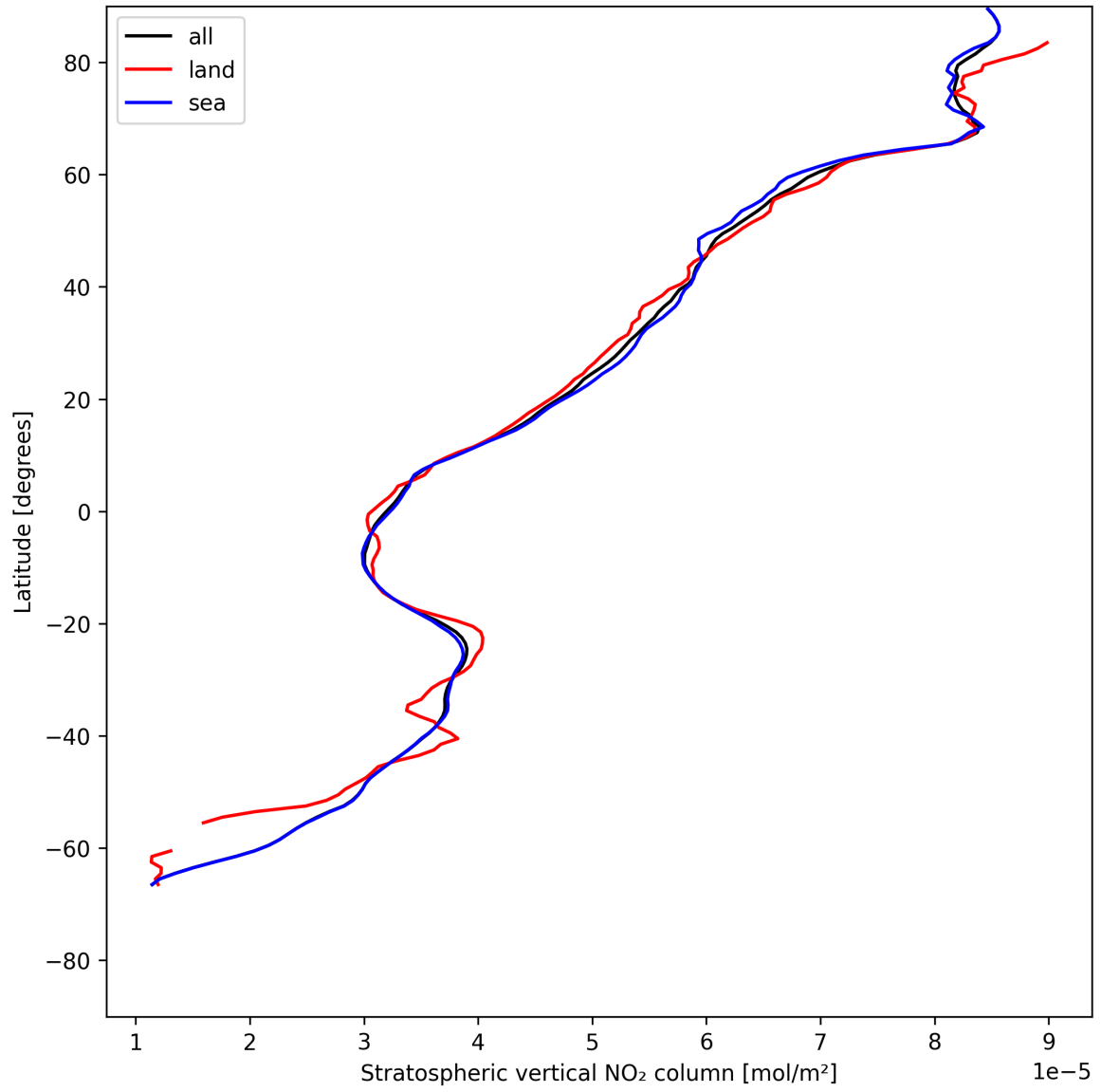
Figure 19: Zonal average of “Stratospheric vertical NO 2 column” for 2025-07-13 to 2025-07-15.
