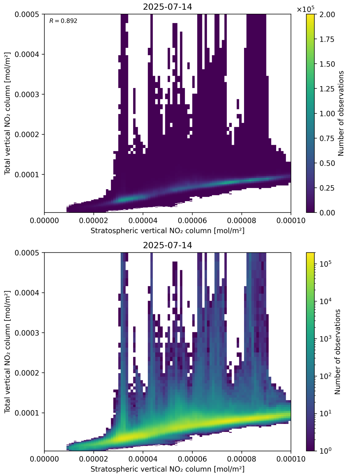
Figure 100: Scatter density plot of “Stratospheric vertical NO 2 column” against “Total vertical NO 2 column” for 2025-07-13 to 2025-07-15.
