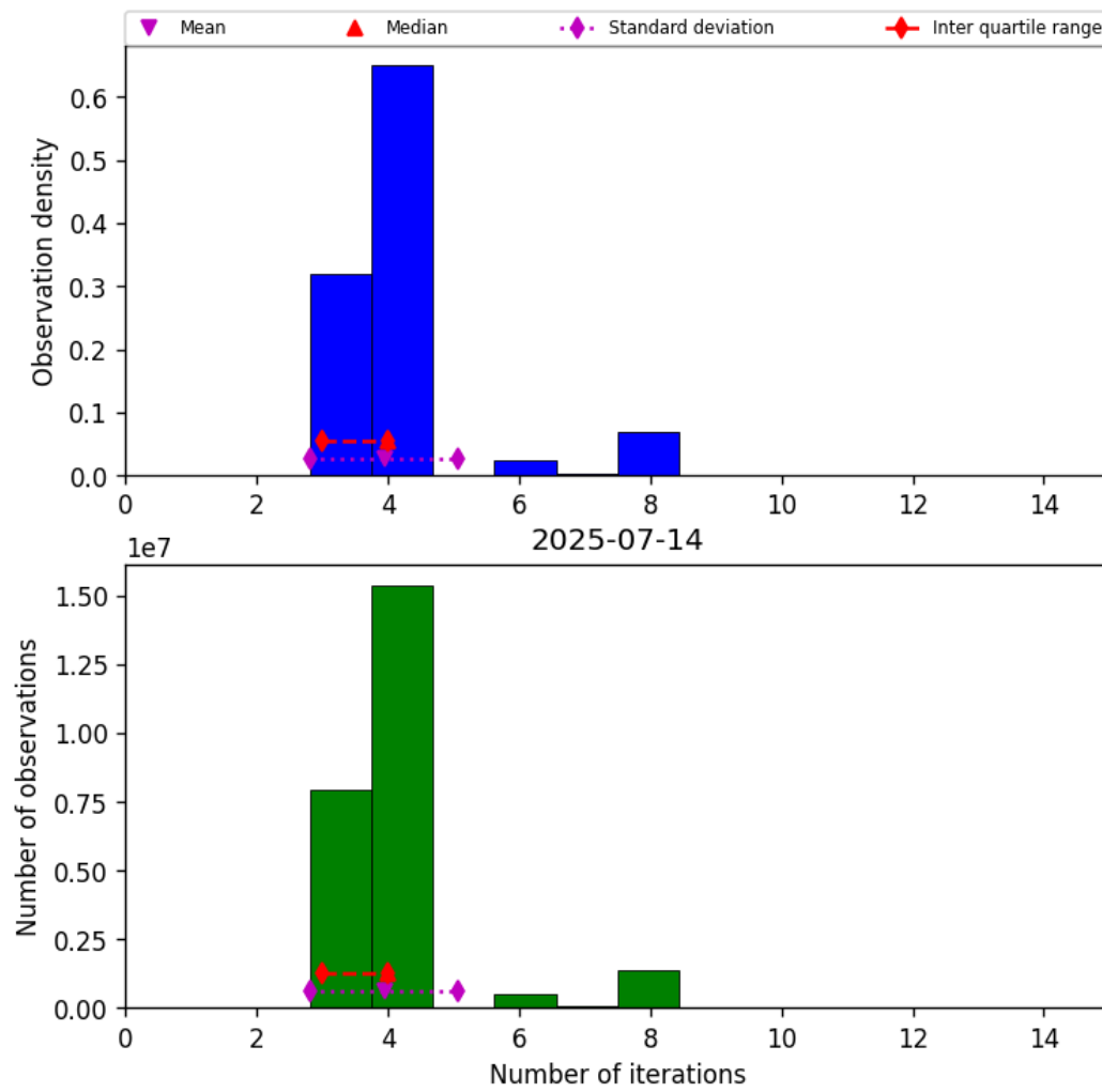
Figure 34: Histogram of “Number of iterations” for 2025-07-13 to 2025-07-15
