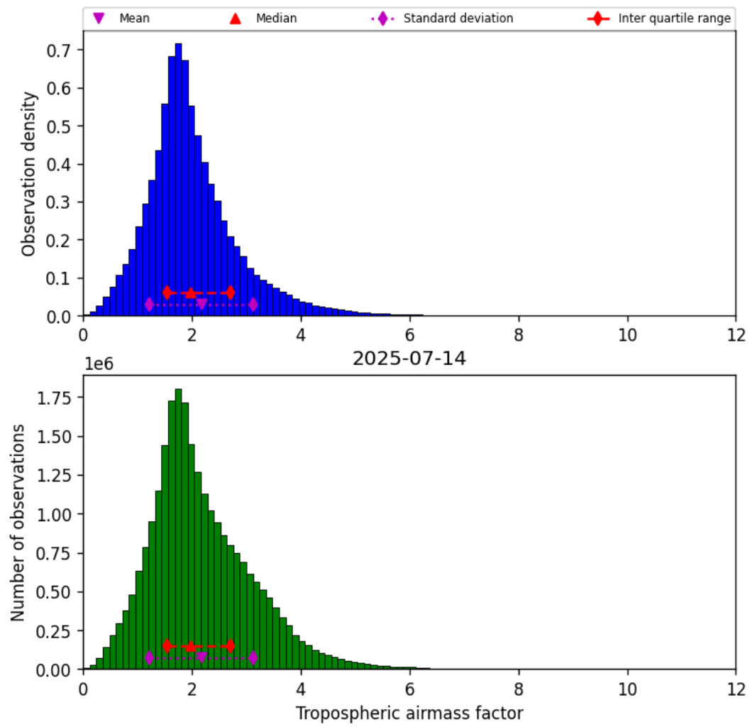
Figure 31: Histogram of “Tropospheric airmass factor” for 2025-07-13 to 2025-07-15
