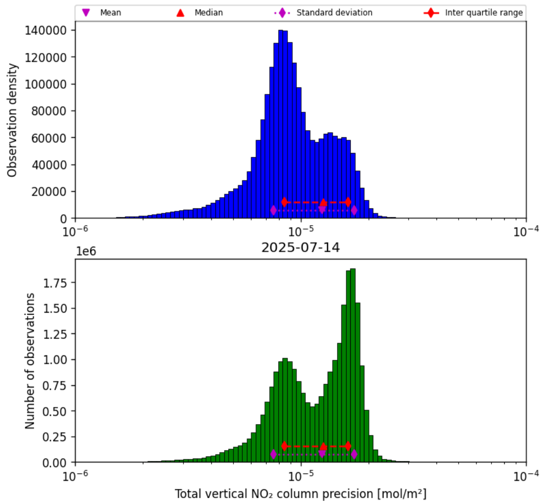
Figure 39: Histogram of “Total vertical NO 2 column precision” for 2025-07-13 to 2025-07-15
