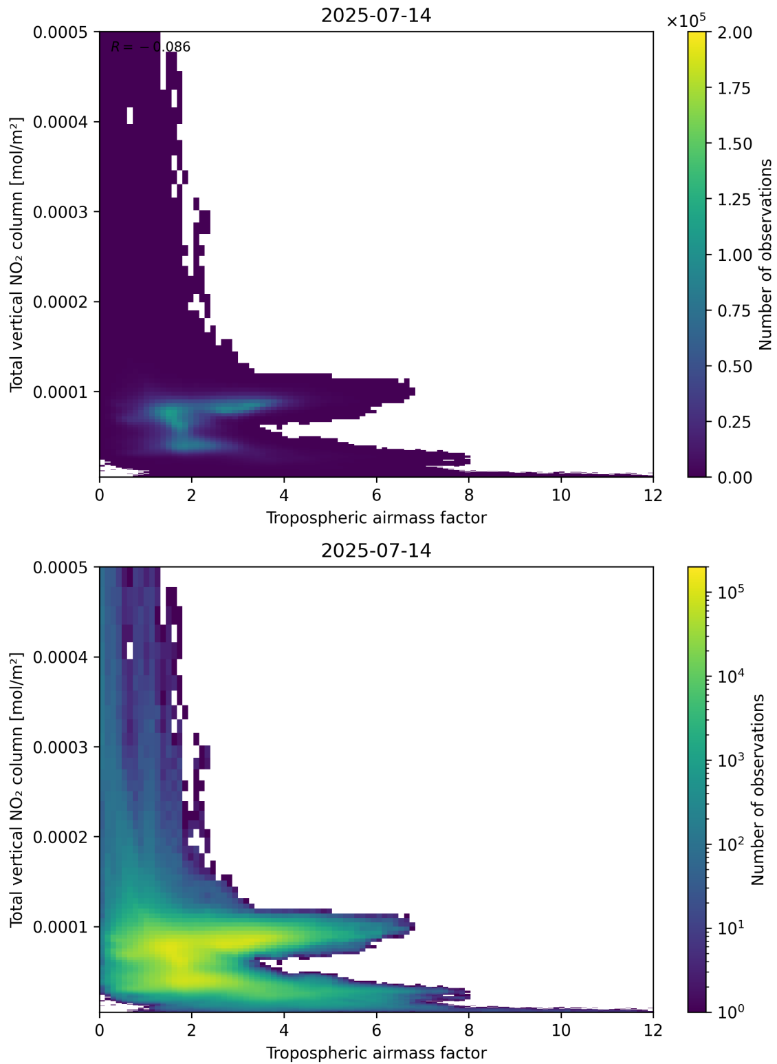
Figure 77: Scatter density plot of “Tropospheric airmass factor” against “Total vertical NO 2 column” for 2025-07-13 to 2025-07-15.
