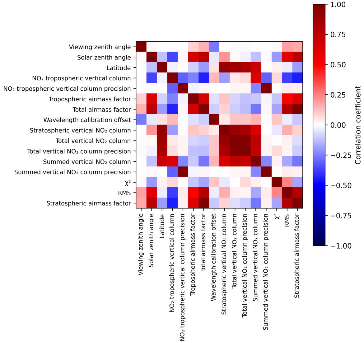
Figure 2: Map of correlation matrix for 2025-07-13 to 2025-07-15.
