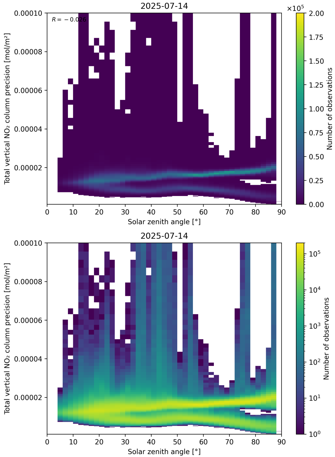
Figure 154: Scatter density plot of “Solar zenith angle” against “Total vertical NO 2 column precision” for 2025-07-13 to 2025-07-15.
