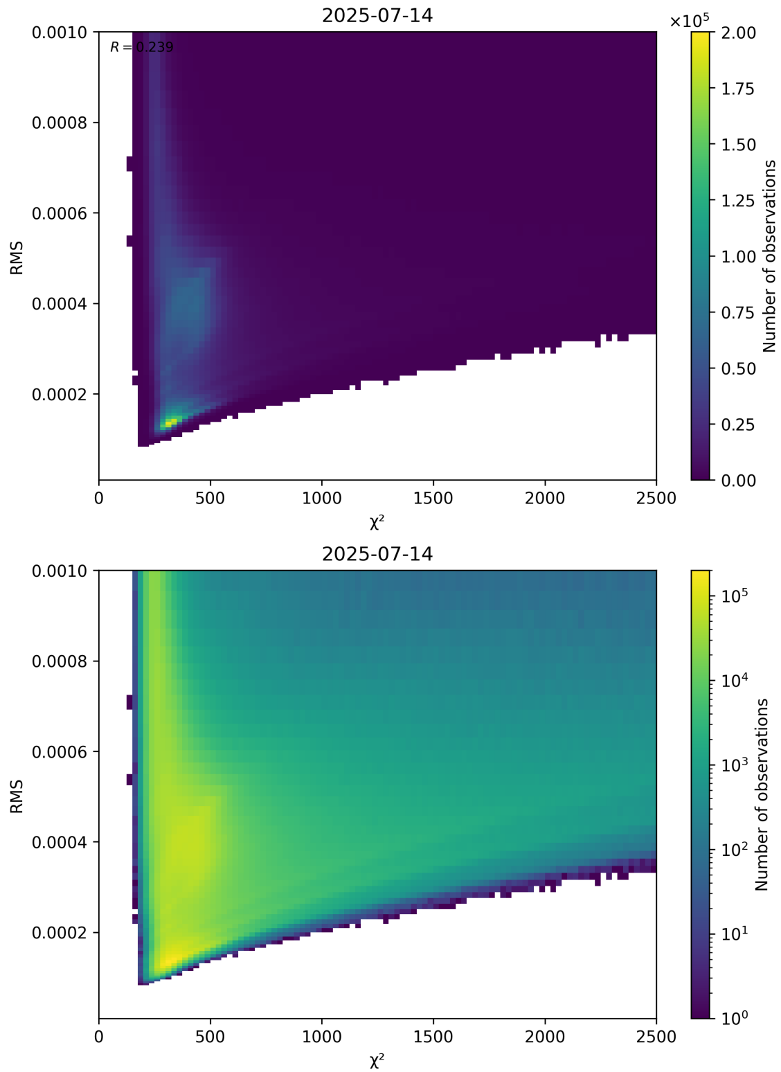
Figure 82: Scatter density plot of “ \chi^2 ” against “RMS” for 2025-07-13 to 2025-07-15.
