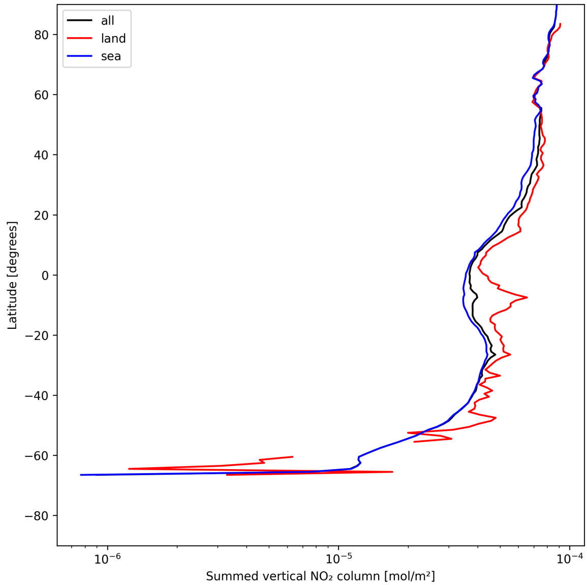
Figure 23: Zonal average of “Summed vertical NO 2 column” for 2025-07-13 to 2025-07-15.
