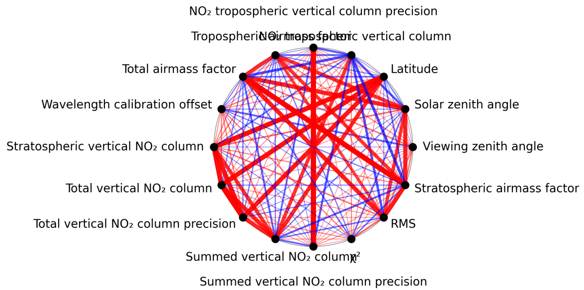
Figure 1: Map of correlation graph for 2025-07-13 to 2025-07-15.
