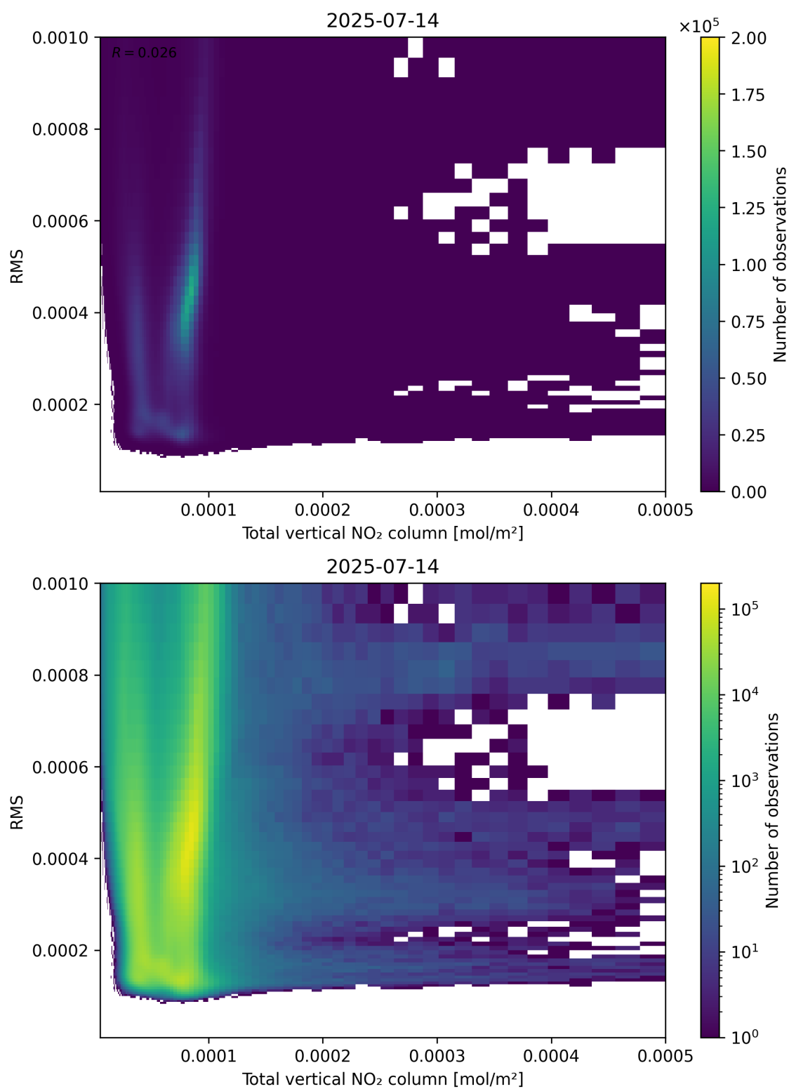
Figure 120: Scatter density plot of “Total vertical NO 2 column” against “RMS” for 2025-07-13 to 2025-07-15.
