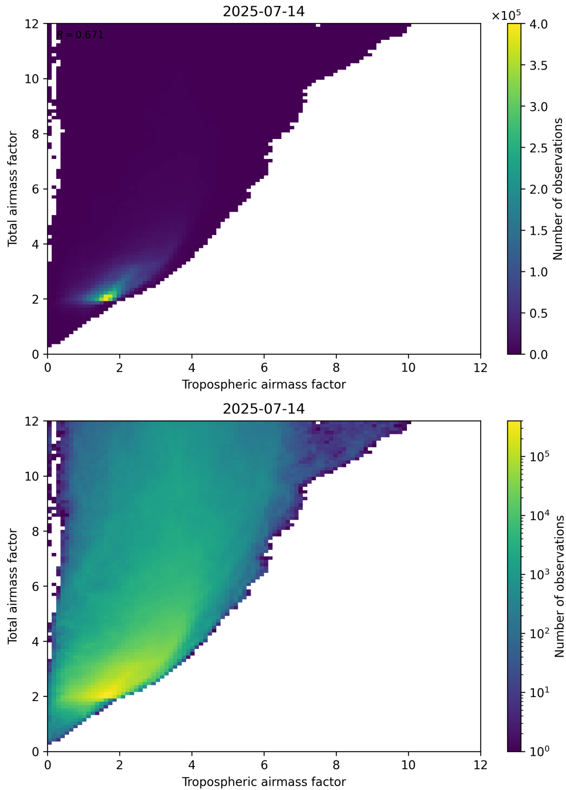
Figure 72: Scatter density plot of “Tropospheric airmass factor” against “Total airmass factor” for 2025-07-13 to 2025-07-15.
