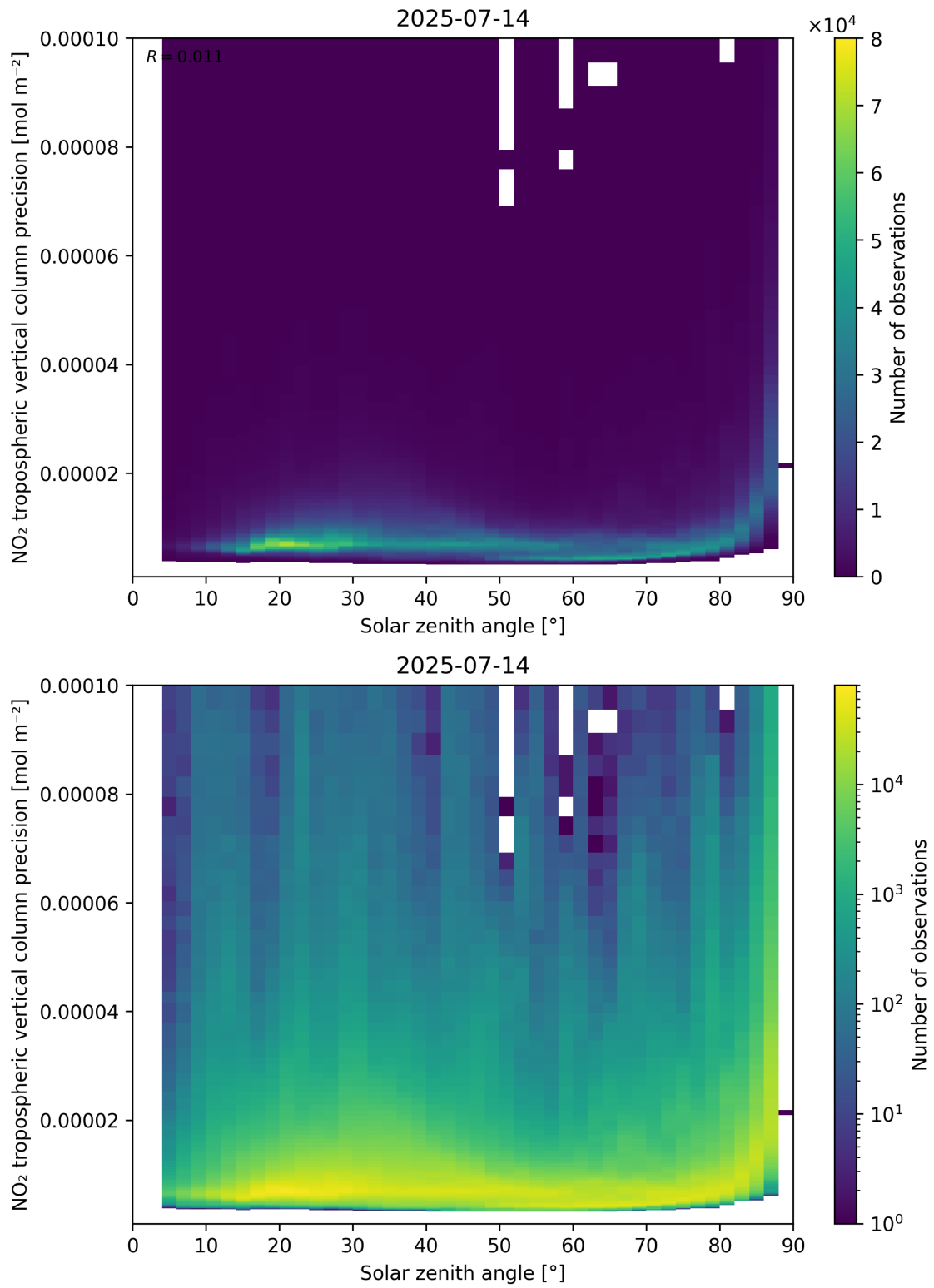
Figure 156: Scatter density plot of “Solar zenith angle” against “NO 2 tropospheric vertical column precision” for 2025-07-13 to 2025-07-15.
