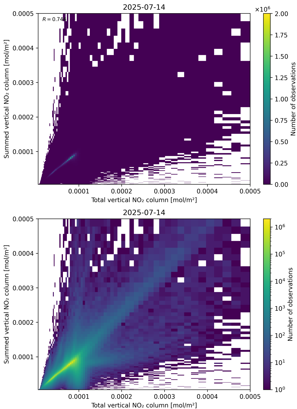
Figure 112: Scatter density plot of “Total vertical NO 2 column” against “Summed vertical NO 2 column” for 2025-07-13 to 2025-07-15.
