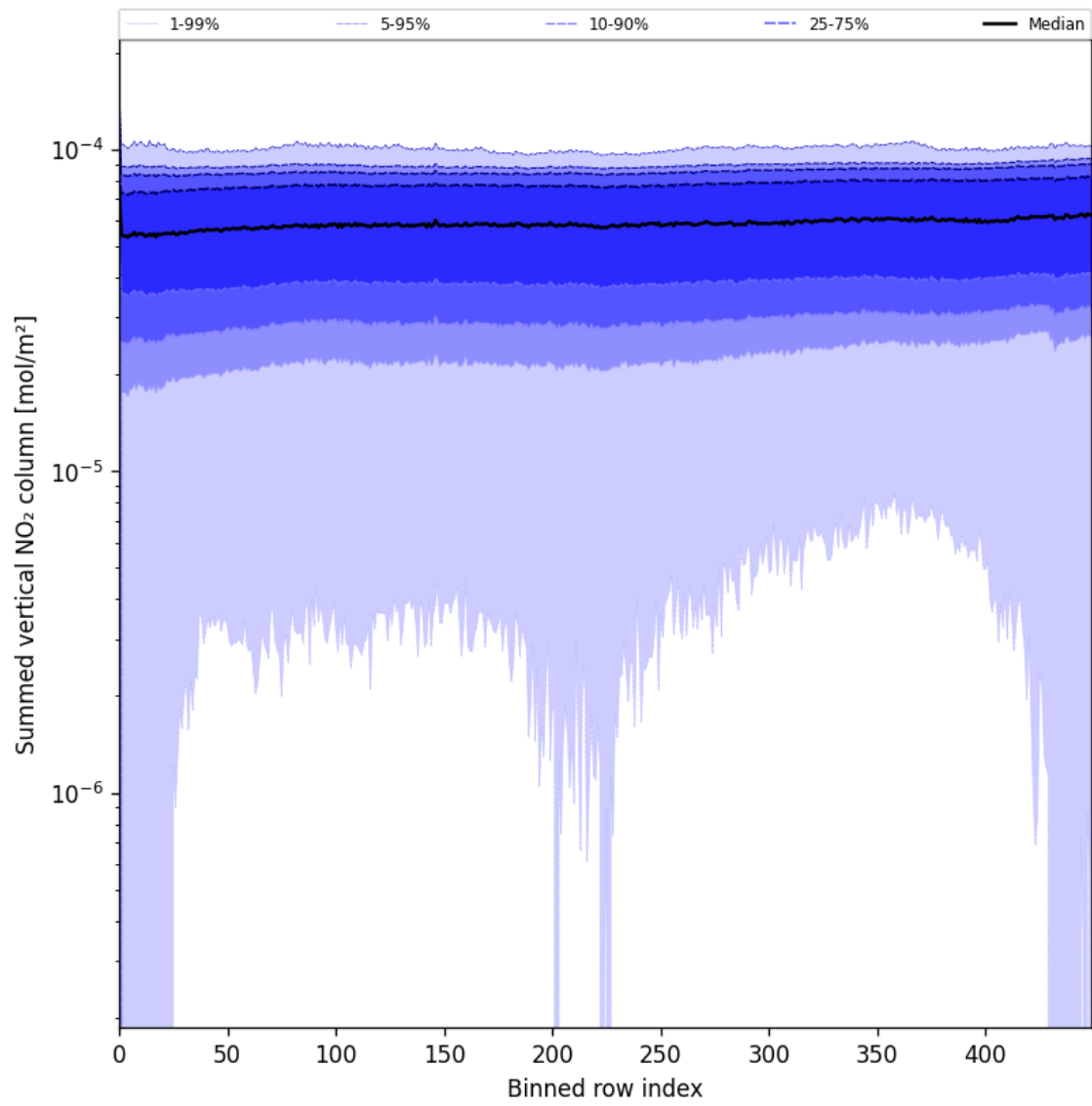
Figure 57: Along track statistics of “Summed vertical NO 2 column” for 2025-07-13 to 2025-07-15
