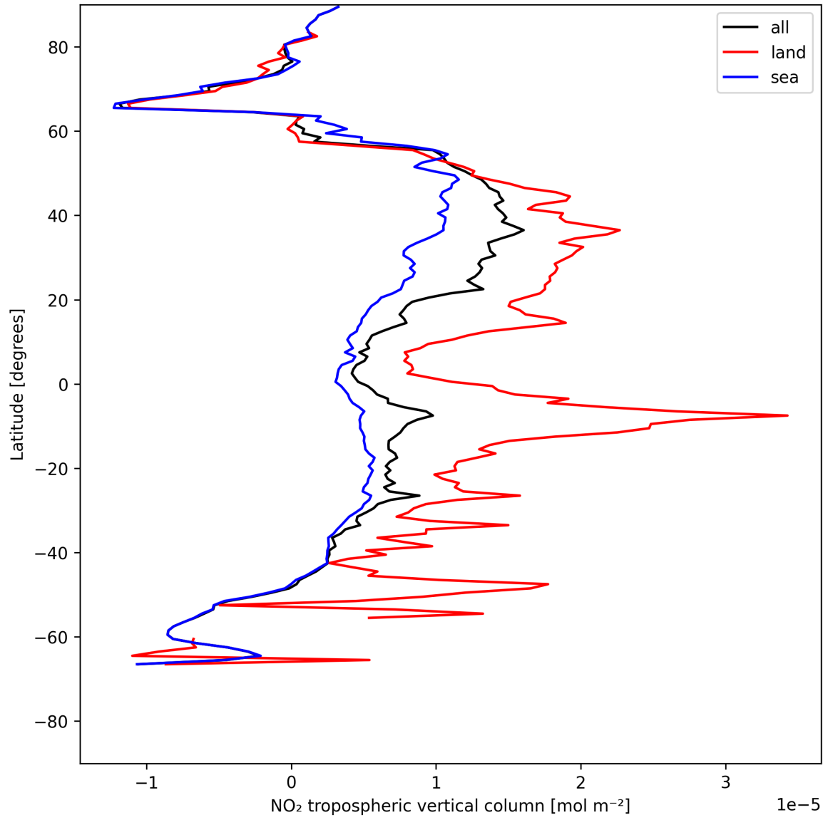
Figure 12: Zonal average of “NO 2 tropospheric vertical column” for 2025-07-13 to 2025-07-15.
