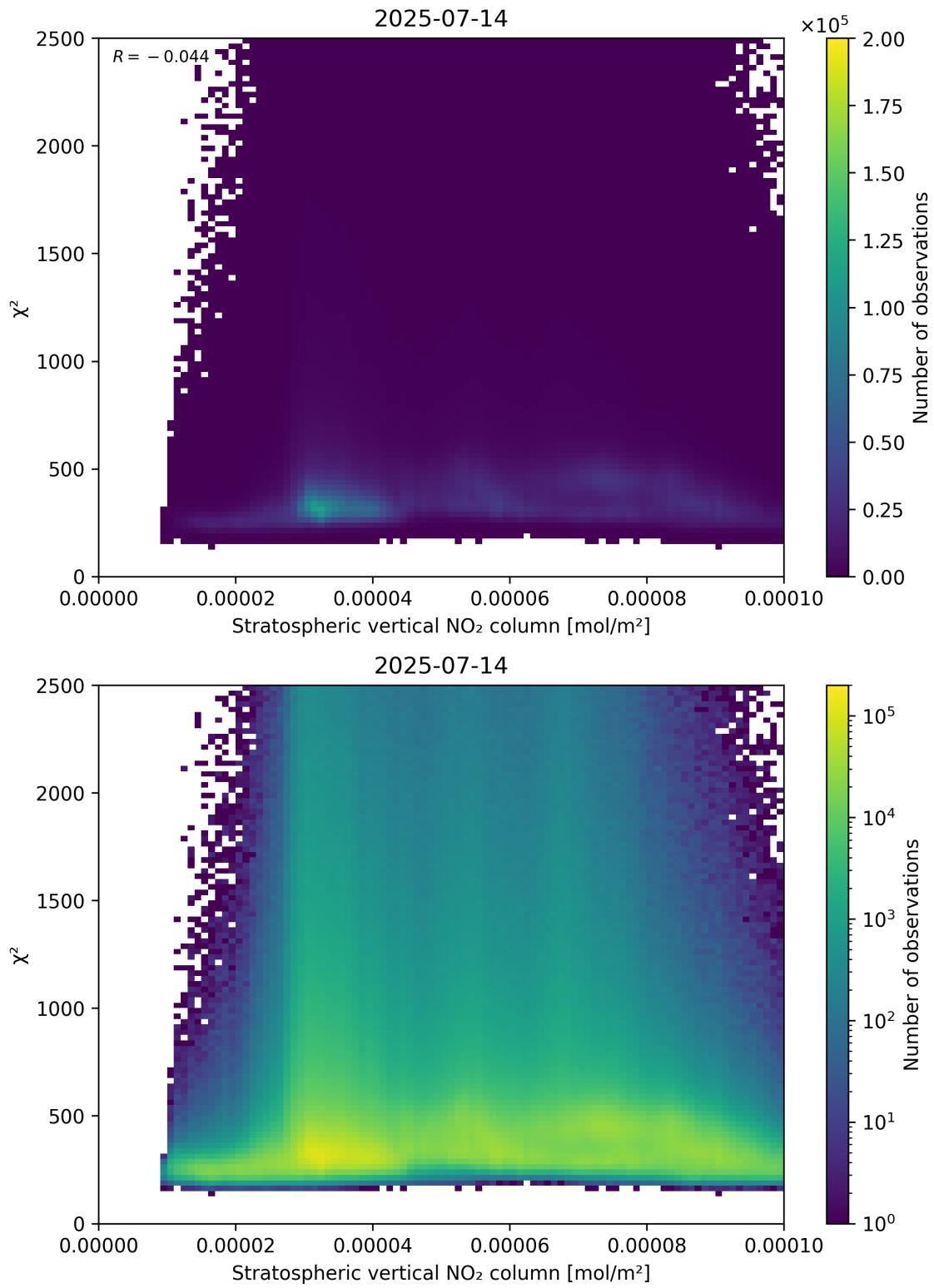
Figure 97: Scatter density plot of “Stratospheric vertical NO 2 column” against “ \chi^2 ” for 2025-07-13 to 2025-07-15.
