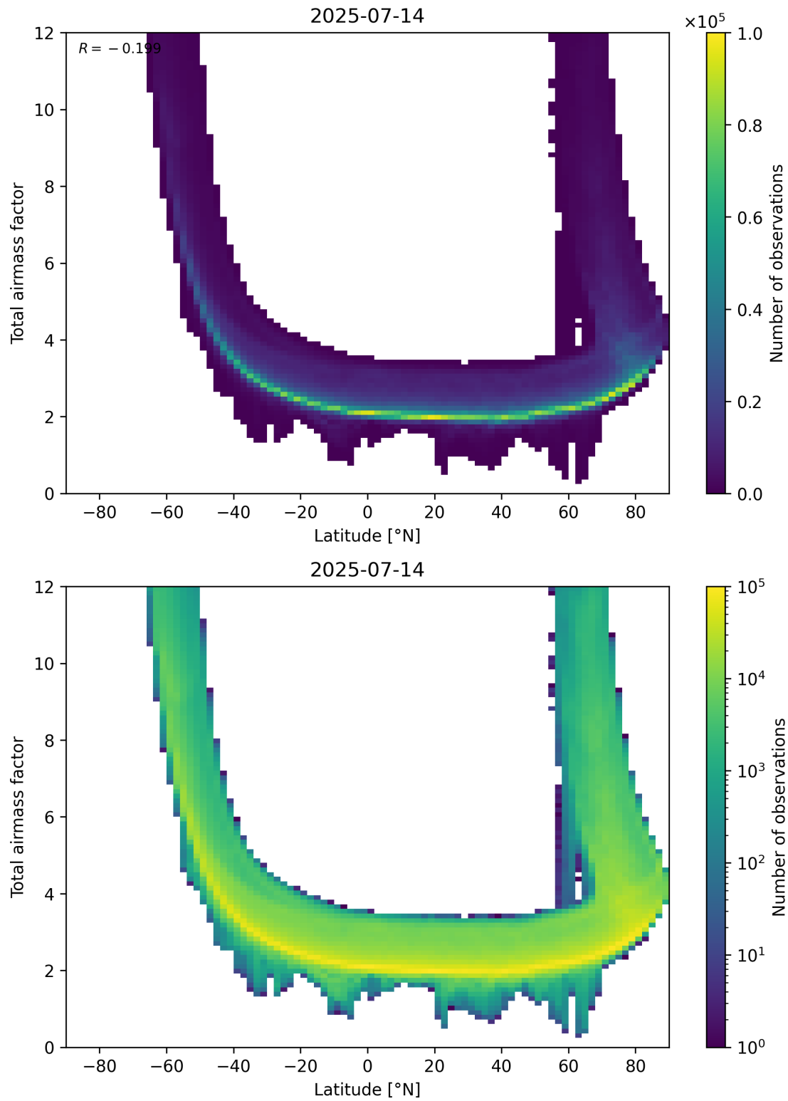
Figure 84: Scatter density plot of “Latitude” against “Total airmass factor” for 2025-07-13 to 2025-07-15.
