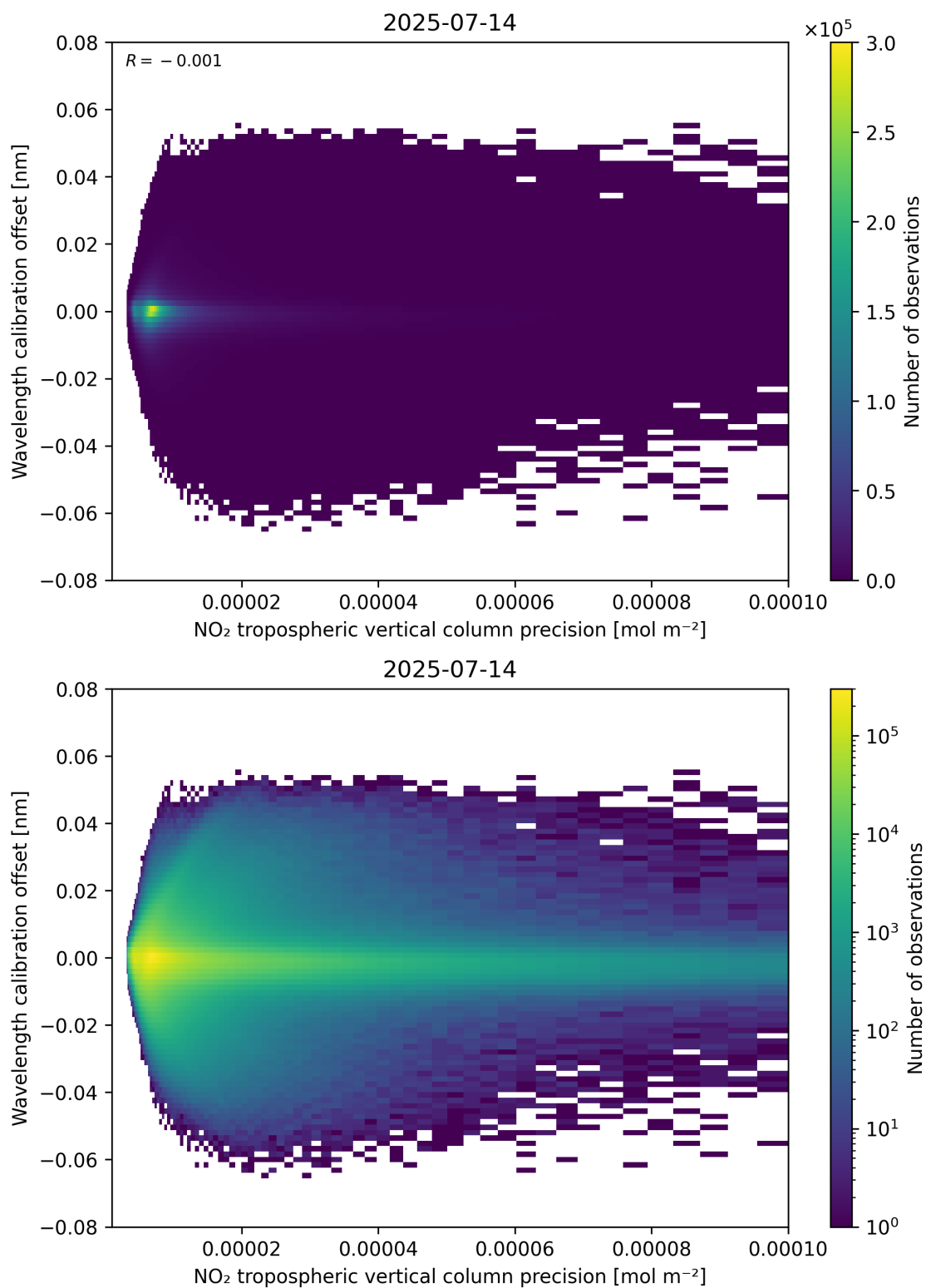
Figure 141: Scatter density plot of “NO 2 tropospheric vertical column precision” against “Wavelength calibration offset” for 2025-07-13 to 2025-07-15.
