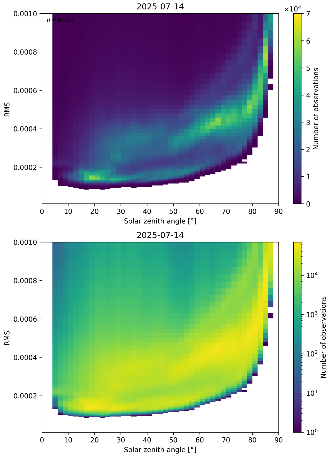
Figure 157: Scatter density plot of “Solar zenith angle” against “RMS” for 2025-07-13 to 2025-07-15.
