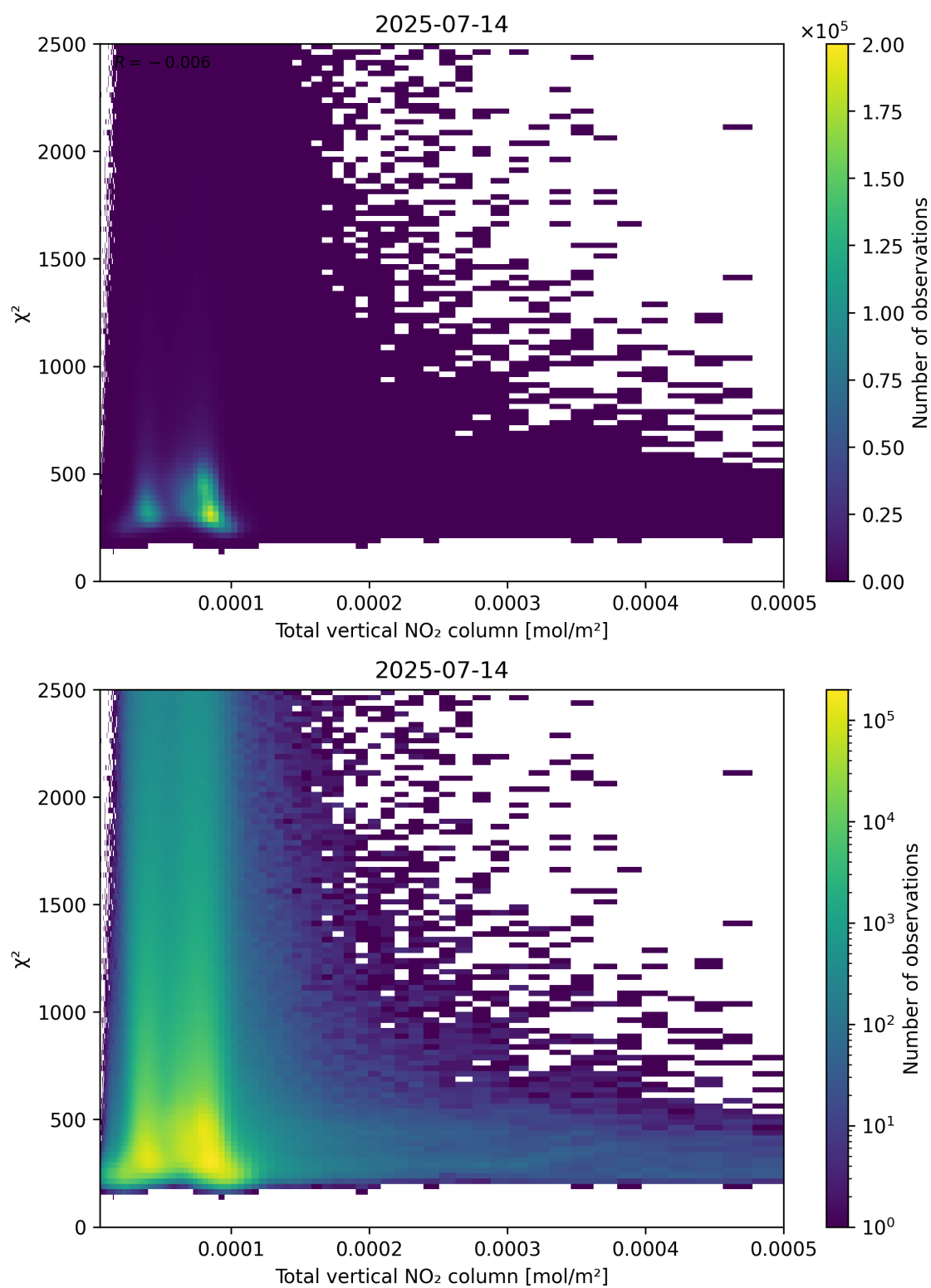
Figure 111: Scatter density plot of “Total vertical NO 2 column” against “ \chi^2 ” for 2025-07-13 to 2025-07-15.
