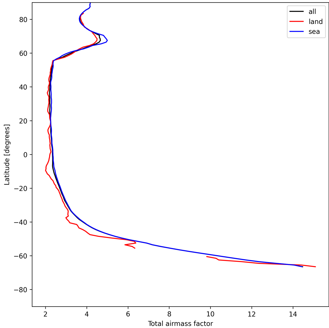
Figure 15: Zonal average of “Total airmass factor” for 2025-07-13 to 2025-07-15.
