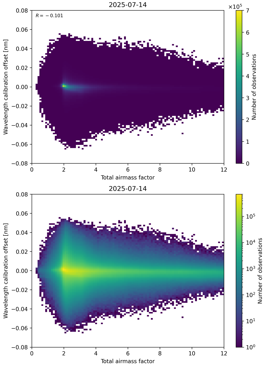
Figure 70: Scatter density plot of “Total airmass factor” against “Wavelength calibration offset” for 2025-07-13 to 2025-07-15.
