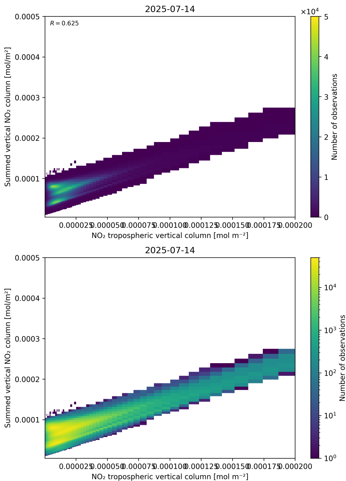
Figure 126: Scatter density plot of “NO 2 tropospheric vertical column” against “Summed vertical NO 2 column” for 2025-07-13 to 2025-07-15.
