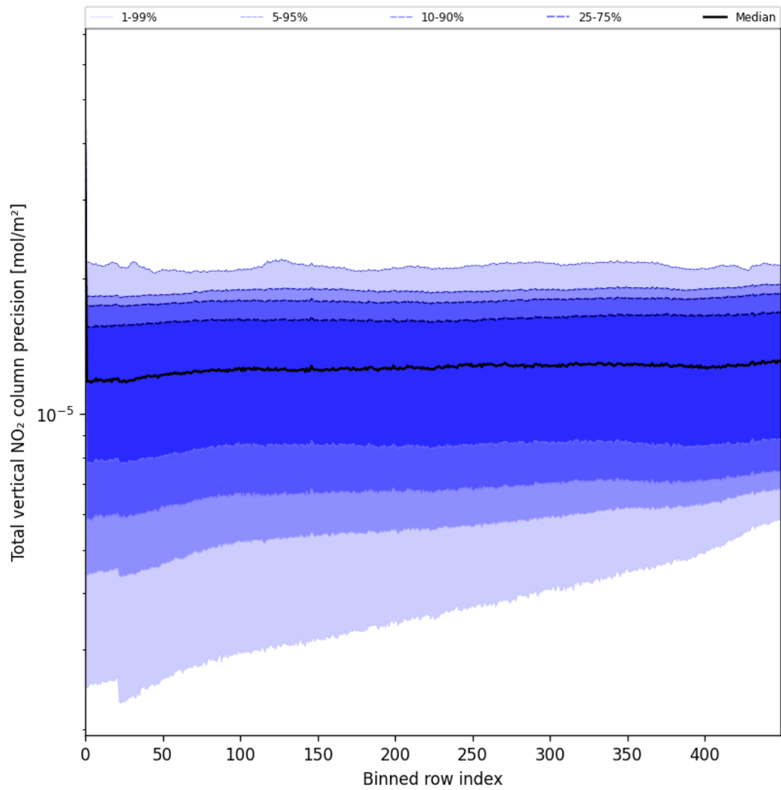
Figure 56: Along track statistics of “Total vertical NO 2 column precision” for 2025-07-13 to 2025-07-15
