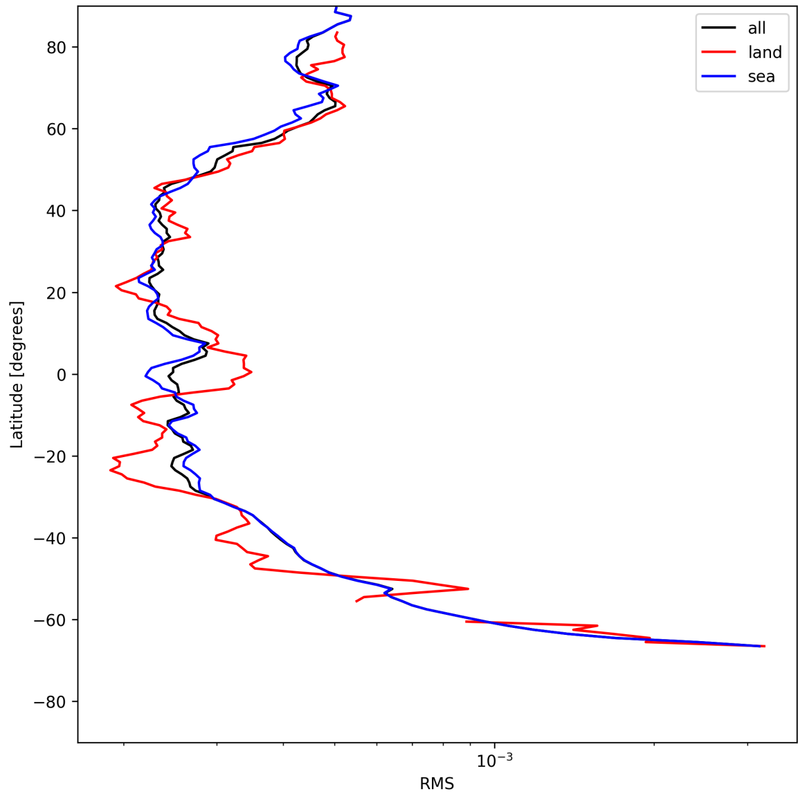
Figure 26: Zonal average of “RMS” for 2025-07-13 to 2025-07-15.
