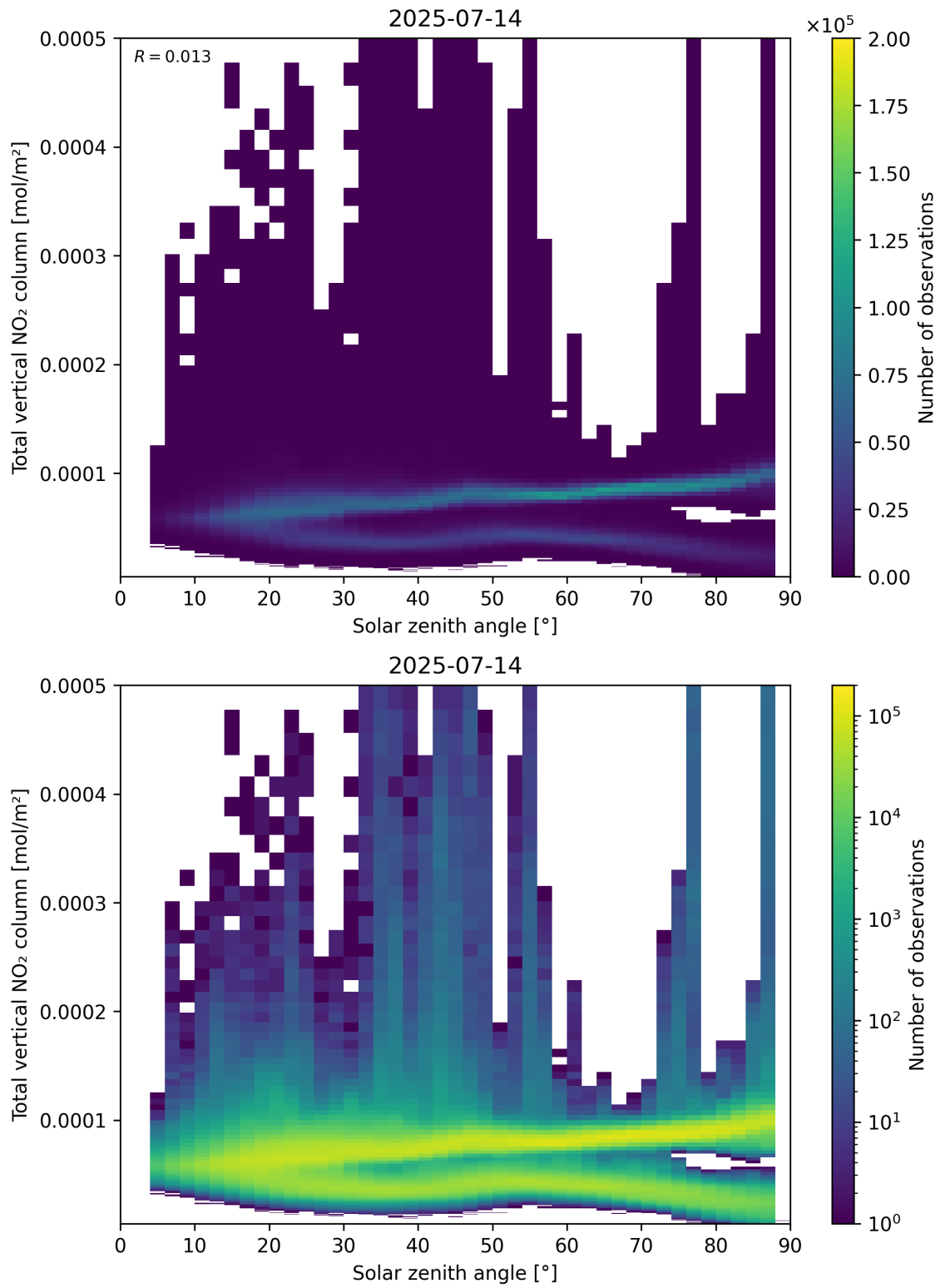
Figure 153: Scatter density plot of “Solar zenith angle” against “Total vertical NO 2 column” for 2025-07-13 to 2025-07-15.
