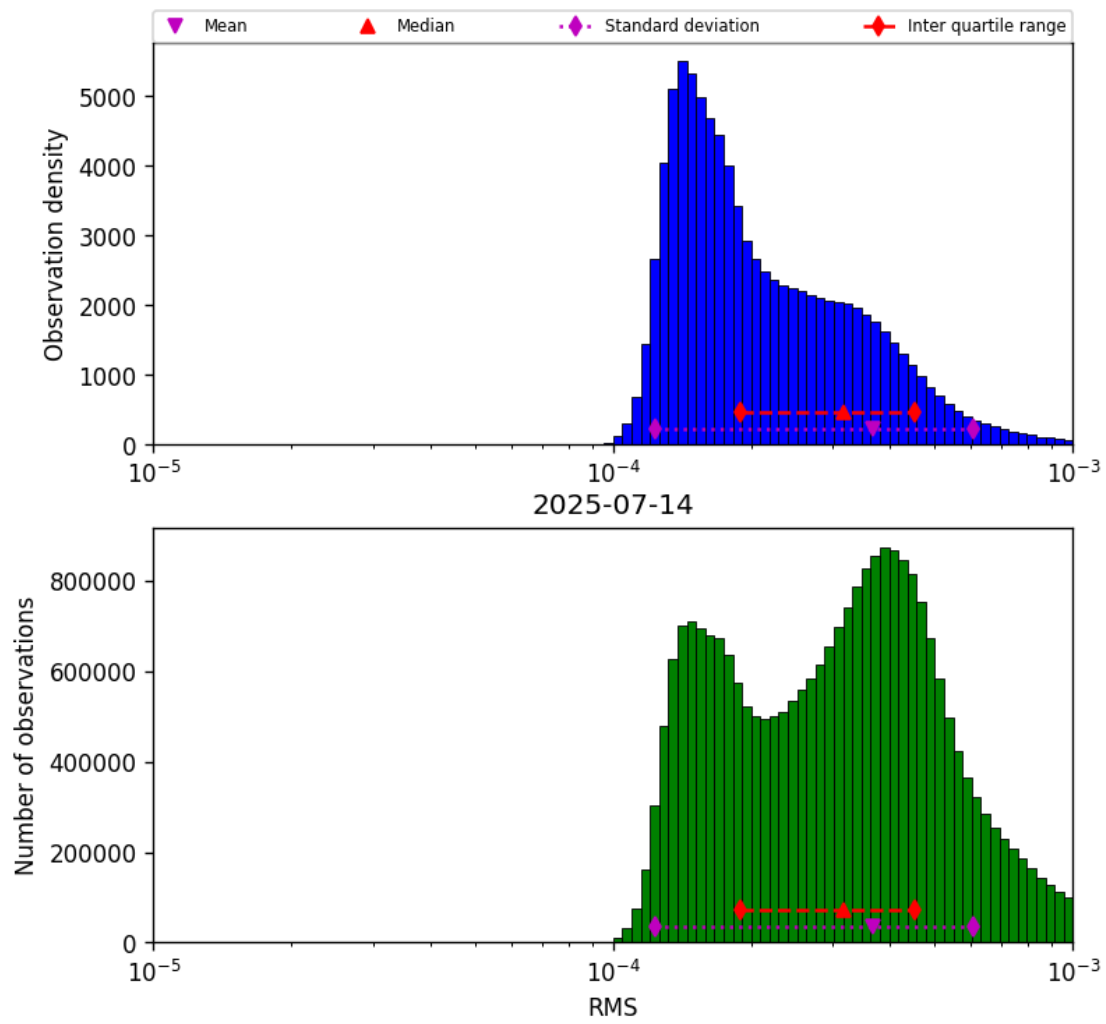
Figure 43: Histogram of “RMS” for 2025-07-13 to 2025-07-15
