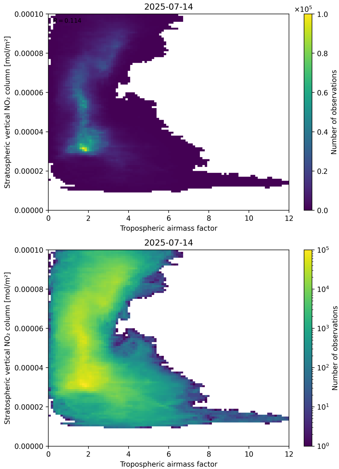
Figure 74: Scatter density plot of “Tropospheric air mass factor” against “Stratospheric vertical NO 2 column” for 2025-07-13 to 2025-07-15.
