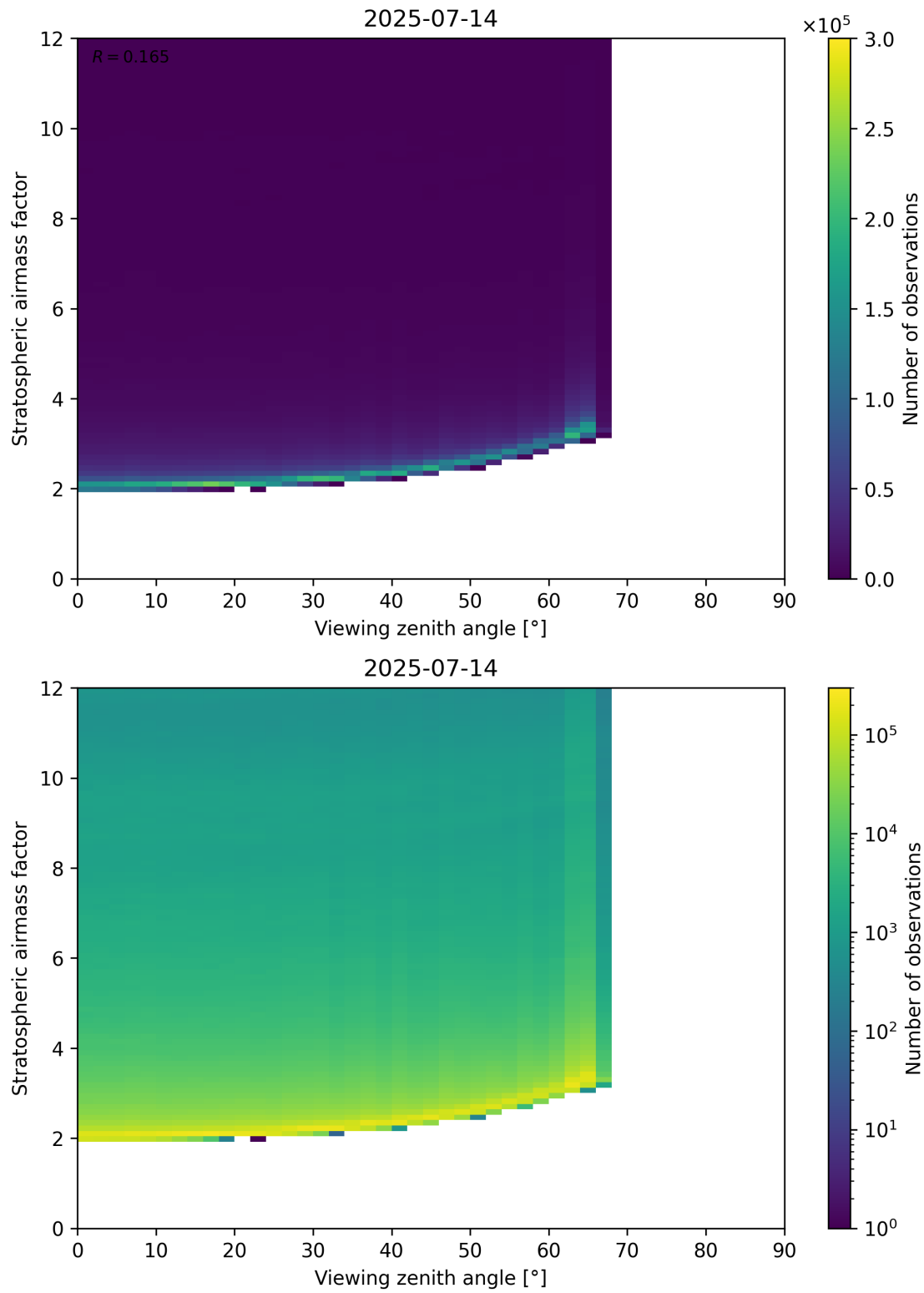
Figure 159: Scatter density plot of “Viewing zenith angle” against “Stratospheric airmass factor” for 2025-07-13 to 2025-07-15.
