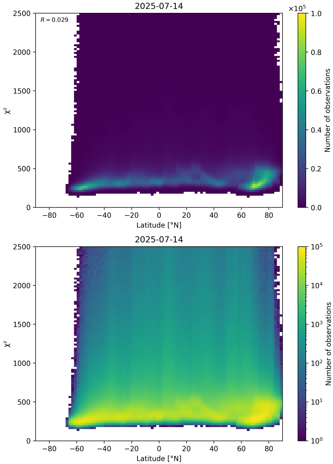
Figure 86: Scatter density plot of “Latitude” against “ \chi^2 ” for 2025-07-13 to 2025-07-15.
