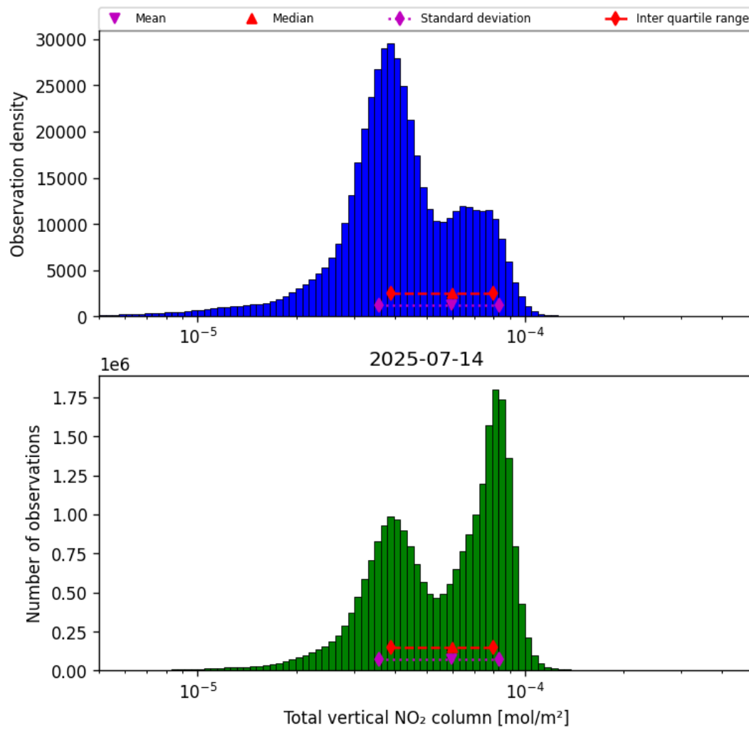
Figure 38: Histogram of “Total vertical NO 2 column” for 2025-07-13 to 2025-07-15
