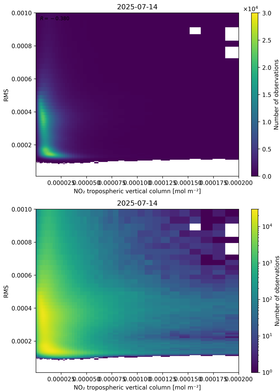
Figure 142: Scatter density plot of “NO 2 tropospheric vertical column” against “RMS” for 2025-07-13 to 2025-07-15.
