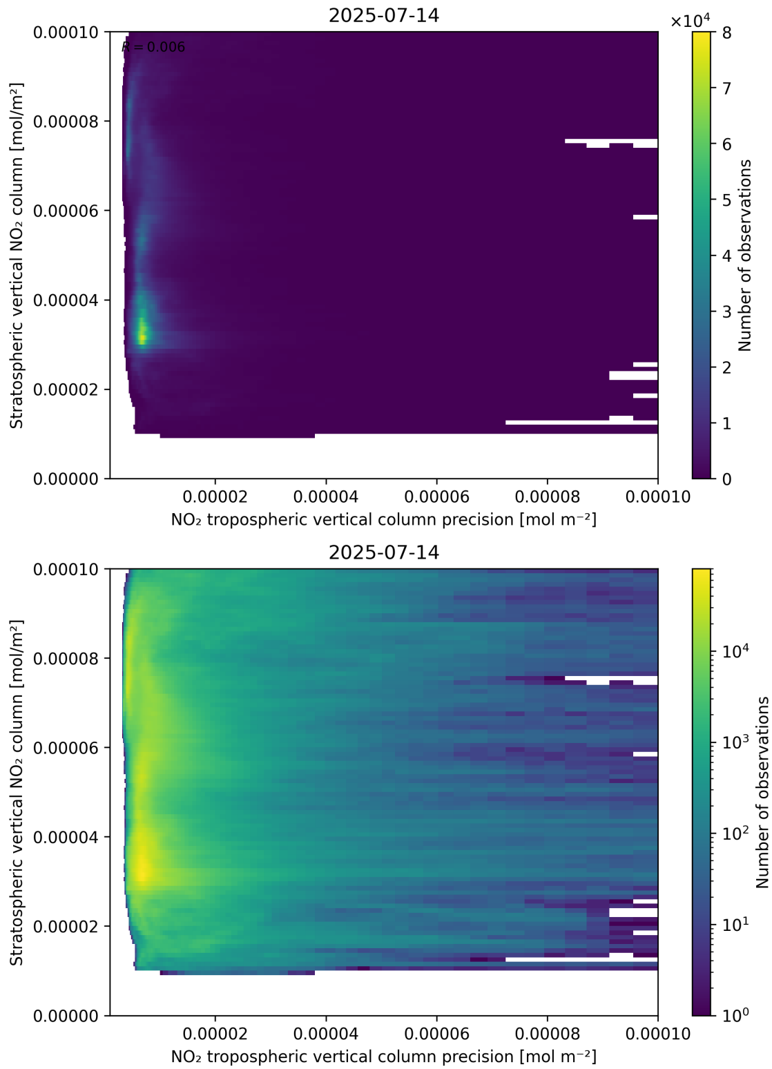
Figure 135: Scatter density plot of “NO 2 tropospheric vertical column precision” against “Stratospheric vertical NO 2 column” for 2025-07-13 to 2025-07-15.
