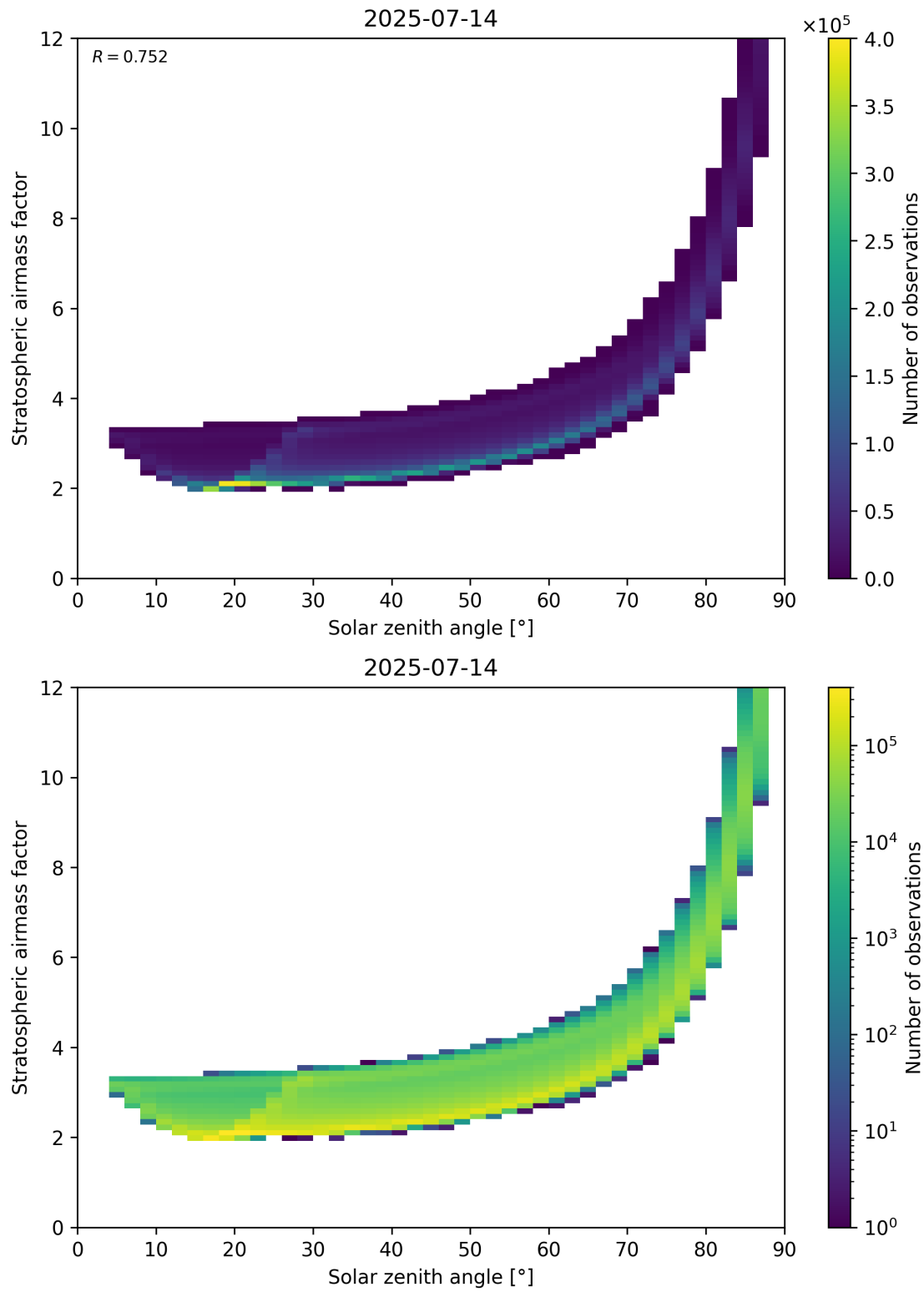
Figure 145: Scatter density plot of “Solar zenith angle” against “Stratospheric airmass factor” for 2025-07-13 to 2025-07-15.
