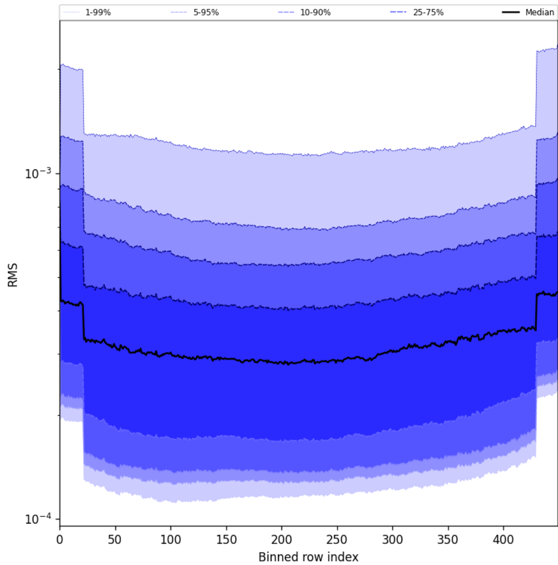
Figure 60: Along track statistics of “RMS” for 2025-07-13 to 2025-07-15
