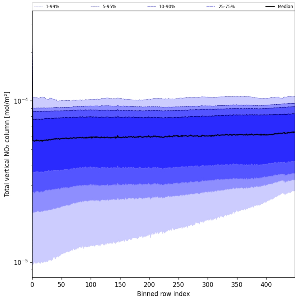
Figure 55: Along track statistics of “Total vertical NO 2 column” for 2025-07-13 to 2025-07-15
