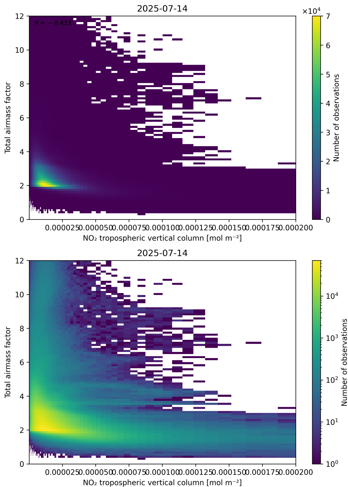
Figure 122: Scatter density plot of “NO 2 tropospheric vertical column” against “Total air mass factor” for 2025-07-13 to 2025-07-15.
