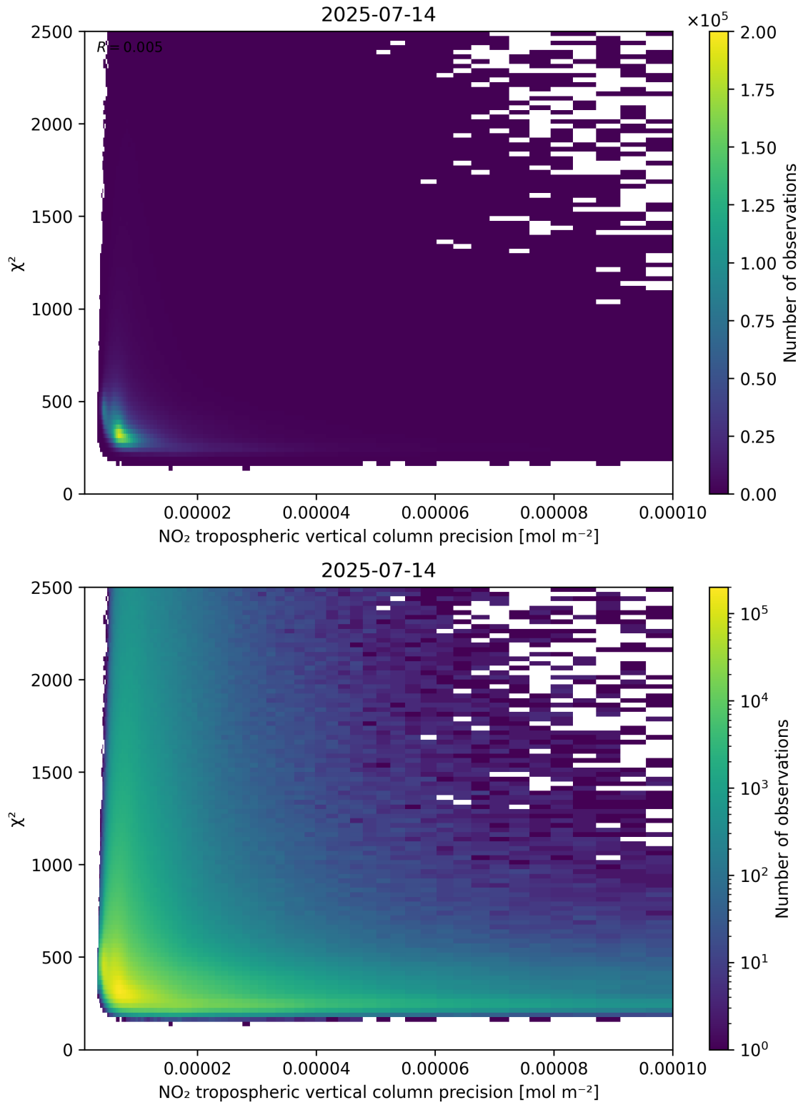
Figure 134: Scatter density plot of “NO 2 tropospheric vertical column precision” against “ \chi^2 ” for 2025-07-13 to 2025-07-15.
