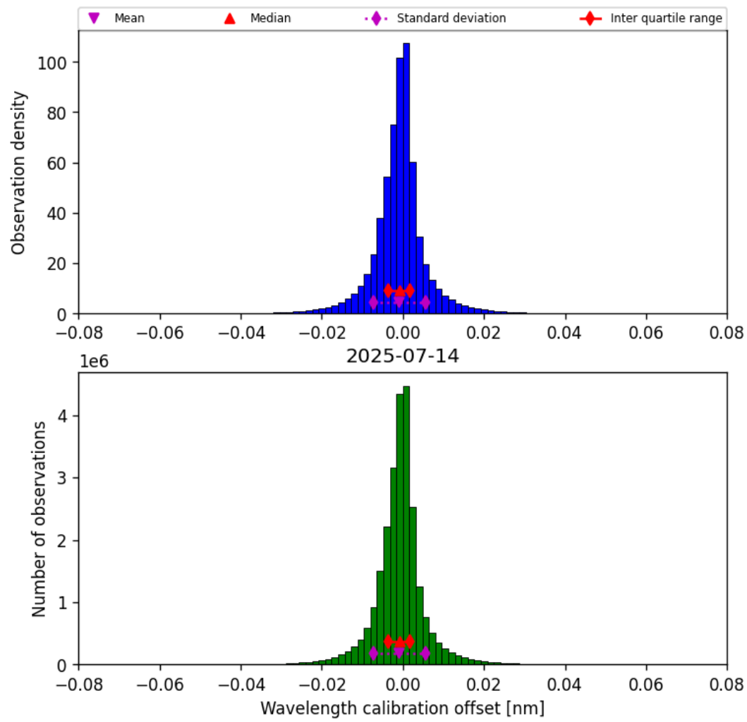
Figure 35: Histogram of “Wavelength calibration offset” for 2025-07-13 to 2025-07-15
