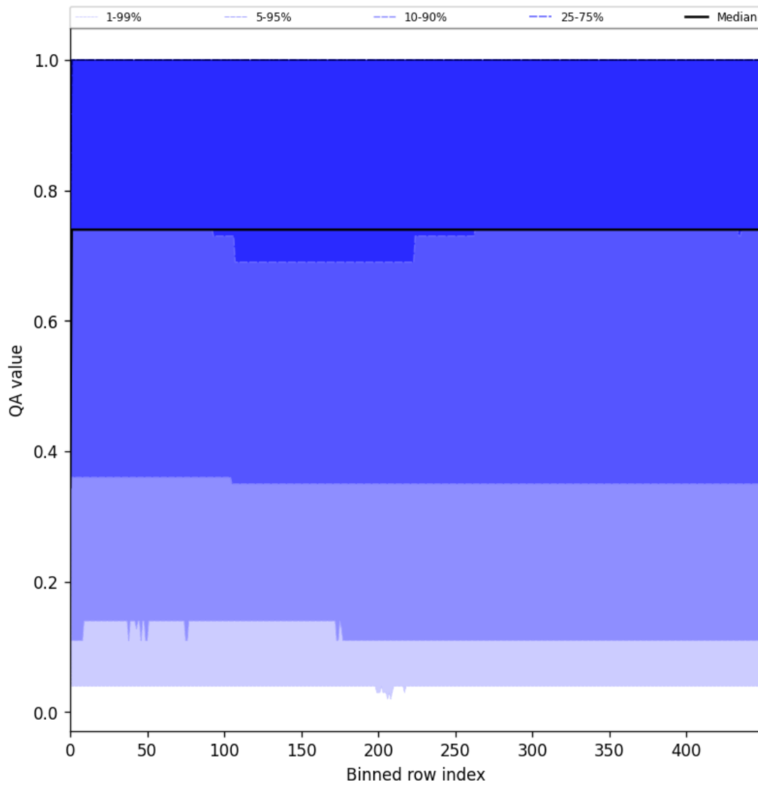
Figure 45: Along track statistics of “QA value” for 2025-07-13 to 2025-07-15
