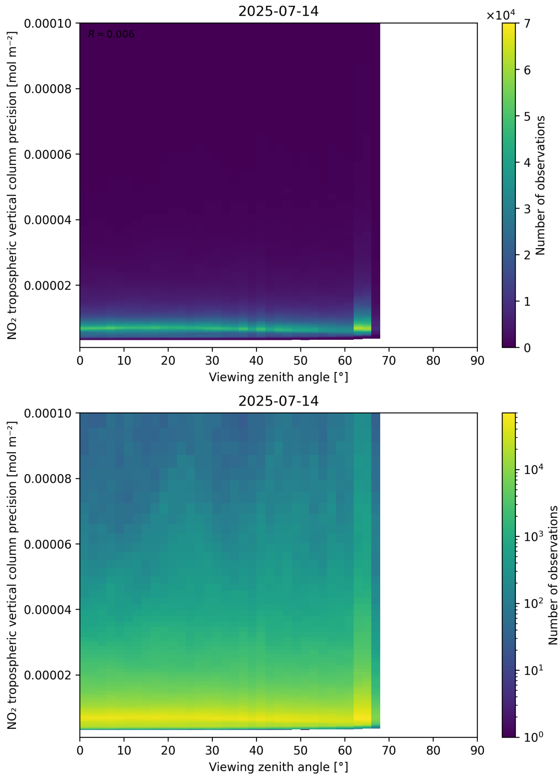
Figure 170: Scatter density plot of “Viewing zenith angle” against “NO 2 tropospheric vertical column precision” for 2025-07-13 to 2025-07-15.
