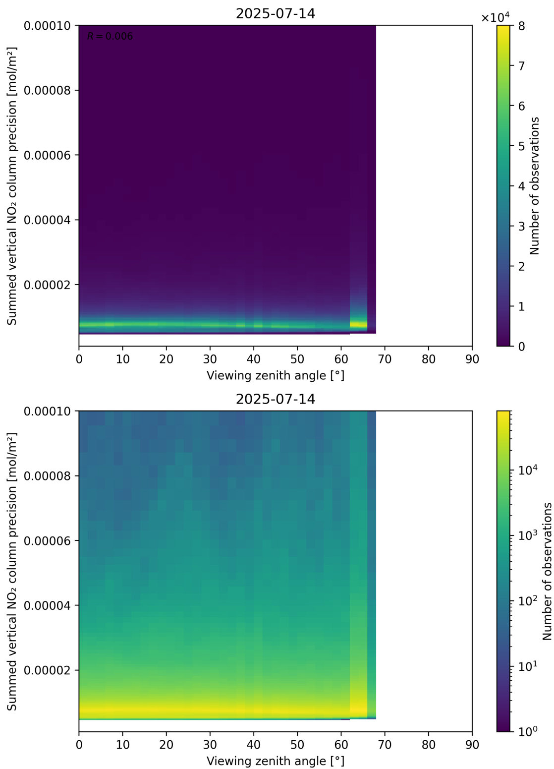
Figure 166: Scatter density plot of “Viewing zenith angle” against “Summed vertical NO 2 column precision” for 2025-07-13 to 2025-07-15.
