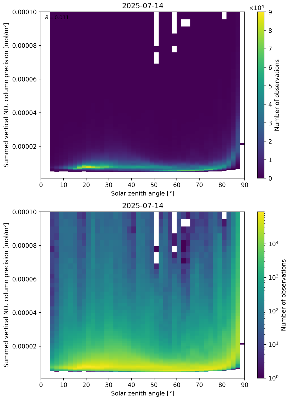
Figure 152: Scatter density plot of “Solar zenith angle” against “Summed vertical NO 2 column precision” for 2025-07-13 to 2025-07-15.
