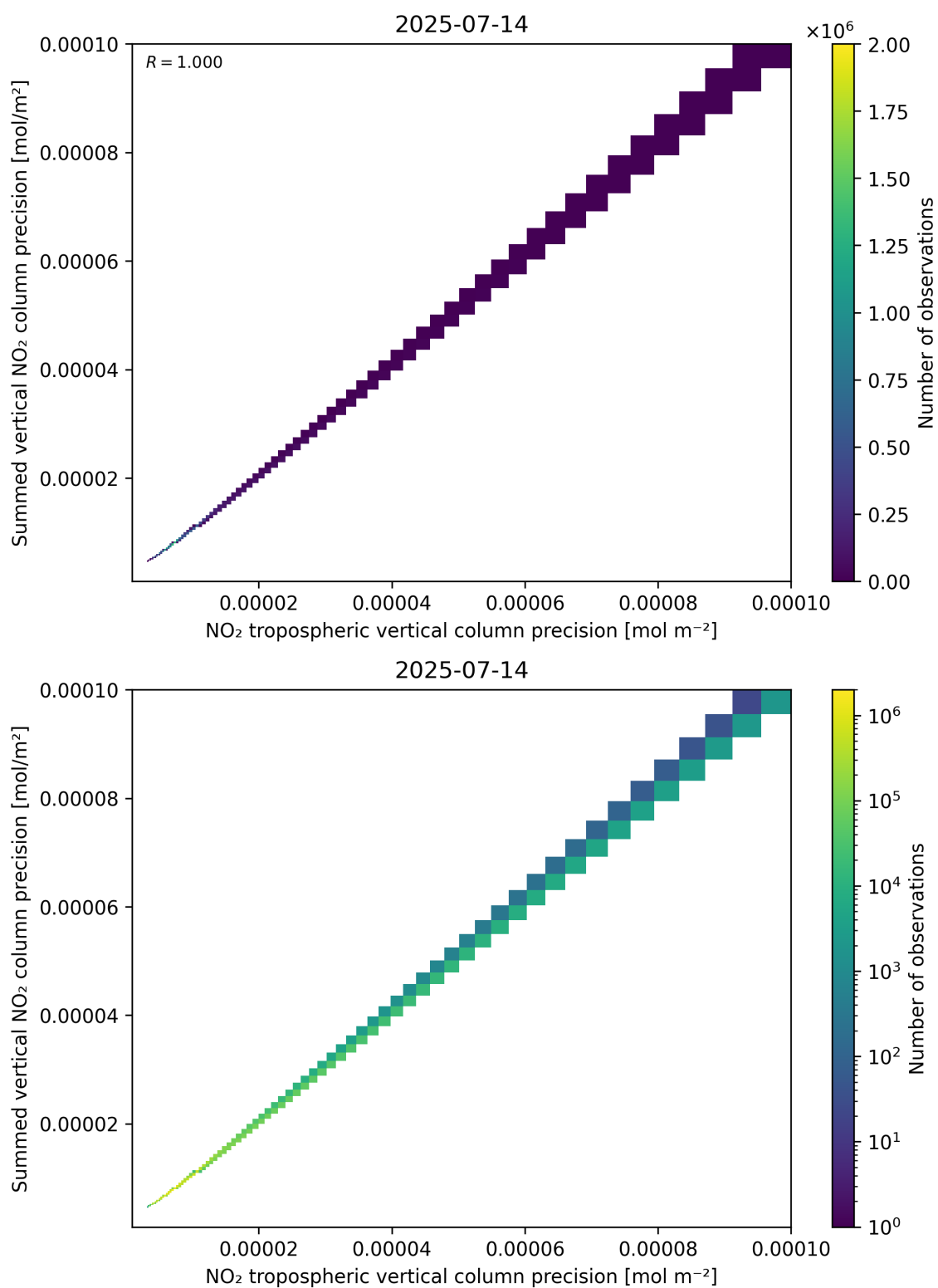
Figure 137: Scatter density plot of “NO 2 tropospheric vertical column precision” against “Summed vertical NO 2 column precision” for 2025-07-13 to 2025-07-15.
