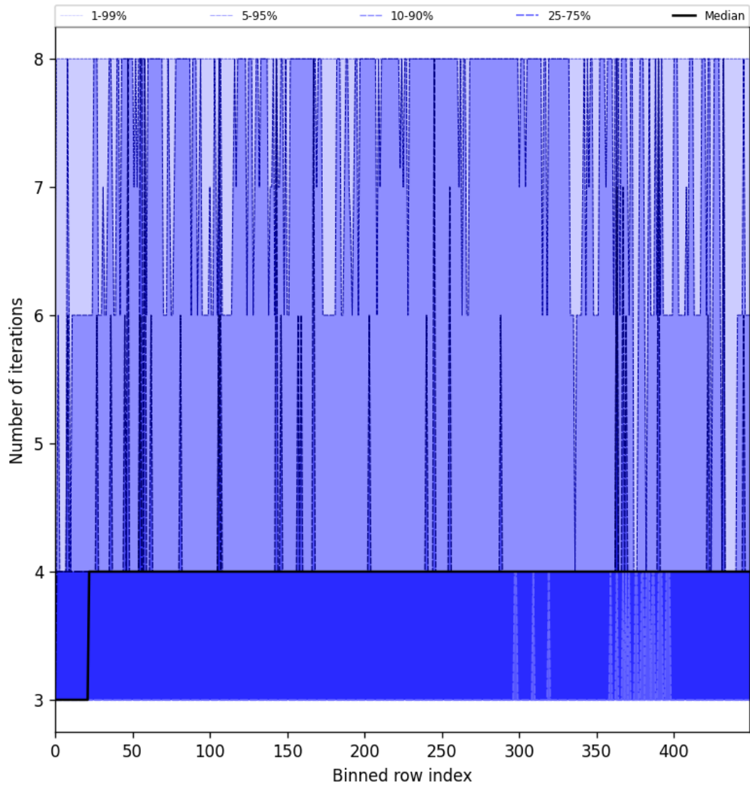
Figure 51: Along track statistics of “Number of iterations” for 2025-07-13 to 2025-07-15
