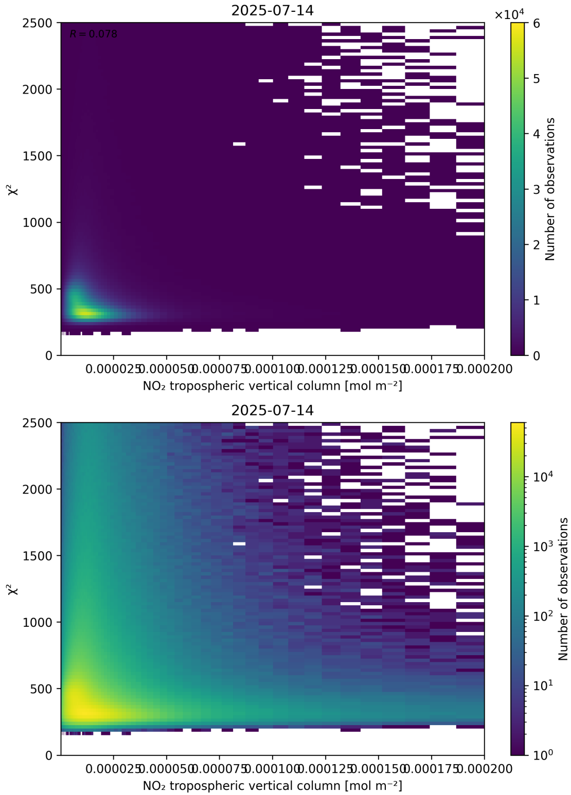
Figure 124: Scatter density plot of “NO 2 tropospheric vertical column” against “ \chi^2 ” for 2025-07-13 to 2025-07-15.
