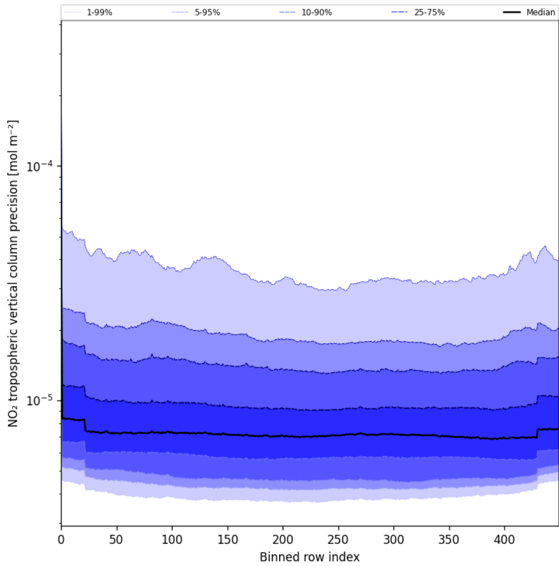
Figure 47: Along track statistics of “NO 2 tropospheric vertical column precision” for 2025-07-13 to 2025-07-15
