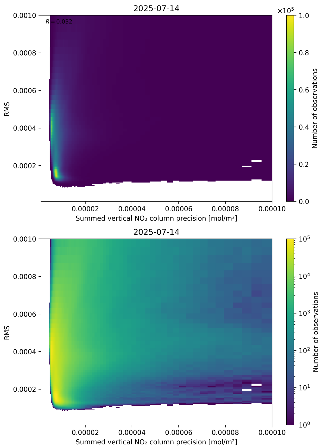
Figure 108: Scatter density plot of “Summed vertical NO 2 column precision” against “RMS” for 2025-07-13 to 2025-07-15.
