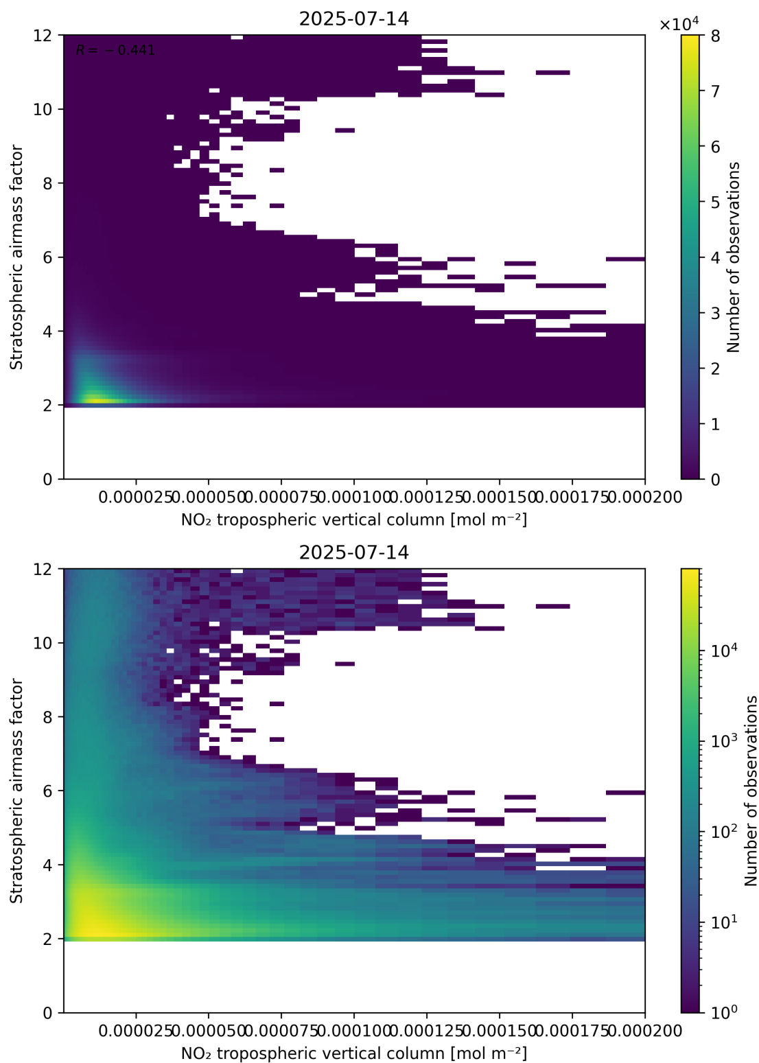
Figure 121: Scatter density plot of “NO 2 tropospheric vertical column” against “Stratospheric air mass factor” for 2025-07-13 to 2025-07-15.
