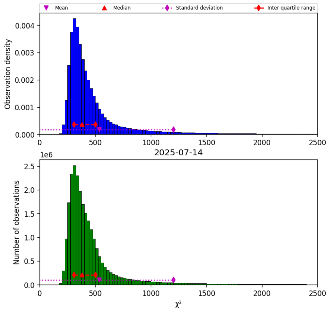
Figure 42: Histogram of “ \chi^2 ” for 2025-07-13 to 2025-07-15
