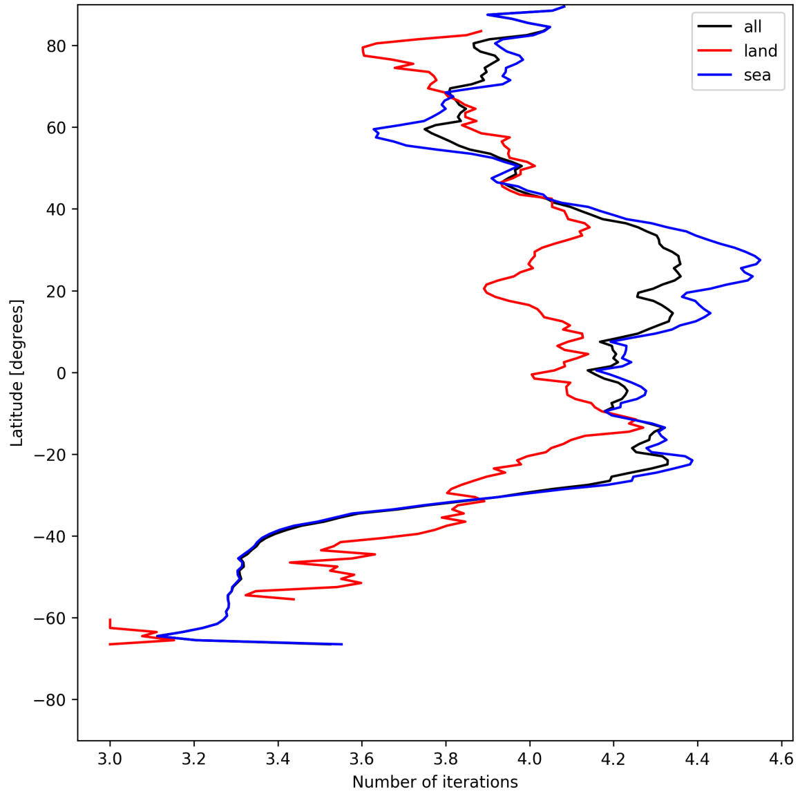
Figure 17: Zonal average of “Number of iterations” for 2025-07-13 to 2025-07-15.
