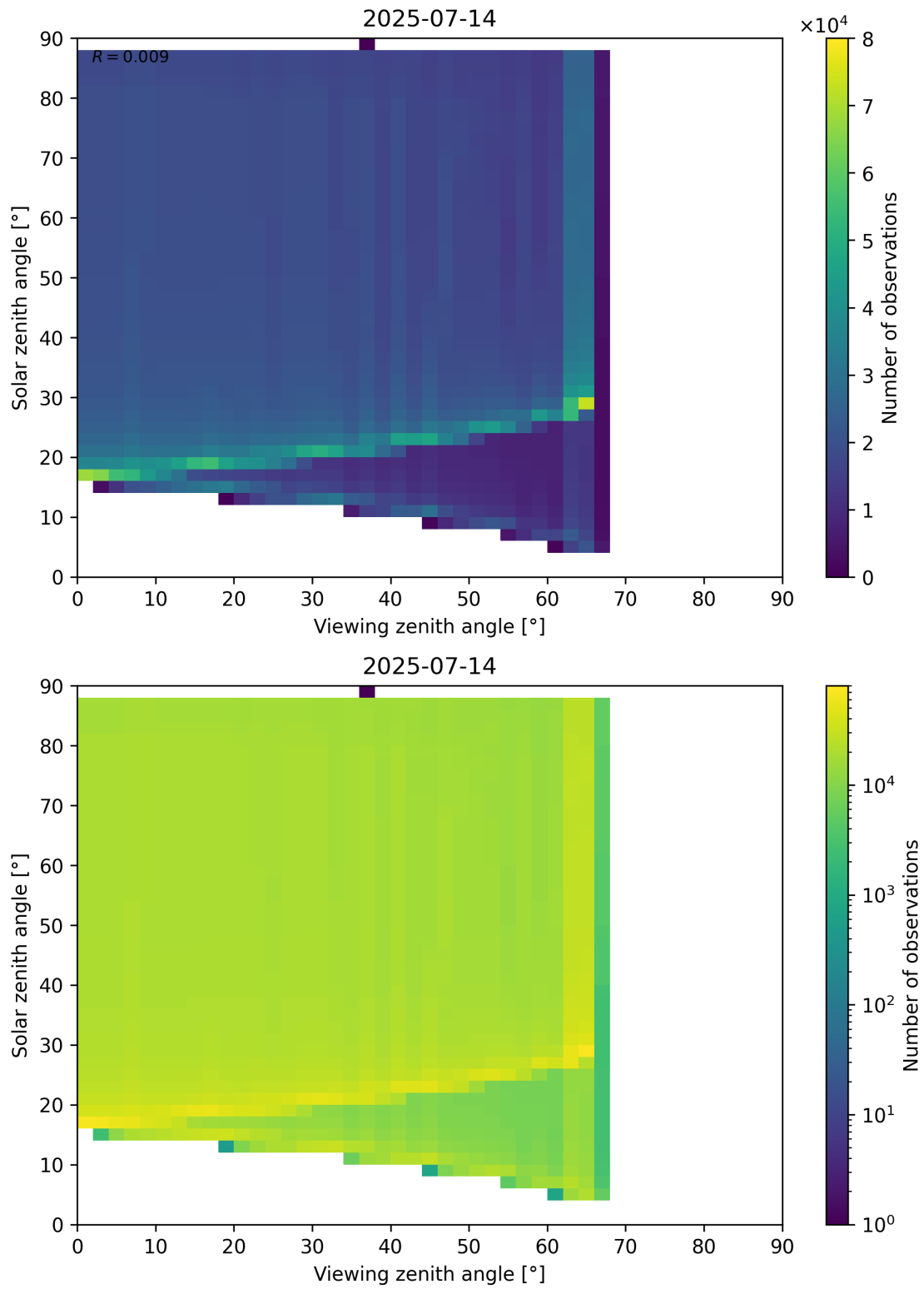
Figure 172: Scatter density plot of “Viewing zenith angle” against “Solar zenith angle” for 2025-07-13 to 2025-07-15.
