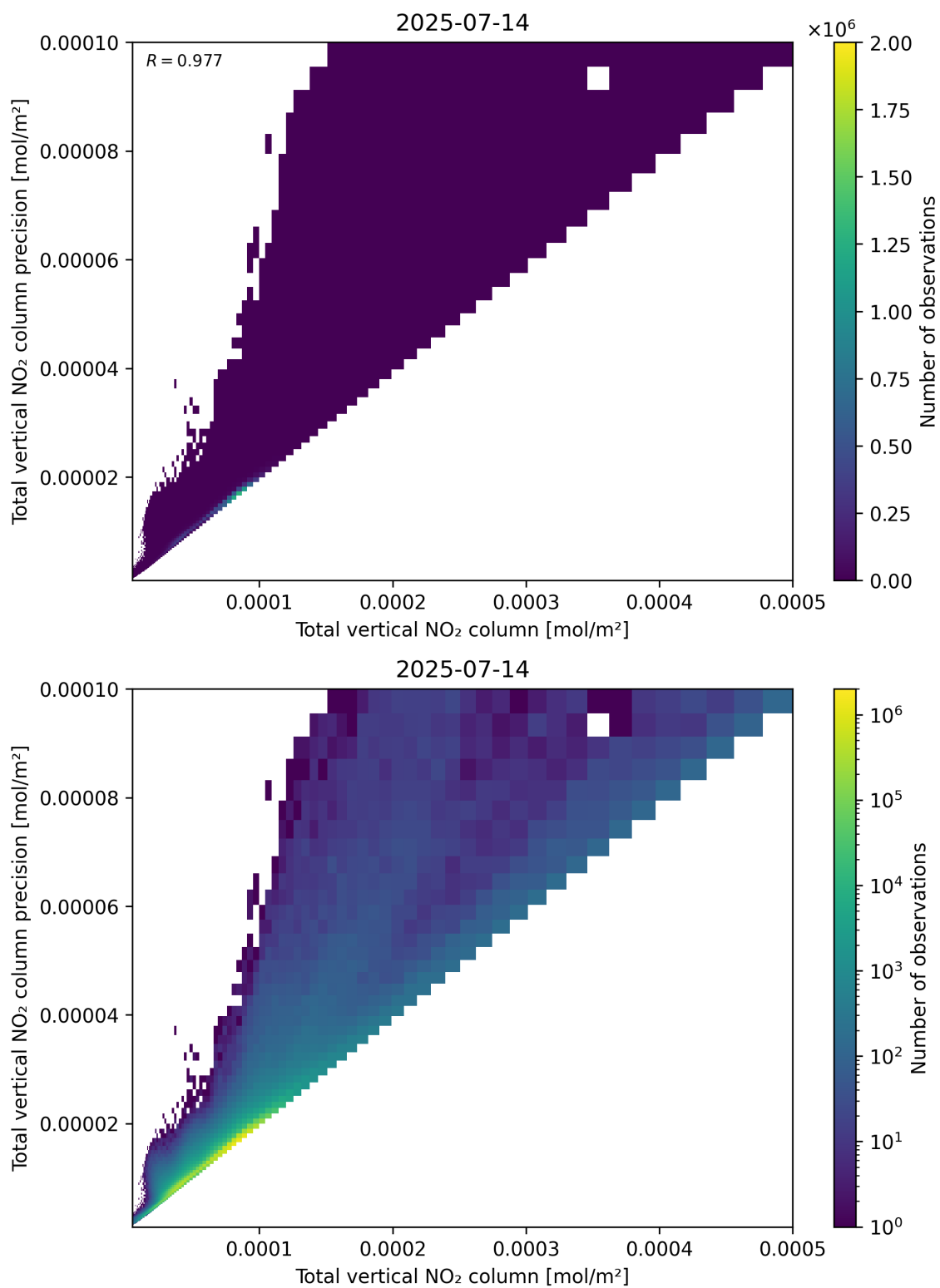
Figure 114: Scatter density plot of “Total vertical NO 2 column” against “Total vertical NO 2 column precision” for 2025-07-13 to 2025-07-15.
