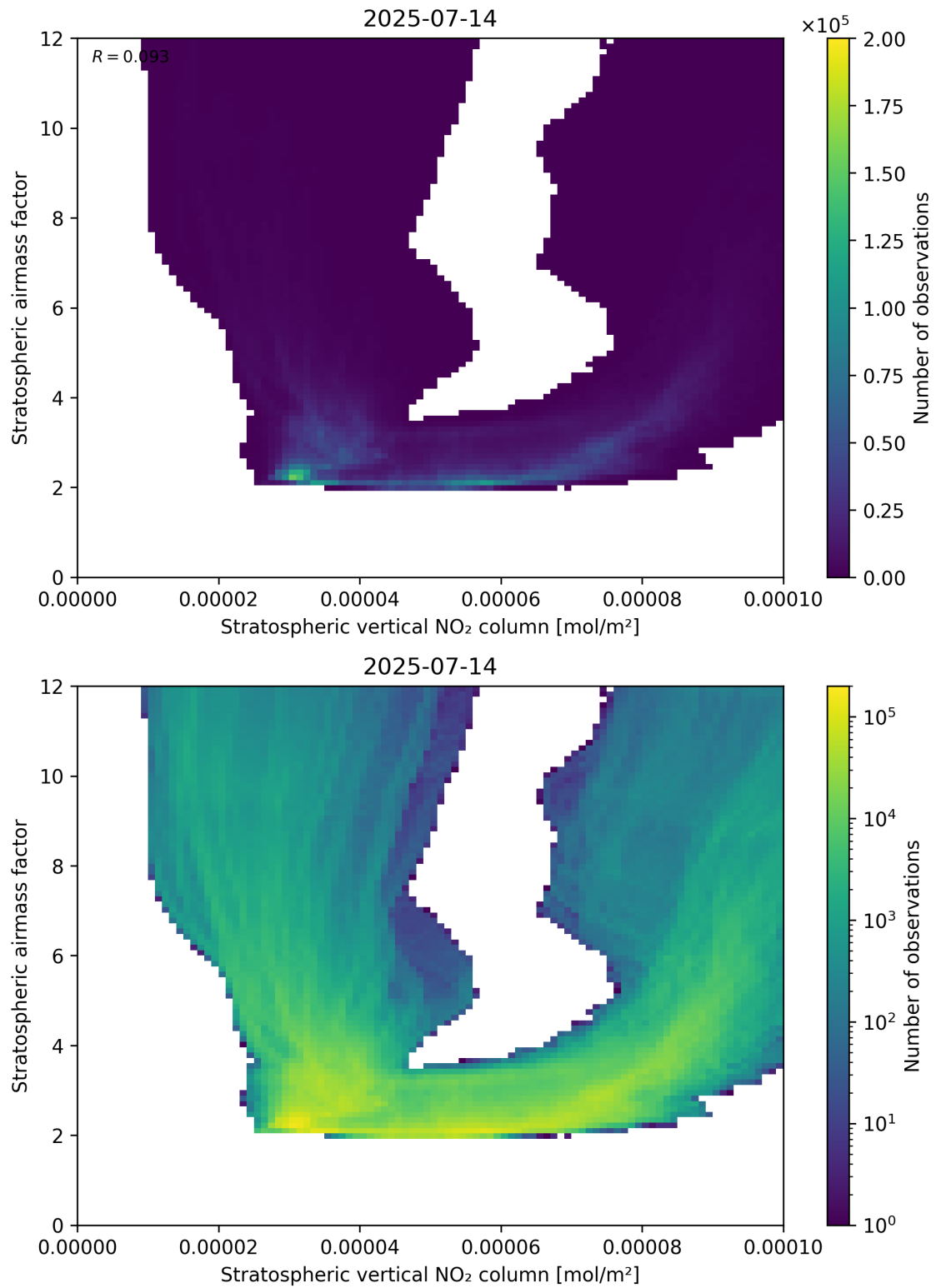
Figure 96: Scatter density plot of “Stratospheric vertical NO 2 column” against “Stratospheric airmass factor” for 2025-07-13 to 2025-07-15.
