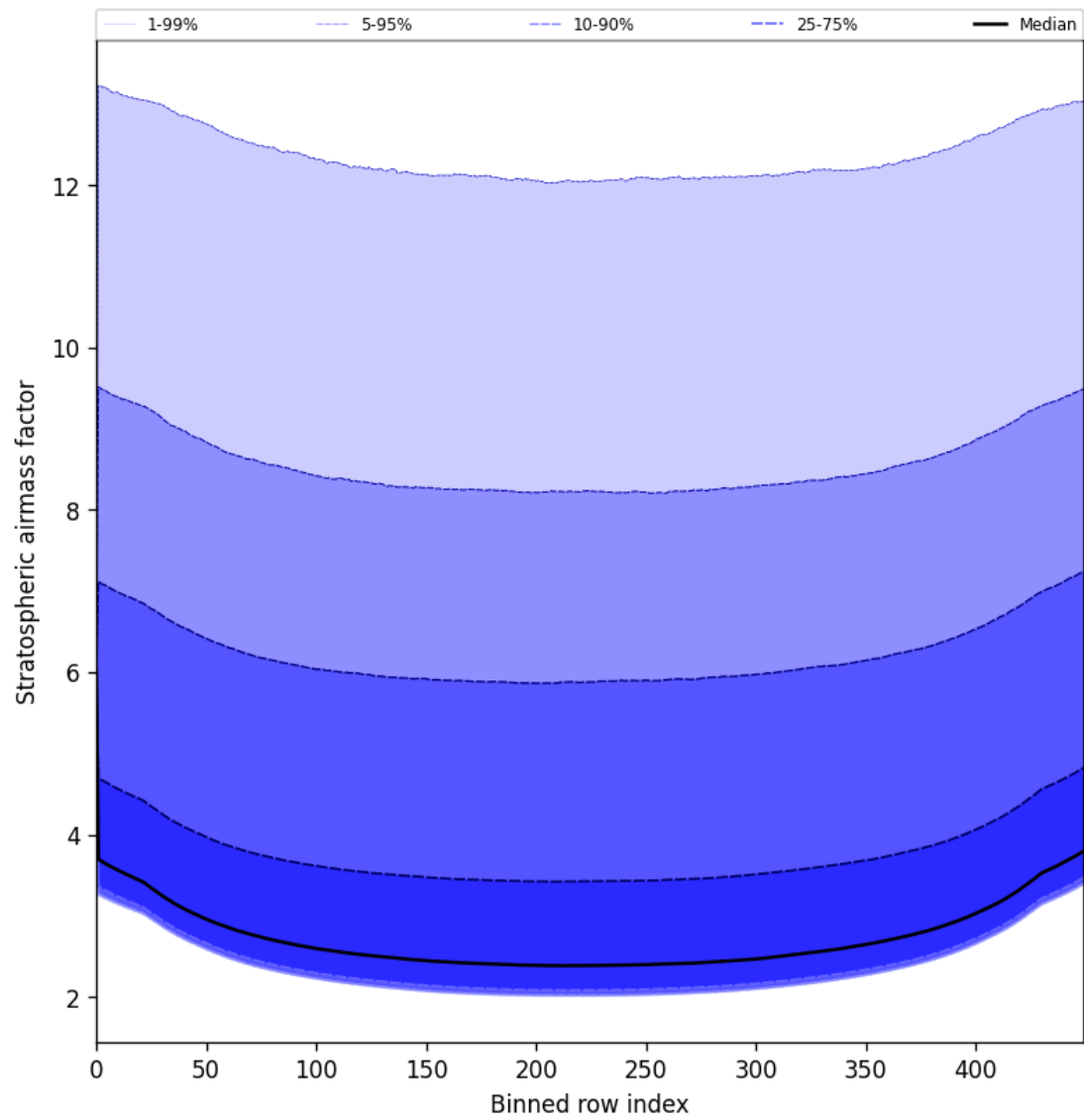
Figure 61: Along track statistics of “Stratospheric airmass factor” for 2025-07-13 to 2025-07-15
