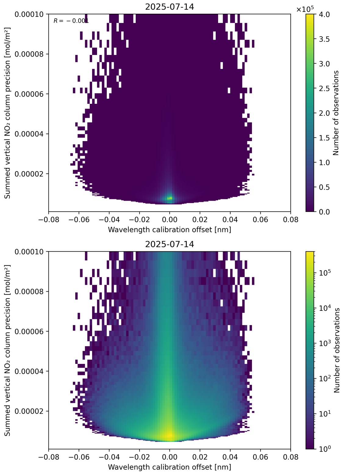
Figure 178: Scatter density plot of “Wavelength calibration offset” against “Summed vertical NO 2 column precision” for 2025-07-13 to 2025-07-15.
