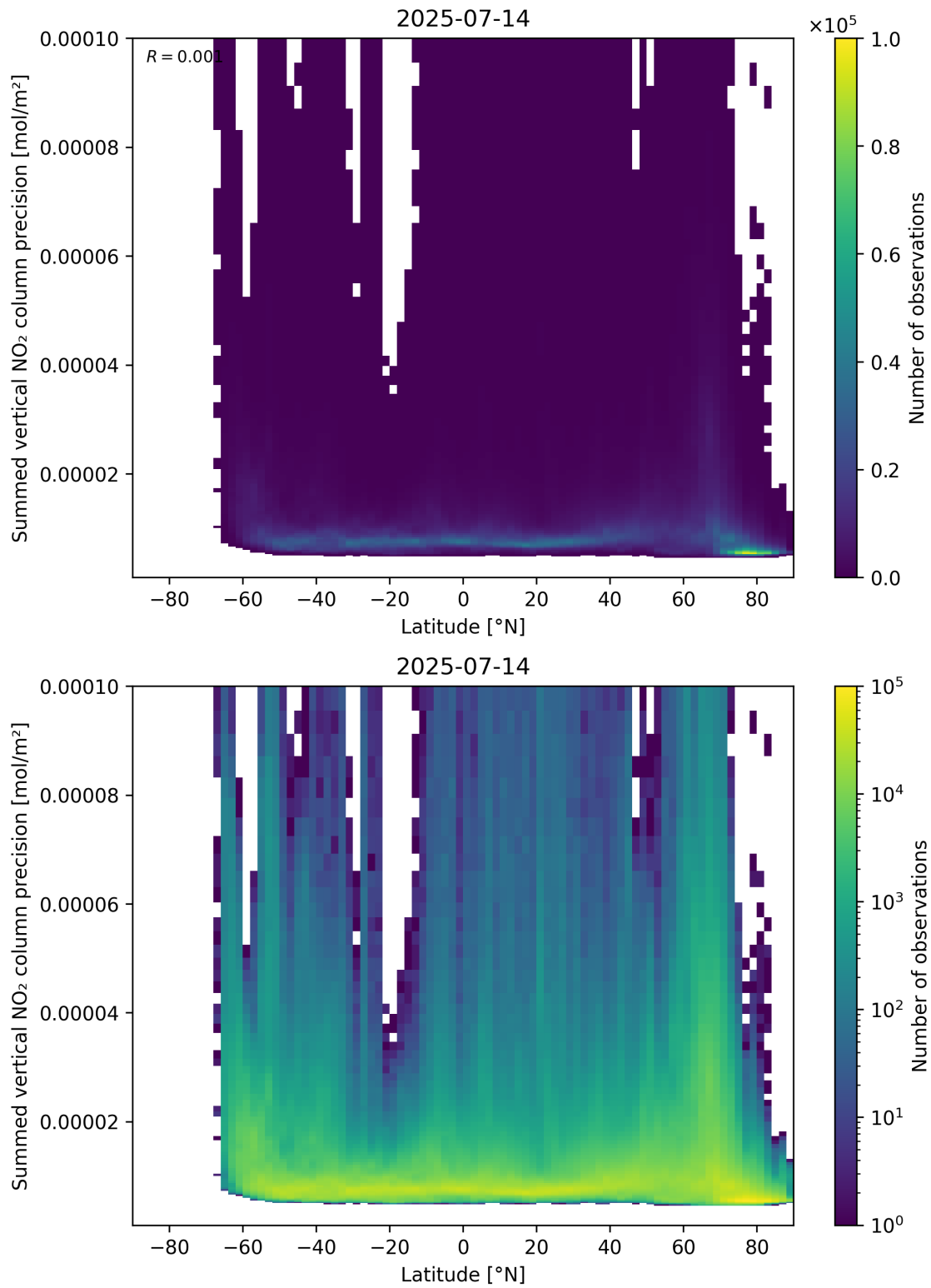
Figure 89: Scatter density plot of “Latitude” against “Summed vertical NO 2 column precision” for 2025-07-13 to 2025-07-15.
