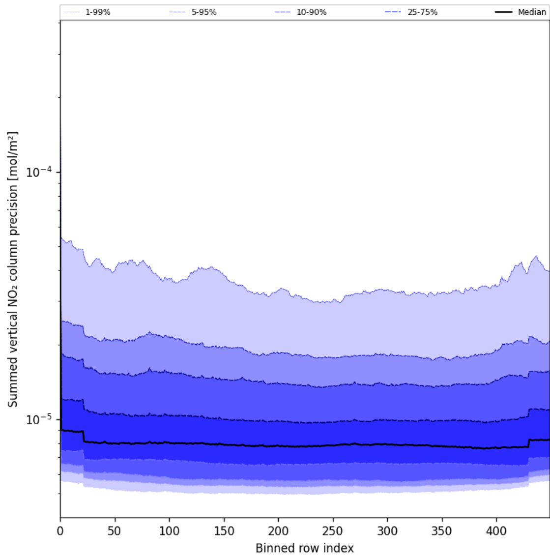
Figure 58: Along track statistics of “Summed vertical NO 2 column precision” for 2025-07-13 to 2025-07-15
