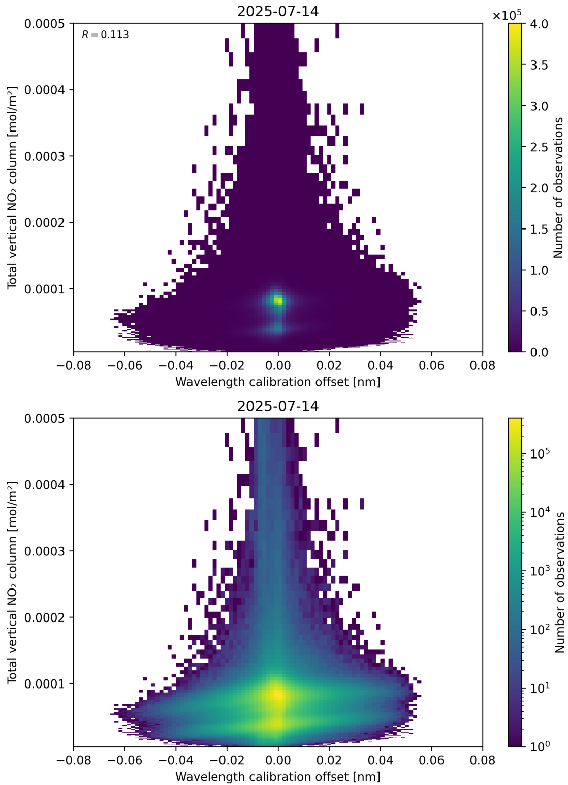
Figure 179: Scatter density plot of “Wavelength calibration offset” against “Total vertical NO 2 column” for 2025-07-13 to 2025-07-15.
