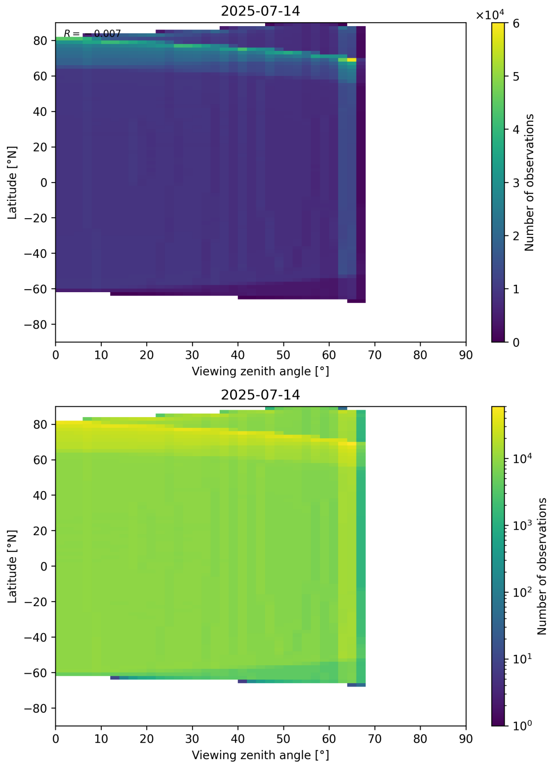
Figure 163: Scatter density plot of “Viewing zenith angle” against “Latitude” for 2025-07-13 to 2025-07-15.
