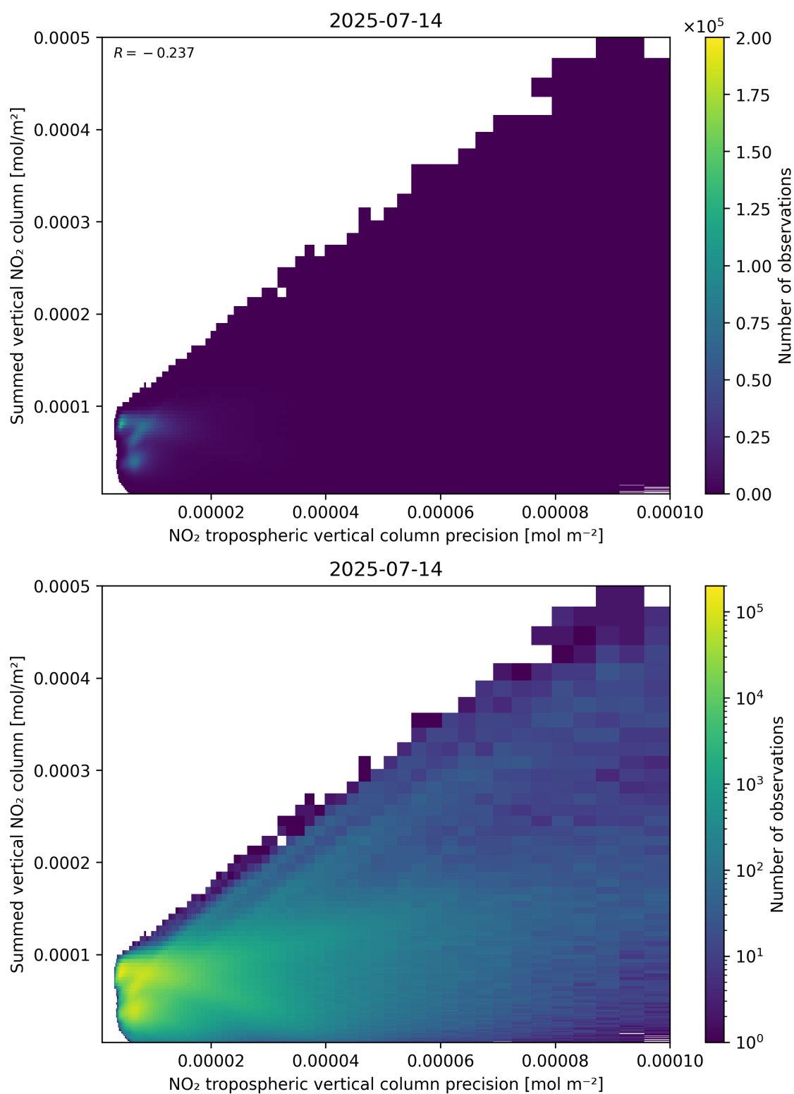
Figure 136: Scatter density plot of “NO 2 tropospheric vertical column precision” against “Summed vertical NO 2 column” for 2025-07-13 to 2025-07-15.
