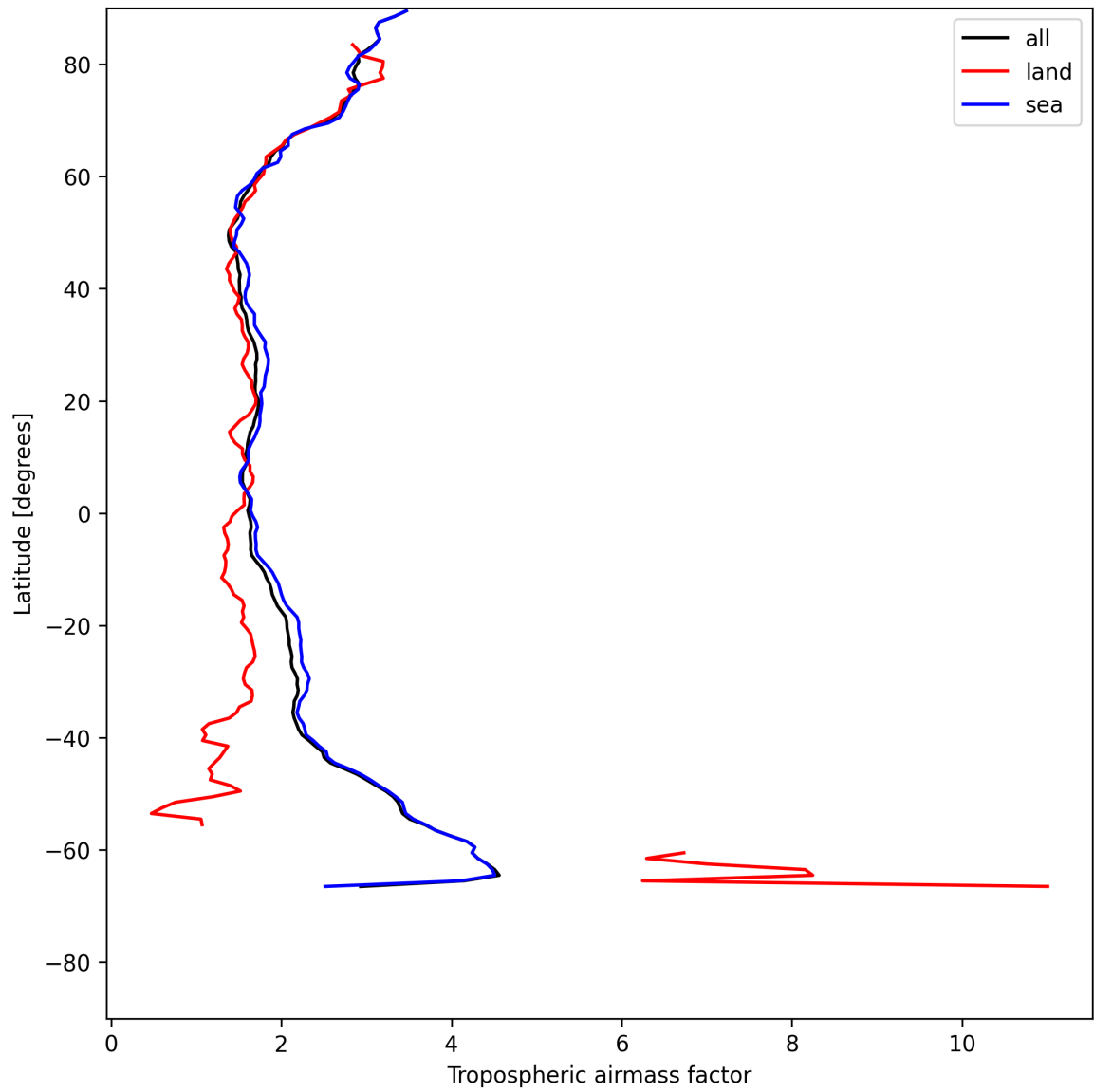
Figure 14: Zonal average of “Tropospheric air mass factor” for 2025-07-13 to 2025-07-15.
