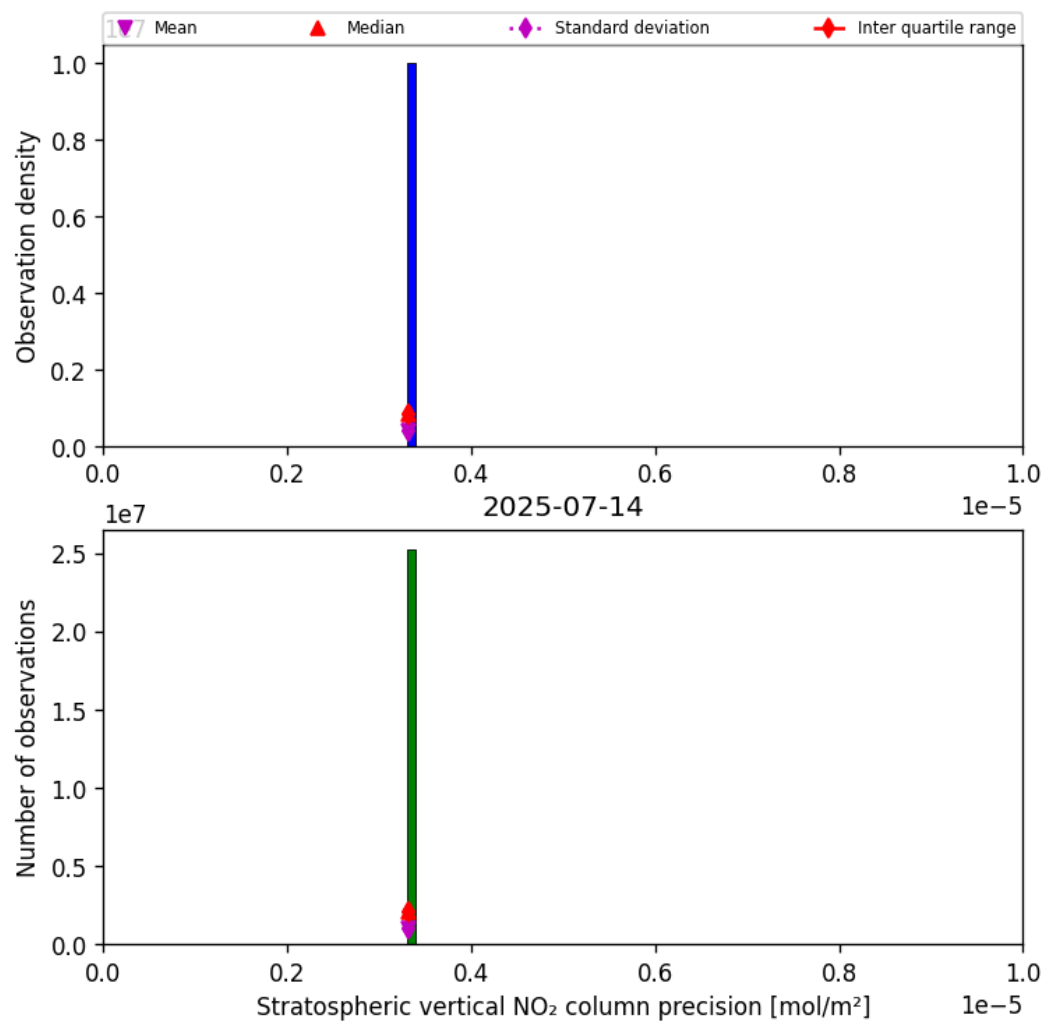
Figure 37: Histogram of “Stratospheric vertical NO 2 column precision” for 2025-07-13 to 2025-07-15
