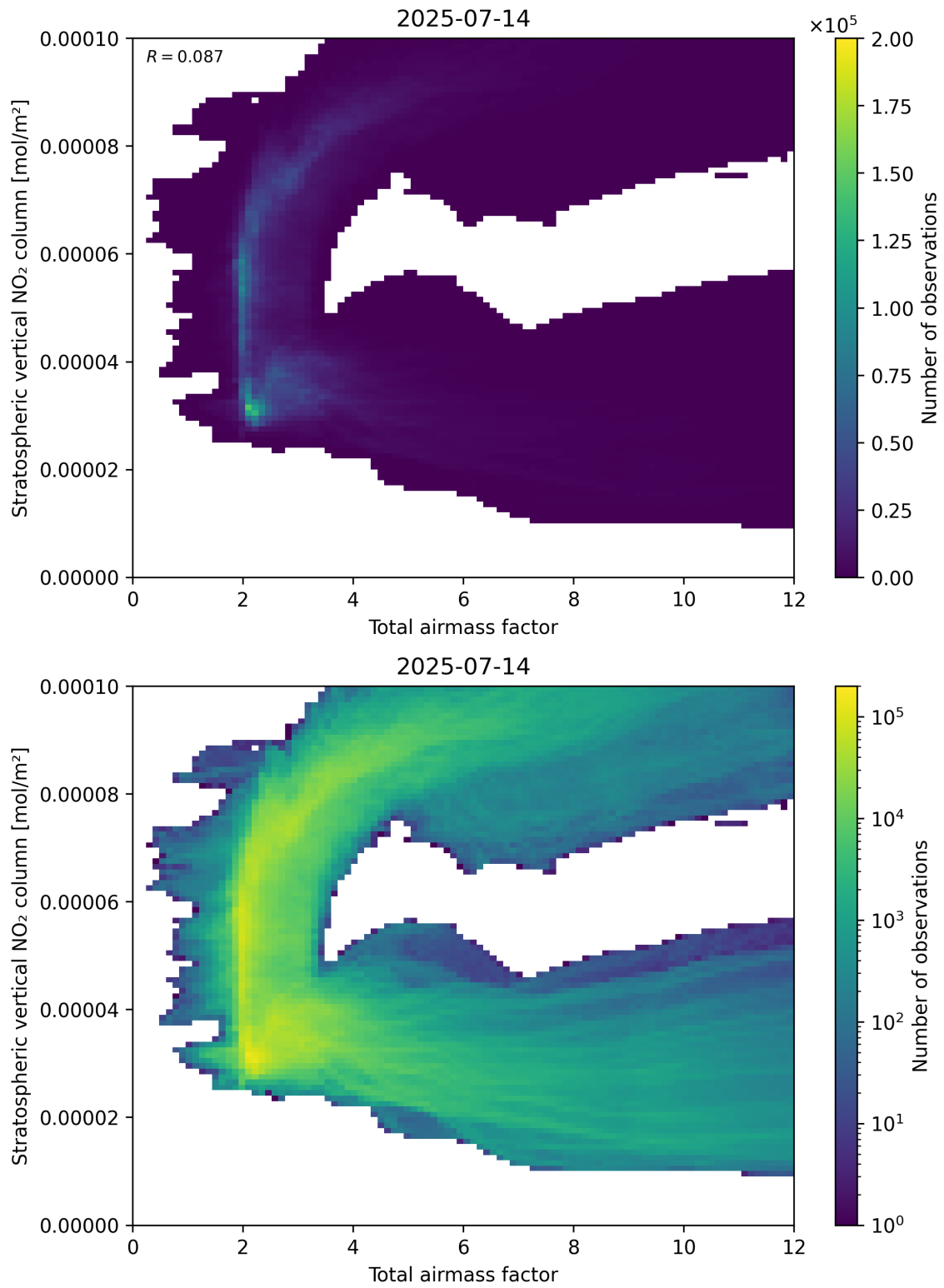
Figure 64: Scatter density plot of “Total airmass factor” against “Stratospheric vertical NO 2 column” for 2025-07-13 to 2025-07-15.
