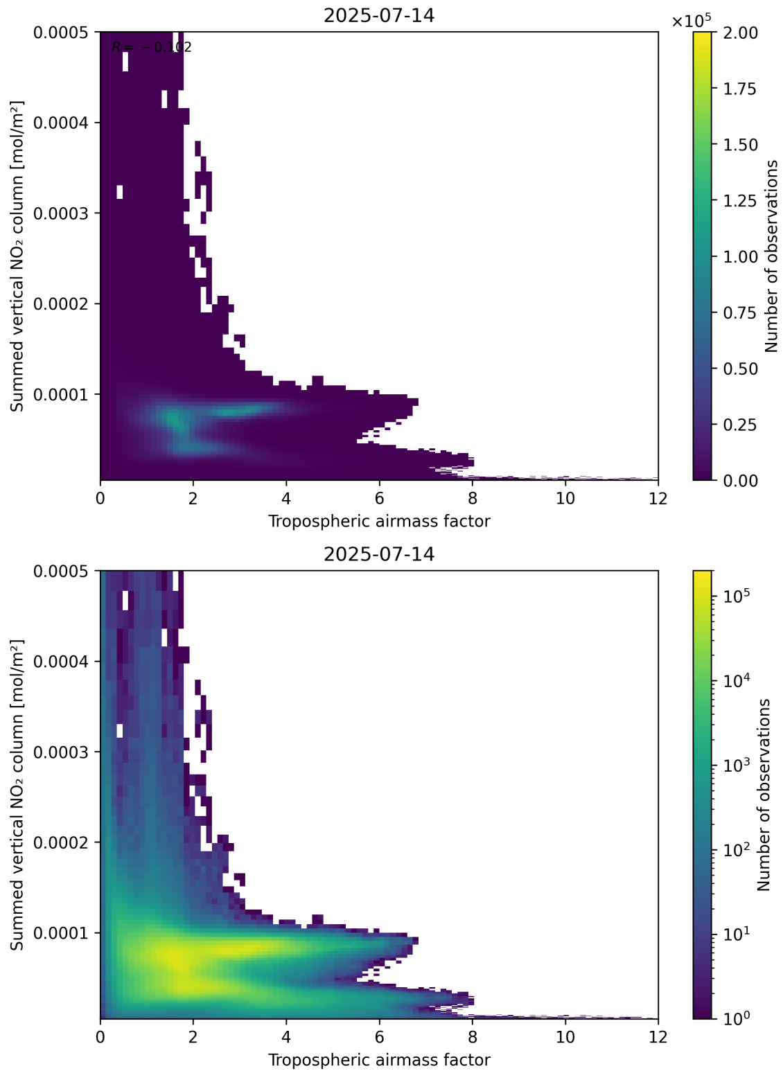
Figure 75: Scatter density plot of “Tropospheric air mass factor” against “Summed vertical NO 2 column” for 2025-07-13 to 2025-07-15.
