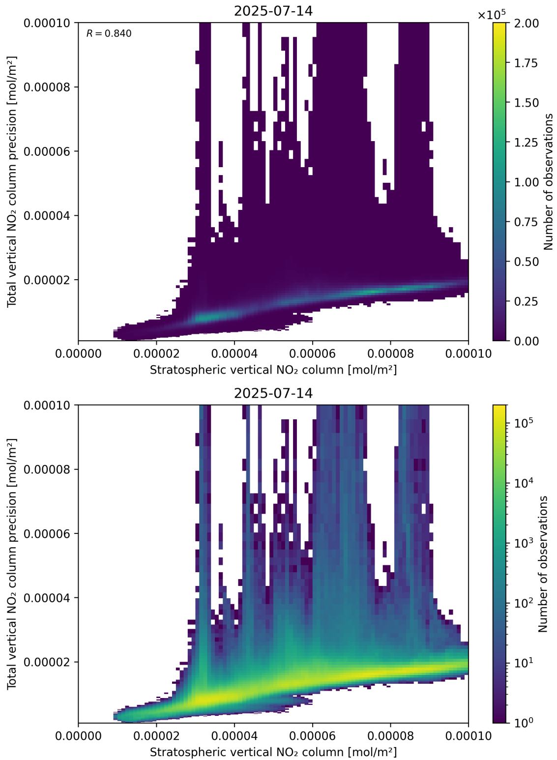
Figure 101: Scatter density plot of “Stratospheric vertical NO 2 column” against “Total vertical NO 2 column precision” for 2025-07-13 to 2025-07-15.
