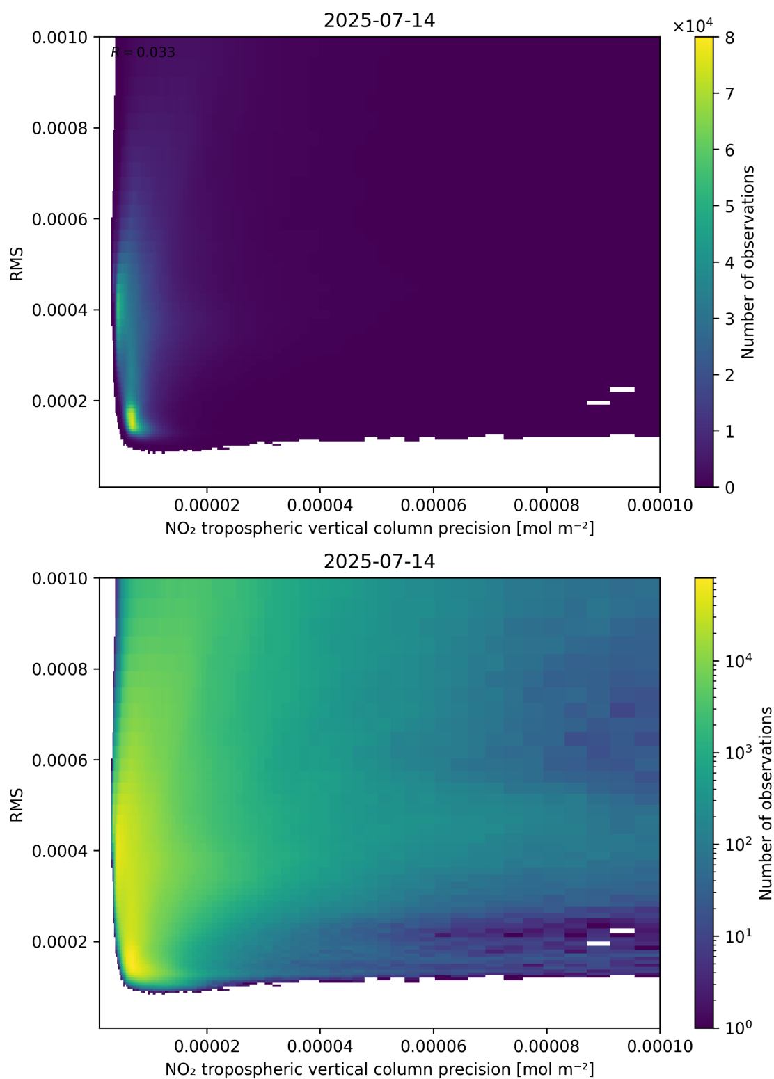
Figure 140: Scatter density plot of “NO 2 tropospheric vertical column precision” against “RMS” for 2025-07-13 to 2025-07-15.
