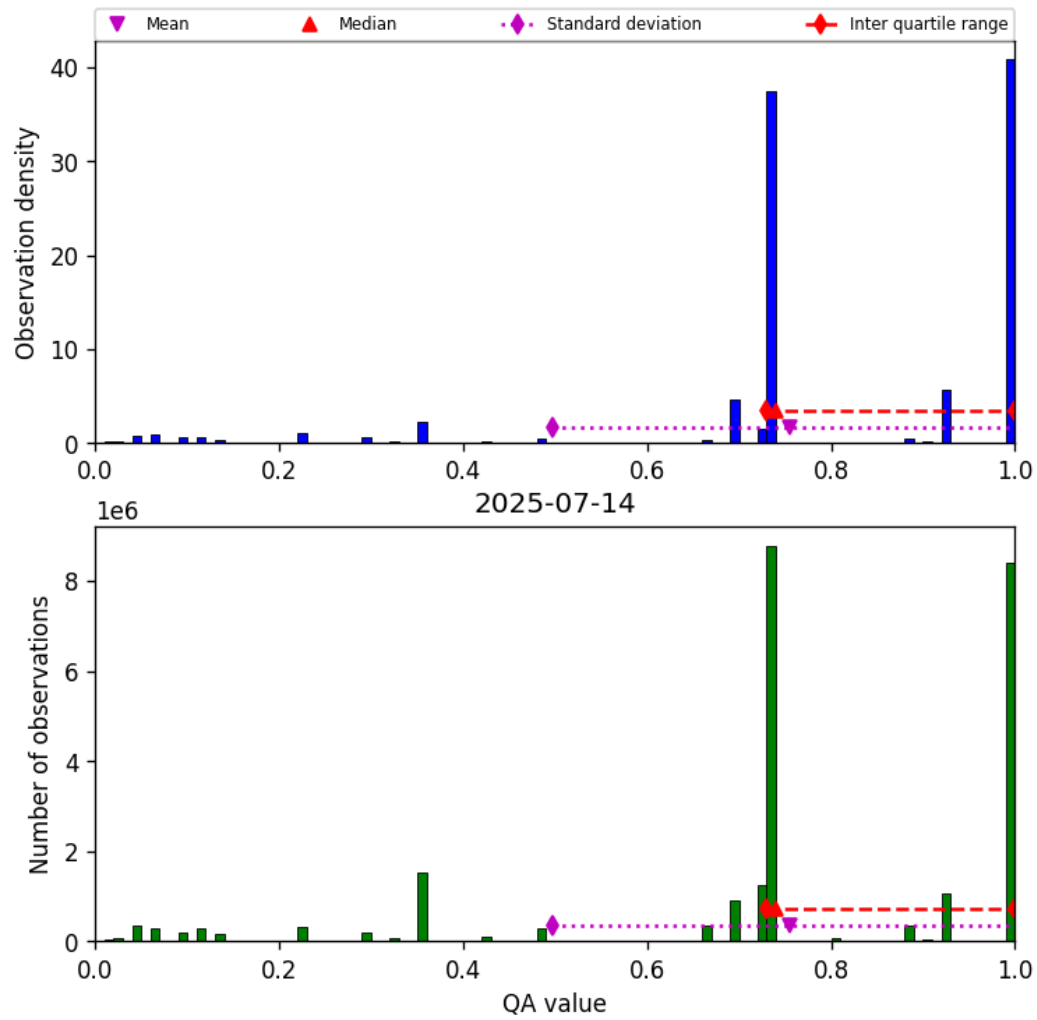
Figure 28: Histogram of “QA value” for 2025-07-13 to 2025-07-15
