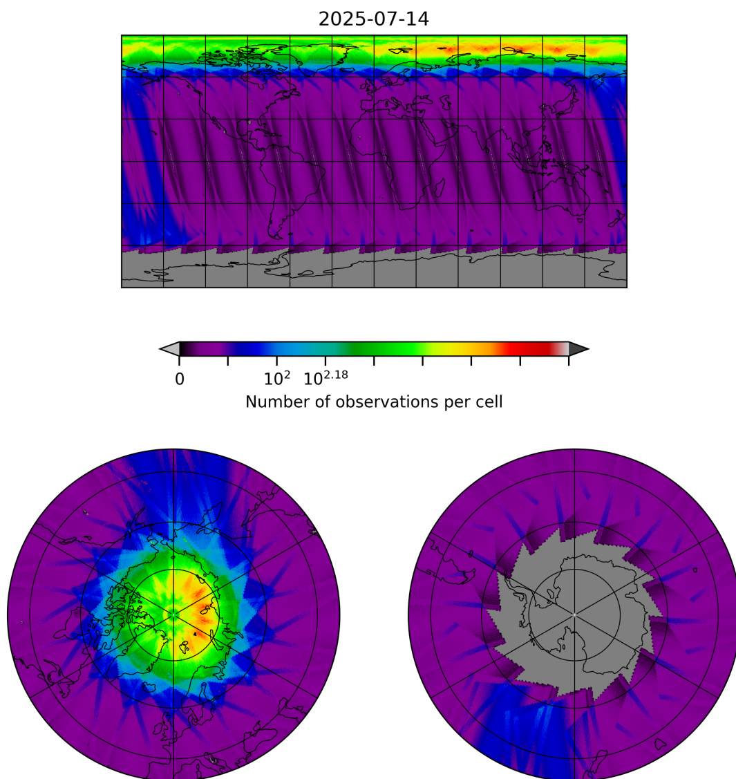
Figure 10: Map of the number of observations for 2025-07-13 to 2025-07-15
