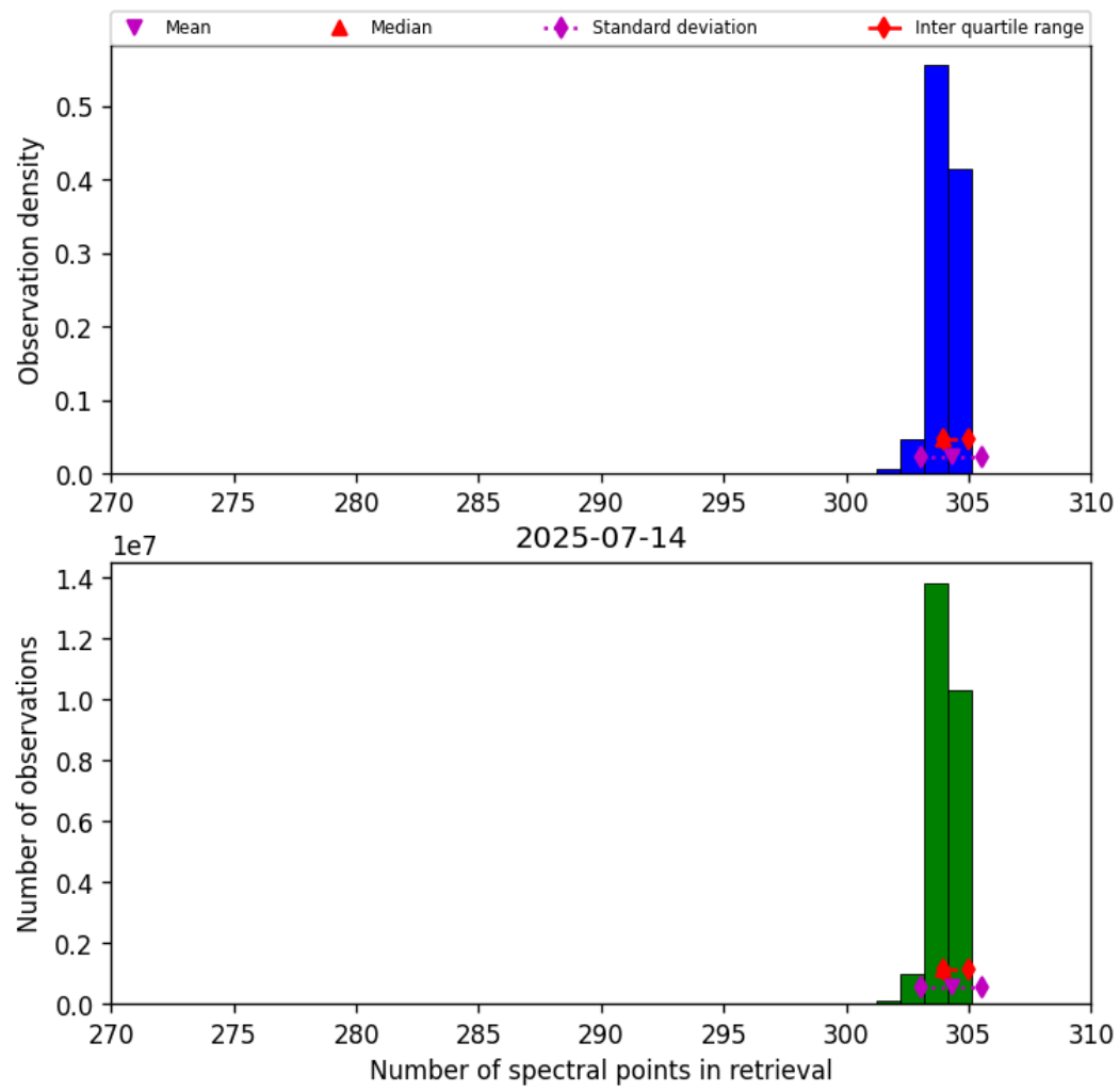
Figure 33: Histogram of “Number of spectral points in retrieval” for 2025-07-13 to 2025-07-15
