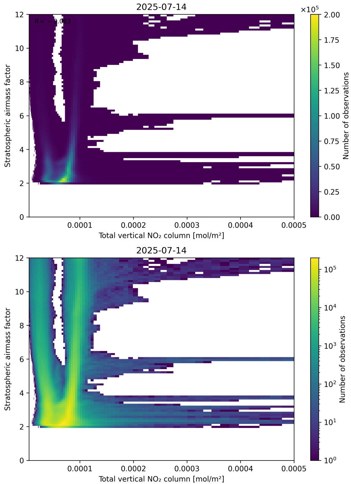
Figure 110: Scatter density plot of “Total vertical NO 2 column” against “Stratospheric airmass factor” for 2025-07-13 to 2025-07-15.
