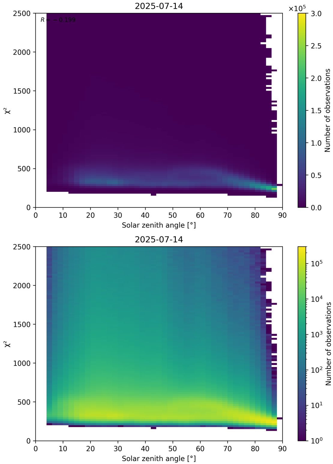
Figure 148: Scatter density plot of “Solar zenith angle” against “ \chi^2 ” for 2025-07-13 to 2025-07-15.
