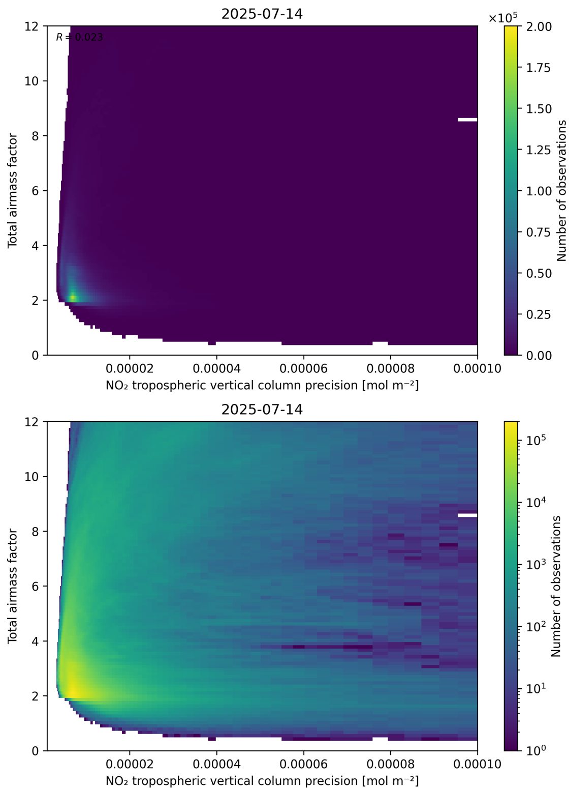
Figure 132: Scatter density plot of “NO 2 tropospheric vertical column precision” against “Total air mass factor” for 2025-07-13 to 2025-07-15.
