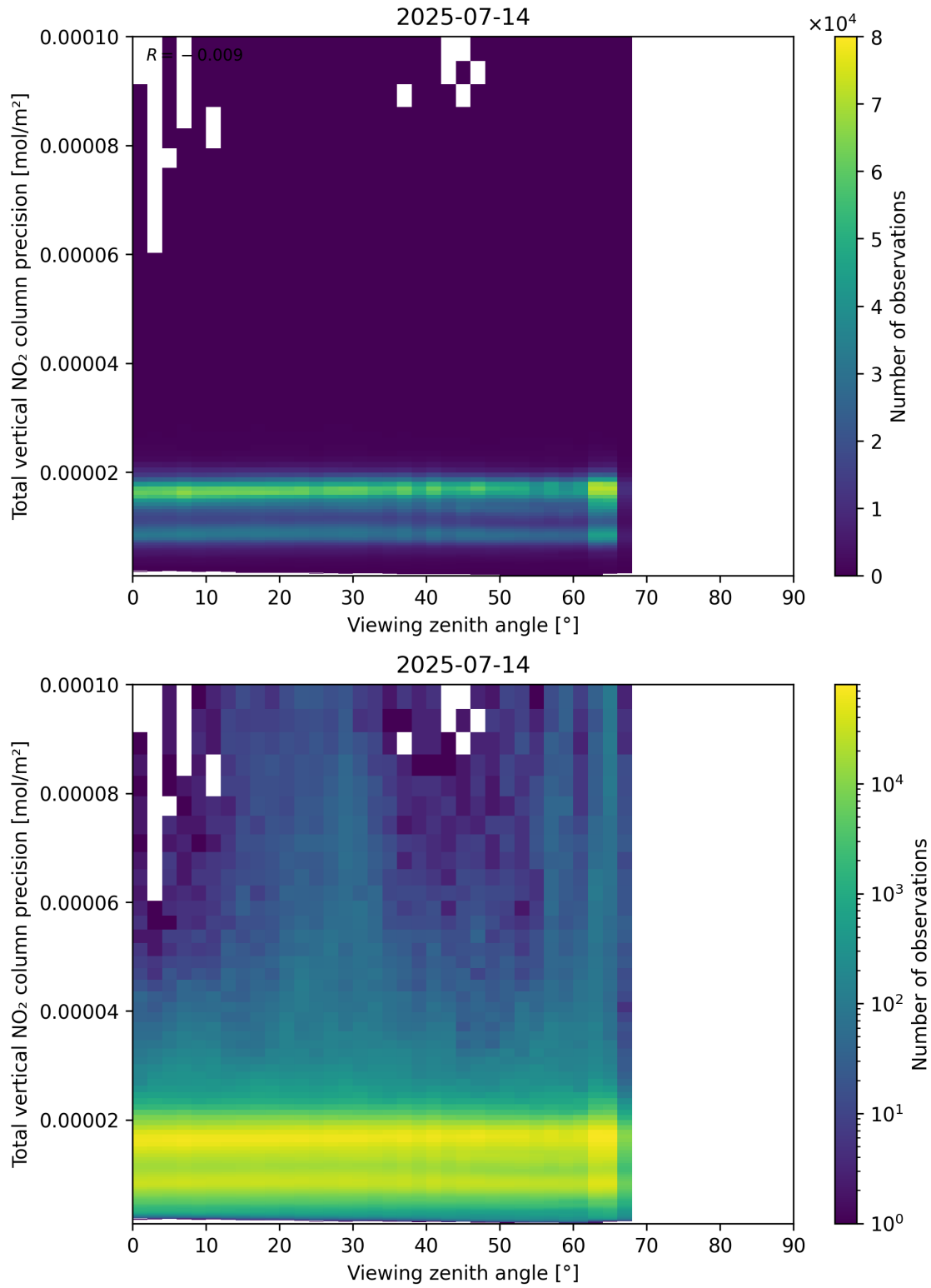
Figure 168: Scatter density plot of “Viewing zenith angle” against “Total vertical NO 2 column precision” for 2025-07-13 to 2025-07-15.
