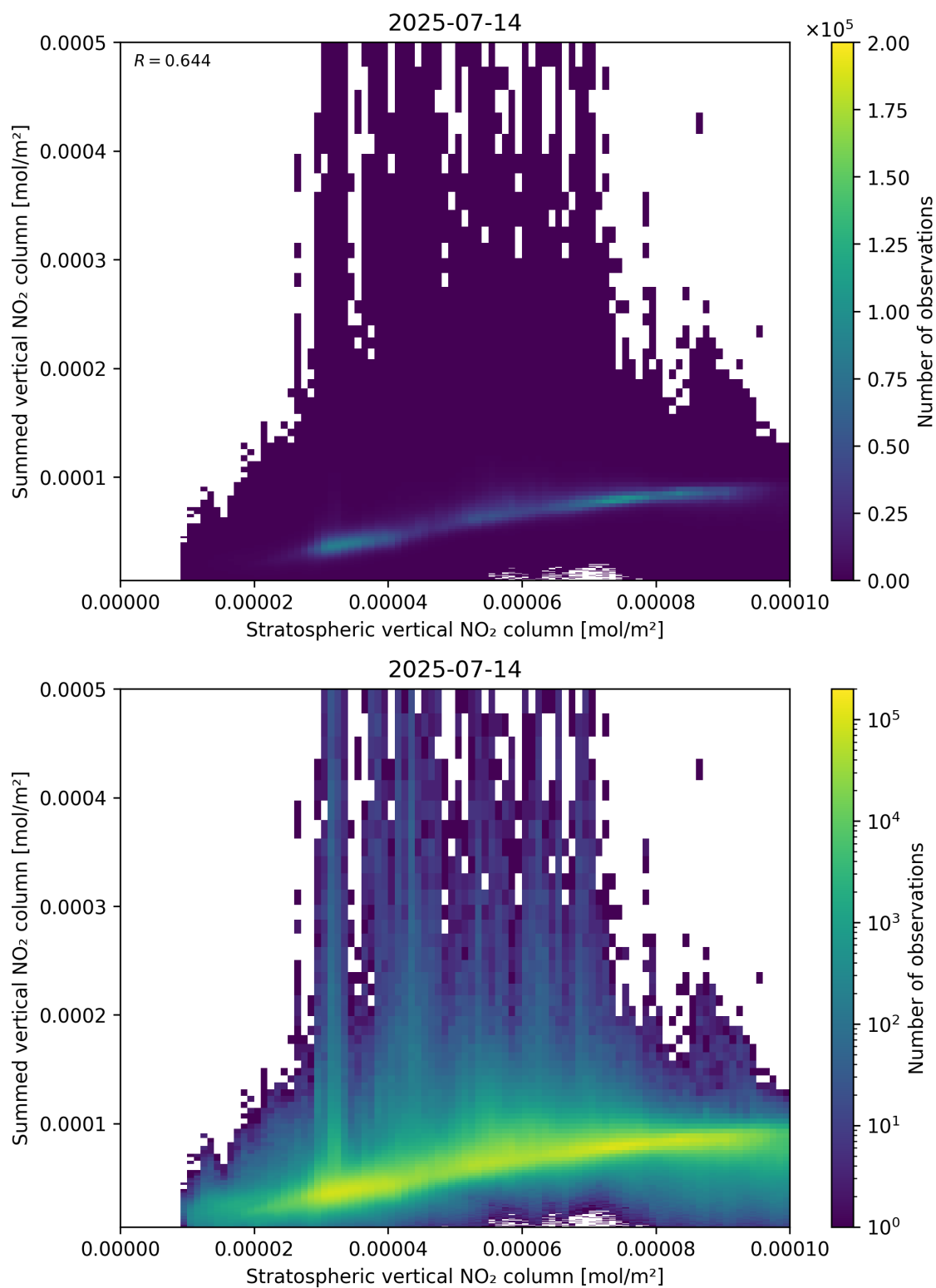
Figure 98: Scatter density plot of “Stratospheric vertical NO 2 column” against “Summed vertical NO 2 column” for 2025-07-13 to 2025-07-15.
