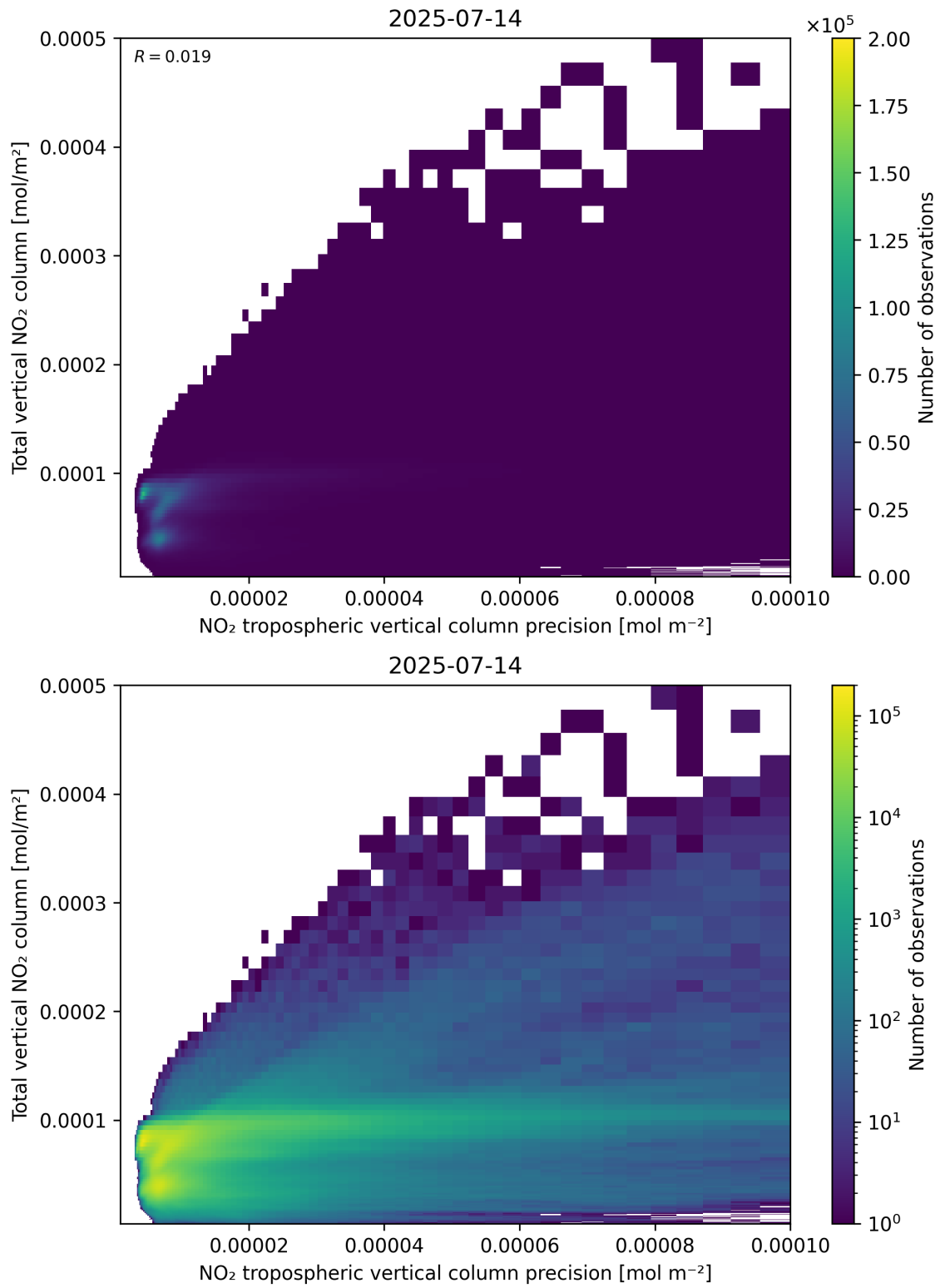
Figure 138: Scatter density plot of “NO 2 tropospheric vertical column precision” against “Total vertical NO 2 column” for 2025-07-13 to 2025-07-15.
