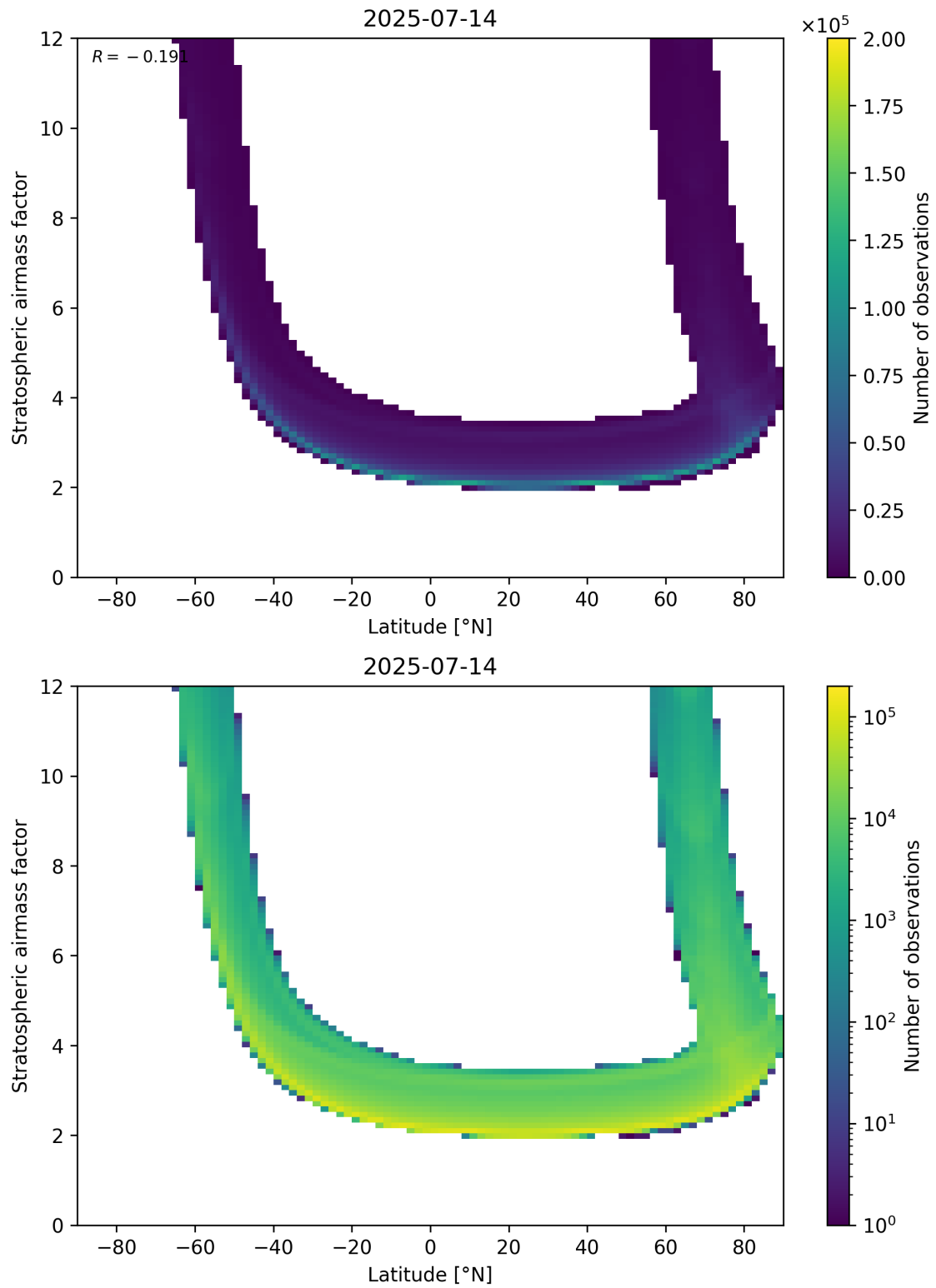
Figure 83: Scatter density plot of “Latitude” against “Stratospheric air mass factor” for 2025-07-13 to 2025-07-15.
