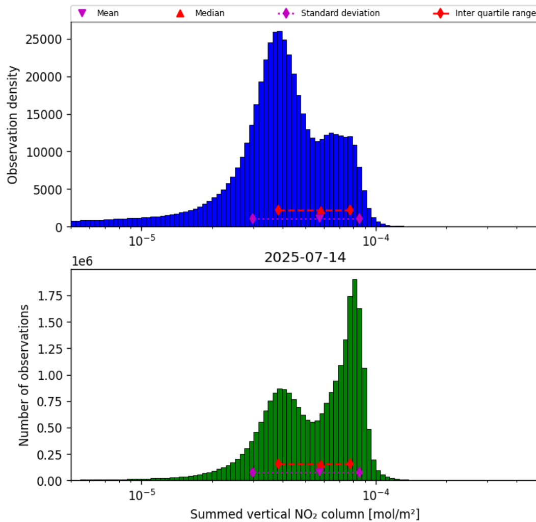
Figure 40: Histogram of “Summed vertical NO 2 column” for 2025-07-13 to 2025-07-15
