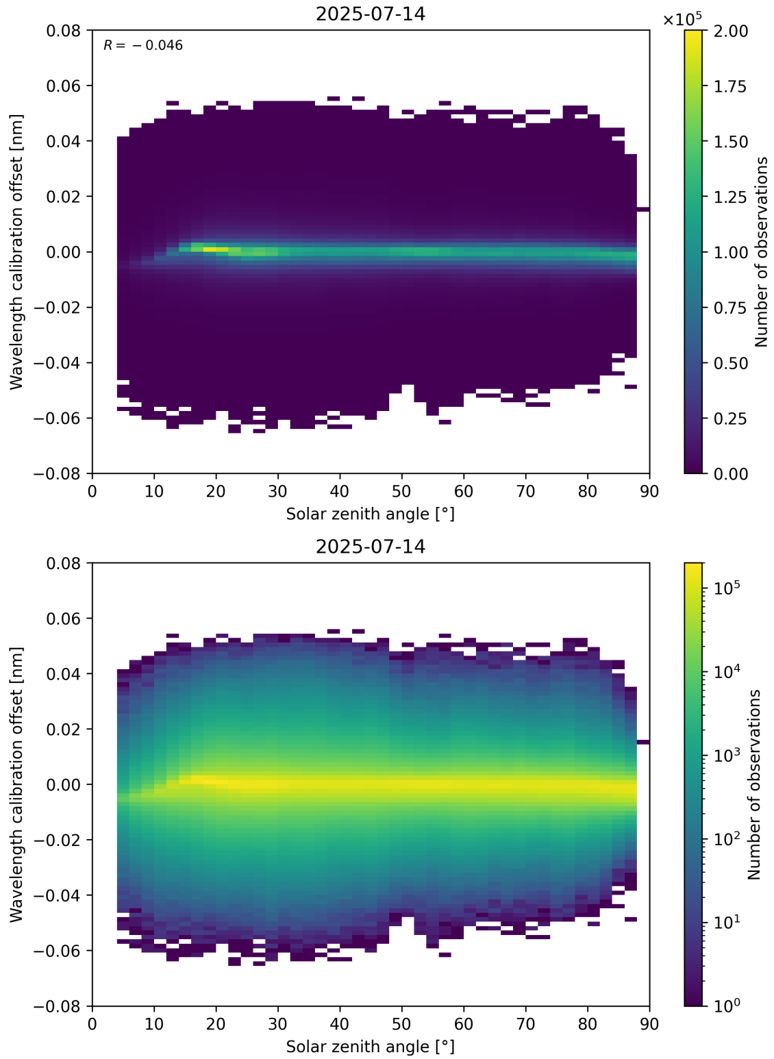
Figure 158: Scatter density plot of “Solar zenith angle” against “Wavelength calibration offset” for 2025-07-13 to 2025-07-15.
