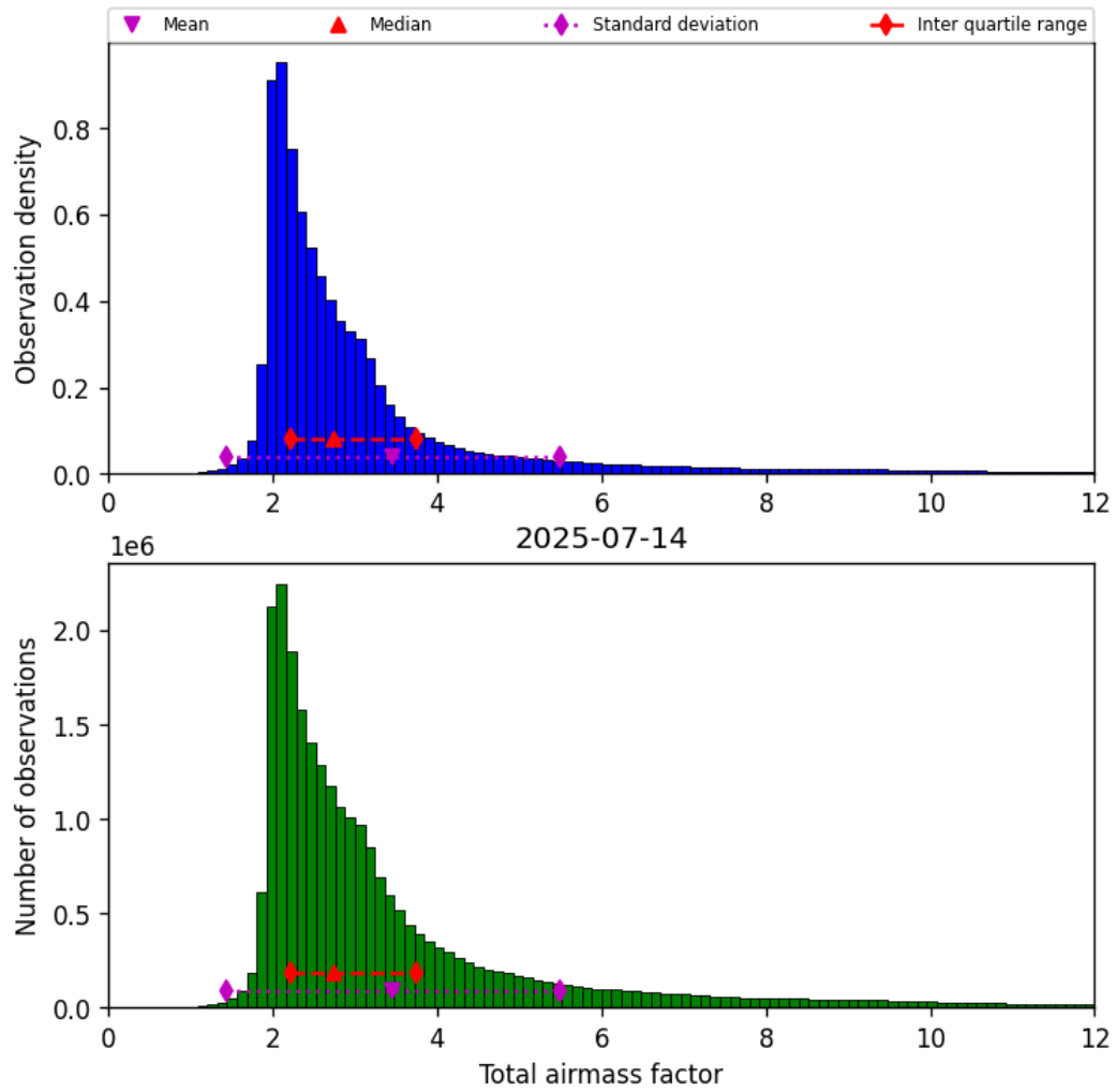
Figure 32: Histogram of “Total airmass factor” for 2025-07-13 to 2025-07-15
