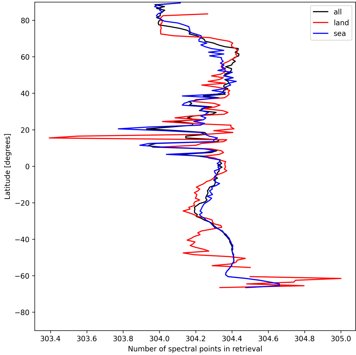
Figure 16: Zonal average of “Number of spectral points in retrieval” for 2025-07-13 to 2025-07-15.
