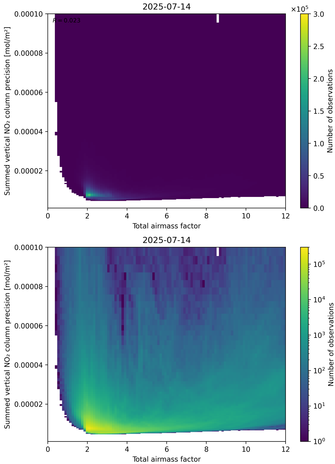
Figure 66: Scatter density plot of “Total airmass factor” against “Summed vertical NO 2 column precision” for 2025-07-13 to 2025-07-15.
