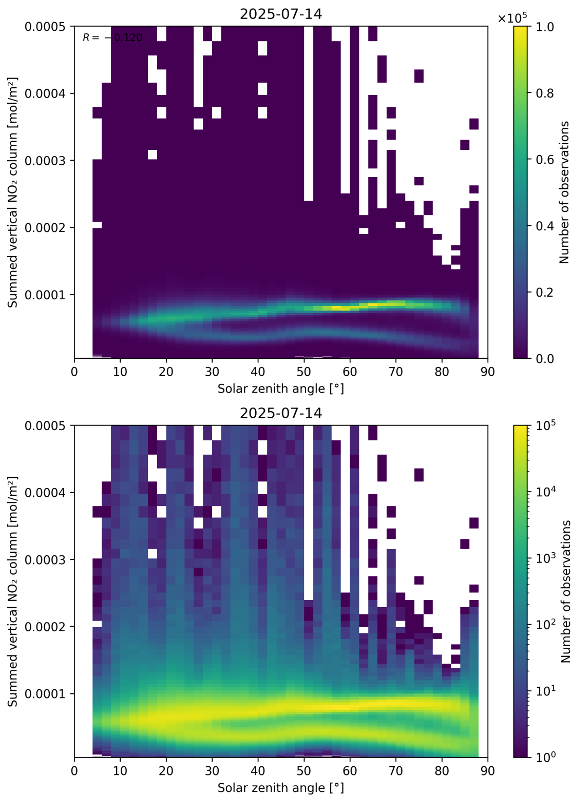
Figure 151: Scatter density plot of “Solar zenith angle” against “Summed vertical NO 2 column” for 2025-07-13 to 2025-07-15.
