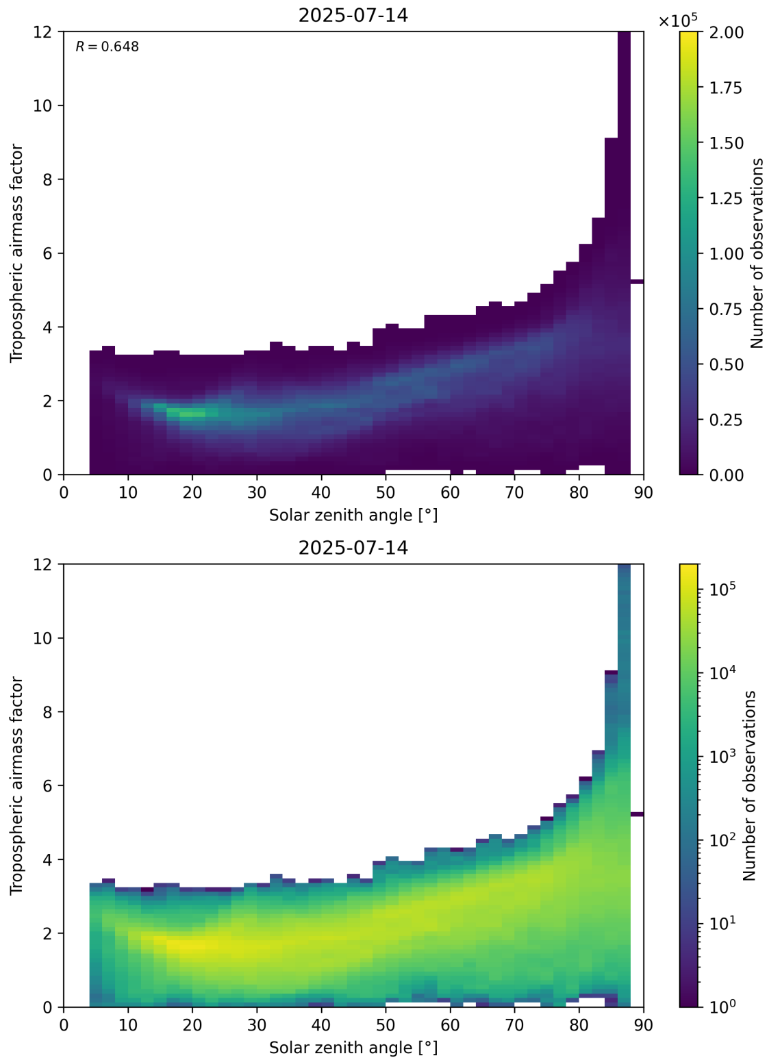
Figure 147: Scatter density plot of “Solar zenith angle” against “Tropospheric airmass factor” for 2025-07-13 to 2025-07-15.
