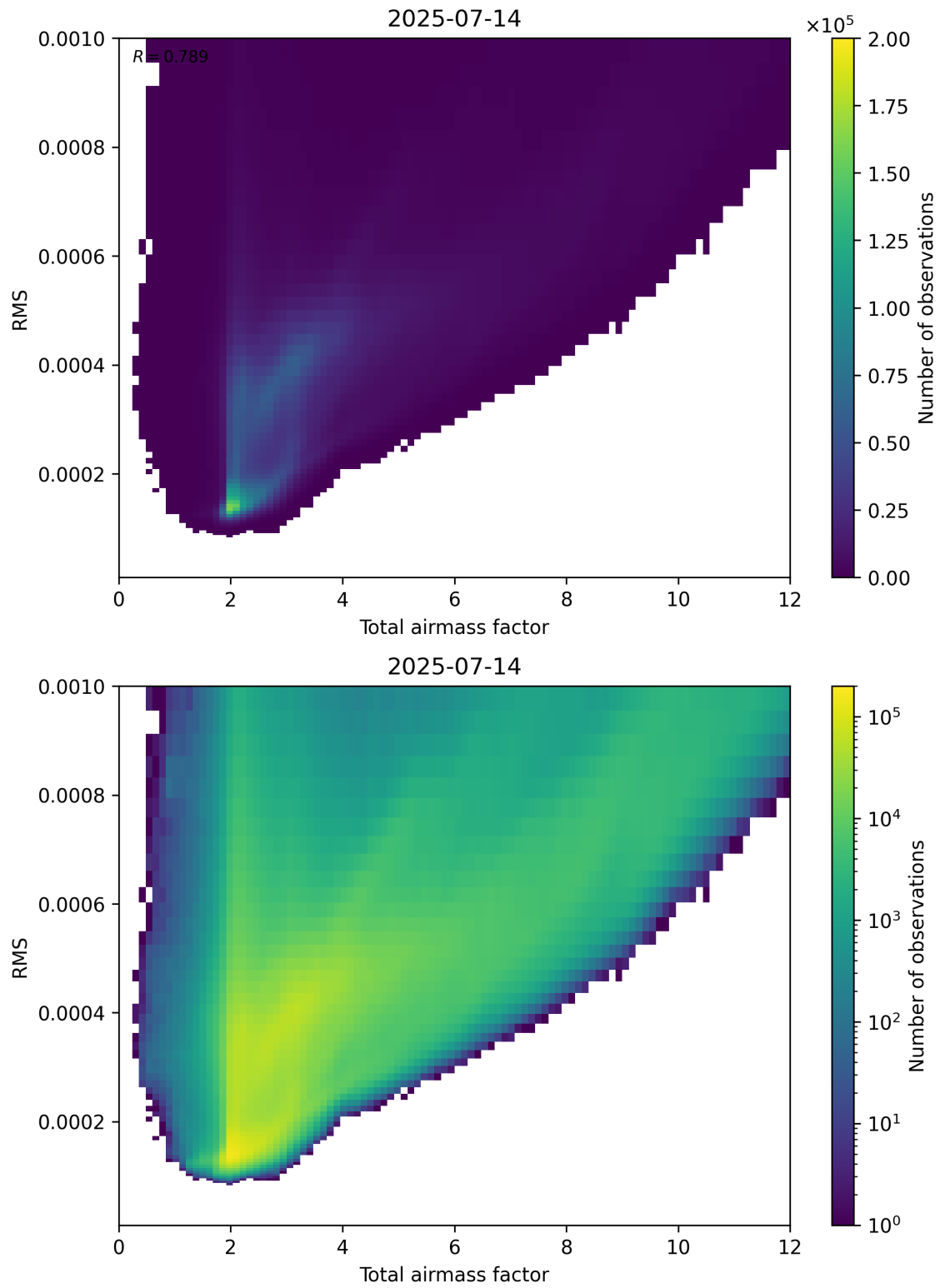
Figure 69: Scatter density plot of “Total airmass factor” against “RMS” for 2025-07-13 to 2025-07-15.
