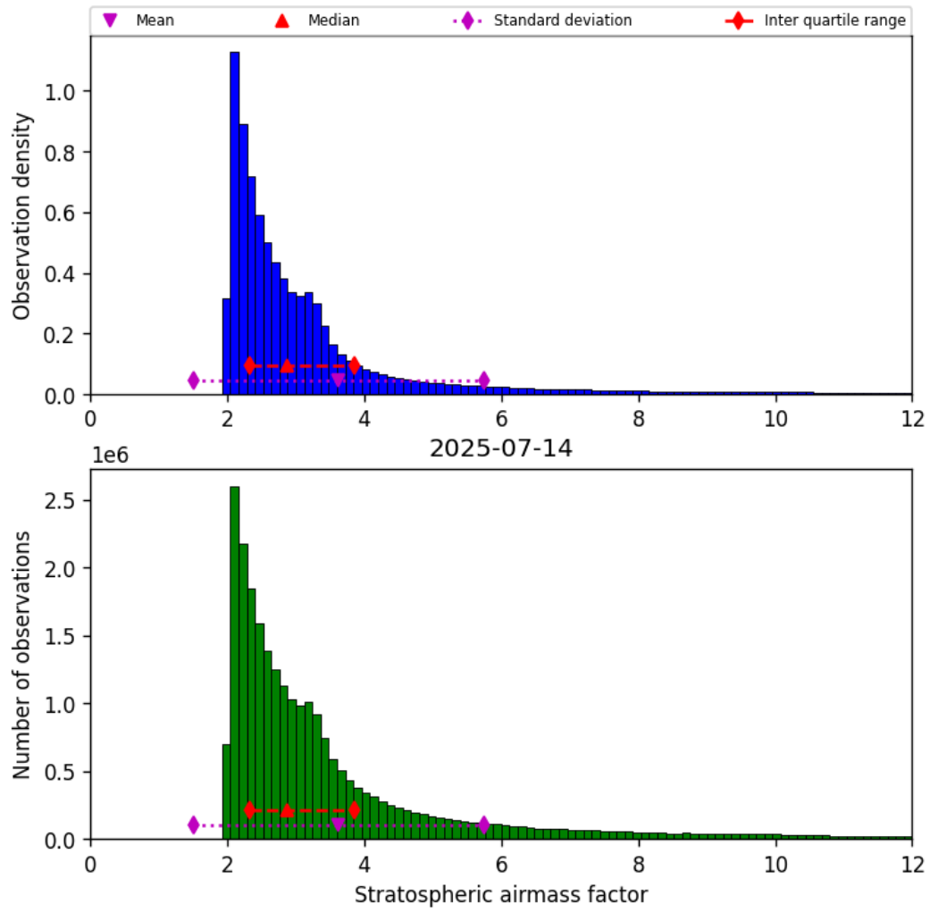
Figure 44: Histogram of “Stratospheric airmass factor” for 2025-07-13 to 2025-07-15
