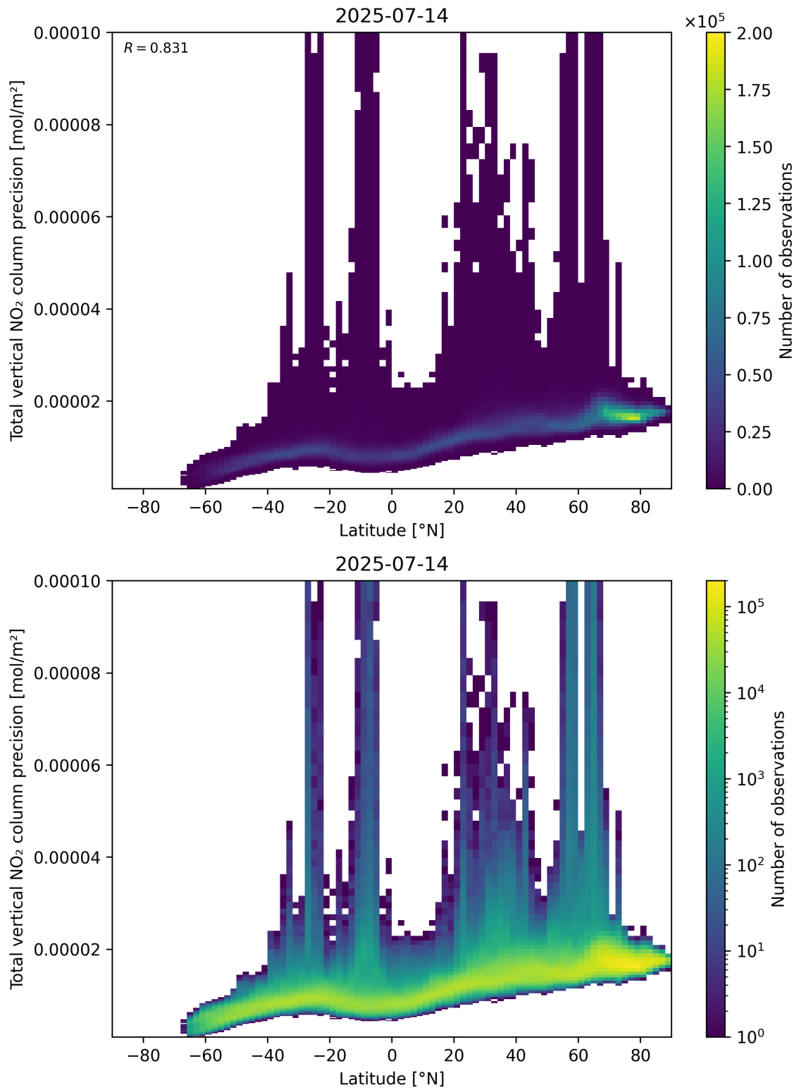
Figure 91: Scatter density plot of “Latitude” against “Total vertical NO 2 column precision” for 2025-07-13 to 2025-07-15.
