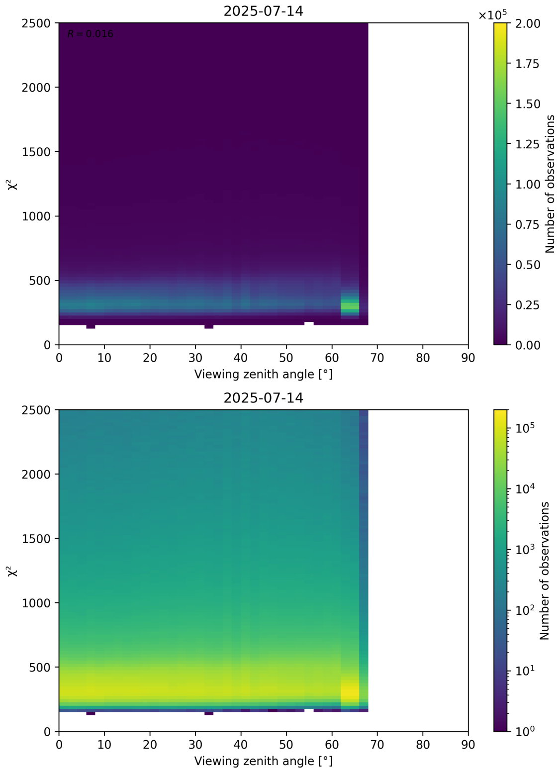
Figure 162: Scatter density plot of “Viewing zenith angle” against “ \chi^2 ” for 2025-07-13 to 2025-07-15.
