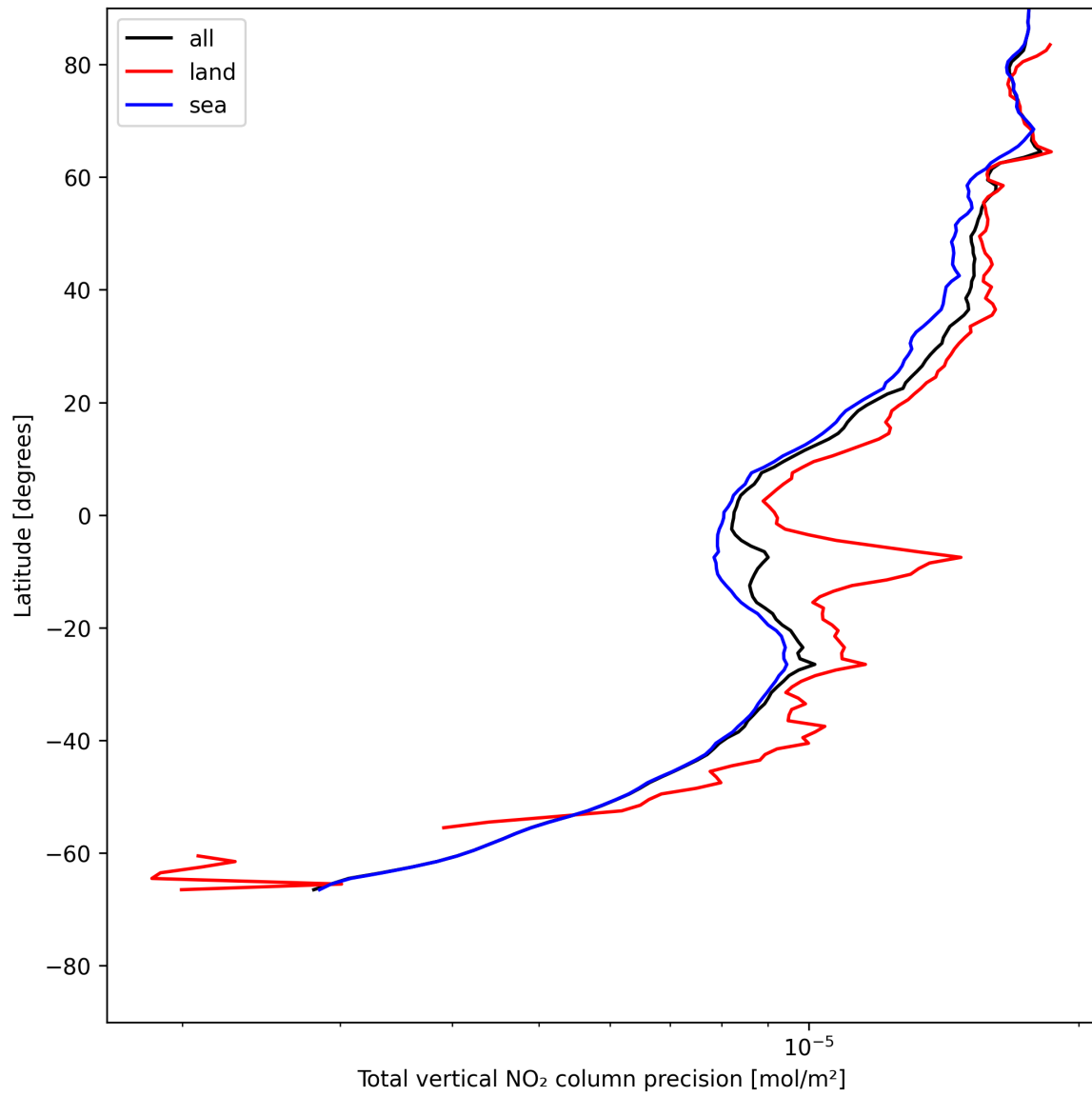
Figure 22: Zonal average of “Total vertical NO 2 column precision” for 2025-07-13 to 2025-07-15.
