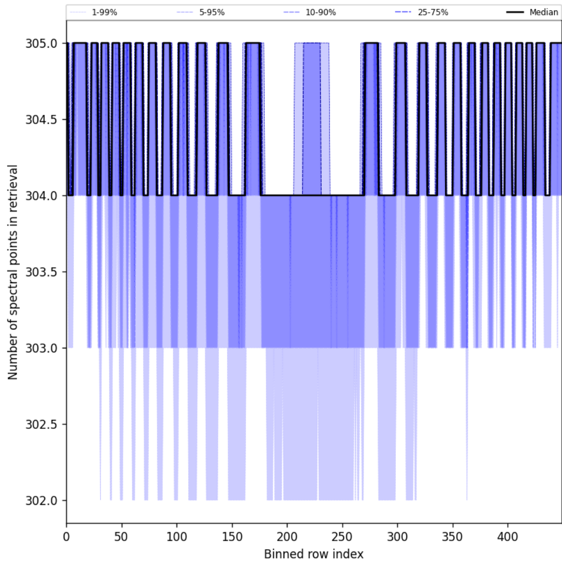
Figure 50: Along track statistics of “Number of spectral points in retrieval” for 2025-07-13 to 2025-07-15
