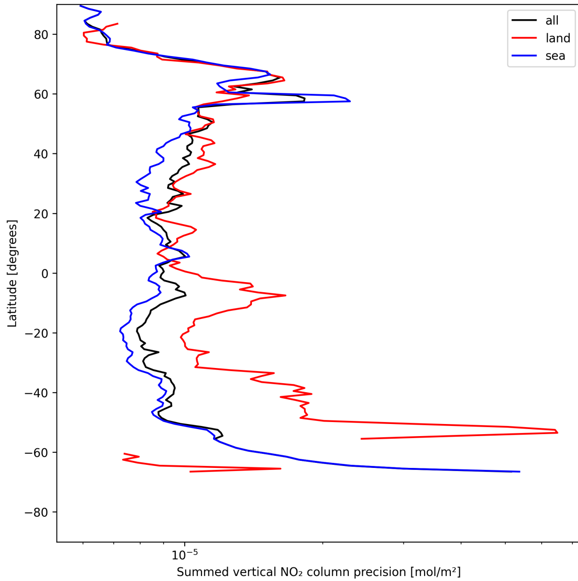
Figure 24: Zonal average of “Summed vertical NO 2 column precision” for 2025-07-13 to 2025-07-15.
