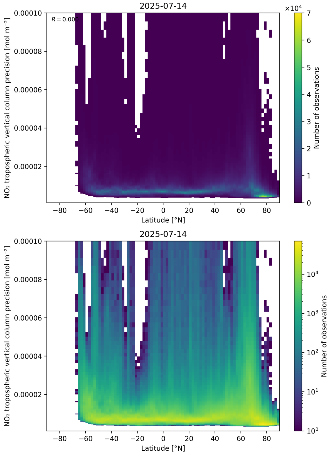
Figure 93: Scatter density plot of “Latitude” against “NO 2 tropospheric vertical column precision” for 2025-07-13 to 2025-07-15.
