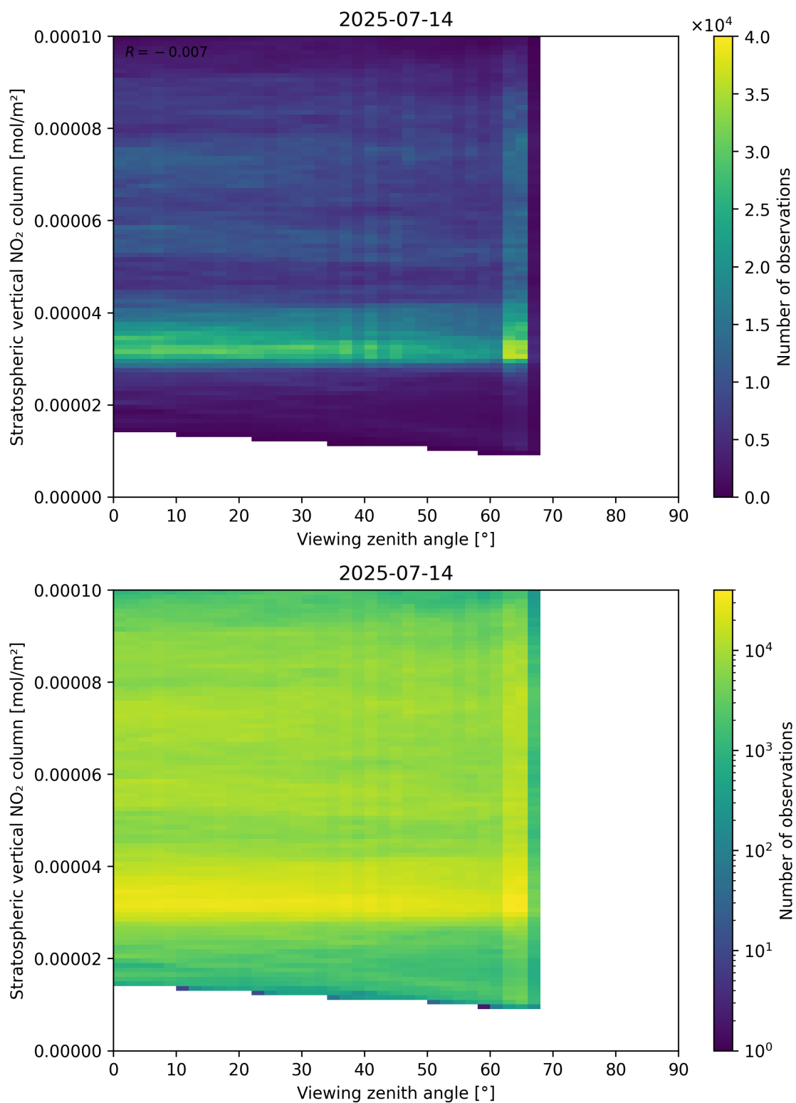
Figure 164: Scatter density plot of “Viewing zenith angle” against “Stratospheric vertical NO 2 column” for 2025-07-13 to 2025-07-15.
