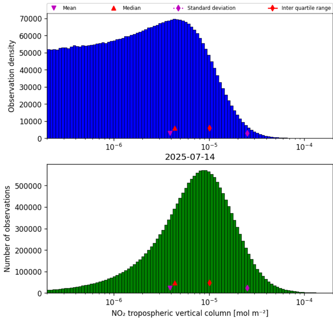
Figure 29: Histogram of “NO 2 tropospheric vertical column” for 2025-07-13 to 2025-07-15
