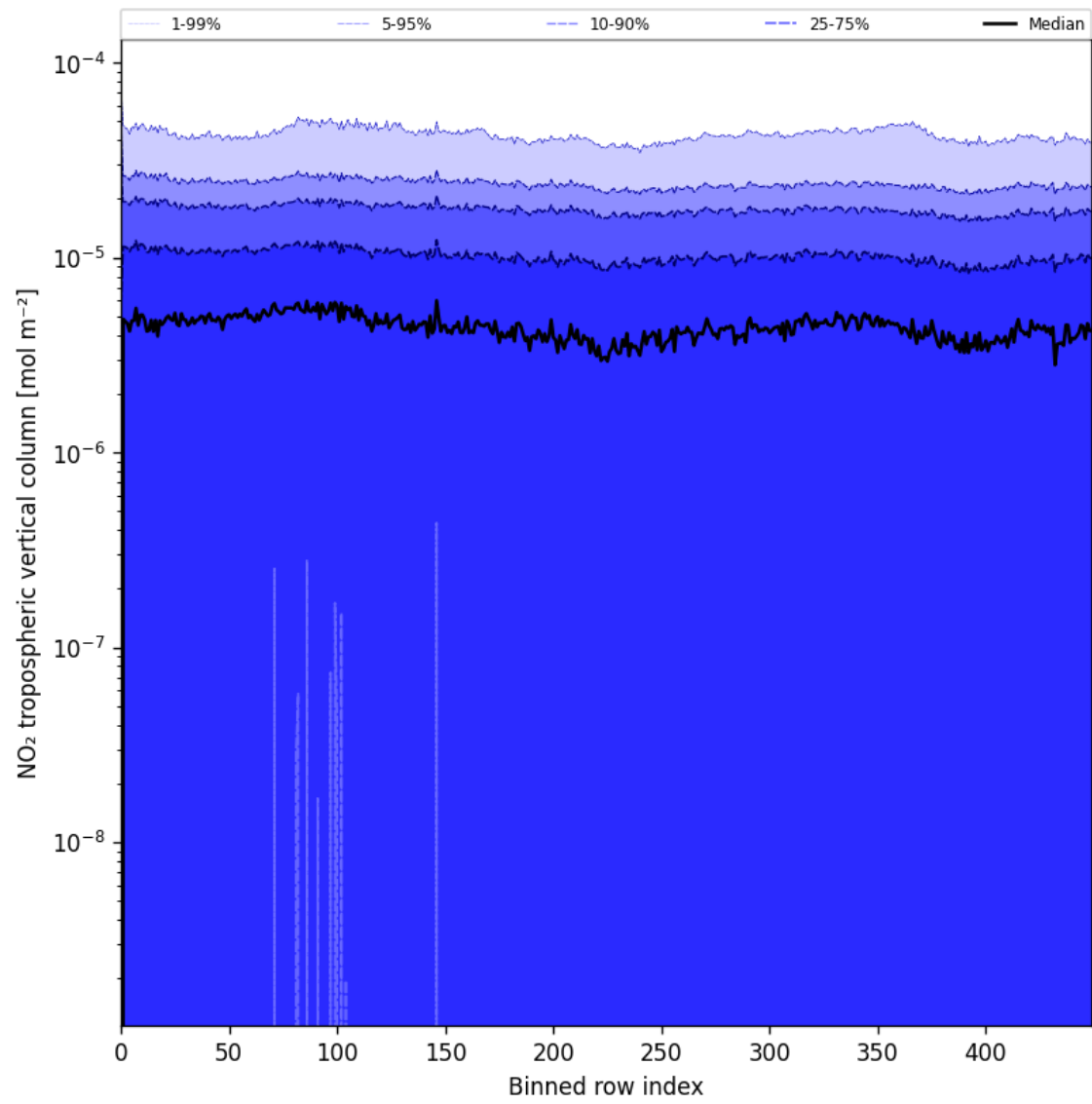
Figure 46: Along track statistics of “NO 2 tropospheric vertical column” for 2025-07-13 to 2025-07-15
