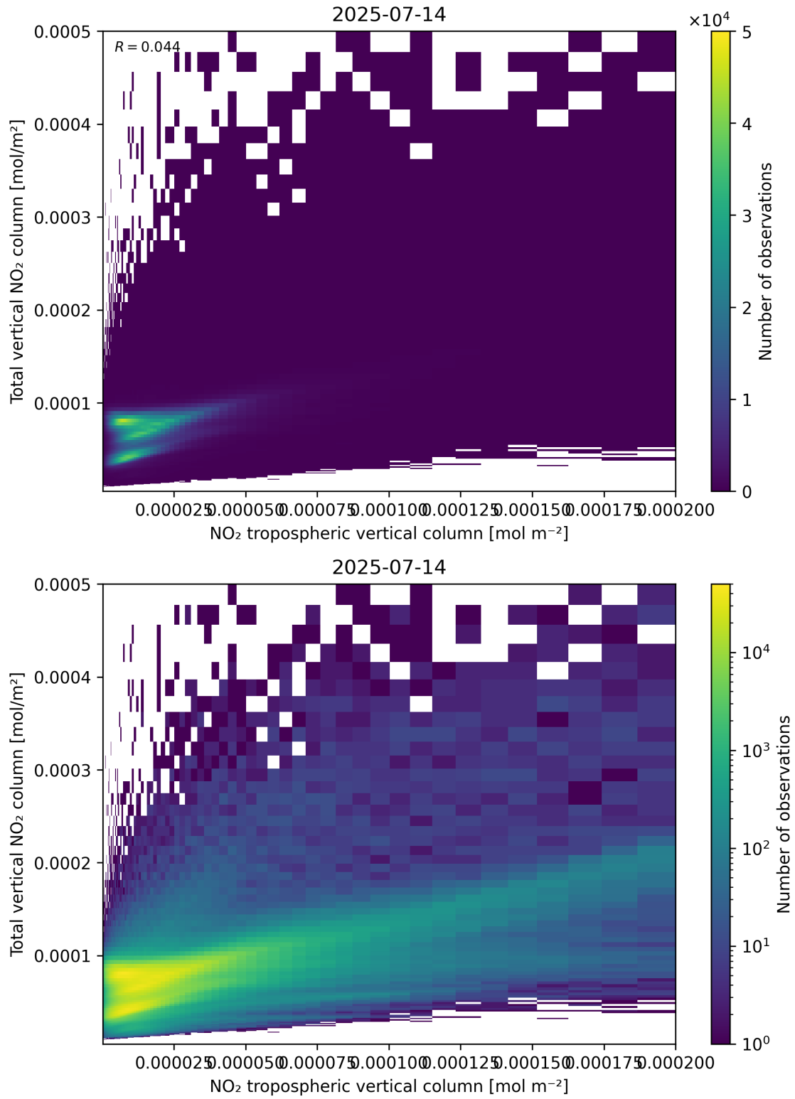
Figure 128: Scatter density plot of “NO 2 tropospheric vertical column” against “Total vertical NO 2 column” for 2025-07-13 to 2025-07-15.
