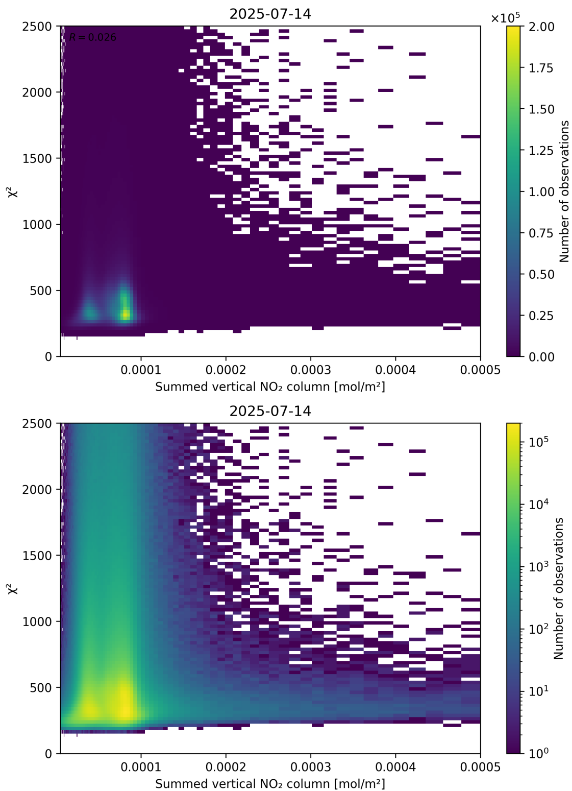
Figure 104: Scatter density plot of “Summed vertical NO 2 column” against “ \chi^2 ” for 2025-07-13 to 2025-07-15.
