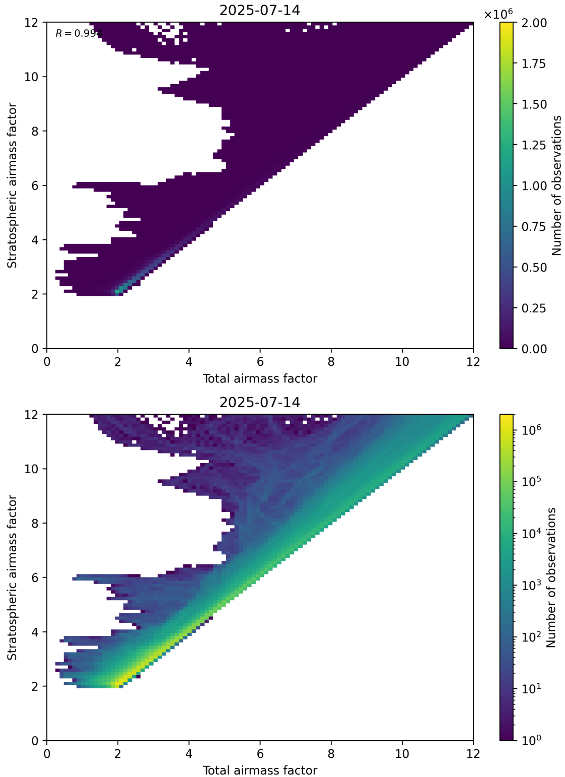
Figure 62: Scatter density plot of “Total airmass factor” against “Stratospheric airmass factor” for 2025-07-13 to 2025-07-15.
