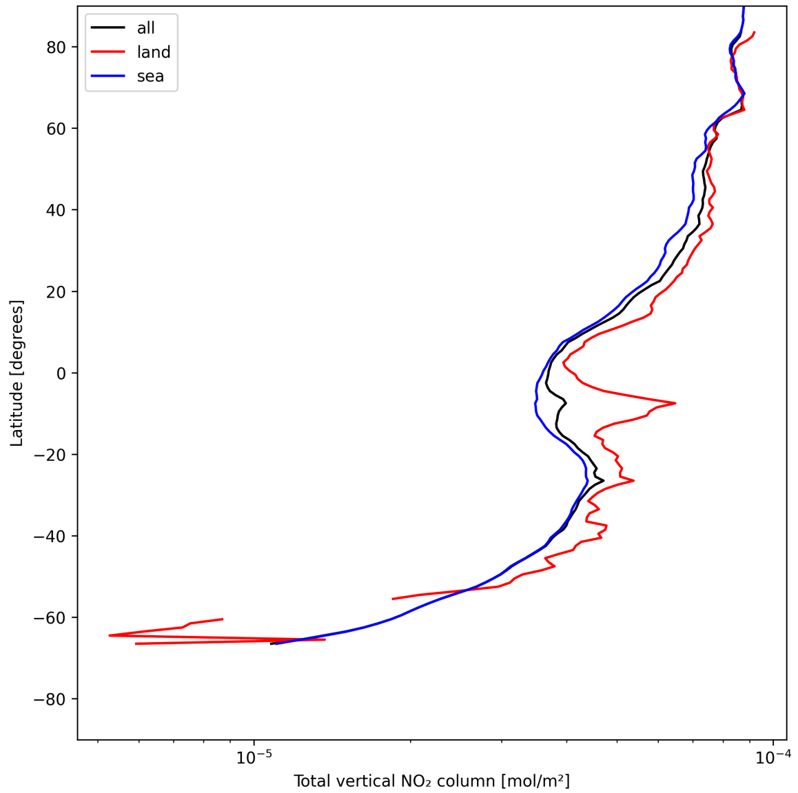
Figure 21: Zonal average of “Total vertical NO 2 column” for 2025-07-13 to 2025-07-15.
