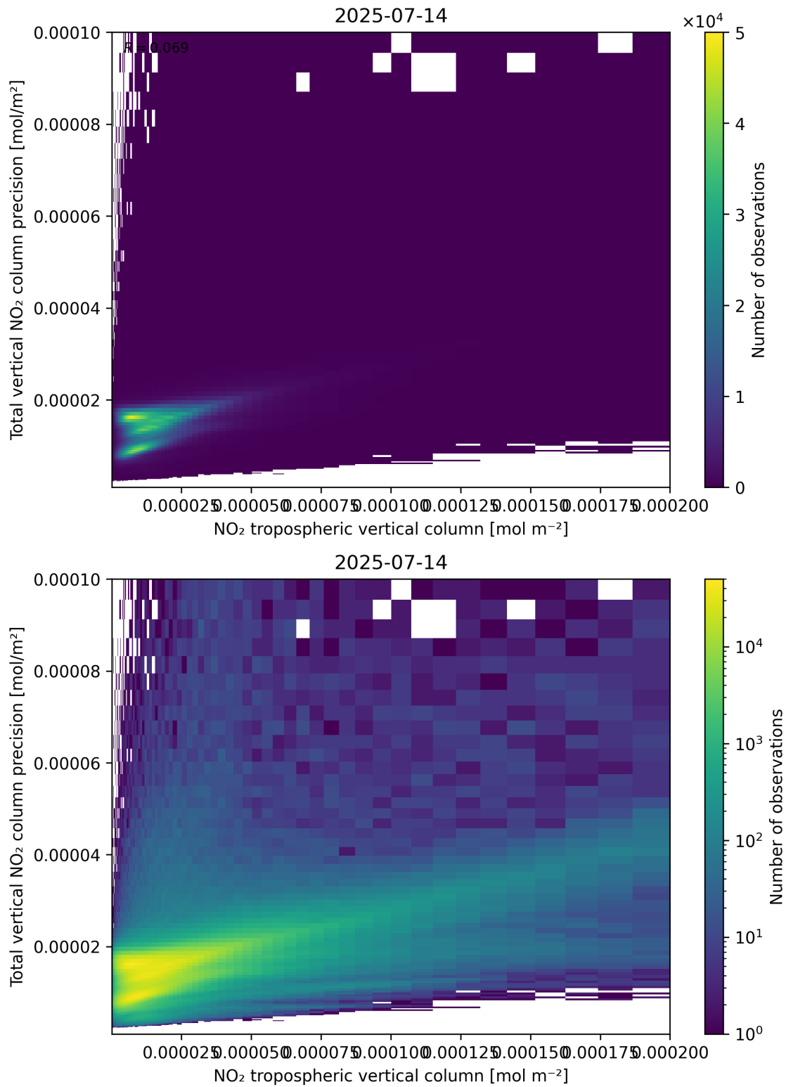
Figure 129: Scatter density plot of “NO 2 tropospheric vertical column” against “Total vertical NO 2 column precision” for 2025-07-13 to 2025-07-15.
