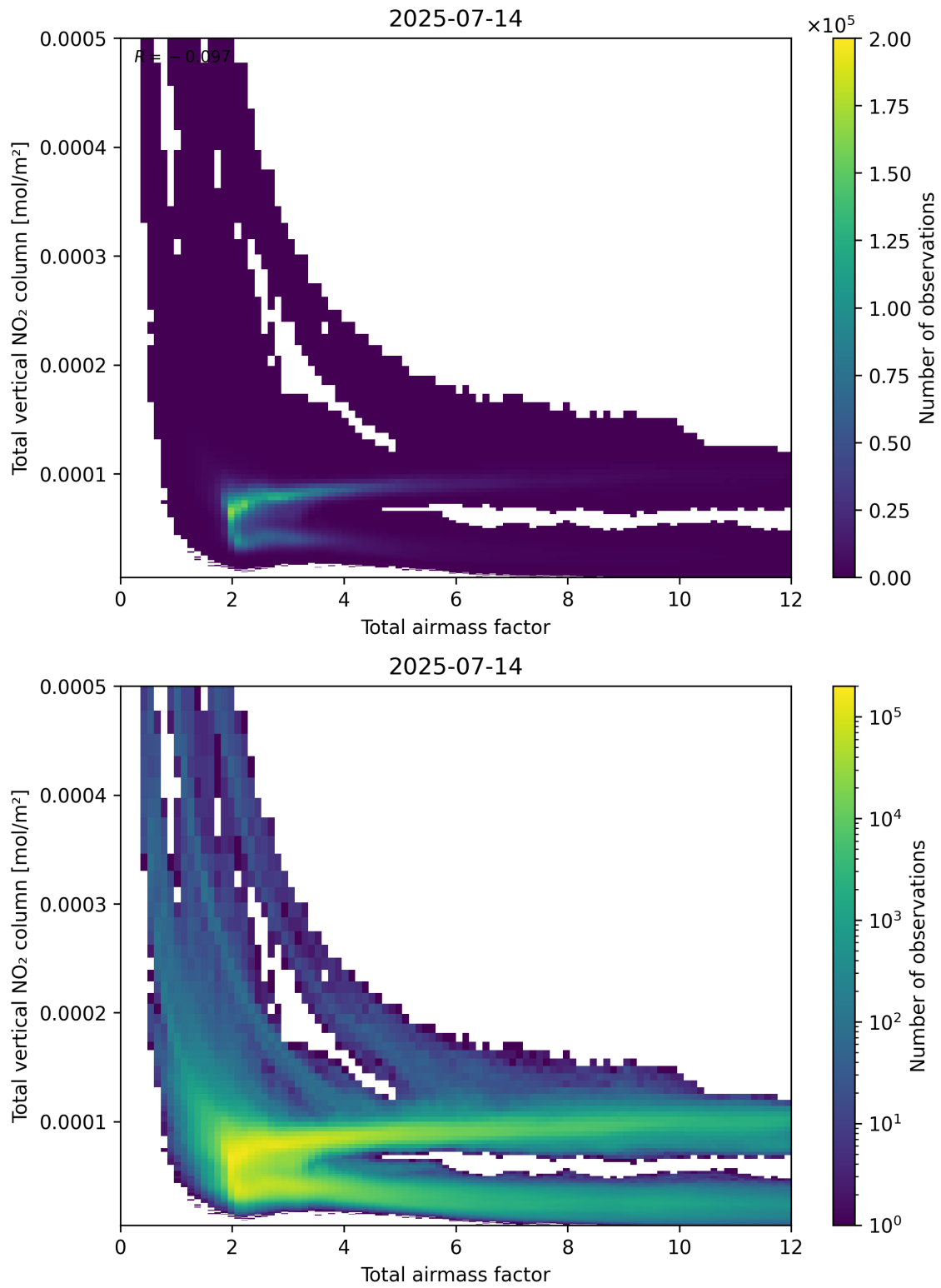
Figure 67: Scatter density plot of “Total airmass factor” against “Total vertical NO 2 column” for 2025-07-13 to 2025-07-15.
