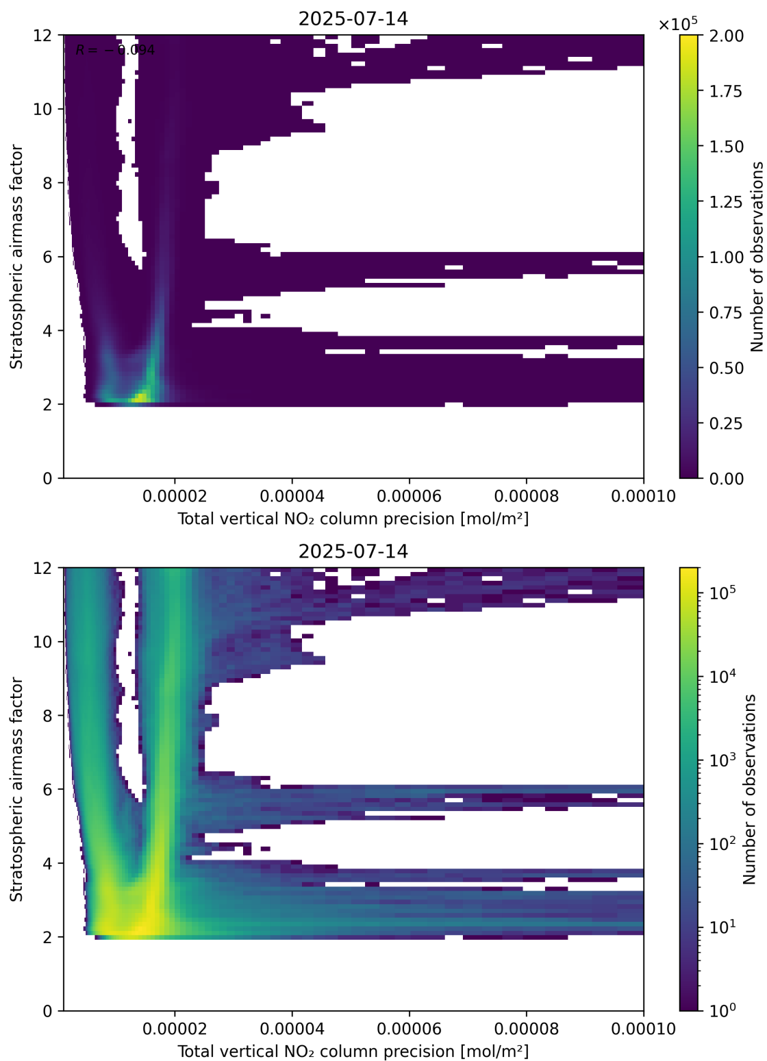
Figure 115: Scatter density plot of “Total vertical NO 2 column precision” against “Stratospheric air mass factor” for 2025-07-13 to 2025-07-15.
