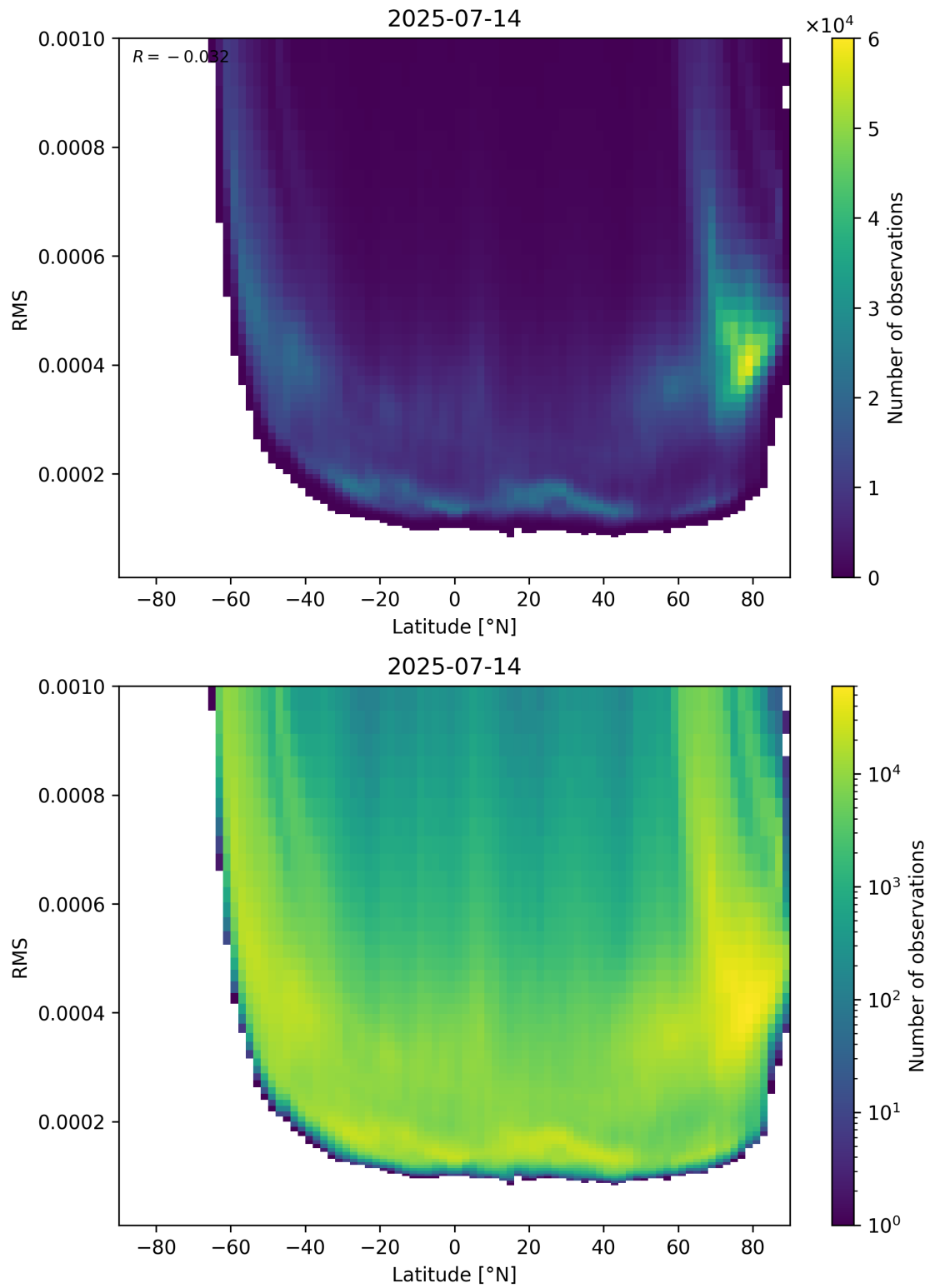
Figure 94: Scatter density plot of “Latitude” against “RMS” for 2025-07-13 to 2025-07-15.
