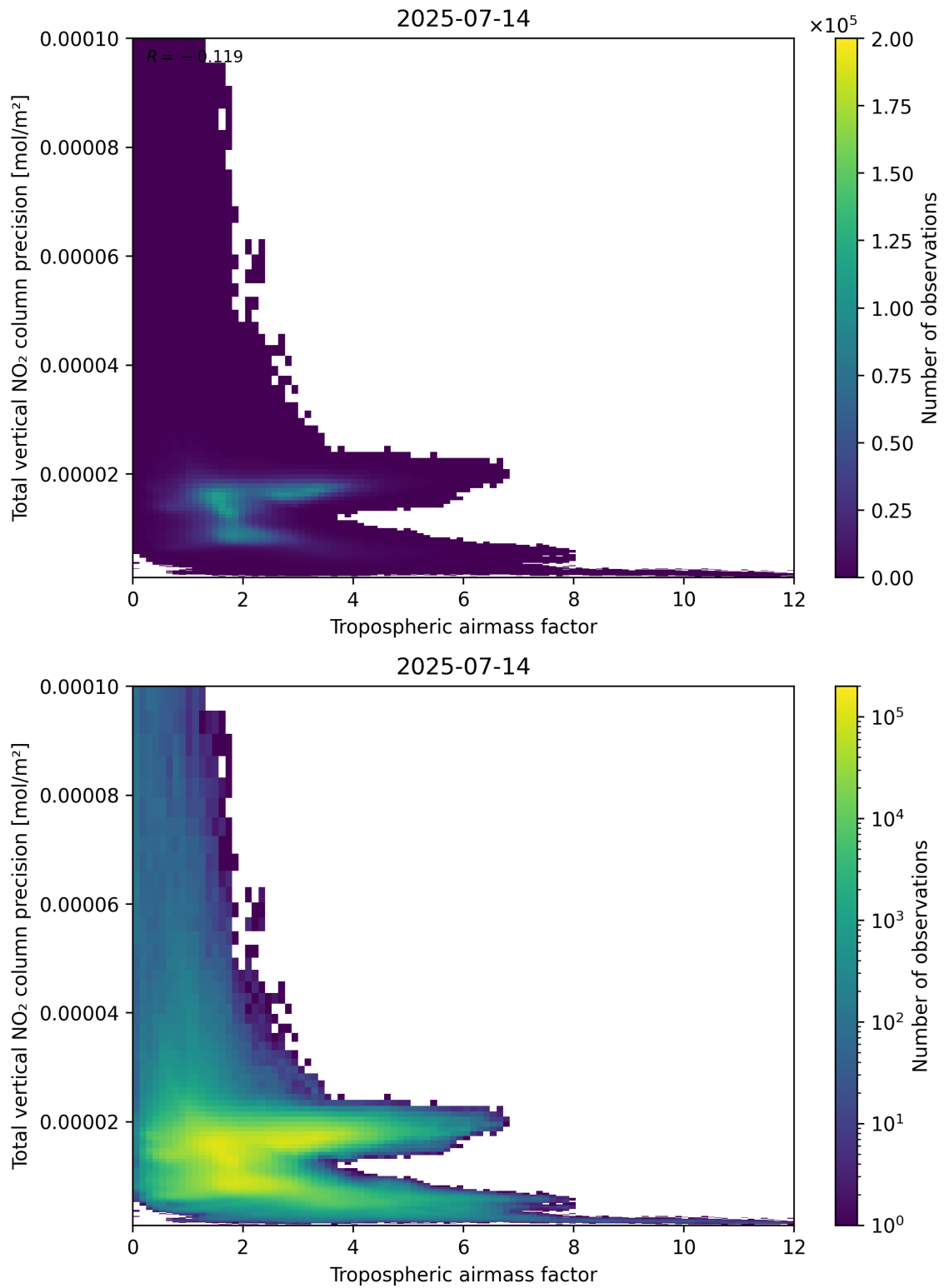
Figure 78: Scatter density plot of “Tropospheric airmass factor” against “Total vertical NO 2 column precision” for 2025-07-13 to 2025-07-15.
