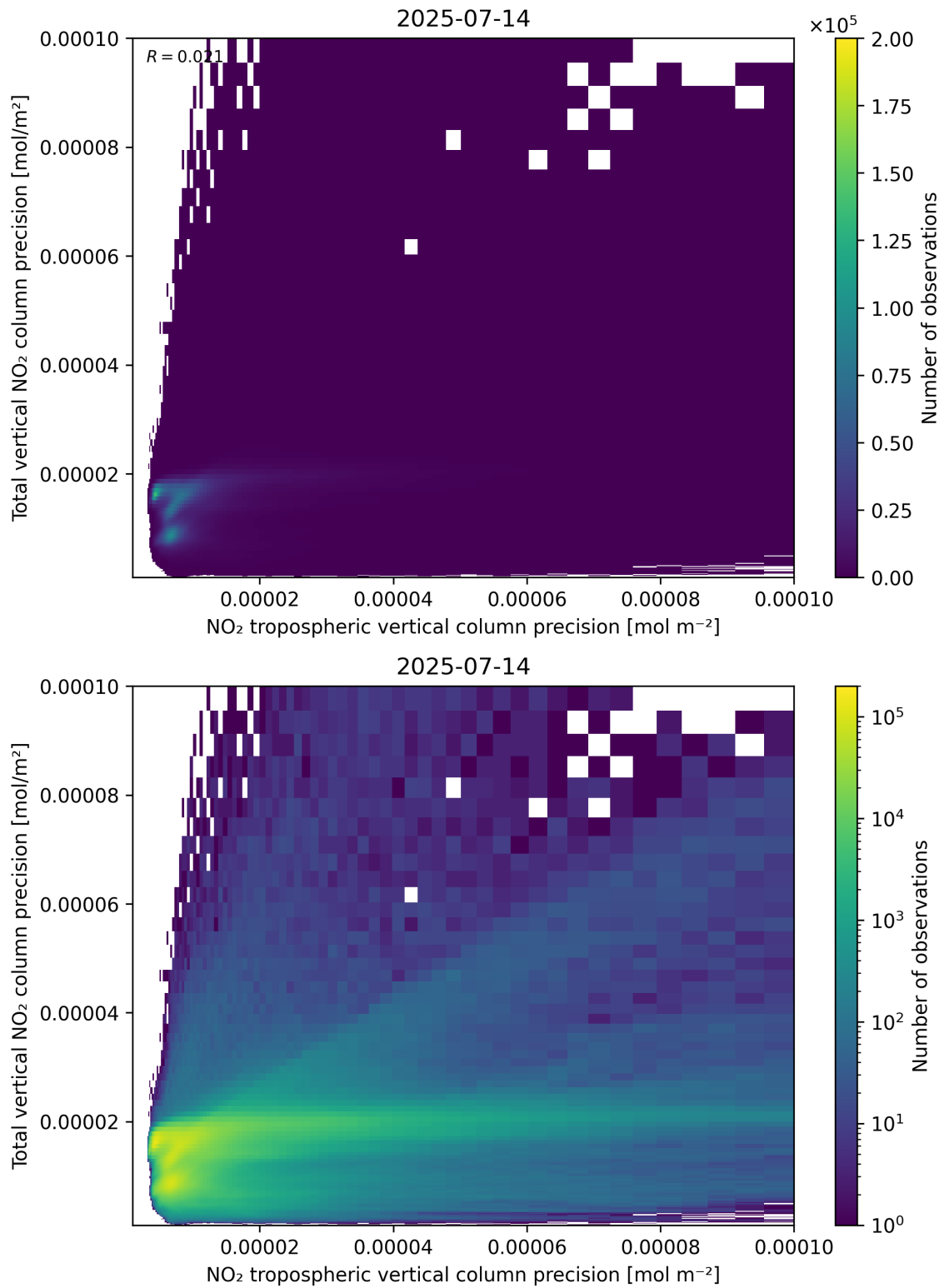
Figure 139: Scatter density plot of “NO 2 tropospheric vertical column precision” against “Total vertical NO 2 column precision” for 2025-07-13 to 2025-07-15.
