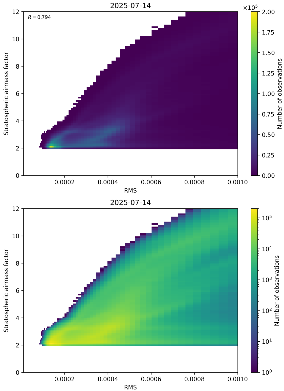
Figure 144: Scatter density plot of “RMS” against “Stratospheric airmass factor” for 2025-07-13 to 2025-07-15.
