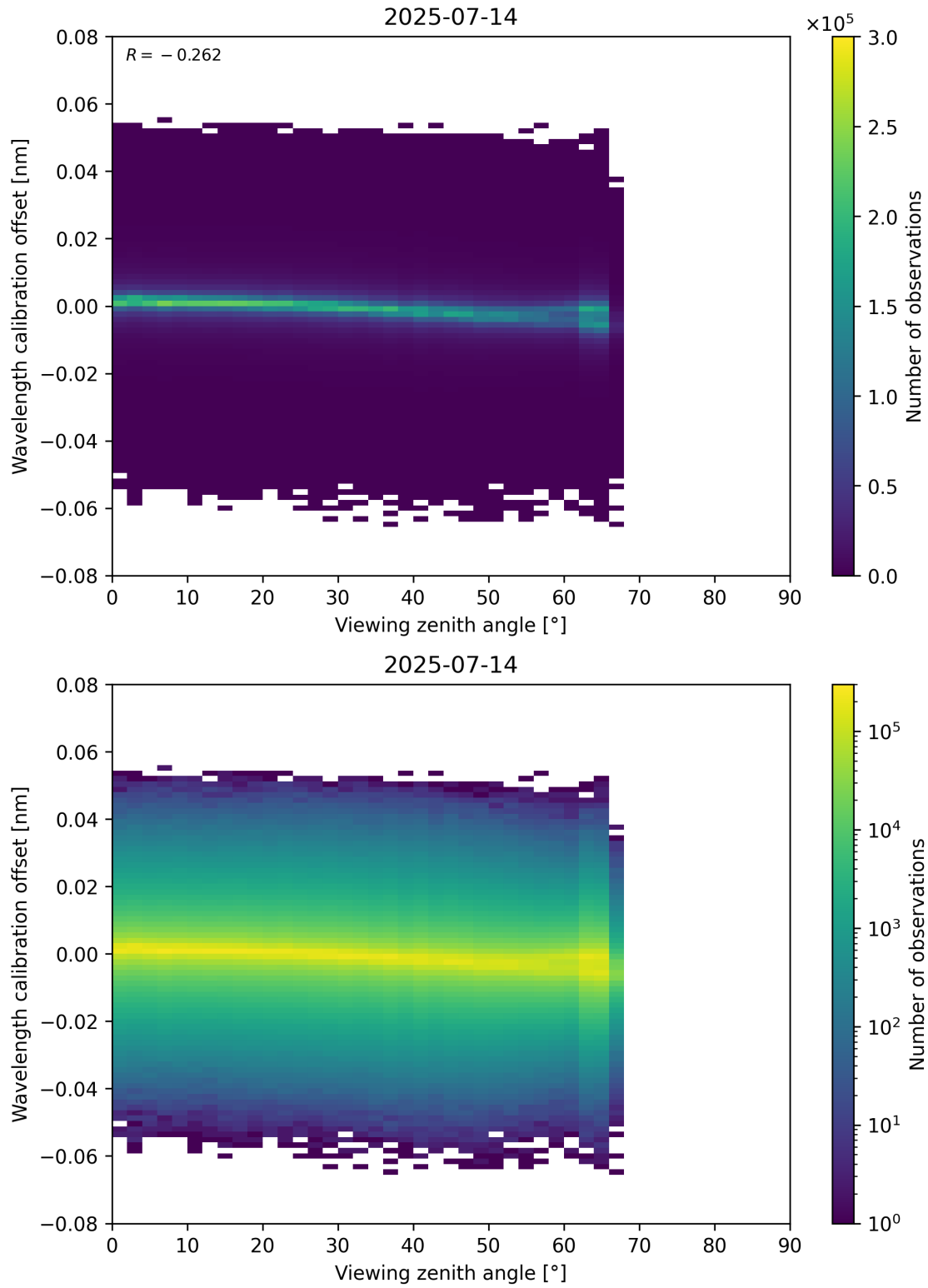
Figure 173: Scatter density plot of “Viewing zenith angle” against “Wavelength calibration offset” for 2025-07-13 to 2025-07-15.
