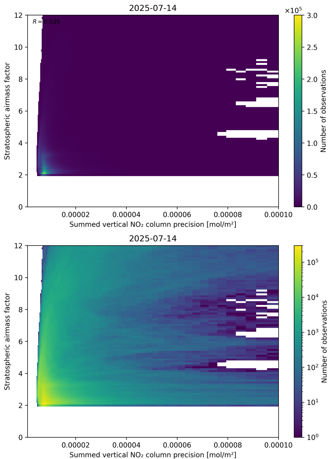
Figure 106: Scatter density plot of “Summed vertical NO 2 column precision” against “Stratospheric airmass factor” for 2025-07-13 to 2025-07-15.
