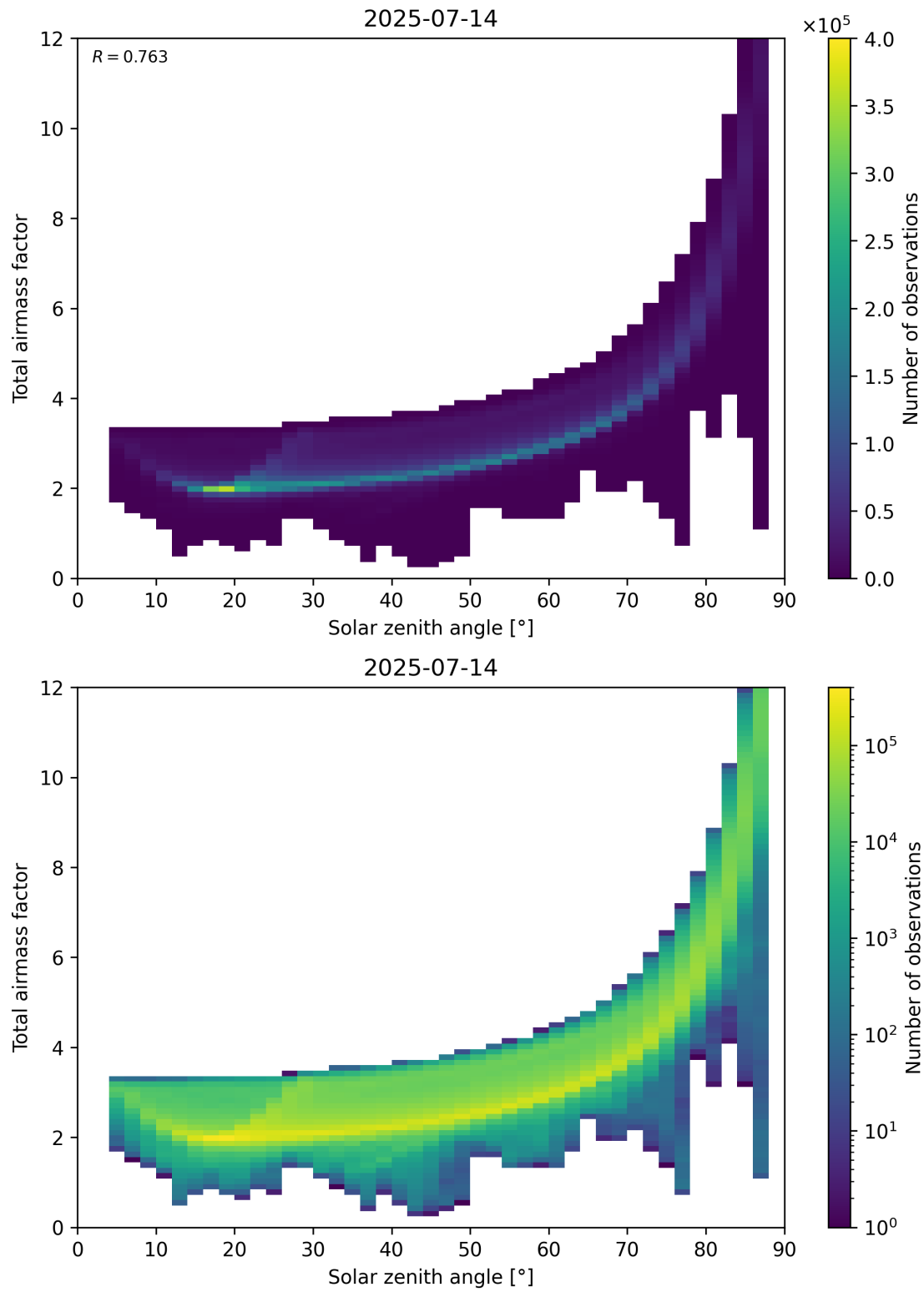
Figure 146: Scatter density plot of “Solar zenith angle” against “Total air mass factor” for 2025-07-13 to 2025-07-15.
