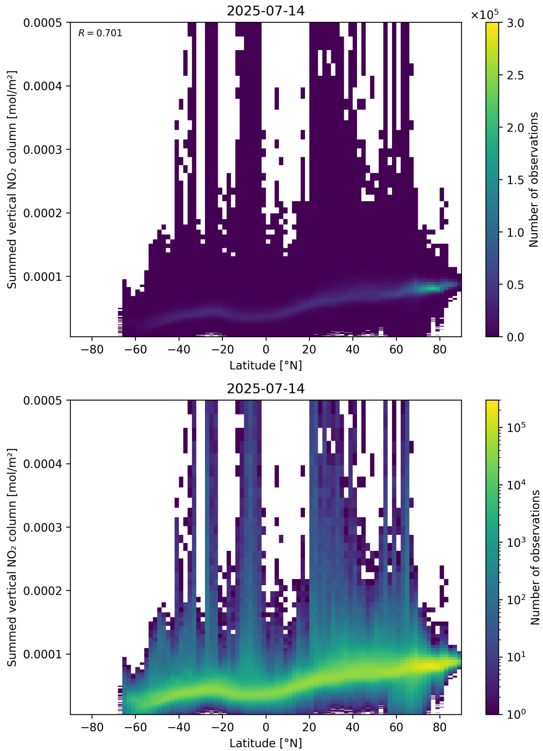
Figure 88: Scatter density plot of “Latitude” against “Summed vertical NO 2 column” for 2025-07-13 to 2025-07-15.
