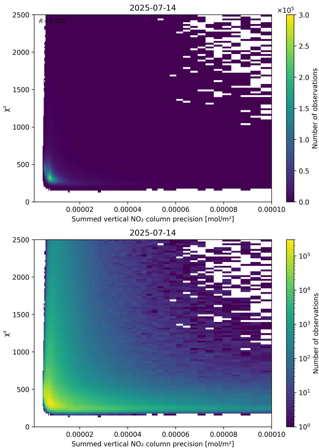
Figure 107: Scatter density plot of “Summed vertical NO 2 column precision” against “ \chi^2 ” for 2025-07-13 to 2025-07-15.
