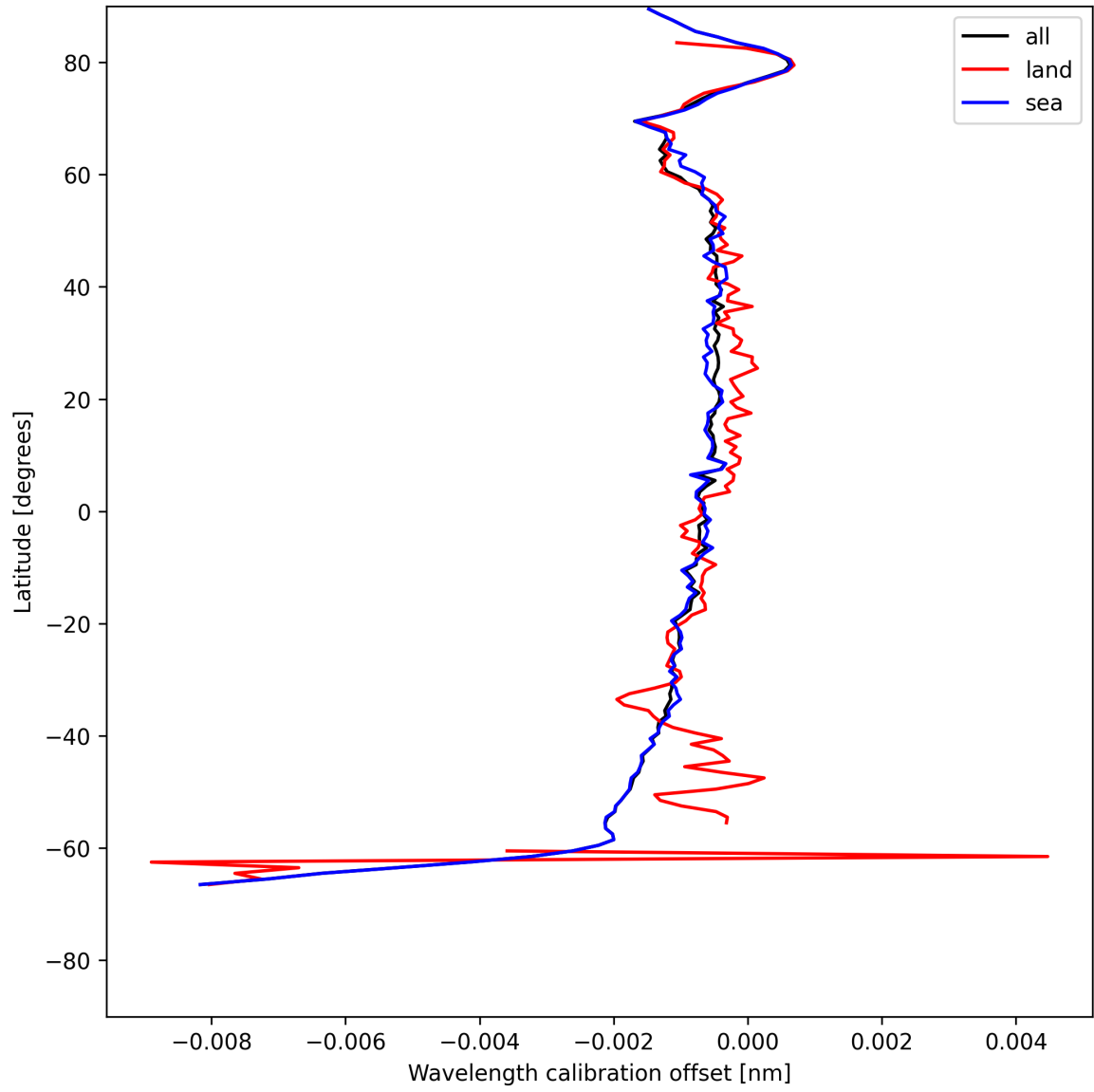
Figure 18: Zonal average of “Wavelength calibration offset” for 2025-07-13 to 2025-07-15.
