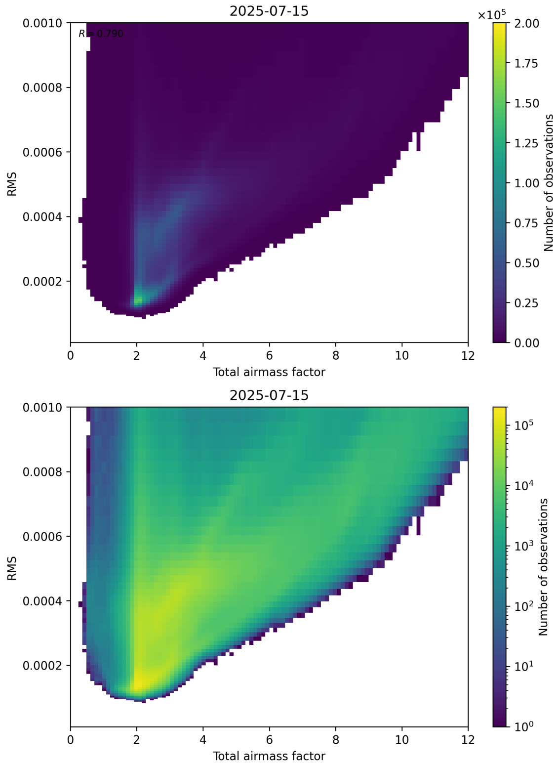
Figure 69: Scatter density plot of “Total airmass factor” against “RMS” for 2025-07-14 to 2025-07-16.
