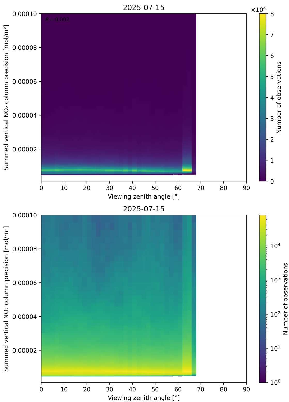
Figure 166: Scatter density plot of “Viewing zenith angle” against “Summed vertical NO 2 column precision” for 2025-07-14 to 2025-07-16.
