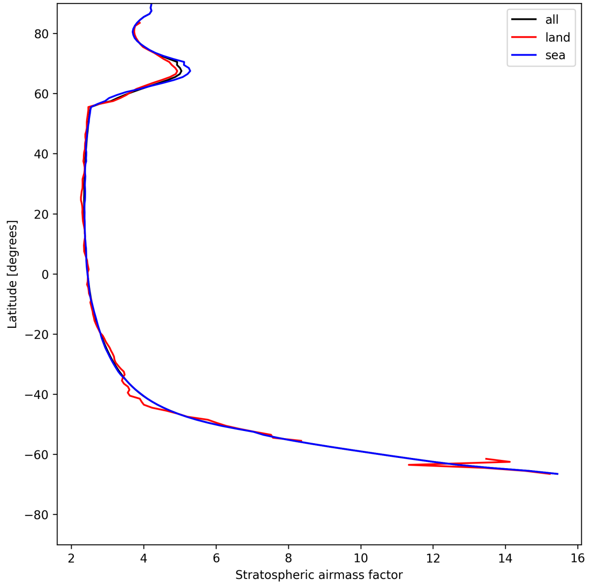
Figure 27: Zonal average of “Stratospheric airmass factor” for 2025-07-14 to 2025-07-16.
