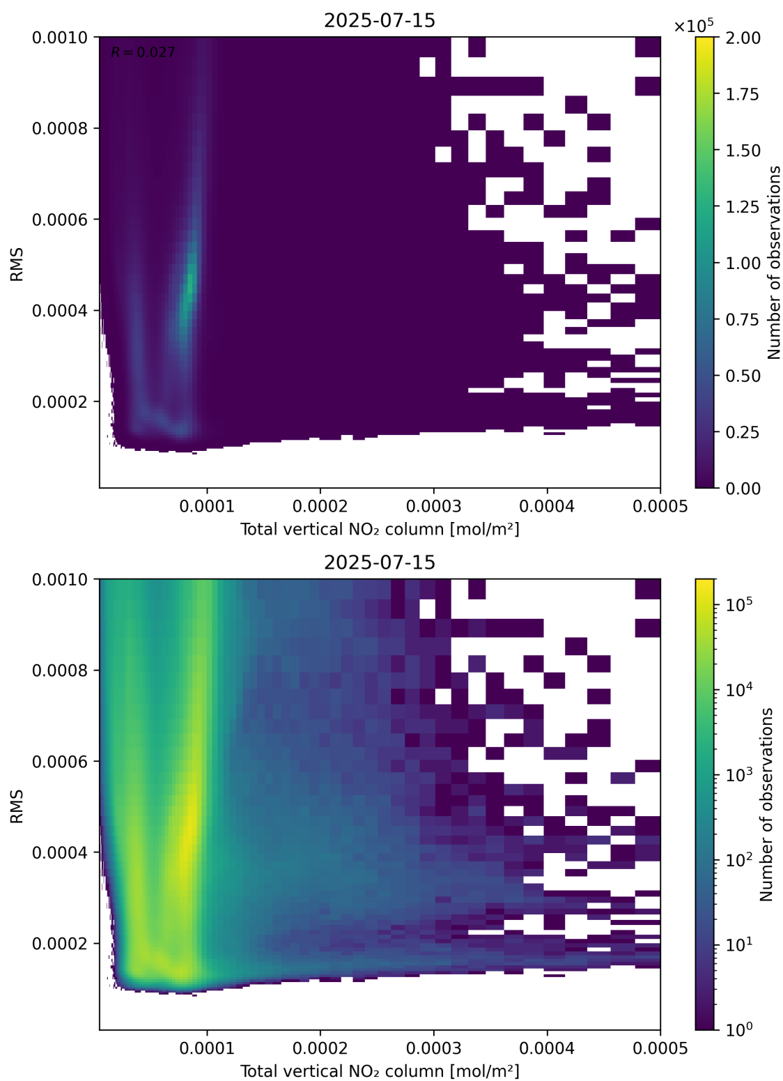
Figure 120: Scatter density plot of “Total vertical NO 2 column” against “RMS” for 2025-07-14 to 2025-07-16.
