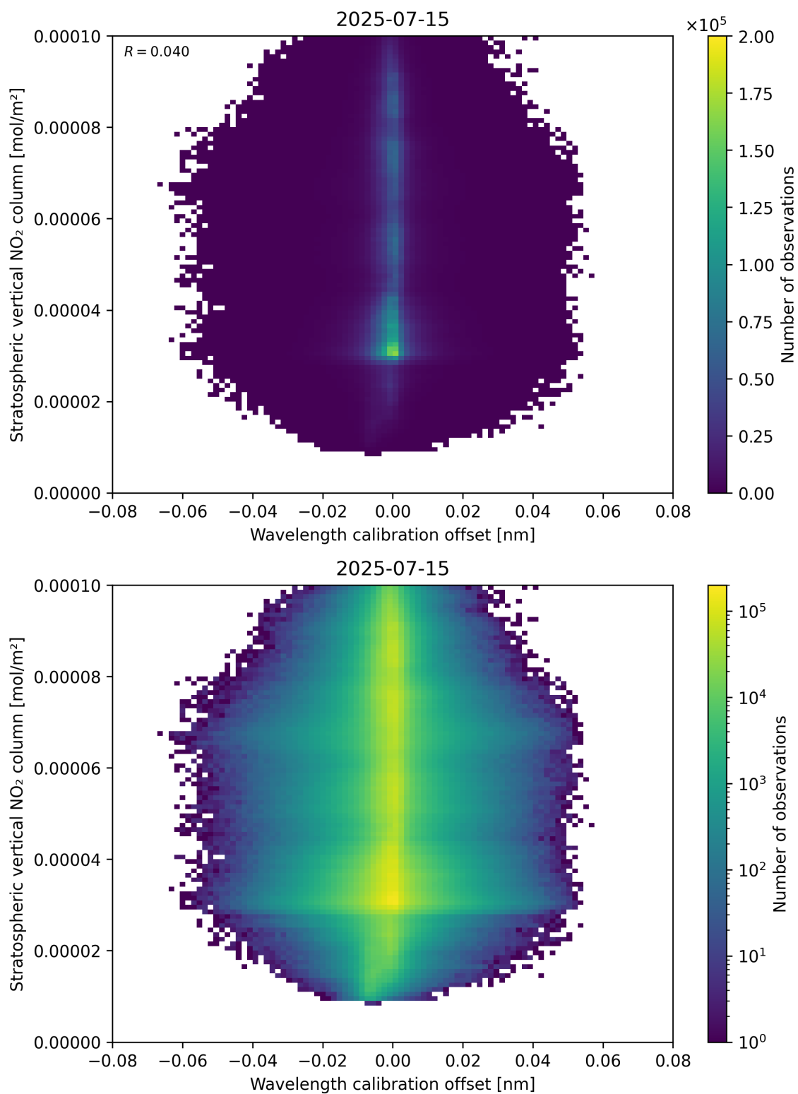
Figure 176: Scatter density plot of “Wavelength calibration offset” against “Stratospheric vertical NO 2 column” for 2025-07-14 to 2025-07-16.
