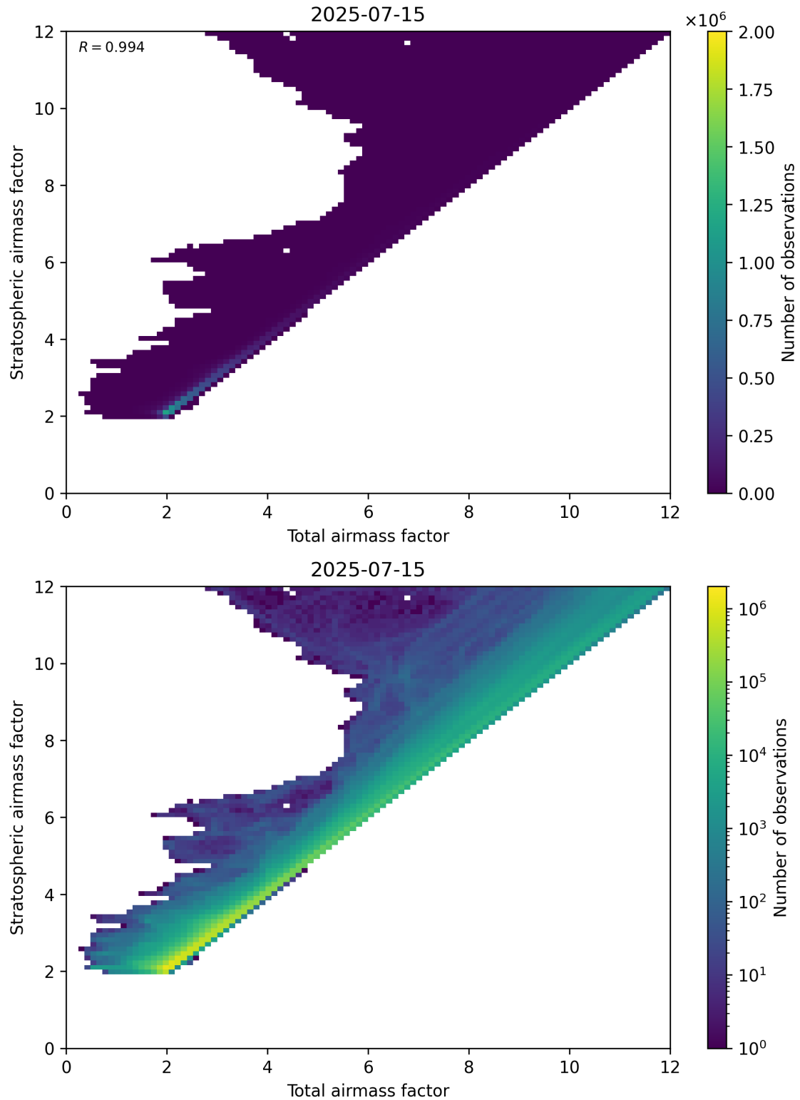
Figure 62: Scatter density plot of “Total airmass factor” against “Stratospheric airmass factor” for 2025-07-14 to 2025-07-16.
