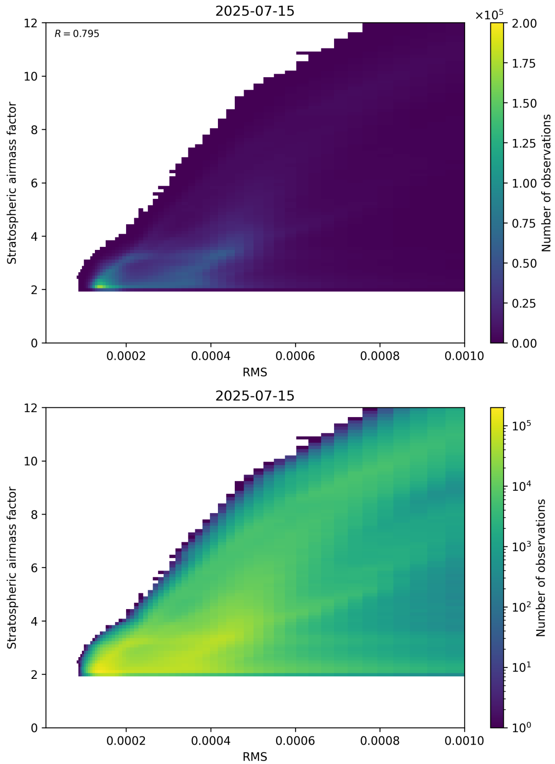
Figure 144: Scatter density plot of “RMS” against “Stratospheric airmass factor” for 2025-07-14 to 2025-07-16.
