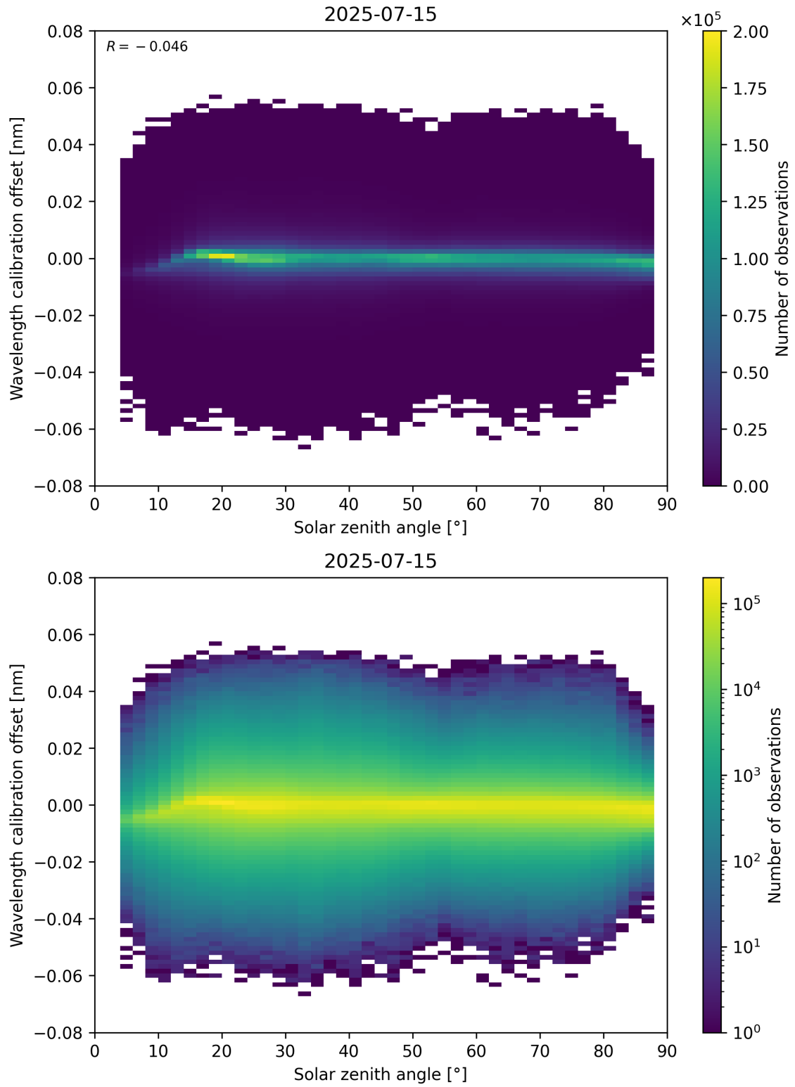
Figure 158: Scatter density plot of “Solar zenith angle” against “Wavelength calibration offset” for 2025-07-14 to 2025-07-16.
