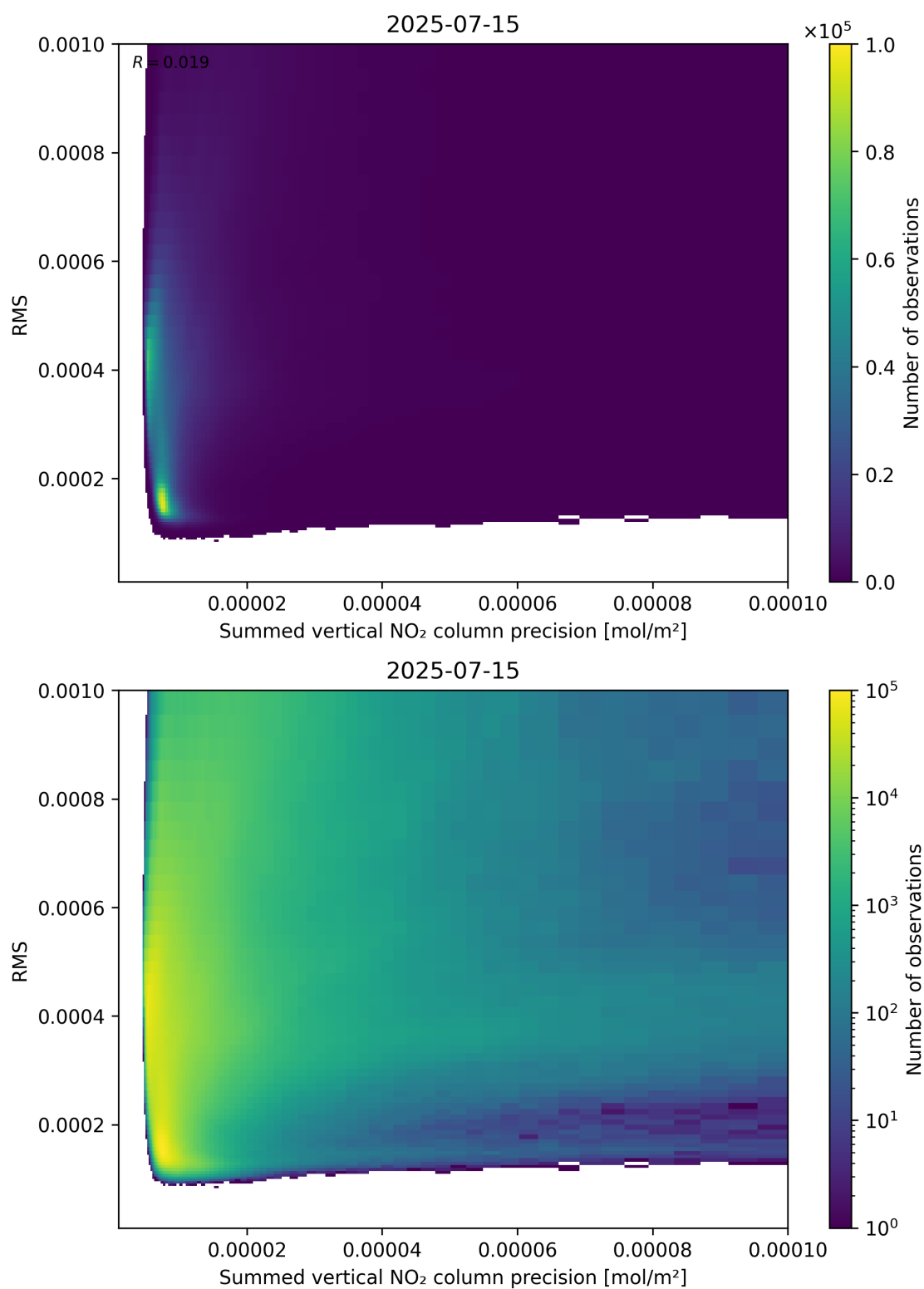
Figure 108: Scatter density plot of “Summed vertical NO 2 column precision” against “RMS” for 2025-07-14 to 2025-07-16.
