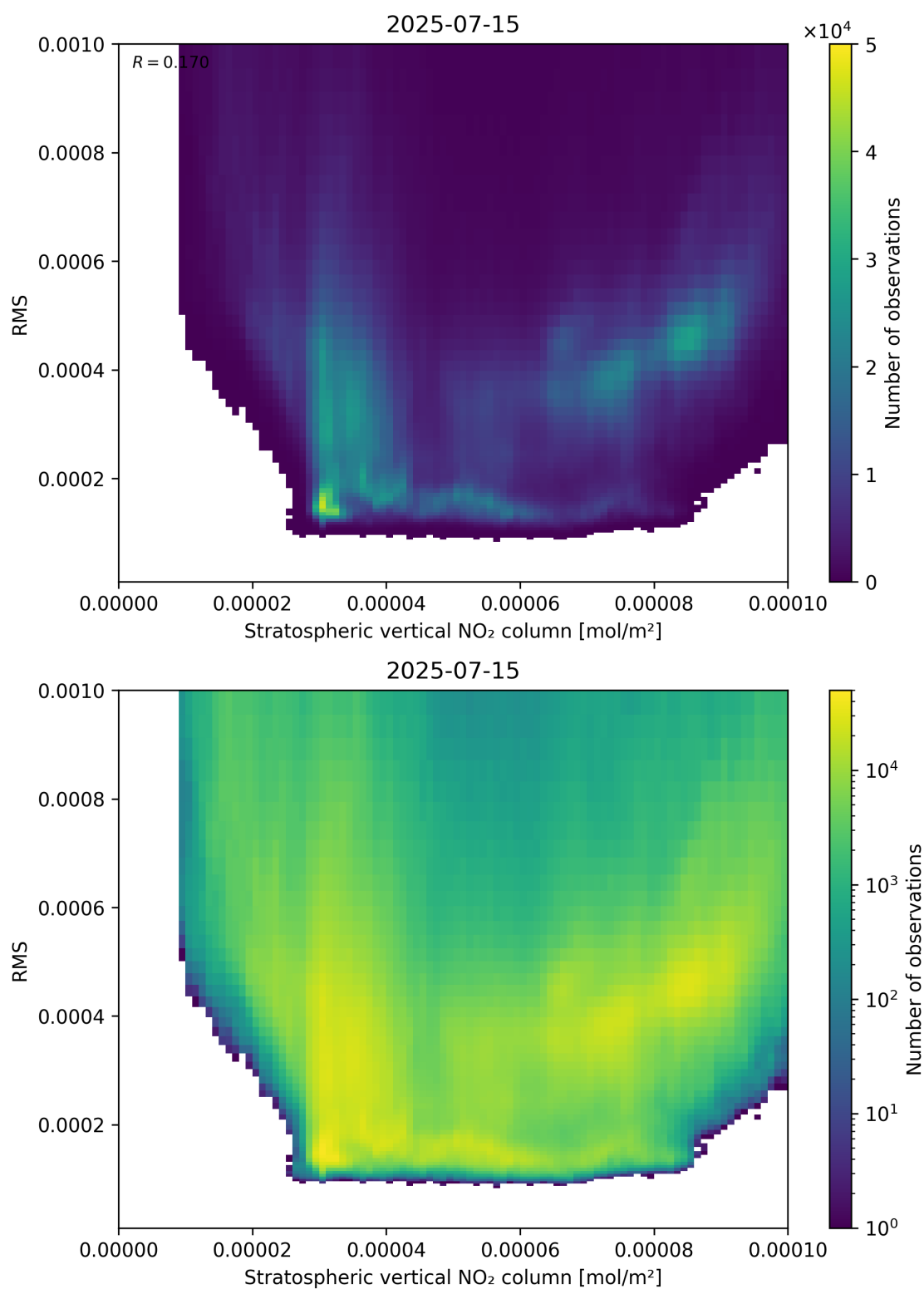
Figure 102: Scatter density plot of “Stratospheric vertical NO 2 column” against “RMS” for 2025-07-14 to 2025-07-16.
