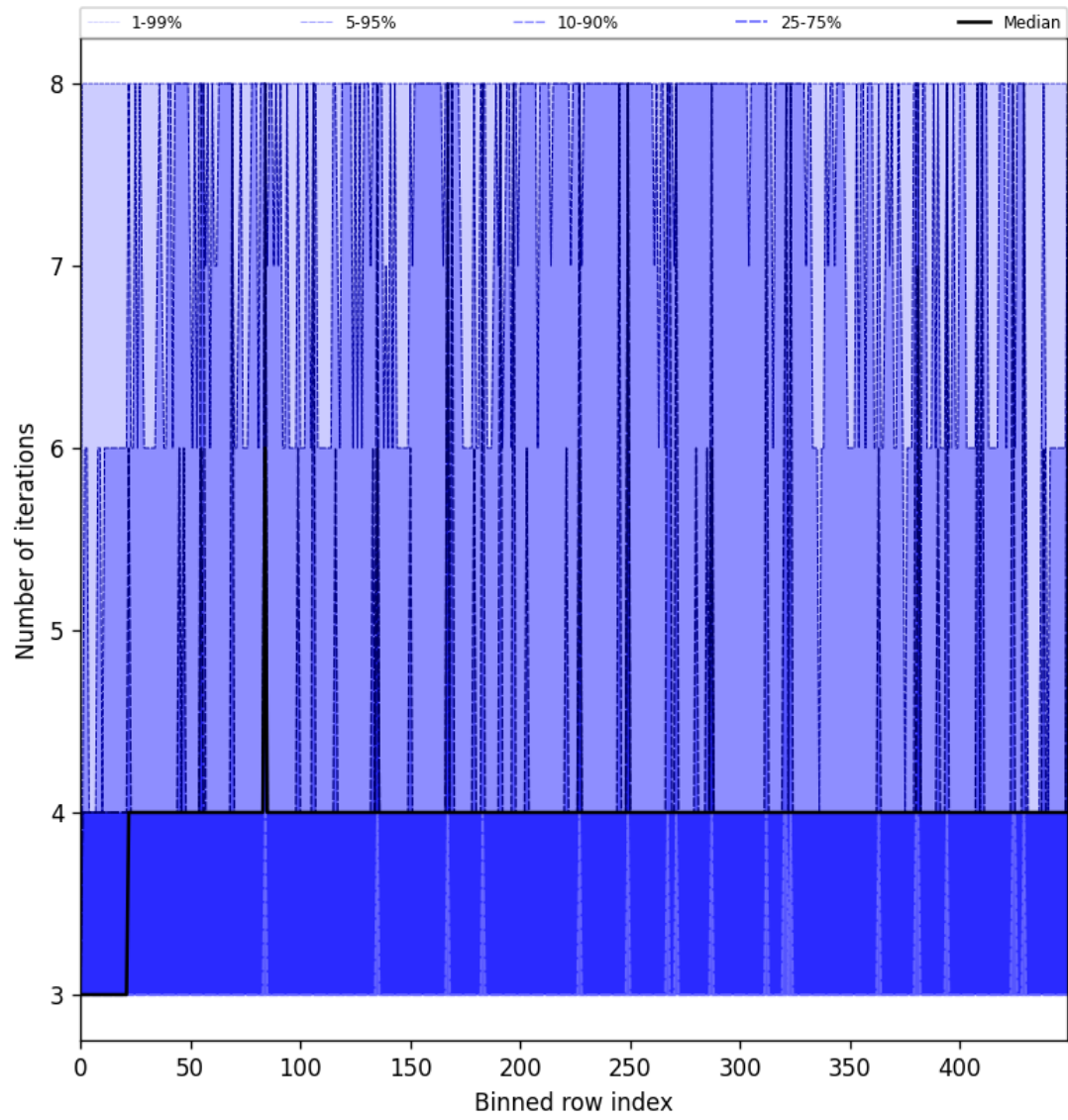
Figure 51: Along track statistics of “Number of iterations” for 2025-07-14 to 2025-07-16
