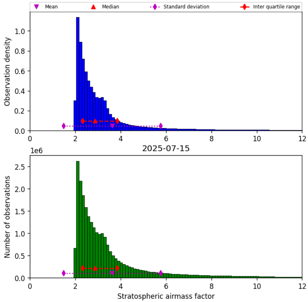
Figure 44: Histogram of “Stratospheric airmass factor” for 2025-07-14 to 2025-07-16
