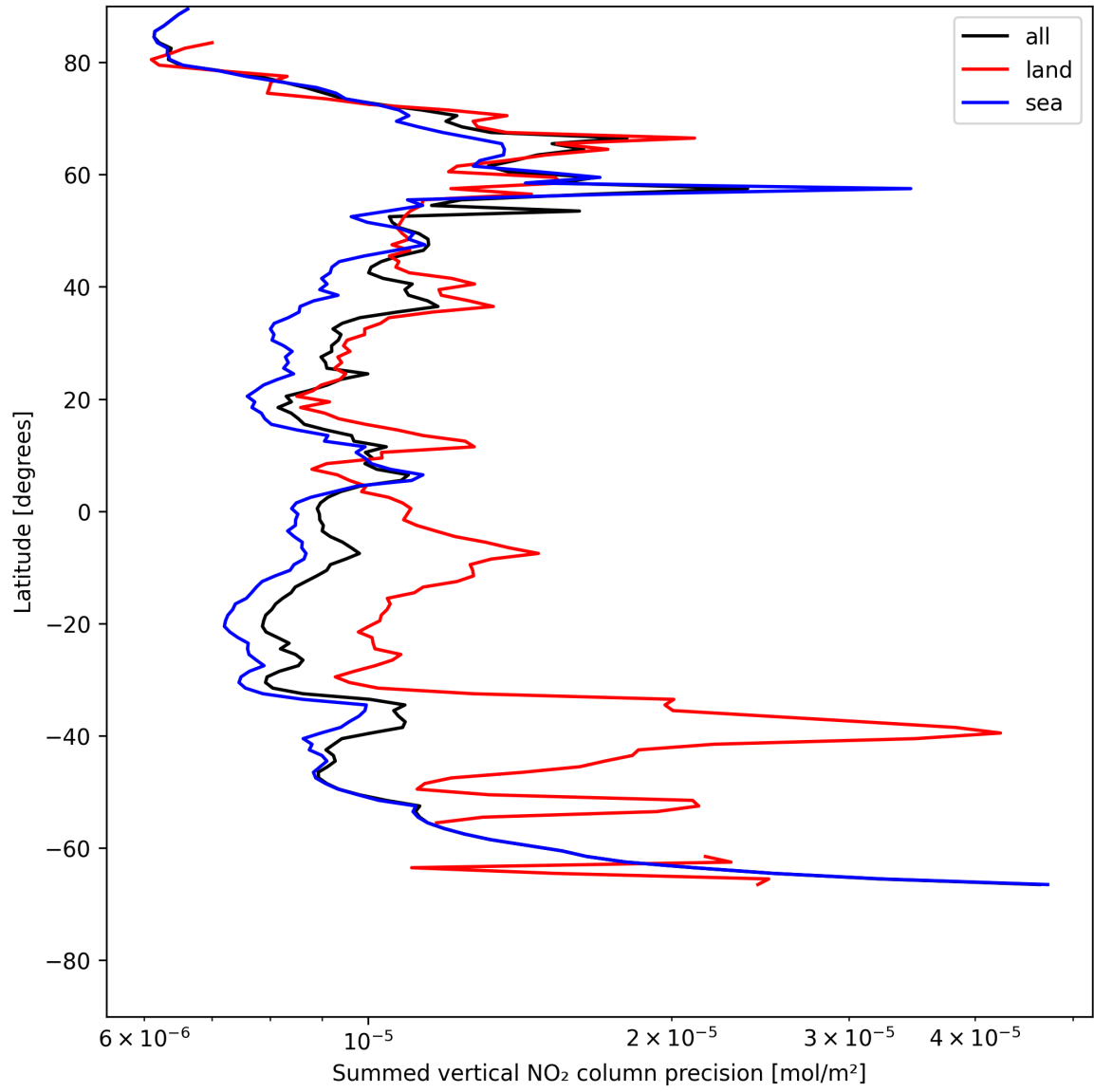
Figure 24: Zonal average of “Summed vertical NO 2 column precision” for 2025-07-14 to 2025-07-16.
