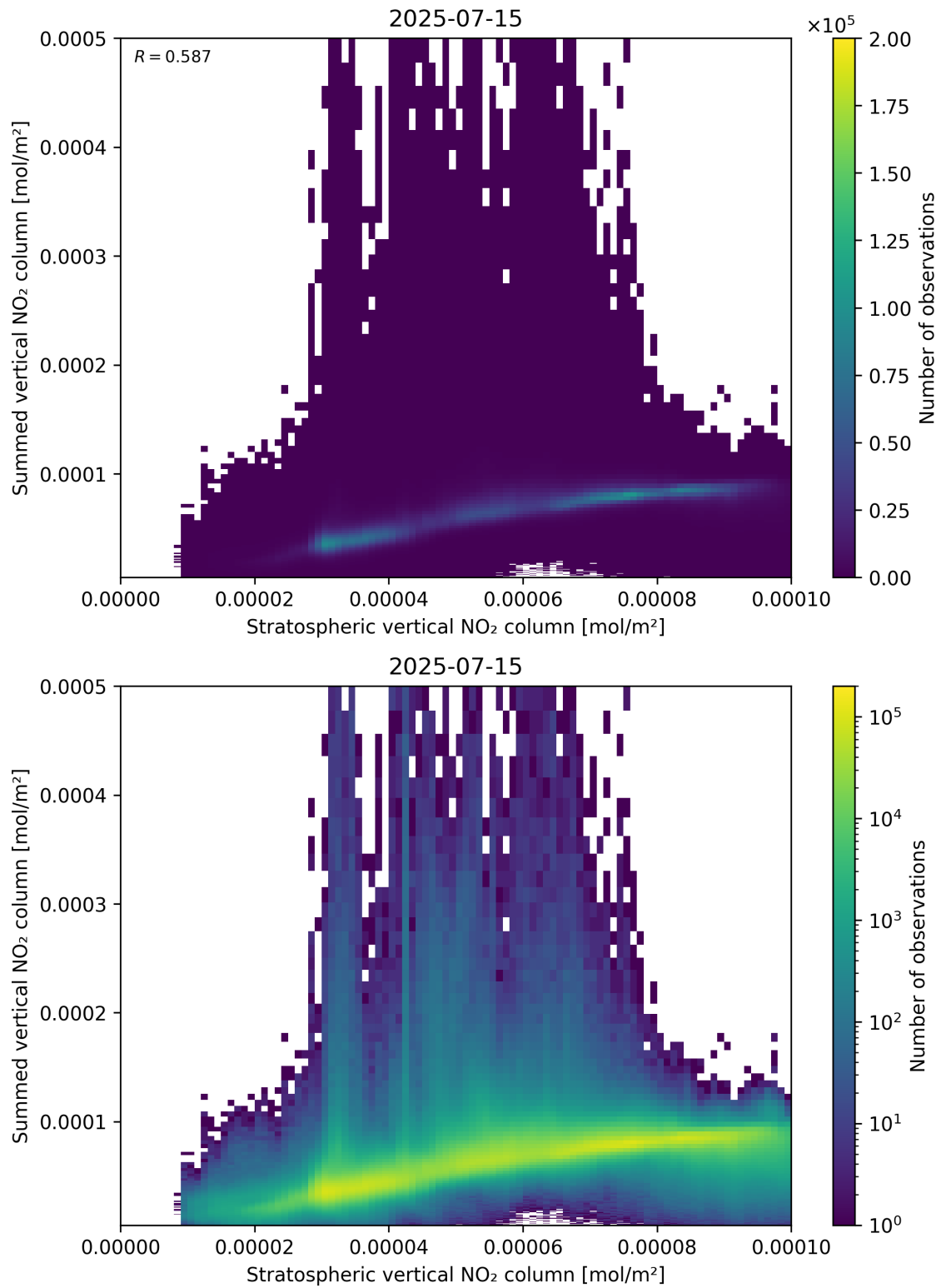
Figure 98: Scatter density plot of “Stratospheric vertical NO 2 column” against “Summed vertical NO 2 column” for 2025-07-14 to 2025-07-16.
