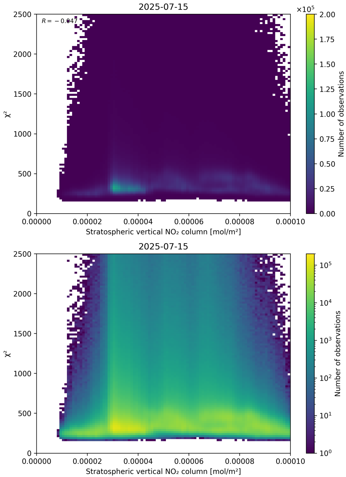
Figure 97: Scatter density plot of “Stratospheric vertical NO 2 column” against “ \chi^2 ” for 2025-07-14 to 2025-07-16.
