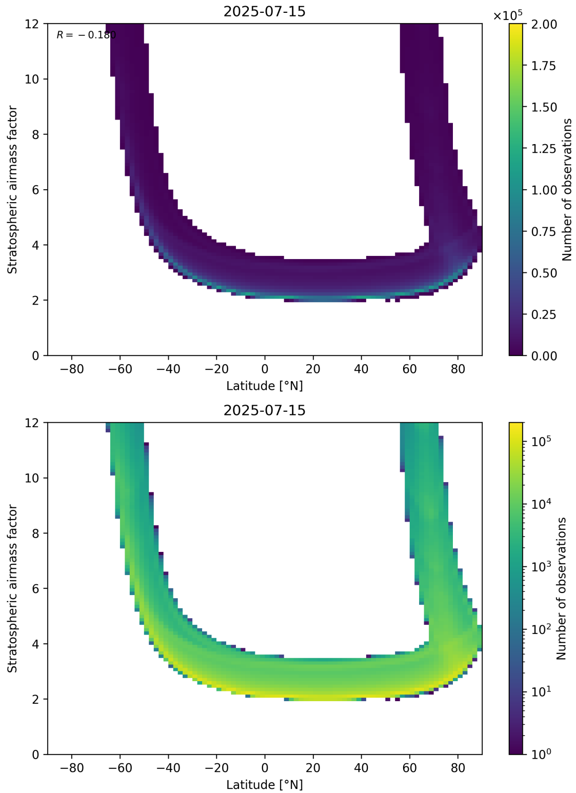
Figure 83: Scatter density plot of “Latitude” against “Stratospheric air mass factor” for 2025-07-14 to 2025-07-16.
