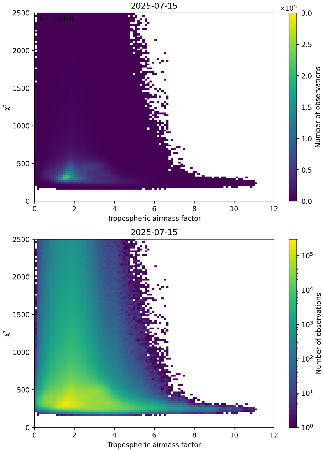
Figure 73: Scatter density plot of “Tropospheric airmass factor” against “ \chi^2 ” for 2025-07-14 to 2025-07-16.
