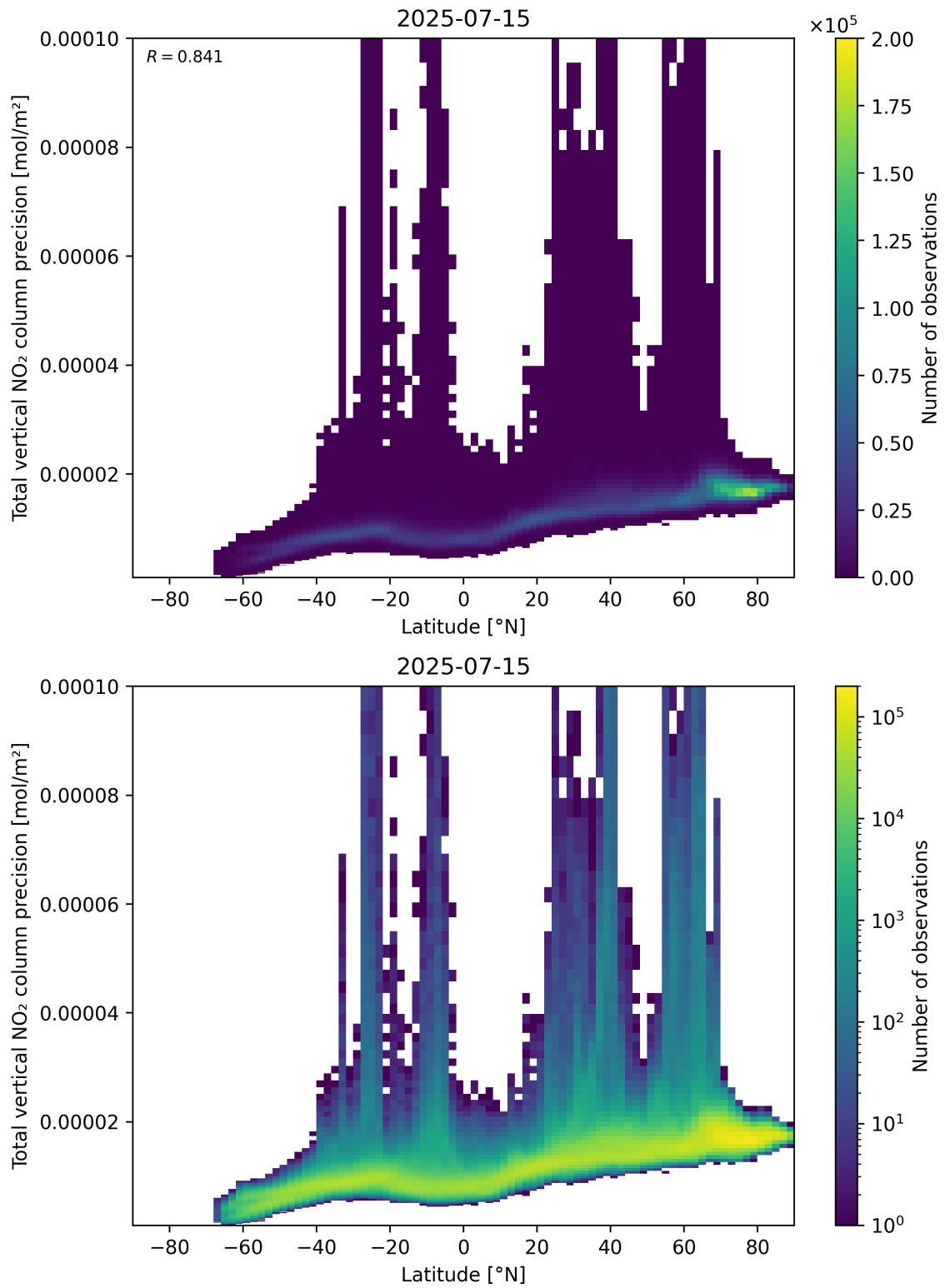
Figure 91: Scatter density plot of “Latitude” against “Total vertical NO 2 column precision” for 2025-07-14 to 2025-07-16.
