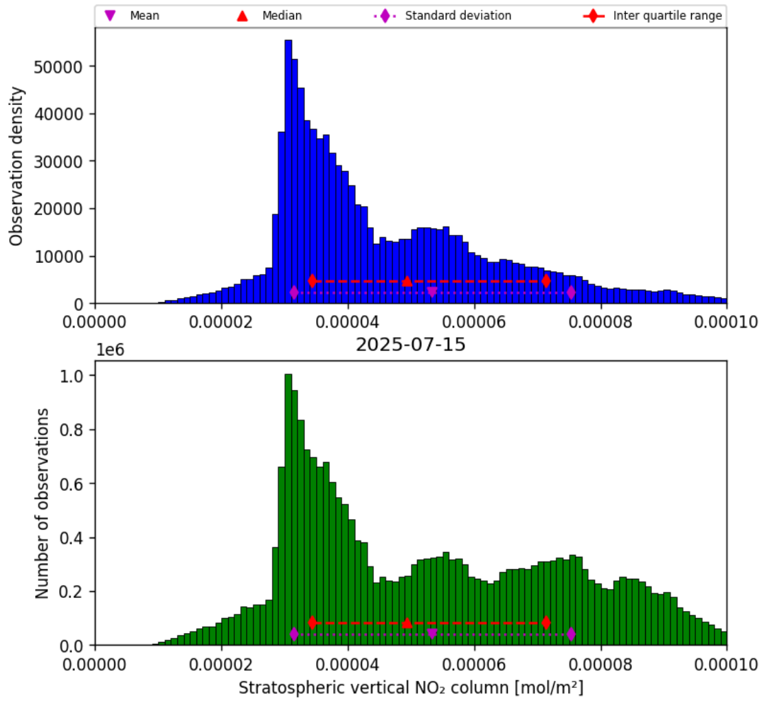
Figure 36: Histogram of “Stratospheric vertical NO 2 column” for 2025-07-14 to 2025-07-16
