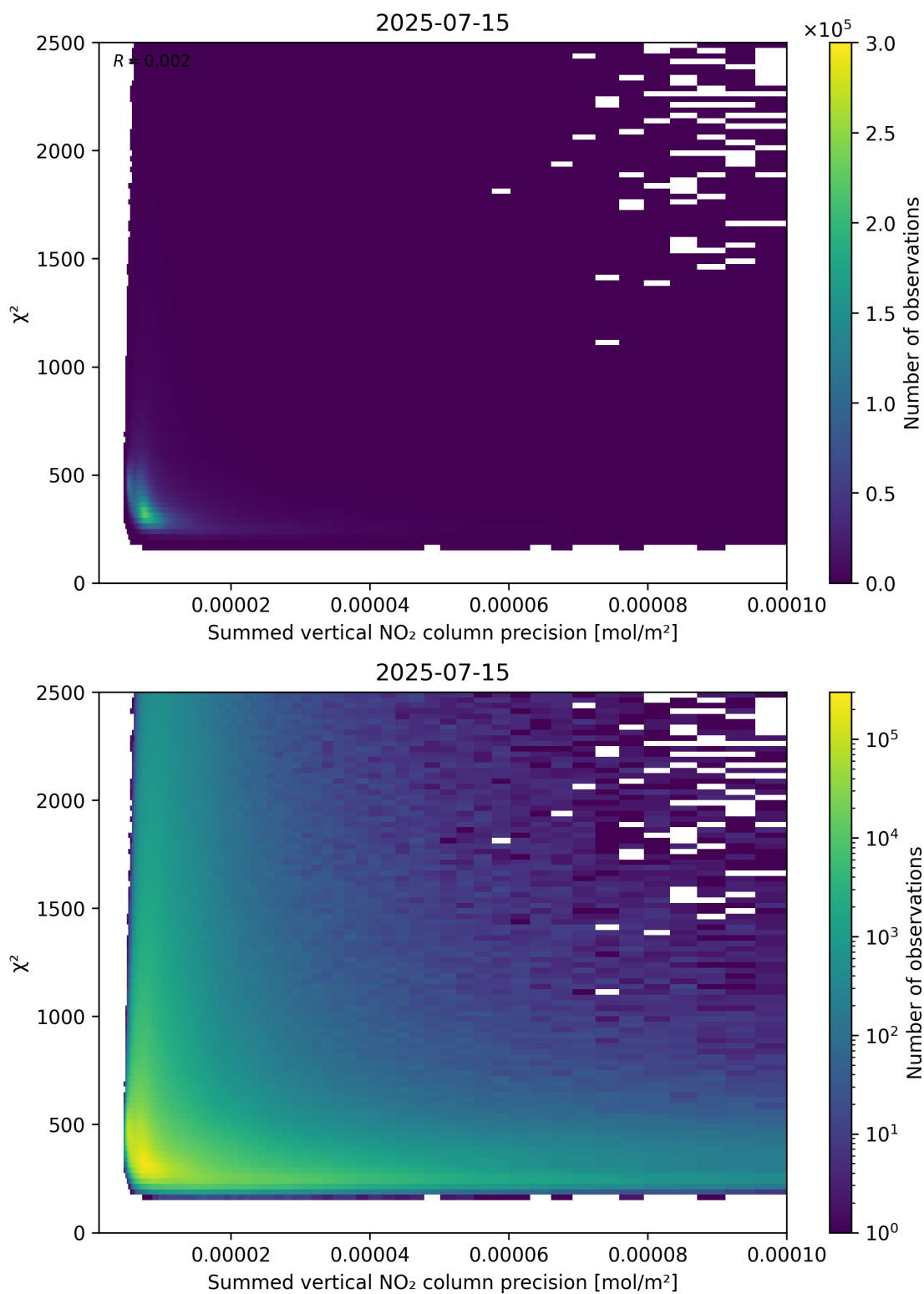
Figure 107: Scatter density plot of “Summed vertical NO 2 column precision” against “ \chi^2 ” for 2025-07-14 to 2025-07-16.
