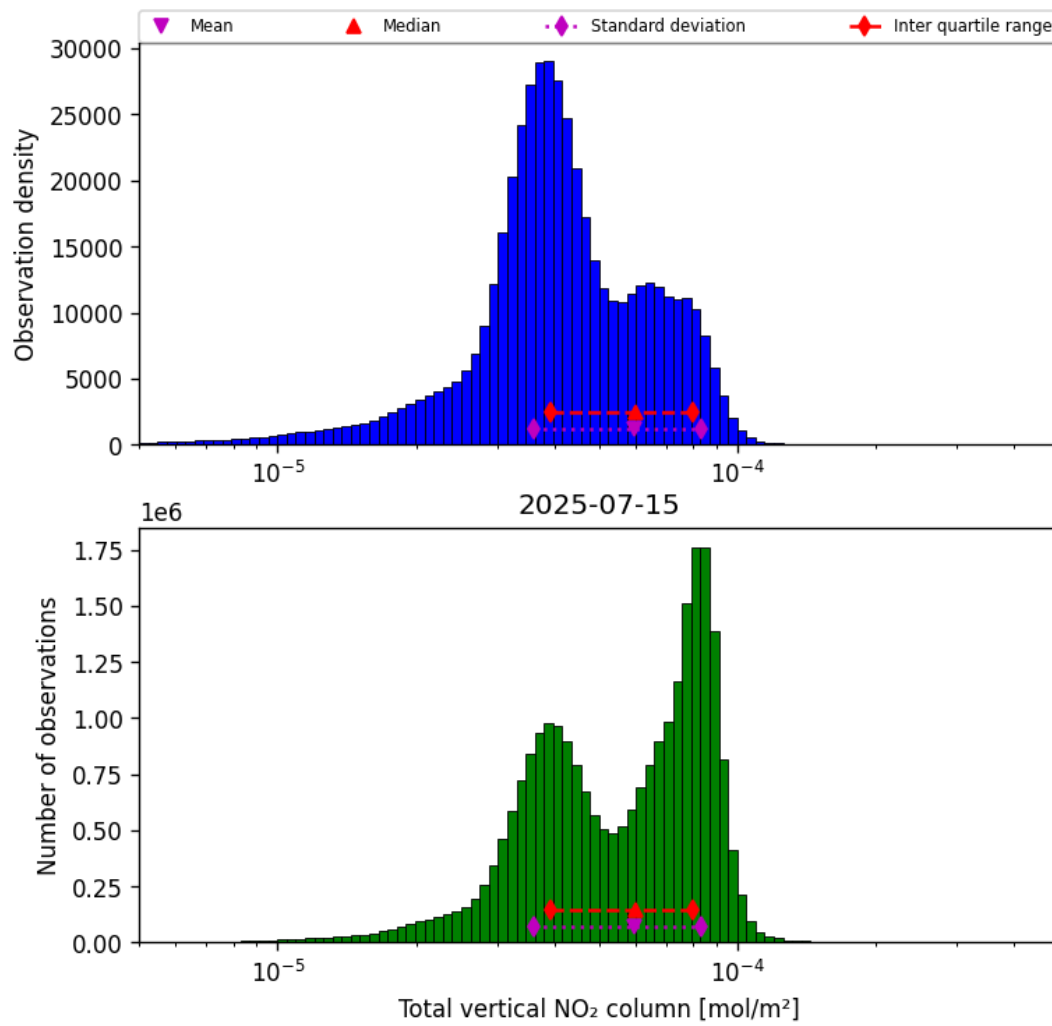
Figure 38: Histogram of “Total vertical NO 2 column” for 2025-07-14 to 2025-07-16
