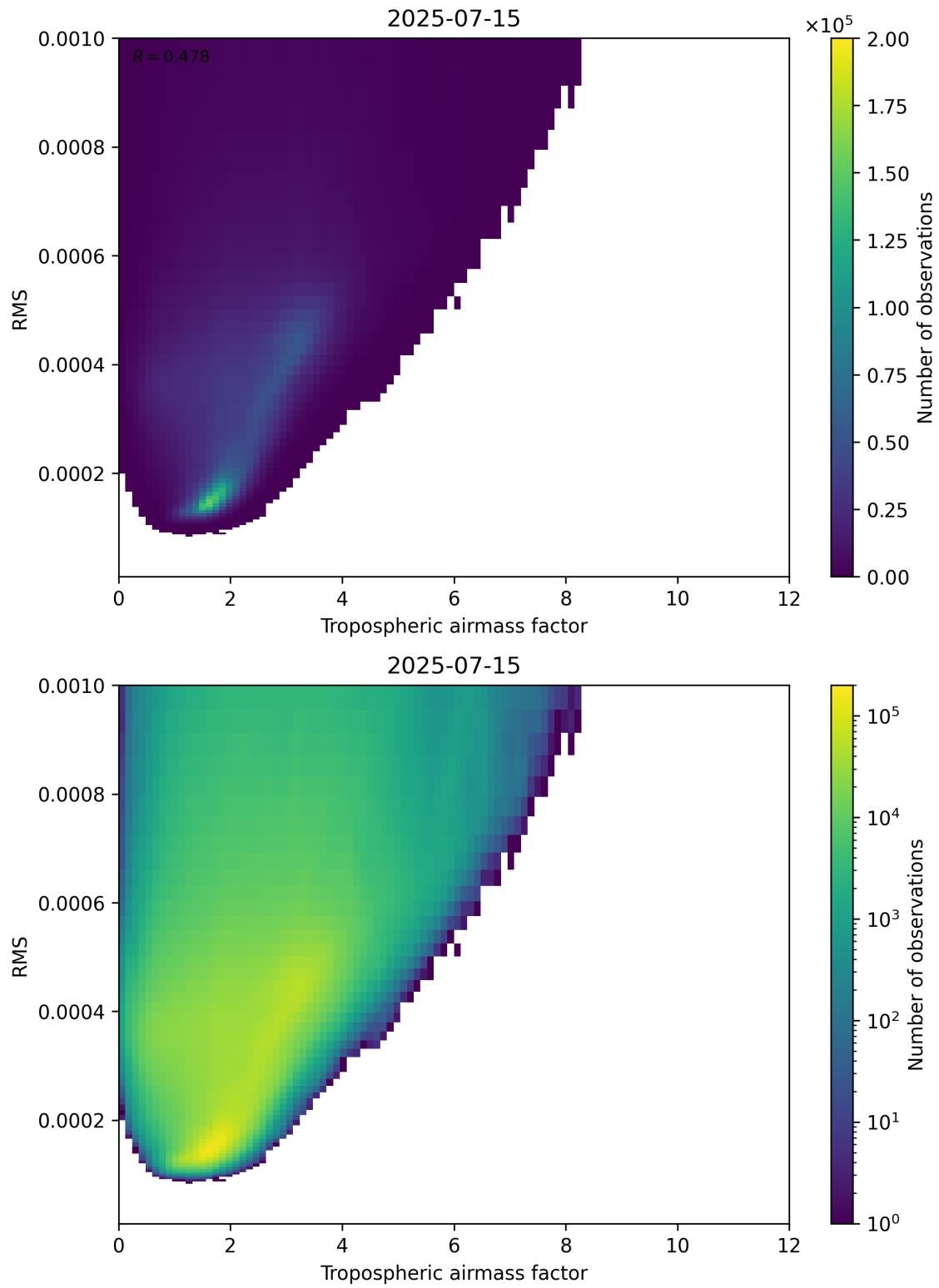
Figure 79: Scatter density plot of “Tropospheric airmass factor” against “RMS” for 2025-07-14 to 2025-07-16.
