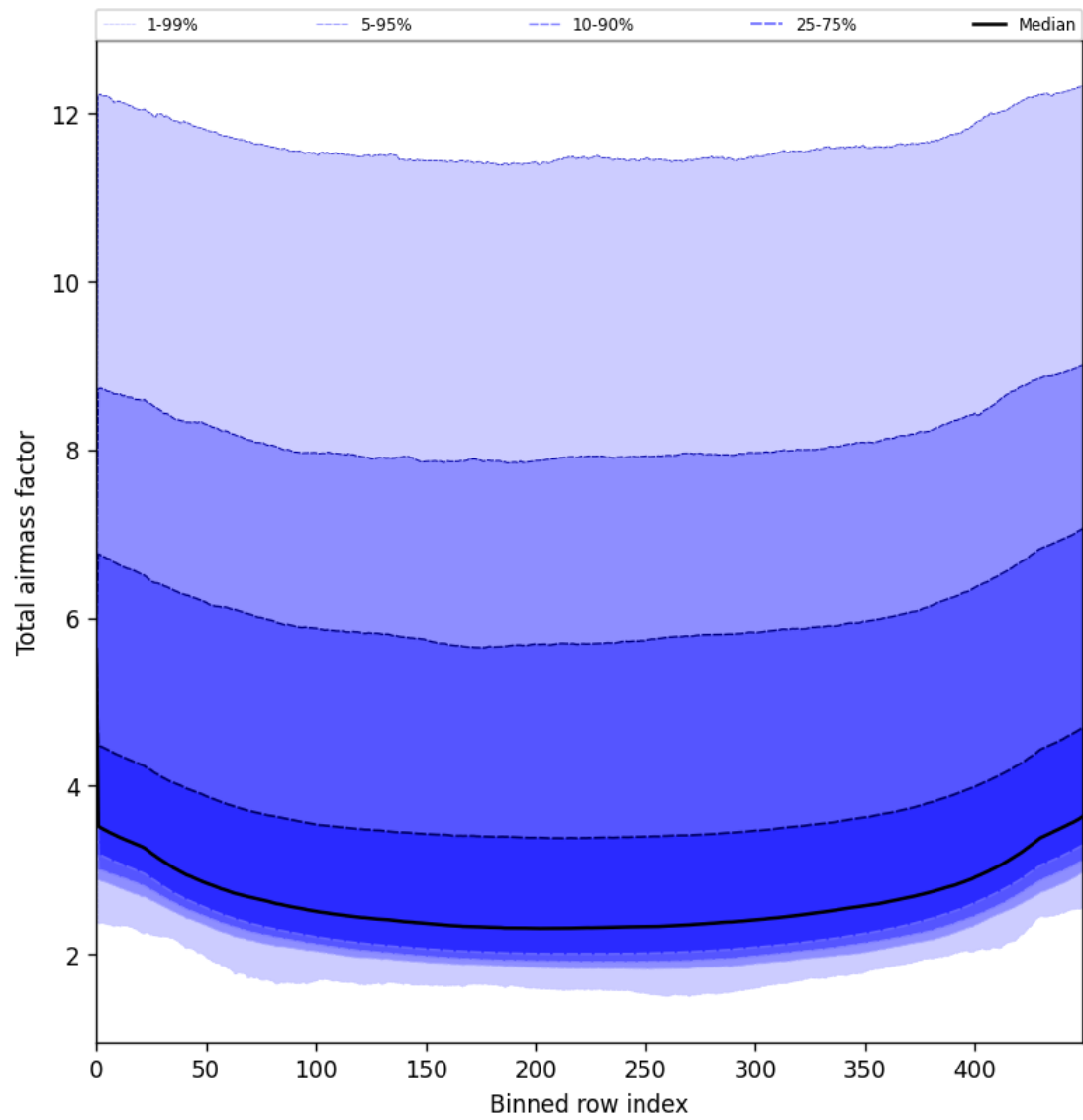
Figure 49: Along track statistics of “Total airmass factor” for 2025-07-14 to 2025-07-16
