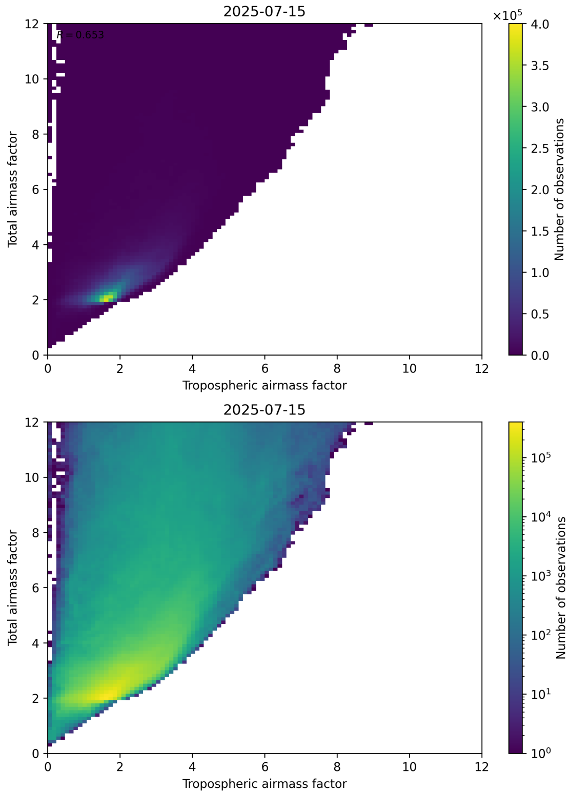
Figure 72: Scatter density plot of “Tropospheric airmass factor” against “Total airmass factor” for 2025-07-14 to 2025-07-16.
