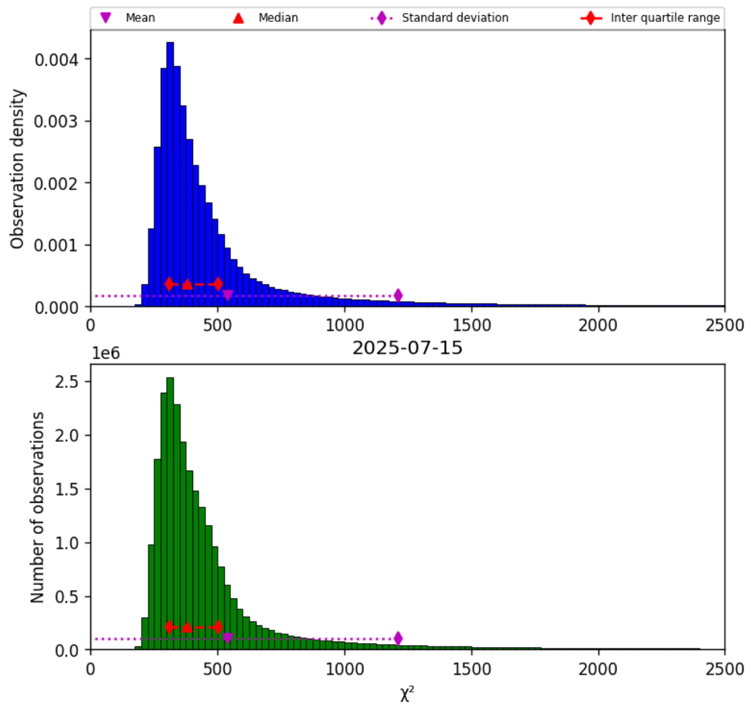
Figure 42: Histogram of “ \chi^2 ” for 2025-07-14 to 2025-07-16
