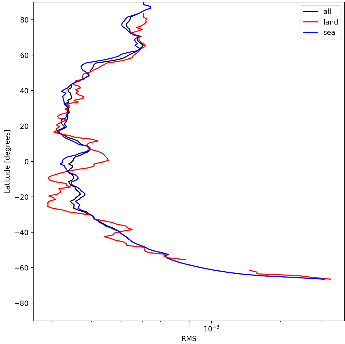
Figure 26: Zonal average of “RMS” for 2025-07-14 to 2025-07-16.
