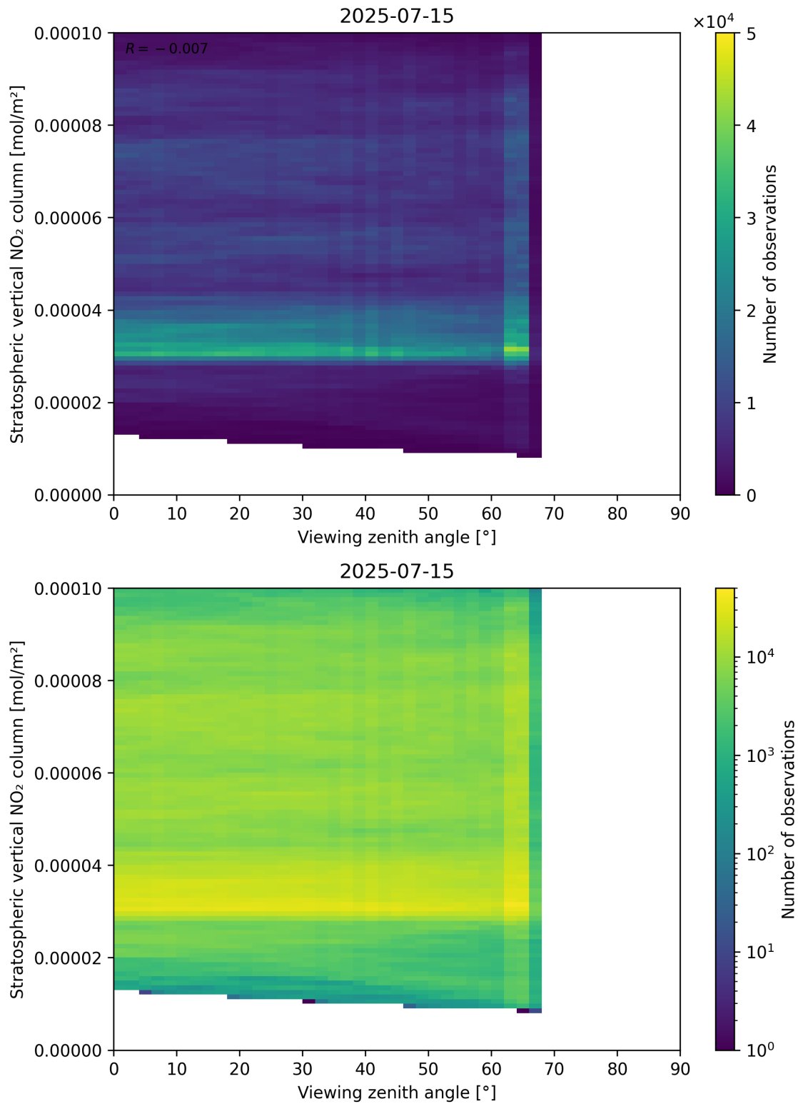
Figure 164: Scatter density plot of “Viewing zenith angle” against “Stratospheric vertical NO 2 column” for 2025-07-14 to 2025-07-16.
