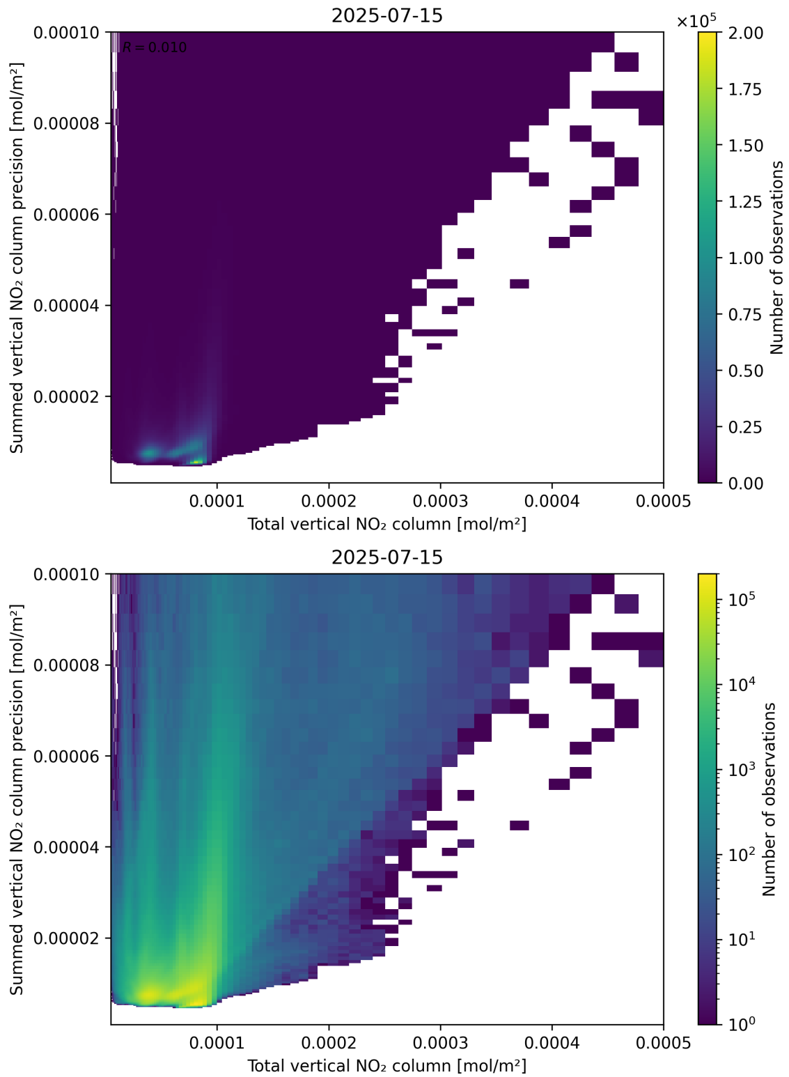
Figure 113: Scatter density plot of “Total vertical NO 2 column” against “Summed vertical NO 2 column precision” for 2025-07-14 to 2025-07-16.
