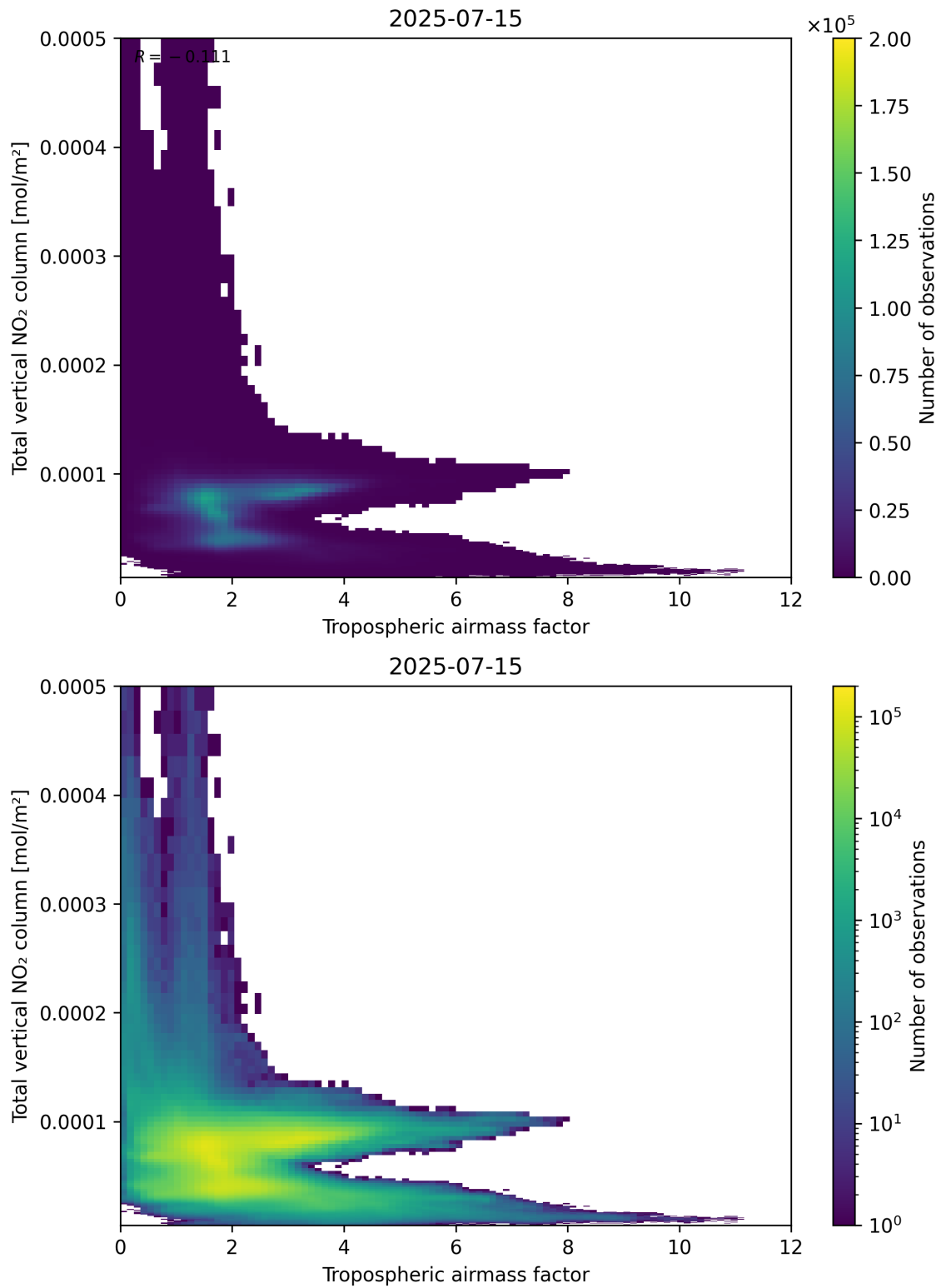
Figure 77: Scatter density plot of “Tropospheric airmass factor” against “Total vertical NO 2 column” for 2025-07-14 to 2025-07-16.
