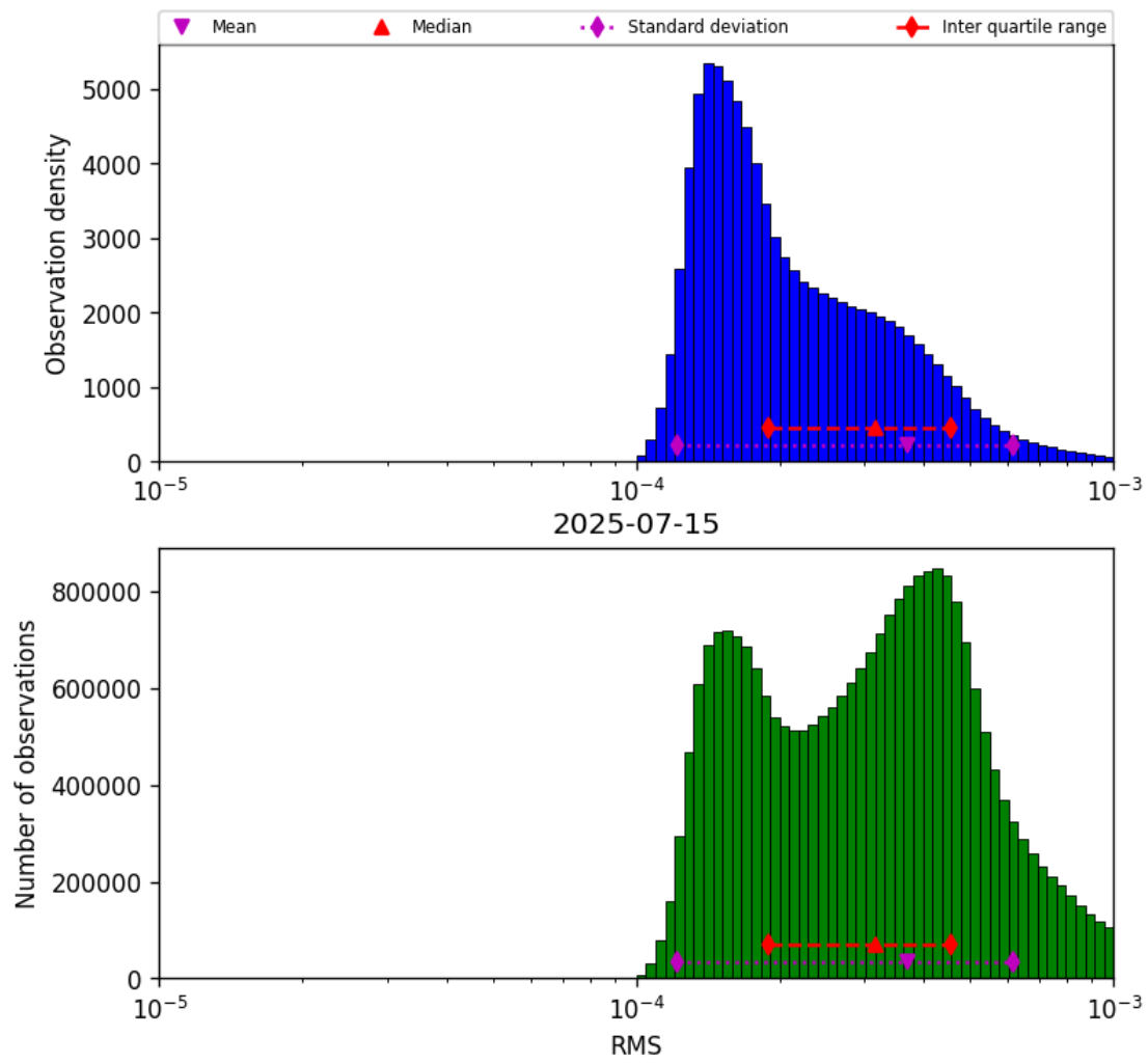
Figure 43: Histogram of “RMS” for 2025-07-14 to 2025-07-16
