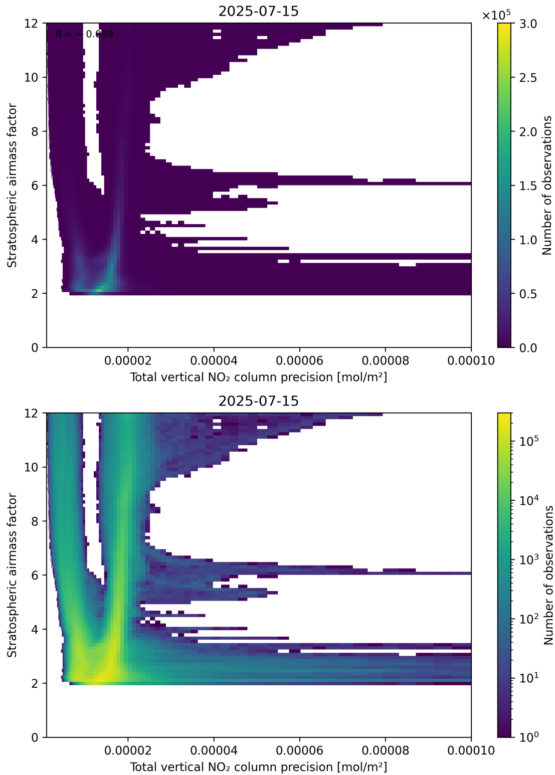
Figure 115: Scatter density plot of “Total vertical NO 2 column precision” against “Stratospheric air mass factor” for 2025-07-14 to 2025-07-16.
