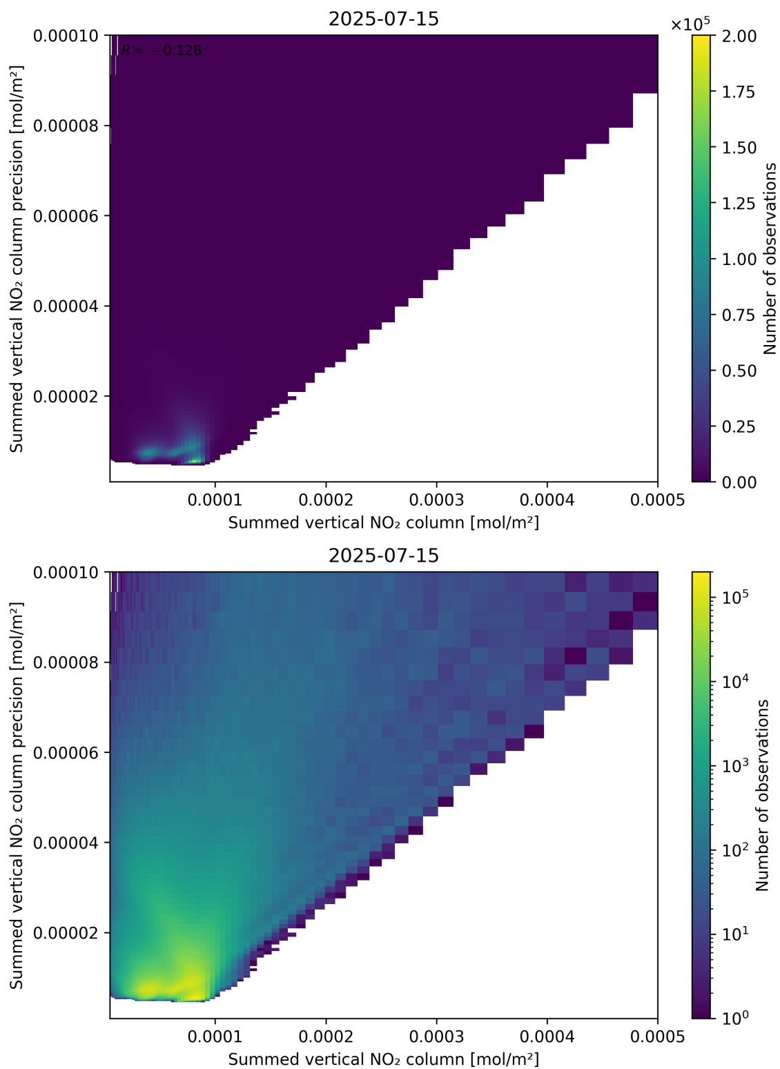
Figure 105: Scatter density plot of “Summed vertical NO 2 column” against “Summed vertical NO 2 column precision” for 2025-07-14 to 2025-07-16.
