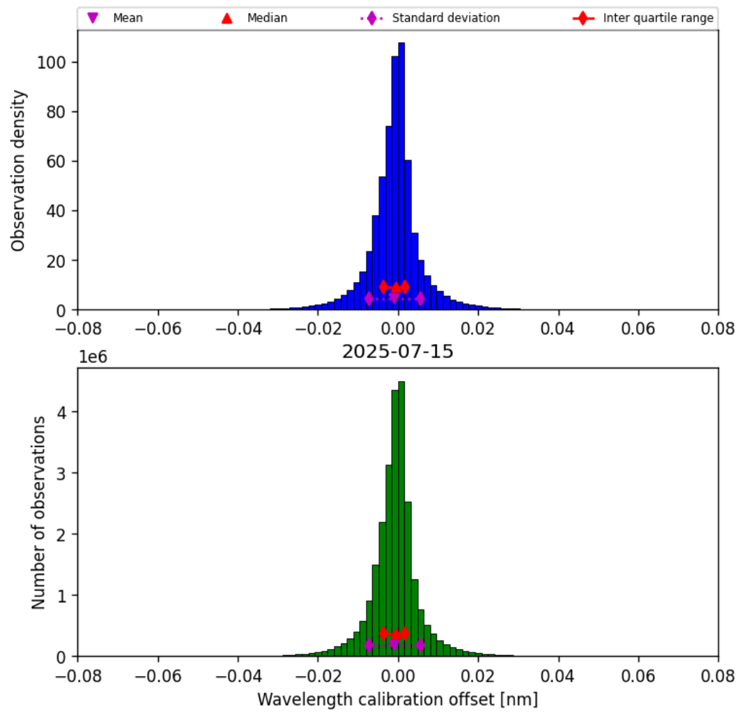
Figure 35: Histogram of “Wavelength calibration offset” for 2025-07-14 to 2025-07-16
