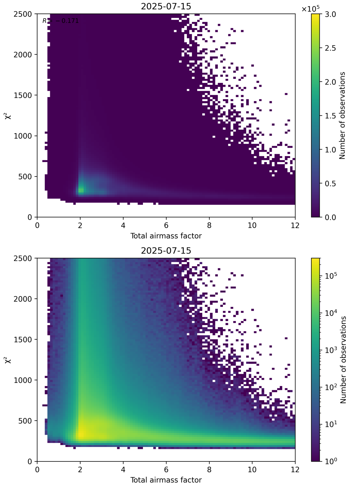
Figure 63: Scatter density plot of “Total airmass factor” against “ \chi^2 ” for 2025-07-14 to 2025-07-16.
