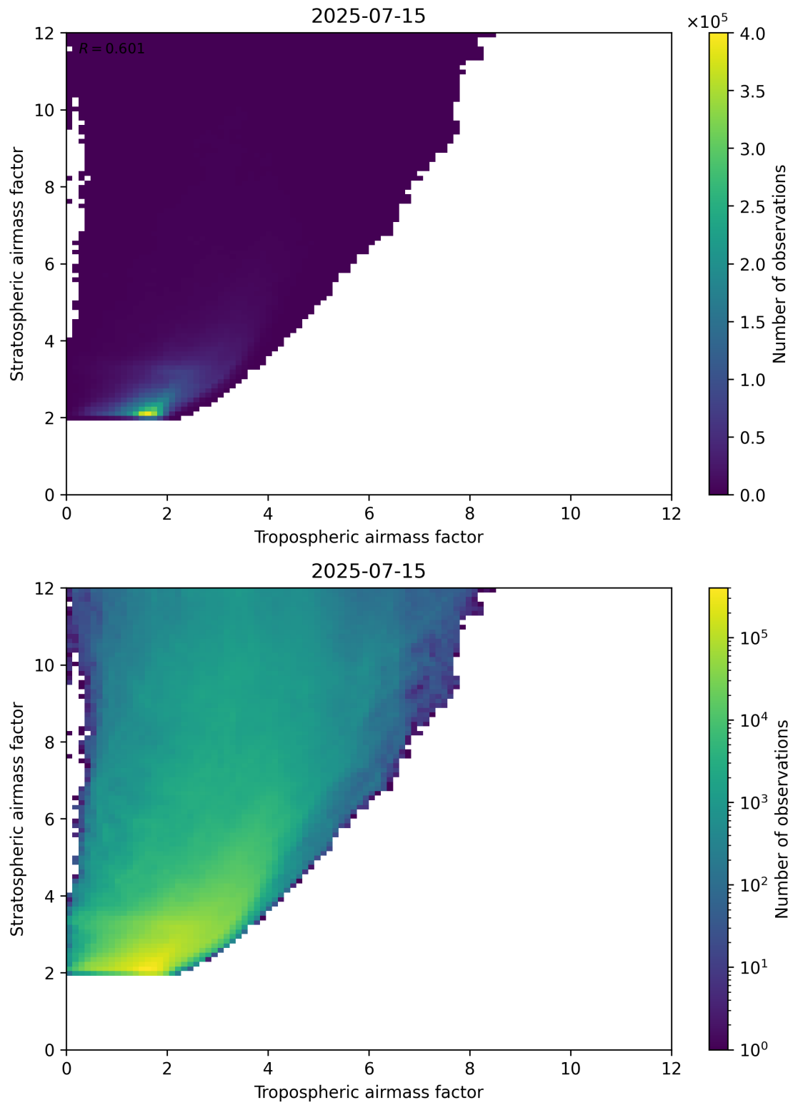
Figure 71: Scatter density plot of “Tropospheric airmass factor” against “Stratospheric airmass factor” for 2025-07-14 to 2025-07-16.
