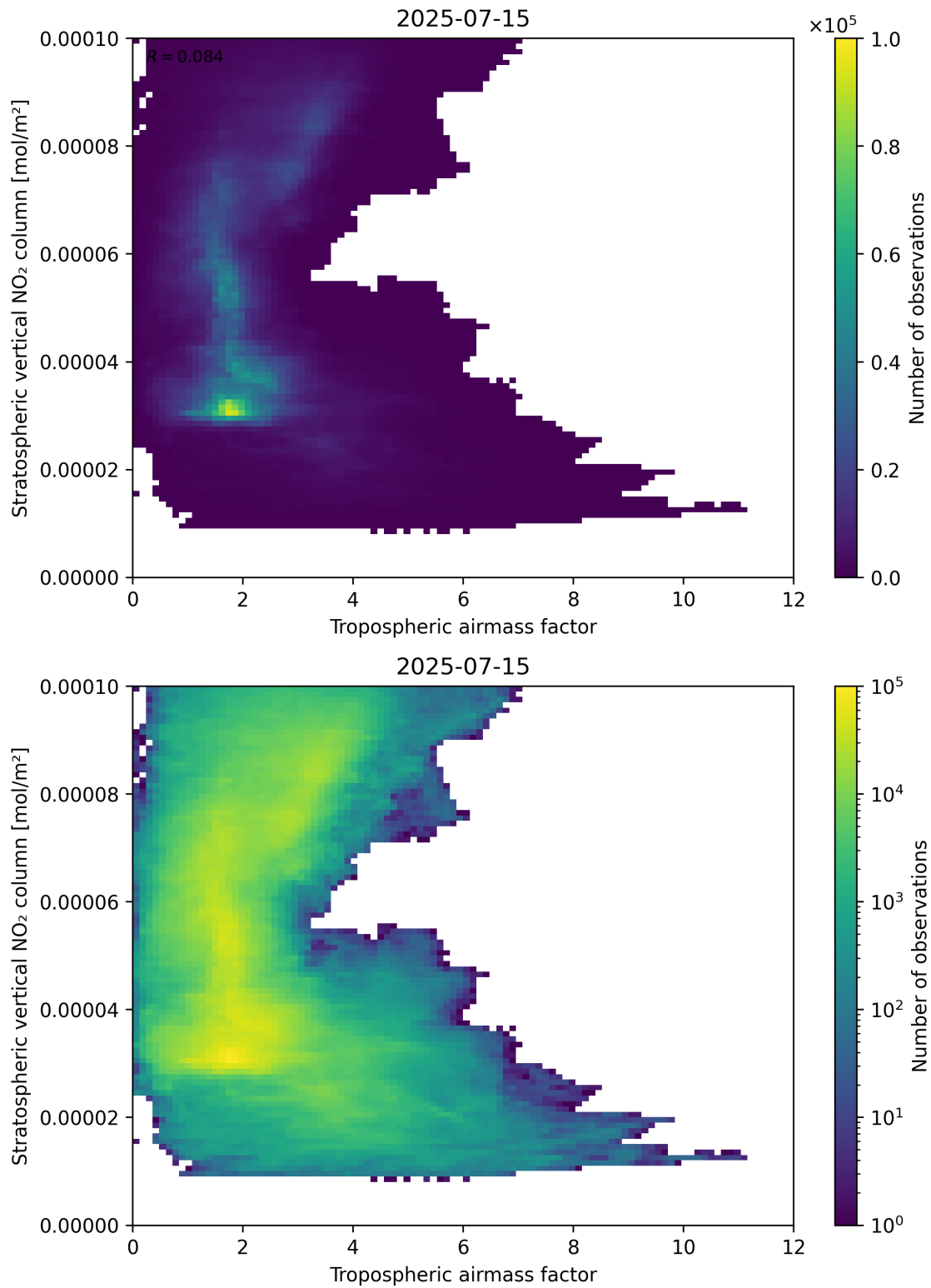
Figure 74: Scatter density plot of “Tropospheric air mass factor” against “Stratospheric vertical NO 2 column” for 2025-07-14 to 2025-07-16.
