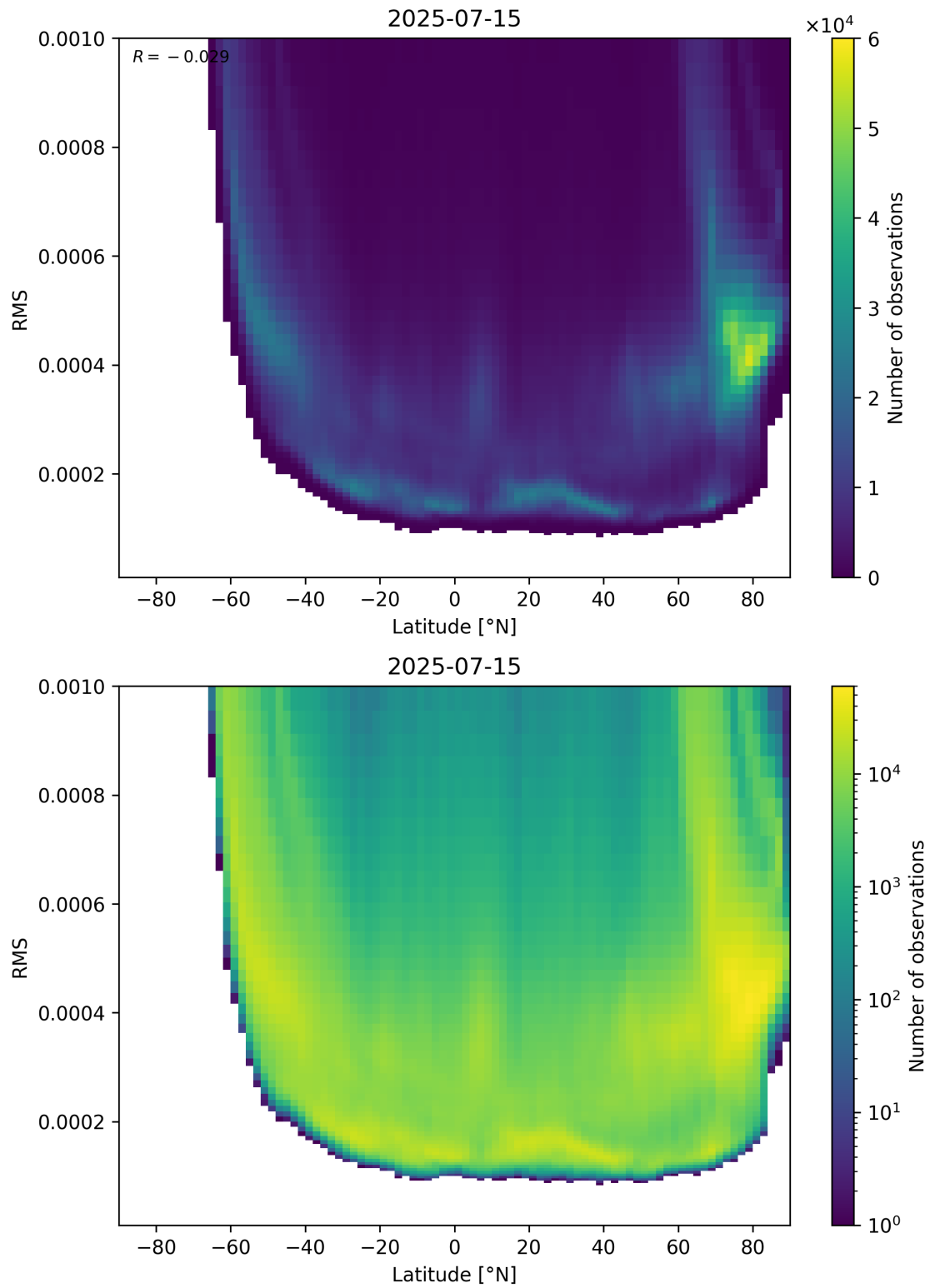
Figure 94: Scatter density plot of “Latitude” against “RMS” for 2025-07-14 to 2025-07-16.
