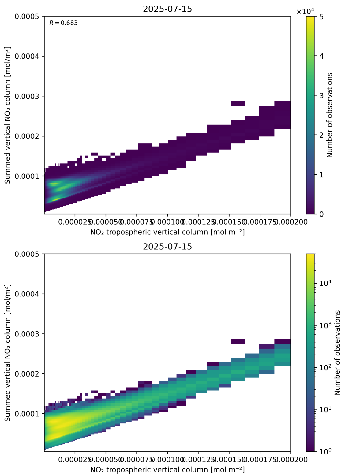
Figure 126: Scatter density plot of “NO 2 tropospheric vertical column” against “Summed vertical NO 2 column” for 2025-07-14 to 2025-07-16.
