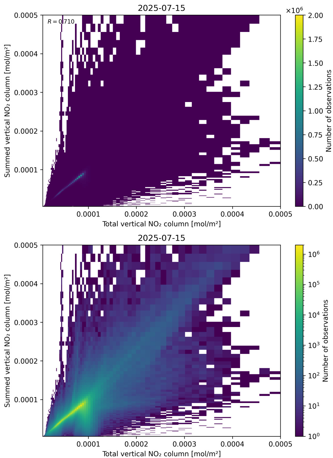
Figure 112: Scatter density plot of “Total vertical NO 2 column” against “Summed vertical NO 2 column” for 2025-07-14 to 2025-07-16.
