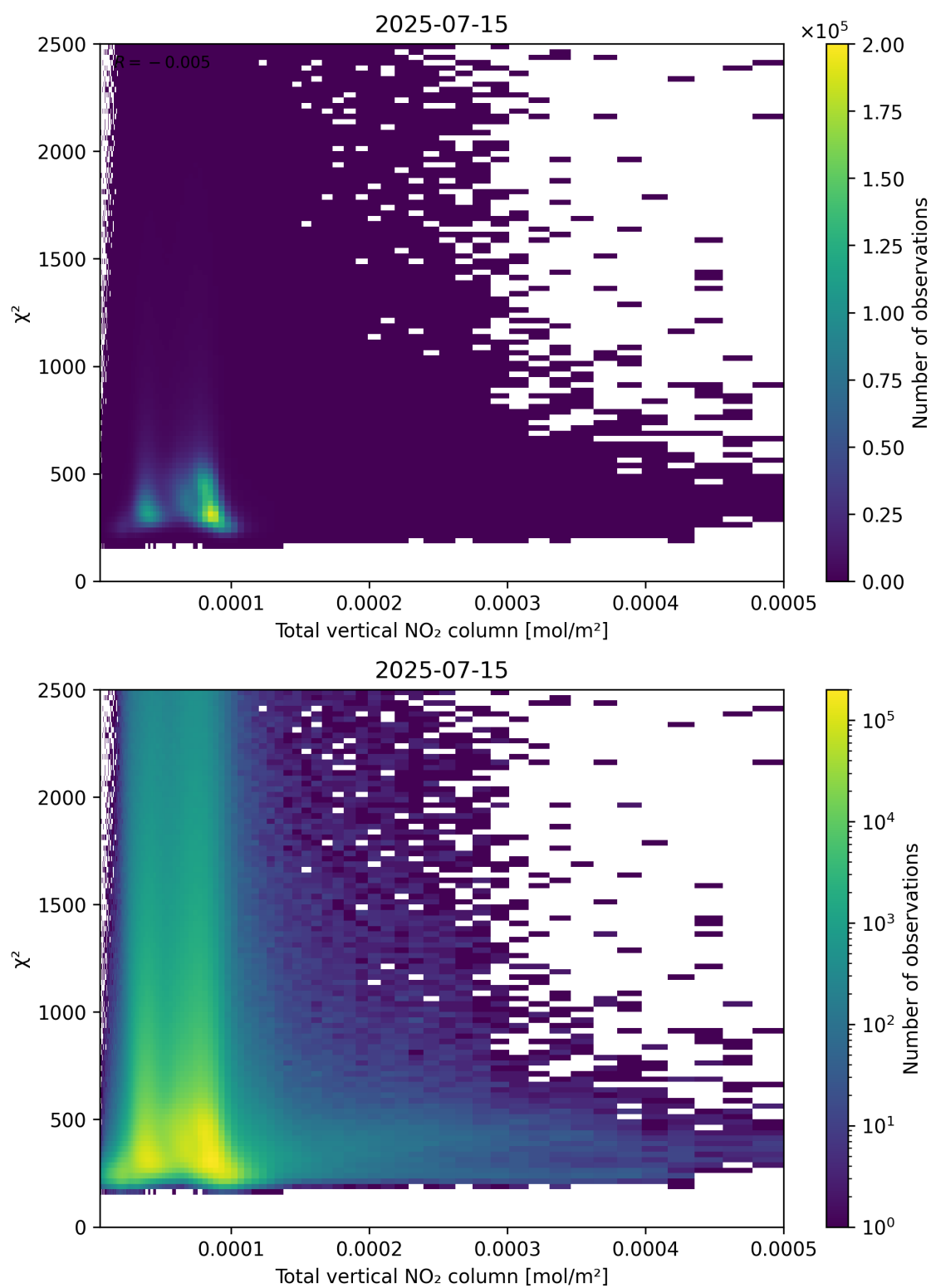
Figure 111: Scatter density plot of “Total vertical NO 2 column” against “ \chi^2 ” for 2025-07-14 to 2025-07-16.
