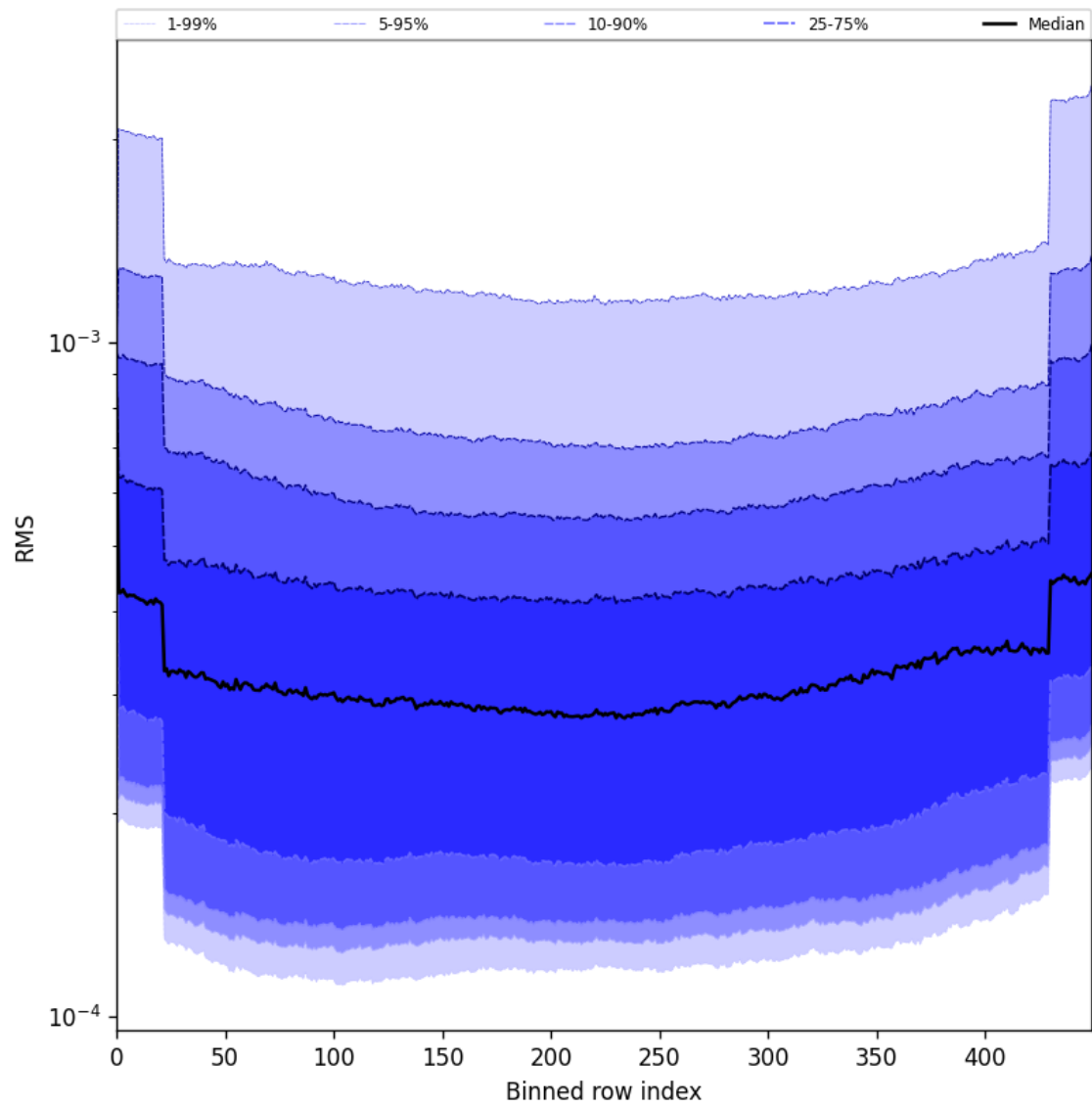
Figure 60: Along track statistics of “RMS” for 2025-07-14 to 2025-07-16
