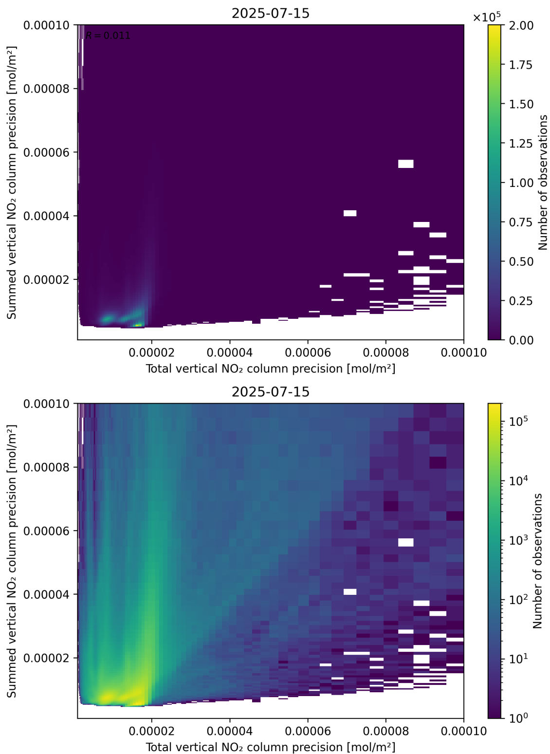
Figure 118: Scatter density plot of “Total vertical NO 2 column precision” against “Summed vertical NO 2 column precision” for 2025-07-14 to 2025-07-16.
