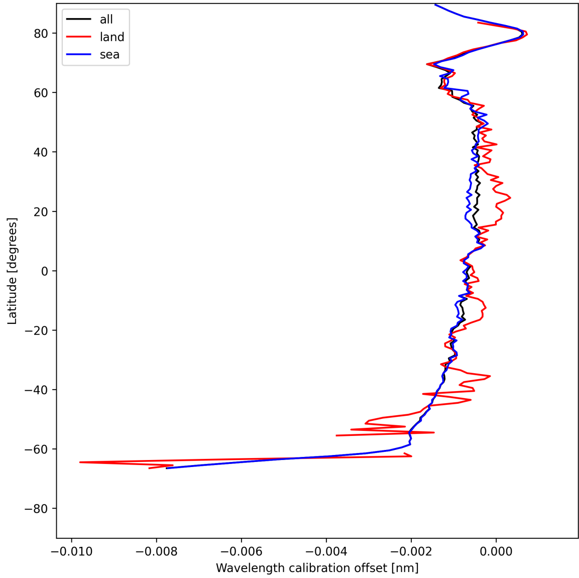
Figure 18: Zonal average of “Wavelength calibration offset” for 2025-07-14 to 2025-07-16.
