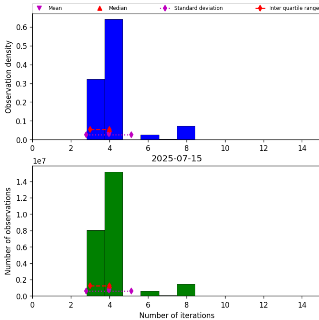
Figure 34: Histogram of “Number of iterations” for 2025-07-14 to 2025-07-16
