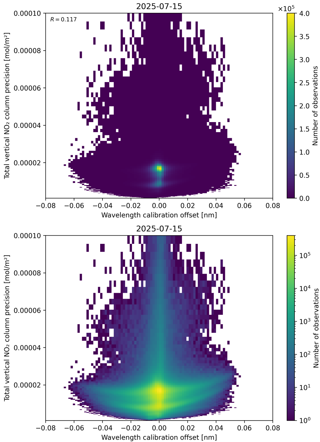
Figure 180: Scatter density plot of “Wavelength calibration offset” against “Total vertical NO 2 column precision” for 2025-07-14 to 2025-07-16.
