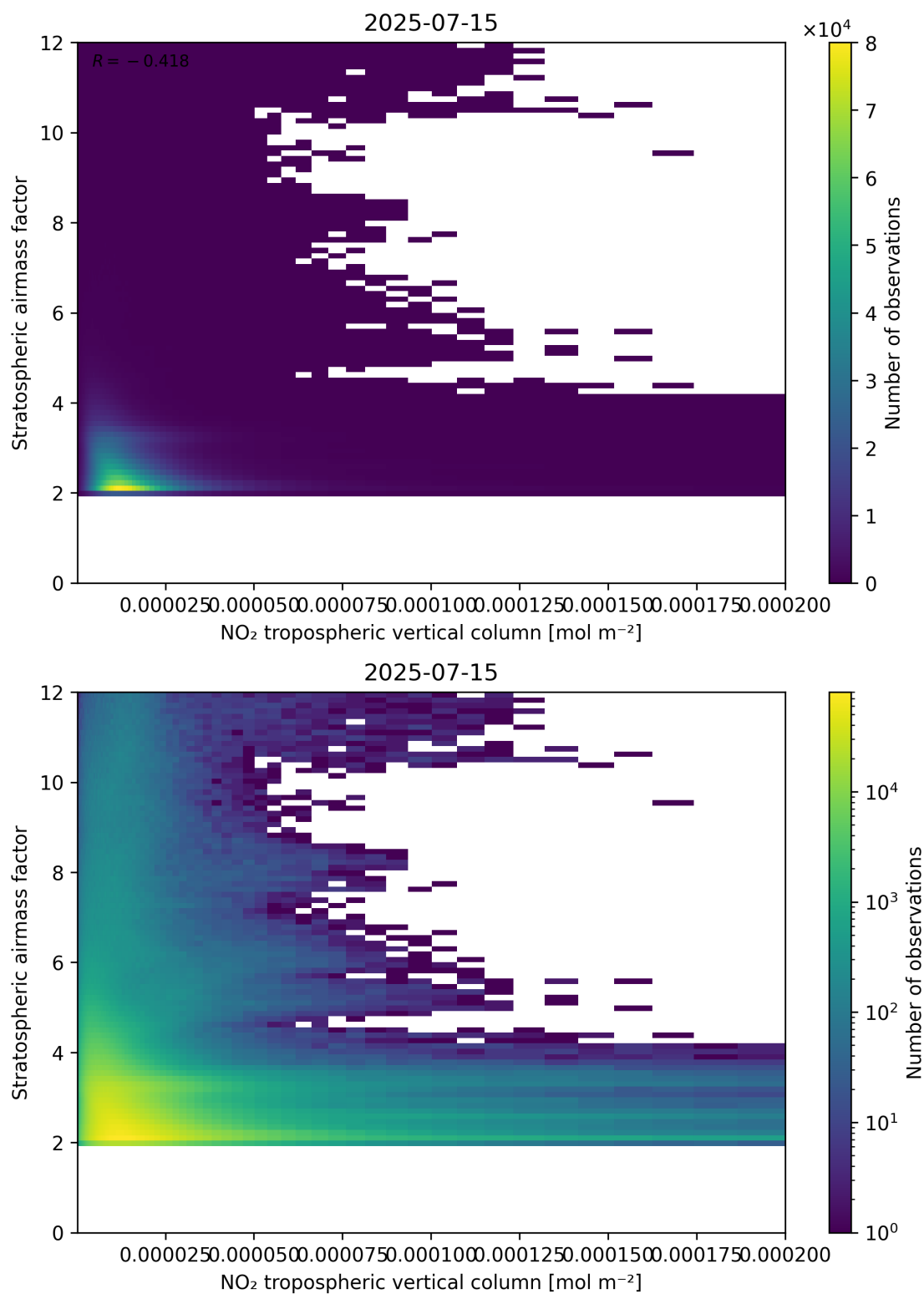
Figure 121: Scatter density plot of “NO 2 tropospheric vertical column” against “Stratospheric air mass factor” for 2025-07-14 to 2025-07-16.
