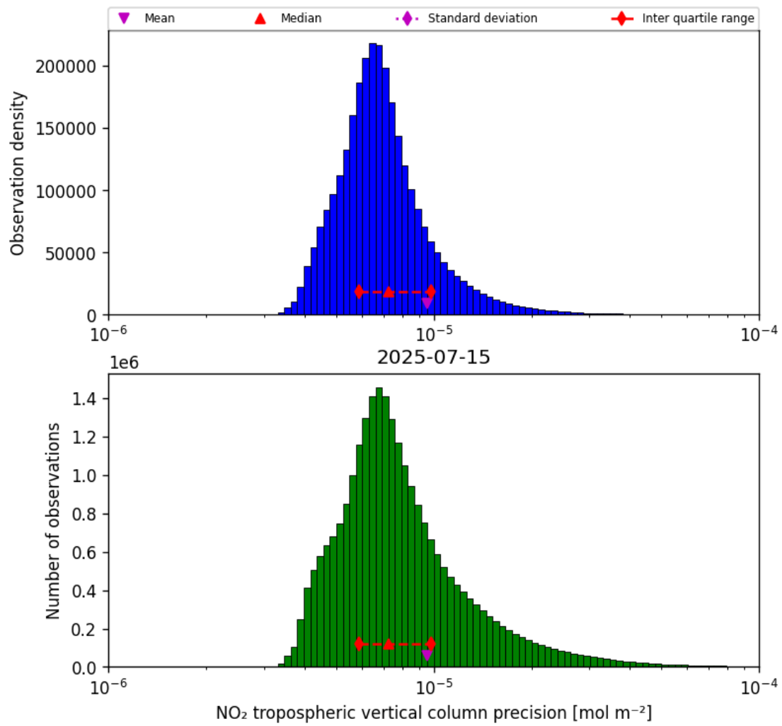
Figure 30: Histogram of "NO 2 tropospheric vertical column precision" for 2025-07-14 to 2025-07-16
