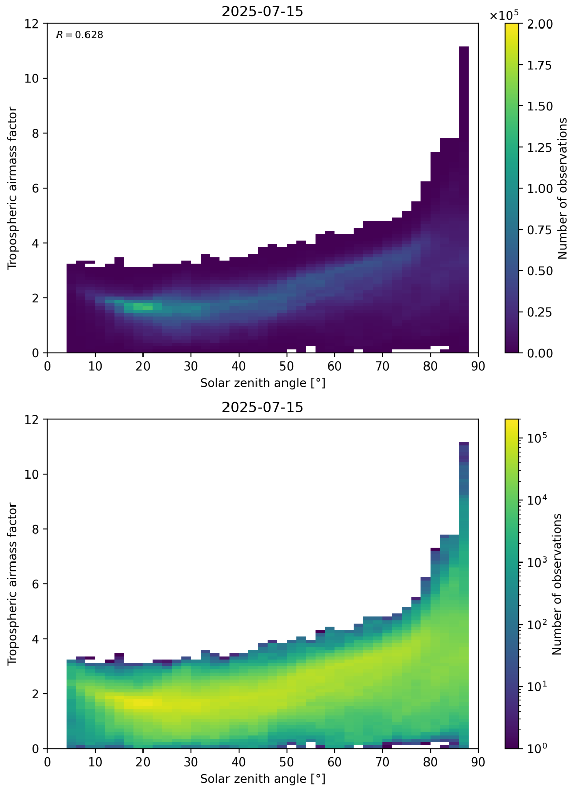
Figure 147: Scatter density plot of “Solar zenith angle” against “Tropospheric airmass factor” for 2025-07-14 to 2025-07-16.
