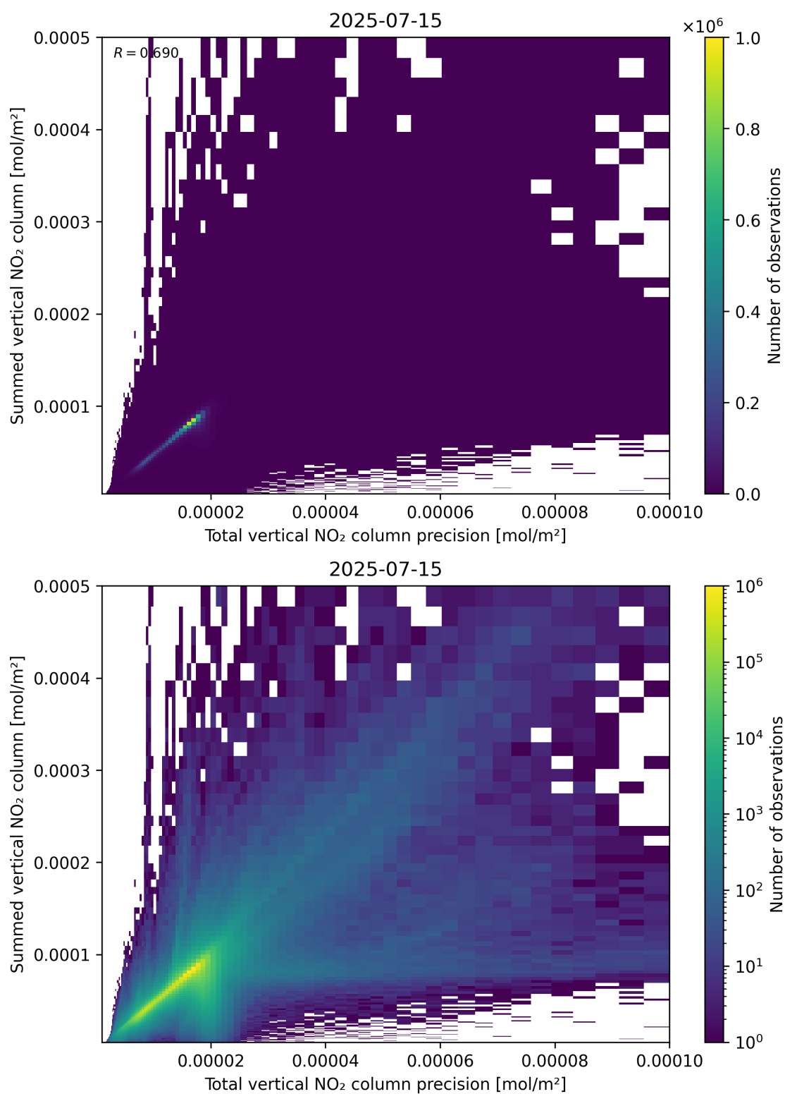
Figure 117: Scatter density plot of “Total vertical NO 2 column precision” against “Summed vertical NO 2 column” for 2025-07-14 to 2025-07-16.
