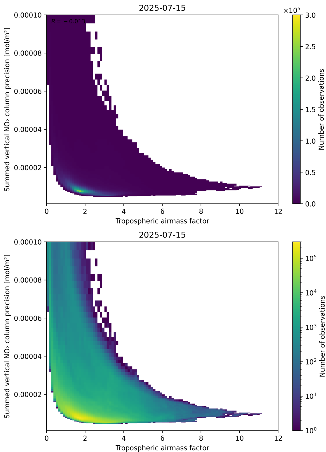
Figure 76: Scatter density plot of “Tropospheric airmass factor” against “Summed vertical NO 2 column precision” for 2025-07-14 to 2025-07-16.
