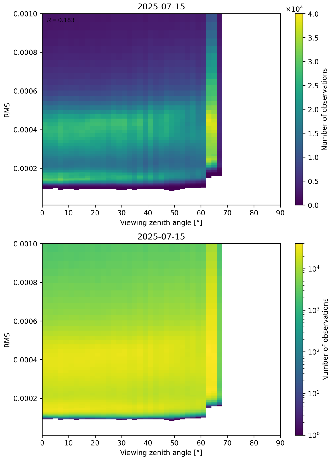
Figure 171: Scatter density plot of “Viewing zenith angle” against “RMS” for 2025-07-14 to 2025-07-16.
