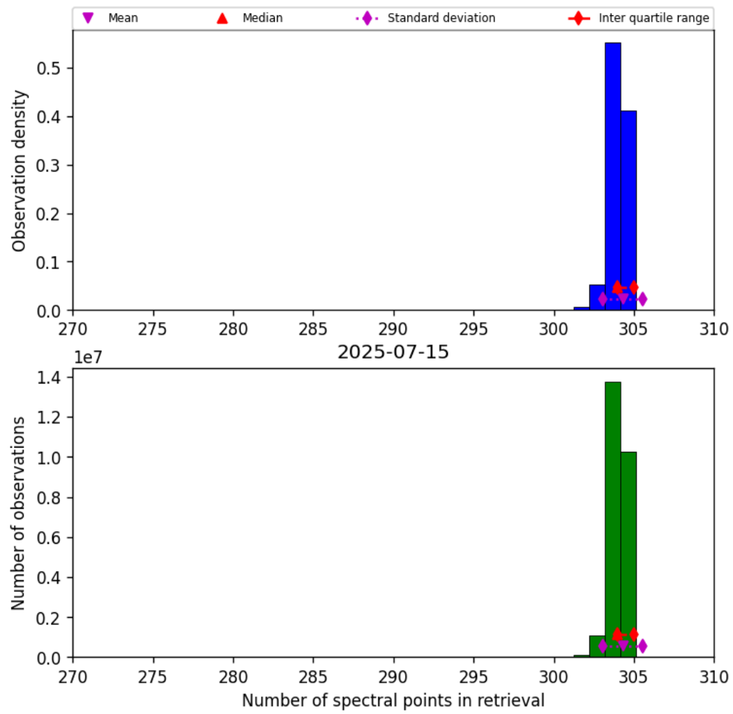
Figure 33: Histogram of “Number of spectral points in retrieval” for 2025-07-14 to 2025-07-16
