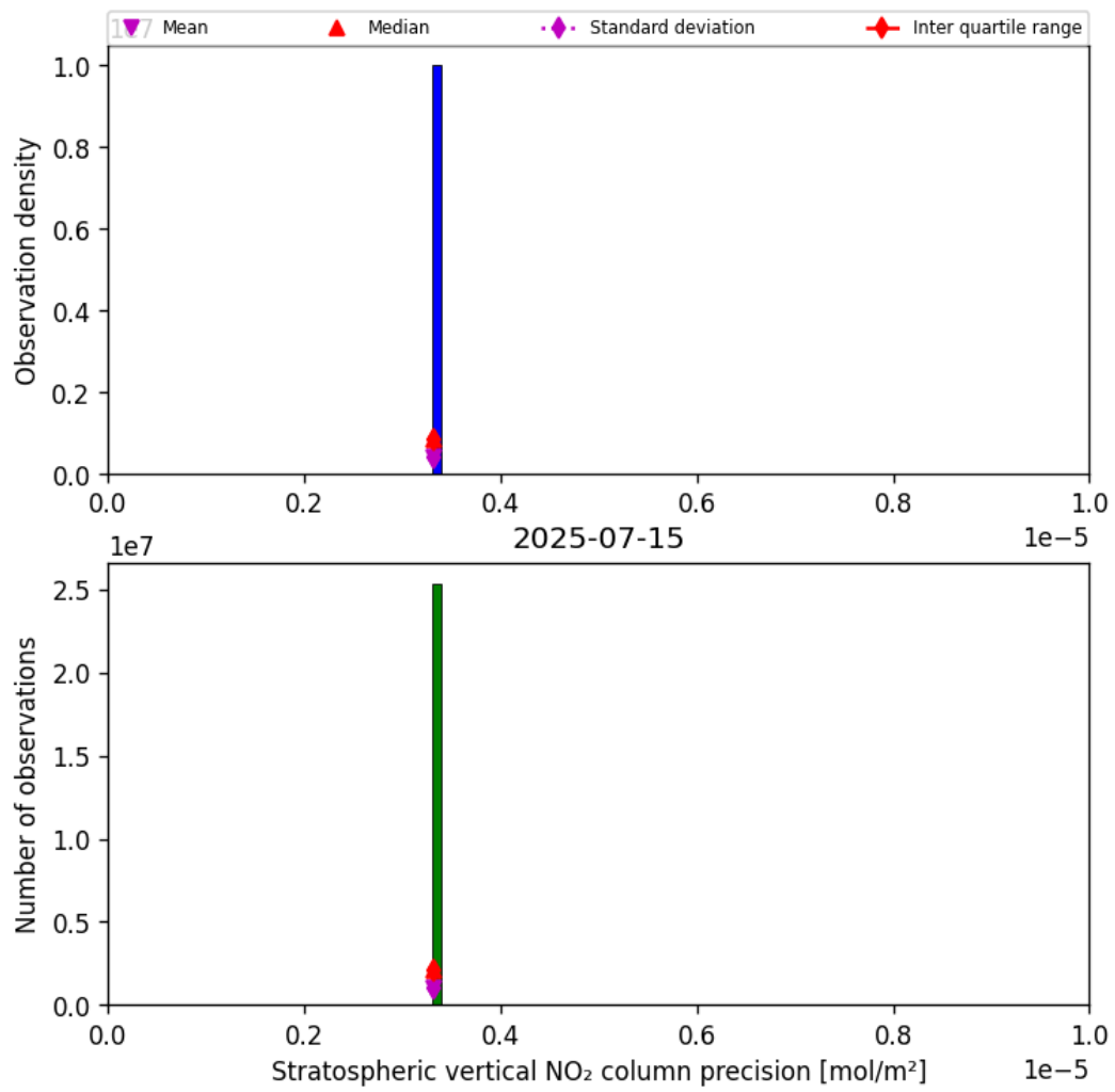
Figure 37: Histogram of “Stratospheric vertical NO 2 column precision” for 2025-07-14 to 2025-07-16
