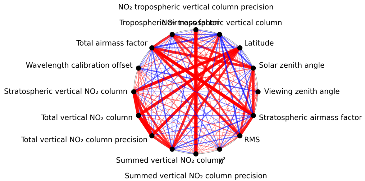
Figure 1: Map of correlation graph for 2025-07-14 to 2025-07-16.
