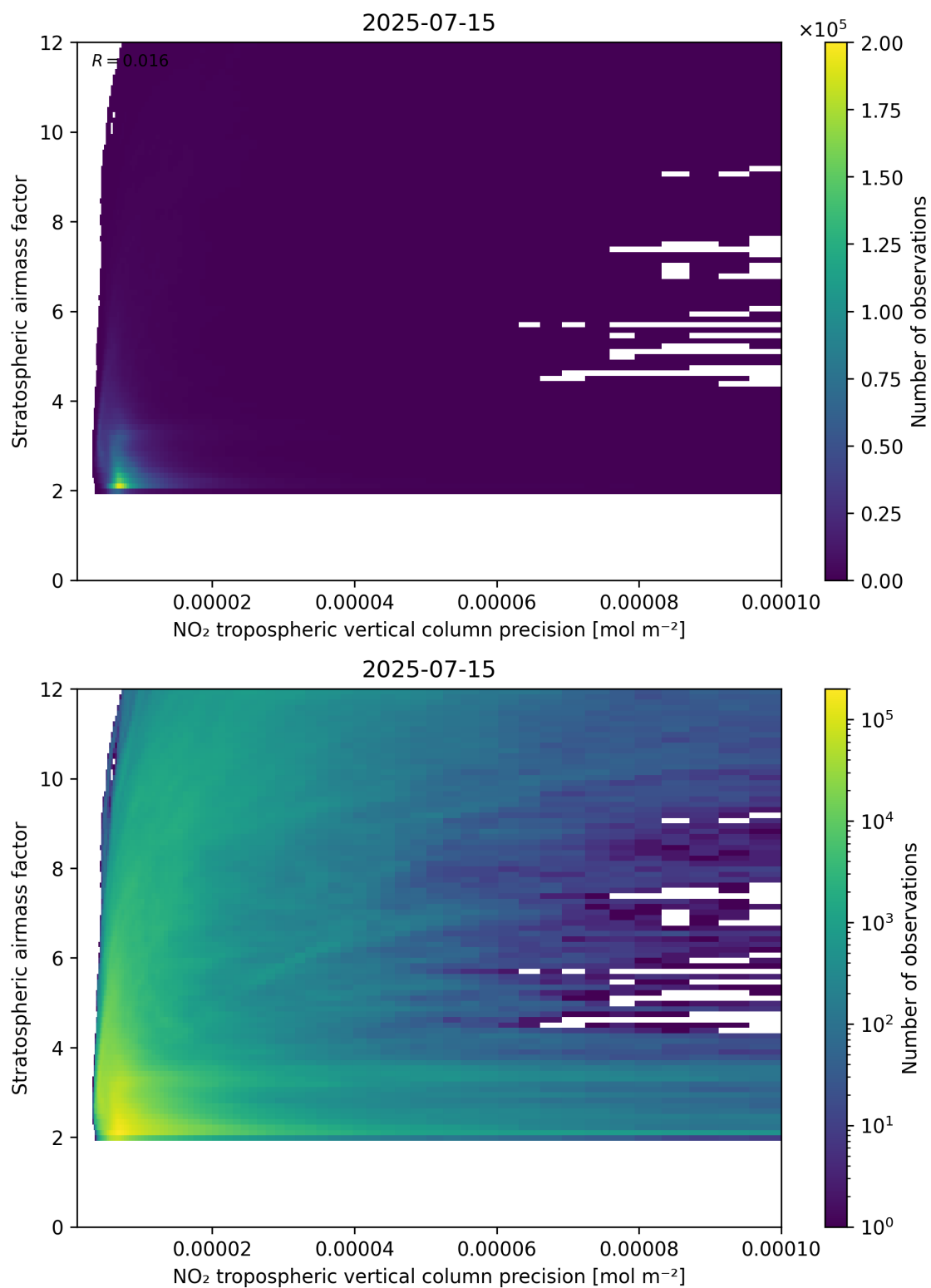
Figure 131: Scatter density plot of “NO 2 tropospheric vertical column precision” against “Stratospheric airmass factor” for 2025-07-14 to 2025-07-16.
