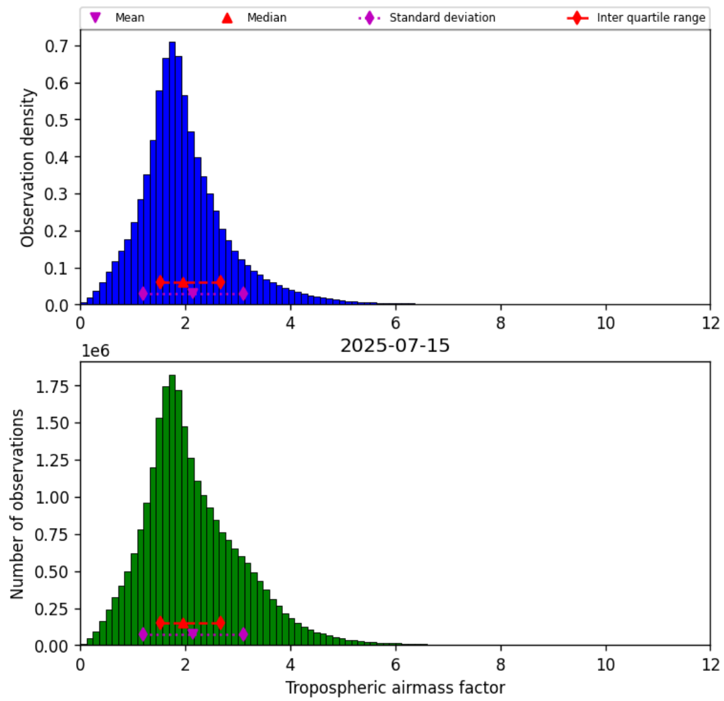
Figure 31: Histogram of “Tropospheric airmass factor” for 2025-07-14 to 2025-07-16
