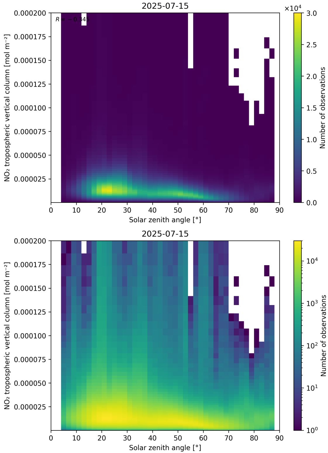
Figure 155: Scatter density plot of “Solar zenith angle” against “NO 2 tropospheric vertical column” for 2025-07-14 to 2025-07-16.
