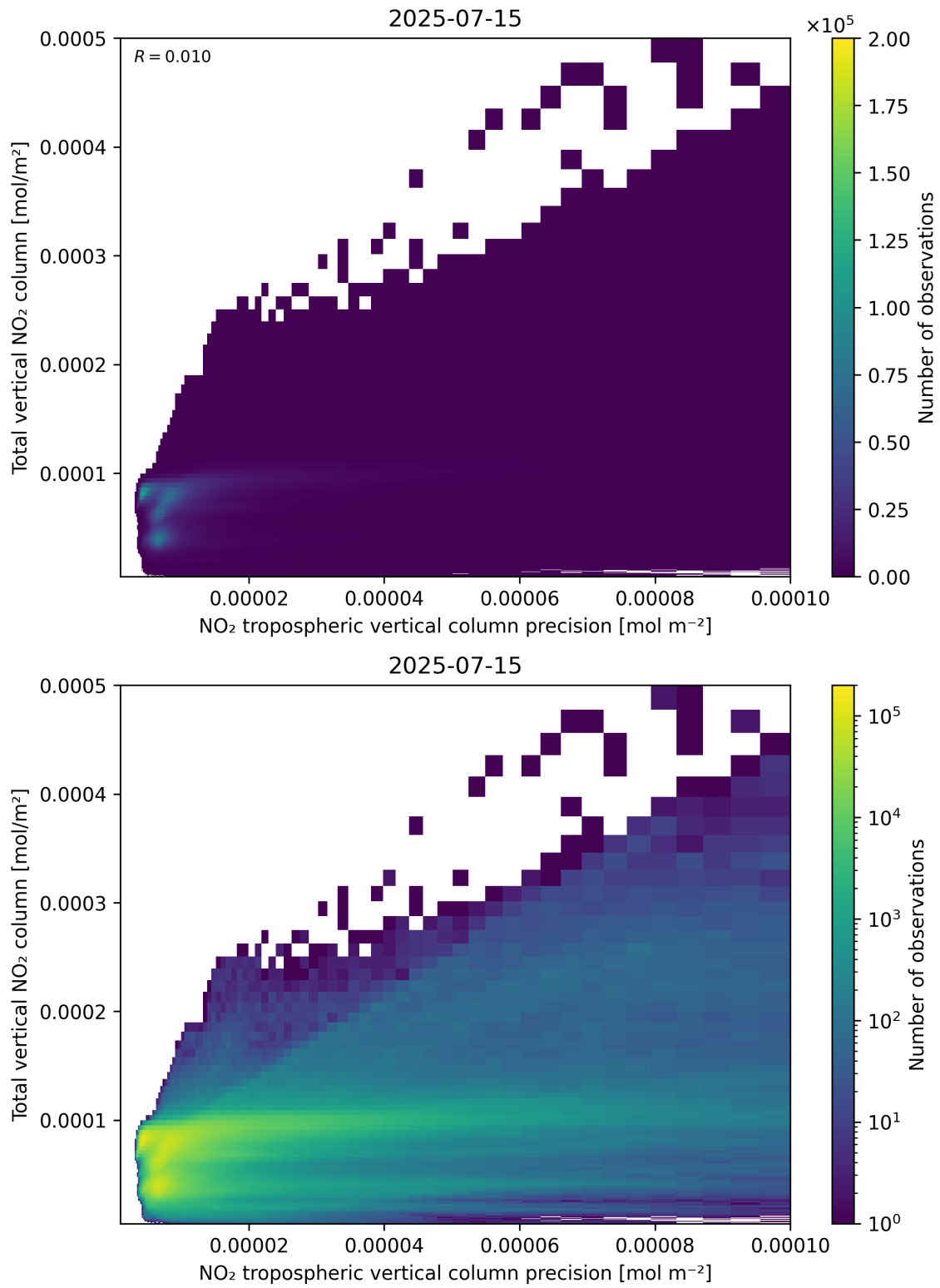
Figure 138: Scatter density plot of “NO 2 tropospheric vertical column precision” against “Total vertical NO 2 column” for 2025-07-14 to 2025-07-16.
