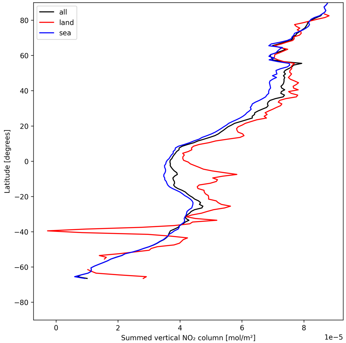
Figure 23: Zonal average of “Summed vertical NO 2 column” for 2025-07-14 to 2025-07-16.
