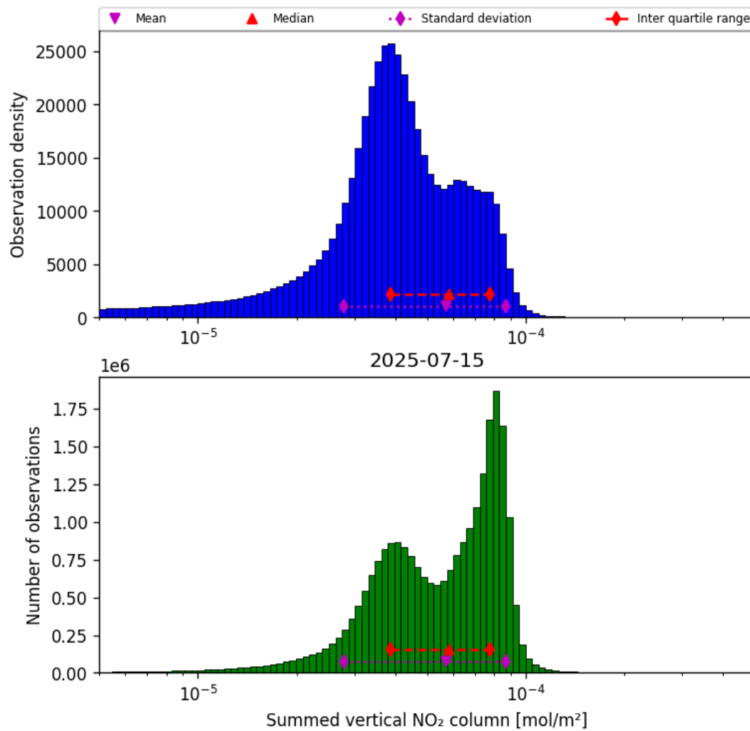
Figure 40: Histogram of “Summed vertical NO 2 column” for 2025-07-14 to 2025-07-16
