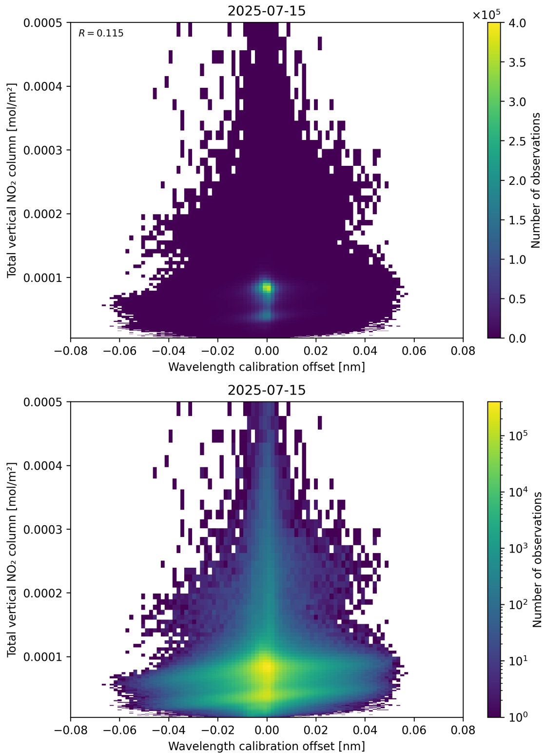
Figure 179: Scatter density plot of “Wavelength calibration offset” against “Total vertical NO 2 column” for 2025-07-14 to 2025-07-16.
