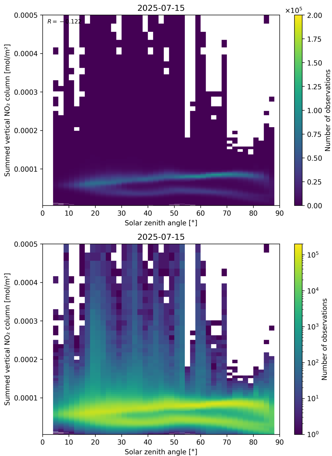
Figure 151: Scatter density plot of “Solar zenith angle” against “Summed vertical NO 2 column” for 2025-07-14 to 2025-07-16.
