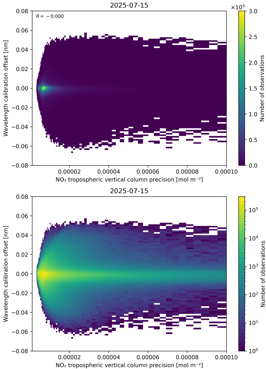
Figure 141: Scatter density plot of “NO 2 tropospheric vertical column precision” against “Wavelength calibration offset” for 2025-07-14 to 2025-07-16.
