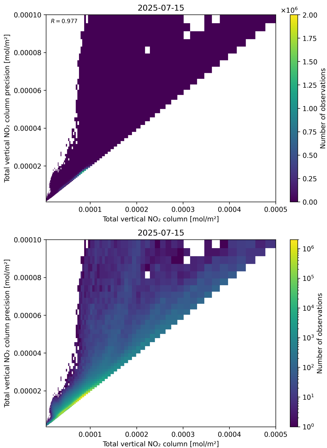
Figure 114: Scatter density plot of “Total vertical NO 2 column” against “Total vertical NO 2 column precision” for 2025-07-14 to 2025-07-16.
