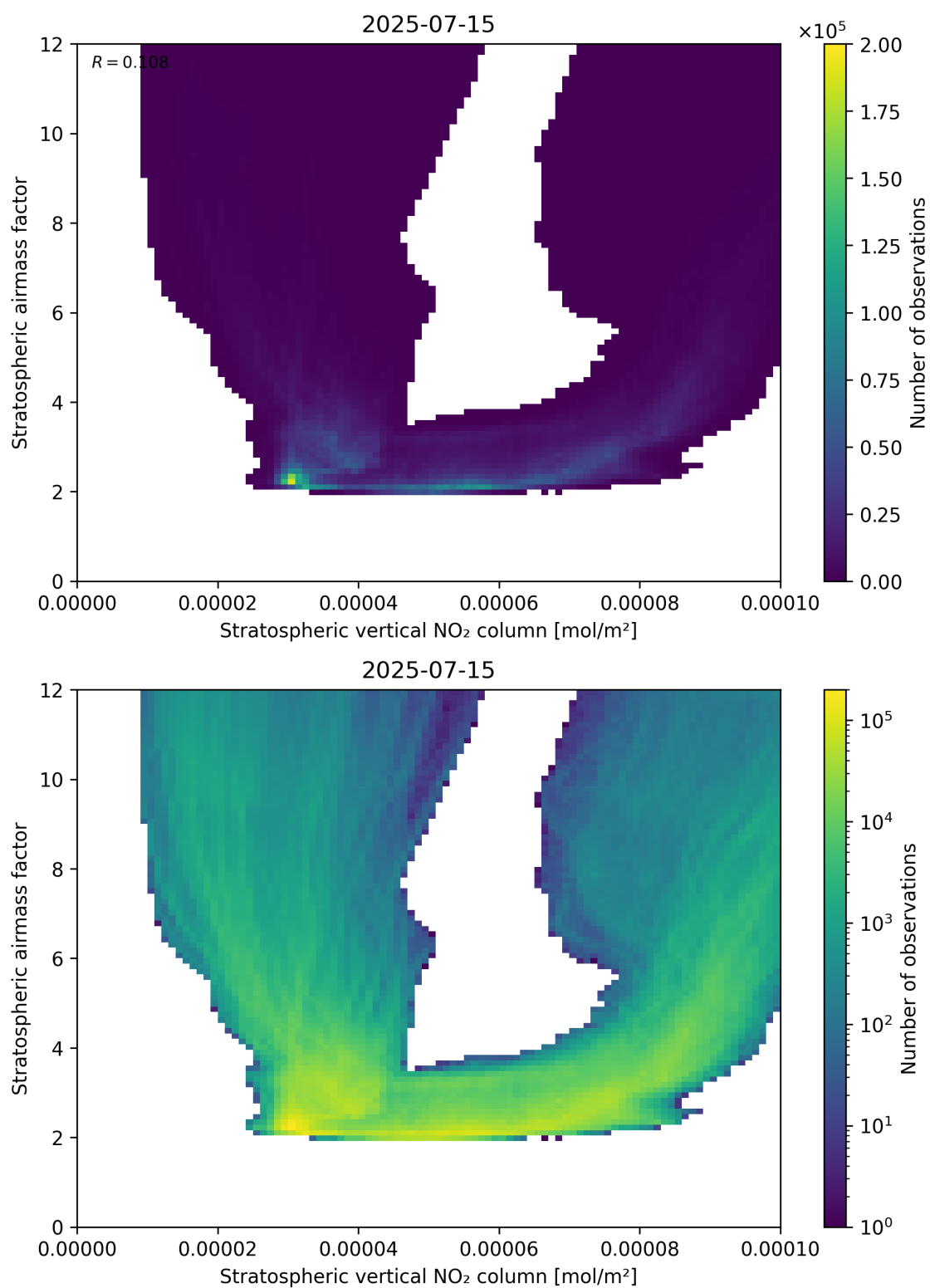
Figure 96: Scatter density plot of “Stratospheric vertical NO 2 column” against “Stratospheric airmass factor” for 2025-07-14 to 2025-07-16.
