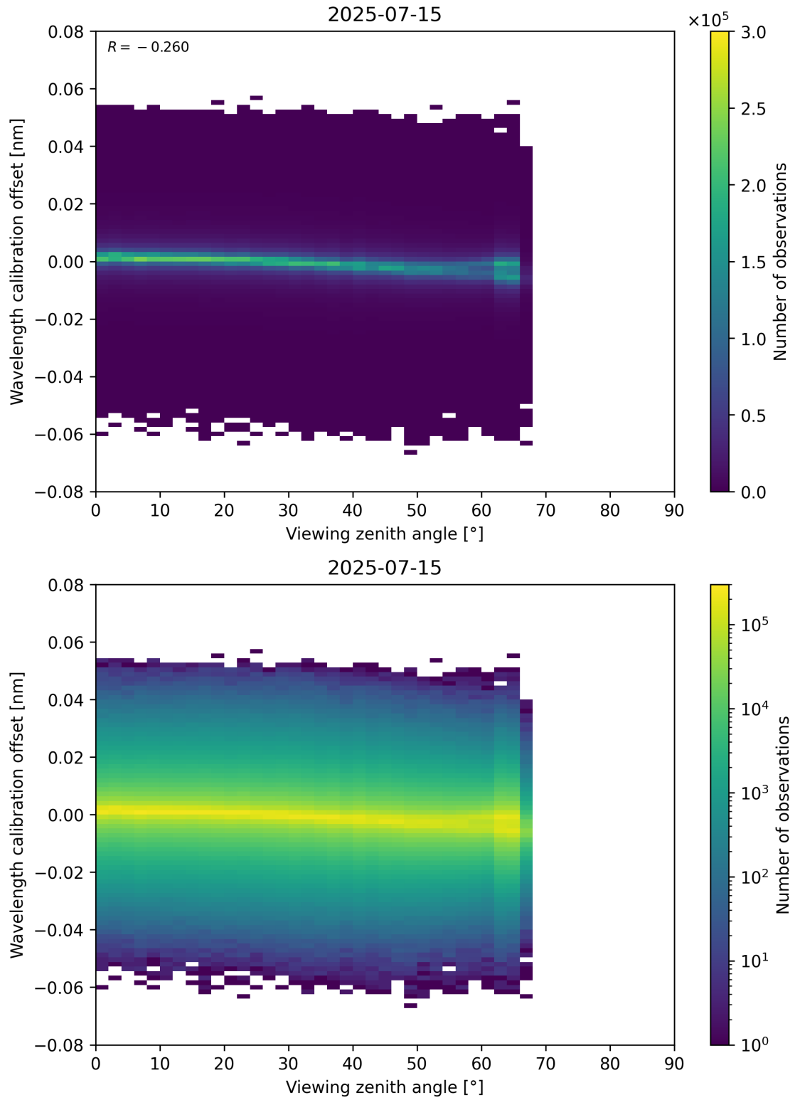
Figure 173: Scatter density plot of “Viewing zenith angle” against “Wavelength calibration offset” for 2025-07-14 to 2025-07-16.
