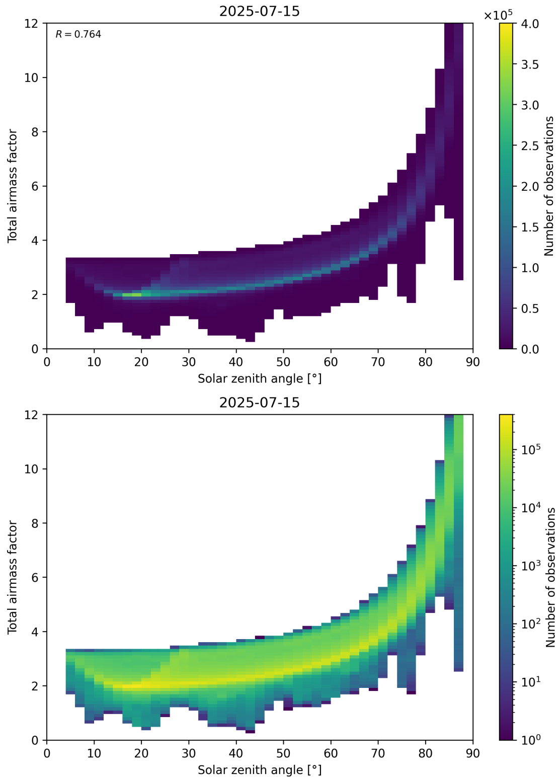
Figure 146: Scatter density plot of “Solar zenith angle” against “Total air mass factor” for 2025-07-14 to 2025-07-16.
