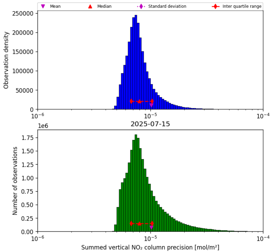
Figure 41: Histogram of “Summed vertical NO 2 column precision” for 2025-07-14 to 2025-07-16
