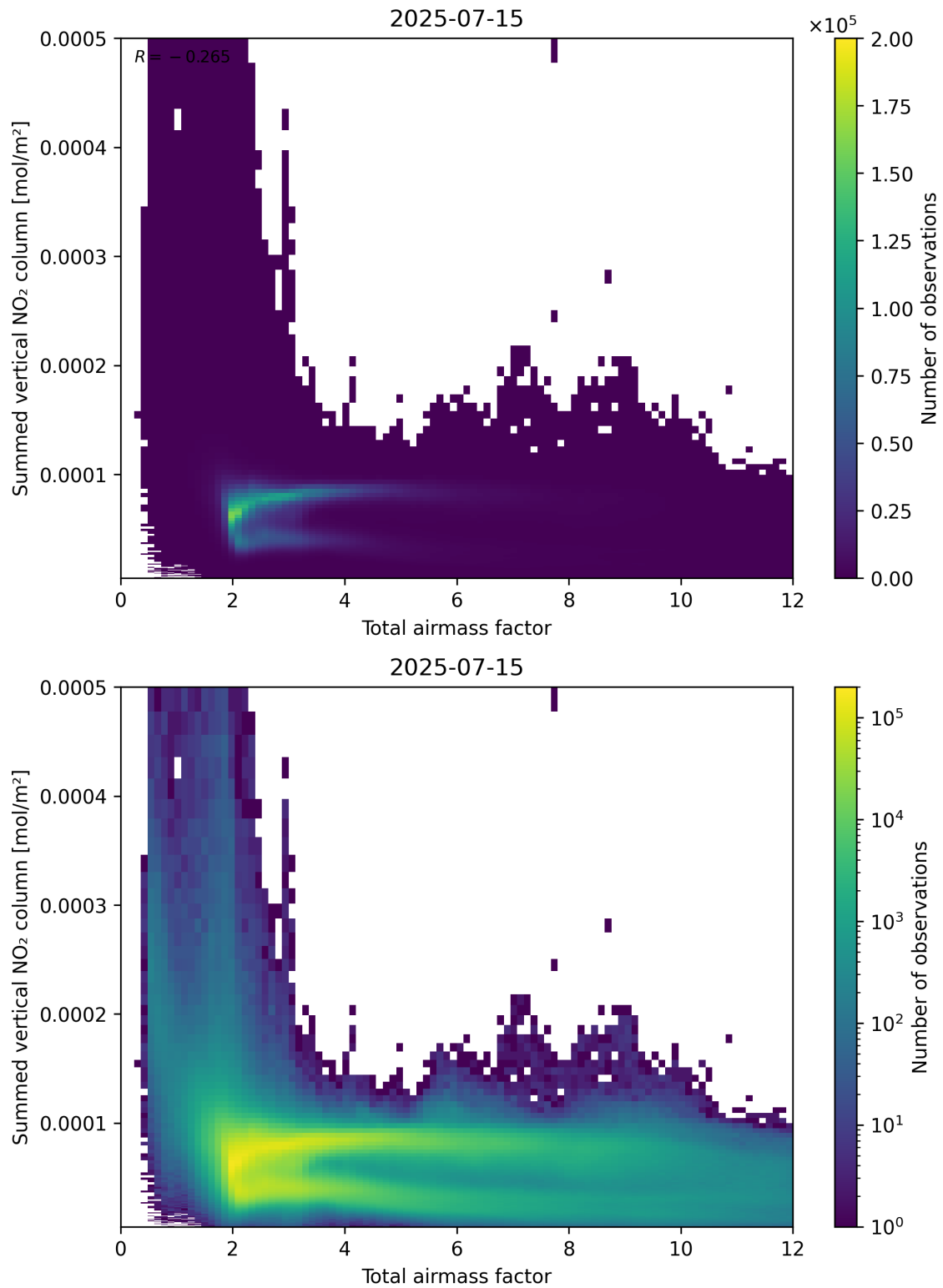
Figure 65: Scatter density plot of “Total airmass factor” against “Summed vertical NO 2 column” for 2025-07-14 to 2025-07-16.
