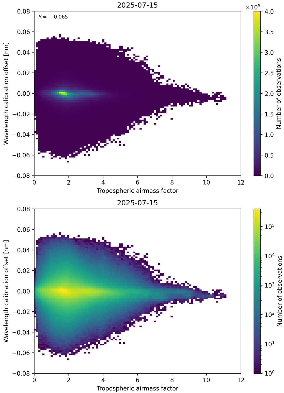
Figure 80: Scatter density plot of “Tropospheric airmass factor” against “Wavelength calibration offset” for 2025-07-14 to 2025-07-16.
