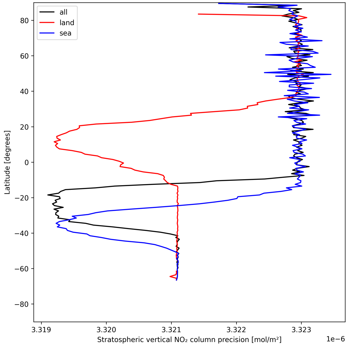
Figure 20: Zonal average of “Stratospheric vertical NO 2 column precision” for 2025-07-14 to 2025-07-16.
