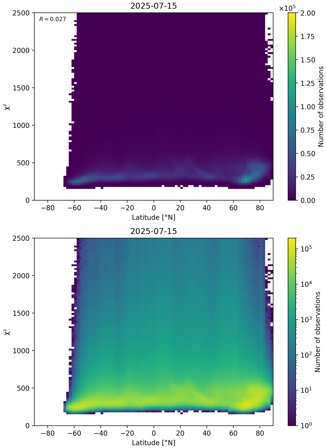
Figure 86: Scatter density plot of “Latitude” against “ \chi^2 ” for 2025-07-14 to 2025-07-16.
