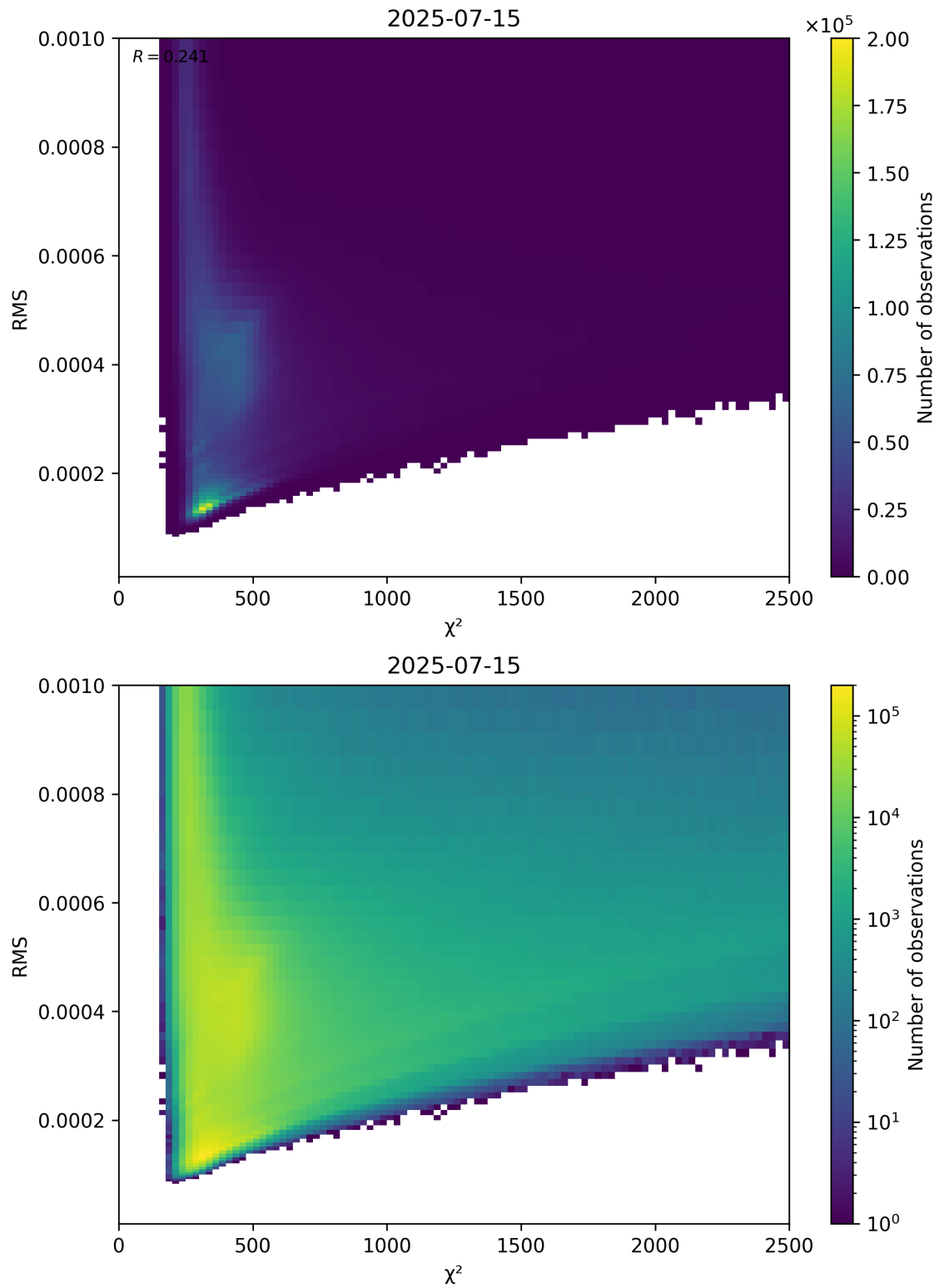
Figure 82: Scatter density plot of “ \chi^2 ” against “RMS” for 2025-07-14 to 2025-07-16.
