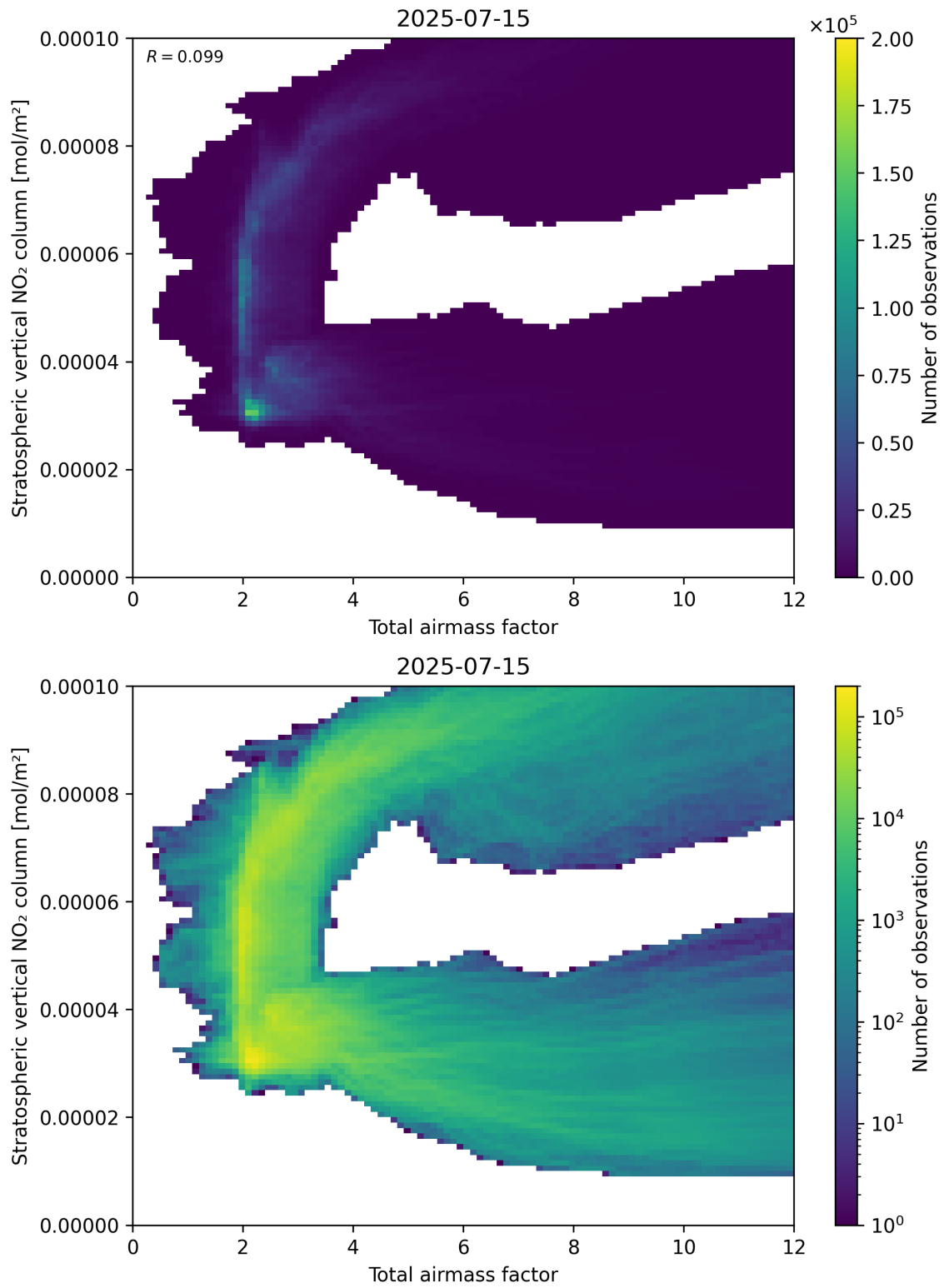
Figure 64: Scatter density plot of “Total airmass factor” against “Stratospheric vertical NO 2 column” for 2025-07-14 to 2025-07-16.
