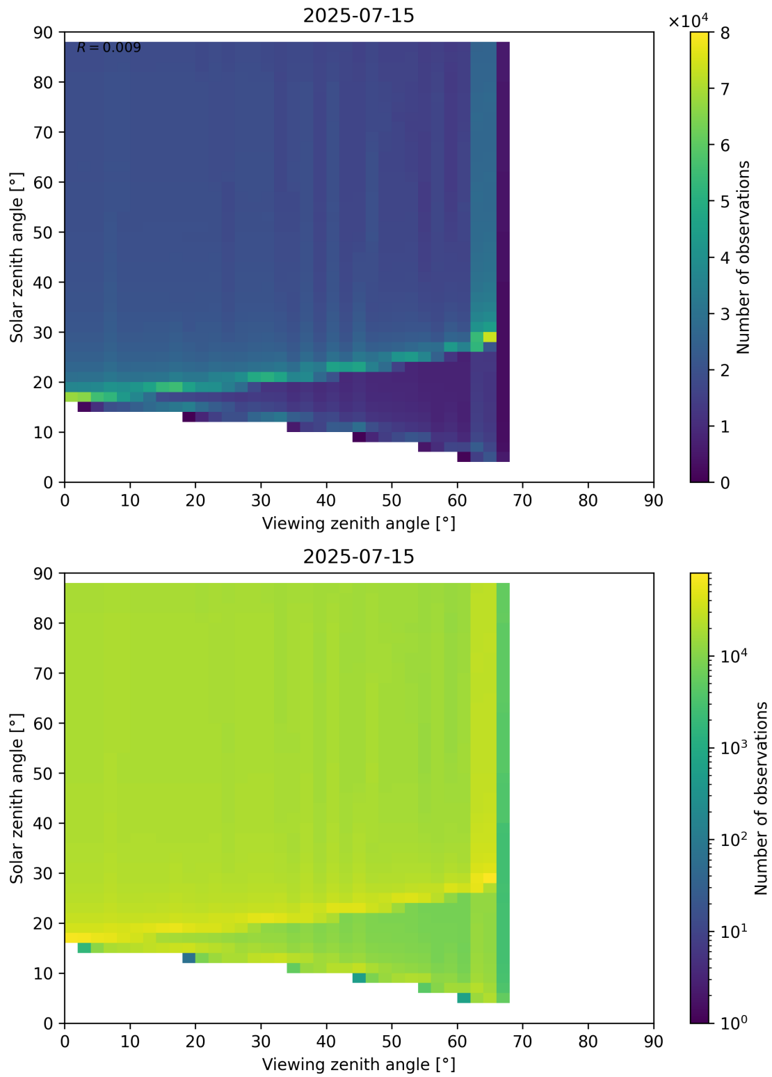
Figure 172: Scatter density plot of “Viewing zenith angle” against “Solar zenith angle” for 2025-07-14 to 2025-07-16.
