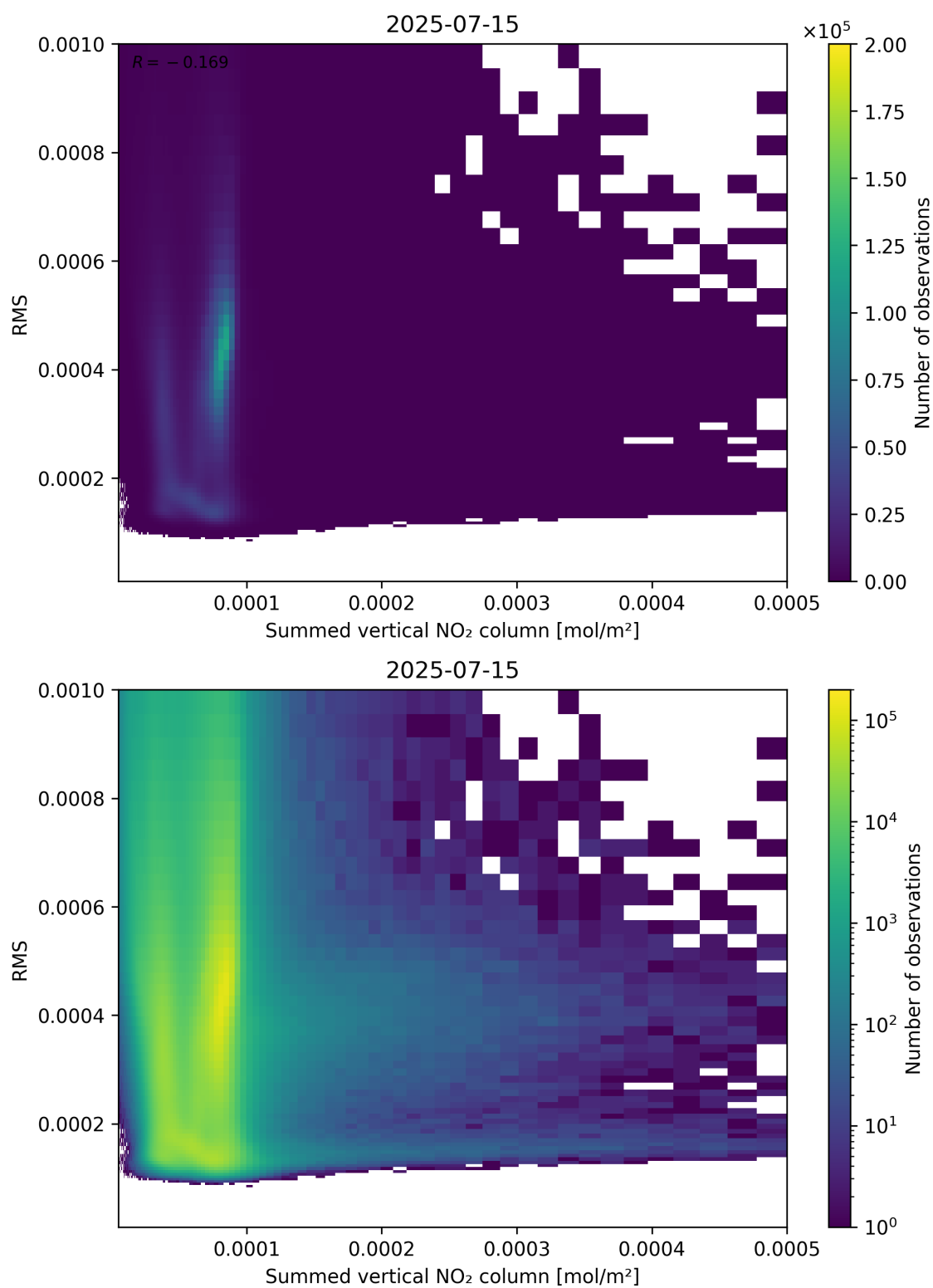
Figure 109: Scatter density plot of “Summed vertical NO 2 column” against “RMS” for 2025-07-14 to 2025-07-16.
