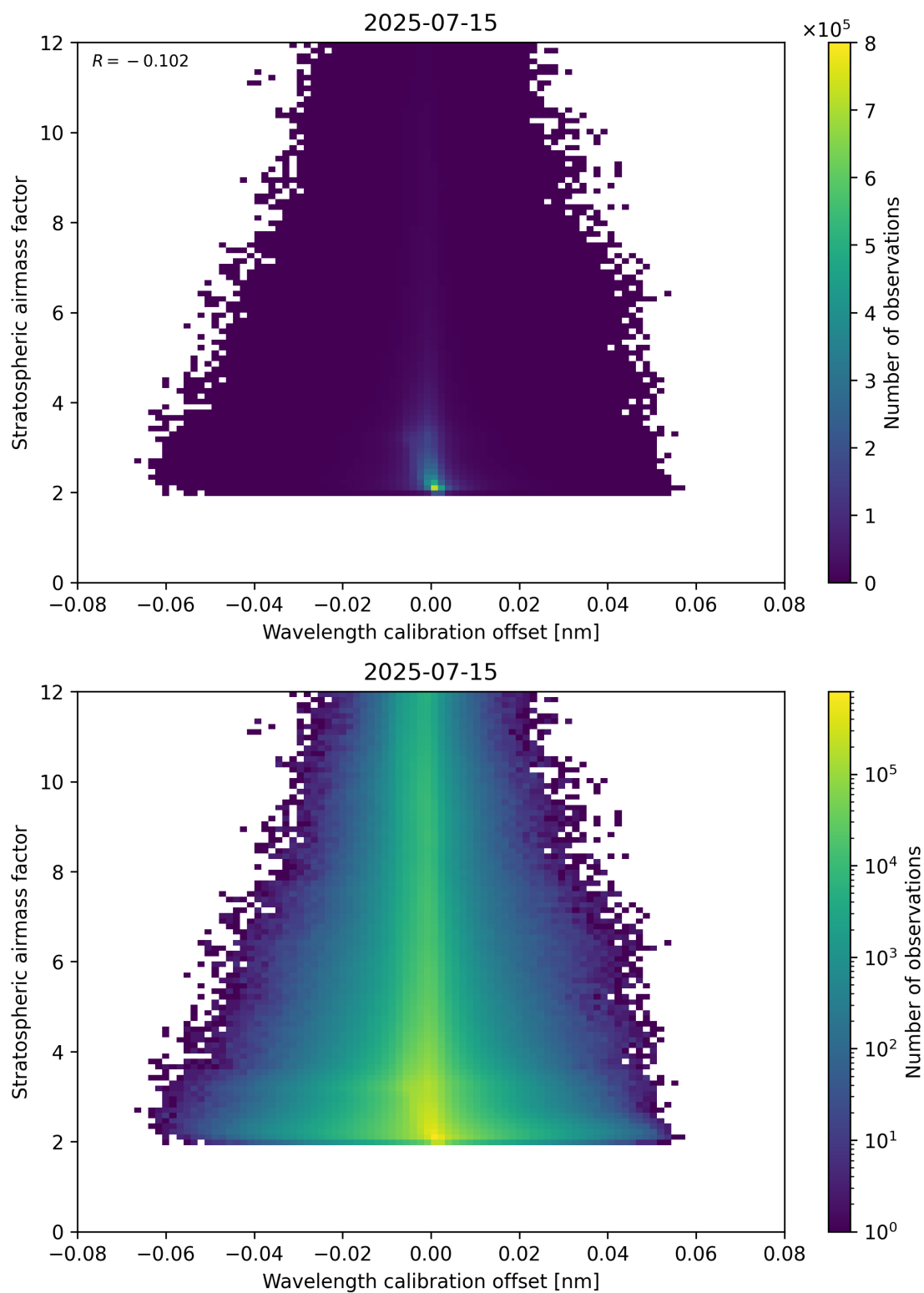
Figure 174: Scatter density plot of “Wavelength calibration offset” against “Stratospheric airmass factor” for 2025-07-14 to 2025-07-16.
