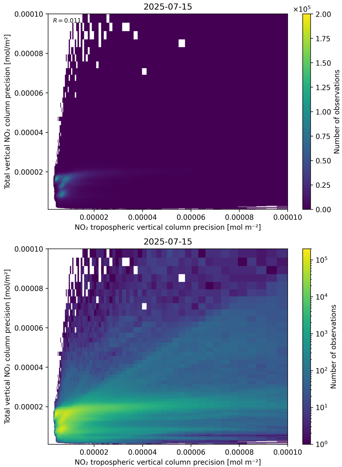
Figure 139: Scatter density plot of “NO 2 tropospheric vertical column precision” against “Total vertical NO 2 column precision” for 2025-07-14 to 2025-07-16.
