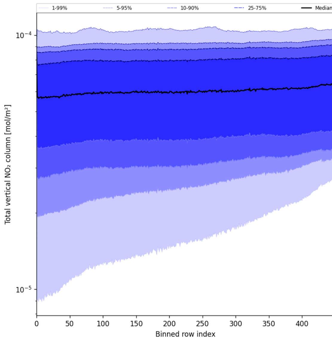
Figure 55: Along track statistics of “Total vertical NO 2 column” for 2025-07-14 to 2025-07-16
