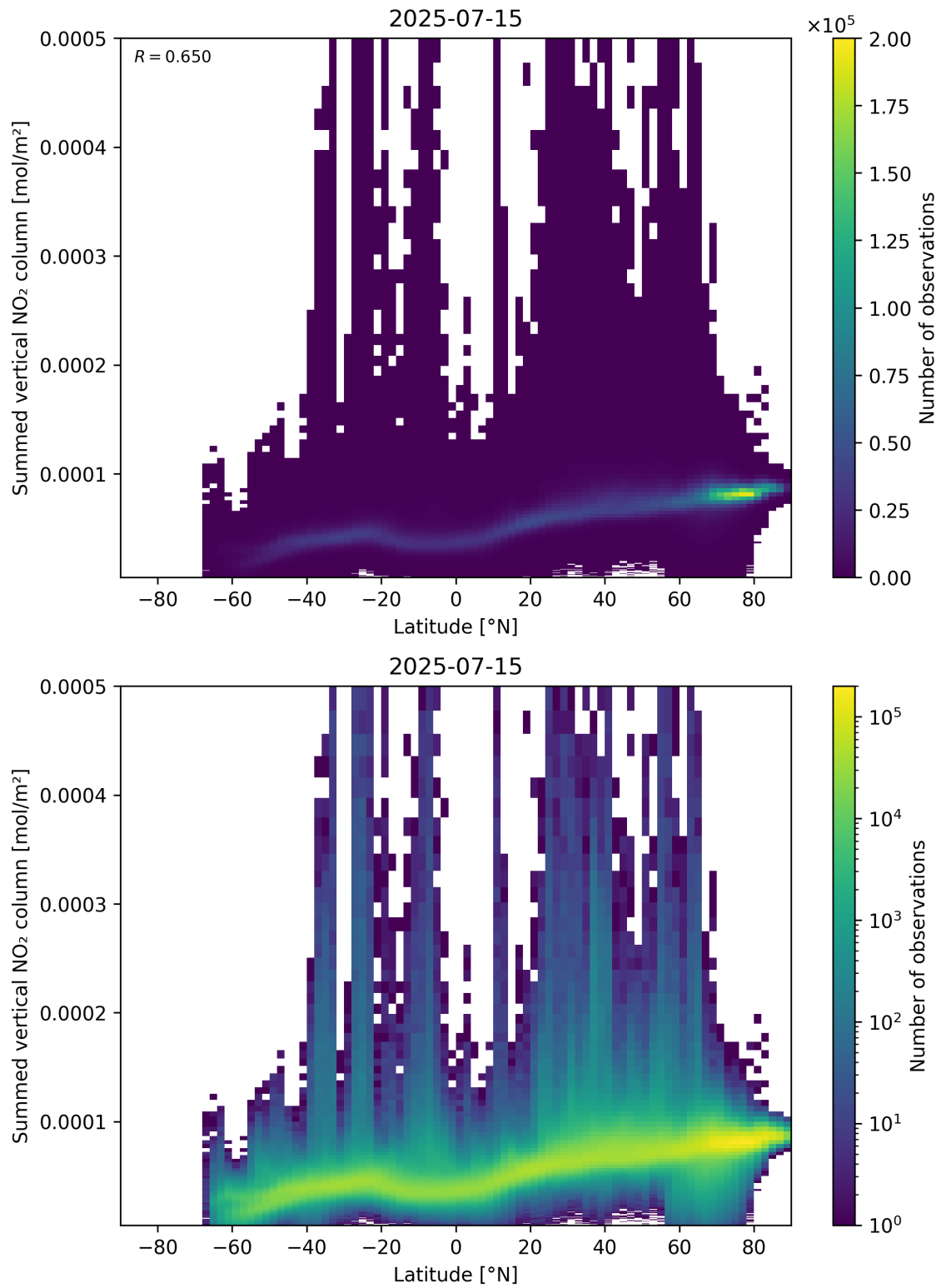
Figure 88: Scatter density plot of “Latitude” against “Summed vertical NO 2 column” for 2025-07-14 to 2025-07-16.
