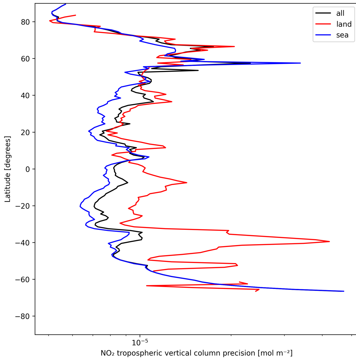
Figure 13: Zonal average of “NO 2 tropospheric vertical column precision” for 2025-07-14 to 2025-07-16.
