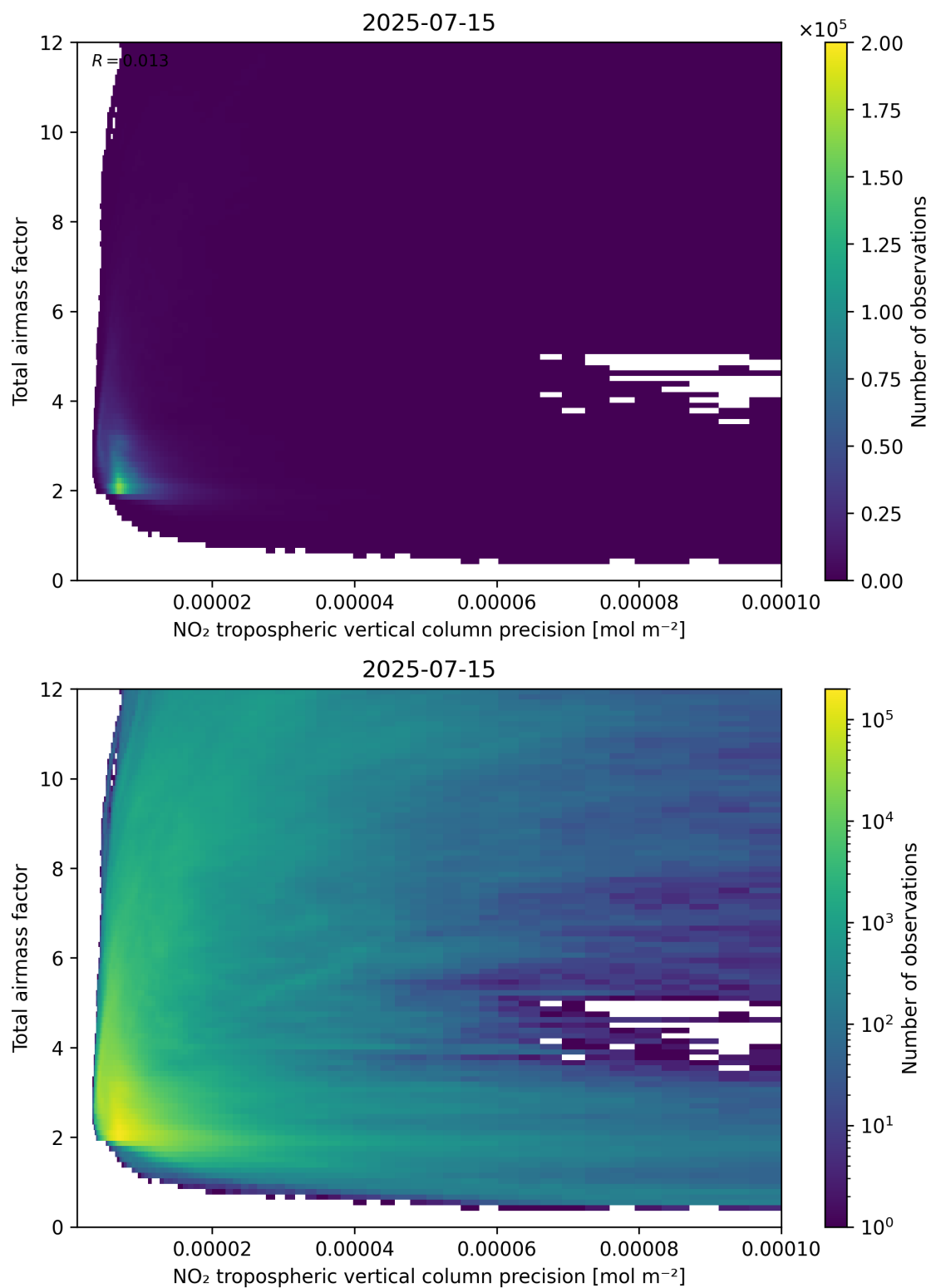
Figure 132: Scatter density plot of “NO 2 tropospheric vertical column precision” against “Total airmass factor” for 2025-07-14 to 2025-07-16.
