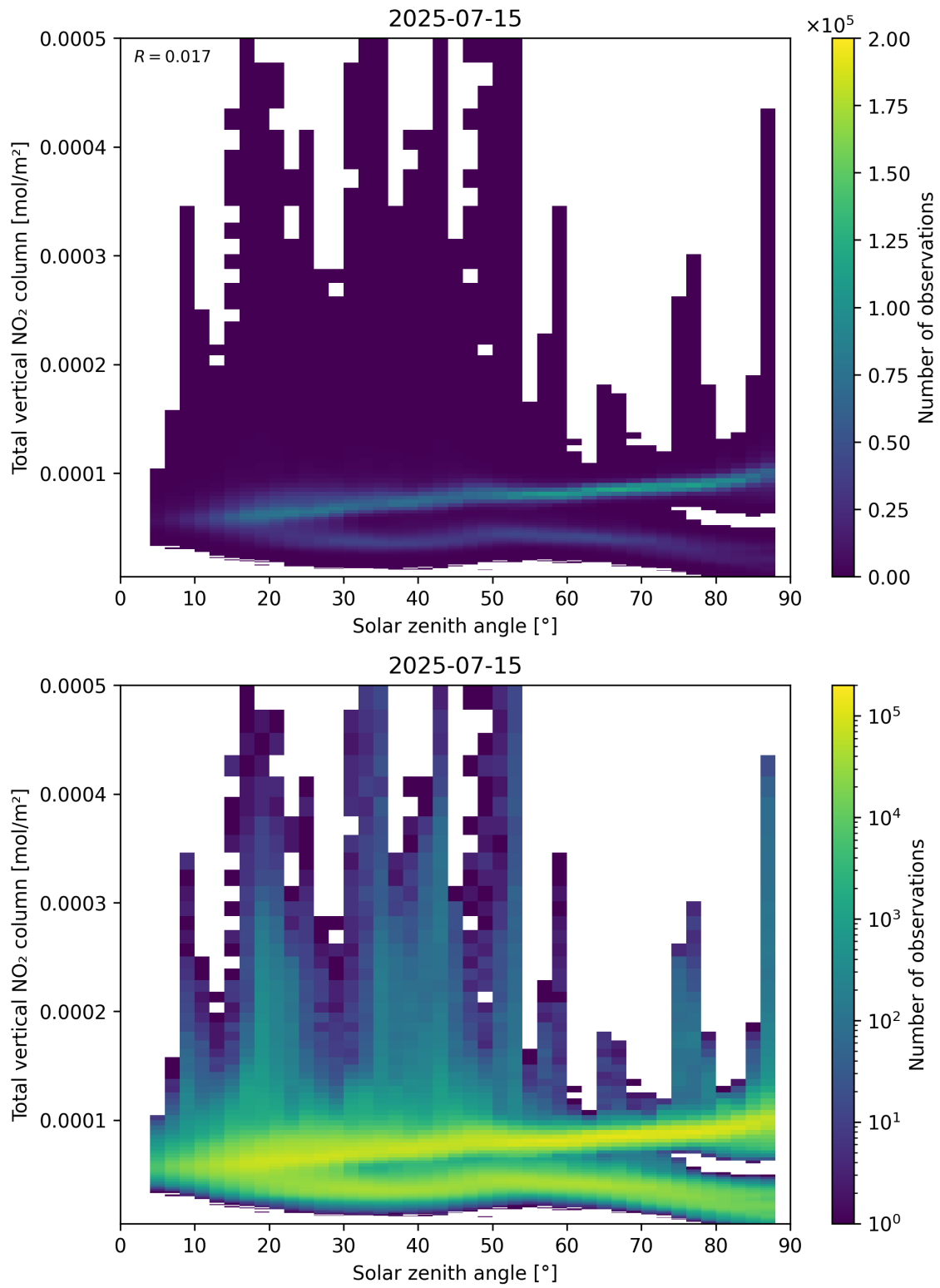
Figure 153: Scatter density plot of “Solar zenith angle” against “Total vertical NO 2 column” for 2025-07-14 to 2025-07-16.
