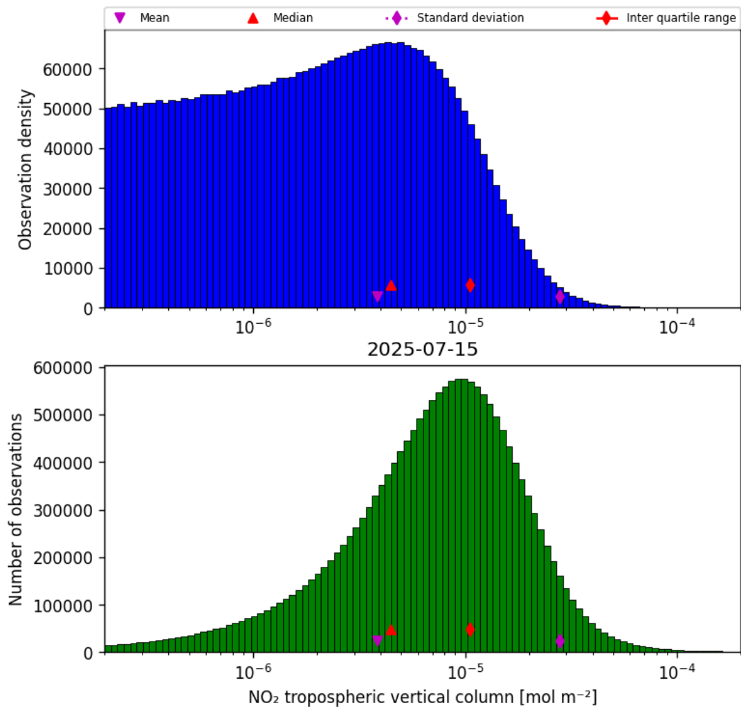
Figure 29: Histogram of “NO 2 tropospheric vertical column” for 2025-07-14 to 2025-07-16
