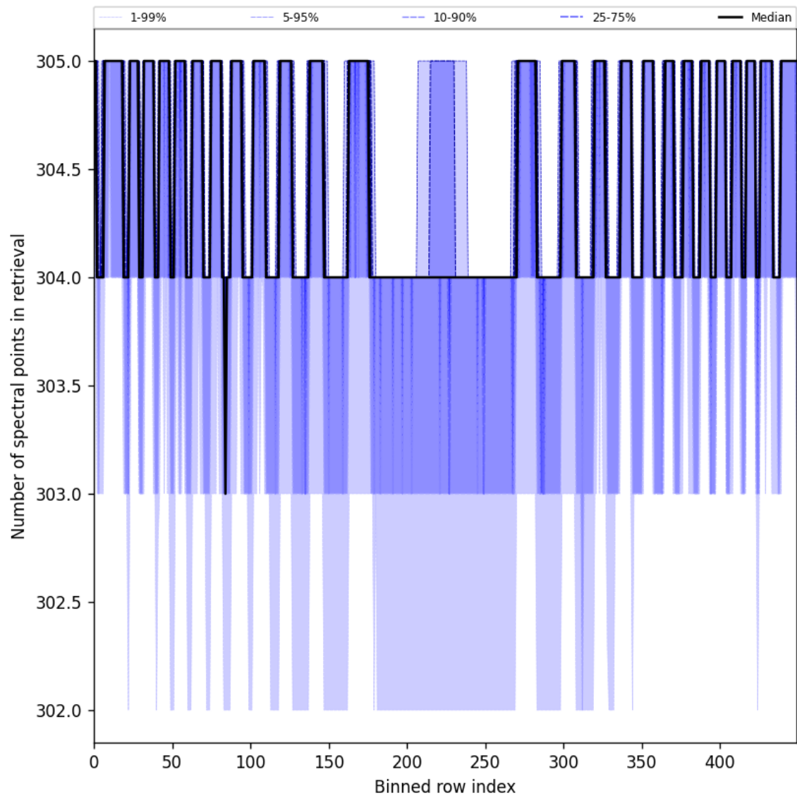
Figure 50: Along track statistics of “Number of spectral points in retrieval” for 2025-07-14 to 2025-07-16
