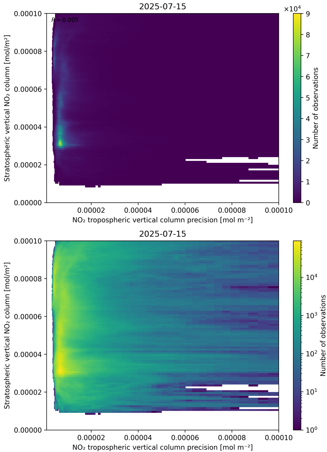
Figure 135: Scatter density plot of “NO 2 tropospheric vertical column precision” against “Stratospheric vertical NO 2 column” for 2025-07-14 to 2025-07-16.
