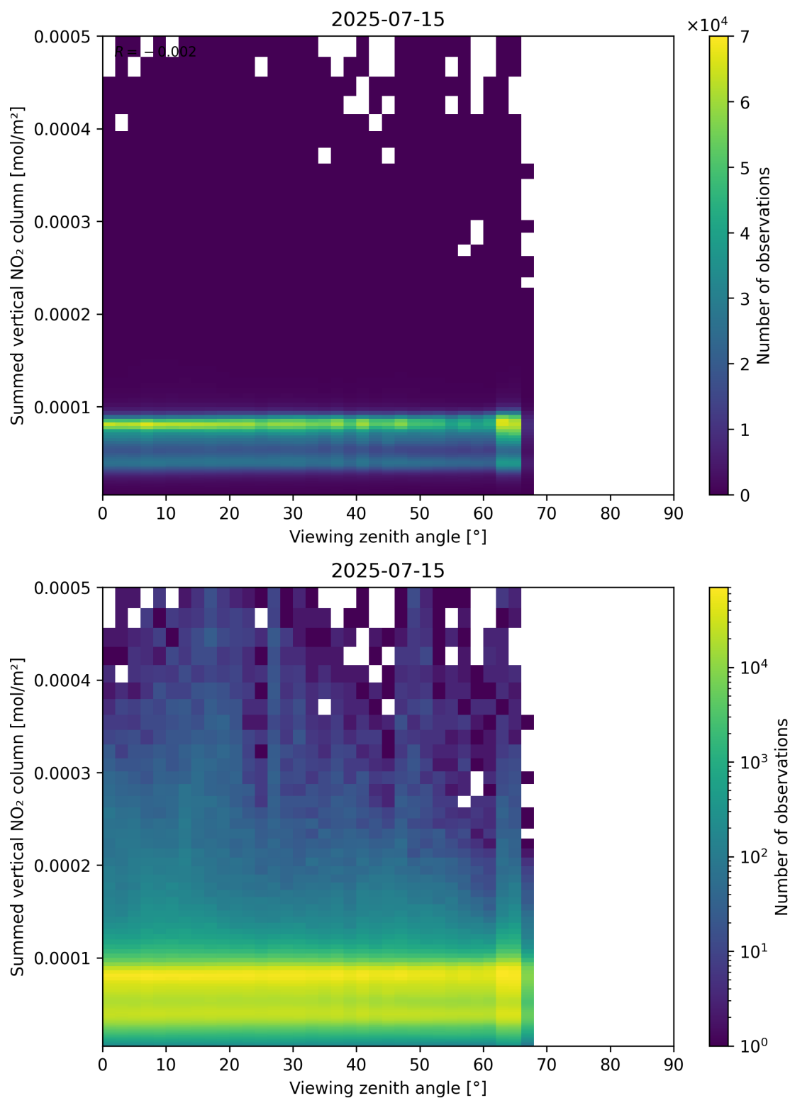
Figure 165: Scatter density plot of “Viewing zenith angle” against “Summed vertical NO 2 column” for 2025-07-14 to 2025-07-16.
