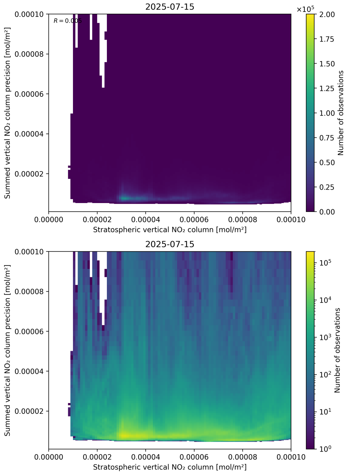
Figure 99: Scatter density plot of “Stratospheric vertical NO 2 column” against “Summed vertical NO 2 column precision” for 2025-07-14 to 2025-07-16.
