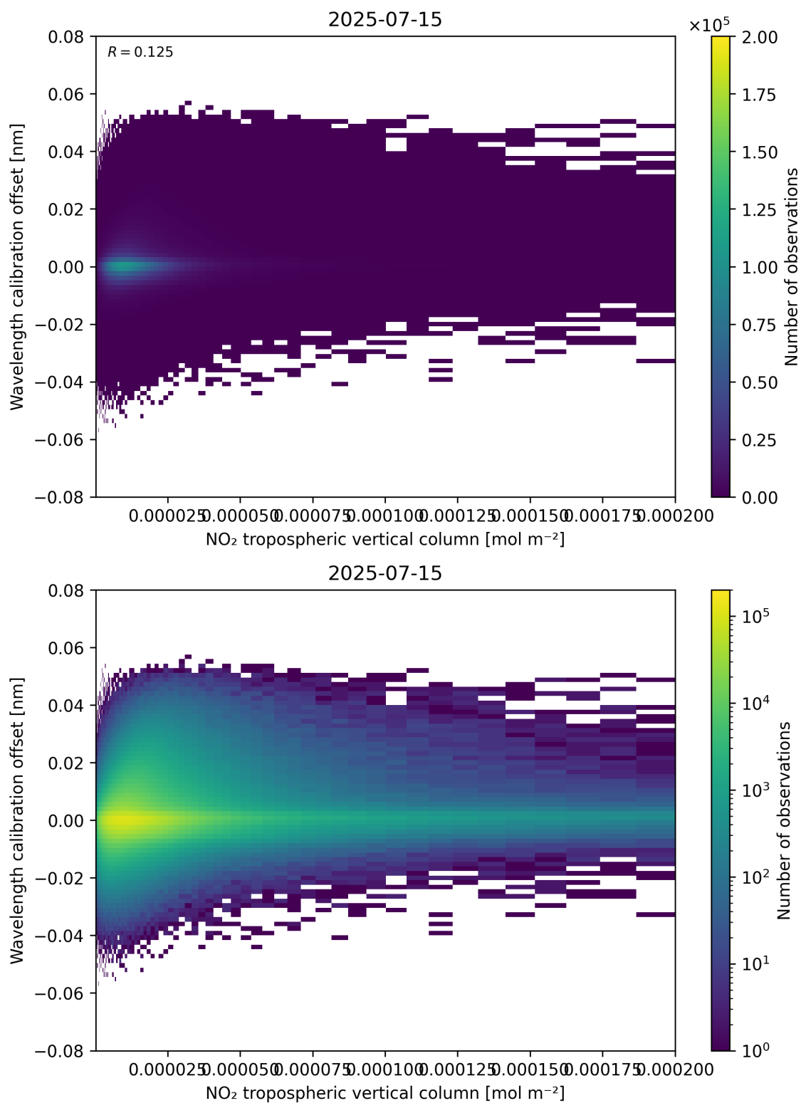
Figure 143: Scatter density plot of “NO 2 tropospheric vertical column” against “Wavelength calibration offset” for 2025-07-14 to 2025-07-16.
