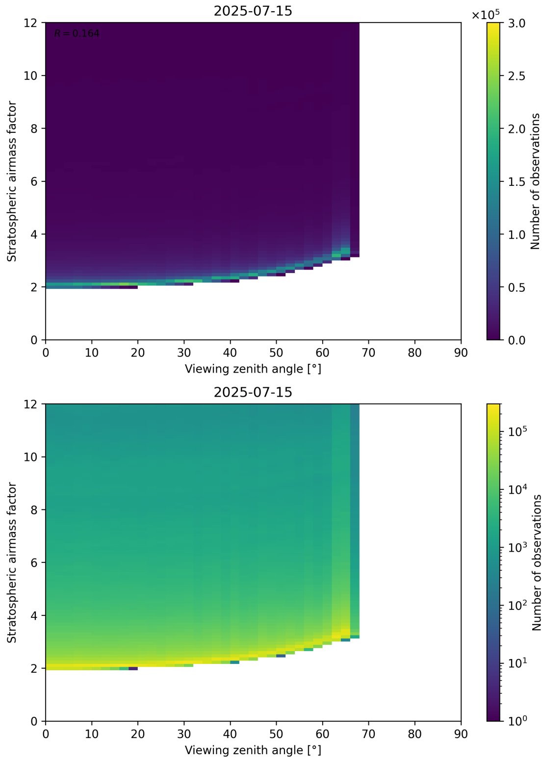
Figure 159: Scatter density plot of “Viewing zenith angle” against “Stratospheric airmass factor” for 2025-07-14 to 2025-07-16.
