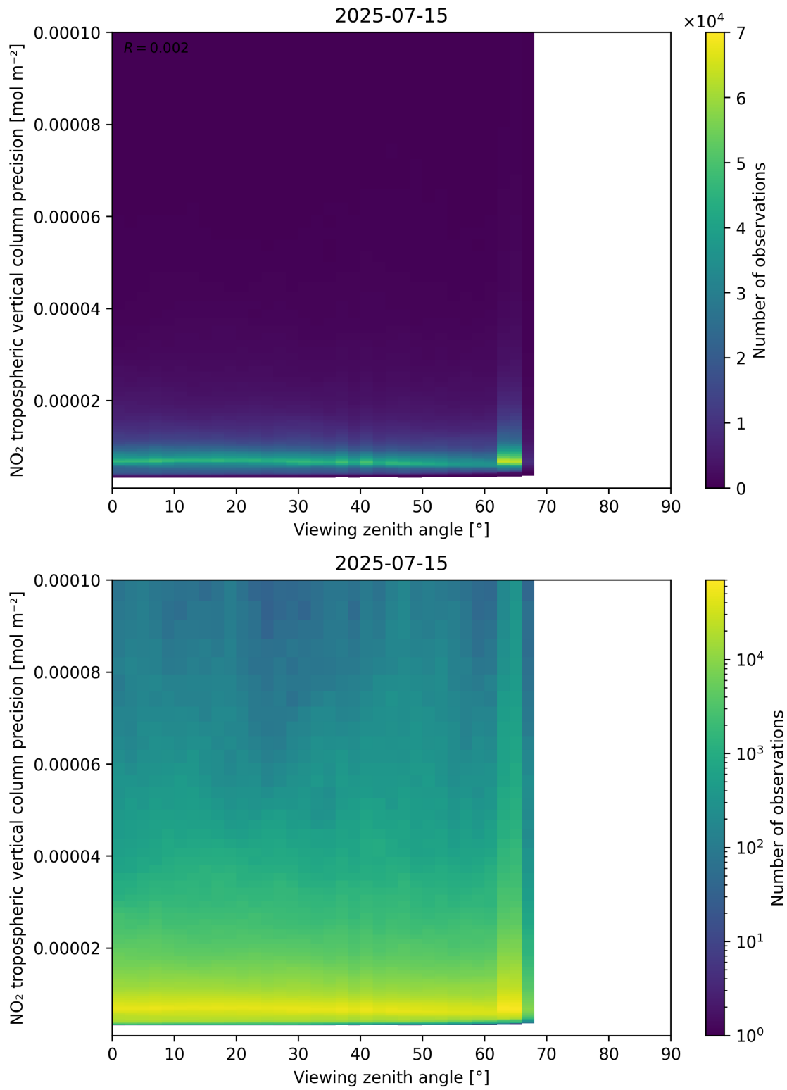
Figure 170: Scatter density plot of “Viewing zenith angle” against “NO 2 tropospheric vertical column precision” for 2025-07-14 to 2025-07-16.
