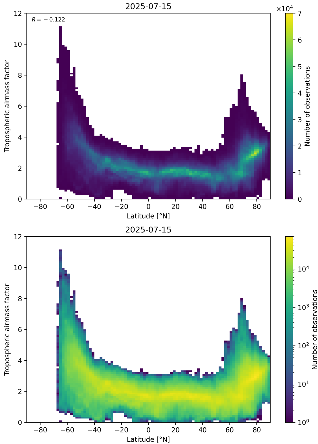
Figure 85: Scatter density plot of “Latitude” against “Tropospheric airmass factor” for 2025-07-14 to 2025-07-16.
