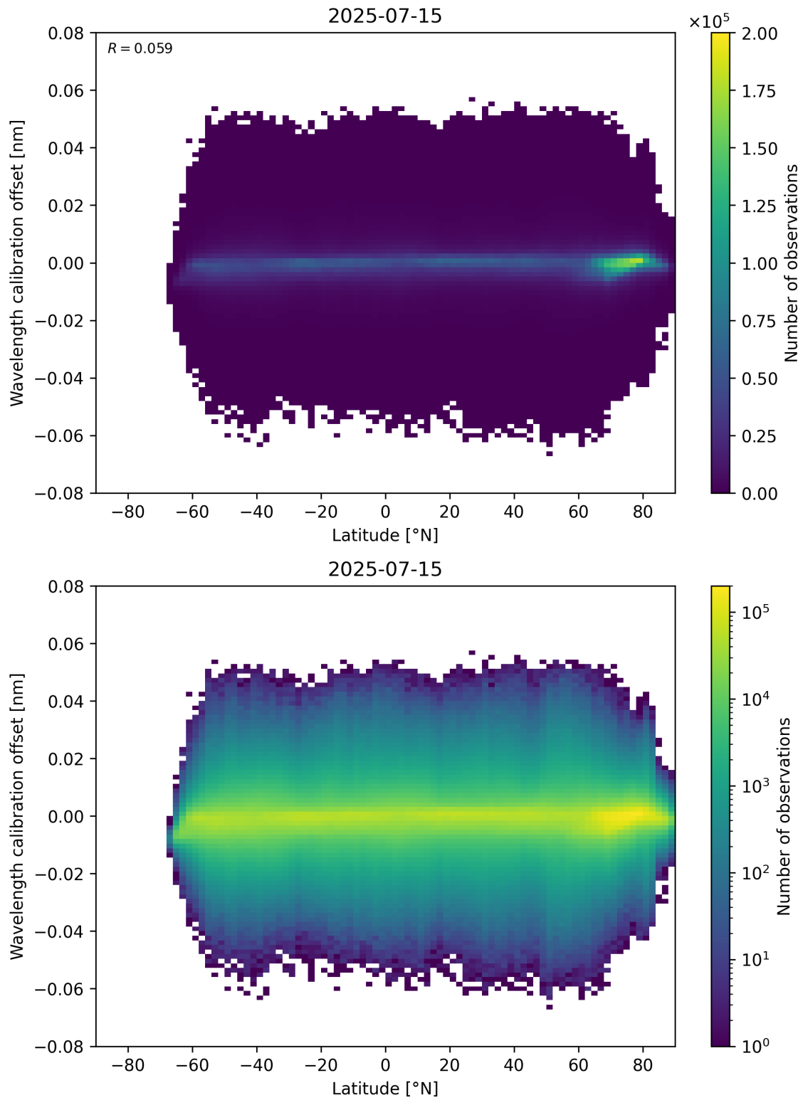
Figure 95: Scatter density plot of “Latitude” against “Wavelength calibration offset” for 2025-07-14 to 2025-07-16.
