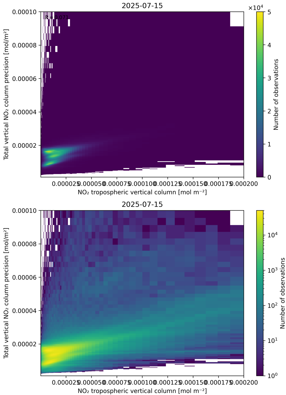
Figure 129: Scatter density plot of “NO 2 tropospheric vertical column” against “Total vertical NO 2 column precision” for 2025-07-14 to 2025-07-16.
