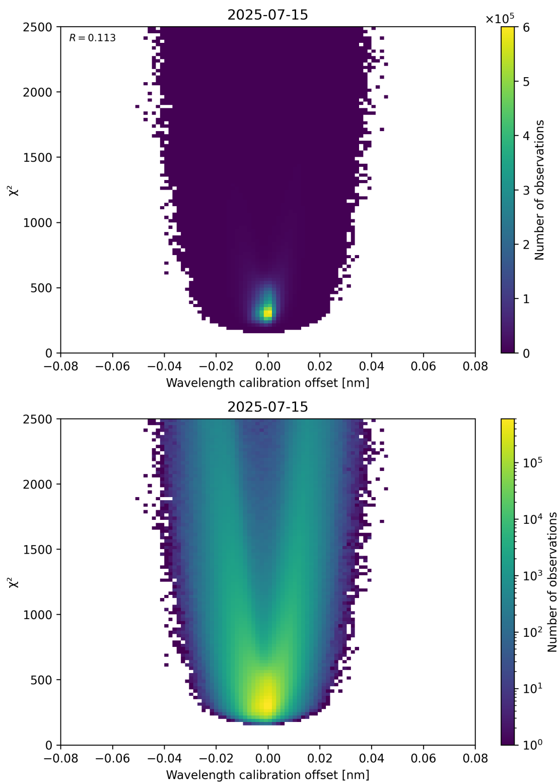
Figure 175: Scatter density plot of “Wavelength calibration offset” against “ \chi^2 ” for 2025-07-14 to 2025-07-16.
