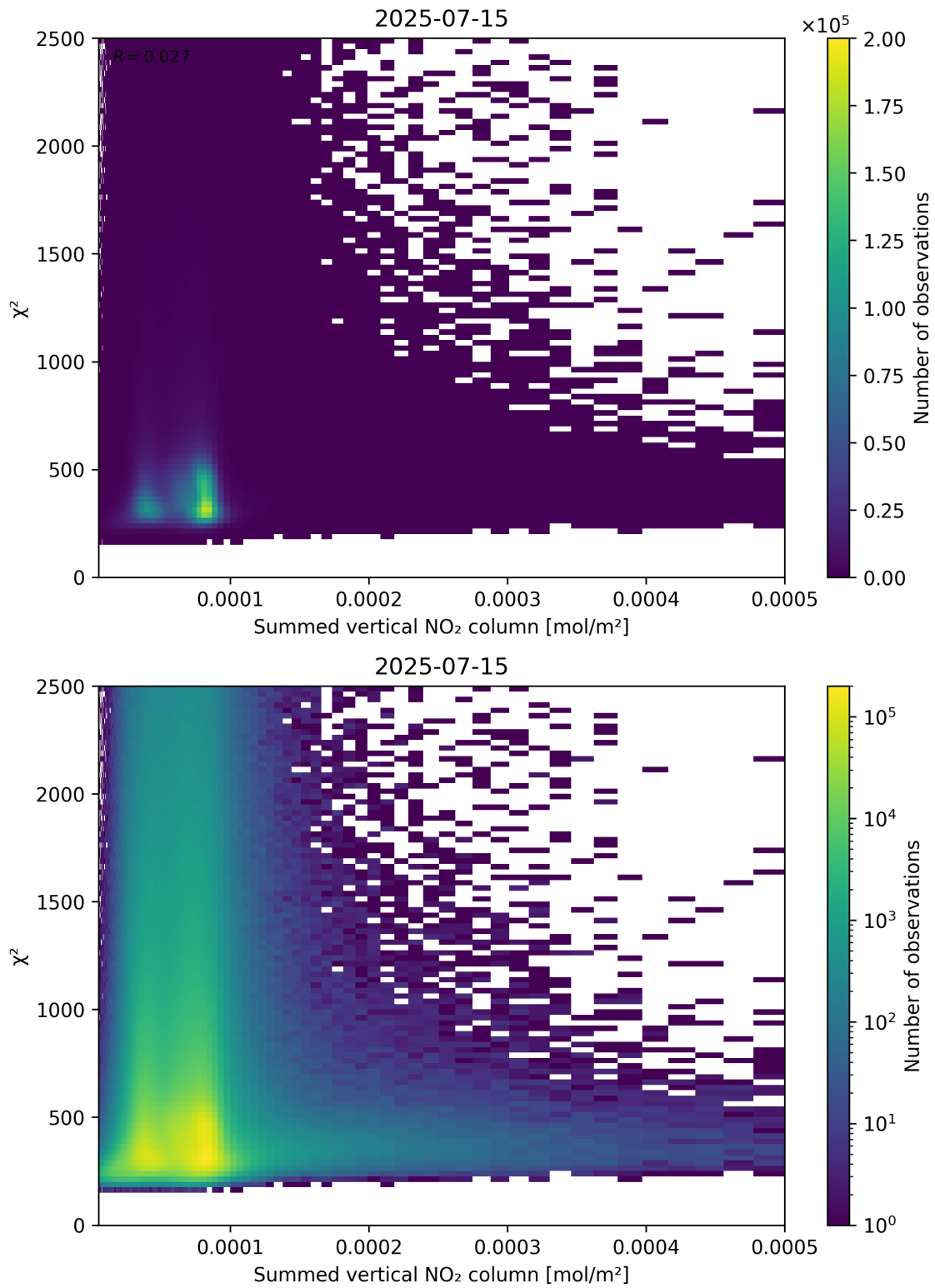
Figure 104: Scatter density plot of “Summed vertical NO 2 column” against “ \chi^2 ” for 2025-07-14 to 2025-07-16.
