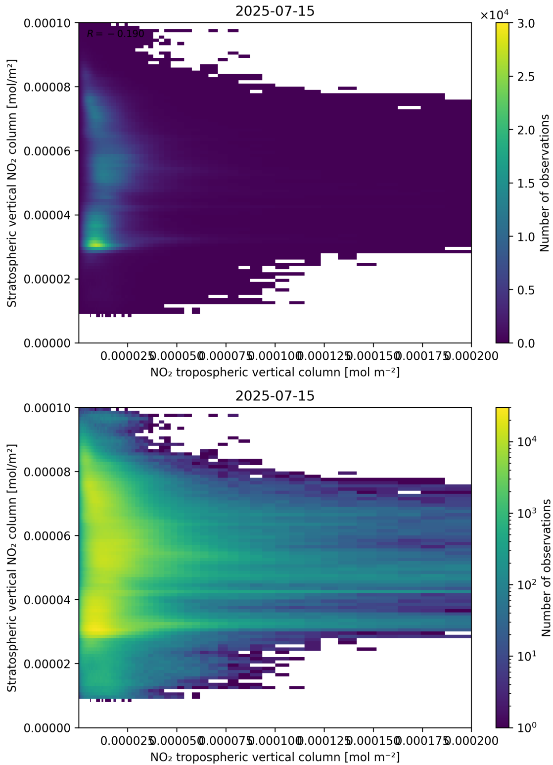
Figure 125: Scatter density plot of “NO 2 tropospheric vertical column” against “Stratospheric vertical NO 2 column” for 2025-07-14 to 2025-07-16.
