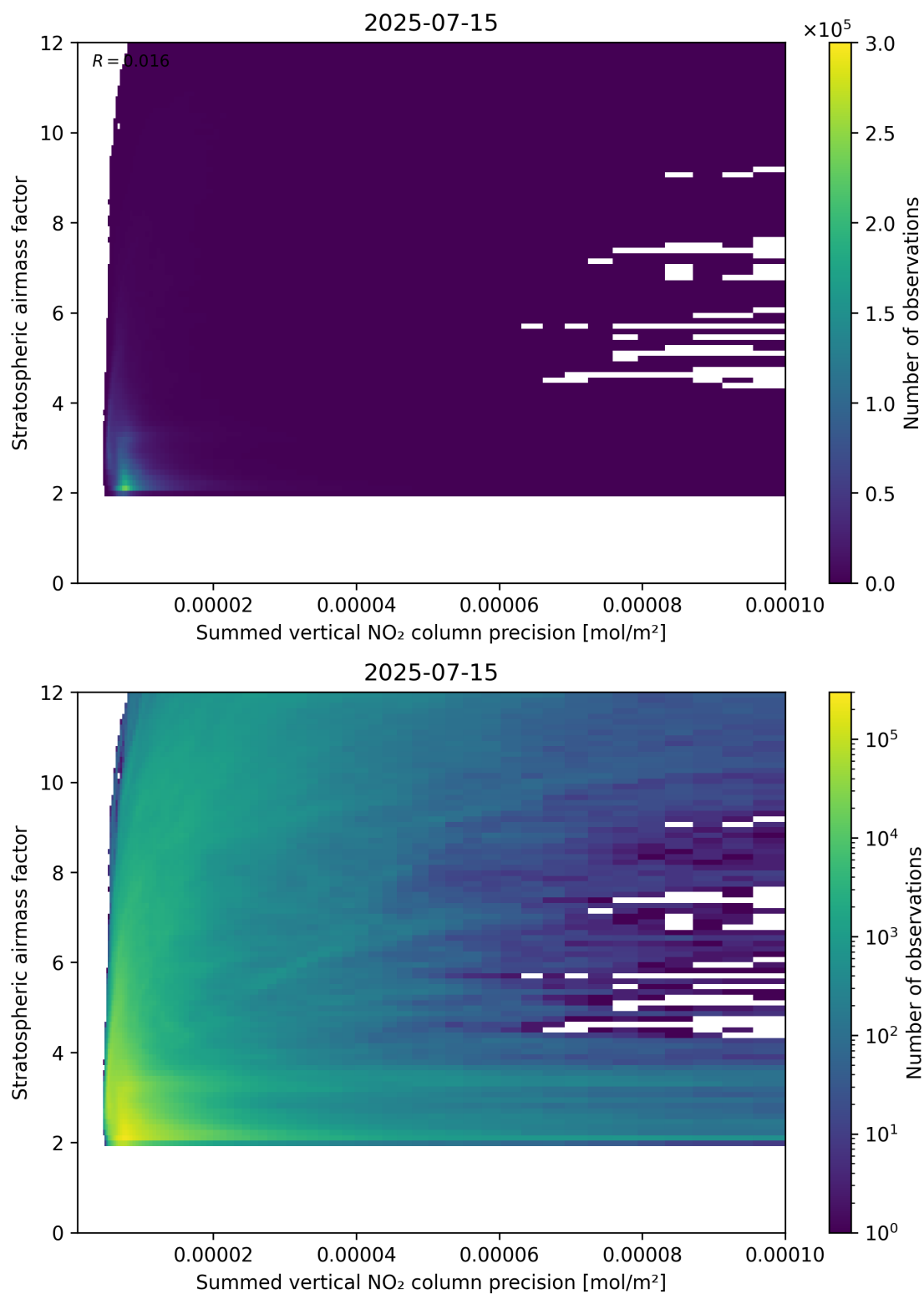
Figure 106: Scatter density plot of “Summed vertical NO 2 column precision” against “Stratospheric airmass factor” for 2025-07-14 to 2025-07-16.
