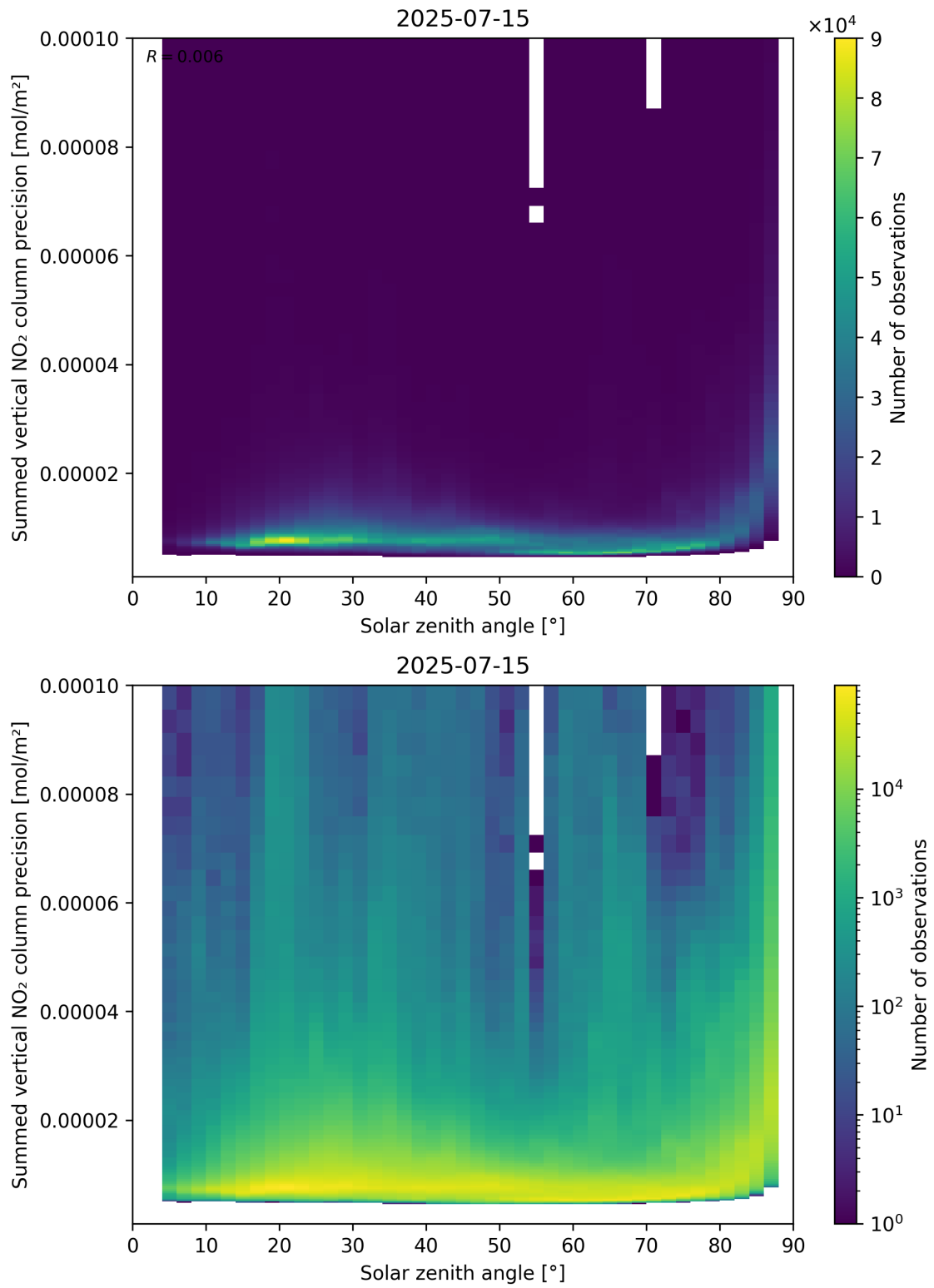
Figure 152: Scatter density plot of “Solar zenith angle” against “Summed vertical NO 2 column precision” for 2025-07-14 to 2025-07-16.
