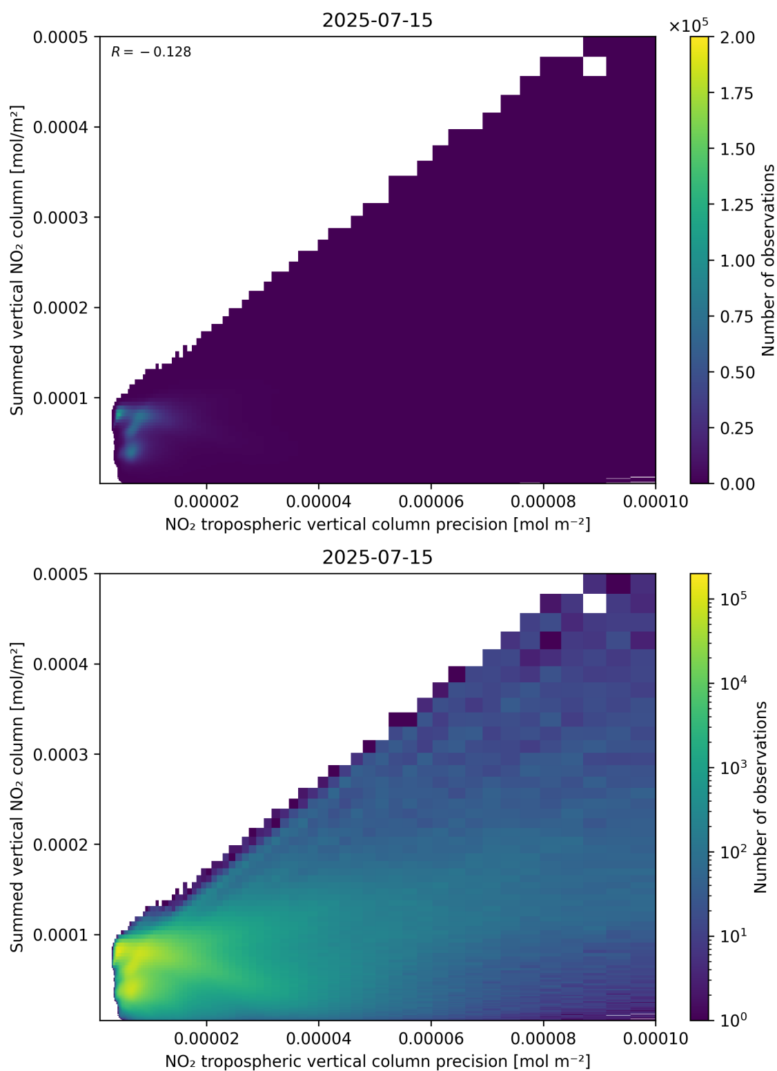
Figure 136: Scatter density plot of “NO 2 tropospheric vertical column precision” against “Summed vertical NO 2 column” for 2025-07-14 to 2025-07-16.
