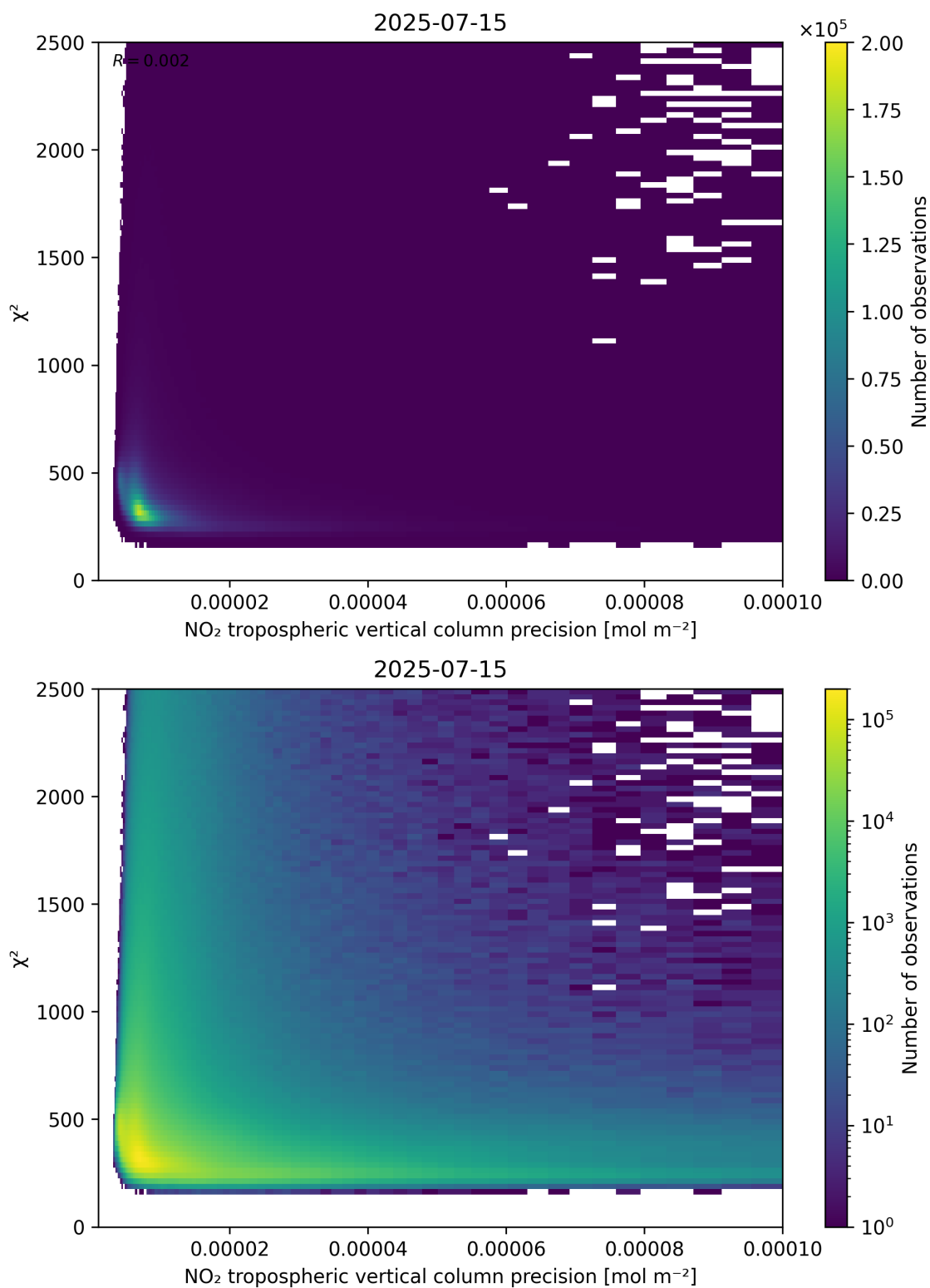
Figure 134: Scatter density plot of “NO 2 tropospheric vertical column precision” against “ \chi^2 ” for 2025-07-14 to 2025-07-16.
