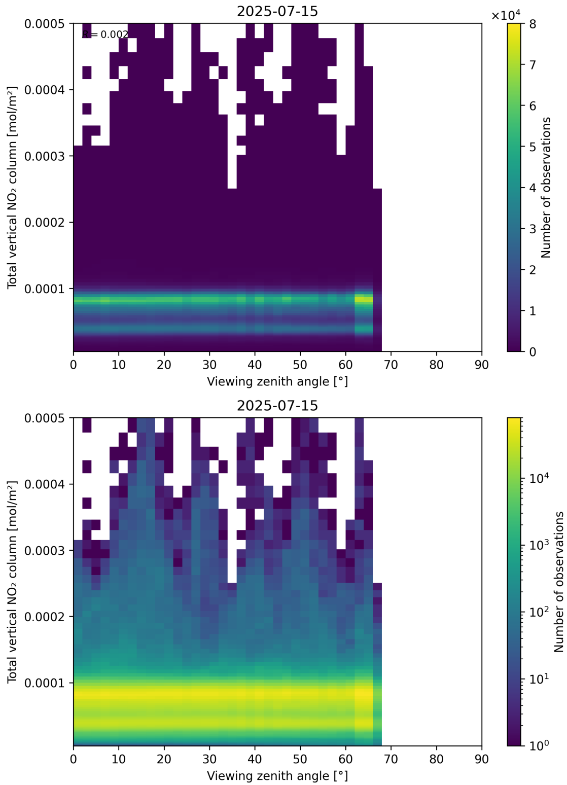
Figure 167: Scatter density plot of “Viewing zenith angle” against “Total vertical NO 2 column” for 2025-07-14 to 2025-07-16.
