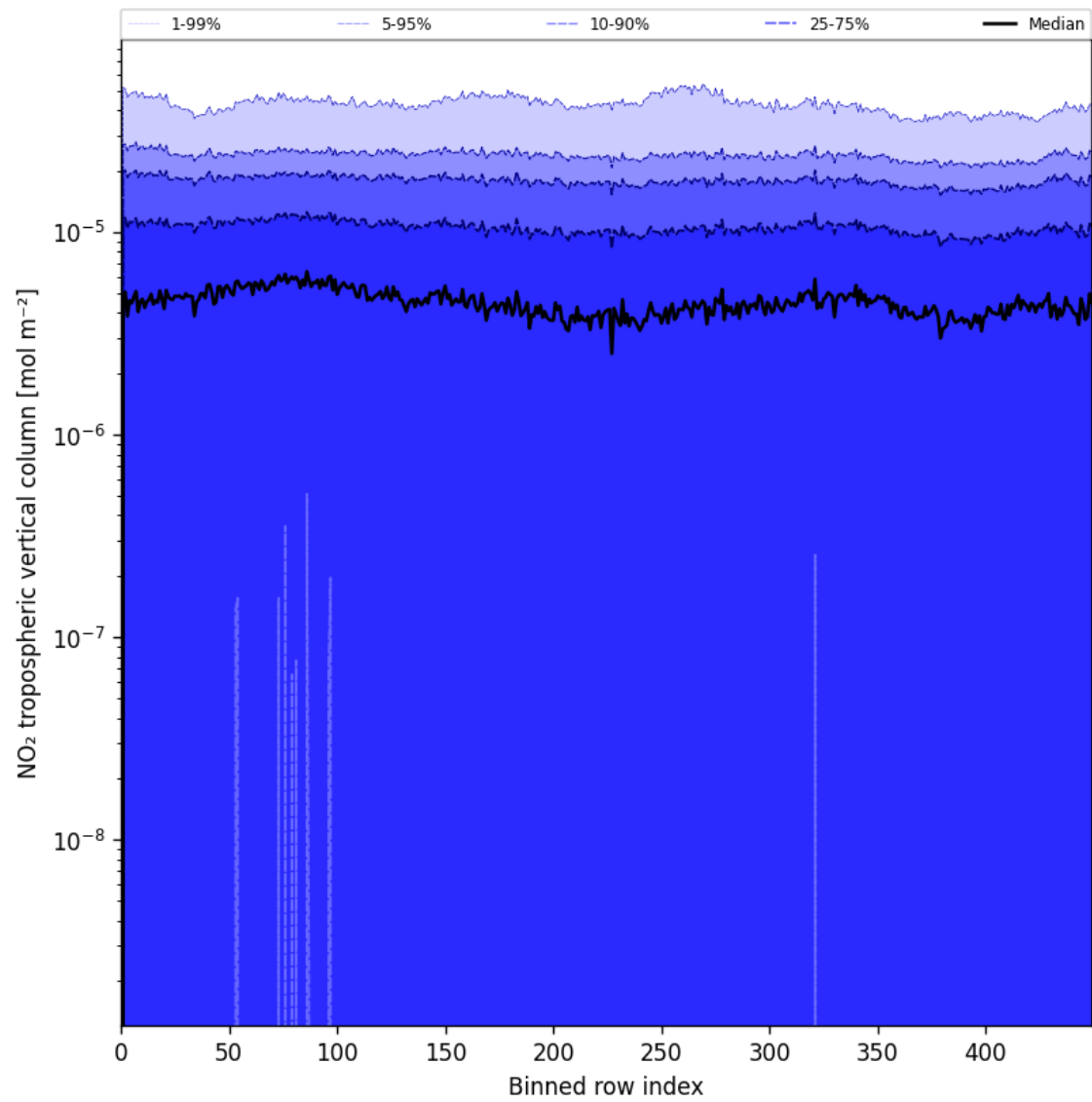
Figure 46: Along track statistics of “NO 2 tropospheric vertical column” for 2025-07-14 to 2025-07-16
