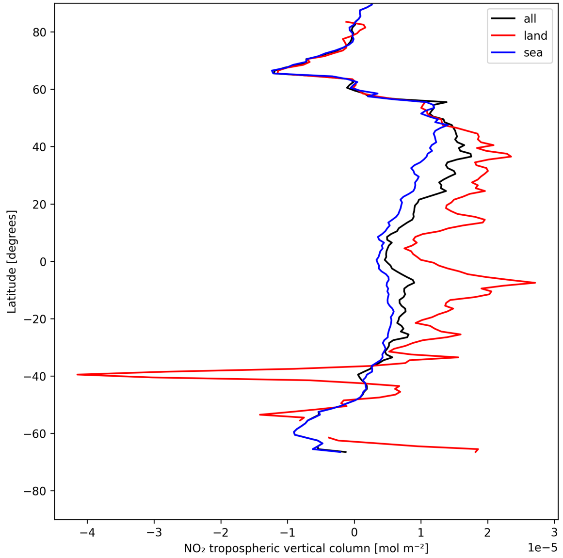
Figure 12: Zonal average of “NO 2 tropospheric vertical column” for 2025-07-14 to 2025-07-16.
