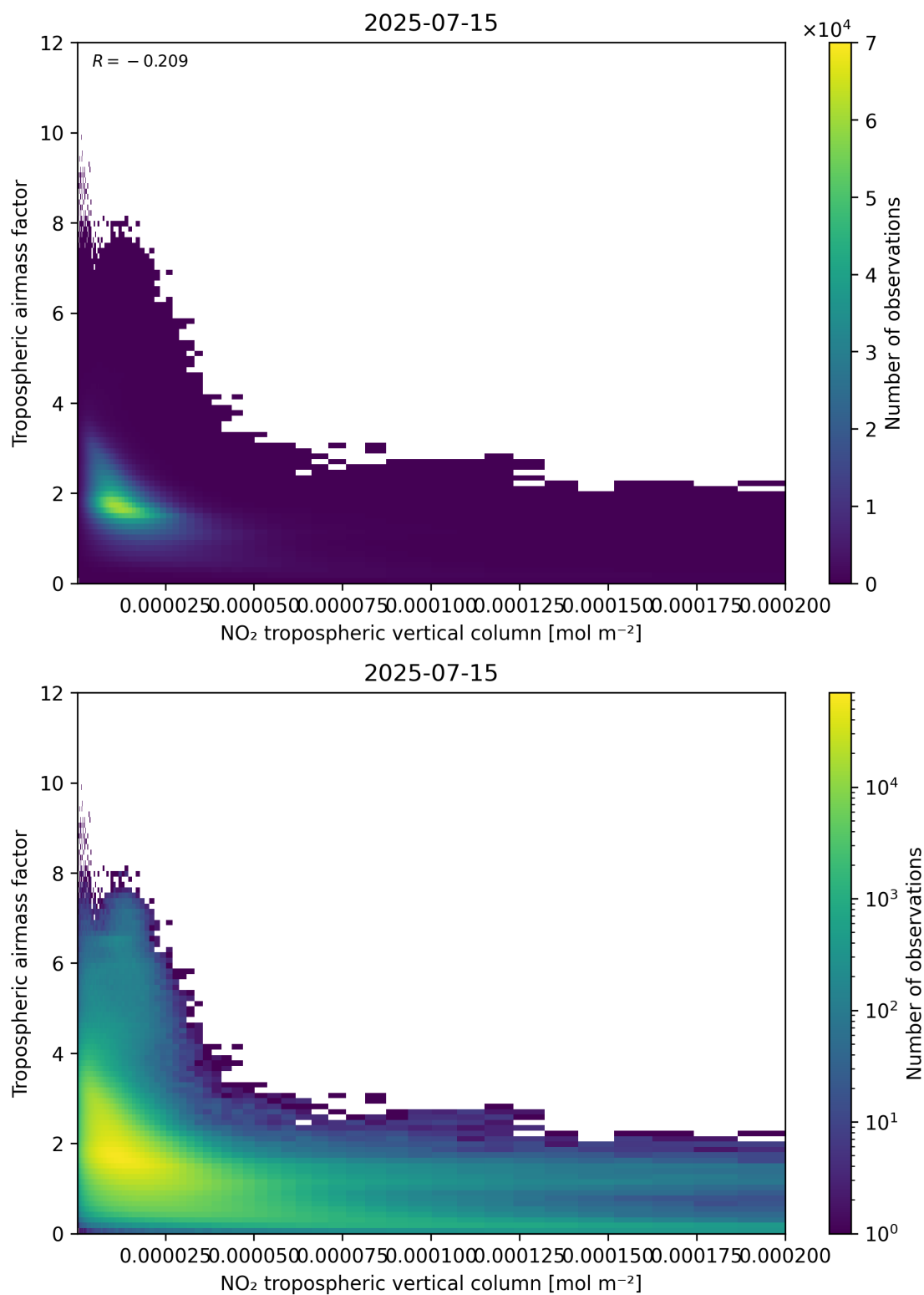
Figure 123: Scatter density plot of “NO 2 tropospheric vertical column” against “Tropospheric air mass factor” for 2025-07-14 to 2025-07-16.
