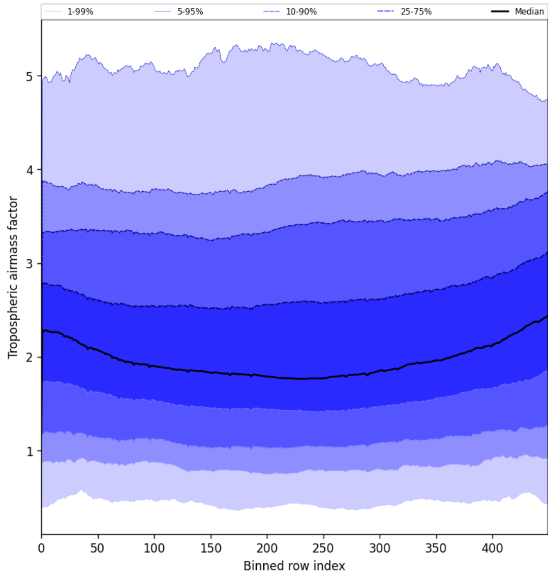
Figure 48: Along track statistics of “Tropospheric airmass factor” for 2025-07-14 to 2025-07-16
