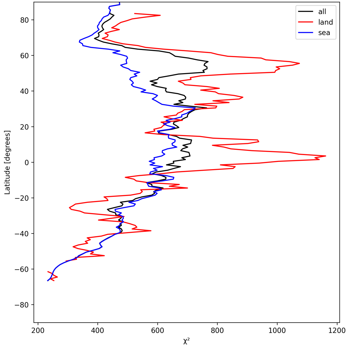
Figure 25: Zonal average of " \chi^2 " for 2025-07-14 to 2025-07-16.
