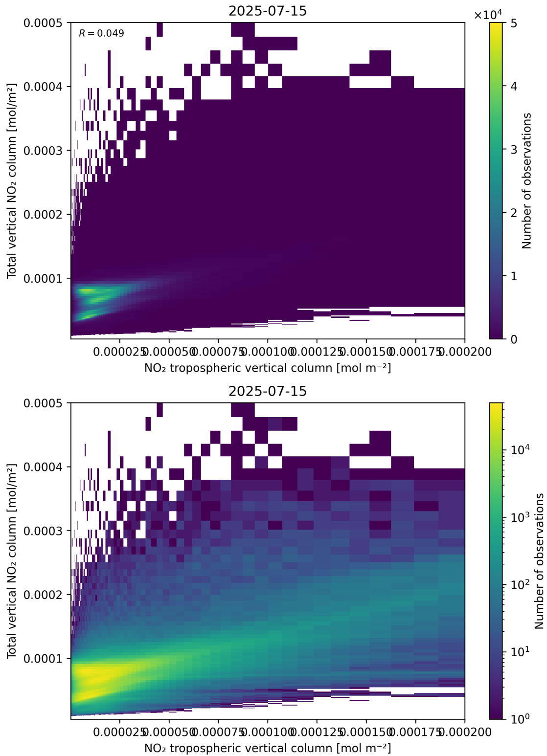
Figure 128: Scatter density plot of “NO 2 tropospheric vertical column” against “Total vertical NO 2 column” for 2025-07-14 to 2025-07-16.
