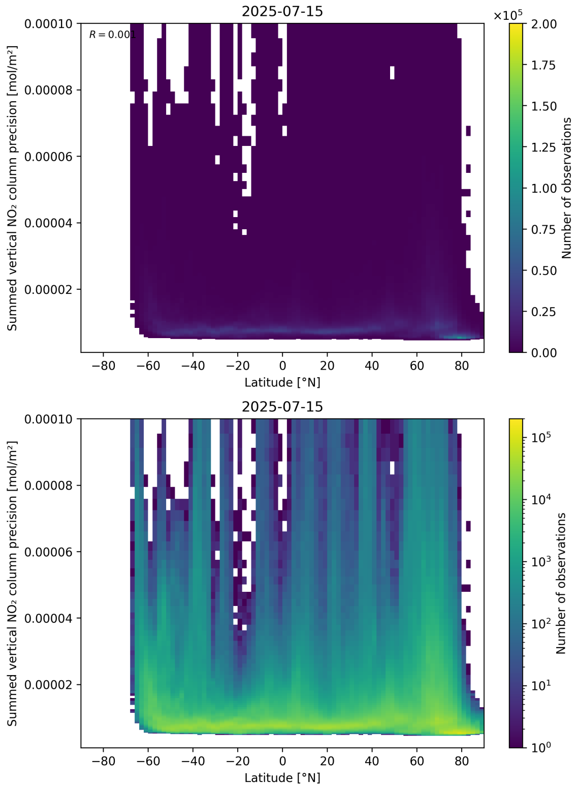
Figure 89: Scatter density plot of “Latitude” against “Summed vertical NO 2 column precision” for 2025-07-14 to 2025-07-16.
