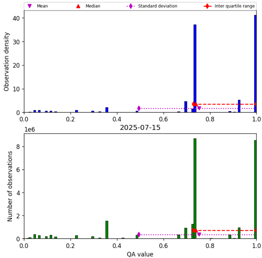
Figure 28: Histogram of “QA value” for 2025-07-14 to 2025-07-16
