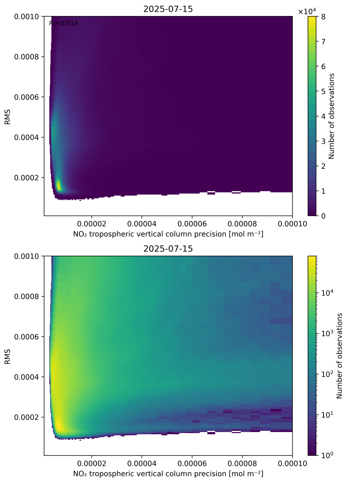
Figure 140: Scatter density plot of “NO 2 tropospheric vertical column precision” against “RMS” for 2025-07-14 to 2025-07-16.
