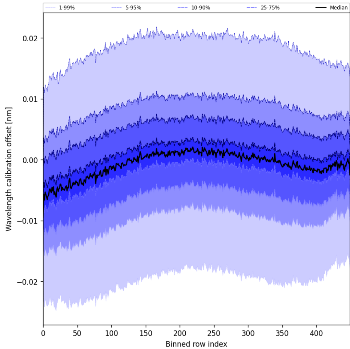
Figure 52: Along track statistics of “Wavelength calibration offset” for 2025-07-14 to 2025-07-16
