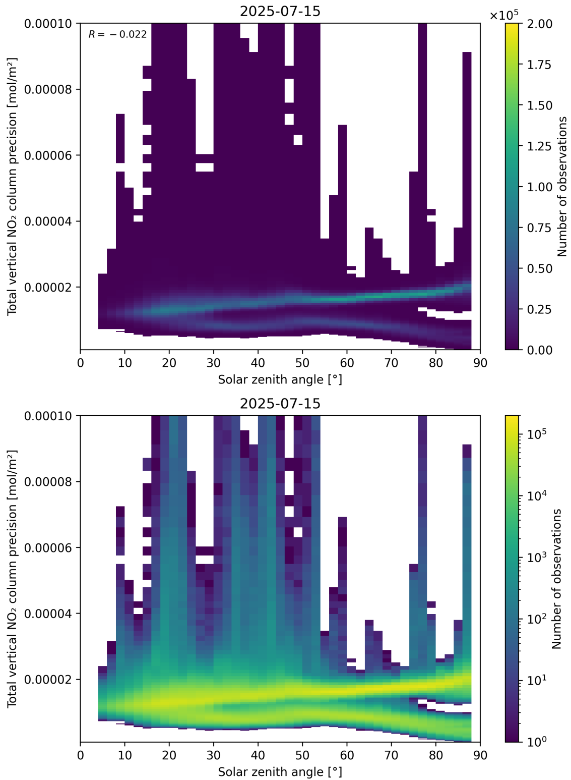
Figure 154: Scatter density plot of “Solar zenith angle” against “Total vertical NO 2 column precision” for 2025-07-14 to 2025-07-16.
