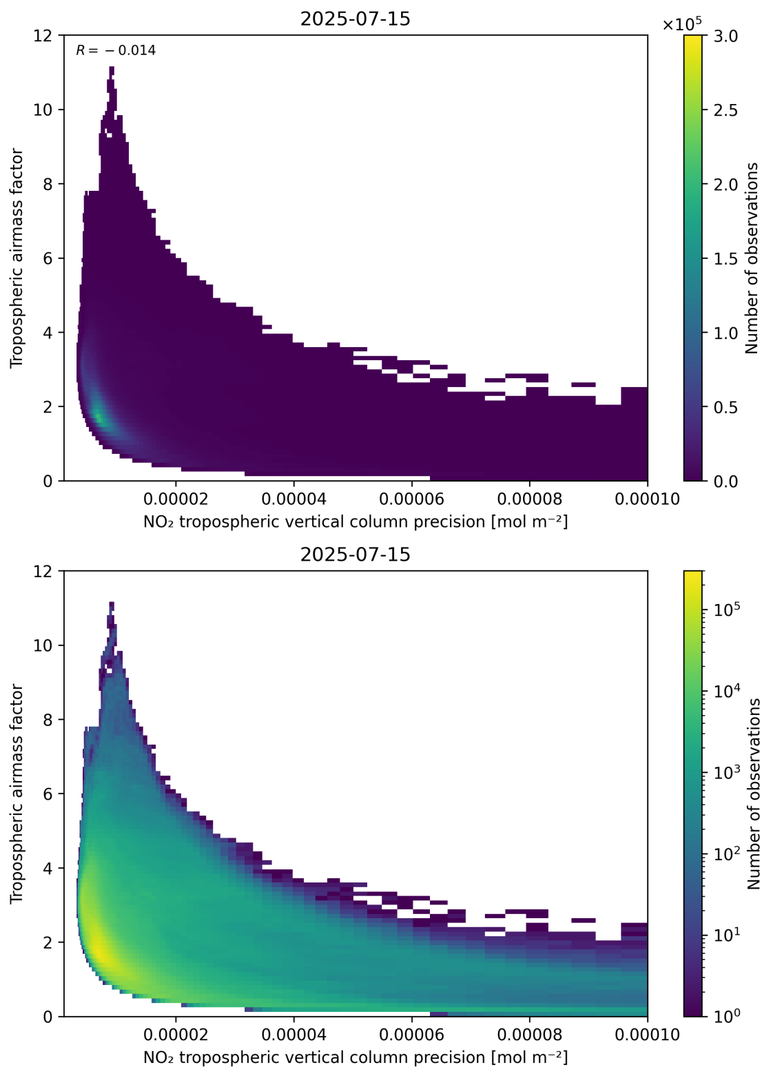
Figure 133: Scatter density plot of “NO 2 tropospheric vertical column precision” against “Tropospheric air mass factor” for 2025-07-14 to 2025-07-16.
