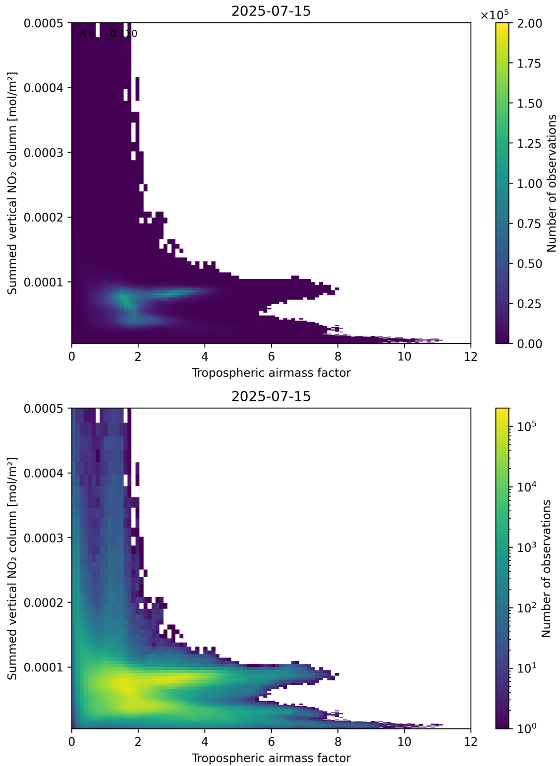
Figure 75: Scatter density plot of “Tropospheric air mass factor” against “Summed vertical NO 2 column” for 2025-07-14 to 2025-07-16.
