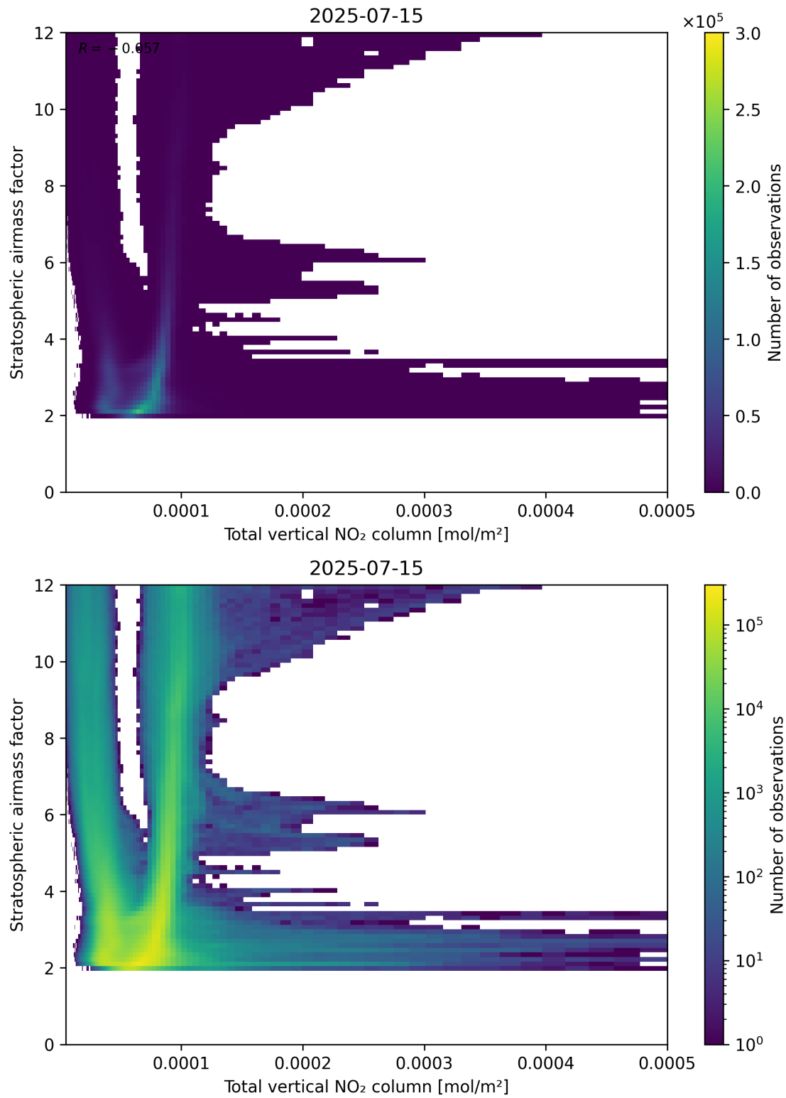
Figure 110: Scatter density plot of “Total vertical NO 2 column” against “Stratospheric airmass factor” for 2025-07-14 to 2025-07-16.
