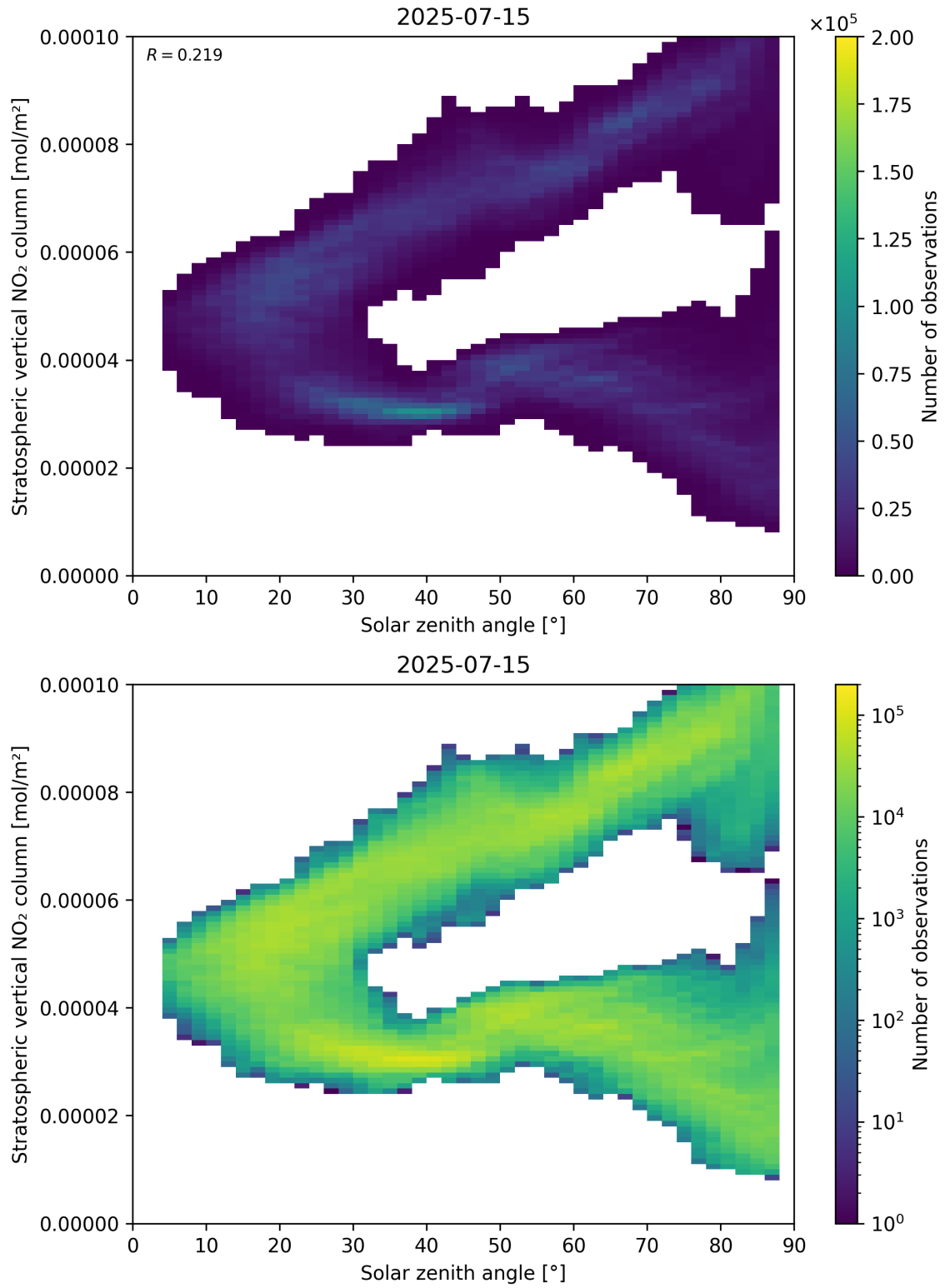
Figure 150: Scatter density plot of “Solar zenith angle” against “Stratospheric vertical NO 2 column” for 2025-07-14 to 2025-07-16.
