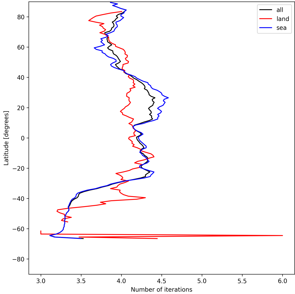
Figure 17: Zonal average of “Number of iterations” for 2025-07-14 to 2025-07-16.
