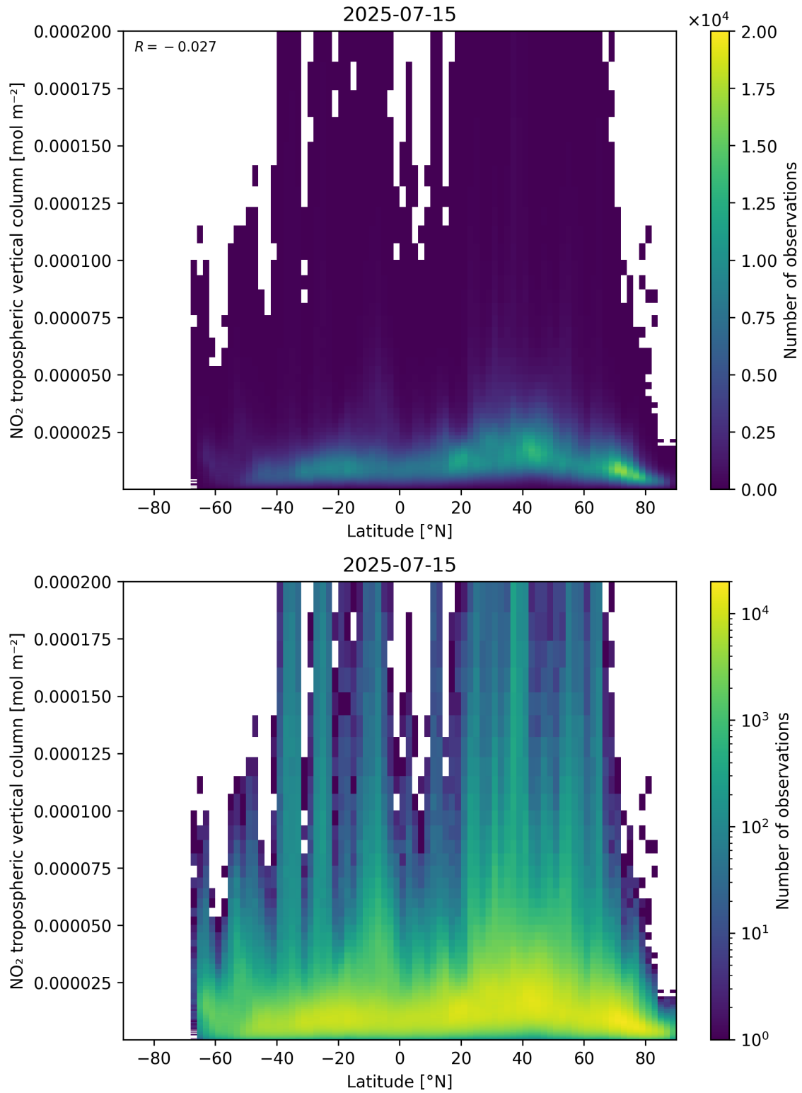
Figure 92: Scatter density plot of “Latitude” against “NO 2 tropospheric vertical column” for 2025-07-14 to 2025-07-16.
