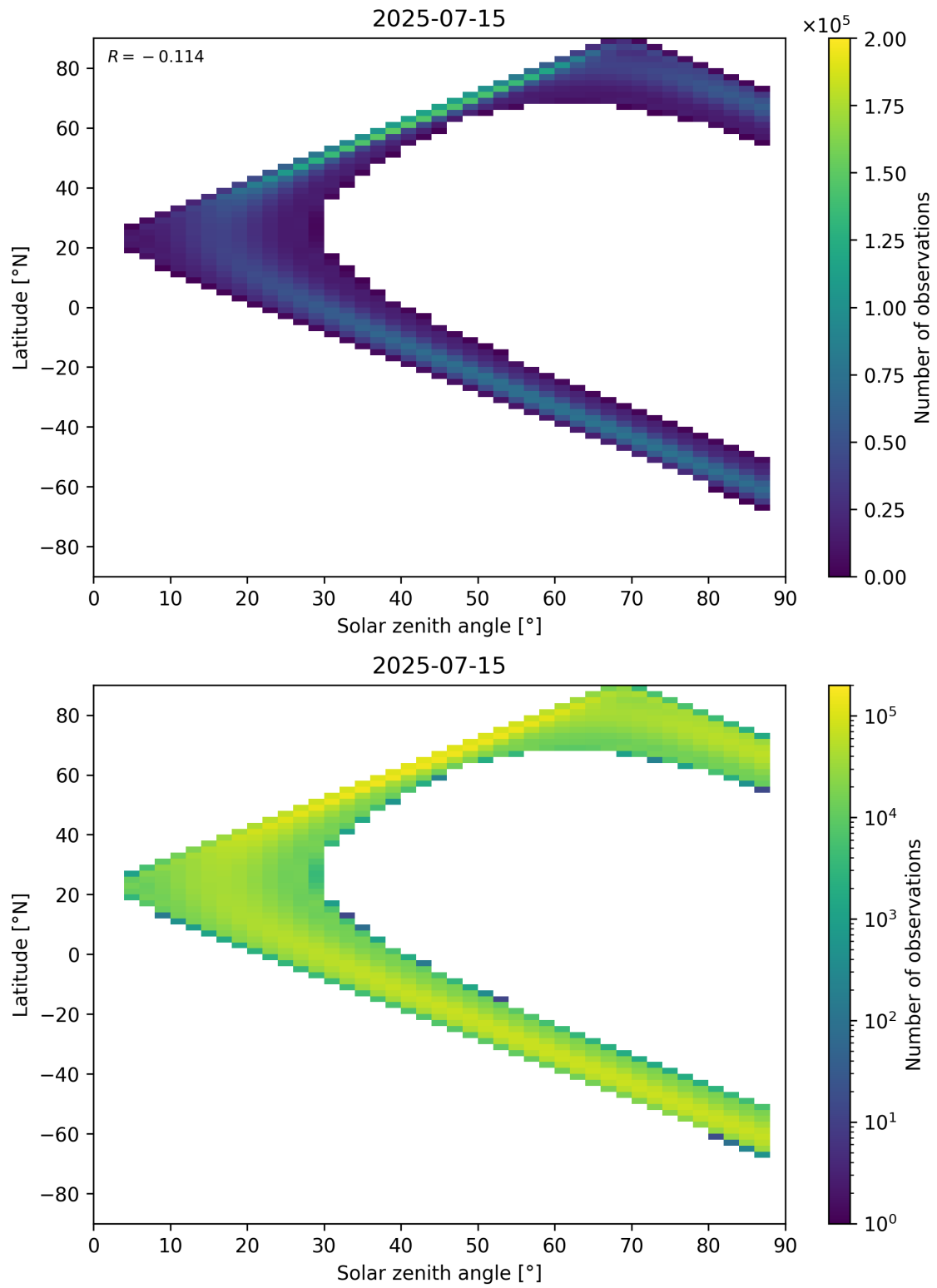
Figure 149: Scatter density plot of “Solar zenith angle” against “Latitude” for 2025-07-14 to 2025-07-16.
