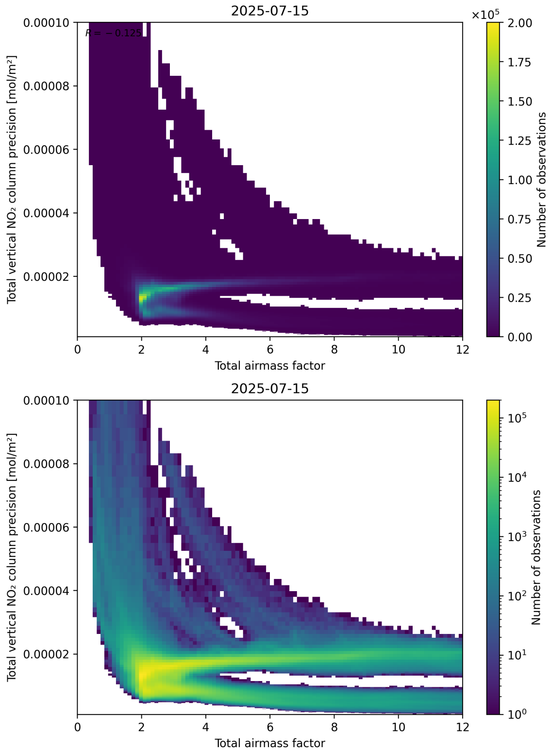
Figure 68: Scatter density plot of “Total airmass factor” against “Total vertical NO 2 column precision” for 2025-07-14 to 2025-07-16.
