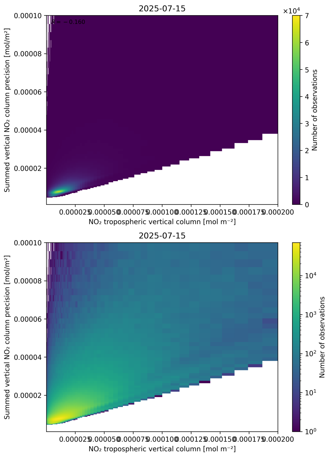
Figure 127: Scatter density plot of “NO 2 tropospheric vertical column” against “Summed vertical NO 2 column precision” for 2025-07-14 to 2025-07-16.
