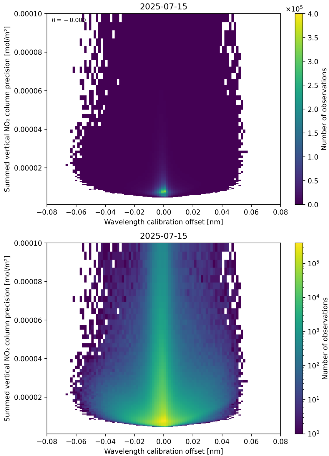
Figure 178: Scatter density plot of “Wavelength calibration offset” against “Summed vertical NO 2 column precision” for 2025-07-14 to 2025-07-16.
