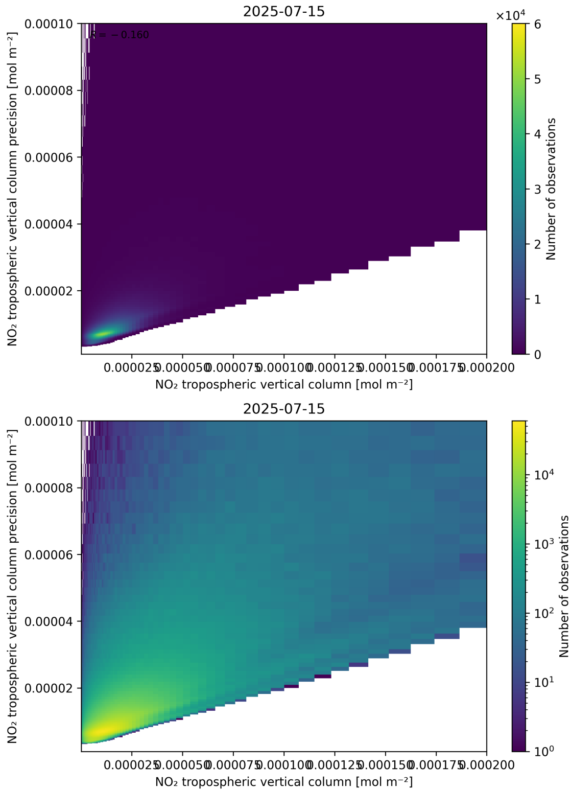
Figure 130: Scatter density plot of “NO 2 tropospheric vertical column” against “NO 2 tropospheric vertical column precision” for 2025-07-14 to 2025-07-16.
