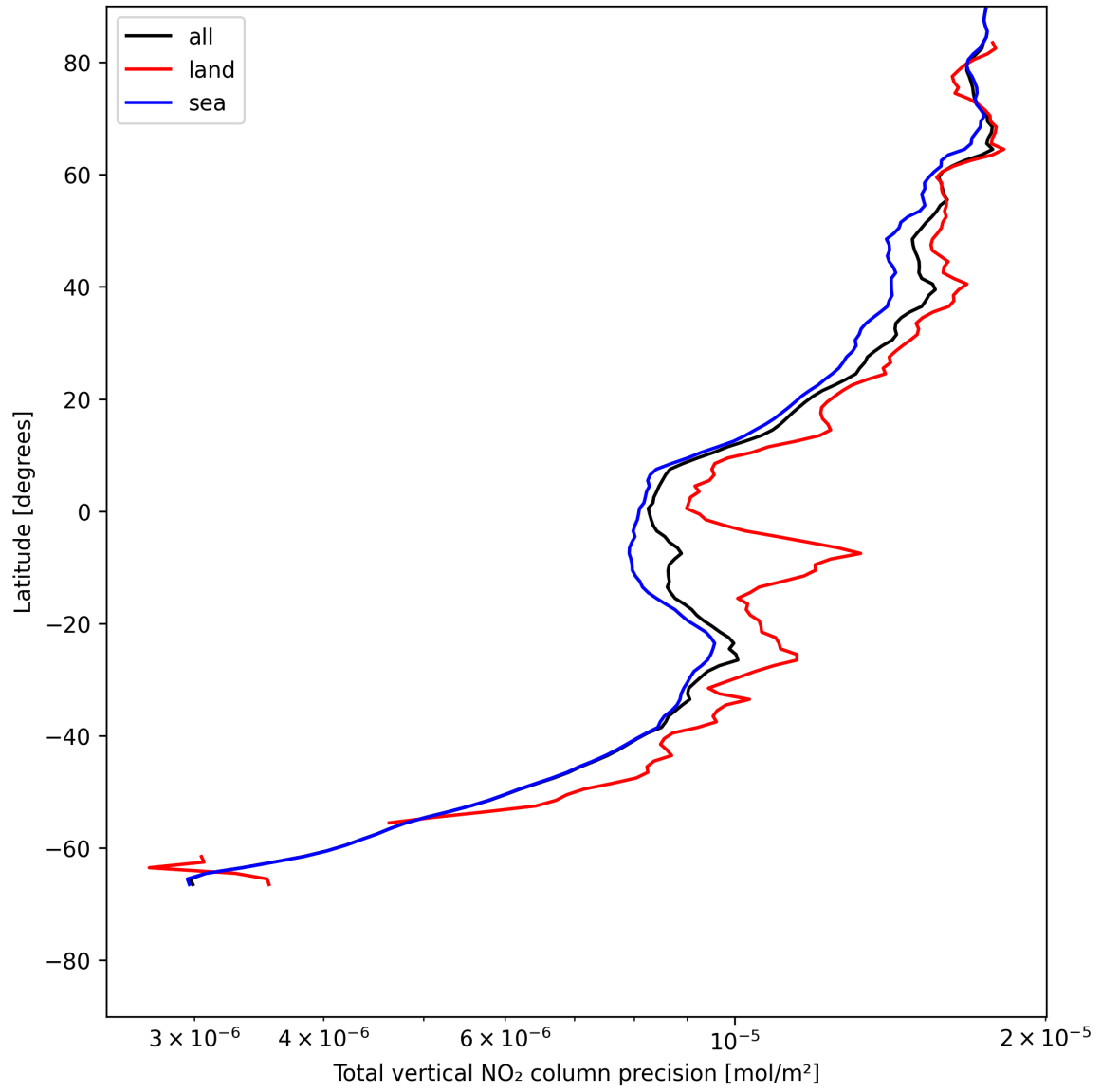
Figure 22: Zonal average of “Total vertical NO 2 column precision” for 2025-07-14 to 2025-07-16.
