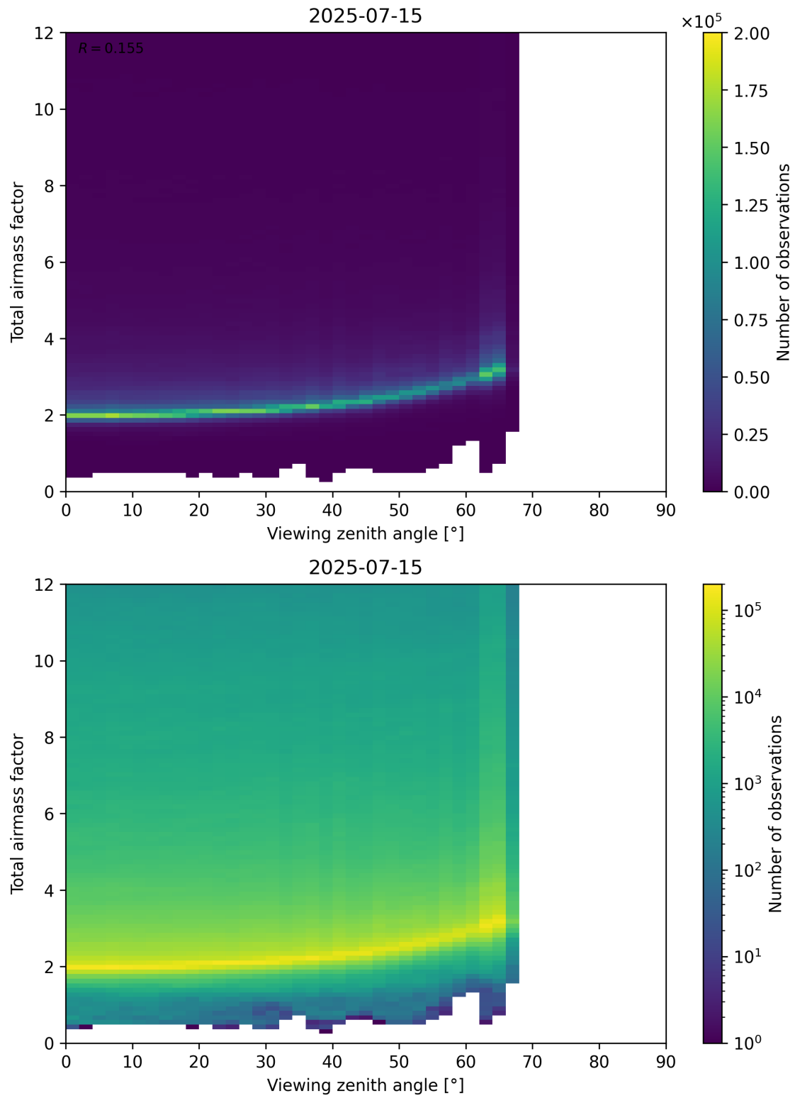
Figure 160: Scatter density plot of “Viewing zenith angle” against “Total airmass factor” for 2025-07-14 to 2025-07-16.
