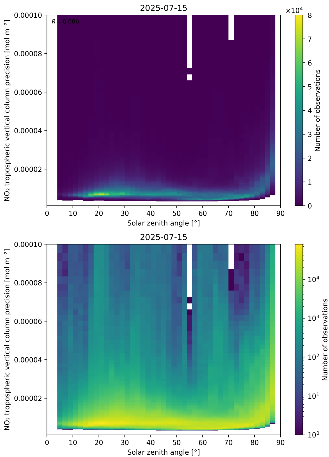
Figure 156: Scatter density plot of “Solar zenith angle” against “NO 2 tropospheric vertical column precision” for 2025-07-14 to 2025-07-16.
