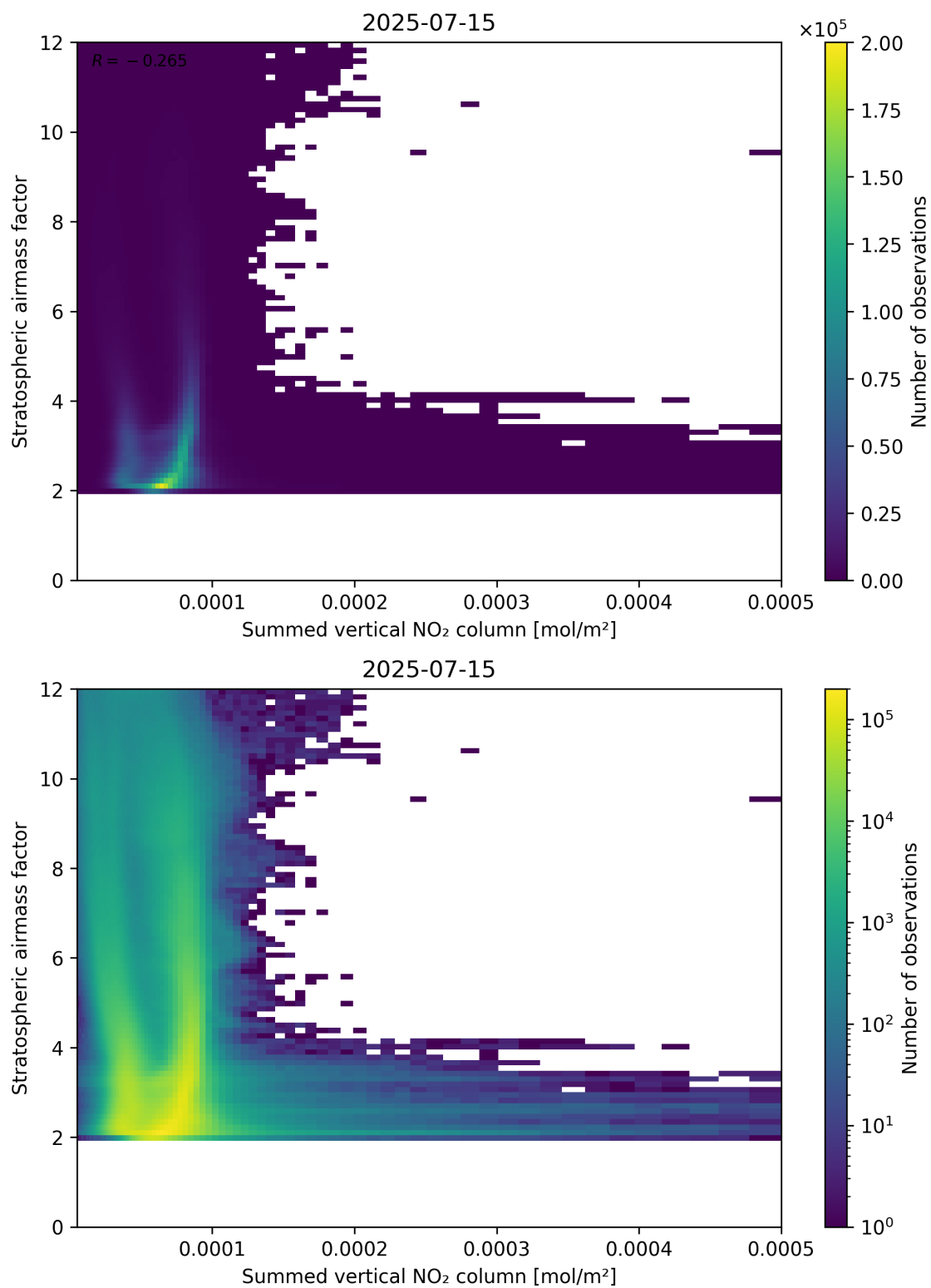
Figure 103: Scatter density plot of “Summed vertical NO 2 column” against “Stratospheric air mass factor” for 2025-07-14 to 2025-07-16.
