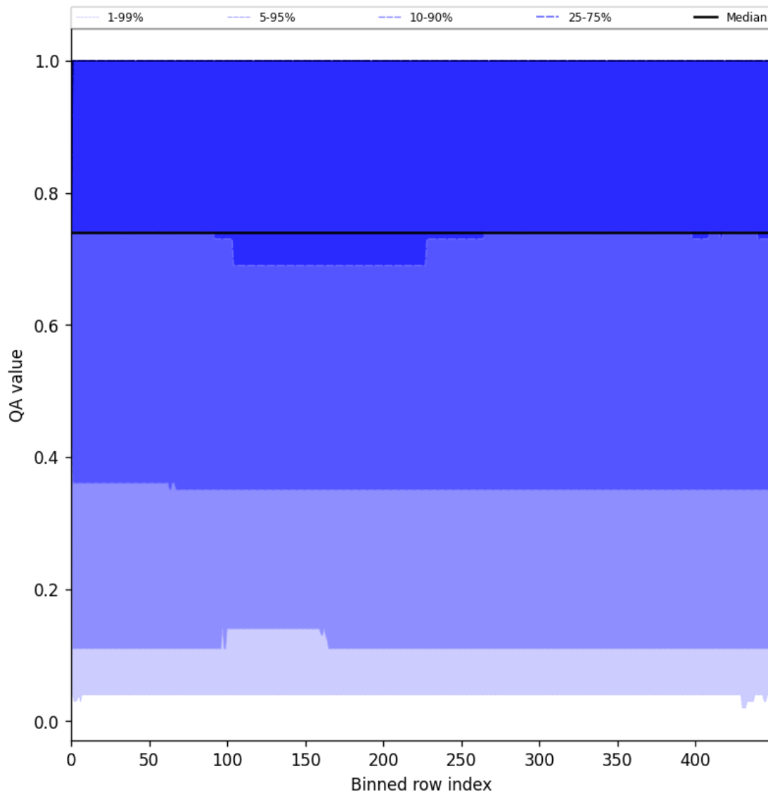
Figure 45: Along track statistics of “QA value” for 2025-07-14 to 2025-07-16
