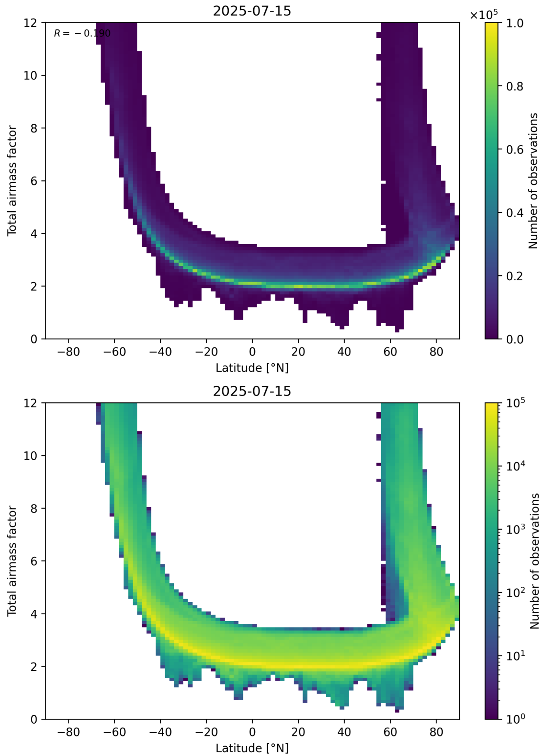
Figure 84: Scatter density plot of “Latitude” against “Total airmass factor” for 2025-07-14 to 2025-07-16.
