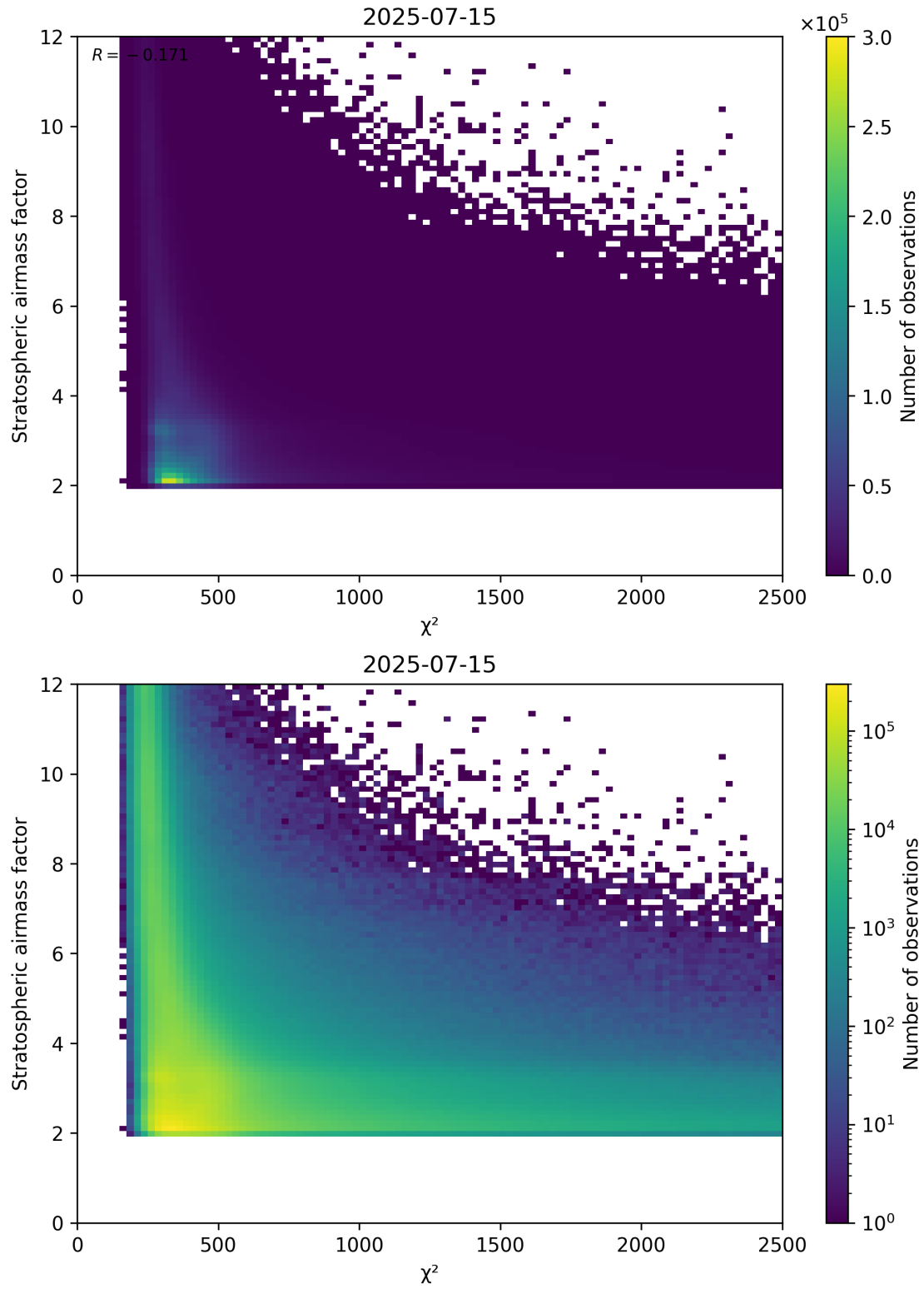
Figure 81: Scatter density plot of “ \chi^2 ” against “Stratospheric airmass factor” for 2025-07-14 to 2025-07-16.
