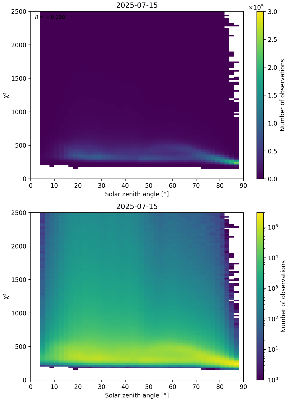
Figure 148: Scatter density plot of “Solar zenith angle” against “ \chi^2 ” for 2025-07-14 to 2025-07-16.
