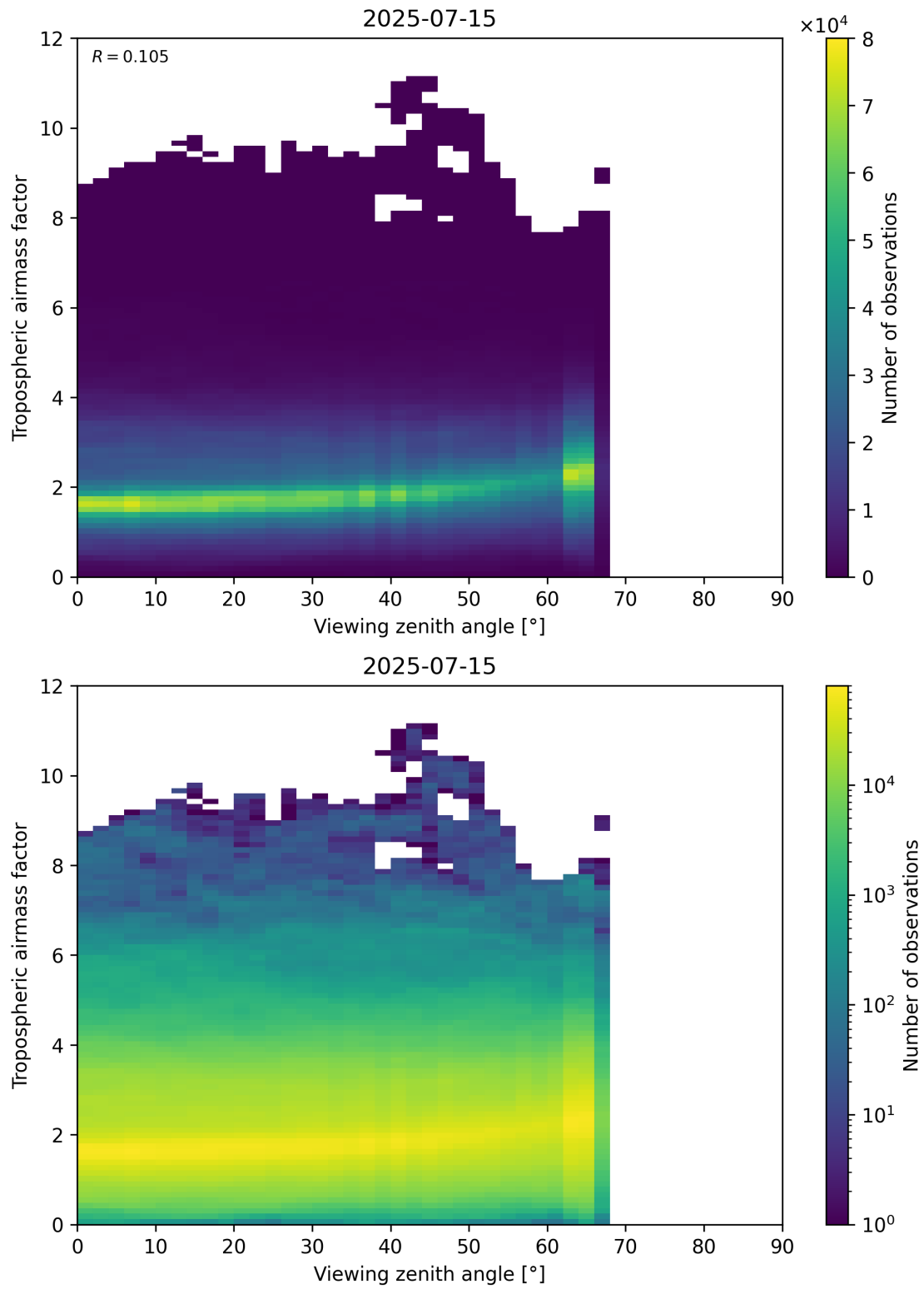
Figure 161: Scatter density plot of “Viewing zenith angle” against “Tropospheric airmass factor” for 2025-07-14 to 2025-07-16.
