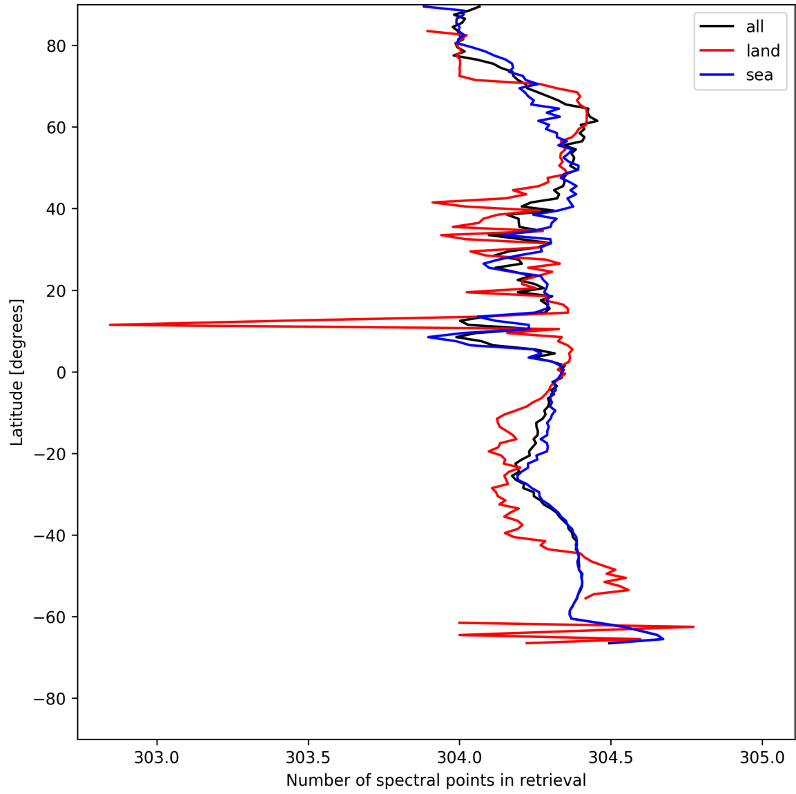
Figure 16: Zonal average of “Number of spectral points in retrieval” for 2025-07-14 to 2025-07-16.
