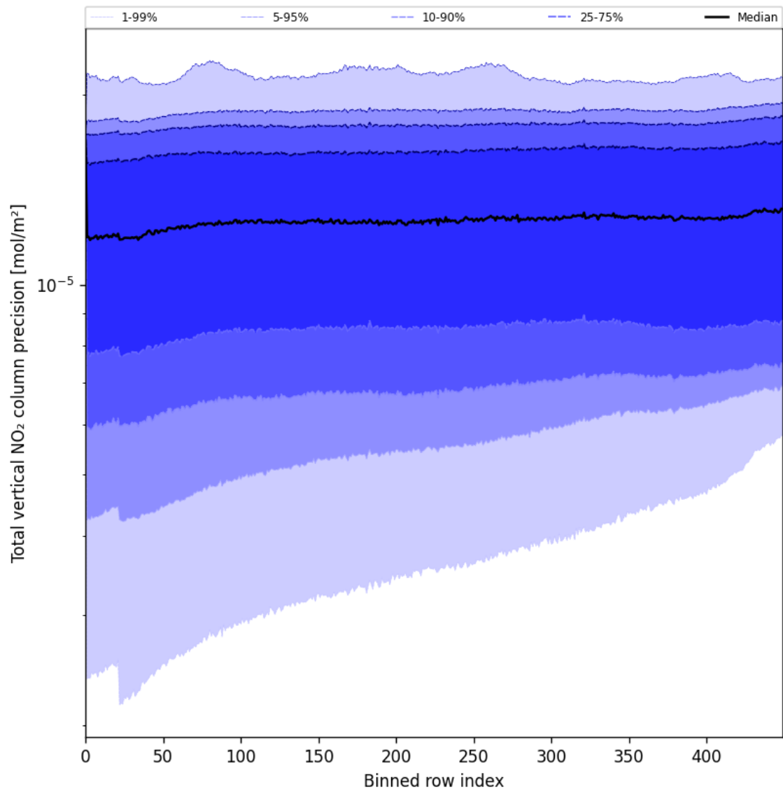
Figure 56: Along track statistics of “Total vertical NO 2 column precision” for 2025-07-14 to 2025-07-16
