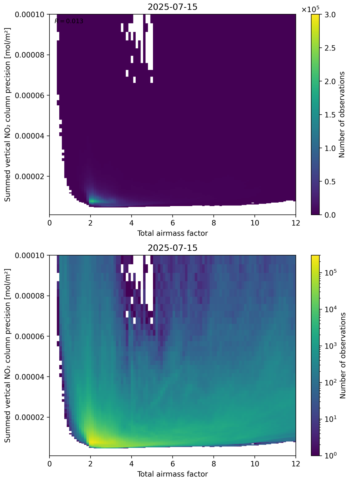
Figure 66: Scatter density plot of “Total airmass factor” against “Summed vertical NO 2 column precision” for 2025-07-14 to 2025-07-16.
