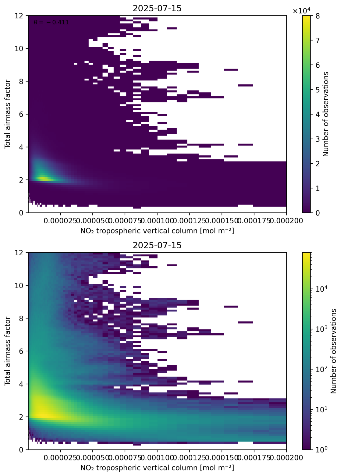
Figure 122: Scatter density plot of “NO 2 tropospheric vertical column” against “Total airmass factor” for 2025-07-14 to 2025-07-16.
