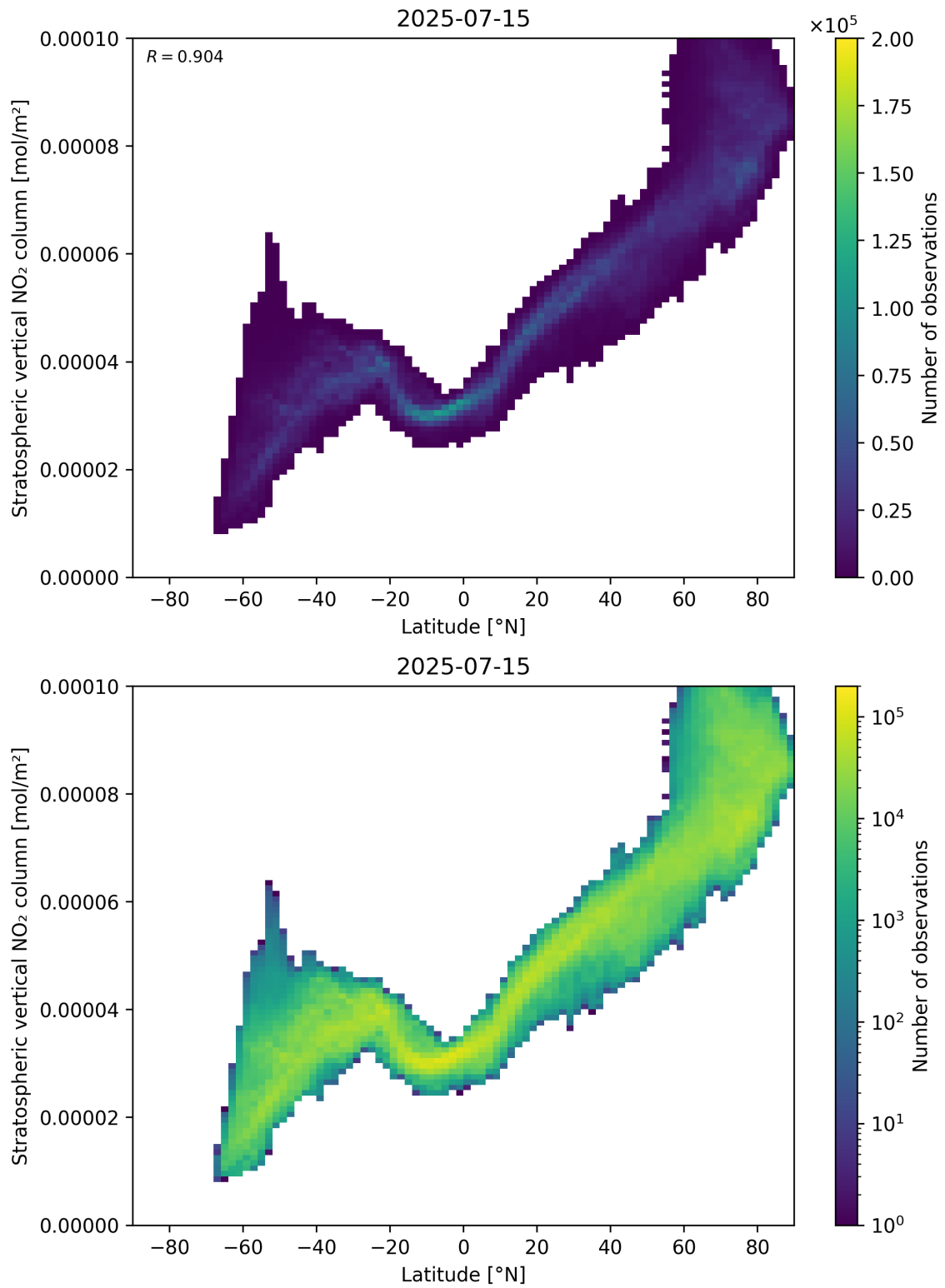
Figure 87: Scatter density plot of “Latitude” against “Stratospheric vertical \text{NO}_2 column” for 2025-07-14 to 2025-07-16.
