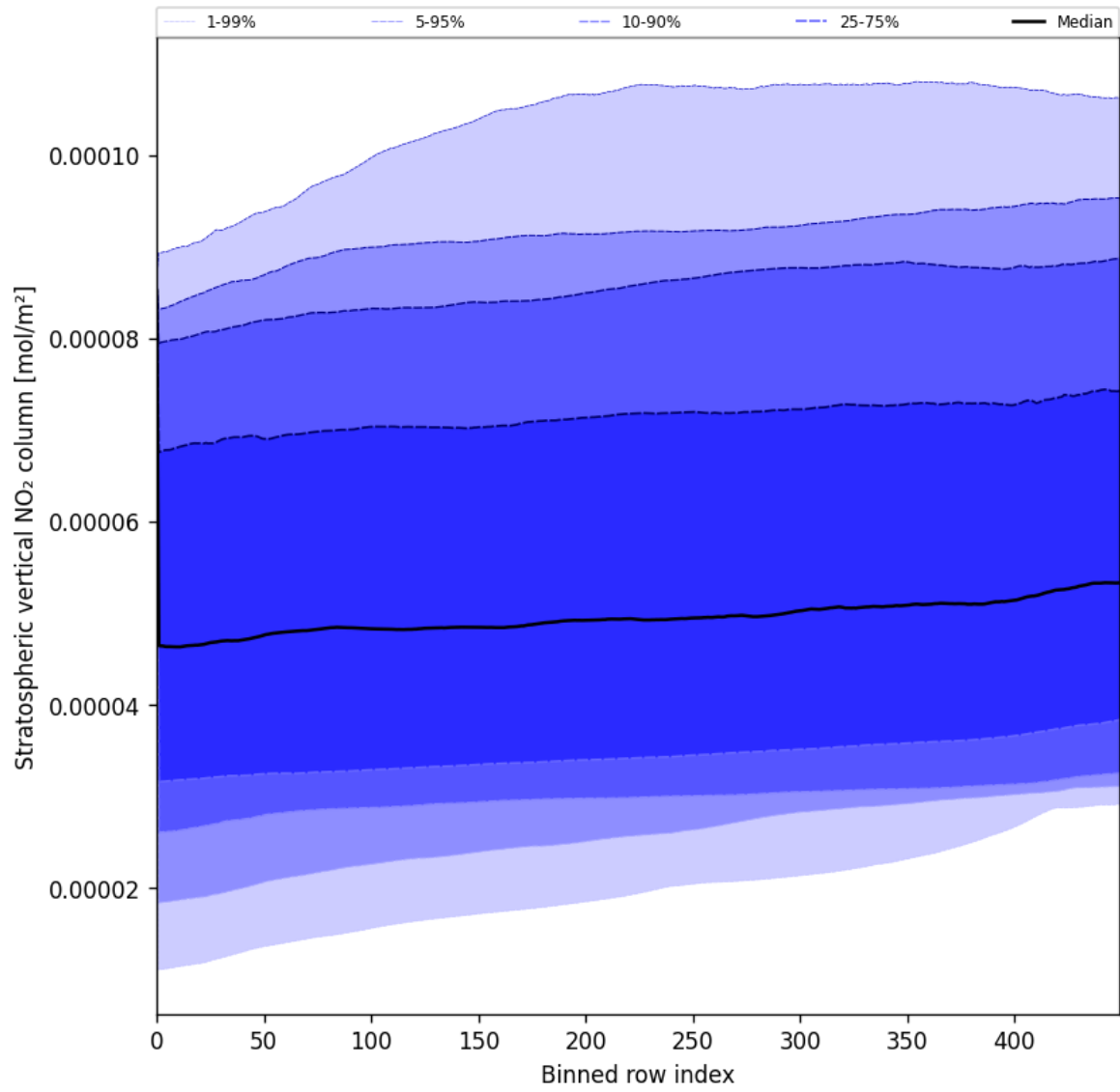
Figure 53: Along track statistics of “Stratospheric vertical NO 2 column” for 2025-07-14 to 2025-07-16
