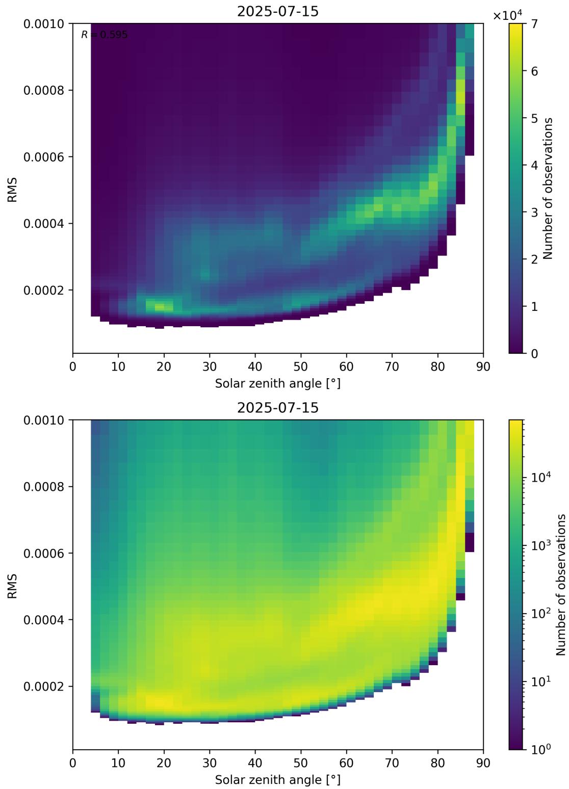
Figure 157: Scatter density plot of “Solar zenith angle” against “RMS” for 2025-07-14 to 2025-07-16.
