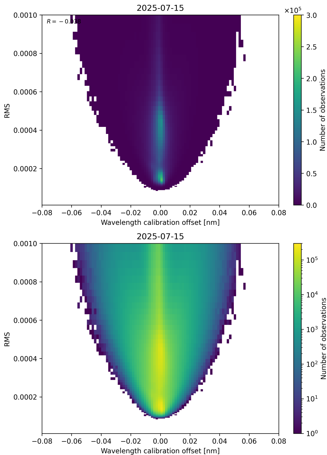
Figure 181: Scatter density plot of “Wavelength calibration offset” against “RMS” for 2025-07-14 to 2025-07-16.
