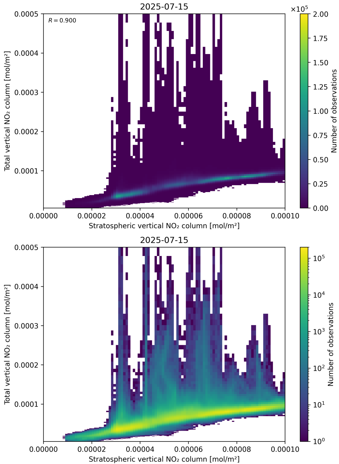
Figure 100: Scatter density plot of “Stratospheric vertical NO 2 column” against “Total vertical NO 2 column” for 2025-07-14 to 2025-07-16.
