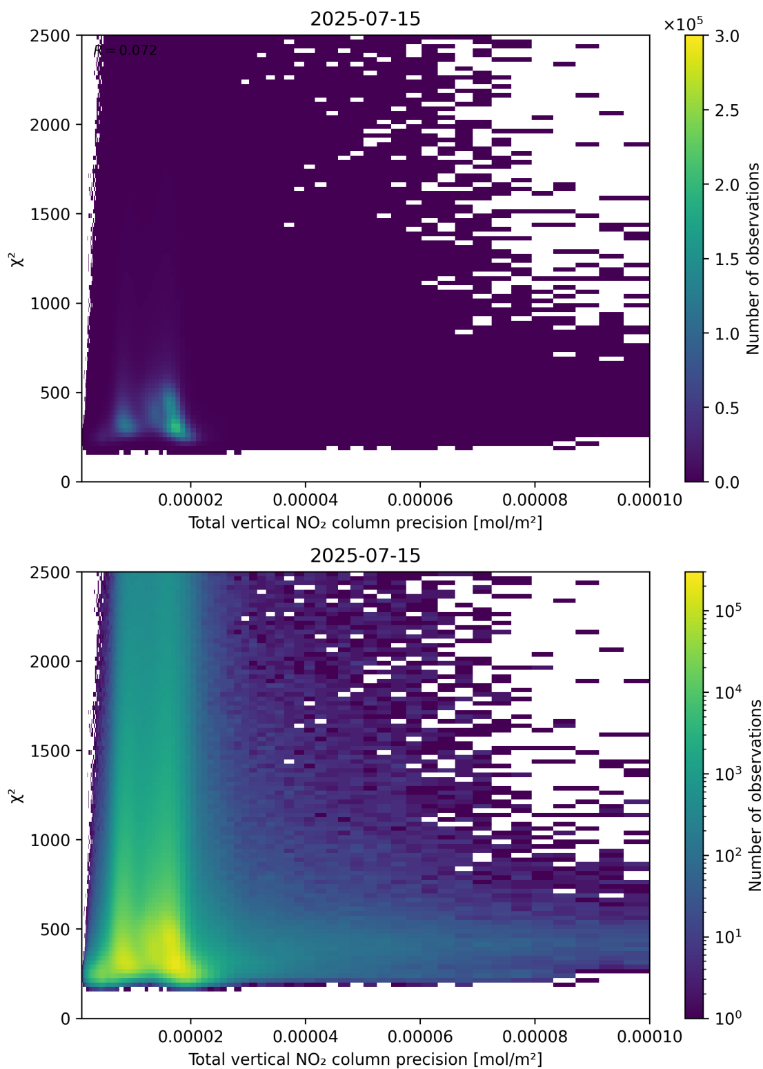
Figure 116: Scatter density plot of “Total vertical NO 2 column precision” against “ \chi^2 ” for 2025-07-14 to 2025-07-16.
