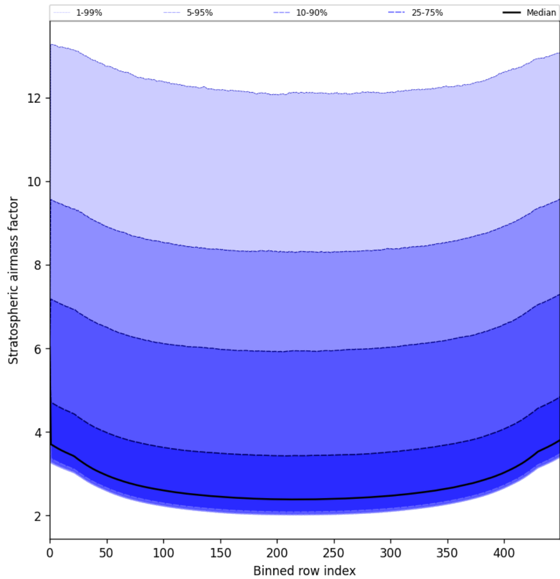
Figure 61: Along track statistics of “Stratospheric airmass factor” for 2025-07-14 to 2025-07-16
