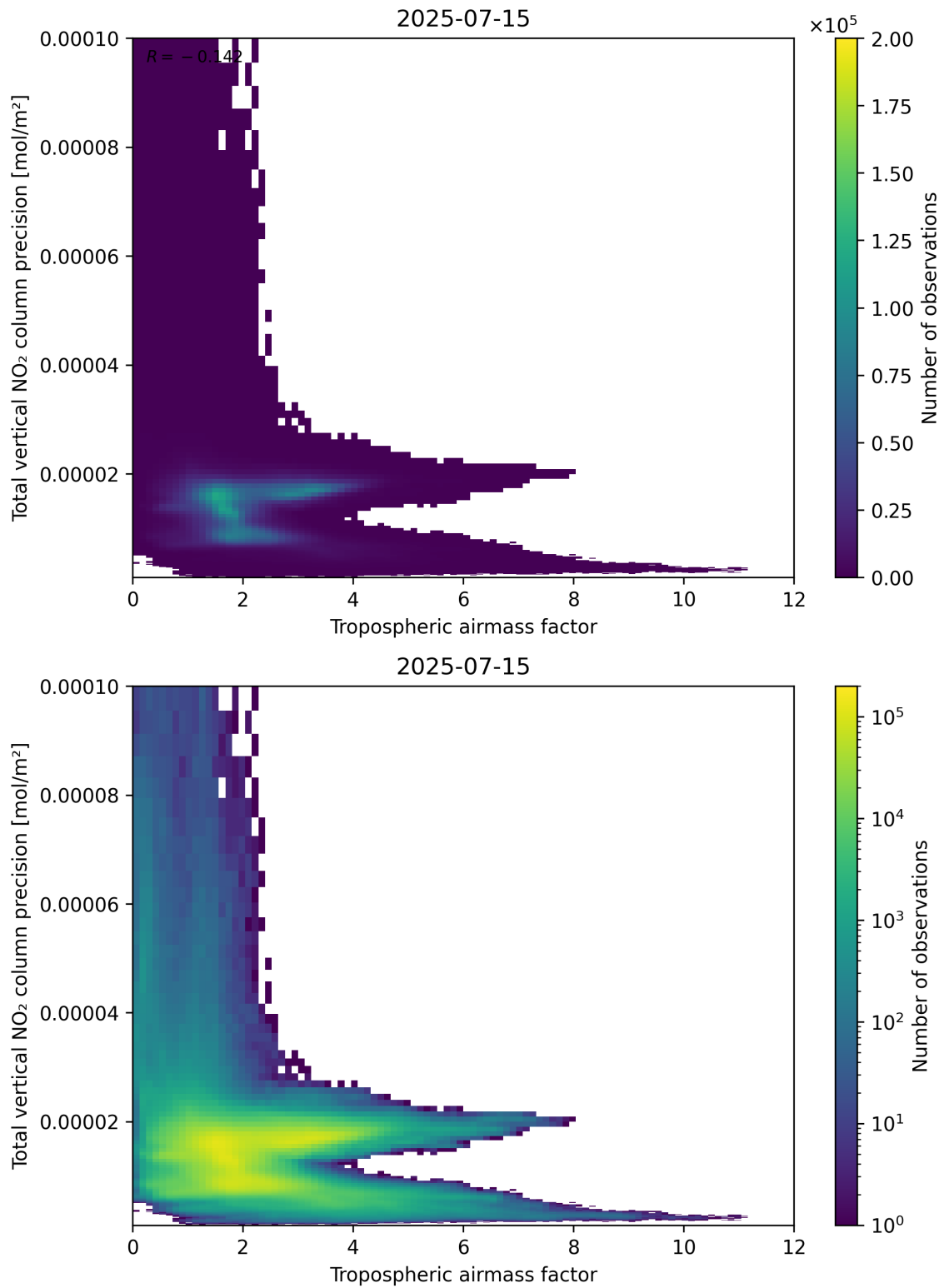
Figure 78: Scatter density plot of “Tropospheric air mass factor” against “Total vertical NO 2 column precision” for 2025-07-14 to 2025-07-16.
