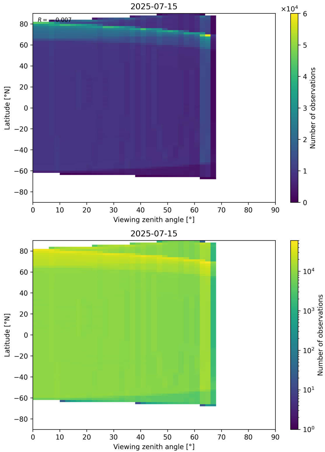
Figure 163: Scatter density plot of “Viewing zenith angle” against “Latitude” for 2025-07-14 to 2025-07-16.
