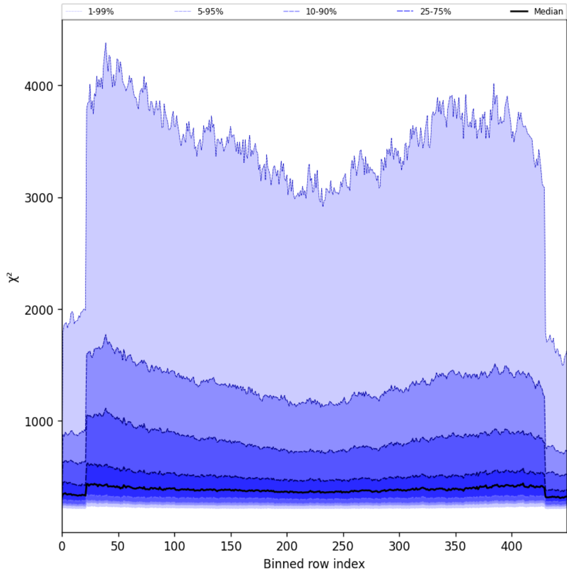
Figure 59: Along track statistics of “ \chi^2 ” for 2025-07-14 to 2025-07-16
