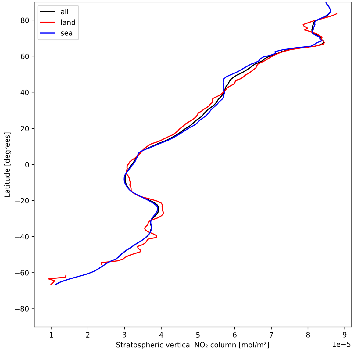
Figure 19: Zonal average of “Stratospheric vertical NO 2 column” for 2025-07-14 to 2025-07-16.
