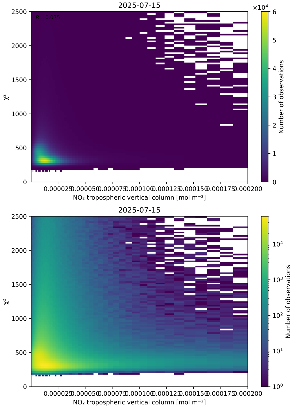
Figure 124: Scatter density plot of “NO 2 tropospheric vertical column” against “ \chi^2 ” for 2025-07-14 to 2025-07-16.
