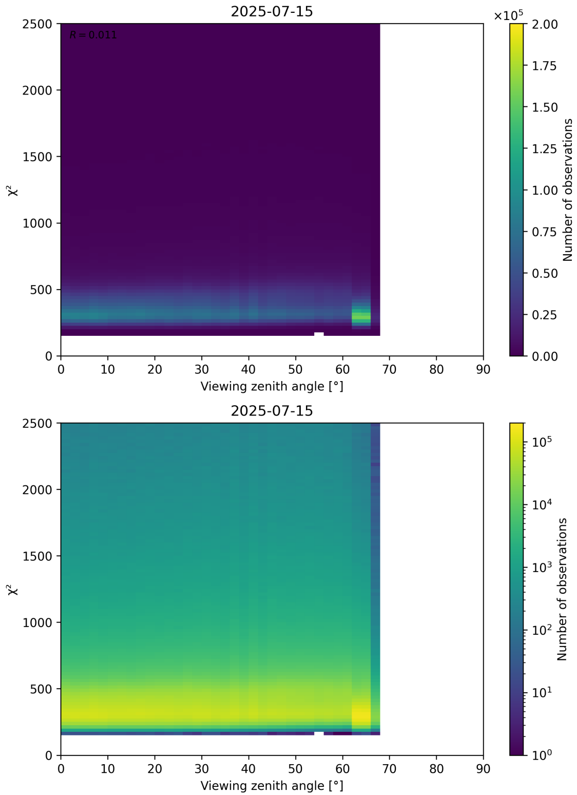
Figure 162: Scatter density plot of “Viewing zenith angle” against “ \chi^2 ” for 2025-07-14 to 2025-07-16.
