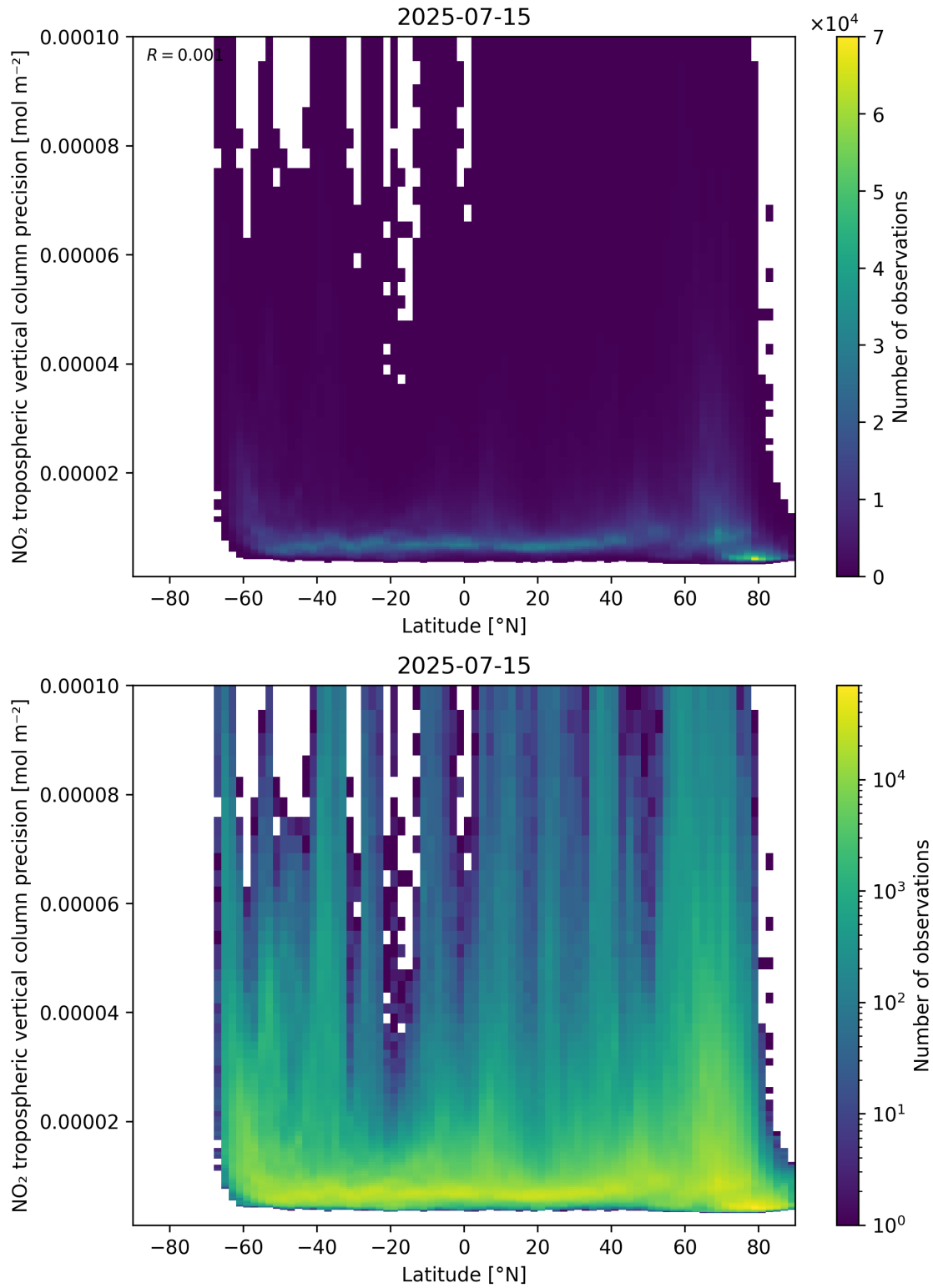
Figure 93: Scatter density plot of “Latitude” against “NO 2 tropospheric vertical column precision” for 2025-07-14 to 2025-07-16.
