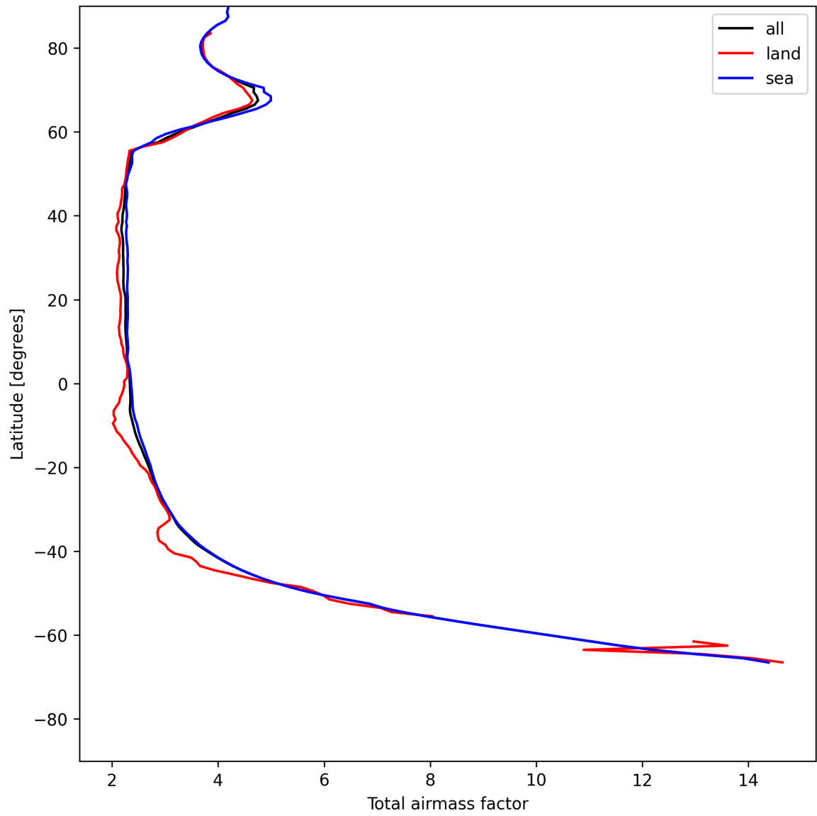
Figure 15: Zonal average of “Total airmass factor” for 2025-07-14 to 2025-07-16.
