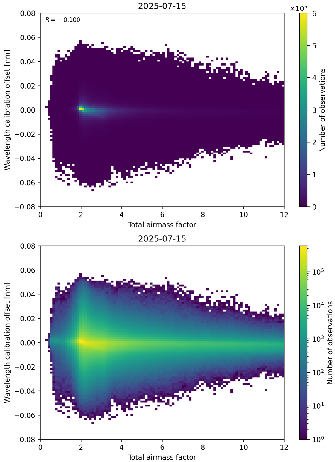
Figure 70: Scatter density plot of “Total airmass factor” against “Wavelength calibration offset” for 2025-07-14 to 2025-07-16.
