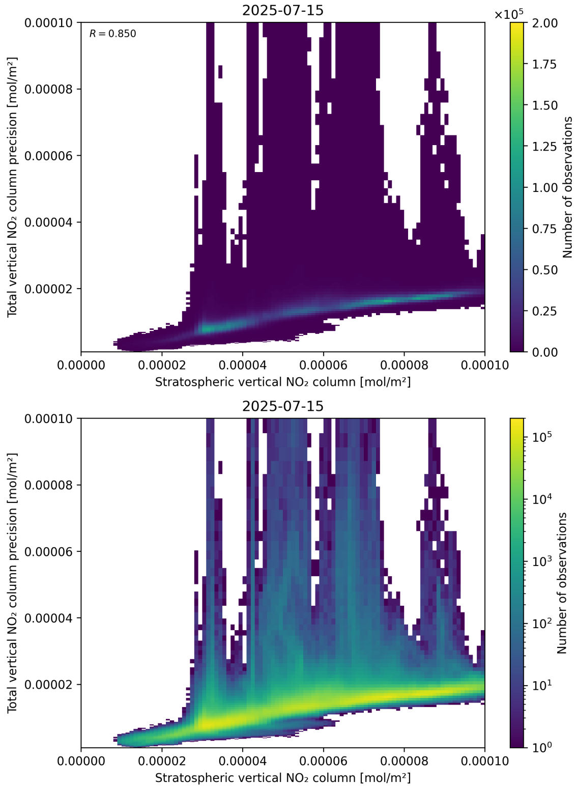
Figure 101: Scatter density plot of “Stratospheric vertical NO 2 column” against “Total vertical NO 2 column precision” for 2025-07-14 to 2025-07-16.
