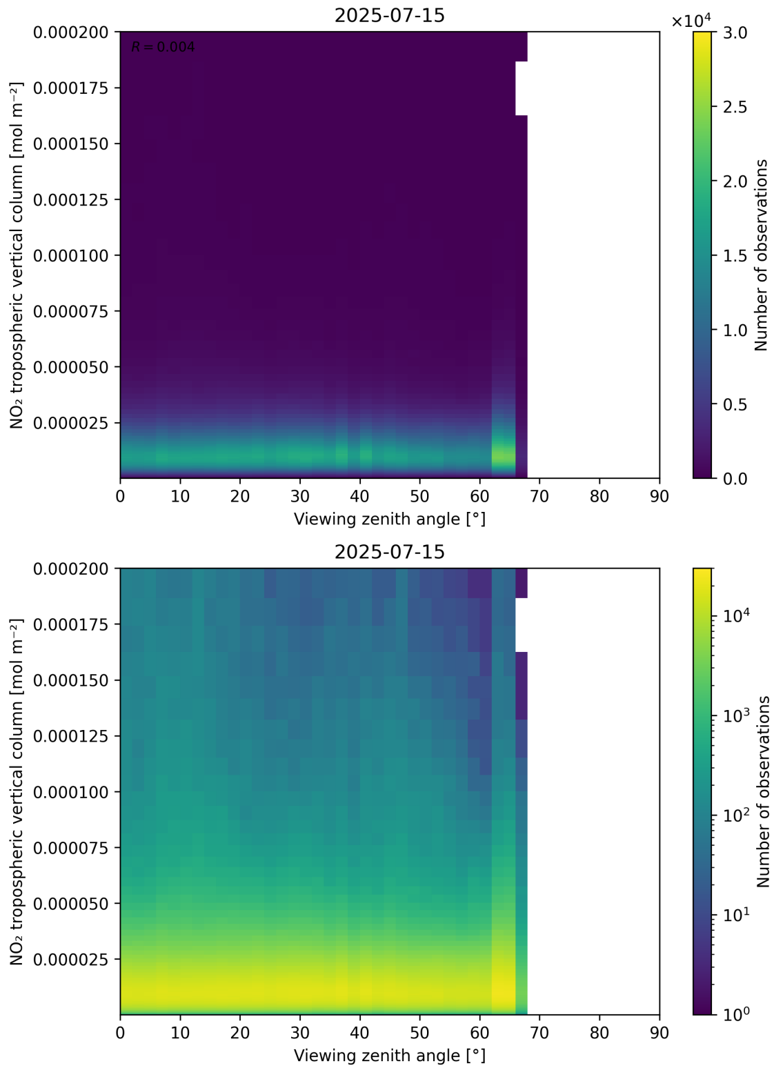
Figure 169: Scatter density plot of “Viewing zenith angle” against “NO 2 tropospheric vertical column” for 2025-07-14 to 2025-07-16.
