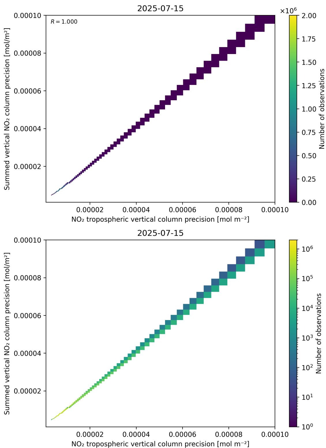
Figure 137: Scatter density plot of “NO 2 tropospheric vertical column precision” against “Summed vertical NO 2 column precision” for 2025-07-14 to 2025-07-16.
