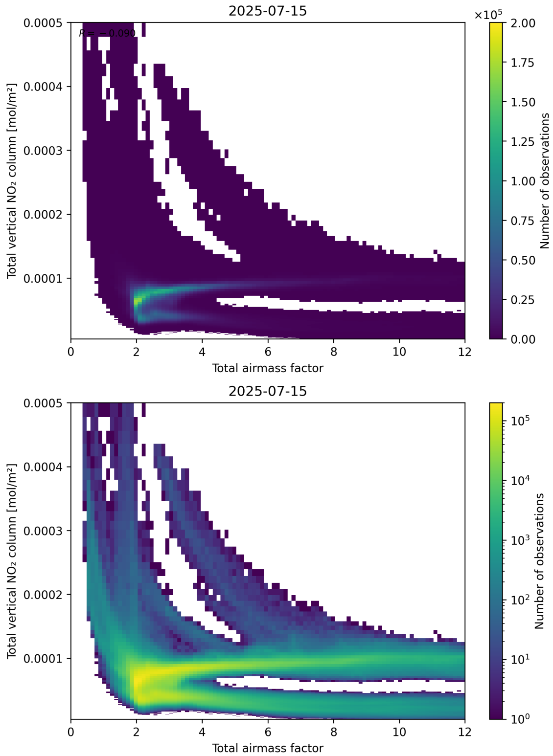
Figure 67: Scatter density plot of “Total airmass factor” against “Total vertical NO 2 column” for 2025-07-14 to 2025-07-16.
