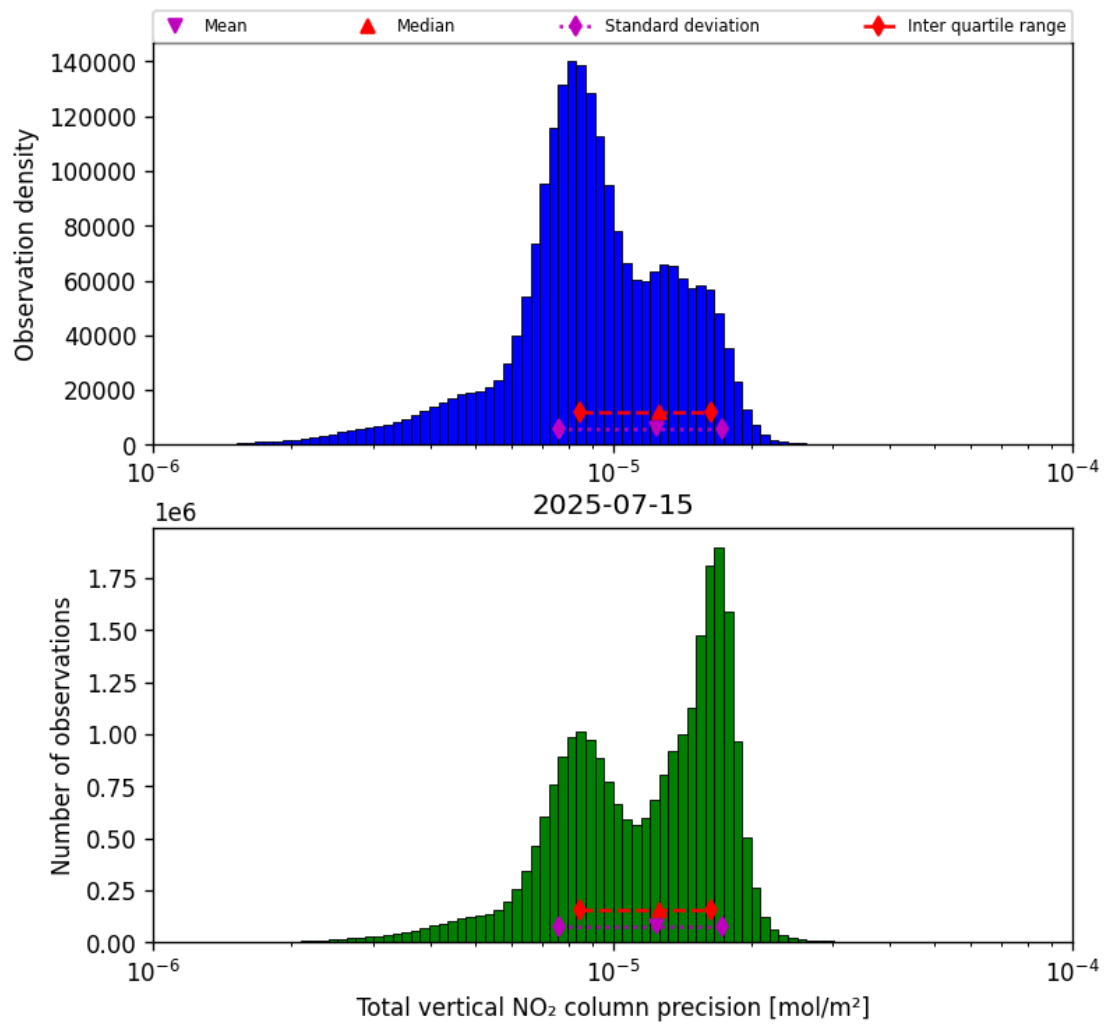
Figure 39: Histogram of “Total vertical NO 2 column precision” for 2025-07-14 to 2025-07-16
