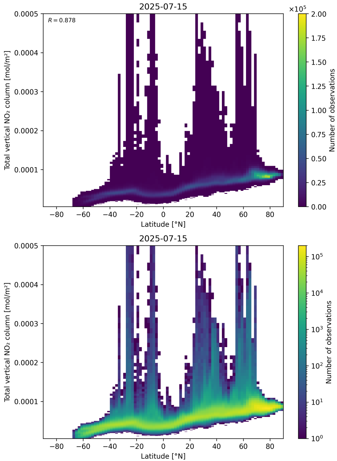
Figure 90: Scatter density plot of “Latitude” against “Total vertical NO 2 column” for 2025-07-14 to 2025-07-16.
