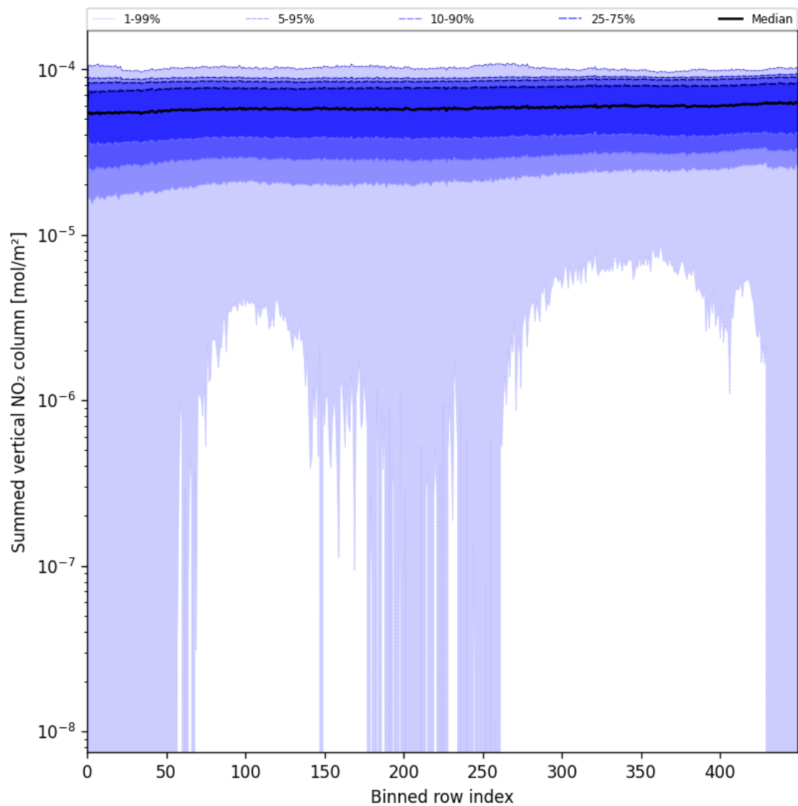
Figure 57: Along track statistics of "Summed vertical NO 2 column" for 2025-07-14 to 2025-07-16
