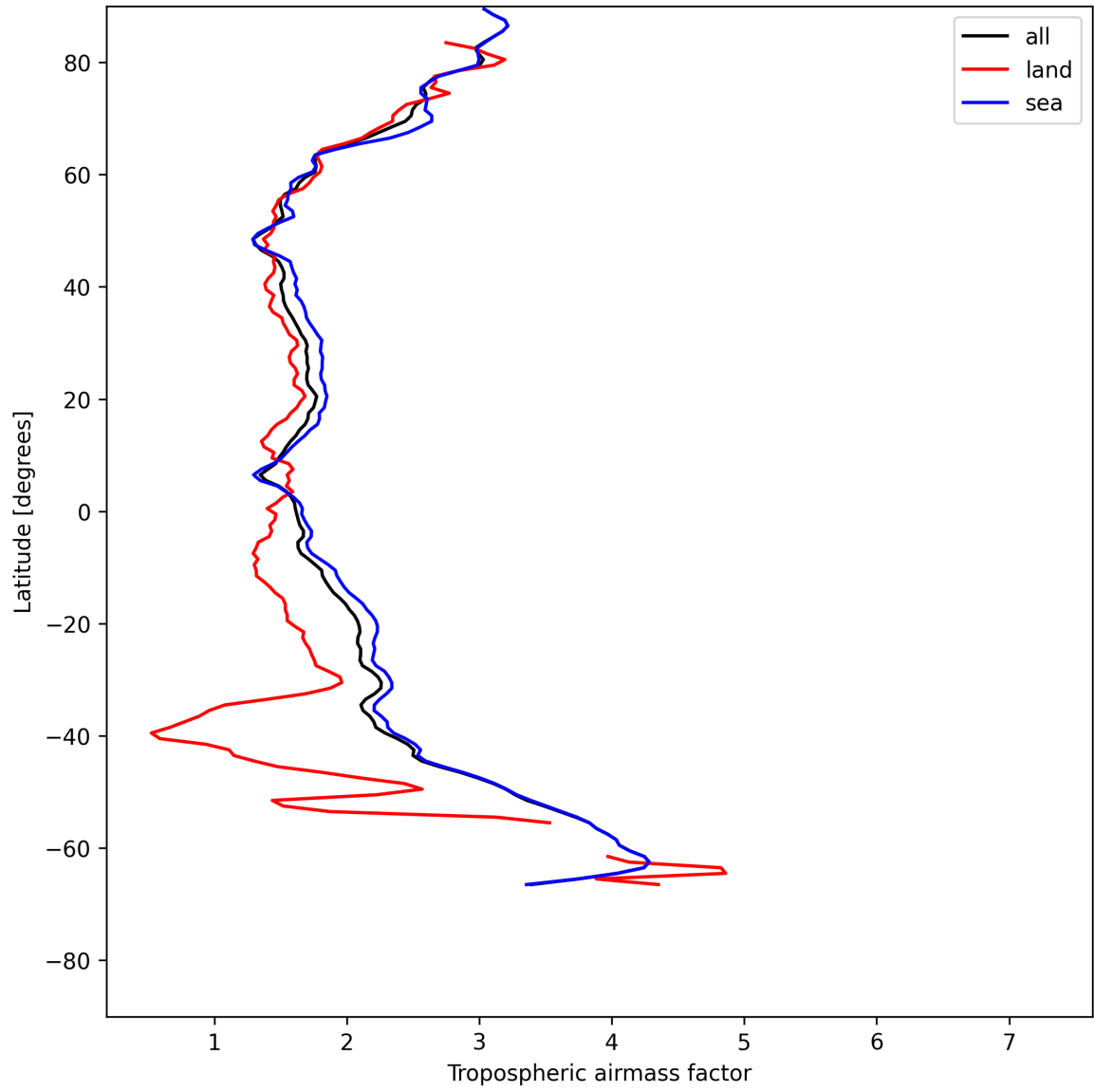
Figure 14: Zonal average of “Tropospheric air mass factor” for 2025-07-14 to 2025-07-16.
