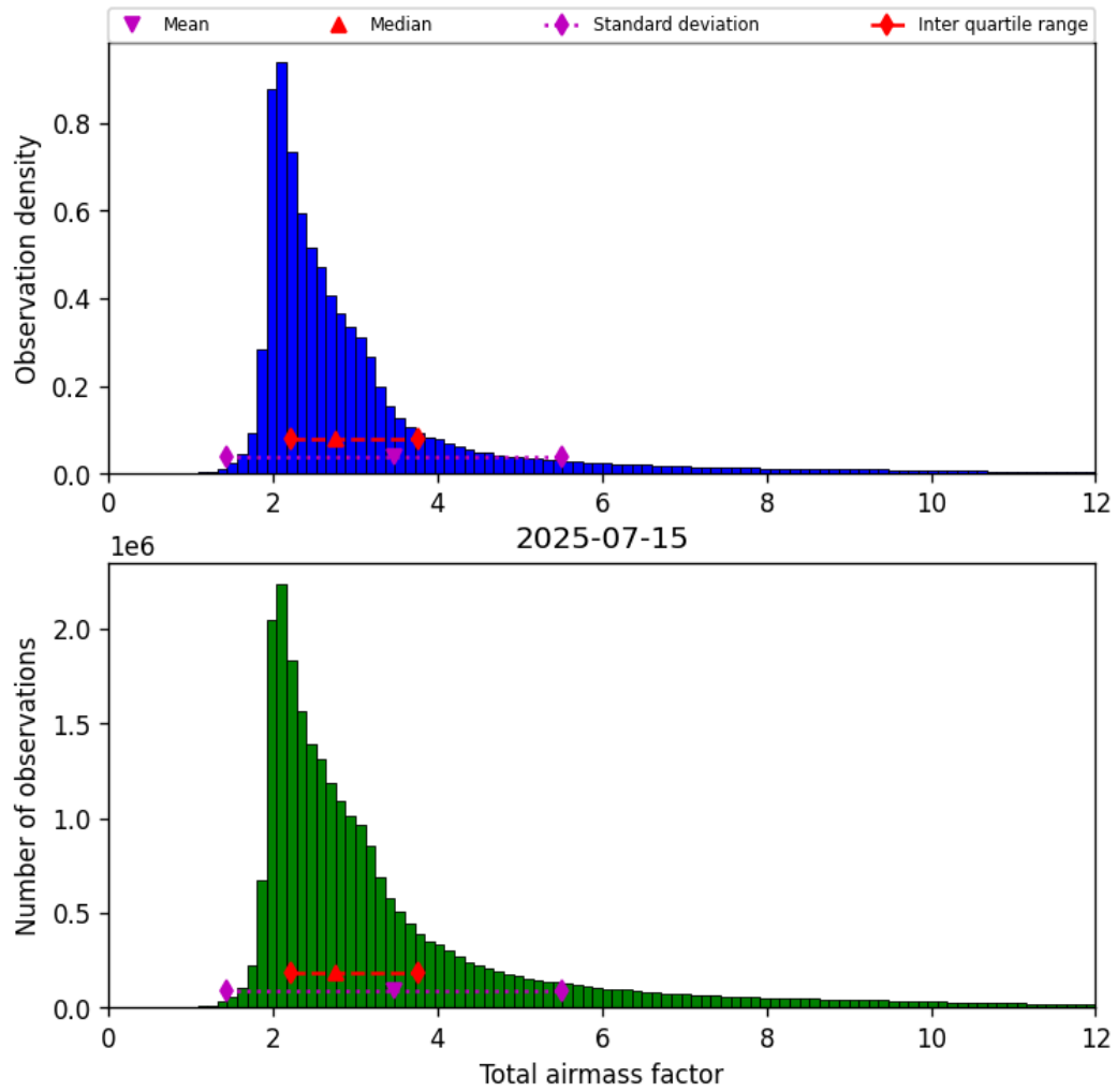
Figure 32: Histogram of “Total airmass factor” for 2025-07-14 to 2025-07-16
