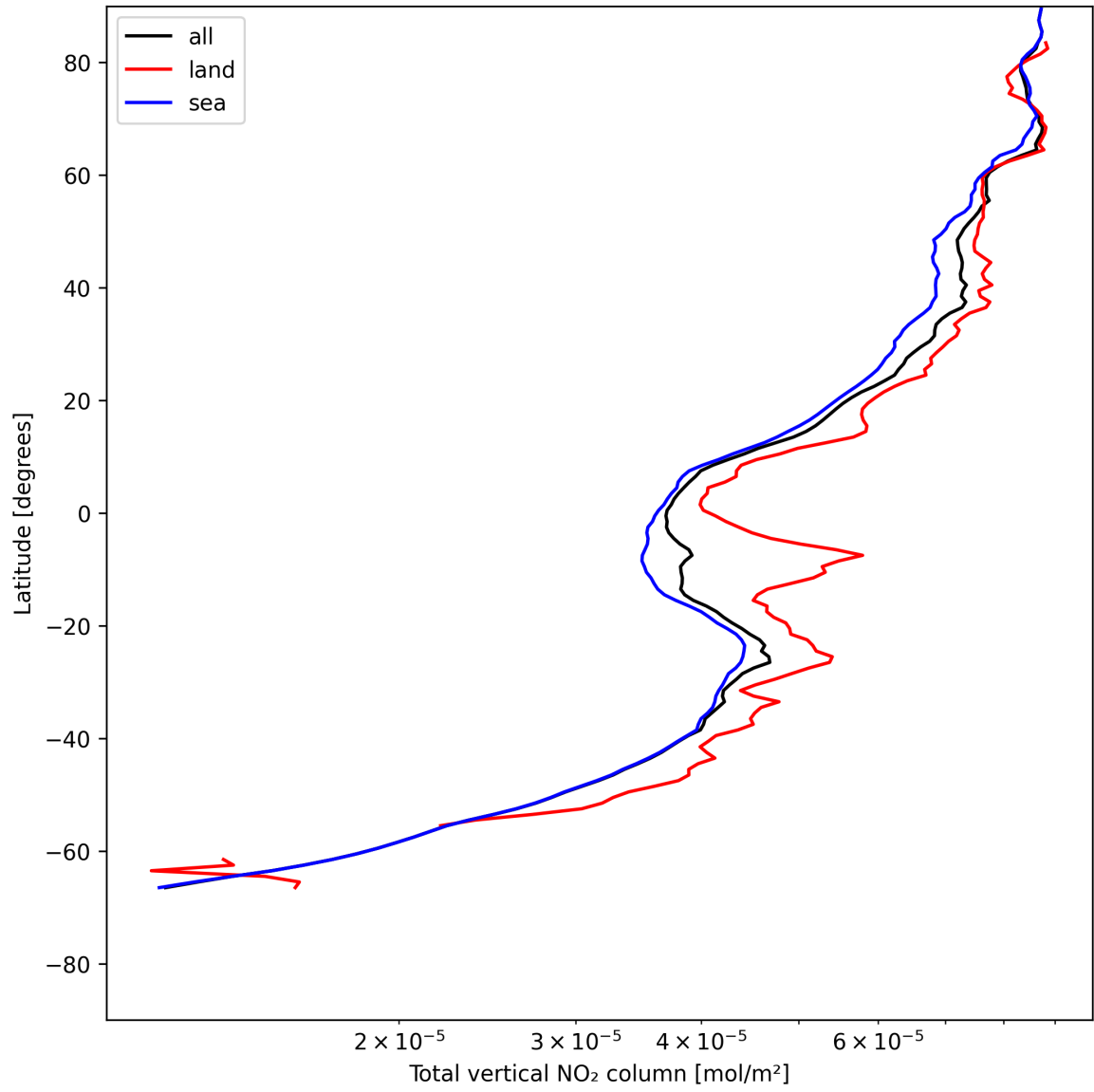
Figure 21: Zonal average of “Total vertical NO 2 column” for 2025-07-14 to 2025-07-16.
