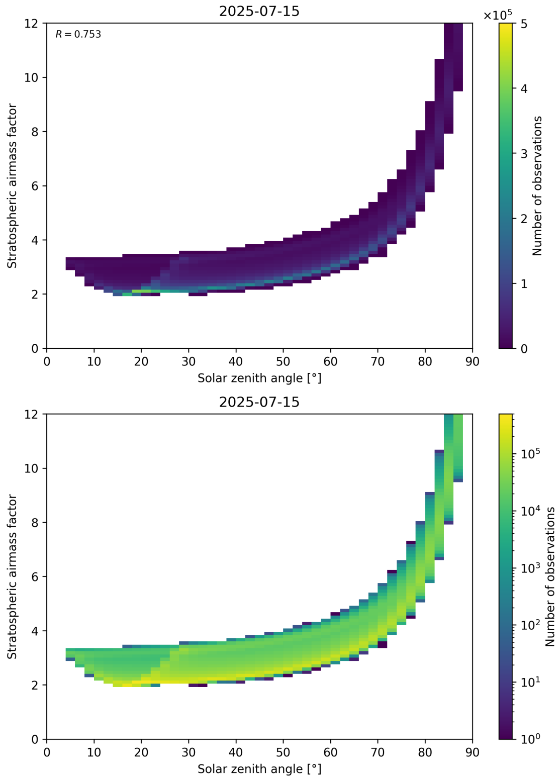
Figure 145: Scatter density plot of “Solar zenith angle” against “Stratospheric airmass factor” for 2025-07-14 to 2025-07-16.
