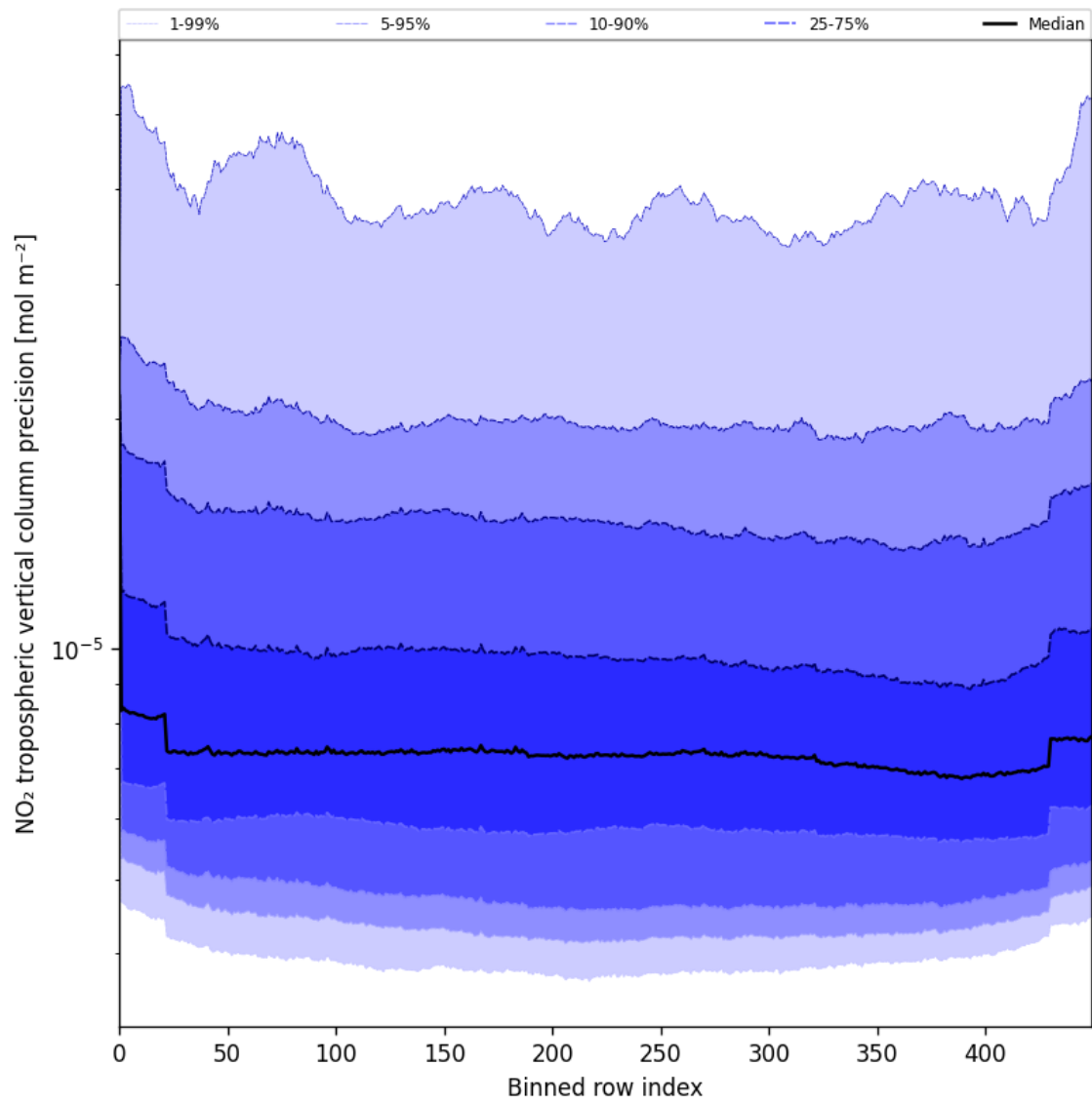
Figure 47: Along track statistics of “NO 2 tropospheric vertical column precision” for 2025-07-14 to 2025-07-16
