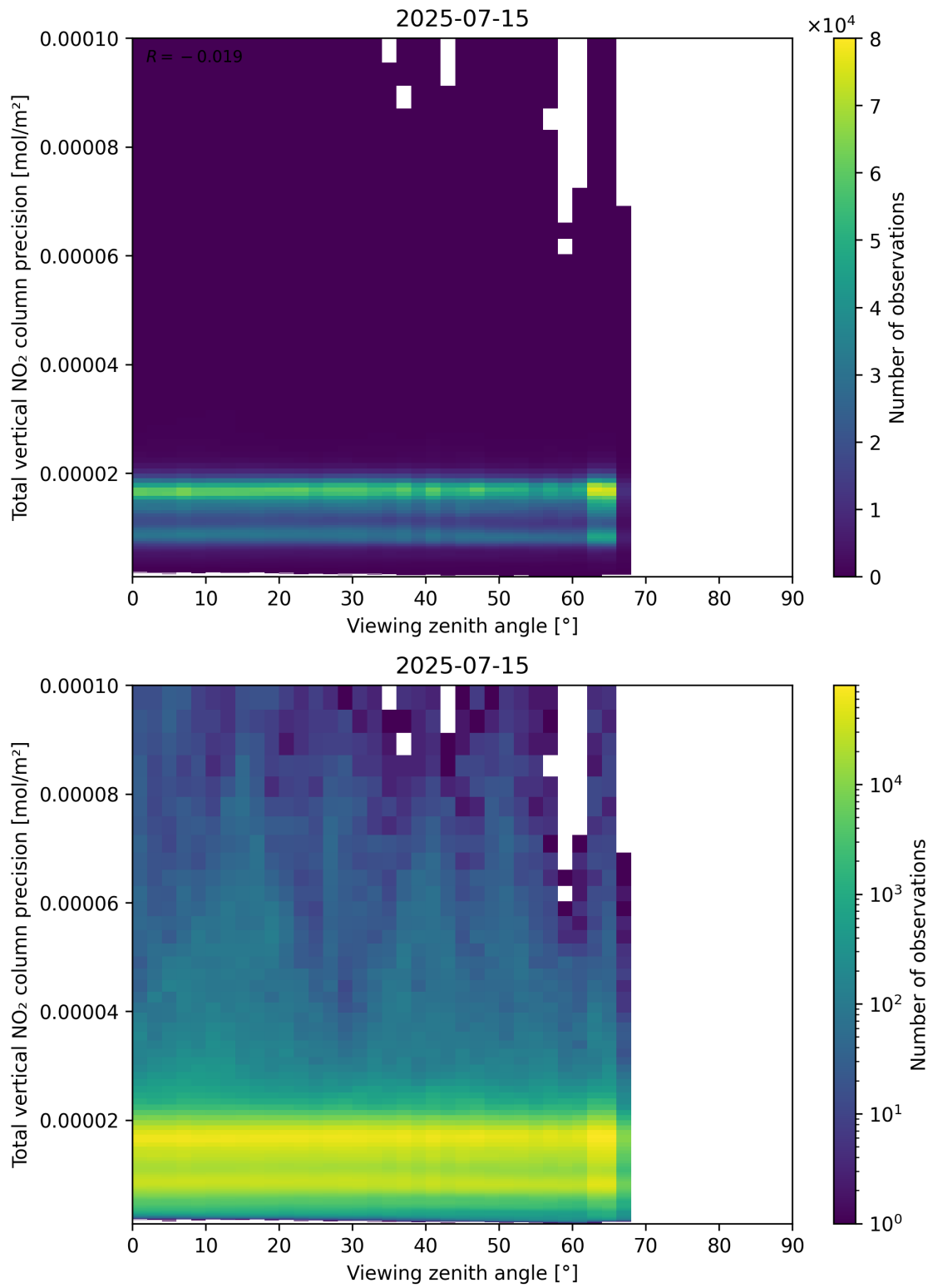
Figure 168: Scatter density plot of “Viewing zenith angle” against “Total vertical NO 2 column precision” for 2025-07-14 to 2025-07-16.
