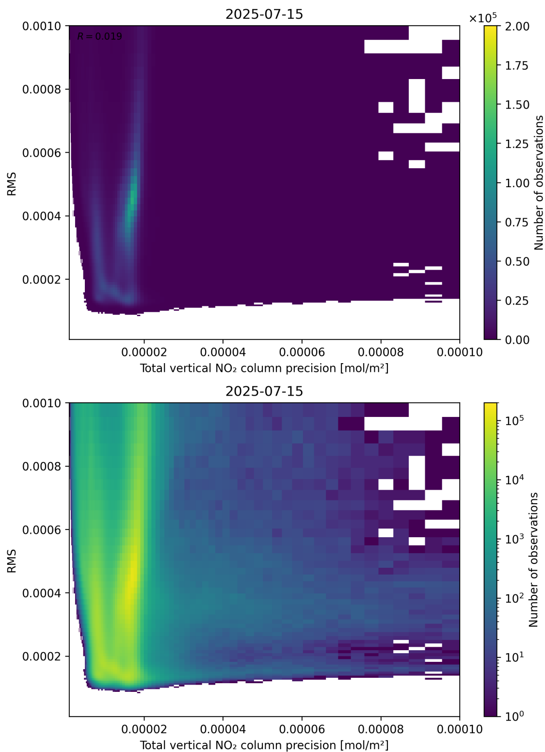
Figure 119: Scatter density plot of “Total vertical NO 2 column precision” against “RMS” for 2025-07-14 to 2025-07-16.
