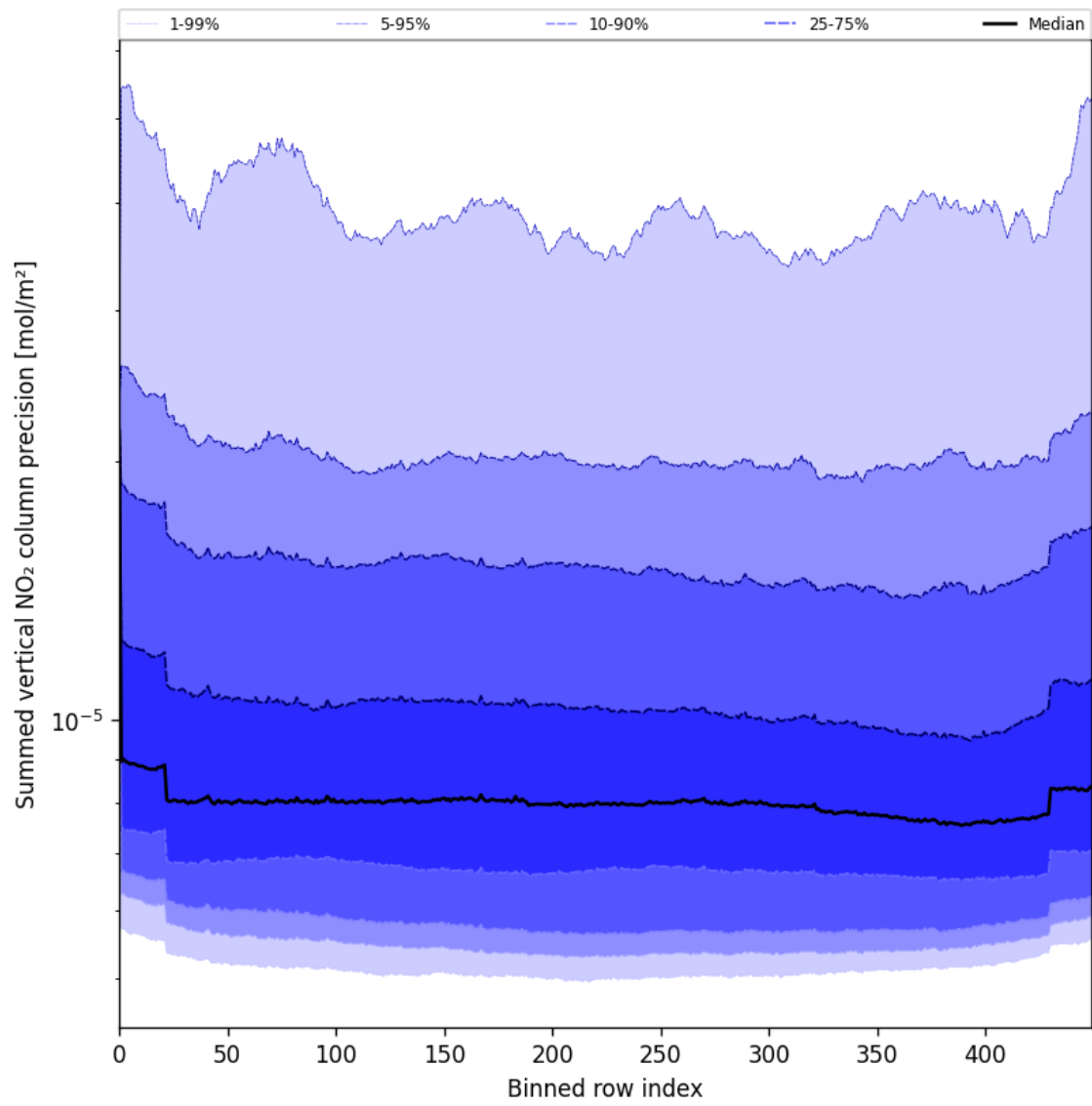
Figure 58: Along track statistics of “Summed vertical NO 2 column precision” for 2025-07-14 to 2025-07-16
