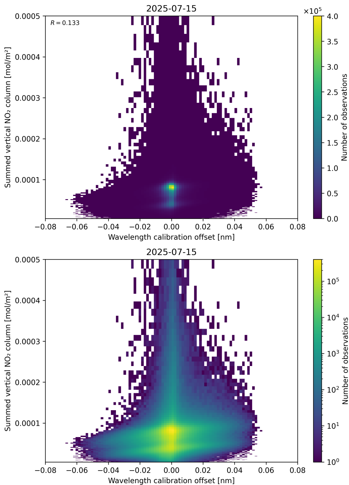
Figure 177: Scatter density plot of “Wavelength calibration offset” against “Summed vertical NO 2 column” for 2025-07-14 to 2025-07-16.
