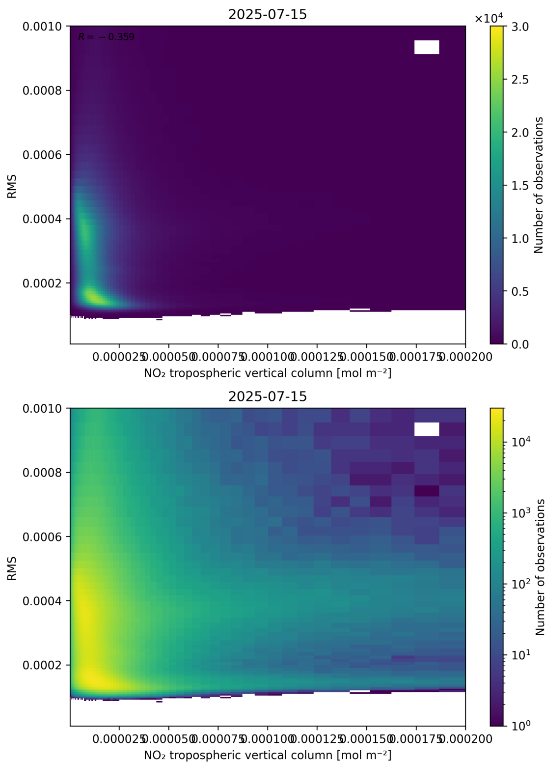
Figure 142: Scatter density plot of “NO 2 tropospheric vertical column” against “RMS” for 2025-07-14 to 2025-07-16.
