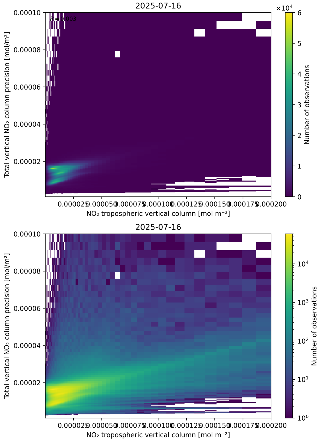
Figure 129: Scatter density plot of “NO 2 tropospheric vertical column” against “Total vertical NO 2 column precision” for 2025-07-15 to 2025-07-17.
