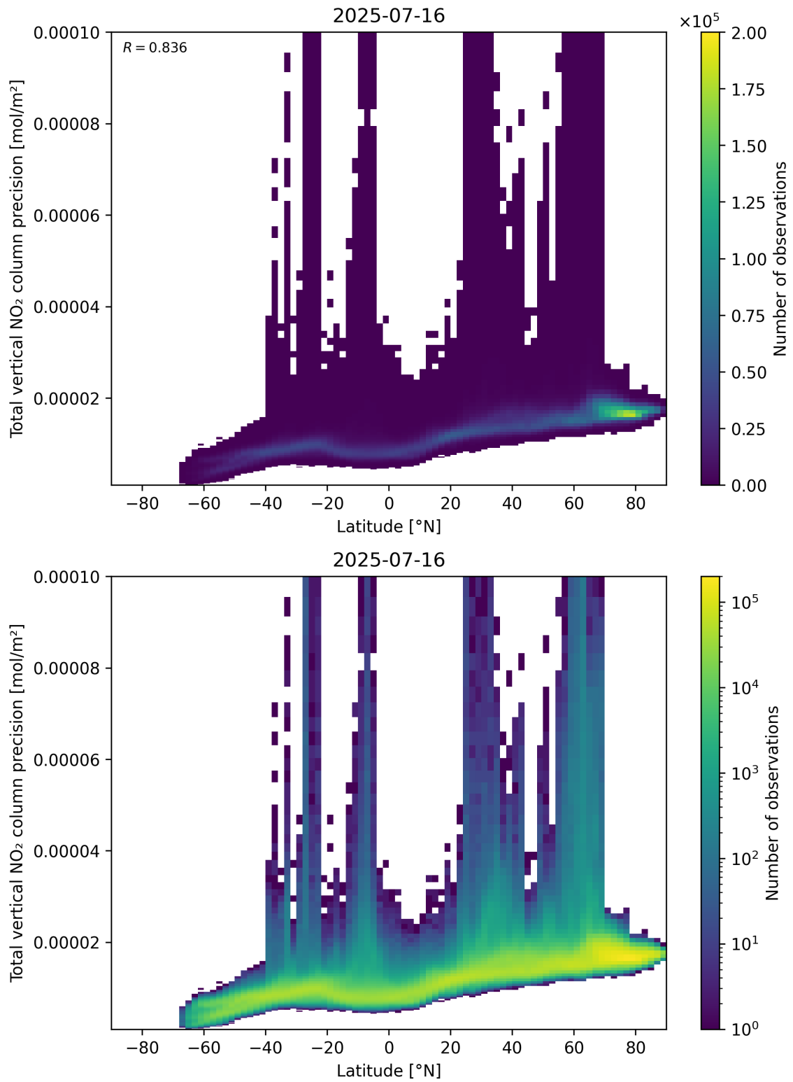
Figure 91: Scatter density plot of “Latitude” against “Total vertical NO 2 column precision” for 2025-07-15 to 2025-07-17.
