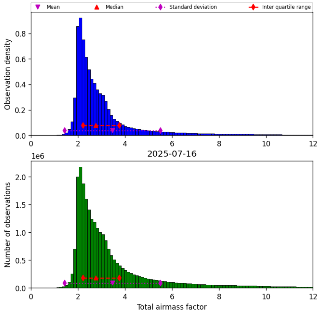
Figure 32: Histogram of “Total airmass factor” for 2025-07-15 to 2025-07-17
