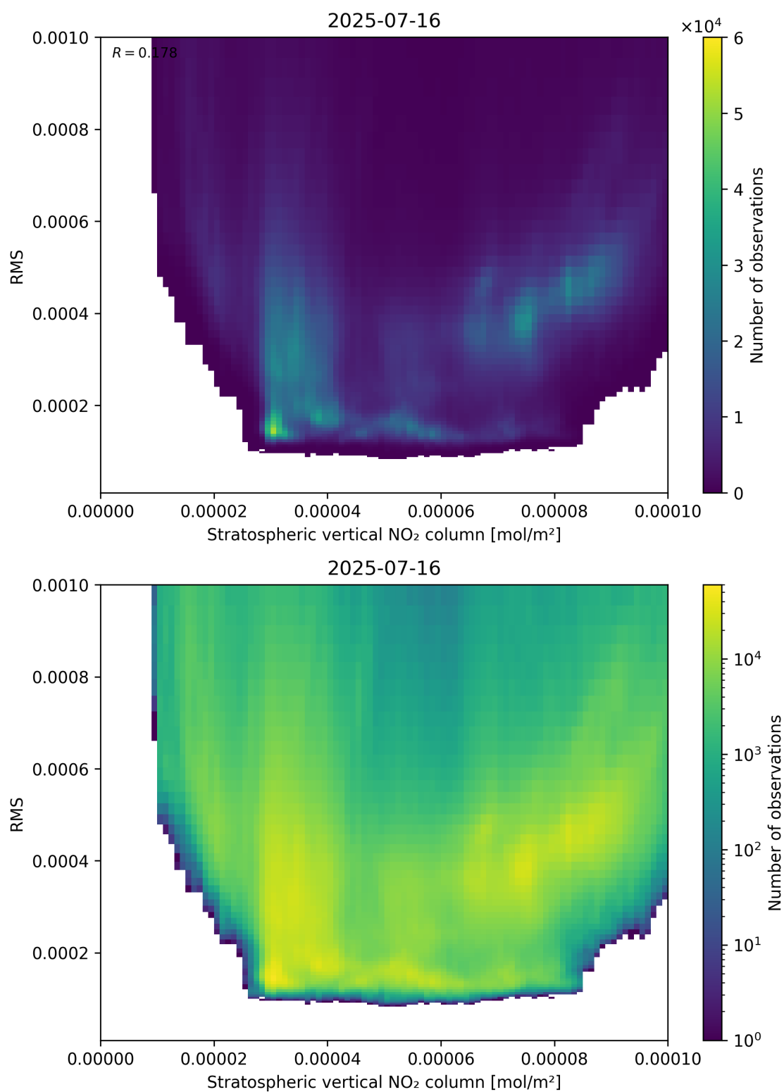
Figure 102: Scatter density plot of “Stratospheric vertical NO 2 column” against “RMS” for 2025-07-15 to 2025-07-17.
