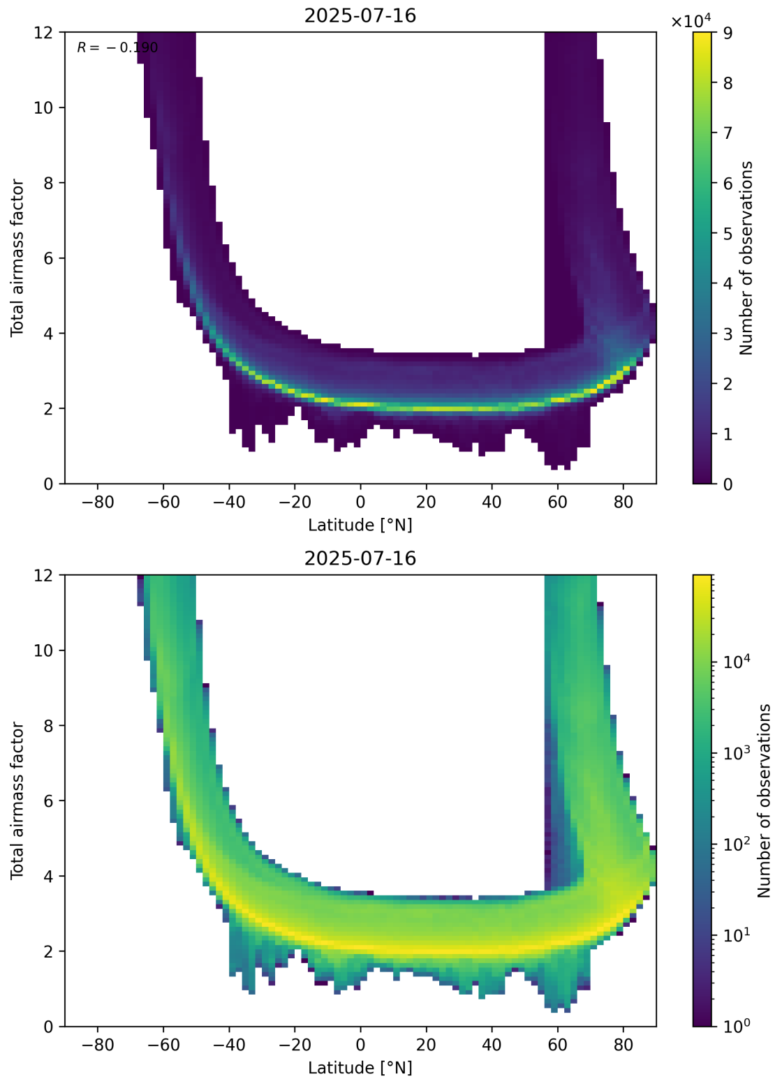
Figure 84: Scatter density plot of “Latitude” against “Total airmass factor” for 2025-07-15 to 2025-07-17.
