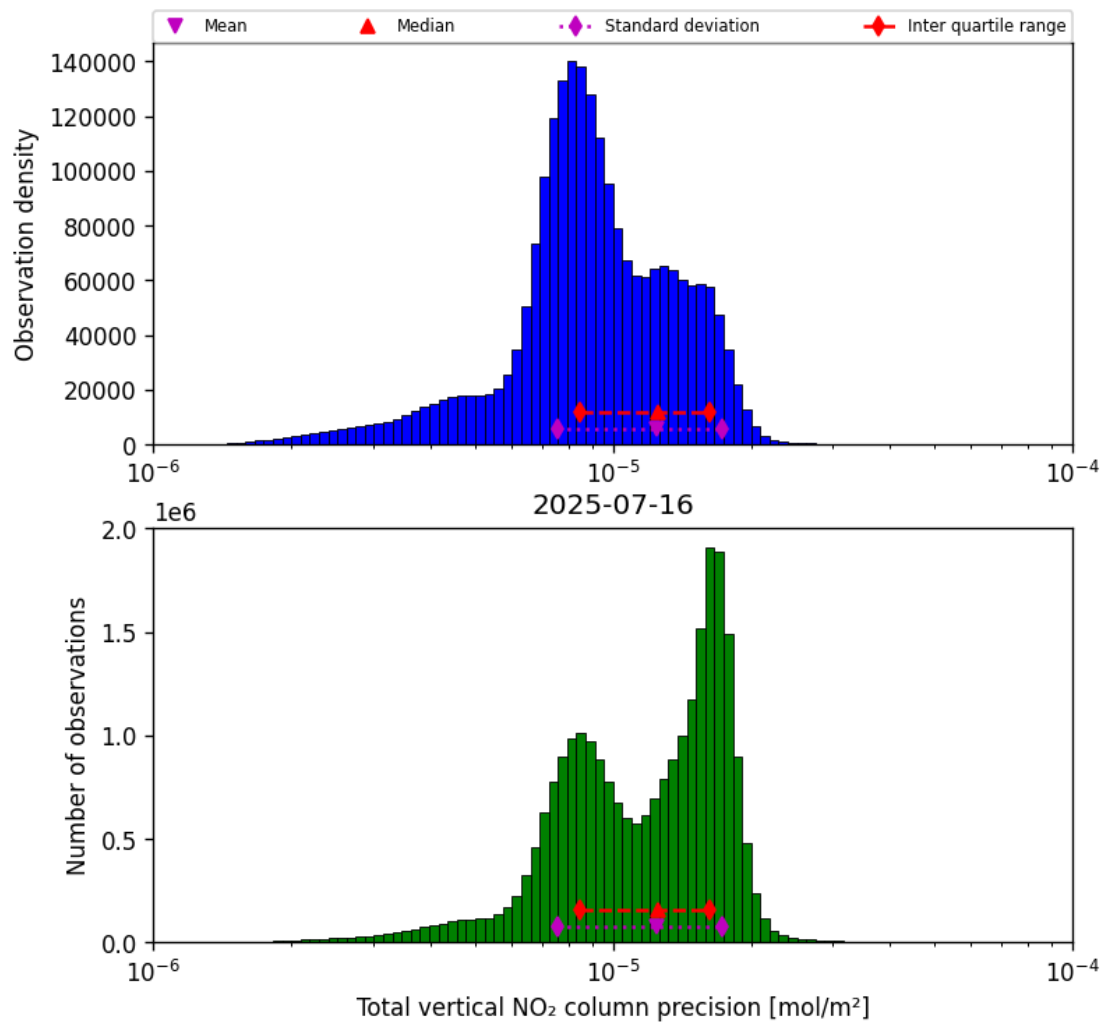
Figure 39: Histogram of “Total vertical NO 2 column precision” for 2025-07-15 to 2025-07-17
