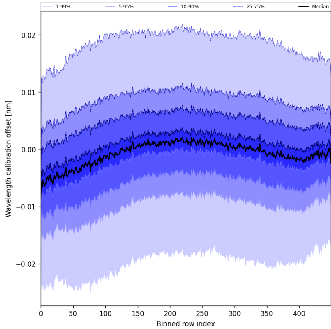
Figure 52: Along track statistics of “Wavelength calibration offset” for 2025-07-15 to 2025-07-17
