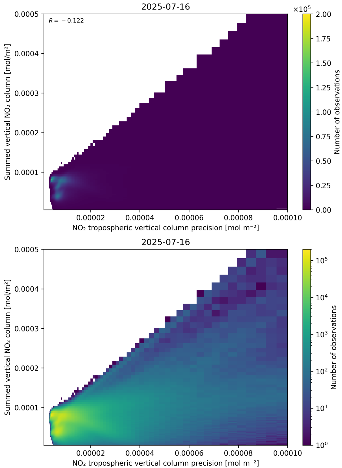
Figure 136: Scatter density plot of “NO 2 tropospheric vertical column precision” against “Summed vertical NO 2 column” for 2025-07-15 to 2025-07-17.
