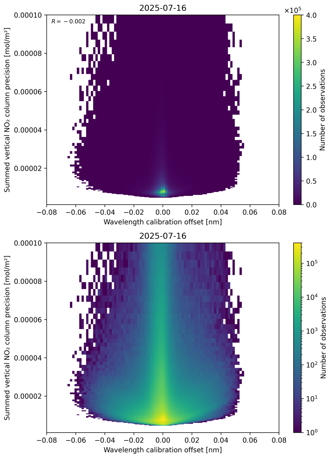
Figure 178: Scatter density plot of “Wavelength calibration offset” against “Summed vertical NO 2 column precision” for 2025-07-15 to 2025-07-17.
