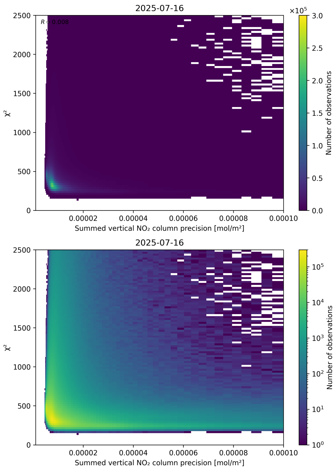
Figure 107: Scatter density plot of “Summed vertical NO 2 column precision” against “ \chi^2 ” for 2025-07-15 to 2025-07-17.
