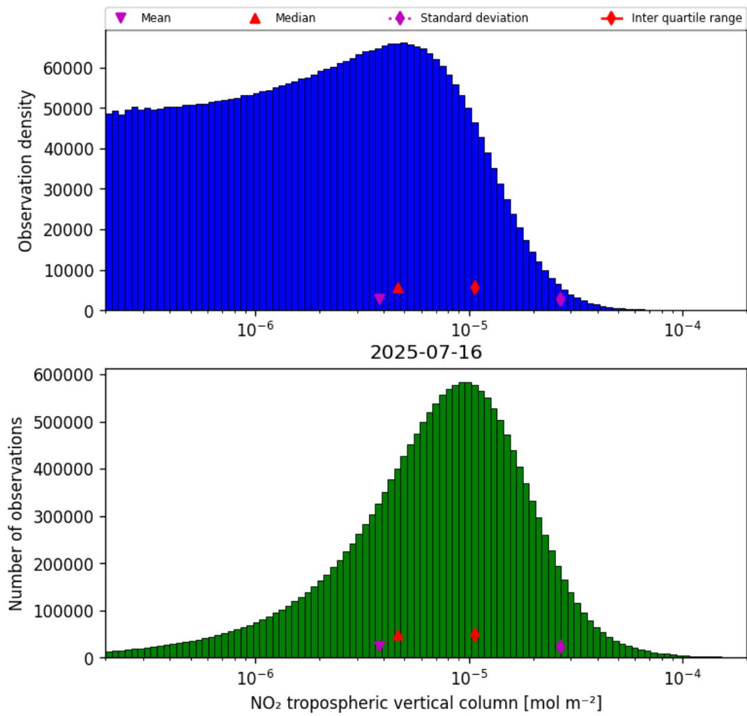
Figure 29: Histogram of “NO 2 tropospheric vertical column” for 2025-07-15 to 2025-07-17
