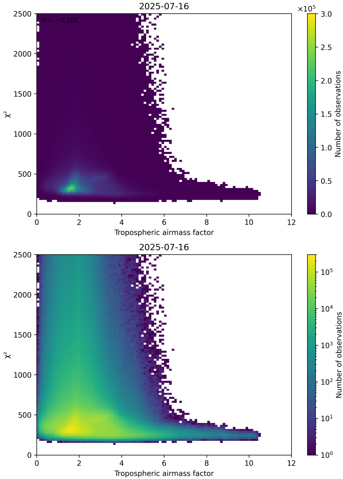
Figure 73: Scatter density plot of “Tropospheric airmass factor” against “ \chi^2 ” for 2025-07-15 to 2025-07-17.
