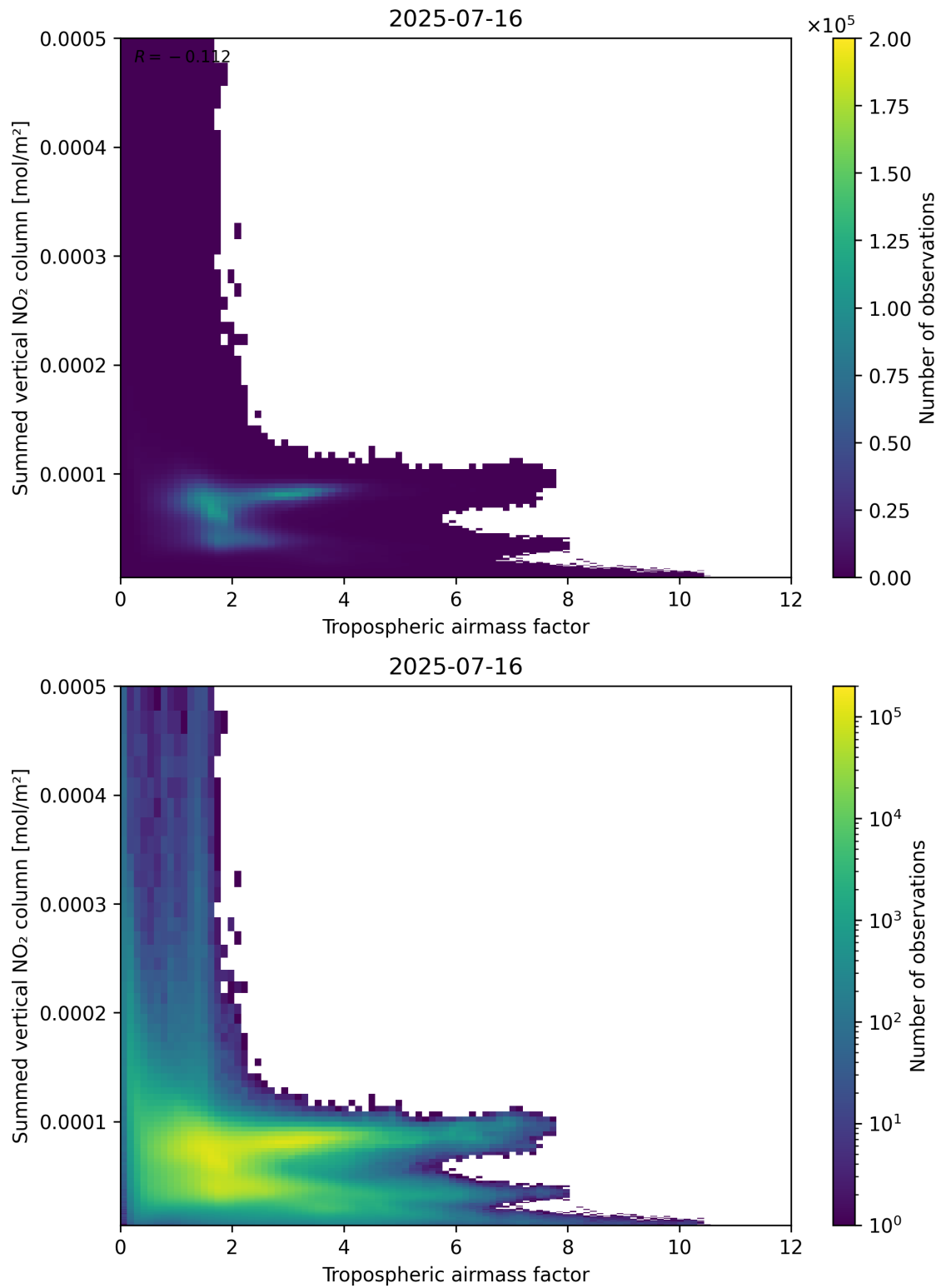
Figure 75: Scatter density plot of “Tropospheric air mass factor” against “Summed vertical NO 2 column” for 2025-07-15 to 2025-07-17.
