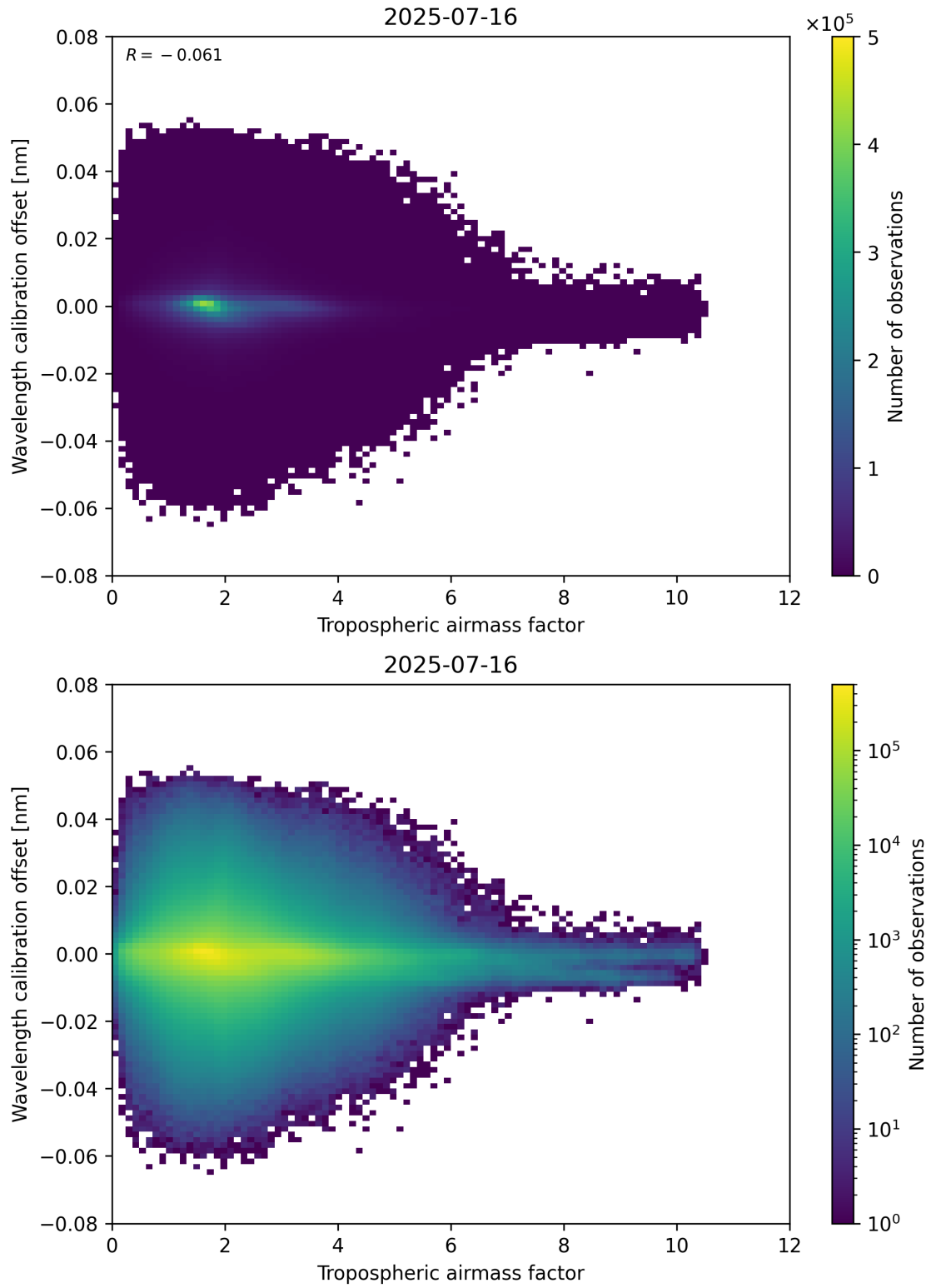
Figure 80: Scatter density plot of “Tropospheric airmass factor” against “Wavelength calibration offset” for 2025-07-15 to 2025-07-17.
