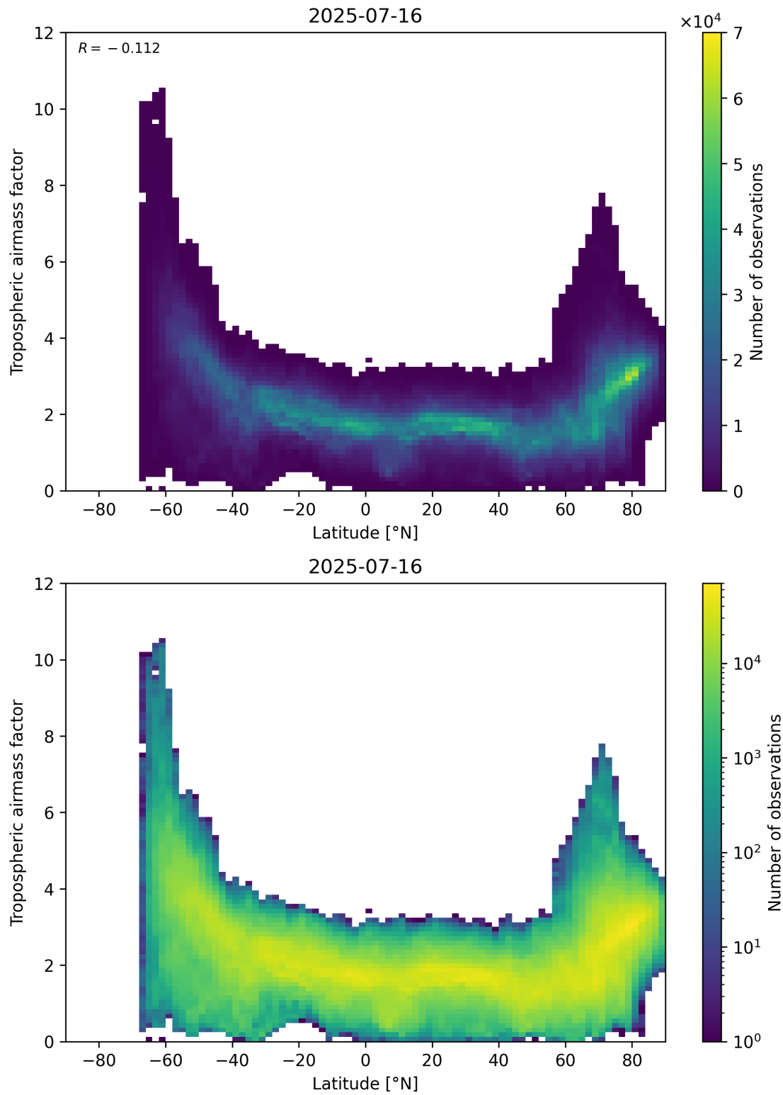
Figure 85: Scatter density plot of “Latitude” against “Tropospheric air mass factor” for 2025-07-15 to 2025-07-17.
