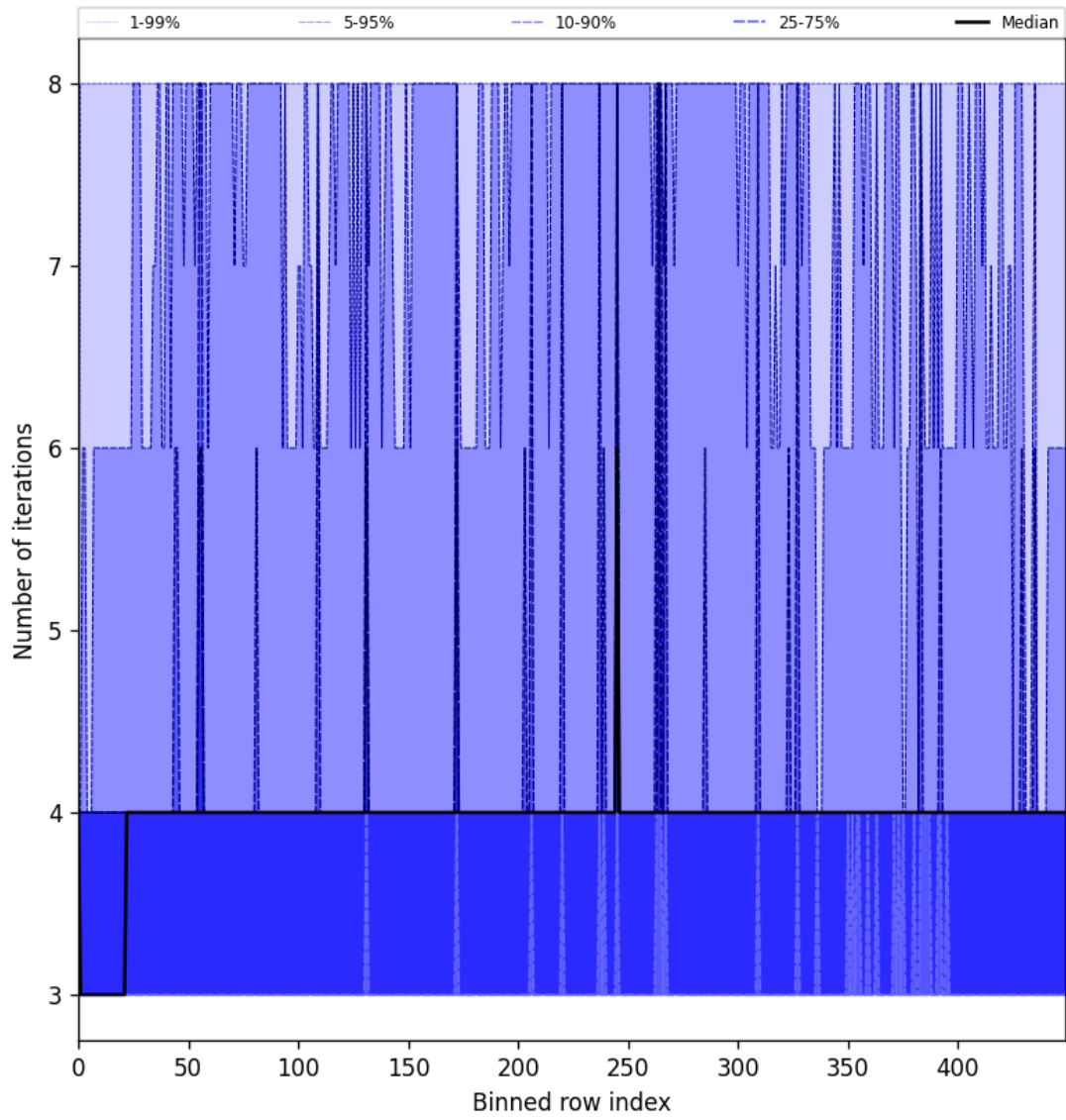
Figure 51: Along track statistics of “Number of iterations” for 2025-07-15 to 2025-07-17
