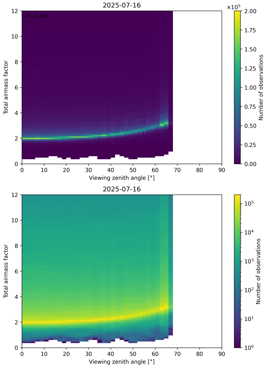
Figure 160: Scatter density plot of “Viewing zenith angle” against “Total airmass factor” for 2025-07-15 to 2025-07-17.
