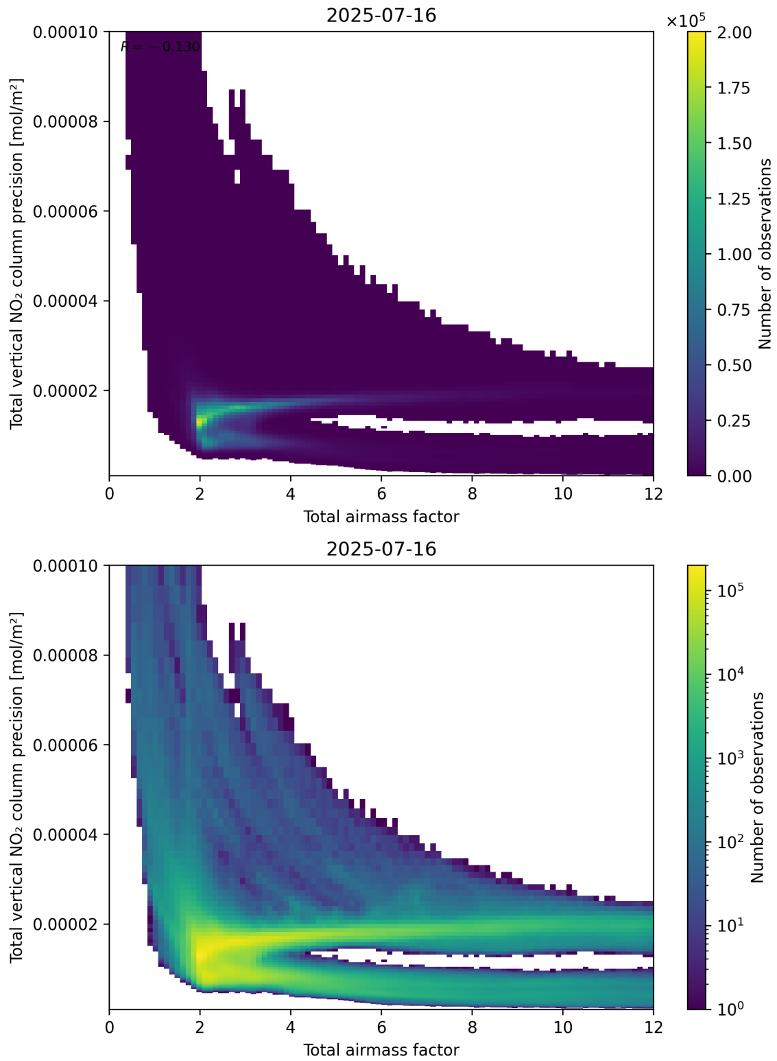
Figure 68: Scatter density plot of “Total airmass factor” against “Total vertical NO 2 column precision” for 2025-07-15 to 2025-07-17.
