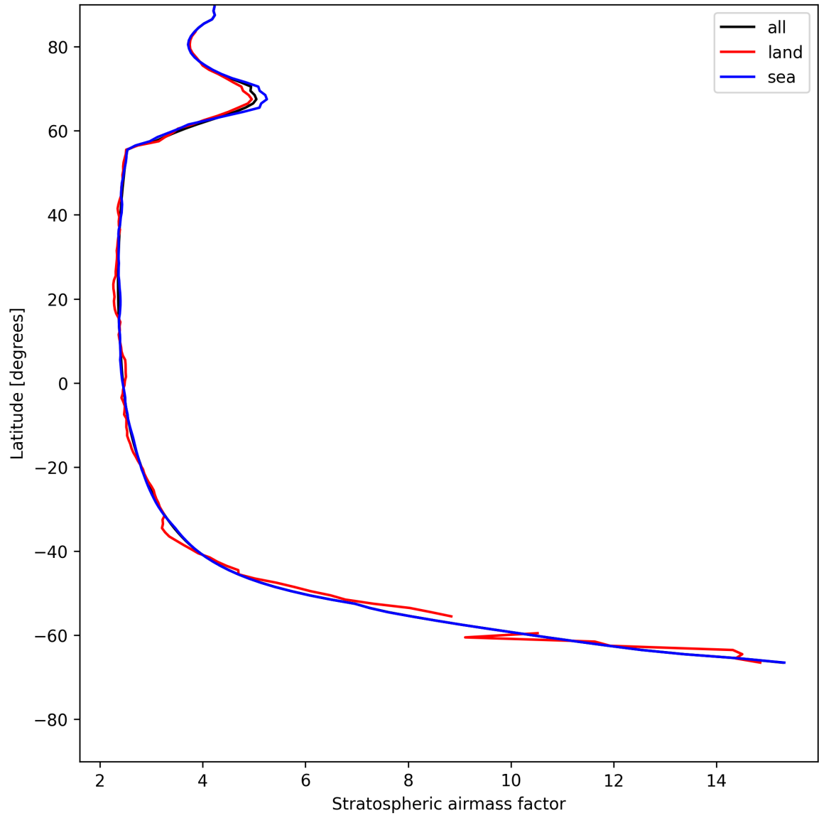
Figure 27: Zonal average of “Stratospheric airmass factor” for 2025-07-15 to 2025-07-17.
