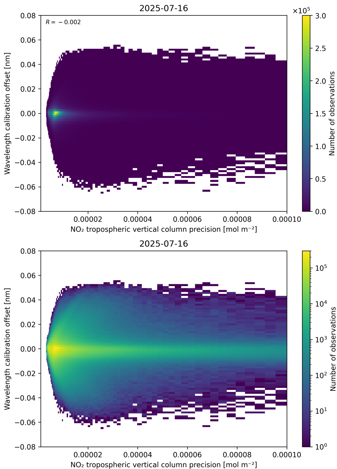
Figure 141: Scatter density plot of “NO 2 tropospheric vertical column precision” against “Wavelength calibration offset” for 2025-07-15 to 2025-07-17.
