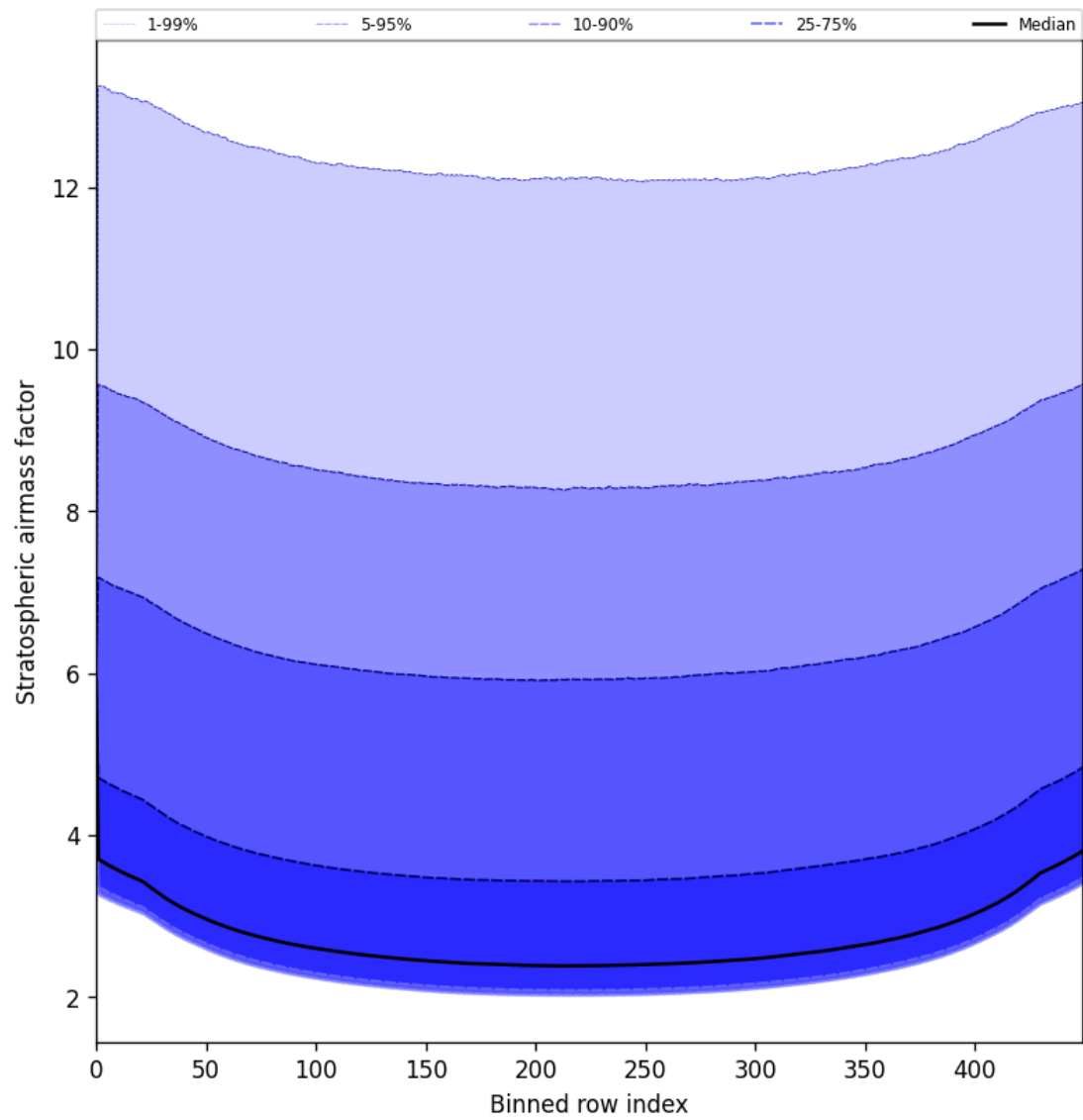
Figure 61: Along track statistics of “Stratospheric airmass factor” for 2025-07-15 to 2025-07-17
