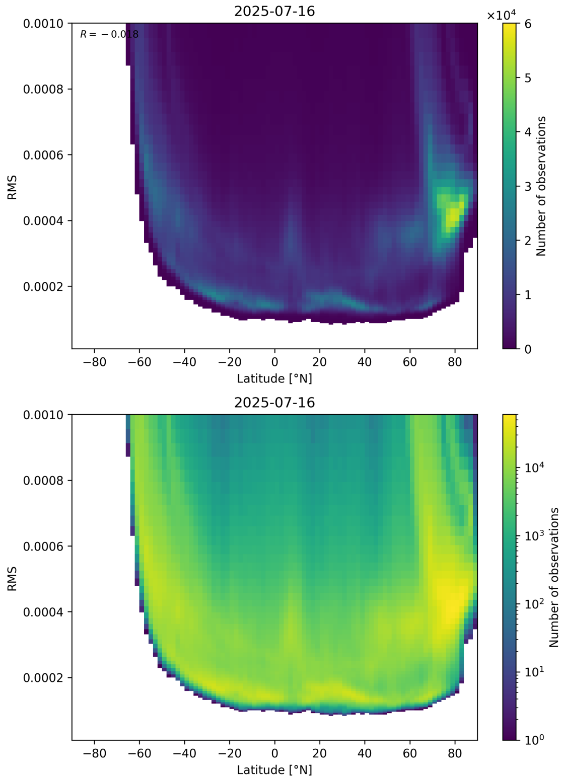
Figure 94: Scatter density plot of “Latitude” against “RMS” for 2025-07-15 to 2025-07-17.
