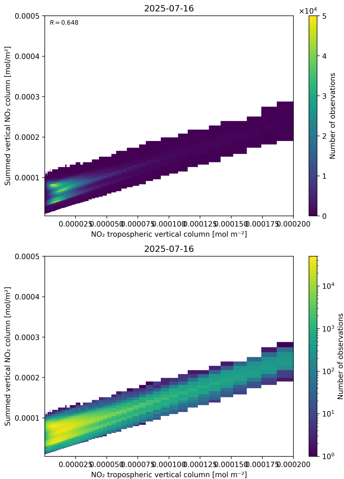
Figure 126: Scatter density plot of “NO 2 tropospheric vertical column” against “Summed vertical NO 2 column” for 2025-07-15 to 2025-07-17.
