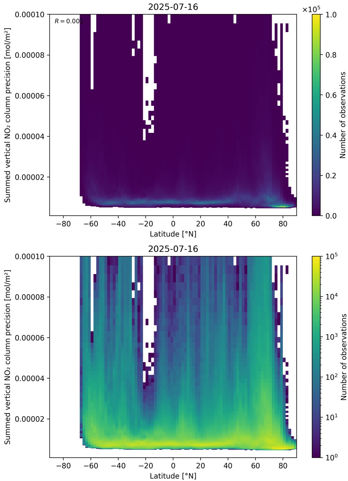
Figure 89: Scatter density plot of “Latitude” against “Summed vertical NO 2 column precision” for 2025-07-15 to 2025-07-17.
