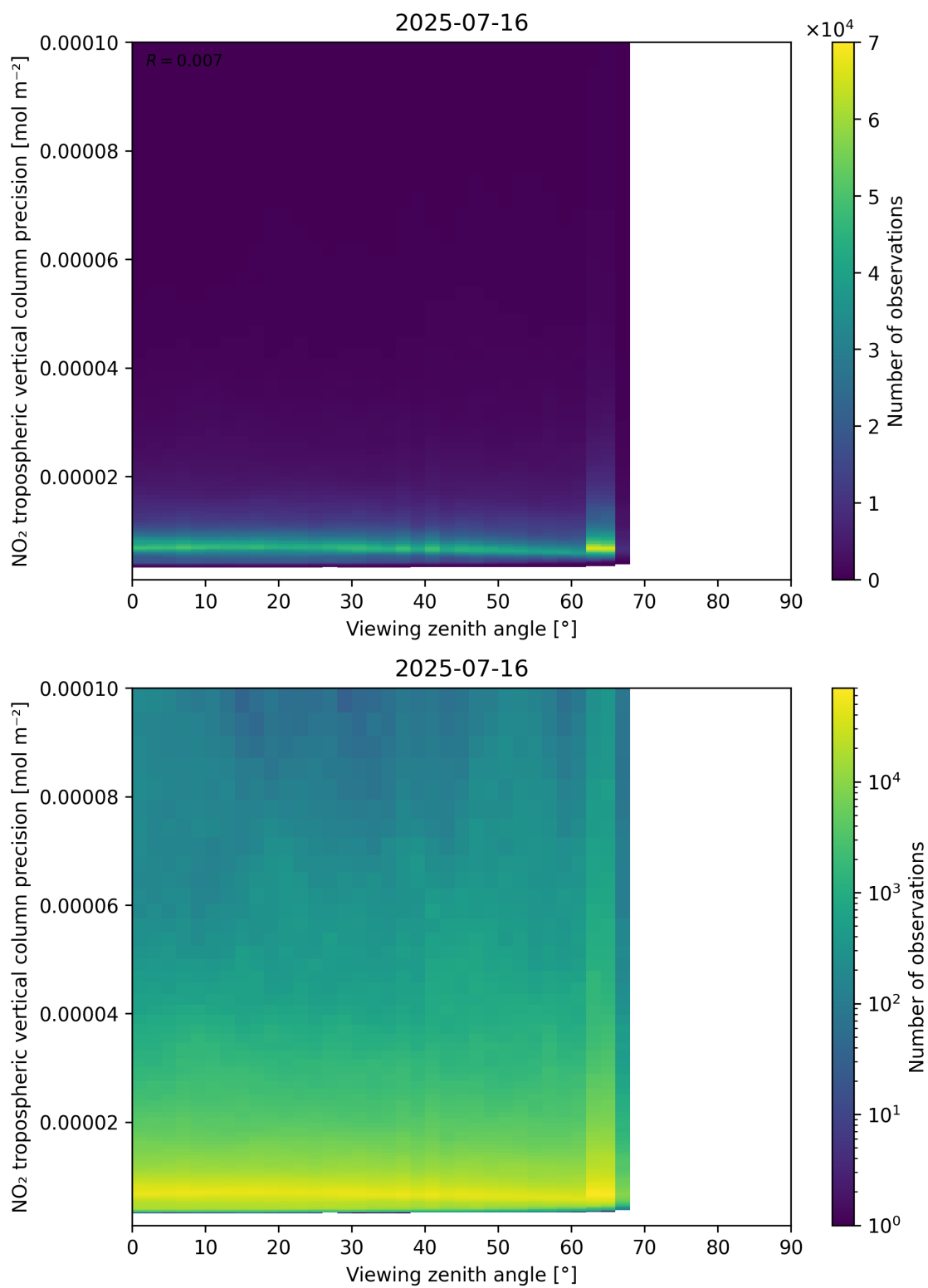
Figure 170: Scatter density plot of “Viewing zenith angle” against “NO 2 tropospheric vertical column precision” for 2025-07-15 to 2025-07-17.
