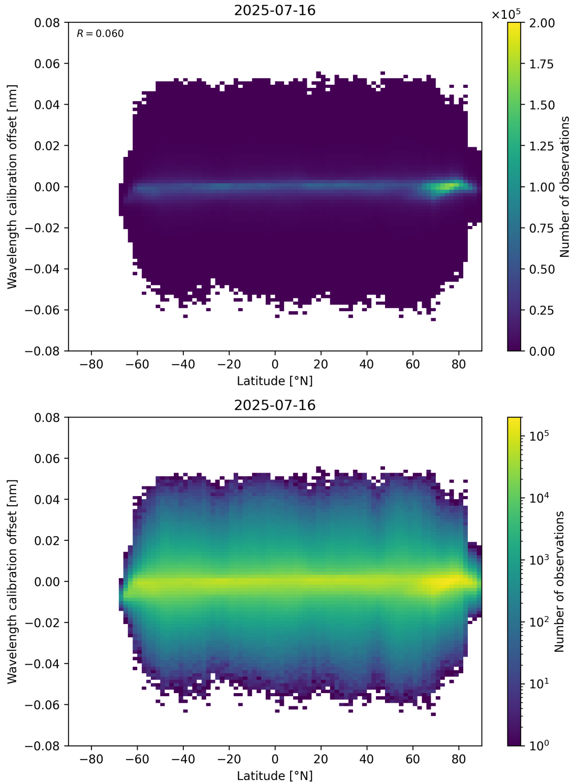
Figure 95: Scatter density plot of “Latitude” against “Wavelength calibration offset” for 2025-07-15 to 2025-07-17.
