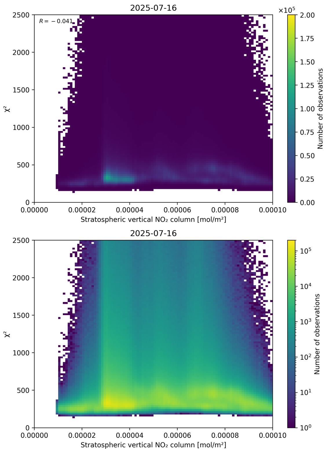
Figure 97: Scatter density plot of “Stratospheric vertical NO 2 column” against “ \chi^2 ” for 2025-07-15 to 2025-07-17.
