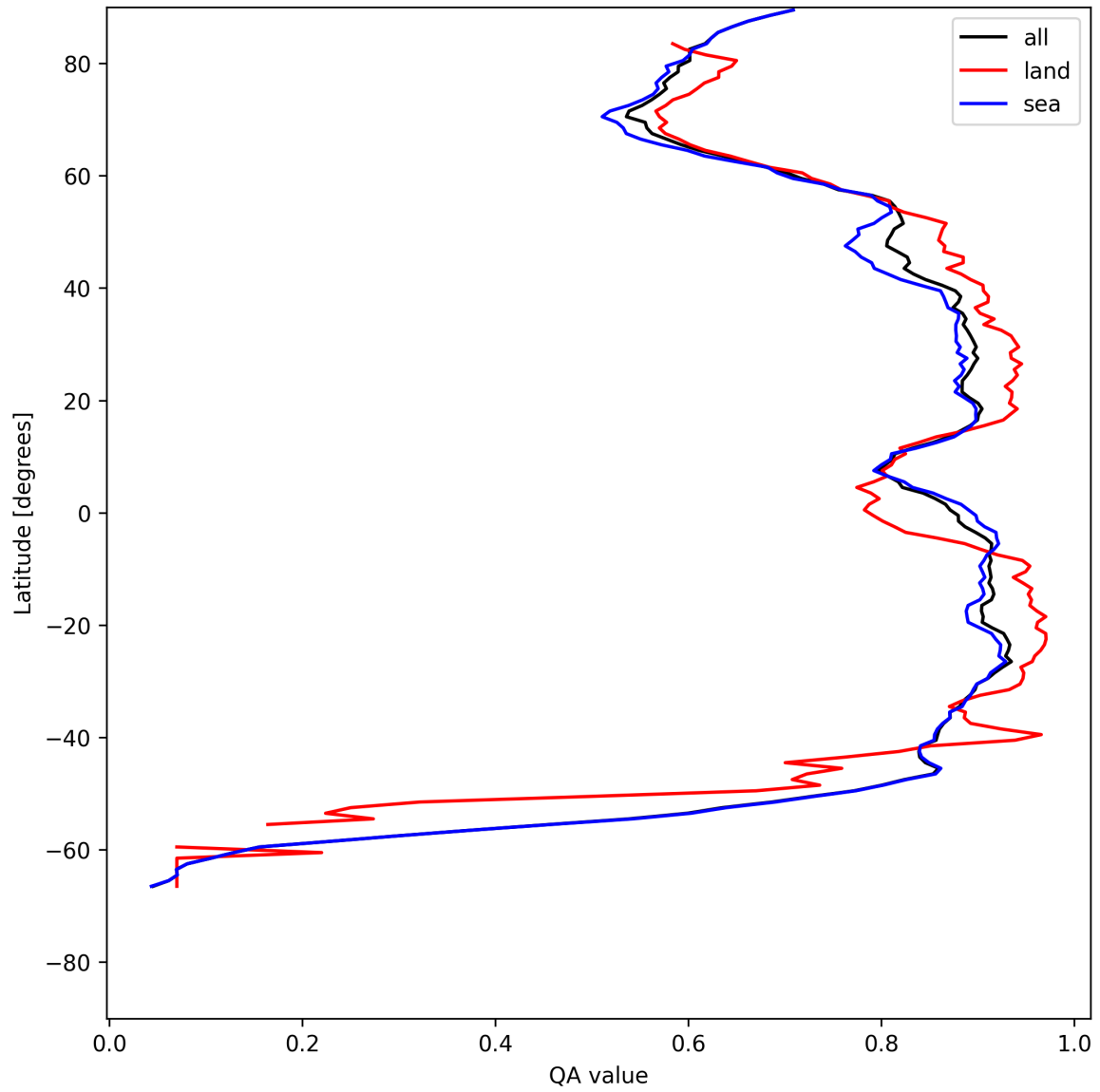
Figure 11: Zonal average of “QA value” for 2025-07-15 to 2025-07-17.
