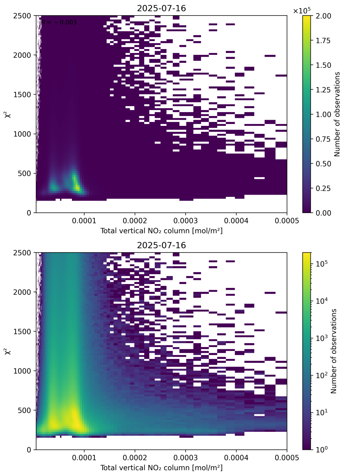
Figure 111: Scatter density plot of “Total vertical NO 2 column” against “ \chi^2 ” for 2025-07-15 to 2025-07-17.
