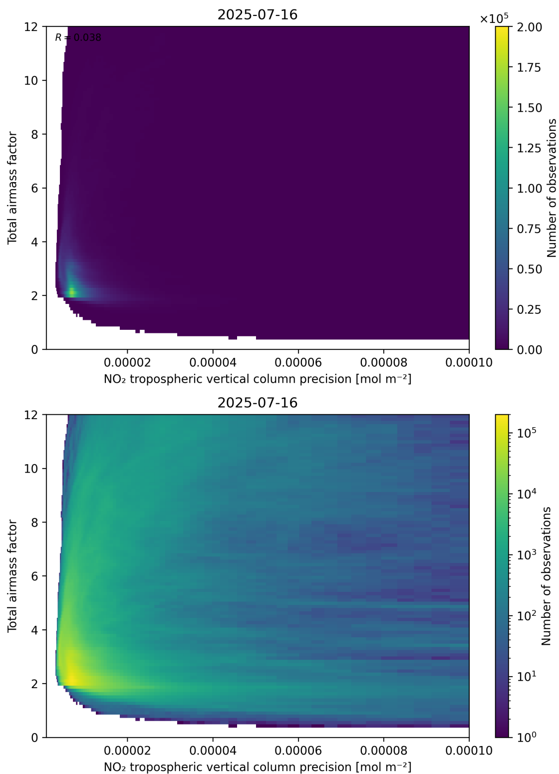
Figure 132: Scatter density plot of “NO 2 tropospheric vertical column precision” against “Total air mass factor” for 2025-07-15 to 2025-07-17.
