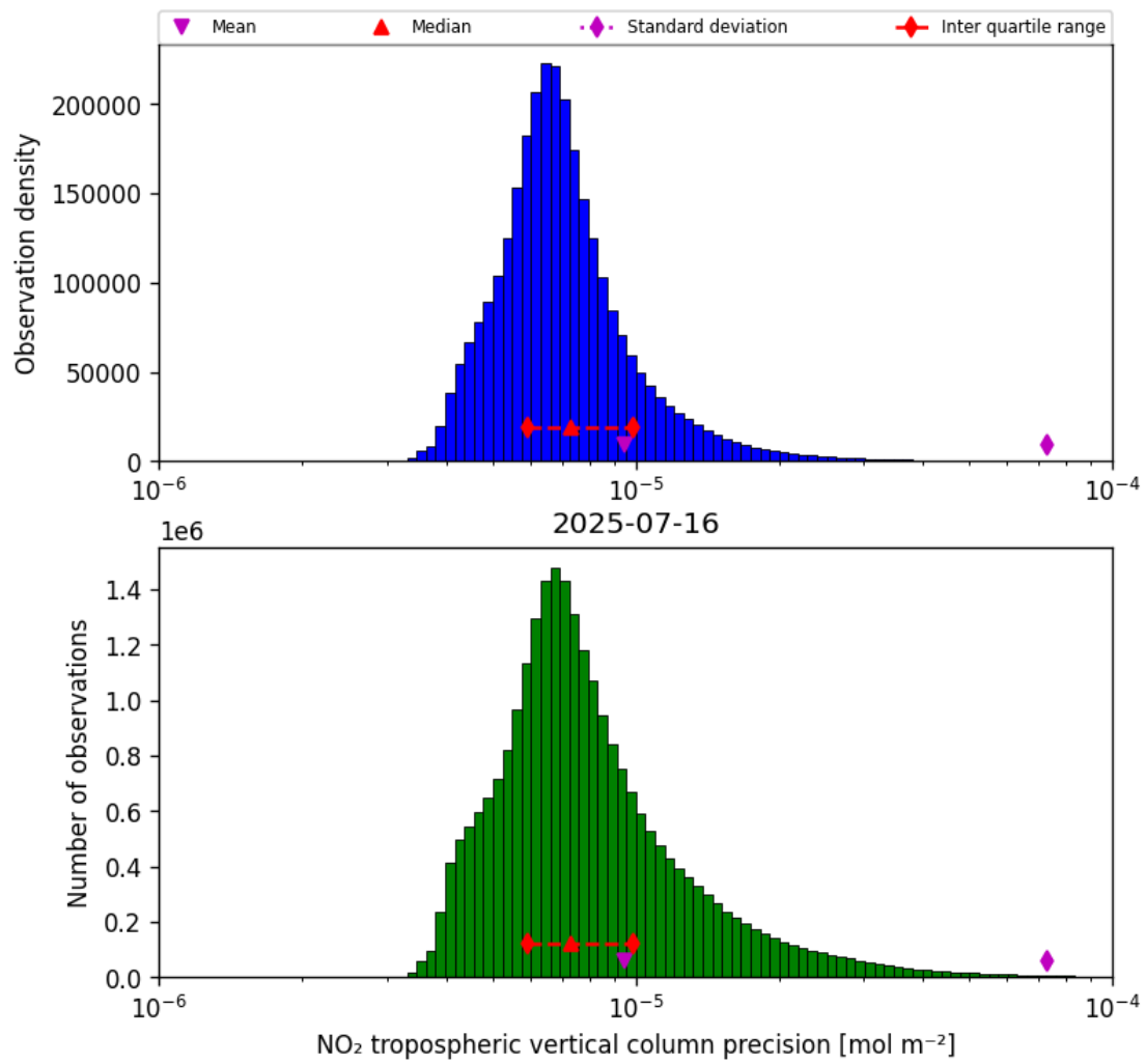
Figure 30: Histogram of “NO 2 tropospheric vertical column precision” for 2025-07-15 to 2025-07-17
