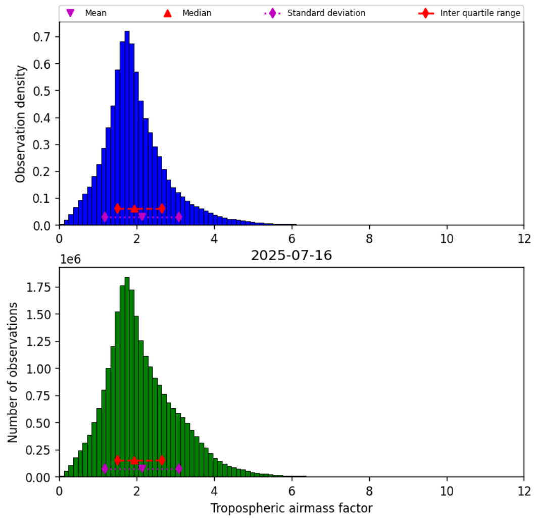
Figure 31: Histogram of “Tropospheric airmass factor” for 2025-07-15 to 2025-07-17
