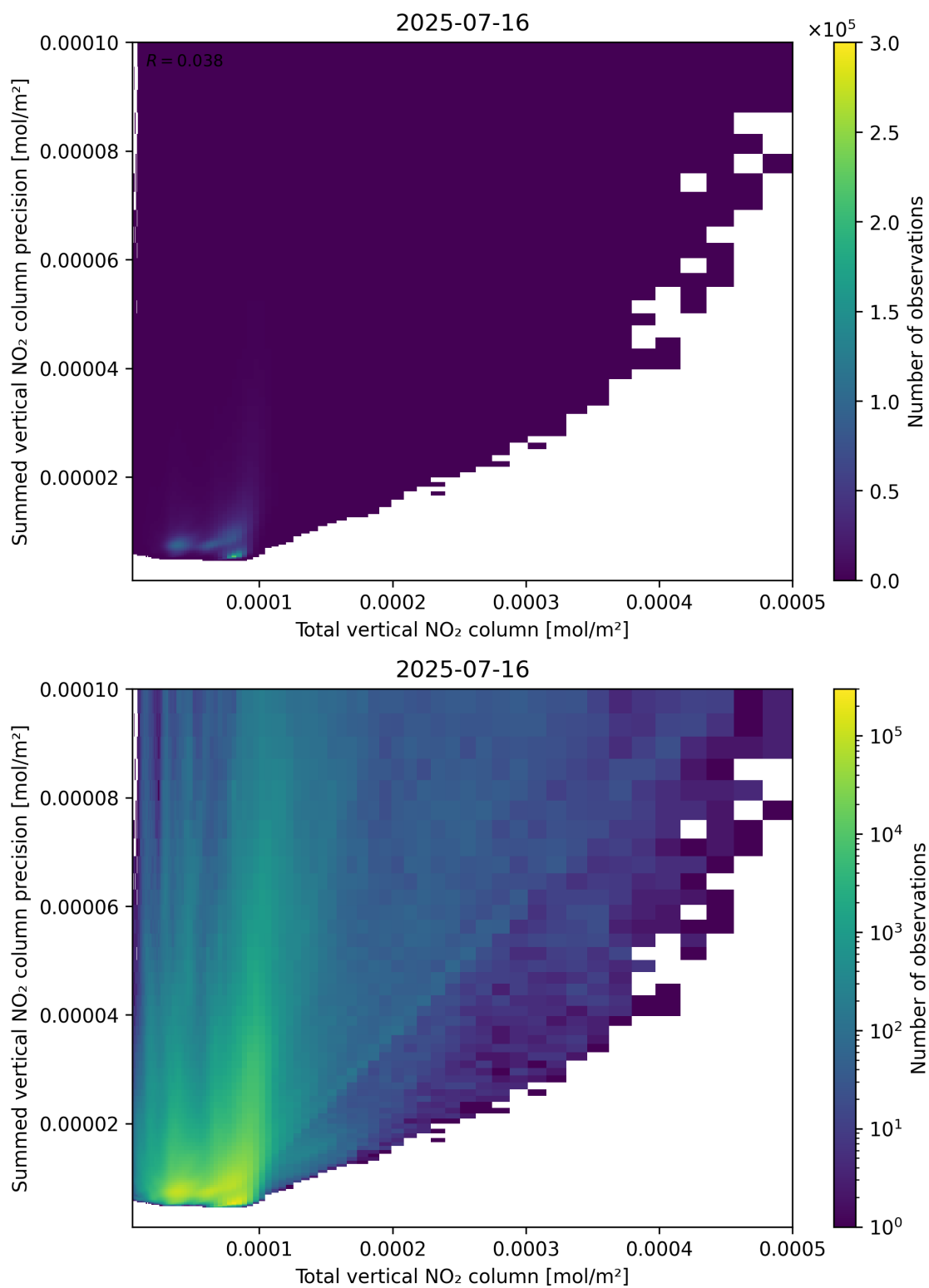
Figure 113: Scatter density plot of “Total vertical NO 2 column” against “Summed vertical NO 2 column precision” for 2025-07-15 to 2025-07-17.
