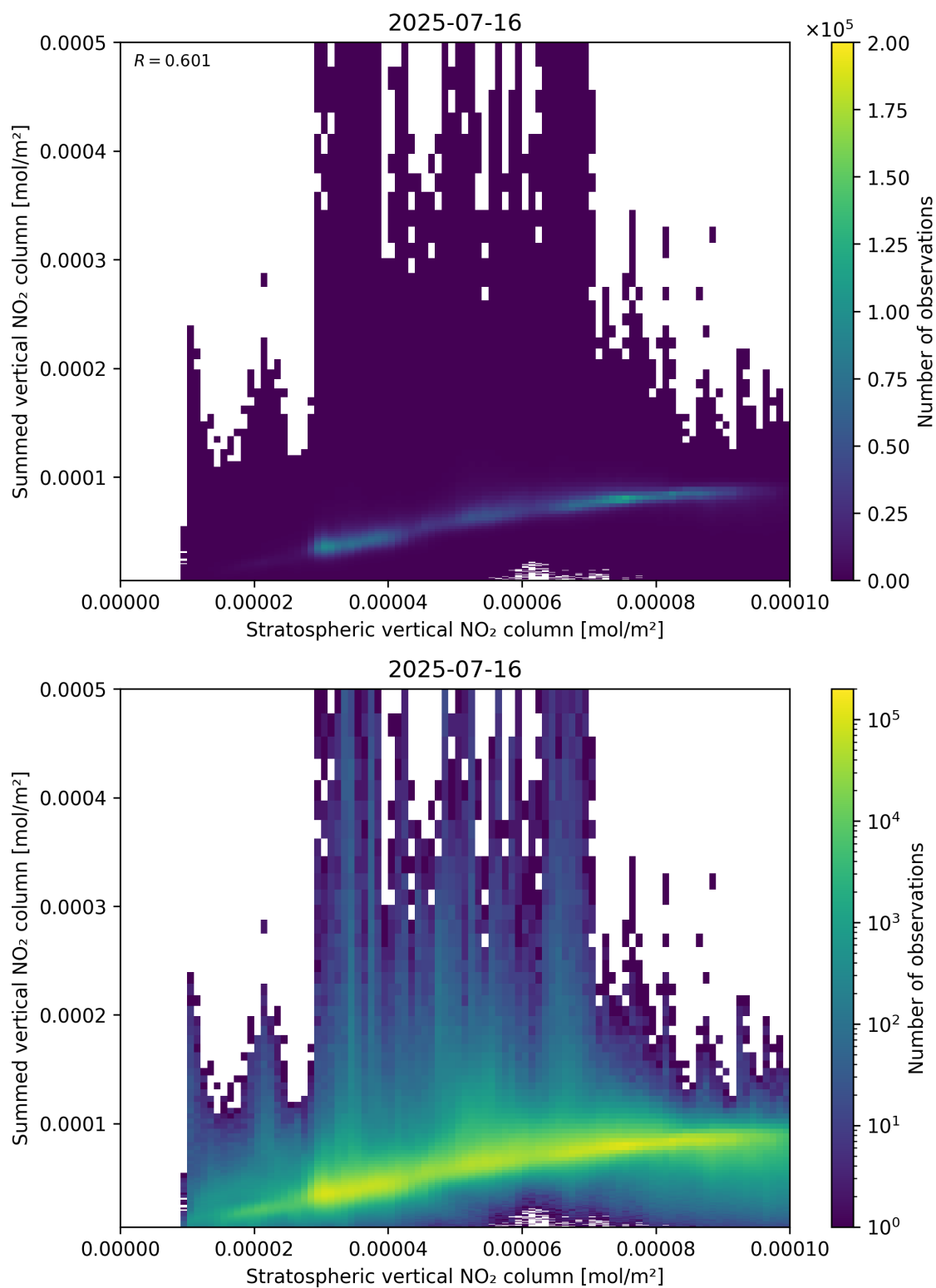
Figure 98: Scatter density plot of “Stratospheric vertical NO 2 column” against “Summed vertical NO 2 column” for 2025-07-15 to 2025-07-17.
