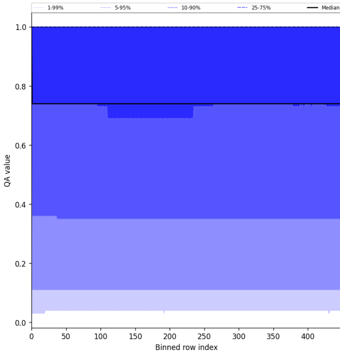
Figure 45: Along track statistics of “QA value” for 2025-07-15 to 2025-07-17
