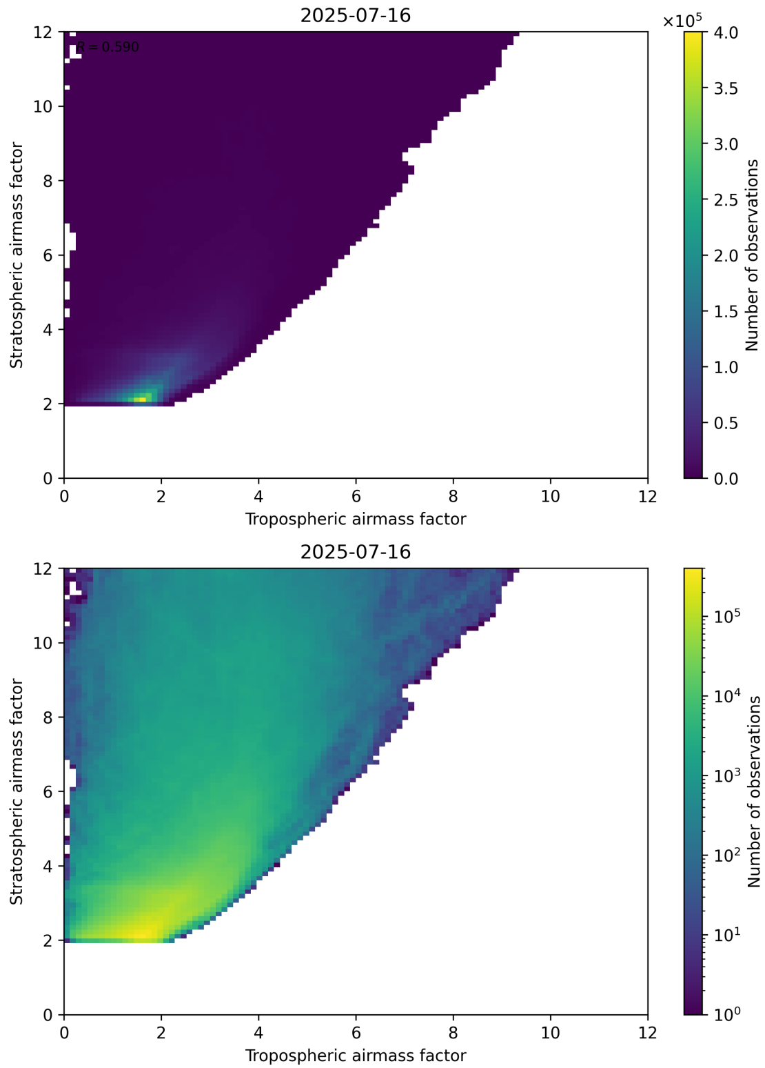
Figure 71: Scatter density plot of “Tropospheric airmass factor” against “Stratospheric airmass factor” for 2025-07-15 to 2025-07-17.
