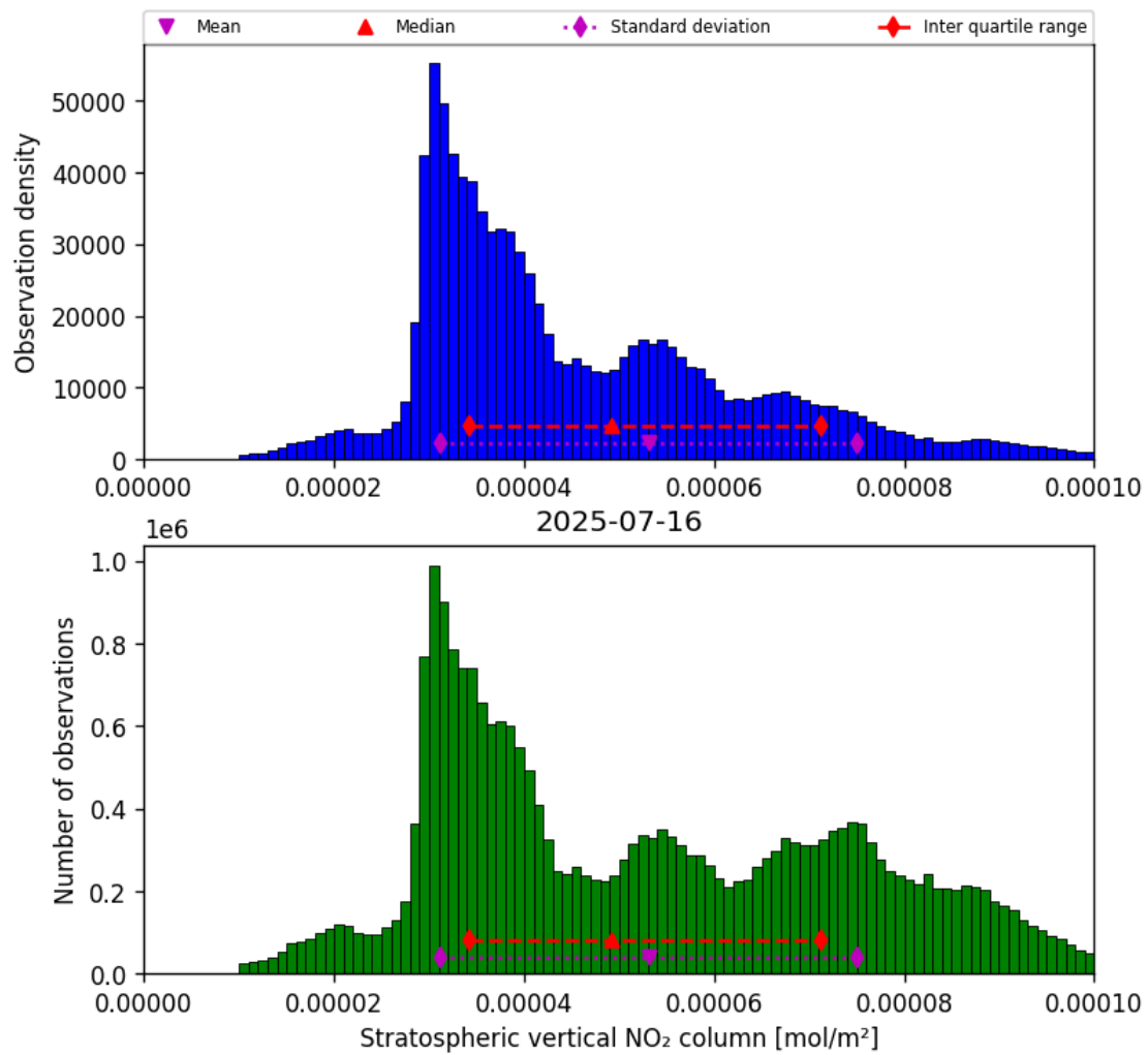
Figure 36: Histogram of “Stratospheric vertical NO 2 column” for 2025-07-15 to 2025-07-17
