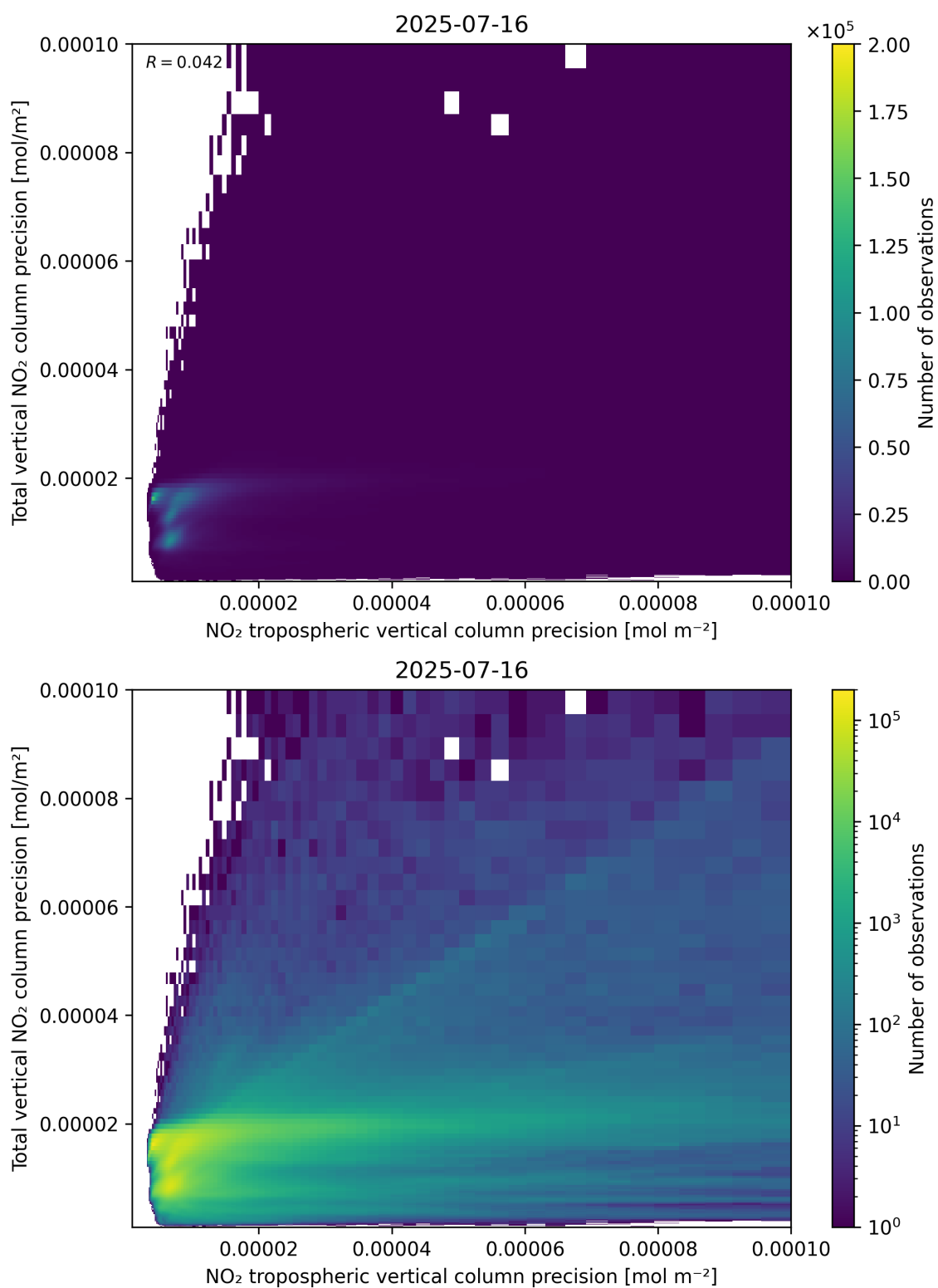
Figure 139: Scatter density plot of “NO 2 tropospheric vertical column precision” against “Total vertical NO 2 column precision” for 2025-07-15 to 2025-07-17.
