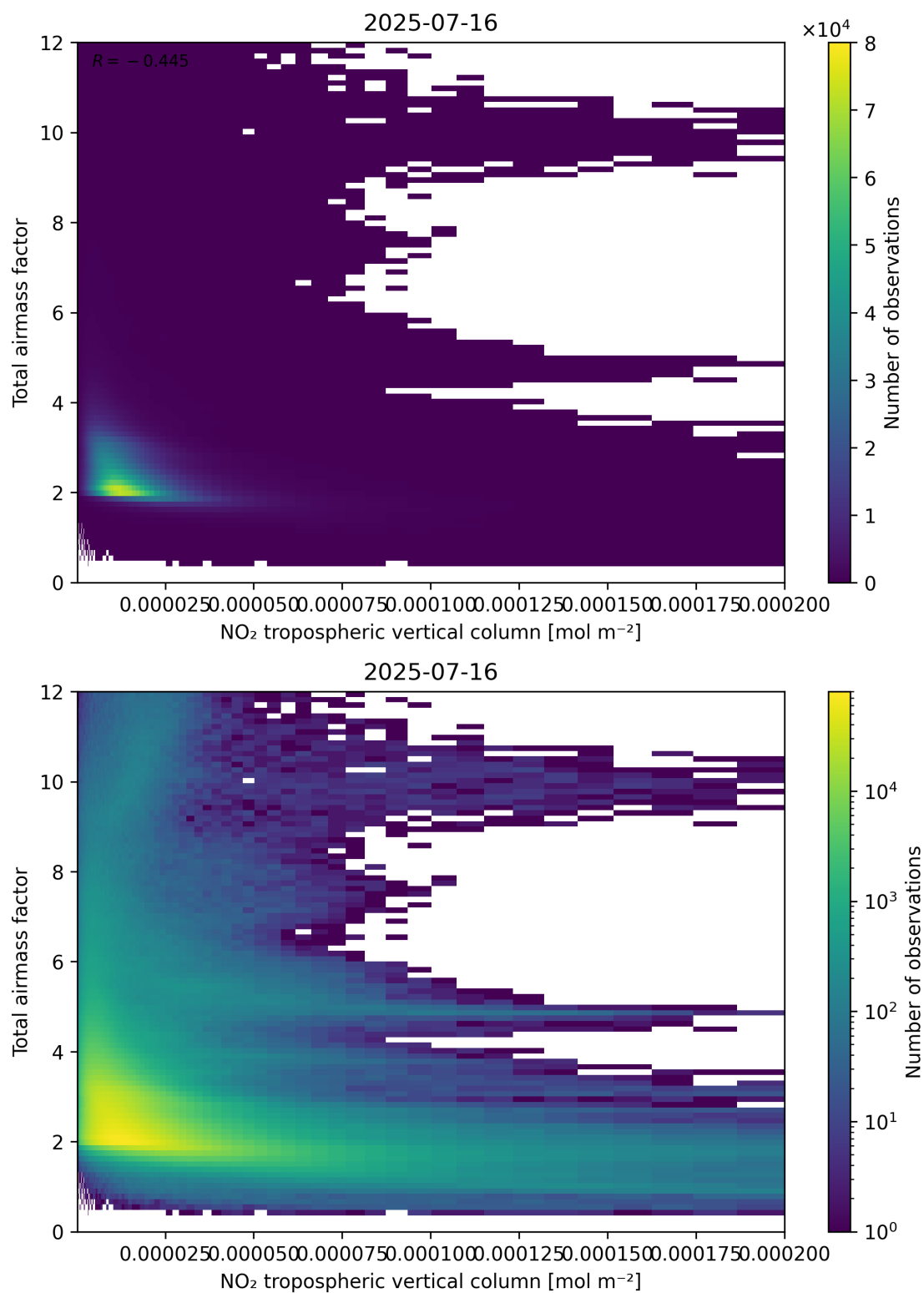
Figure 122: Scatter density plot of “NO 2 tropospheric vertical column” against “Total air mass factor” for 2025-07-15 to 2025-07-17.
