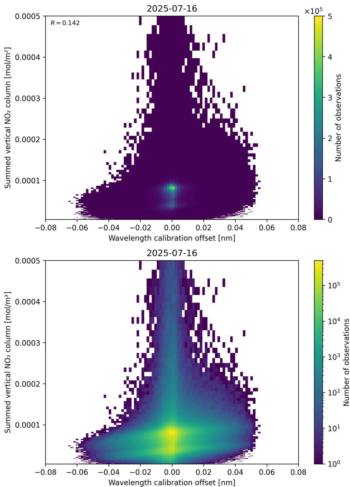
Figure 177: Scatter density plot of “Wavelength calibration offset” against “Summed vertical NO 2 column” for 2025-07-15 to 2025-07-17.
