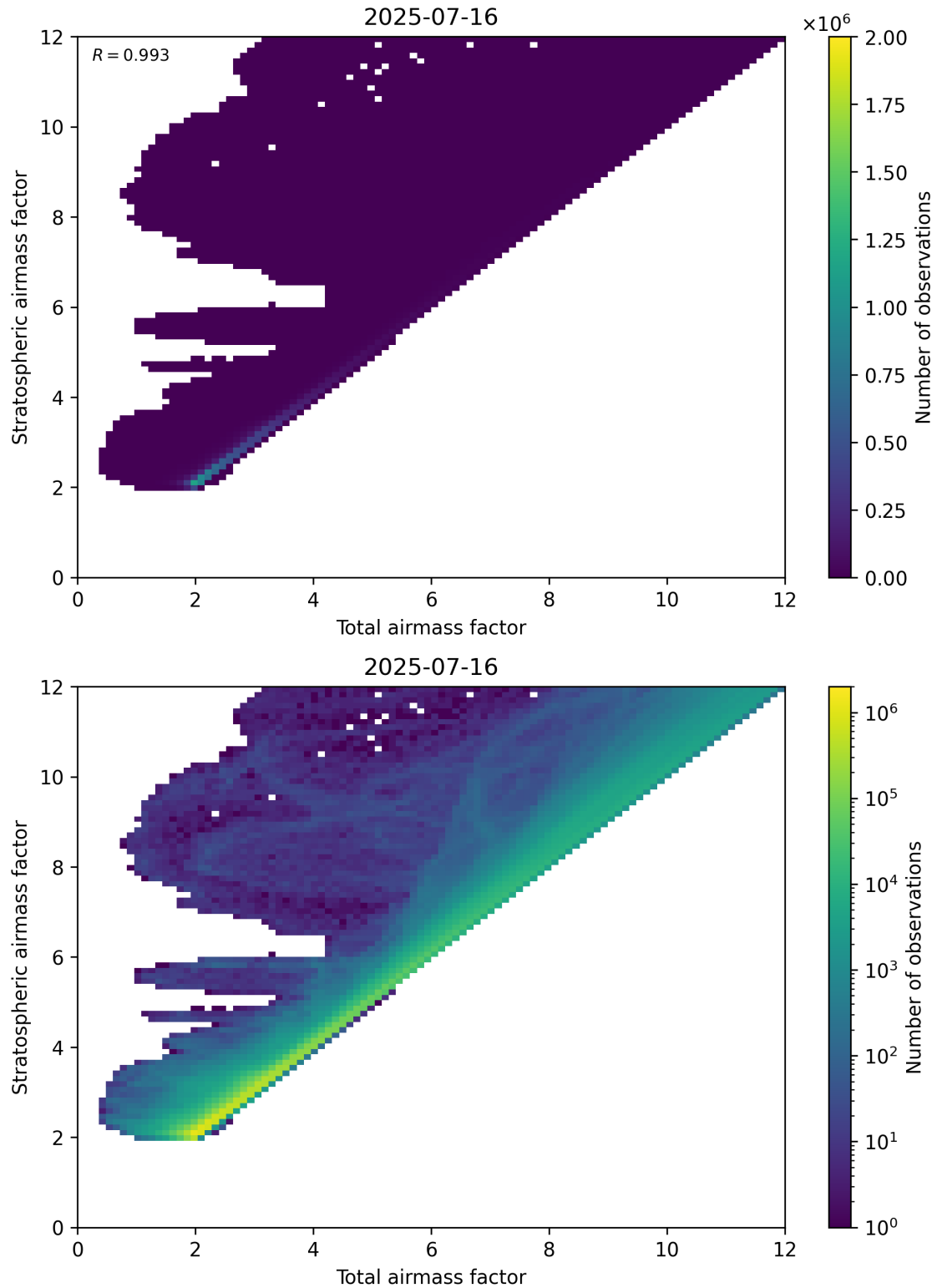
Figure 62: Scatter density plot of “Total airmass factor” against “Stratospheric airmass factor” for 2025-07-15 to 2025-07-17.
