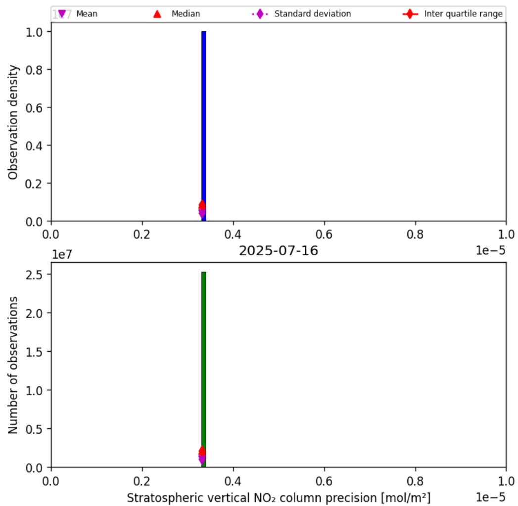
Figure 37: Histogram of “Stratospheric vertical NO 2 column precision” for 2025-07-15 to 2025-07-17
