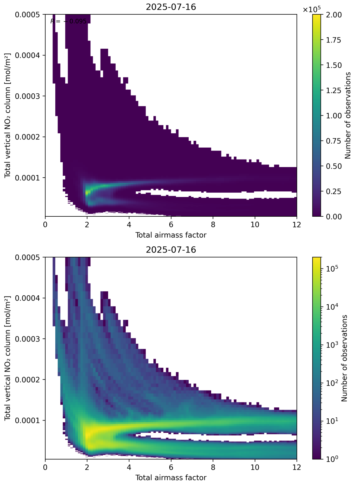
Figure 67: Scatter density plot of “Total airmass factor” against “Total vertical NO 2 column” for 2025-07-15 to 2025-07-17.
