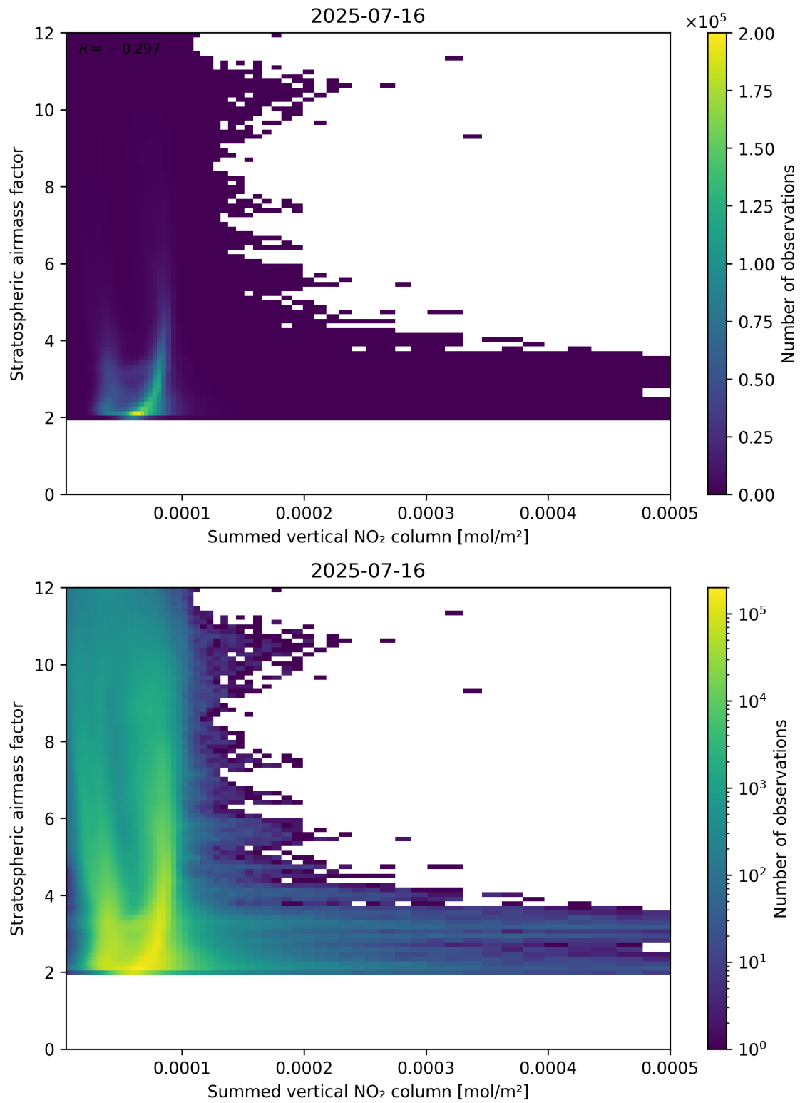
Figure 103: Scatter density plot of “Summed vertical NO 2 column” against “Stratospheric air mass factor” for 2025-07-15 to 2025-07-17.
