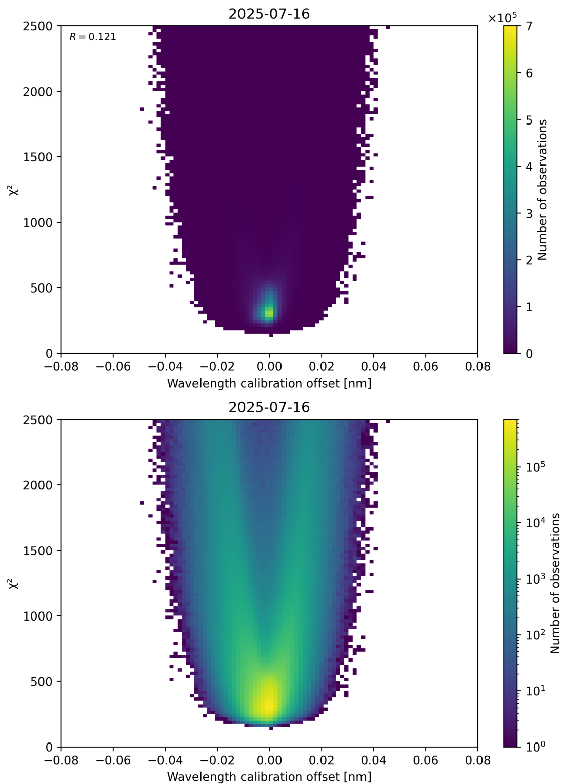
Figure 175: Scatter density plot of “Wavelength calibration offset” against “ \chi^2 ” for 2025-07-15 to 2025-07-17.
