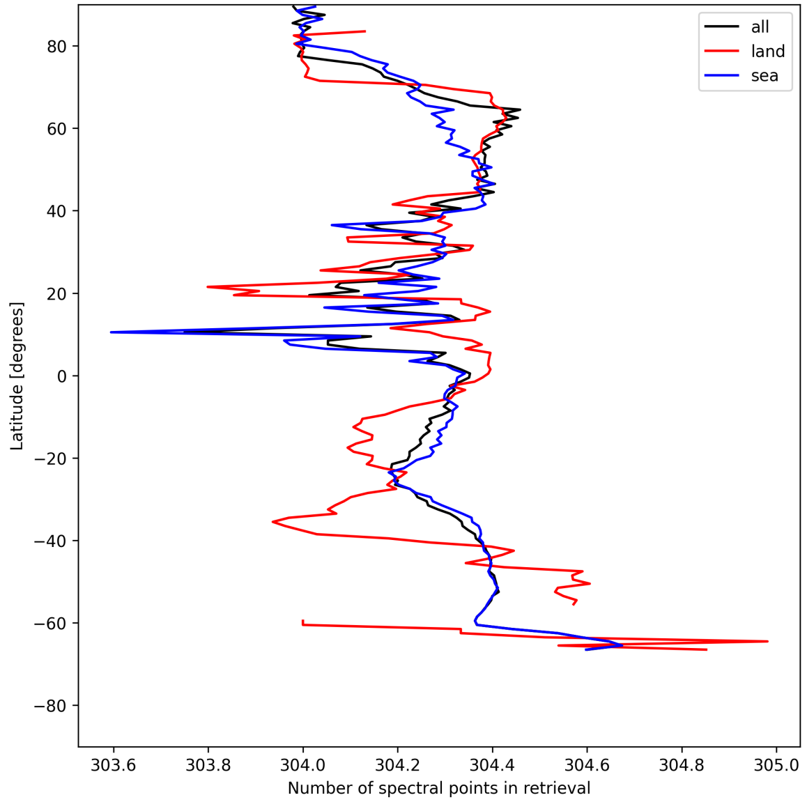
Figure 16: Zonal average of “Number of spectral points in retrieval” for 2025-07-15 to 2025-07-17.
