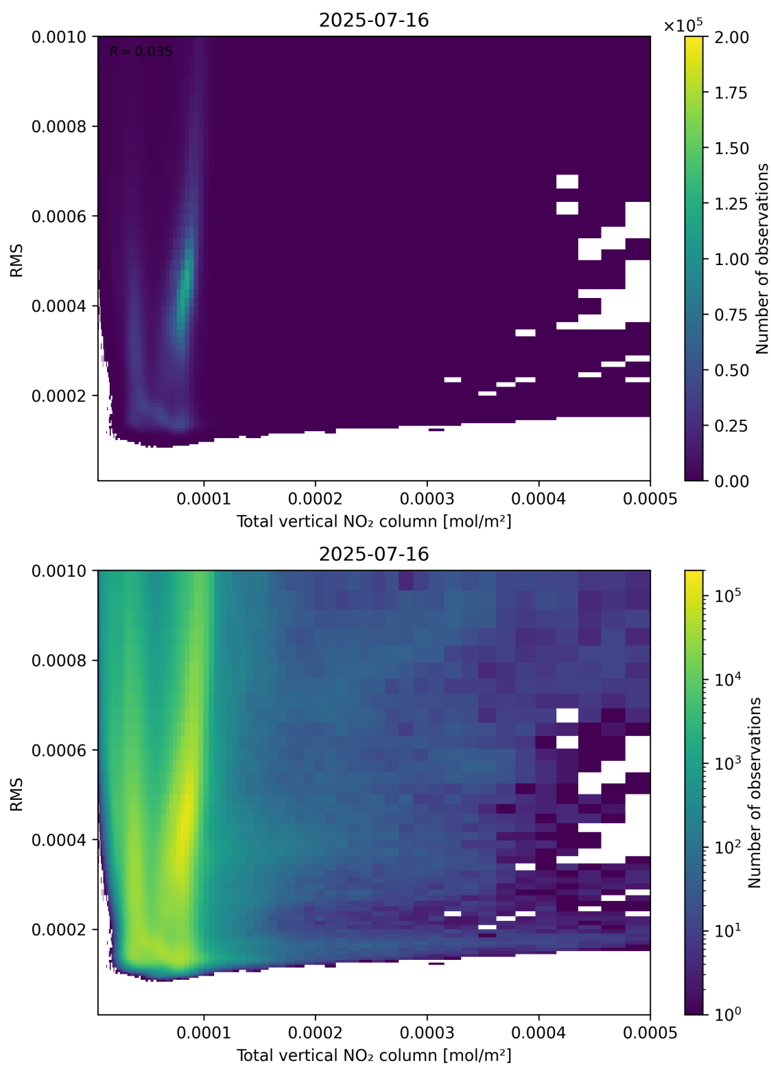
Figure 120: Scatter density plot of “Total vertical NO 2 column” against “RMS” for 2025-07-15 to 2025-07-17.
