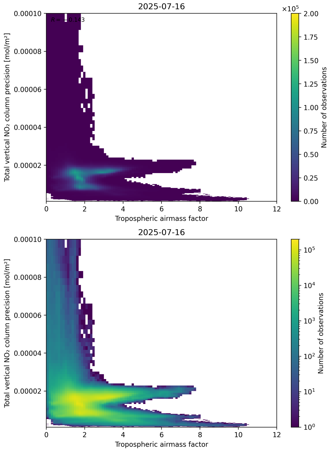
Figure 78: Scatter density plot of “Tropospheric air mass factor” against “Total vertical NO 2 column precision” for 2025-07-15 to 2025-07-17.
