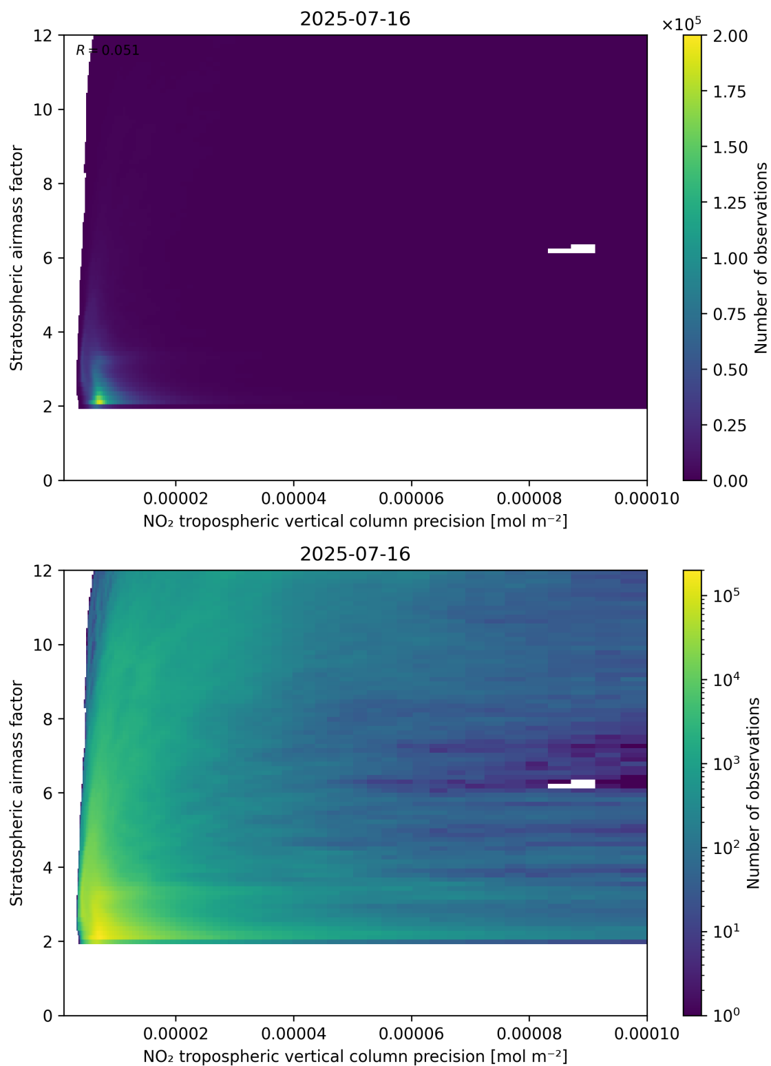
Figure 131: Scatter density plot of “NO 2 tropospheric vertical column precision” against “Stratospheric airmass factor” for 2025-07-15 to 2025-07-17.
