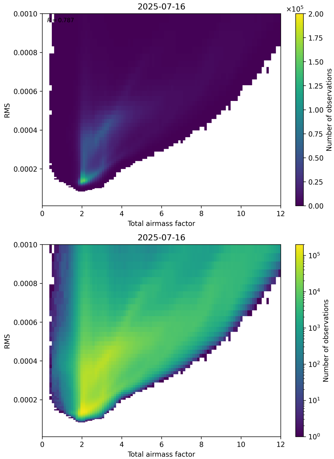
Figure 69: Scatter density plot of “Total airmass factor” against “RMS” for 2025-07-15 to 2025-07-17.
