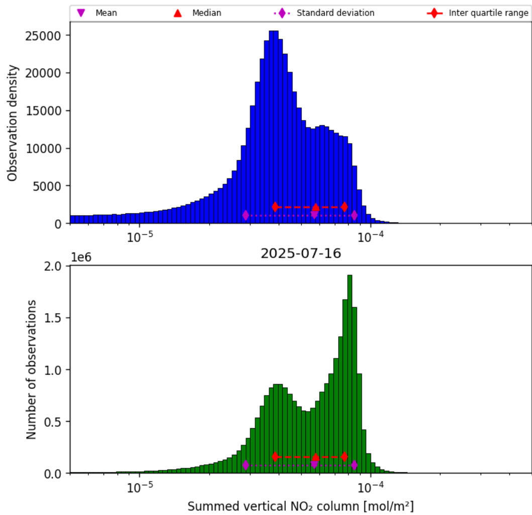
Figure 40: Histogram of “Summed vertical NO 2 column” for 2025-07-15 to 2025-07-17
