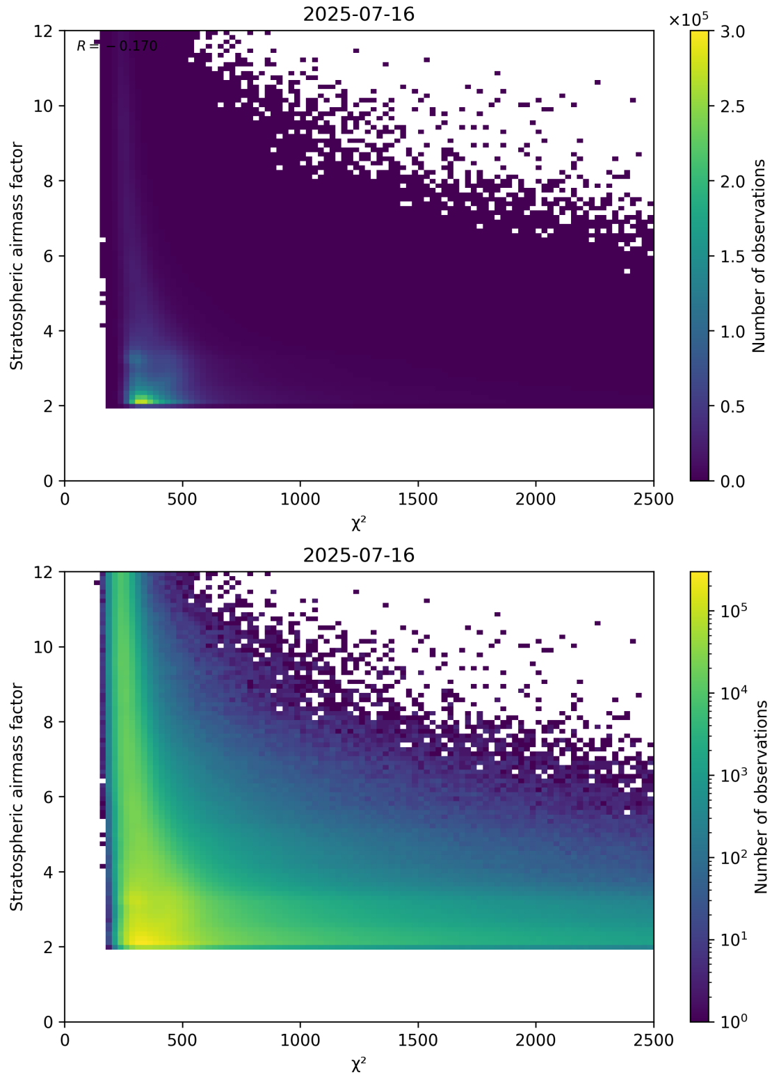
Figure 81: Scatter density plot of “ \chi^2 ” against “Stratospheric airmass factor” for 2025-07-15 to 2025-07-17.
