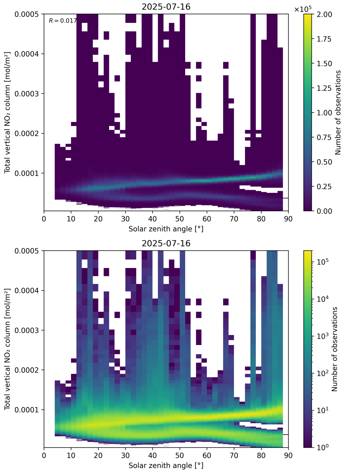
Figure 153: Scatter density plot of “Solar zenith angle” against “Total vertical NO 2 column” for 2025-07-15 to 2025-07-17.
