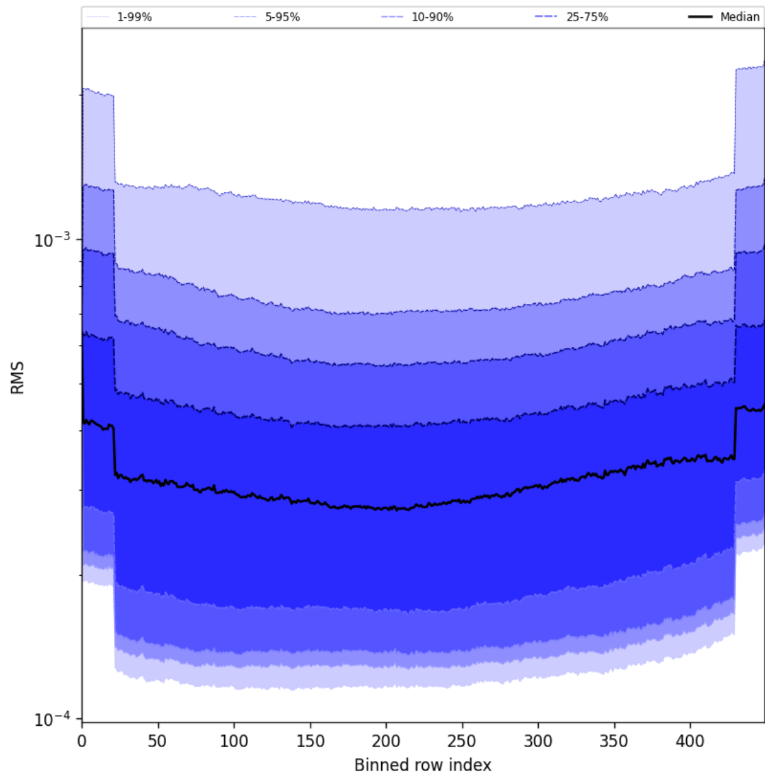
Figure 60: Along track statistics of “RMS” for 2025-07-15 to 2025-07-17
