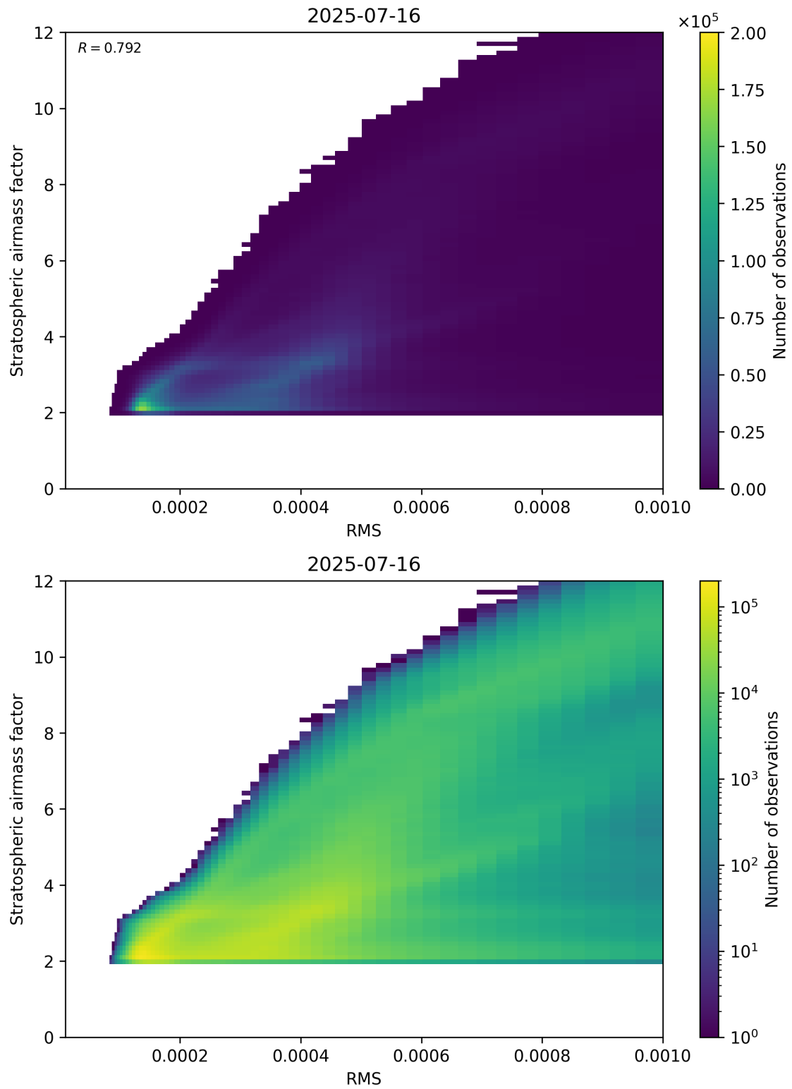
Figure 144: Scatter density plot of “RMS” against “Stratospheric airmass factor” for 2025-07-15 to 2025-07-17.
