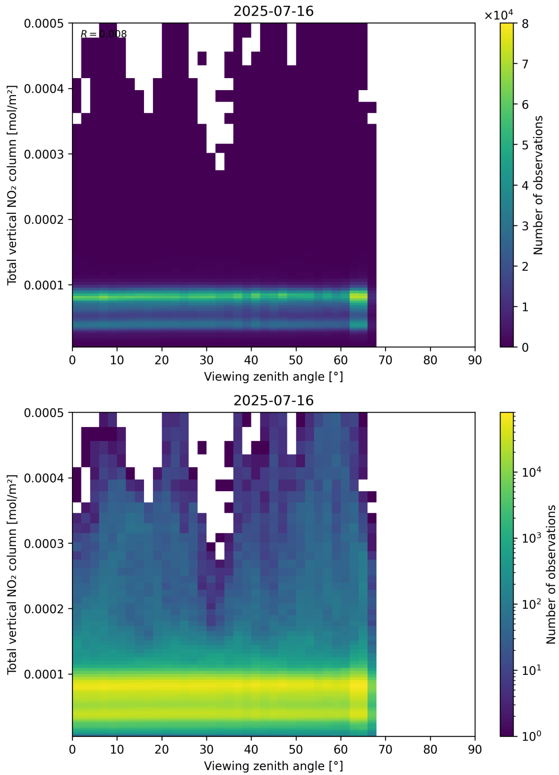
Figure 167: Scatter density plot of “Viewing zenith angle” against “Total vertical NO 2 column” for 2025-07-15 to 2025-07-17.
