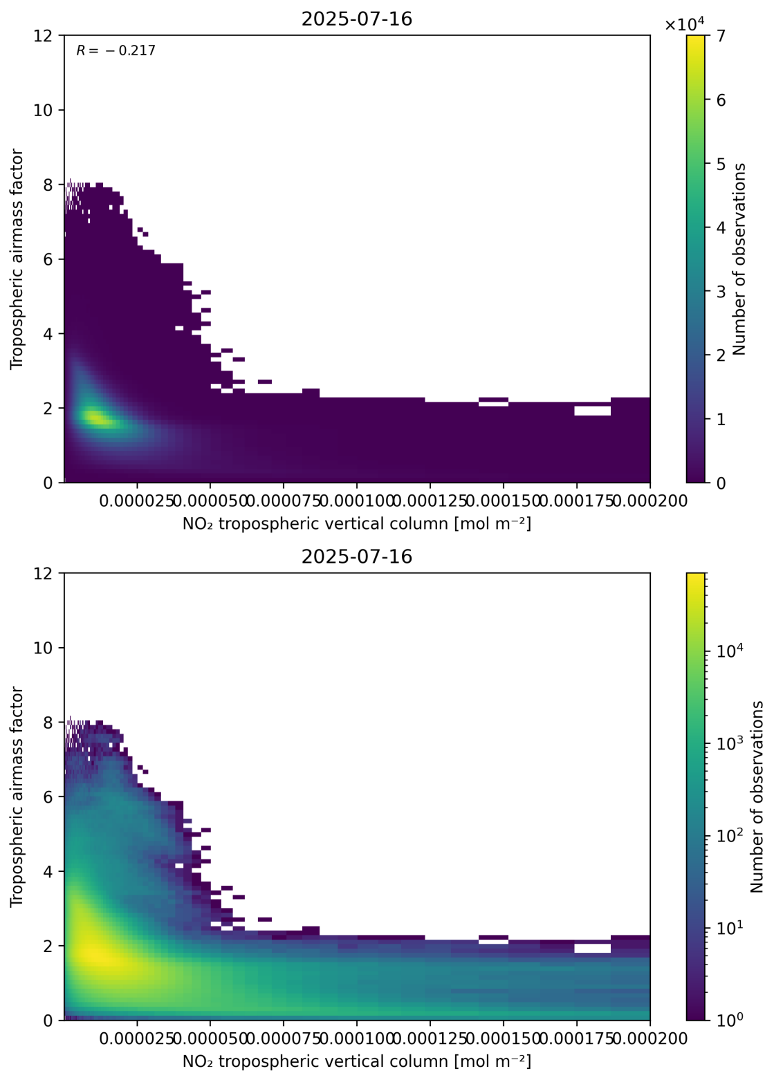
Figure 123: Scatter density plot of “NO 2 tropospheric vertical column” against “Tropospheric air mass factor” for 2025-07-15 to 2025-07-17.
