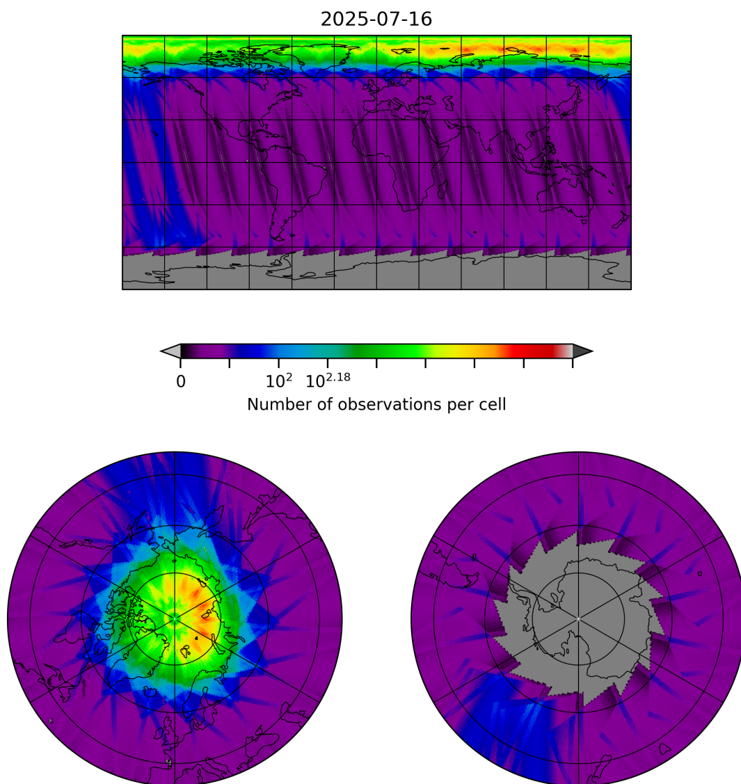
Figure 10: Map of the number of observations for 2025-07-15 to 2025-07-17
