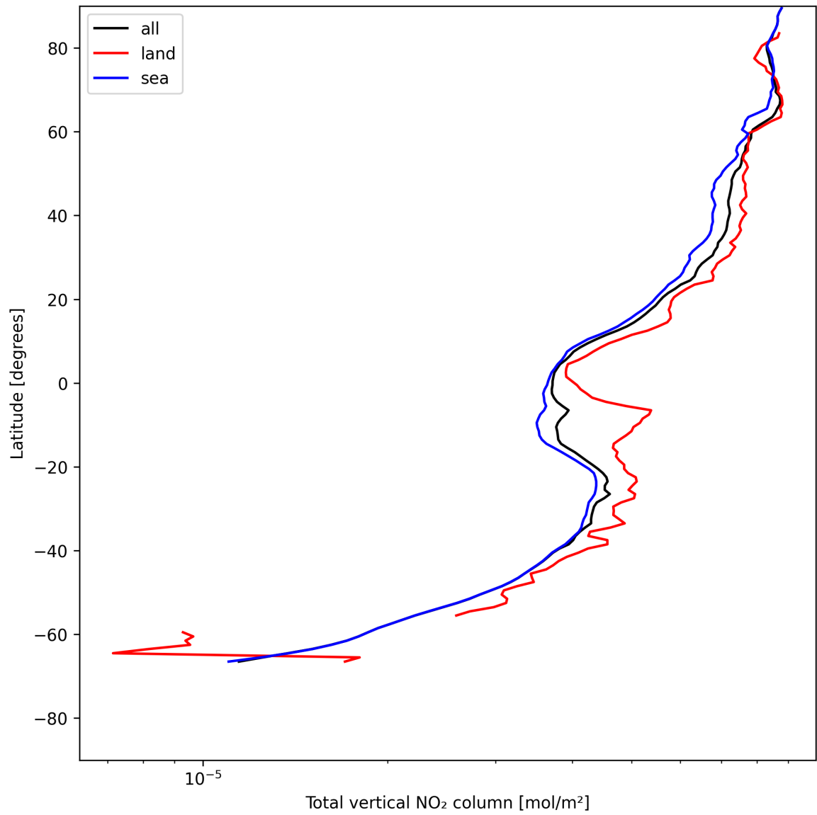
Figure 21: Zonal average of “Total vertical NO 2 column” for 2025-07-15 to 2025-07-17.
