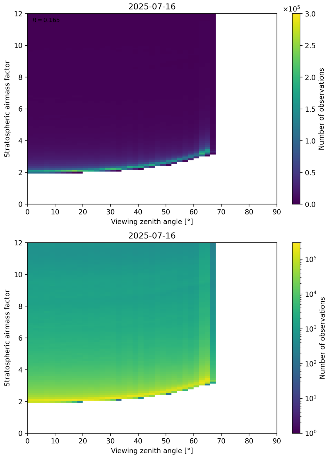
Figure 159: Scatter density plot of “Viewing zenith angle” against “Stratospheric airmass factor” for 2025-07-15 to 2025-07-17.
