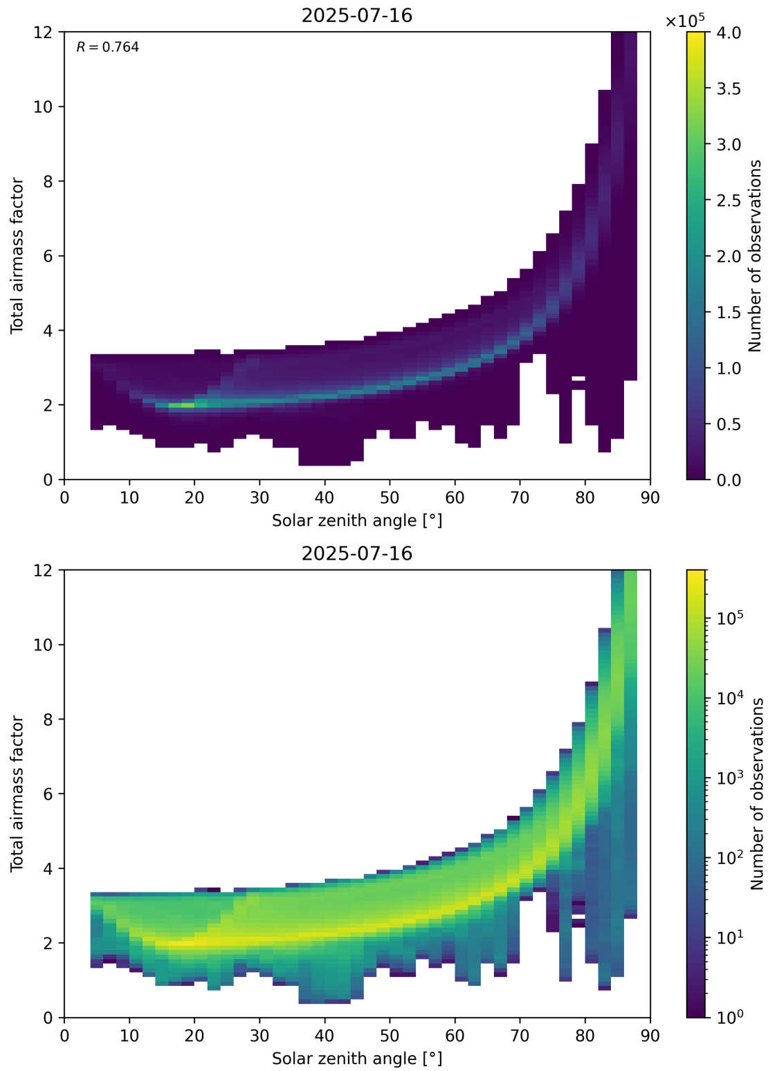
Figure 146: Scatter density plot of “Solar zenith angle” against “Total air mass factor” for 2025-07-15 to 2025-07-17.
