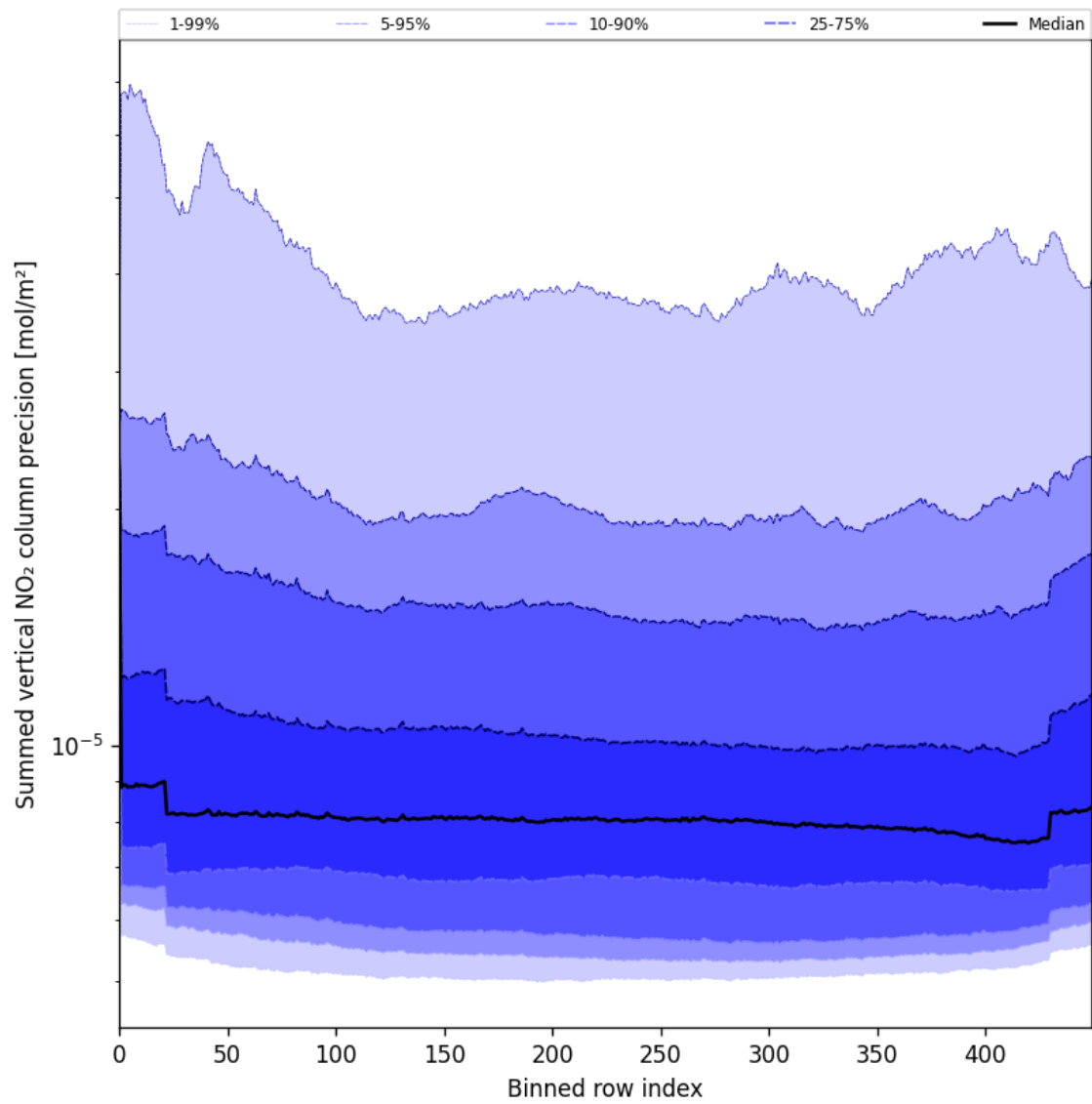
Figure 58: Along track statistics of “Summed vertical NO 2 column precision” for 2025-07-15 to 2025-07-17
