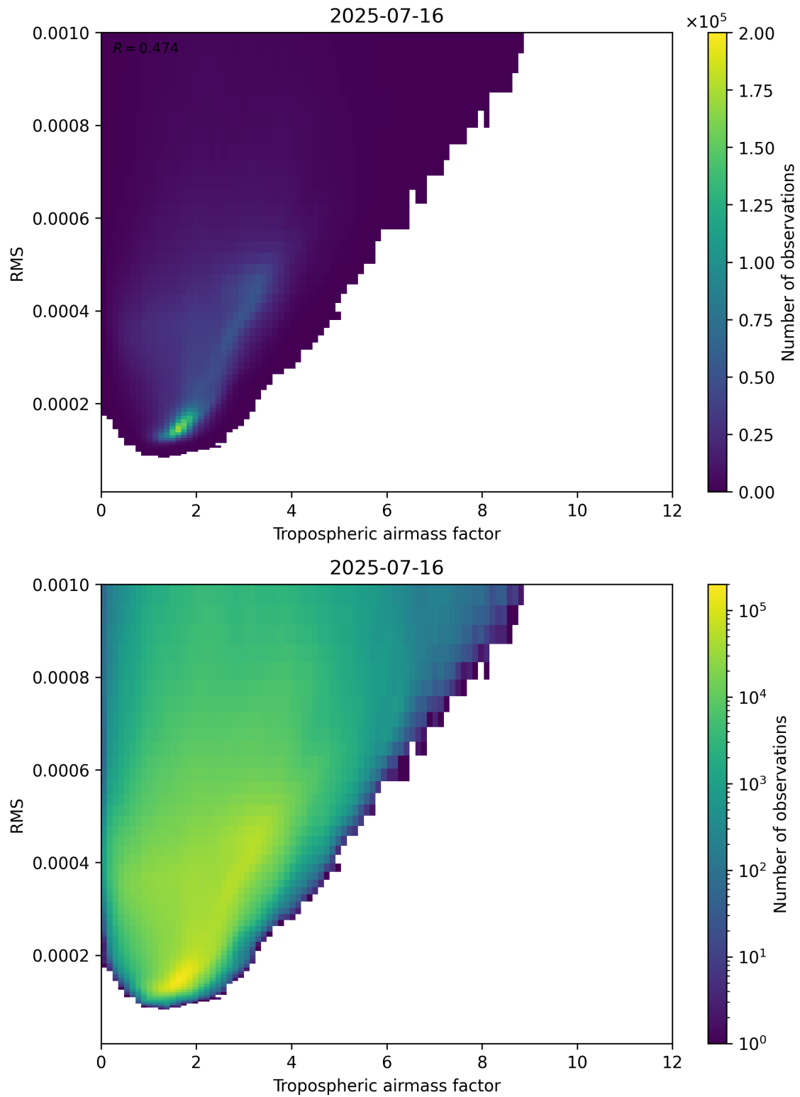
Figure 79: Scatter density plot of “Tropospheric airmass factor” against “RMS” for 2025-07-15 to 2025-07-17.
