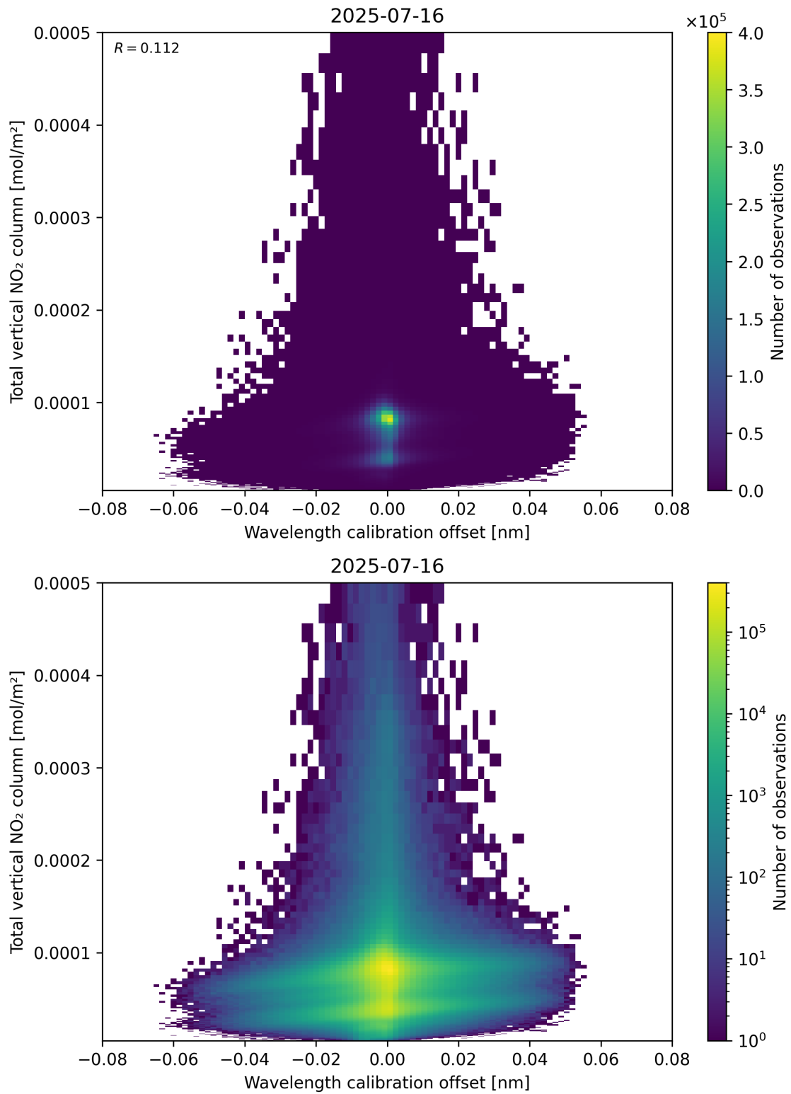
Figure 179: Scatter density plot of “Wavelength calibration offset” against “Total vertical NO 2 column” for 2025-07-15 to 2025-07-17.
