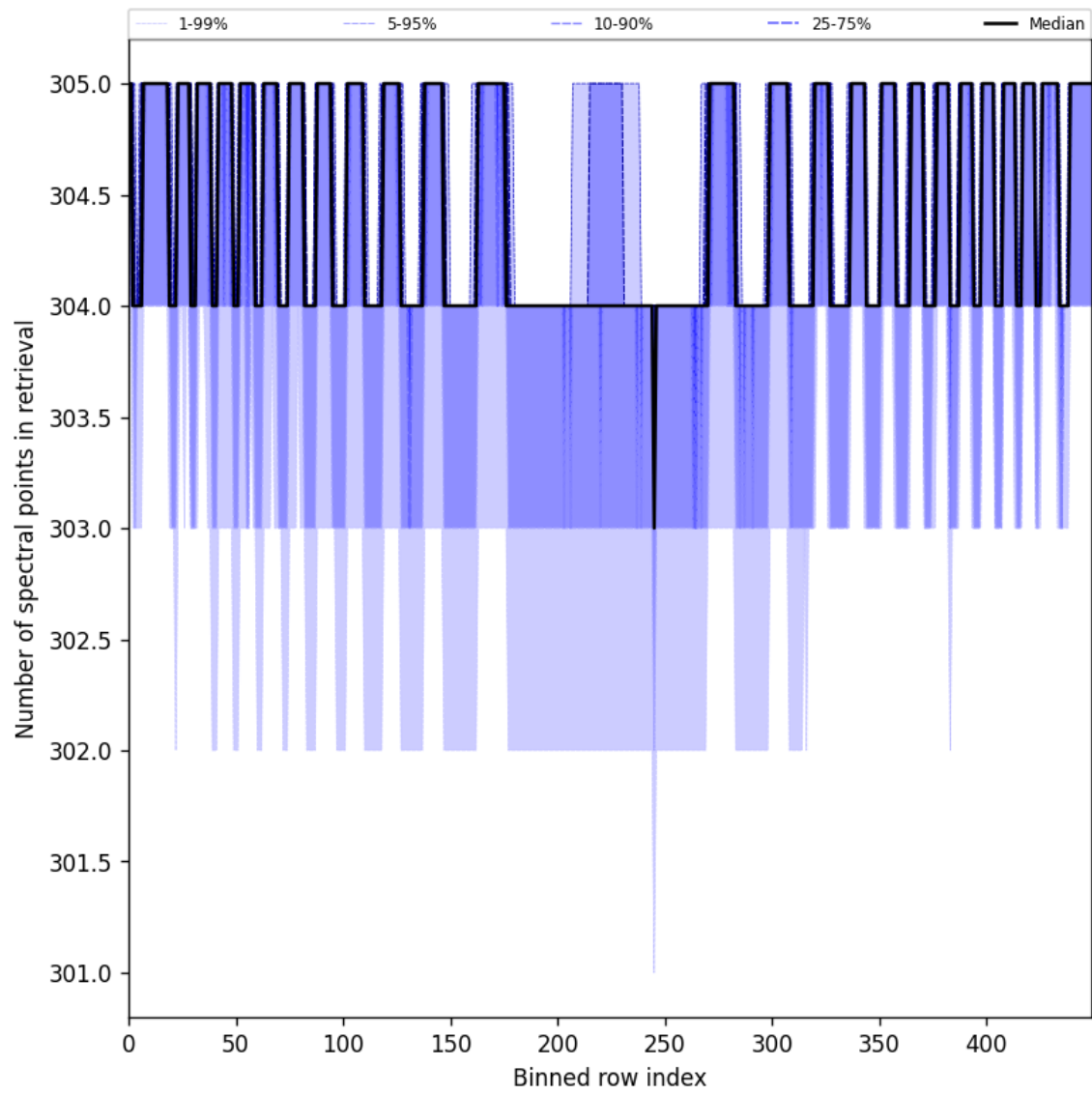
Figure 50: Along track statistics of “Number of spectral points in retrieval” for 2025-07-15 to 2025-07-17
