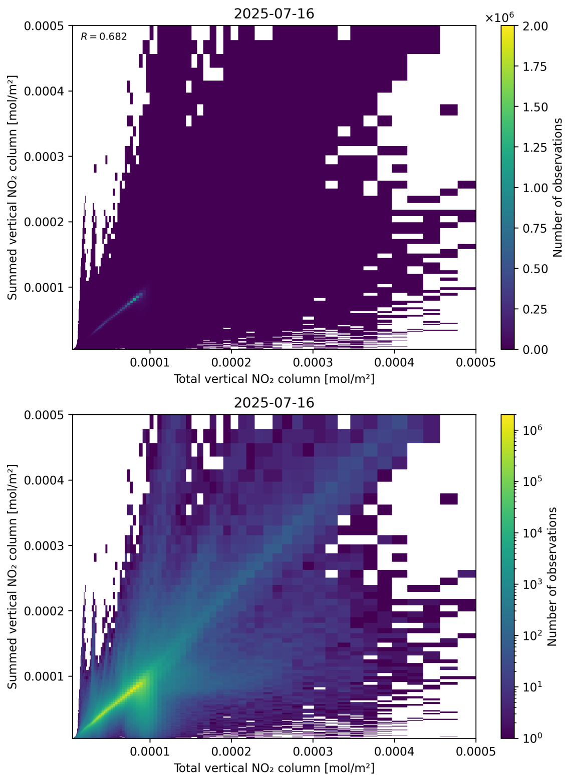
Figure 112: Scatter density plot of “Total vertical NO 2 column” against “Summed vertical NO 2 column” for 2025-07-15 to 2025-07-17.
