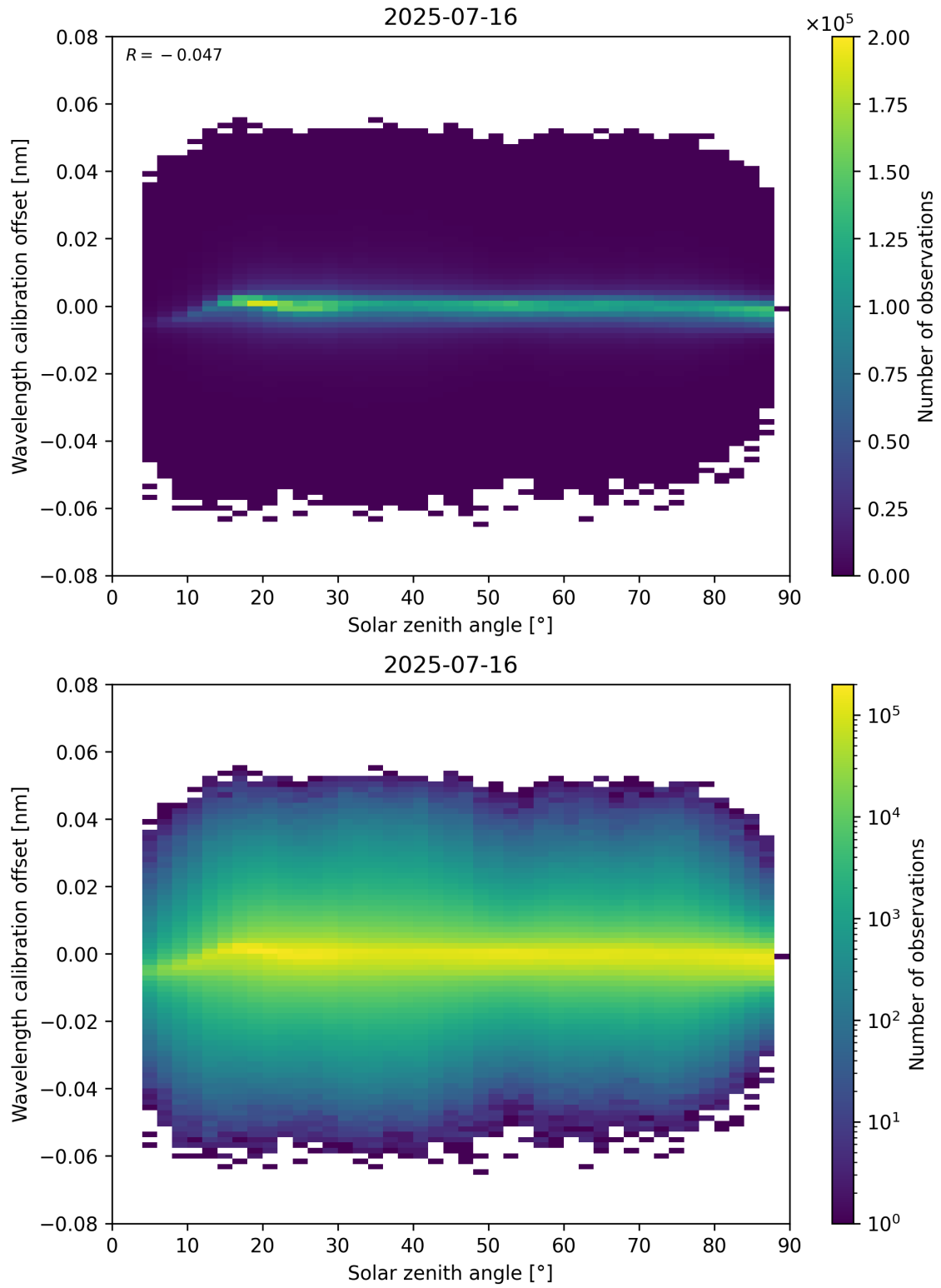
Figure 158: Scatter density plot of “Solar zenith angle” against “Wavelength calibration offset” for 2025-07-15 to 2025-07-17.
