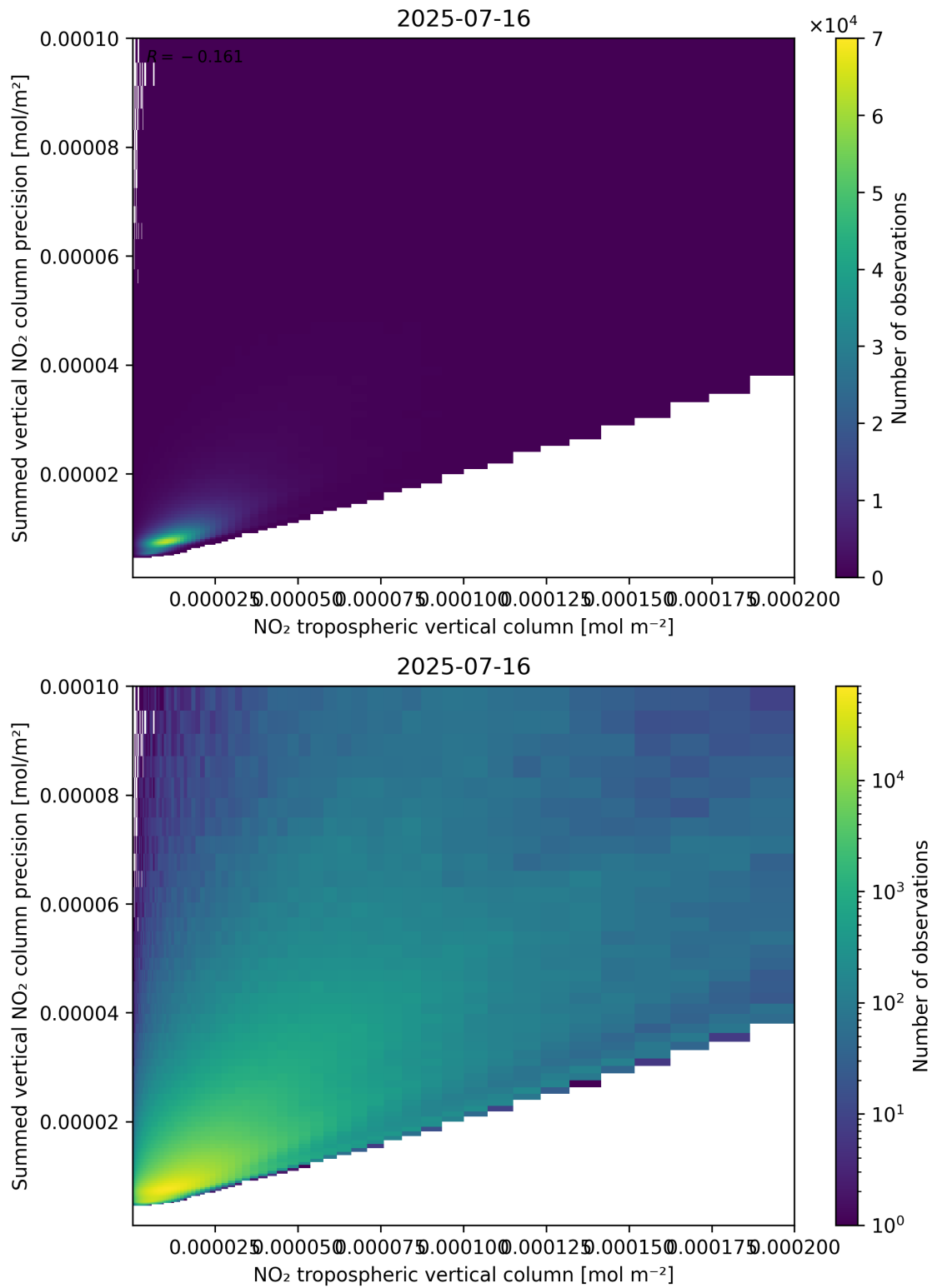
Figure 127: Scatter density plot of “NO 2 tropospheric vertical column” against “Summed vertical NO 2 column precision” for 2025-07-15 to 2025-07-17.
