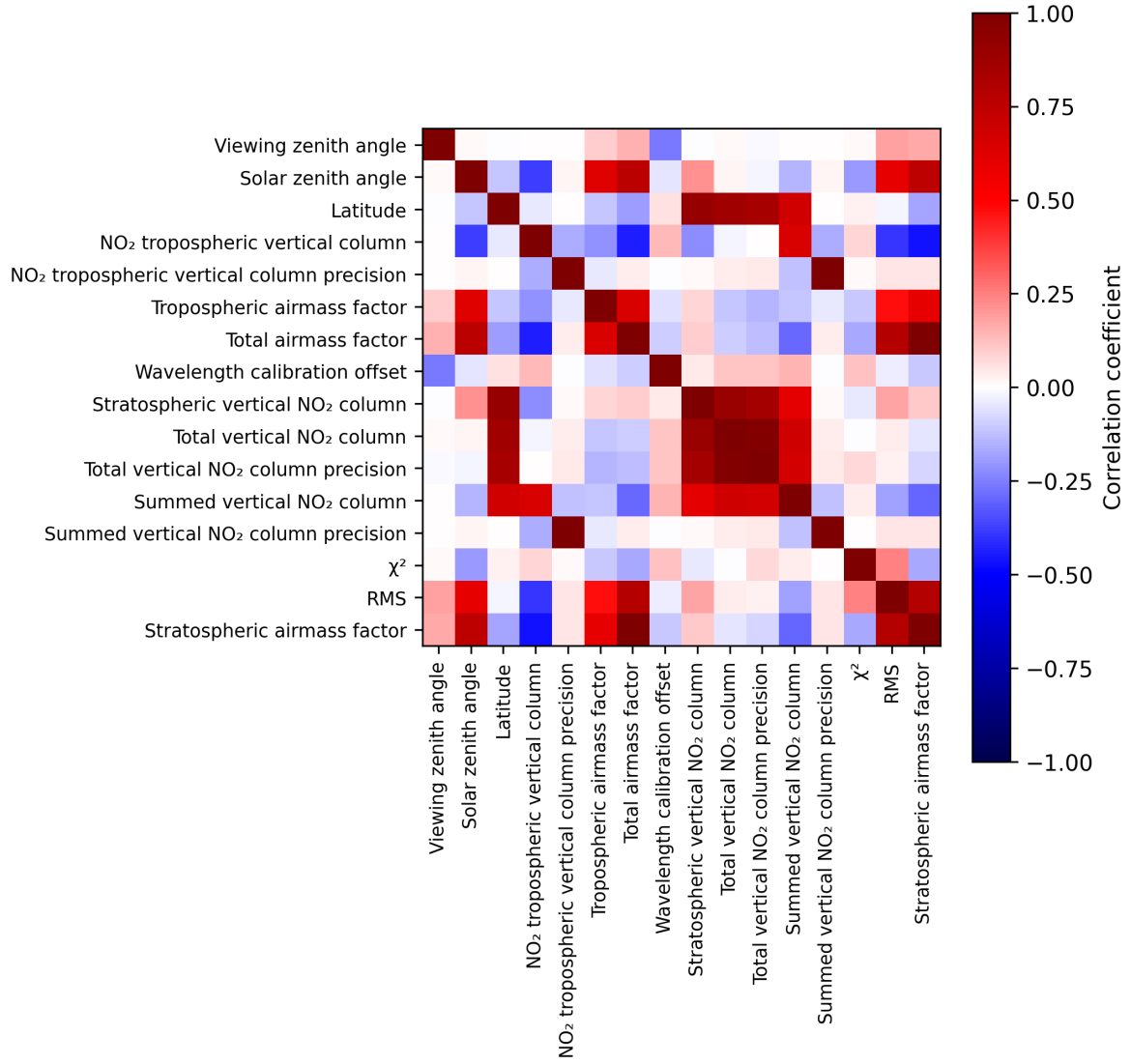
Figure 2: Map of correlation matrix for 2025-07-15 to 2025-07-17.
