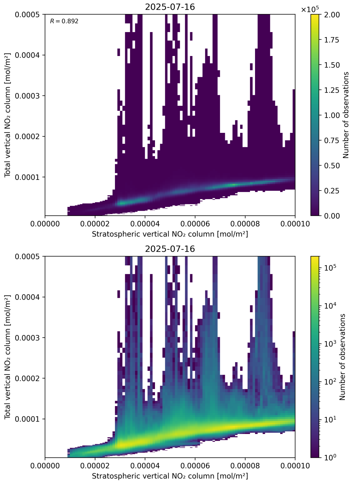
Figure 100: Scatter density plot of “Stratospheric vertical NO 2 column” against “Total vertical NO 2 column” for 2025-07-15 to 2025-07-17.
