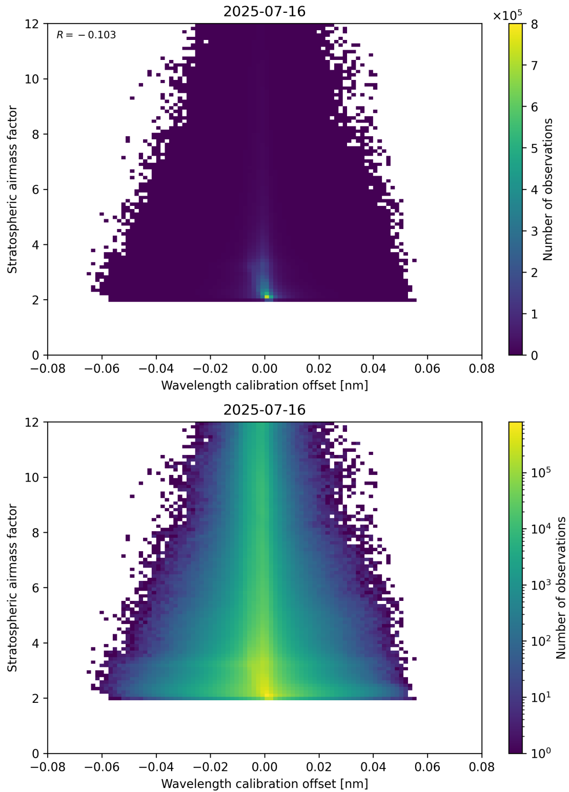
Figure 174: Scatter density plot of “Wavelength calibration offset” against “Stratospheric airmass factor” for 2025-07-15 to 2025-07-17.
