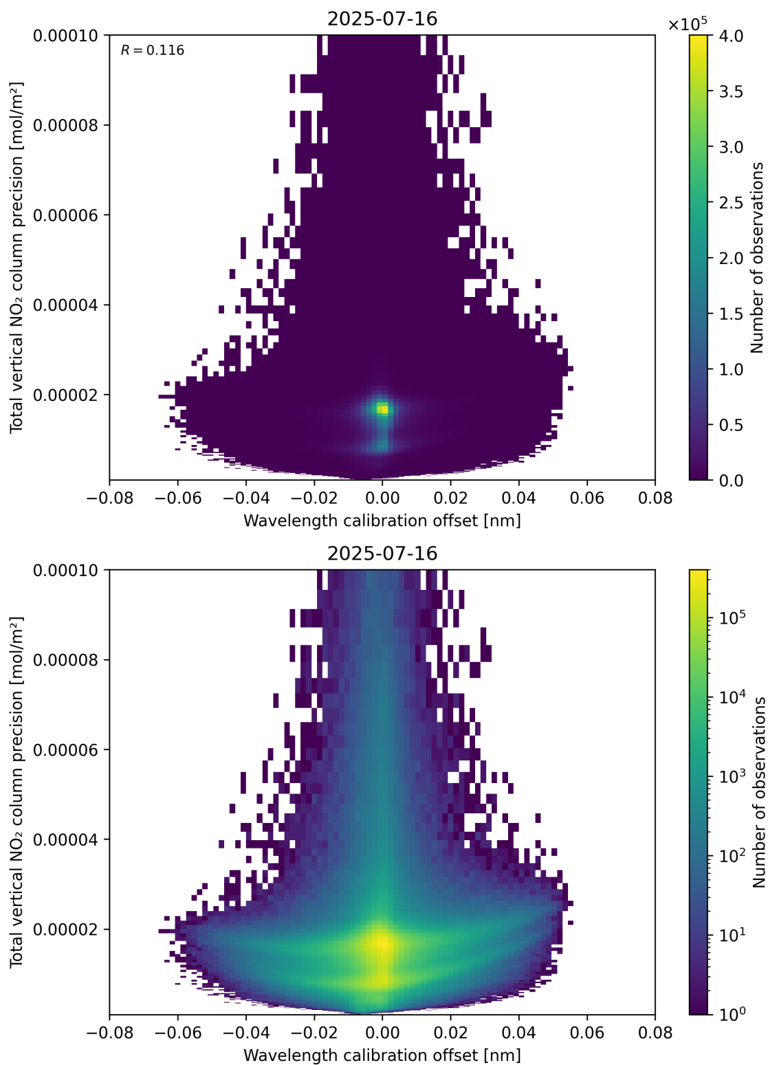
Figure 180: Scatter density plot of “Wavelength calibration offset” against “Total vertical NO 2 column precision” for 2025-07-15 to 2025-07-17.
