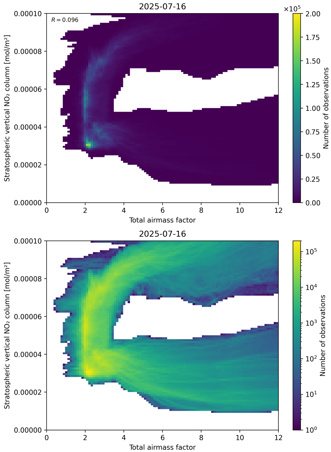
Figure 64: Scatter density plot of “Total airmass factor” against “Stratospheric vertical \text{NO}_2 column” for 2025-07-15 to 2025-07-17.
