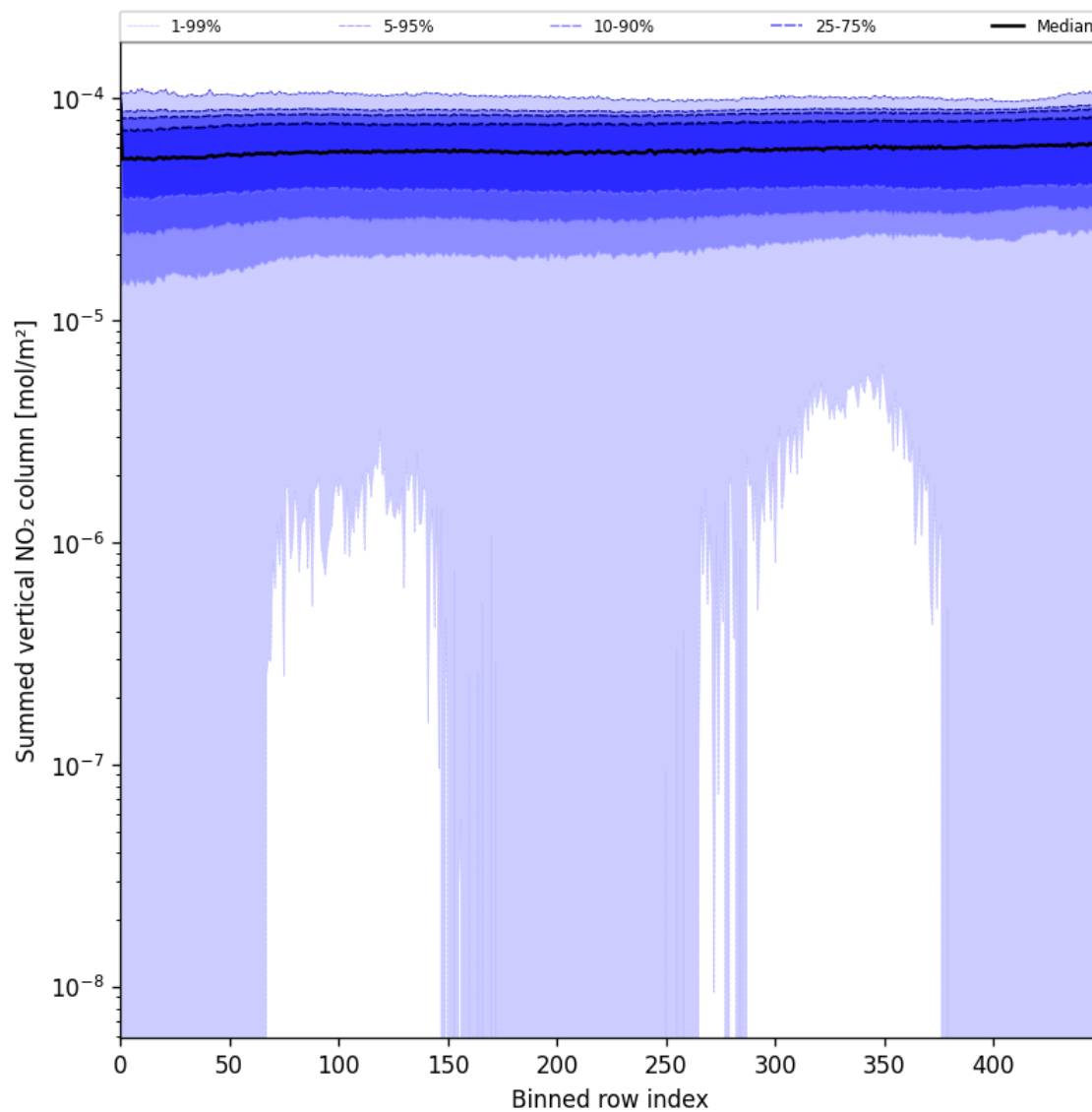
Figure 57: Along track statistics of “Summed vertical NO 2 column” for 2025-07-15 to 2025-07-17
