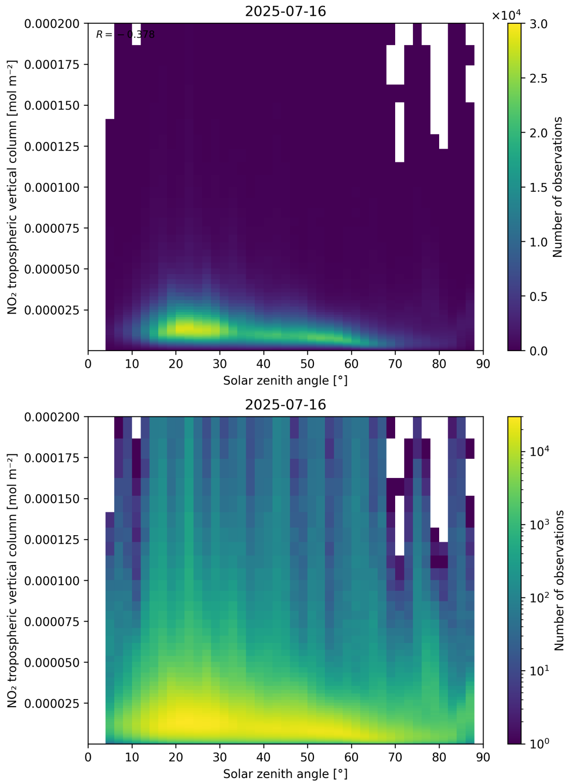
Figure 155: Scatter density plot of “Solar zenith angle” against “NO 2 tropospheric vertical column” for 2025-07-15 to 2025-07-17.
