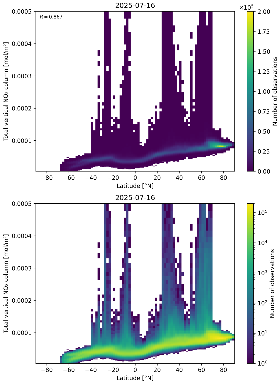
Figure 90: Scatter density plot of “Latitude” against “Total vertical NO 2 column” for 2025-07-15 to 2025-07-17.
