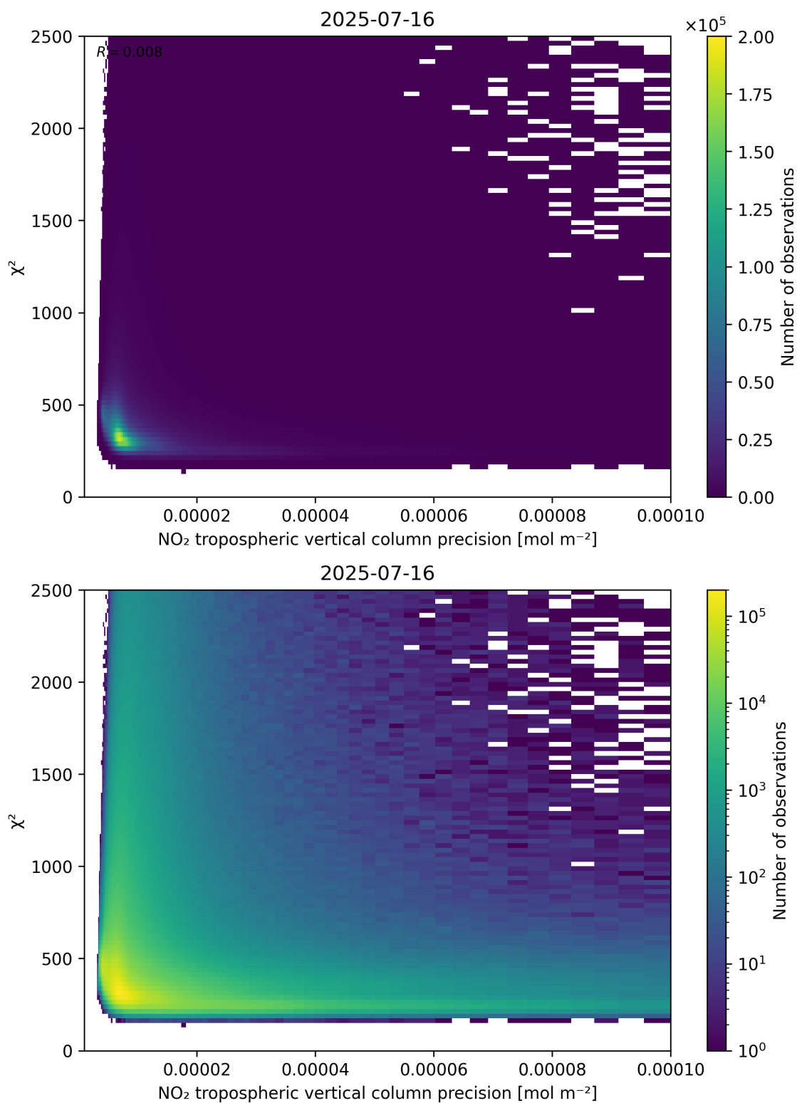
Figure 134: Scatter density plot of “NO 2 tropospheric vertical column precision” against “ \chi^2 ” for 2025-07-15 to 2025-07-17.
