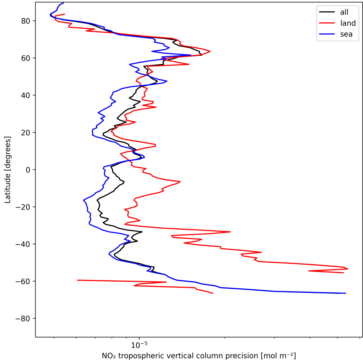
Figure 13: Zonal average of “NO 2 tropospheric vertical column precision” for 2025-07-15 to 2025-07-17.
