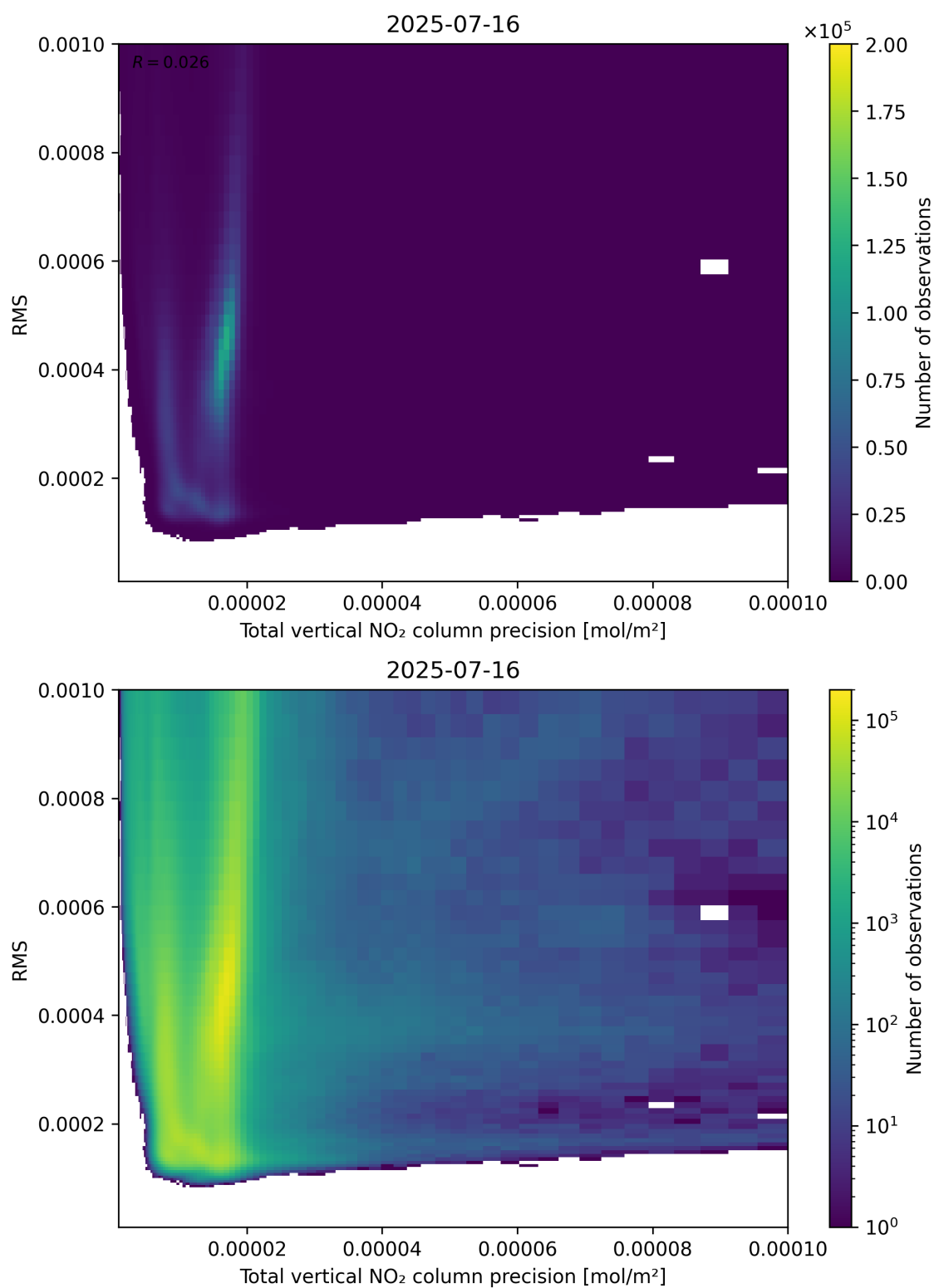
Figure 119: Scatter density plot of “Total vertical NO 2 column precision” against “RMS” for 2025-07-15 to 2025-07-17.
