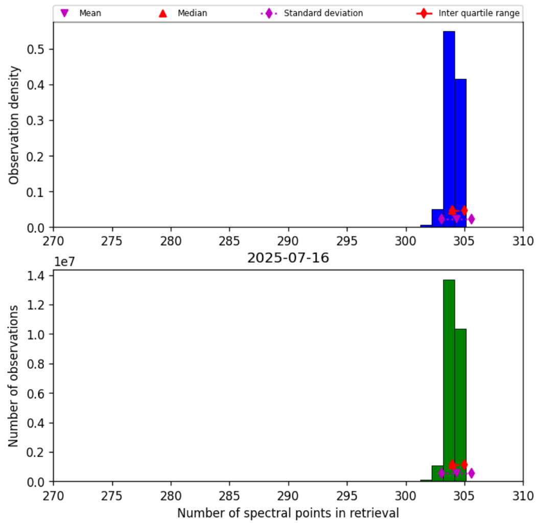
Figure 33: Histogram of “Number of spectral points in retrieval” for 2025-07-15 to 2025-07-17
