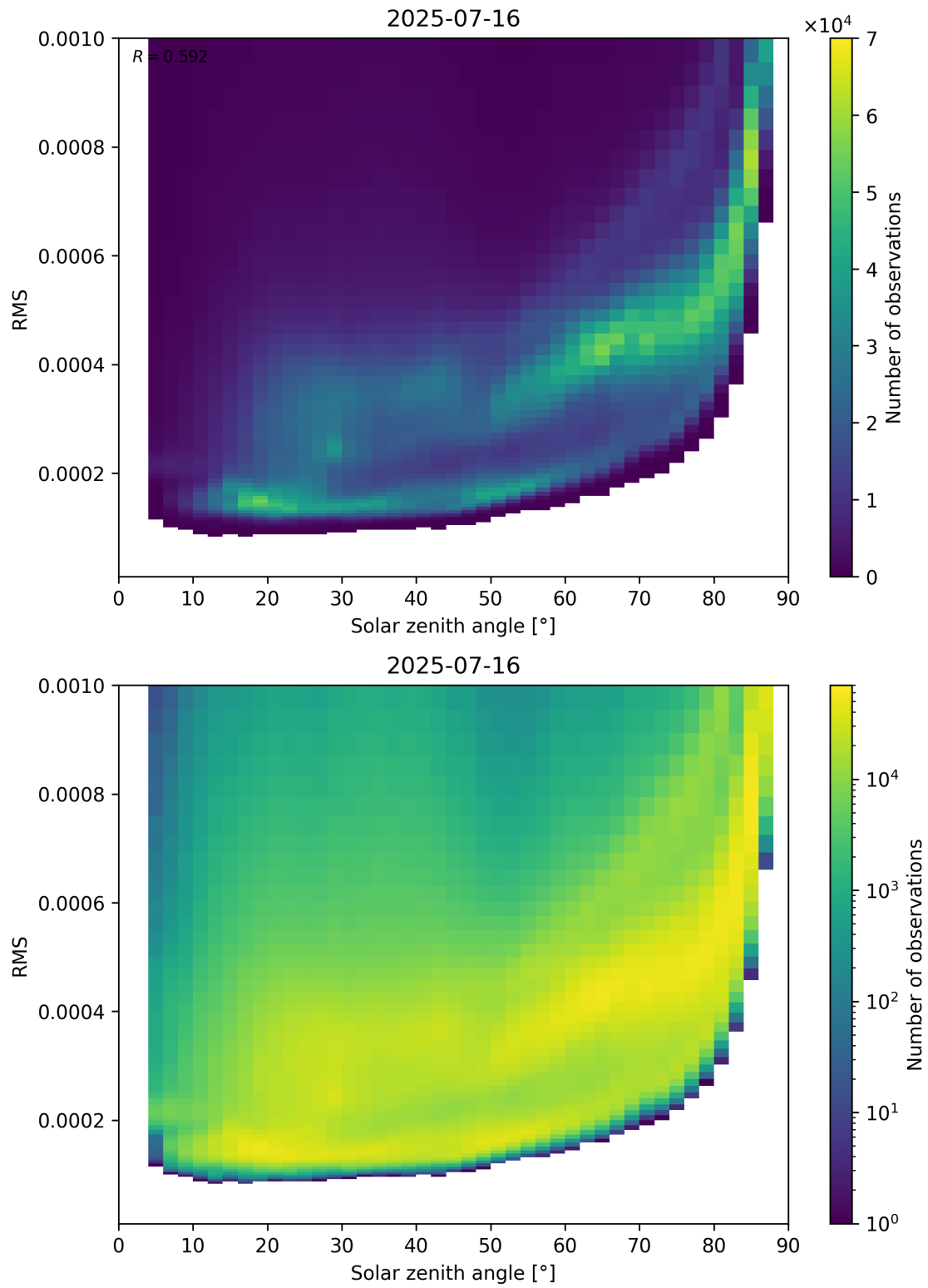
Figure 157: Scatter density plot of “Solar zenith angle” against “RMS” for 2025-07-15 to 2025-07-17.
