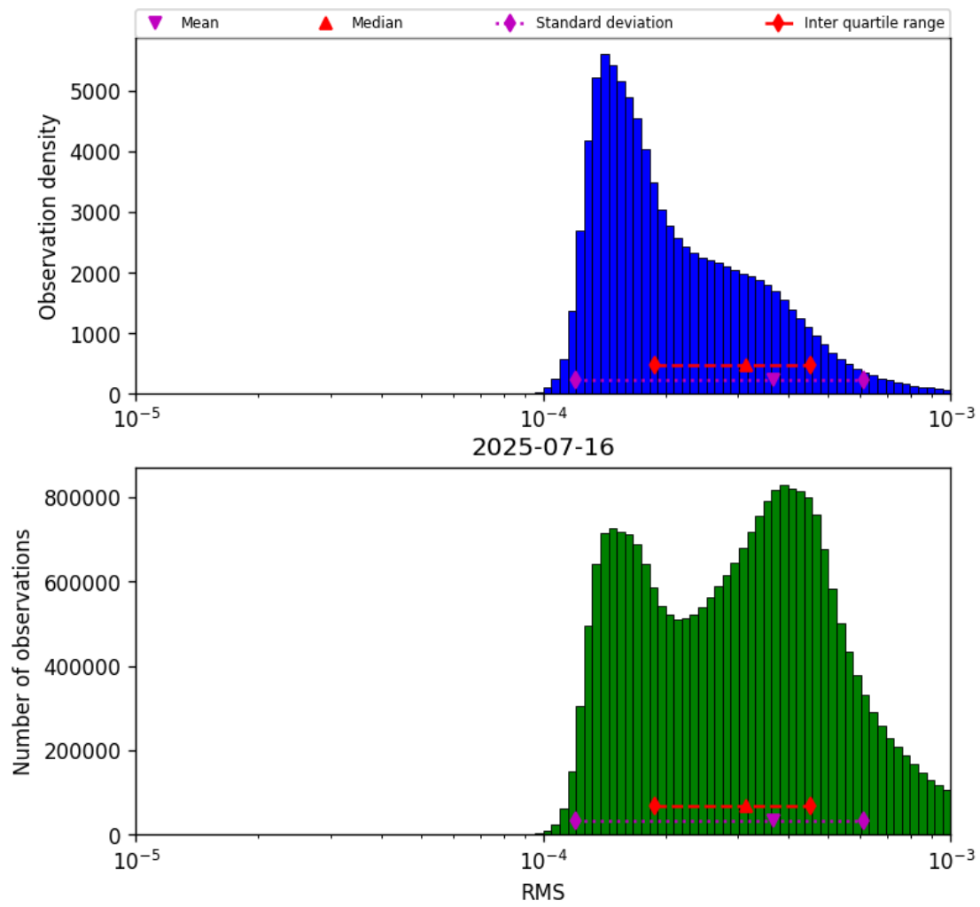
Figure 43: Histogram of “RMS” for 2025-07-15 to 2025-07-17
