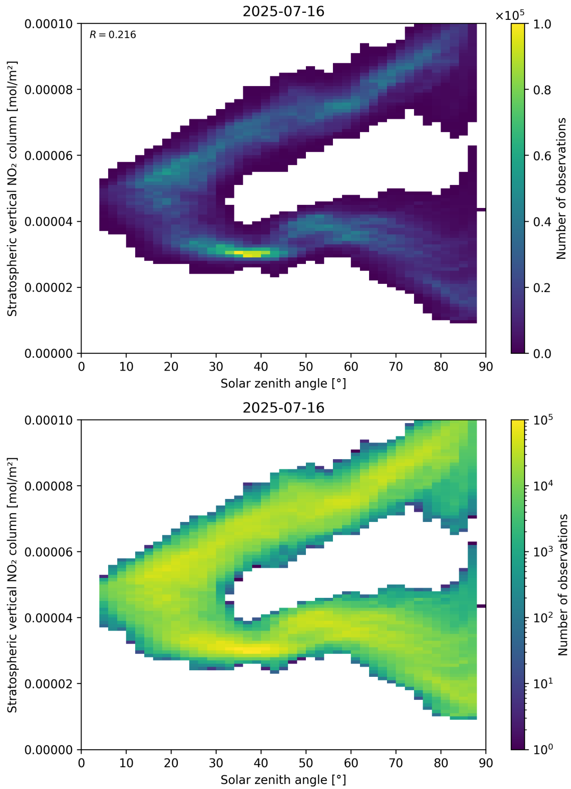
Figure 150: Scatter density plot of “Solar zenith angle” against “Stratospheric vertical NO 2 column” for 2025-07-15 to 2025-07-17.
