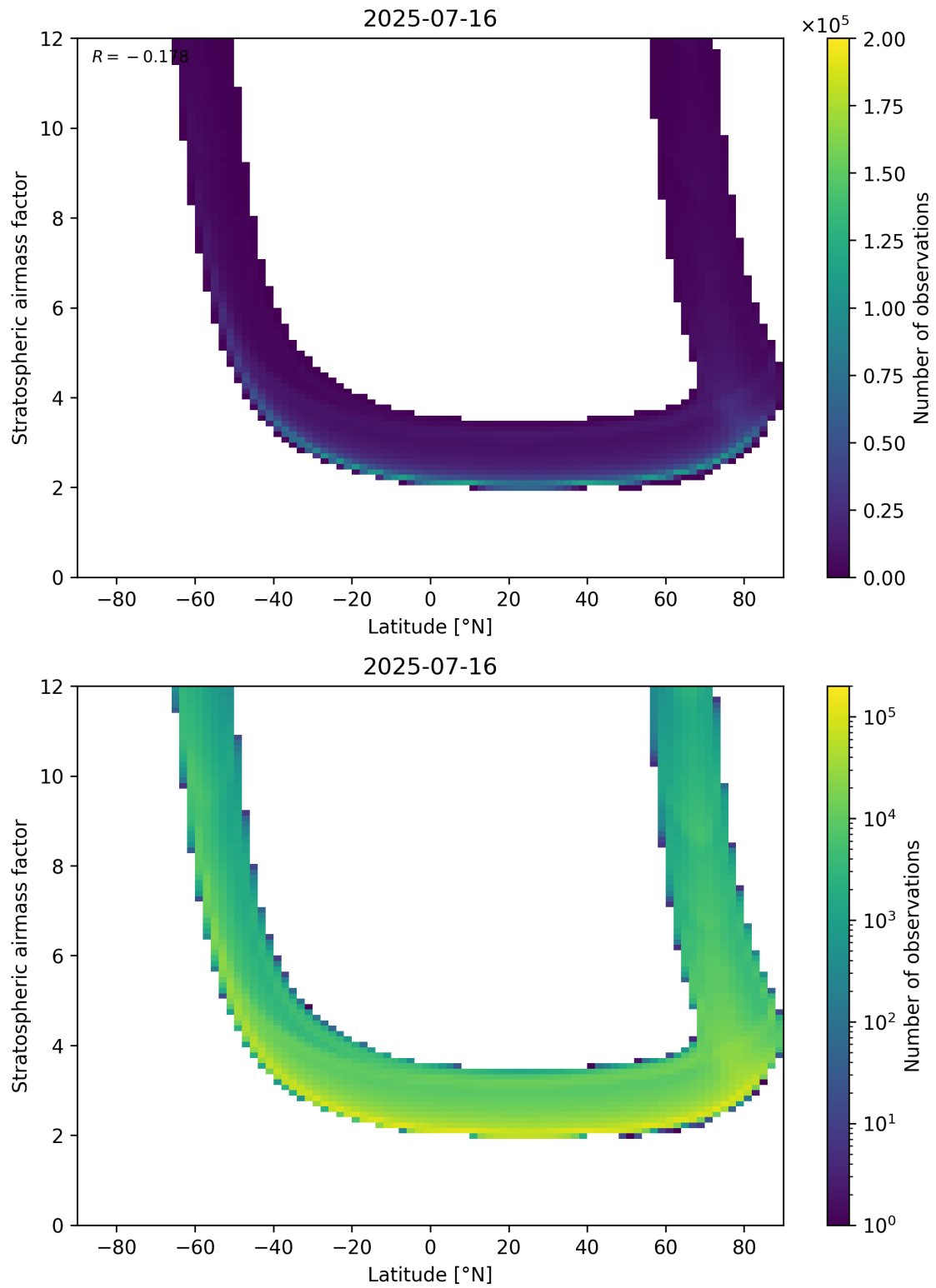
Figure 83: Scatter density plot of “Latitude” against “Stratospheric air mass factor” for 2025-07-15 to 2025-07-17.
