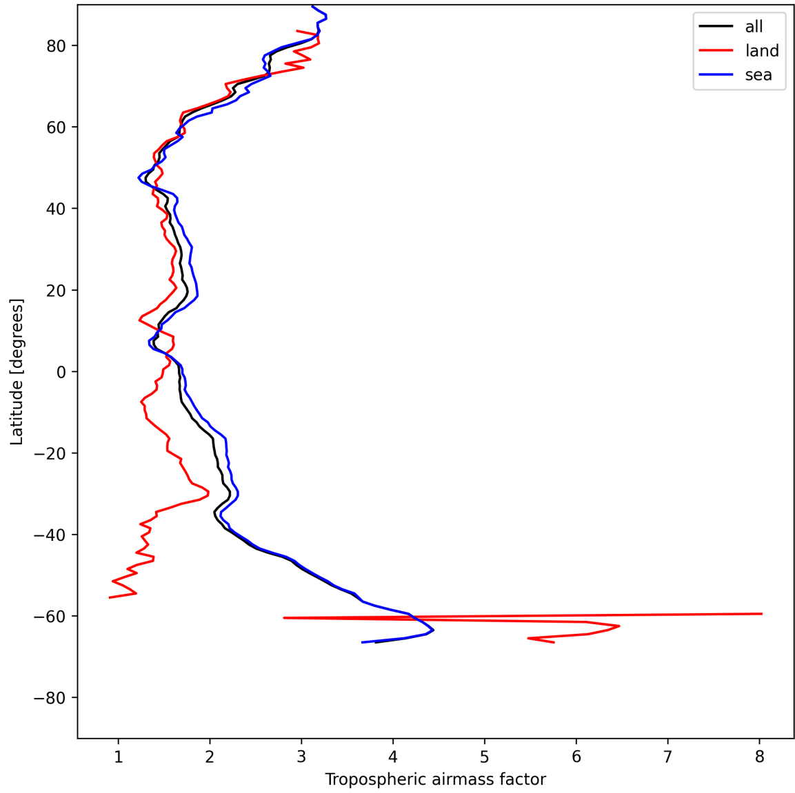
Figure 14: Zonal average of “Tropospheric air mass factor” for 2025-07-15 to 2025-07-17.
