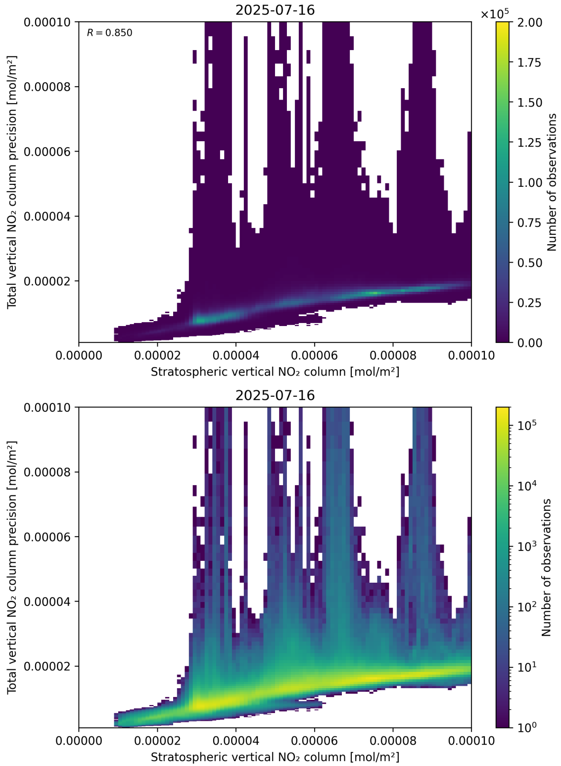
Figure 101: Scatter density plot of “Stratospheric vertical NO 2 column” against “Total vertical NO 2 column precision” for 2025-07-15 to 2025-07-17.
