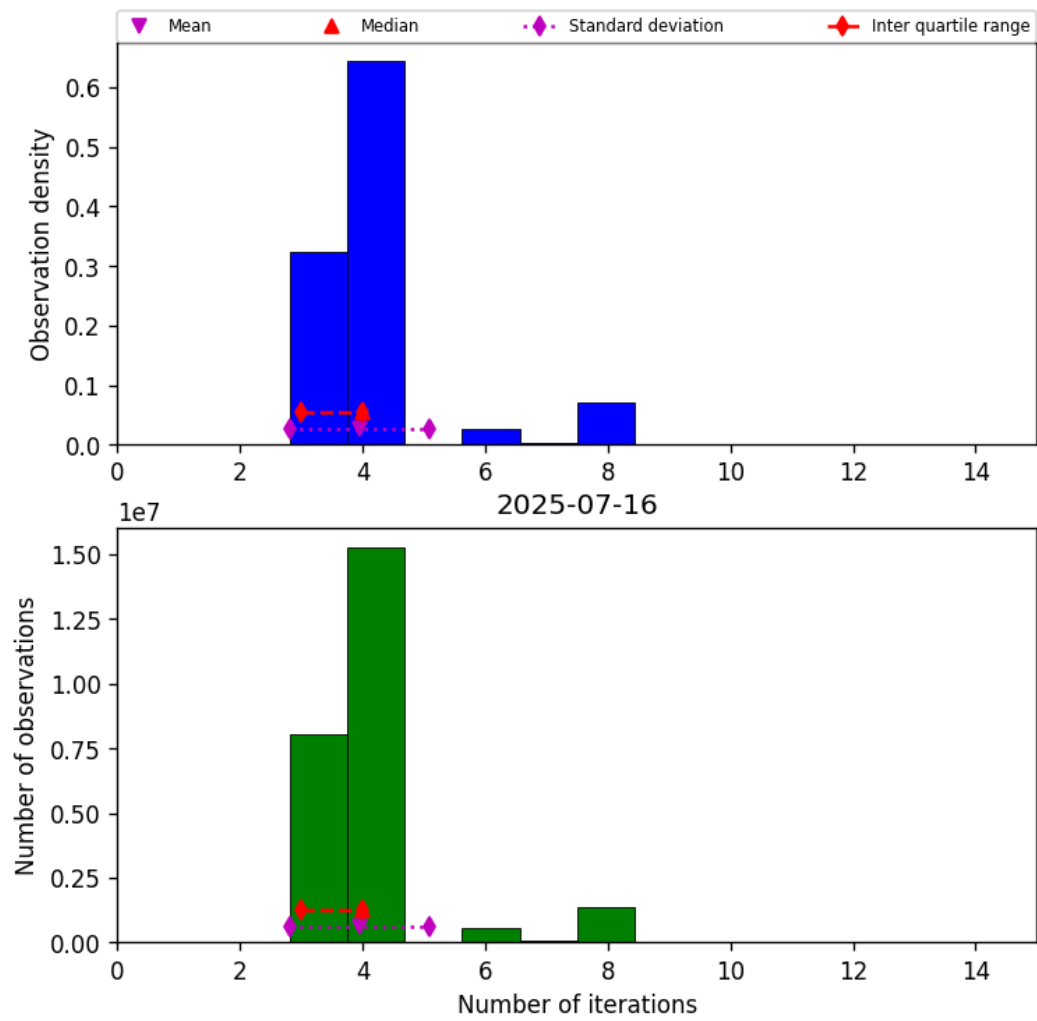
Figure 34: Histogram of “Number of iterations” for 2025-07-15 to 2025-07-17
