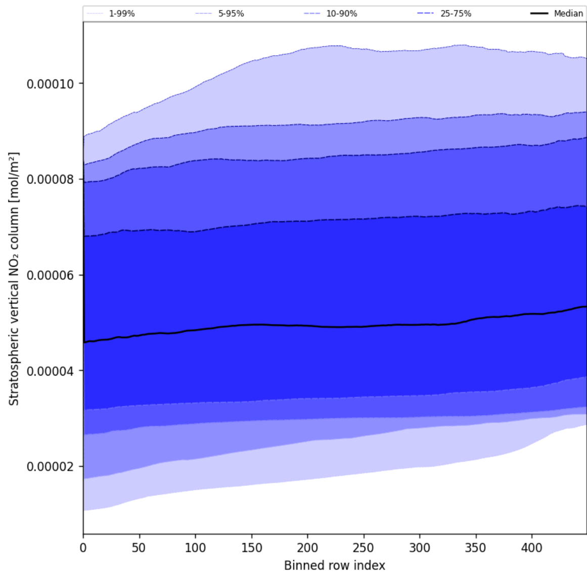
Figure 53: Along track statistics of “Stratospheric vertical NO 2 column” for 2025-07-15 to 2025-07-17
