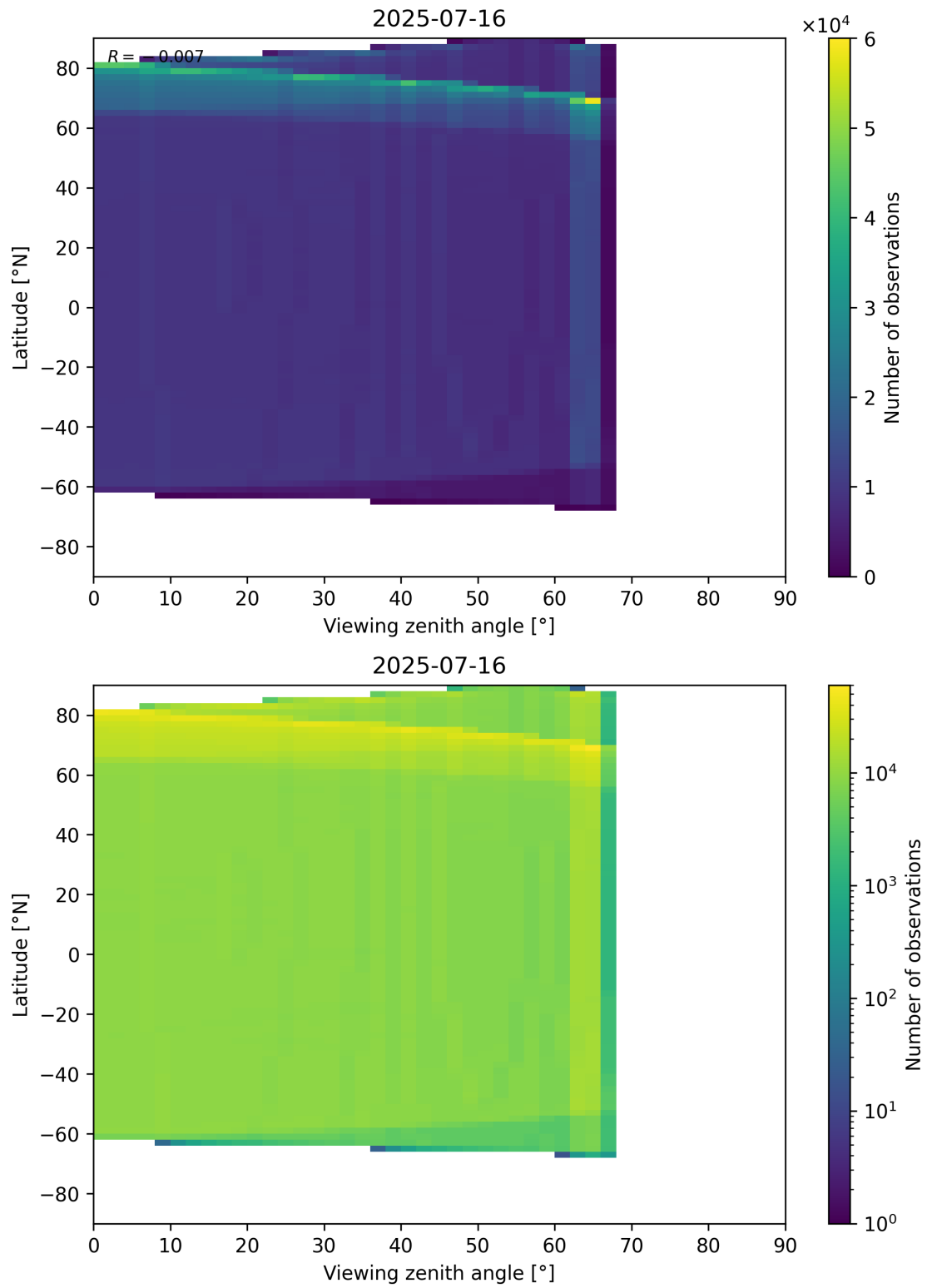
Figure 163: Scatter density plot of “Viewing zenith angle” against “Latitude” for 2025-07-15 to 2025-07-17.
