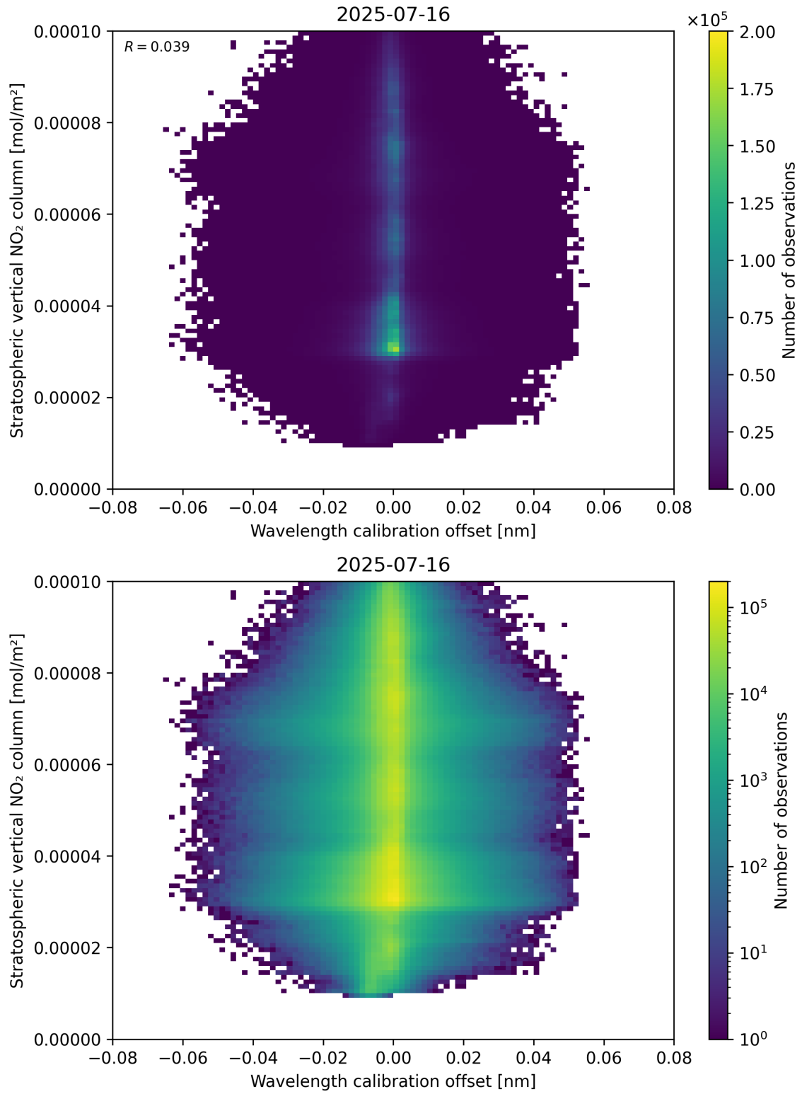
Figure 176: Scatter density plot of “Wavelength calibration offset” against “Stratospheric vertical NO 2 column” for 2025-07-15 to 2025-07-17.
