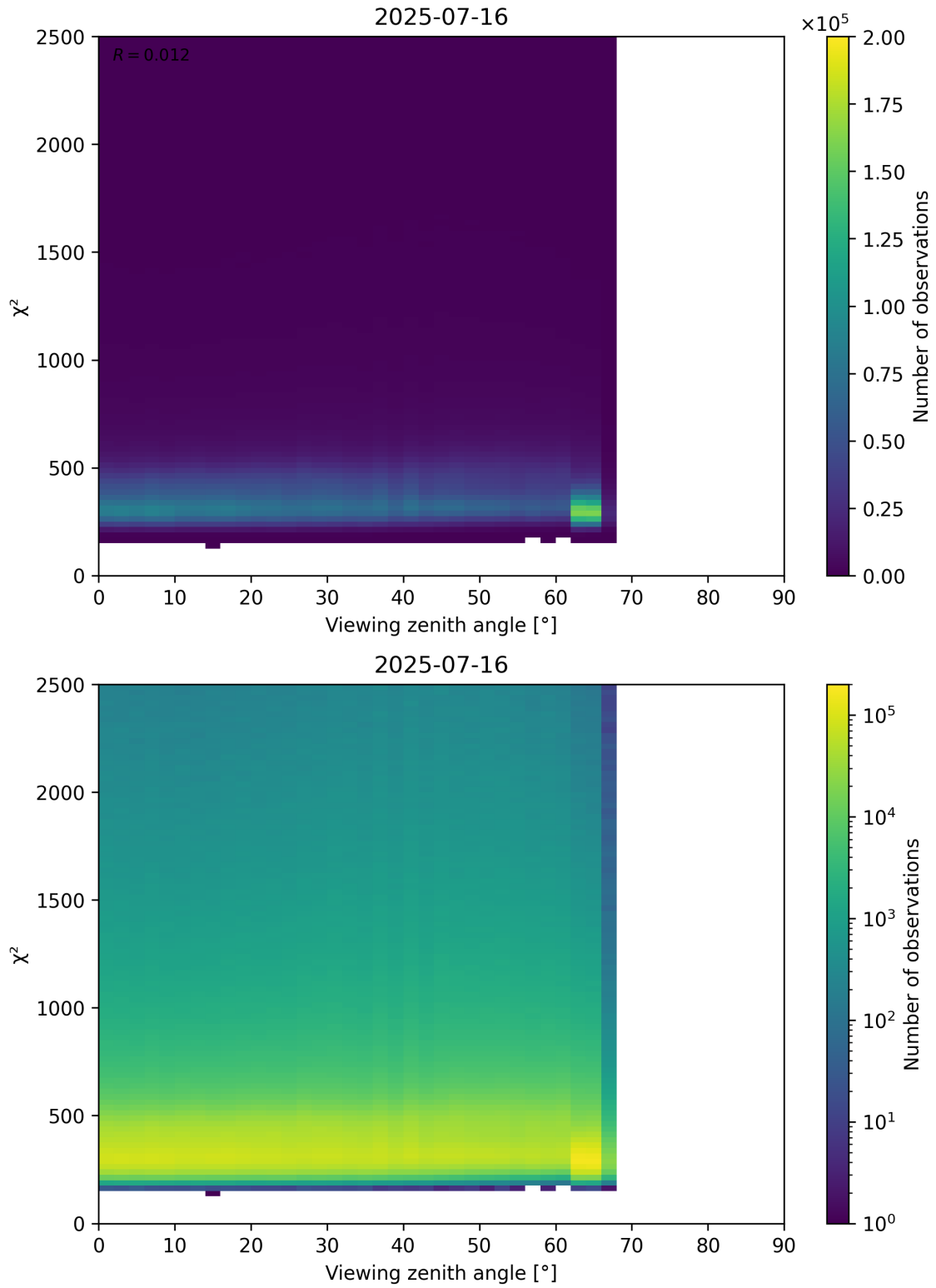
Figure 162: Scatter density plot of “Viewing zenith angle” against “ \chi^2 ” for 2025-07-15 to 2025-07-17.
