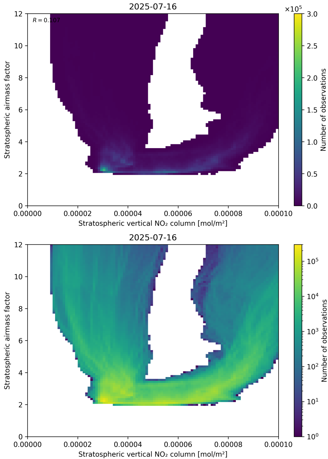
Figure 96: Scatter density plot of “Stratospheric vertical NO 2 column” against “Stratospheric airmass factor” for 2025-07-15 to 2025-07-17.
