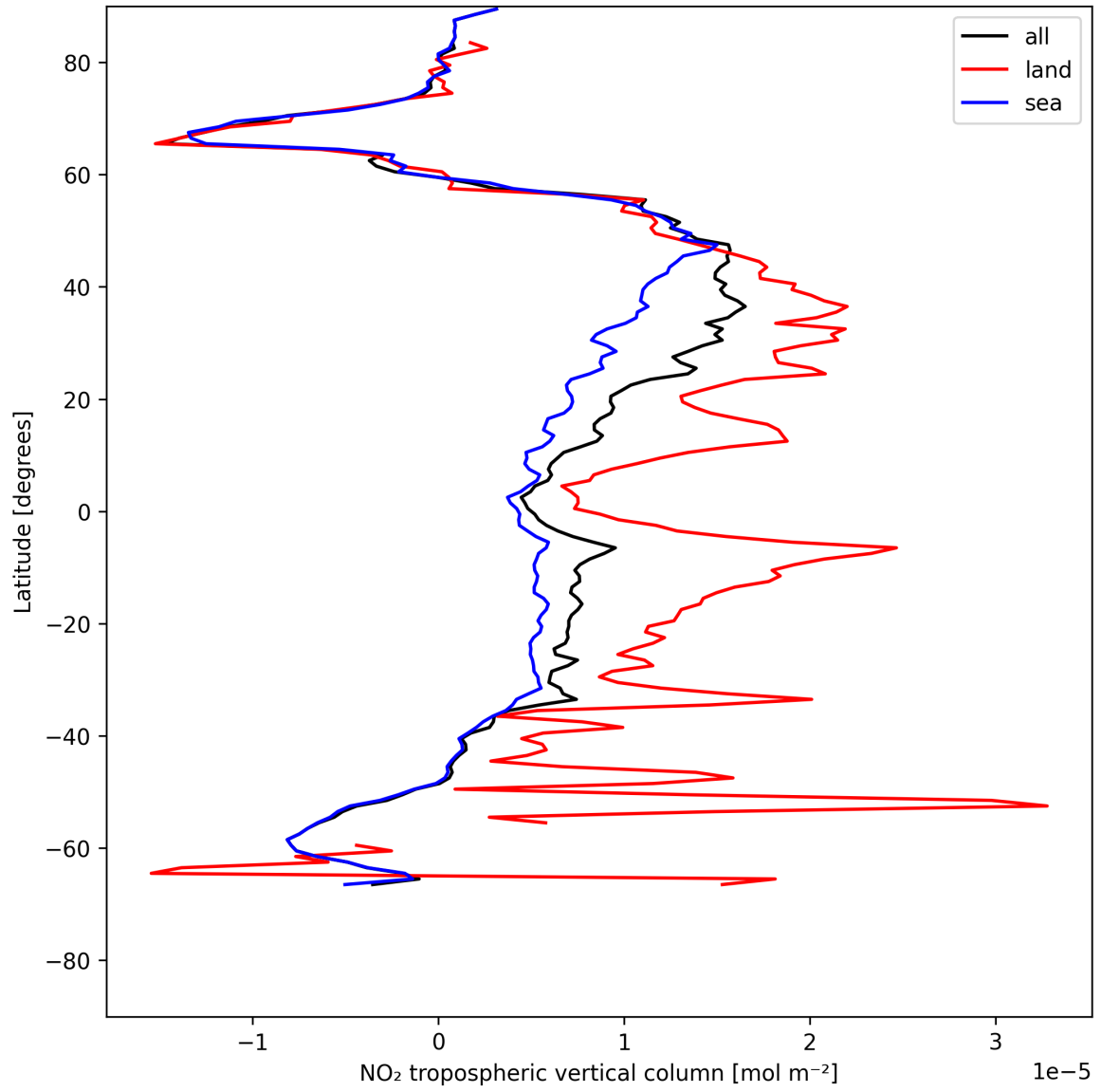
Figure 12: Zonal average of “NO 2 tropospheric vertical column” for 2025-07-15 to 2025-07-17.
