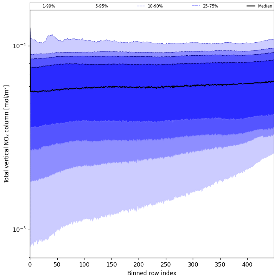
Figure 55: Along track statistics of “Total vertical NO 2 column” for 2025-07-15 to 2025-07-17
