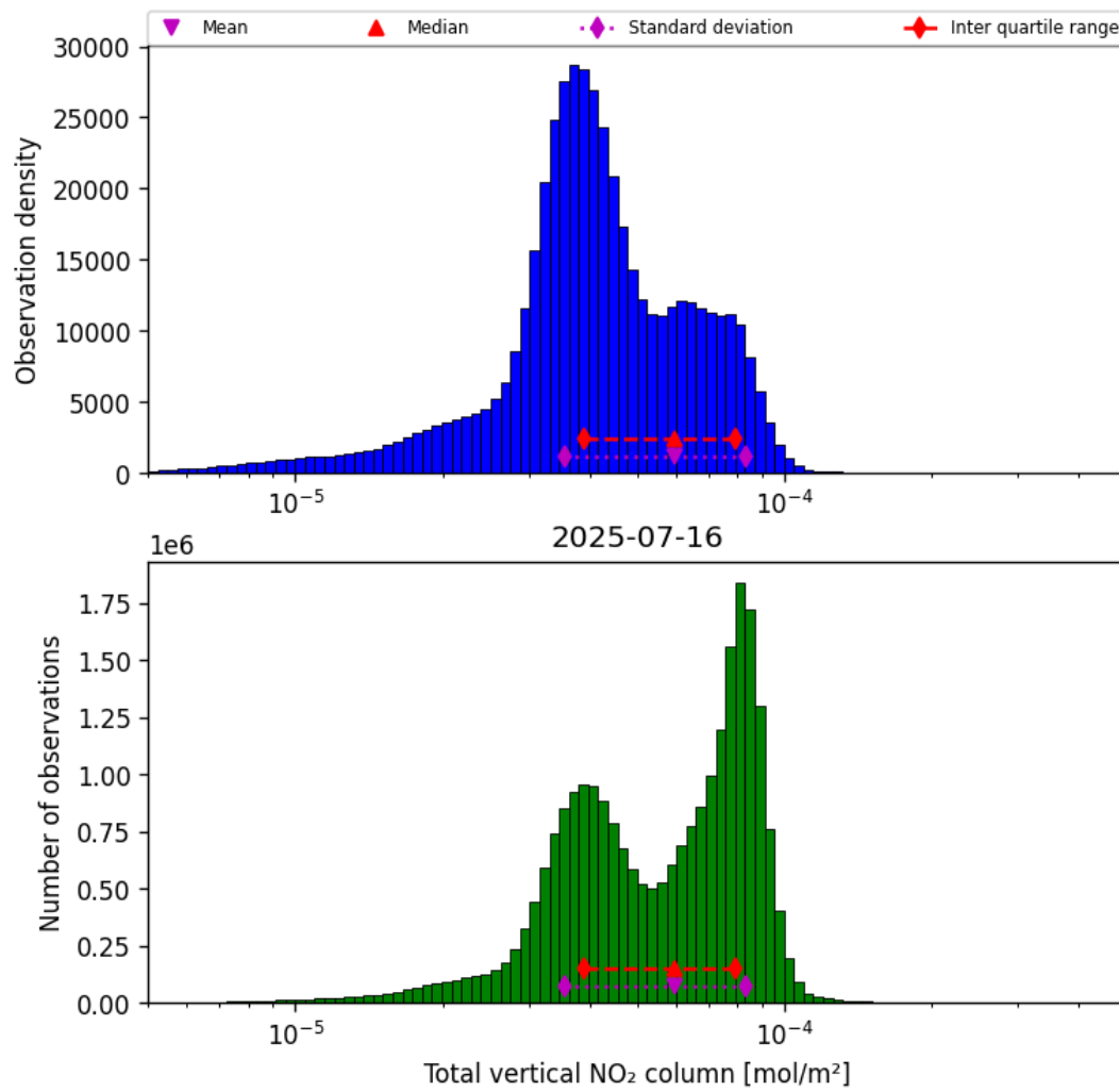
Figure 38: Histogram of “Total vertical NO 2 column” for 2025-07-15 to 2025-07-17
