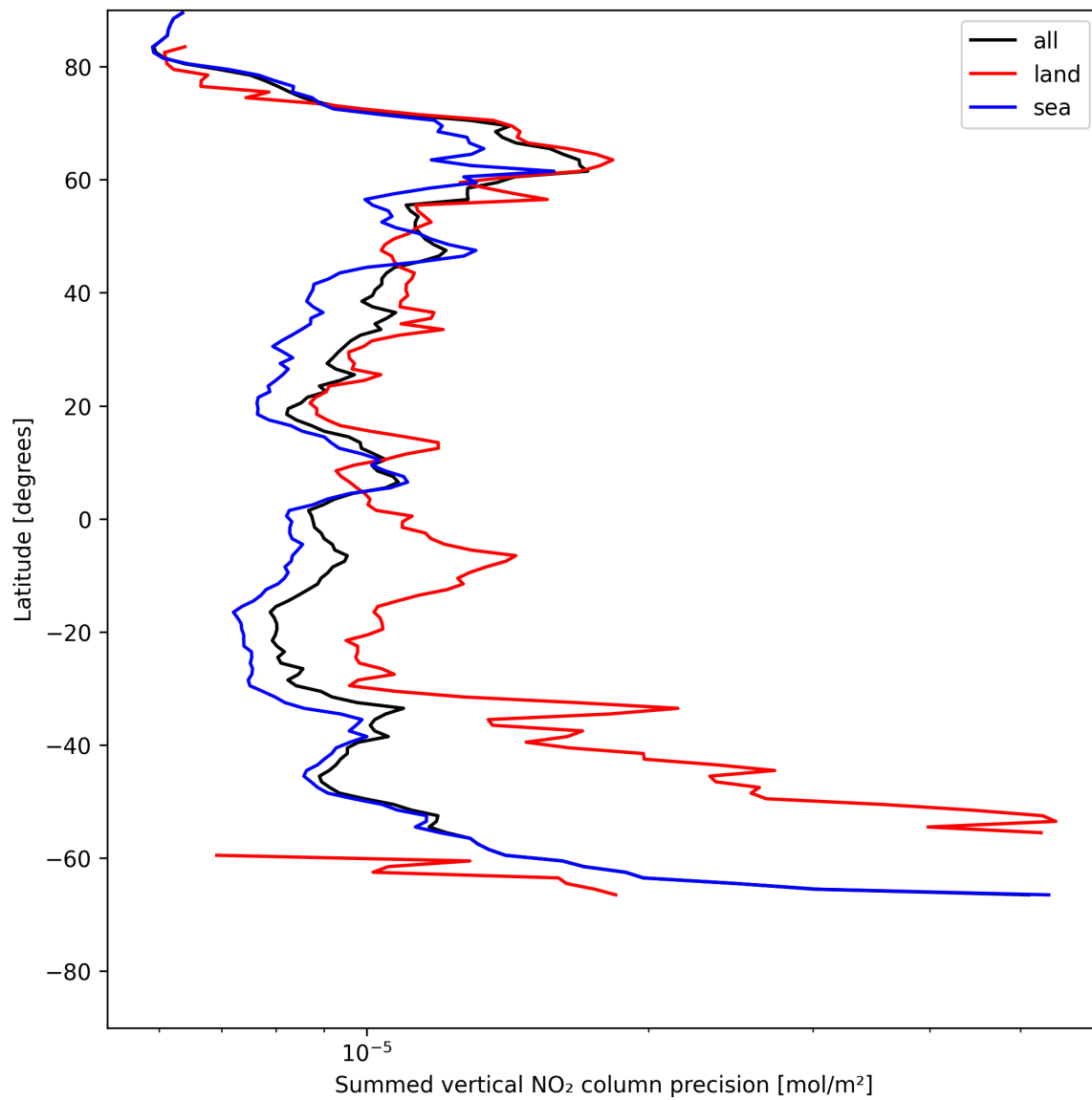
Figure 24: Zonal average of “Summed vertical NO 2 column precision” for 2025-07-15 to 2025-07-17.
