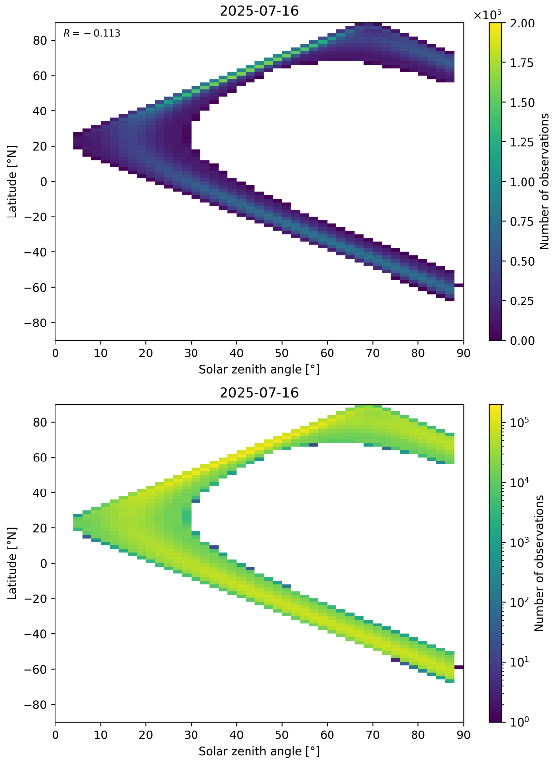
Figure 149: Scatter density plot of “Solar zenith angle” against “Latitude” for 2025-07-15 to 2025-07-17.
