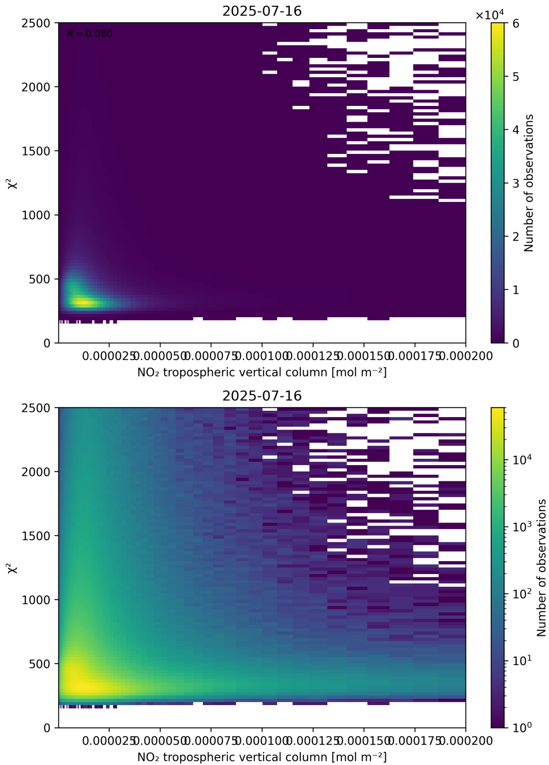
Figure 124: Scatter density plot of “NO 2 tropospheric vertical column” against “ \chi^2 ” for 2025-07-15 to 2025-07-17.
