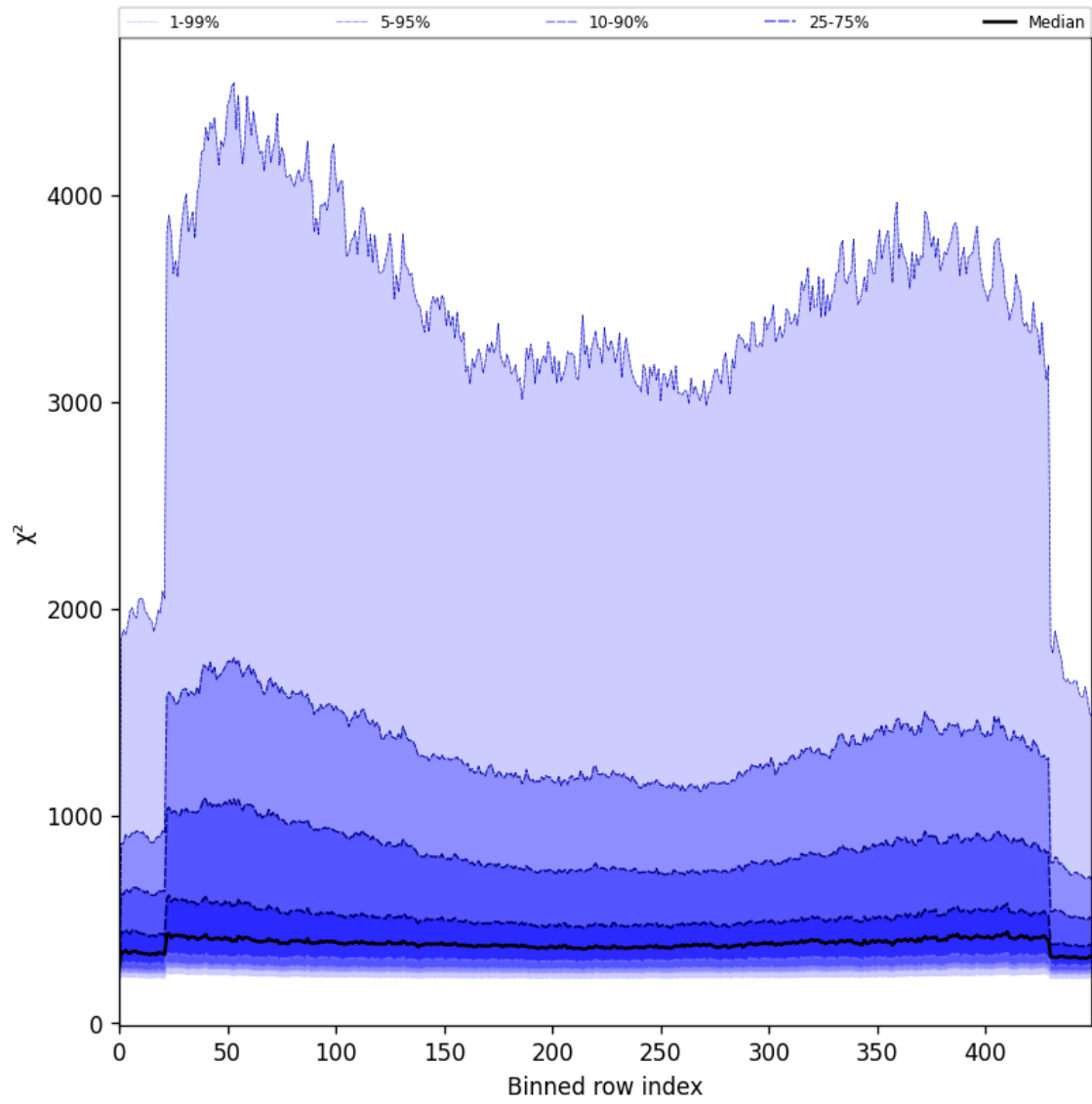
Figure 59: Along track statistics of “ \chi^2 ” for 2025-07-15 to 2025-07-17
