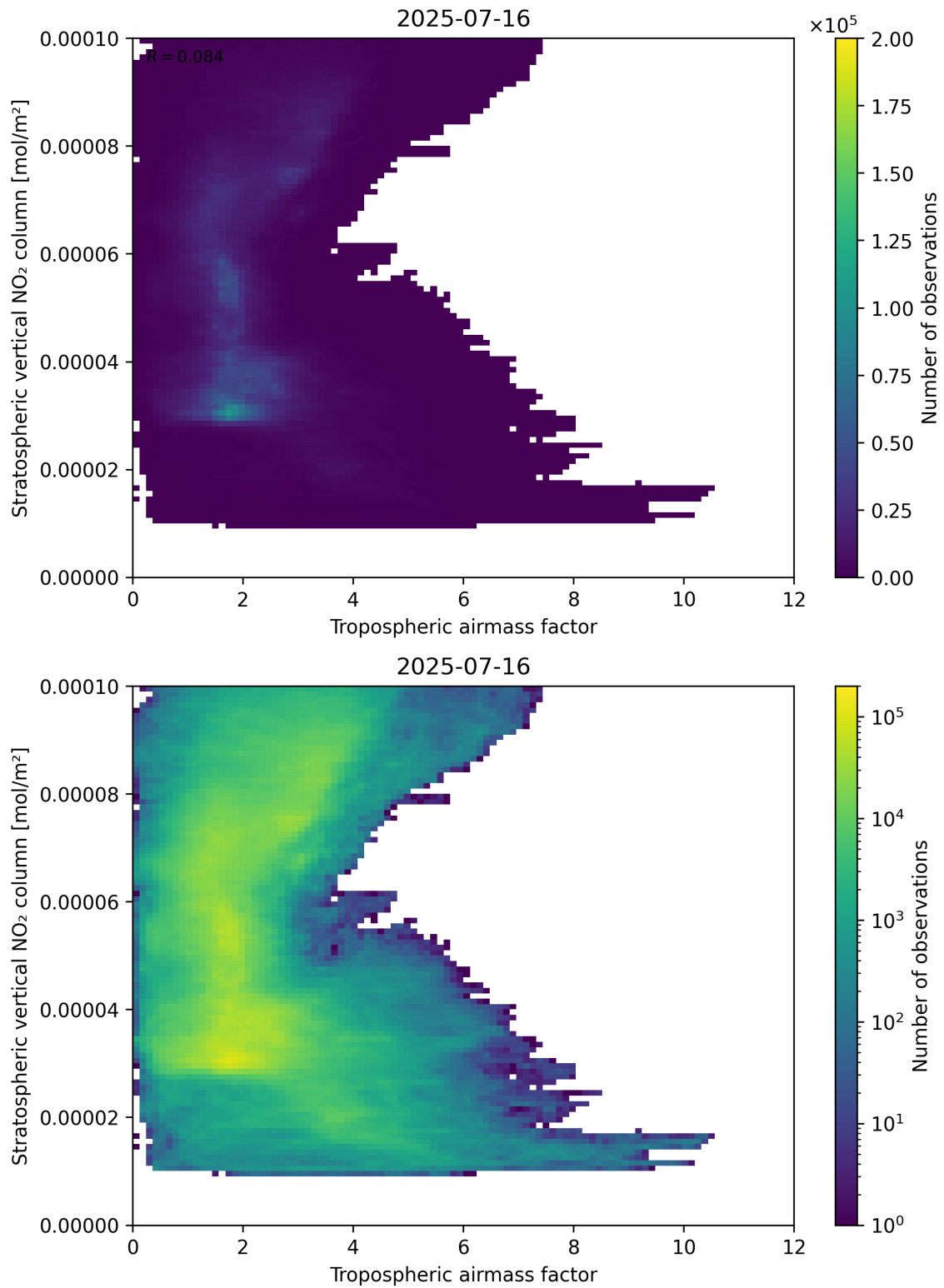
Figure 74: Scatter density plot of “Tropospheric air mass factor” against “Stratospheric vertical NO 2 column” for 2025-07-15 to 2025-07-17.
