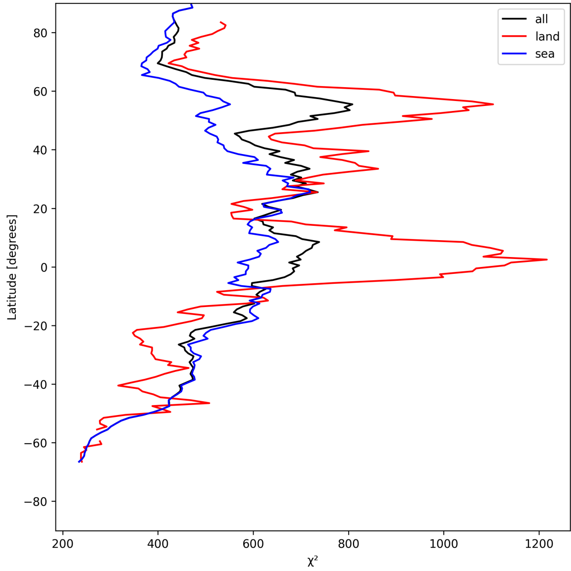
Figure 25: Zonal average of “ \chi^2 ” for 2025-07-15 to 2025-07-17.
