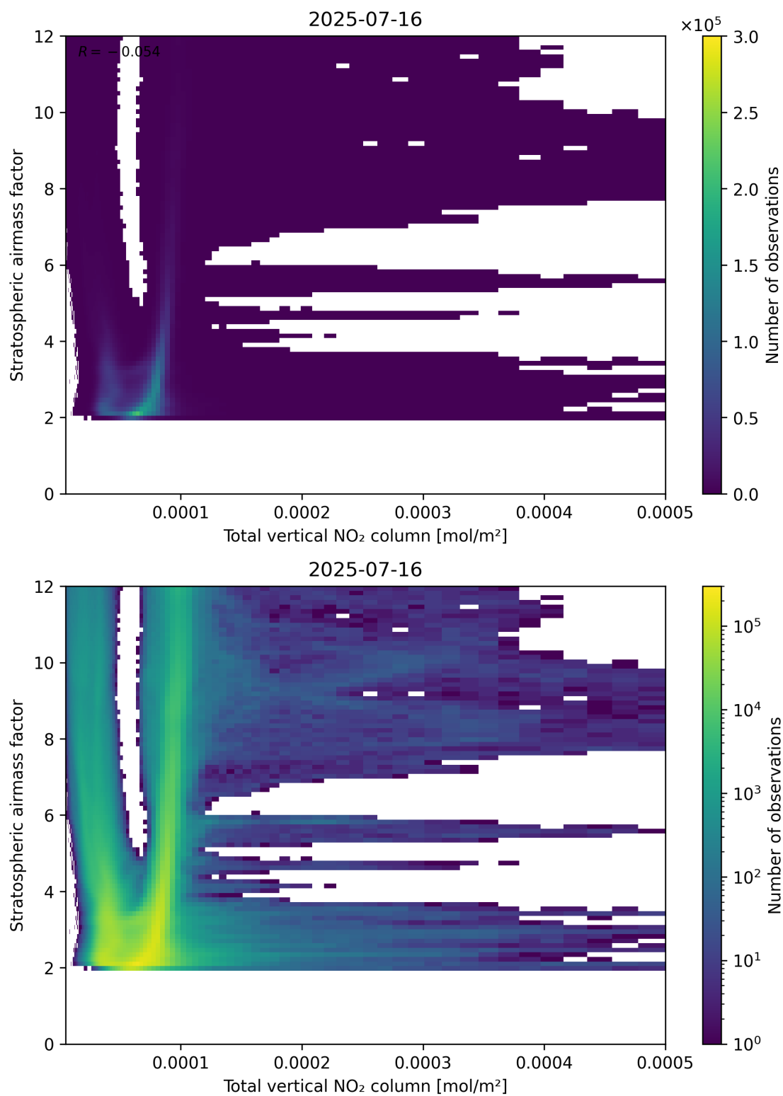
Figure 110: Scatter density plot of “Total vertical NO 2 column” against “Stratospheric airmass factor” for 2025-07-15 to 2025-07-17.
