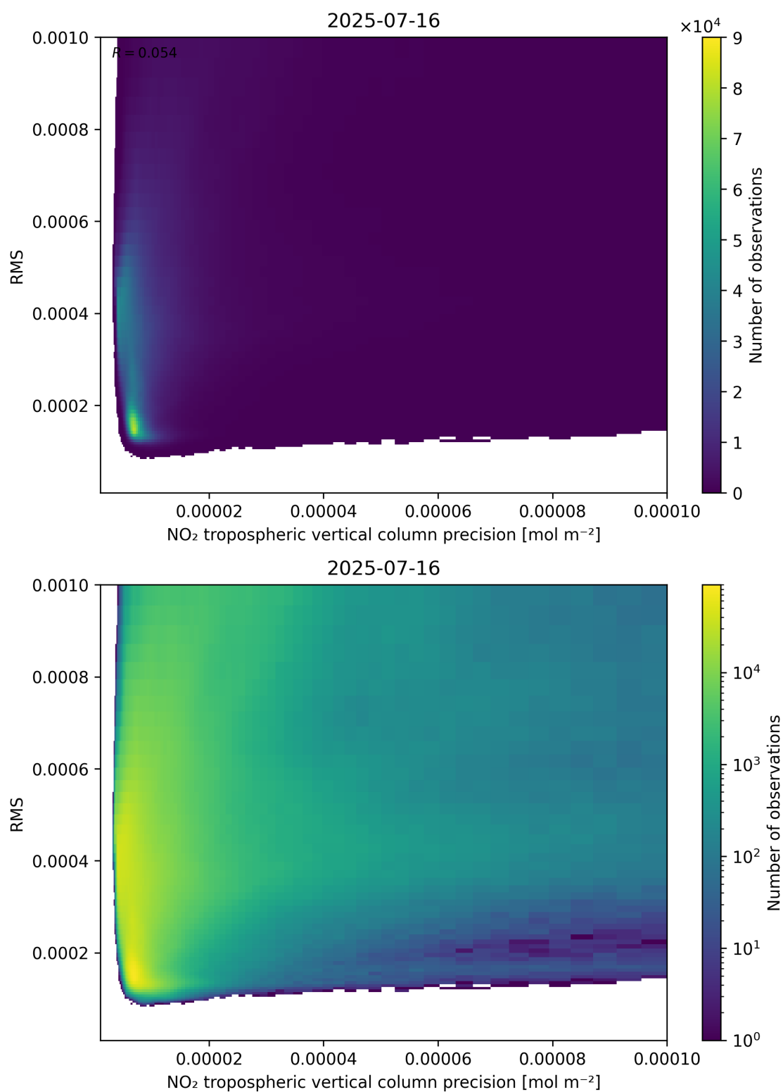
Figure 140: Scatter density plot of “NO 2 tropospheric vertical column precision” against “RMS” for 2025-07-15 to 2025-07-17.
