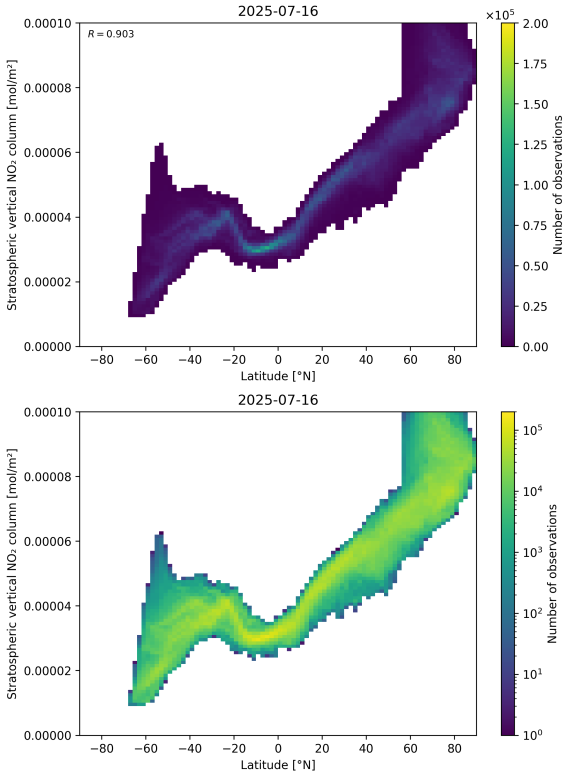
Figure 87: Scatter density plot of “Latitude” against “Stratospheric vertical NO 2 column” for 2025-07-15 to 2025-07-17.
