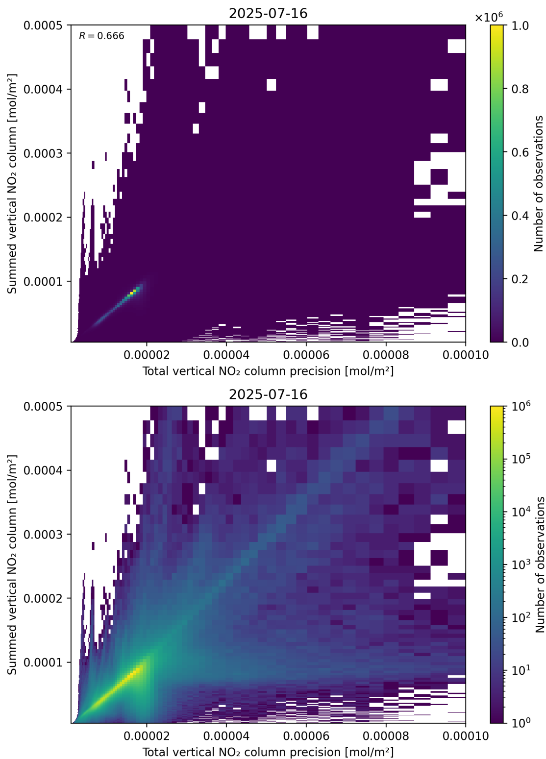
Figure 117: Scatter density plot of “Total vertical NO 2 column precision” against “Summed vertical NO 2 column” for 2025-07-15 to 2025-07-17.
