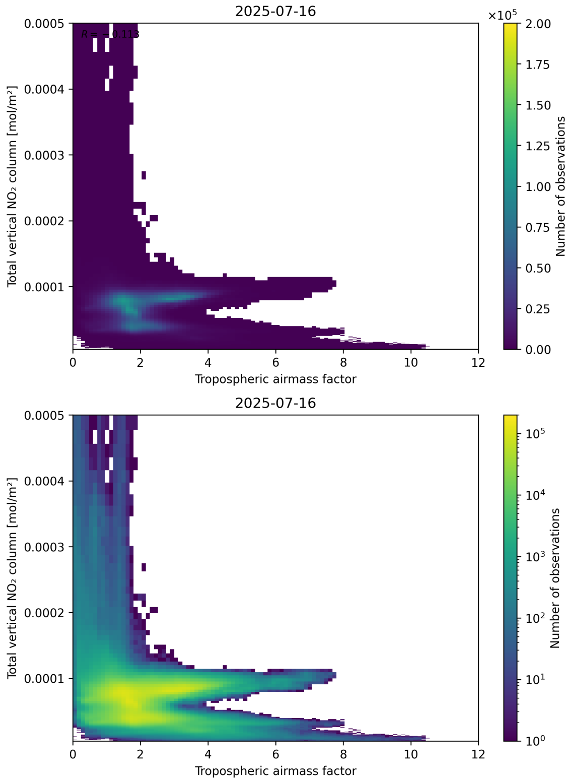
Figure 77: Scatter density plot of “Tropospheric airmass factor” against “Total vertical NO 2 column” for 2025-07-15 to 2025-07-17.
