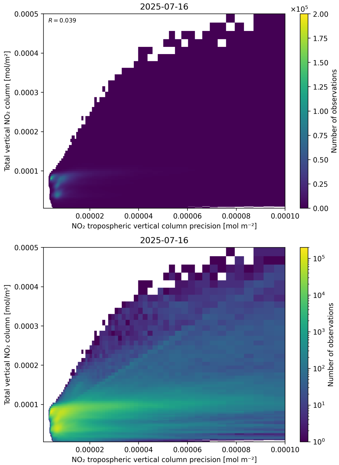
Figure 138: Scatter density plot of “NO 2 tropospheric vertical column precision” against “Total vertical NO 2 column” for 2025-07-15 to 2025-07-17.
