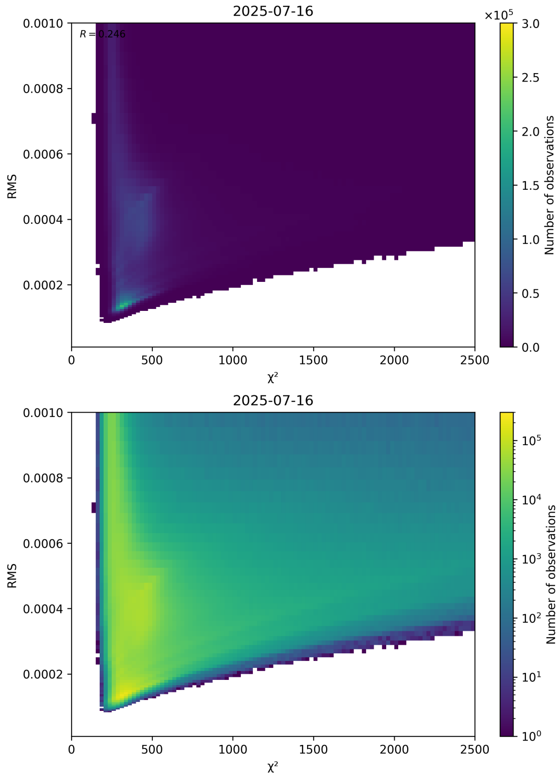
Figure 82: Scatter density plot of “ \chi^2 ” against “RMS” for 2025-07-15 to 2025-07-17.
