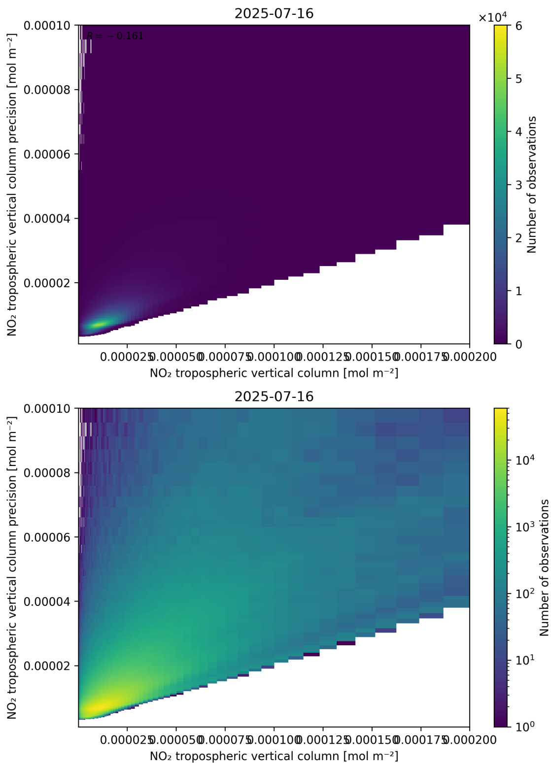
Figure 130: Scatter density plot of “NO 2 tropospheric vertical column” against “NO 2 tropospheric vertical column precision” for 2025-07-15 to 2025-07-17.
