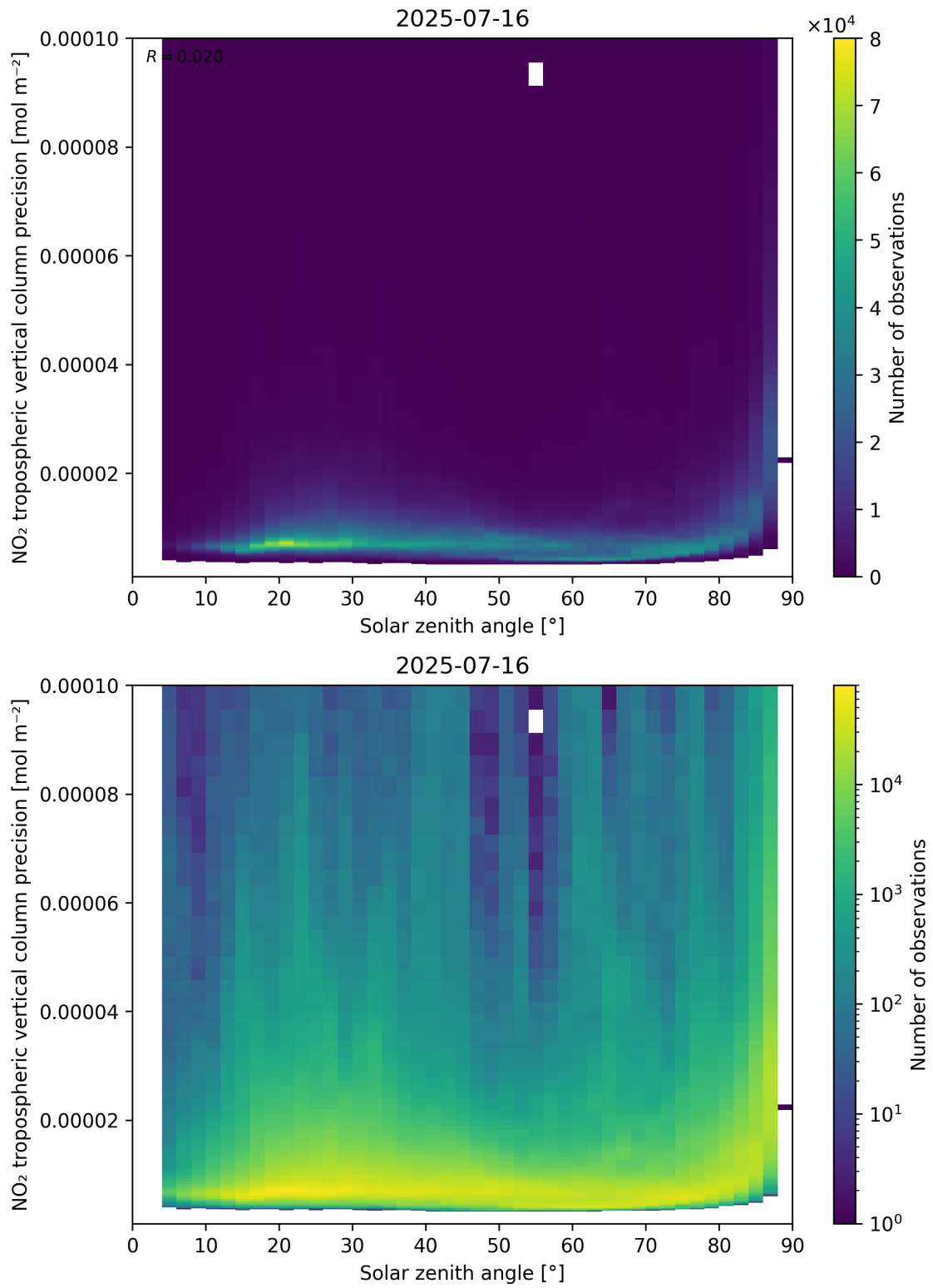
Figure 156: Scatter density plot of “Solar zenith angle” against “NO 2 tropospheric vertical column precision” for 2025-07-15 to 2025-07-17.
