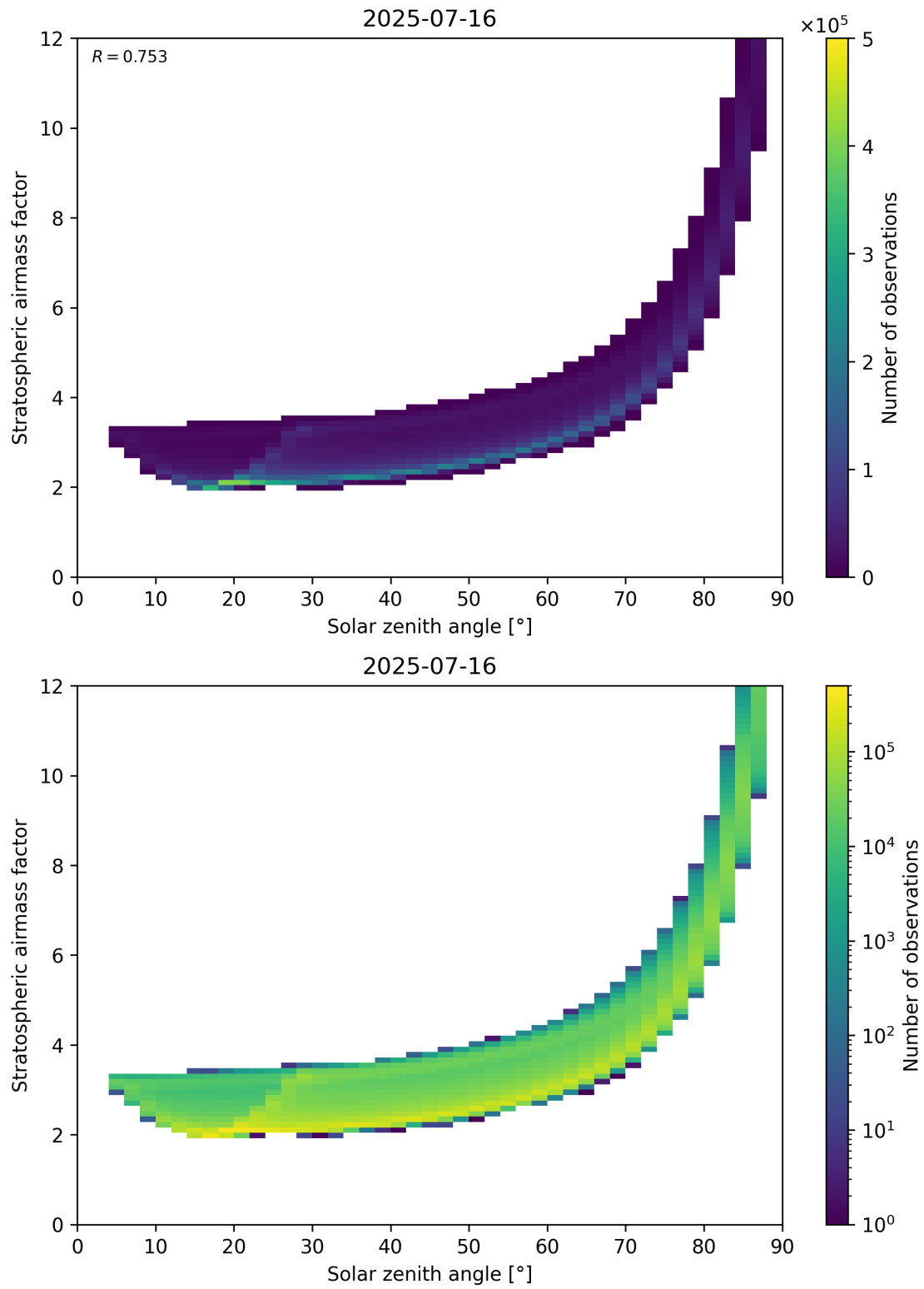
Figure 145: Scatter density plot of “Solar zenith angle” against “Stratospheric airmass factor” for 2025-07-15 to 2025-07-17.
