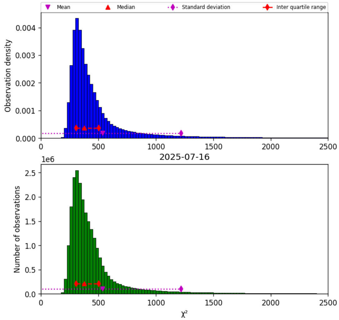
Figure 42: Histogram of “ \chi^2 ” for 2025-07-15 to 2025-07-17
