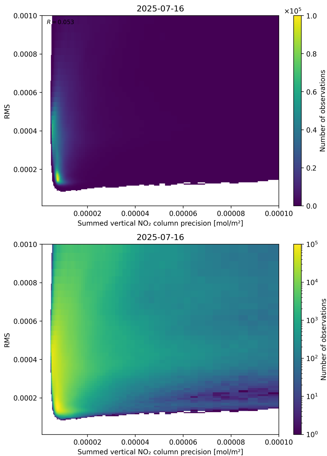
Figure 108: Scatter density plot of “Summed vertical NO 2 column precision” against “RMS” for 2025-07-15 to 2025-07-17.
