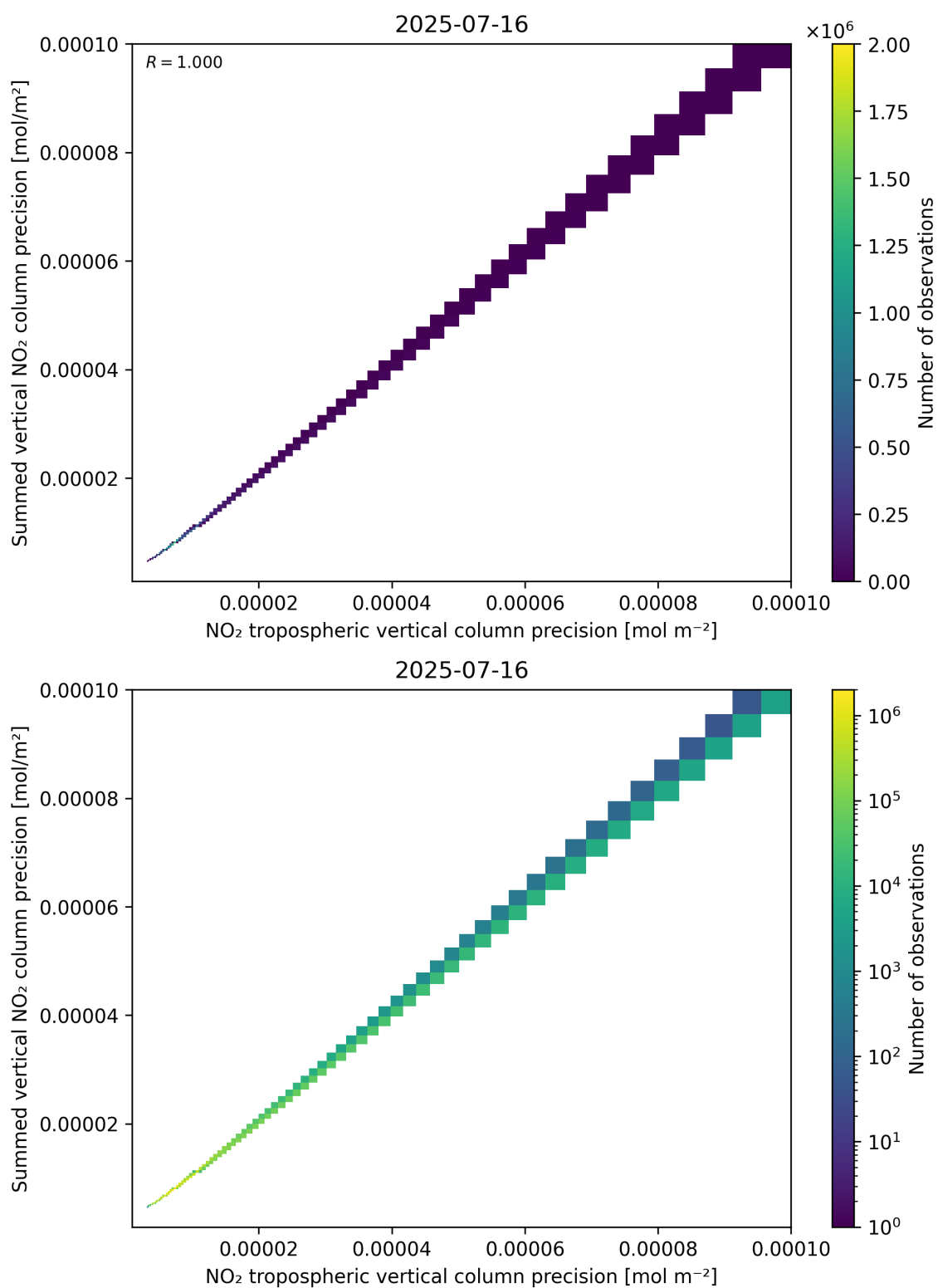
Figure 137: Scatter density plot of “NO 2 tropospheric vertical column precision” against “Summed vertical NO 2 column precision” for 2025-07-15 to 2025-07-17.
