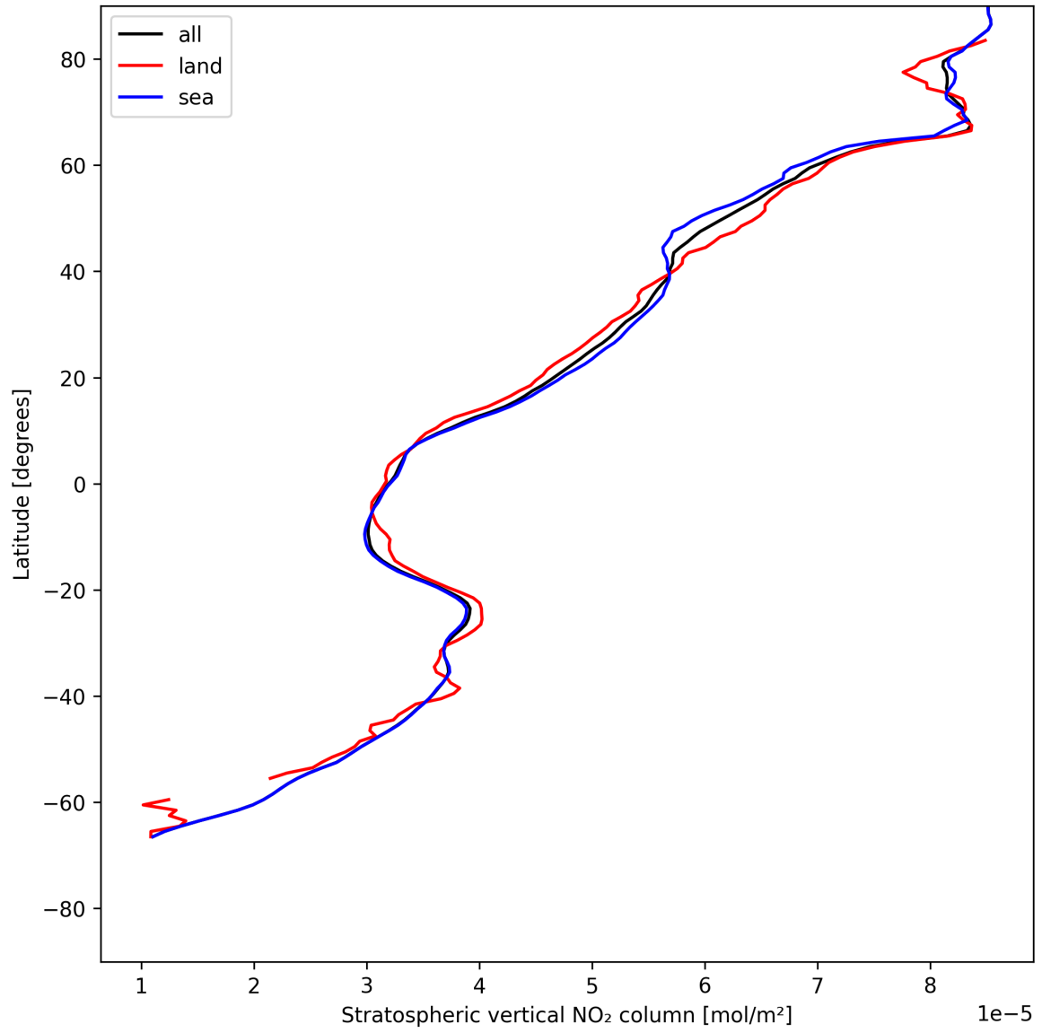
Figure 19: Zonal average of “Stratospheric vertical NO 2 column” for 2025-07-15 to 2025-07-17.
