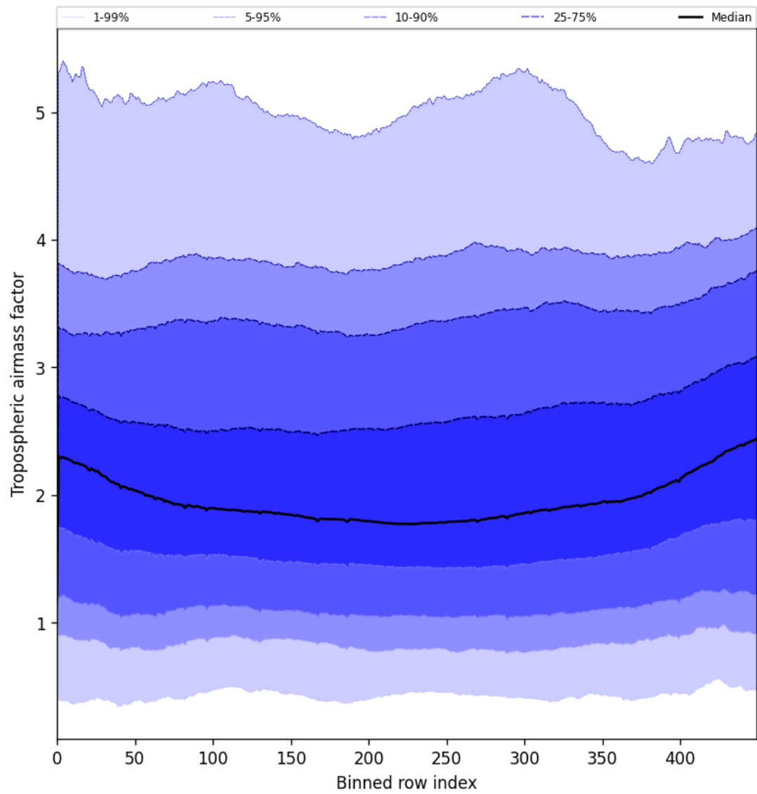
Figure 48: Along track statistics of “Tropospheric air mass factor” for 2025-07-15 to 2025-07-17
