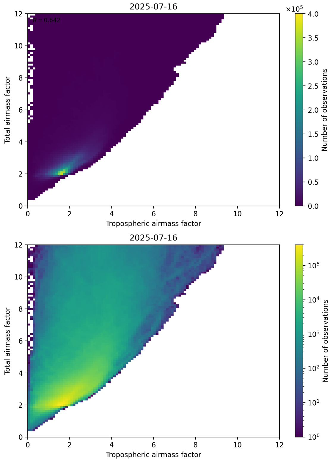
Figure 72: Scatter density plot of “Tropospheric airmass factor” against “Total airmass factor” for 2025-07-15 to 2025-07-17.
