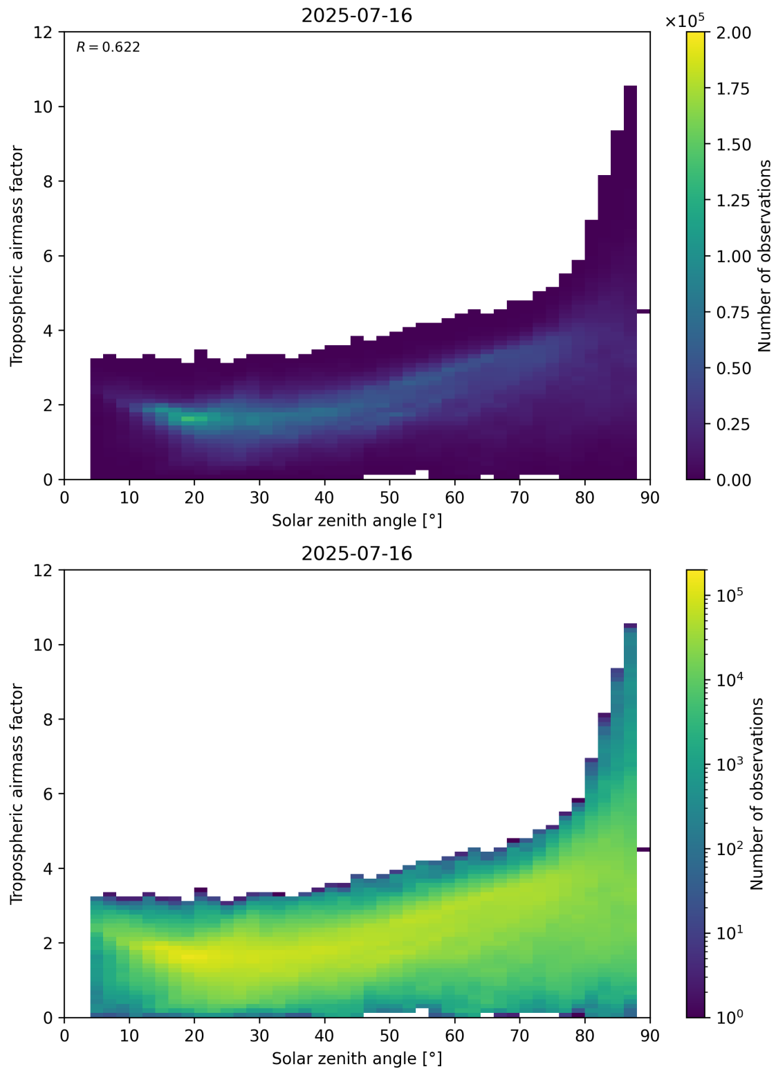
Figure 147: Scatter density plot of “Solar zenith angle” against “Tropospheric airmass factor” for 2025-07-15 to 2025-07-17.
