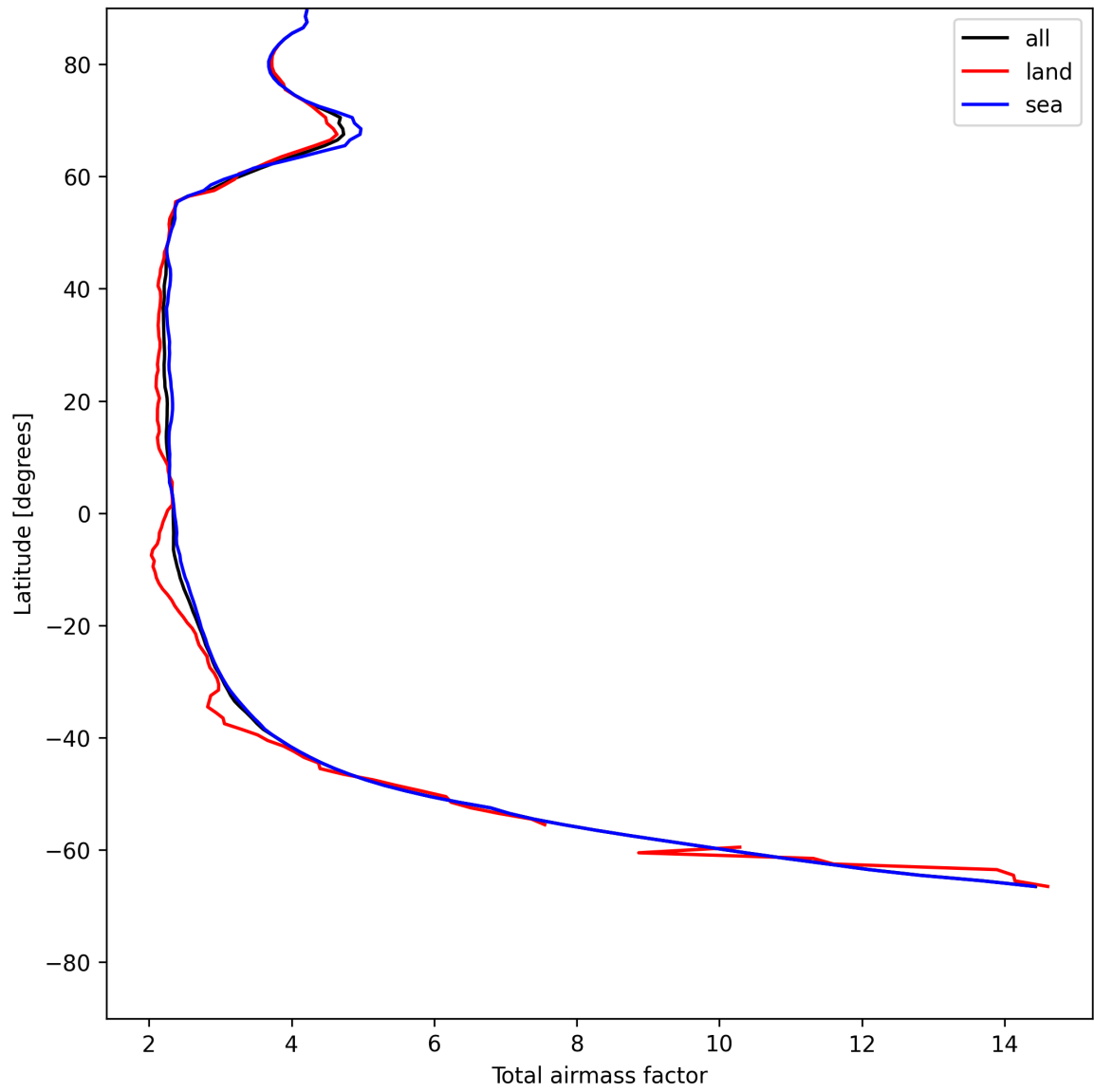
Figure 15: Zonal average of “Total airmass factor” for 2025-07-15 to 2025-07-17.
