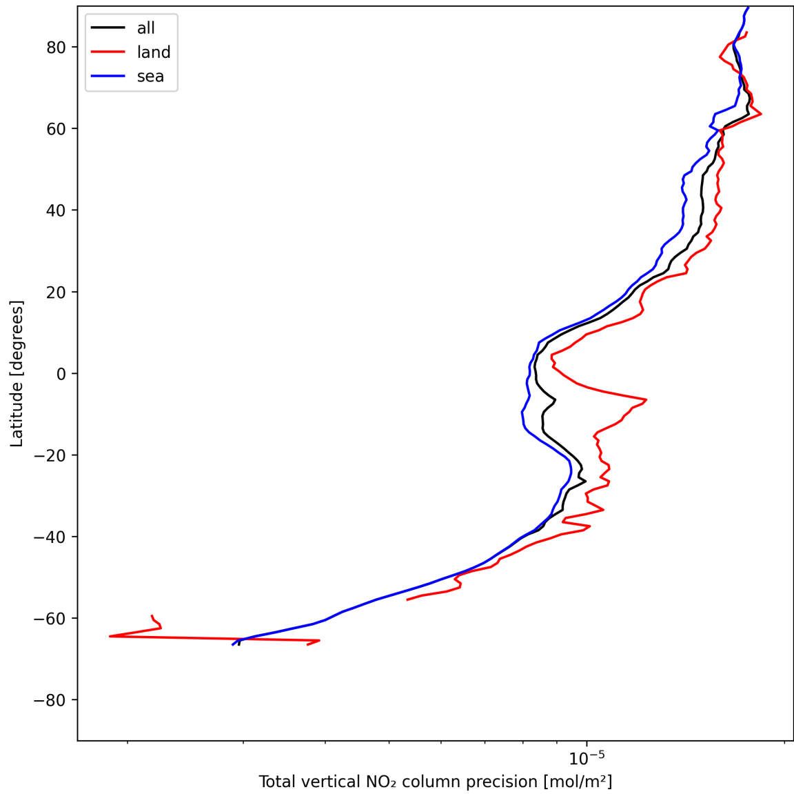
Figure 22: Zonal average of “Total vertical NO 2 column precision” for 2025-07-15 to 2025-07-17.
