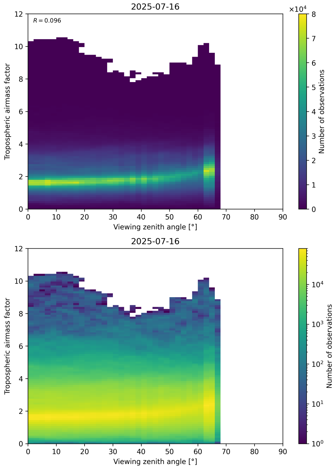
Figure 161: Scatter density plot of “Viewing zenith angle” against “Tropospheric airmass factor” for 2025-07-15 to 2025-07-17.
