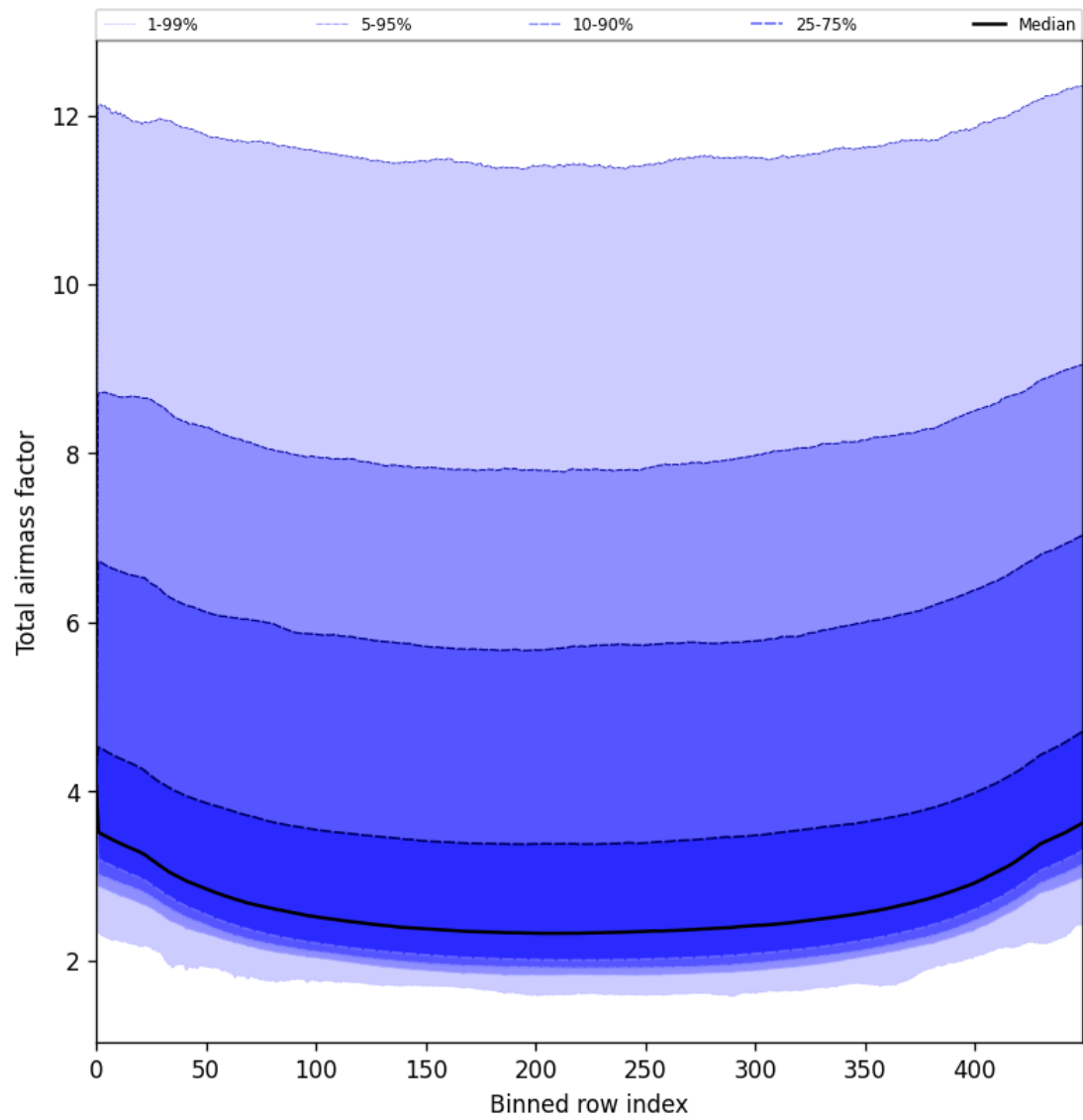
Figure 49: Along track statistics of “Total airmass factor” for 2025-07-15 to 2025-07-17
