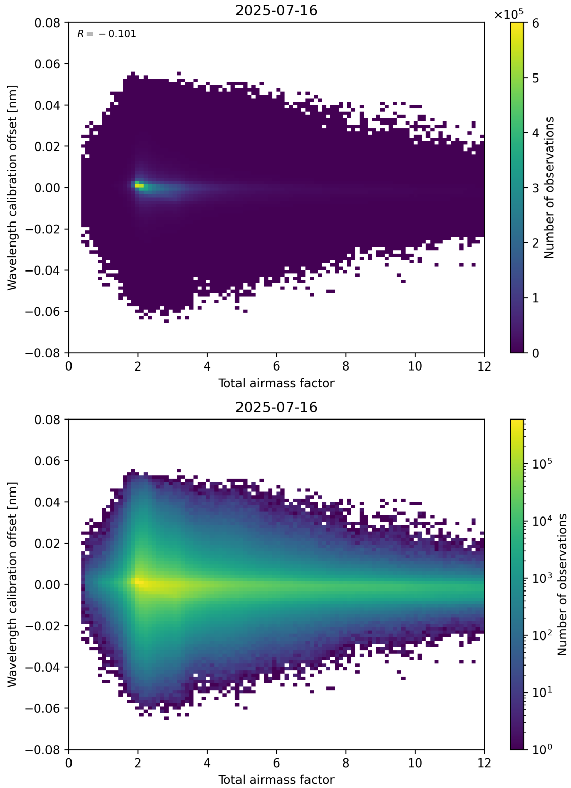
Figure 70: Scatter density plot of “Total airmass factor” against “Wavelength calibration offset” for 2025-07-15 to 2025-07-17.
