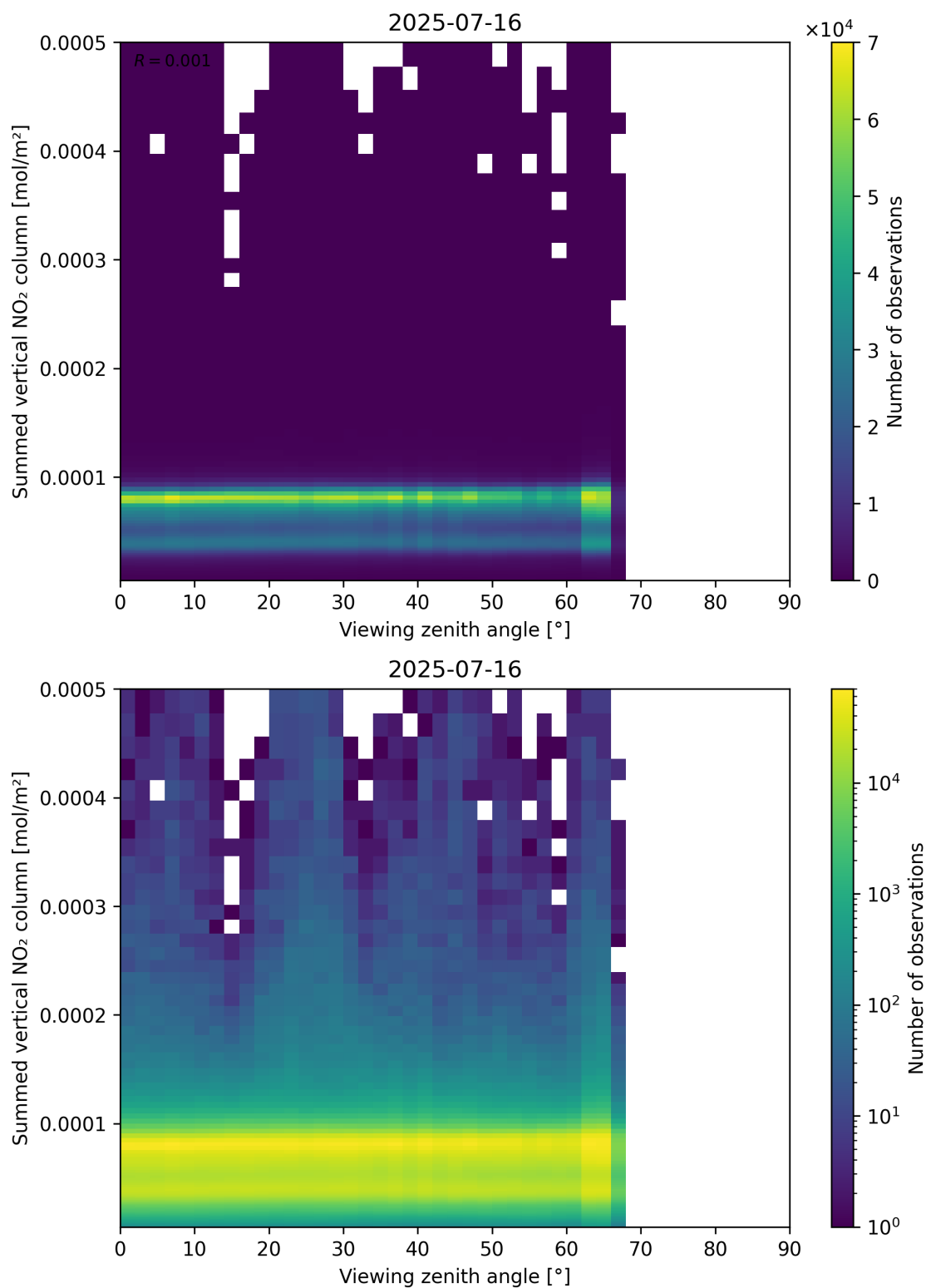
Figure 165: Scatter density plot of “Viewing zenith angle” against “Summed vertical NO 2 column” for 2025-07-15 to 2025-07-17.
