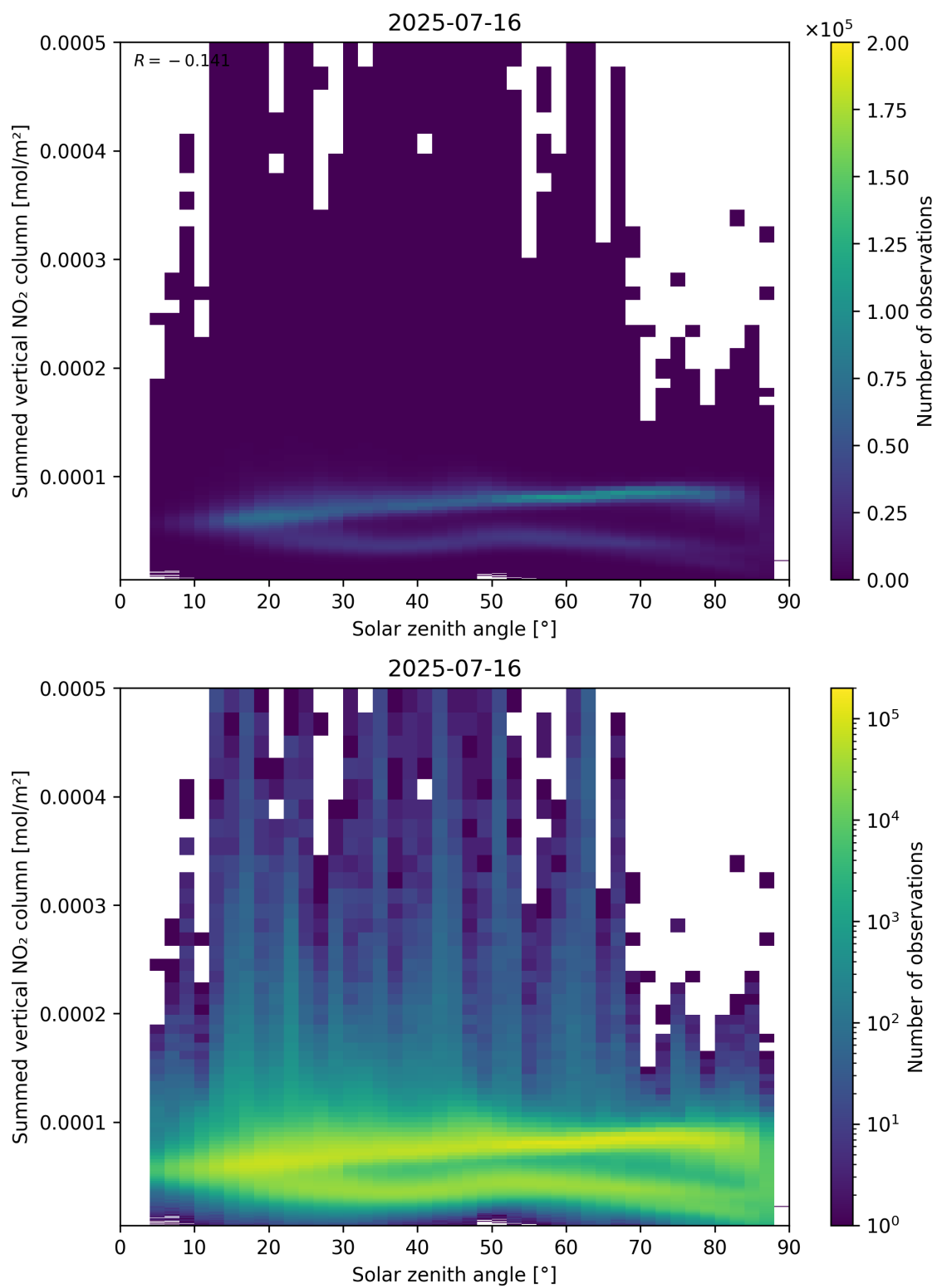
Figure 151: Scatter density plot of “Solar zenith angle” against “Summed vertical NO 2 column” for 2025-07-15 to 2025-07-17.
