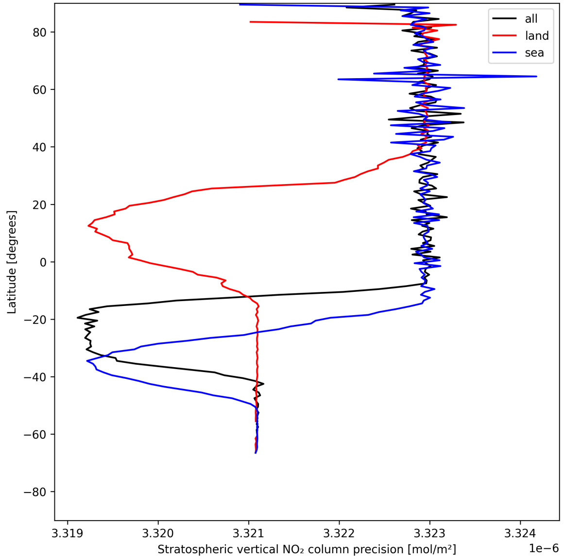
Figure 20: Zonal average of “Stratospheric vertical NO 2 column precision” for 2025-07-15 to 2025-07-17.
