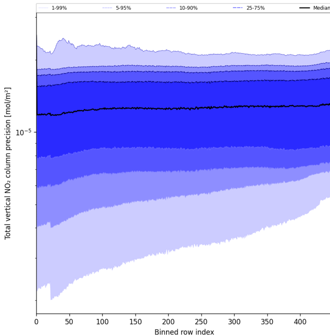
Figure 56: Along track statistics of “Total vertical NO 2 column precision” for 2025-07-15 to 2025-07-17
