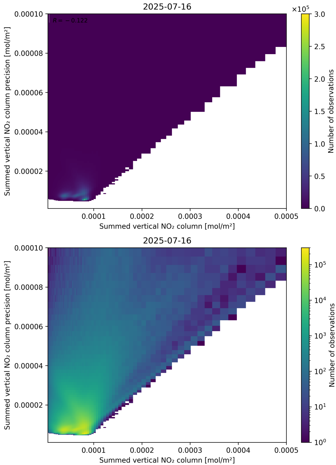
Figure 105: Scatter density plot of “Summed vertical NO 2 column” against “Summed vertical NO 2 column precision” for 2025-07-15 to 2025-07-17.
