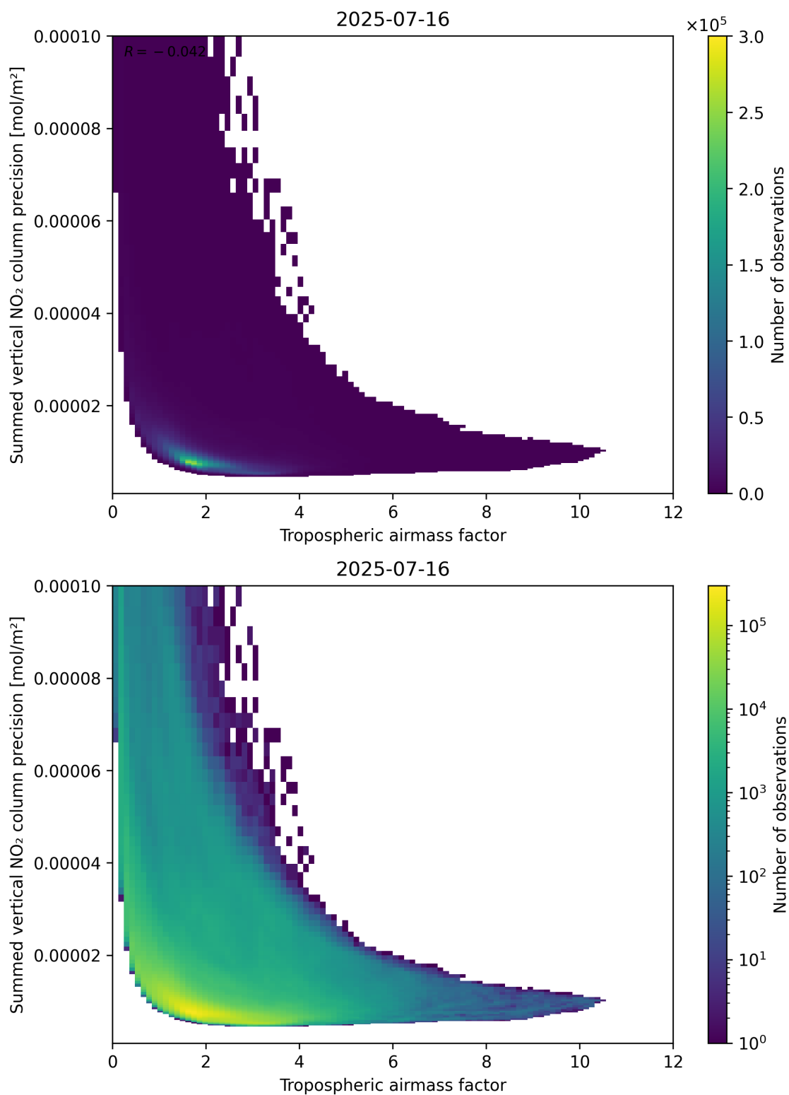
Figure 76: Scatter density plot of “Tropospheric air mass factor” against “Summed vertical NO 2 column precision” for 2025-07-15 to 2025-07-17.
