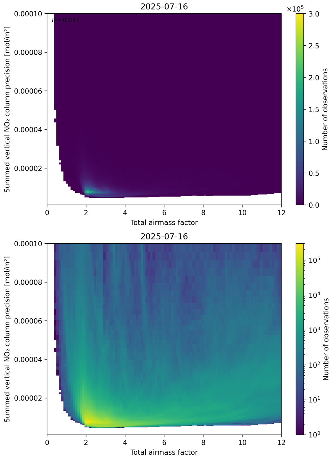
Figure 66: Scatter density plot of “Total airmass factor” against “Summed vertical NO 2 column precision” for 2025-07-15 to 2025-07-17.
