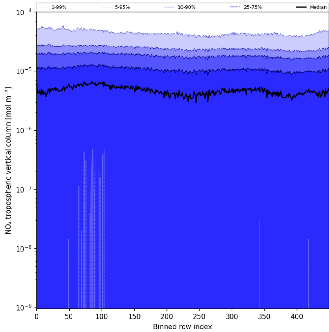
Figure 46: Along track statistics of “NO 2 tropospheric vertical column” for 2025-07-15 to 2025-07-17
