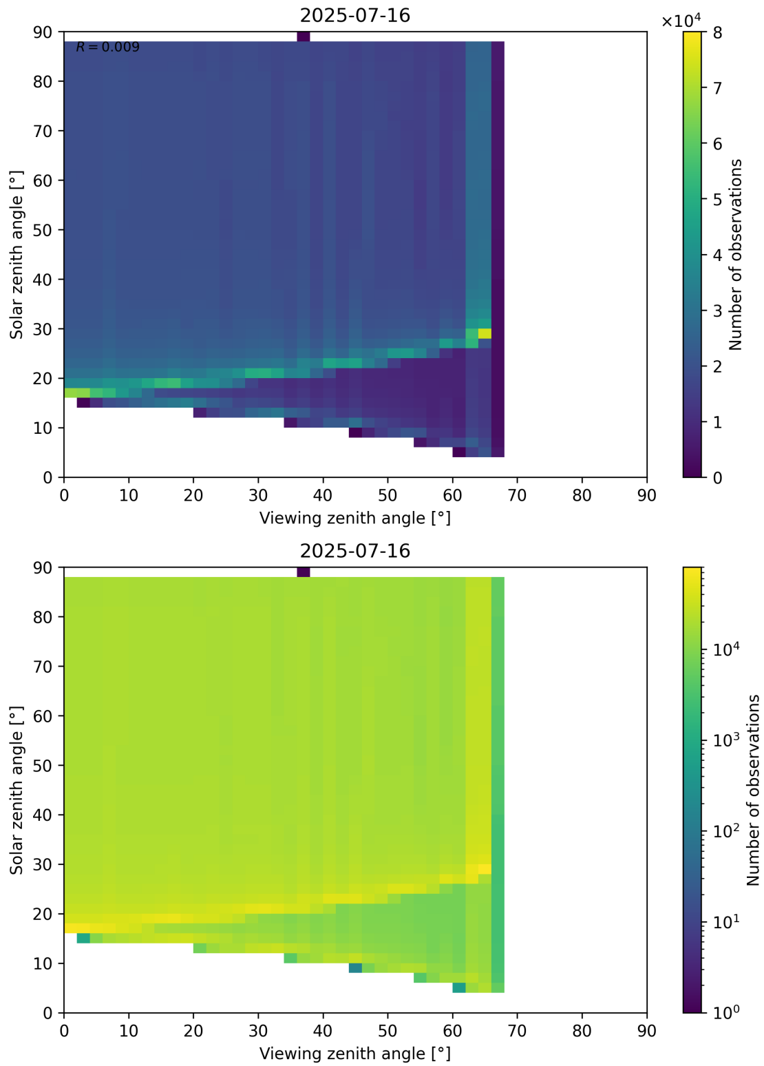
Figure 172: Scatter density plot of “Viewing zenith angle” against “Solar zenith angle” for 2025-07-15 to 2025-07-17.
