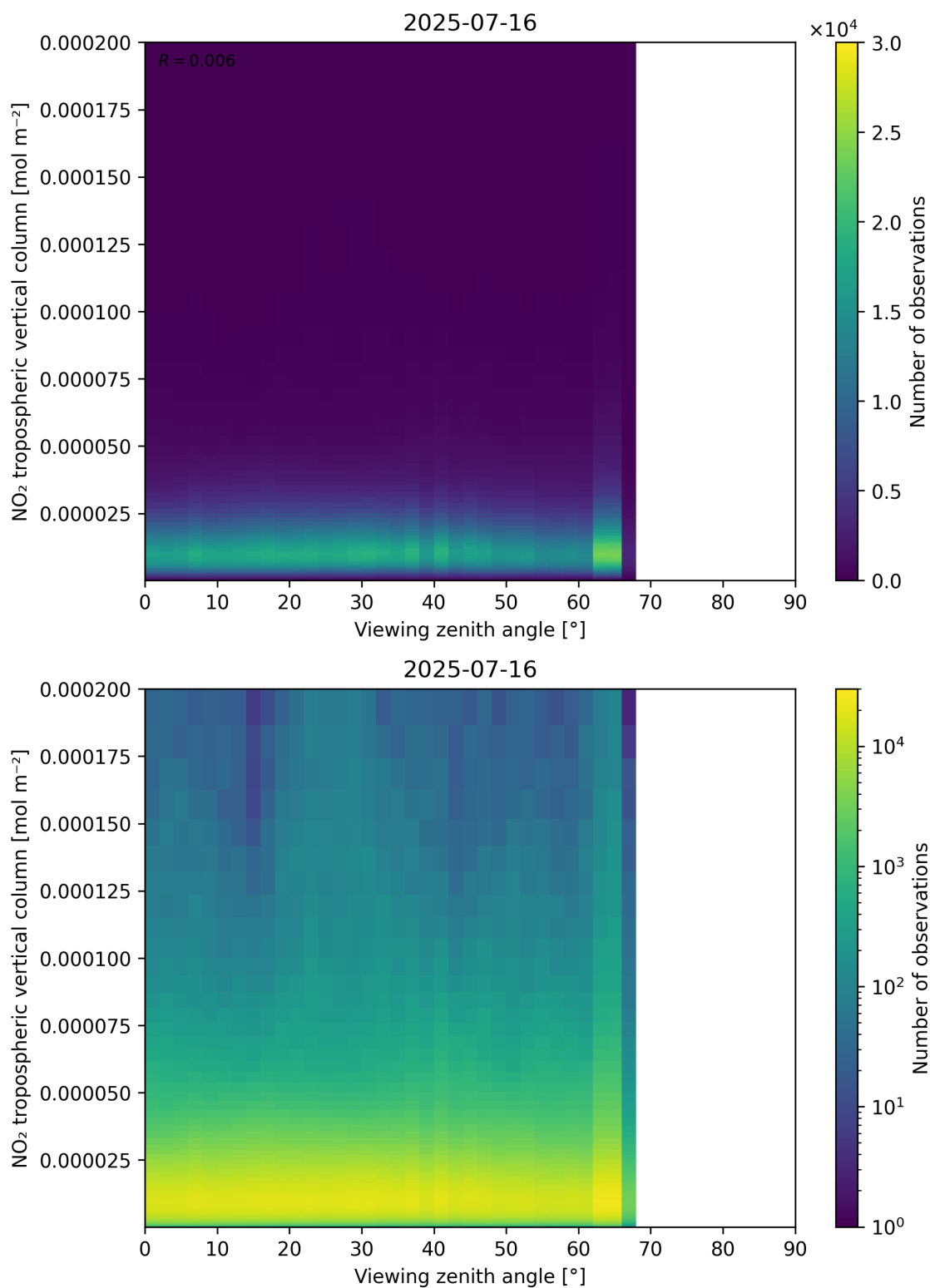
Figure 169: Scatter density plot of “Viewing zenith angle” against “NO 2 tropospheric vertical column” for 2025-07-15 to 2025-07-17.
