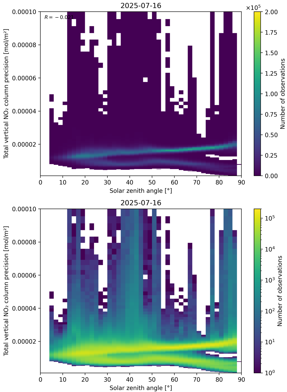
Figure 154: Scatter density plot of “Solar zenith angle” against “Total vertical NO 2 column precision” for 2025-07-15 to 2025-07-17.
