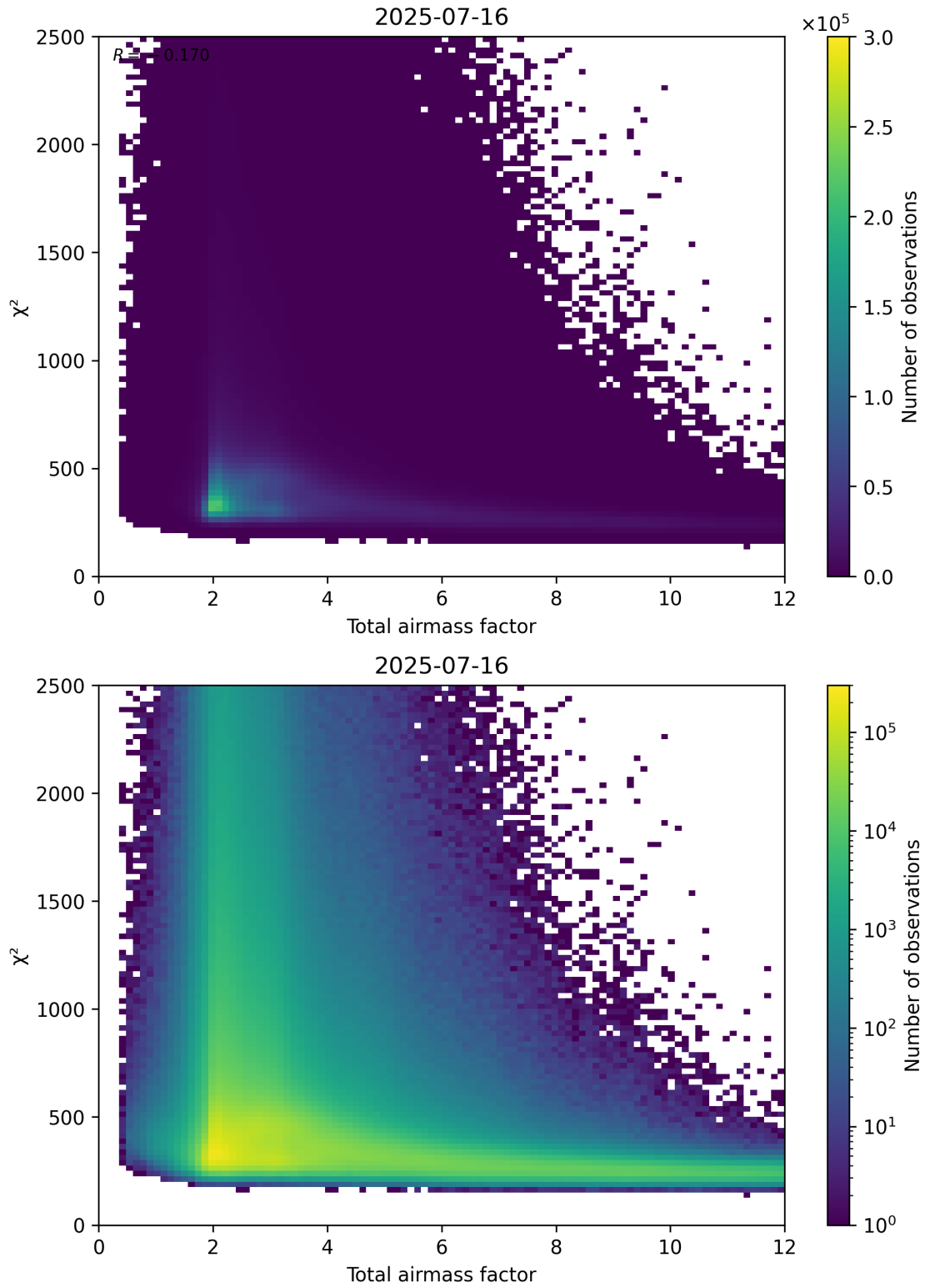
Figure 63: Scatter density plot of “Total airmass factor” against “ \chi^2 ” for 2025-07-15 to 2025-07-17.
