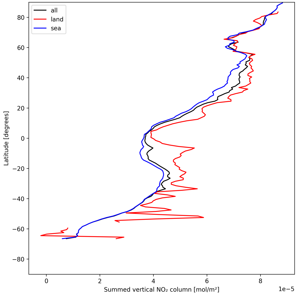
Figure 23: Zonal average of “Summed vertical NO 2 column” for 2025-07-15 to 2025-07-17.
