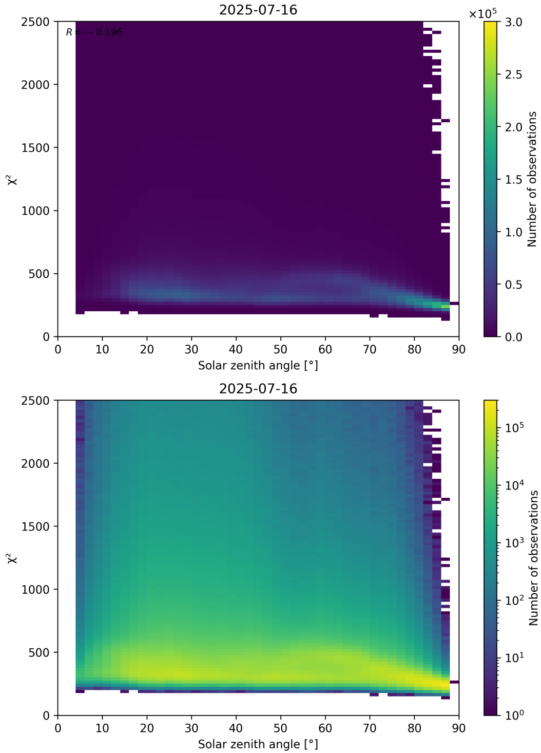
Figure 148: Scatter density plot of “Solar zenith angle” against “ \chi^2 ” for 2025-07-15 to 2025-07-17.
