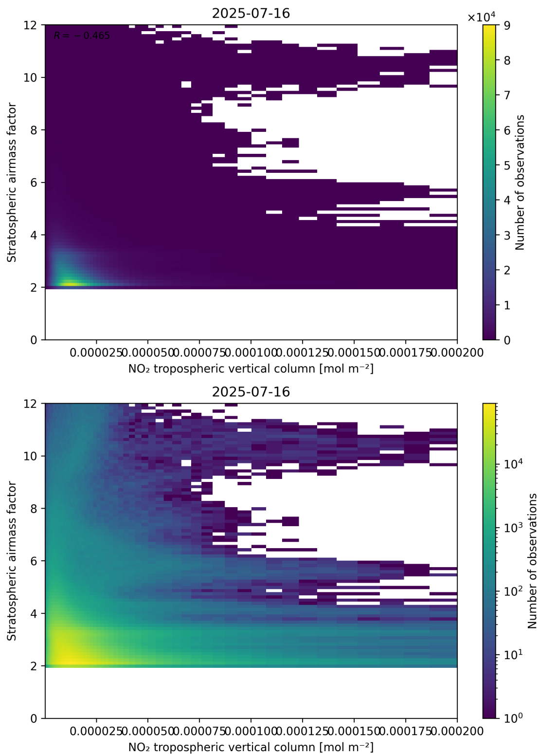
Figure 121: Scatter density plot of “NO 2 tropospheric vertical column” against “Stratospheric air mass factor” for 2025-07-15 to 2025-07-17.
