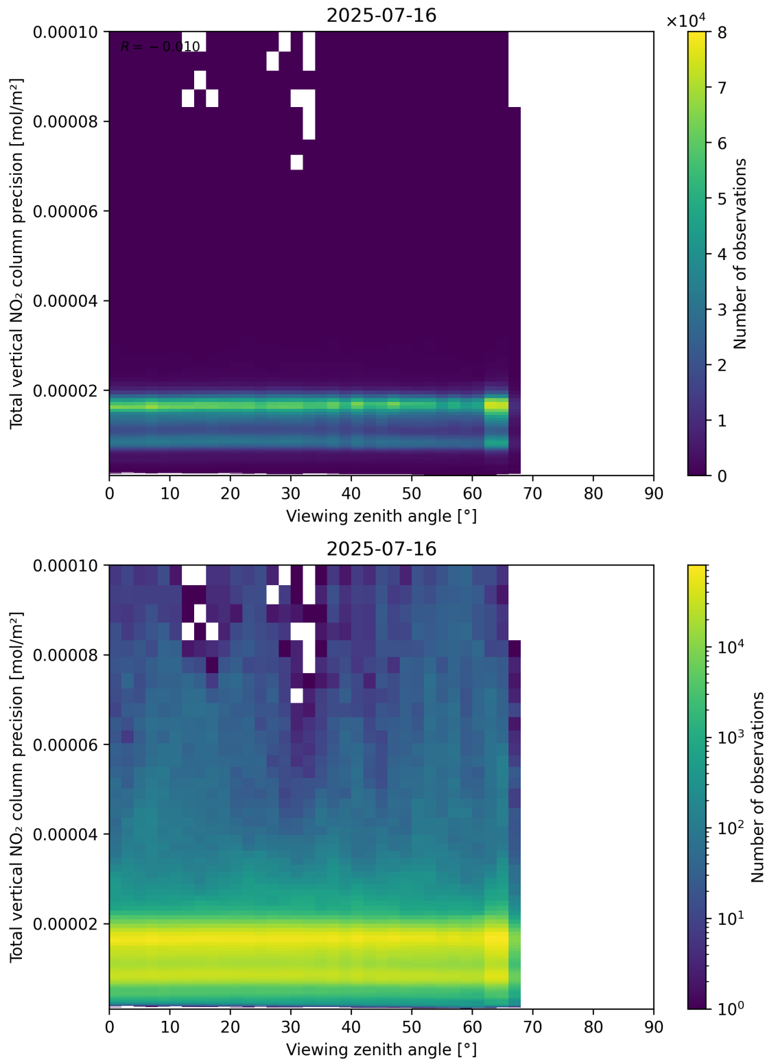
Figure 168: Scatter density plot of “Viewing zenith angle” against “Total vertical NO 2 column precision” for 2025-07-15 to 2025-07-17.
