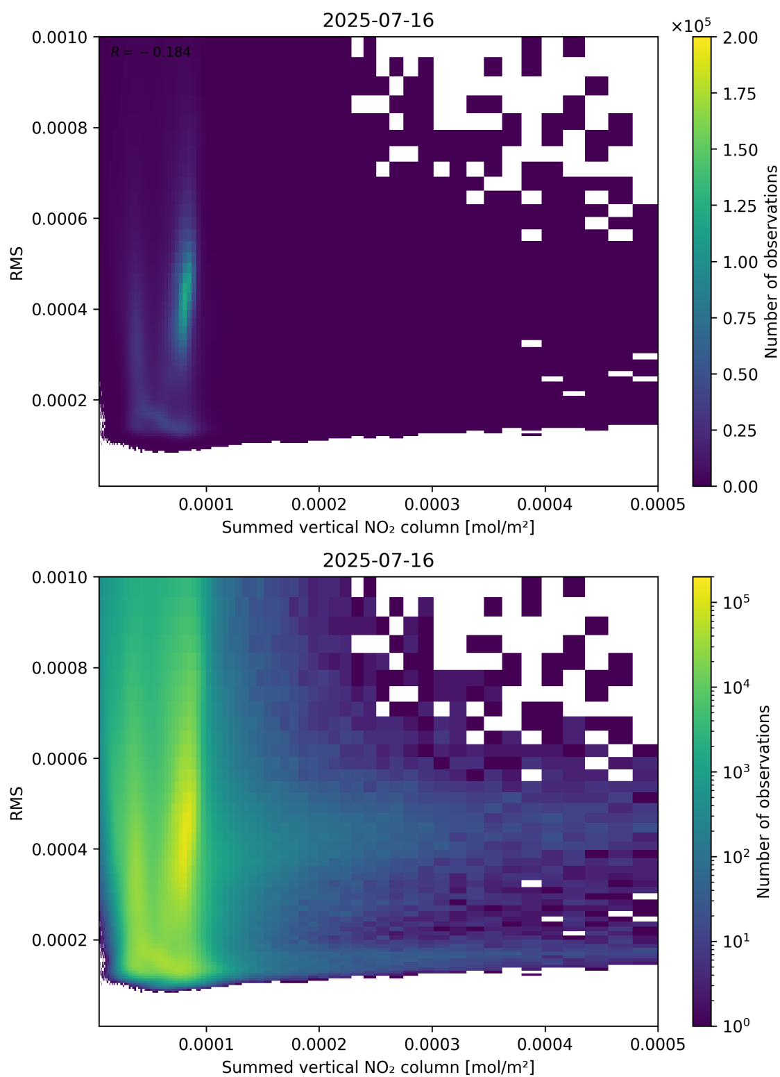
Figure 109: Scatter density plot of “Summed vertical NO 2 column” against “RMS” for 2025-07-15 to 2025-07-17.
