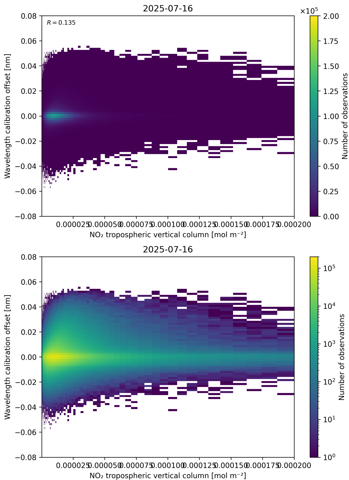
Figure 143: Scatter density plot of “NO 2 tropospheric vertical column” against “Wavelength calibration offset” for 2025-07-15 to 2025-07-17.
