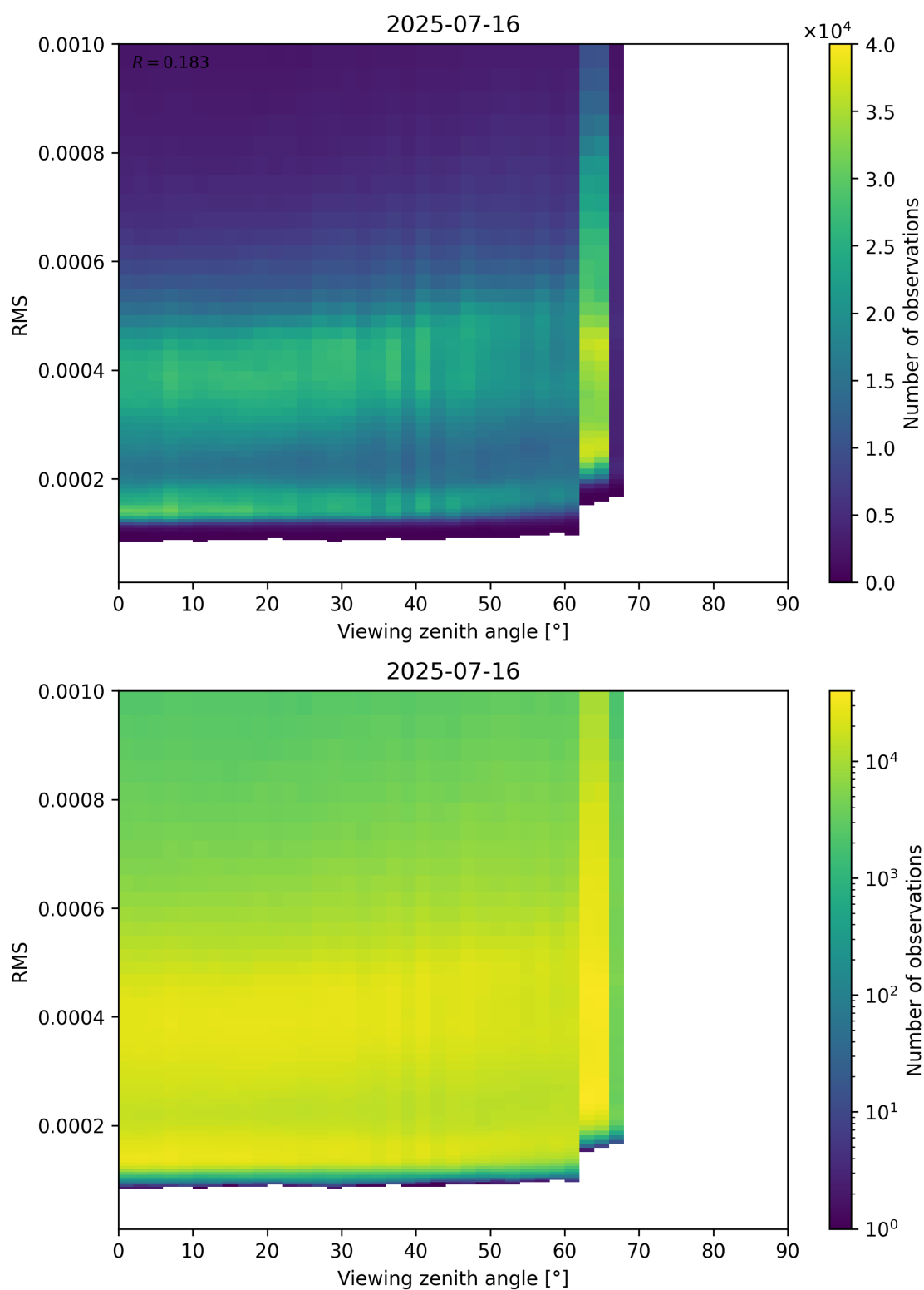
Figure 171: Scatter density plot of “Viewing zenith angle” against “RMS” for 2025-07-15 to 2025-07-17.
