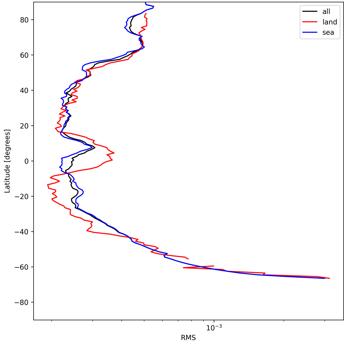
Figure 26: Zonal average of “RMS” for 2025-07-15 to 2025-07-17.
