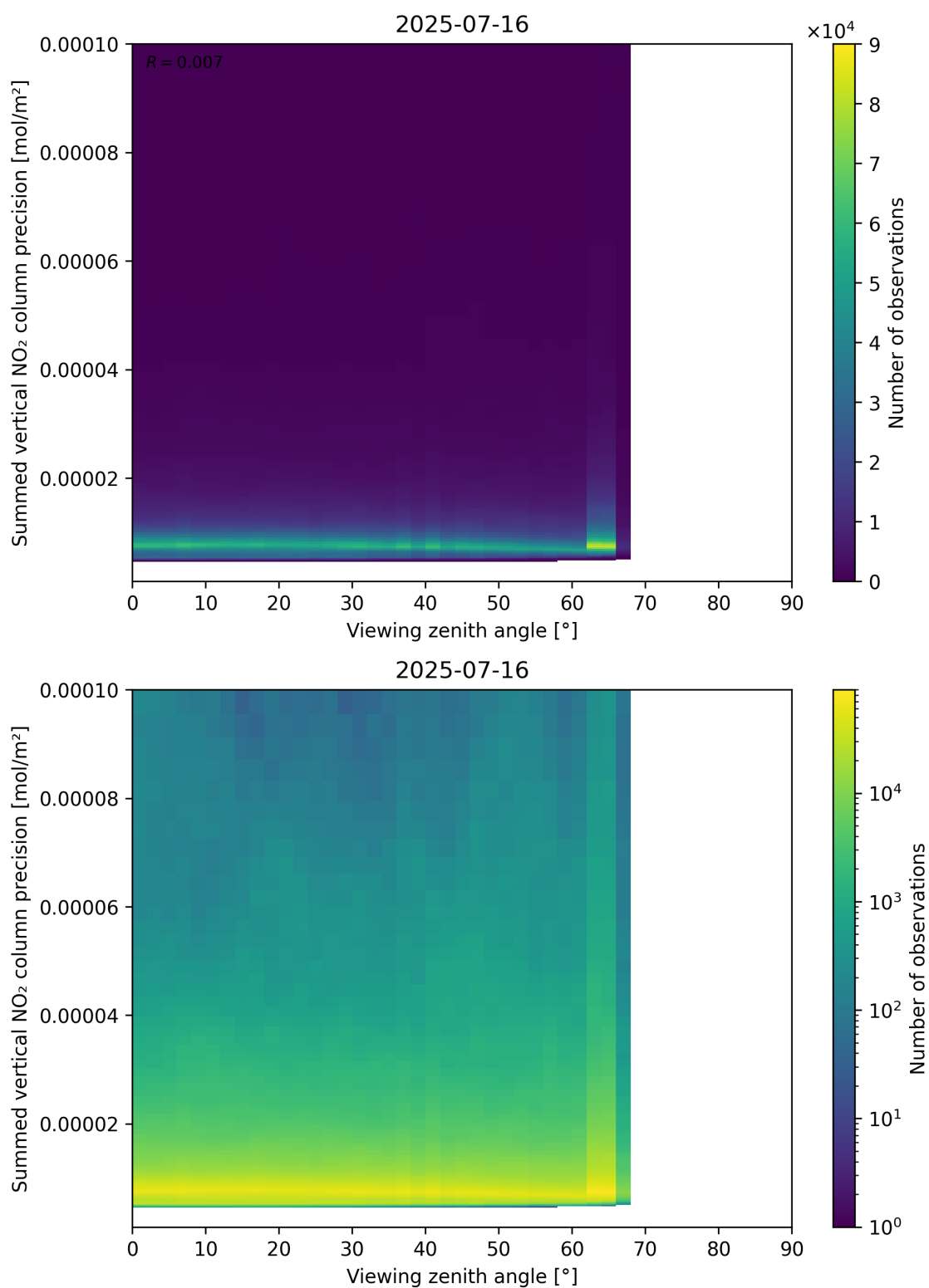
Figure 166: Scatter density plot of “Viewing zenith angle” against “Summed vertical NO 2 column precision” for 2025-07-15 to 2025-07-17.
