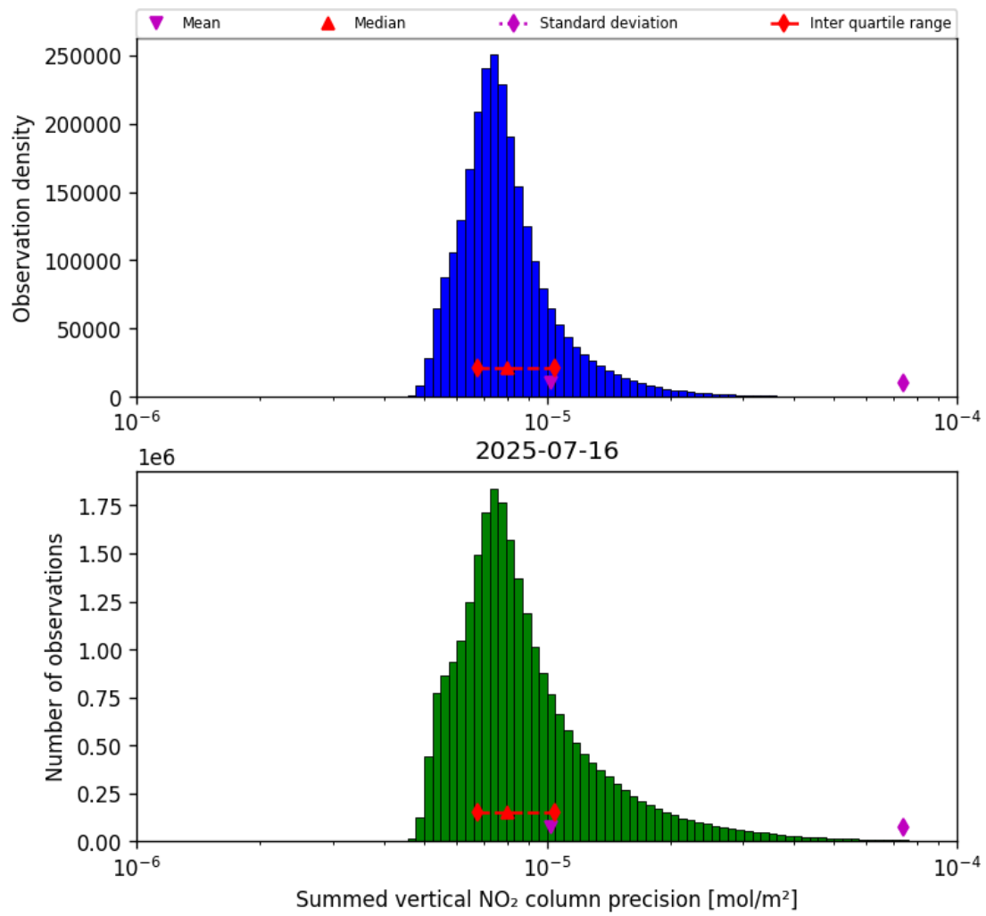
Figure 41: Histogram of "Summed vertical NO 2 column precision" for 2025-07-15 to 2025-07-17
