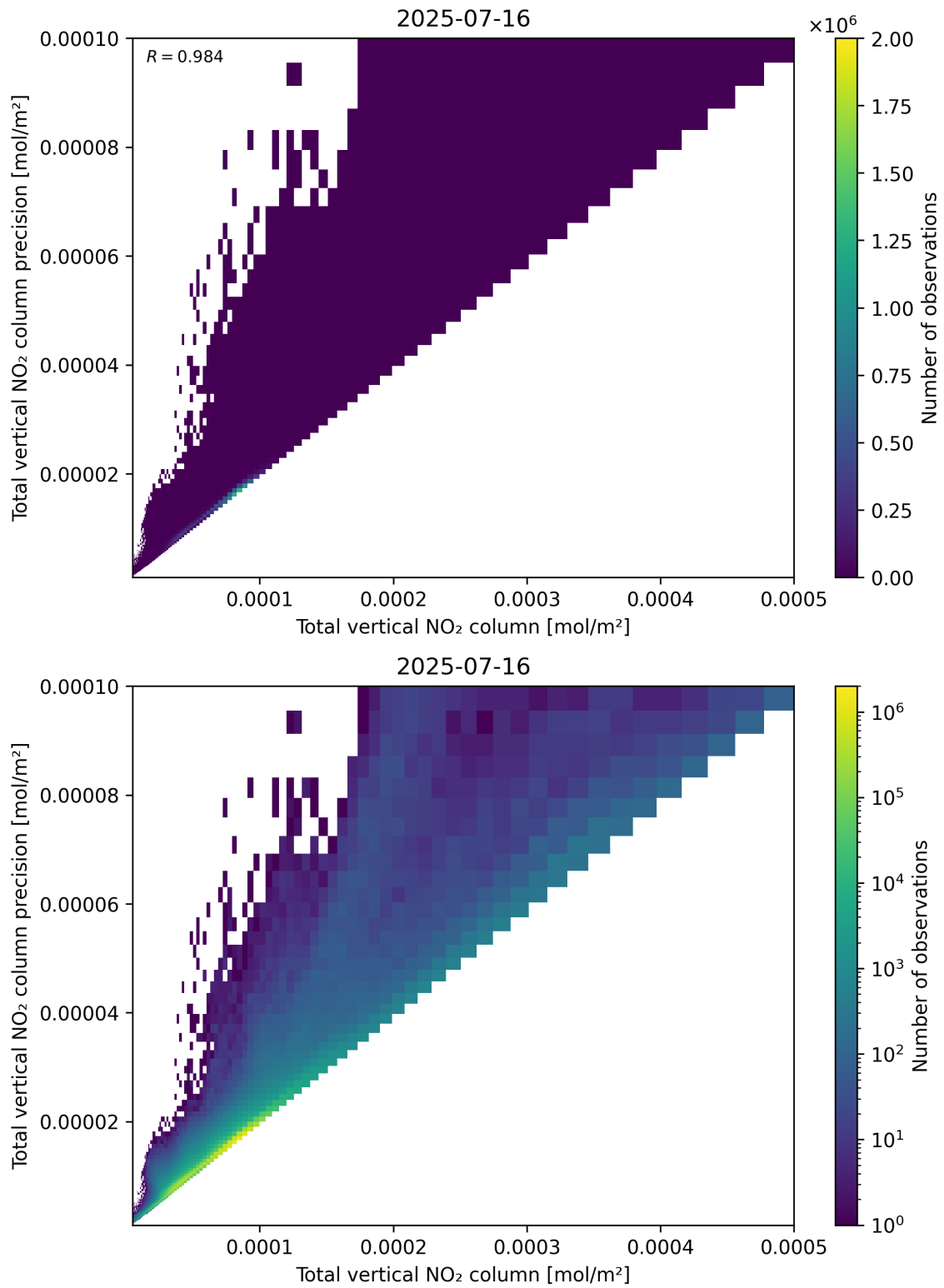
Figure 114: Scatter density plot of “Total vertical NO 2 column” against “Total vertical NO 2 column precision” for 2025-07-15 to 2025-07-17.
