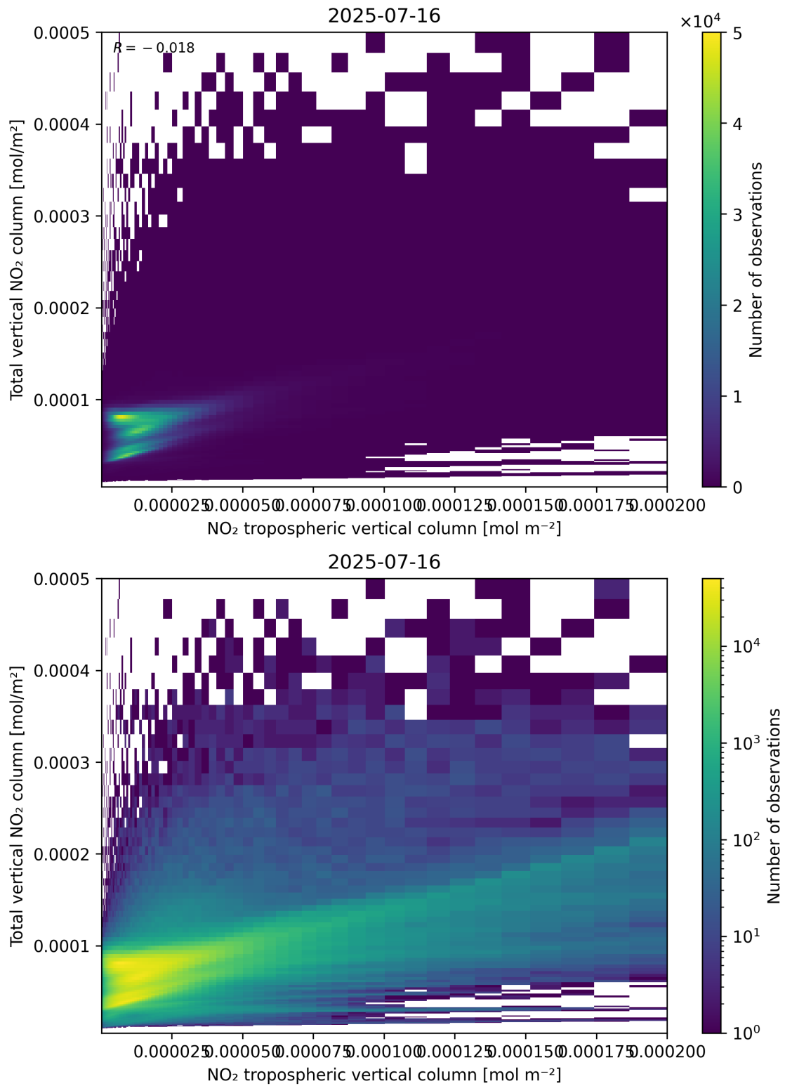
Figure 128: Scatter density plot of “NO 2 tropospheric vertical column” against “Total vertical NO 2 column” for 2025-07-15 to 2025-07-17.
