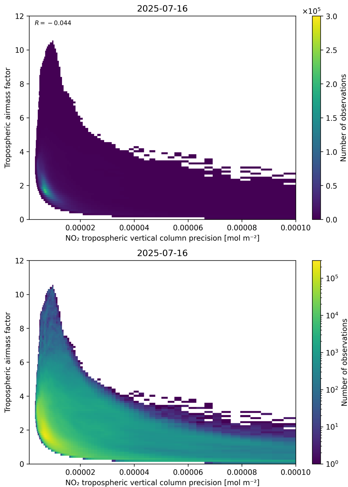
Figure 133: Scatter density plot of “NO 2 tropospheric vertical column precision” against “Tropospheric air mass factor” for 2025-07-15 to 2025-07-17.
