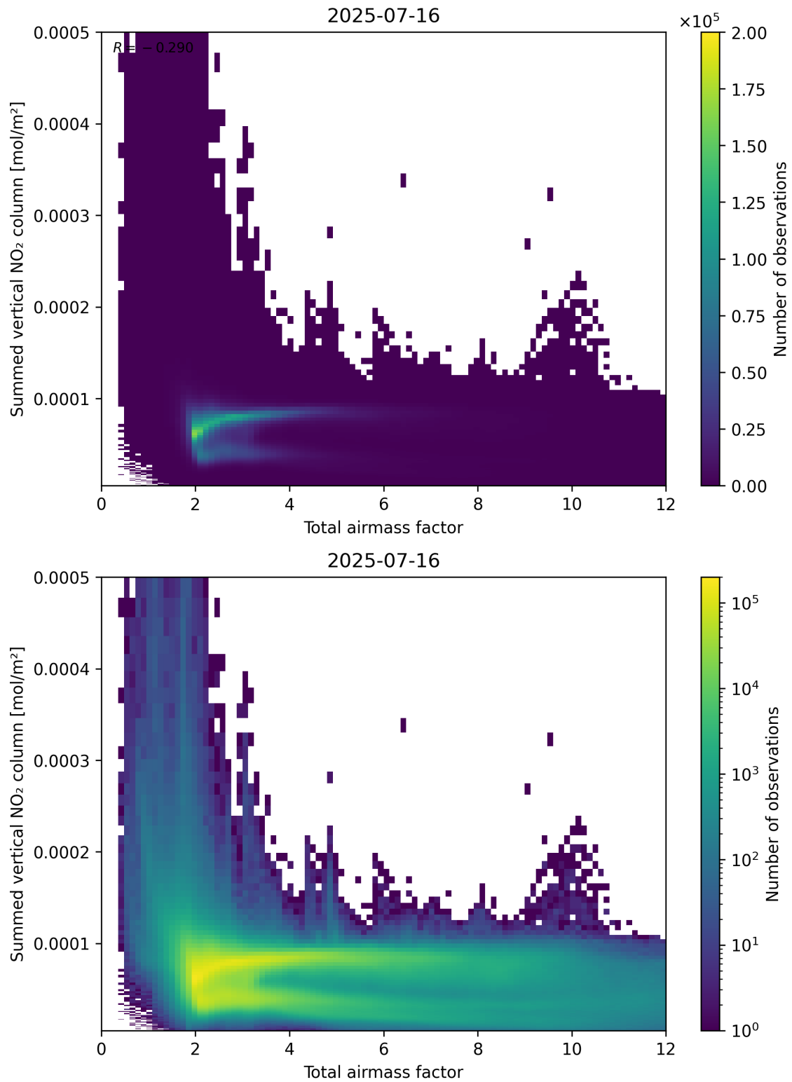
Figure 65: Scatter density plot of “Total airmass factor” against “Summed vertical NO 2 column” for 2025-07-15 to 2025-07-17.
