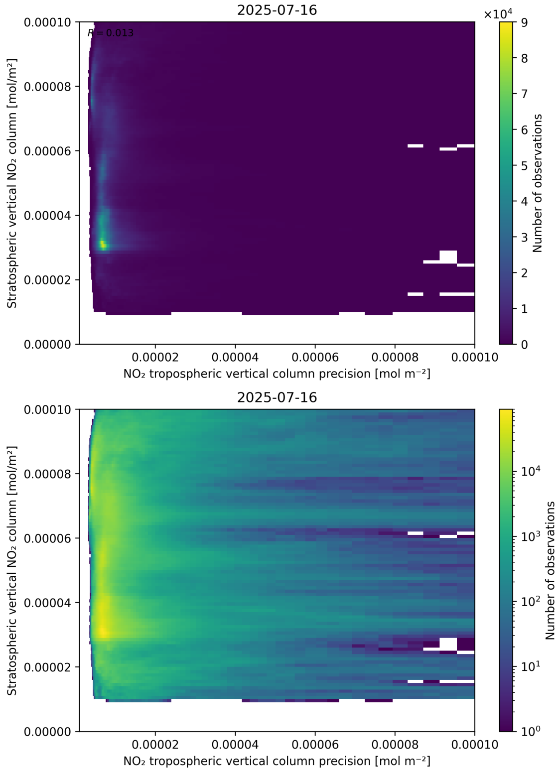
Figure 135: Scatter density plot of “NO 2 tropospheric vertical column precision” against “Stratospheric vertical NO 2 column” for 2025-07-15 to 2025-07-17.
