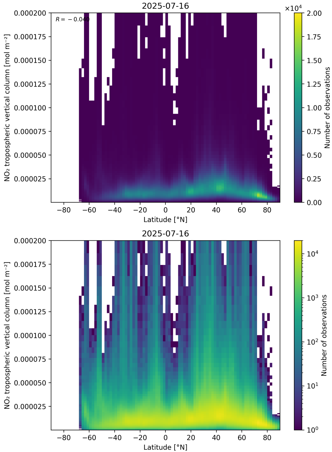
Figure 92: Scatter density plot of “Latitude” against “NO 2 tropospheric vertical column” for 2025-07-15 to 2025-07-17.
