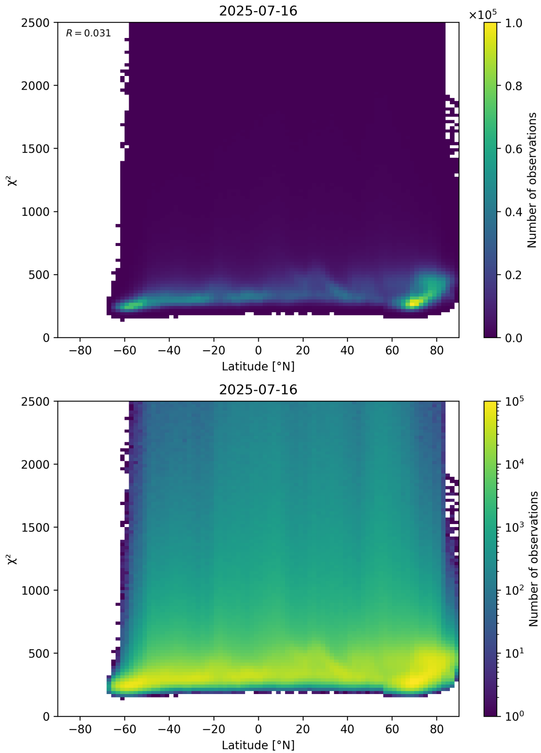
Figure 86: Scatter density plot of “Latitude” against “ \chi^2 ” for 2025-07-15 to 2025-07-17.
