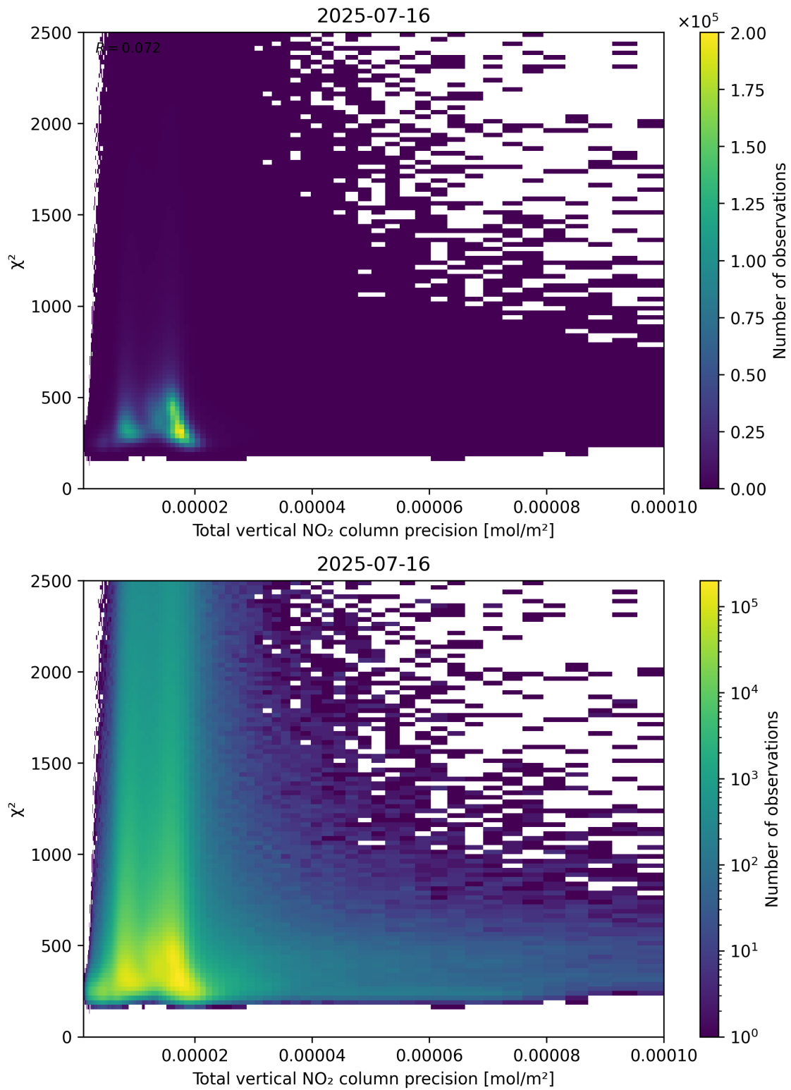
Figure 116: Scatter density plot of “Total vertical NO 2 column precision” against “ \chi^2 ” for 2025-07-15 to 2025-07-17.
