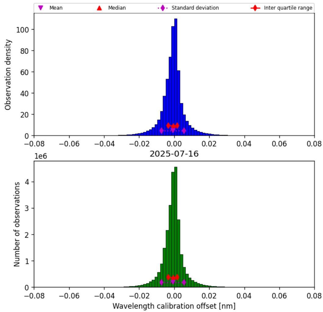
Figure 35: Histogram of “Wavelength calibration offset” for 2025-07-15 to 2025-07-17
