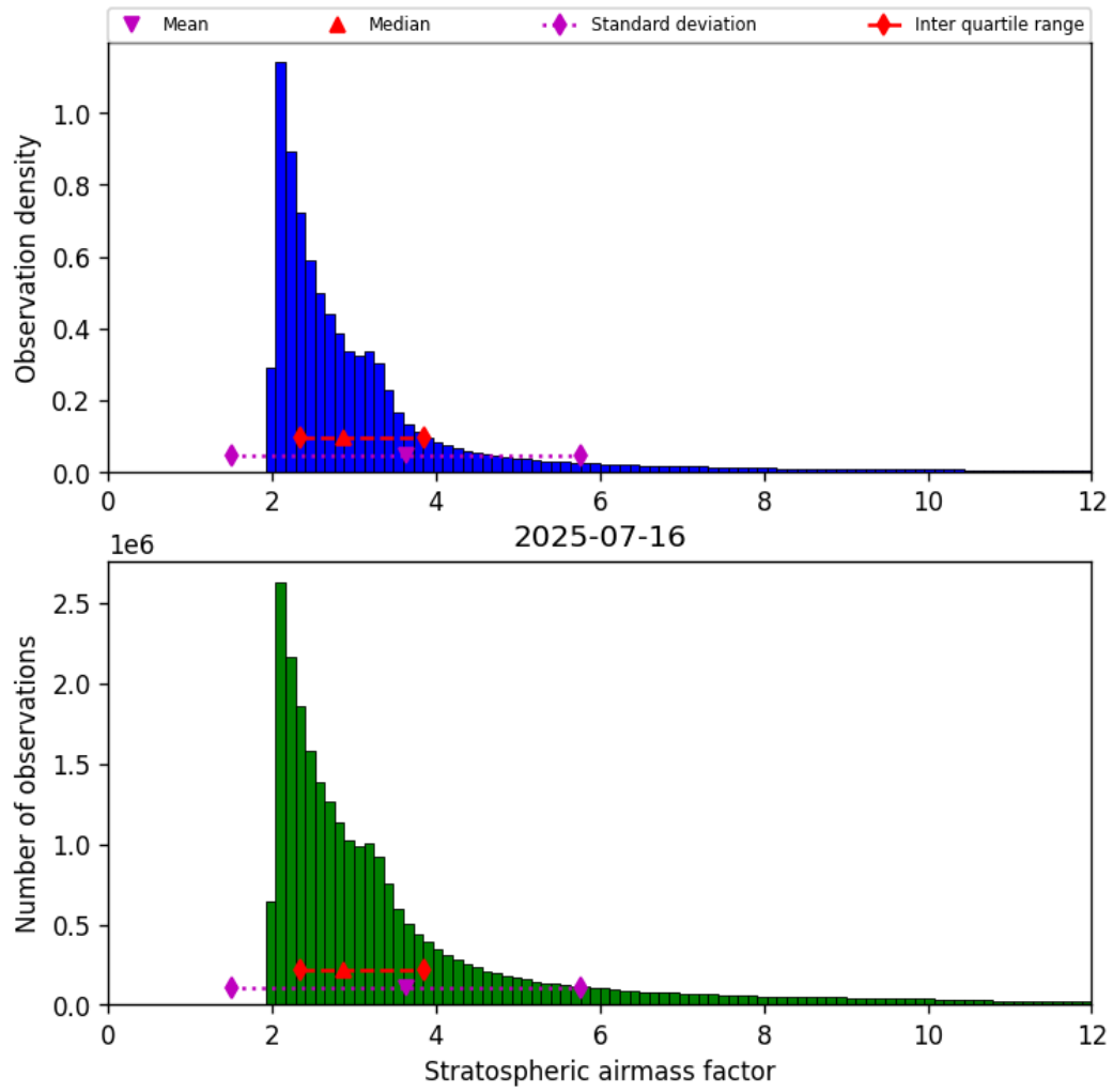
Figure 44: Histogram of “Stratospheric airmass factor” for 2025-07-15 to 2025-07-17
