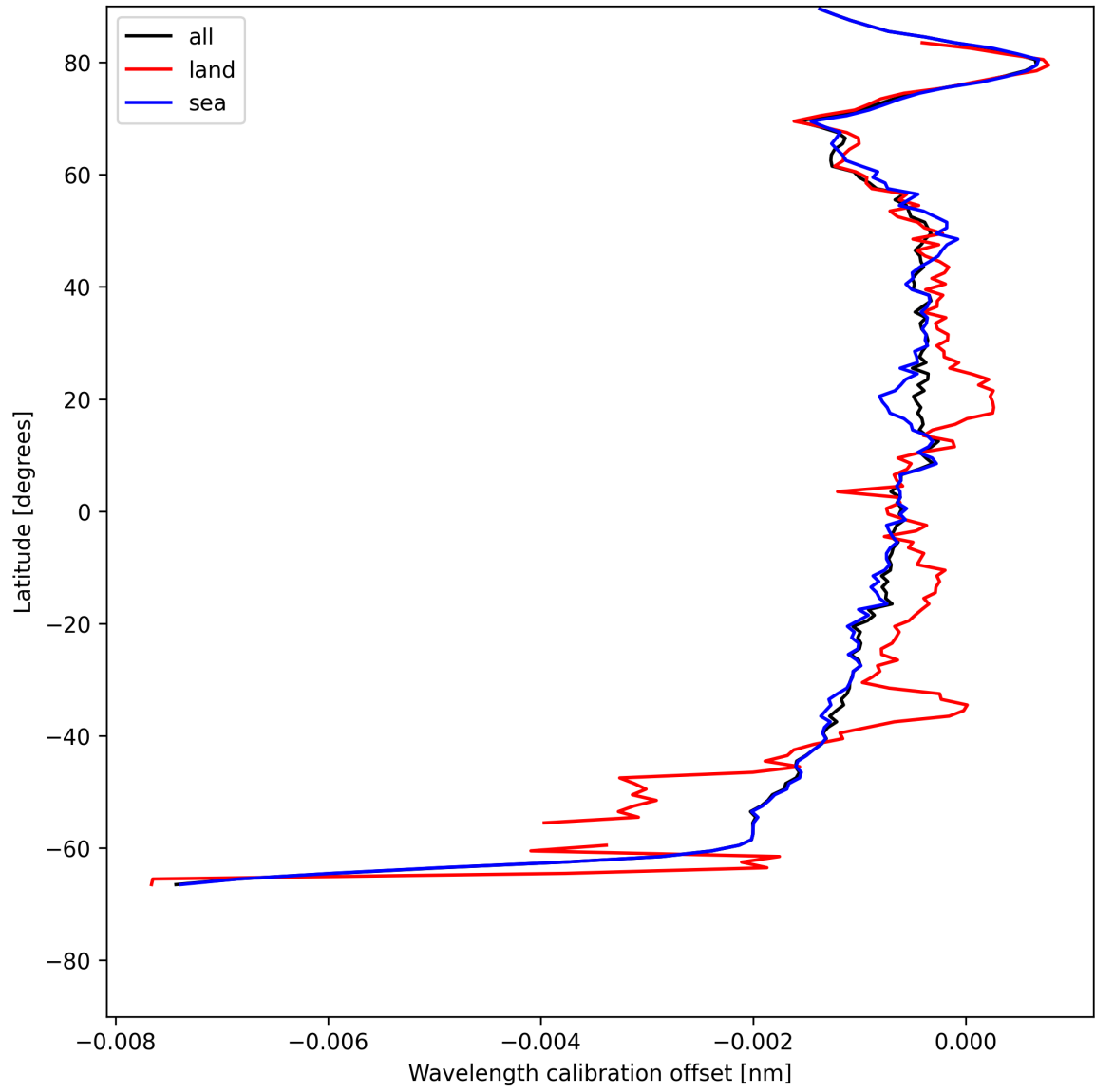
Figure 18: Zonal average of “Wavelength calibration offset” for 2025-07-15 to 2025-07-17.
