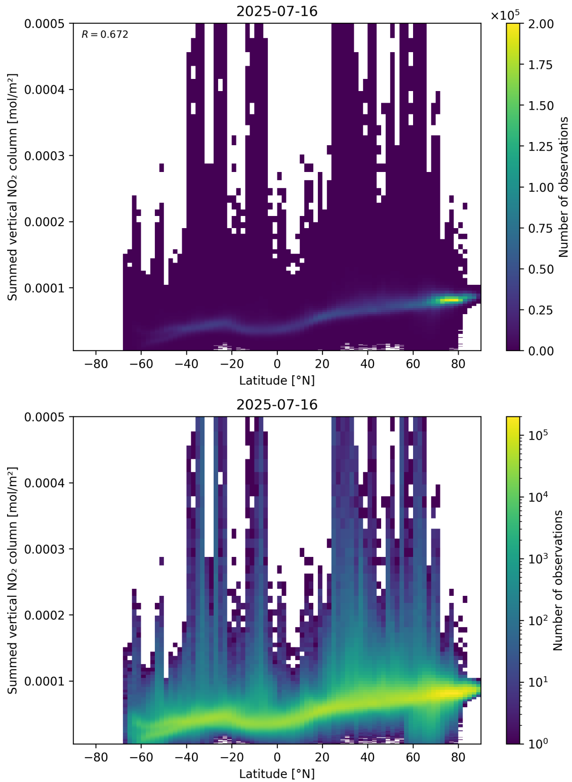
Figure 88: Scatter density plot of “Latitude” against “Summed vertical NO 2 column” for 2025-07-15 to 2025-07-17.
