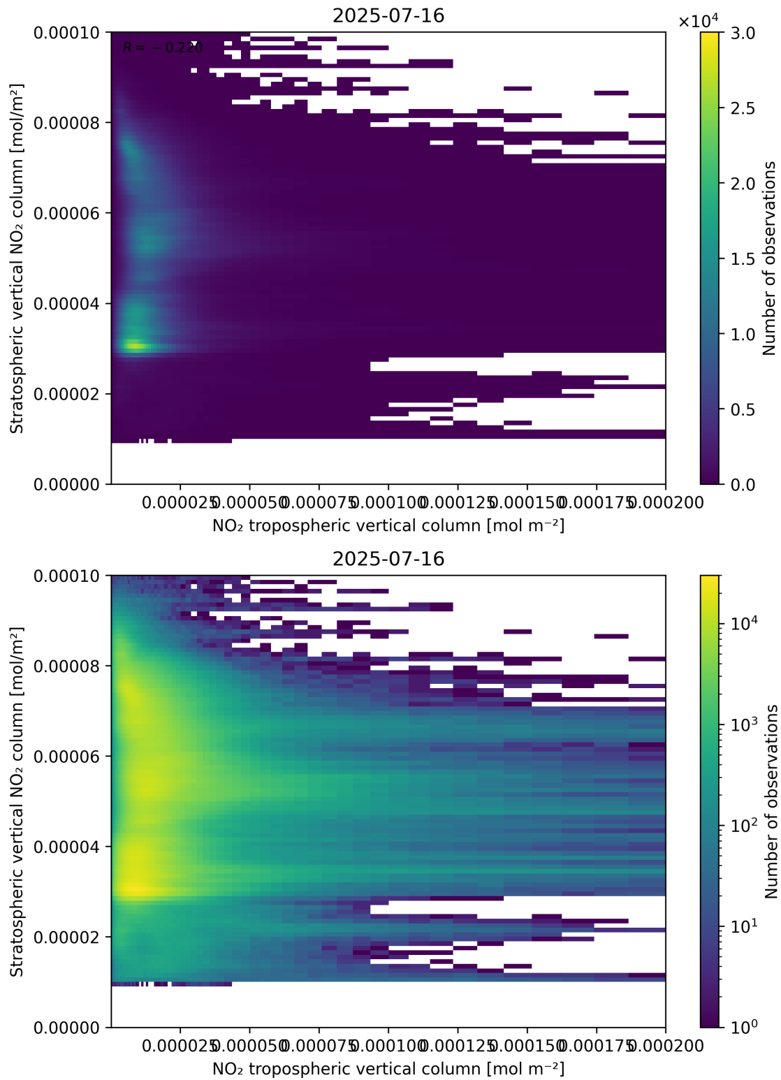
Figure 125: Scatter density plot of “NO 2 tropospheric vertical column” against “Stratospheric vertical NO 2 column” for 2025-07-15 to 2025-07-17.
