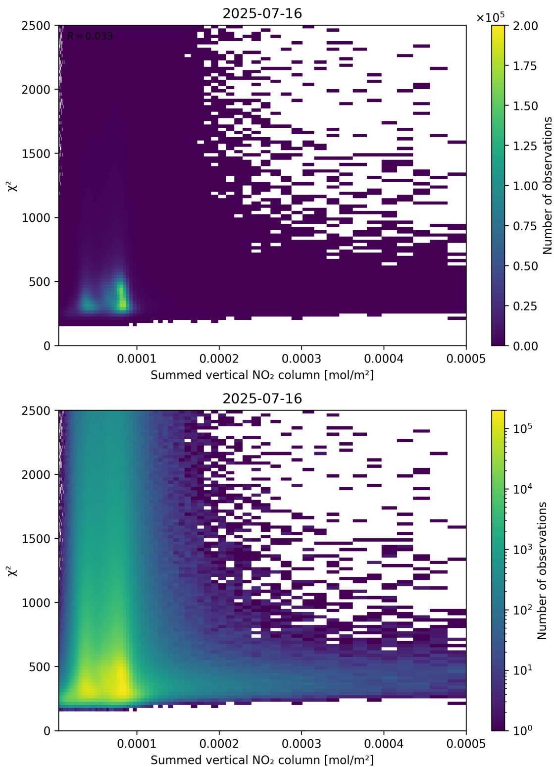
Figure 104: Scatter density plot of “Summed vertical NO 2 column” against “ \chi^2 ” for 2025-07-15 to 2025-07-17.
