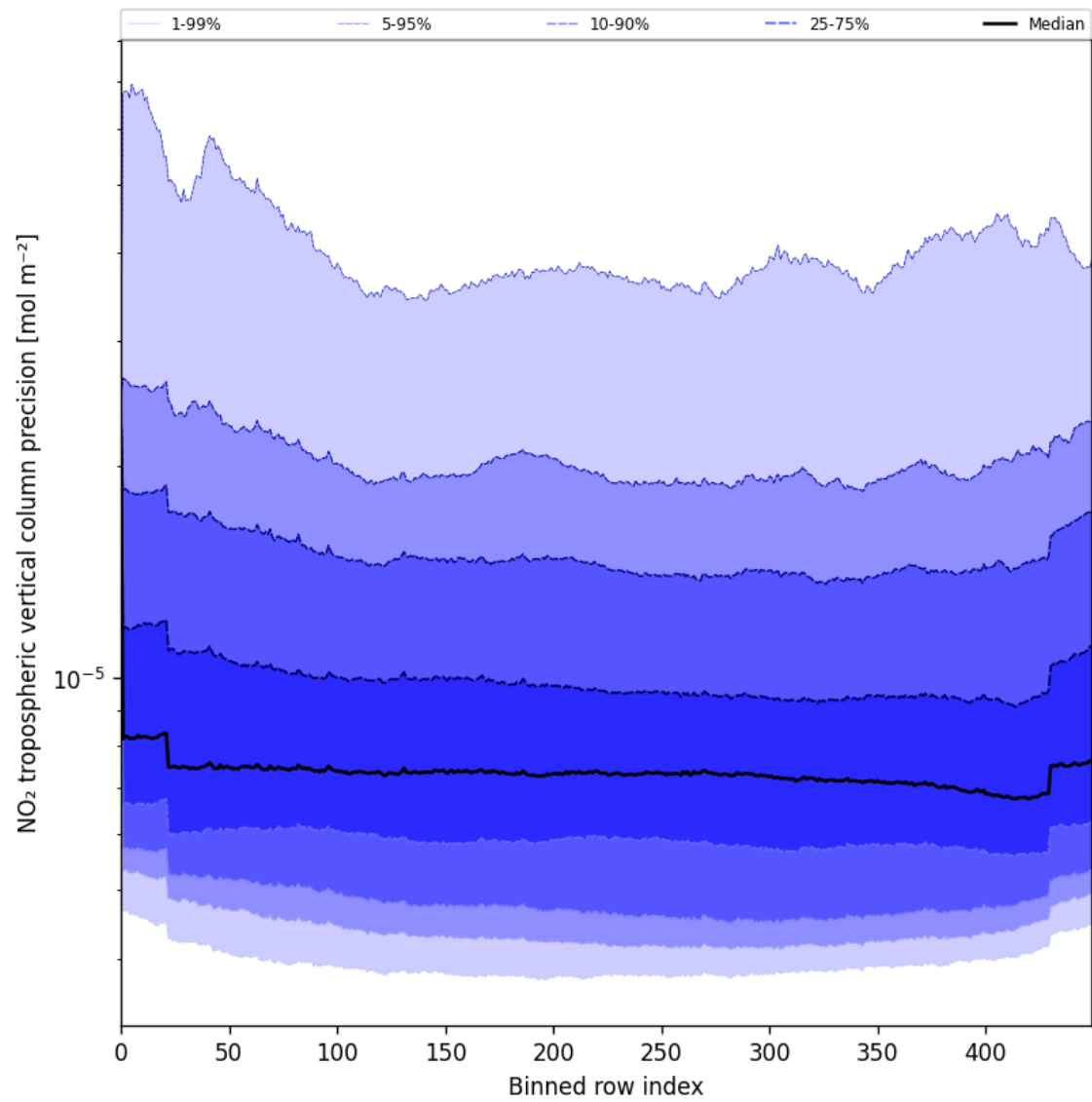
Figure 47: Along track statistics of “NO 2 tropospheric vertical column precision” for 2025-07-15 to 2025-07-17
