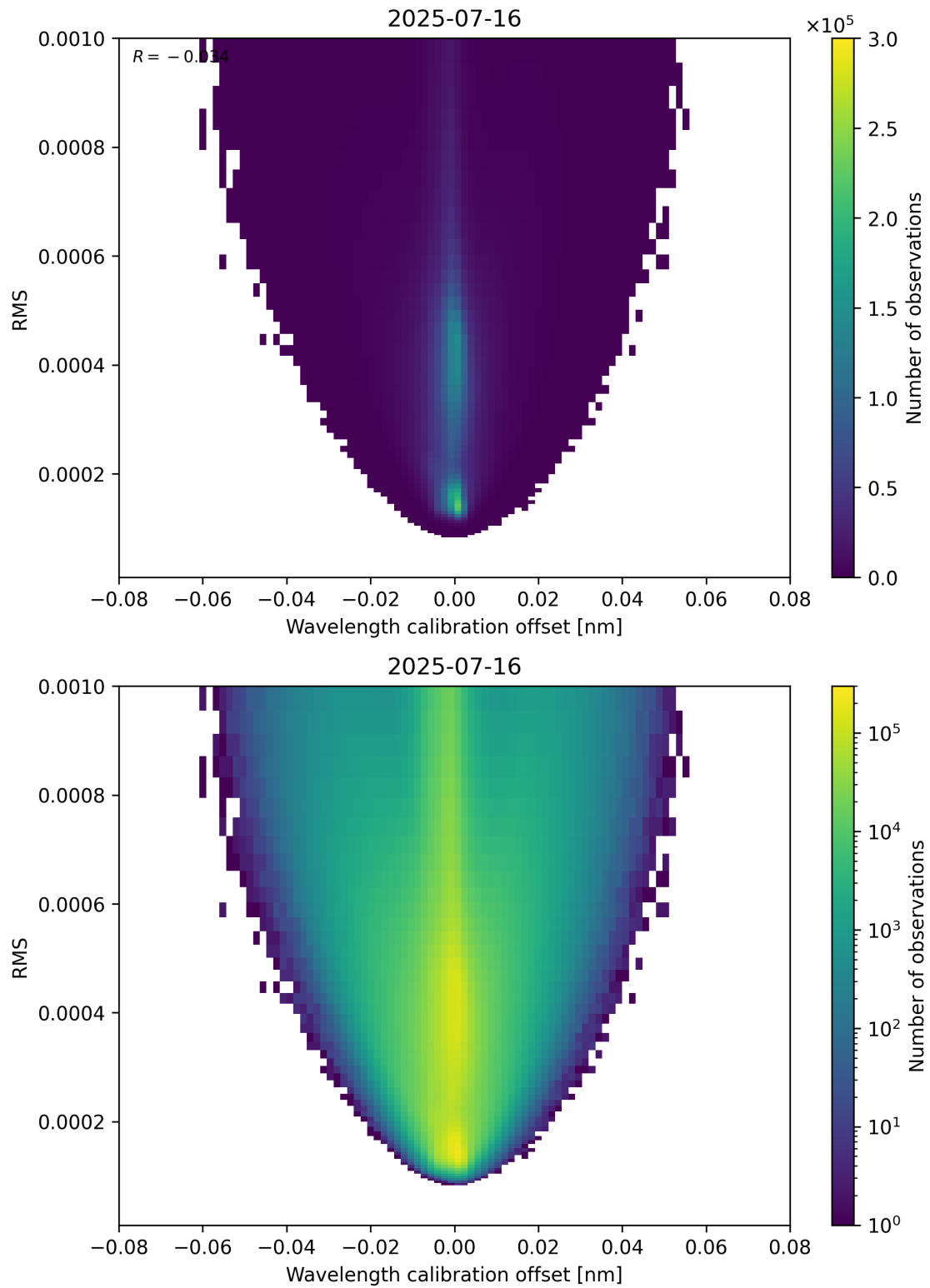
Figure 181: Scatter density plot of “Wavelength calibration offset” against “RMS” for 2025-07-15 to 2025-07-17.
