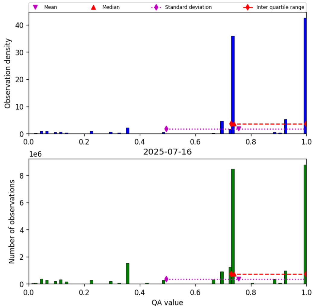
Figure 28: Histogram of “QA value” for 2025-07-15 to 2025-07-17
