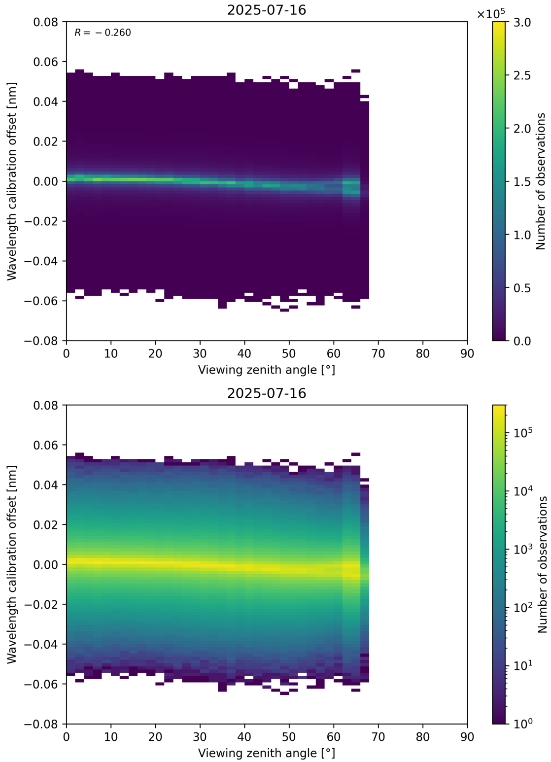
Figure 173: Scatter density plot of “Viewing zenith angle” against “Wavelength calibration offset” for 2025-07-15 to 2025-07-17.
