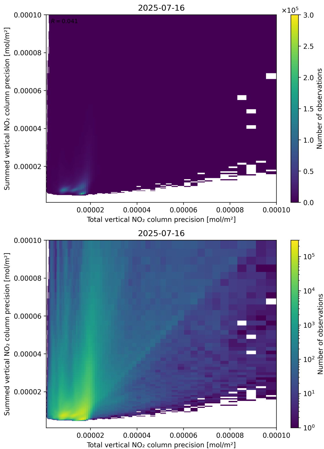
Figure 118: Scatter density plot of “Total vertical NO 2 column precision” against “Summed vertical NO 2 column precision” for 2025-07-15 to 2025-07-17.
