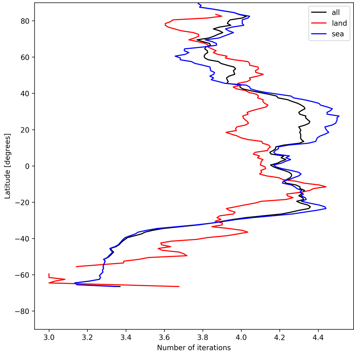
Figure 17: Zonal average of “Number of iterations” for 2025-07-15 to 2025-07-17.
