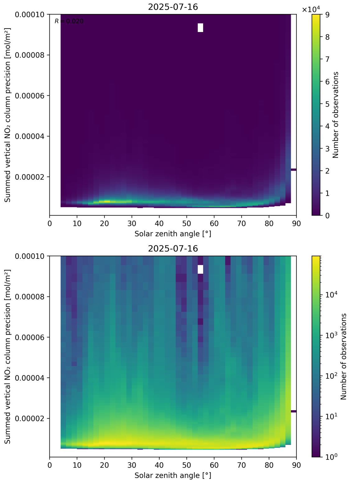
Figure 152: Scatter density plot of “Solar zenith angle” against “Summed vertical NO 2 column precision” for 2025-07-15 to 2025-07-17.
