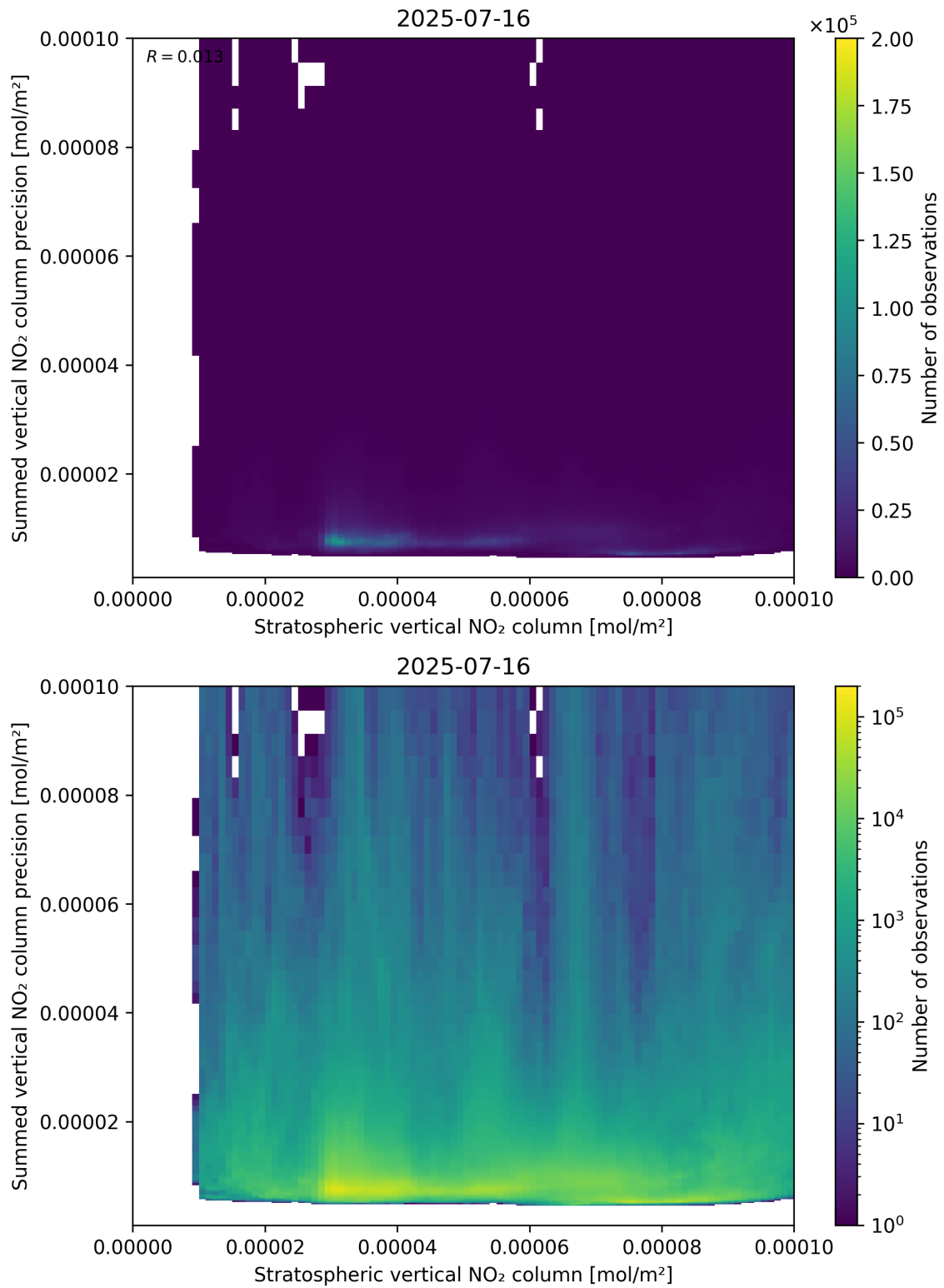
Figure 99: Scatter density plot of “Stratospheric vertical NO 2 column” against “Summed vertical NO 2 column precision” for 2025-07-15 to 2025-07-17.
