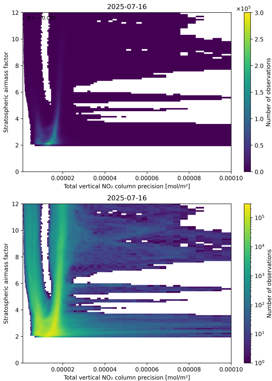
Figure 115: Scatter density plot of “Total vertical NO 2 column precision” against “Stratospheric air mass factor” for 2025-07-15 to 2025-07-17.
