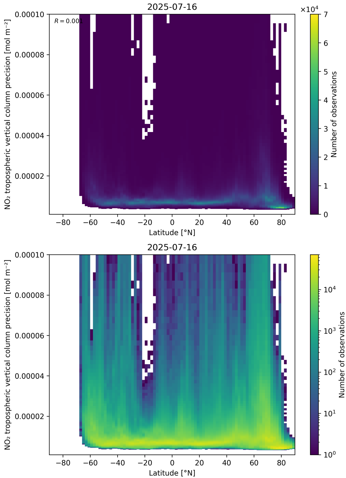
Figure 93: Scatter density plot of “Latitude” against “NO 2 tropospheric vertical column precision” for 2025-07-15 to 2025-07-17.
