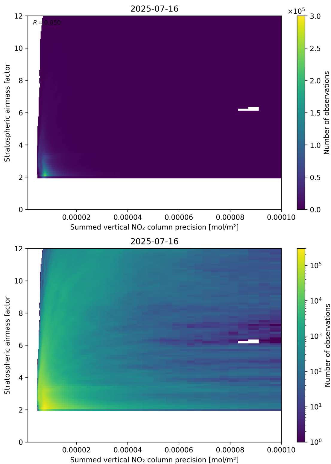
Figure 106: Scatter density plot of “Summed vertical NO 2 column precision” against “Stratospheric airmass factor” for 2025-07-15 to 2025-07-17.
