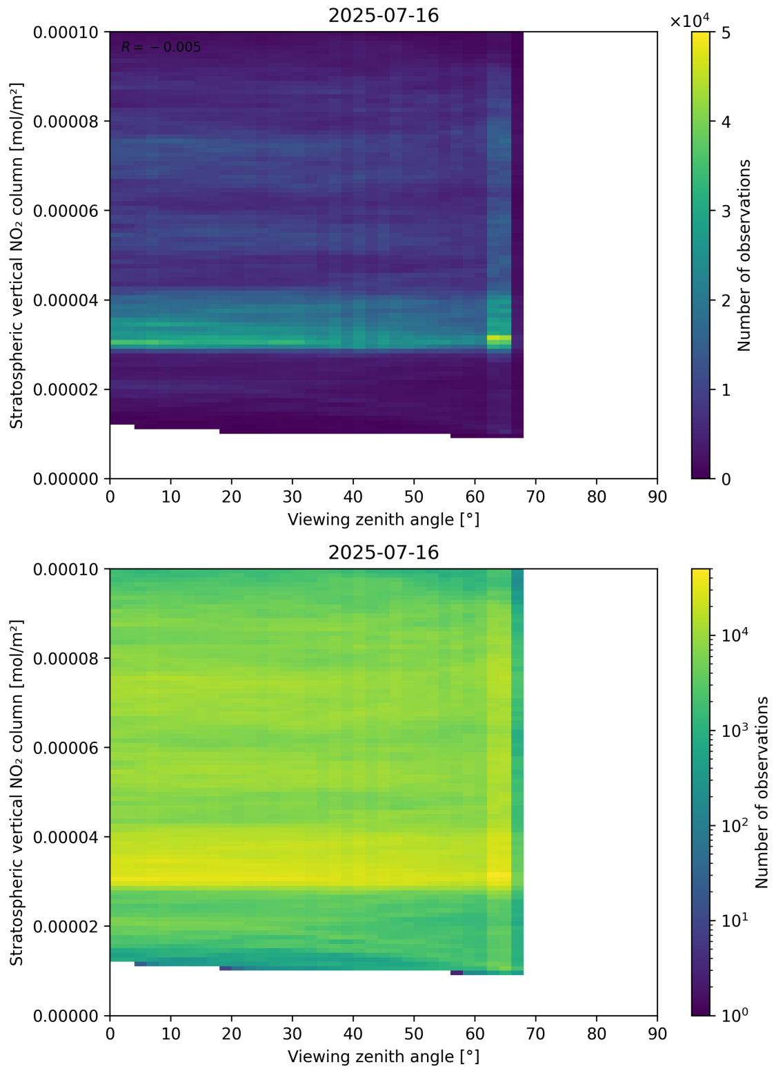
Figure 164: Scatter density plot of “Viewing zenith angle” against “Stratospheric vertical NO 2 column” for 2025-07-15 to 2025-07-17.
