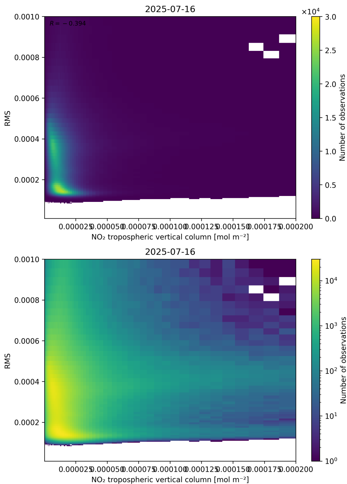
Figure 142: Scatter density plot of “NO 2 tropospheric vertical column” against “RMS” for 2025-07-15 to 2025-07-17.
