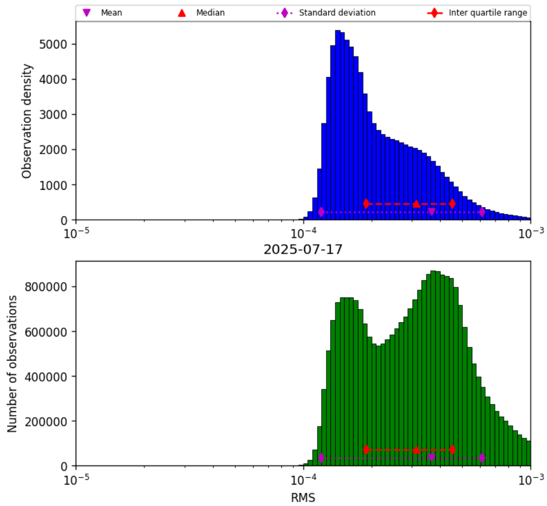
Figure 43: Histogram of “RMS” for 2025-07-16 to 2025-07-18
