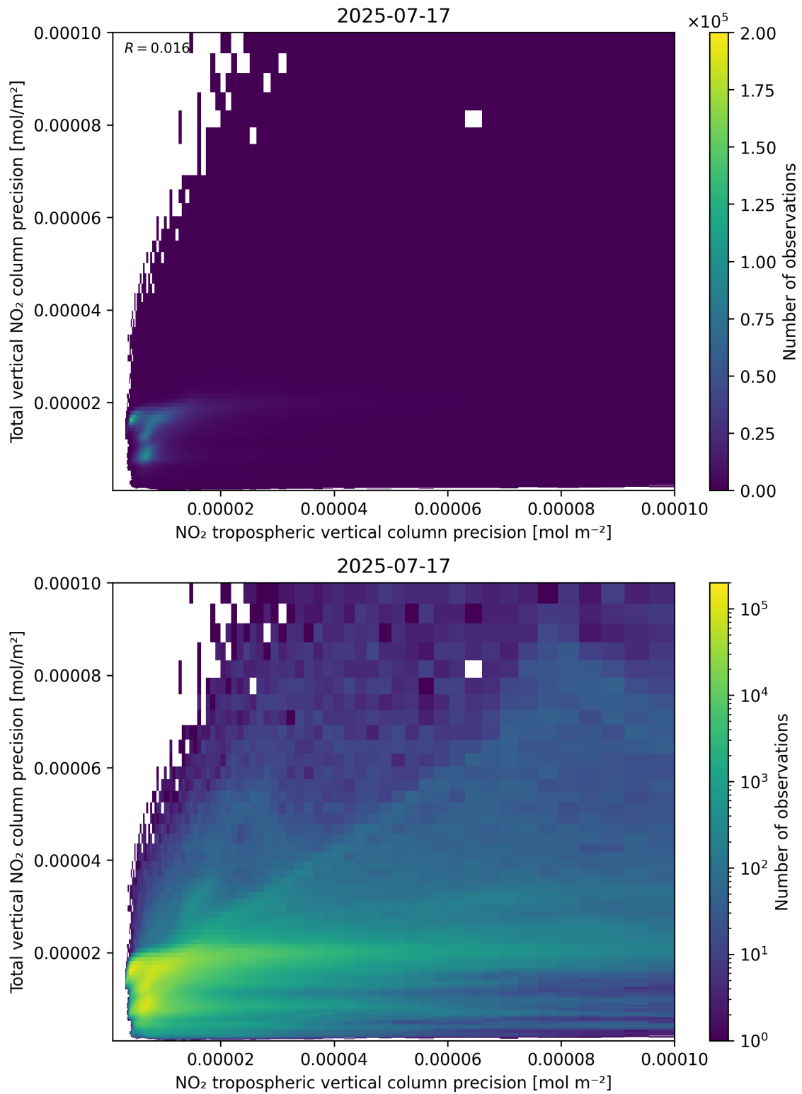
Figure 139: Scatter density plot of “NO 2 tropospheric vertical column precision” against “Total vertical NO 2 column precision” for 2025-07-16 to 2025-07-18.
