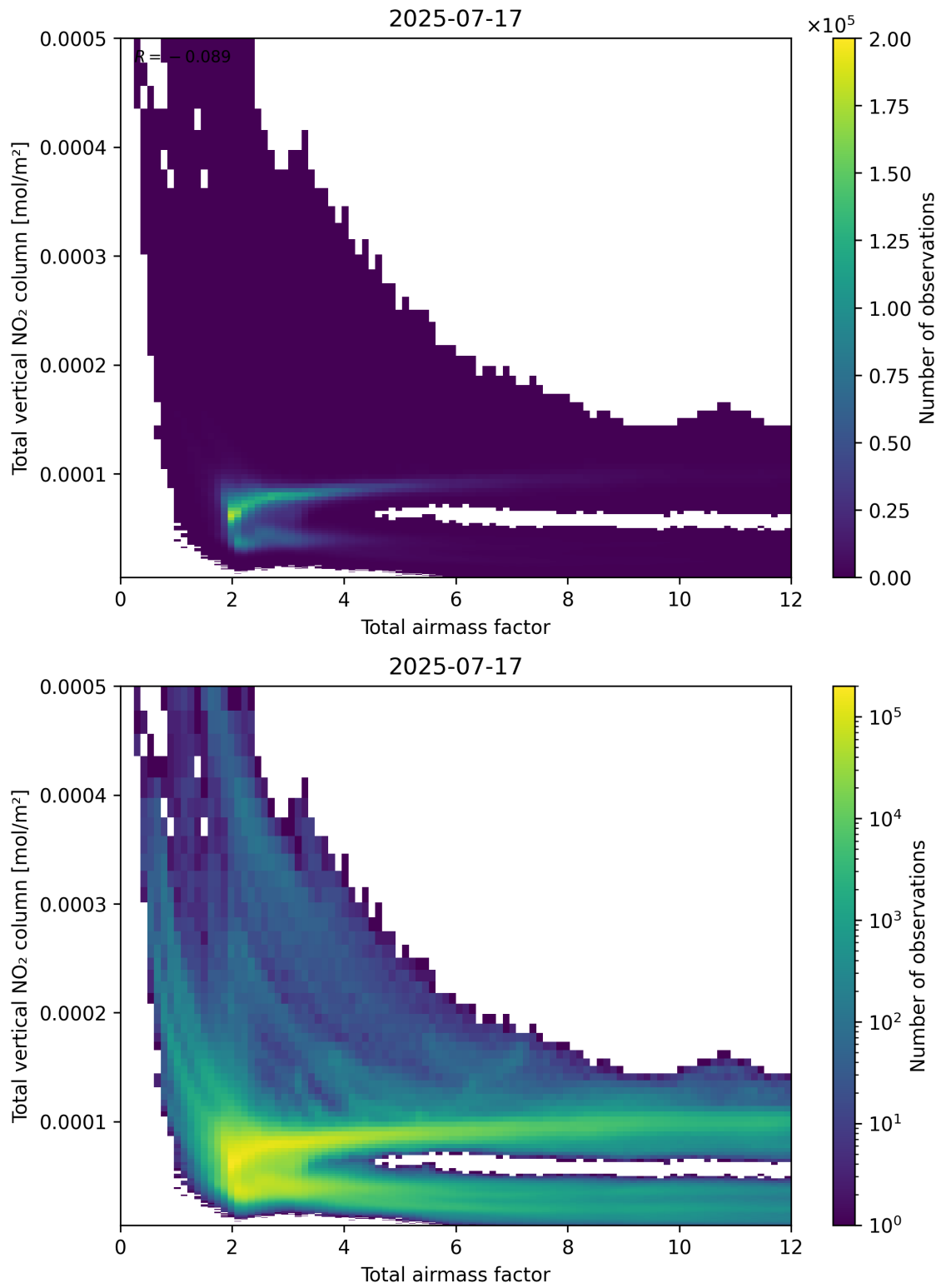
Figure 67: Scatter density plot of “Total airmass factor” against “Total vertical NO 2 column” for 2025-07-16 to 2025-07-18.
