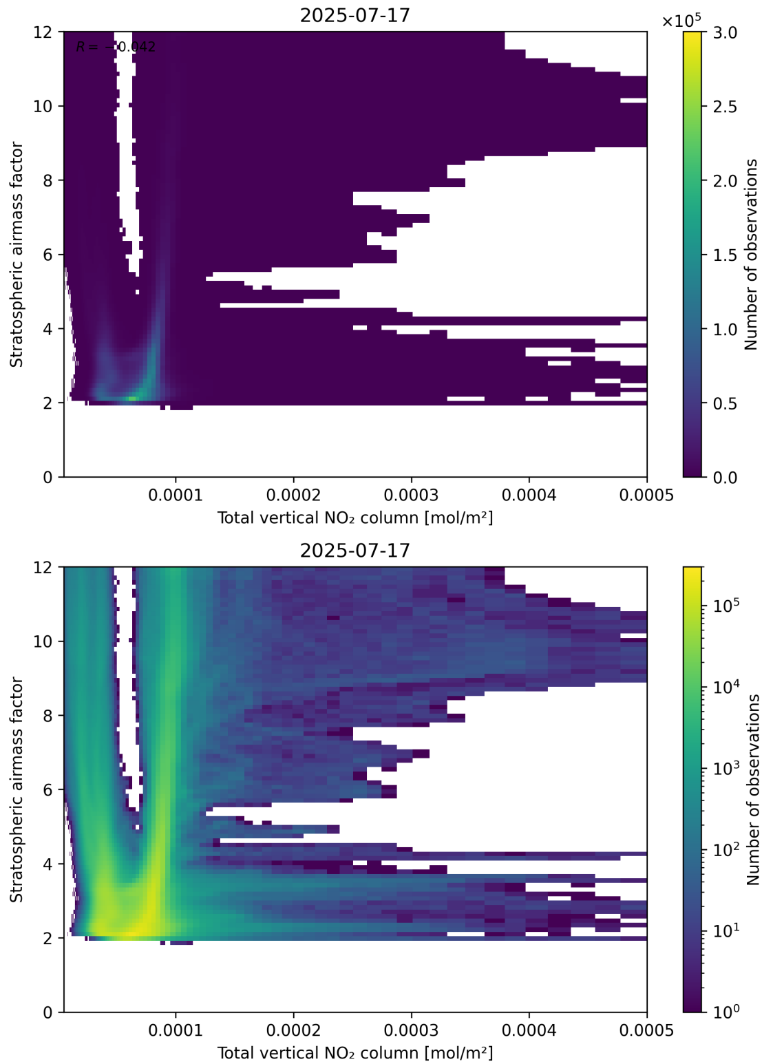
Figure 110: Scatter density plot of “Total vertical NO 2 column” against “Stratospheric airmass factor” for 2025-07-16 to 2025-07-18.
