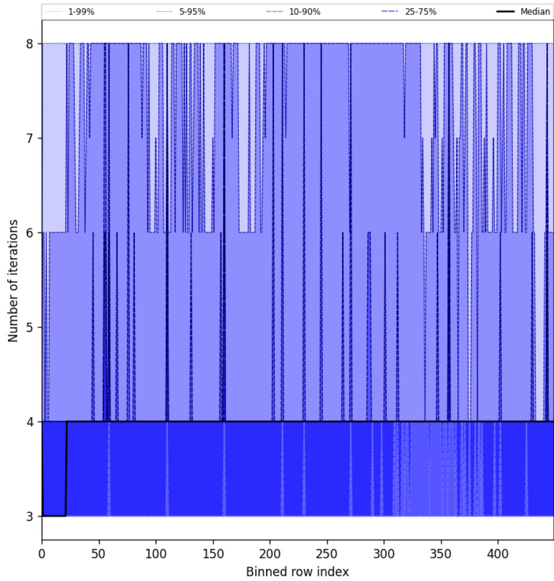
Figure 51: Along track statistics of “Number of iterations” for 2025-07-16 to 2025-07-18
