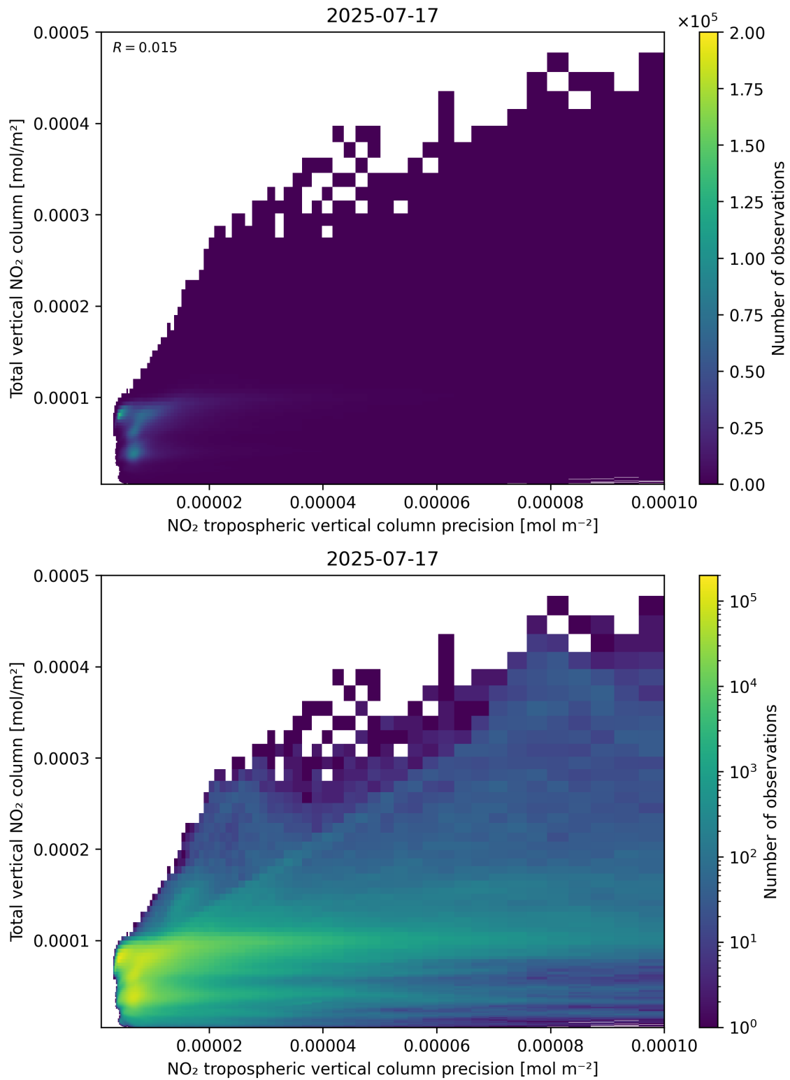
Figure 138: Scatter density plot of “NO 2 tropospheric vertical column precision” against “Total vertical NO 2 column” for 2025-07-16 to 2025-07-18.
