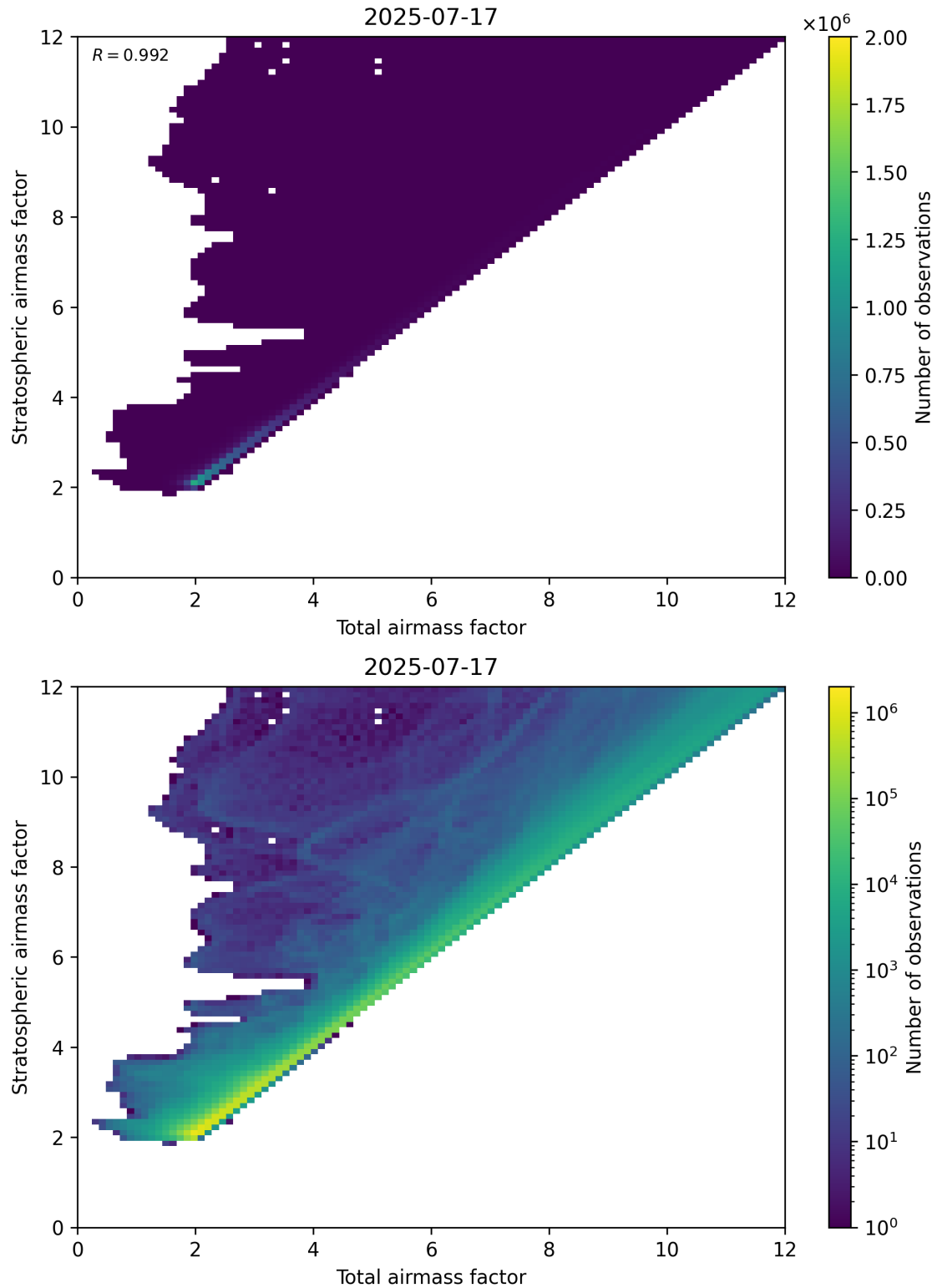
Figure 62: Scatter density plot of “Total air mass factor” against “Stratospheric air mass factor” for 2025-07-16 to 2025-07-18.
