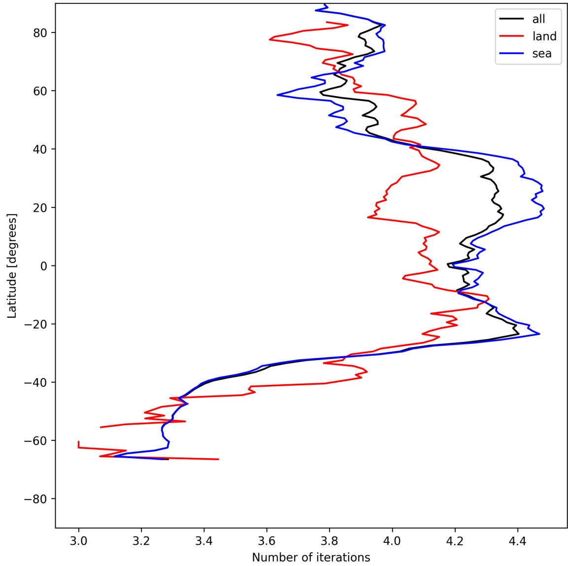
Figure 17: Zonal average of “Number of iterations” for 2025-07-16 to 2025-07-18.
