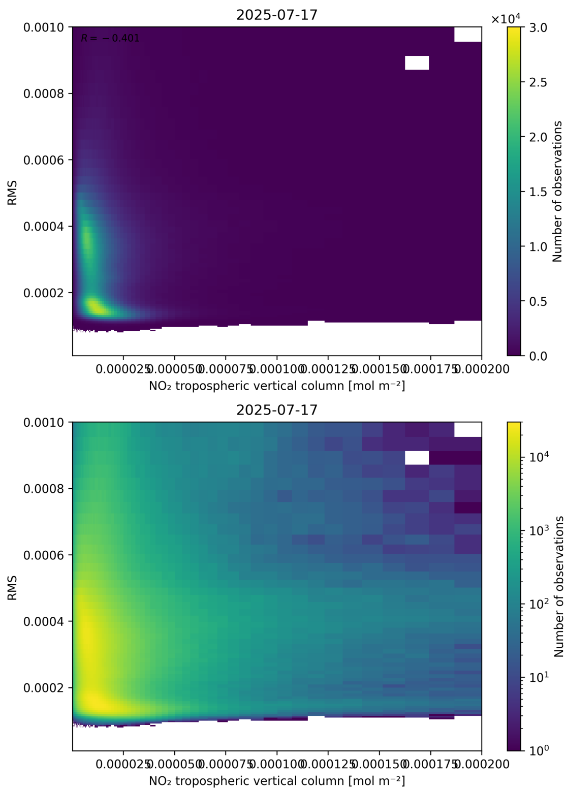
Figure 142: Scatter density plot of “NO 2 tropospheric vertical column” against “RMS” for 2025-07-16 to 2025-07-18.
