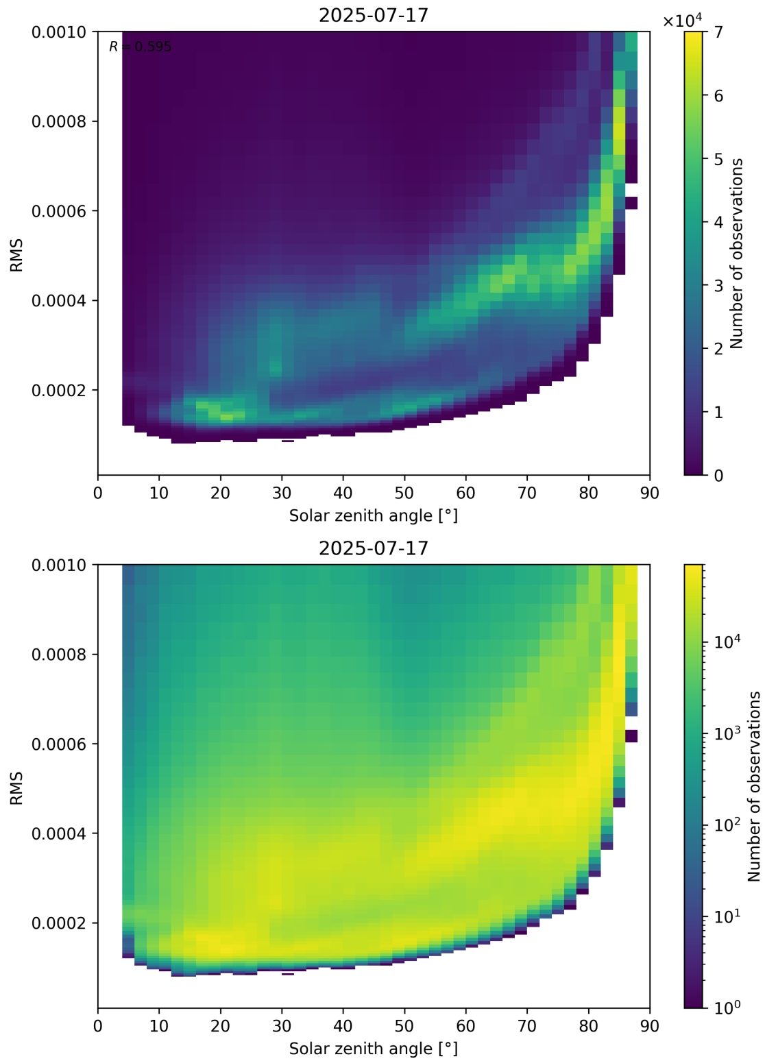
Figure 157: Scatter density plot of “Solar zenith angle” against “RMS” for 2025-07-16 to 2025-07-18.
