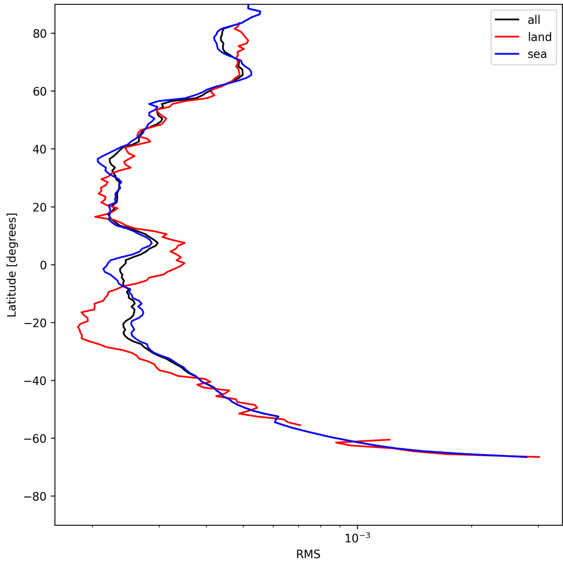
Figure 26: Zonal average of “RMS” for 2025-07-16 to 2025-07-18.
