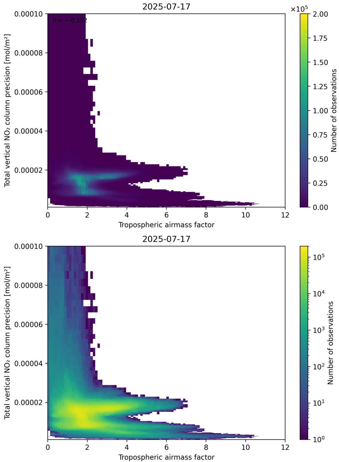
Figure 78: Scatter density plot of “Tropospheric air mass factor” against “Total vertical NO 2 column precision” for 2025-07-16 to 2025-07-18.
