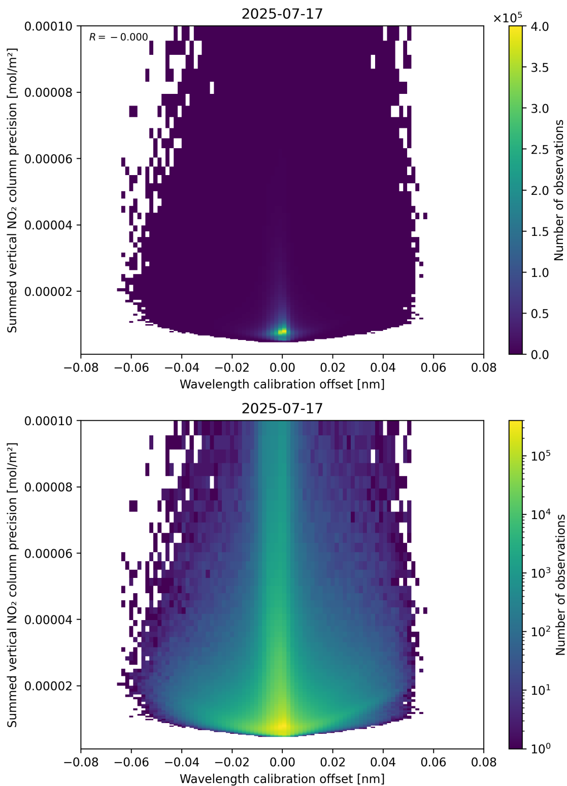
Figure 178: Scatter density plot of “Wavelength calibration offset” against “Summed vertical NO 2 column precision” for 2025-07-16 to 2025-07-18.
