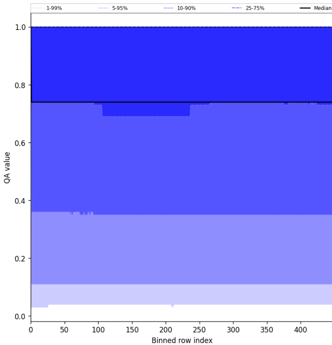
Figure 45: Along track statistics of “QA value” for 2025-07-16 to 2025-07-18
