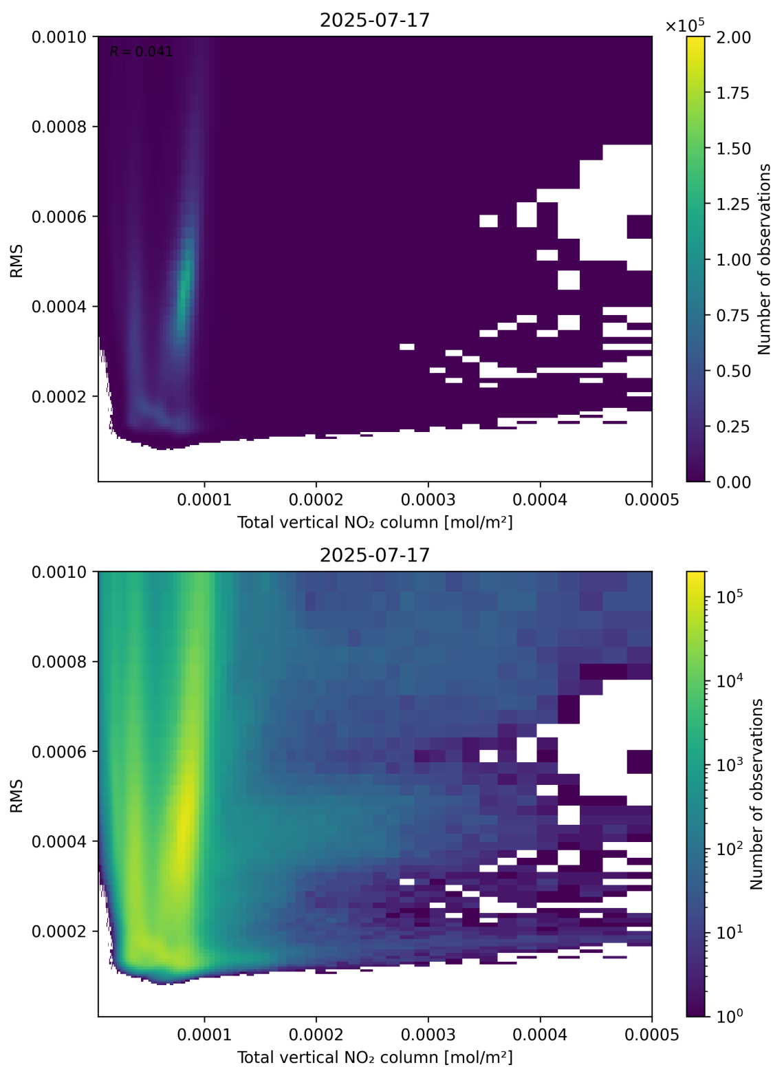
Figure 120: Scatter density plot of “Total vertical NO 2 column” against “RMS” for 2025-07-16 to 2025-07-18.
