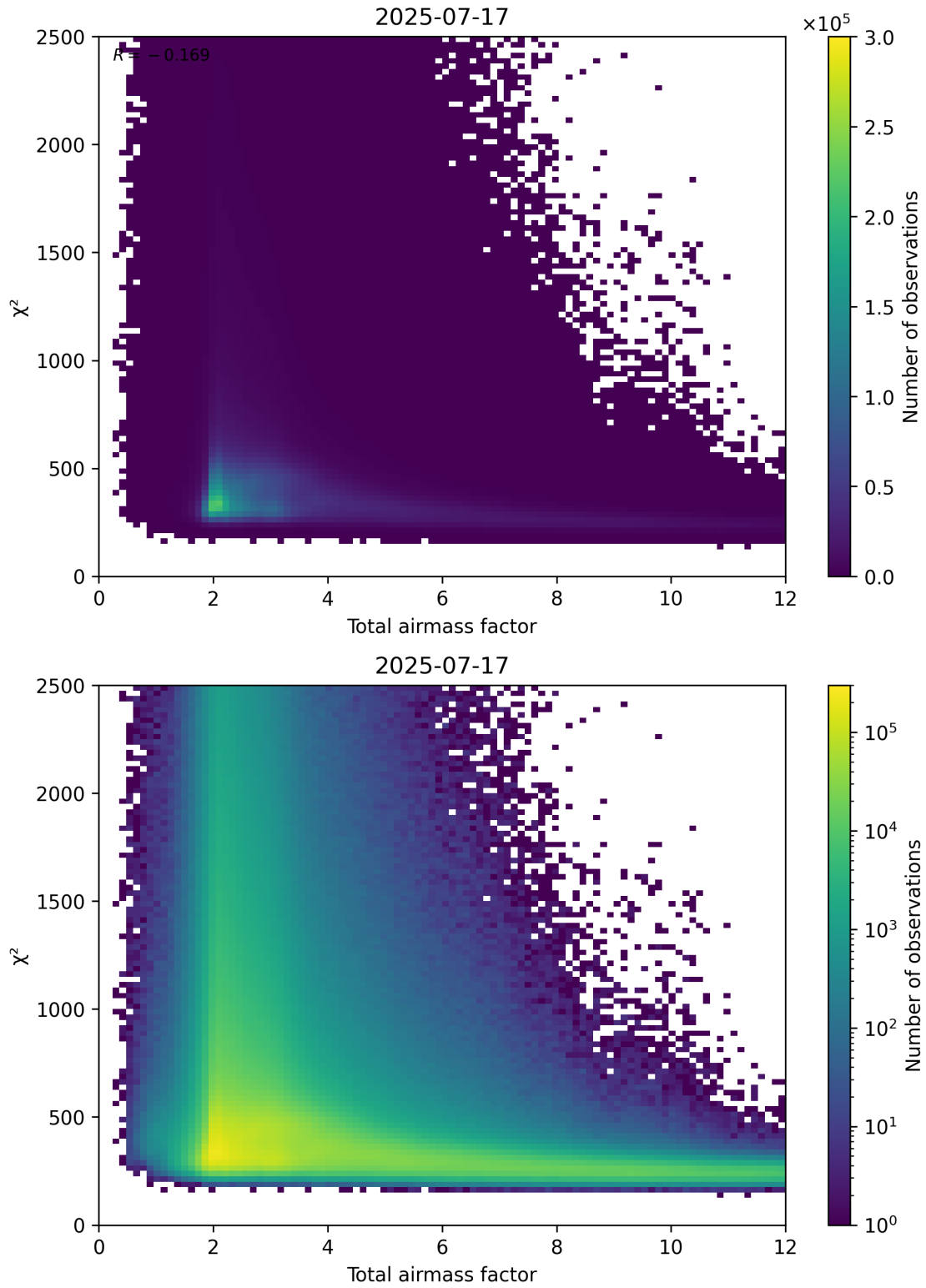
Figure 63: Scatter density plot of “Total airmass factor” against “ \chi^2 ” for 2025-07-16 to 2025-07-18.
