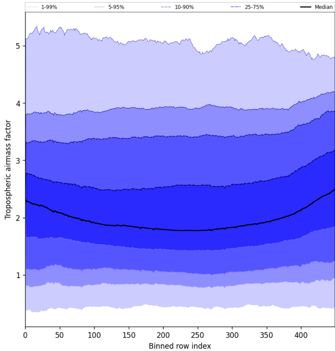
Figure 48: Along track statistics of “Tropospheric airmass factor” for 2025-07-16 to 2025-07-18
