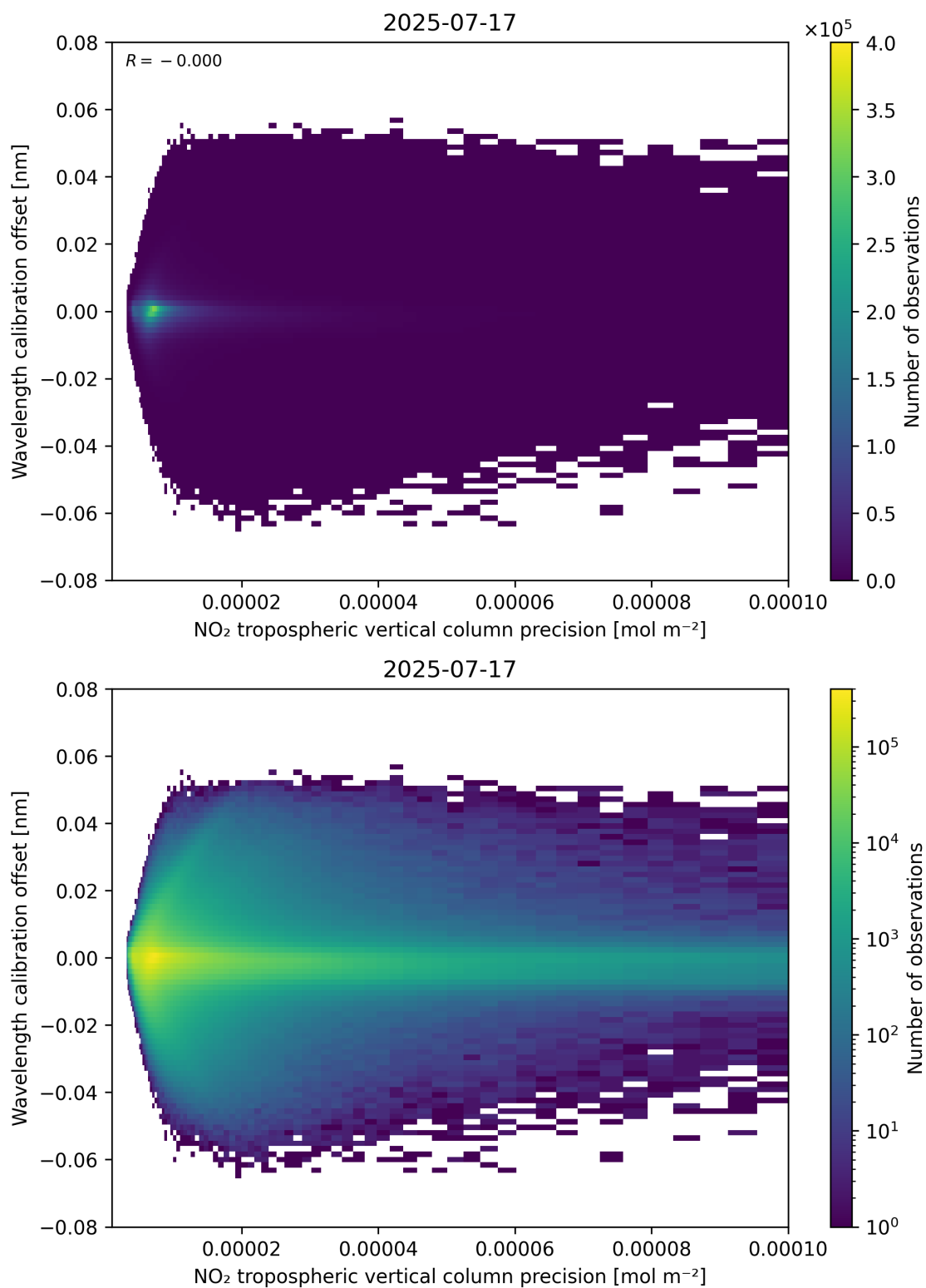
Figure 141: Scatter density plot of “NO 2 tropospheric vertical column precision” against “Wavelength calibration offset” for 2025-07-16 to 2025-07-18.
