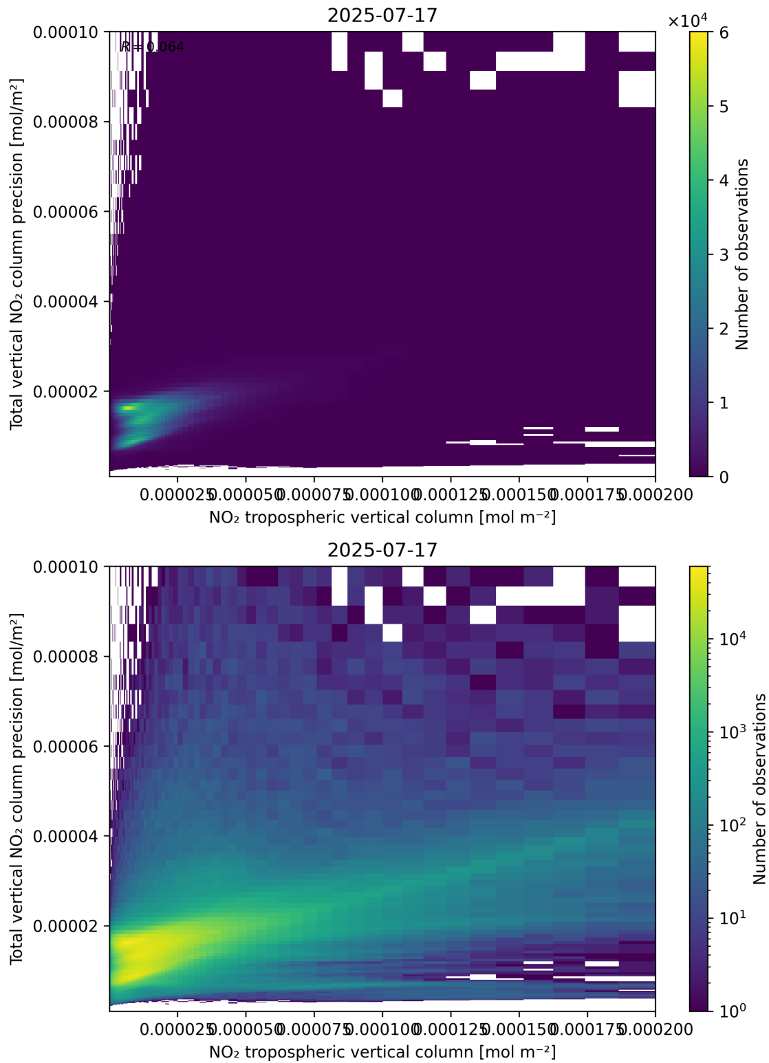
Figure 129: Scatter density plot of “NO 2 tropospheric vertical column” against “Total vertical NO 2 column precision” for 2025-07-16 to 2025-07-18.
