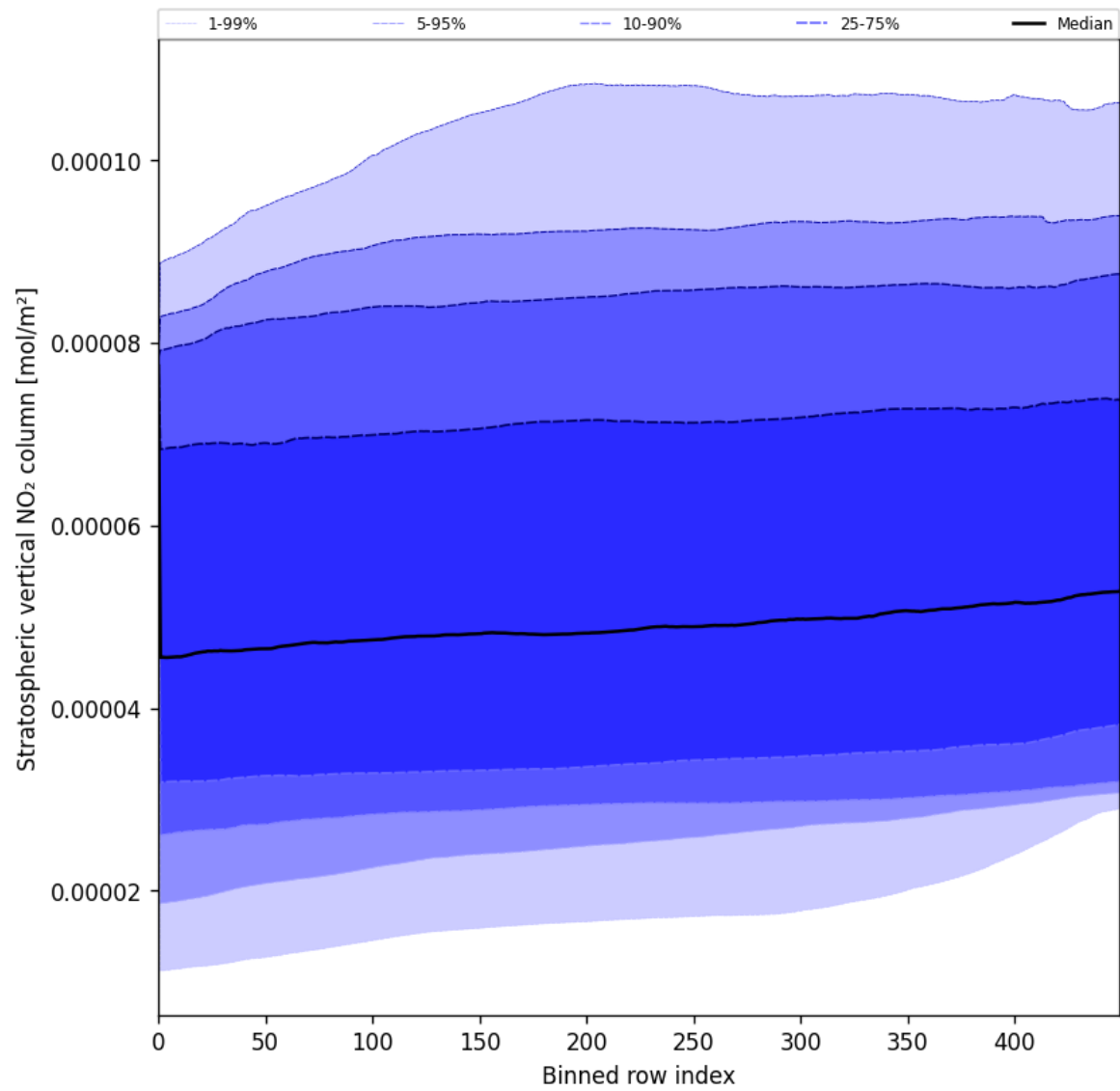
Figure 53: Along track statistics of “Stratospheric vertical NO 2 column” for 2025-07-16 to 2025-07-18
