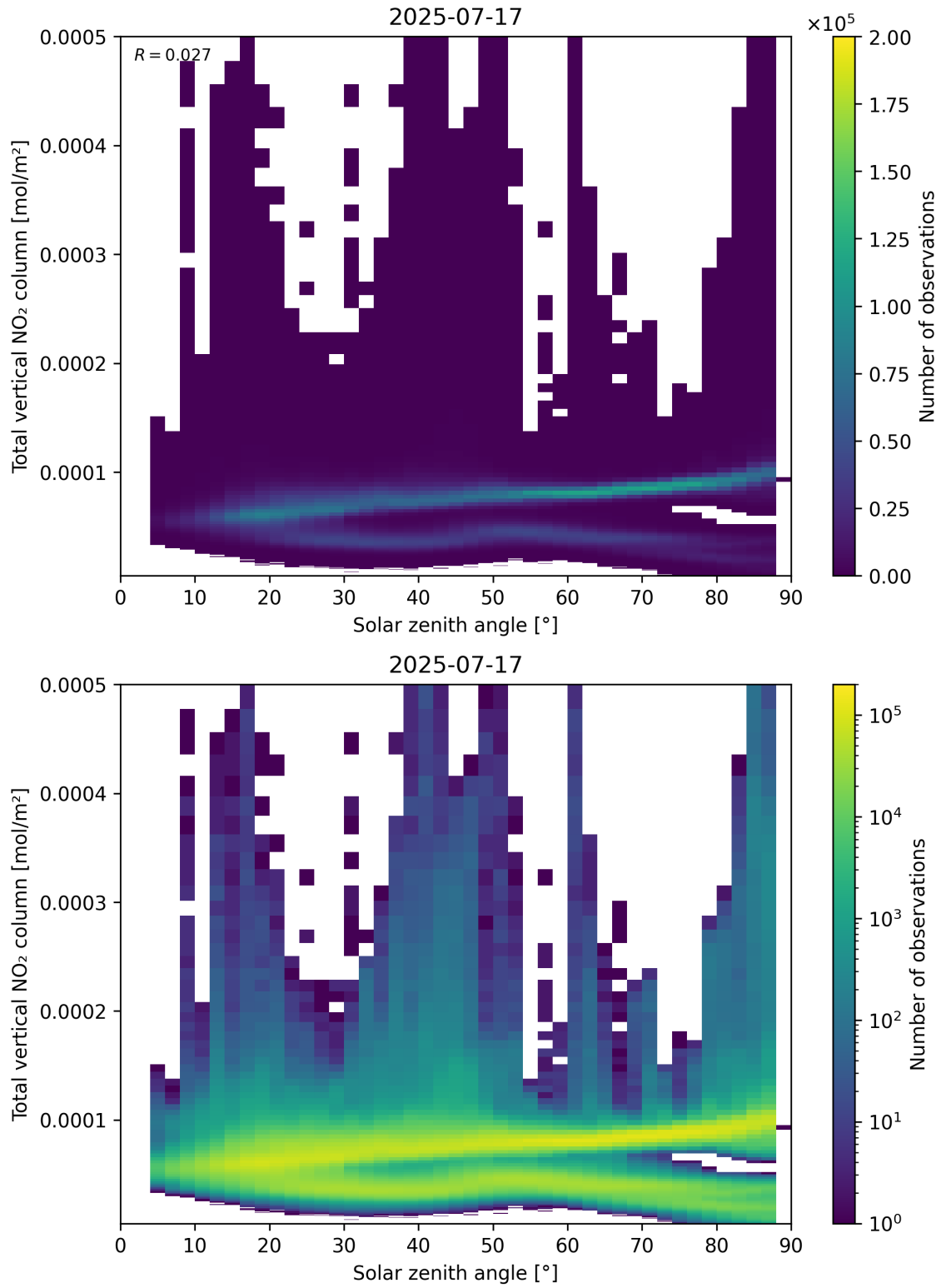
Figure 153: Scatter density plot of “Solar zenith angle” against “Total vertical NO 2 column” for 2025-07-16 to 2025-07-18.
