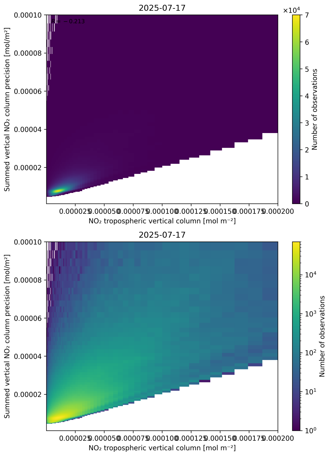
Figure 127: Scatter density plot of “NO 2 tropospheric vertical column” against “Summed vertical NO 2 column precision” for 2025-07-16 to 2025-07-18.
