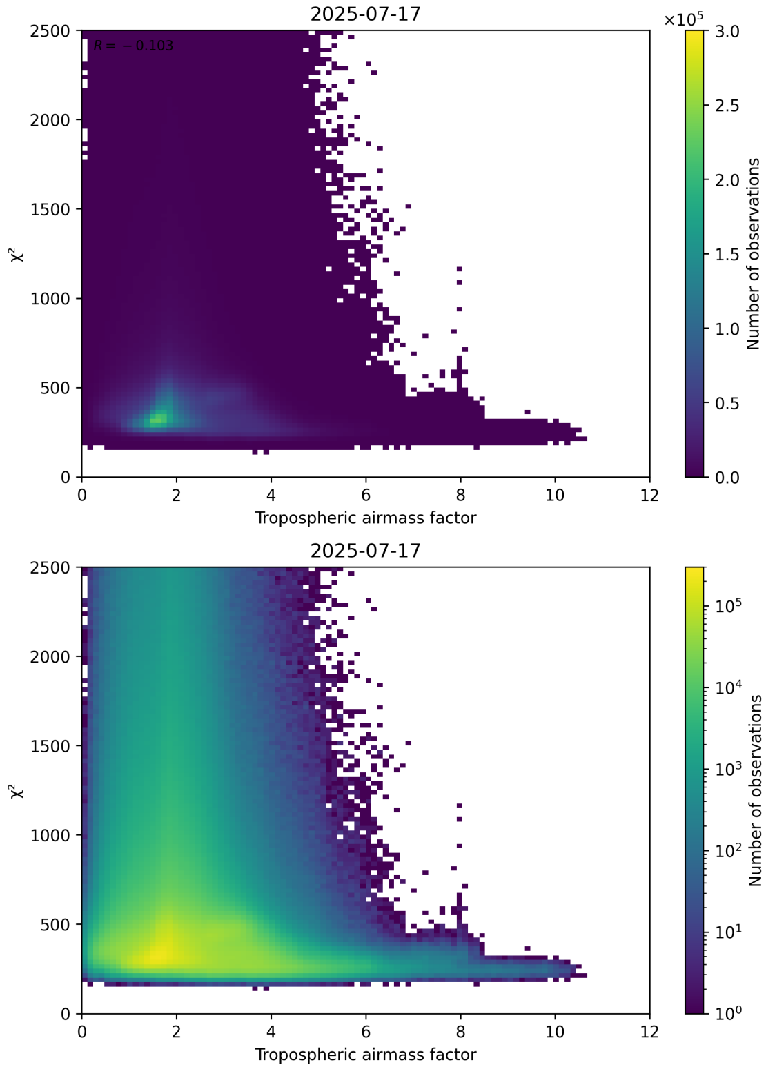
Figure 73: Scatter density plot of “Tropospheric airmass factor” against “ \chi^2 ” for 2025-07-16 to 2025-07-18.
