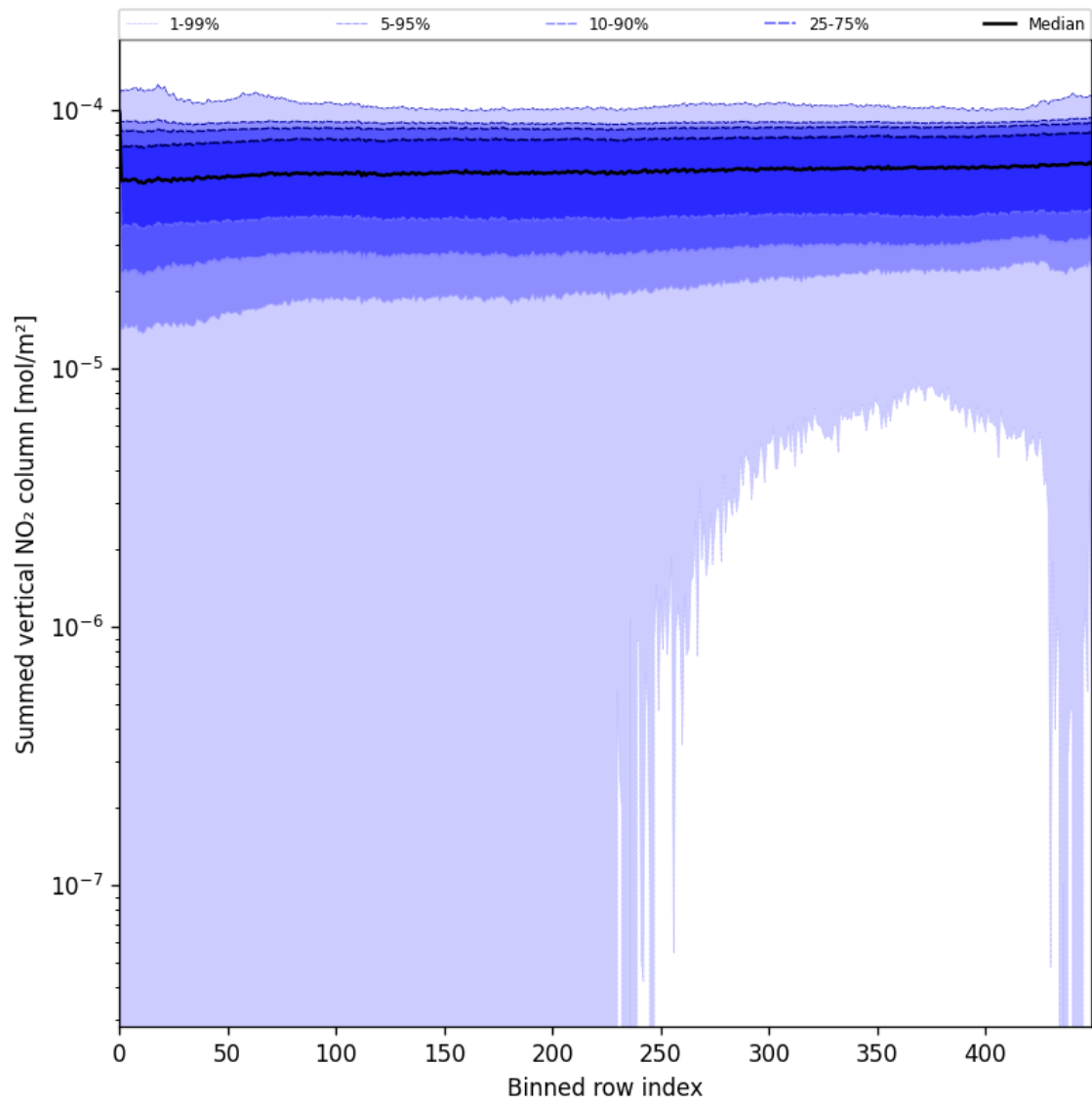
Figure 57: Along track statistics of “Summed vertical NO 2 column” for 2025-07-16 to 2025-07-18
