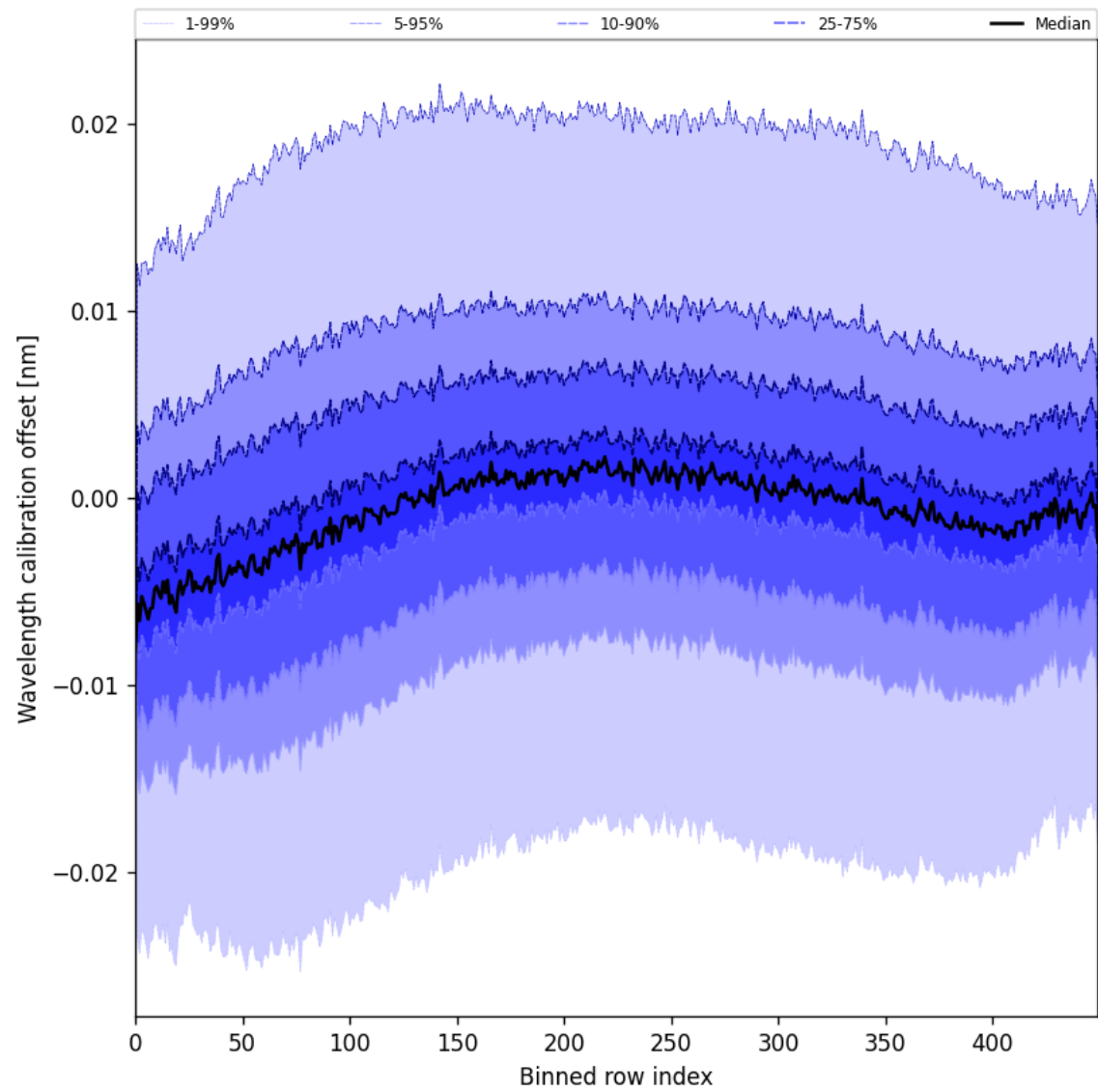
Figure 52: Along track statistics of “Wavelength calibration offset” for 2025-07-16 to 2025-07-18
