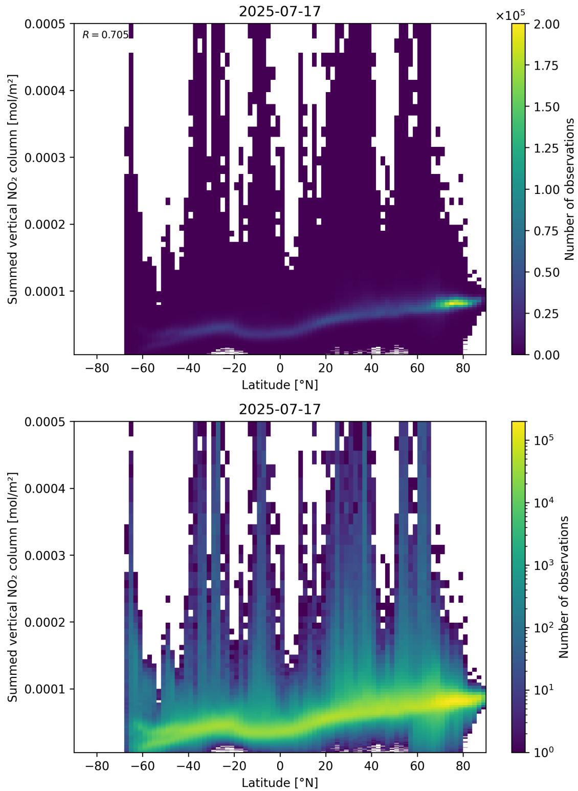
Figure 88: Scatter density plot of “Latitude” against “Summed vertical NO 2 column” for 2025-07-16 to 2025-07-18.
