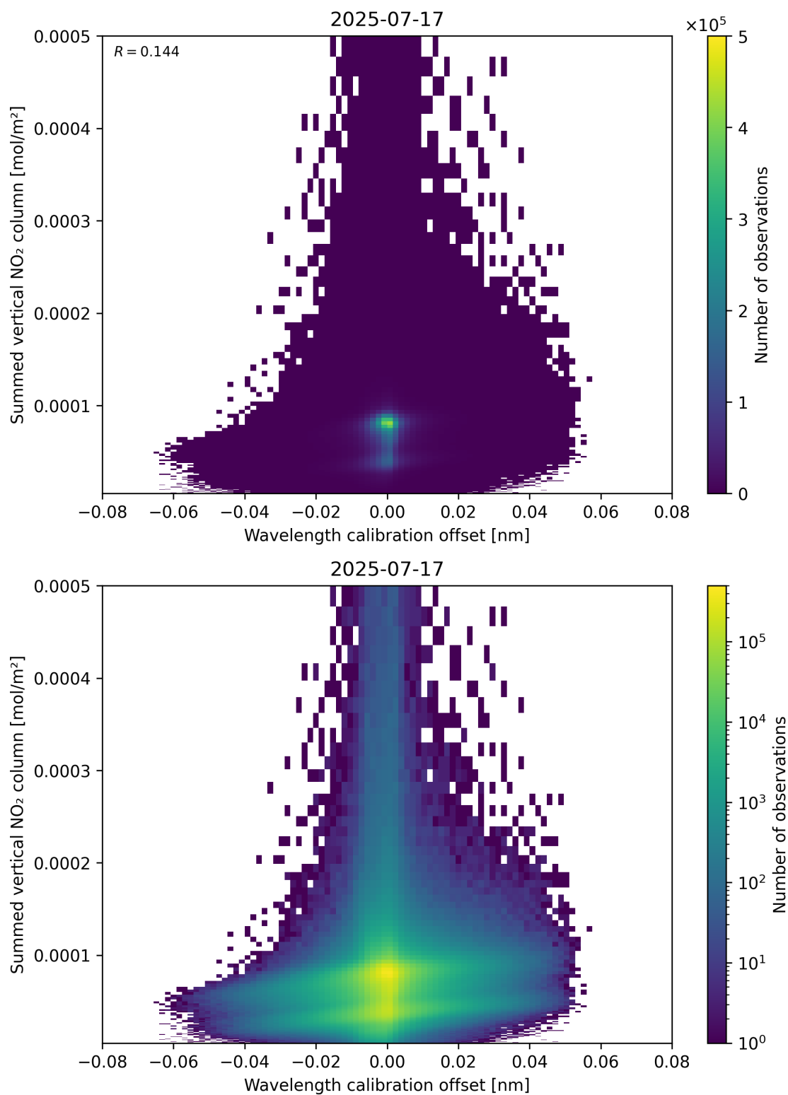
Figure 177: Scatter density plot of “Wavelength calibration offset” against “Summed vertical NO 2 column” for 2025-07-16 to 2025-07-18.
