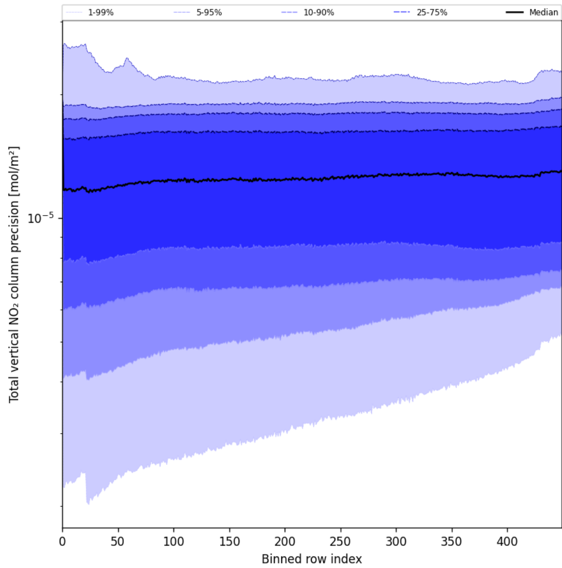
Figure 56: Along track statistics of “Total vertical NO 2 column precision” for 2025-07-16 to 2025-07-18
