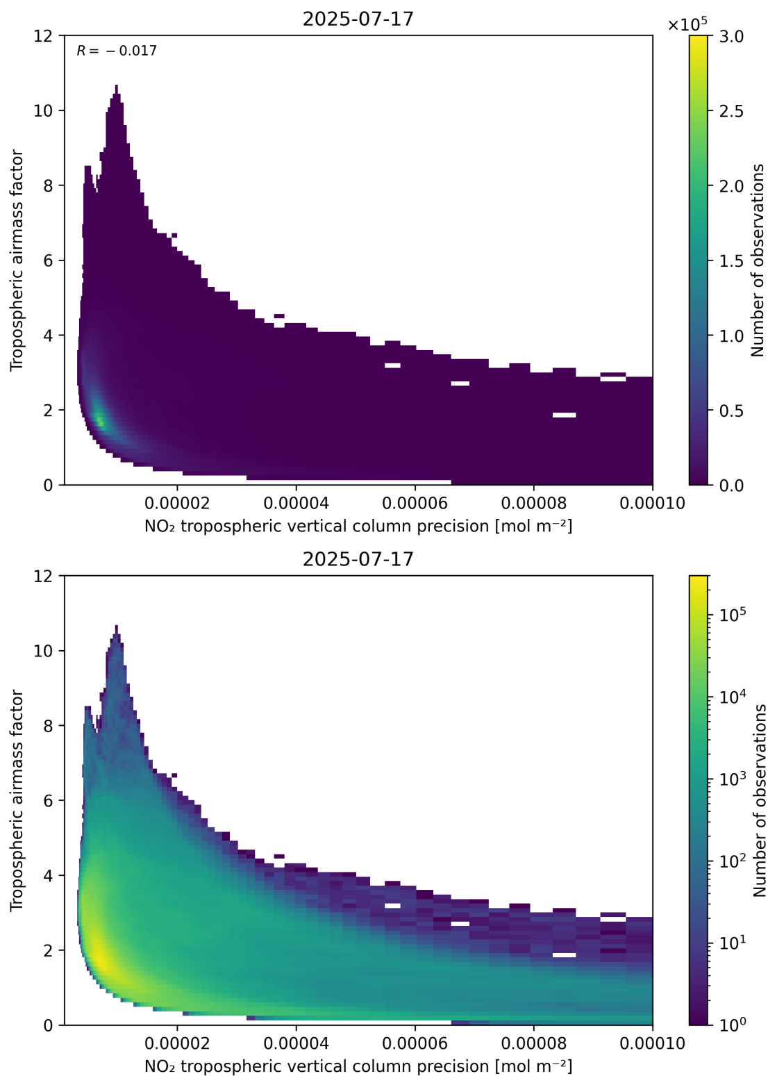
Figure 133: Scatter density plot of “NO 2 tropospheric vertical column precision” against “Tropospheric airmass factor” for 2025-07-16 to 2025-07-18.
