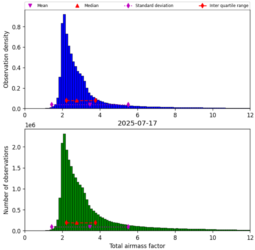
Figure 32: Histogram of “Total airmass factor” for 2025-07-16 to 2025-07-18
