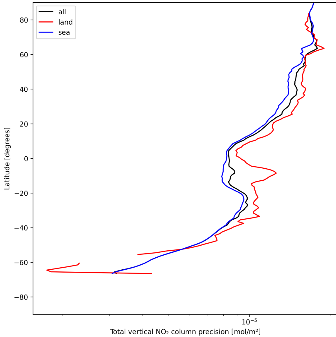
Figure 22: Zonal average of “Total vertical NO 2 column precision” for 2025-07-16 to 2025-07-18.
