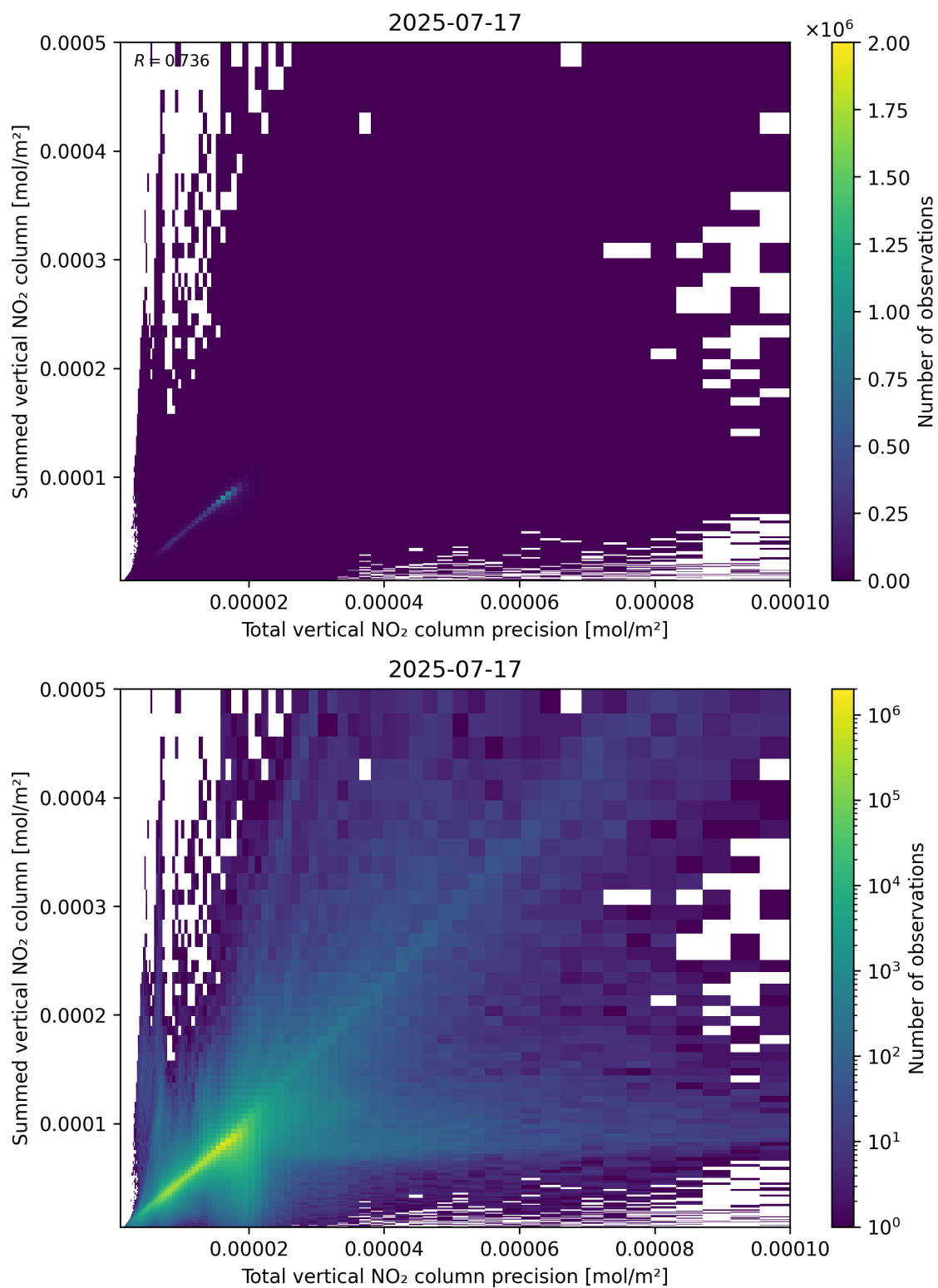
Figure 117: Scatter density plot of “Total vertical NO 2 column precision” against “Summed vertical NO 2 column” for 2025-07-16 to 2025-07-18.
