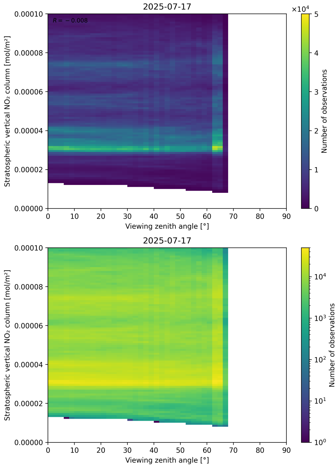
Figure 164: Scatter density plot of “Viewing zenith angle” against “Stratospheric vertical NO 2 column” for 2025-07-16 to 2025-07-18.
