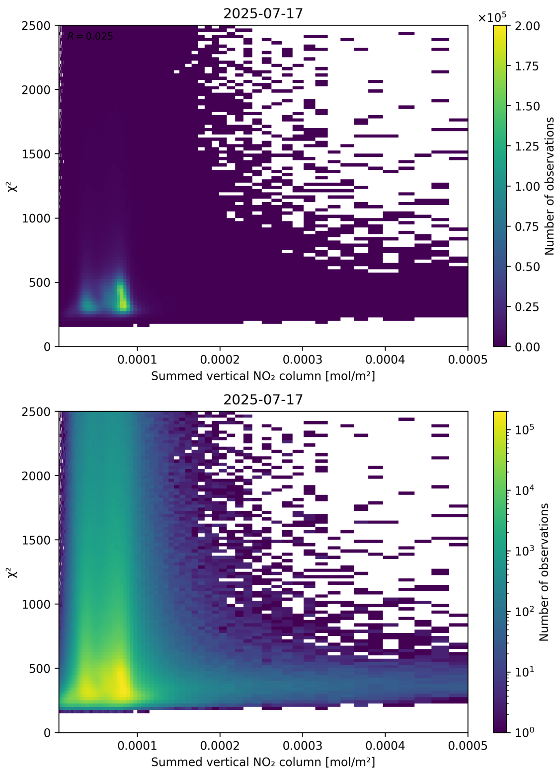
Figure 104: Scatter density plot of “Summed vertical NO 2 column” against “ \chi^2 ” for 2025-07-16 to 2025-07-18.
