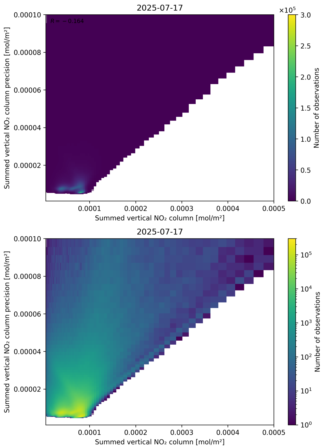
Figure 105: Scatter density plot of “Summed vertical NO 2 column” against “Summed vertical NO 2 column precision” for 2025-07-16 to 2025-07-18.
