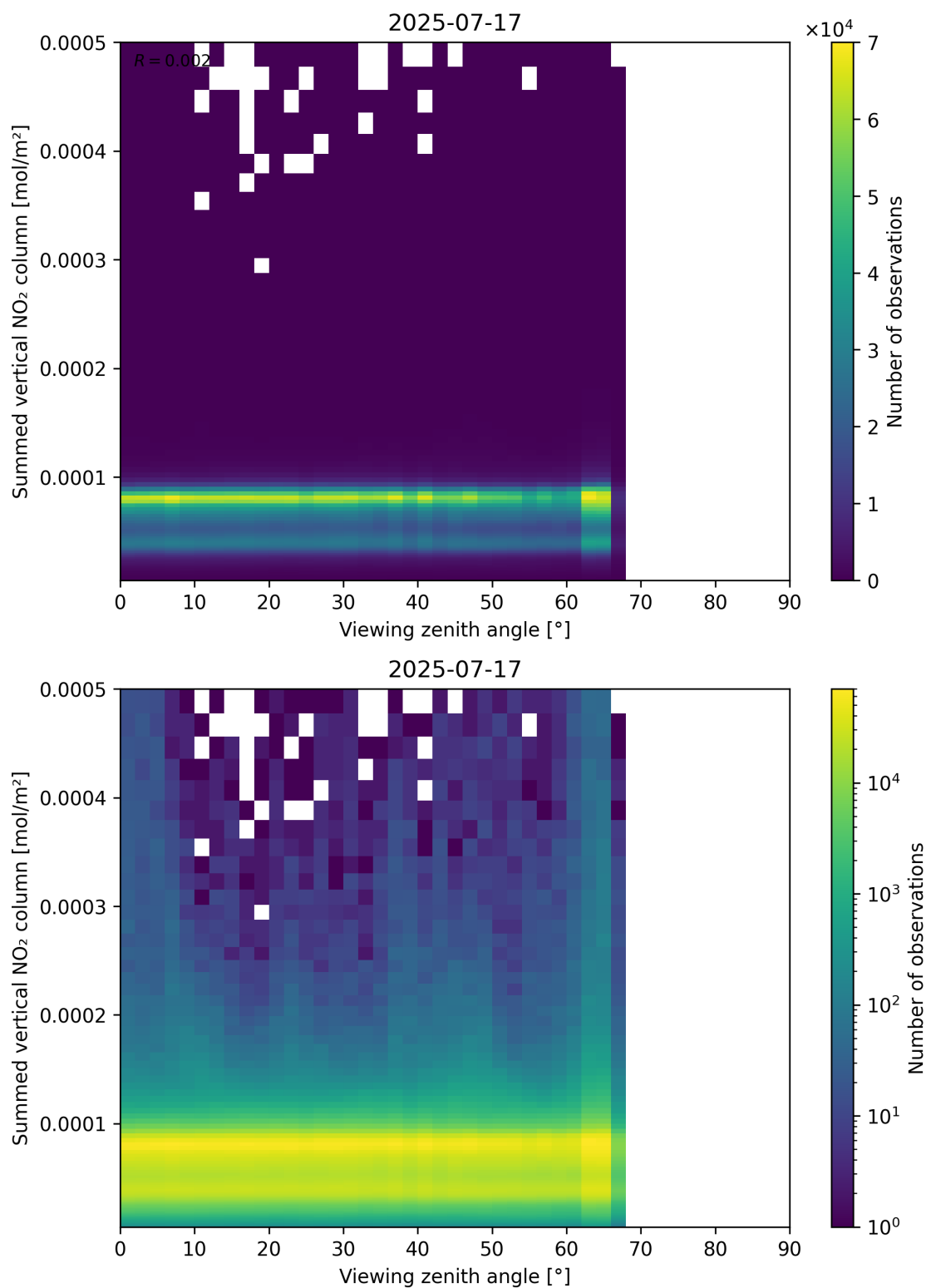
Figure 165: Scatter density plot of “Viewing zenith angle” against “Summed vertical NO 2 column” for 2025-07-16 to 2025-07-18.
