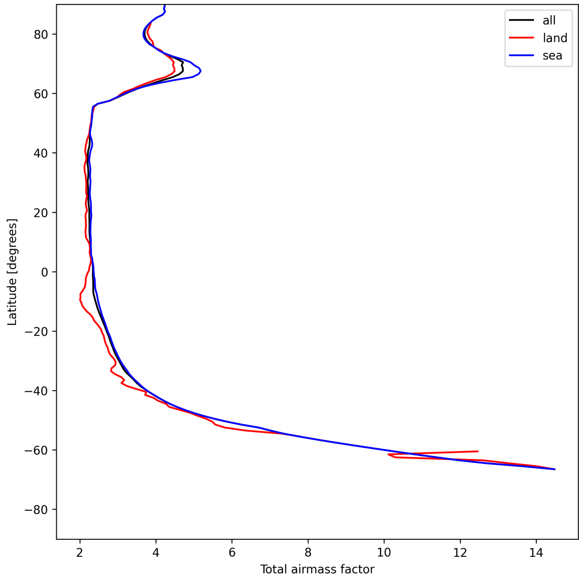
Figure 15: Zonal average of “Total airmass factor” for 2025-07-16 to 2025-07-18.
