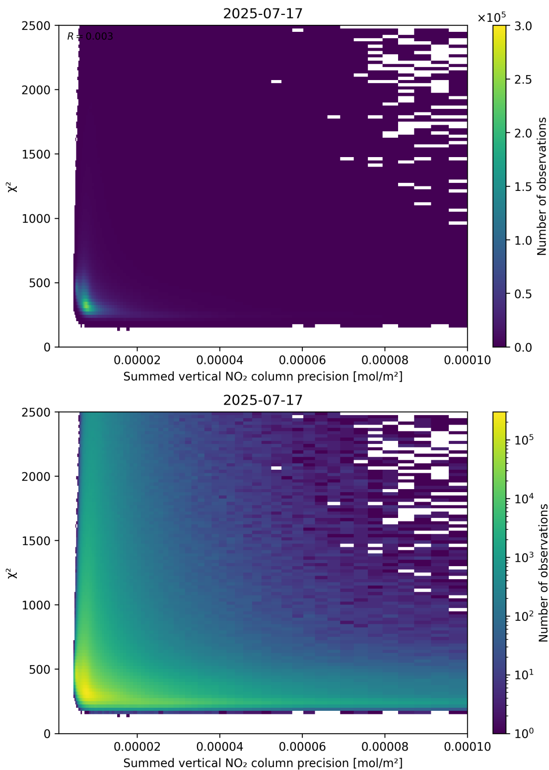
Figure 107: Scatter density plot of “Summed vertical NO 2 column precision” against “ \chi^2 ” for 2025-07-16 to 2025-07-18.
