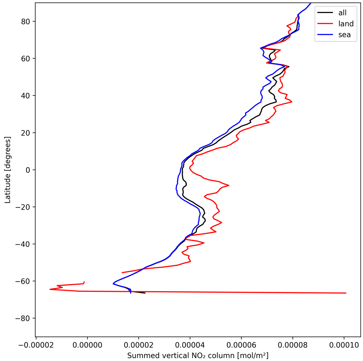
Figure 23: Zonal average of “Summed vertical NO 2 column” for 2025-07-16 to 2025-07-18.
