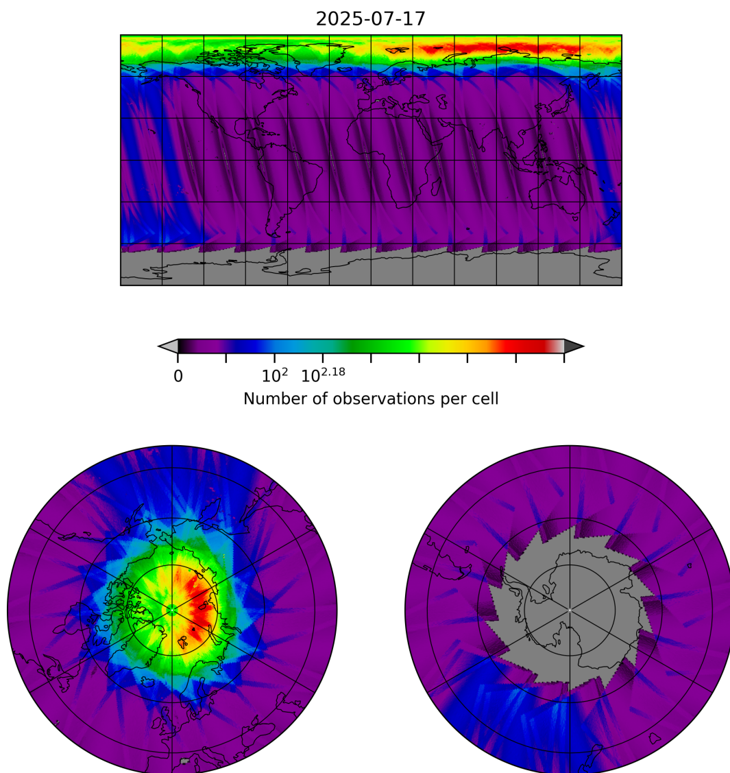
Figure 10: Map of the number of observations for 2025-07-16 to 2025-07-18
