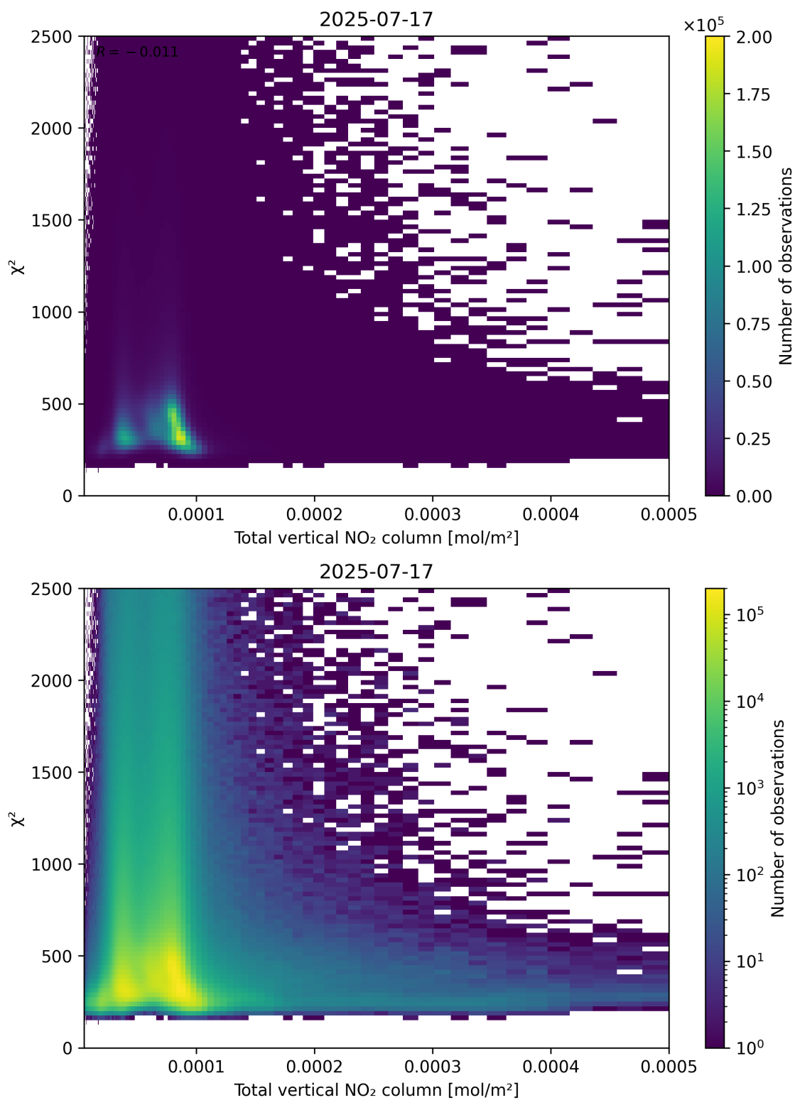
Figure 111: Scatter density plot of “Total vertical NO 2 column” against “ \chi^2 ” for 2025-07-16 to 2025-07-18.
