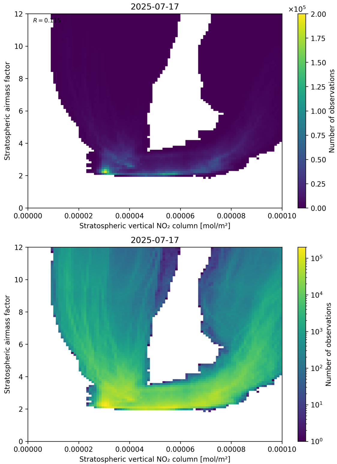
Figure 96: Scatter density plot of “Stratospheric vertical NO 2 column” against “Stratospheric airmass factor” for 2025-07-16 to 2025-07-18.
