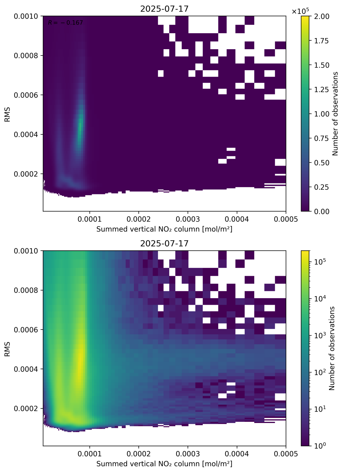
Figure 109: Scatter density plot of “Summed vertical NO 2 column” against “RMS” for 2025-07-16 to 2025-07-18.
