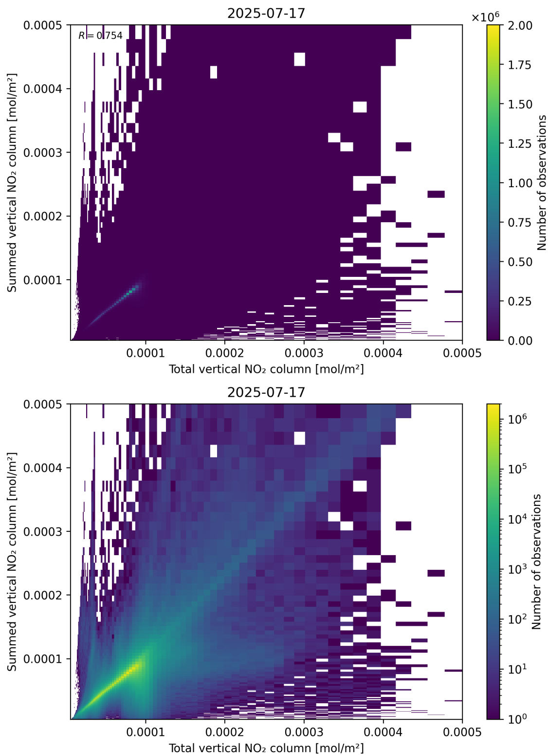
Figure 112: Scatter density plot of “Total vertical NO 2 column” against “Summed vertical NO 2 column” for 2025-07-16 to 2025-07-18.
