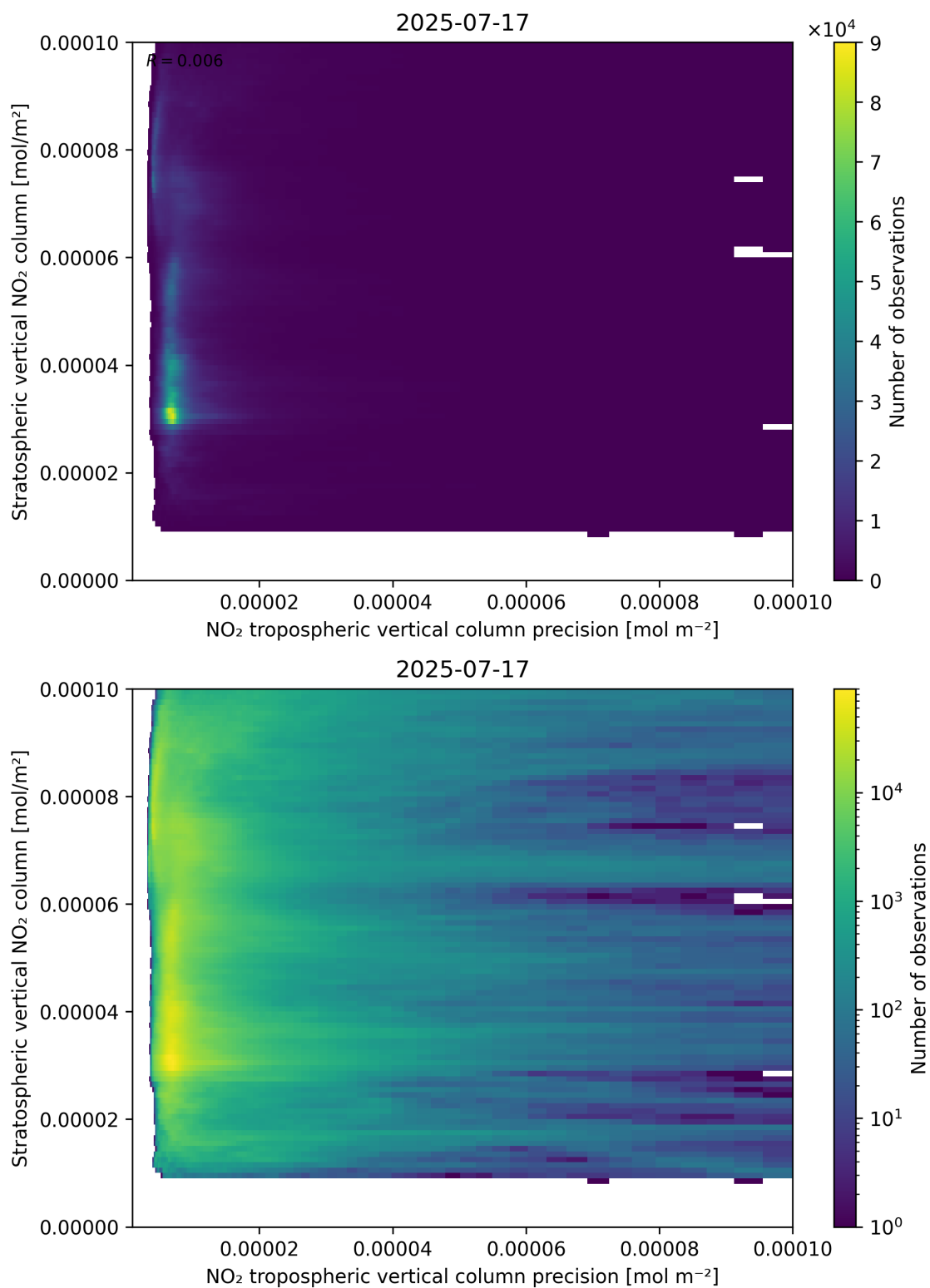
Figure 135: Scatter density plot of “NO 2 tropospheric vertical column precision” against “Stratospheric vertical NO 2 column” for 2025-07-16 to 2025-07-18.
