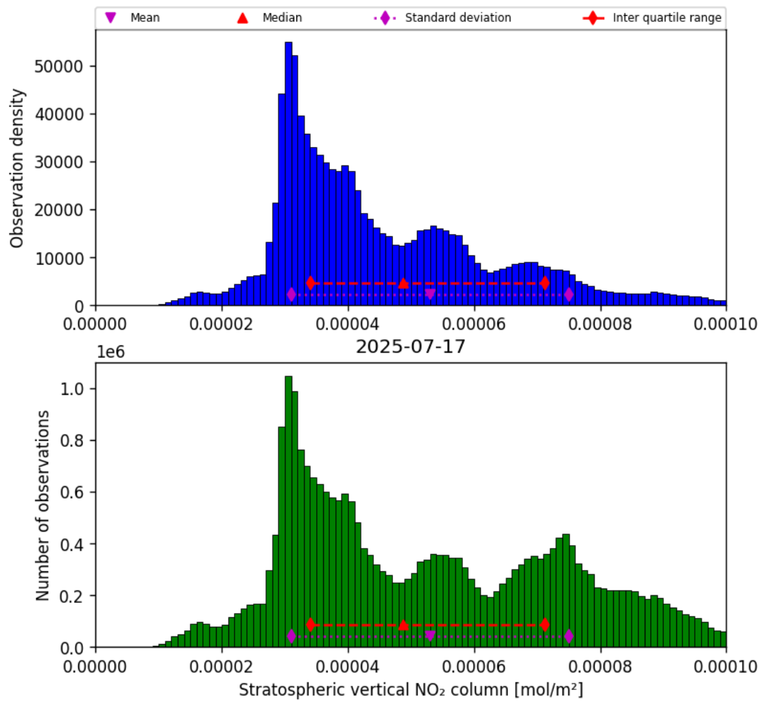
Figure 36: Histogram of “Stratospheric vertical NO 2 column” for 2025-07-16 to 2025-07-18
