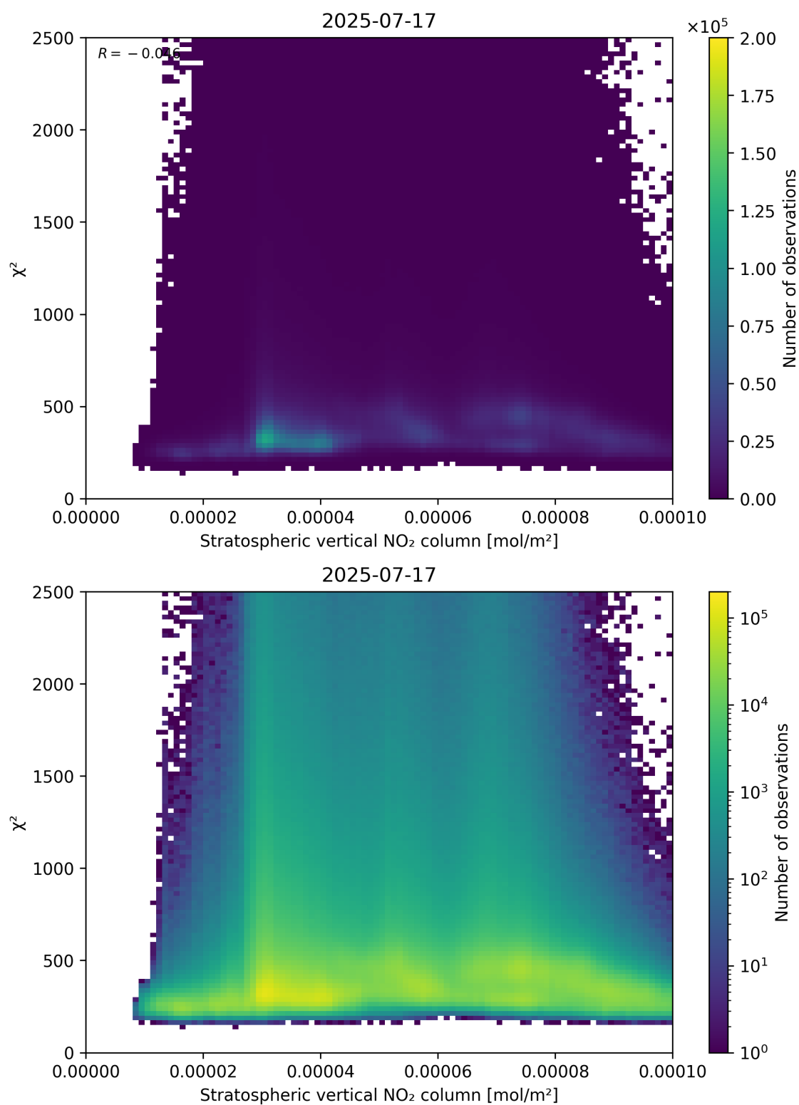
Figure 97: Scatter density plot of “Stratospheric vertical NO 2 column” against “ \chi^2 ” for 2025-07-16 to 2025-07-18.
