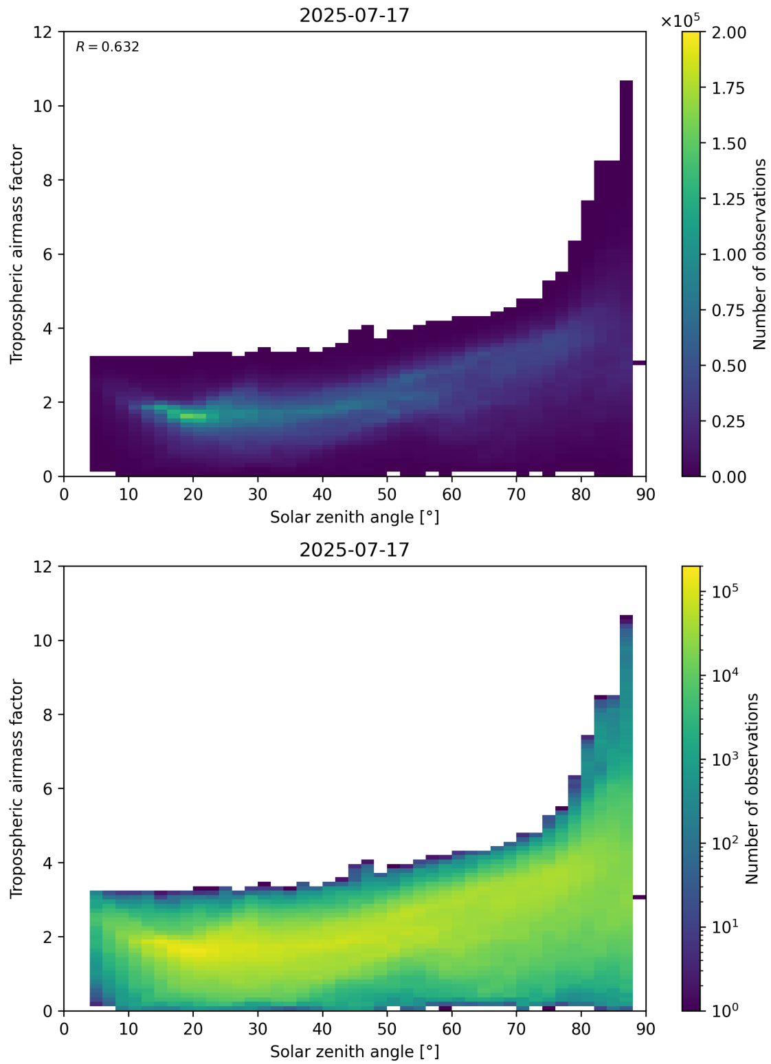
Figure 147: Scatter density plot of “Solar zenith angle” against “Tropospheric airmass factor” for 2025-07-16 to 2025-07-18.
