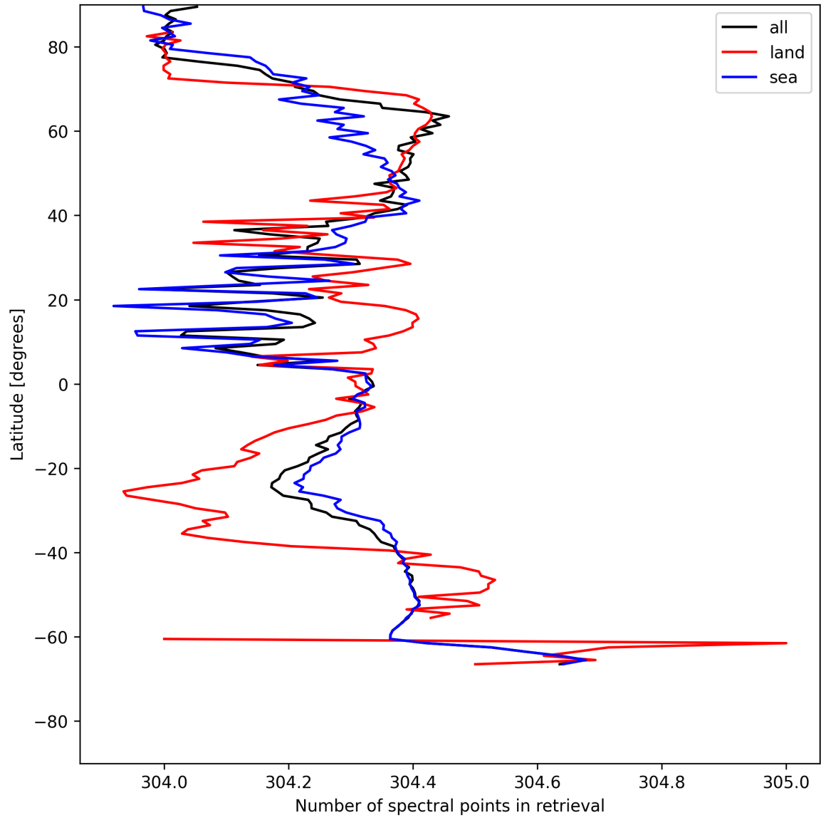
Figure 16: Zonal average of “Number of spectral points in retrieval” for 2025-07-16 to 2025-07-18.
