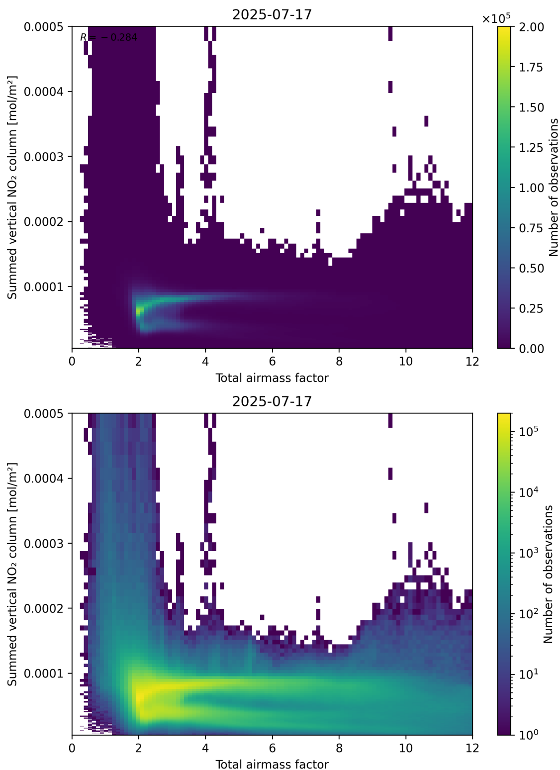
Figure 65: Scatter density plot of “Total airmass factor” against “Summed vertical NO 2 column” for 2025-07-16 to 2025-07-18.
