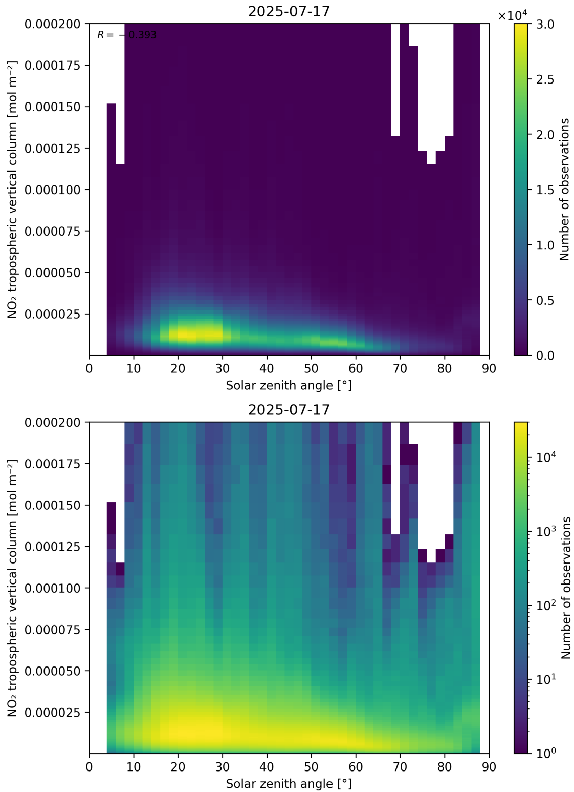
Figure 155: Scatter density plot of “Solar zenith angle” against “NO 2 tropospheric vertical column” for 2025-07-16 to 2025-07-18.
