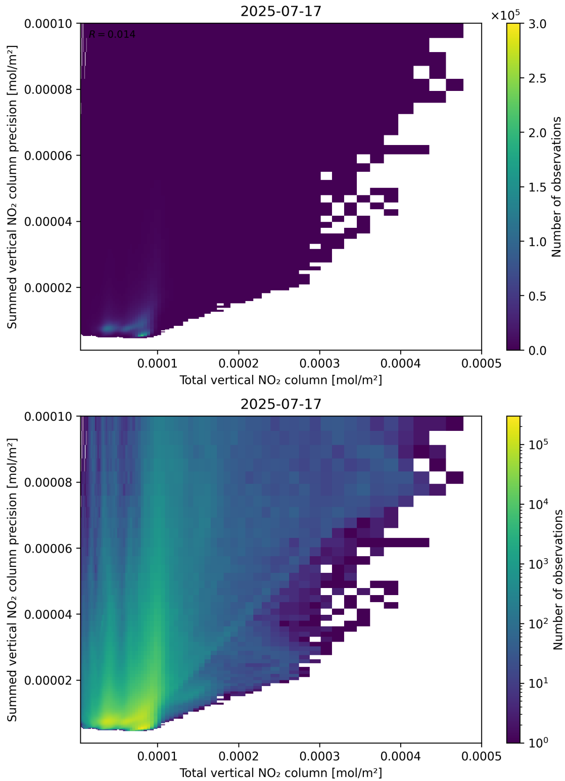
Figure 113: Scatter density plot of “Total vertical NO 2 column” against “Summed vertical NO 2 column precision” for 2025-07-16 to 2025-07-18.
