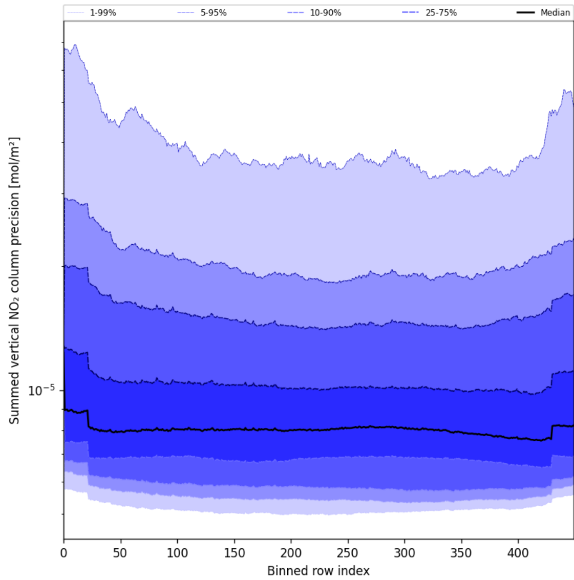
Figure 58: Along track statistics of “Summed vertical NO 2 column precision” for 2025-07-16 to 2025-07-18
