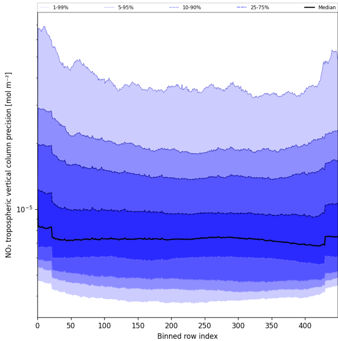
Figure 47: Along track statistics of “NO 2 tropospheric vertical column precision” for 2025-07-16 to 2025-07-18
