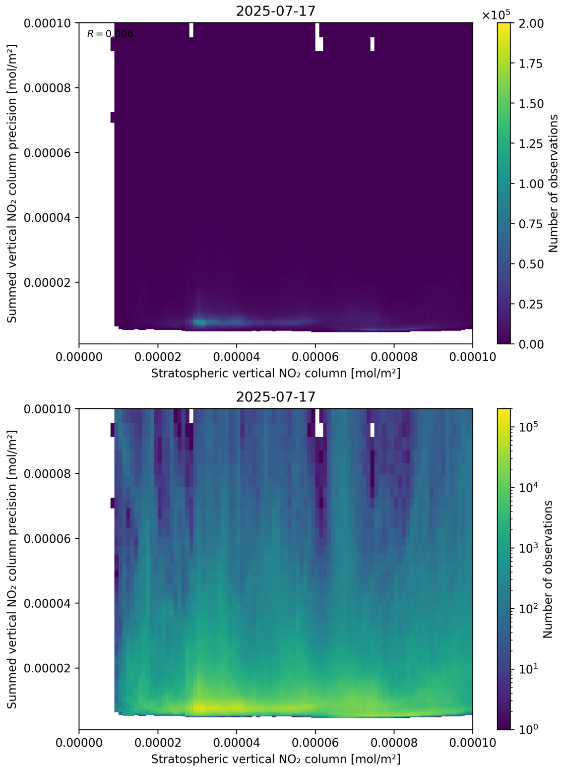
Figure 99: Scatter density plot of “Stratospheric vertical NO 2 column” against “Summed vertical NO 2 column precision” for 2025-07-16 to 2025-07-18.
