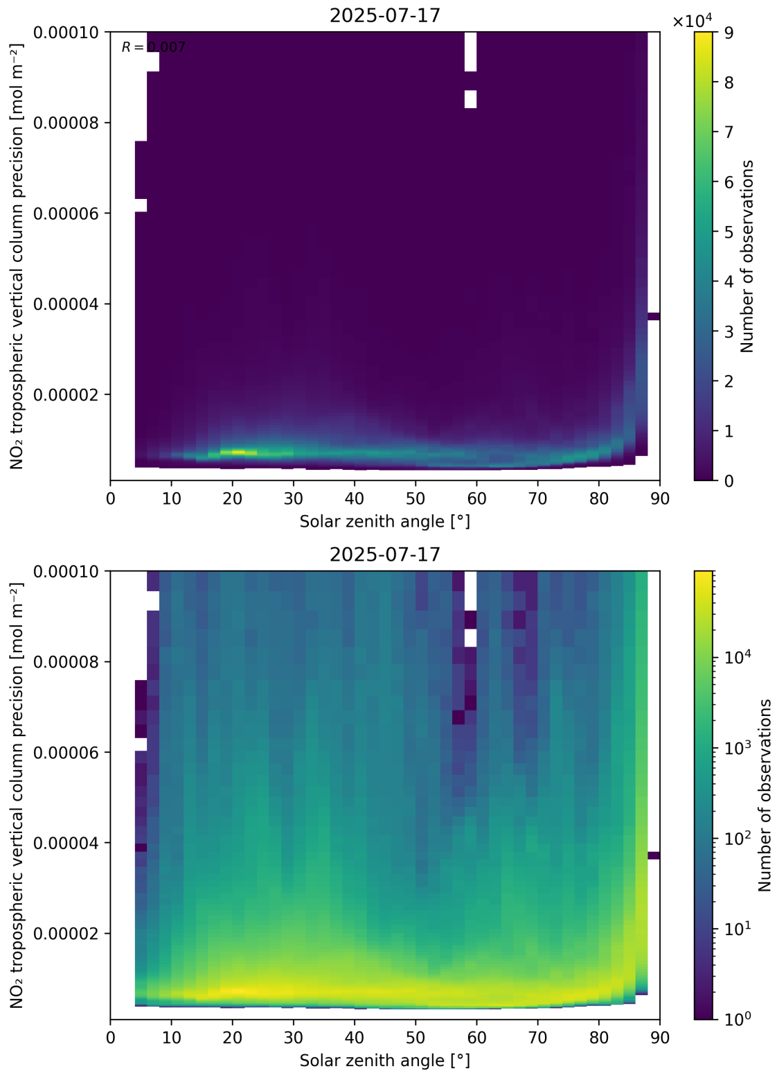
Figure 156: Scatter density plot of “Solar zenith angle” against “NO 2 tropospheric vertical column precision” for 2025-07-16 to 2025-07-18.
