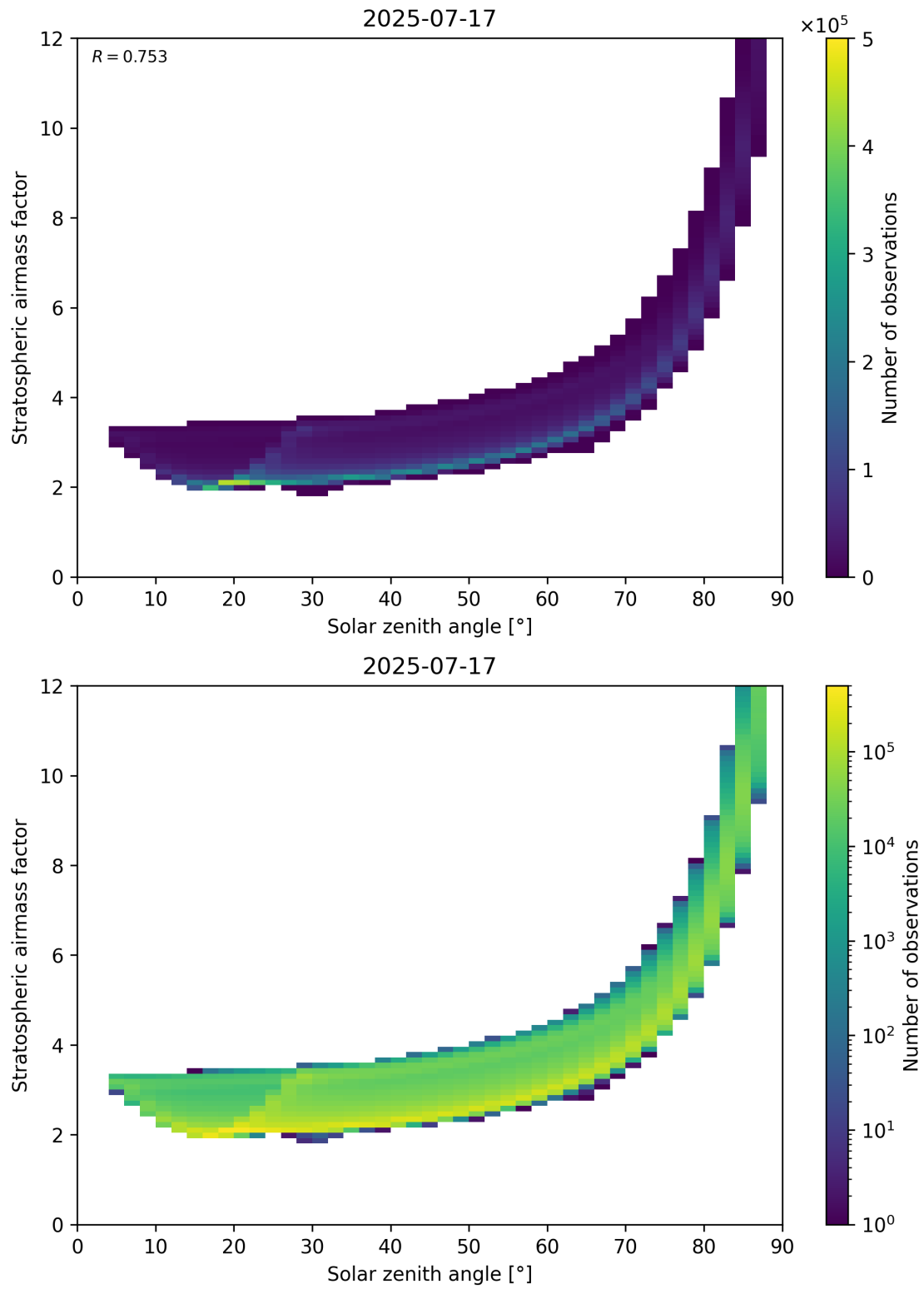
Figure 145: Scatter density plot of “Solar zenith angle” against “Stratospheric airmass factor” for 2025-07-16 to 2025-07-18.
