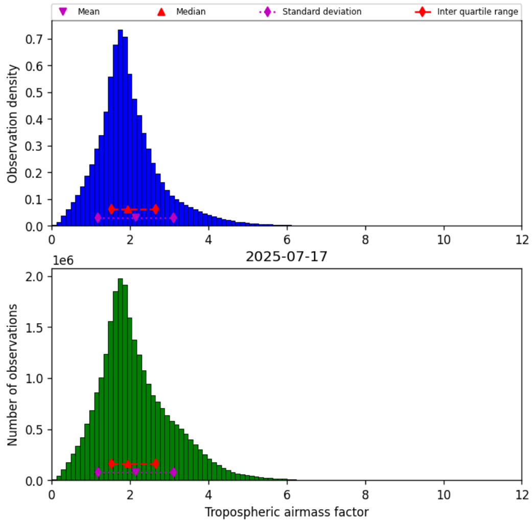
Figure 31: Histogram of “Tropospheric airmass factor” for 2025-07-16 to 2025-07-18
