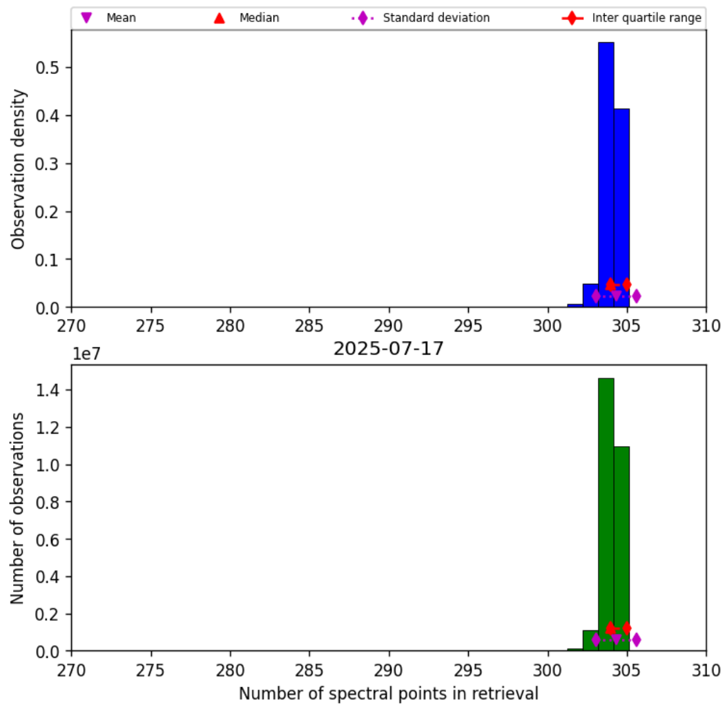
Figure 33: Histogram of "Number of spectral points in retrieval" for 2025-07-16 to 2025-07-18
