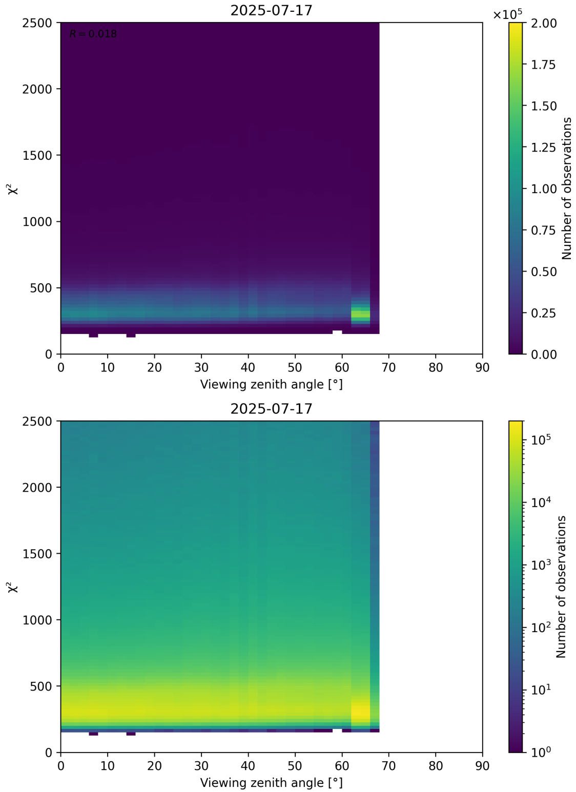
Figure 162: Scatter density plot of “Viewing zenith angle” against “ \chi^2 ” for 2025-07-16 to 2025-07-18.
