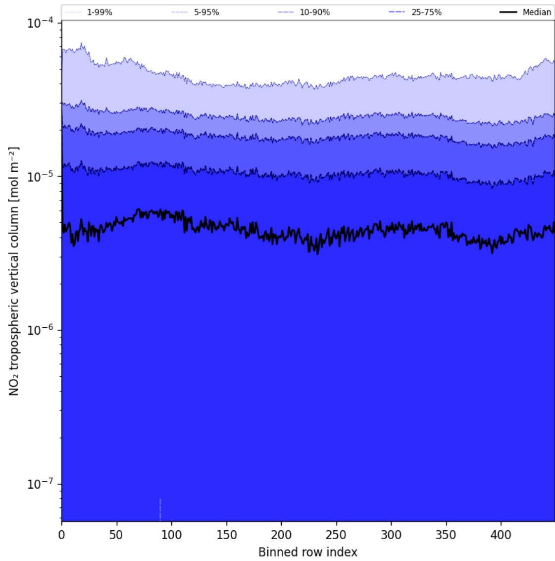
Figure 46: Along track statistics of "NO 2 tropospheric vertical column" for 2025-07-16 to 2025-07-18
