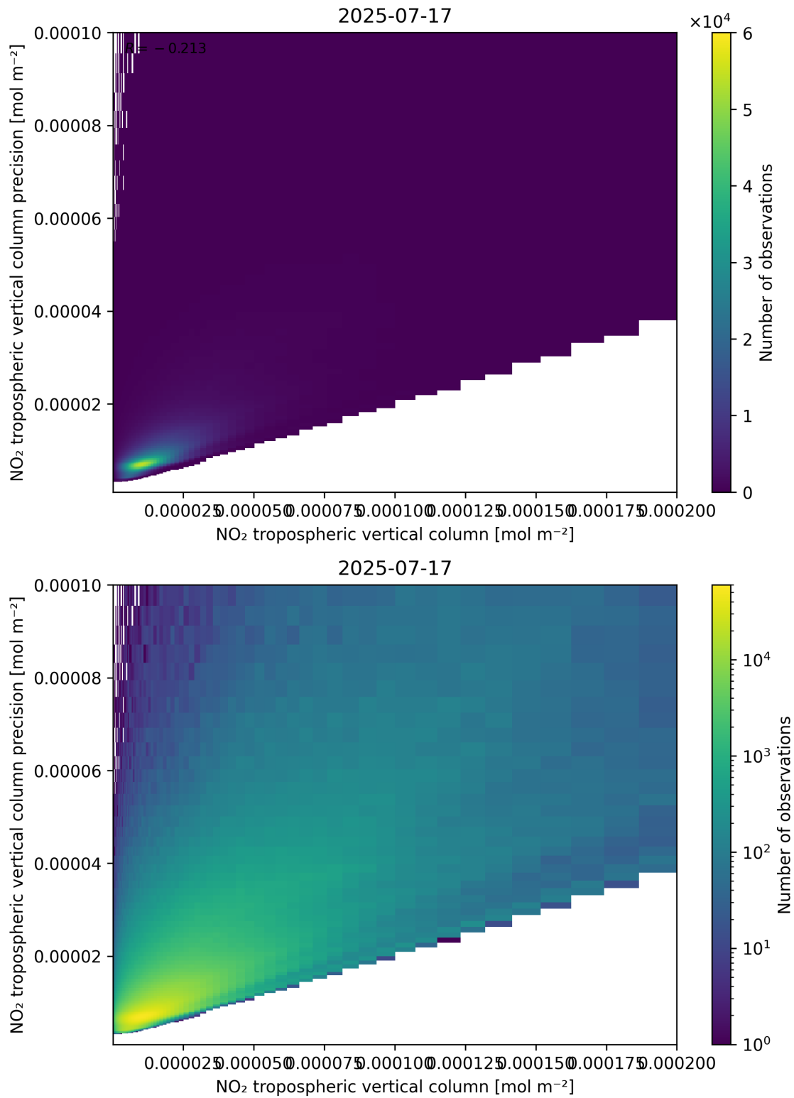
Figure 130: Scatter density plot of “NO 2 tropospheric vertical column” against “NO 2 tropospheric vertical column precision” for 2025-07-16 to 2025-07-18.
