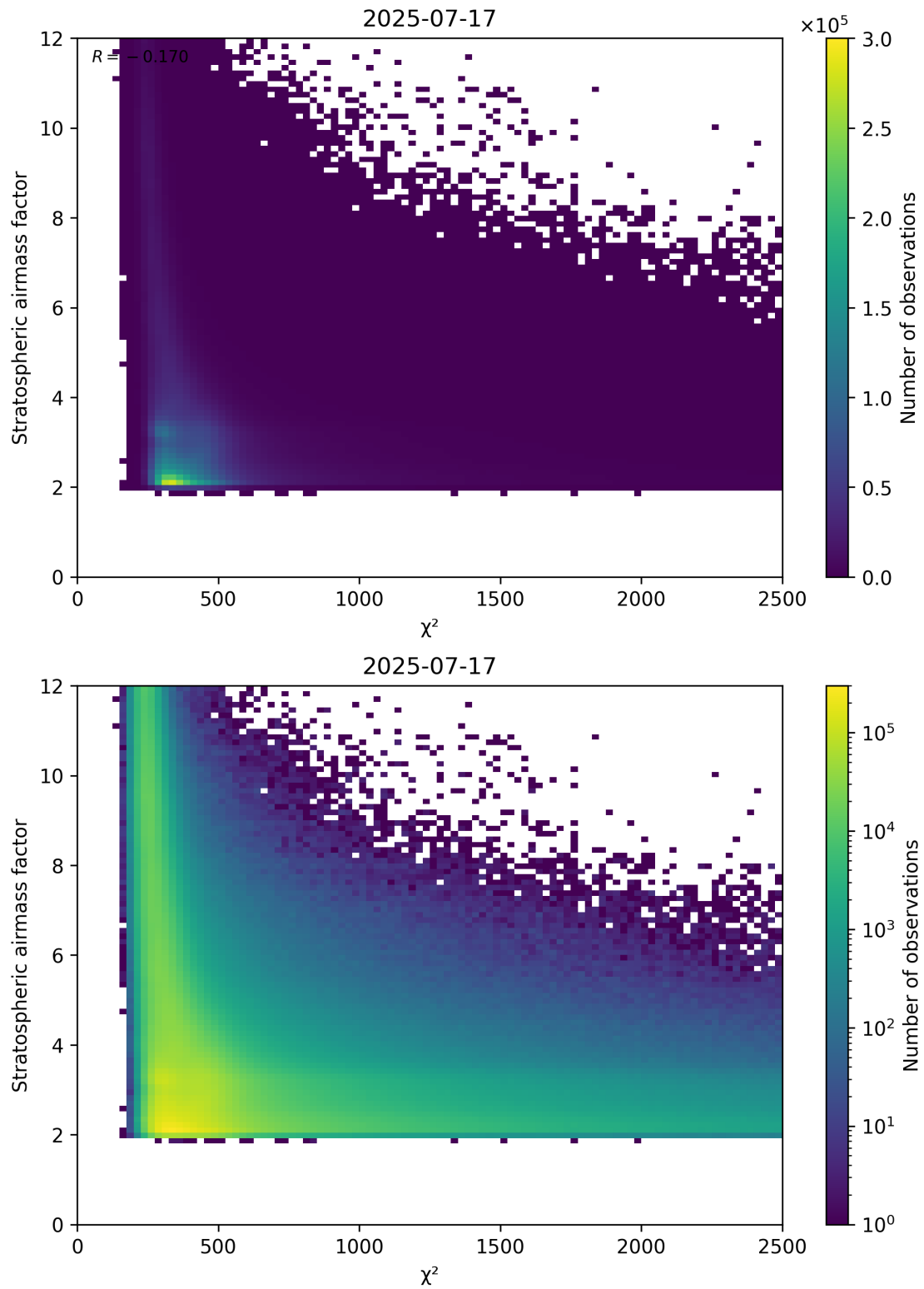
Figure 81: Scatter density plot of “ \chi^2 ” against “Stratospheric airmass factor” for 2025-07-16 to 2025-07-18.
