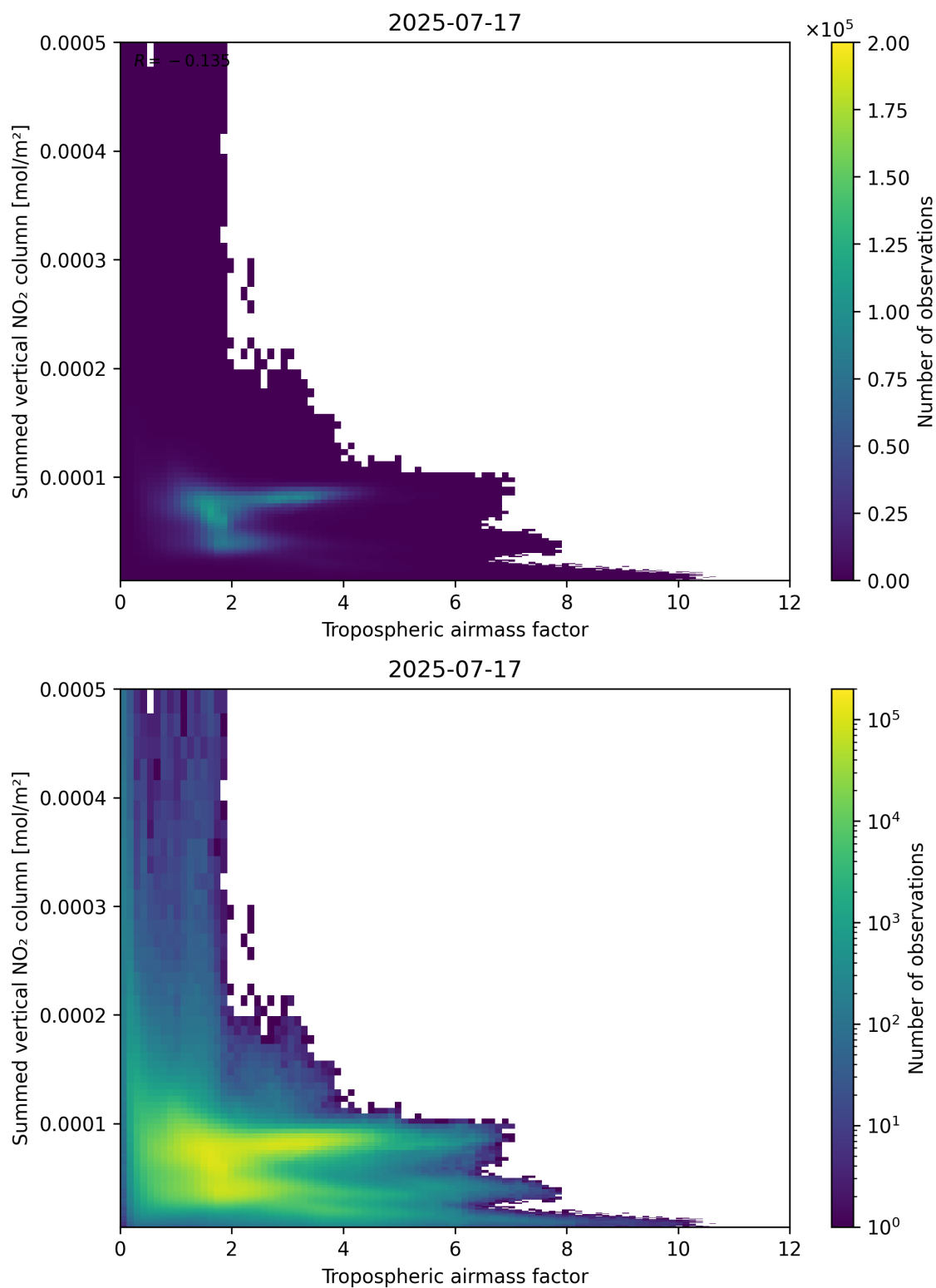
Figure 75: Scatter density plot of “Tropospheric air mass factor” against “Summed vertical NO 2 column” for 2025-07-16 to 2025-07-18.
