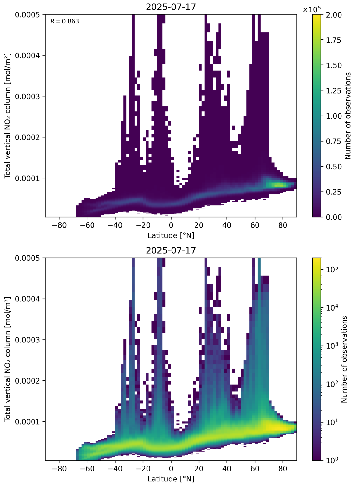
Figure 90: Scatter density plot of “Latitude” against “Total vertical NO 2 column” for 2025-07-16 to 2025-07-18.
