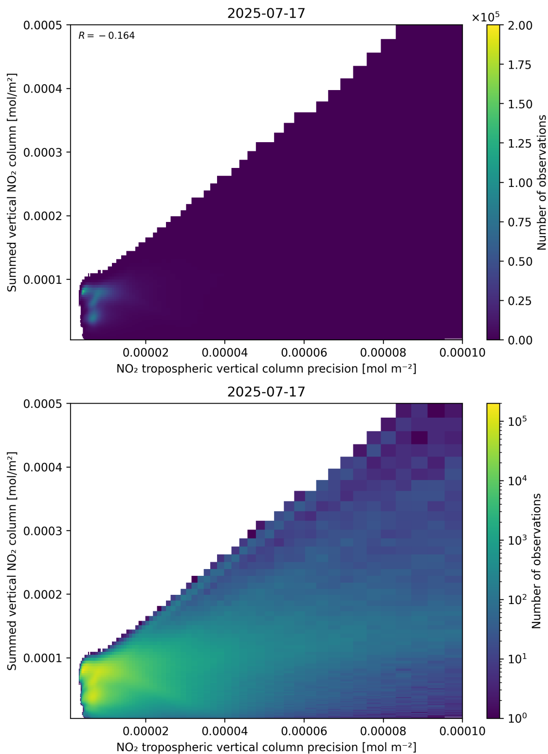
Figure 136: Scatter density plot of “NO 2 tropospheric vertical column precision” against “Summed vertical NO 2 column” for 2025-07-16 to 2025-07-18.
