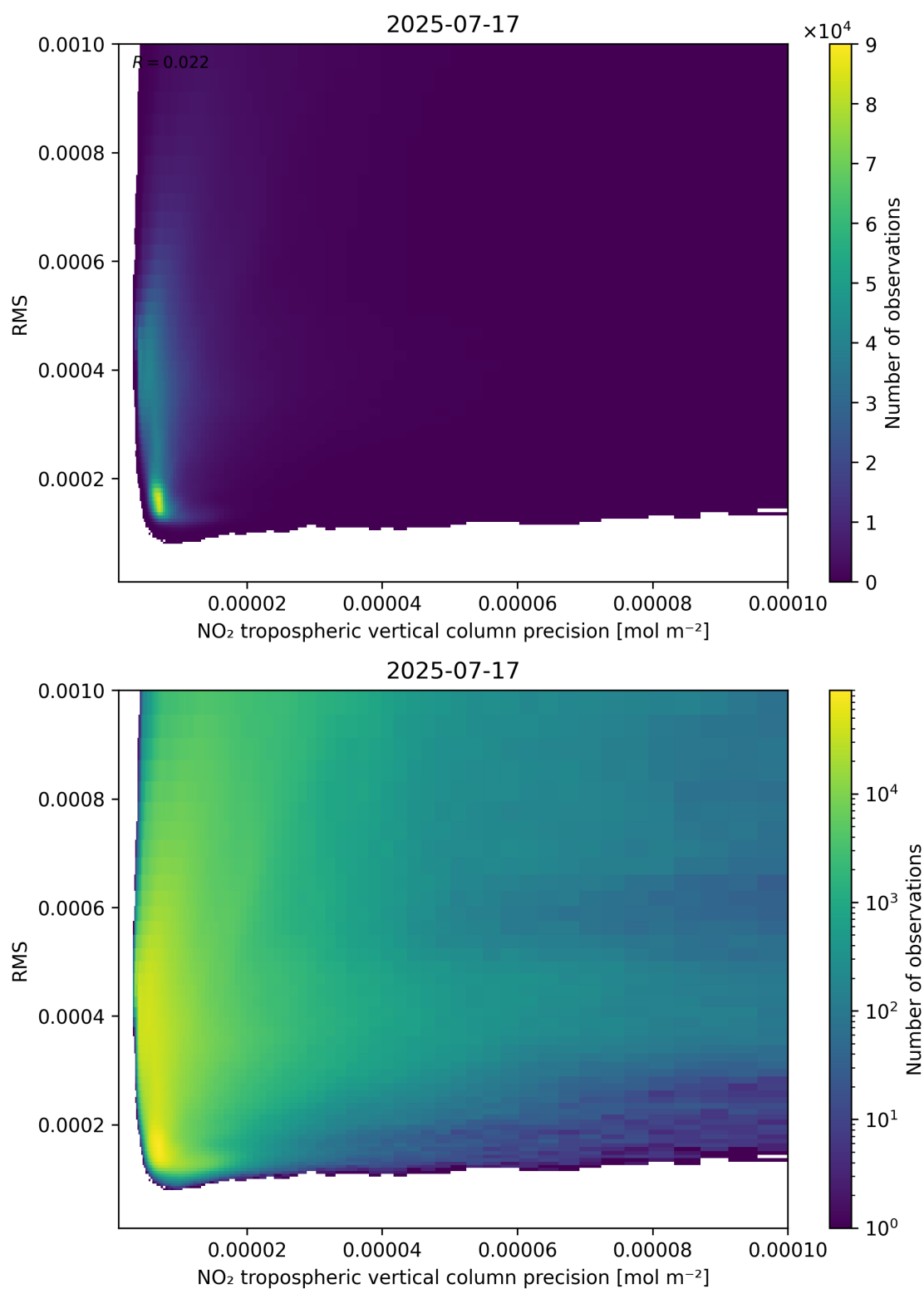
Figure 140: Scatter density plot of “NO 2 tropospheric vertical column precision” against “RMS” for 2025-07-16 to 2025-07-18.
