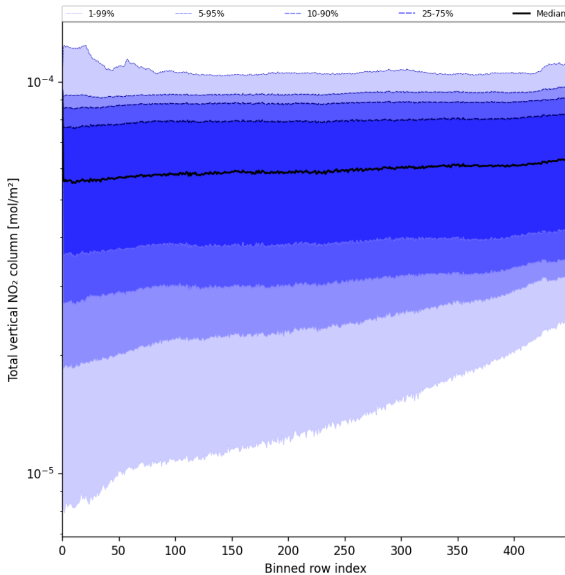
Figure 55: Along track statistics of “Total vertical NO 2 column” for 2025-07-16 to 2025-07-18
