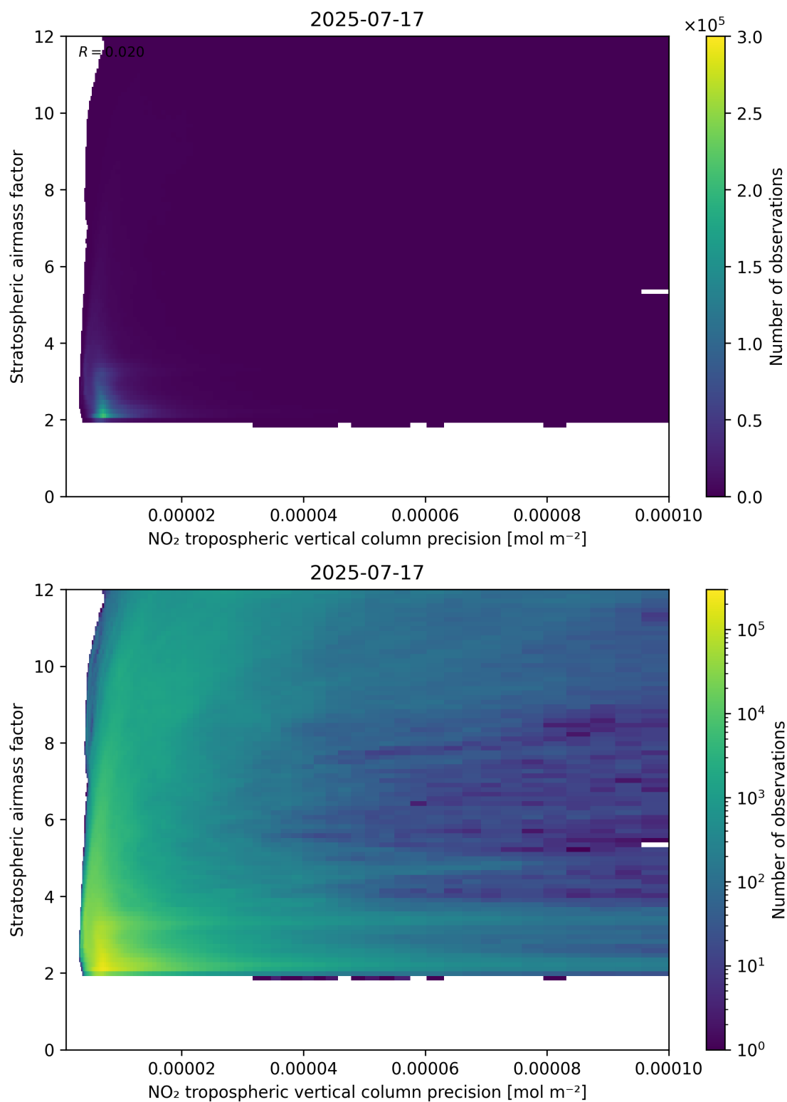
Figure 131: Scatter density plot of “NO 2 tropospheric vertical column precision” against “Stratospheric airmass factor” for 2025-07-16 to 2025-07-18.
