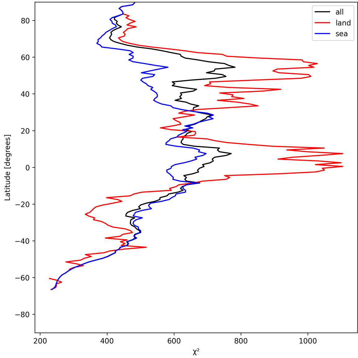
Figure 25: Zonal average of “ \chi^2 ” for 2025-07-16 to 2025-07-18.
