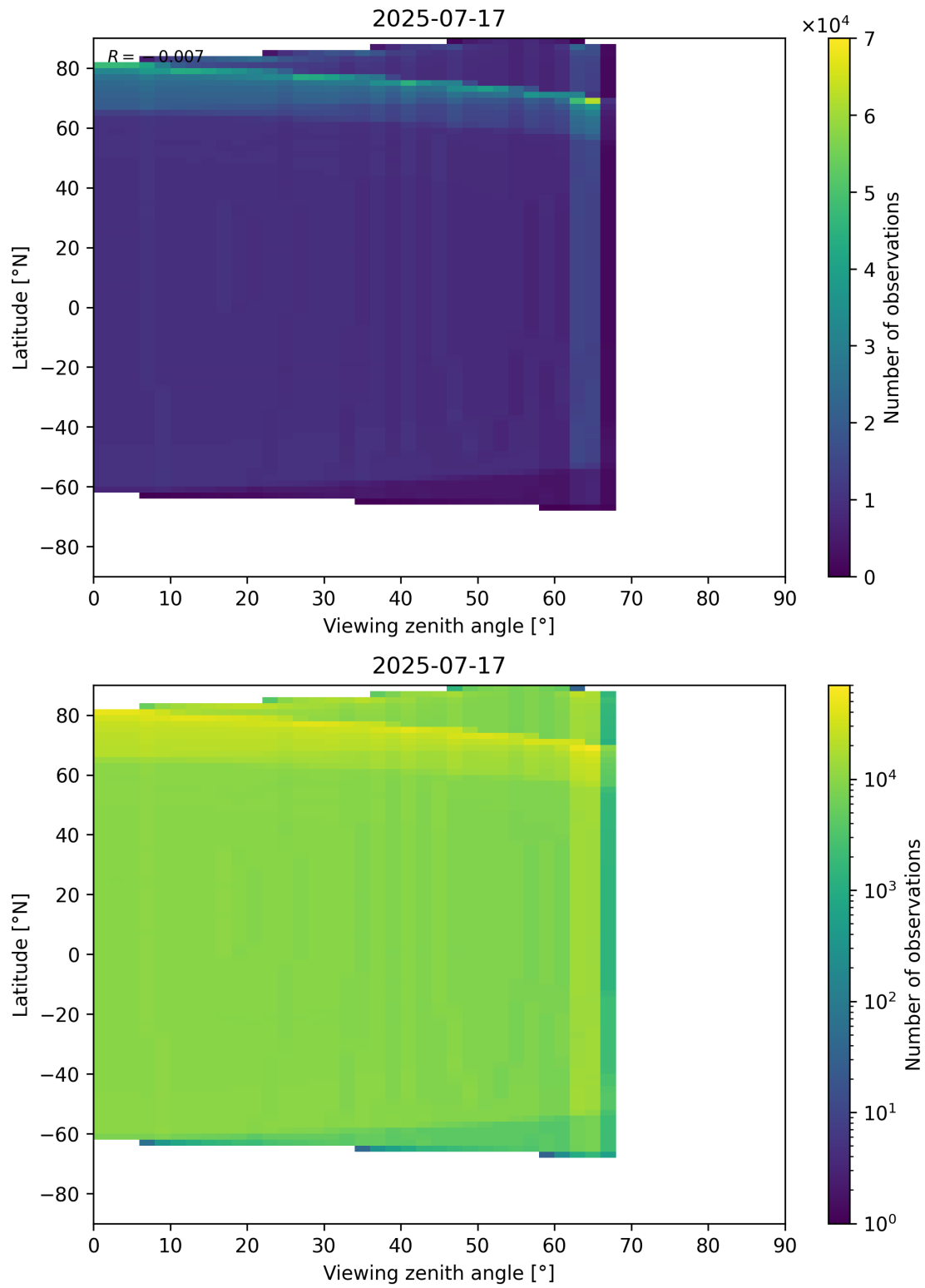
Figure 163: Scatter density plot of “Viewing zenith angle” against “Latitude” for 2025-07-16 to 2025-07-18.
