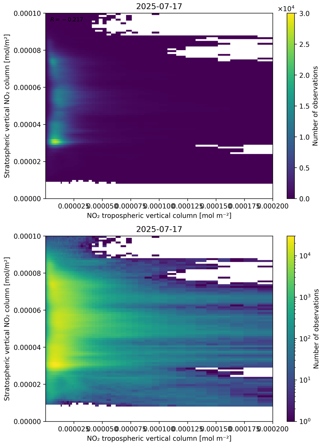
Figure 125: Scatter density plot of “NO 2 tropospheric vertical column” against “Stratospheric vertical NO 2 column” for 2025-07-16 to 2025-07-18.
