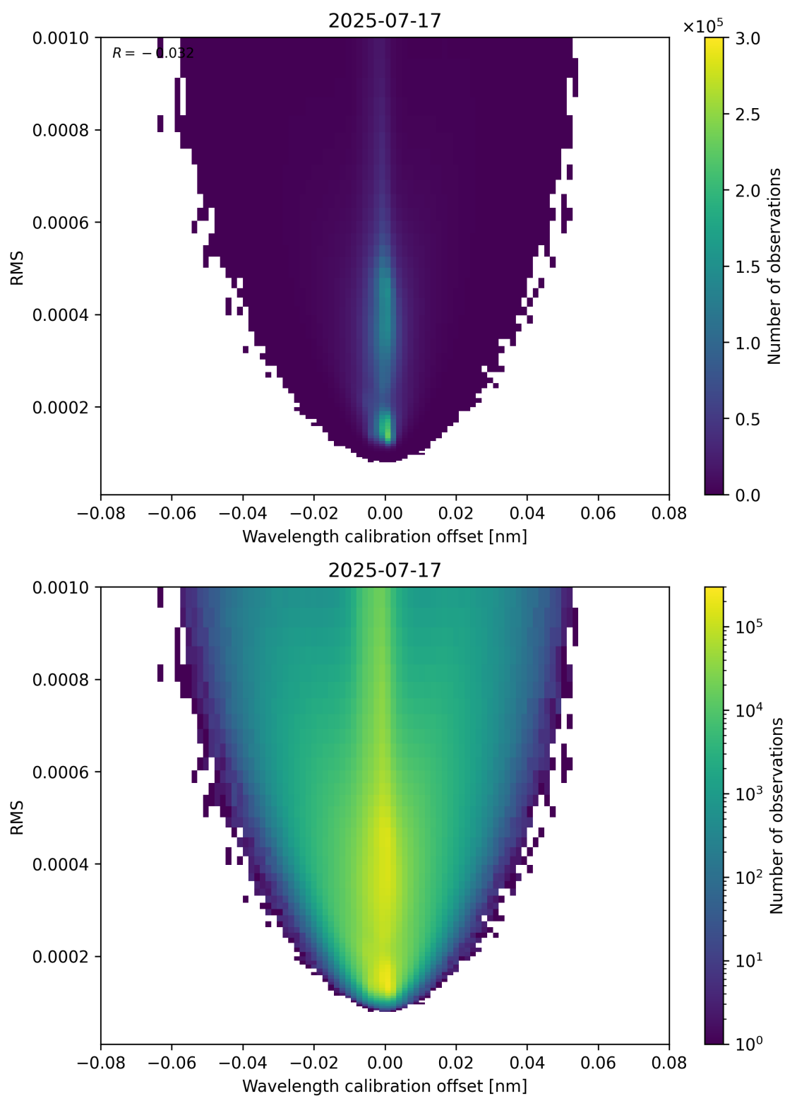
Figure 181: Scatter density plot of “Wavelength calibration offset” against “RMS” for 2025-07-16 to 2025-07-18.
