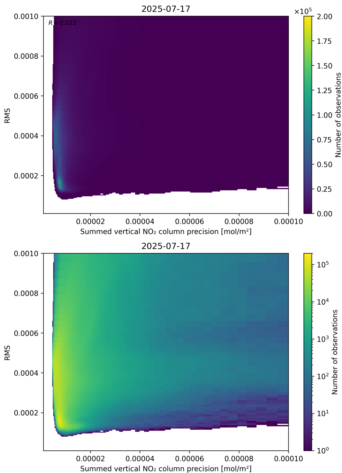
Figure 108: Scatter density plot of “Summed vertical NO 2 column precision” against “RMS” for 2025-07-16 to 2025-07-18.
