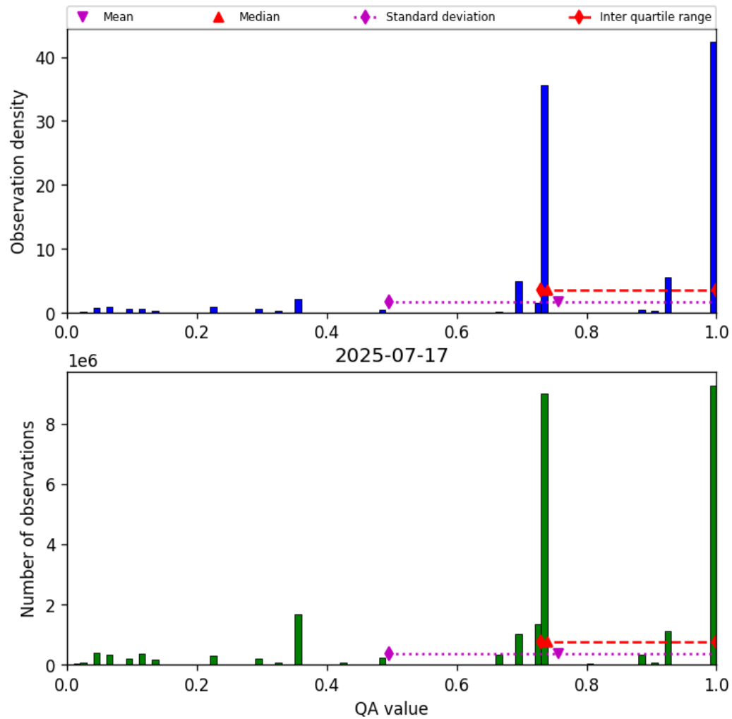
Figure 28: Histogram of “QA value” for 2025-07-16 to 2025-07-18
