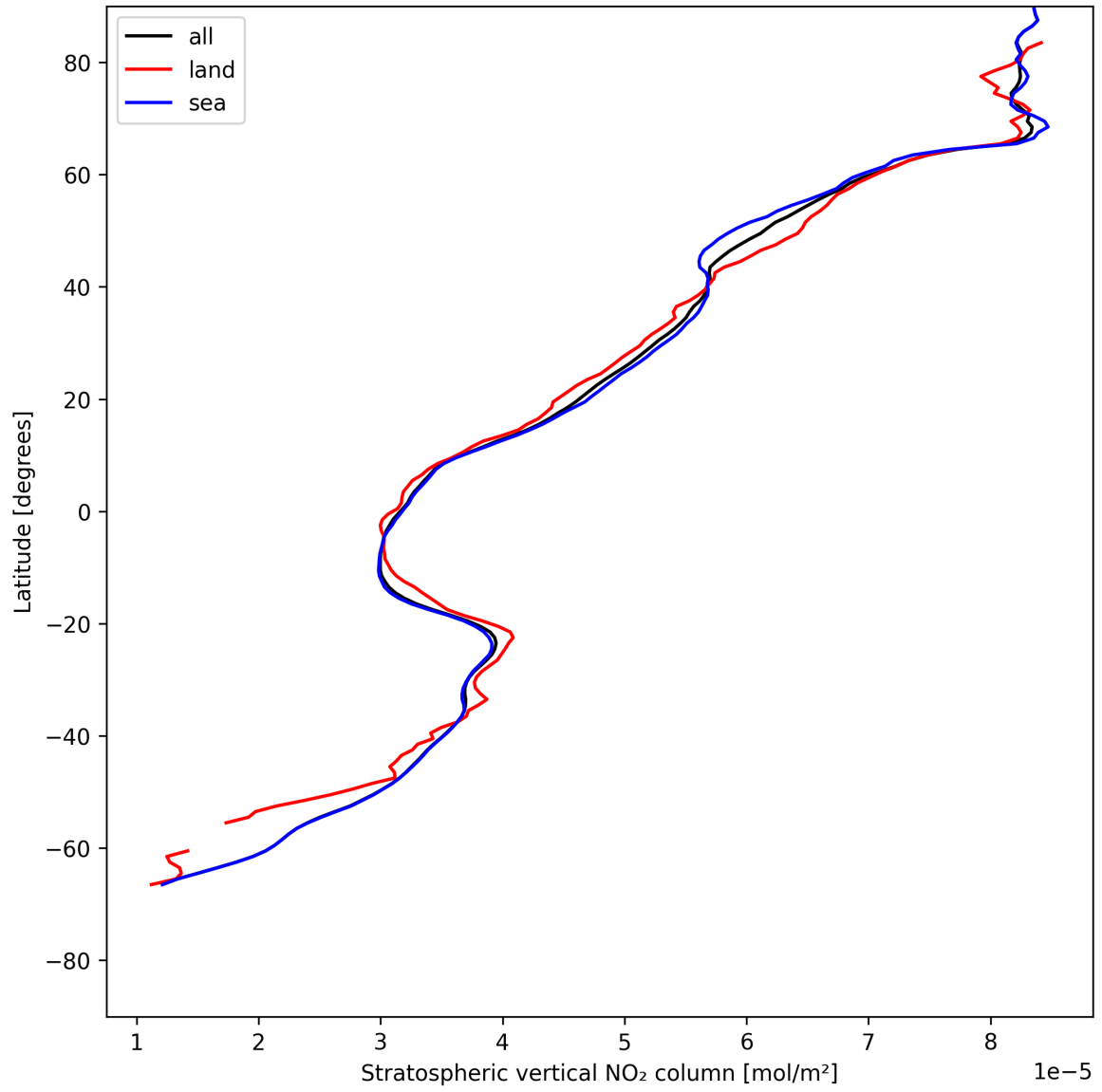
Figure 19: Zonal average of “Stratospheric vertical NO 2 column” for 2025-07-16 to 2025-07-18.
