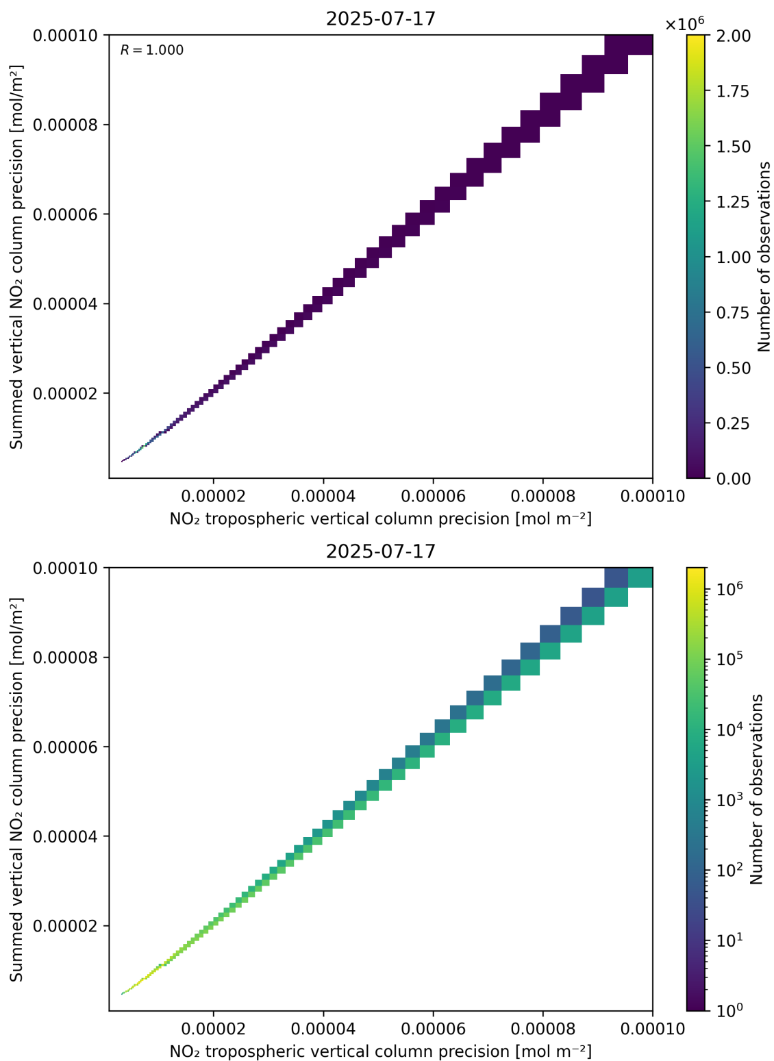
Figure 137: Scatter density plot of “NO 2 tropospheric vertical column precision” against “Summed vertical NO 2 column precision” for 2025-07-16 to 2025-07-18.
