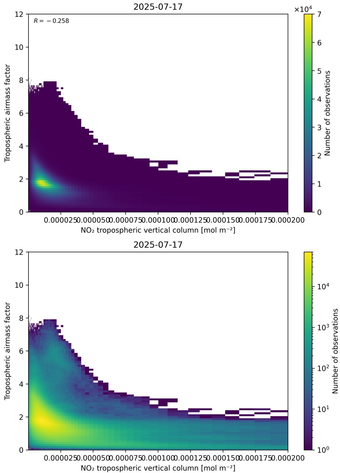
Figure 123: Scatter density plot of “NO 2 tropospheric vertical column” against “Tropospheric air mass factor” for 2025-07-16 to 2025-07-18.
