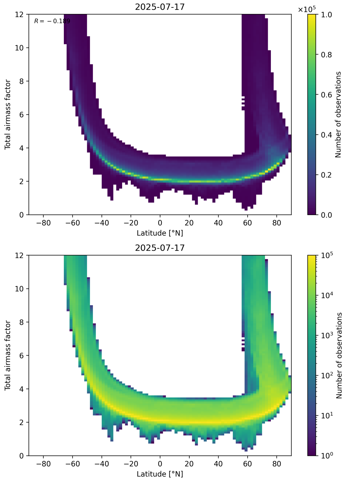
Figure 84: Scatter density plot of “Latitude” against “Total airmass factor” for 2025-07-16 to 2025-07-18.
