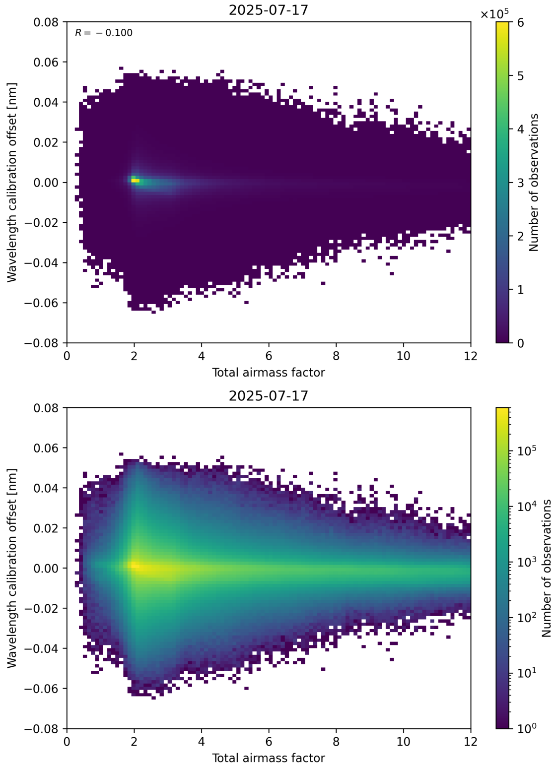
Figure 70: Scatter density plot of “Total airmass factor” against “Wavelength calibration offset” for 2025-07-16 to 2025-07-18.
