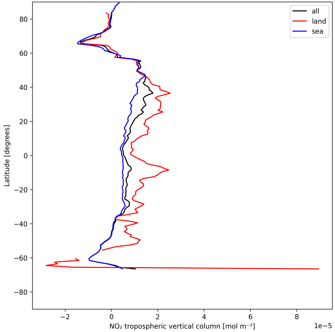
Figure 12: Zonal average of “NO 2 tropospheric vertical column” for 2025-07-16 to 2025-07-18.
