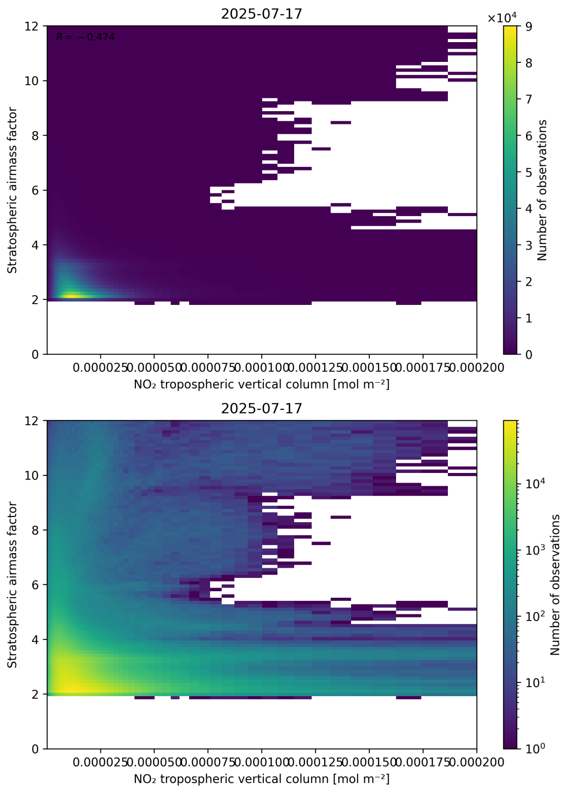
Figure 121: Scatter density plot of “NO 2 tropospheric vertical column” against “Stratospheric air mass factor” for 2025-07-16 to 2025-07-18.
