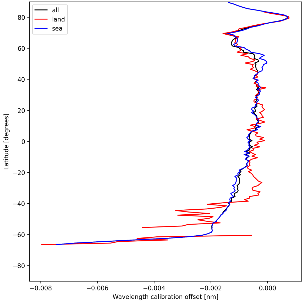
Figure 18: Zonal average of “Wavelength calibration offset” for 2025-07-16 to 2025-07-18.
