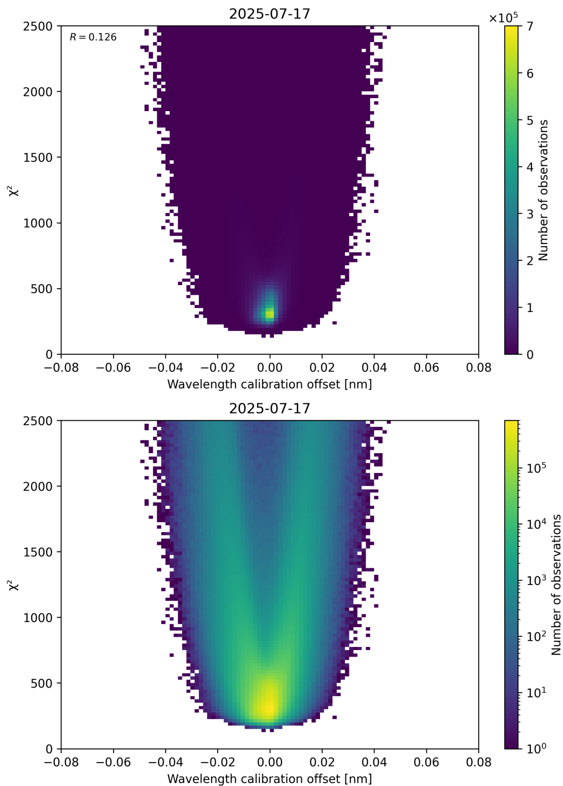
Figure 175: Scatter density plot of “Wavelength calibration offset” against “ \chi^2 ” for 2025-07-16 to 2025-07-18.
