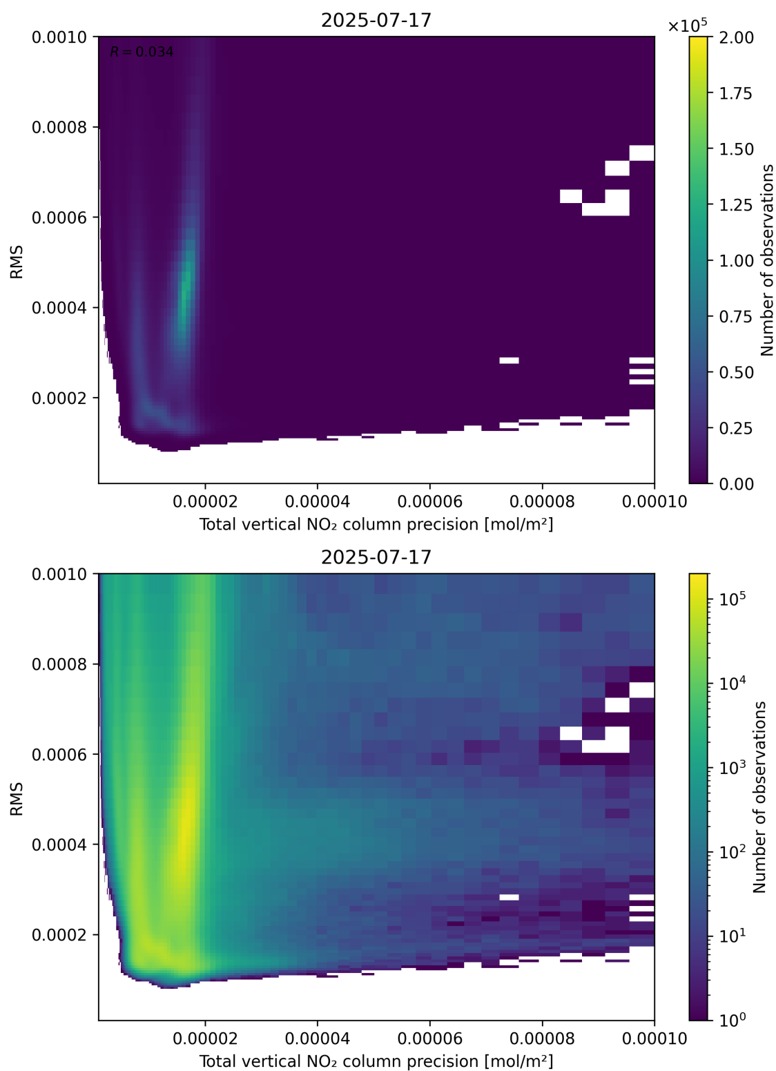
Figure 119: Scatter density plot of “Total vertical NO 2 column precision” against “RMS” for 2025-07-16 to 2025-07-18.
