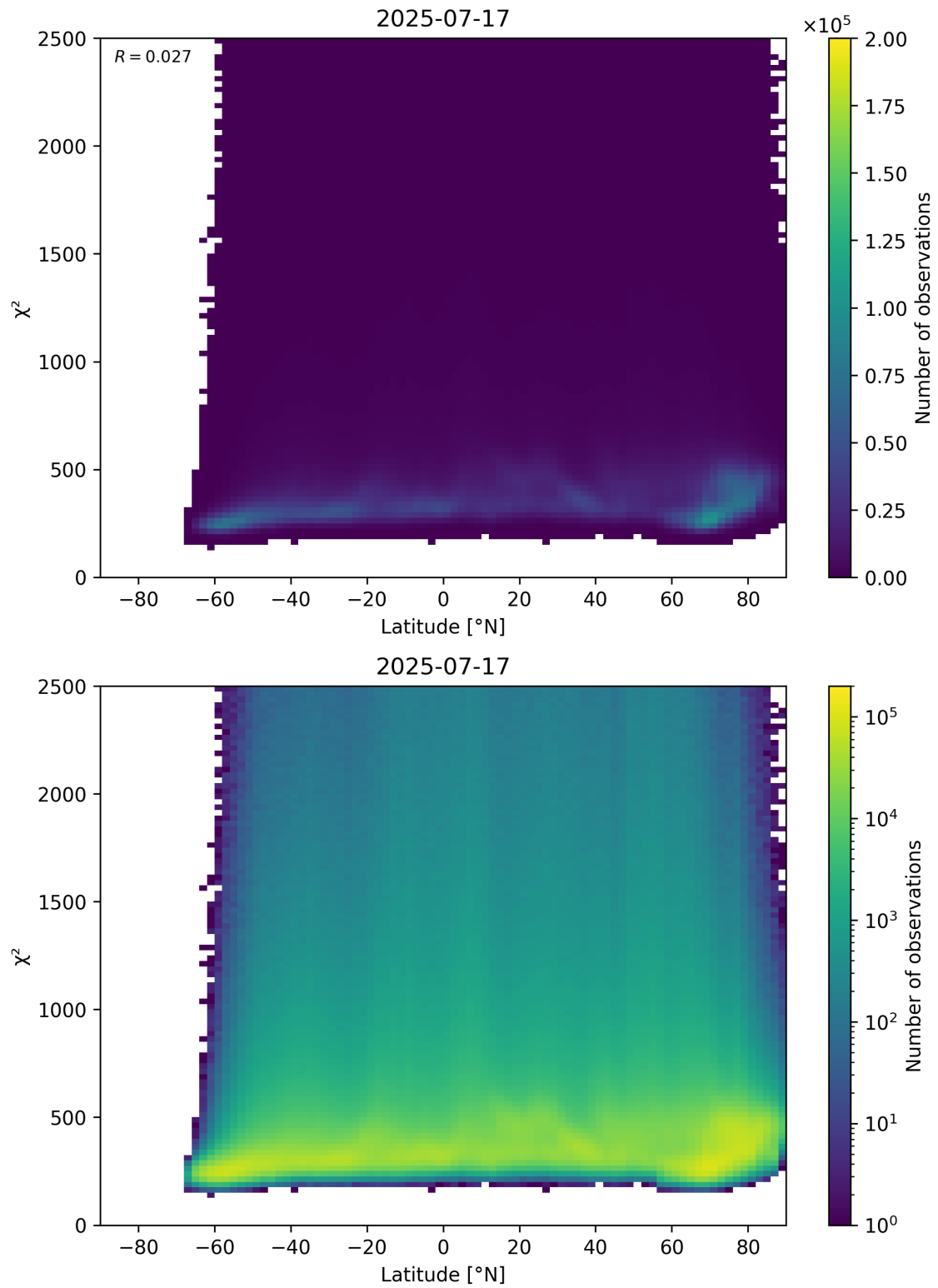
Figure 86: Scatter density plot of “Latitude” against “ \chi^2 ” for 2025-07-16 to 2025-07-18.
