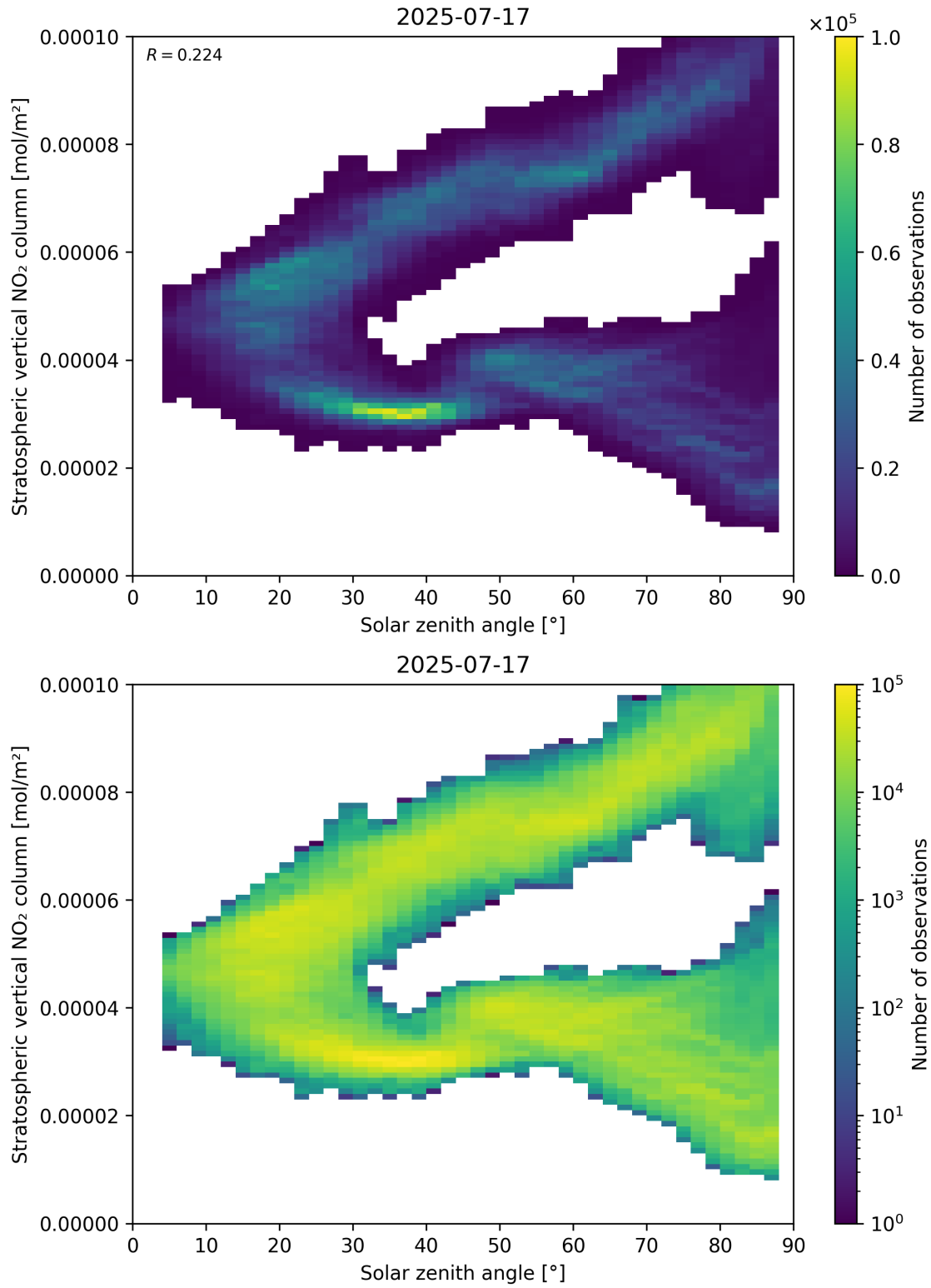
Figure 150: Scatter density plot of “Solar zenith angle” against “Stratospheric vertical NO 2 column” for 2025-07-16 to 2025-07-18.
