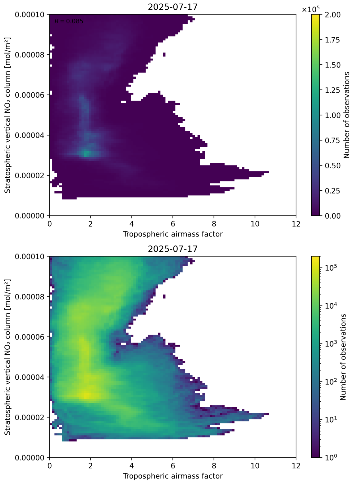
Figure 74: Scatter density plot of “Tropospheric airmass factor” against “Stratospheric vertical NO 2 column” for 2025-07-16 to 2025-07-18.
