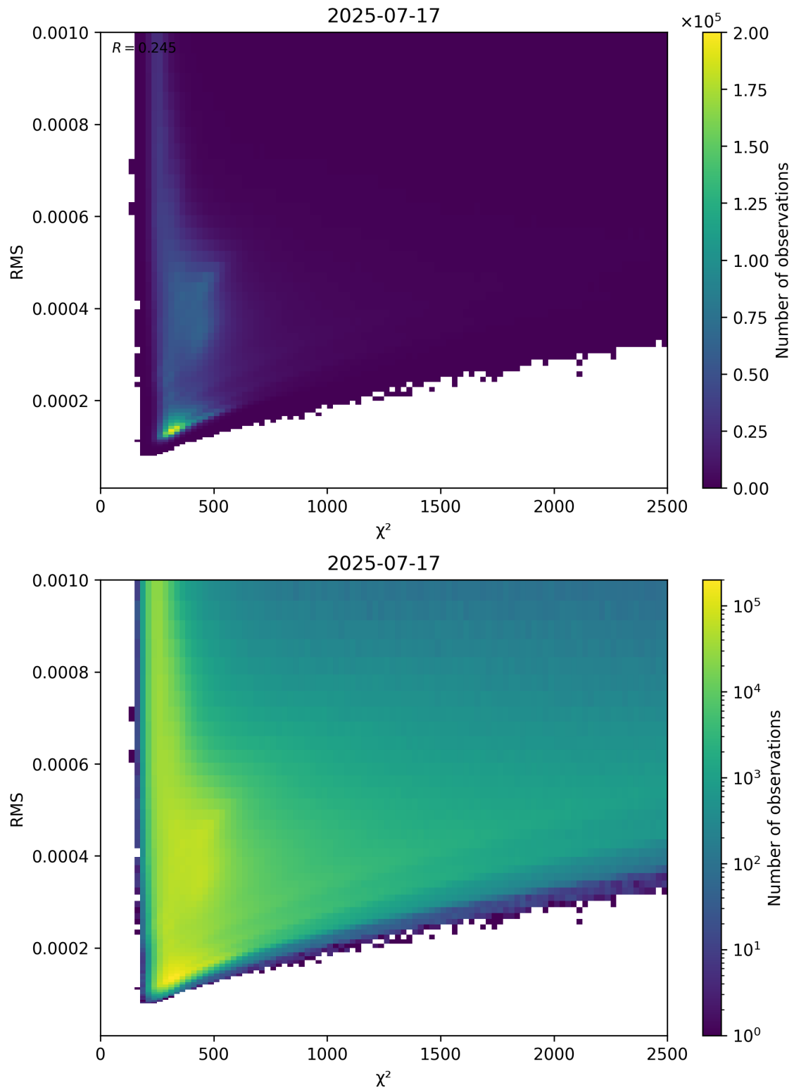
Figure 82: Scatter density plot of “ \chi^2 ” against “RMS” for 2025-07-16 to 2025-07-18.
