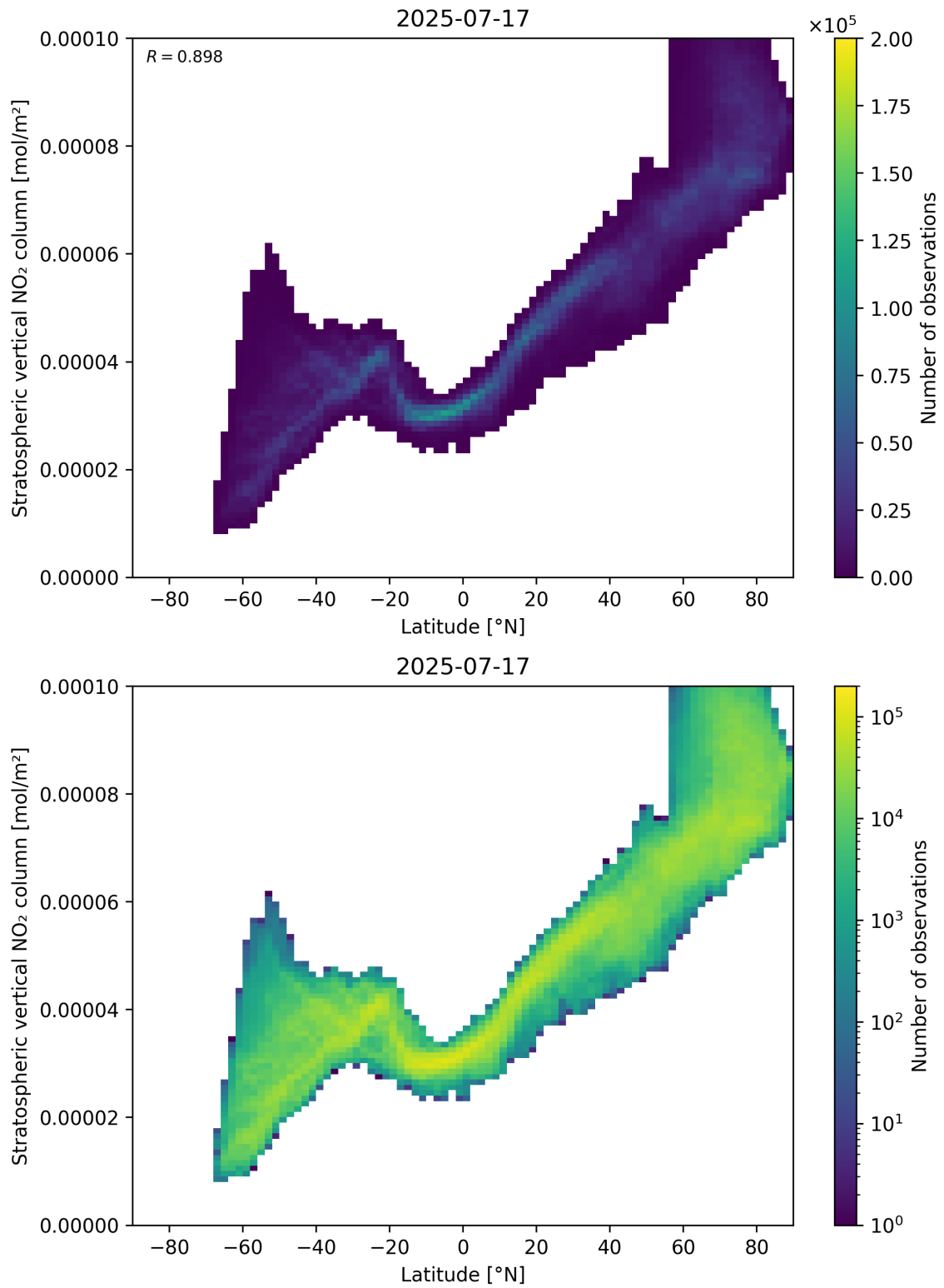
Figure 87: Scatter density plot of “Latitude” against “Stratospheric vertical \text{NO}_2 column” for 2025-07-16 to 2025-07-18.
