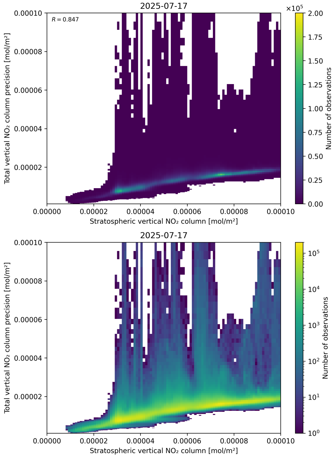
Figure 101: Scatter density plot of “Stratospheric vertical NO 2 column” against “Total vertical NO 2 column precision” for 2025-07-16 to 2025-07-18.
