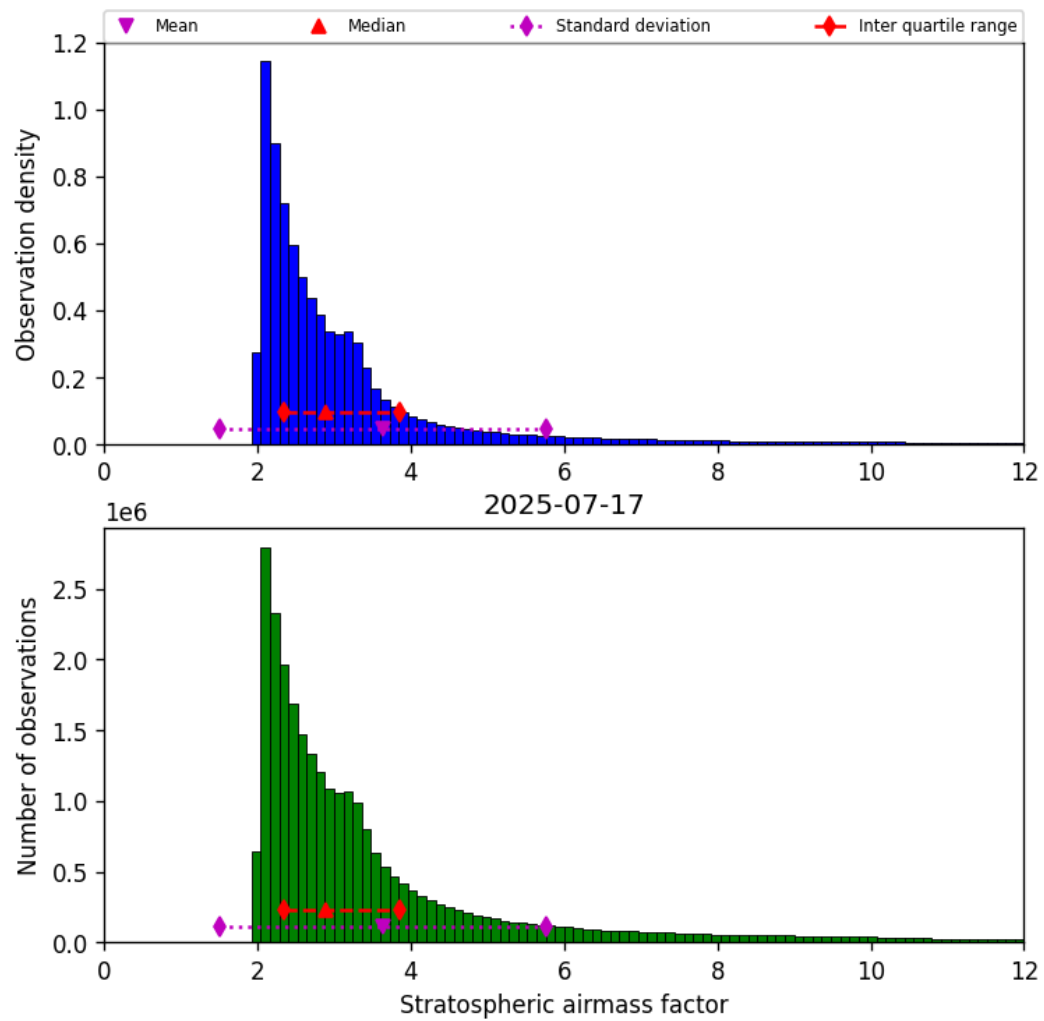
Figure 44: Histogram of “Stratospheric airmass factor” for 2025-07-16 to 2025-07-18
