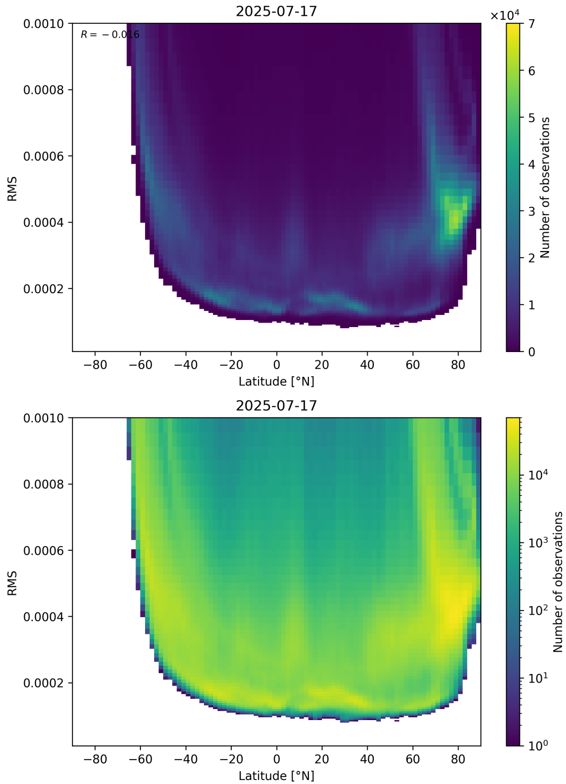
Figure 94: Scatter density plot of “Latitude” against “RMS” for 2025-07-16 to 2025-07-18.
