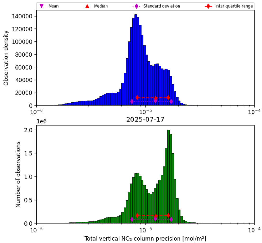
Figure 39: Histogram of “Total vertical NO 2 column precision” for 2025-07-16 to 2025-07-18
