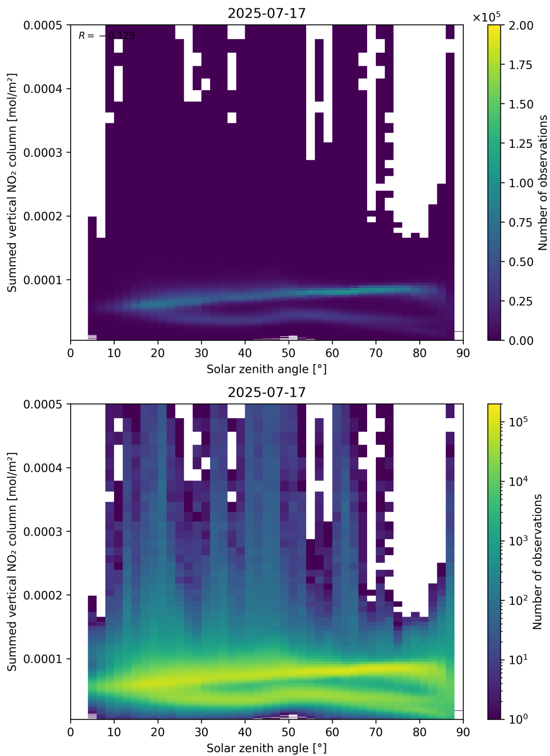
Figure 151: Scatter density plot of “Solar zenith angle” against “Summed vertical NO 2 column” for 2025-07-16 to 2025-07-18.
