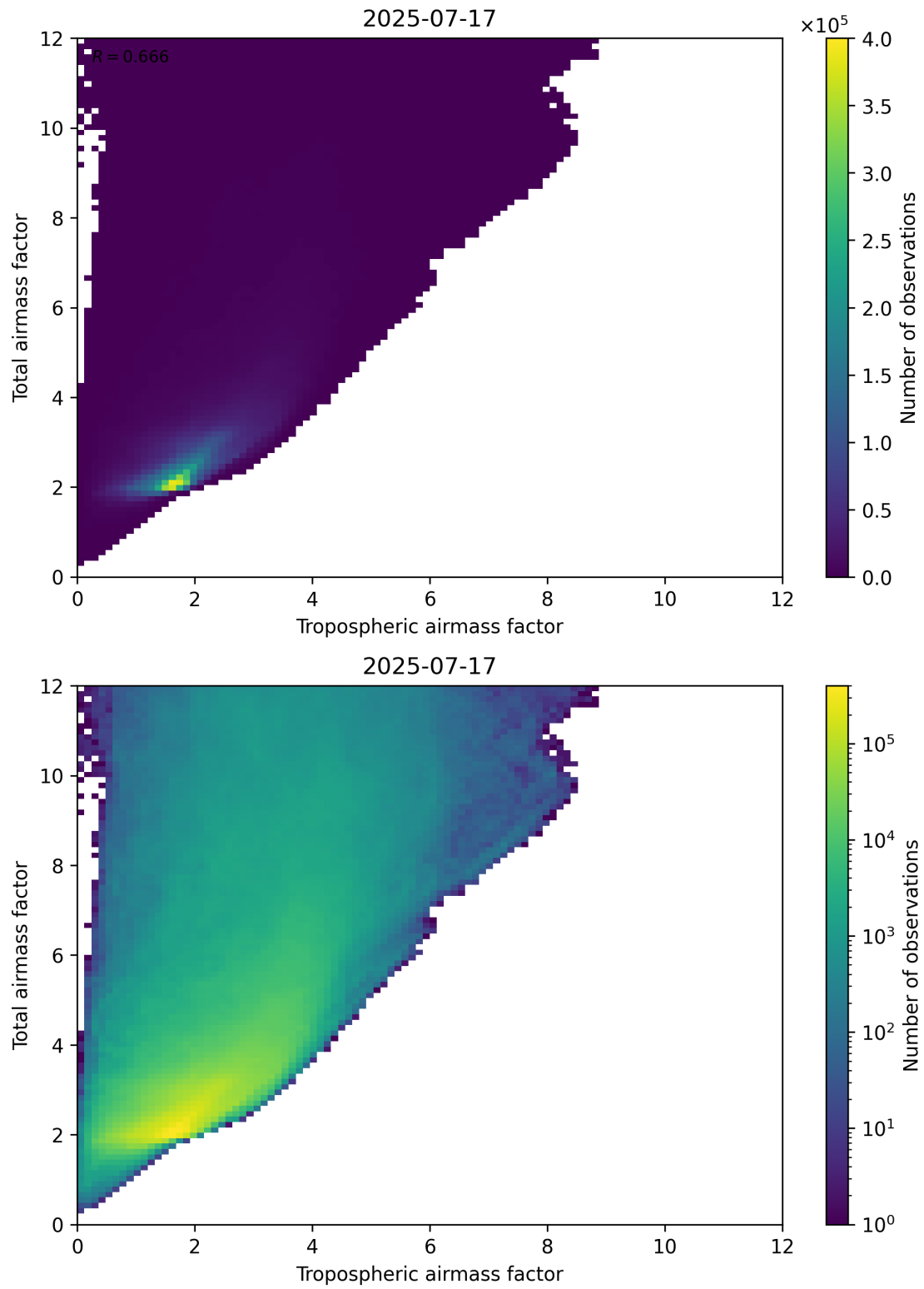
Figure 72: Scatter density plot of “Tropospheric airmass factor” against “Total airmass factor” for 2025-07-16 to 2025-07-18.
