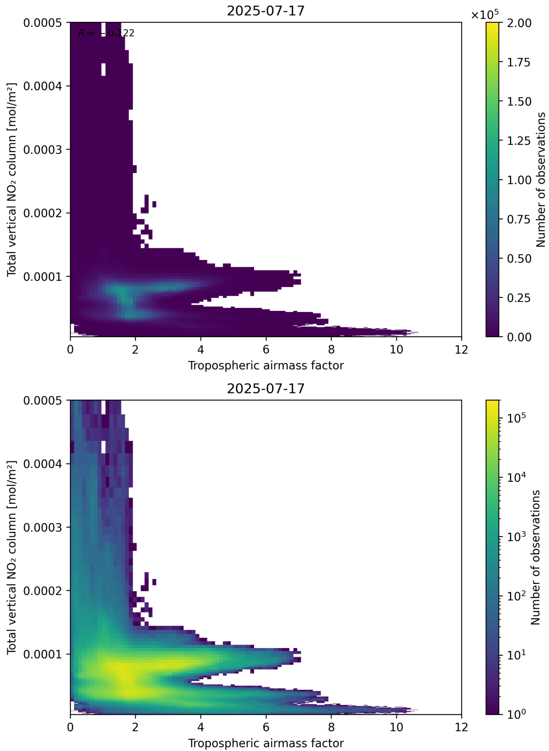
Figure 77: Scatter density plot of “Tropospheric airmass factor” against “Total vertical NO 2 column” for 2025-07-16 to 2025-07-18.
