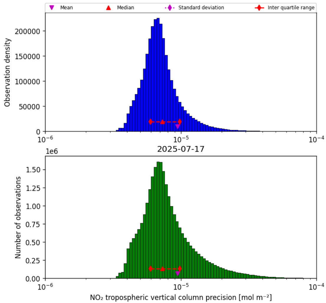
Figure 30: Histogram of “NO 2 tropospheric vertical column precision” for 2025-07-16 to 2025-07-18
