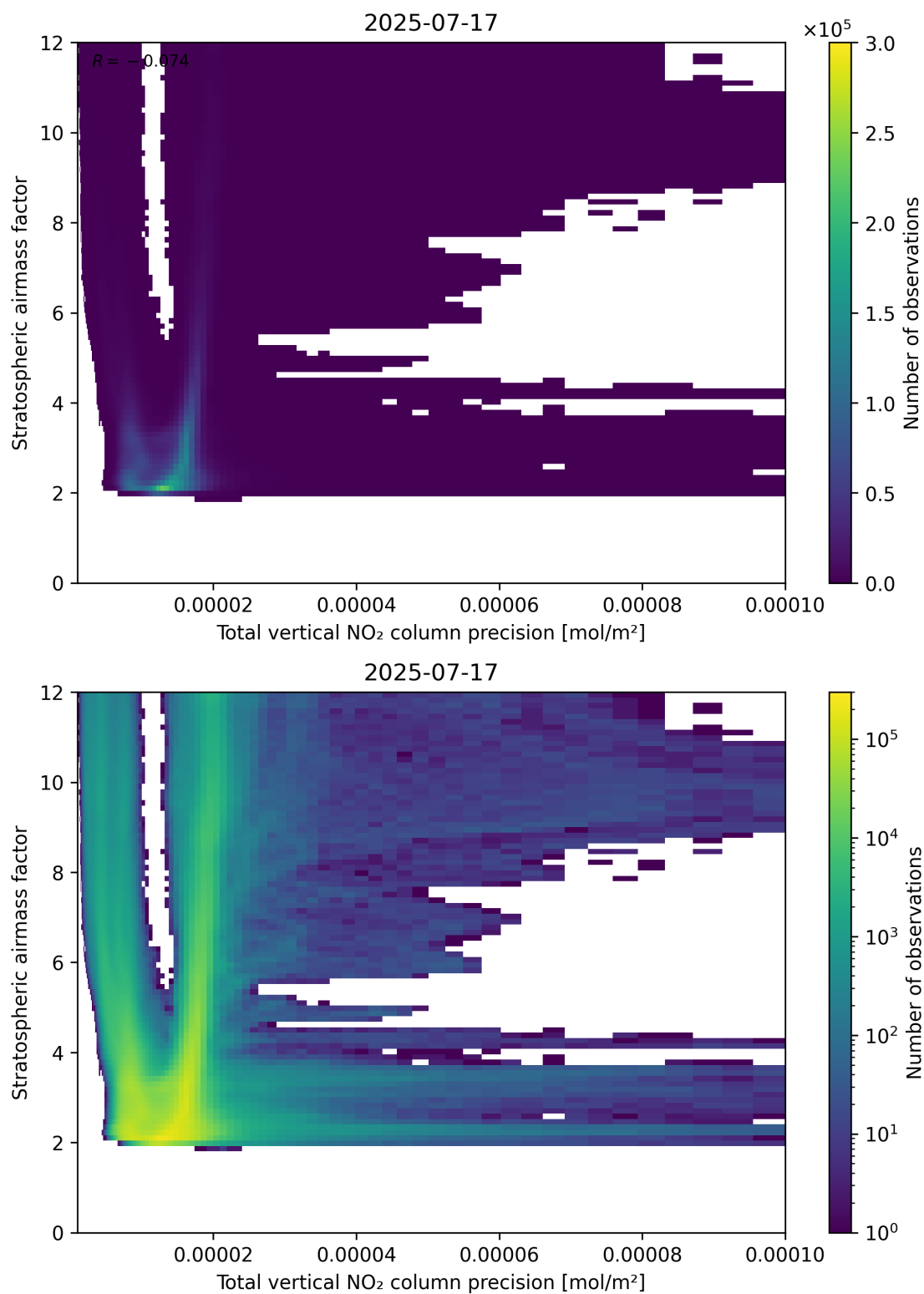
Figure 115: Scatter density plot of “Total vertical NO 2 column precision” against “Stratospheric air mass factor” for 2025-07-16 to 2025-07-18.
