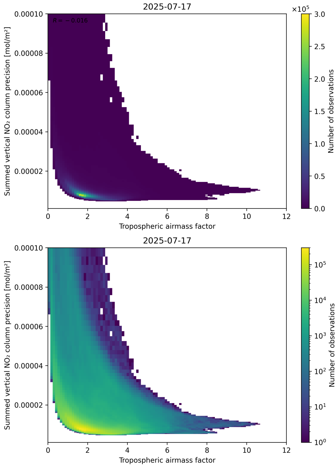
Figure 76: Scatter density plot of “Tropospheric airmass factor” against “Summed vertical NO 2 column precision” for 2025-07-16 to 2025-07-18.
