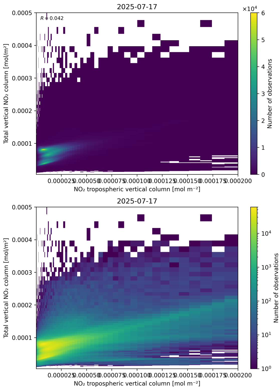
Figure 128: Scatter density plot of “NO 2 tropospheric vertical column” against “Total vertical NO 2 column” for 2025-07-16 to 2025-07-18.
