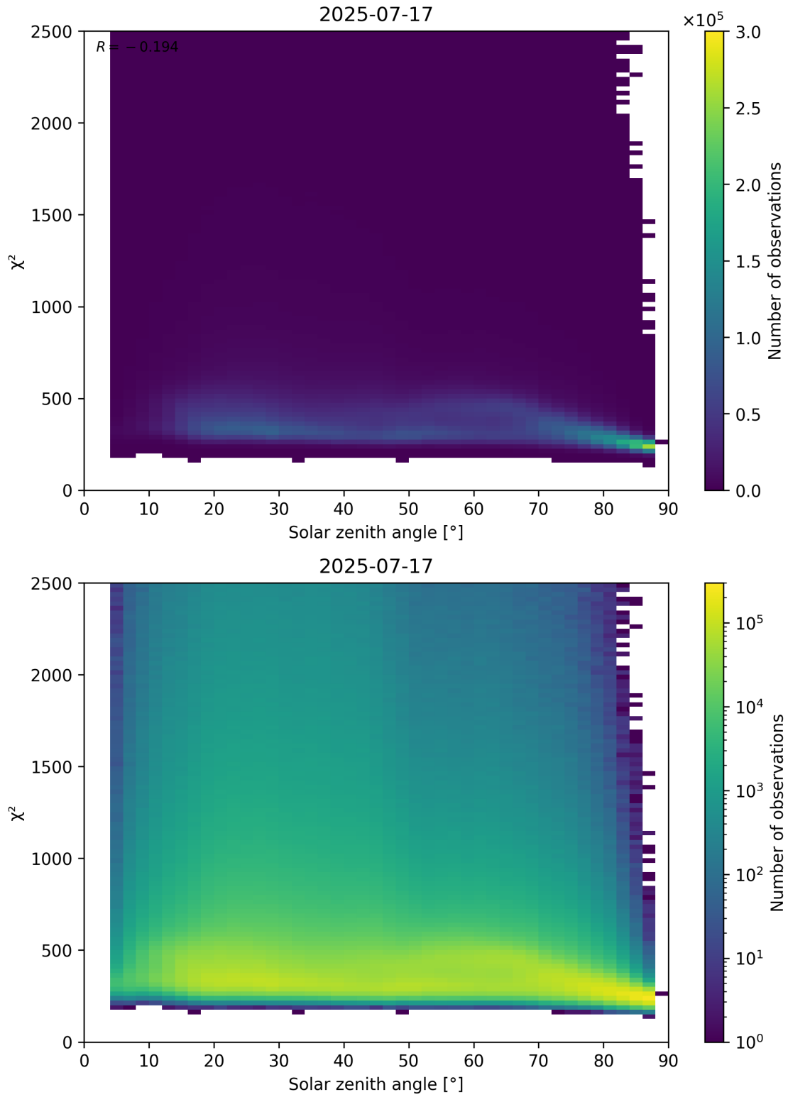
Figure 148: Scatter density plot of “Solar zenith angle” against “ \chi^2 ” for 2025-07-16 to 2025-07-18.
