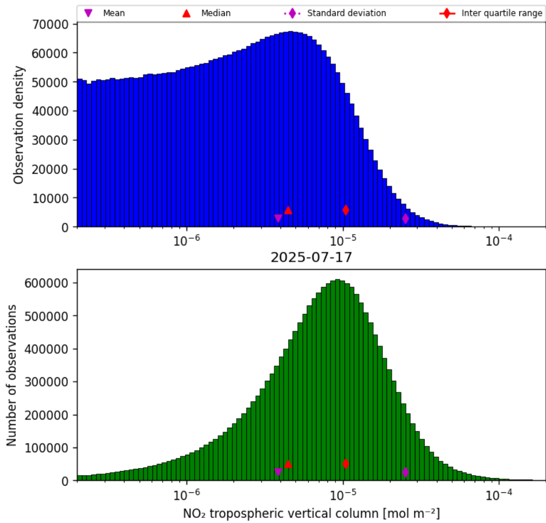
Figure 29: Histogram of “NO 2 tropospheric vertical column” for 2025-07-16 to 2025-07-18
