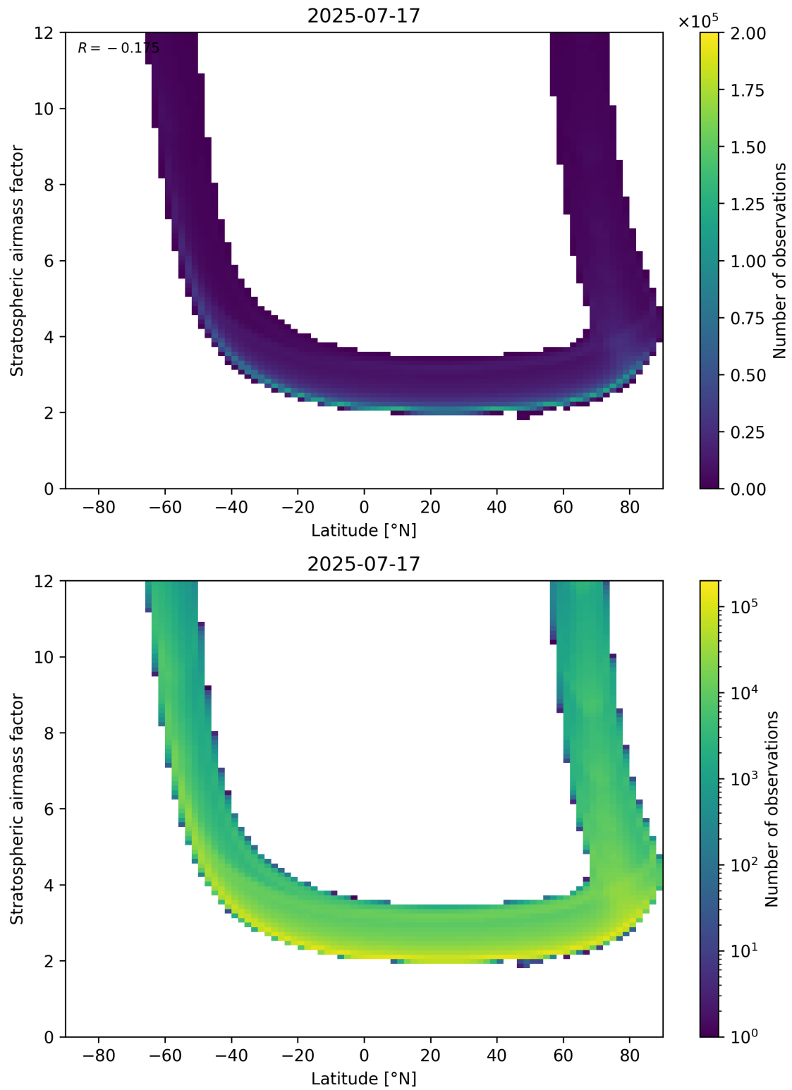
Figure 83: Scatter density plot of “Latitude” against “Stratospheric air mass factor” for 2025-07-16 to 2025-07-18.
