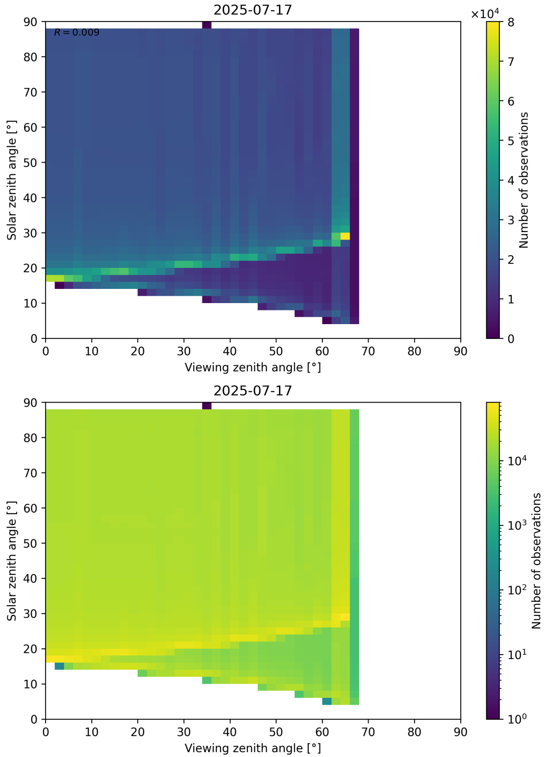
Figure 172: Scatter density plot of “Viewing zenith angle” against “Solar zenith angle” for 2025-07-16 to 2025-07-18.
