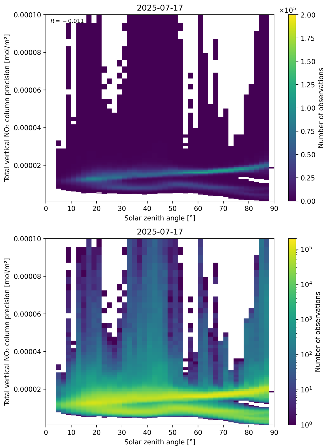
Figure 154: Scatter density plot of “Solar zenith angle” against “Total vertical NO 2 column precision” for 2025-07-16 to 2025-07-18.
