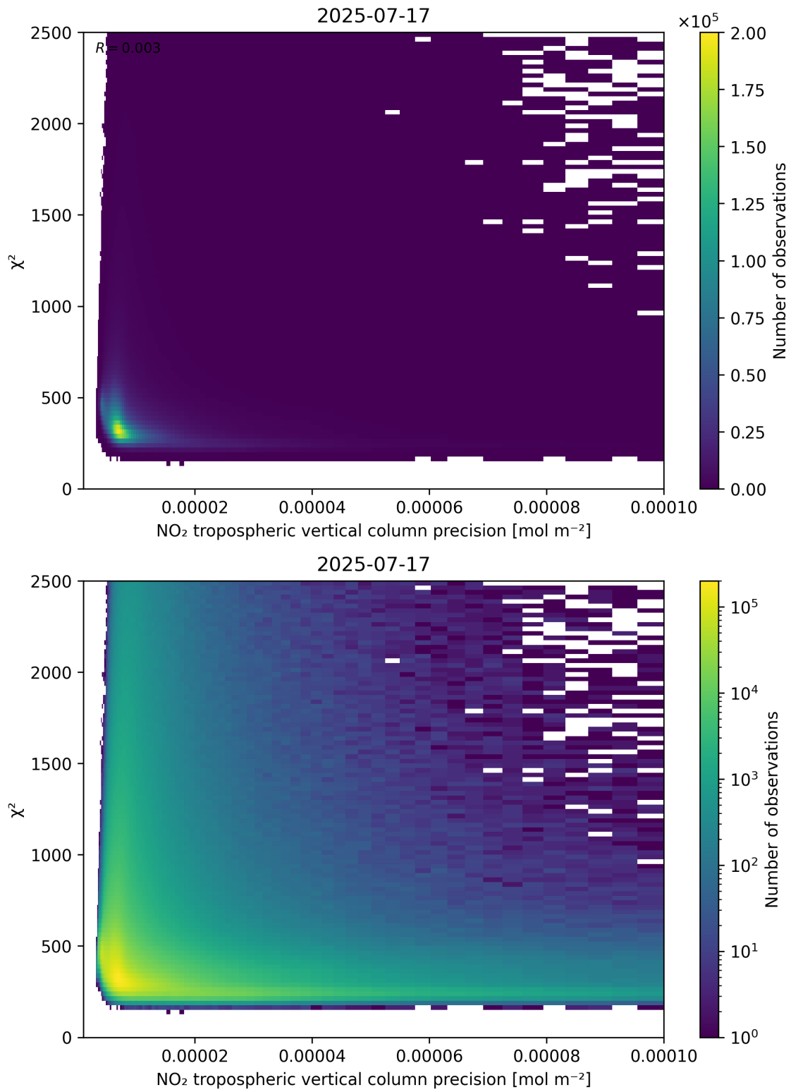
Figure 134: Scatter density plot of “NO 2 tropospheric vertical column precision” against “ \chi^2 ” for 2025-07-16 to 2025-07-18.
