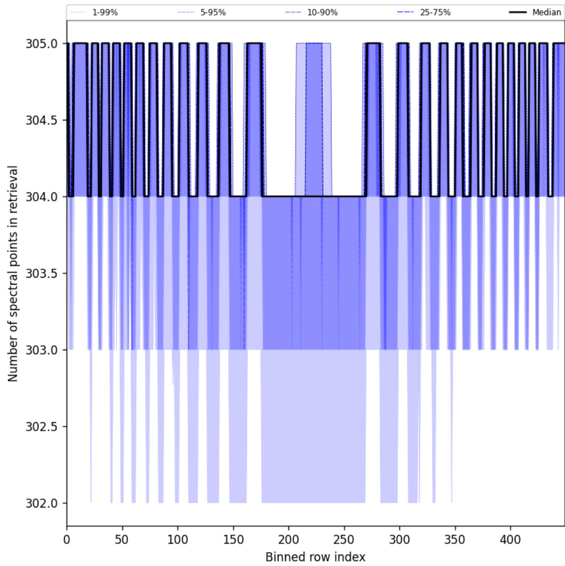
Figure 50: Along track statistics of “Number of spectral points in retrieval” for 2025-07-16 to 2025-07-18
