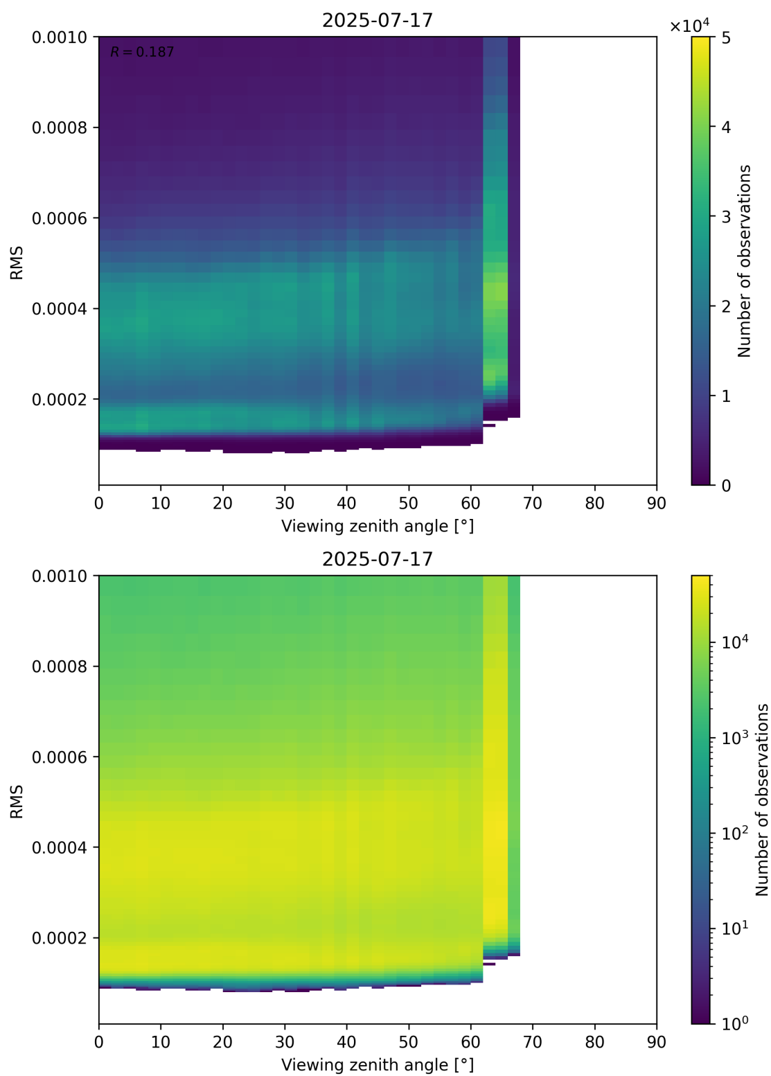
Figure 171: Scatter density plot of “Viewing zenith angle” against “RMS” for 2025-07-16 to 2025-07-18.
