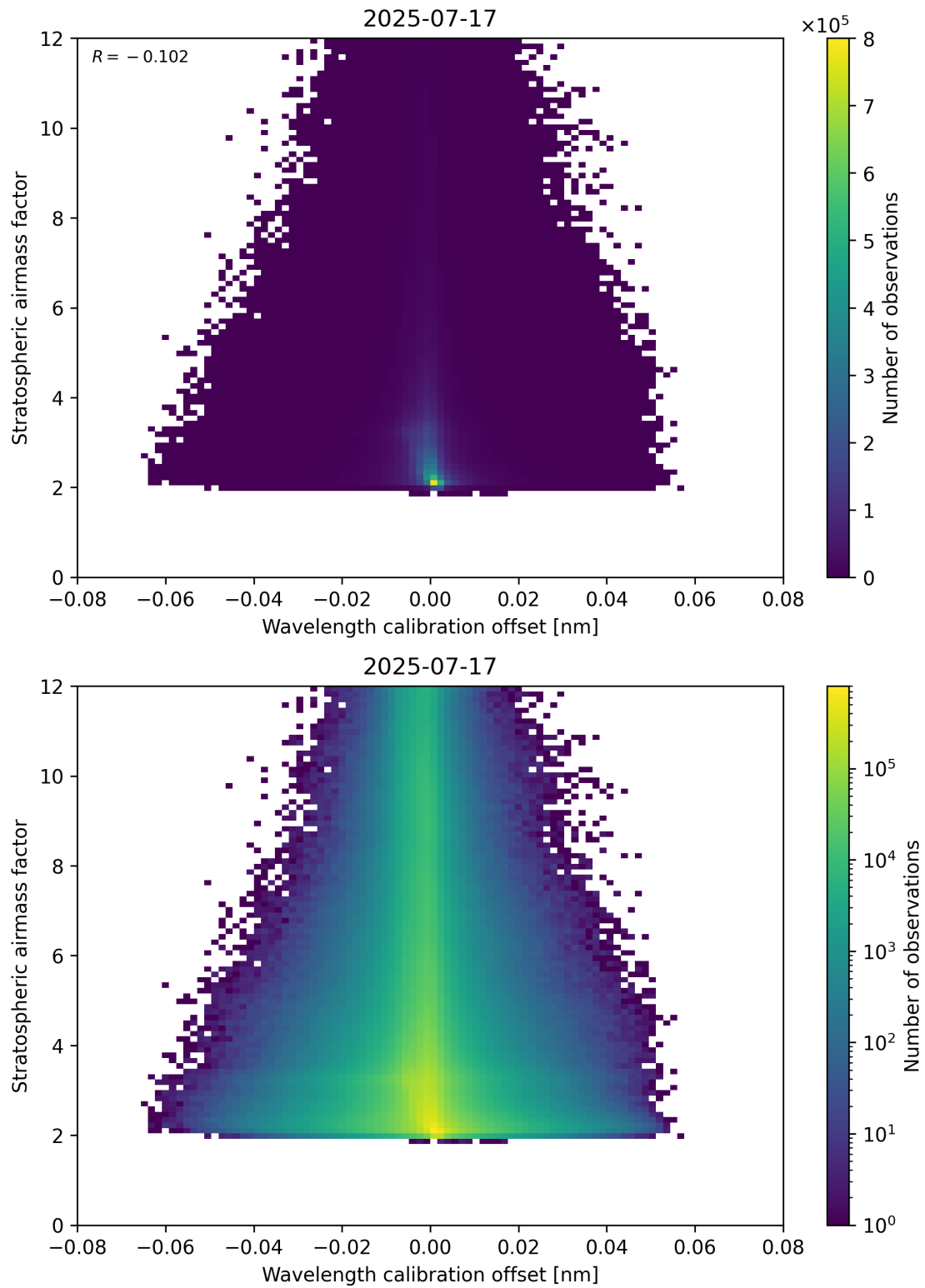
Figure 174: Scatter density plot of “Wavelength calibration offset” against “Stratospheric airmass factor” for 2025-07-16 to 2025-07-18.
