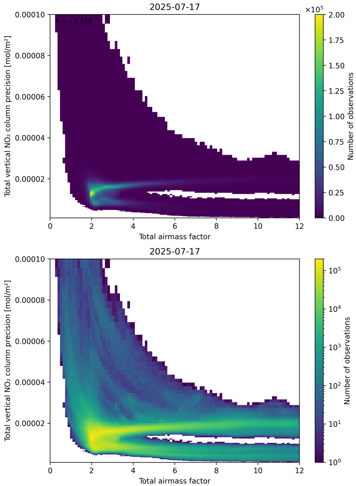
Figure 68: Scatter density plot of “Total airmass factor” against “Total vertical NO 2 column precision” for 2025-07-16 to 2025-07-18.
