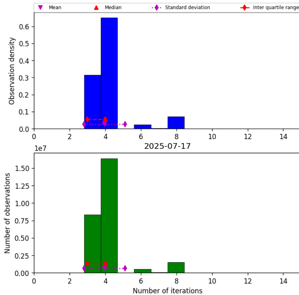
Figure 34: Histogram of “Number of iterations” for 2025-07-16 to 2025-07-18
