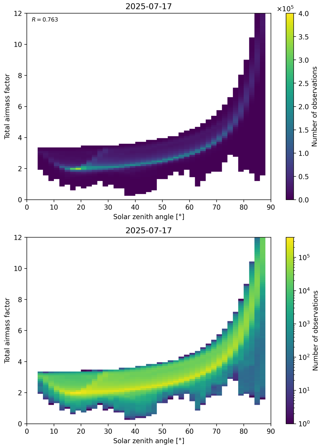
Figure 146: Scatter density plot of “Solar zenith angle” against “Total air mass factor” for 2025-07-16 to 2025-07-18.
