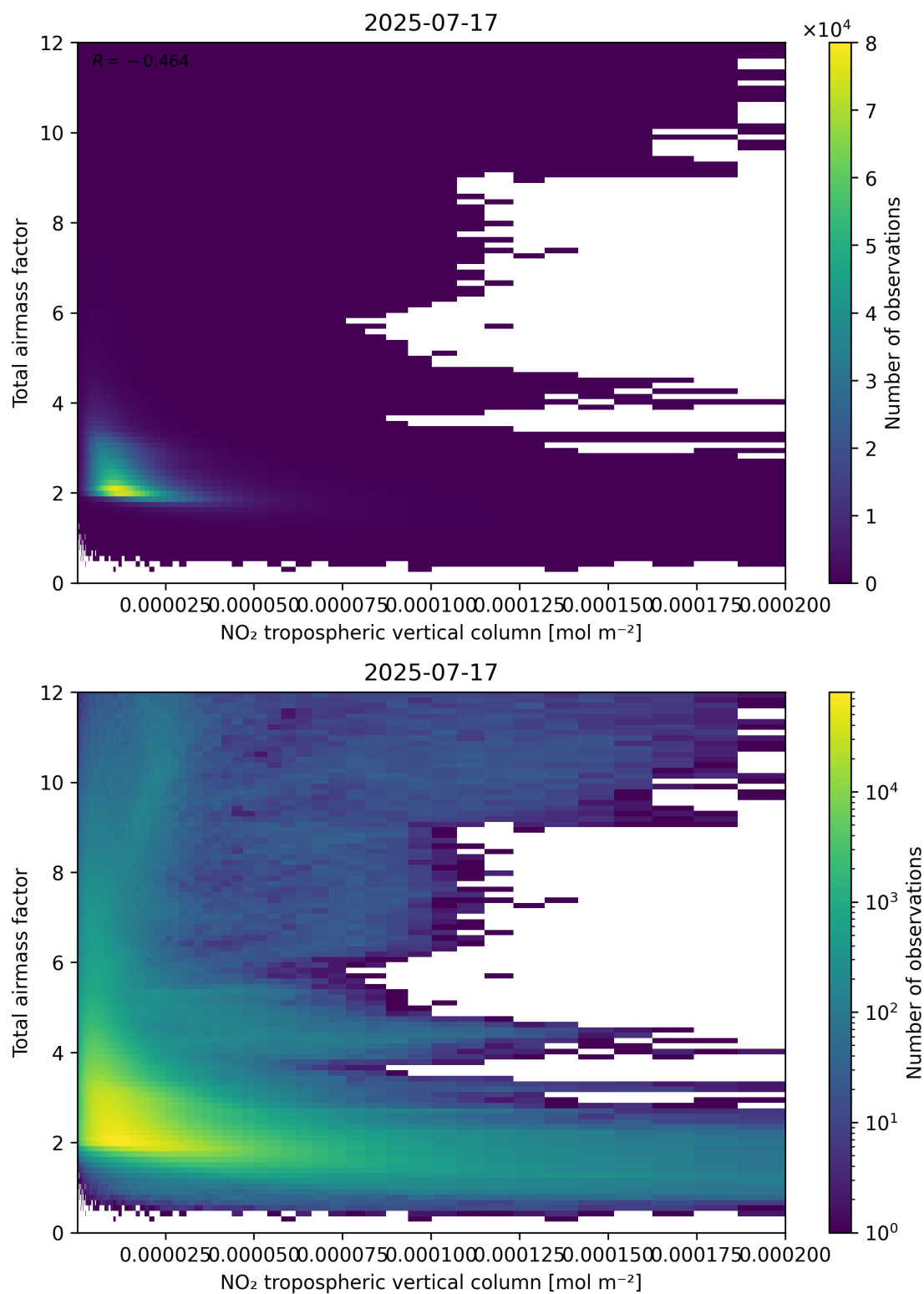
Figure 122: Scatter density plot of “NO 2 tropospheric vertical column” against “Total air mass factor” for 2025-07-16 to 2025-07-18.
