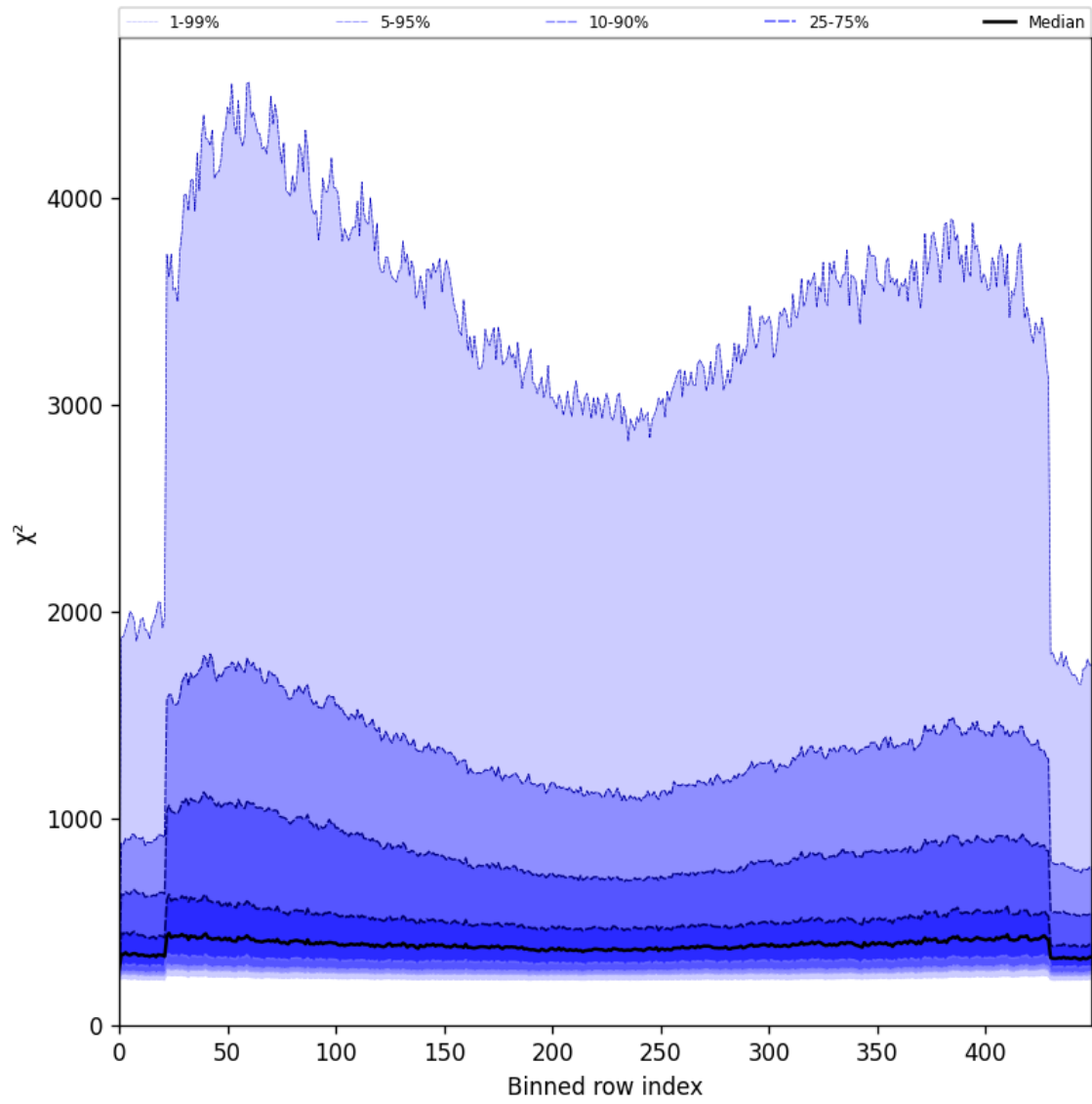
Figure 59: Along track statistics of “ \chi^2 ” for 2025-07-16 to 2025-07-18
