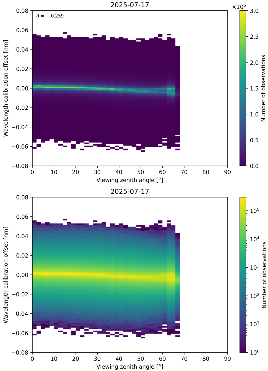
Figure 173: Scatter density plot of “Viewing zenith angle” against “Wavelength calibration offset” for 2025-07-16 to 2025-07-18.
