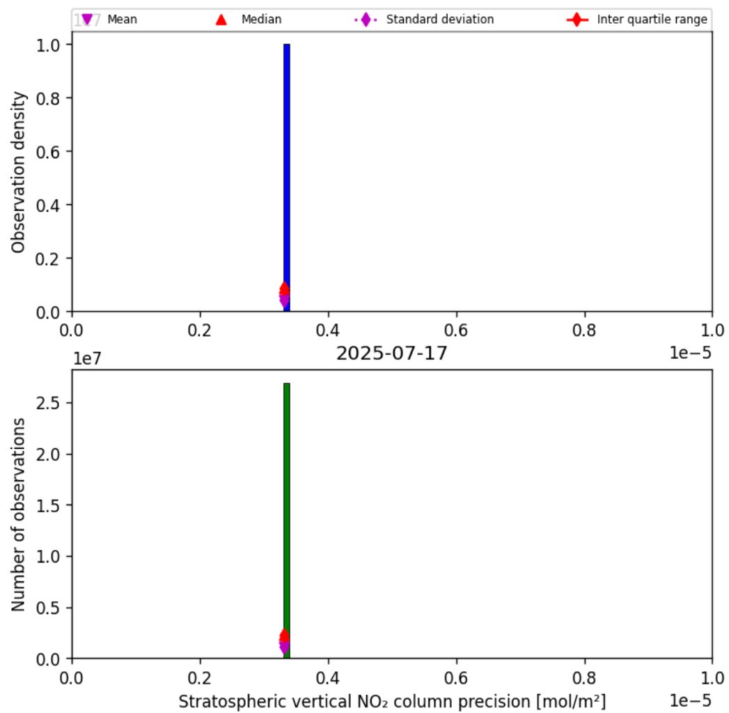
Figure 37: Histogram of “Stratospheric vertical NO 2 column precision” for 2025-07-16 to 2025-07-18
