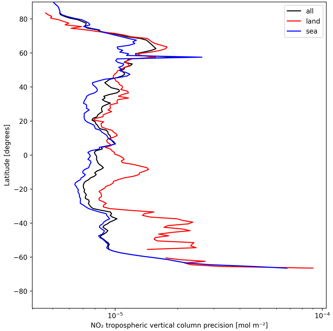
Figure 13: Zonal average of "NO 2 tropospheric vertical column precision" for 2025-07-16 to 2025-07-18.
