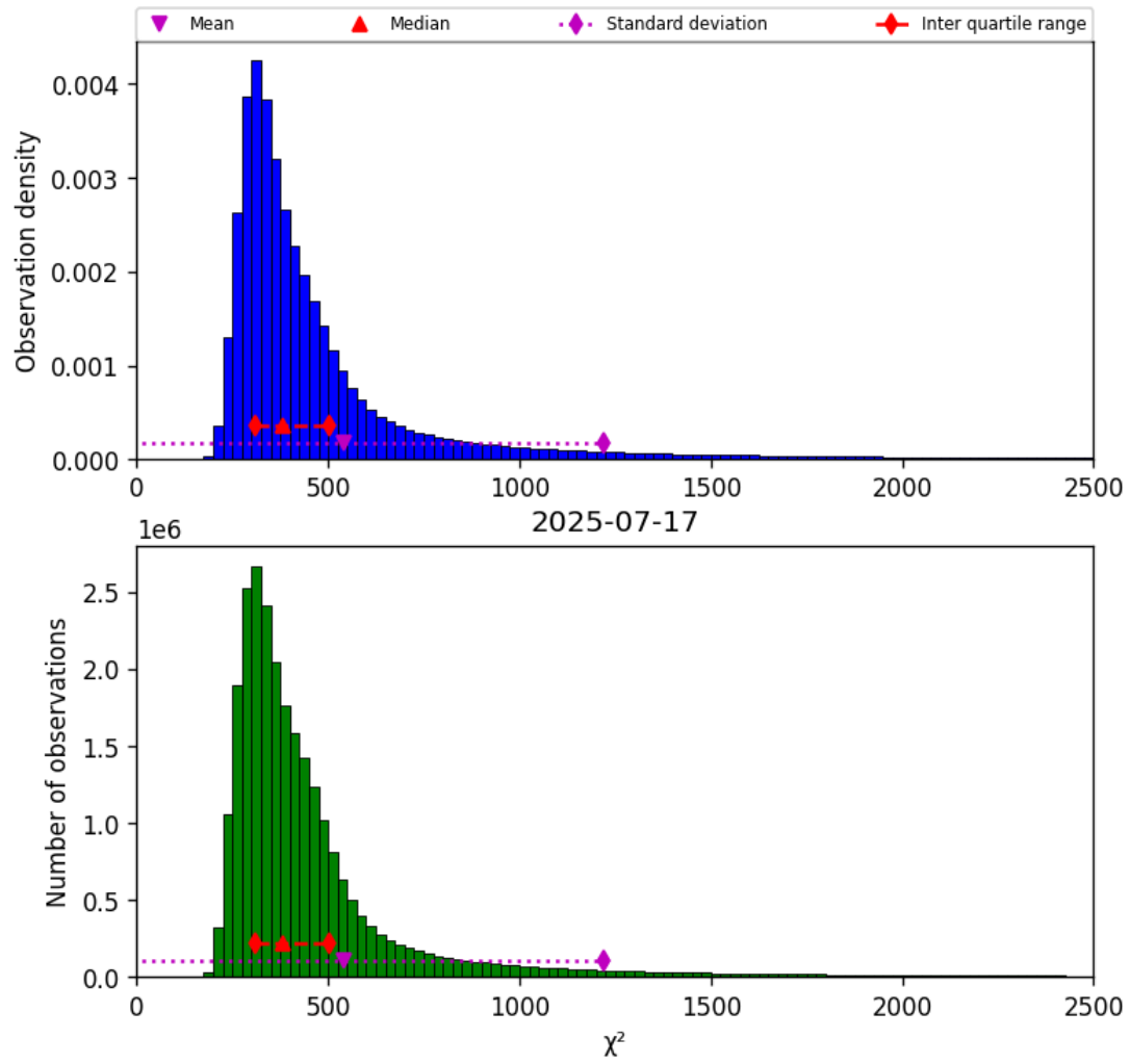
Figure 42: Histogram of “ \chi^2 ” for 2025-07-16 to 2025-07-18
