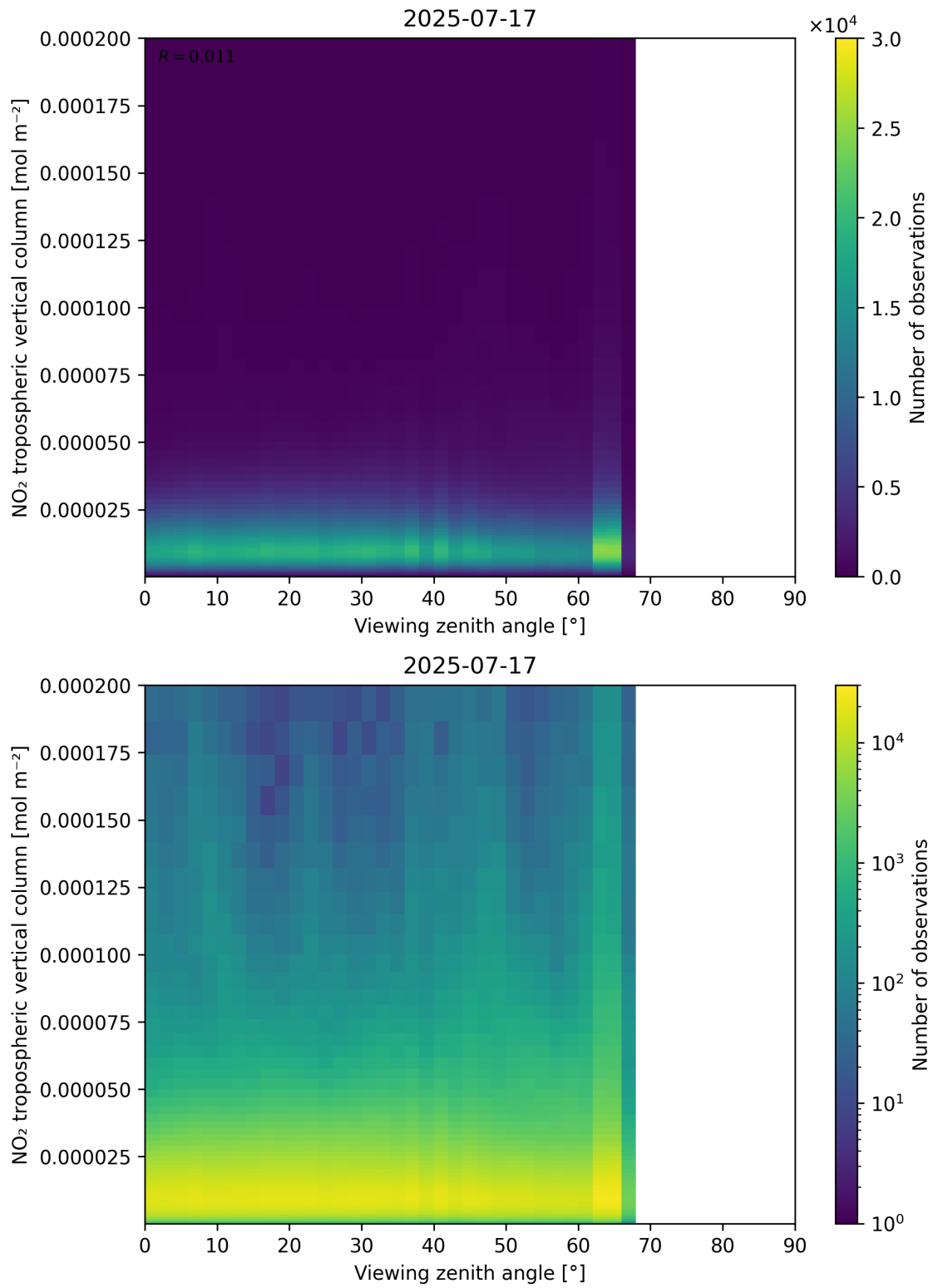
Figure 169: Scatter density plot of “Viewing zenith angle” against “NO 2 tropospheric vertical column” for 2025-07-16 to 2025-07-18.
