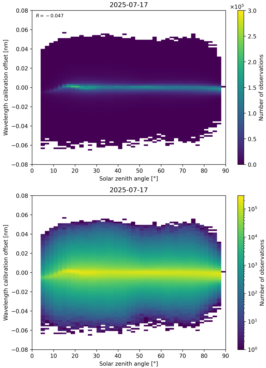
Figure 158: Scatter density plot of “Solar zenith angle” against “Wavelength calibration offset” for 2025-07-16 to 2025-07-18.
