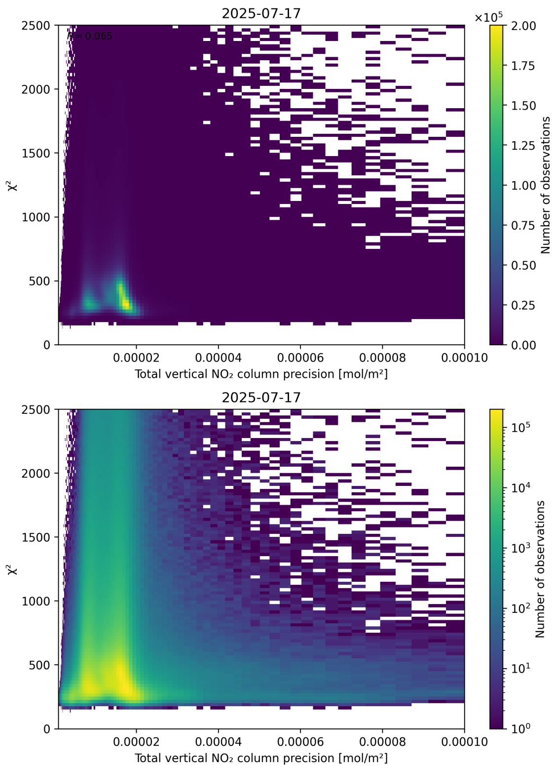
Figure 116: Scatter density plot of “Total vertical NO 2 column precision” against “ \chi^2 ” for 2025-07-16 to 2025-07-18.
