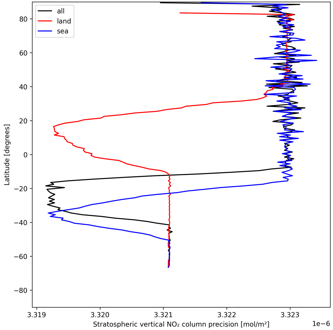
Figure 20: Zonal average of “Stratospheric vertical NO 2 column precision” for 2025-07-16 to 2025-07-18.
