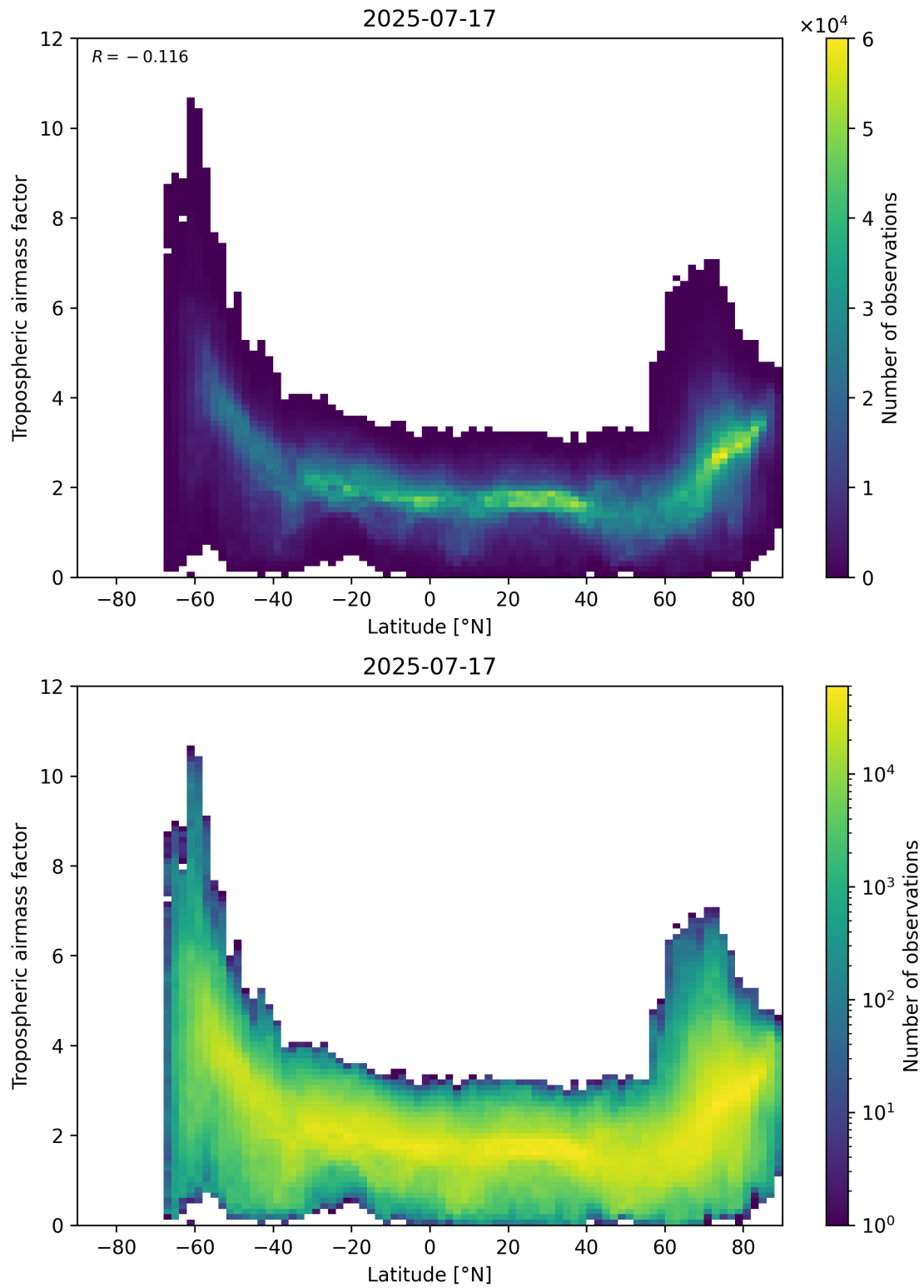
Figure 85: Scatter density plot of “Latitude” against “Tropospheric air mass factor” for 2025-07-16 to 2025-07-18.
