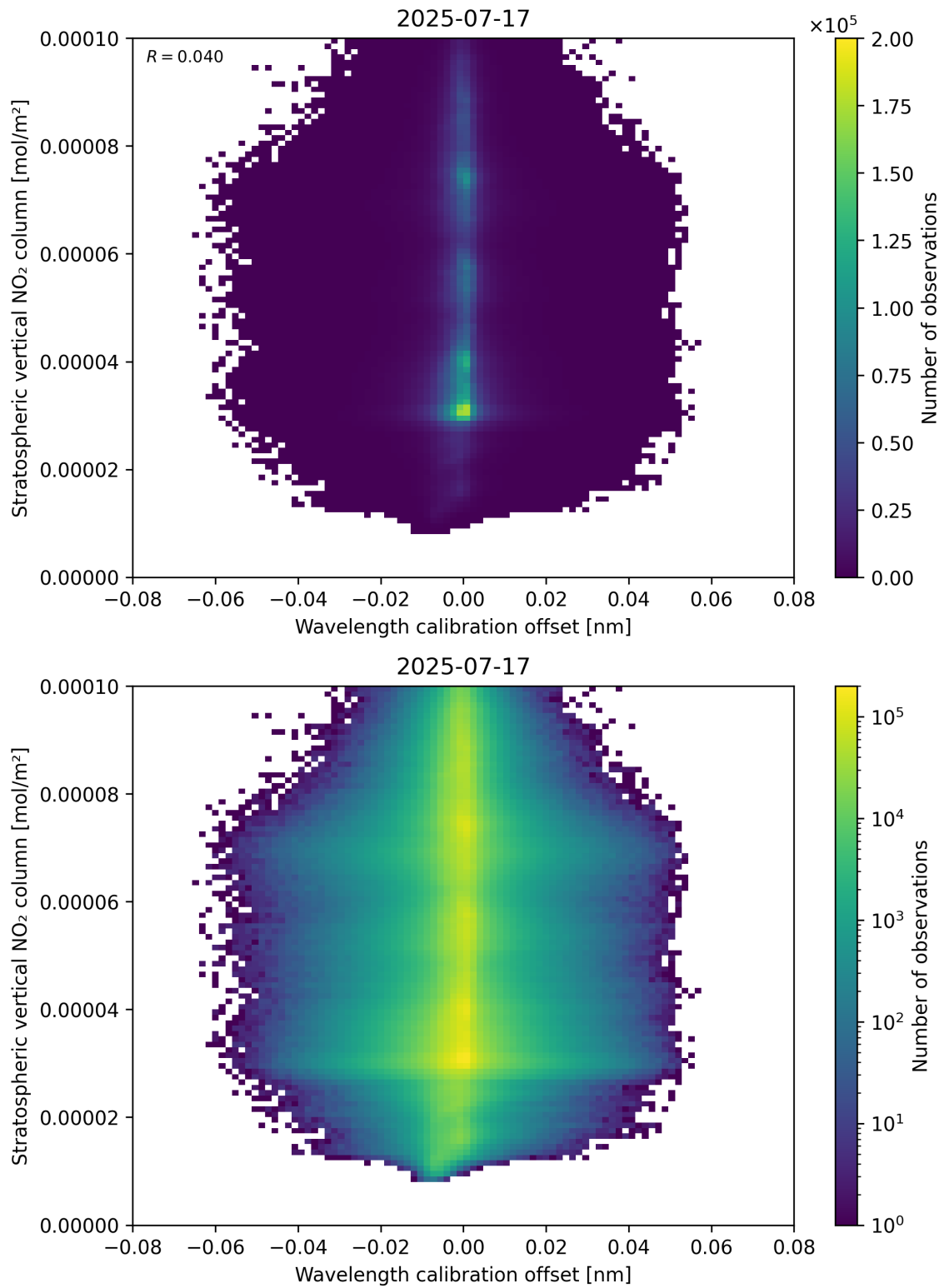
Figure 176: Scatter density plot of “Wavelength calibration offset” against “Stratospheric vertical NO 2 column” for 2025-07-16 to 2025-07-18.
