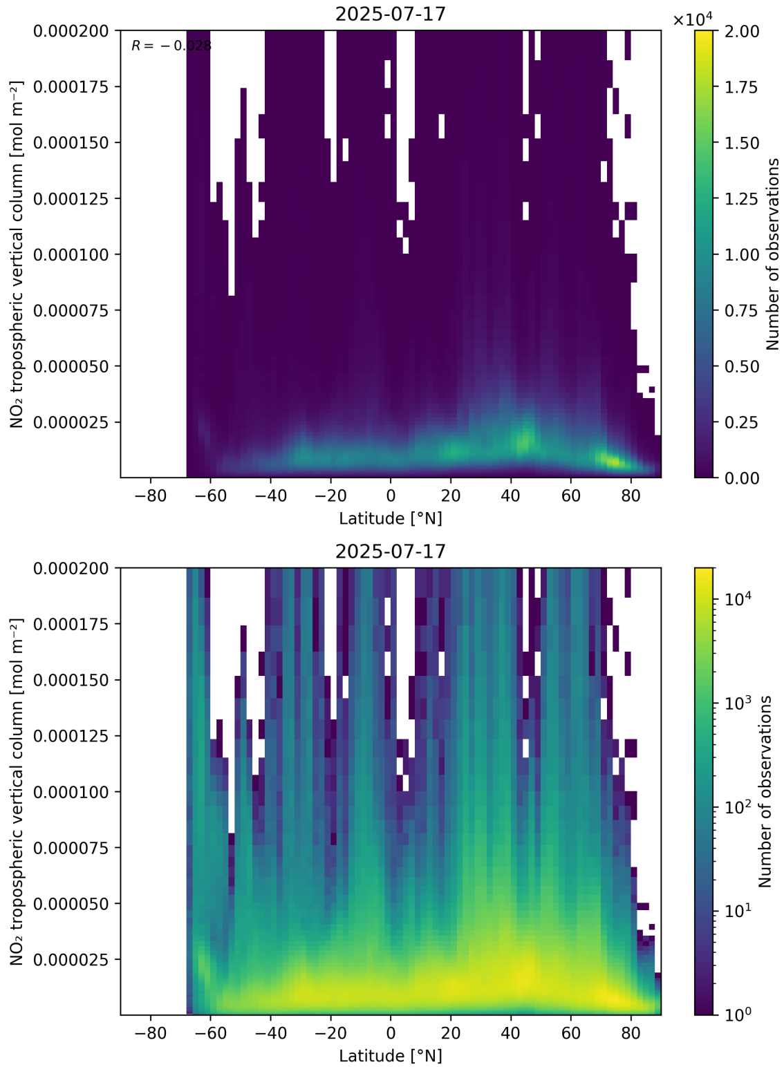
Figure 92: Scatter density plot of “Latitude” against “NO 2 tropospheric vertical column” for 2025-07-16 to 2025-07-18.
