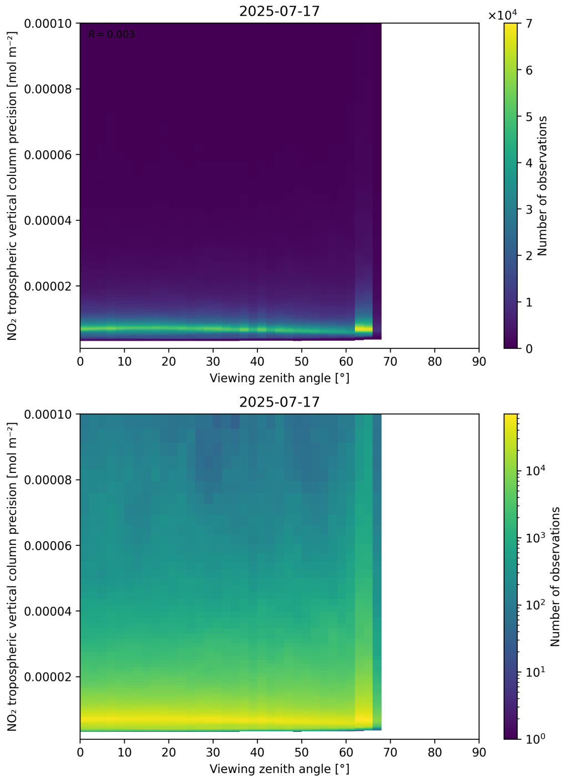
Figure 170: Scatter density plot of “Viewing zenith angle” against “NO 2 tropospheric vertical column precision” for 2025-07-16 to 2025-07-18.
