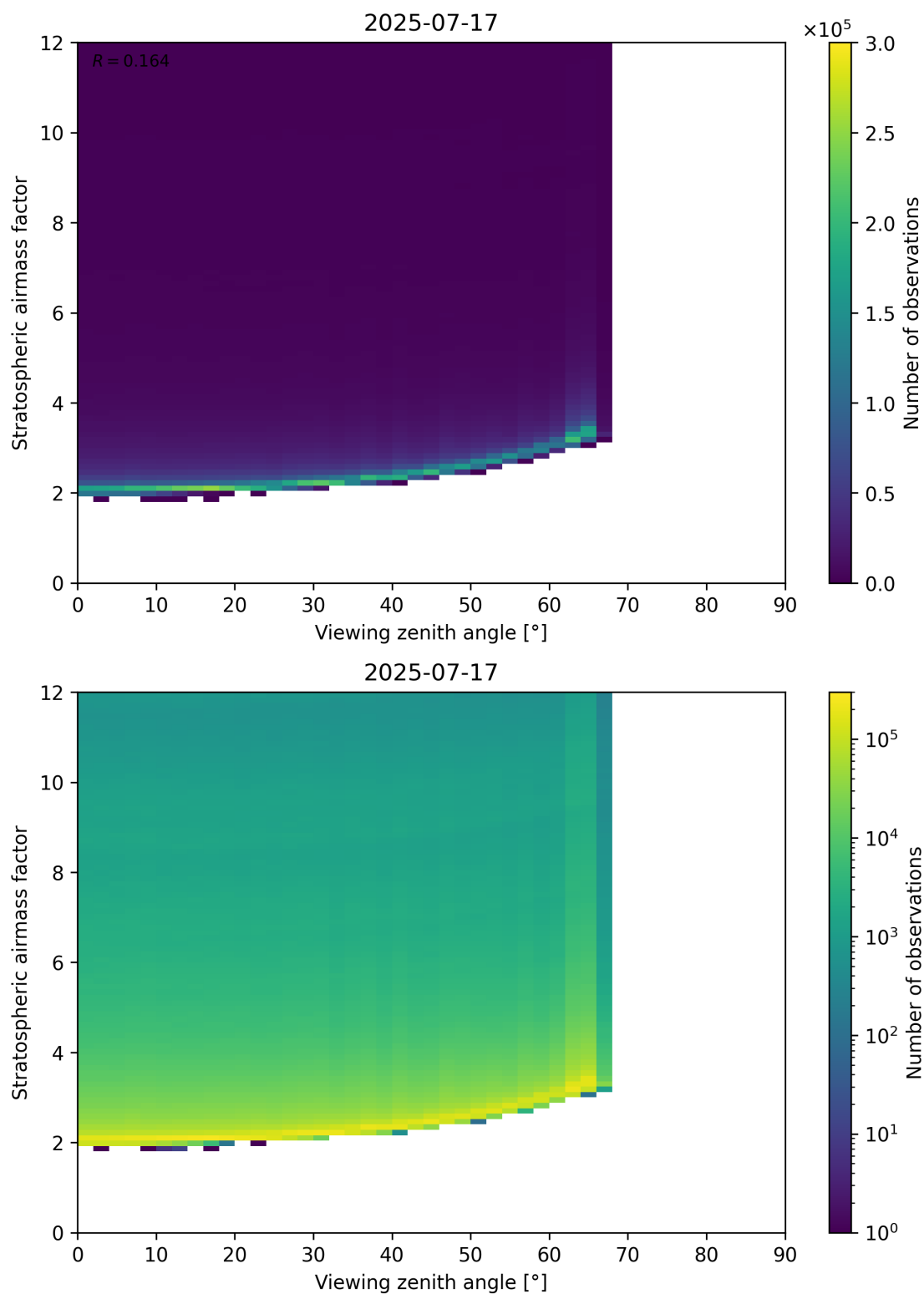
Figure 159: Scatter density plot of “Viewing zenith angle” against “Stratospheric airmass factor” for 2025-07-16 to 2025-07-18.
