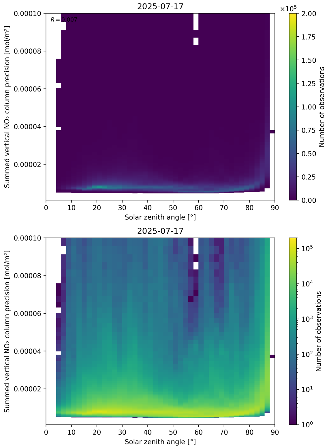
Figure 152: Scatter density plot of “Solar zenith angle” against “Summed vertical NO 2 column precision” for 2025-07-16 to 2025-07-18.
