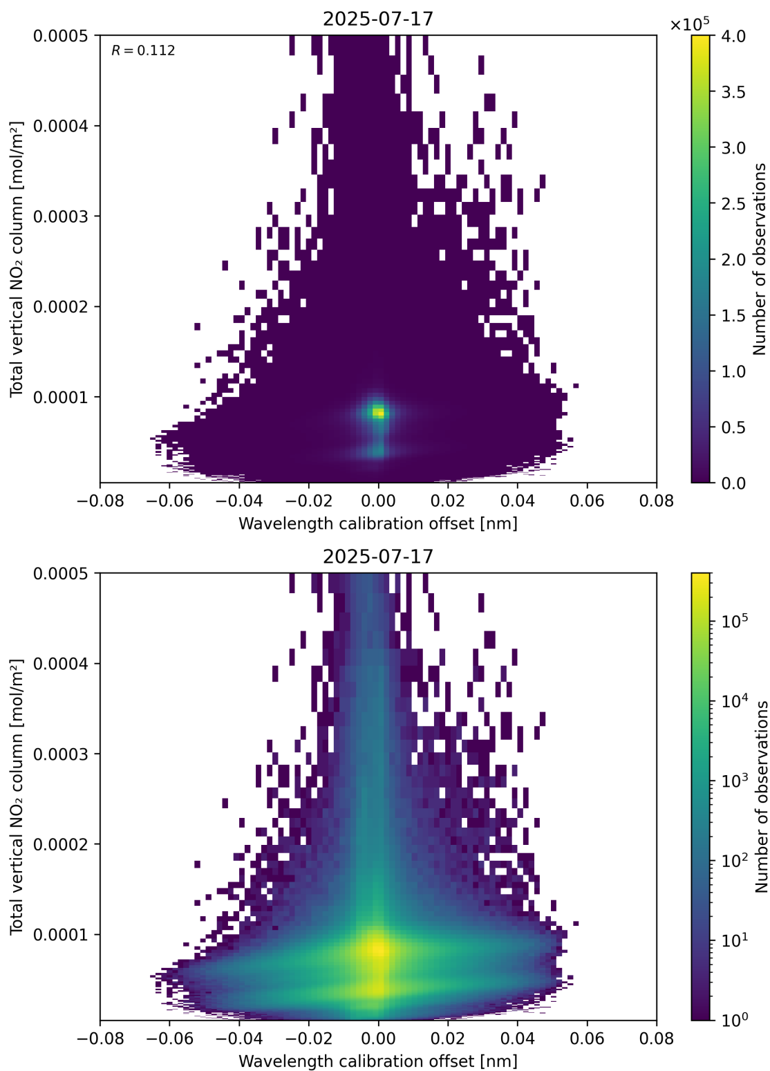
Figure 179: Scatter density plot of “Wavelength calibration offset” against “Total vertical NO 2 column” for 2025-07-16 to 2025-07-18.
