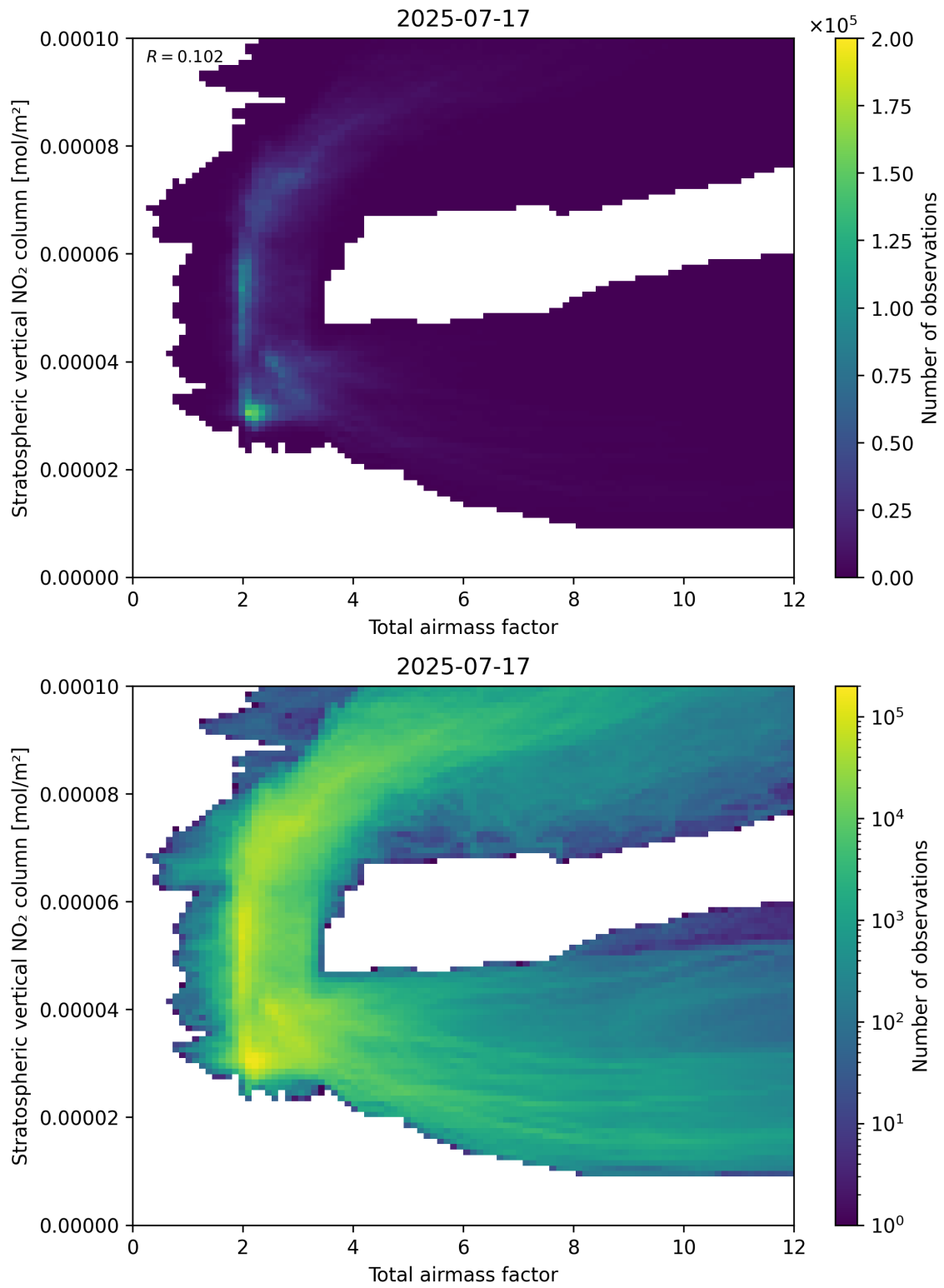
Figure 64: Scatter density plot of “Total airmass factor” against “Stratospheric vertical NO 2 column” for 2025-07-16 to 2025-07-18.
