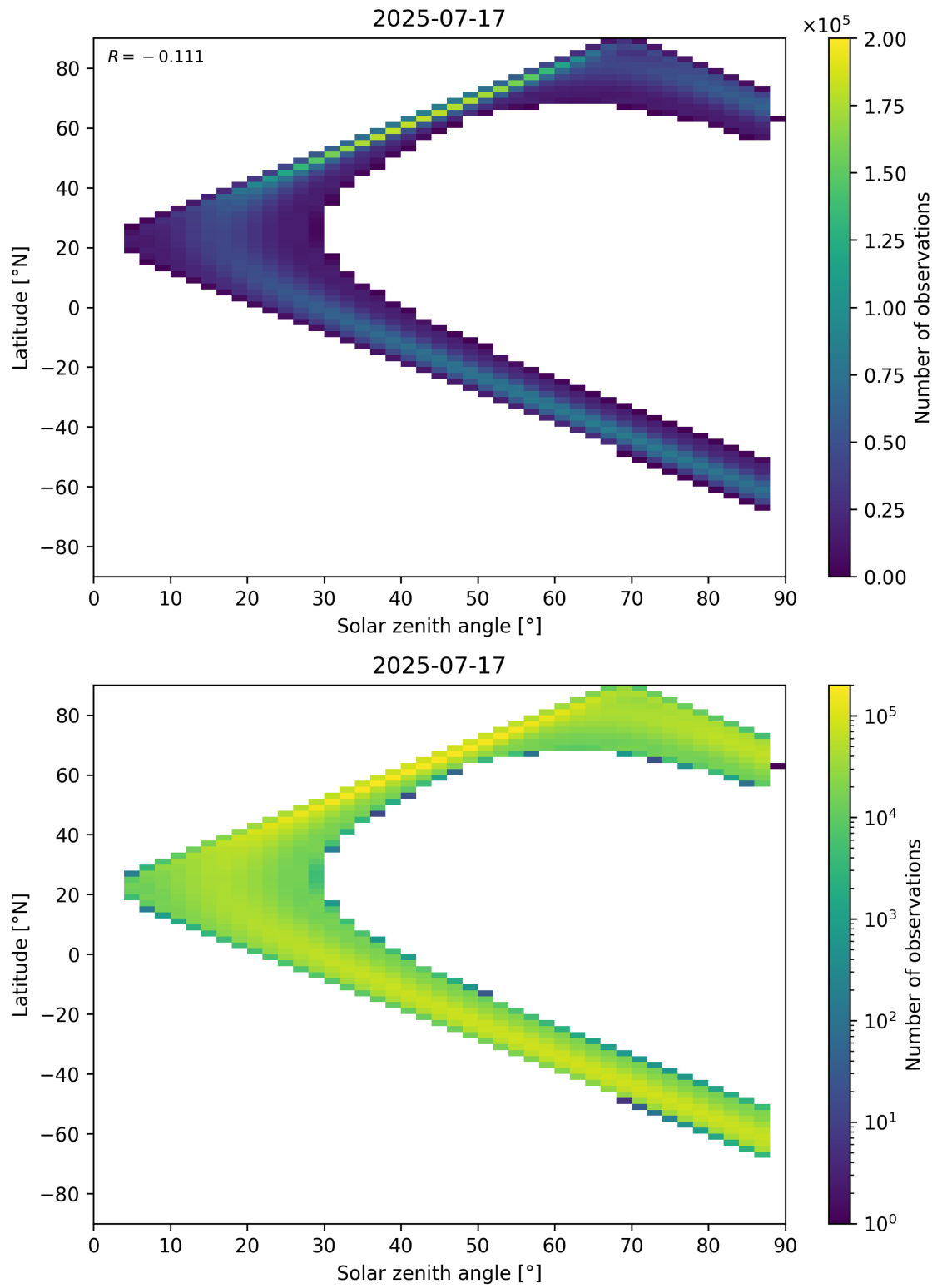
Figure 149: Scatter density plot of “Solar zenith angle” against “Latitude” for 2025-07-16 to 2025-07-18.
