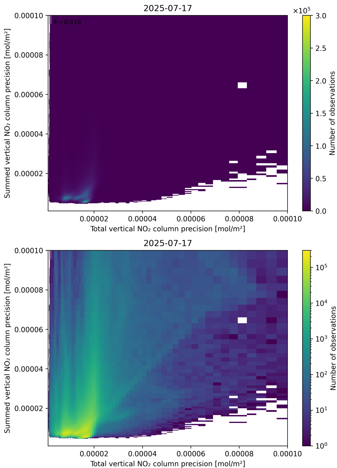
Figure 118: Scatter density plot of “Total vertical NO 2 column precision” against “Summed vertical NO 2 column precision” for 2025-07-16 to 2025-07-18.
