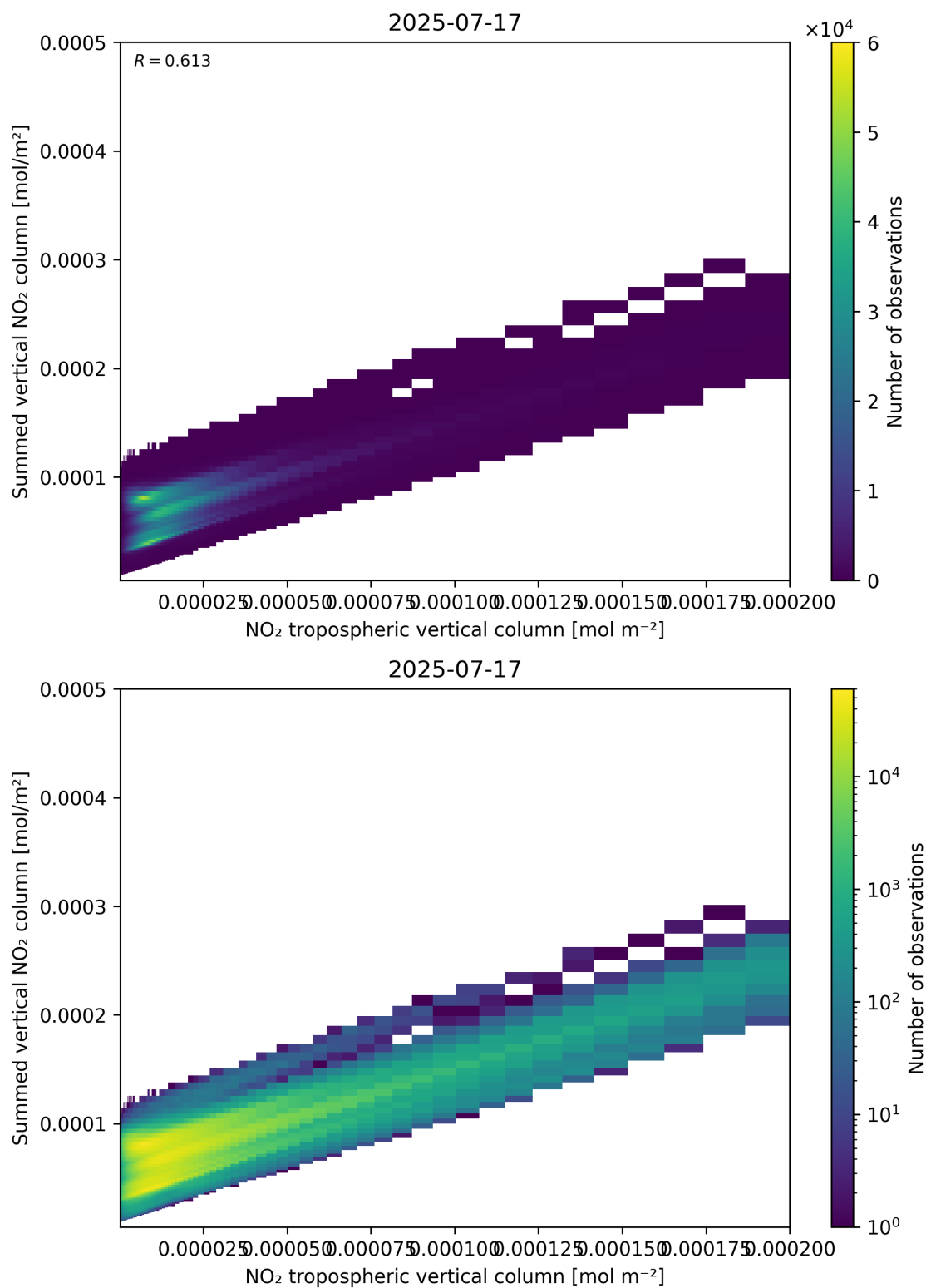
Figure 126: Scatter density plot of “NO 2 tropospheric vertical column” against “Summed vertical NO 2 column” for 2025-07-16 to 2025-07-18.
