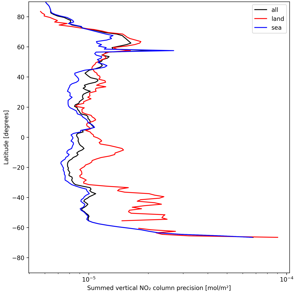
Figure 24: Zonal average of “Summed vertical NO 2 column precision” for 2025-07-16 to 2025-07-18.
