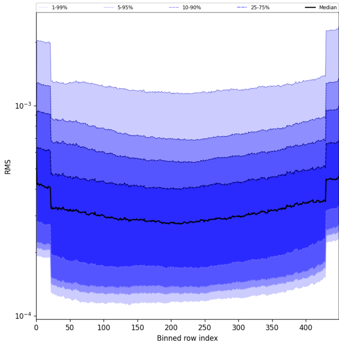
Figure 60: Along track statistics of “RMS” for 2025-07-16 to 2025-07-18
