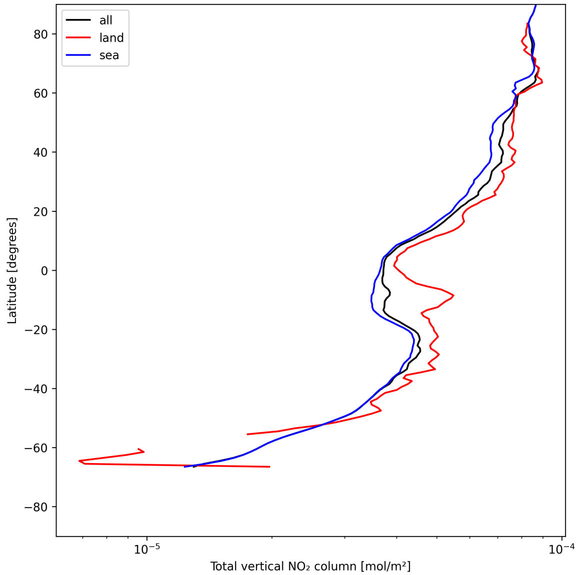
Figure 21: Zonal average of “Total vertical NO 2 column” for 2025-07-16 to 2025-07-18.
