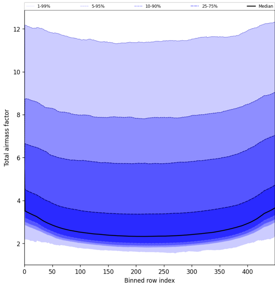
Figure 49: Along track statistics of “Total airmass factor” for 2025-07-16 to 2025-07-18
