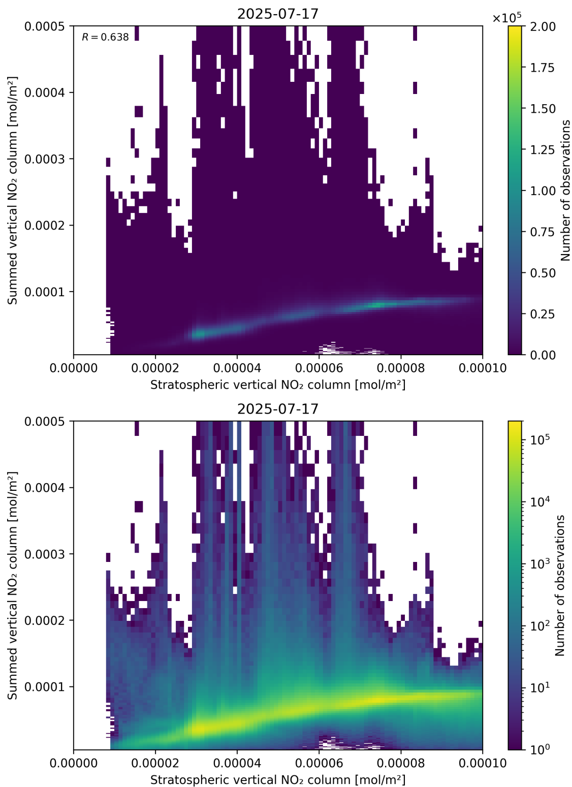
Figure 98: Scatter density plot of “Stratospheric vertical NO 2 column” against “Summed vertical NO 2 column” for 2025-07-16 to 2025-07-18.
