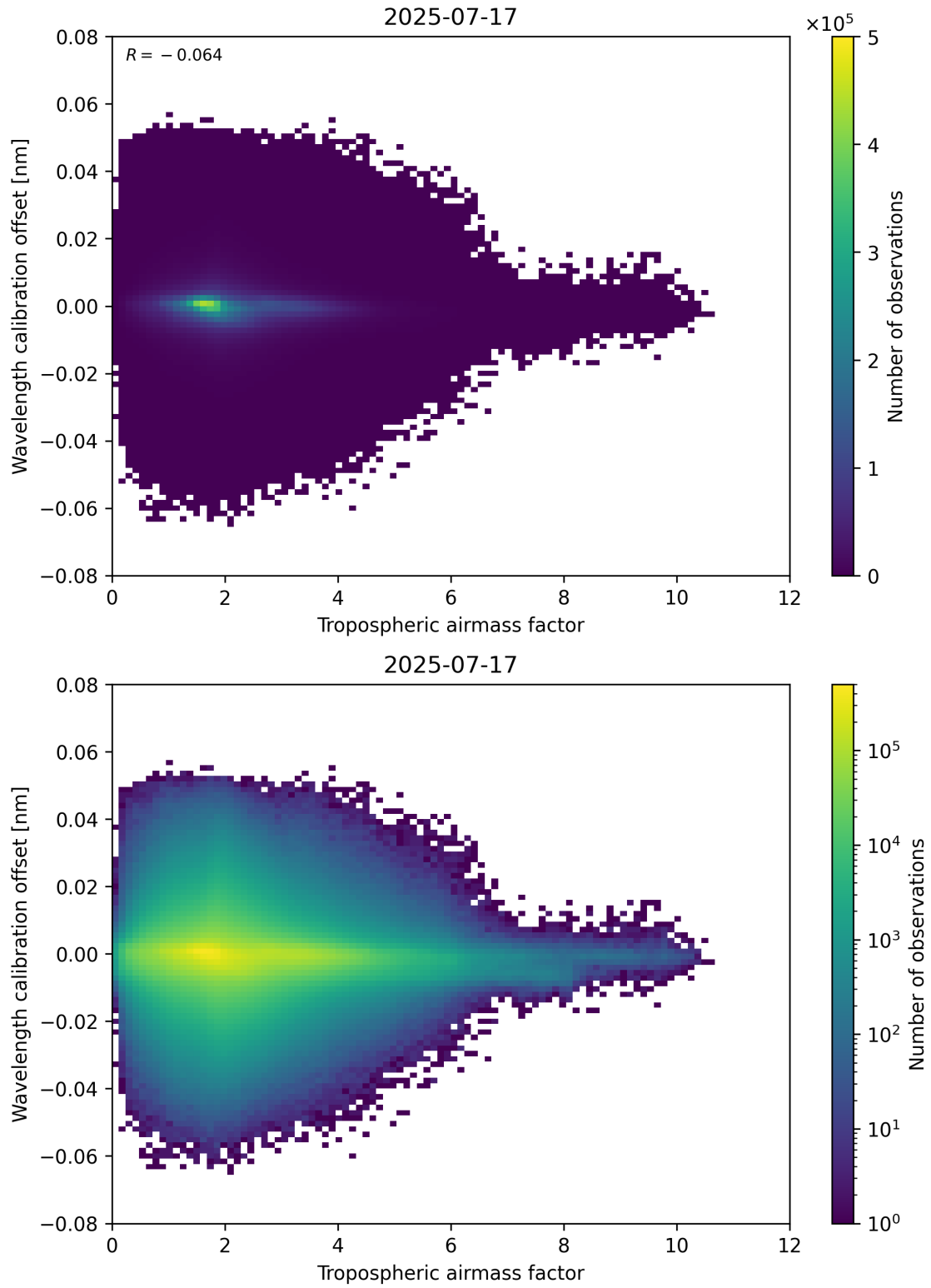
Figure 80: Scatter density plot of “Tropospheric airmass factor” against “Wavelength calibration offset” for 2025-07-16 to 2025-07-18.
