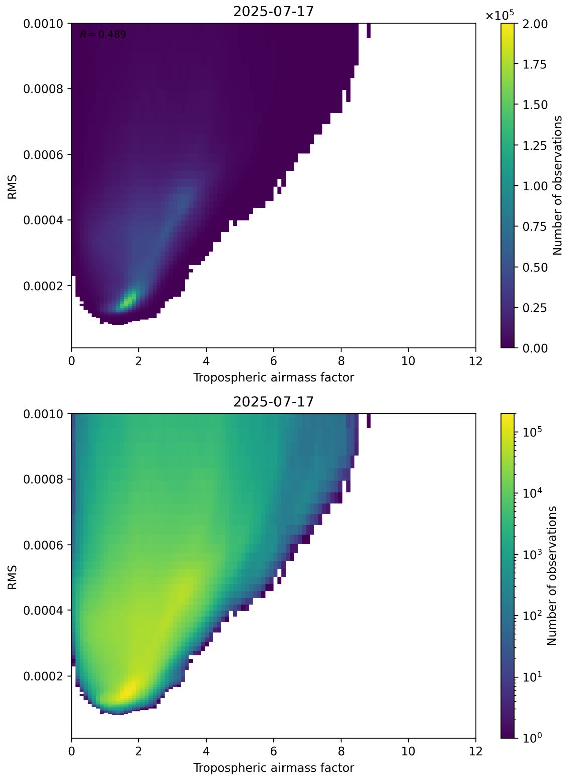
Figure 79: Scatter density plot of “Tropospheric airmass factor” against “RMS” for 2025-07-16 to 2025-07-18.
