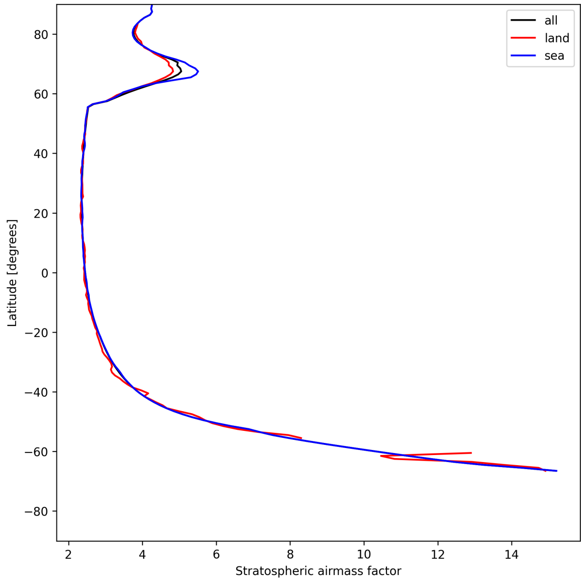
Figure 27: Zonal average of “Stratospheric airmass factor” for 2025-07-16 to 2025-07-18.
