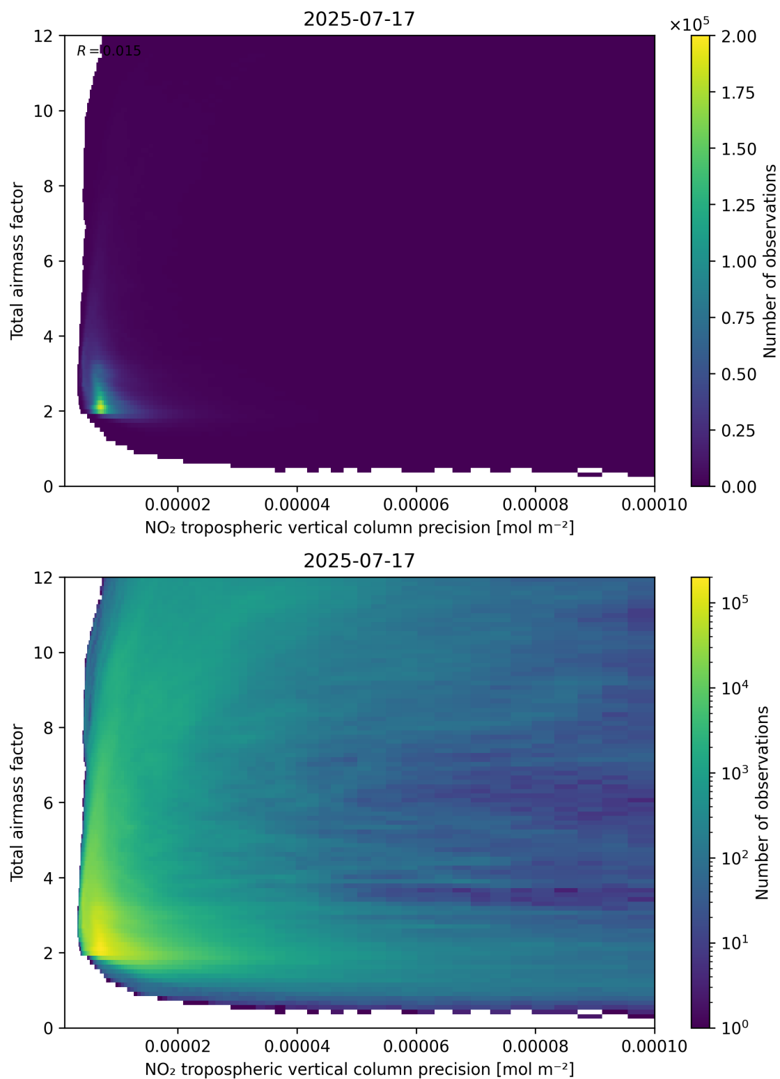
Figure 132: Scatter density plot of “NO 2 tropospheric vertical column precision” against “Total air mass factor” for 2025-07-16 to 2025-07-18.
