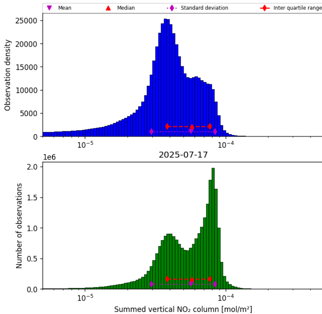
Figure 40: Histogram of “Summed vertical NO 2 column” for 2025-07-16 to 2025-07-18
