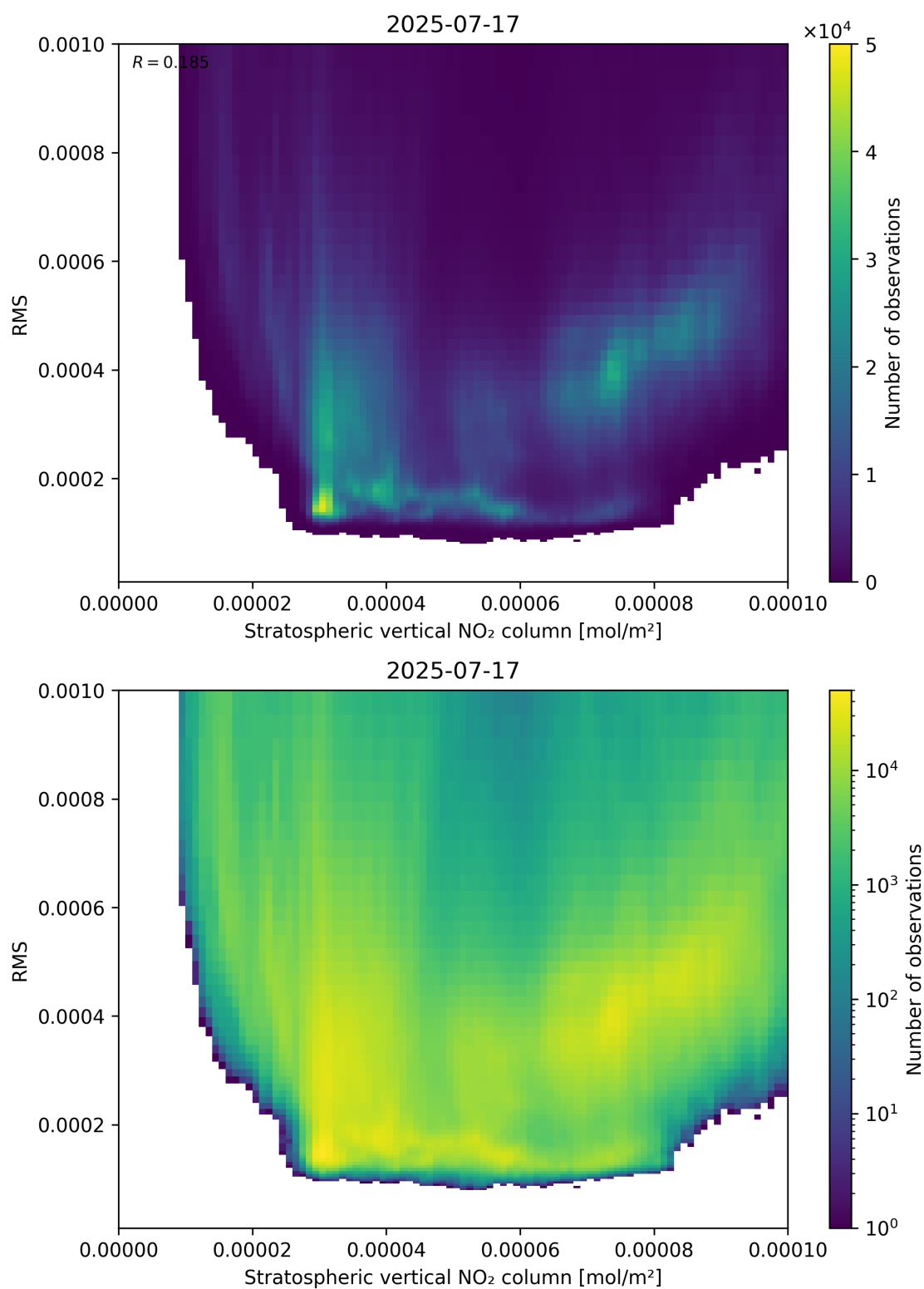
Figure 102: Scatter density plot of “Stratospheric vertical NO 2 column” against “RMS” for 2025-07-16 to 2025-07-18.
