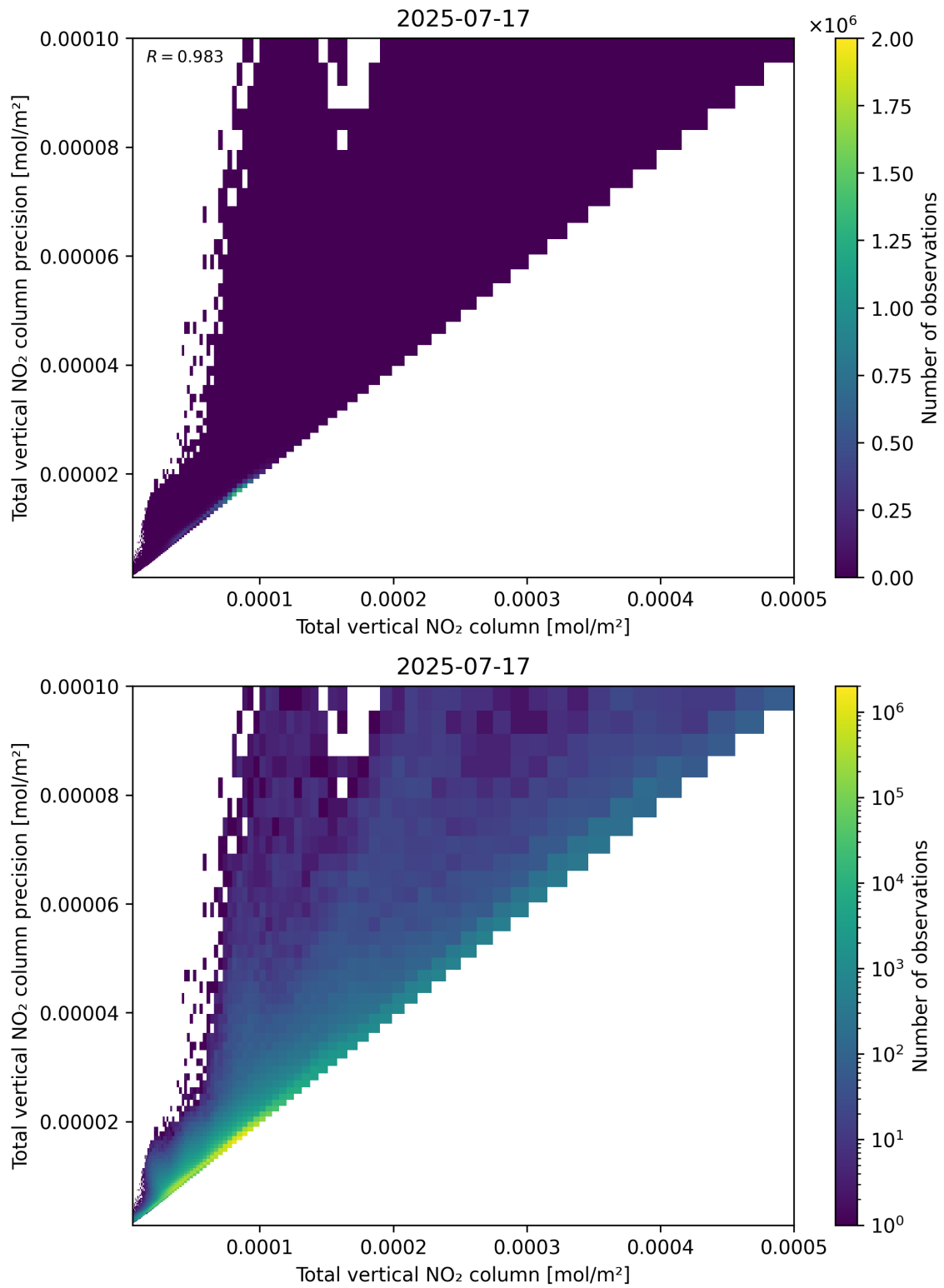
Figure 114: Scatter density plot of “Total vertical NO 2 column” against “Total vertical NO 2 column precision” for 2025-07-16 to 2025-07-18.
