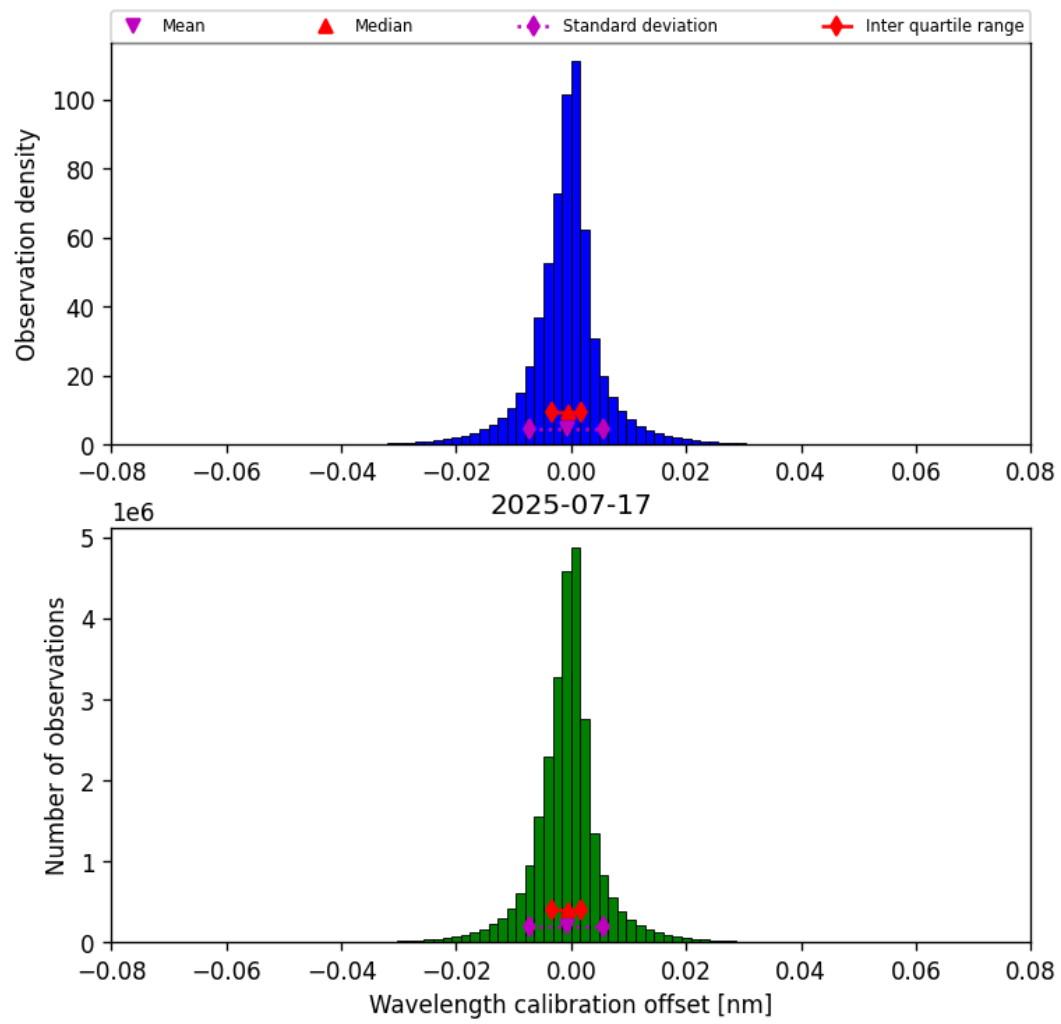
Figure 35: Histogram of “Wavelength calibration offset” for 2025-07-16 to 2025-07-18
