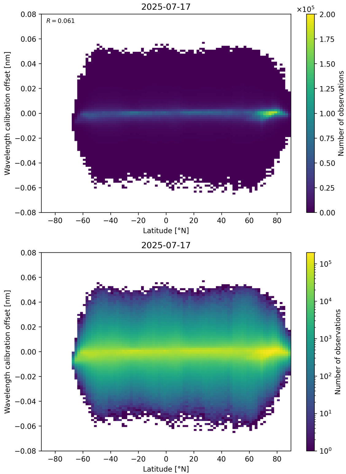
Figure 95: Scatter density plot of “Latitude” against “Wavelength calibration offset” for 2025-07-16 to 2025-07-18.
