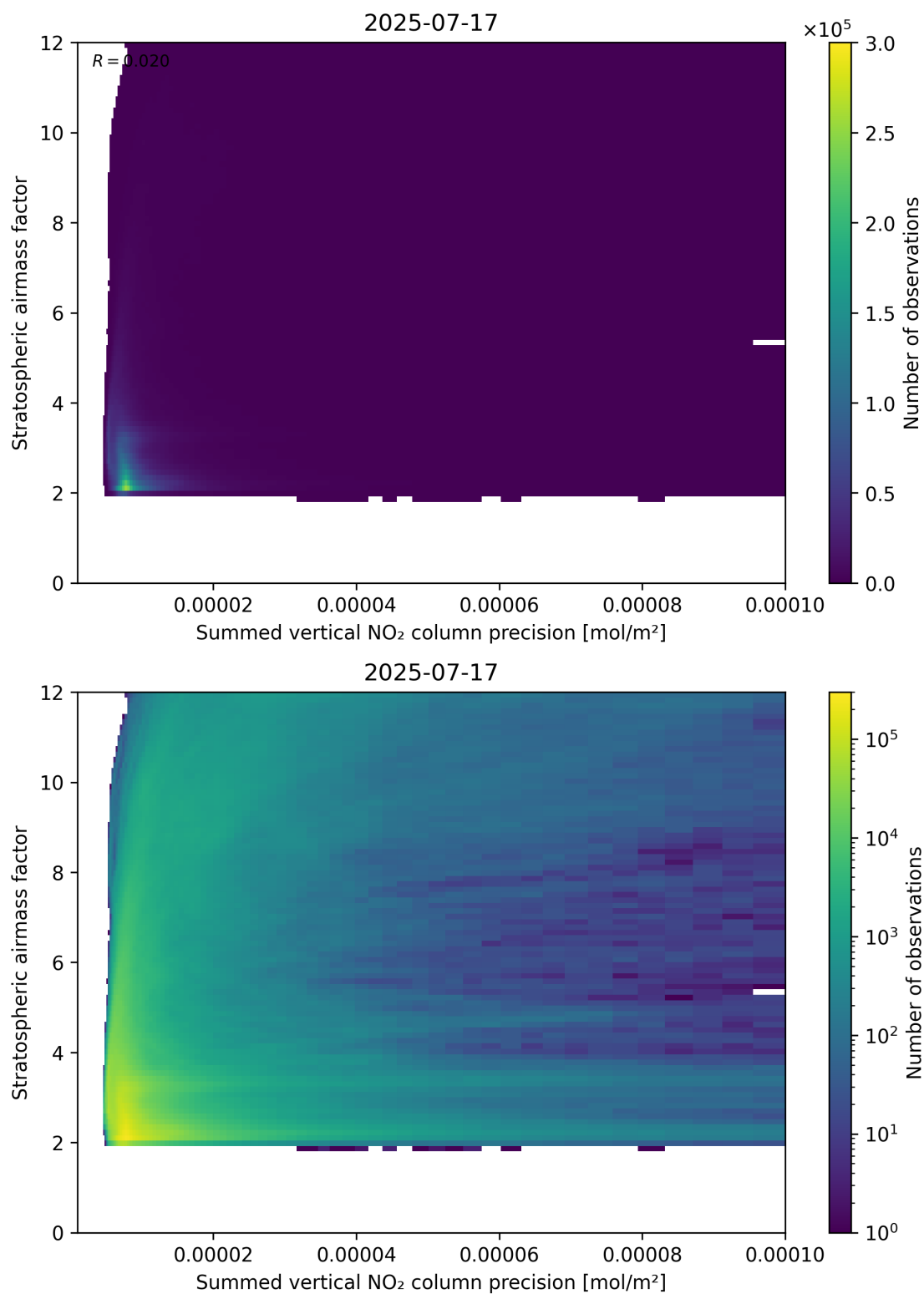
Figure 106: Scatter density plot of “Summed vertical NO 2 column precision” against “Stratospheric airmass factor” for 2025-07-16 to 2025-07-18.
