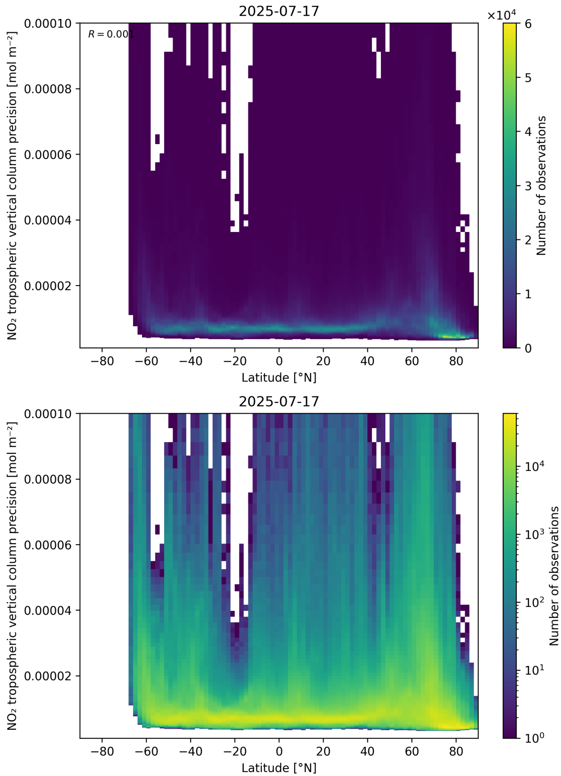
Figure 93: Scatter density plot of “Latitude” against “NO 2 tropospheric vertical column precision” for 2025-07-16 to 2025-07-18.
