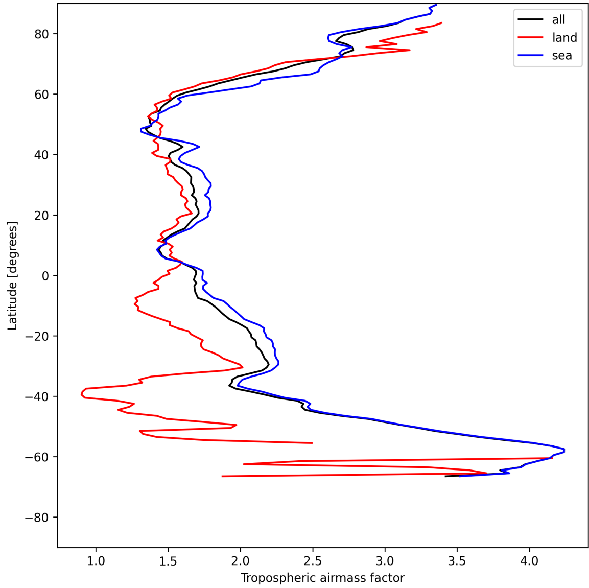
Figure 14: Zonal average of “Tropospheric airmass factor” for 2025-07-16 to 2025-07-18.
