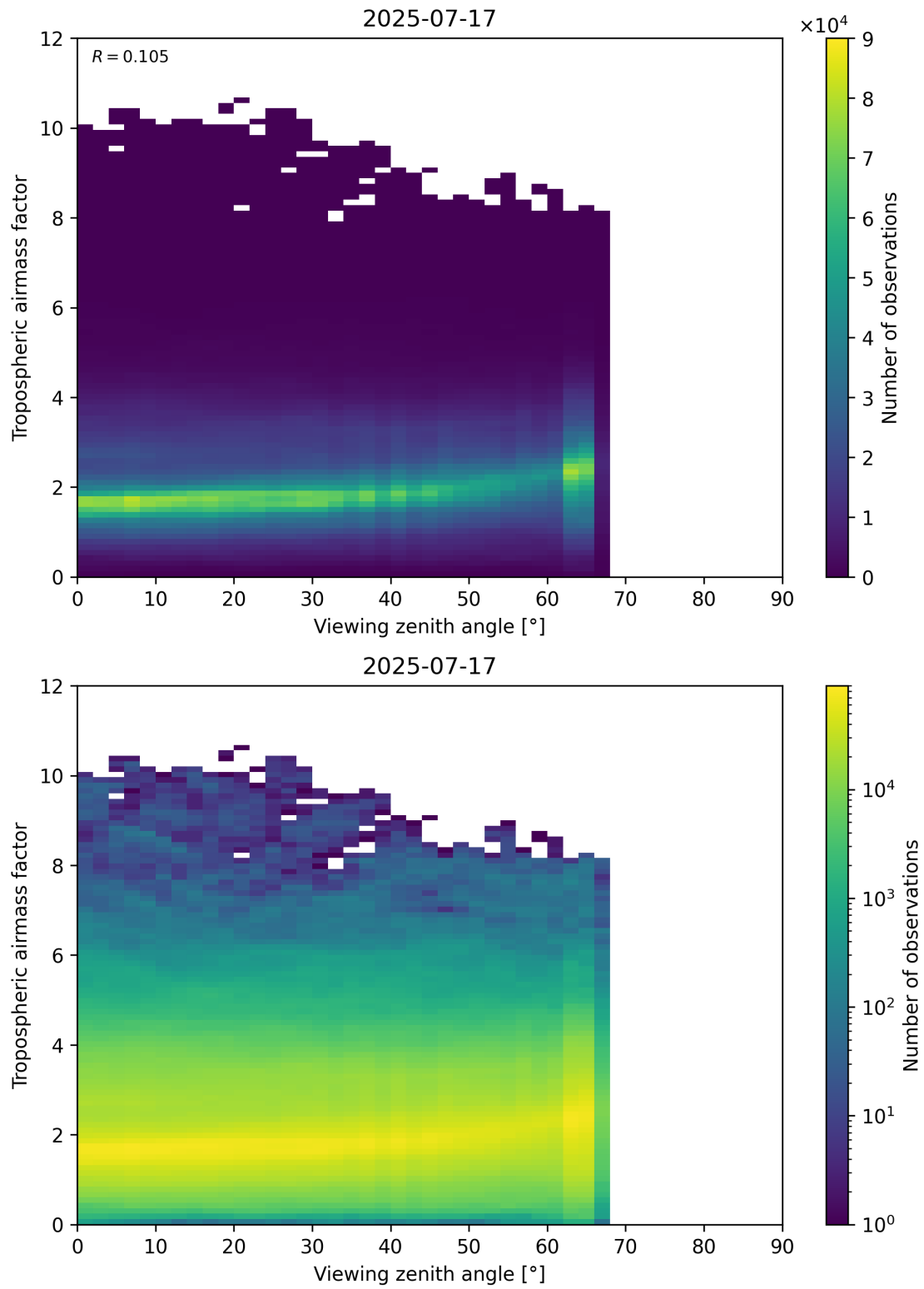
Figure 161: Scatter density plot of “Viewing zenith angle” against “Tropospheric airmass factor” for 2025-07-16 to 2025-07-18.
