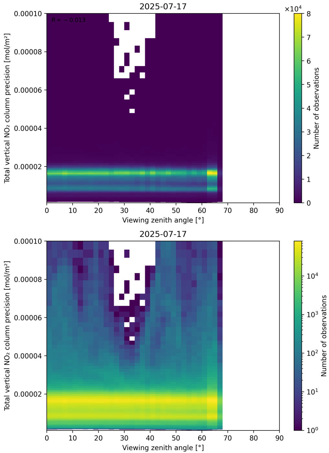
Figure 168: Scatter density plot of “Viewing zenith angle” against “Total vertical NO 2 column precision” for 2025-07-16 to 2025-07-18.
