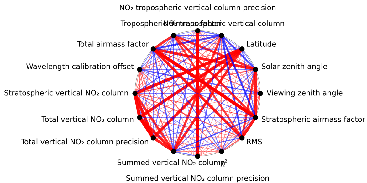
Figure 1: Map of correlation graph for 2025-07-16 to 2025-07-18.
