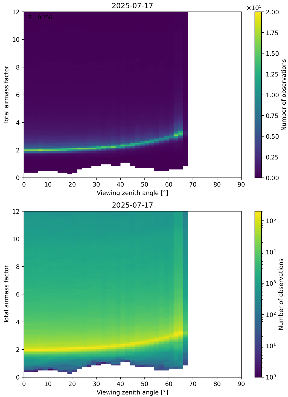
Figure 160: Scatter density plot of “Viewing zenith angle” against “Total airmass factor” for 2025-07-16 to 2025-07-18.
