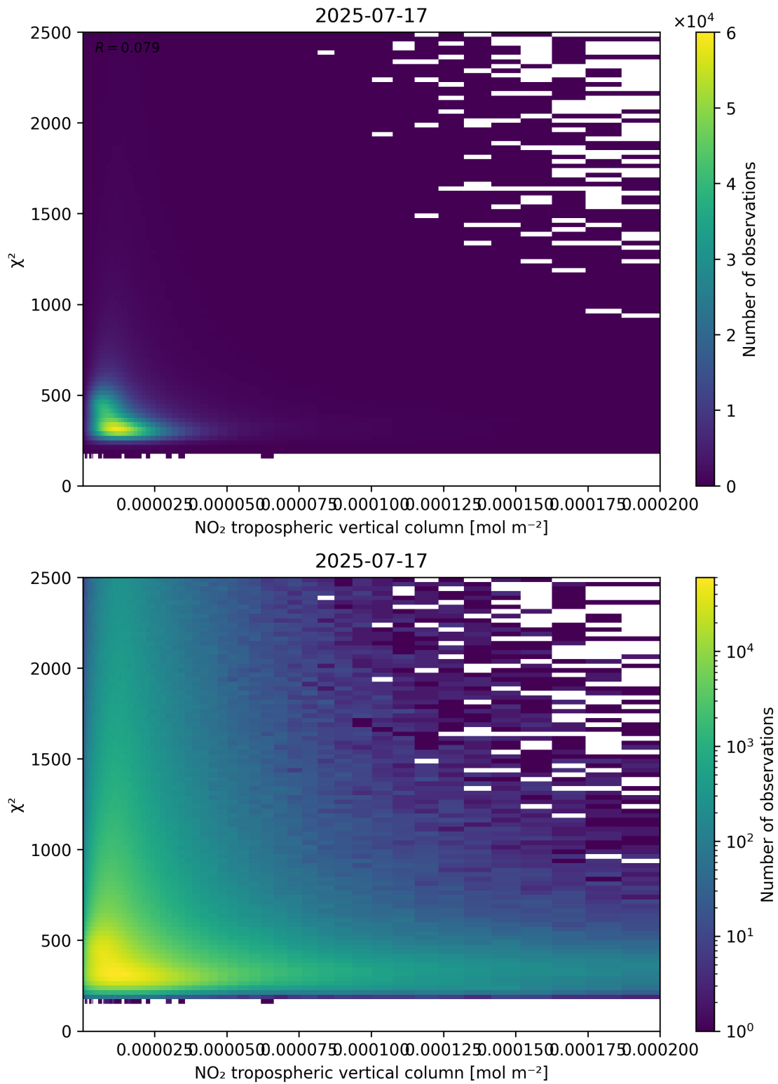
Figure 124: Scatter density plot of “NO 2 tropospheric vertical column” against “ \chi^2 ” for 2025-07-16 to 2025-07-18.
