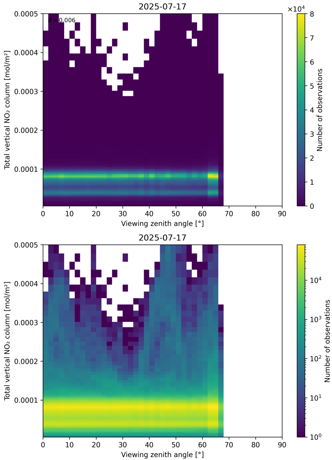
Figure 167: Scatter density plot of “Viewing zenith angle” against “Total vertical NO 2 column” for 2025-07-16 to 2025-07-18.
