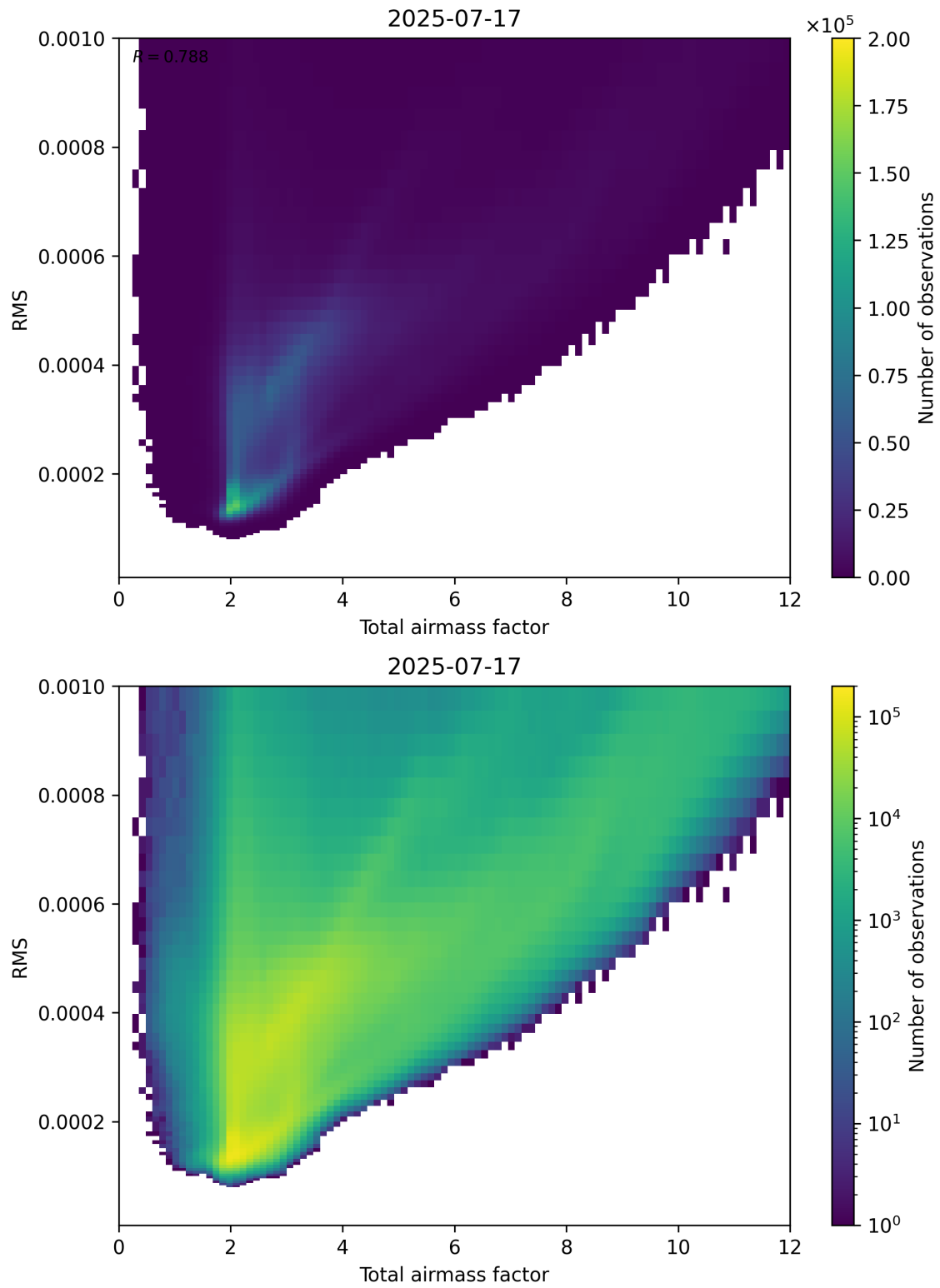
Figure 69: Scatter density plot of “Total airmass factor” against “RMS” for 2025-07-16 to 2025-07-18.
