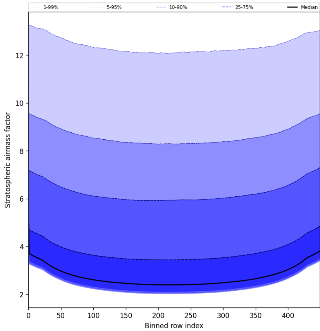
Figure 61: Along track statistics of “Stratospheric airmass factor” for 2025-07-16 to 2025-07-18
