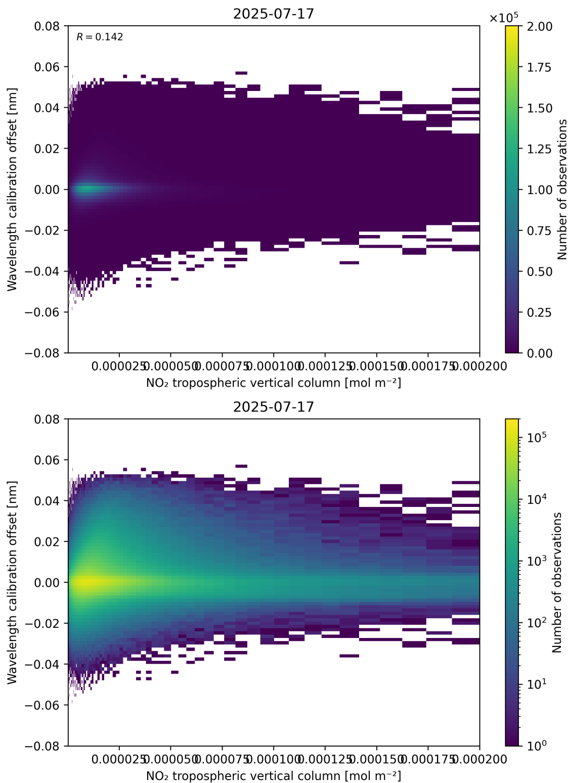
Figure 143: Scatter density plot of “NO 2 tropospheric vertical column” against “Wavelength calibration offset” for 2025-07-16 to 2025-07-18.
