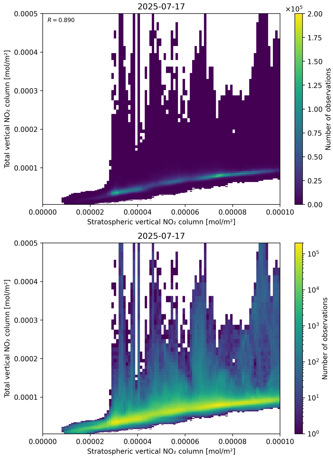
Figure 100: Scatter density plot of “Stratospheric vertical NO 2 column” against “Total vertical NO 2 column” for 2025-07-16 to 2025-07-18.
