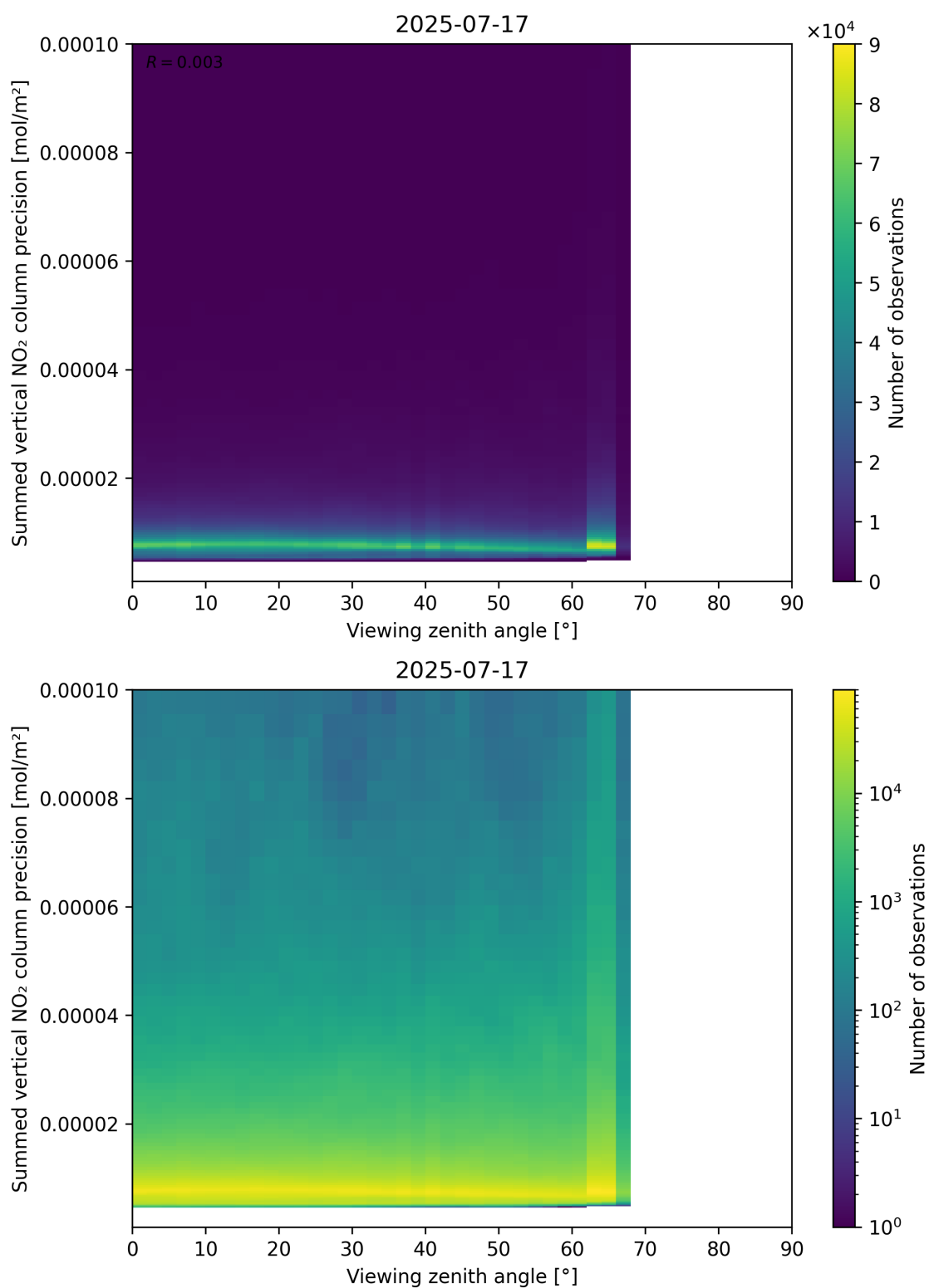
Figure 166: Scatter density plot of “Viewing zenith angle” against “Summed vertical NO 2 column precision” for 2025-07-16 to 2025-07-18.
