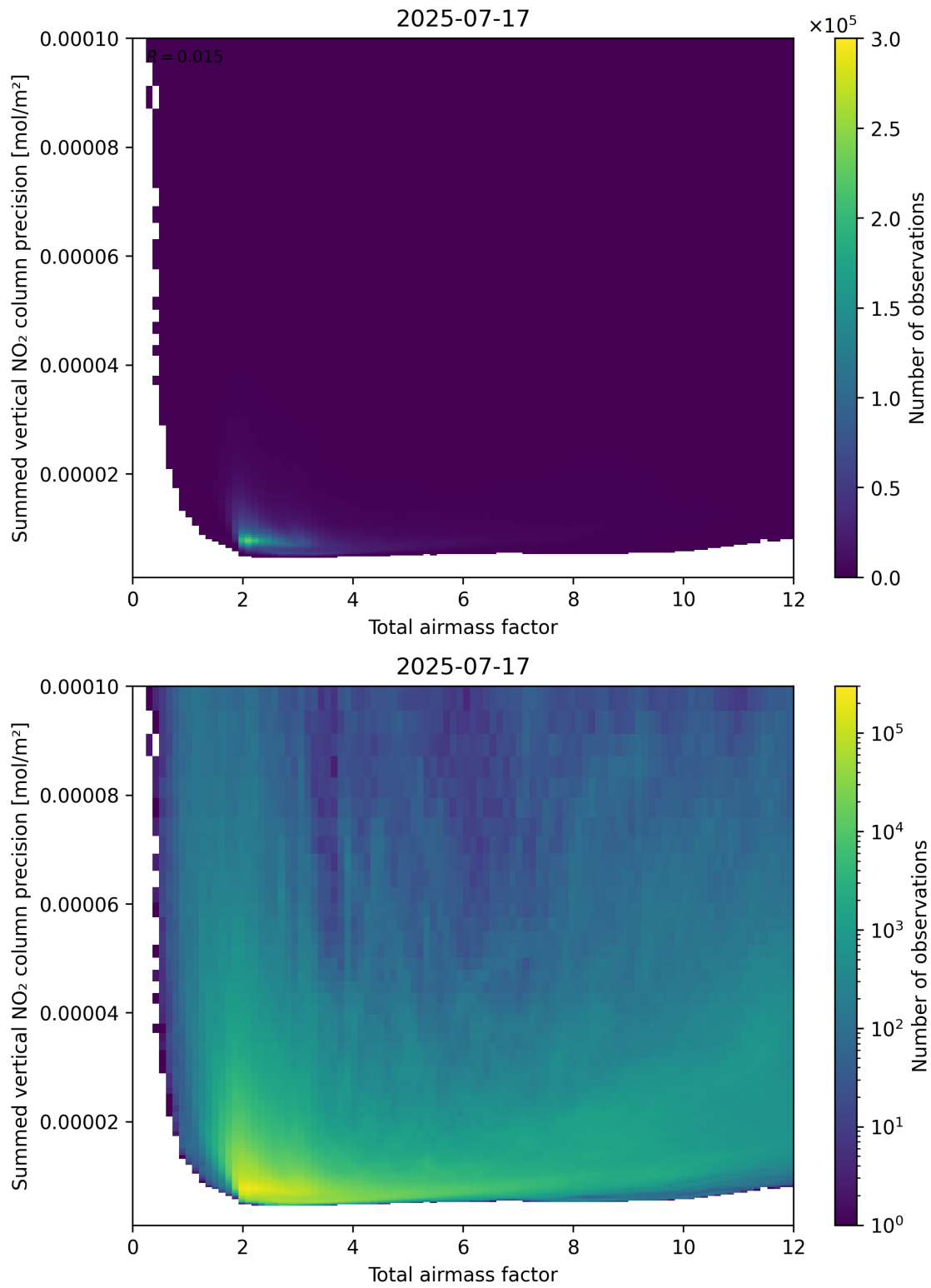
Figure 66: Scatter density plot of “Total airmass factor” against “Summed vertical NO 2 column precision” for 2025-07-16 to 2025-07-18.
