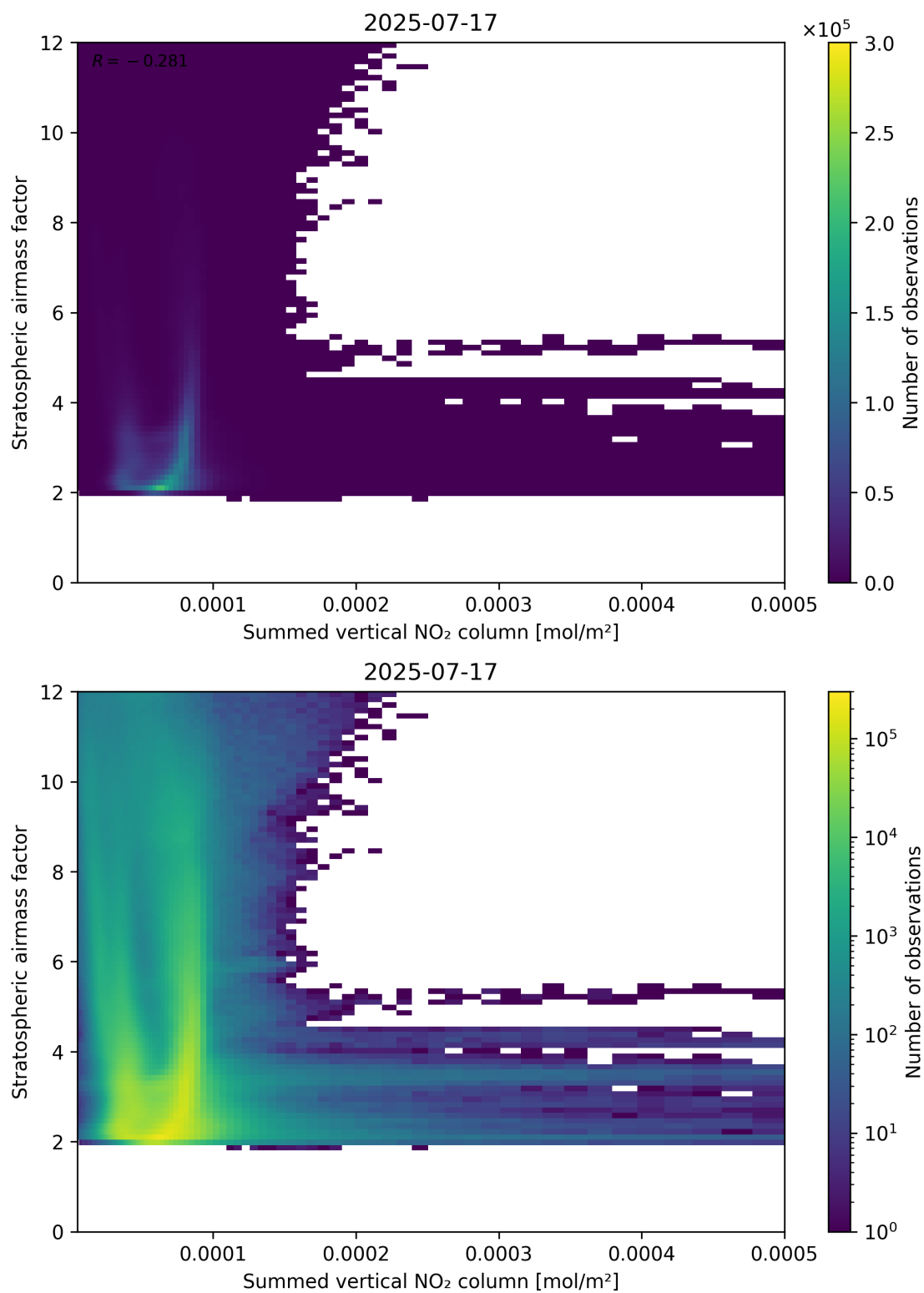
Figure 103: Scatter density plot of “Summed vertical NO 2 column” against “Stratospheric air mass factor” for 2025-07-16 to 2025-07-18.
