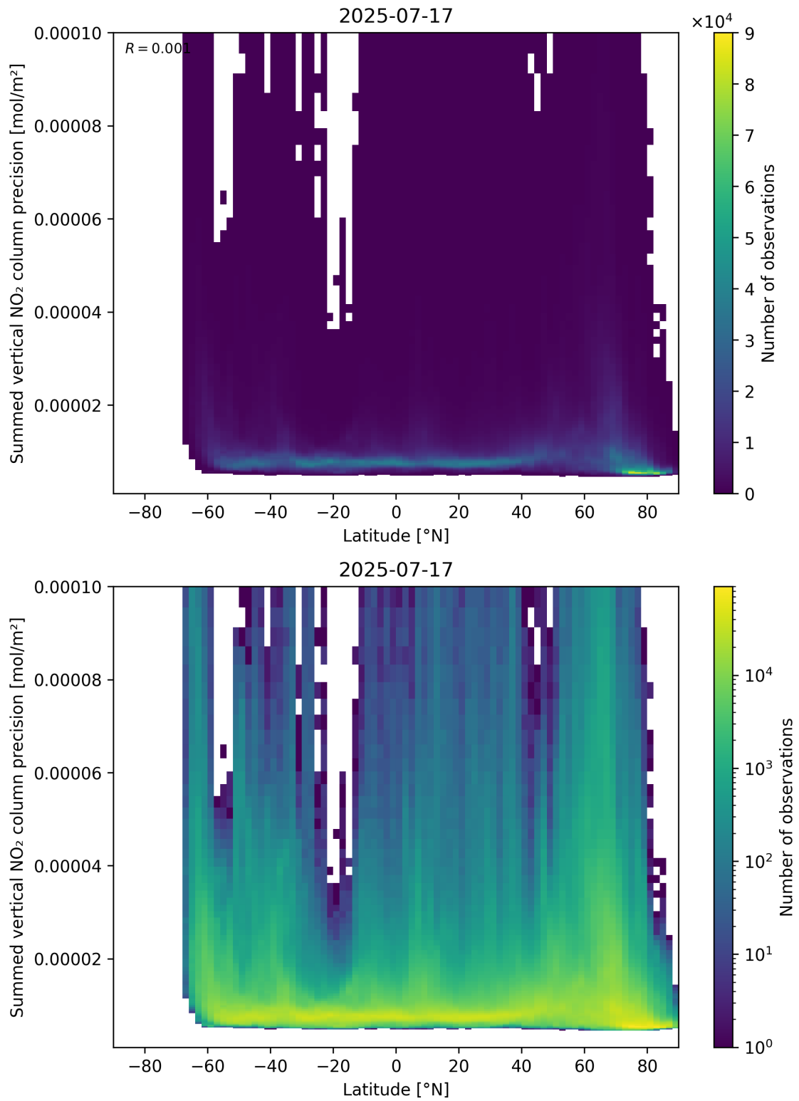
Figure 89: Scatter density plot of “Latitude” against “Summed vertical NO 2 column precision” for 2025-07-16 to 2025-07-18.
