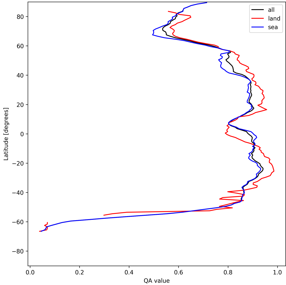
Figure 11: Zonal average of “QA value” for 2025-07-16 to 2025-07-18.
