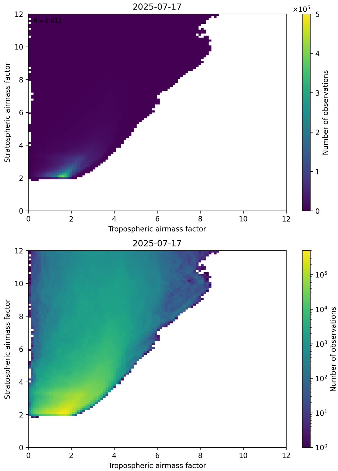
Figure 71: Scatter density plot of “Tropospheric airmass factor” against “Stratospheric airmass factor” for 2025-07-16 to 2025-07-18.
