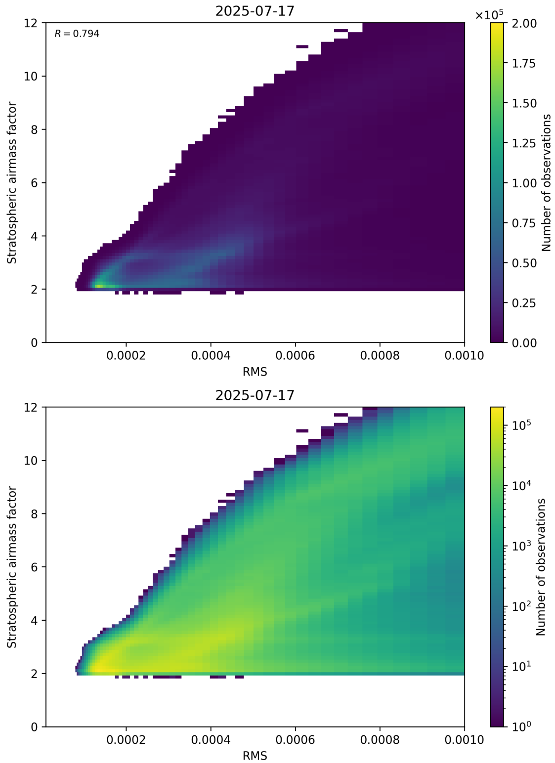
Figure 144: Scatter density plot of “RMS” against “Stratospheric airmass factor” for 2025-07-16 to 2025-07-18.
