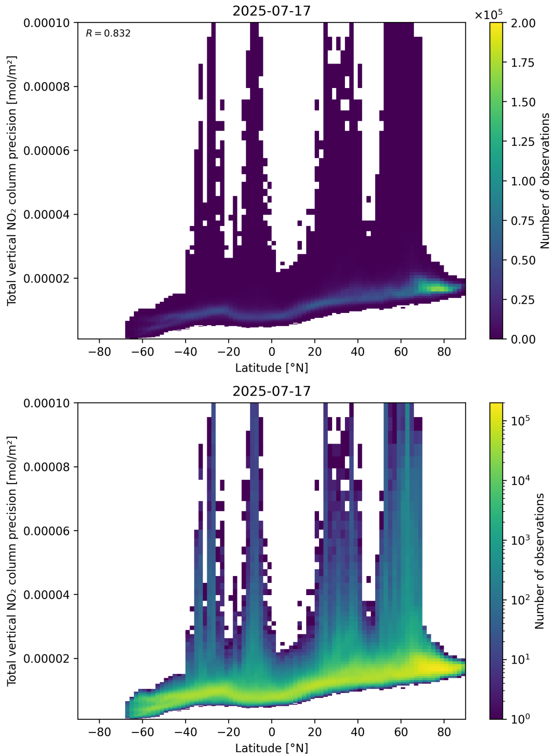
Figure 91: Scatter density plot of “Latitude” against “Total vertical NO 2 column precision” for 2025-07-16 to 2025-07-18.
