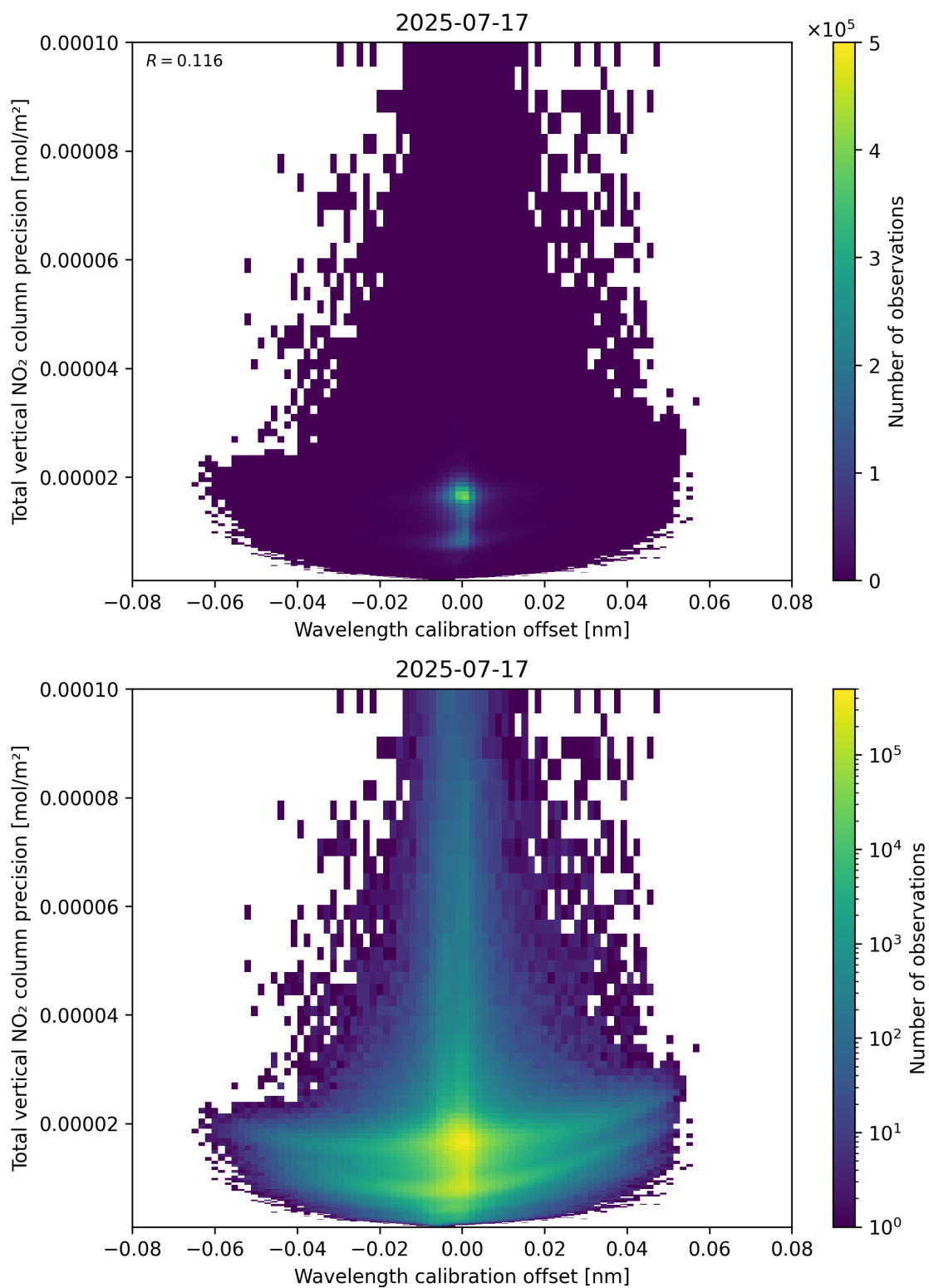
Figure 180: Scatter density plot of “Wavelength calibration offset” against “Total vertical NO 2 column precision” for 2025-07-16 to 2025-07-18.
