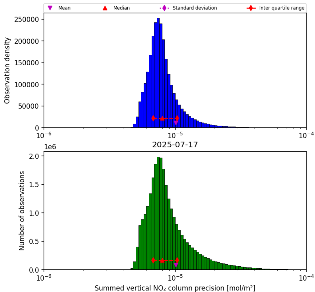
Figure 41: Histogram of "Summed vertical NO 2 column precision" for 2025-07-16 to 2025-07-18
