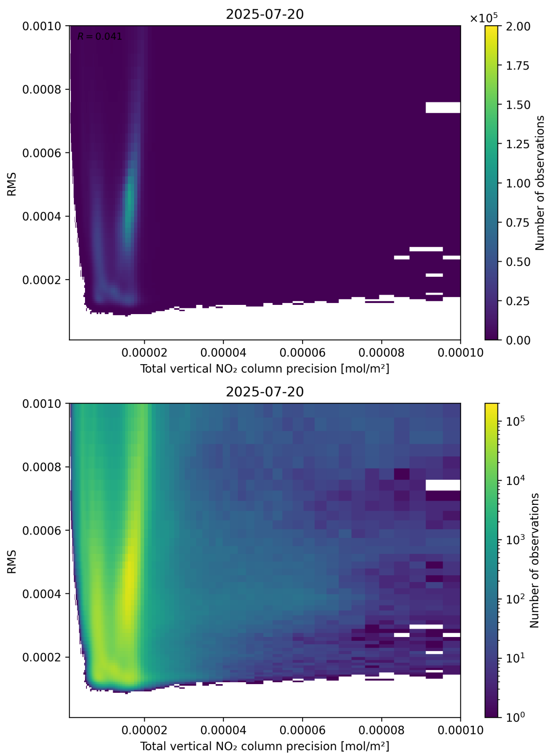
Figure 119: Scatter density plot of “Total vertical NO 2 column precision” against “RMS” for 2025-07-19 to 2025-07-21.
