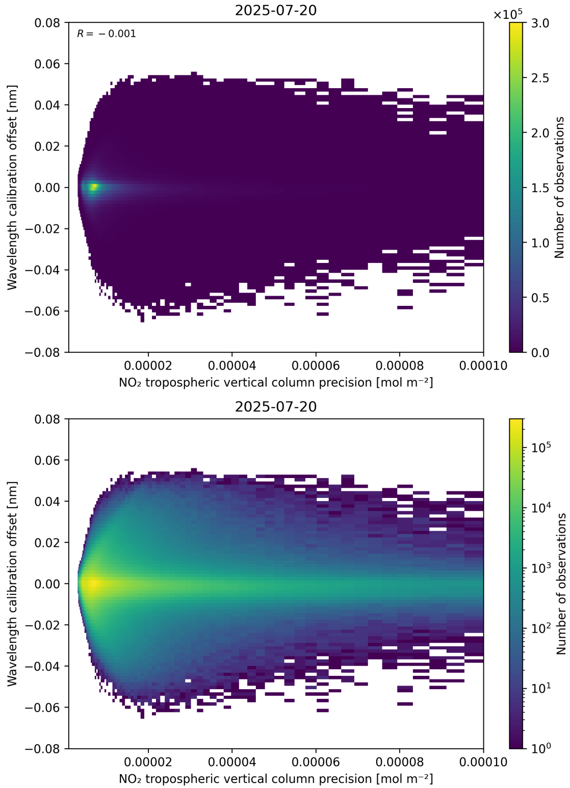
Figure 141: Scatter density plot of “NO 2 tropospheric vertical column precision” against “Wavelength calibration offset” for 2025-07-19 to 2025-07-21.
