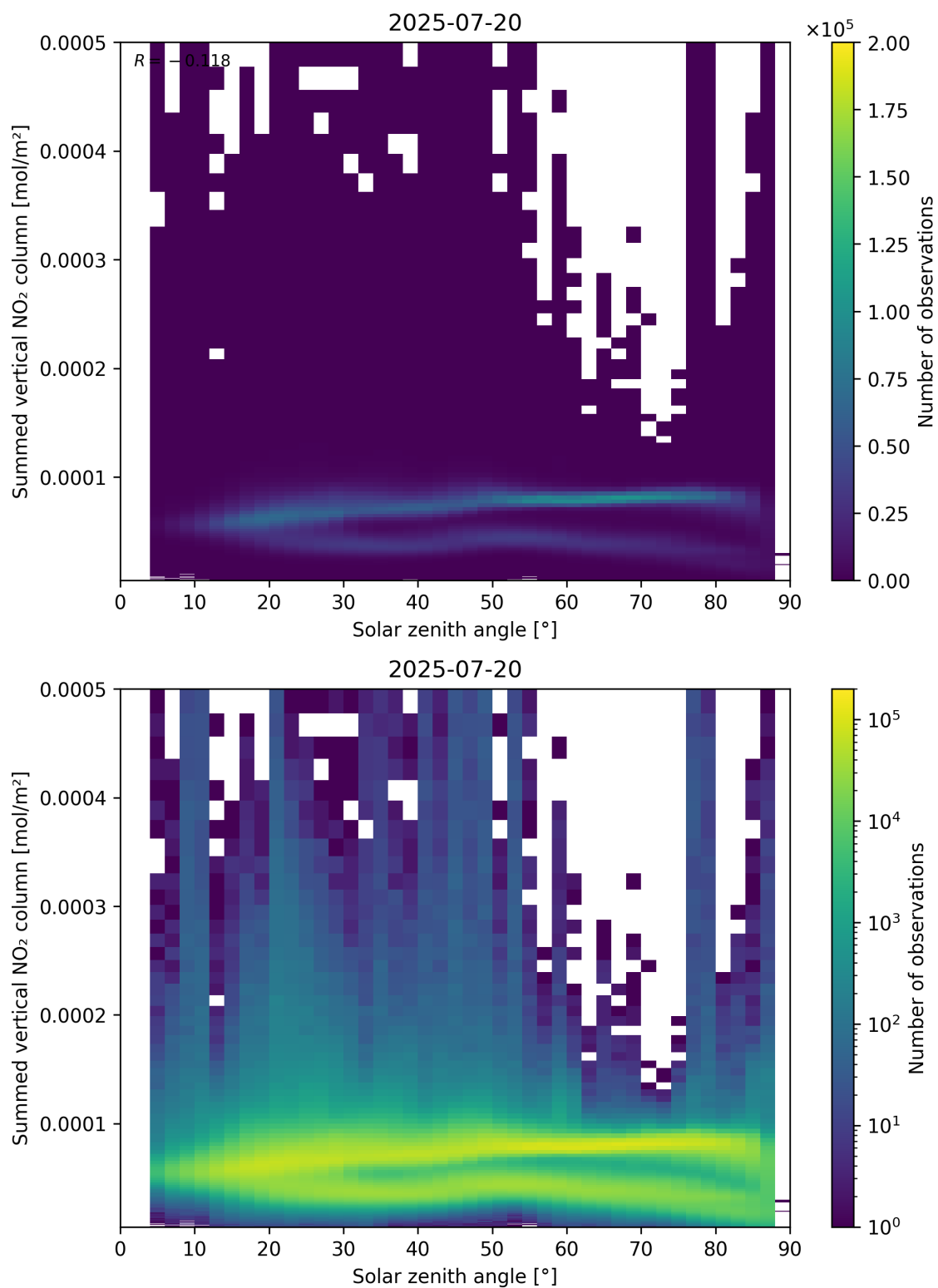
Figure 151: Scatter density plot of “Solar zenith angle” against “Summed vertical NO 2 column” for 2025-07-19 to 2025-07-21.
