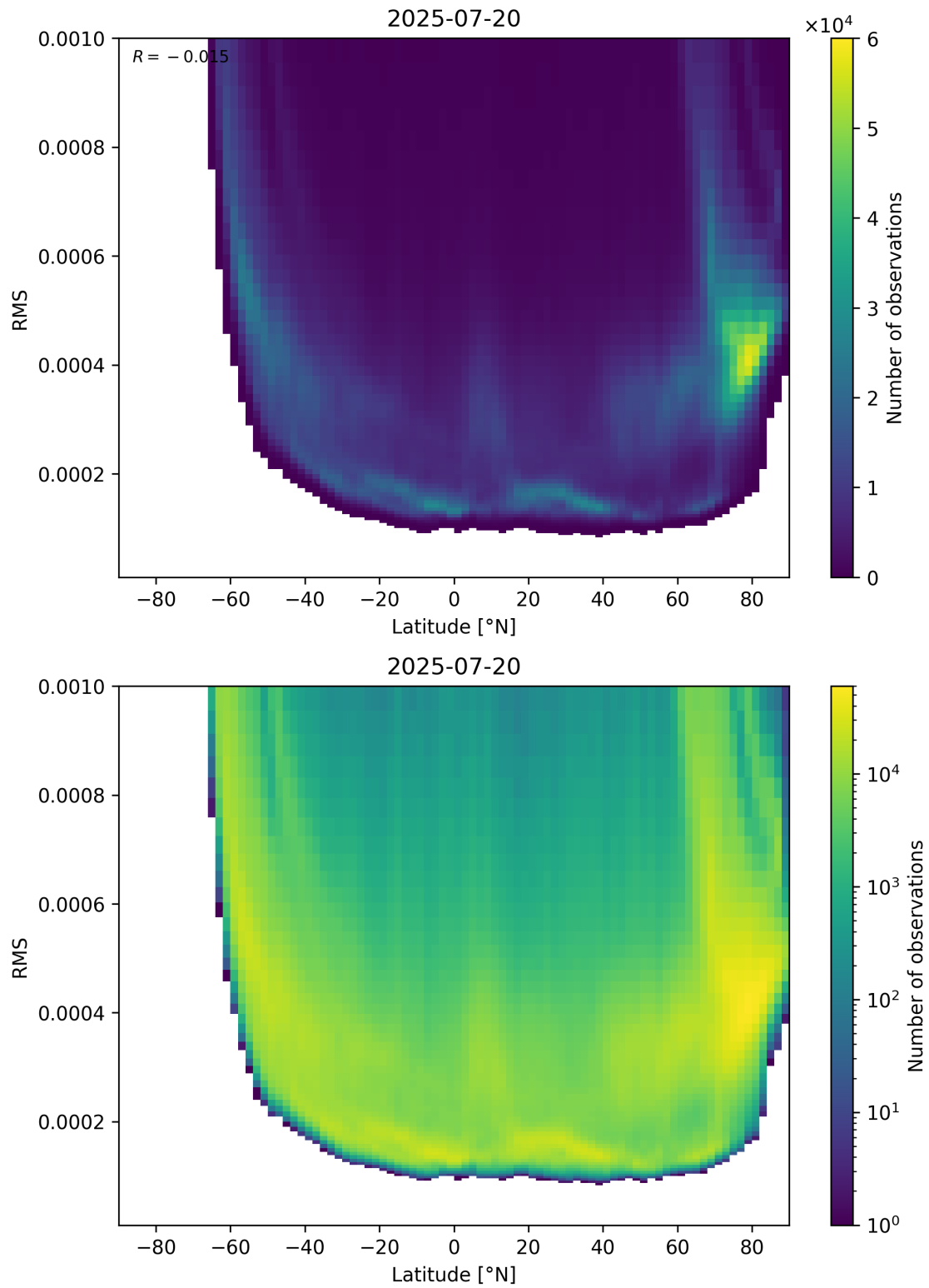
Figure 94: Scatter density plot of “Latitude” against “RMS” for 2025-07-19 to 2025-07-21.
