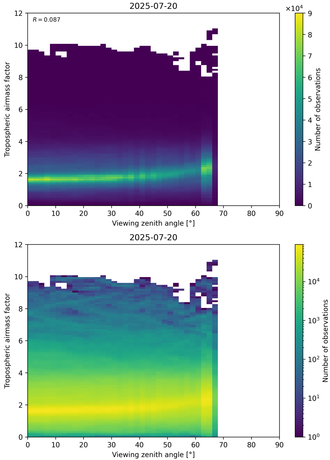
Figure 161: Scatter density plot of “Viewing zenith angle” against “Tropospheric airmass factor” for 2025-07-19 to 2025-07-21.
