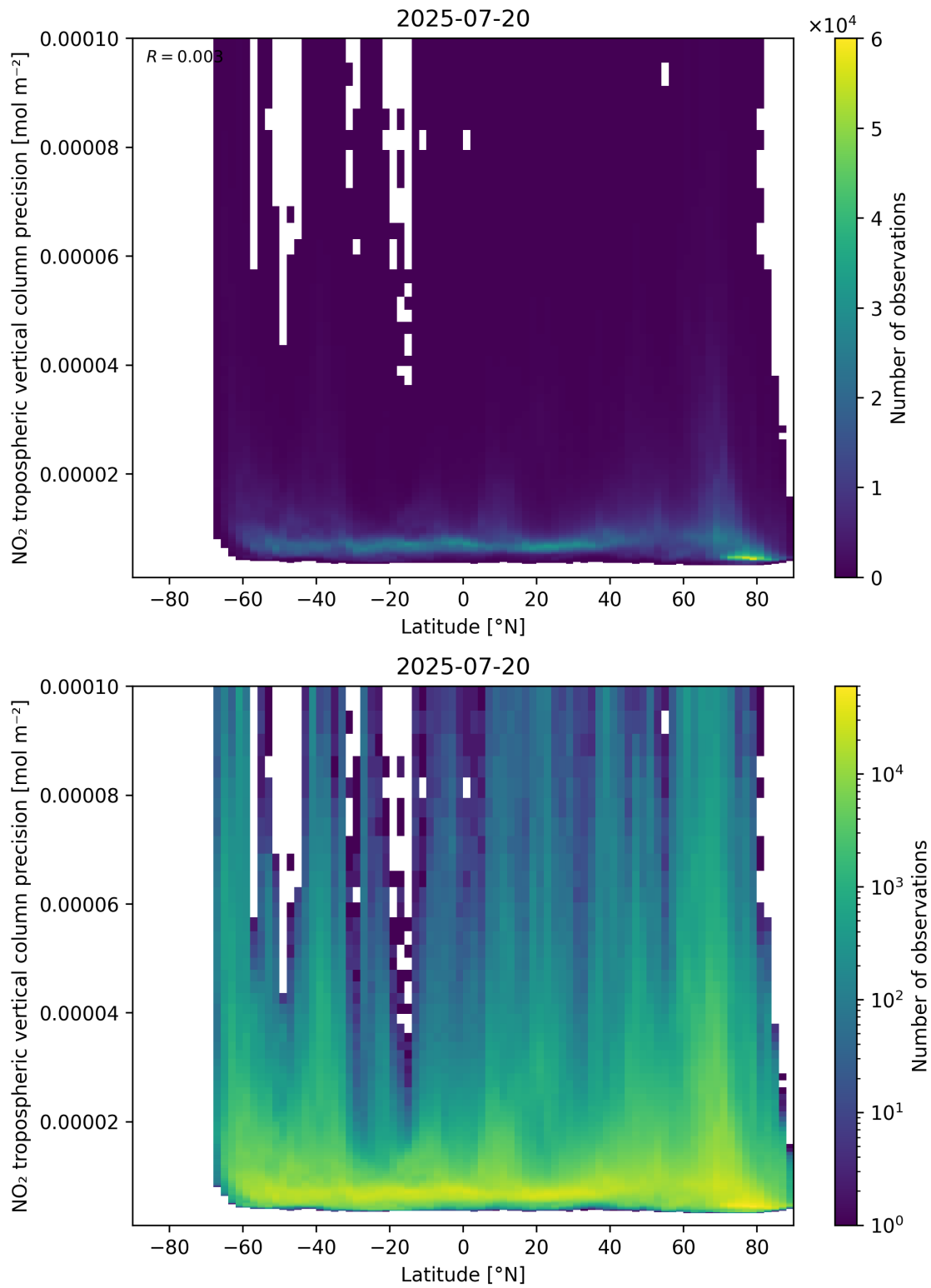
Figure 93: Scatter density plot of “Latitude” against “NO 2 tropospheric vertical column precision” for 2025-07-19 to 2025-07-21.
