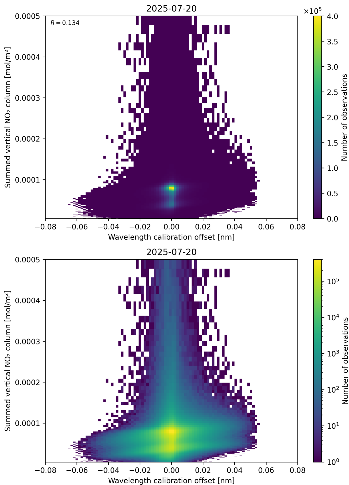
Figure 177: Scatter density plot of “Wavelength calibration offset” against “Summed vertical NO 2 column” for 2025-07-19 to 2025-07-21.
