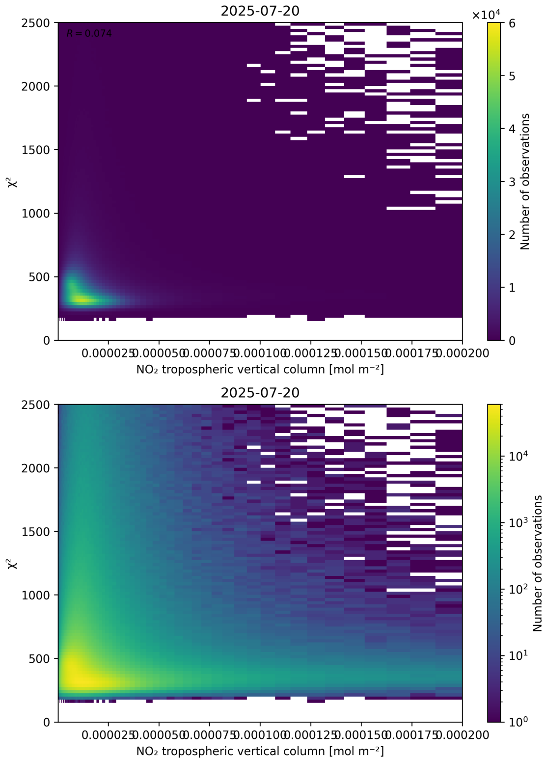
Figure 124: Scatter density plot of “NO 2 tropospheric vertical column” against “ \chi^2 ” for 2025-07-19 to 2025-07-21.
