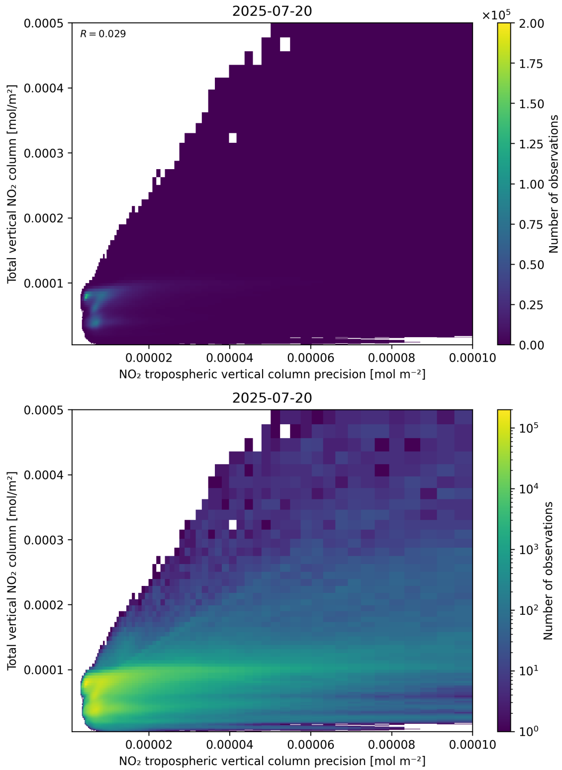
Figure 138: Scatter density plot of “NO 2 tropospheric vertical column precision” against “Total vertical NO 2 column” for 2025-07-19 to 2025-07-21.
