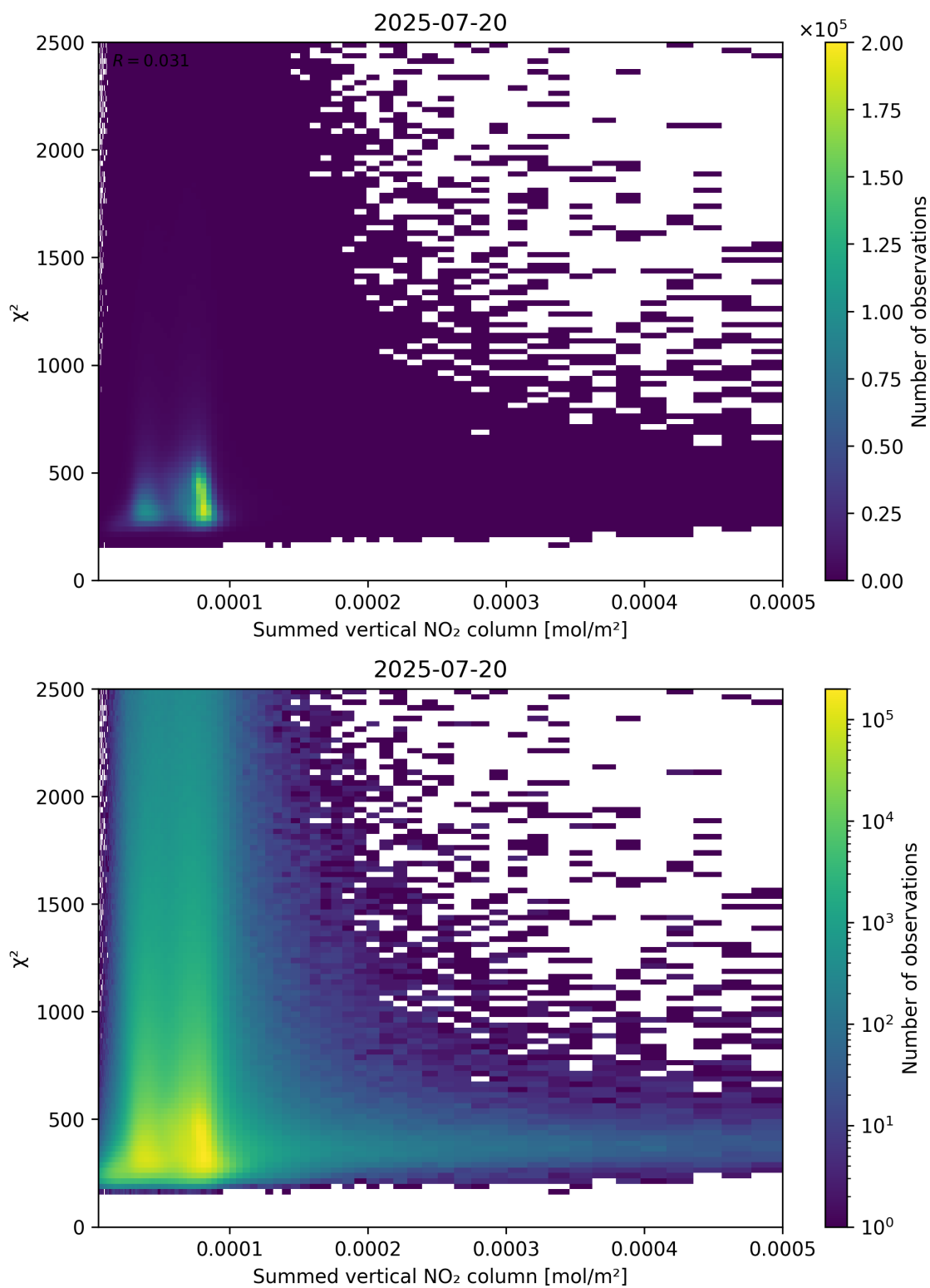
Figure 104: Scatter density plot of “Summed vertical NO 2 column” against “ \chi^2 ” for 2025-07-19 to 2025-07-21.
