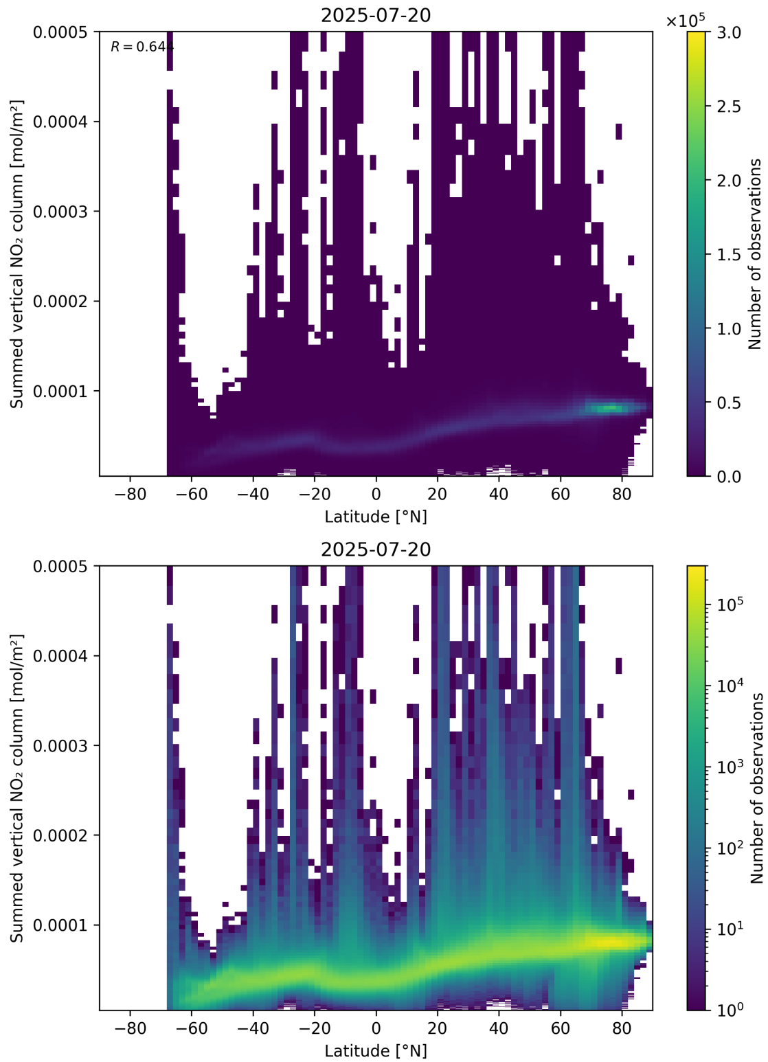
Figure 88: Scatter density plot of “Latitude” against “Summed vertical NO 2 column” for 2025-07-19 to 2025-07-21.
