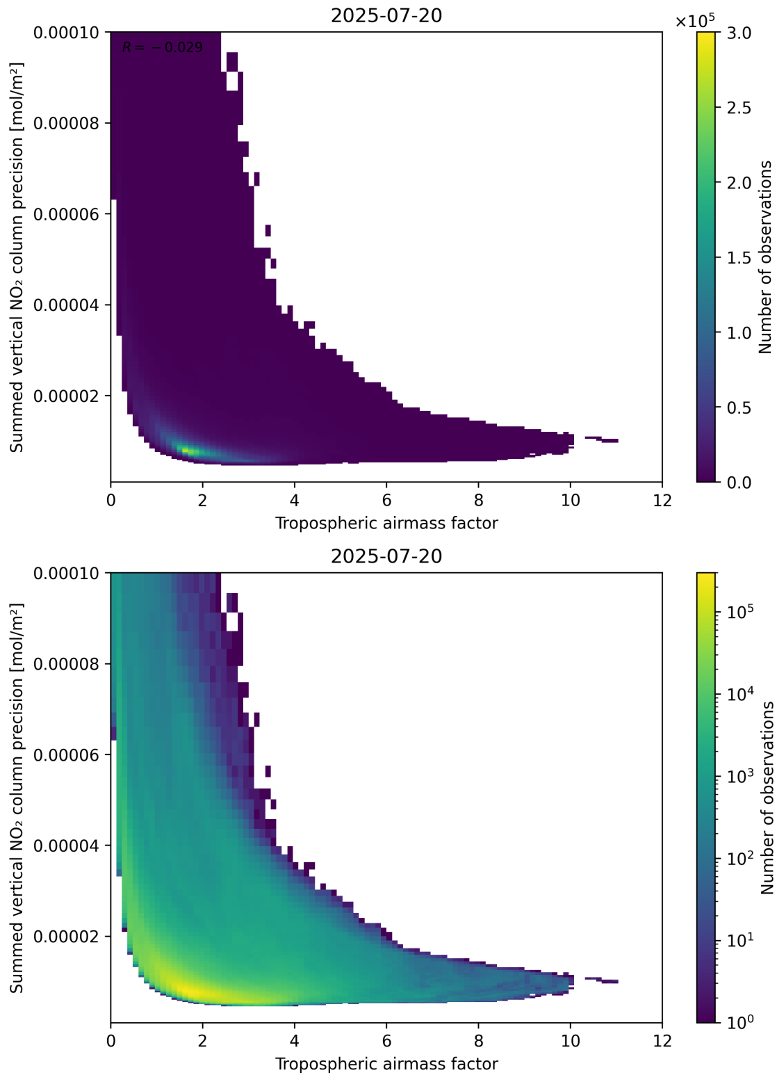
Figure 76: Scatter density plot of “Tropospheric air mass factor” against “Summed vertical NO 2 column precision” for 2025-07-19 to 2025-07-21.
