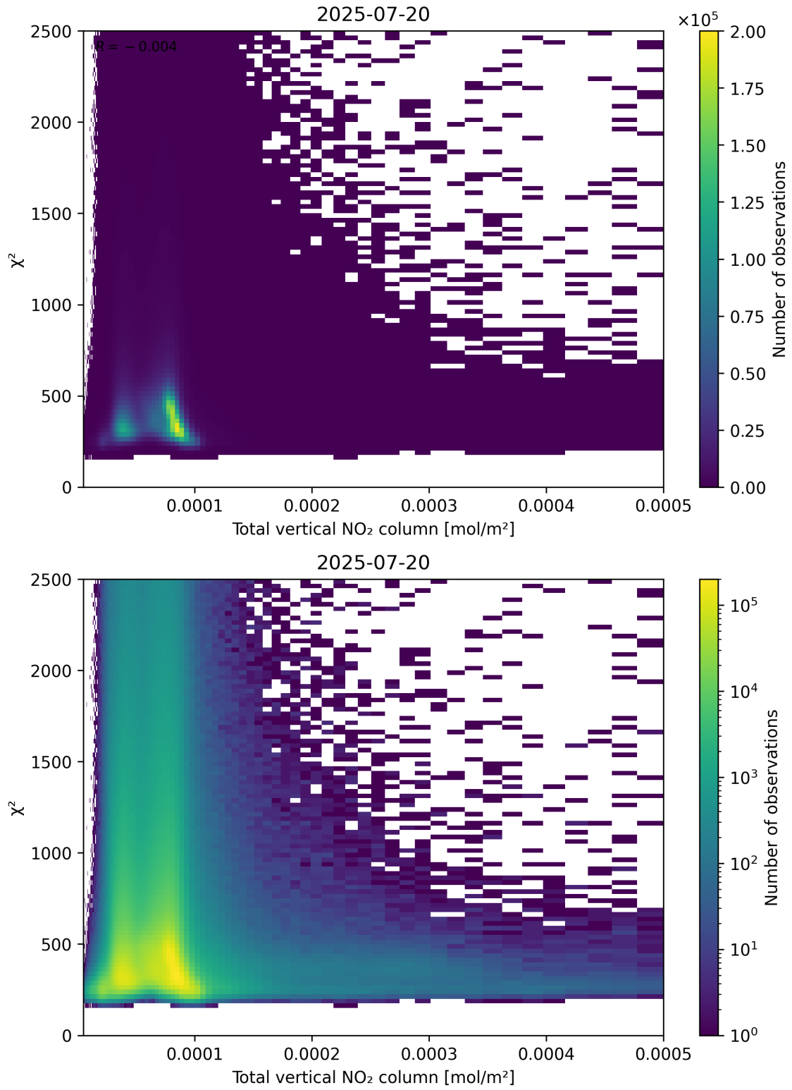
Figure 111: Scatter density plot of “Total vertical NO 2 column” against “ \chi^2 ” for 2025-07-19 to 2025-07-21.
