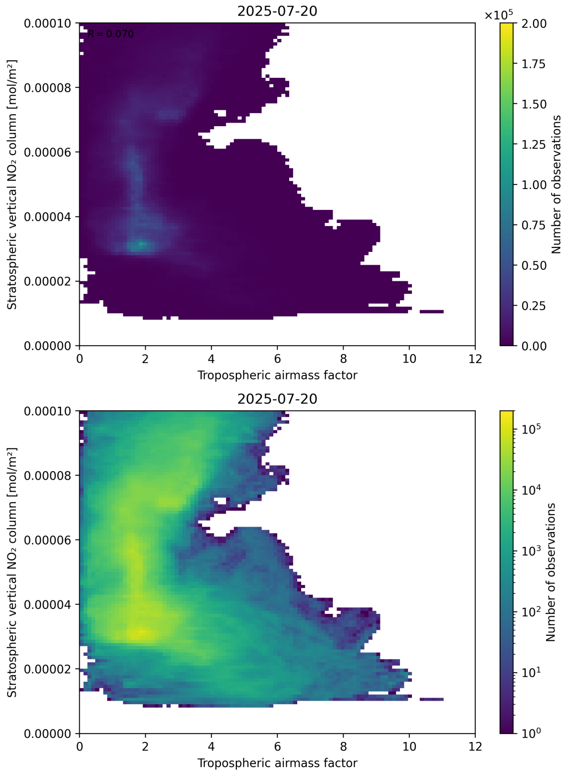
Figure 74: Scatter density plot of “Tropospheric air mass factor” against “Stratospheric vertical NO 2 column” for 2025-07-19 to 2025-07-21.
