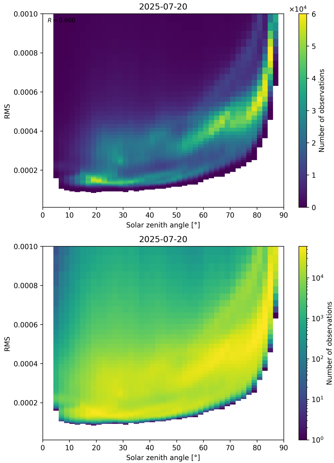
Figure 157: Scatter density plot of “Solar zenith angle” against “RMS” for 2025-07-19 to 2025-07-21.
