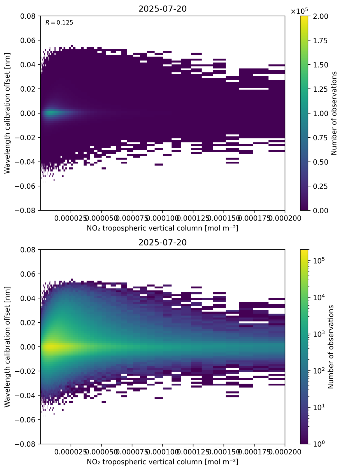
Figure 143: Scatter density plot of “NO 2 tropospheric vertical column” against “Wavelength calibration offset” for 2025-07-19 to 2025-07-21.
