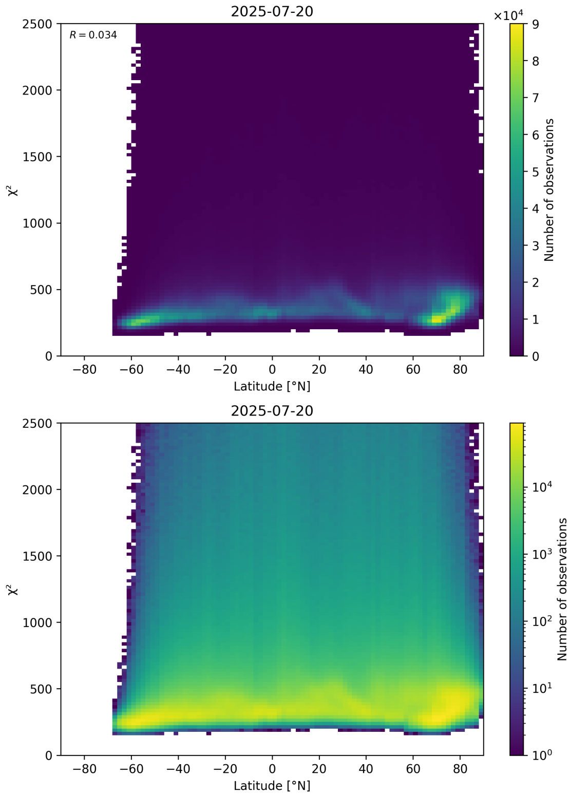
Figure 86: Scatter density plot of “Latitude” against “ \chi^2 ” for 2025-07-19 to 2025-07-21.
