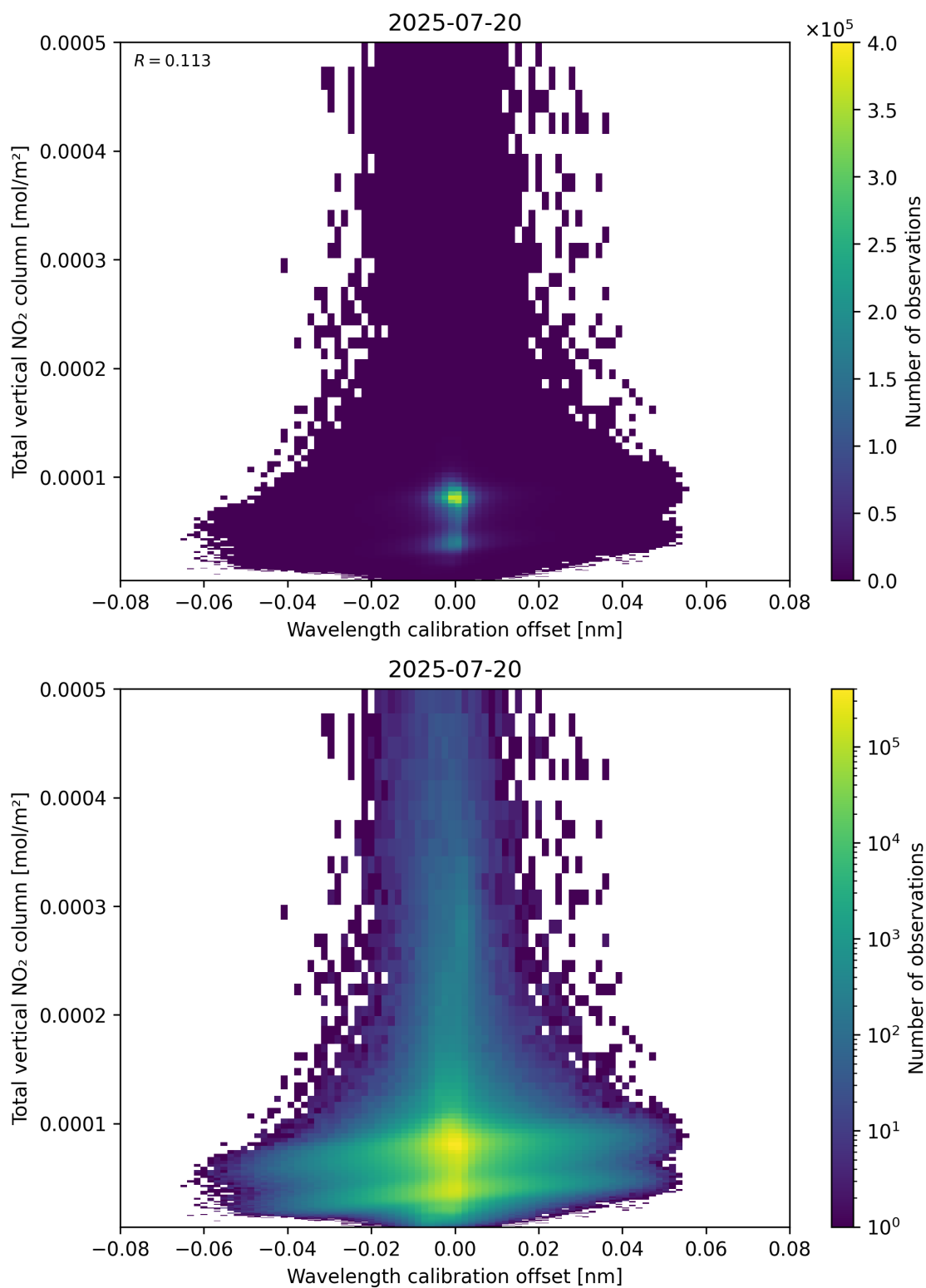
Figure 179: Scatter density plot of “Wavelength calibration offset” against “Total vertical NO 2 column” for 2025-07-19 to 2025-07-21.
