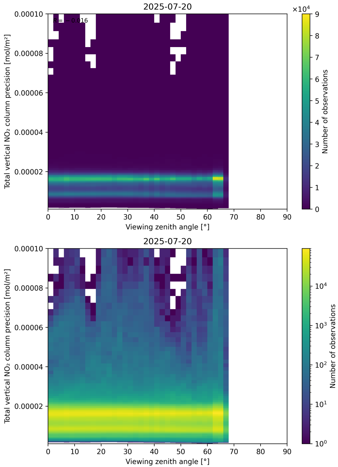
Figure 168: Scatter density plot of “Viewing zenith angle” against “Total vertical NO 2 column precision” for 2025-07-19 to 2025-07-21.
