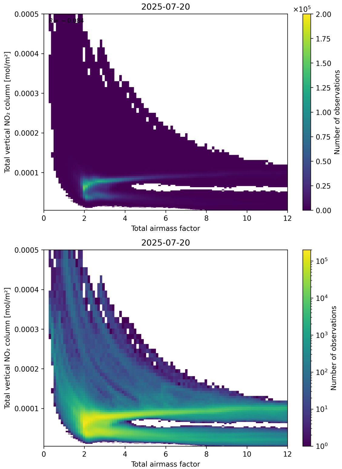
Figure 67: Scatter density plot of “Total airmass factor” against “Total vertical NO 2 column” for 2025-07-19 to 2025-07-21.
