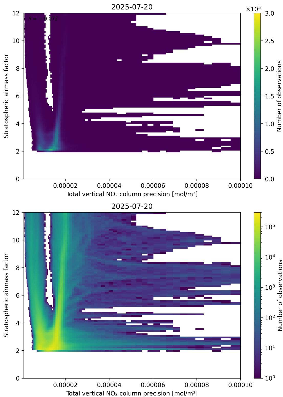
Figure 115: Scatter density plot of “Total vertical NO 2 column precision” against “Stratospheric airmass factor” for 2025-07-19 to 2025-07-21.
