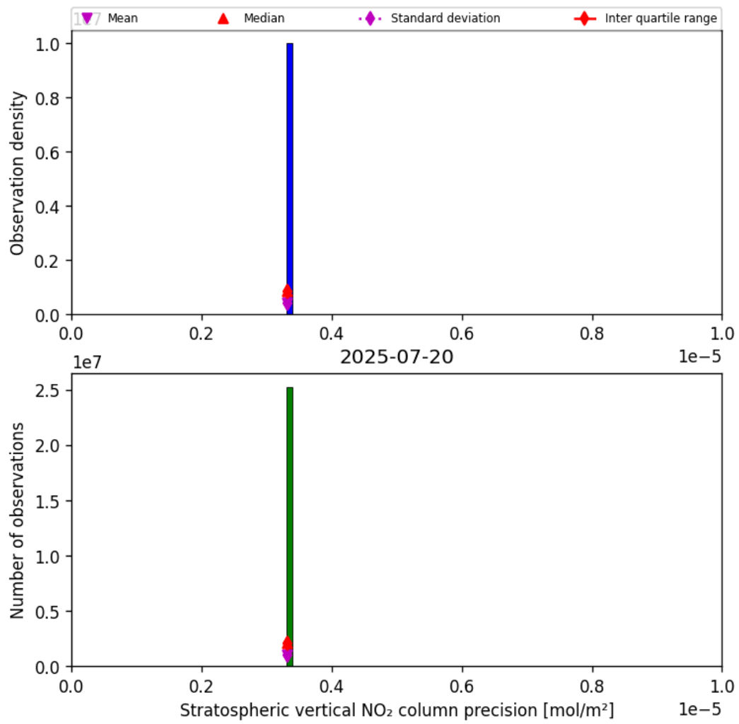
Figure 37: Histogram of “Stratospheric vertical NO 2 column precision” for 2025-07-19 to 2025-07-21
