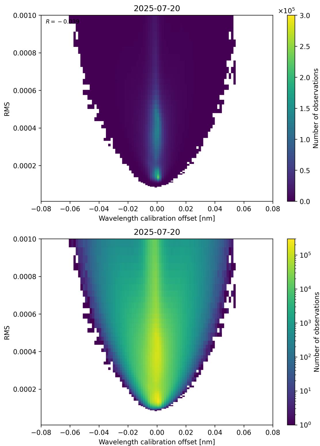
Figure 181: Scatter density plot of “Wavelength calibration offset” against “RMS” for 2025-07-19 to 2025-07-21.
