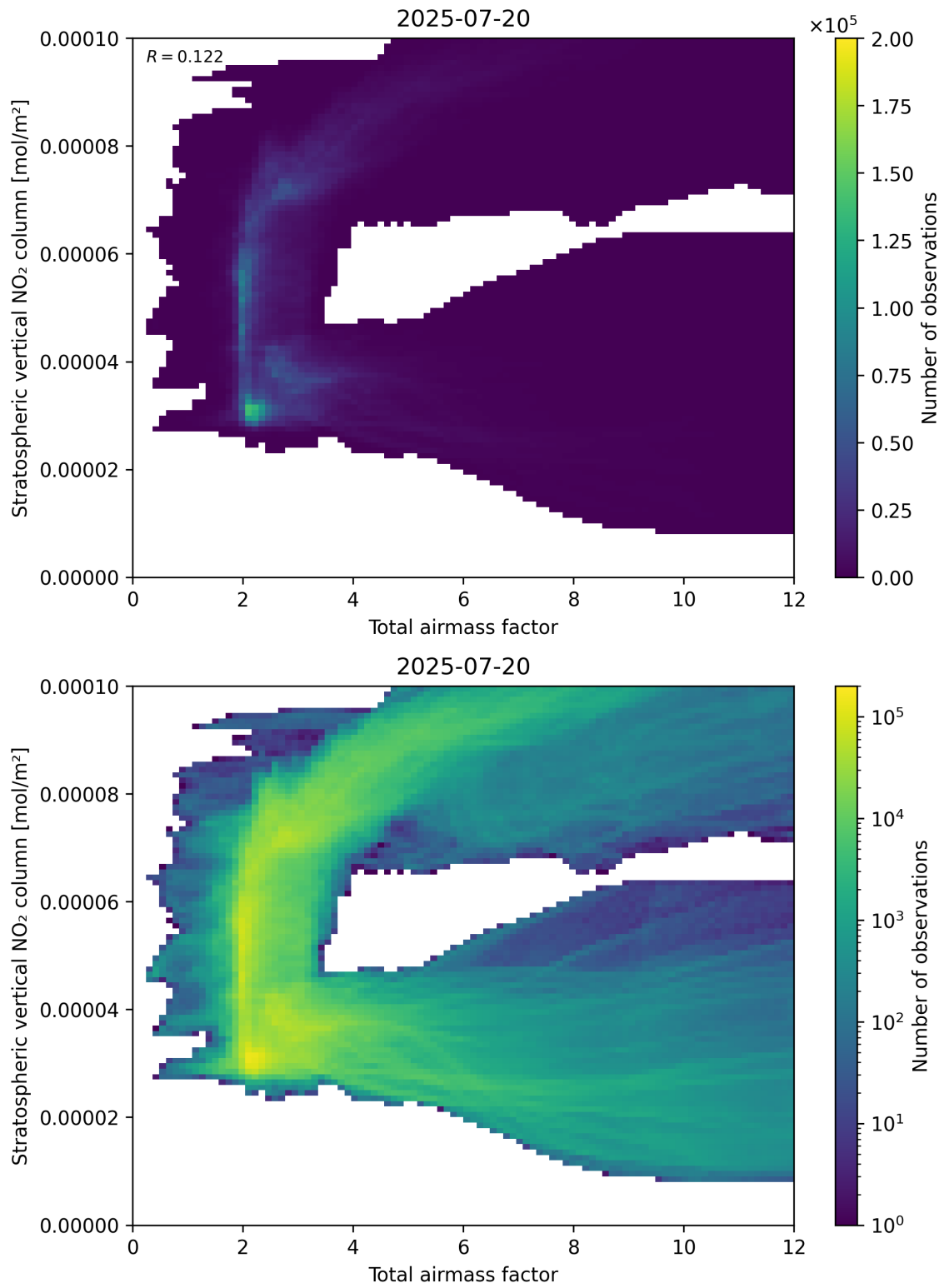
Figure 64: Scatter density plot of “Total airmass factor” against “Stratospheric vertical NO 2 column” for 2025-07-19 to 2025-07-21.
