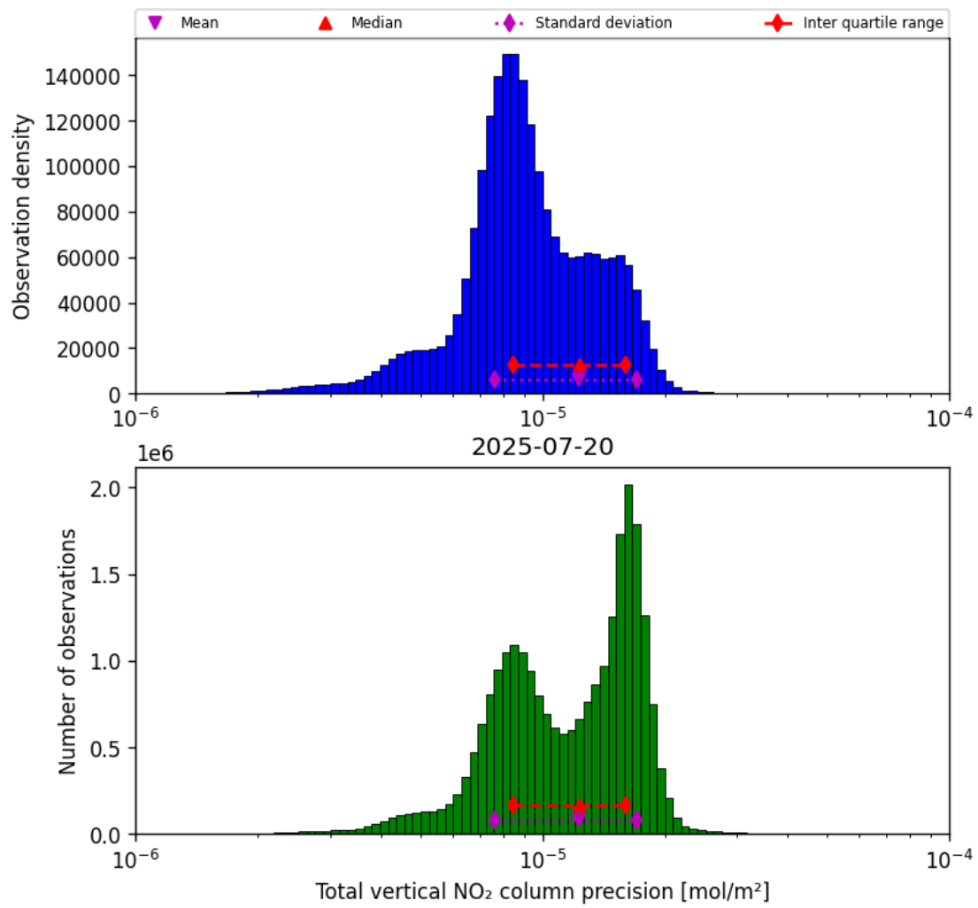
Figure 39: Histogram of “Total vertical NO 2 column precision” for 2025-07-19 to 2025-07-21
