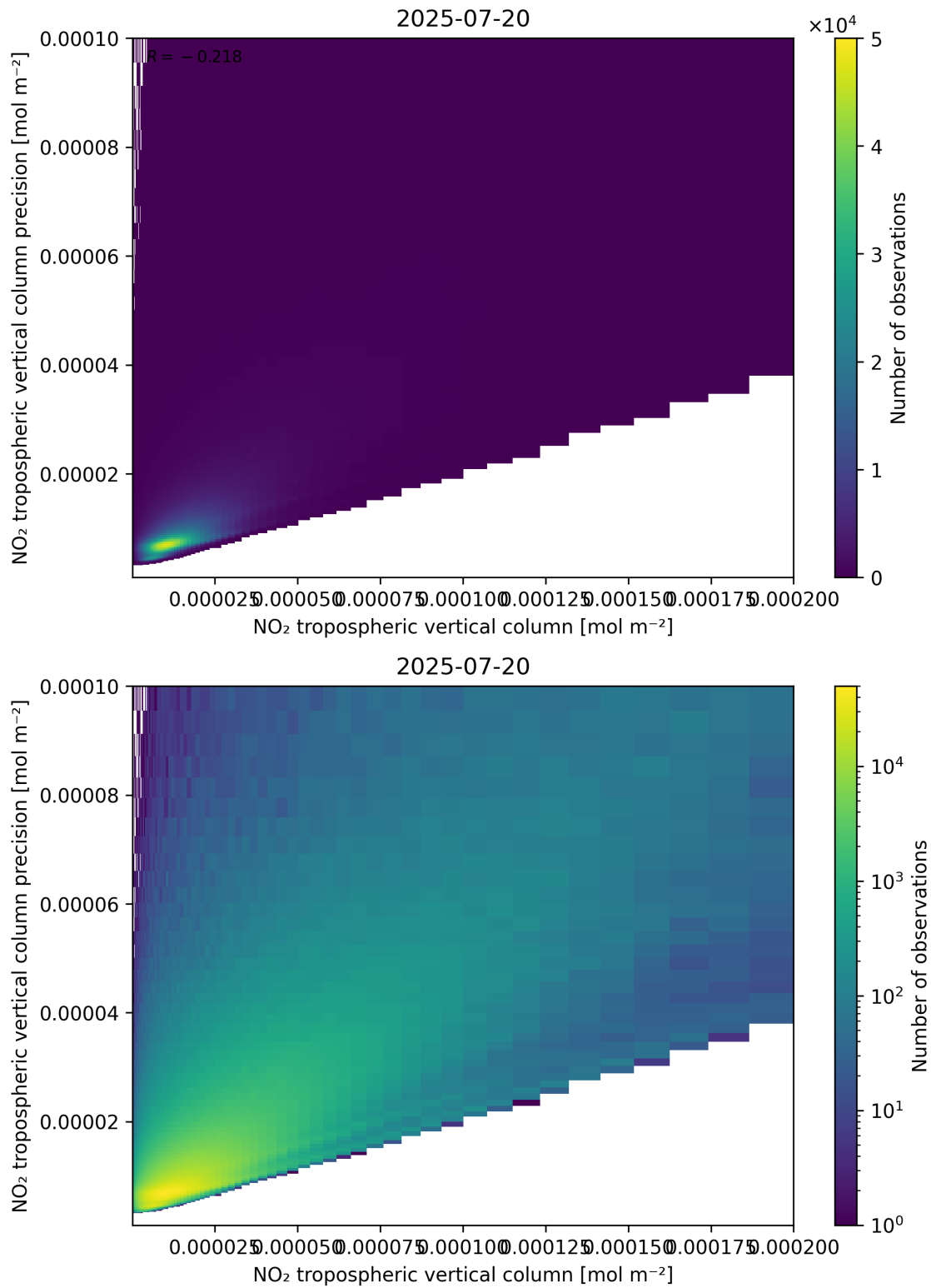
Figure 130: Scatter density plot of “NO 2 tropospheric vertical column” against “NO 2 tropospheric vertical column precision” for 2025-07-19 to 2025-07-21.
