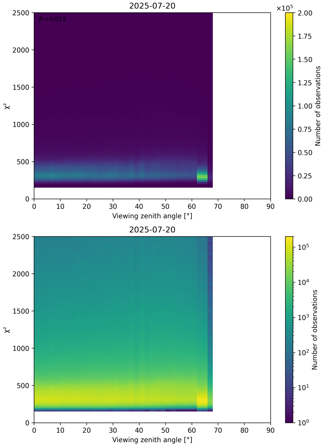
Figure 162: Scatter density plot of “Viewing zenith angle” against “ \chi^2 ” for 2025-07-19 to 2025-07-21.
