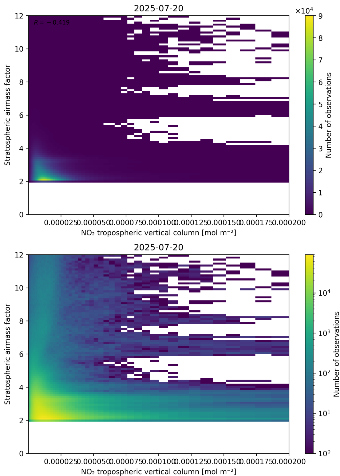
Figure 121: Scatter density plot of “NO 2 tropospheric vertical column” against “Stratospheric air mass factor” for 2025-07-19 to 2025-07-21.
