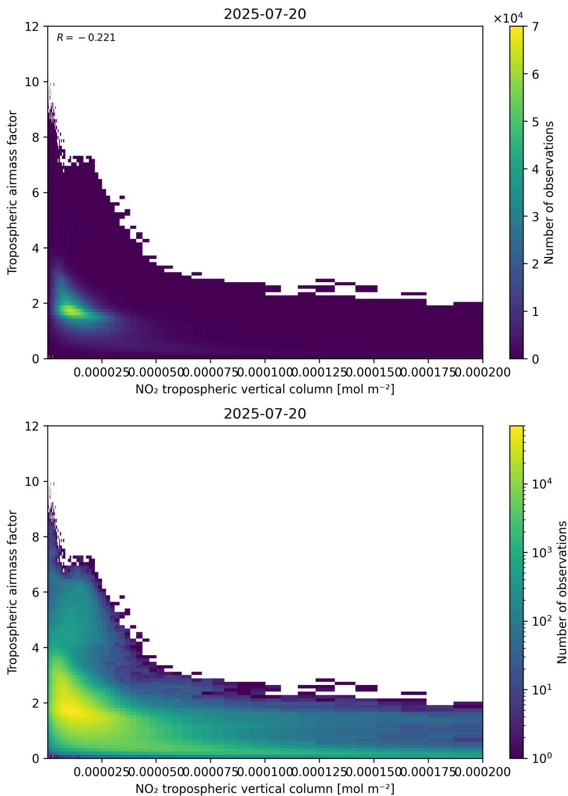
Figure 123: Scatter density plot of “NO 2 tropospheric vertical column” against “Tropospheric air mass factor” for 2025-07-19 to 2025-07-21.
