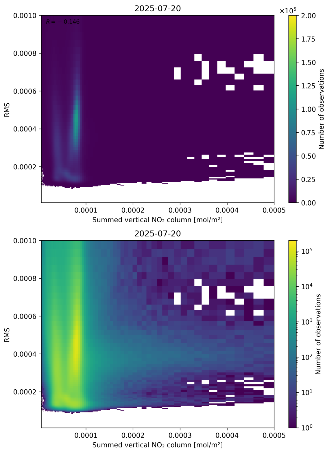
Figure 109: Scatter density plot of “Summed vertical NO 2 column” against “RMS” for 2025-07-19 to 2025-07-21.
