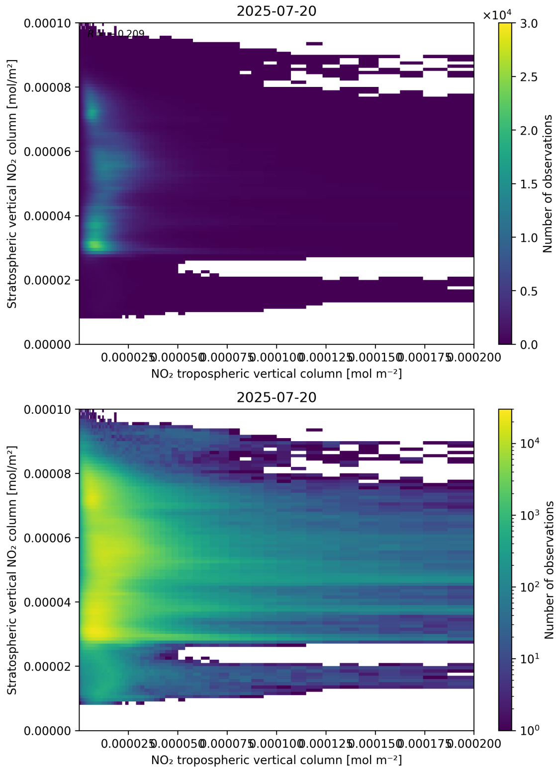
Figure 125: Scatter density plot of “NO 2 tropospheric vertical column” against “Stratospheric vertical NO 2 column” for 2025-07-19 to 2025-07-21.
