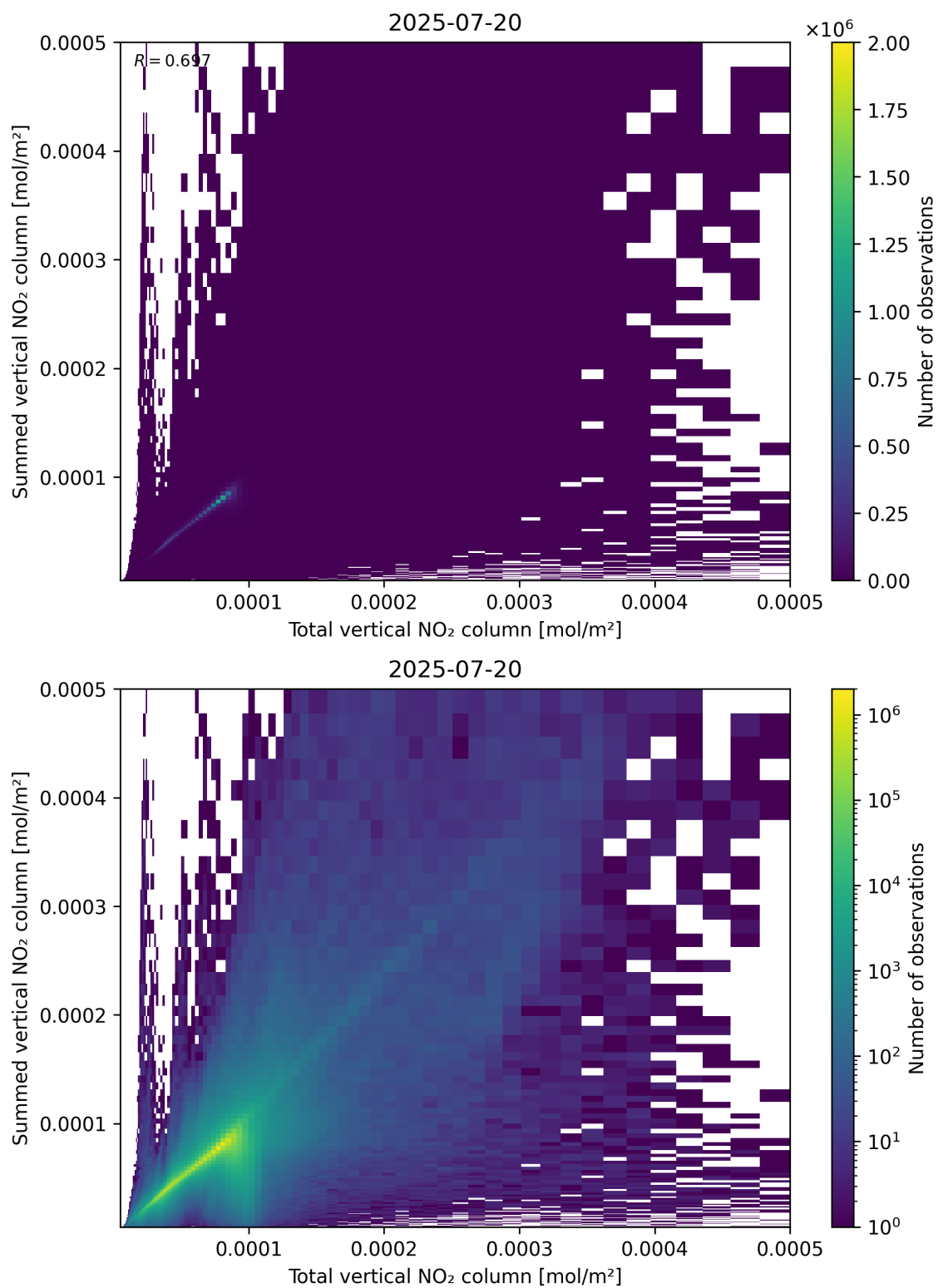
Figure 112: Scatter density plot of “Total vertical NO 2 column” against “Summed vertical NO 2 column” for 2025-07-19 to 2025-07-21.
