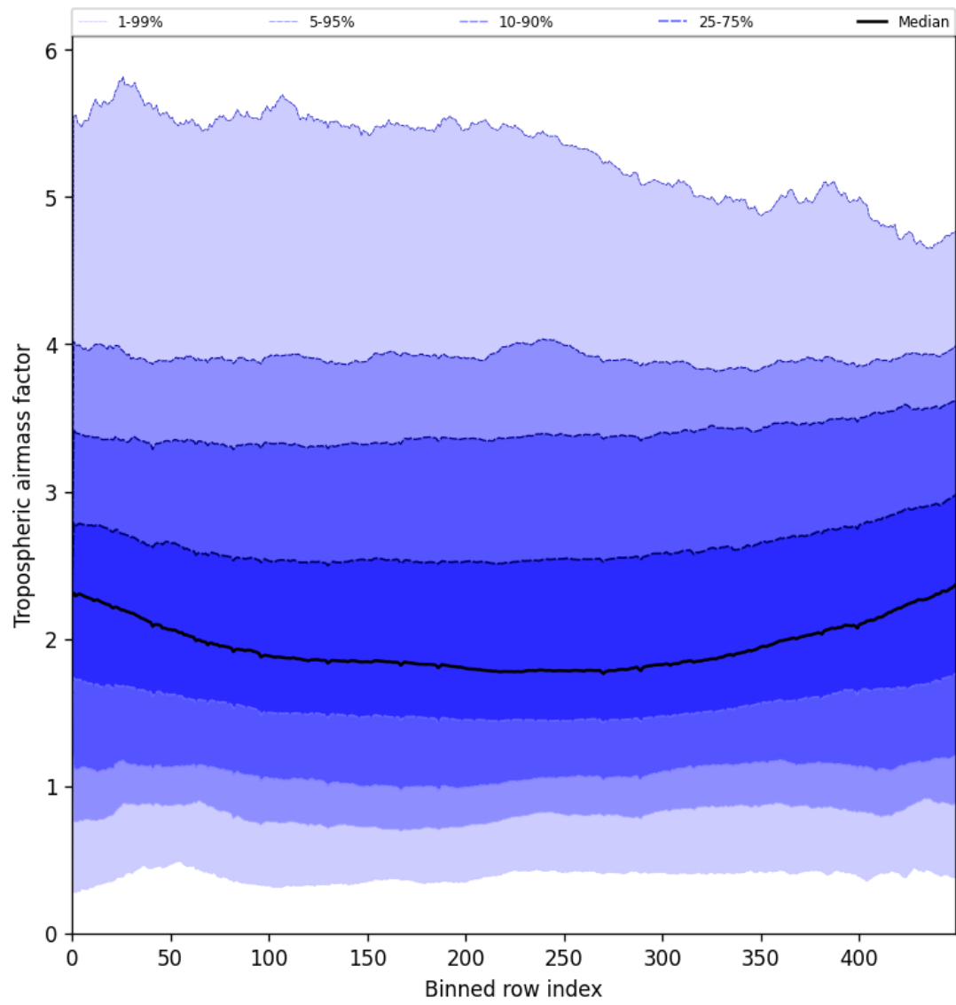
Figure 48: Along track statistics of “Tropospheric airmass factor” for 2025-07-19 to 2025-07-21
