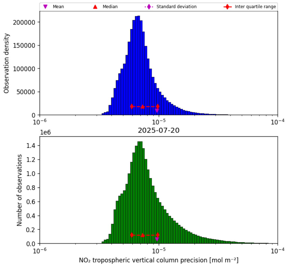
Figure 30: Histogram of “NO 2 tropospheric vertical column precision” for 2025-07-19 to 2025-07-21
