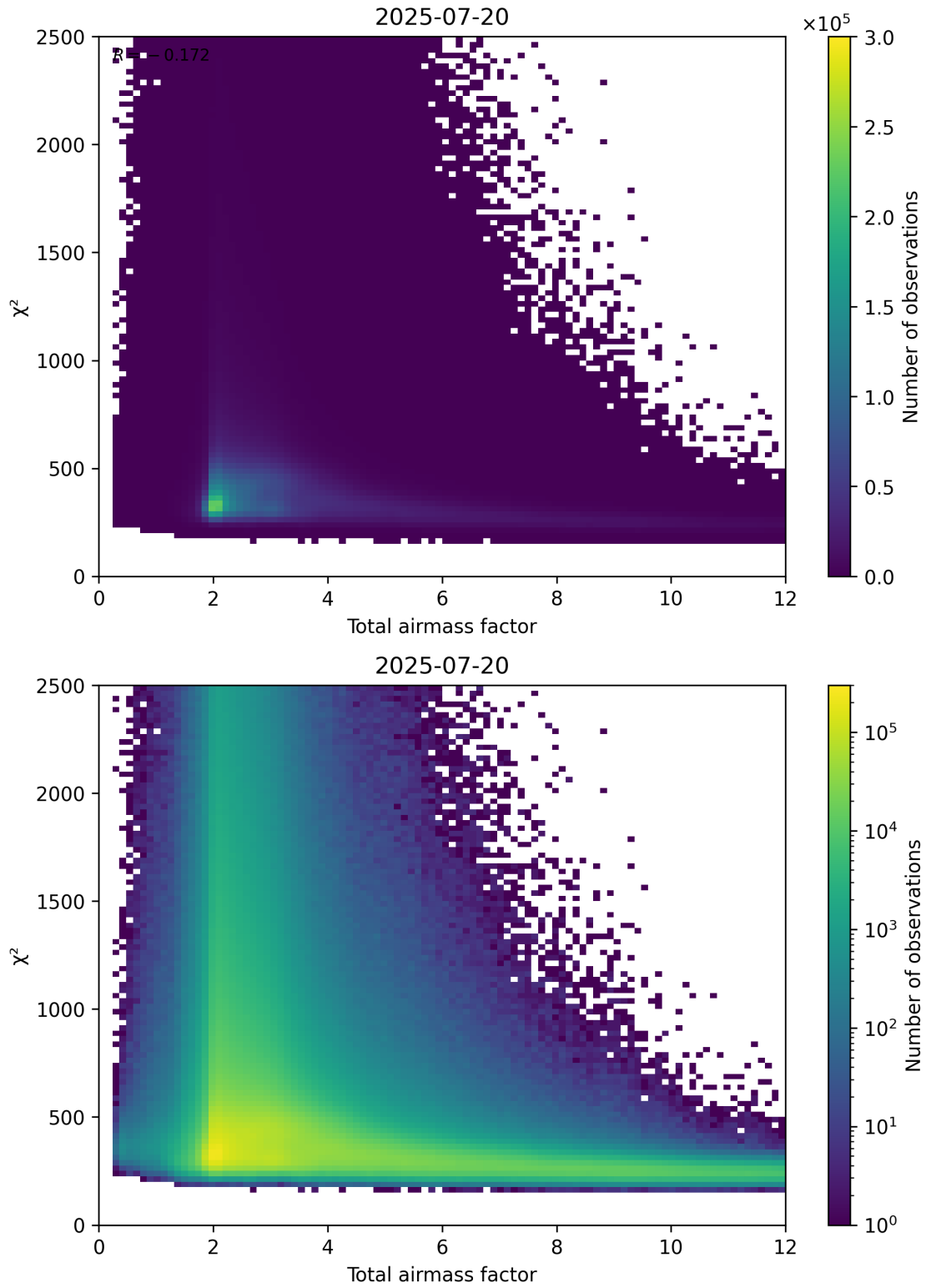
Figure 63: Scatter density plot of “Total airmass factor” against “ \chi^2 ” for 2025-07-19 to 2025-07-21.
