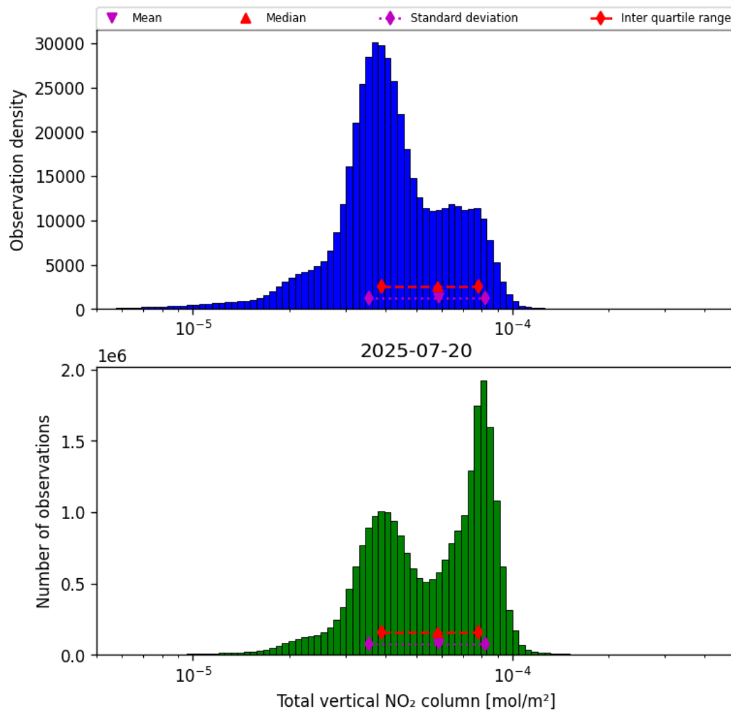
Figure 38: Histogram of "Total vertical NO 2 column" for 2025-07-19 to 2025-07-21
