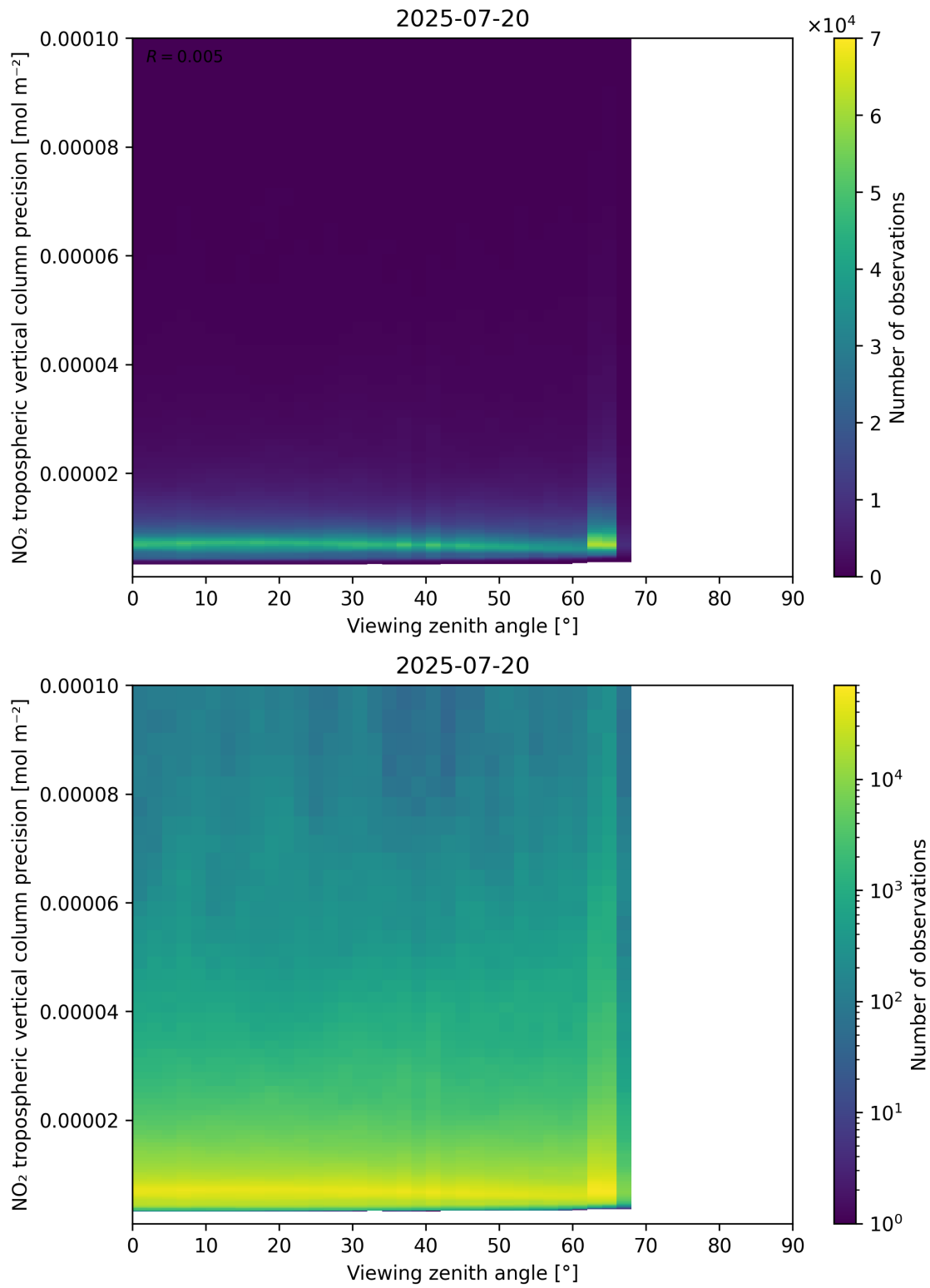
Figure 170: Scatter density plot of “Viewing zenith angle” against “NO 2 tropospheric vertical column precision” for 2025-07-19 to 2025-07-21.
