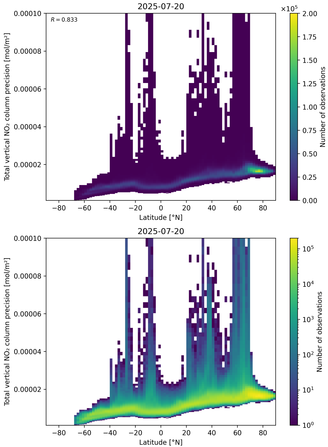
Figure 91: Scatter density plot of “Latitude” against “Total vertical NO 2 column precision” for 2025-07-19 to 2025-07-21.
