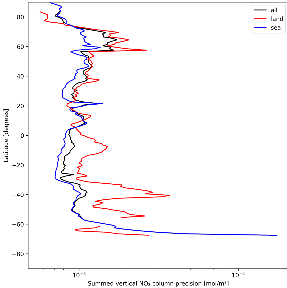
Figure 24: Zonal average of “Summed vertical NO 2 column precision” for 2025-07-19 to 2025-07-21.
