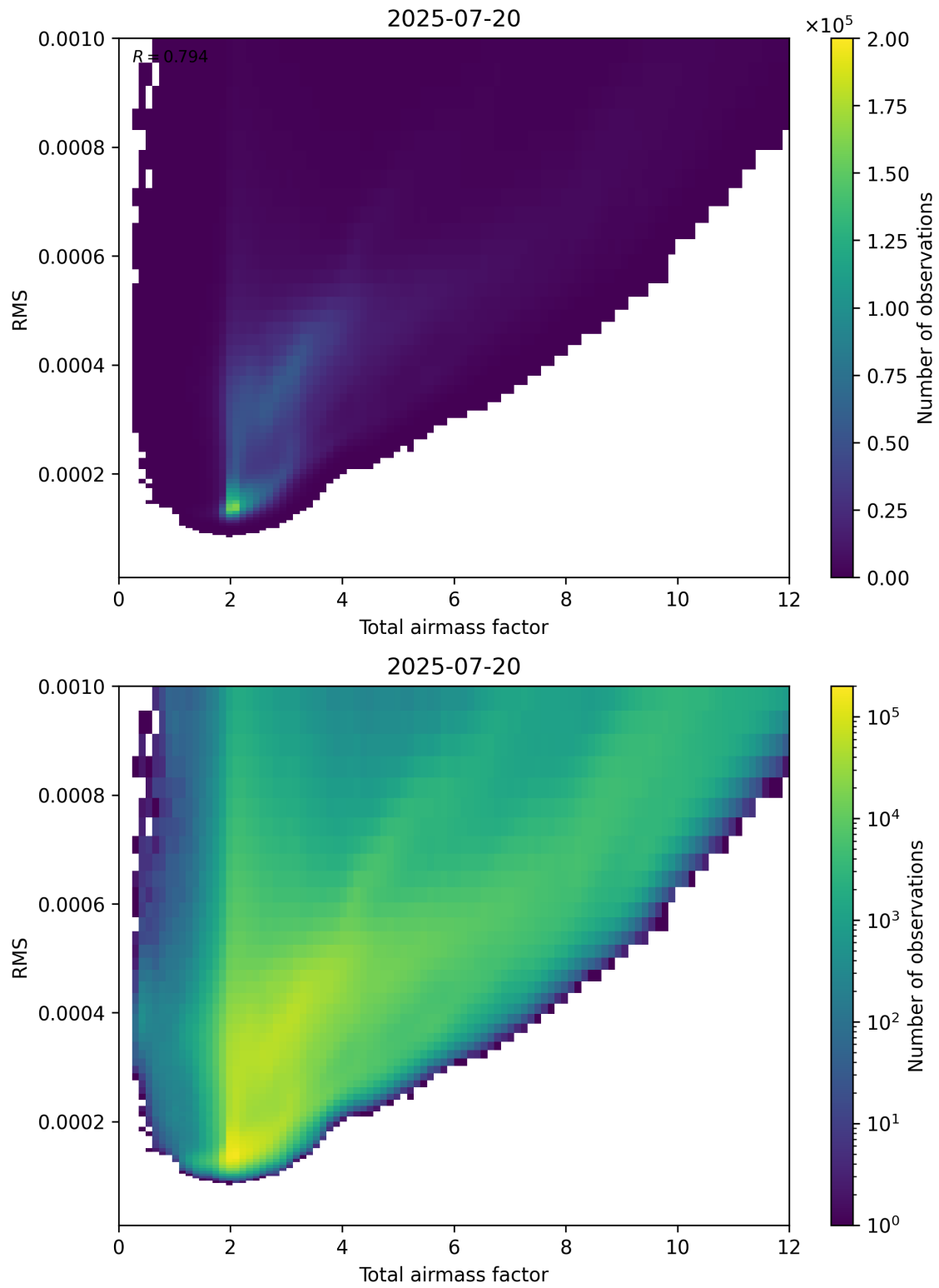
Figure 69: Scatter density plot of “Total airmass factor” against “RMS” for 2025-07-19 to 2025-07-21.
