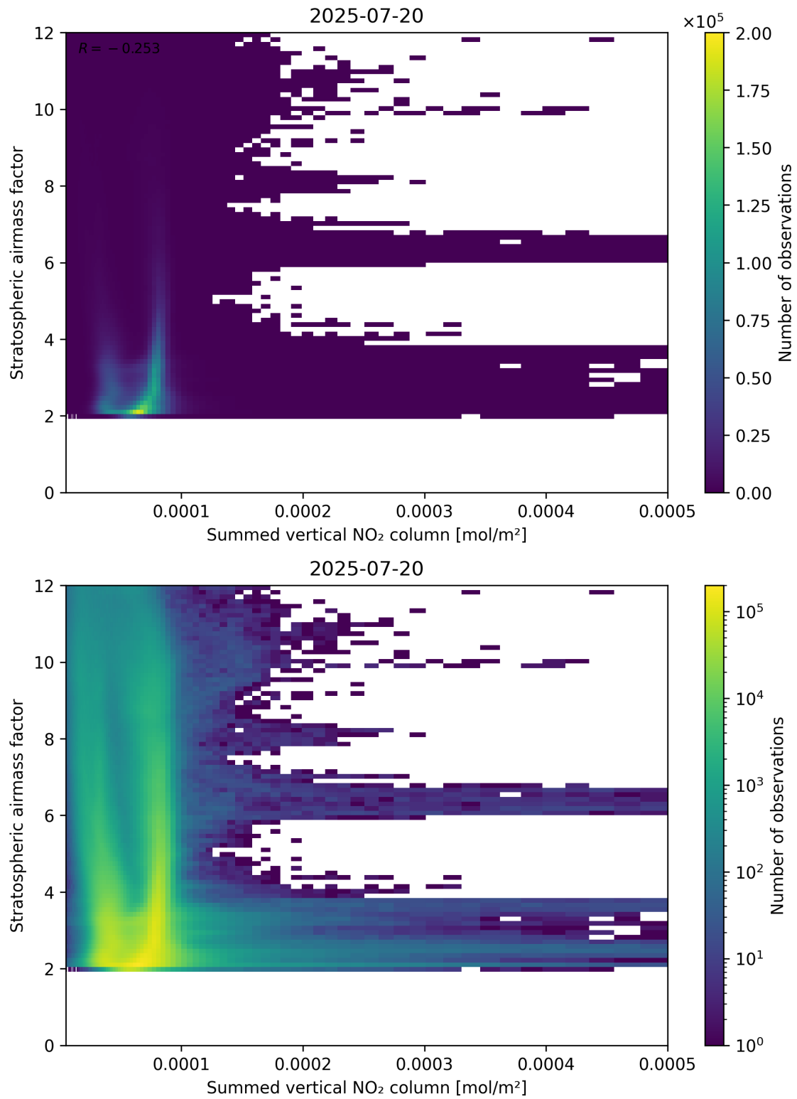
Figure 103: Scatter density plot of “Summed vertical NO 2 column” against “Stratospheric airmass factor” for 2025-07-19 to 2025-07-21.
