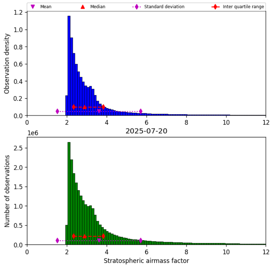
Figure 44: Histogram of “Stratospheric airmass factor” for 2025-07-19 to 2025-07-21
