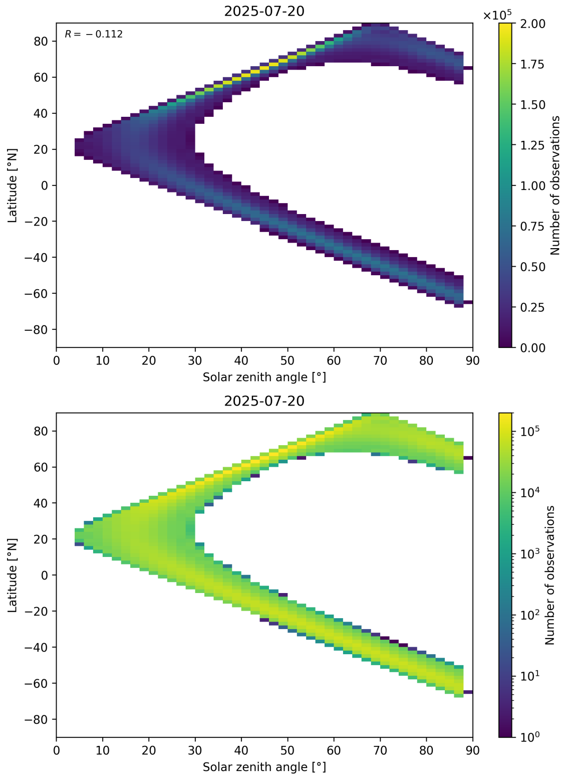
Figure 149: Scatter density plot of “Solar zenith angle” against “Latitude” for 2025-07-19 to 2025-07-21.
