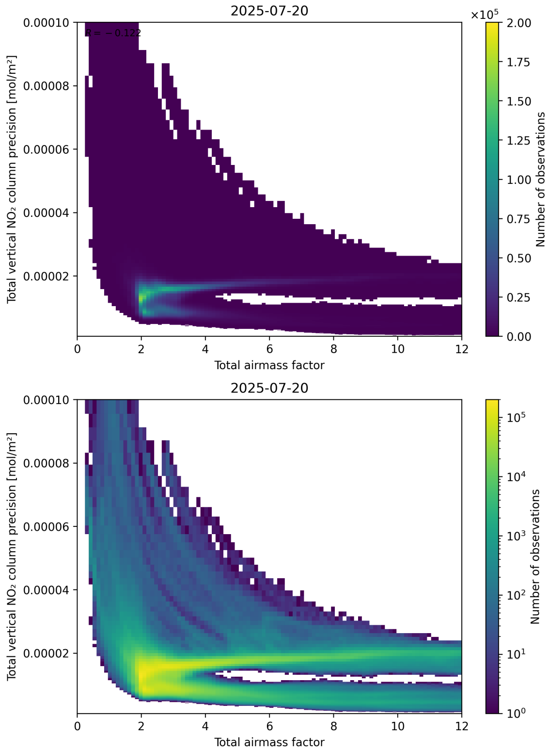
Figure 68: Scatter density plot of “Total airmass factor” against “Total vertical NO 2 column precision” for 2025-07-19 to 2025-07-21.
