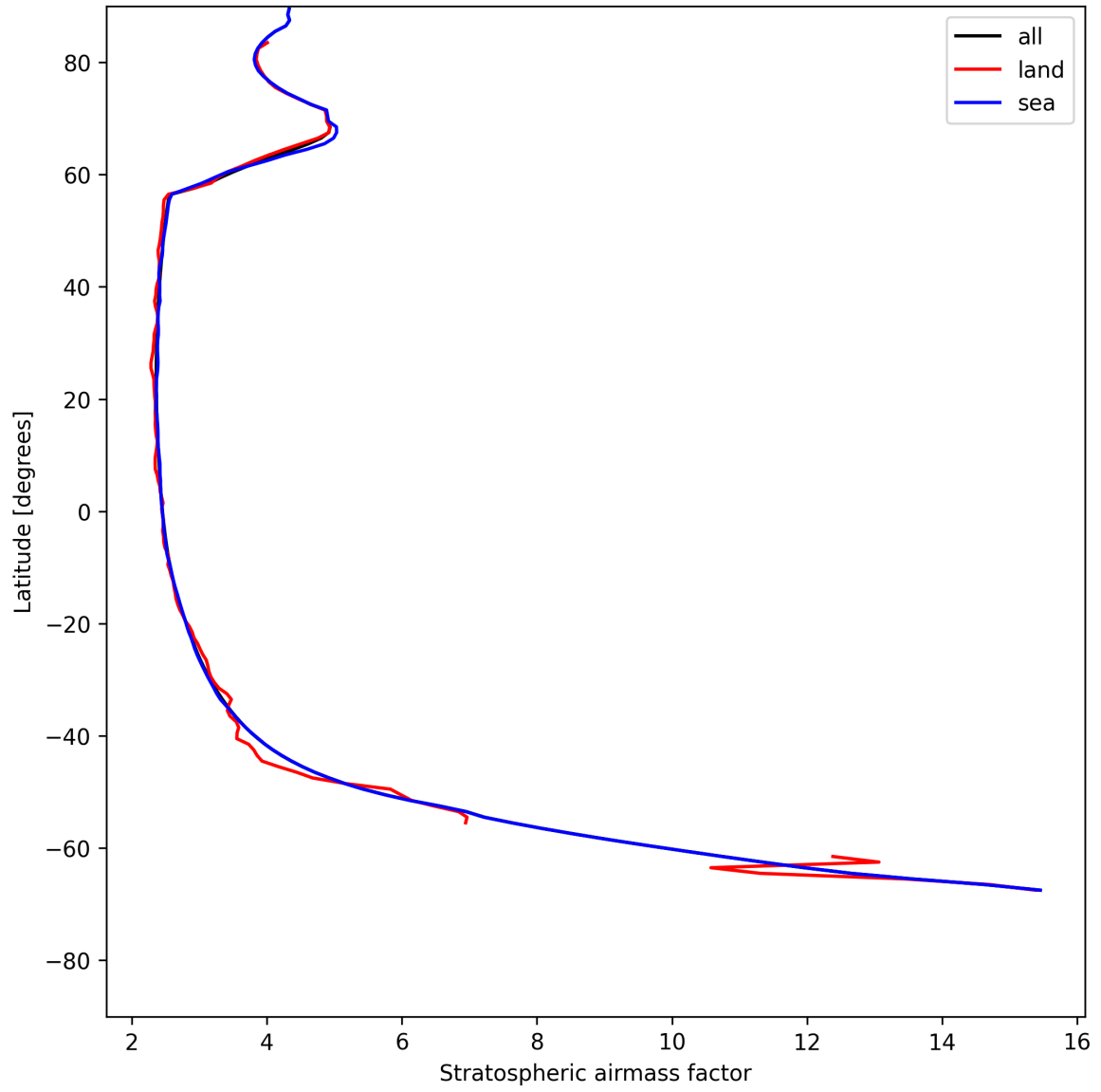
Figure 27: Zonal average of “Stratospheric airmass factor” for 2025-07-19 to 2025-07-21.
