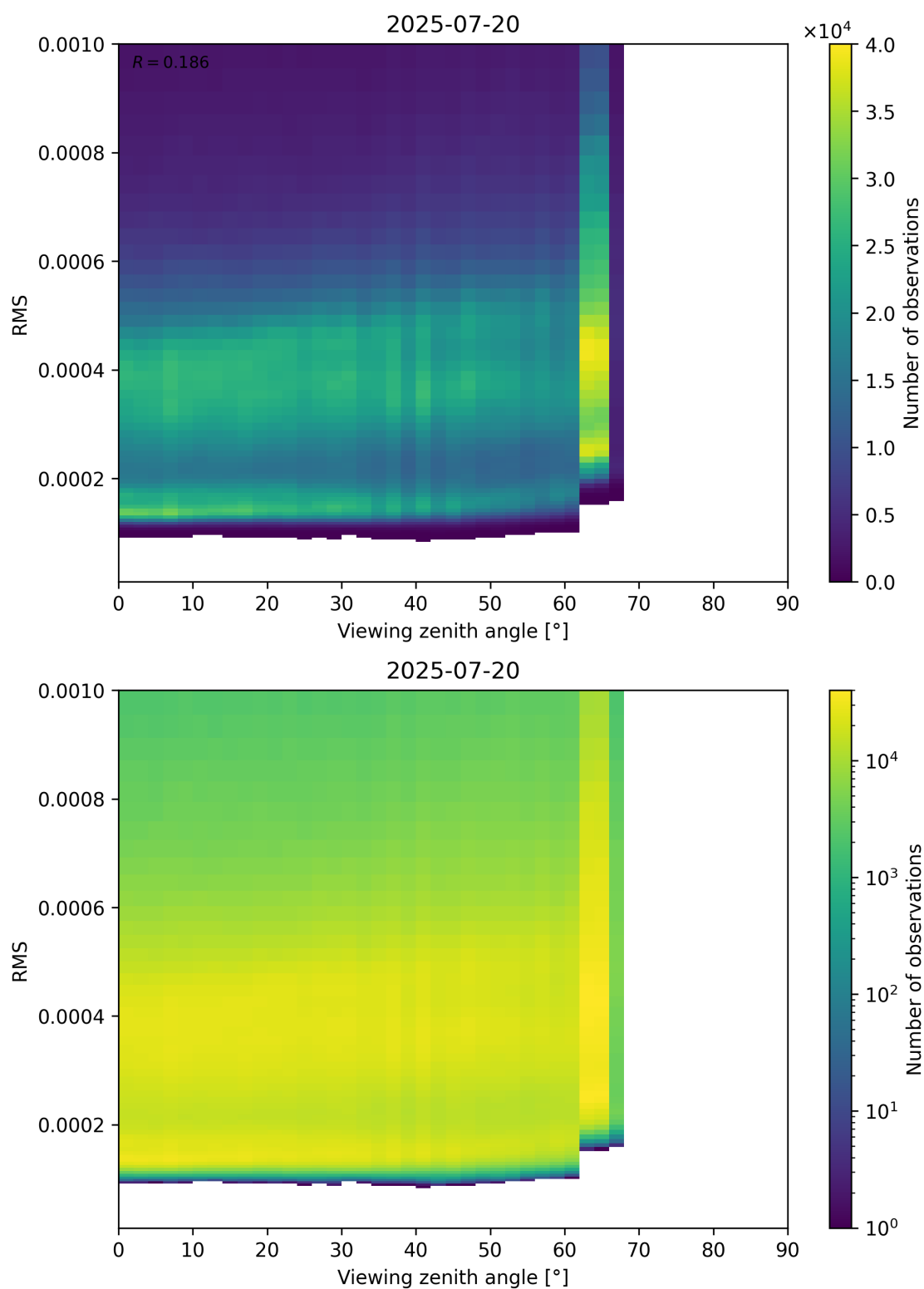
Figure 171: Scatter density plot of “Viewing zenith angle” against “RMS” for 2025-07-19 to 2025-07-21.
