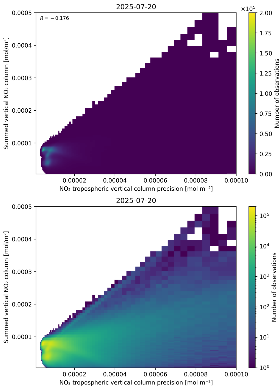
Figure 136: Scatter density plot of “NO 2 tropospheric vertical column precision” against “Summed vertical NO 2 column” for 2025-07-19 to 2025-07-21.
