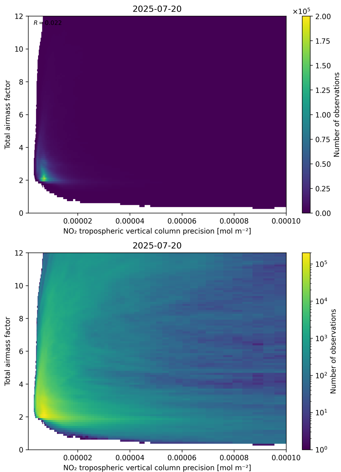
Figure 132: Scatter density plot of “NO 2 tropospheric vertical column precision” against “Total air mass factor” for 2025-07-19 to 2025-07-21.
