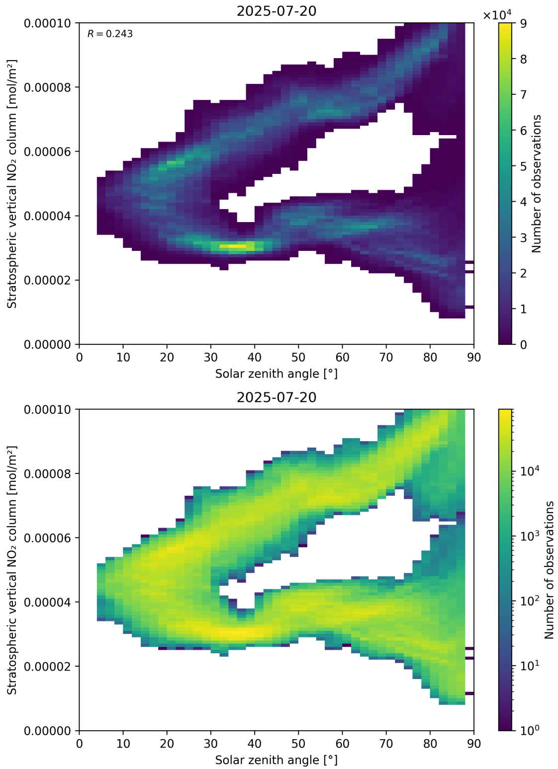
Figure 150: Scatter density plot of “Solar zenith angle” against “Stratospheric vertical NO 2 column” for 2025-07-19 to 2025-07-21.
