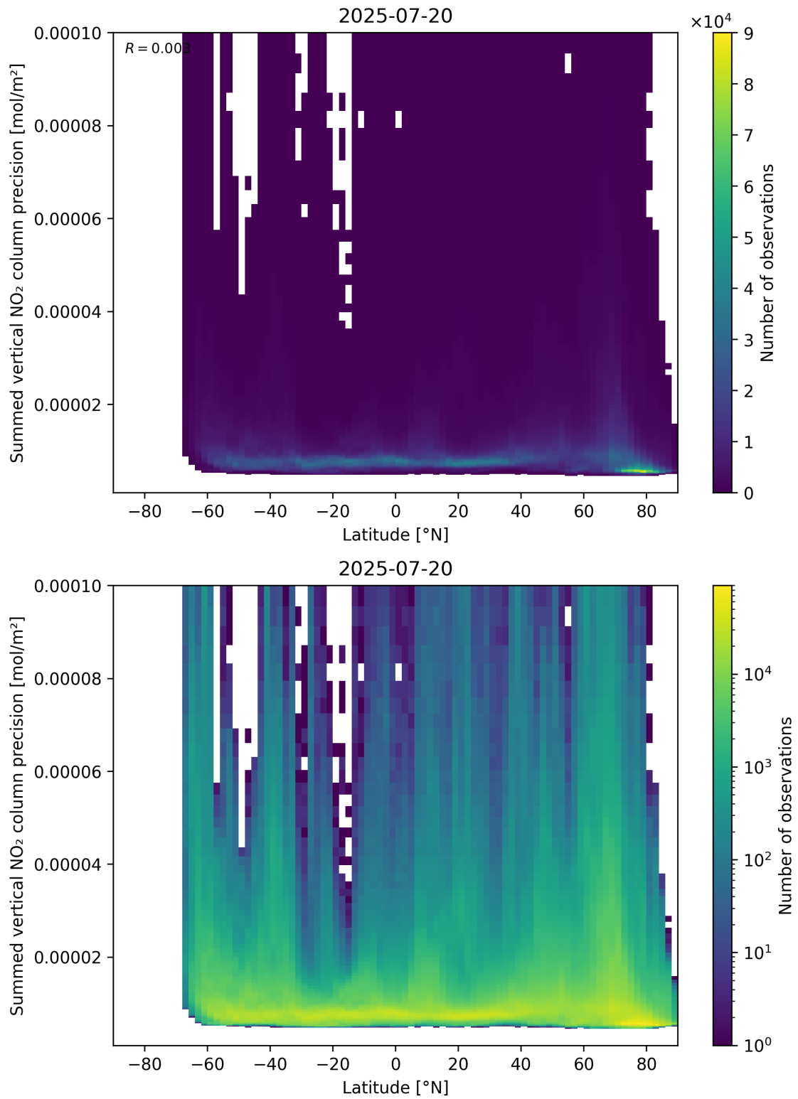
Figure 89: Scatter density plot of “Latitude” against “Summed vertical NO 2 column precision” for 2025-07-19 to 2025-07-21.
