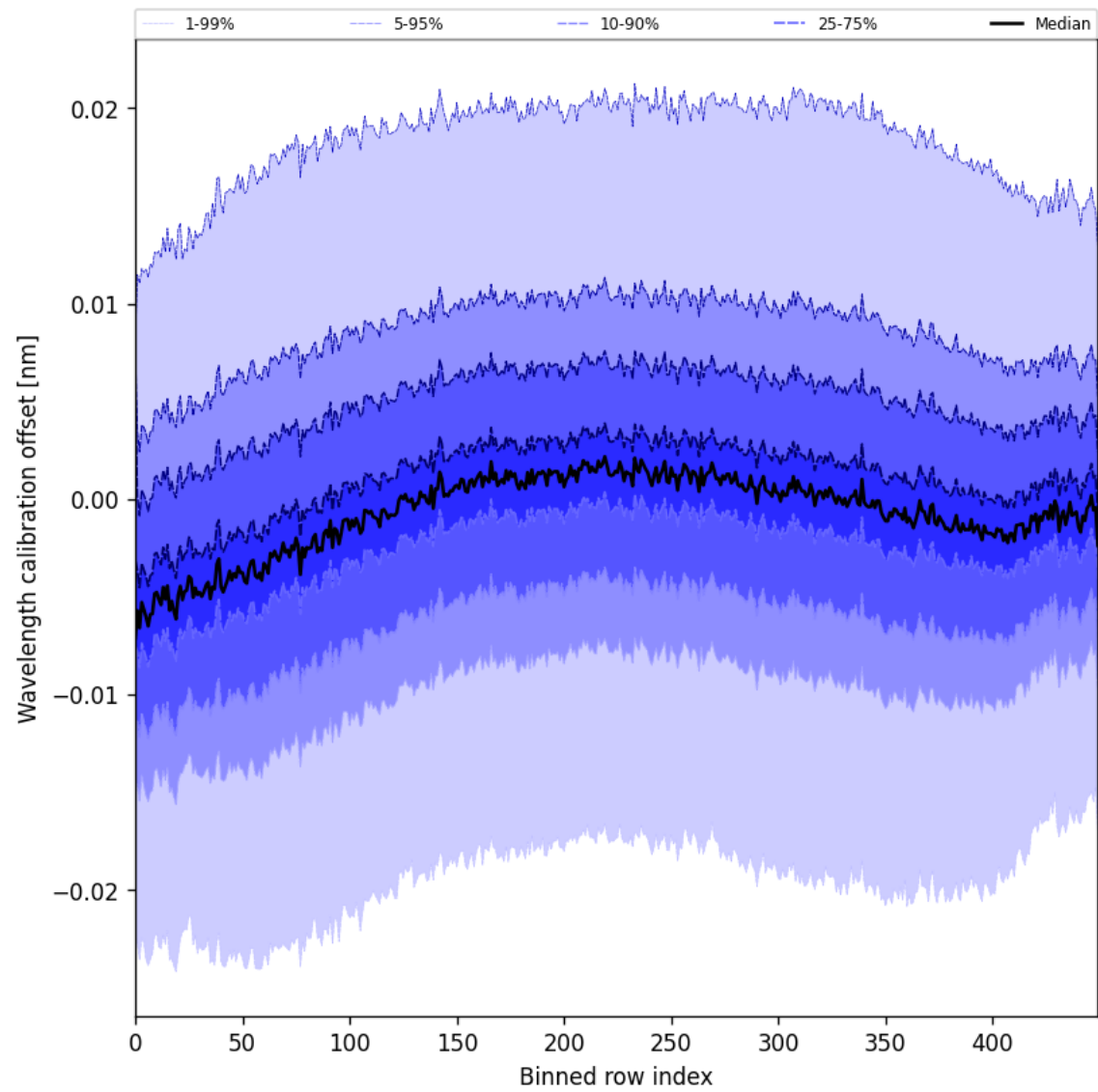
Figure 52: Along track statistics of “Wavelength calibration offset” for 2025-07-19 to 2025-07-21
