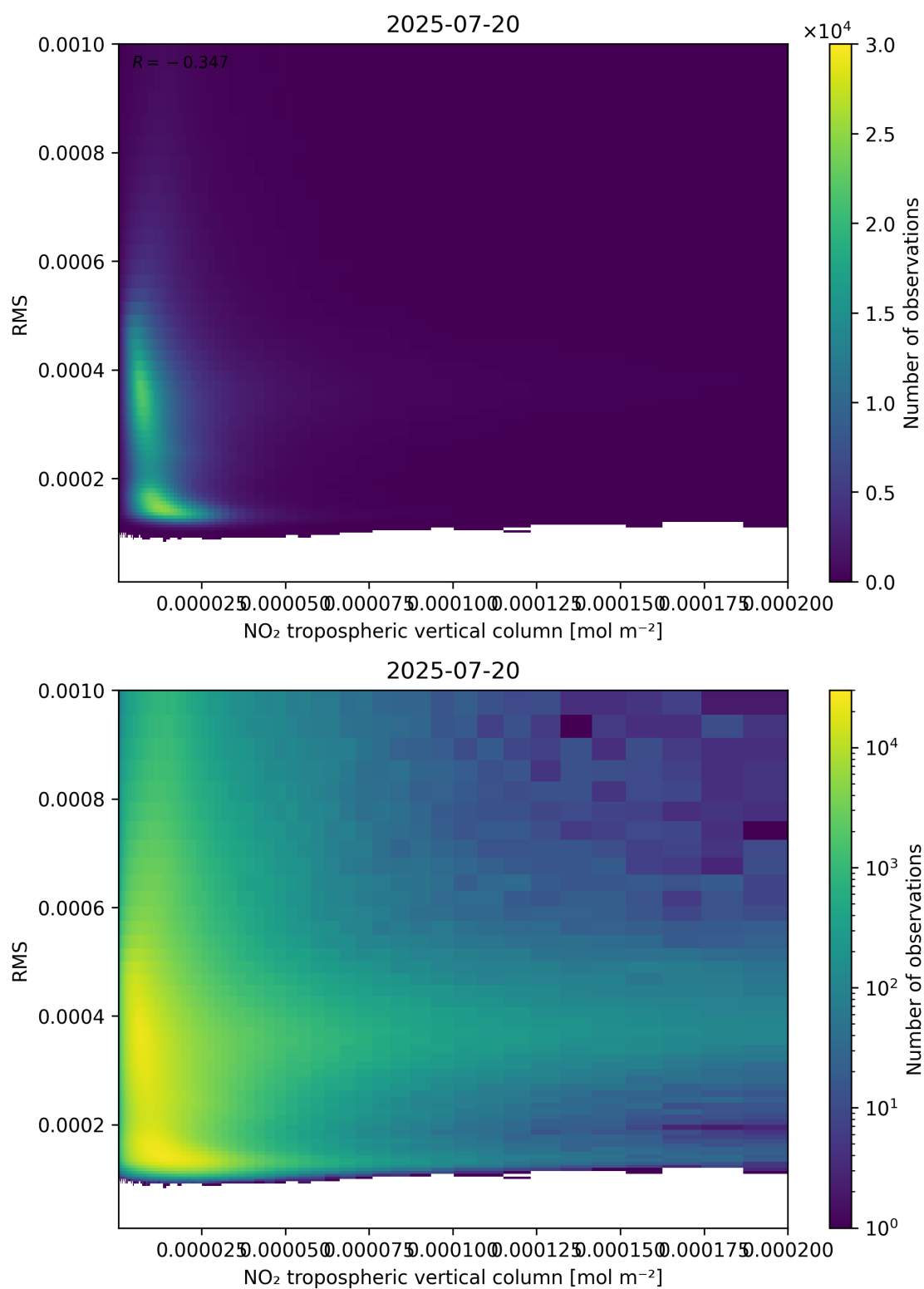
Figure 142: Scatter density plot of “NO 2 tropospheric vertical column” against “RMS” for 2025-07-19 to 2025-07-21.
