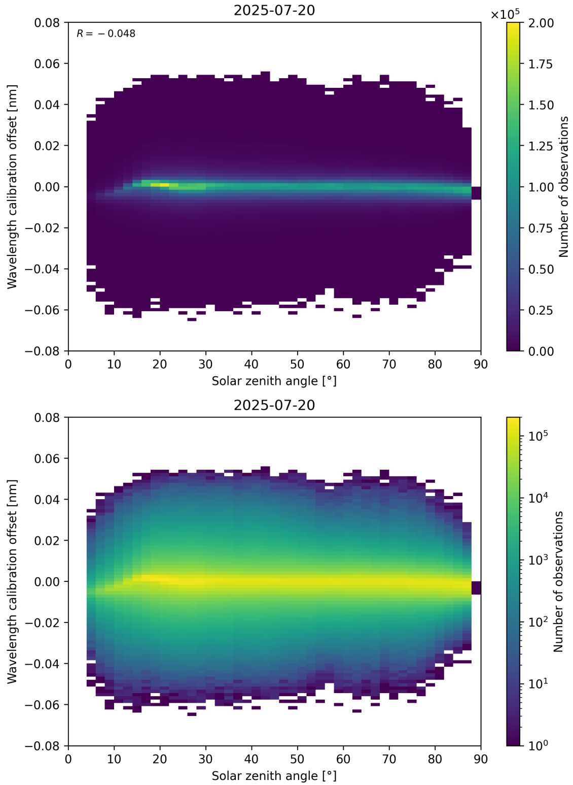
Figure 158: Scatter density plot of “Solar zenith angle” against “Wavelength calibration offset” for 2025-07-19 to 2025-07-21.
