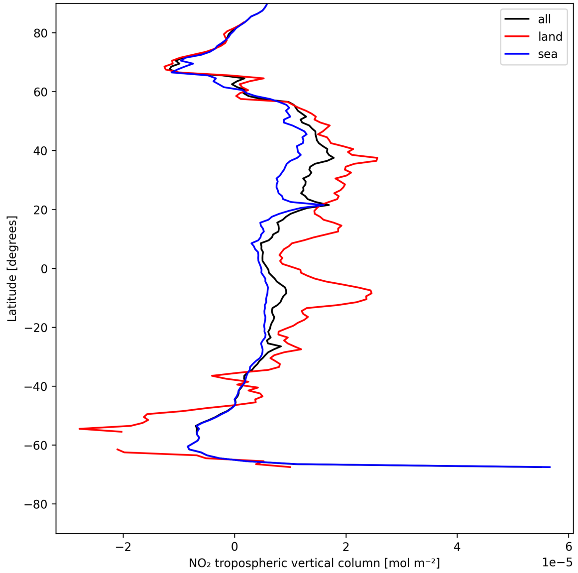
Figure 12: Zonal average of “NO 2 tropospheric vertical column” for 2025-07-19 to 2025-07-21.
