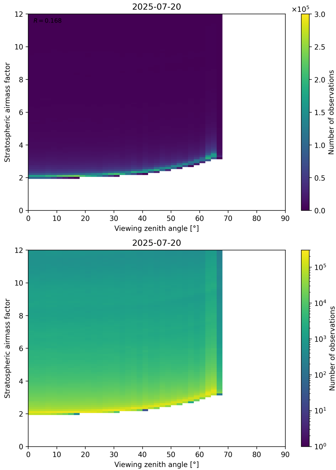
Figure 159: Scatter density plot of “Viewing zenith angle” against “Stratospheric airmass factor” for 2025-07-19 to 2025-07-21.
