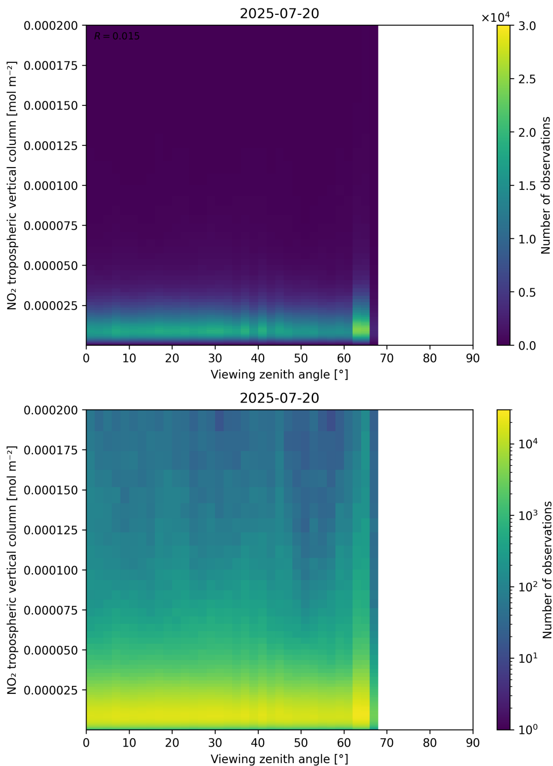
Figure 169: Scatter density plot of “Viewing zenith angle” against “NO 2 tropospheric vertical column” for 2025-07-19 to 2025-07-21.
