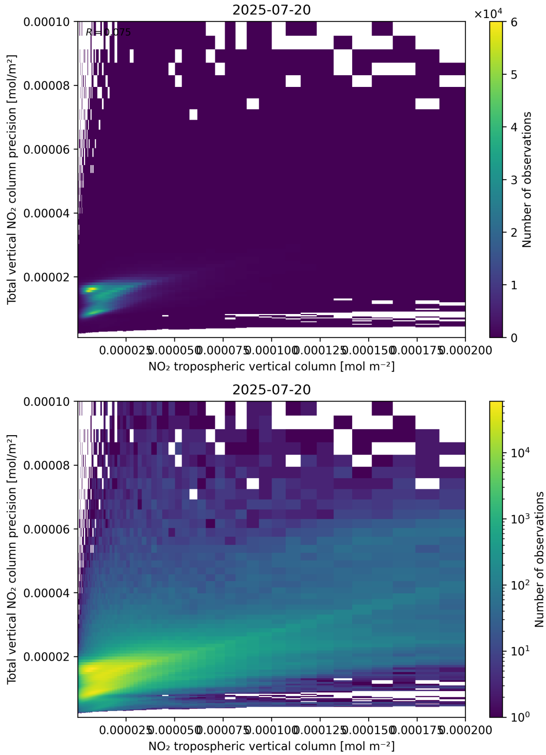
Figure 129: Scatter density plot of “NO 2 tropospheric vertical column” against “Total vertical NO 2 column precision” for 2025-07-19 to 2025-07-21.
