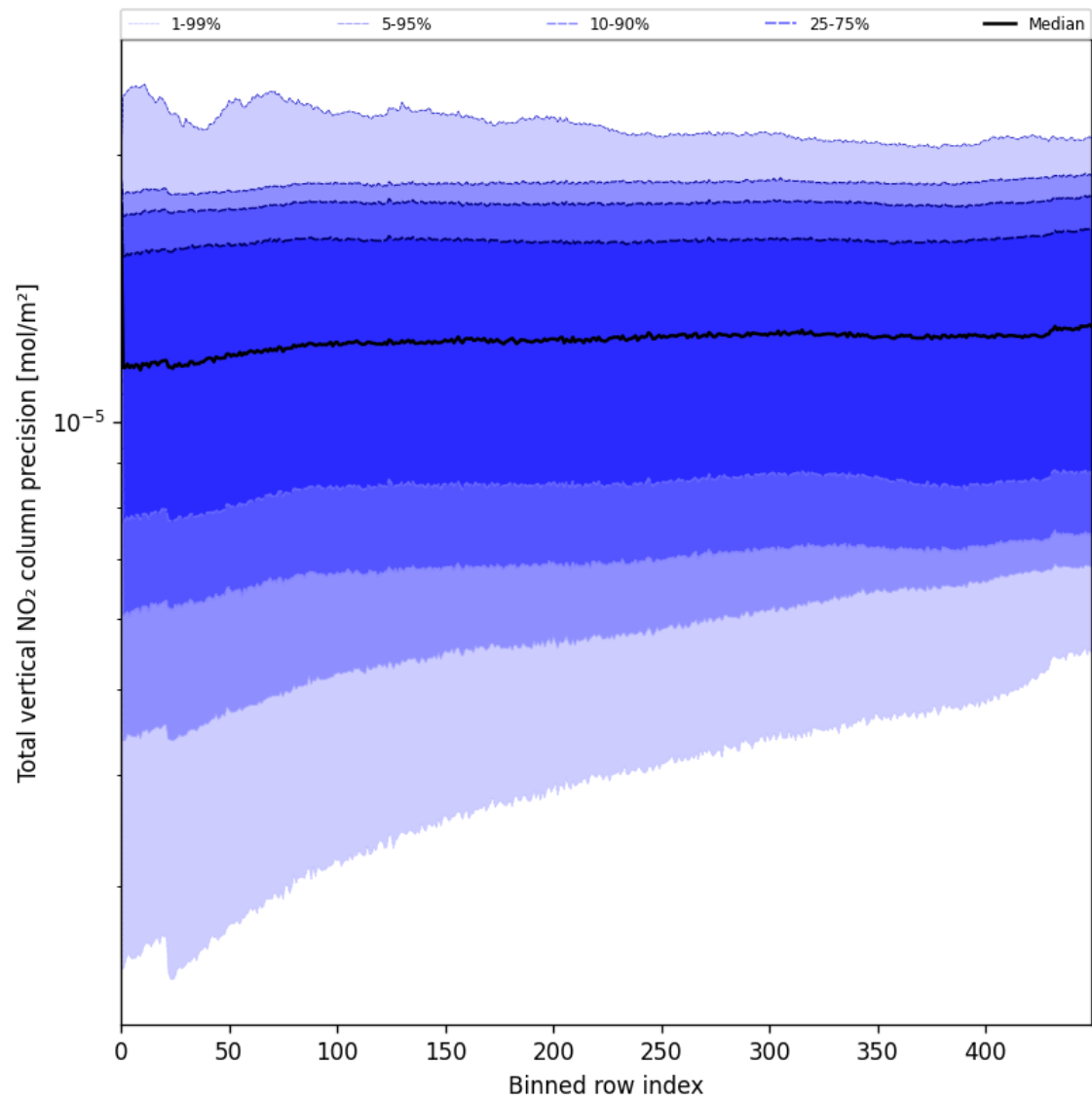
Figure 56: Along track statistics of “Total vertical NO 2 column precision” for 2025-07-19 to 2025-07-21
