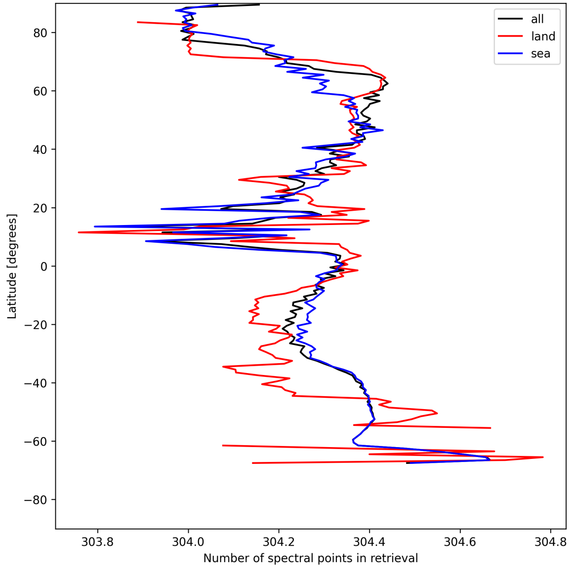
Figure 16: Zonal average of “Number of spectral points in retrieval” for 2025-07-19 to 2025-07-21.
