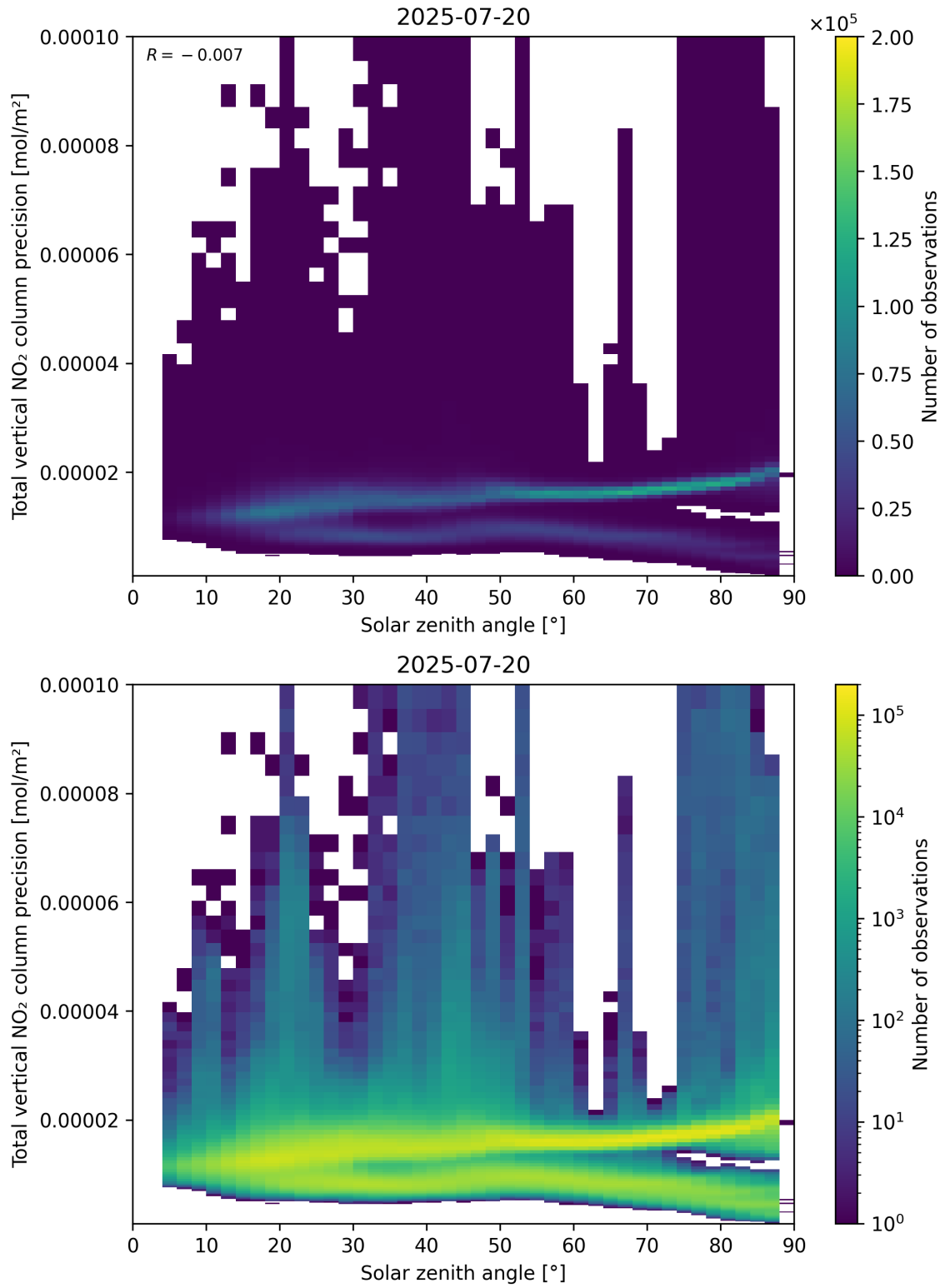
Figure 154: Scatter density plot of “Solar zenith angle” against “Total vertical NO 2 column precision” for 2025-07-19 to 2025-07-21.
