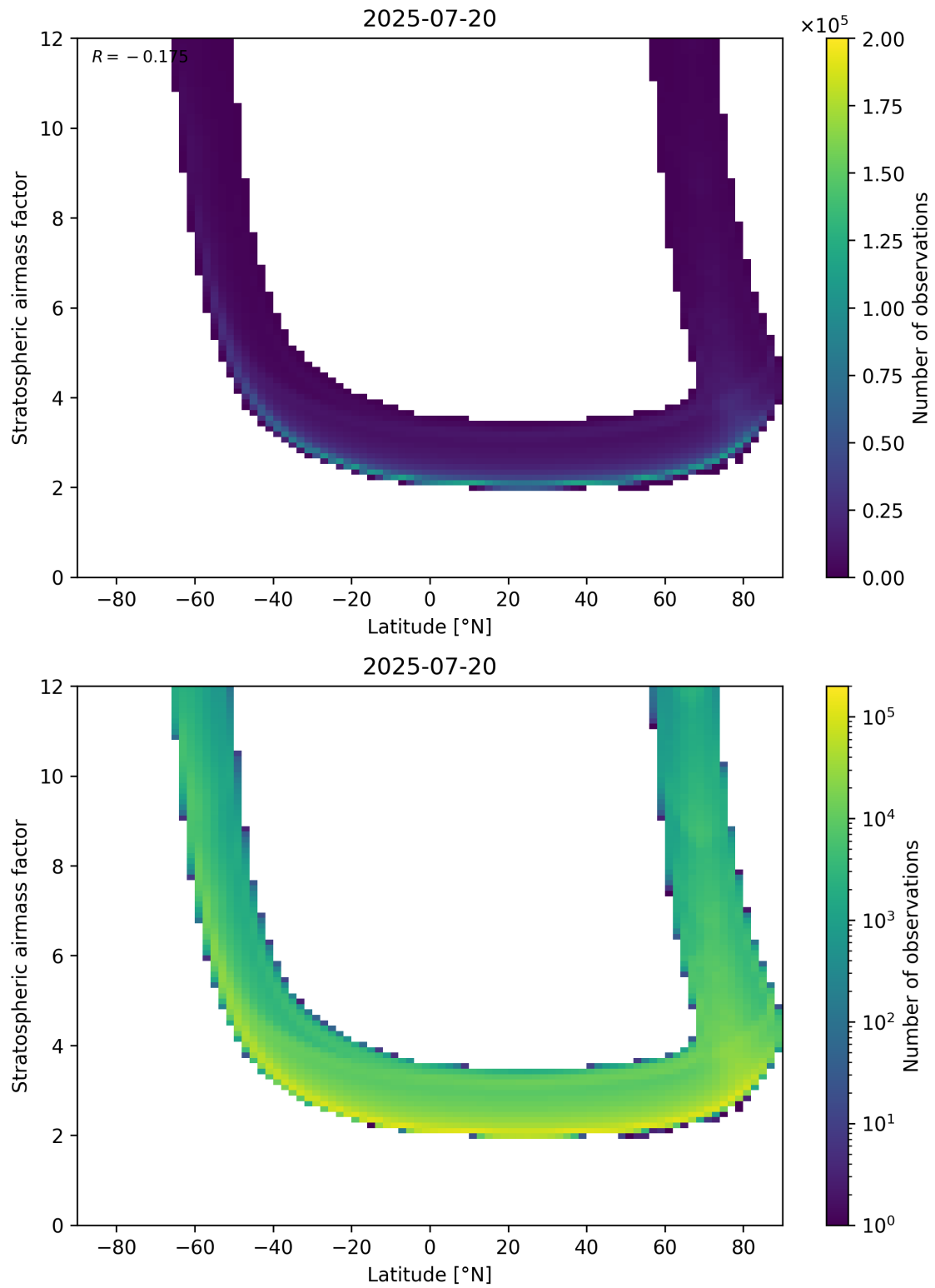
Figure 83: Scatter density plot of “Latitude” against “Stratospheric air mass factor” for 2025-07-19 to 2025-07-21.
