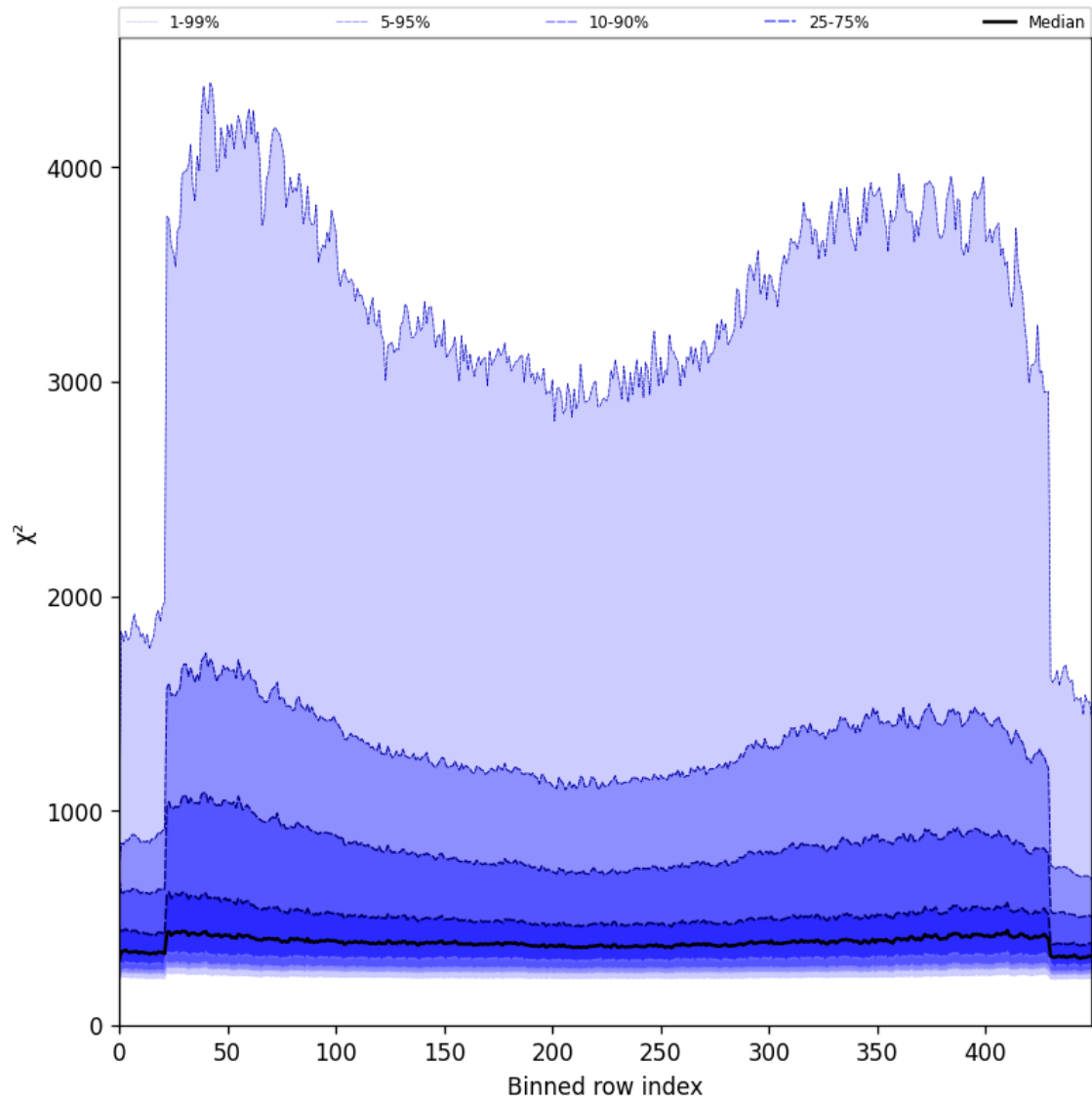
Figure 59: Along track statistics of “ \chi^2 ” for 2025-07-19 to 2025-07-21
