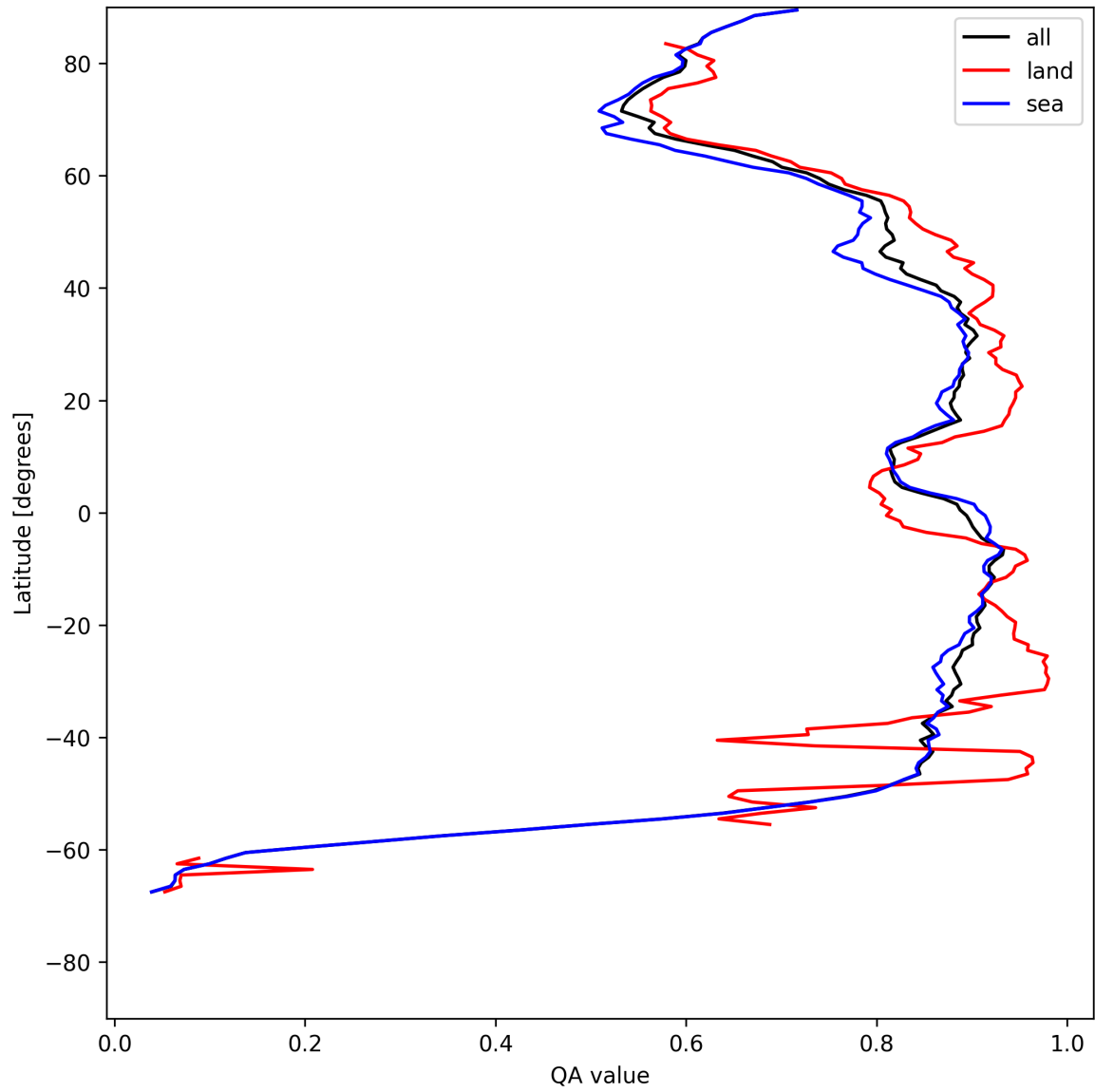
Figure 11: Zonal average of “QA value” for 2025-07-19 to 2025-07-21.
