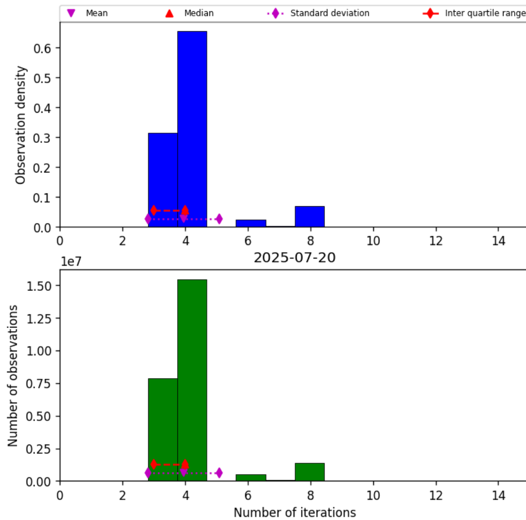
Figure 34: Histogram of “Number of iterations” for 2025-07-19 to 2025-07-21
