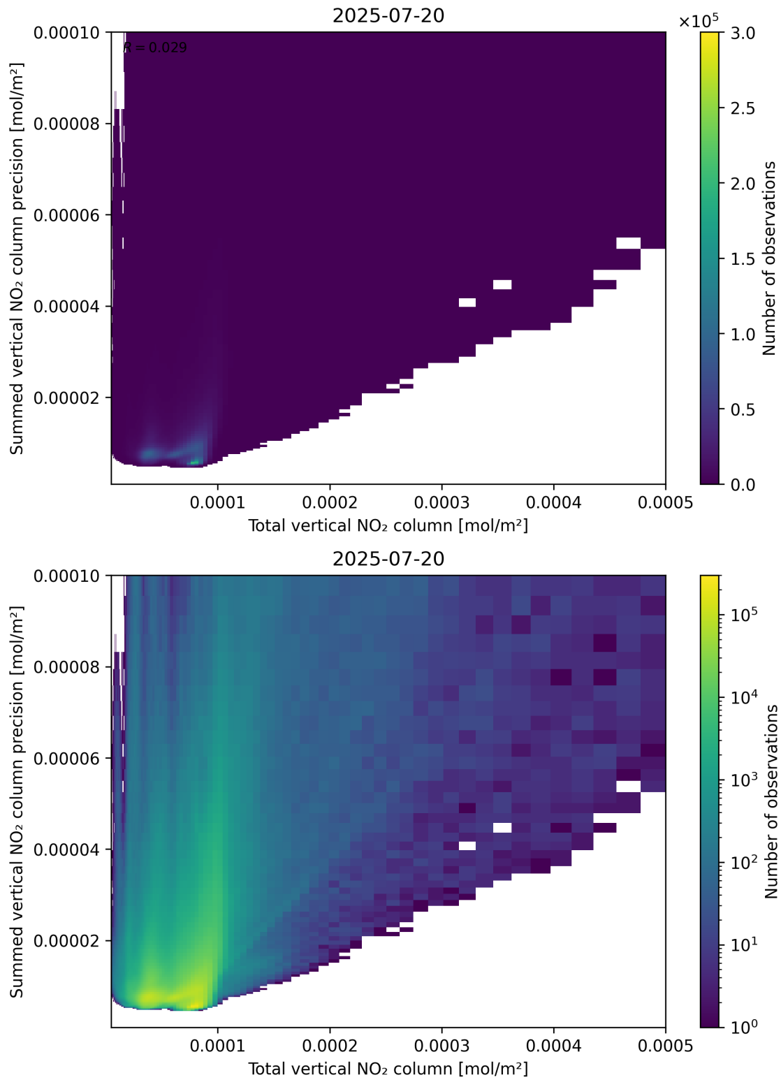
Figure 113: Scatter density plot of “Total vertical NO 2 column” against “Summed vertical NO 2 column precision” for 2025-07-19 to 2025-07-21.
