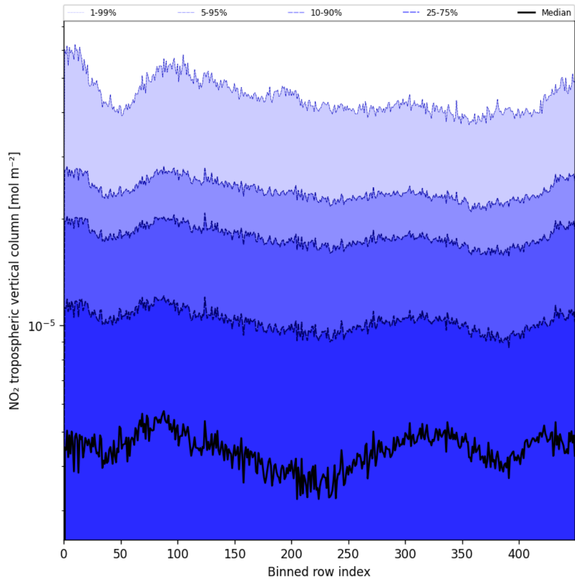
Figure 46: Along track statistics of “NO 2 tropospheric vertical column” for 2025-07-19 to 2025-07-21
