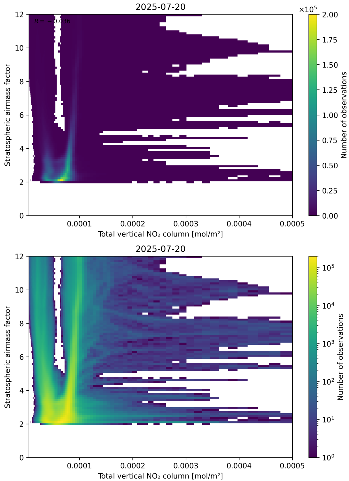
Figure 110: Scatter density plot of “Total vertical NO 2 column” against “Stratospheric air mass factor” for 2025-07-19 to 2025-07-21.
