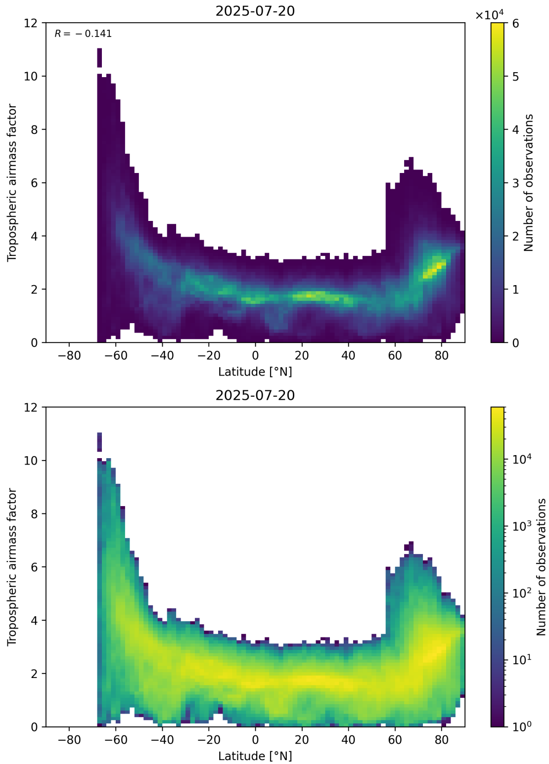
Figure 85: Scatter density plot of “Latitude” against “Tropospheric airmass factor” for 2025-07-19 to 2025-07-21.
