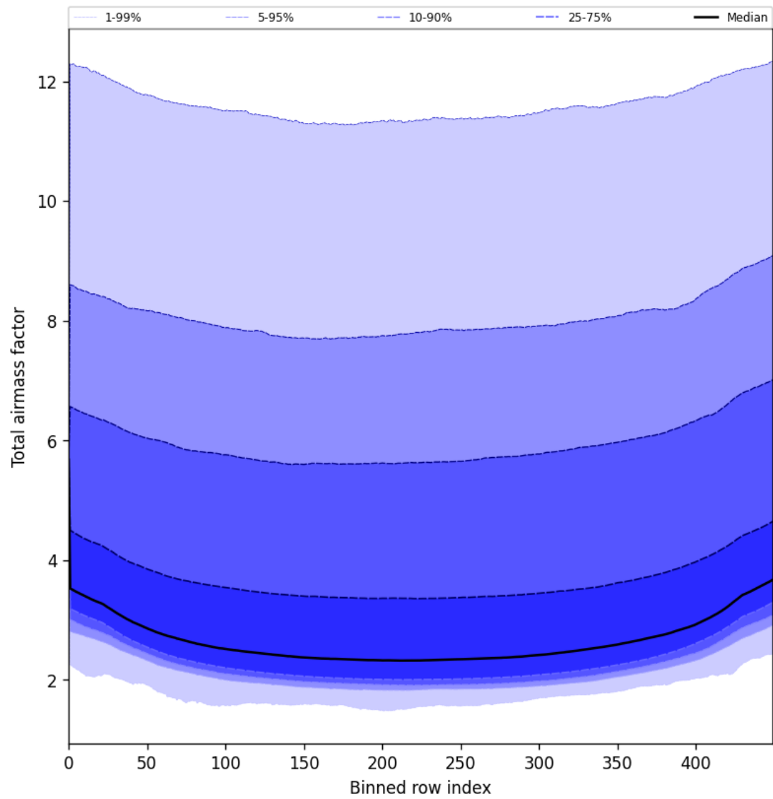
Figure 49: Along track statistics of “Total airmass factor” for 2025-07-19 to 2025-07-21
