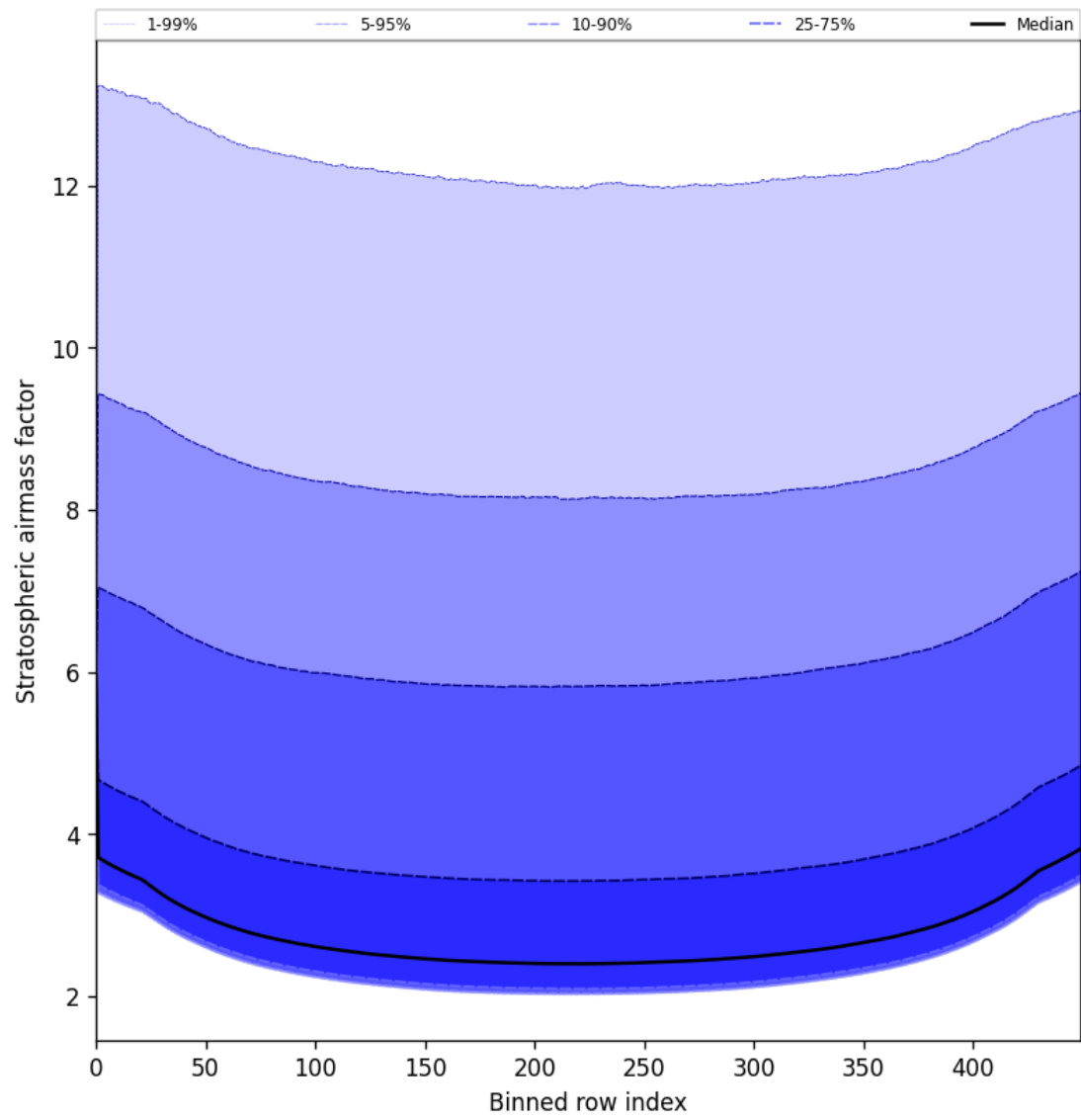
Figure 61: Along track statistics of “Stratospheric airmass factor” for 2025-07-19 to 2025-07-21
