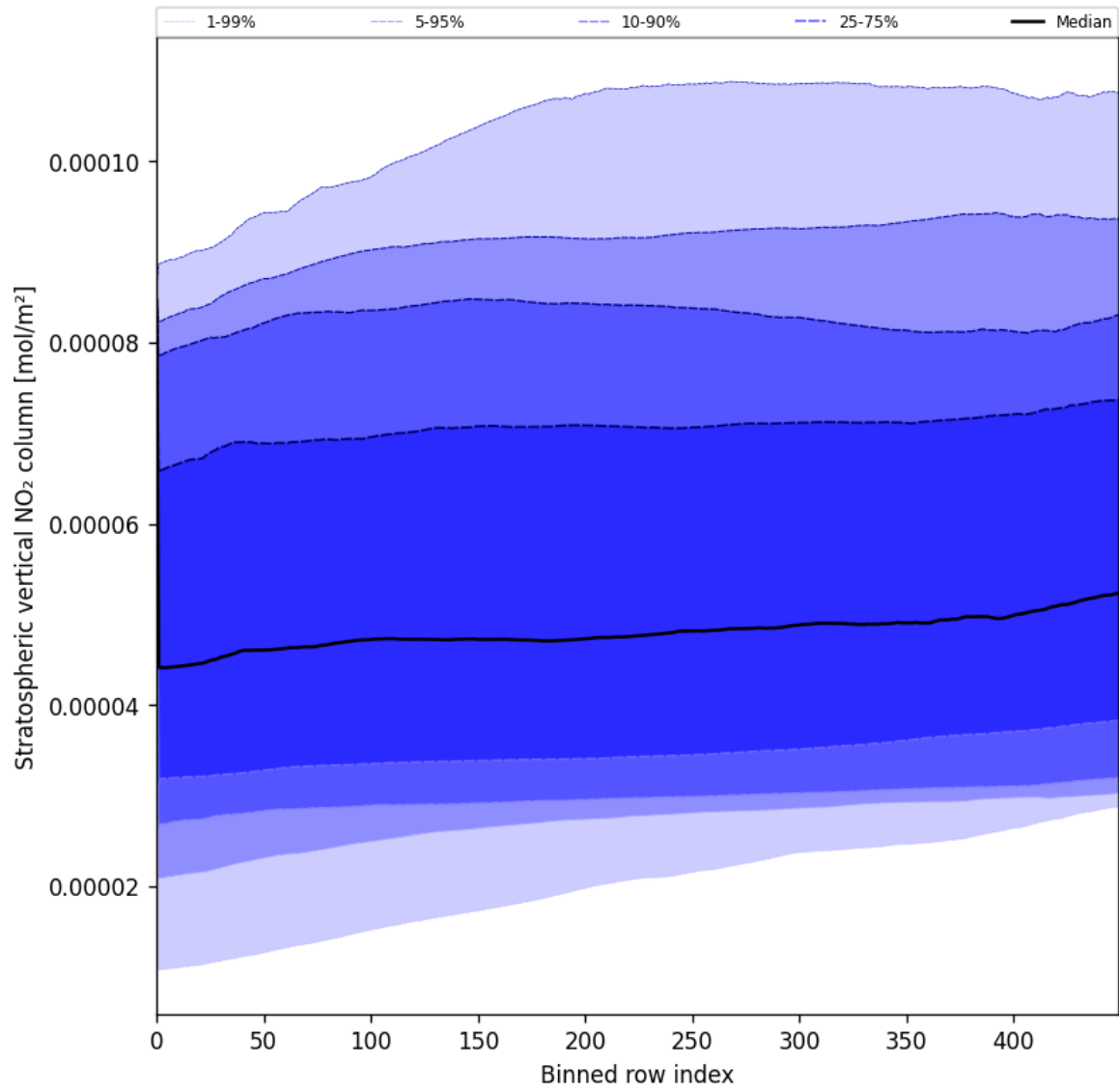
Figure 53: Along track statistics of “Stratospheric vertical NO 2 column” for 2025-07-19 to 2025-07-21
