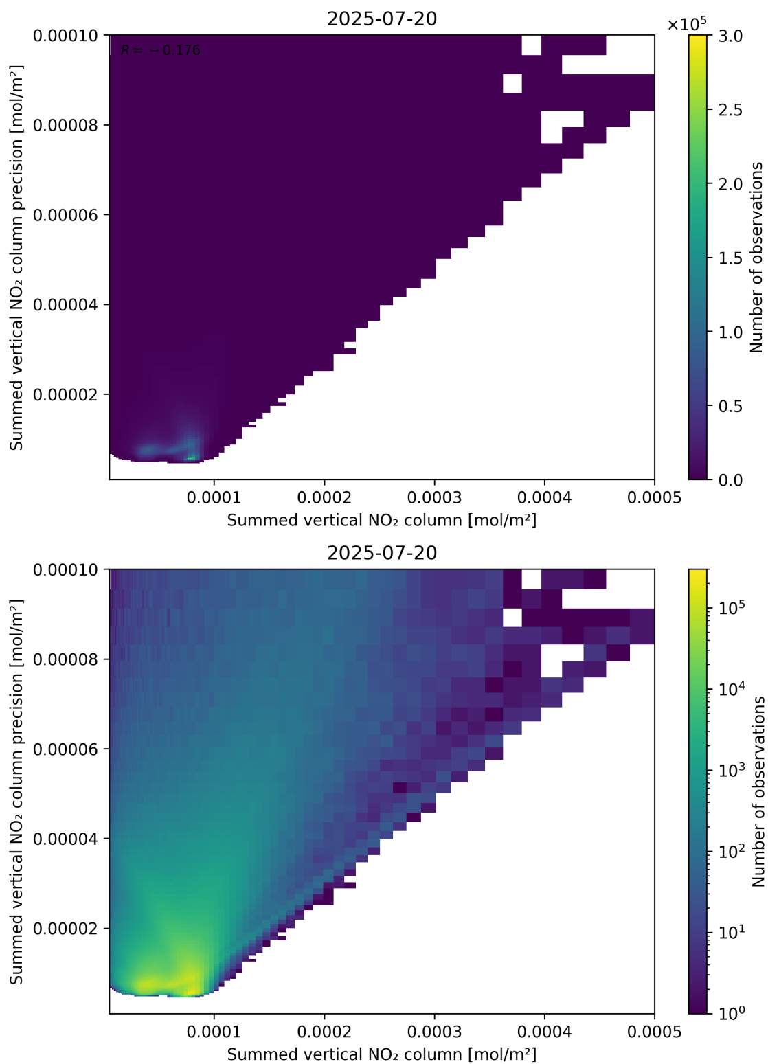
Figure 105: Scatter density plot of “Summed vertical NO 2 column” against “Summed vertical NO 2 column precision” for 2025-07-19 to 2025-07-21.
