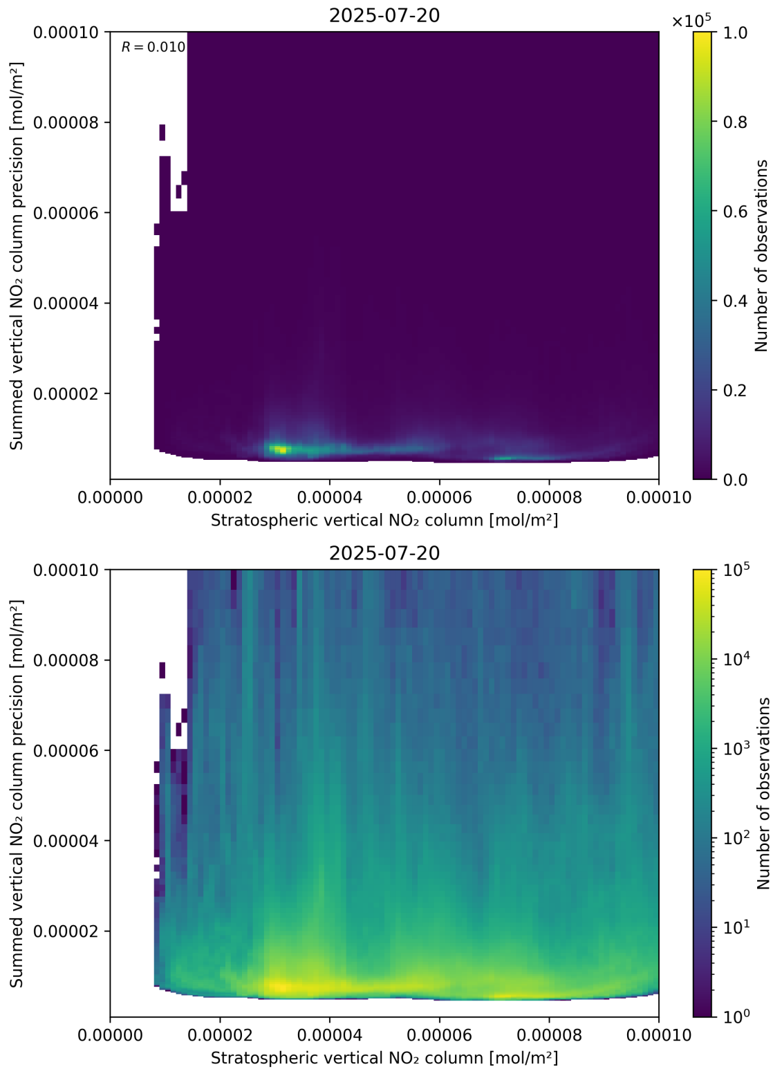
Figure 99: Scatter density plot of “Stratospheric vertical NO 2 column” against “Summed vertical NO 2 column precision” for 2025-07-19 to 2025-07-21.
