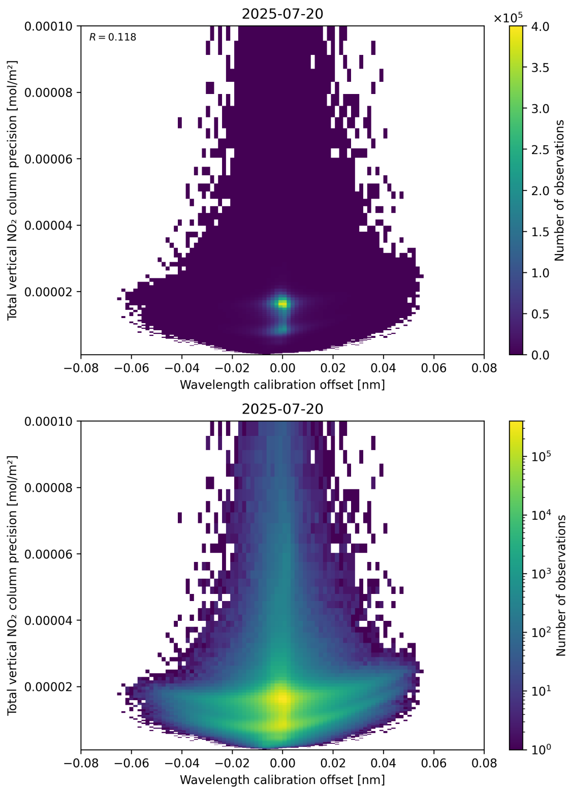
Figure 180: Scatter density plot of “Wavelength calibration offset” against “Total vertical NO 2 column precision” for 2025-07-19 to 2025-07-21.
