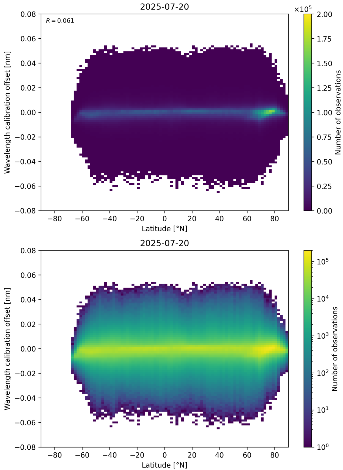
Figure 95: Scatter density plot of “Latitude” against “Wavelength calibration offset” for 2025-07-19 to 2025-07-21.
