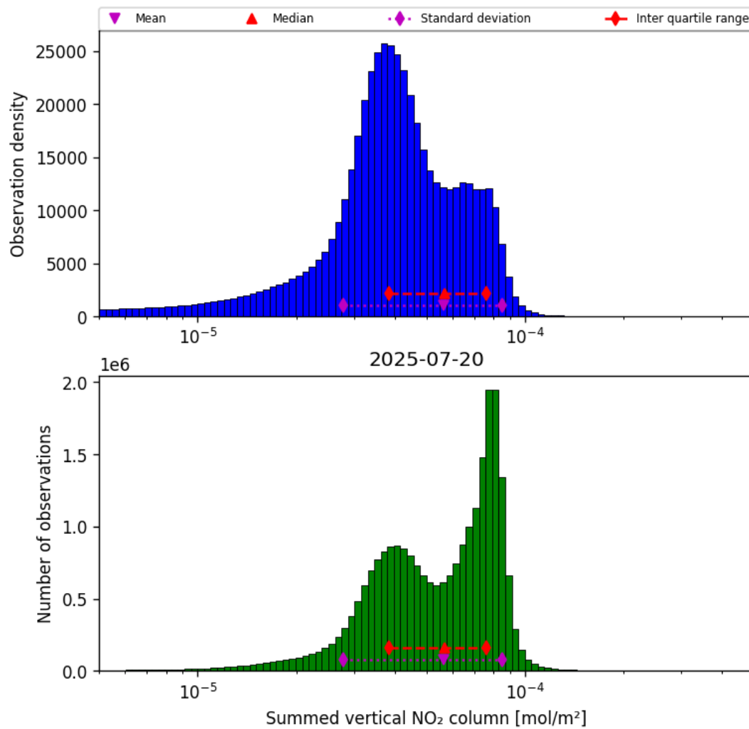
Figure 40: Histogram of “Summed vertical NO 2 column” for 2025-07-19 to 2025-07-21
