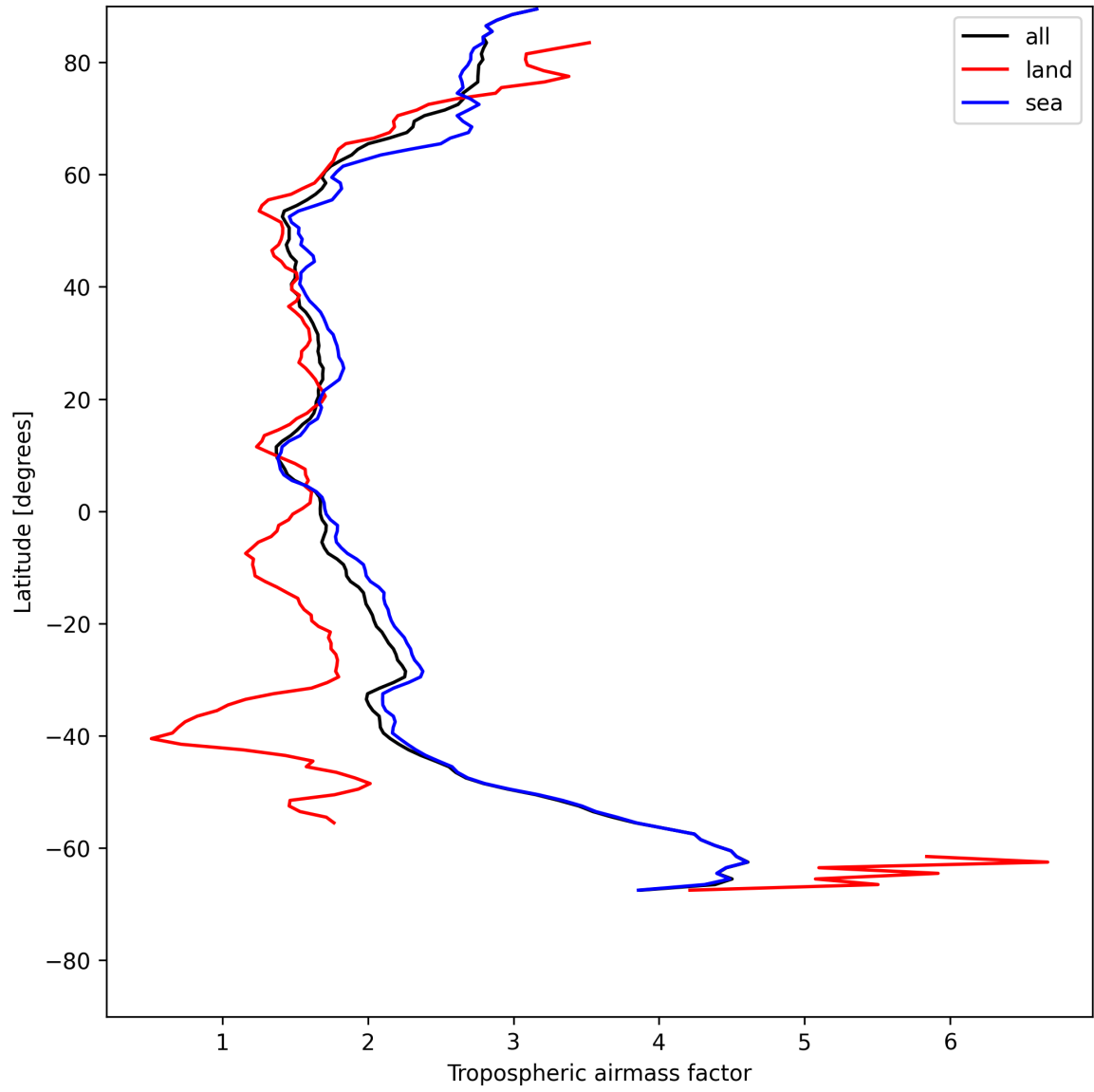
Figure 14: Zonal average of “Tropospheric airmass factor” for 2025-07-19 to 2025-07-21.
