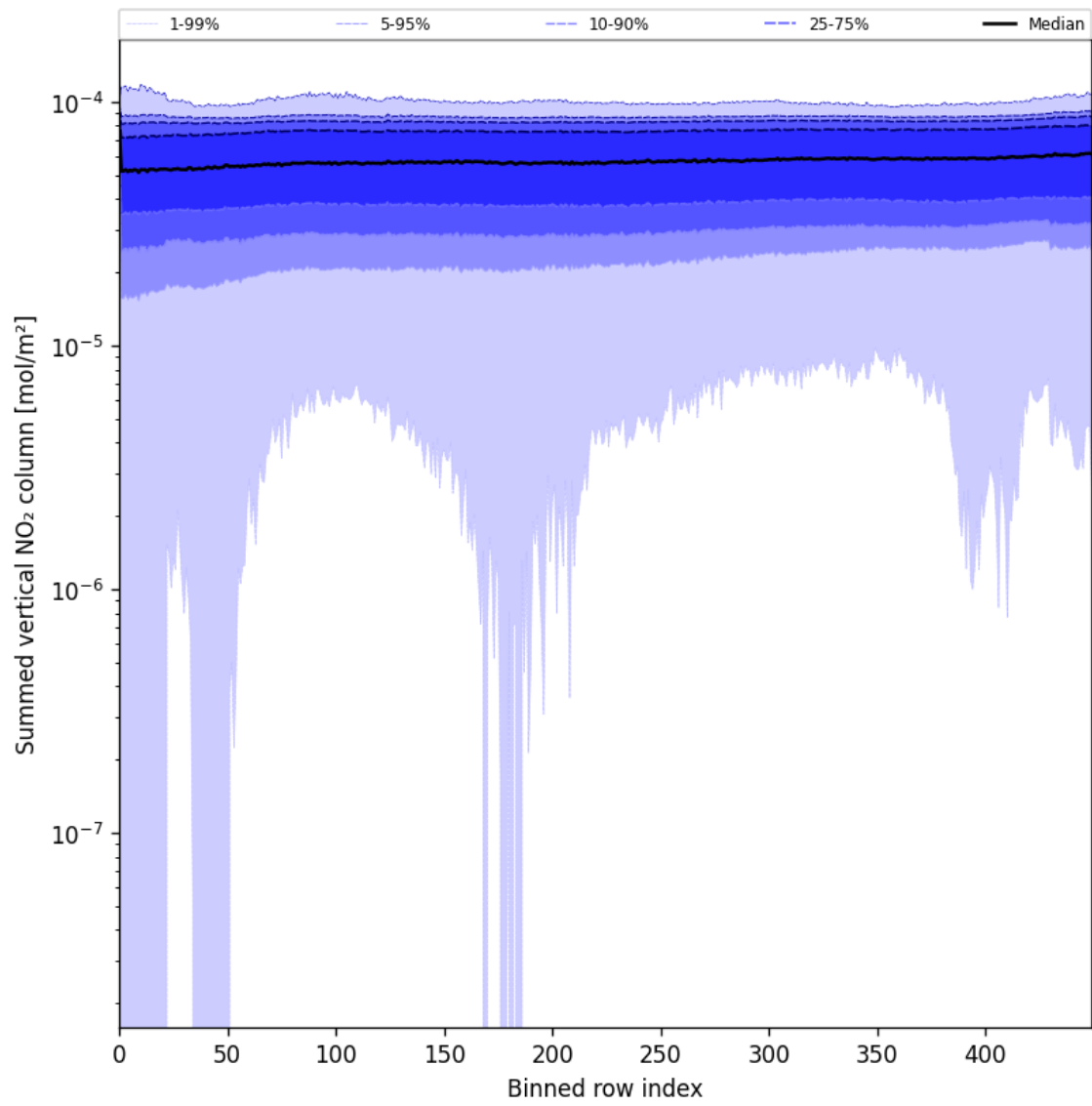
Figure 57: Along track statistics of “Summed vertical NO 2 column” for 2025-07-19 to 2025-07-21
