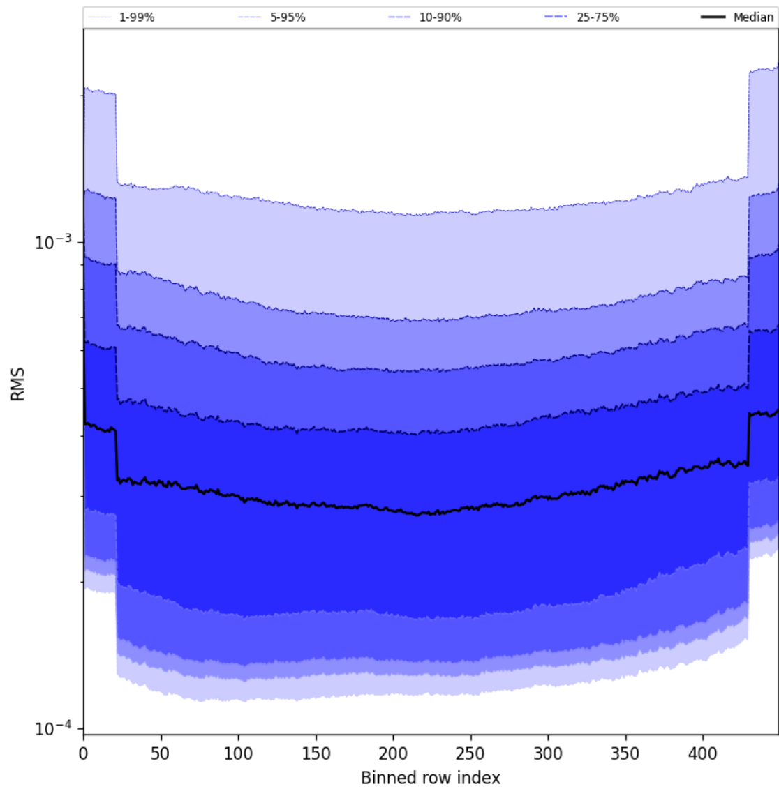
Figure 60: Along track statistics of “RMS” for 2025-07-19 to 2025-07-21
