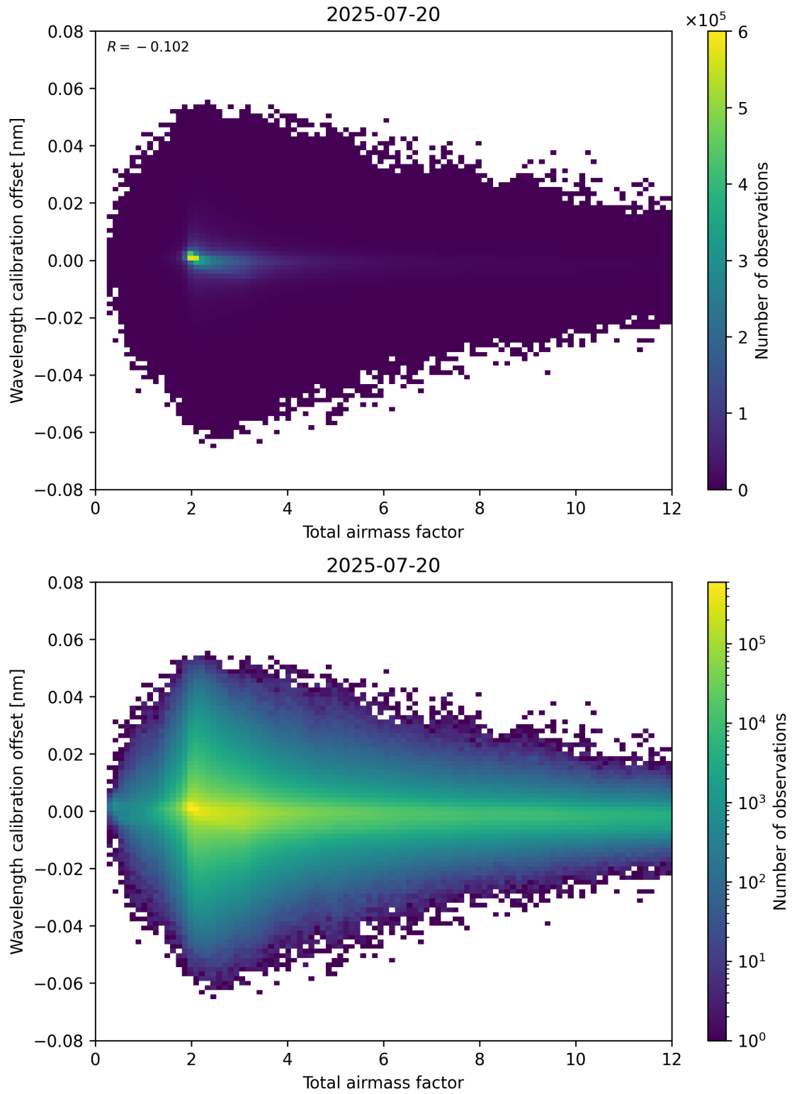
Figure 70: Scatter density plot of “Total airmass factor” against “Wavelength calibration offset” for 2025-07-19 to 2025-07-21.
