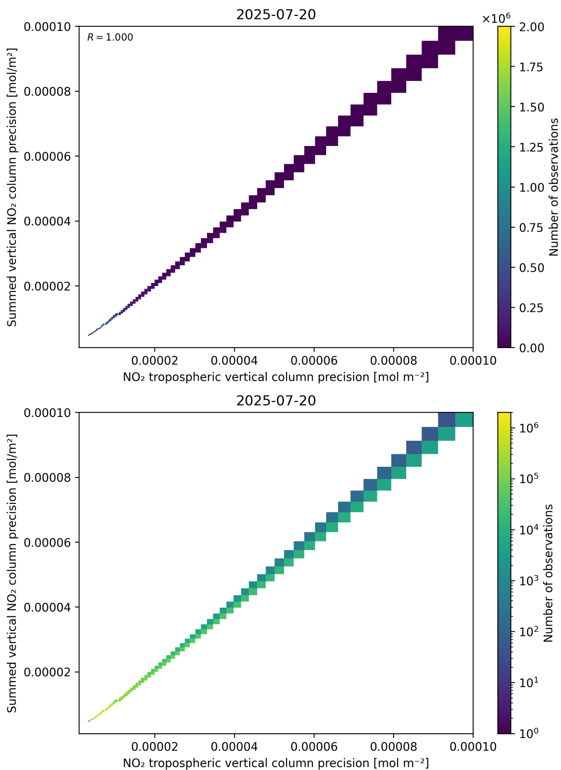
Figure 137: Scatter density plot of “NO 2 tropospheric vertical column precision” against “Summed vertical NO 2 column precision” for 2025-07-19 to 2025-07-21.
