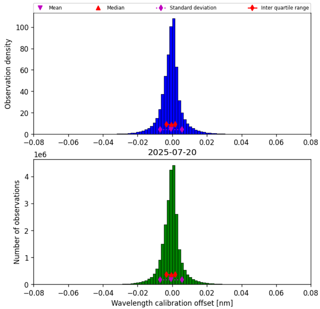
Figure 35: Histogram of “Wavelength calibration offset” for 2025-07-19 to 2025-07-21
