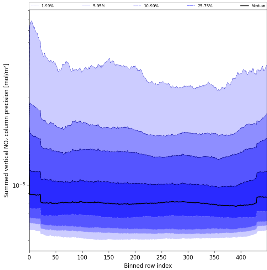
Figure 58: Along track statistics of “Summed vertical NO 2 column precision” for 2025-07-19 to 2025-07-21
