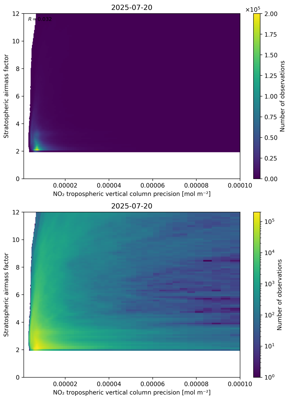
Figure 131: Scatter density plot of “NO 2 tropospheric vertical column precision” against “Stratospheric airmass factor” for 2025-07-19 to 2025-07-21.
