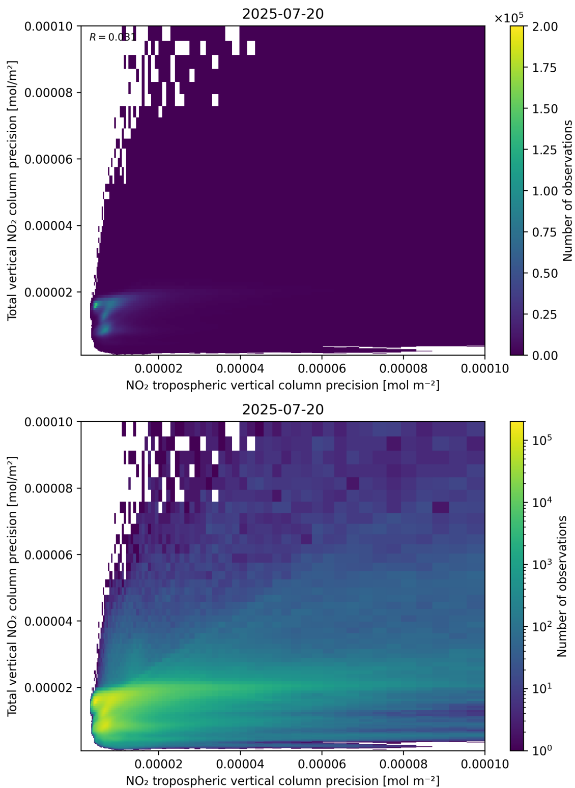
Figure 139: Scatter density plot of “NO 2 tropospheric vertical column precision” against “Total vertical NO 2 column precision” for 2025-07-19 to 2025-07-21.
