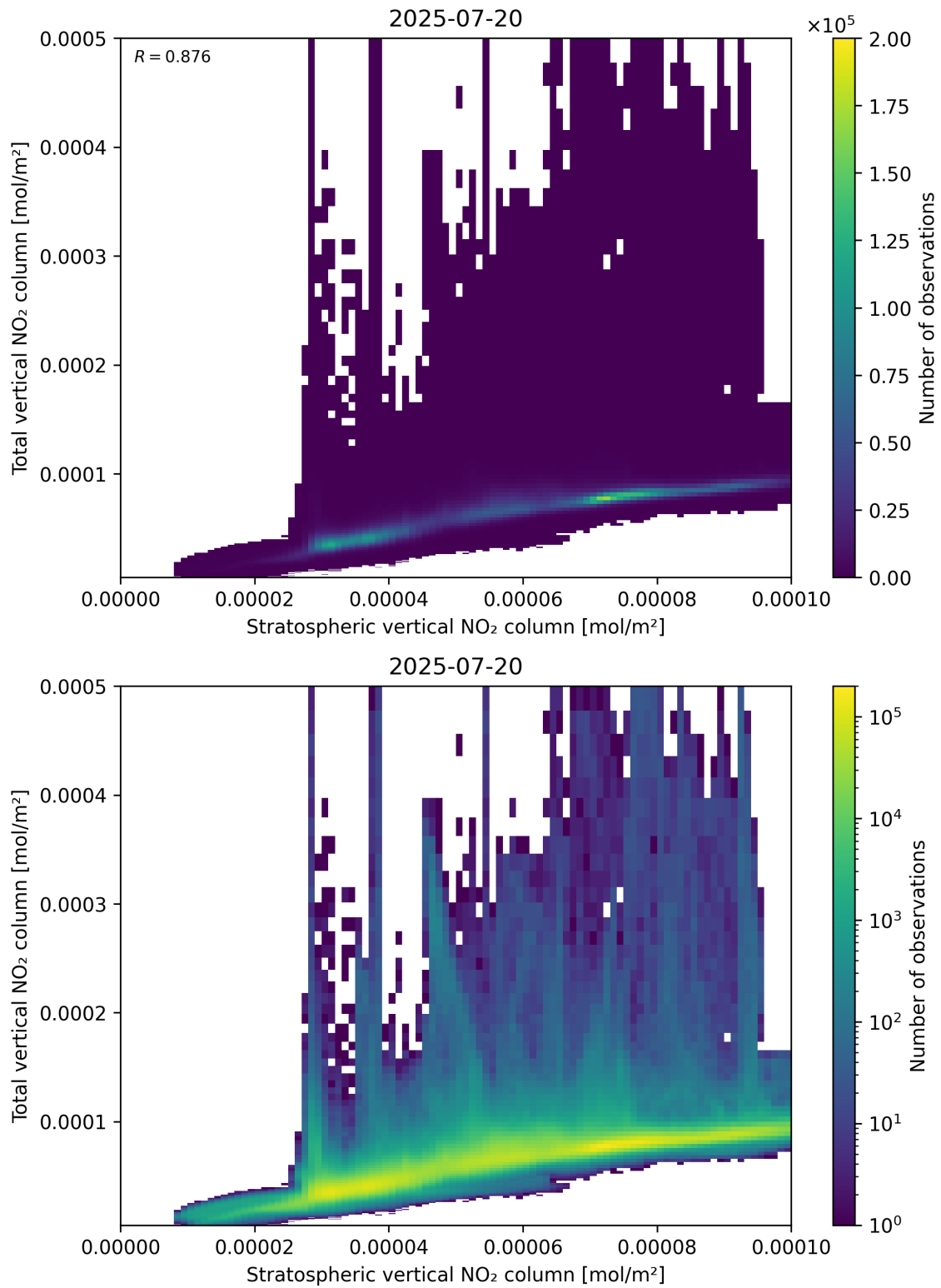
Figure 100: Scatter density plot of “Stratospheric vertical NO 2 column” against “Total vertical NO 2 column” for 2025-07-19 to 2025-07-21.
