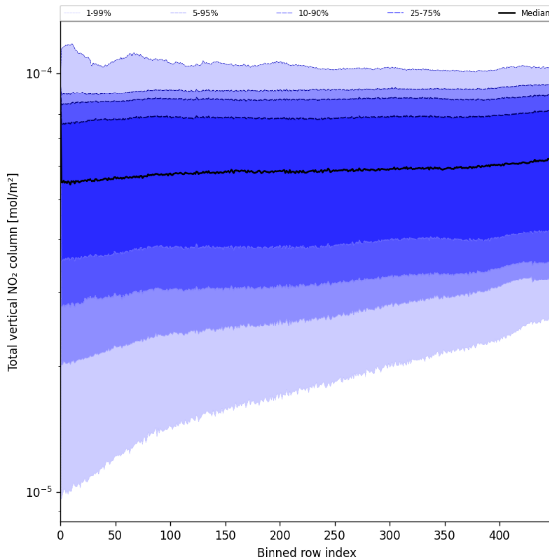
Figure 55: Along track statistics of “Total vertical NO 2 column” for 2025-07-19 to 2025-07-21
