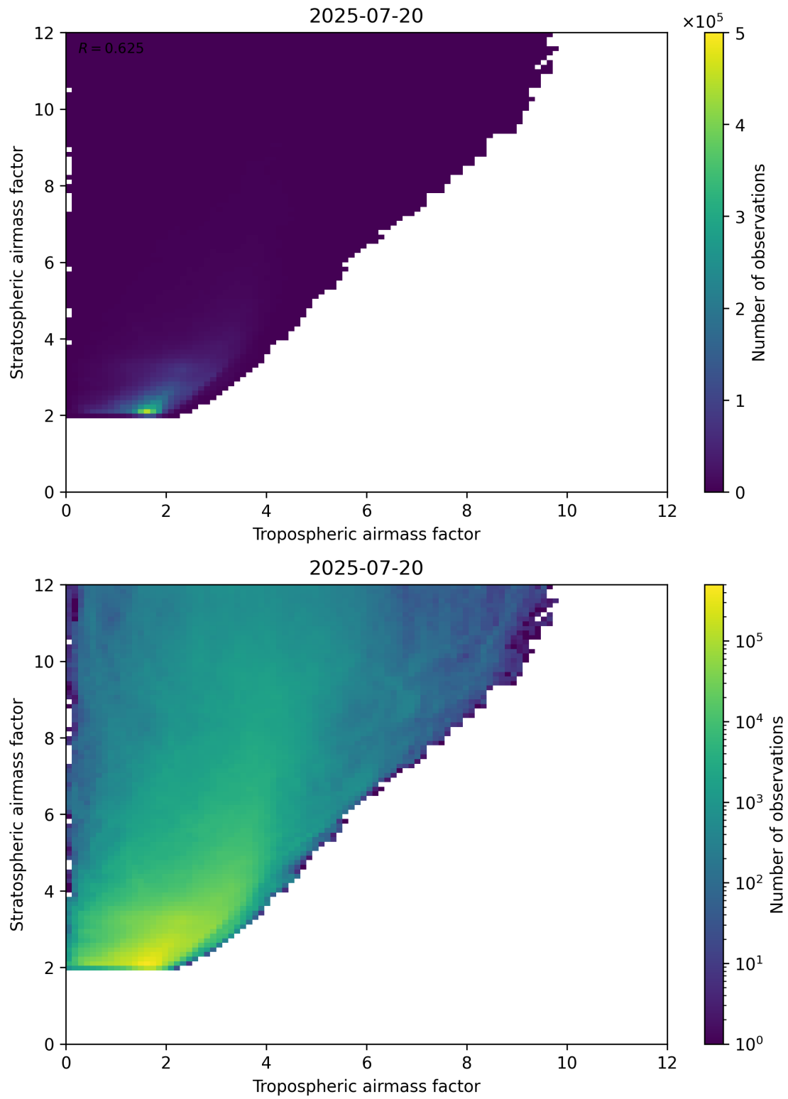
Figure 71: Scatter density plot of “Tropospheric airmass factor” against “Stratospheric airmass factor” for 2025-07-19 to 2025-07-21.
