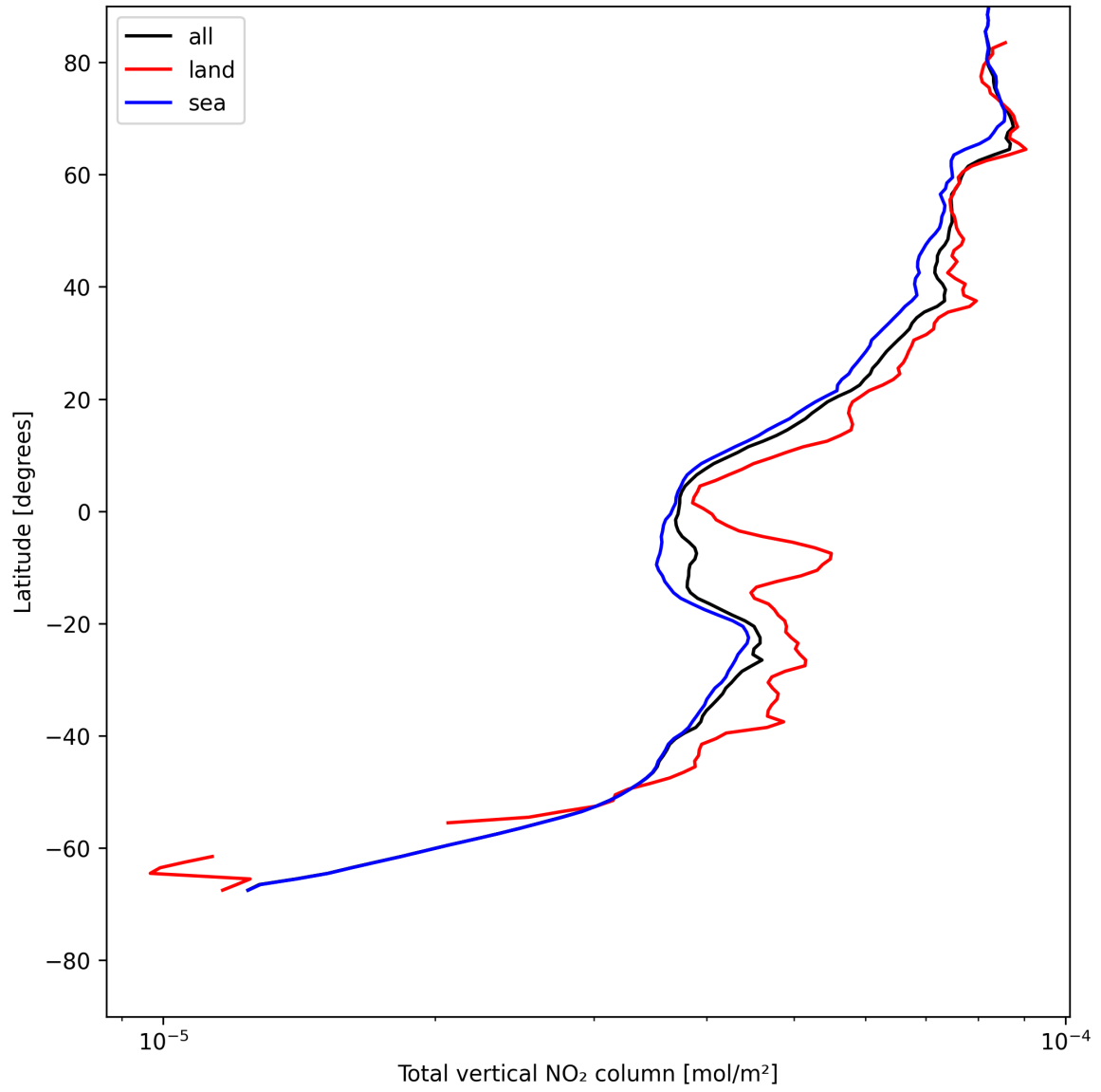
Figure 21: Zonal average of “Total vertical NO 2 column” for 2025-07-19 to 2025-07-21.
