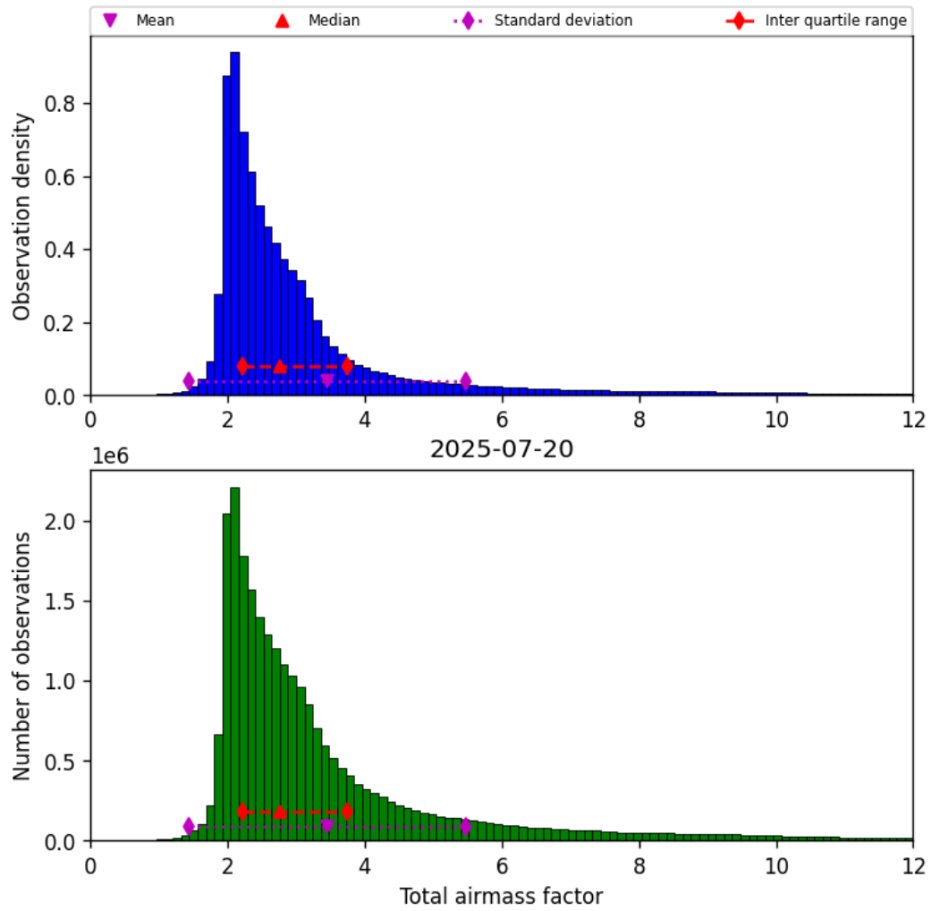
Figure 32: Histogram of “Total airmass factor” for 2025-07-19 to 2025-07-21
