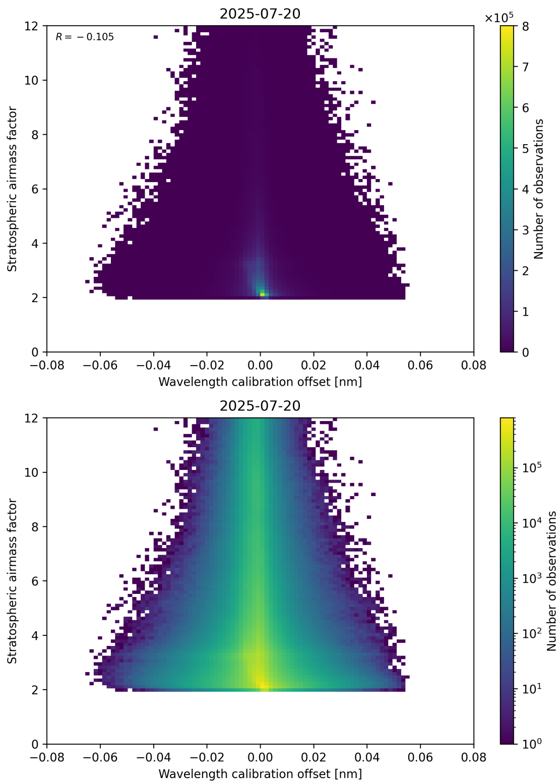
Figure 174: Scatter density plot of “Wavelength calibration offset” against “Stratospheric airmass factor” for 2025-07-19 to 2025-07-21.
