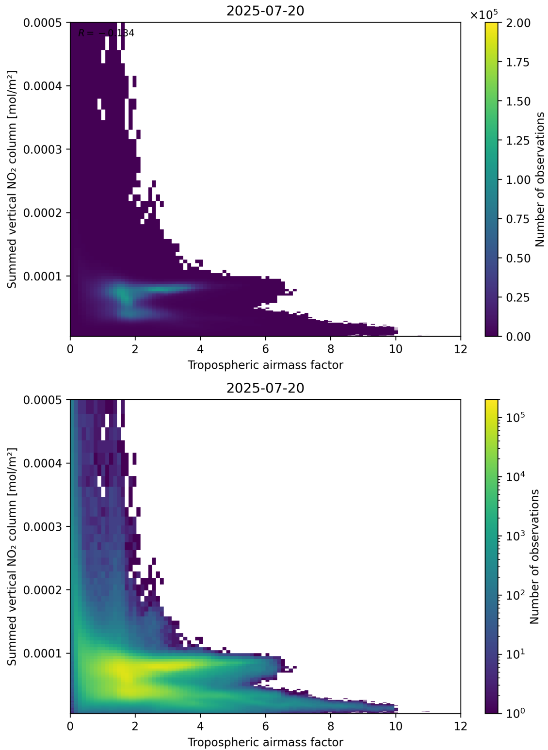
Figure 75: Scatter density plot of “Tropospheric air mass factor” against “Summed vertical NO 2 column” for 2025-07-19 to 2025-07-21.
