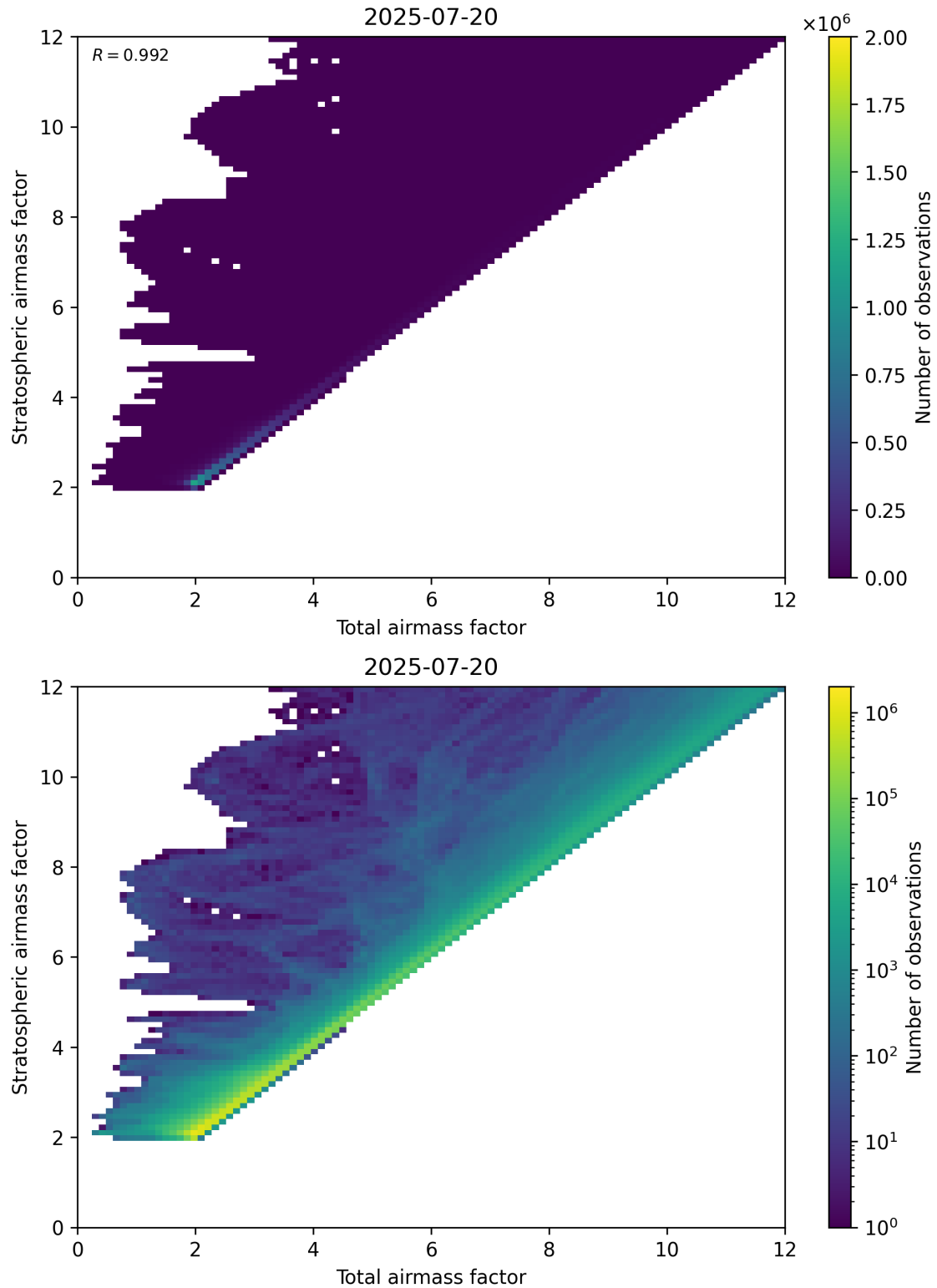
Figure 62: Scatter density plot of “Total airmass factor” against “Stratospheric airmass factor” for 2025-07-19 to 2025-07-21.
