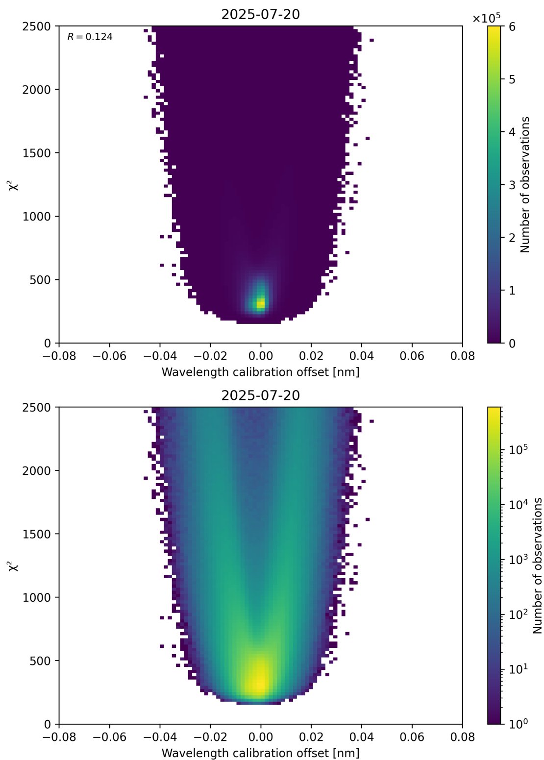
Figure 175: Scatter density plot of “Wavelength calibration offset” against “ \chi^2 ” for 2025-07-19 to 2025-07-21.
