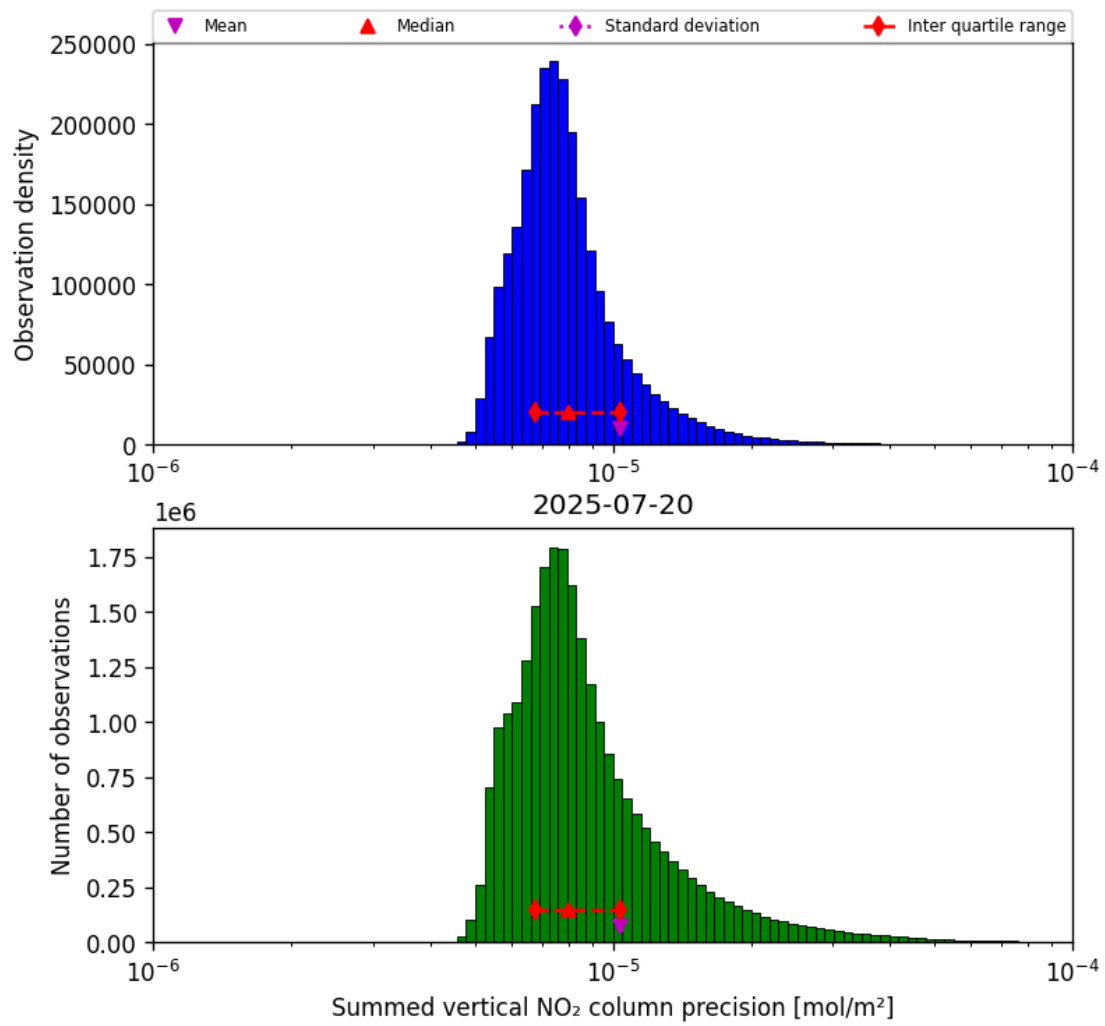
Figure 41: Histogram of "Summed vertical NO 2 column precision" for 2025-07-19 to 2025-07-21
