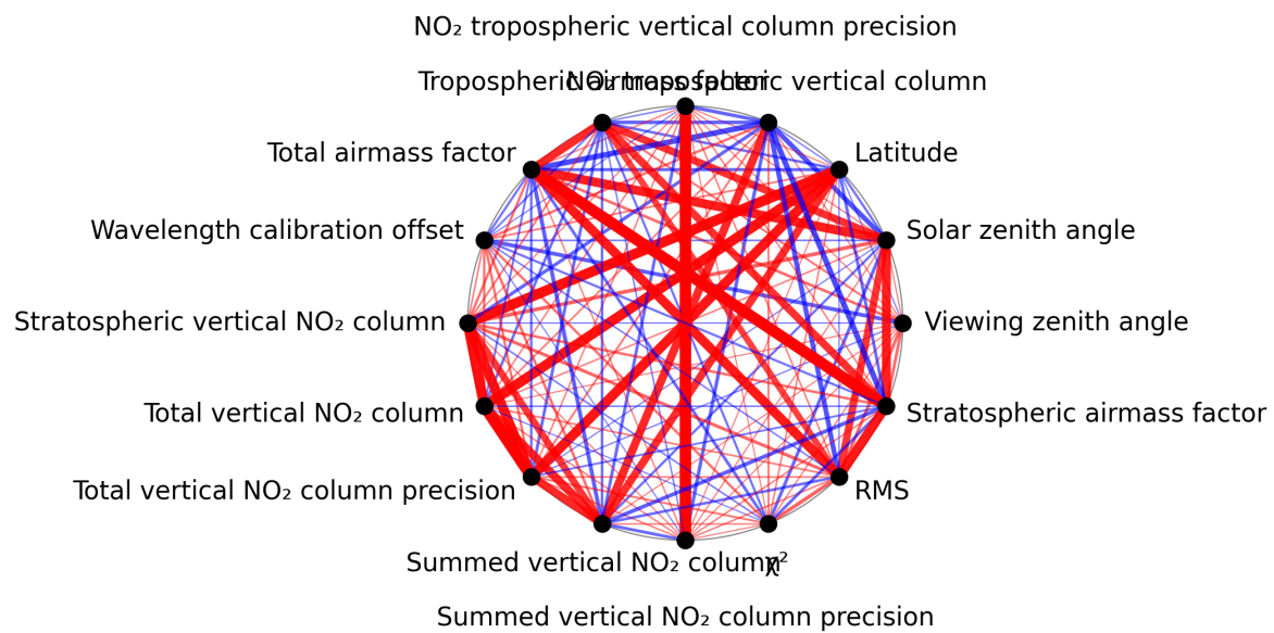
Figure 1: Map of correlation graph for 2025-07-19 to 2025-07-21.
