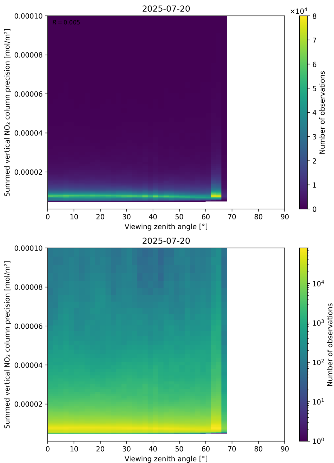
Figure 166: Scatter density plot of “Viewing zenith angle” against “Summed vertical NO 2 column precision” for 2025-07-19 to 2025-07-21.
