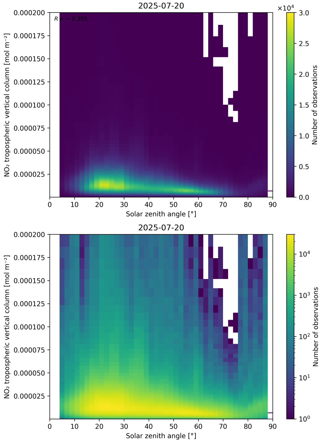
Figure 155: Scatter density plot of “Solar zenith angle” against “NO 2 tropospheric vertical column” for 2025-07-19 to 2025-07-21.
