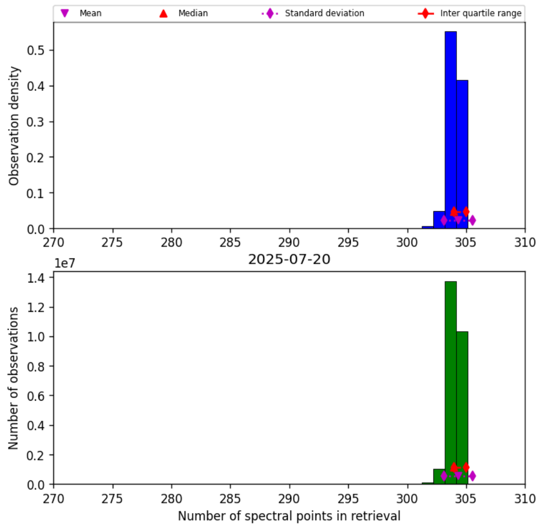
Figure 33: Histogram of “Number of spectral points in retrieval” for 2025-07-19 to 2025-07-21
