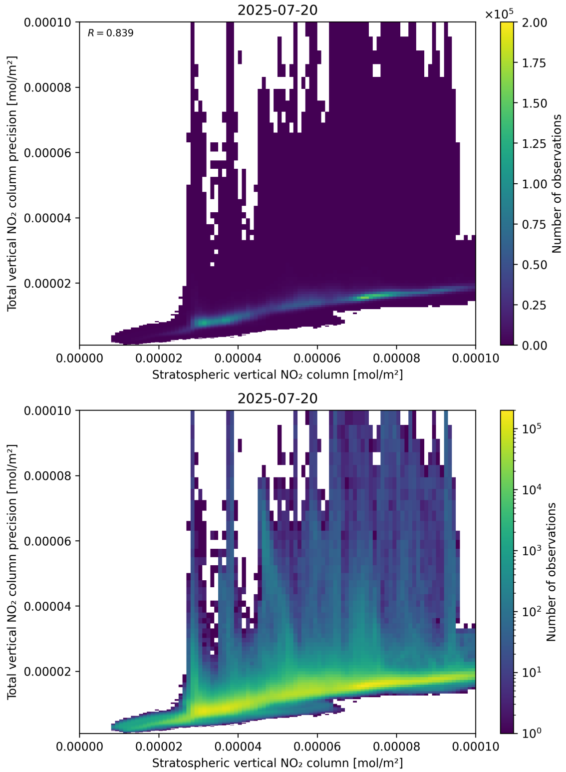
Figure 101: Scatter density plot of “Stratospheric vertical NO 2 column” against “Total vertical NO 2 column precision” for 2025-07-19 to 2025-07-21.
