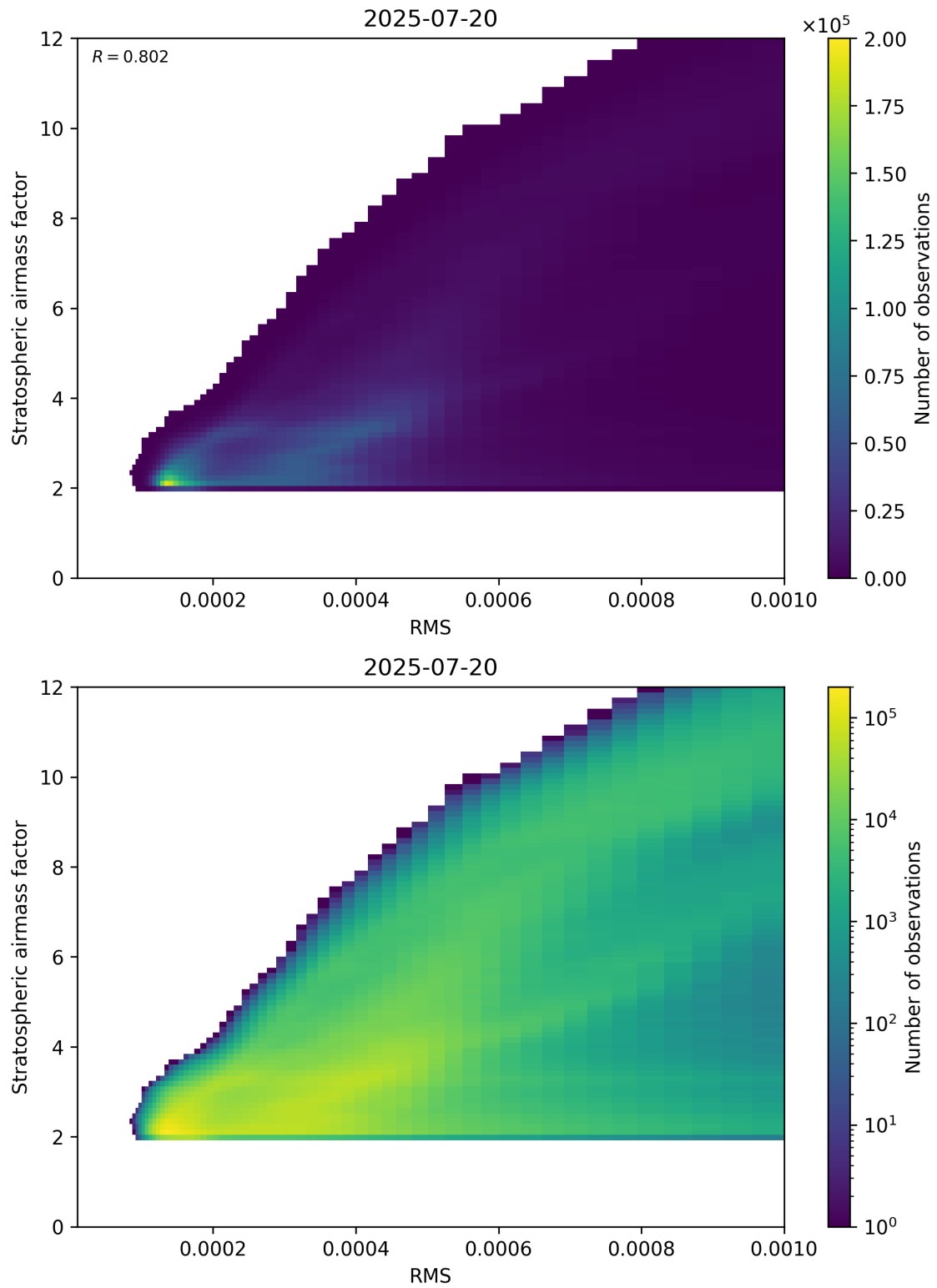
Figure 144: Scatter density plot of “RMS” against “Stratospheric airmass factor” for 2025-07-19 to 2025-07-21.
