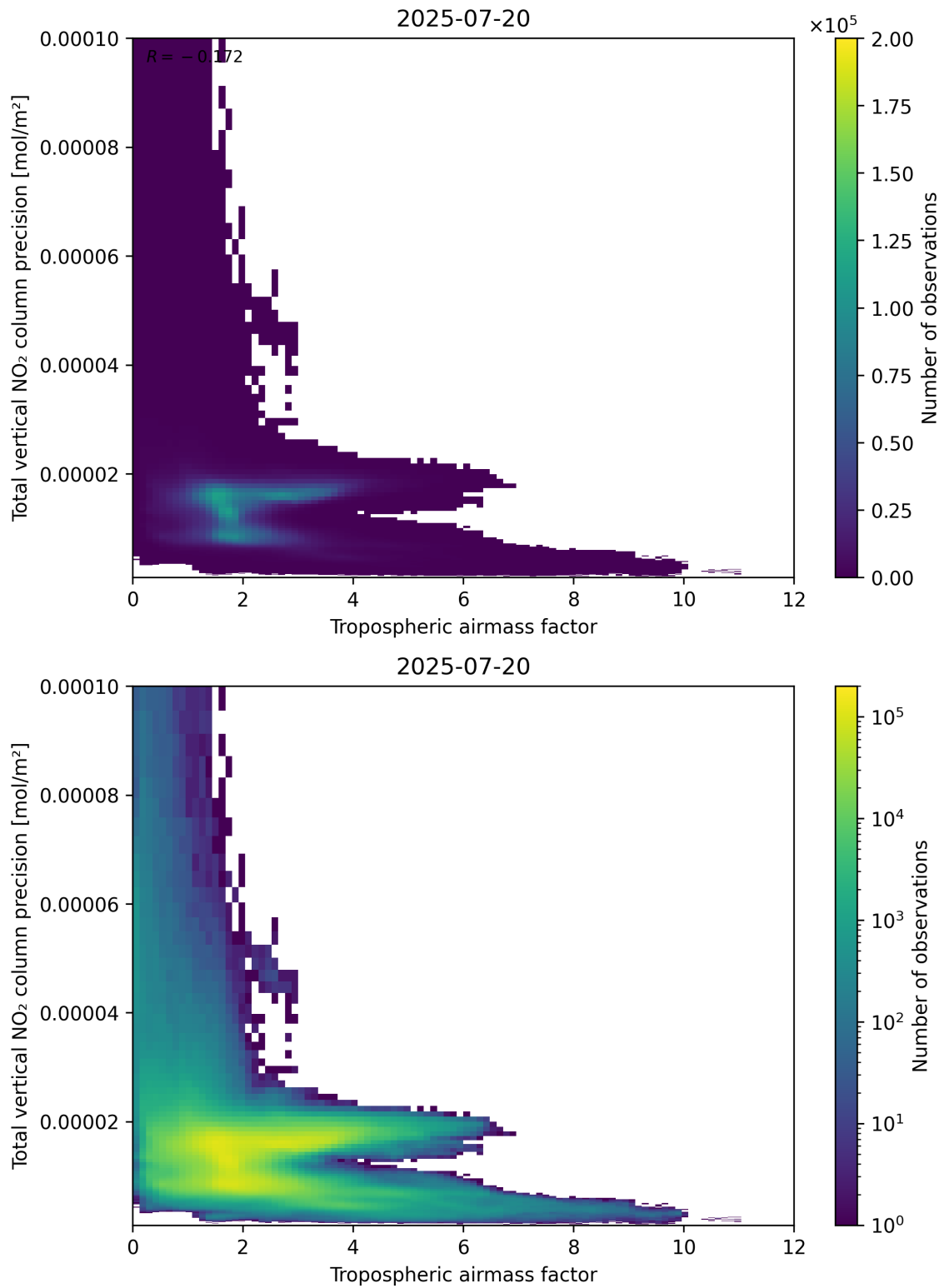
Figure 78: Scatter density plot of “Tropospheric air mass factor” against “Total vertical NO 2 column precision” for 2025-07-19 to 2025-07-21.
