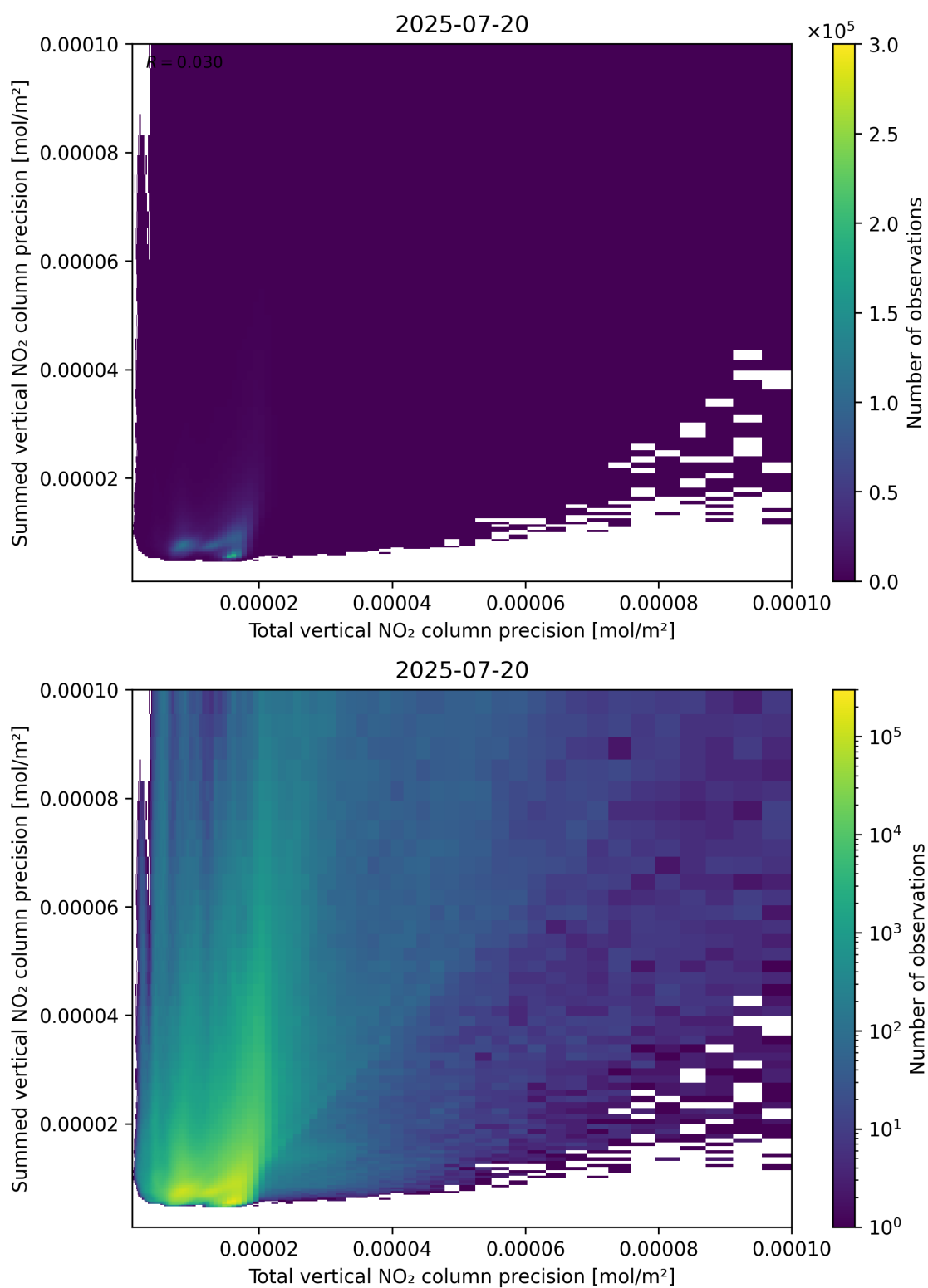
Figure 118: Scatter density plot of “Total vertical NO 2 column precision” against “Summed vertical NO 2 column precision” for 2025-07-19 to 2025-07-21.
