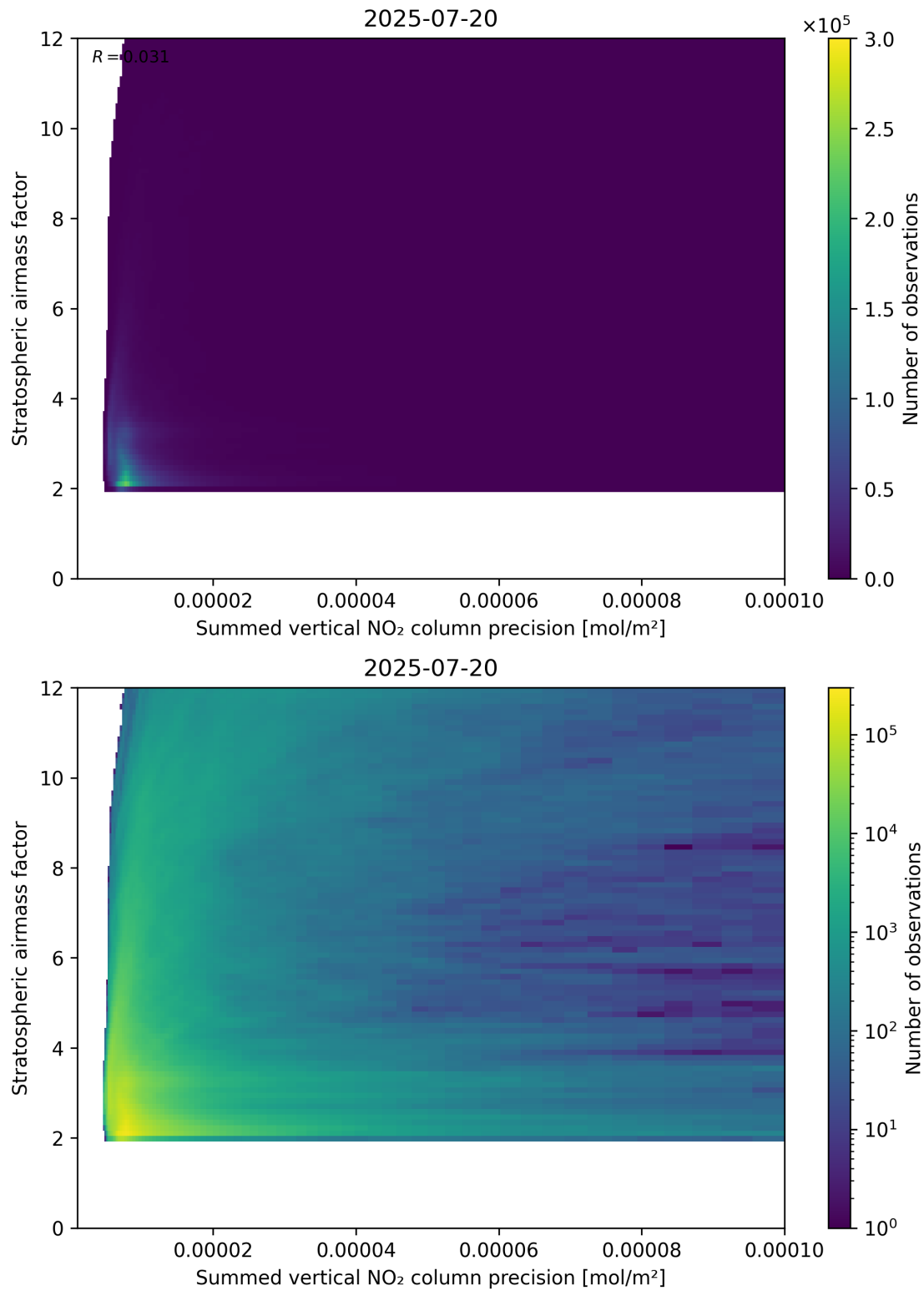
Figure 106: Scatter density plot of “Summed vertical NO 2 column precision” against “Stratospheric airmass factor” for 2025-07-19 to 2025-07-21.
