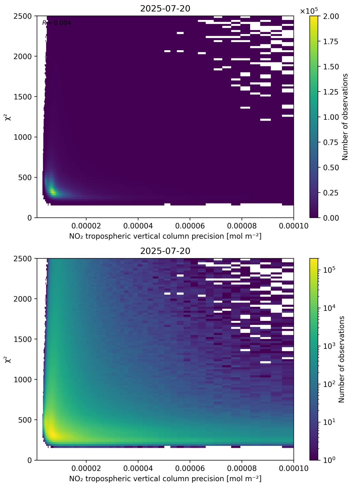
Figure 134: Scatter density plot of “NO 2 tropospheric vertical column precision” against “ \chi^2 ” for 2025-07-19 to 2025-07-21.
