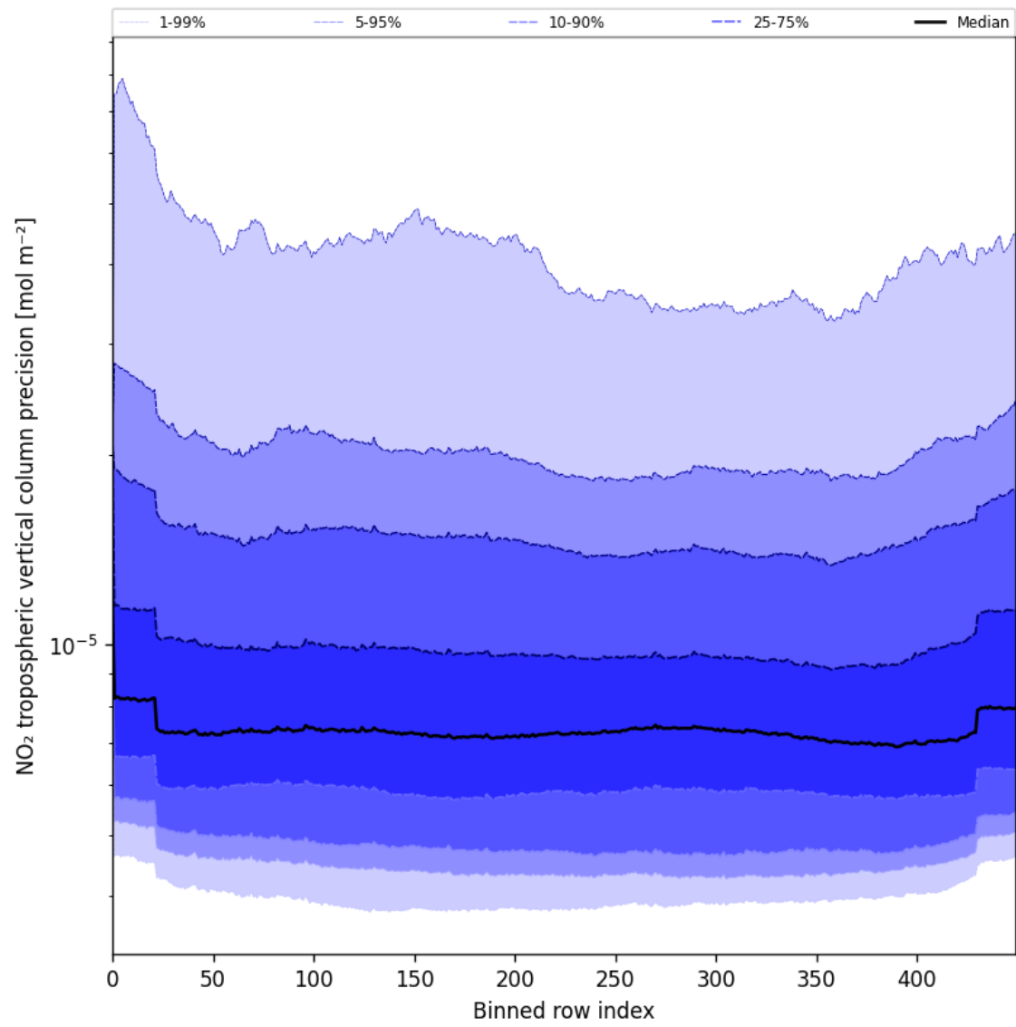
Figure 47: Along track statistics of “NO 2 tropospheric vertical column precision” for 2025-07-19 to 2025-07-21
