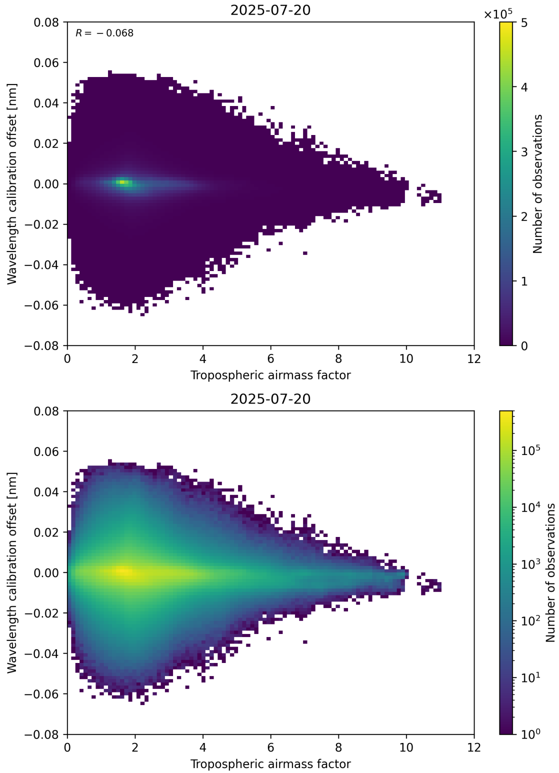
Figure 80: Scatter density plot of “Tropospheric airmass factor” against “Wavelength calibration offset” for 2025-07-19 to 2025-07-21.
