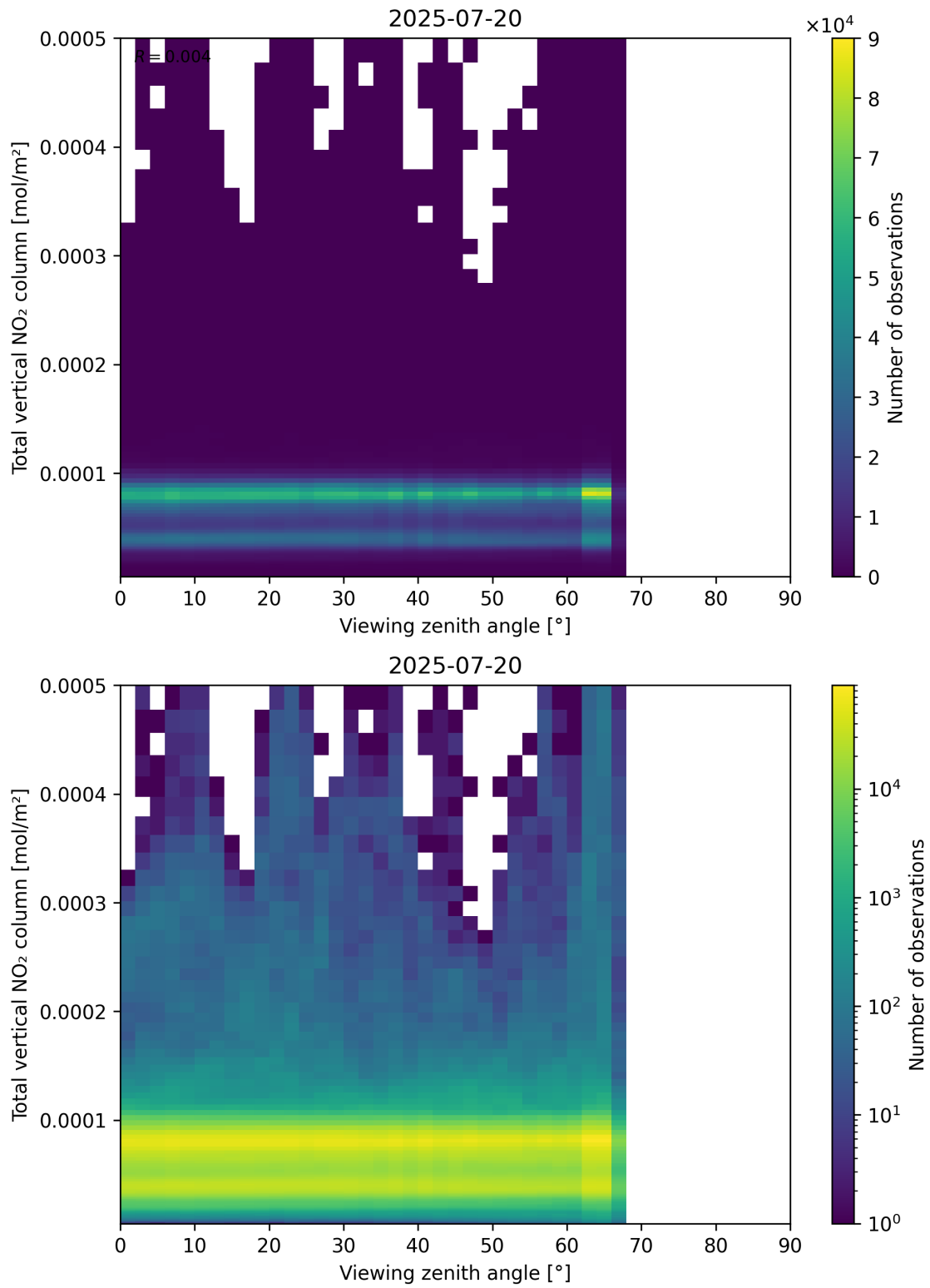
Figure 167: Scatter density plot of “Viewing zenith angle” against “Total vertical NO 2 column” for 2025-07-19 to 2025-07-21.
