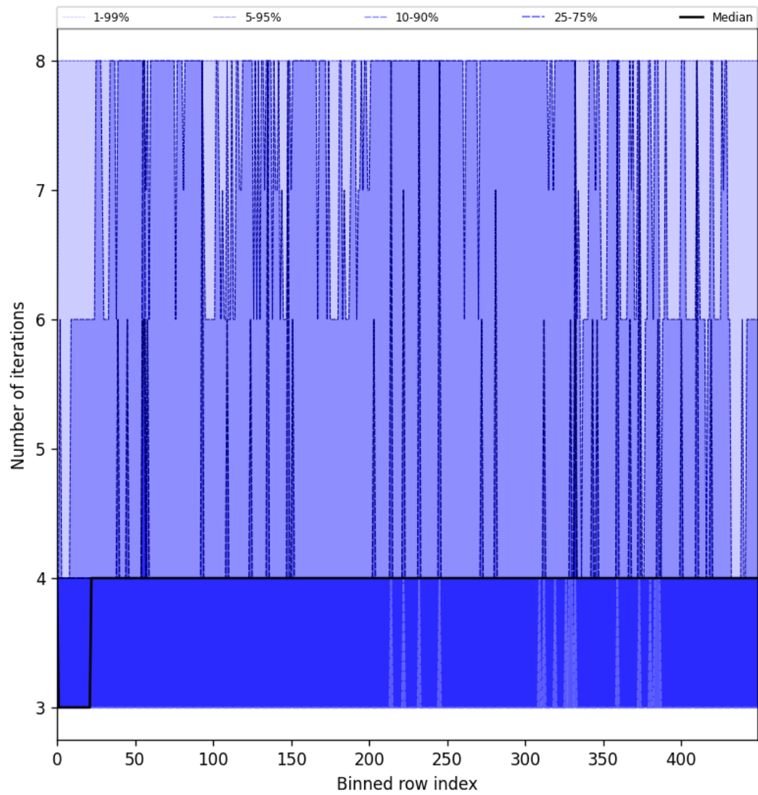
Figure 51: Along track statistics of “Number of iterations” for 2025-07-19 to 2025-07-21
