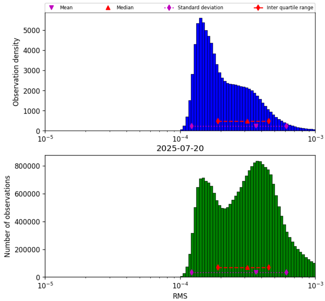
Figure 43: Histogram of “RMS” for 2025-07-19 to 2025-07-21
