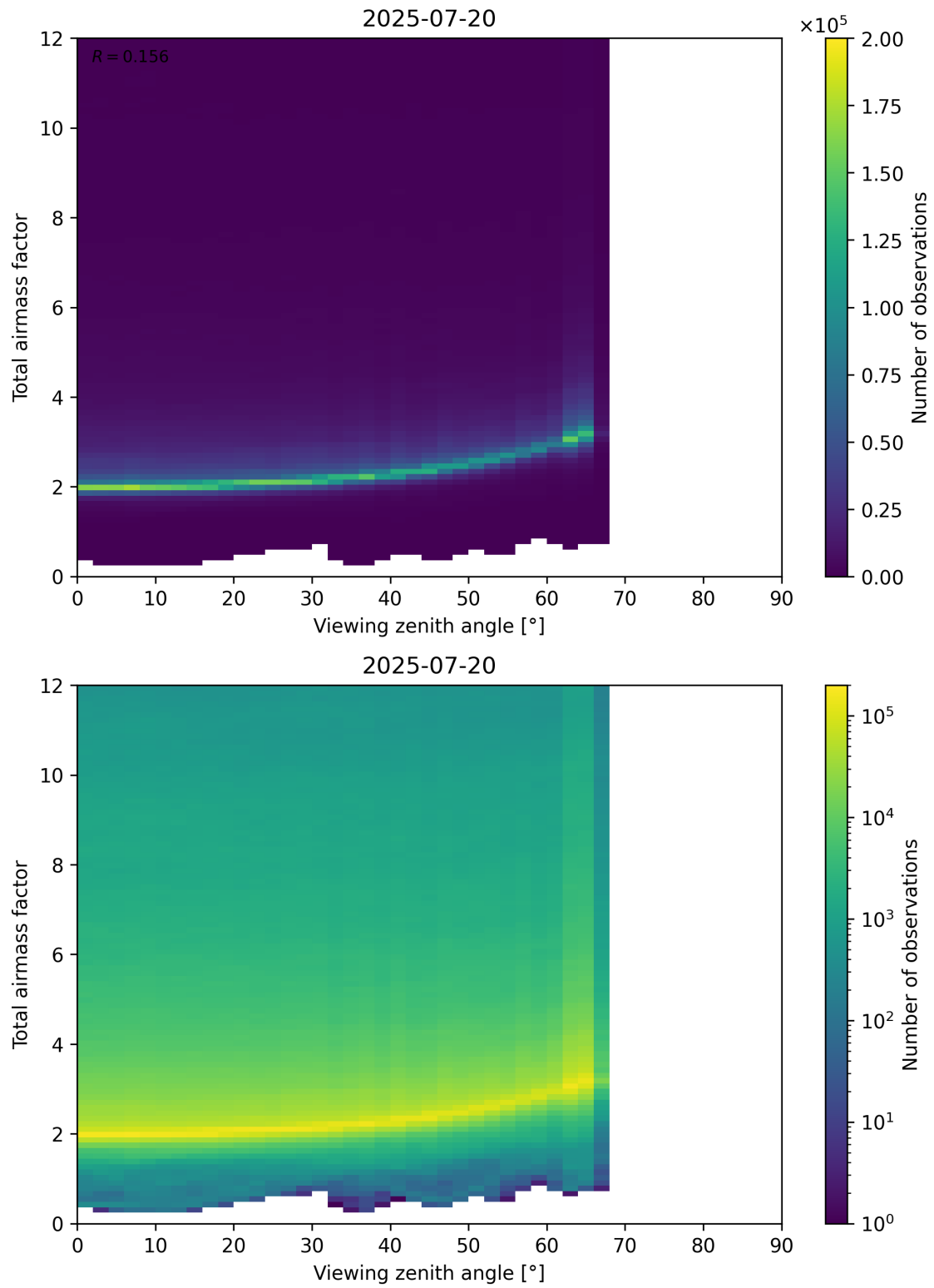
Figure 160: Scatter density plot of “Viewing zenith angle” against “Total airmass factor” for 2025-07-19 to 2025-07-21.
