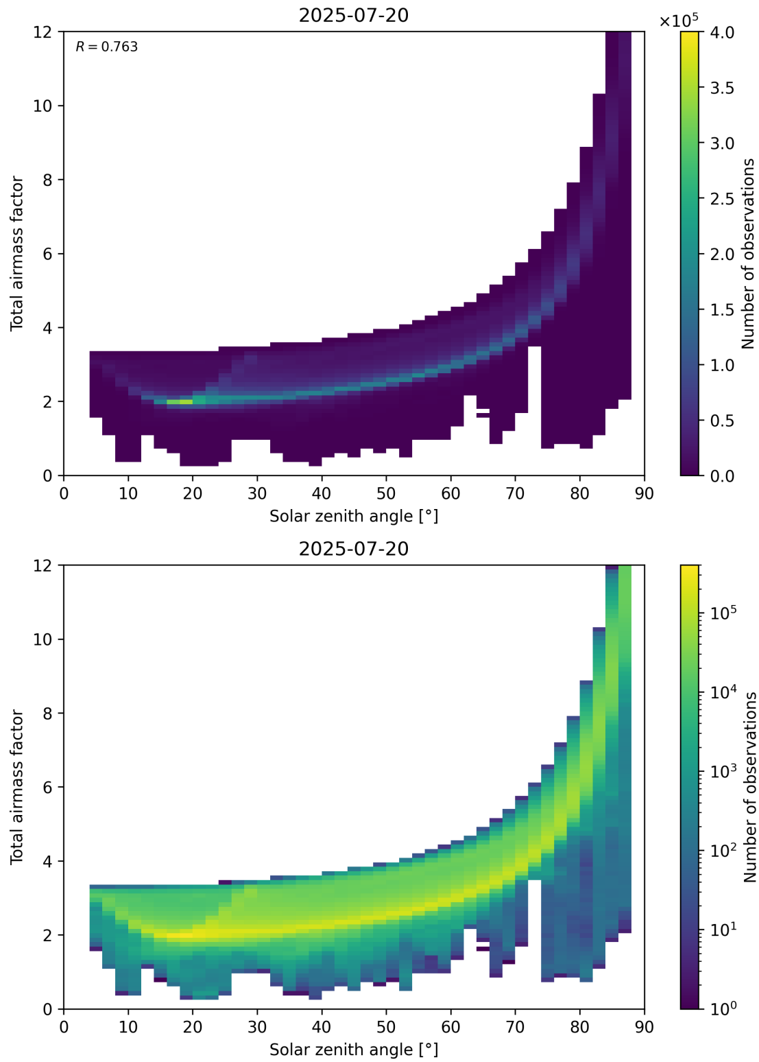
Figure 146: Scatter density plot of “Solar zenith angle” against “Total air mass factor” for 2025-07-19 to 2025-07-21.
