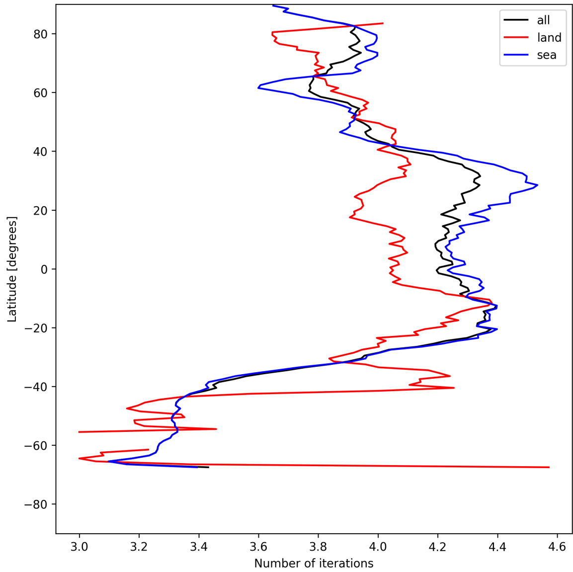
Figure 17: Zonal average of “Number of iterations” for 2025-07-19 to 2025-07-21.
