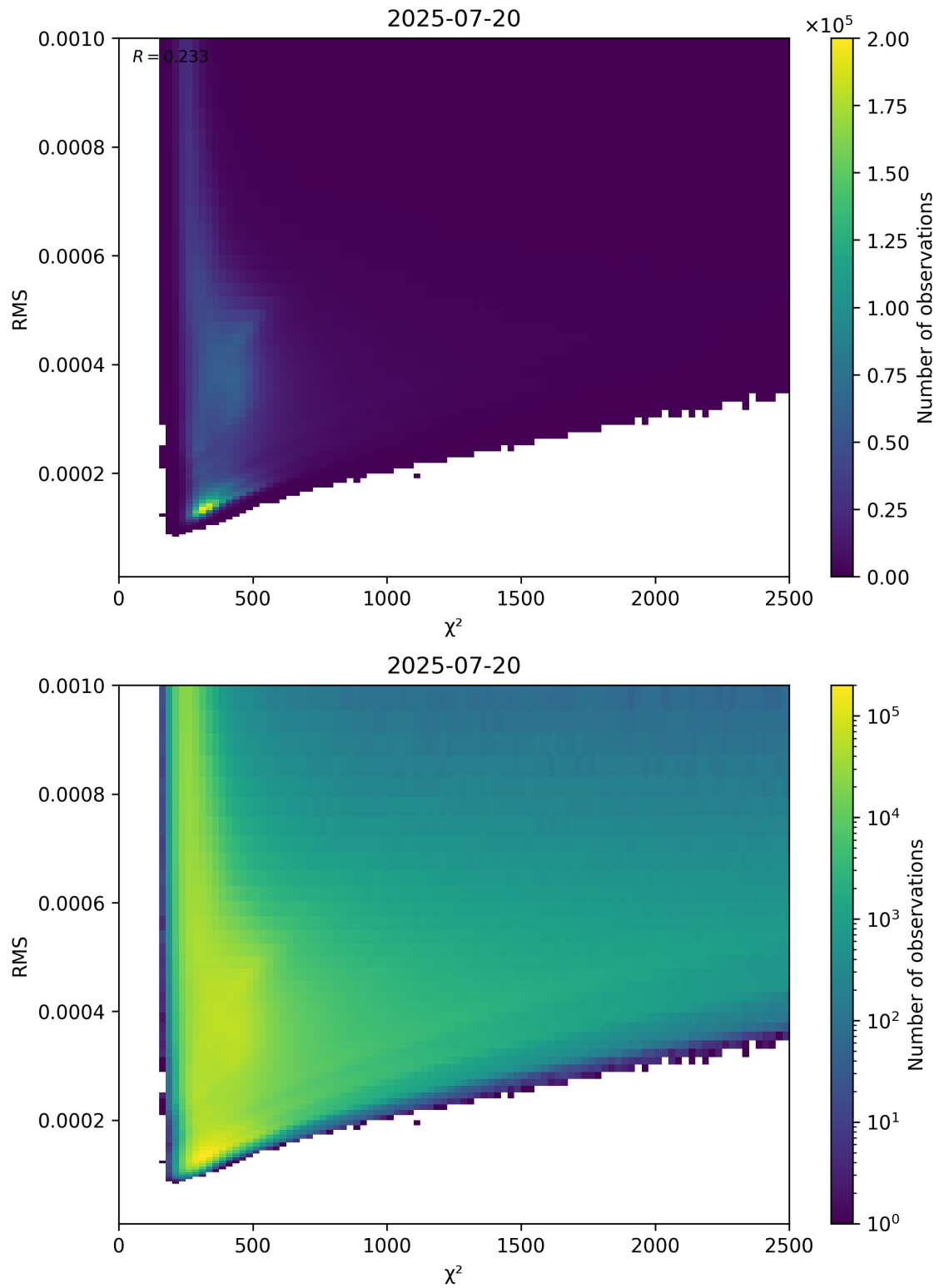
Figure 82: Scatter density plot of “ \chi^2 ” against “RMS” for 2025-07-19 to 2025-07-21.
