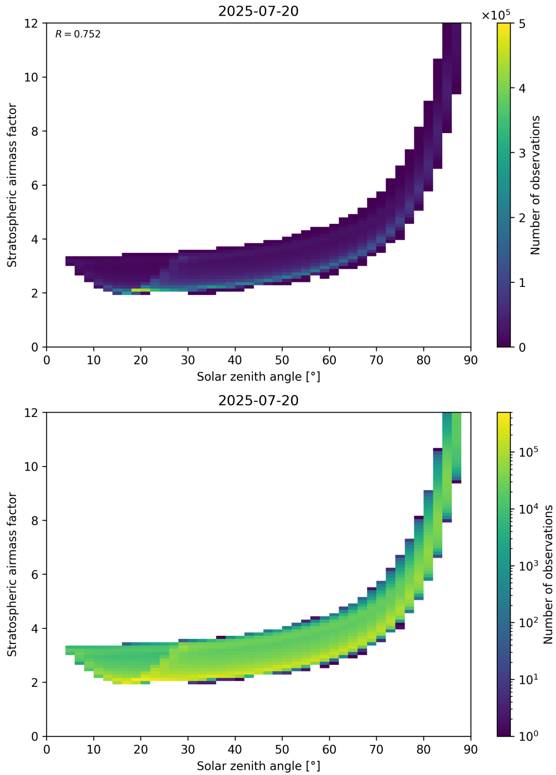
Figure 145: Scatter density plot of “Solar zenith angle” against “Stratospheric airmass factor” for 2025-07-19 to 2025-07-21.
