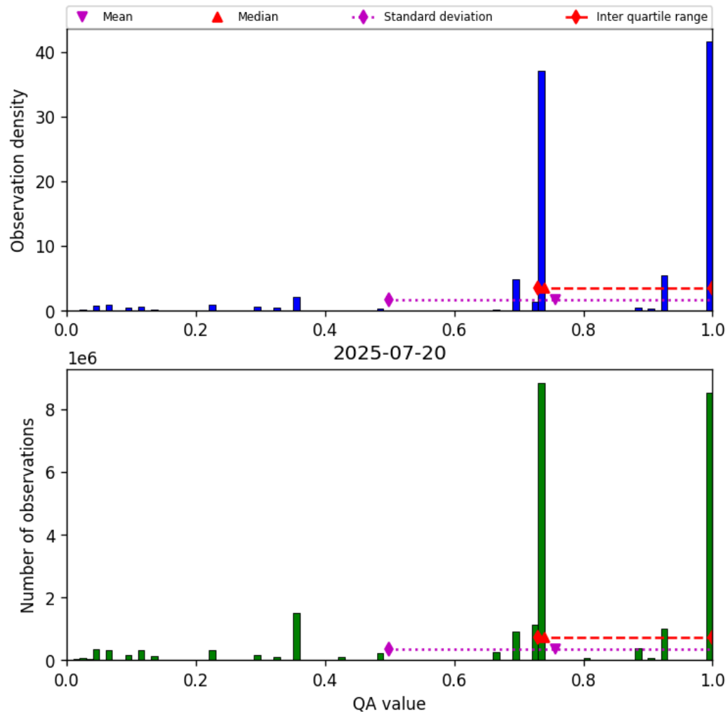
Figure 28: Histogram of “QA value” for 2025-07-19 to 2025-07-21
