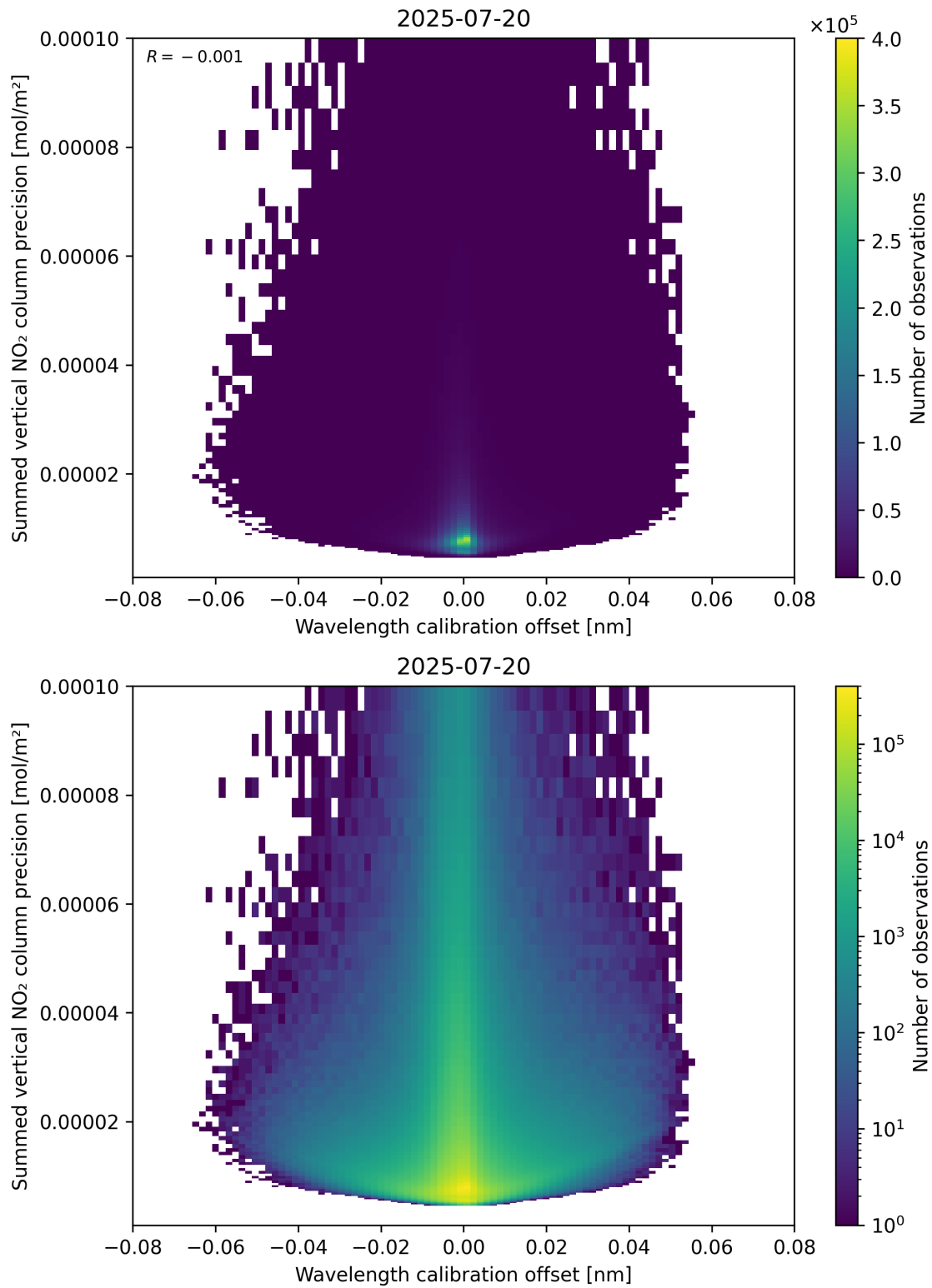
Figure 178: Scatter density plot of “Wavelength calibration offset” against “Summed vertical NO 2 column precision” for 2025-07-19 to 2025-07-21.
