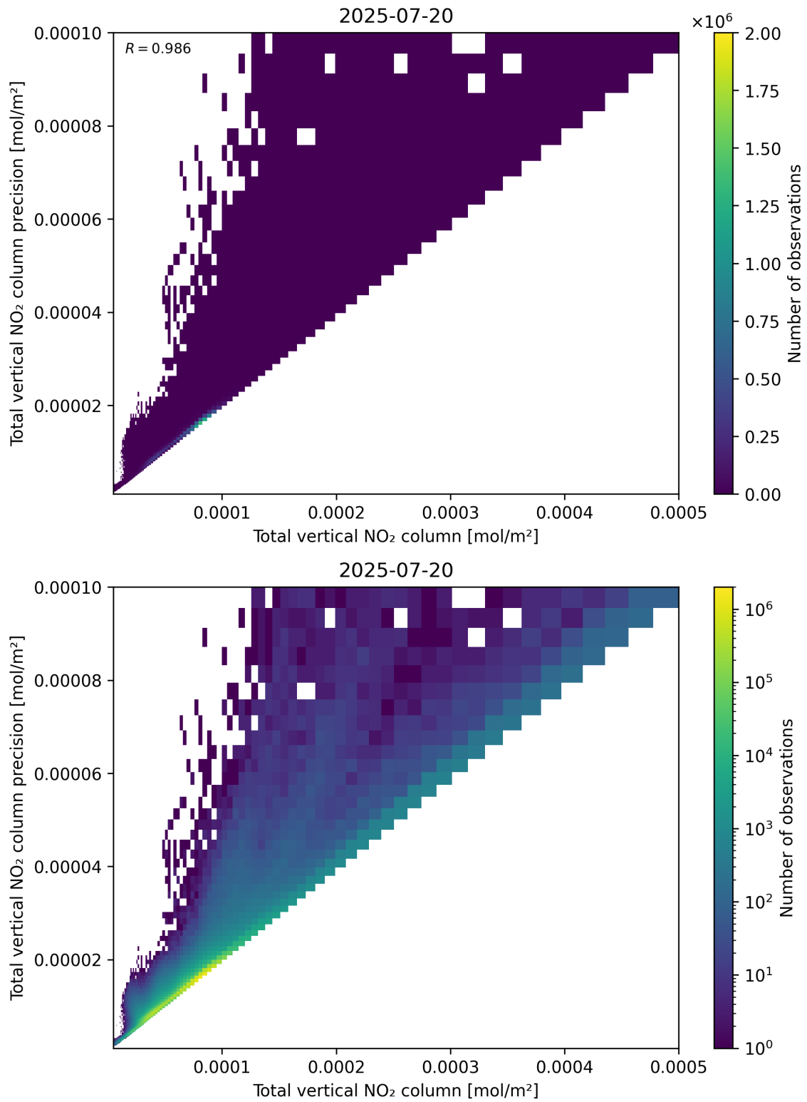
Figure 114: Scatter density plot of “Total vertical NO 2 column” against “Total vertical NO 2 column precision” for 2025-07-19 to 2025-07-21.
