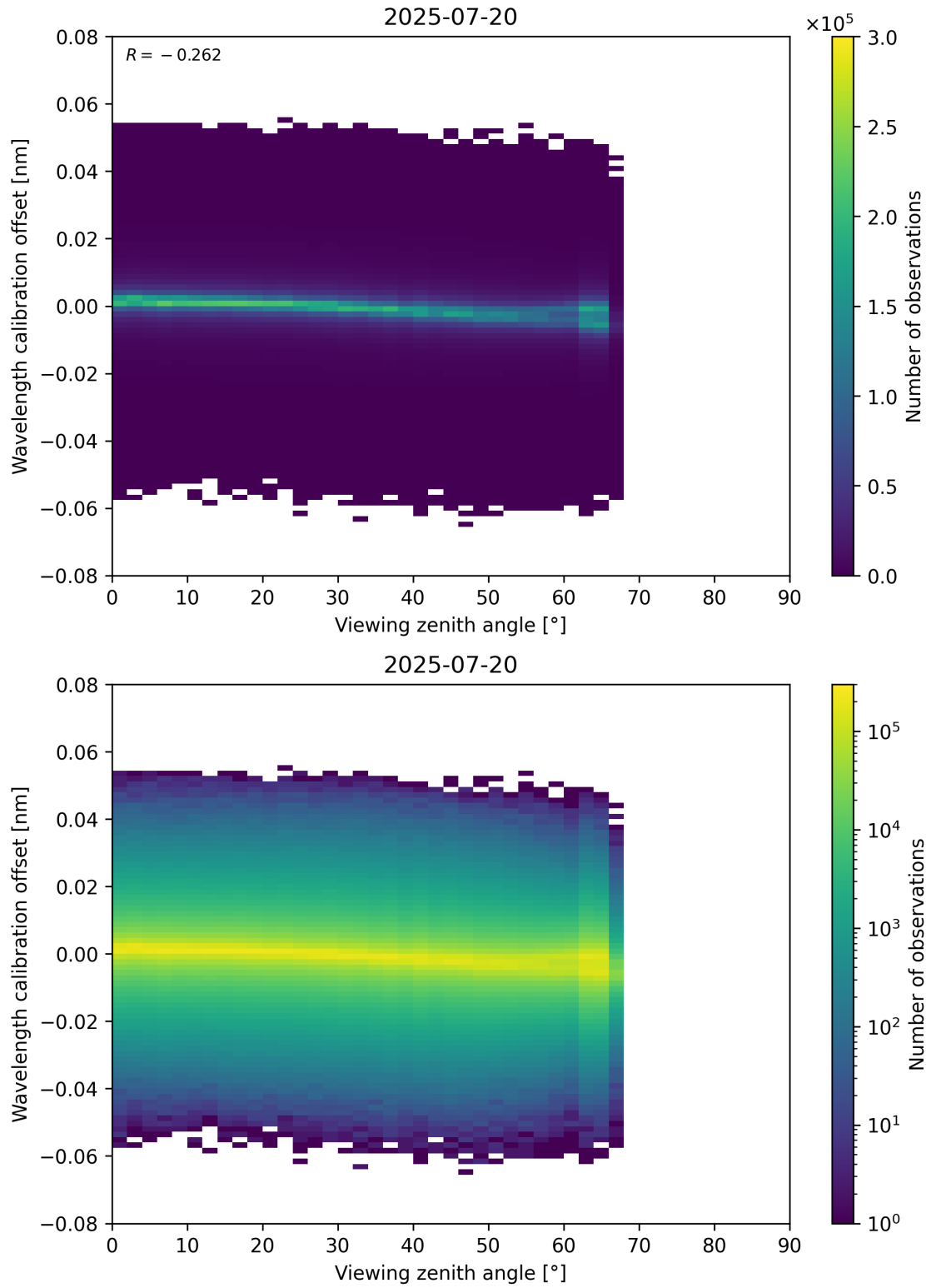
Figure 173: Scatter density plot of “Viewing zenith angle” against “Wavelength calibration offset” for 2025-07-19 to 2025-07-21.
