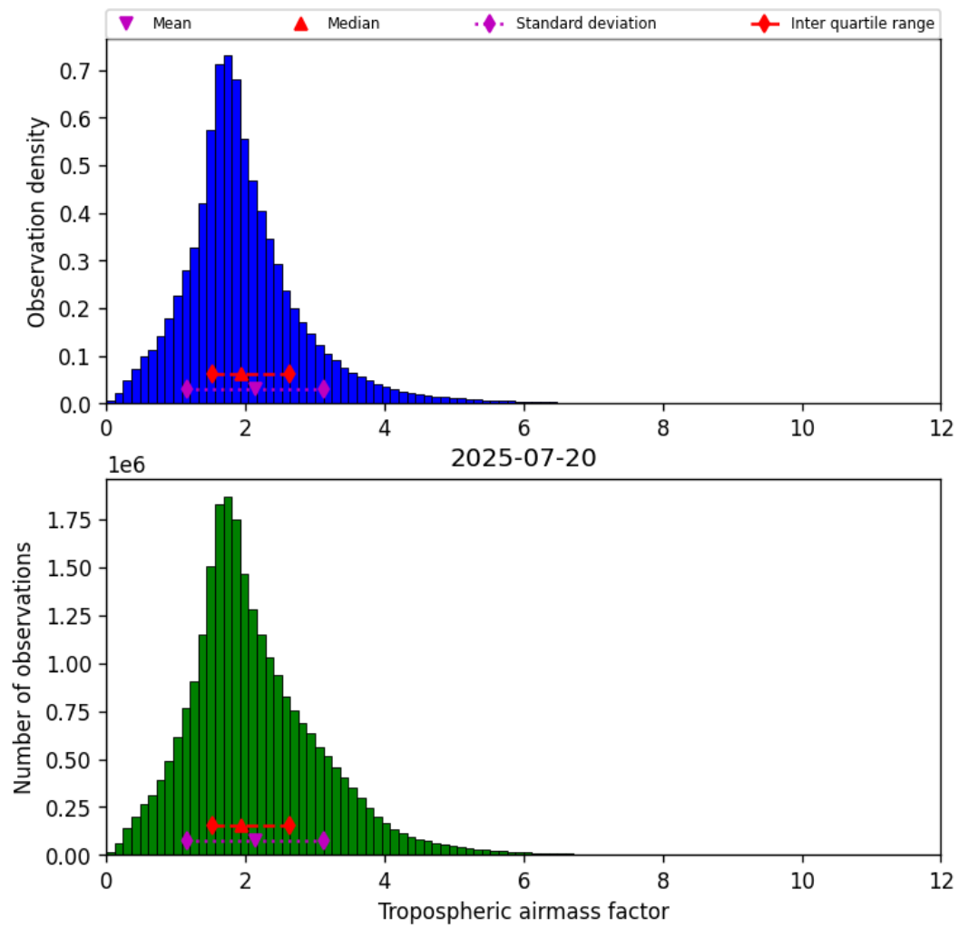
Figure 31: Histogram of “Tropospheric airmass factor” for 2025-07-19 to 2025-07-21
