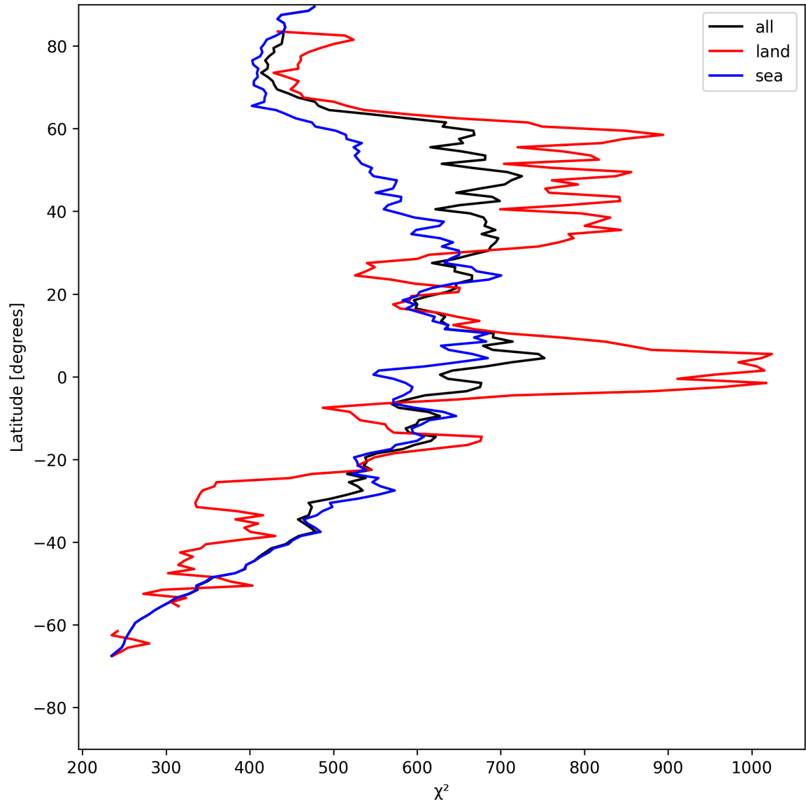
Figure 25: Zonal average of “ \chi^2 ” for 2025-07-19 to 2025-07-21.
