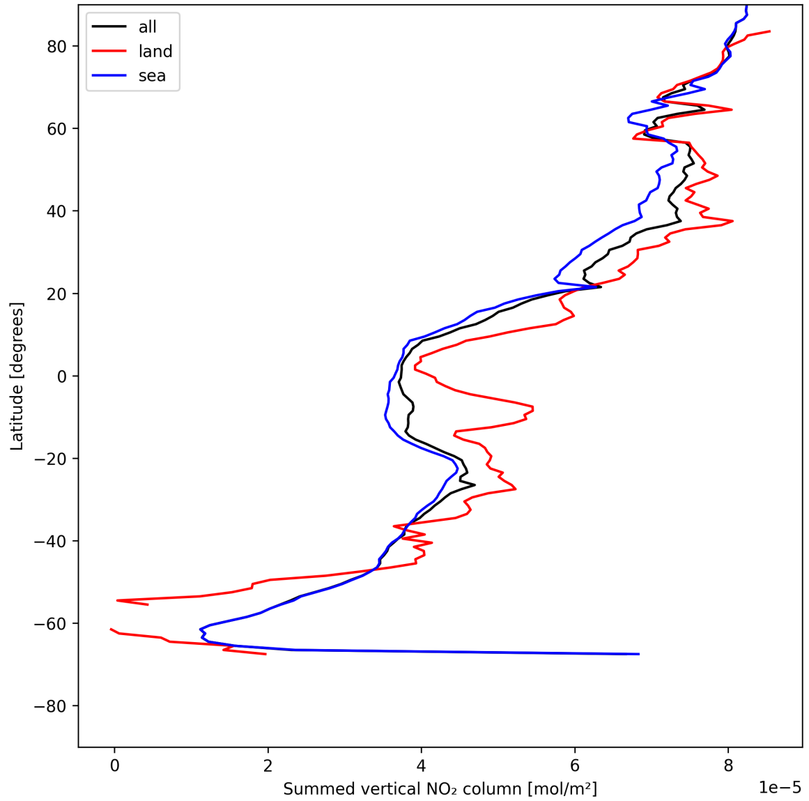
Figure 23: Zonal average of “Summed vertical NO 2 column” for 2025-07-19 to 2025-07-21.
