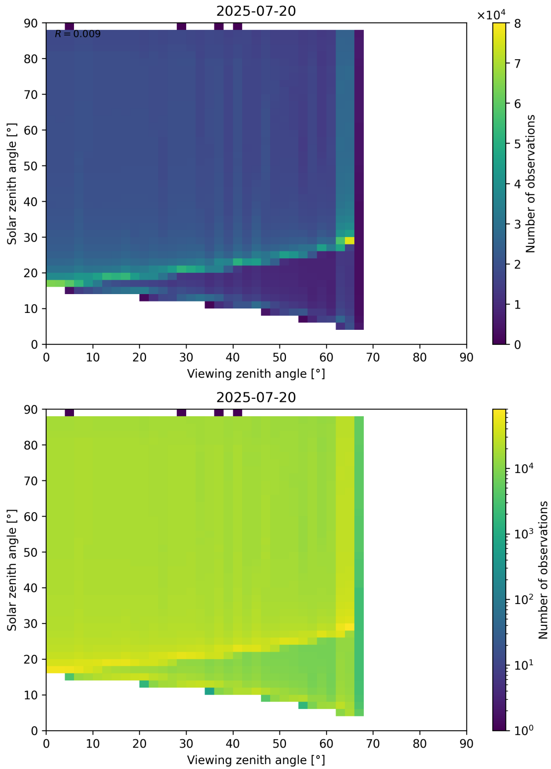
Figure 172: Scatter density plot of “Viewing zenith angle” against “Solar zenith angle” for 2025-07-19 to 2025-07-21.
