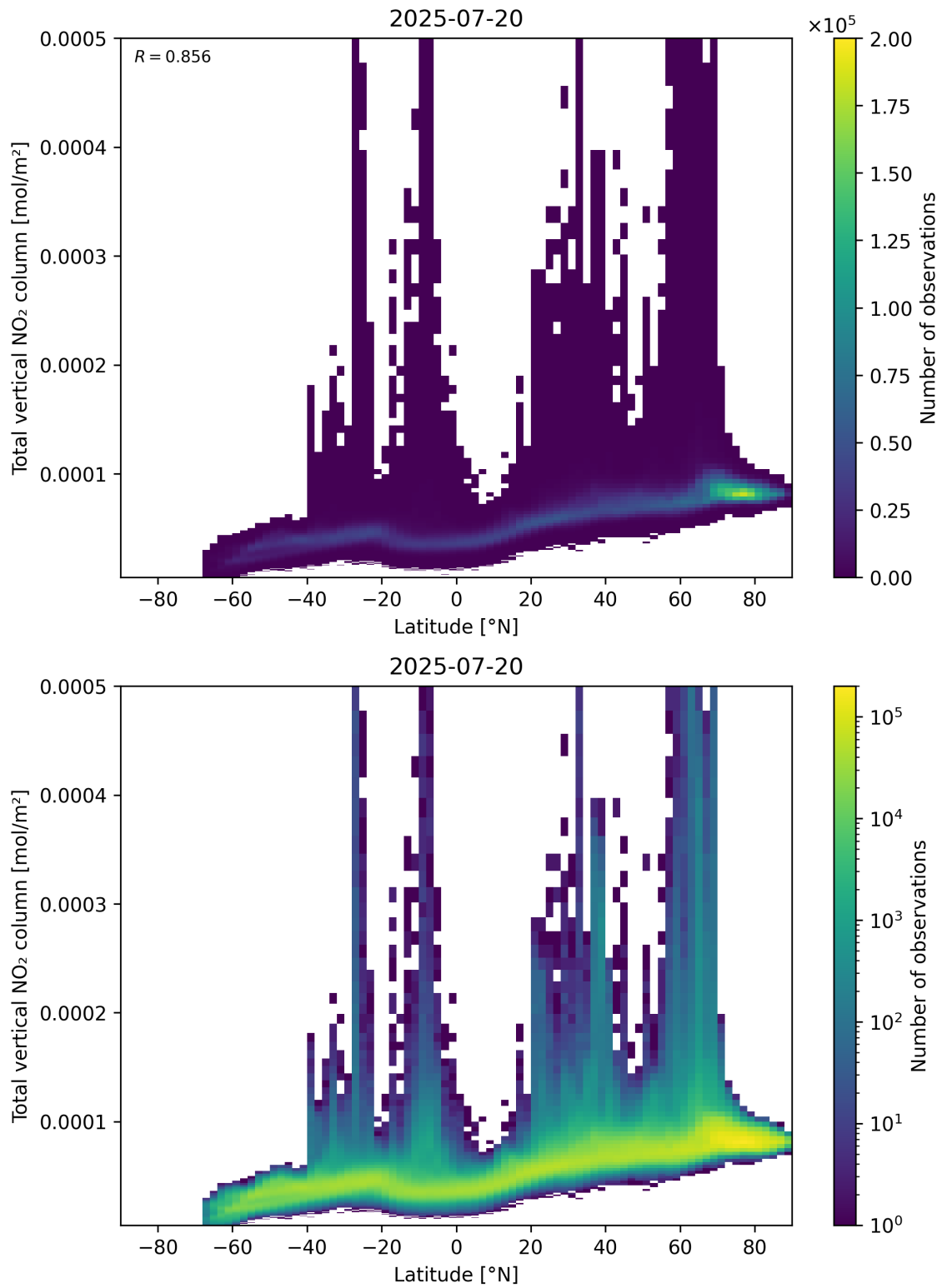
Figure 90: Scatter density plot of “Latitude” against “Total vertical NO 2 column” for 2025-07-19 to 2025-07-21.
