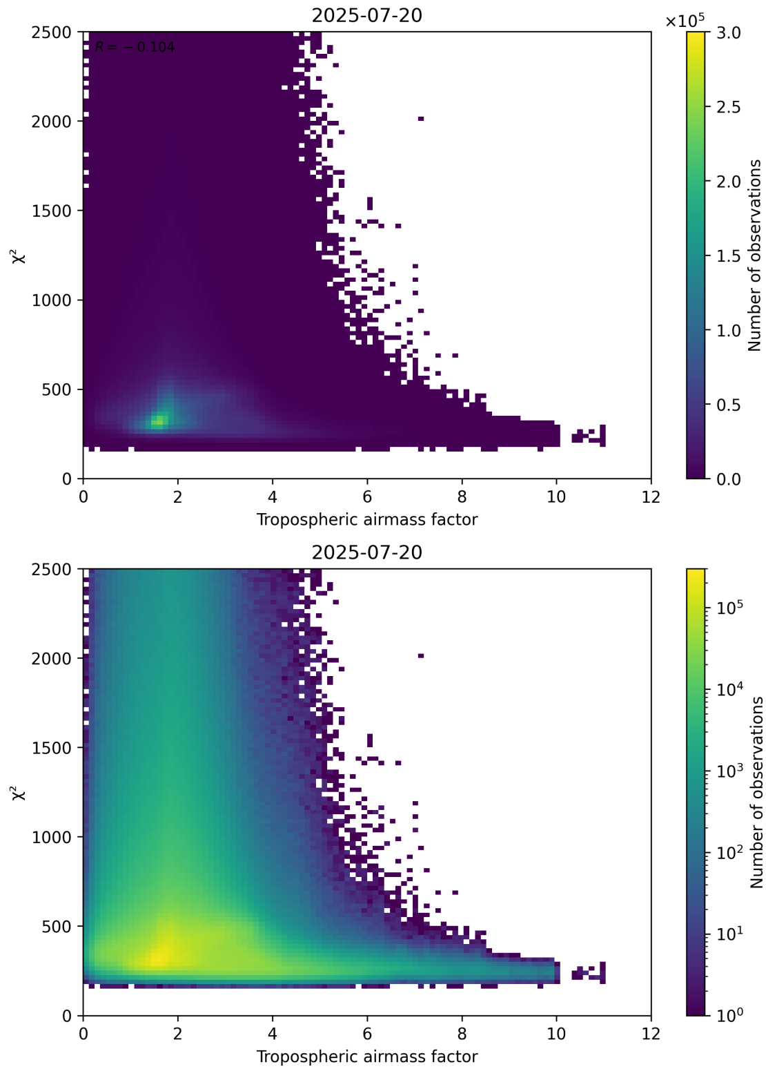
Figure 73: Scatter density plot of “Tropospheric airmass factor” against “ \chi^2 ” for 2025-07-19 to 2025-07-21.
