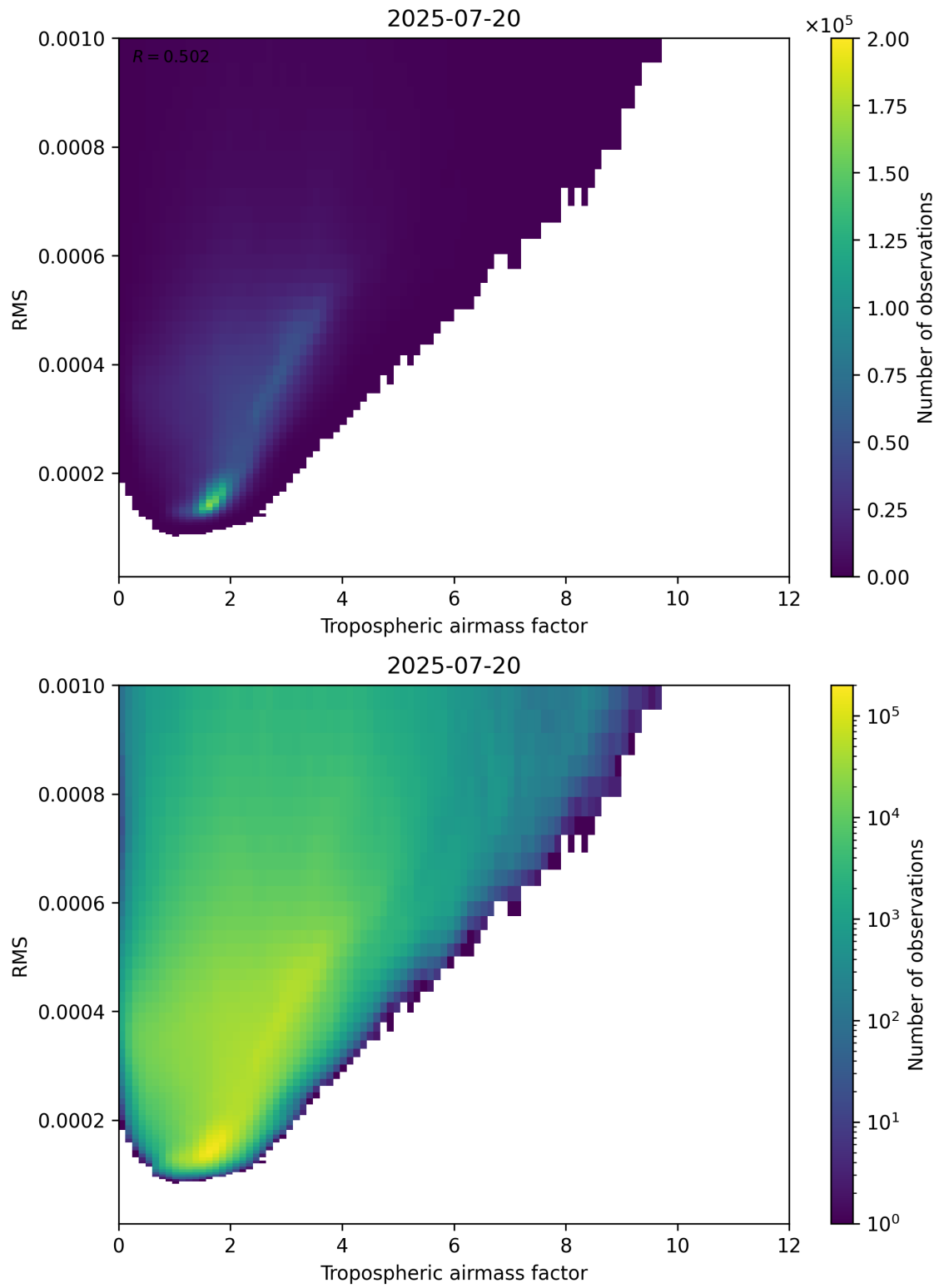
Figure 79: Scatter density plot of “Tropospheric airmass factor” against “RMS” for 2025-07-19 to 2025-07-21.
