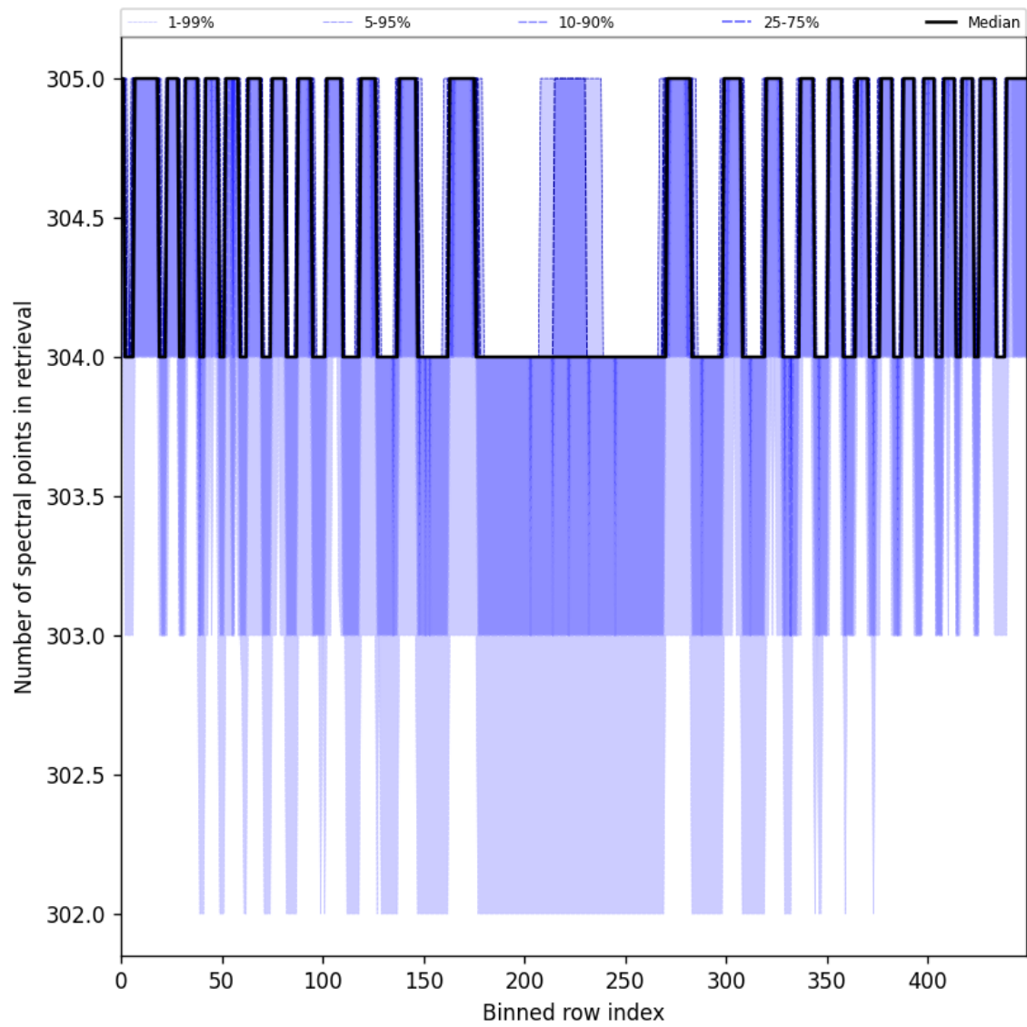
Figure 50: Along track statistics of “Number of spectral points in retrieval” for 2025-07-19 to 2025-07-21
