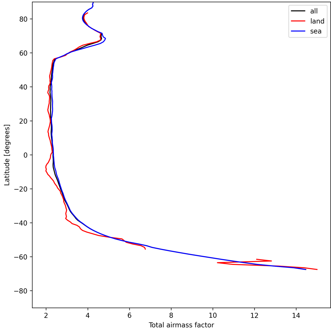
Figure 15: Zonal average of “Total airmass factor” for 2025-07-19 to 2025-07-21.
