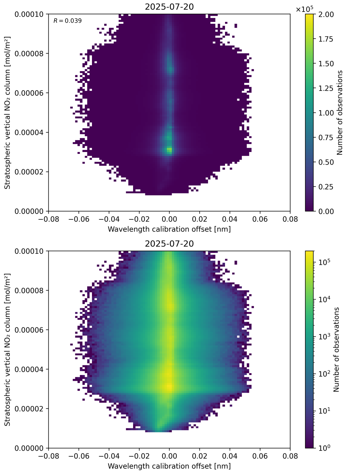
Figure 176: Scatter density plot of “Wavelength calibration offset” against “Stratospheric vertical NO 2 column” for 2025-07-19 to 2025-07-21.
