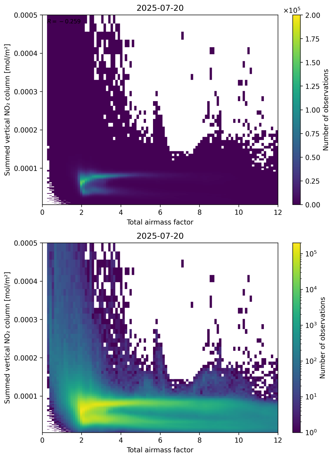
Figure 65: Scatter density plot of “Total airmass factor” against “Summed vertical NO 2 column” for 2025-07-19 to 2025-07-21.
