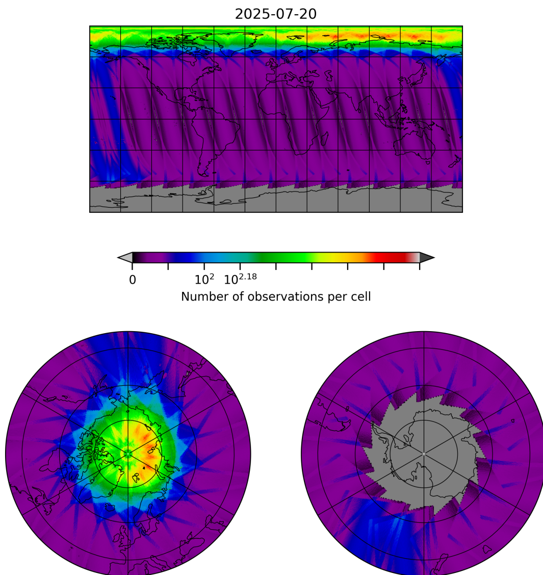
Figure 10: Map of the number of observations for 2025-07-19 to 2025-07-21
