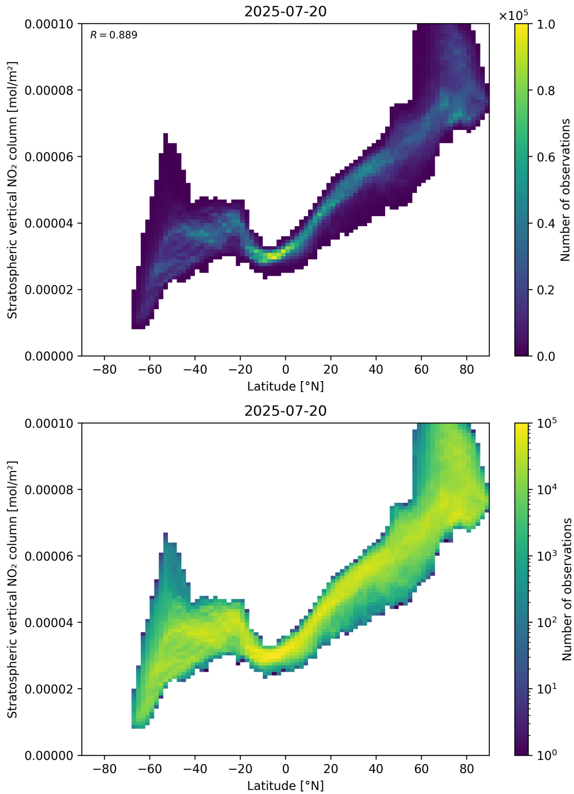
Figure 87: Scatter density plot of “Latitude” against “Stratospheric vertical NO 2 column” for 2025-07-19 to 2025-07-21.
