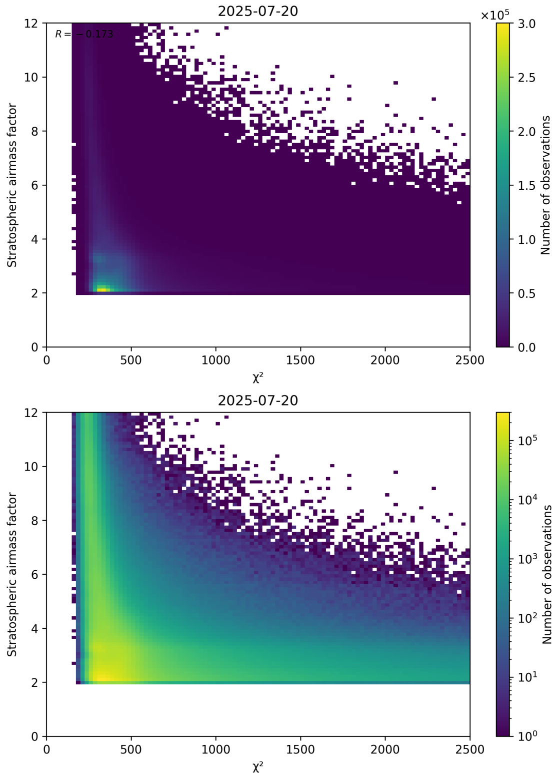
Figure 81: Scatter density plot of “ \chi^2 ” against “Stratospheric airmass factor” for 2025-07-19 to 2025-07-21.
