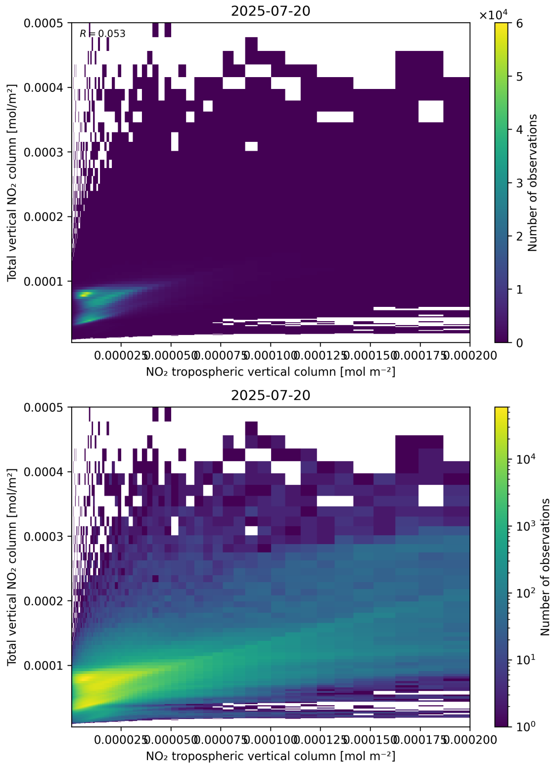
Figure 128: Scatter density plot of “NO 2 tropospheric vertical column” against “Total vertical NO 2 column” for 2025-07-19 to 2025-07-21.
