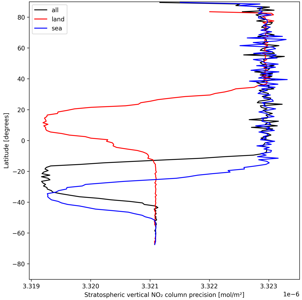
Figure 20: Zonal average of “Stratospheric vertical NO 2 column precision” for 2025-07-19 to 2025-07-21.
