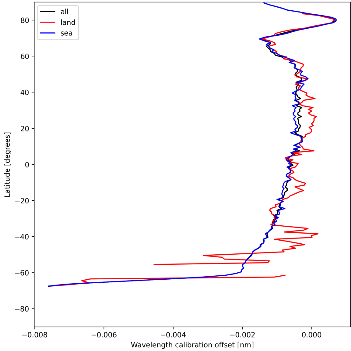
Figure 18: Zonal average of “Wavelength calibration offset” for 2025-07-19 to 2025-07-21.
