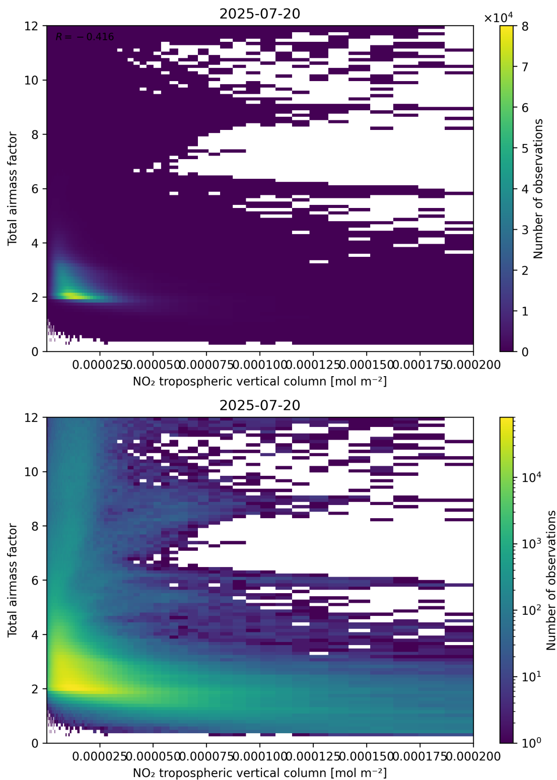
Figure 122: Scatter density plot of “NO 2 tropospheric vertical column” against “Total air mass factor” for 2025-07-19 to 2025-07-21.
