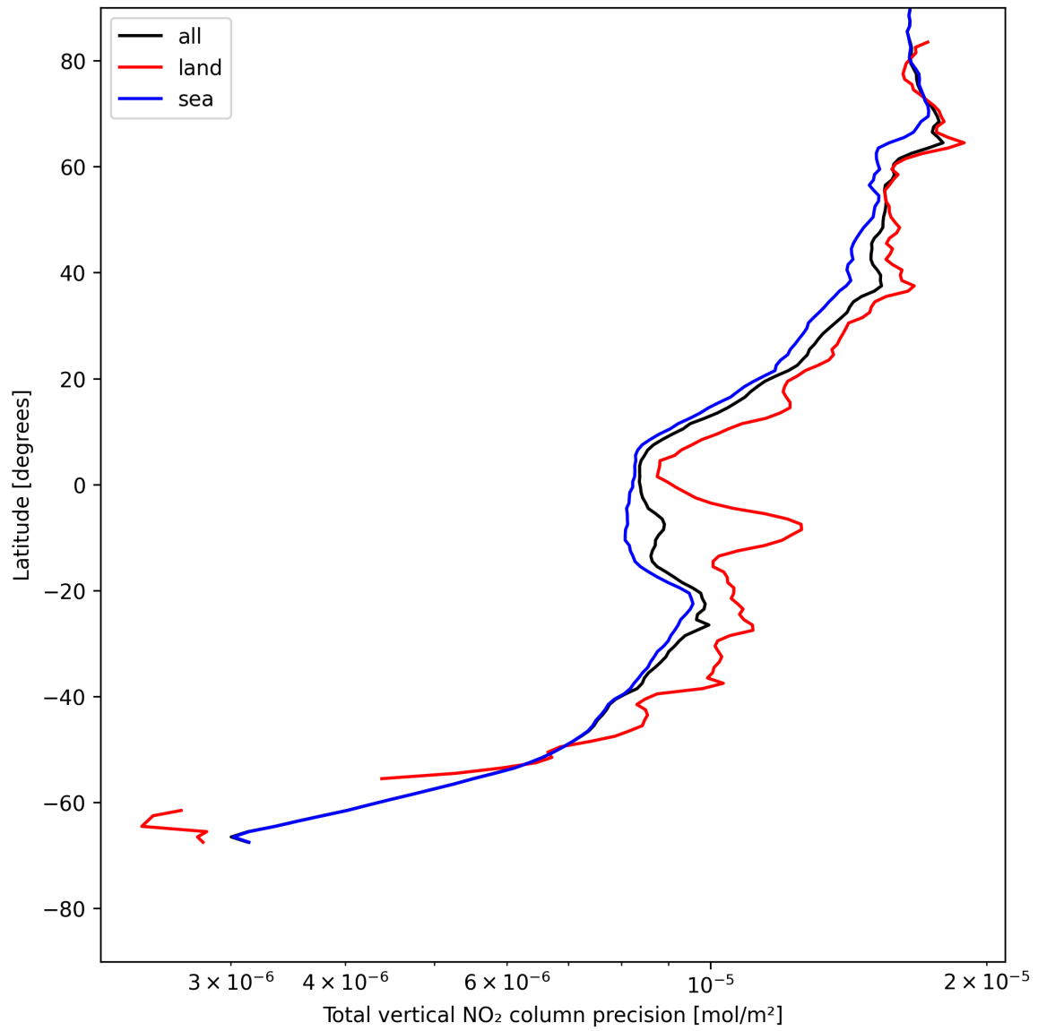
Figure 22: Zonal average of “Total vertical NO 2 column precision” for 2025-07-19 to 2025-07-21.
