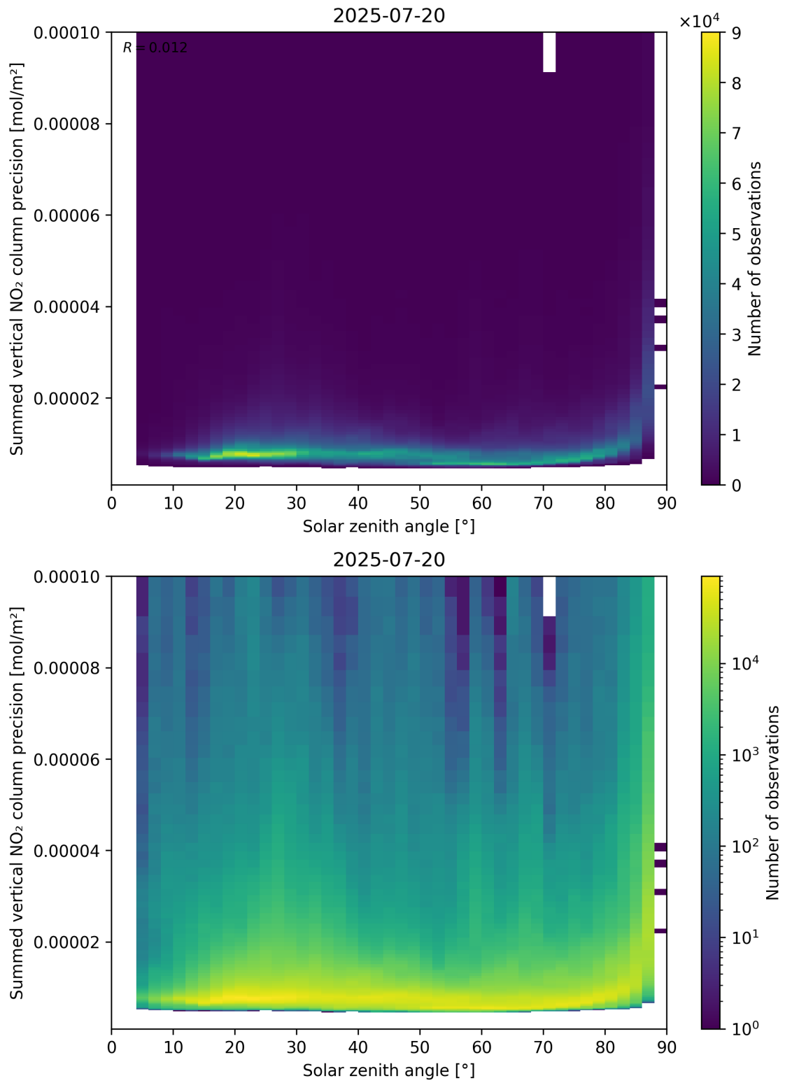
Figure 152: Scatter density plot of “Solar zenith angle” against “Summed vertical NO 2 column precision” for 2025-07-19 to 2025-07-21.
