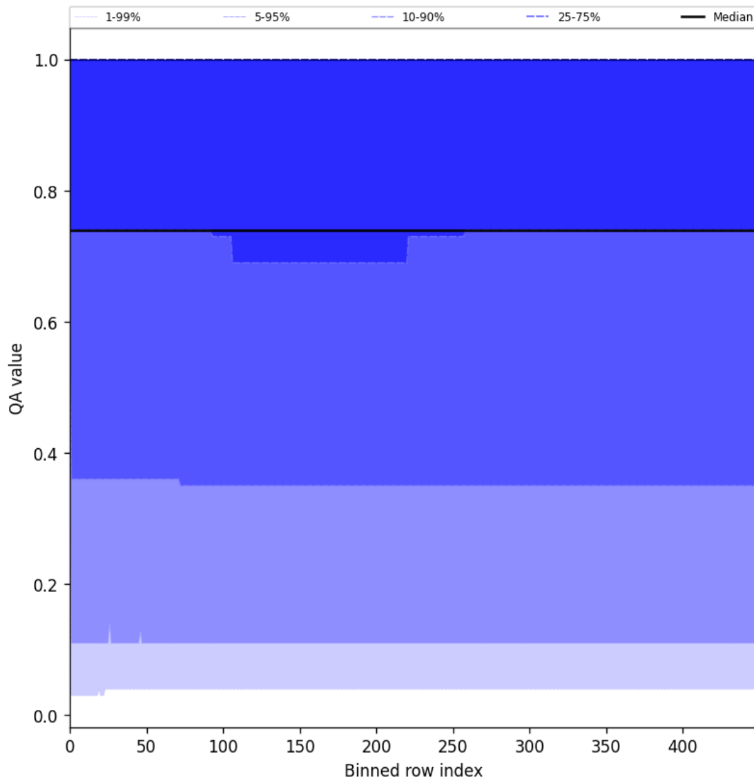
Figure 45: Along track statistics of “QA value” for 2025-07-19 to 2025-07-21
