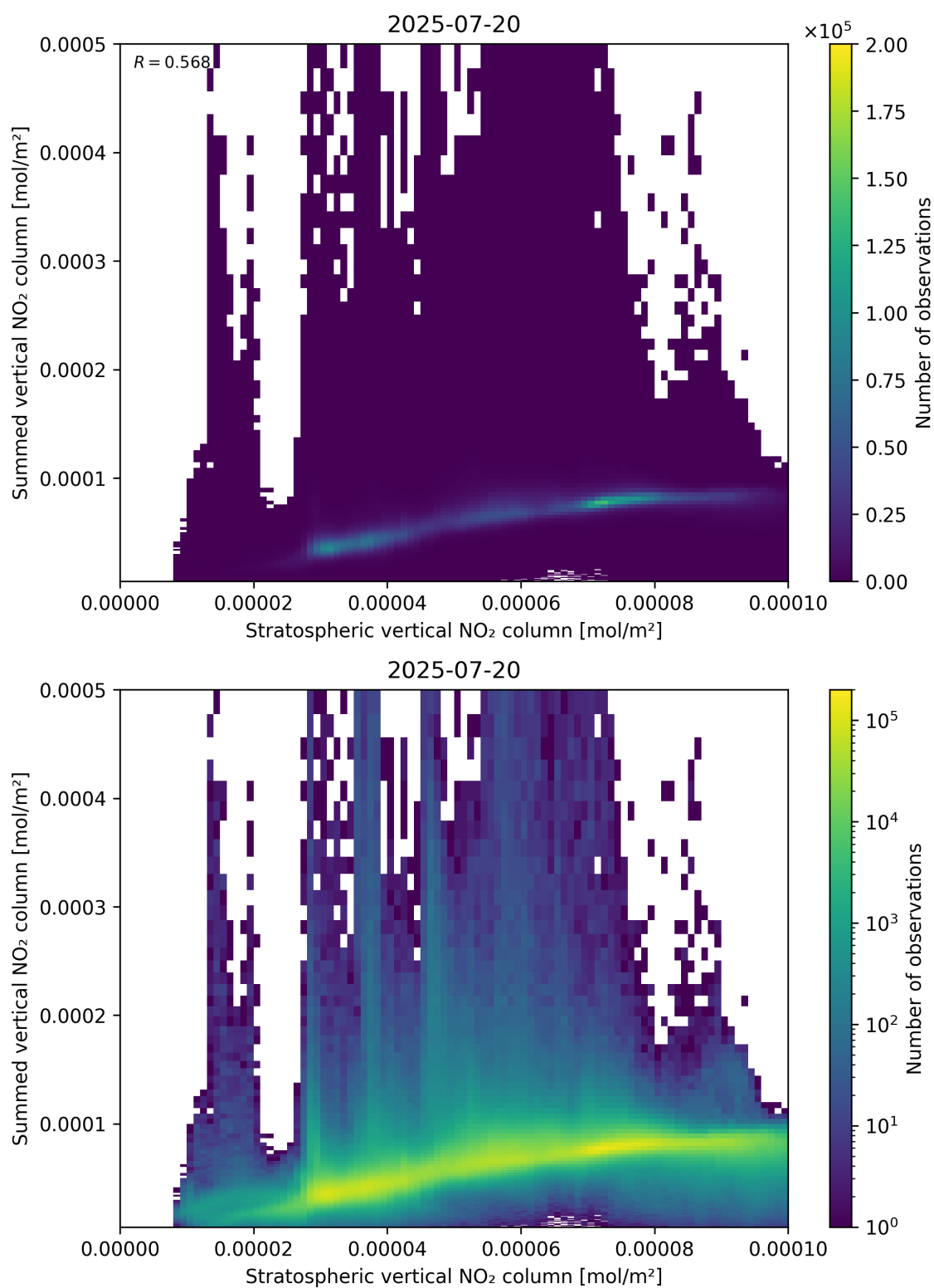
Figure 98: Scatter density plot of “Stratospheric vertical NO 2 column” against “Summed vertical NO 2 column” for 2025-07-19 to 2025-07-21.
