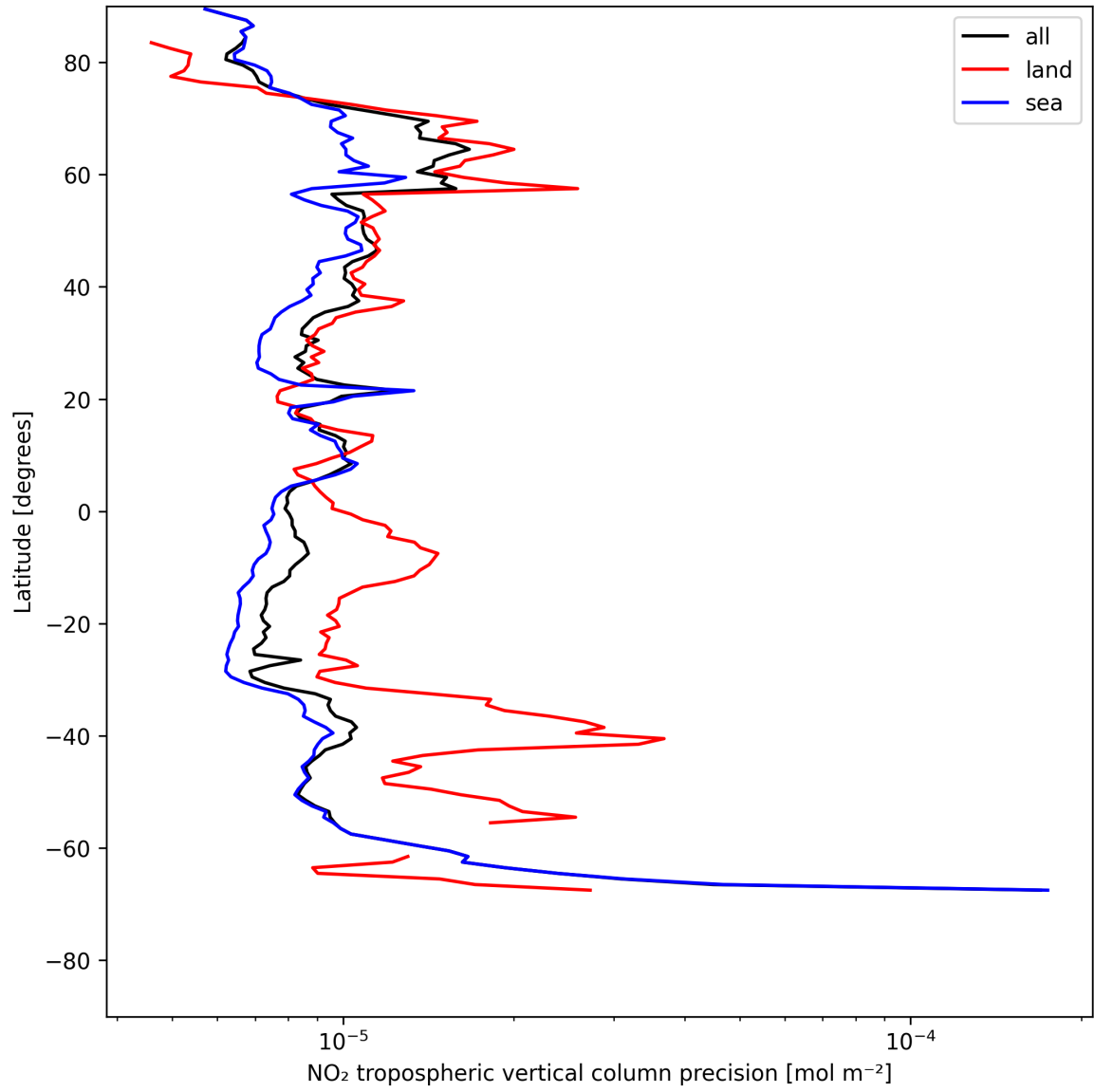
Figure 13: Zonal average of “NO 2 tropospheric vertical column precision” for 2025-07-19 to 2025-07-21.
