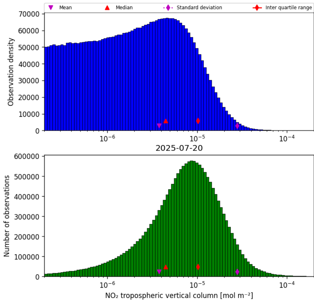
Figure 29: Histogram of “NO 2 tropospheric vertical column” for 2025-07-19 to 2025-07-21
