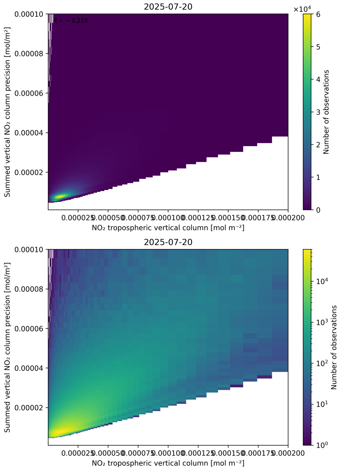
Figure 127: Scatter density plot of “NO 2 tropospheric vertical column” against “Summed vertical NO 2 column precision” for 2025-07-19 to 2025-07-21.
