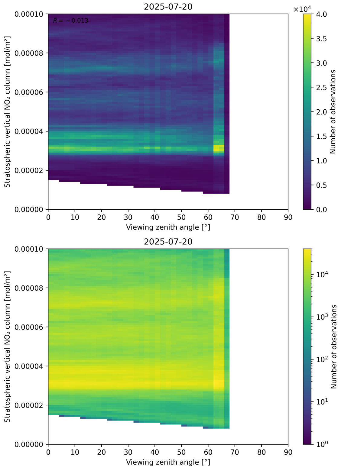
Figure 164: Scatter density plot of “Viewing zenith angle” against “Stratospheric vertical NO 2 column” for 2025-07-19 to 2025-07-21.
