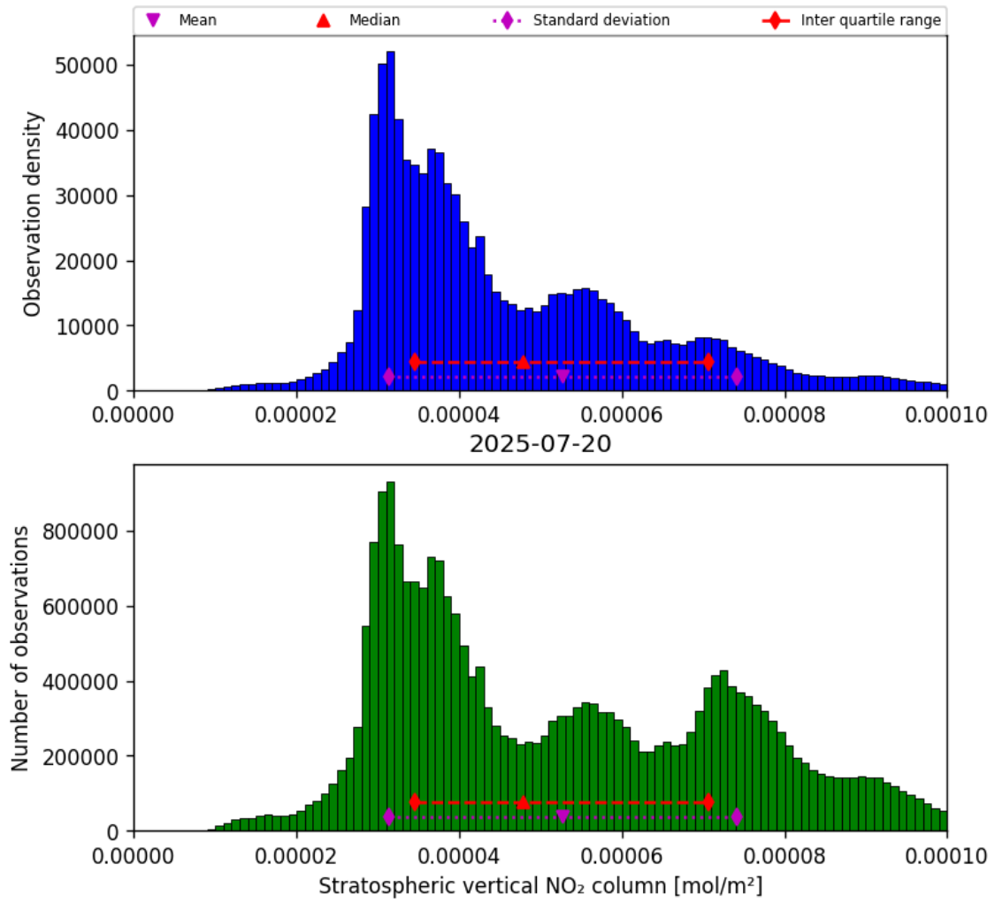
Figure 36: Histogram of “Stratospheric vertical NO 2 column” for 2025-07-19 to 2025-07-21
