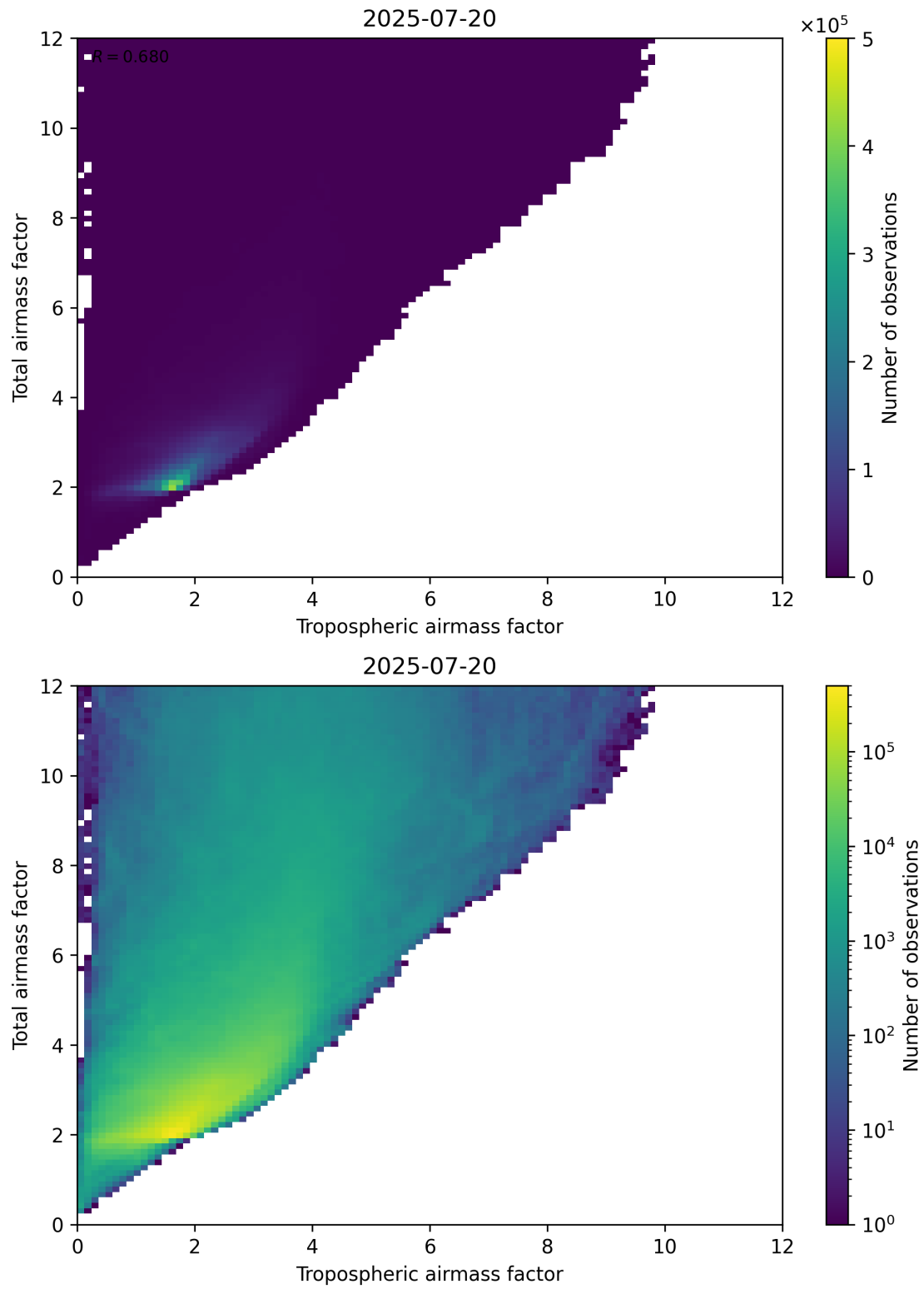
Figure 72: Scatter density plot of “Tropospheric airmass factor” against “Total airmass factor” for 2025-07-19 to 2025-07-21.
