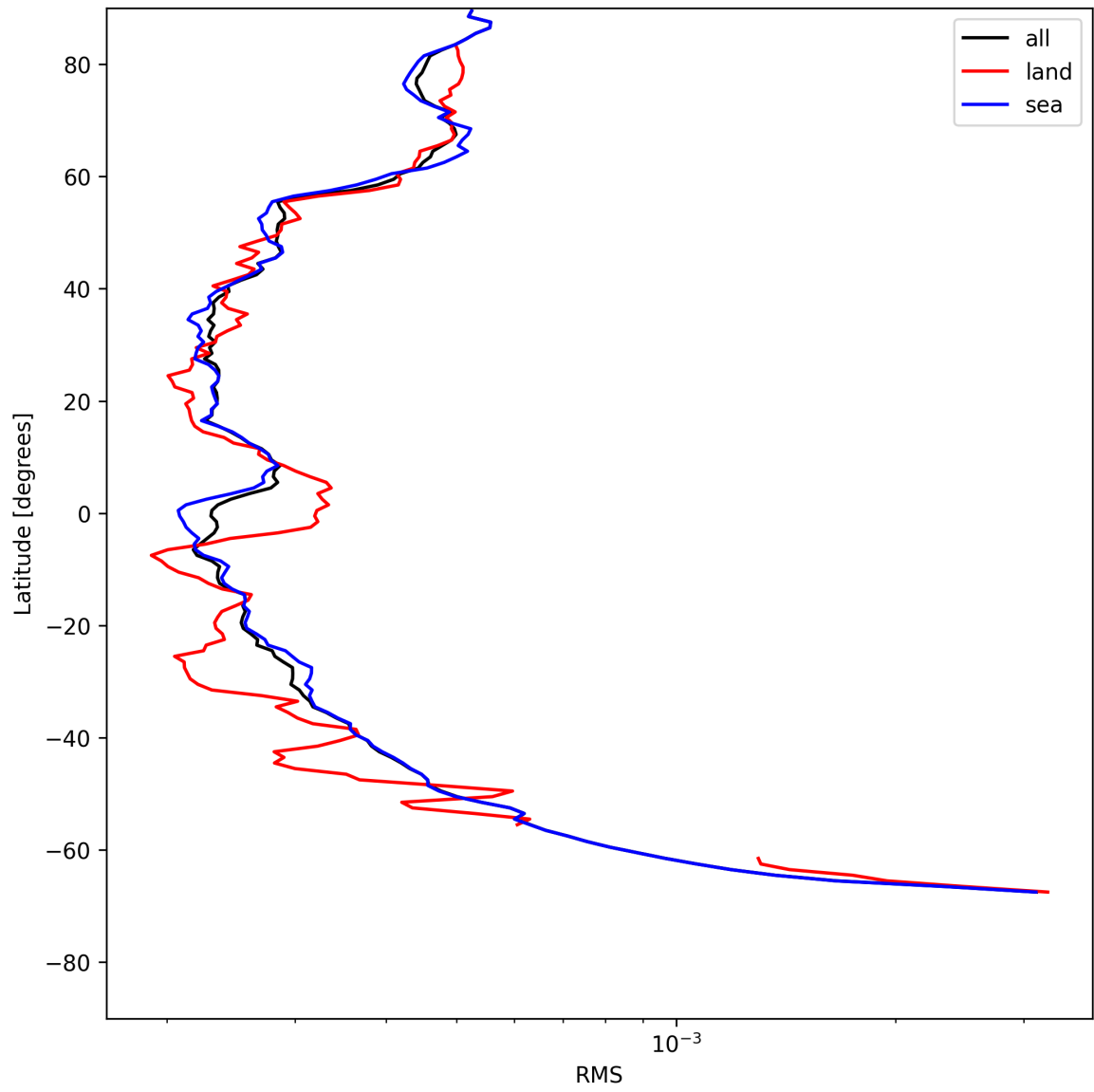
Figure 26: Zonal average of “RMS” for 2025-07-19 to 2025-07-21.
