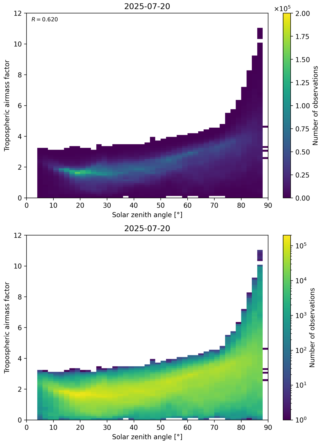
Figure 147: Scatter density plot of “Solar zenith angle” against “Tropospheric airmass factor” for 2025-07-19 to 2025-07-21.
