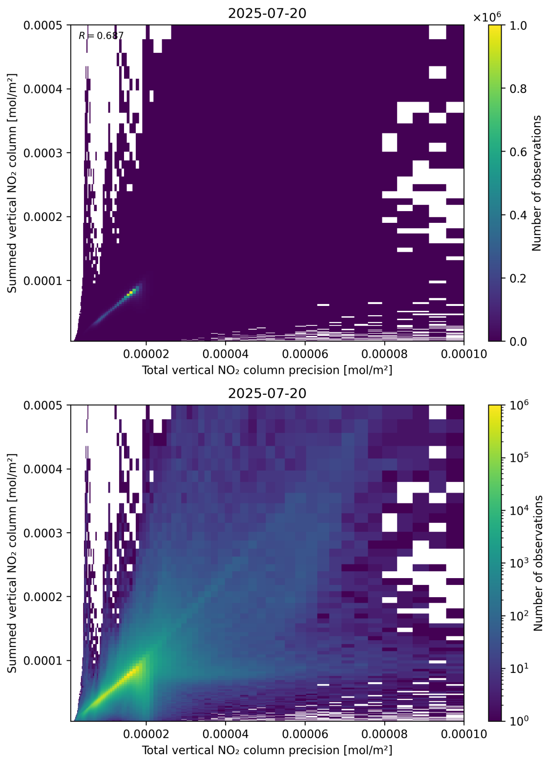
Figure 117: Scatter density plot of “Total vertical NO 2 column precision” against “Summed vertical NO 2 column” for 2025-07-19 to 2025-07-21.
