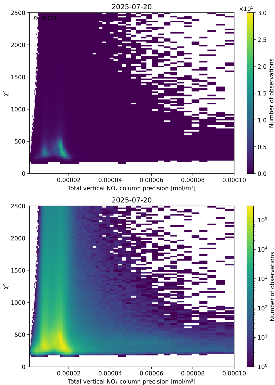
Figure 116: Scatter density plot of “Total vertical NO 2 column precision” against “ \chi^2 ” for 2025-07-19 to 2025-07-21.
