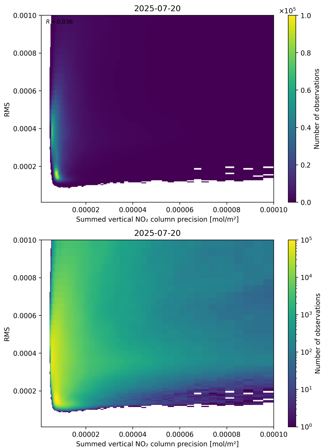
Figure 108: Scatter density plot of “Summed vertical NO 2 column precision” against “RMS” for 2025-07-19 to 2025-07-21.
