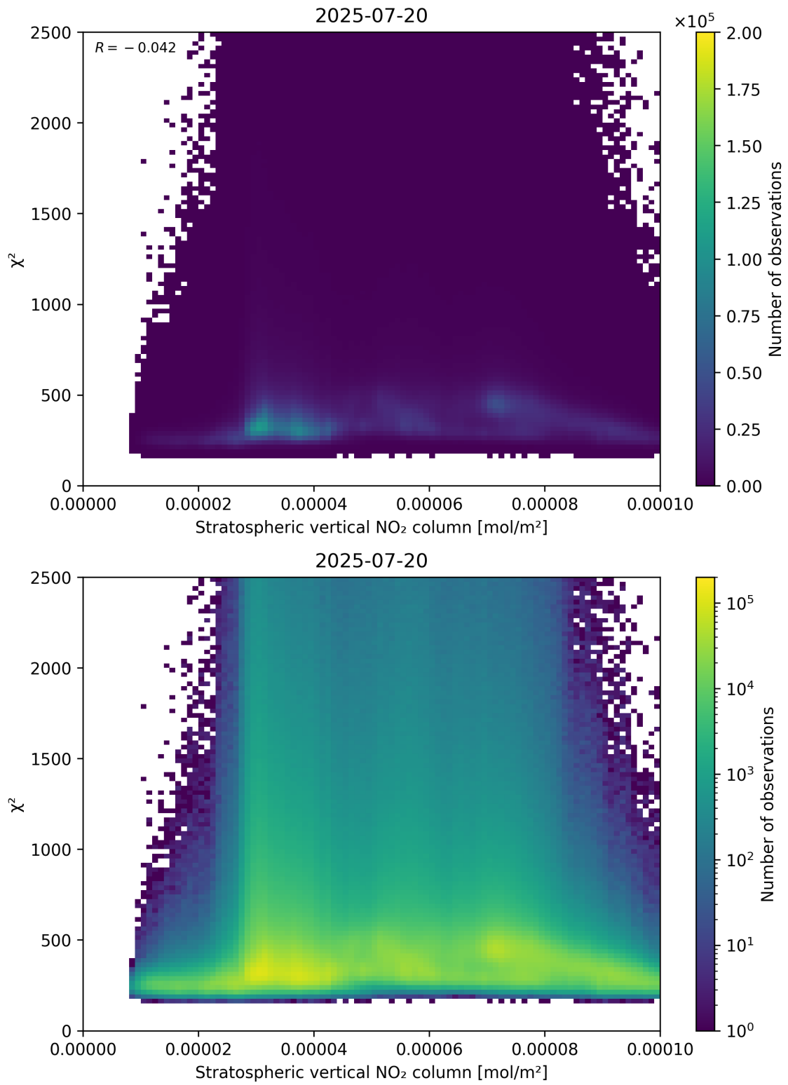
Figure 97: Scatter density plot of “Stratospheric vertical NO 2 column” against “ \chi^2 ” for 2025-07-19 to 2025-07-21.
