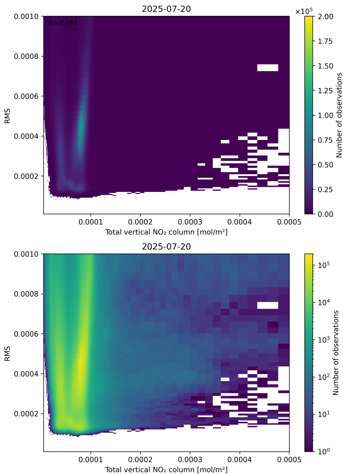
Figure 120: Scatter density plot of “Total vertical NO 2 column” against “RMS” for 2025-07-19 to 2025-07-21.
