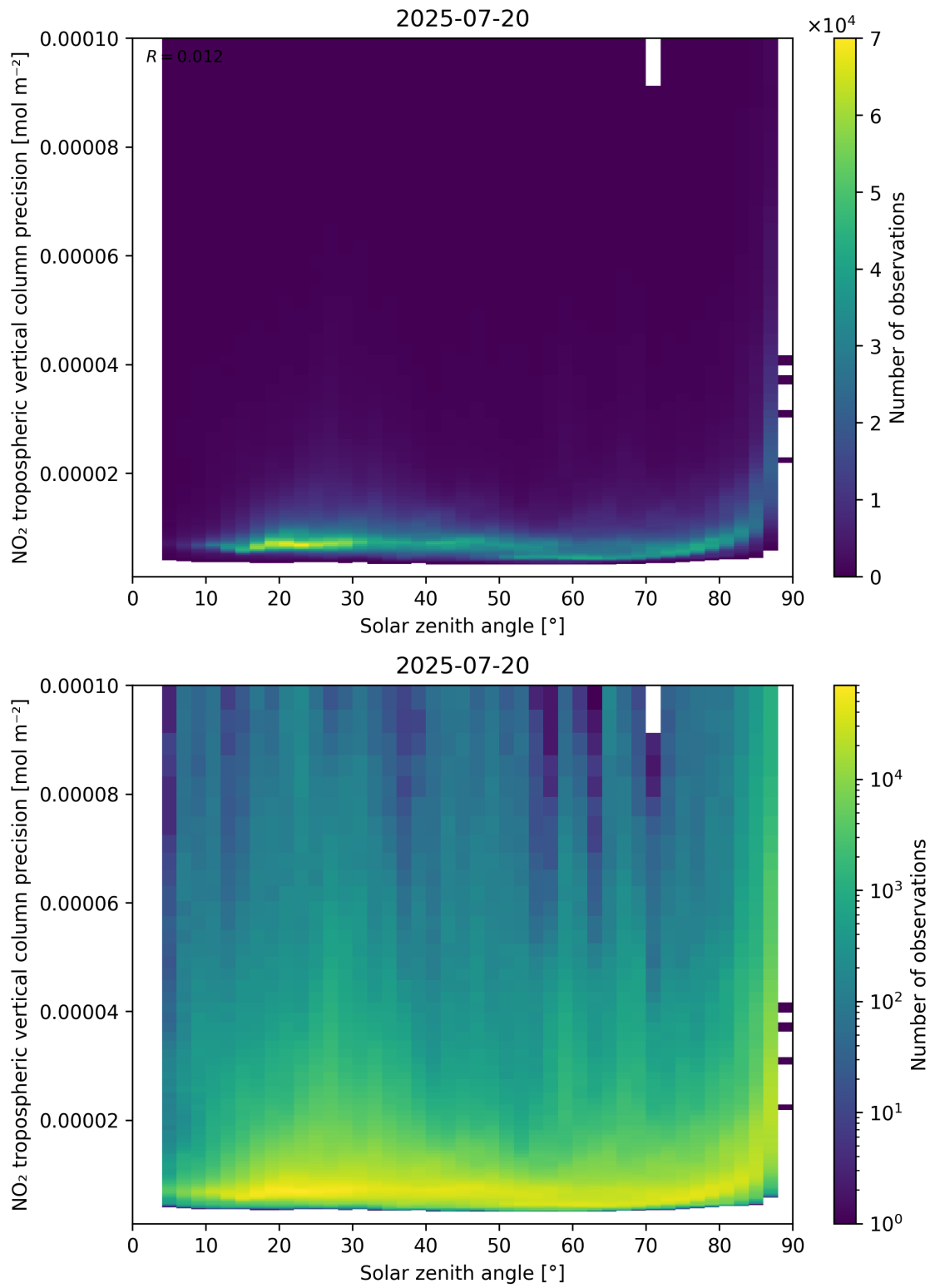
Figure 156: Scatter density plot of “Solar zenith angle” against “NO 2 tropospheric vertical column precision” for 2025-07-19 to 2025-07-21.
