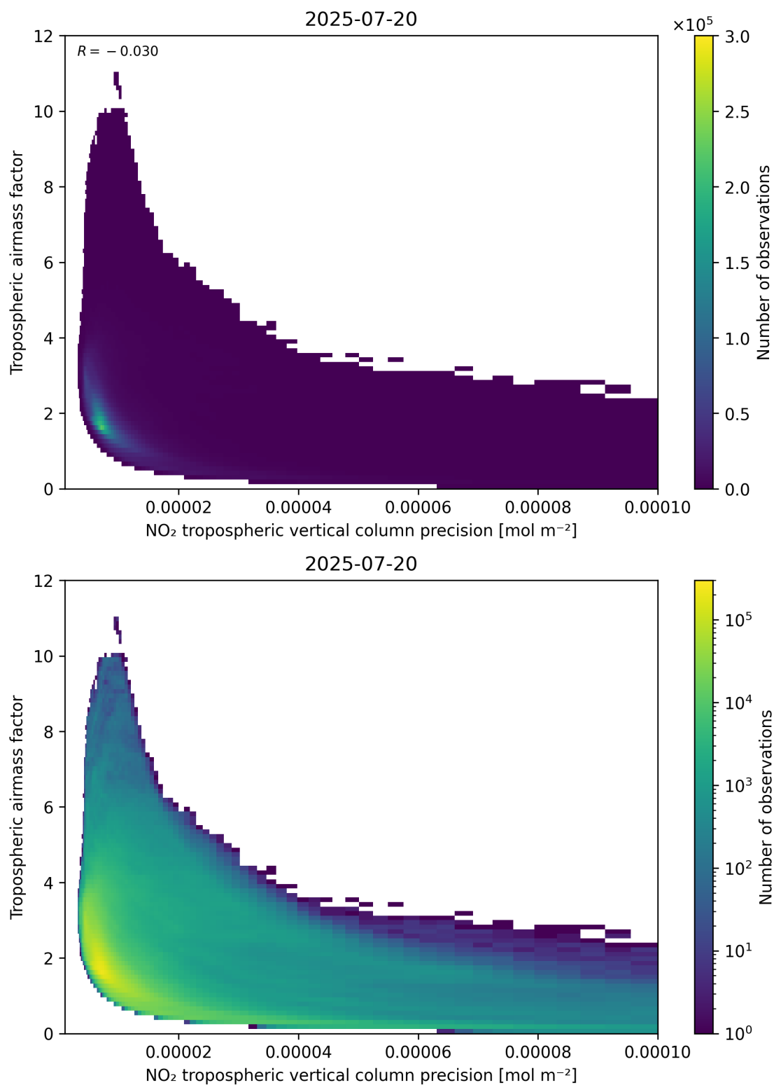
Figure 133: Scatter density plot of “NO 2 tropospheric vertical column precision” against “Tropospheric airmass factor” for 2025-07-19 to 2025-07-21.
