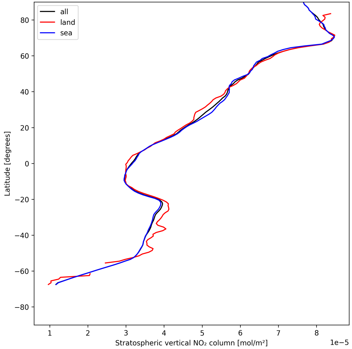
Figure 19: Zonal average of “Stratospheric vertical NO 2 column” for 2025-07-19 to 2025-07-21.
