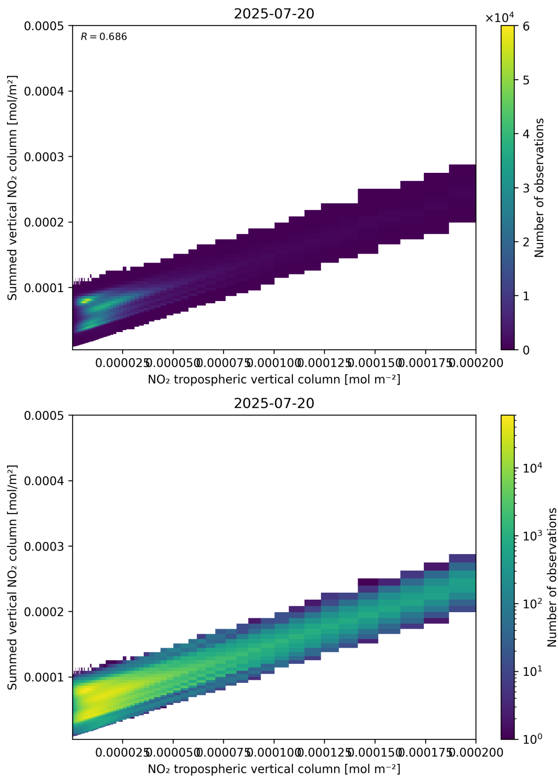
Figure 126: Scatter density plot of “NO 2 tropospheric vertical column” against “Summed vertical NO 2 column” for 2025-07-19 to 2025-07-21.
