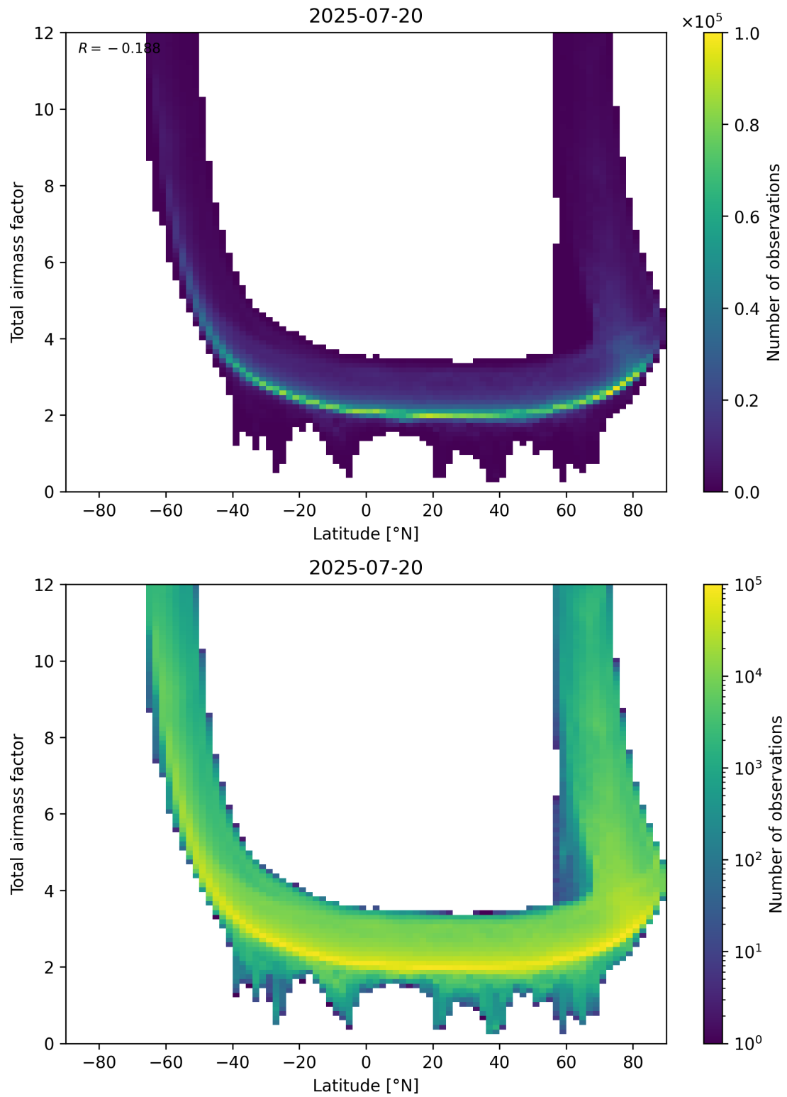
Figure 84: Scatter density plot of “Latitude” against “Total airmass factor” for 2025-07-19 to 2025-07-21.
