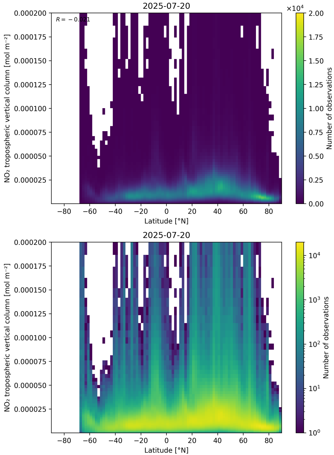
Figure 92: Scatter density plot of “Latitude” against “NO 2 tropospheric vertical column” for 2025-07-19 to 2025-07-21.
