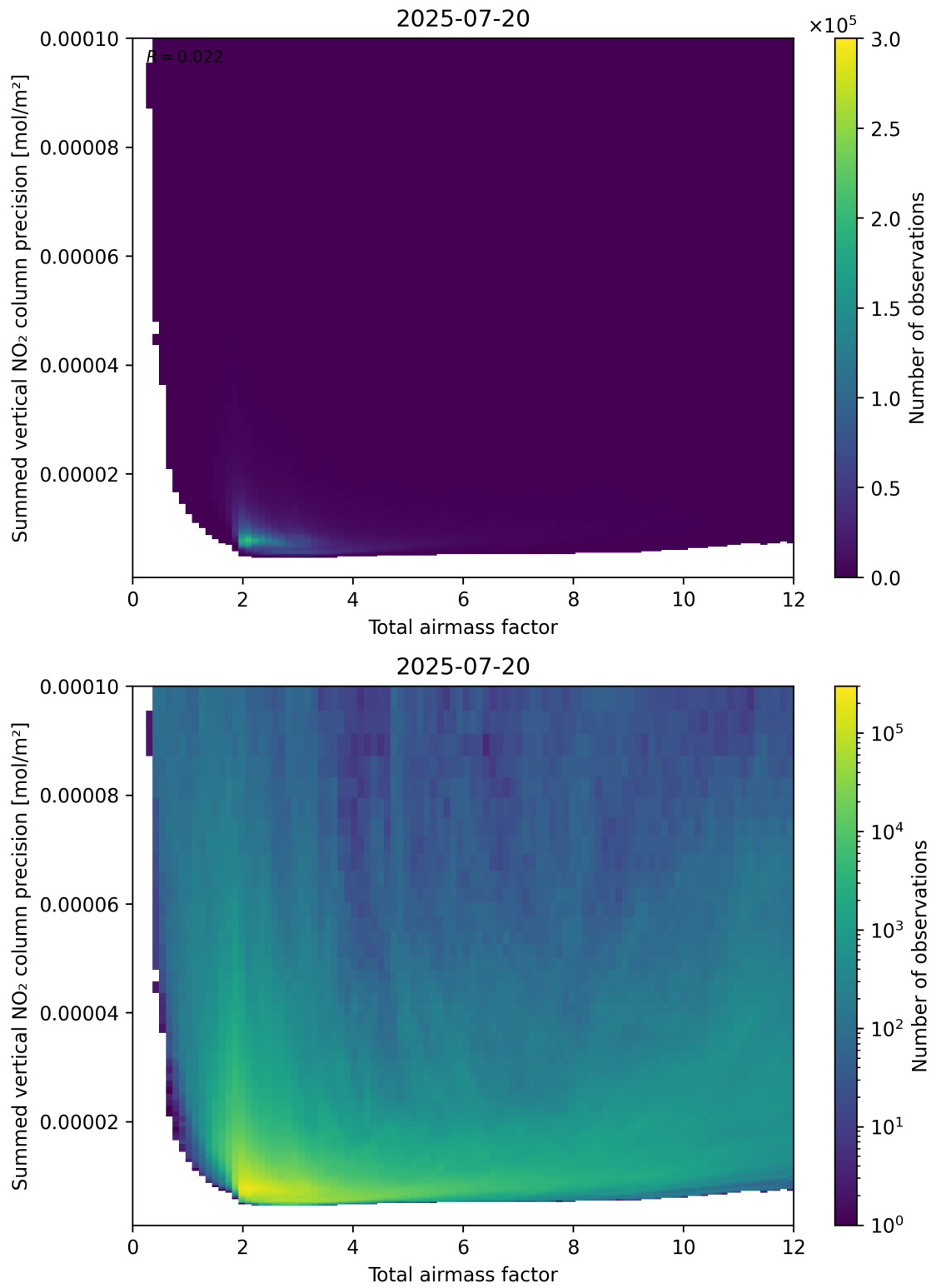
Figure 66: Scatter density plot of “Total airmass factor” against “Summed vertical NO 2 column precision” for 2025-07-19 to 2025-07-21.
