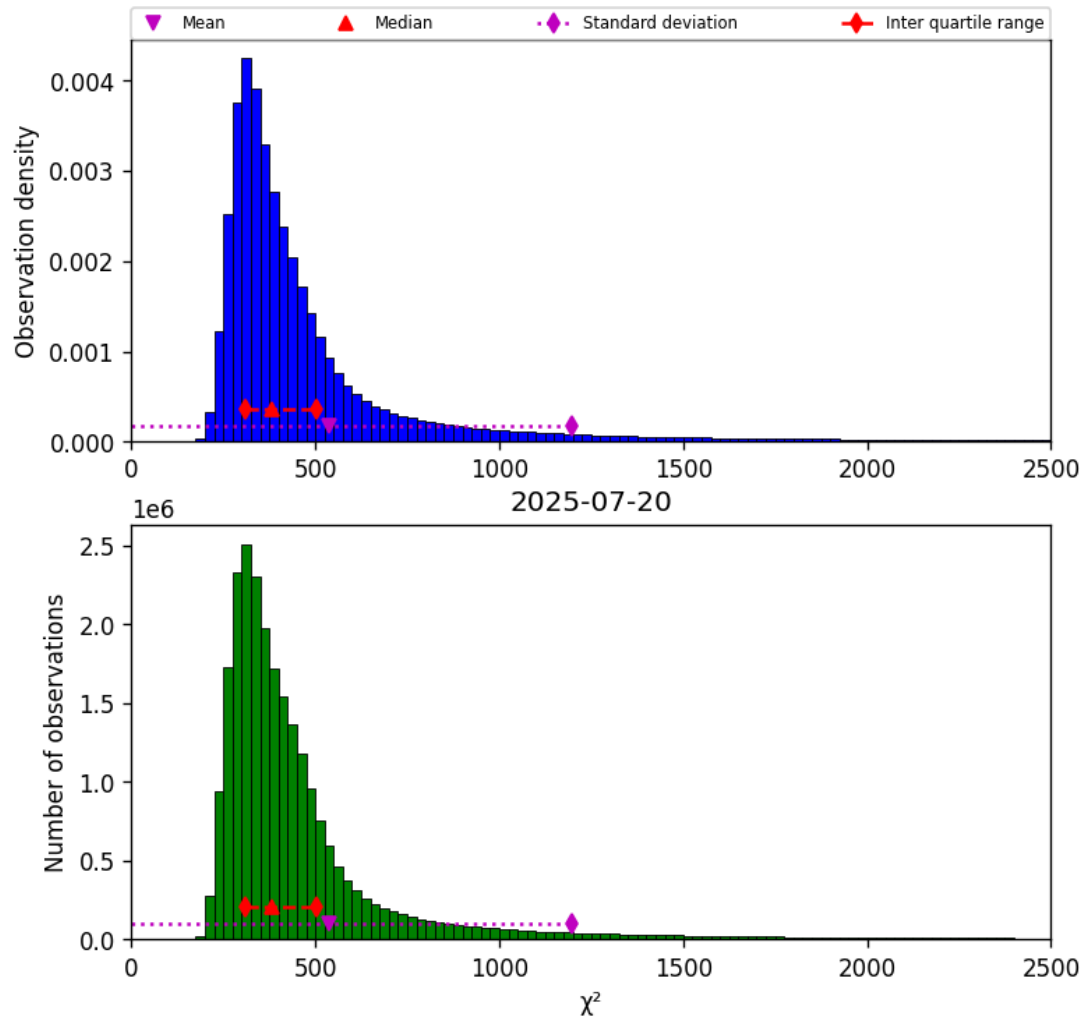
Figure 42: Histogram of " \chi^2 " for 2025-07-19 to 2025-07-21
