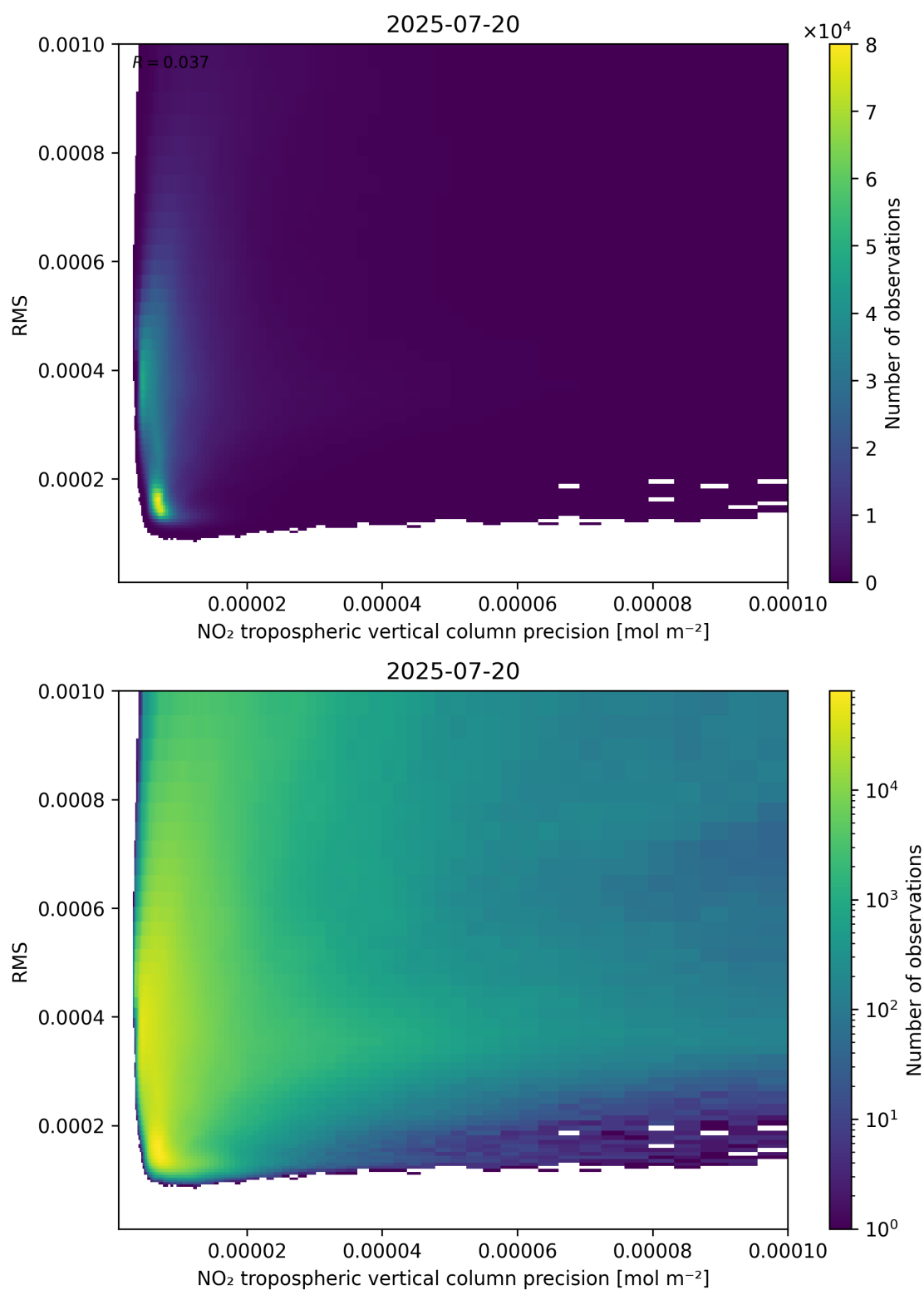
Figure 140: Scatter density plot of “NO 2 tropospheric vertical column precision” against “RMS” for 2025-07-19 to 2025-07-21.
