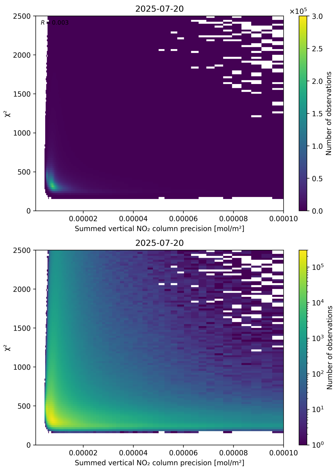
Figure 107: Scatter density plot of “Summed vertical NO 2 column precision” against “ \chi^2 ” for 2025-07-19 to 2025-07-21.
