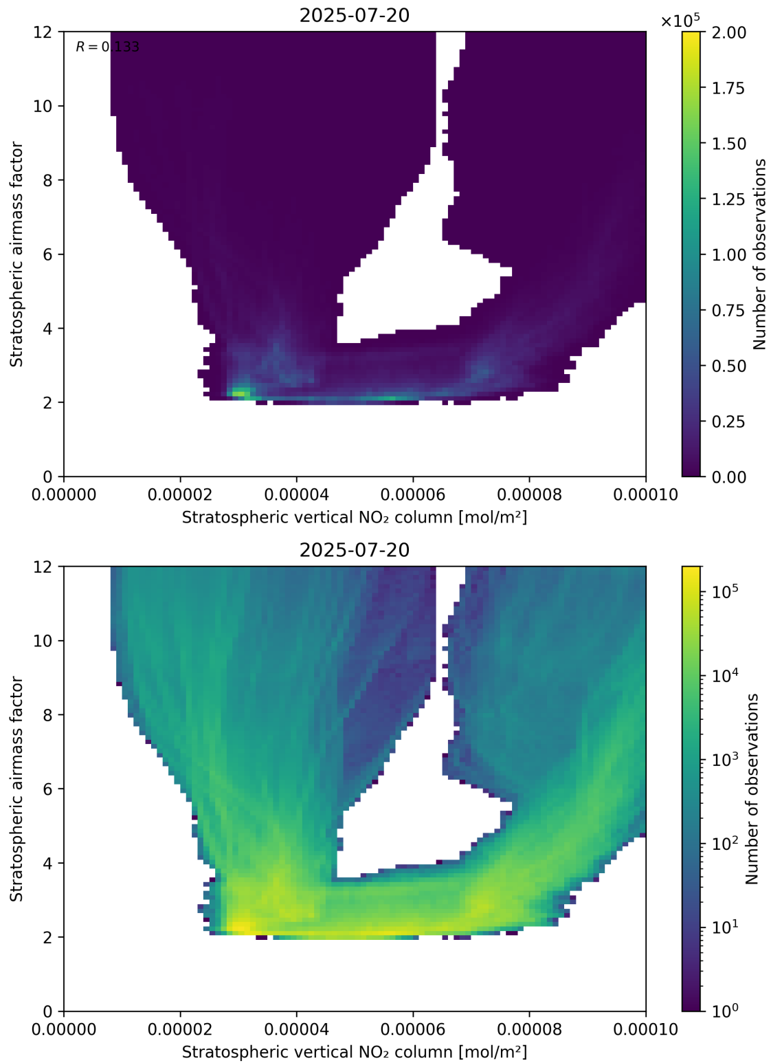
Figure 96: Scatter density plot of “Stratospheric vertical NO 2 column” against “Stratospheric airmass factor” for 2025-07-19 to 2025-07-21.
