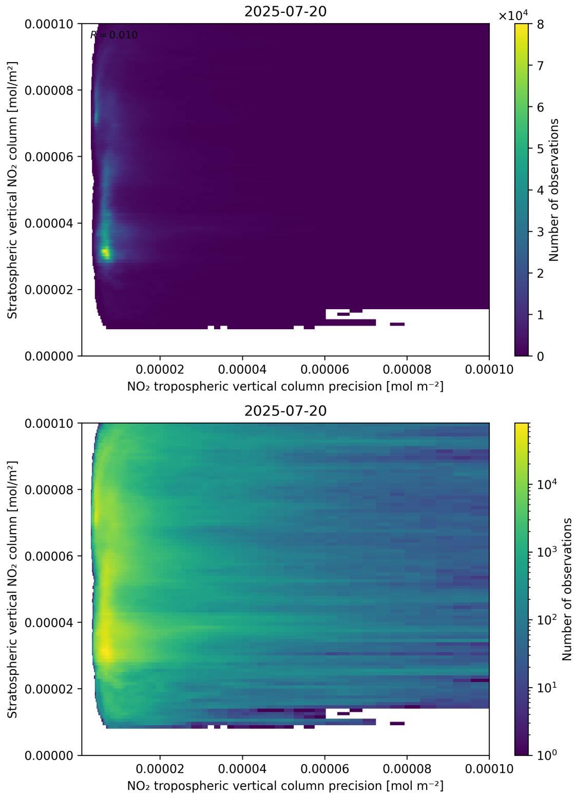
Figure 135: Scatter density plot of “NO 2 tropospheric vertical column precision” against “Stratospheric vertical NO 2 column” for 2025-07-19 to 2025-07-21.
