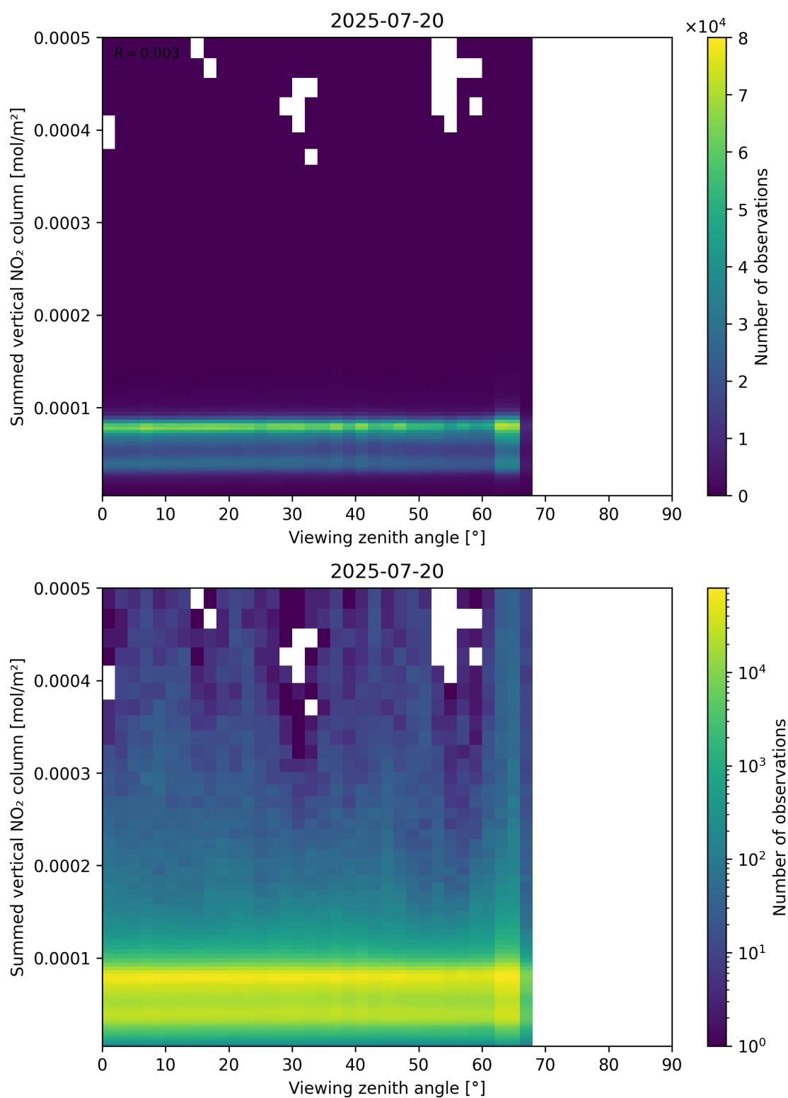
Figure 165: Scatter density plot of “Viewing zenith angle” against “Summed vertical NO 2 column” for 2025-07-19 to 2025-07-21.
