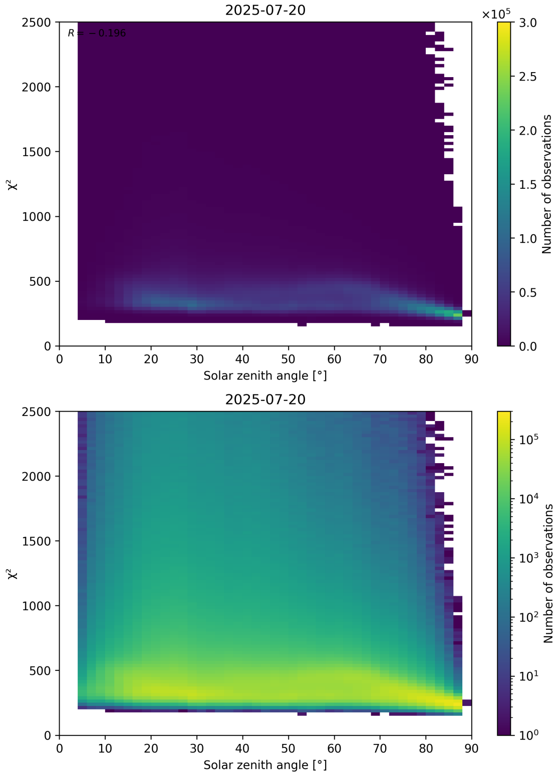
Figure 148: Scatter density plot of “Solar zenith angle” against “ \chi^2 ” for 2025-07-19 to 2025-07-21.
