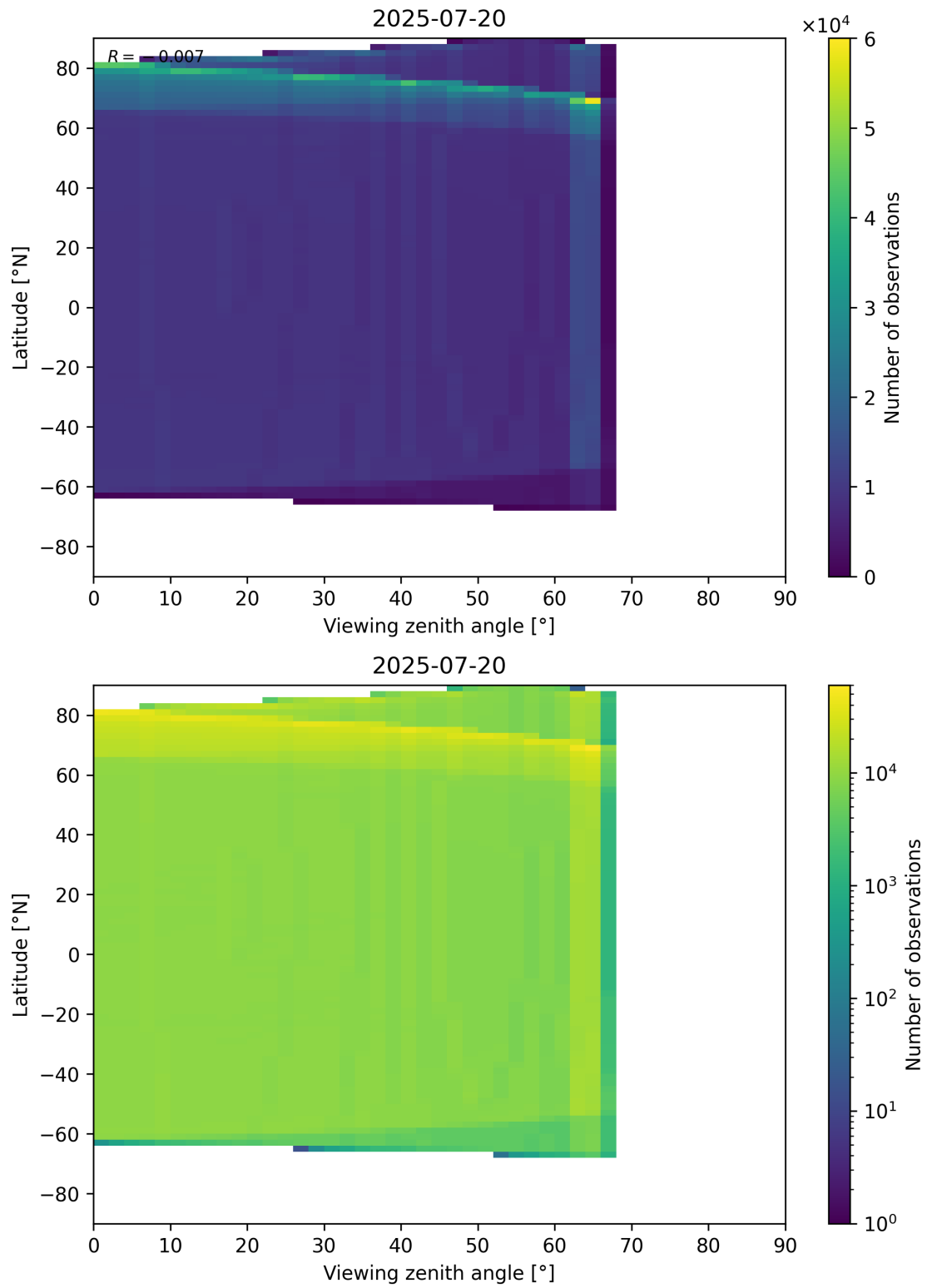
Figure 163: Scatter density plot of “Viewing zenith angle” against “Latitude” for 2025-07-19 to 2025-07-21.
