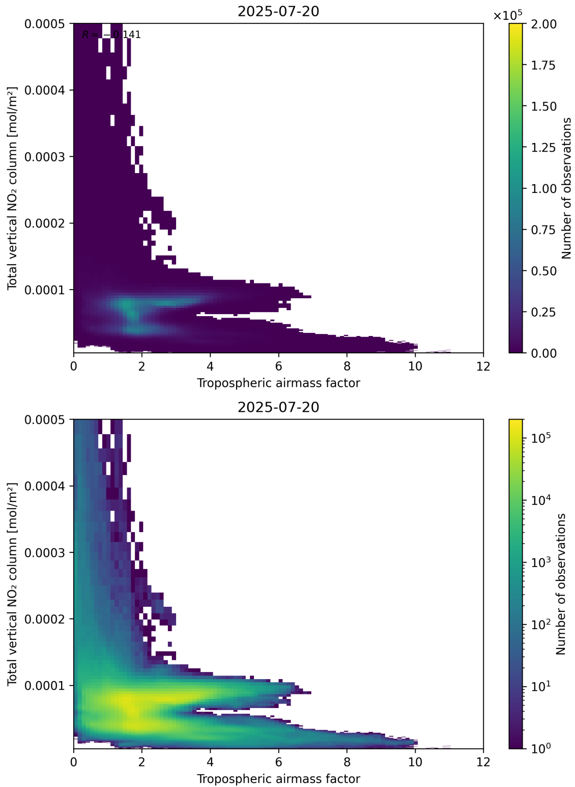
Figure 77: Scatter density plot of “Tropospheric airmass factor” against “Total vertical NO 2 column” for 2025-07-19 to 2025-07-21.
