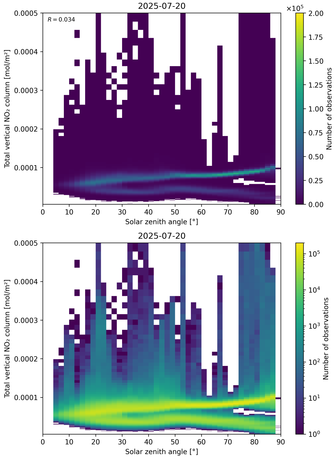
Figure 153: Scatter density plot of “Solar zenith angle” against “Total vertical NO 2 column” for 2025-07-19 to 2025-07-21.
