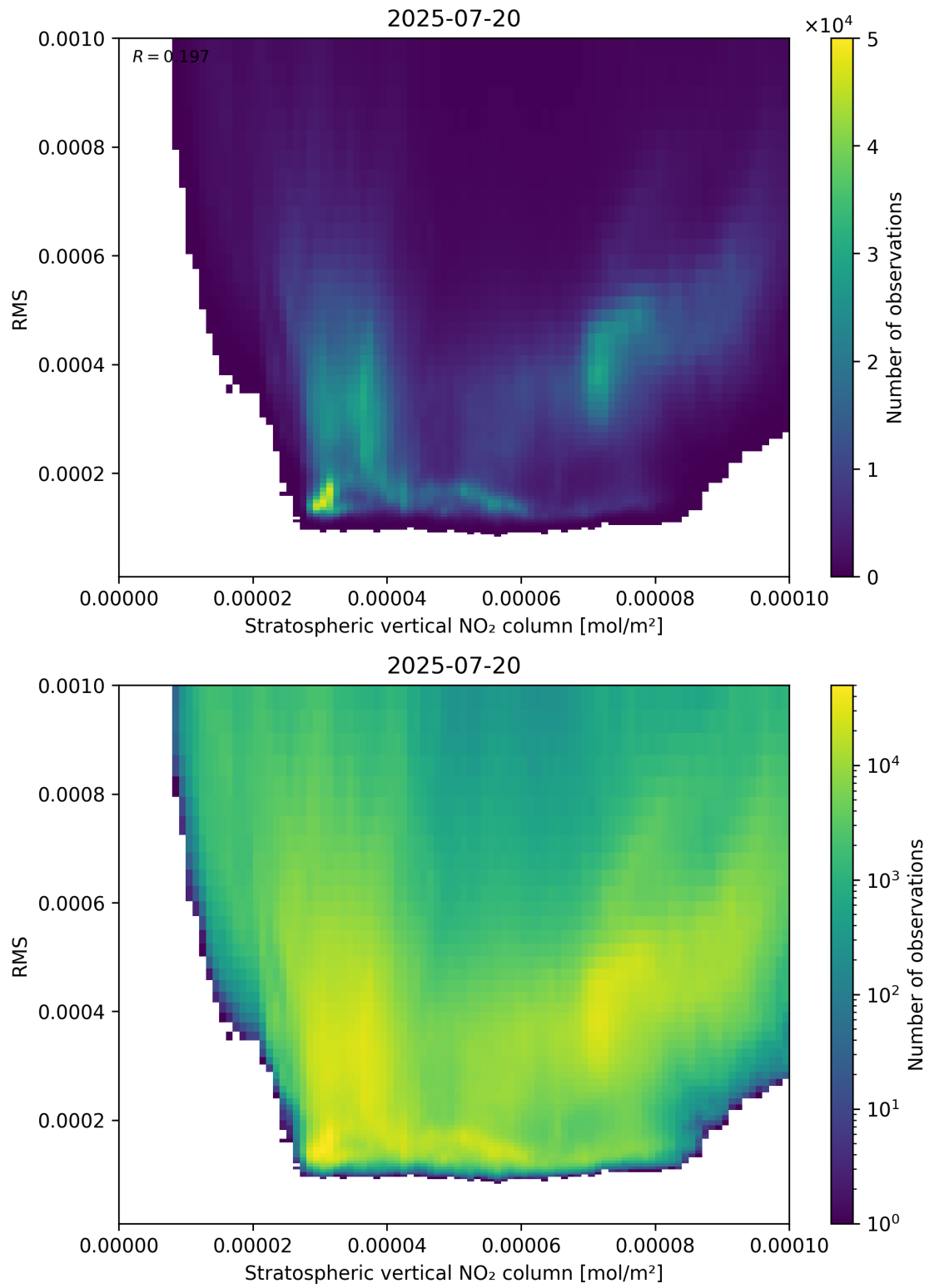
Figure 102: Scatter density plot of “Stratospheric vertical NO 2 column” against “RMS” for 2025-07-19 to 2025-07-21.
