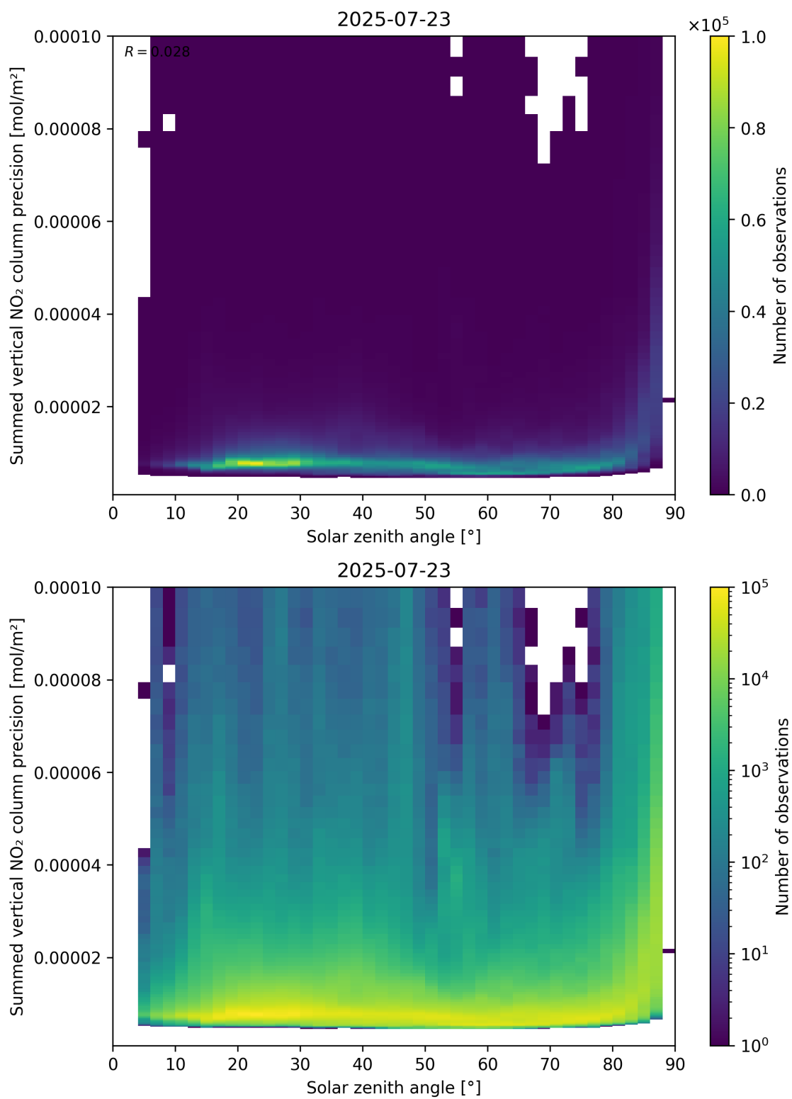
Figure 152: Scatter density plot of “Solar zenith angle” against “Summed vertical NO 2 column precision” for 2025-07-22 to 2025-07-24.
