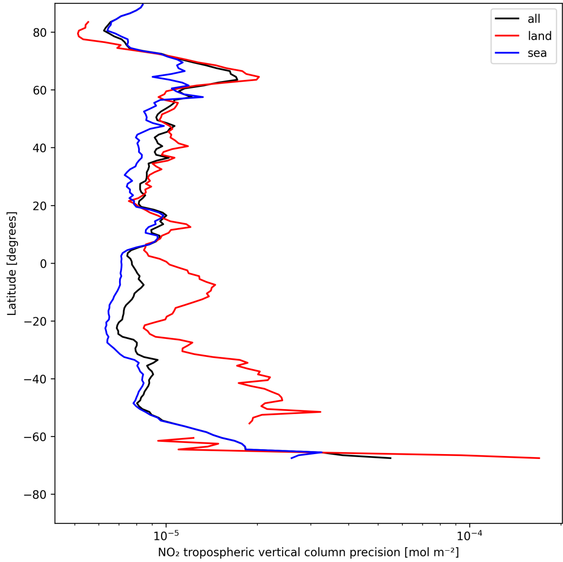
Figure 13: Zonal average of “NO 2 tropospheric vertical column precision” for 2025-07-22 to 2025-07-24.
