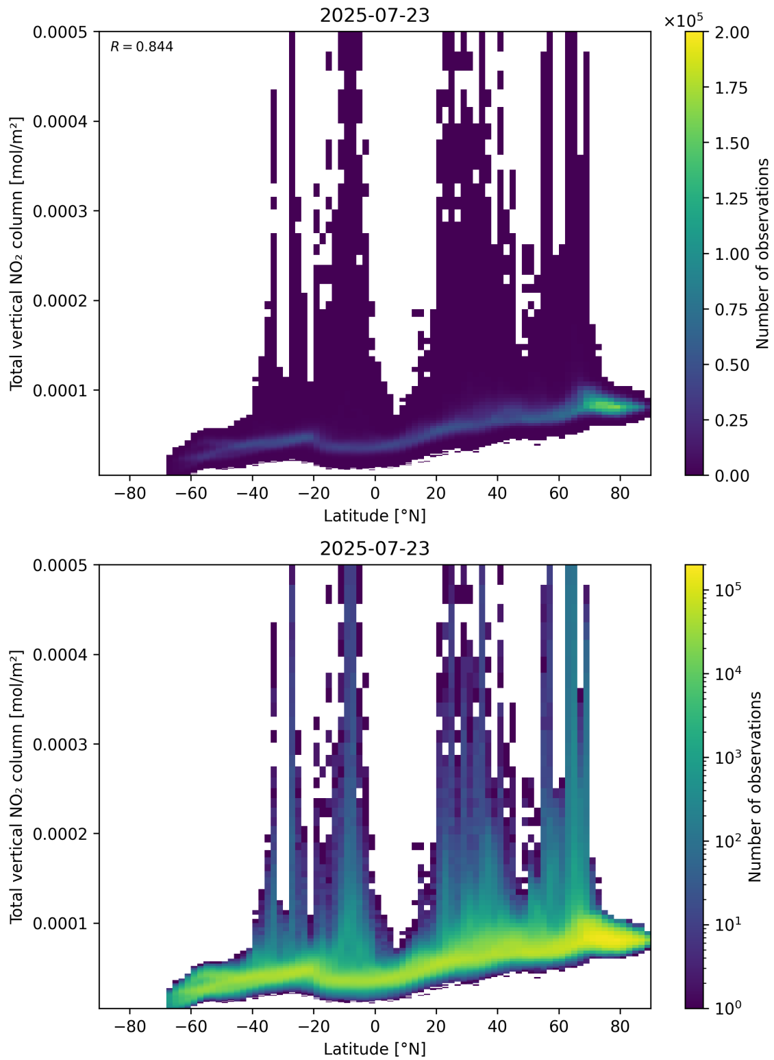
Figure 90: Scatter density plot of “Latitude” against “Total vertical NO 2 column” for 2025-07-22 to 2025-07-24.
