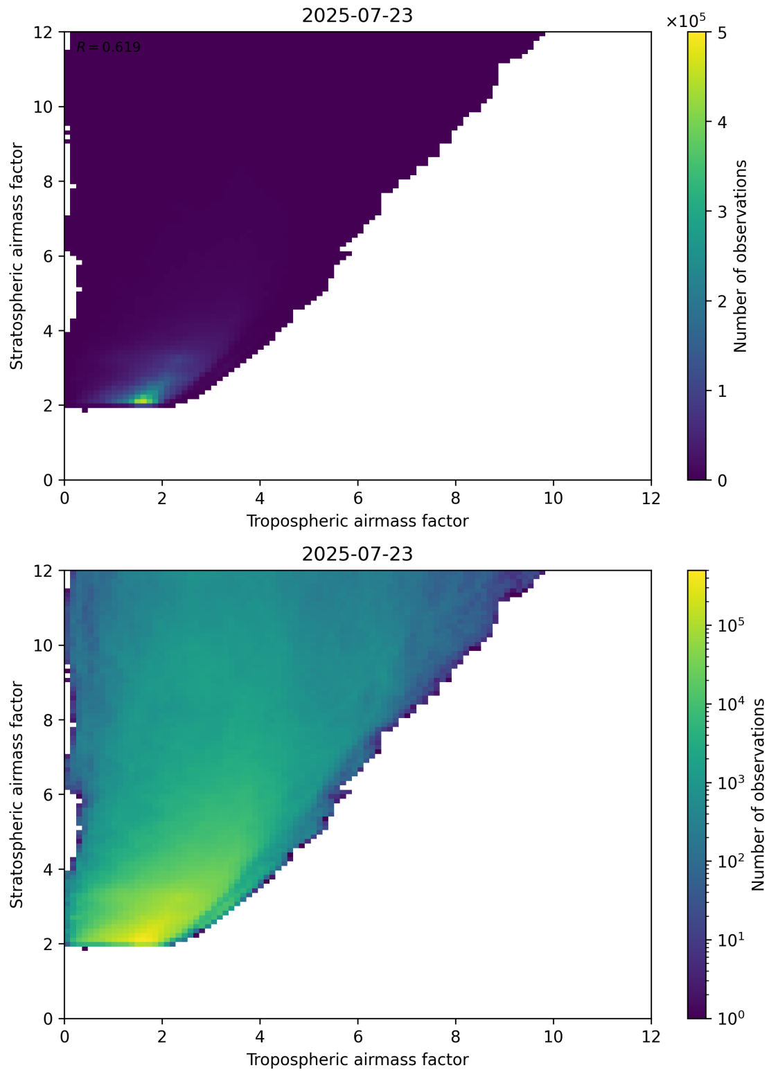
Figure 71: Scatter density plot of “Tropospheric airmass factor” against “Stratospheric airmass factor” for 2025-07-22 to 2025-07-24.
