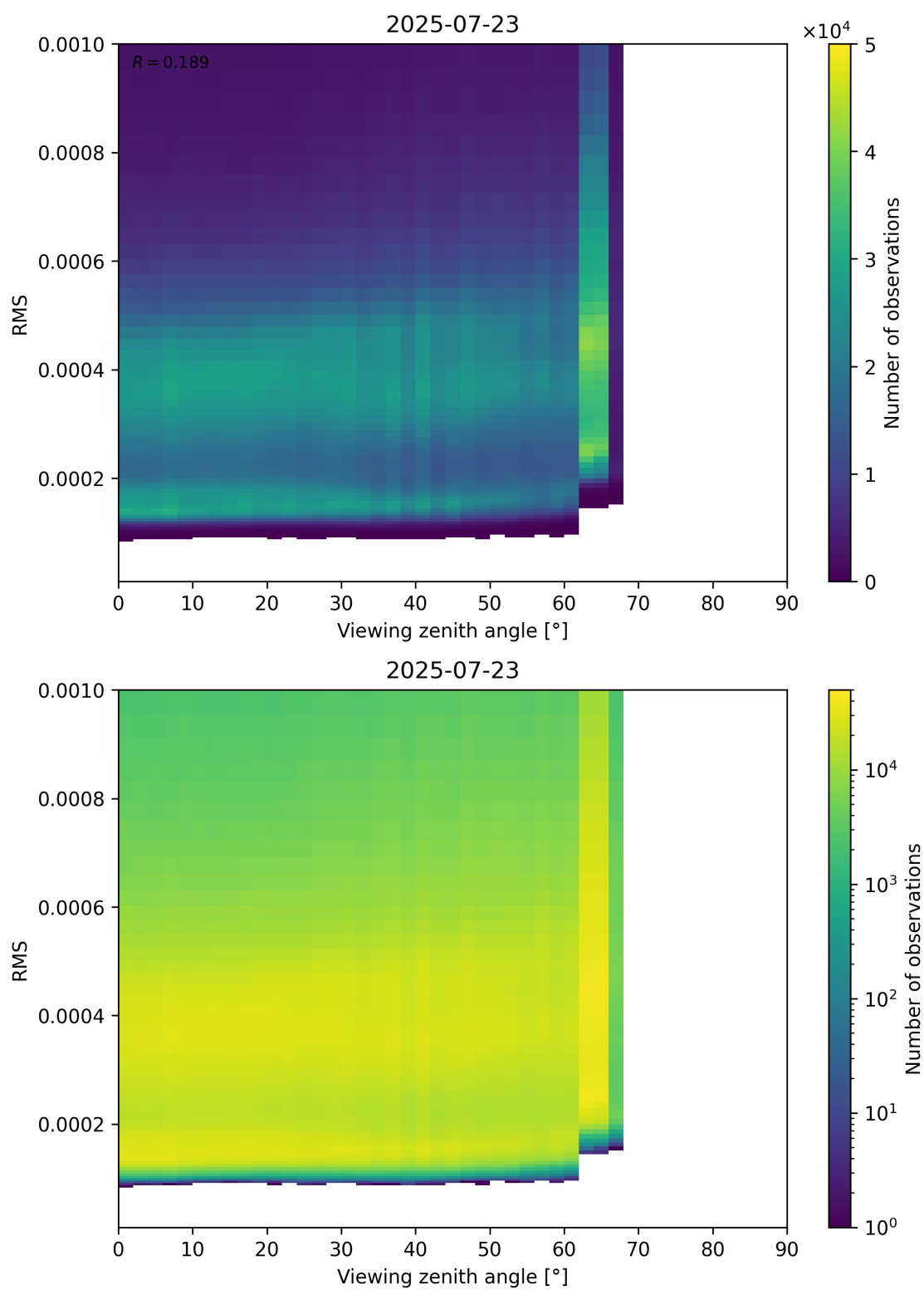
Figure 171: Scatter density plot of “Viewing zenith angle” against “RMS” for 2025-07-22 to 2025-07-24.
