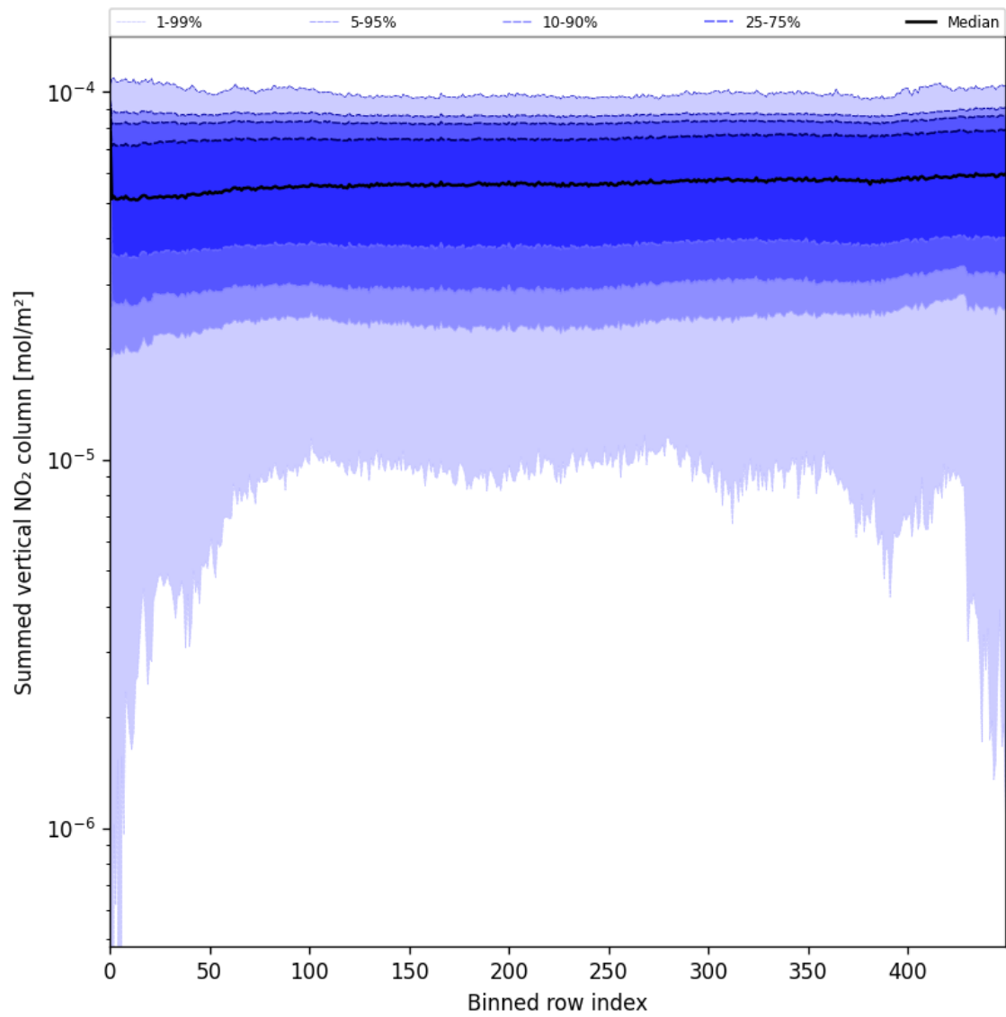
Figure 57: Along track statistics of “Summed vertical NO 2 column” for 2025-07-22 to 2025-07-24
