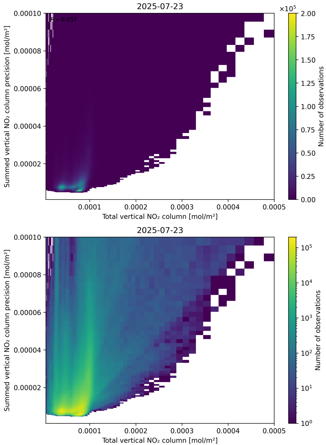
Figure 113: Scatter density plot of “Total vertical NO 2 column” against “Summed vertical NO 2 column precision” for 2025-07-22 to 2025-07-24.
