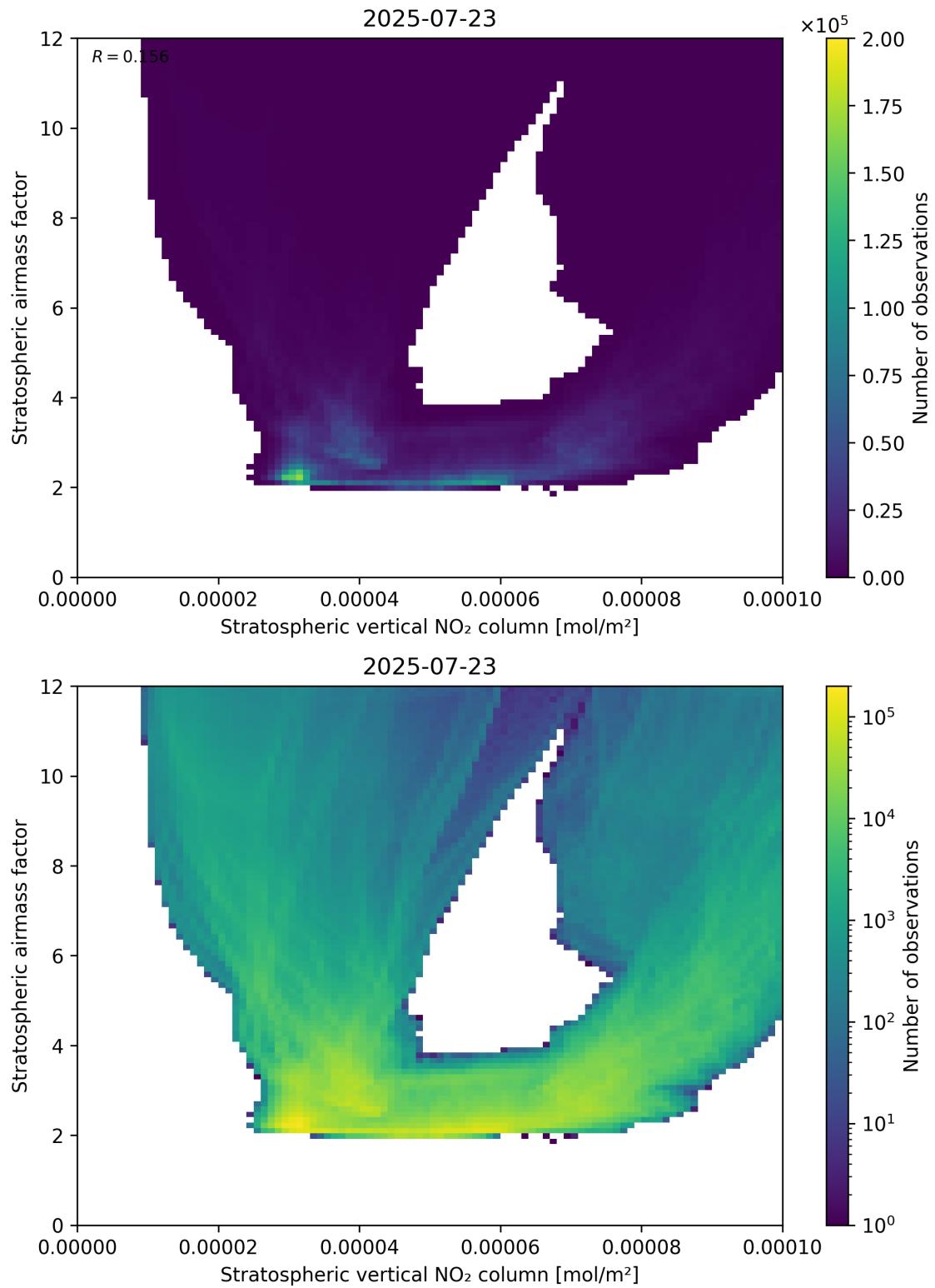
Figure 96: Scatter density plot of “Stratospheric vertical NO 2 column” against “Stratospheric airmass factor” for 2025-07-22 to 2025-07-24.
