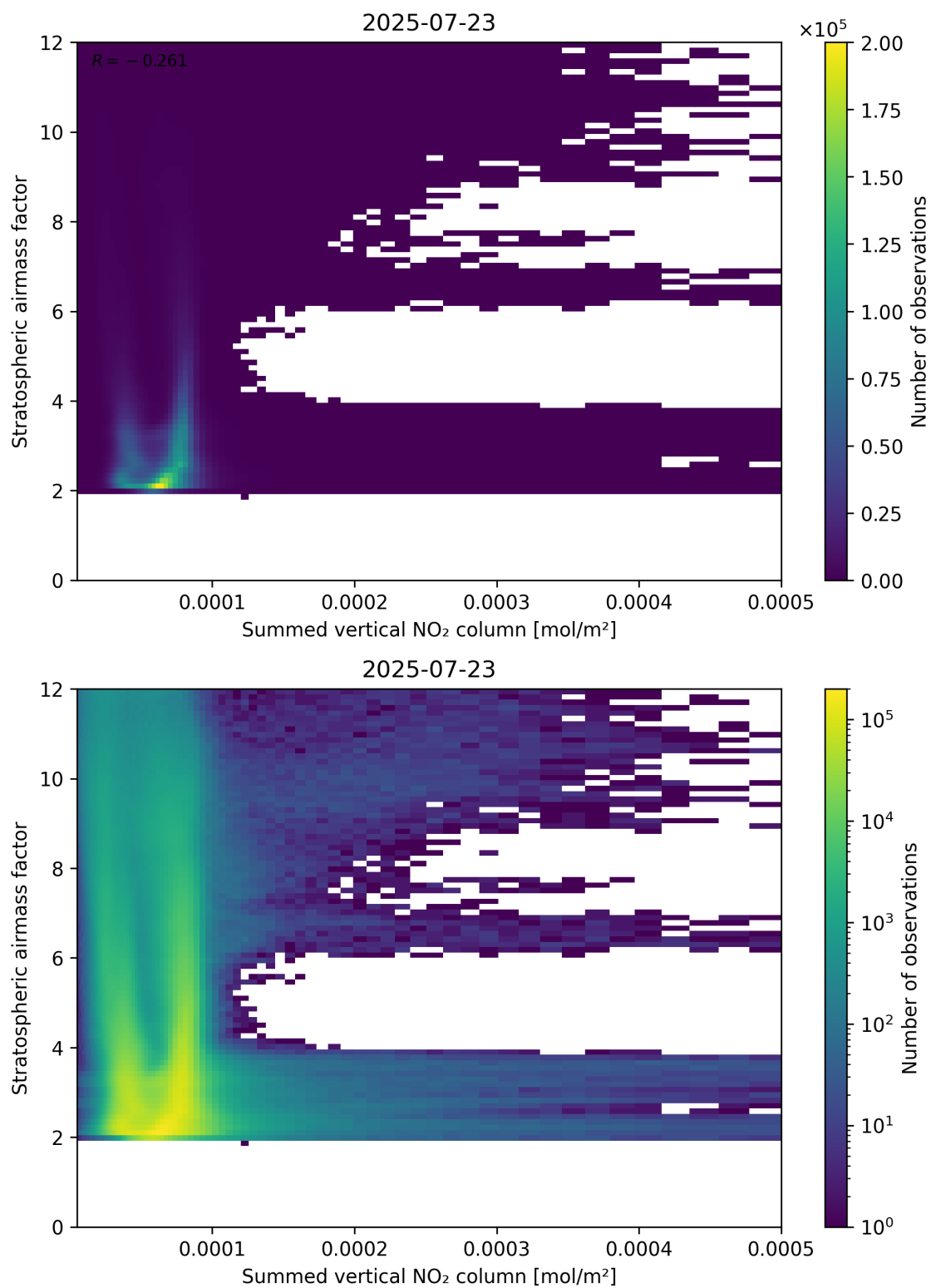
Figure 103: Scatter density plot of “Summed vertical NO 2 column” against “Stratospheric airmass factor” for 2025-07-22 to 2025-07-24.
