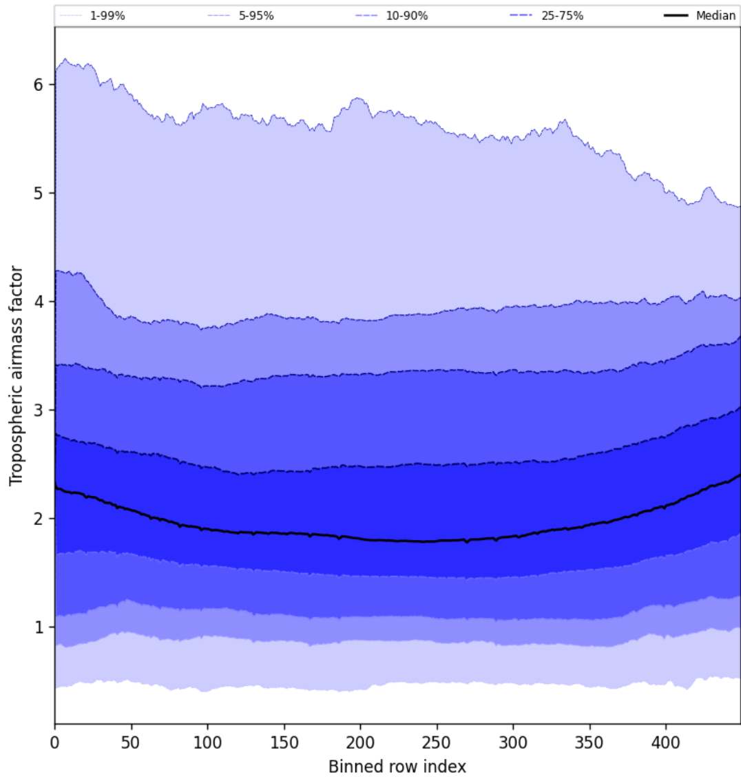
Figure 48: Along track statistics of “Tropospheric airmass factor” for 2025-07-22 to 2025-07-24
