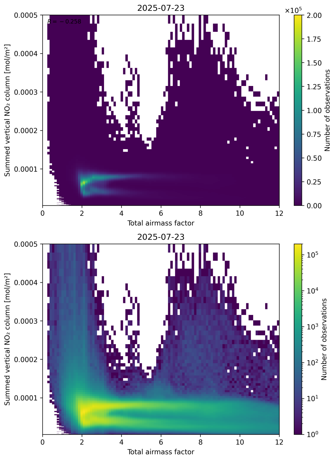
Figure 65: Scatter density plot of “Total airmass factor” against “Summed vertical NO 2 column” for 2025-07-22 to 2025-07-24.
