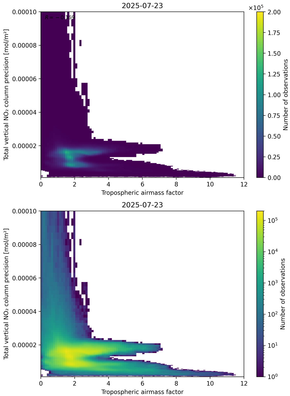
Figure 78: Scatter density plot of “Tropospheric air mass factor” against “Total vertical NO 2 column precision” for 2025-07-22 to 2025-07-24.
