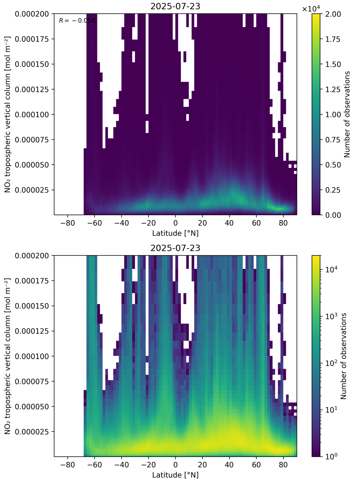
Figure 92: Scatter density plot of “Latitude” against “NO 2 tropospheric vertical column” for 2025-07-22 to 2025-07-24.
