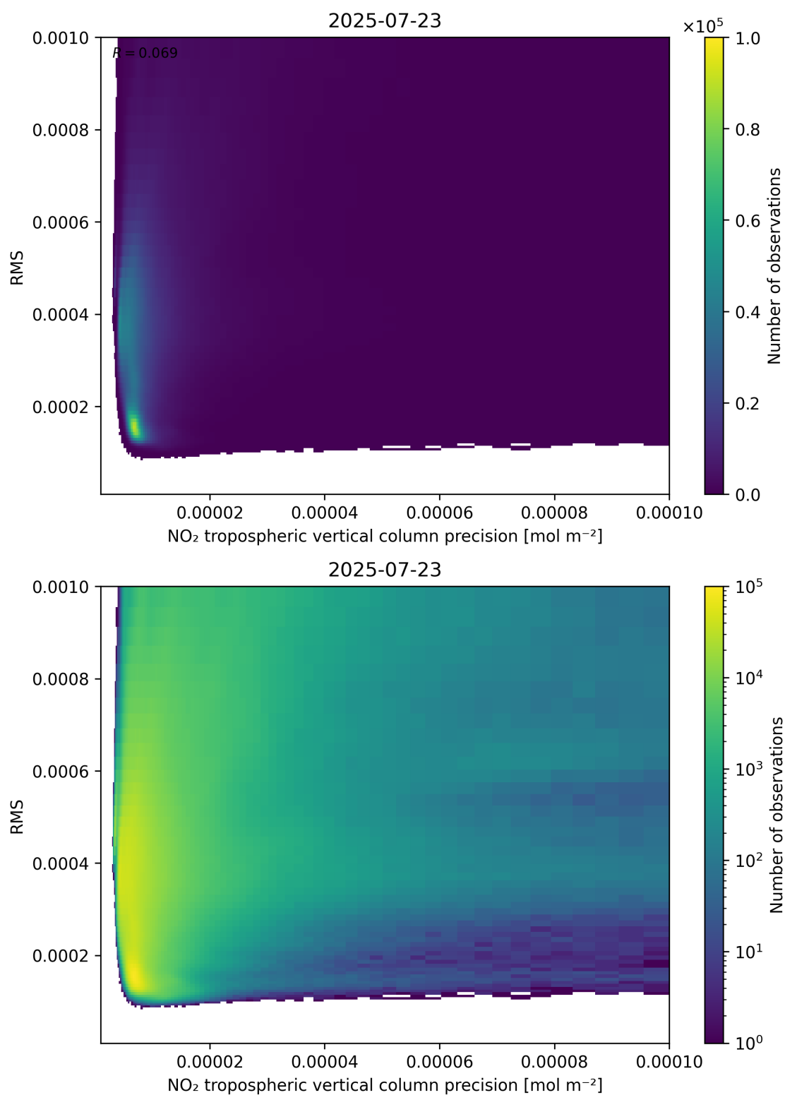
Figure 140: Scatter density plot of “NO 2 tropospheric vertical column precision” against “RMS” for 2025-07-22 to 2025-07-24.
