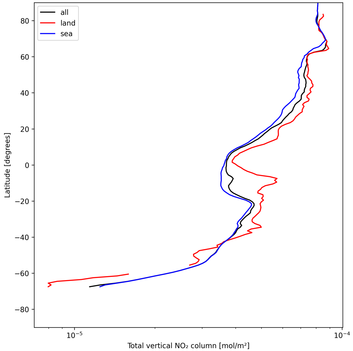
Figure 21: Zonal average of “Total vertical NO 2 column” for 2025-07-22 to 2025-07-24.
