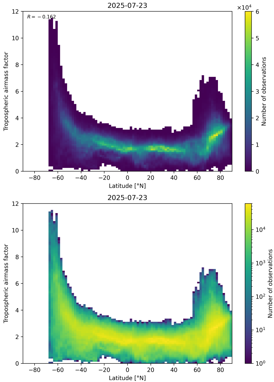
Figure 85: Scatter density plot of “Latitude” against “Tropospheric air mass factor” for 2025-07-22 to 2025-07-24.
