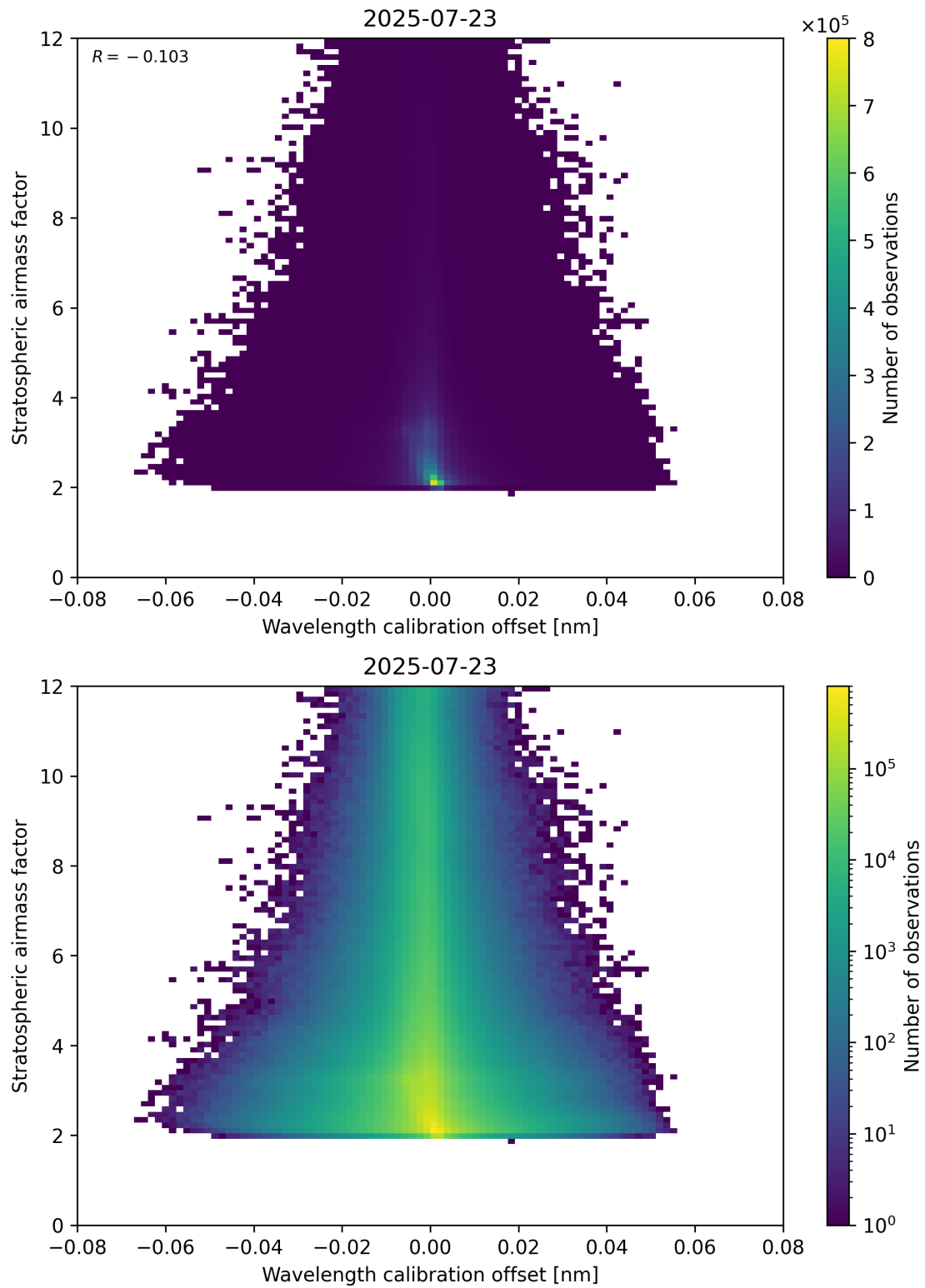
Figure 174: Scatter density plot of “Wavelength calibration offset” against “Stratospheric airmass factor” for 2025-07-22 to 2025-07-24.
