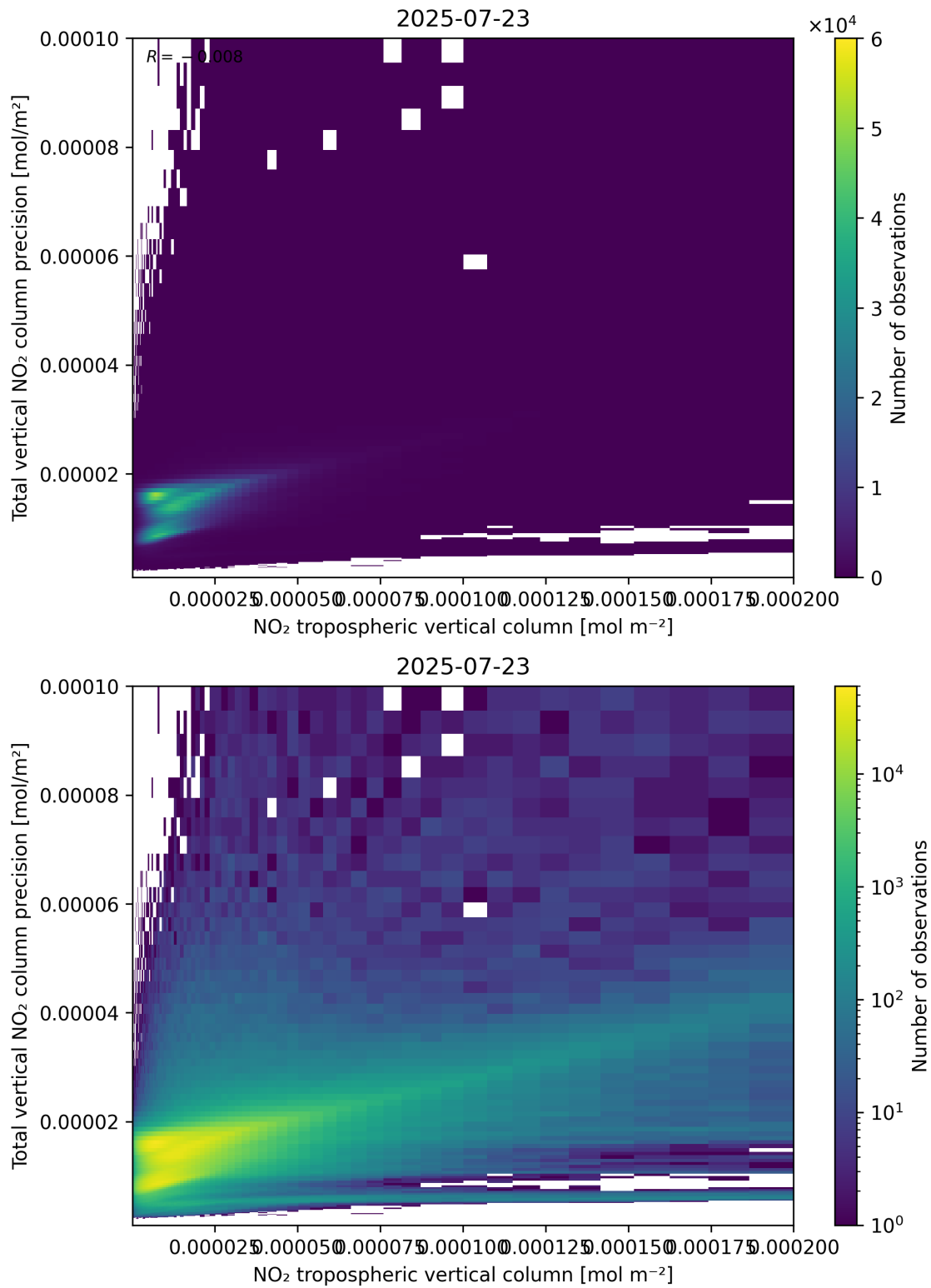
Figure 129: Scatter density plot of “NO 2 tropospheric vertical column” against “Total vertical NO 2 column precision” for 2025-07-22 to 2025-07-24.
