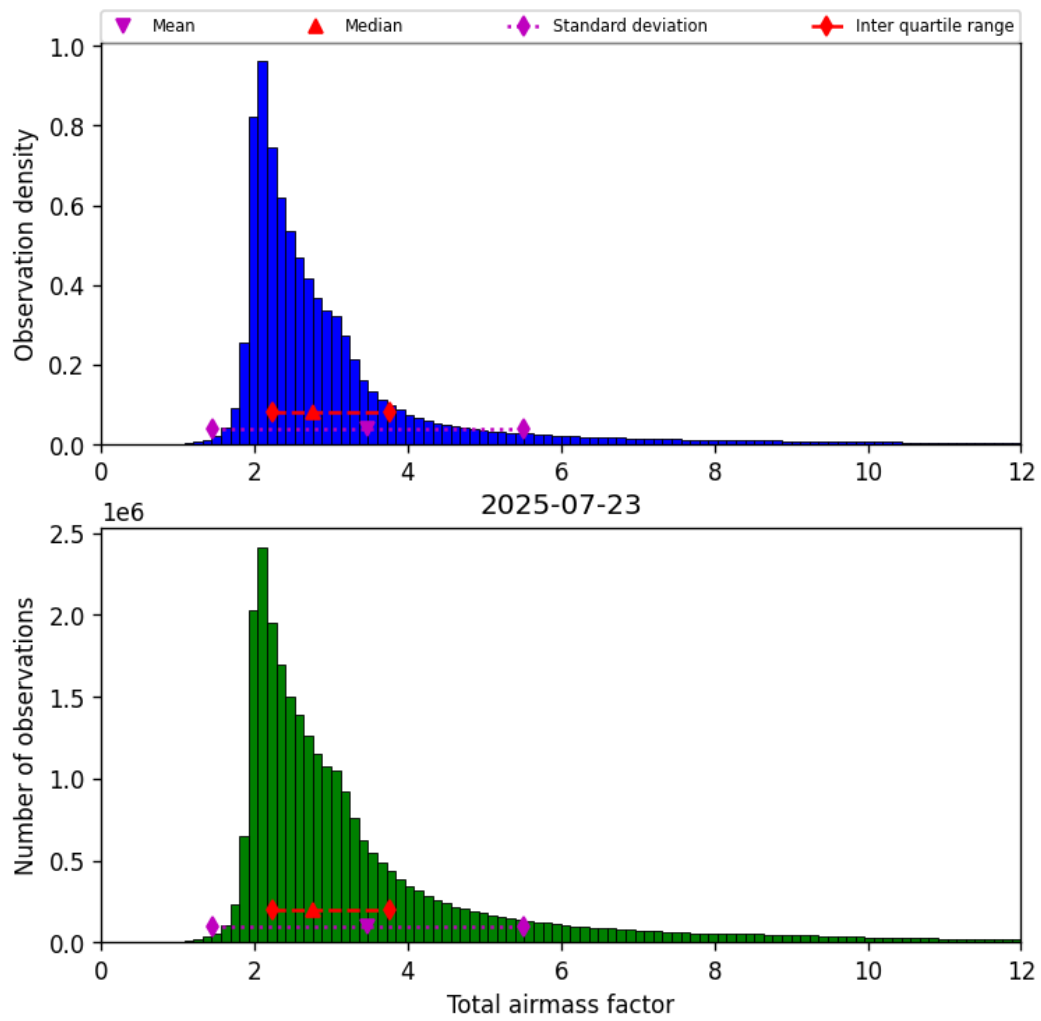
Figure 32: Histogram of “Total airmass factor” for 2025-07-22 to 2025-07-24
