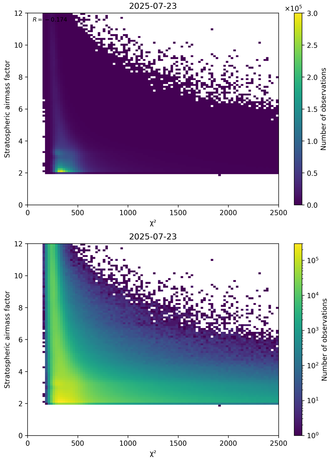
Figure 81: Scatter density plot of “ \chi^2 ” against “Stratospheric airmass factor” for 2025-07-22 to 2025-07-24.
