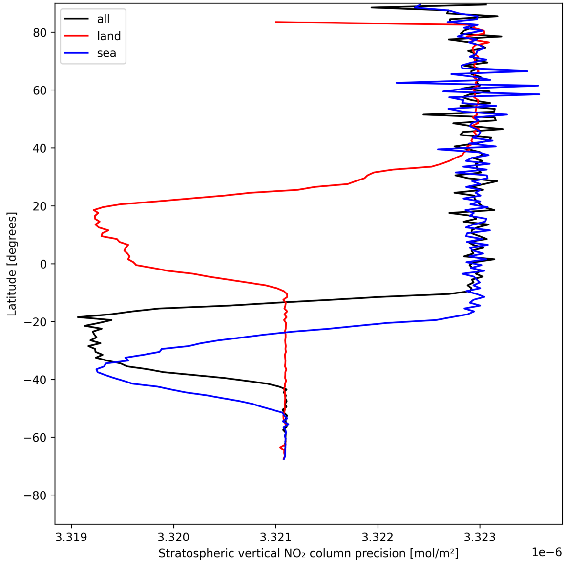
Figure 20: Zonal average of “Stratospheric vertical NO 2 column precision” for 2025-07-22 to 2025-07-24.
