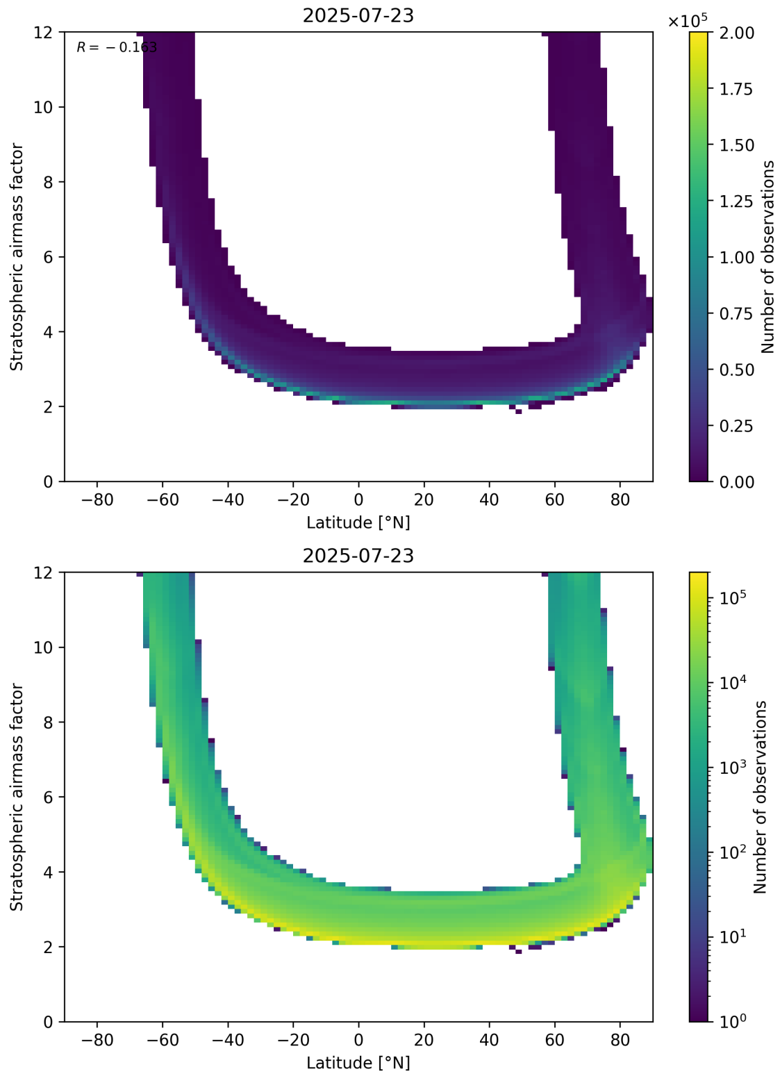
Figure 83: Scatter density plot of “Latitude” against “Stratospheric air mass factor” for 2025-07-22 to 2025-07-24.
