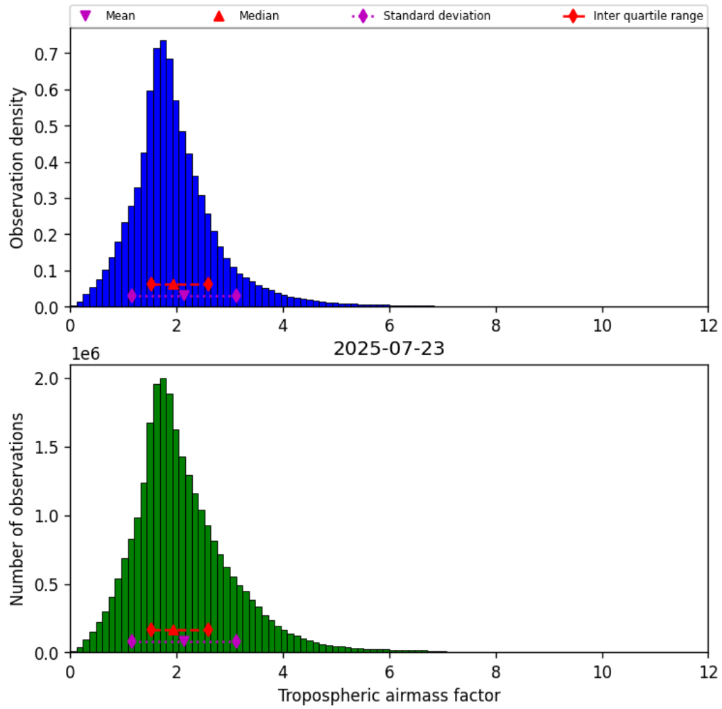
Figure 31: Histogram of “Tropospheric airmass factor” for 2025-07-22 to 2025-07-24
