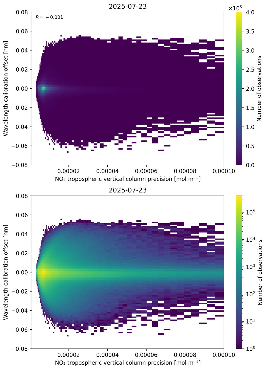
Figure 141: Scatter density plot of “NO 2 tropospheric vertical column precision” against “Wavelength calibration offset” for 2025-07-22 to 2025-07-24.
