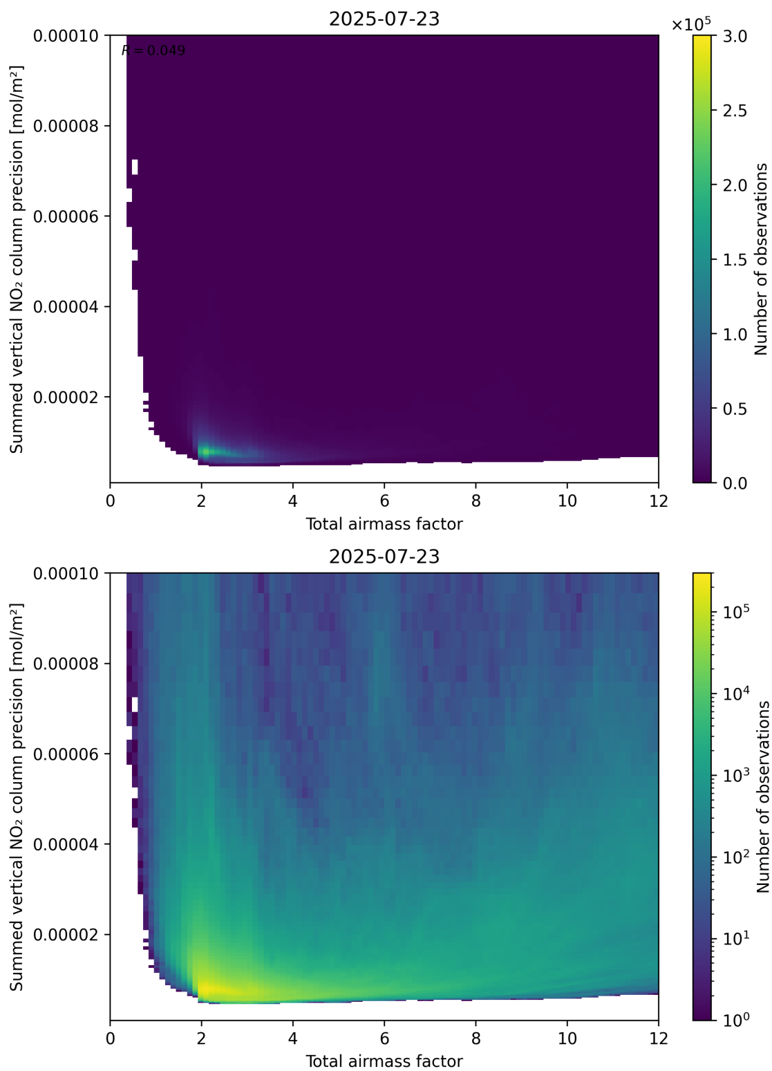
Figure 66: Scatter density plot of “Total airmass factor” against “Summed vertical NO 2 column precision” for 2025-07-22 to 2025-07-24.
