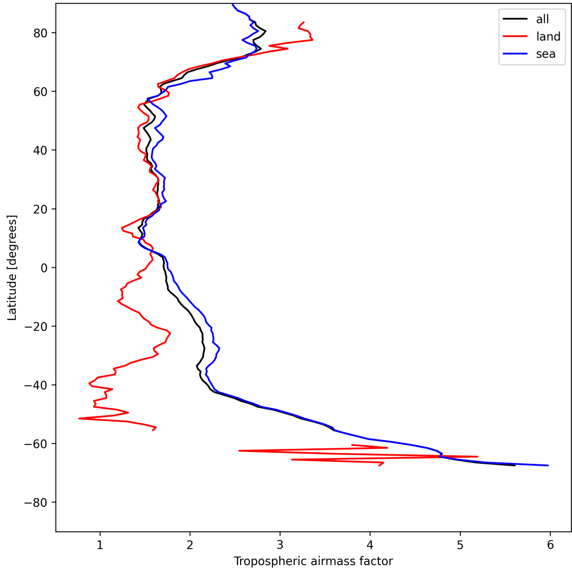
Figure 14: Zonal average of “Tropospheric airmass factor” for 2025-07-22 to 2025-07-24.
