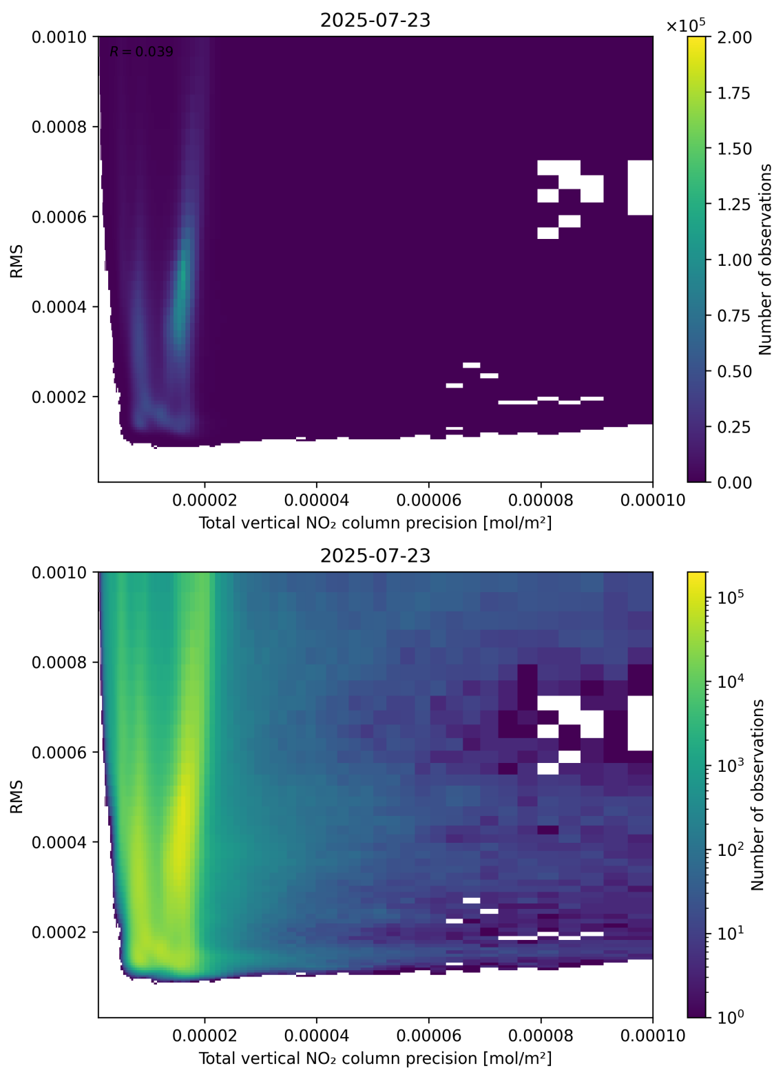
Figure 119: Scatter density plot of “Total vertical NO 2 column precision” against “RMS” for 2025-07-22 to 2025-07-24.
