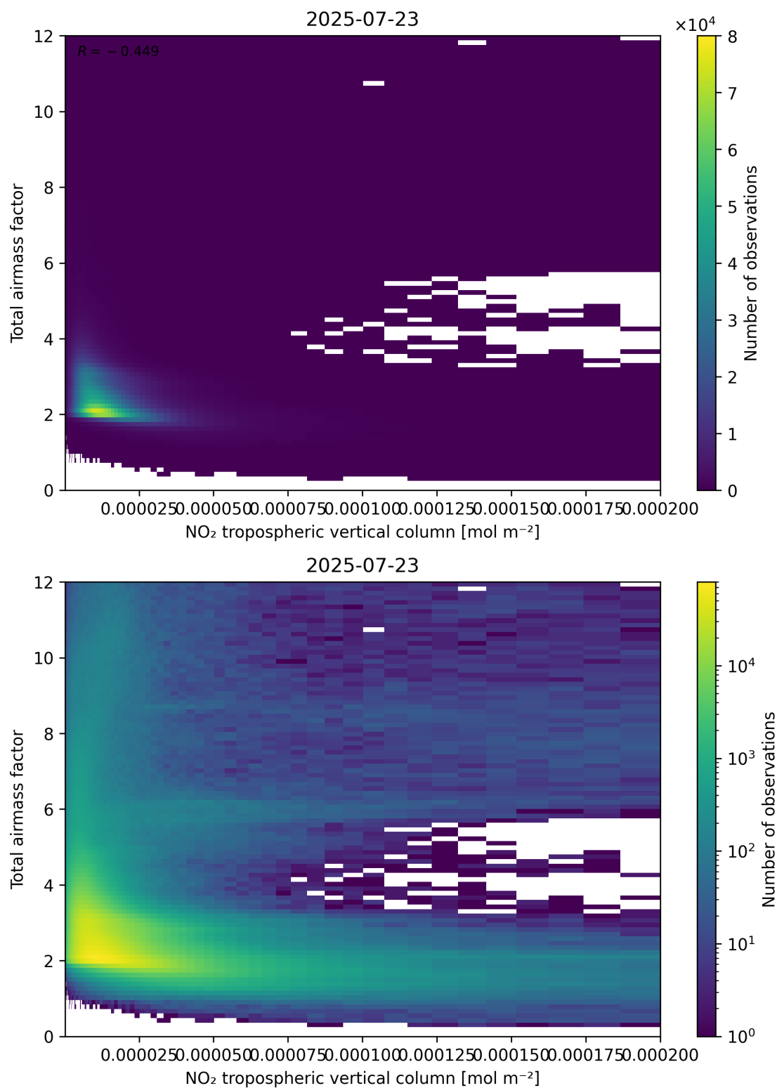
Figure 122: Scatter density plot of “NO 2 tropospheric vertical column” against “Total air mass factor” for 2025-07-22 to 2025-07-24.
