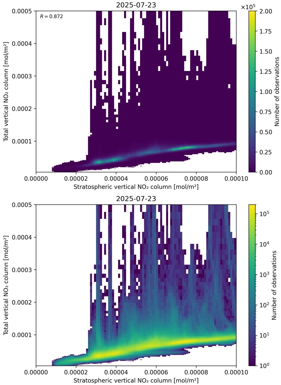
Figure 100: Scatter density plot of “Stratospheric vertical NO 2 column” against “Total vertical NO 2 column” for 2025-07-22 to 2025-07-24.
