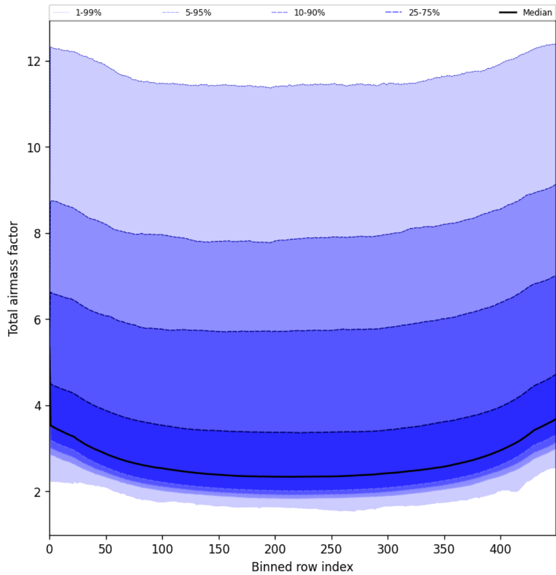
Figure 49: Along track statistics of “Total airmass factor” for 2025-07-22 to 2025-07-24
