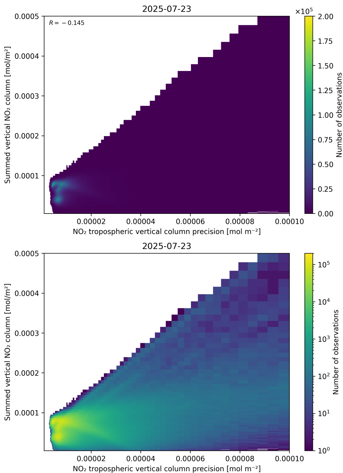
Figure 136: Scatter density plot of “NO 2 tropospheric vertical column precision” against “Summed vertical NO 2 column” for 2025-07-22 to 2025-07-24.
