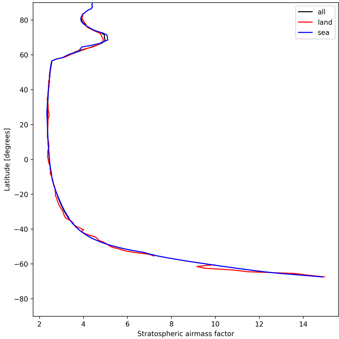
Figure 27: Zonal average of “Stratospheric air mass factor” for 2025-07-22 to 2025-07-24.
