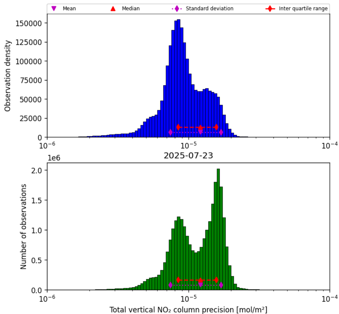
Figure 39: Histogram of “Total vertical NO 2 column precision” for 2025-07-22 to 2025-07-24
