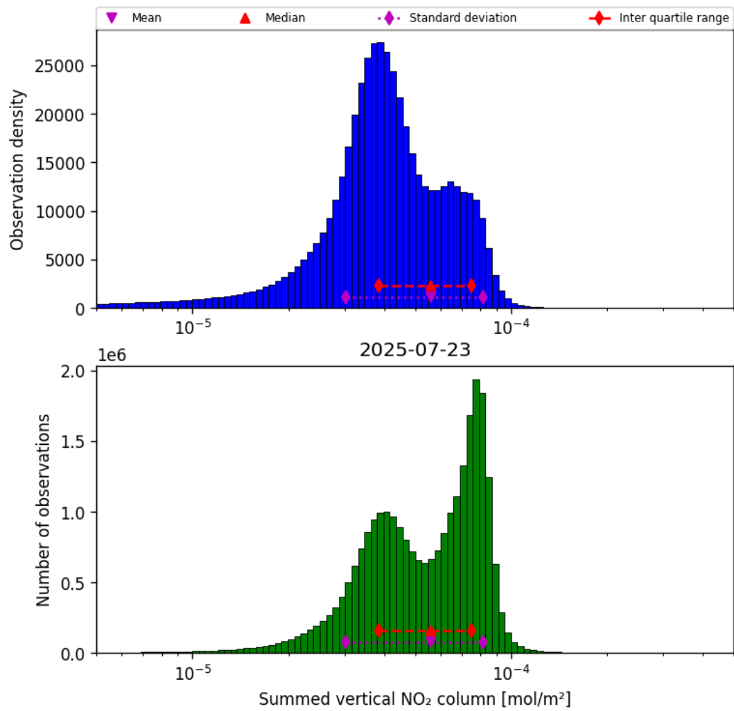
Figure 40: Histogram of “Summed vertical NO 2 column” for 2025-07-22 to 2025-07-24
