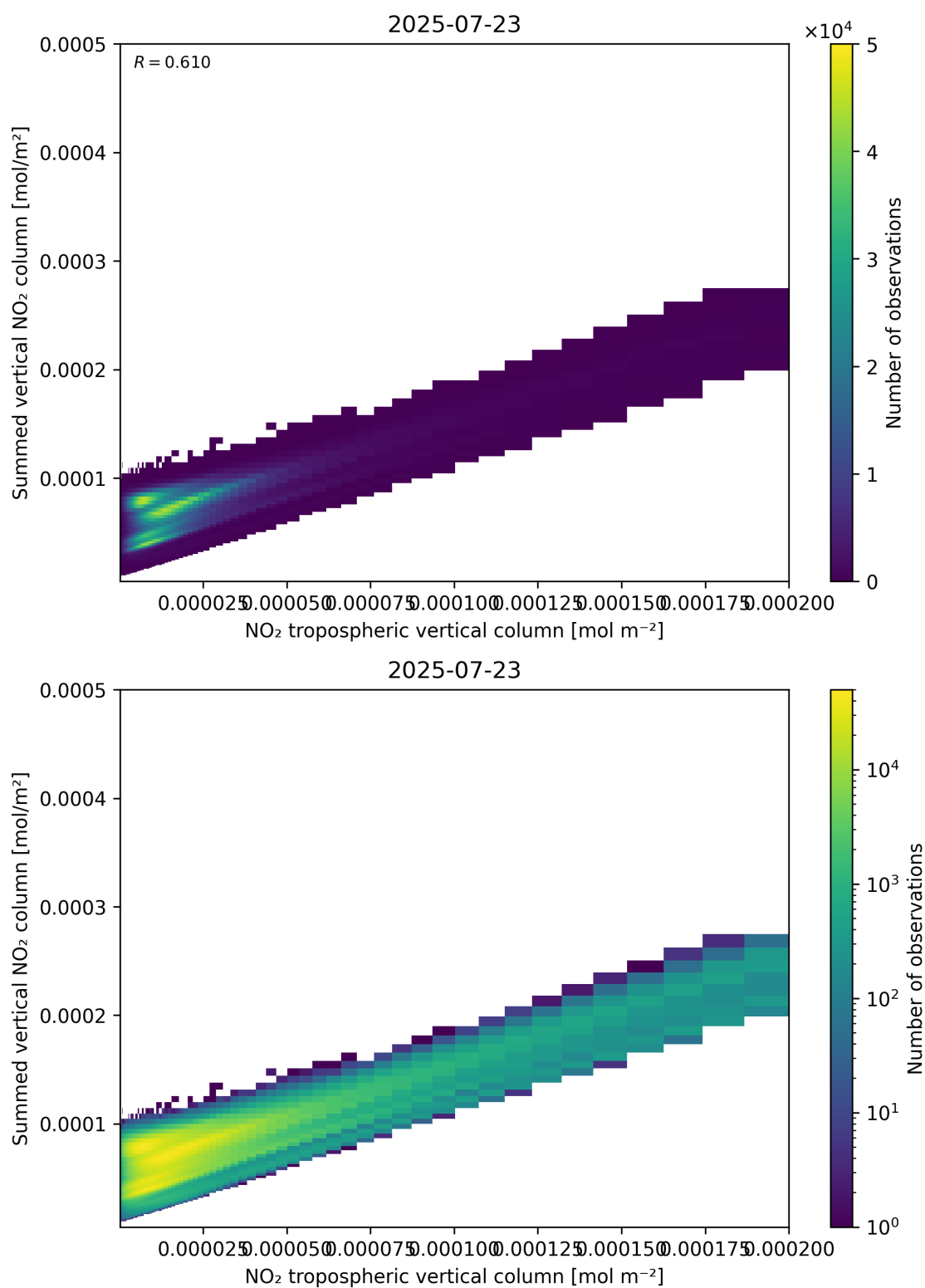
Figure 126: Scatter density plot of “NO 2 tropospheric vertical column” against “Summed vertical NO 2 column” for 2025-07-22 to 2025-07-24.
