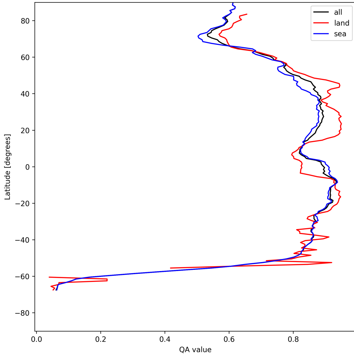
Figure 11: Zonal average of “QA value” for 2025-07-22 to 2025-07-24.
