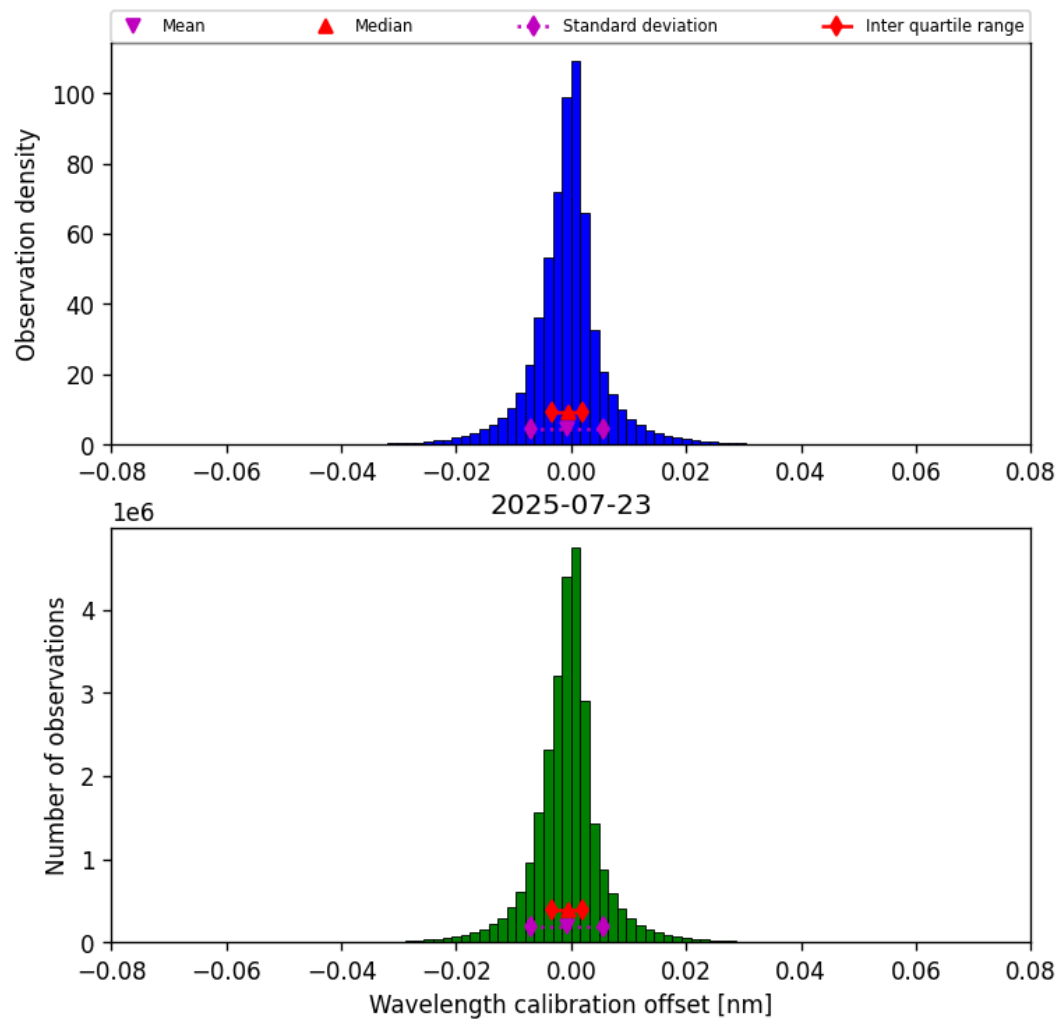
Figure 35: Histogram of “Wavelength calibration offset” for 2025-07-22 to 2025-07-24
