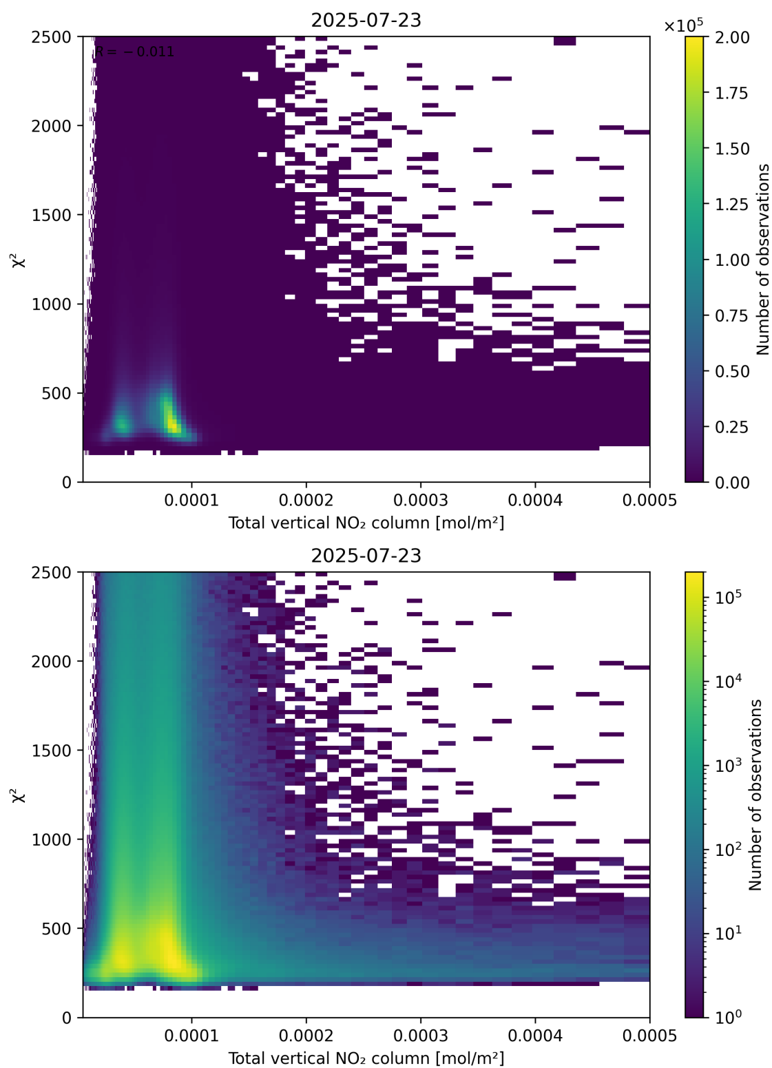
Figure 111: Scatter density plot of “Total vertical NO 2 column” against “ \chi^2 ” for 2025-07-22 to 2025-07-24.
