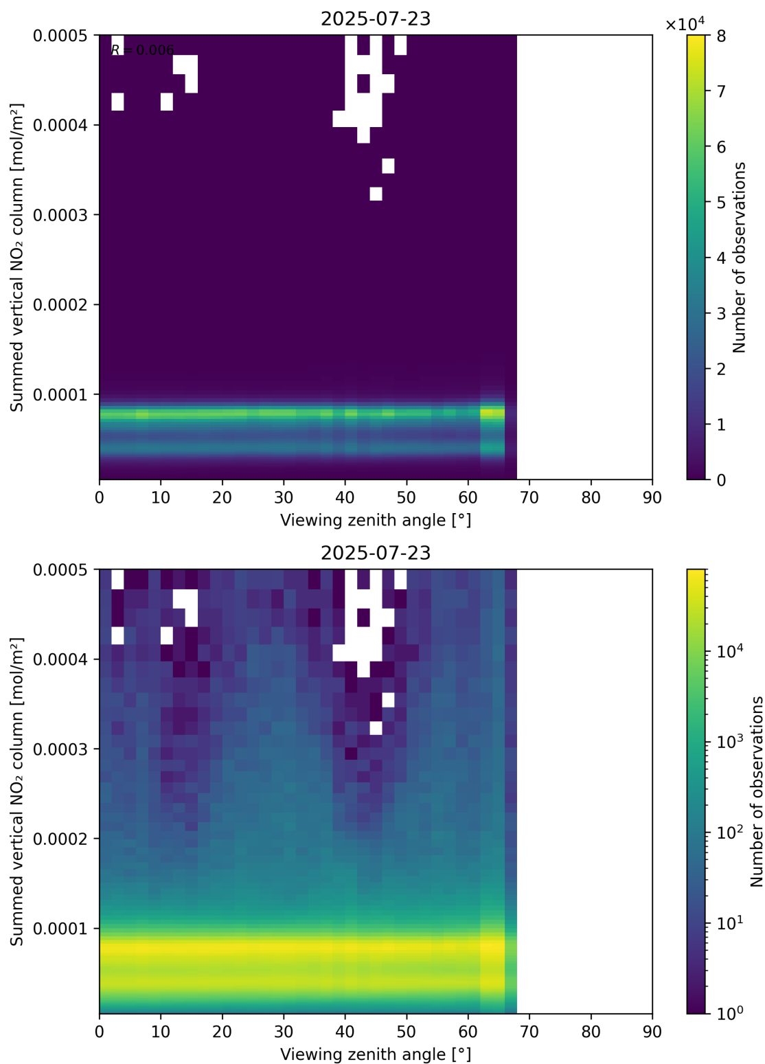
Figure 165: Scatter density plot of “Viewing zenith angle” against “Summed vertical NO 2 column” for 2025-07-22 to 2025-07-24.
