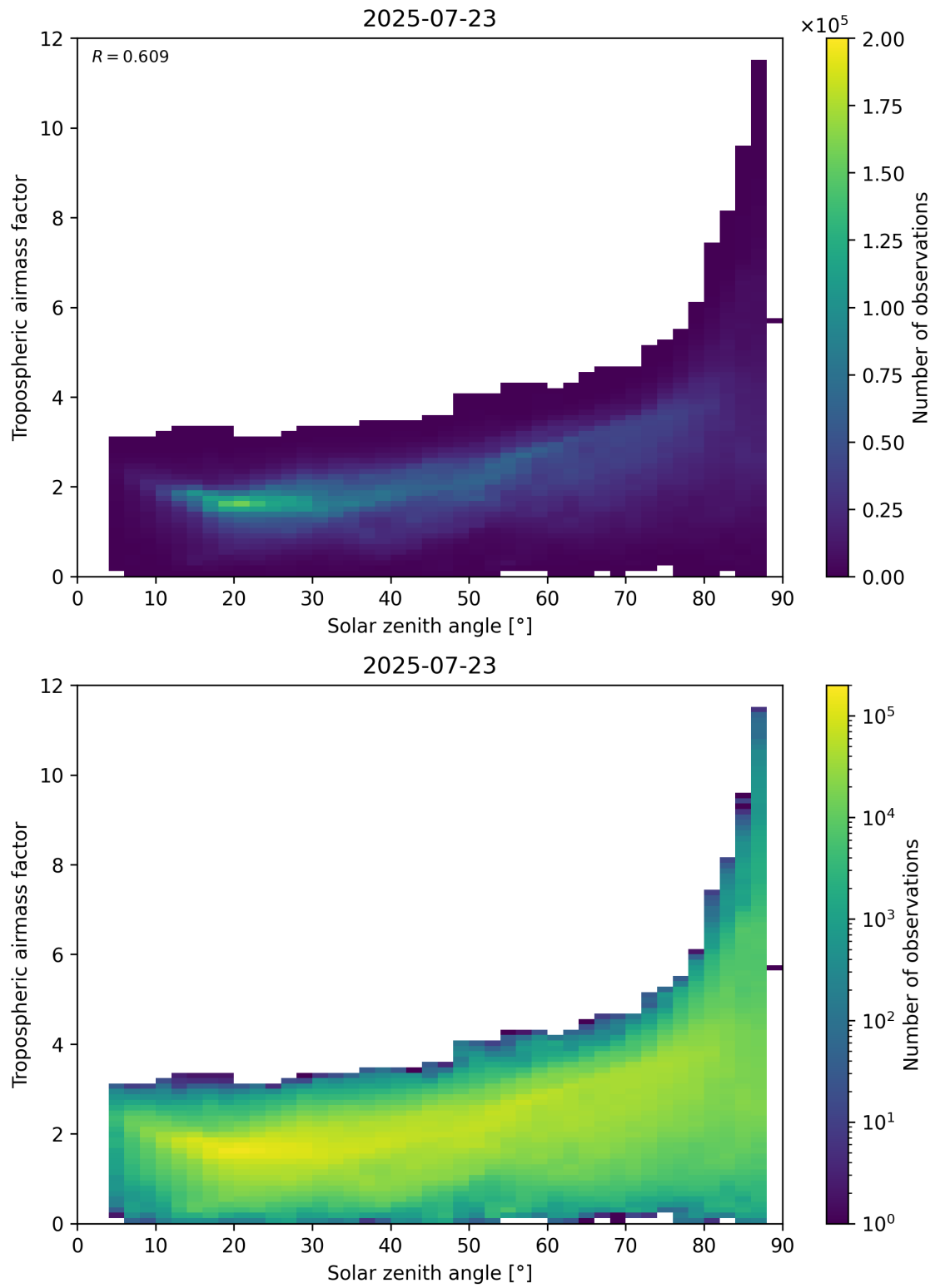
Figure 147: Scatter density plot of “Solar zenith angle” against “Tropospheric airmass factor” for 2025-07-22 to 2025-07-24.
