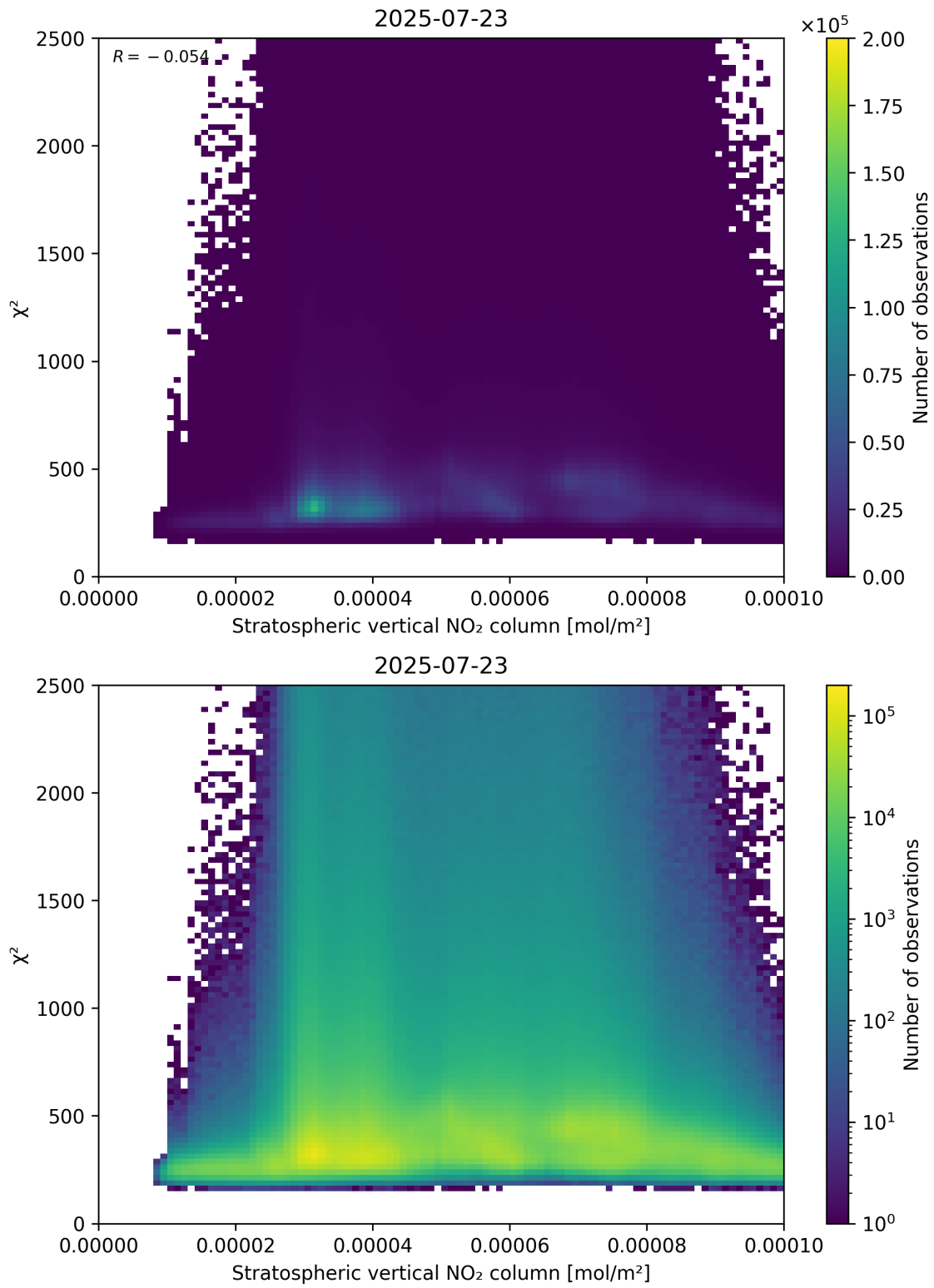
Figure 97: Scatter density plot of “Stratospheric vertical NO 2 column” against “ \chi^2 ” for 2025-07-22 to 2025-07-24.
