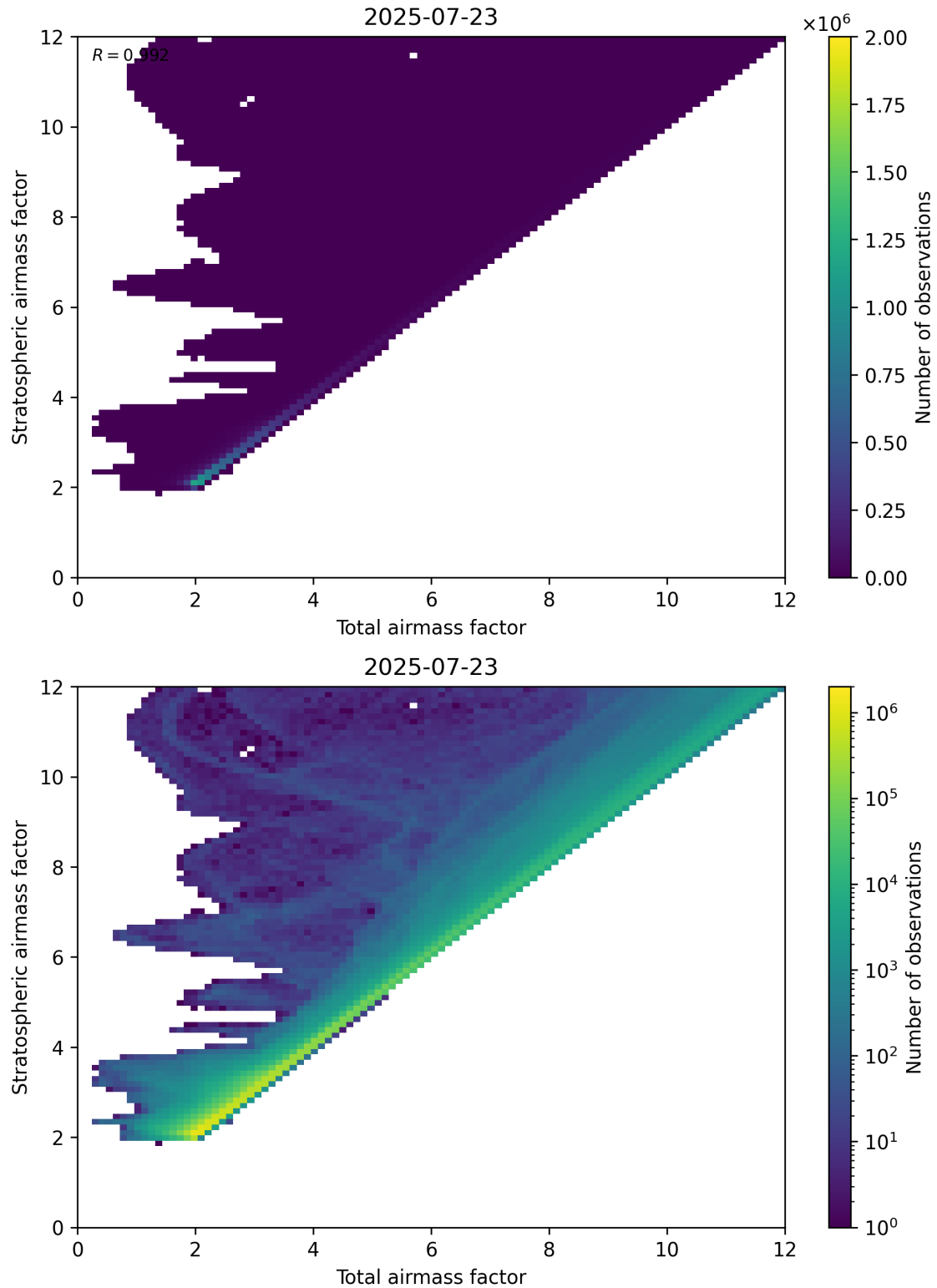
Figure 62: Scatter density plot of “Total airmass factor” against “Stratospheric airmass factor” for 2025-07-22 to 2025-07-24.
