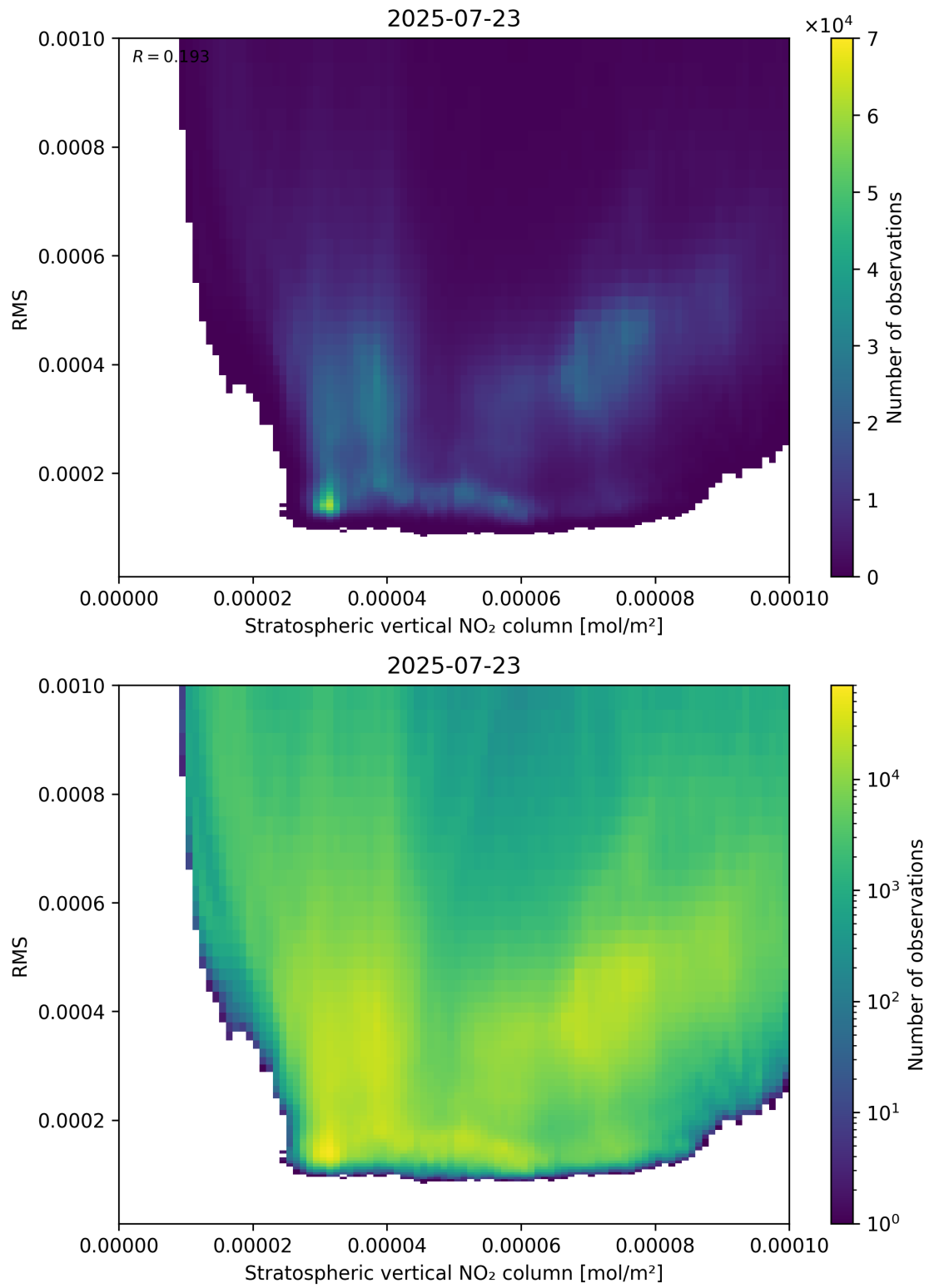
Figure 102: Scatter density plot of “Stratospheric vertical NO 2 column” against “RMS” for 2025-07-22 to 2025-07-24.
