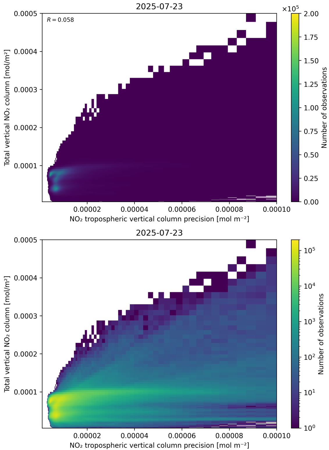
Figure 138: Scatter density plot of “NO 2 tropospheric vertical column precision” against “Total vertical NO 2 column” for 2025-07-22 to 2025-07-24.
