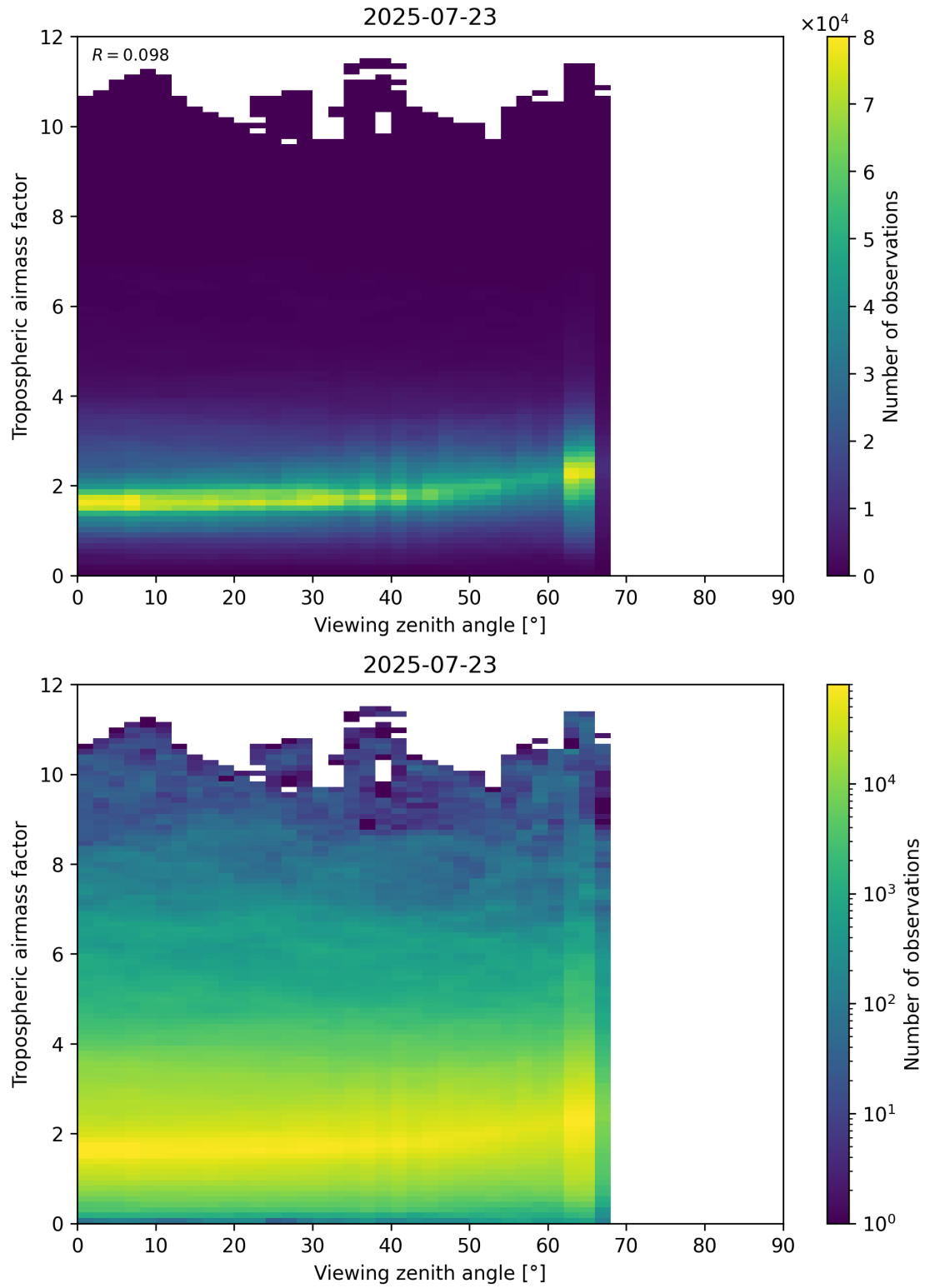
Figure 161: Scatter density plot of “Viewing zenith angle” against “Tropospheric airmass factor” for 2025-07-22 to 2025-07-24.
