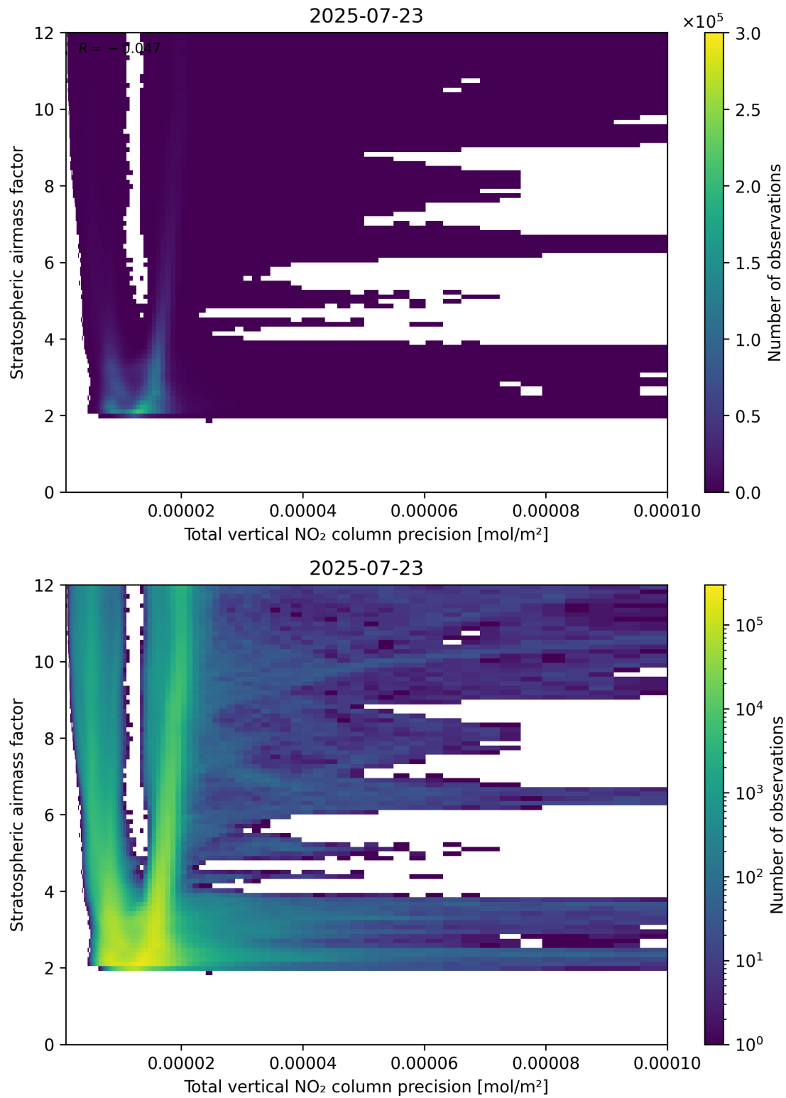
Figure 115: Scatter density plot of “Total vertical NO 2 column precision” against “Stratospheric air mass factor” for 2025-07-22 to 2025-07-24.
