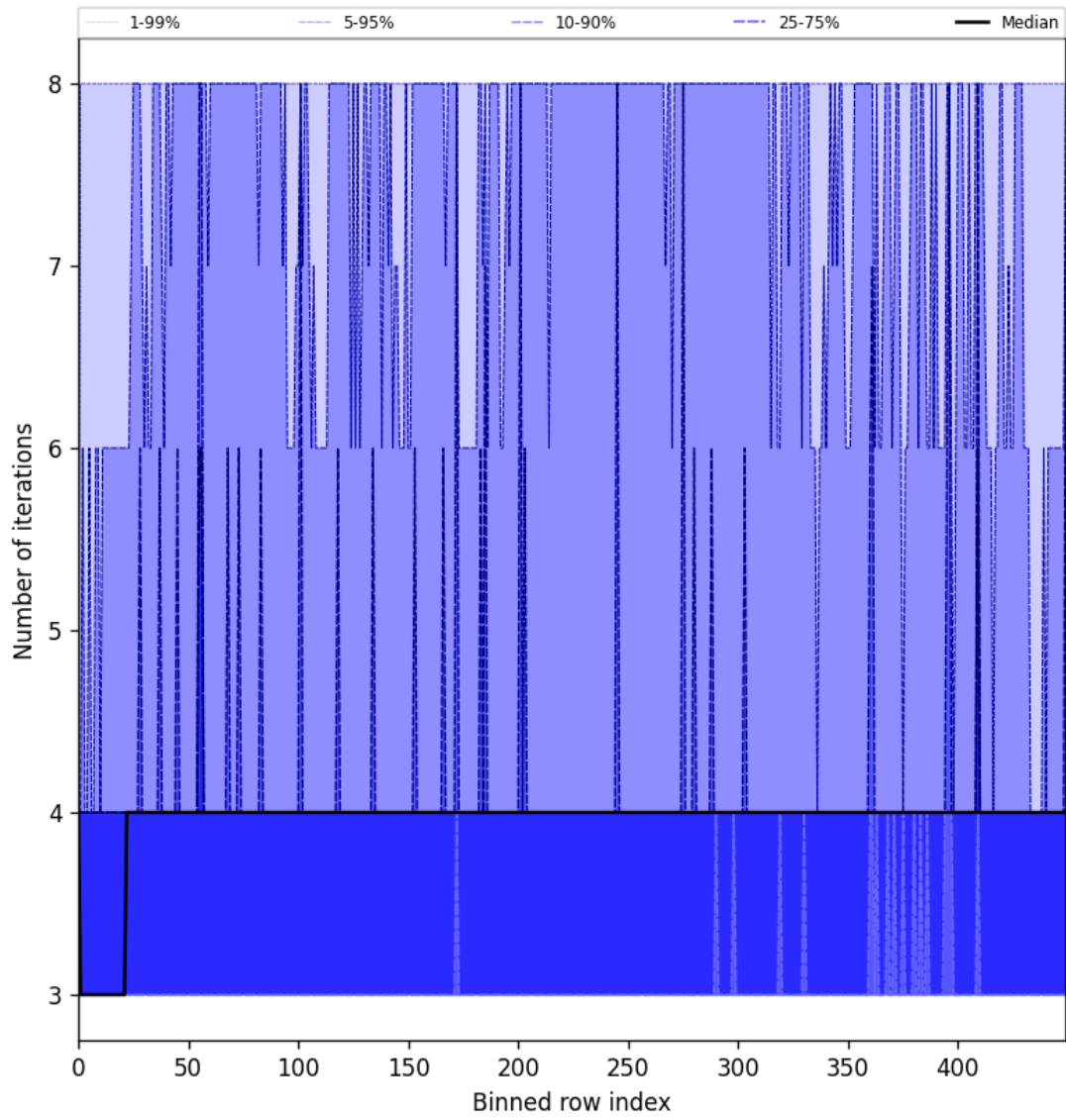
Figure 51: Along track statistics of “Number of iterations” for 2025-07-22 to 2025-07-24
