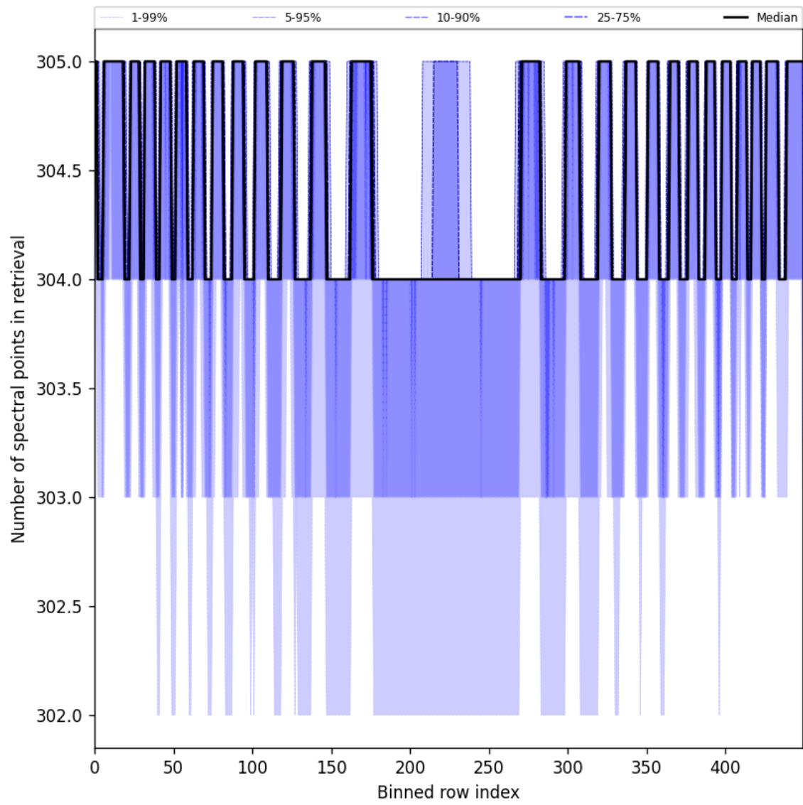
Figure 50: Along track statistics of “Number of spectral points in retrieval” for 2025-07-22 to 2025-07-24
