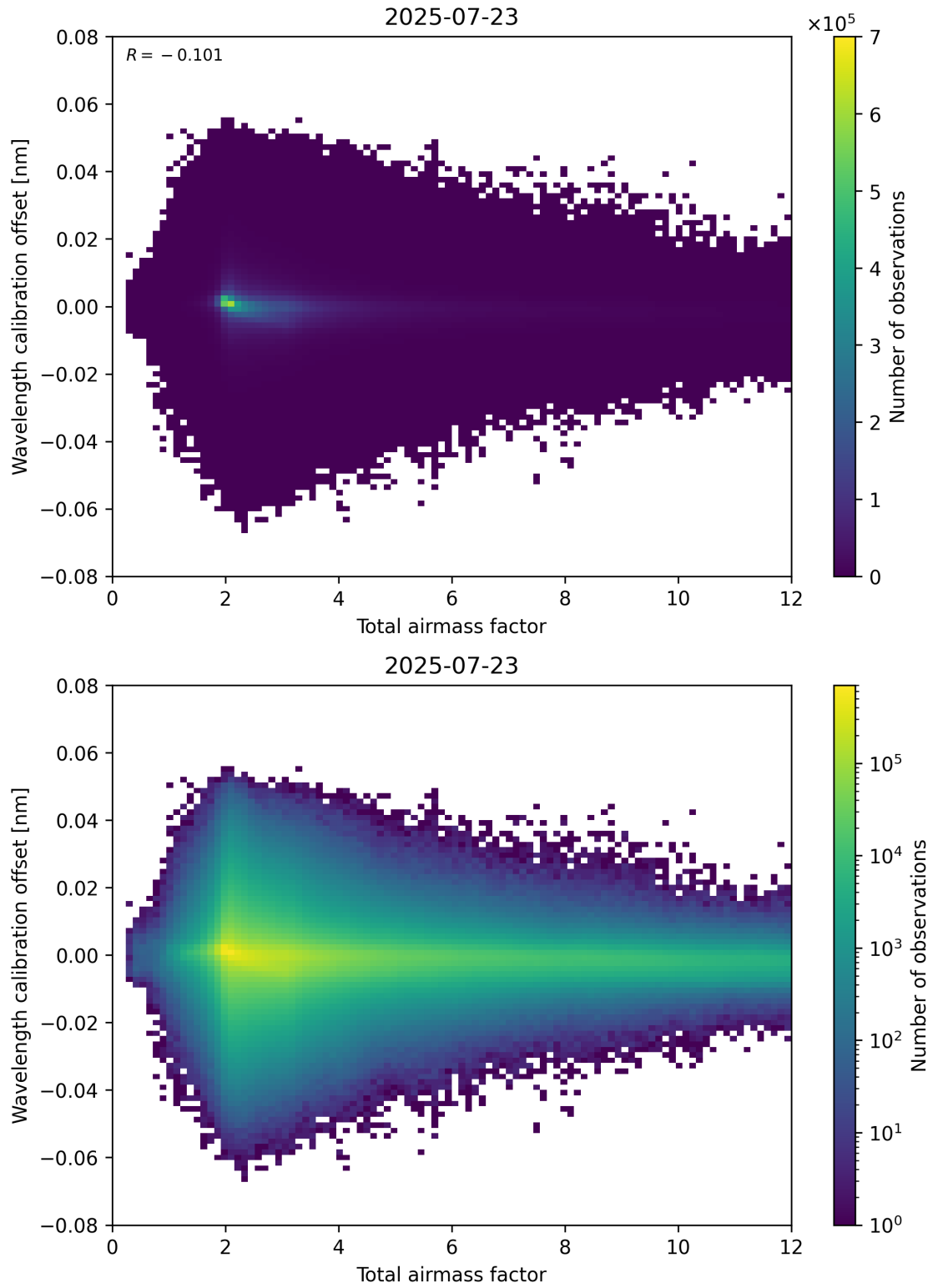
Figure 70: Scatter density plot of “Total airmass factor” against “Wavelength calibration offset” for 2025-07-22 to 2025-07-24.
