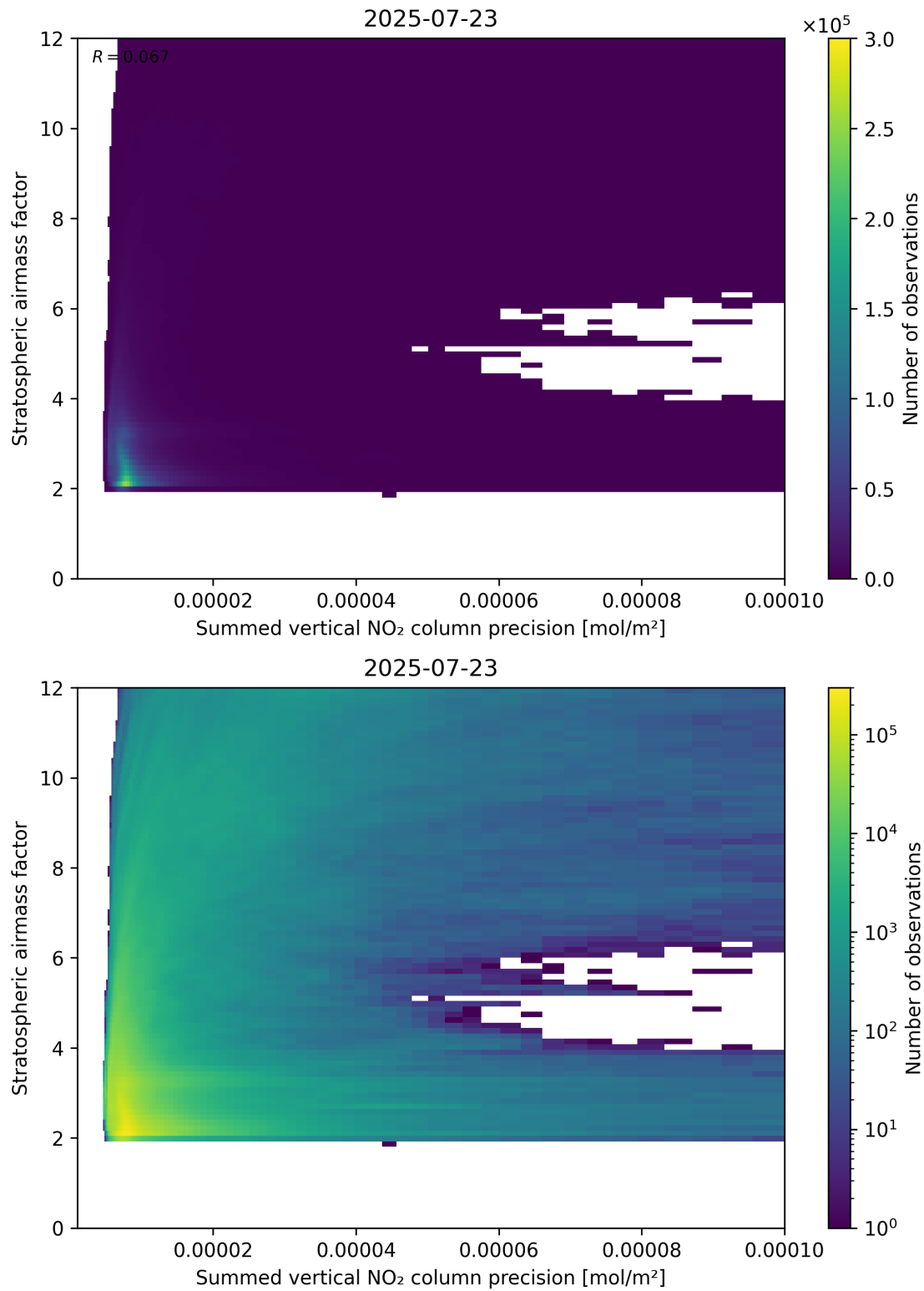
Figure 106: Scatter density plot of “Summed vertical NO 2 column precision” against “Stratospheric airmass factor” for 2025-07-22 to 2025-07-24.
