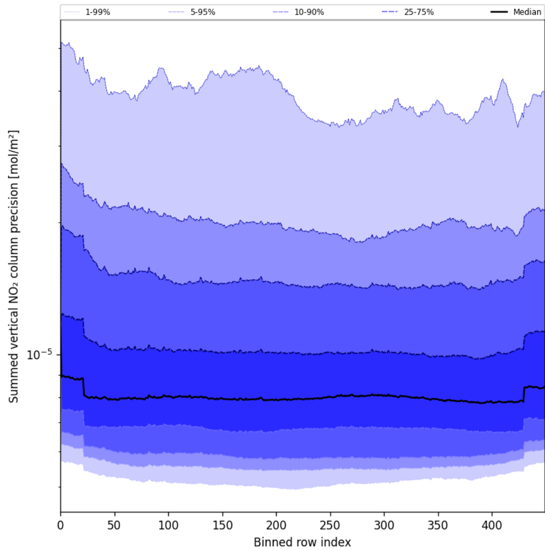
Figure 58: Along track statistics of “Summed vertical NO 2 column precision” for 2025-07-22 to 2025-07-24
