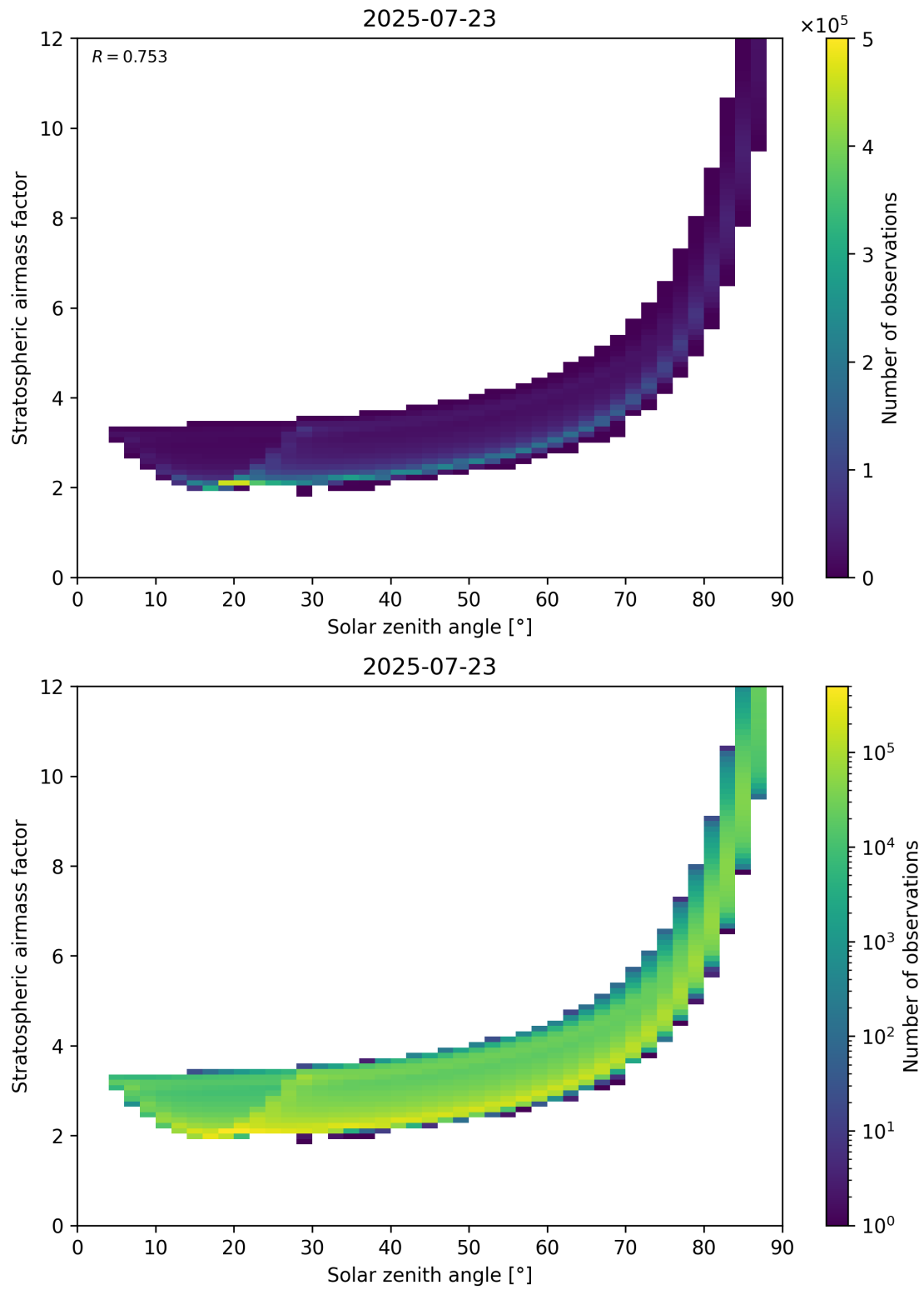
Figure 145: Scatter density plot of “Solar zenith angle” against “Stratospheric airmass factor” for 2025-07-22 to 2025-07-24.
