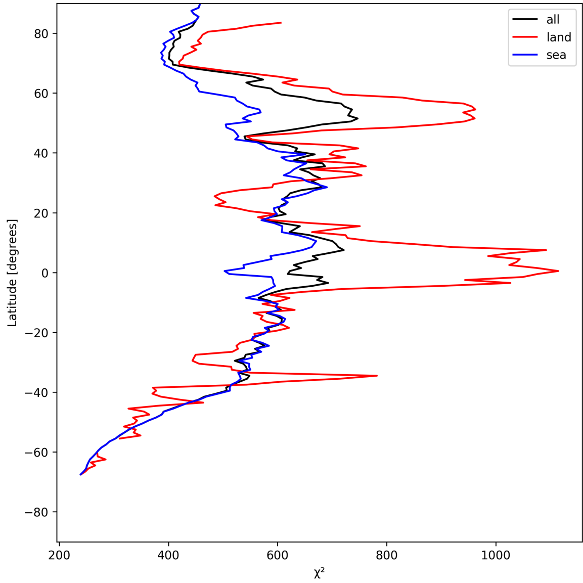
Figure 25: Zonal average of “ \chi^2 ” for 2025-07-22 to 2025-07-24.
