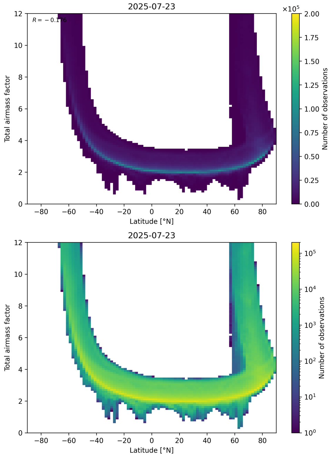
Figure 84: Scatter density plot of “Latitude” against “Total airmass factor” for 2025-07-22 to 2025-07-24.
