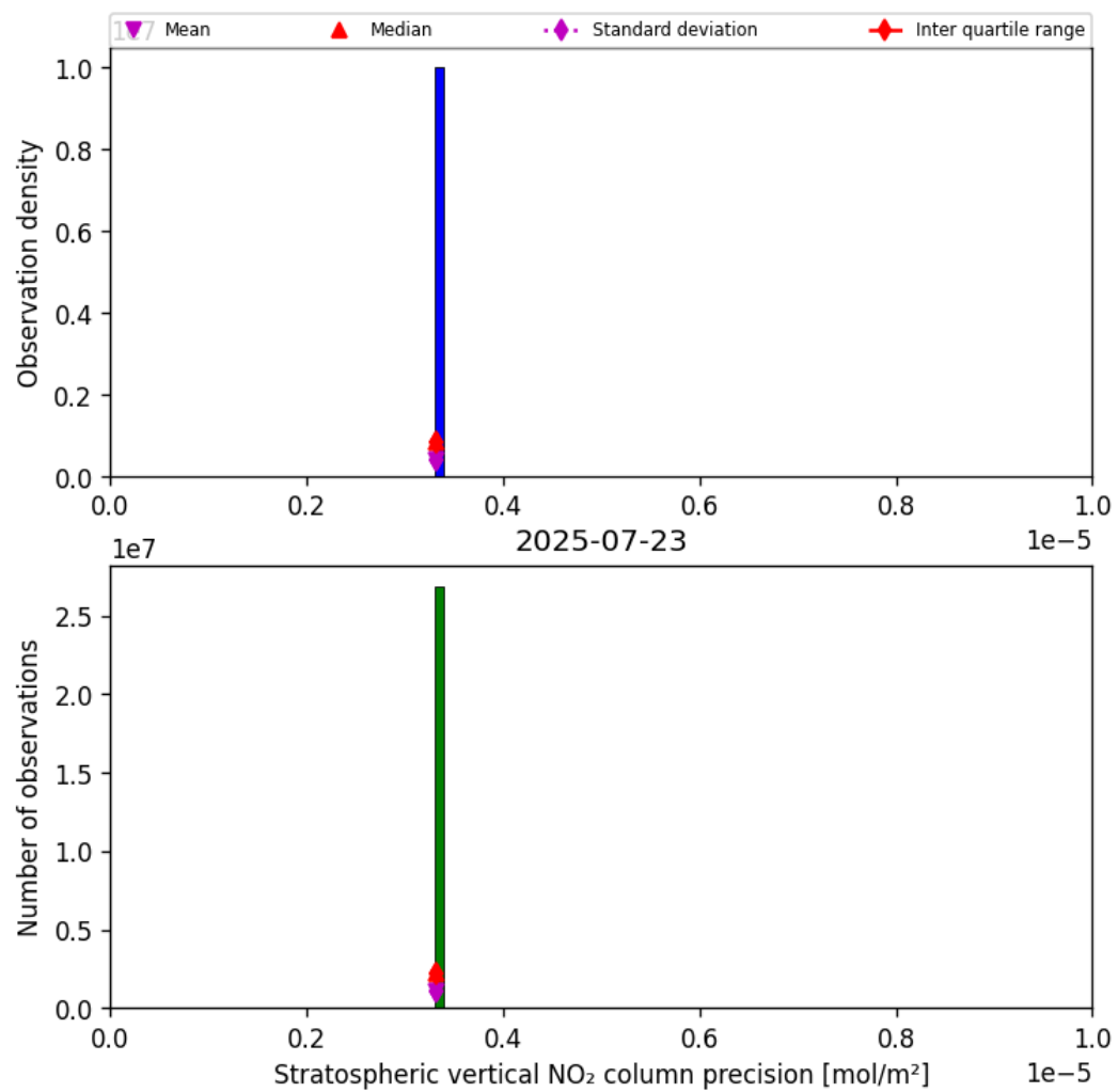
Figure 37: Histogram of “Stratospheric vertical NO 2 column precision” for 2025-07-22 to 2025-07-24
