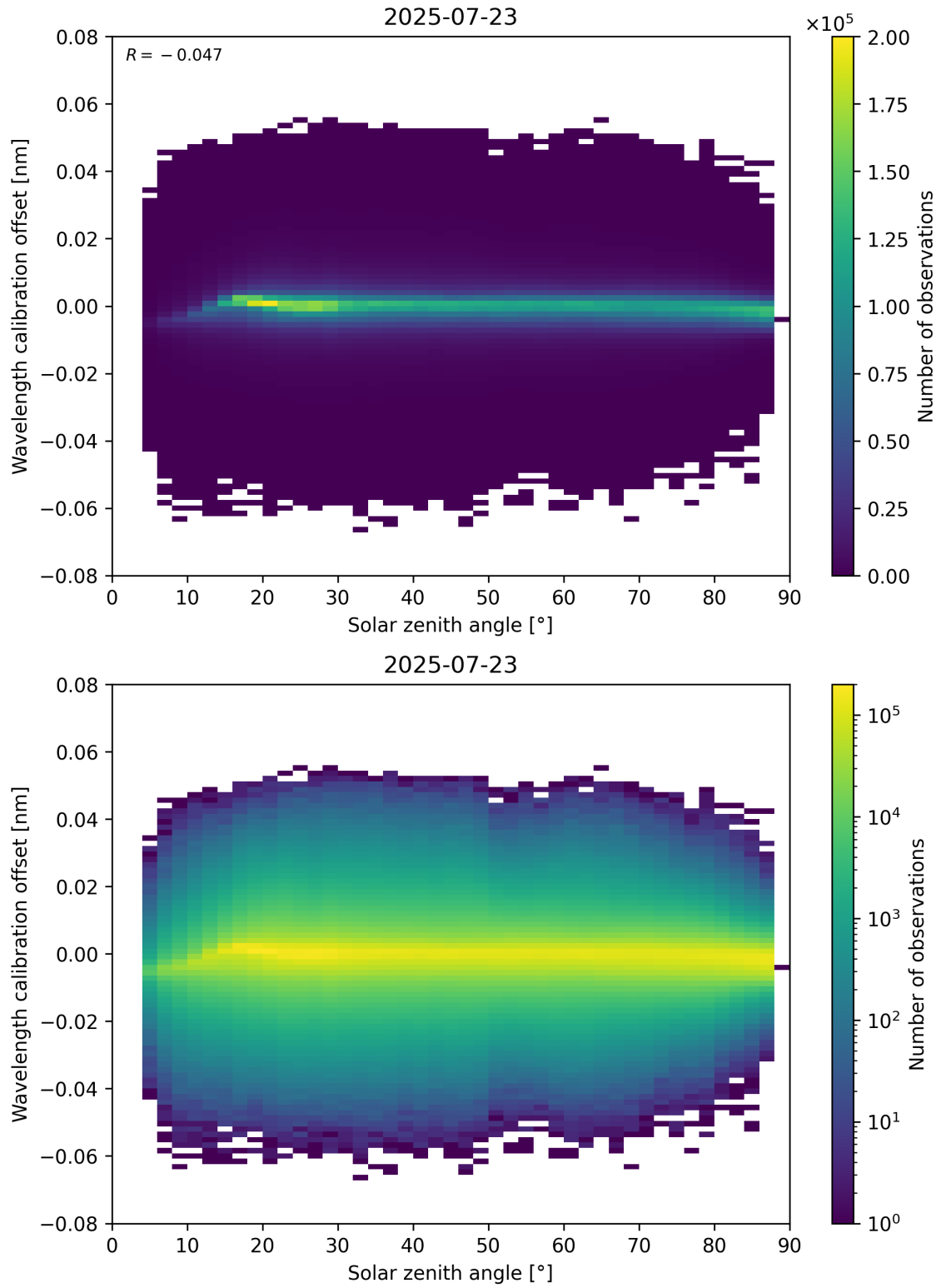
Figure 158: Scatter density plot of “Solar zenith angle” against “Wavelength calibration offset” for 2025-07-22 to 2025-07-24.
