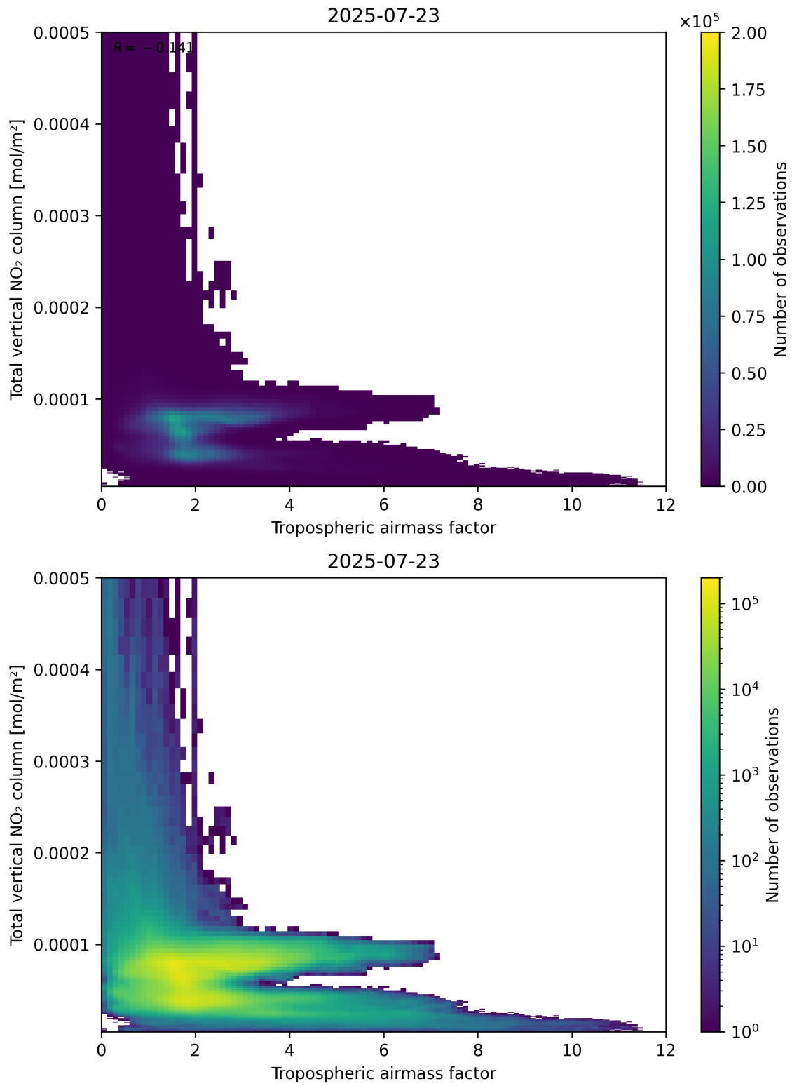
Figure 77: Scatter density plot of “Tropospheric airmass factor” against “Total vertical NO 2 column” for 2025-07-22 to 2025-07-24.
