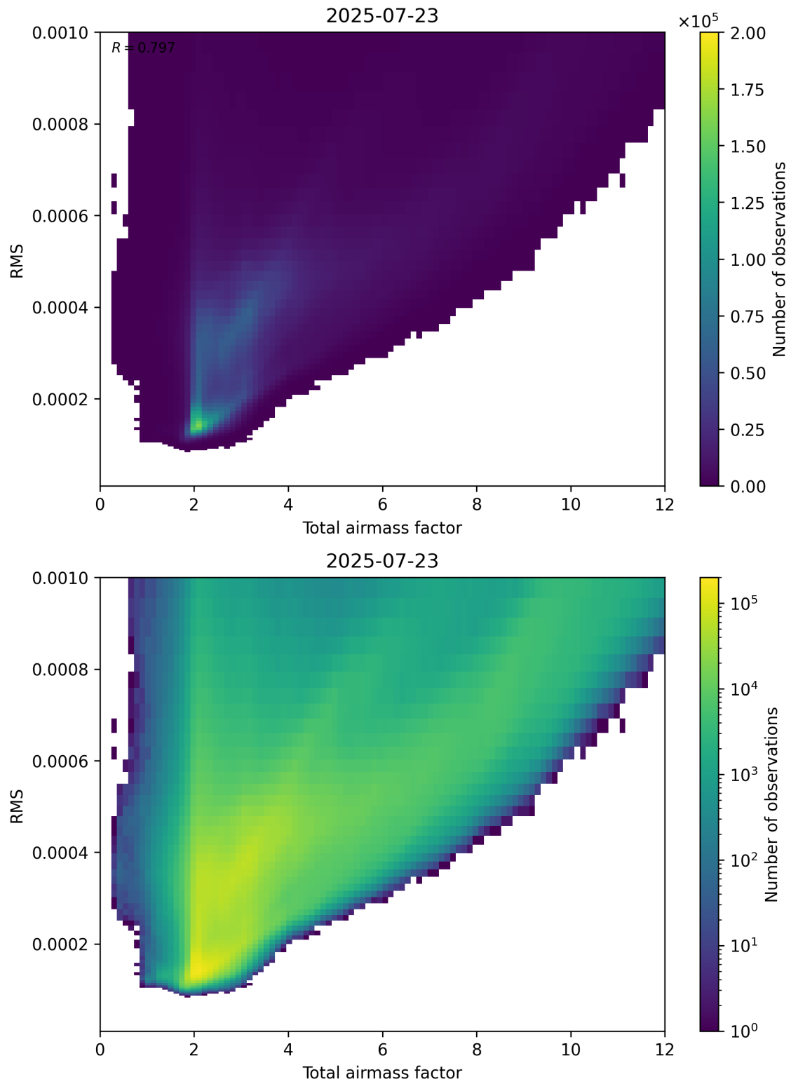
Figure 69: Scatter density plot of “Total airmass factor” against “RMS” for 2025-07-22 to 2025-07-24.
