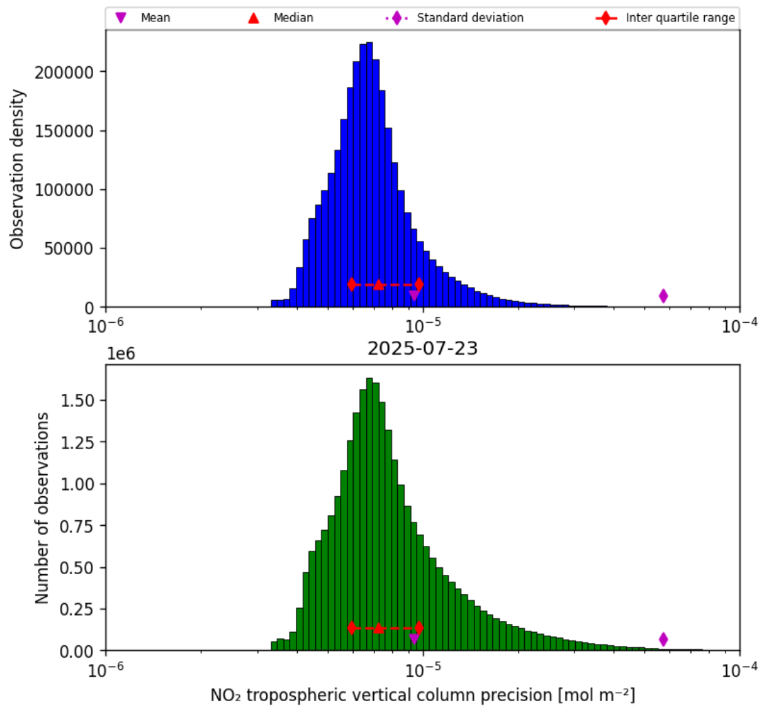
Figure 30: Histogram of “NO 2 tropospheric vertical column precision” for 2025-07-22 to 2025-07-24
