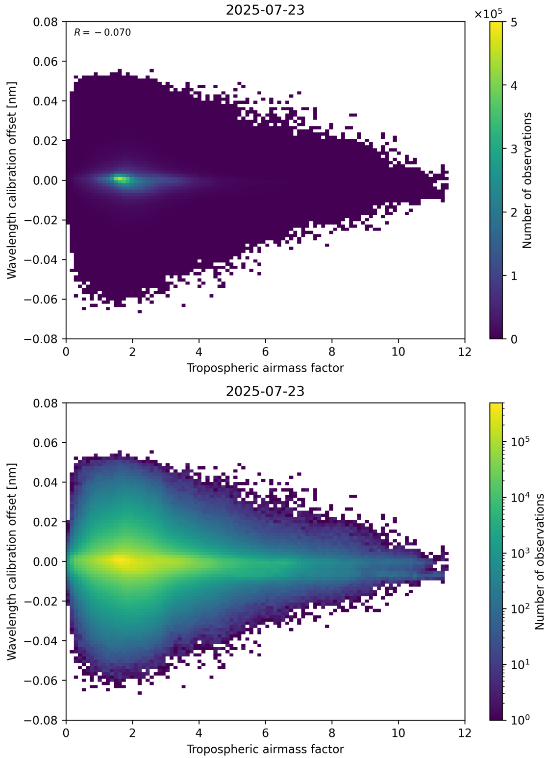
Figure 80: Scatter density plot of “Tropospheric airmass factor” against “Wavelength calibration offset” for 2025-07-22 to 2025-07-24.
