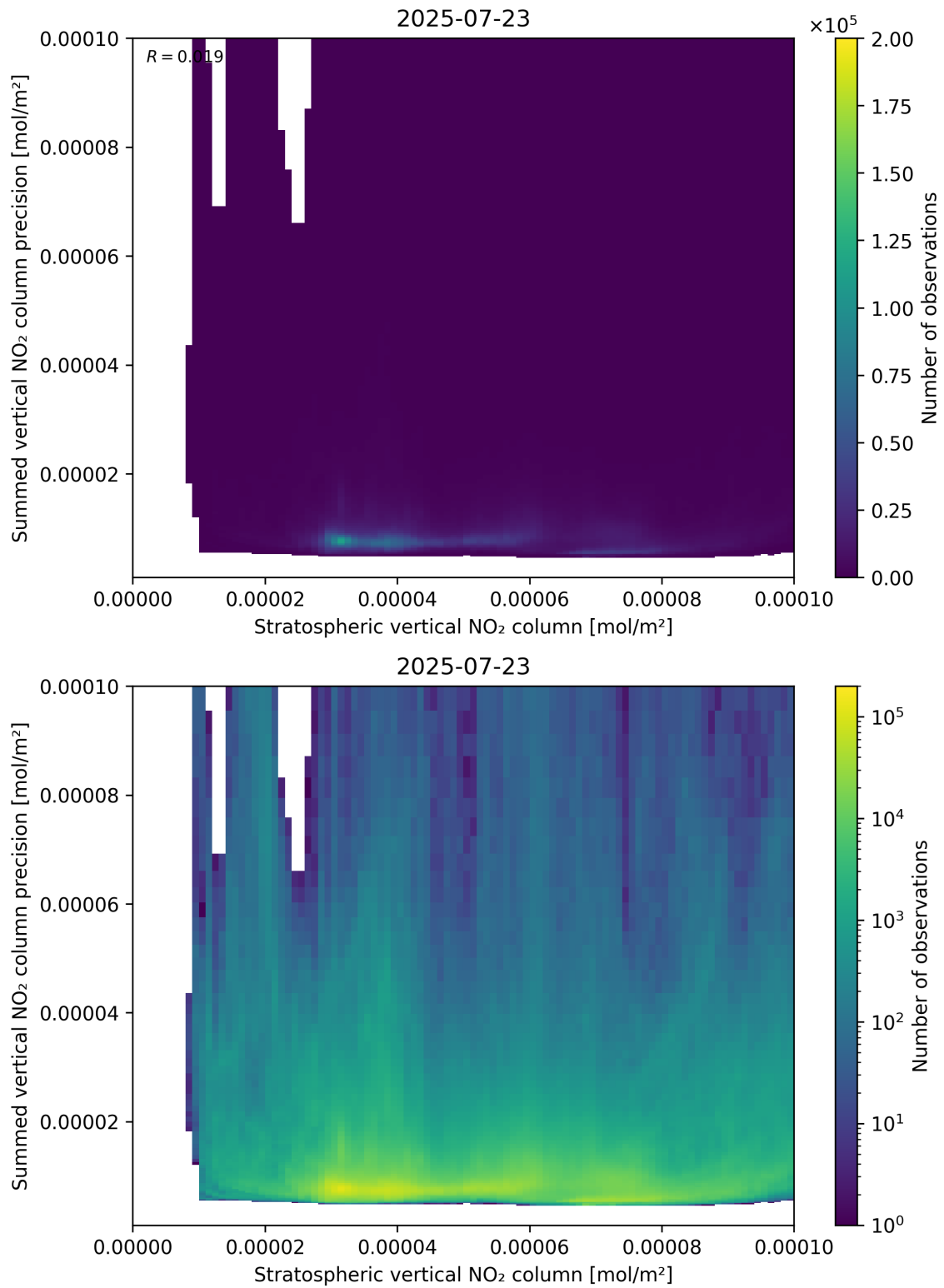
Figure 99: Scatter density plot of “Stratospheric vertical NO 2 column” against “Summed vertical NO 2 column precision” for 2025-07-22 to 2025-07-24.
