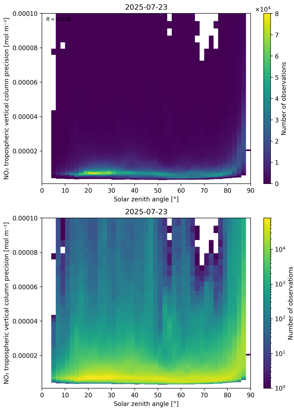
Figure 156: Scatter density plot of “Solar zenith angle” against “NO 2 tropospheric vertical column precision” for 2025-07-22 to 2025-07-24.
