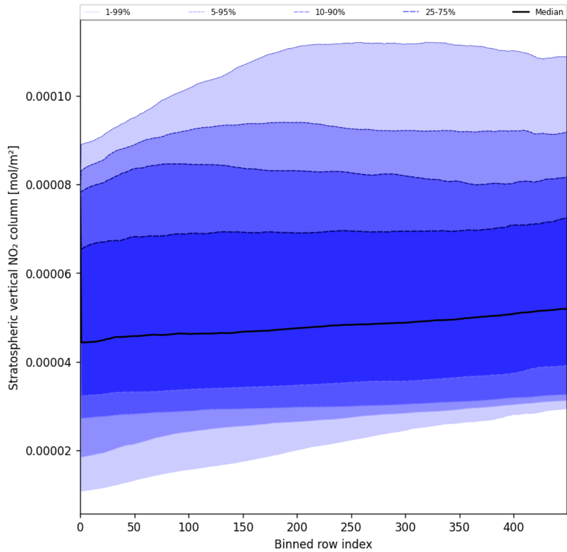
Figure 53: Along track statistics of “Stratospheric vertical NO 2 column” for 2025-07-22 to 2025-07-24
