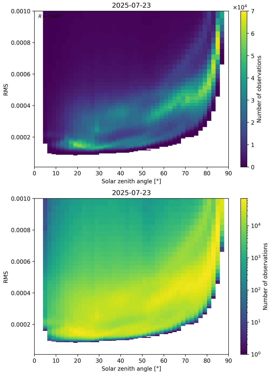
Figure 157: Scatter density plot of “Solar zenith angle” against “RMS” for 2025-07-22 to 2025-07-24.
