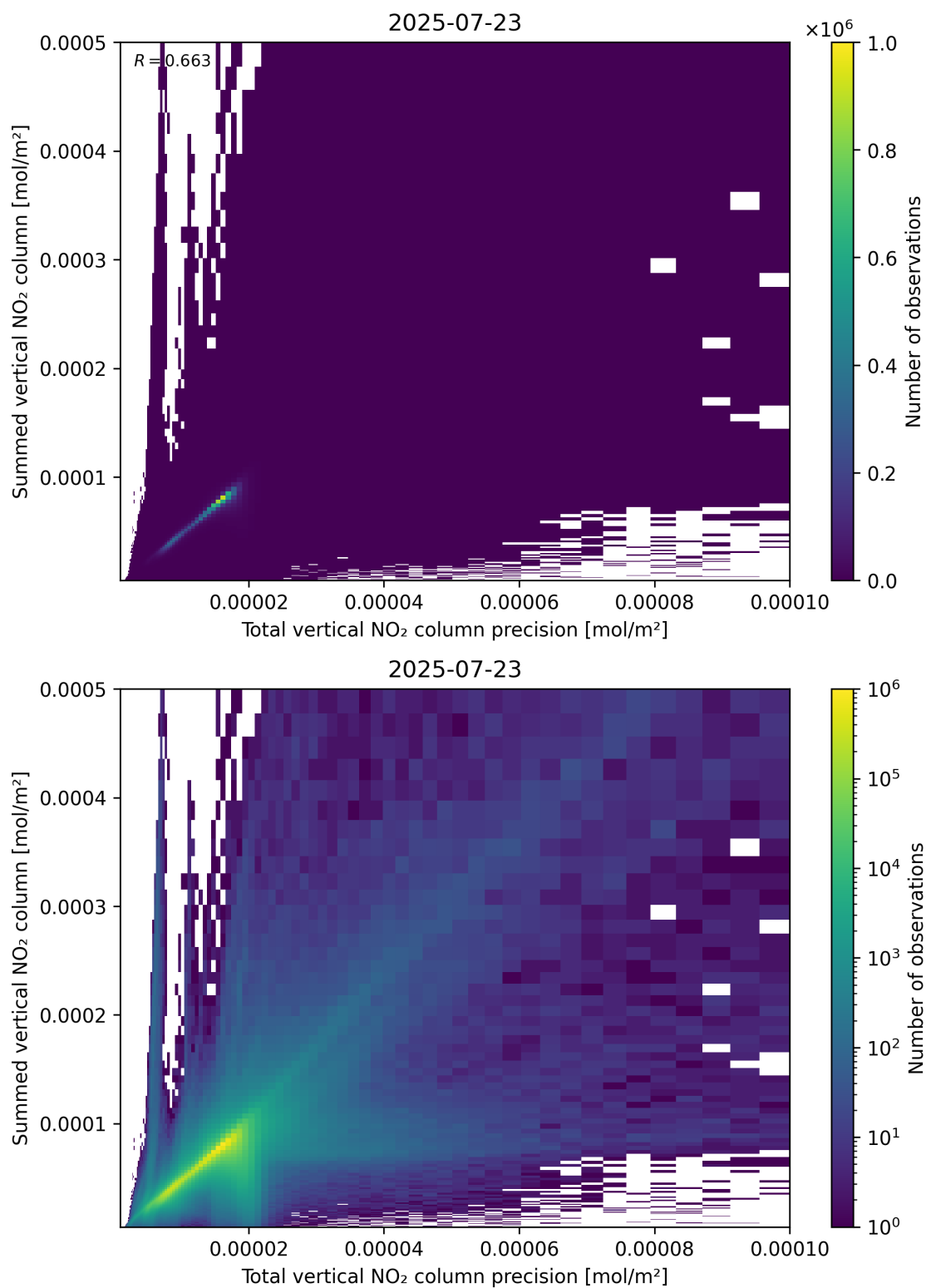
Figure 117: Scatter density plot of “Total vertical NO 2 column precision” against “Summed vertical NO 2 column” for 2025-07-22 to 2025-07-24.
