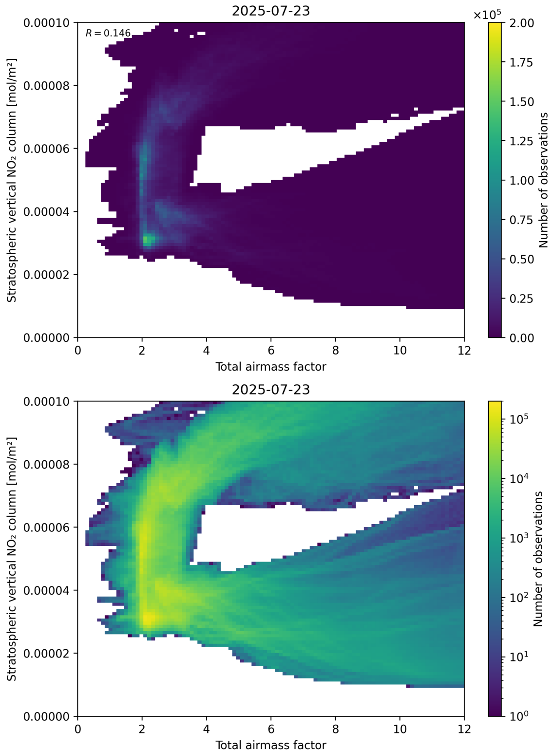
Figure 64: Scatter density plot of “Total airmass factor” against “Stratospheric vertical NO 2 column” for 2025-07-22 to 2025-07-24.
