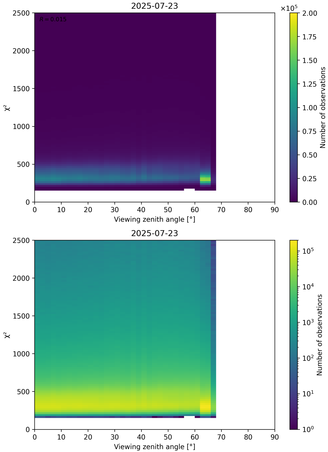
Figure 162: Scatter density plot of “Viewing zenith angle” against “ \chi^2 ” for 2025-07-22 to 2025-07-24.
