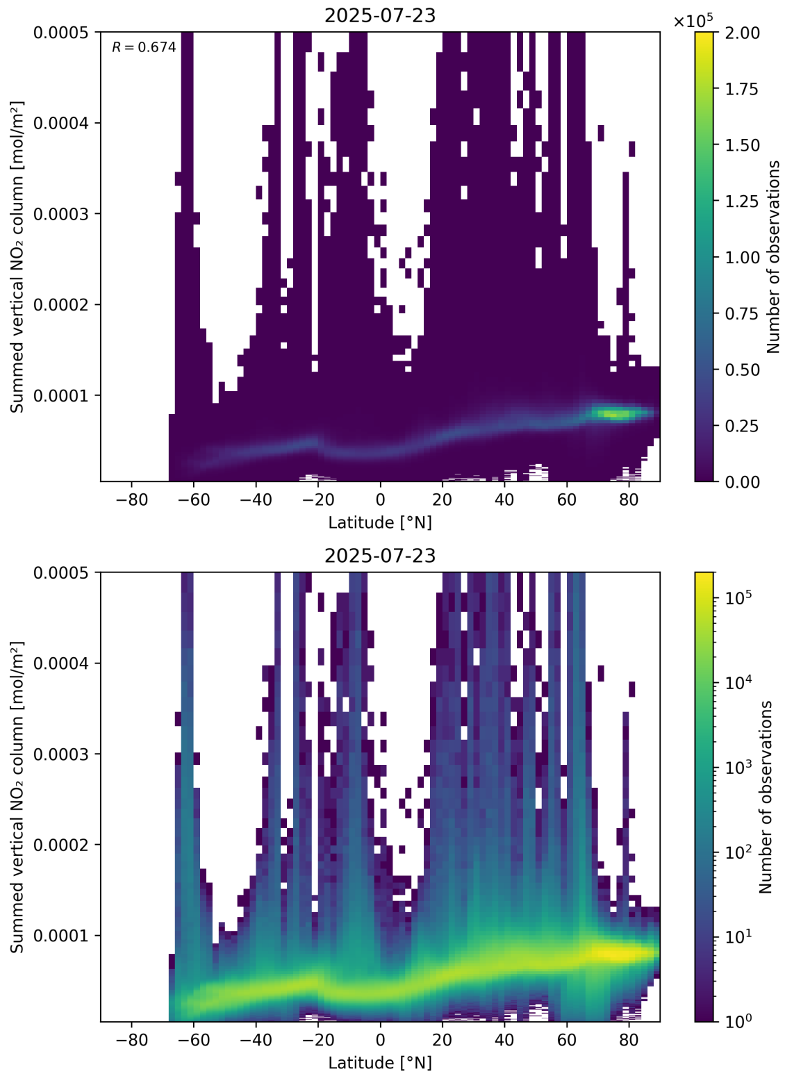
Figure 88: Scatter density plot of “Latitude” against “Summed vertical NO 2 column” for 2025-07-22 to 2025-07-24.
