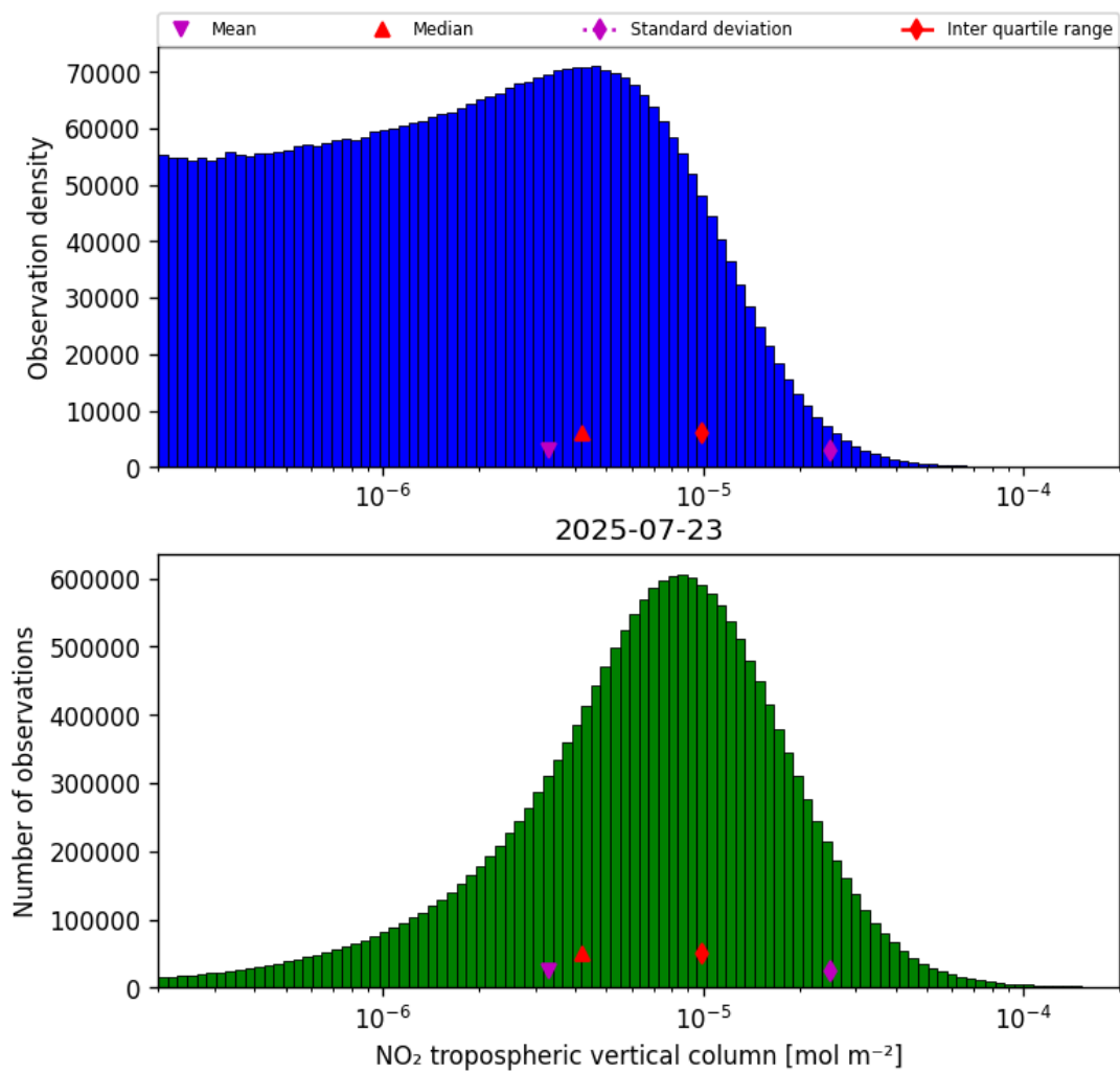
Figure 29: Histogram of “NO 2 tropospheric vertical column” for 2025-07-22 to 2025-07-24
