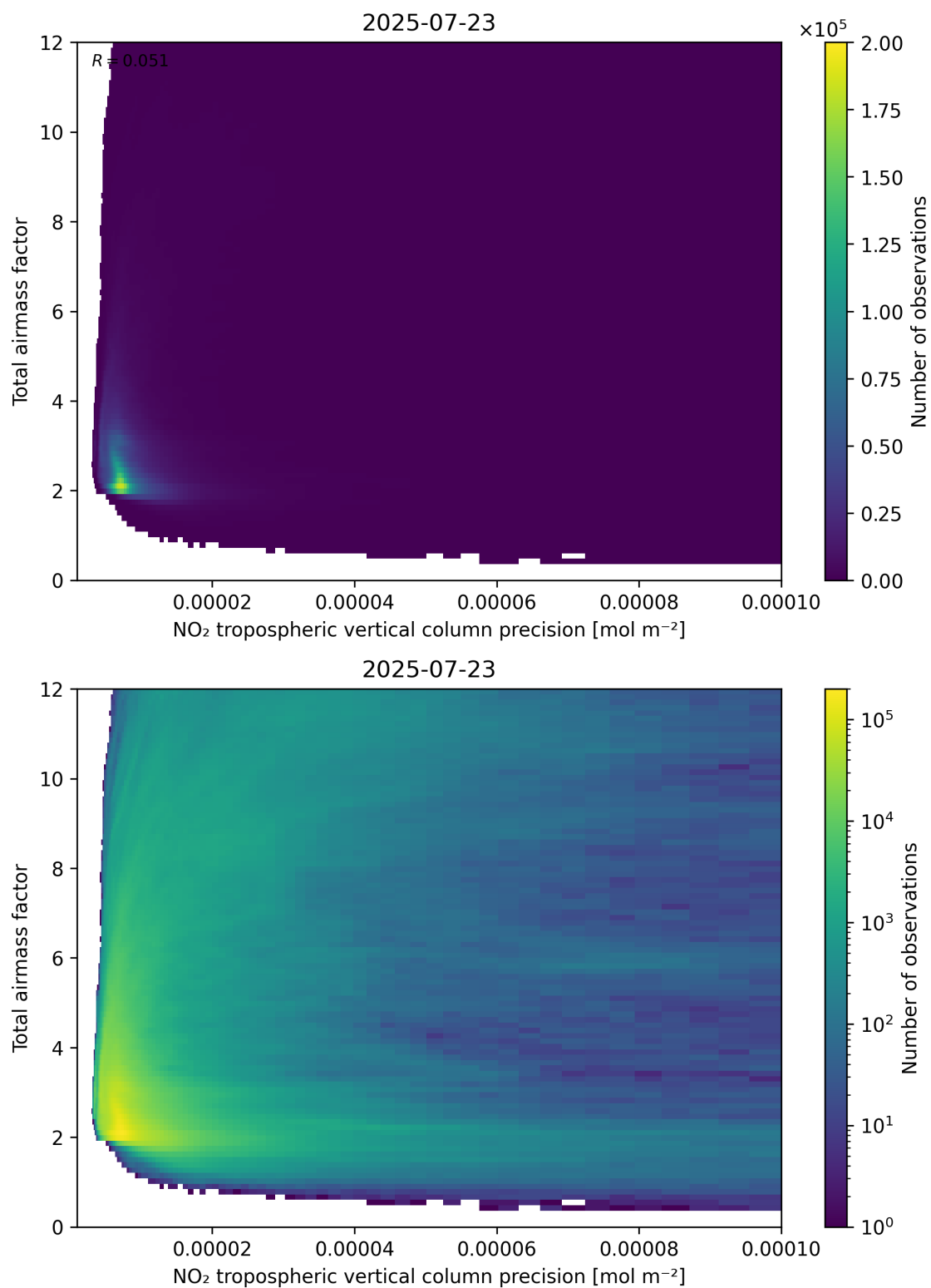
Figure 132: Scatter density plot of “NO 2 tropospheric vertical column precision” against “Total air mass factor” for 2025-07-22 to 2025-07-24.
