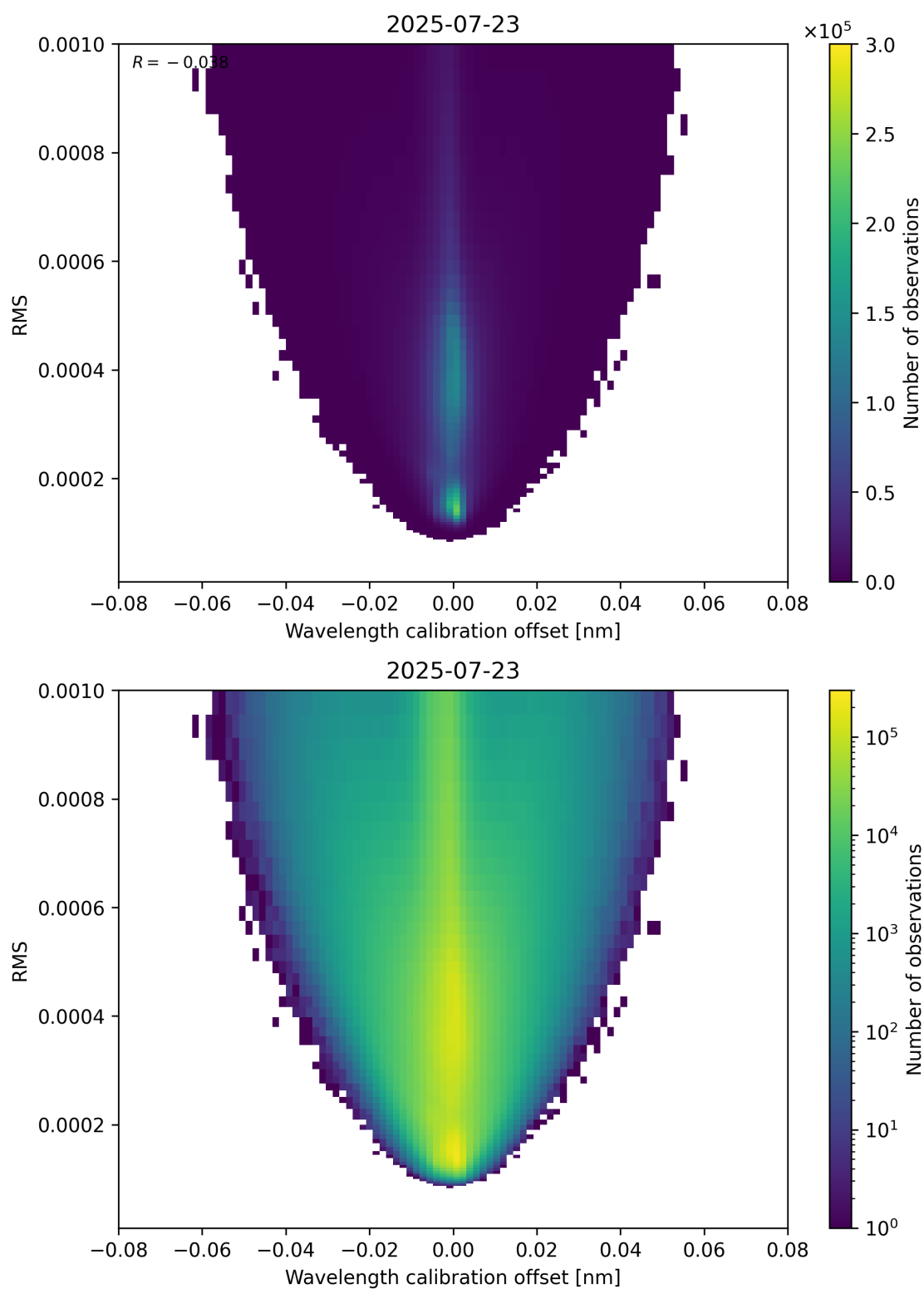
Figure 181: Scatter density plot of “Wavelength calibration offset” against “RMS” for 2025-07-22 to 2025-07-24.
