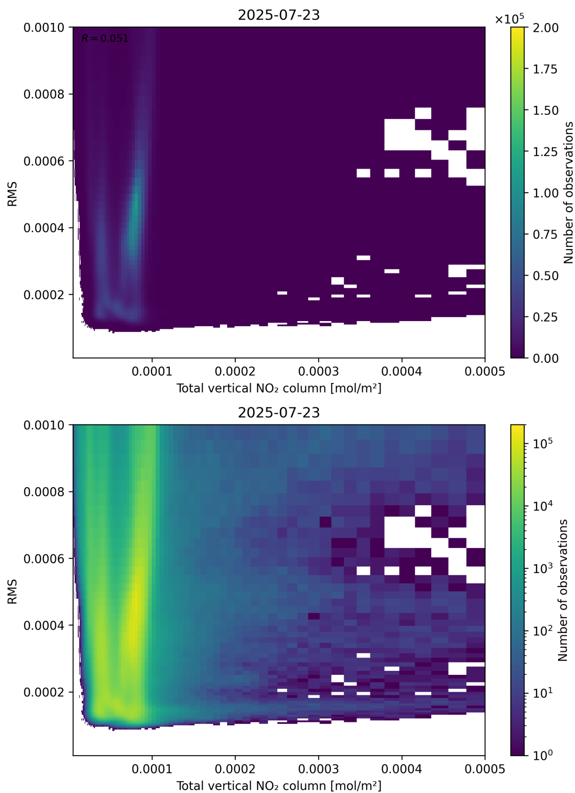
Figure 120: Scatter density plot of “Total vertical NO 2 column” against “RMS” for 2025-07-22 to 2025-07-24.
