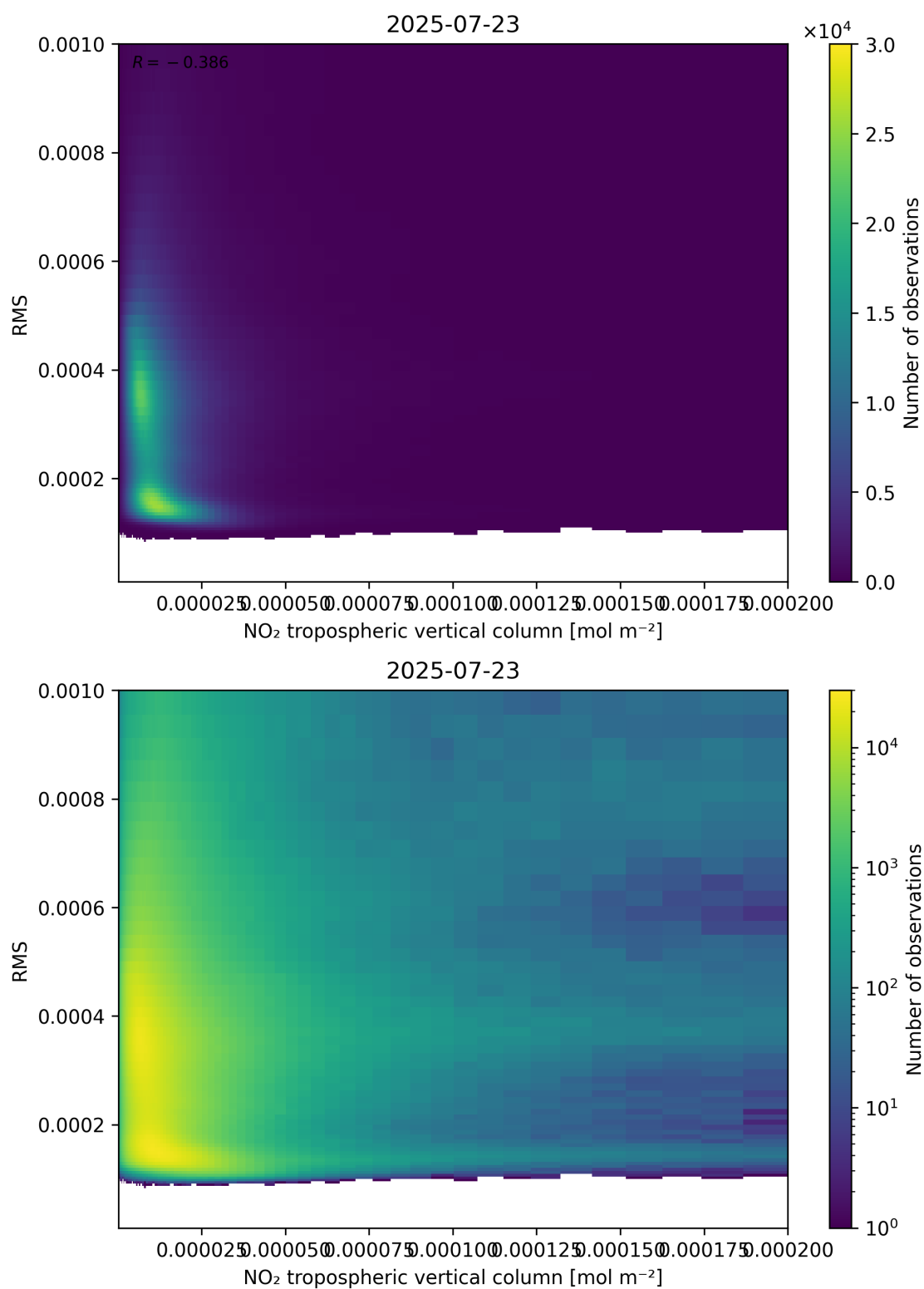
Figure 142: Scatter density plot of “NO 2 tropospheric vertical column” against “RMS” for 2025-07-22 to 2025-07-24.
