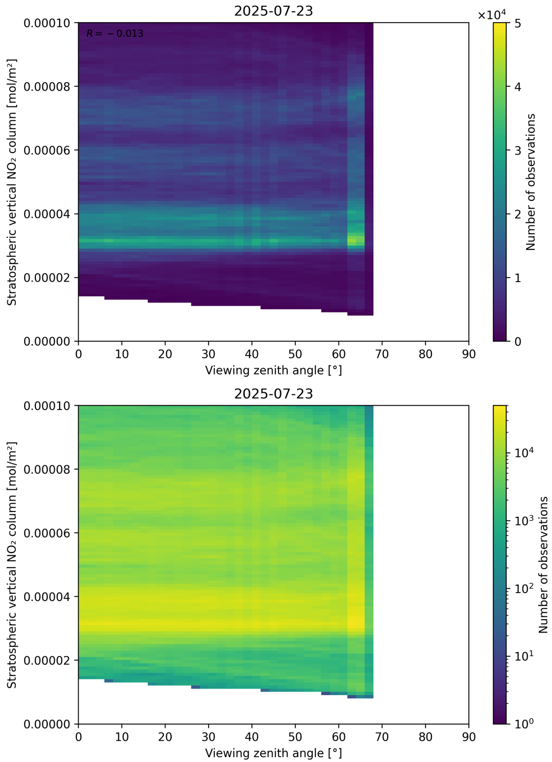
Figure 164: Scatter density plot of “Viewing zenith angle” against “Stratospheric vertical NO 2 column” for 2025-07-22 to 2025-07-24.
