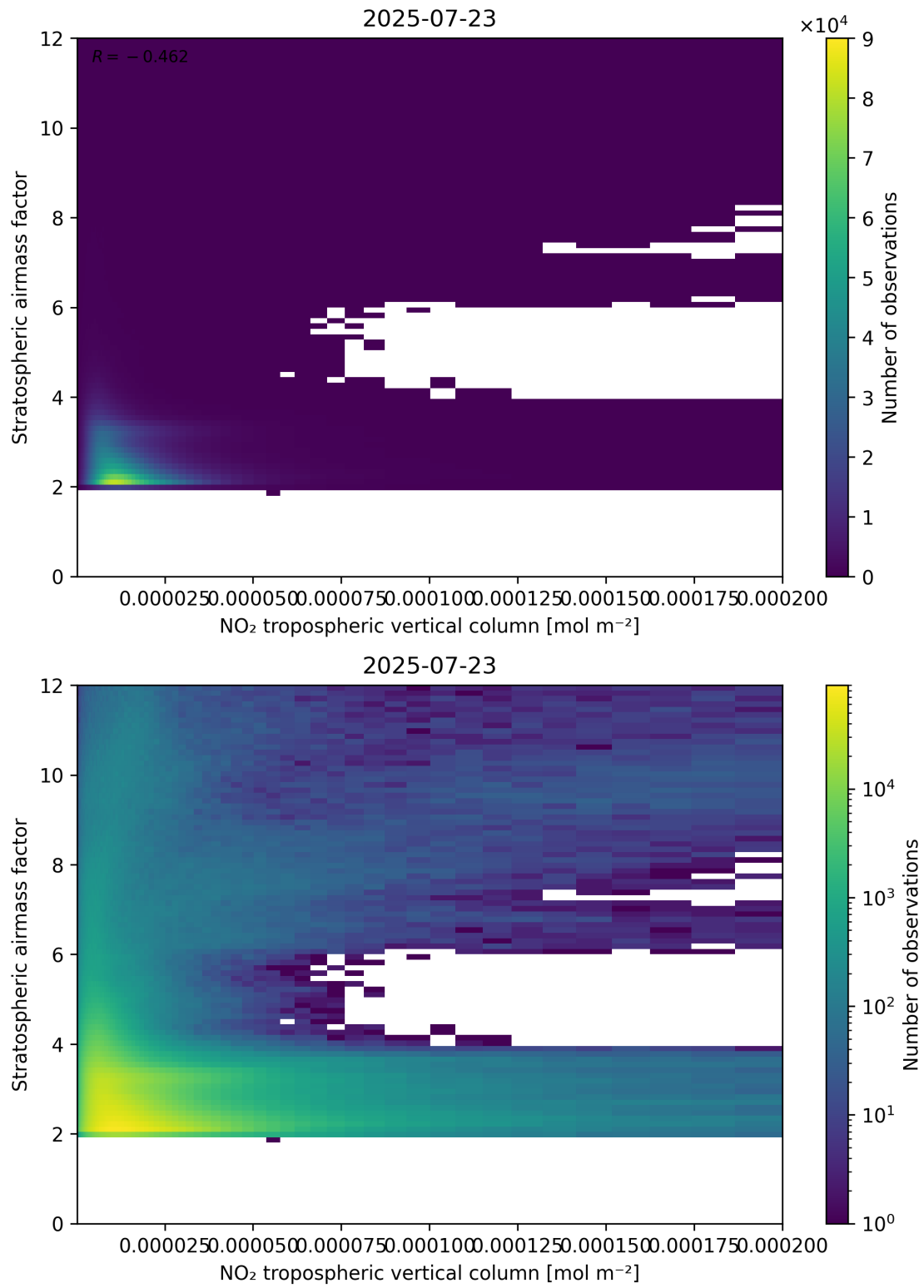
Figure 121: Scatter density plot of “NO 2 tropospheric vertical column” against “Stratospheric air mass factor” for 2025-07-22 to 2025-07-24.
