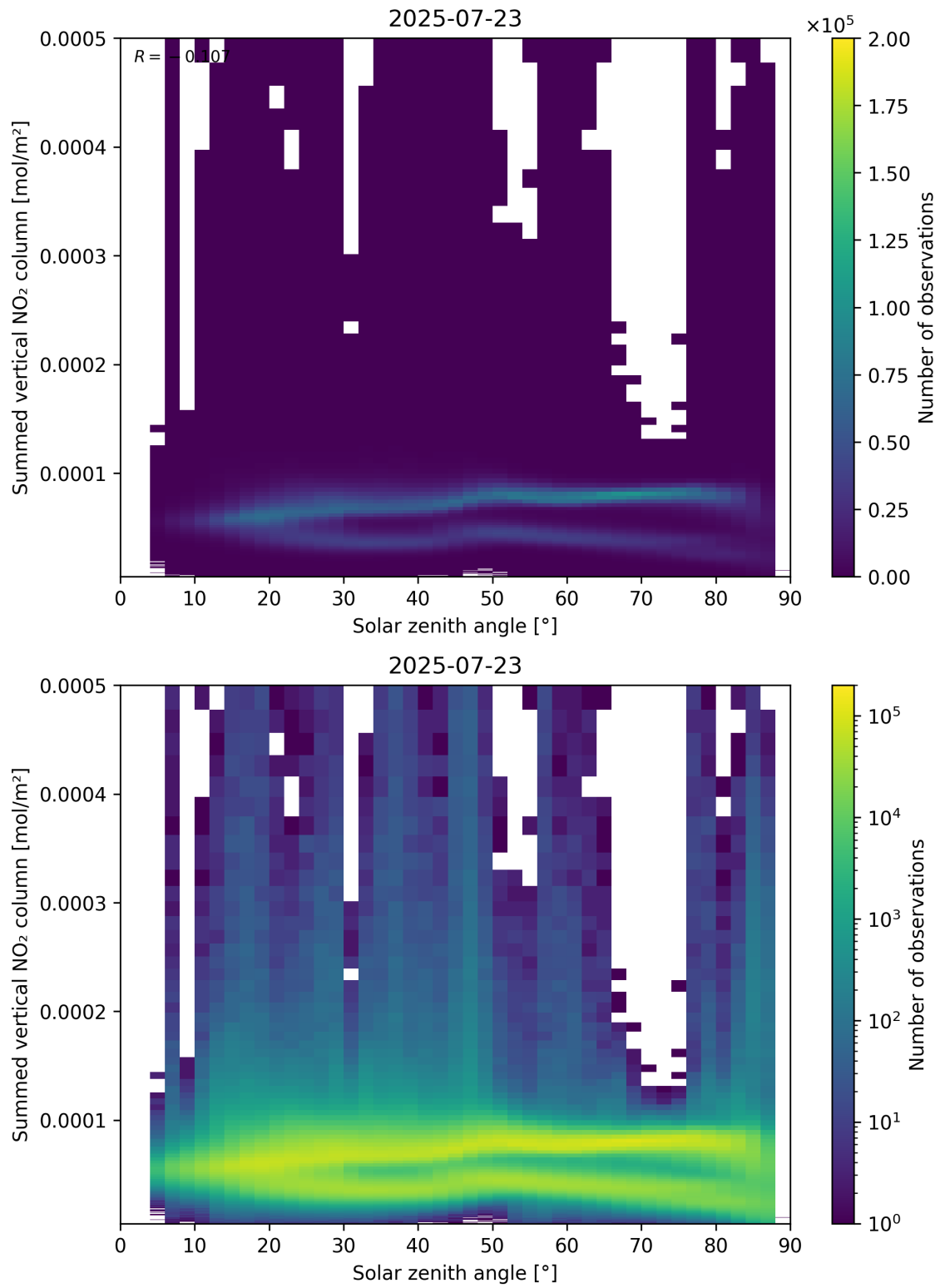
Figure 151: Scatter density plot of “Solar zenith angle” against “Summed vertical NO 2 column” for 2025-07-22 to 2025-07-24.
