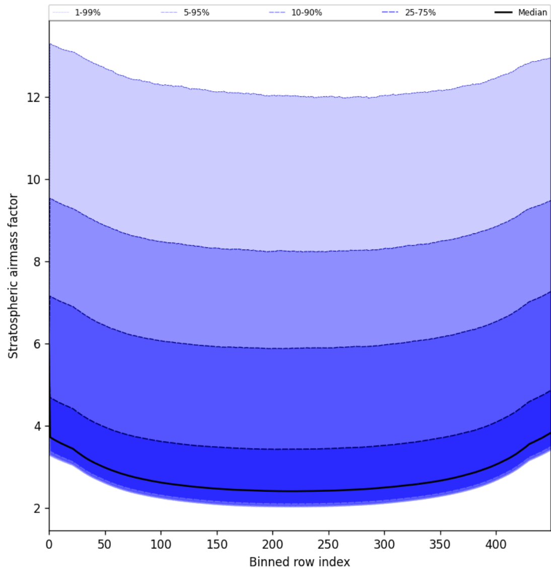
Figure 61: Along track statistics of “Stratospheric airmass factor” for 2025-07-22 to 2025-07-24
