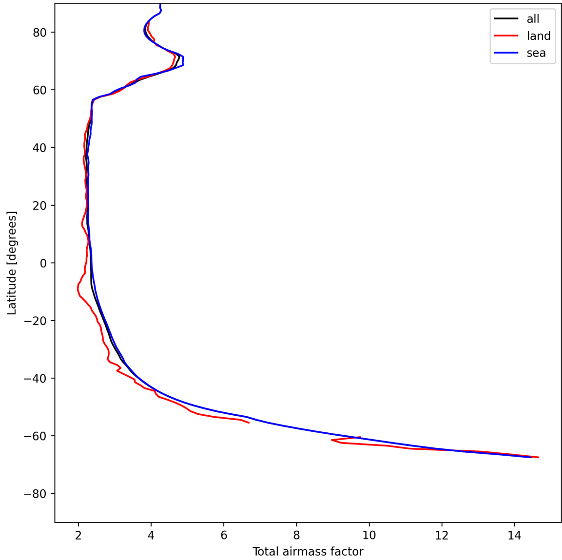
Figure 15: Zonal average of “Total airmass factor” for 2025-07-22 to 2025-07-24.
