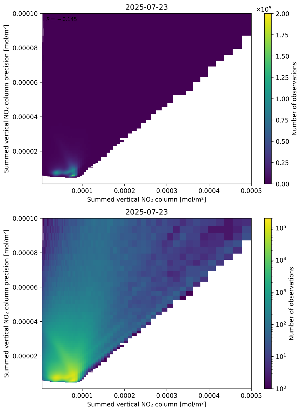
Figure 105: Scatter density plot of “Summed vertical NO 2 column” against “Summed vertical NO 2 column precision” for 2025-07-22 to 2025-07-24.
