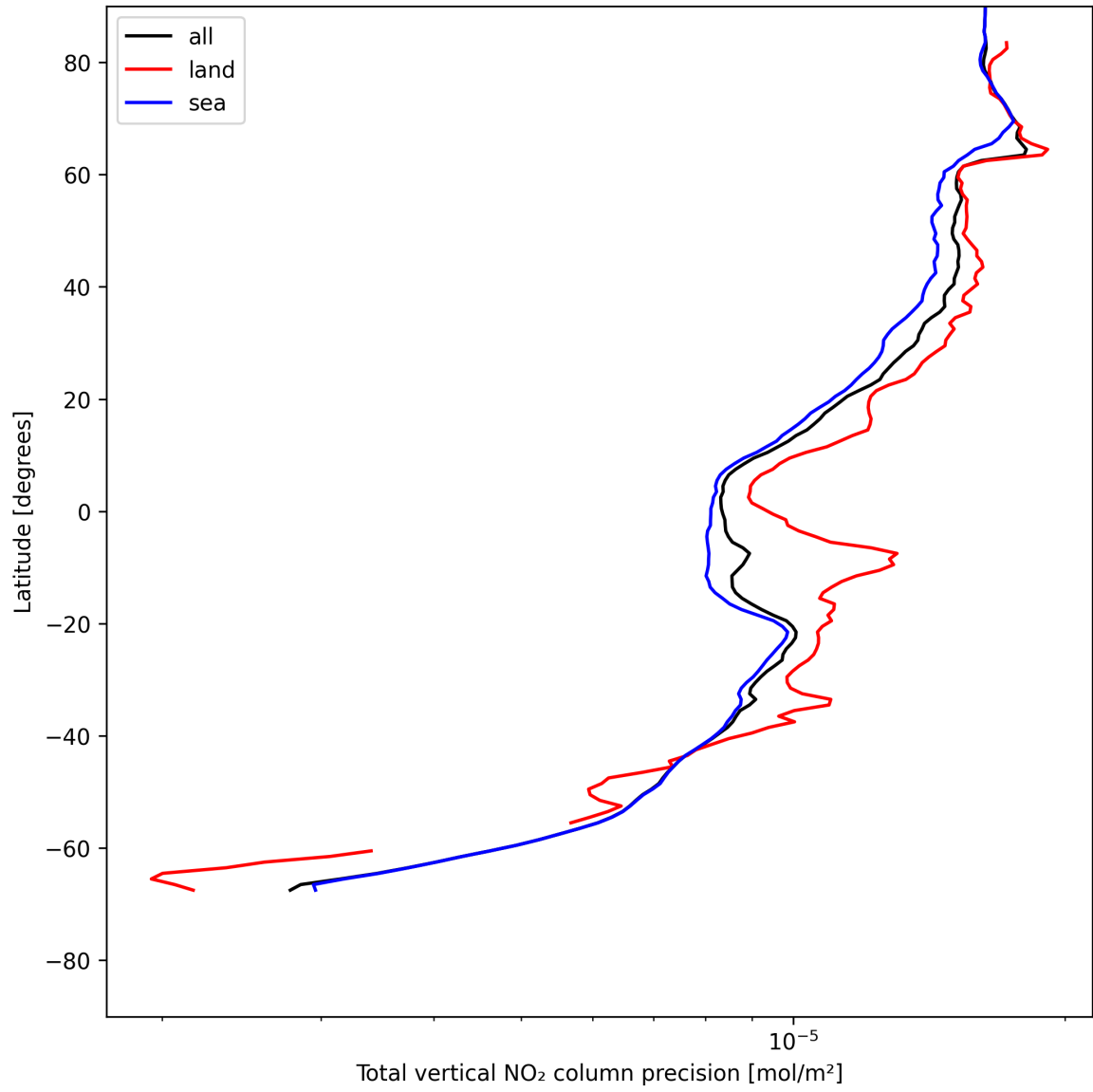
Figure 22: Zonal average of “Total vertical NO 2 column precision” for 2025-07-22 to 2025-07-24.
