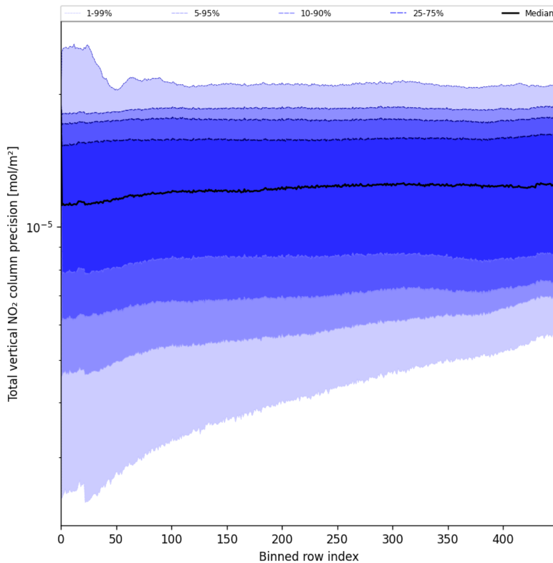
Figure 56: Along track statistics of “Total vertical NO 2 column precision” for 2025-07-22 to 2025-07-24
