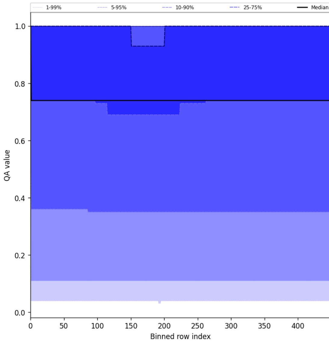
Figure 45: Along track statistics of “QA value” for 2025-07-22 to 2025-07-24
