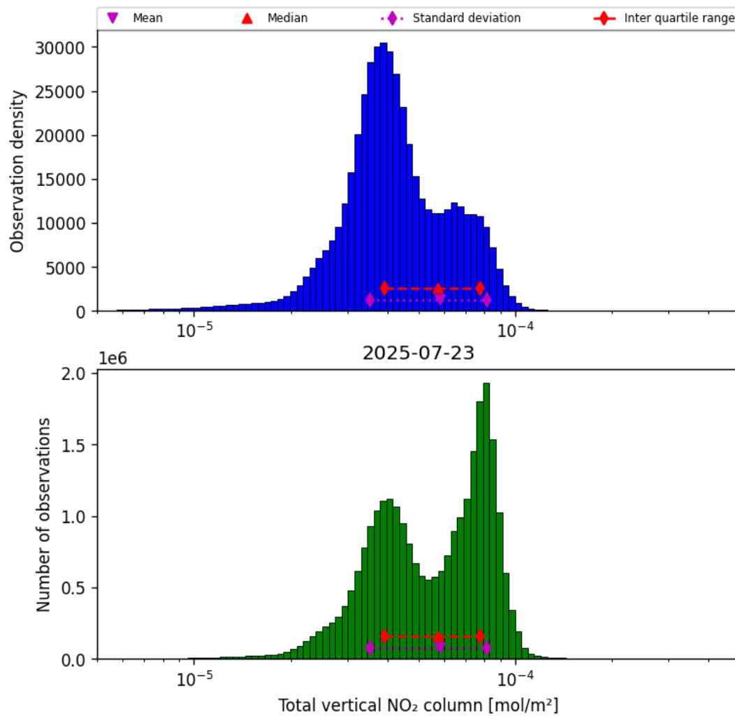
Figure 38: Histogram of “Total vertical NO 2 column” for 2025-07-22 to 2025-07-24
