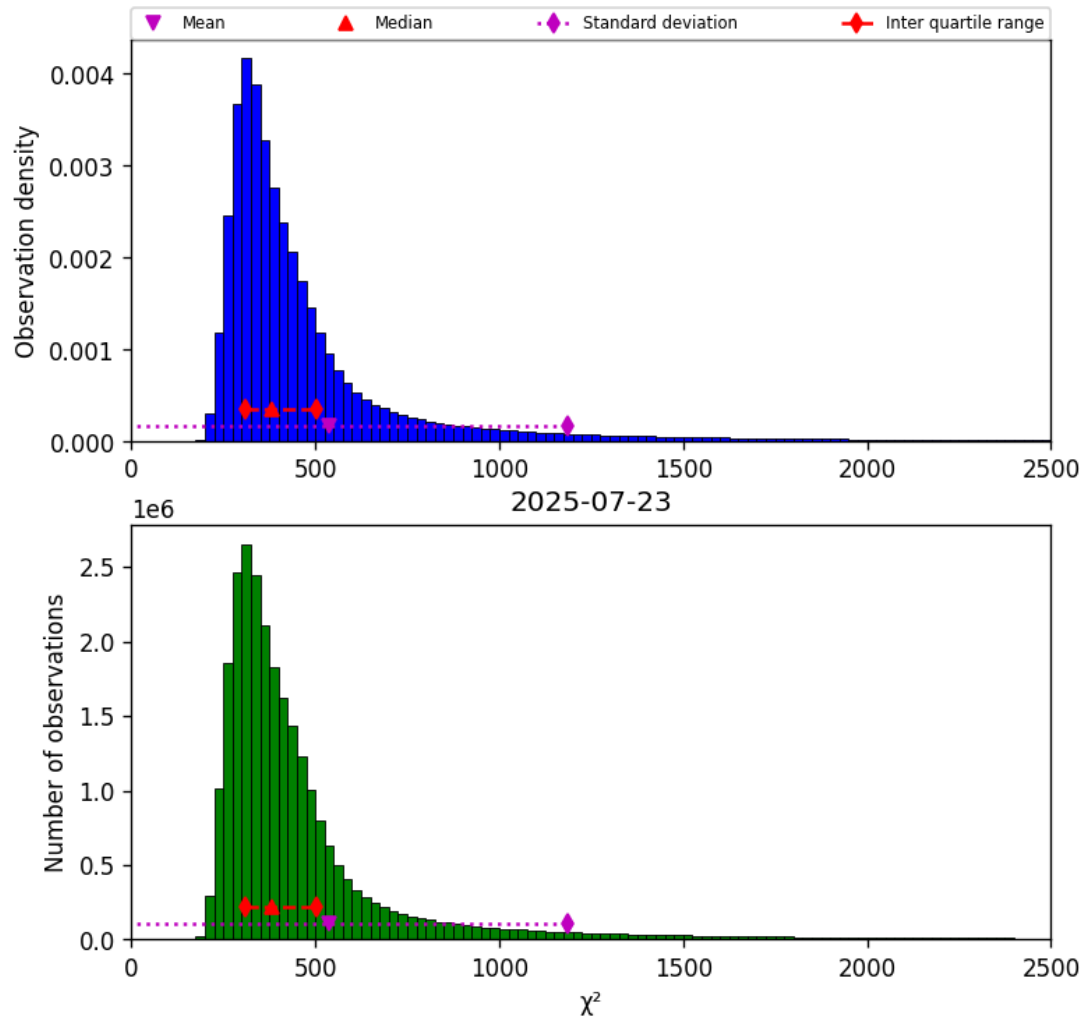
Figure 42: Histogram of “ \chi^2 ” for 2025-07-22 to 2025-07-24
