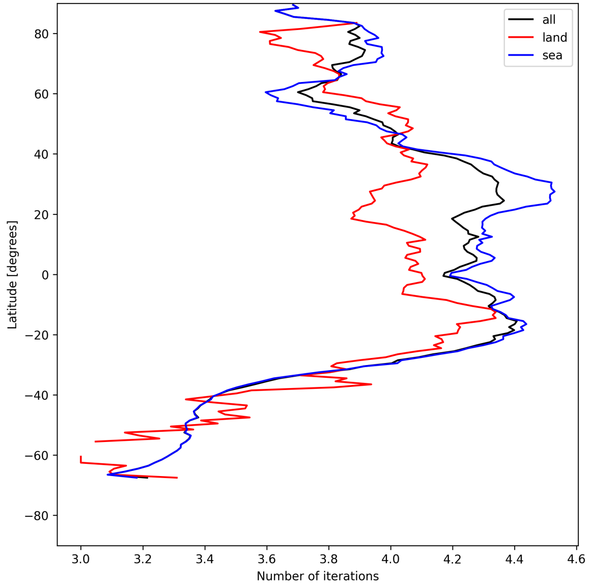
Figure 17: Zonal average of “Number of iterations” for 2025-07-22 to 2025-07-24.
