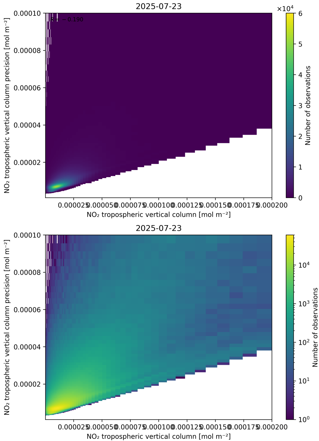
Figure 130: Scatter density plot of “NO 2 tropospheric vertical column” against “NO 2 tropospheric vertical column precision” for 2025-07-22 to 2025-07-24.
