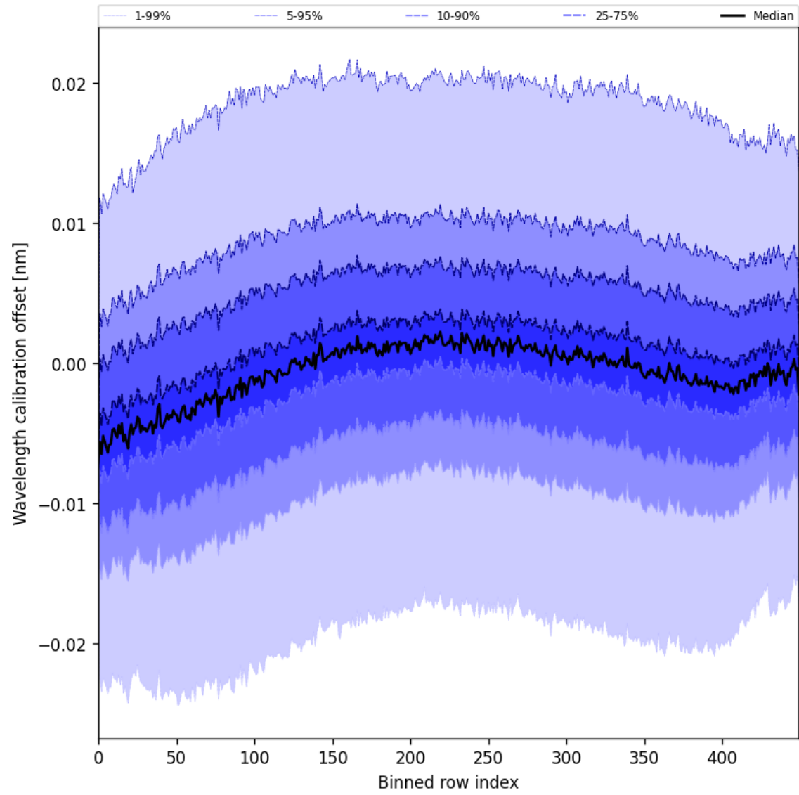
Figure 52: Along track statistics of “Wavelength calibration offset” for 2025-07-22 to 2025-07-24
