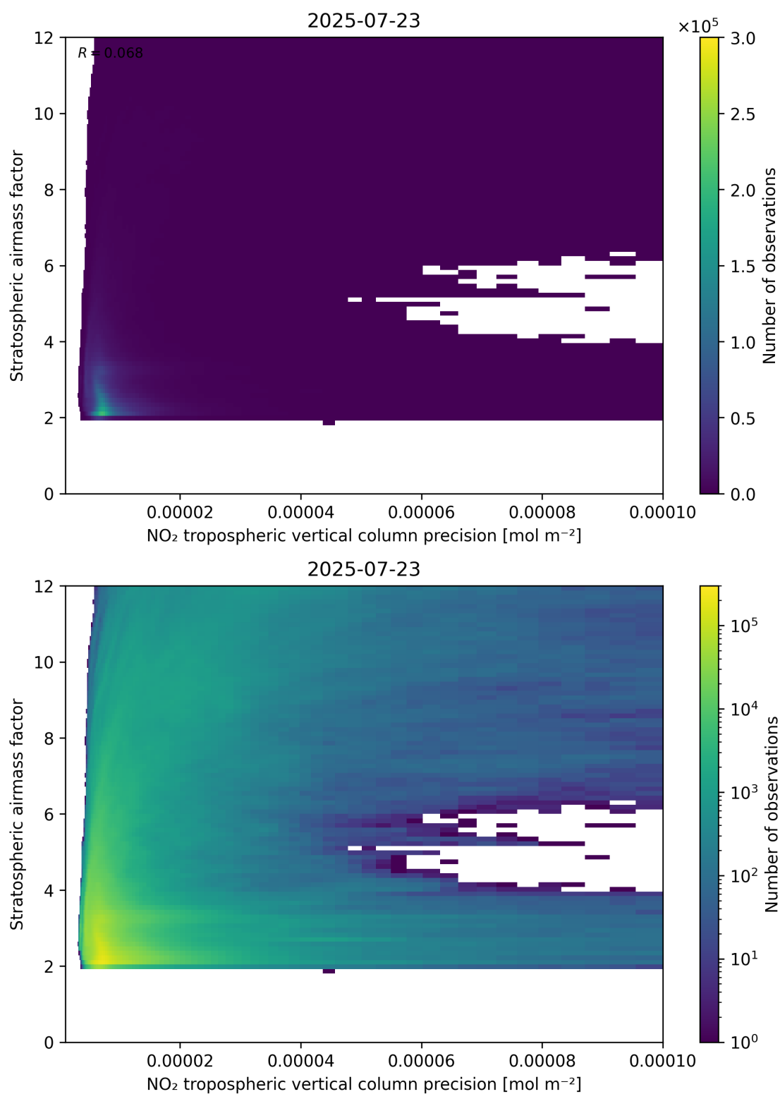
Figure 131: Scatter density plot of “NO 2 tropospheric vertical column precision” against “Stratospheric airmass factor” for 2025-07-22 to 2025-07-24.
