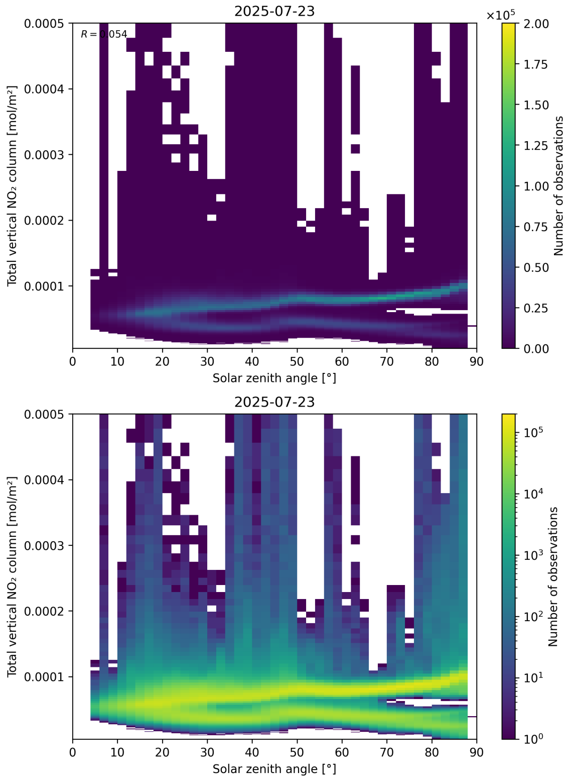
Figure 153: Scatter density plot of “Solar zenith angle” against “Total vertical NO 2 column” for 2025-07-22 to 2025-07-24.
