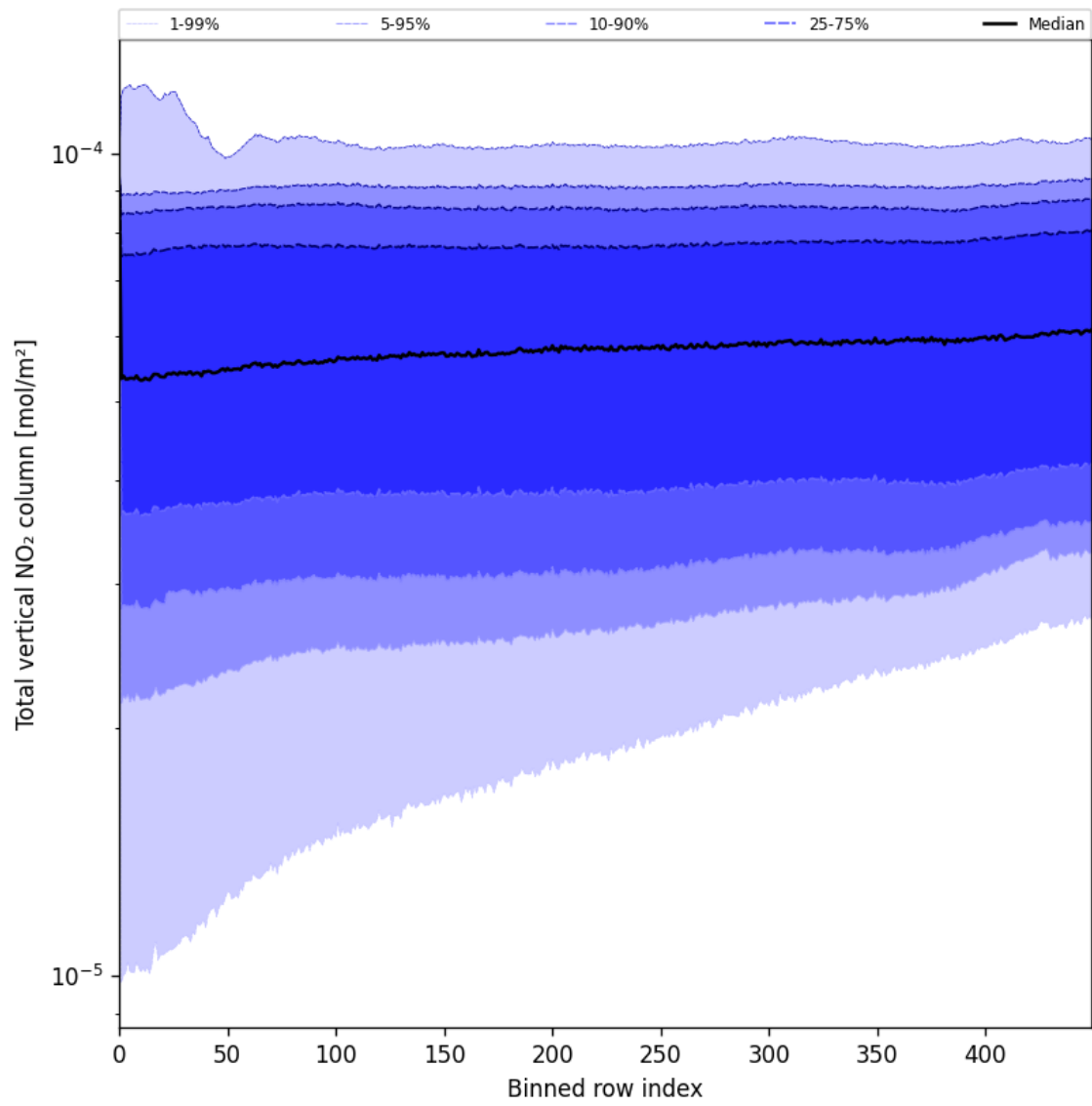
Figure 55: Along track statistics of “Total vertical NO 2 column” for 2025-07-22 to 2025-07-24
