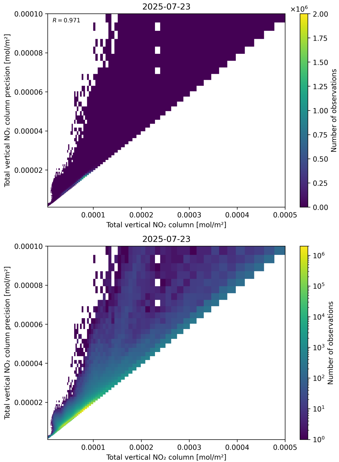
Figure 114: Scatter density plot of “Total vertical NO 2 column” against “Total vertical NO 2 column precision” for 2025-07-22 to 2025-07-24.
