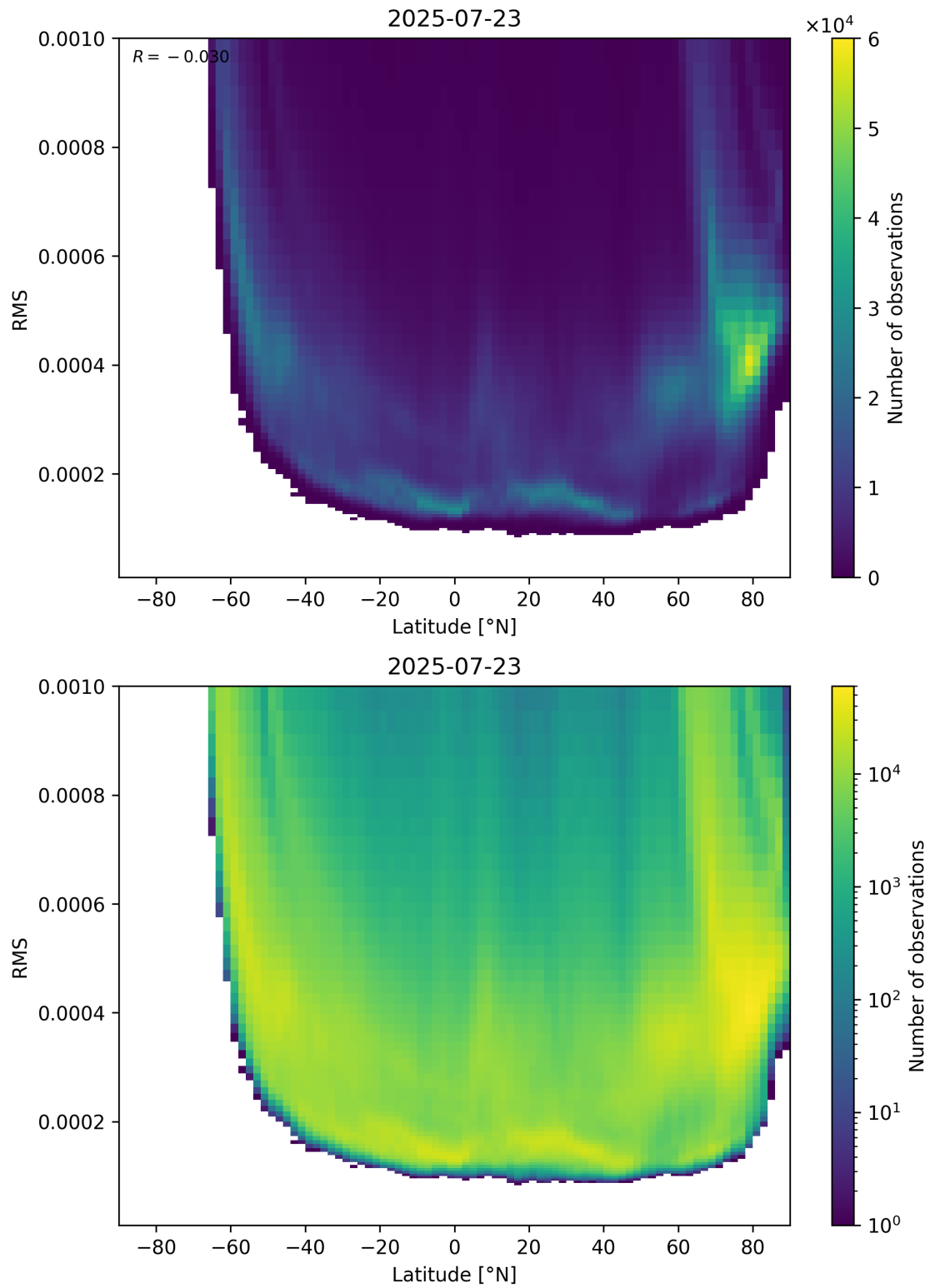
Figure 94: Scatter density plot of “Latitude” against “RMS” for 2025-07-22 to 2025-07-24.
