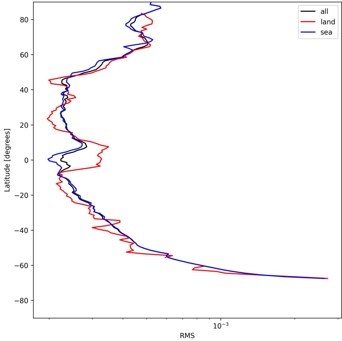
Figure 26: Zonal average of “RMS” for 2025-07-22 to 2025-07-24.
