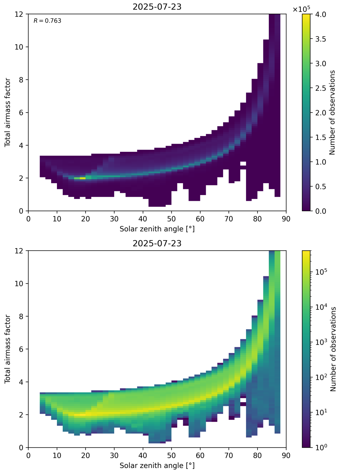
Figure 146: Scatter density plot of “Solar zenith angle” against “Total air mass factor” for 2025-07-22 to 2025-07-24.
