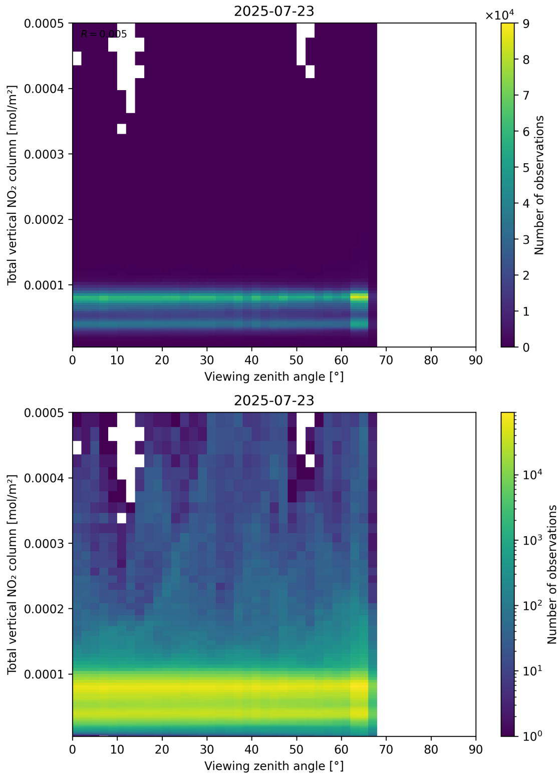
Figure 167: Scatter density plot of “Viewing zenith angle” against “Total vertical NO 2 column” for 2025-07-22 to 2025-07-24.
