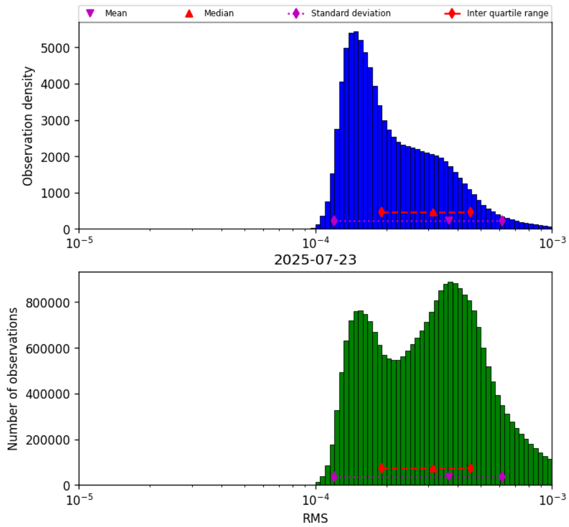
Figure 43: Histogram of “RMS” for 2025-07-22 to 2025-07-24
