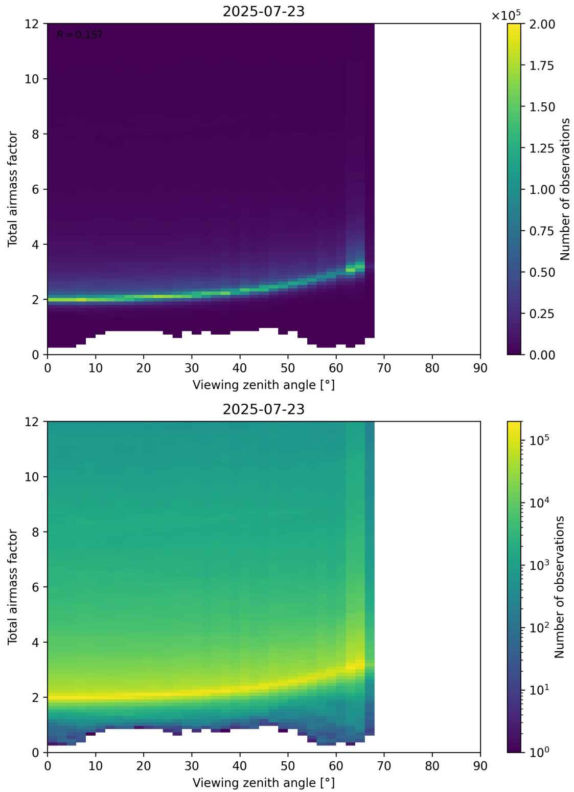
Figure 160: Scatter density plot of “Viewing zenith angle” against “Total airmass factor” for 2025-07-22 to 2025-07-24.
