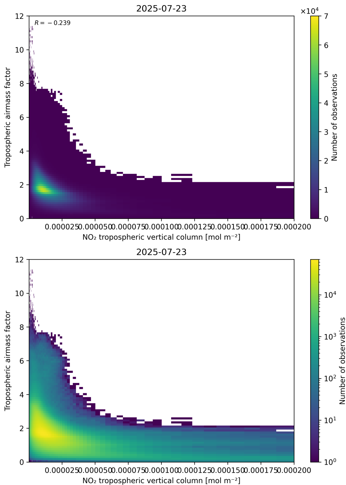
Figure 123: Scatter density plot of “NO 2 tropospheric vertical column” against “Tropospheric air mass factor” for 2025-07-22 to 2025-07-24.
