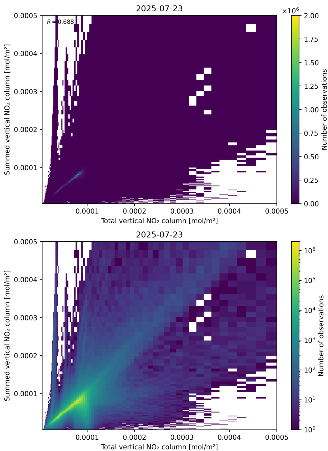
Figure 112: Scatter density plot of “Total vertical NO 2 column” against “Summed vertical NO 2 column” for 2025-07-22 to 2025-07-24.
