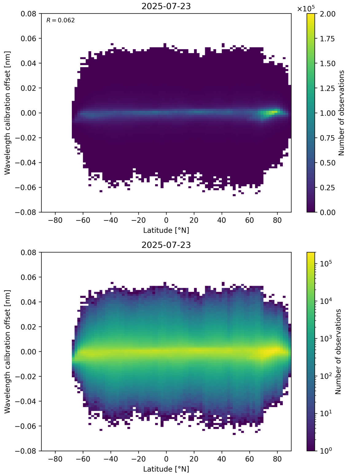
Figure 95: Scatter density plot of “Latitude” against “Wavelength calibration offset” for 2025-07-22 to 2025-07-24.
