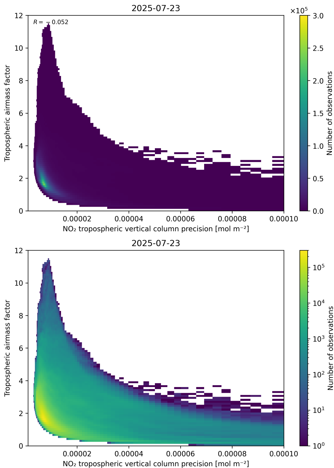
Figure 133: Scatter density plot of “NO 2 tropospheric vertical column precision” against “Tropospheric airmass factor” for 2025-07-22 to 2025-07-24.
