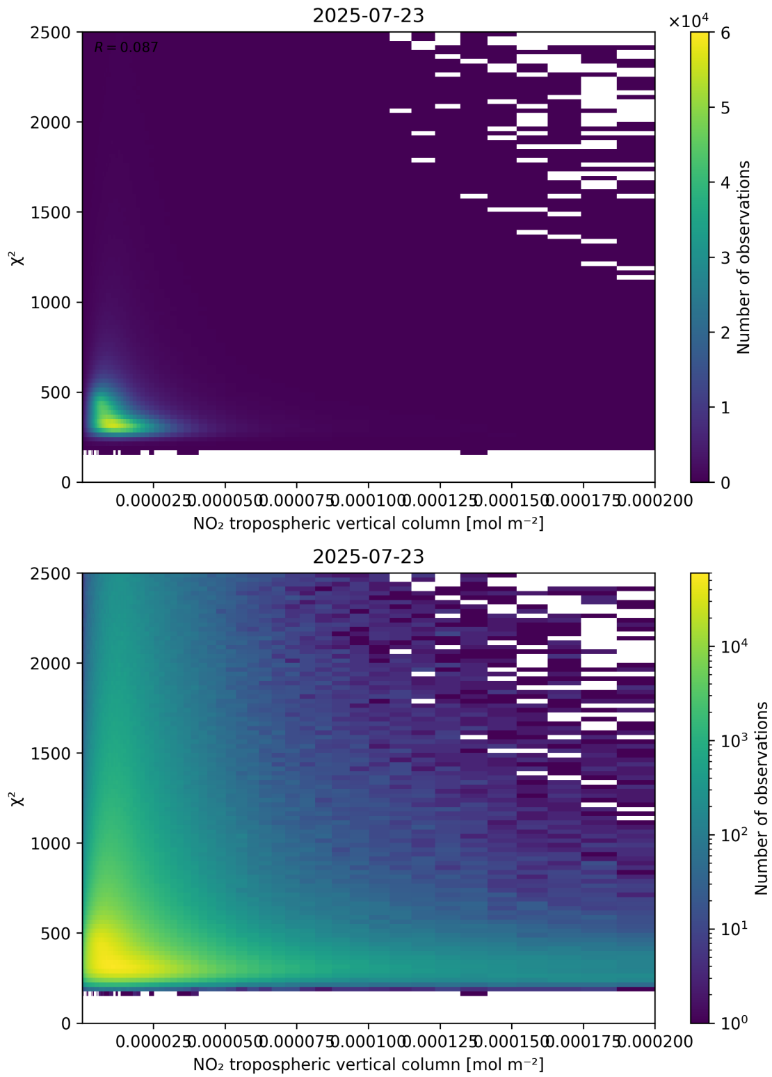
Figure 124: Scatter density plot of “NO 2 tropospheric vertical column” against “ \chi^2 ” for 2025-07-22 to 2025-07-24.
