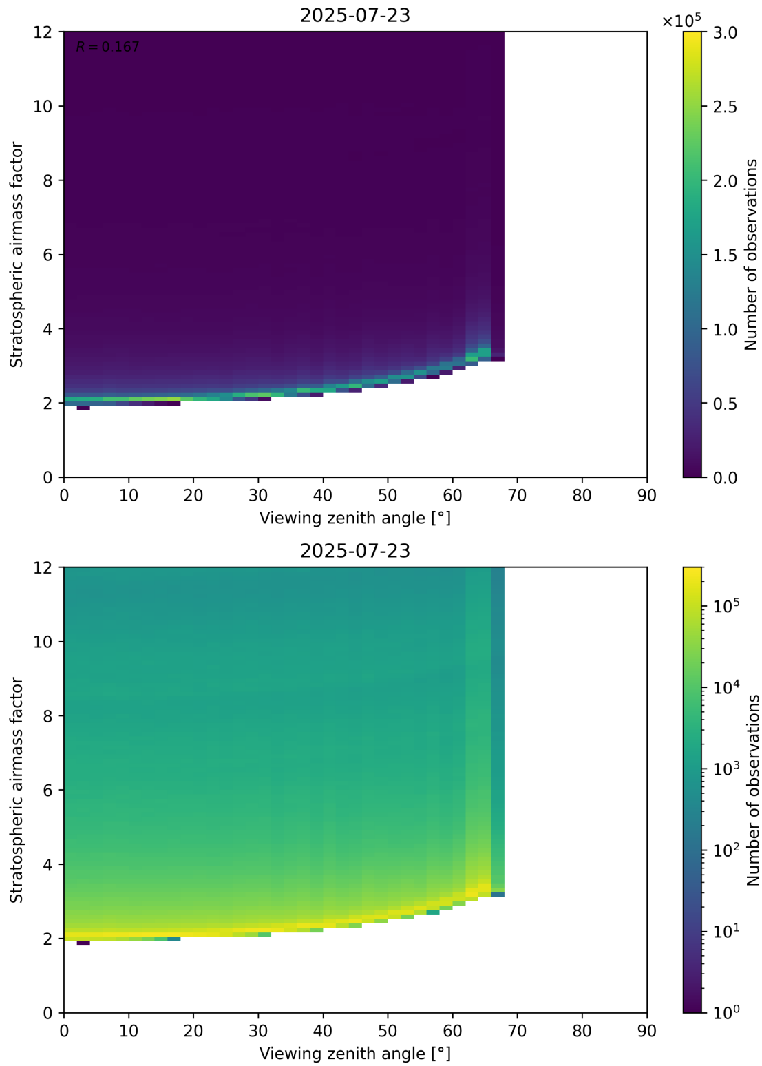
Figure 159: Scatter density plot of “Viewing zenith angle” against “Stratospheric airmass factor” for 2025-07-22 to 2025-07-24.
