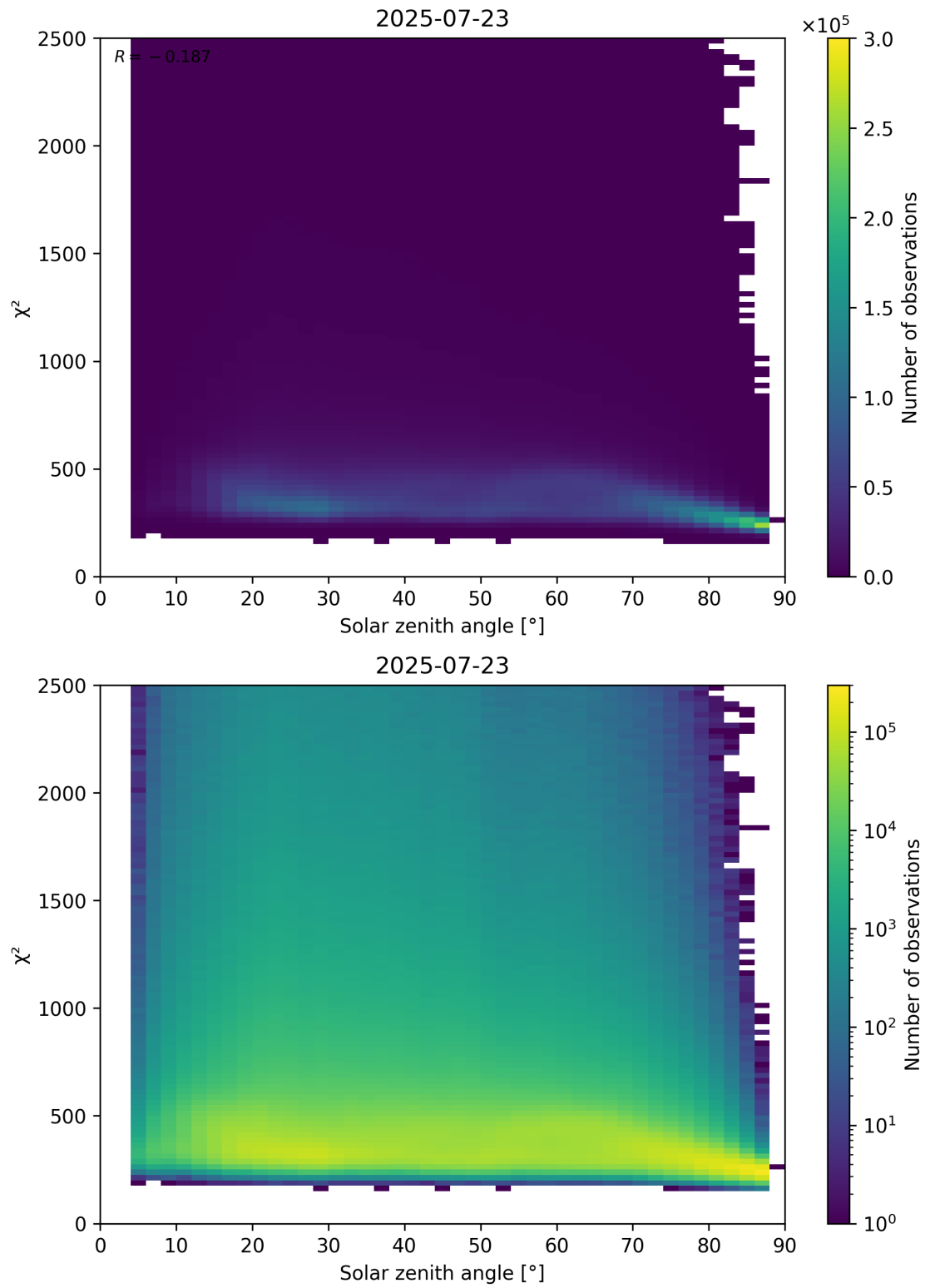
Figure 148: Scatter density plot of “Solar zenith angle” against “ \chi^2 ” for 2025-07-22 to 2025-07-24.
