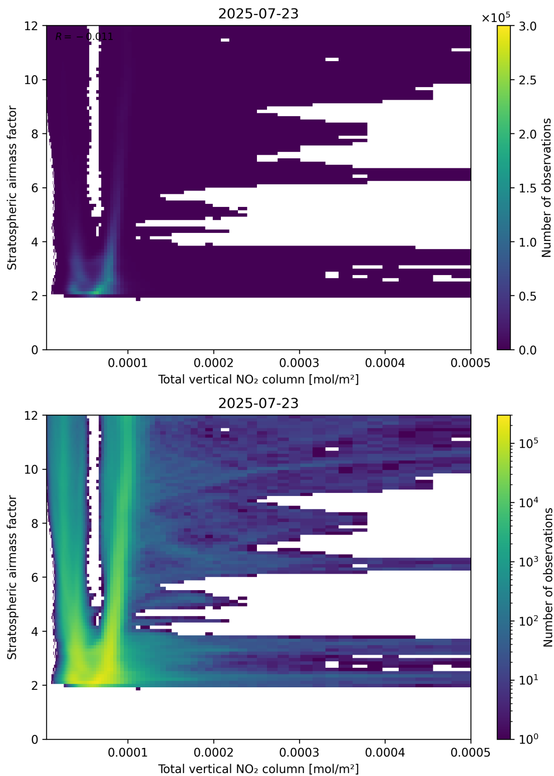
Figure 110: Scatter density plot of “Total vertical NO 2 column” against “Stratospheric air mass factor” for 2025-07-22 to 2025-07-24.
