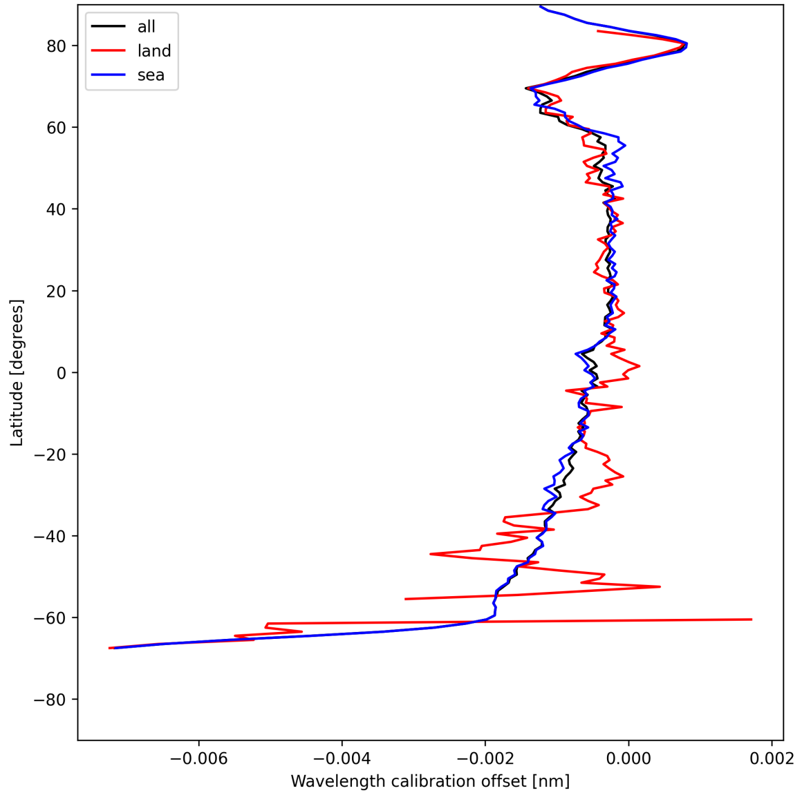
Figure 18: Zonal average of “Wavelength calibration offset” for 2025-07-22 to 2025-07-24.
