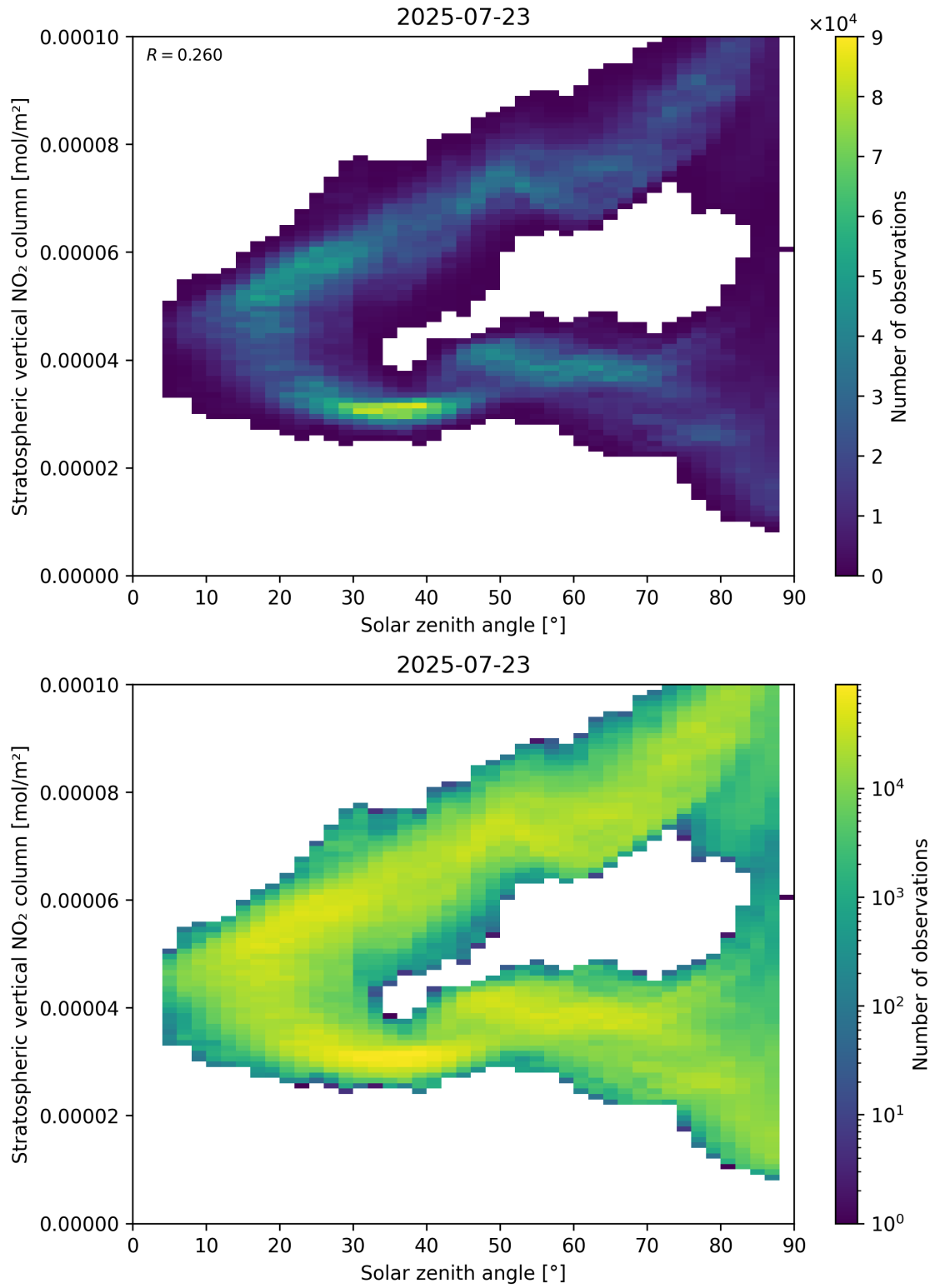
Figure 150: Scatter density plot of “Solar zenith angle” against “Stratospheric vertical NO 2 column” for 2025-07-22 to 2025-07-24.
