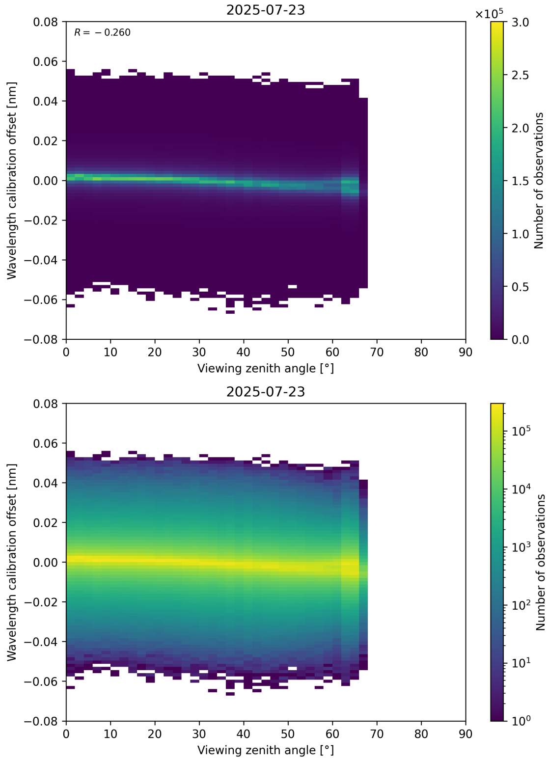
Figure 173: Scatter density plot of “Viewing zenith angle” against “Wavelength calibration offset” for 2025-07-22 to 2025-07-24.
