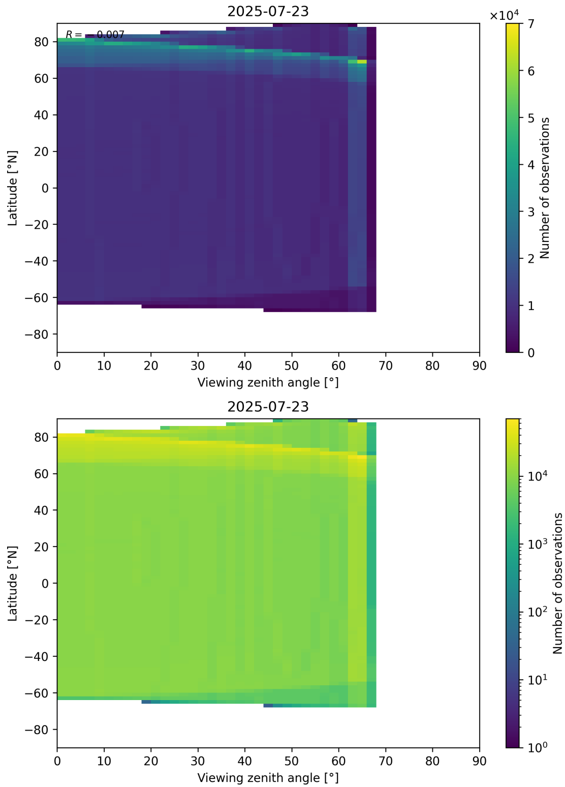
Figure 163: Scatter density plot of “Viewing zenith angle” against “Latitude” for 2025-07-22 to 2025-07-24.
