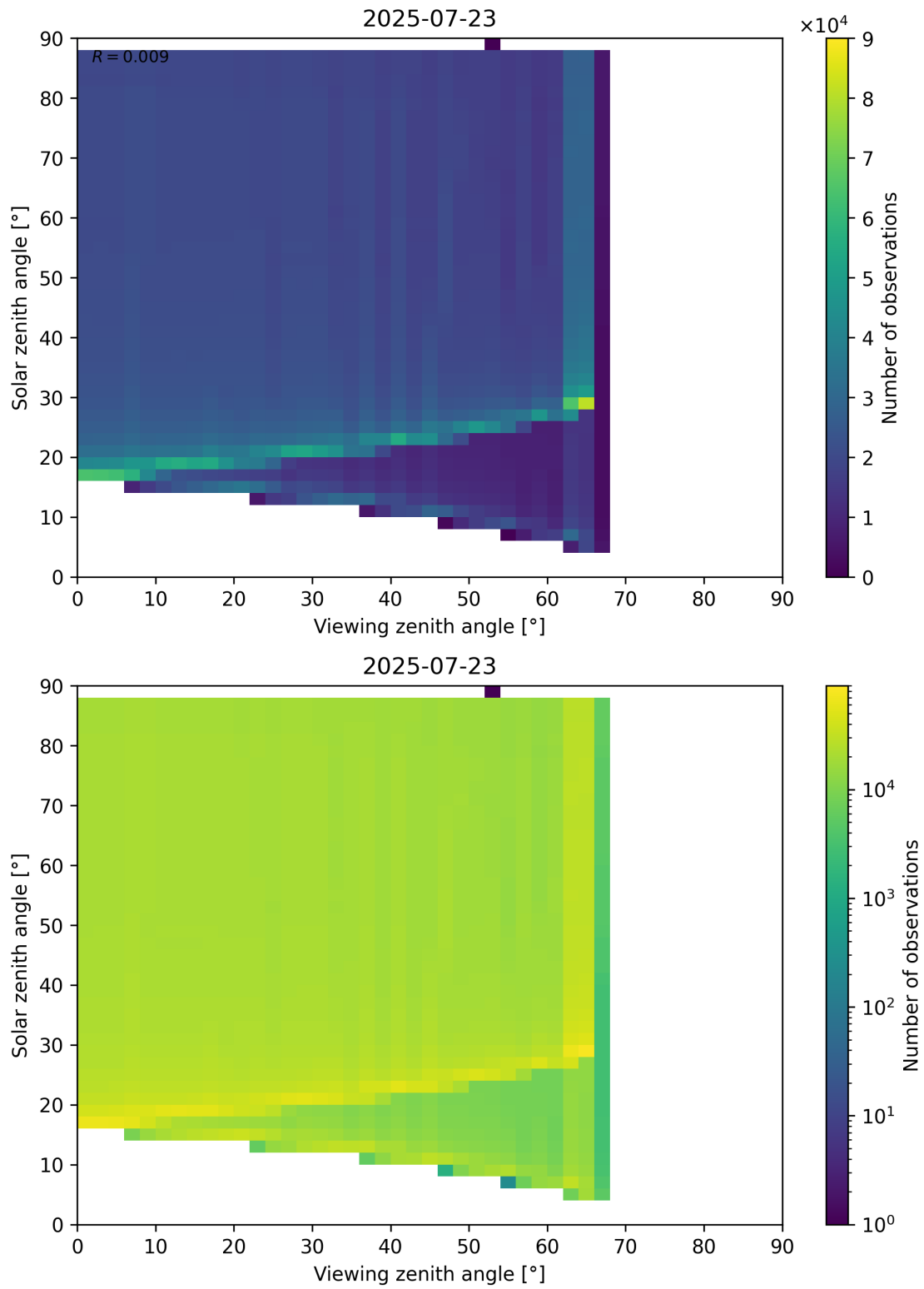
Figure 172: Scatter density plot of “Viewing zenith angle” against “Solar zenith angle” for 2025-07-22 to 2025-07-24.
