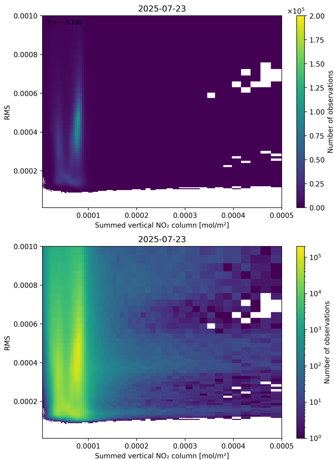
Figure 109: Scatter density plot of “Summed vertical NO 2 column” against “RMS” for 2025-07-22 to 2025-07-24.
