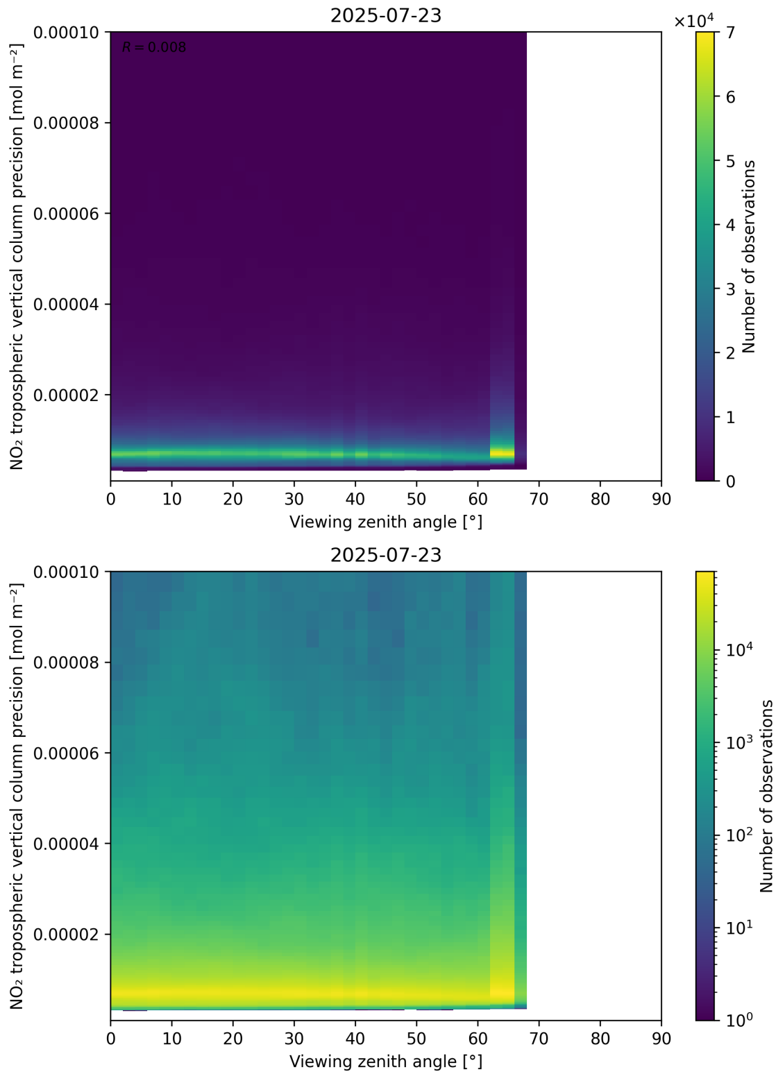
Figure 170: Scatter density plot of “Viewing zenith angle” against “NO 2 tropospheric vertical column precision” for 2025-07-22 to 2025-07-24.
