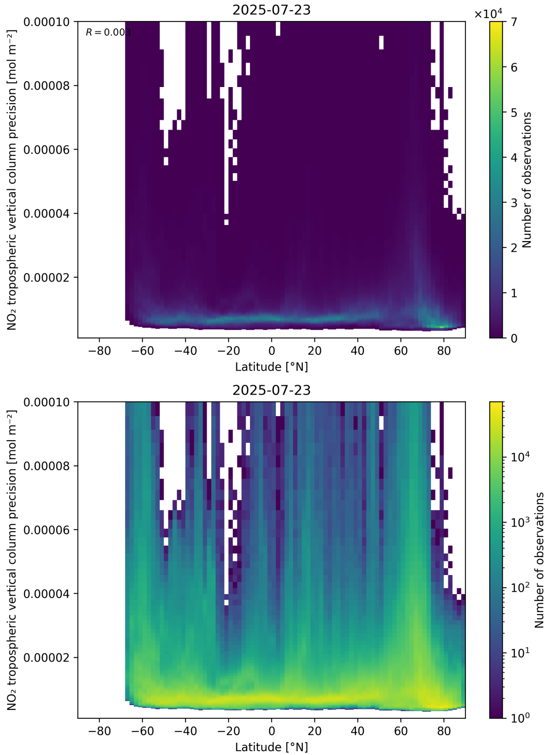
Figure 93: Scatter density plot of “Latitude” against “NO 2 tropospheric vertical column precision” for 2025-07-22 to 2025-07-24.
