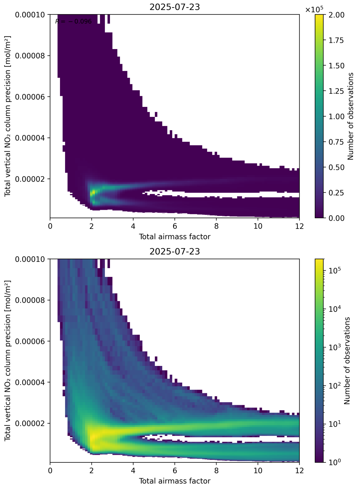
Figure 68: Scatter density plot of “Total airmass factor” against “Total vertical NO 2 column precision” for 2025-07-22 to 2025-07-24.
