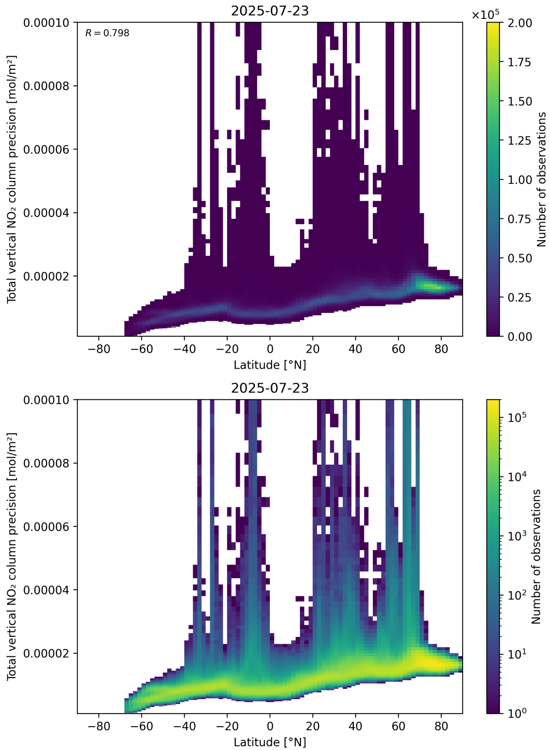
Figure 91: Scatter density plot of “Latitude” against “Total vertical NO 2 column precision” for 2025-07-22 to 2025-07-24.
