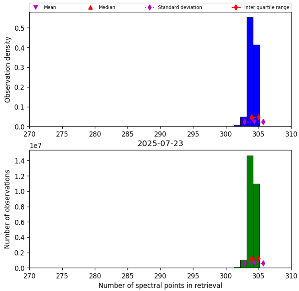
Figure 33: Histogram of “Number of spectral points in retrieval” for 2025-07-22 to 2025-07-24
