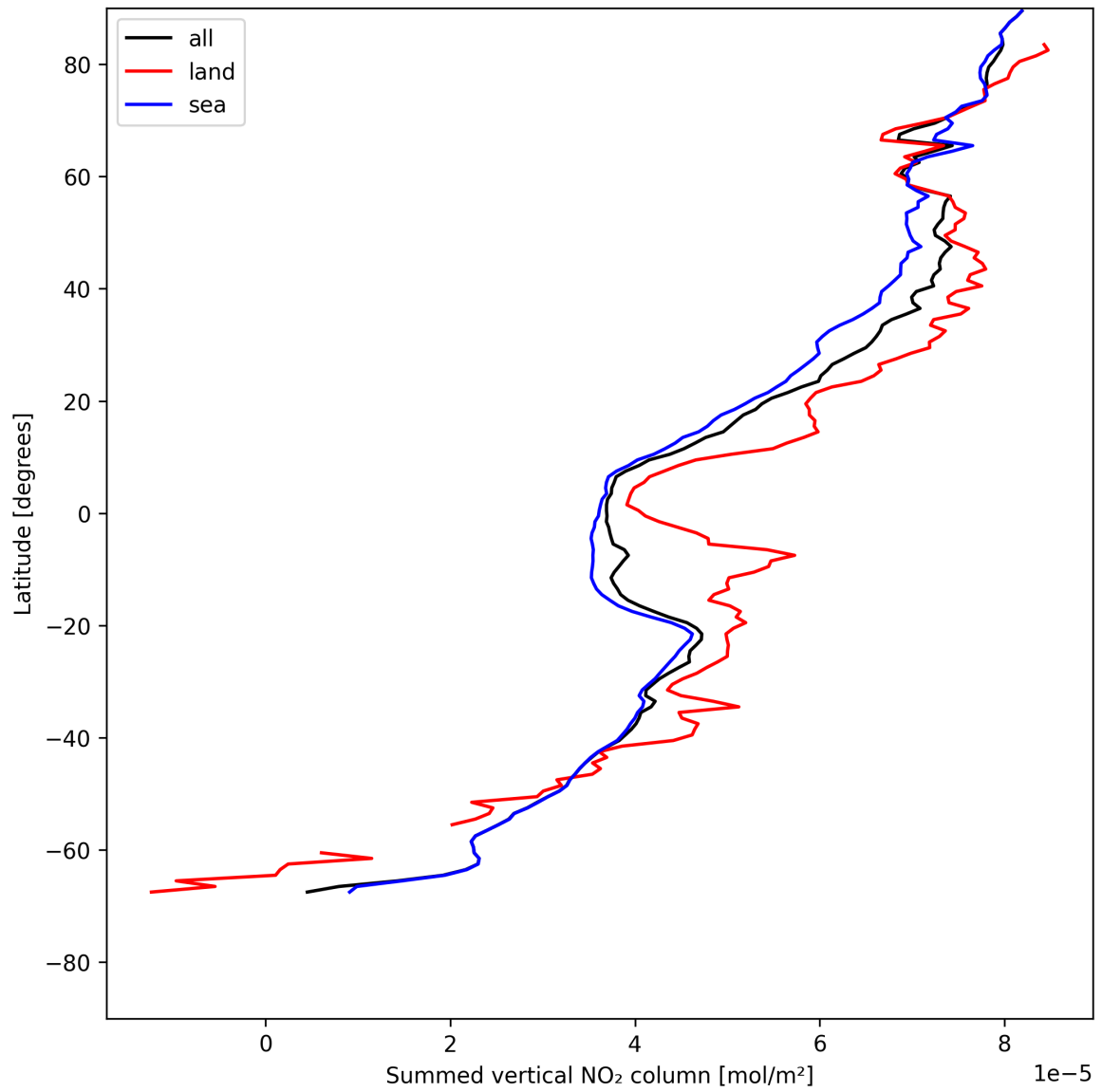
Figure 23: Zonal average of “Summed vertical NO 2 column” for 2025-07-22 to 2025-07-24.
