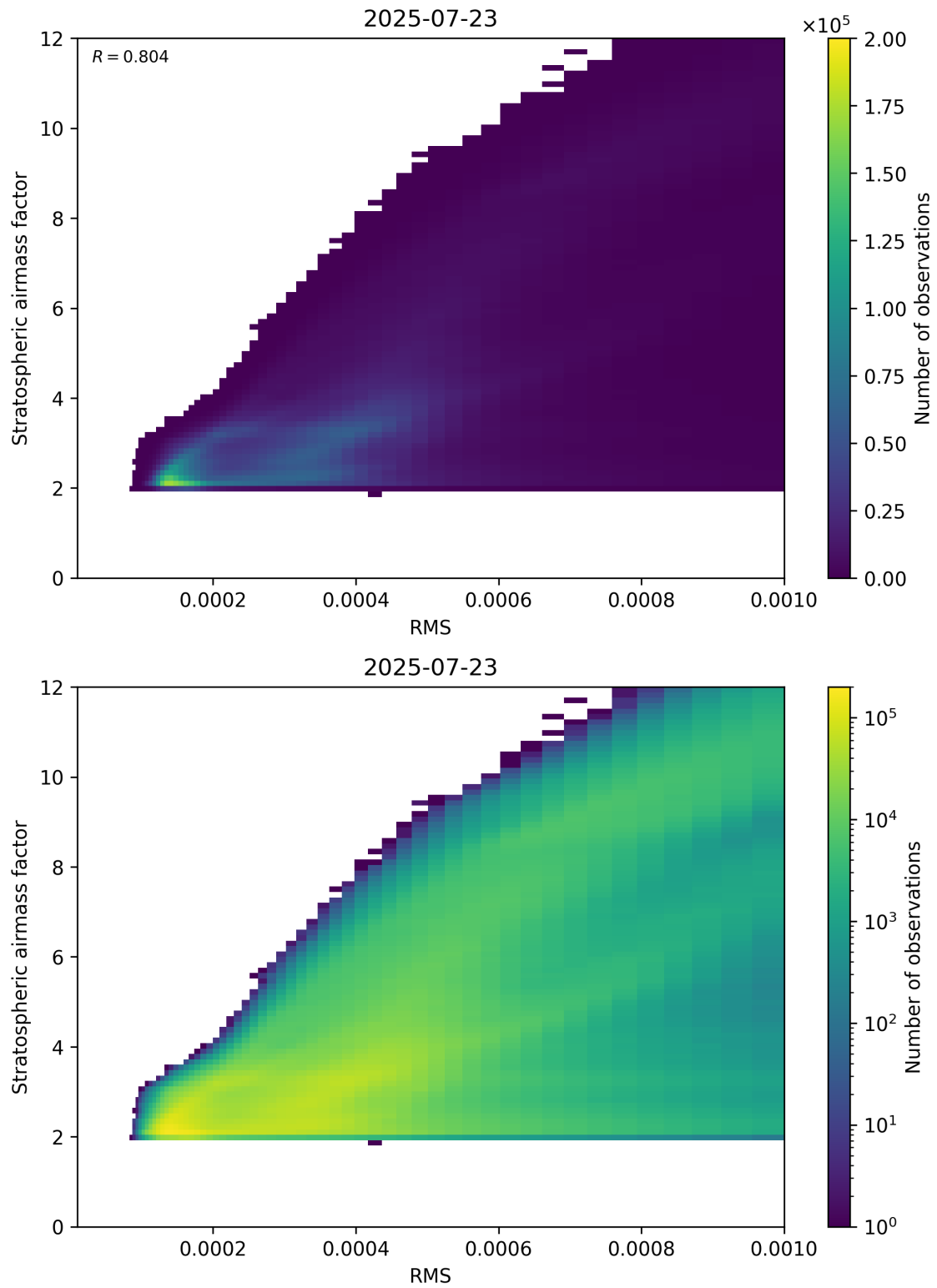
Figure 144: Scatter density plot of “RMS” against “Stratospheric airmass factor” for 2025-07-22 to 2025-07-24.
