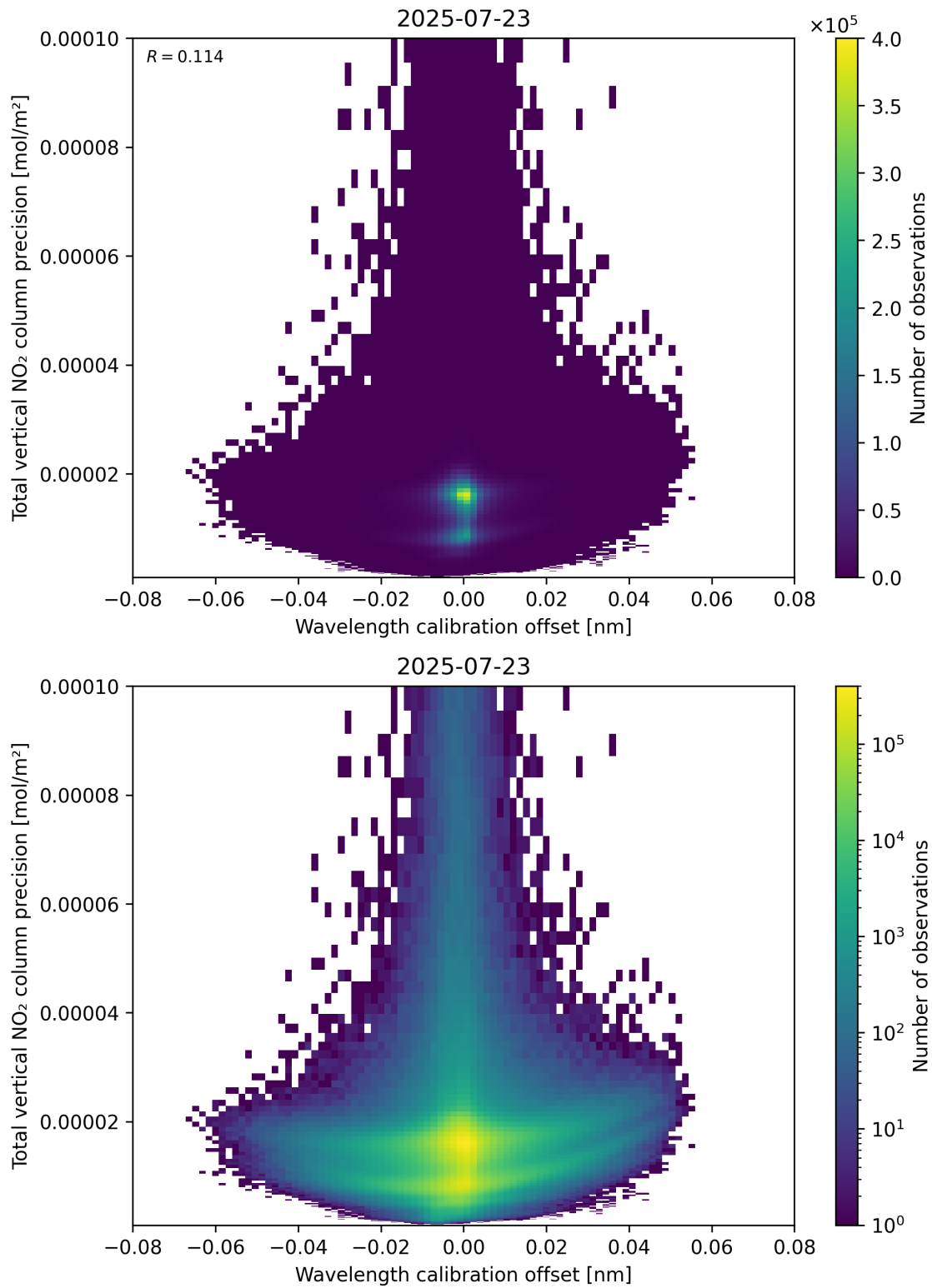
Figure 180: Scatter density plot of “Wavelength calibration offset” against “Total vertical NO 2 column precision” for 2025-07-22 to 2025-07-24.
