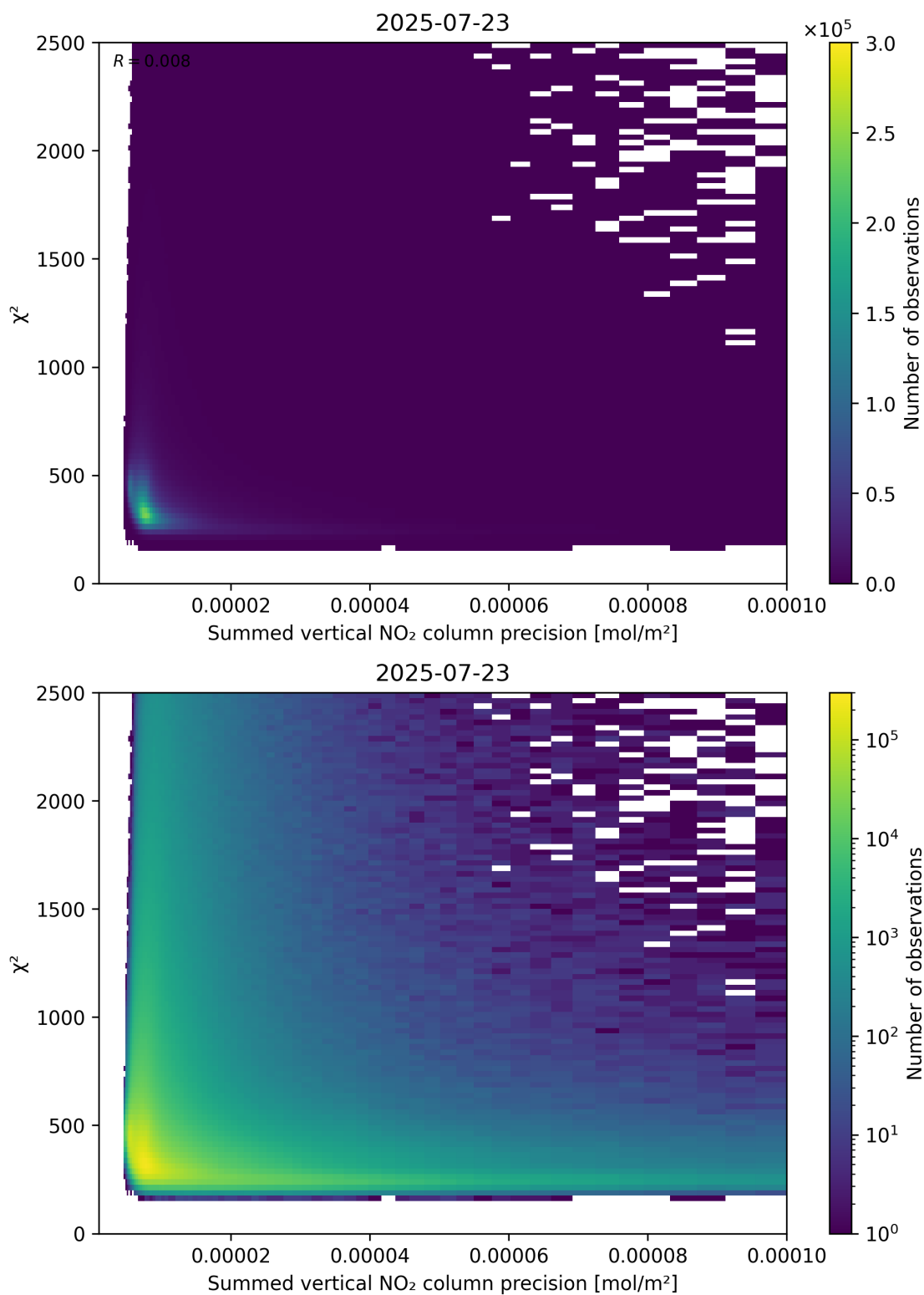
Figure 107: Scatter density plot of “Summed vertical NO 2 column precision” against “ \chi^2 ” for 2025-07-22 to 2025-07-24.
