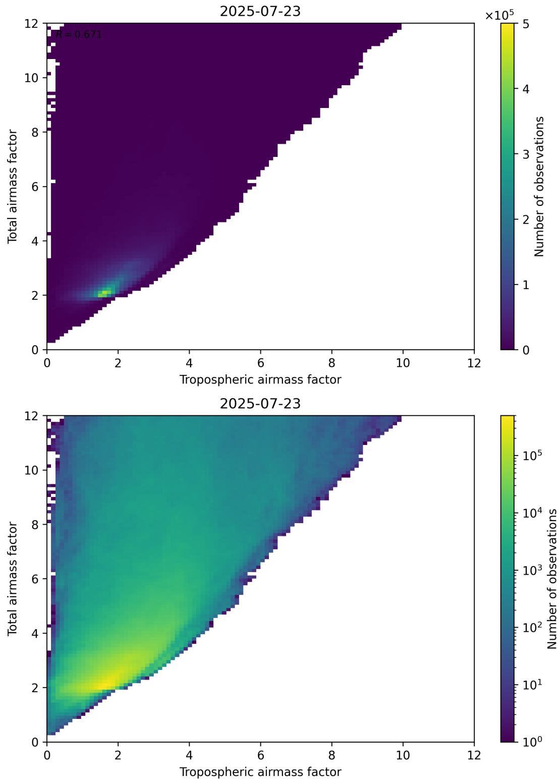
Figure 72: Scatter density plot of “Tropospheric airmass factor” against “Total airmass factor” for 2025-07-22 to 2025-07-24.
