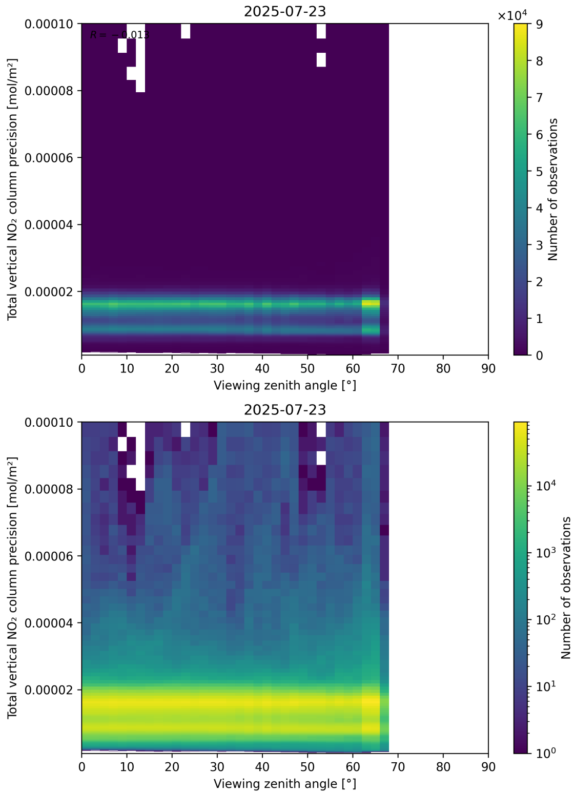
Figure 168: Scatter density plot of “Viewing zenith angle” against “Total vertical NO 2 column precision” for 2025-07-22 to 2025-07-24.
