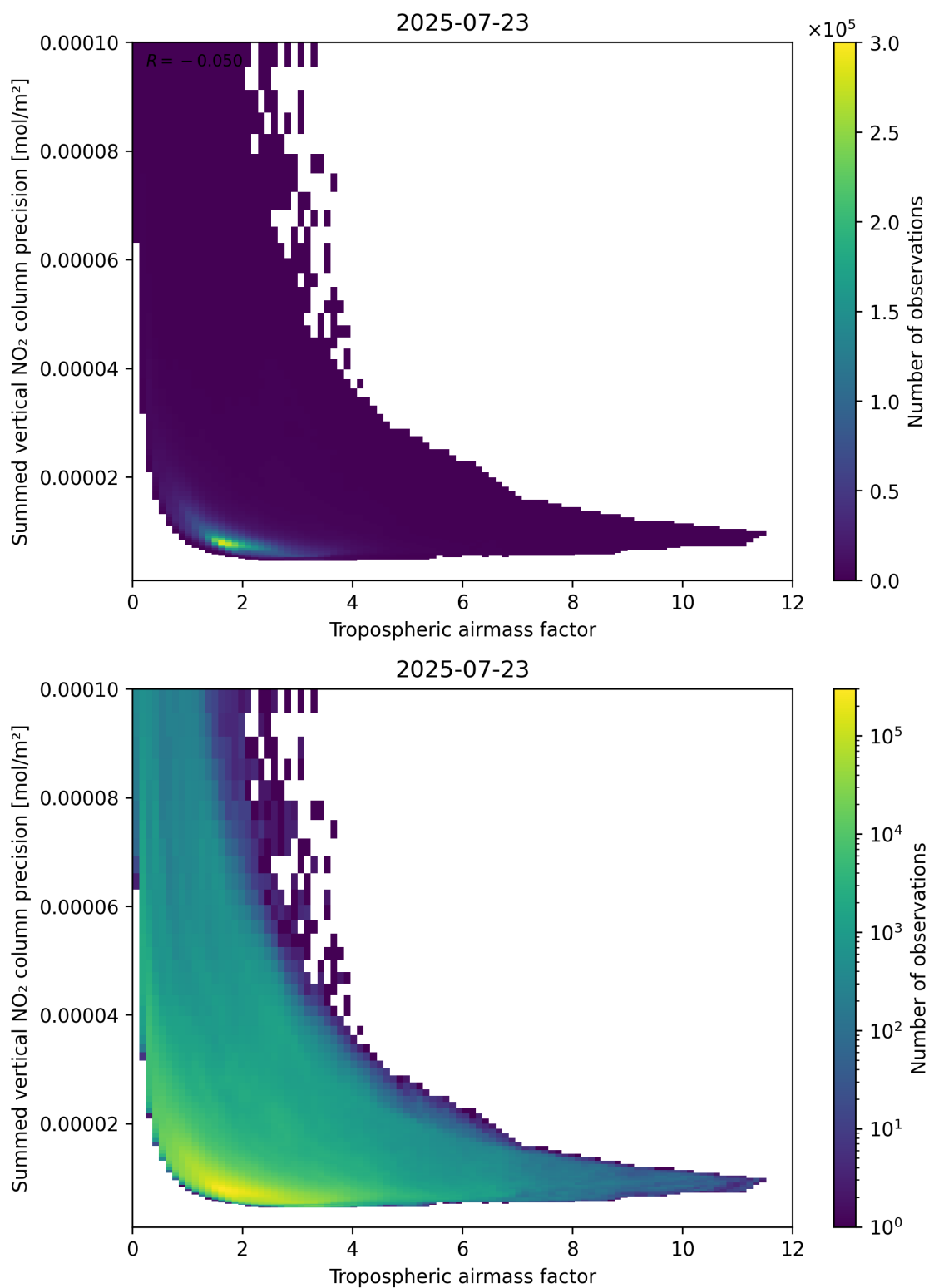
Figure 76: Scatter density plot of “Tropospheric air mass factor” against “Summed vertical NO 2 column precision” for 2025-07-22 to 2025-07-24.
