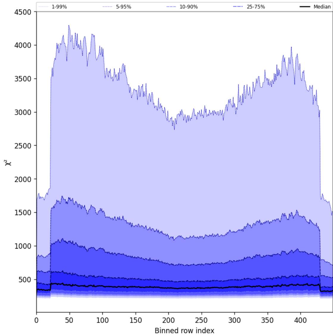
Figure 59: Along track statistics of “ \chi^2 ” for 2025-07-22 to 2025-07-24
