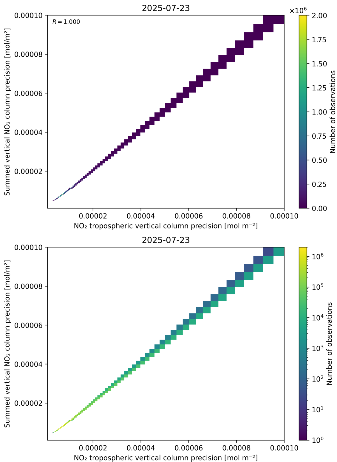
Figure 137: Scatter density plot of “NO 2 tropospheric vertical column precision” against “Summed vertical NO 2 column precision” for 2025-07-22 to 2025-07-24.
