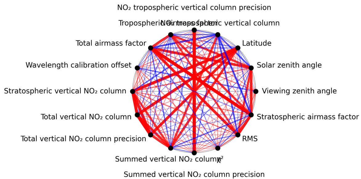
Figure 1: Map of correlation graph for 2025-07-22 to 2025-07-24.
