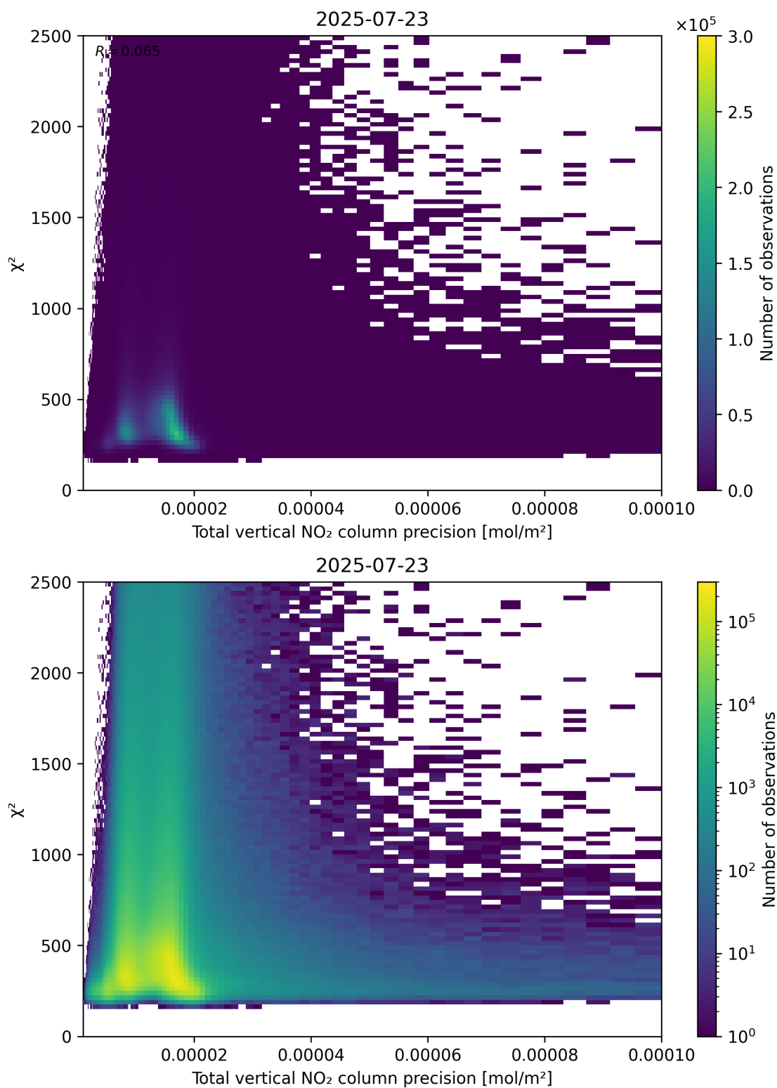
Figure 116: Scatter density plot of “Total vertical NO 2 column precision” against “ \chi^2 ” for 2025-07-22 to 2025-07-24.
