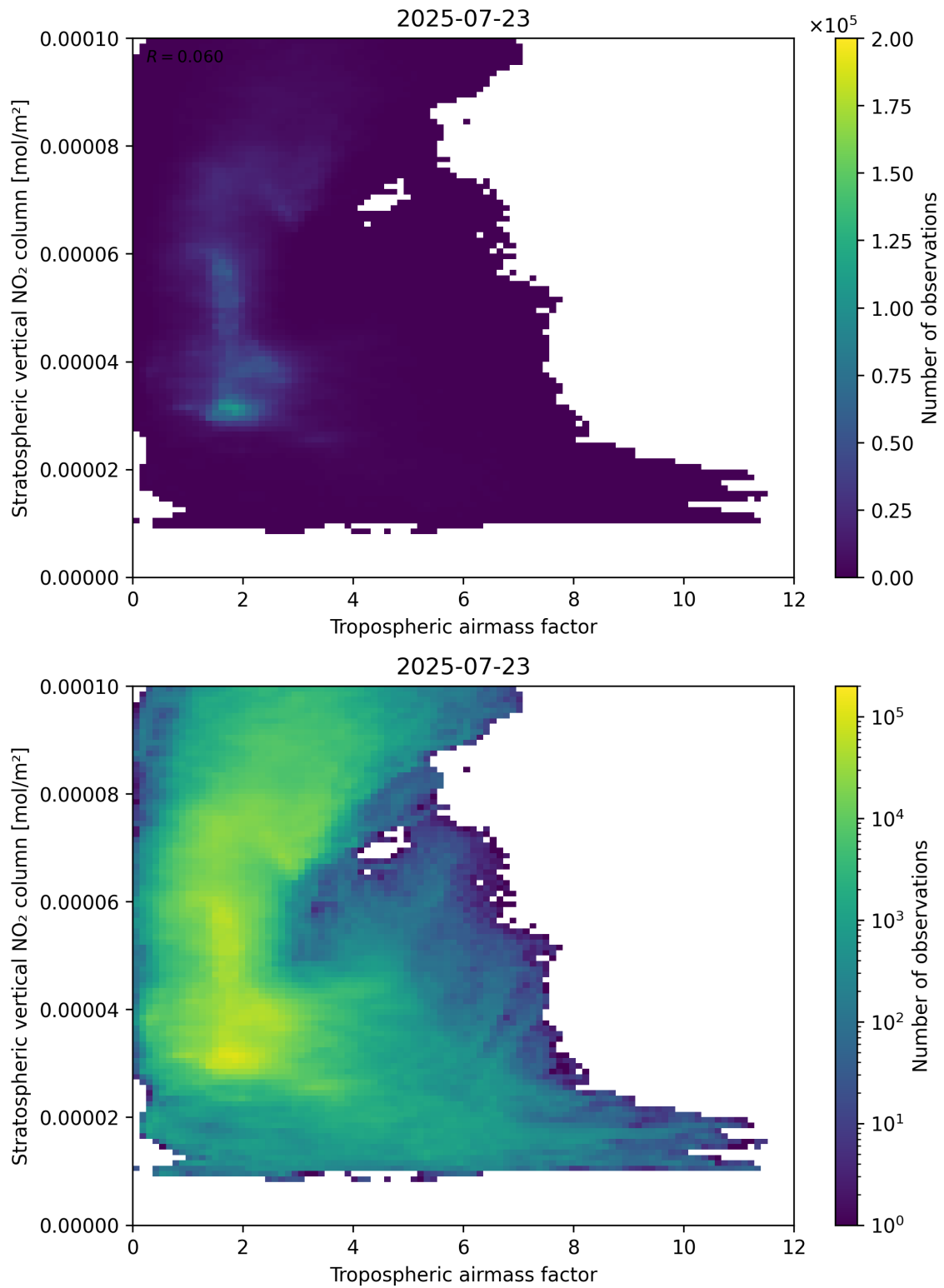
Figure 74: Scatter density plot of “Tropospheric air mass factor” against “Stratospheric vertical NO 2 column” for 2025-07-22 to 2025-07-24.
