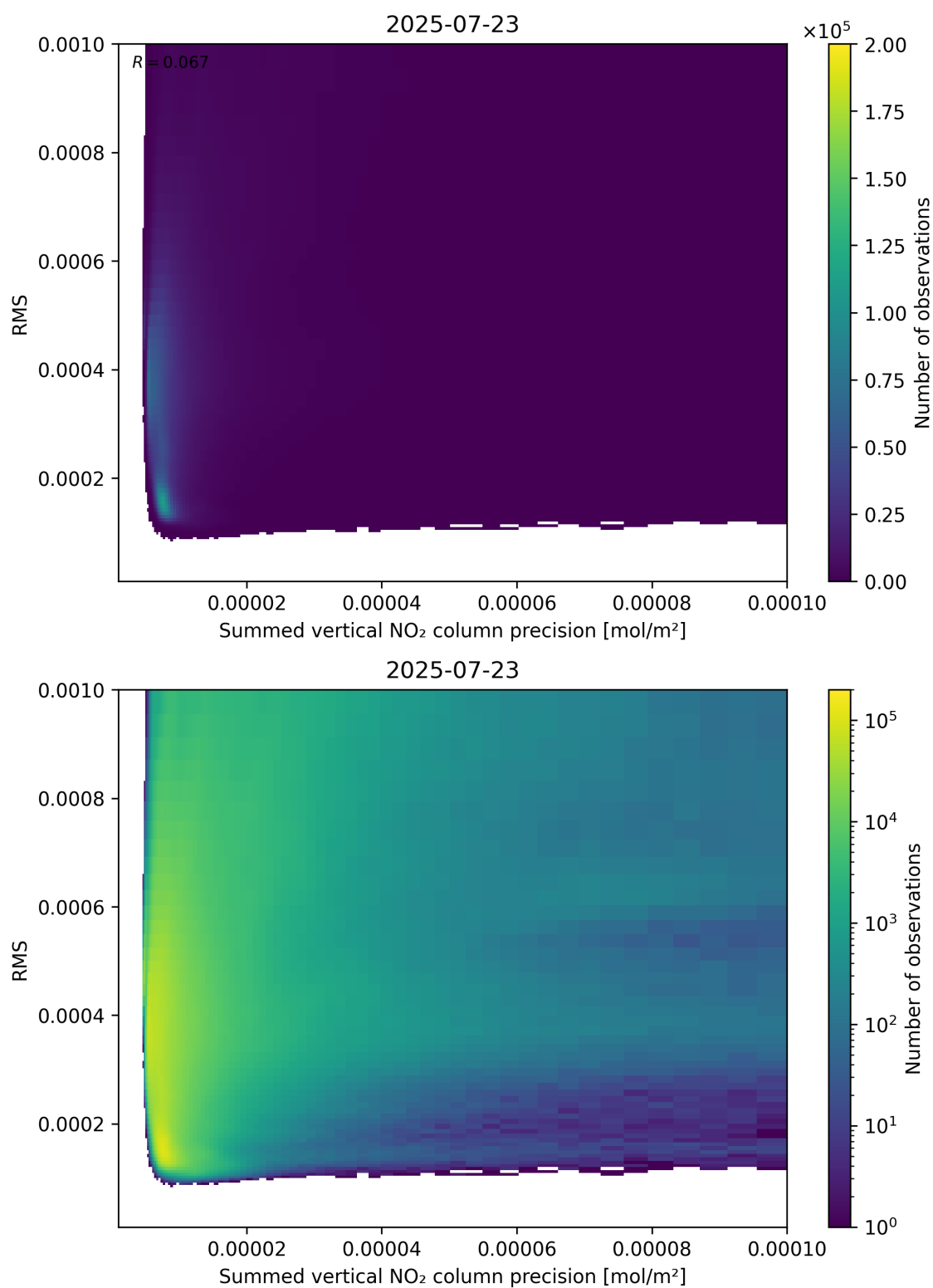
Figure 108: Scatter density plot of “Summed vertical NO 2 column precision” against “RMS” for 2025-07-22 to 2025-07-24.
