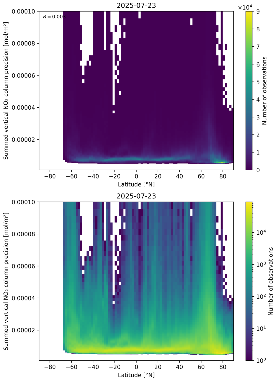
Figure 89: Scatter density plot of “Latitude” against “Summed vertical NO 2 column precision” for 2025-07-22 to 2025-07-24.
