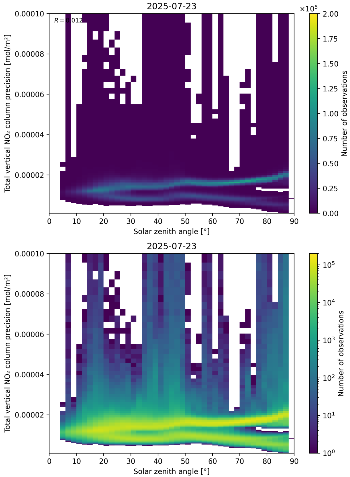
Figure 154: Scatter density plot of “Solar zenith angle” against “Total vertical NO 2 column precision” for 2025-07-22 to 2025-07-24.
