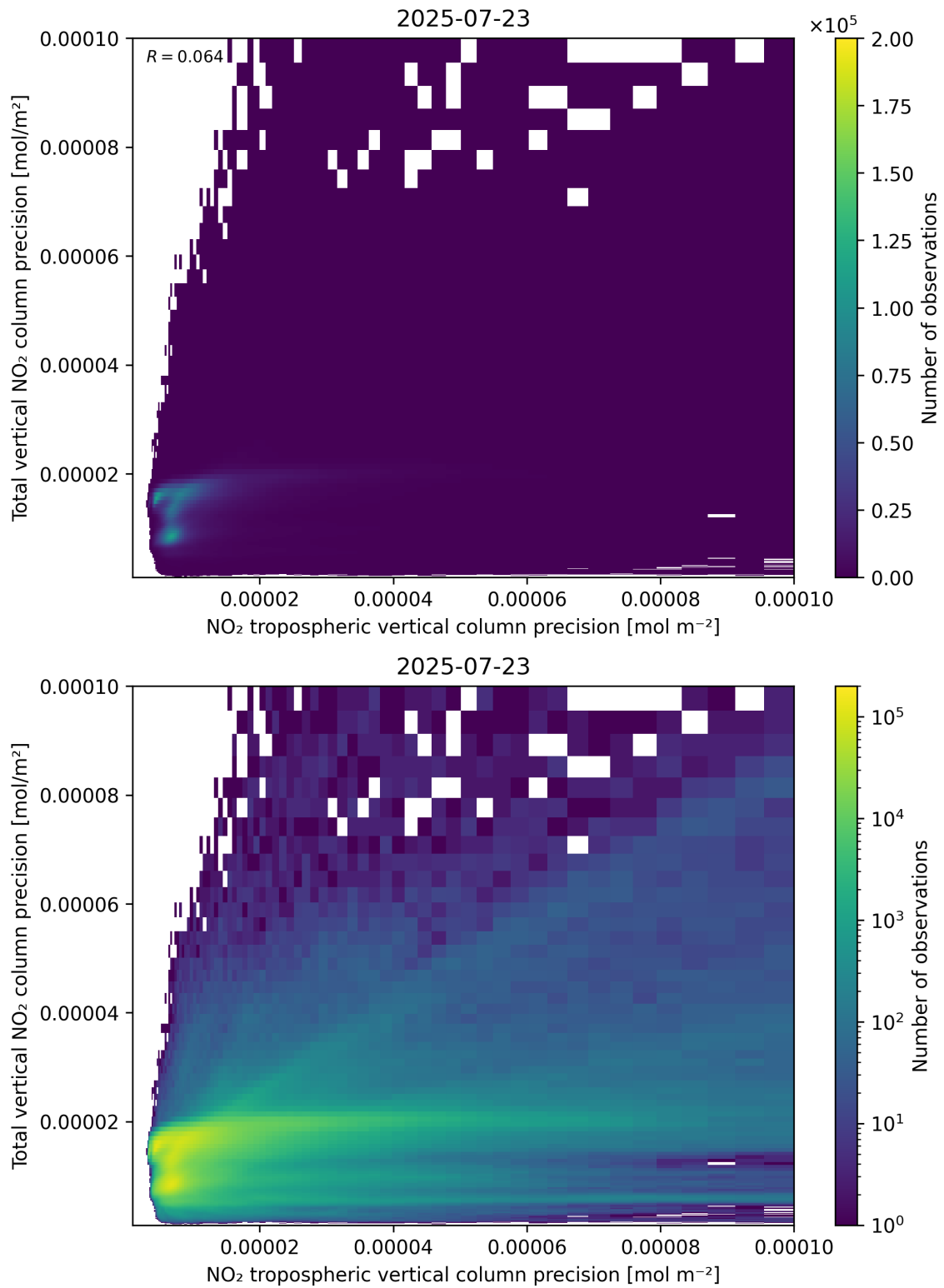
Figure 139: Scatter density plot of “NO 2 tropospheric vertical column precision” against “Total vertical NO 2 column precision” for 2025-07-22 to 2025-07-24.
