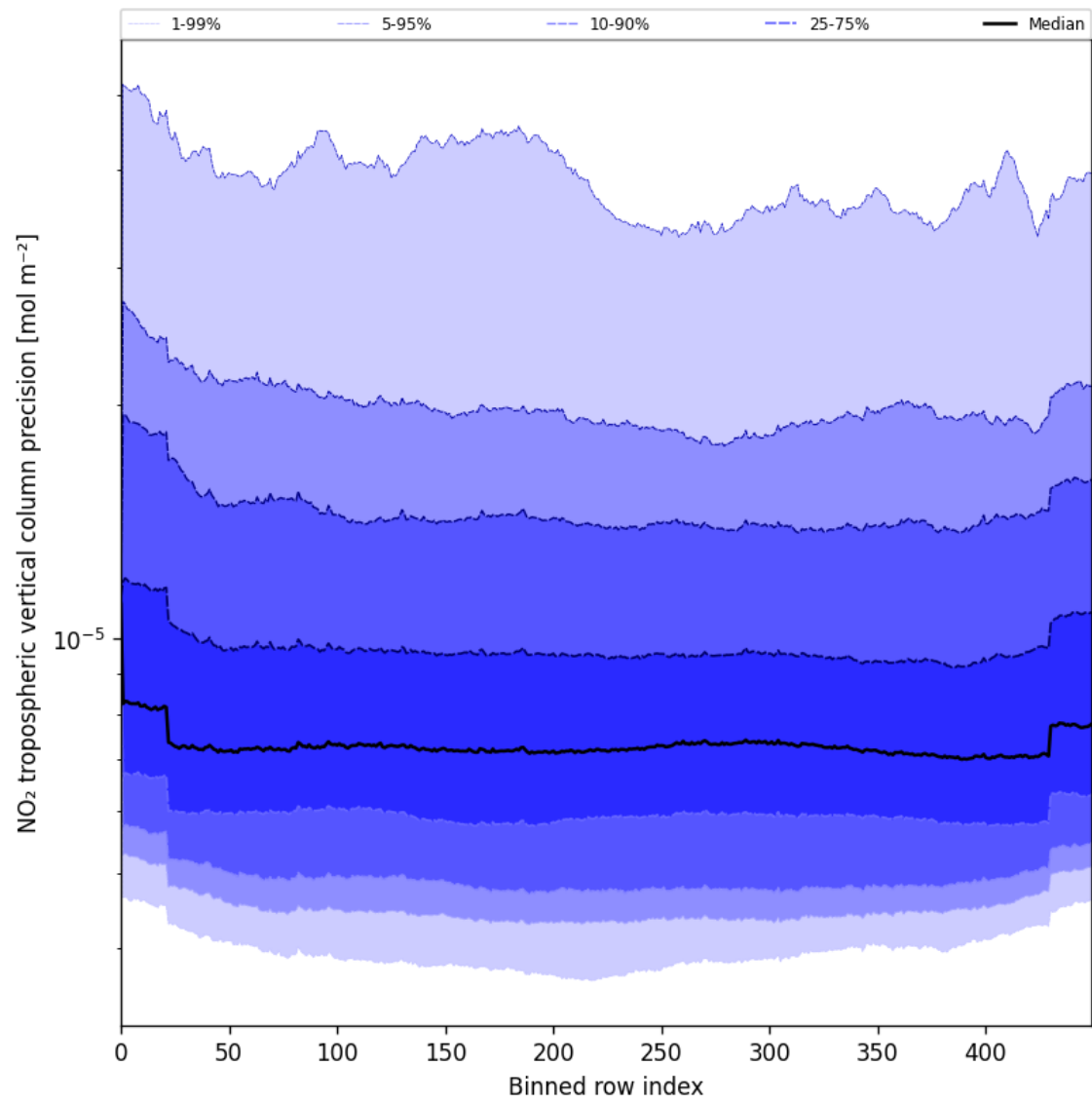
Figure 47: Along track statistics of “NO 2 tropospheric vertical column precision” for 2025-07-22 to 2025-07-24
