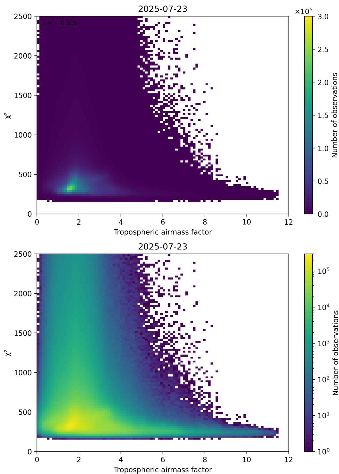
Figure 73: Scatter density plot of “Tropospheric airmass factor” against “ \chi^2 ” for 2025-07-22 to 2025-07-24.
