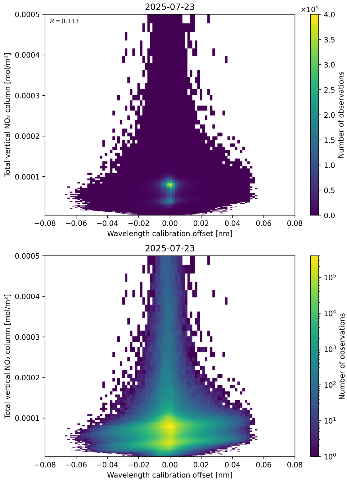
Figure 179: Scatter density plot of “Wavelength calibration offset” against “Total vertical NO 2 column” for 2025-07-22 to 2025-07-24.
