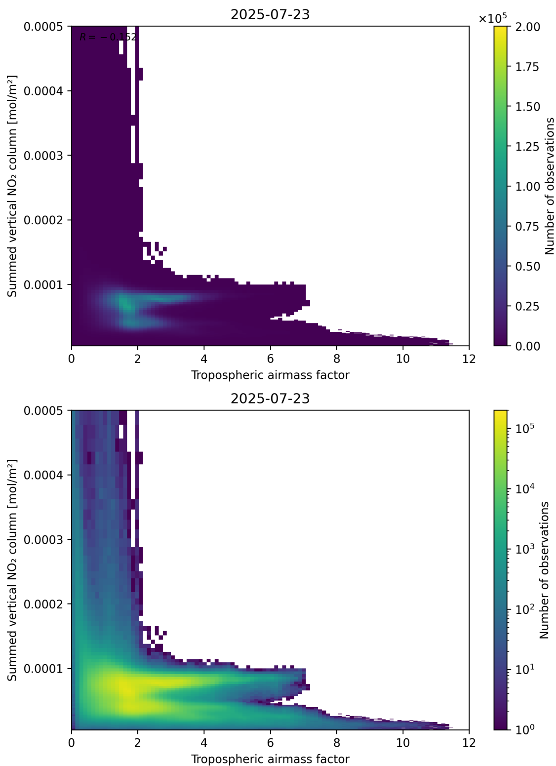
Figure 75: Scatter density plot of “Tropospheric airmass factor” against “Summed vertical NO 2 column” for 2025-07-22 to 2025-07-24.
