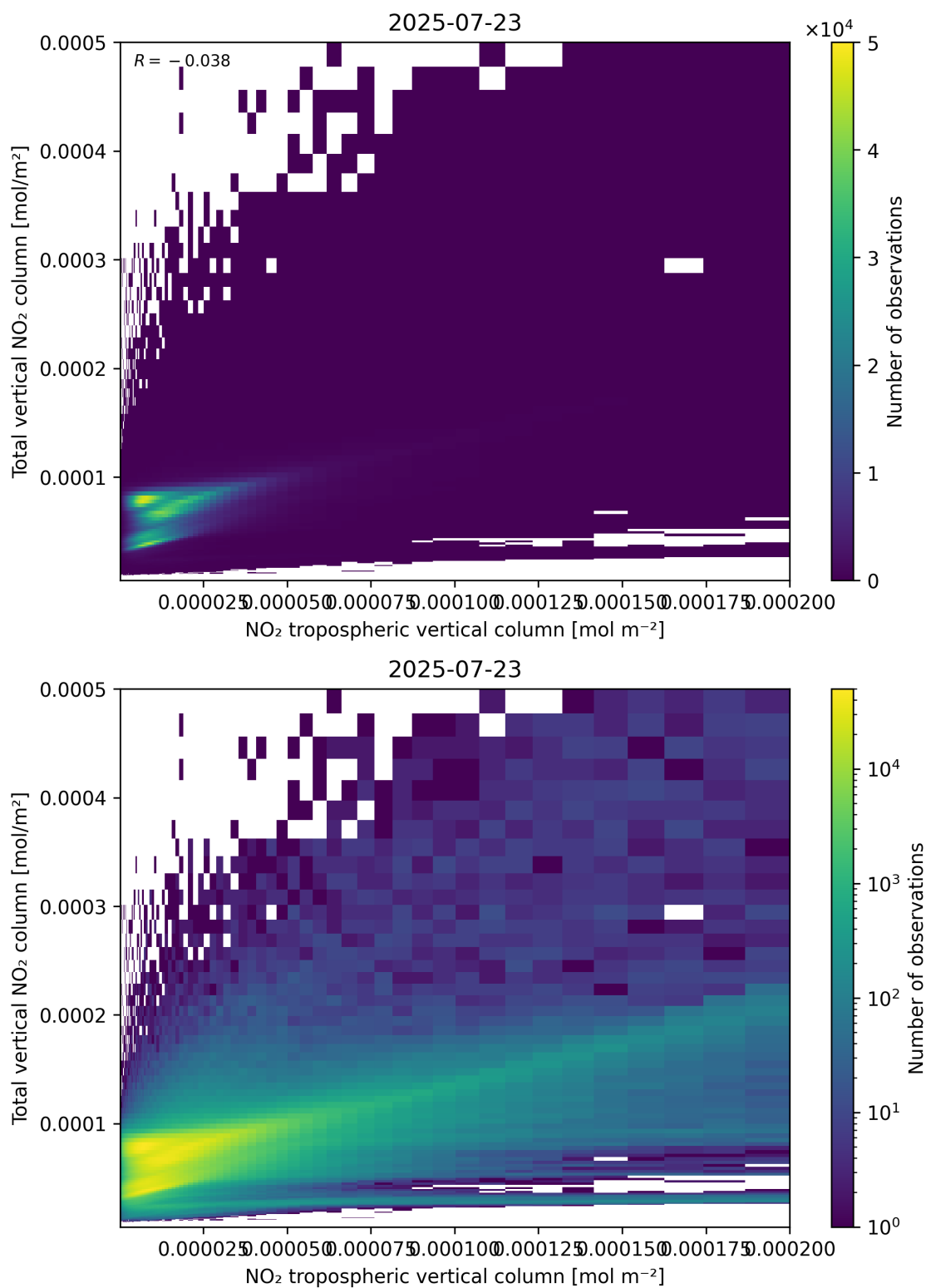
Figure 128: Scatter density plot of “NO 2 tropospheric vertical column” against “Total vertical NO 2 column” for 2025-07-22 to 2025-07-24.
