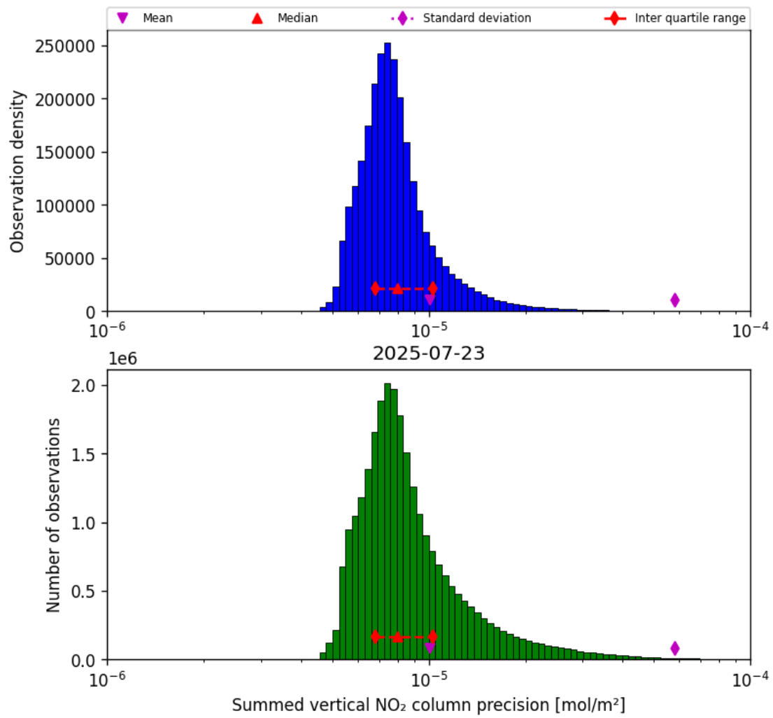
Figure 41: Histogram of “Summed vertical NO 2 column precision” for 2025-07-22 to 2025-07-24
