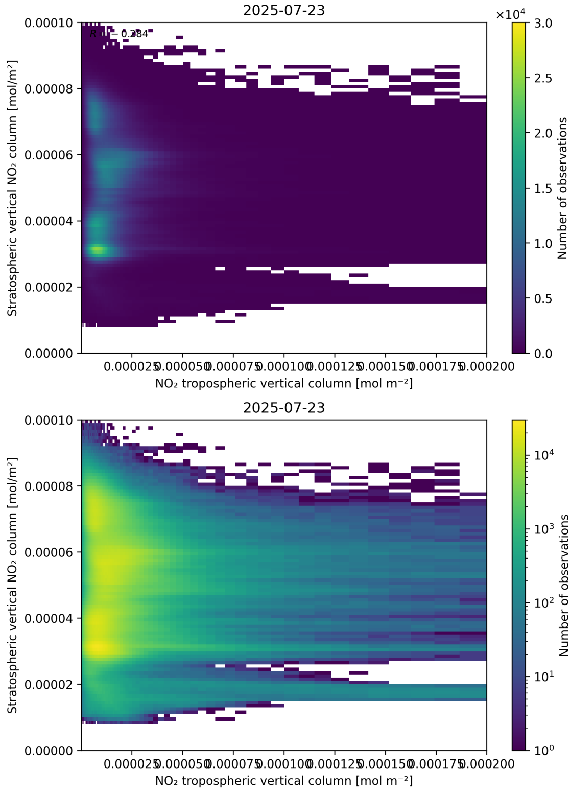
Figure 125: Scatter density plot of “NO 2 tropospheric vertical column” against “Stratospheric vertical NO 2 column” for 2025-07-22 to 2025-07-24.
