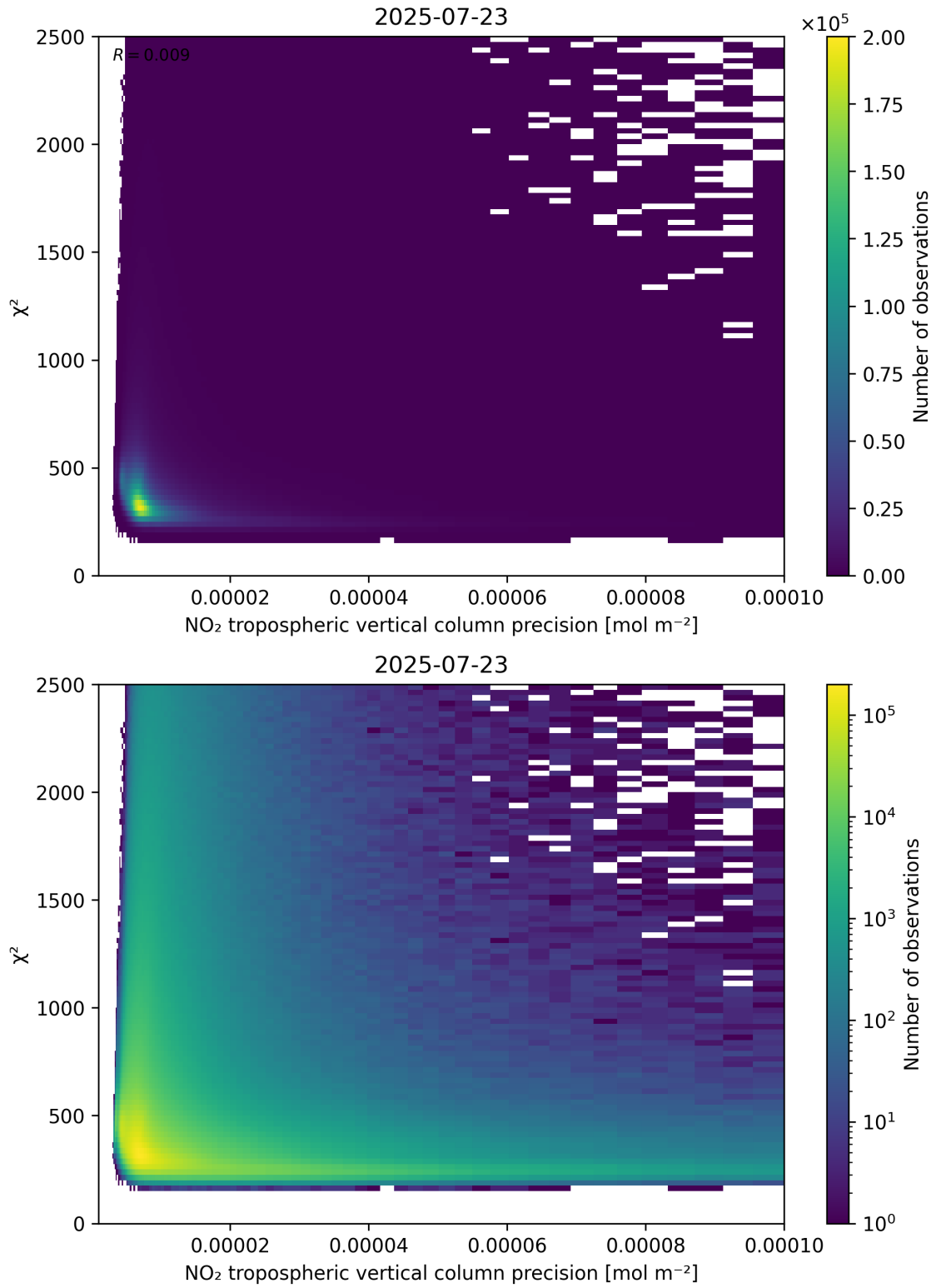
Figure 134: Scatter density plot of “NO 2 tropospheric vertical column precision” against “ \chi^2 ” for 2025-07-22 to 2025-07-24.
