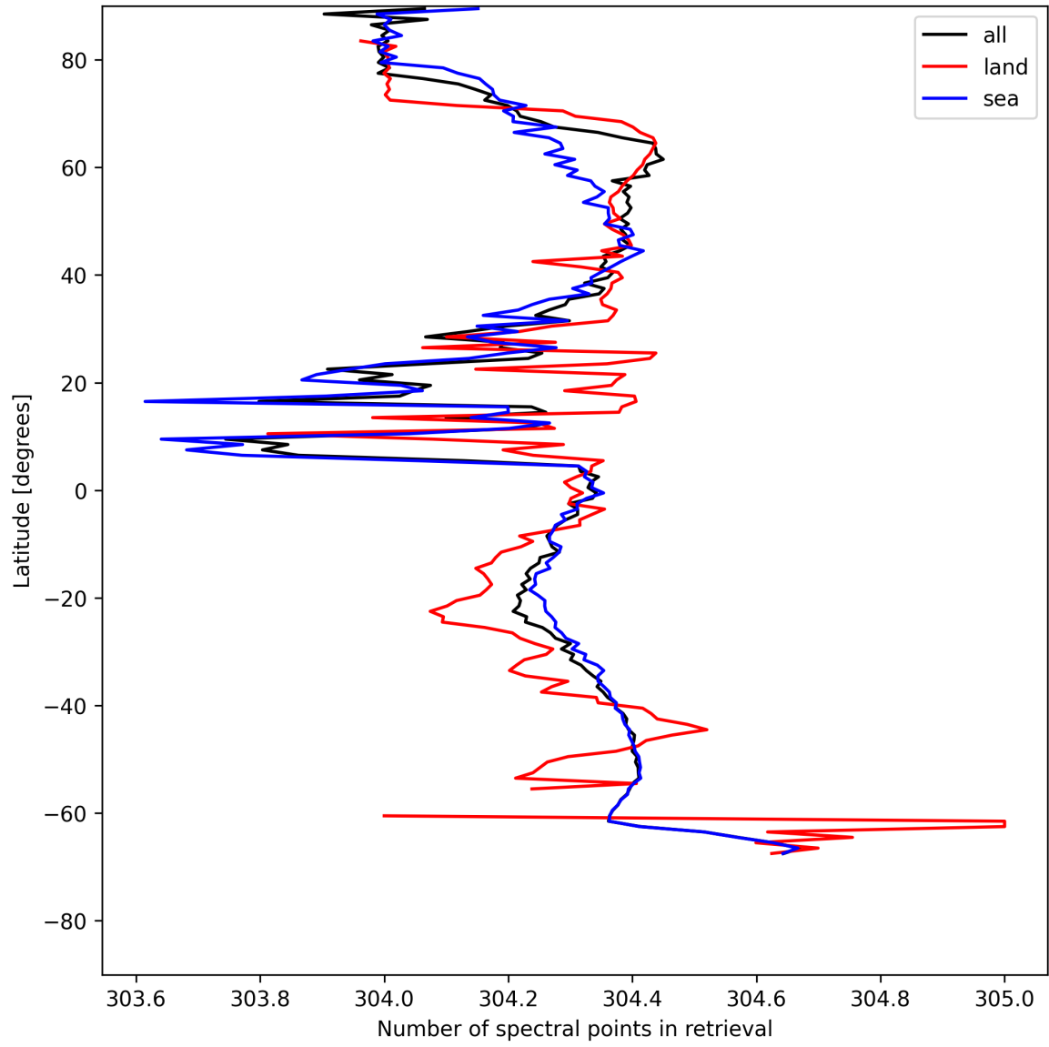
Figure 16: Zonal average of “Number of spectral points in retrieval” for 2025-07-22 to 2025-07-24.
