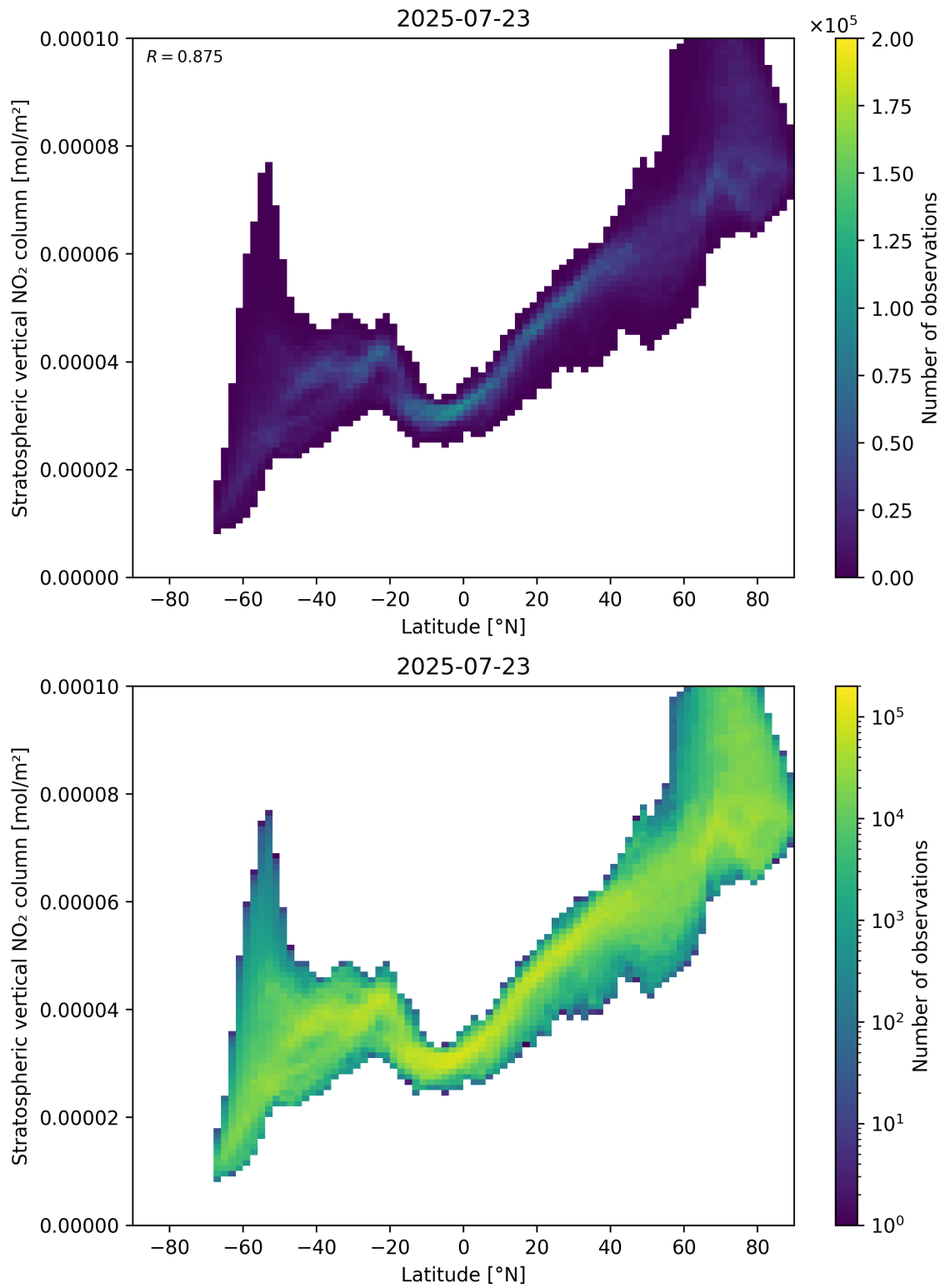
Figure 87: Scatter density plot of “Latitude” against “Stratospheric vertical \text{NO}_2 column” for 2025-07-22 to 2025-07-24.
