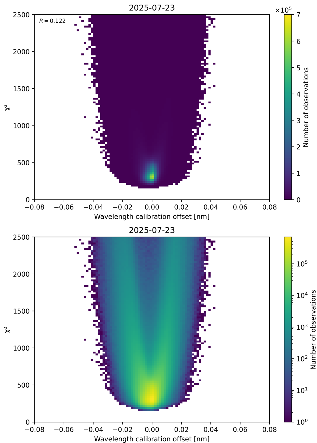
Figure 175: Scatter density plot of “Wavelength calibration offset” against “ \chi^2 ” for 2025-07-22 to 2025-07-24.
