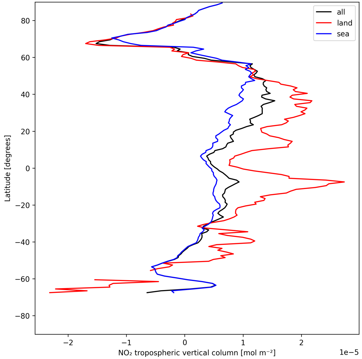
Figure 12: Zonal average of “NO 2 tropospheric vertical column” for 2025-07-22 to 2025-07-24.
