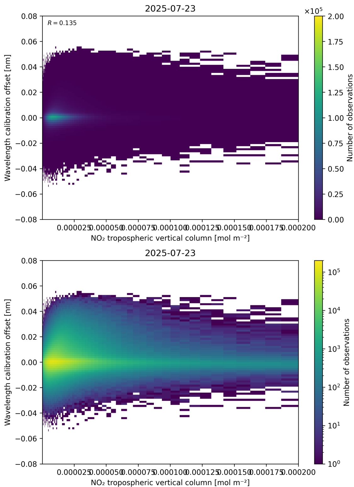
Figure 143: Scatter density plot of “NO 2 tropospheric vertical column” against “Wavelength calibration offset” for 2025-07-22 to 2025-07-24.
