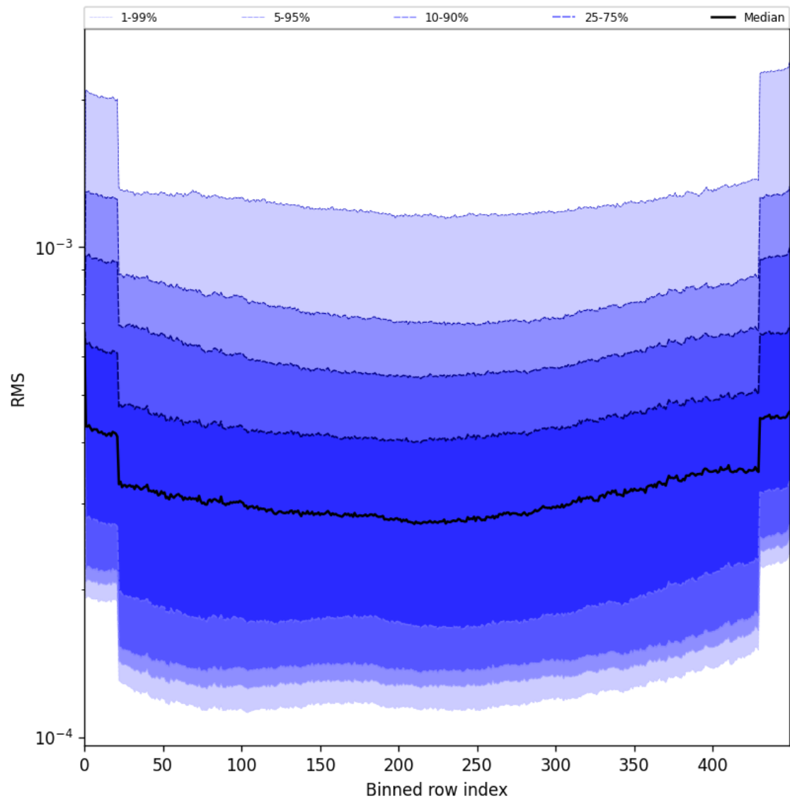
Figure 60: Along track statistics of “RMS” for 2025-07-22 to 2025-07-24
