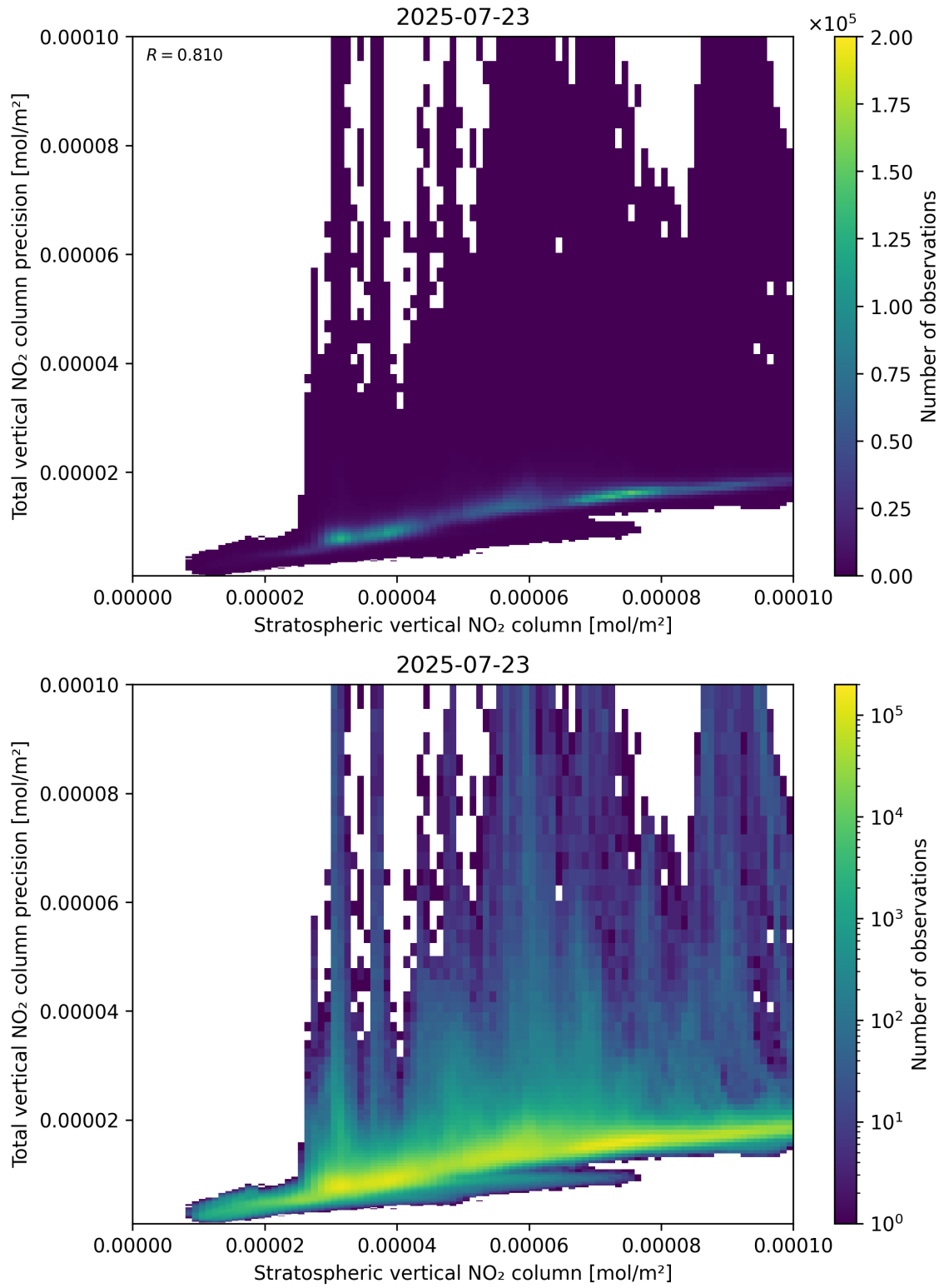
Figure 101: Scatter density plot of “Stratospheric vertical NO 2 column” against “Total vertical NO 2 column precision” for 2025-07-22 to 2025-07-24.
