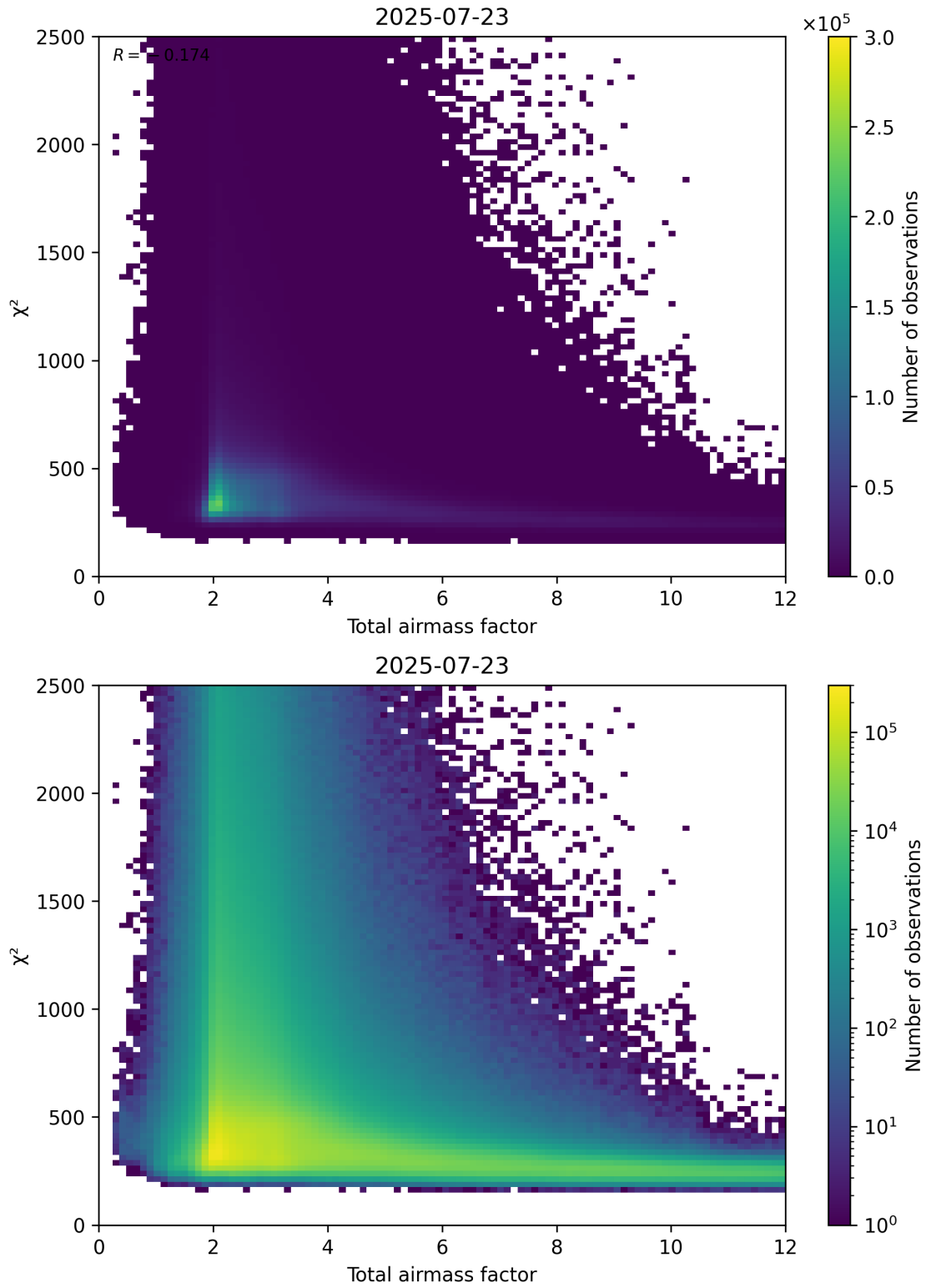
Figure 63: Scatter density plot of “Total airmass factor” against “ \chi^2 ” for 2025-07-22 to 2025-07-24.
