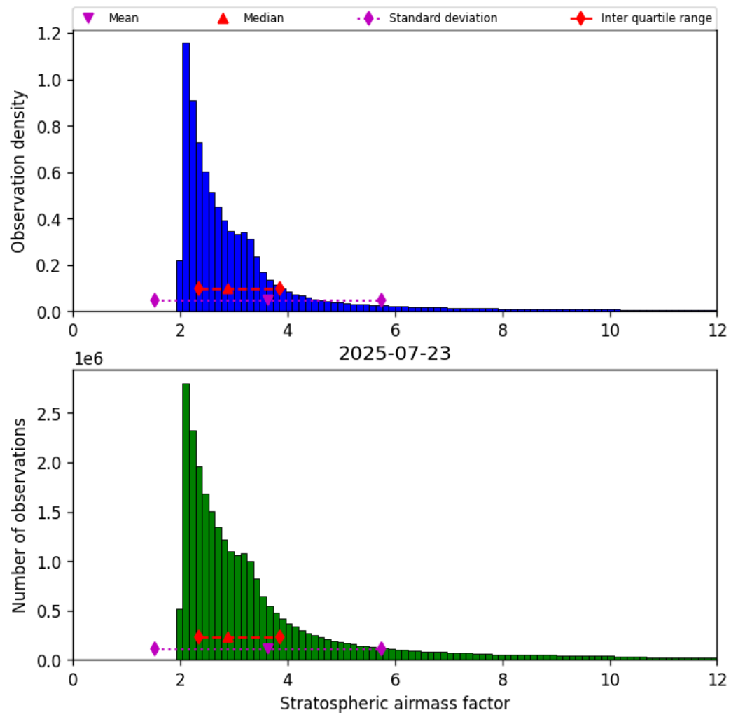
Figure 44: Histogram of “Stratospheric airmass factor” for 2025-07-22 to 2025-07-24
