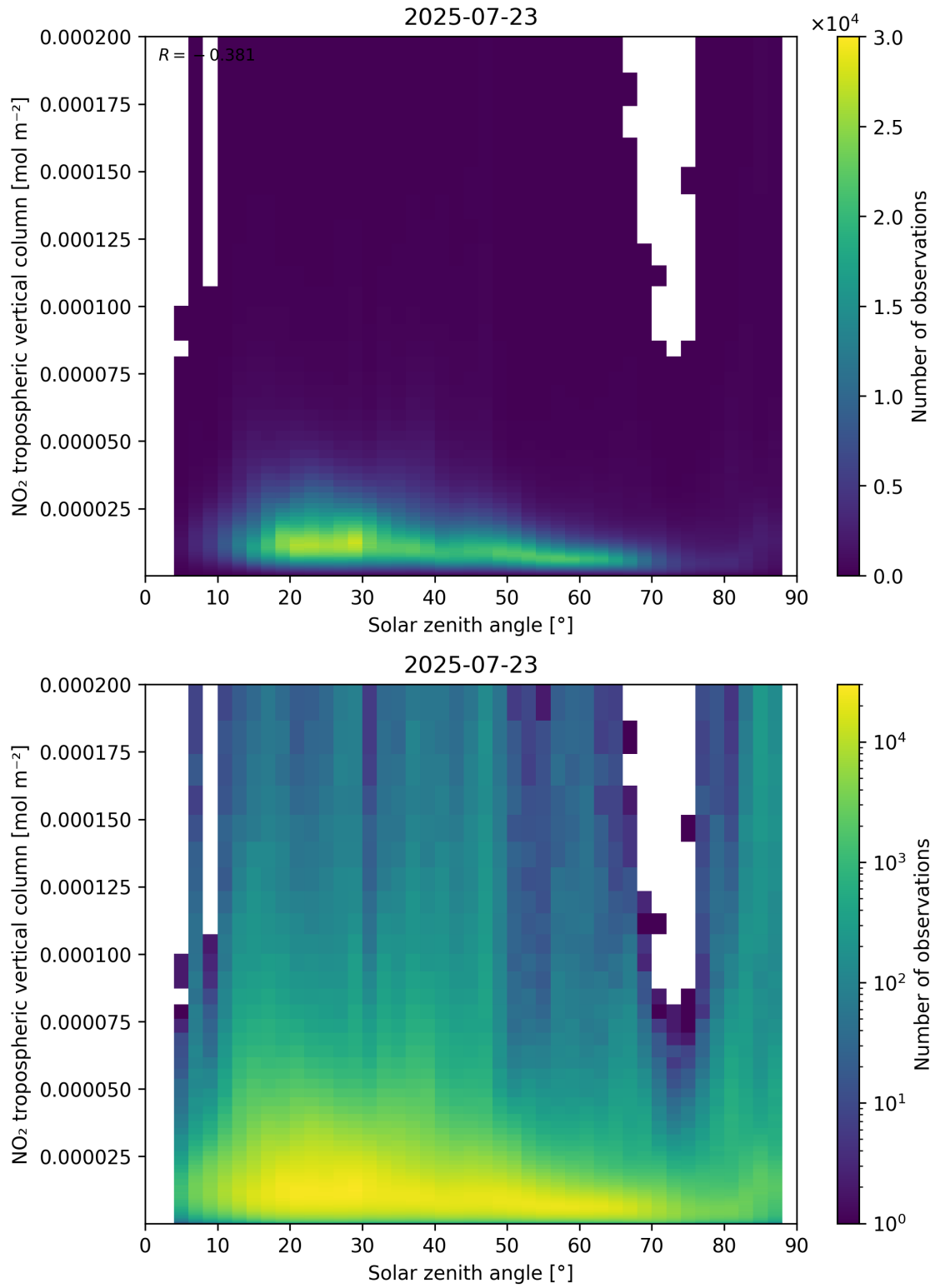
Figure 155: Scatter density plot of “Solar zenith angle” against “NO 2 tropospheric vertical column” for 2025-07-22 to 2025-07-24.
