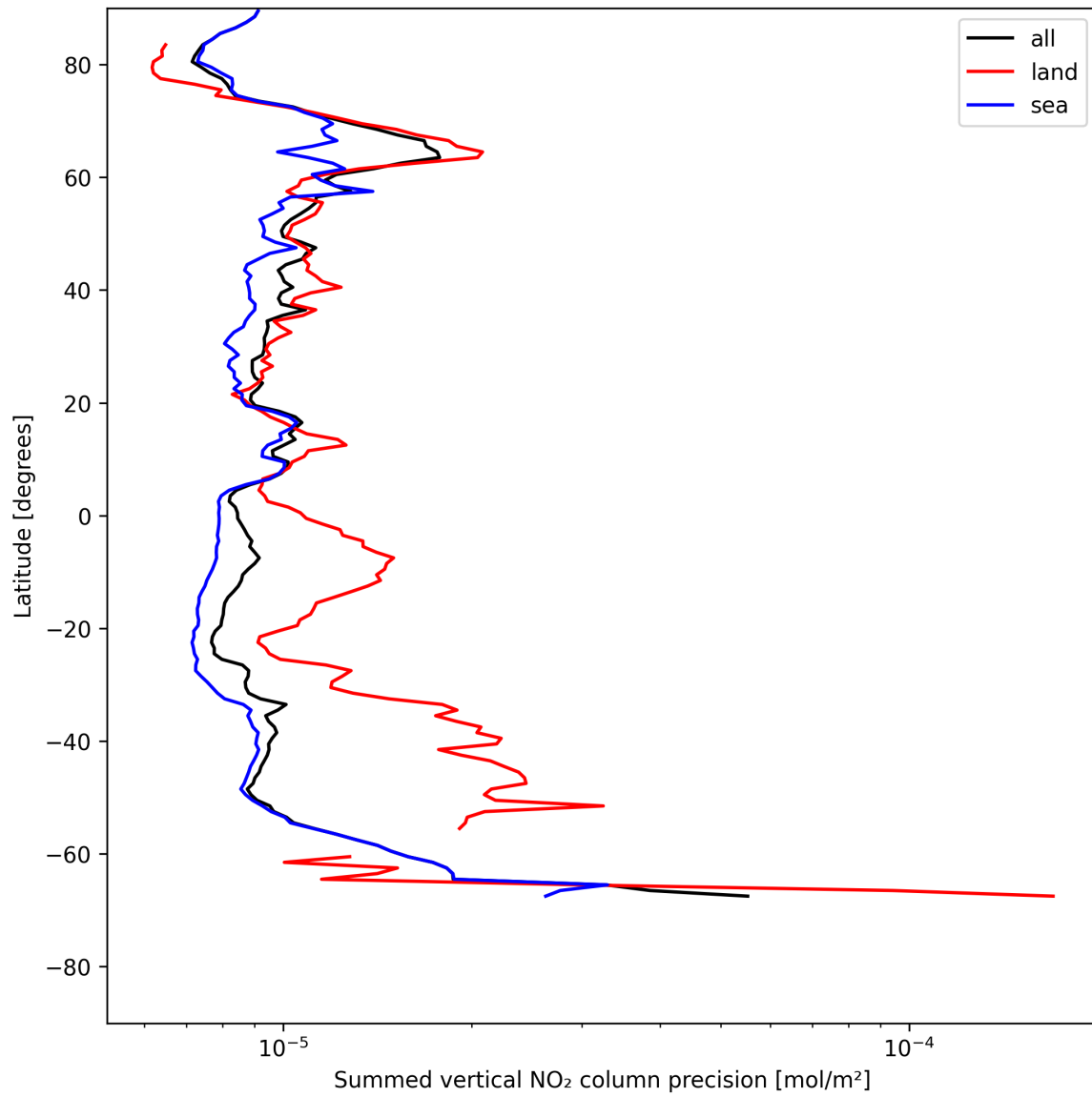
Figure 24: Zonal average of “Summed vertical NO 2 column precision” for 2025-07-22 to 2025-07-24.
