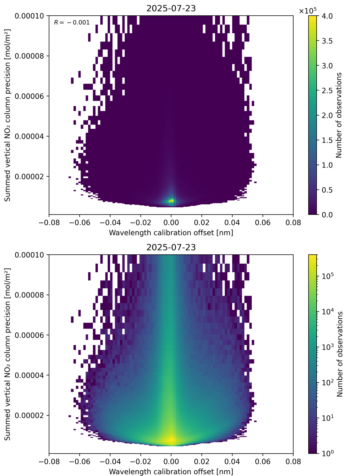
Figure 178: Scatter density plot of “Wavelength calibration offset” against “Summed vertical NO 2 column precision” for 2025-07-22 to 2025-07-24.
