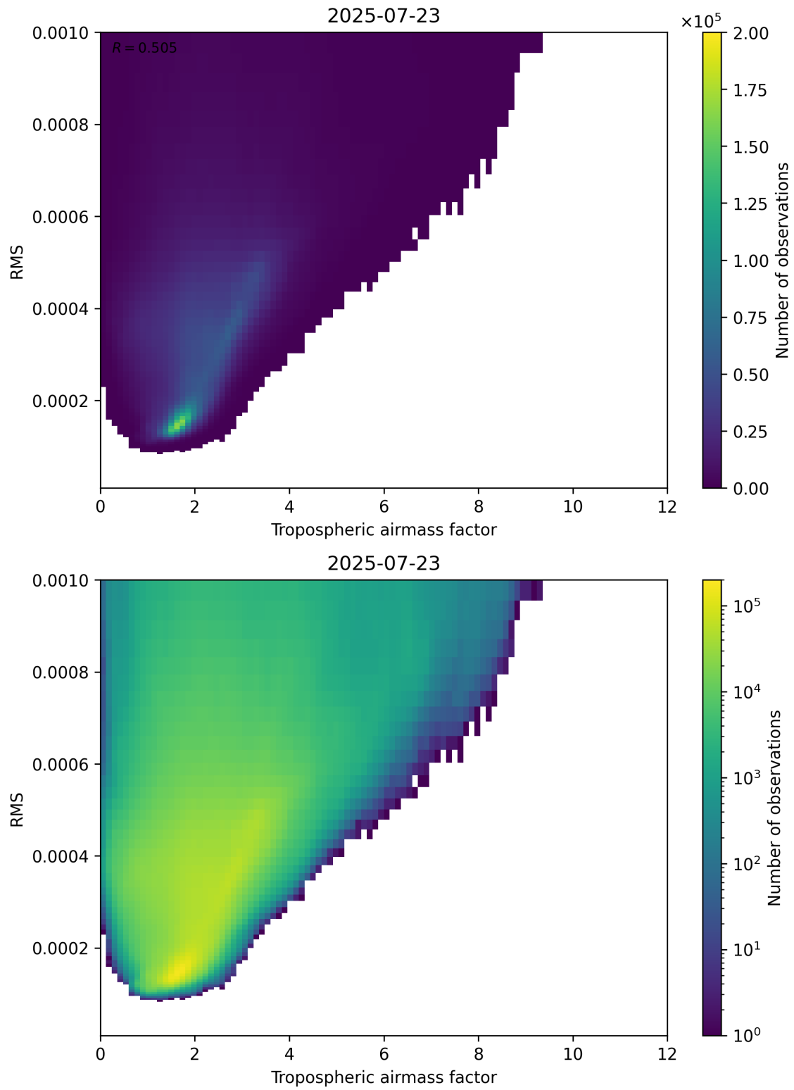
Figure 79: Scatter density plot of “Tropospheric airmass factor” against “RMS” for 2025-07-22 to 2025-07-24.
