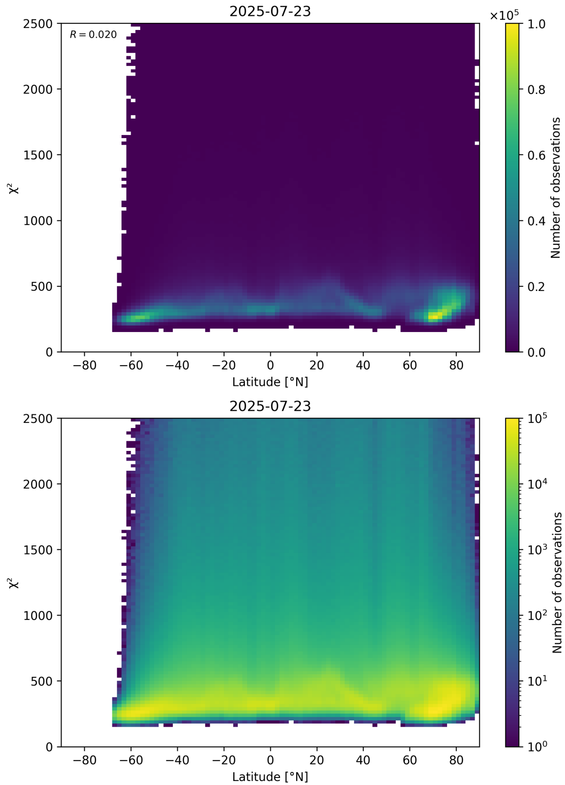
Figure 86: Scatter density plot of “Latitude” against “ \chi^2 ” for 2025-07-22 to 2025-07-24.
