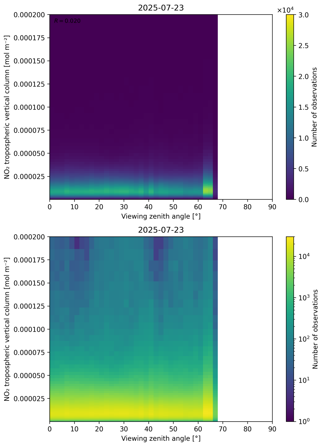
Figure 169: Scatter density plot of “Viewing zenith angle” against “NO 2 tropospheric vertical column” for 2025-07-22 to 2025-07-24.
