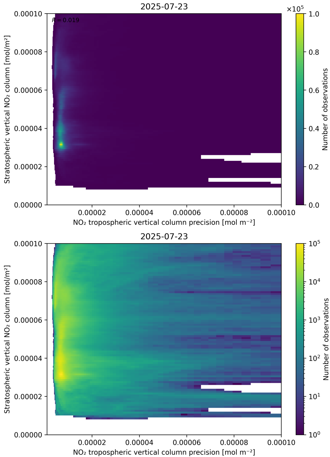
Figure 135: Scatter density plot of “NO 2 tropospheric vertical column precision” against “Stratospheric vertical NO 2 column” for 2025-07-22 to 2025-07-24.
