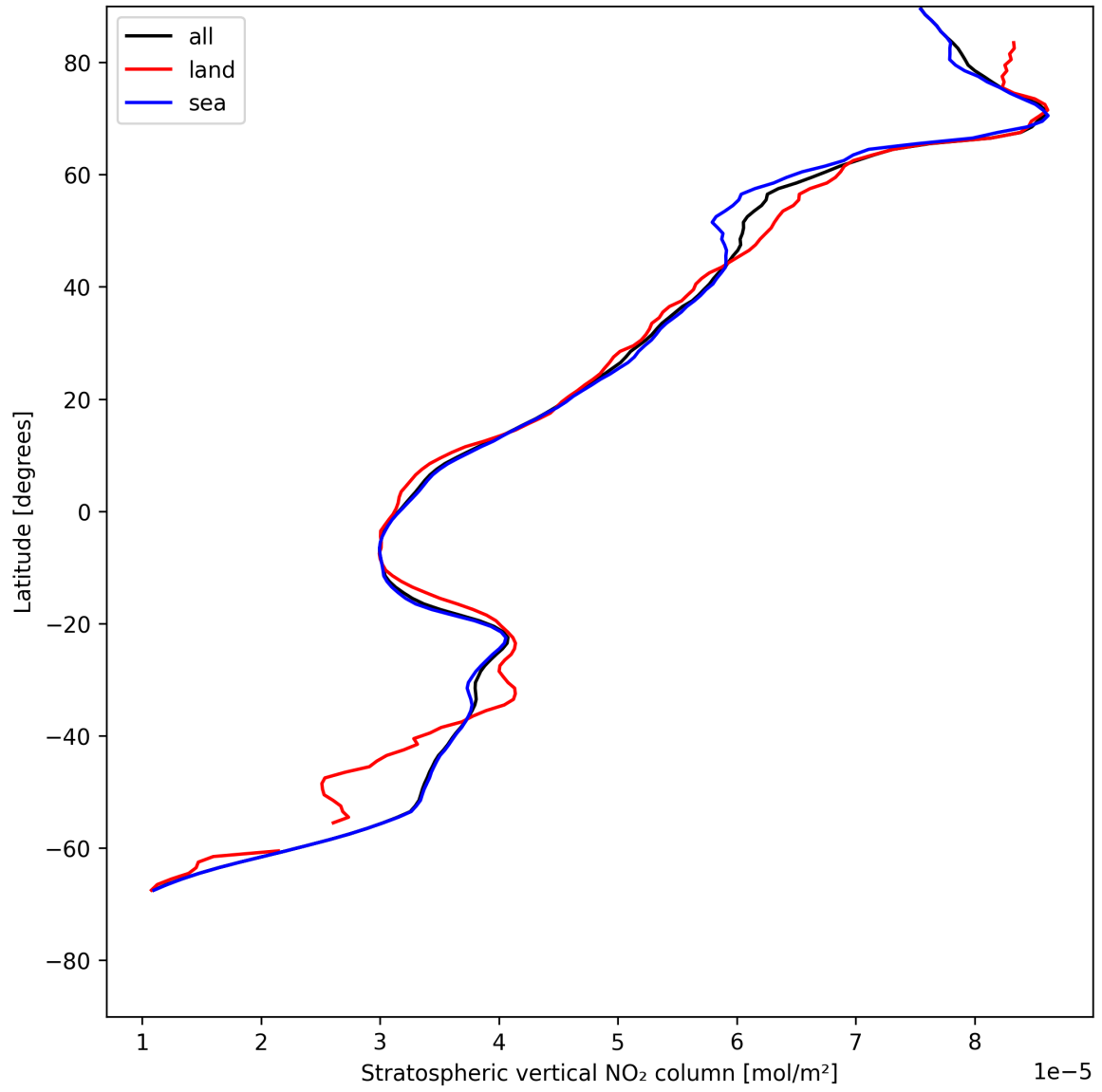
Figure 19: Zonal average of “Stratospheric vertical NO 2 column” for 2025-07-22 to 2025-07-24.
