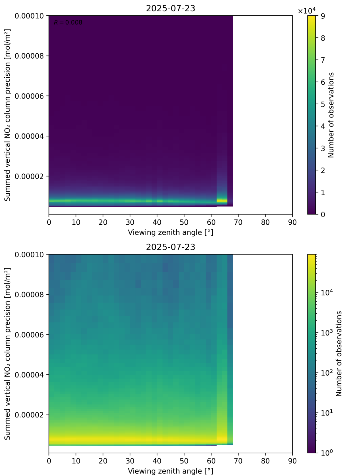
Figure 166: Scatter density plot of “Viewing zenith angle” against “Summed vertical NO 2 column precision” for 2025-07-22 to 2025-07-24.
