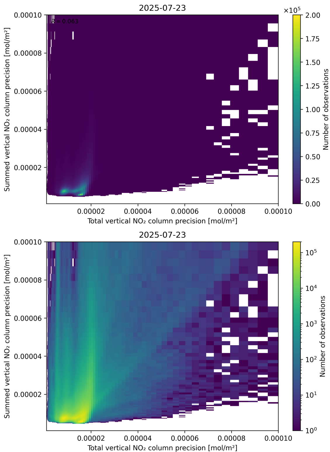
Figure 118: Scatter density plot of “Total vertical NO 2 column precision” against “Summed vertical NO 2 column precision” for 2025-07-22 to 2025-07-24.
