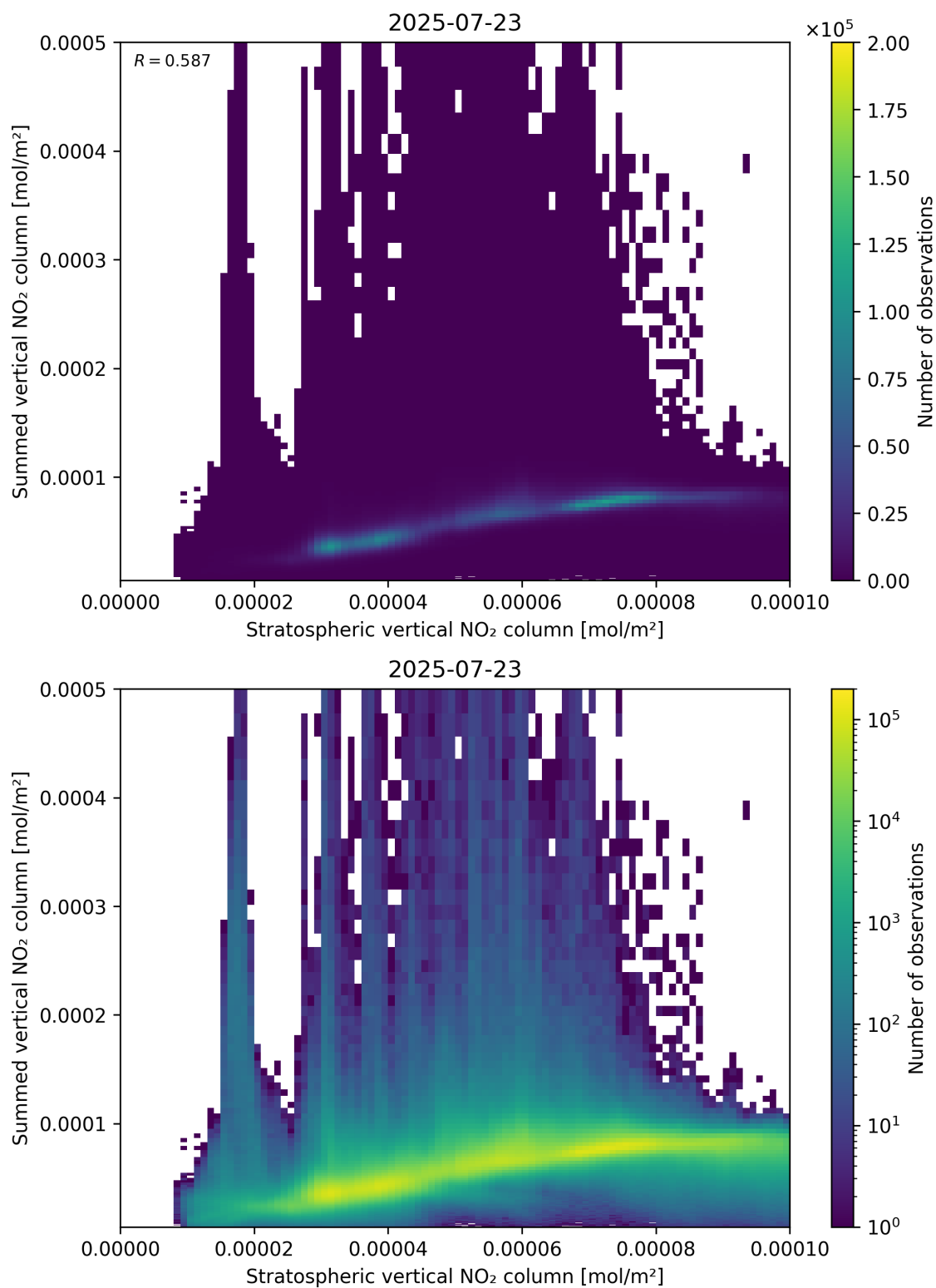
Figure 98: Scatter density plot of “Stratospheric vertical NO 2 column” against “Summed vertical NO 2 column” for 2025-07-22 to 2025-07-24.
