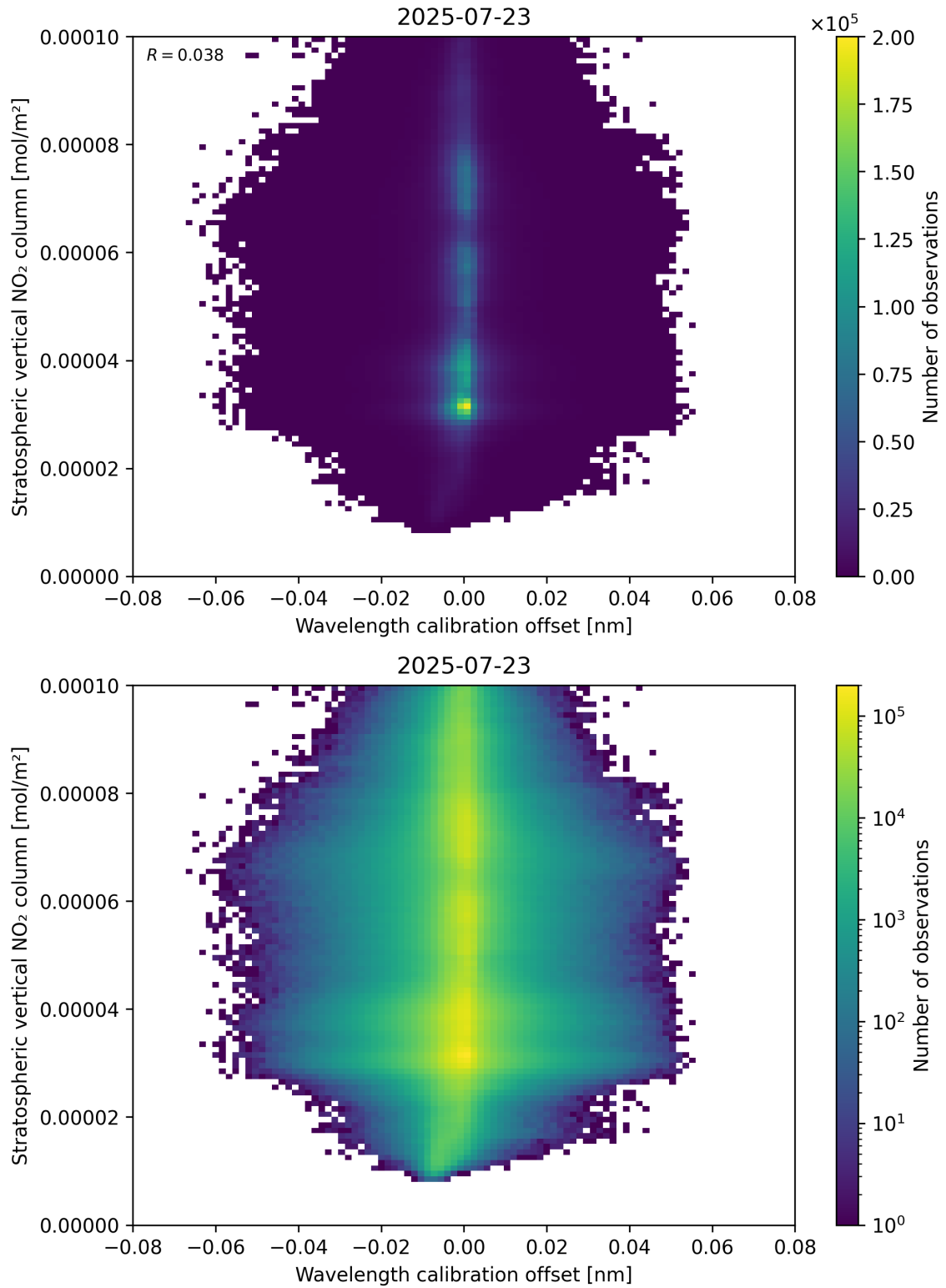
Figure 176: Scatter density plot of “Wavelength calibration offset” against “Stratospheric vertical NO 2 column” for 2025-07-22 to 2025-07-24.
