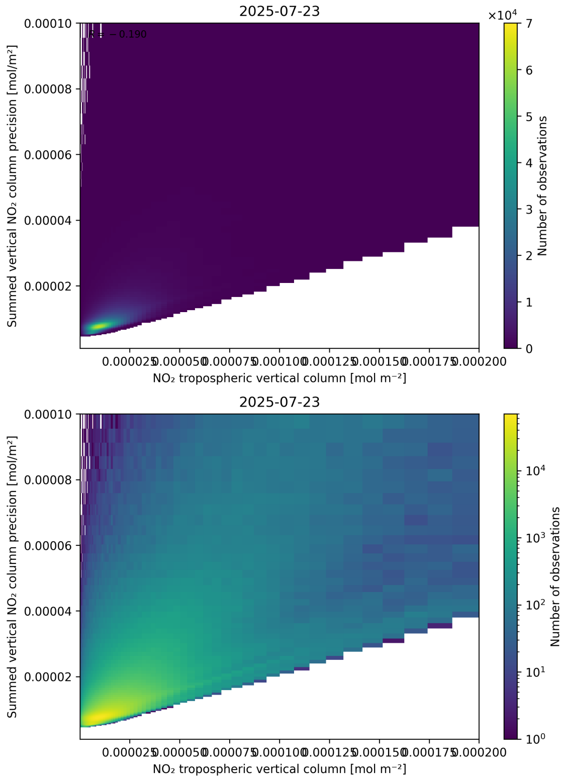
Figure 127: Scatter density plot of “NO 2 tropospheric vertical column” against “Summed vertical NO 2 column precision” for 2025-07-22 to 2025-07-24.
