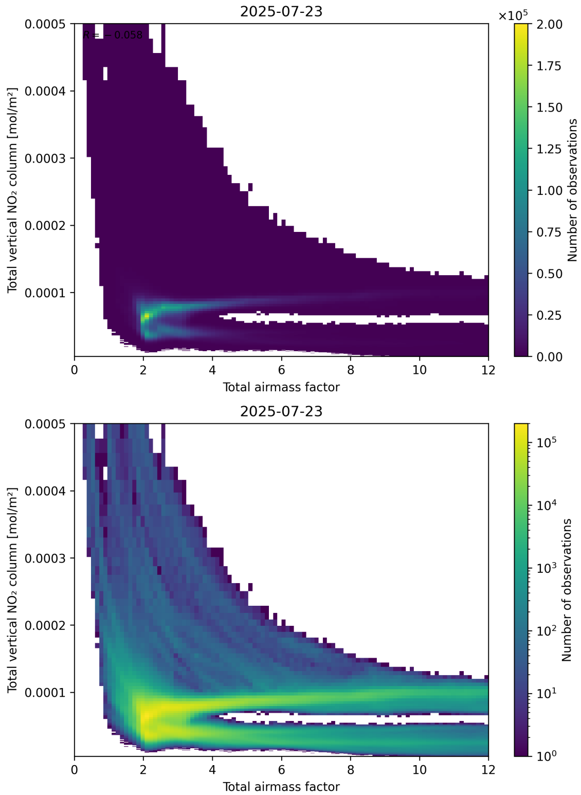
Figure 67: Scatter density plot of “Total airmass factor” against “Total vertical NO 2 column” for 2025-07-22 to 2025-07-24.
