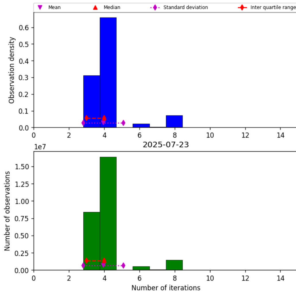
Figure 34: Histogram of “Number of iterations” for 2025-07-22 to 2025-07-24
