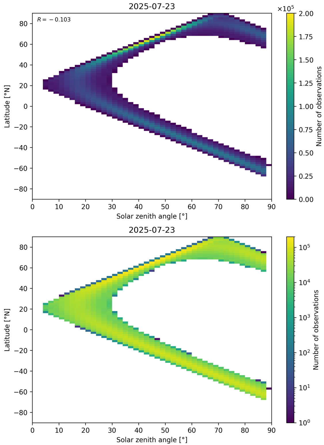
Figure 149: Scatter density plot of “Solar zenith angle” against “Latitude” for 2025-07-22 to 2025-07-24.
