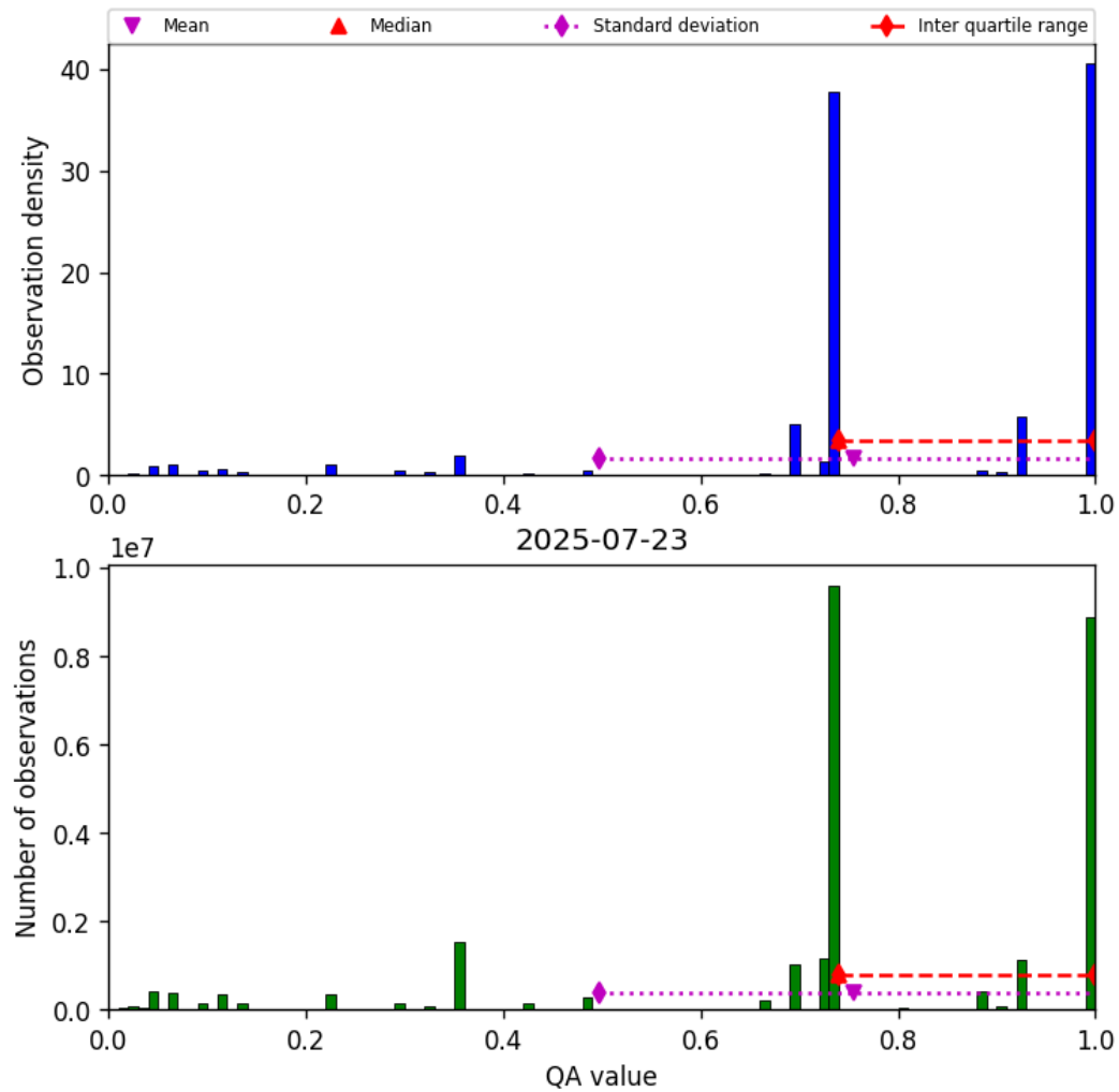
Figure 28: Histogram of “QA value” for 2025-07-22 to 2025-07-24
