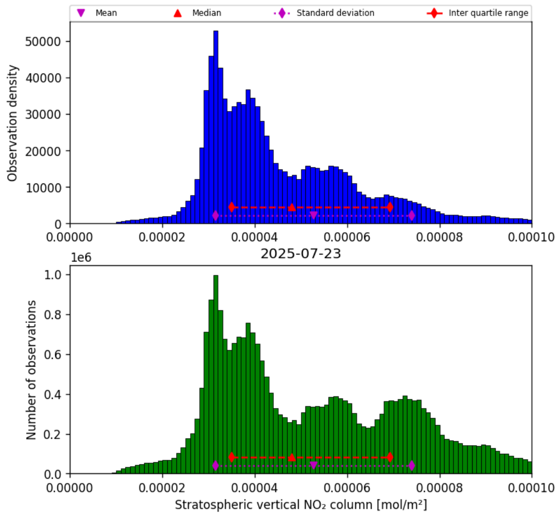
Figure 36: Histogram of “Stratospheric vertical NO 2 column” for 2025-07-22 to 2025-07-24
