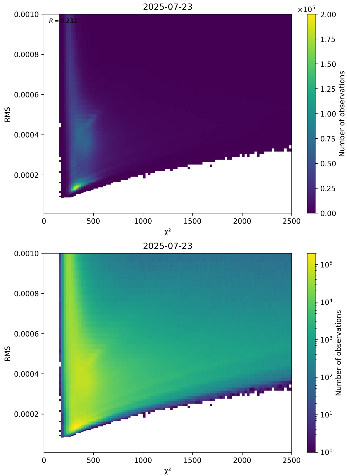
Figure 82: Scatter density plot of “ \chi^2 ” against “RMS” for 2025-07-22 to 2025-07-24.
