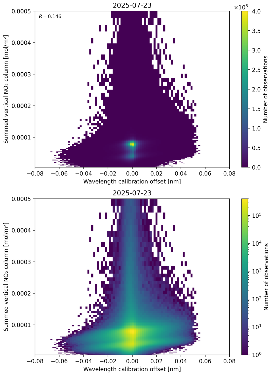
Figure 177: Scatter density plot of “Wavelength calibration offset” against “Summed vertical NO 2 column” for 2025-07-22 to 2025-07-24.
