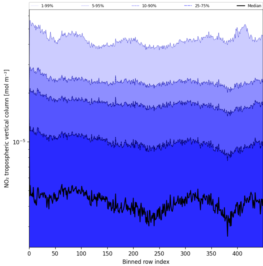
Figure 46: Along track statistics of “NO 2 tropospheric vertical column” for 2025-07-22 to 2025-07-24
