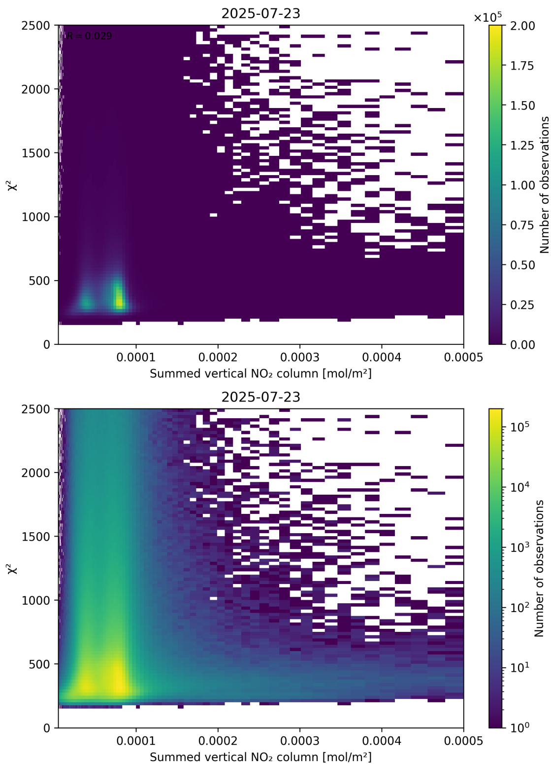
Figure 104: Scatter density plot of “Summed vertical NO 2 column” against “ \chi^2 ” for 2025-07-22 to 2025-07-24.
