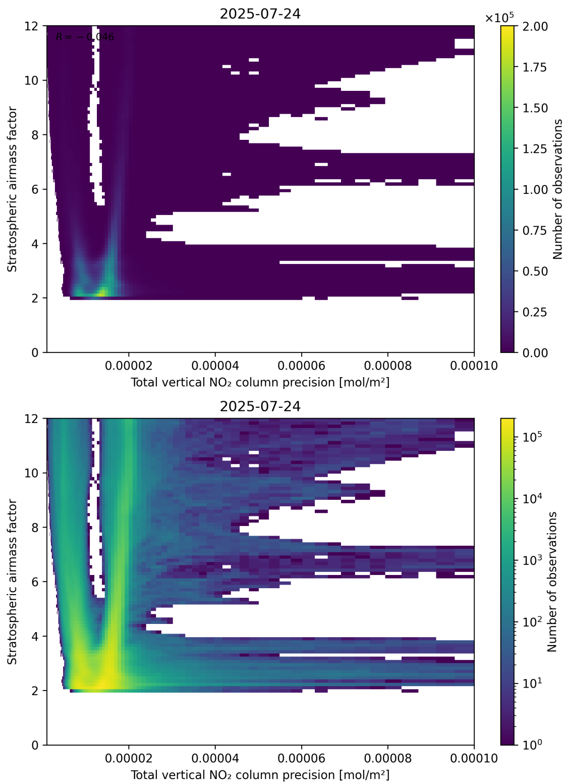
Figure 115: Scatter density plot of “Total vertical NO 2 column precision” against “Stratospheric air mass factor” for 2025-07-24 to 2025-07-25.
