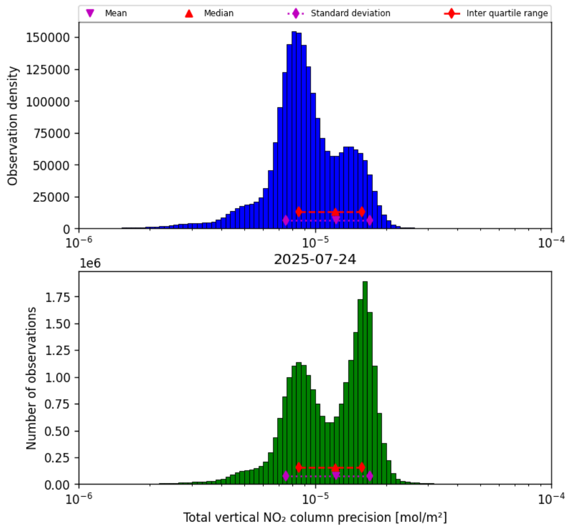
Figure 39: Histogram of “Total vertical NO 2 column precision” for 2025-07-24 to 2025-07-25
