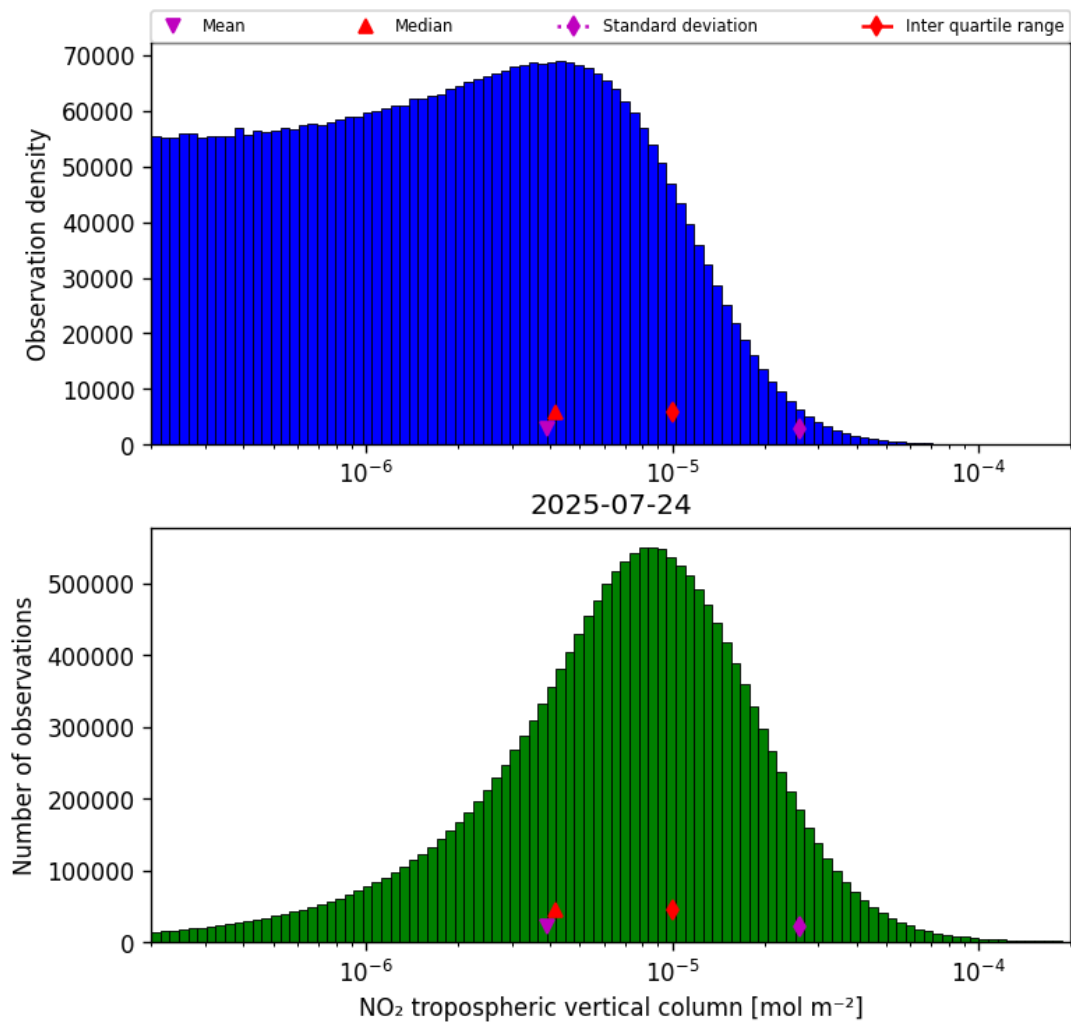
Figure 29: Histogram of “NO 2 tropospheric vertical column” for 2025-07-24 to 2025-07-25
