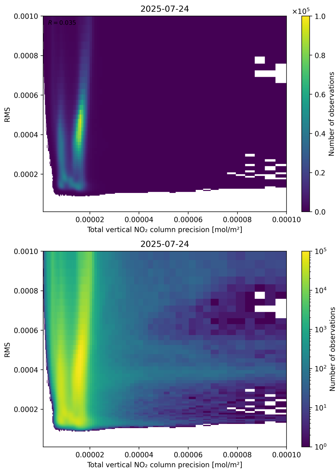
Figure 119: Scatter density plot of “Total vertical NO 2 column precision” against “RMS” for 2025-07-24 to 2025-07-25.
