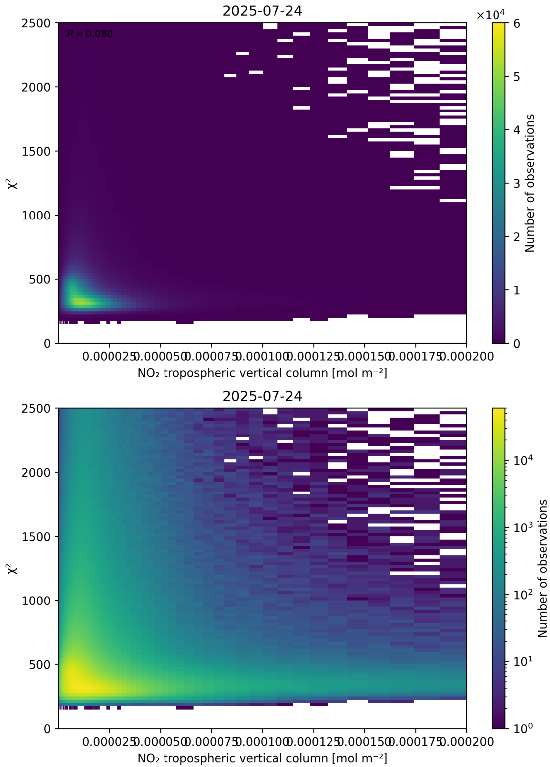
Figure 124: Scatter density plot of “NO 2 tropospheric vertical column” against “ \chi^2 ” for 2025-07-24 to 2025-07-25.
