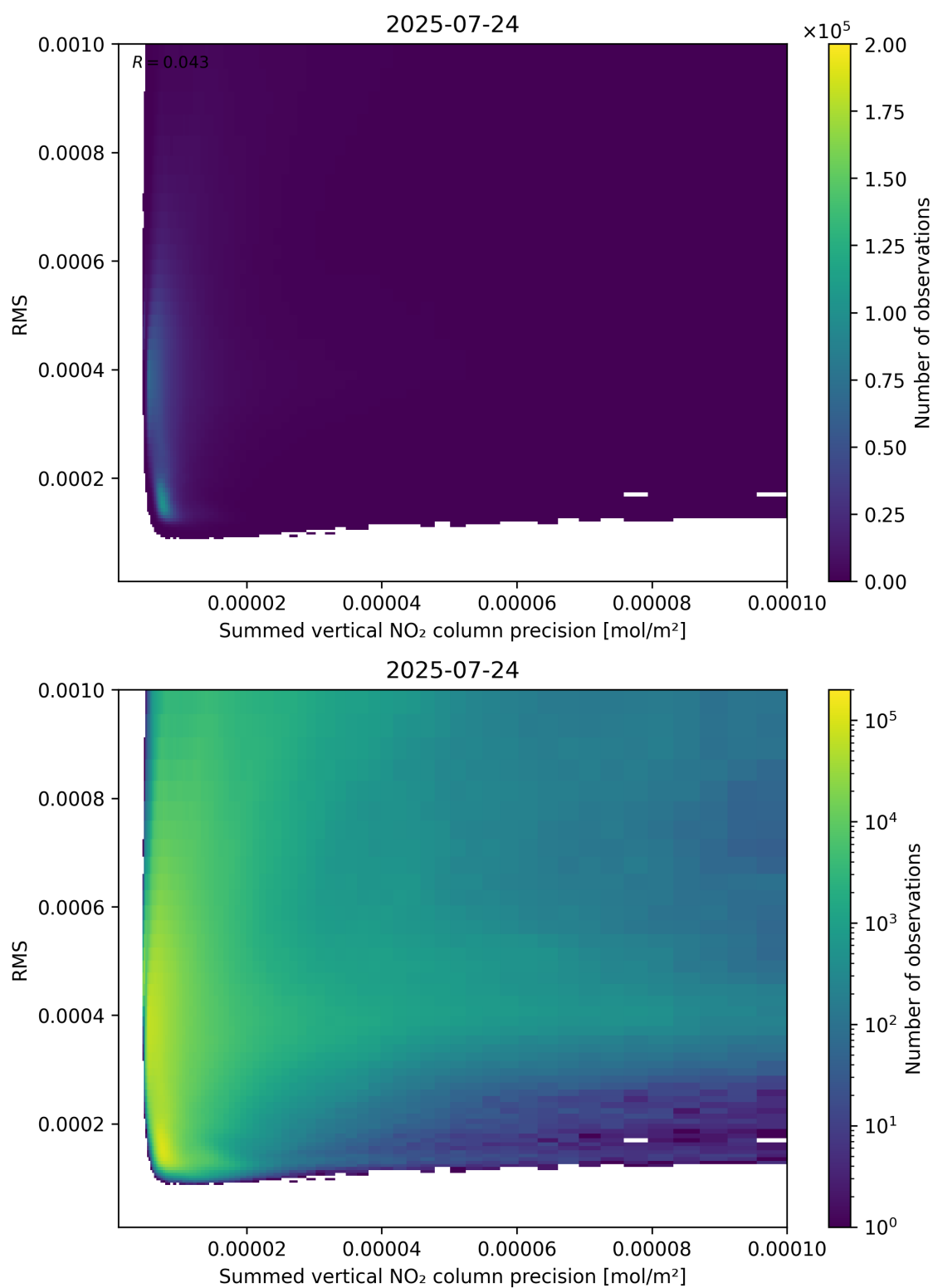
Figure 108: Scatter density plot of “Summed vertical NO 2 column precision” against “RMS” for 2025-07-24 to 2025-07-25.
