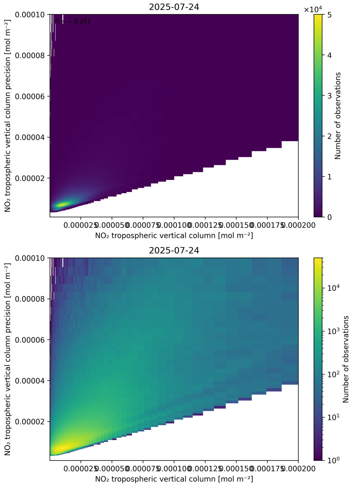
Figure 130: Scatter density plot of “NO 2 tropospheric vertical column” against “NO 2 tropospheric vertical column precision” for 2025-07-24 to 2025-07-25.
