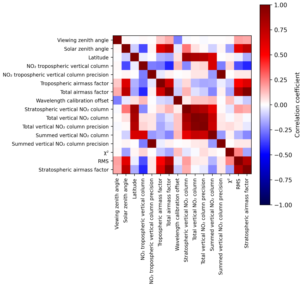
Figure 2: Map of correlation matrix for 2025-07-24 to 2025-07-25.
