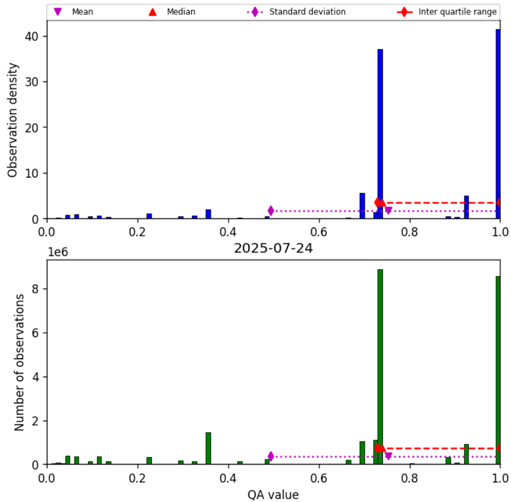
Figure 28: Histogram of “QA value” for 2025-07-24 to 2025-07-25
