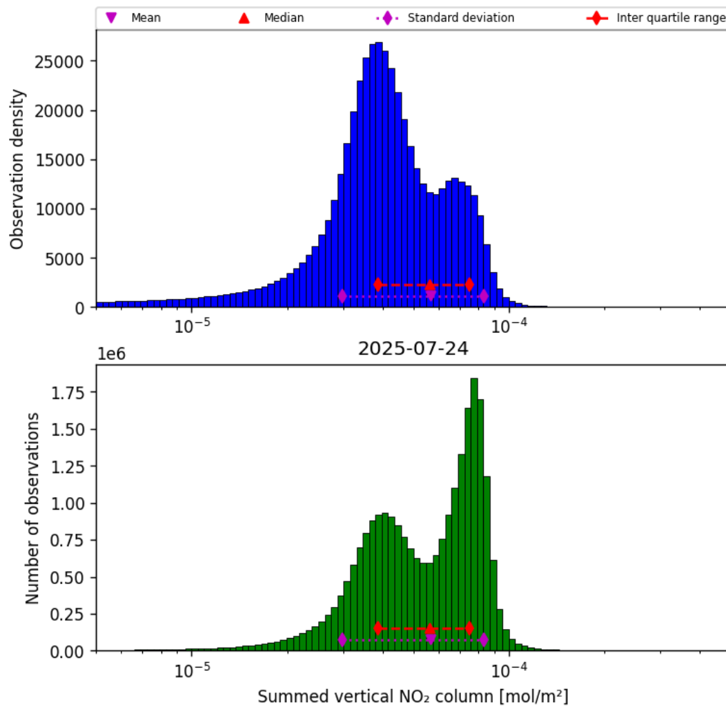
Figure 40: Histogram of “Summed vertical NO 2 column” for 2025-07-24 to 2025-07-25
