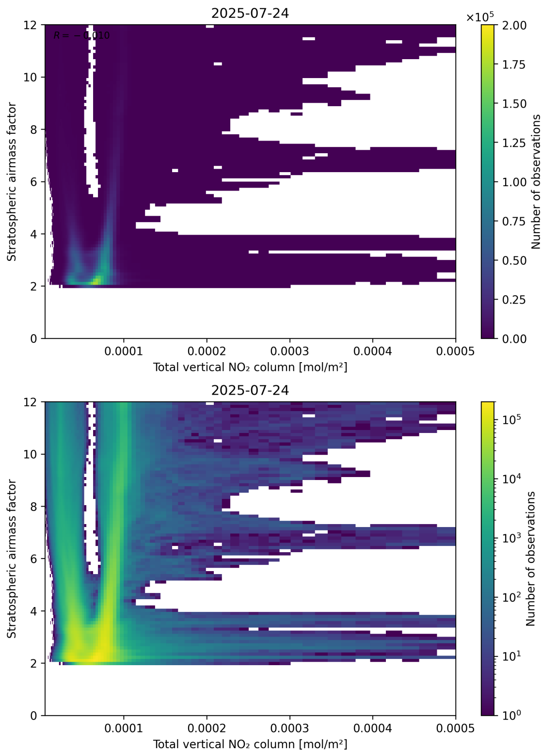
Figure 110: Scatter density plot of “Total vertical NO 2 column” against “Stratospheric air mass factor” for 2025-07-24 to 2025-07-25.
