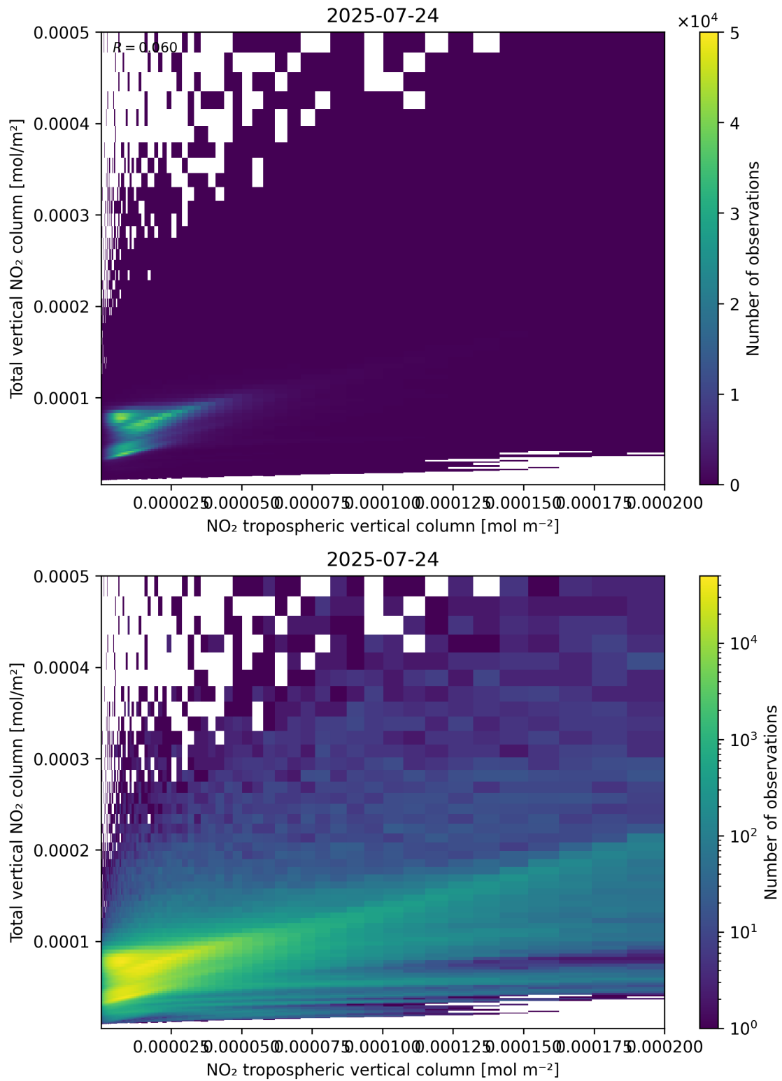
Figure 128: Scatter density plot of “NO 2 tropospheric vertical column” against “Total vertical NO 2 column” for 2025-07-24 to 2025-07-25.
