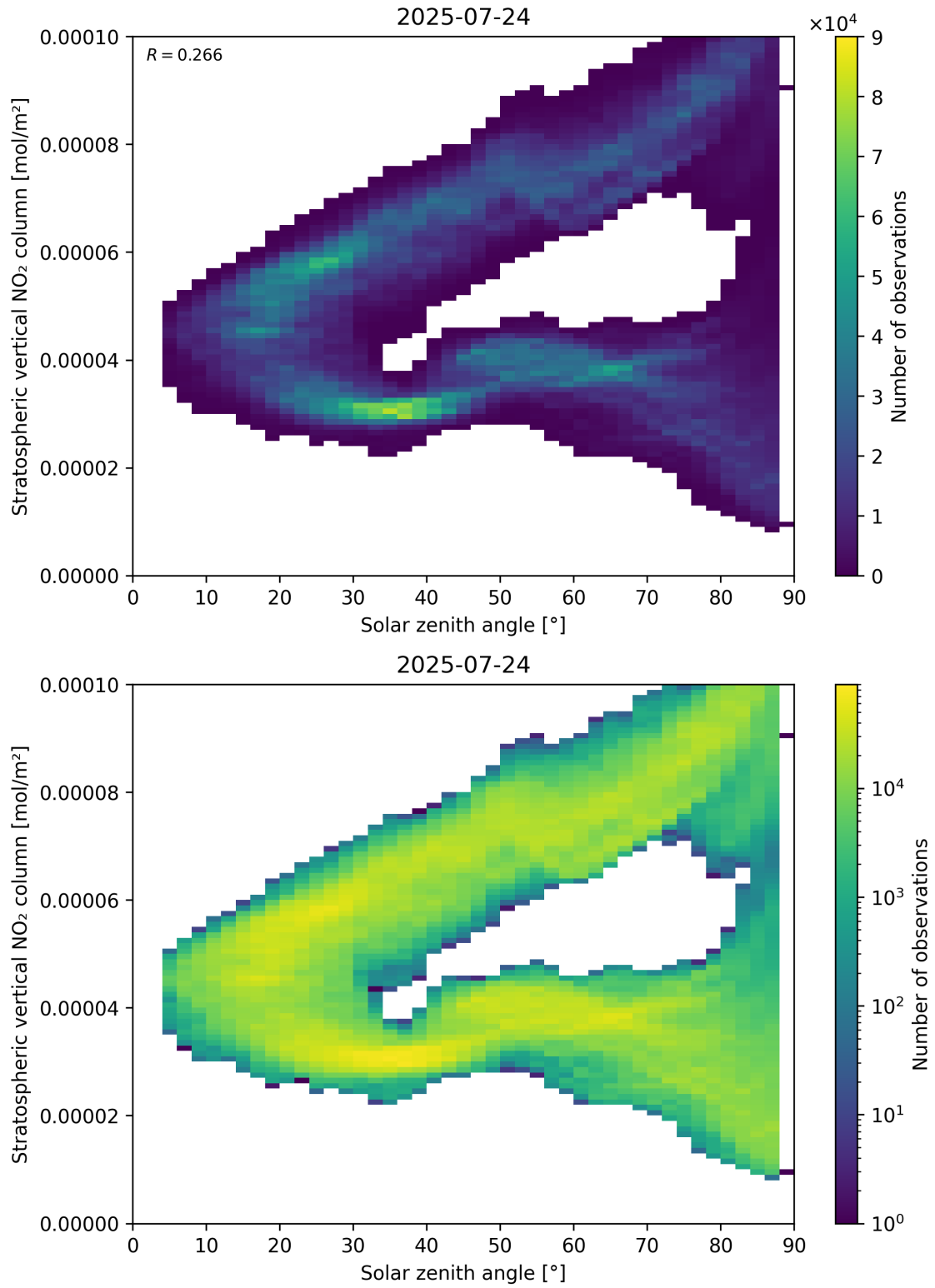
Figure 150: Scatter density plot of “Solar zenith angle” against “Stratospheric vertical NO 2 column” for 2025-07-24 to 2025-07-25.
