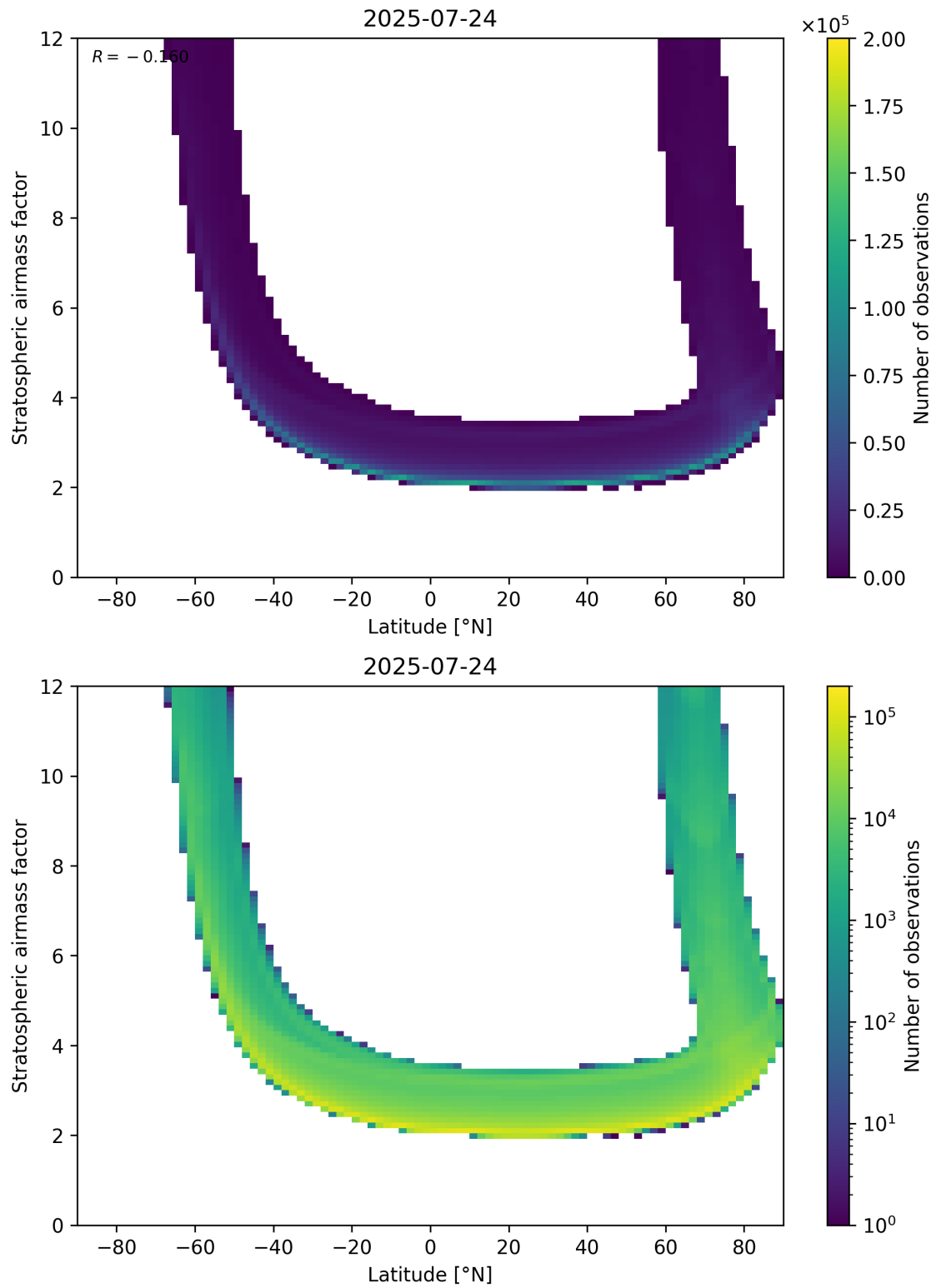
Figure 83: Scatter density plot of “Latitude” against “Stratospheric air mass factor” for 2025-07-24 to 2025-07-25.
