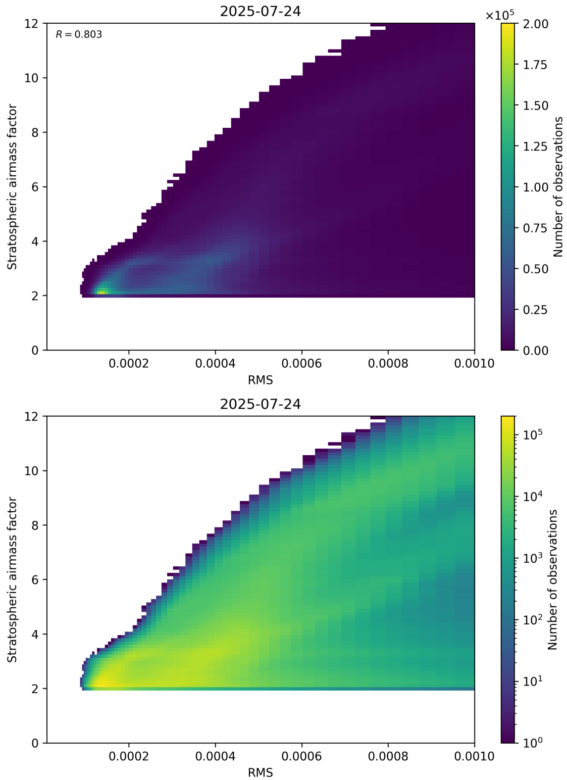
Figure 144: Scatter density plot of “RMS” against “Stratospheric airmass factor” for 2025-07-24 to 2025-07-25.
