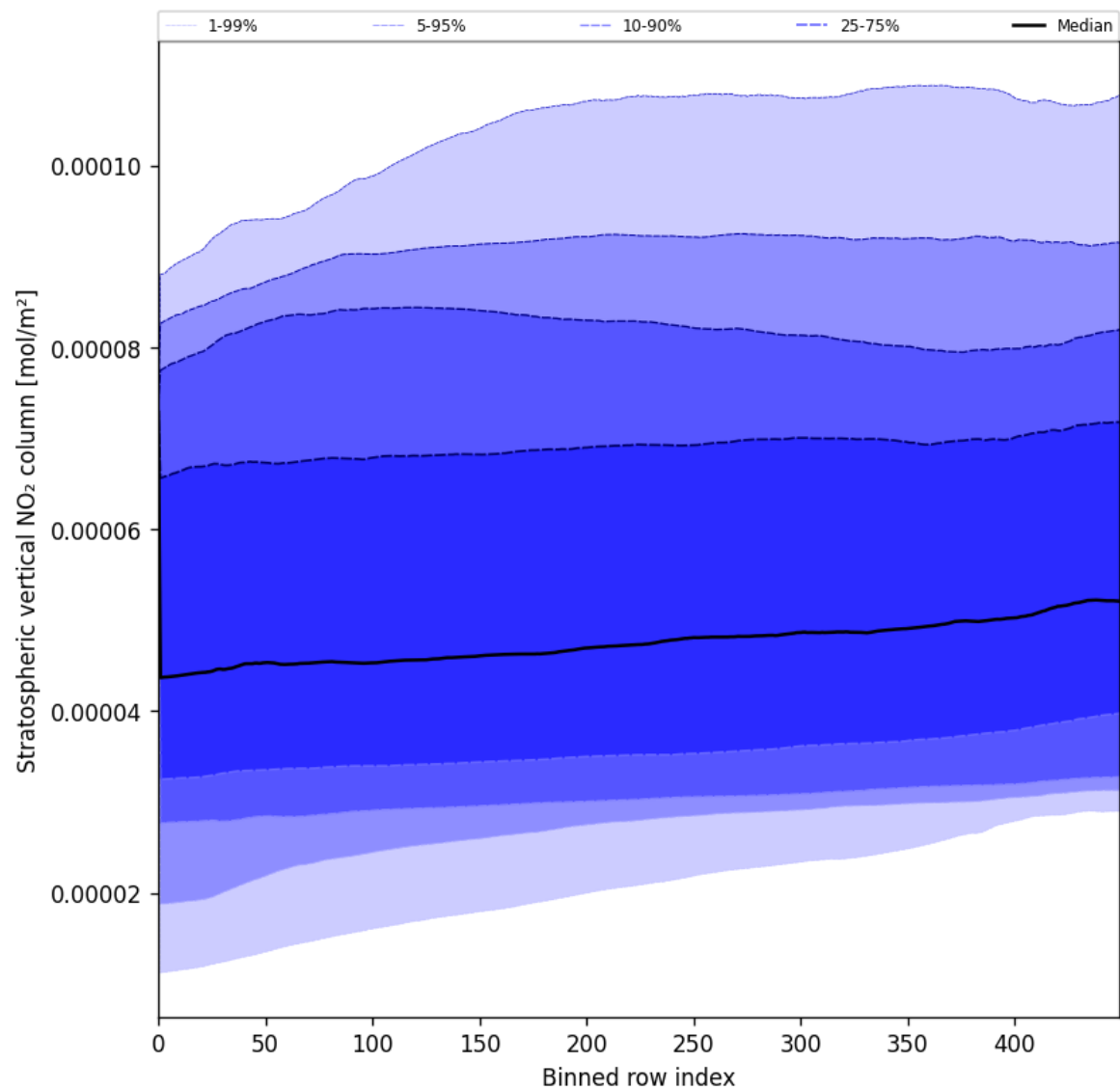
Figure 53: Along track statistics of “Stratospheric vertical NO 2 column” for 2025-07-24 to 2025-07-25
