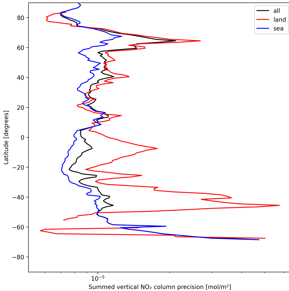
Figure 24: Zonal average of “Summed vertical NO 2 column precision” for 2025-07-24 to 2025-07-25.
