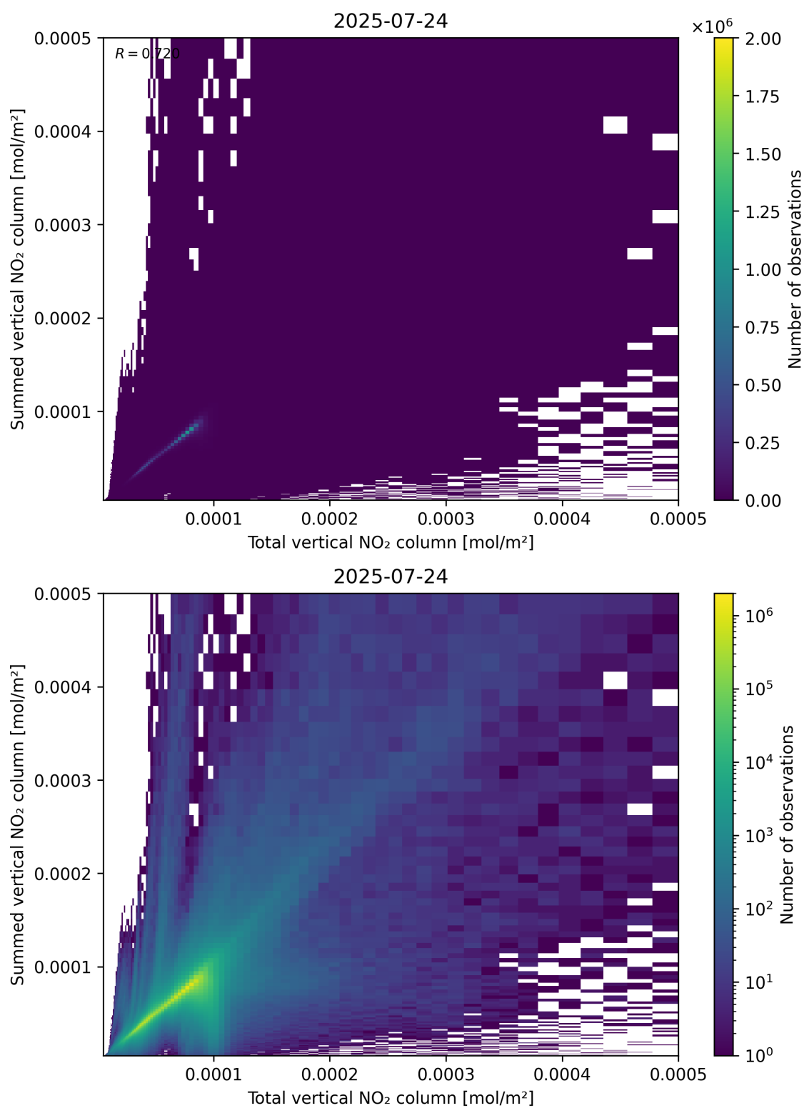
Figure 112: Scatter density plot of “Total vertical NO 2 column” against “Summed vertical NO 2 column” for 2025-07-24 to 2025-07-25.
