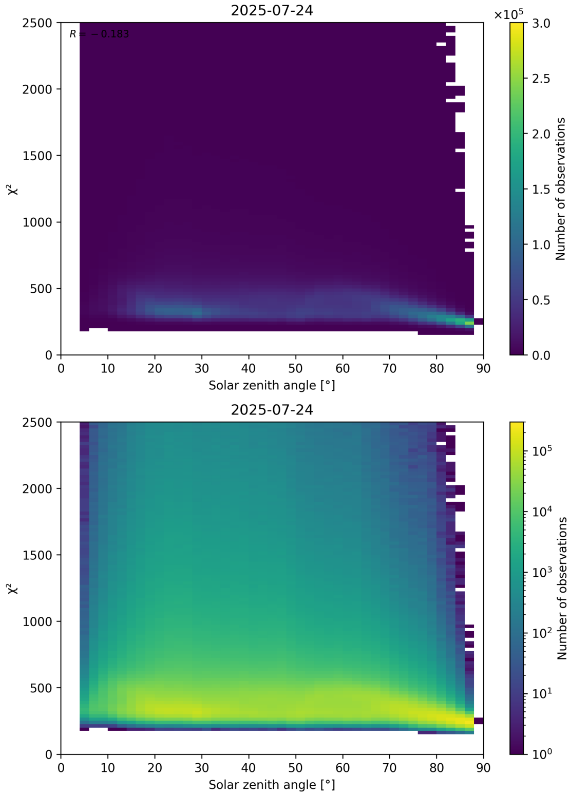
Figure 148: Scatter density plot of “Solar zenith angle” against “ \chi^2 ” for 2025-07-24 to 2025-07-25.
