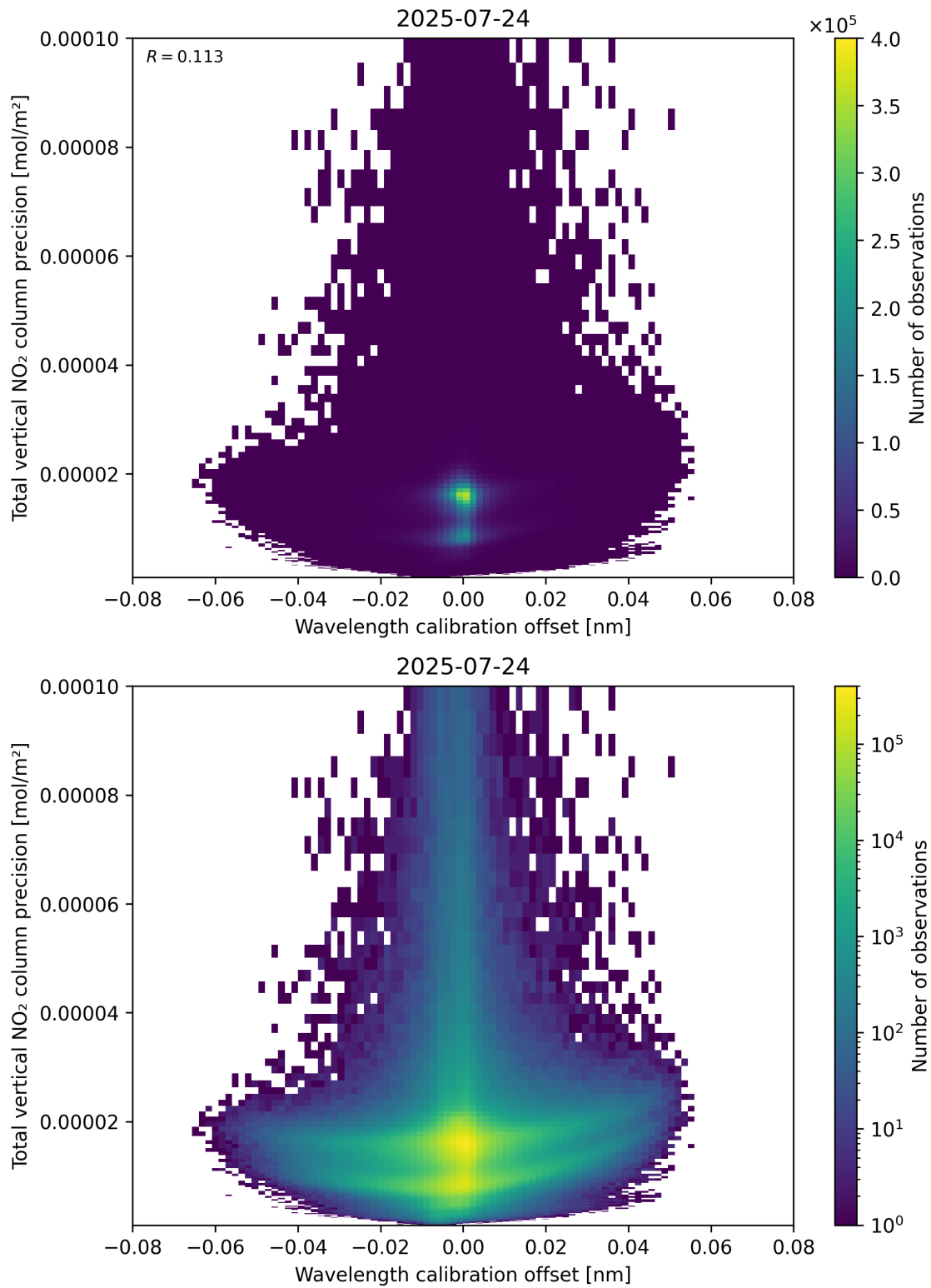
Figure 180: Scatter density plot of “Wavelength calibration offset” against “Total vertical NO 2 column precision” for 2025-07-24 to 2025-07-25.
