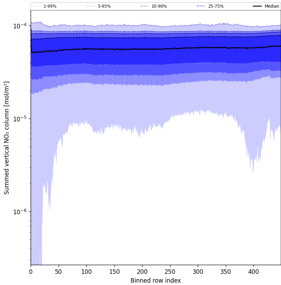
Figure 57: Along track statistics of “Summed vertical NO 2 column” for 2025-07-24 to 2025-07-25
