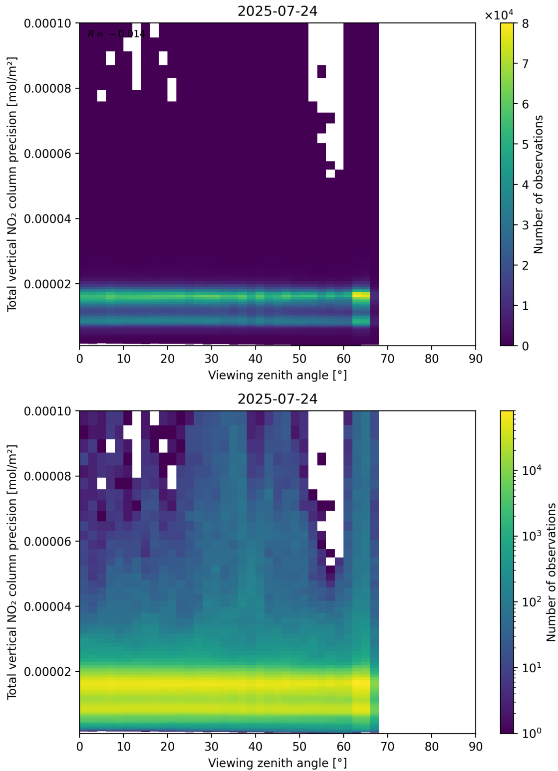
Figure 168: Scatter density plot of “Viewing zenith angle” against “Total vertical NO 2 column precision” for 2025-07-24 to 2025-07-25.
