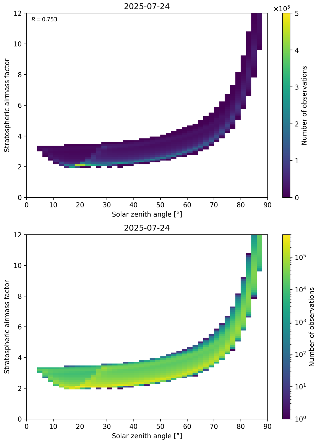
Figure 145: Scatter density plot of “Solar zenith angle” against “Stratospheric airmass factor” for 2025-07-24 to 2025-07-25.
