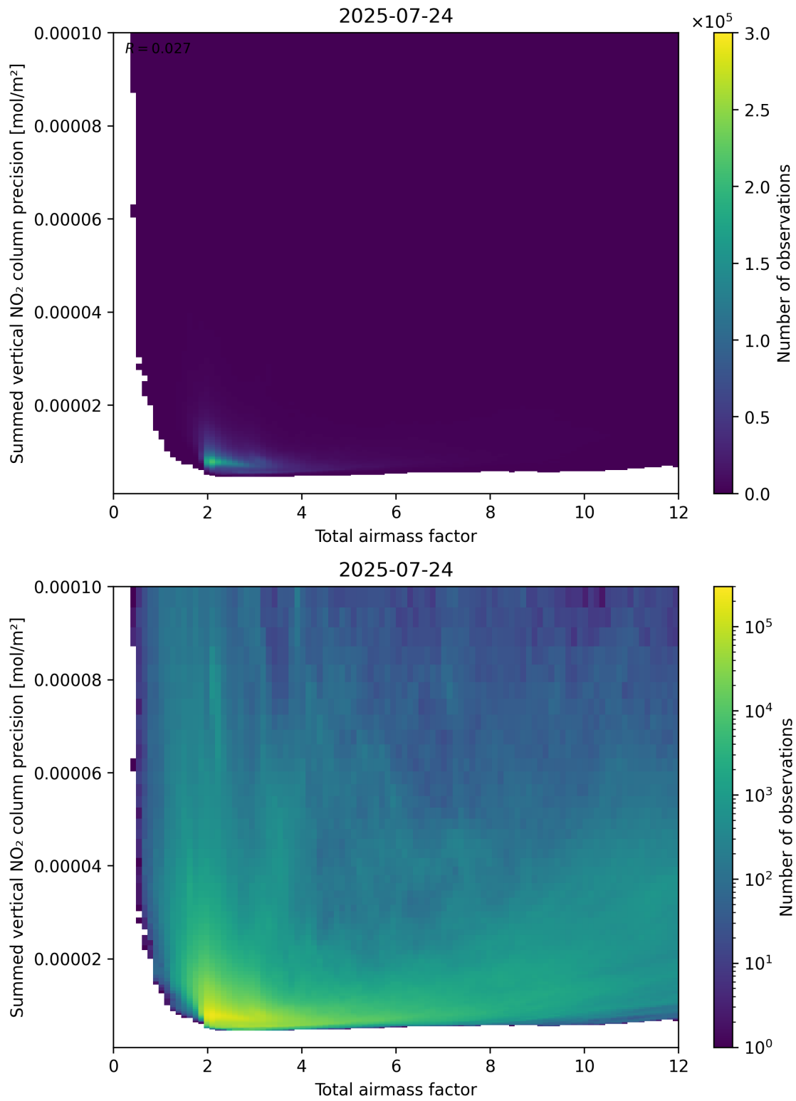
Figure 66: Scatter density plot of “Total airmass factor” against “Summed vertical NO 2 column precision” for 2025-07-24 to 2025-07-25.
