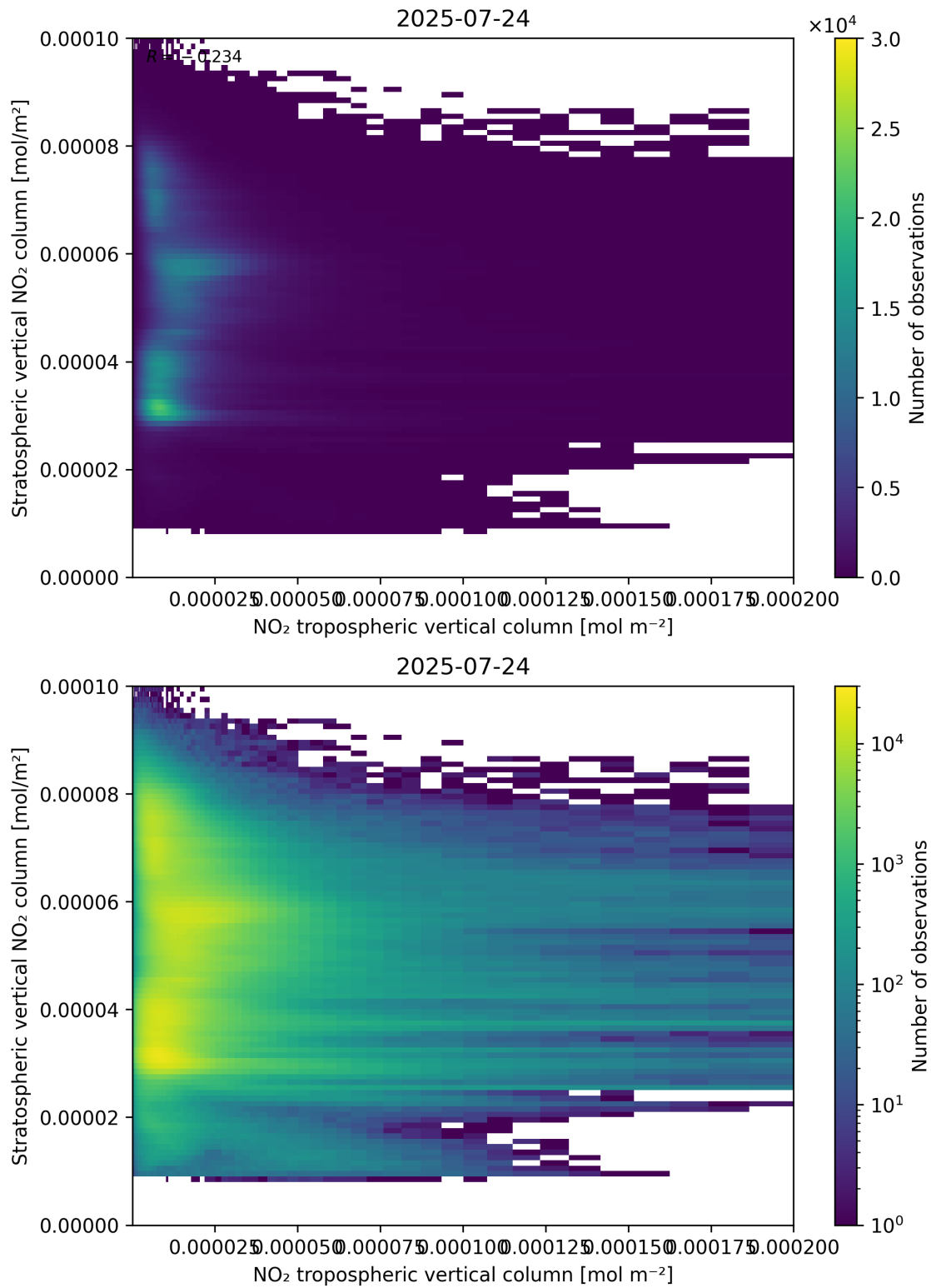
Figure 125: Scatter density plot of “NO 2 tropospheric vertical column” against “Stratospheric vertical NO 2 column” for 2025-07-24 to 2025-07-25.
