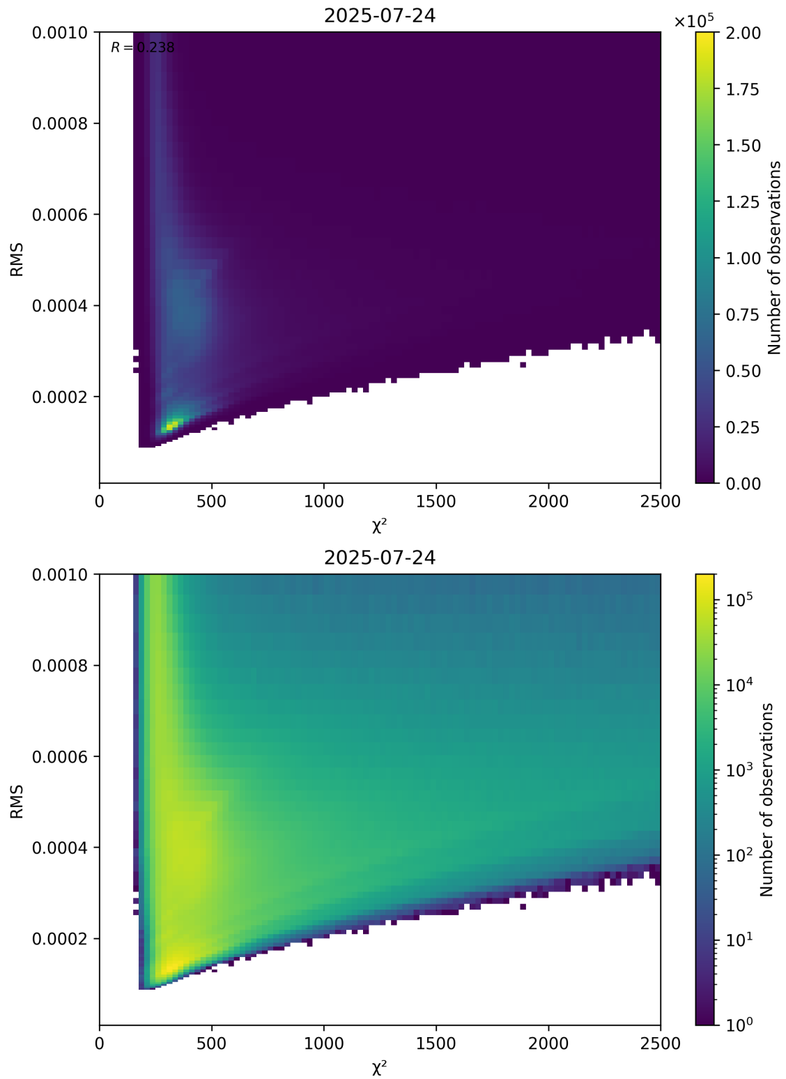
Figure 82: Scatter density plot of “ \chi^2 ” against “RMS” for 2025-07-24 to 2025-07-25.
