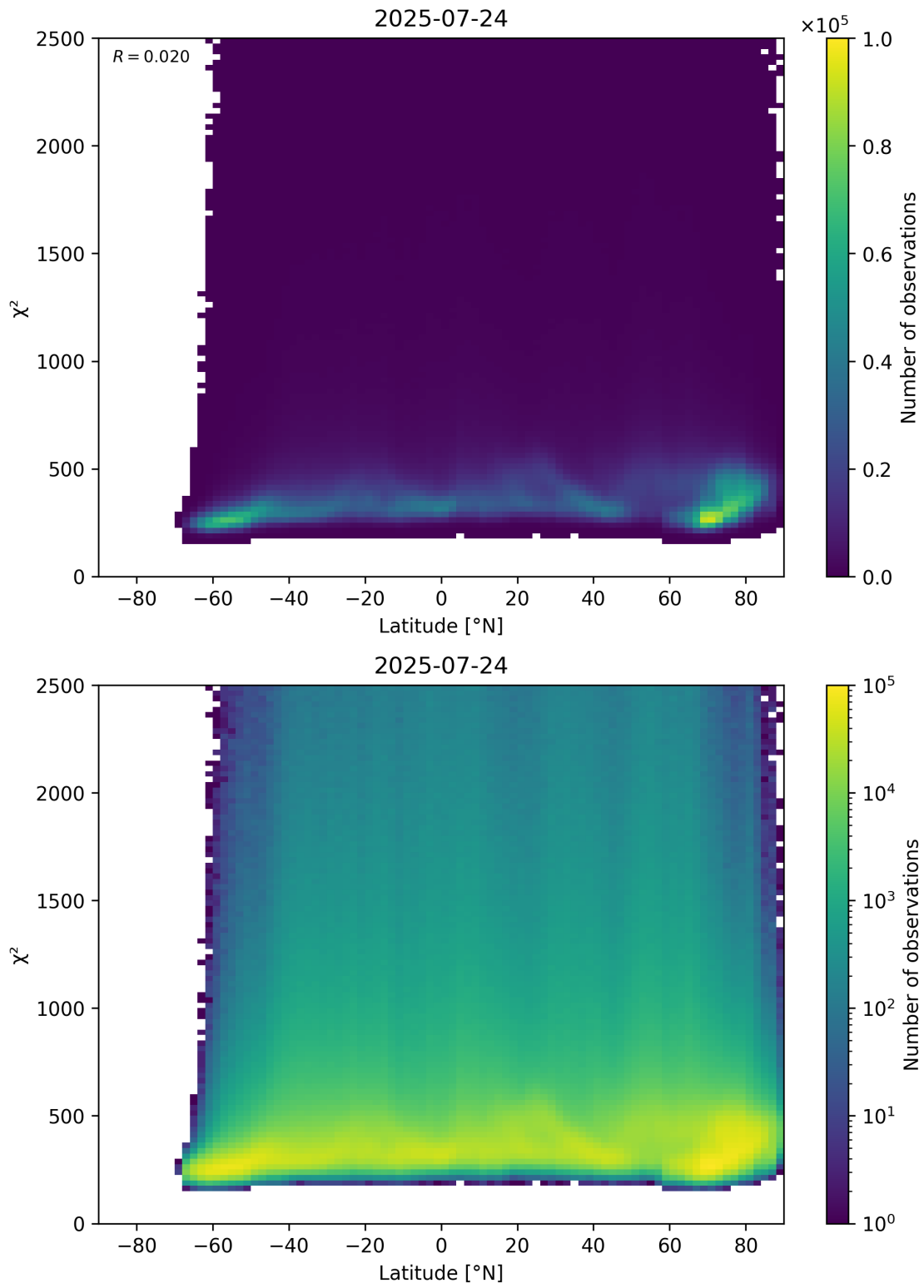
Figure 86: Scatter density plot of “Latitude” against “ \chi^2 ” for 2025-07-24 to 2025-07-25.
