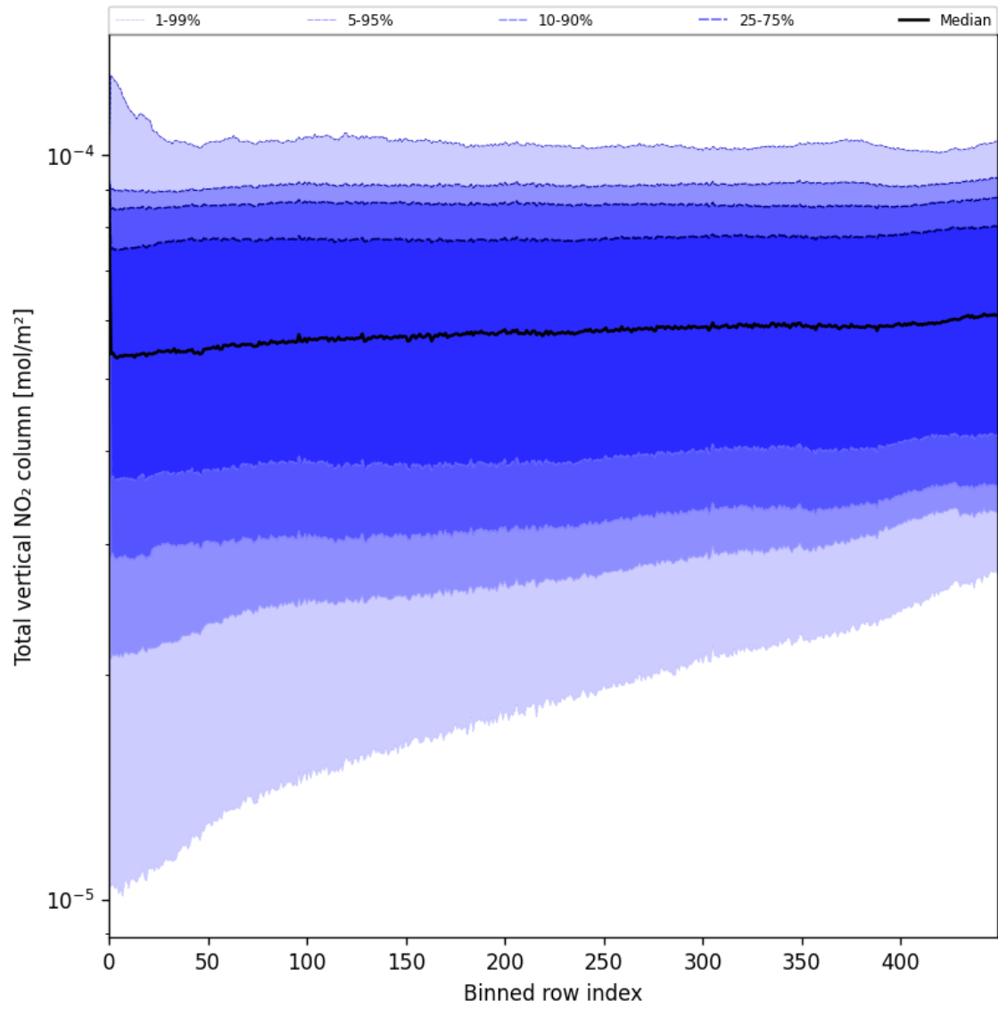
Figure 55: Along track statistics of “Total vertical NO 2 column” for 2025-07-24 to 2025-07-25
