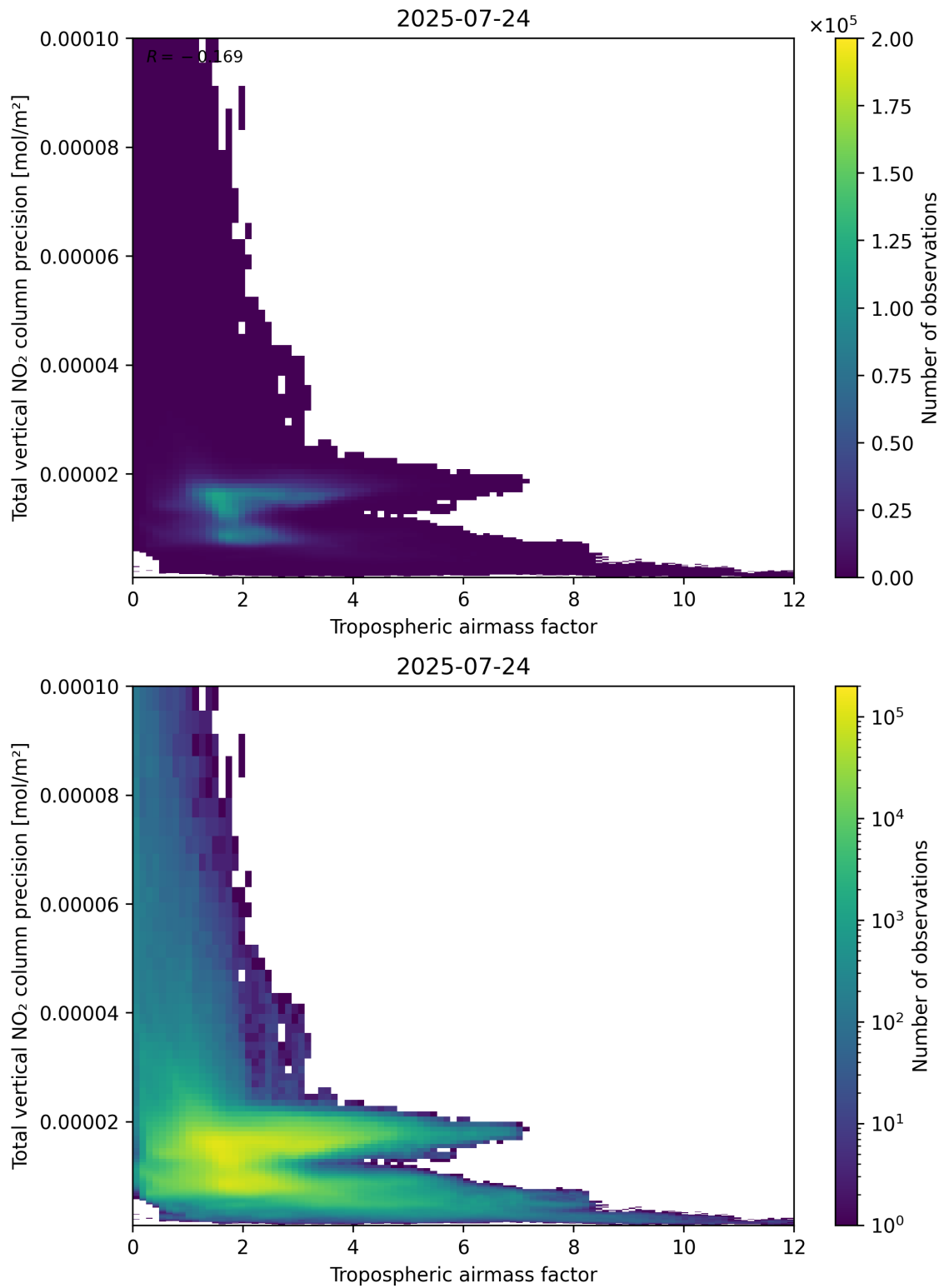
Figure 78: Scatter density plot of “Tropospheric airmass factor” against “Total vertical NO 2 column precision” for 2025-07-24 to 2025-07-25.
