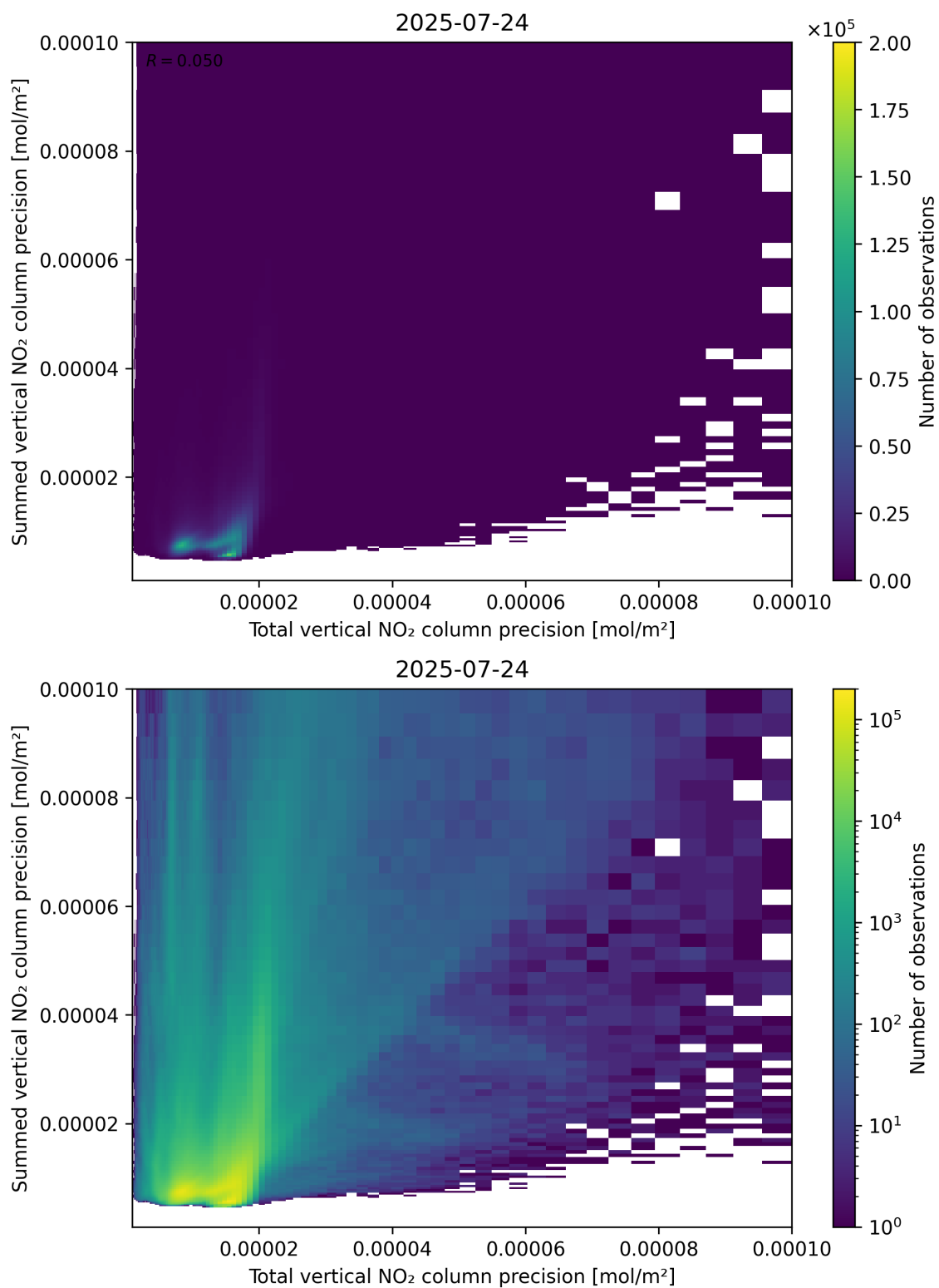
Figure 118: Scatter density plot of “Total vertical NO 2 column precision” against “Summed vertical NO 2 column precision” for 2025-07-24 to 2025-07-25.
