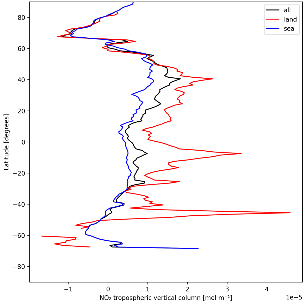
Figure 12: Zonal average of “NO 2 tropospheric vertical column” for 2025-07-24 to 2025-07-25.
