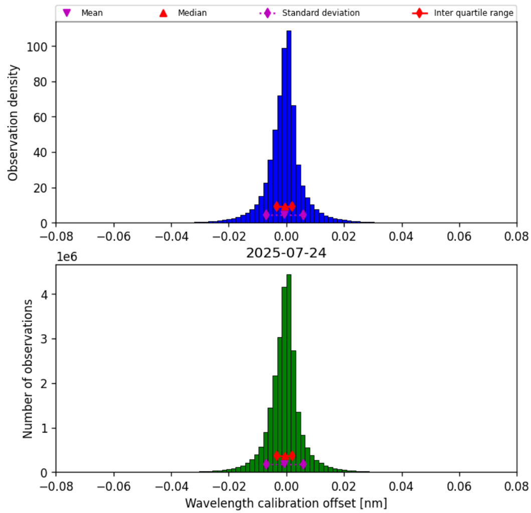
Figure 35: Histogram of “Wavelength calibration offset” for 2025-07-24 to 2025-07-25
