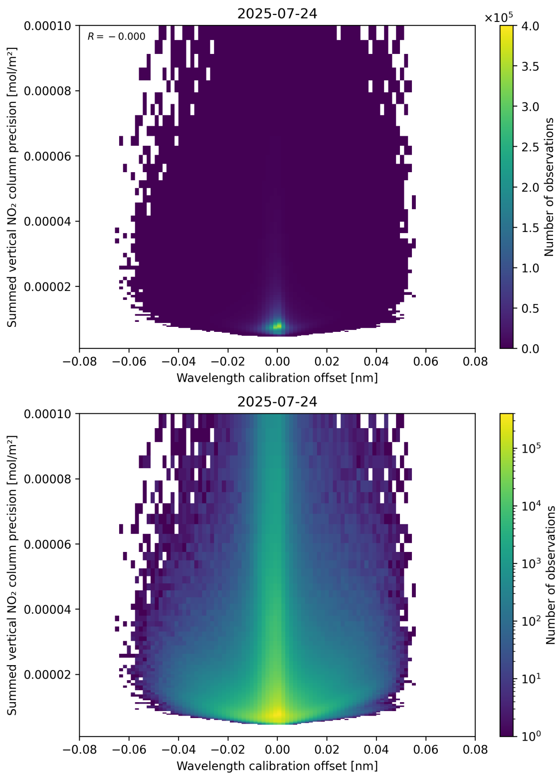
Figure 178: Scatter density plot of “Wavelength calibration offset” against “Summed vertical NO 2 column precision” for 2025-07-24 to 2025-07-25.
