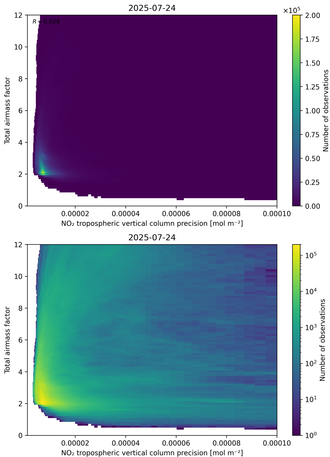
Figure 132: Scatter density plot of “NO 2 tropospheric vertical column precision” against “Total air mass factor” for 2025-07-24 to 2025-07-25.
