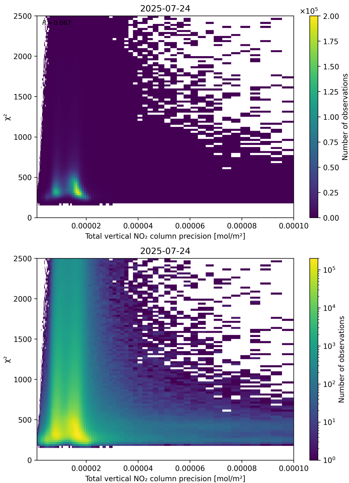
Figure 116: Scatter density plot of “Total vertical NO 2 column precision” against “ \chi^2 ” for 2025-07-24 to 2025-07-25.
