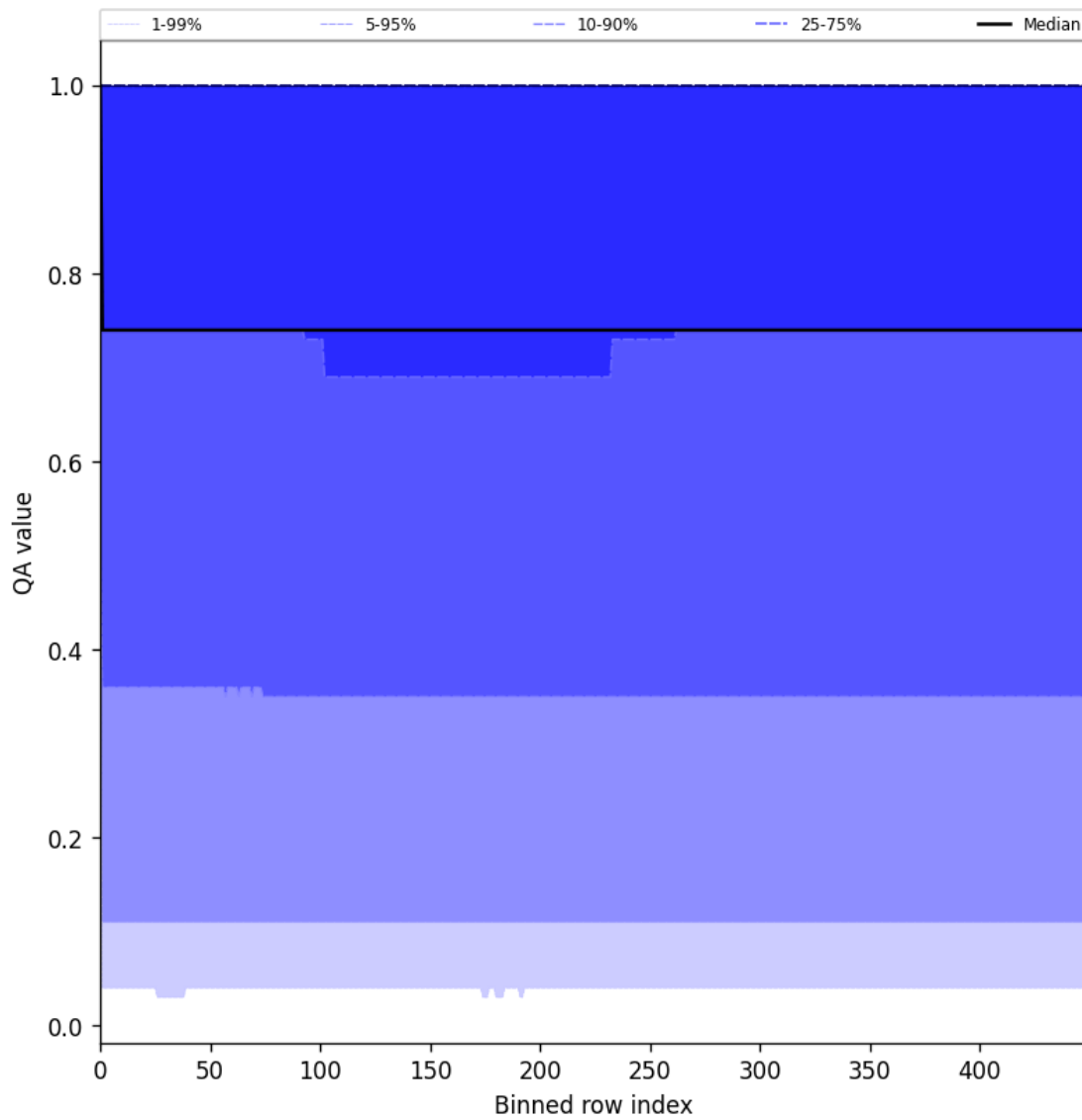
Figure 45: Along track statistics of “QA value” for 2025-07-24 to 2025-07-25
