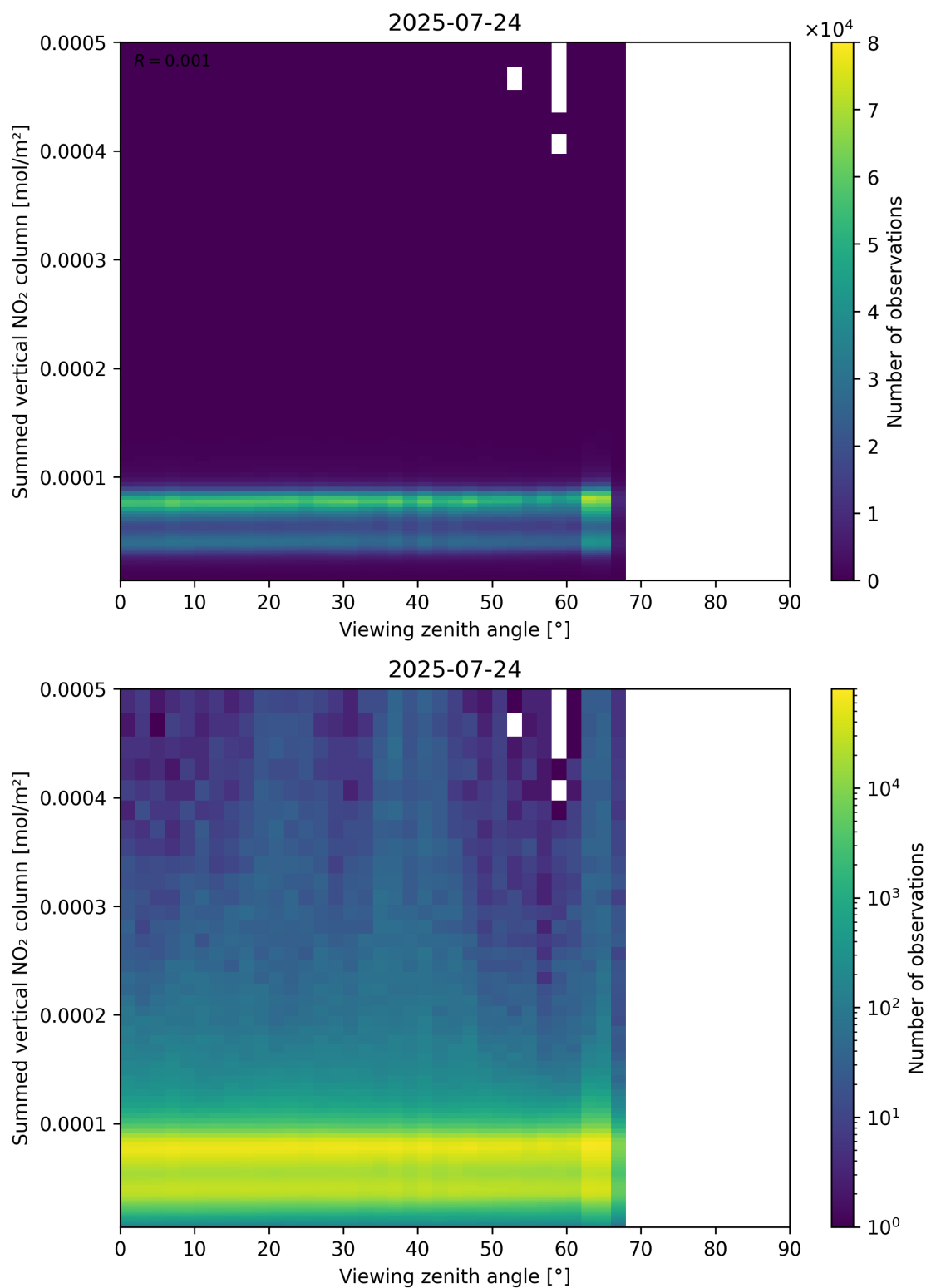
Figure 165: Scatter density plot of “Viewing zenith angle” against “Summed vertical NO 2 column” for 2025-07-24 to 2025-07-25.
