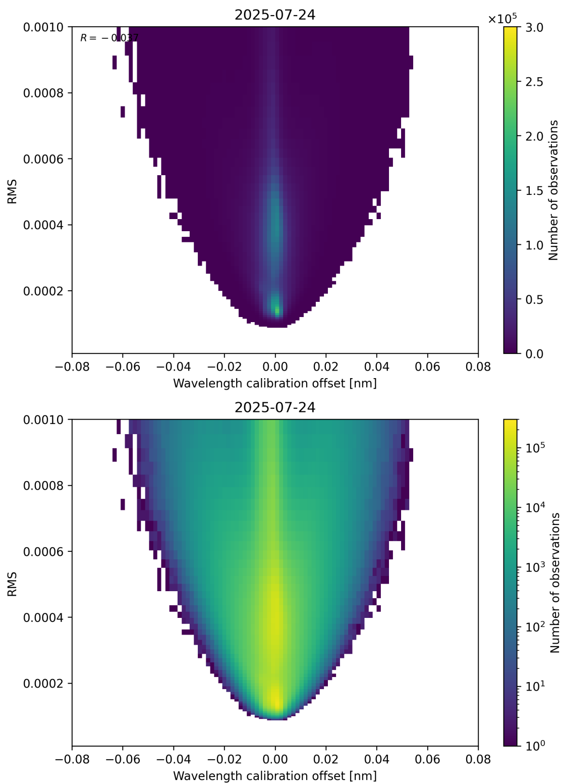
Figure 181: Scatter density plot of “Wavelength calibration offset” against “RMS” for 2025-07-24 to 2025-07-25.
