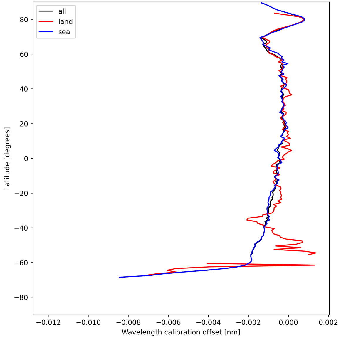
Figure 18: Zonal average of “Wavelength calibration offset” for 2025-07-24 to 2025-07-25.
