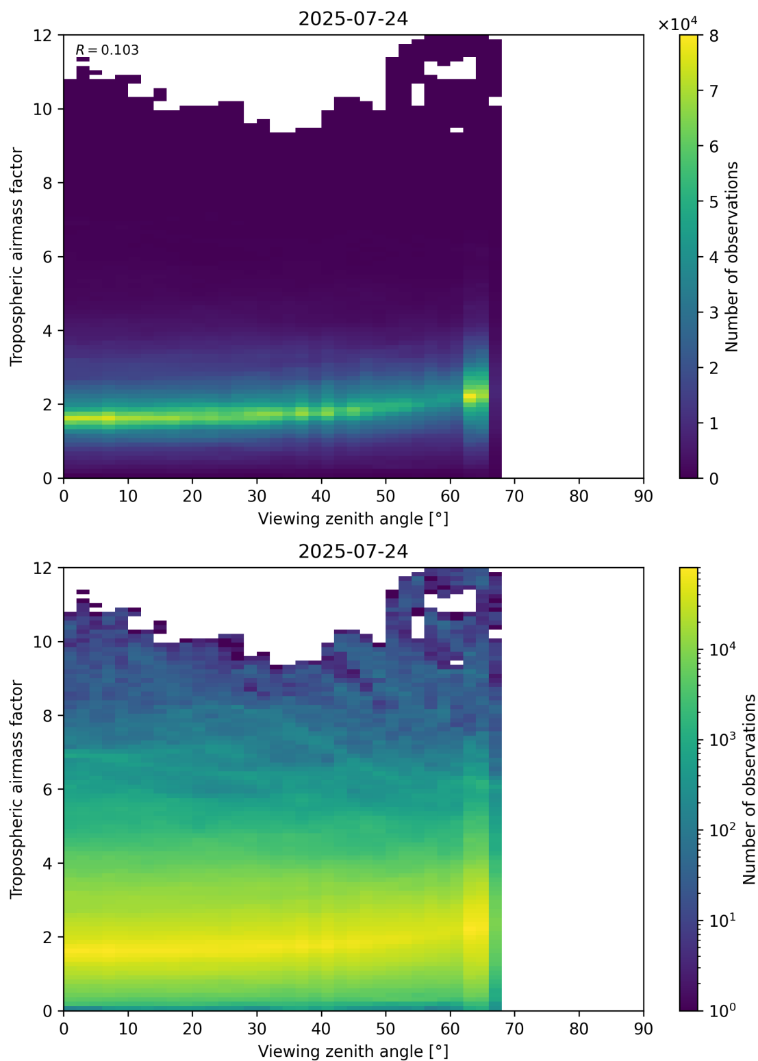
Figure 161: Scatter density plot of “Viewing zenith angle” against “Tropospheric airmass factor” for 2025-07-24 to 2025-07-25.
