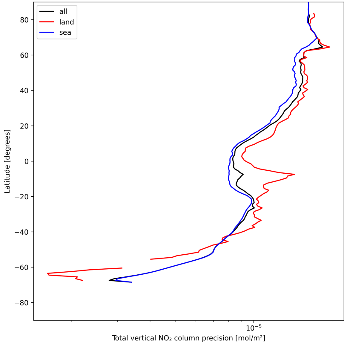
Figure 22: Zonal average of “Total vertical NO 2 column precision” for 2025-07-24 to 2025-07-25.
