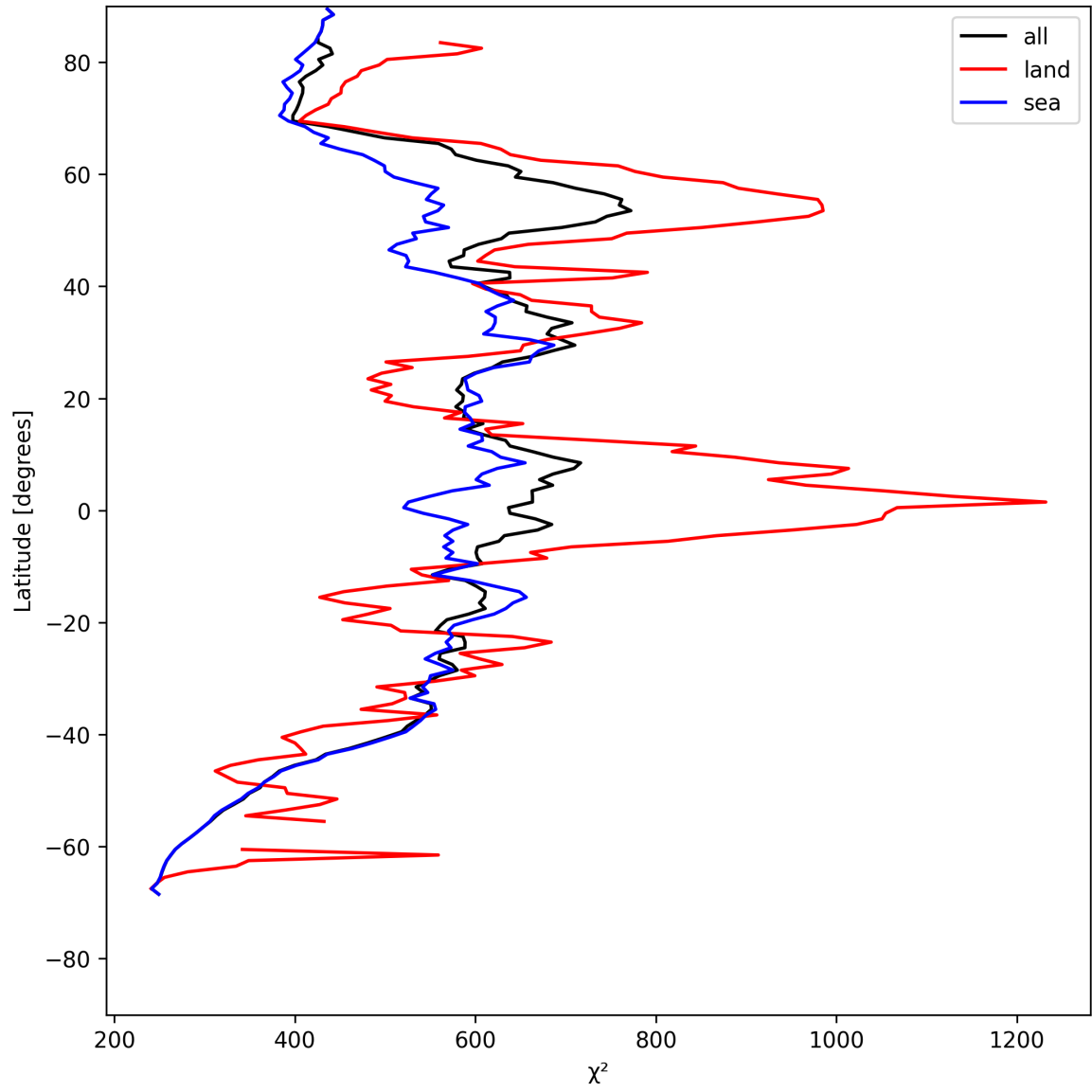
Figure 25: Zonal average of “ \chi^2 ” for 2025-07-24 to 2025-07-25.
