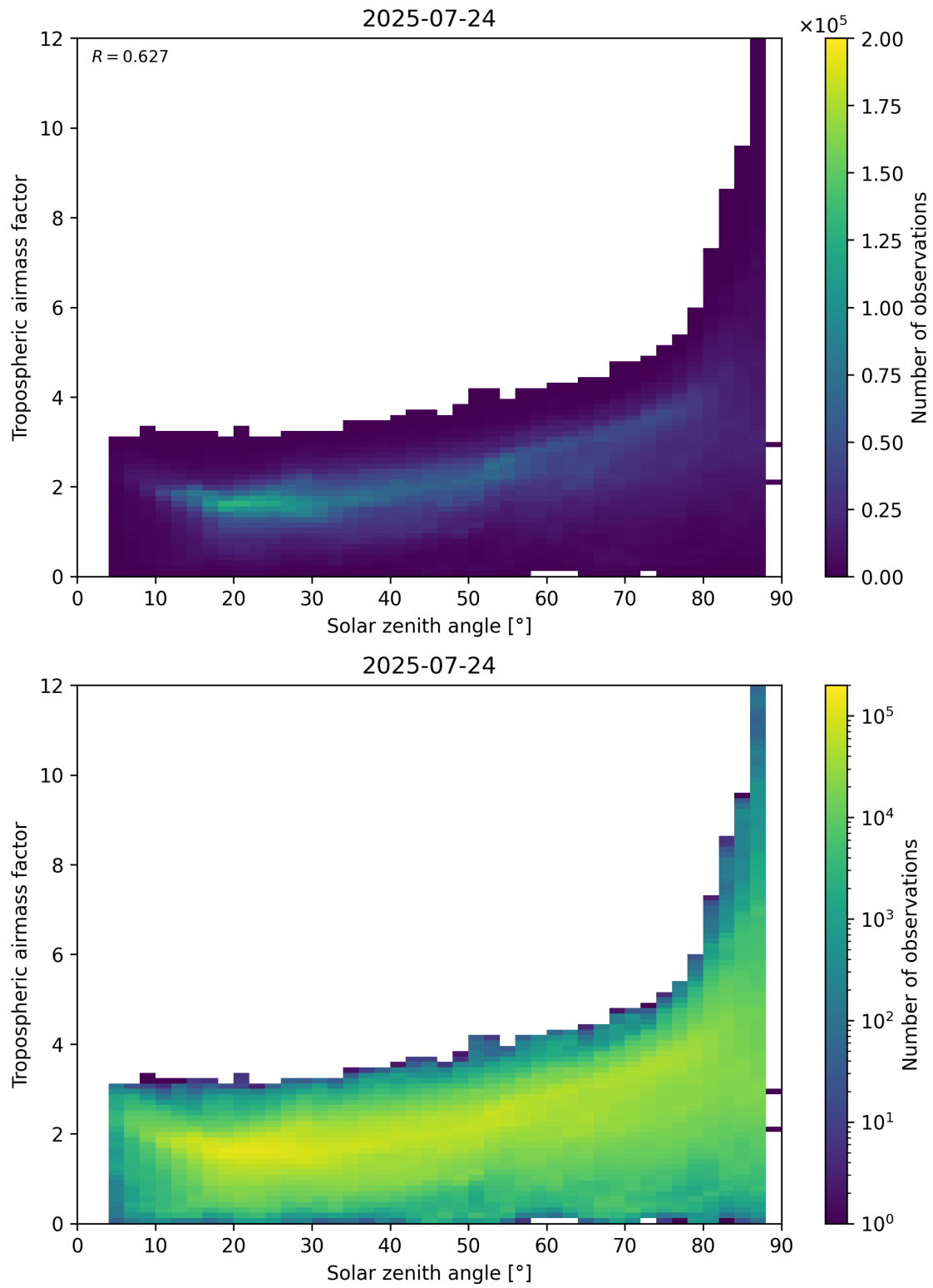
Figure 147: Scatter density plot of “Solar zenith angle” against “Tropospheric airmass factor” for 2025-07-24 to 2025-07-25.
