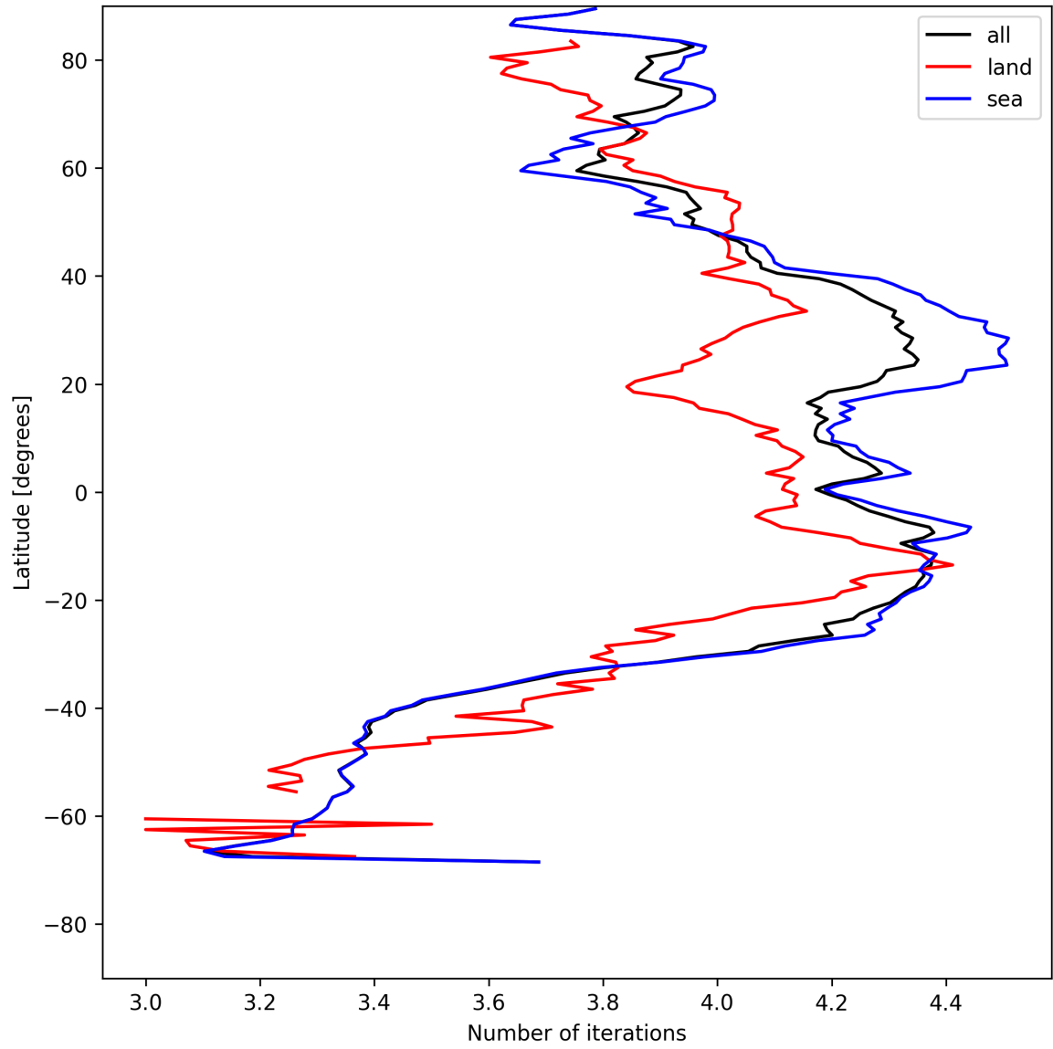
Figure 17: Zonal average of “Number of iterations” for 2025-07-24 to 2025-07-25.
