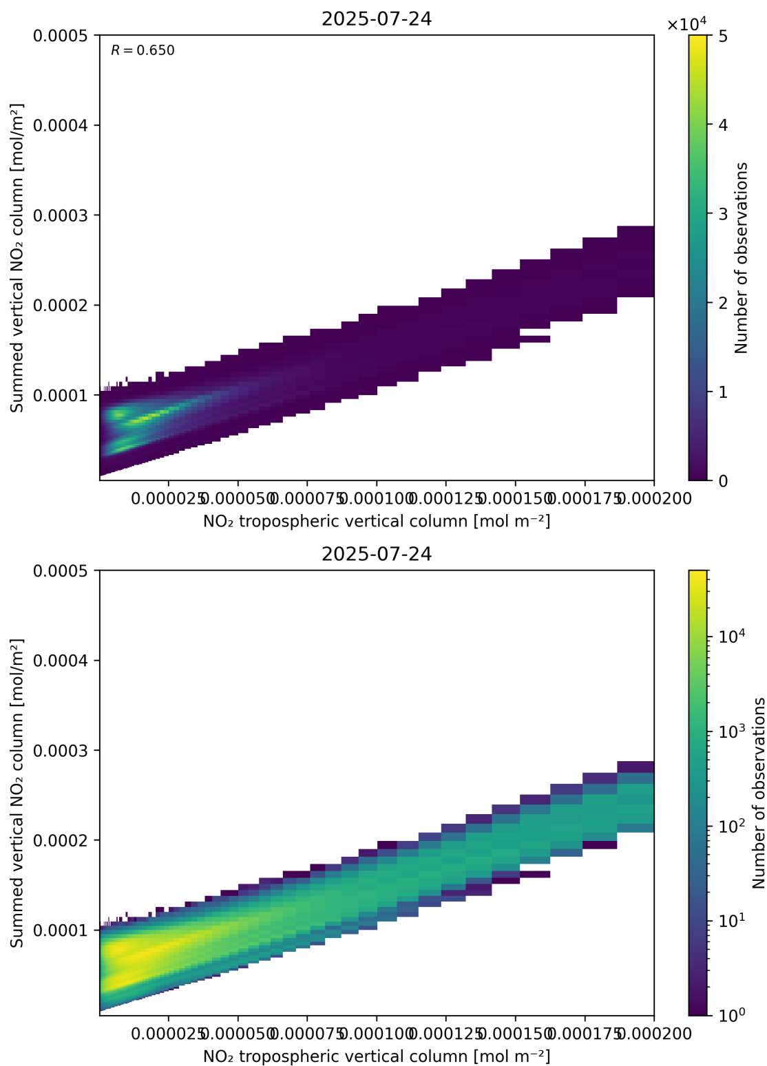
Figure 126: Scatter density plot of “NO 2 tropospheric vertical column” against “Summed vertical NO 2 column” for 2025-07-24 to 2025-07-25.
