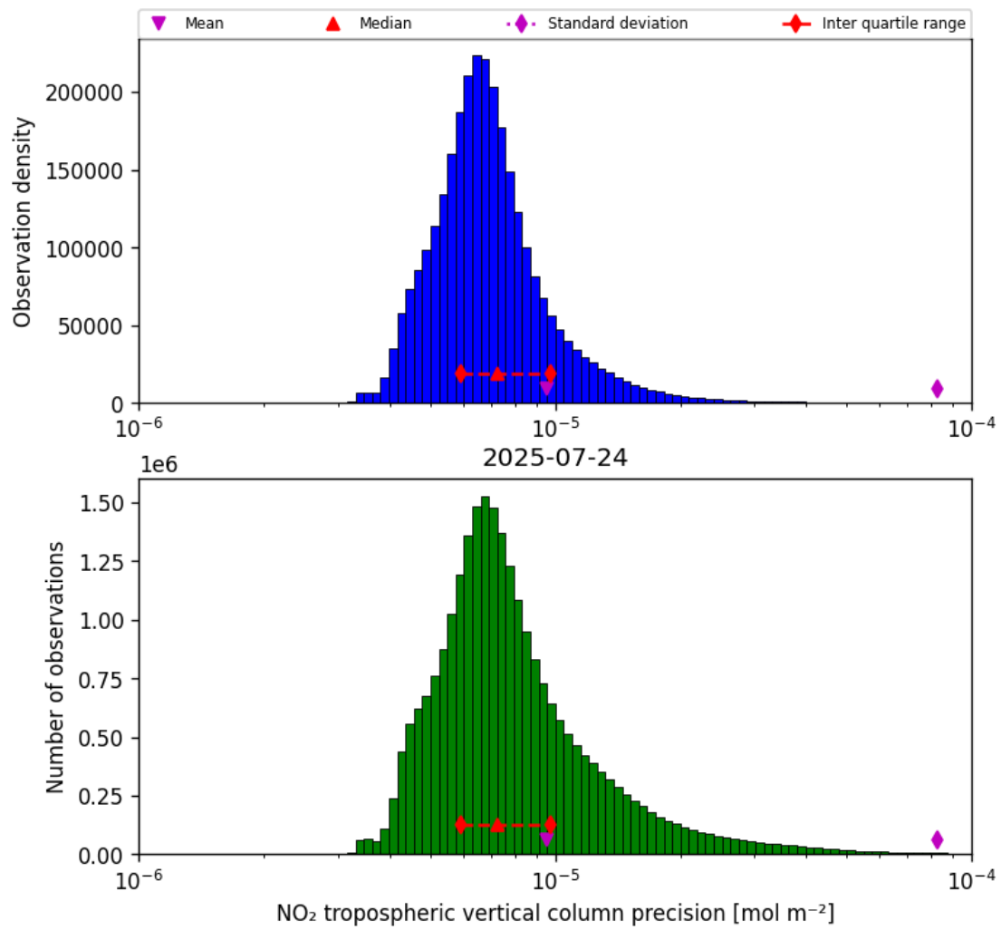
Figure 30: Histogram of “NO 2 tropospheric vertical column precision” for 2025-07-24 to 2025-07-25
