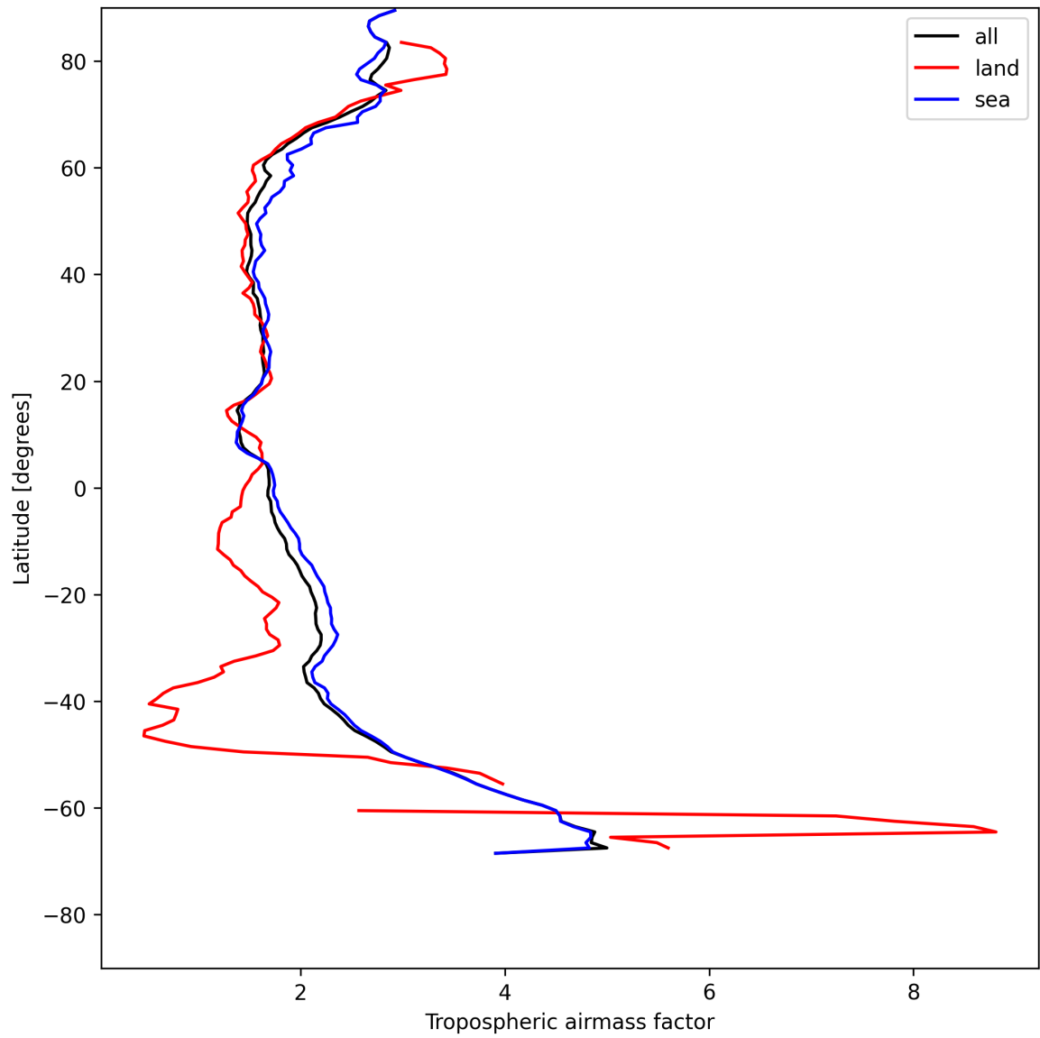
Figure 14: Zonal average of “Tropospheric air mass factor” for 2025-07-24 to 2025-07-25.
