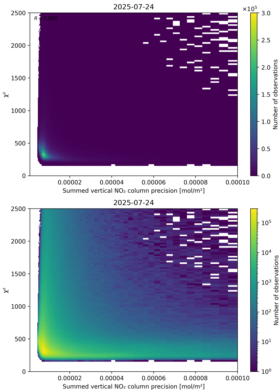
Figure 107: Scatter density plot of “Summed vertical NO 2 column precision” against “ \chi^2 ” for 2025-07-24 to 2025-07-25.
