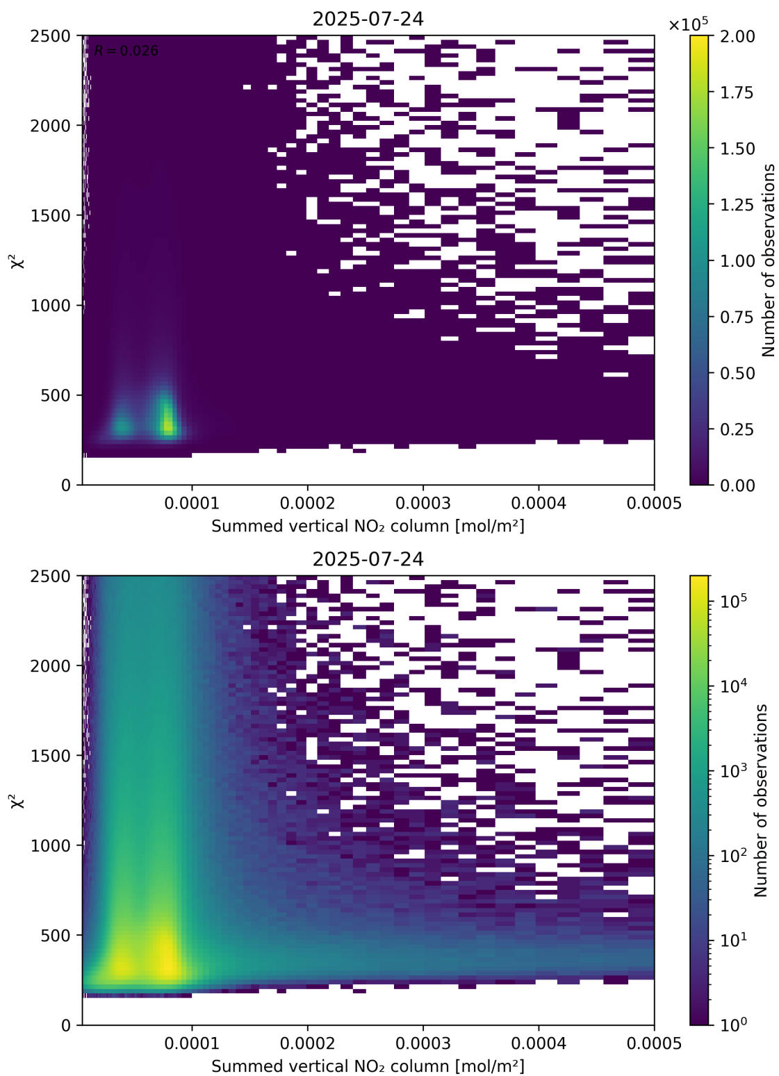
Figure 104: Scatter density plot of “Summed vertical NO 2 column” against “ \chi^2 ” for 2025-07-24 to 2025-07-25.
