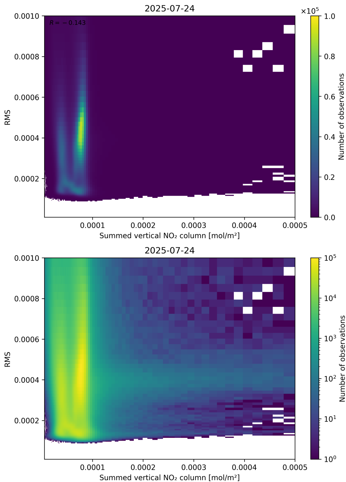
Figure 109: Scatter density plot of “Summed vertical NO 2 column” against “RMS” for 2025-07-24 to 2025-07-25.
