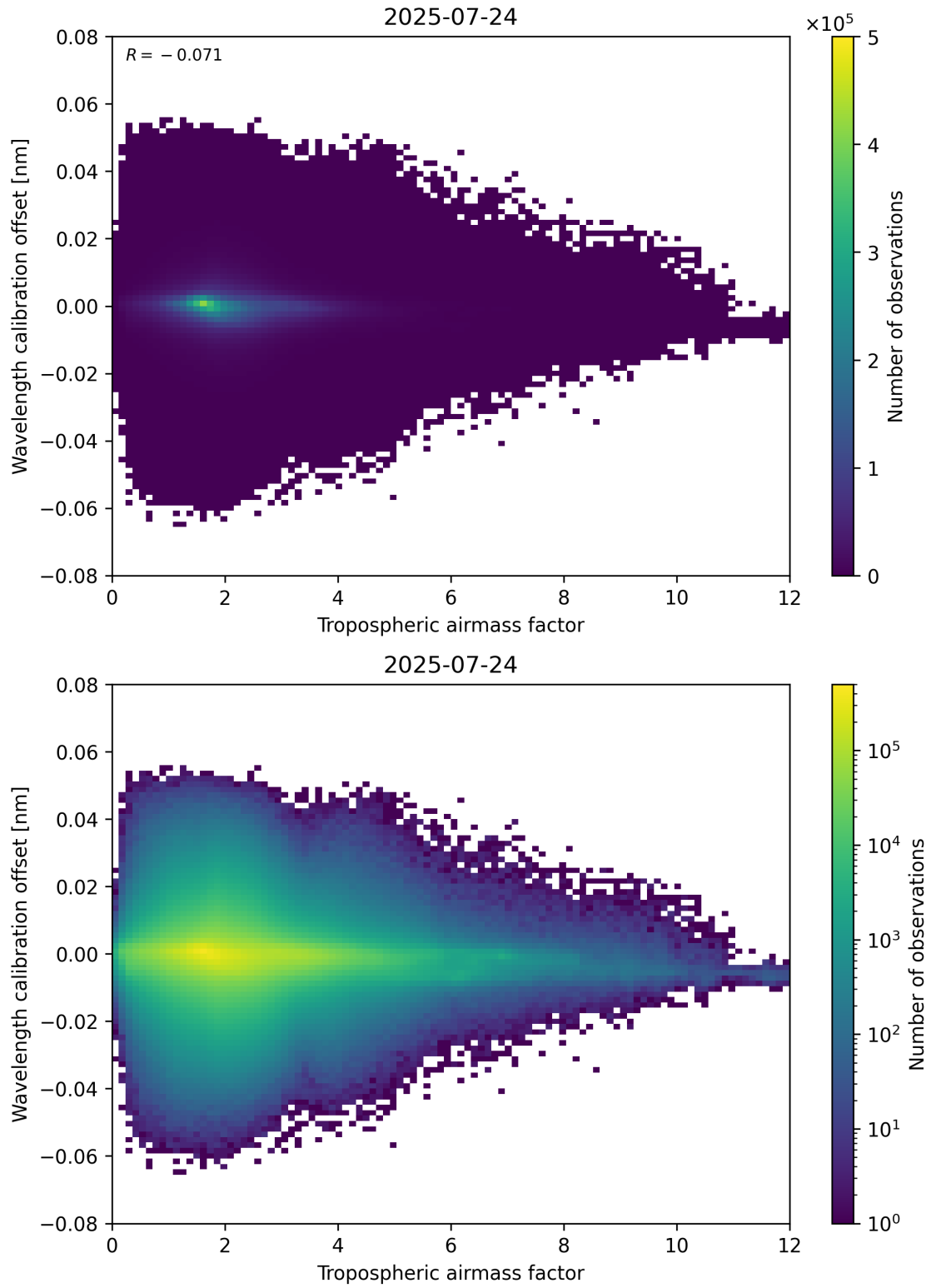
Figure 80: Scatter density plot of “Tropospheric airmass factor” against “Wavelength calibration offset” for 2025-07-24 to 2025-07-25.
