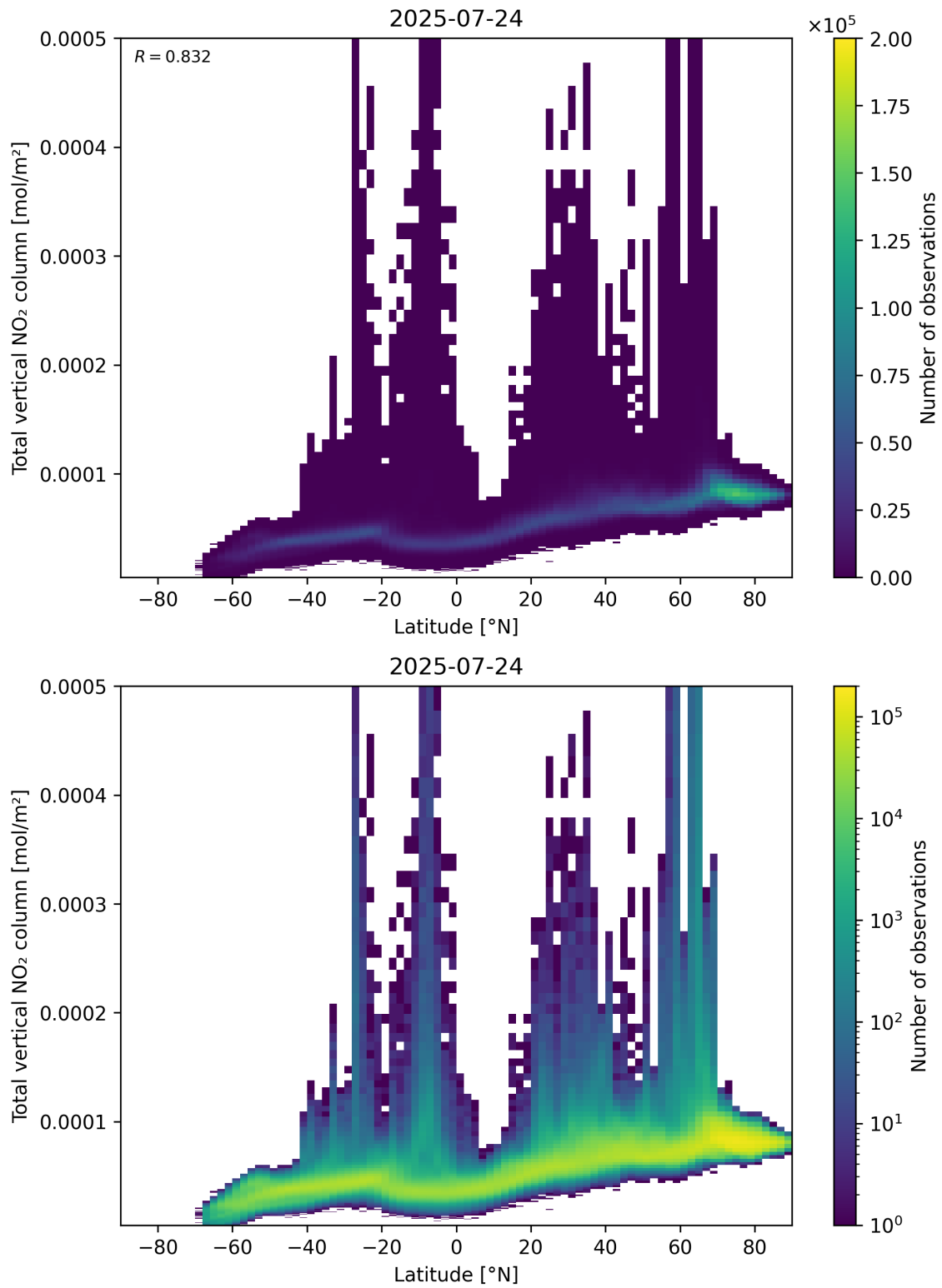
Figure 90: Scatter density plot of “Latitude” against “Total vertical NO 2 column” for 2025-07-24 to 2025-07-25.
