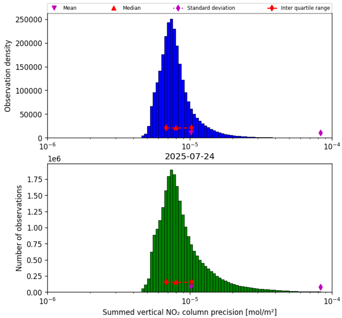
Figure 41: Histogram of “Summed vertical NO 2 column precision” for 2025-07-24 to 2025-07-25
