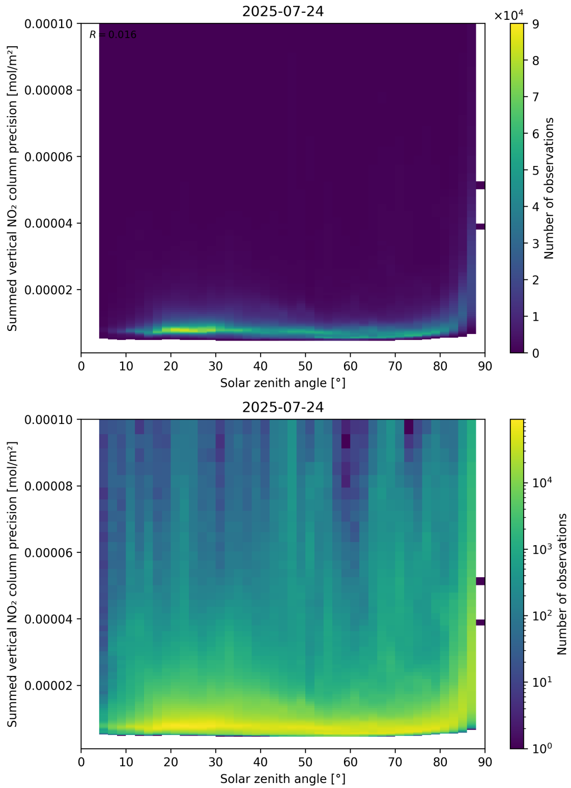
Figure 152: Scatter density plot of “Solar zenith angle” against “Summed vertical NO 2 column precision” for 2025-07-24 to 2025-07-25.
