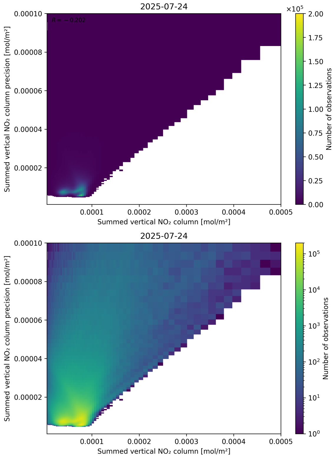
Figure 105: Scatter density plot of “Summed vertical NO 2 column” against “Summed vertical NO 2 column precision” for 2025-07-24 to 2025-07-25.
