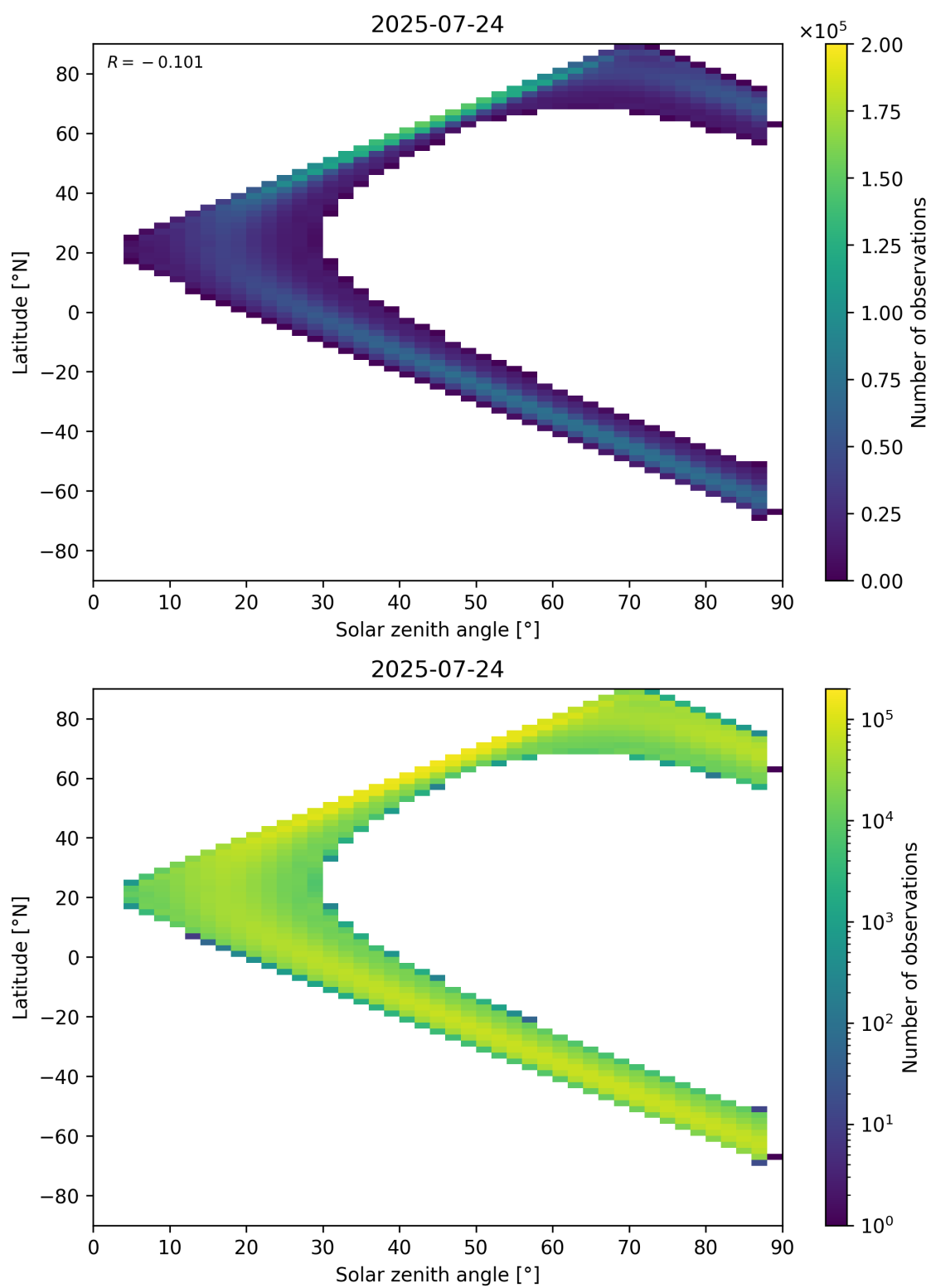
Figure 149: Scatter density plot of “Solar zenith angle” against “Latitude” for 2025-07-24 to 2025-07-25.
