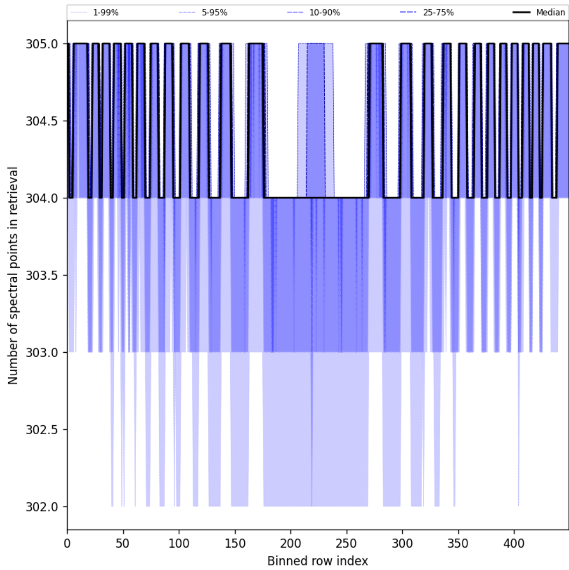
Figure 50: Along track statistics of “Number of spectral points in retrieval” for 2025-07-24 to 2025-07-25
