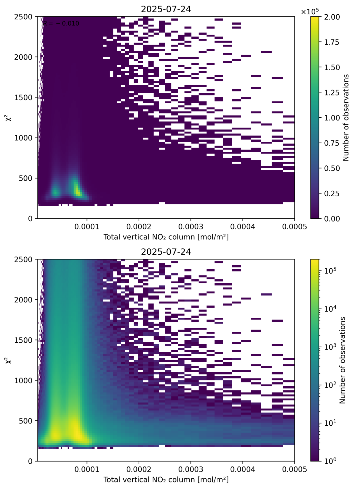
Figure 111: Scatter density plot of “Total vertical NO 2 column” against “ \chi^2 ” for 2025-07-24 to 2025-07-25.
