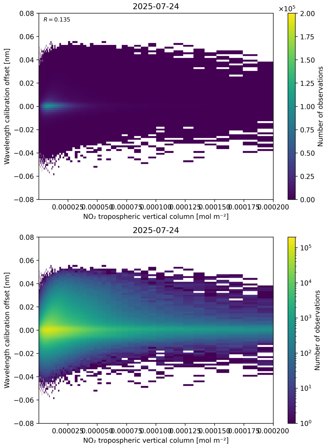
Figure 143: Scatter density plot of “NO 2 tropospheric vertical column” against “Wavelength calibration offset” for 2025-07-24 to 2025-07-25.
