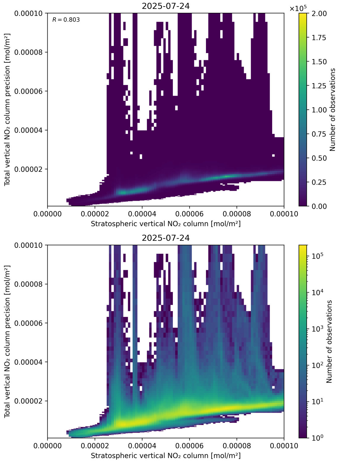
Figure 101: Scatter density plot of “Stratospheric vertical NO 2 column” against “Total vertical NO 2 column precision” for 2025-07-24 to 2025-07-25.
