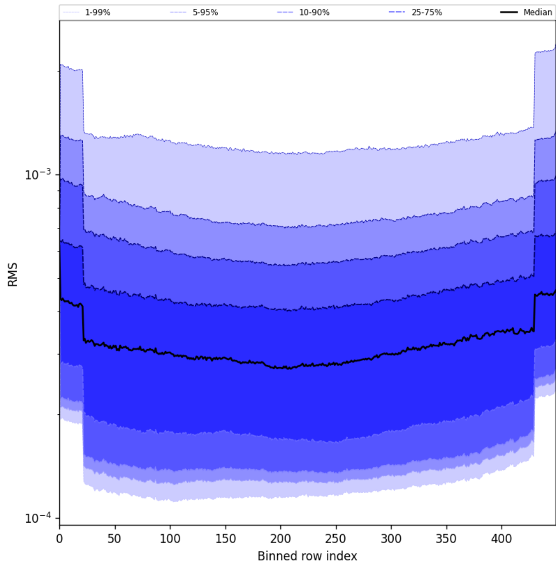
Figure 60: Along track statistics of “RMS” for 2025-07-24 to 2025-07-25
