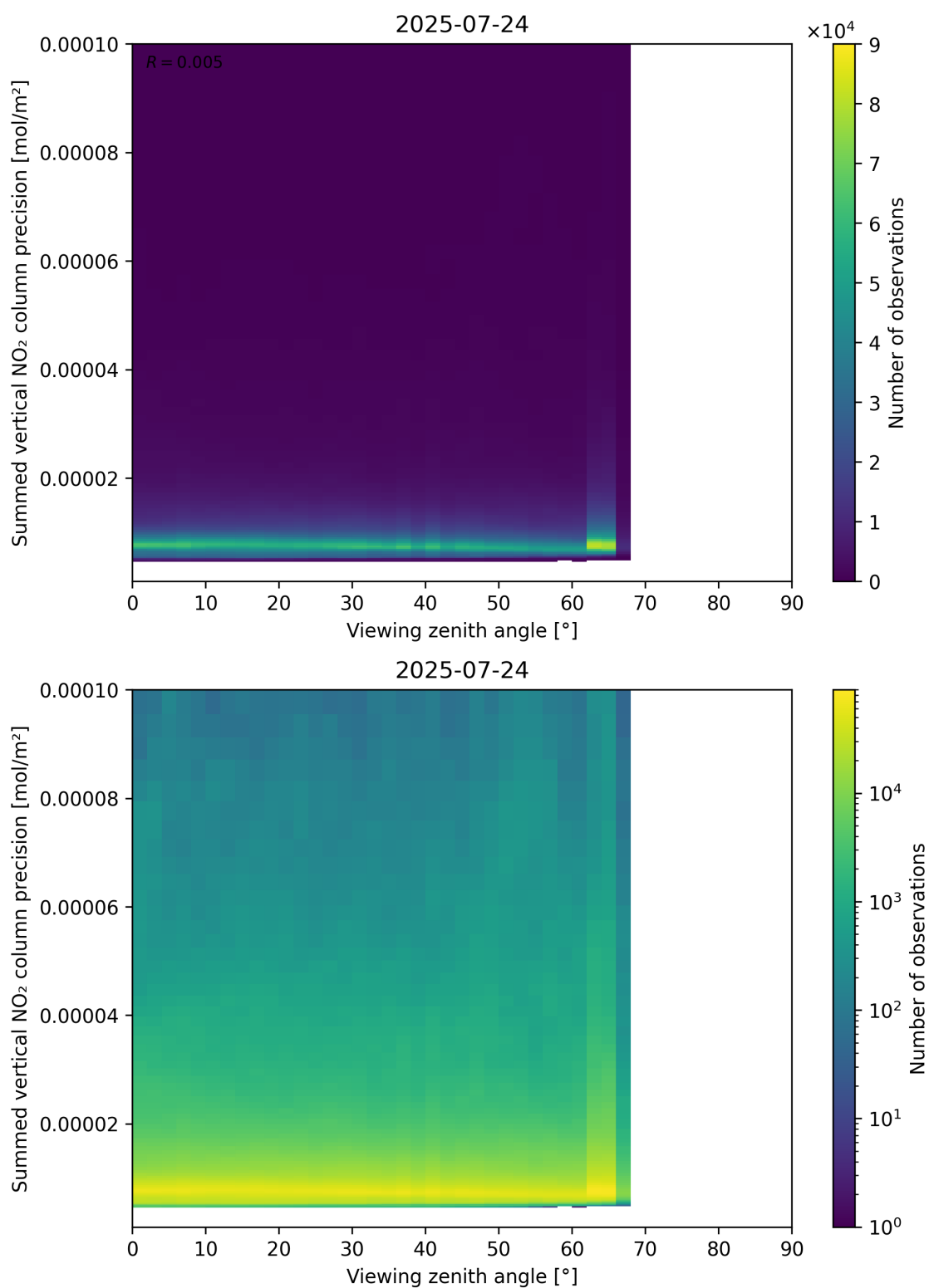
Figure 166: Scatter density plot of “Viewing zenith angle” against “Summed vertical NO 2 column precision” for 2025-07-24 to 2025-07-25.
