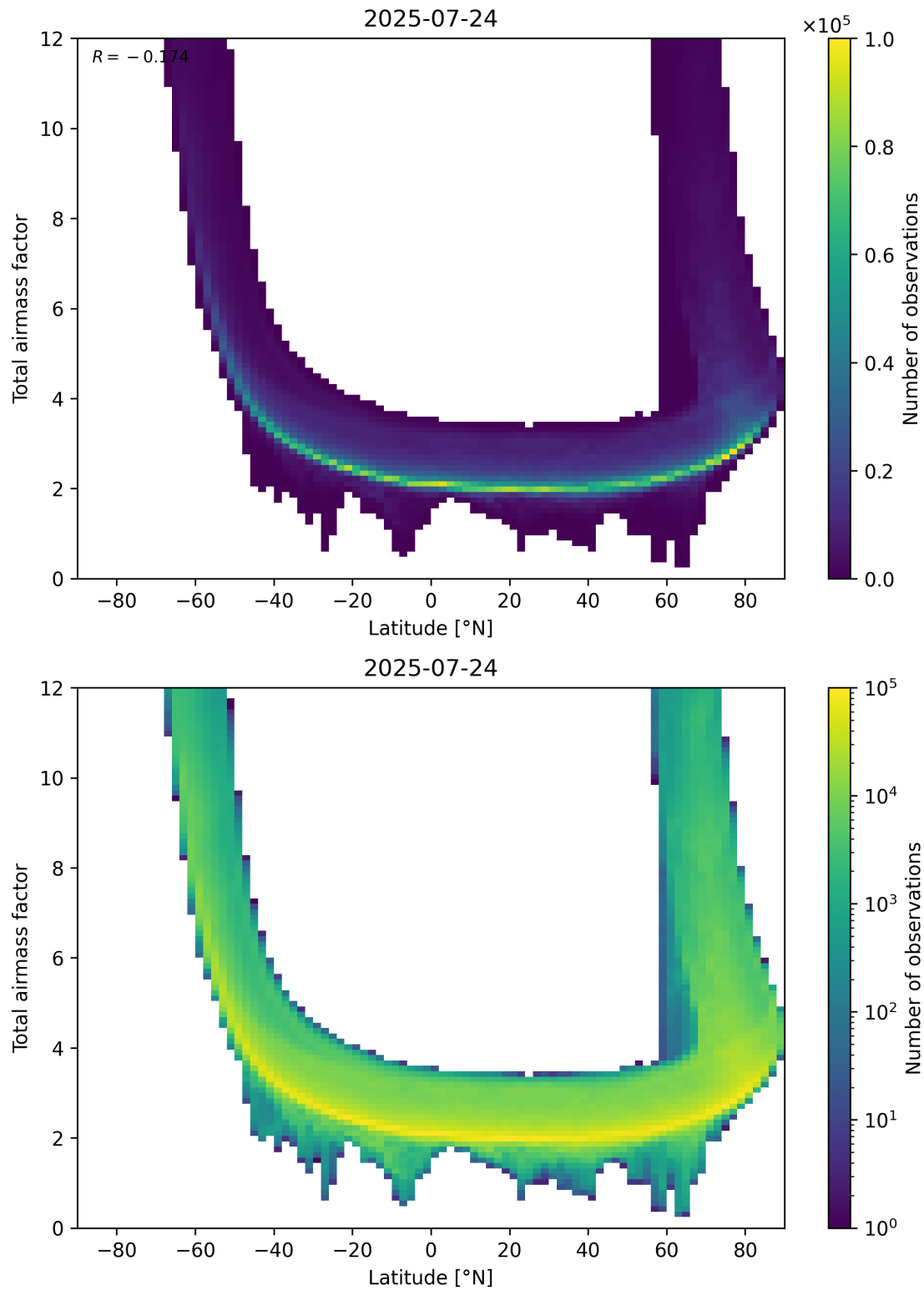
Figure 84: Scatter density plot of “Latitude” against “Total airmass factor” for 2025-07-24 to 2025-07-25.
