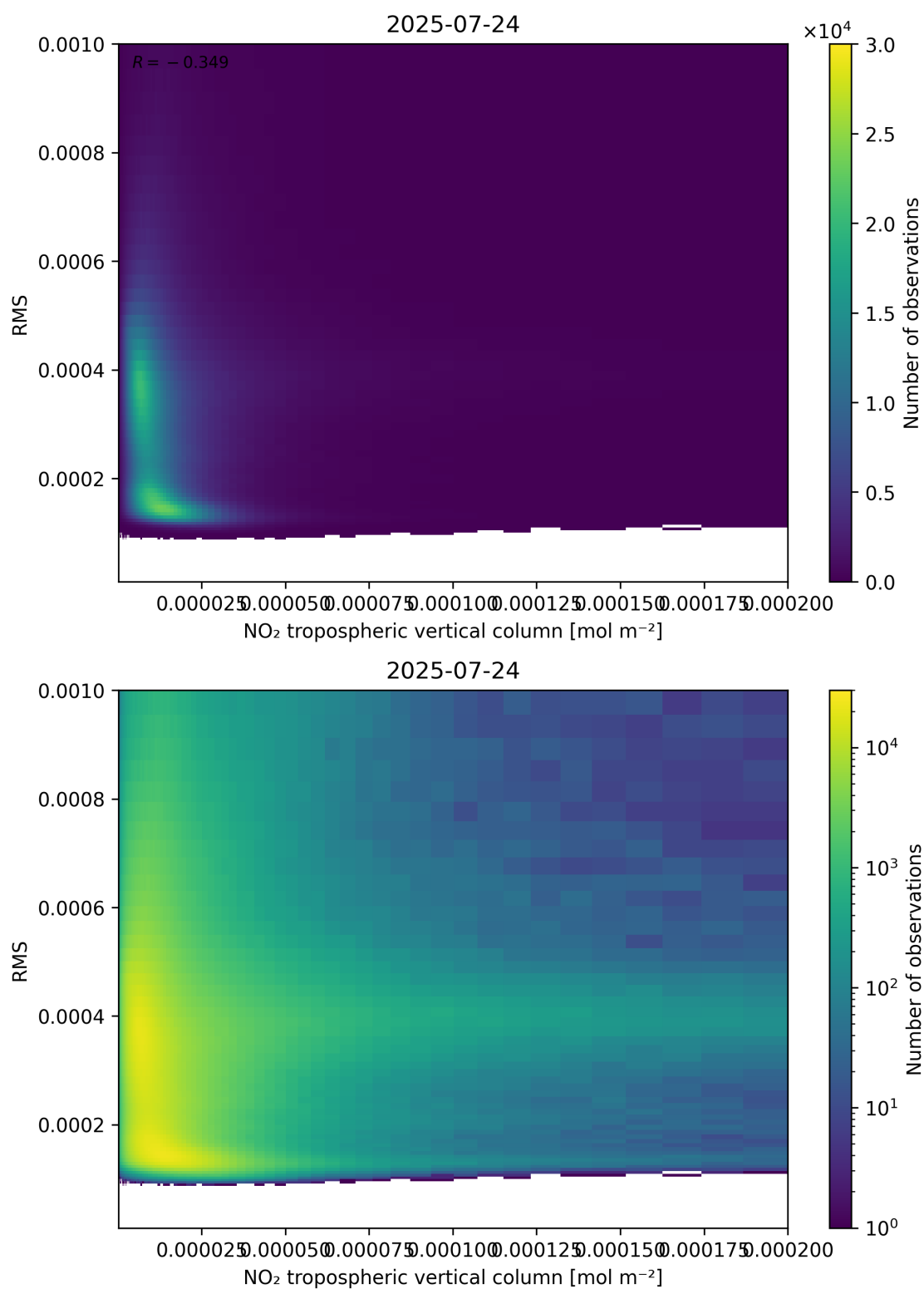
Figure 142: Scatter density plot of “NO 2 tropospheric vertical column” against “RMS” for 2025-07-24 to 2025-07-25.
