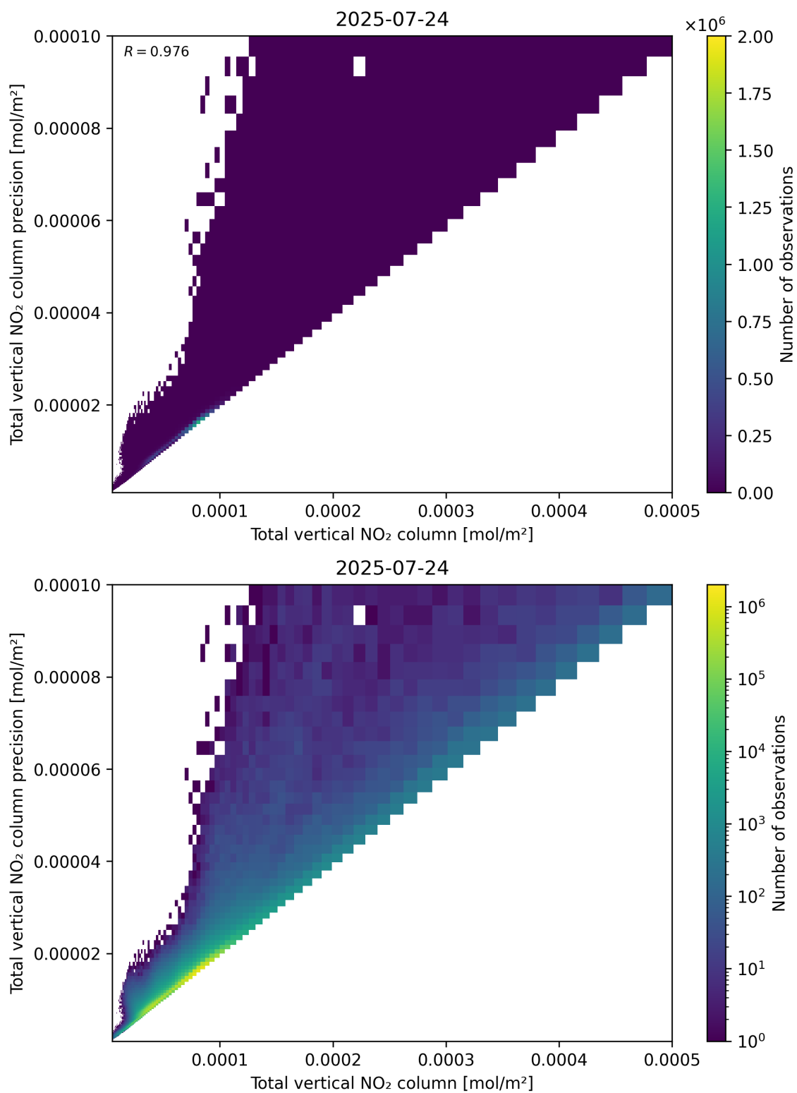
Figure 114: Scatter density plot of “Total vertical NO 2 column” against “Total vertical NO 2 column precision” for 2025-07-24 to 2025-07-25.
