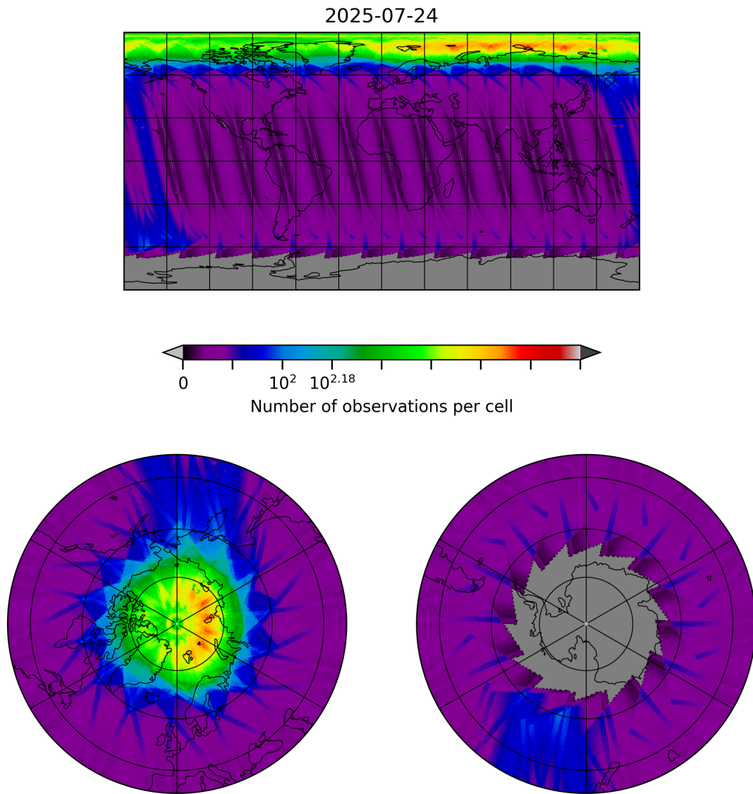
Figure 10: Map of the number of observations for 2025-07-24 to 2025-07-25
