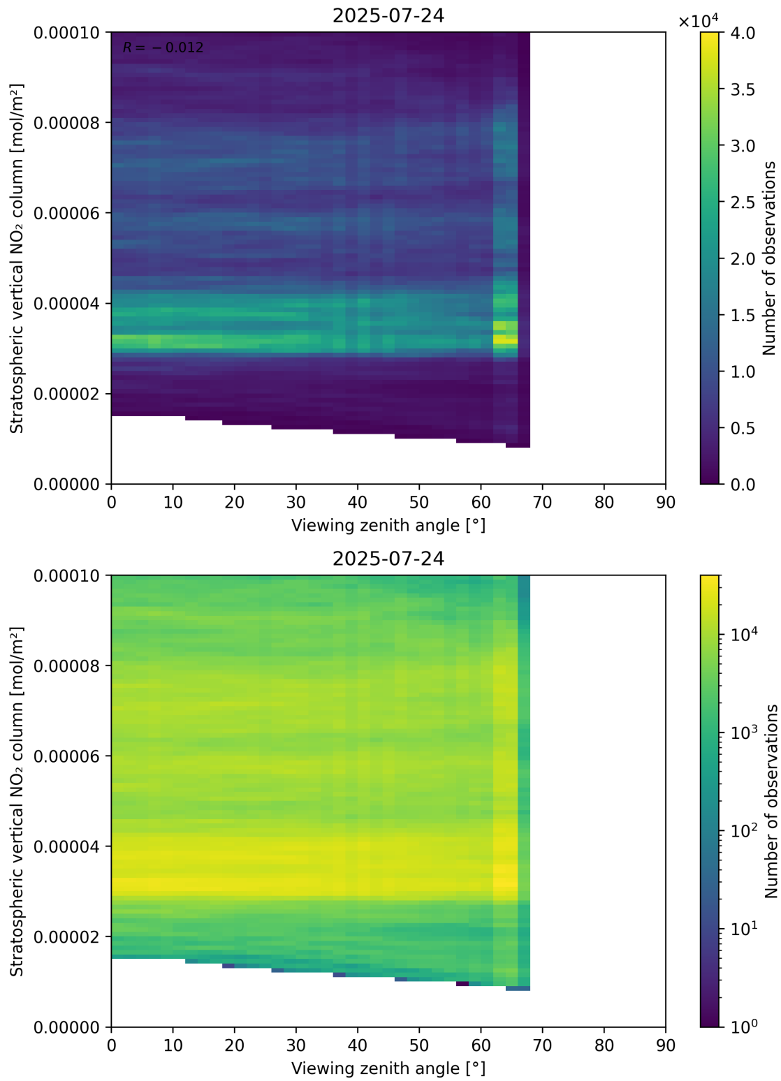
Figure 164: Scatter density plot of “Viewing zenith angle” against “Stratospheric vertical NO 2 column” for 2025-07-24 to 2025-07-25.
