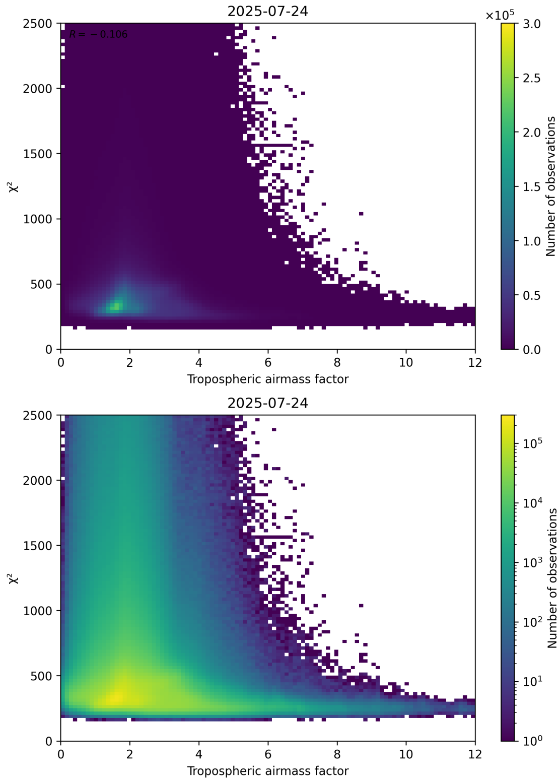
Figure 73: Scatter density plot of “Tropospheric airmass factor” against “ \chi^2 ” for 2025-07-24 to 2025-07-25.
