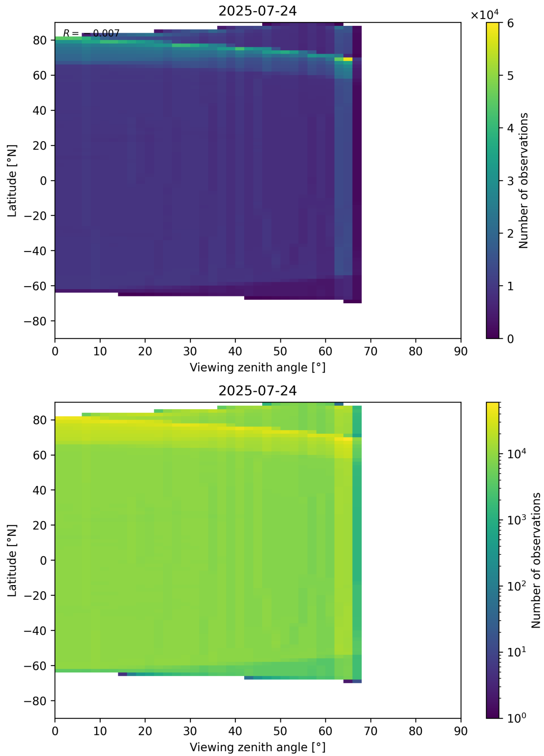
Figure 163: Scatter density plot of “Viewing zenith angle” against “Latitude” for 2025-07-24 to 2025-07-25.
