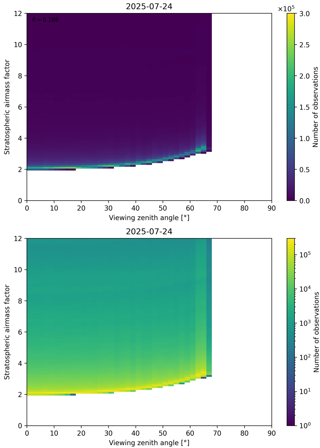
Figure 159: Scatter density plot of “Viewing zenith angle” against “Stratospheric airmass factor” for 2025-07-24 to 2025-07-25.
