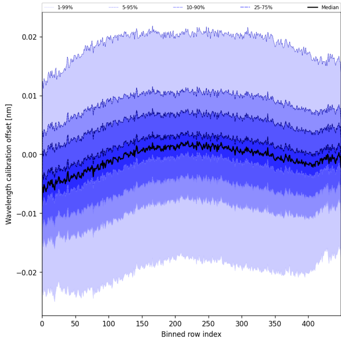
Figure 52: Along track statistics of “Wavelength calibration offset” for 2025-07-24 to 2025-07-25
