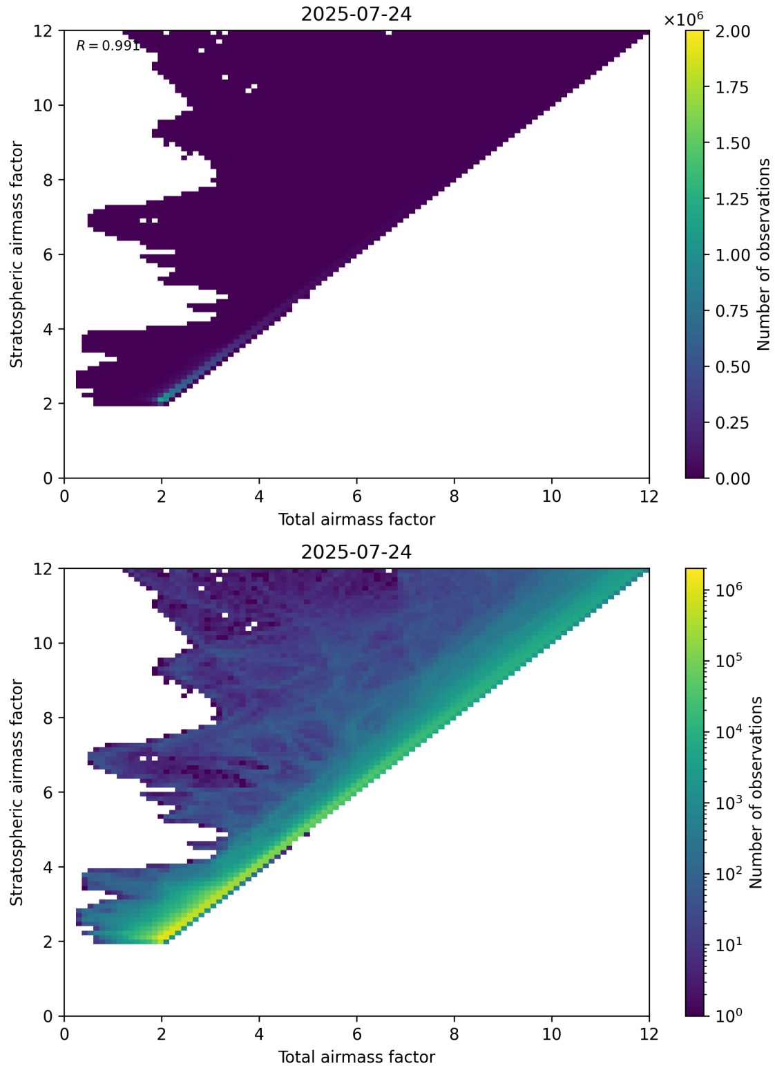
Figure 62: Scatter density plot of “Total airmass factor” against “Stratospheric airmass factor” for 2025-07-24 to 2025-07-25.
