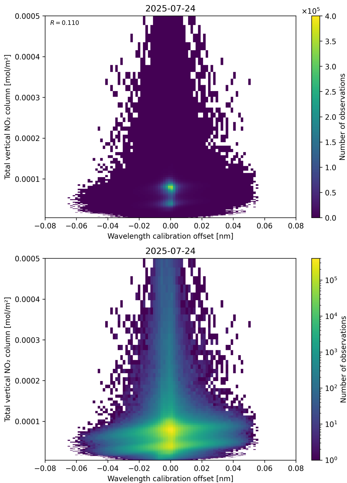
Figure 179: Scatter density plot of “Wavelength calibration offset” against “Total vertical NO 2 column” for 2025-07-24 to 2025-07-25.
