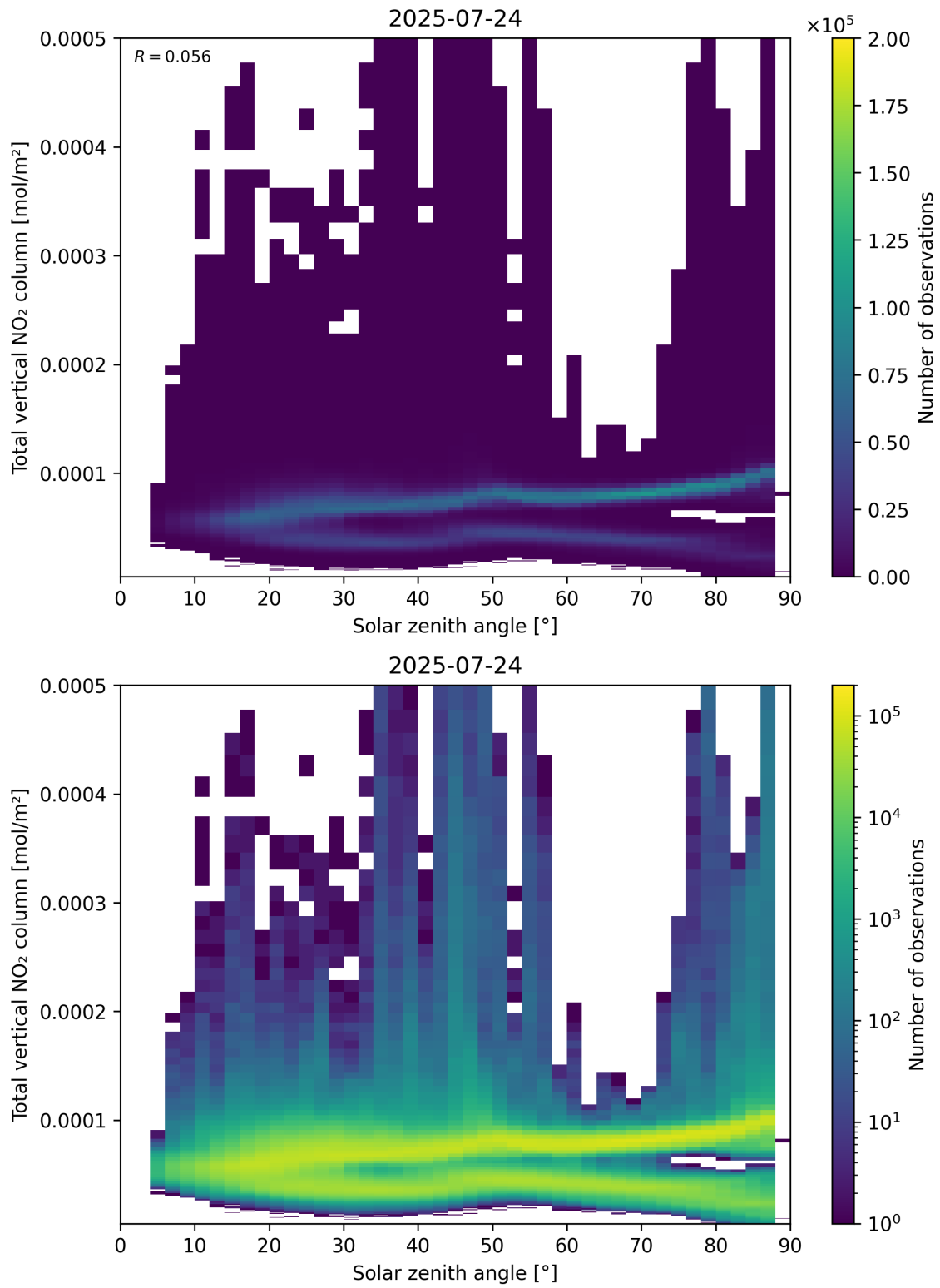
Figure 153: Scatter density plot of “Solar zenith angle” against “Total vertical NO 2 column” for 2025-07-24 to 2025-07-25.
