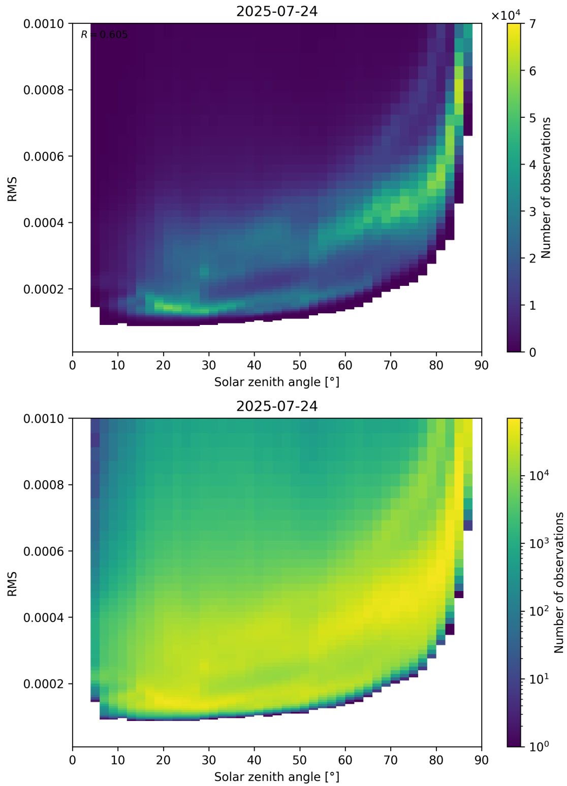
Figure 157: Scatter density plot of “Solar zenith angle” against “RMS” for 2025-07-24 to 2025-07-25.
