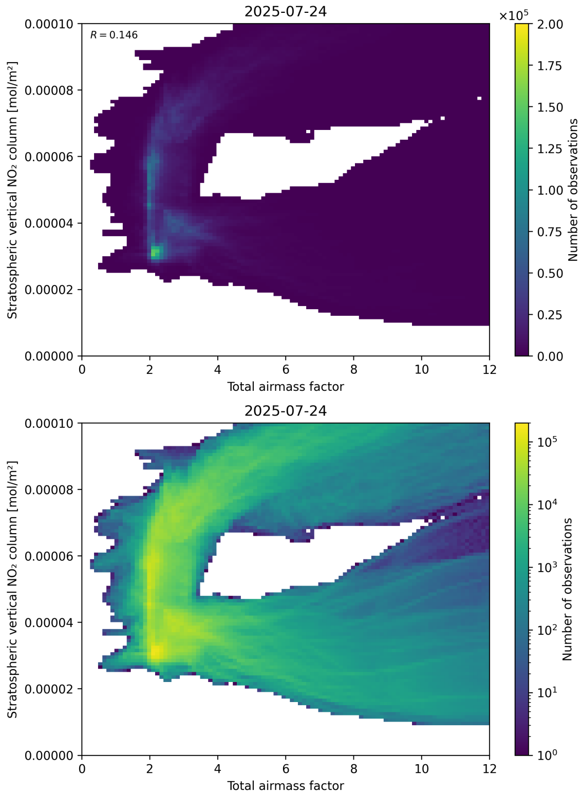
Figure 64: Scatter density plot of “Total airmass factor” against “Stratospheric vertical \text{NO}_2 column” for 2025-07-24 to 2025-07-25.
