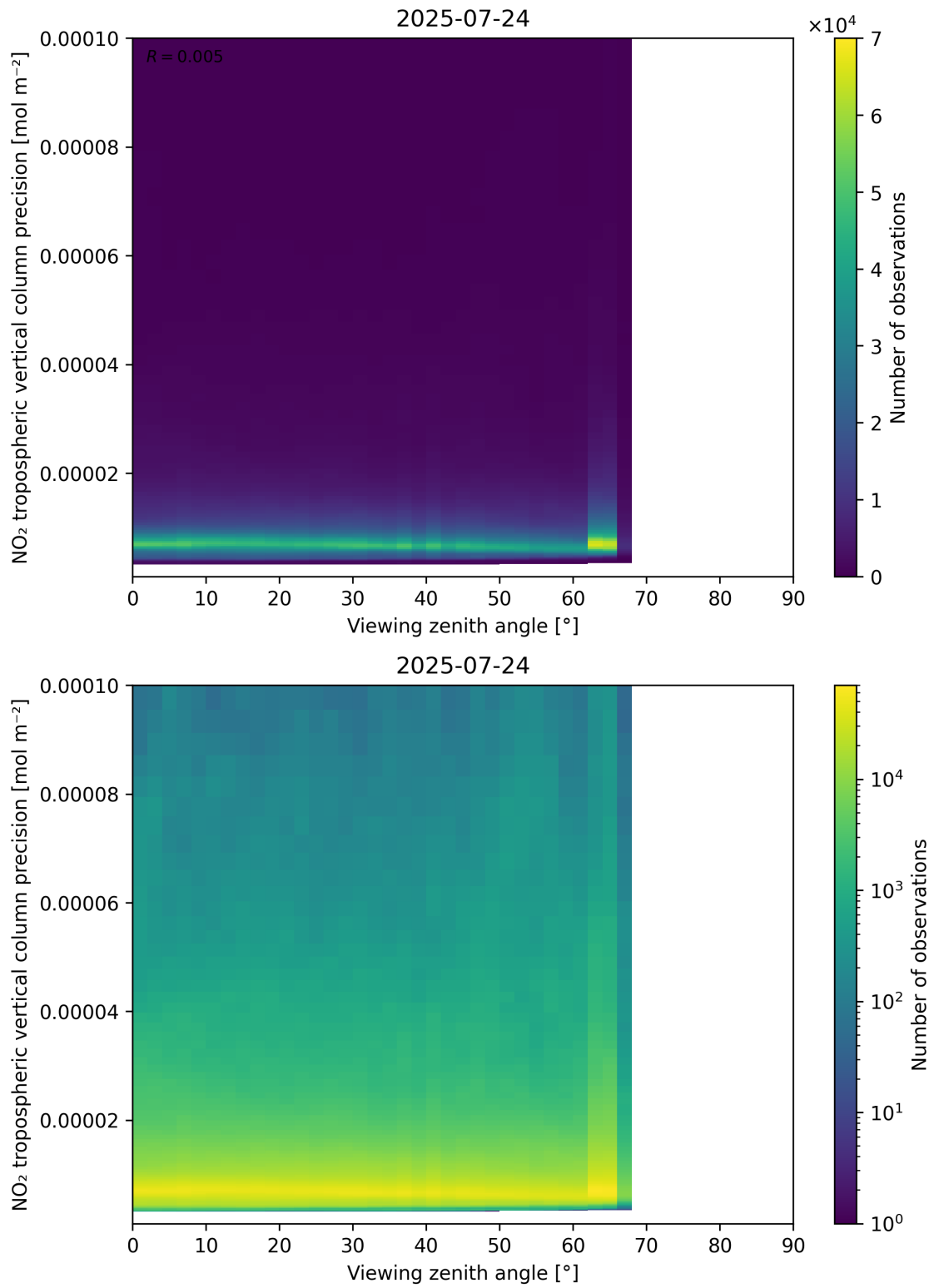
Figure 170: Scatter density plot of “Viewing zenith angle” against “NO 2 tropospheric vertical column precision” for 2025-07-24 to 2025-07-25.
