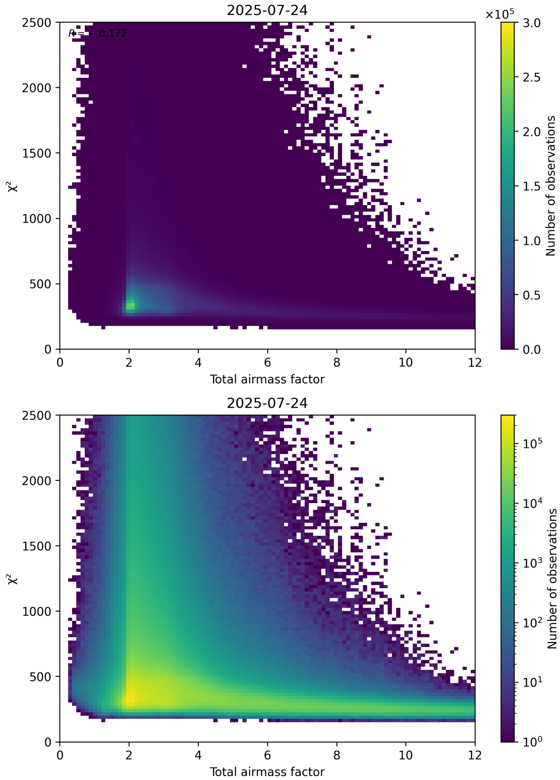
Figure 63: Scatter density plot of “Total airmass factor” against “ \chi^2 ” for 2025-07-24 to 2025-07-25.
