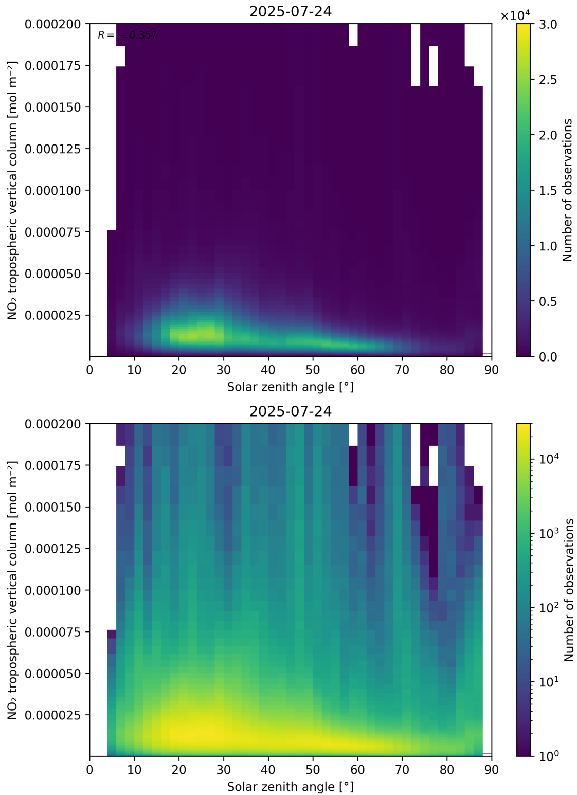
Figure 155: Scatter density plot of “Solar zenith angle” against “NO 2 tropospheric vertical column” for 2025-07-24 to 2025-07-25.
