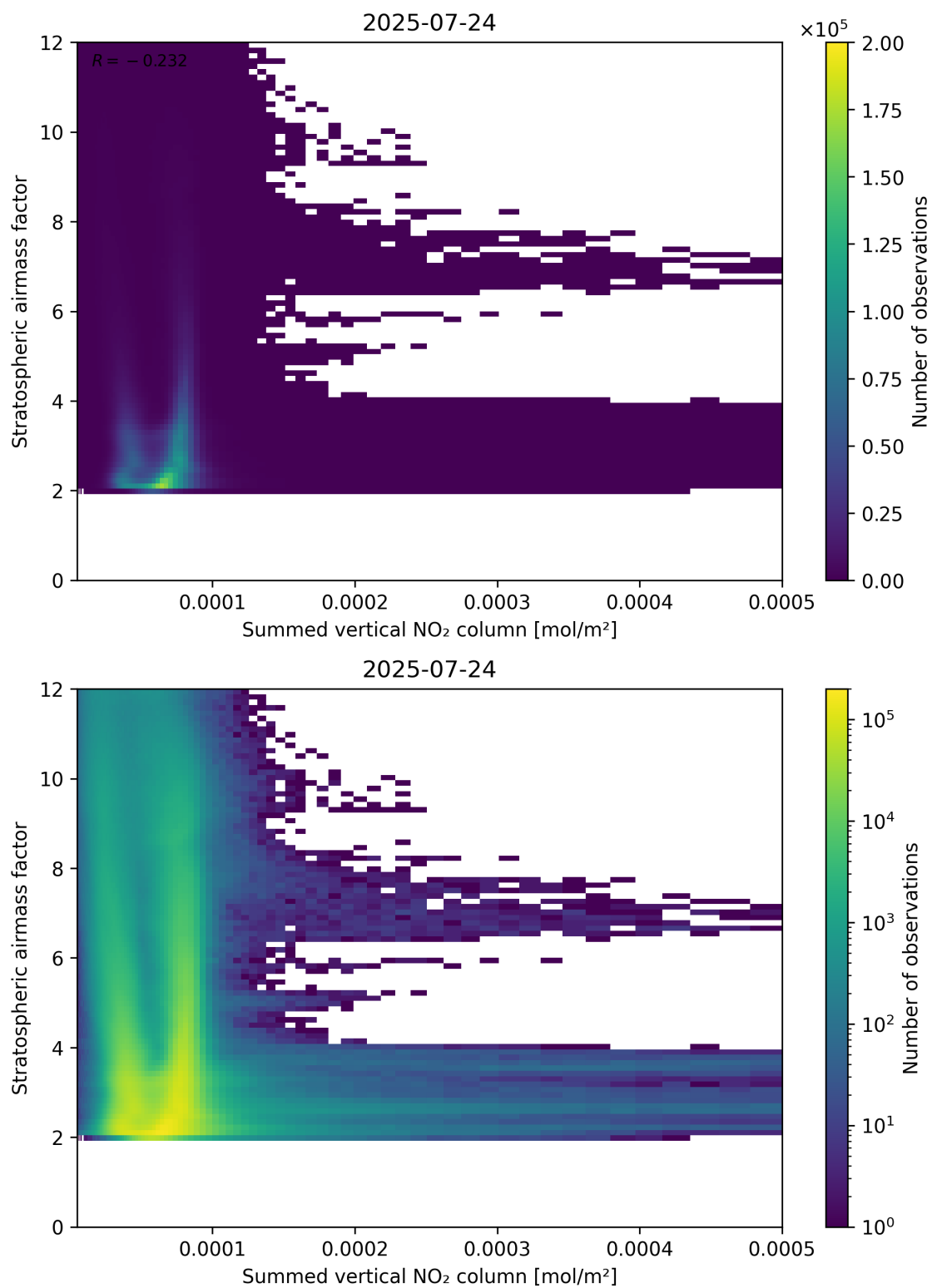
Figure 103: Scatter density plot of “Summed vertical NO 2 column” against “Stratospheric airmass factor” for 2025-07-24 to 2025-07-25.
