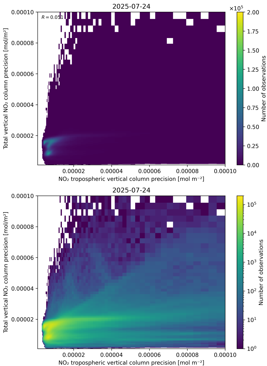
Figure 139: Scatter density plot of “NO 2 tropospheric vertical column precision” against “Total vertical NO 2 column precision” for 2025-07-24 to 2025-07-25.
