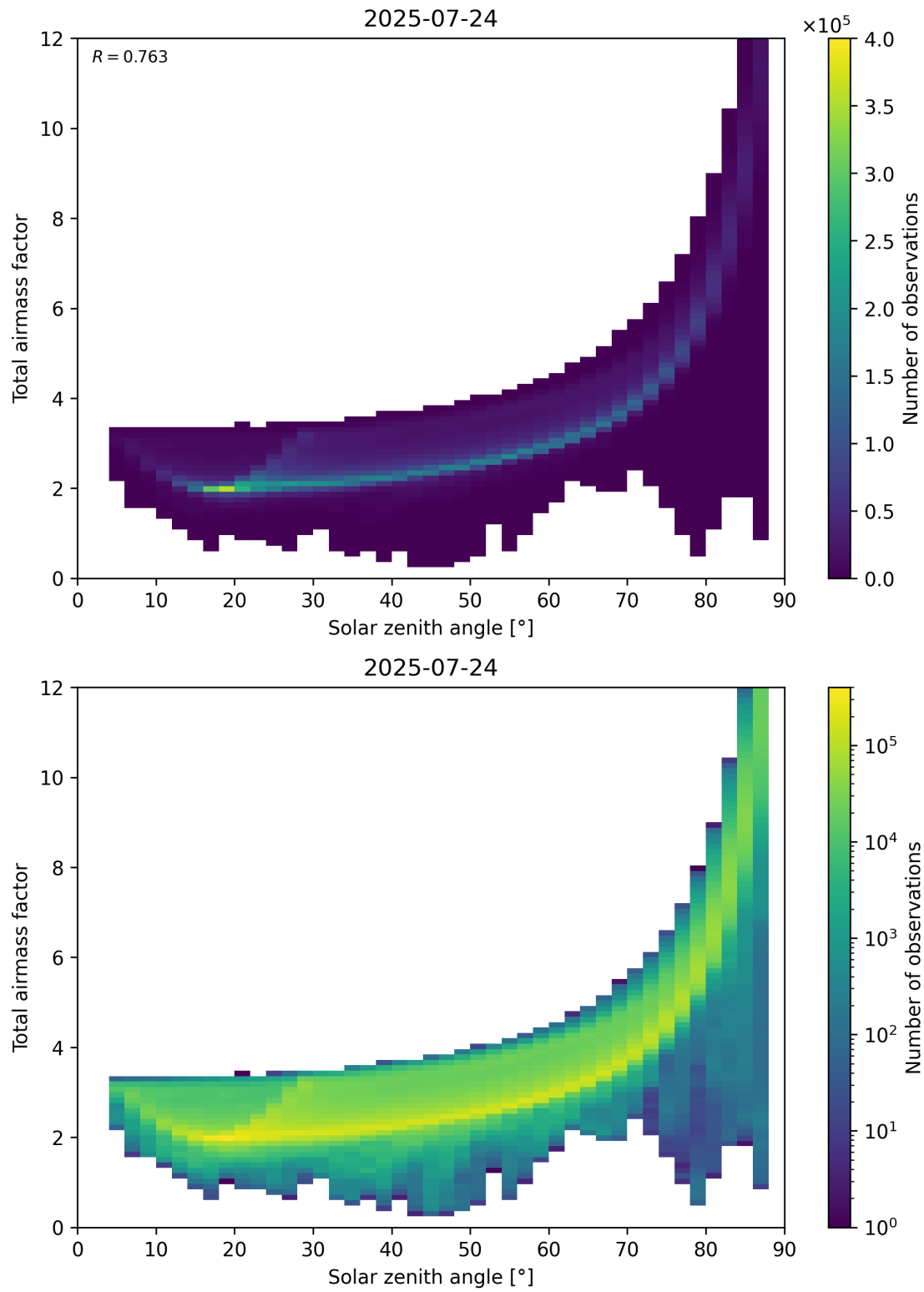
Figure 146: Scatter density plot of “Solar zenith angle” against “Total air mass factor” for 2025-07-24 to 2025-07-25.
