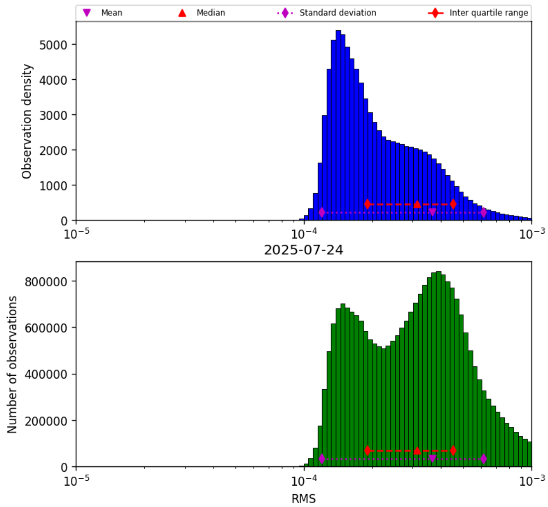
Figure 43: Histogram of “RMS” for 2025-07-24 to 2025-07-25
