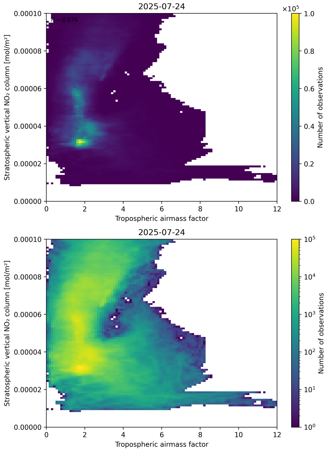
Figure 74: Scatter density plot of “Tropospheric air mass factor” against “Stratospheric vertical NO 2 column” for 2025-07-24 to 2025-07-25.
