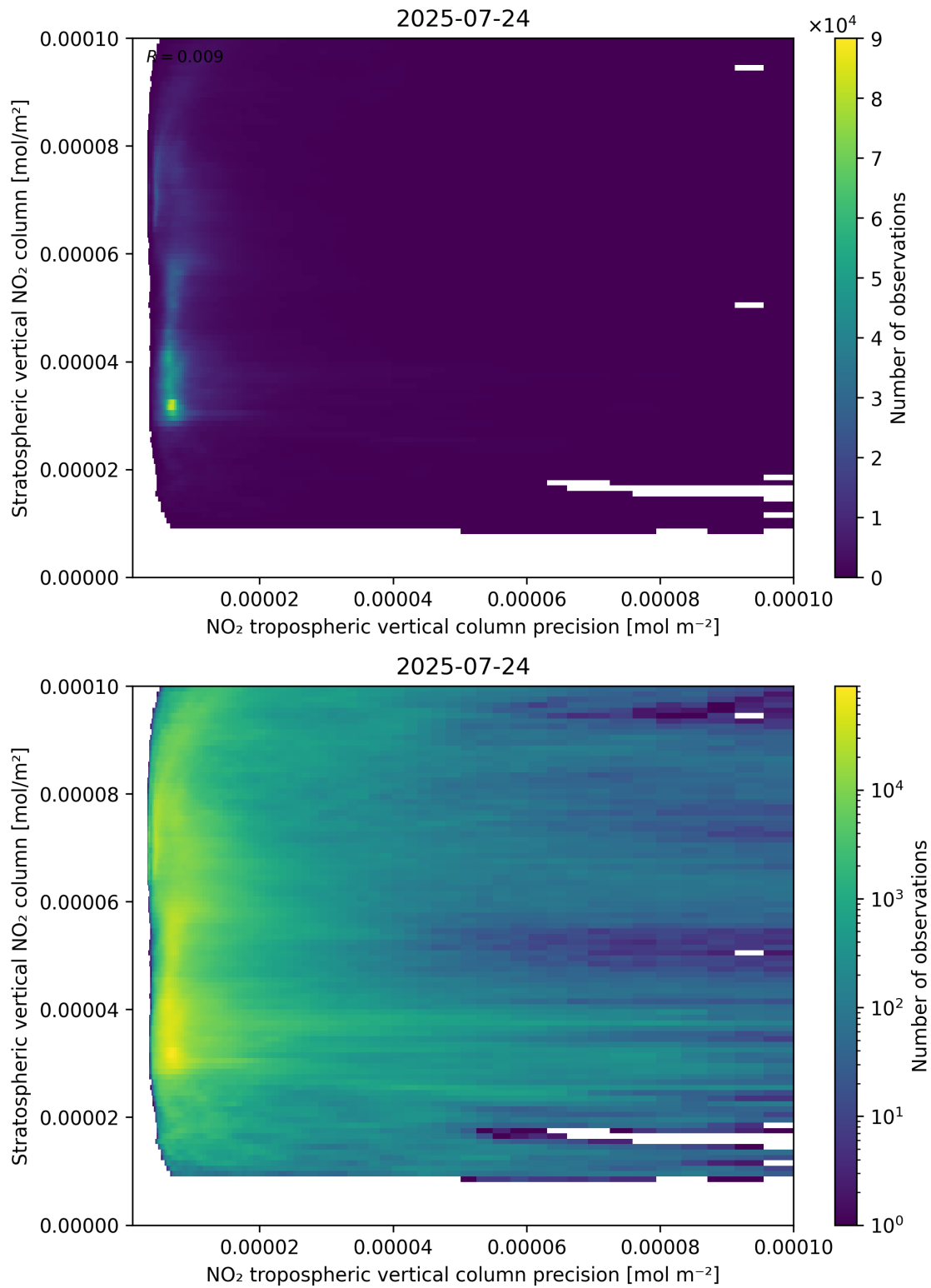
Figure 135: Scatter density plot of “NO 2 tropospheric vertical column precision” against “Stratospheric vertical NO 2 column” for 2025-07-24 to 2025-07-25.
