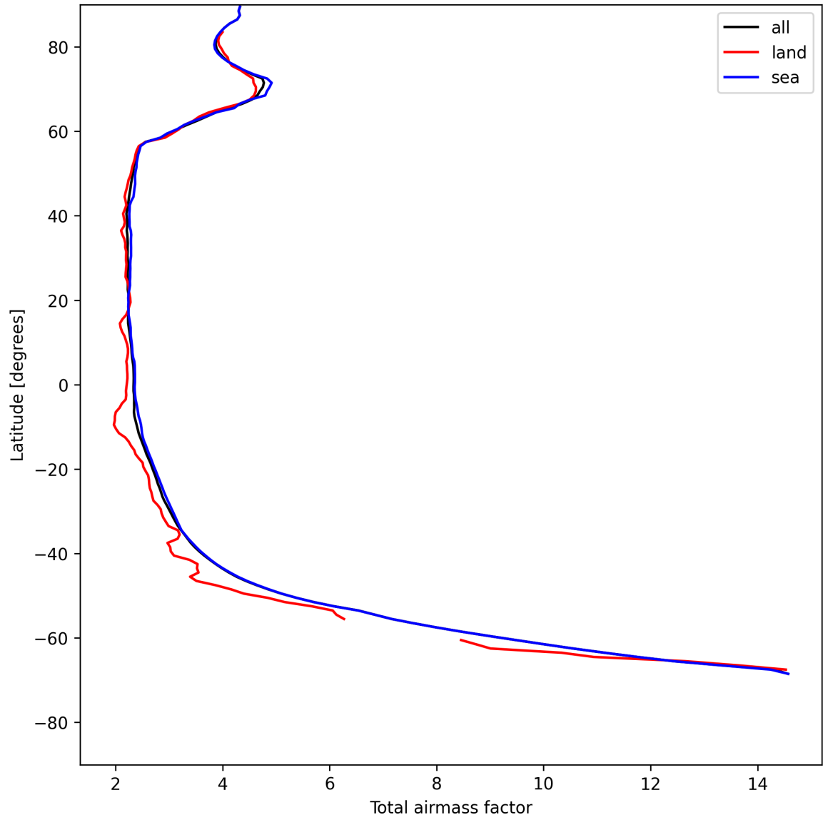
Figure 15: Zonal average of “Total airmass factor” for 2025-07-24 to 2025-07-25.
