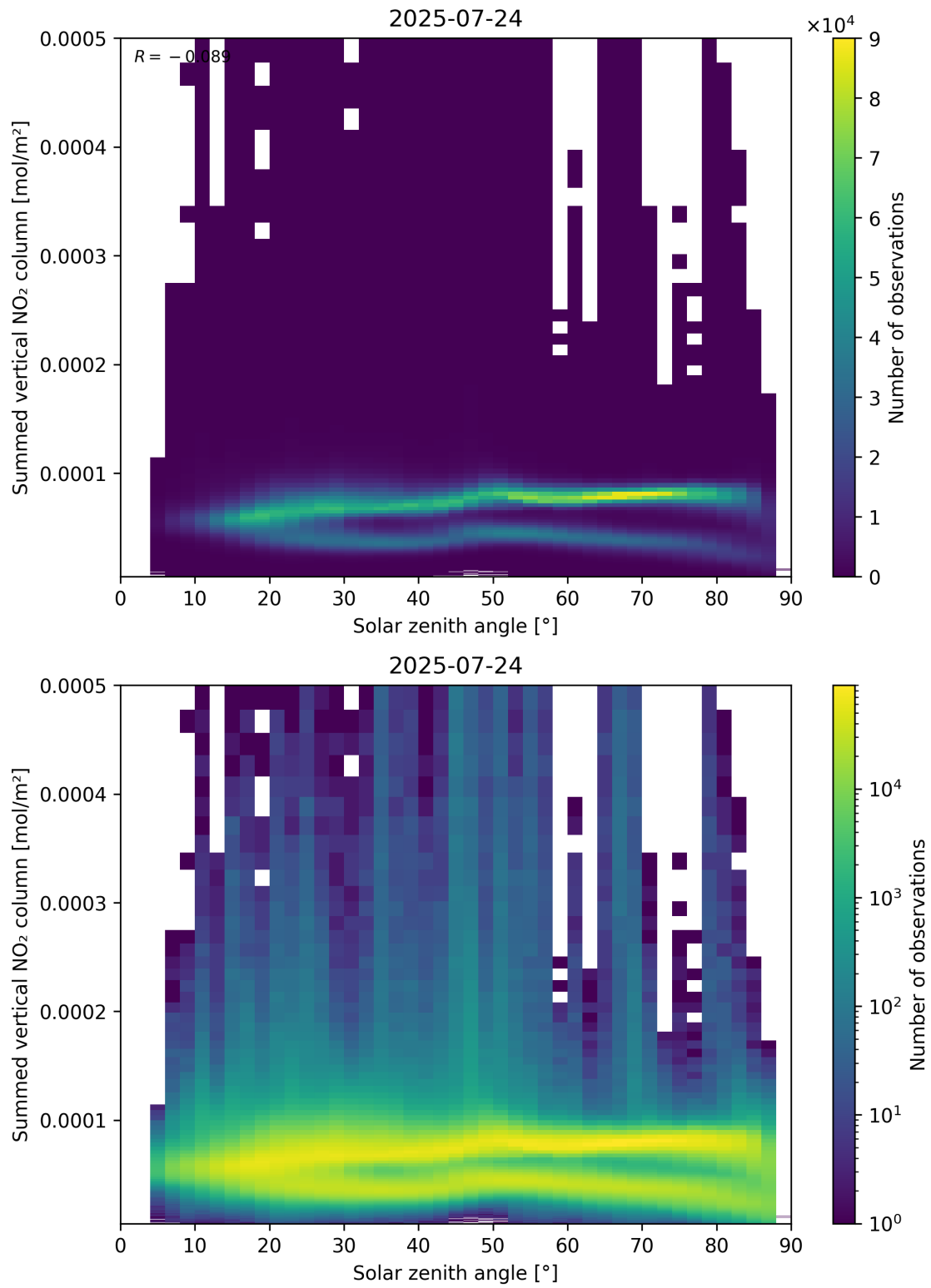
Figure 151: Scatter density plot of “Solar zenith angle” against “Summed vertical NO 2 column” for 2025-07-24 to 2025-07-25.
