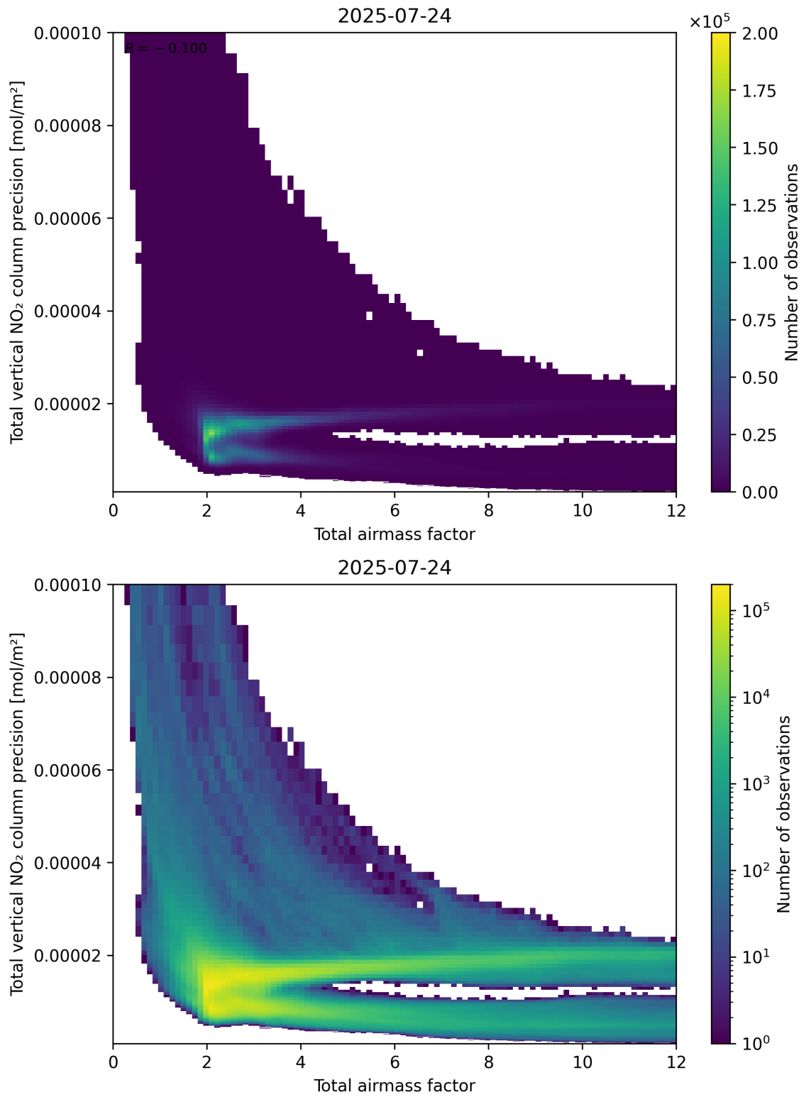
Figure 68: Scatter density plot of “Total airmass factor” against “Total vertical NO 2 column precision” for 2025-07-24 to 2025-07-25.
