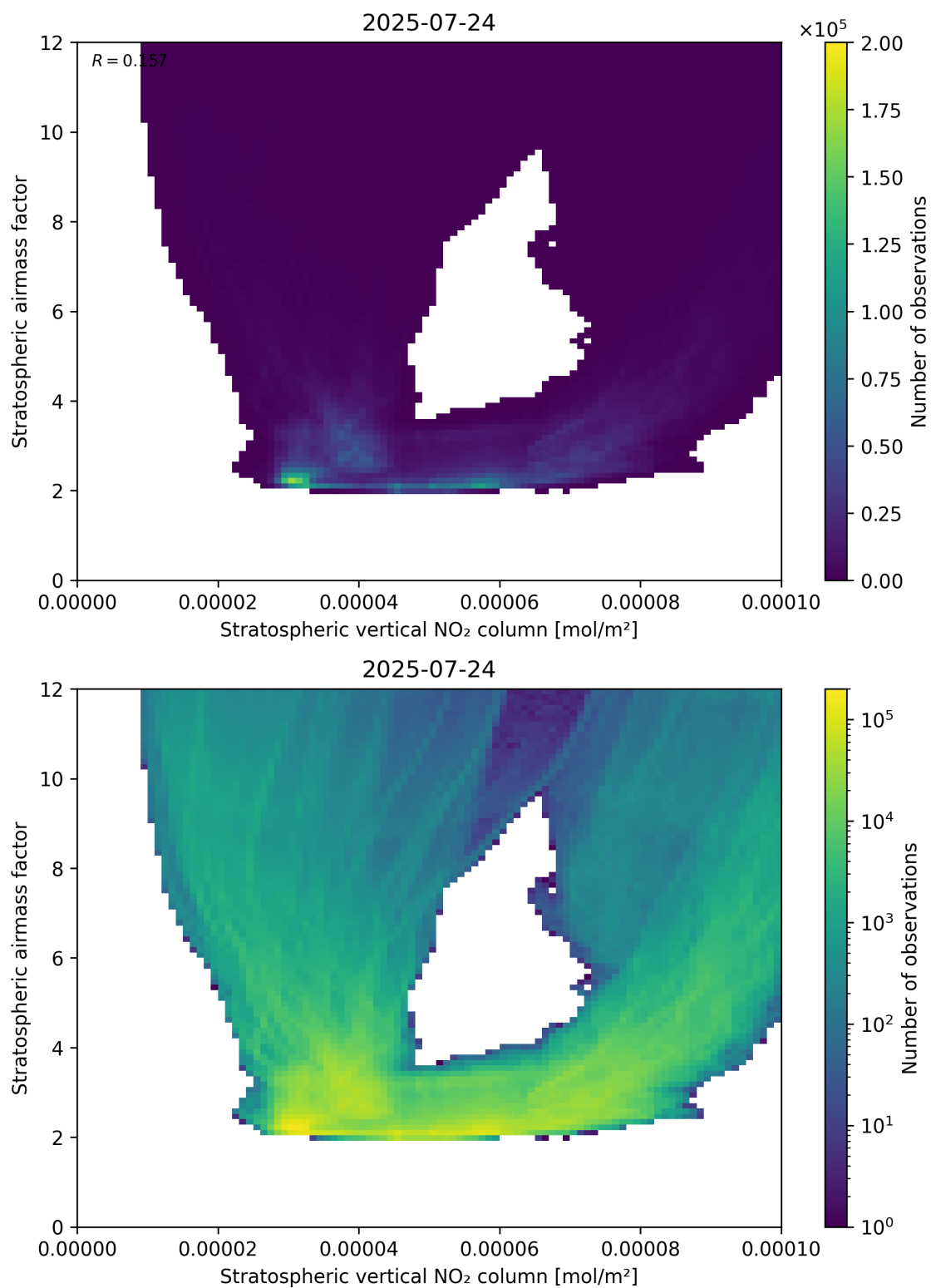
Figure 96: Scatter density plot of “Stratospheric vertical NO 2 column” against “Stratospheric airmass factor” for 2025-07-24 to 2025-07-25.
