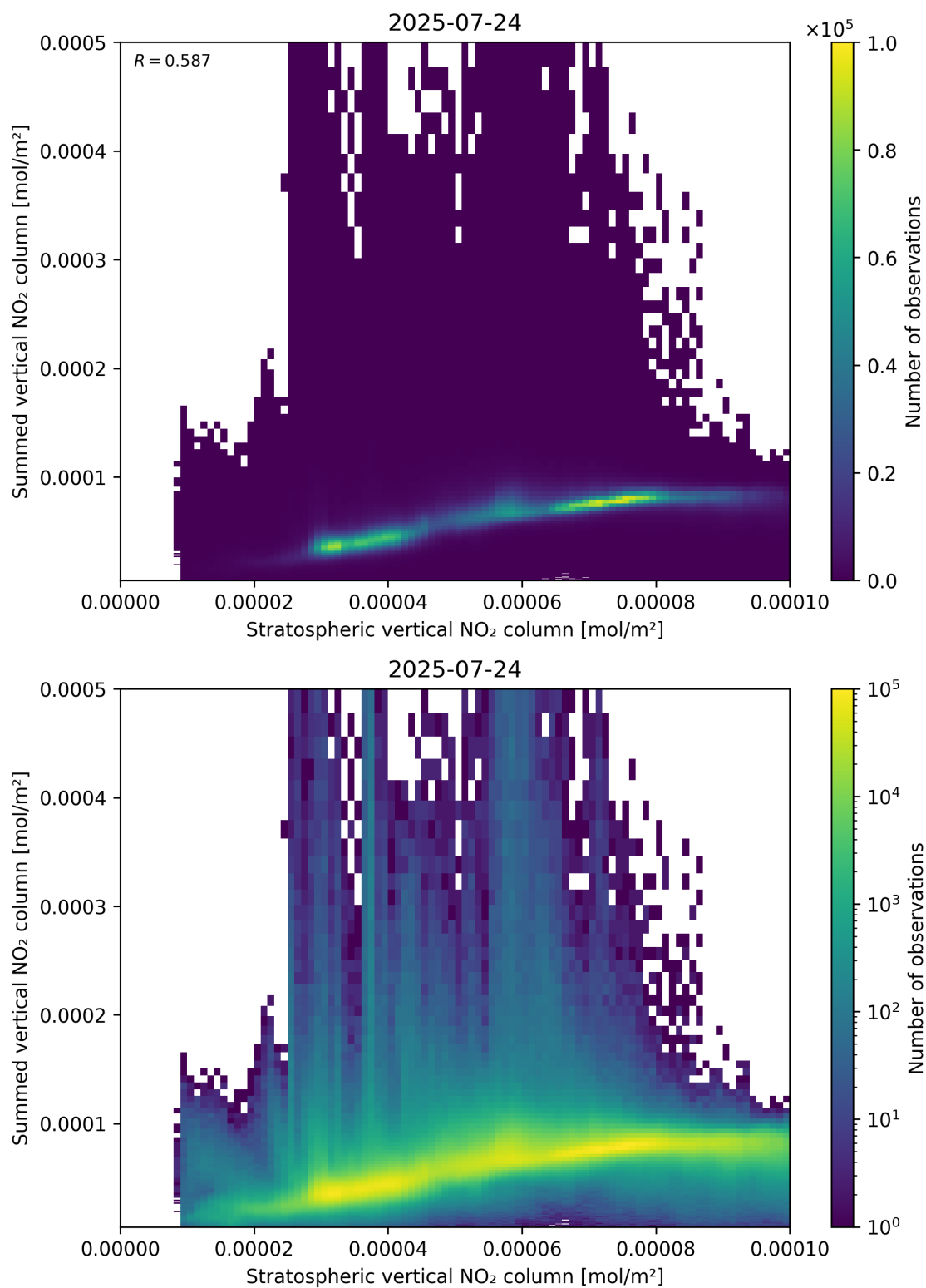
Figure 98: Scatter density plot of “Stratospheric vertical NO 2 column” against “Summed vertical NO 2 column” for 2025-07-24 to 2025-07-25.
