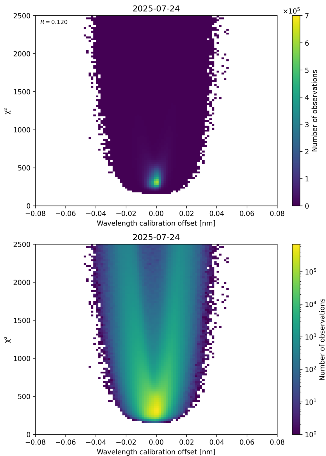
Figure 175: Scatter density plot of “Wavelength calibration offset” against “ \chi^2 ” for 2025-07-24 to 2025-07-25.
