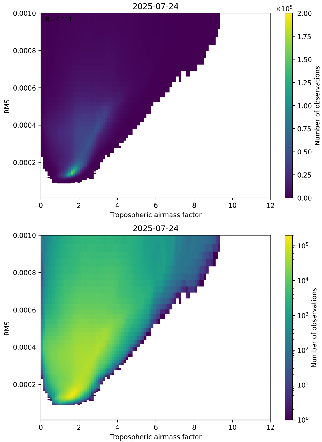
Figure 79: Scatter density plot of “Tropospheric airmass factor” against “RMS” for 2025-07-24 to 2025-07-25.
