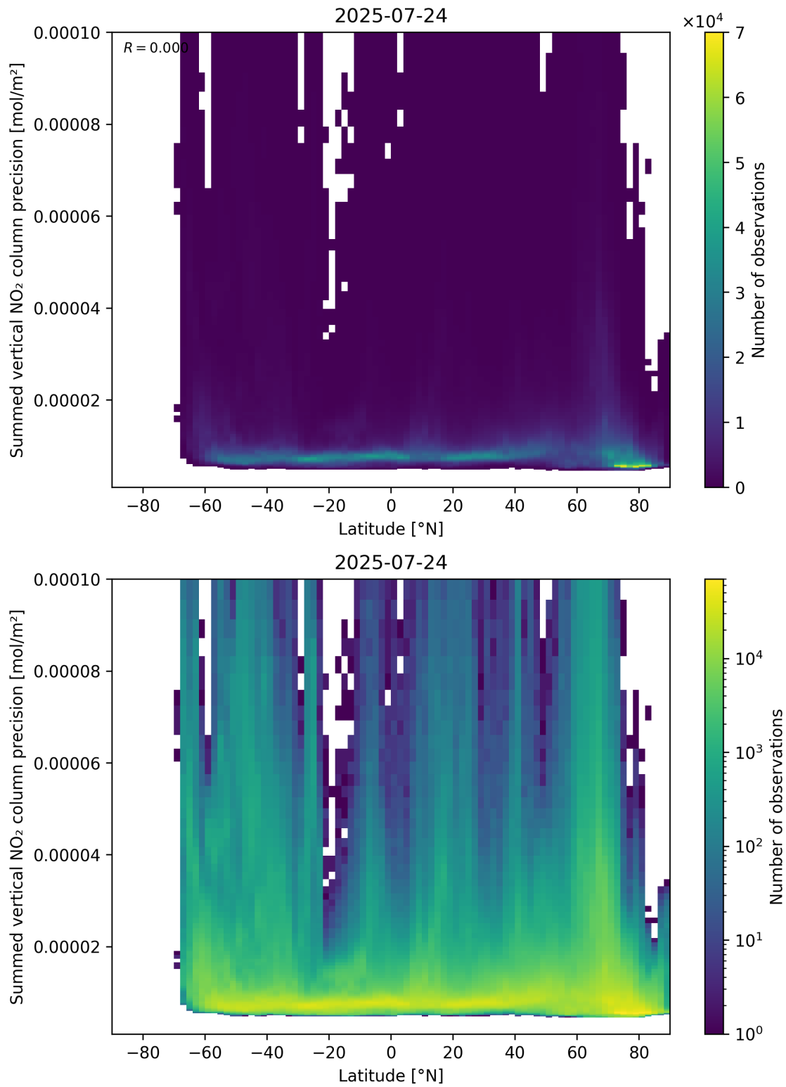
Figure 89: Scatter density plot of “Latitude” against “Summed vertical NO 2 column precision” for 2025-07-24 to 2025-07-25.
