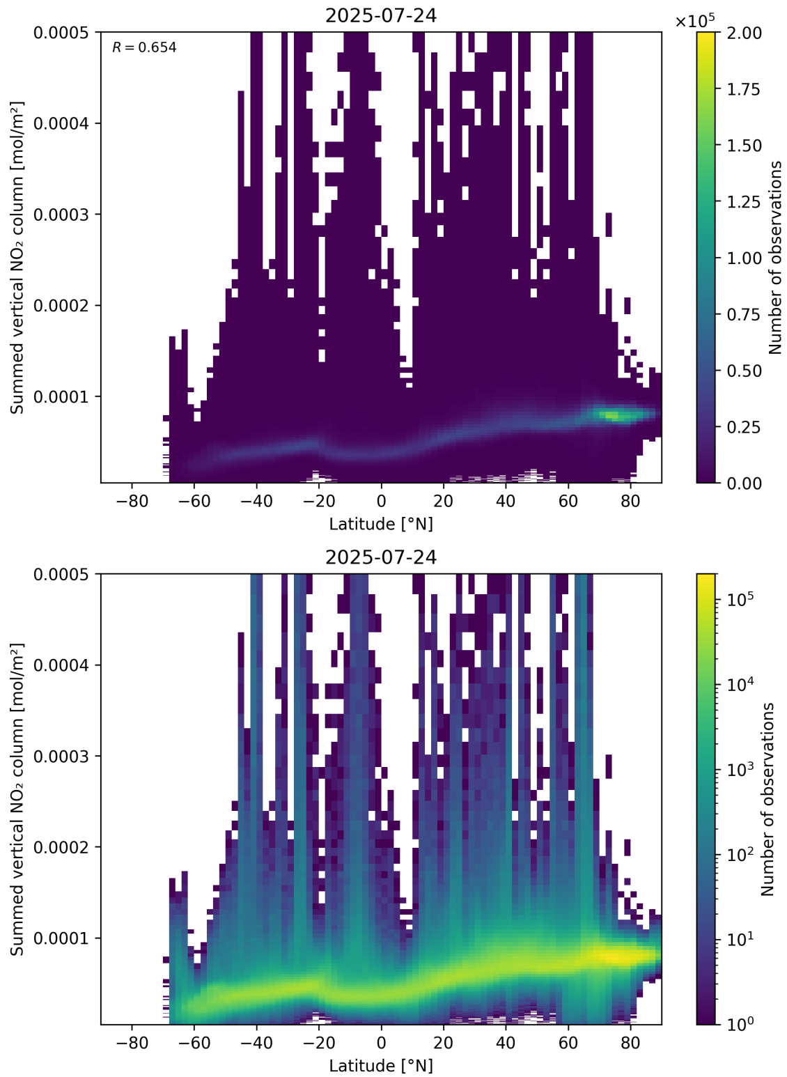
Figure 88: Scatter density plot of “Latitude” against “Summed vertical NO 2 column” for 2025-07-24 to 2025-07-25.
