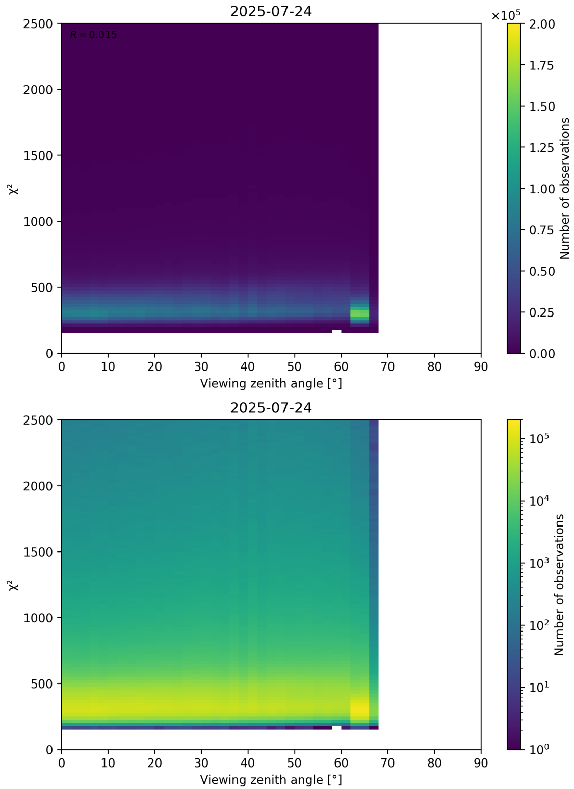
Figure 162: Scatter density plot of “Viewing zenith angle” against “ \chi^2 ” for 2025-07-24 to 2025-07-25.
