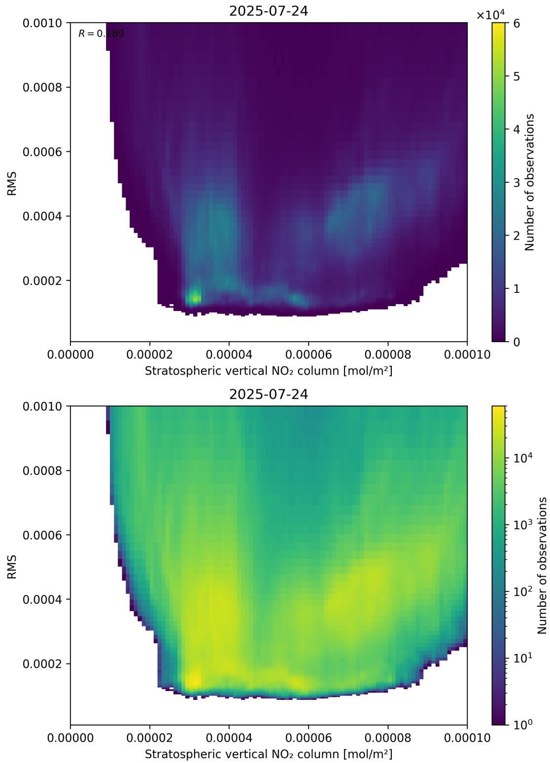
Figure 102: Scatter density plot of “Stratospheric vertical NO 2 column” against “RMS” for 2025-07-24 to 2025-07-25.
