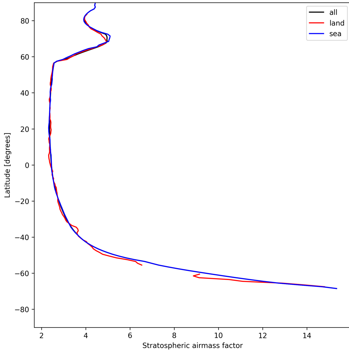
Figure 27: Zonal average of “Stratospheric air mass factor” for 2025-07-24 to 2025-07-25.
