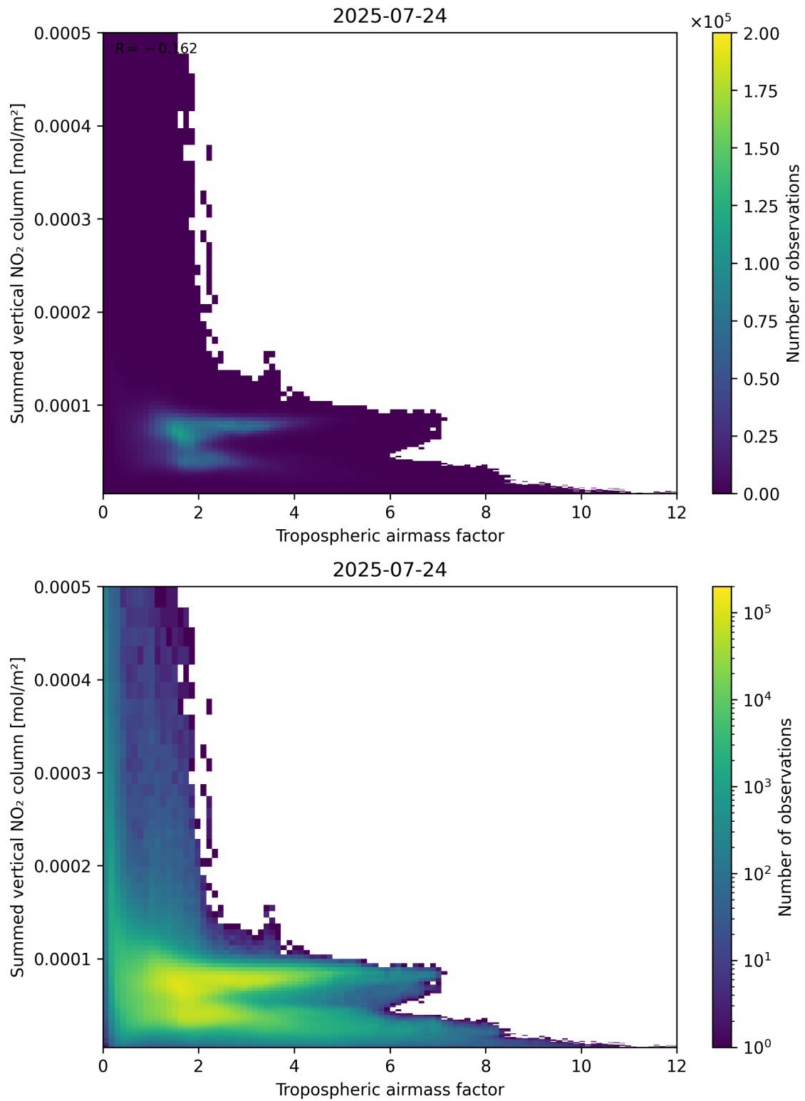
Figure 75: Scatter density plot of “Tropospheric airmass factor” against “Summed vertical NO 2 column” for 2025-07-24 to 2025-07-25.
