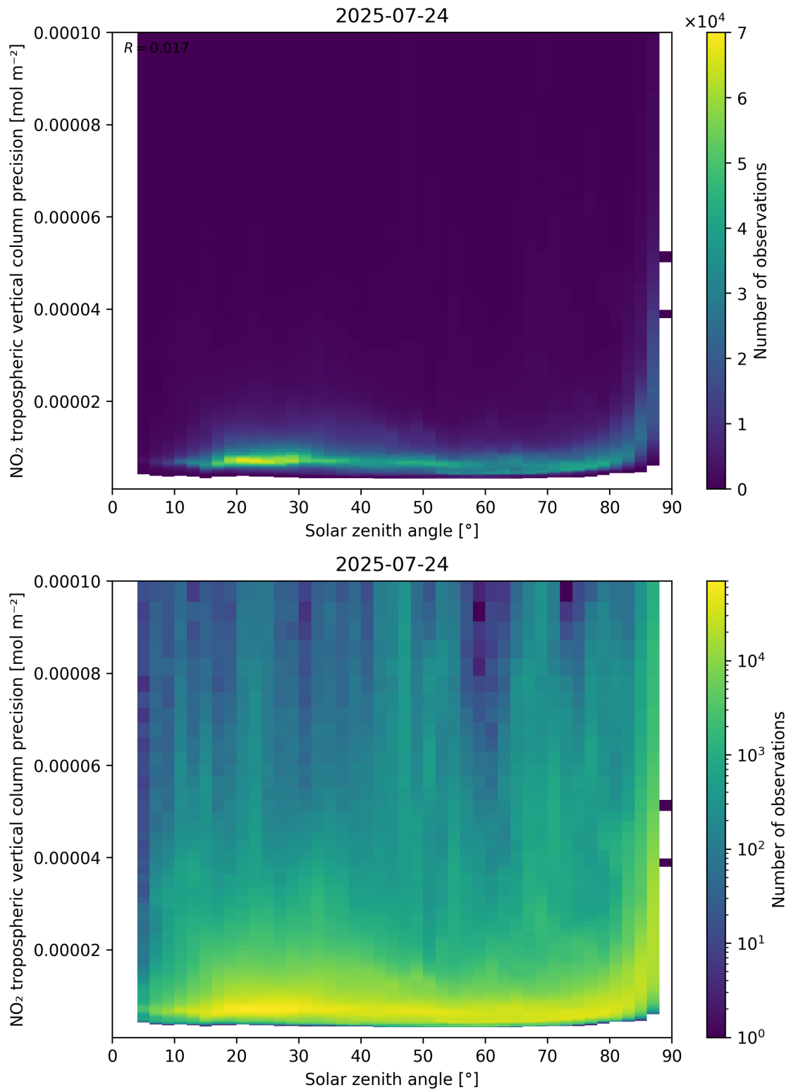
Figure 156: Scatter density plot of “Solar zenith angle” against “NO 2 tropospheric vertical column precision” for 2025-07-24 to 2025-07-25.
