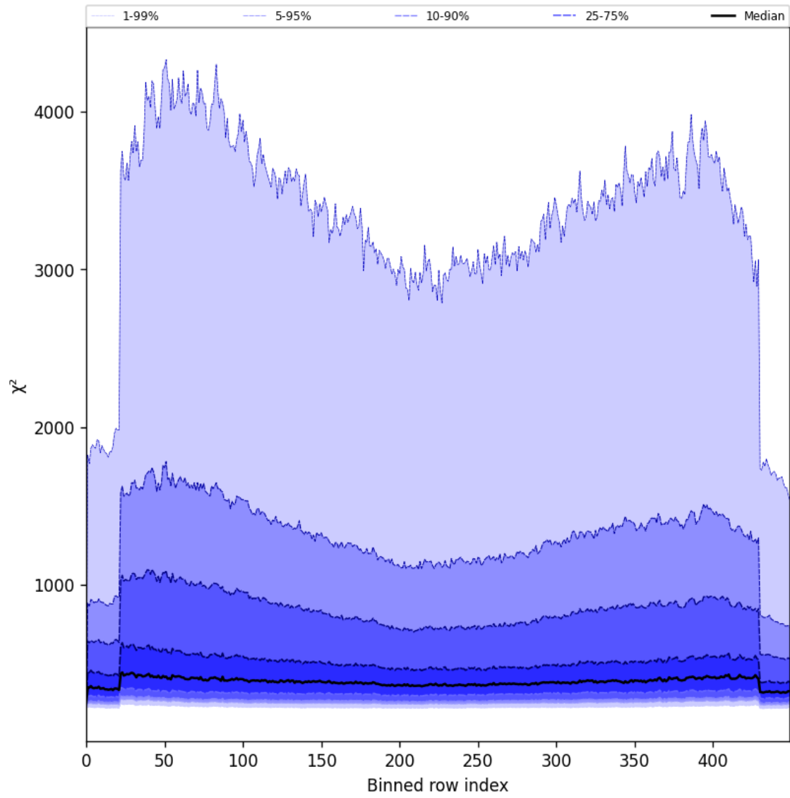
Figure 59: Along track statistics of “ \chi^2 ” for 2025-07-24 to 2025-07-25
