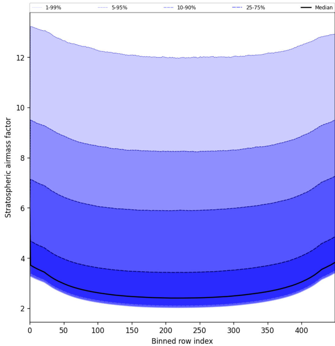
Figure 61: Along track statistics of “Stratospheric air mass factor” for 2025-07-24 to 2025-07-25
