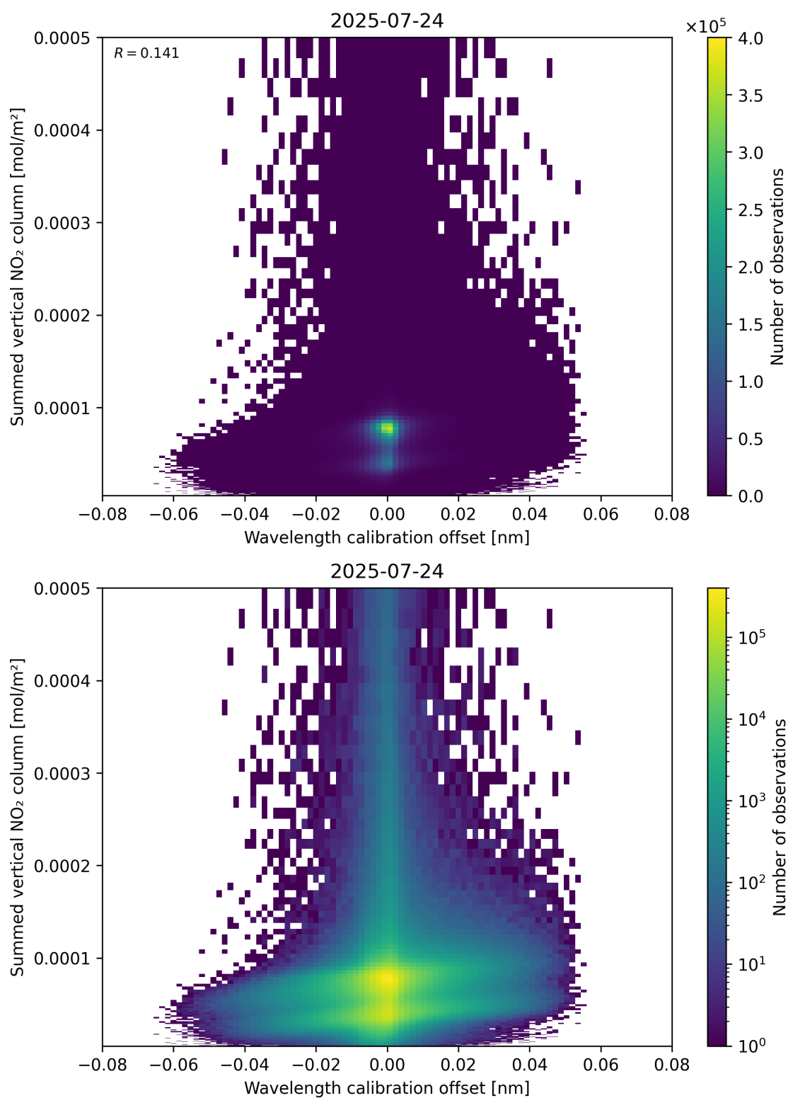
Figure 177: Scatter density plot of “Wavelength calibration offset” against “Summed vertical NO 2 column” for 2025-07-24 to 2025-07-25.
