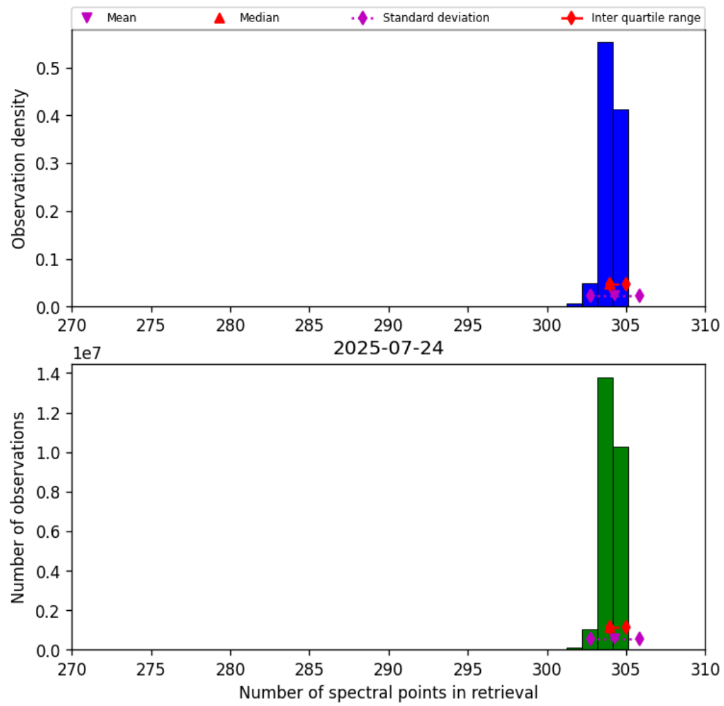
Figure 33: Histogram of “Number of spectral points in retrieval” for 2025-07-24 to 2025-07-25
