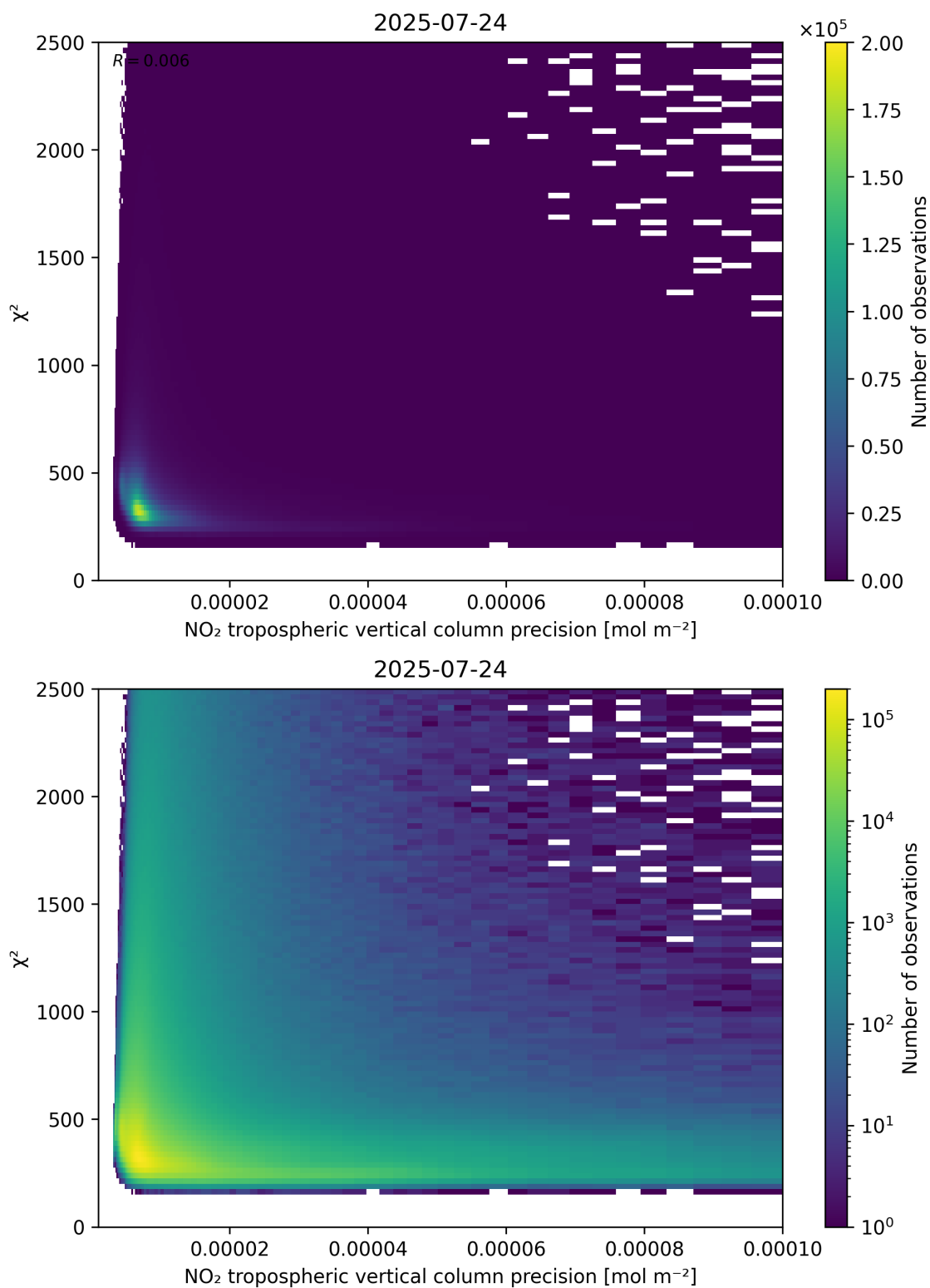
Figure 134: Scatter density plot of “NO 2 tropospheric vertical column precision” against “ \chi^2 ” for 2025-07-24 to 2025-07-25.
