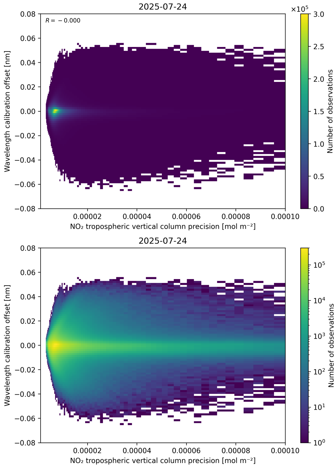
Figure 141: Scatter density plot of “NO 2 tropospheric vertical column precision” against “Wavelength calibration offset” for 2025-07-24 to 2025-07-25.
