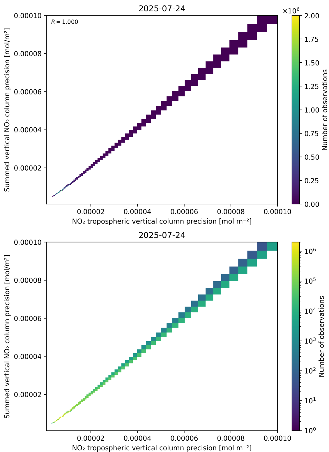
Figure 137: Scatter density plot of “NO 2 tropospheric vertical column precision” against “Summed vertical NO 2 column precision” for 2025-07-24 to 2025-07-25.
