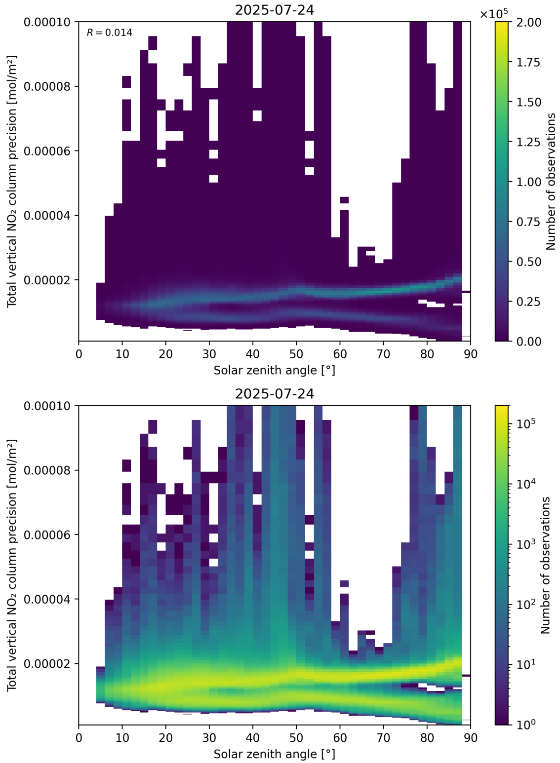
Figure 154: Scatter density plot of “Solar zenith angle” against “Total vertical NO 2 column precision” for 2025-07-24 to 2025-07-25.
