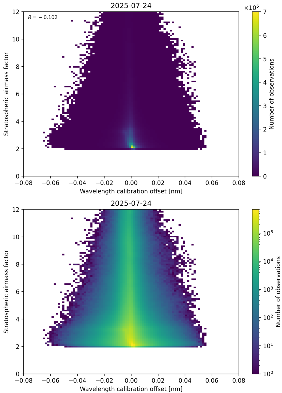
Figure 174: Scatter density plot of “Wavelength calibration offset” against “Stratospheric airmass factor” for 2025-07-24 to 2025-07-25.
