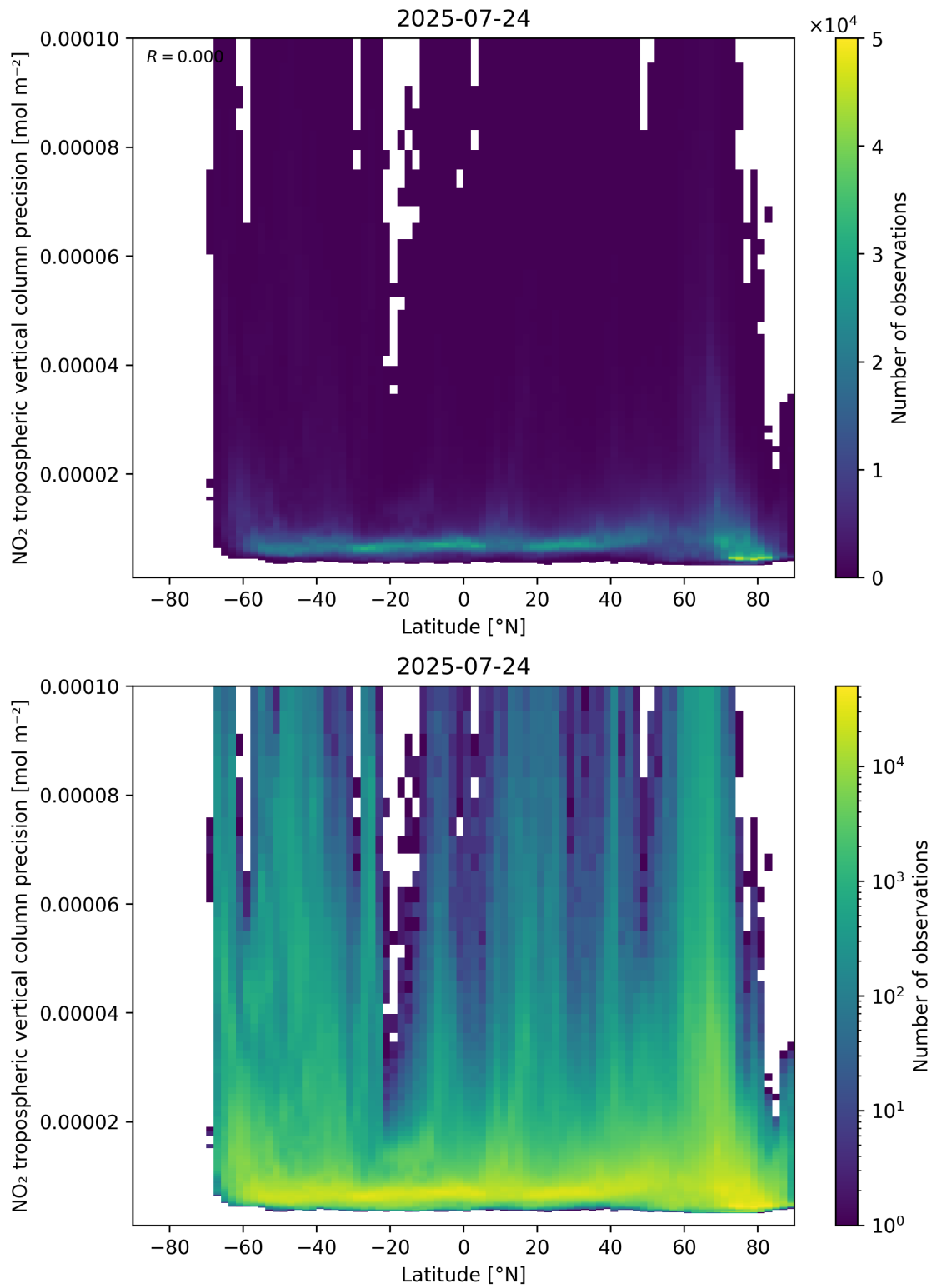
Figure 93: Scatter density plot of “Latitude” against “NO 2 tropospheric vertical column precision” for 2025-07-24 to 2025-07-25.
