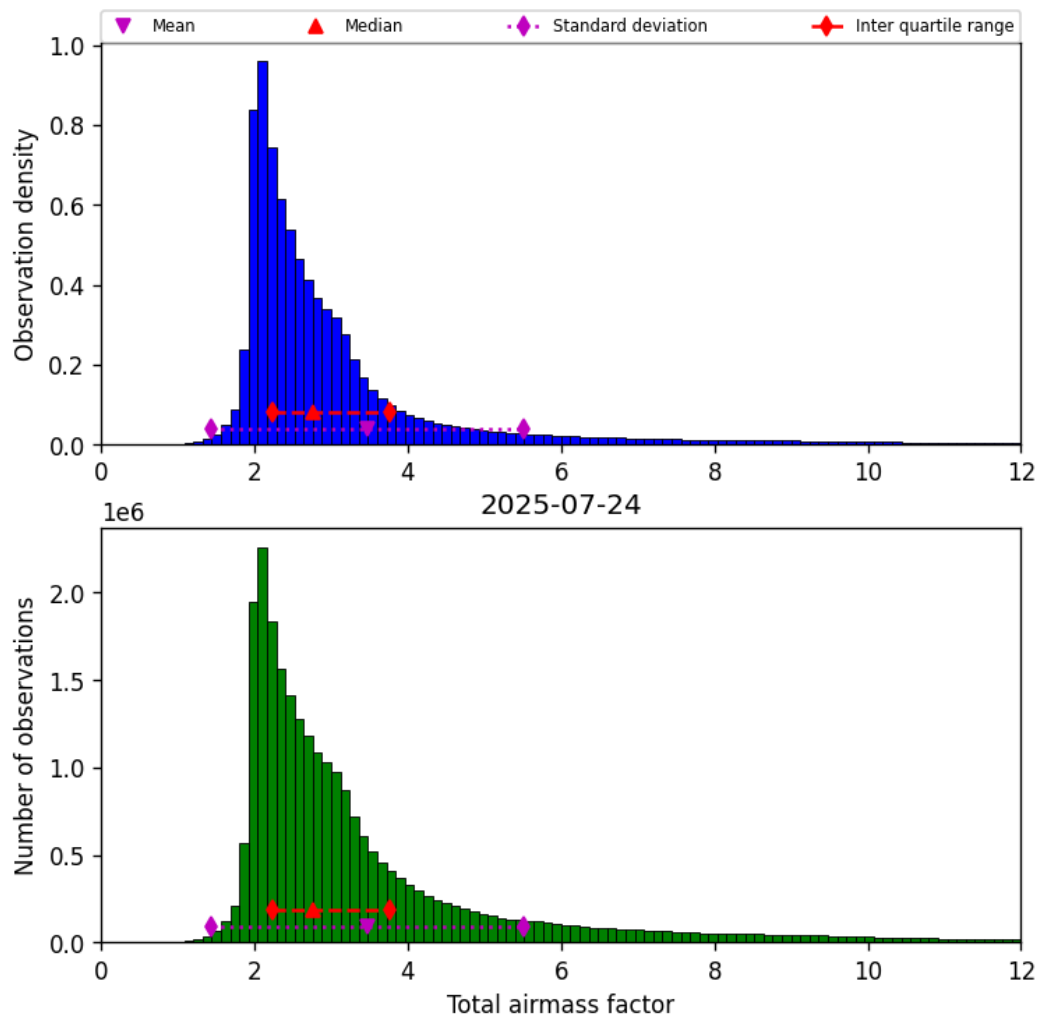
Figure 32: Histogram of “Total airmass factor” for 2025-07-24 to 2025-07-25
