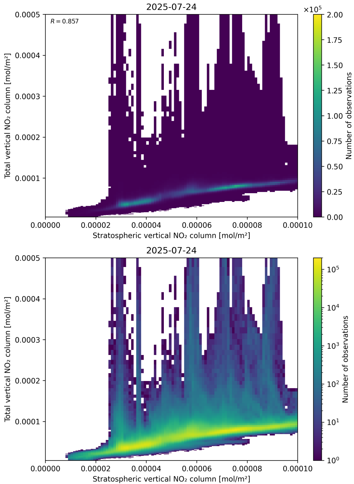
Figure 100: Scatter density plot of “Stratospheric vertical NO 2 column” against “Total vertical NO 2 column” for 2025-07-24 to 2025-07-25.
