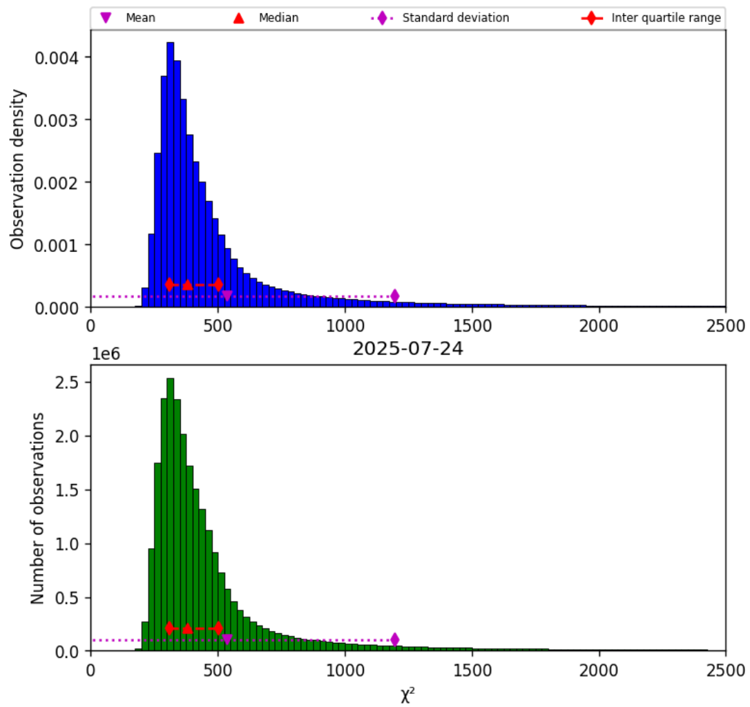
Figure 42: Histogram of “ \chi^2 ” for 2025-07-24 to 2025-07-25
