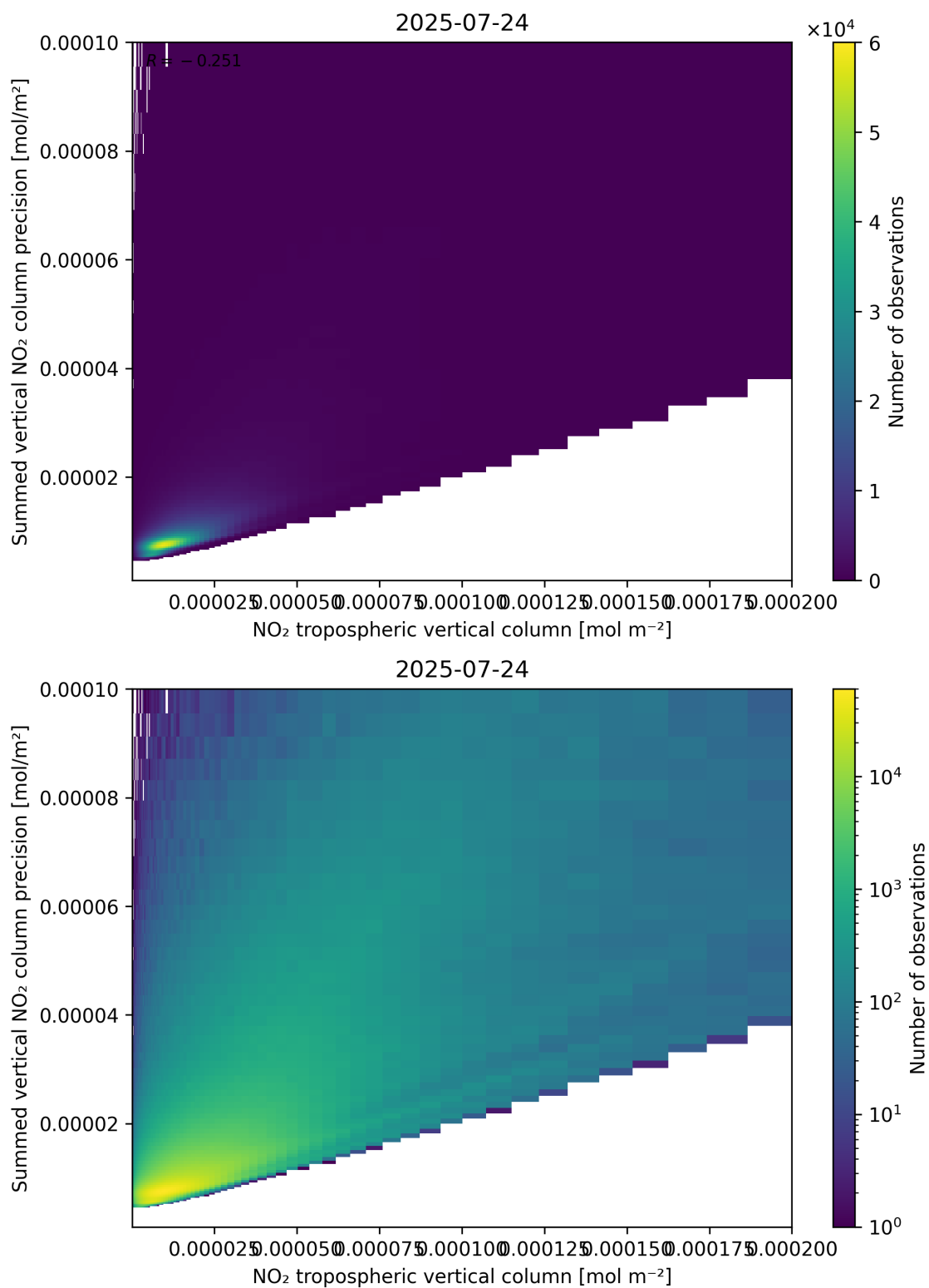
Figure 127: Scatter density plot of “NO 2 tropospheric vertical column” against “Summed vertical NO 2 column precision” for 2025-07-24 to 2025-07-25.
