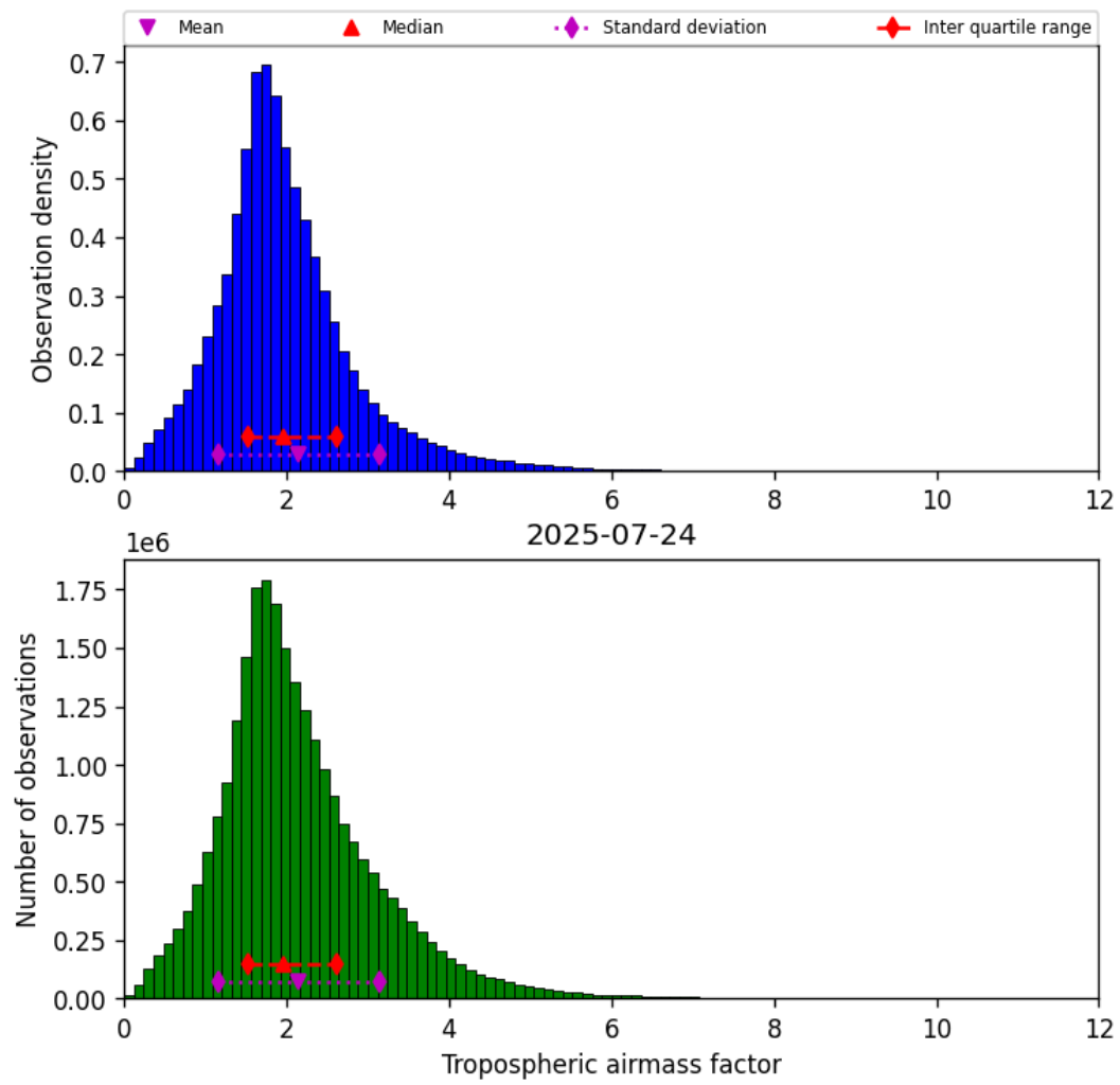
Figure 31: Histogram of “Tropospheric airmass factor” for 2025-07-24 to 2025-07-25
