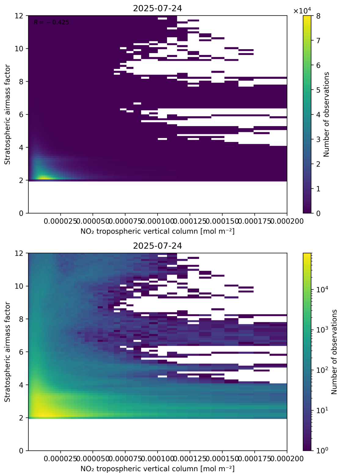
Figure 121: Scatter density plot of “NO 2 tropospheric vertical column” against “Stratospheric air mass factor” for 2025-07-24 to 2025-07-25.
