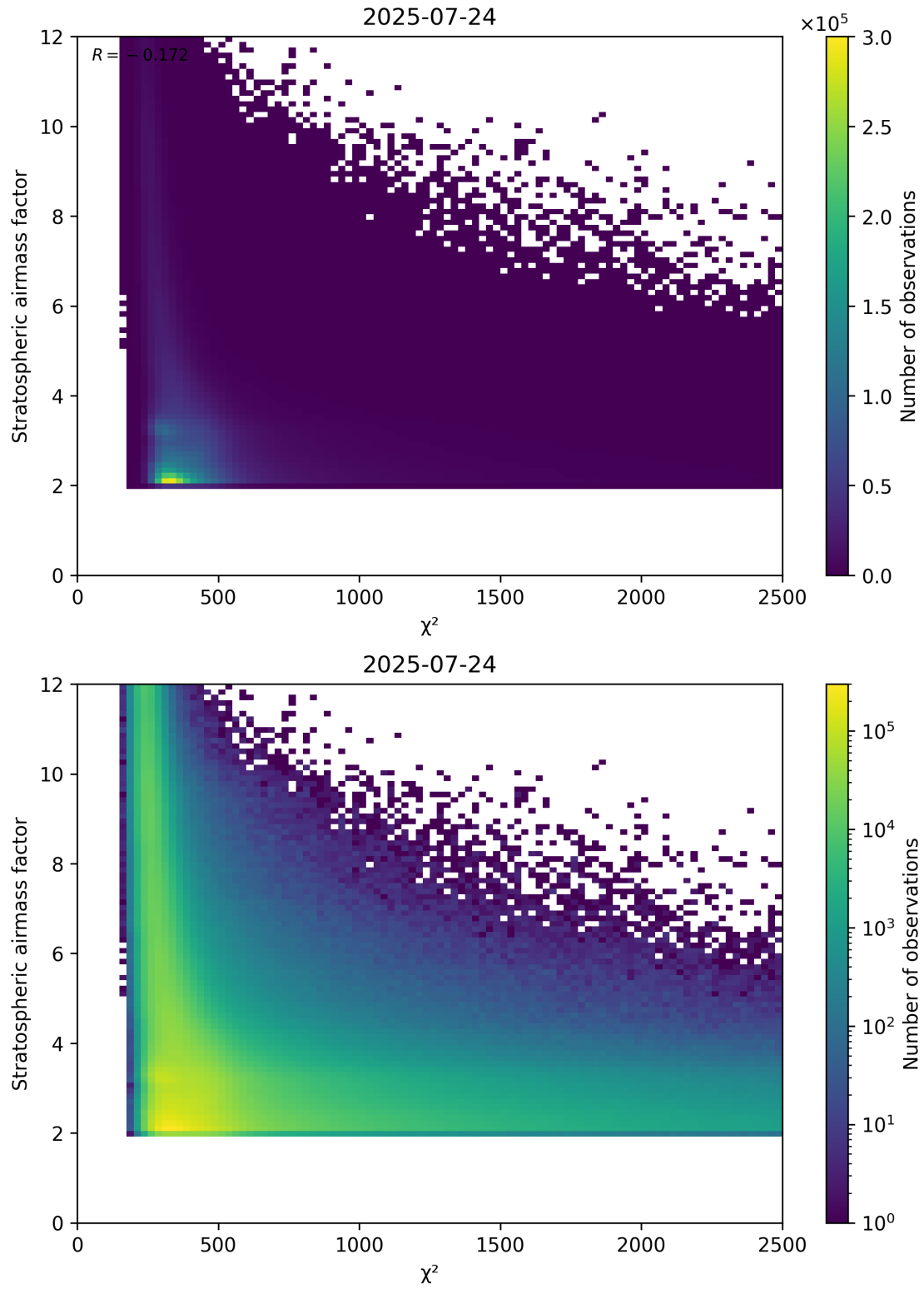
Figure 81: Scatter density plot of “ \chi^2 ” against “Stratospheric airmass factor” for 2025-07-24 to 2025-07-25.
