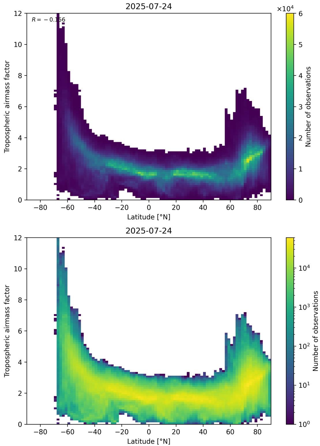
Figure 85: Scatter density plot of “Latitude” against “Tropospheric air mass factor” for 2025-07-24 to 2025-07-25.
