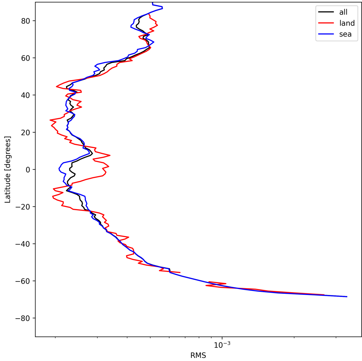
Figure 26: Zonal average of “RMS” for 2025-07-24 to 2025-07-25.
