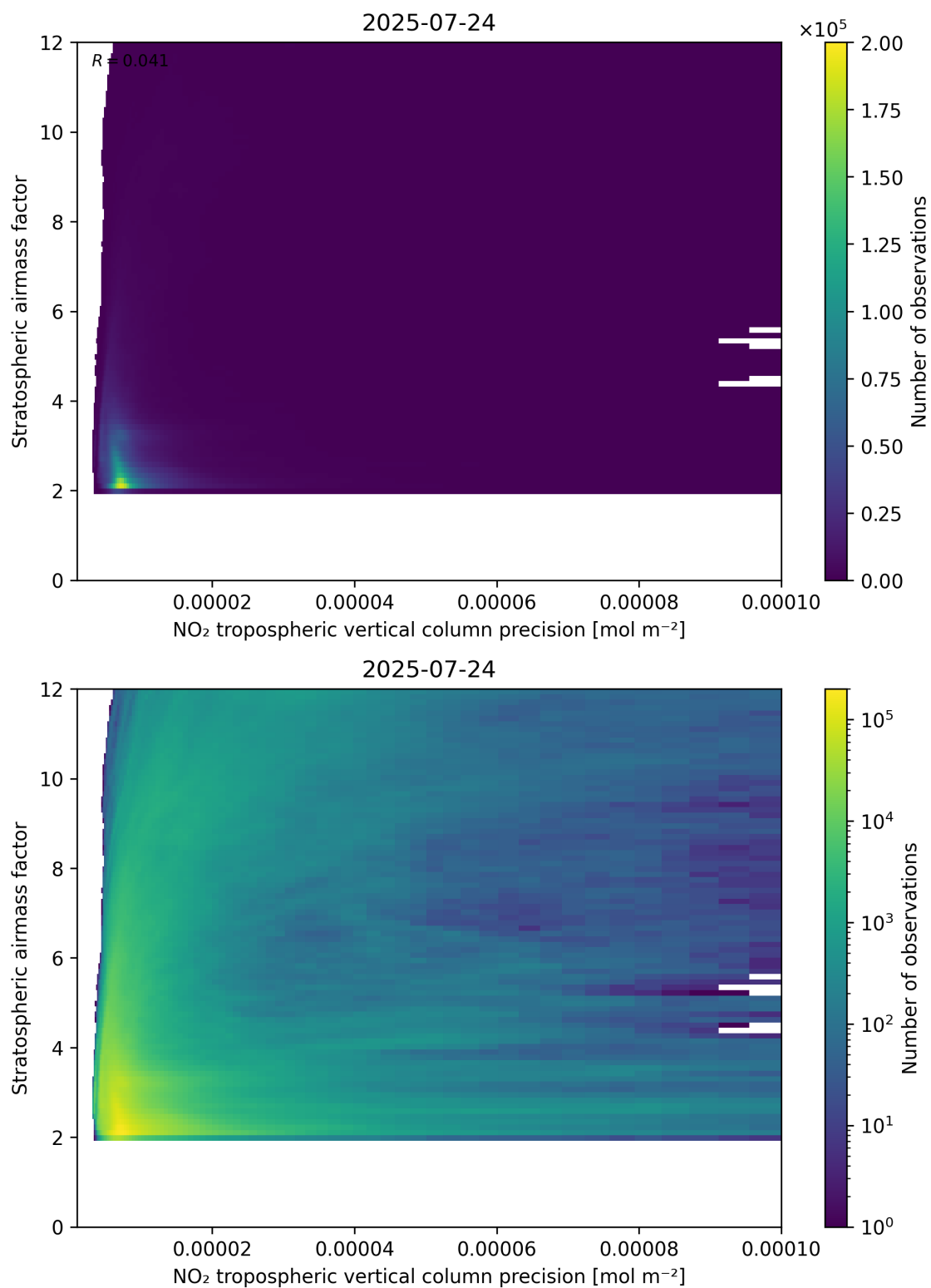
Figure 131: Scatter density plot of “NO 2 tropospheric vertical column precision” against “Stratospheric airmass factor” for 2025-07-24 to 2025-07-25.
