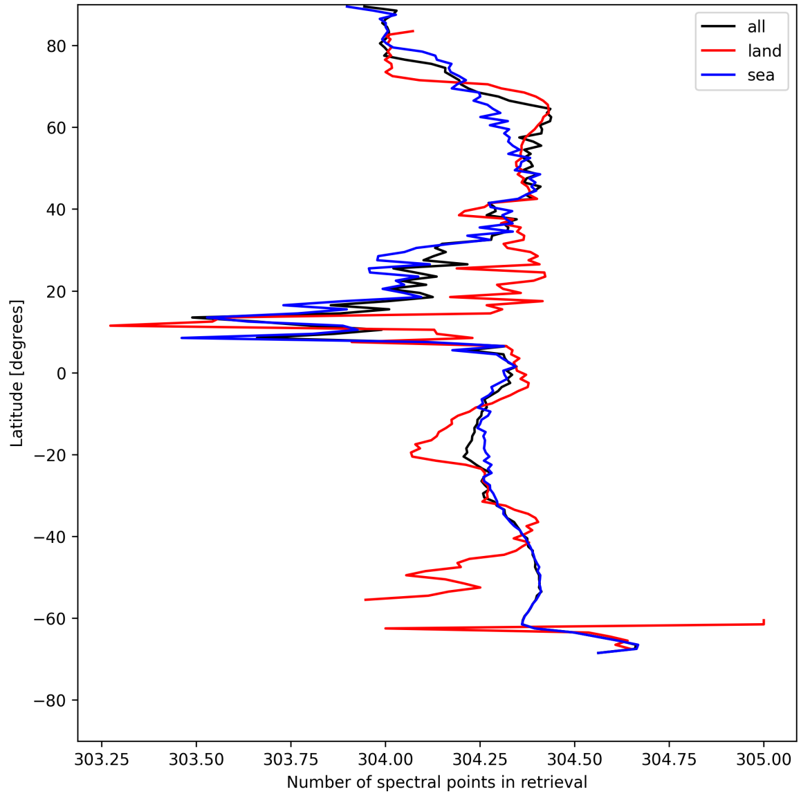
Figure 16: Zonal average of “Number of spectral points in retrieval” for 2025-07-24 to 2025-07-25.
