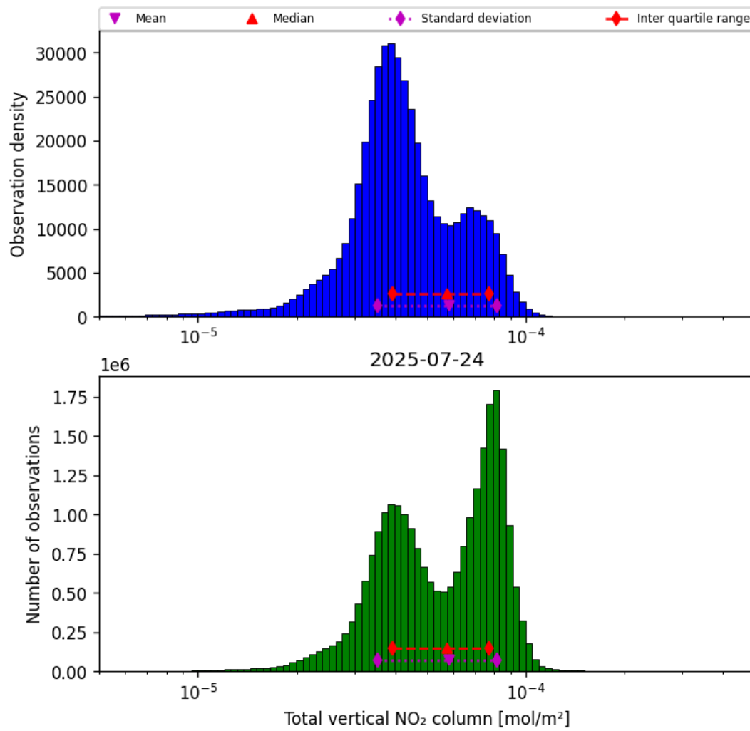
Figure 38: Histogram of “Total vertical NO 2 column” for 2025-07-24 to 2025-07-25
