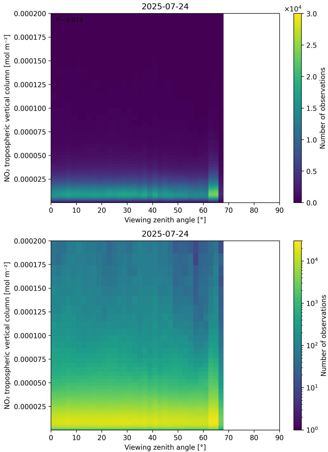
Figure 169: Scatter density plot of “Viewing zenith angle” against “NO 2 tropospheric vertical column” for 2025-07-24 to 2025-07-25.
