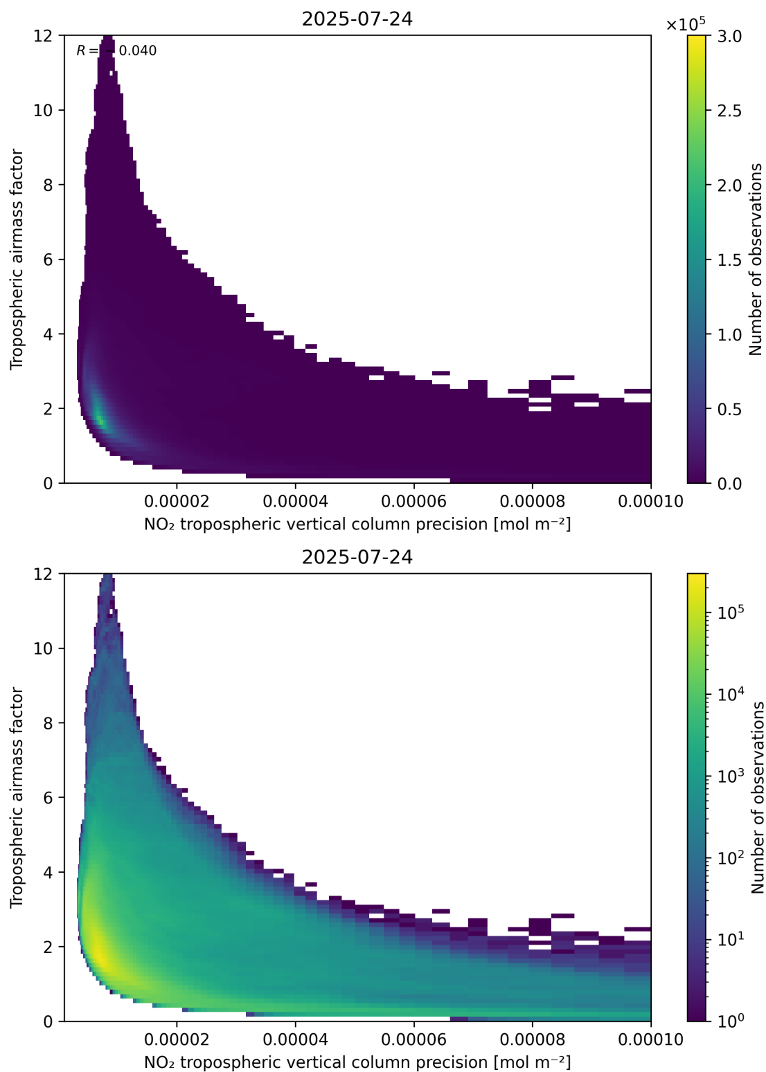
Figure 133: Scatter density plot of “NO 2 tropospheric vertical column precision” against “Tropospheric air mass factor” for 2025-07-24 to 2025-07-25.
