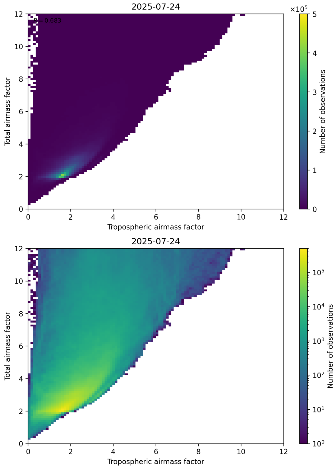
Figure 72: Scatter density plot of “Tropospheric airmass factor” against “Total airmass factor” for 2025-07-24 to 2025-07-25.
