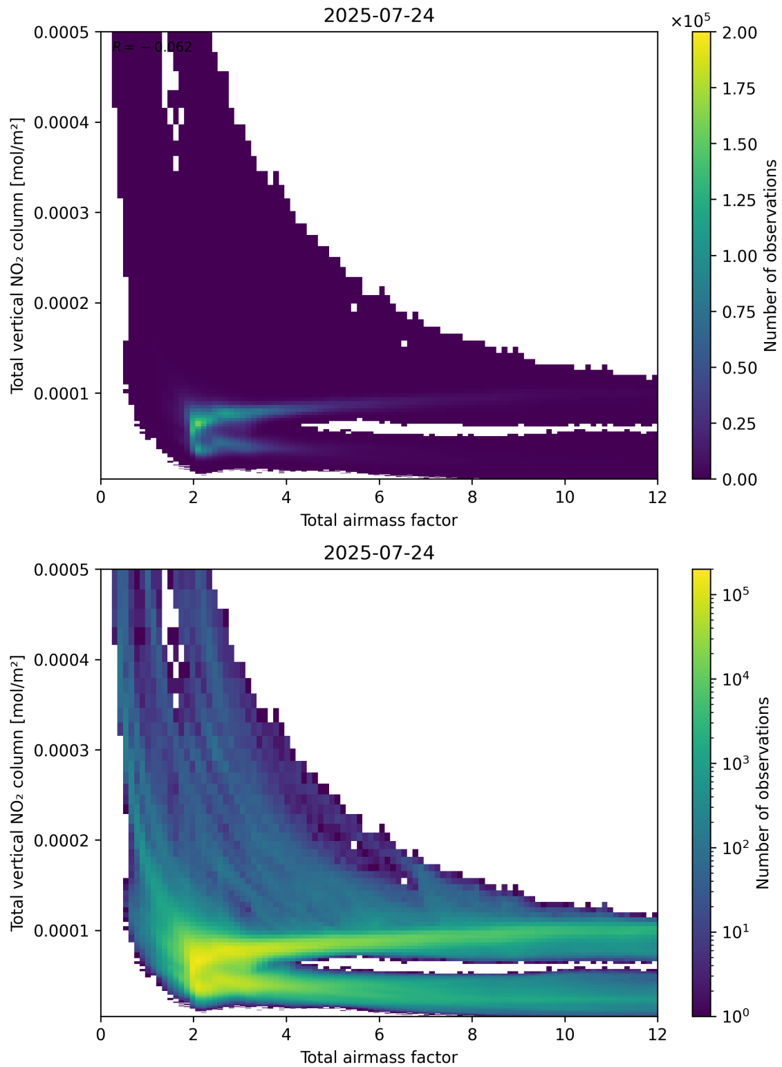
Figure 67: Scatter density plot of “Total airmass factor” against “Total vertical NO 2 column” for 2025-07-24 to 2025-07-25.
