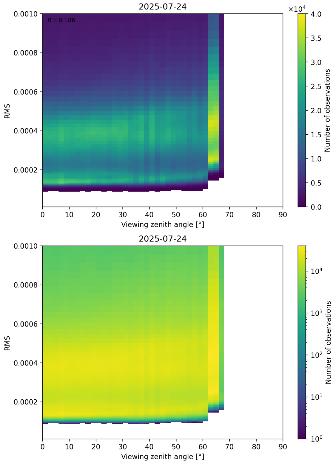
Figure 171: Scatter density plot of “Viewing zenith angle” against “RMS” for 2025-07-24 to 2025-07-25.
