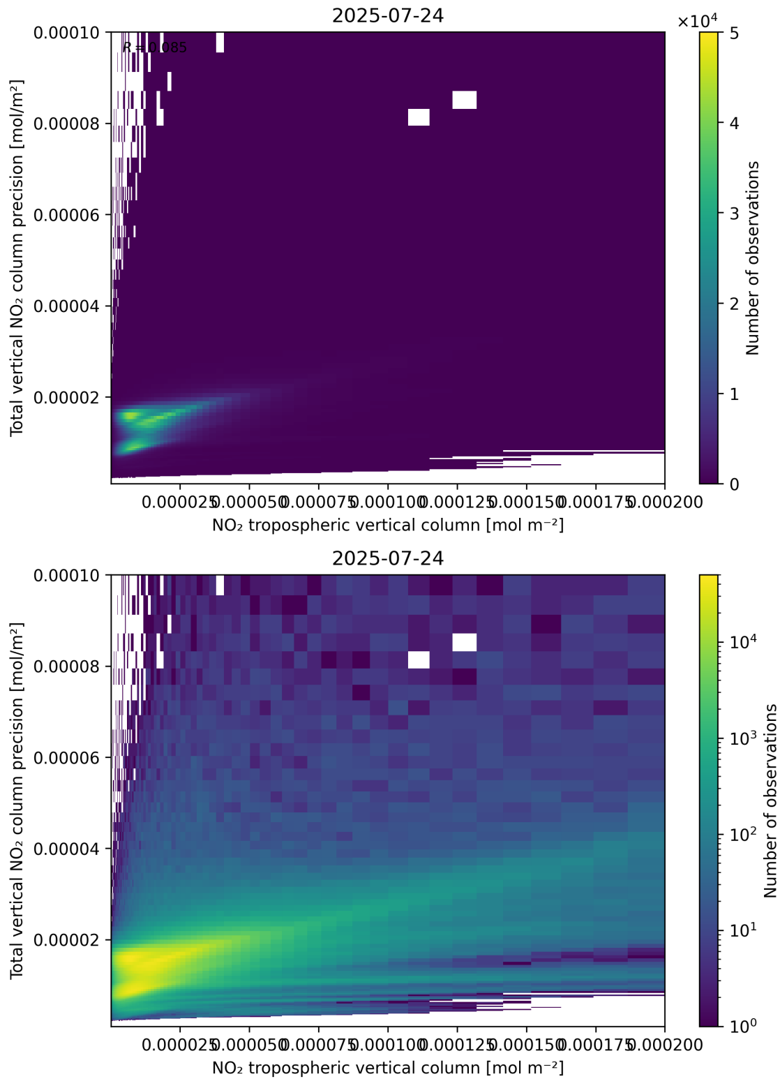
Figure 129: Scatter density plot of “NO 2 tropospheric vertical column” against “Total vertical NO 2 column precision” for 2025-07-24 to 2025-07-25.
