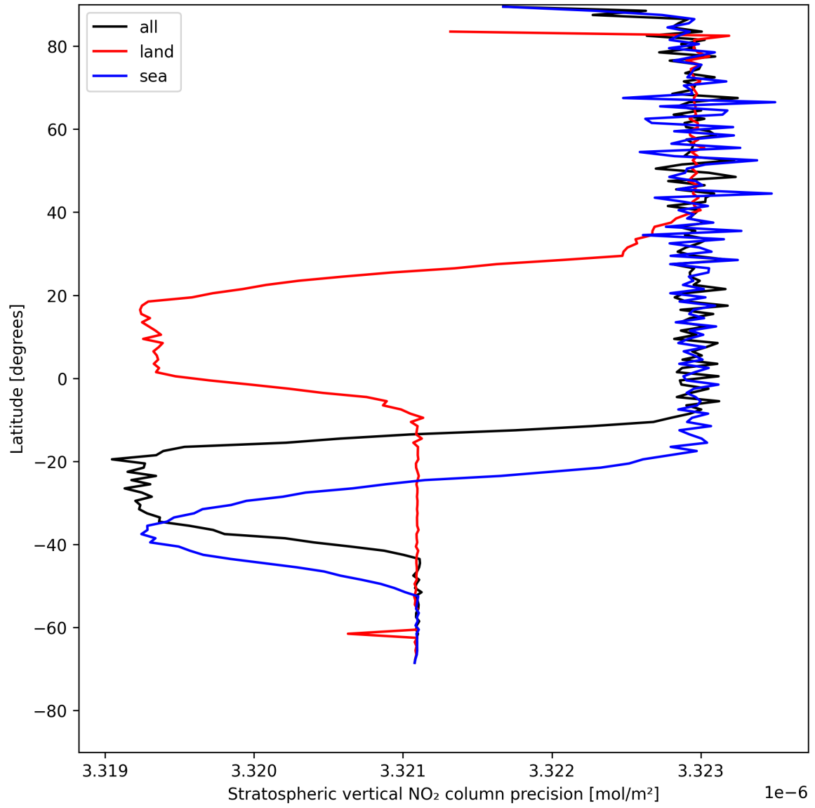
Figure 20: Zonal average of “Stratospheric vertical NO 2 column precision” for 2025-07-24 to 2025-07-25.
