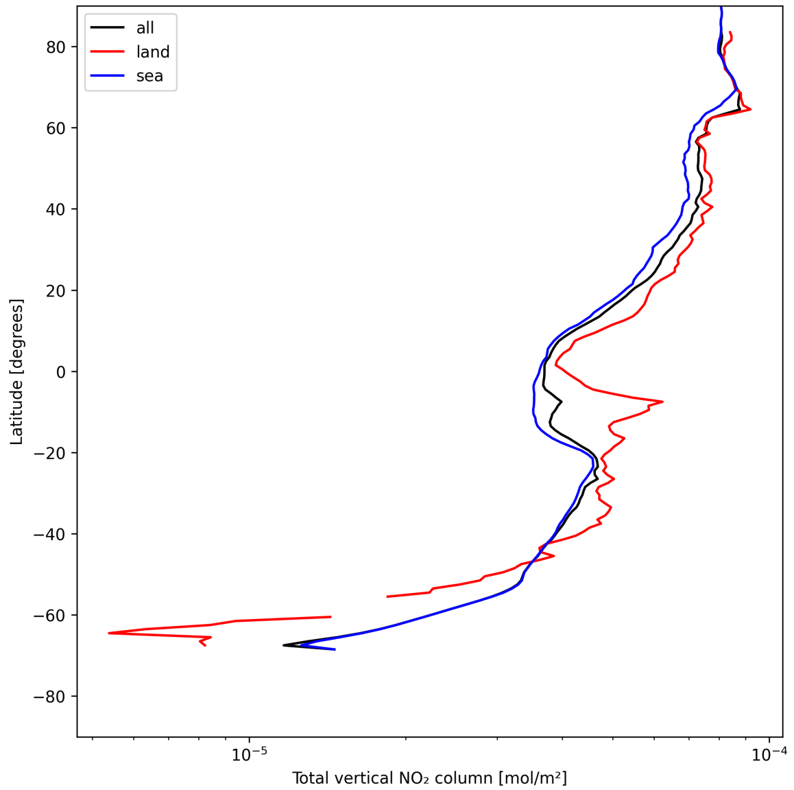
Figure 21: Zonal average of “Total vertical NO 2 column” for 2025-07-24 to 2025-07-25.
