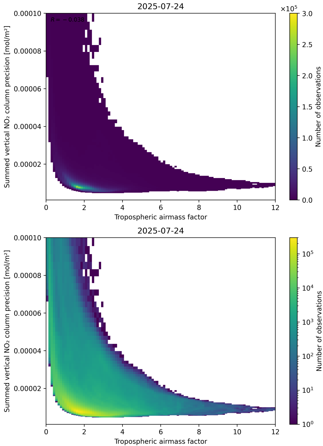
Figure 76: Scatter density plot of “Tropospheric air mass factor” against “Summed vertical NO 2 column precision” for 2025-07-24 to 2025-07-25.
