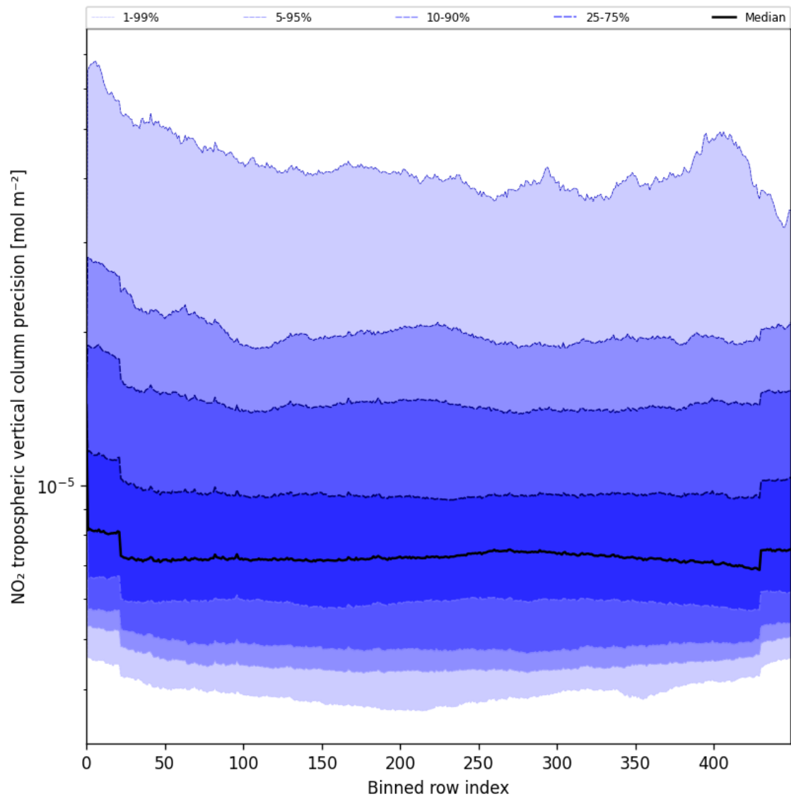
Figure 47: Along track statistics of “NO 2 tropospheric vertical column precision” for 2025-07-24 to 2025-07-25
