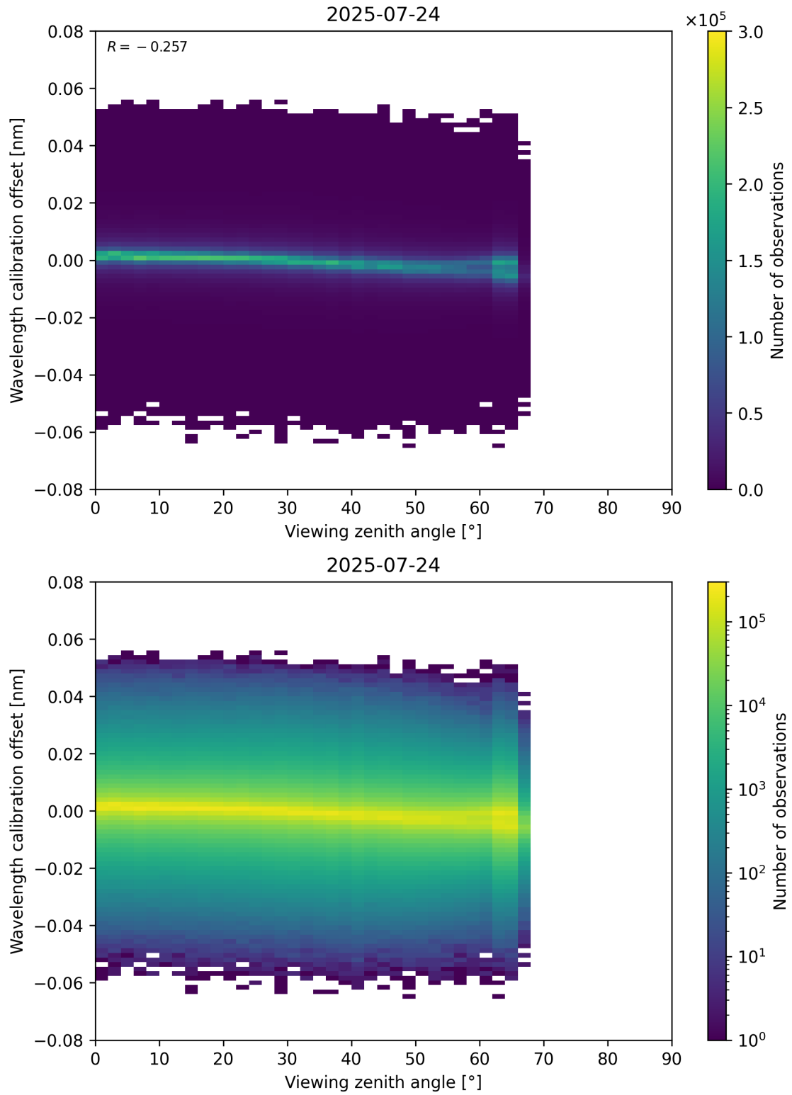
Figure 173: Scatter density plot of “Viewing zenith angle” against “Wavelength calibration offset” for 2025-07-24 to 2025-07-25.
