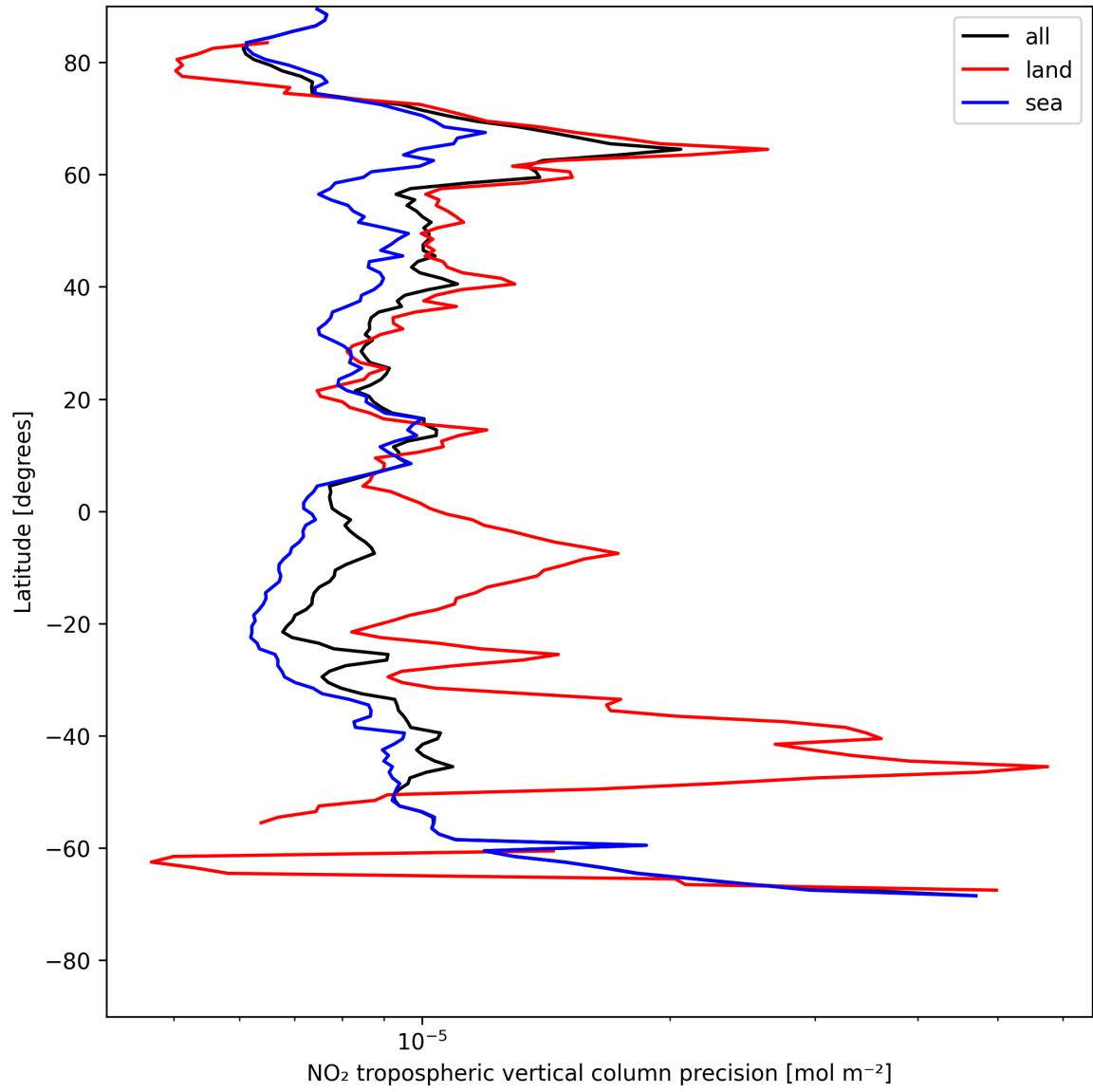
Figure 13: Zonal average of “NO 2 tropospheric vertical column precision” for 2025-07-24 to 2025-07-25.
