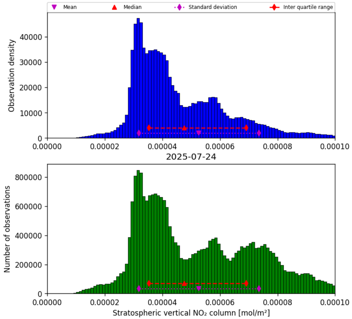
Figure 36: Histogram of “Stratospheric vertical NO 2 column” for 2025-07-24 to 2025-07-25
