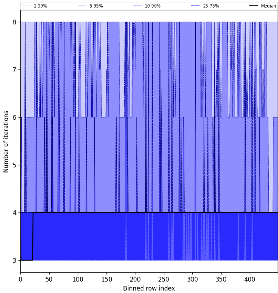
Figure 51: Along track statistics of “Number of iterations” for 2025-07-24 to 2025-07-25
