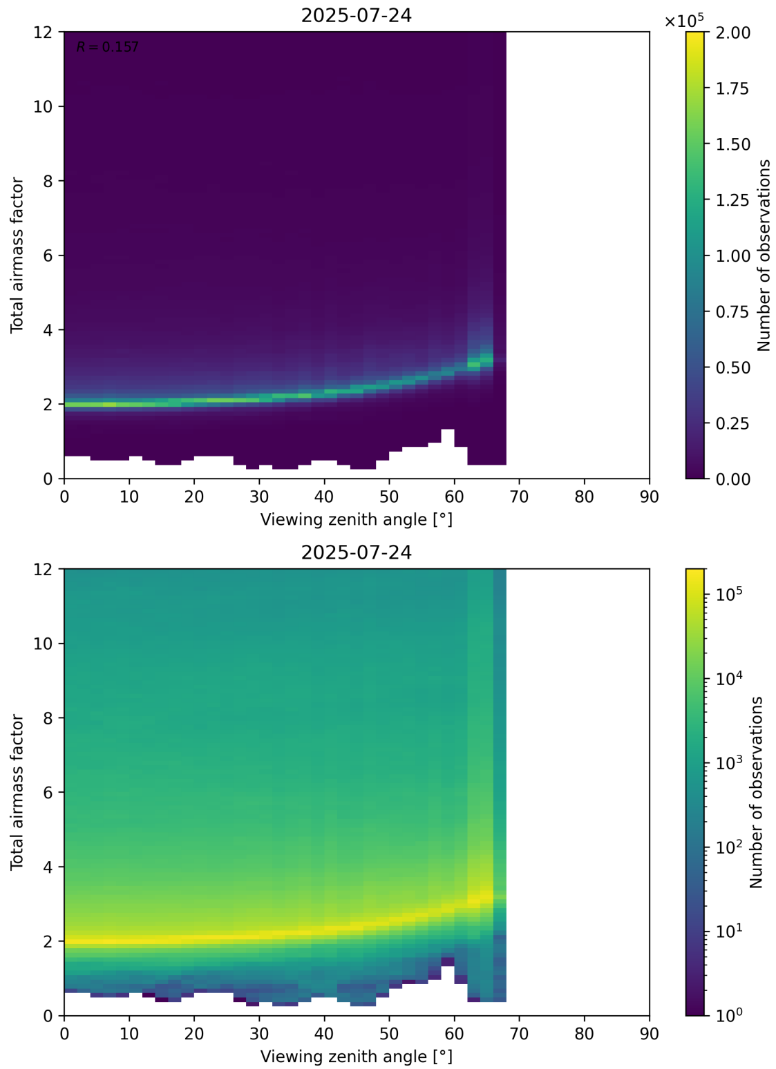
Figure 160: Scatter density plot of “Viewing zenith angle” against “Total airmass factor” for 2025-07-24 to 2025-07-25.
