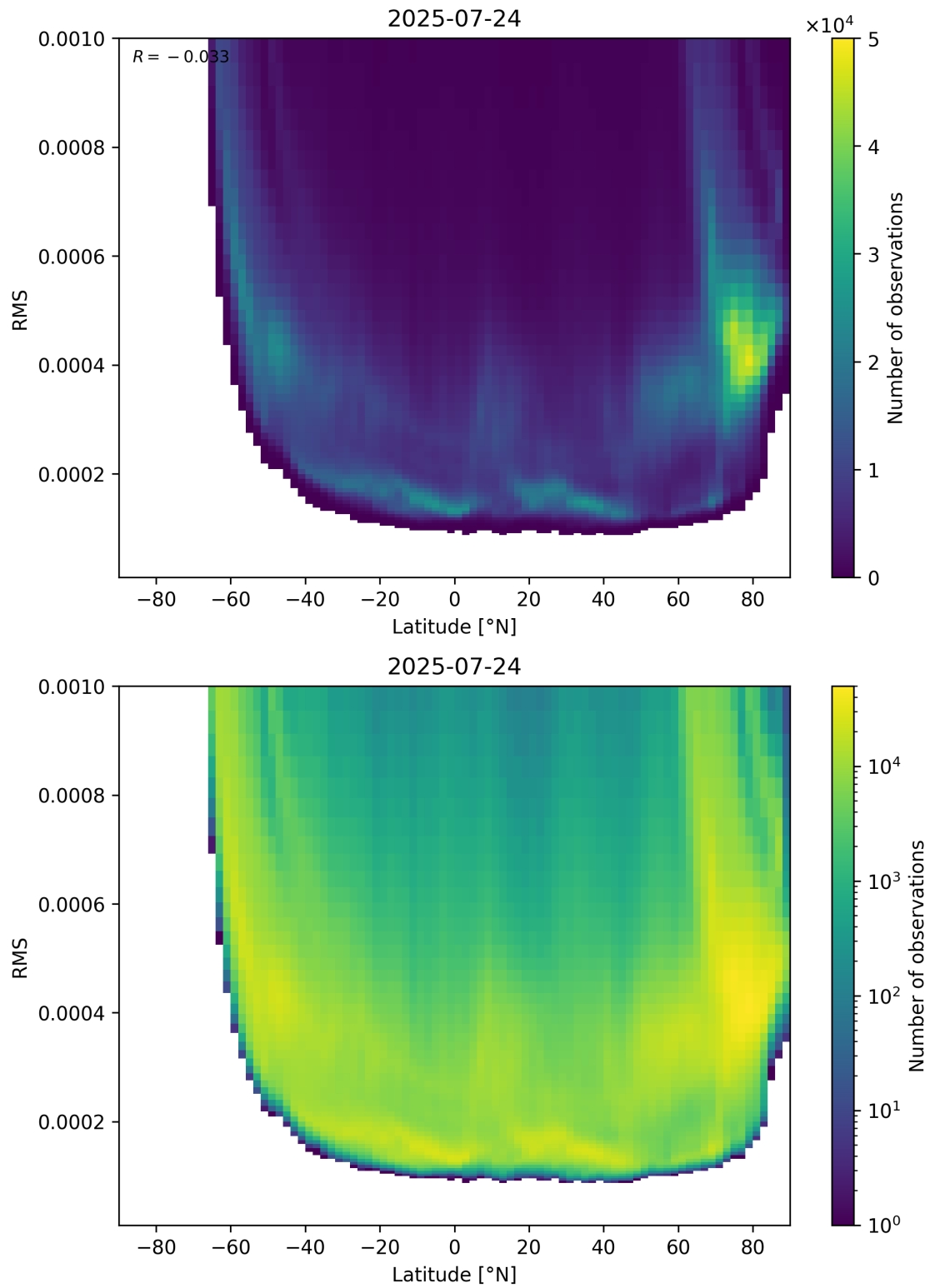
Figure 94: Scatter density plot of “Latitude” against “RMS” for 2025-07-24 to 2025-07-25.
