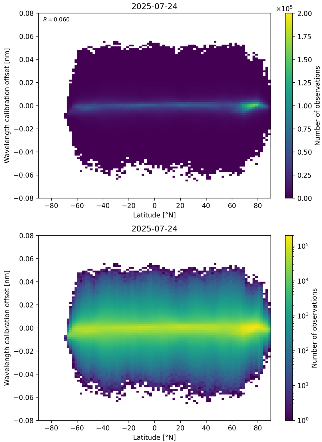
Figure 95: Scatter density plot of “Latitude” against “Wavelength calibration offset” for 2025-07-24 to 2025-07-25.
