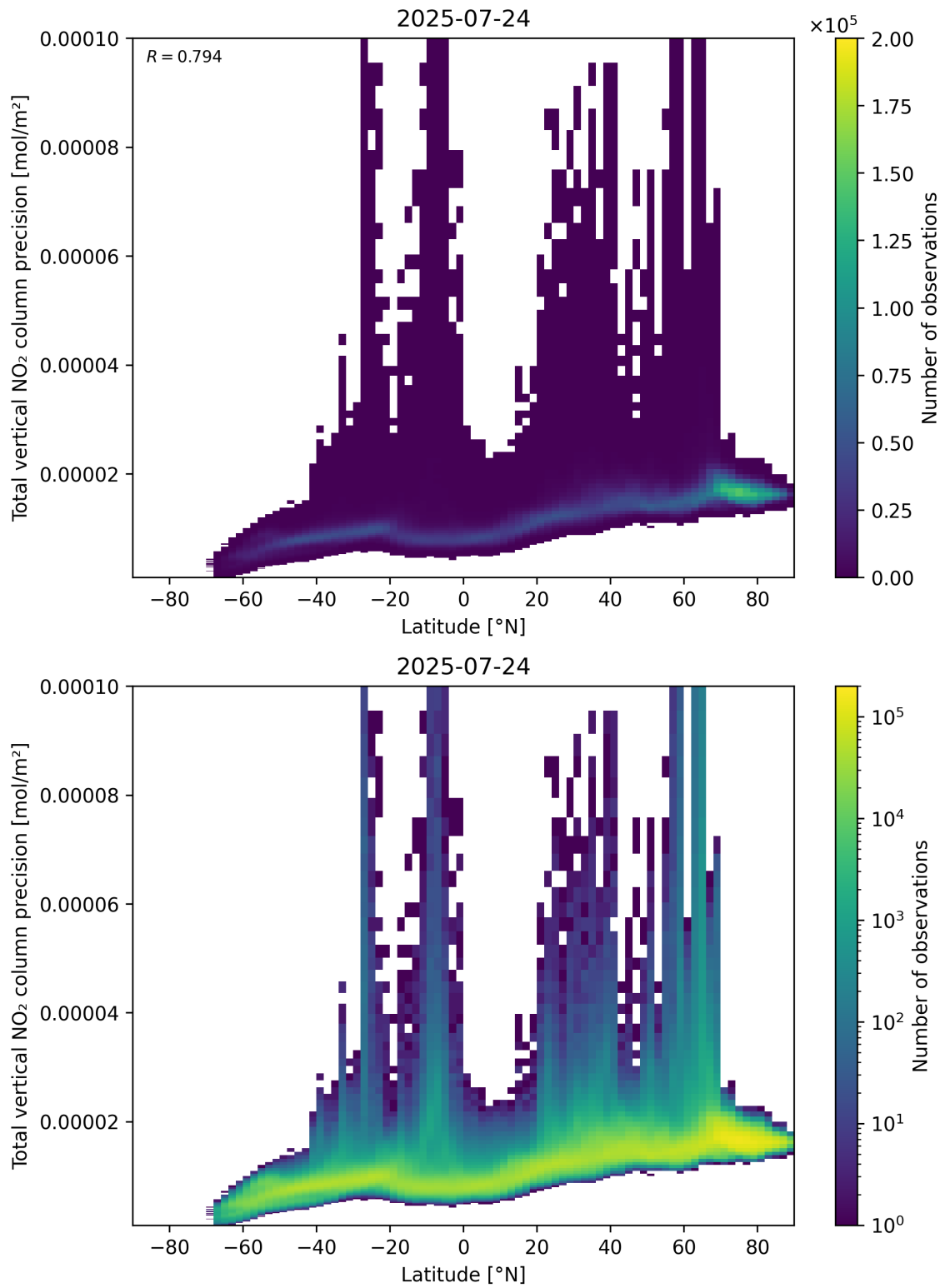
Figure 91: Scatter density plot of “Latitude” against “Total vertical NO 2 column precision” for 2025-07-24 to 2025-07-25.
