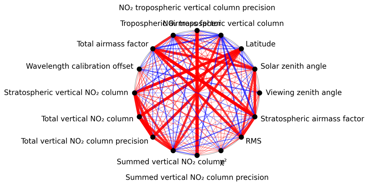
Figure 1: Map of correlation graph for 2025-07-24 to 2025-07-25.
