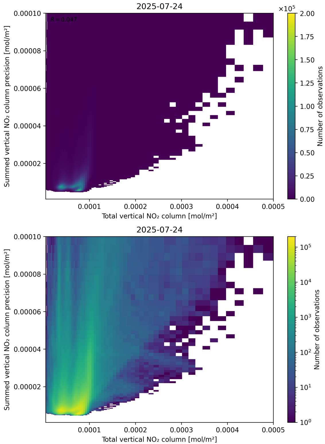
Figure 113: Scatter density plot of “Total vertical NO 2 column” against “Summed vertical NO 2 column precision” for 2025-07-24 to 2025-07-25.
