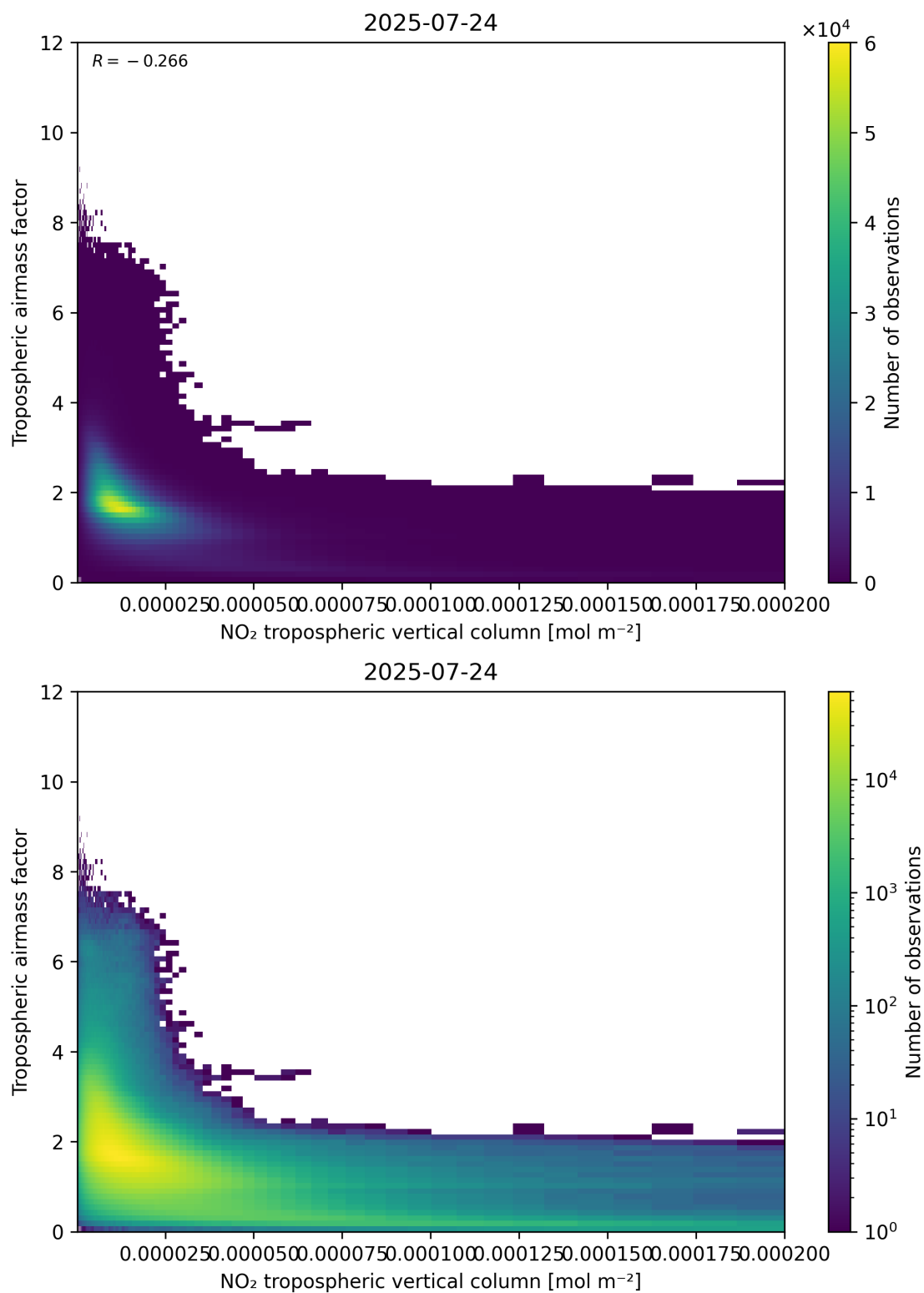
Figure 123: Scatter density plot of “NO 2 tropospheric vertical column” against “Tropospheric air mass factor” for 2025-07-24 to 2025-07-25.
