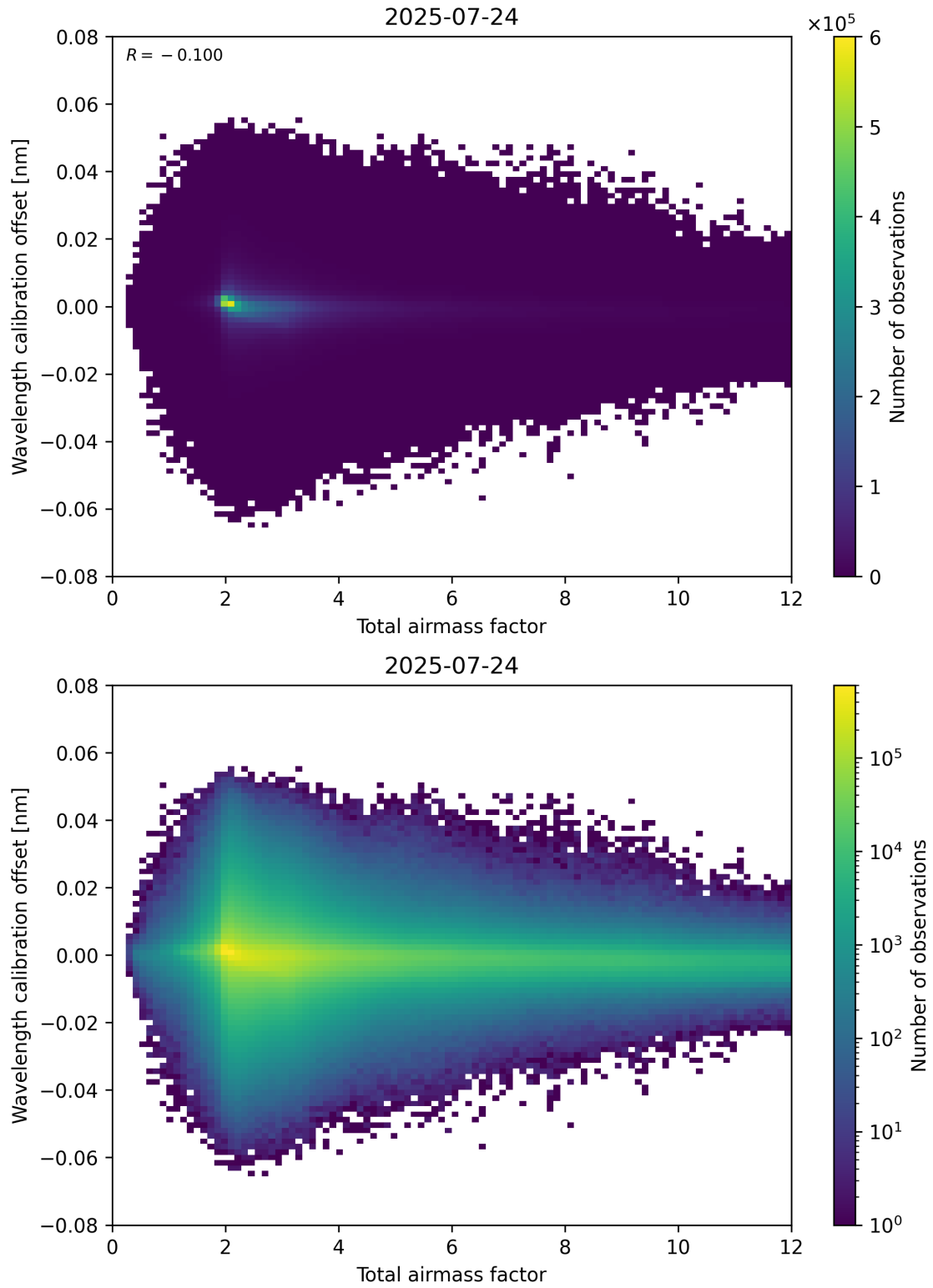
Figure 70: Scatter density plot of “Total airmass factor” against “Wavelength calibration offset” for 2025-07-24 to 2025-07-25.
