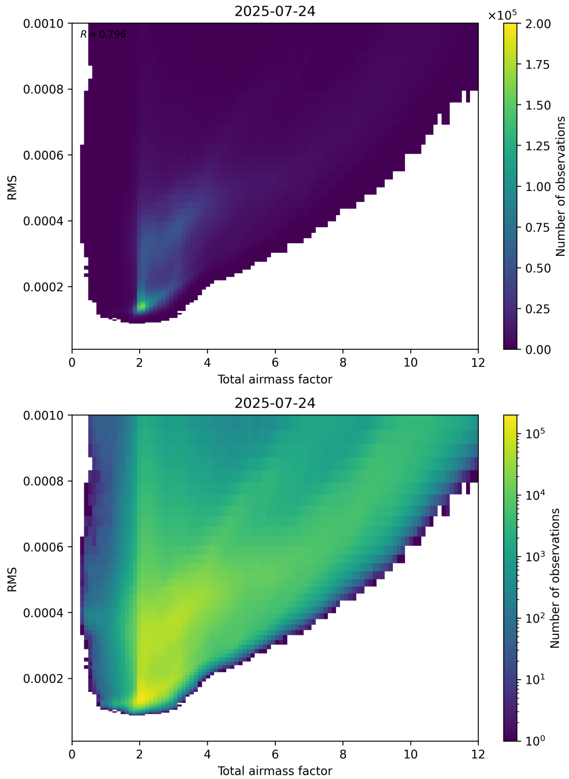
Figure 69: Scatter density plot of “Total airmass factor” against “RMS” for 2025-07-24 to 2025-07-25.
