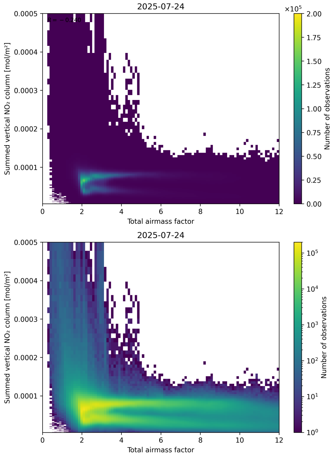
Figure 65: Scatter density plot of “Total airmass factor” against “Summed vertical NO 2 column” for 2025-07-24 to 2025-07-25.
