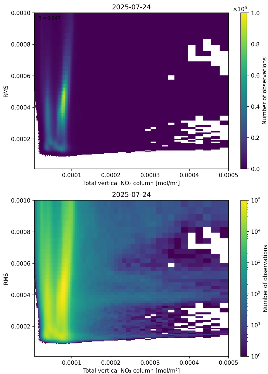
Figure 120: Scatter density plot of “Total vertical NO 2 column” against “RMS” for 2025-07-24 to 2025-07-25.
