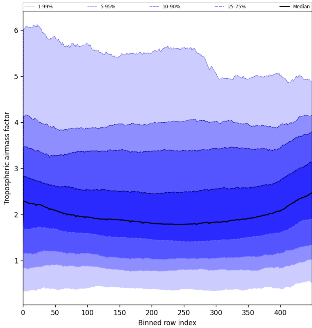
Figure 48: Along track statistics of “Tropospheric airmass factor” for 2025-07-24 to 2025-07-25
