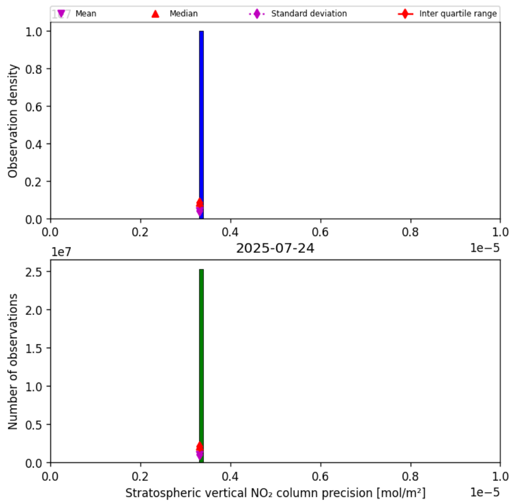
Figure 37: Histogram of “Stratospheric vertical NO 2 column precision” for 2025-07-24 to 2025-07-25
