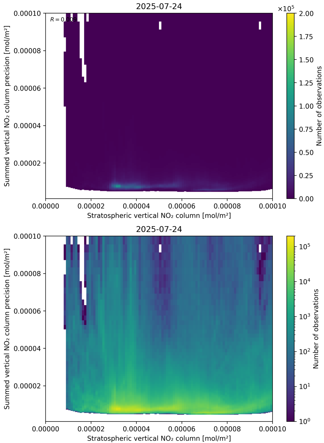
Figure 99: Scatter density plot of “Stratospheric vertical NO 2 column” against “Summed vertical NO 2 column precision” for 2025-07-24 to 2025-07-25.
