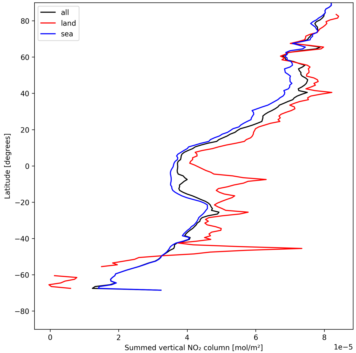
Figure 23: Zonal average of “Summed vertical NO 2 column” for 2025-07-24 to 2025-07-25.
