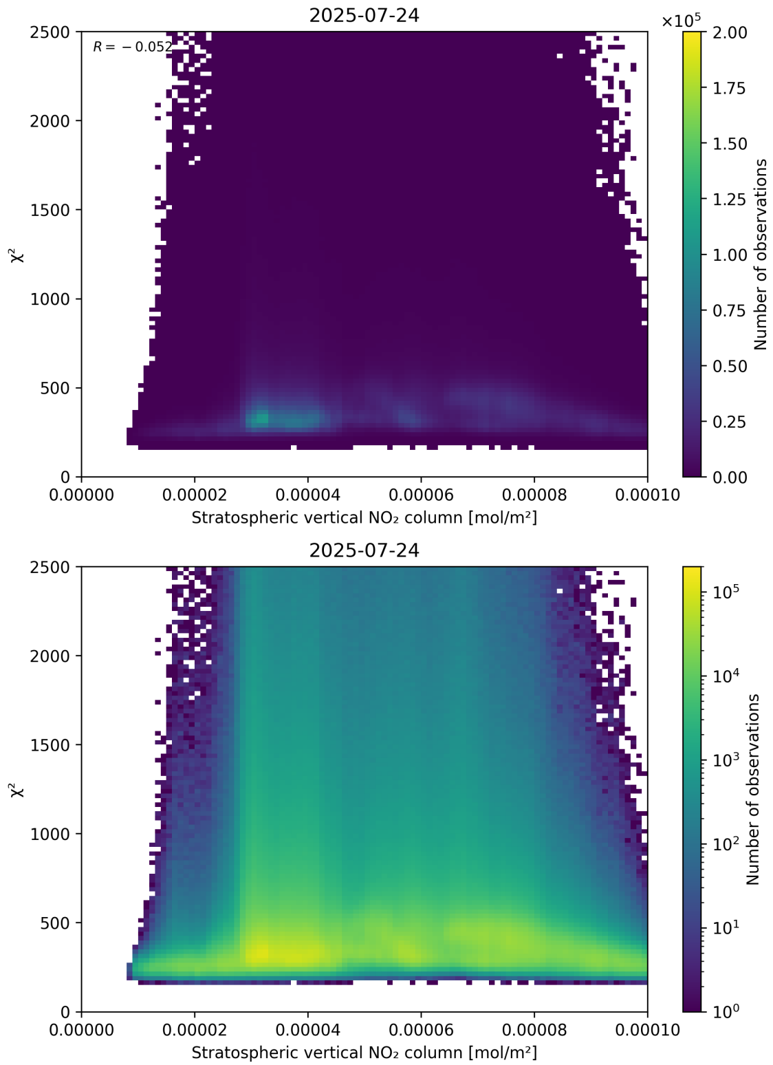
Figure 97: Scatter density plot of “Stratospheric vertical NO 2 column” against “ \chi^2 ” for 2025-07-24 to 2025-07-25.
