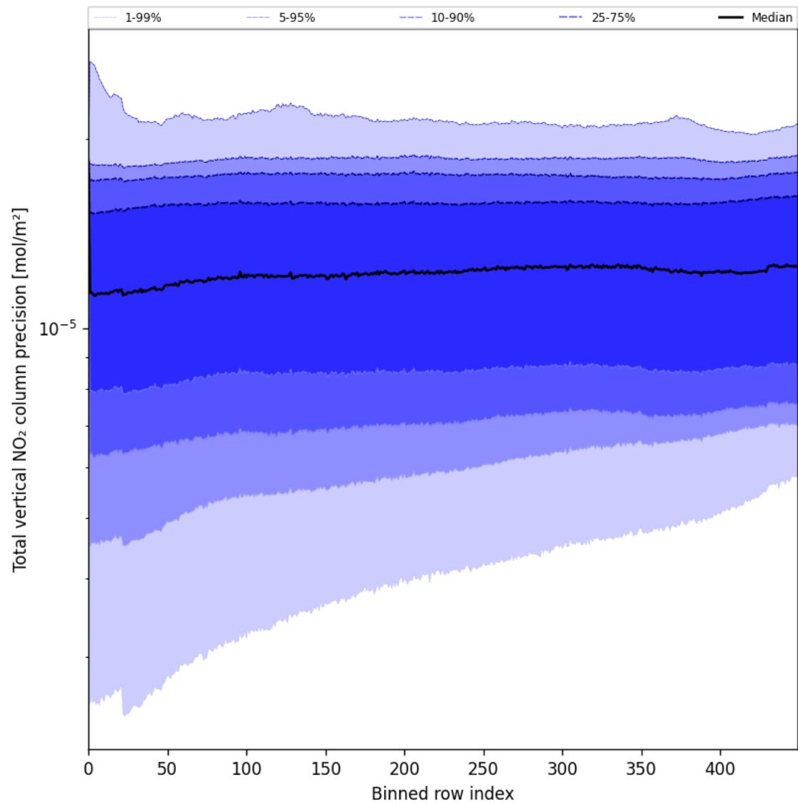
Figure 56: Along track statistics of “Total vertical NO 2 column precision” for 2025-07-24 to 2025-07-25
