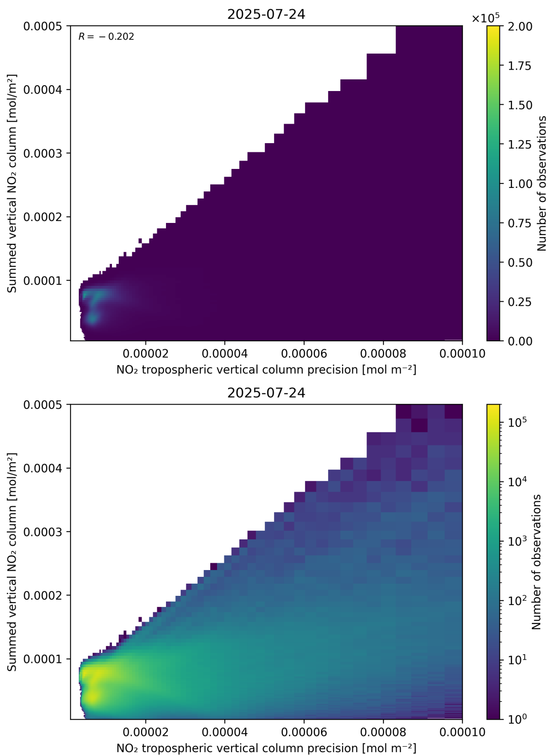
Figure 136: Scatter density plot of “NO 2 tropospheric vertical column precision” against “Summed vertical NO 2 column” for 2025-07-24 to 2025-07-25.
