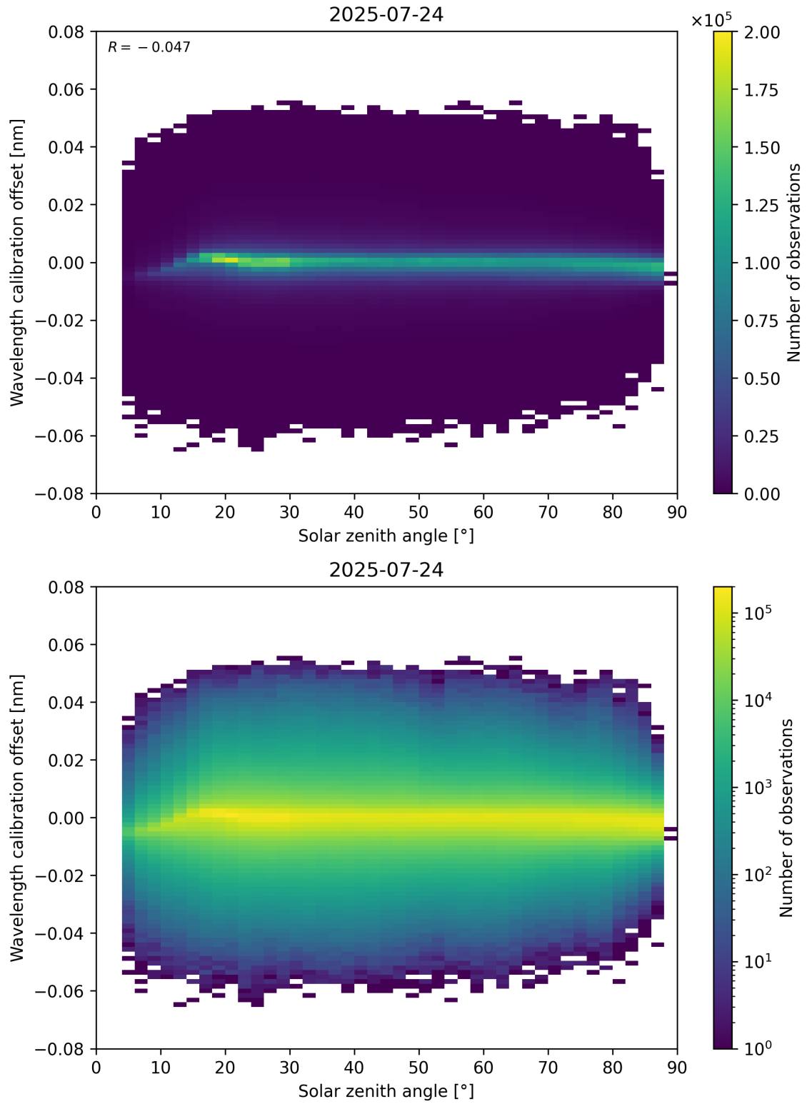
Figure 158: Scatter density plot of “Solar zenith angle” against “Wavelength calibration offset” for 2025-07-24 to 2025-07-25.
