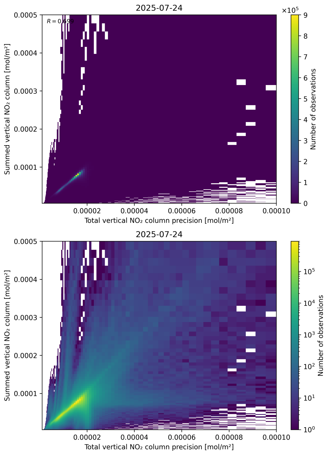
Figure 117: Scatter density plot of “Total vertical NO 2 column precision” against “Summed vertical NO 2 column” for 2025-07-24 to 2025-07-25.
