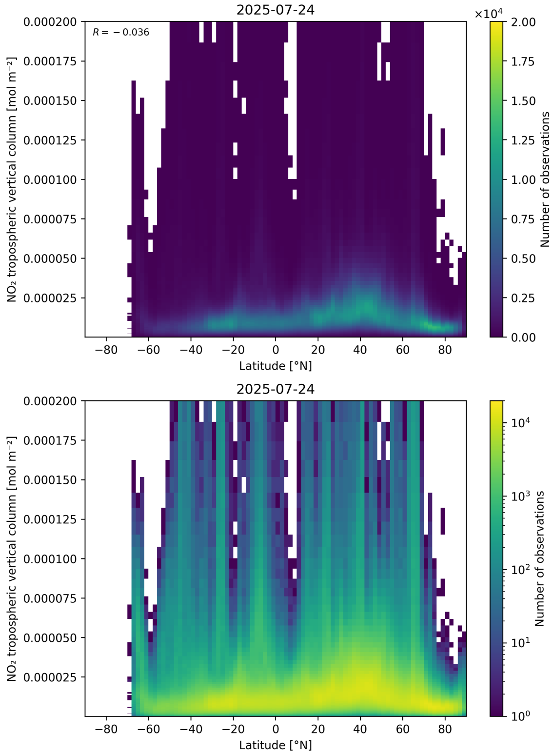
Figure 92: Scatter density plot of “Latitude” against “NO 2 tropospheric vertical column” for 2025-07-24 to 2025-07-25.
