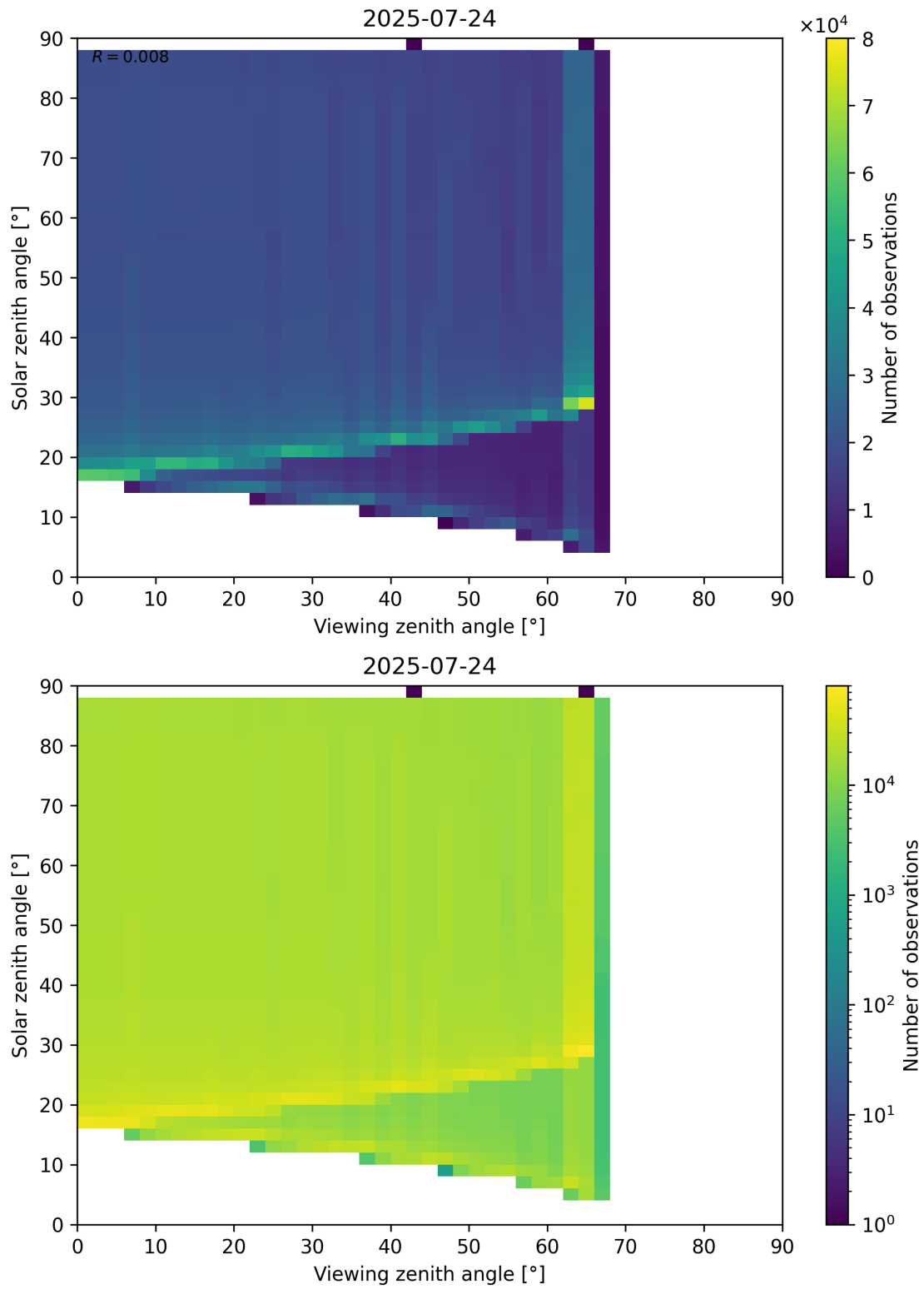
Figure 172: Scatter density plot of “Viewing zenith angle” against “Solar zenith angle” for 2025-07-24 to 2025-07-25.
