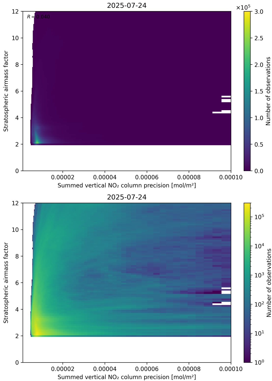
Figure 106: Scatter density plot of “Summed vertical NO 2 column precision” against “Stratospheric airmass factor” for 2025-07-24 to 2025-07-25.
