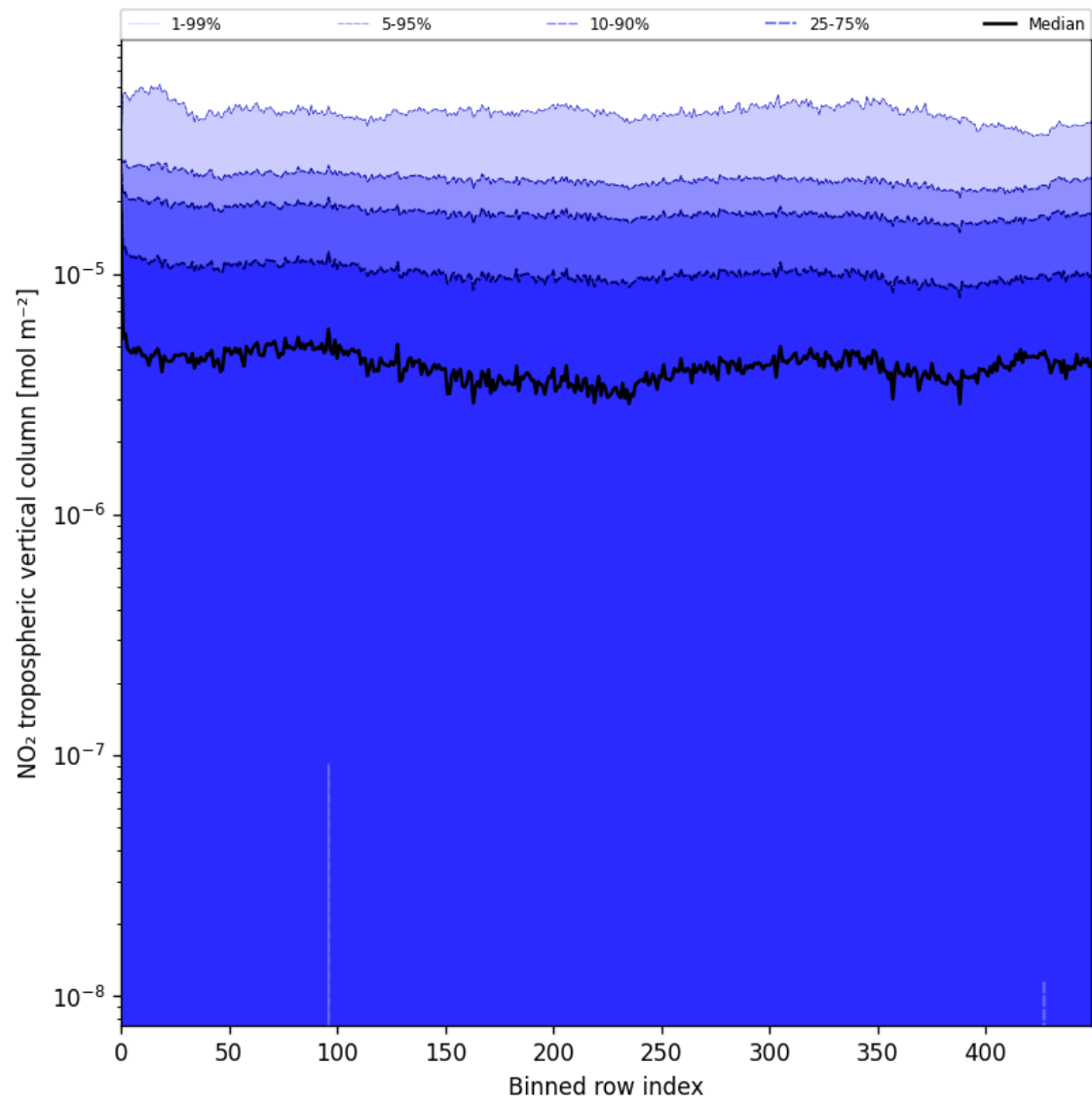
Figure 46: Along track statistics of “NO 2 tropospheric vertical column” for 2025-07-24 to 2025-07-25
