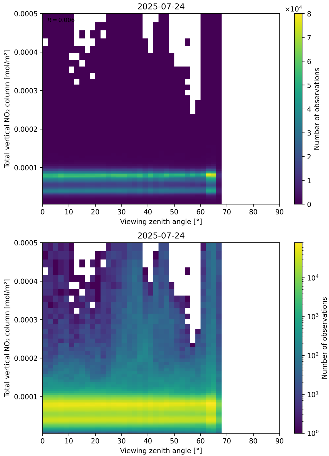
Figure 167: Scatter density plot of “Viewing zenith angle” against “Total vertical NO 2 column” for 2025-07-24 to 2025-07-25.
