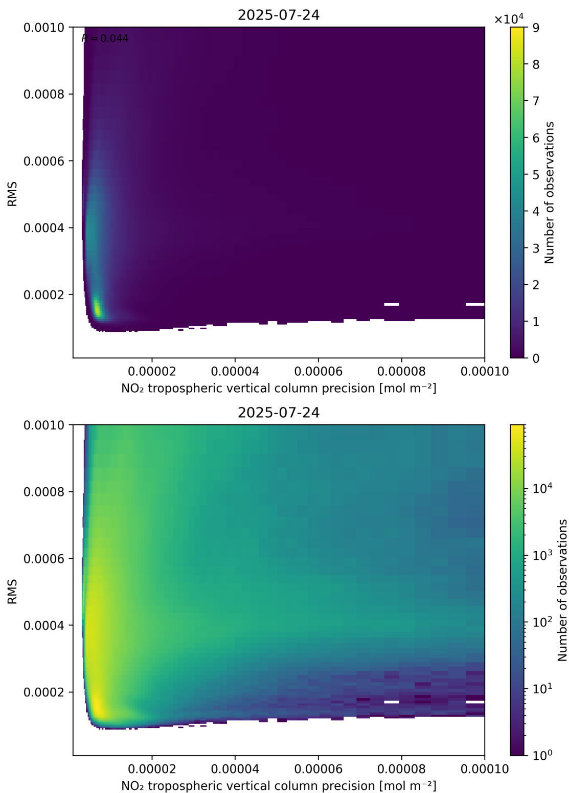
Figure 140: Scatter density plot of “NO 2 tropospheric vertical column precision” against “RMS” for 2025-07-24 to 2025-07-25.
