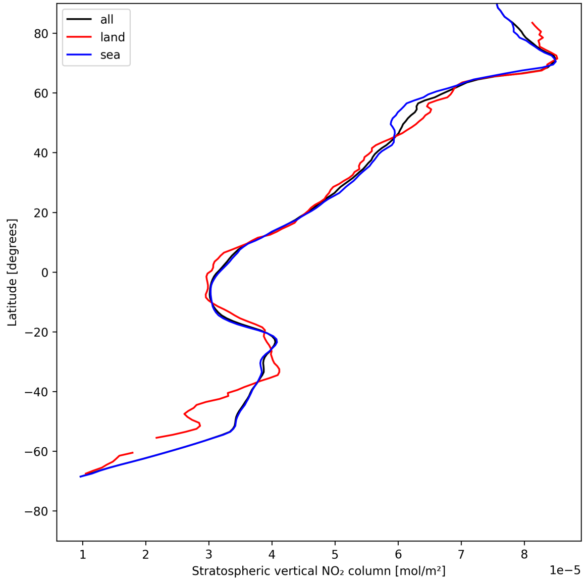
Figure 19: Zonal average of “Stratospheric vertical NO 2 column” for 2025-07-24 to 2025-07-25.
