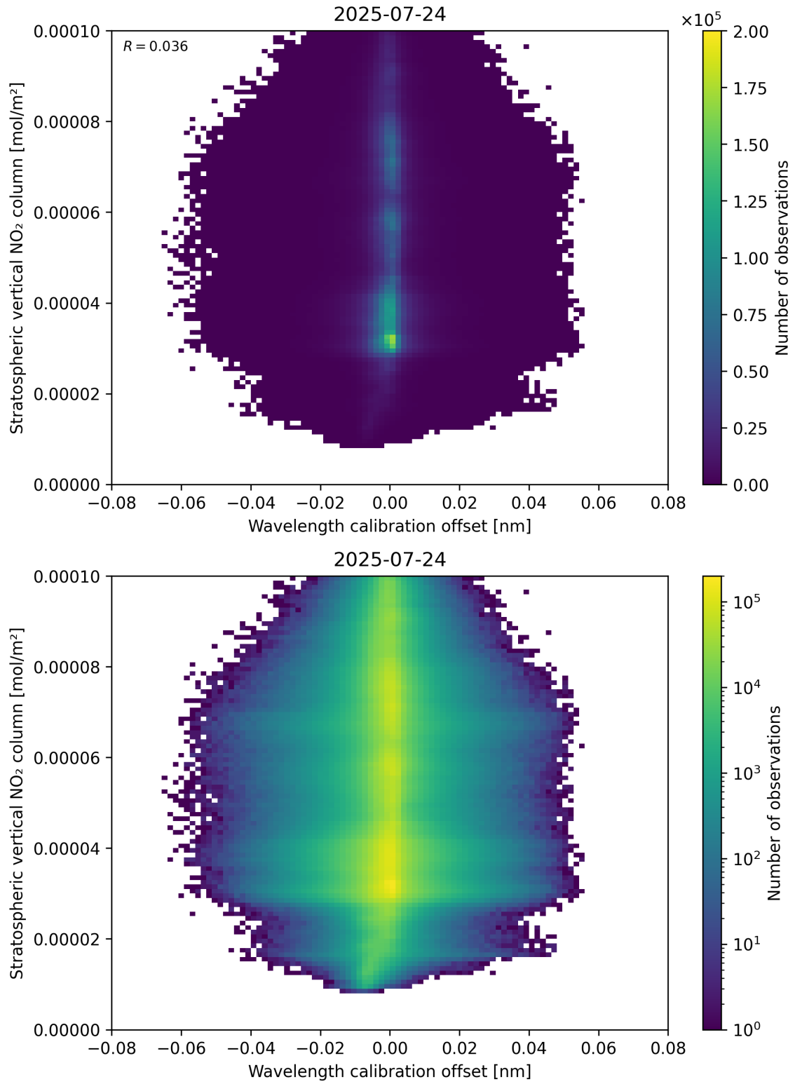
Figure 176: Scatter density plot of “Wavelength calibration offset” against “Stratospheric vertical NO 2 column” for 2025-07-24 to 2025-07-25.
