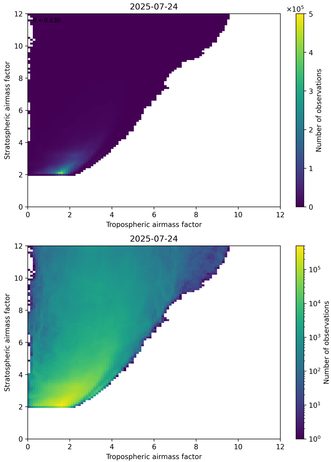
Figure 71: Scatter density plot of “Tropospheric airmass factor” against “Stratospheric airmass factor” for 2025-07-24 to 2025-07-25.
