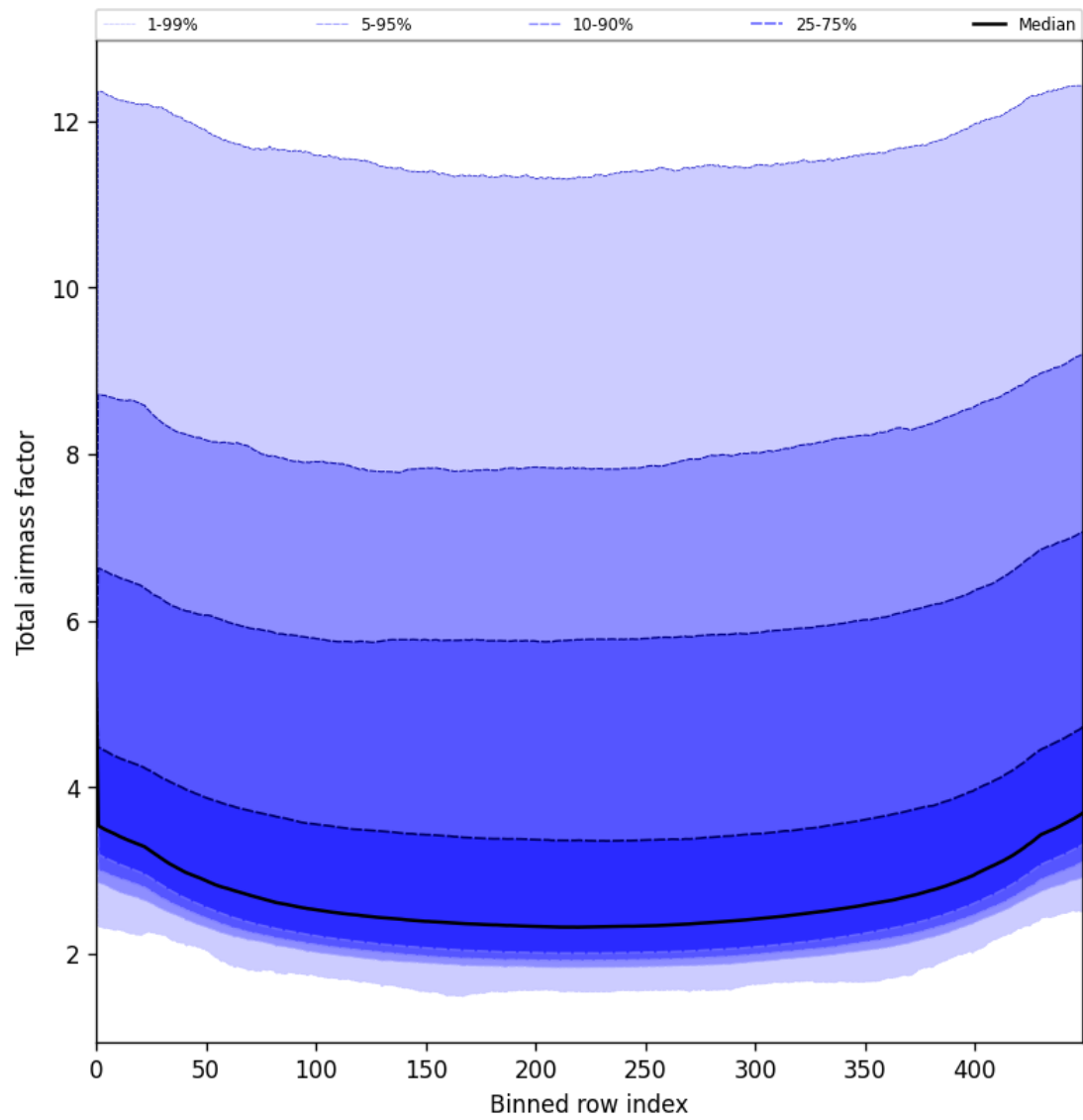
Figure 49: Along track statistics of “Total airmass factor” for 2025-07-24 to 2025-07-25
