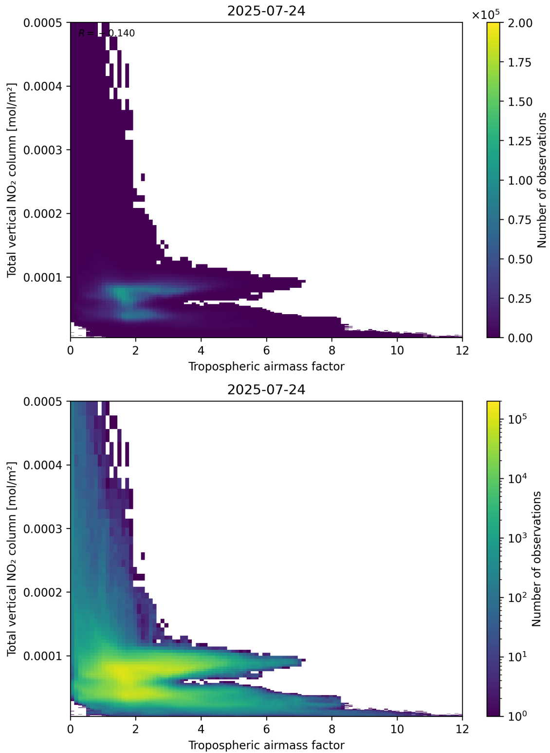
Figure 77: Scatter density plot of “Tropospheric airmass factor” against “Total vertical NO 2 column” for 2025-07-24 to 2025-07-25.
