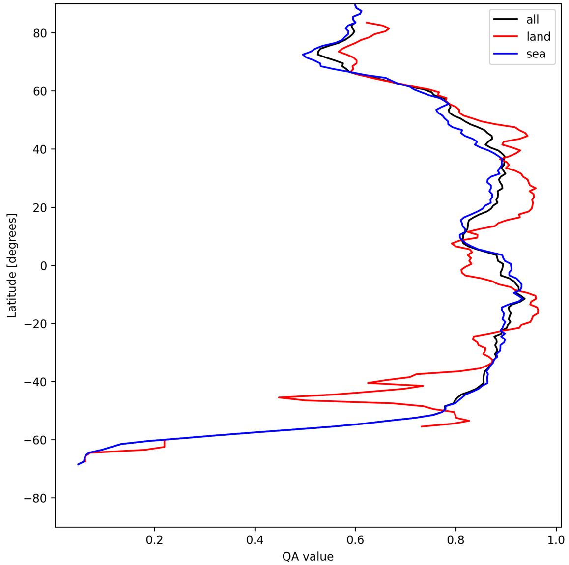
Figure 11: Zonal average of “QA value” for 2025-07-24 to 2025-07-25.
