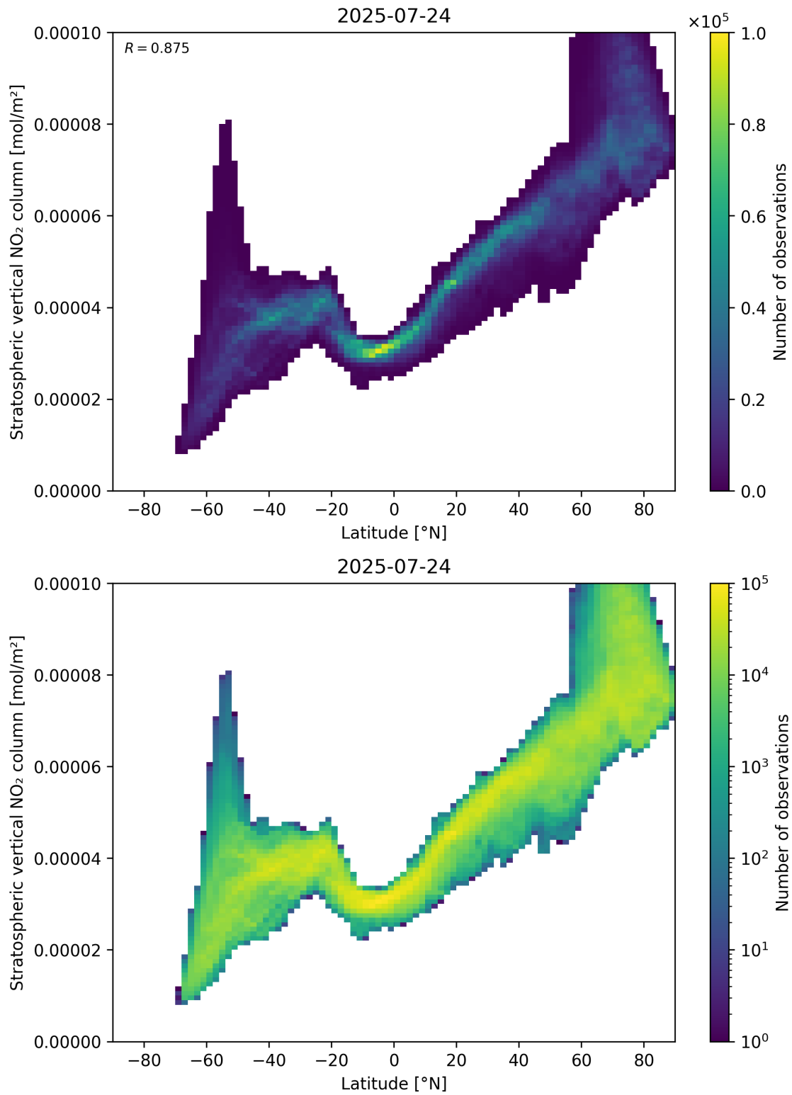
Figure 87: Scatter density plot of “Latitude” against “Stratospheric vertical NO 2 column” for 2025-07-24 to 2025-07-25.
