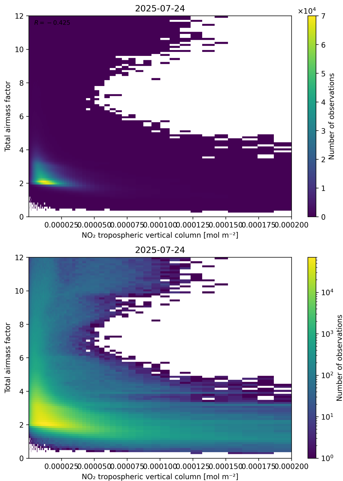
Figure 122: Scatter density plot of “NO 2 tropospheric vertical column” against “Total air mass factor” for 2025-07-24 to 2025-07-25.
