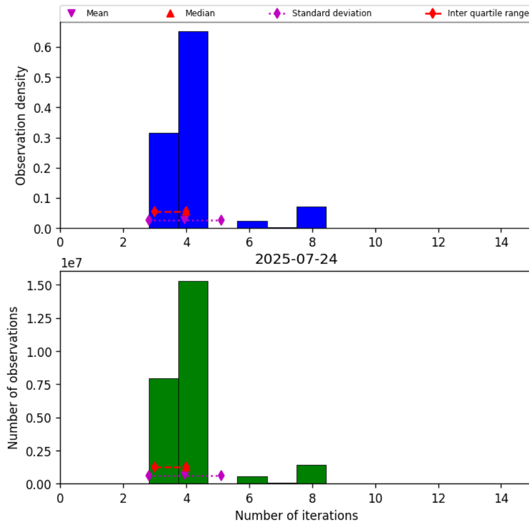
Figure 34: Histogram of “Number of iterations” for 2025-07-24 to 2025-07-25
