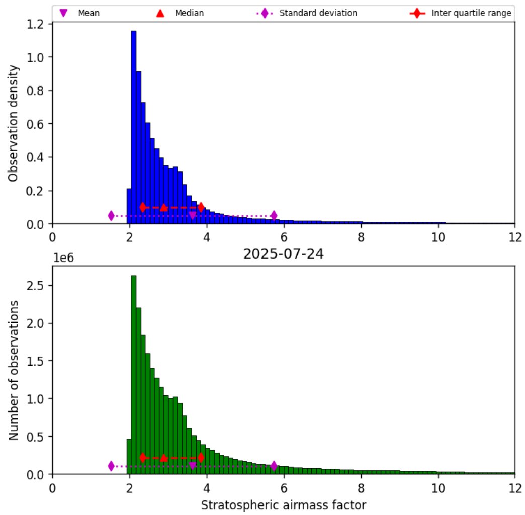
Figure 44: Histogram of “Stratospheric airmass factor” for 2025-07-24 to 2025-07-25
