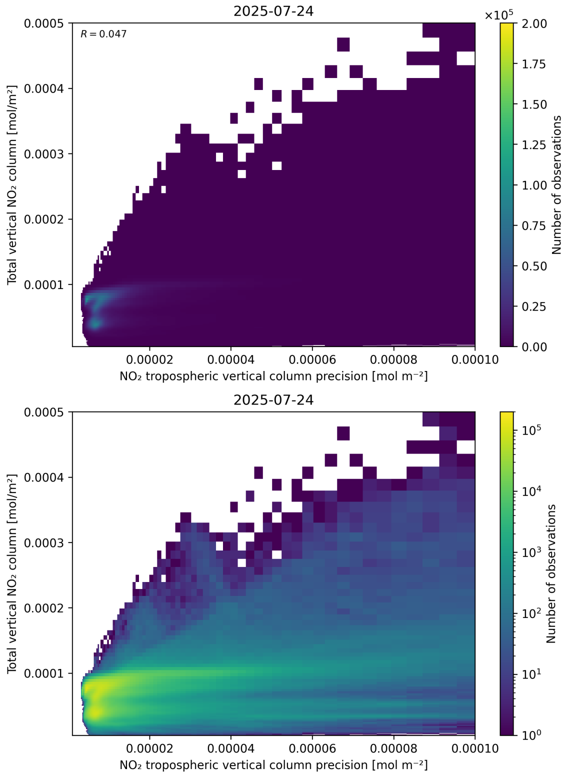
Figure 138: Scatter density plot of “NO 2 tropospheric vertical column precision” against “Total vertical NO 2 column” for 2025-07-24 to 2025-07-25.
