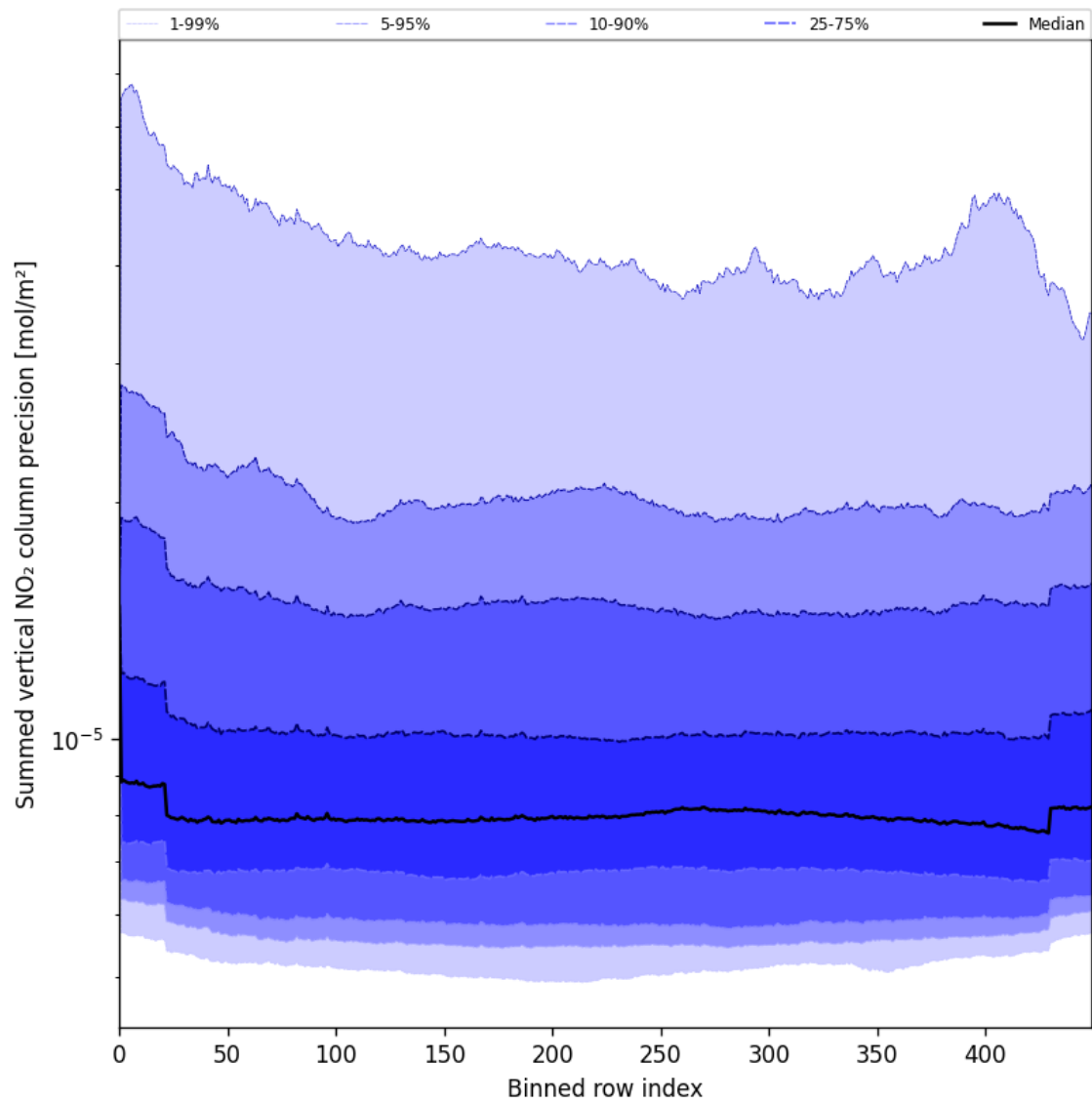
Figure 58: Along track statistics of “Summed vertical NO 2 column precision” for 2025-07-24 to 2025-07-25
