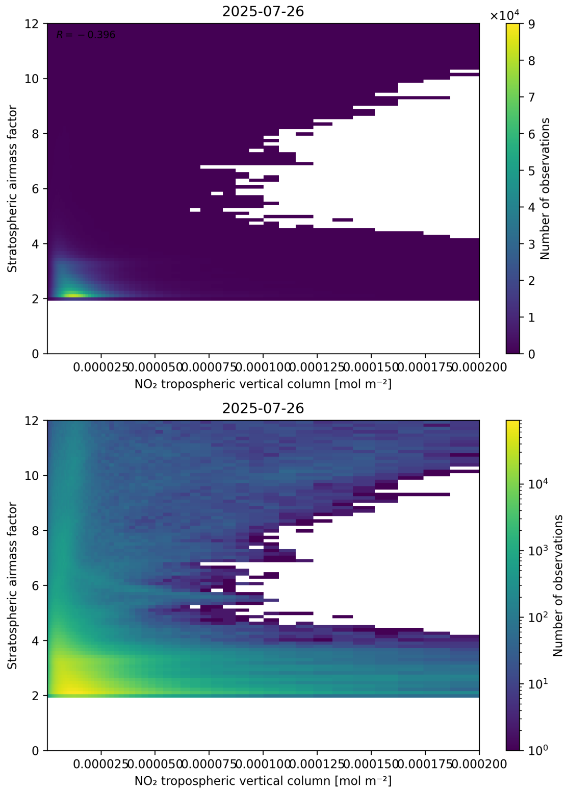
Figure 121: Scatter density plot of “NO 2 tropospheric vertical column” against “Stratospheric air mass factor” for 2025-07-25 to 2025-07-27.
