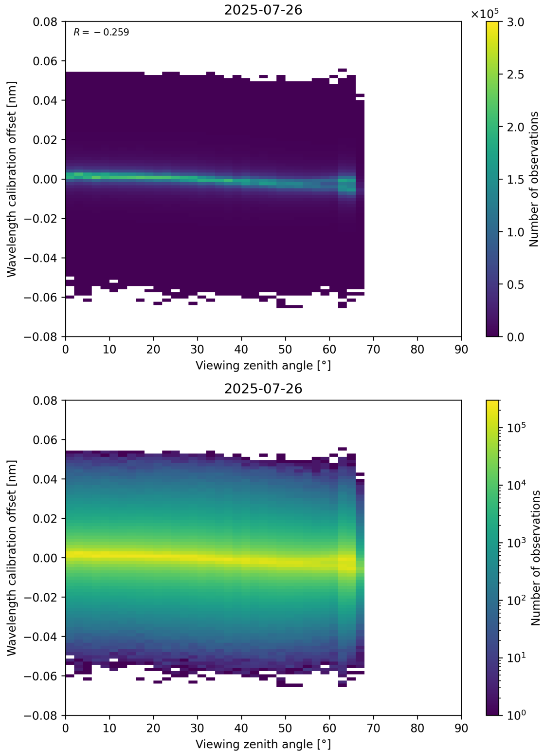
Figure 173: Scatter density plot of “Viewing zenith angle” against “Wavelength calibration offset” for 2025-07-25 to 2025-07-27.
