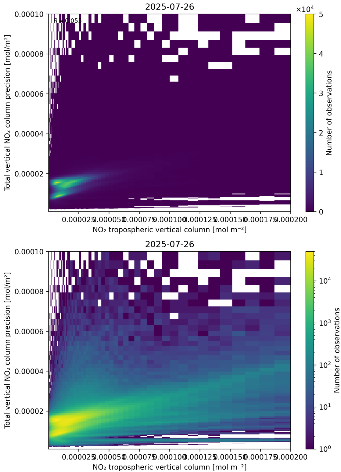
Figure 129: Scatter density plot of “NO 2 tropospheric vertical column” against “Total vertical NO 2 column precision” for 2025-07-25 to 2025-07-27.
