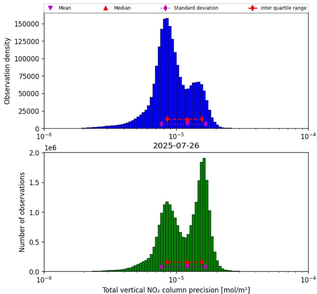
Figure 39: Histogram of "Total vertical NO 2 column precision" for 2025-07-25 to 2025-07-27
