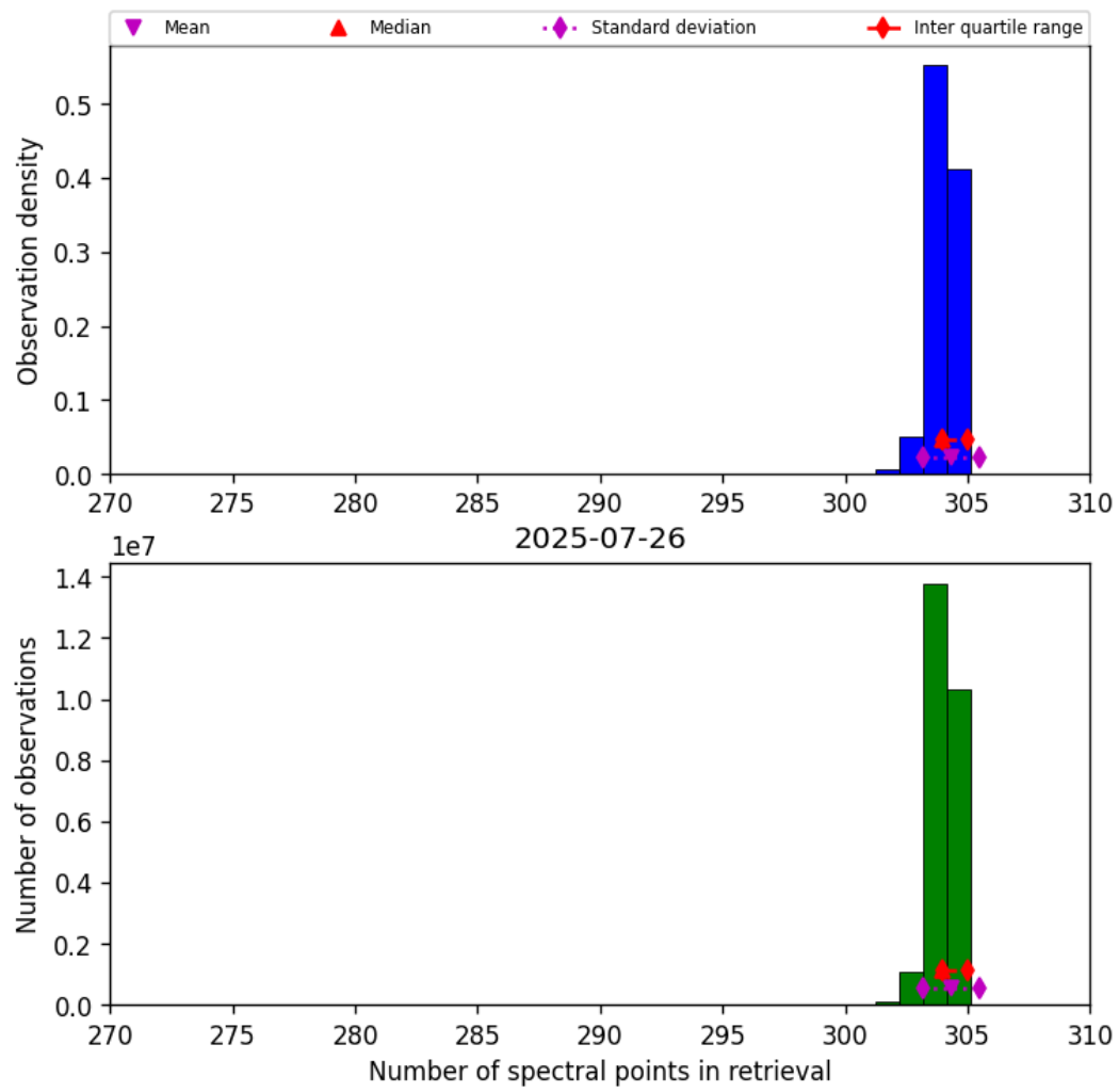
Figure 33: Histogram of “Number of spectral points in retrieval” for 2025-07-25 to 2025-07-27
