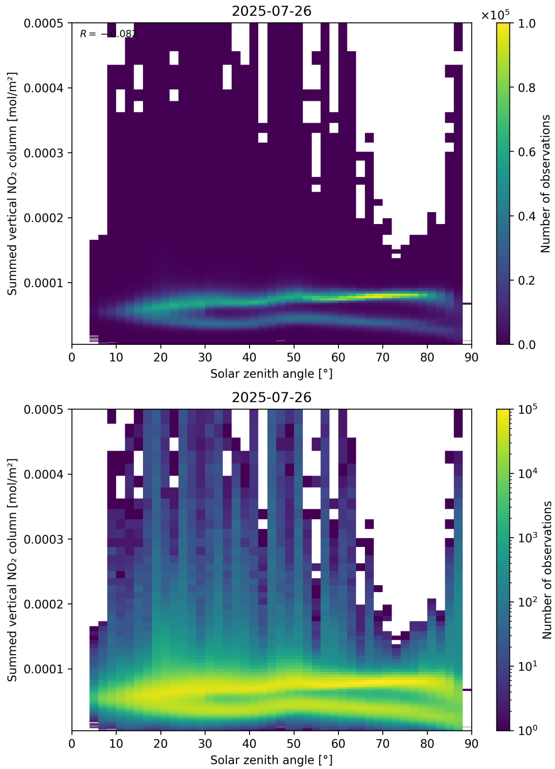
Figure 151: Scatter density plot of “Solar zenith angle” against “Summed vertical NO 2 column” for 2025-07-25 to 2025-07-27.
