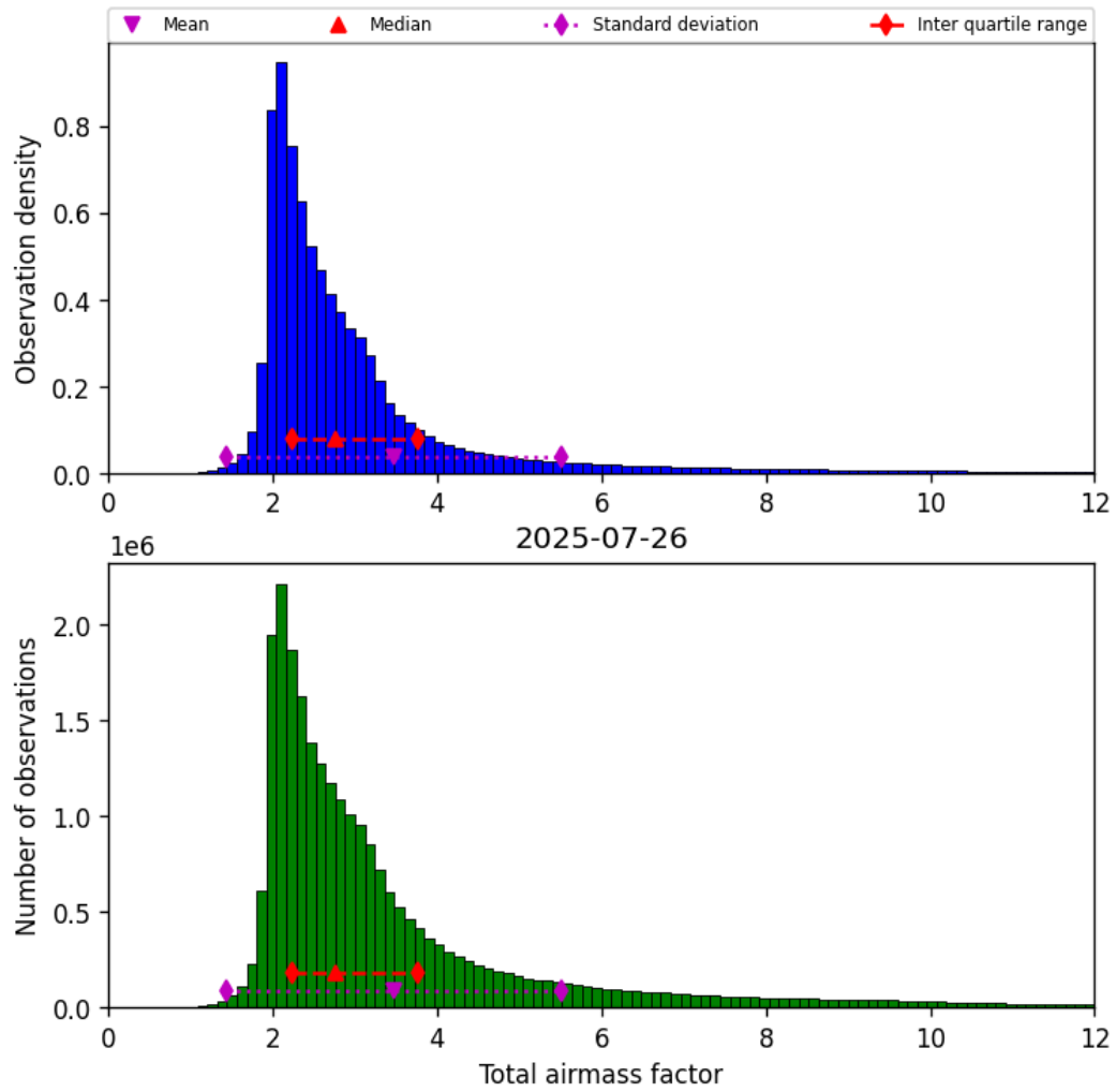
Figure 32: Histogram of “Total airmass factor” for 2025-07-25 to 2025-07-27
