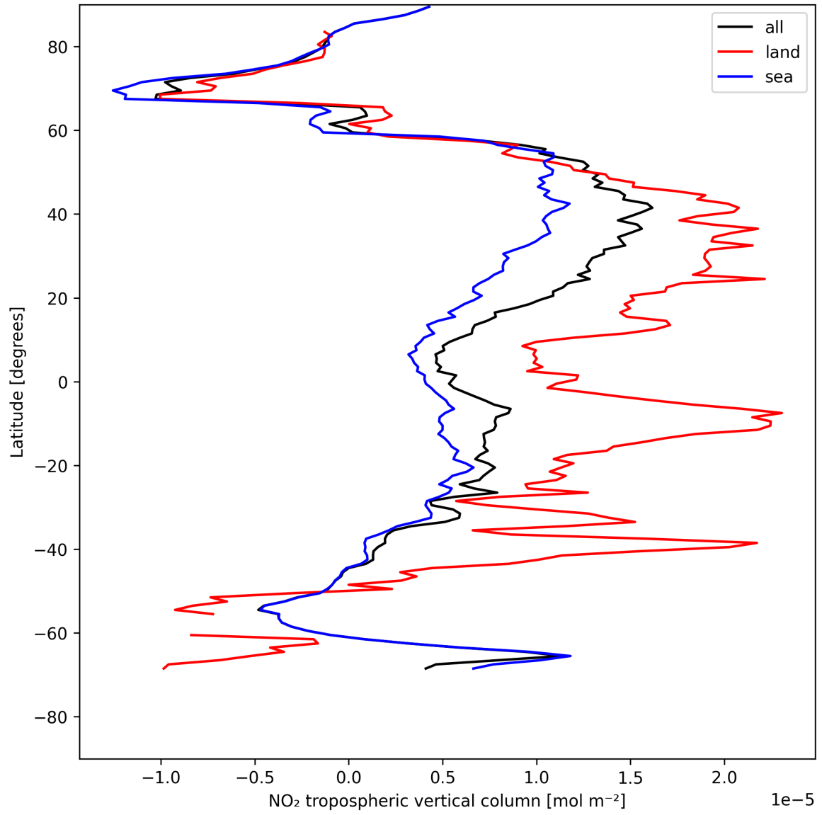
Figure 12: Zonal average of “NO 2 tropospheric vertical column” for 2025-07-25 to 2025-07-27.
