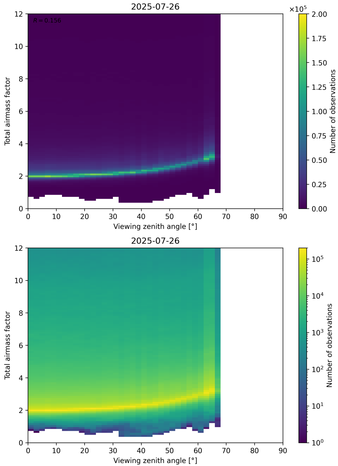
Figure 160: Scatter density plot of “Viewing zenith angle” against “Total airmass factor” for 2025-07-25 to 2025-07-27.
