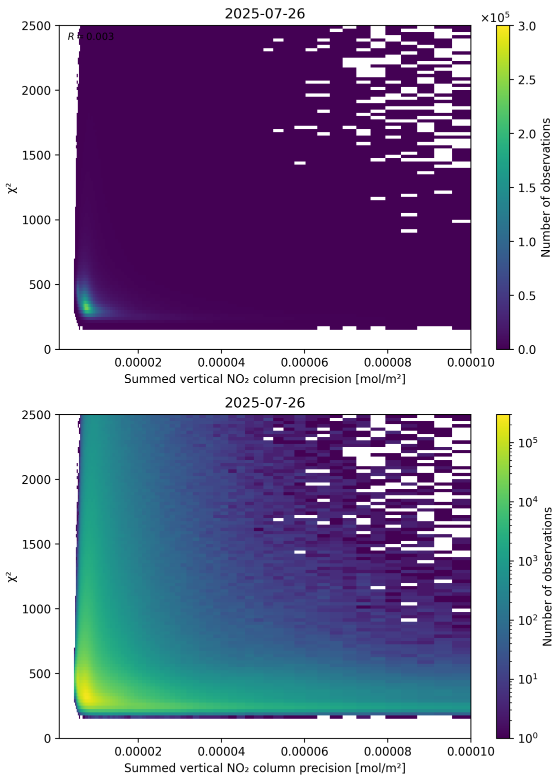
Figure 107: Scatter density plot of “Summed vertical NO 2 column precision” against “ \chi^2 ” for 2025-07-25 to 2025-07-27.
