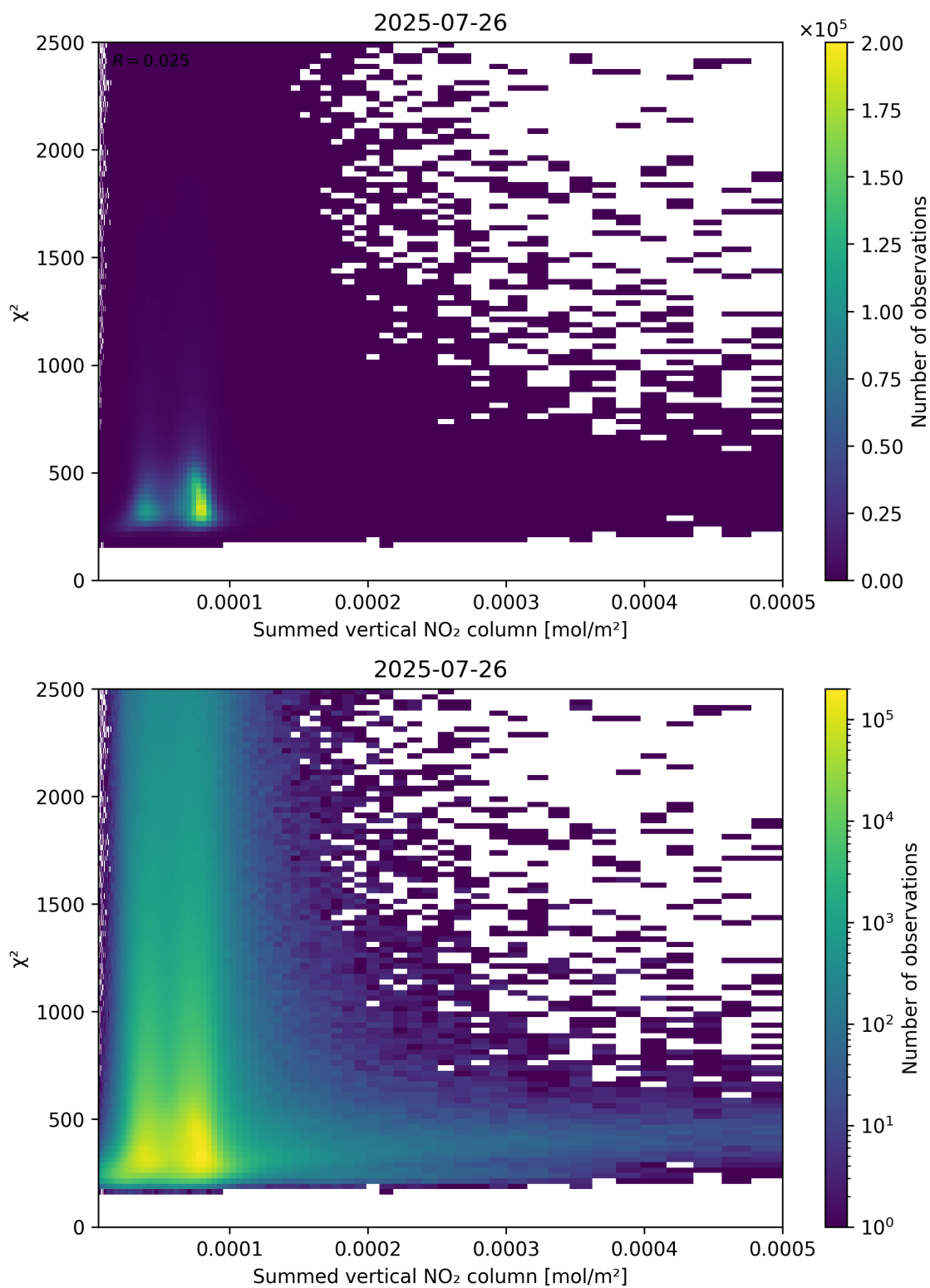
Figure 104: Scatter density plot of “Summed vertical NO 2 column” against “ \chi^2 ” for 2025-07-25 to 2025-07-27.
