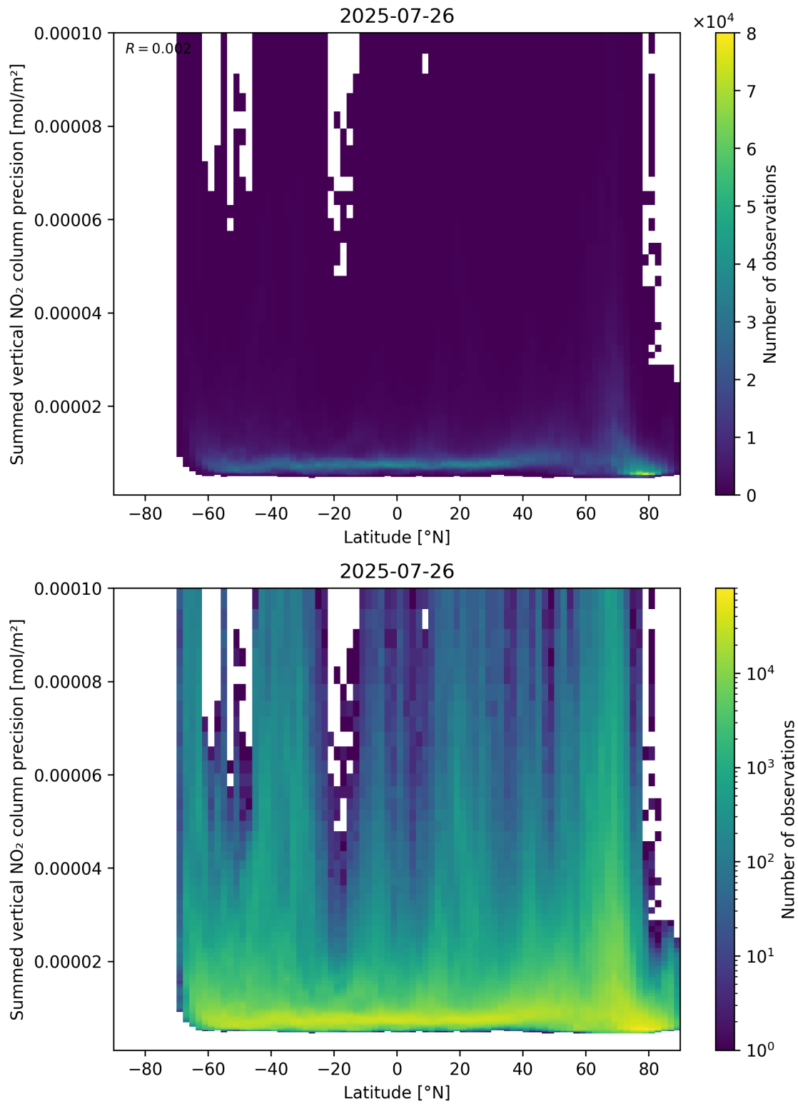
Figure 89: Scatter density plot of “Latitude” against “Summed vertical NO 2 column precision” for 2025-07-25 to 2025-07-27.
