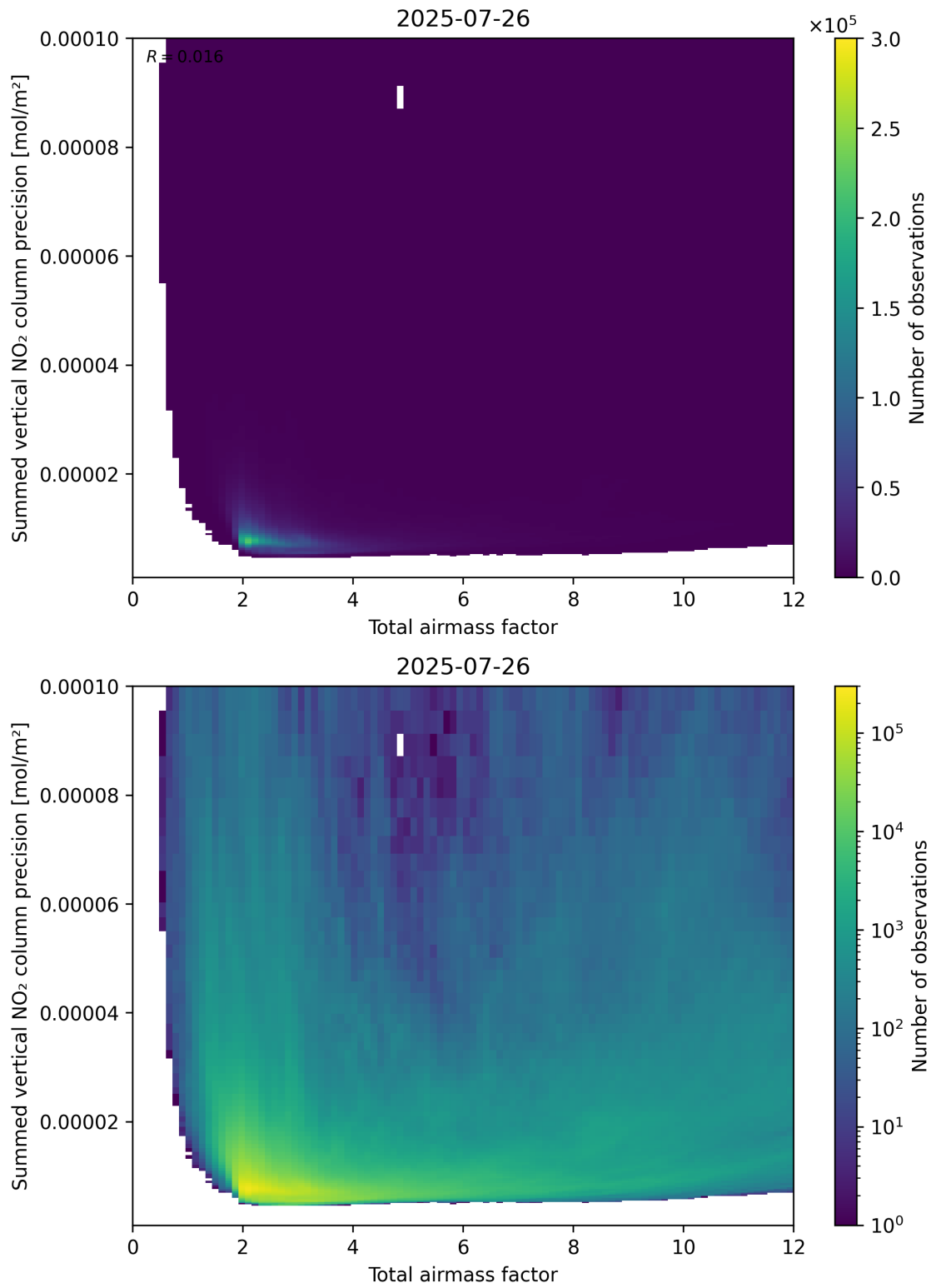
Figure 66: Scatter density plot of “Total airmass factor” against “Summed vertical NO 2 column precision” for 2025-07-25 to 2025-07-27.
