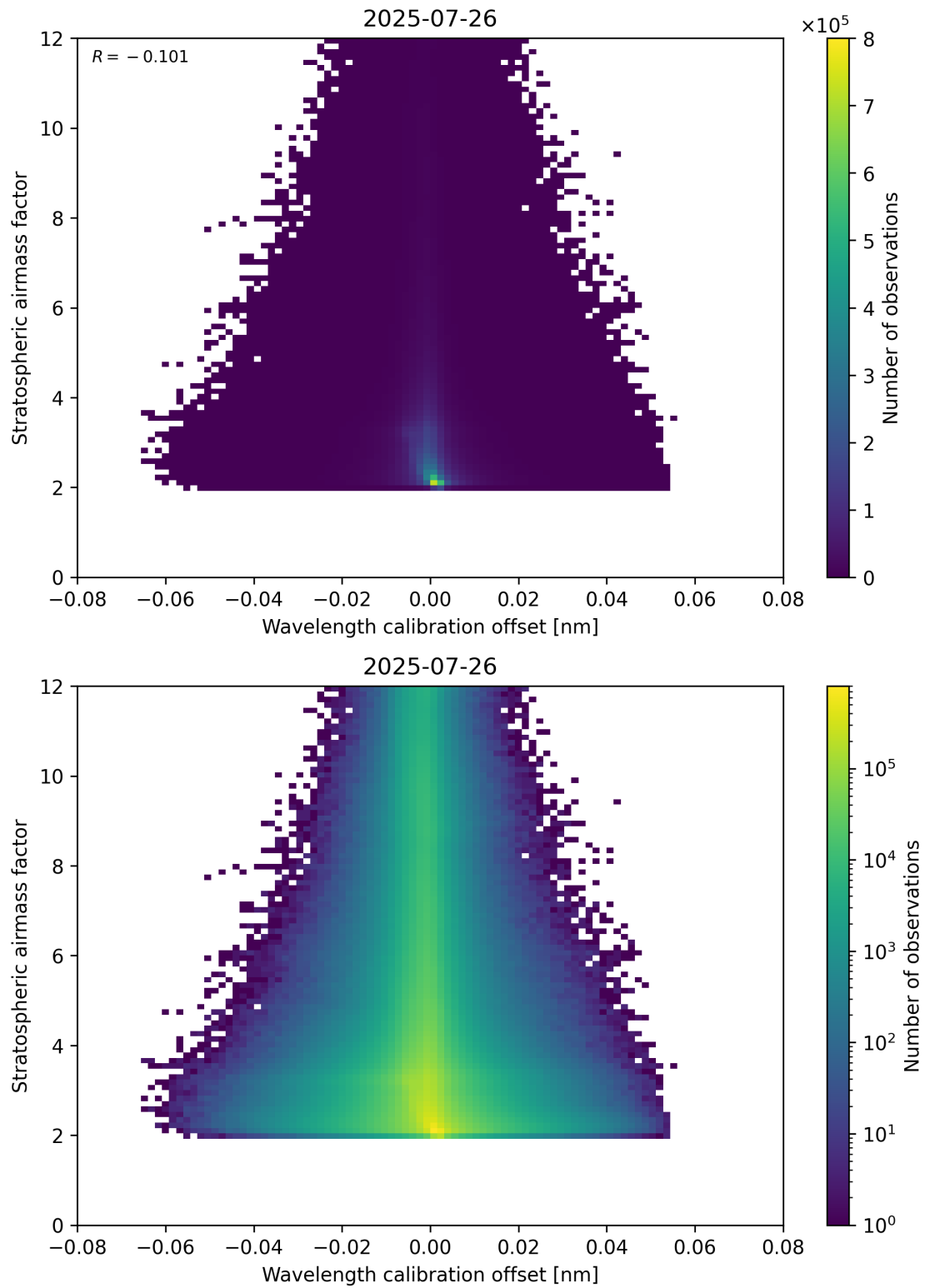
Figure 174: Scatter density plot of “Wavelength calibration offset” against “Stratospheric airmass factor” for 2025-07-25 to 2025-07-27.
