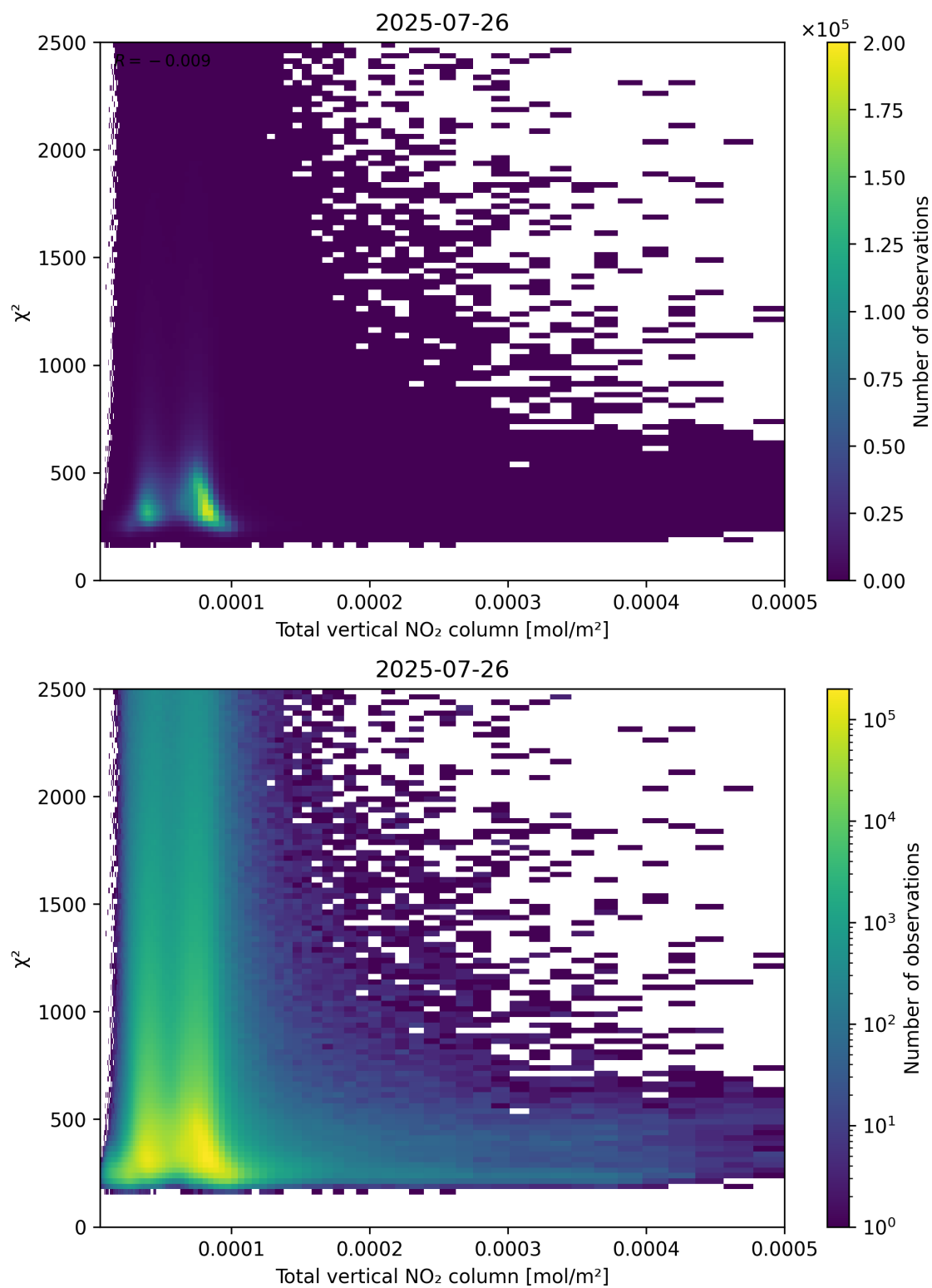
Figure 111: Scatter density plot of “Total vertical NO 2 column” against “ \chi^2 ” for 2025-07-25 to 2025-07-27.
