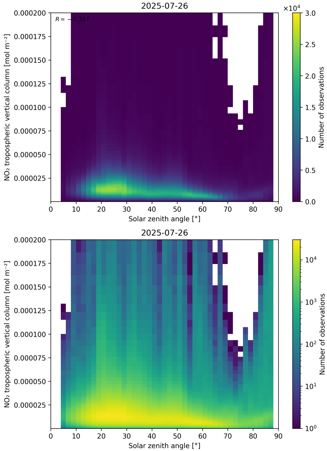
Figure 155: Scatter density plot of “Solar zenith angle” against “NO 2 tropospheric vertical column” for 2025-07-25 to 2025-07-27.
