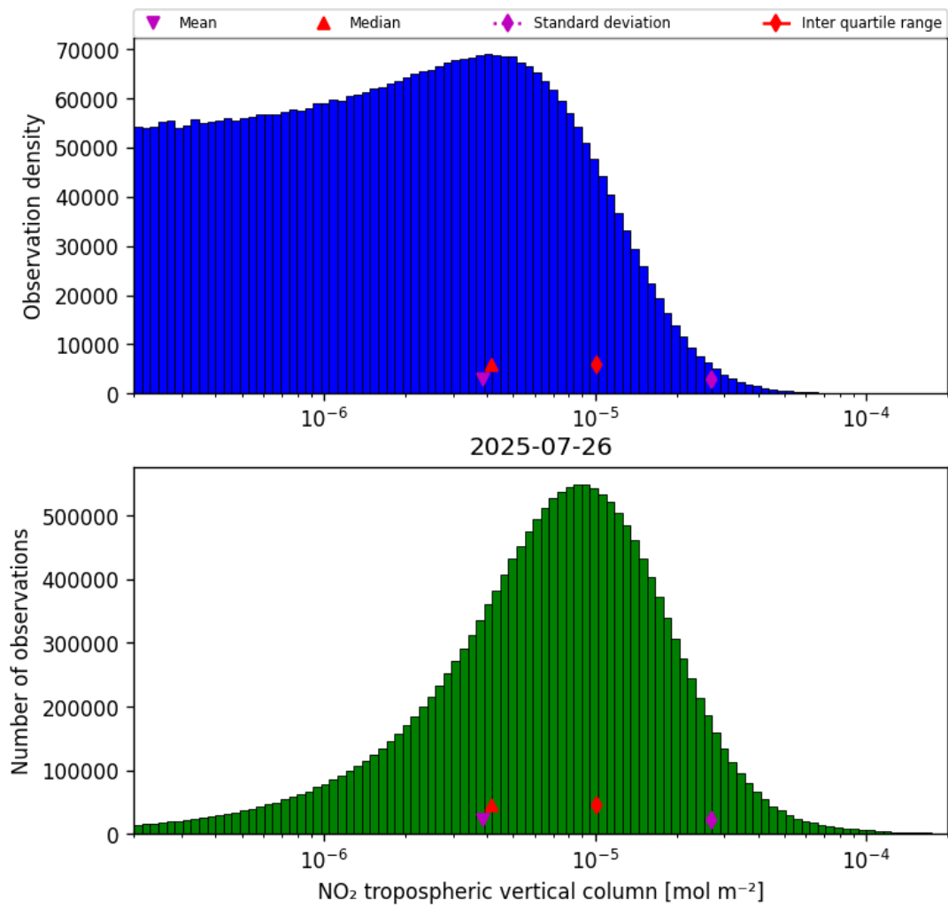
Figure 29: Histogram of “NO 2 tropospheric vertical column” for 2025-07-25 to 2025-07-27
