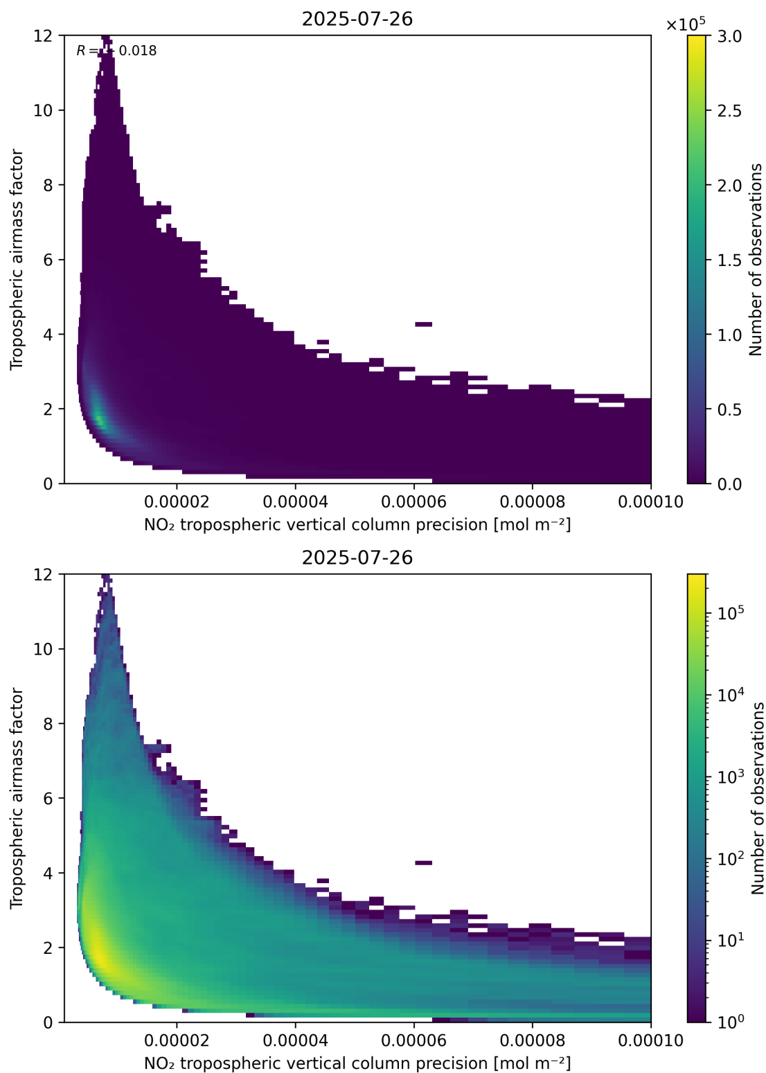
Figure 133: Scatter density plot of “NO 2 tropospheric vertical column precision” against “Tropospheric airmass factor” for 2025-07-25 to 2025-07-27.
