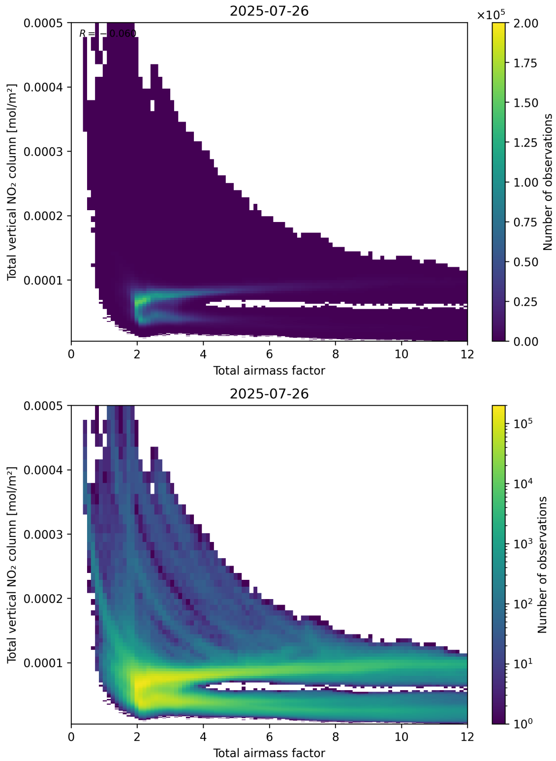
Figure 67: Scatter density plot of “Total airmass factor” against “Total vertical NO 2 column” for 2025-07-25 to 2025-07-27.
