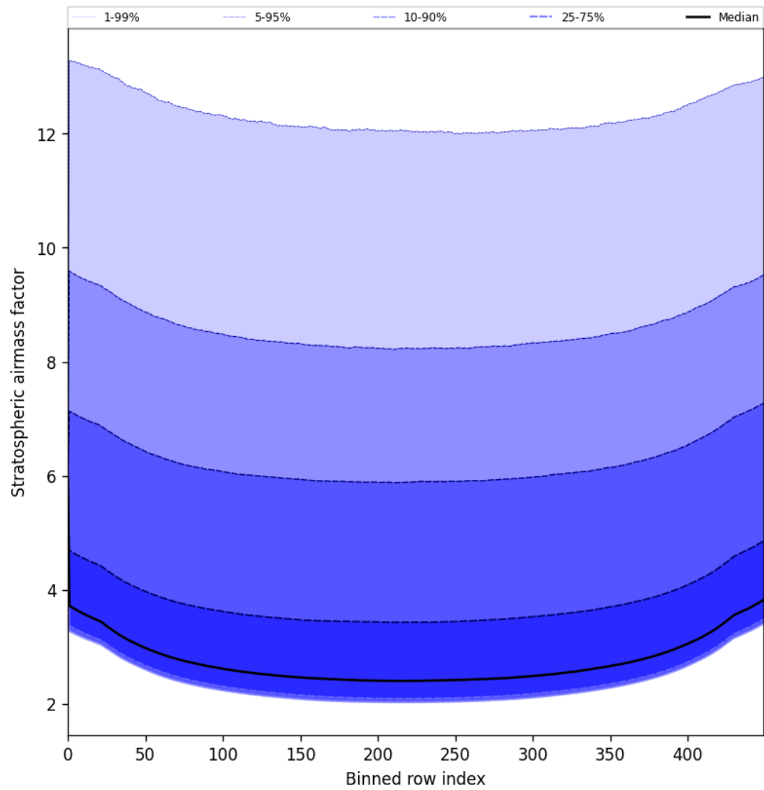
Figure 61: Along track statistics of “Stratospheric airmass factor” for 2025-07-25 to 2025-07-27
