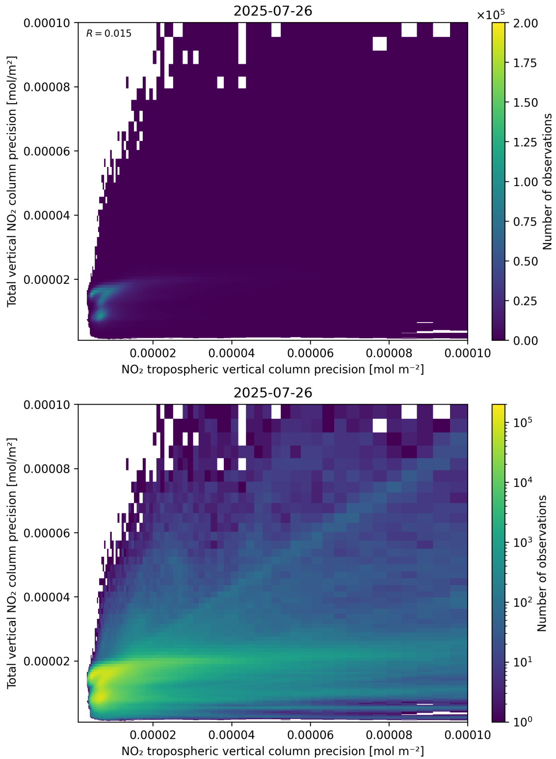
Figure 139: Scatter density plot of “NO 2 tropospheric vertical column precision” against “Total vertical NO 2 column precision” for 2025-07-25 to 2025-07-27.
