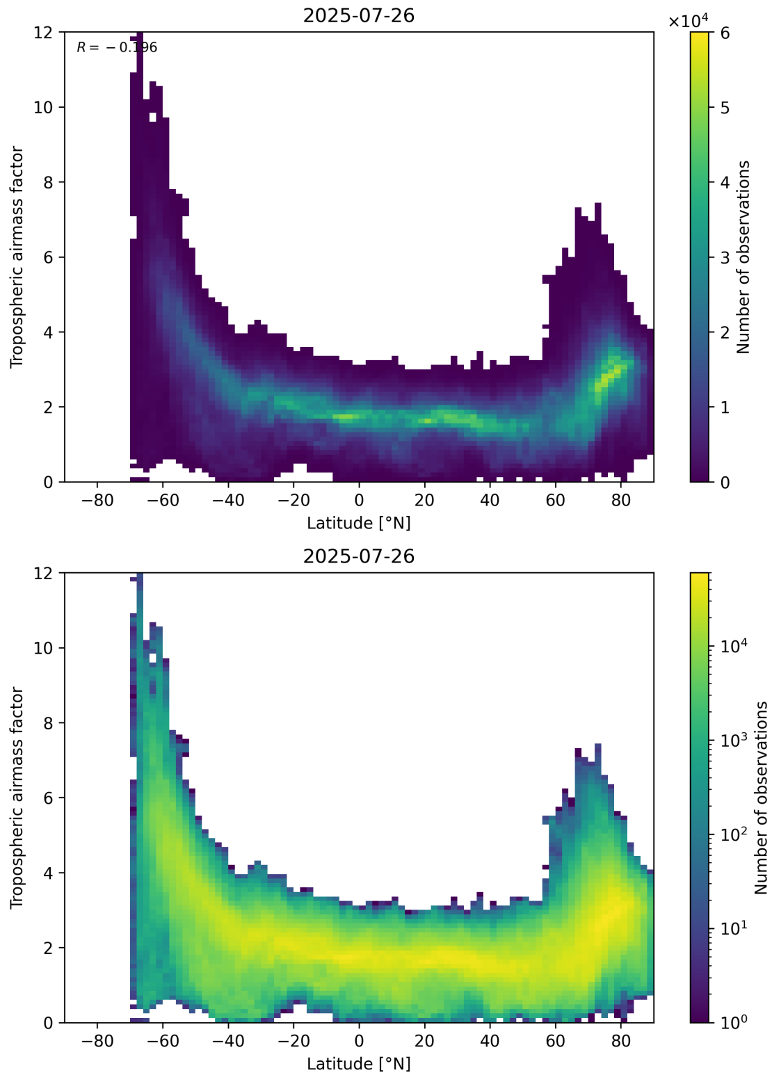
Figure 85: Scatter density plot of “Latitude” against “Tropospheric air mass factor” for 2025-07-25 to 2025-07-27.
