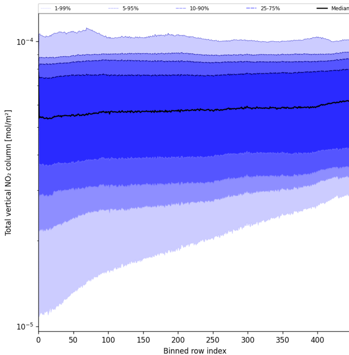
Figure 55: Along track statistics of “Total vertical NO 2 column” for 2025-07-25 to 2025-07-27
