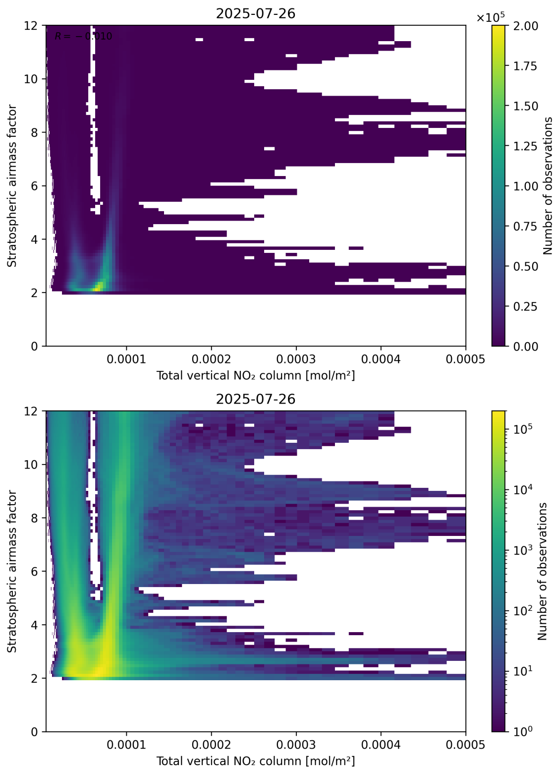
Figure 110: Scatter density plot of “Total vertical NO 2 column” against “Stratospheric airmass factor” for 2025-07-25 to 2025-07-27.
