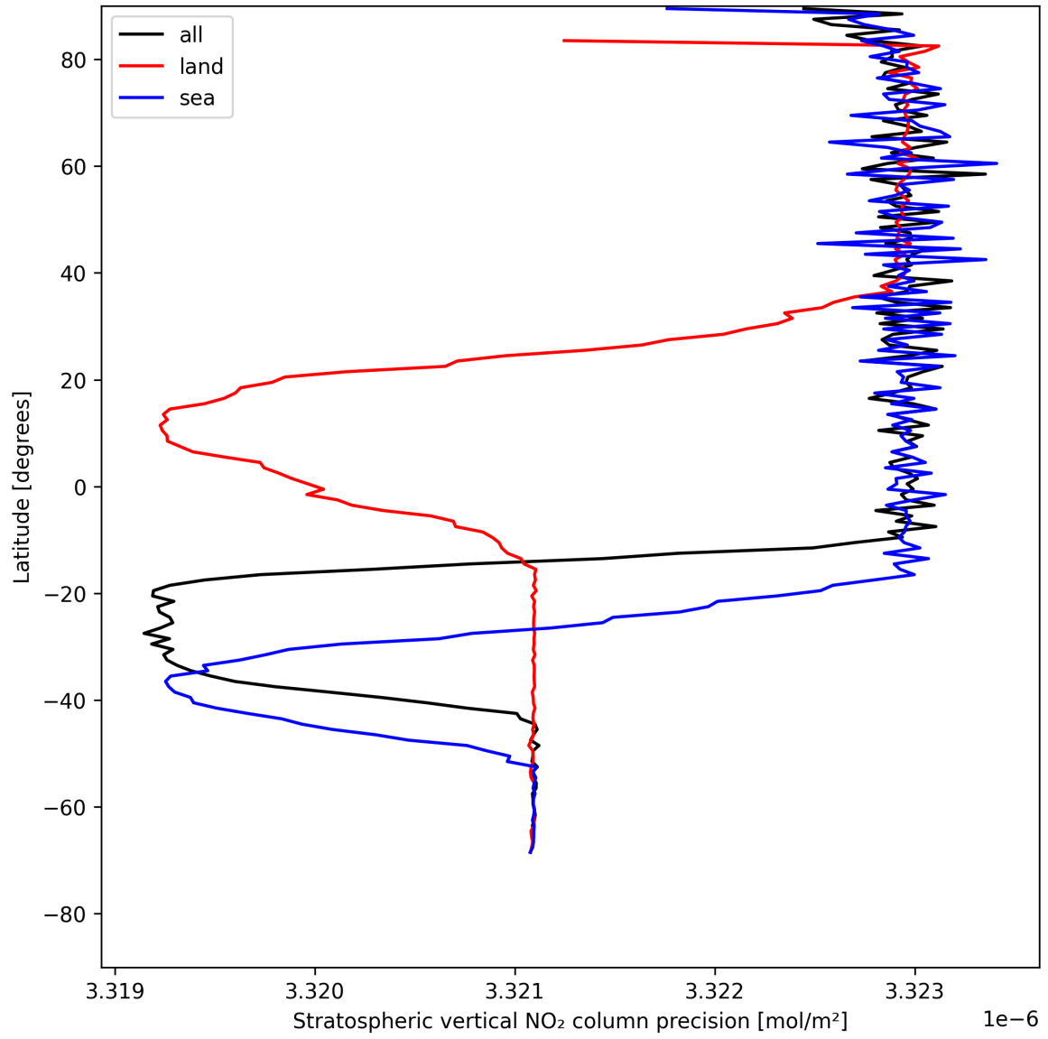
Figure 20: Zonal average of “Stratospheric vertical NO 2 column precision” for 2025-07-25 to 2025-07-27.
