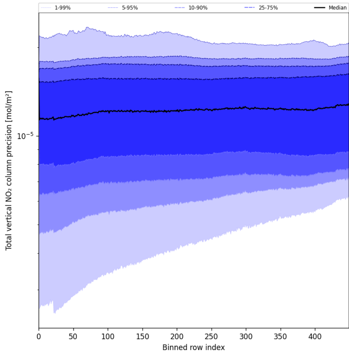
Figure 56: Along track statistics of “Total vertical NO 2 column precision” for 2025-07-25 to 2025-07-27
