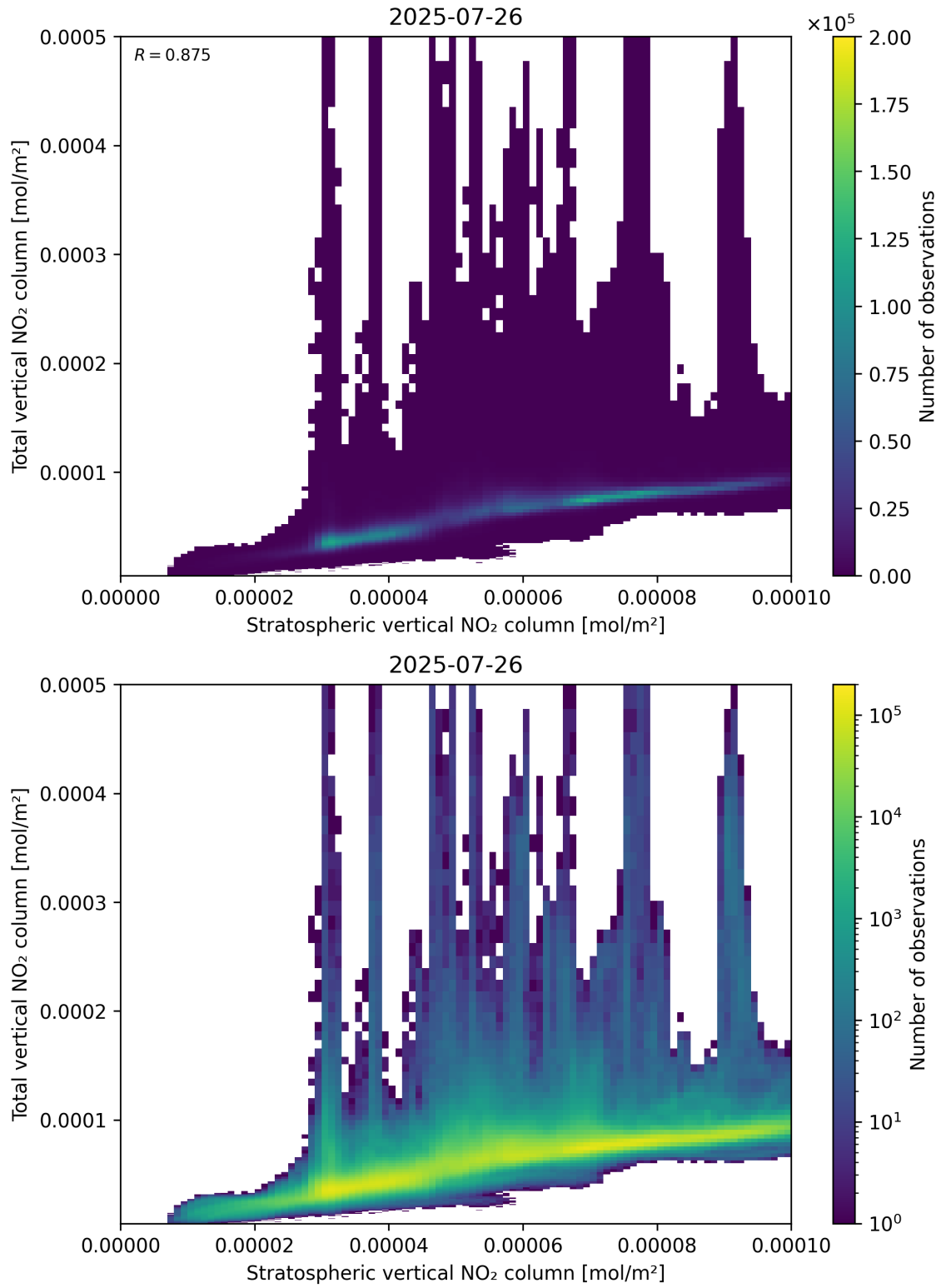
Figure 100: Scatter density plot of “Stratospheric vertical NO 2 column” against “Total vertical NO 2 column” for 2025-07-25 to 2025-07-27.
