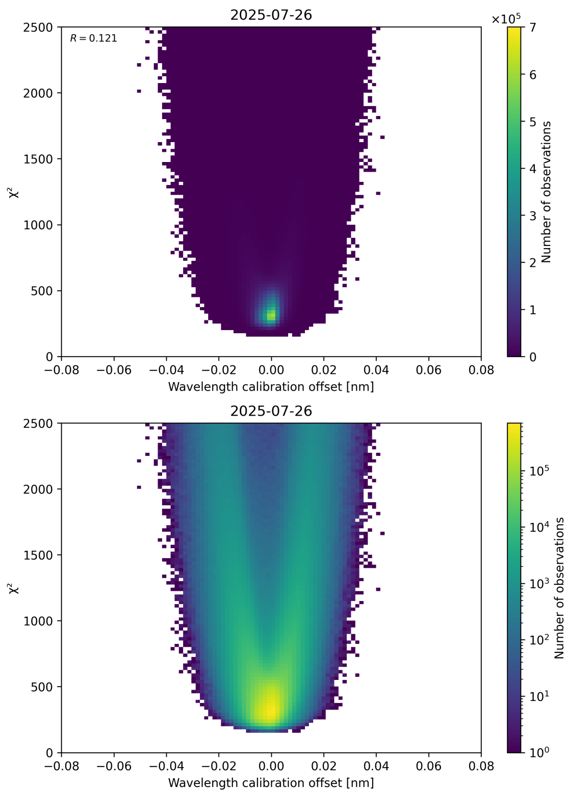
Figure 175: Scatter density plot of “Wavelength calibration offset” against “ \chi^2 ” for 2025-07-25 to 2025-07-27.
