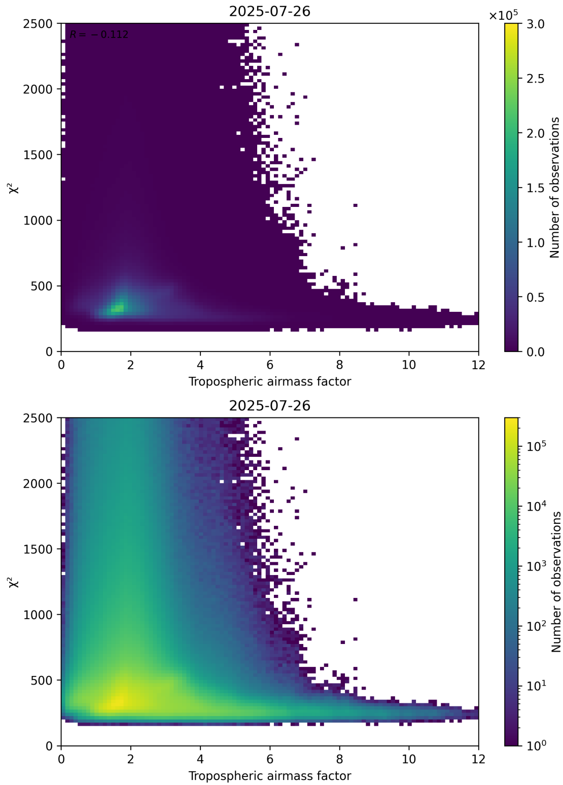
Figure 73: Scatter density plot of “Tropospheric airmass factor” against “ \chi^2 ” for 2025-07-25 to 2025-07-27.
