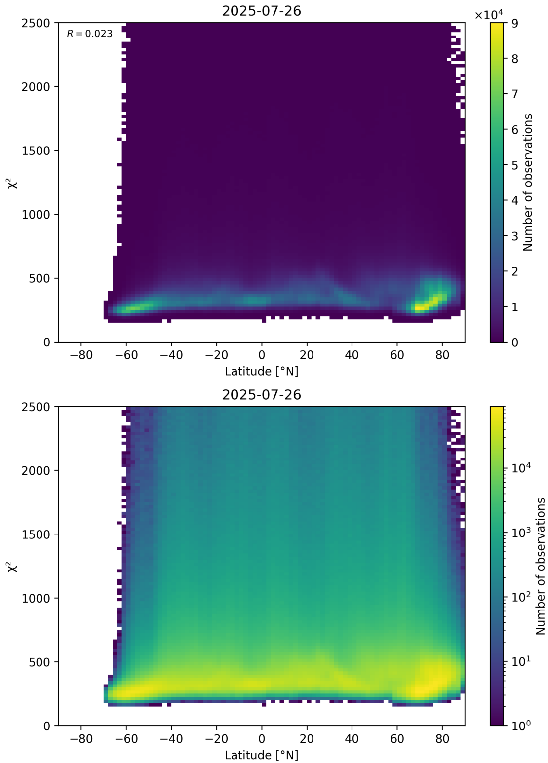
Figure 86: Scatter density plot of “Latitude” against “ \chi^2 ” for 2025-07-25 to 2025-07-27.
