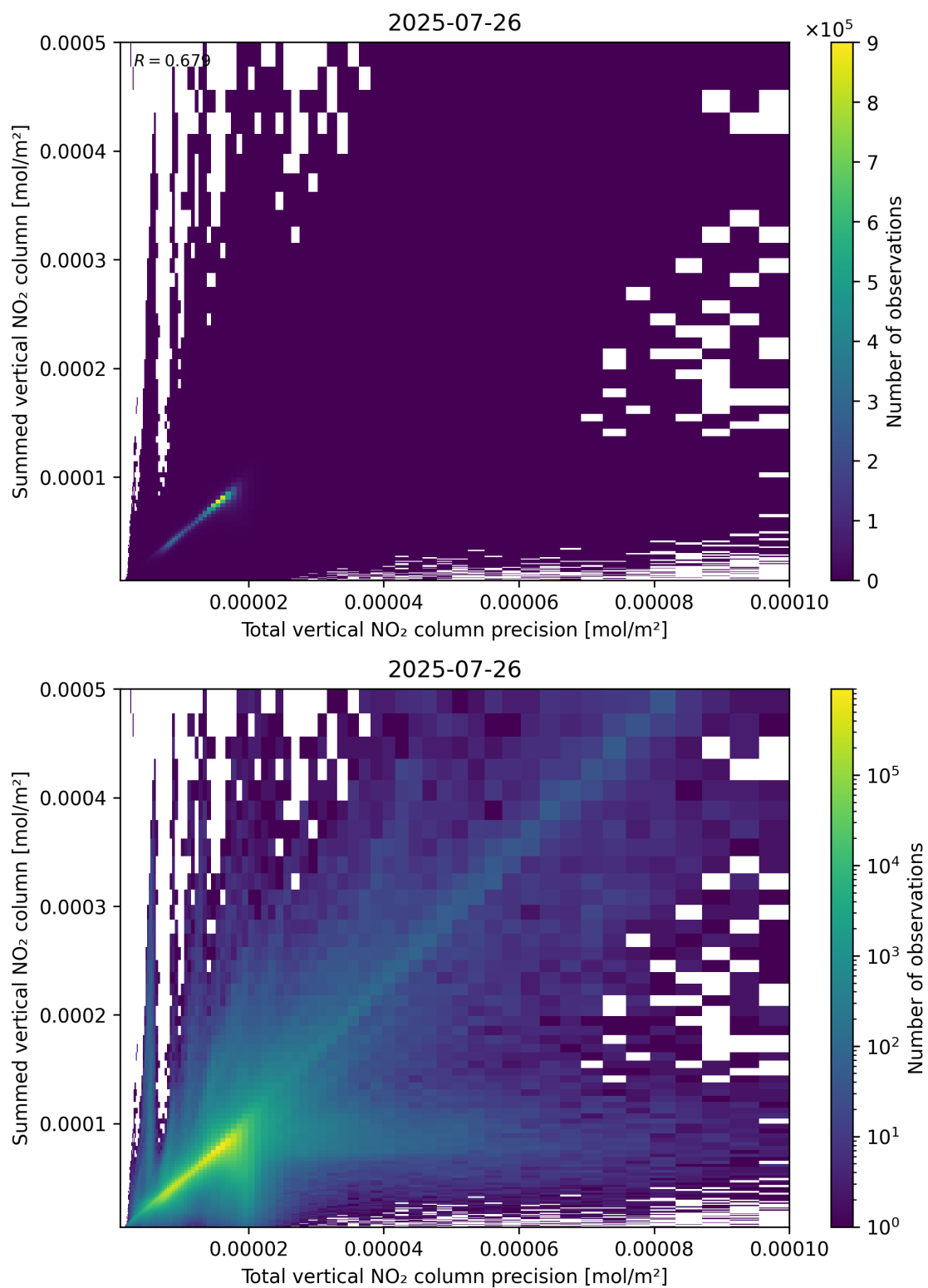
Figure 117: Scatter density plot of “Total vertical NO 2 column precision” against “Summed vertical NO 2 column” for 2025-07-25 to 2025-07-27.
