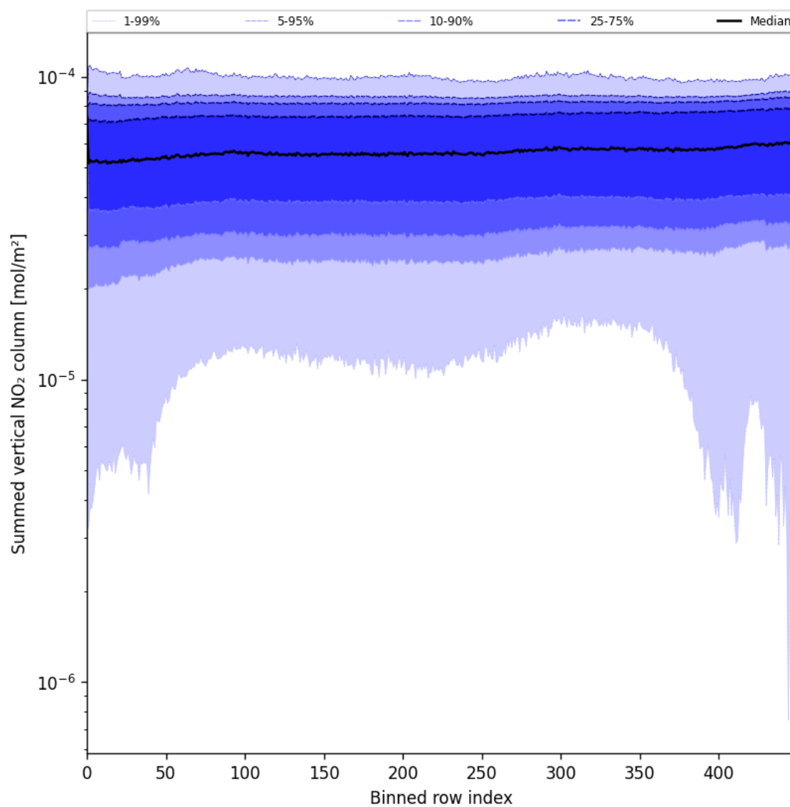
Figure 57: Along track statistics of “Summed vertical NO 2 column” for 2025-07-25 to 2025-07-27
