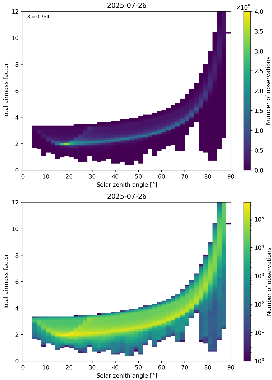
Figure 146: Scatter density plot of “Solar zenith angle” against “Total air mass factor” for 2025-07-25 to 2025-07-27.
