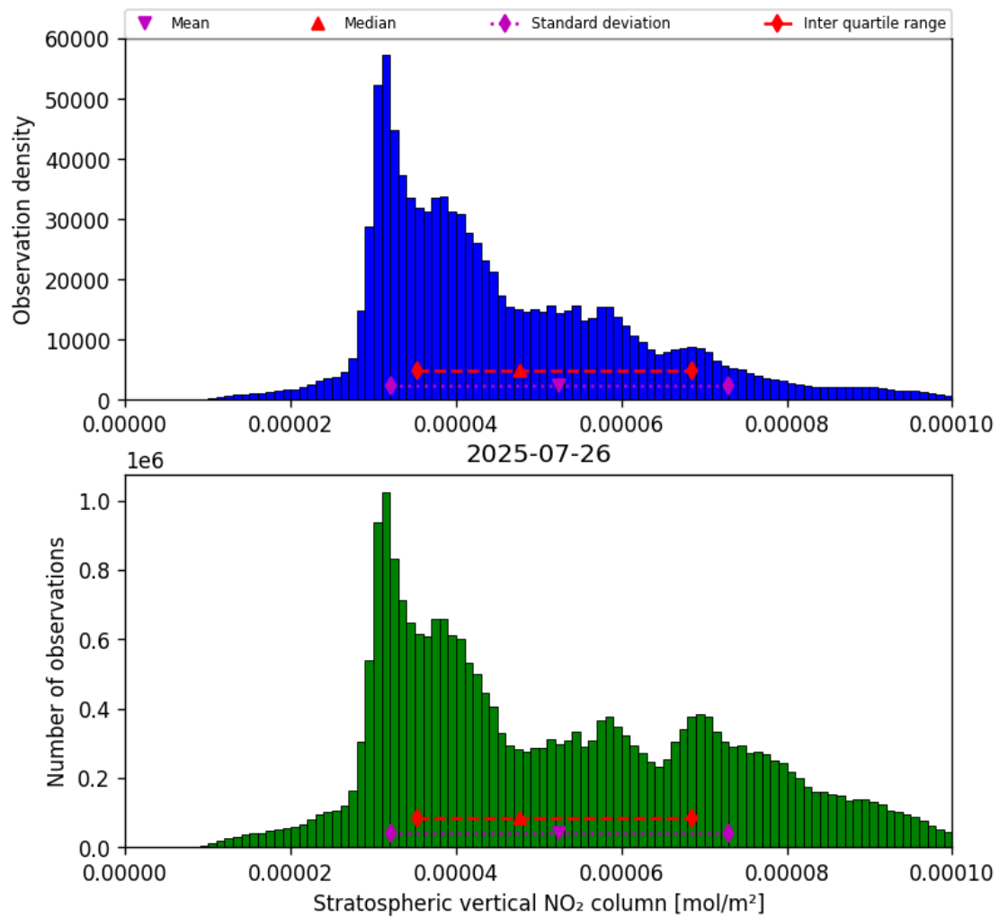
Figure 36: Histogram of “Stratospheric vertical NO 2 column” for 2025-07-25 to 2025-07-27
