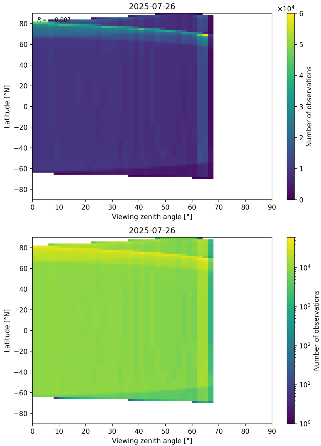
Figure 163: Scatter density plot of “Viewing zenith angle” against “Latitude” for 2025-07-25 to 2025-07-27.
