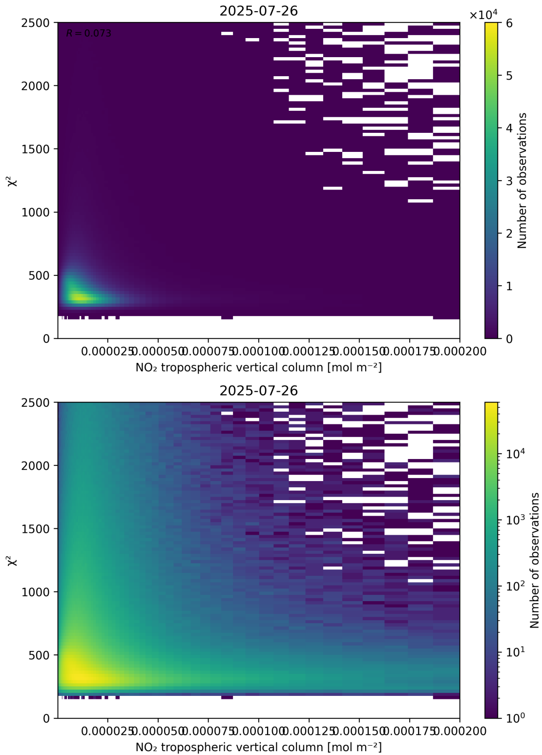
Figure 124: Scatter density plot of “NO 2 tropospheric vertical column” against “ \chi^2 ” for 2025-07-25 to 2025-07-27.
