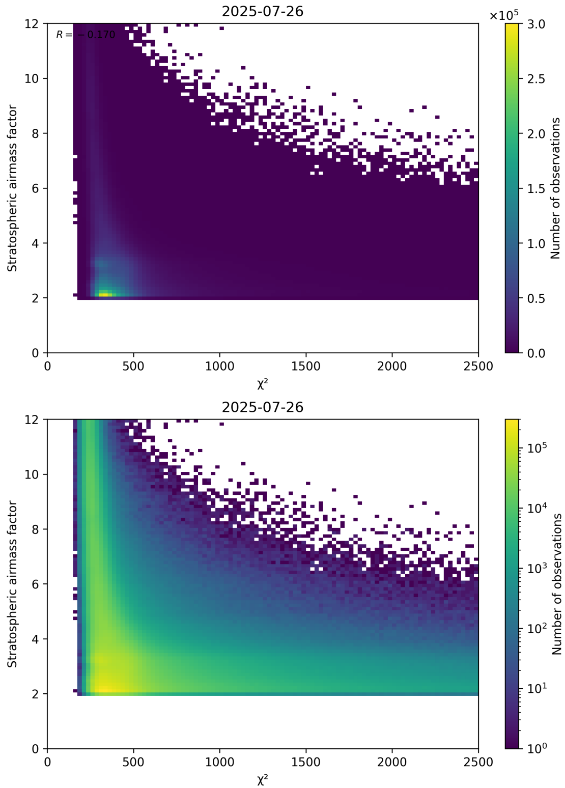
Figure 81: Scatter density plot of “ \chi^2 ” against “Stratospheric airmass factor” for 2025-07-25 to 2025-07-27.
