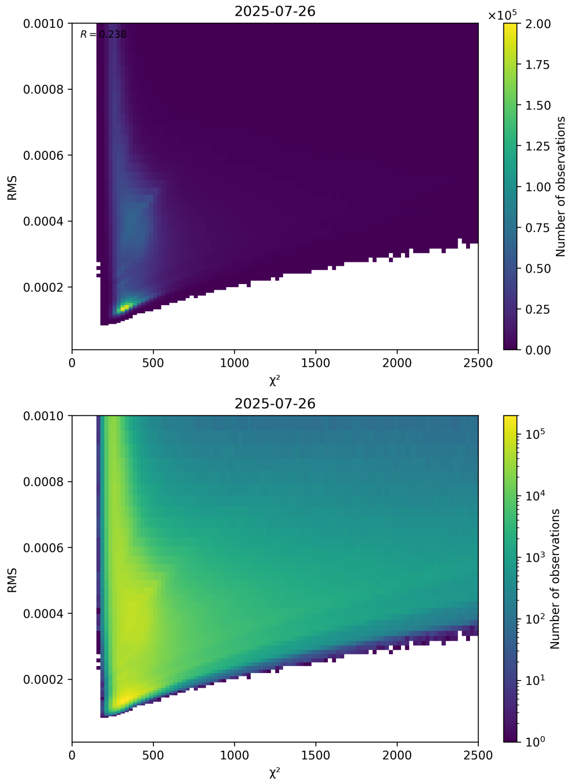
Figure 82: Scatter density plot of “ \chi^2 ” against “RMS” for 2025-07-25 to 2025-07-27.
