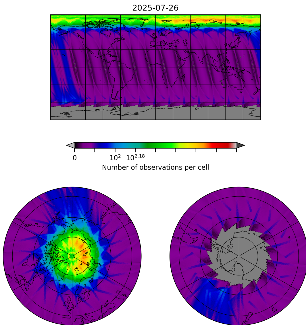
Figure 10: Map of the number of observations for 2025-07-25 to 2025-07-27
