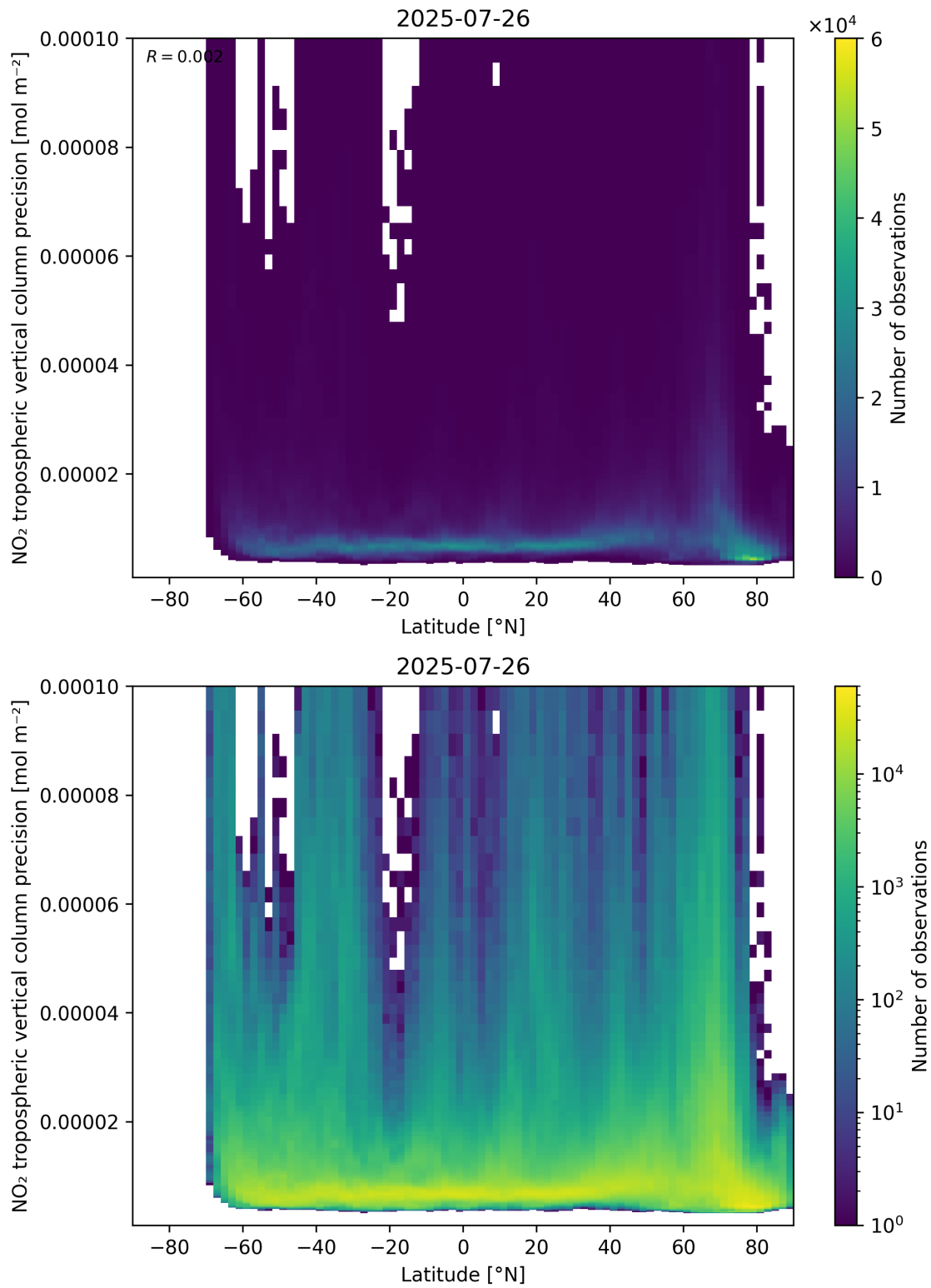
Figure 93: Scatter density plot of “Latitude” against “NO 2 tropospheric vertical column precision” for 2025-07-25 to 2025-07-27.
