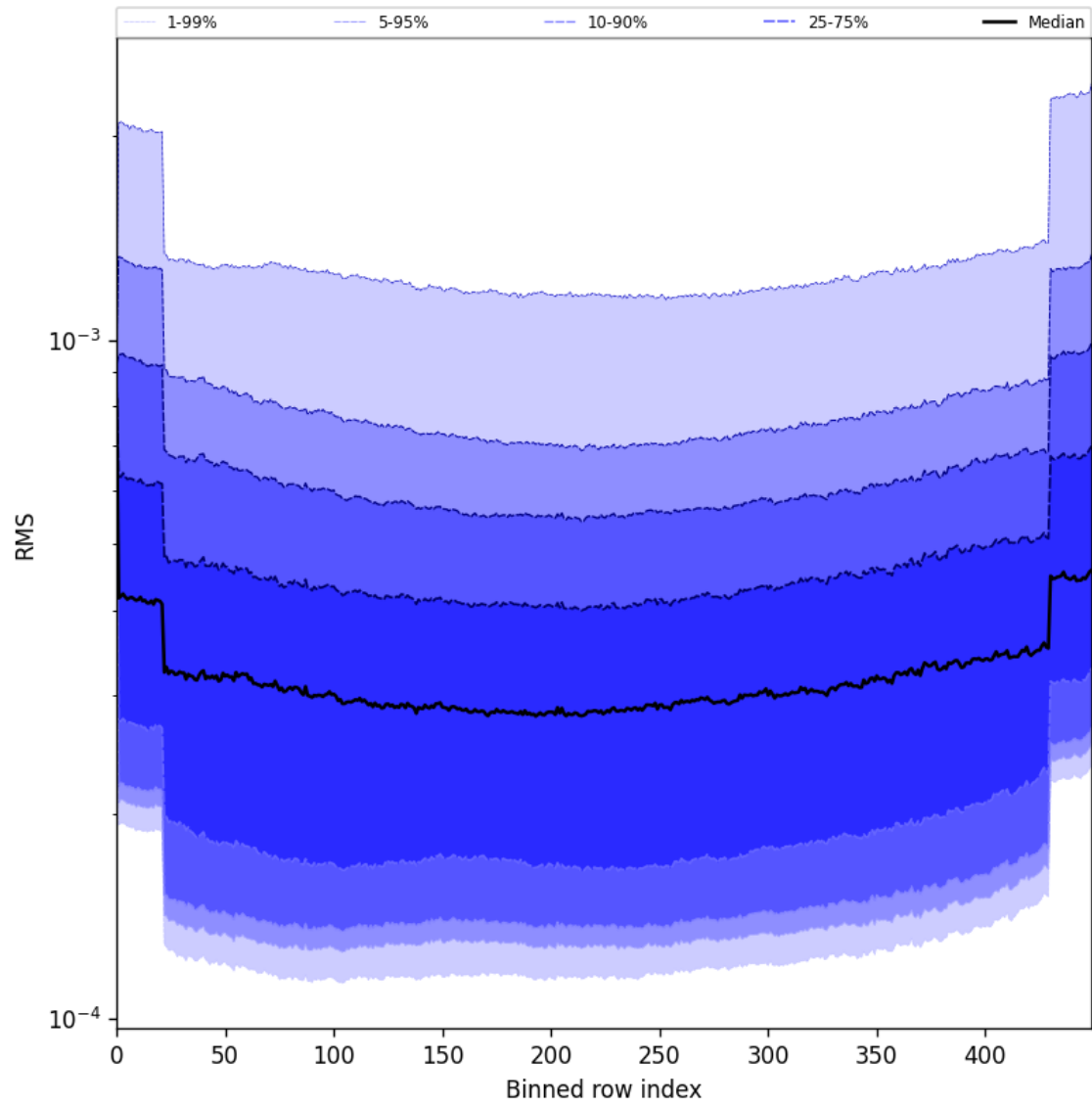
Figure 60: Along track statistics of “RMS” for 2025-07-25 to 2025-07-27
