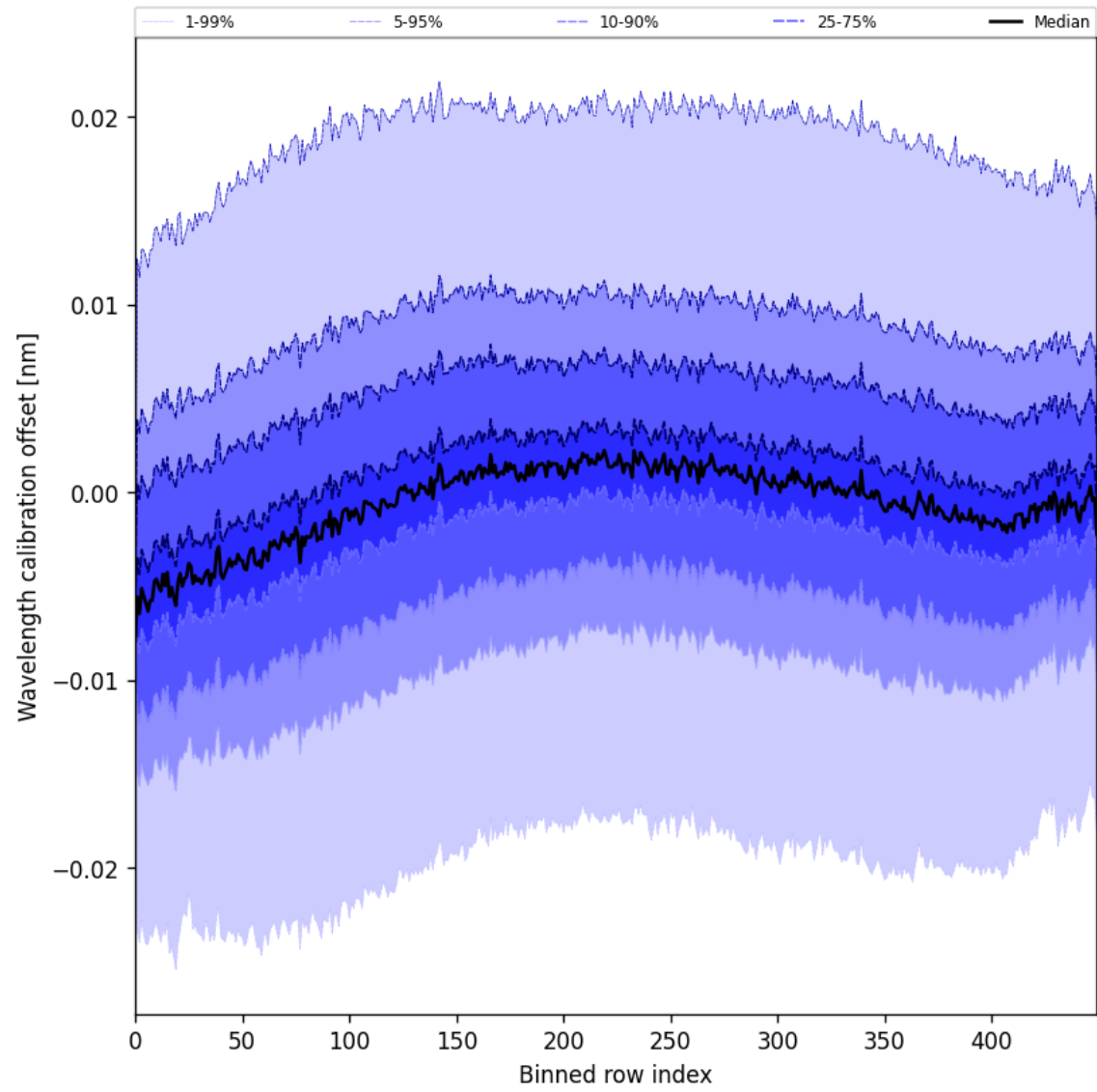
Figure 52: Along track statistics of “Wavelength calibration offset” for 2025-07-25 to 2025-07-27
