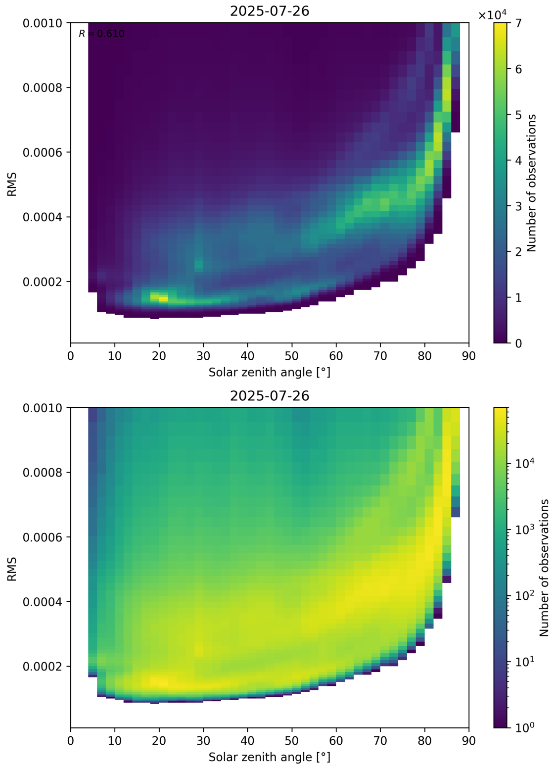
Figure 157: Scatter density plot of “Solar zenith angle” against “RMS” for 2025-07-25 to 2025-07-27.
