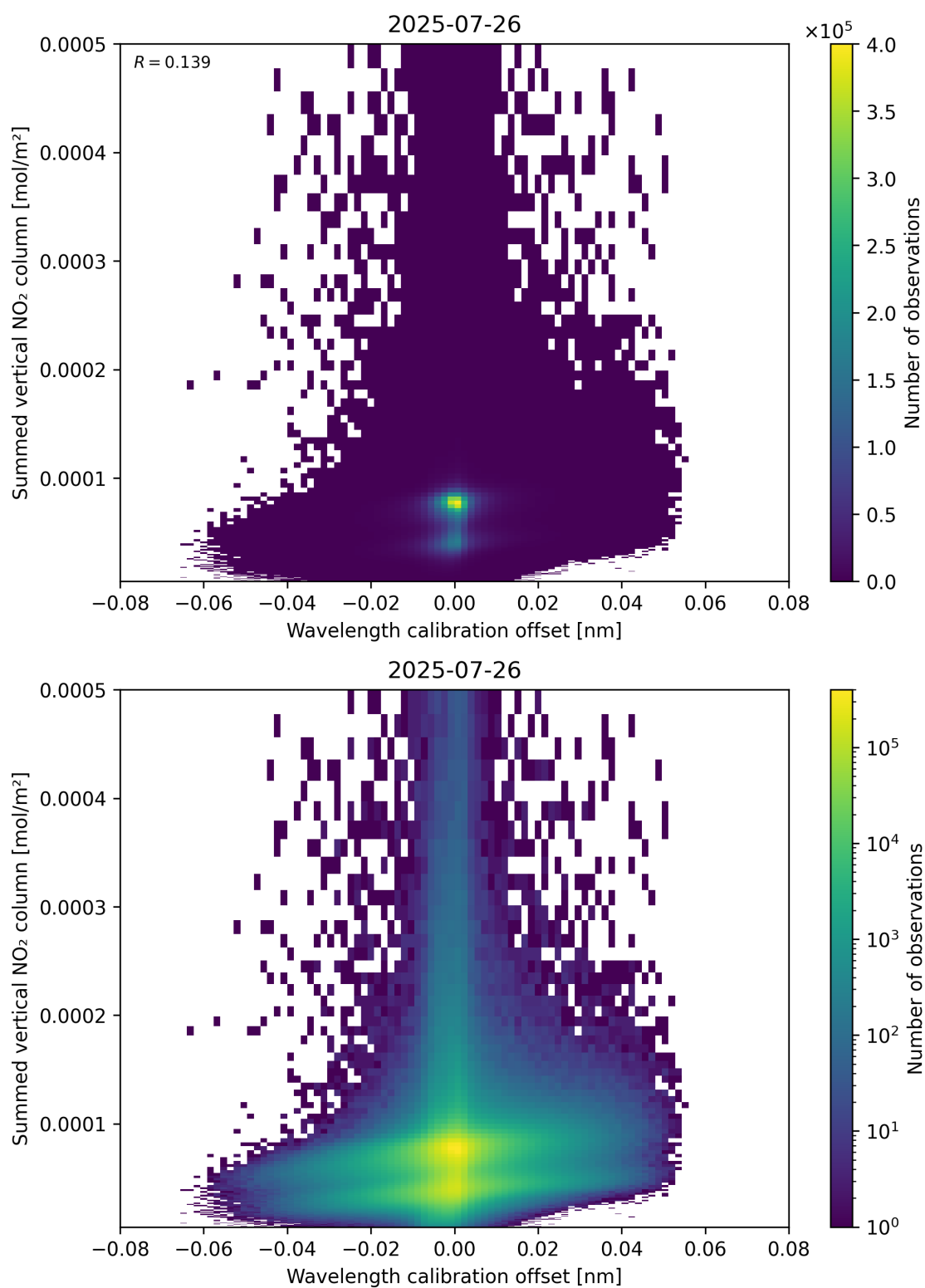
Figure 177: Scatter density plot of “Wavelength calibration offset” against “Summed vertical NO 2 column” for 2025-07-25 to 2025-07-27.
