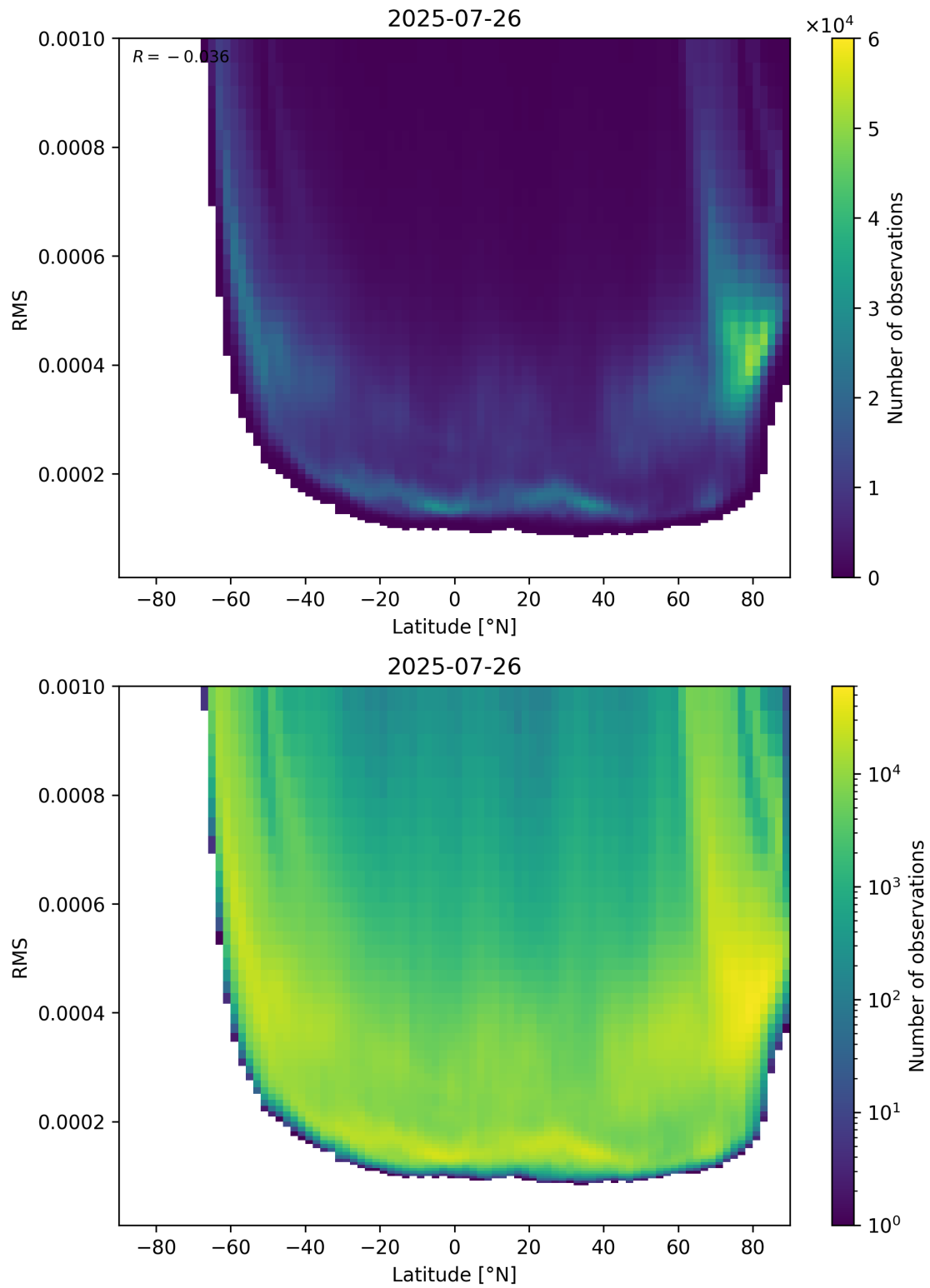
Figure 94: Scatter density plot of “Latitude” against “RMS” for 2025-07-25 to 2025-07-27.
