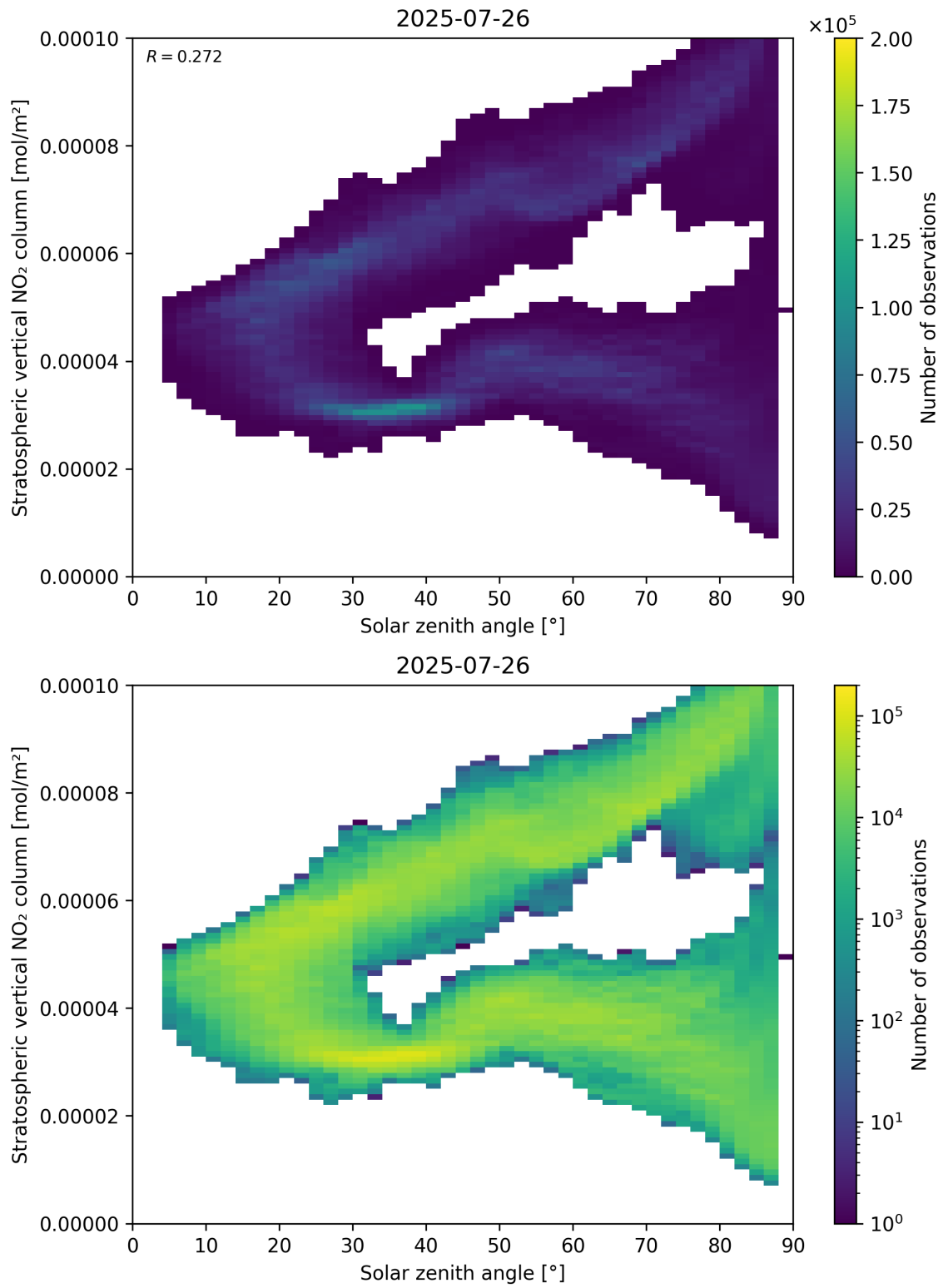
Figure 150: Scatter density plot of “Solar zenith angle” against “Stratospheric vertical NO 2 column” for 2025-07-25 to 2025-07-27.
