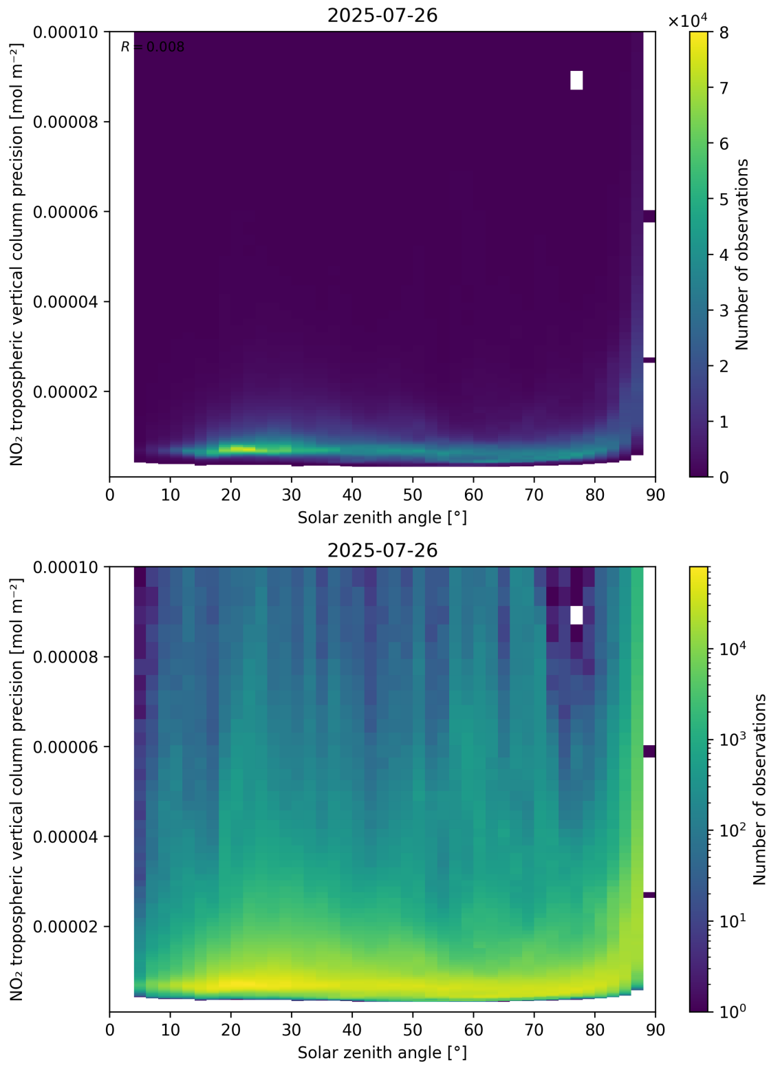
Figure 156: Scatter density plot of “Solar zenith angle” against “NO 2 tropospheric vertical column precision” for 2025-07-25 to 2025-07-27.
