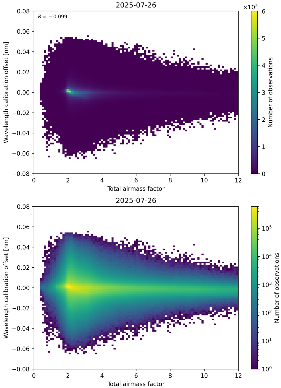
Figure 70: Scatter density plot of “Total airmass factor” against “Wavelength calibration offset” for 2025-07-25 to 2025-07-27.
