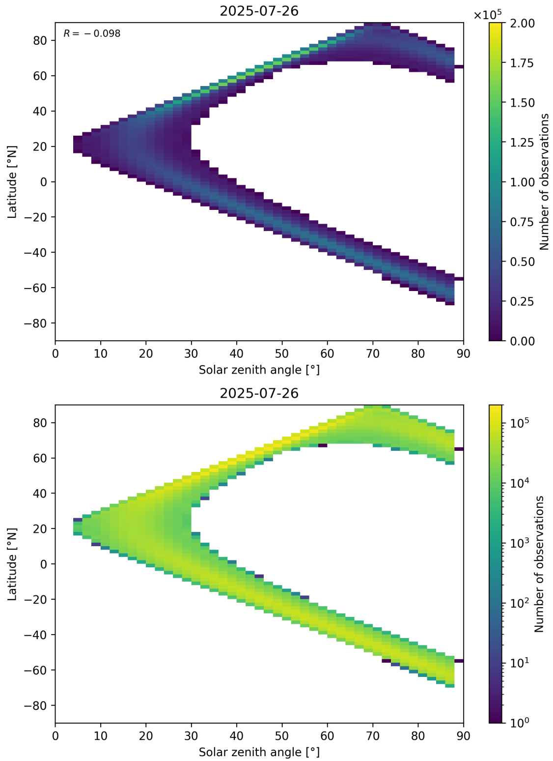
Figure 149: Scatter density plot of “Solar zenith angle” against “Latitude” for 2025-07-25 to 2025-07-27.
