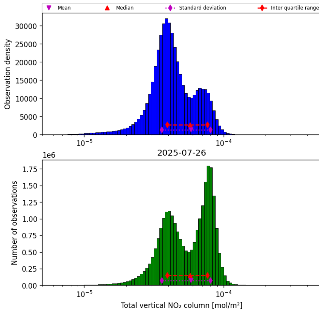
Figure 38: Histogram of “Total vertical NO 2 column” for 2025-07-25 to 2025-07-27
