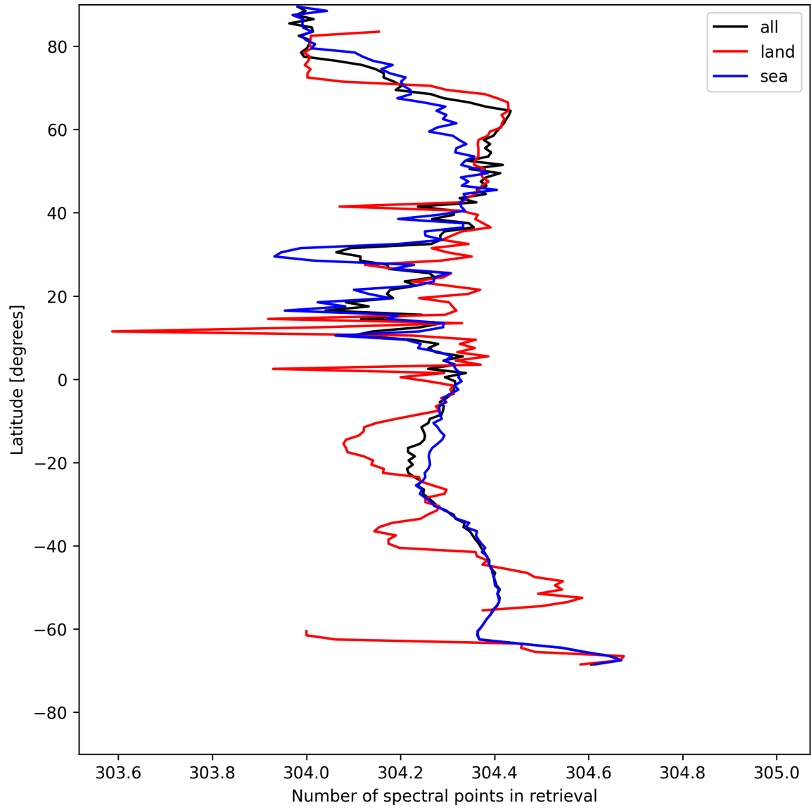
Figure 16: Zonal average of “Number of spectral points in retrieval” for 2025-07-25 to 2025-07-27.
