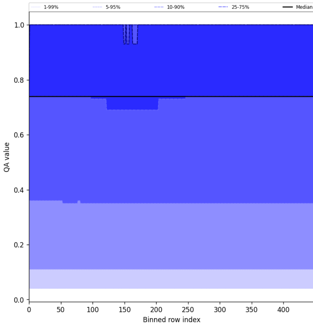
Figure 45: Along track statistics of “QA value” for 2025-07-25 to 2025-07-27
