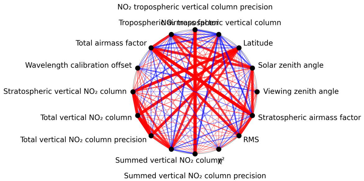
Figure 1: Map of correlation graph for 2025-07-25 to 2025-07-27.
