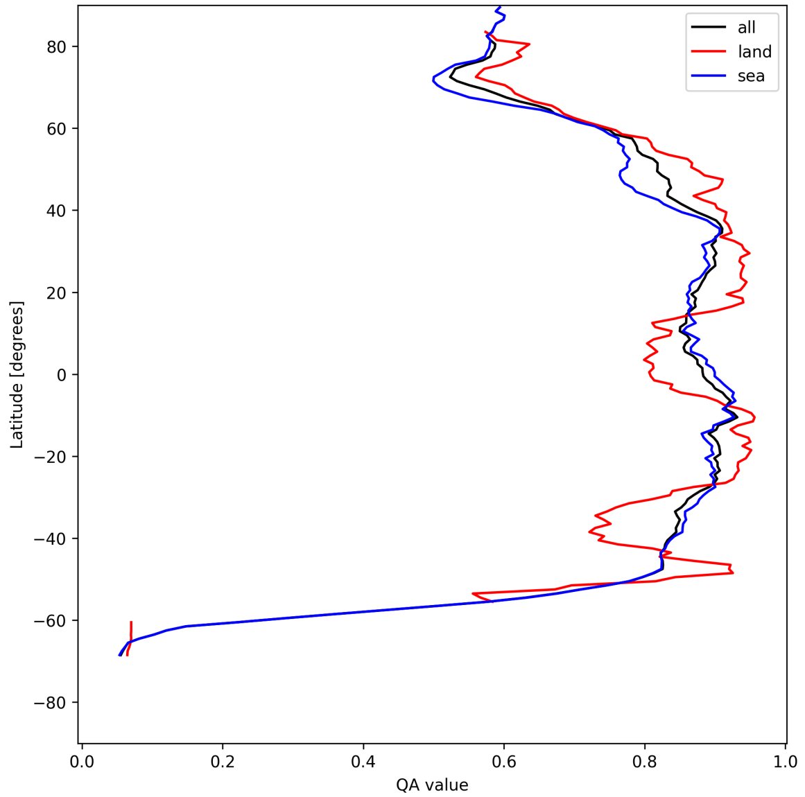
Figure 11: Zonal average of “QA value” for 2025-07-25 to 2025-07-27.
