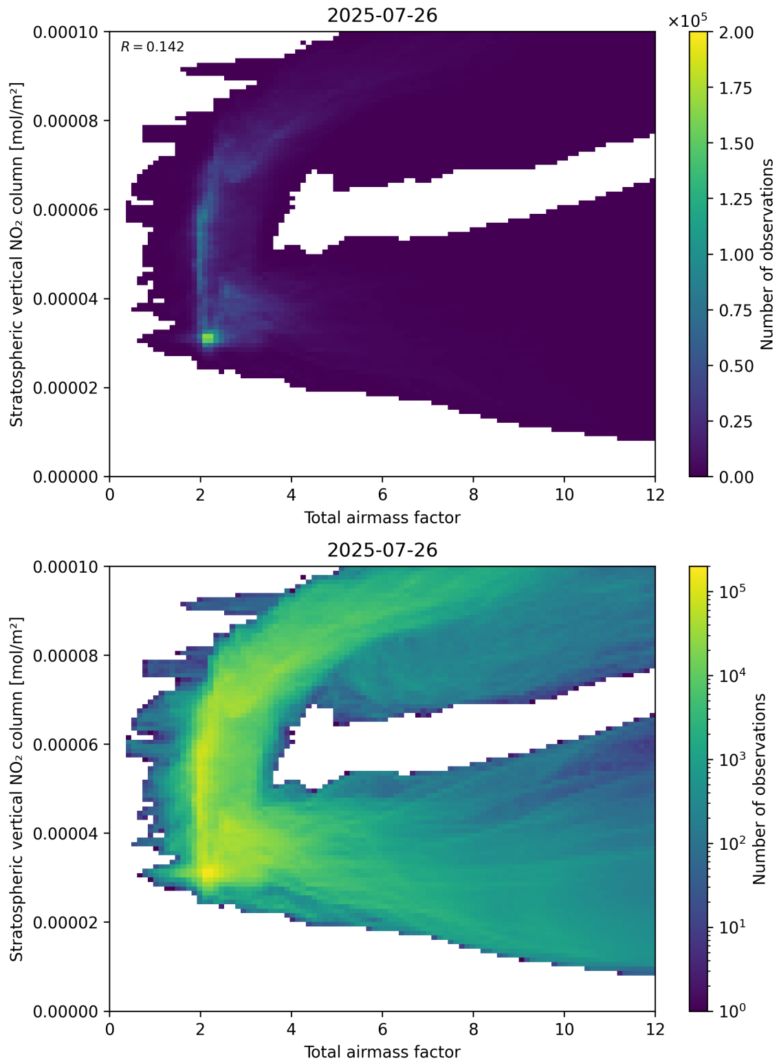
Figure 64: Scatter density plot of “Total airmass factor” against “Stratospheric vertical \text{NO}_2 column” for 2025-07-25 to 2025-07-27.
