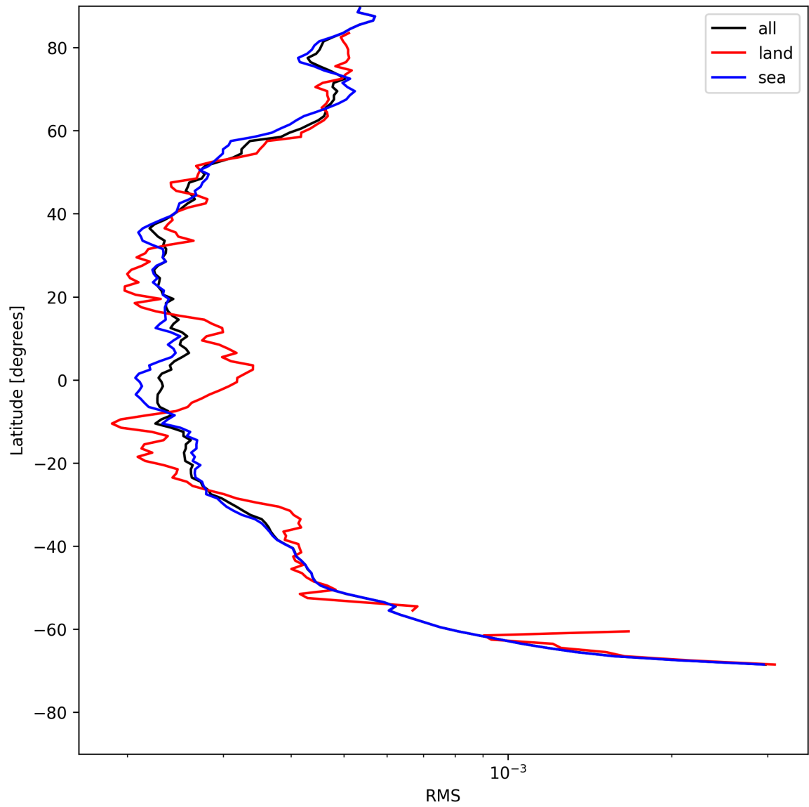
Figure 26: Zonal average of “RMS” for 2025-07-25 to 2025-07-27.
