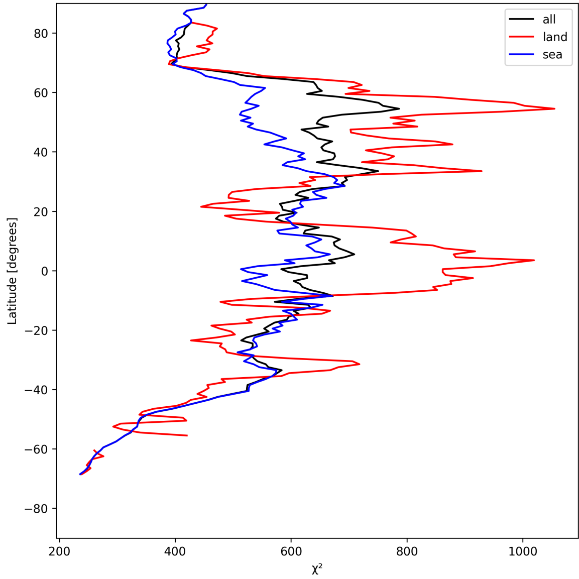
Figure 25: Zonal average of “ \chi^2 ” for 2025-07-25 to 2025-07-27.
