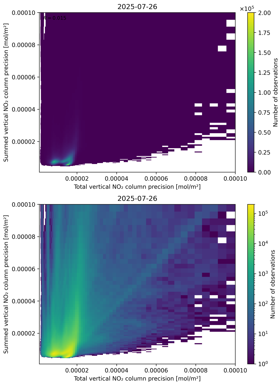
Figure 118: Scatter density plot of “Total vertical NO 2 column precision” against “Summed vertical NO 2 column precision” for 2025-07-25 to 2025-07-27.
