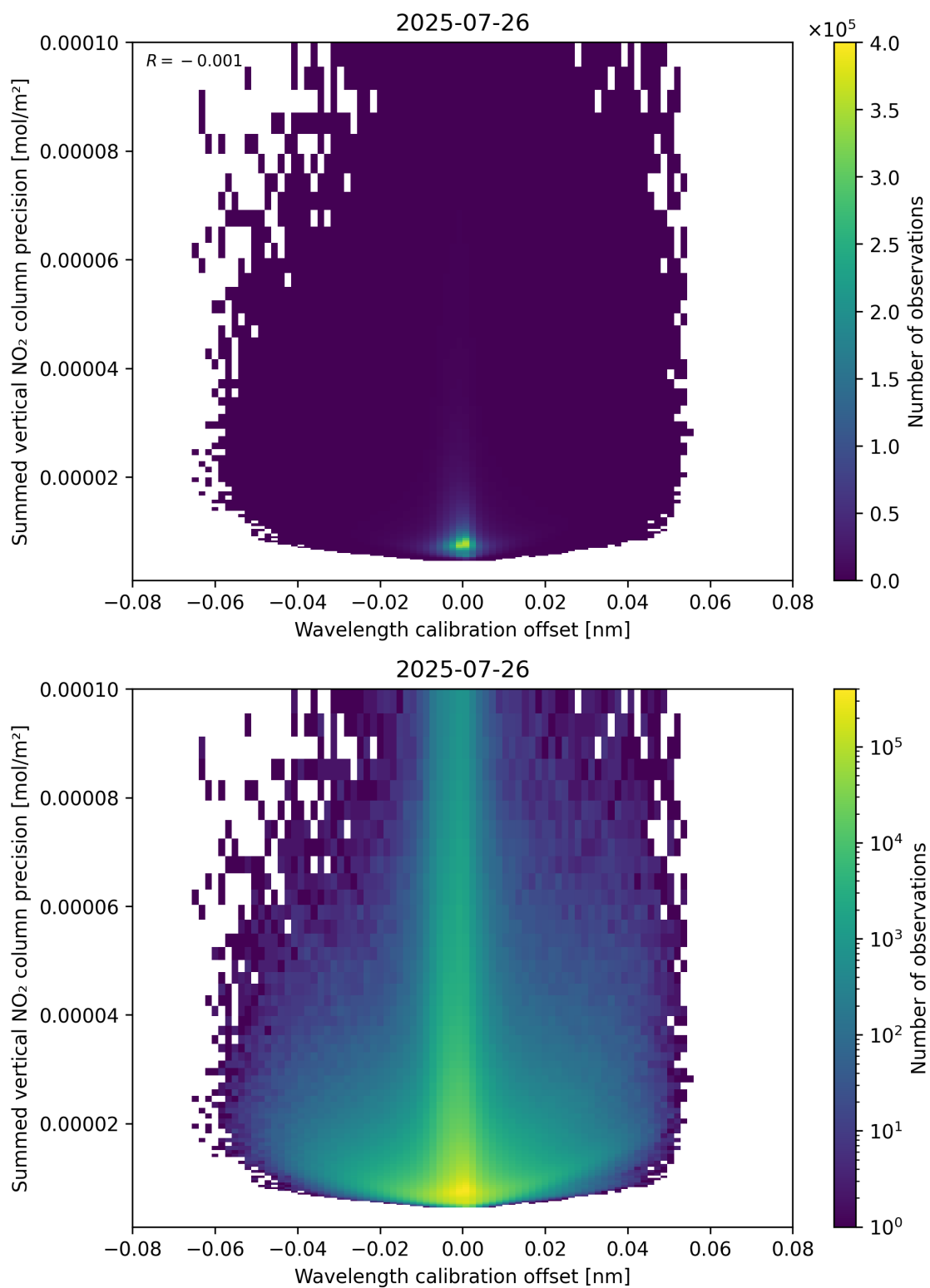
Figure 178: Scatter density plot of “Wavelength calibration offset” against “Summed vertical NO 2 column precision” for 2025-07-25 to 2025-07-27.
