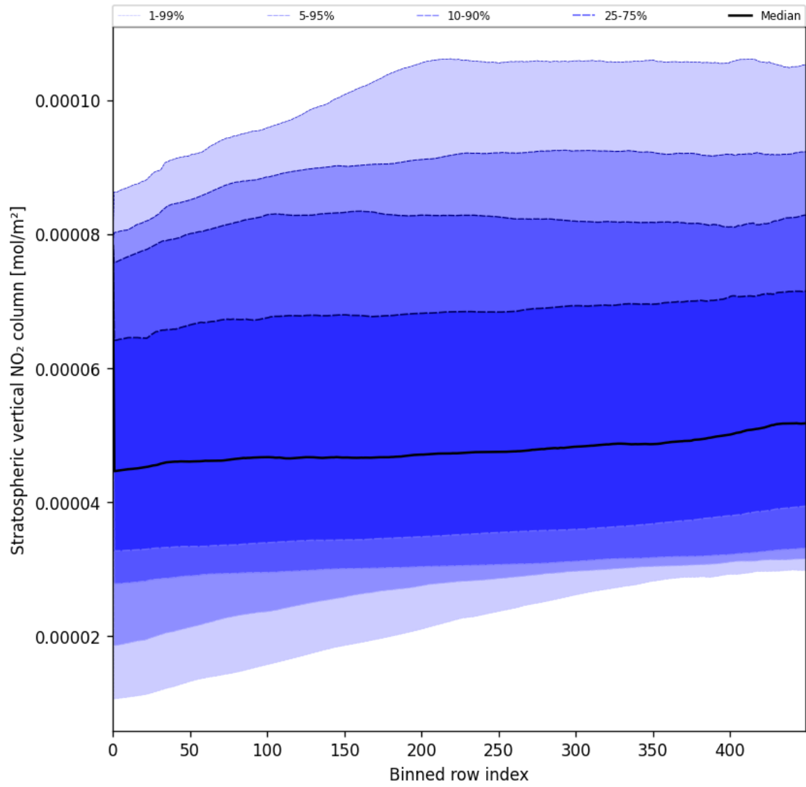
Figure 53: Along track statistics of “Stratospheric vertical NO 2 column” for 2025-07-25 to 2025-07-27
