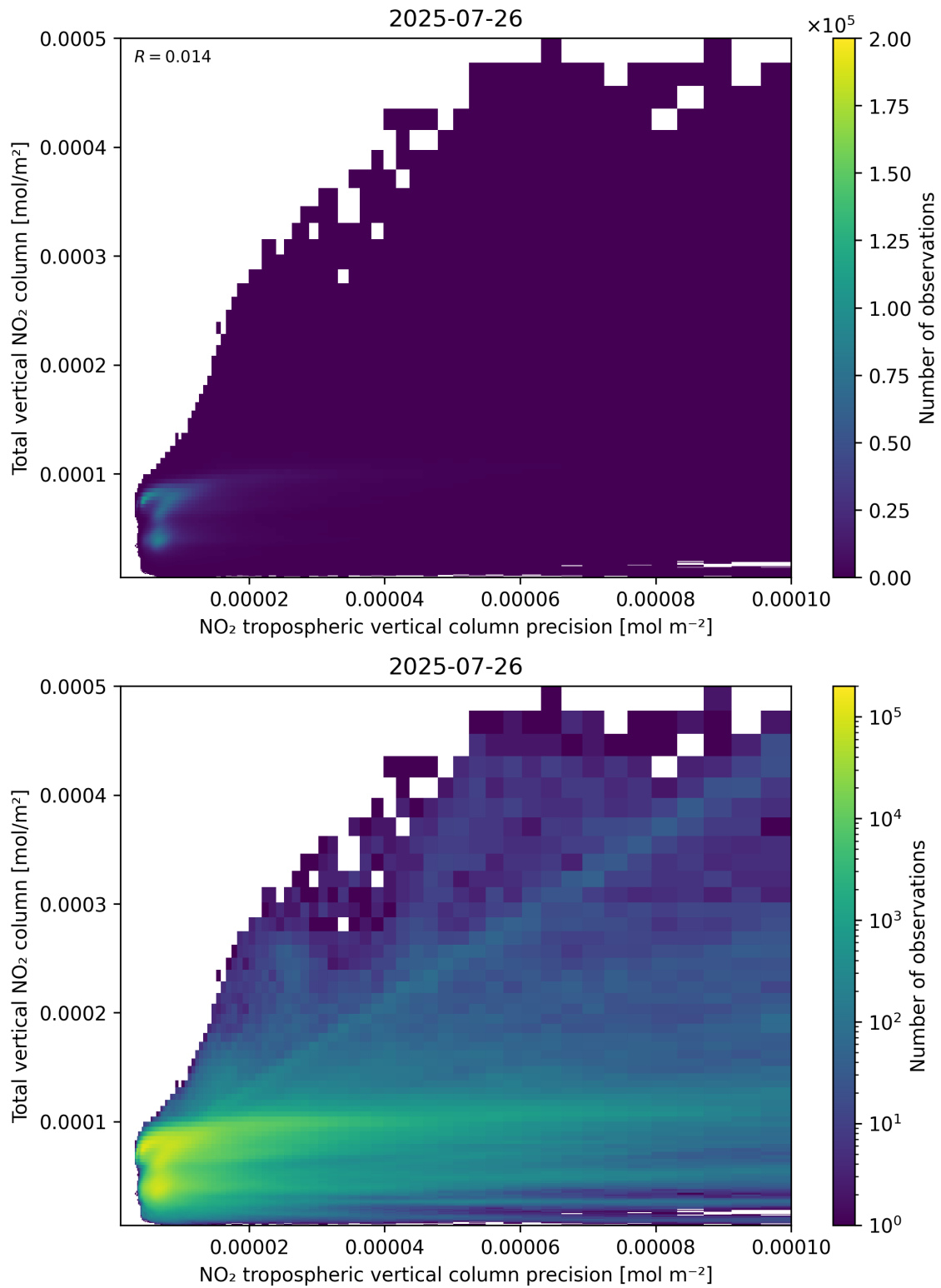
Figure 138: Scatter density plot of “NO 2 tropospheric vertical column precision” against “Total vertical NO 2 column” for 2025-07-25 to 2025-07-27.
