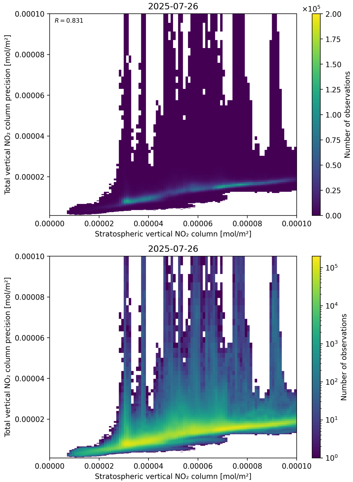
Figure 101: Scatter density plot of “Stratospheric vertical NO 2 column” against “Total vertical NO 2 column precision” for 2025-07-25 to 2025-07-27.
