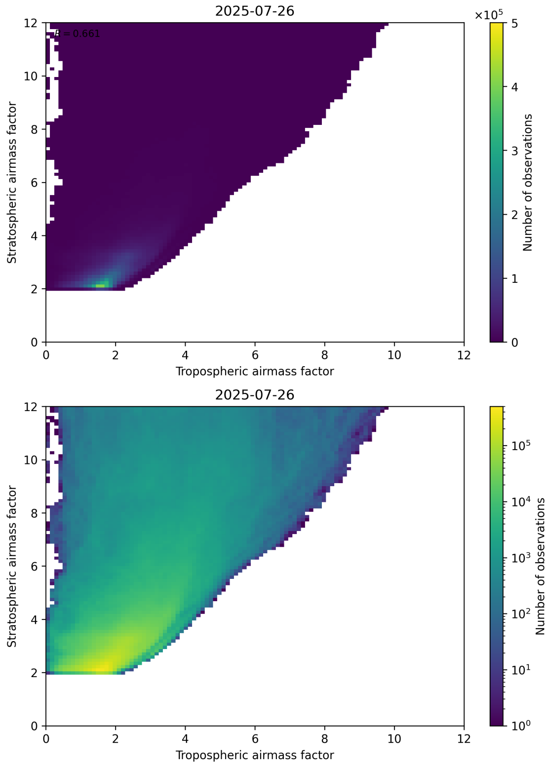
Figure 71: Scatter density plot of “Tropospheric airmass factor” against “Stratospheric airmass factor” for 2025-07-25 to 2025-07-27.
