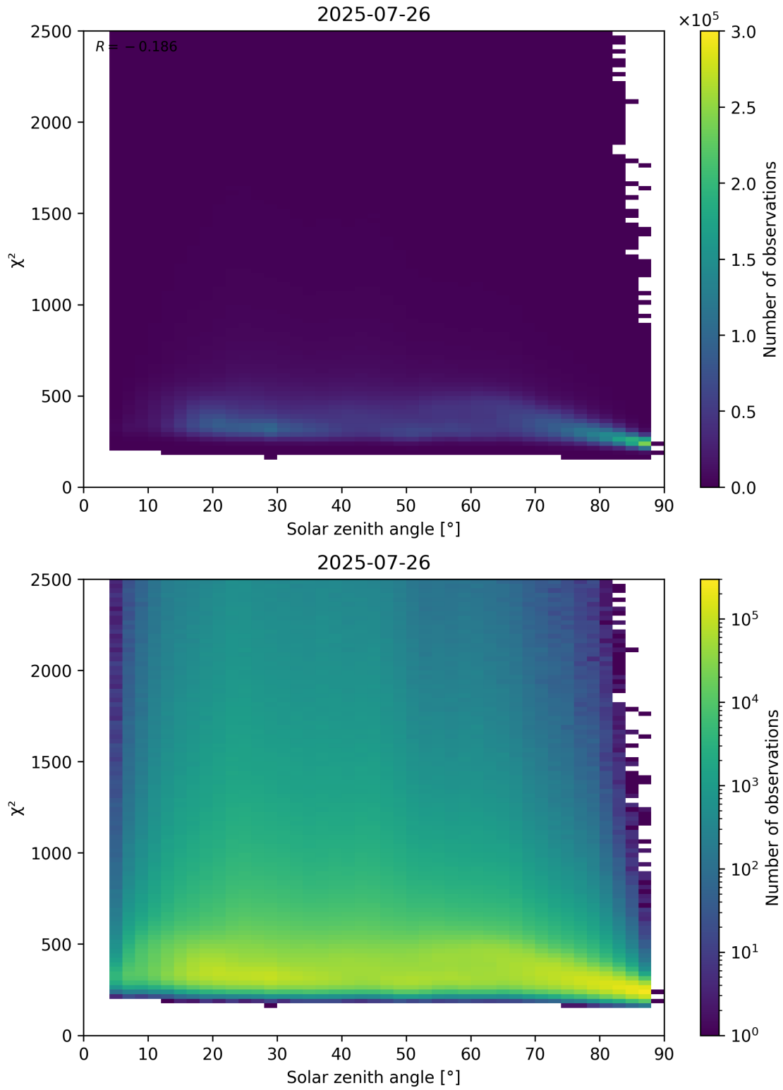
Figure 148: Scatter density plot of “Solar zenith angle” against “ \chi^2 ” for 2025-07-25 to 2025-07-27.
