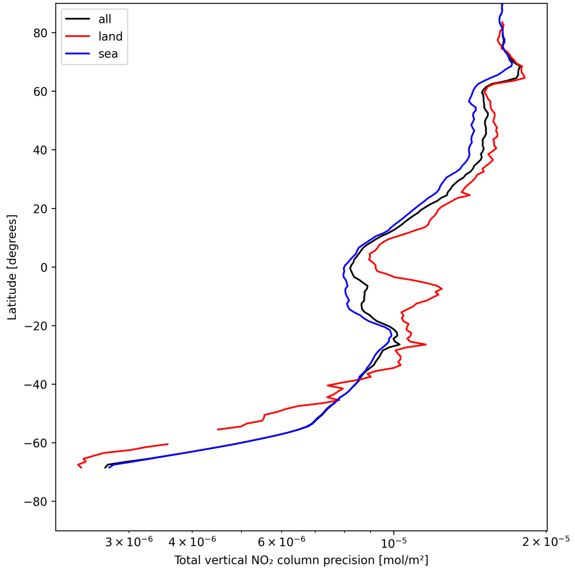
Figure 22: Zonal average of “Total vertical NO 2 column precision” for 2025-07-25 to 2025-07-27.
