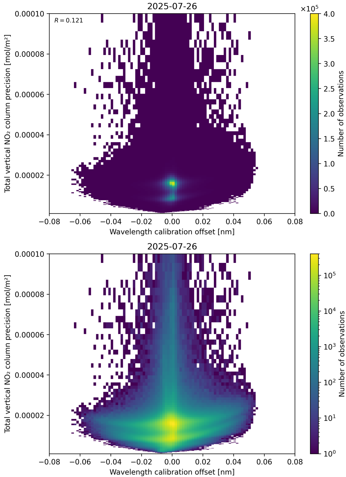
Figure 180: Scatter density plot of “Wavelength calibration offset” against “Total vertical NO 2 column precision” for 2025-07-25 to 2025-07-27.
