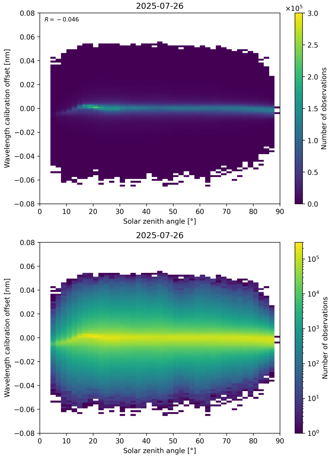
Figure 158: Scatter density plot of “Solar zenith angle” against “Wavelength calibration offset” for 2025-07-25 to 2025-07-27.
