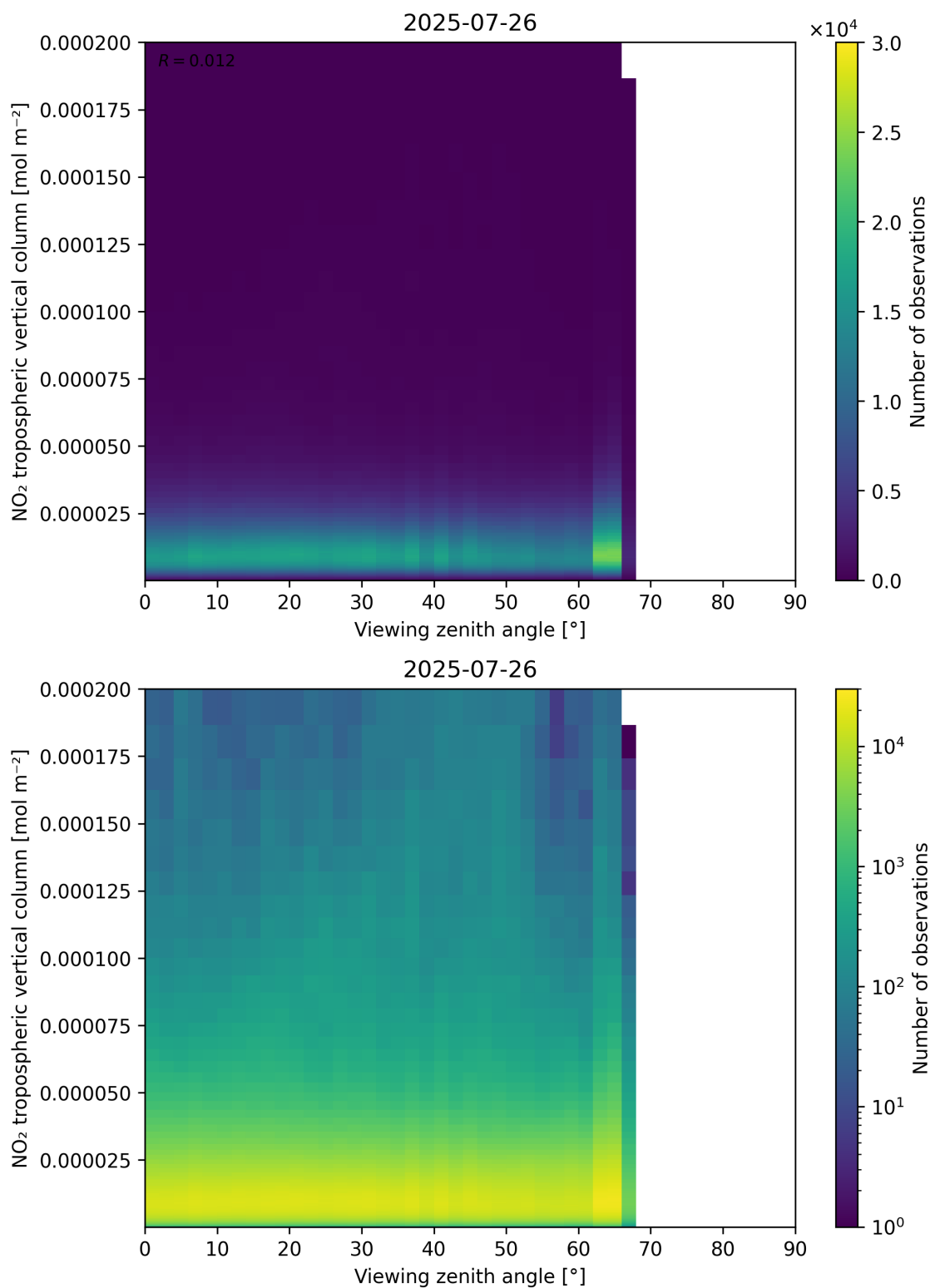
Figure 169: Scatter density plot of “Viewing zenith angle” against “NO 2 tropospheric vertical column” for 2025-07-25 to 2025-07-27.
