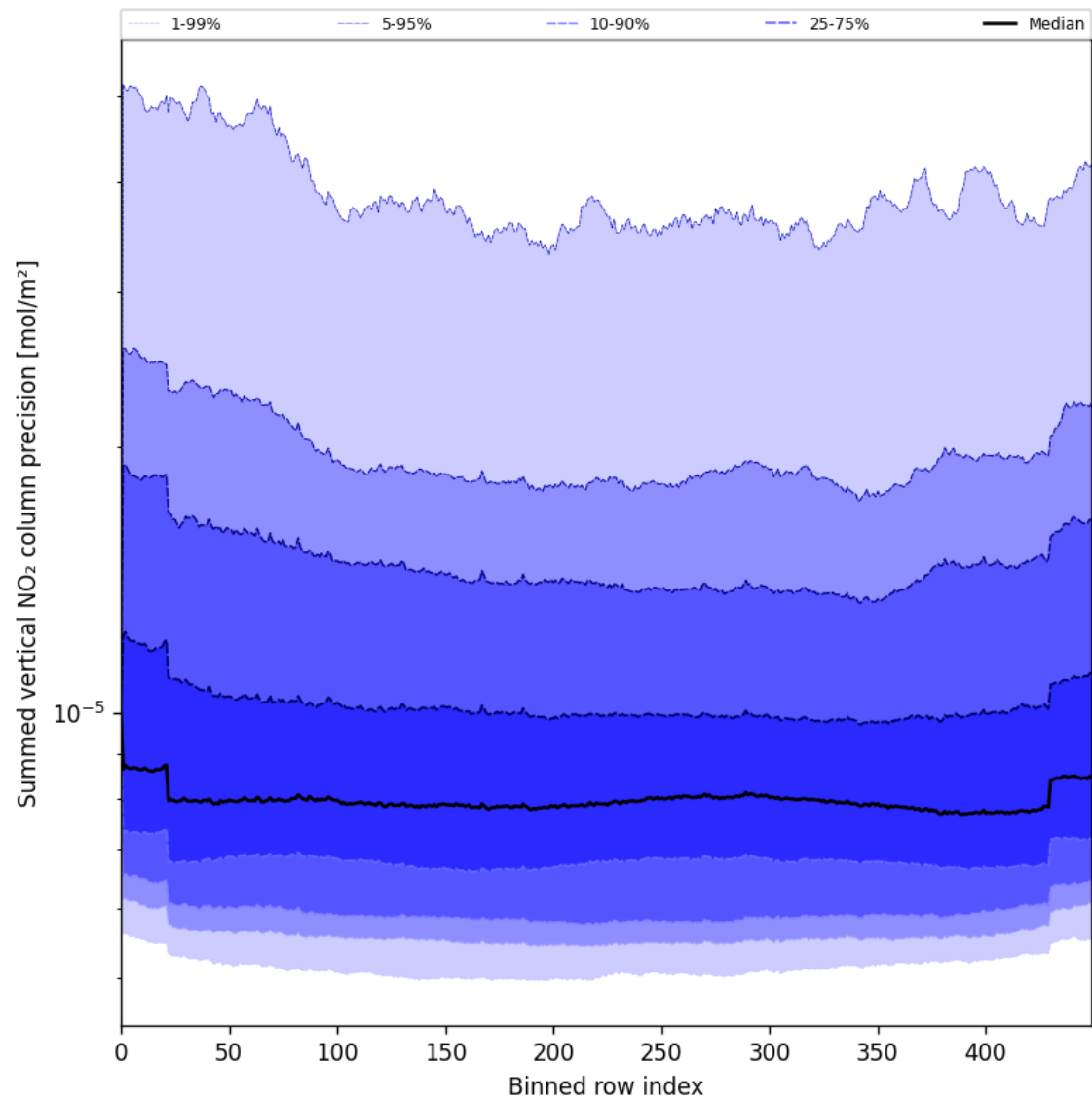
Figure 58: Along track statistics of “Summed vertical NO 2 column precision” for 2025-07-25 to 2025-07-27
