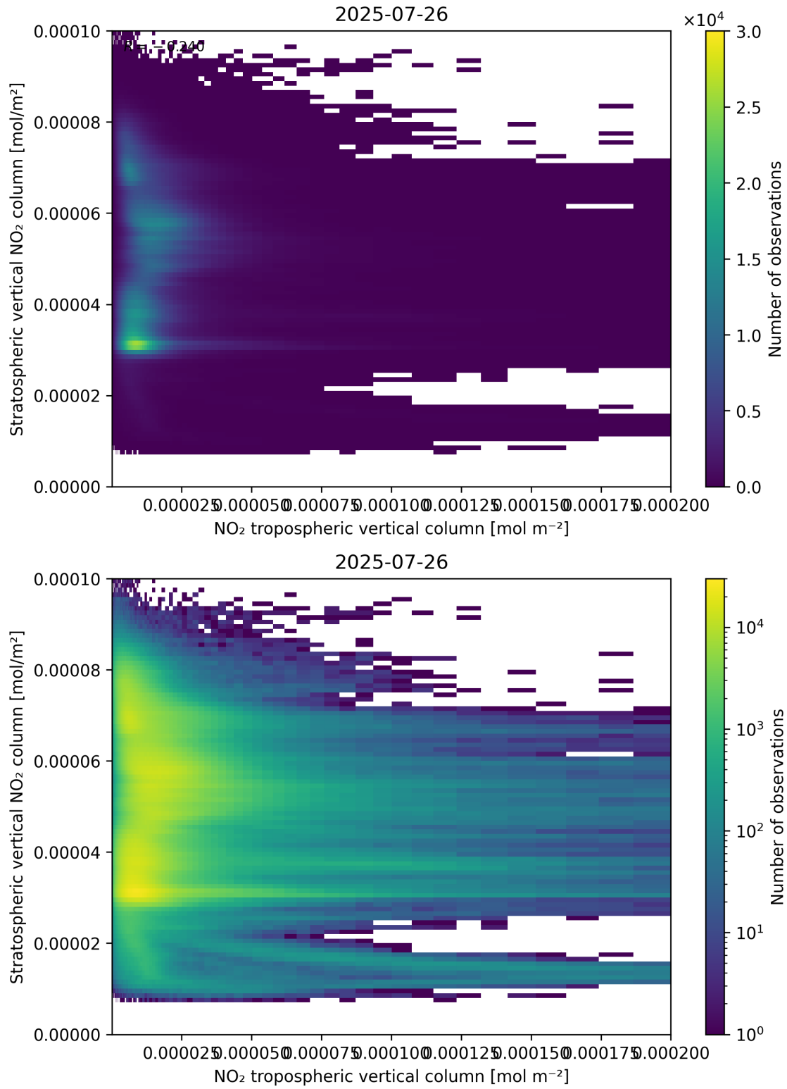
Figure 125: Scatter density plot of “NO 2 tropospheric vertical column” against “Stratospheric vertical NO 2 column” for 2025-07-25 to 2025-07-27.
