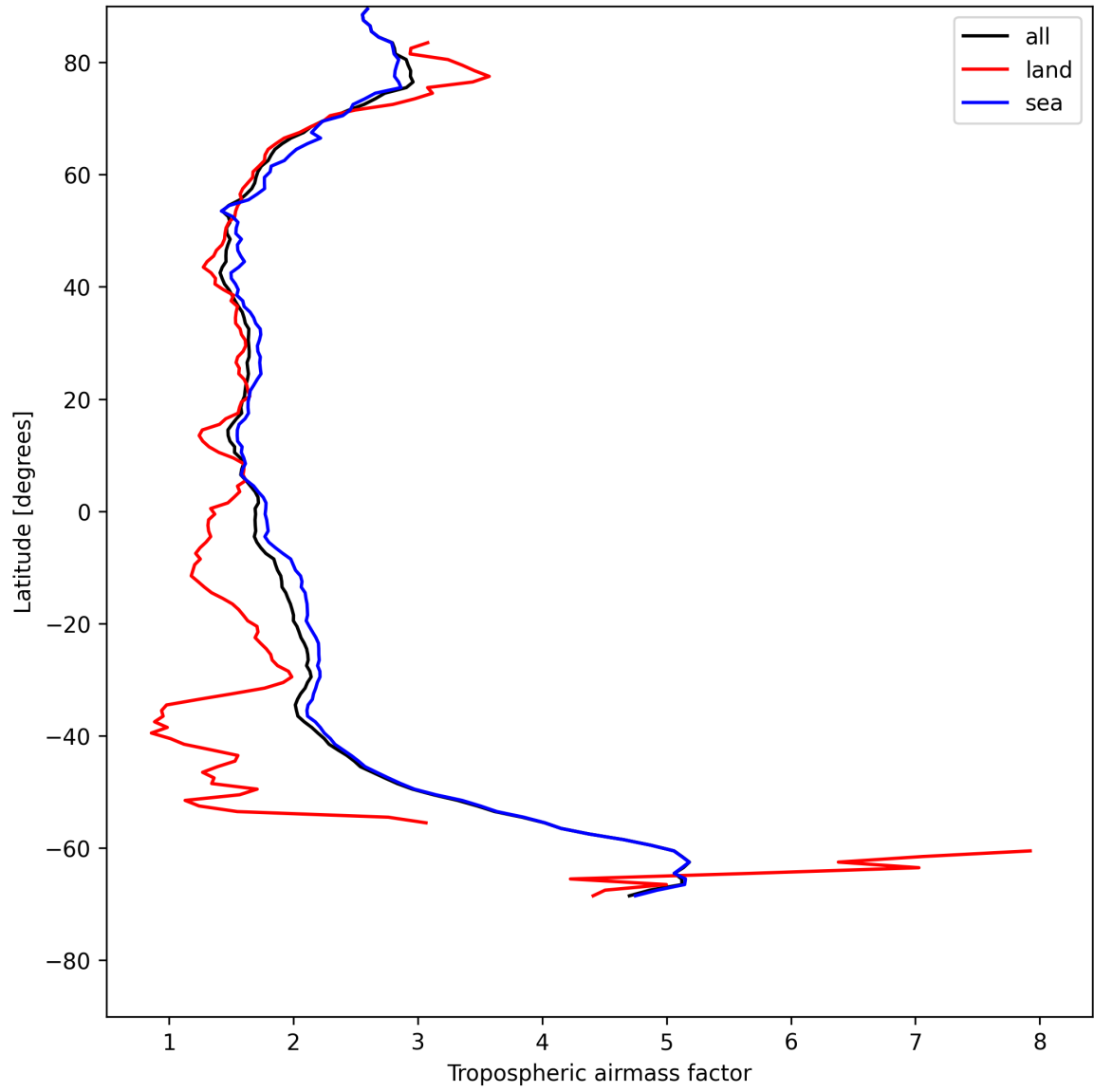
Figure 14: Zonal average of “Tropospheric airmass factor” for 2025-07-25 to 2025-07-27.
