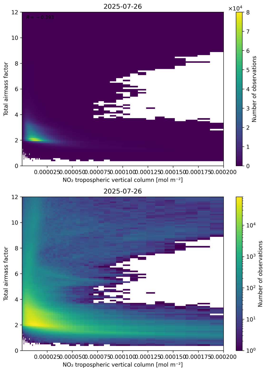
Figure 122: Scatter density plot of “NO 2 tropospheric vertical column” against “Total air mass factor” for 2025-07-25 to 2025-07-27.
