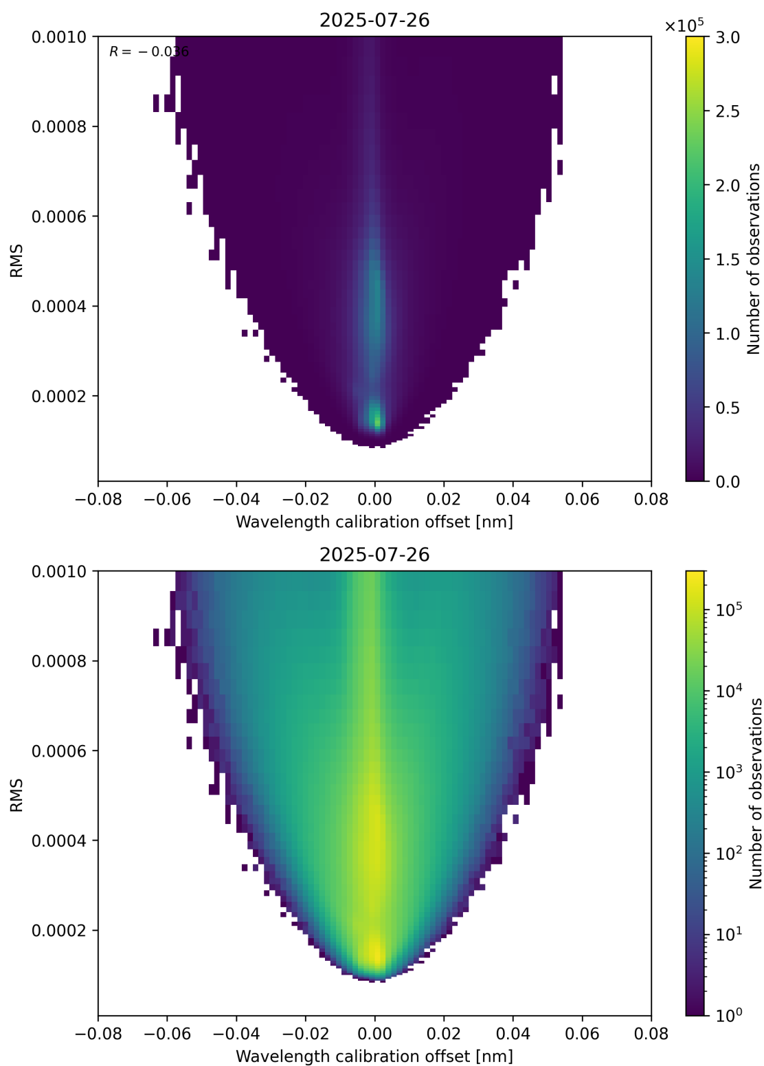
Figure 181: Scatter density plot of “Wavelength calibration offset” against “RMS” for 2025-07-25 to 2025-07-27.
