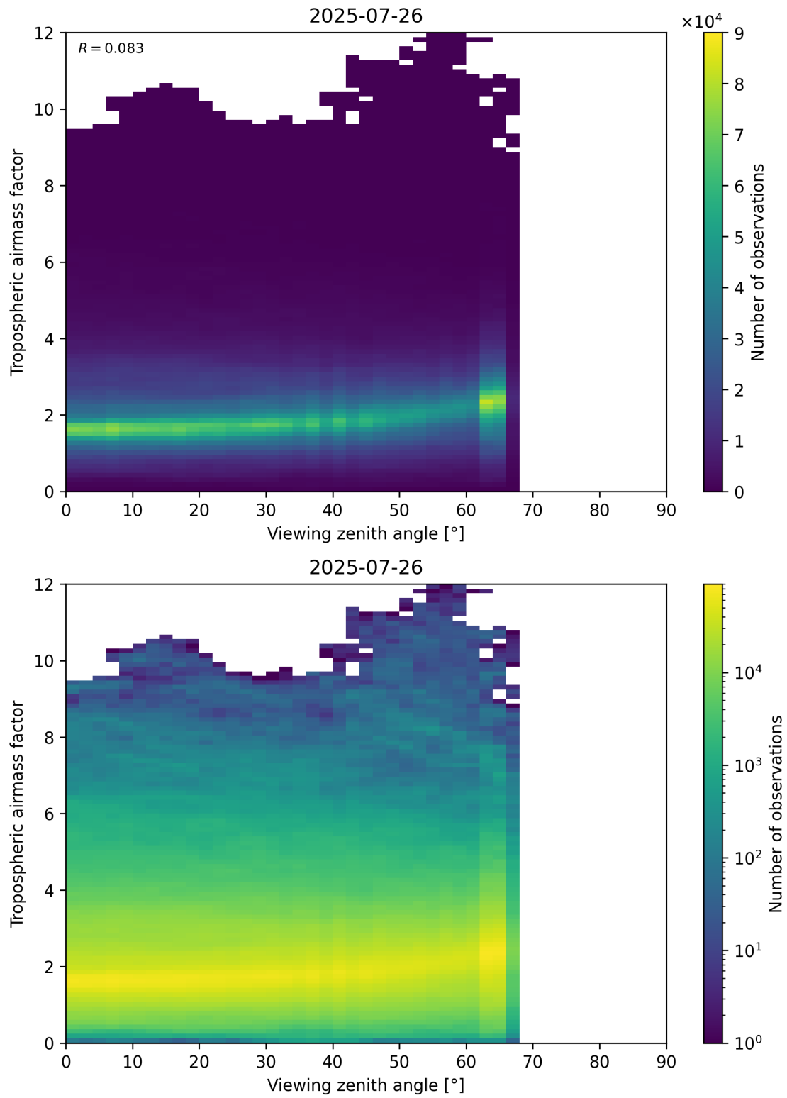
Figure 161: Scatter density plot of “Viewing zenith angle” against “Tropospheric airmass factor” for 2025-07-25 to 2025-07-27.
