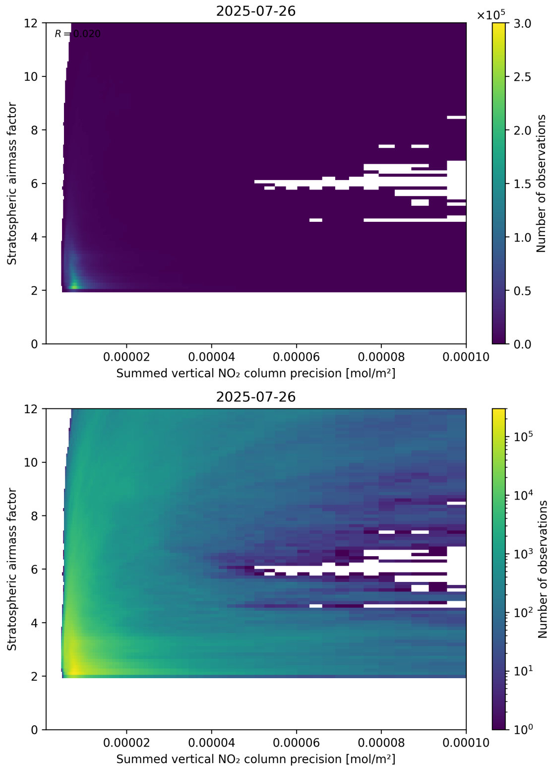
Figure 106: Scatter density plot of “Summed vertical NO 2 column precision” against “Stratospheric airmass factor” for 2025-07-25 to 2025-07-27.
