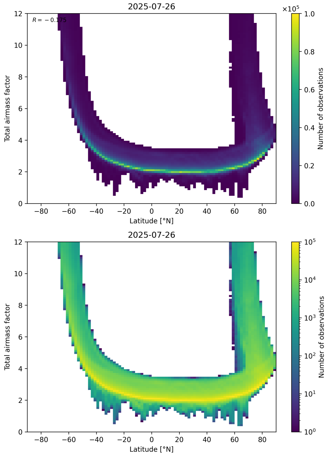
Figure 84: Scatter density plot of “Latitude” against “Total airmass factor” for 2025-07-25 to 2025-07-27.
