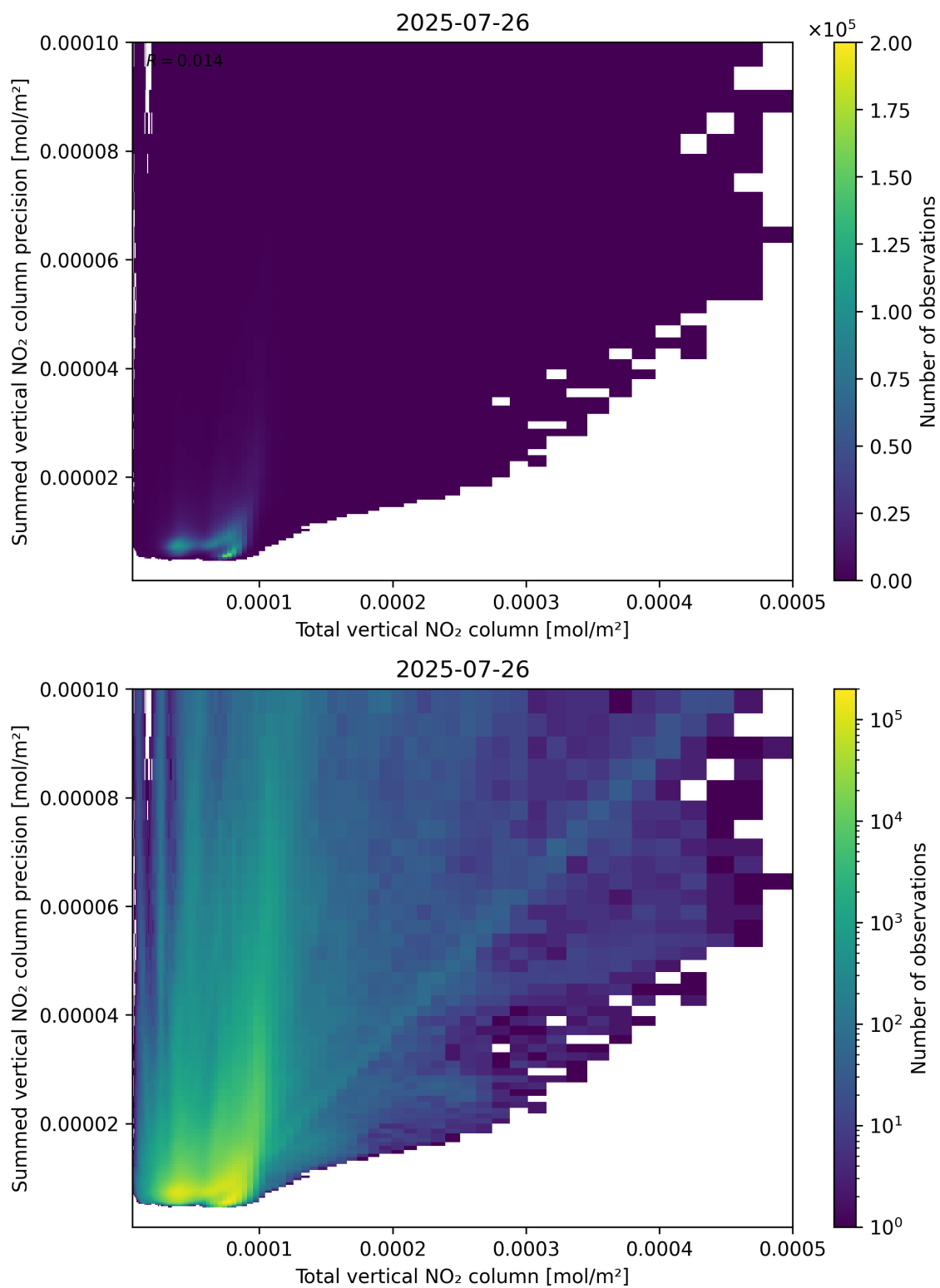
Figure 113: Scatter density plot of “Total vertical NO 2 column” against “Summed vertical NO 2 column precision” for 2025-07-25 to 2025-07-27.
