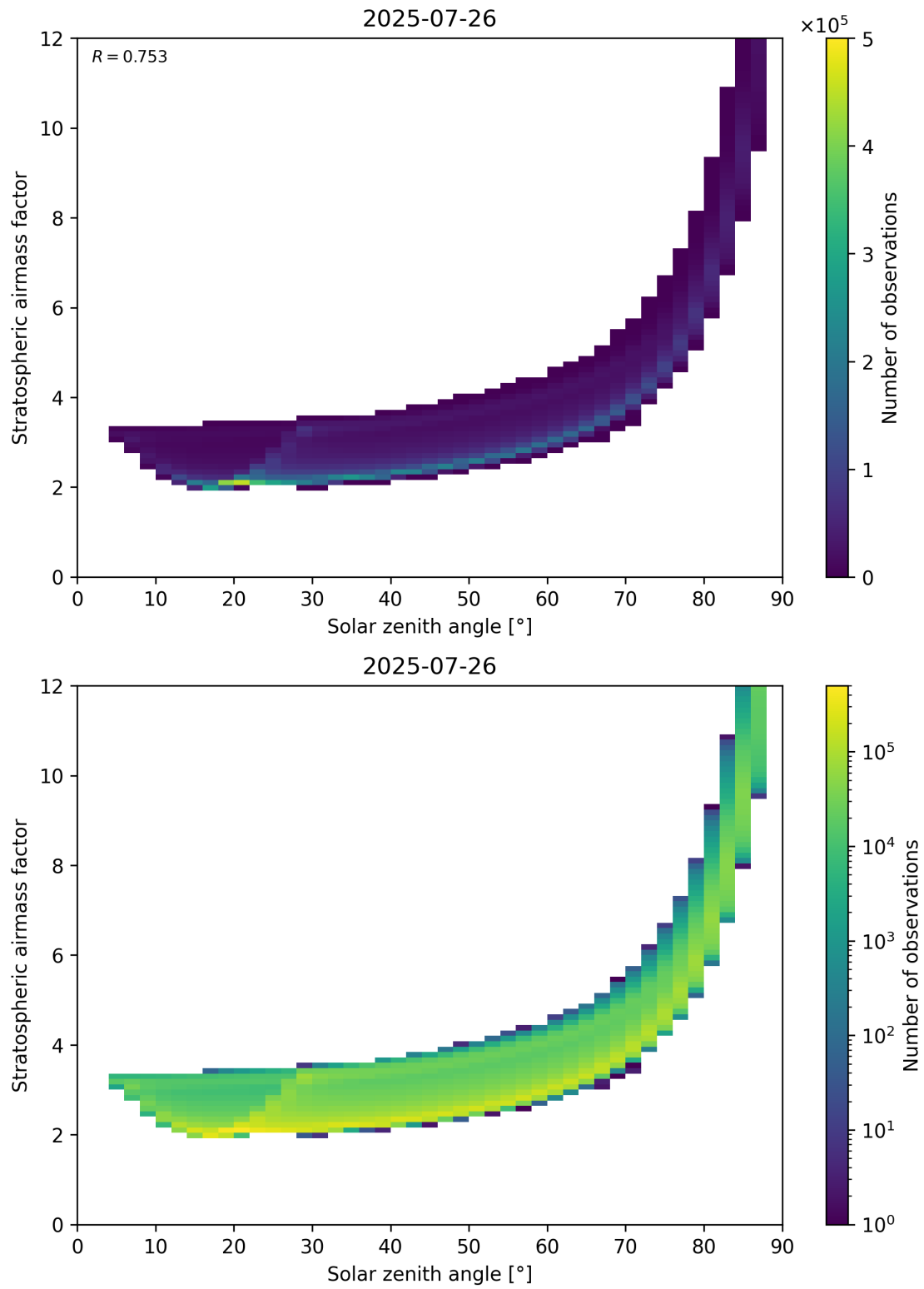
Figure 145: Scatter density plot of “Solar zenith angle” against “Stratospheric airmass factor” for 2025-07-25 to 2025-07-27.
