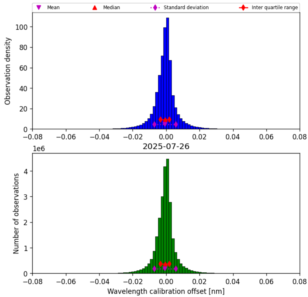
Figure 35: Histogram of “Wavelength calibration offset” for 2025-07-25 to 2025-07-27
