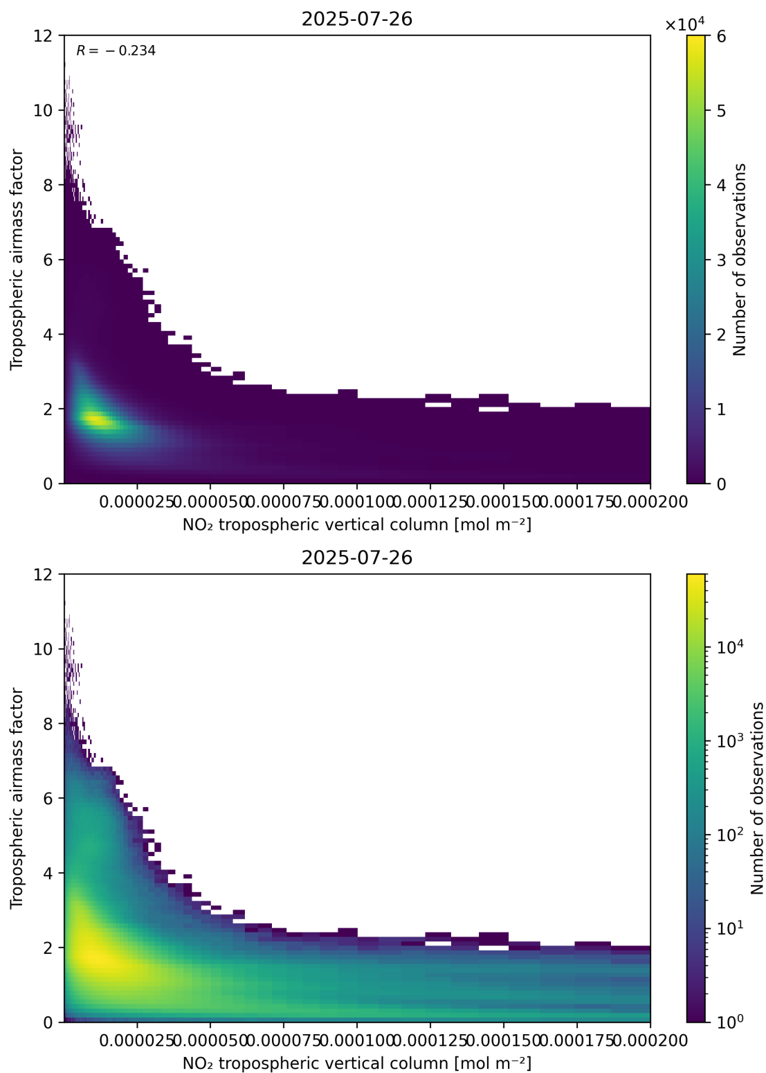
Figure 123: Scatter density plot of “NO 2 tropospheric vertical column” against “Tropospheric air mass factor” for 2025-07-25 to 2025-07-27.
