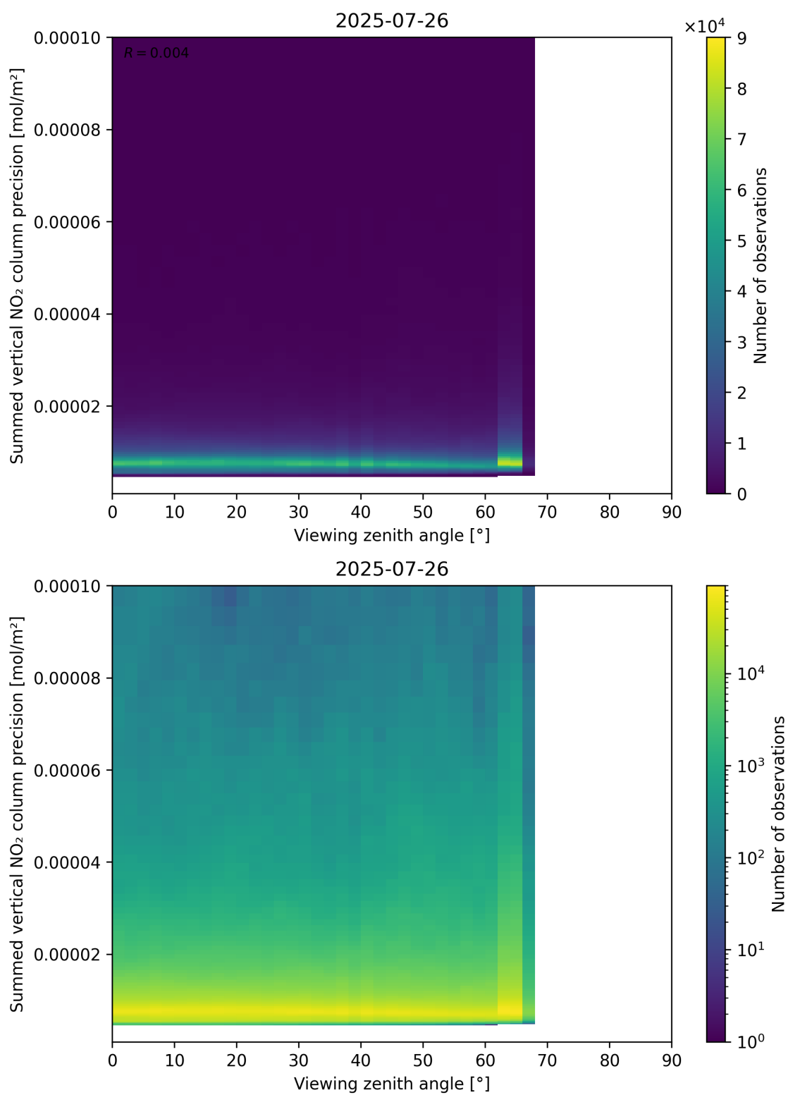
Figure 166: Scatter density plot of “Viewing zenith angle” against “Summed vertical NO 2 column precision” for 2025-07-25 to 2025-07-27.
