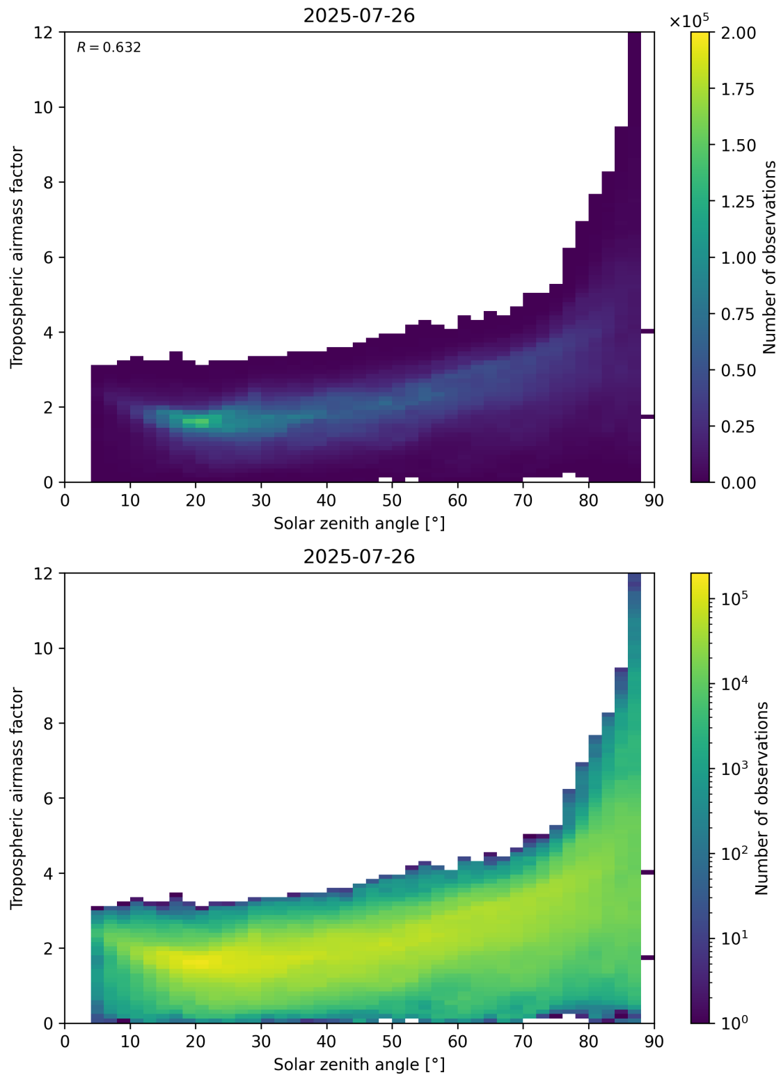
Figure 147: Scatter density plot of “Solar zenith angle” against “Tropospheric airmass factor” for 2025-07-25 to 2025-07-27.
