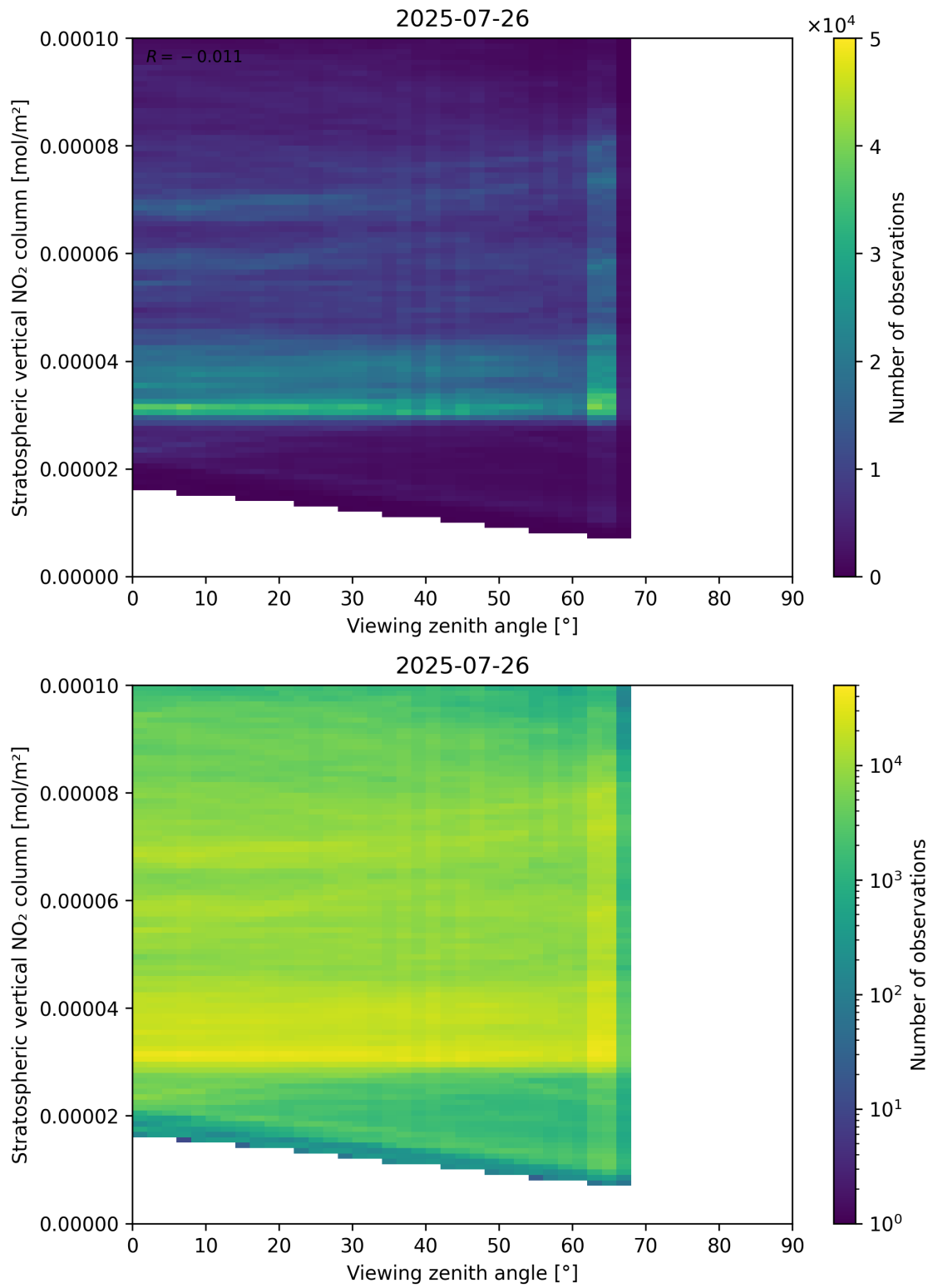
Figure 164: Scatter density plot of “Viewing zenith angle” against “Stratospheric vertical NO 2 column” for 2025-07-25 to 2025-07-27.
