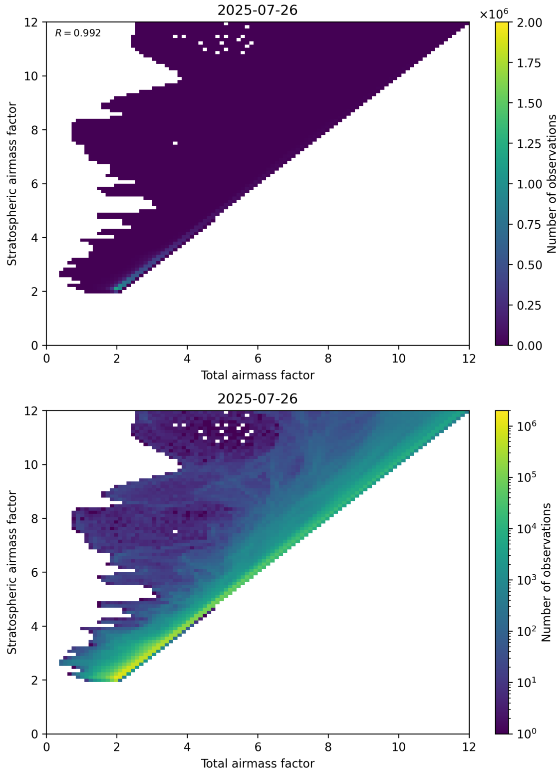
Figure 62: Scatter density plot of “Total airmass factor” against “Stratospheric airmass factor” for 2025-07-25 to 2025-07-27.
