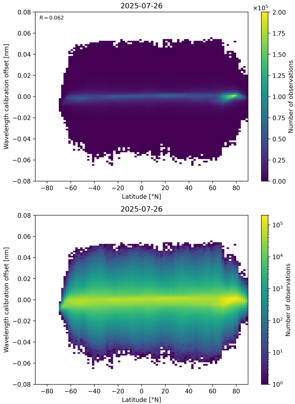
Figure 95: Scatter density plot of “Latitude” against “Wavelength calibration offset” for 2025-07-25 to 2025-07-27.
