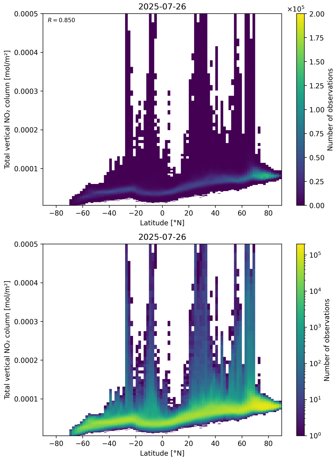
Figure 90: Scatter density plot of “Latitude” against “Total vertical NO 2 column” for 2025-07-25 to 2025-07-27.
