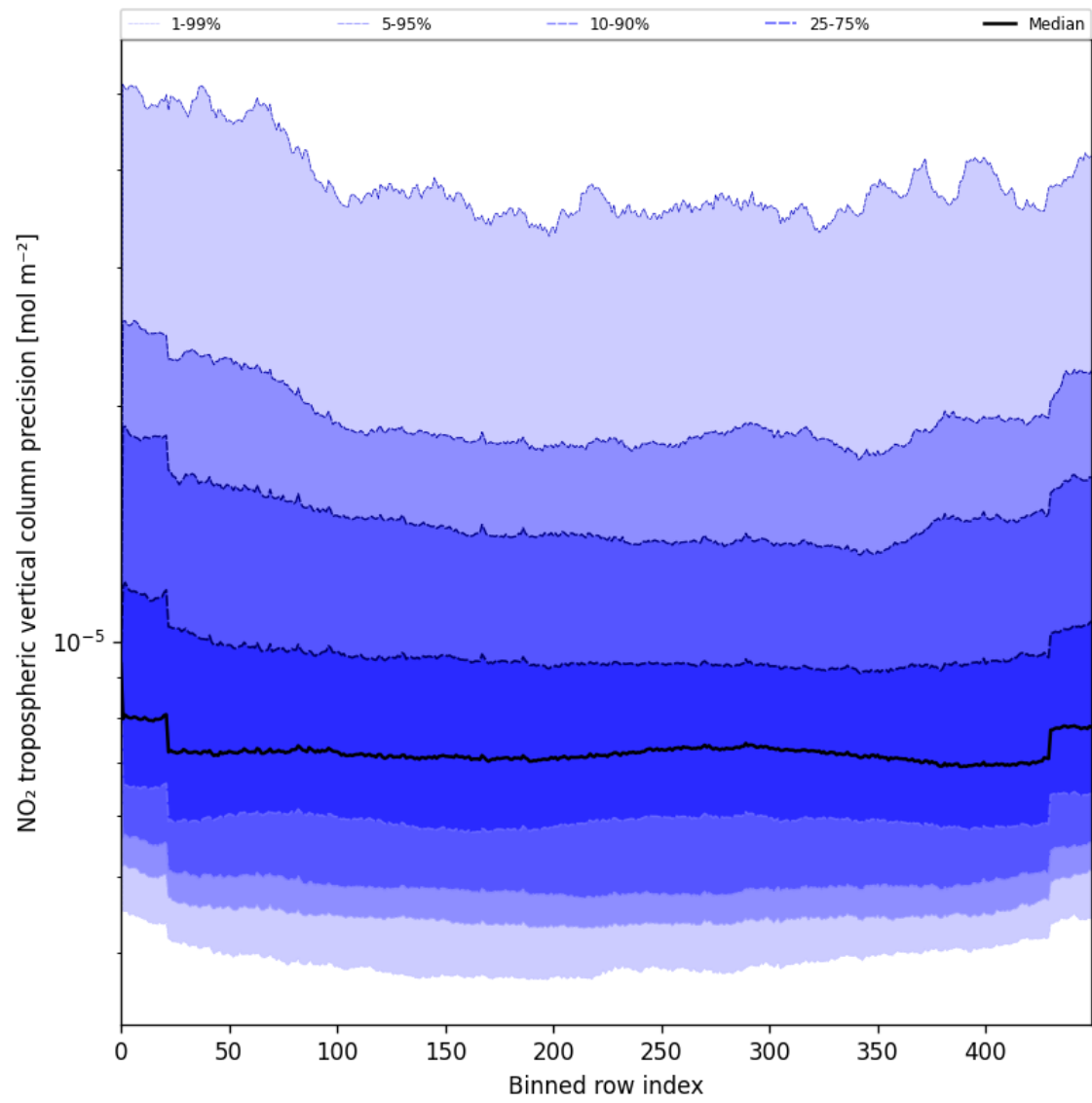
Figure 47: Along track statistics of “NO 2 tropospheric vertical column precision” for 2025-07-25 to 2025-07-27
