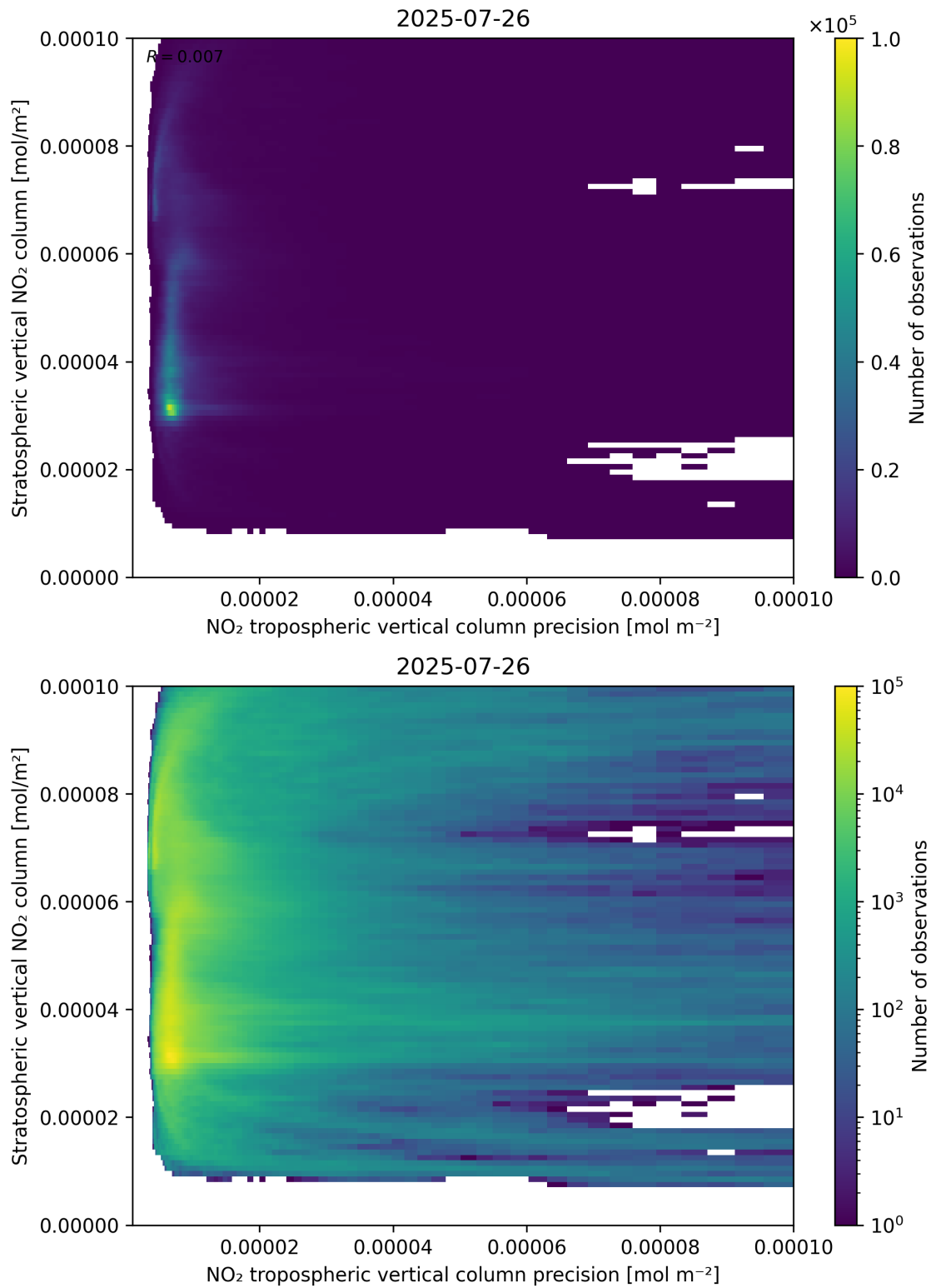
Figure 135: Scatter density plot of “NO 2 tropospheric vertical column precision” against “Stratospheric vertical NO 2 column” for 2025-07-25 to 2025-07-27.
