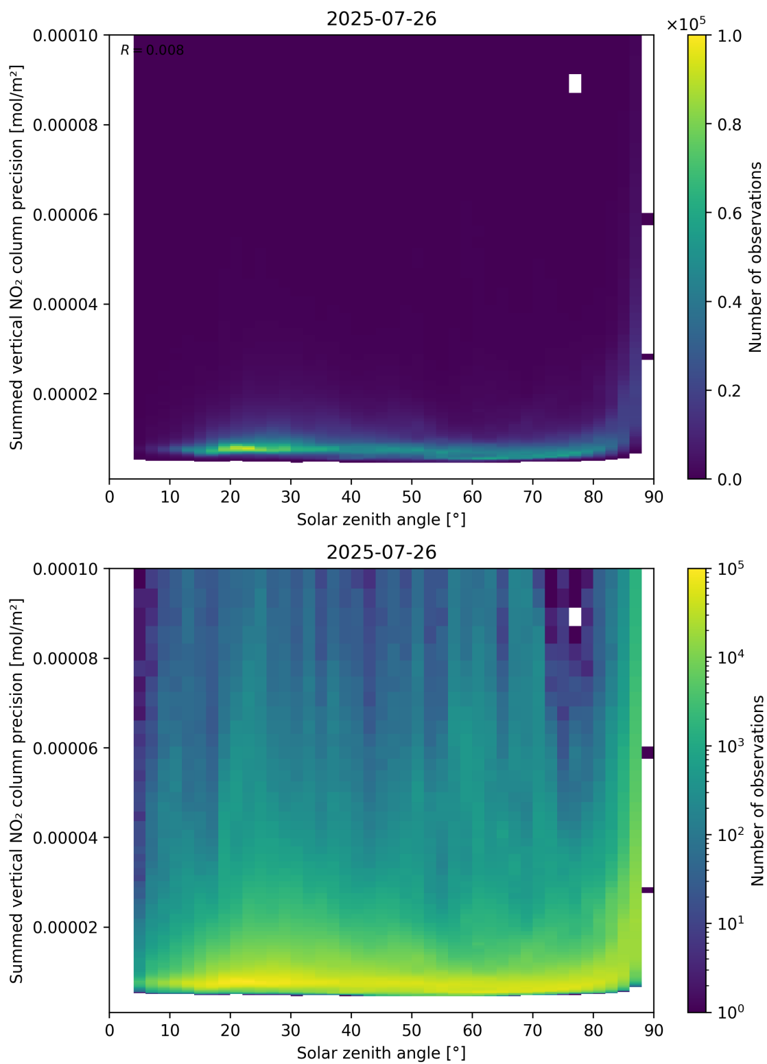
Figure 152: Scatter density plot of “Solar zenith angle” against “Summed vertical NO 2 column precision” for 2025-07-25 to 2025-07-27.
