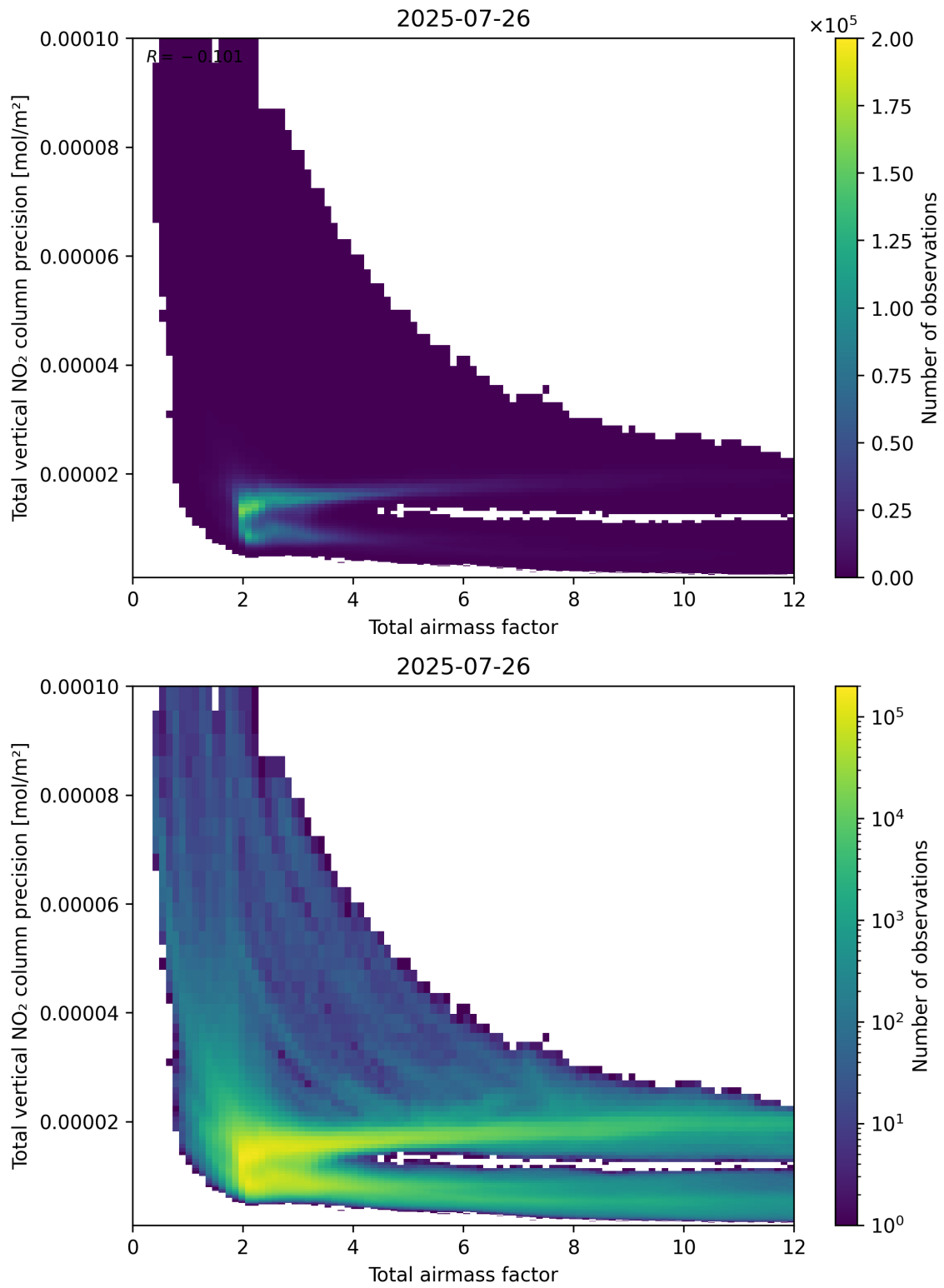
Figure 68: Scatter density plot of “Total airmass factor” against “Total vertical NO 2 column precision” for 2025-07-25 to 2025-07-27.
