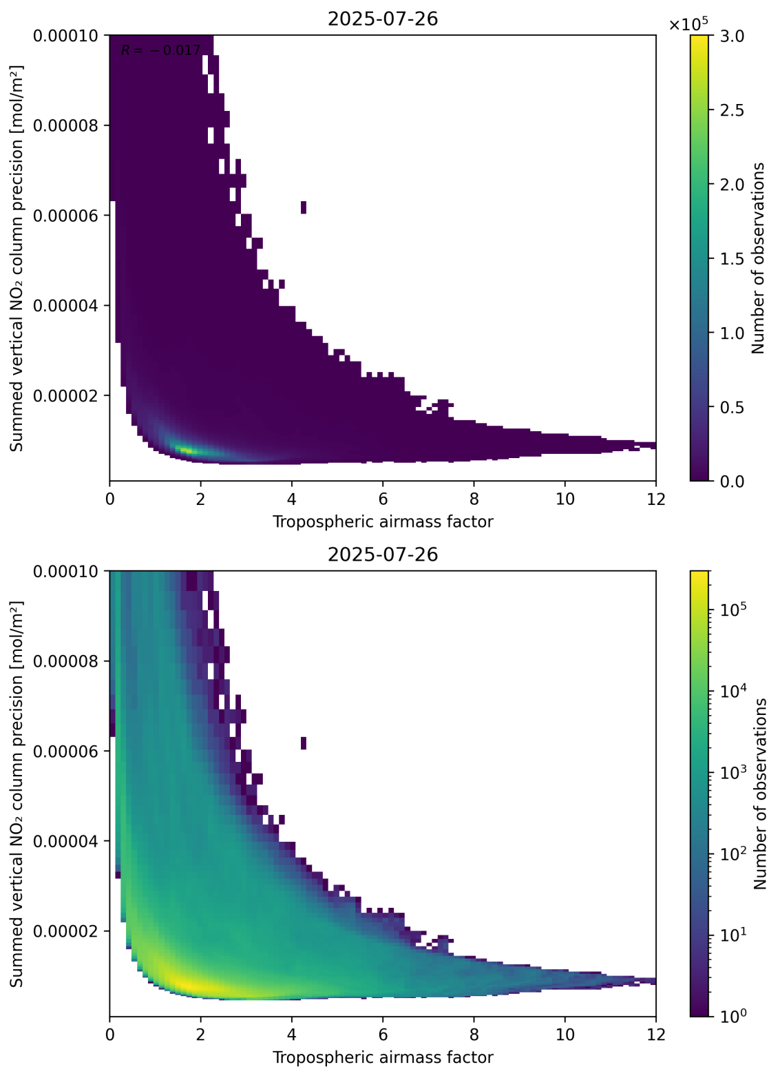
Figure 76: Scatter density plot of “Tropospheric air mass factor” against “Summed vertical NO 2 column precision” for 2025-07-25 to 2025-07-27.
