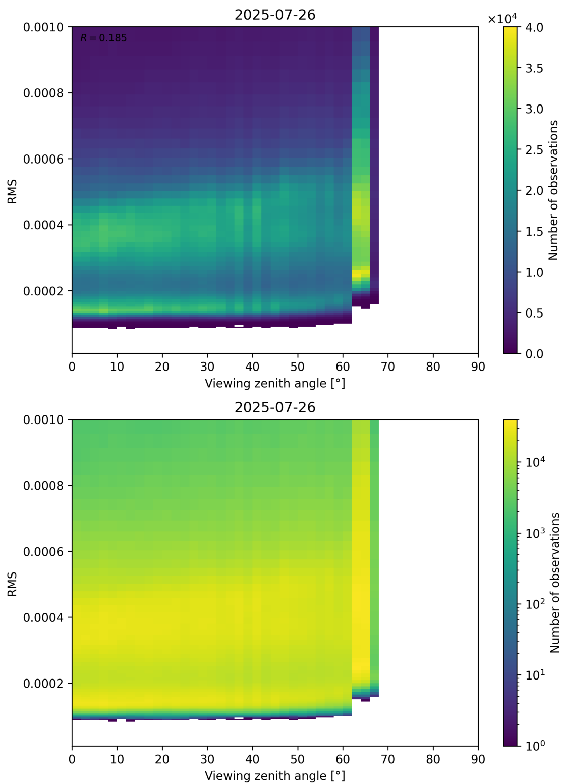
Figure 171: Scatter density plot of “Viewing zenith angle” against “RMS” for 2025-07-25 to 2025-07-27.
