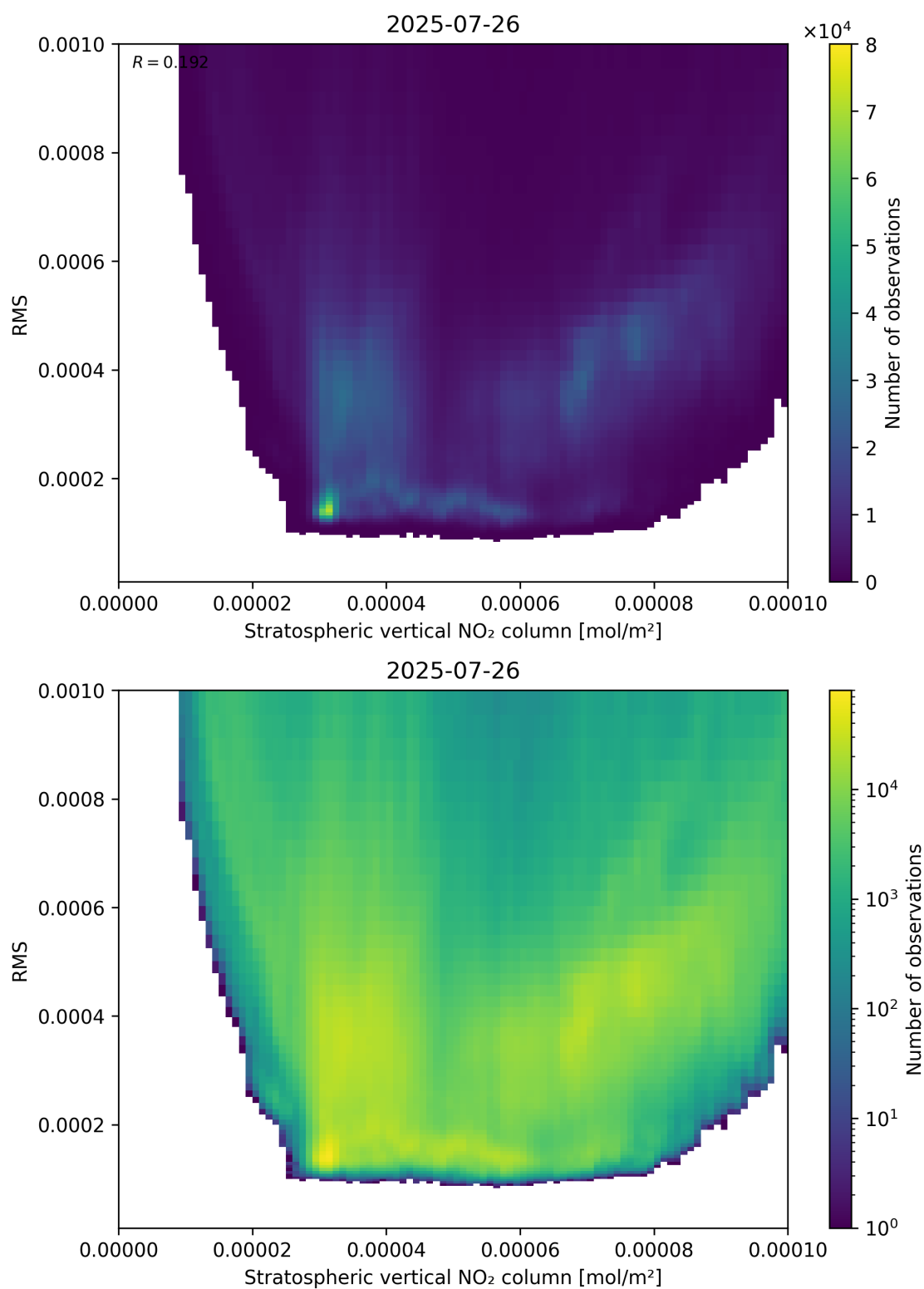
Figure 102: Scatter density plot of “Stratospheric vertical NO 2 column” against “RMS” for 2025-07-25 to 2025-07-27.
