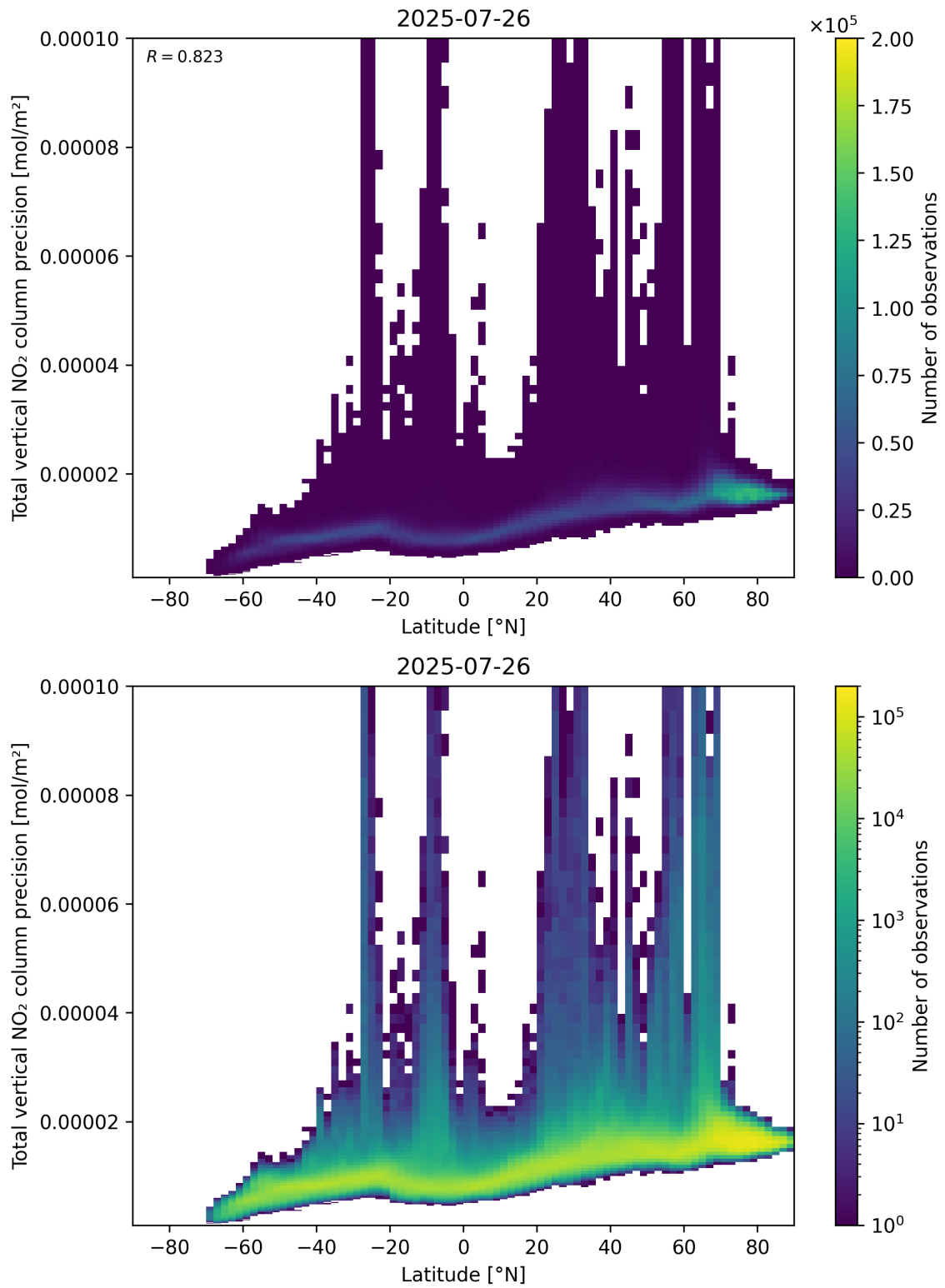
Figure 91: Scatter density plot of “Latitude” against “Total vertical NO 2 column precision” for 2025-07-25 to 2025-07-27.
