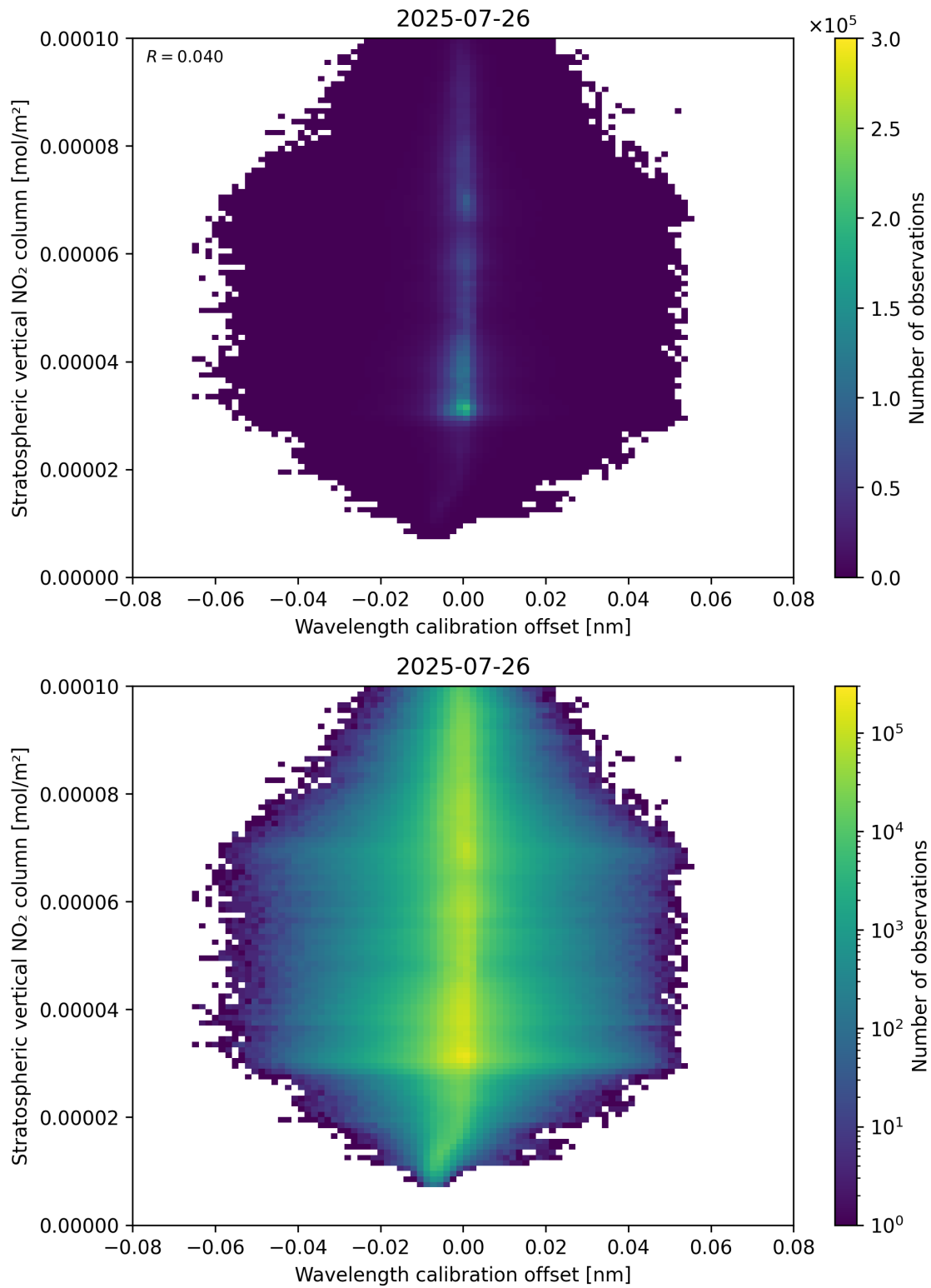
Figure 176: Scatter density plot of “Wavelength calibration offset” against “Stratospheric vertical NO 2 column” for 2025-07-25 to 2025-07-27.
