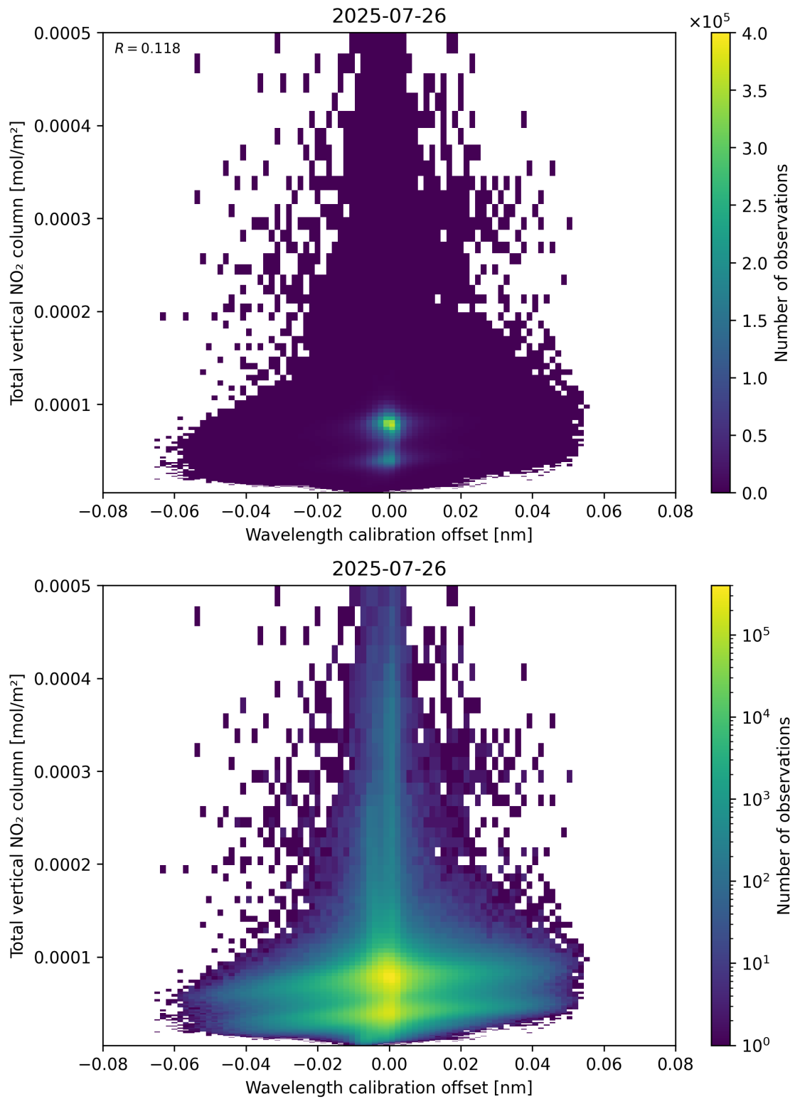
Figure 179: Scatter density plot of “Wavelength calibration offset” against “Total vertical NO 2 column” for 2025-07-25 to 2025-07-27.
