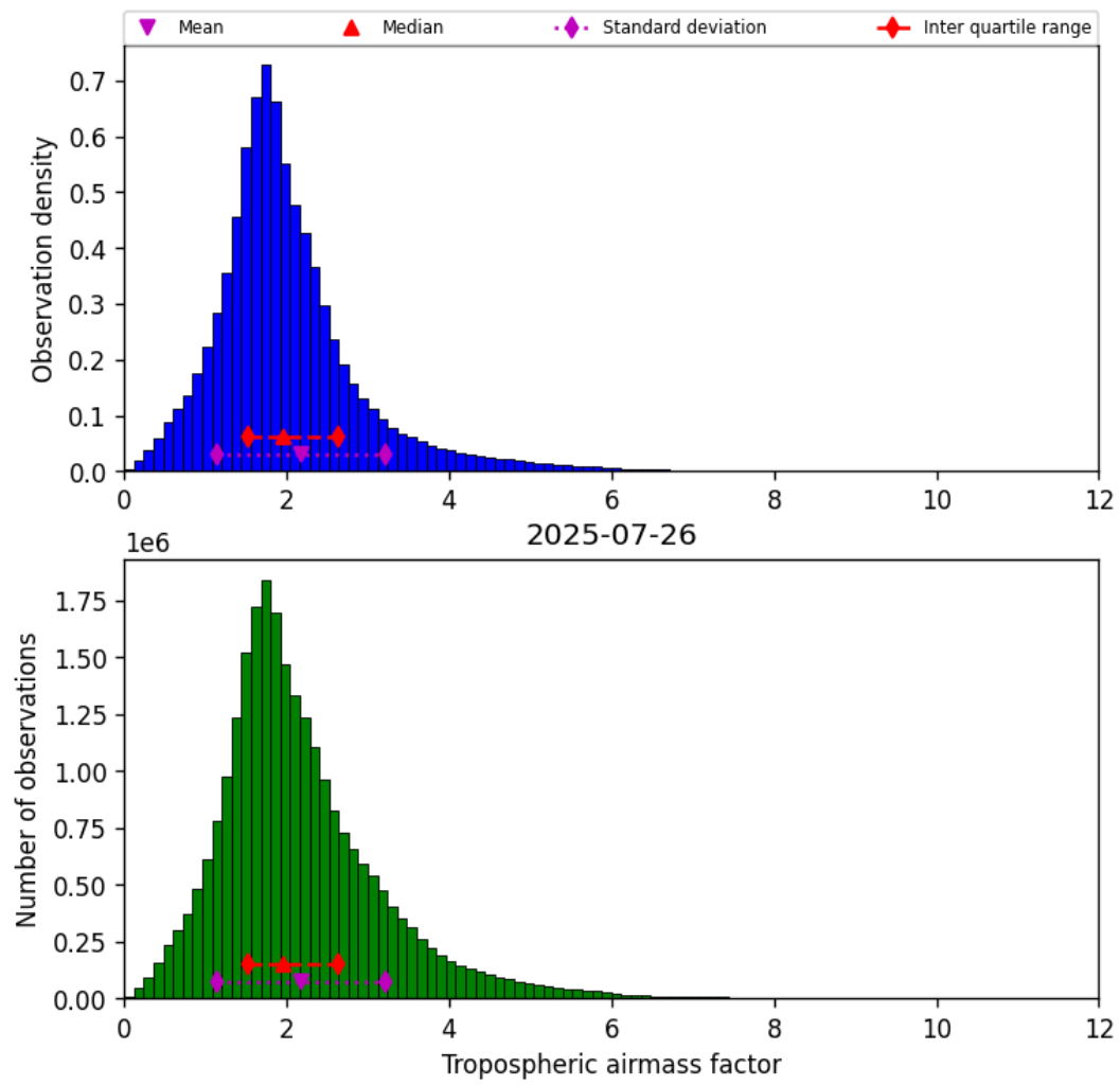
Figure 31: Histogram of “Tropospheric airmass factor” for 2025-07-25 to 2025-07-27
