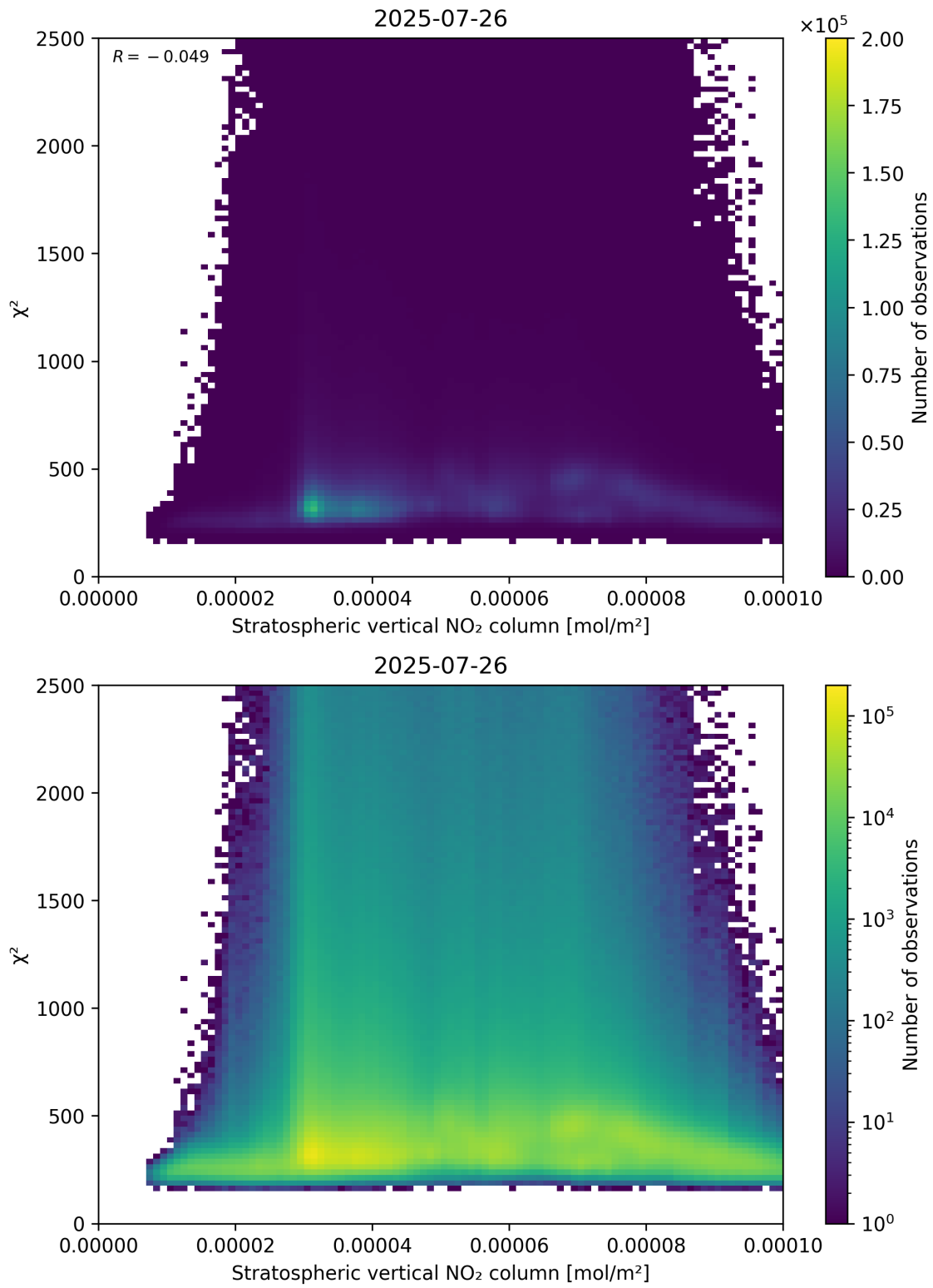
Figure 97: Scatter density plot of “Stratospheric vertical NO 2 column” against “ \chi^2 ” for 2025-07-25 to 2025-07-27.
