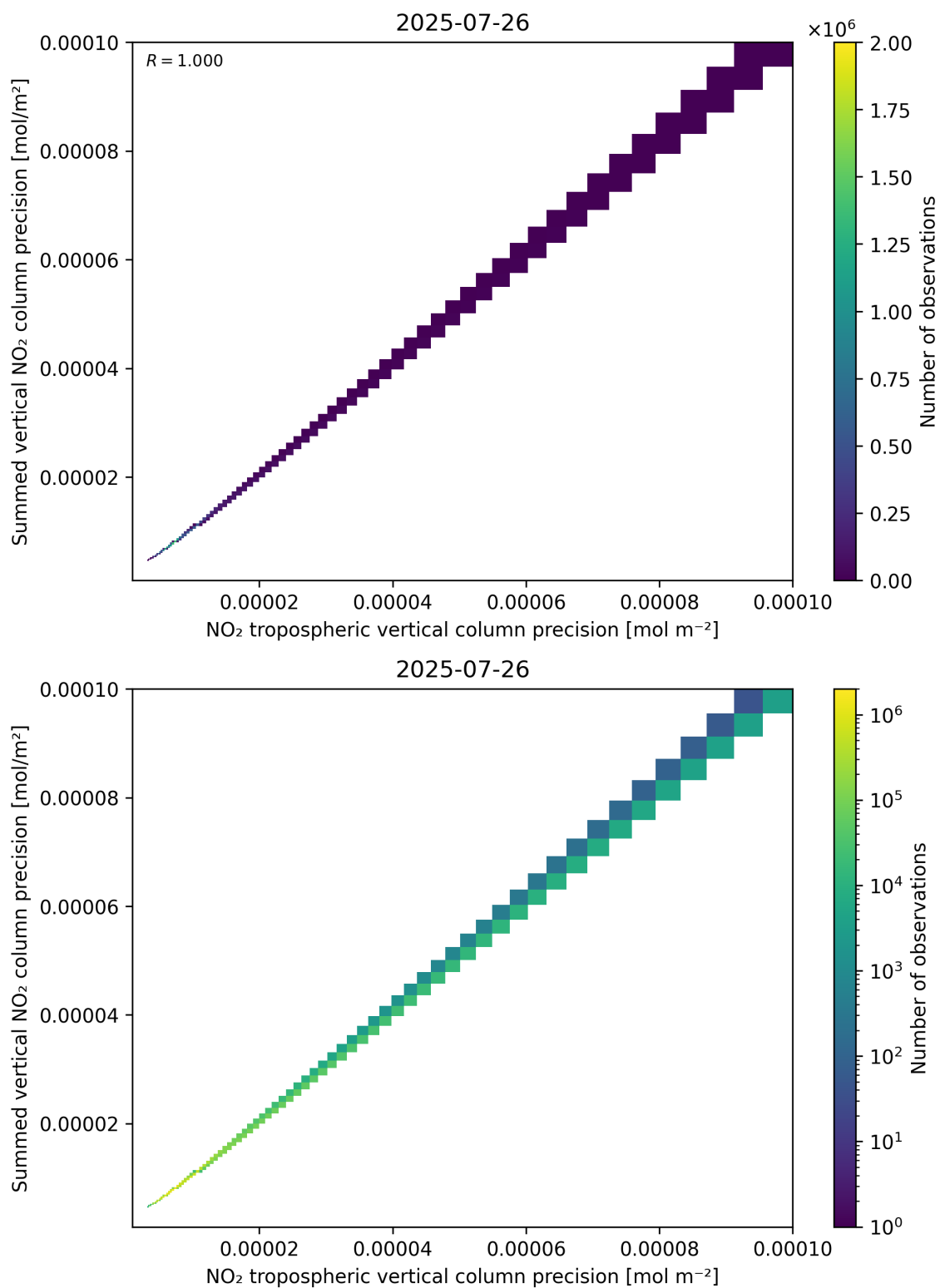
Figure 137: Scatter density plot of “NO 2 tropospheric vertical column precision” against “Summed vertical NO 2 column precision” for 2025-07-25 to 2025-07-27.
