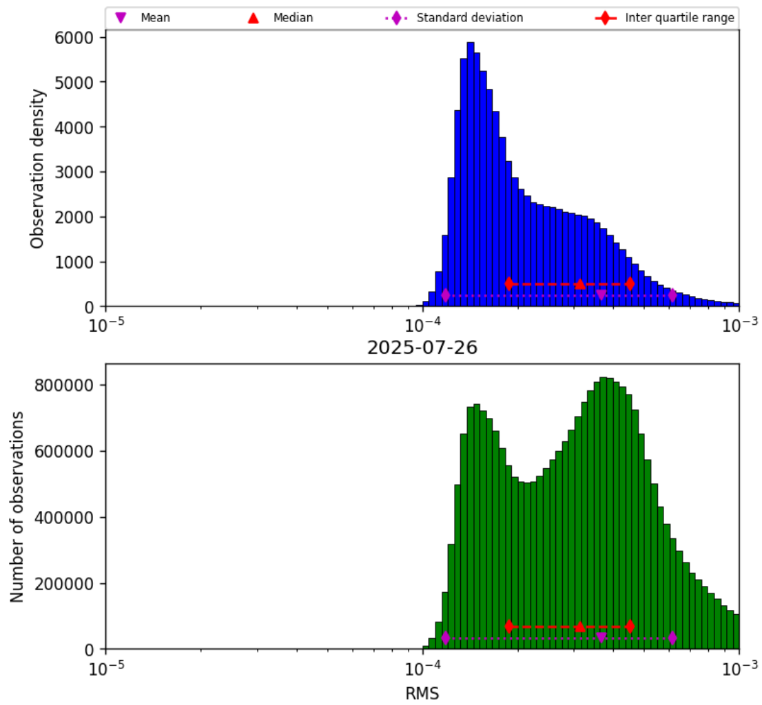
Figure 43: Histogram of “RMS” for 2025-07-25 to 2025-07-27
