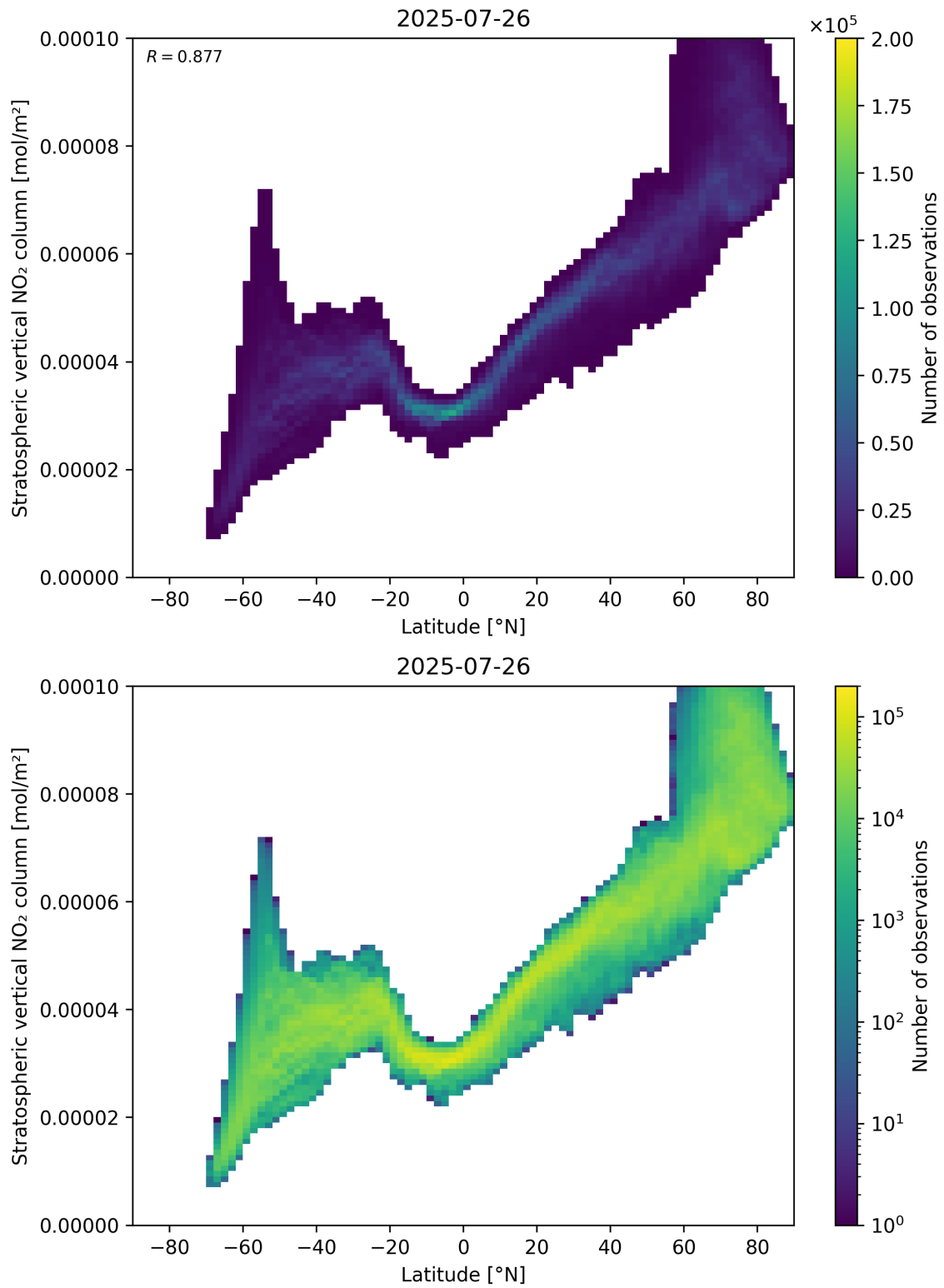
Figure 87: Scatter density plot of “Latitude” against “Stratospheric vertical NO 2 column” for 2025-07-25 to 2025-07-27.
