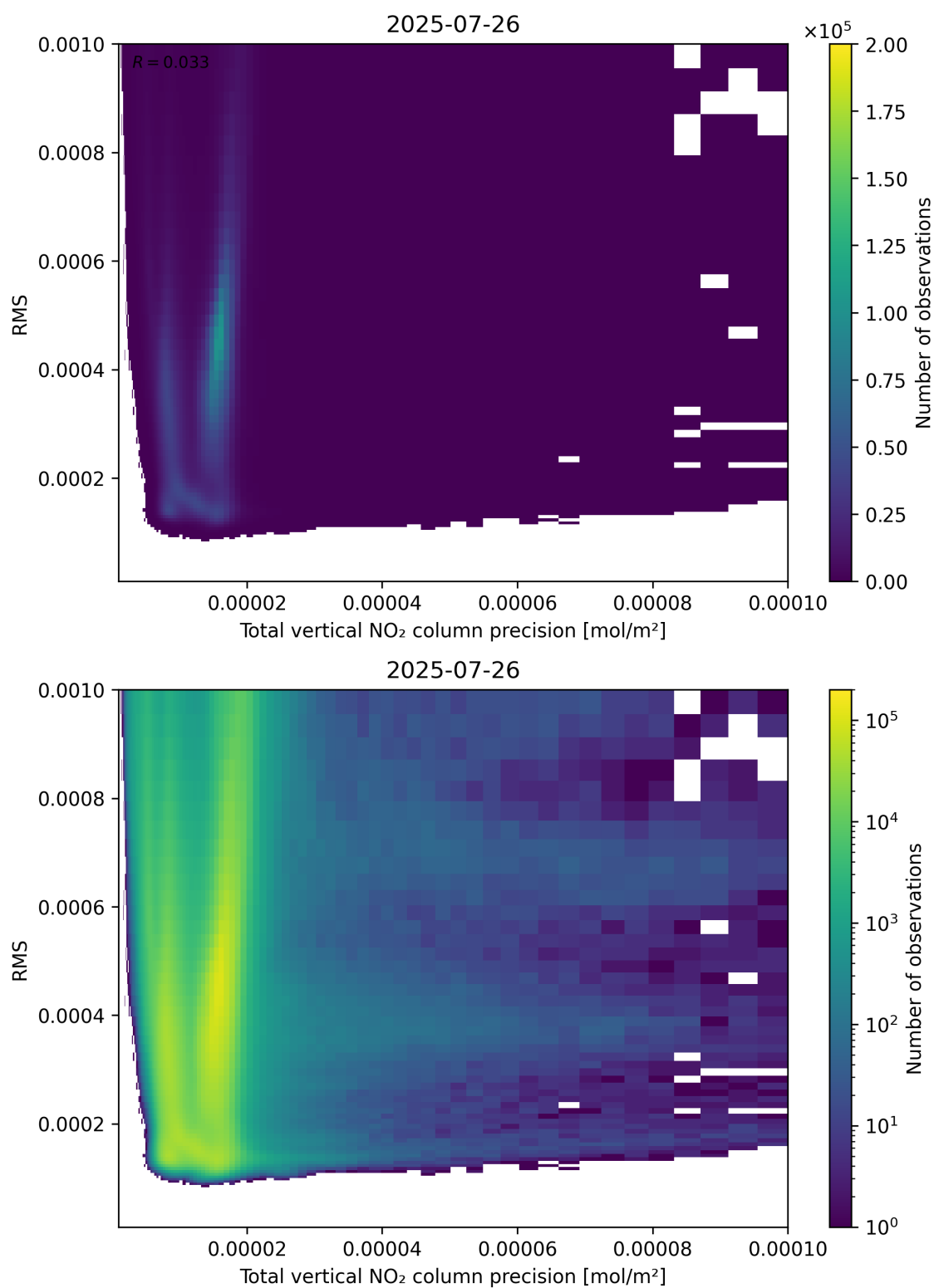
Figure 119: Scatter density plot of “Total vertical NO 2 column precision” against “RMS” for 2025-07-25 to 2025-07-27.
