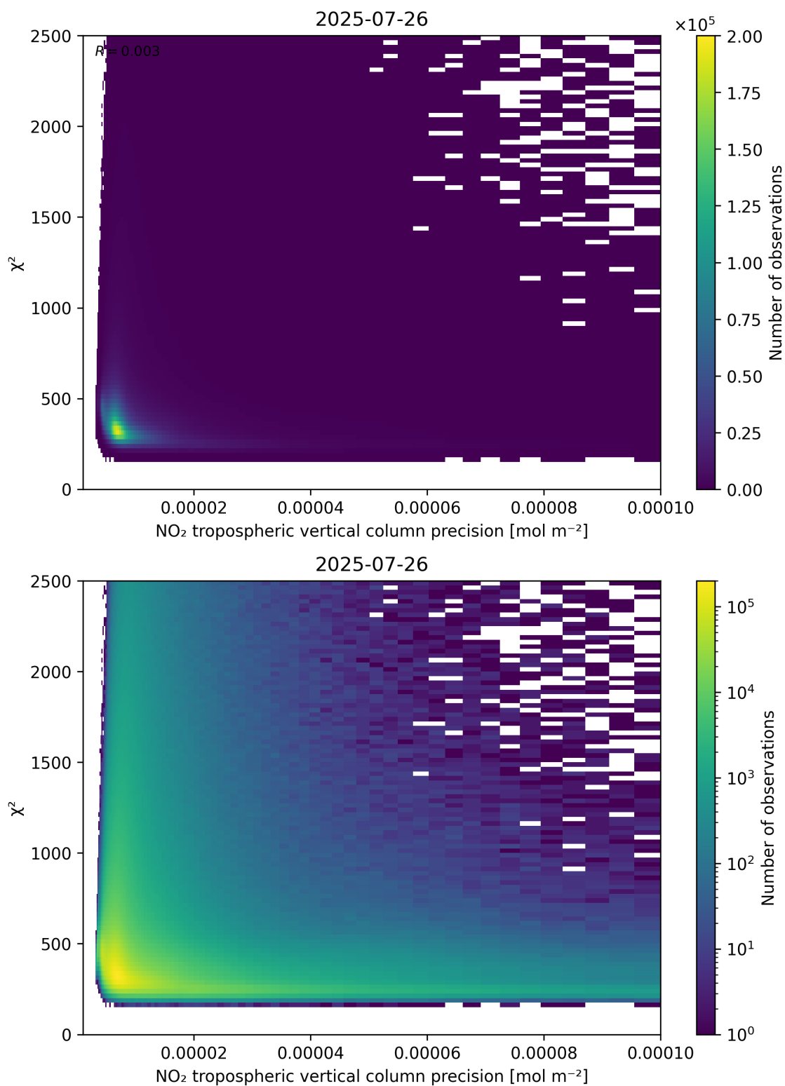
Figure 134: Scatter density plot of “NO 2 tropospheric vertical column precision” against “ \chi^2 ” for 2025-07-25 to 2025-07-27.
