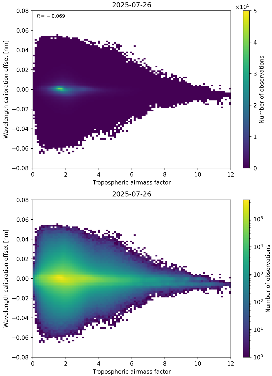
Figure 80: Scatter density plot of “Tropospheric air mass factor” against “Wavelength calibration offset” for 2025-07-25 to 2025-07-27.
