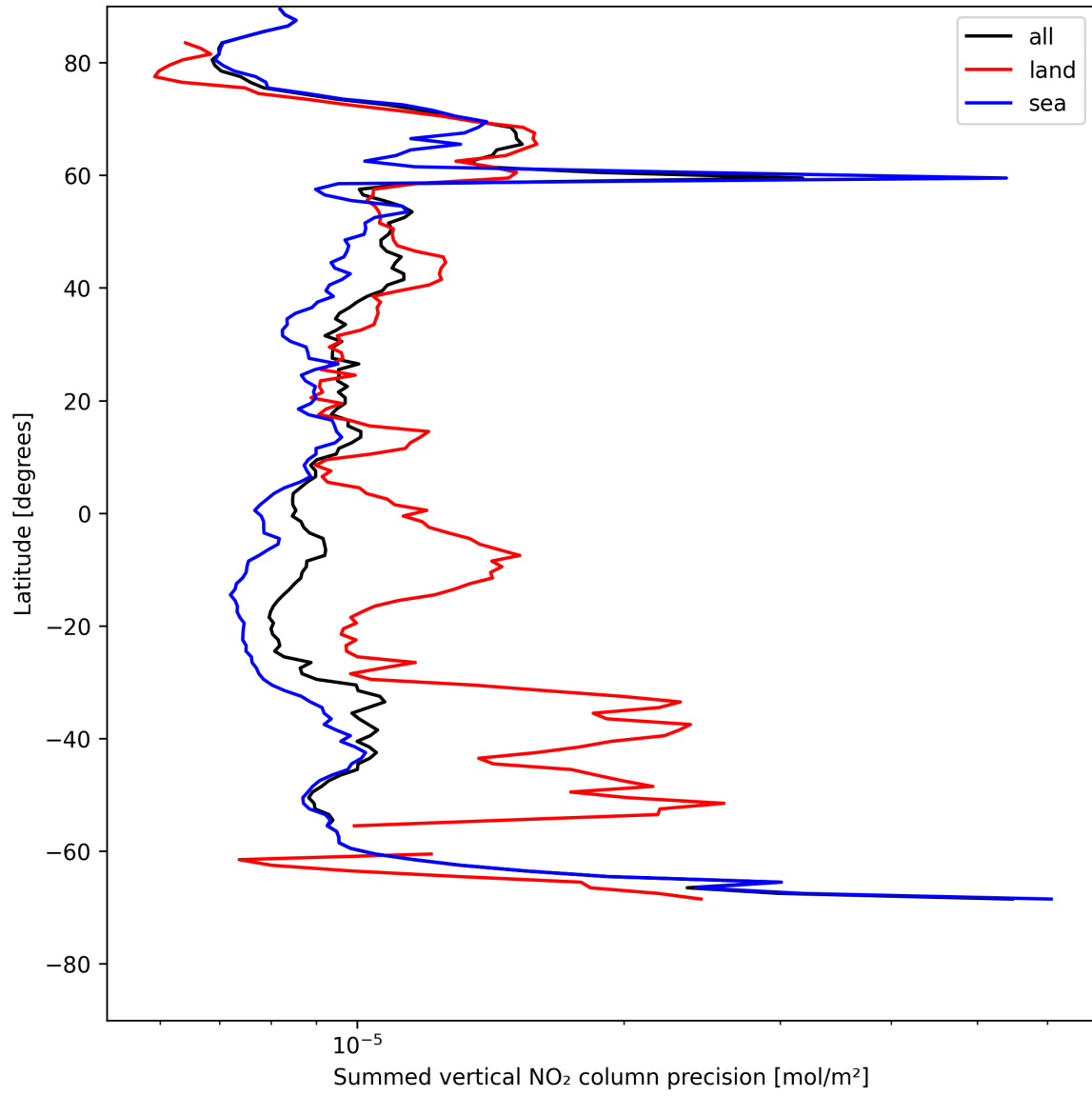
Figure 24: Zonal average of “Summed vertical NO 2 column precision” for 2025-07-25 to 2025-07-27.
