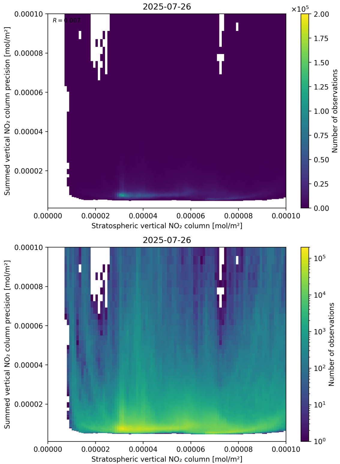
Figure 99: Scatter density plot of “Stratospheric vertical NO 2 column” against “Summed vertical NO 2 column precision” for 2025-07-25 to 2025-07-27.
