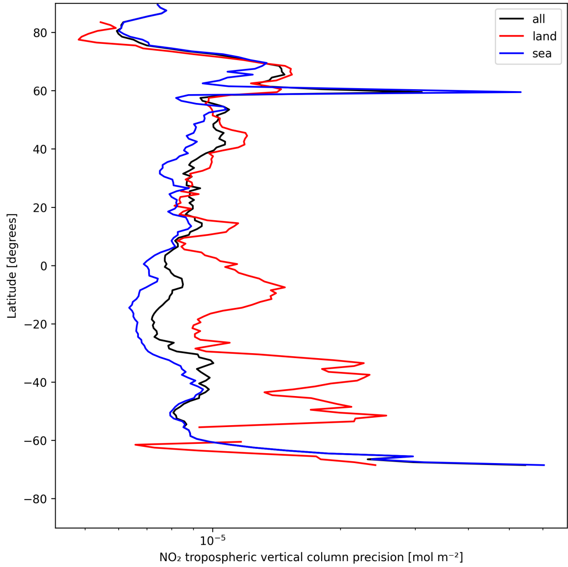
Figure 13: Zonal average of “NO 2 tropospheric vertical column precision” for 2025-07-25 to 2025-07-27.
