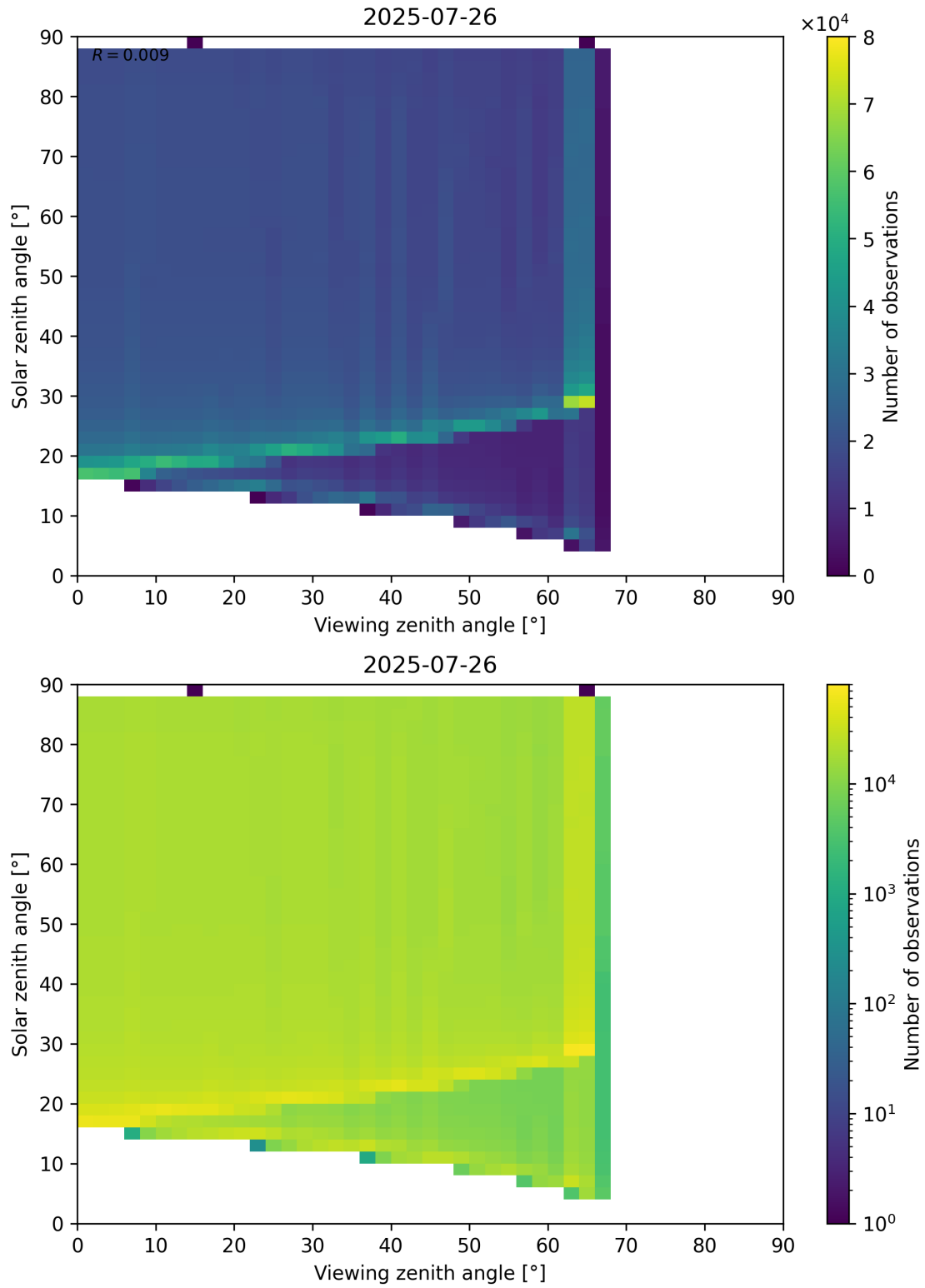
Figure 172: Scatter density plot of “Viewing zenith angle” against “Solar zenith angle” for 2025-07-25 to 2025-07-27.
