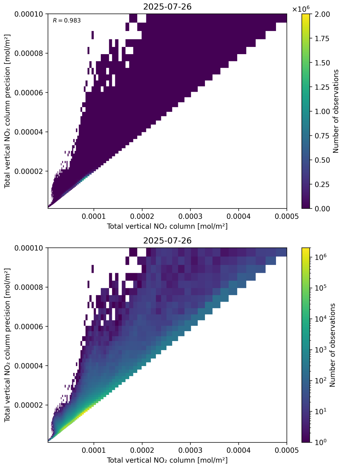
Figure 114: Scatter density plot of “Total vertical NO 2 column” against “Total vertical NO 2 column precision” for 2025-07-25 to 2025-07-27.
