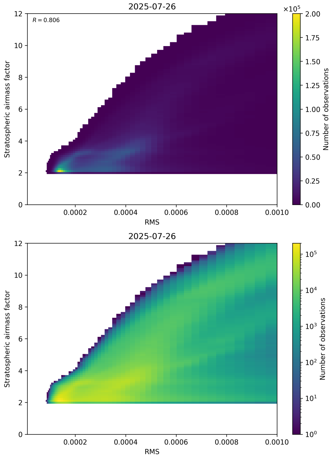
Figure 144: Scatter density plot of “RMS” against “Stratospheric airmass factor” for 2025-07-25 to 2025-07-27.
