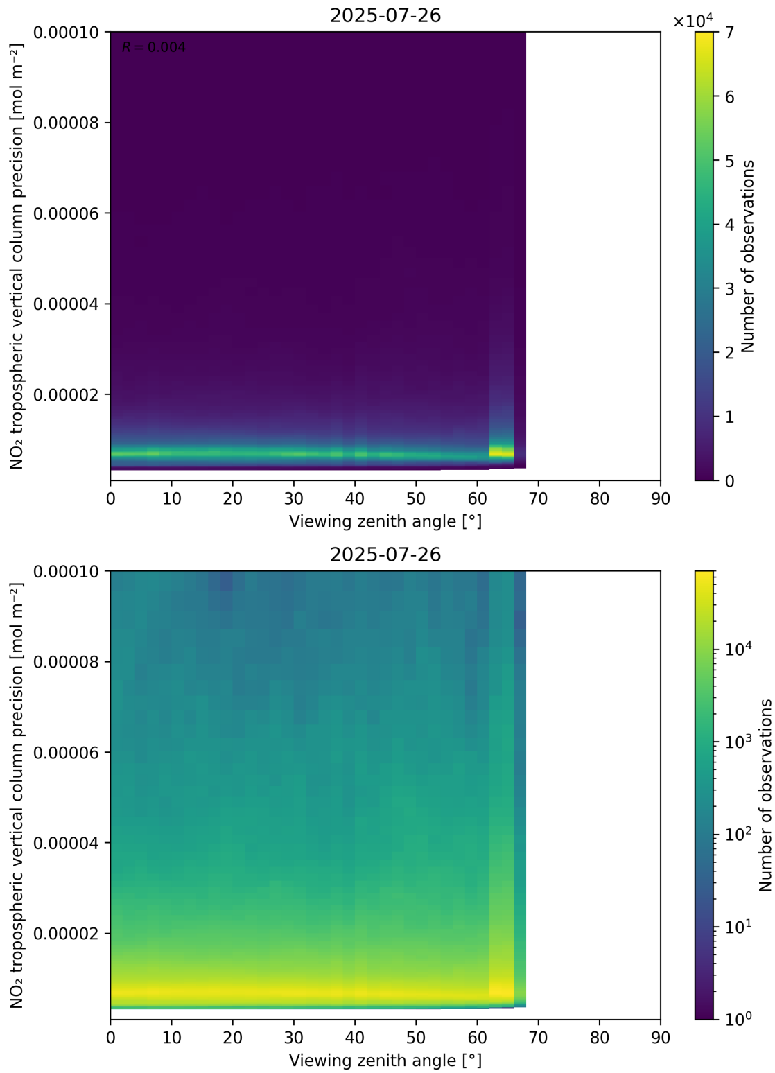
Figure 170: Scatter density plot of “Viewing zenith angle” against “NO 2 tropospheric vertical column precision” for 2025-07-25 to 2025-07-27.
