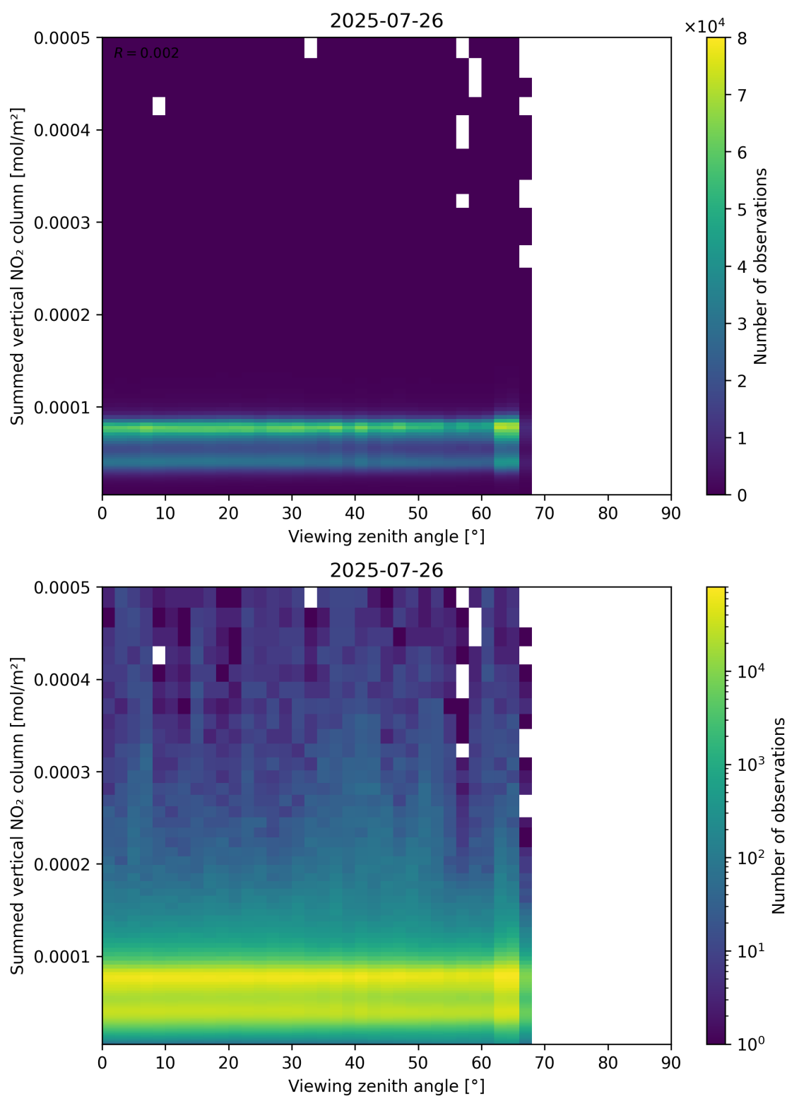
Figure 165: Scatter density plot of “Viewing zenith angle” against “Summed vertical NO 2 column” for 2025-07-25 to 2025-07-27.
