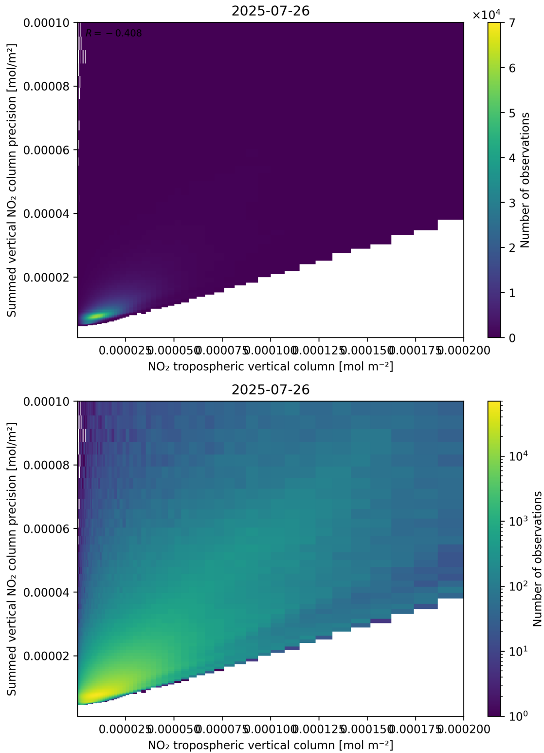
Figure 127: Scatter density plot of “NO 2 tropospheric vertical column” against “Summed vertical NO 2 column precision” for 2025-07-25 to 2025-07-27.
