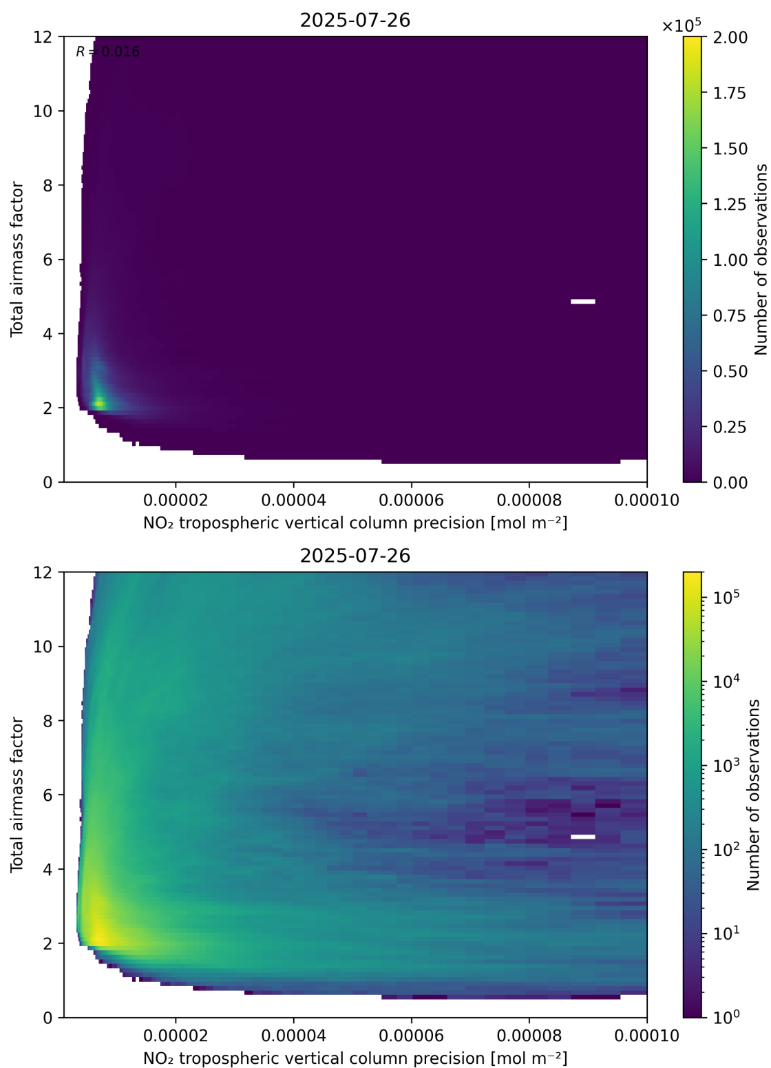
Figure 132: Scatter density plot of “NO 2 tropospheric vertical column precision” against “Total air mass factor” for 2025-07-25 to 2025-07-27.
