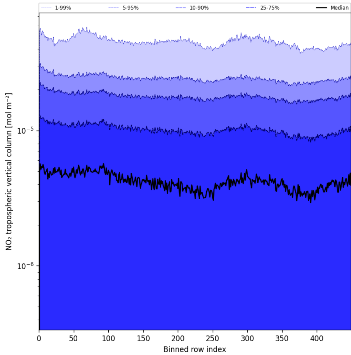
Figure 46: Along track statistics of “NO 2 tropospheric vertical column” for 2025-07-25 to 2025-07-27
