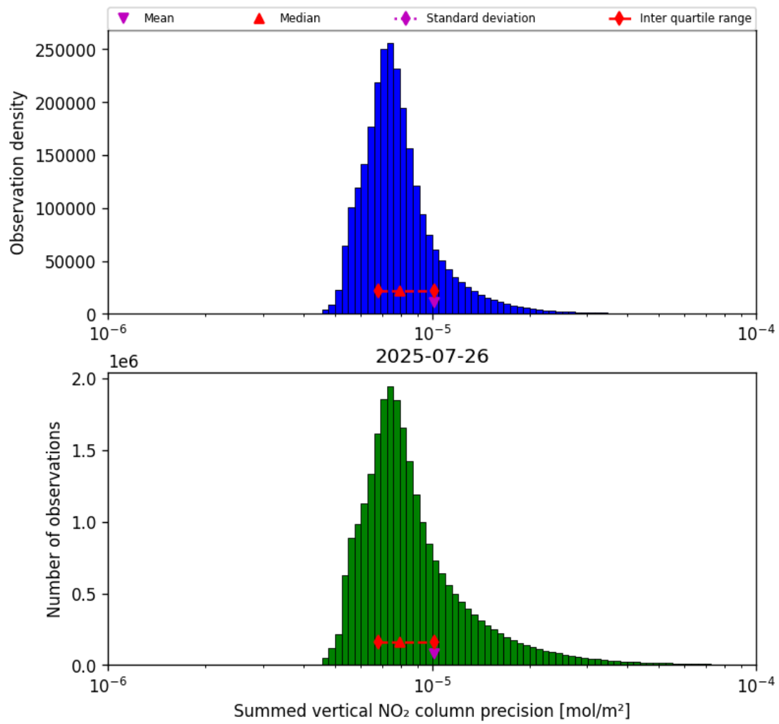
Figure 41: Histogram of "Summed vertical NO 2 column precision" for 2025-07-25 to 2025-07-27
