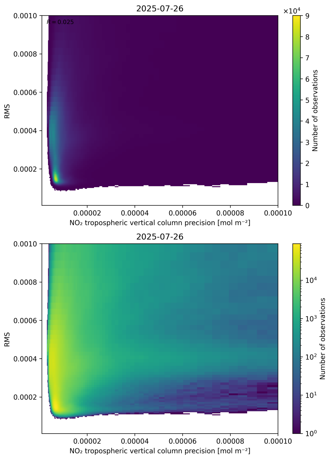
Figure 140: Scatter density plot of “NO 2 tropospheric vertical column precision” against “RMS” for 2025-07-25 to 2025-07-27.
