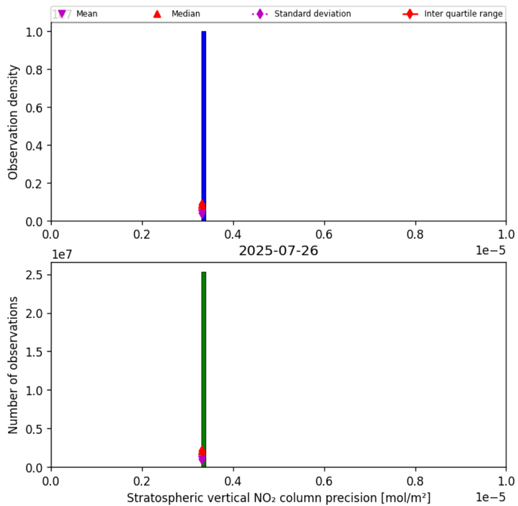
Figure 37: Histogram of “Stratospheric vertical NO 2 column precision” for 2025-07-25 to 2025-07-27
