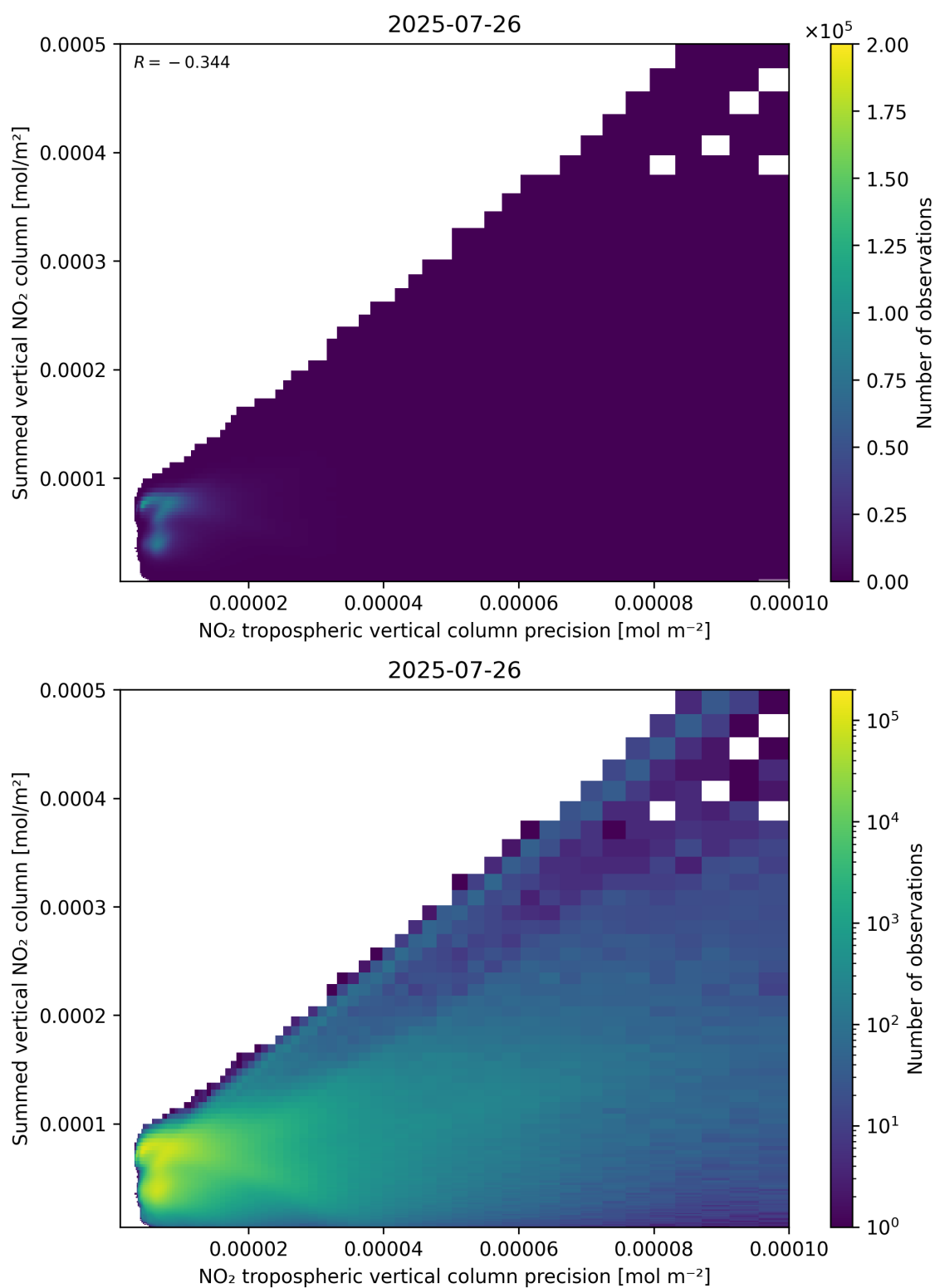
Figure 136: Scatter density plot of “NO 2 tropospheric vertical column precision” against “Summed vertical NO 2 column” for 2025-07-25 to 2025-07-27.
