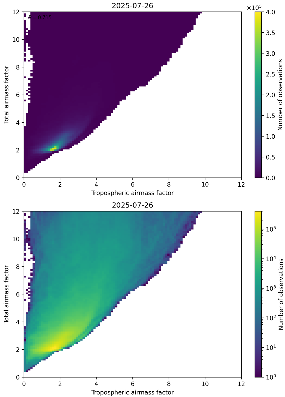
Figure 72: Scatter density plot of “Tropospheric airmass factor” against “Total airmass factor” for 2025-07-25 to 2025-07-27.
