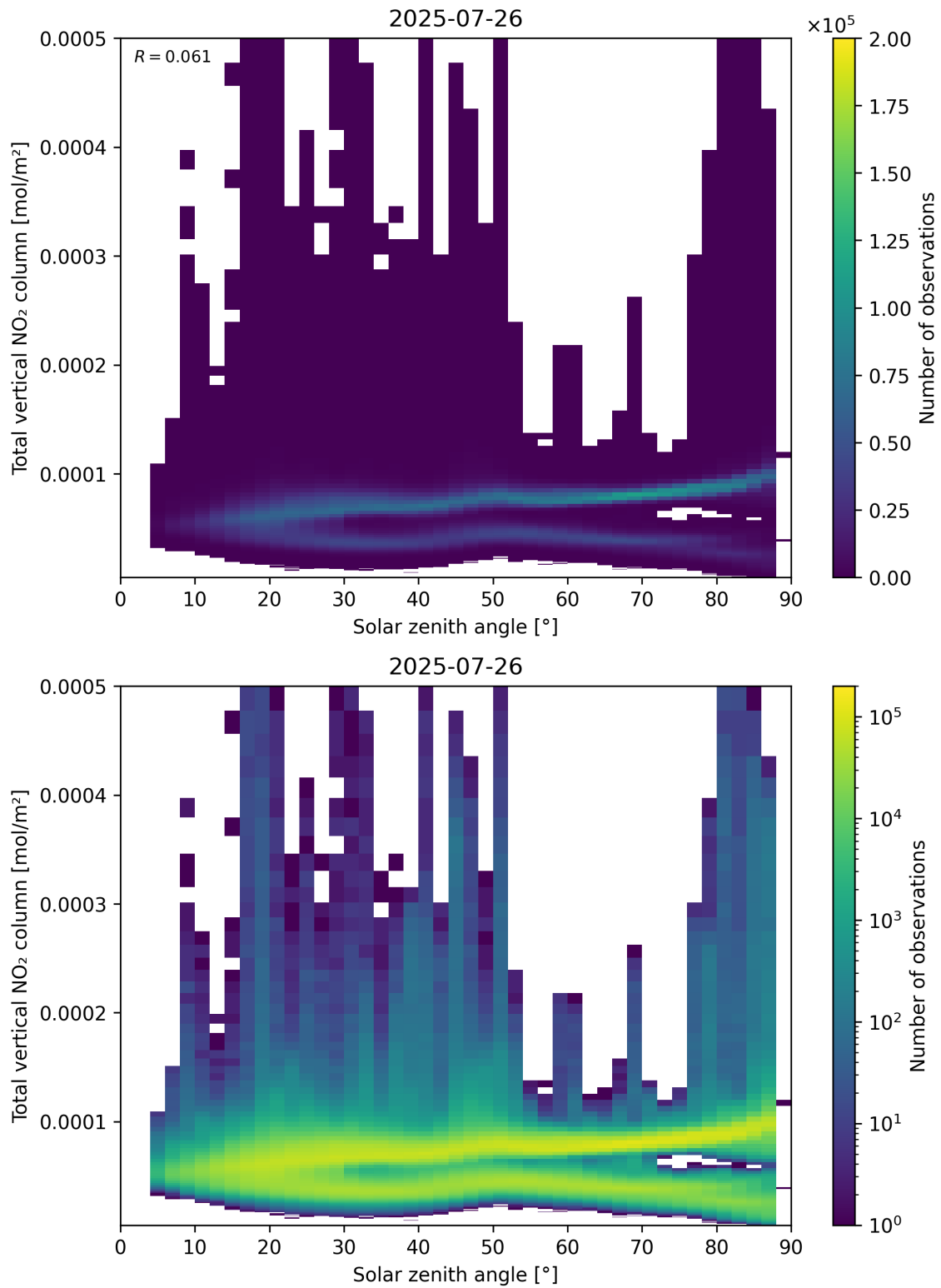
Figure 153: Scatter density plot of “Solar zenith angle” against “Total vertical \text{NO}_2 column” for 2025-07-25 to 2025-07-27.
