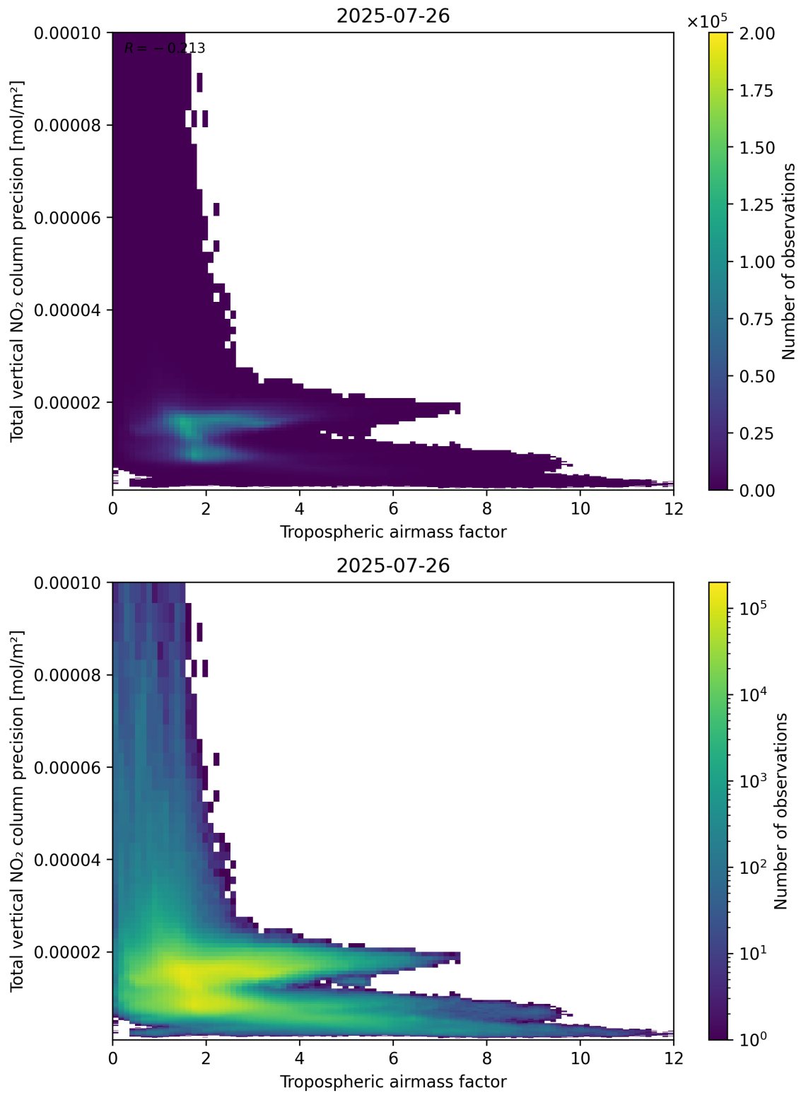
Figure 78: Scatter density plot of “Tropospheric air mass factor” against “Total vertical NO 2 column precision” for 2025-07-25 to 2025-07-27.
