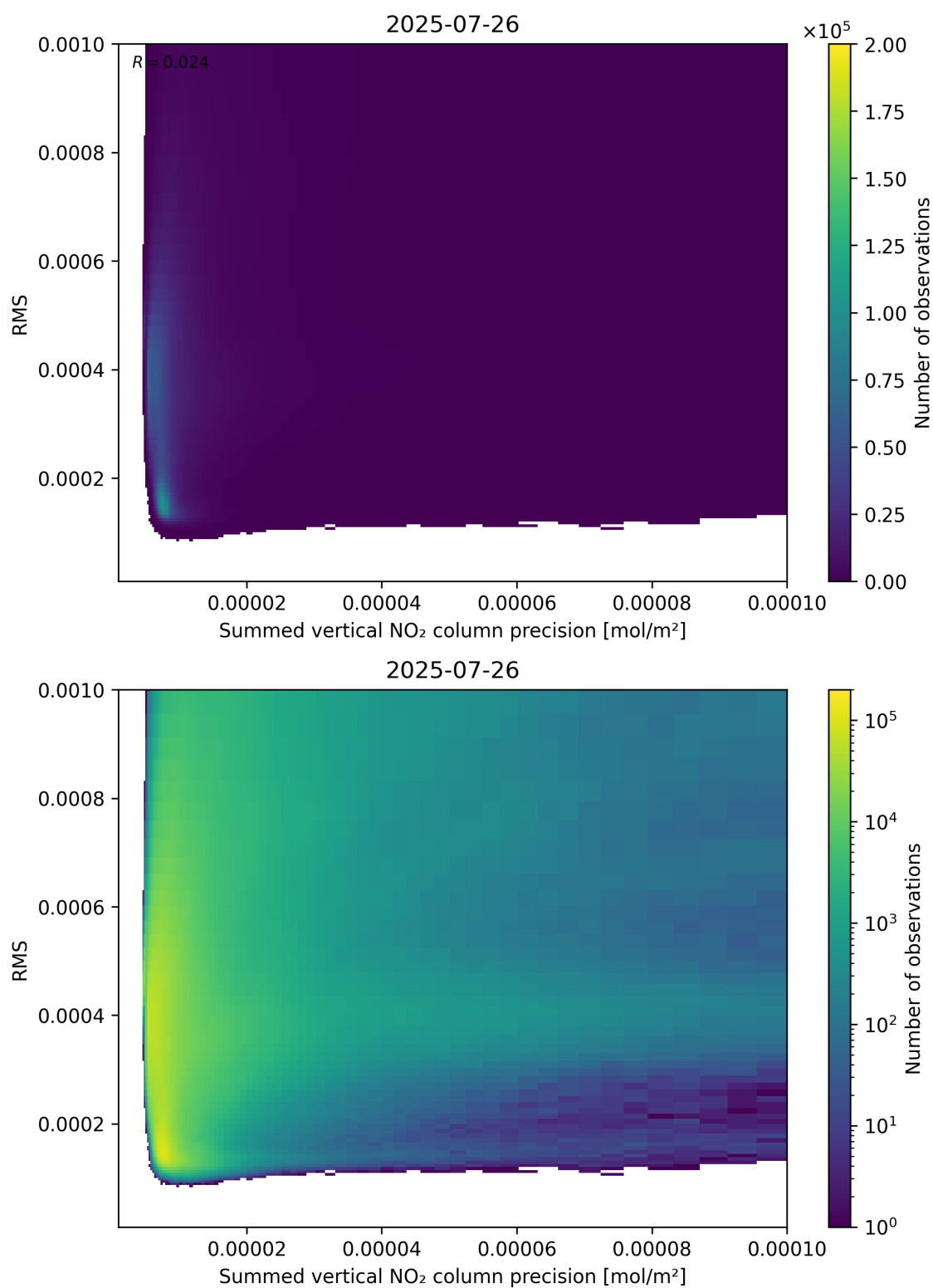
Figure 108: Scatter density plot of “Summed vertical NO 2 column precision” against “RMS” for 2025-07-25 to 2025-07-27.
