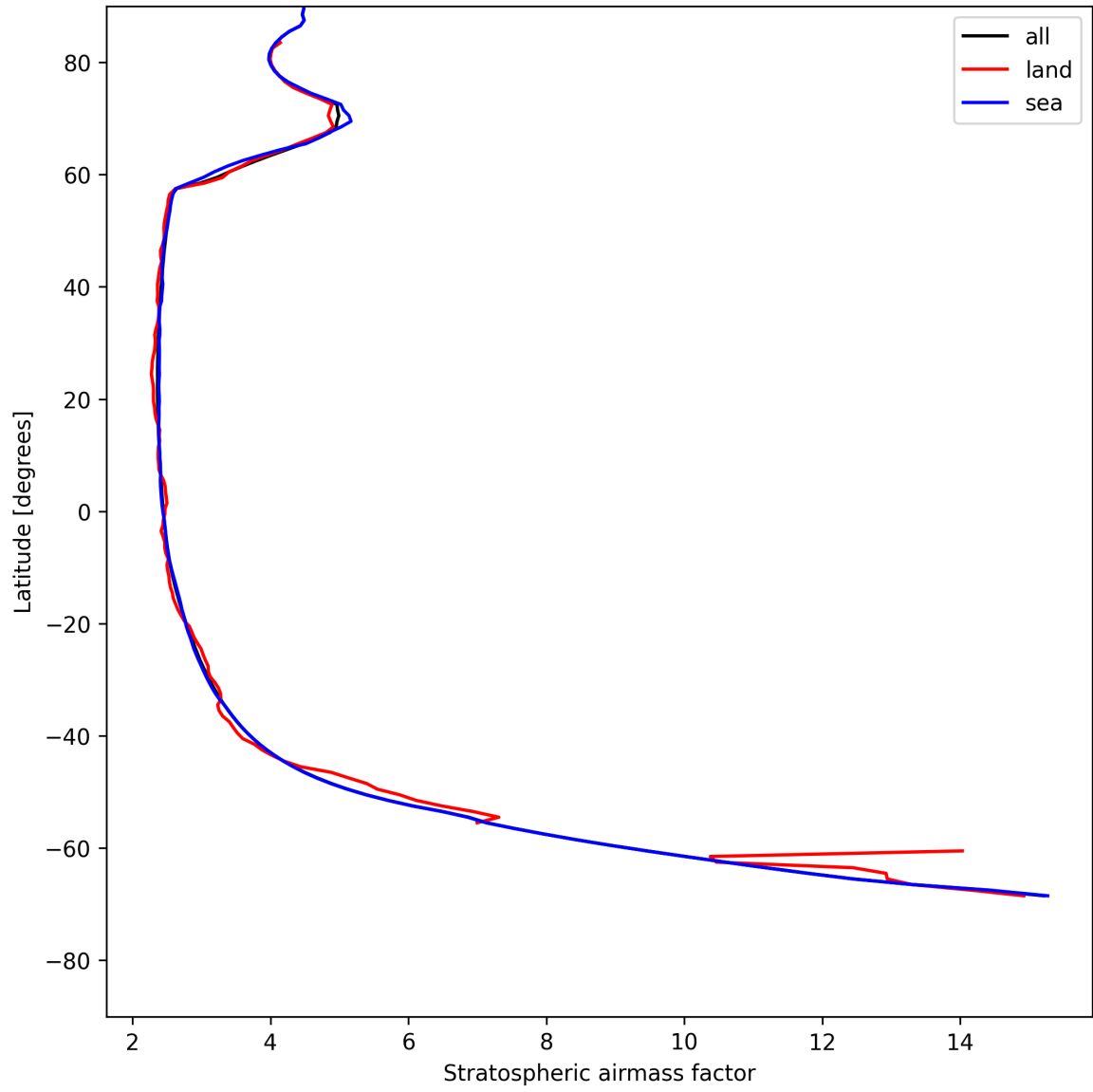
Figure 27: Zonal average of “Stratospheric airmass factor” for 2025-07-25 to 2025-07-27.
