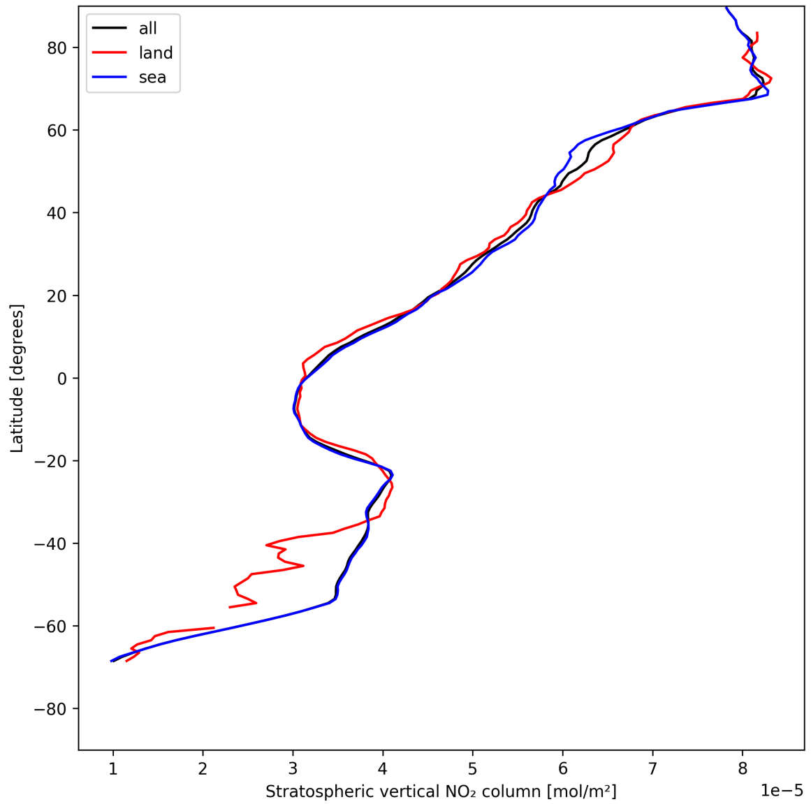
Figure 19: Zonal average of “Stratospheric vertical NO 2 column” for 2025-07-25 to 2025-07-27.
