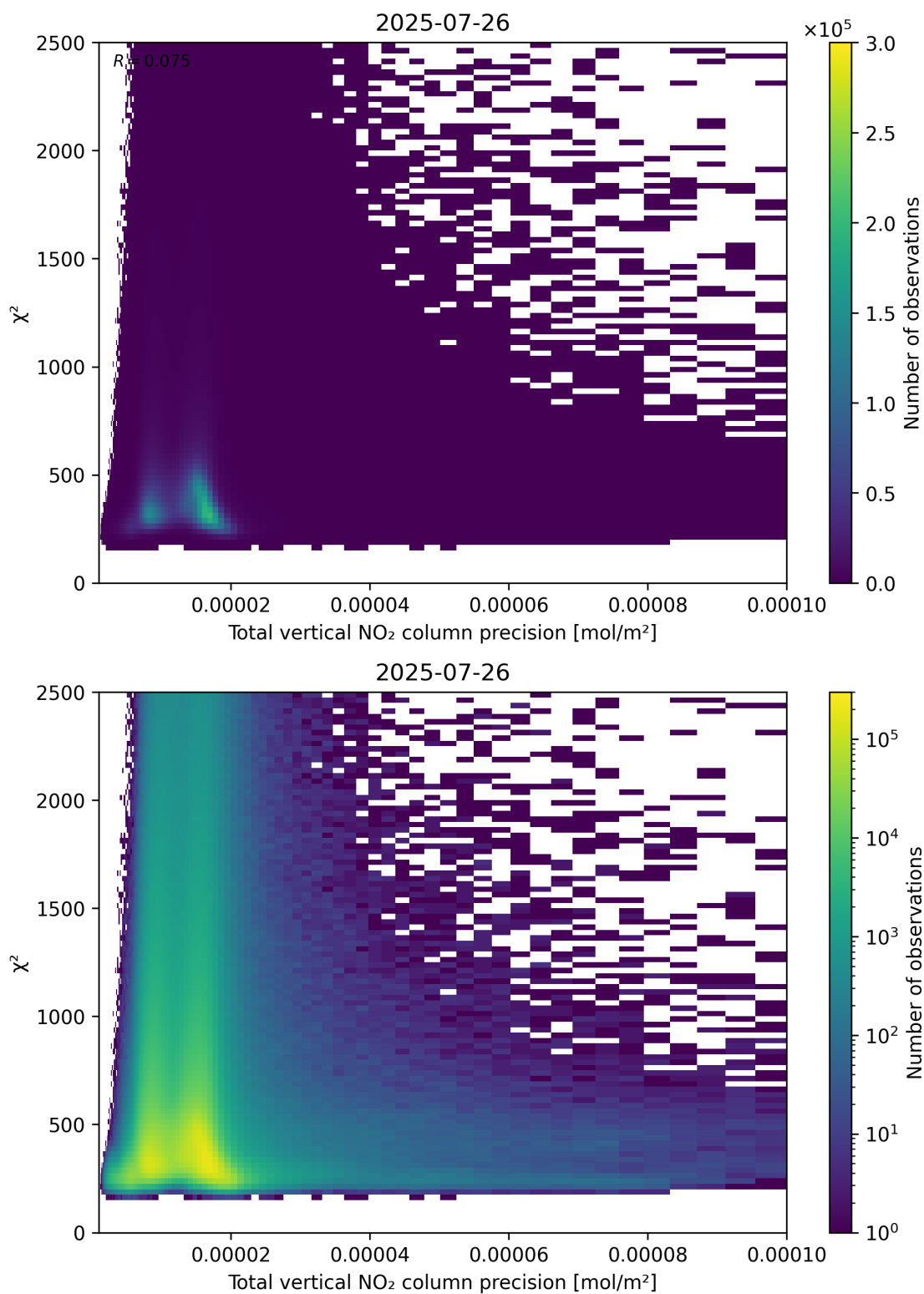
Figure 116: Scatter density plot of “Total vertical NO 2 column precision” against “ \chi^2 ” for 2025-07-25 to 2025-07-27.
