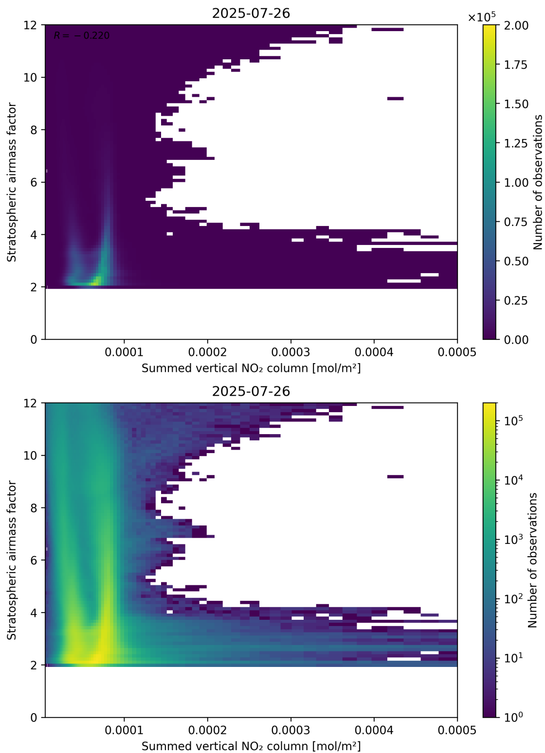
Figure 103: Scatter density plot of “Summed vertical NO 2 column” against “Stratospheric air mass factor” for 2025-07-25 to 2025-07-27.
