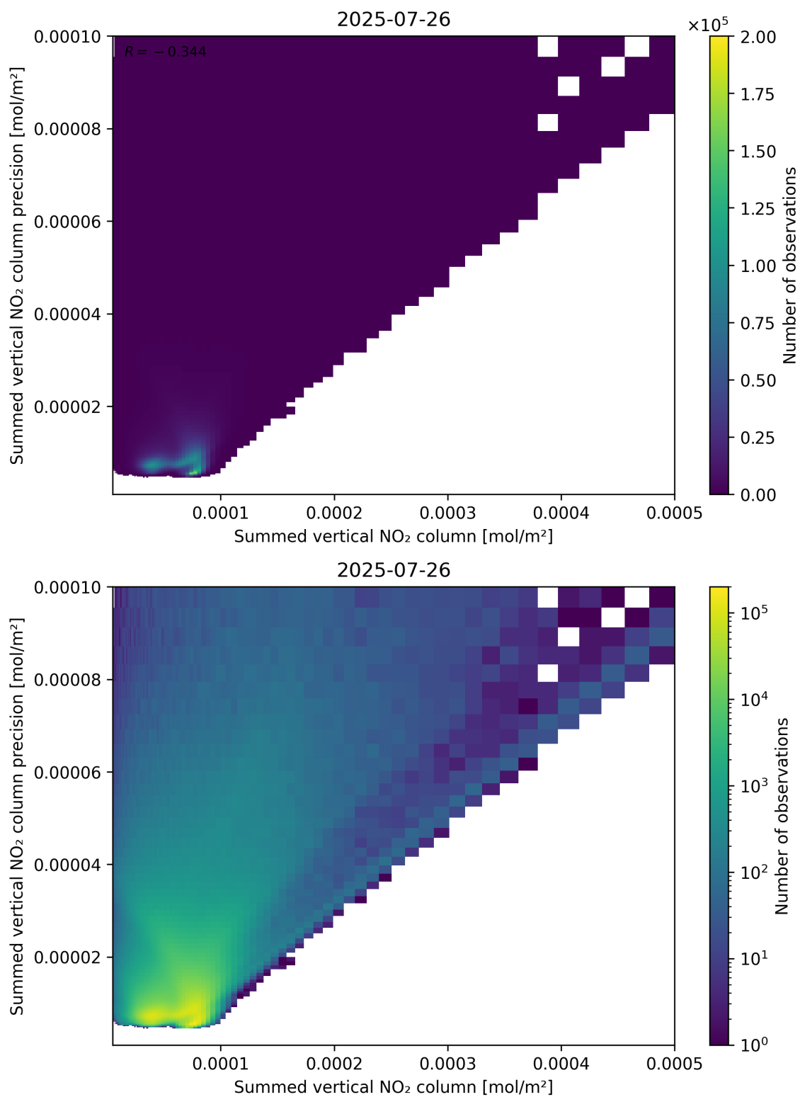
Figure 105: Scatter density plot of “Summed vertical NO 2 column” against “Summed vertical NO 2 column precision” for 2025-07-25 to 2025-07-27.
