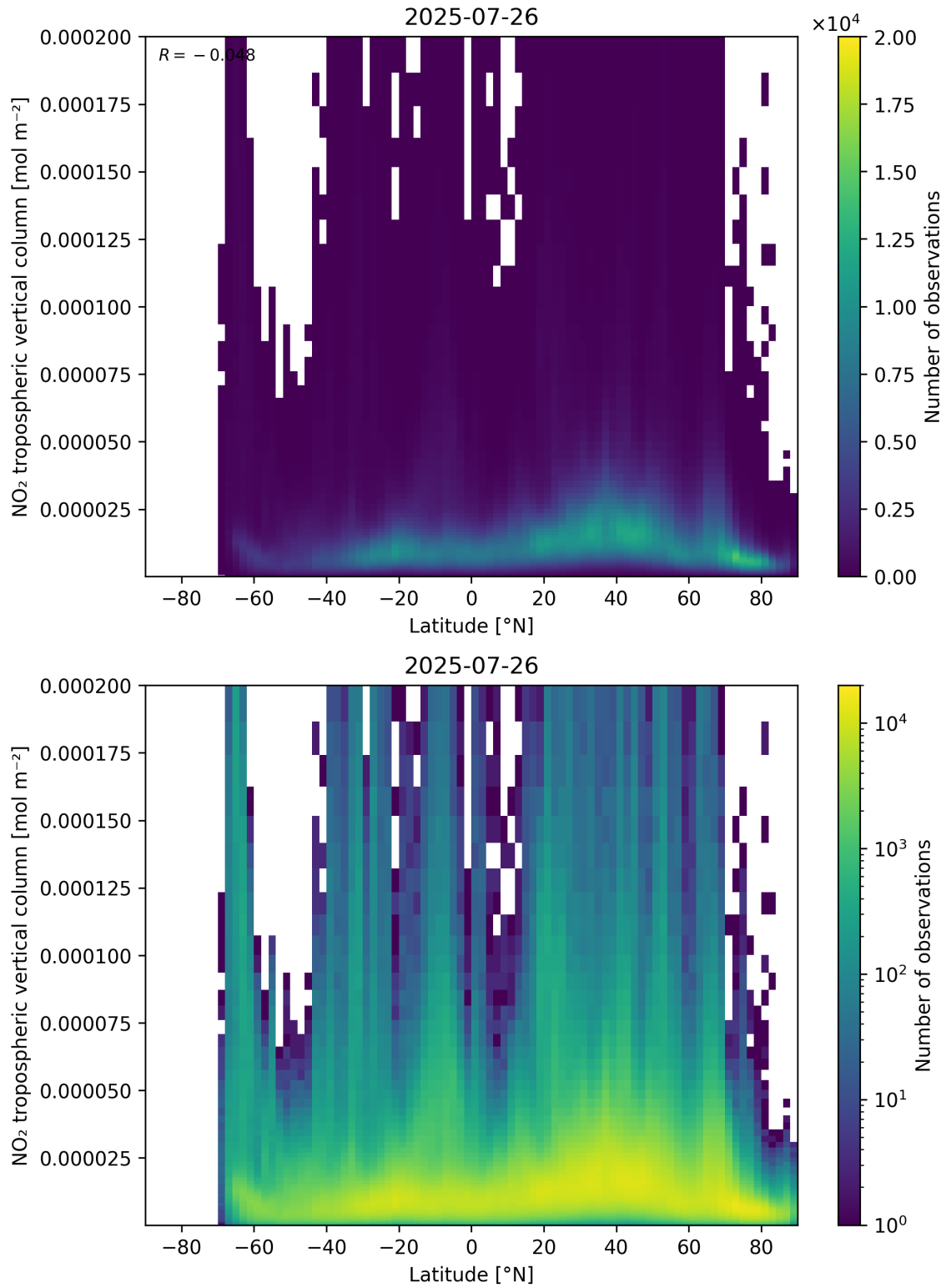
Figure 92: Scatter density plot of “Latitude” against “NO 2 tropospheric vertical column” for 2025-07-25 to 2025-07-27.
