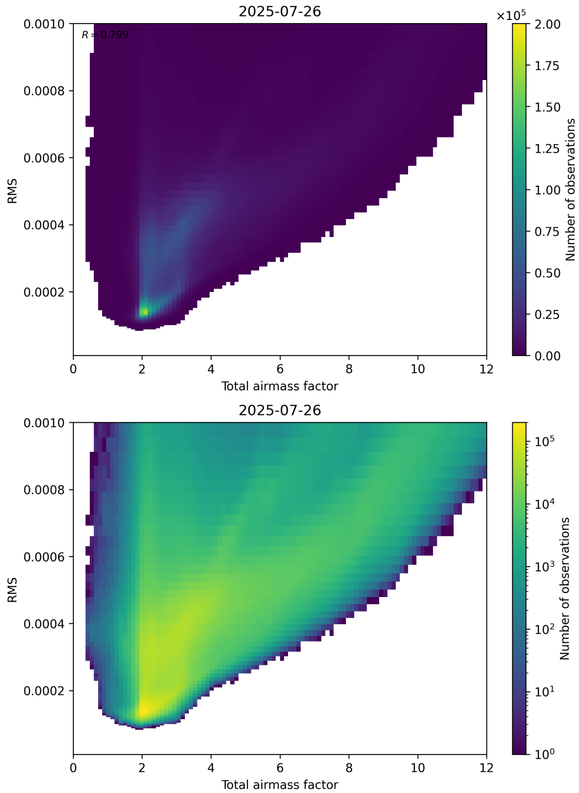
Figure 69: Scatter density plot of “Total airmass factor” against “RMS” for 2025-07-25 to 2025-07-27.
