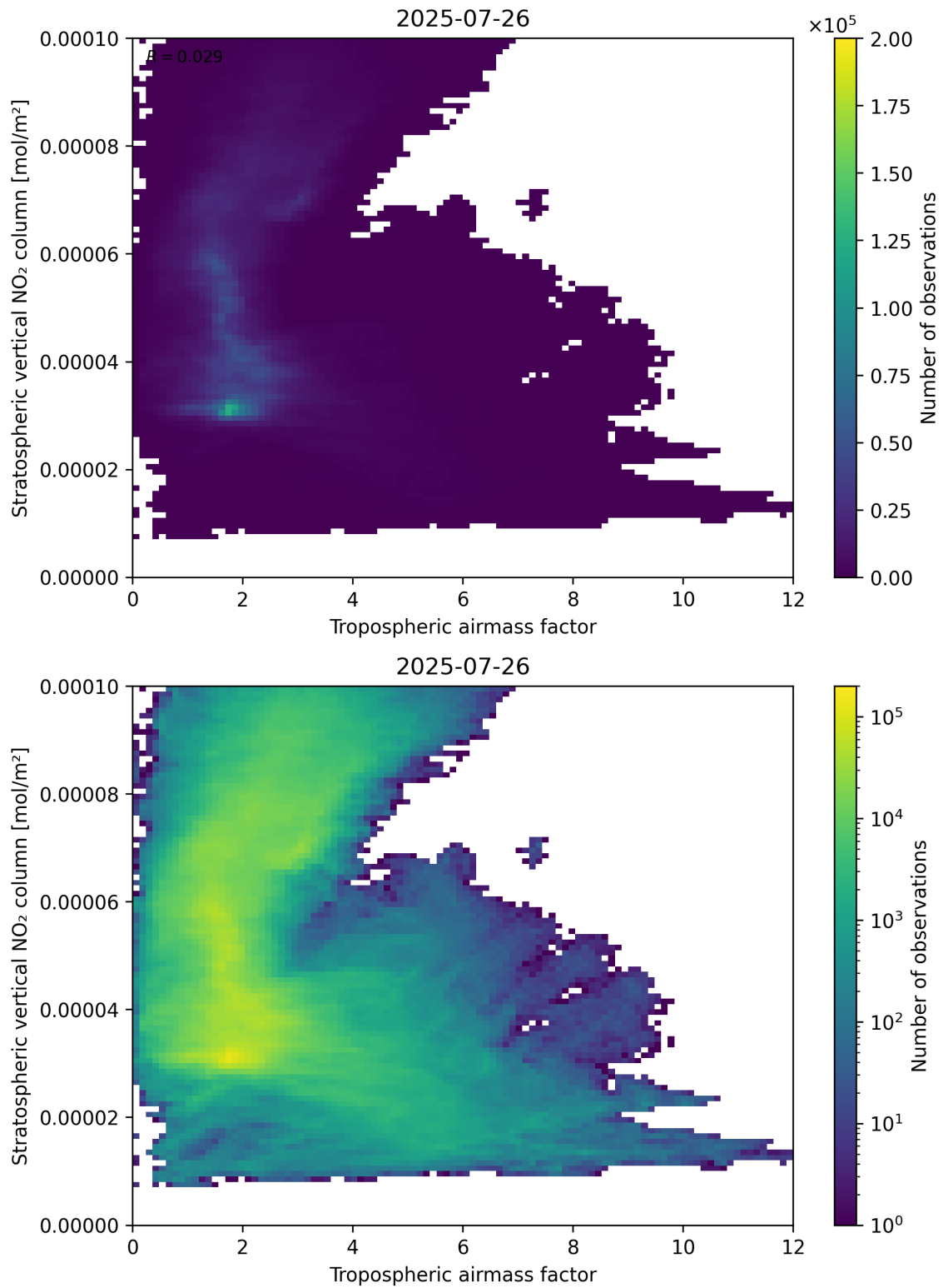
Figure 74: Scatter density plot of “Tropospheric air mass factor” against “Stratospheric vertical NO 2 column” for 2025-07-25 to 2025-07-27.
