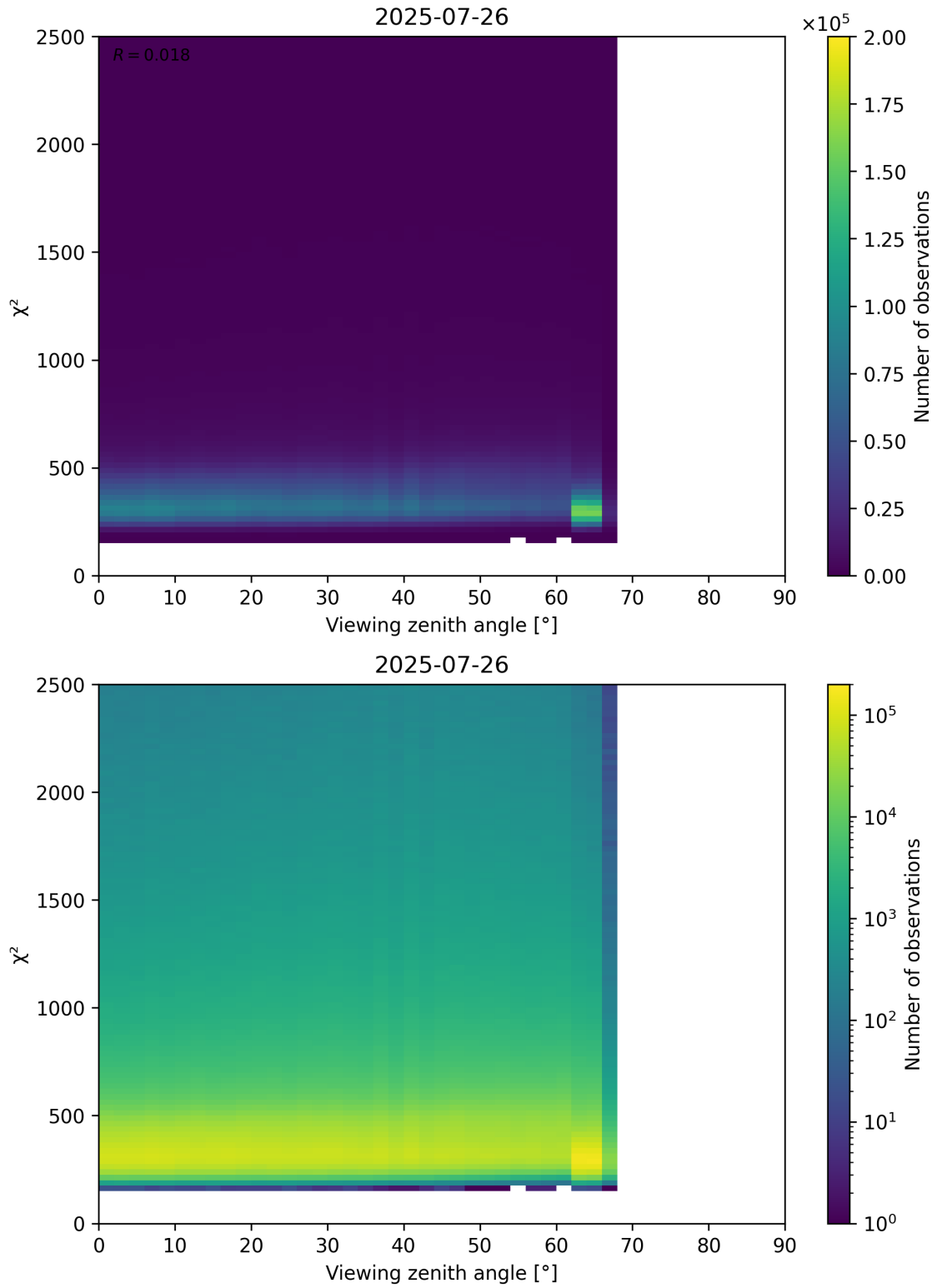
Figure 162: Scatter density plot of “Viewing zenith angle” against “ \chi^2 ” for 2025-07-25 to 2025-07-27.
