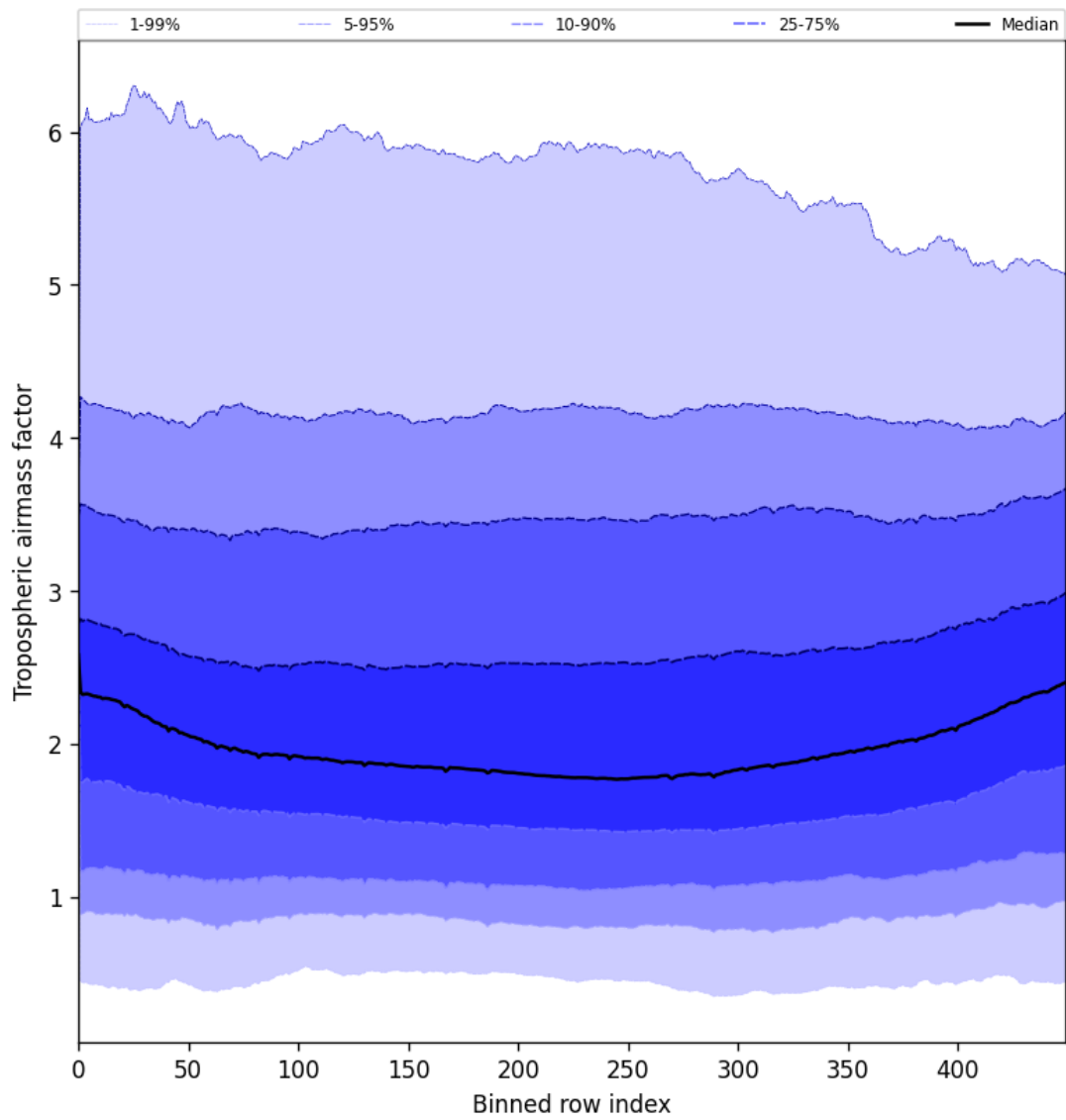
Figure 48: Along track statistics of “Tropospheric airmass factor” for 2025-07-25 to 2025-07-27
