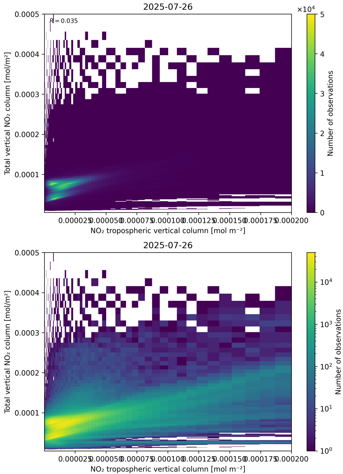
Figure 128: Scatter density plot of “NO 2 tropospheric vertical column” against “Total vertical NO 2 column” for 2025-07-25 to 2025-07-27.
