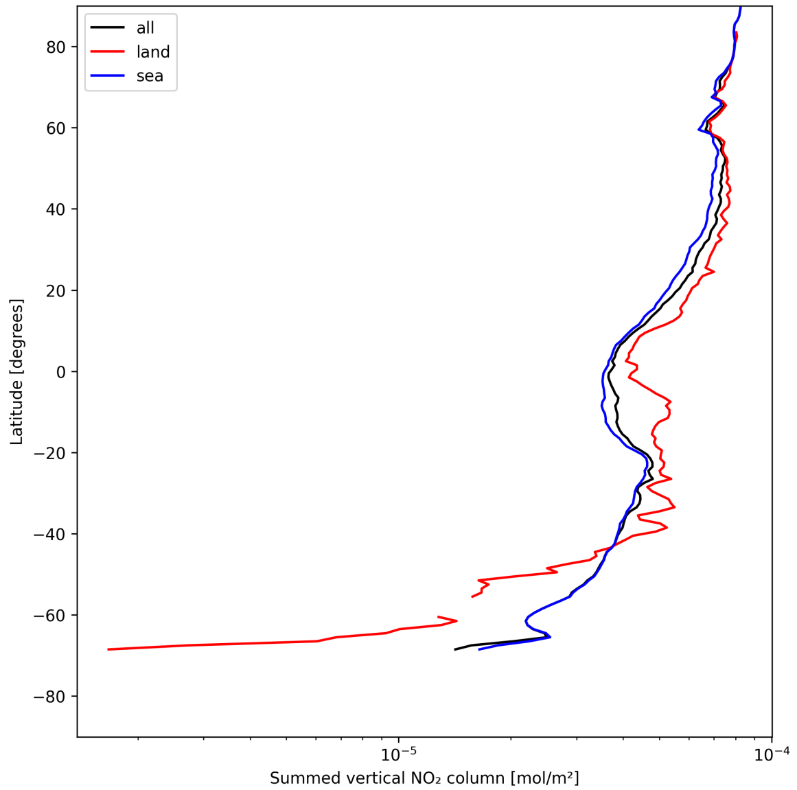
Figure 23: Zonal average of “Summed vertical NO 2 column” for 2025-07-25 to 2025-07-27.
