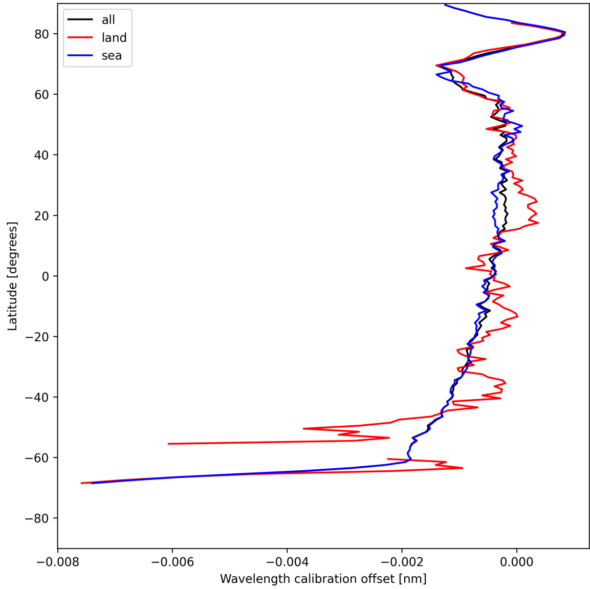
Figure 18: Zonal average of “Wavelength calibration offset” for 2025-07-25 to 2025-07-27.
