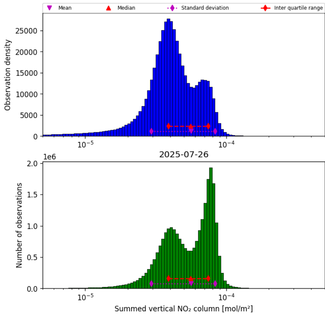
Figure 40: Histogram of “Summed vertical NO 2 column” for 2025-07-25 to 2025-07-27
