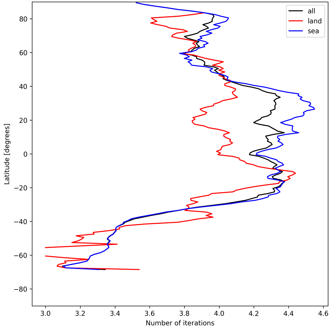
Figure 17: Zonal average of “Number of iterations” for 2025-07-25 to 2025-07-27.
