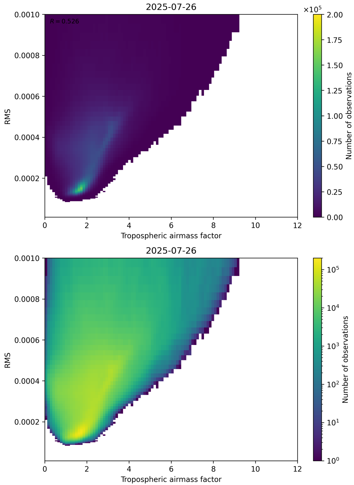
Figure 79: Scatter density plot of “Tropospheric airmass factor” against “RMS” for 2025-07-25 to 2025-07-27.
