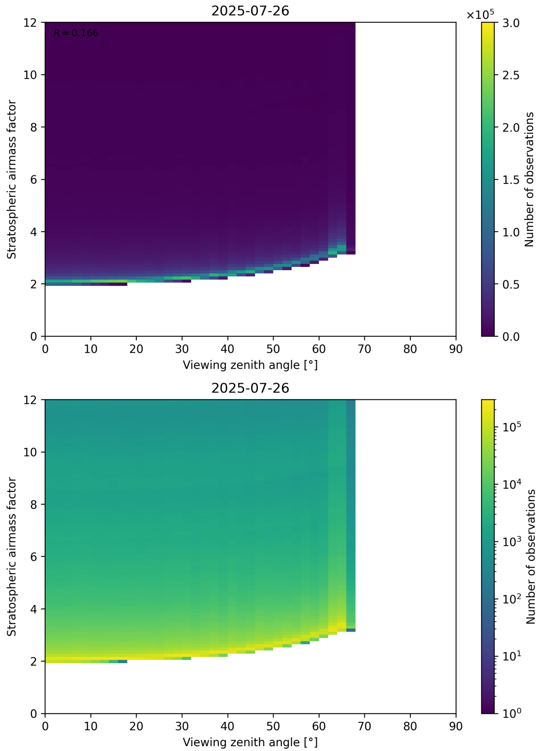
Figure 159: Scatter density plot of “Viewing zenith angle” against “Stratospheric airmass factor” for 2025-07-25 to 2025-07-27.
