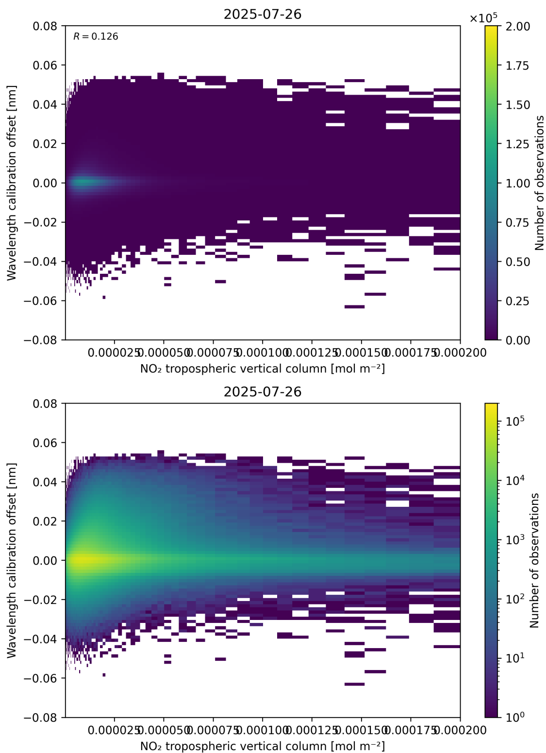
Figure 143: Scatter density plot of “NO 2 tropospheric vertical column” against “Wavelength calibration offset” for 2025-07-25 to 2025-07-27.
