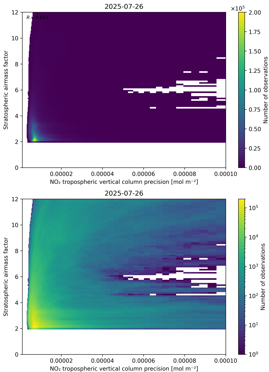
Figure 131: Scatter density plot of “NO 2 tropospheric vertical column precision” against “Stratospheric airmass factor” for 2025-07-25 to 2025-07-27.
