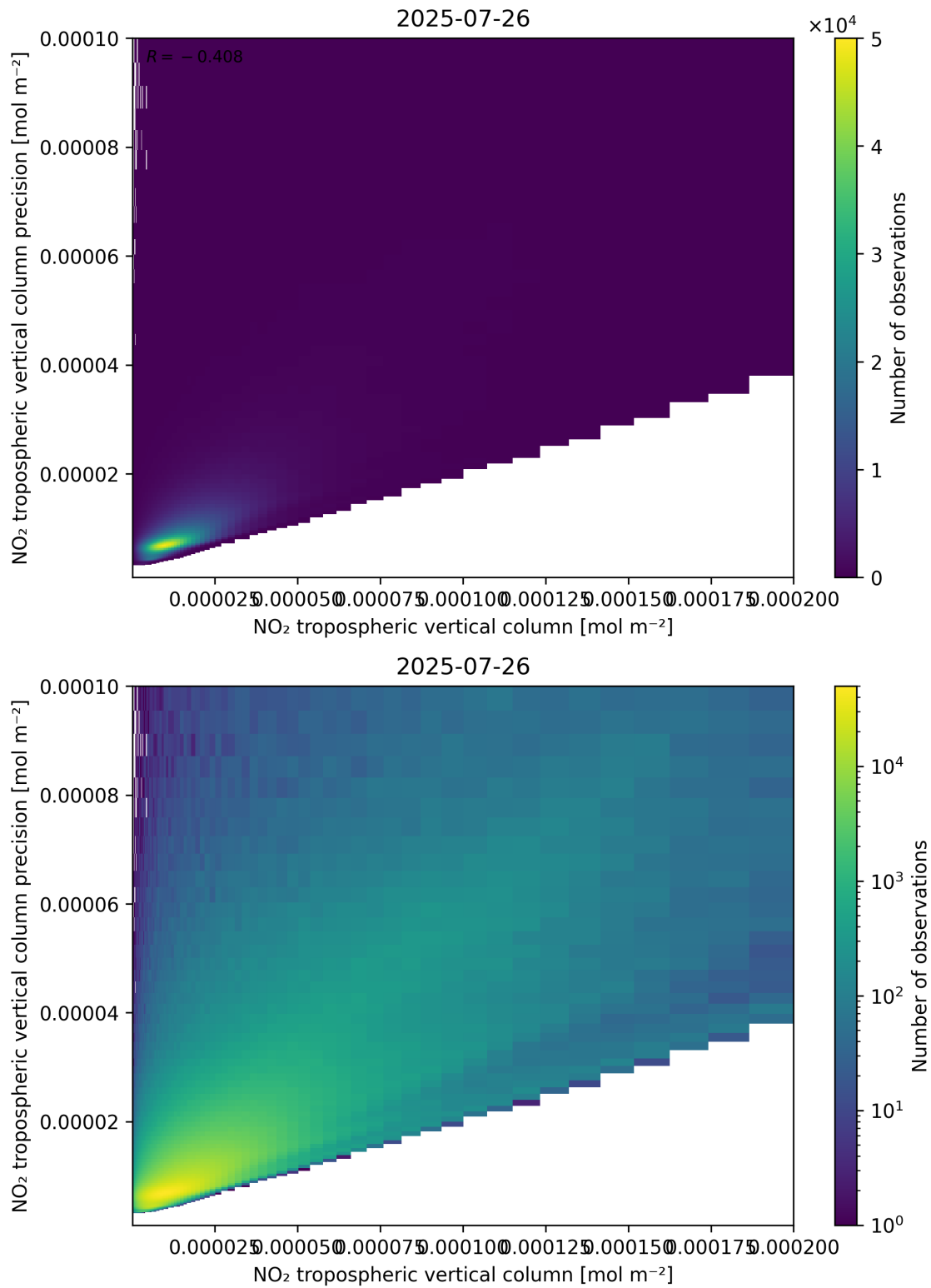
Figure 130: Scatter density plot of “NO 2 tropospheric vertical column” against “NO 2 tropospheric vertical column precision” for 2025-07-25 to 2025-07-27.
