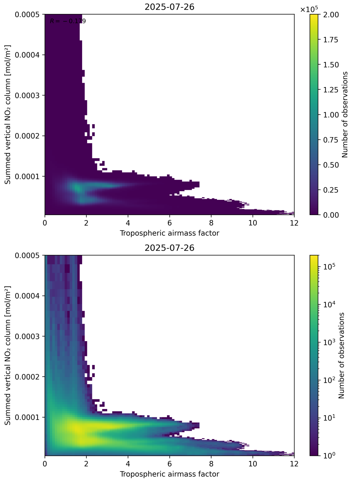
Figure 75: Scatter density plot of “Tropospheric airmass factor” against “Summed vertical NO 2 column” for 2025-07-25 to 2025-07-27.
