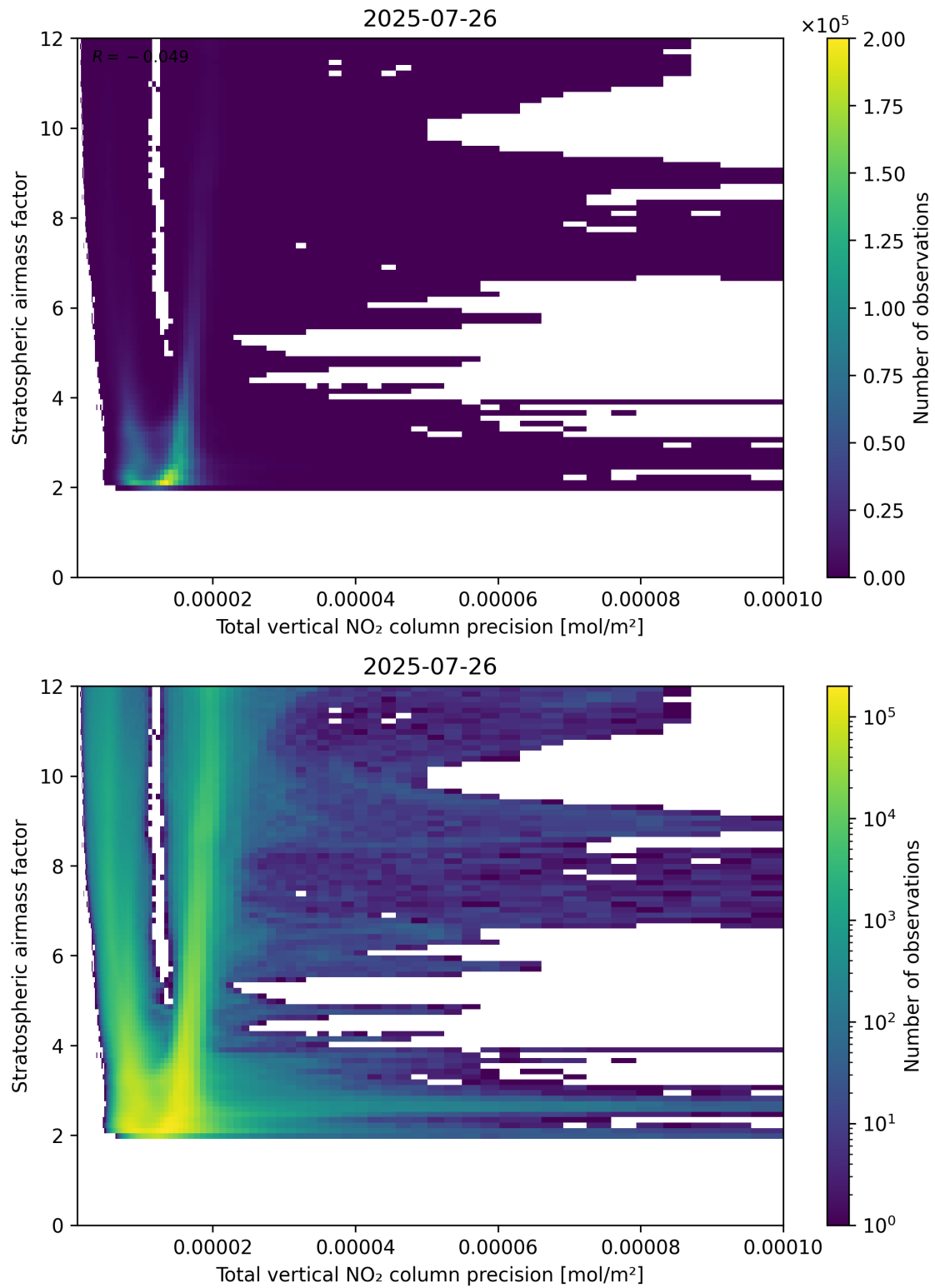
Figure 115: Scatter density plot of “Total vertical NO 2 column precision” against “Stratospheric air mass factor” for 2025-07-25 to 2025-07-27.
