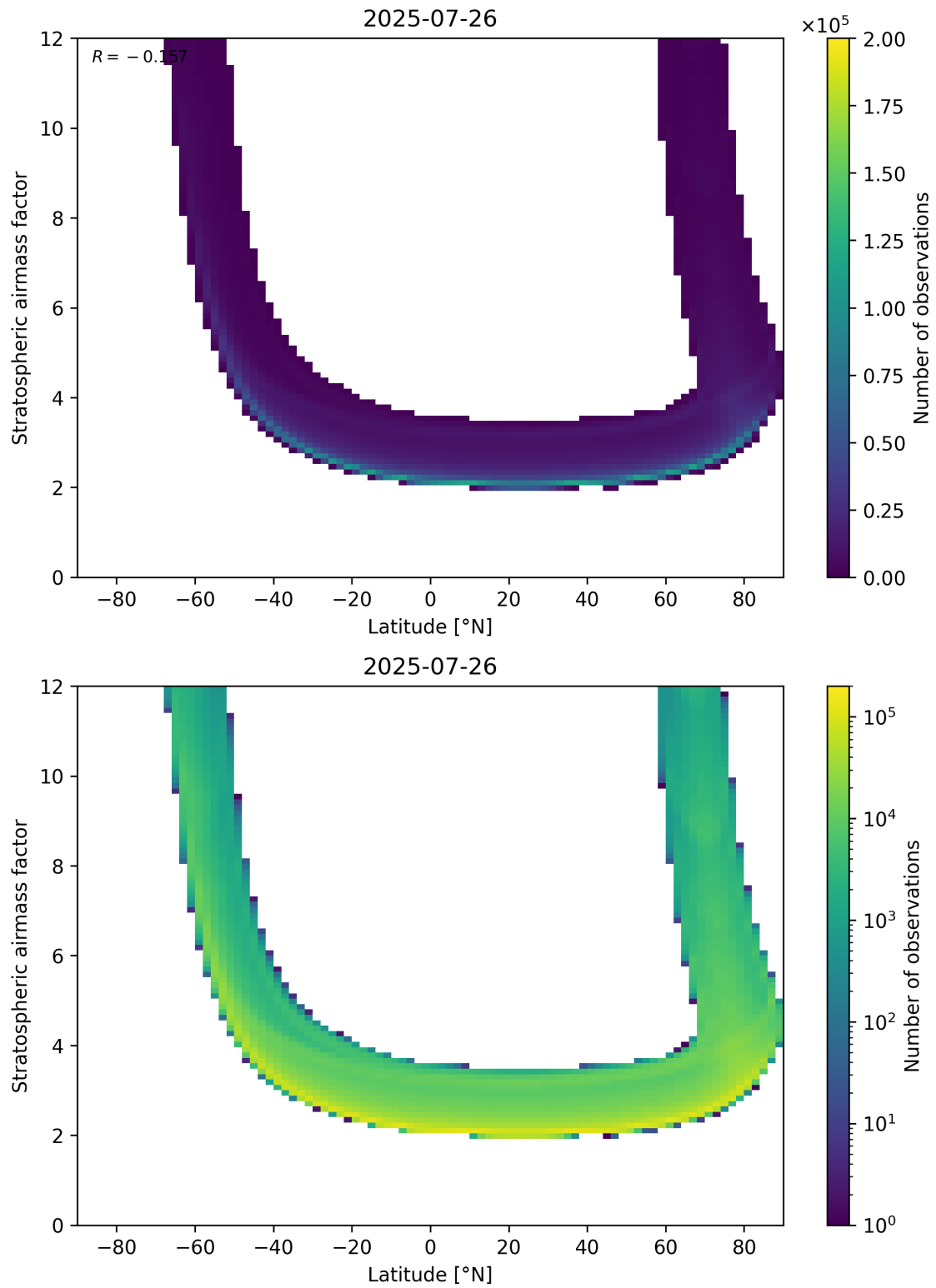
Figure 83: Scatter density plot of “Latitude” against “Stratospheric air mass factor” for 2025-07-25 to 2025-07-27.
