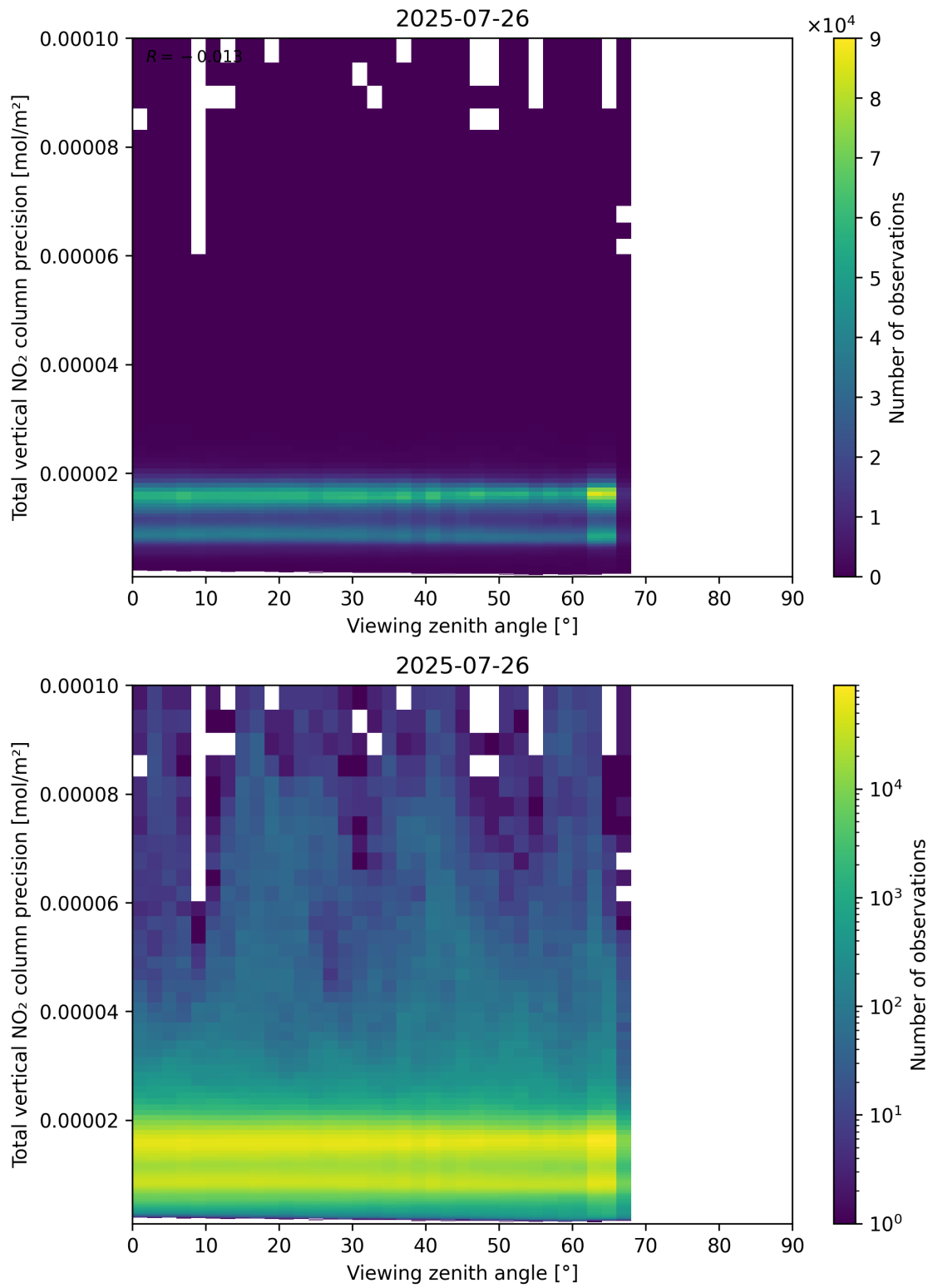
Figure 168: Scatter density plot of “Viewing zenith angle” against “Total vertical NO 2 column precision” for 2025-07-25 to 2025-07-27.
