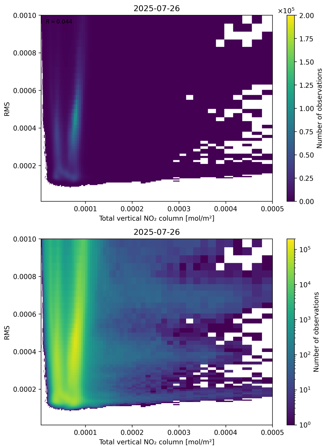
Figure 120: Scatter density plot of “Total vertical NO 2 column” against “RMS” for 2025-07-25 to 2025-07-27.
