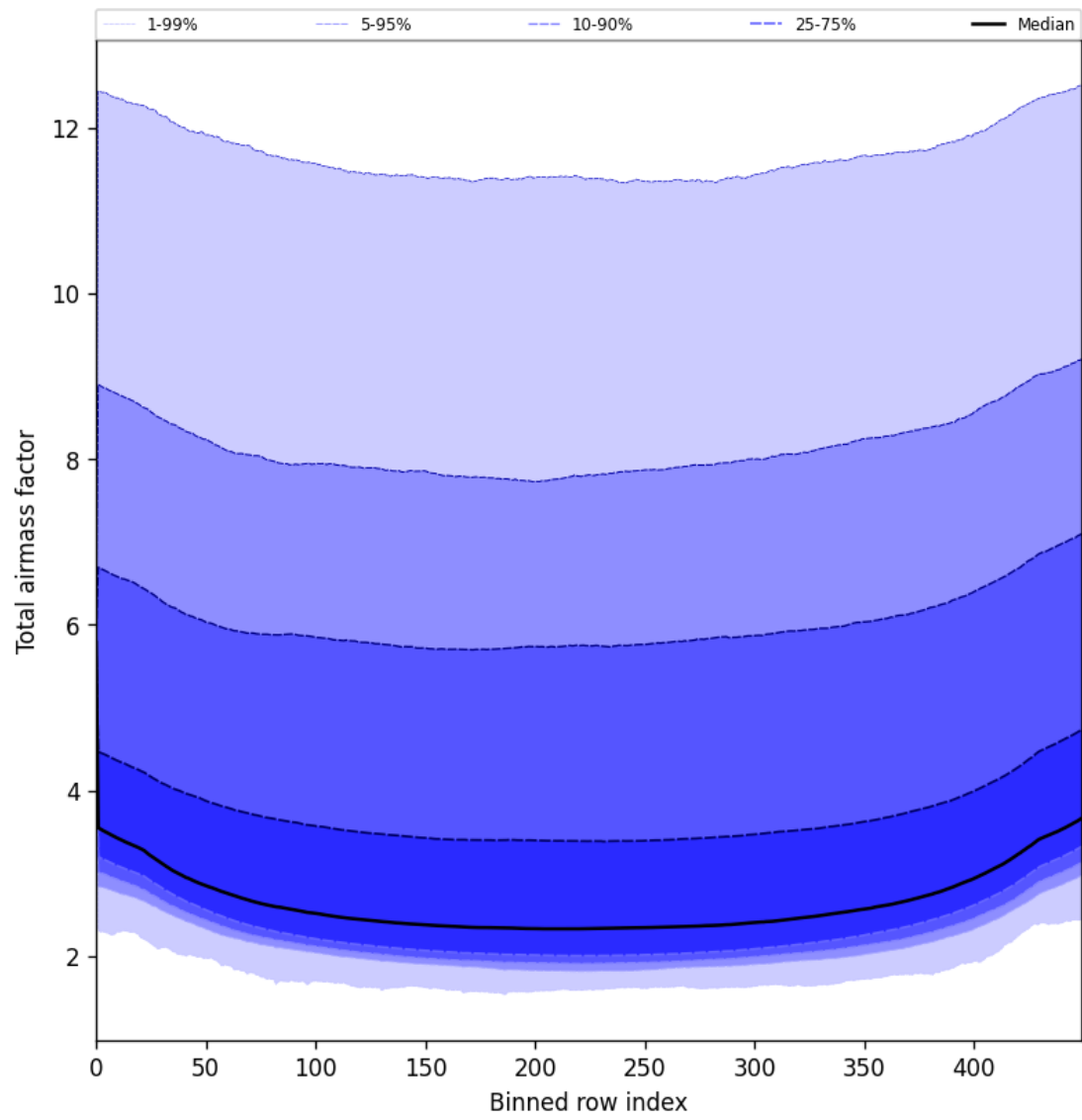
Figure 49: Along track statistics of “Total airmass factor” for 2025-07-25 to 2025-07-27
