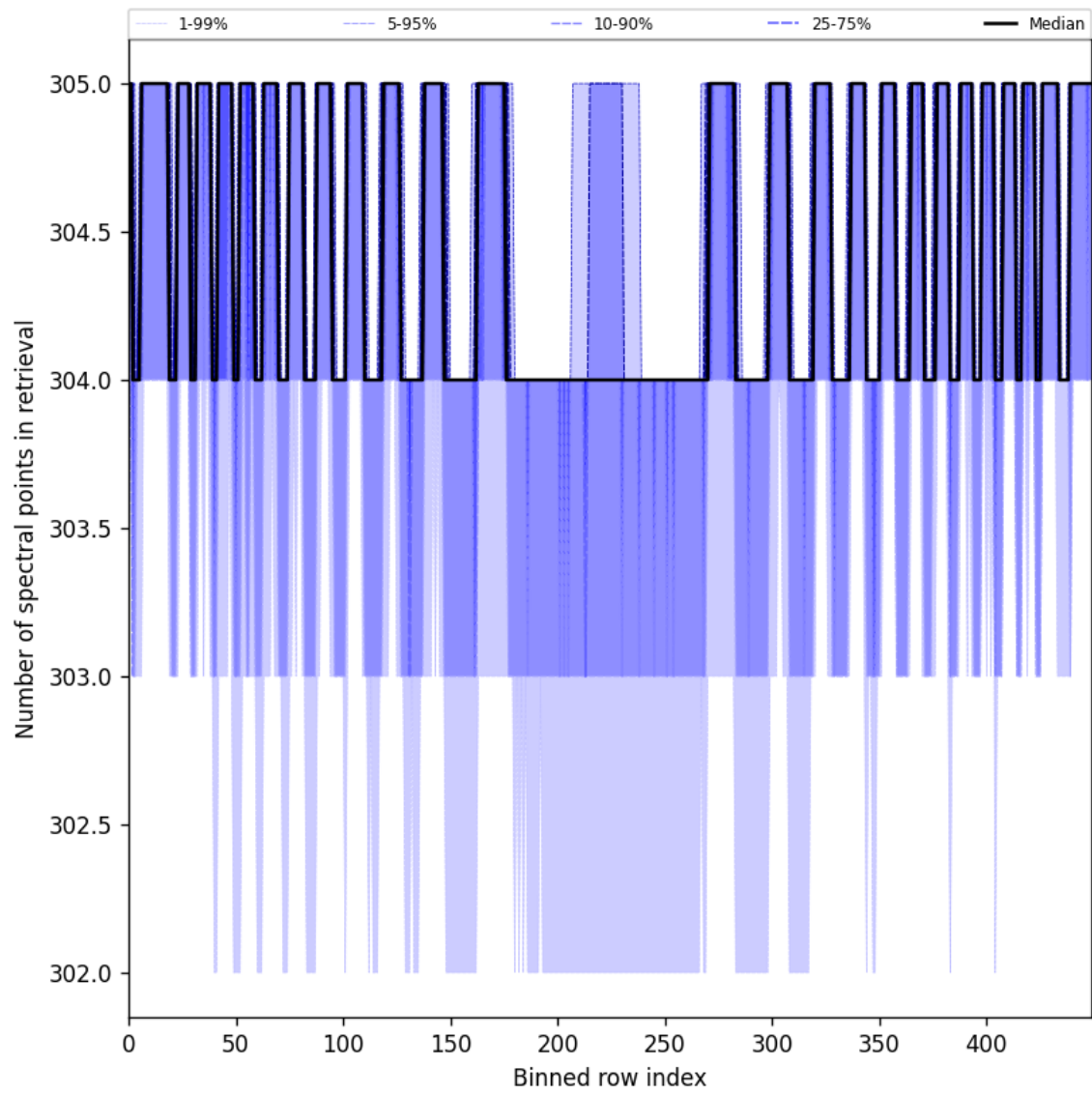
Figure 50: Along track statistics of “Number of spectral points in retrieval” for 2025-07-25 to 2025-07-27
