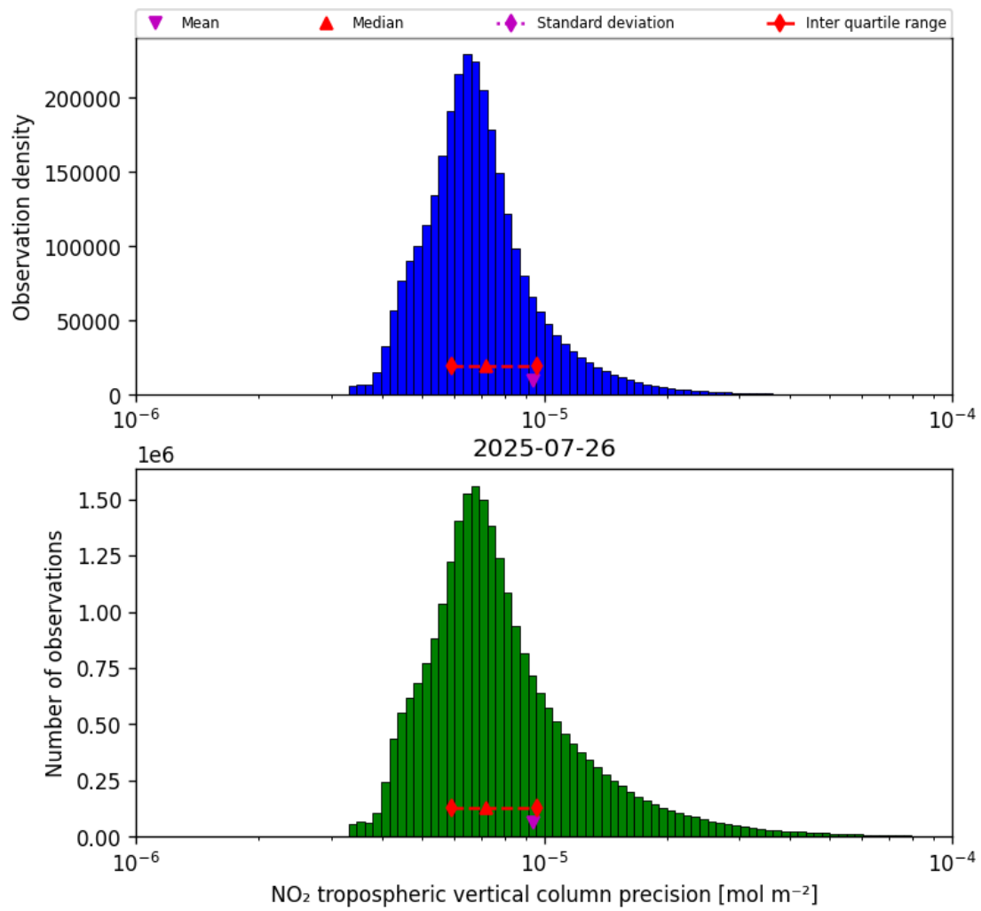
Figure 30: Histogram of “NO 2 tropospheric vertical column precision” for 2025-07-25 to 2025-07-27
