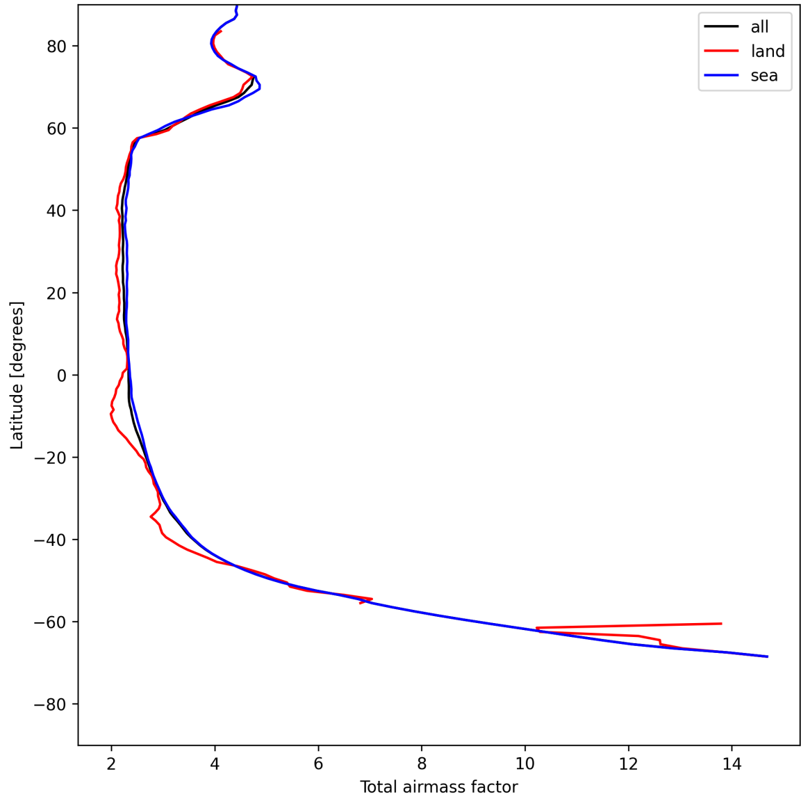
Figure 15: Zonal average of “Total airmass factor” for 2025-07-25 to 2025-07-27.
