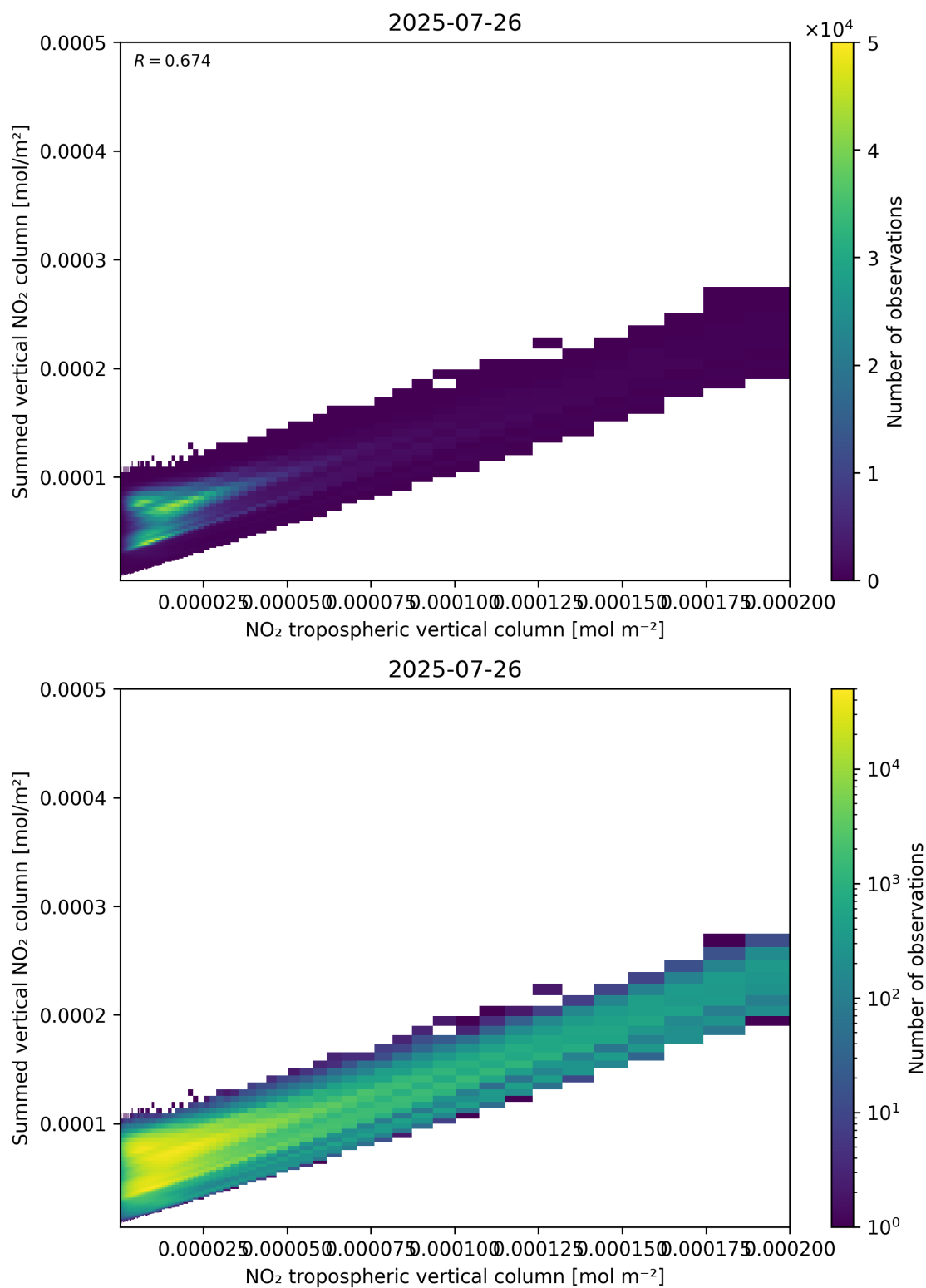
Figure 126: Scatter density plot of “NO 2 tropospheric vertical column” against “Summed vertical NO 2 column” for 2025-07-25 to 2025-07-27.
