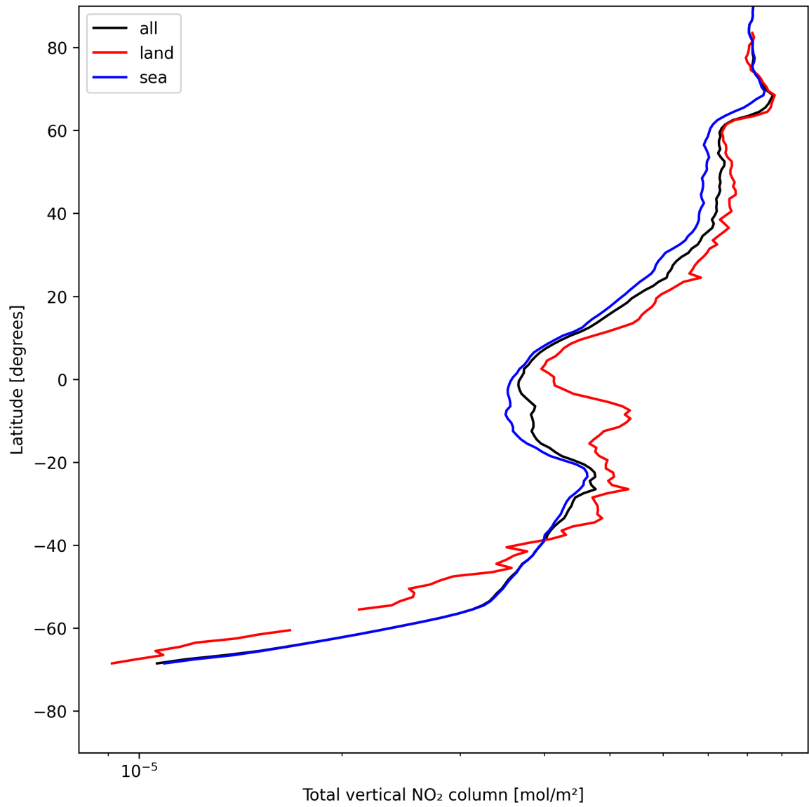
Figure 21: Zonal average of “Total vertical NO 2 column” for 2025-07-25 to 2025-07-27.
