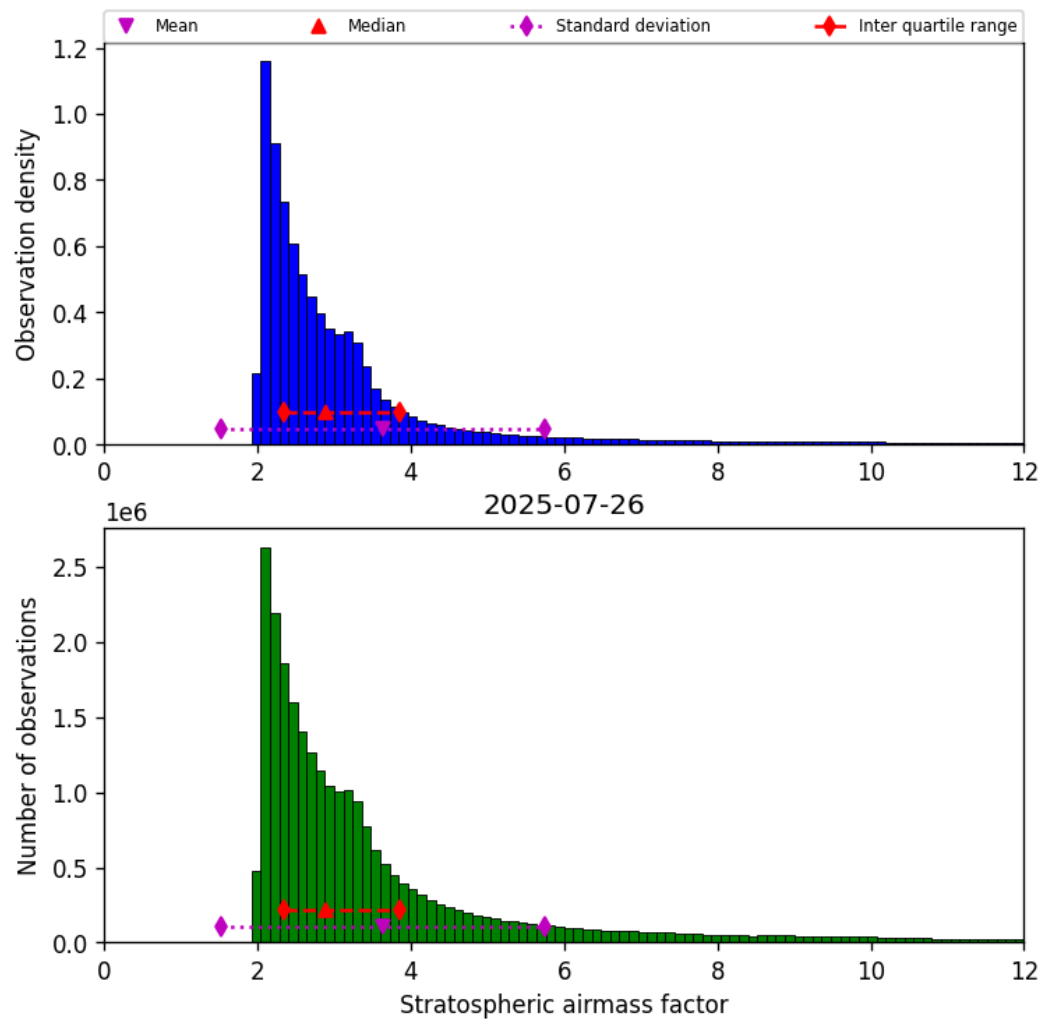
Figure 44: Histogram of “Stratospheric airmass factor” for 2025-07-25 to 2025-07-27
