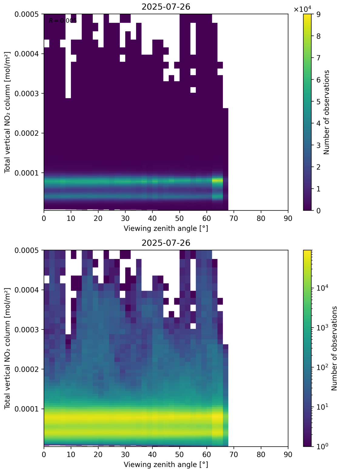
Figure 167: Scatter density plot of “Viewing zenith angle” against “Total vertical NO 2 column” for 2025-07-25 to 2025-07-27.
