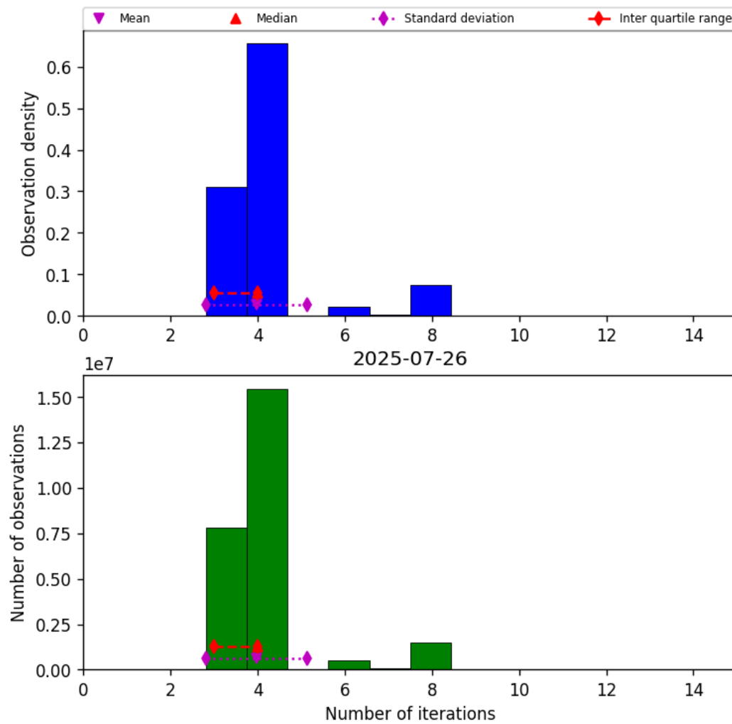
Figure 34: Histogram of “Number of iterations” for 2025-07-25 to 2025-07-27
