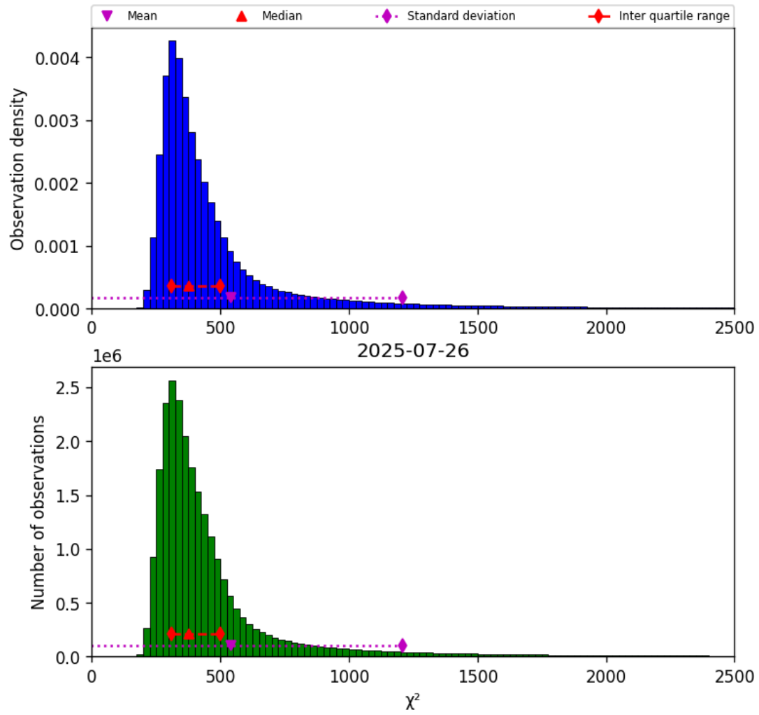
Figure 42: Histogram of " \chi^2 " for 2025-07-25 to 2025-07-27
