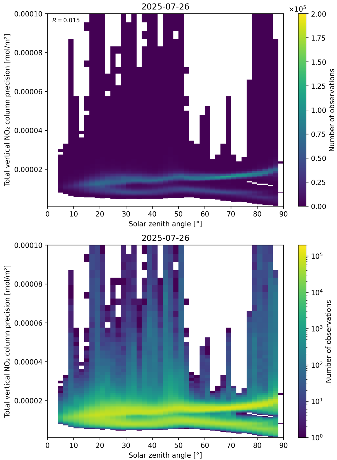
Figure 154: Scatter density plot of “Solar zenith angle” against “Total vertical NO 2 column precision” for 2025-07-25 to 2025-07-27.
