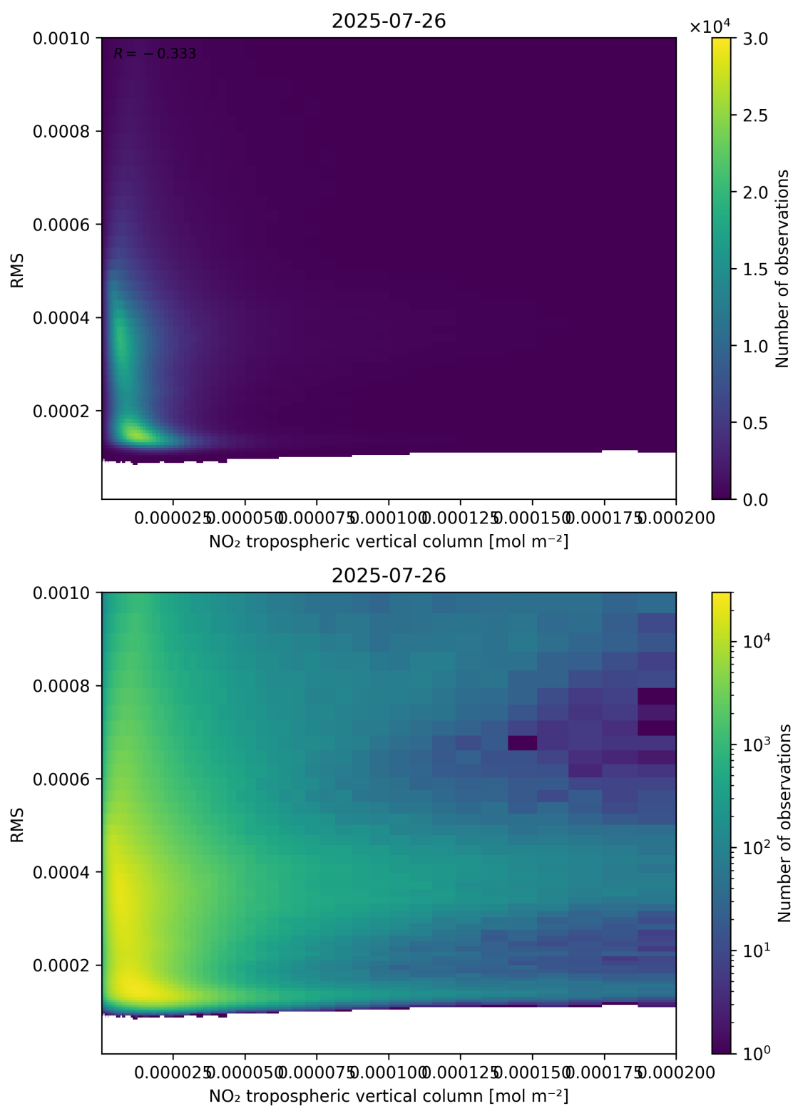
Figure 142: Scatter density plot of “NO 2 tropospheric vertical column” against “RMS” for 2025-07-25 to 2025-07-27.
