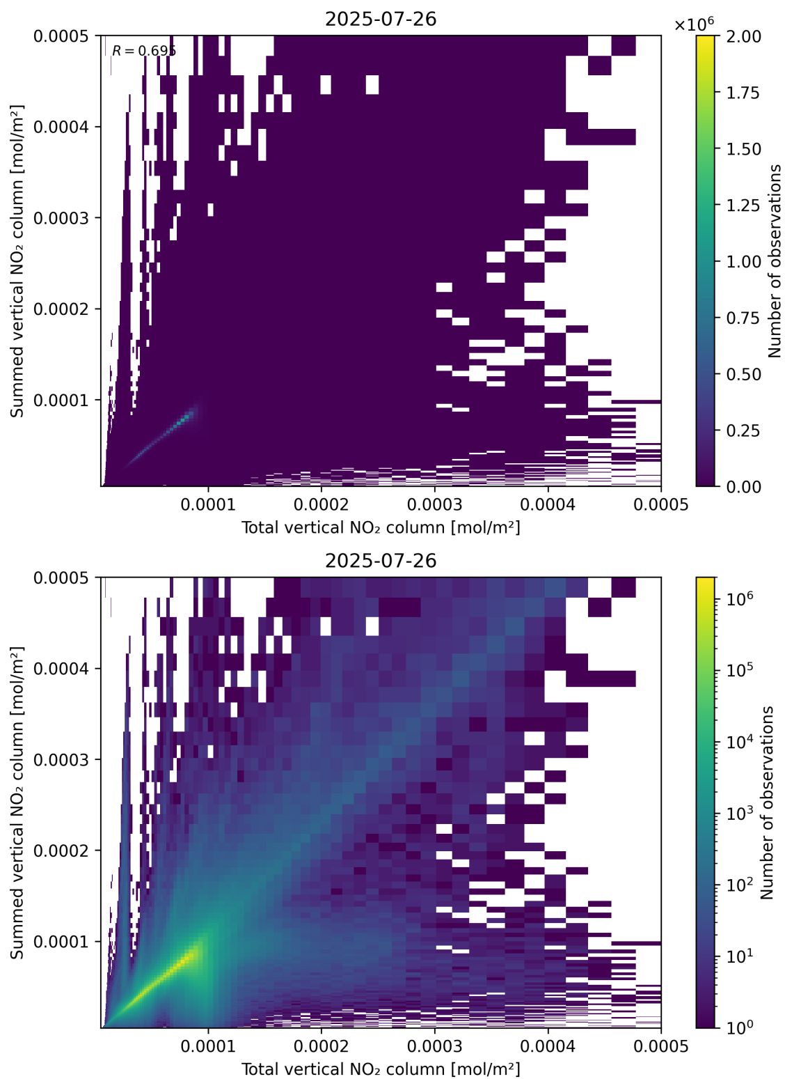
Figure 112: Scatter density plot of “Total vertical NO 2 column” against “Summed vertical NO 2 column” for 2025-07-25 to 2025-07-27.
