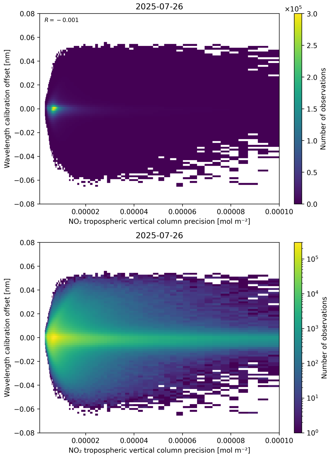
Figure 141: Scatter density plot of “NO 2 tropospheric vertical column precision” against “Wavelength calibration offset” for 2025-07-25 to 2025-07-27.
