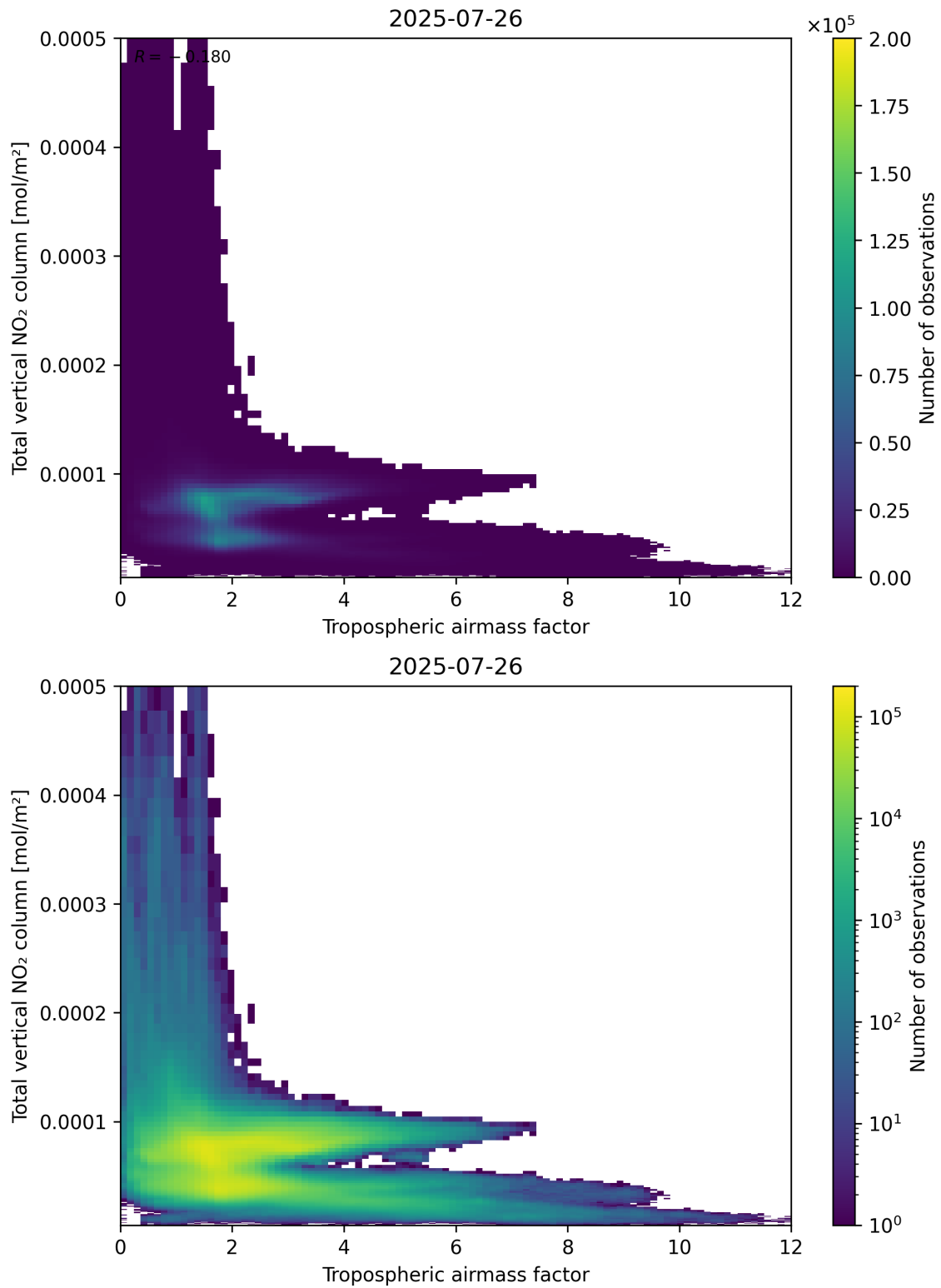
Figure 77: Scatter density plot of “Tropospheric airmass factor” against “Total vertical NO 2 column” for 2025-07-25 to 2025-07-27.
