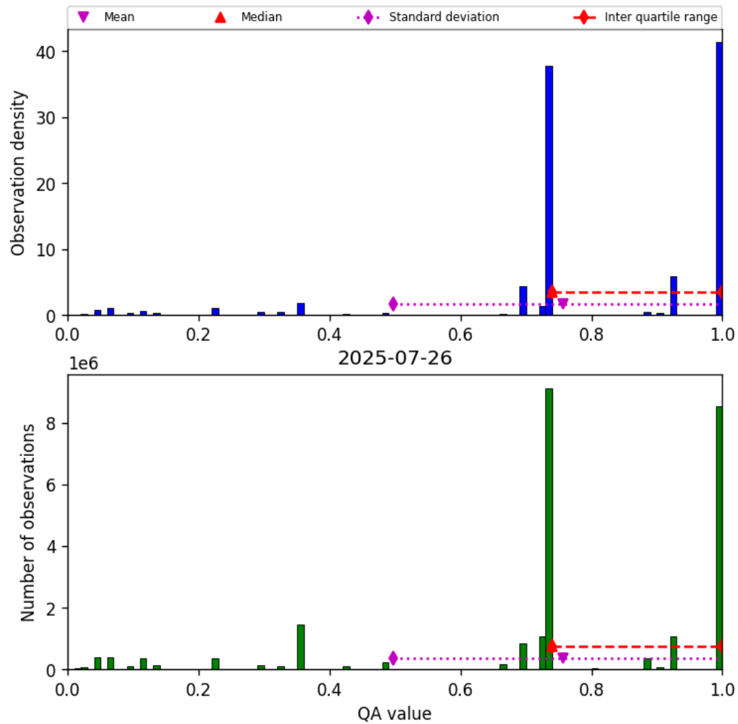
Figure 28: Histogram of “QA value” for 2025-07-25 to 2025-07-27
