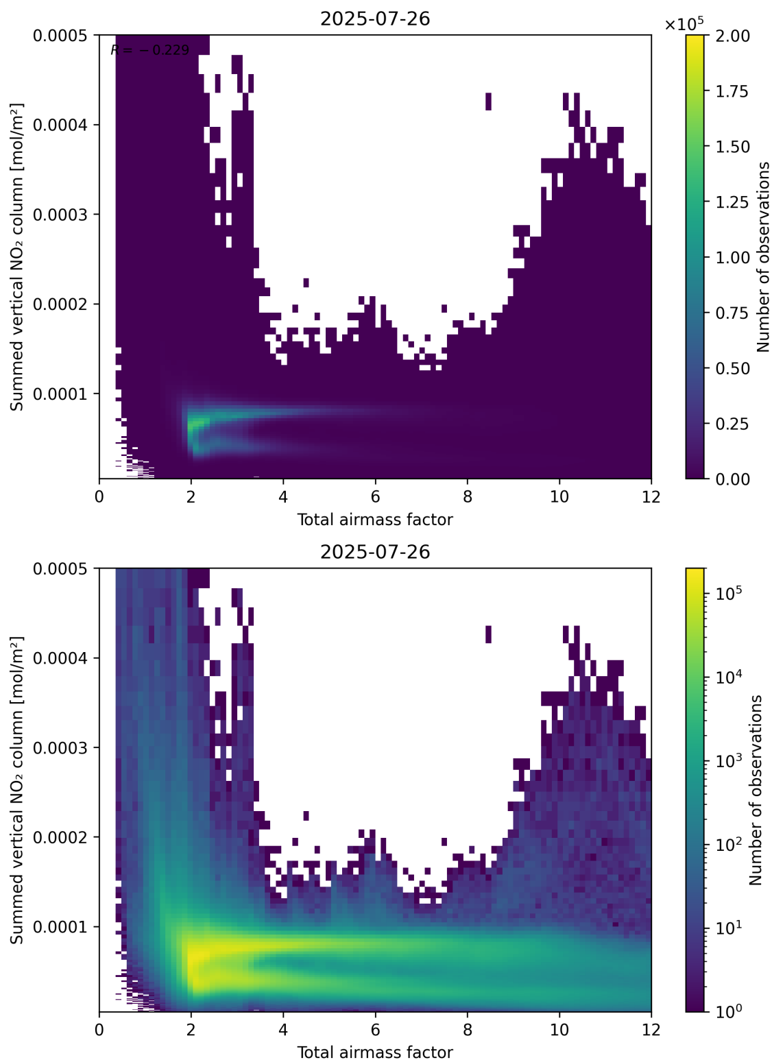
Figure 65: Scatter density plot of “Total airmass factor” against “Summed vertical NO 2 column” for 2025-07-25 to 2025-07-27.
