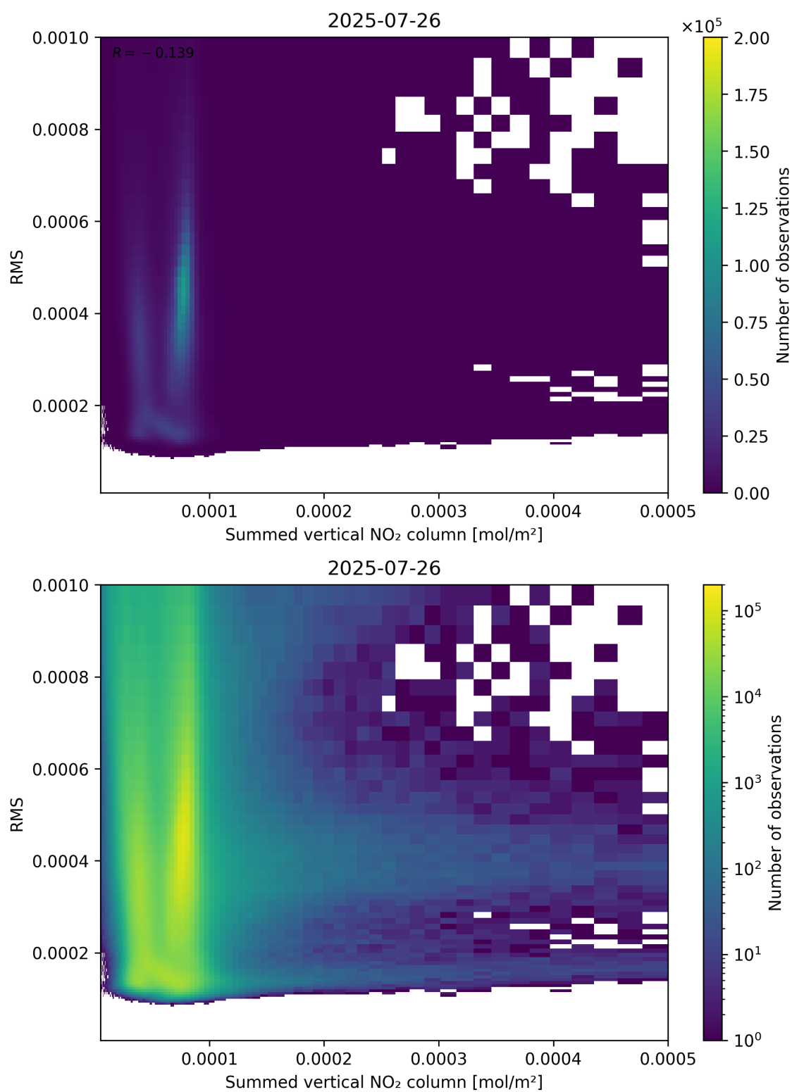
Figure 109: Scatter density plot of “Summed vertical NO 2 column” against “RMS” for 2025-07-25 to 2025-07-27.
