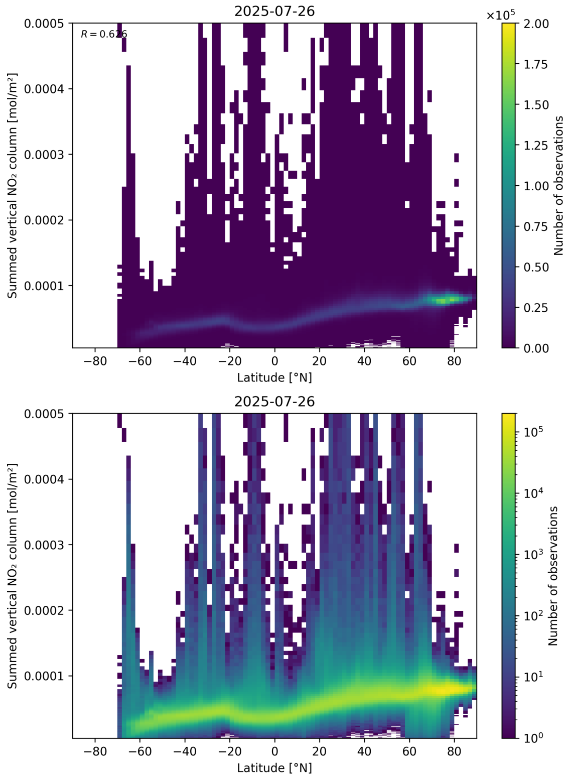
Figure 88: Scatter density plot of “Latitude” against “Summed vertical NO 2 column” for 2025-07-25 to 2025-07-27.
