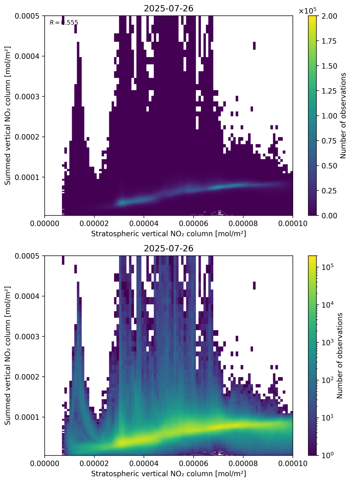
Figure 98: Scatter density plot of “Stratospheric vertical NO 2 column” against “Summed vertical NO 2 column” for 2025-07-25 to 2025-07-27.
