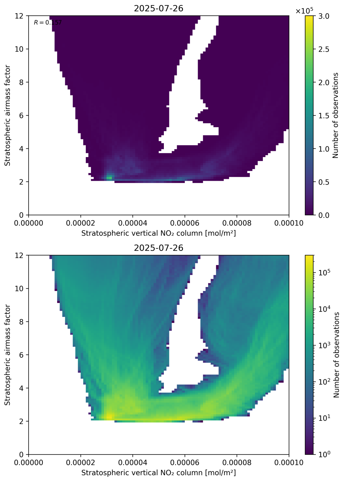
Figure 96: Scatter density plot of “Stratospheric vertical NO 2 column” against “Stratospheric airmass factor” for 2025-07-25 to 2025-07-27.
