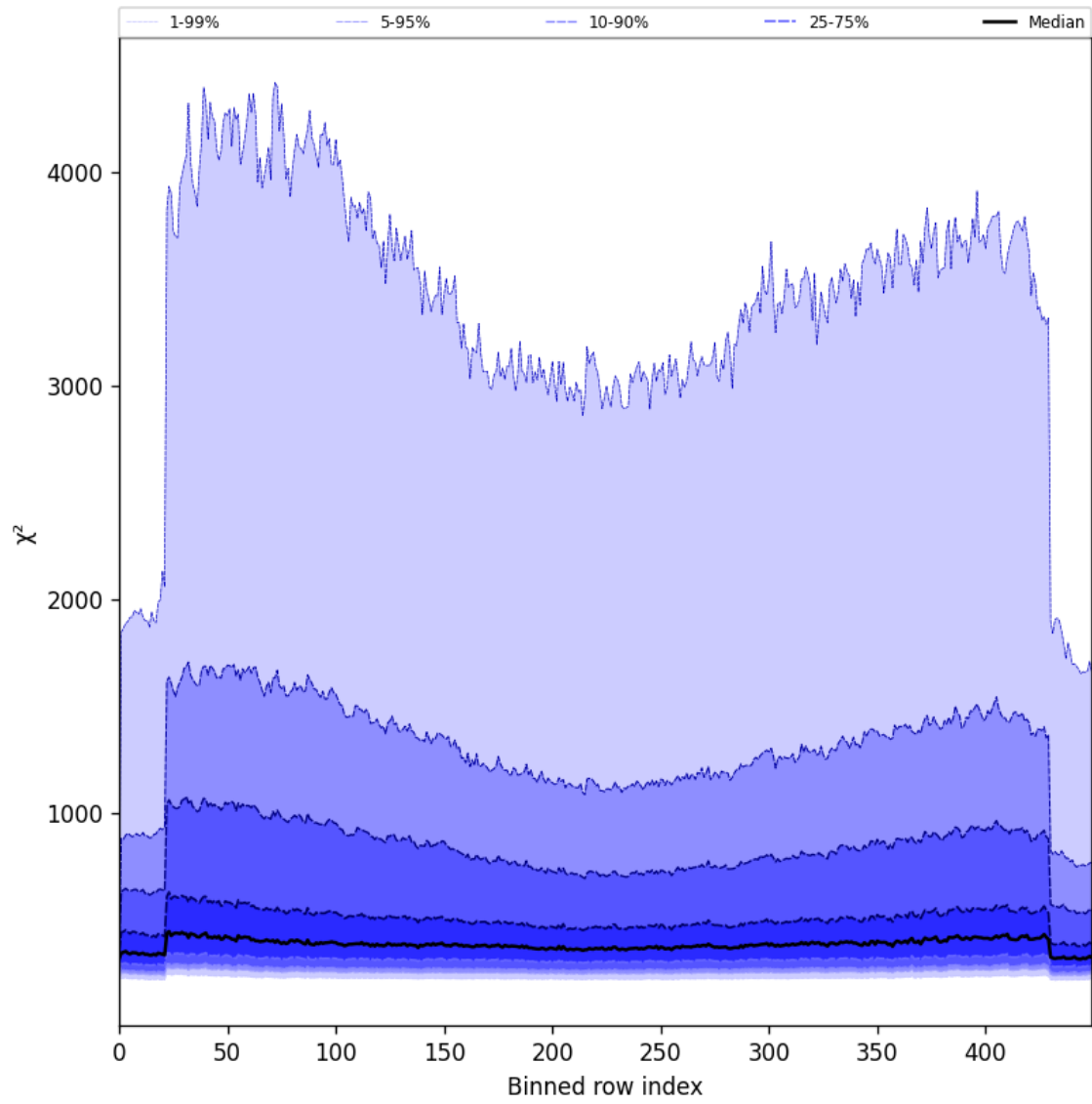
Figure 59: Along track statistics of “ \chi^2 ” for 2025-07-25 to 2025-07-27
