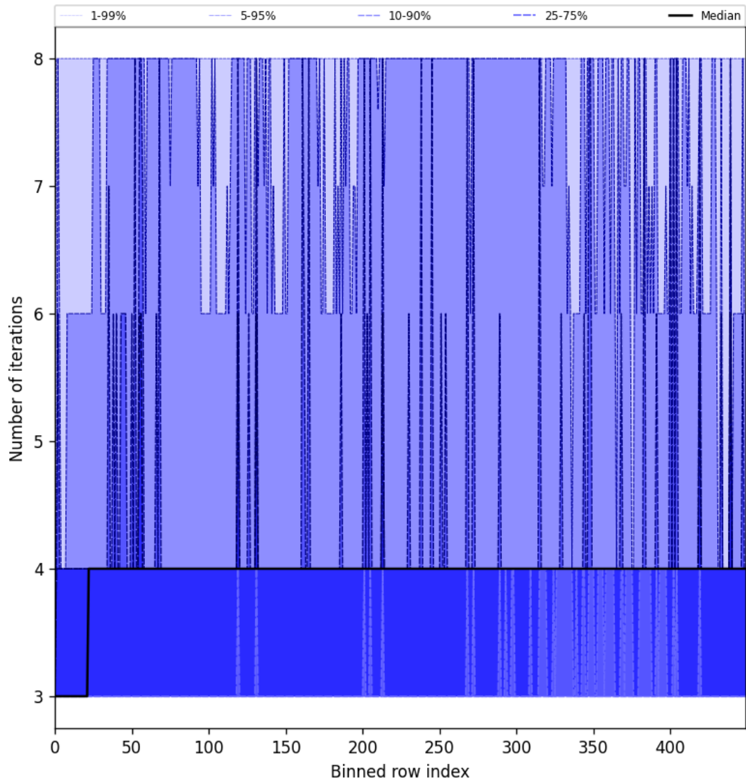
Figure 51: Along track statistics of “Number of iterations” for 2025-07-25 to 2025-07-27
