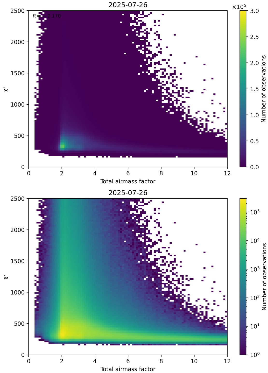
Figure 63: Scatter density plot of “Total airmass factor” against “ \chi^2 ” for 2025-07-25 to 2025-07-27.
