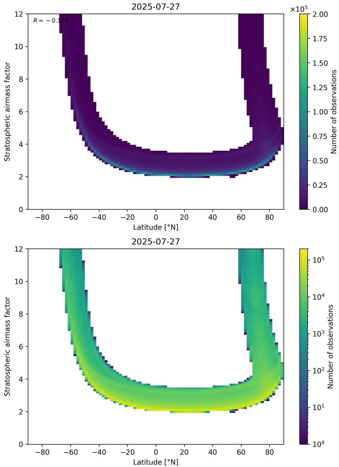
Figure 83: Scatter density plot of “Latitude” against “Stratospheric air mass factor” for 2025-07-26 to 2025-07-28.
