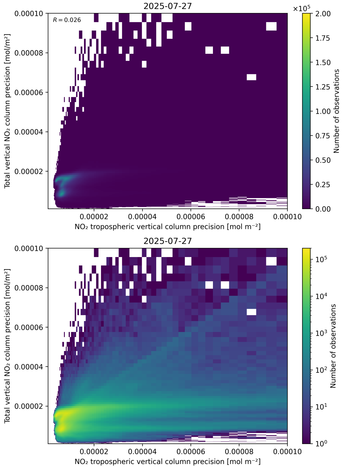
Figure 139: Scatter density plot of “NO 2 tropospheric vertical column precision” against “Total vertical NO 2 column precision” for 2025-07-26 to 2025-07-28.
