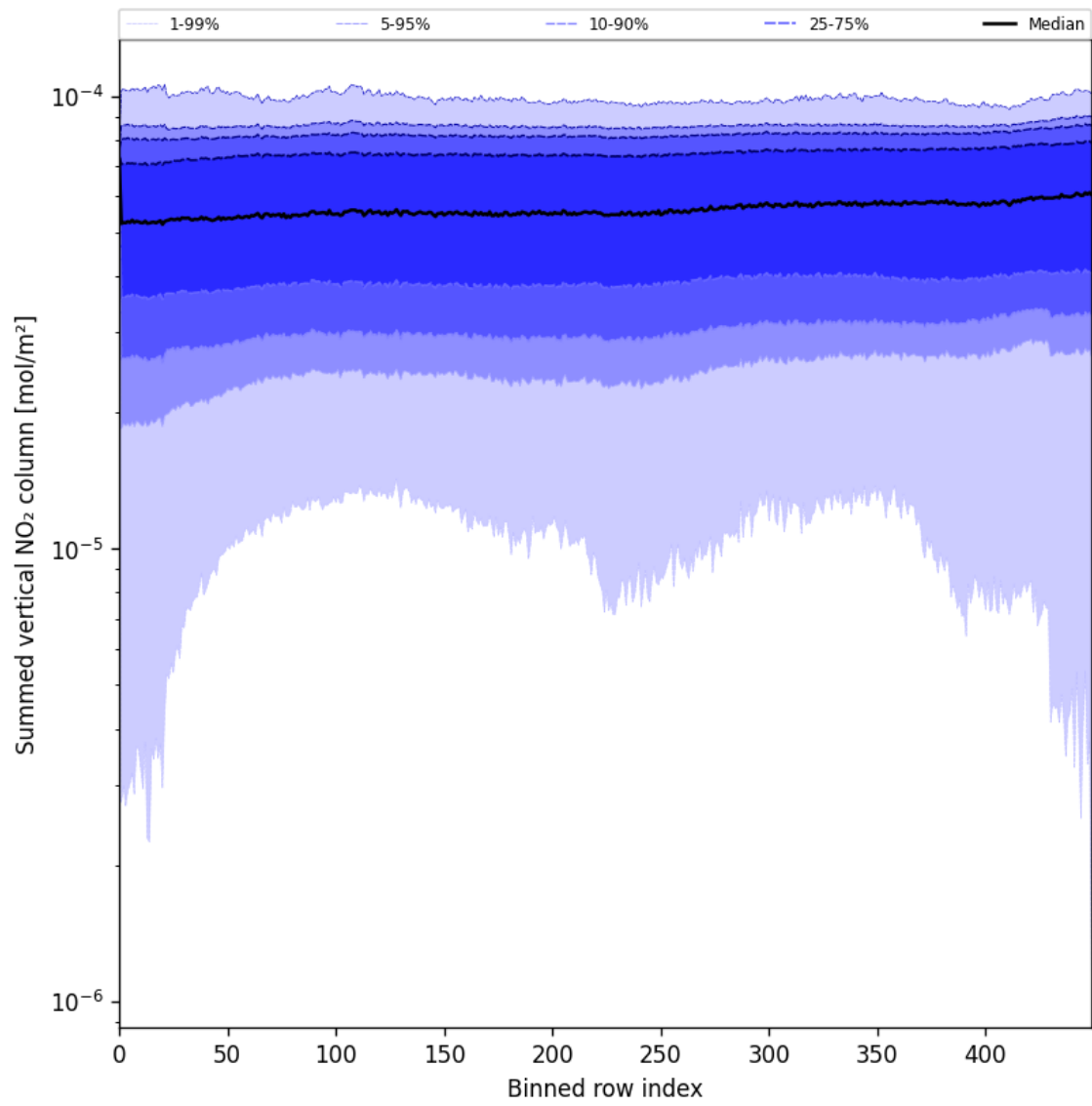
Figure 57: Along track statistics of “Summed vertical NO 2 column” for 2025-07-26 to 2025-07-28
