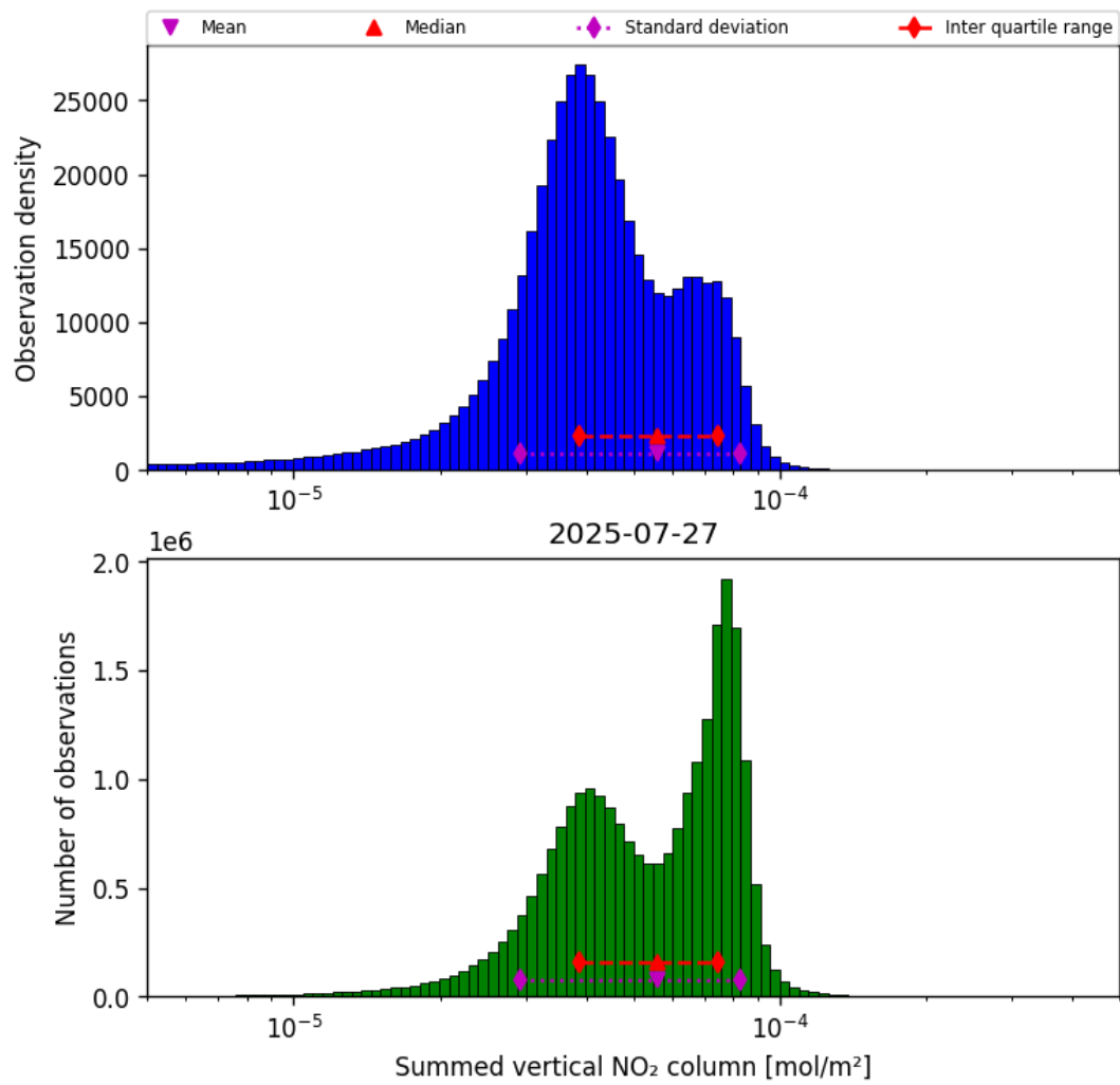
Figure 40: Histogram of “Summed vertical NO 2 column” for 2025-07-26 to 2025-07-28
