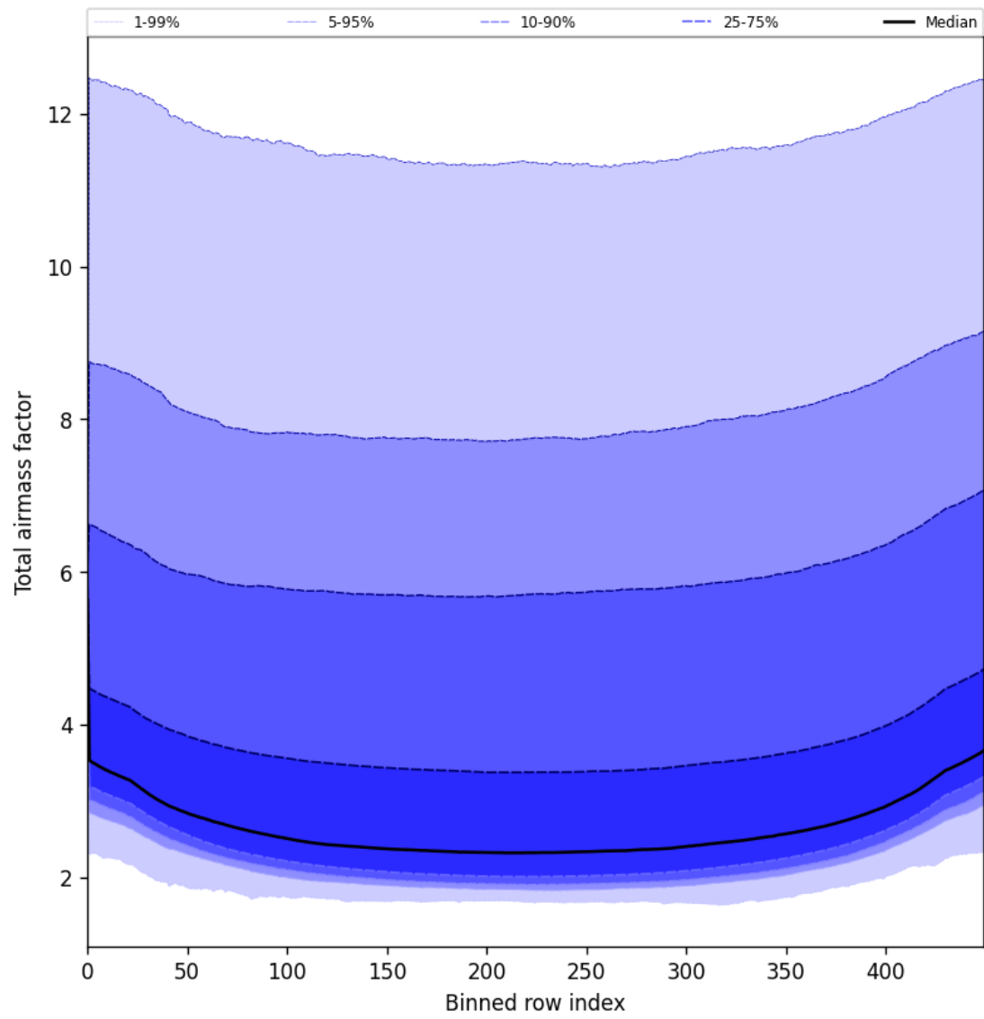
Figure 49: Along track statistics of “Total airmass factor” for 2025-07-26 to 2025-07-28
