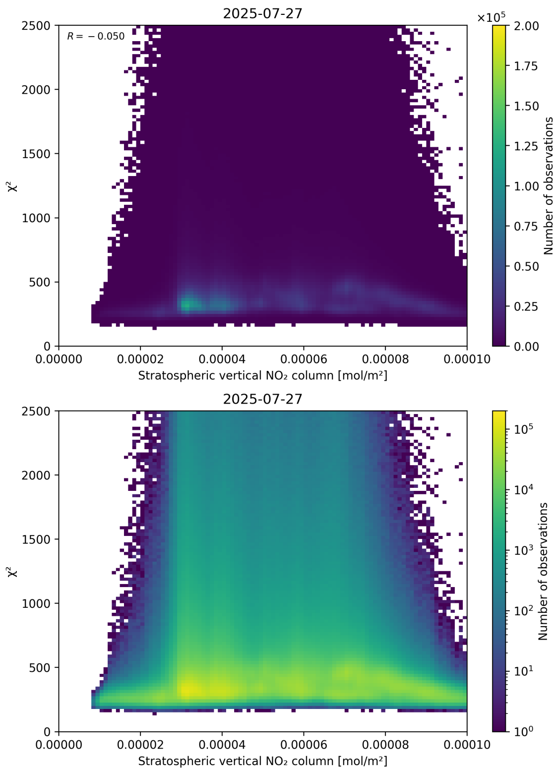
Figure 97: Scatter density plot of “Stratospheric vertical NO 2 column” against “ \chi^2 ” for 2025-07-26 to 2025-07-28.
