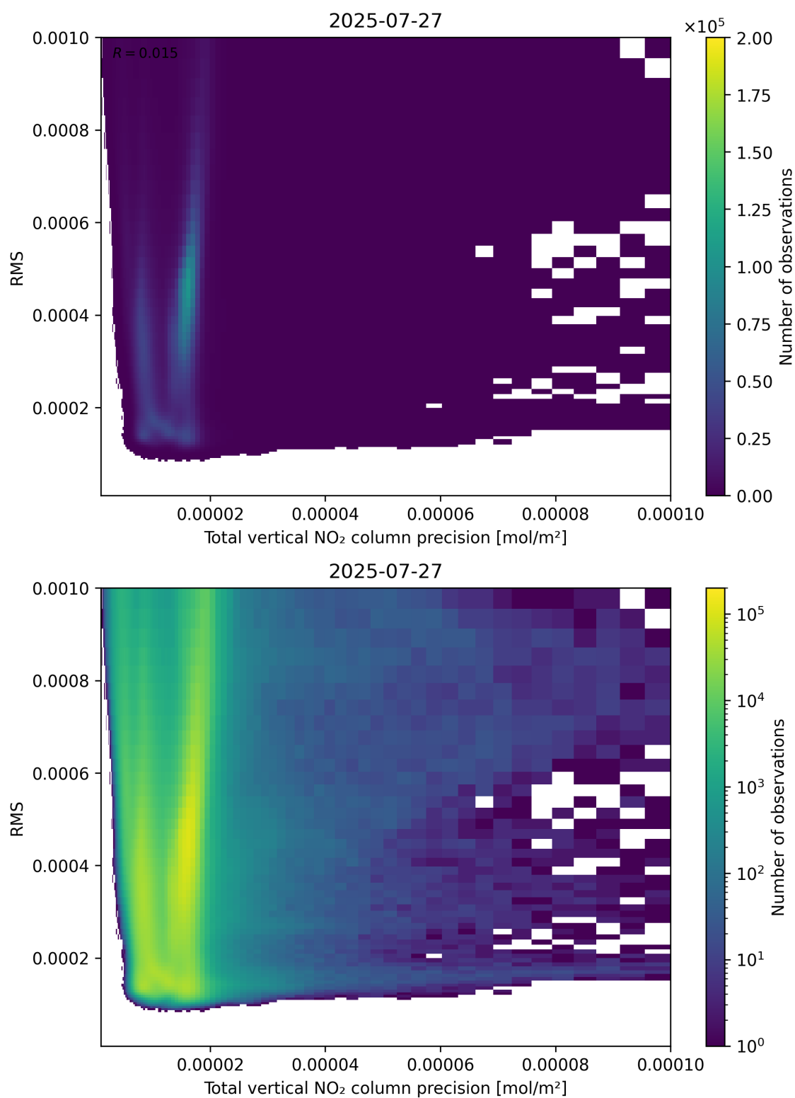
Figure 119: Scatter density plot of “Total vertical NO 2 column precision” against “RMS” for 2025-07-26 to 2025-07-28.
