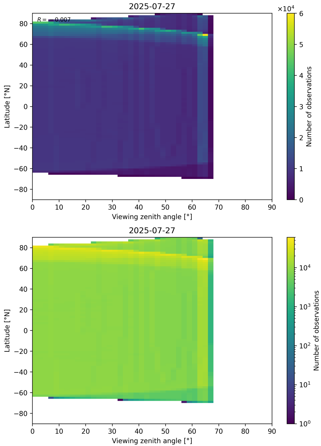
Figure 163: Scatter density plot of “Viewing zenith angle” against “Latitude” for 2025-07-26 to 2025-07-28.
