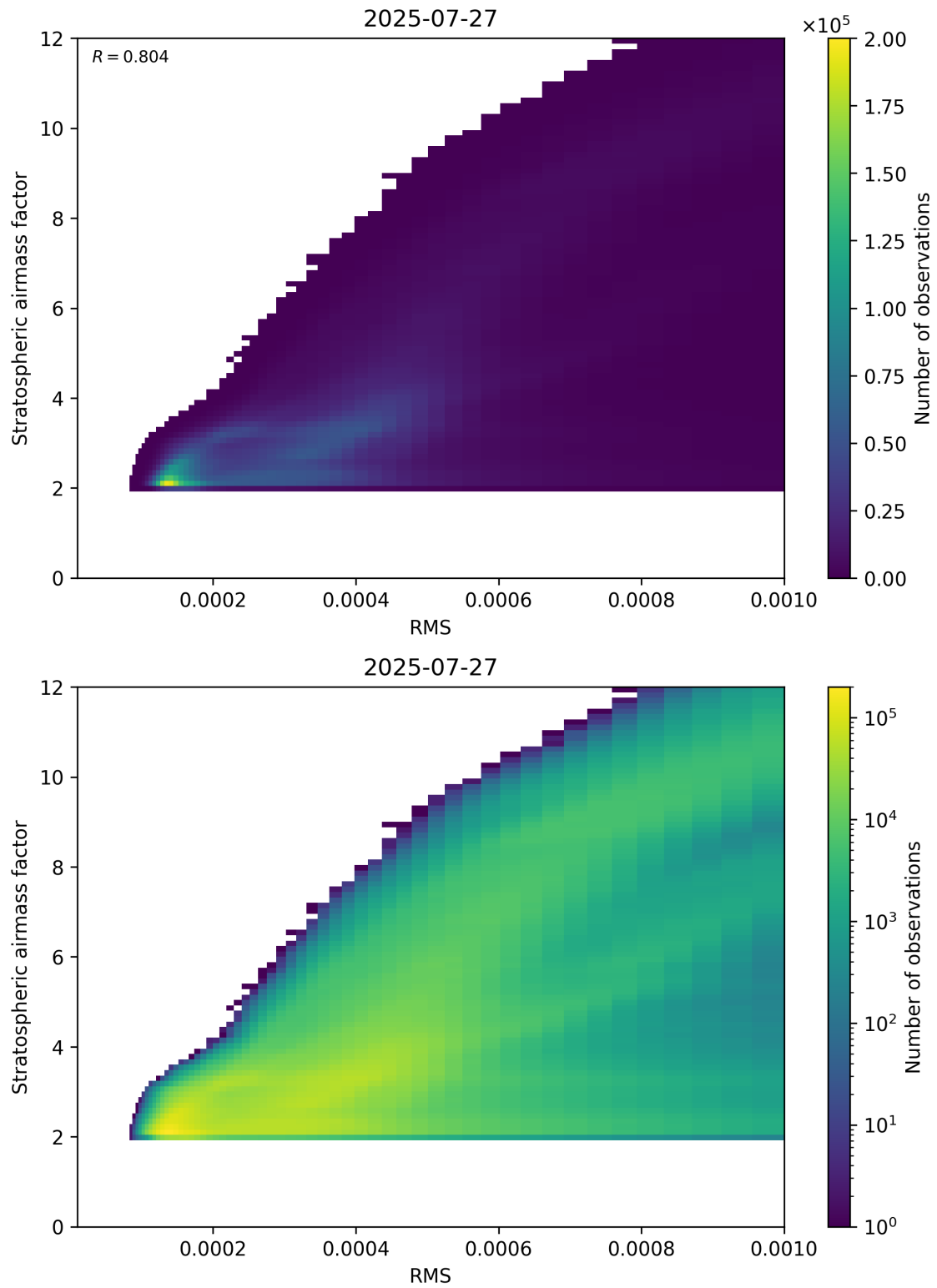
Figure 144: Scatter density plot of “RMS” against “Stratospheric airmass factor” for 2025-07-26 to 2025-07-28.
