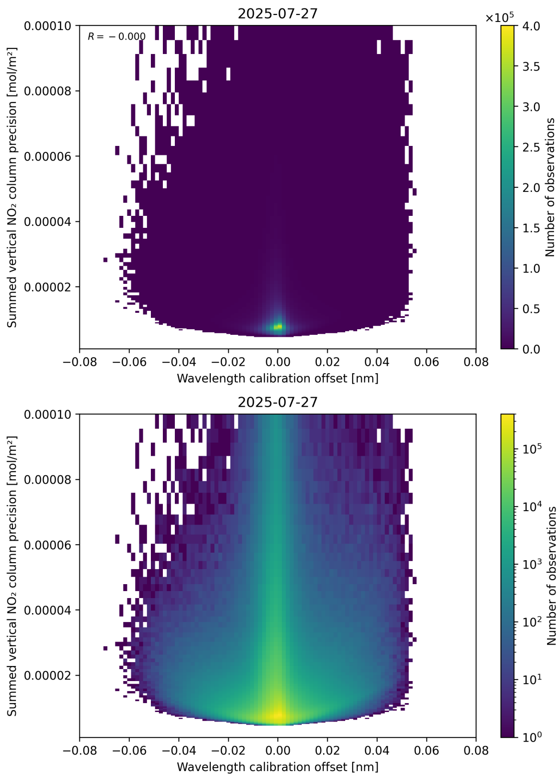
Figure 178: Scatter density plot of “Wavelength calibration offset” against “Summed vertical NO 2 column precision” for 2025-07-26 to 2025-07-28.
