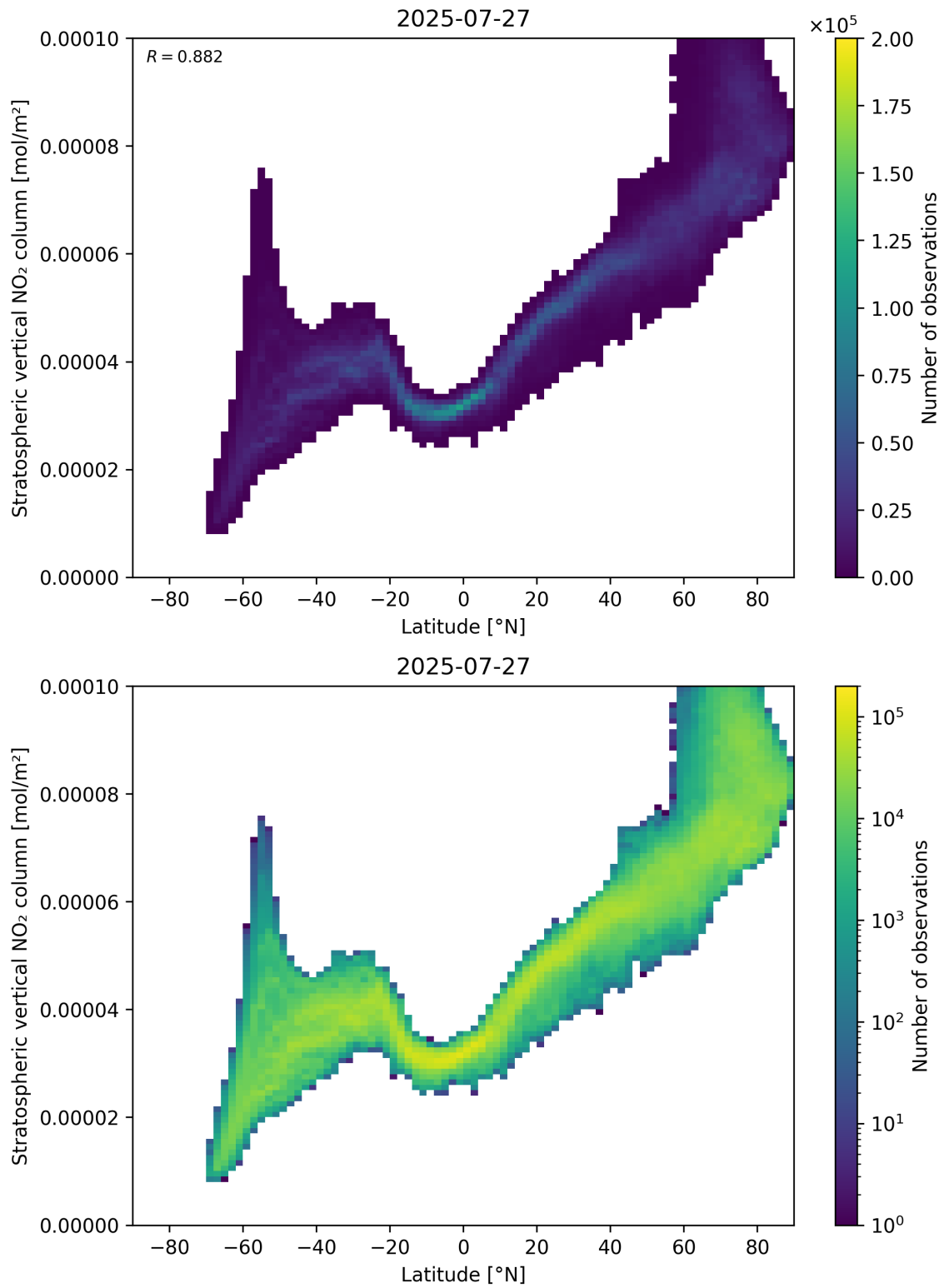
Figure 87: Scatter density plot of “Latitude” against “Stratospheric vertical \text{NO}_2 column” for 2025-07-26 to 2025-07-28.
