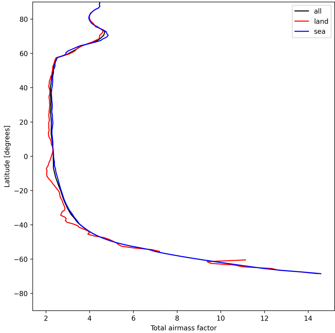
Figure 15: Zonal average of “Total airmass factor” for 2025-07-26 to 2025-07-28.
