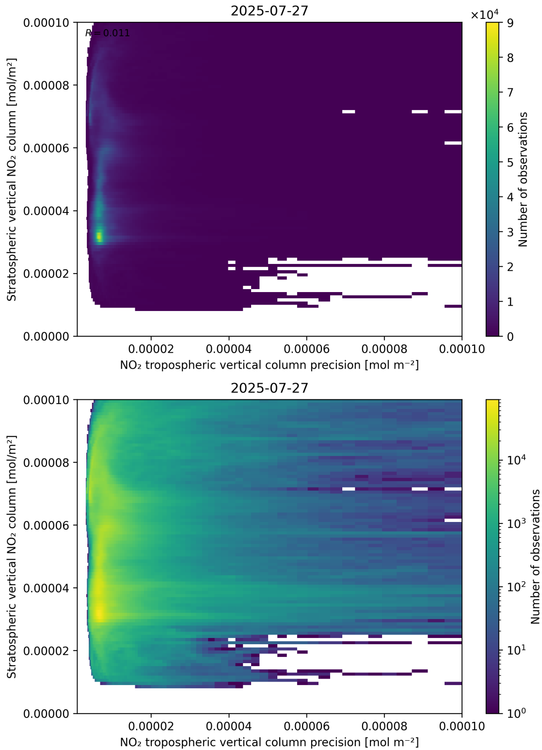
Figure 135: Scatter density plot of “NO 2 tropospheric vertical column precision” against “Stratospheric vertical NO 2 column” for 2025-07-26 to 2025-07-28.
