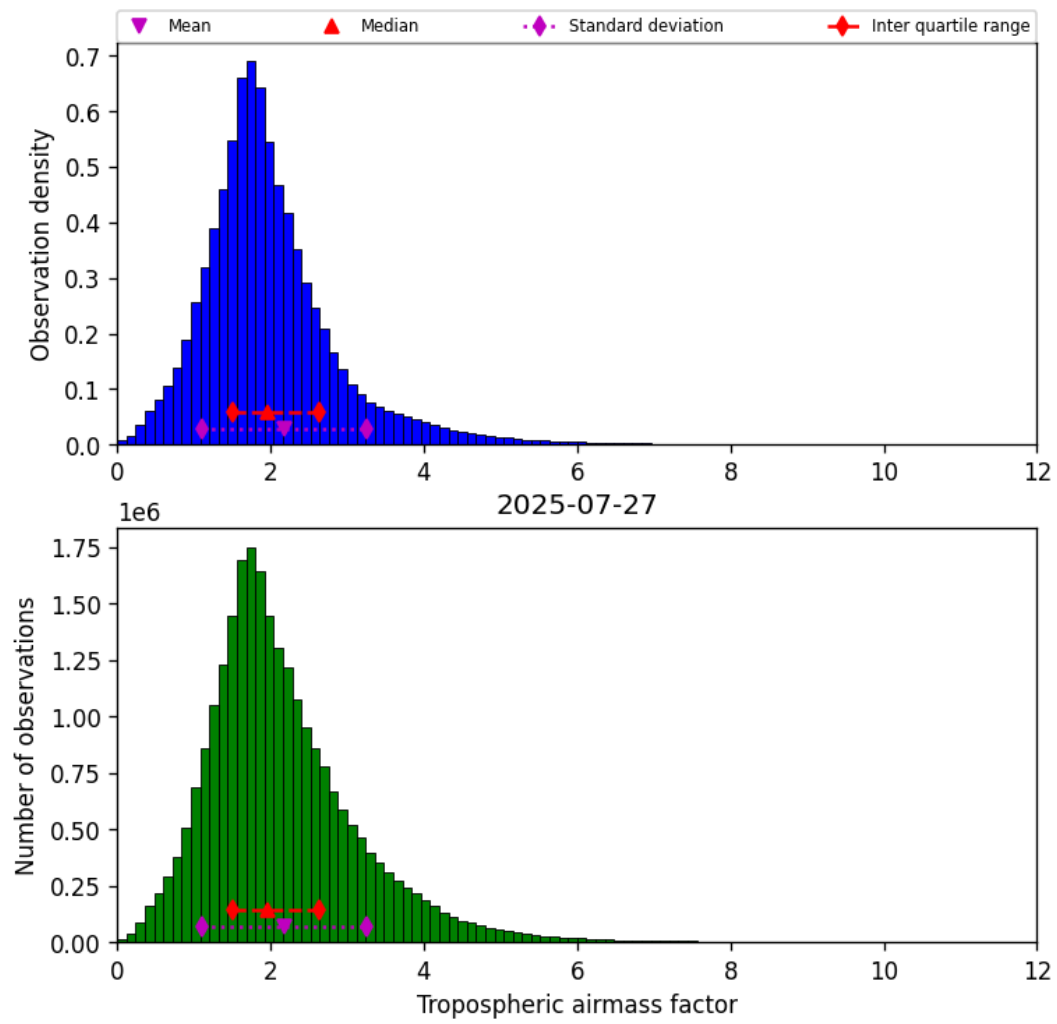
Figure 31: Histogram of “Tropospheric airmass factor” for 2025-07-26 to 2025-07-28
