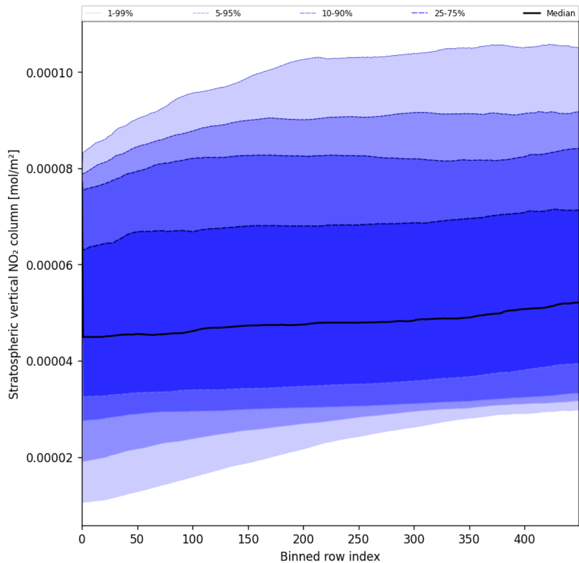
Figure 53: Along track statistics of “Stratospheric vertical NO 2 column” for 2025-07-26 to 2025-07-28
