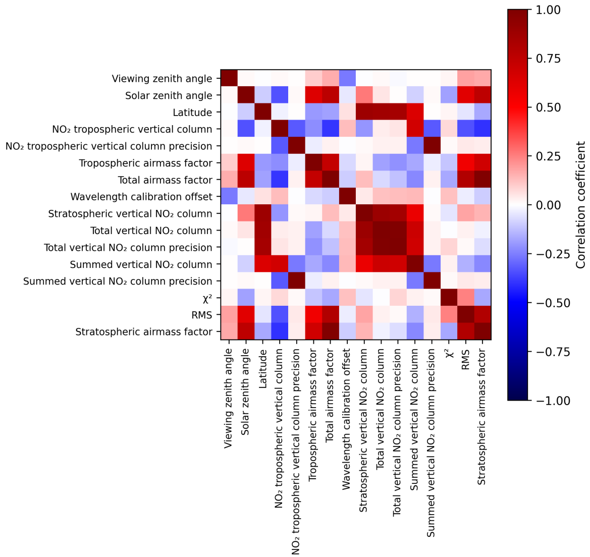
Figure 2: Map of correlation matrix for 2025-07-26 to 2025-07-28.
