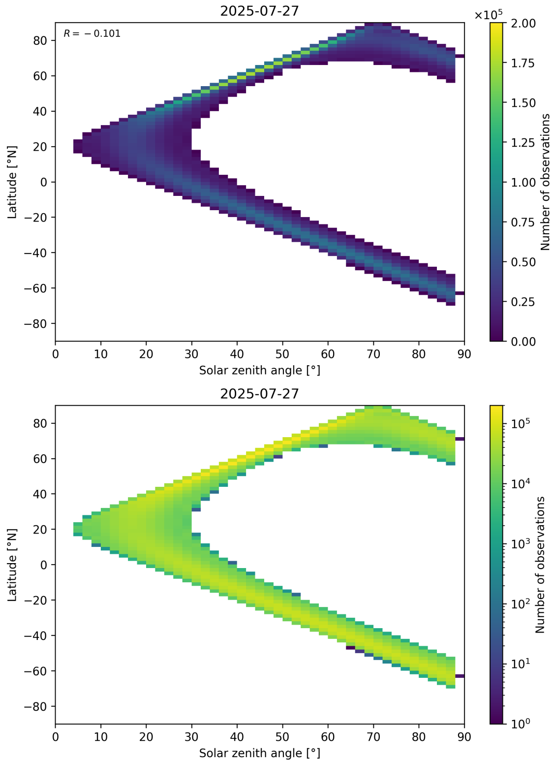
Figure 149: Scatter density plot of “Solar zenith angle” against “Latitude” for 2025-07-26 to 2025-07-28.
