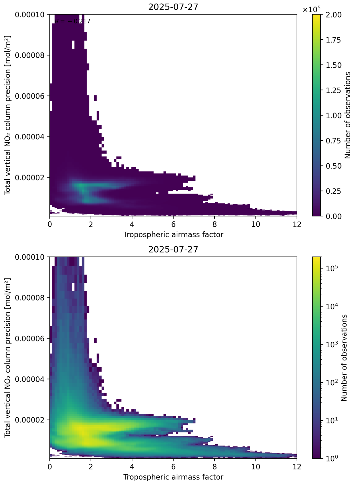
Figure 78: Scatter density plot of “Tropospheric airmass factor” against “Total vertical NO 2 column precision” for 2025-07-26 to 2025-07-28.
