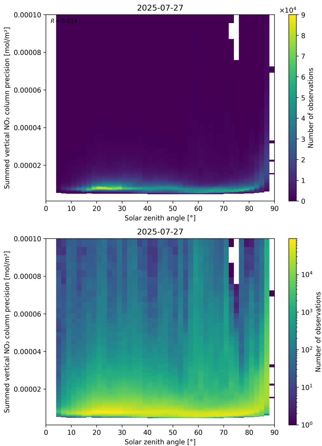
Figure 152: Scatter density plot of “Solar zenith angle” against “Summed vertical NO 2 column precision” for 2025-07-26 to 2025-07-28.
