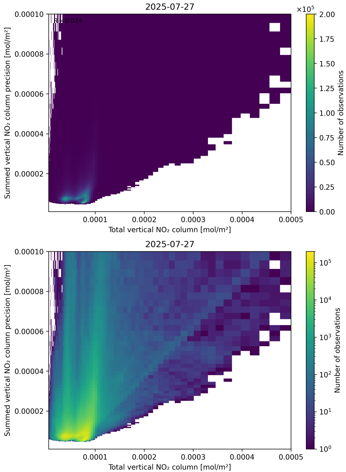
Figure 113: Scatter density plot of “Total vertical NO 2 column” against “Summed vertical NO 2 column precision” for 2025-07-26 to 2025-07-28.
