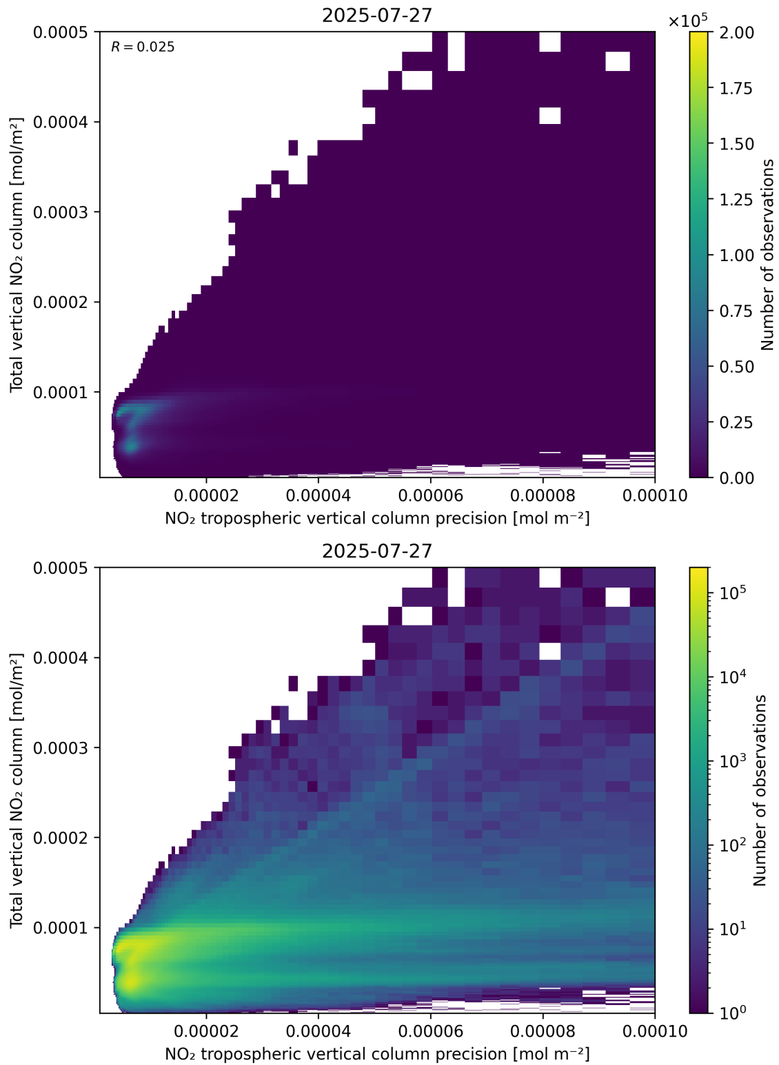
Figure 138: Scatter density plot of “NO 2 tropospheric vertical column precision” against “Total vertical NO 2 column” for 2025-07-26 to 2025-07-28.
