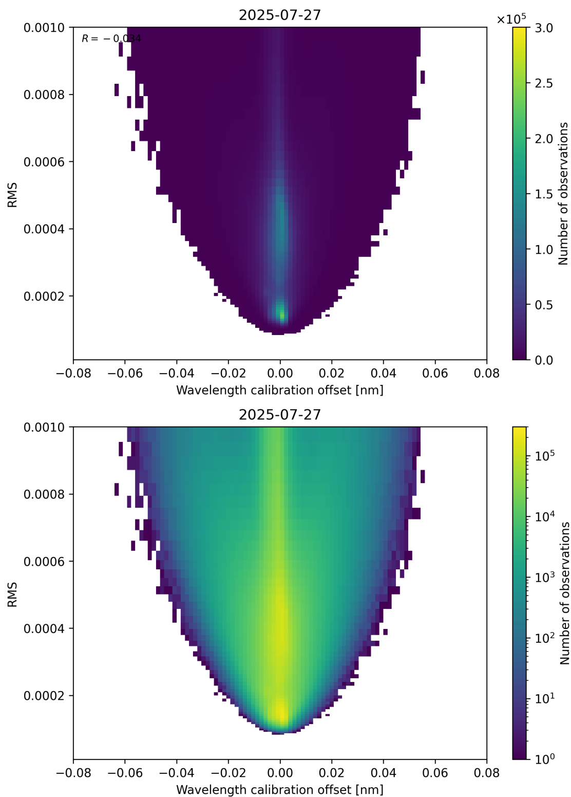
Figure 181: Scatter density plot of “Wavelength calibration offset” against “RMS” for 2025-07-26 to 2025-07-28.
