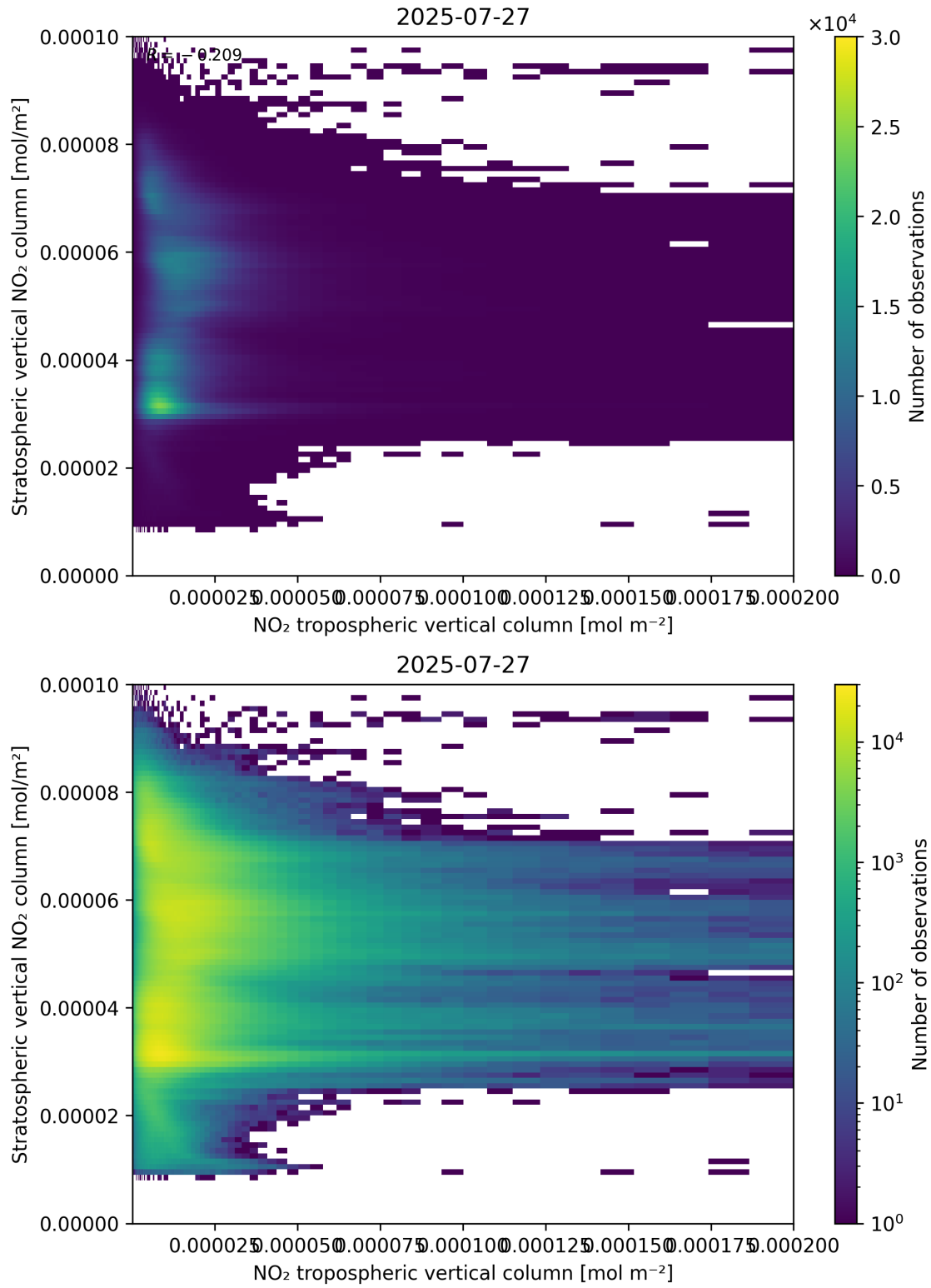
Figure 125: Scatter density plot of “NO 2 tropospheric vertical column” against “Stratospheric vertical NO 2 column” for 2025-07-26 to 2025-07-28.
