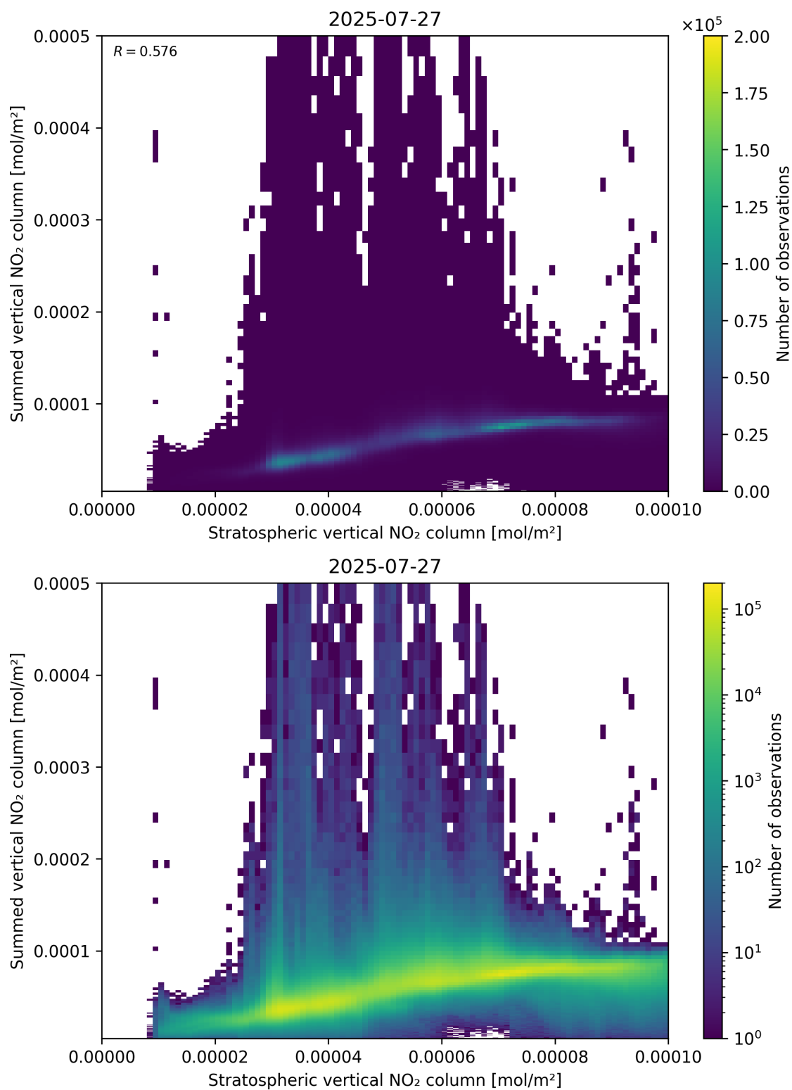
Figure 98: Scatter density plot of “Stratospheric vertical NO 2 column” against “Summed vertical NO 2 column” for 2025-07-26 to 2025-07-28.
