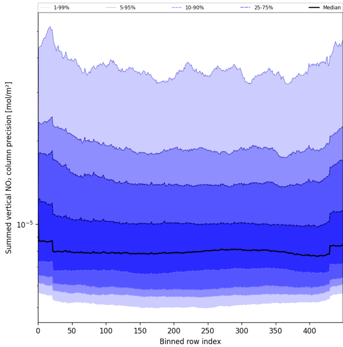
Figure 58: Along track statistics of “Summed vertical NO 2 column precision” for 2025-07-26 to 2025-07-28
