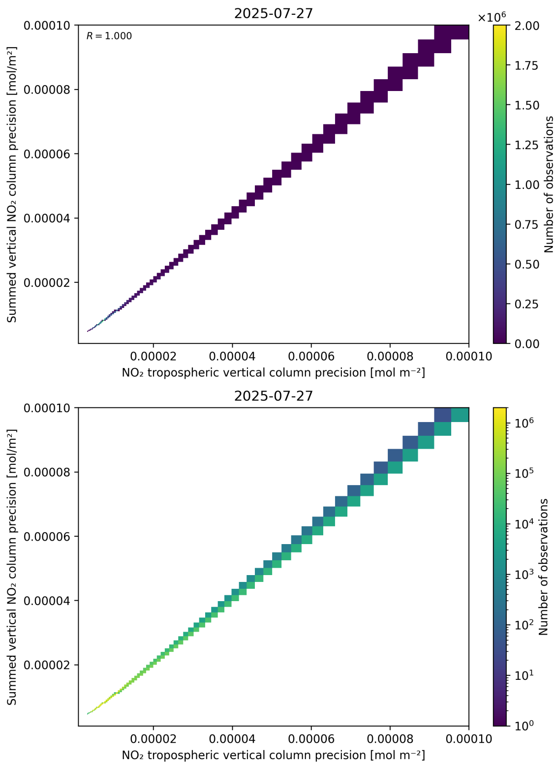
Figure 137: Scatter density plot of “NO 2 tropospheric vertical column precision” against “Summed vertical NO 2 column precision” for 2025-07-26 to 2025-07-28.
