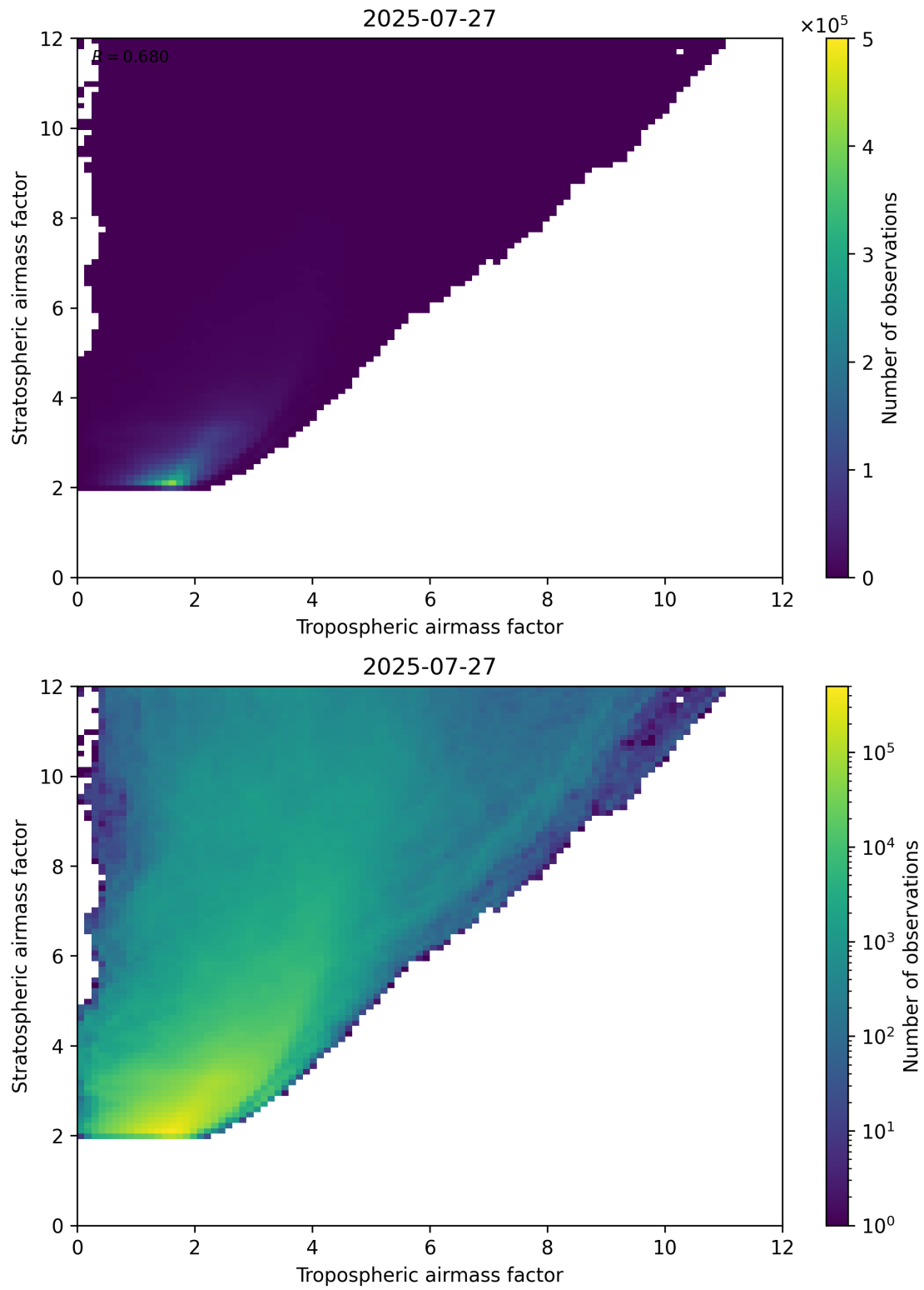
Figure 71: Scatter density plot of “Tropospheric airmass factor” against “Stratospheric airmass factor” for 2025-07-26 to 2025-07-28.
