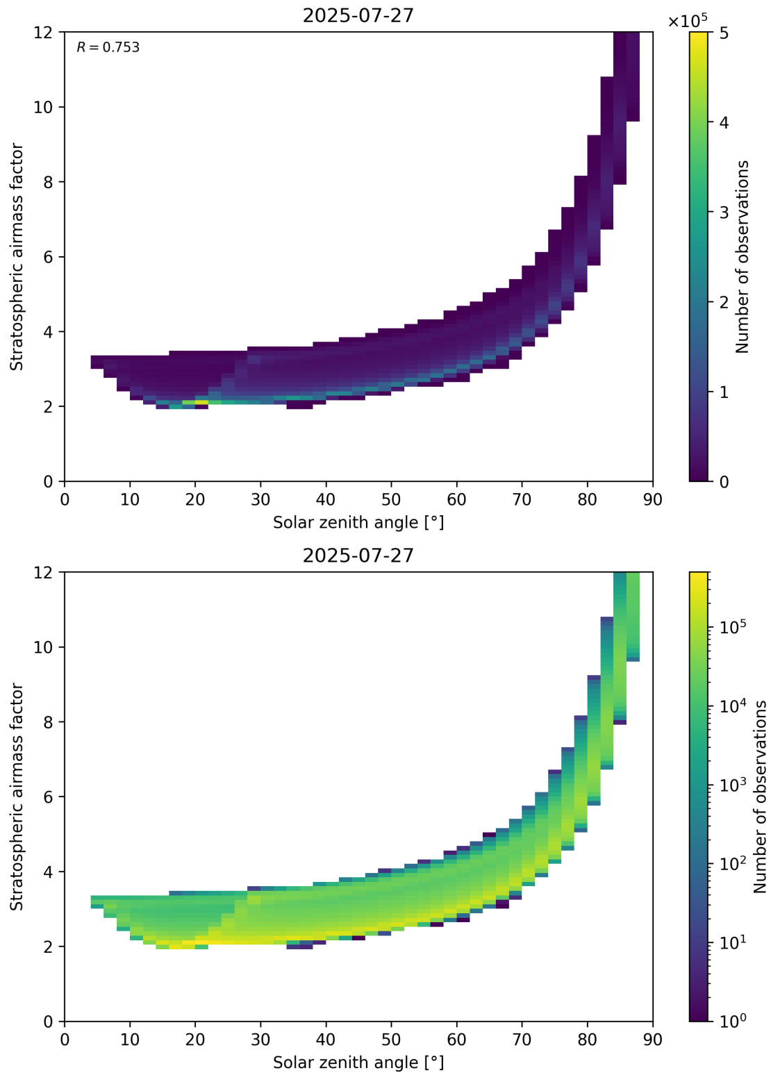
Figure 145: Scatter density plot of “Solar zenith angle” against “Stratospheric airmass factor” for 2025-07-26 to 2025-07-28.
