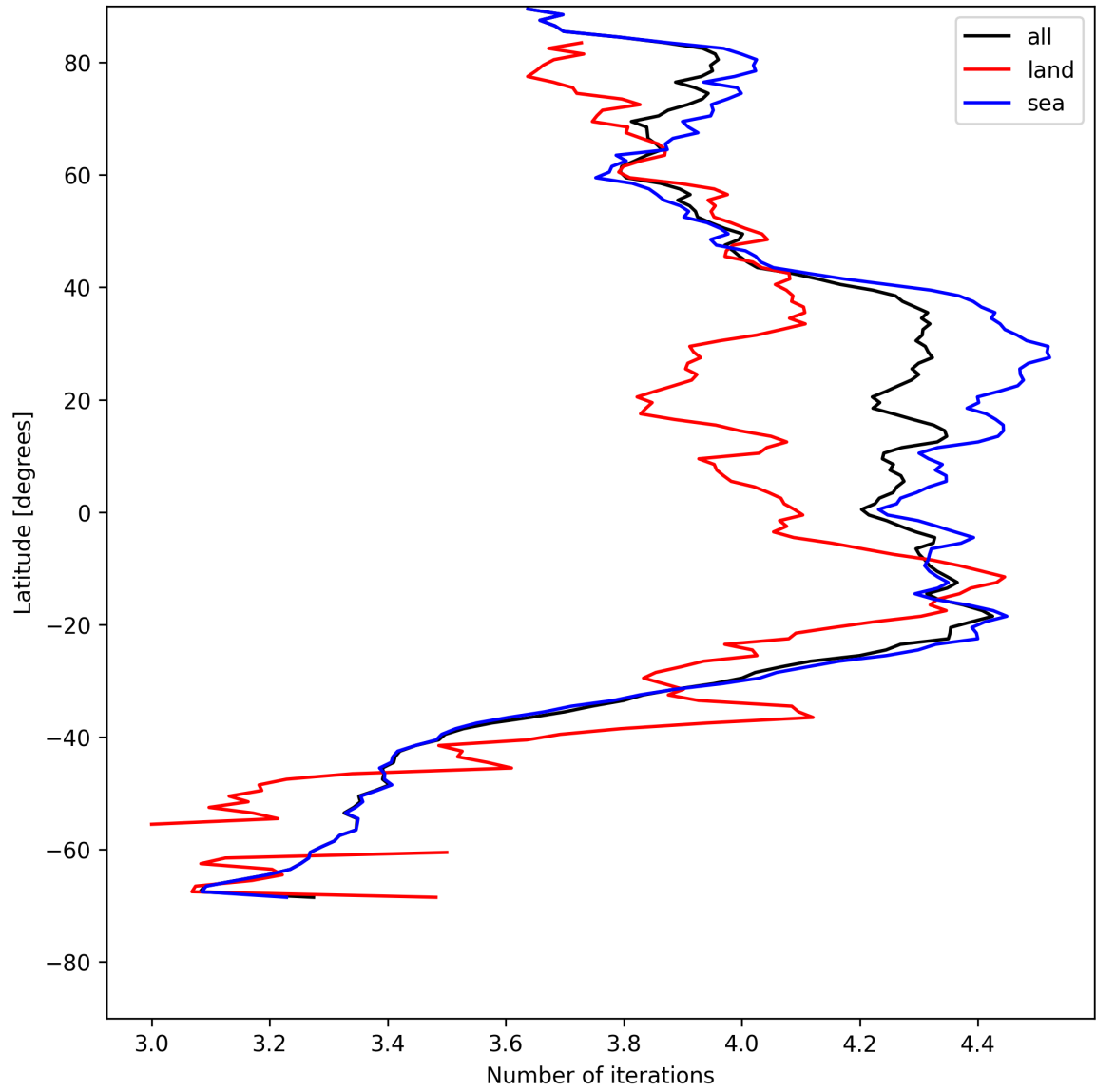
Figure 17: Zonal average of “Number of iterations” for 2025-07-26 to 2025-07-28.
