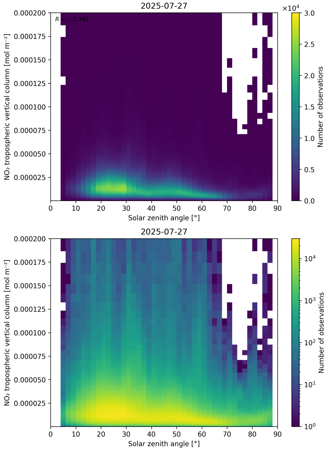
Figure 155: Scatter density plot of “Solar zenith angle” against “NO 2 tropospheric vertical column” for 2025-07-26 to 2025-07-28.
