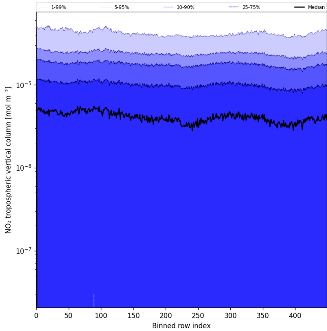
Figure 46: Along track statistics of “NO 2 tropospheric vertical column” for 2025-07-26 to 2025-07-28
