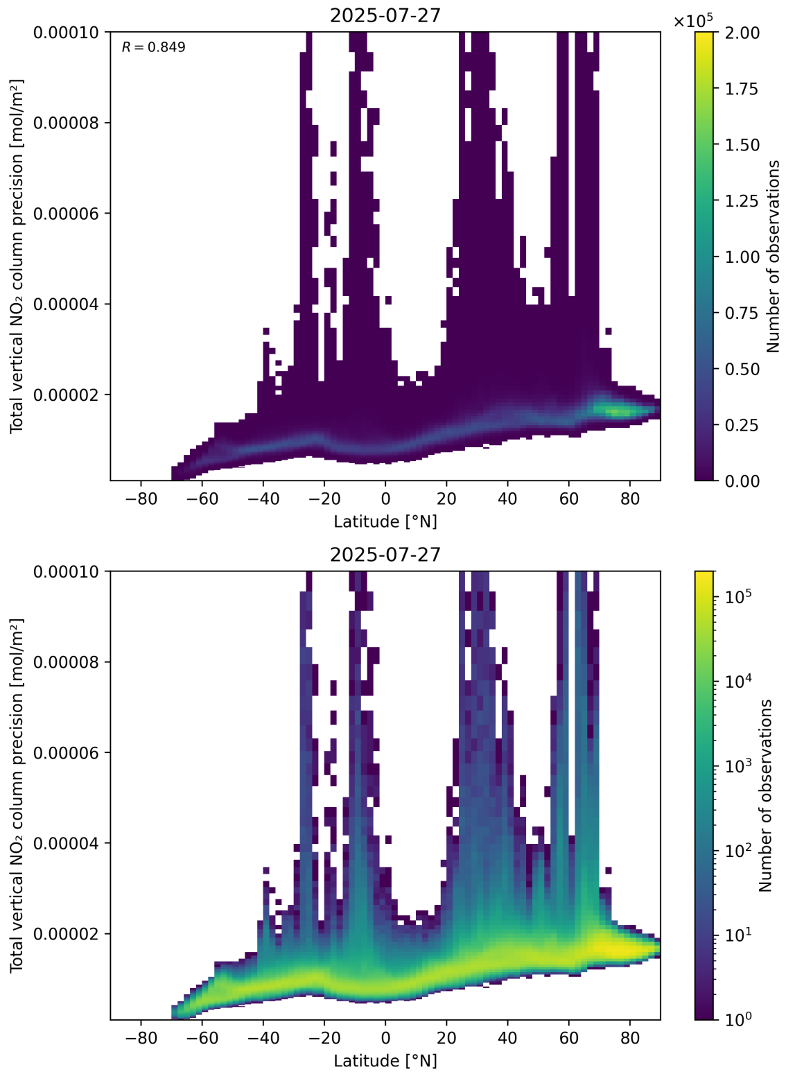
Figure 91: Scatter density plot of “Latitude” against “Total vertical NO 2 column precision” for 2025-07-26 to 2025-07-28.
