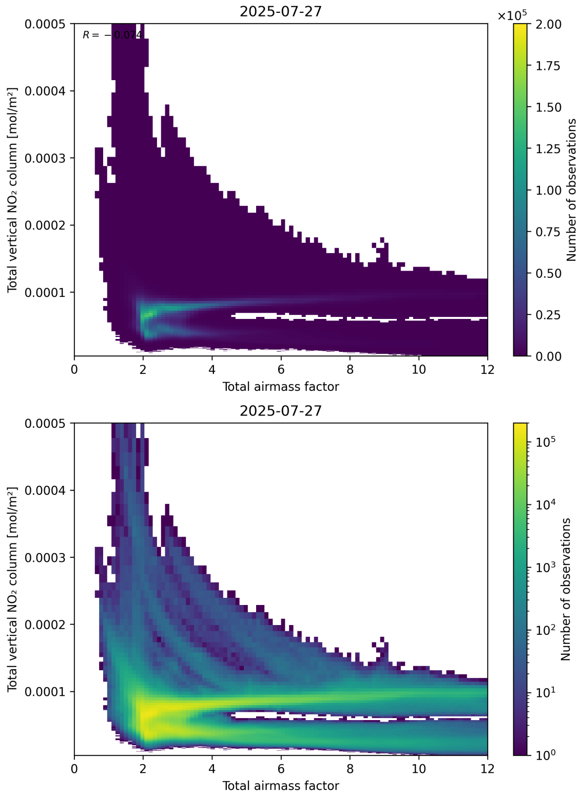
Figure 67: Scatter density plot of “Total airmass factor” against “Total vertical NO 2 column” for 2025-07-26 to 2025-07-28.
