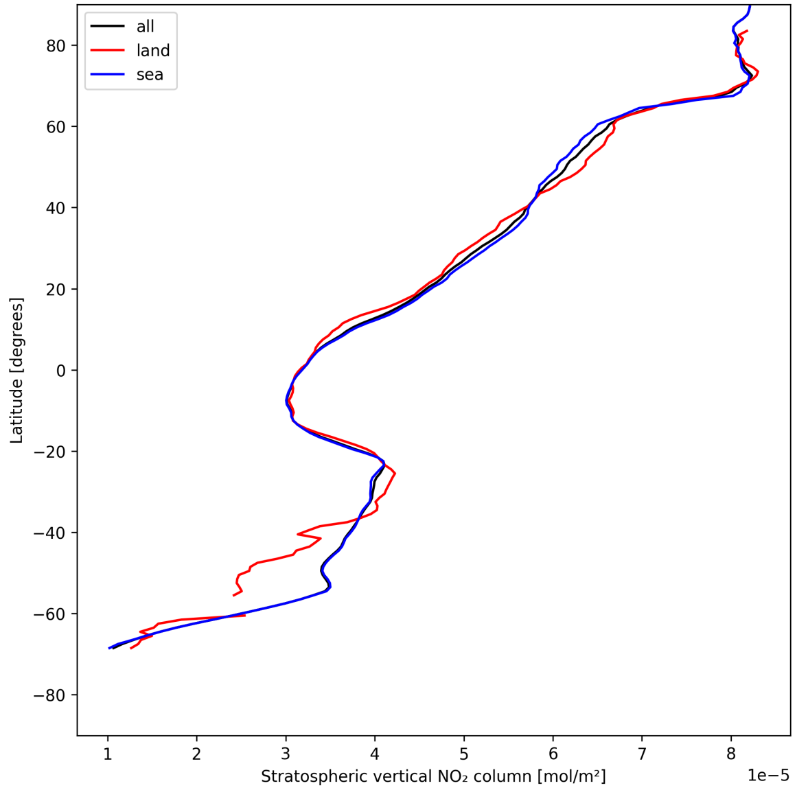
Figure 19: Zonal average of “Stratospheric vertical NO 2 column” for 2025-07-26 to 2025-07-28.
