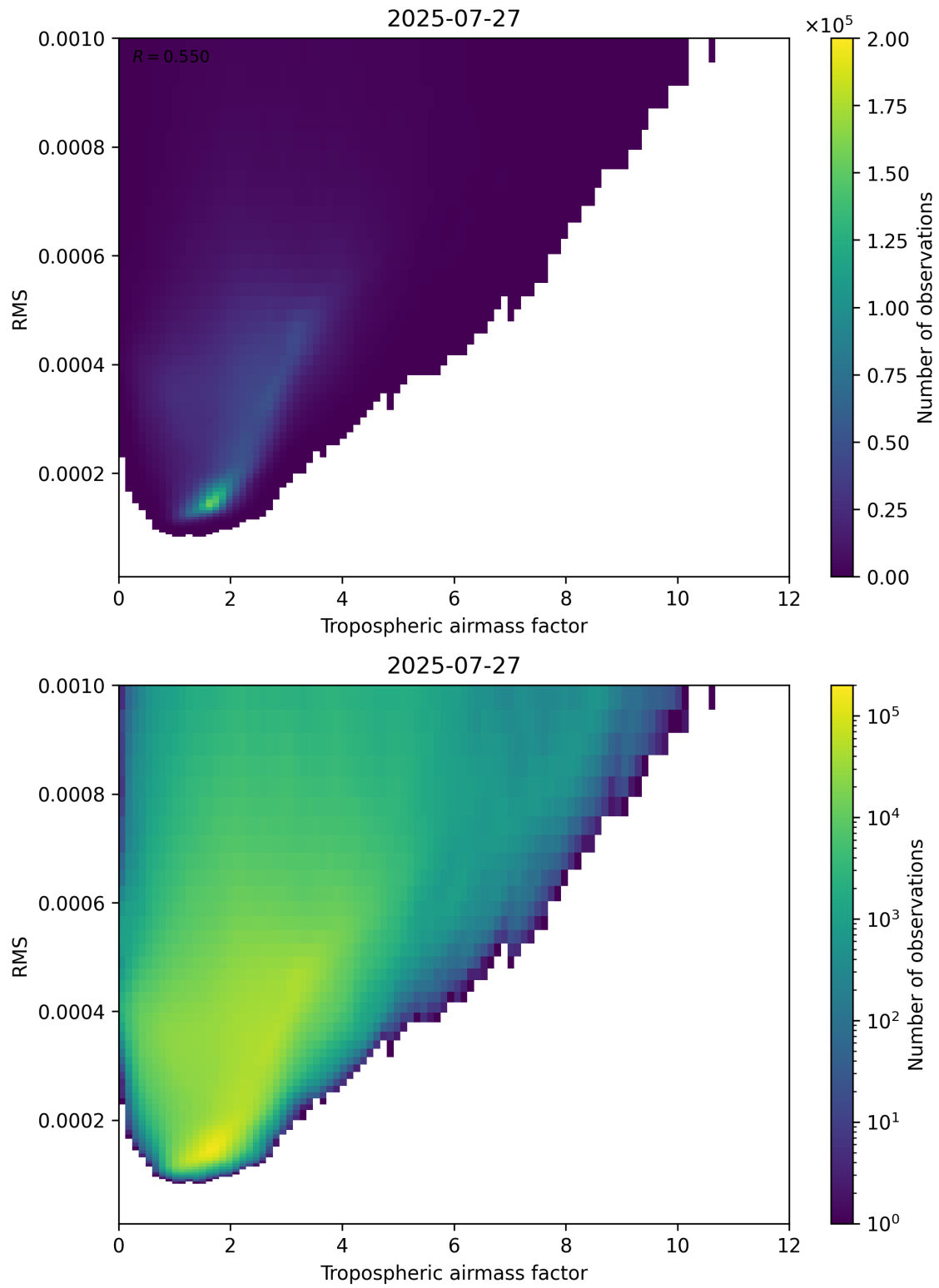
Figure 79: Scatter density plot of “Tropospheric airmass factor” against “RMS” for 2025-07-26 to 2025-07-28.
