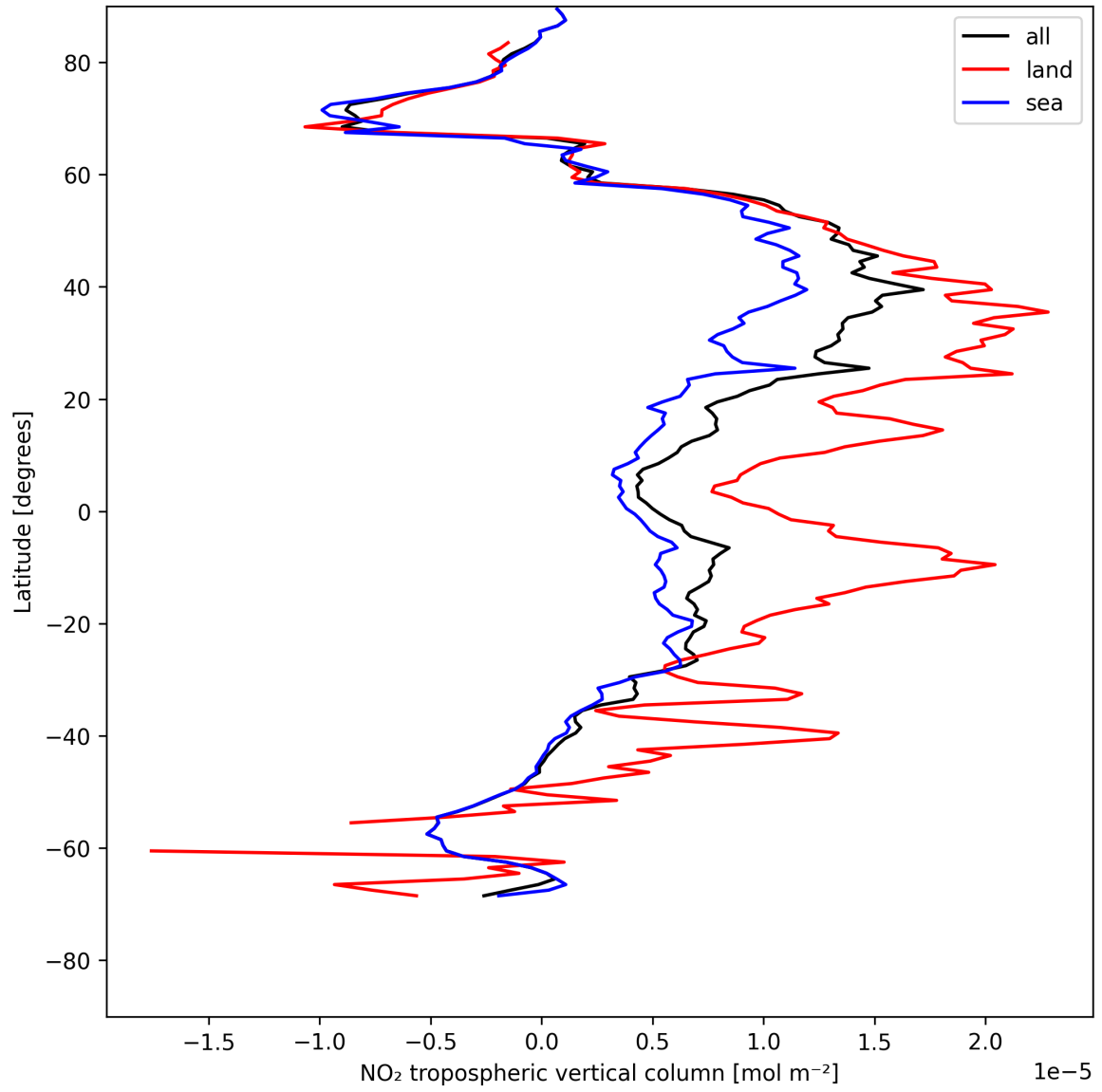
Figure 12: Zonal average of “NO 2 tropospheric vertical column” for 2025-07-26 to 2025-07-28.
