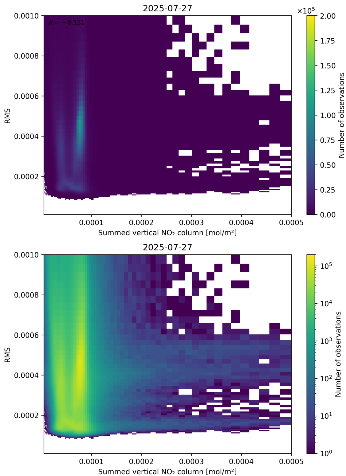
Figure 109: Scatter density plot of “Summed vertical NO 2 column” against “RMS” for 2025-07-26 to 2025-07-28.
