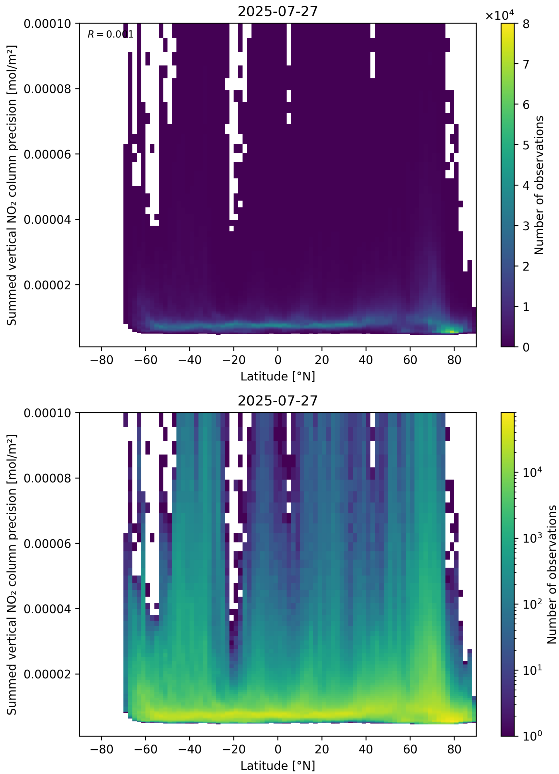
Figure 89: Scatter density plot of “Latitude” against “Summed vertical NO 2 column precision” for 2025-07-26 to 2025-07-28.
