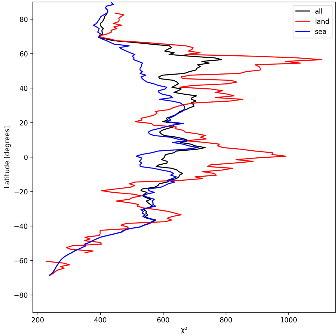
Figure 25: Zonal average of “ \chi^2 ” for 2025-07-26 to 2025-07-28.
