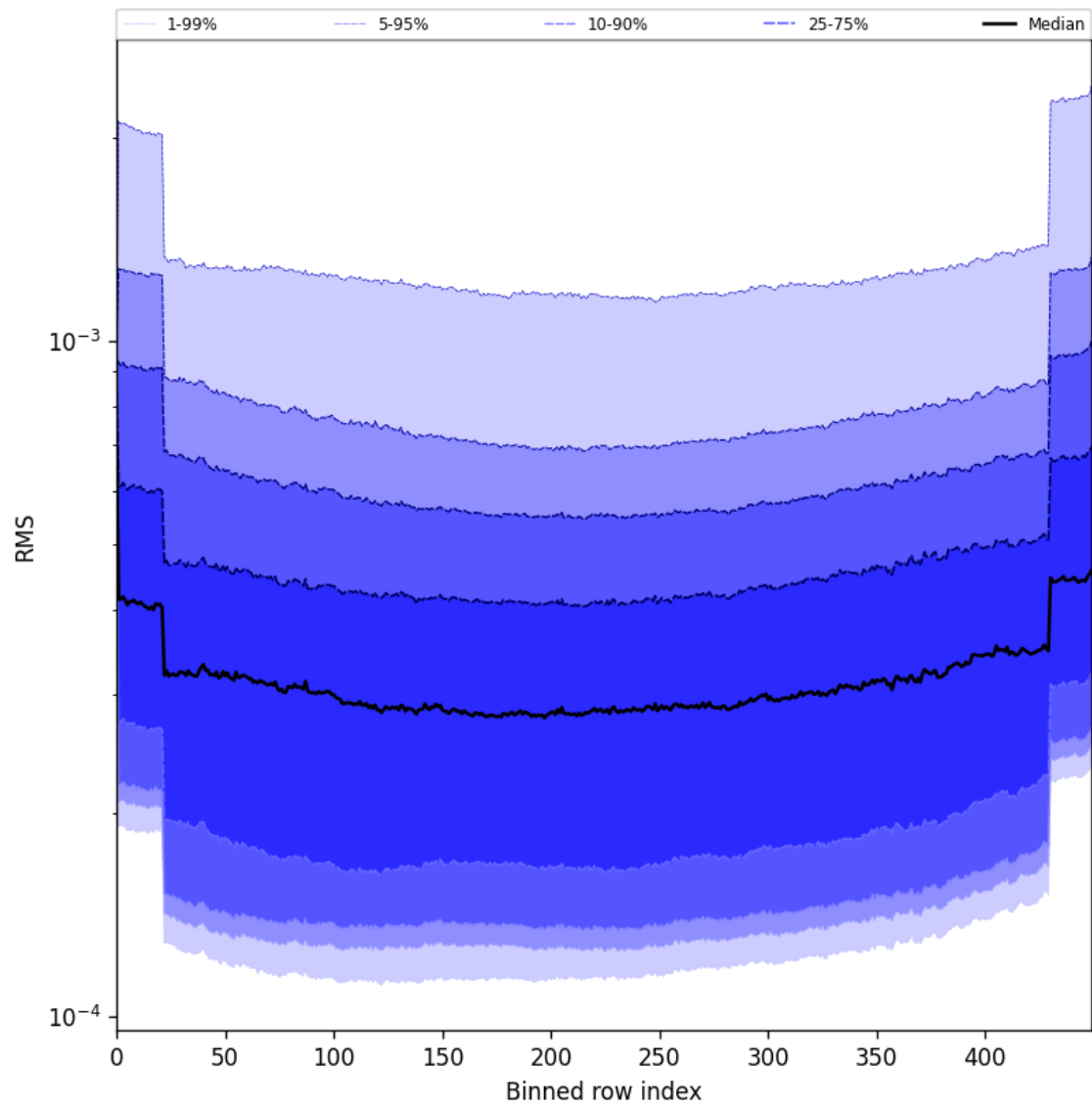
Figure 60: Along track statistics of “RMS” for 2025-07-26 to 2025-07-28
