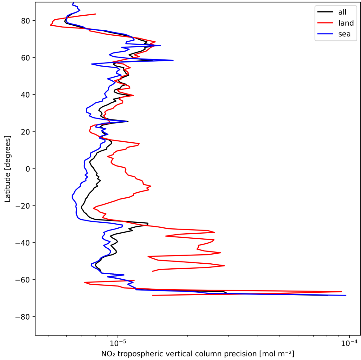
Figure 13: Zonal average of “NO 2 tropospheric vertical column precision” for 2025-07-26 to 2025-07-28.
