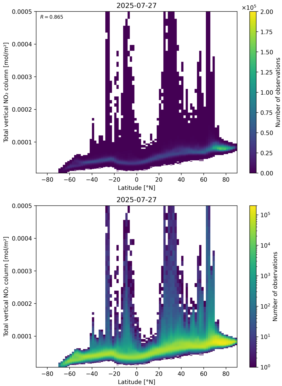
Figure 90: Scatter density plot of “Latitude” against “Total vertical NO 2 column” for 2025-07-26 to 2025-07-28.
