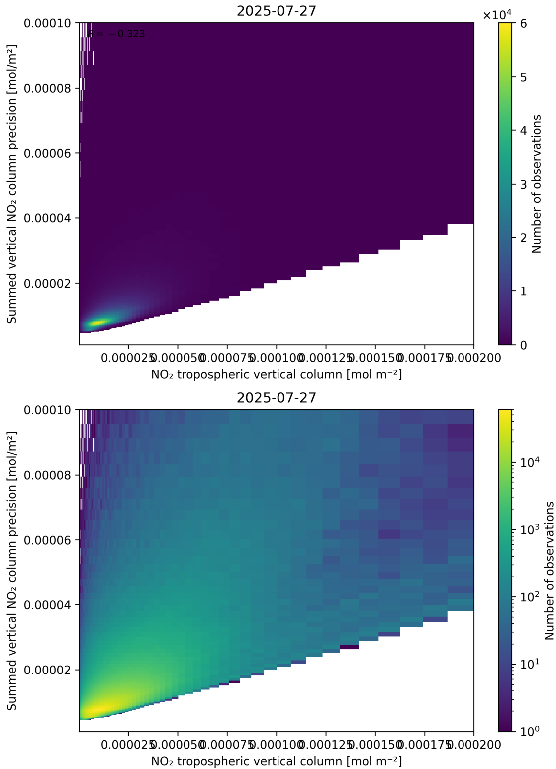
Figure 127: Scatter density plot of “NO 2 tropospheric vertical column” against “Summed vertical NO 2 column precision” for 2025-07-26 to 2025-07-28.
