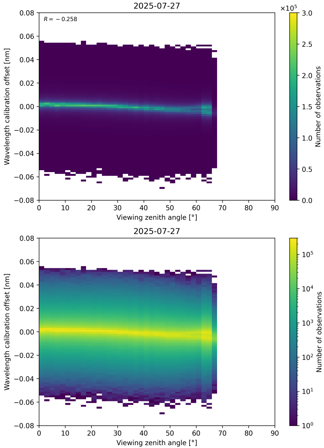
Figure 173: Scatter density plot of “Viewing zenith angle” against “Wavelength calibration offset” for 2025-07-26 to 2025-07-28.
