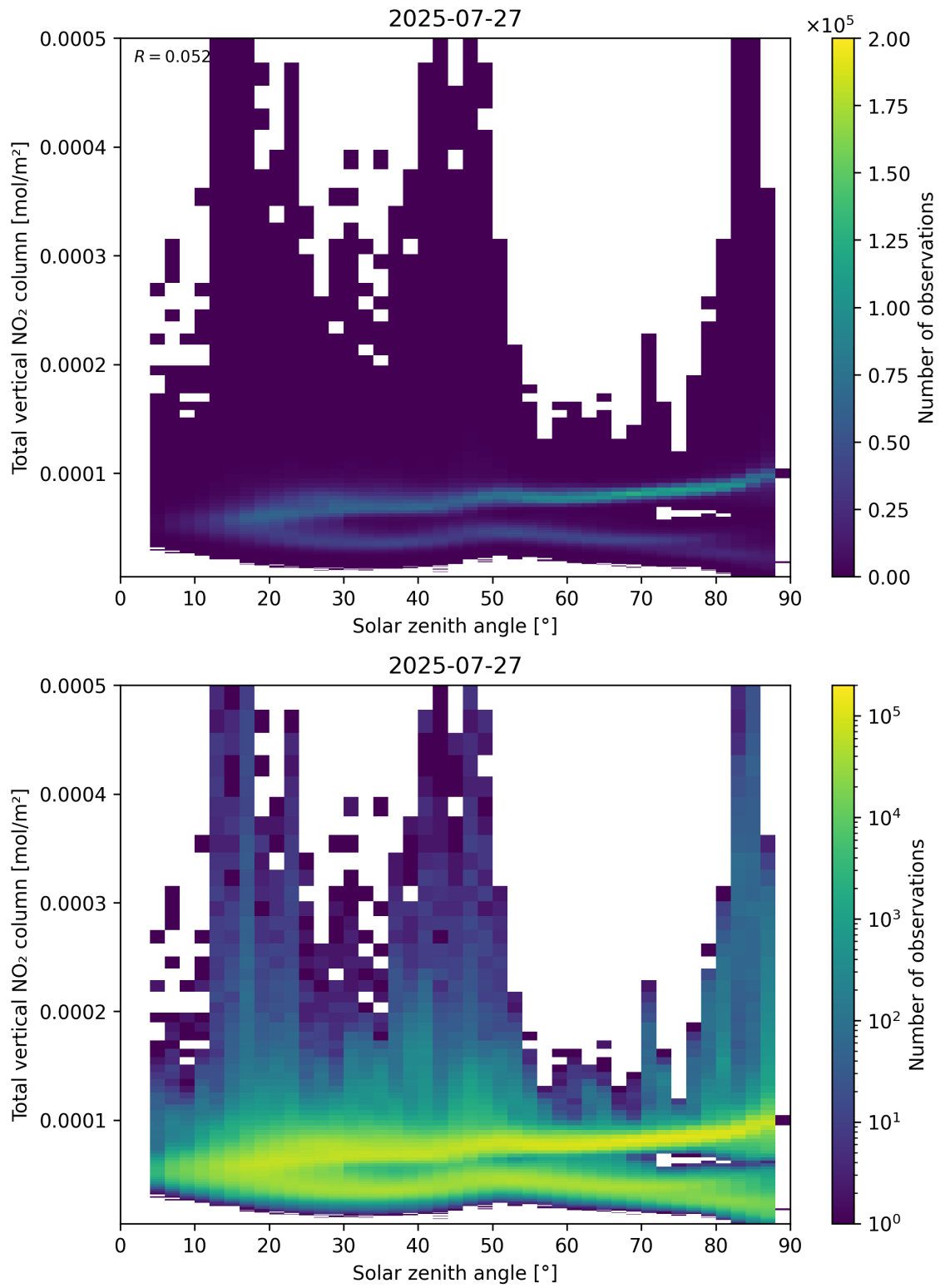
Figure 153: Scatter density plot of “Solar zenith angle” against “Total vertical NO 2 column” for 2025-07-26 to 2025-07-28.
