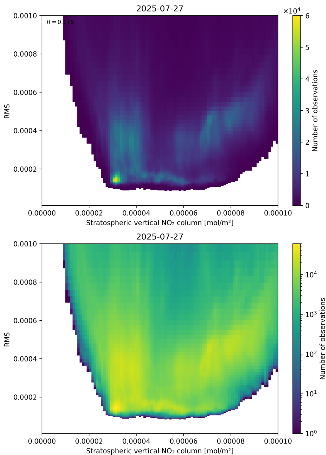
Figure 102: Scatter density plot of “Stratospheric vertical NO 2 column” against “RMS” for 2025-07-26 to 2025-07-28.
