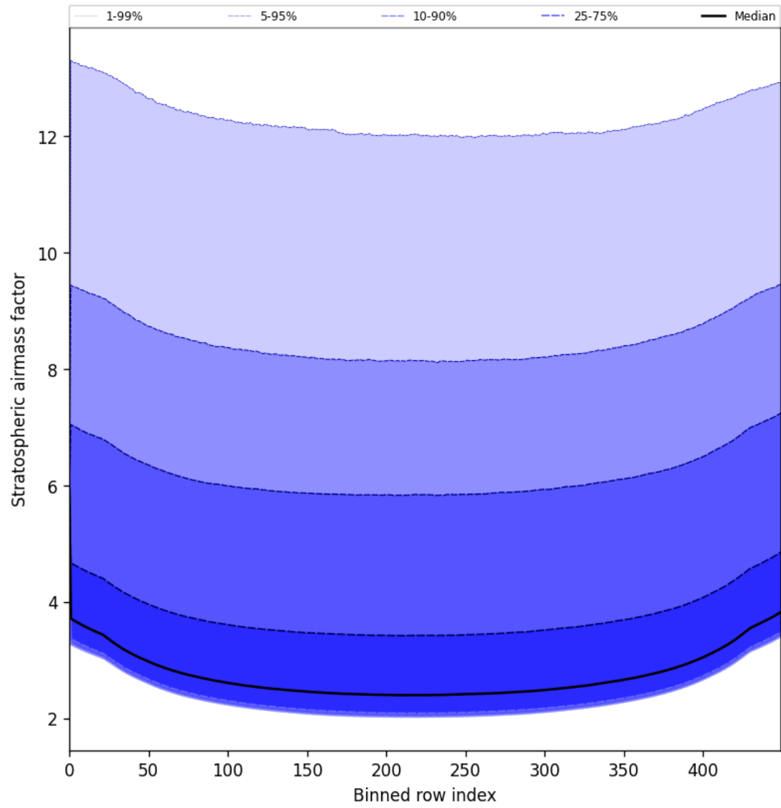
Figure 61: Along track statistics of “Stratospheric airmass factor” for 2025-07-26 to 2025-07-28
