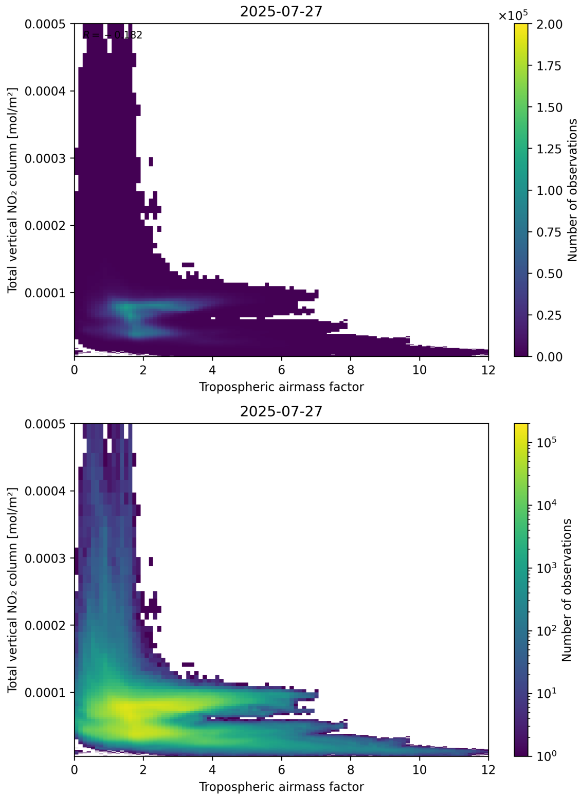
Figure 77: Scatter density plot of “Tropospheric airmass factor” against “Total vertical NO 2 column” for 2025-07-26 to 2025-07-28.
