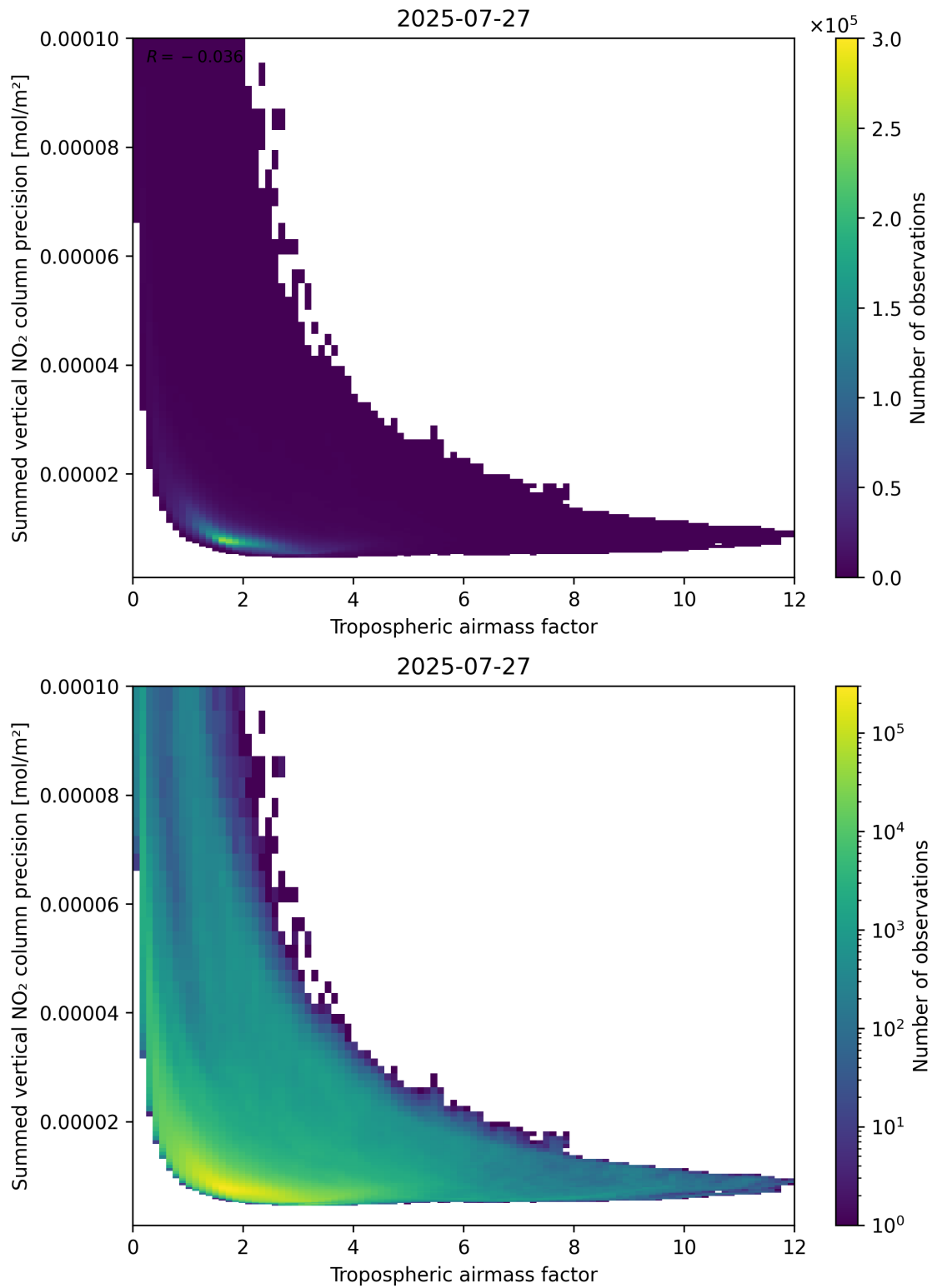
Figure 76: Scatter density plot of “Tropospheric air mass factor” against “Summed vertical NO 2 column precision” for 2025-07-26 to 2025-07-28.
