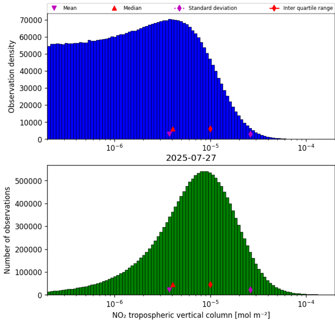
Figure 29: Histogram of “NO 2 tropospheric vertical column” for 2025-07-26 to 2025-07-28
