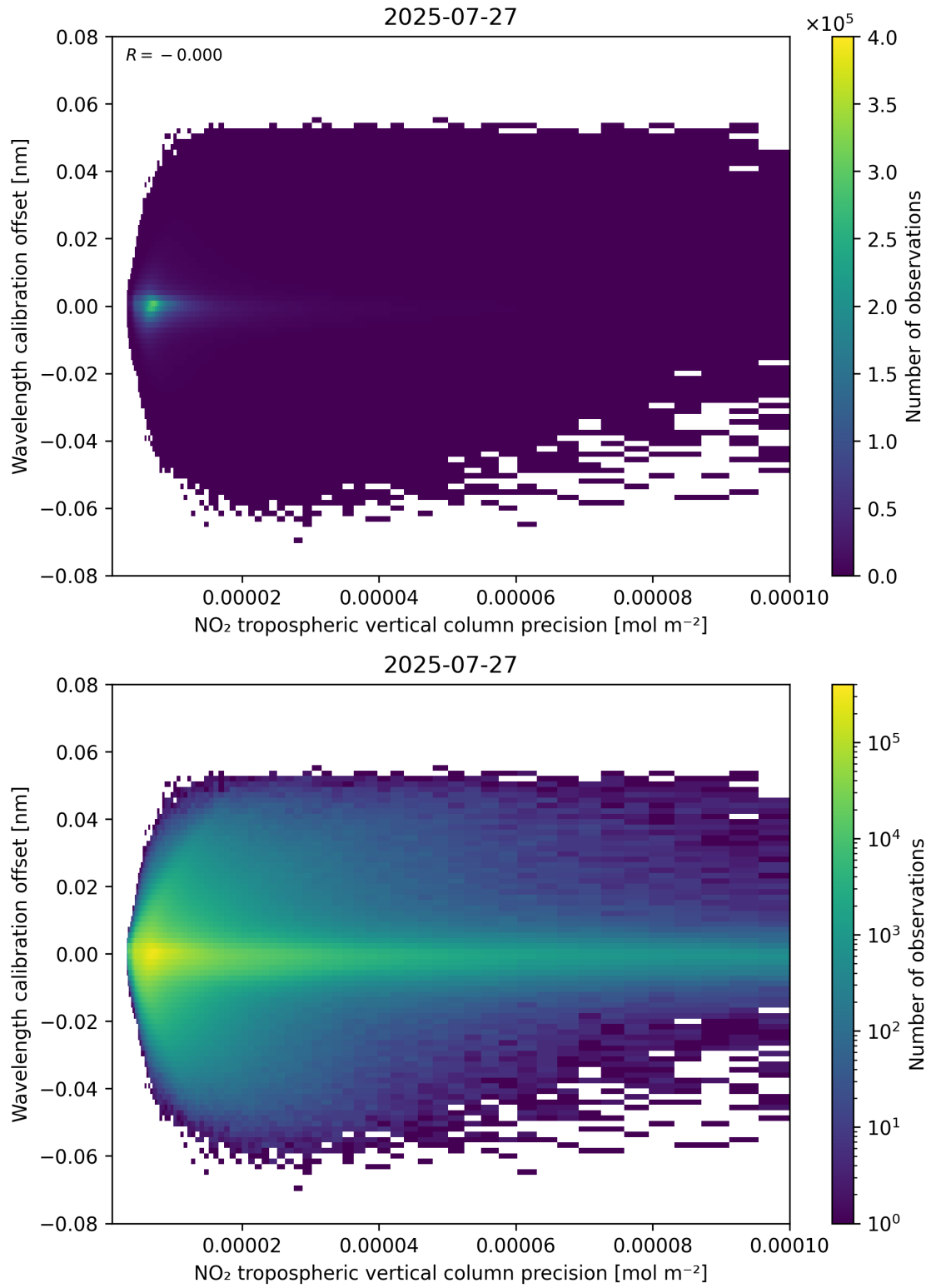
Figure 141: Scatter density plot of “NO 2 tropospheric vertical column precision” against “Wavelength calibration offset” for 2025-07-26 to 2025-07-28.
