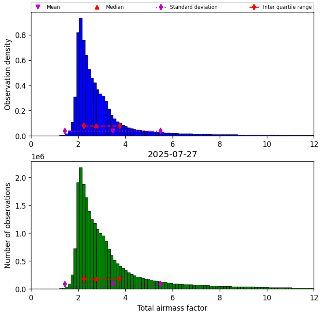
Figure 32: Histogram of “Total airmass factor” for 2025-07-26 to 2025-07-28
