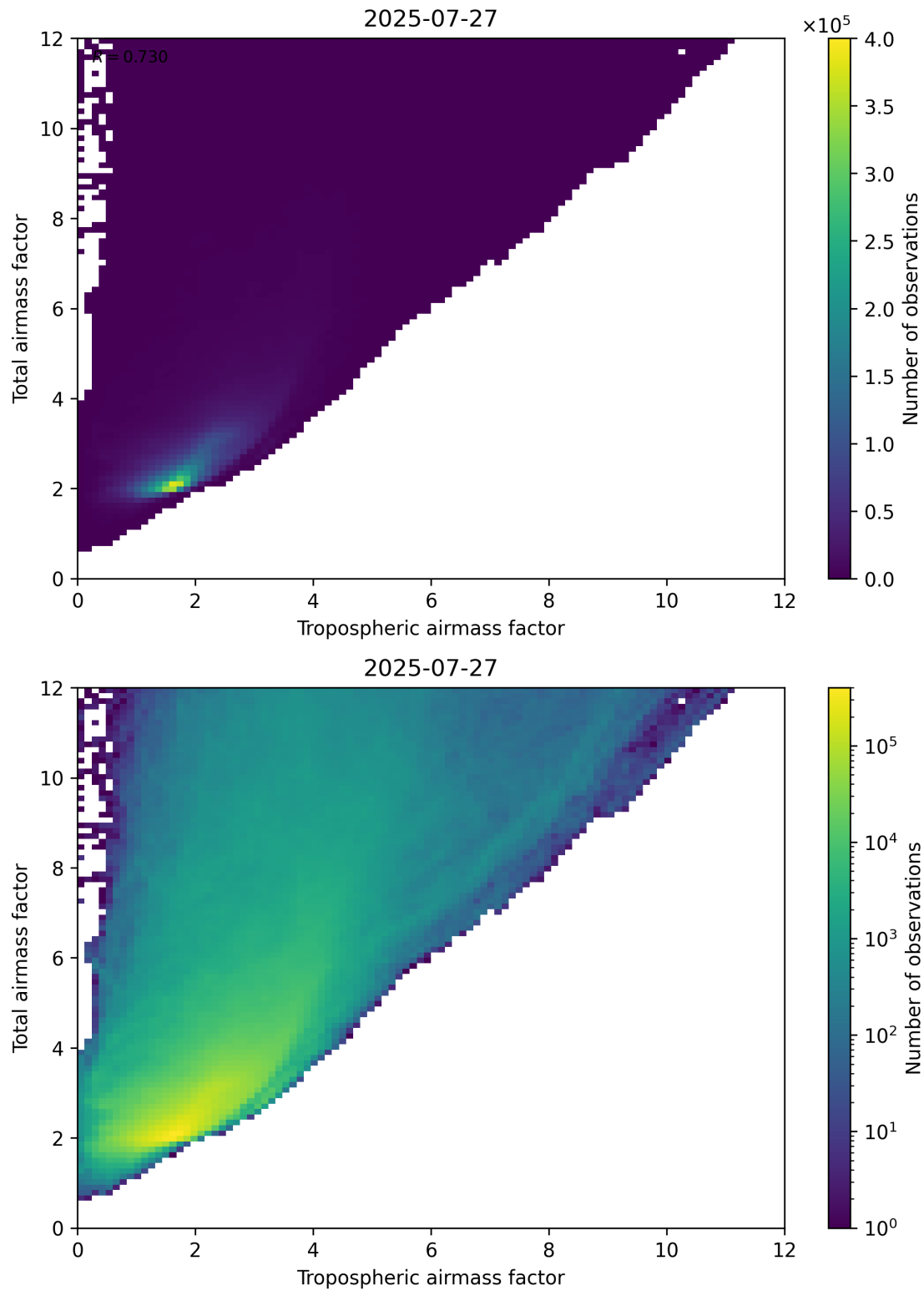
Figure 72: Scatter density plot of “Tropospheric airmass factor” against “Total airmass factor” for 2025-07-26 to 2025-07-28.
