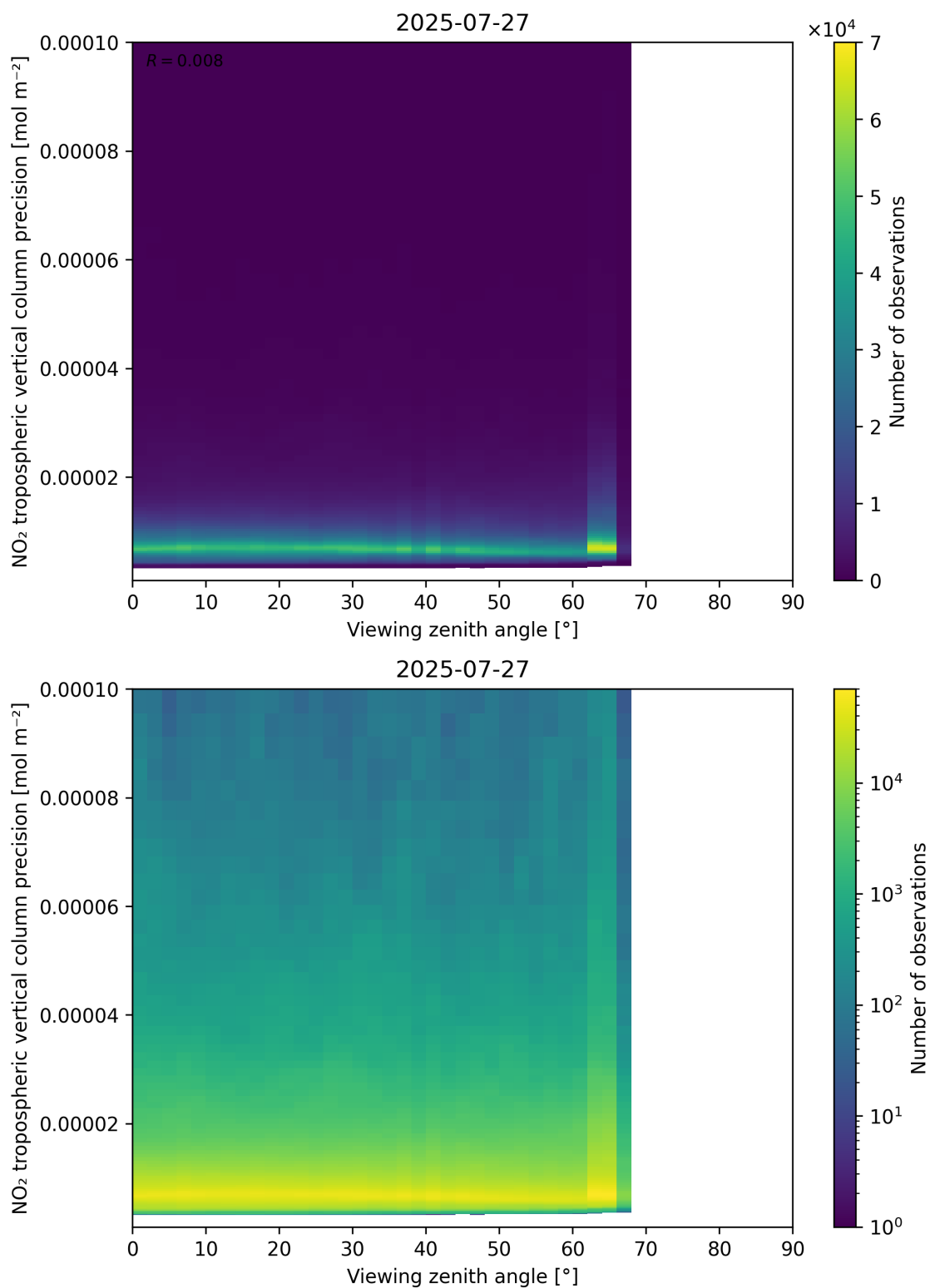
Figure 170: Scatter density plot of “Viewing zenith angle” against “NO 2 tropospheric vertical column precision” for 2025-07-26 to 2025-07-28.
