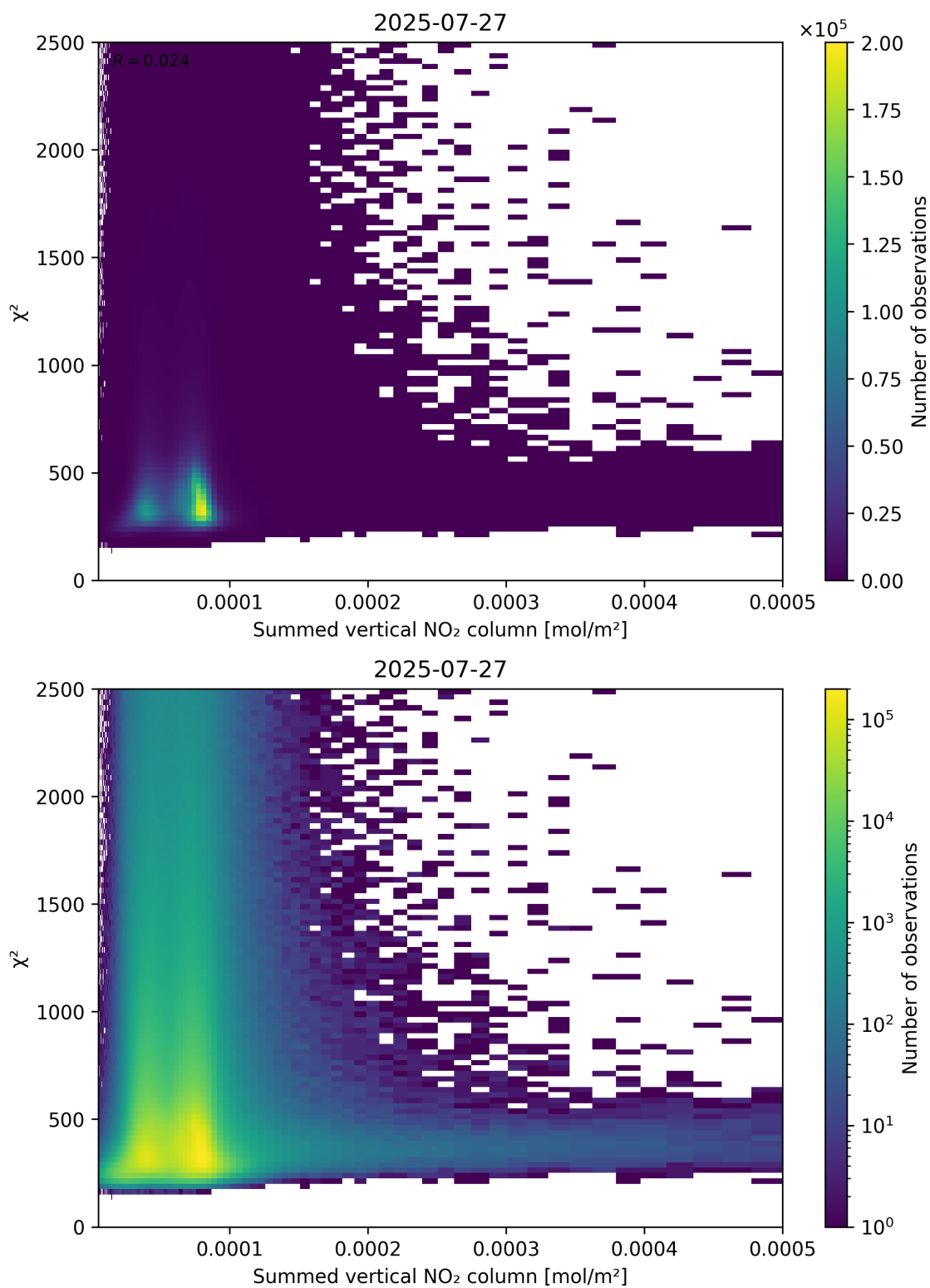
Figure 104: Scatter density plot of “Summed vertical NO 2 column” against “ \chi^2 ” for 2025-07-26 to 2025-07-28.
