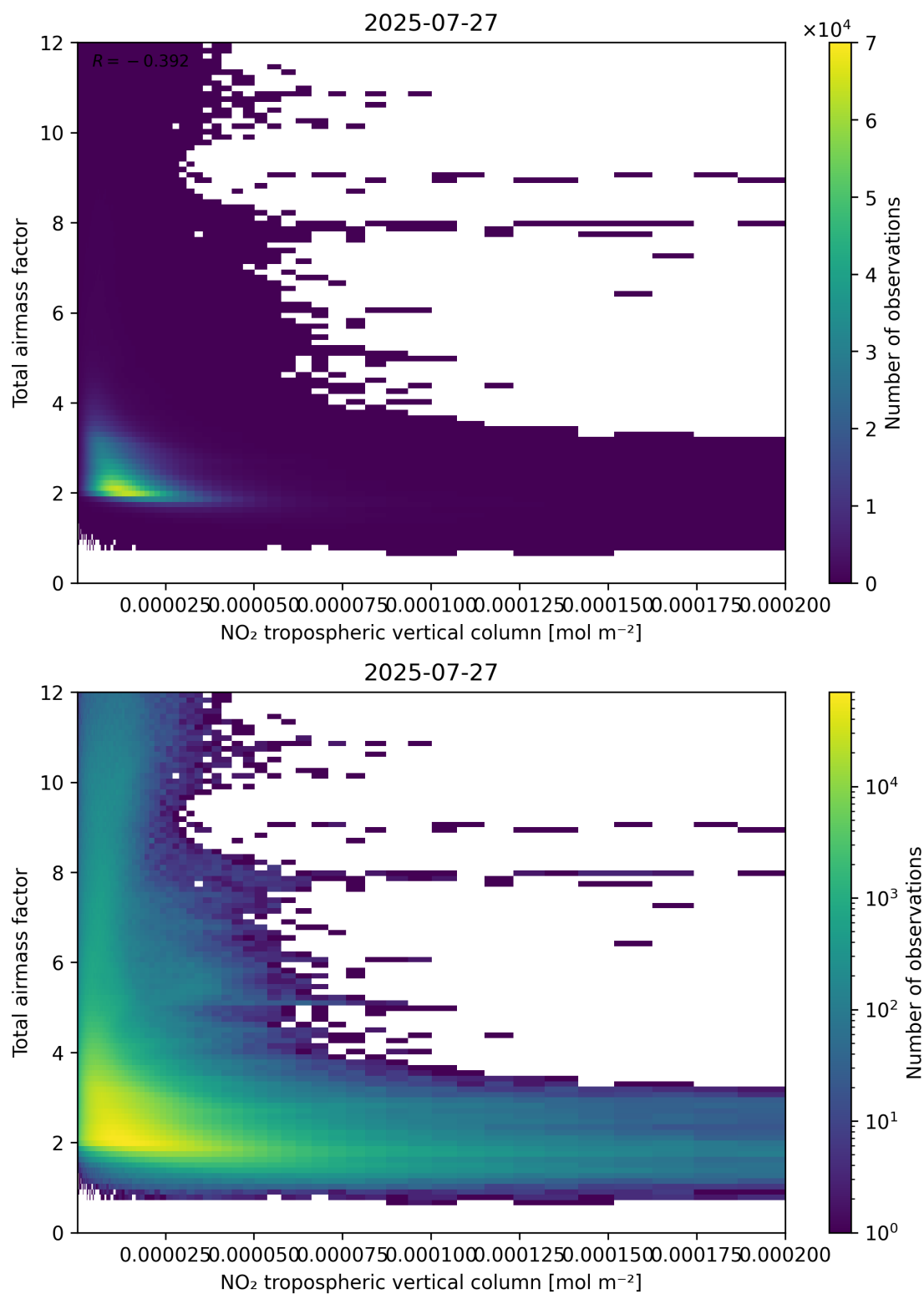
Figure 122: Scatter density plot of “NO 2 tropospheric vertical column” against “Total air mass factor” for 2025-07-26 to 2025-07-28.
