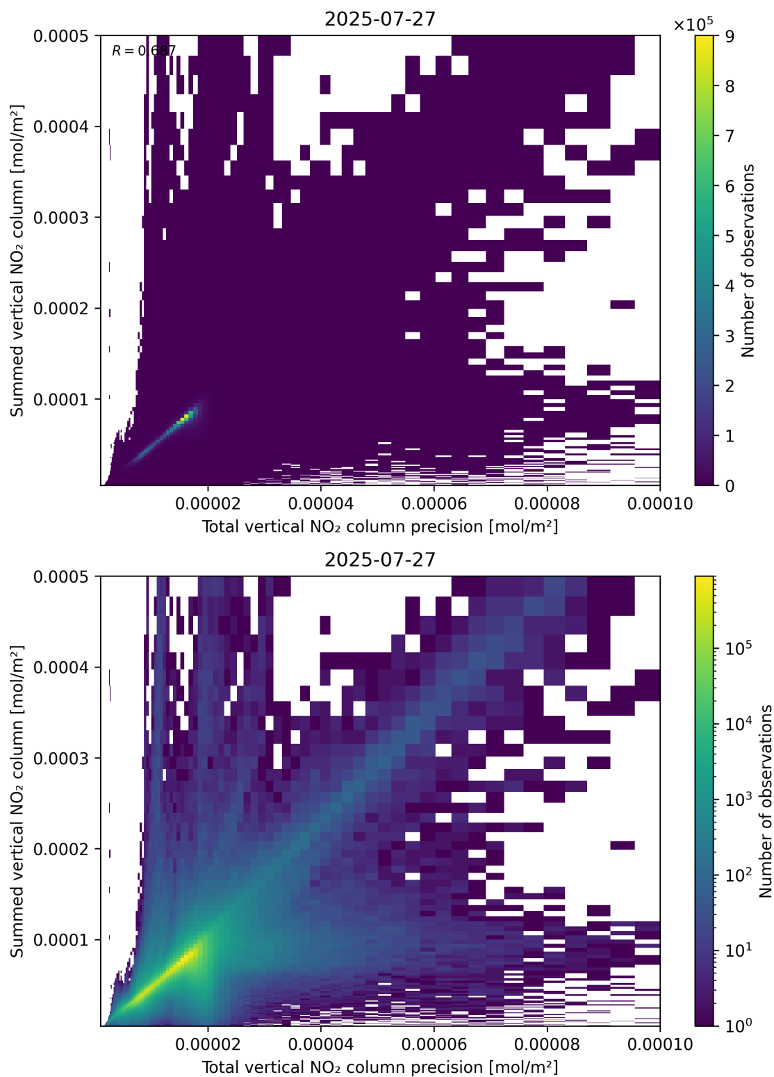
Figure 117: Scatter density plot of “Total vertical NO 2 column precision” against “Summed vertical NO 2 column” for 2025-07-26 to 2025-07-28.
