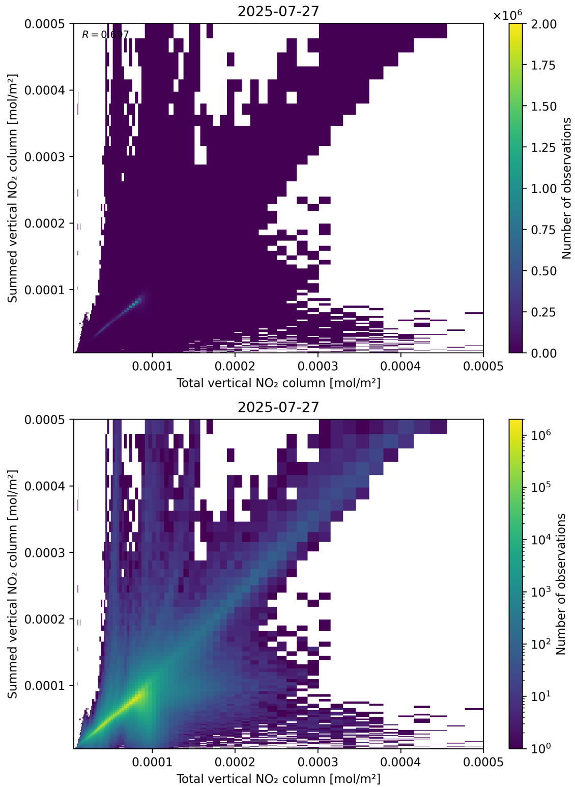
Figure 112: Scatter density plot of “Total vertical NO 2 column” against “Summed vertical NO 2 column” for 2025-07-26 to 2025-07-28.
