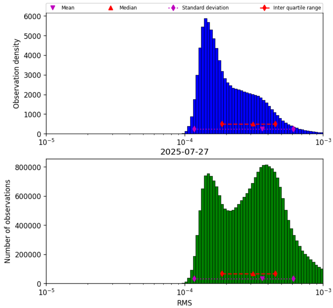
Figure 43: Histogram of “RMS” for 2025-07-26 to 2025-07-28
