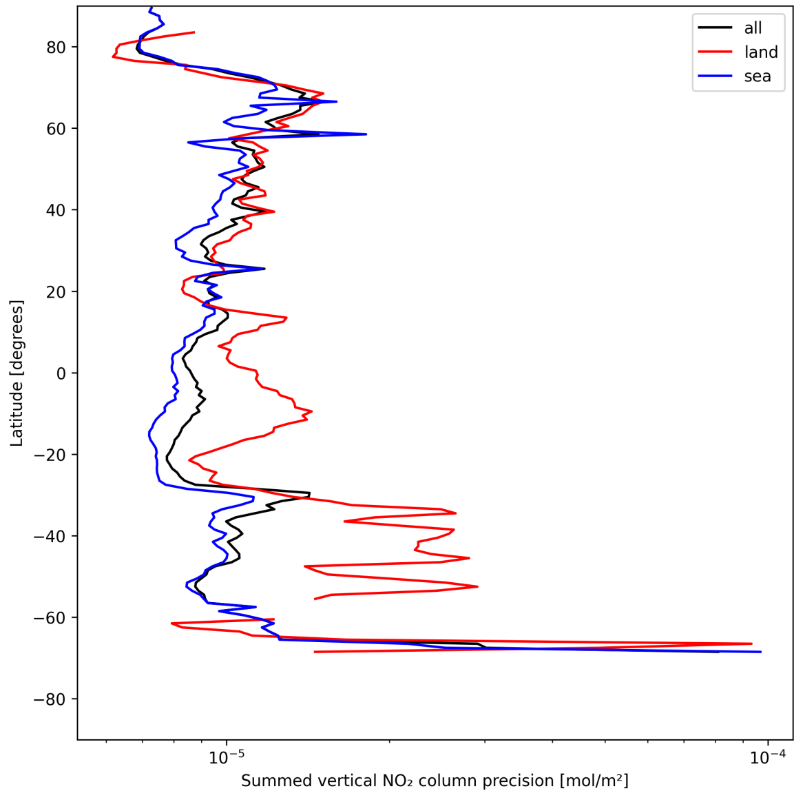
Figure 24: Zonal average of “Summed vertical NO 2 column precision” for 2025-07-26 to 2025-07-28.
