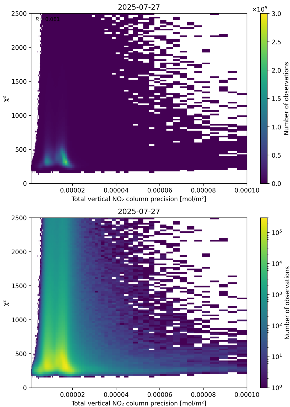
Figure 116: Scatter density plot of “Total vertical NO 2 column precision” against “ \chi^2 ” for 2025-07-26 to 2025-07-28.
