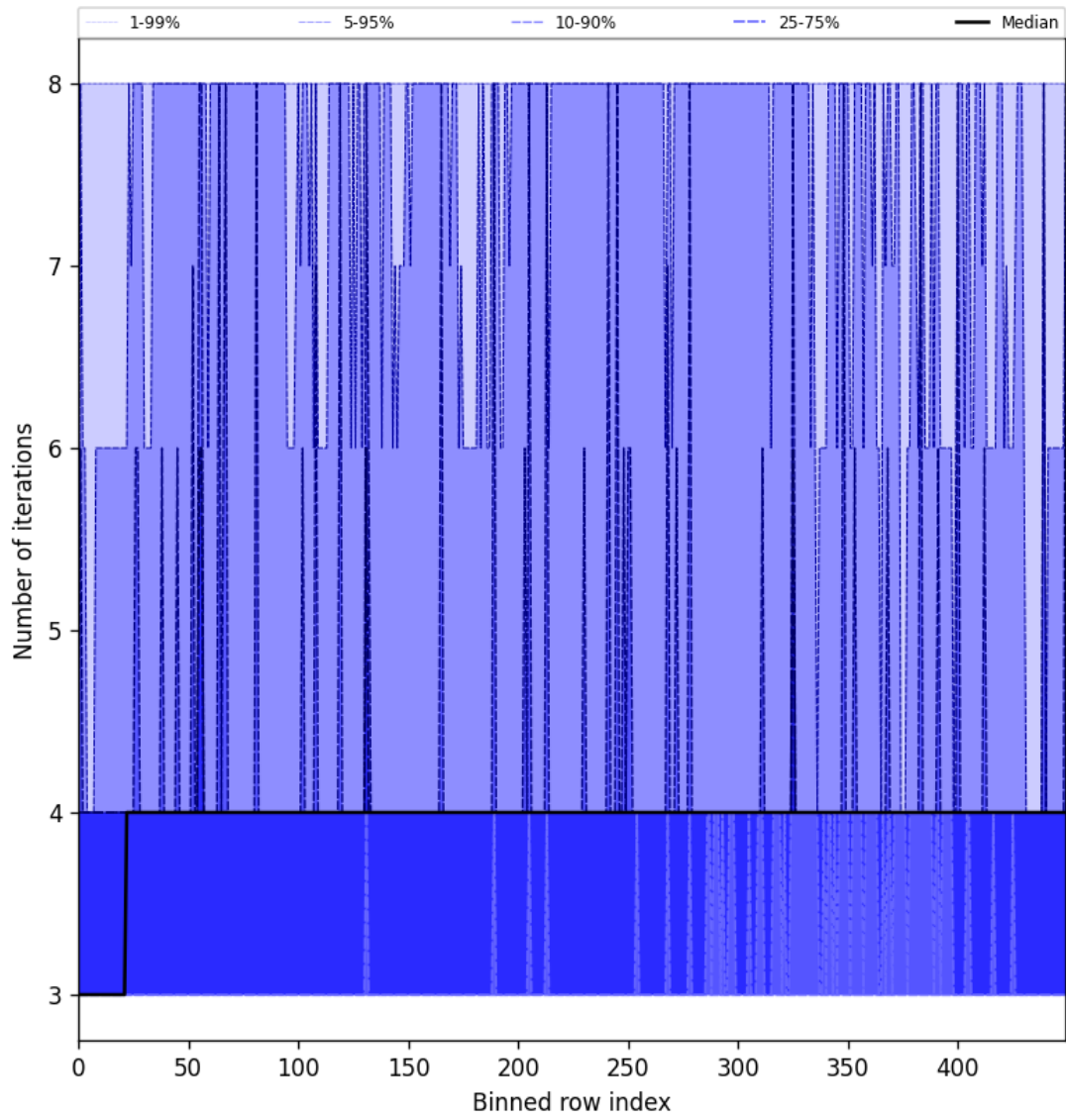
Figure 51: Along track statistics of “Number of iterations” for 2025-07-26 to 2025-07-28
