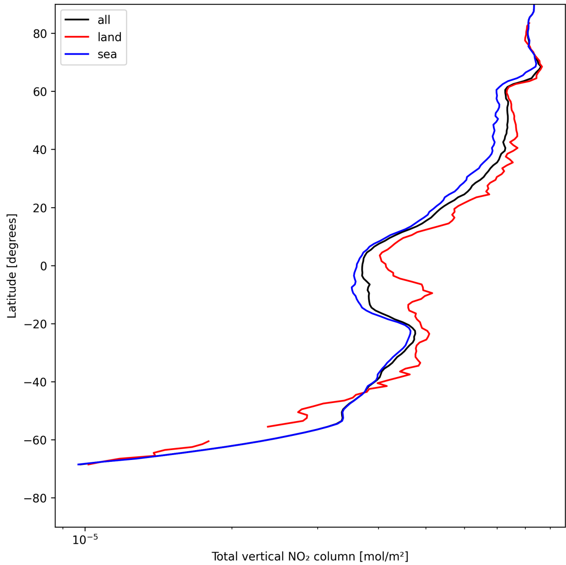
Figure 21: Zonal average of “Total vertical NO 2 column” for 2025-07-26 to 2025-07-28.
