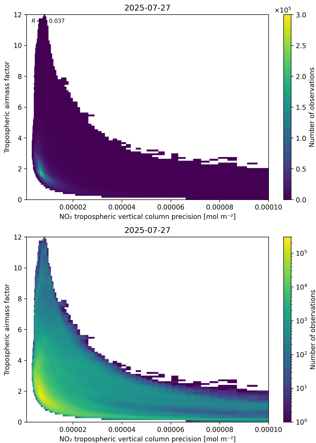
Figure 133: Scatter density plot of “NO 2 tropospheric vertical column precision” against “Tropospheric air mass factor” for 2025-07-26 to 2025-07-28.
