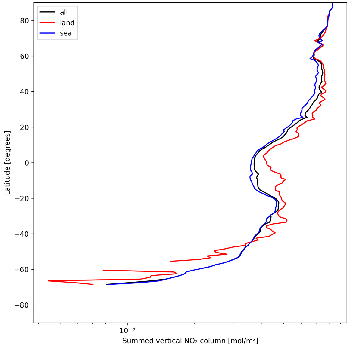
Figure 23: Zonal average of “Summed vertical NO 2 column” for 2025-07-26 to 2025-07-28.
