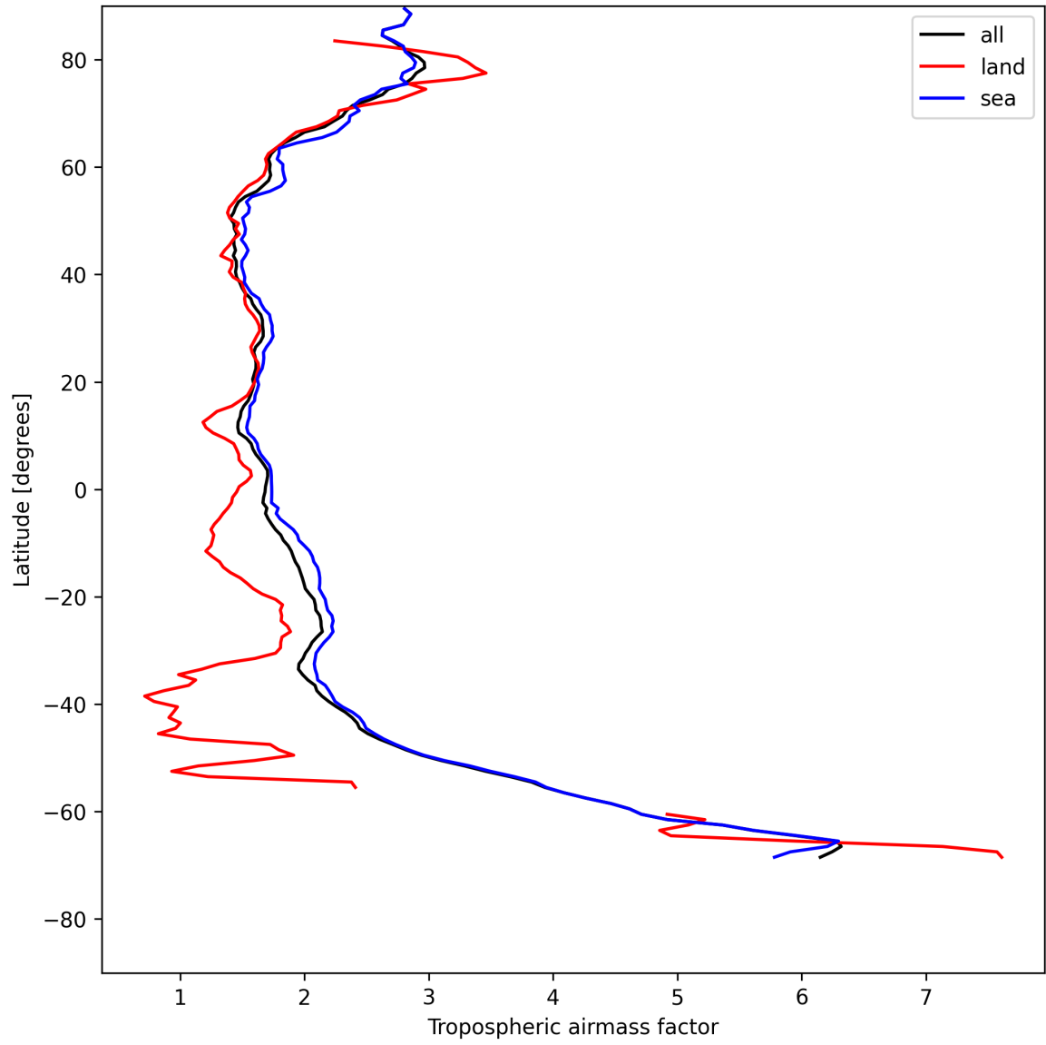
Figure 14: Zonal average of “Tropospheric air mass factor” for 2025-07-26 to 2025-07-28.
