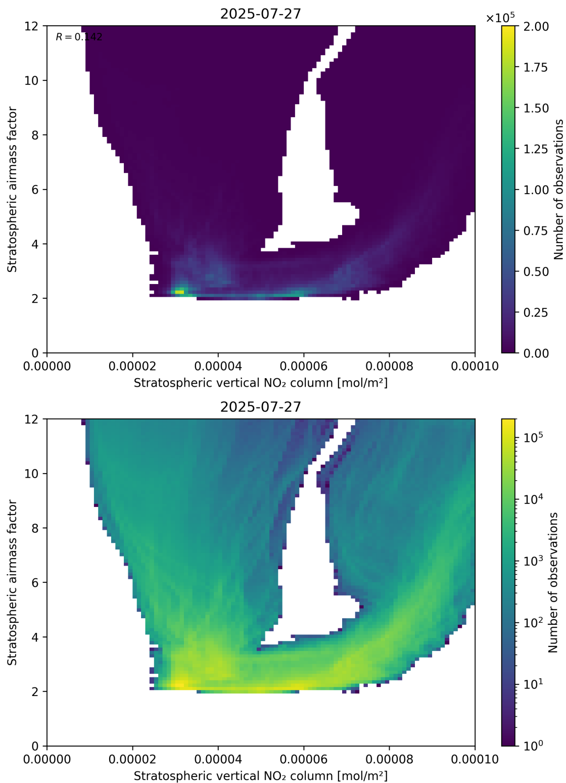
Figure 96: Scatter density plot of “Stratospheric vertical NO 2 column” against “Stratospheric airmass factor” for 2025-07-26 to 2025-07-28.
