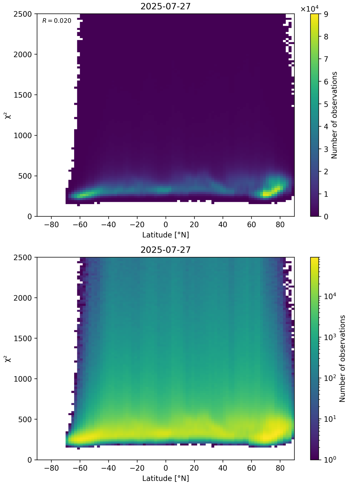
Figure 86: Scatter density plot of “Latitude” against “ \chi^2 ” for 2025-07-26 to 2025-07-28.
