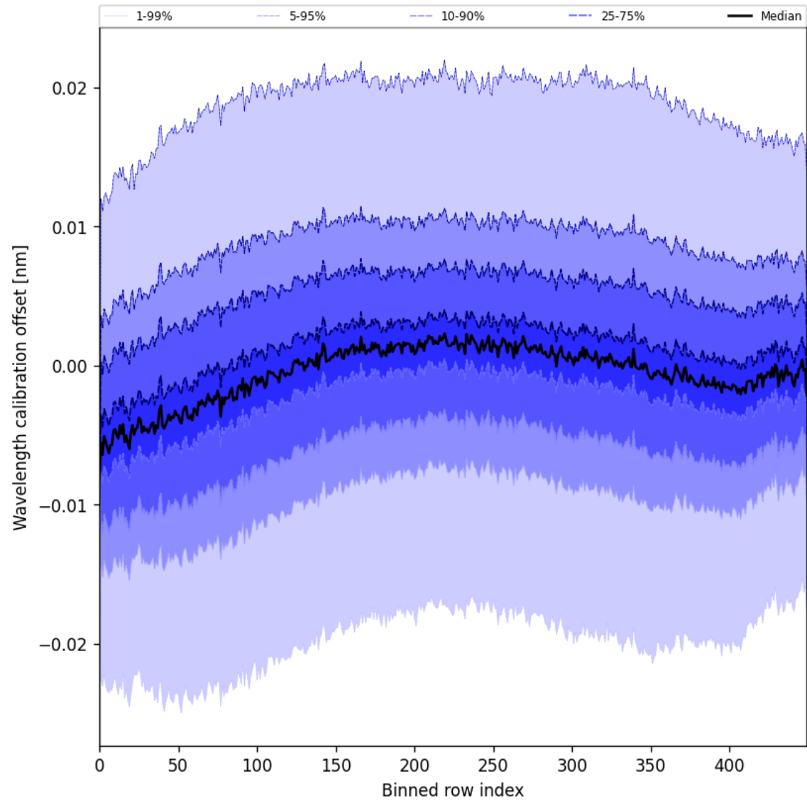
Figure 52: Along track statistics of “Wavelength calibration offset” for 2025-07-26 to 2025-07-28
