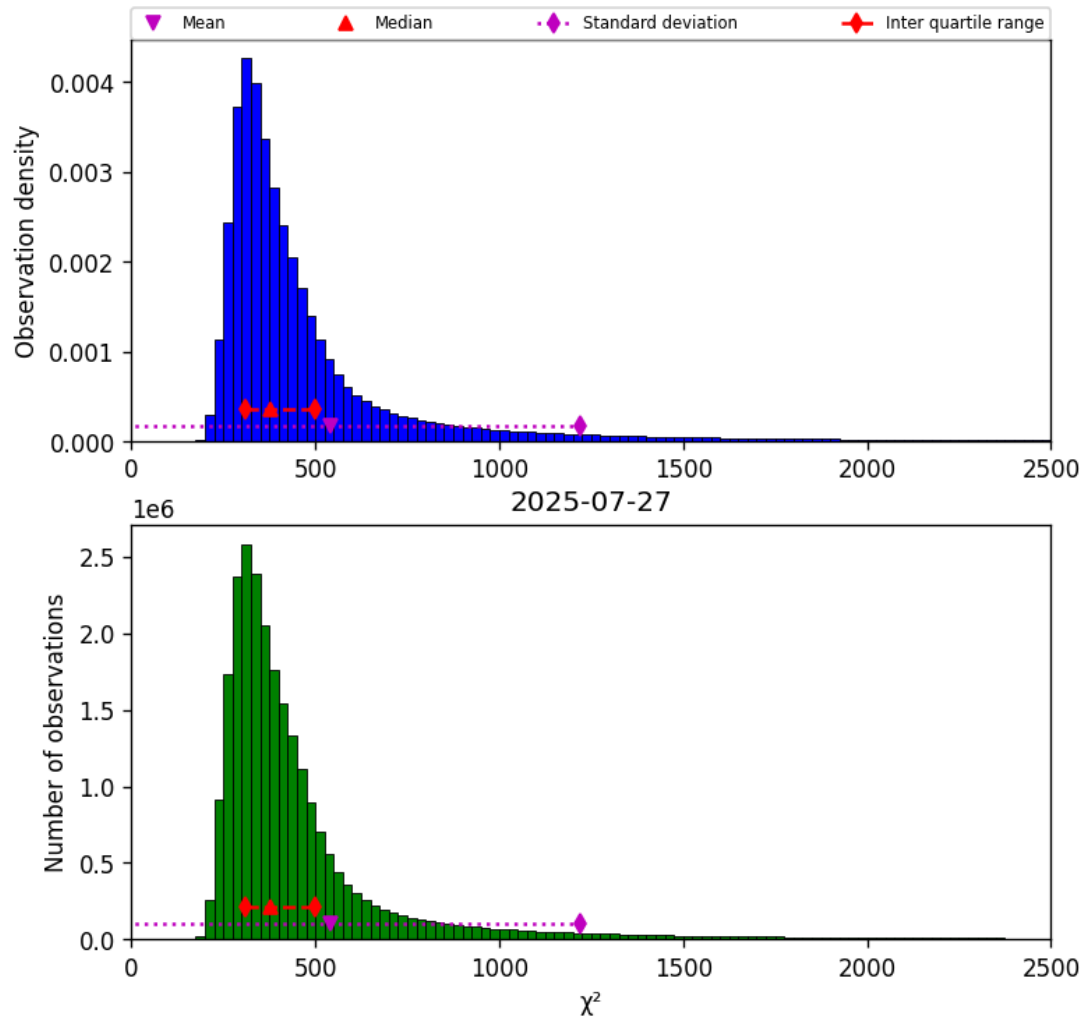
Figure 42: Histogram of “ \chi^2 ” for 2025-07-26 to 2025-07-28
