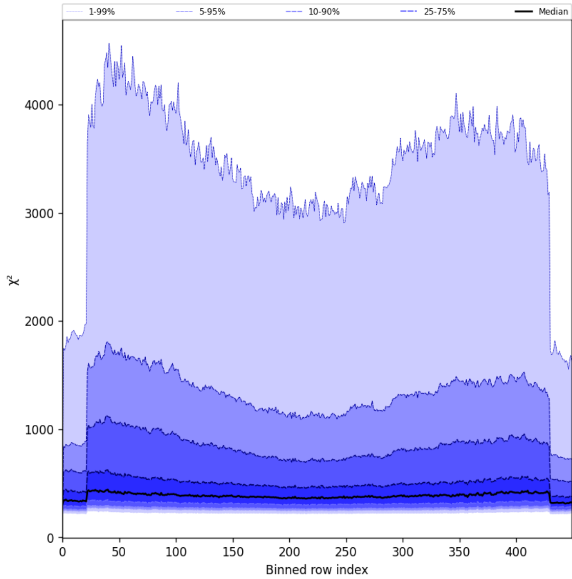
Figure 59: Along track statistics of “ \chi^2 ” for 2025-07-26 to 2025-07-28
