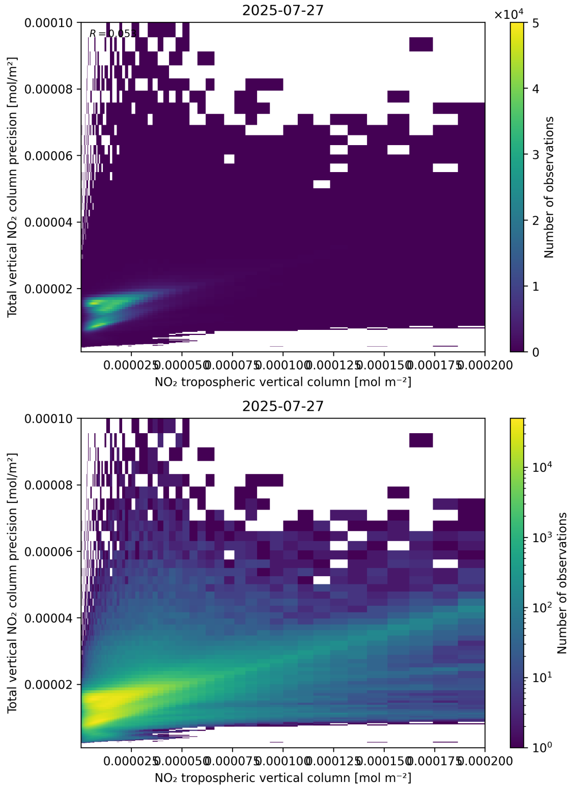
Figure 129: Scatter density plot of “NO 2 tropospheric vertical column” against “Total vertical NO 2 column precision” for 2025-07-26 to 2025-07-28.
