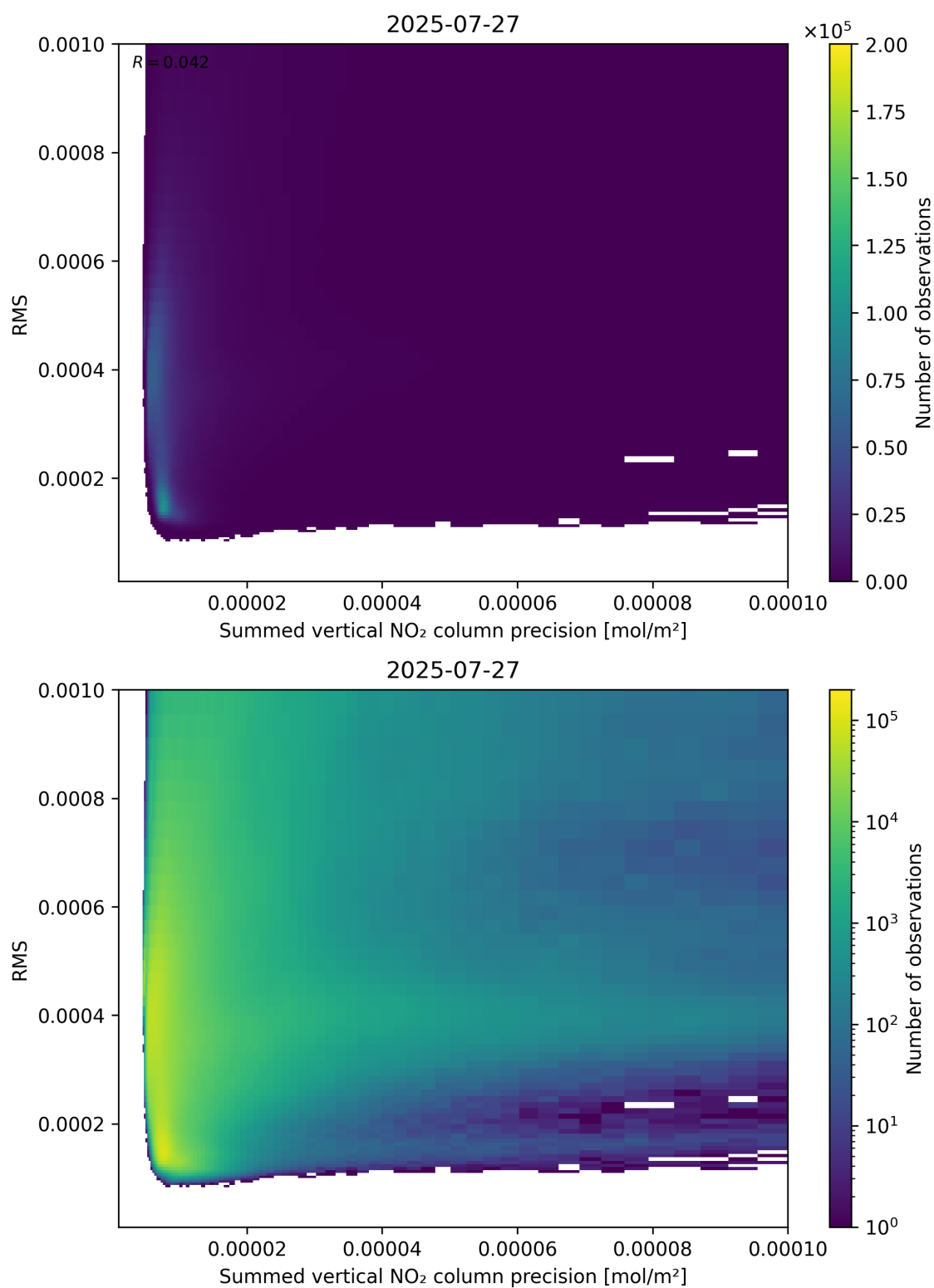
Figure 108: Scatter density plot of “Summed vertical NO 2 column precision” against “RMS” for 2025-07-26 to 2025-07-28.
