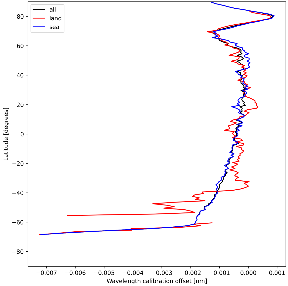
Figure 18: Zonal average of “Wavelength calibration offset” for 2025-07-26 to 2025-07-28.
