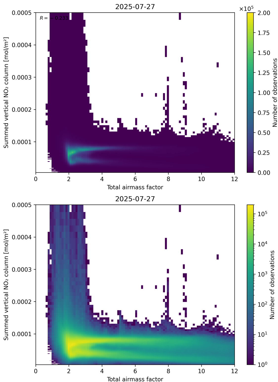
Figure 65: Scatter density plot of “Total airmass factor” against “Summed vertical NO 2 column” for 2025-07-26 to 2025-07-28.
