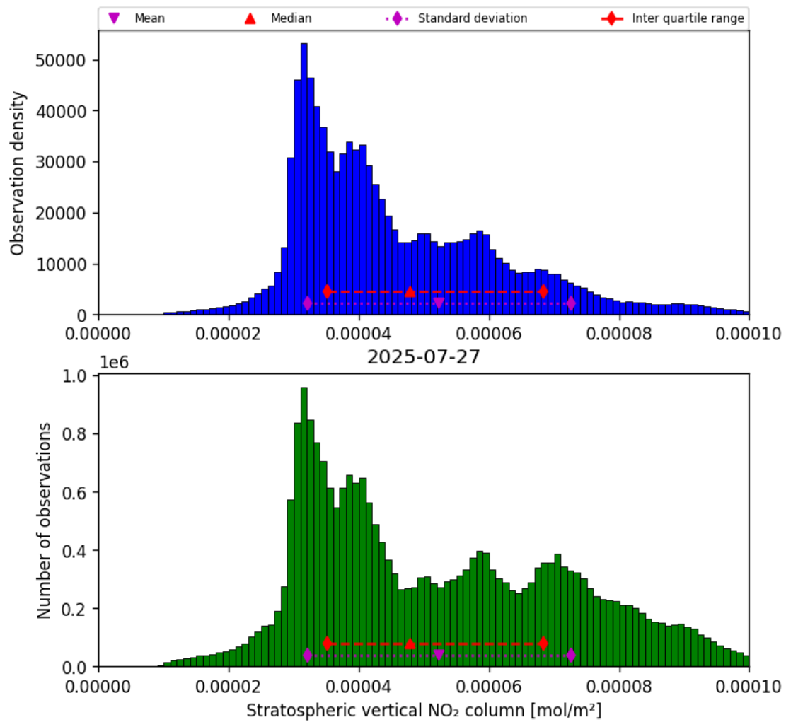
Figure 36: Histogram of “Stratospheric vertical NO 2 column” for 2025-07-26 to 2025-07-28
