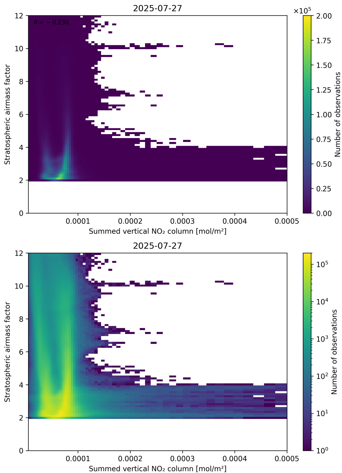
Figure 103: Scatter density plot of “Summed vertical NO 2 column” against “Stratospheric air mass factor” for 2025-07-26 to 2025-07-28.
