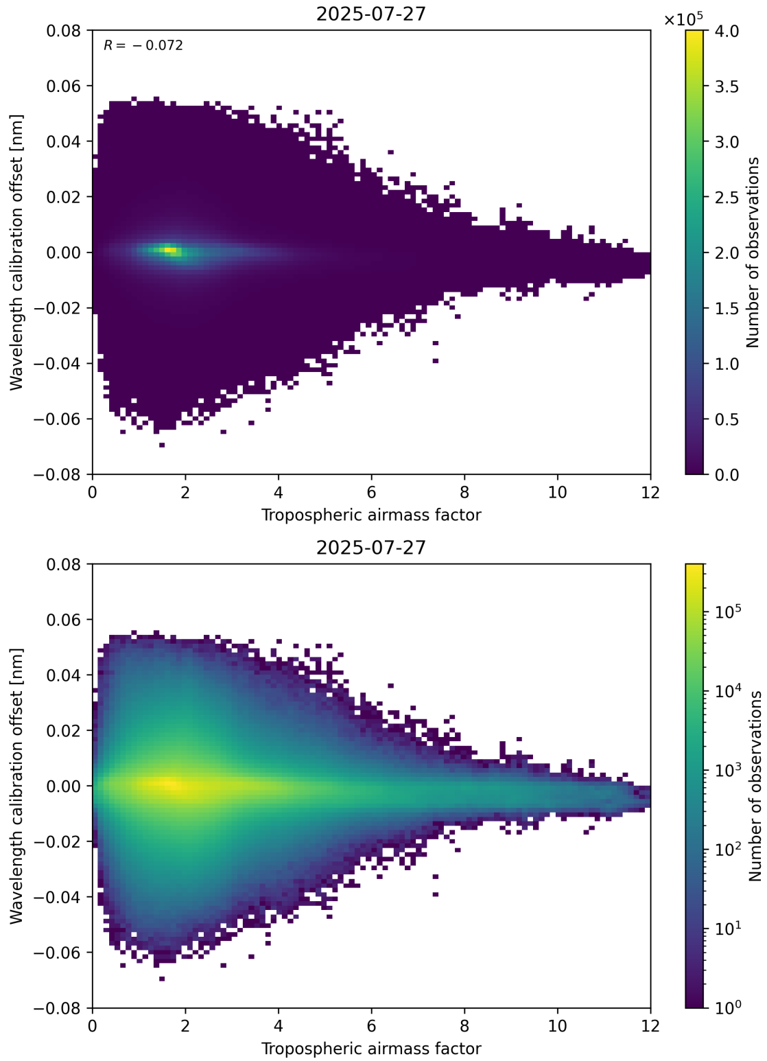
Figure 80: Scatter density plot of “Tropospheric air mass factor” against “Wavelength calibration offset” for 2025-07-26 to 2025-07-28.
