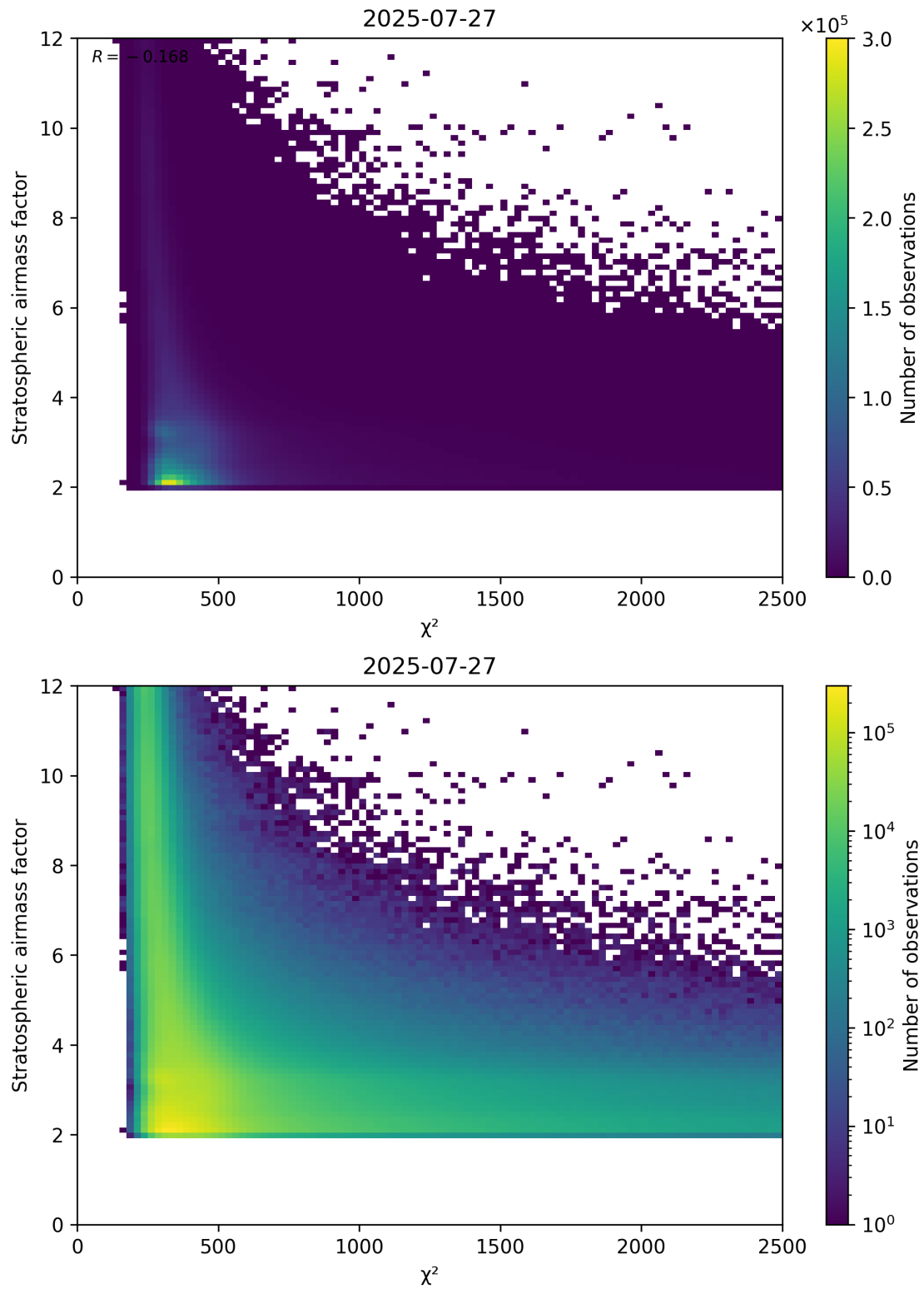
Figure 81: Scatter density plot of “ \chi^2 ” against “Stratospheric airmass factor” for 2025-07-26 to 2025-07-28.
