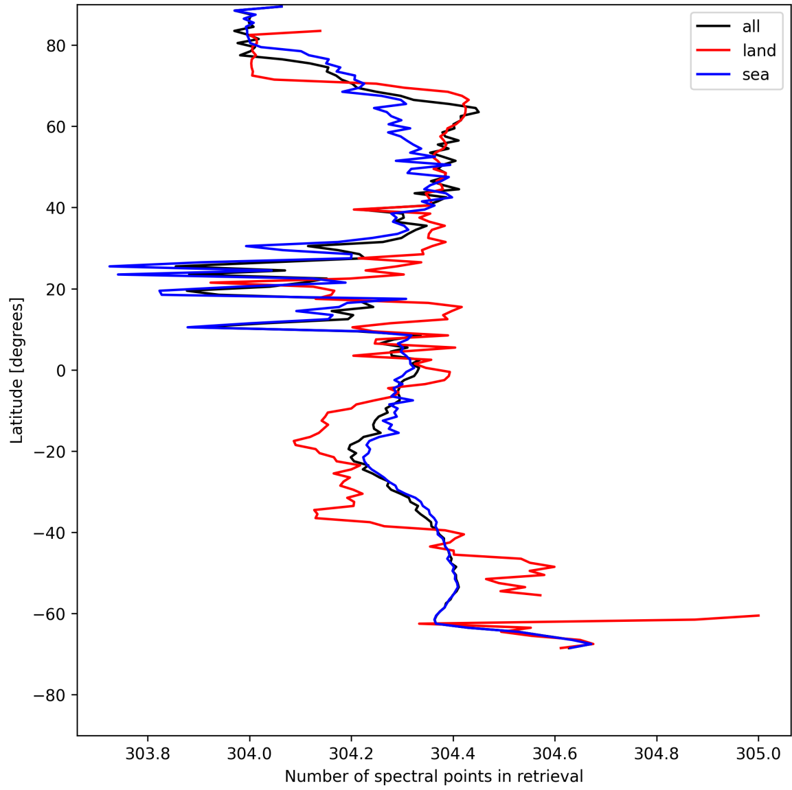
Figure 16: Zonal average of “Number of spectral points in retrieval” for 2025-07-26 to 2025-07-28.
