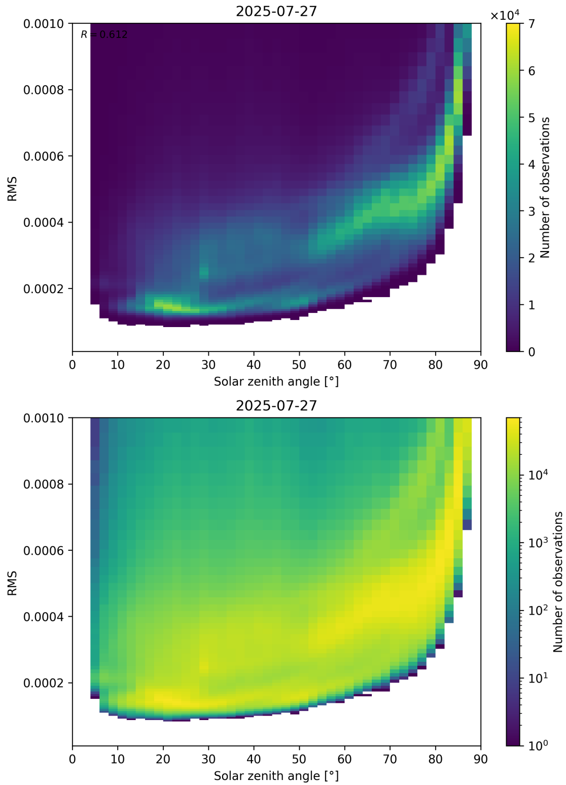
Figure 157: Scatter density plot of “Solar zenith angle” against “RMS” for 2025-07-26 to 2025-07-28.
