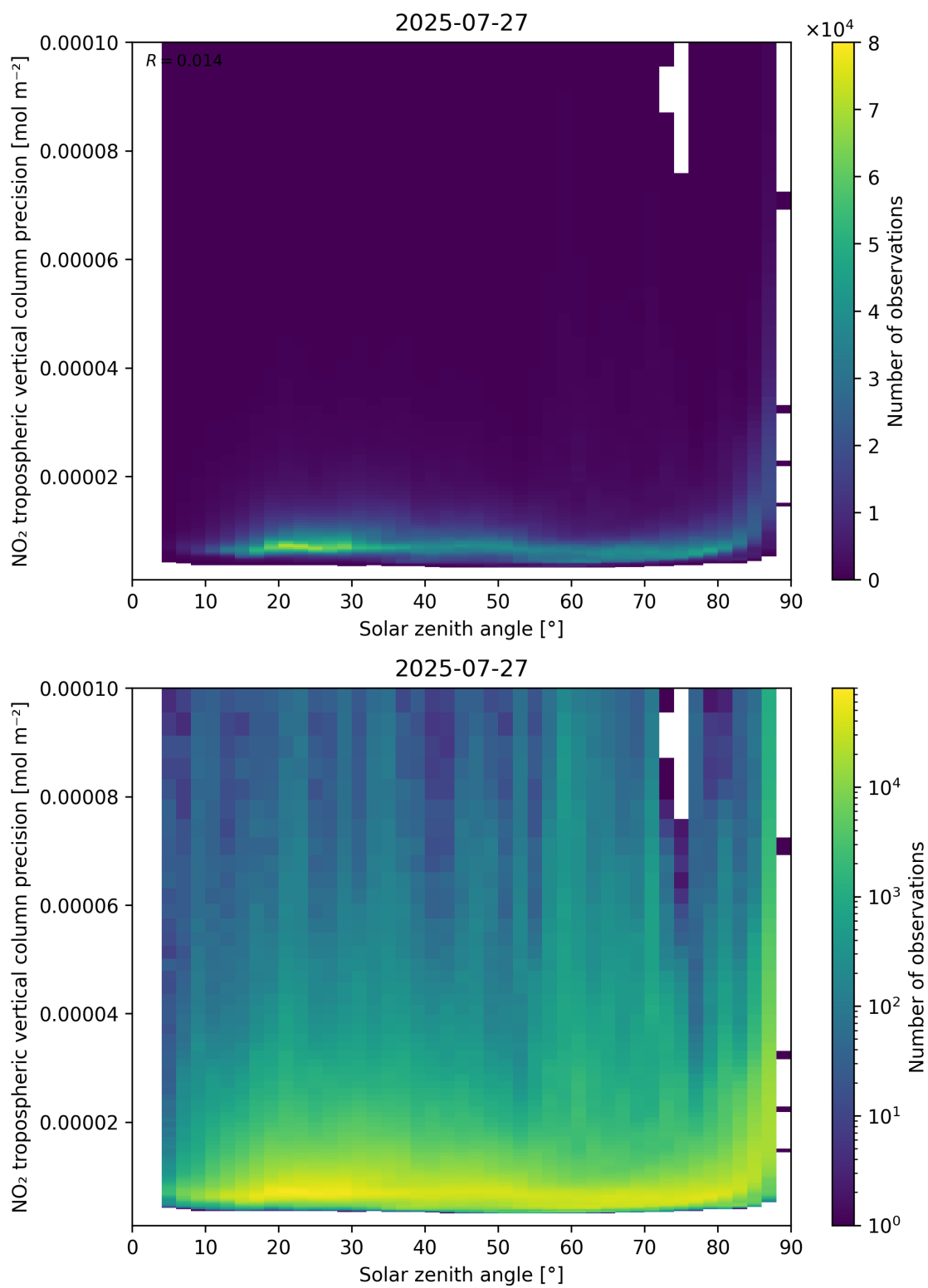
Figure 156: Scatter density plot of “Solar zenith angle” against “NO 2 tropospheric vertical column precision” for 2025-07-26 to 2025-07-28.
