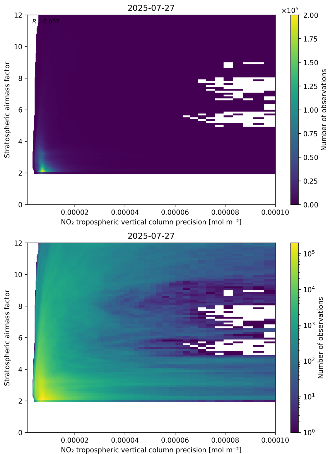
Figure 131: Scatter density plot of “NO 2 tropospheric vertical column precision” against “Stratospheric airmass factor” for 2025-07-26 to 2025-07-28.
