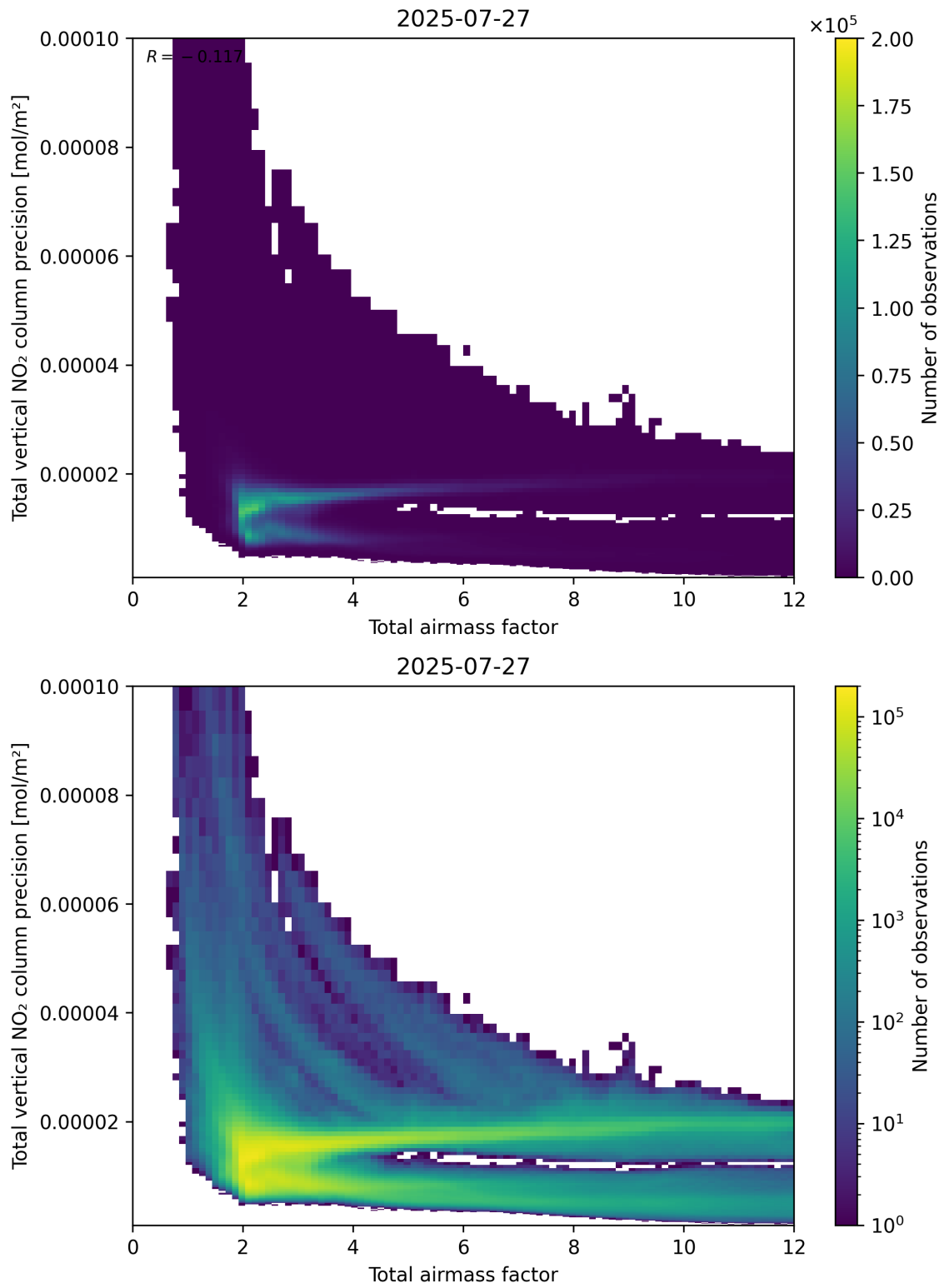
Figure 68: Scatter density plot of “Total airmass factor” against “Total vertical NO 2 column precision” for 2025-07-26 to 2025-07-28.
