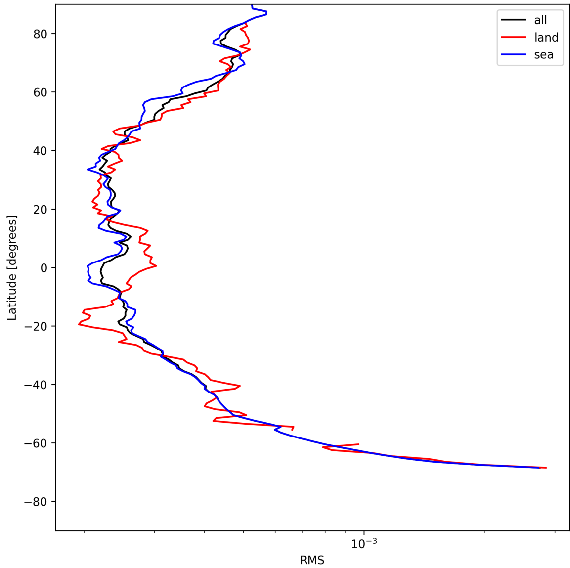
Figure 26: Zonal average of “RMS” for 2025-07-26 to 2025-07-28.
