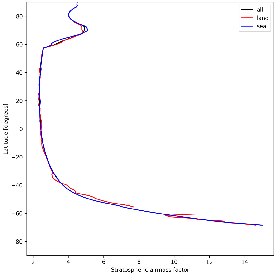
Figure 27: Zonal average of “Stratospheric airmass factor” for 2025-07-26 to 2025-07-28.
