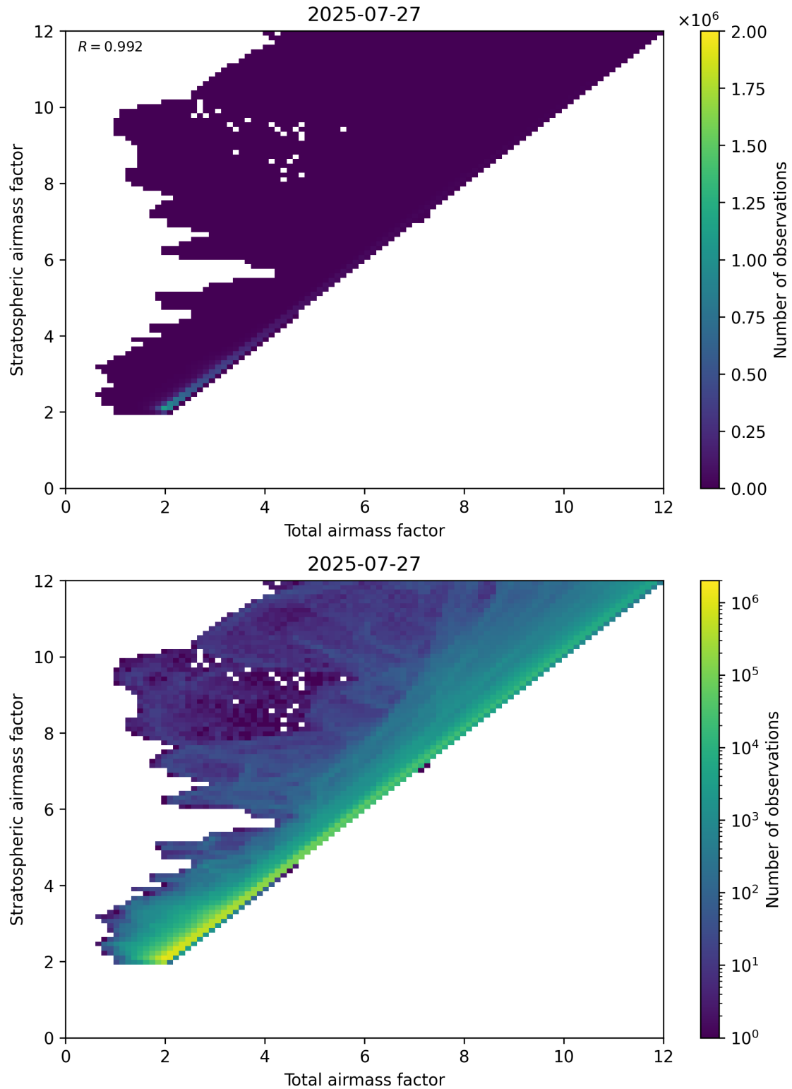
Figure 62: Scatter density plot of “Total air mass factor” against “Stratospheric air mass factor” for 2025-07-26 to 2025-07-28.
