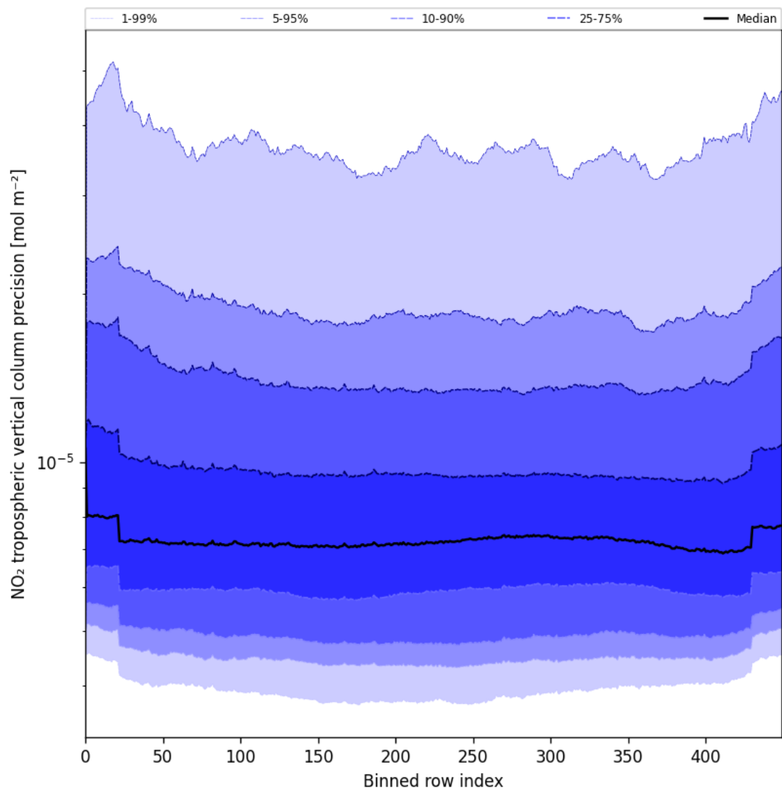
Figure 47: Along track statistics of “NO 2 tropospheric vertical column precision” for 2025-07-26 to 2025-07-28
