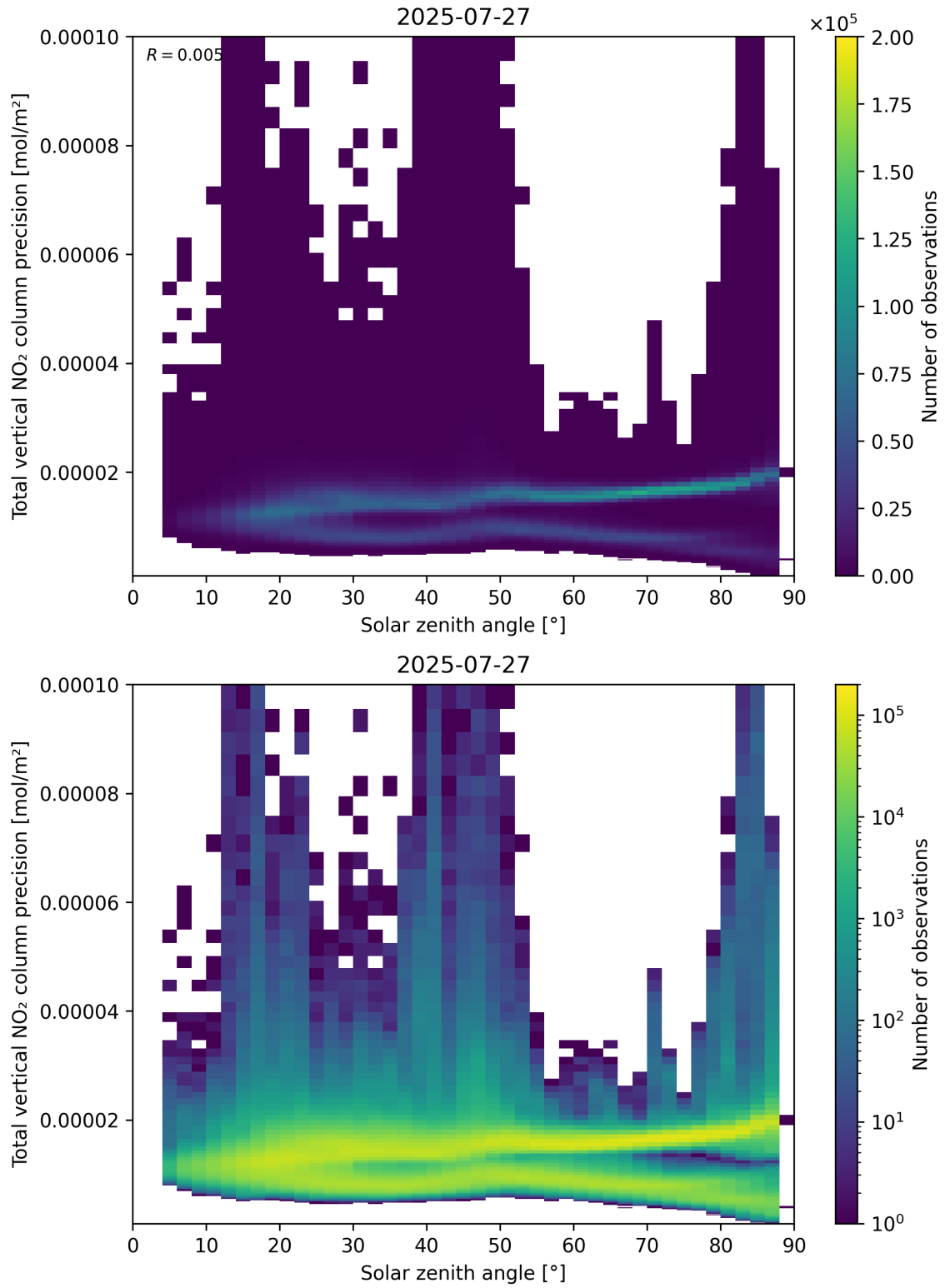
Figure 154: Scatter density plot of “Solar zenith angle” against “Total vertical NO 2 column precision” for 2025-07-26 to 2025-07-28.
