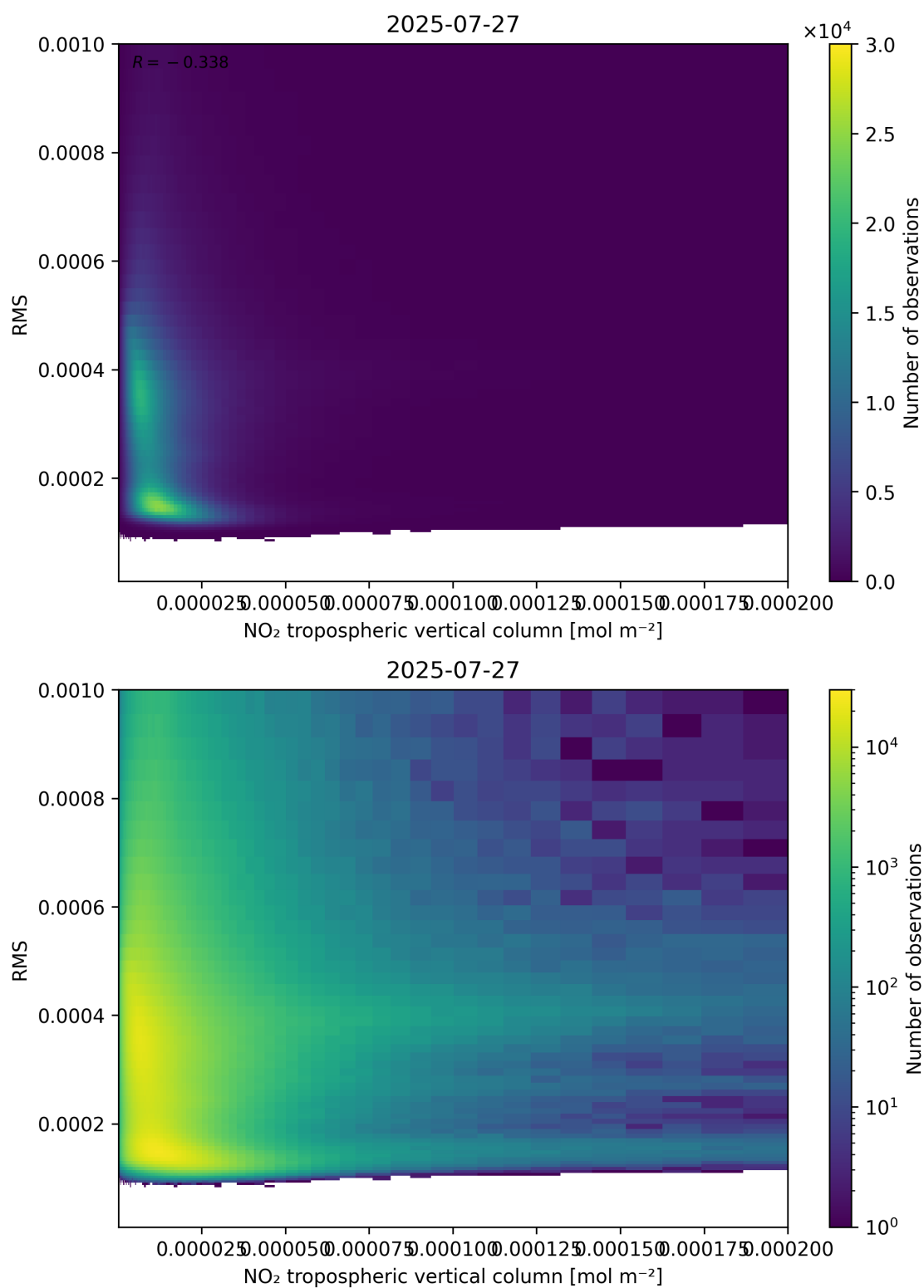
Figure 142: Scatter density plot of “NO 2 tropospheric vertical column” against “RMS” for 2025-07-26 to 2025-07-28.
