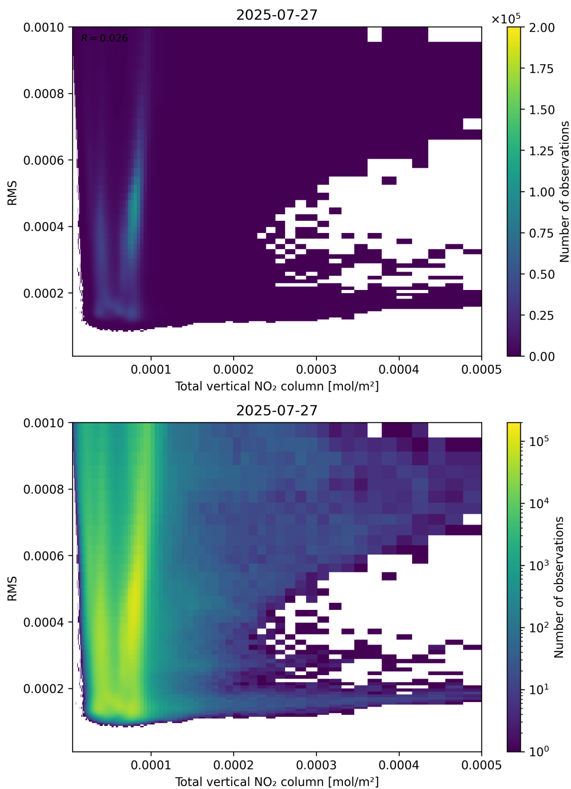
Figure 120: Scatter density plot of “Total vertical NO 2 column” against “RMS” for 2025-07-26 to 2025-07-28.
