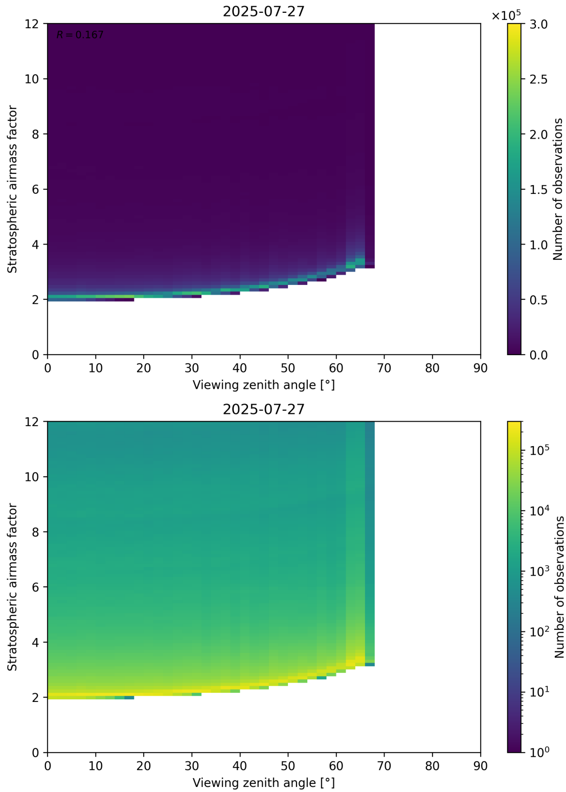
Figure 159: Scatter density plot of “Viewing zenith angle” against “Stratospheric airmass factor” for 2025-07-26 to 2025-07-28.
