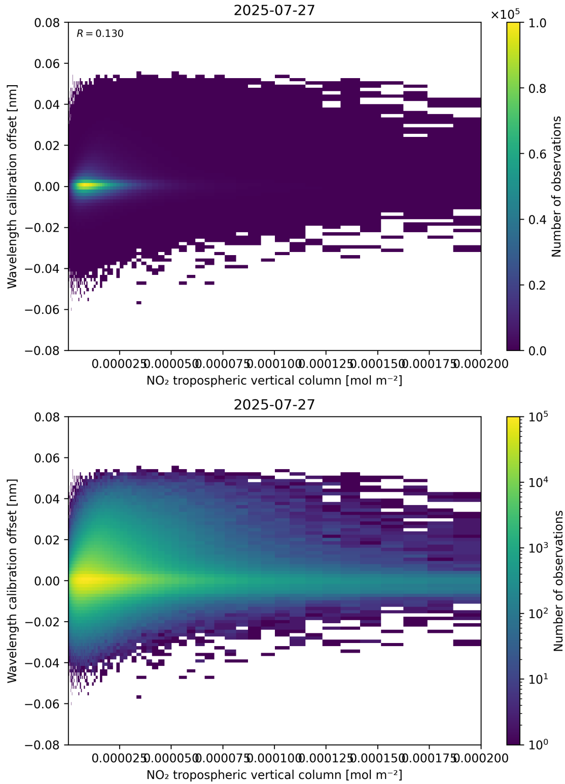
Figure 143: Scatter density plot of “NO 2 tropospheric vertical column” against “Wavelength calibration offset” for 2025-07-26 to 2025-07-28.
