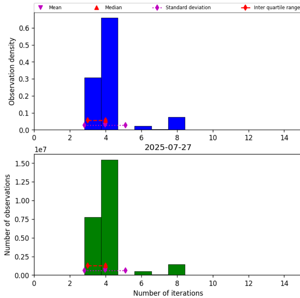
Figure 34: Histogram of “Number of iterations” for 2025-07-26 to 2025-07-28
