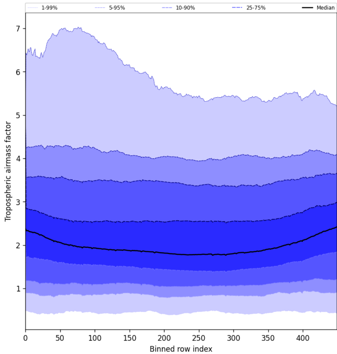
Figure 48: Along track statistics of “Tropospheric air mass factor” for 2025-07-26 to 2025-07-28
