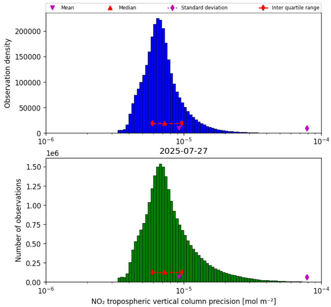
Figure 30: Histogram of “NO 2 tropospheric vertical column precision” for 2025-07-26 to 2025-07-28
