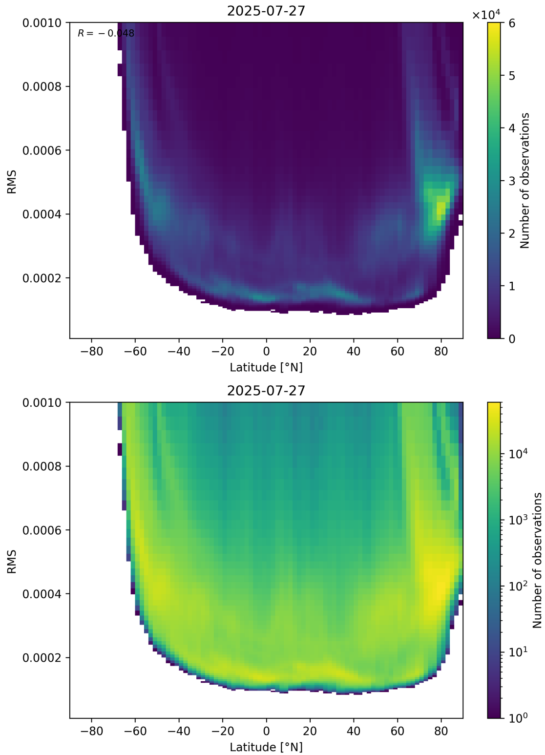
Figure 94: Scatter density plot of “Latitude” against “RMS” for 2025-07-26 to 2025-07-28.
