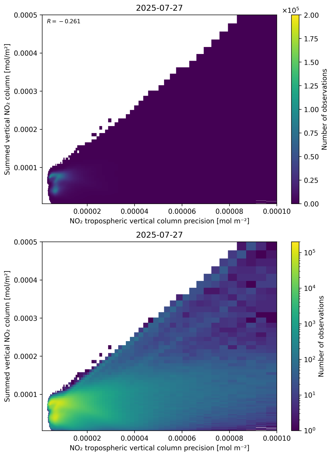
Figure 136: Scatter density plot of “NO 2 tropospheric vertical column precision” against “Summed vertical NO 2 column” for 2025-07-26 to 2025-07-28.
