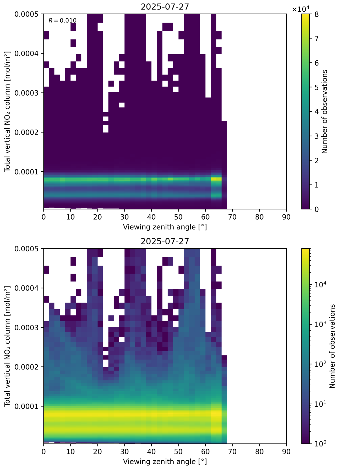
Figure 167: Scatter density plot of “Viewing zenith angle” against “Total vertical NO 2 column” for 2025-07-26 to 2025-07-28.
