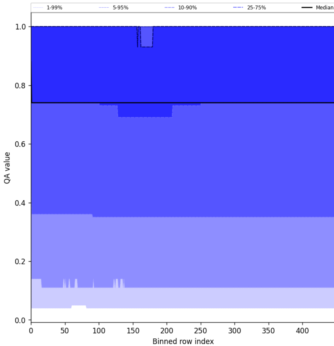
Figure 45: Along track statistics of “QA value” for 2025-07-26 to 2025-07-28
