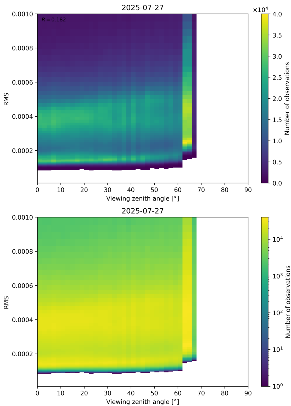
Figure 171: Scatter density plot of “Viewing zenith angle” against “RMS” for 2025-07-26 to 2025-07-28.
