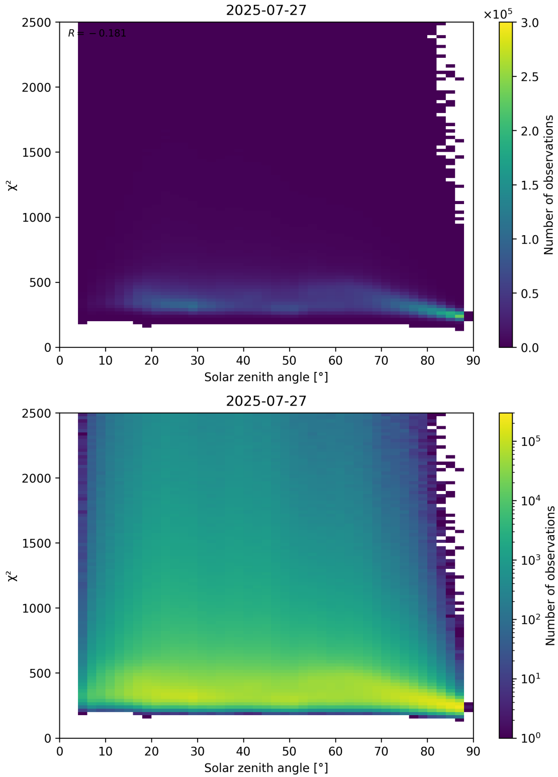
Figure 148: Scatter density plot of “Solar zenith angle” against “ \chi^2 ” for 2025-07-26 to 2025-07-28.
