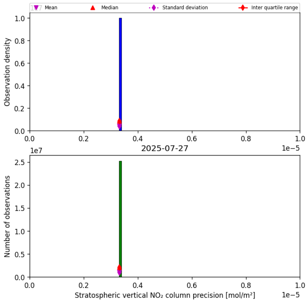
Figure 37: Histogram of “Stratospheric vertical NO 2 column precision” for 2025-07-26 to 2025-07-28
