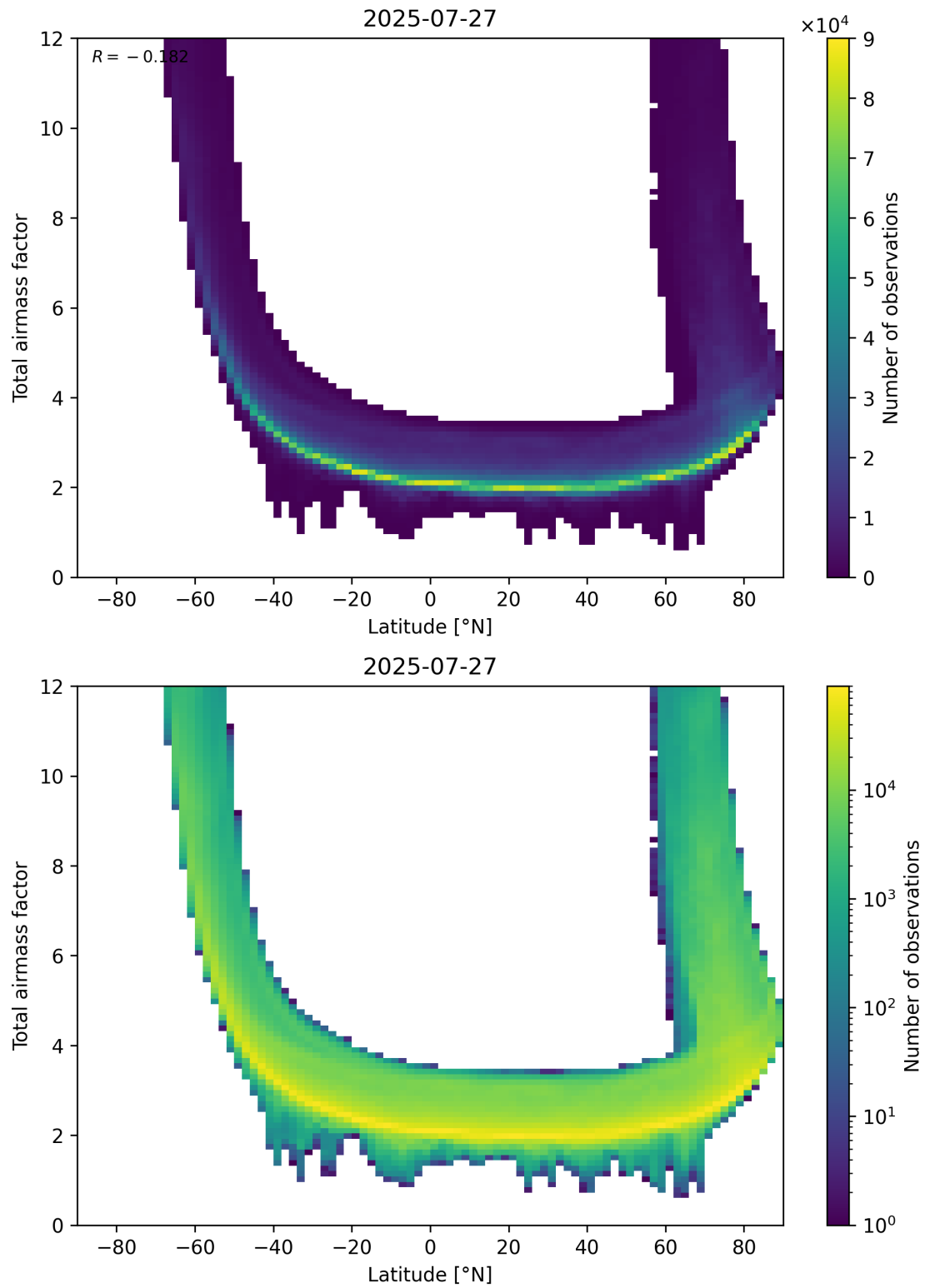
Figure 84: Scatter density plot of “Latitude” against “Total airmass factor” for 2025-07-26 to 2025-07-28.
