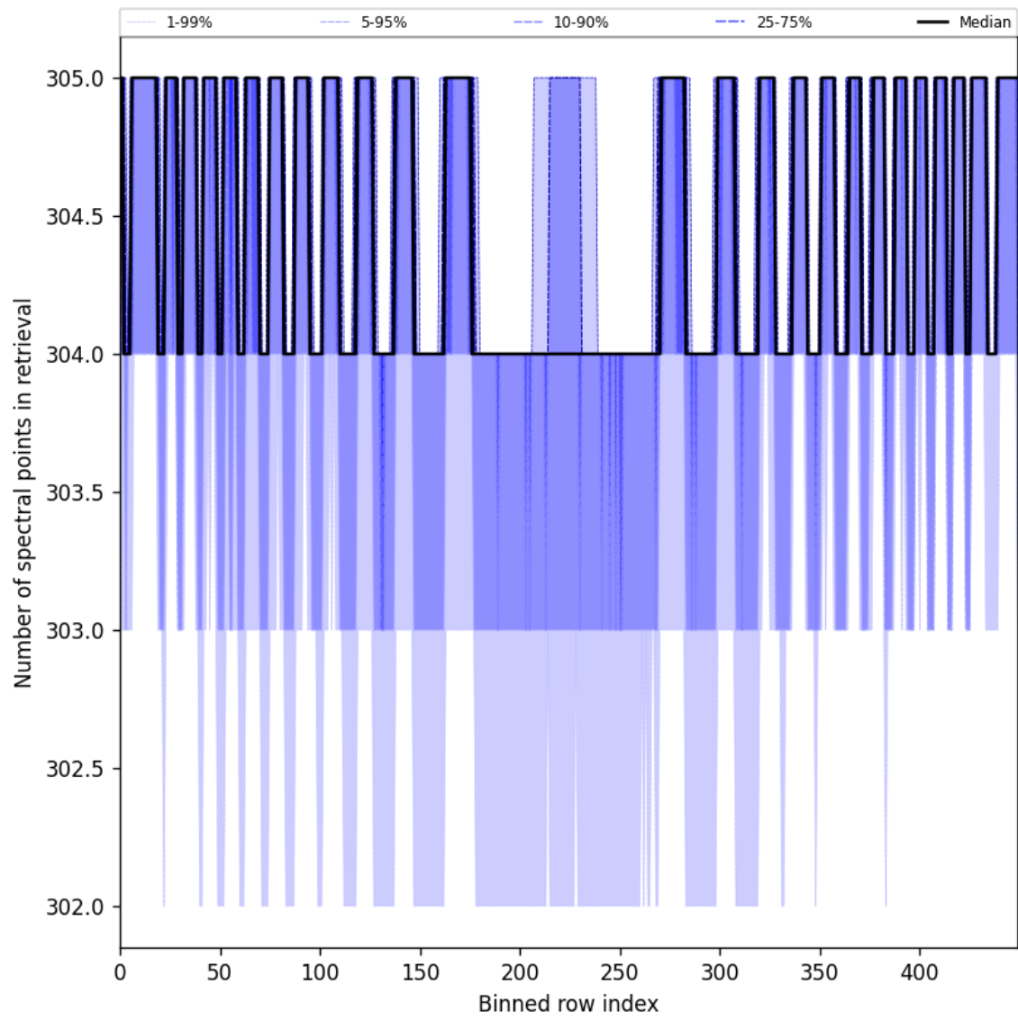
Figure 50: Along track statistics of “Number of spectral points in retrieval” for 2025-07-26 to 2025-07-28
