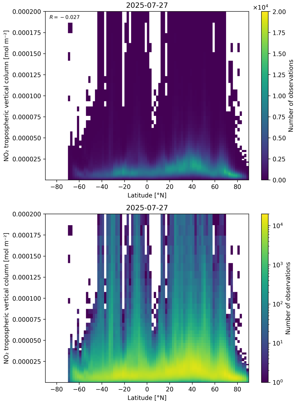
Figure 92: Scatter density plot of “Latitude” against “NO 2 tropospheric vertical column” for 2025-07-26 to 2025-07-28.
