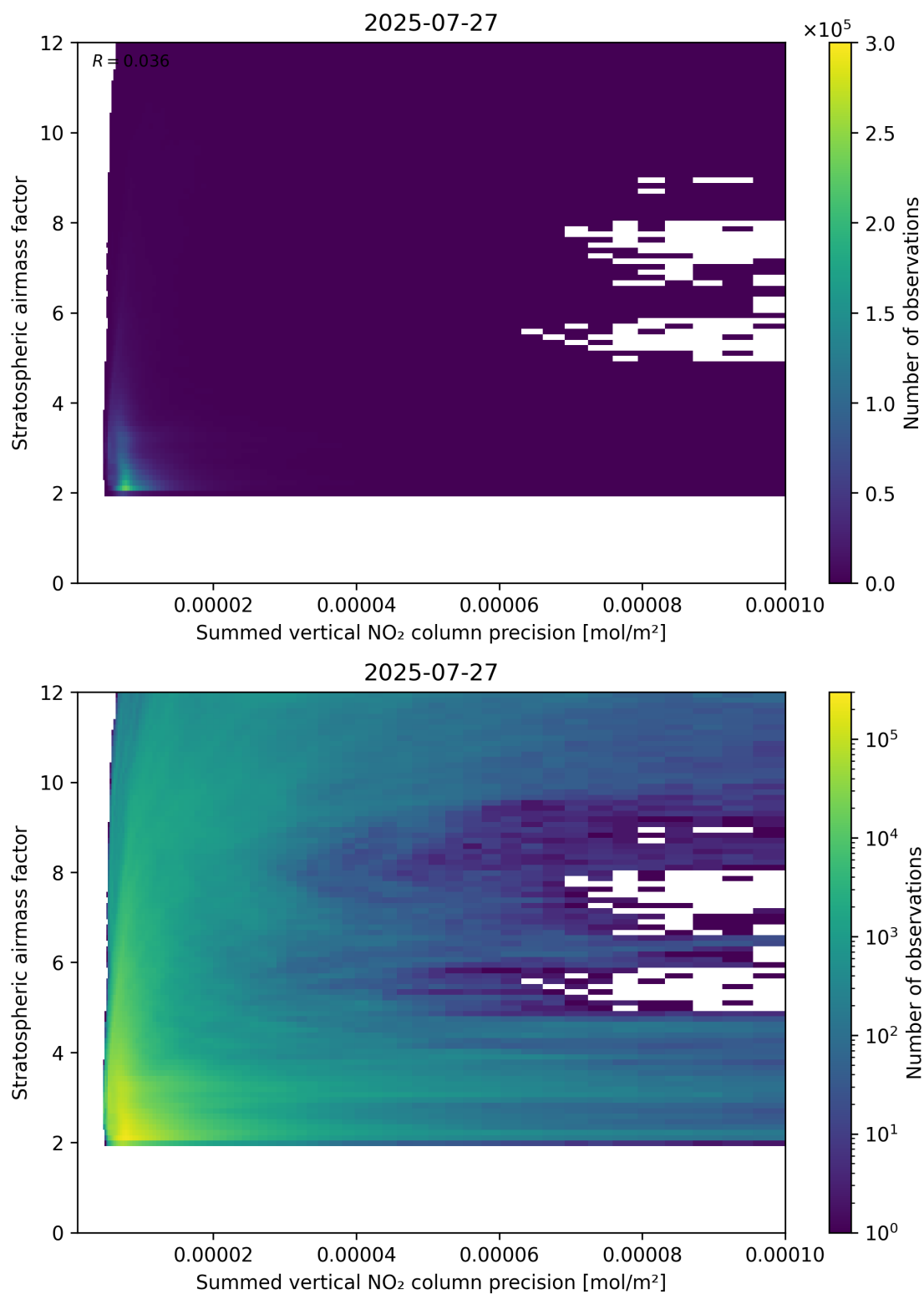
Figure 106: Scatter density plot of “Summed vertical NO 2 column precision” against “Stratospheric airmass factor” for 2025-07-26 to 2025-07-28.
