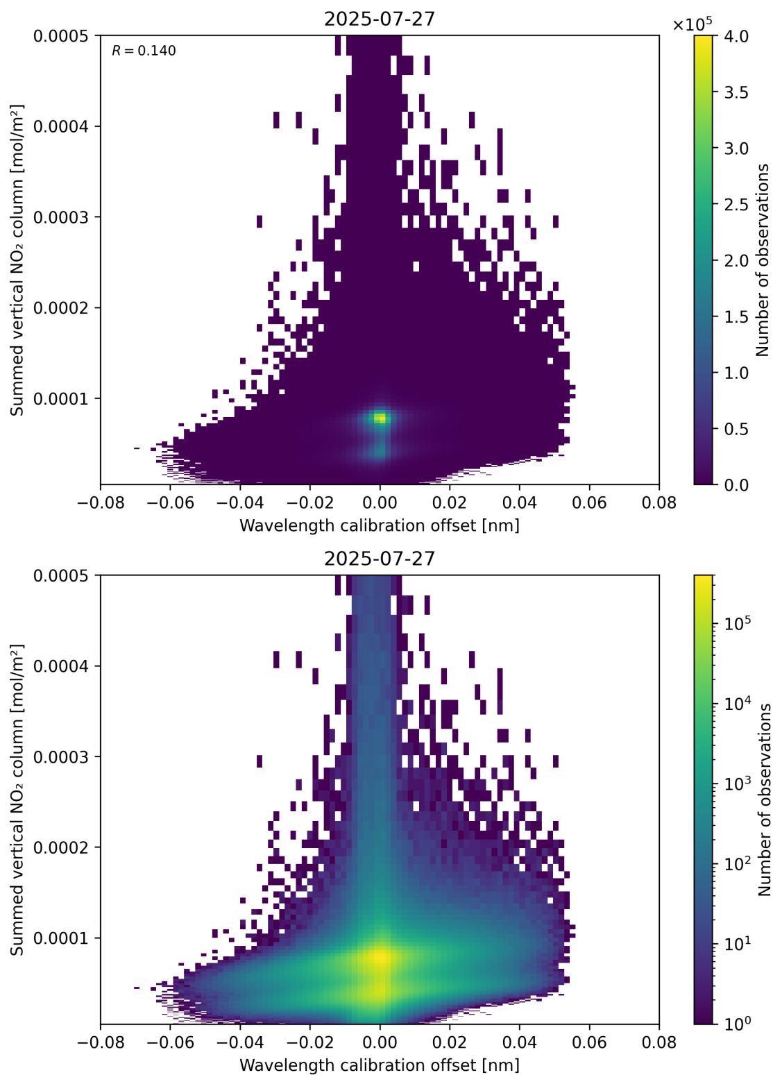
Figure 177: Scatter density plot of “Wavelength calibration offset” against “Summed vertical NO 2 column” for 2025-07-26 to 2025-07-28.
