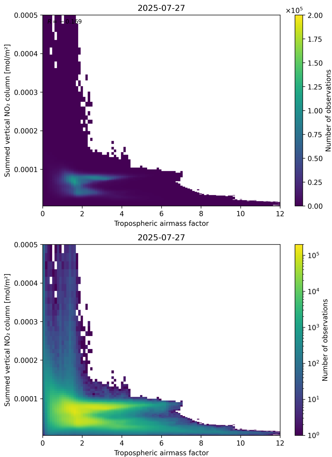
Figure 75: Scatter density plot of “Tropospheric airmass factor” against “Summed vertical NO 2 column” for 2025-07-26 to 2025-07-28.
