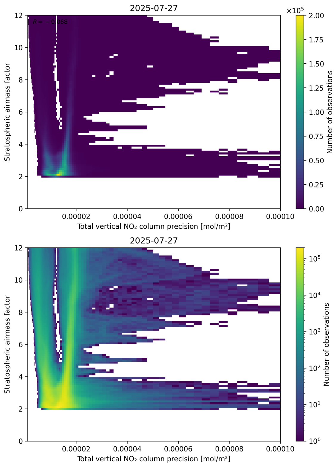
Figure 115: Scatter density plot of “Total vertical NO 2 column precision” against “Stratospheric air mass factor” for 2025-07-26 to 2025-07-28.
