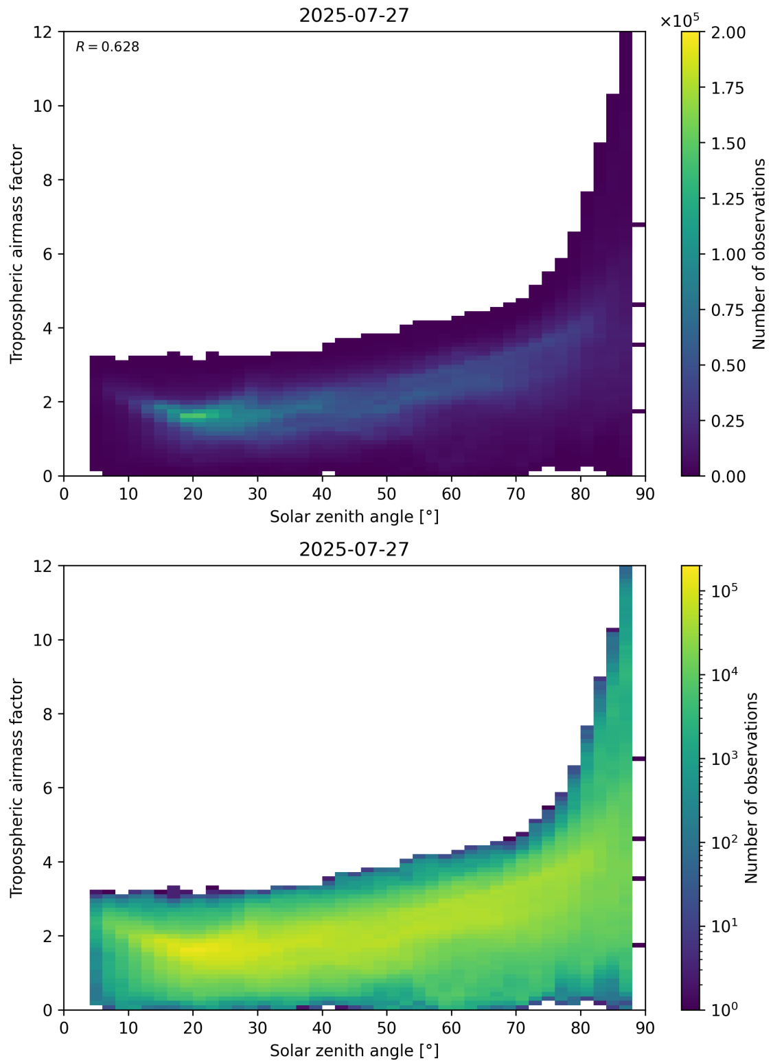
Figure 147: Scatter density plot of “Solar zenith angle” against “Tropospheric airmass factor” for 2025-07-26 to 2025-07-28.
