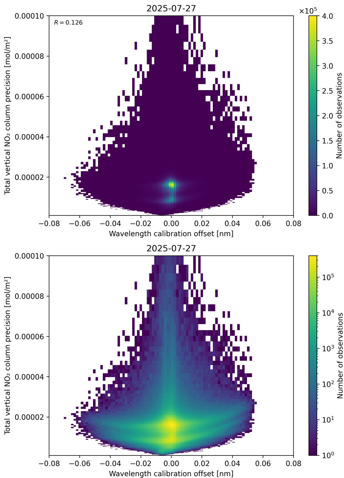
Figure 180: Scatter density plot of “Wavelength calibration offset” against “Total vertical NO 2 column precision” for 2025-07-26 to 2025-07-28.
