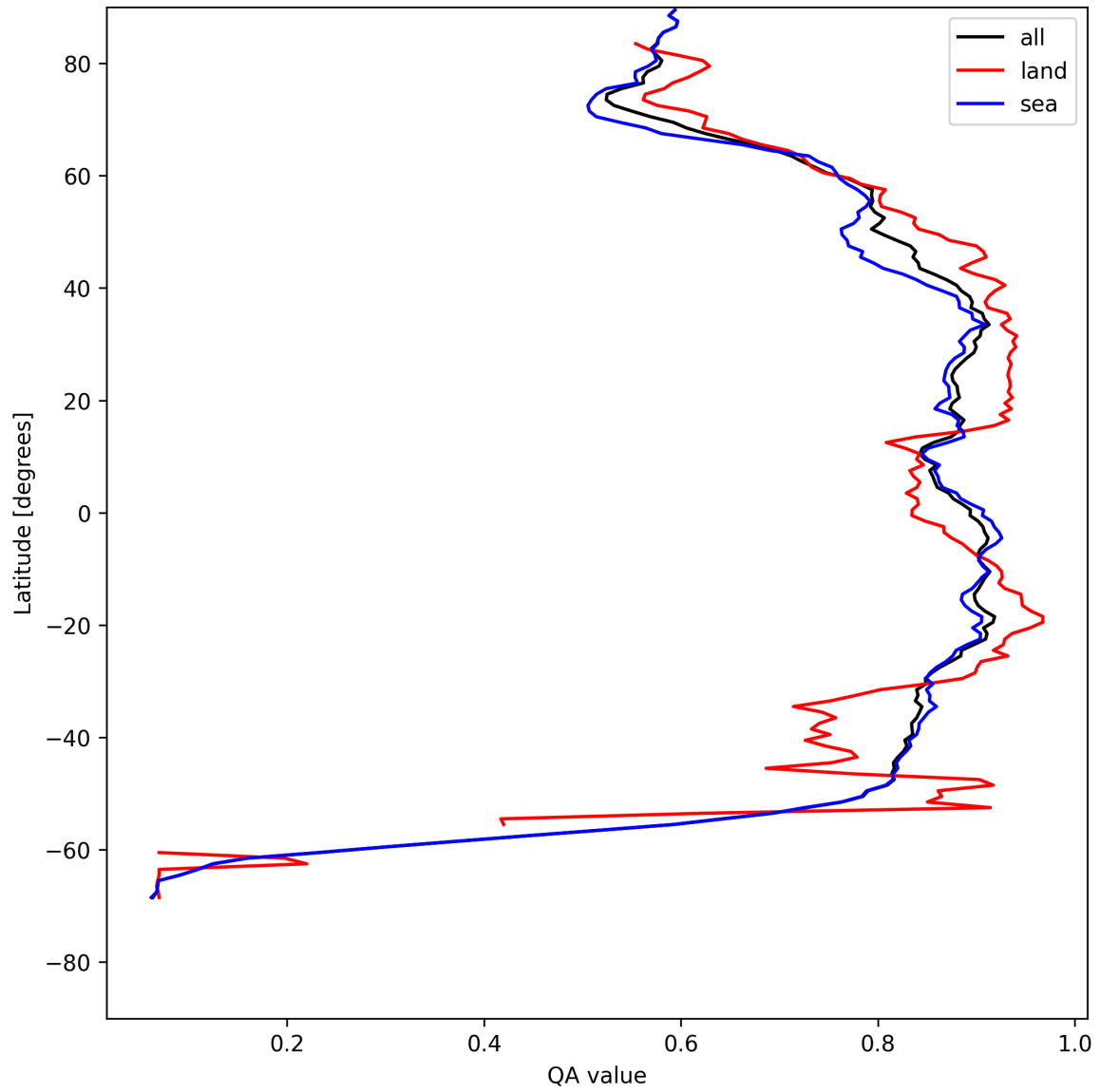
Figure 11: Zonal average of “QA value” for 2025-07-26 to 2025-07-28.
