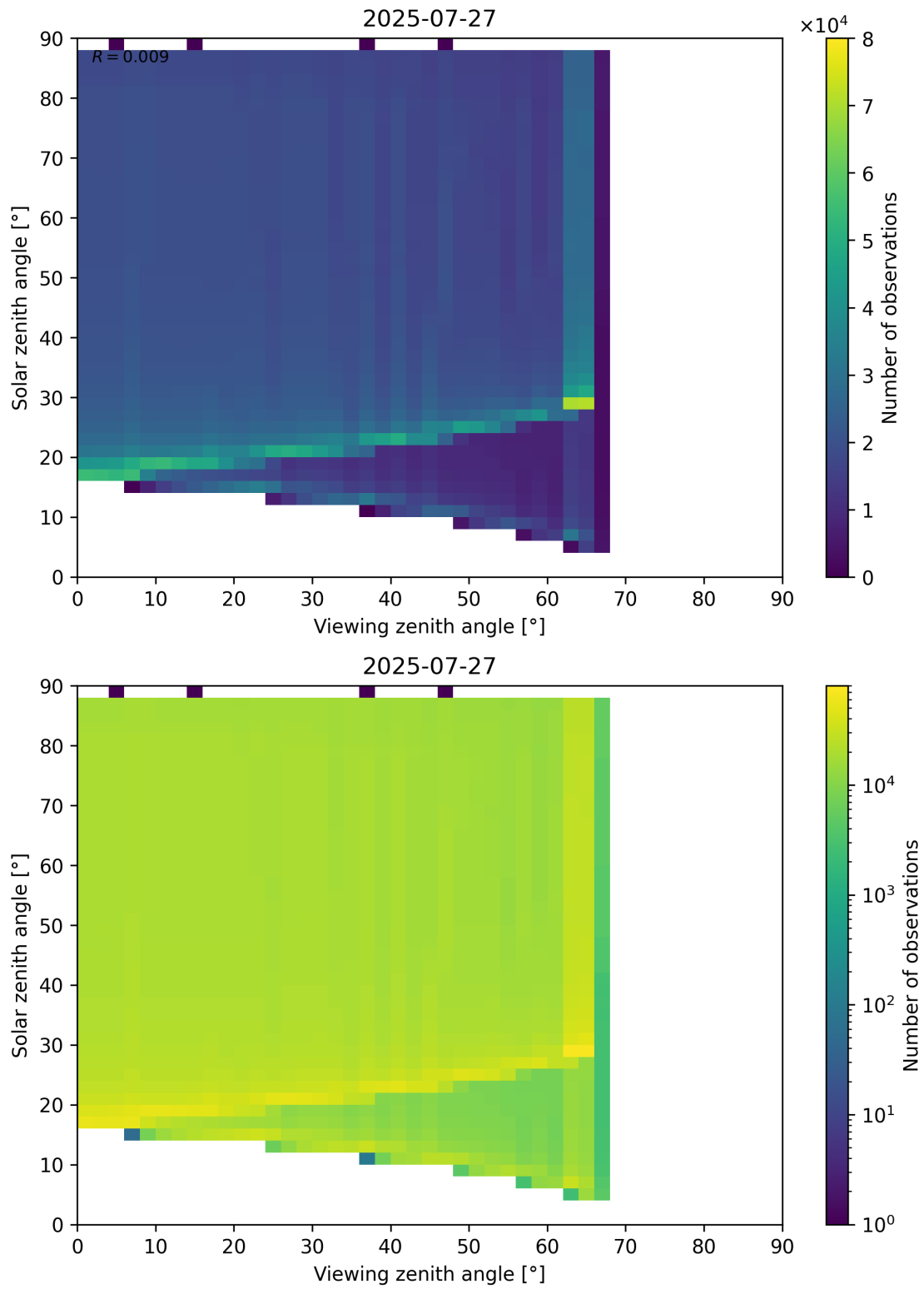
Figure 172: Scatter density plot of “Viewing zenith angle” against “Solar zenith angle” for 2025-07-26 to 2025-07-28.
