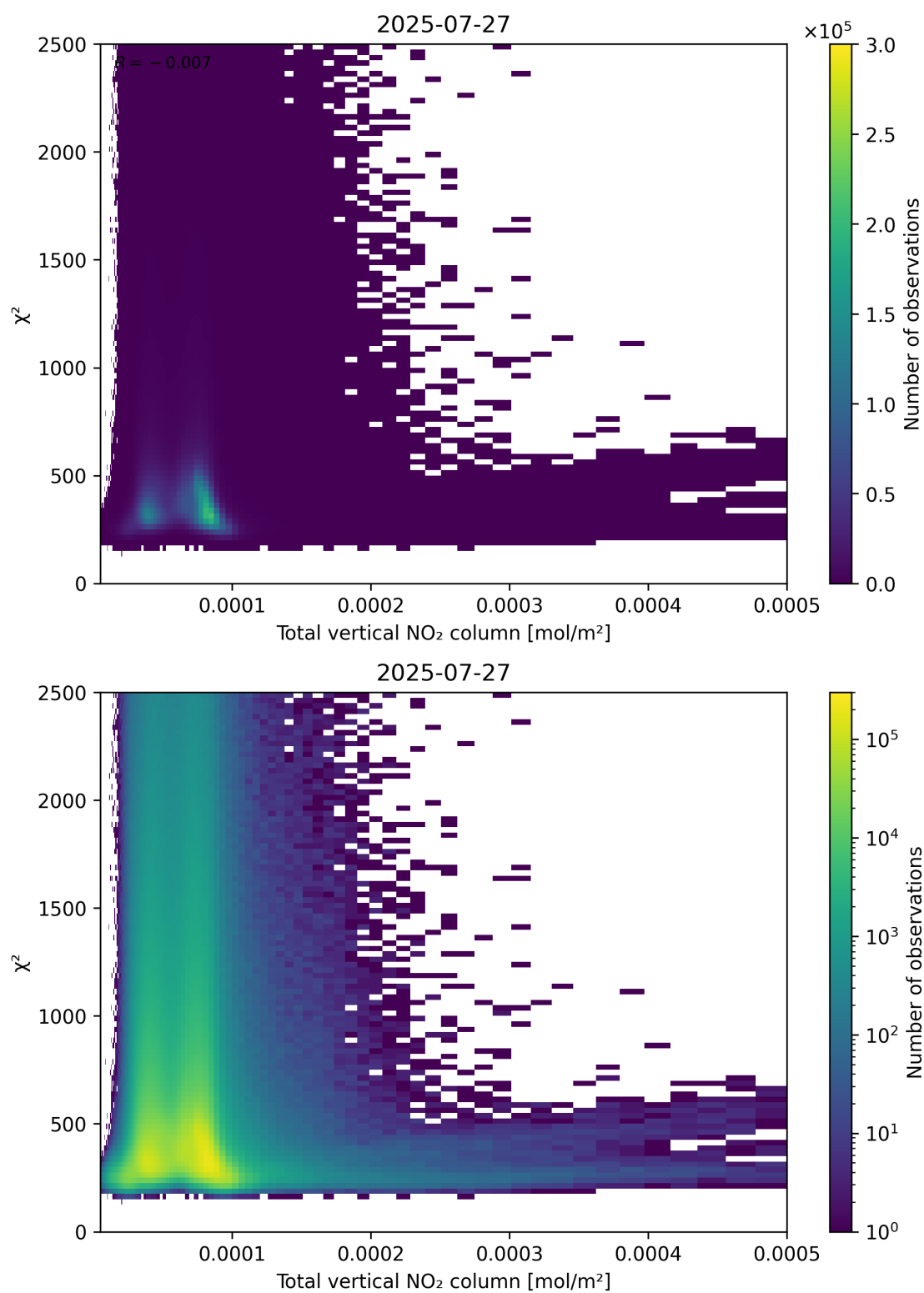
Figure 111: Scatter density plot of “Total vertical NO 2 column” against “ \chi^2 ” for 2025-07-26 to 2025-07-28.
