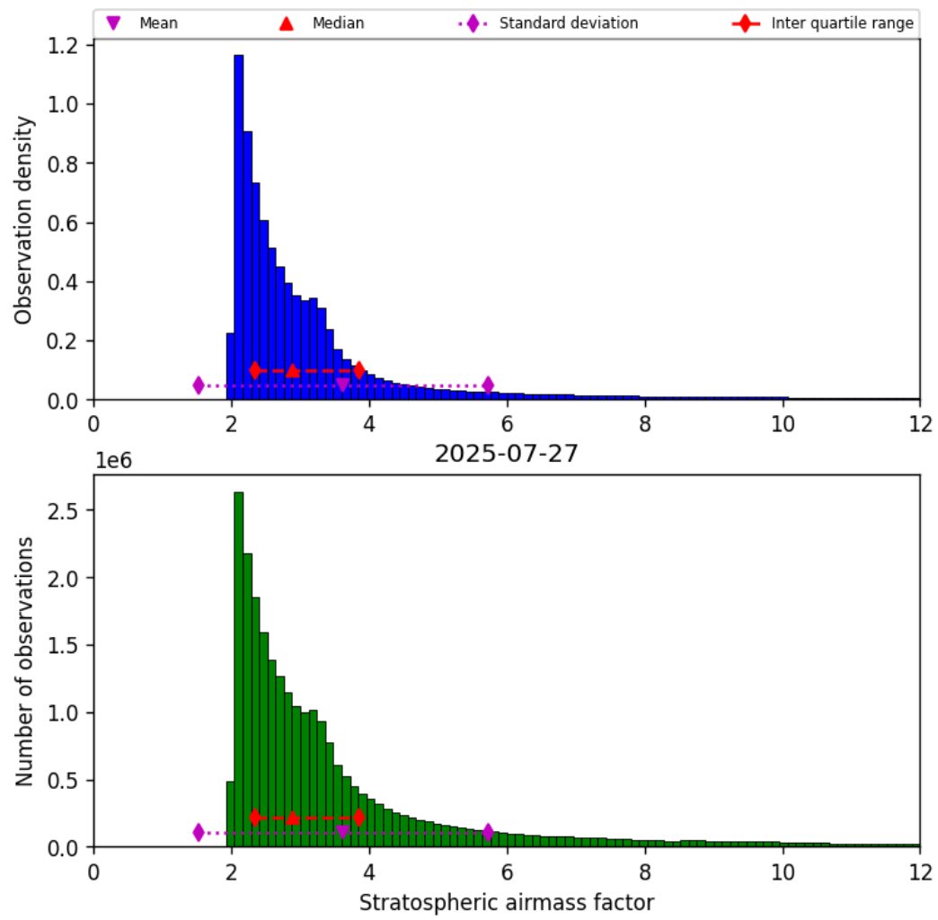
Figure 44: Histogram of “Stratospheric airmass factor” for 2025-07-26 to 2025-07-28
