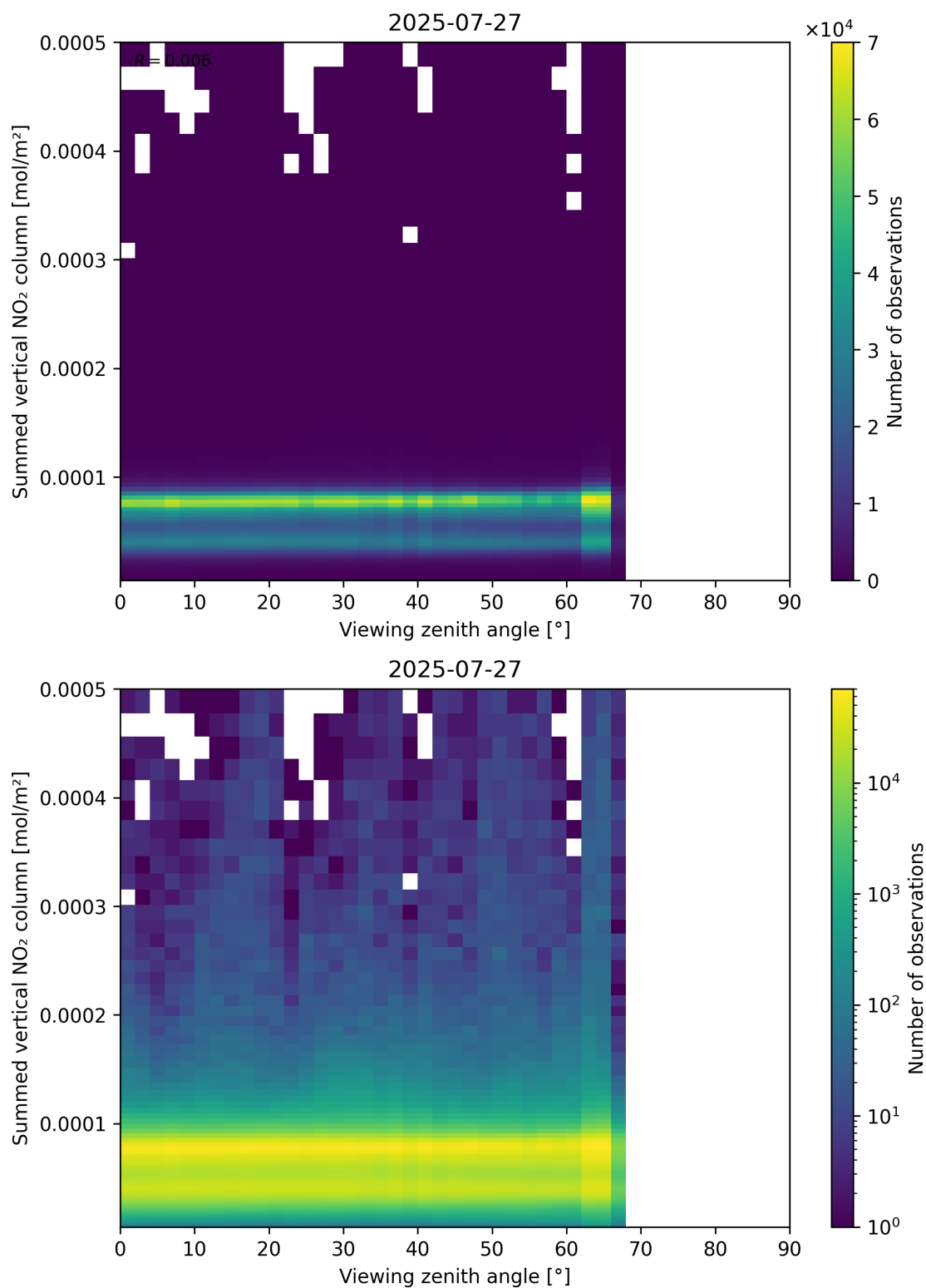
Figure 165: Scatter density plot of “Viewing zenith angle” against “Summed vertical NO 2 column” for 2025-07-26 to 2025-07-28.
