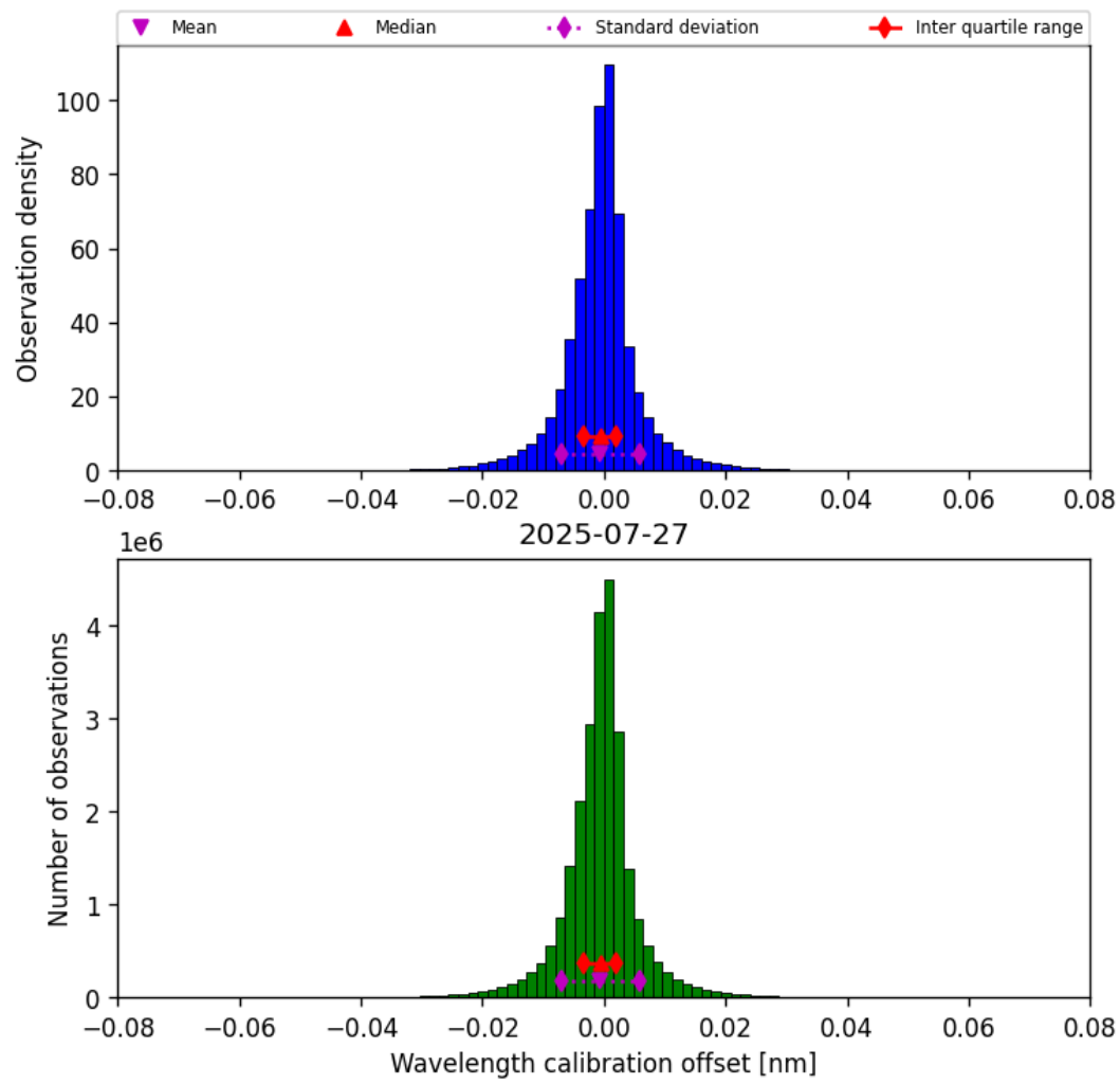
Figure 35: Histogram of “Wavelength calibration offset” for 2025-07-26 to 2025-07-28
