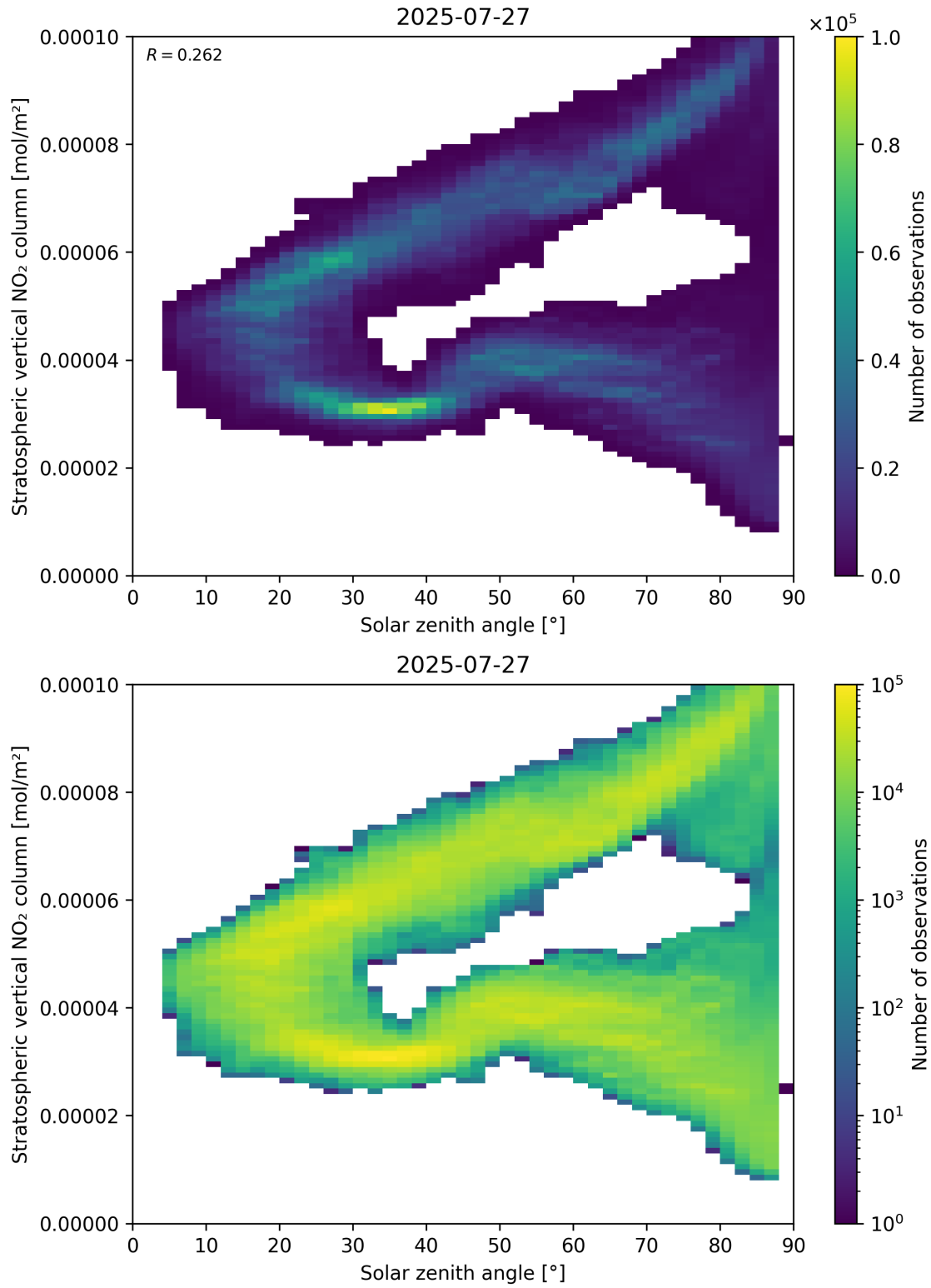
Figure 150: Scatter density plot of “Solar zenith angle” against “Stratospheric vertical NO 2 column” for 2025-07-26 to 2025-07-28.
