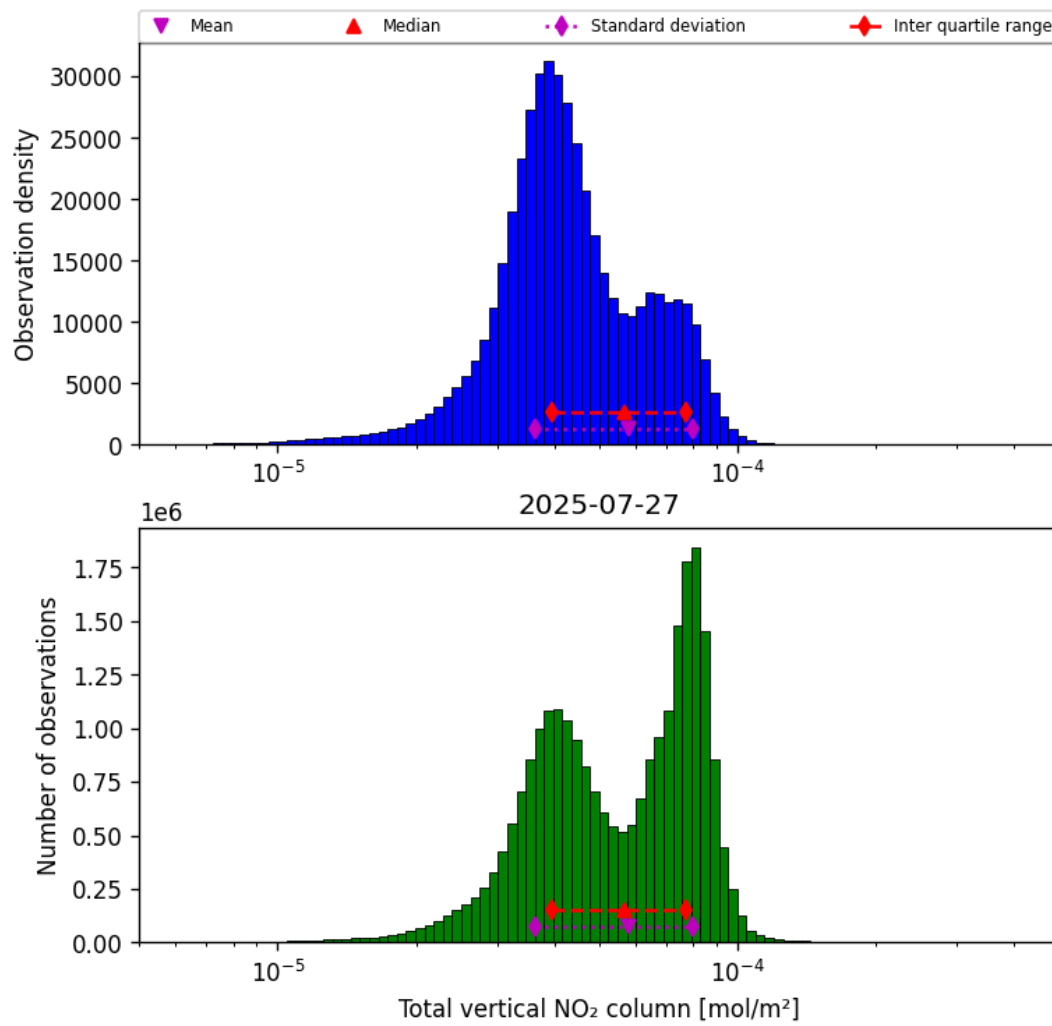
Figure 38: Histogram of “Total vertical NO 2 column” for 2025-07-26 to 2025-07-28
