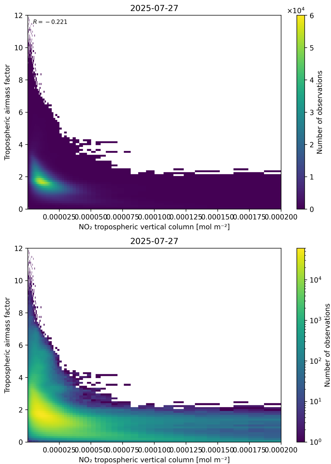
Figure 123: Scatter density plot of “NO 2 tropospheric vertical column” against “Tropospheric air mass factor” for 2025-07-26 to 2025-07-28.
