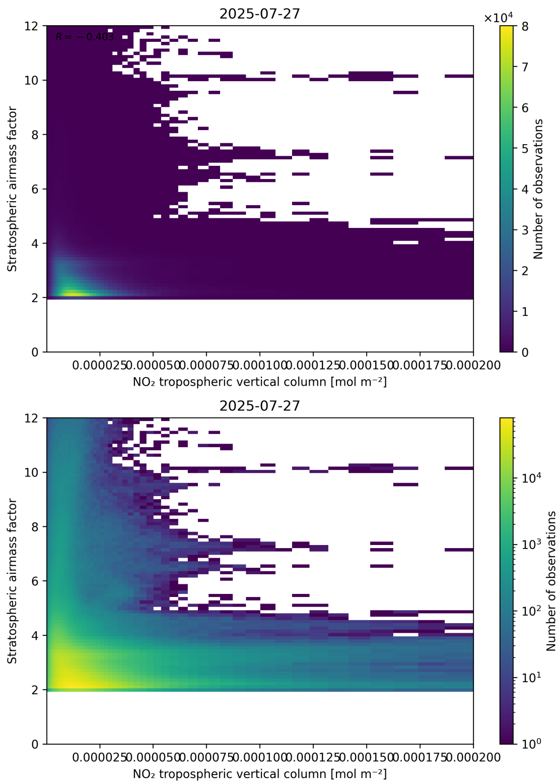
Figure 121: Scatter density plot of “NO 2 tropospheric vertical column” against “Stratospheric air mass factor” for 2025-07-26 to 2025-07-28.
