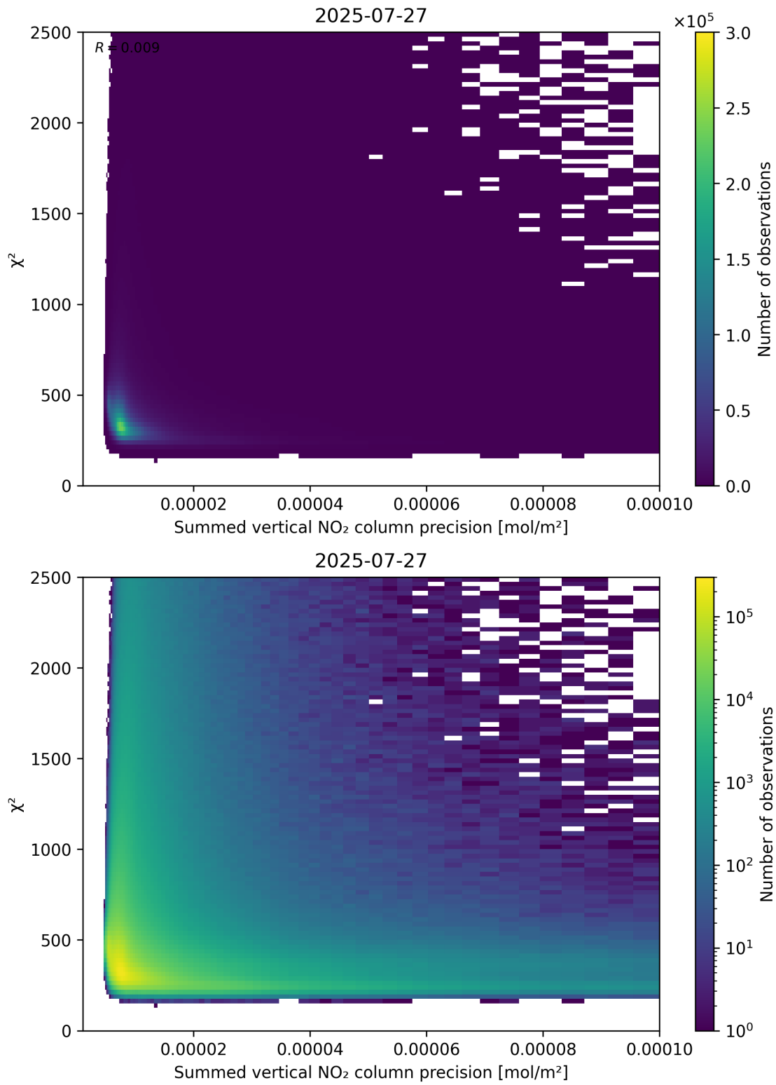
Figure 107: Scatter density plot of “Summed vertical NO 2 column precision” against “ \chi^2 ” for 2025-07-26 to 2025-07-28.
