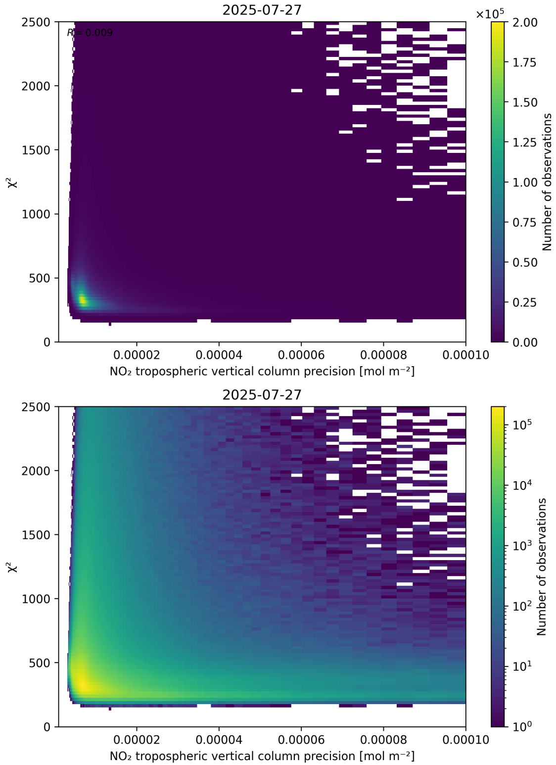
Figure 134: Scatter density plot of “NO 2 tropospheric vertical column precision” against “ \chi^2 ” for 2025-07-26 to 2025-07-28.
