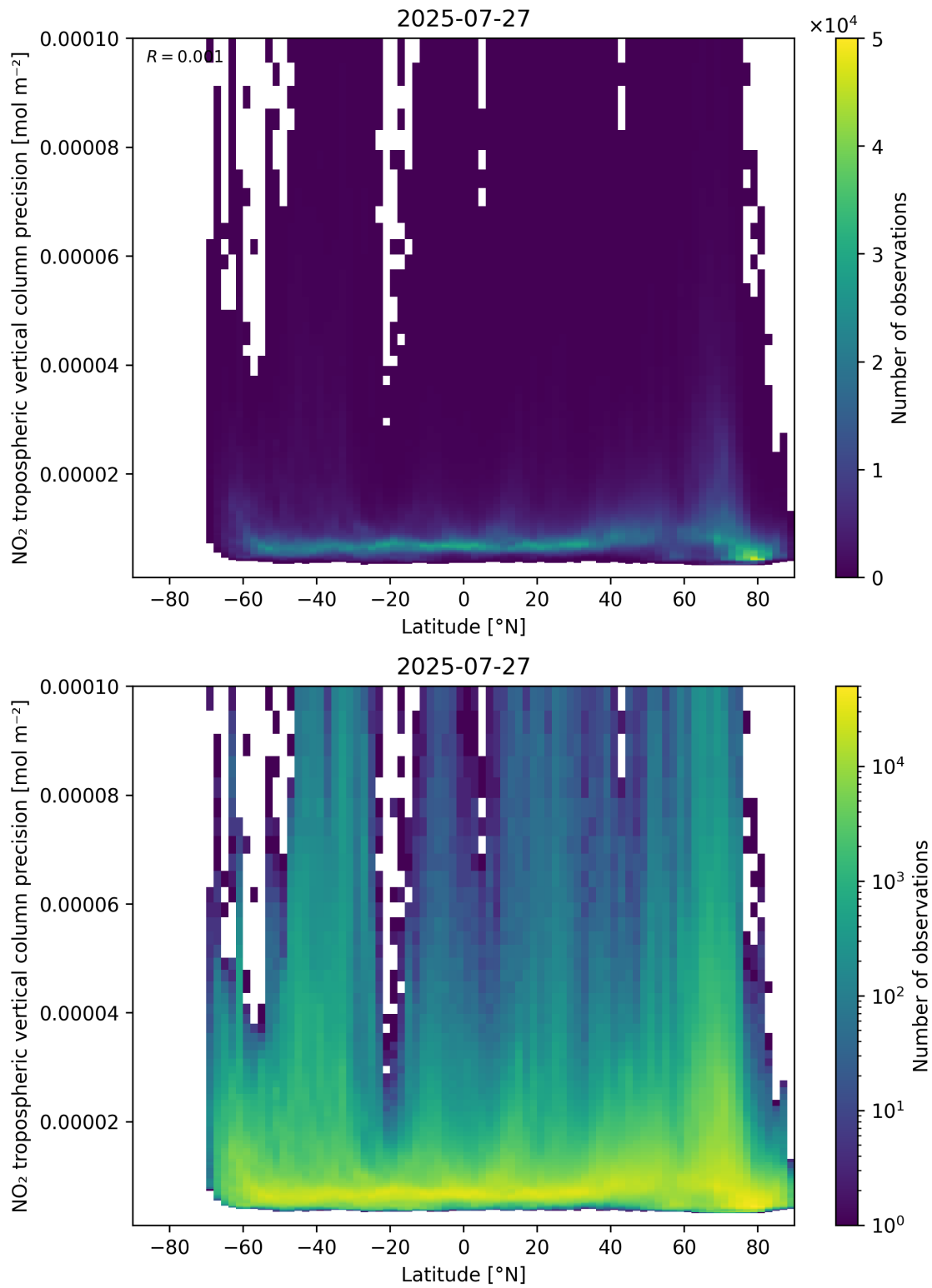
Figure 93: Scatter density plot of “Latitude” against “NO 2 tropospheric vertical column precision” for 2025-07-26 to 2025-07-28.
