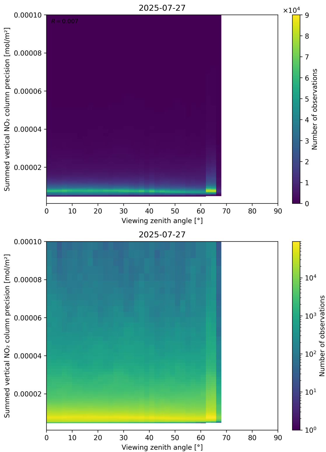
Figure 166: Scatter density plot of “Viewing zenith angle” against “Summed vertical NO 2 column precision” for 2025-07-26 to 2025-07-28.
