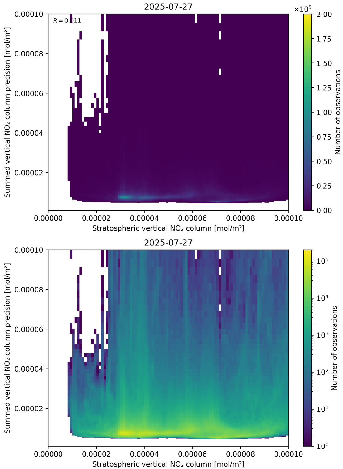
Figure 99: Scatter density plot of “Stratospheric vertical NO 2 column” against “Summed vertical NO 2 column precision” for 2025-07-26 to 2025-07-28.
