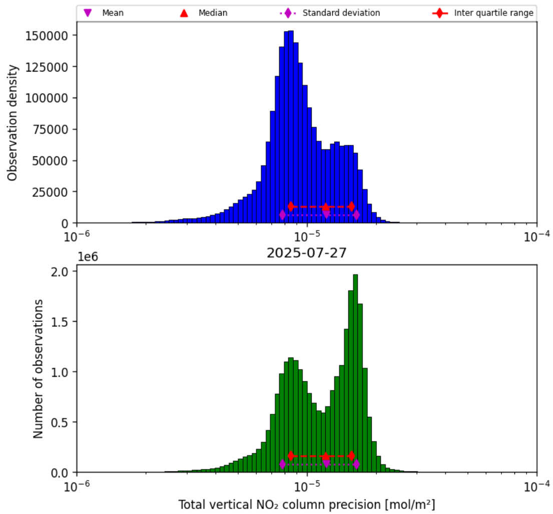
Figure 39: Histogram of "Total vertical NO 2 column precision" for 2025-07-26 to 2025-07-28
