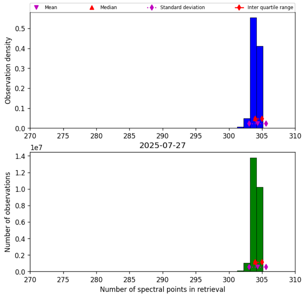
Figure 33: Histogram of “Number of spectral points in retrieval” for 2025-07-26 to 2025-07-28
