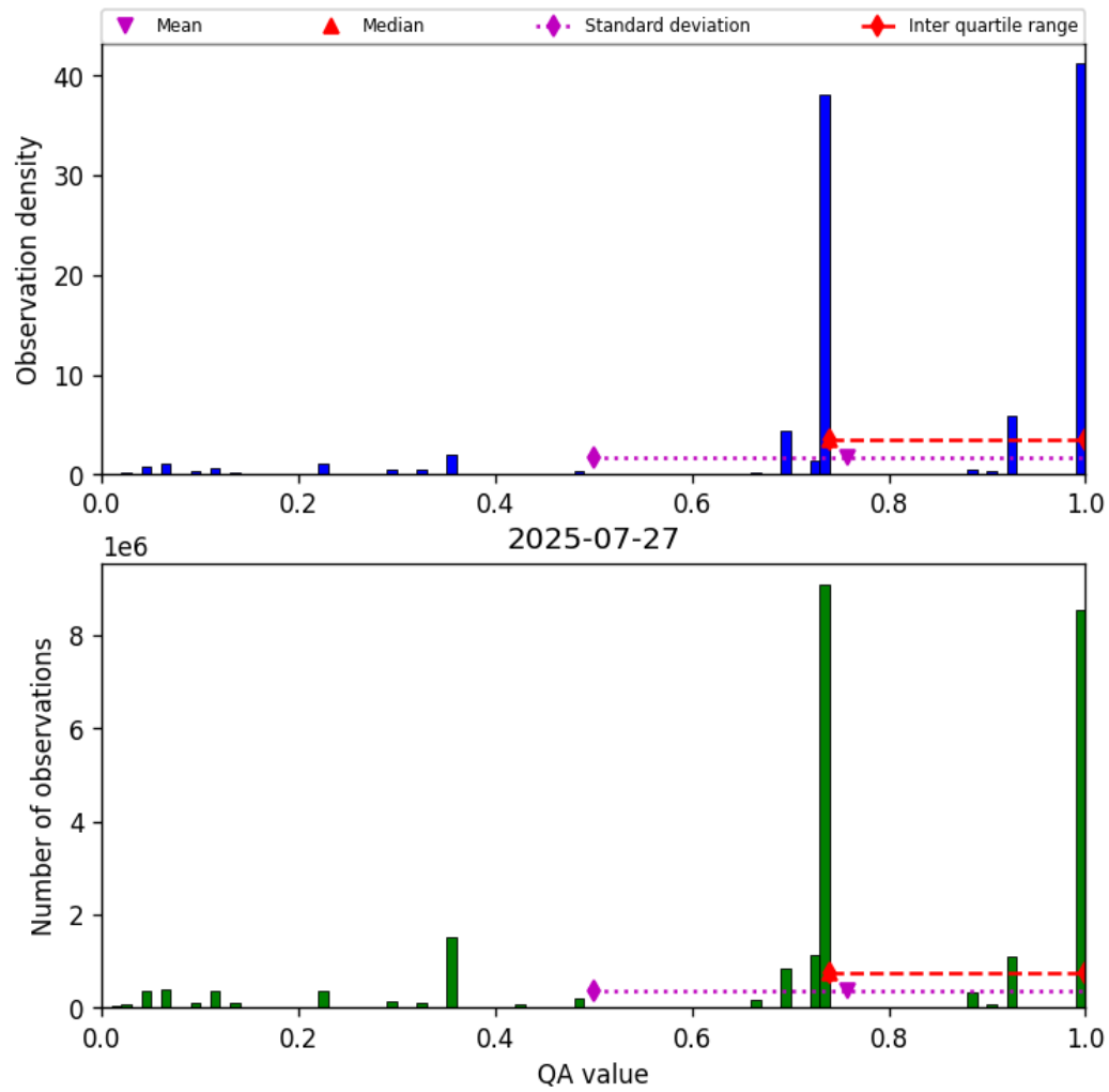
Figure 28: Histogram of “QA value” for 2025-07-26 to 2025-07-28
