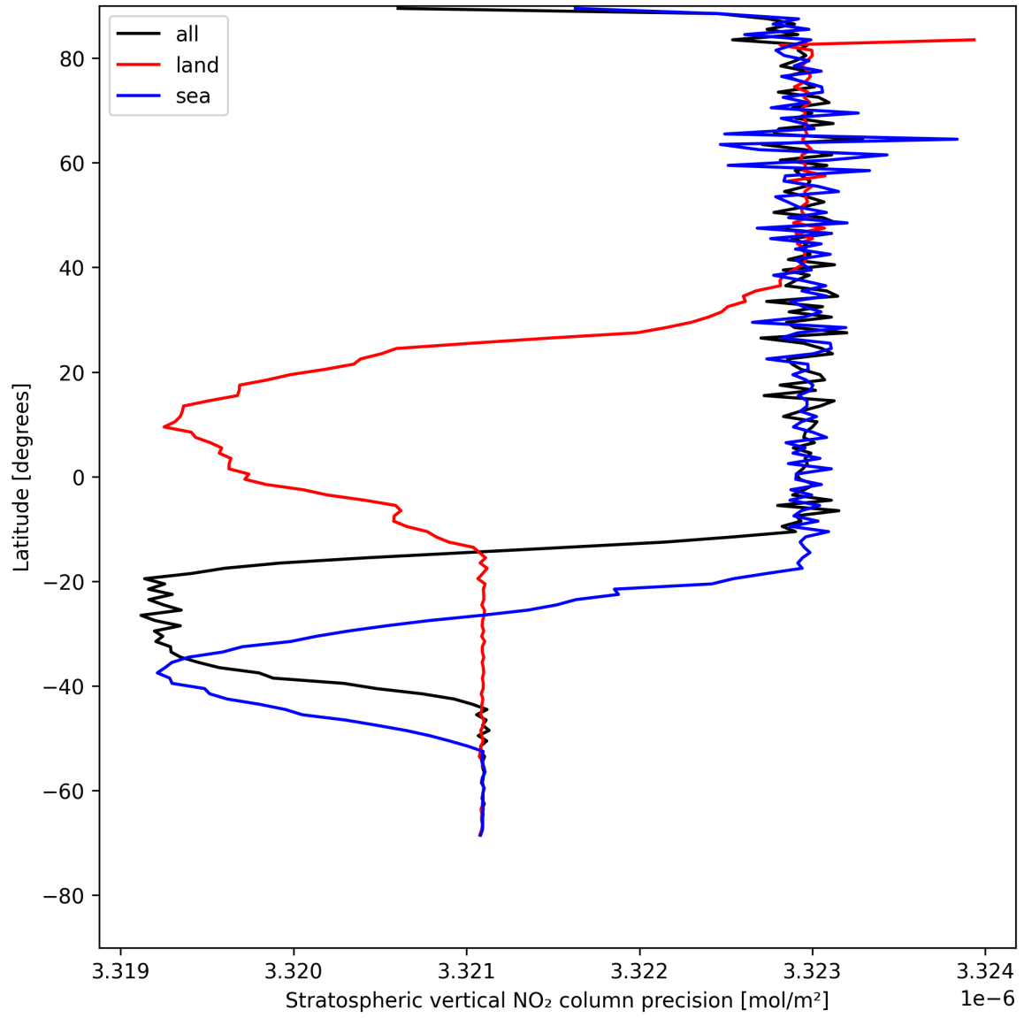
Figure 20: Zonal average of “Stratospheric vertical NO 2 column precision” for 2025-07-26 to 2025-07-28.
