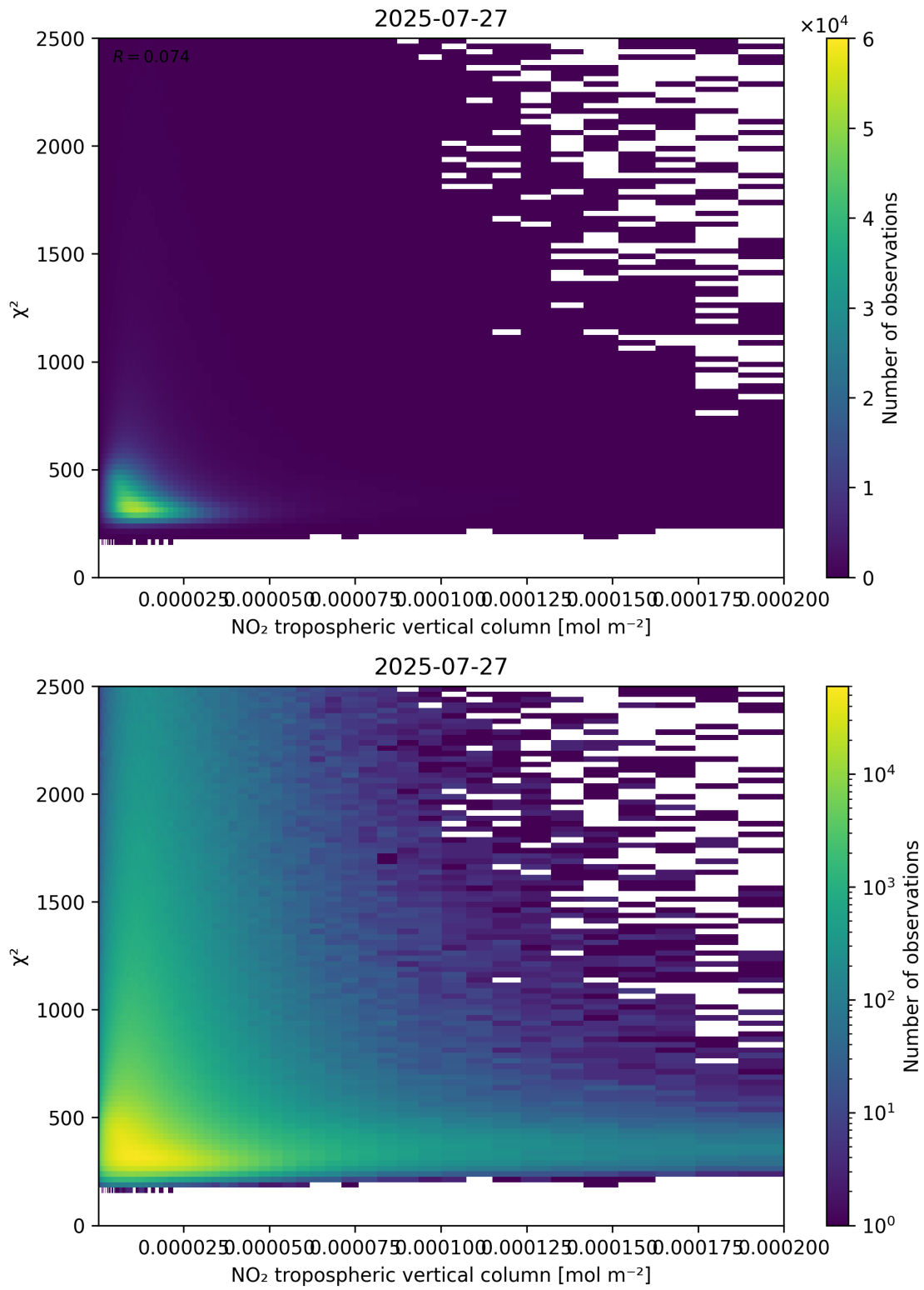
Figure 124: Scatter density plot of “NO 2 tropospheric vertical column” against “ \chi^2 ” for 2025-07-26 to 2025-07-28.
