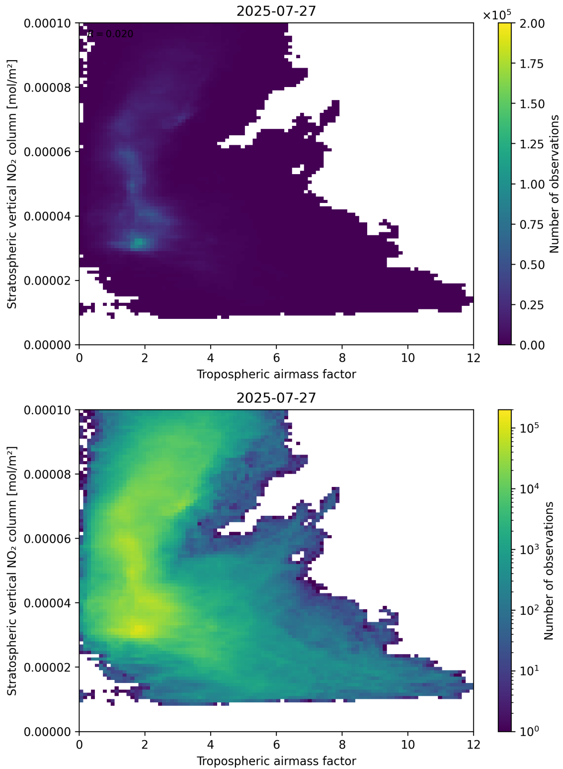
Figure 74: Scatter density plot of “Tropospheric air mass factor” against “Stratospheric vertical NO 2 column” for 2025-07-26 to 2025-07-28.
