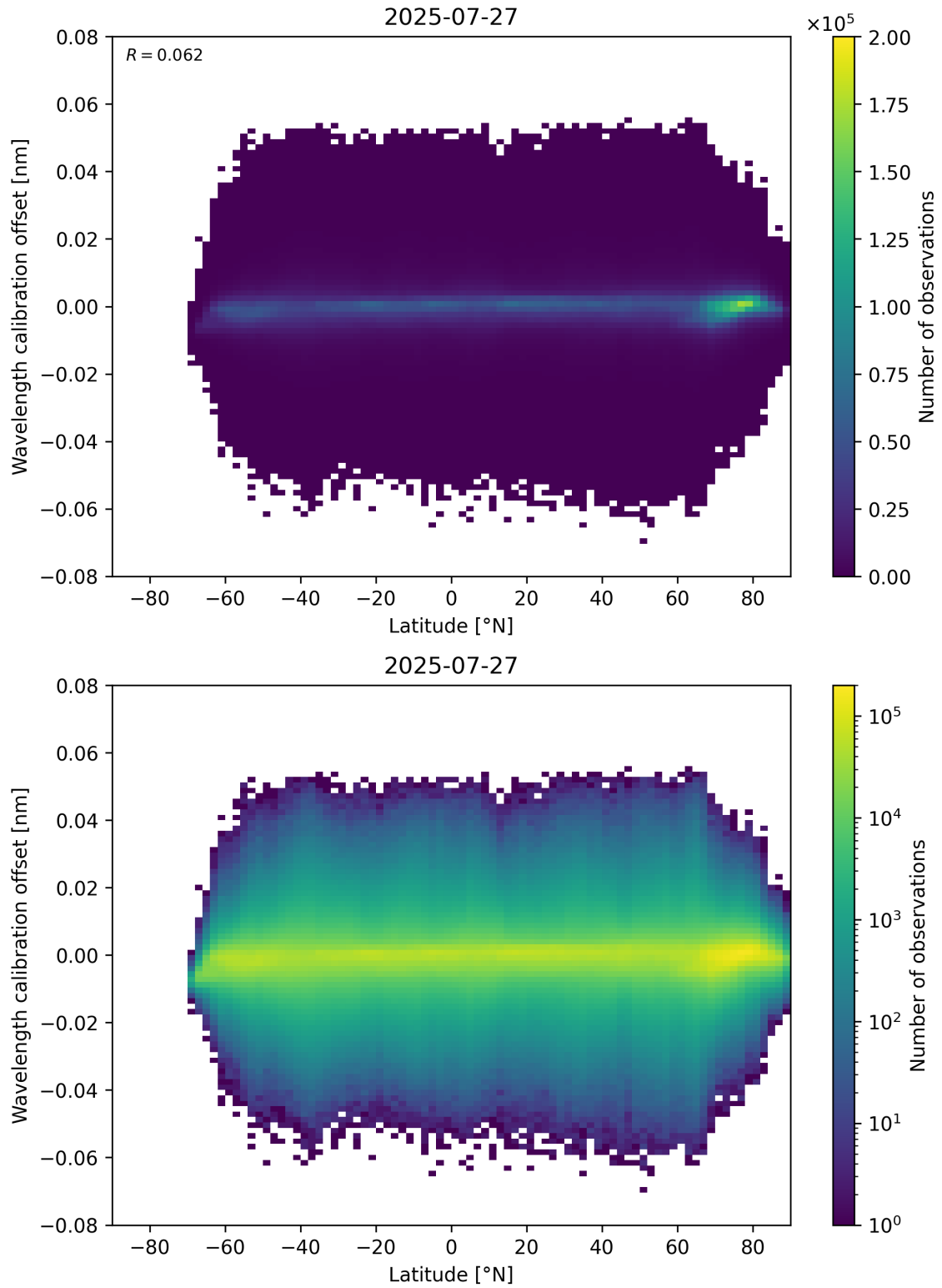
Figure 95: Scatter density plot of “Latitude” against “Wavelength calibration offset” for 2025-07-26 to 2025-07-28.
