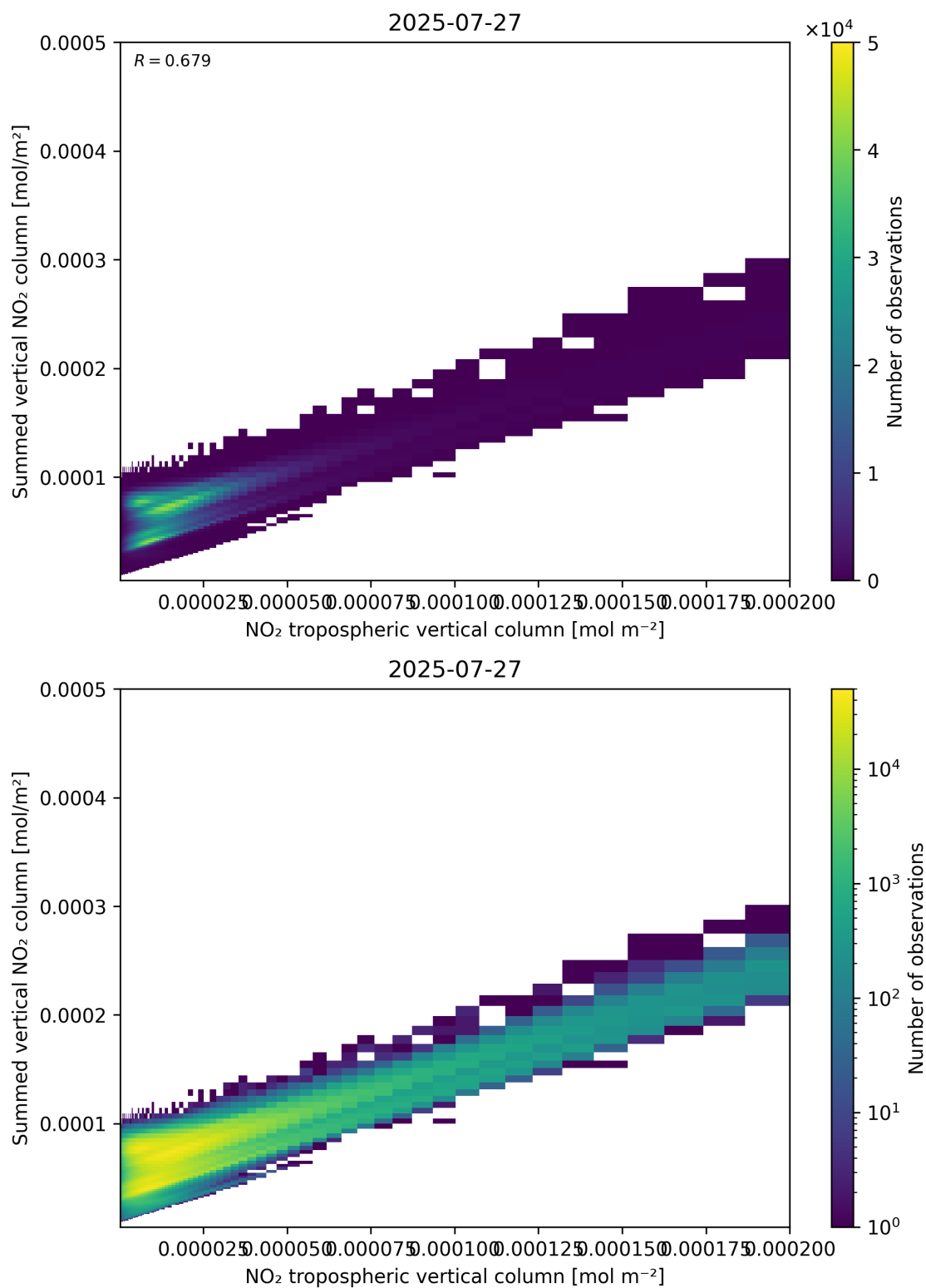
Figure 126: Scatter density plot of “NO 2 tropospheric vertical column” against “Summed vertical NO 2 column” for 2025-07-26 to 2025-07-28.
