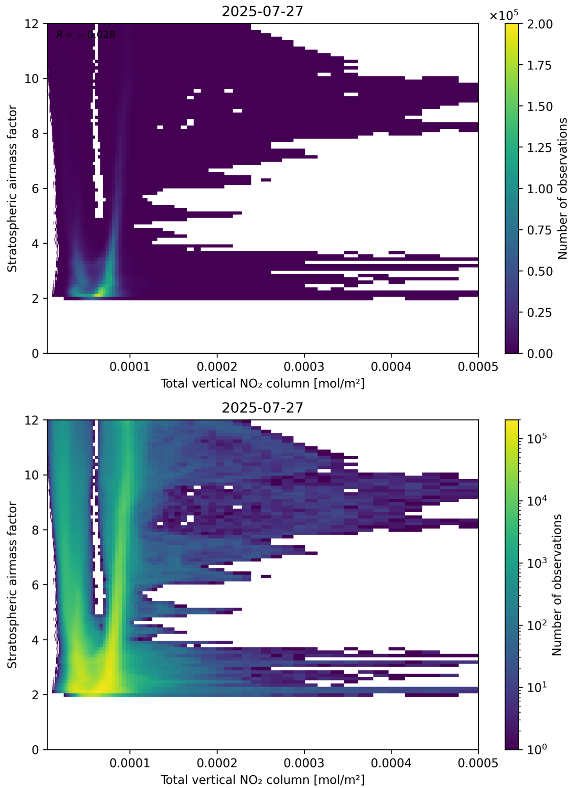
Figure 110: Scatter density plot of “Total vertical NO 2 column” against “Stratospheric airmass factor” for 2025-07-26 to 2025-07-28.
