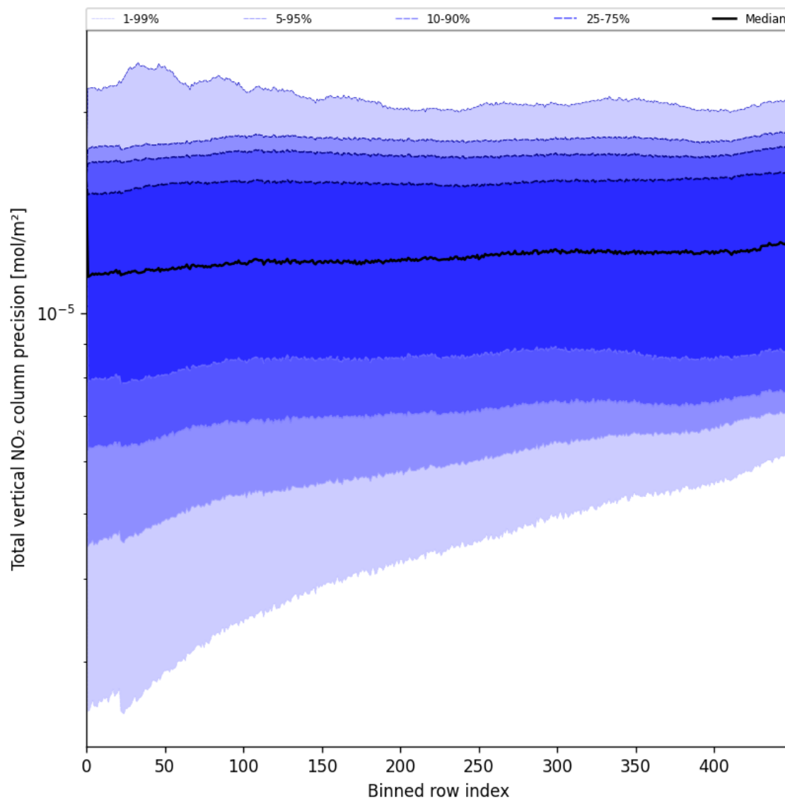
Figure 56: Along track statistics of “Total vertical NO 2 column precision” for 2025-07-26 to 2025-07-28
