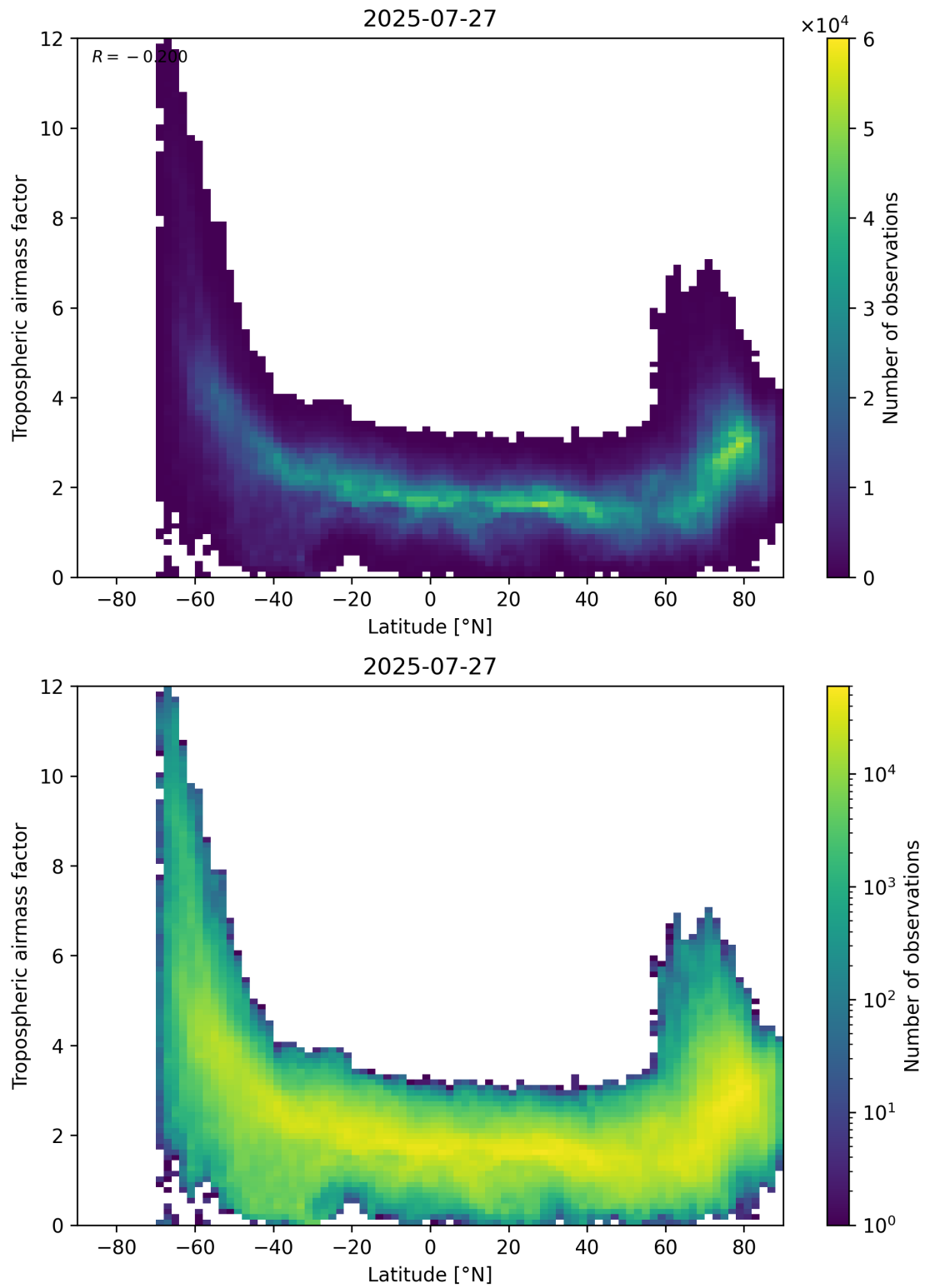
Figure 85: Scatter density plot of “Latitude” against “Tropospheric air mass factor” for 2025-07-26 to 2025-07-28.
