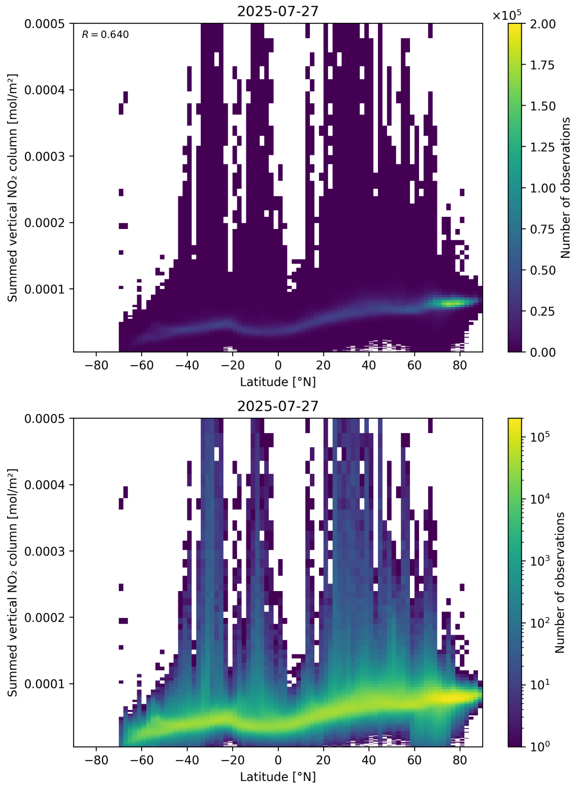
Figure 88: Scatter density plot of “Latitude” against “Summed vertical NO 2 column” for 2025-07-26 to 2025-07-28.
