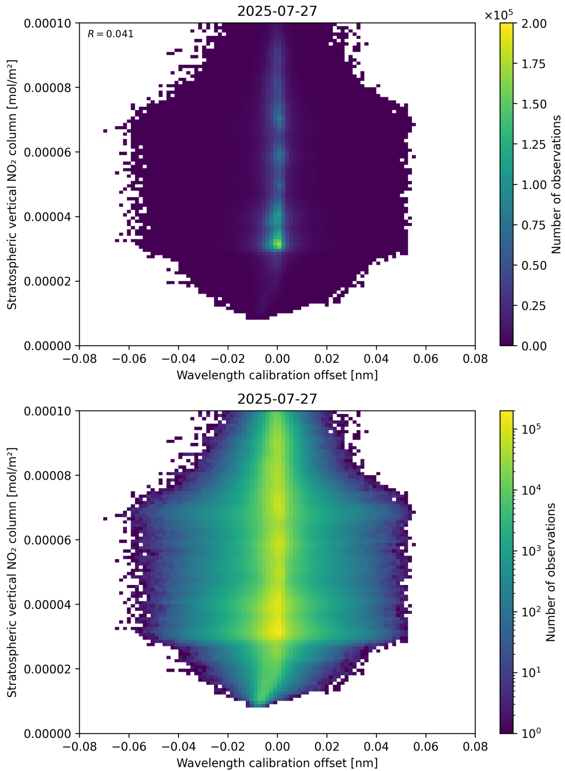
Figure 176: Scatter density plot of “Wavelength calibration offset” against “Stratospheric vertical NO 2 column” for 2025-07-26 to 2025-07-28.
