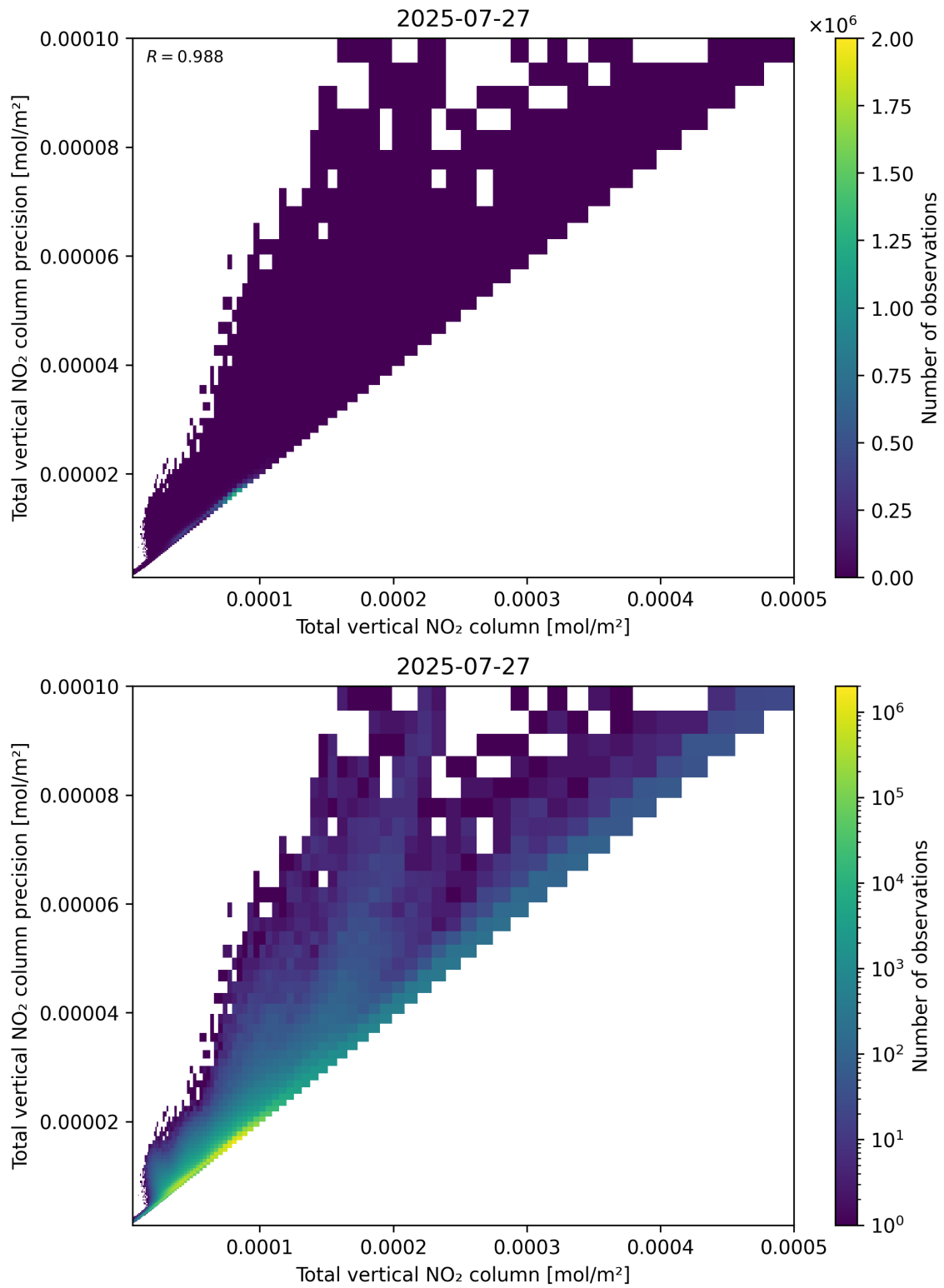
Figure 114: Scatter density plot of “Total vertical NO 2 column” against “Total vertical NO 2 column precision” for 2025-07-26 to 2025-07-28.
