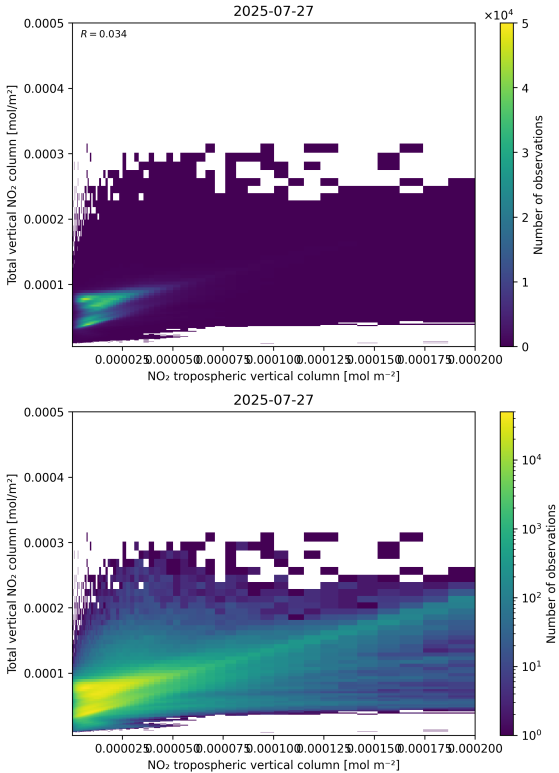
Figure 128: Scatter density plot of “NO 2 tropospheric vertical column” against “Total vertical NO 2 column” for 2025-07-26 to 2025-07-28.
