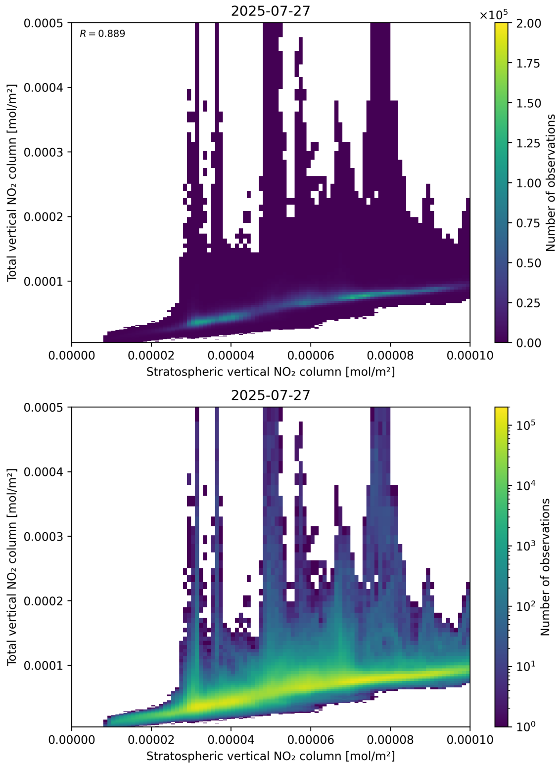
Figure 100: Scatter density plot of “Stratospheric vertical NO 2 column” against “Total vertical NO 2 column” for 2025-07-26 to 2025-07-28.
