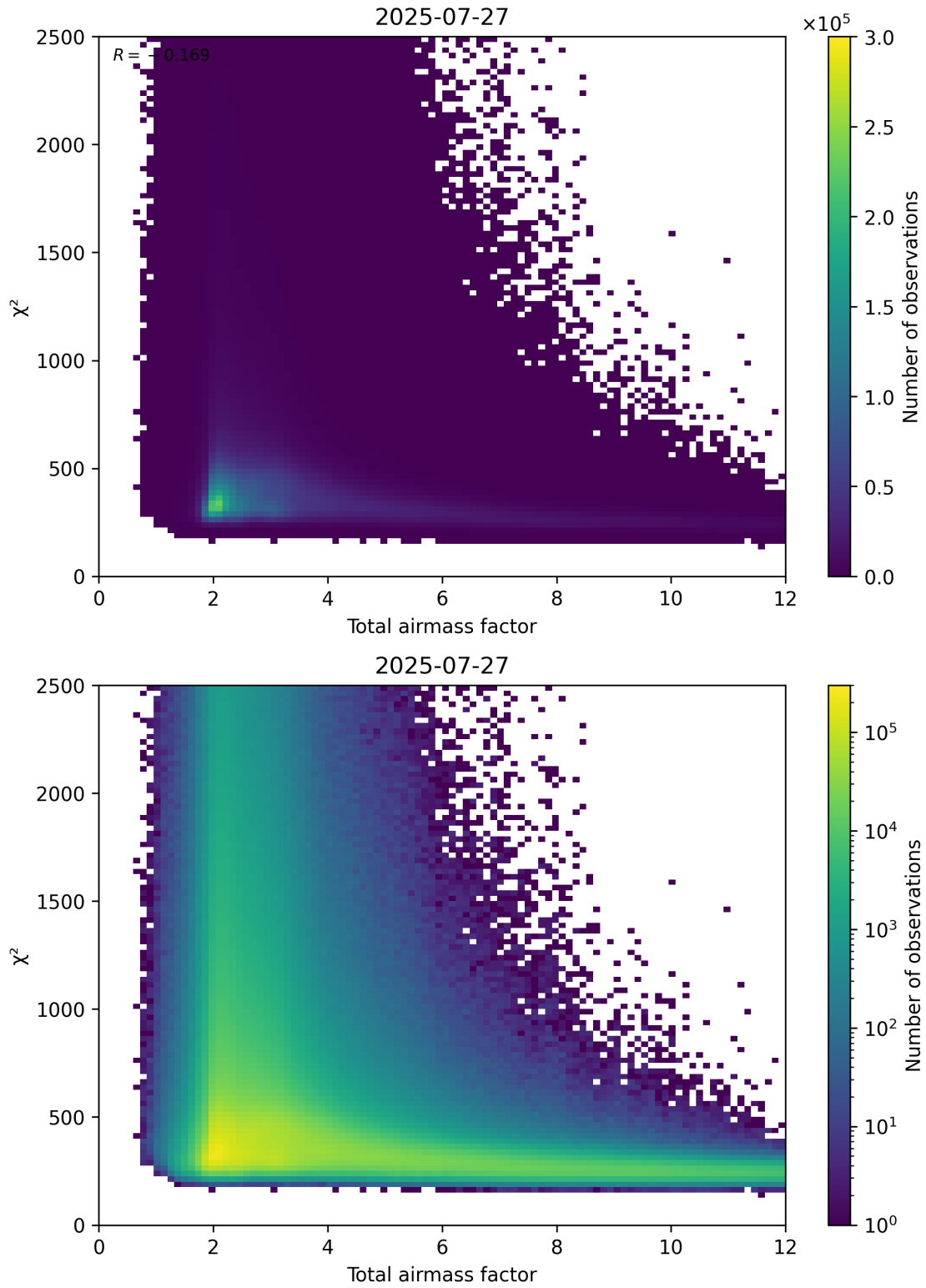
Figure 63: Scatter density plot of “Total airmass factor” against “ \chi^2 ” for 2025-07-26 to 2025-07-28.
