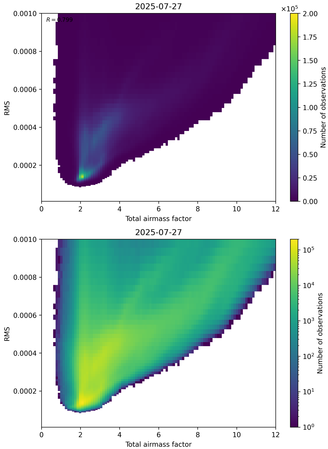
Figure 69: Scatter density plot of “Total airmass factor” against “RMS” for 2025-07-26 to 2025-07-28.
