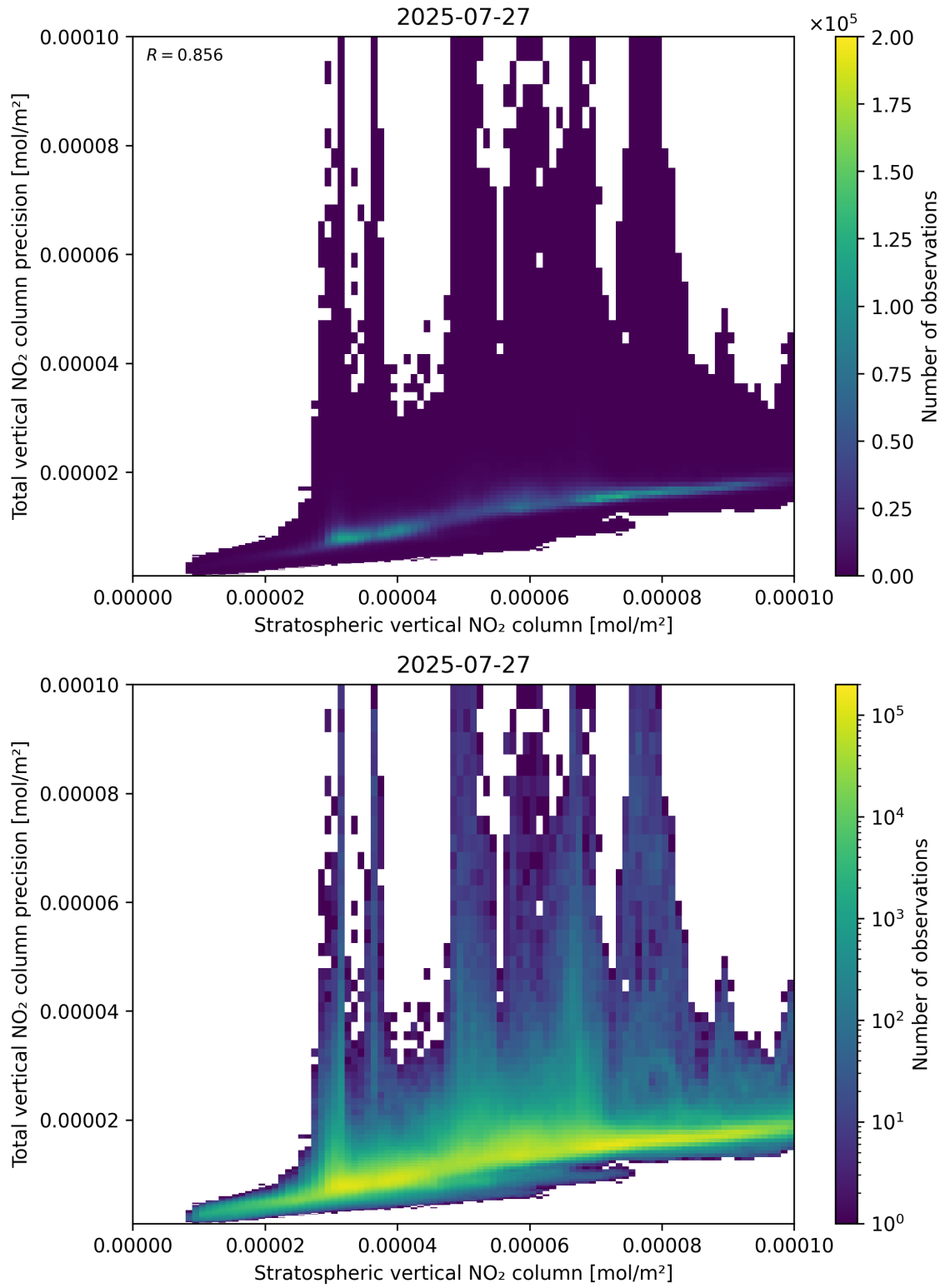
Figure 101: Scatter density plot of “Stratospheric vertical NO 2 column” against “Total vertical NO 2 column precision” for 2025-07-26 to 2025-07-28.
