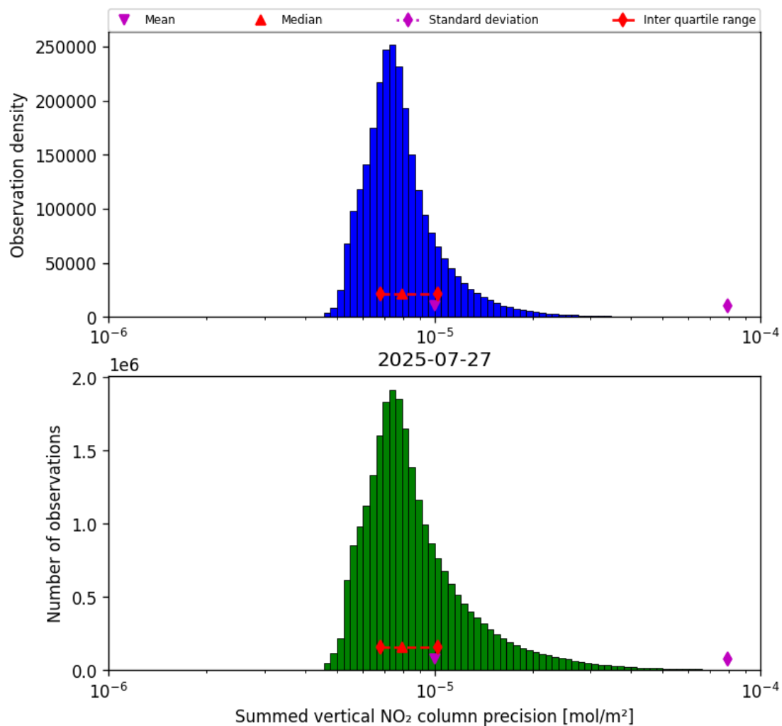
Figure 41: Histogram of “Summed vertical NO 2 column precision” for 2025-07-26 to 2025-07-28
