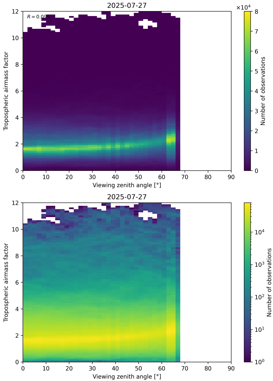
Figure 161: Scatter density plot of “Viewing zenith angle” against “Tropospheric airmass factor” for 2025-07-26 to 2025-07-28.
