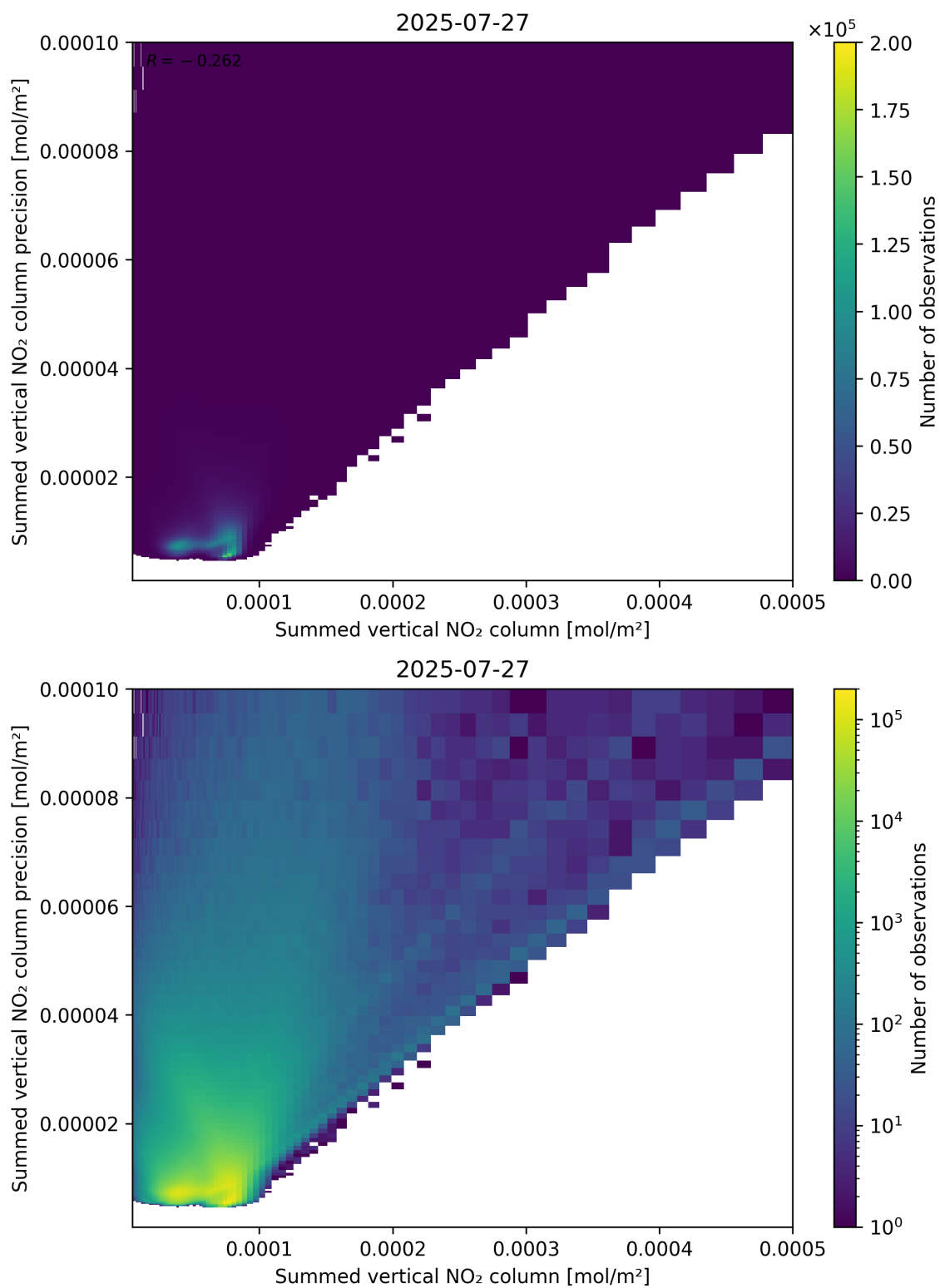
Figure 105: Scatter density plot of “Summed vertical NO 2 column” against “Summed vertical NO 2 column precision” for 2025-07-26 to 2025-07-28.
