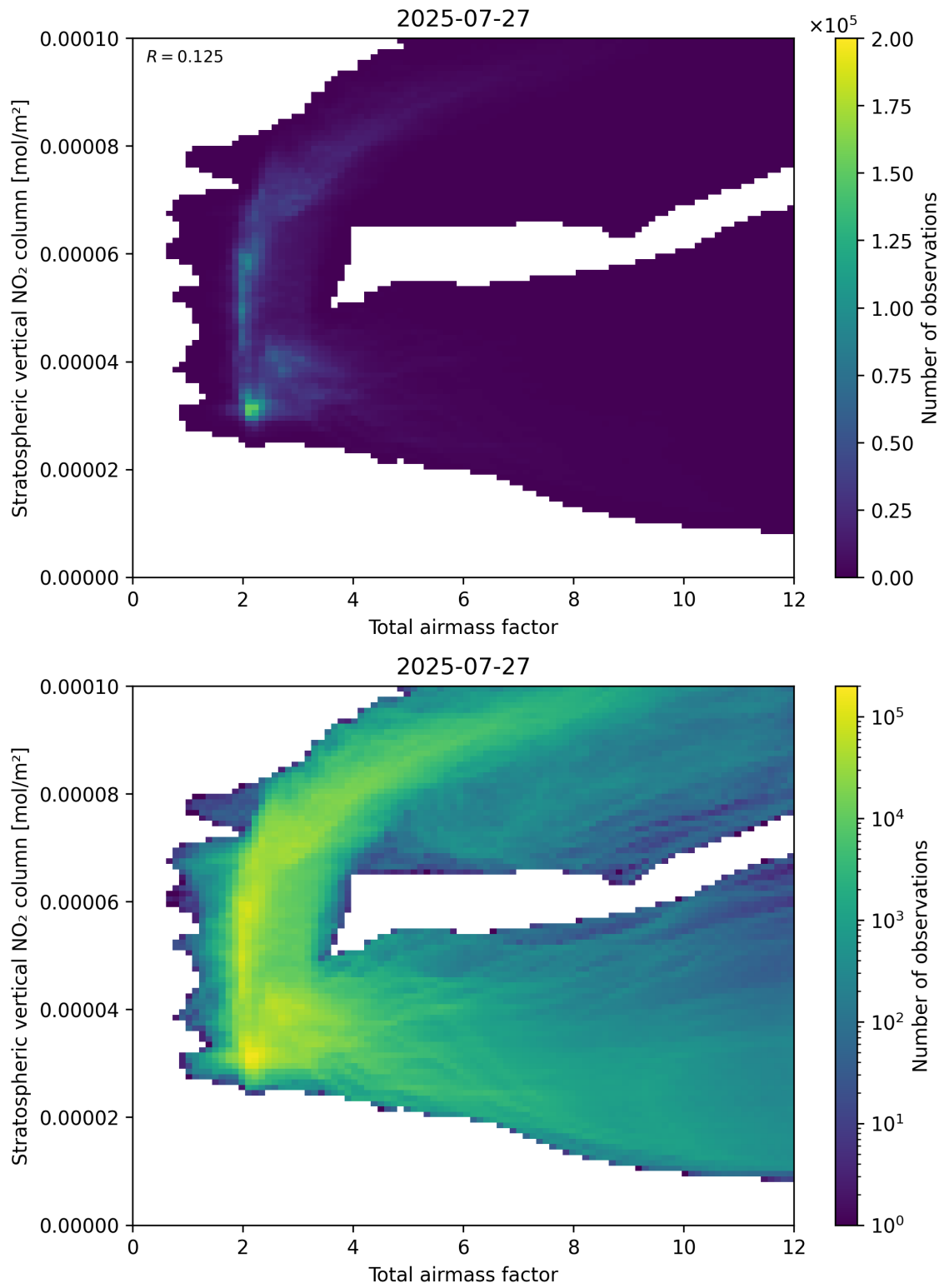
Figure 64: Scatter density plot of “Total airmass factor” against “Stratospheric vertical NO 2 column” for 2025-07-26 to 2025-07-28.
