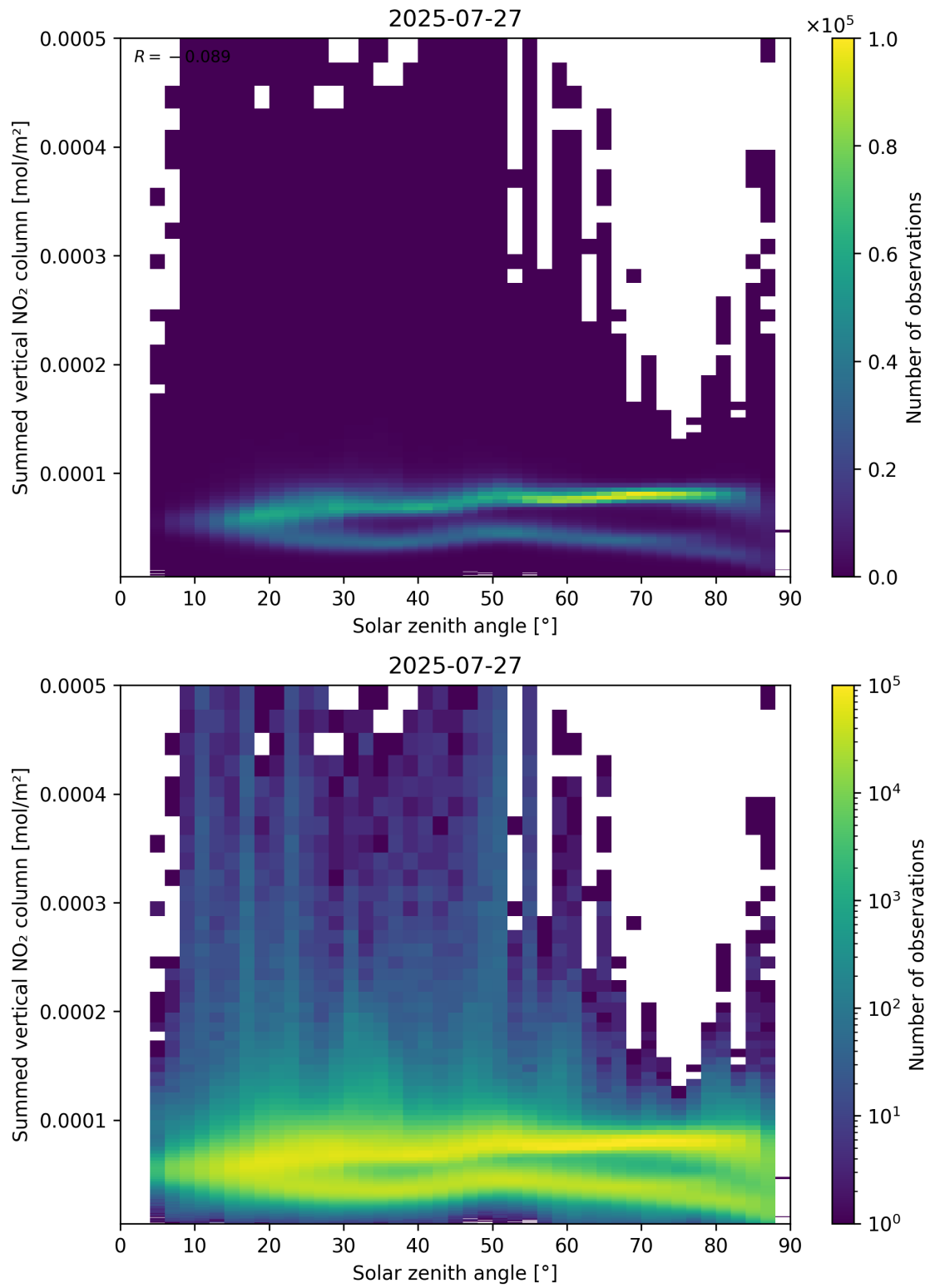
Figure 151: Scatter density plot of “Solar zenith angle” against “Summed vertical NO 2 column” for 2025-07-26 to 2025-07-28.
