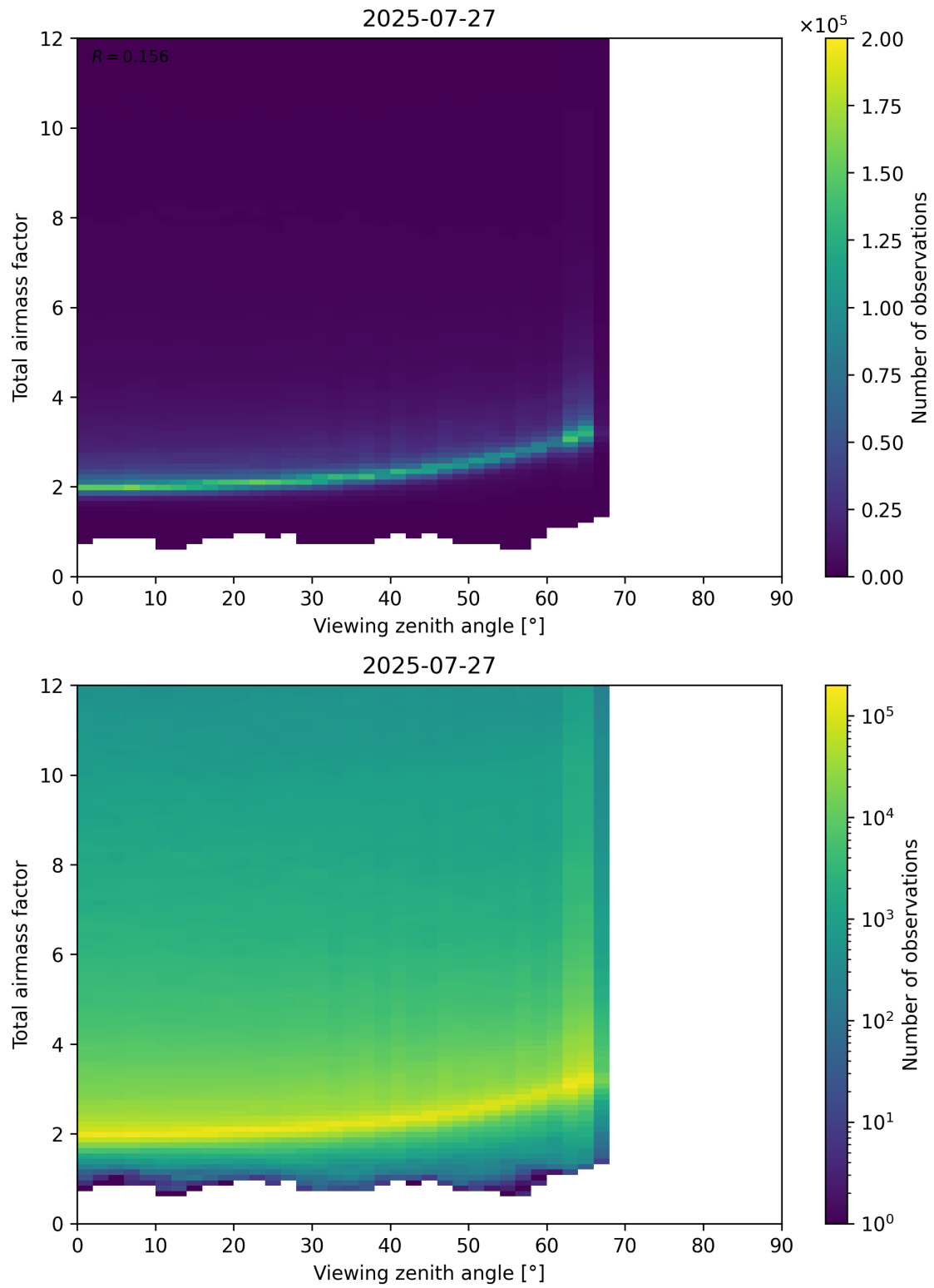
Figure 160: Scatter density plot of “Viewing zenith angle” against “Total airmass factor” for 2025-07-26 to 2025-07-28.
