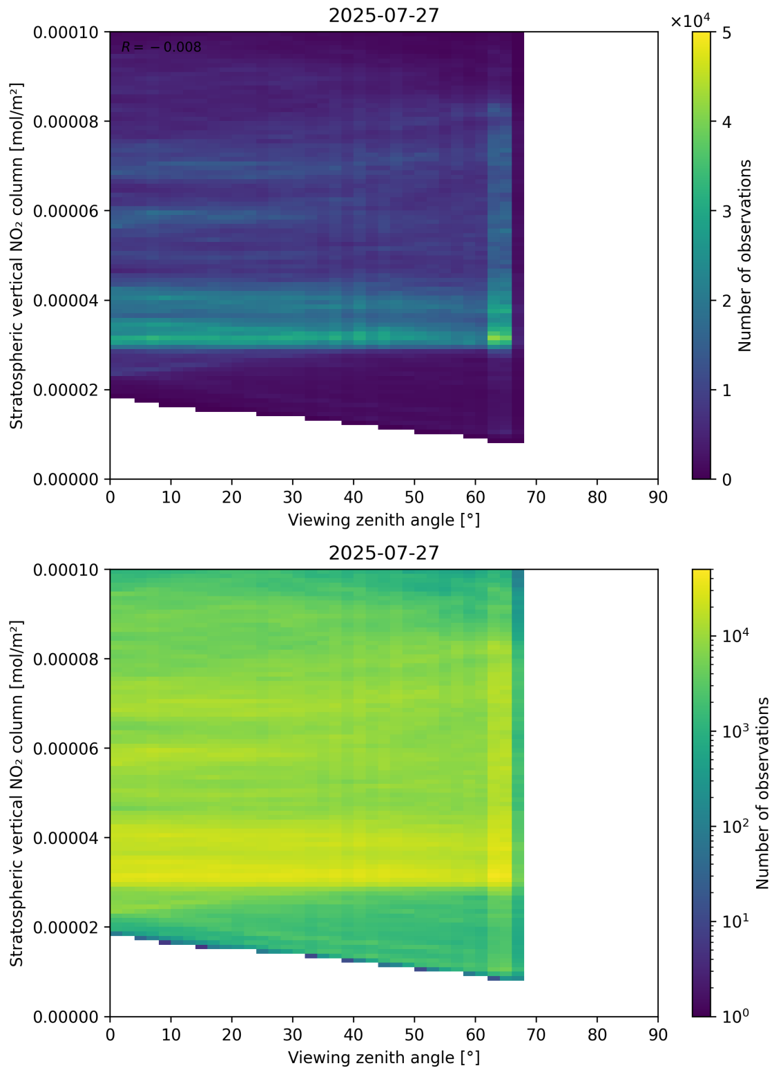
Figure 164: Scatter density plot of “Viewing zenith angle” against “Stratospheric vertical NO 2 column” for 2025-07-26 to 2025-07-28.
