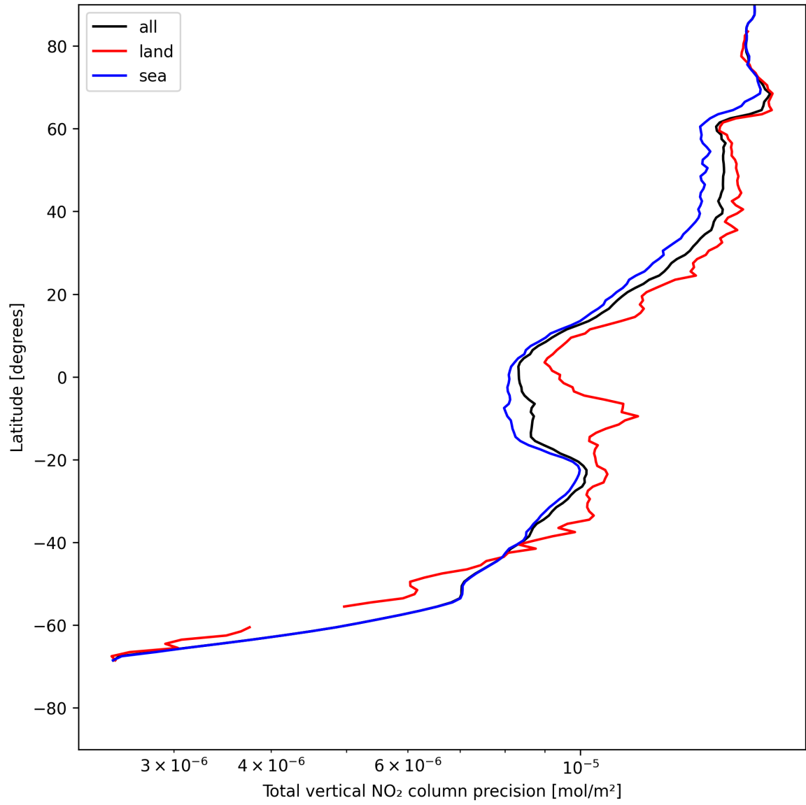
Figure 22: Zonal average of “Total vertical NO 2 column precision” for 2025-07-26 to 2025-07-28.
