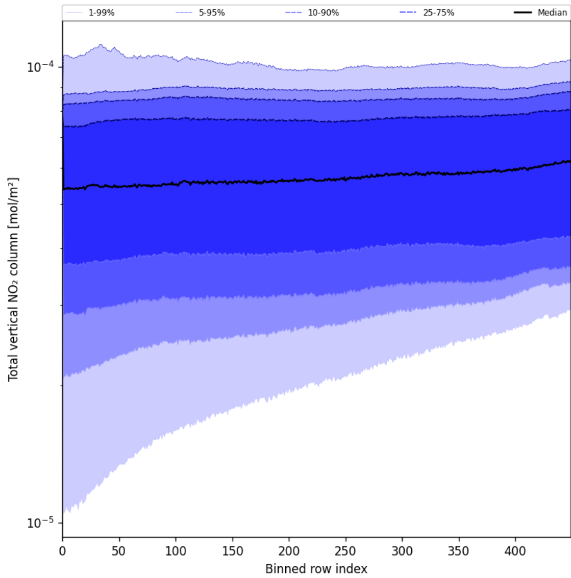
Figure 55: Along track statistics of “Total vertical NO 2 column” for 2025-07-26 to 2025-07-28
