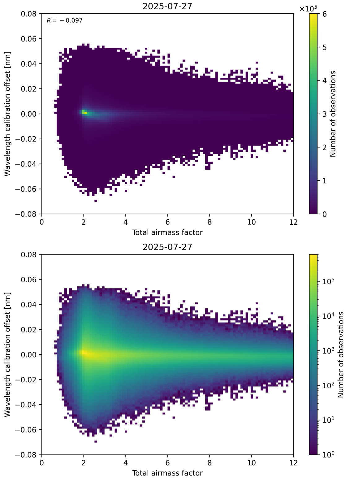
Figure 70: Scatter density plot of “Total airmass factor” against “Wavelength calibration offset” for 2025-07-26 to 2025-07-28.
