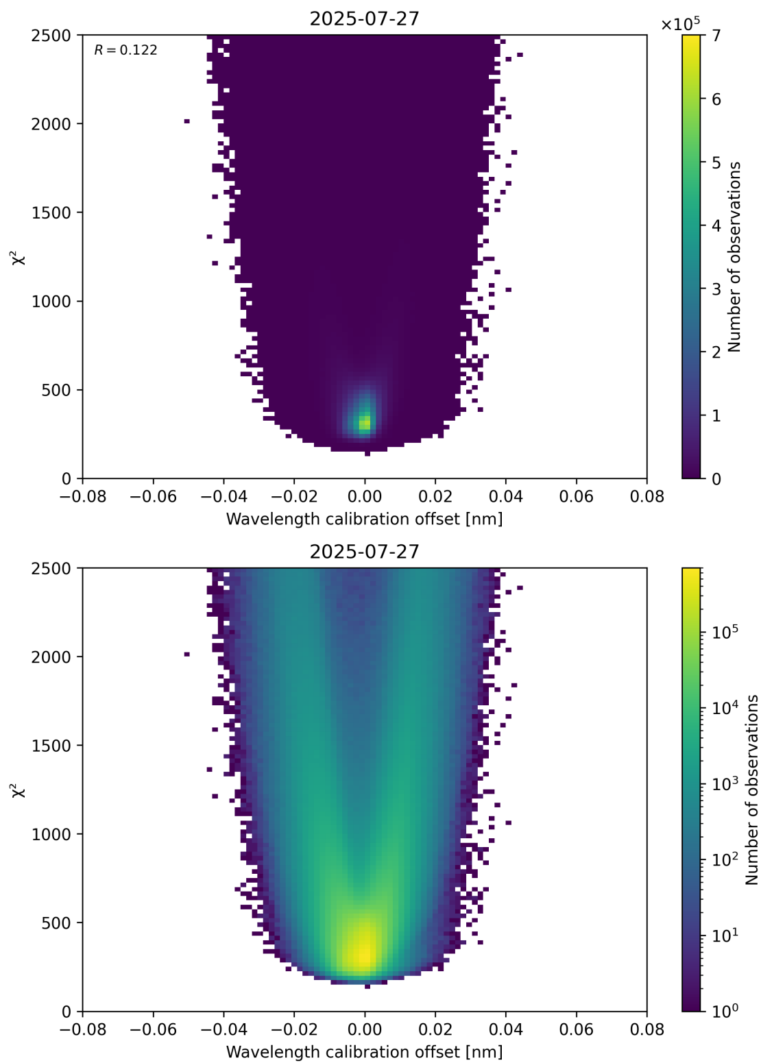
Figure 175: Scatter density plot of “Wavelength calibration offset” against “ \chi^2 ” for 2025-07-26 to 2025-07-28.
