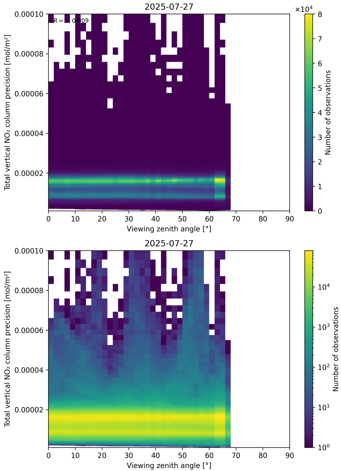
Figure 168: Scatter density plot of “Viewing zenith angle” against “Total vertical NO 2 column precision” for 2025-07-26 to 2025-07-28.
