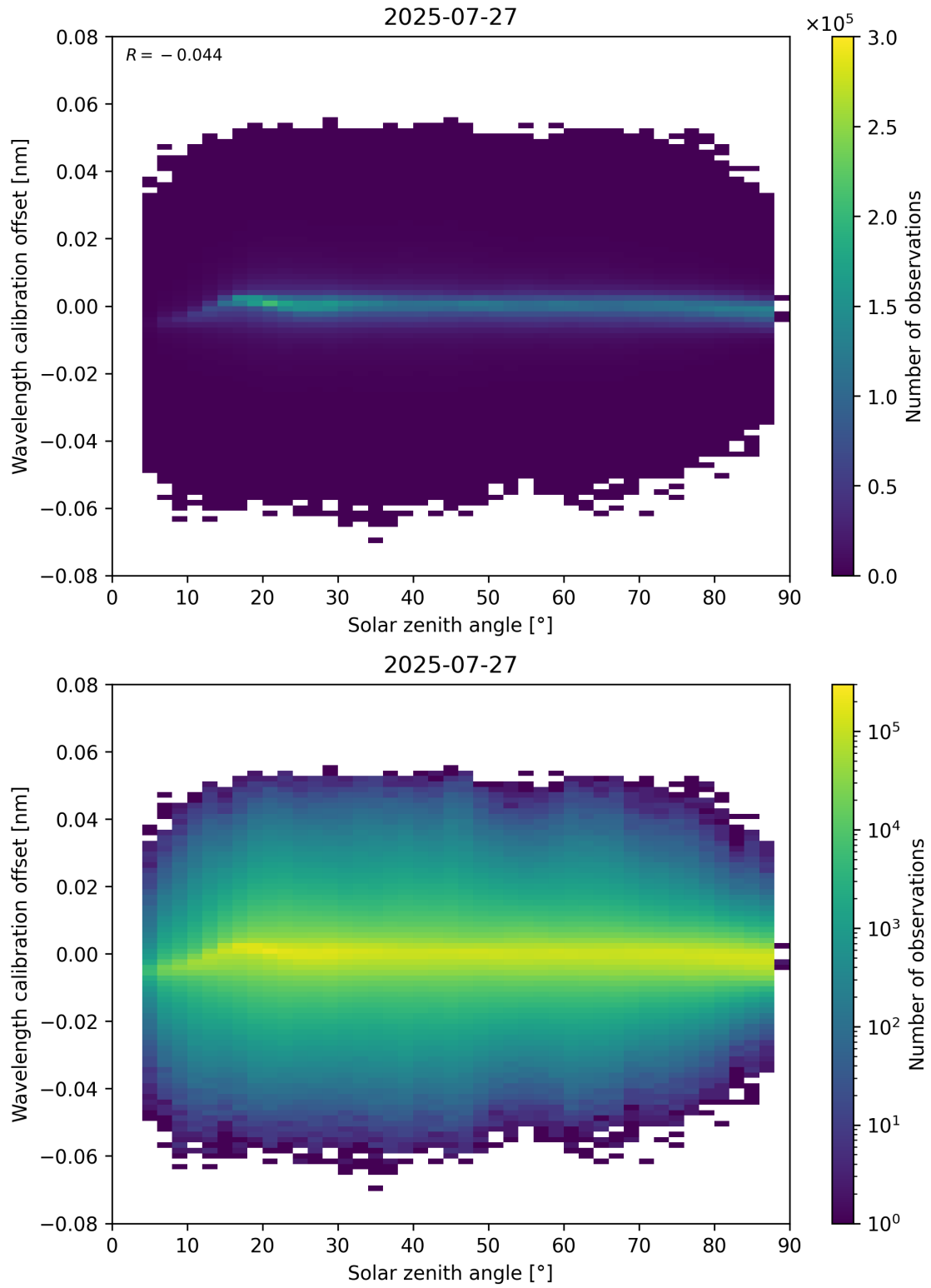
Figure 158: Scatter density plot of “Solar zenith angle” against “Wavelength calibration offset” for 2025-07-26 to 2025-07-28.
