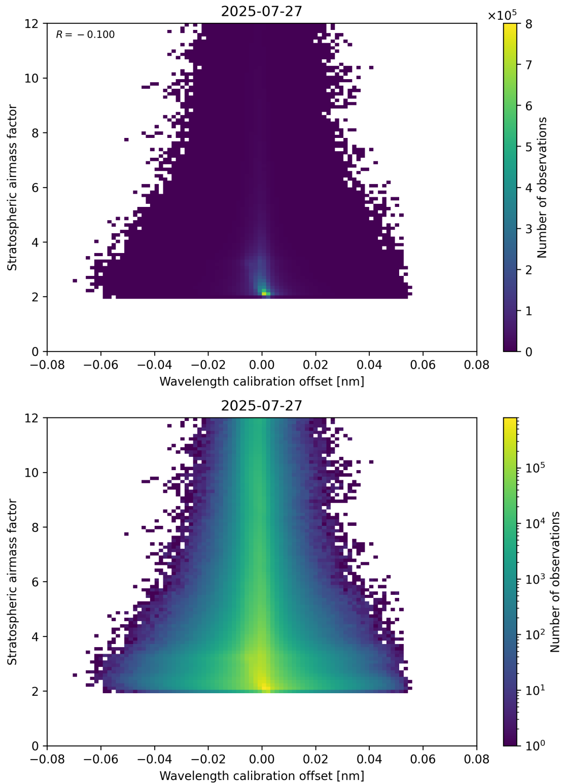
Figure 174: Scatter density plot of “Wavelength calibration offset” against “Stratospheric airmass factor” for 2025-07-26 to 2025-07-28.
