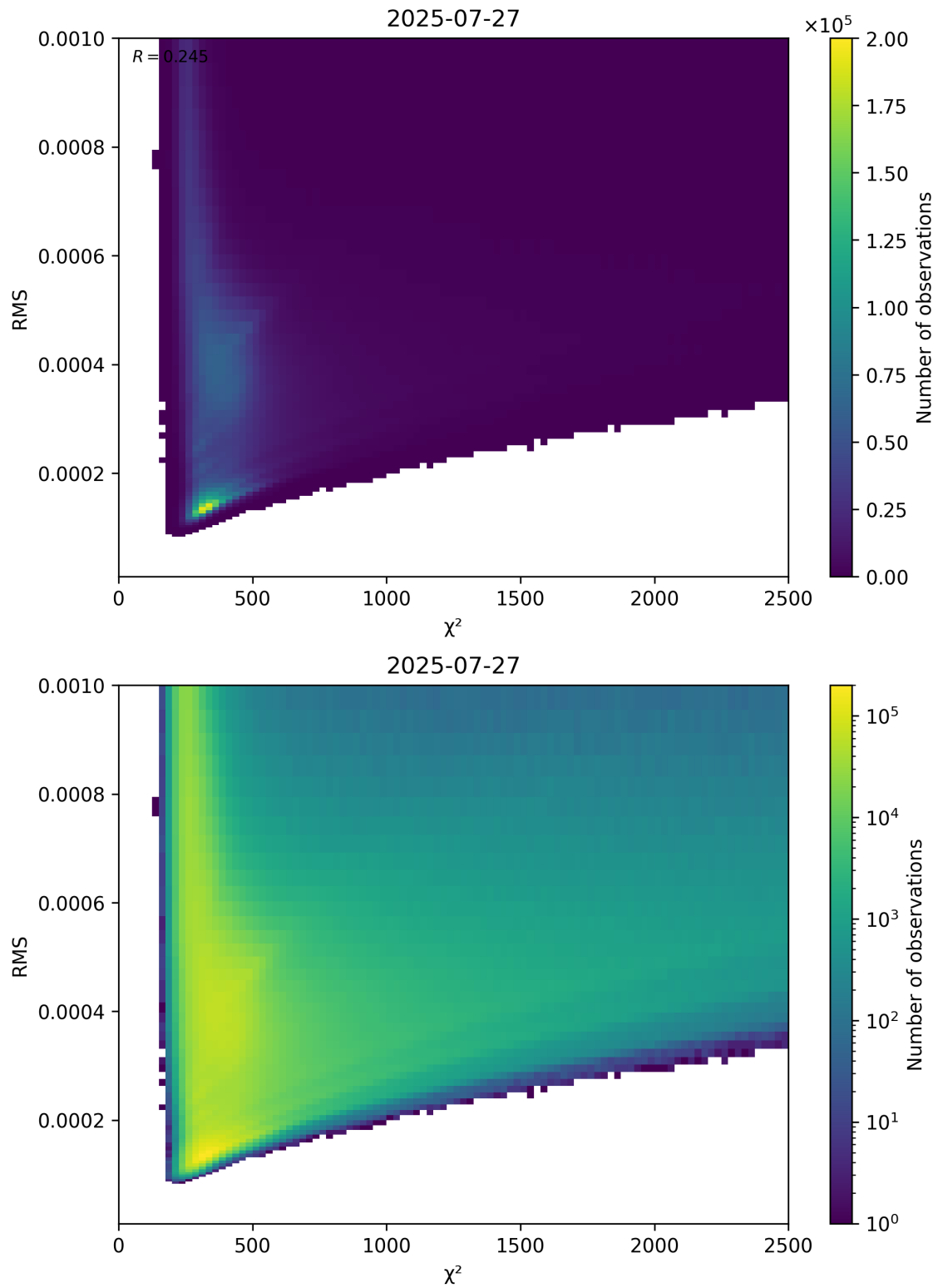
Figure 82: Scatter density plot of “ \chi^2 ” against “RMS” for 2025-07-26 to 2025-07-28.
