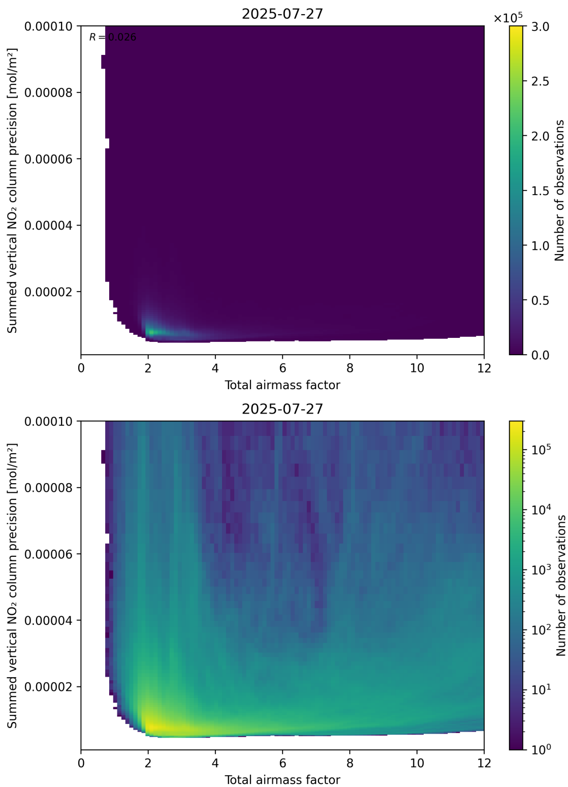
Figure 66: Scatter density plot of “Total airmass factor” against “Summed vertical NO 2 column precision” for 2025-07-26 to 2025-07-28.
