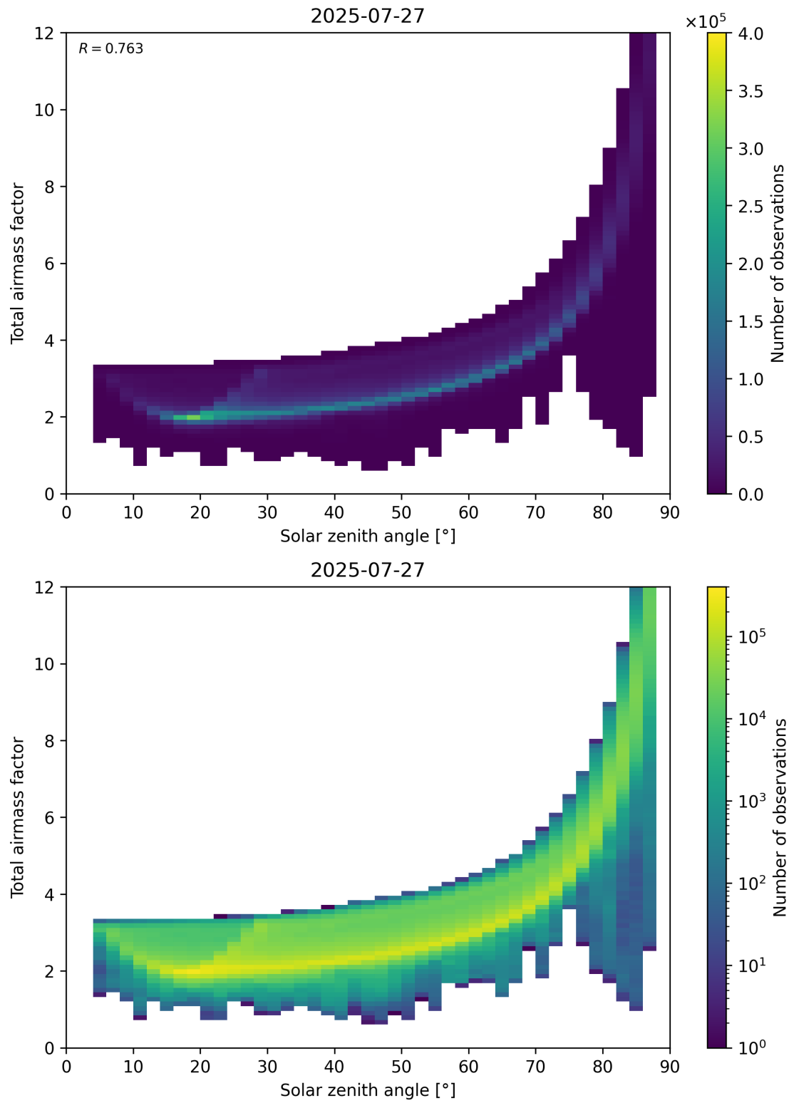
Figure 146: Scatter density plot of “Solar zenith angle” against “Total air mass factor” for 2025-07-26 to 2025-07-28.
