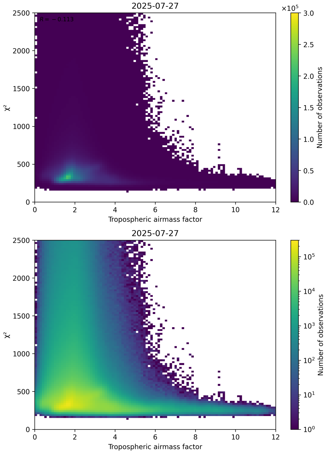
Figure 73: Scatter density plot of “Tropospheric airmass factor” against “ \chi^2 ” for 2025-07-26 to 2025-07-28.
