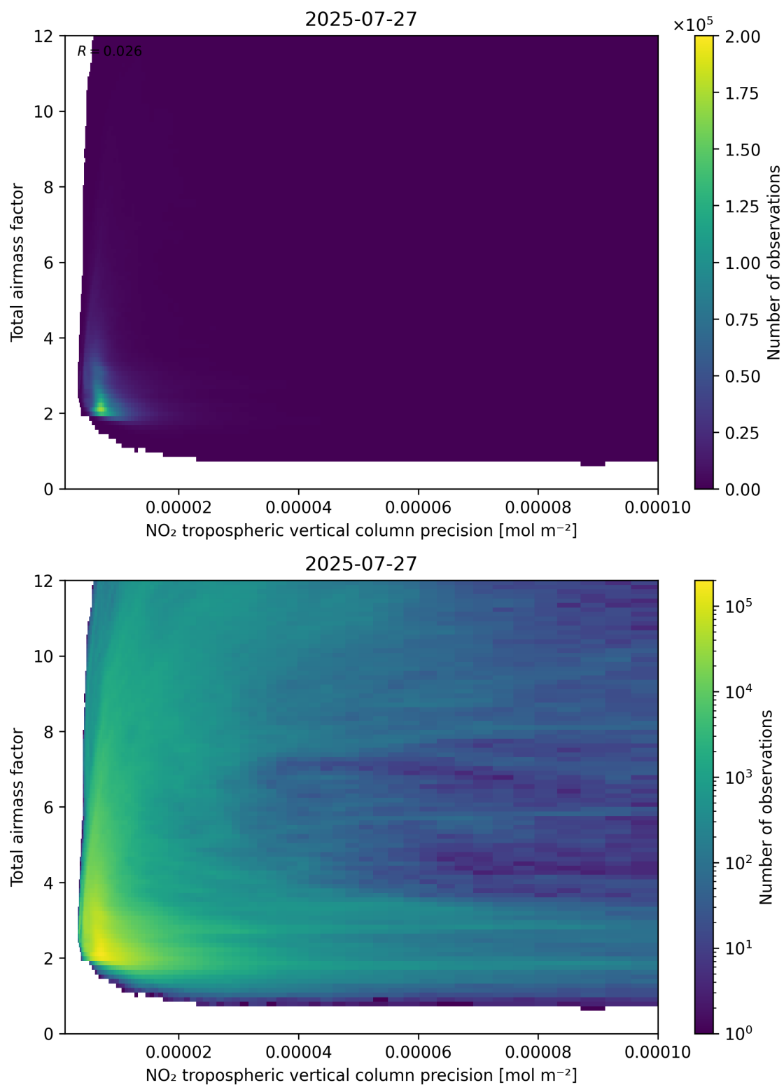
Figure 132: Scatter density plot of “NO 2 tropospheric vertical column precision” against “Total air mass factor” for 2025-07-26 to 2025-07-28.
