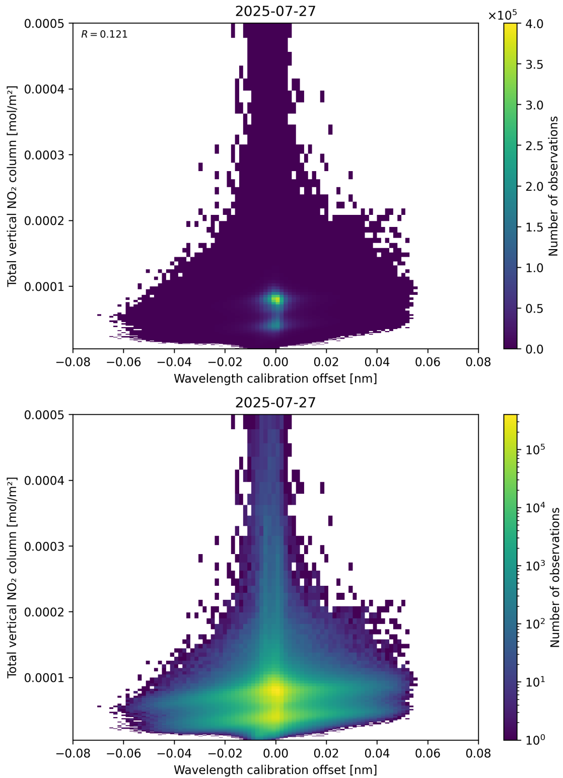
Figure 179: Scatter density plot of “Wavelength calibration offset” against “Total vertical NO 2 column” for 2025-07-26 to 2025-07-28.
