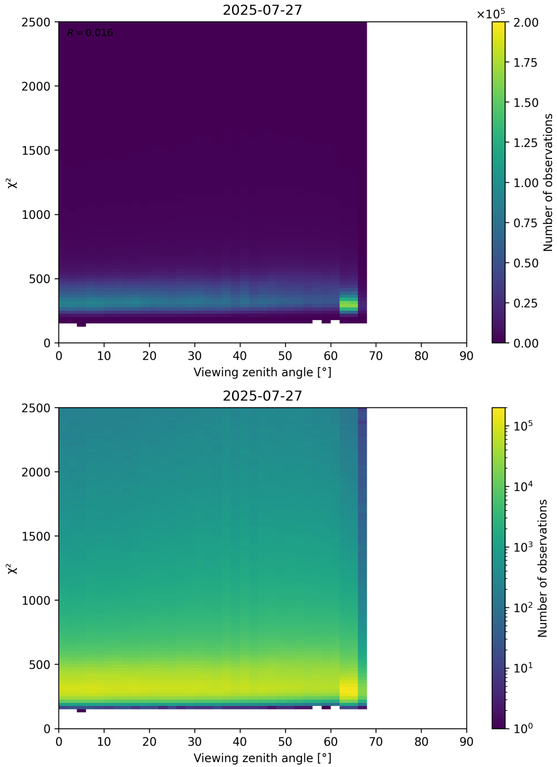
Figure 162: Scatter density plot of “Viewing zenith angle” against “ \chi^2 ” for 2025-07-26 to 2025-07-28.
