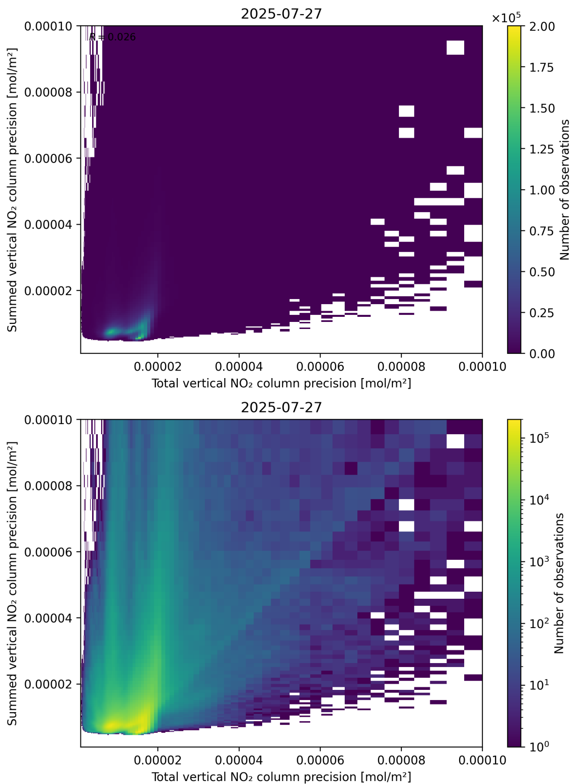
Figure 118: Scatter density plot of “Total vertical NO 2 column precision” against “Summed vertical NO 2 column precision” for 2025-07-26 to 2025-07-28.
