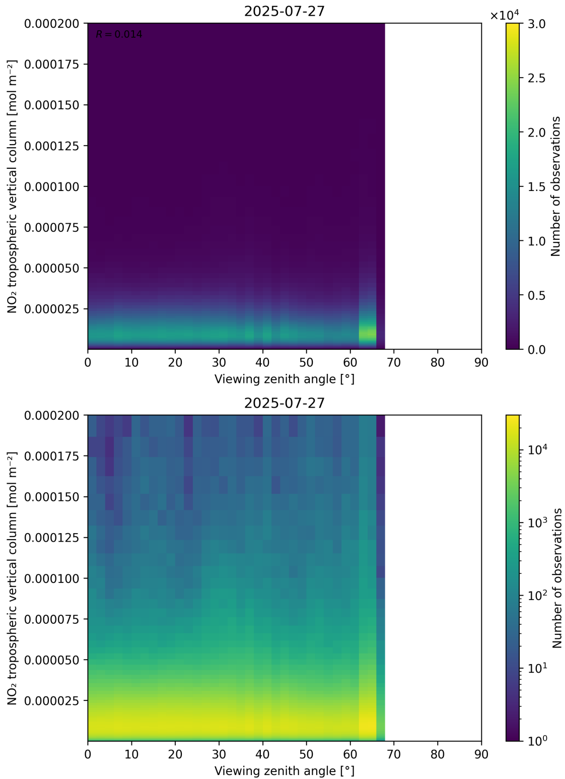
Figure 169: Scatter density plot of “Viewing zenith angle” against “NO 2 tropospheric vertical column” for 2025-07-26 to 2025-07-28.
