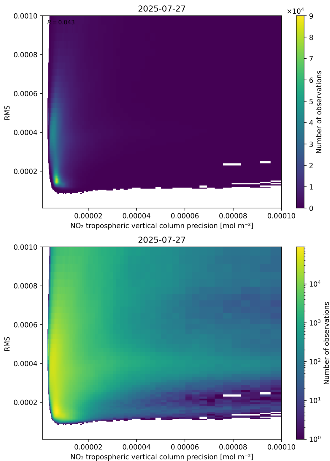
Figure 140: Scatter density plot of “NO 2 tropospheric vertical column precision” against “RMS” for 2025-07-26 to 2025-07-28.
