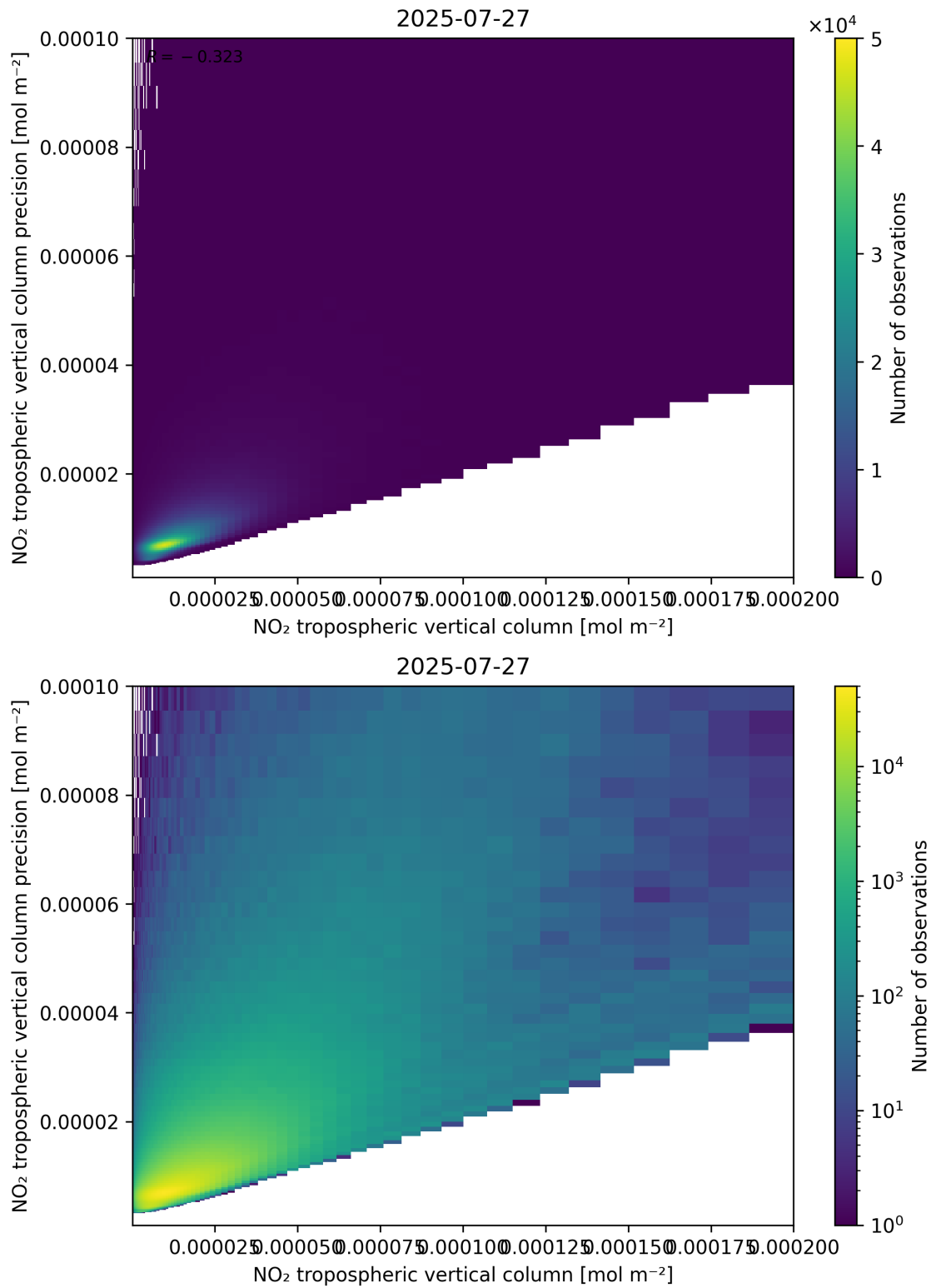
Figure 130: Scatter density plot of “NO 2 tropospheric vertical column” against “NO 2 tropospheric vertical column precision” for 2025-07-26 to 2025-07-28.
