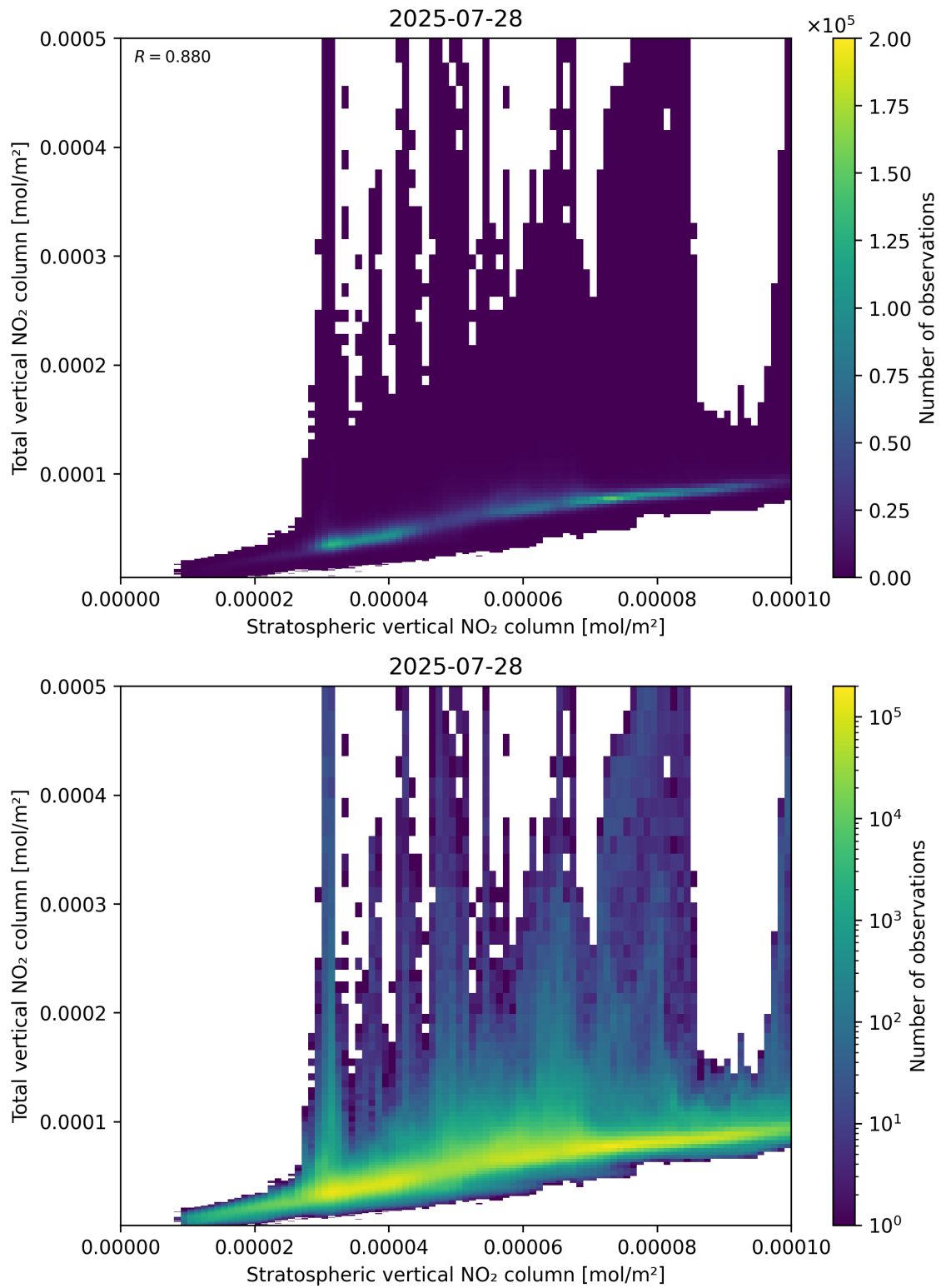
Figure 100: Scatter density plot of “Stratospheric vertical NO 2 column” against “Total vertical NO 2 column” for 2025-07-27 to 2025-07-29.
