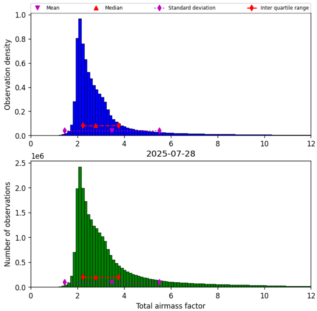
Figure 32: Histogram of “Total airmass factor” for 2025-07-27 to 2025-07-29
