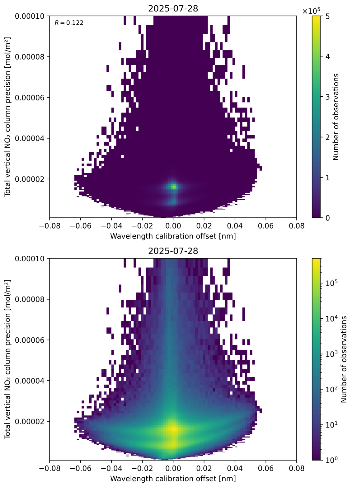
Figure 180: Scatter density plot of “Wavelength calibration offset” against “Total vertical NO 2 column precision” for 2025-07-27 to 2025-07-29.
