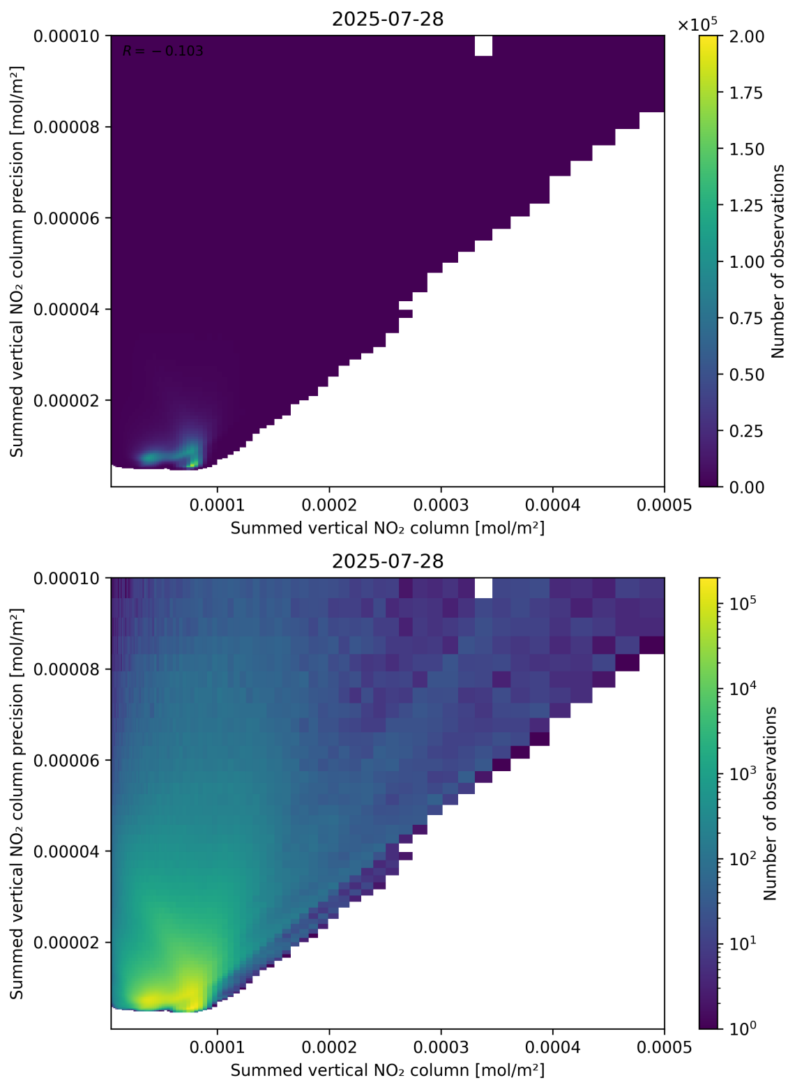
Figure 105: Scatter density plot of “Summed vertical NO 2 column” against “Summed vertical NO 2 column precision” for 2025-07-27 to 2025-07-29.
