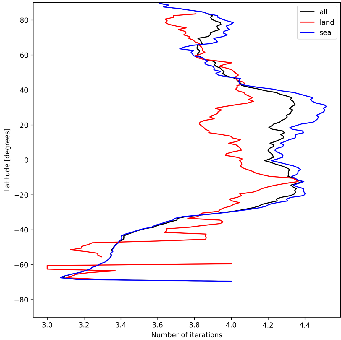
Figure 17: Zonal average of “Number of iterations” for 2025-07-27 to 2025-07-29.
