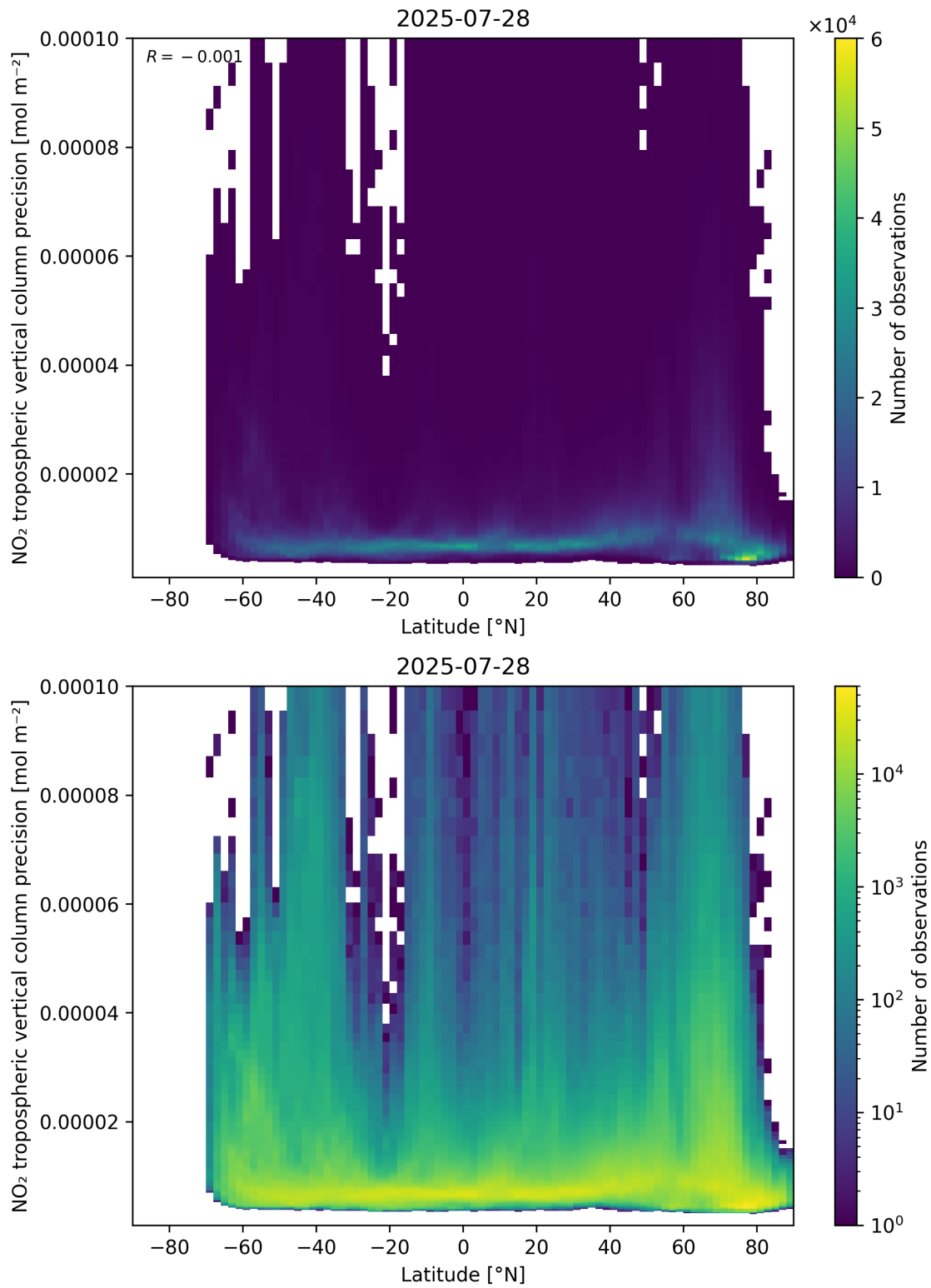
Figure 93: Scatter density plot of “Latitude” against “NO 2 tropospheric vertical column precision” for 2025-07-27 to 2025-07-29.
