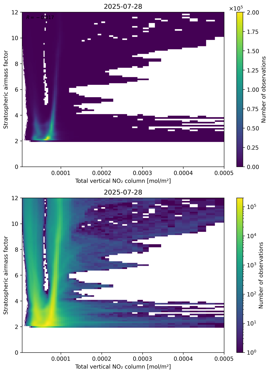
Figure 110: Scatter density plot of “Total vertical NO 2 column” against “Stratospheric airmass factor” for 2025-07-27 to 2025-07-29.
