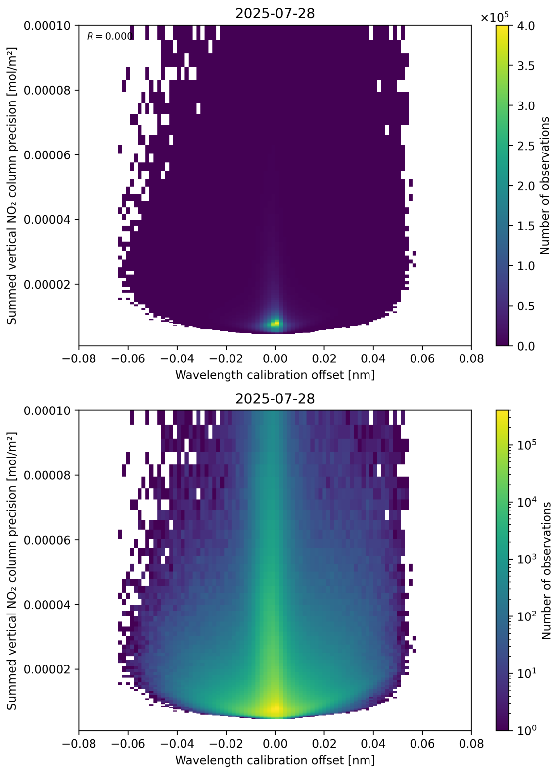
Figure 178: Scatter density plot of “Wavelength calibration offset” against “Summed vertical NO 2 column precision” for 2025-07-27 to 2025-07-29.
