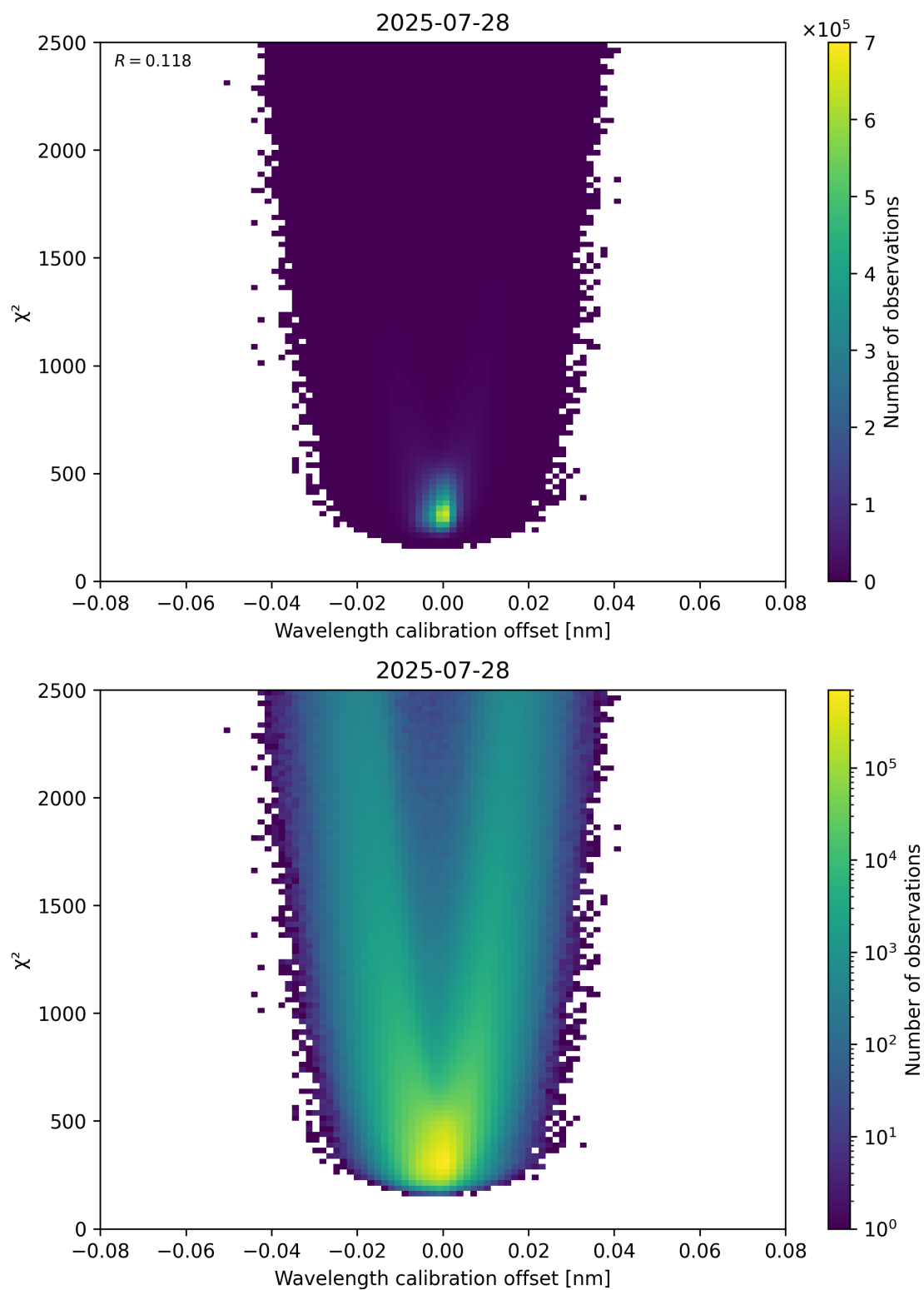
Figure 175: Scatter density plot of “Wavelength calibration offset” against “ \chi^2 ” for 2025-07-27 to 2025-07-29.
