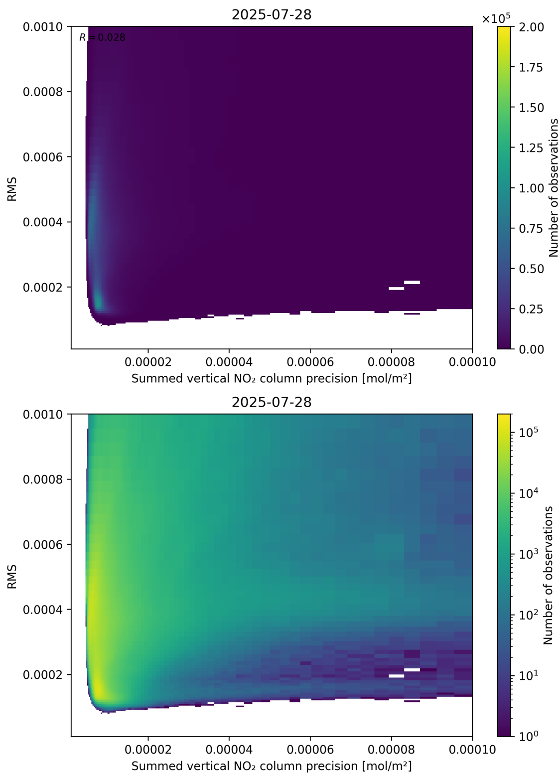
Figure 108: Scatter density plot of “Summed vertical NO 2 column precision” against “RMS” for 2025-07-27 to 2025-07-29.
