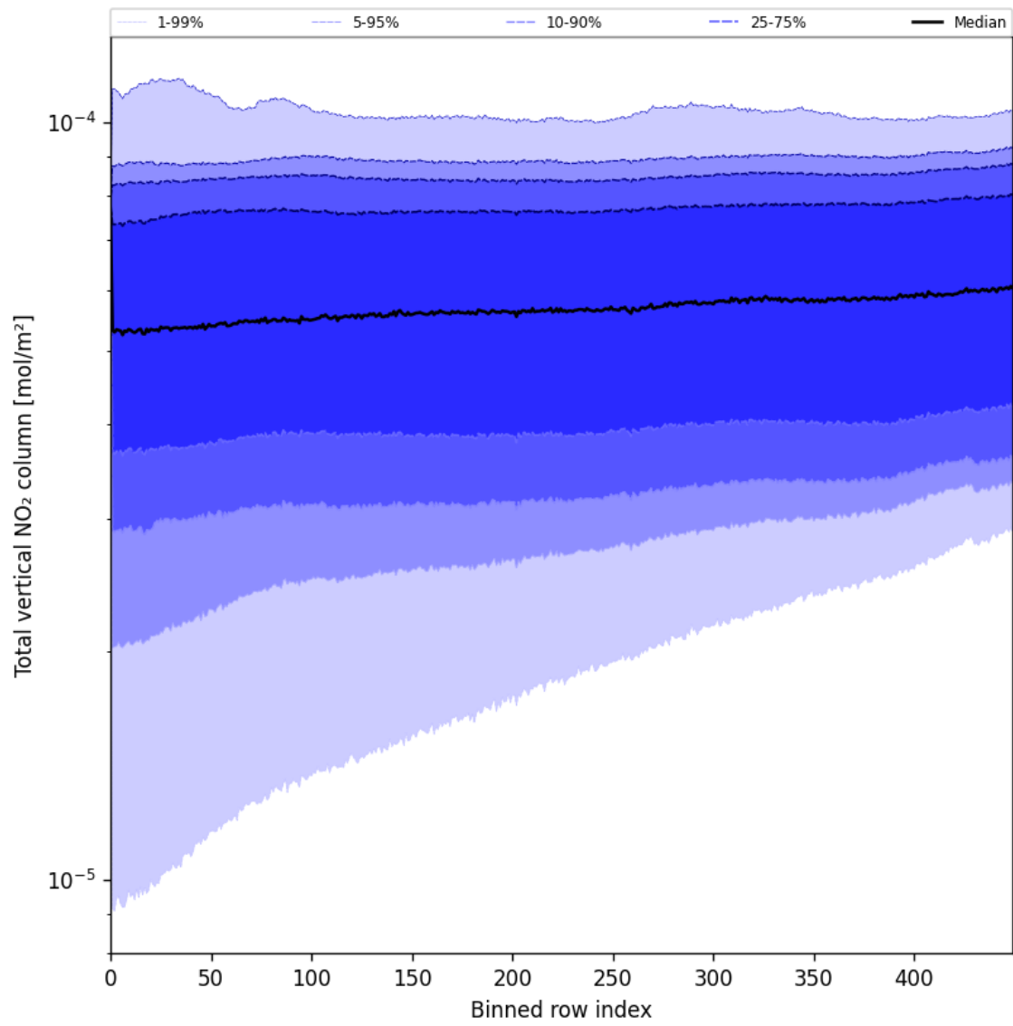
Figure 55: Along track statistics of “Total vertical NO 2 column” for 2025-07-27 to 2025-07-29
