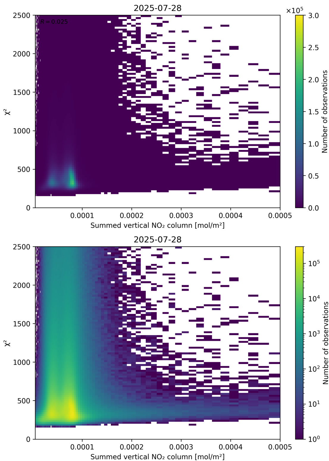
Figure 104: Scatter density plot of “Summed vertical NO 2 column” against “ \chi^2 ” for 2025-07-27 to 2025-07-29.
