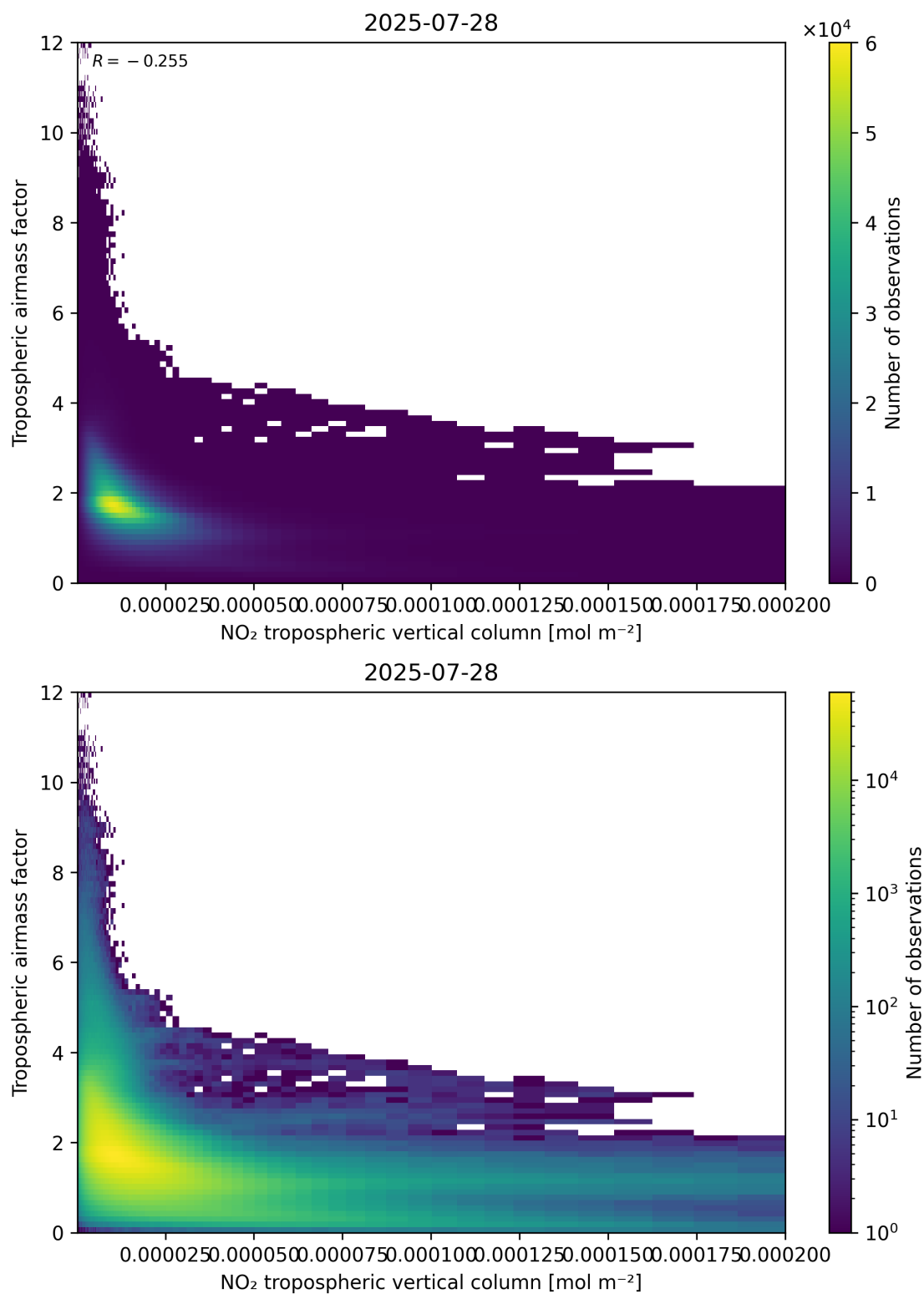
Figure 123: Scatter density plot of “NO 2 tropospheric vertical column” against “Tropospheric air mass factor” for 2025-07-27 to 2025-07-29.
