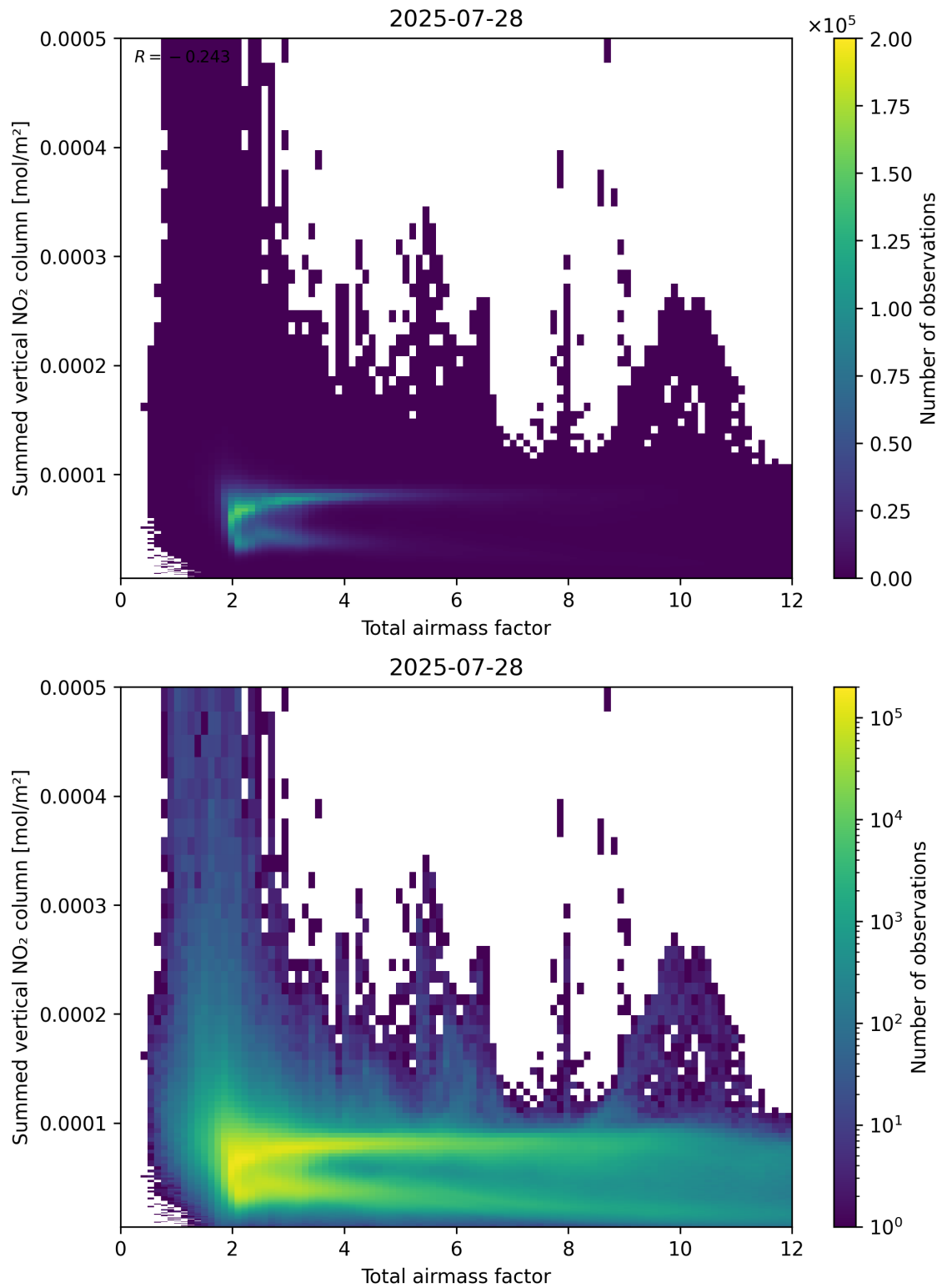
Figure 65: Scatter density plot of “Total airmass factor” against “Summed vertical NO 2 column” for 2025-07-27 to 2025-07-29.
