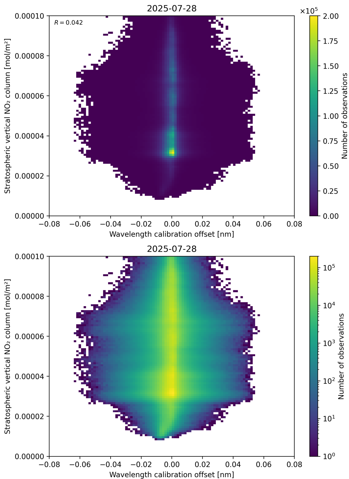
Figure 176: Scatter density plot of “Wavelength calibration offset” against “Stratospheric vertical NO 2 column” for 2025-07-27 to 2025-07-29.
