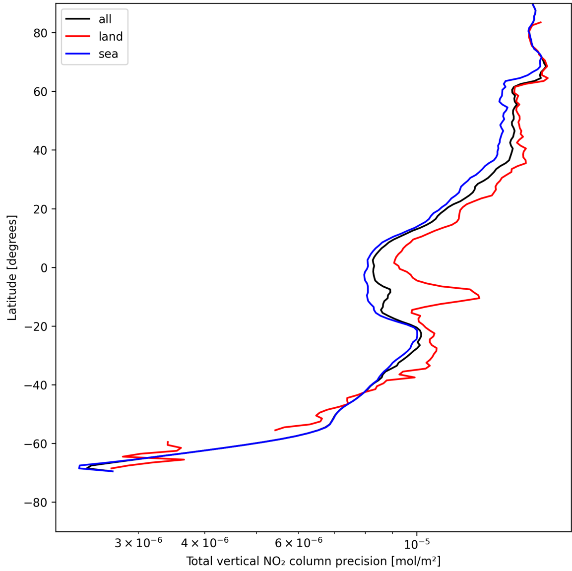
Figure 22: Zonal average of “Total vertical NO 2 column precision” for 2025-07-27 to 2025-07-29.
