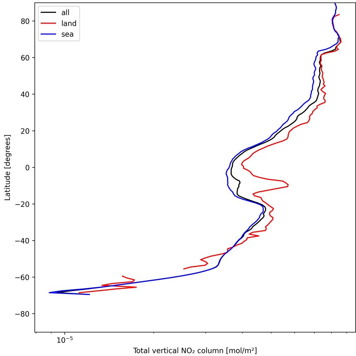
Figure 21: Zonal average of “Total vertical NO 2 column” for 2025-07-27 to 2025-07-29.
