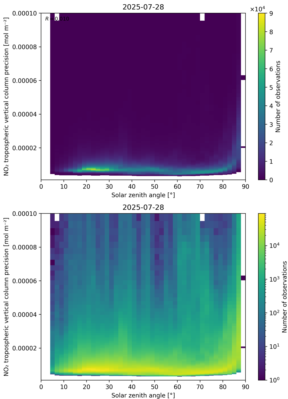
Figure 156: Scatter density plot of “Solar zenith angle” against “NO 2 tropospheric vertical column precision” for 2025-07-27 to 2025-07-29.
