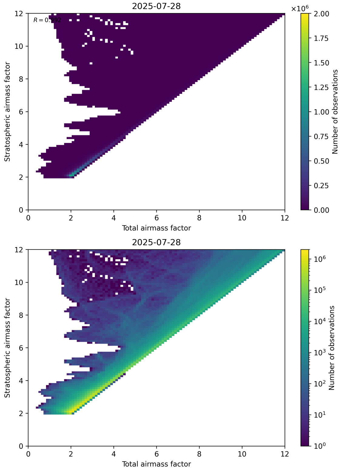
Figure 62: Scatter density plot of “Total airmass factor” against “Stratospheric airmass factor” for 2025-07-27 to 2025-07-29.
