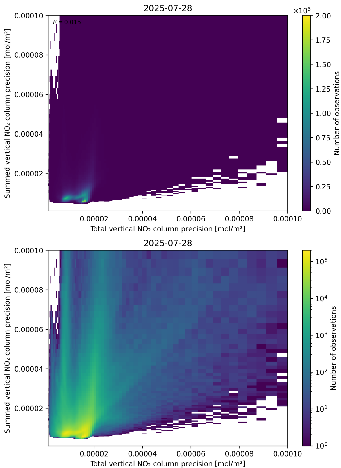
Figure 118: Scatter density plot of “Total vertical NO 2 column precision” against “Summed vertical NO 2 column precision” for 2025-07-27 to 2025-07-29.
