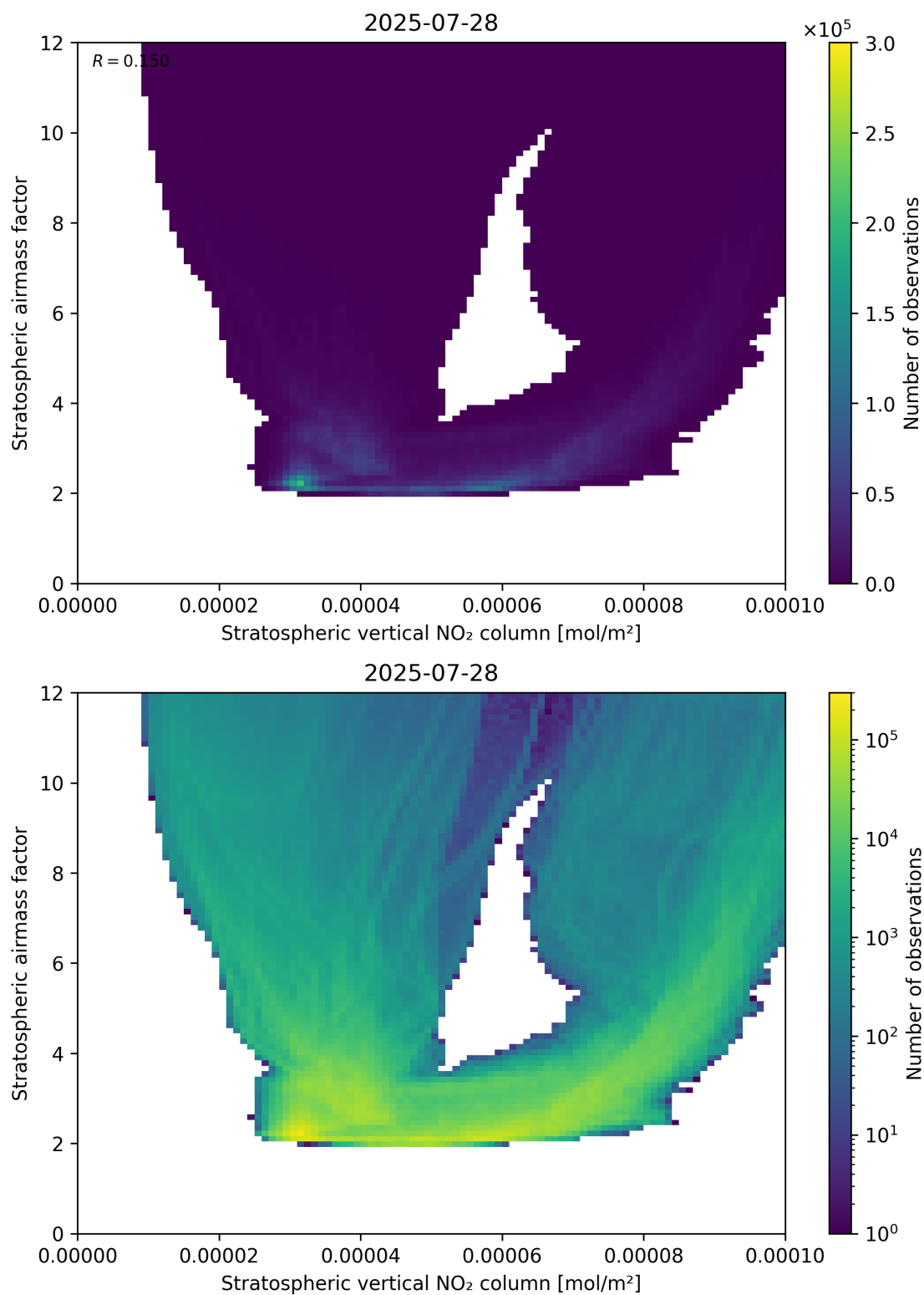
Figure 96: Scatter density plot of “Stratospheric vertical NO 2 column” against “Stratospheric airmass factor” for 2025-07-27 to 2025-07-29.
