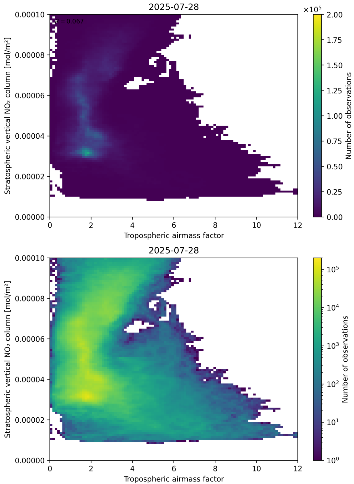
Figure 74: Scatter density plot of “Tropospheric air mass factor” against “Stratospheric vertical NO 2 column” for 2025-07-27 to 2025-07-29.
