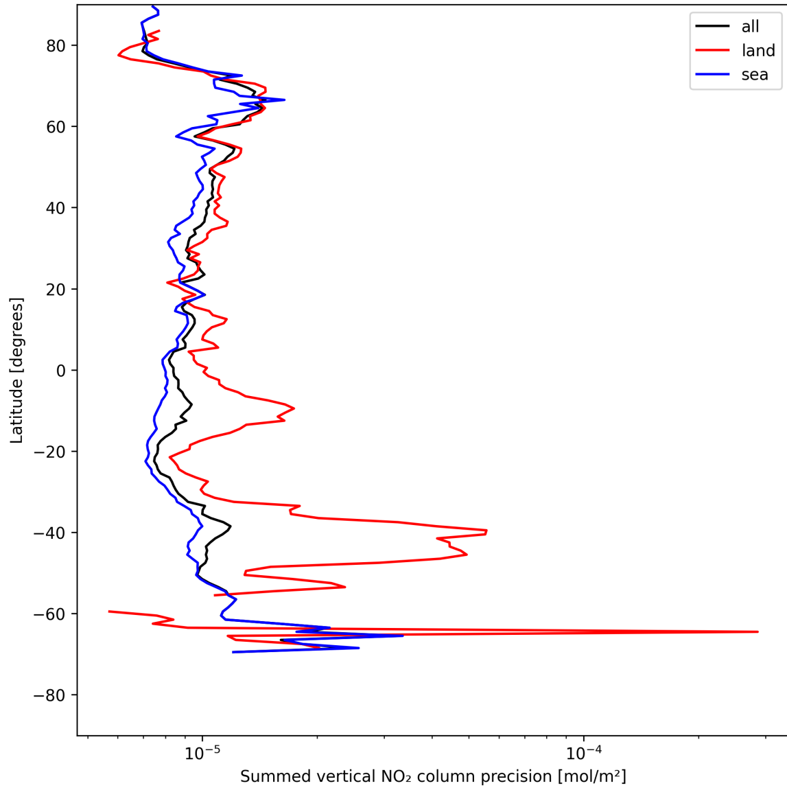
Figure 24: Zonal average of “Summed vertical NO 2 column precision” for 2025-07-27 to 2025-07-29.
