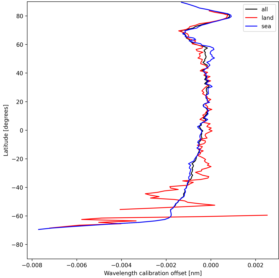
Figure 18: Zonal average of “Wavelength calibration offset” for 2025-07-27 to 2025-07-29.
