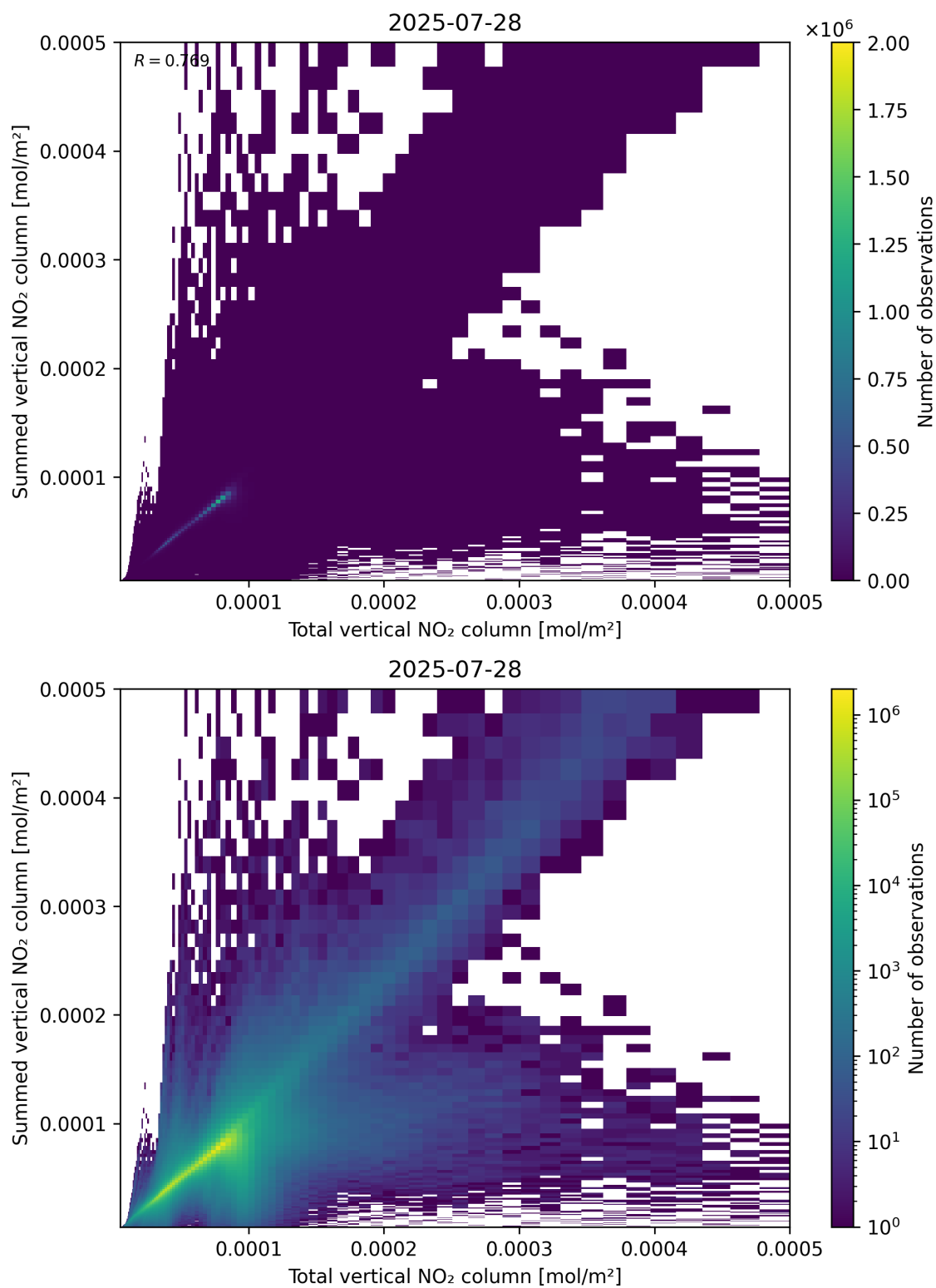
Figure 112: Scatter density plot of “Total vertical NO 2 column” against “Summed vertical NO 2 column” for 2025-07-27 to 2025-07-29.
