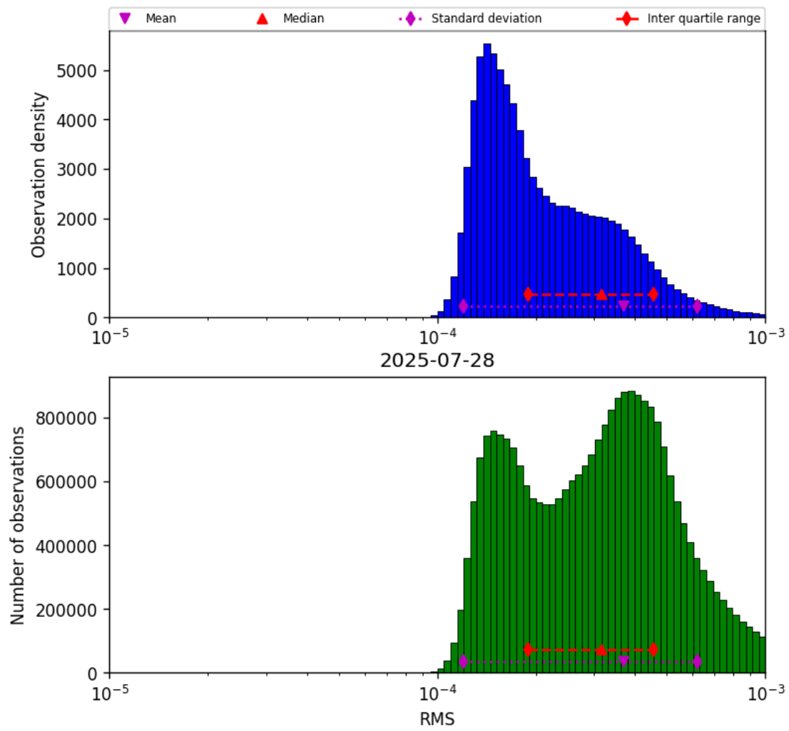
Figure 43: Histogram of “RMS” for 2025-07-27 to 2025-07-29
