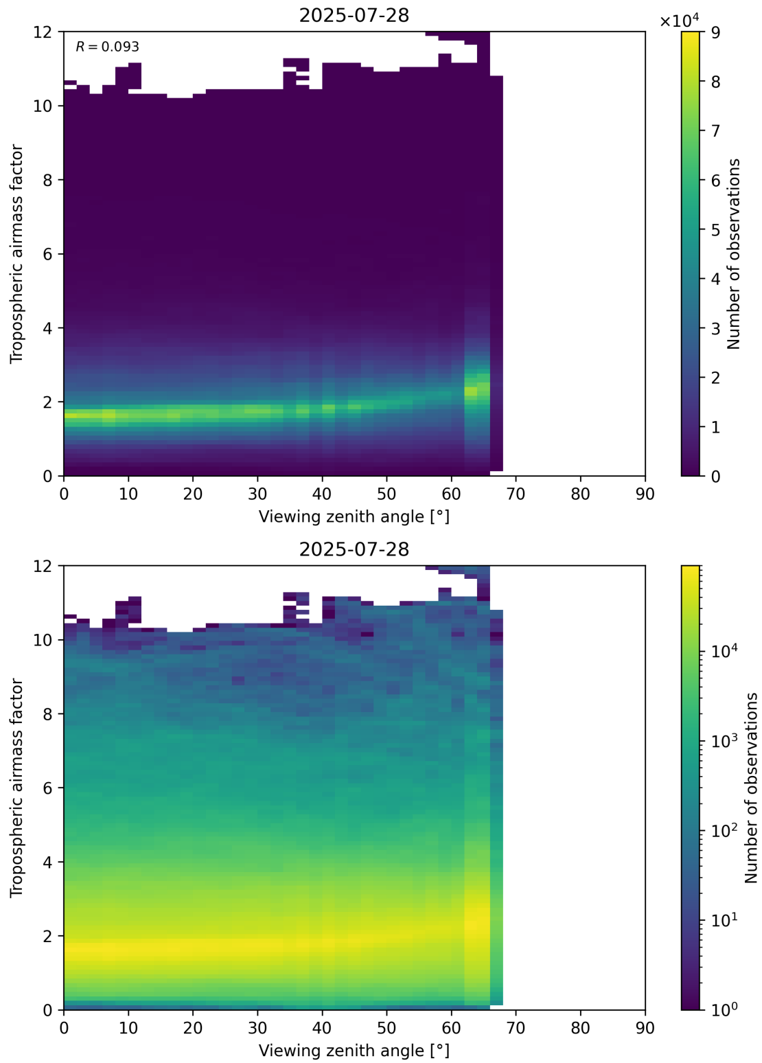
Figure 161: Scatter density plot of “Viewing zenith angle” against “Tropospheric airmass factor” for 2025-07-27 to 2025-07-29.
