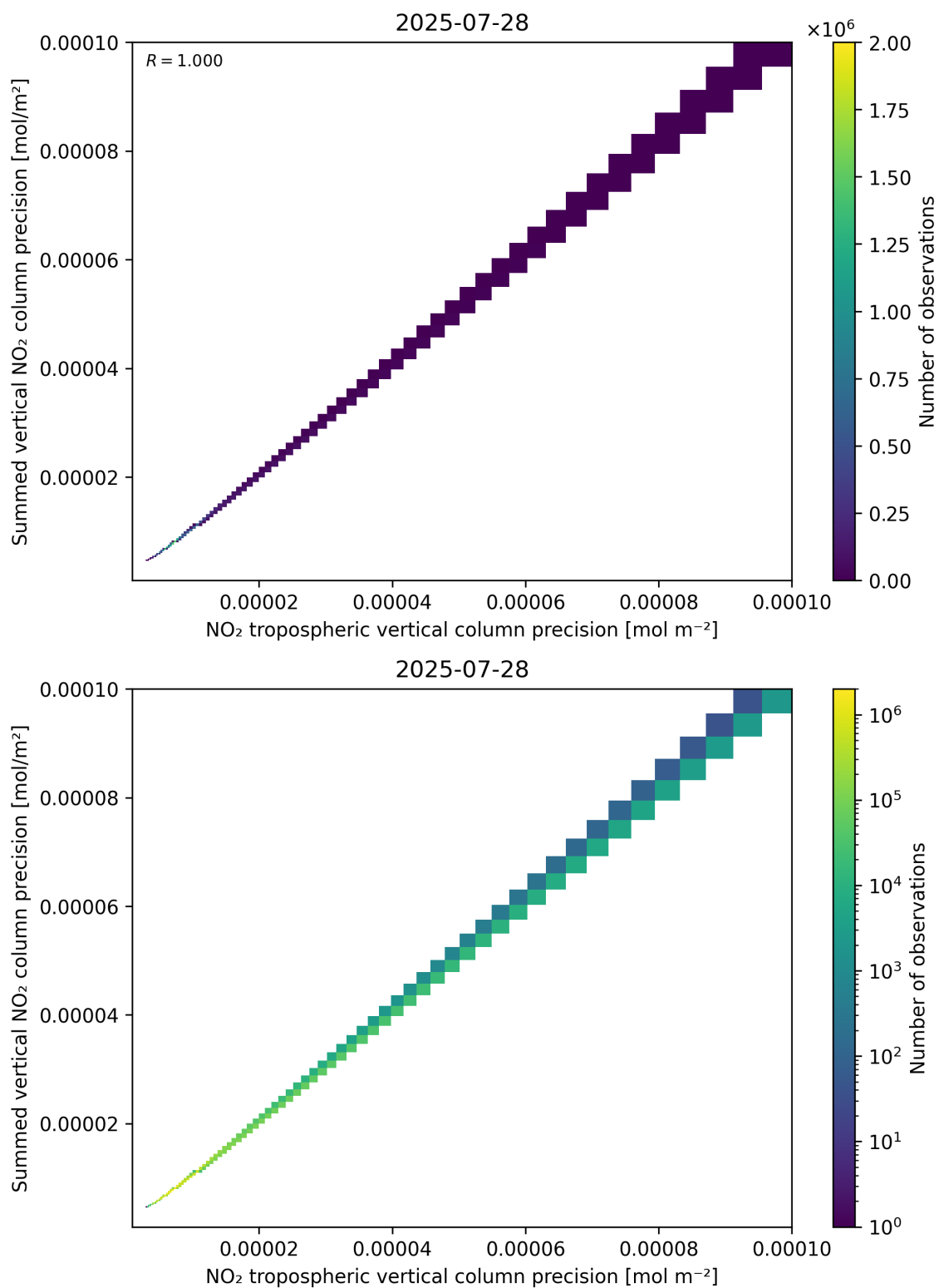
Figure 137: Scatter density plot of “NO 2 tropospheric vertical column precision” against “Summed vertical NO 2 column precision” for 2025-07-27 to 2025-07-29.
