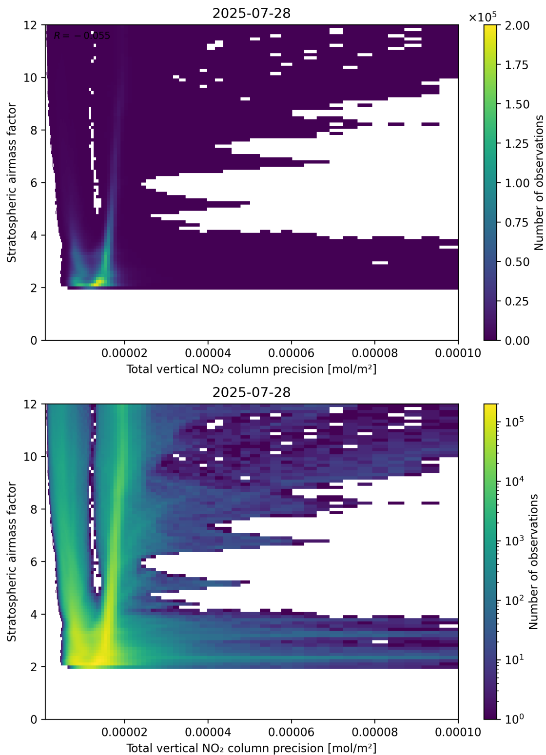
Figure 115: Scatter density plot of “Total vertical NO 2 column precision” against “Stratospheric air mass factor” for 2025-07-27 to 2025-07-29.
