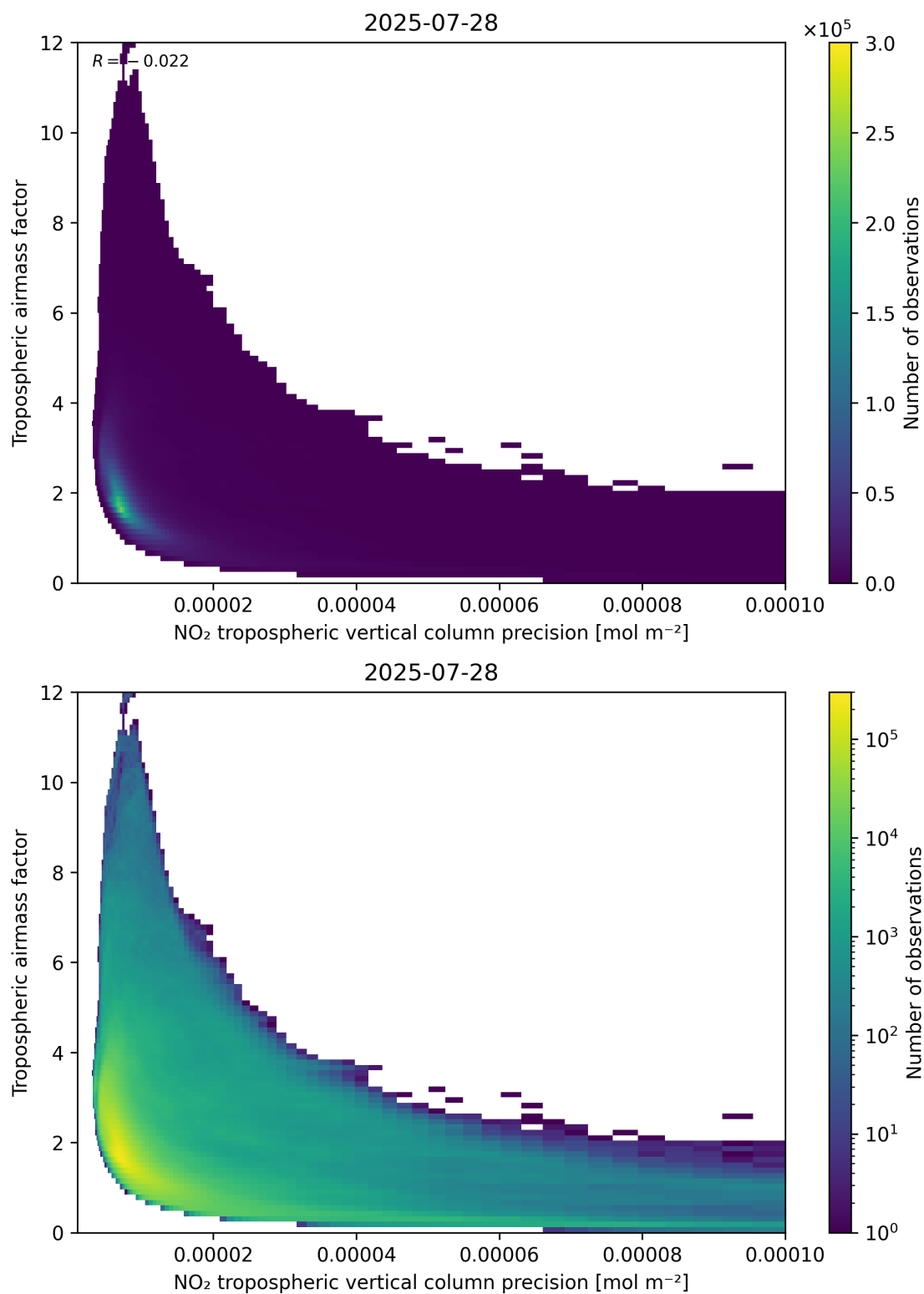
Figure 133: Scatter density plot of “NO 2 tropospheric vertical column precision” against “Tropospheric airmass factor” for 2025-07-27 to 2025-07-29.
