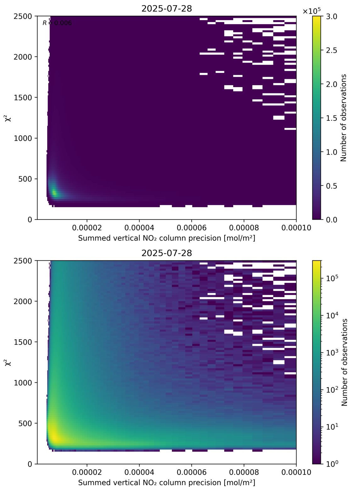
Figure 107: Scatter density plot of “Summed vertical NO 2 column precision” against “ \chi^2 ” for 2025-07-27 to 2025-07-29.
