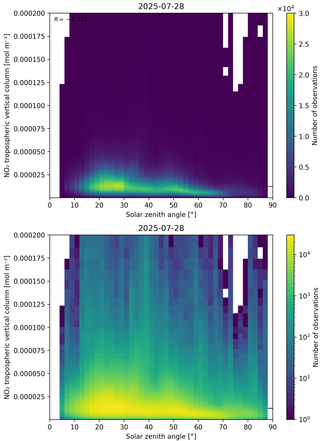
Figure 155: Scatter density plot of “Solar zenith angle” against “NO 2 tropospheric vertical column” for 2025-07-27 to 2025-07-29.
