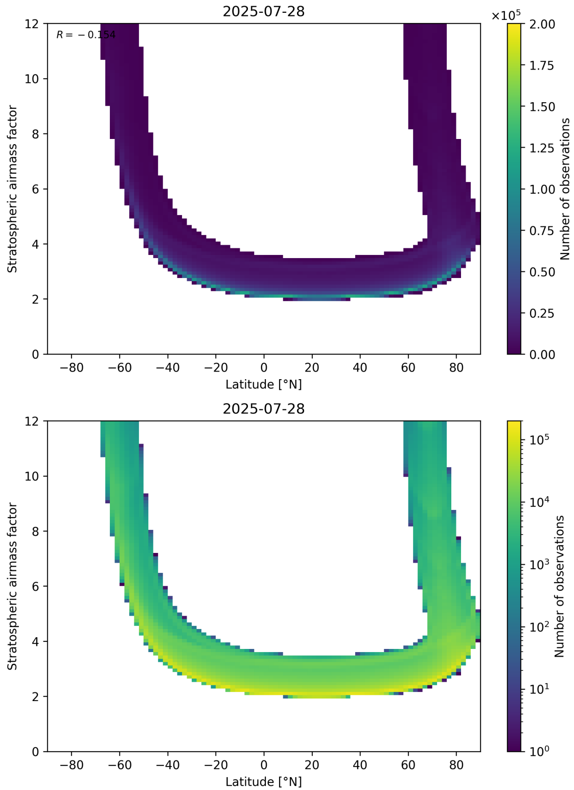
Figure 83: Scatter density plot of “Latitude” against “Stratospheric air mass factor” for 2025-07-27 to 2025-07-29.
