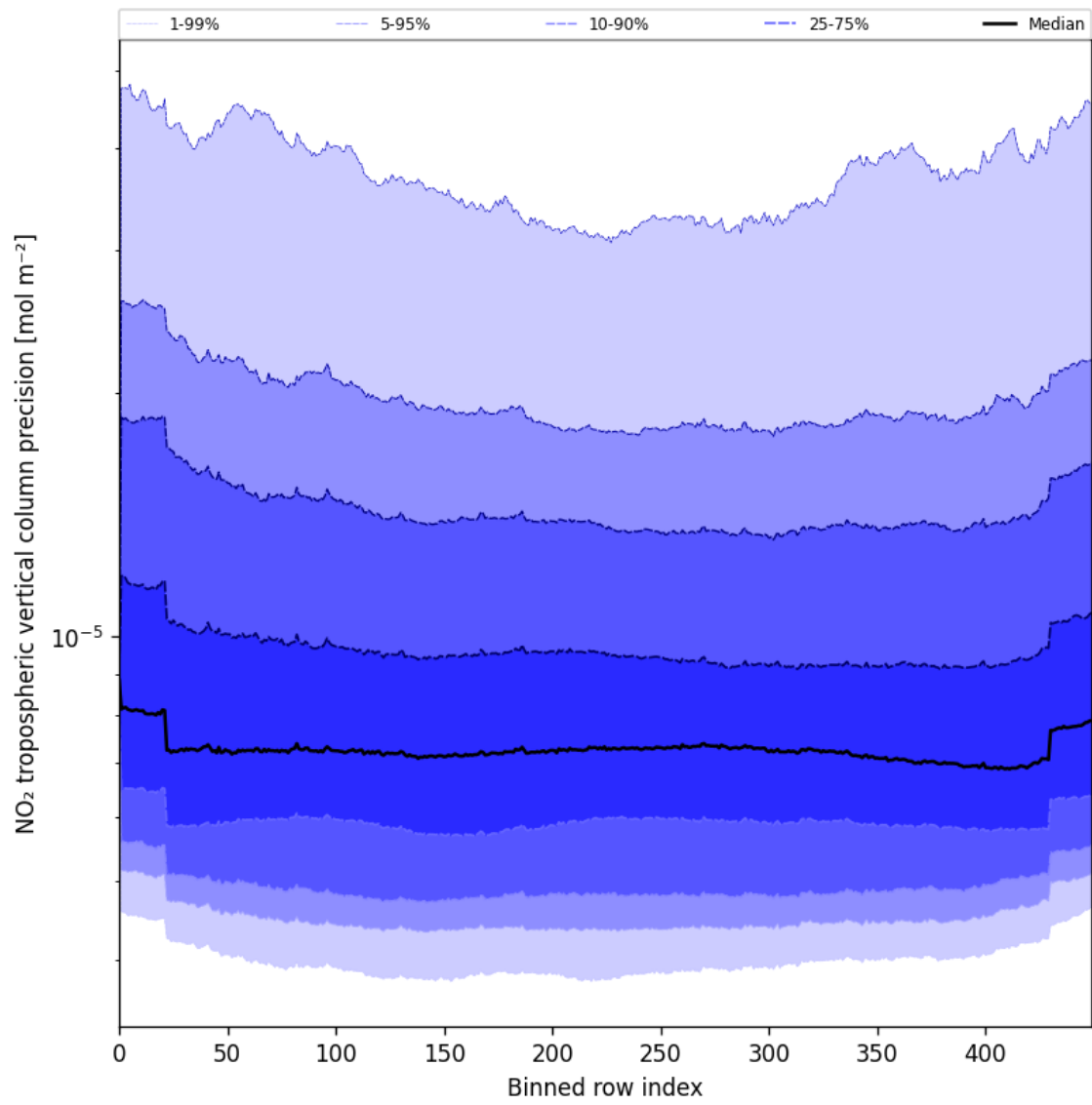
Figure 47: Along track statistics of “NO 2 tropospheric vertical column precision” for 2025-07-27 to 2025-07-29
