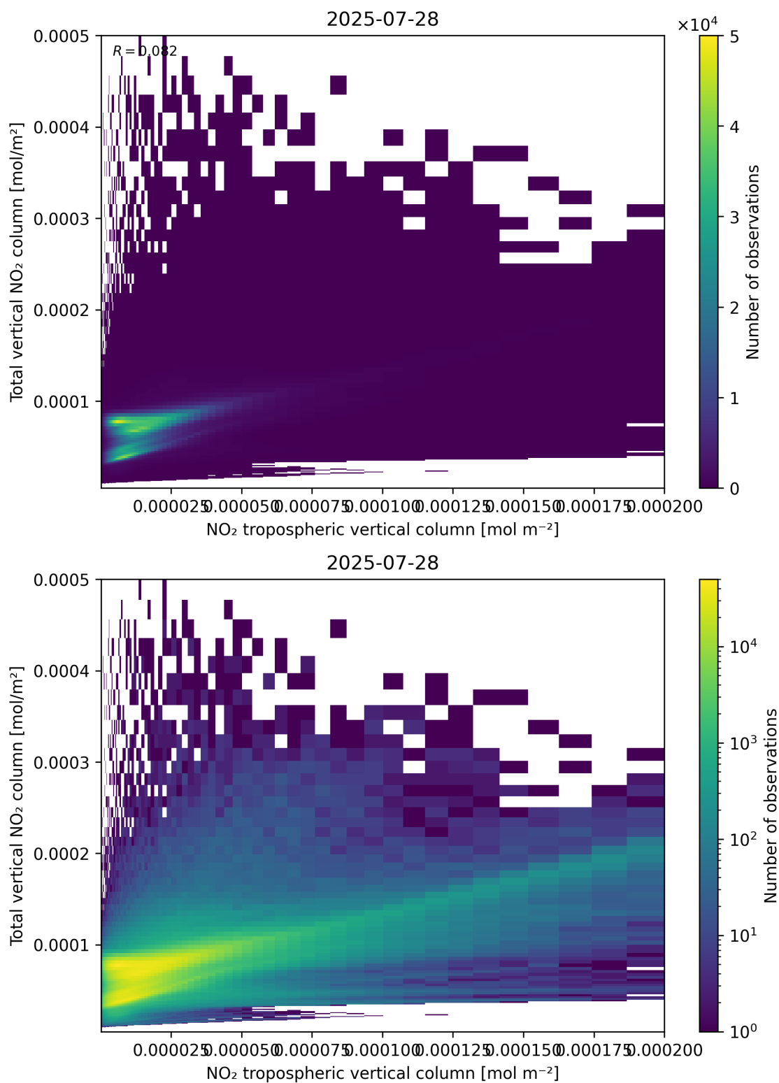
Figure 128: Scatter density plot of “NO 2 tropospheric vertical column” against “Total vertical NO 2 column” for 2025-07-27 to 2025-07-29.
