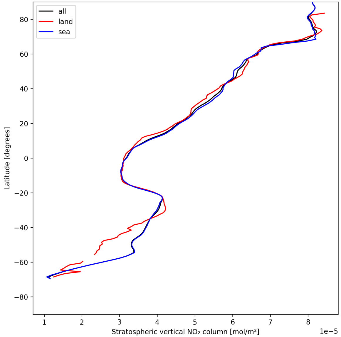
Figure 19: Zonal average of “Stratospheric vertical NO 2 column” for 2025-07-27 to 2025-07-29.
