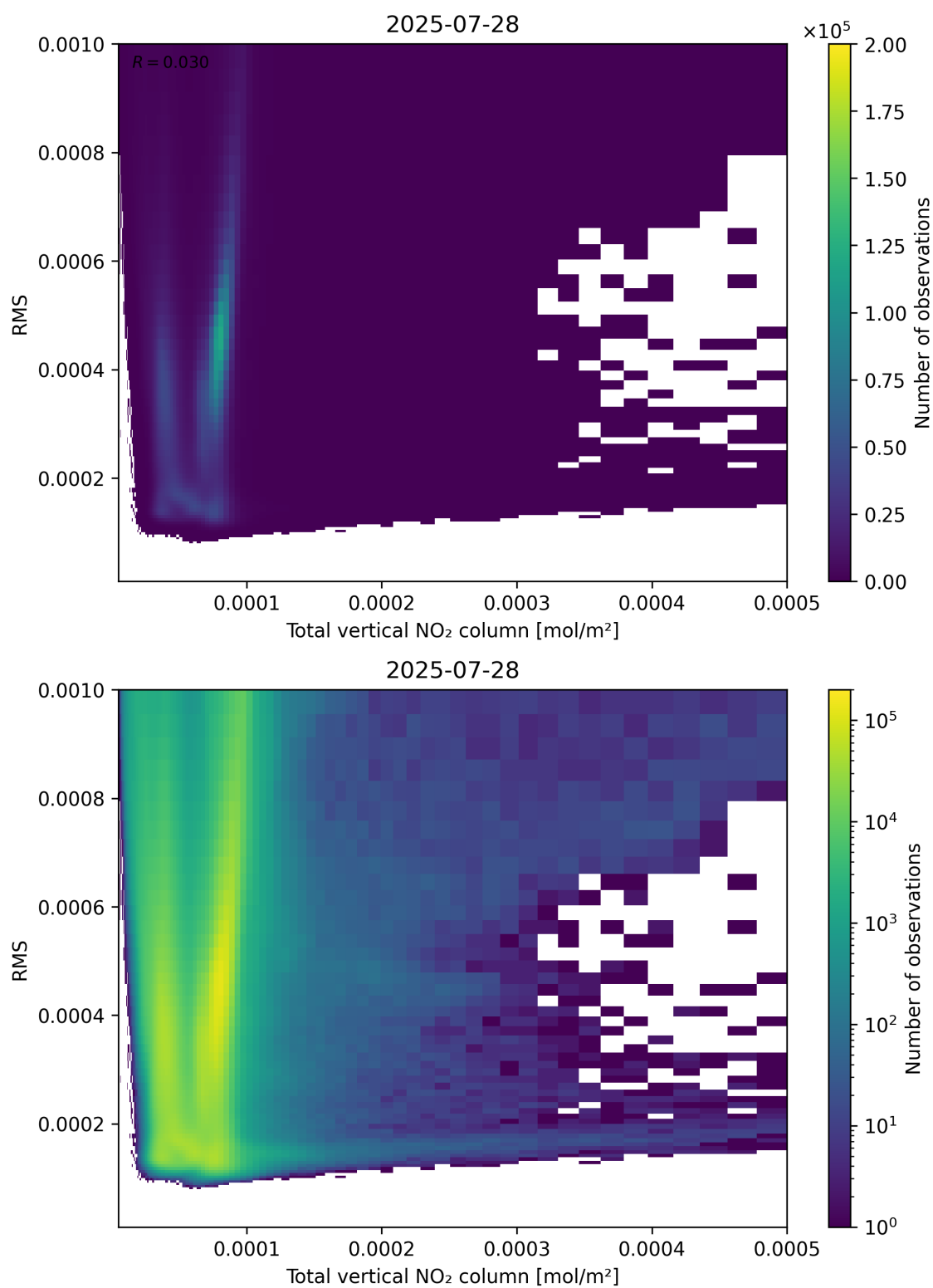
Figure 120: Scatter density plot of “Total vertical NO 2 column” against “RMS” for 2025-07-27 to 2025-07-29.
