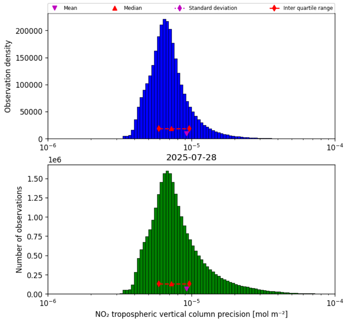
Figure 30: Histogram of “NO 2 tropospheric vertical column precision” for 2025-07-27 to 2025-07-29
