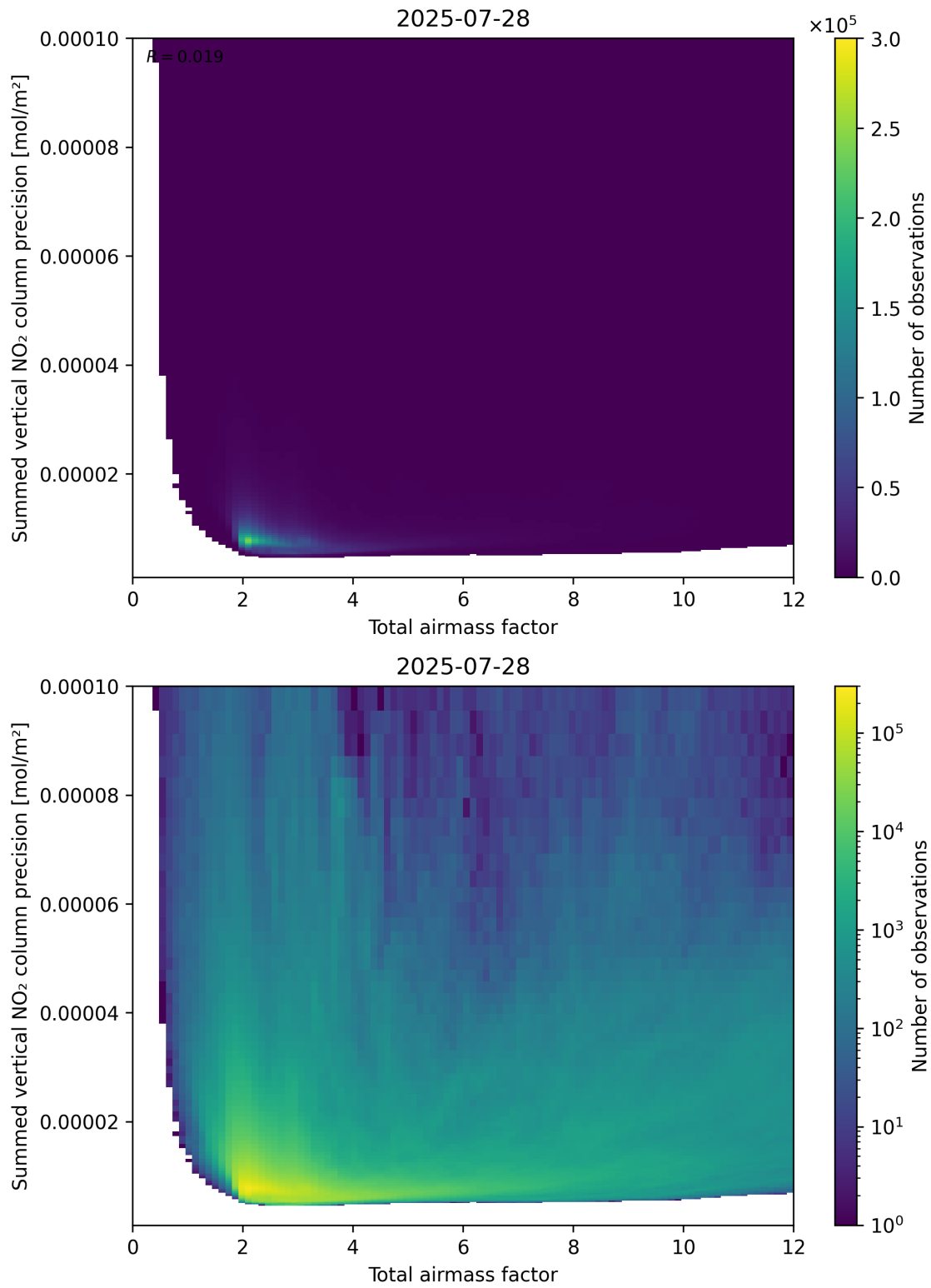
Figure 66: Scatter density plot of “Total airmass factor” against “Summed vertical NO 2 column precision” for 2025-07-27 to 2025-07-29.
