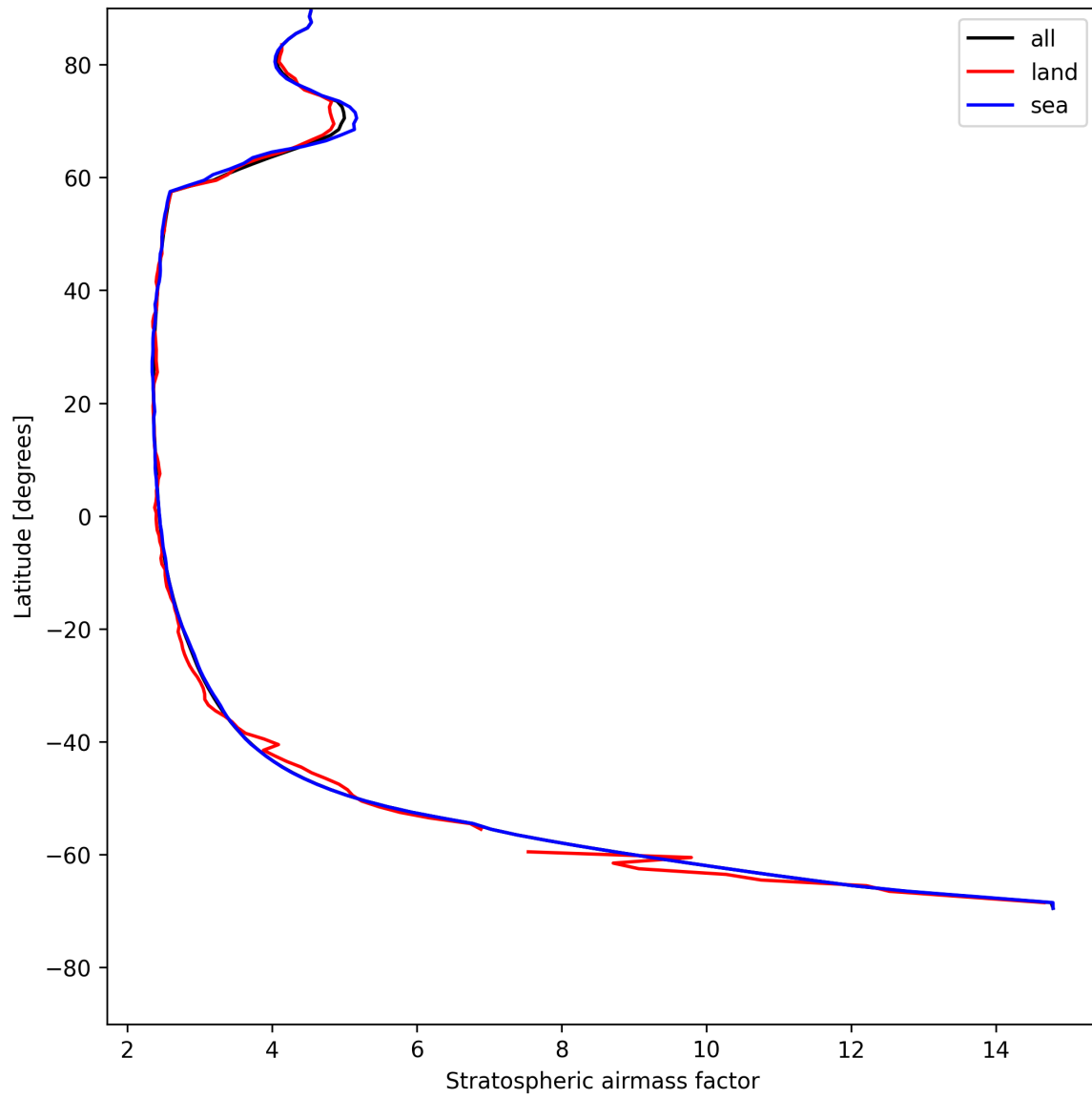
Figure 27: Zonal average of “Stratospheric air mass factor” for 2025-07-27 to 2025-07-29.
