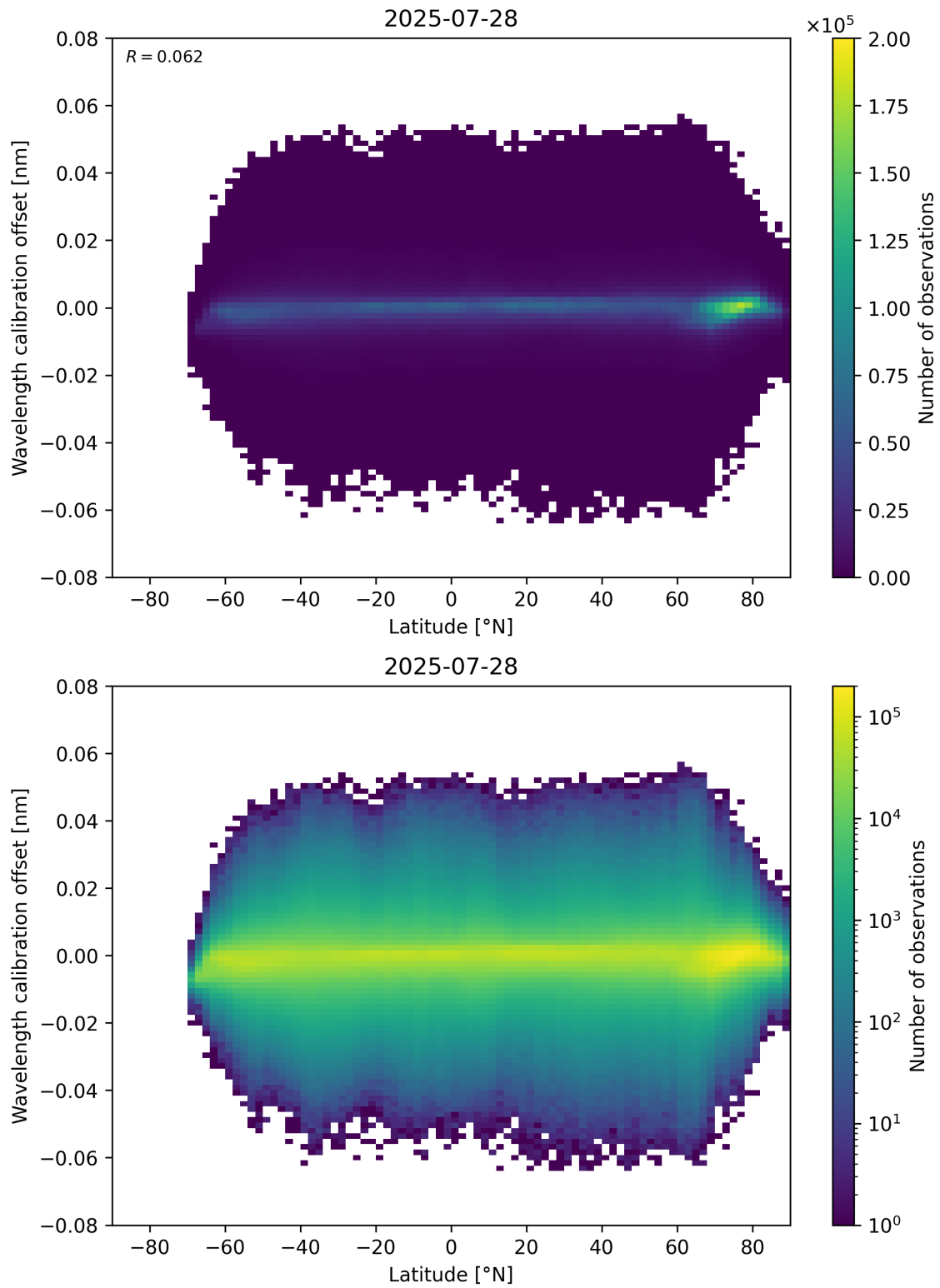
Figure 95: Scatter density plot of “Latitude” against “Wavelength calibration offset” for 2025-07-27 to 2025-07-29.
