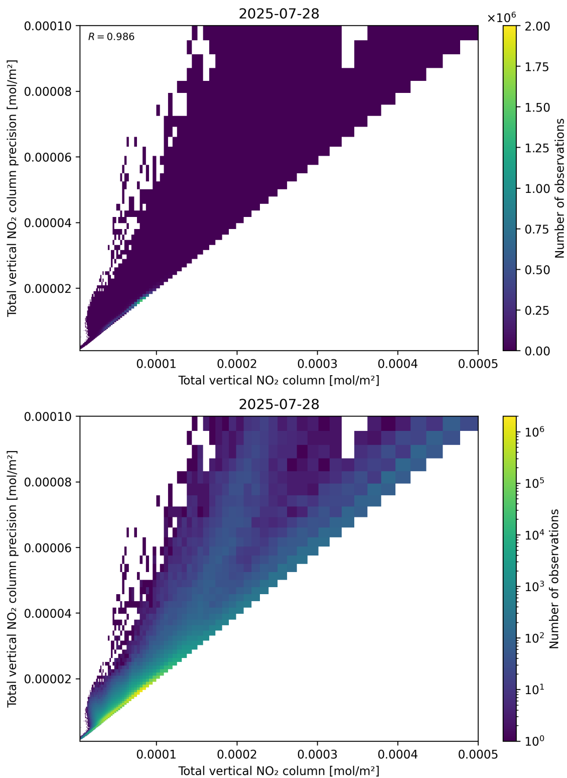
Figure 114: Scatter density plot of “Total vertical NO 2 column” against “Total vertical NO 2 column precision” for 2025-07-27 to 2025-07-29.
