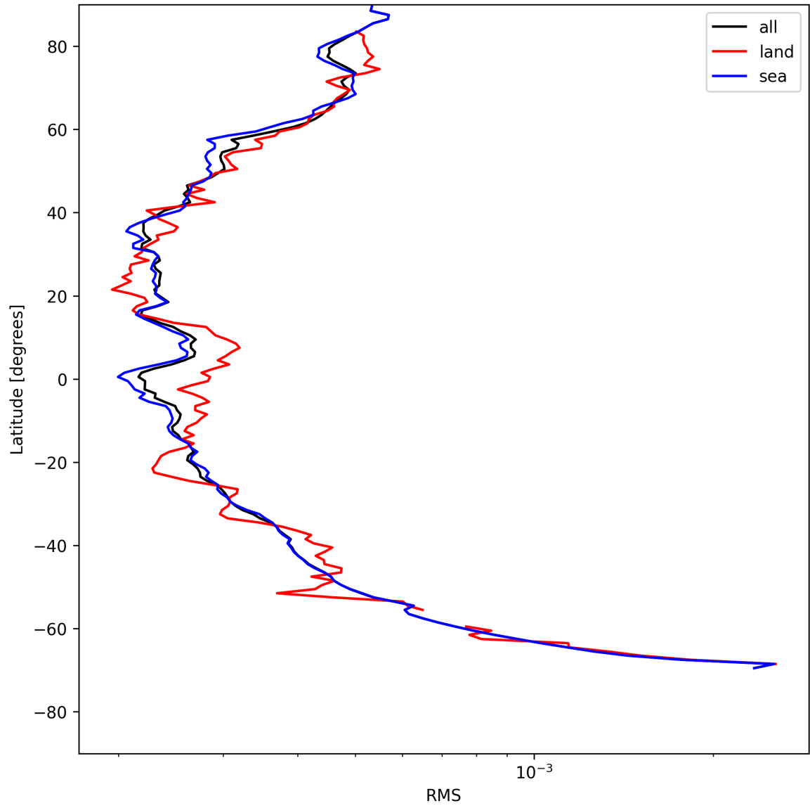
Figure 26: Zonal average of “RMS” for 2025-07-27 to 2025-07-29.
