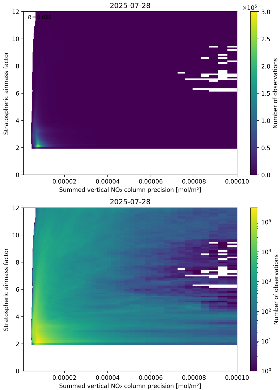
Figure 106: Scatter density plot of “Summed vertical NO 2 column precision” against “Stratospheric airmass factor” for 2025-07-27 to 2025-07-29.
