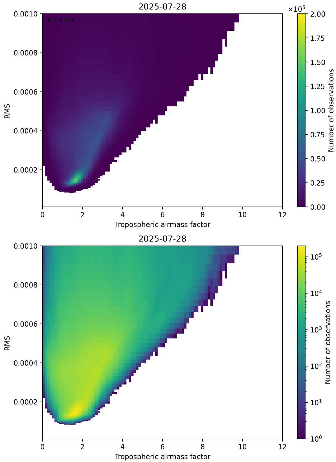
Figure 79: Scatter density plot of “Tropospheric airmass factor” against “RMS” for 2025-07-27 to 2025-07-29.
