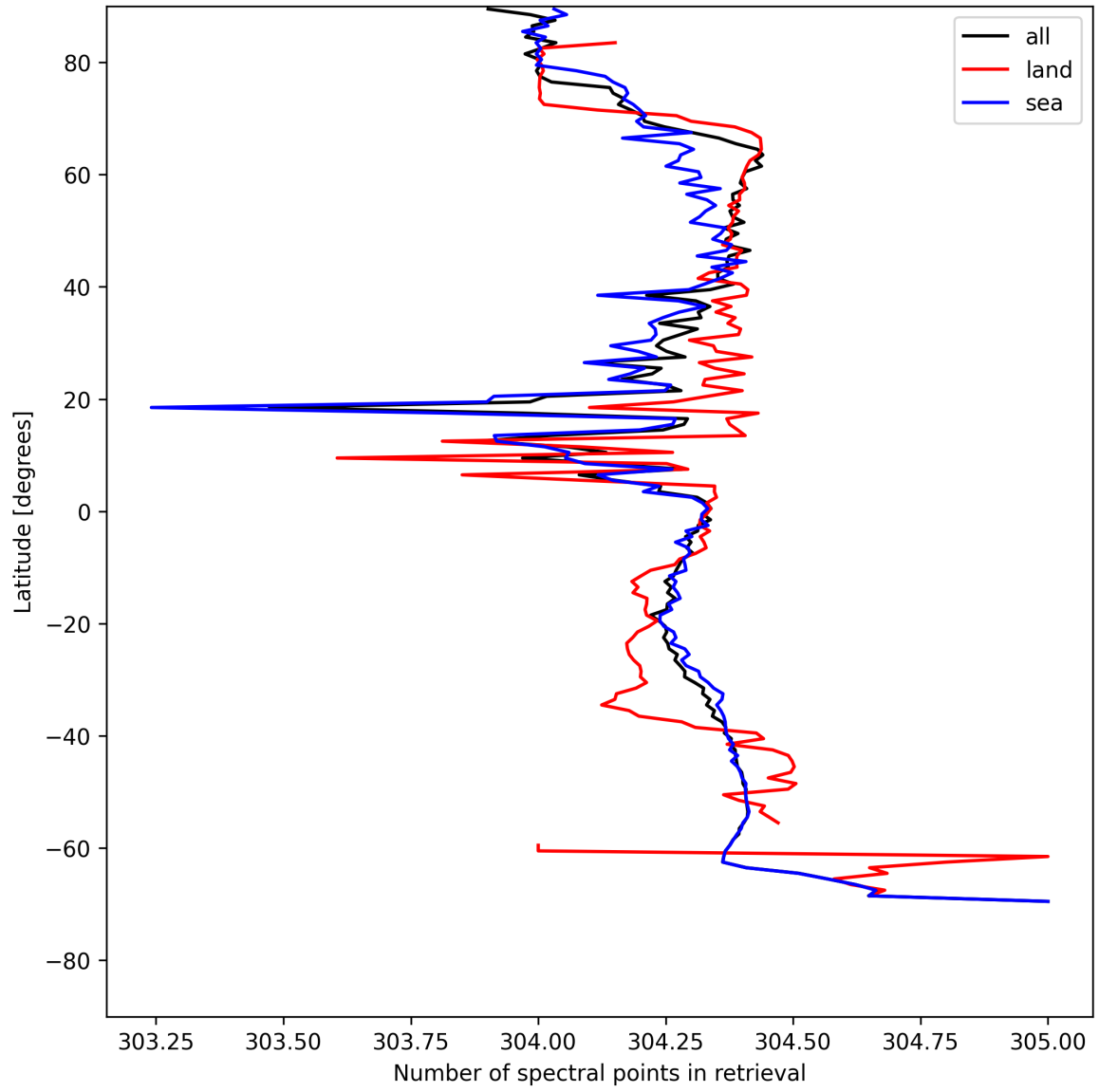
Figure 16: Zonal average of “Number of spectral points in retrieval” for 2025-07-27 to 2025-07-29.
