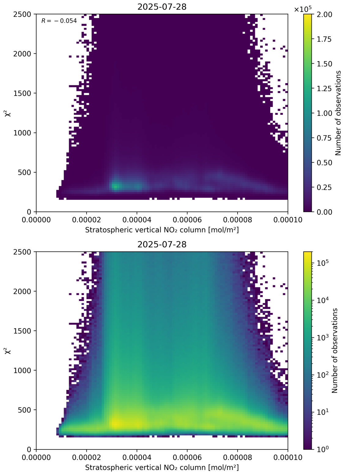
Figure 97: Scatter density plot of “Stratospheric vertical NO 2 column” against “ \chi^2 ” for 2025-07-27 to 2025-07-29.
