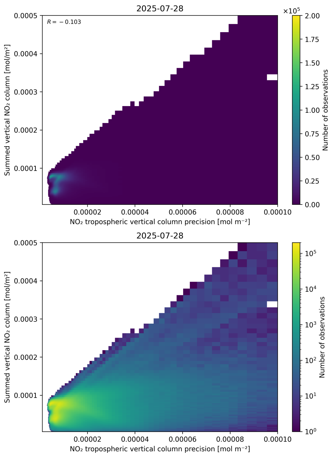
Figure 136: Scatter density plot of “NO 2 tropospheric vertical column precision” against “Summed vertical NO 2 column” for 2025-07-27 to 2025-07-29.
