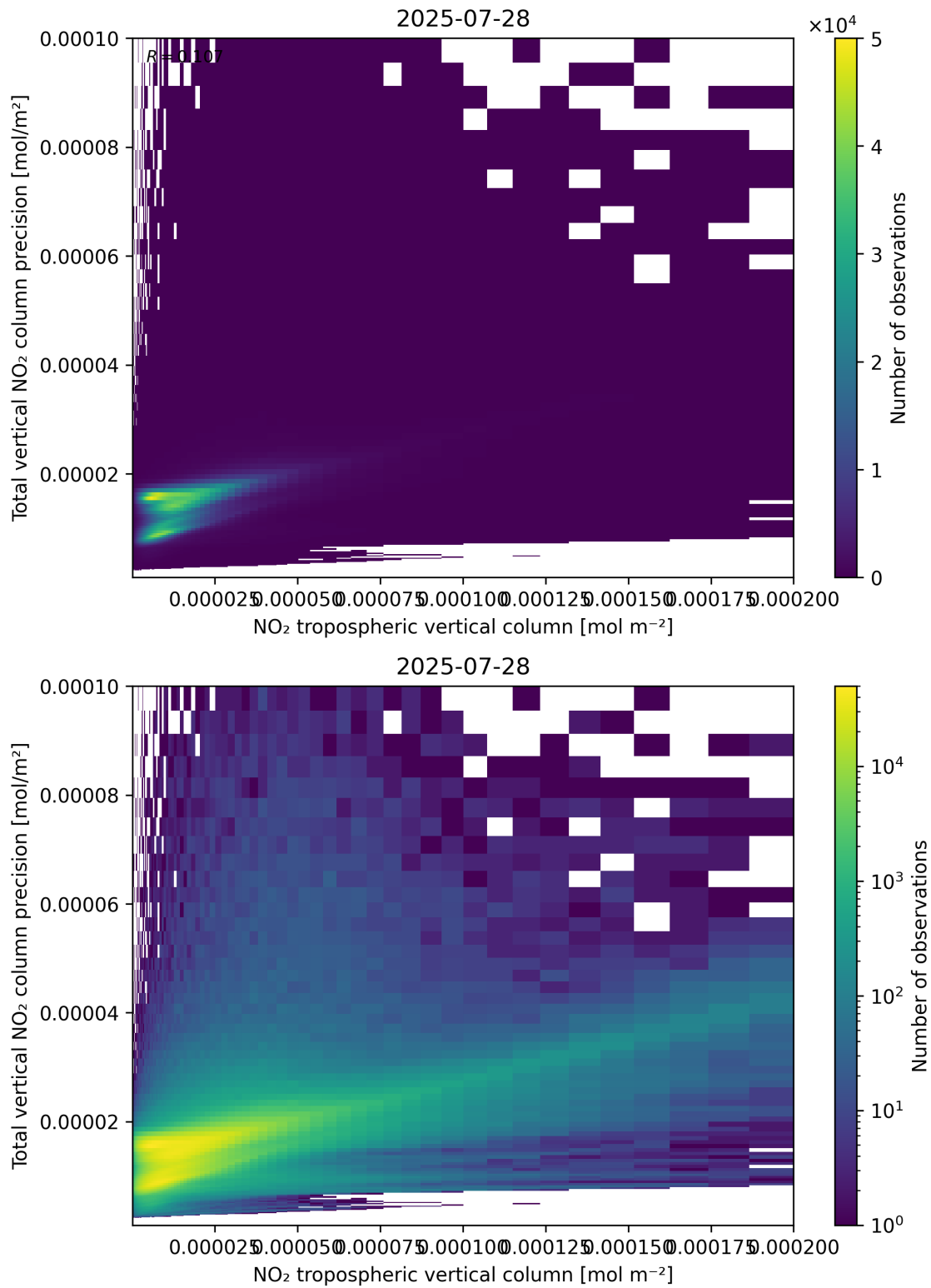
Figure 129: Scatter density plot of “NO 2 tropospheric vertical column” against “Total vertical NO 2 column precision” for 2025-07-27 to 2025-07-29.
