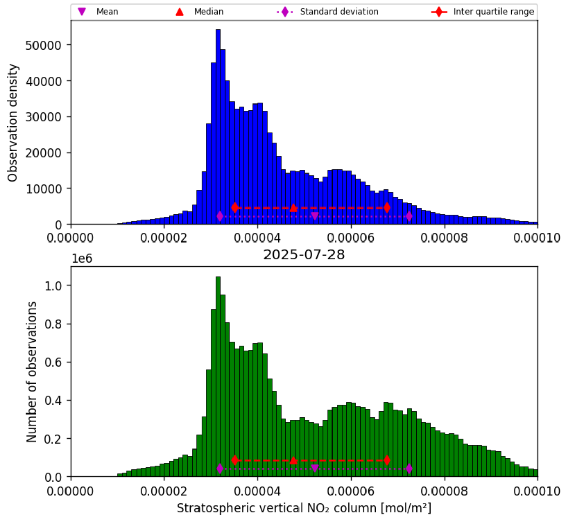
Figure 36: Histogram of “Stratospheric vertical NO 2 column” for 2025-07-27 to 2025-07-29
