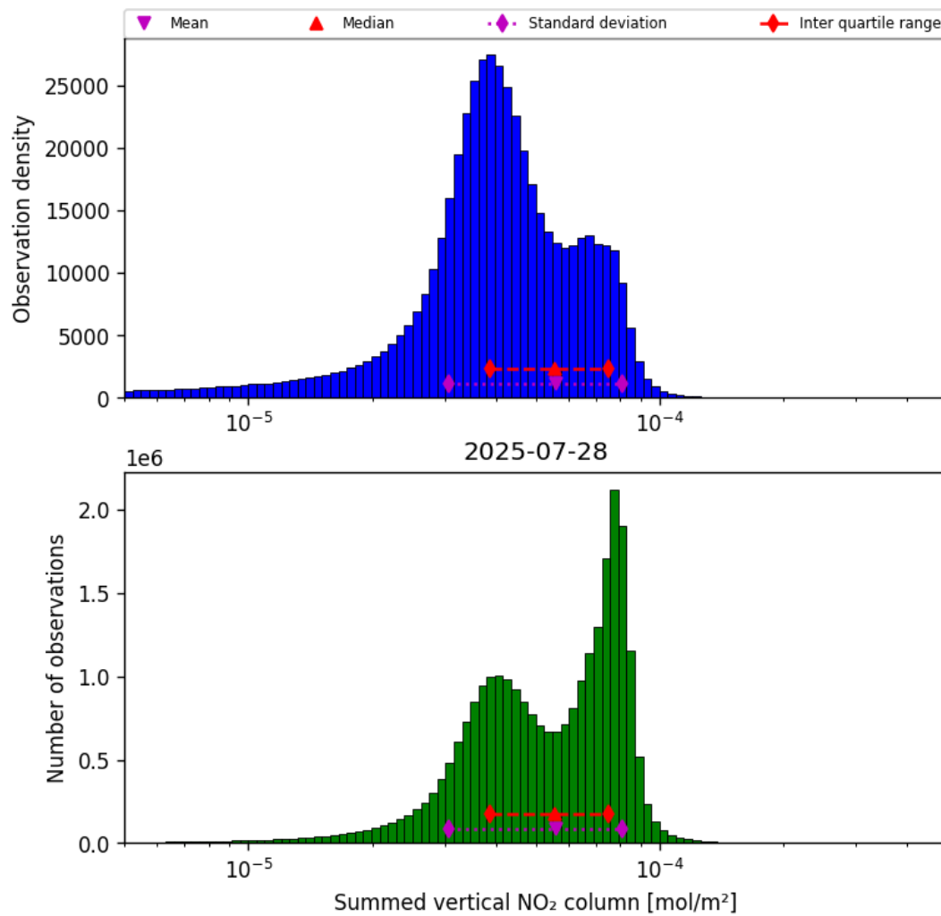
Figure 40: Histogram of “Summed vertical NO 2 column” for 2025-07-27 to 2025-07-29
