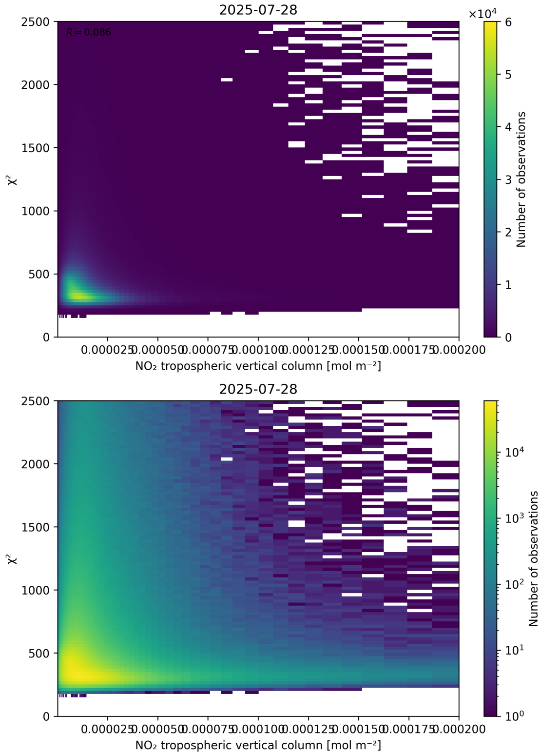
Figure 124: Scatter density plot of “NO 2 tropospheric vertical column” against “ \chi^2 ” for 2025-07-27 to 2025-07-29.
