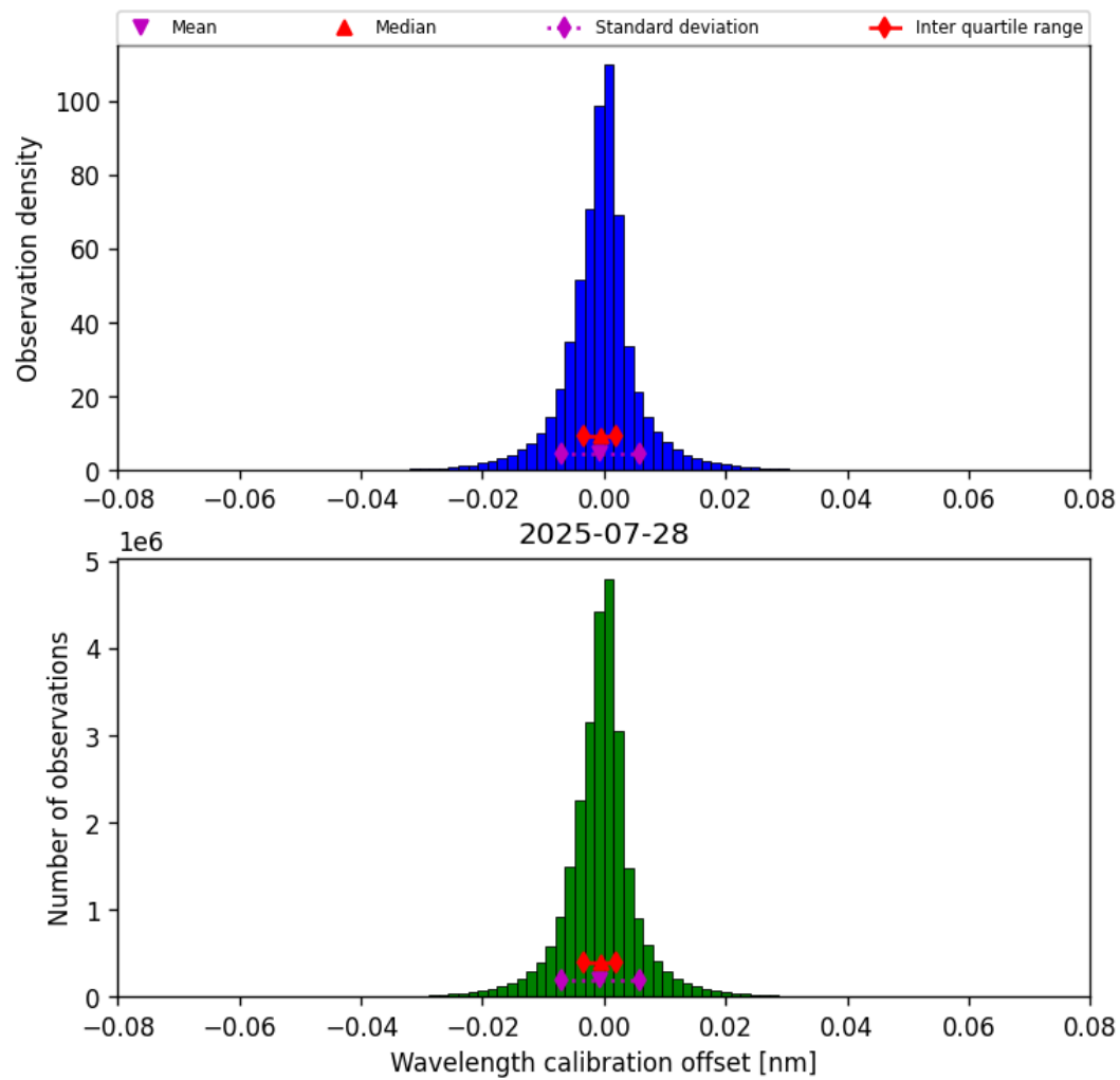
Figure 35: Histogram of “Wavelength calibration offset” for 2025-07-27 to 2025-07-29
