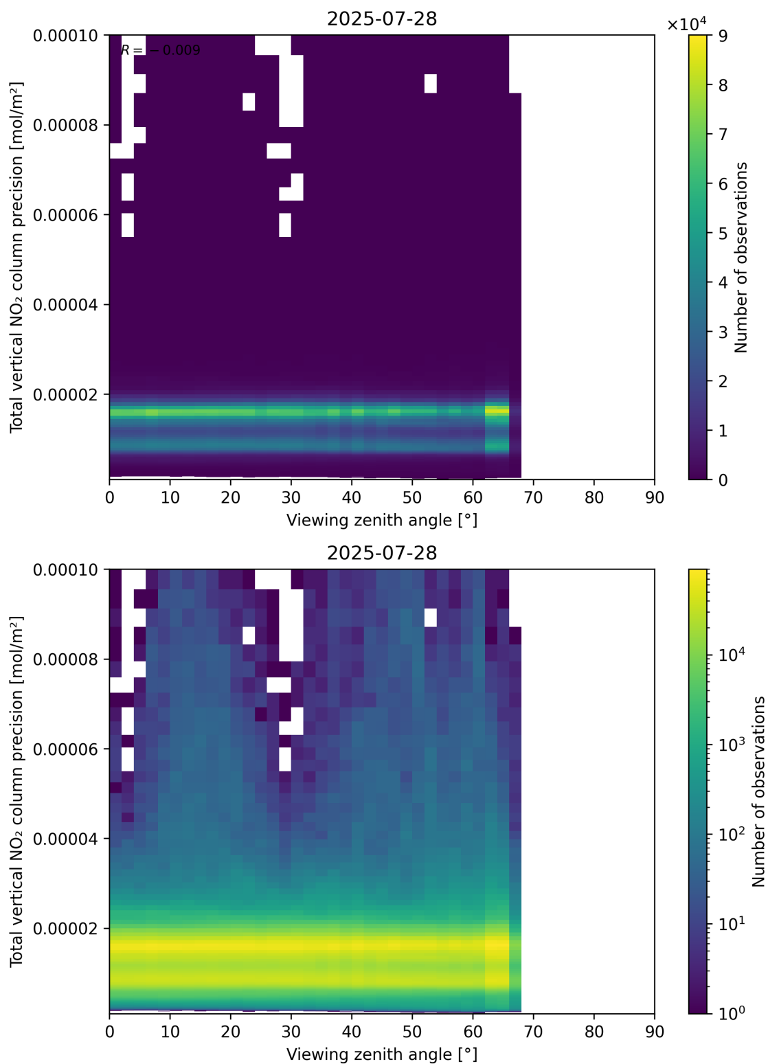
Figure 168: Scatter density plot of “Viewing zenith angle” against “Total vertical NO 2 column precision” for 2025-07-27 to 2025-07-29.
