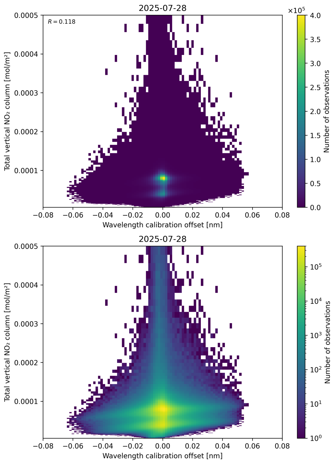
Figure 179: Scatter density plot of “Wavelength calibration offset” against “Total vertical NO 2 column” for 2025-07-27 to 2025-07-29.
