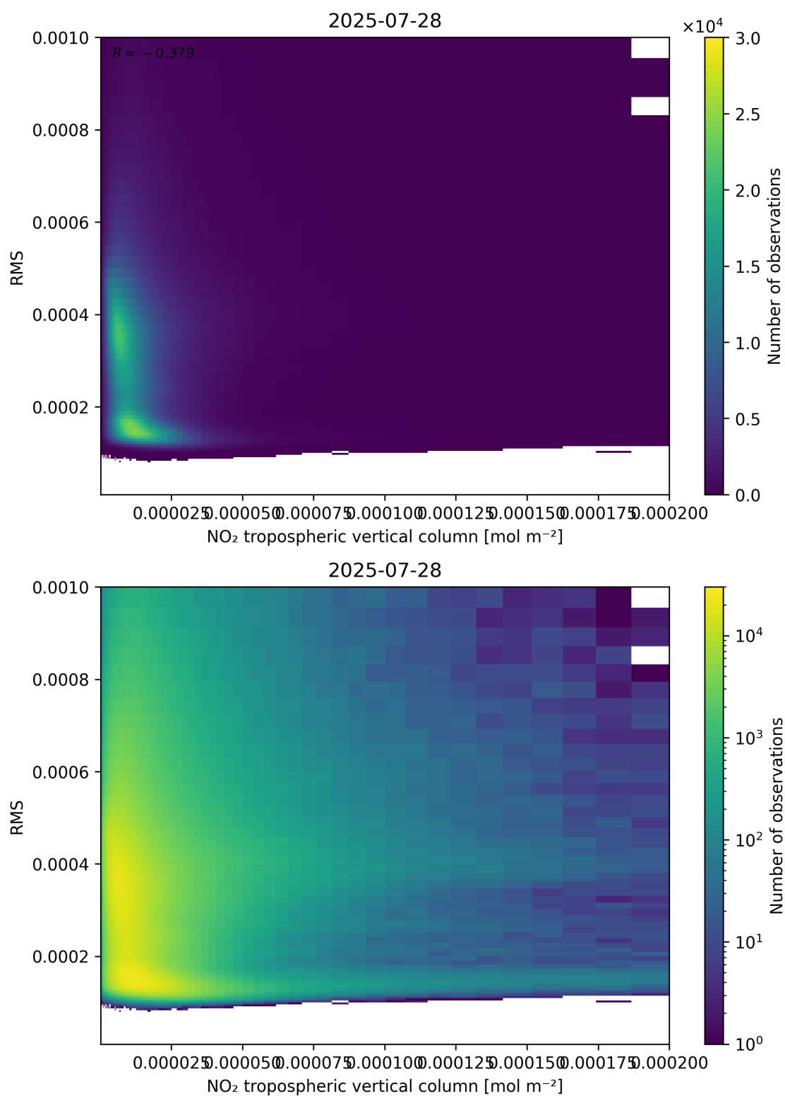
Figure 142: Scatter density plot of “NO 2 tropospheric vertical column” against “RMS” for 2025-07-27 to 2025-07-29.
