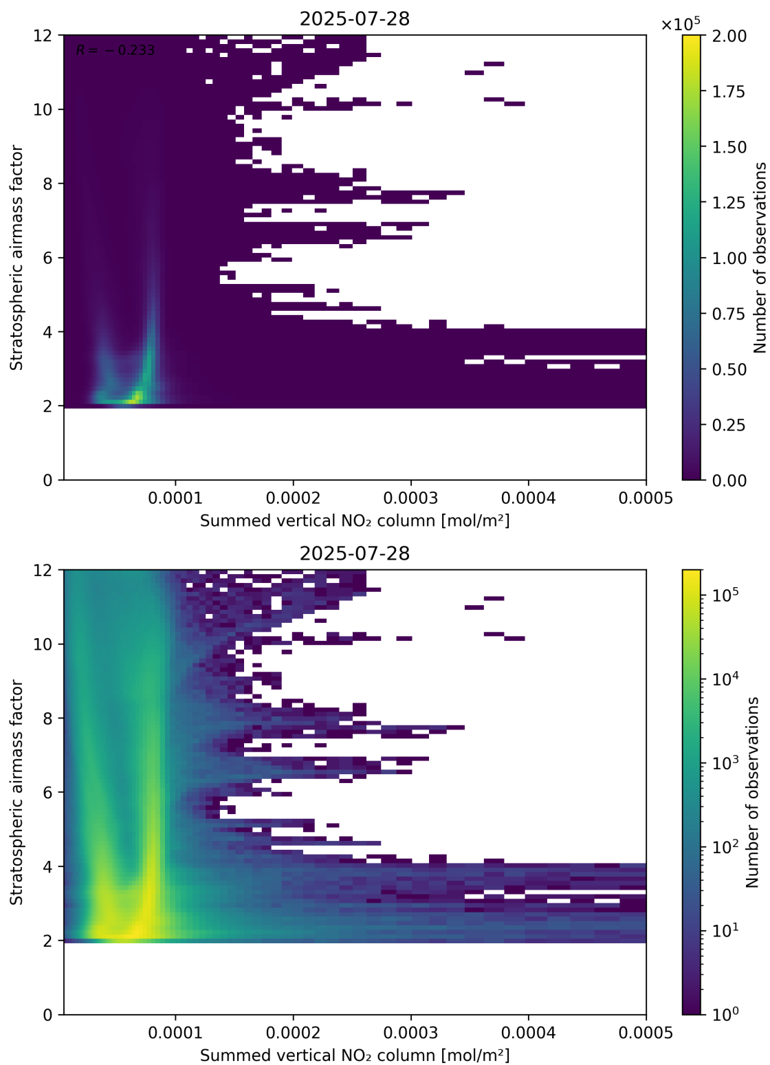
Figure 103: Scatter density plot of “Summed vertical NO 2 column” against “Stratospheric air mass factor” for 2025-07-27 to 2025-07-29.
