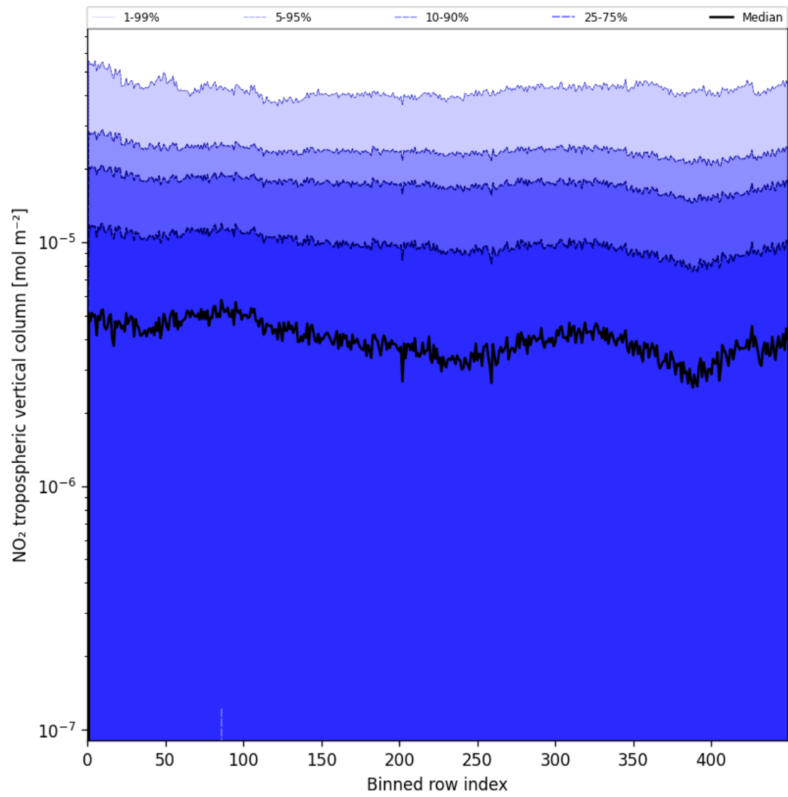
Figure 46: Along track statistics of "NO 2 tropospheric vertical column" for 2025-07-27 to 2025-07-29
