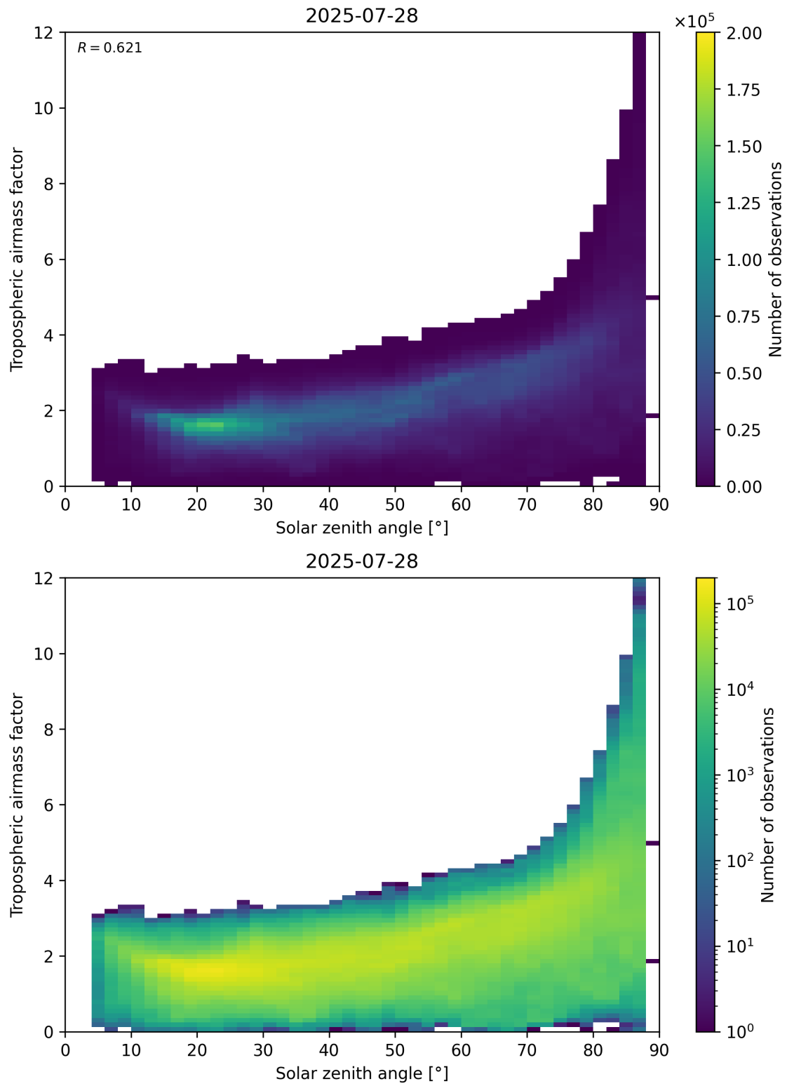
Figure 147: Scatter density plot of “Solar zenith angle” against “Tropospheric airmass factor” for 2025-07-27 to 2025-07-29.
