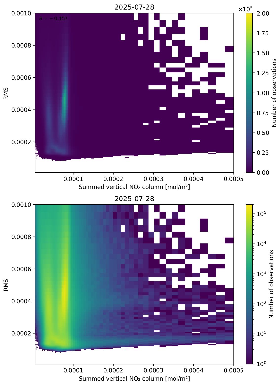
Figure 109: Scatter density plot of “Summed vertical NO 2 column” against “RMS” for 2025-07-27 to 2025-07-29.
