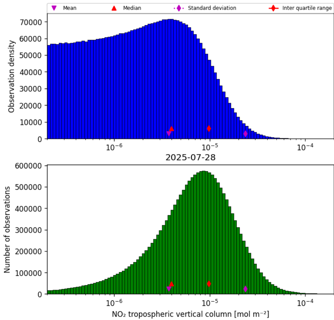
Figure 29: Histogram of “NO 2 tropospheric vertical column” for 2025-07-27 to 2025-07-29
