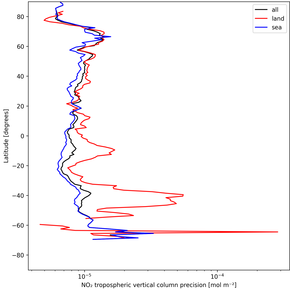
Figure 13: Zonal average of “NO 2 tropospheric vertical column precision” for 2025-07-27 to 2025-07-29.
