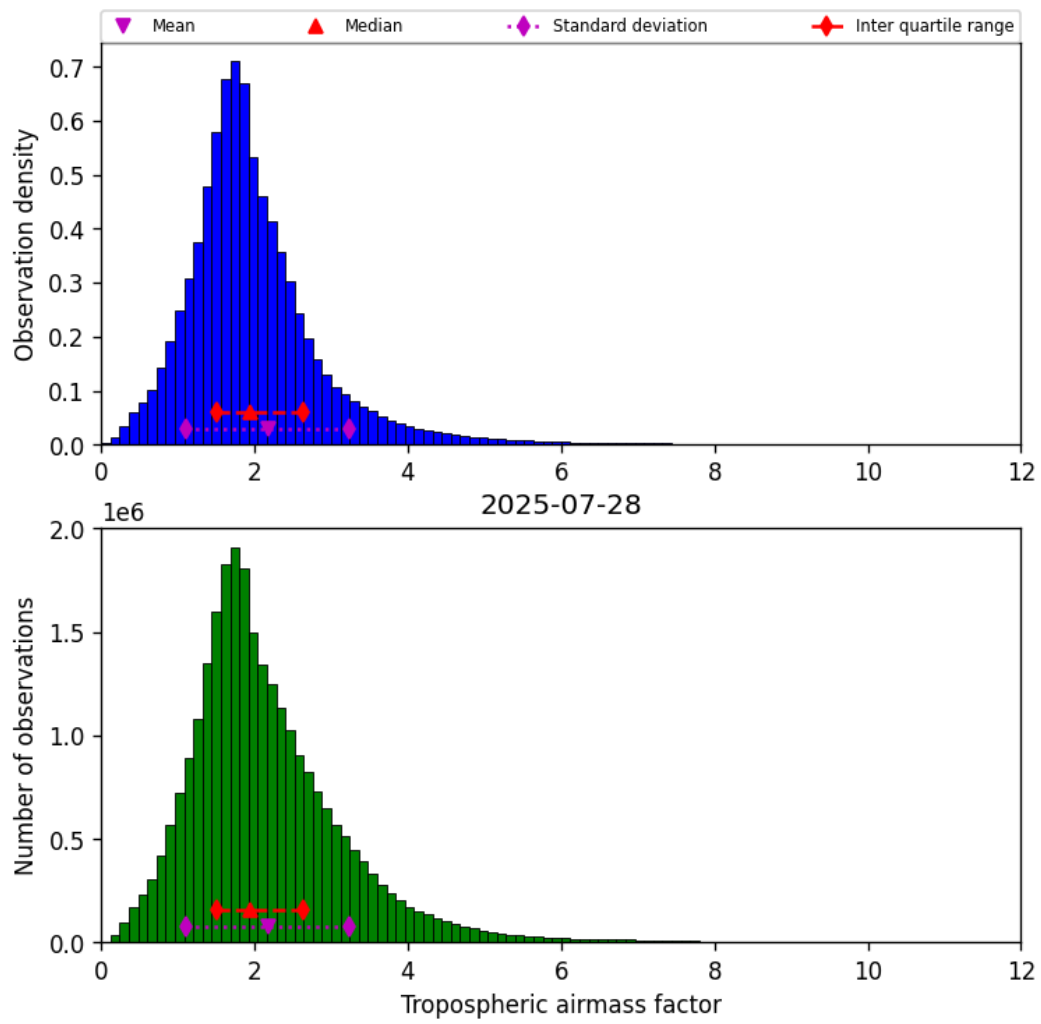
Figure 31: Histogram of “Tropospheric airmass factor” for 2025-07-27 to 2025-07-29
