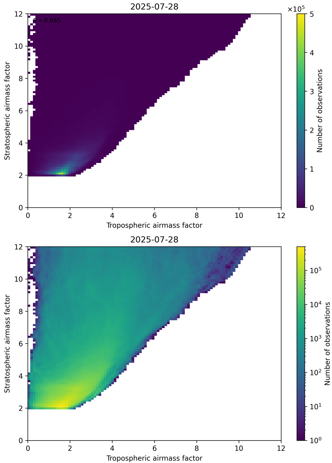
Figure 71: Scatter density plot of “Tropospheric airmass factor” against “Stratospheric airmass factor” for 2025-07-27 to 2025-07-29.
