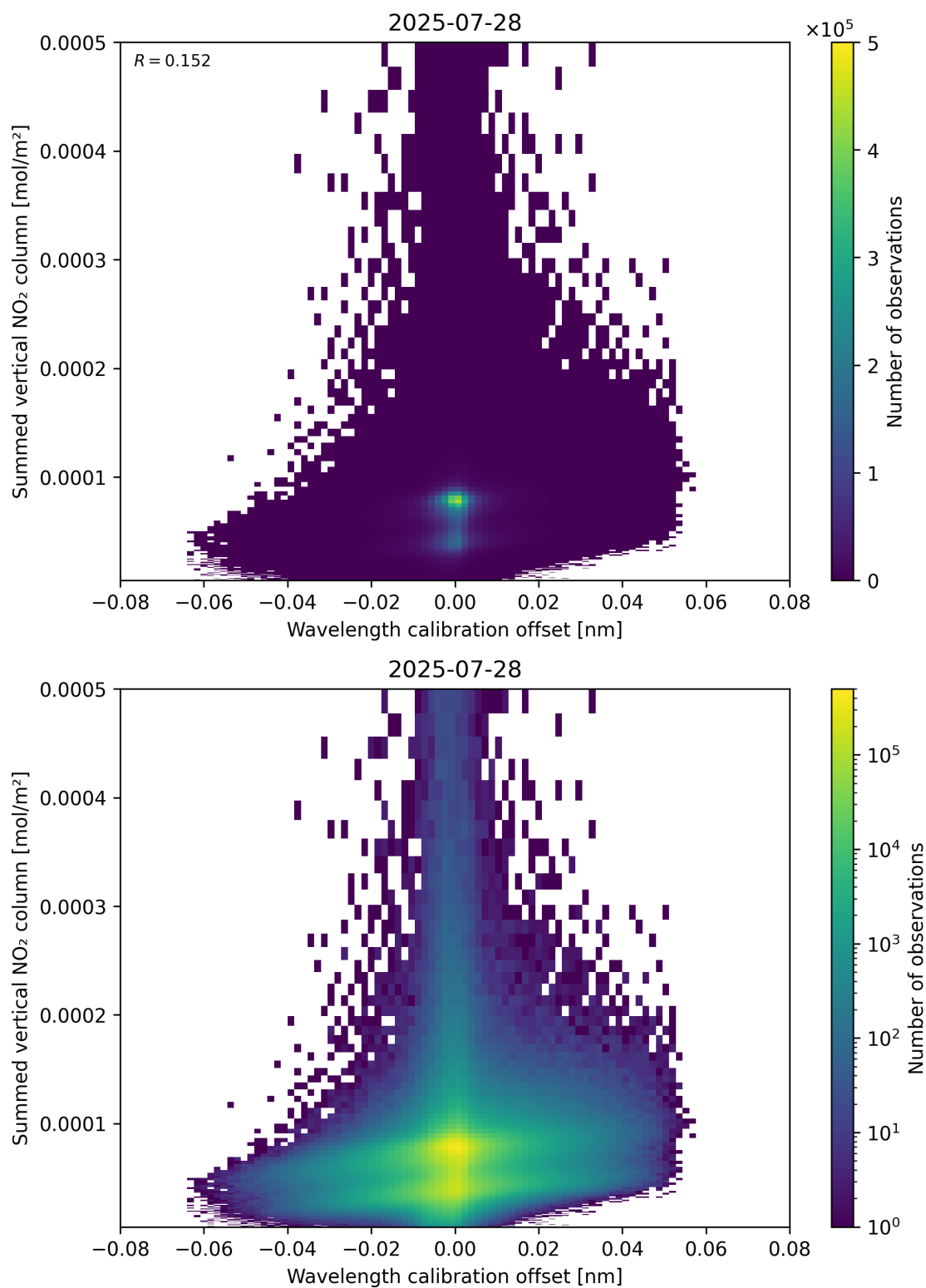
Figure 177: Scatter density plot of “Wavelength calibration offset” against “Summed vertical NO 2 column” for 2025-07-27 to 2025-07-29.
