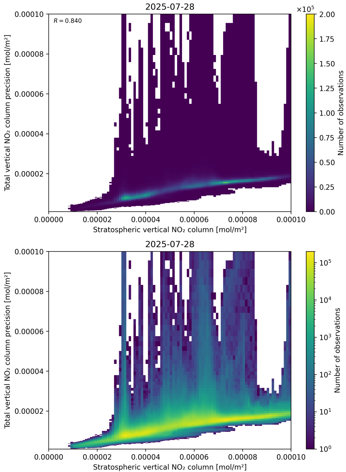
Figure 101: Scatter density plot of “Stratospheric vertical NO 2 column” against “Total vertical NO 2 column precision” for 2025-07-27 to 2025-07-29.
