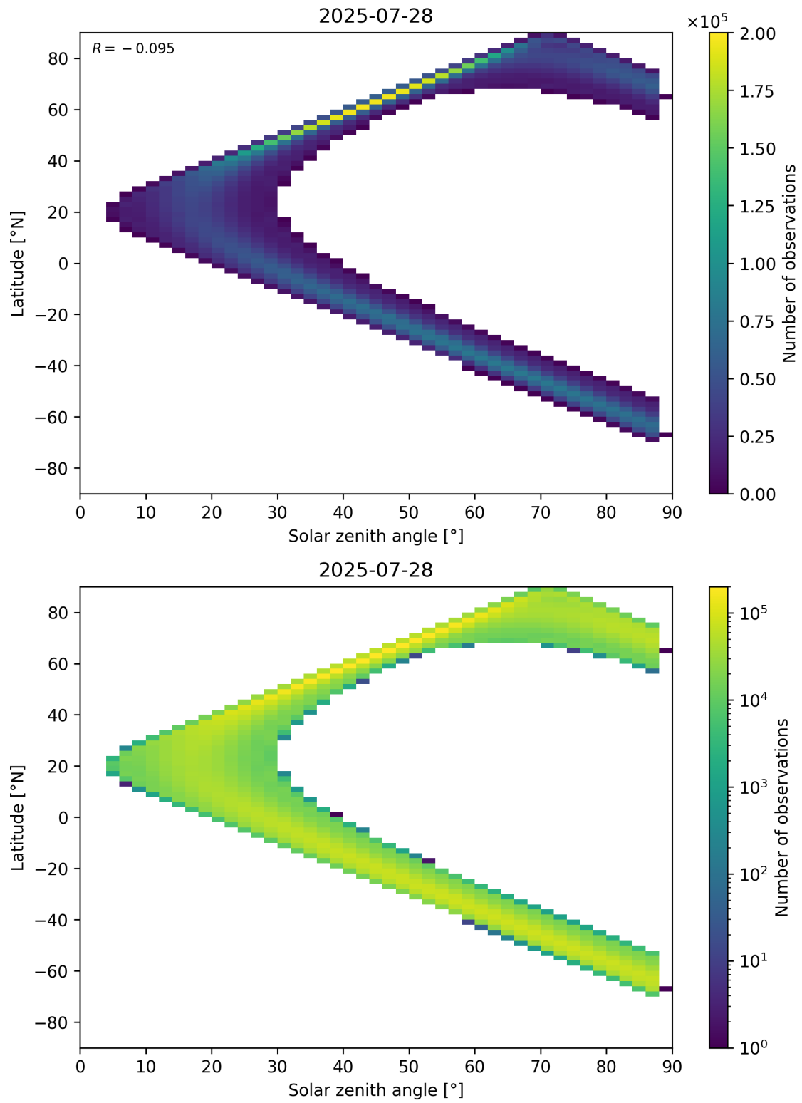
Figure 149: Scatter density plot of “Solar zenith angle” against “Latitude” for 2025-07-27 to 2025-07-29.
