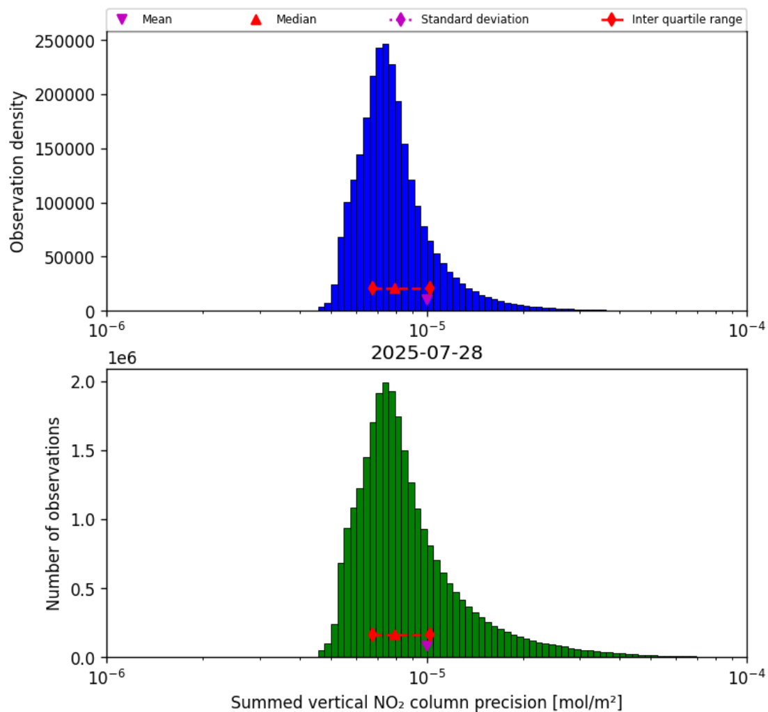
Figure 41: Histogram of "Summed vertical NO 2 column precision" for 2025-07-27 to 2025-07-29
