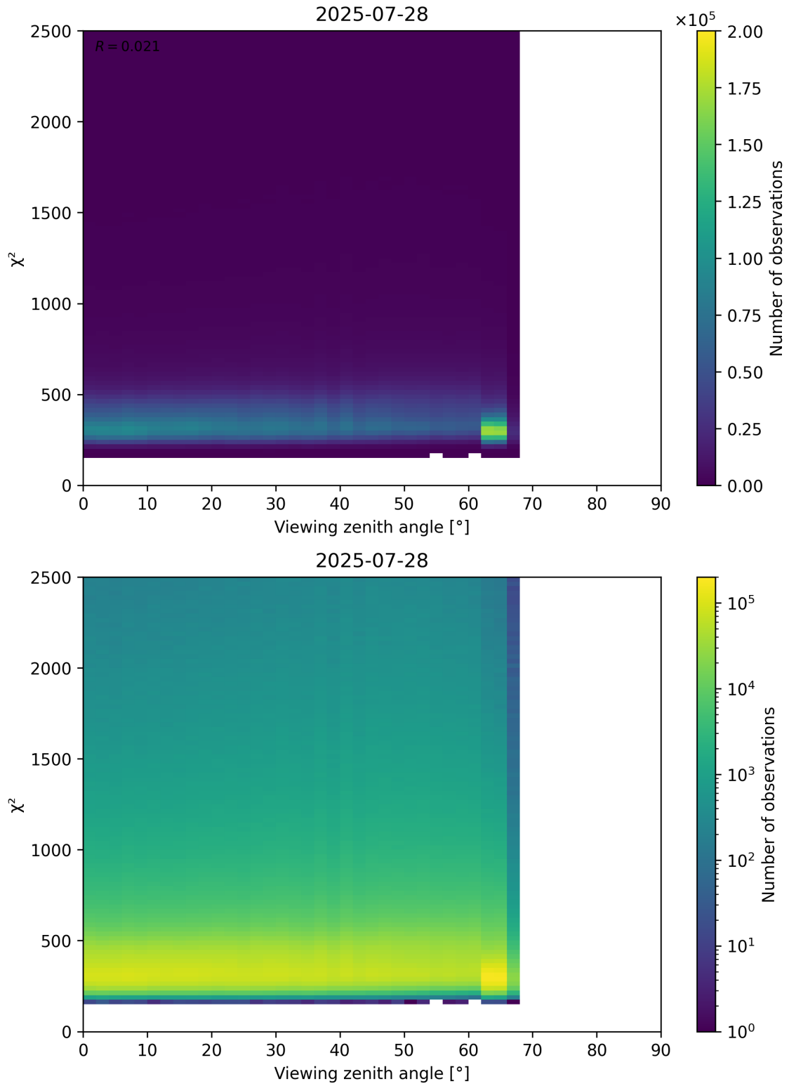
Figure 162: Scatter density plot of “Viewing zenith angle” against “ \chi^2 ” for 2025-07-27 to 2025-07-29.
