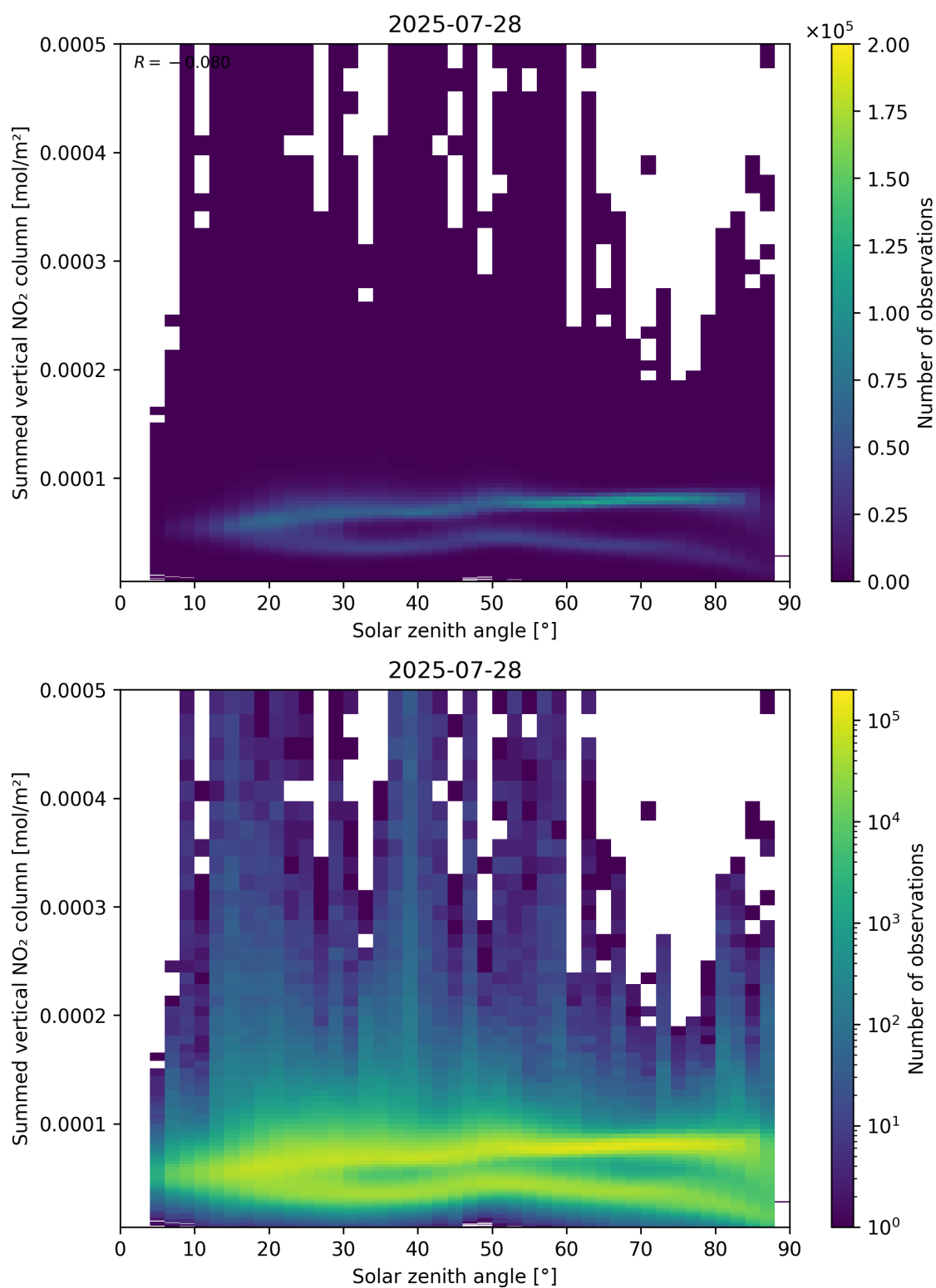
Figure 151: Scatter density plot of “Solar zenith angle” against “Summed vertical NO 2 column” for 2025-07-27 to 2025-07-29.
