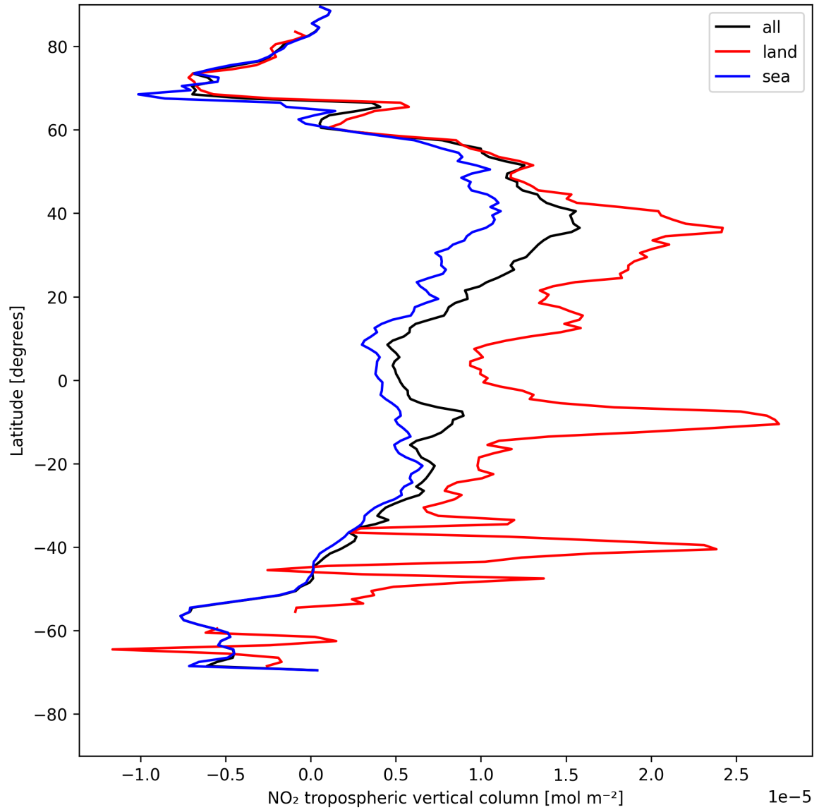
Figure 12: Zonal average of “NO 2 tropospheric vertical column” for 2025-07-27 to 2025-07-29.
