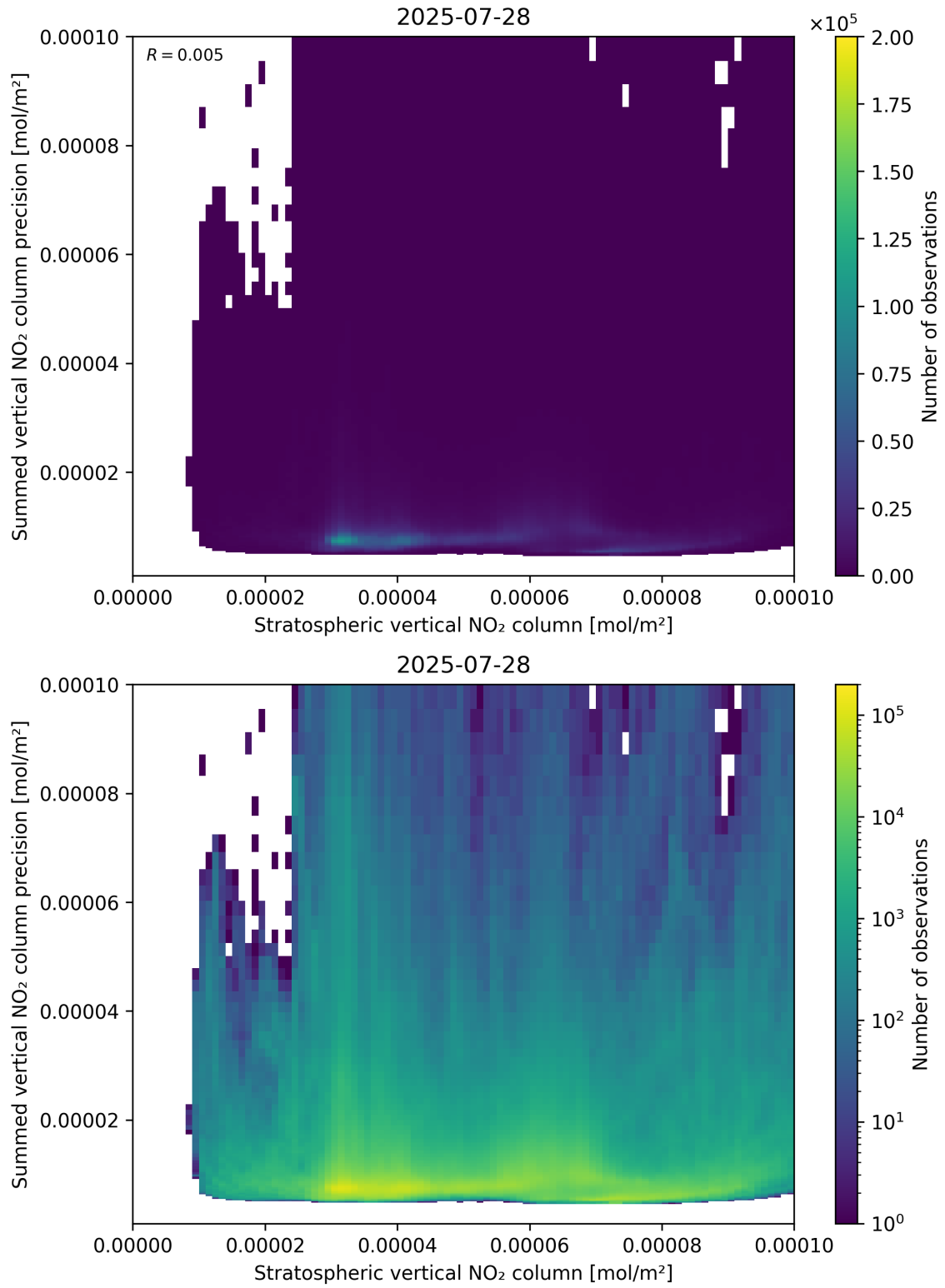
Figure 99: Scatter density plot of “Stratospheric vertical NO 2 column” against “Summed vertical NO 2 column precision” for 2025-07-27 to 2025-07-29.
