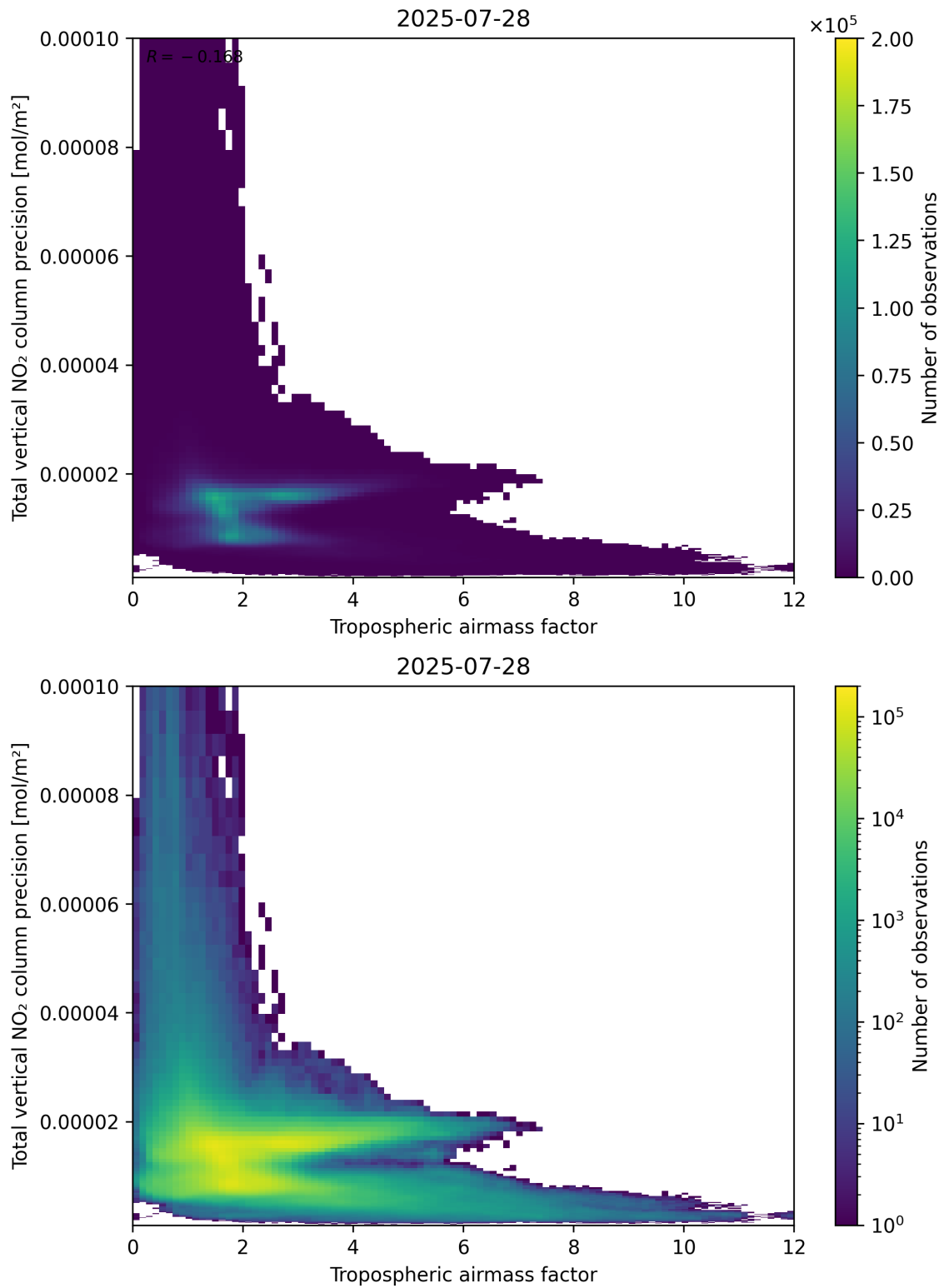
Figure 78: Scatter density plot of “Tropospheric air mass factor” against “Total vertical NO 2 column precision” for 2025-07-27 to 2025-07-29.
