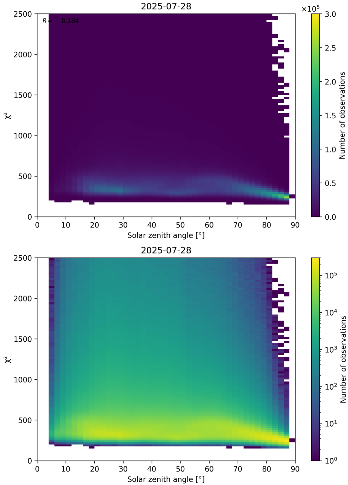
Figure 148: Scatter density plot of “Solar zenith angle” against “ \chi^2 ” for 2025-07-27 to 2025-07-29.
