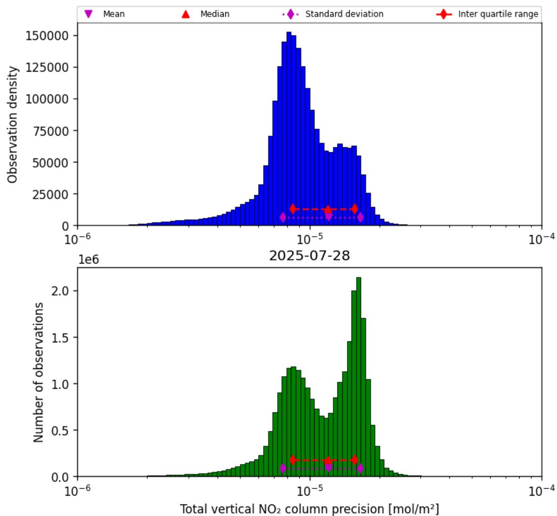
Figure 39: Histogram of “Total vertical NO 2 column precision” for 2025-07-27 to 2025-07-29
