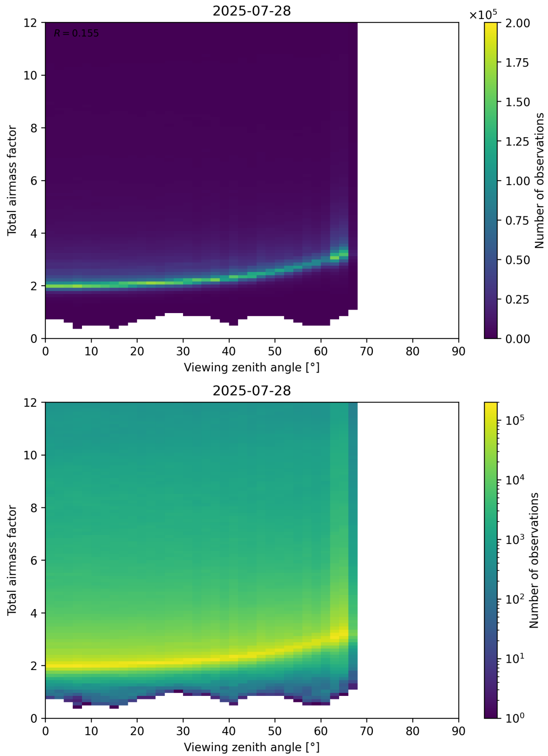
Figure 160: Scatter density plot of “Viewing zenith angle” against “Total airmass factor” for 2025-07-27 to 2025-07-29.
