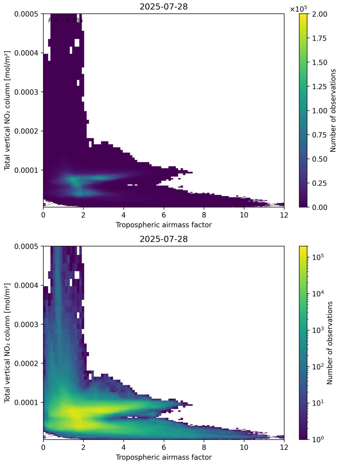
Figure 77: Scatter density plot of “Tropospheric airmass factor” against “Total vertical \text{NO}_2 column” for 2025-07-27 to 2025-07-29.
