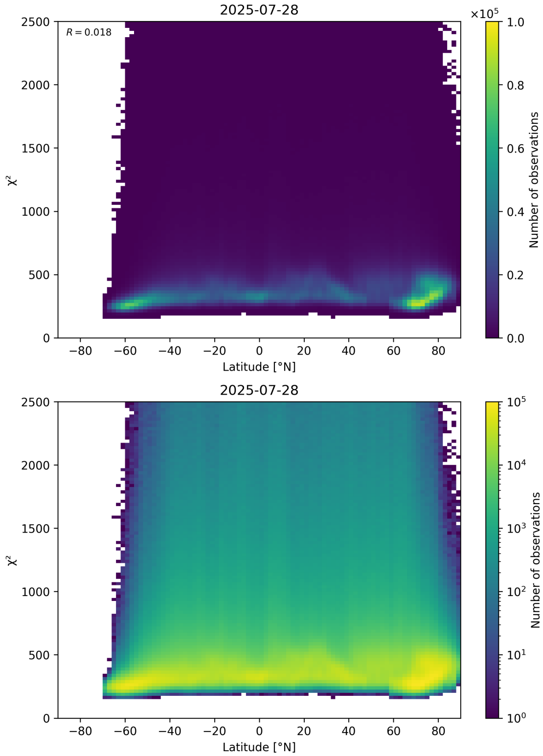
Figure 86: Scatter density plot of “Latitude” against “ \chi^2 ” for 2025-07-27 to 2025-07-29.
