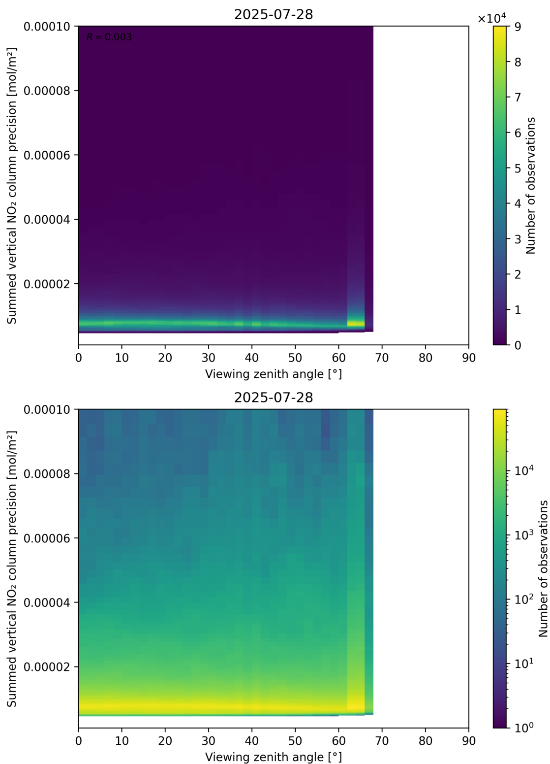
Figure 166: Scatter density plot of “Viewing zenith angle” against “Summed vertical NO 2 column precision” for 2025-07-27 to 2025-07-29.
