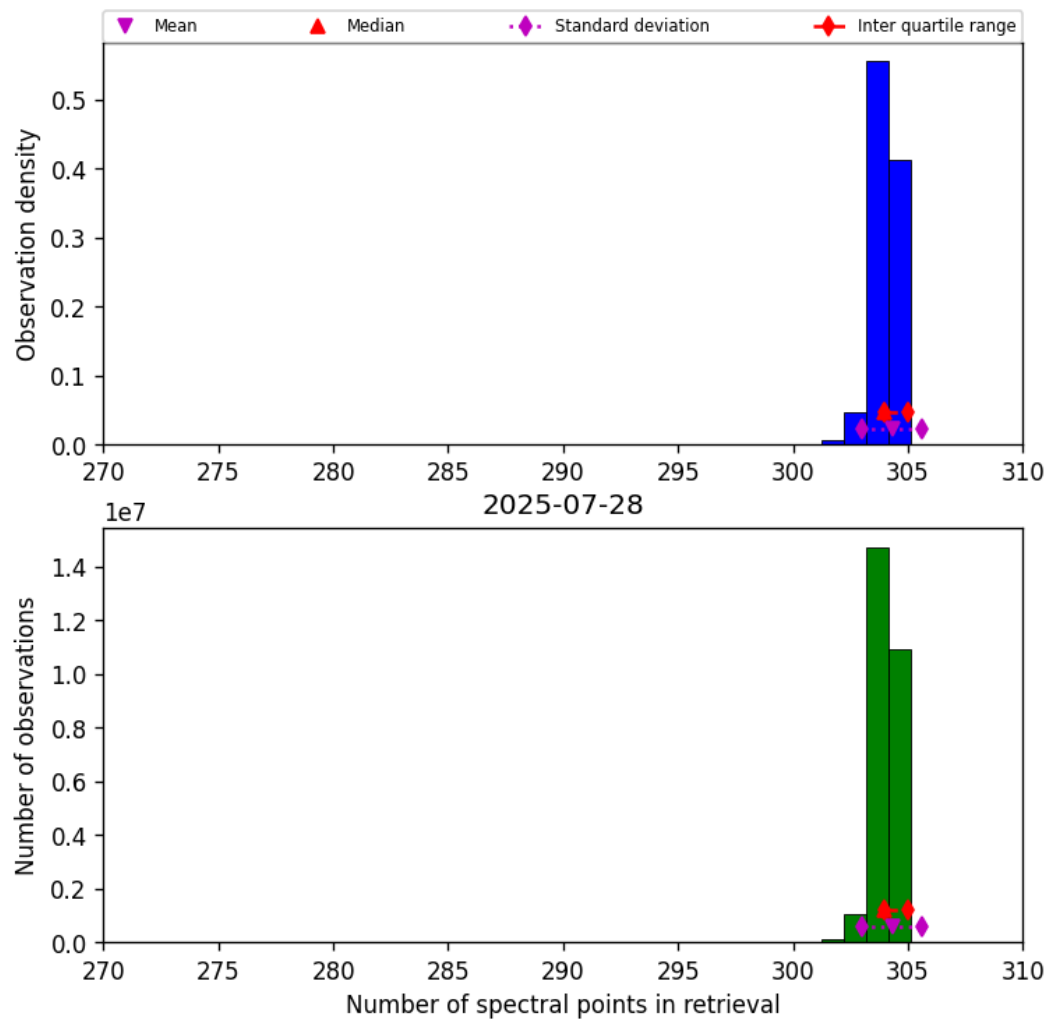
Figure 33: Histogram of “Number of spectral points in retrieval” for 2025-07-27 to 2025-07-29
