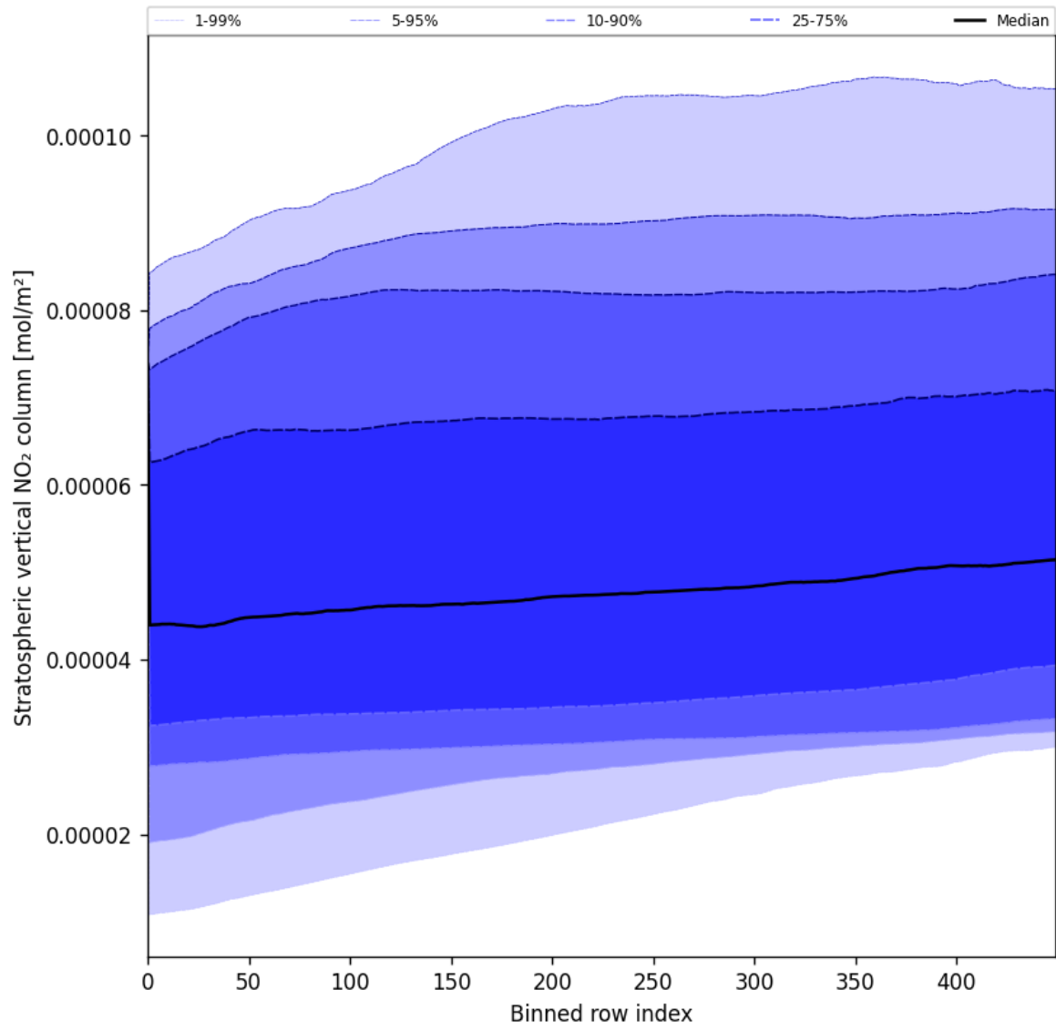
Figure 53: Along track statistics of “Stratospheric vertical NO 2 column” for 2025-07-27 to 2025-07-29
