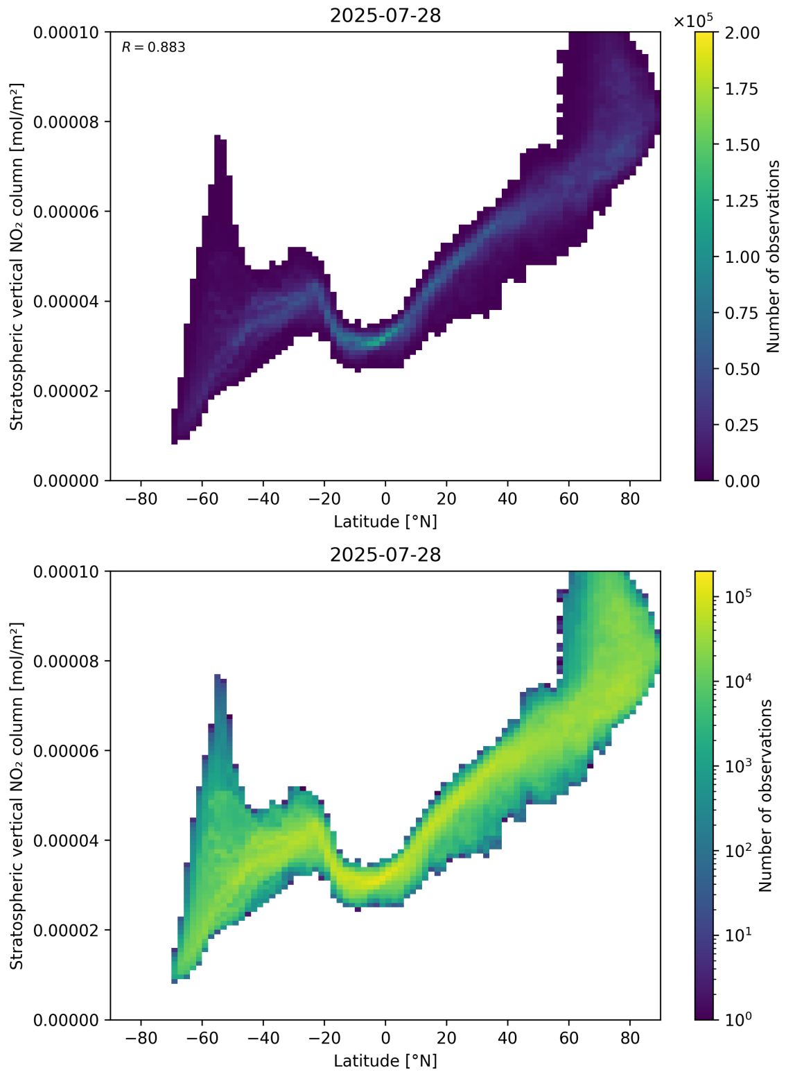
Figure 87: Scatter density plot of “Latitude” against “Stratospheric vertical \text{NO}_2 column” for 2025-07-27 to 2025-07-29.
