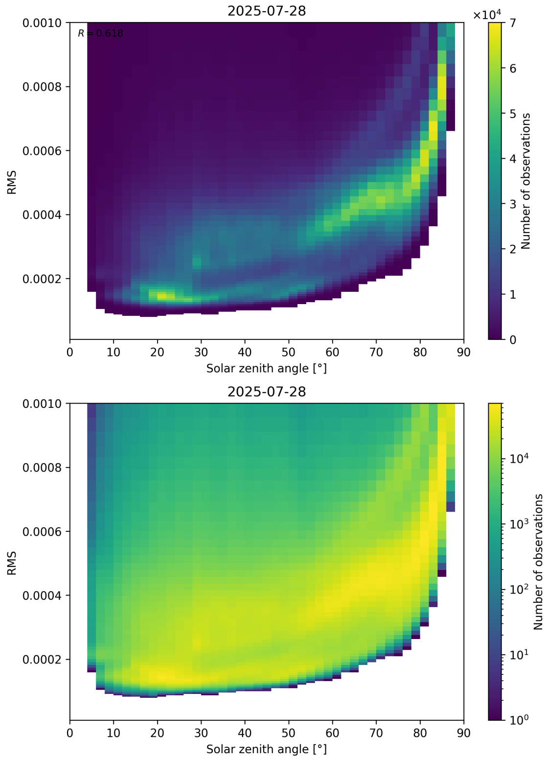
Figure 157: Scatter density plot of “Solar zenith angle” against “RMS” for 2025-07-27 to 2025-07-29.
