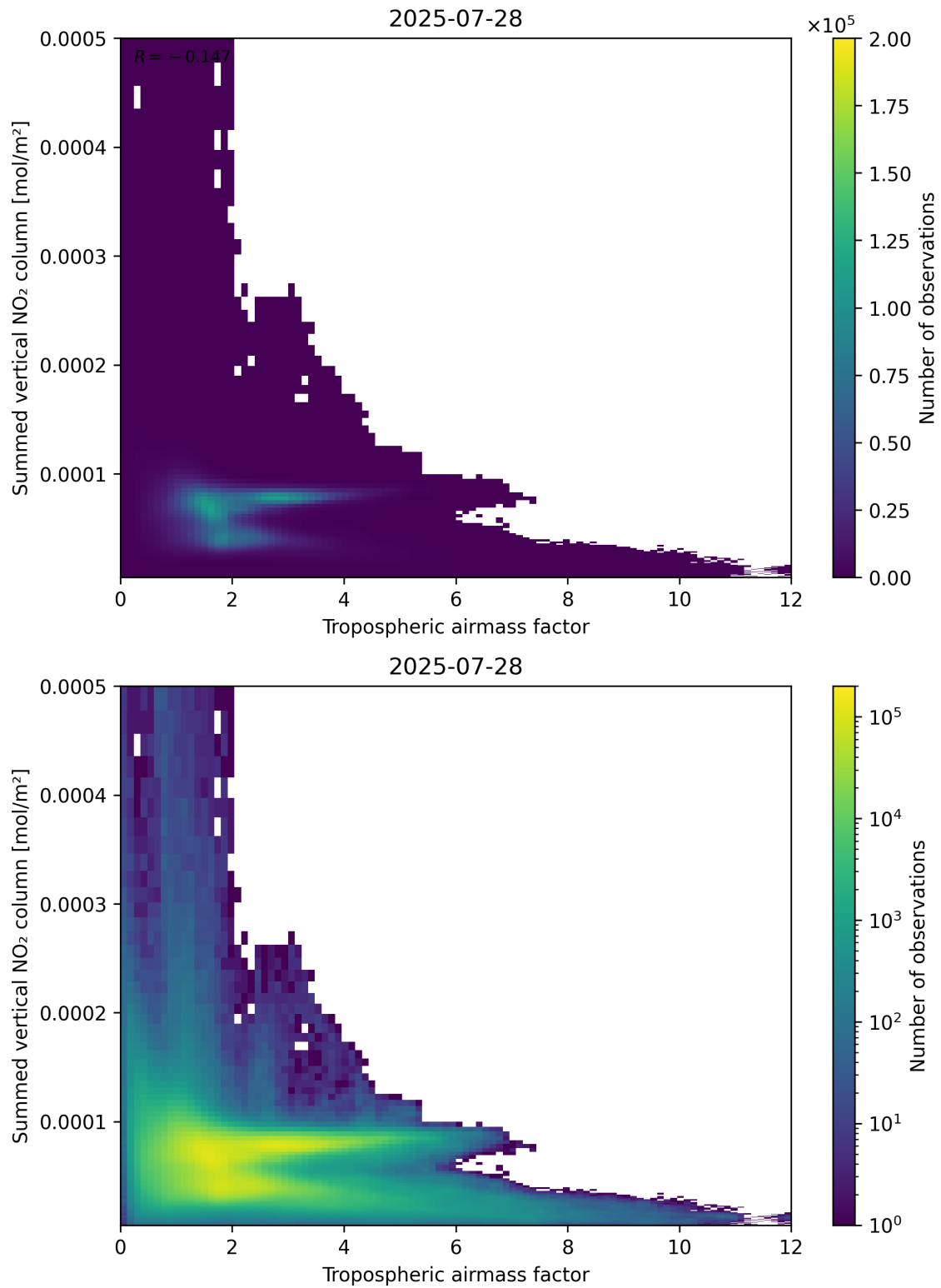
Figure 75: Scatter density plot of “Tropospheric air mass factor” against “Summed vertical NO 2 column” for 2025-07-27 to 2025-07-29.
