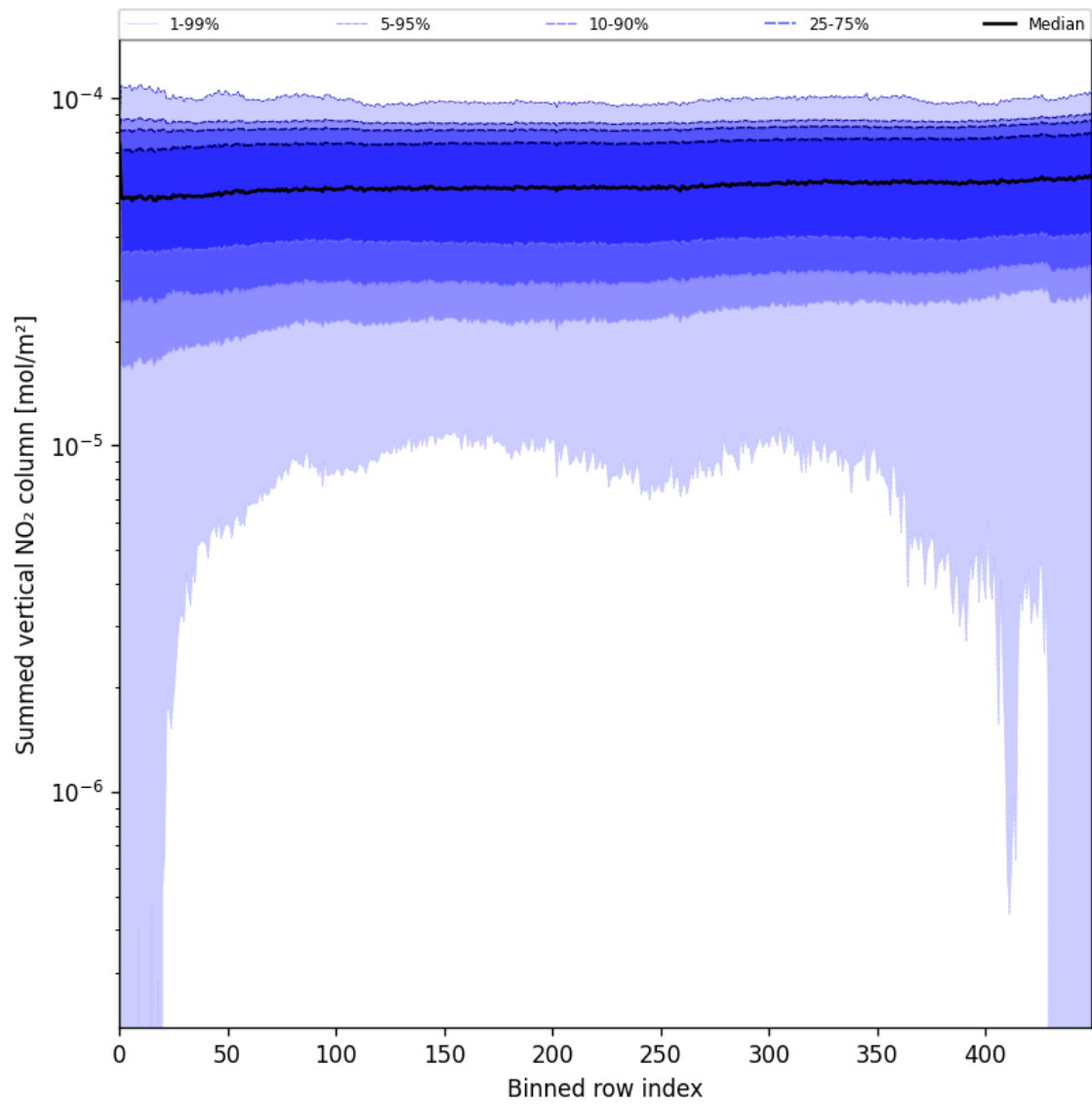
Figure 57: Along track statistics of “Summed vertical NO 2 column” for 2025-07-27 to 2025-07-29
