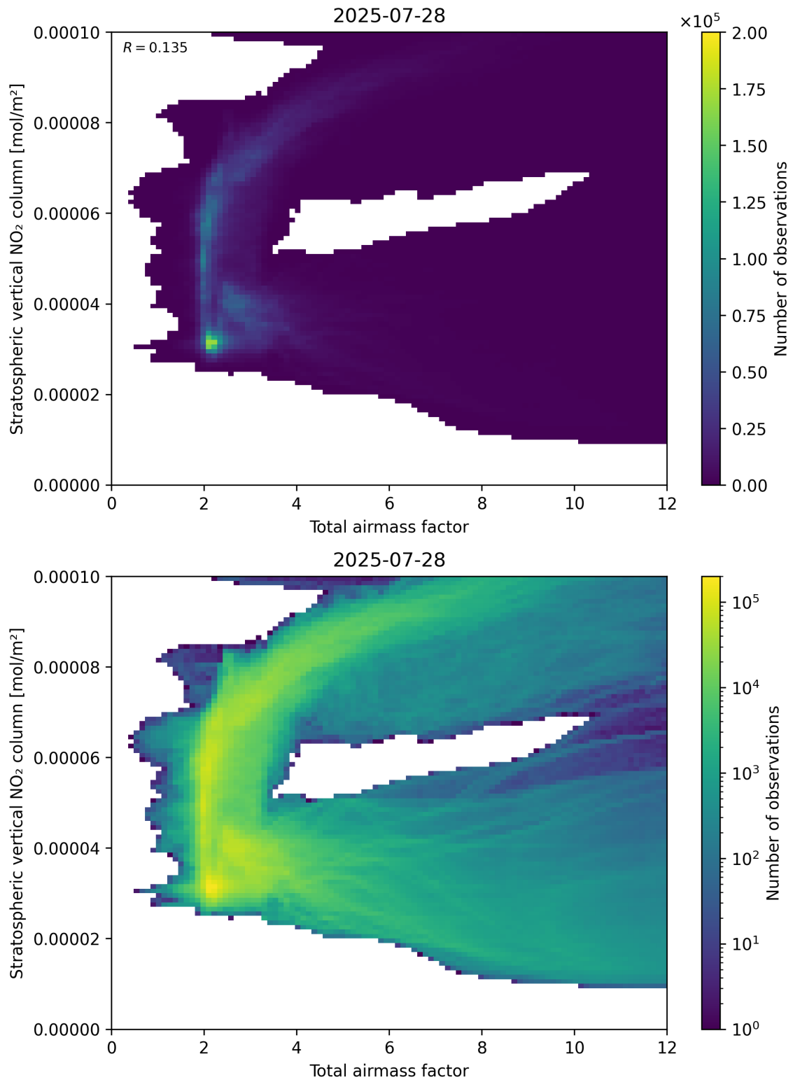
Figure 64: Scatter density plot of “Total airmass factor” against “Stratospheric vertical \text{NO}_2 column” for 2025-07-27 to 2025-07-29.
