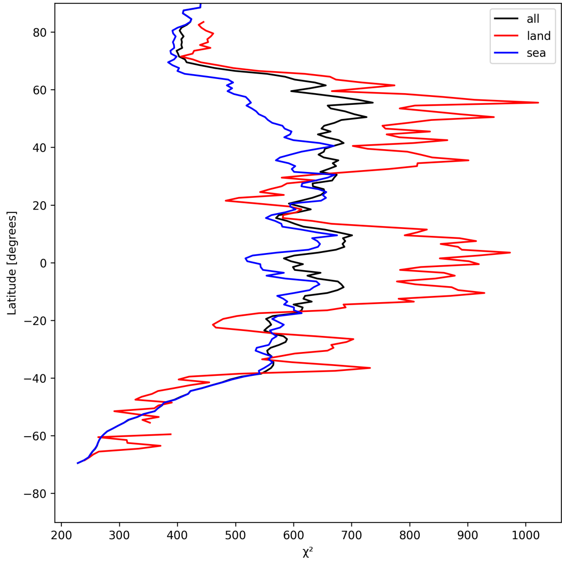
Figure 25: Zonal average of " \chi^2 " for 2025-07-27 to 2025-07-29.
