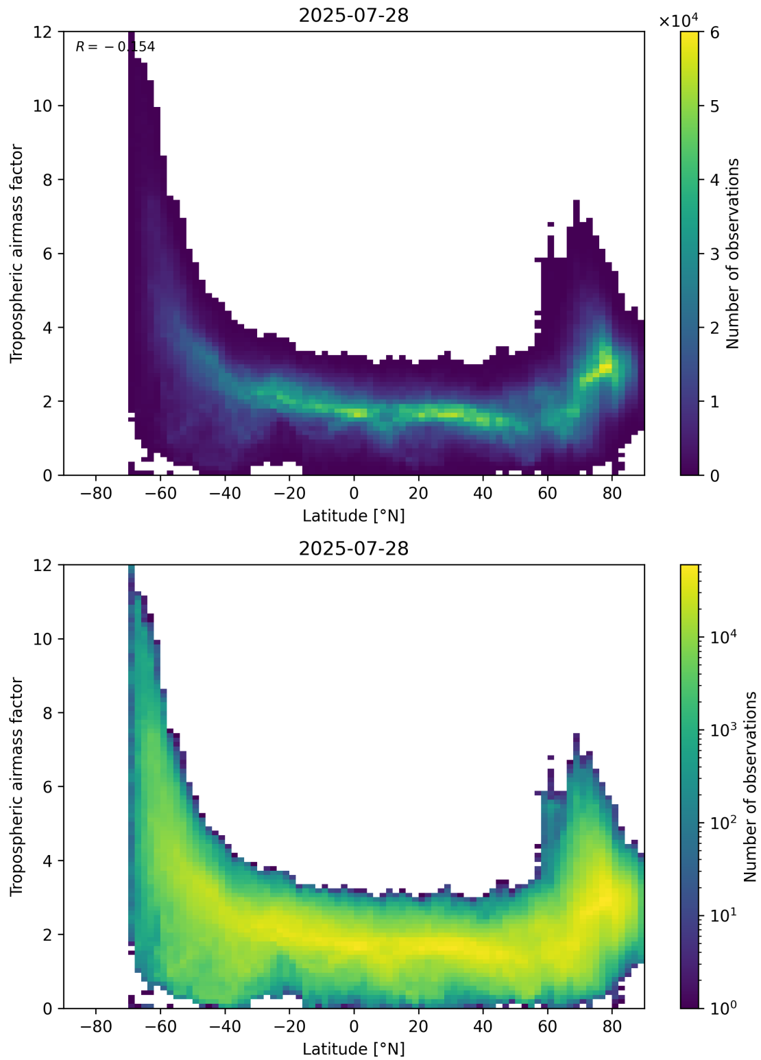
Figure 85: Scatter density plot of “Latitude” against “Tropospheric air mass factor” for 2025-07-27 to 2025-07-29.
