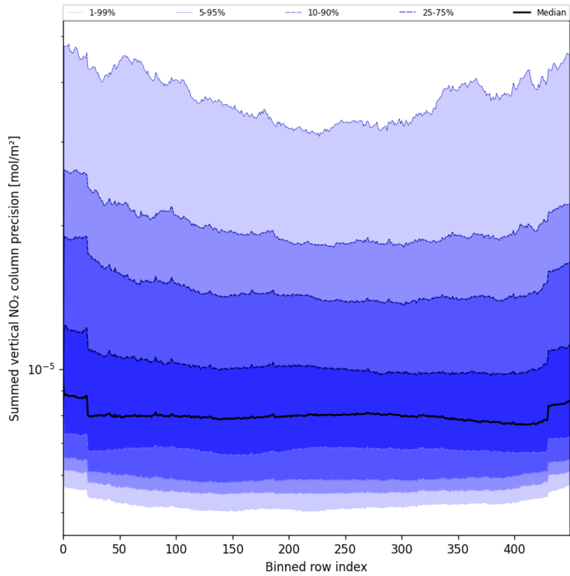
Figure 58: Along track statistics of “Summed vertical NO 2 column precision” for 2025-07-27 to 2025-07-29
