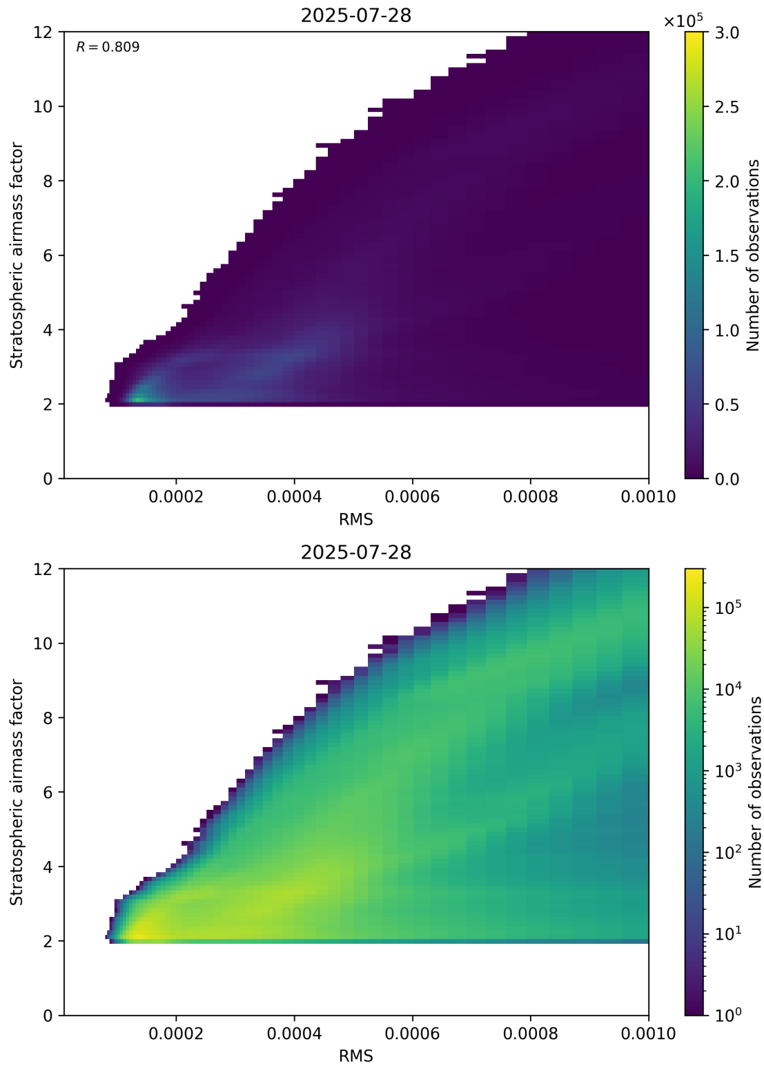
Figure 144: Scatter density plot of “RMS” against “Stratospheric airmass factor” for 2025-07-27 to 2025-07-29.
