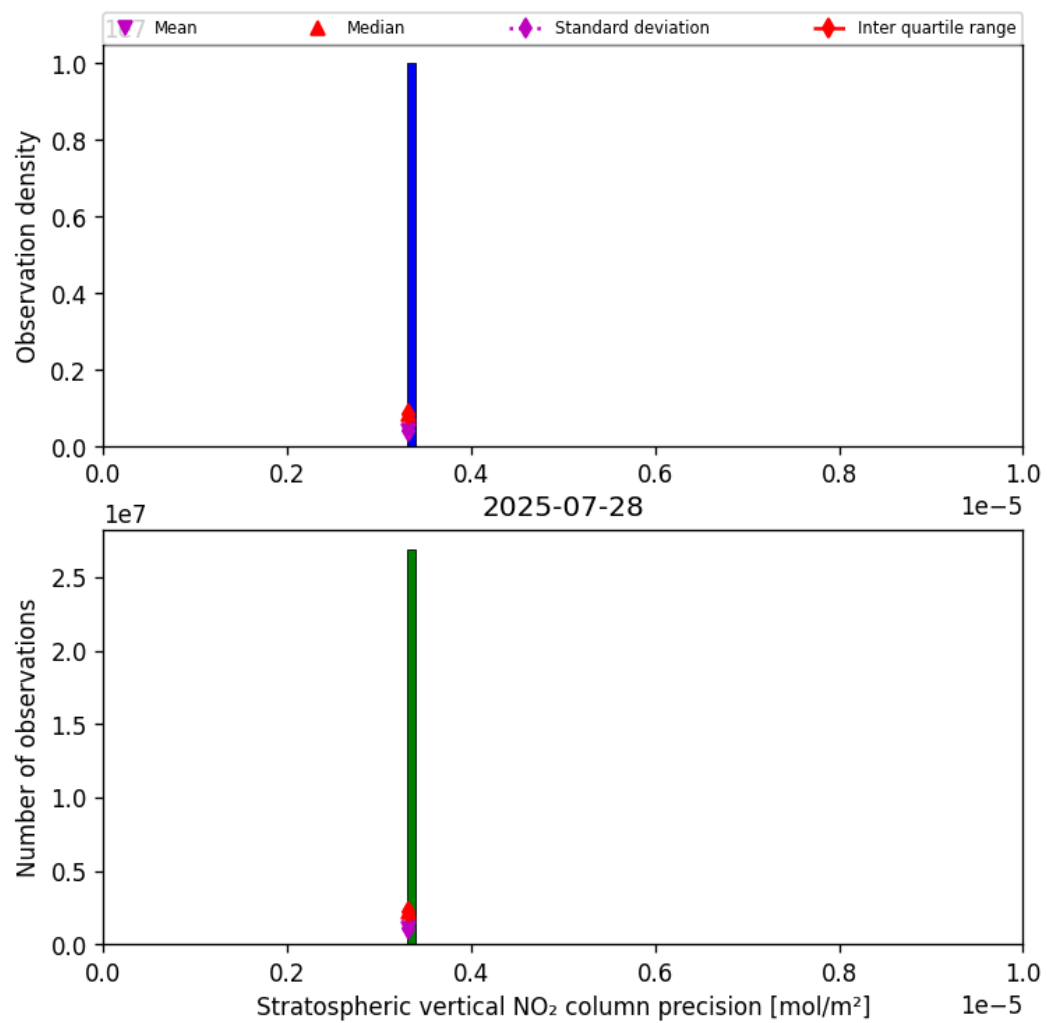
Figure 37: Histogram of “Stratospheric vertical NO 2 column precision” for 2025-07-27 to 2025-07-29
