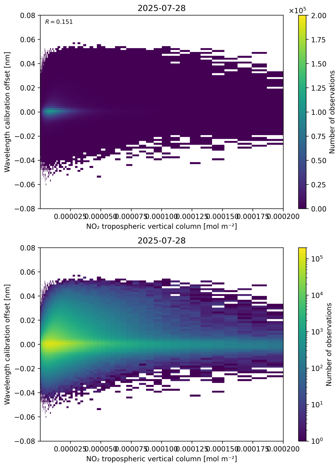
Figure 143: Scatter density plot of “NO 2 tropospheric vertical column” against “Wavelength calibration offset” for 2025-07-27 to 2025-07-29.
