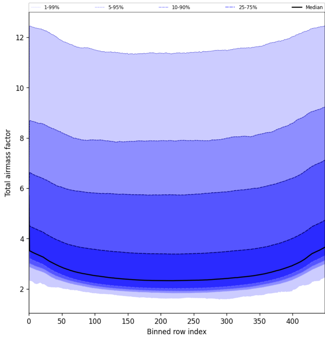
Figure 49: Along track statistics of “Total airmass factor” for 2025-07-27 to 2025-07-29
