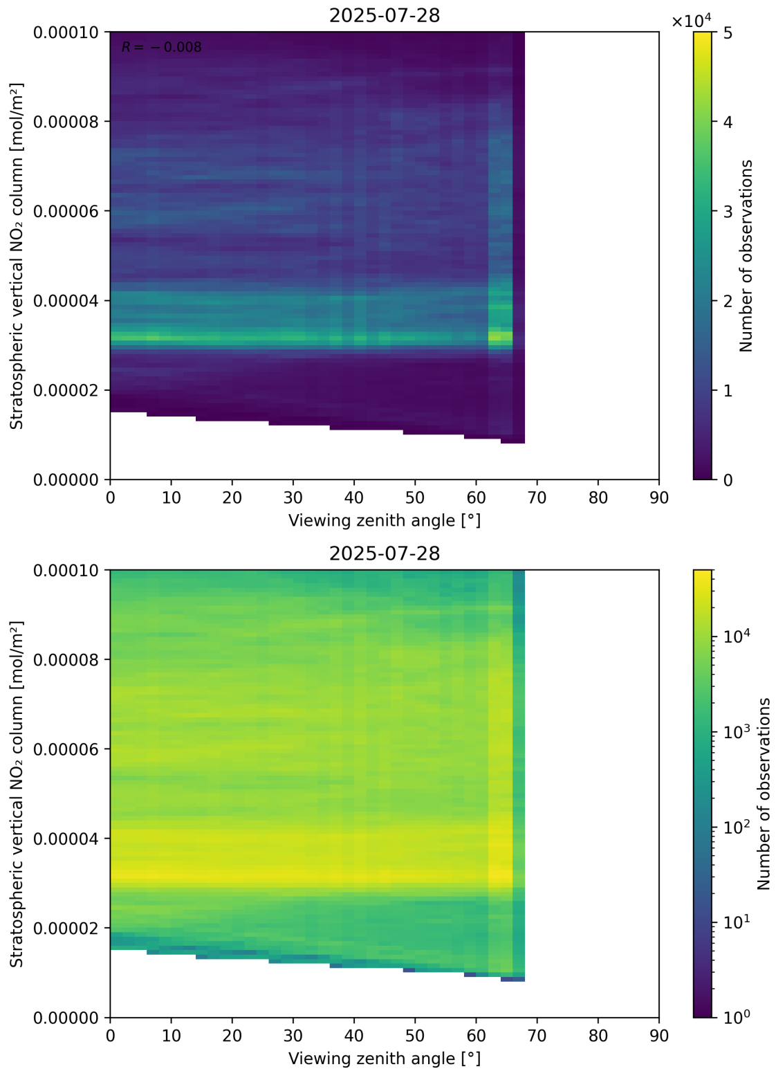
Figure 164: Scatter density plot of “Viewing zenith angle” against “Stratospheric vertical NO 2 column” for 2025-07-27 to 2025-07-29.
