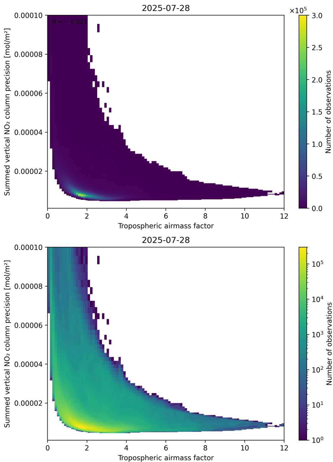
Figure 76: Scatter density plot of “Tropospheric air mass factor” against “Summed vertical NO 2 column precision” for 2025-07-27 to 2025-07-29.
