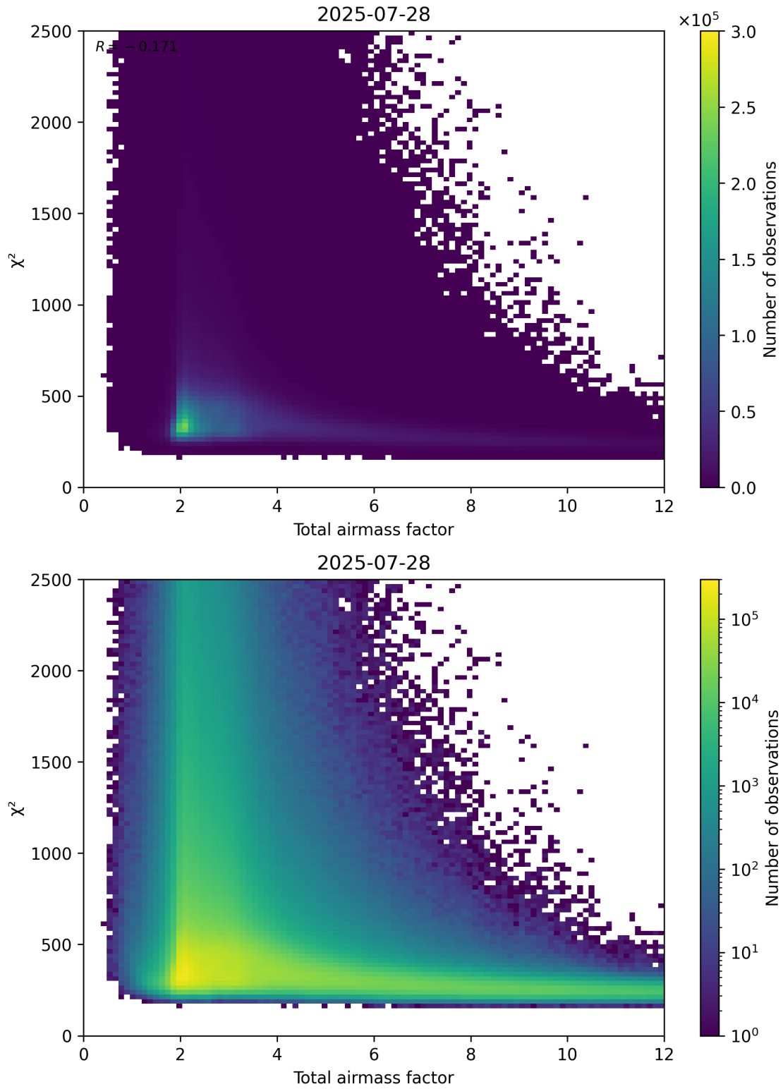
Figure 63: Scatter density plot of “Total airmass factor” against “ \chi^2 ” for 2025-07-27 to 2025-07-29.
