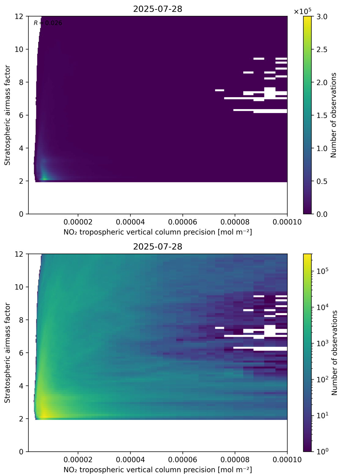
Figure 131: Scatter density plot of “NO 2 tropospheric vertical column precision” against “Stratospheric airmass factor” for 2025-07-27 to 2025-07-29.
