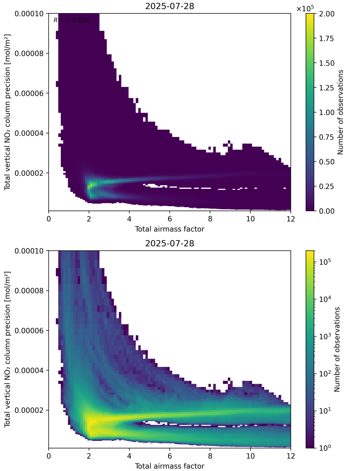
Figure 68: Scatter density plot of “Total airmass factor” against “Total vertical NO 2 column precision” for 2025-07-27 to 2025-07-29.
