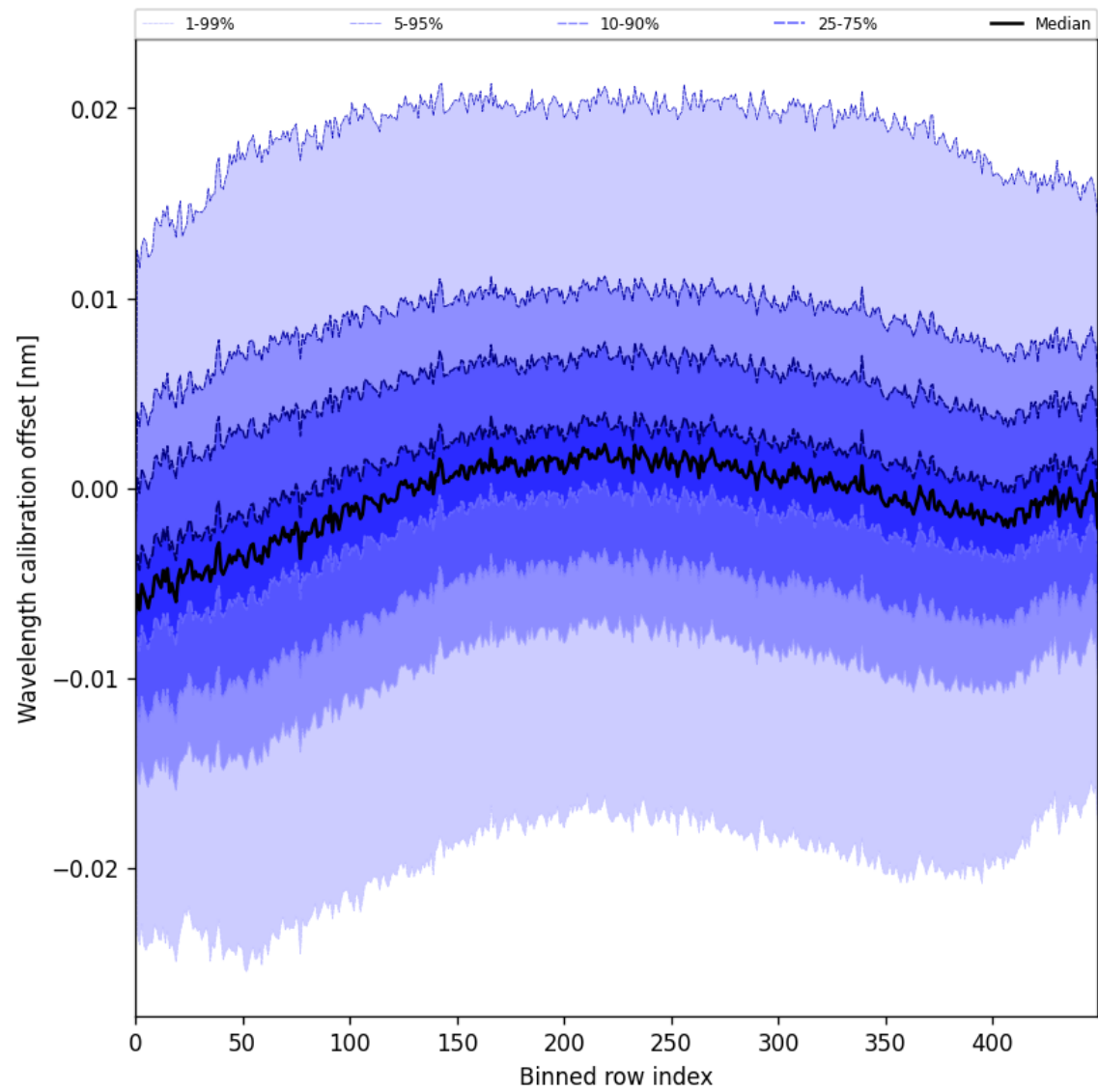
Figure 52: Along track statistics of “Wavelength calibration offset” for 2025-07-27 to 2025-07-29
