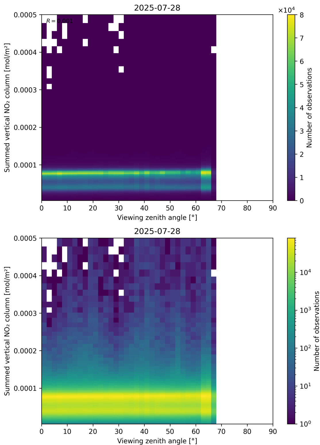
Figure 165: Scatter density plot of “Viewing zenith angle” against “Summed vertical NO 2 column” for 2025-07-27 to 2025-07-29.
