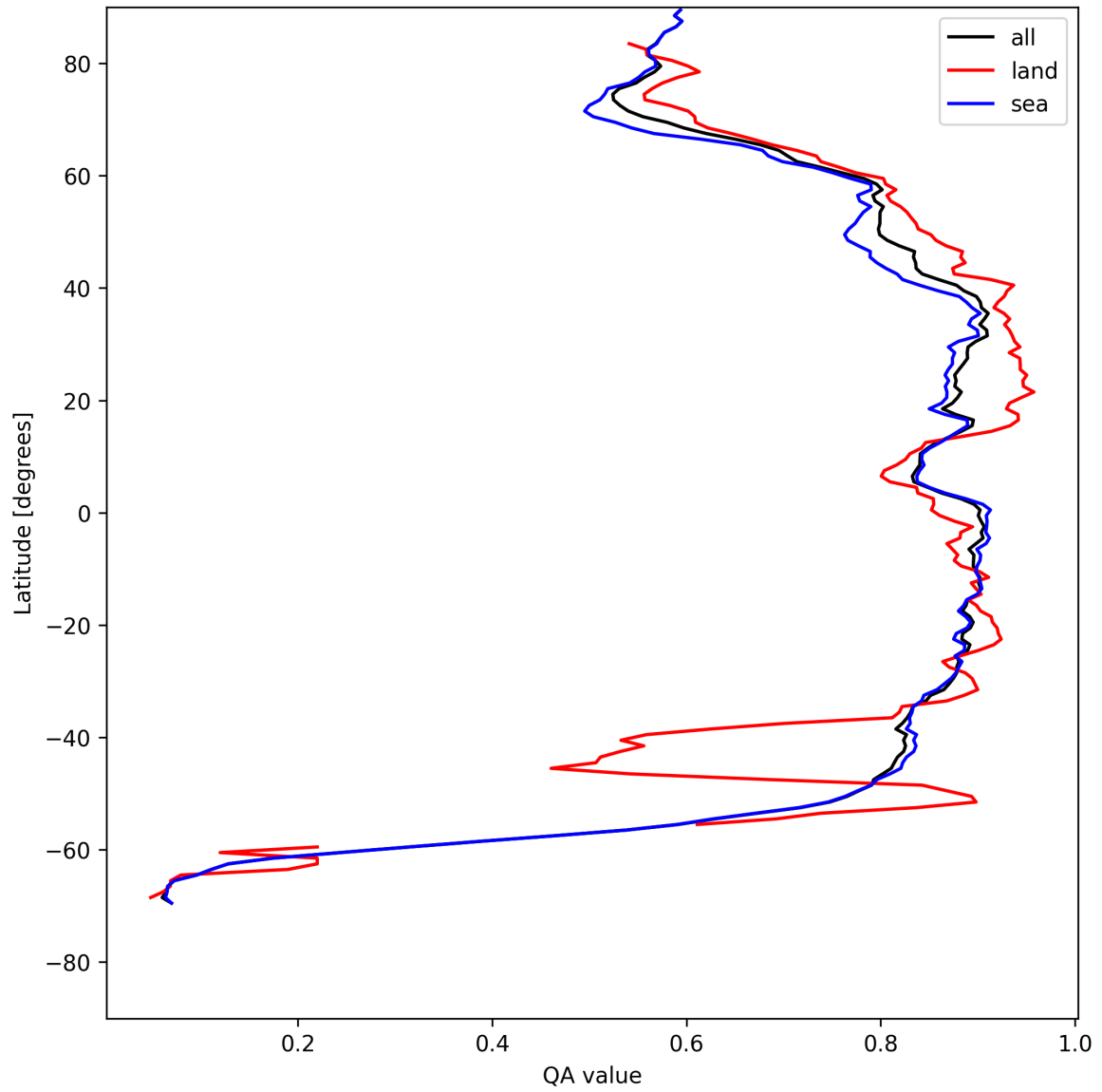
Figure 11: Zonal average of “QA value” for 2025-07-27 to 2025-07-29.
