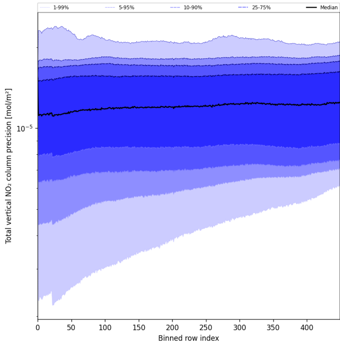
Figure 56: Along track statistics of “Total vertical NO 2 column precision” for 2025-07-27 to 2025-07-29
