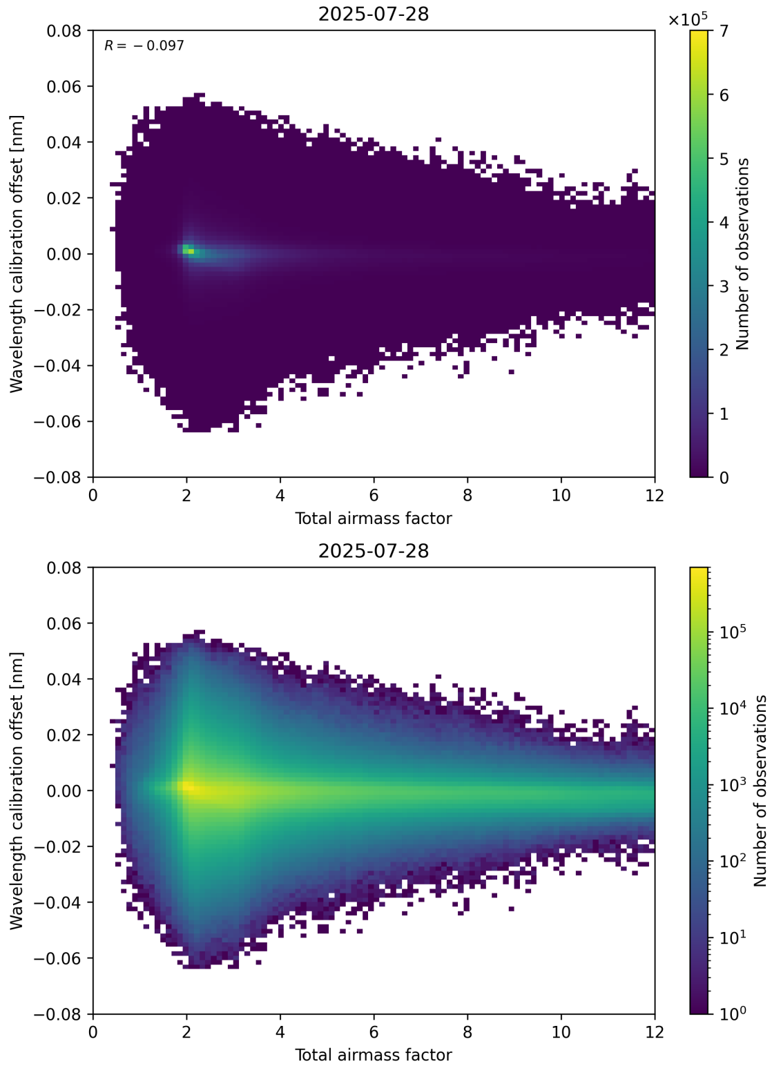
Figure 70: Scatter density plot of “Total airmass factor” against “Wavelength calibration offset” for 2025-07-27 to 2025-07-29.
