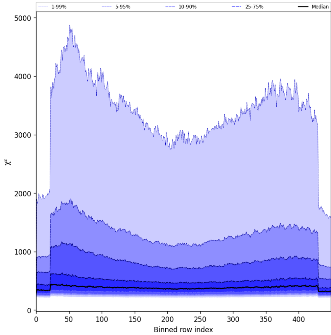
Figure 59: Along track statistics of “ \chi^2 ” for 2025-07-27 to 2025-07-29
