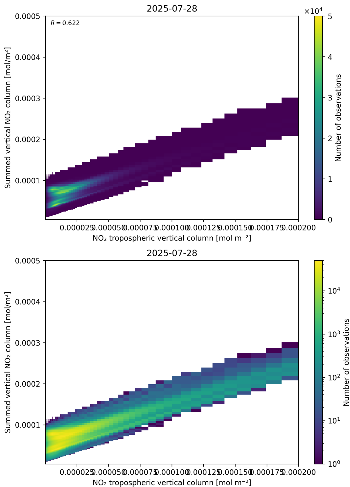
Figure 126: Scatter density plot of “NO 2 tropospheric vertical column” against “Summed vertical NO 2 column” for 2025-07-27 to 2025-07-29.
