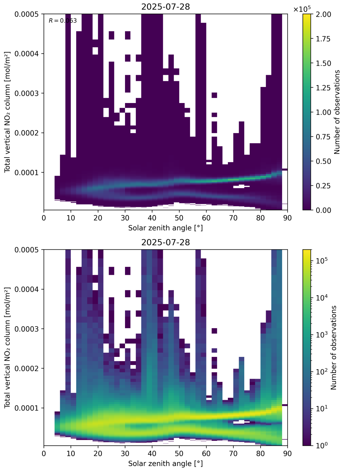
Figure 153: Scatter density plot of “Solar zenith angle” against “Total vertical NO 2 column” for 2025-07-27 to 2025-07-29.
