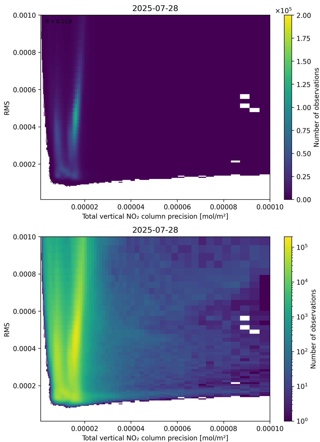
Figure 119: Scatter density plot of “Total vertical NO 2 column precision” against “RMS” for 2025-07-27 to 2025-07-29.
