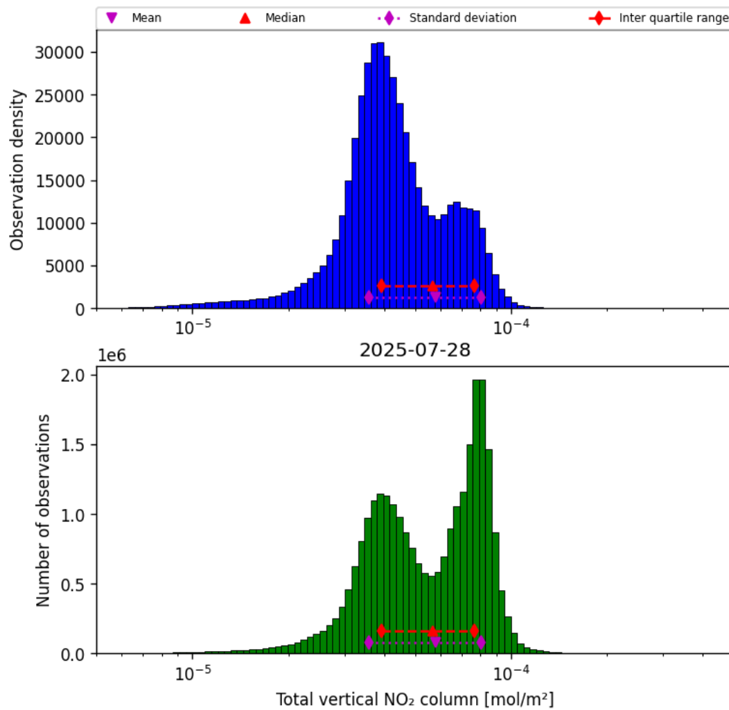
Figure 38: Histogram of “Total vertical NO 2 column” for 2025-07-27 to 2025-07-29
