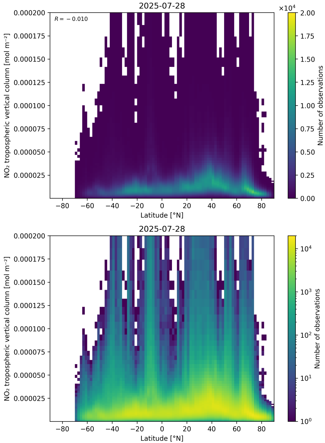
Figure 92: Scatter density plot of “Latitude” against “NO 2 tropospheric vertical column” for 2025-07-27 to 2025-07-29.
