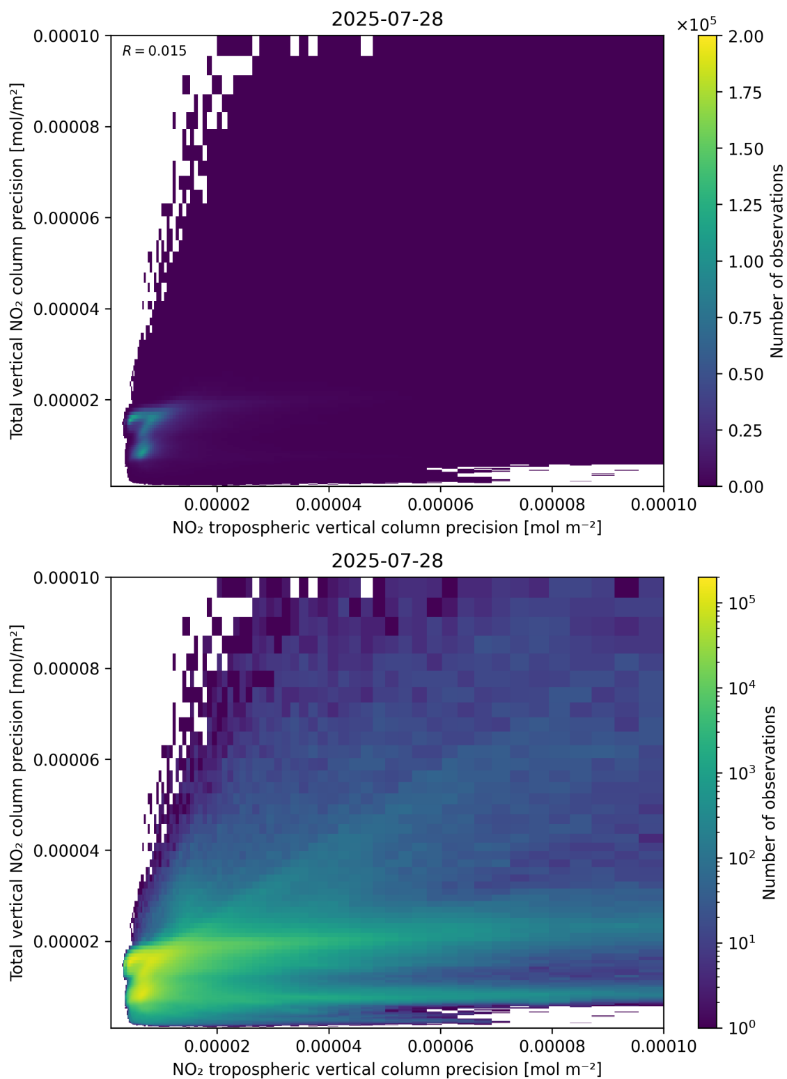
Figure 139: Scatter density plot of “NO 2 tropospheric vertical column precision” against “Total vertical NO 2 column precision” for 2025-07-27 to 2025-07-29.
