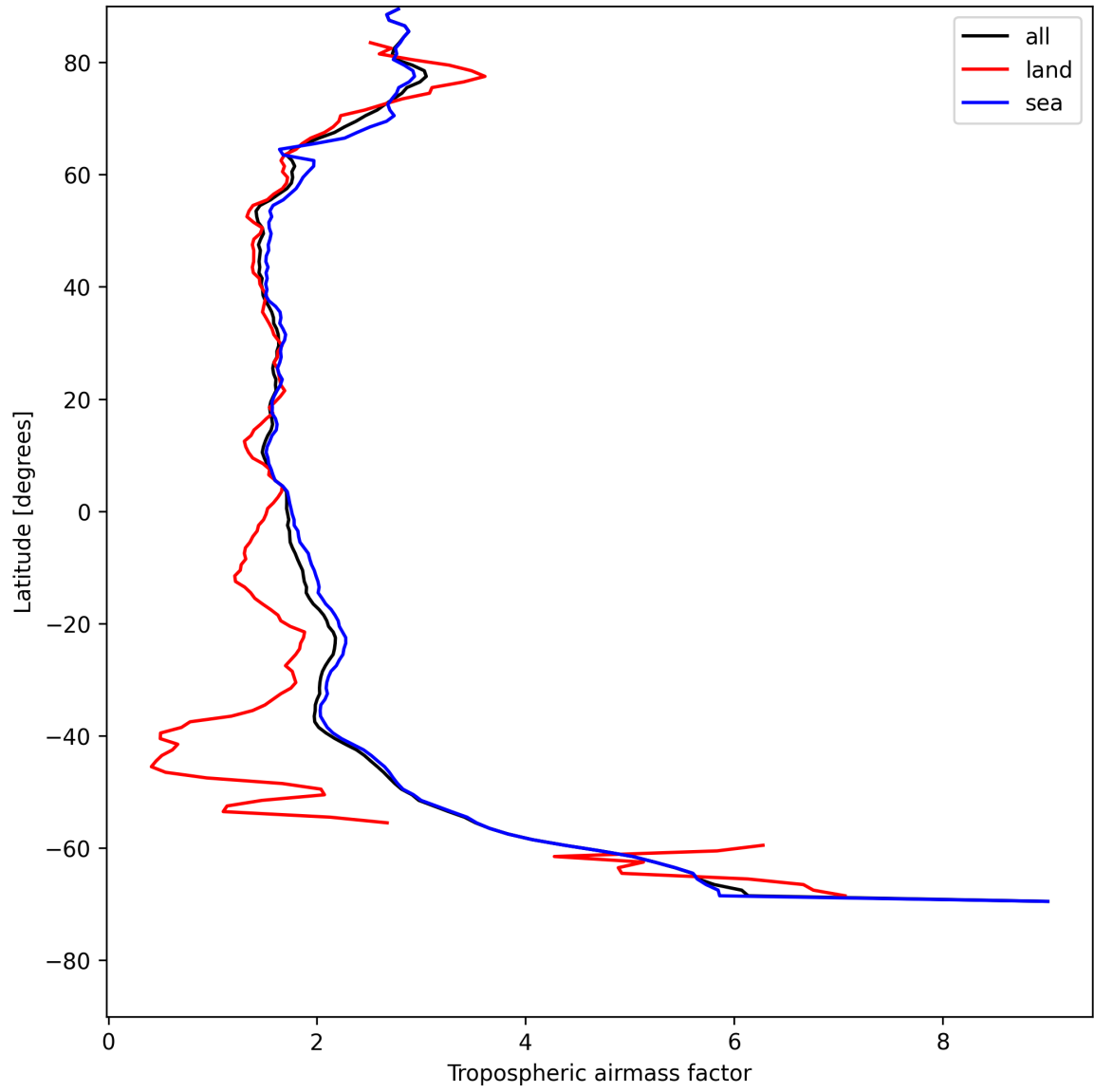
Figure 14: Zonal average of “Tropospheric airmass factor” for 2025-07-27 to 2025-07-29.
