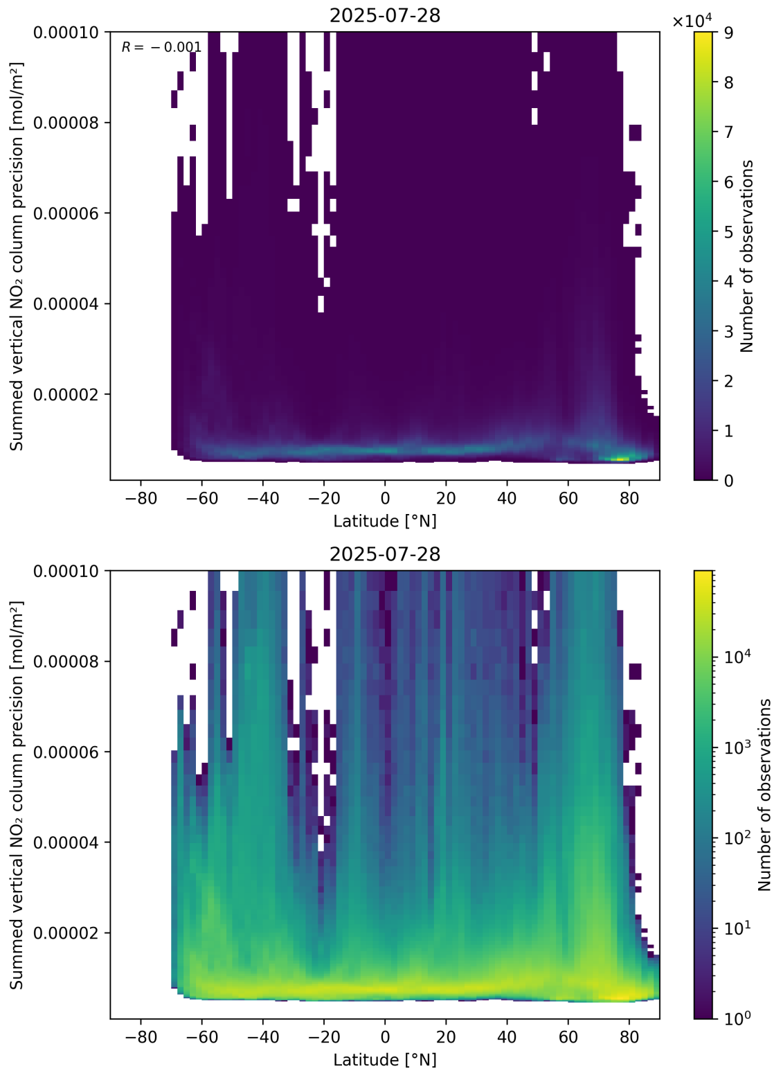
Figure 89: Scatter density plot of “Latitude” against “Summed vertical NO 2 column precision” for 2025-07-27 to 2025-07-29.
