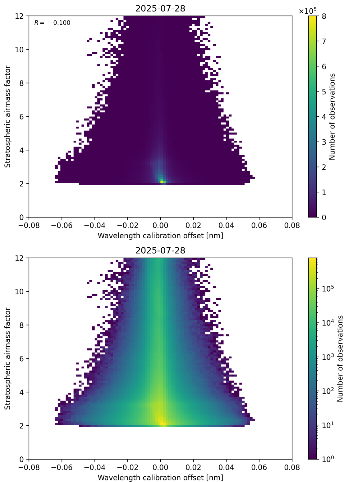
Figure 174: Scatter density plot of “Wavelength calibration offset” against “Stratospheric airmass factor” for 2025-07-27 to 2025-07-29.
