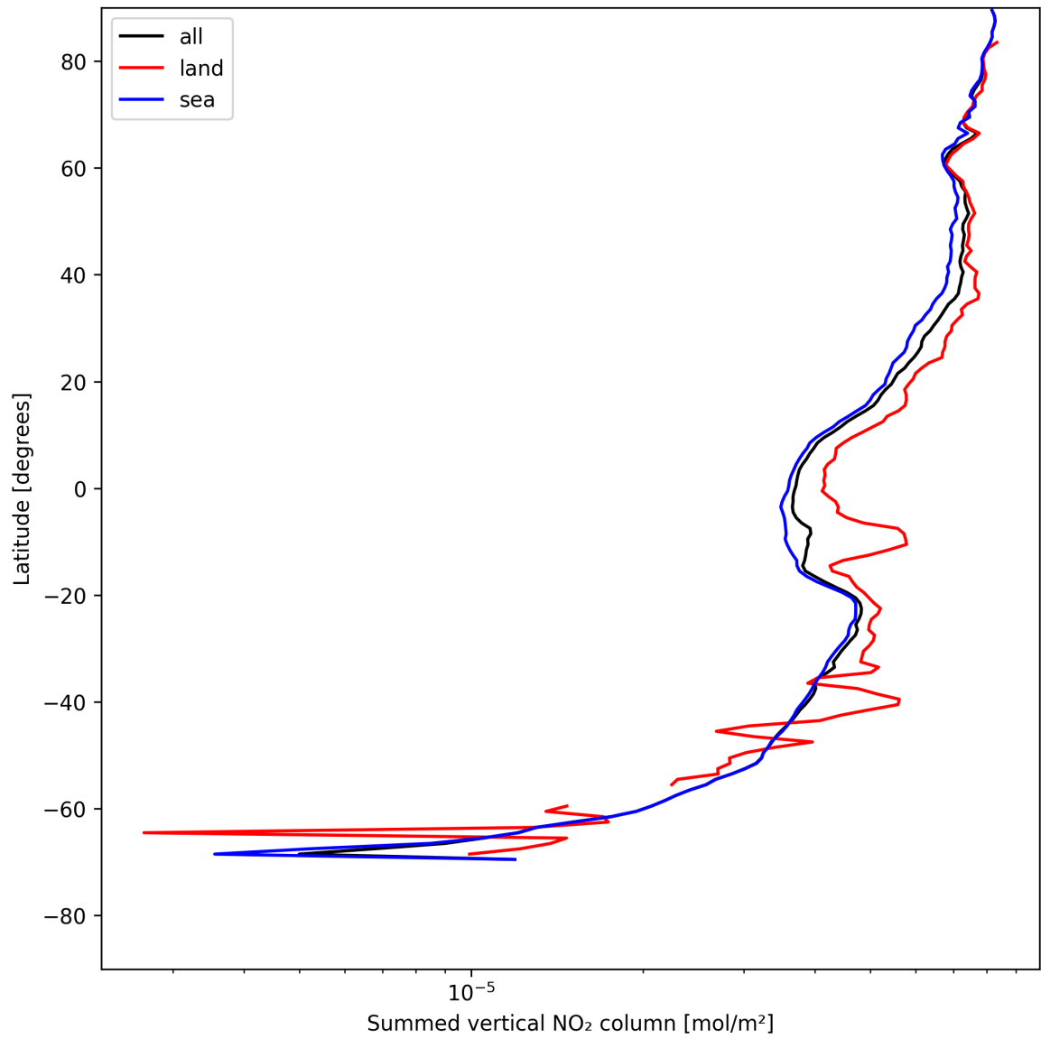
Figure 23: Zonal average of “Summed vertical NO 2 column” for 2025-07-27 to 2025-07-29.
