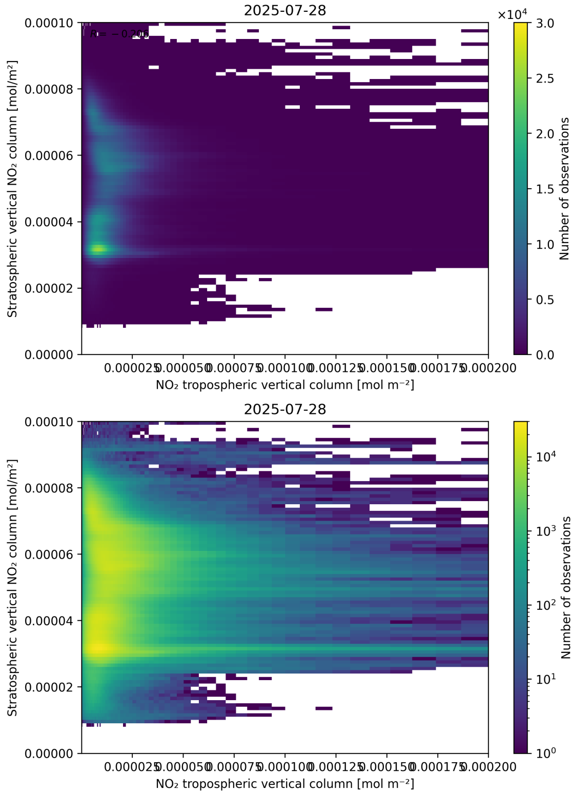
Figure 125: Scatter density plot of “NO 2 tropospheric vertical column” against “Stratospheric vertical NO 2 column” for 2025-07-27 to 2025-07-29.
