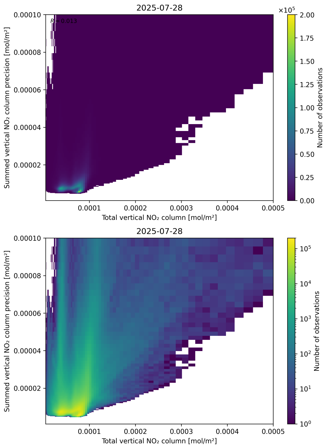
Figure 113: Scatter density plot of “Total vertical NO 2 column” against “Summed vertical NO 2 column precision” for 2025-07-27 to 2025-07-29.
