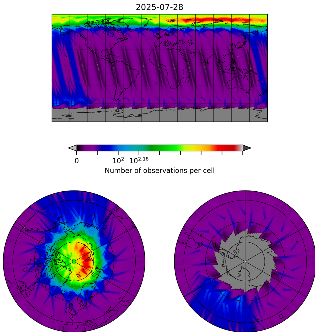
Figure 10: Map of the number of observations for 2025-07-27 to 2025-07-29
