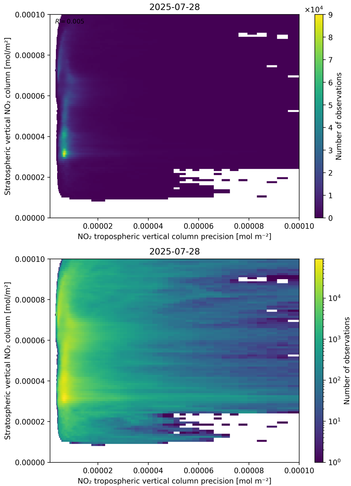
Figure 135: Scatter density plot of “NO 2 tropospheric vertical column precision” against “Stratospheric vertical NO 2 column” for 2025-07-27 to 2025-07-29.
