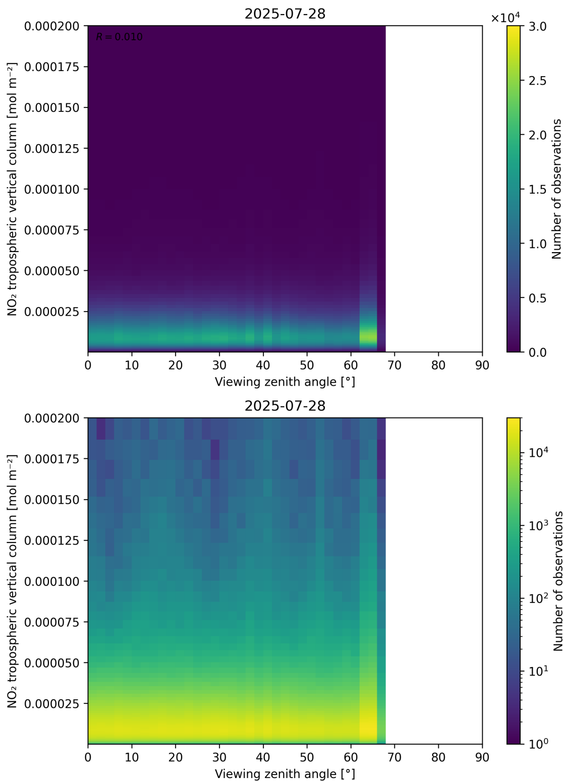
Figure 169: Scatter density plot of “Viewing zenith angle” against “NO 2 tropospheric vertical column” for 2025-07-27 to 2025-07-29.
