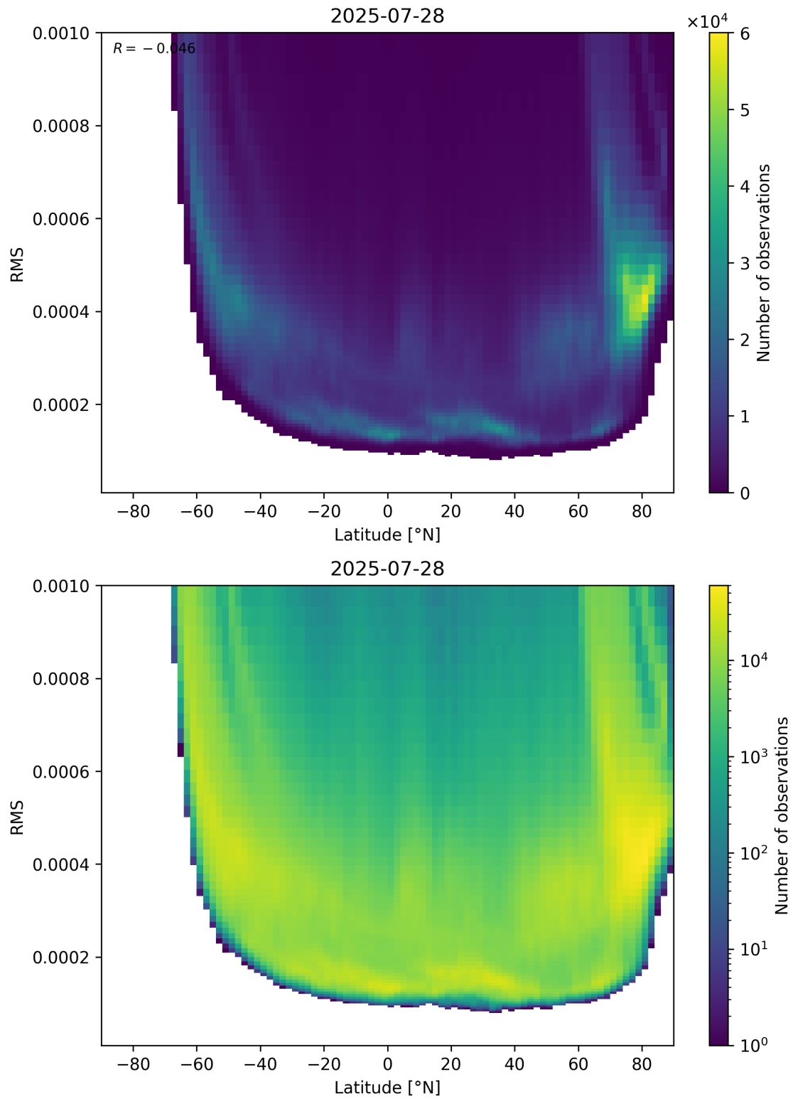
Figure 94: Scatter density plot of “Latitude” against “RMS” for 2025-07-27 to 2025-07-29.
