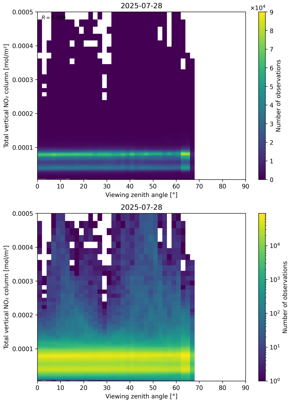
Figure 167: Scatter density plot of “Viewing zenith angle” against “Total vertical NO 2 column” for 2025-07-27 to 2025-07-29.
