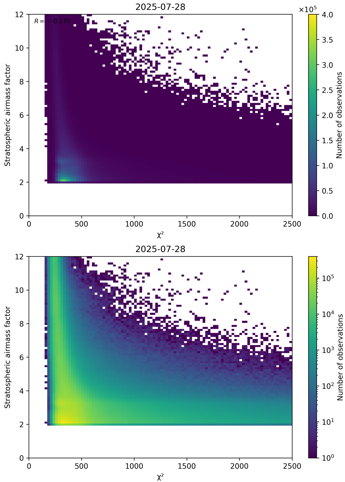
Figure 81: Scatter density plot of " \chi^2 " against "Stratospheric airmass factor" for 2025-07-27 to 2025-07-29.
