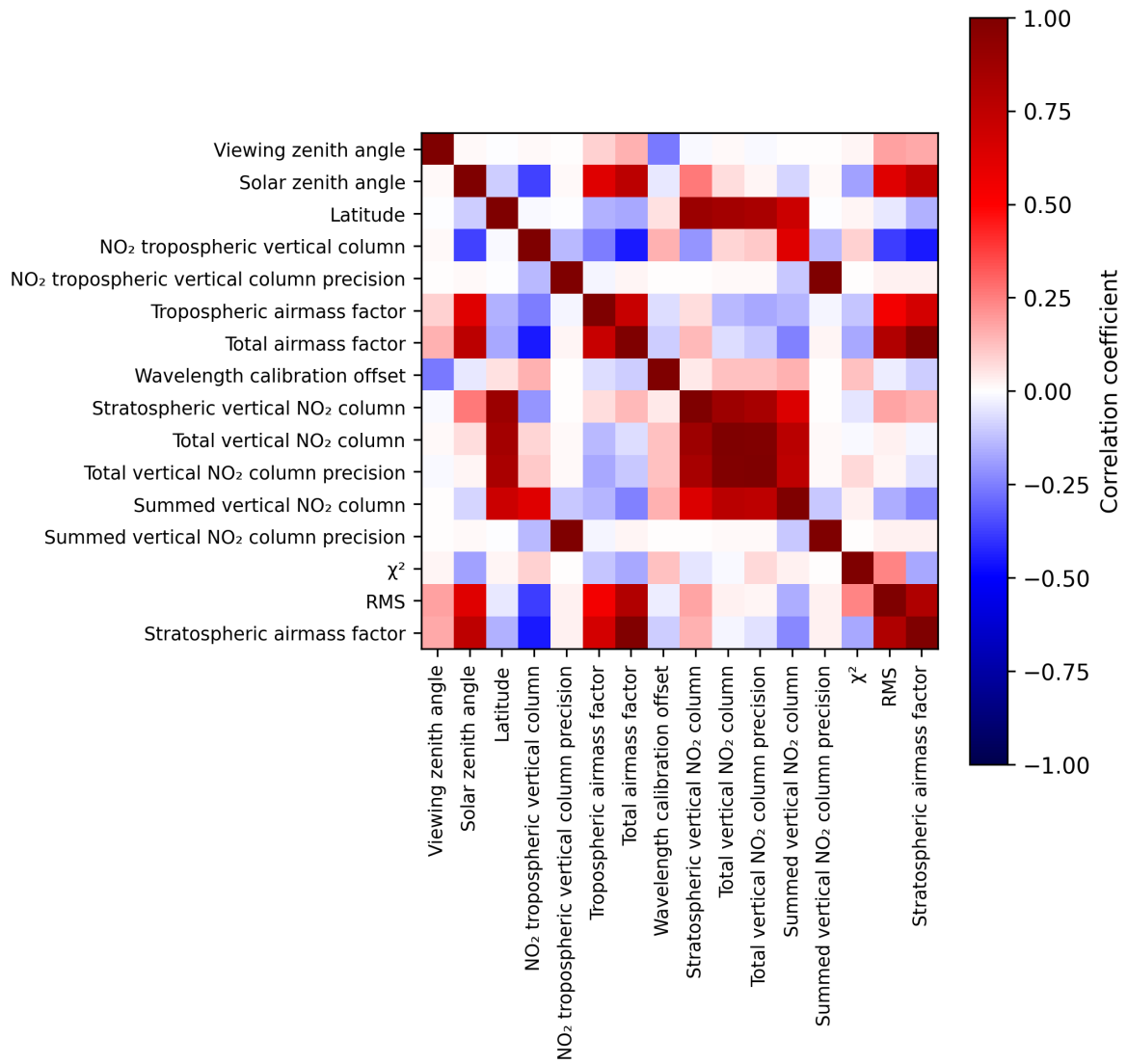
Figure 2: Map of correlation matrix for 2025-07-27 to 2025-07-29.
