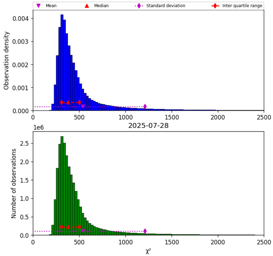
Figure 42: Histogram of “ \chi^2 ” for 2025-07-27 to 2025-07-29
