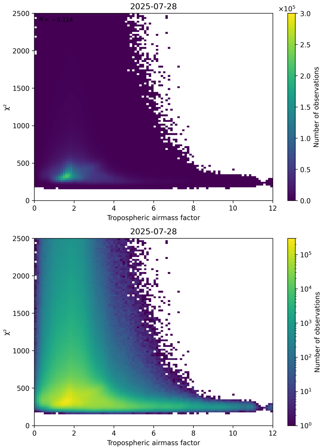
Figure 73: Scatter density plot of “Tropospheric airmass factor” against “ \chi^2 ” for 2025-07-27 to 2025-07-29.
