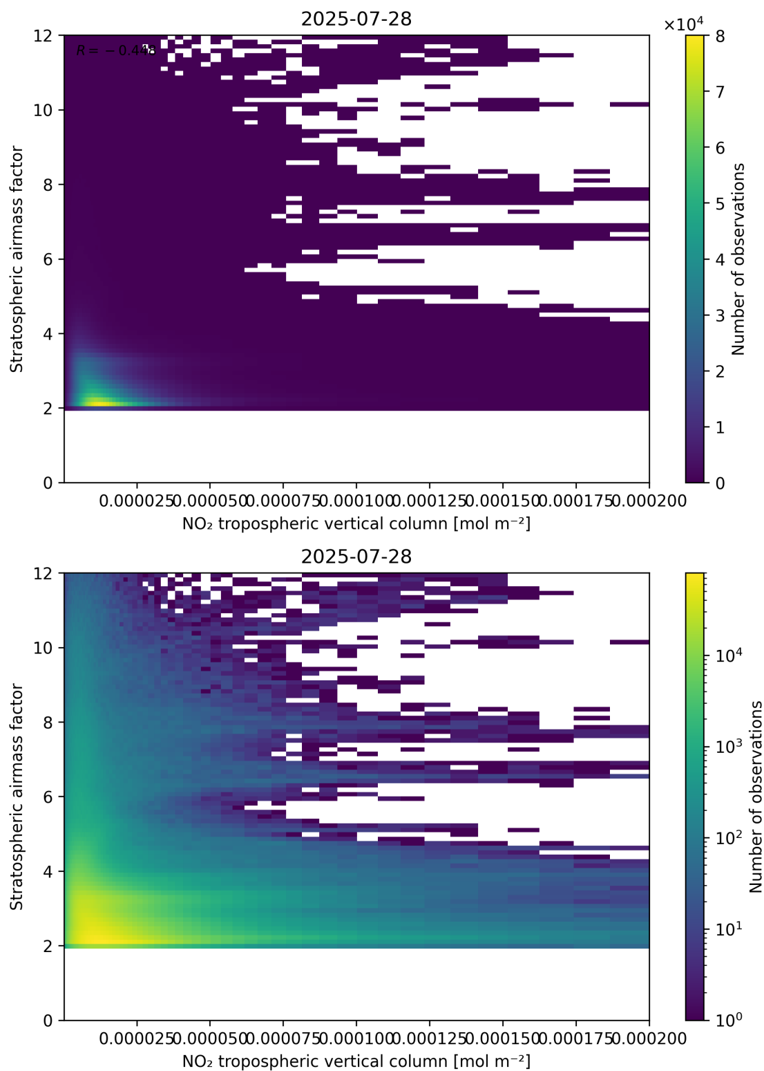
Figure 121: Scatter density plot of “NO 2 tropospheric vertical column” against “Stratospheric air mass factor” for 2025-07-27 to 2025-07-29.
