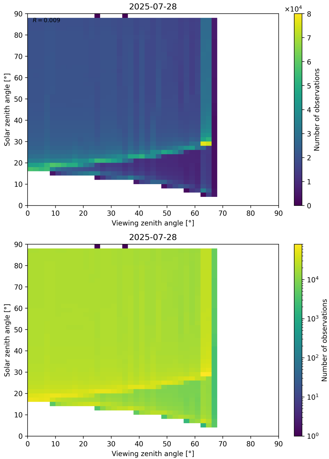
Figure 172: Scatter density plot of “Viewing zenith angle” against “Solar zenith angle” for 2025-07-27 to 2025-07-29.
