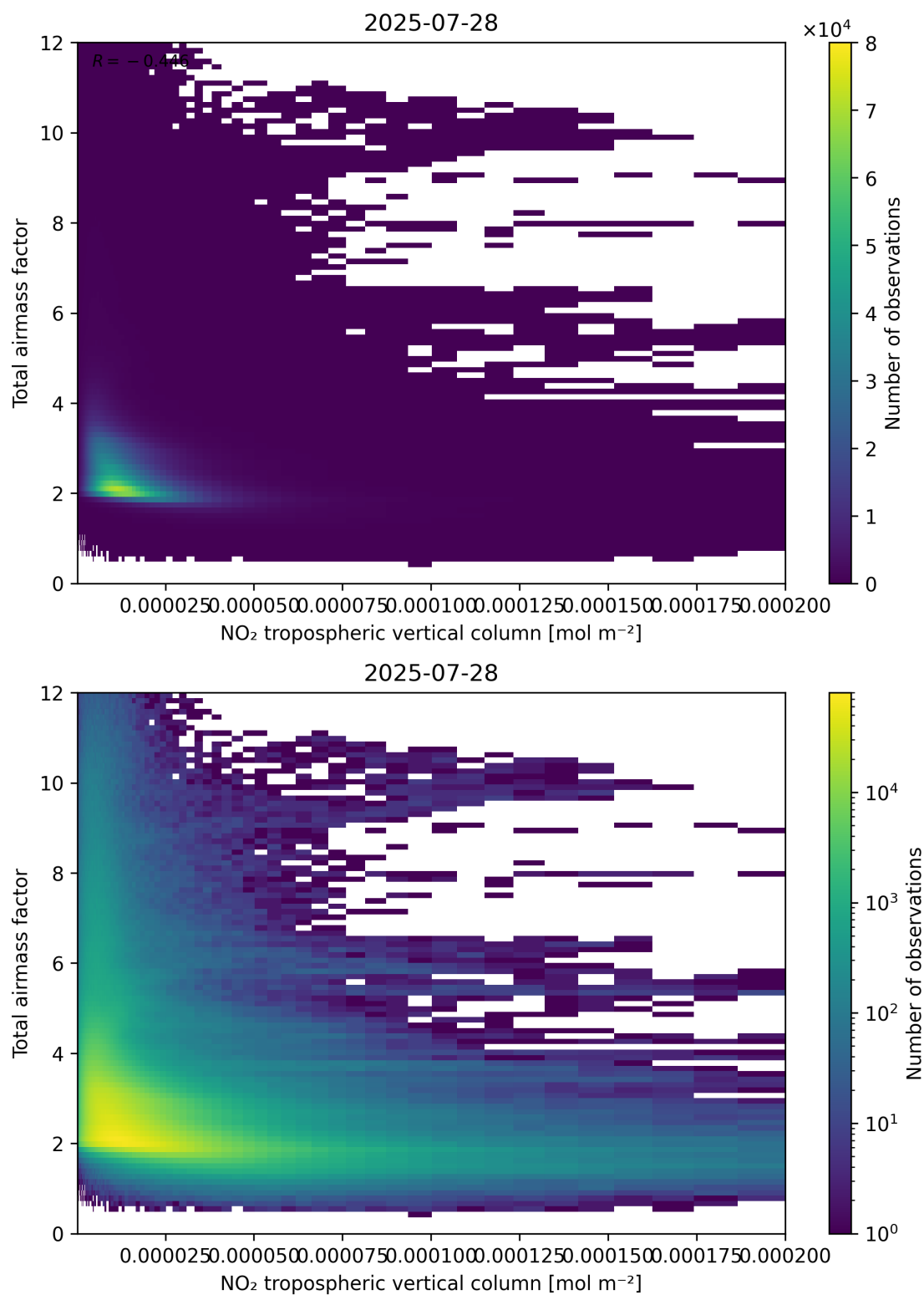
Figure 122: Scatter density plot of “NO 2 tropospheric vertical column” against “Total air mass factor” for 2025-07-27 to 2025-07-29.
