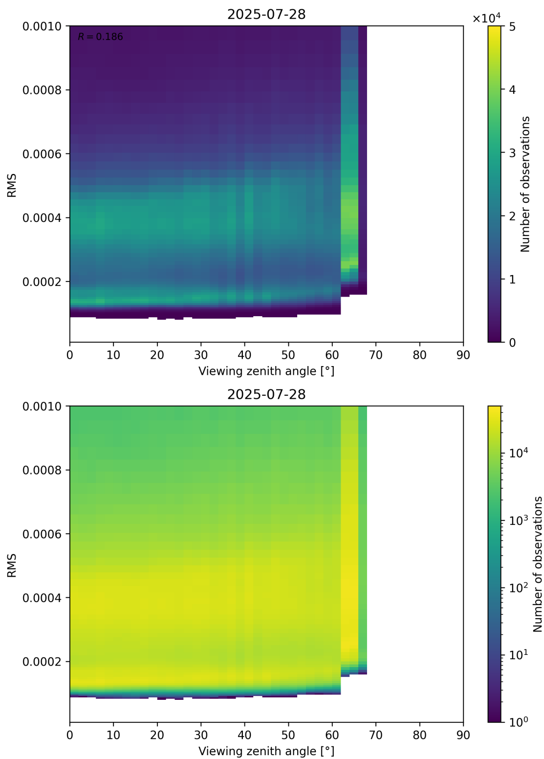
Figure 171: Scatter density plot of “Viewing zenith angle” against “RMS” for 2025-07-27 to 2025-07-29.
