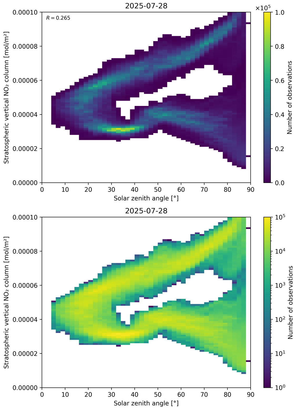
Figure 150: Scatter density plot of “Solar zenith angle” against “Stratospheric vertical NO 2 column” for 2025-07-27 to 2025-07-29.
