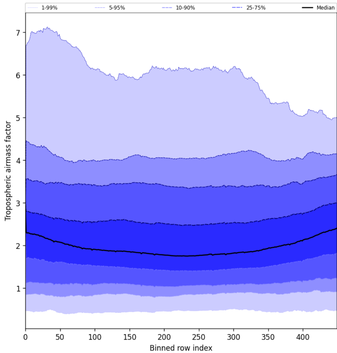
Figure 48: Along track statistics of “Tropospheric air mass factor” for 2025-07-27 to 2025-07-29
