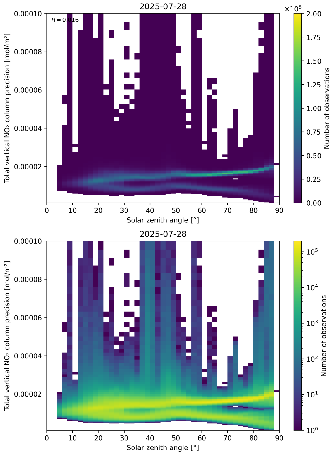
Figure 154: Scatter density plot of “Solar zenith angle” against “Total vertical NO 2 column precision” for 2025-07-27 to 2025-07-29.
