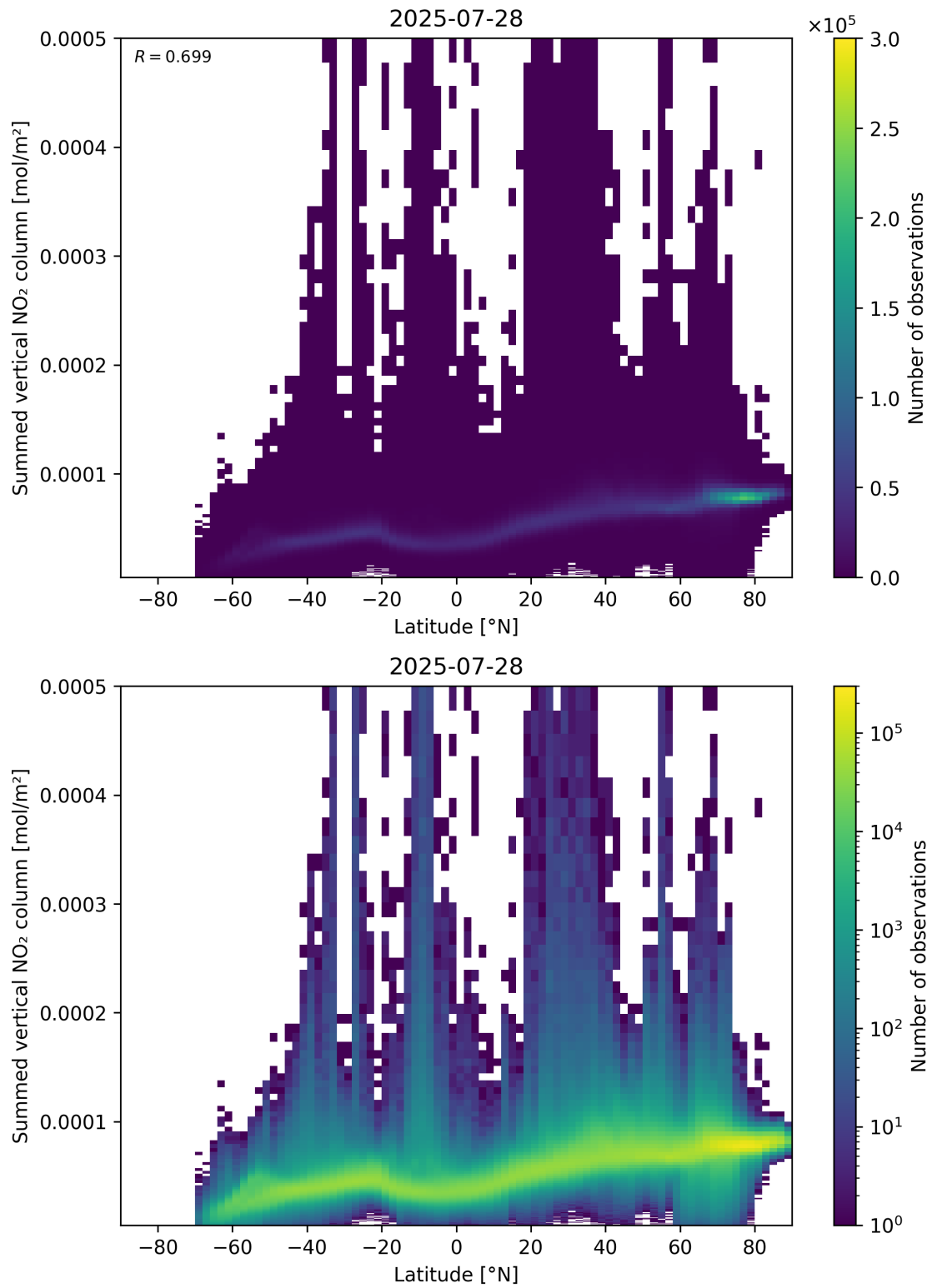
Figure 88: Scatter density plot of “Latitude” against “Summed vertical NO 2 column” for 2025-07-27 to 2025-07-29.
