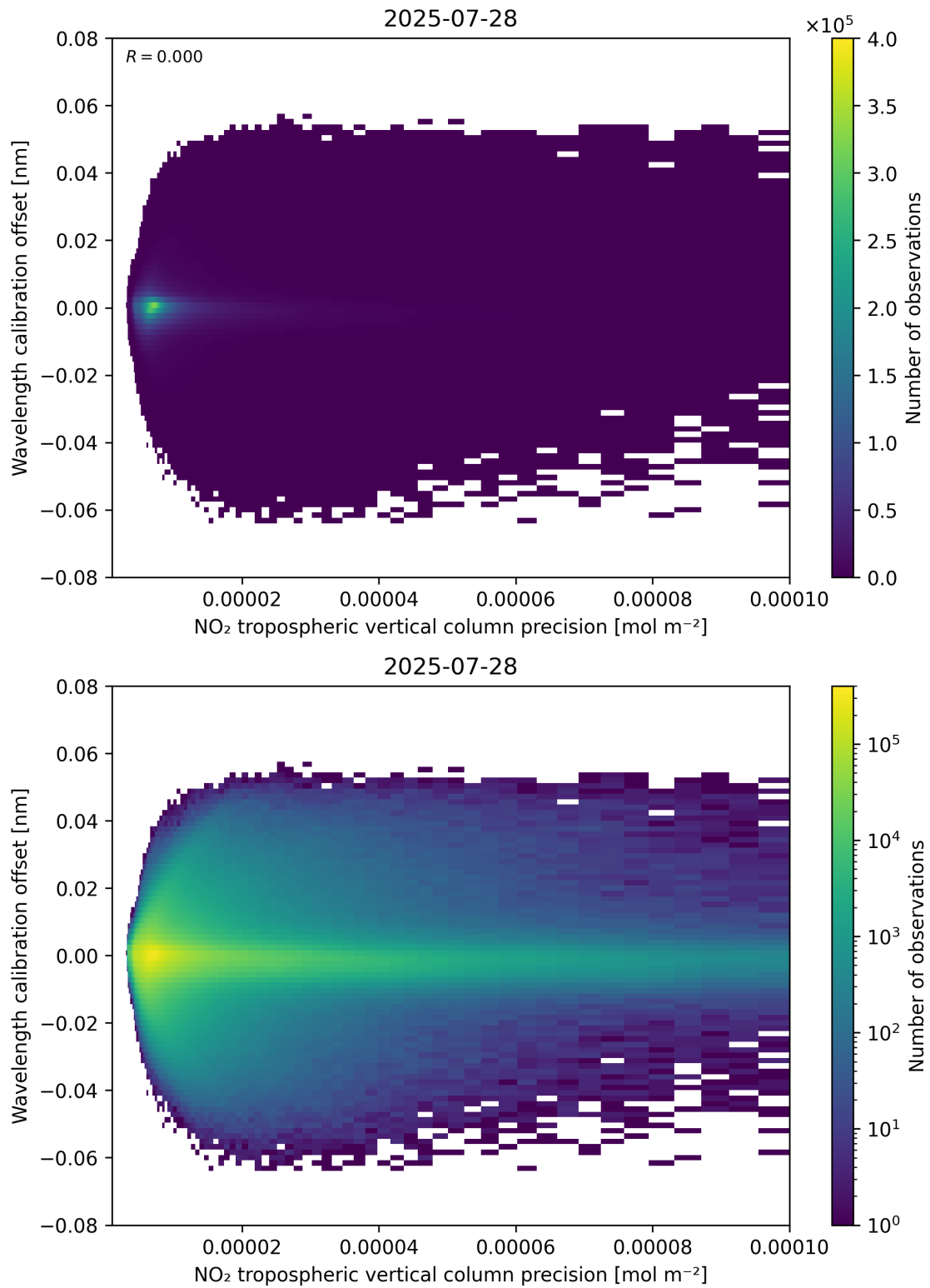
Figure 141: Scatter density plot of “NO 2 tropospheric vertical column precision” against “Wavelength calibration offset” for 2025-07-27 to 2025-07-29.
