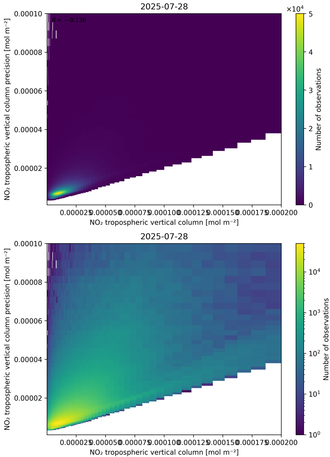
Figure 130: Scatter density plot of “NO 2 tropospheric vertical column” against “NO 2 tropospheric vertical column precision” for 2025-07-27 to 2025-07-29.
