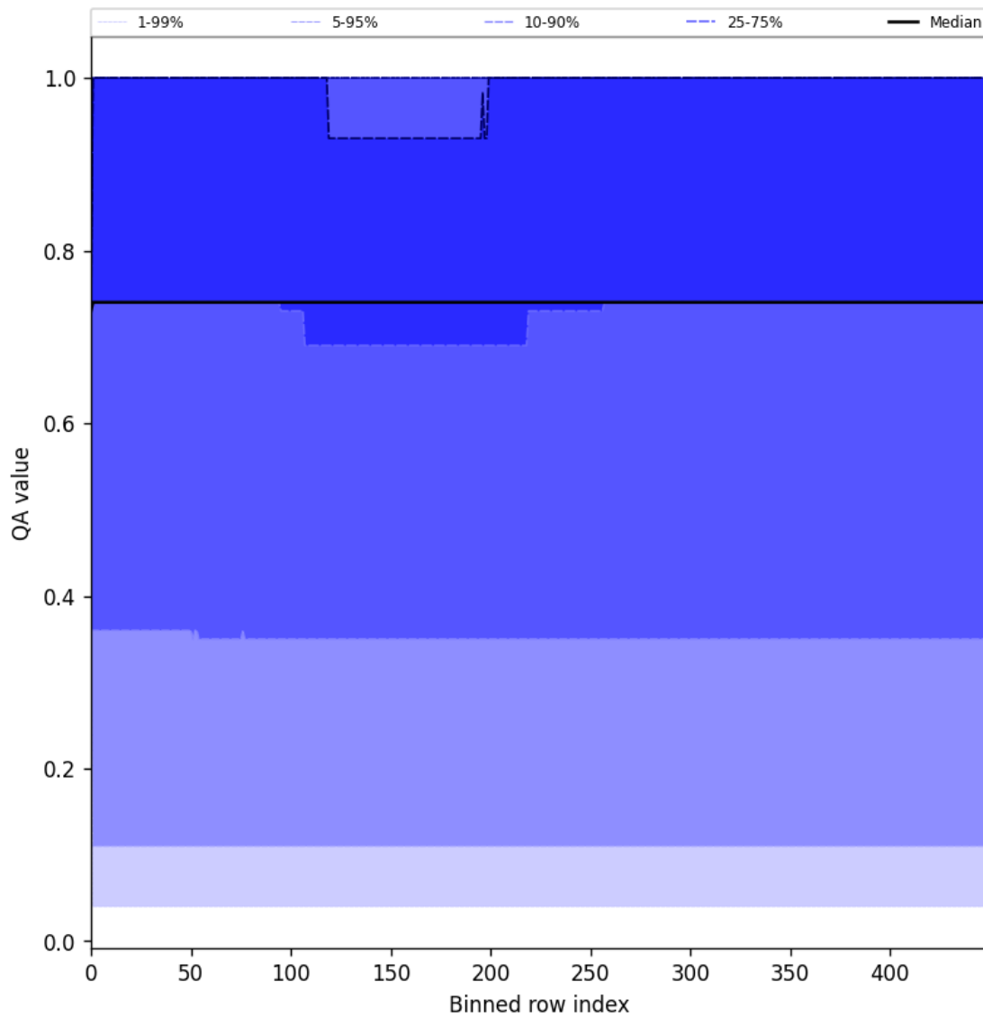
Figure 45: Along track statistics of “QA value” for 2025-07-27 to 2025-07-29
