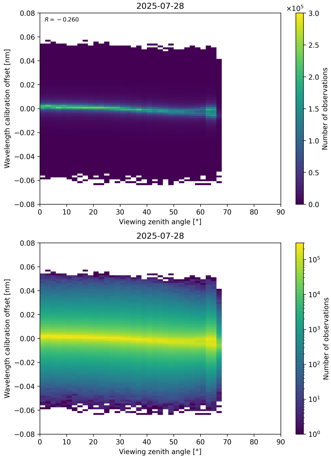
Figure 173: Scatter density plot of “Viewing zenith angle” against “Wavelength calibration offset” for 2025-07-27 to 2025-07-29.
