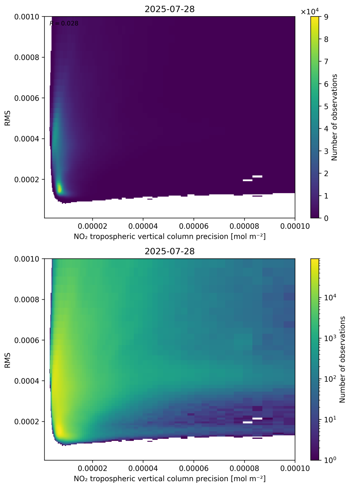
Figure 140: Scatter density plot of “NO 2 tropospheric vertical column precision” against “RMS” for 2025-07-27 to 2025-07-29.
