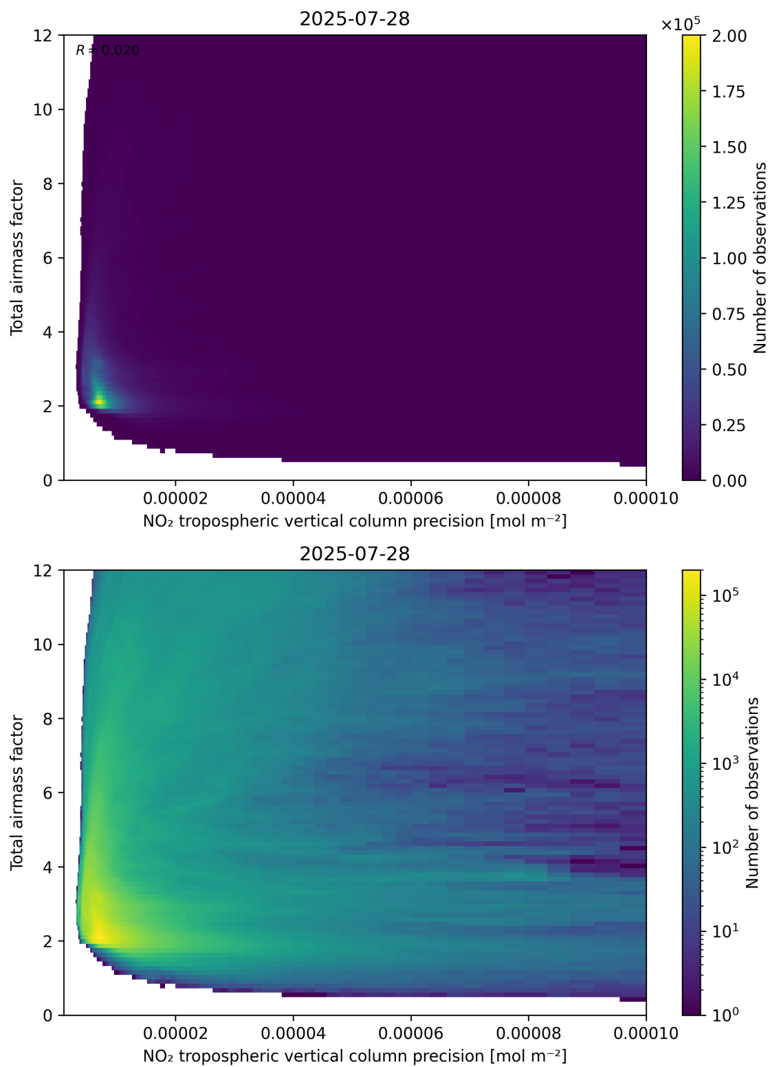
Figure 132: Scatter density plot of “NO 2 tropospheric vertical column precision” against “Total air mass factor” for 2025-07-27 to 2025-07-29.
