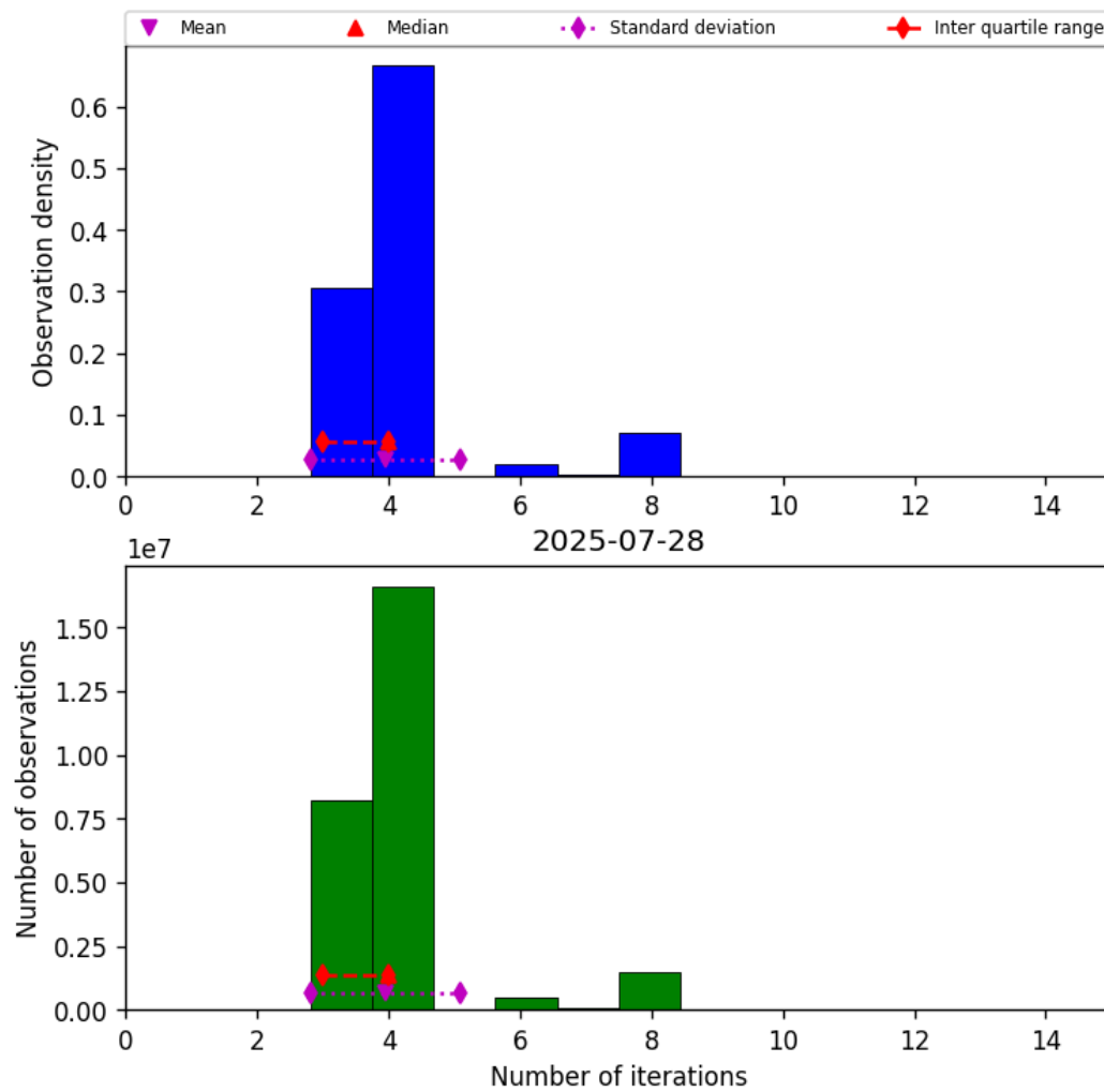
Figure 34: Histogram of “Number of iterations” for 2025-07-27 to 2025-07-29
