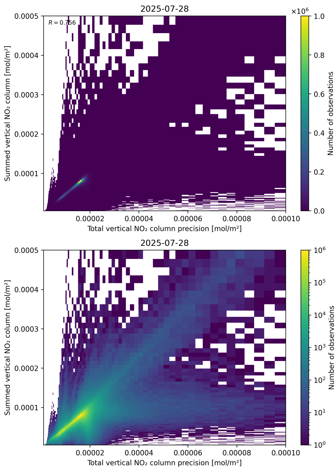
Figure 117: Scatter density plot of “Total vertical NO 2 column precision” against “Summed vertical NO 2 column” for 2025-07-27 to 2025-07-29.
