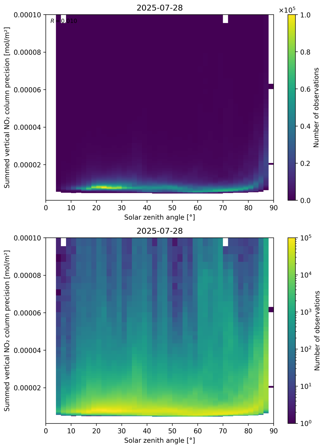
Figure 152: Scatter density plot of “Solar zenith angle” against “Summed vertical NO 2 column precision” for 2025-07-27 to 2025-07-29.
