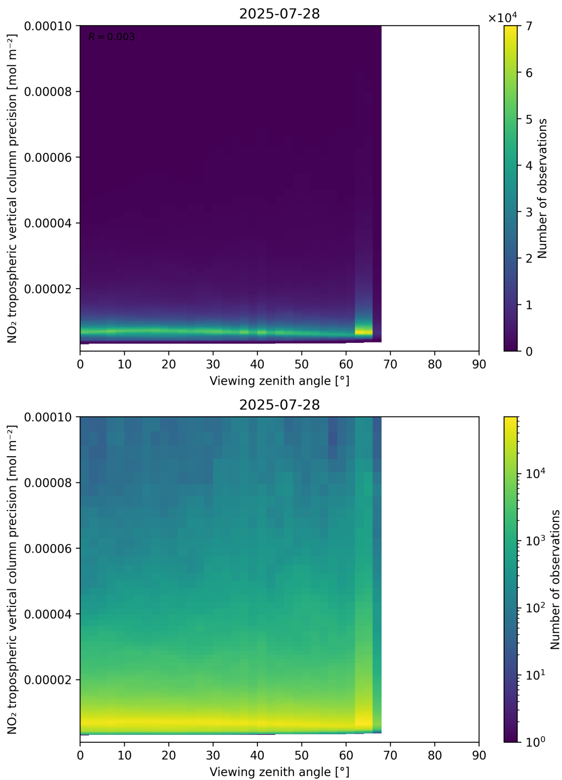
Figure 170: Scatter density plot of “Viewing zenith angle” against “NO 2 tropospheric vertical column precision” for 2025-07-27 to 2025-07-29.
