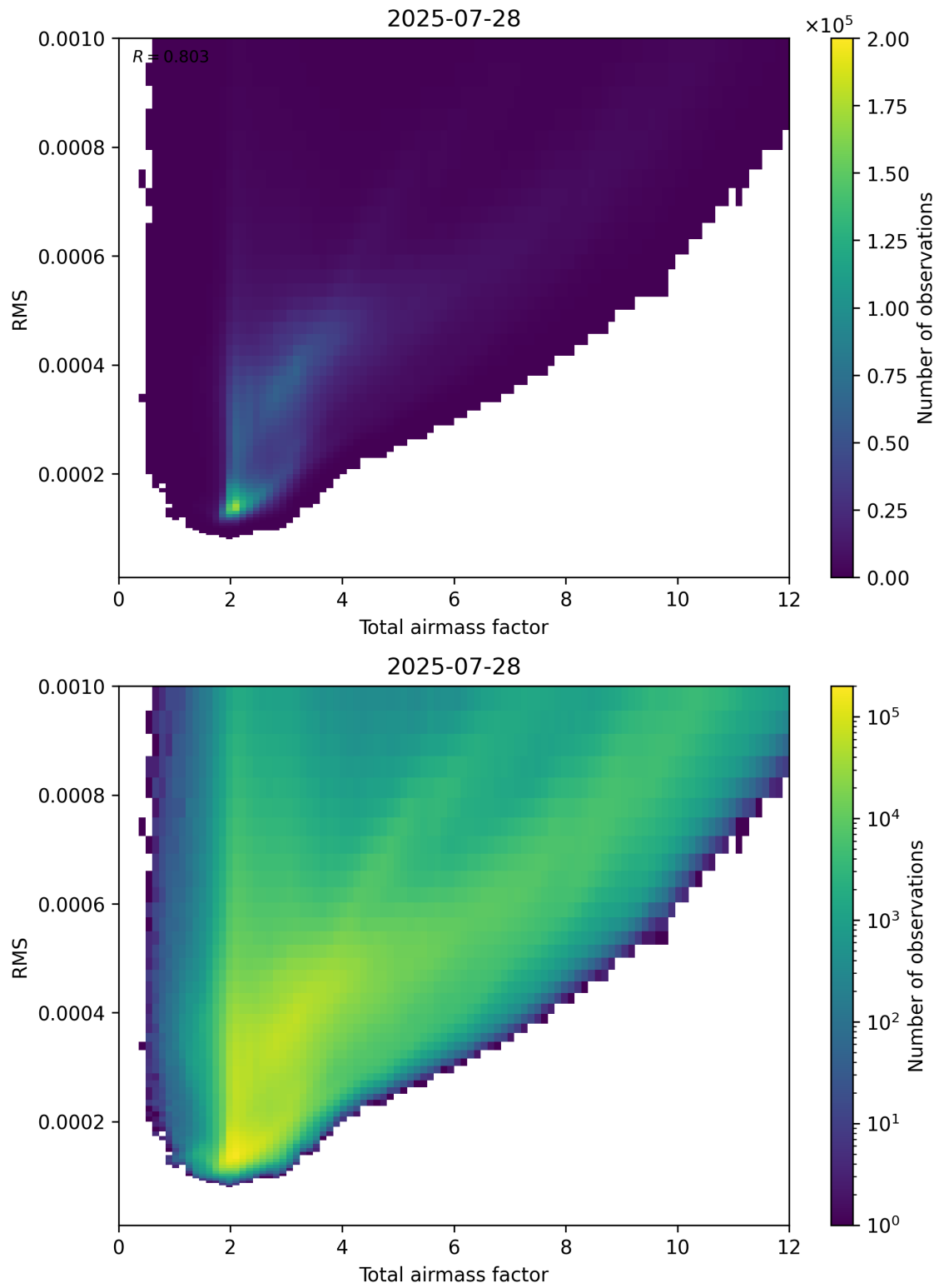
Figure 69: Scatter density plot of “Total airmass factor” against “RMS” for 2025-07-27 to 2025-07-29.
