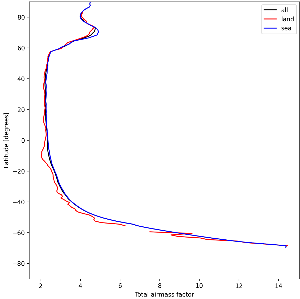
Figure 15: Zonal average of “Total airmass factor” for 2025-07-27 to 2025-07-29.
