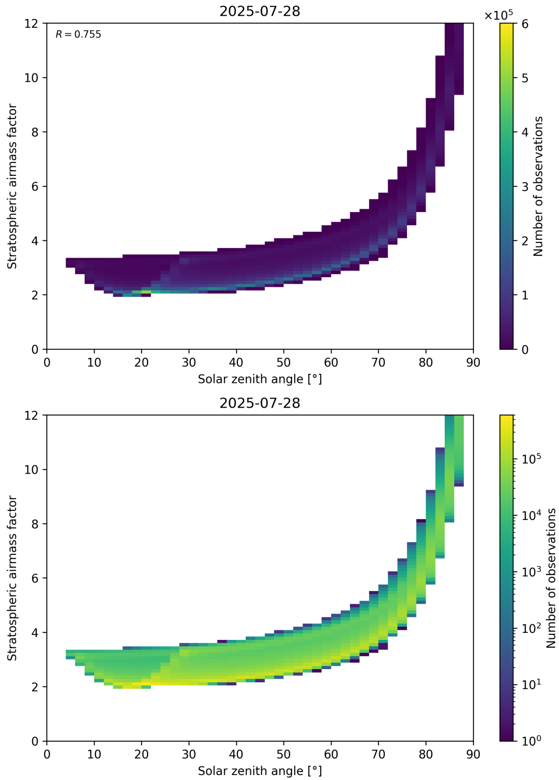
Figure 145: Scatter density plot of “Solar zenith angle” against “Stratospheric airmass factor” for 2025-07-27 to 2025-07-29.
