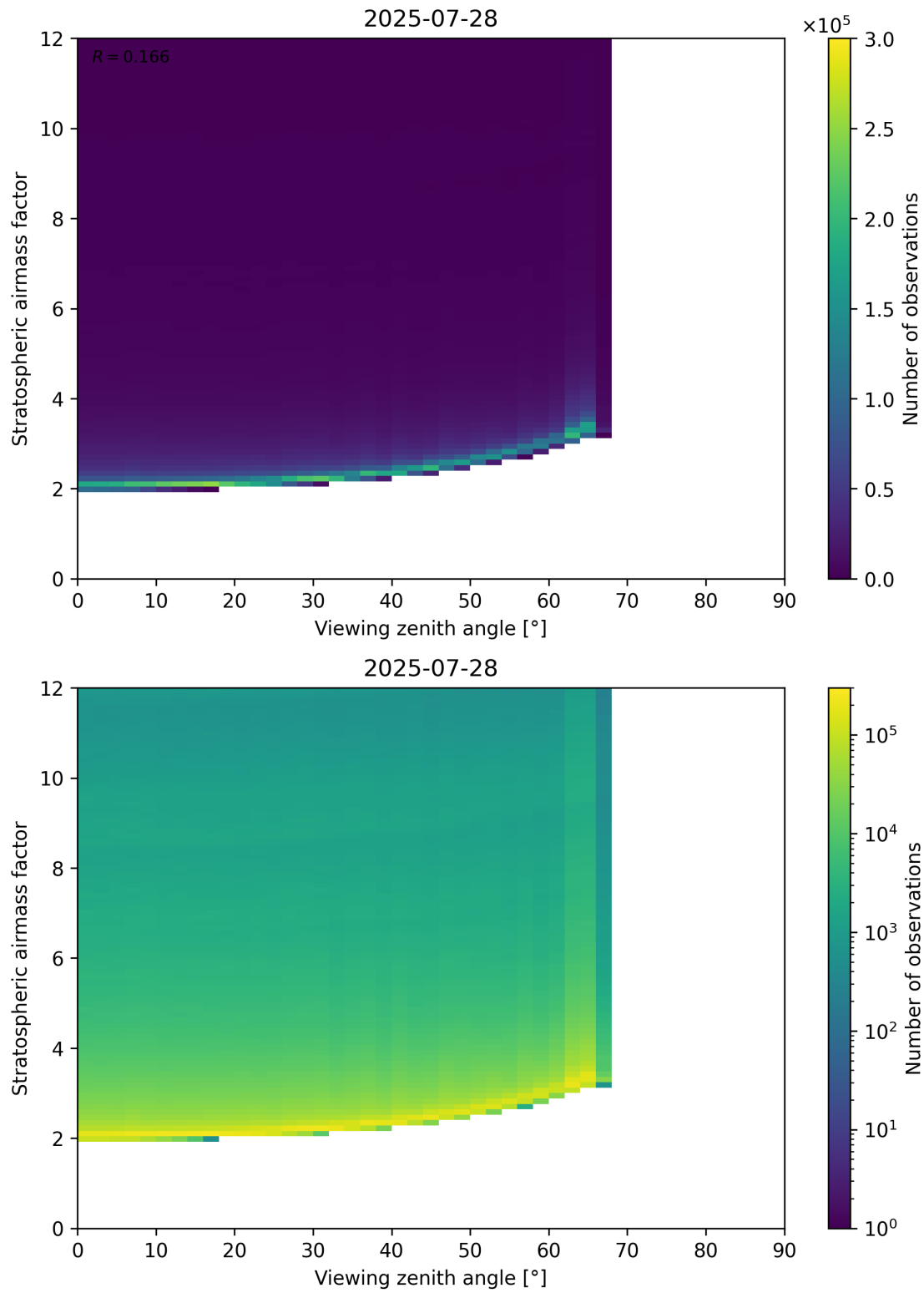
Figure 159: Scatter density plot of “Viewing zenith angle” against “Stratospheric airmass factor” for 2025-07-27 to 2025-07-29.
