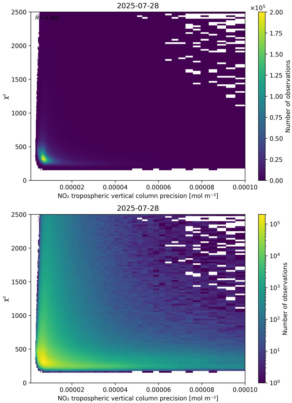
Figure 134: Scatter density plot of “NO 2 tropospheric vertical column precision” against “ \chi^2 ” for 2025-07-27 to 2025-07-29.
