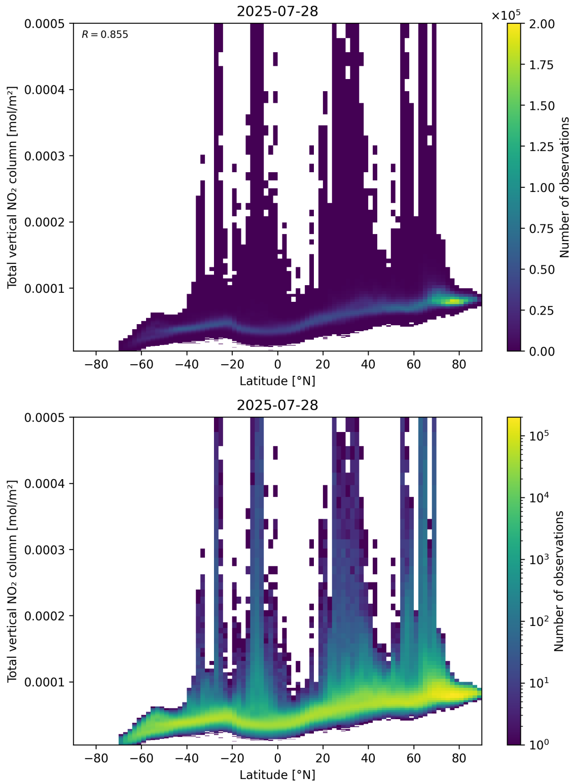
Figure 90: Scatter density plot of “Latitude” against “Total vertical NO 2 column” for 2025-07-27 to 2025-07-29.
