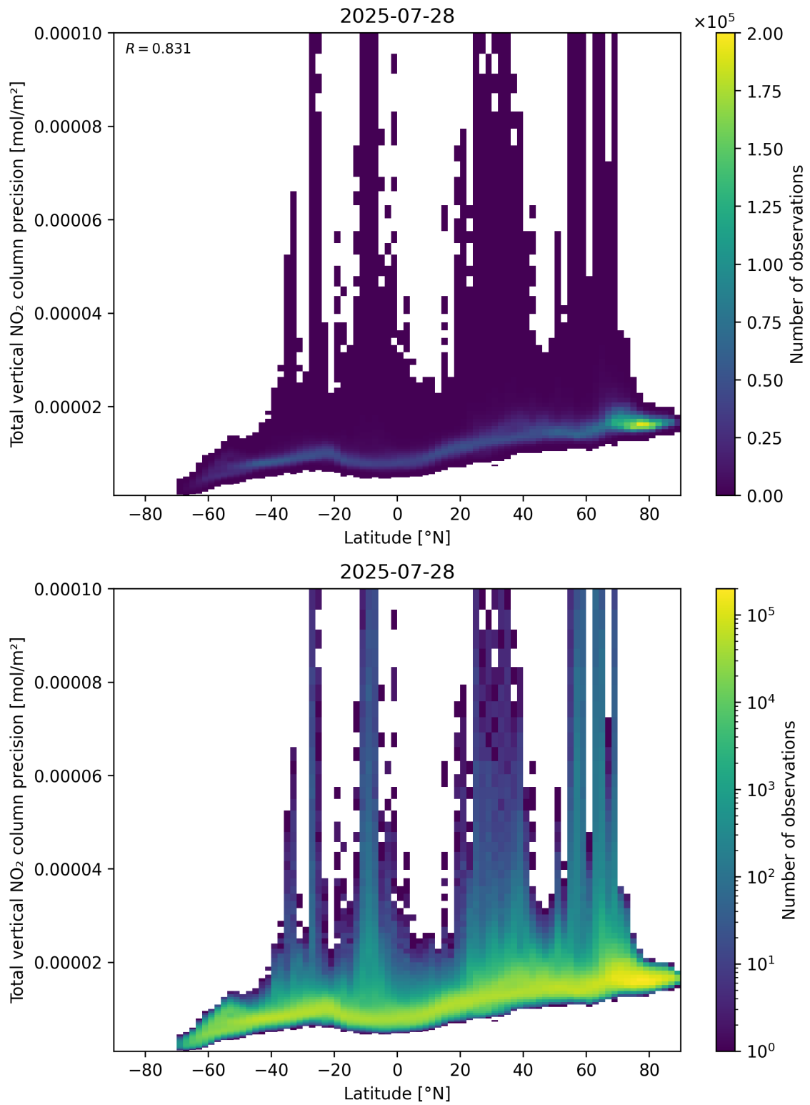
Figure 91: Scatter density plot of “Latitude” against “Total vertical NO 2 column precision” for 2025-07-27 to 2025-07-29.
