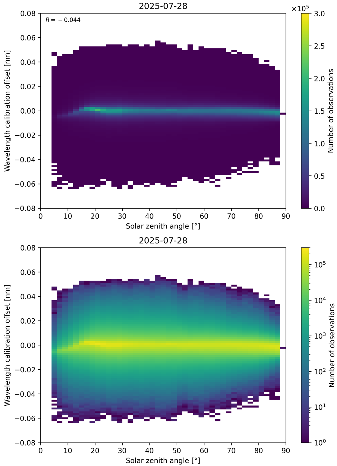
Figure 158: Scatter density plot of “Solar zenith angle” against “Wavelength calibration offset” for 2025-07-27 to 2025-07-29.
