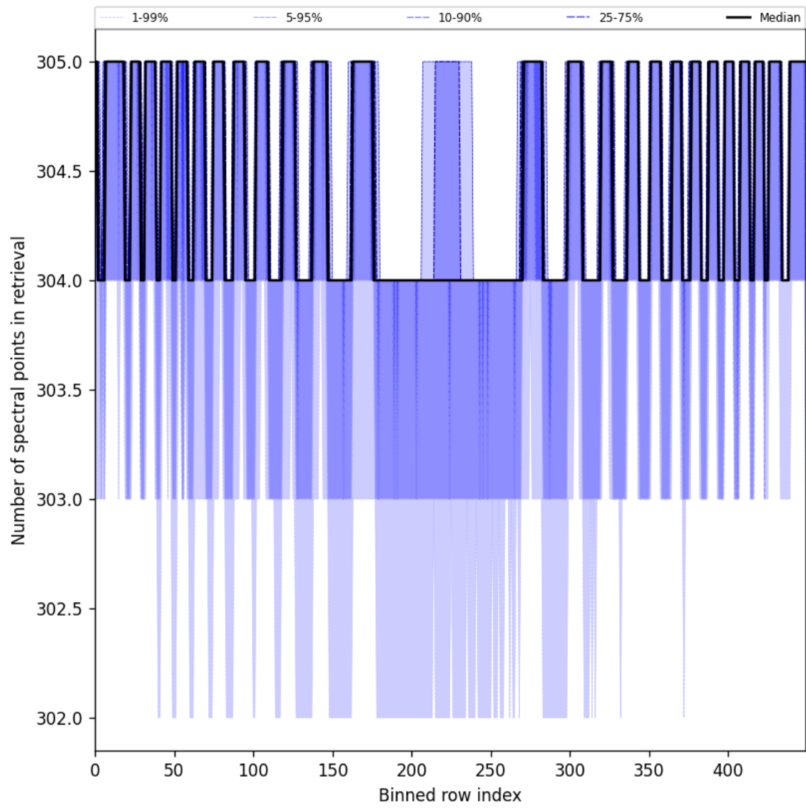
Figure 50: Along track statistics of “Number of spectral points in retrieval” for 2025-07-27 to 2025-07-29
