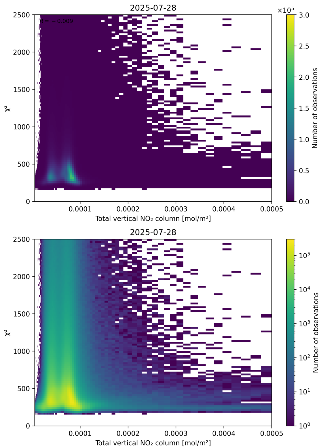
Figure 111: Scatter density plot of “Total vertical NO 2 column” against “ \chi^2 ” for 2025-07-27 to 2025-07-29.
