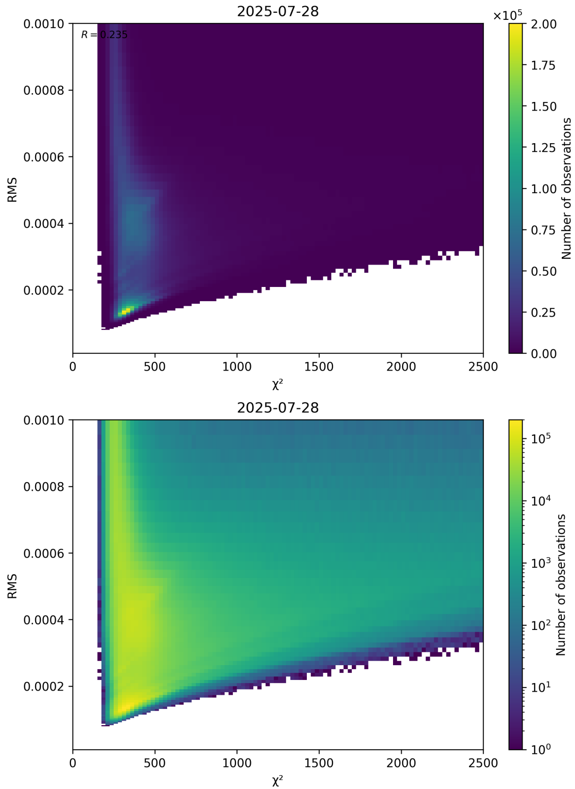
Figure 82: Scatter density plot of “ \chi^2 ” against “RMS” for 2025-07-27 to 2025-07-29.
