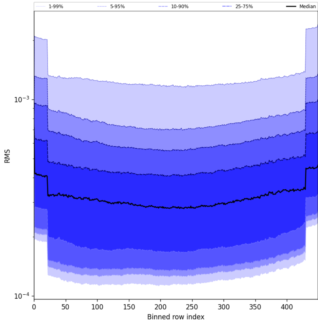
Figure 60: Along track statistics of “RMS” for 2025-07-27 to 2025-07-29
