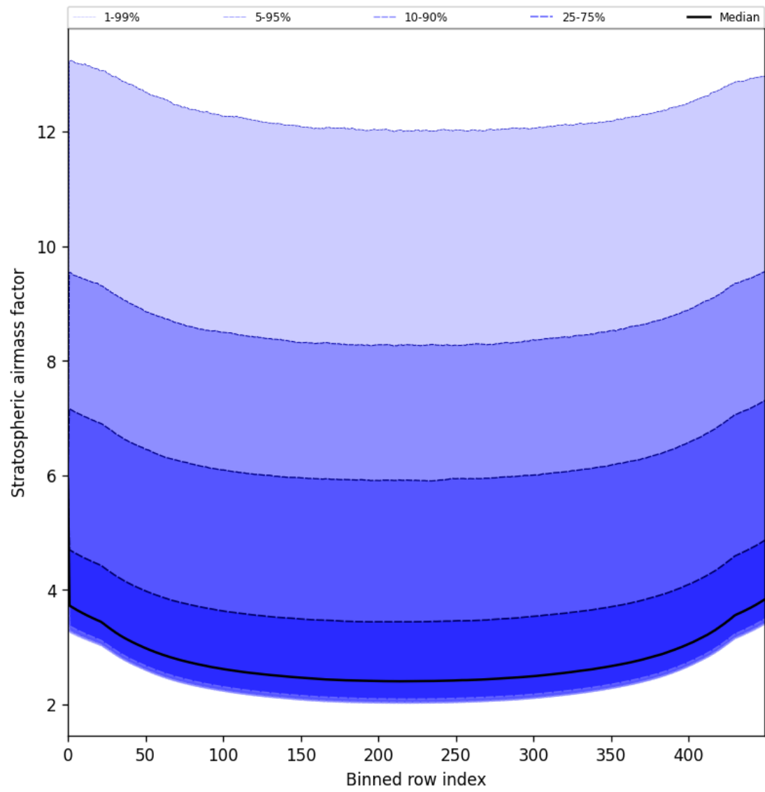
Figure 61: Along track statistics of “Stratospheric airmass factor” for 2025-07-27 to 2025-07-29
