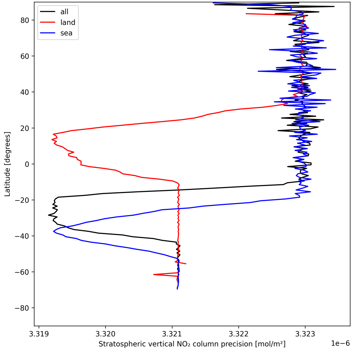
Figure 20: Zonal average of “Stratospheric vertical NO 2 column precision” for 2025-07-27 to 2025-07-29.
