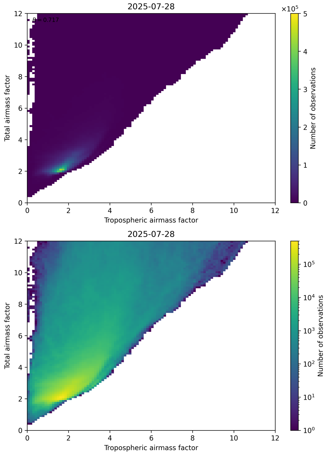
Figure 72: Scatter density plot of “Tropospheric airmass factor” against “Total airmass factor” for 2025-07-27 to 2025-07-29.
