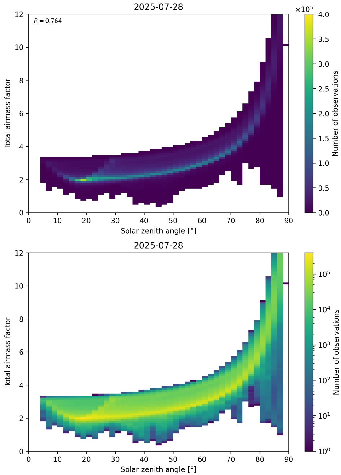
Figure 146: Scatter density plot of “Solar zenith angle” against “Total air mass factor” for 2025-07-27 to 2025-07-29.
