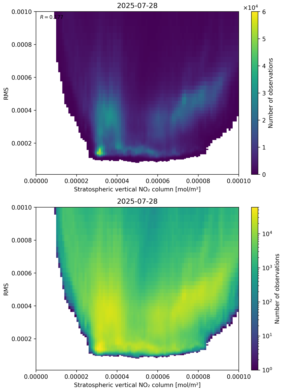
Figure 102: Scatter density plot of “Stratospheric vertical NO 2 column” against “RMS” for 2025-07-27 to 2025-07-29.
