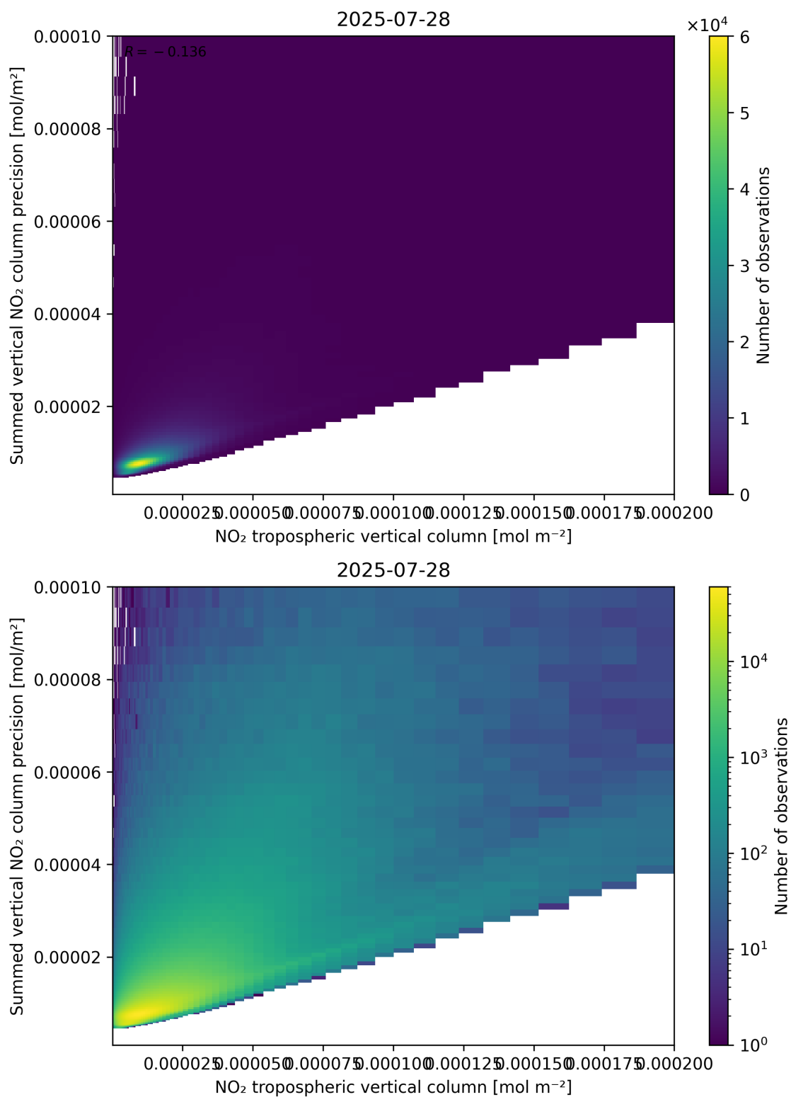
Figure 127: Scatter density plot of “NO 2 tropospheric vertical column” against “Summed vertical NO 2 column precision” for 2025-07-27 to 2025-07-29.
