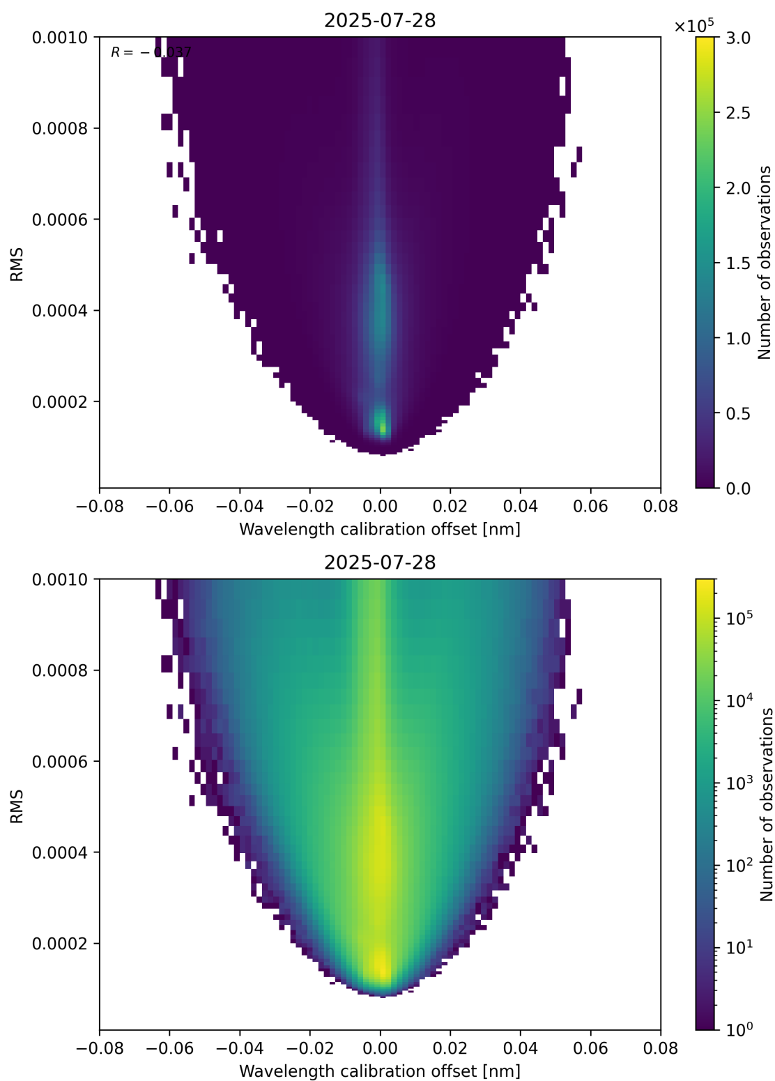
Figure 181: Scatter density plot of “Wavelength calibration offset” against “RMS” for 2025-07-27 to 2025-07-29.
