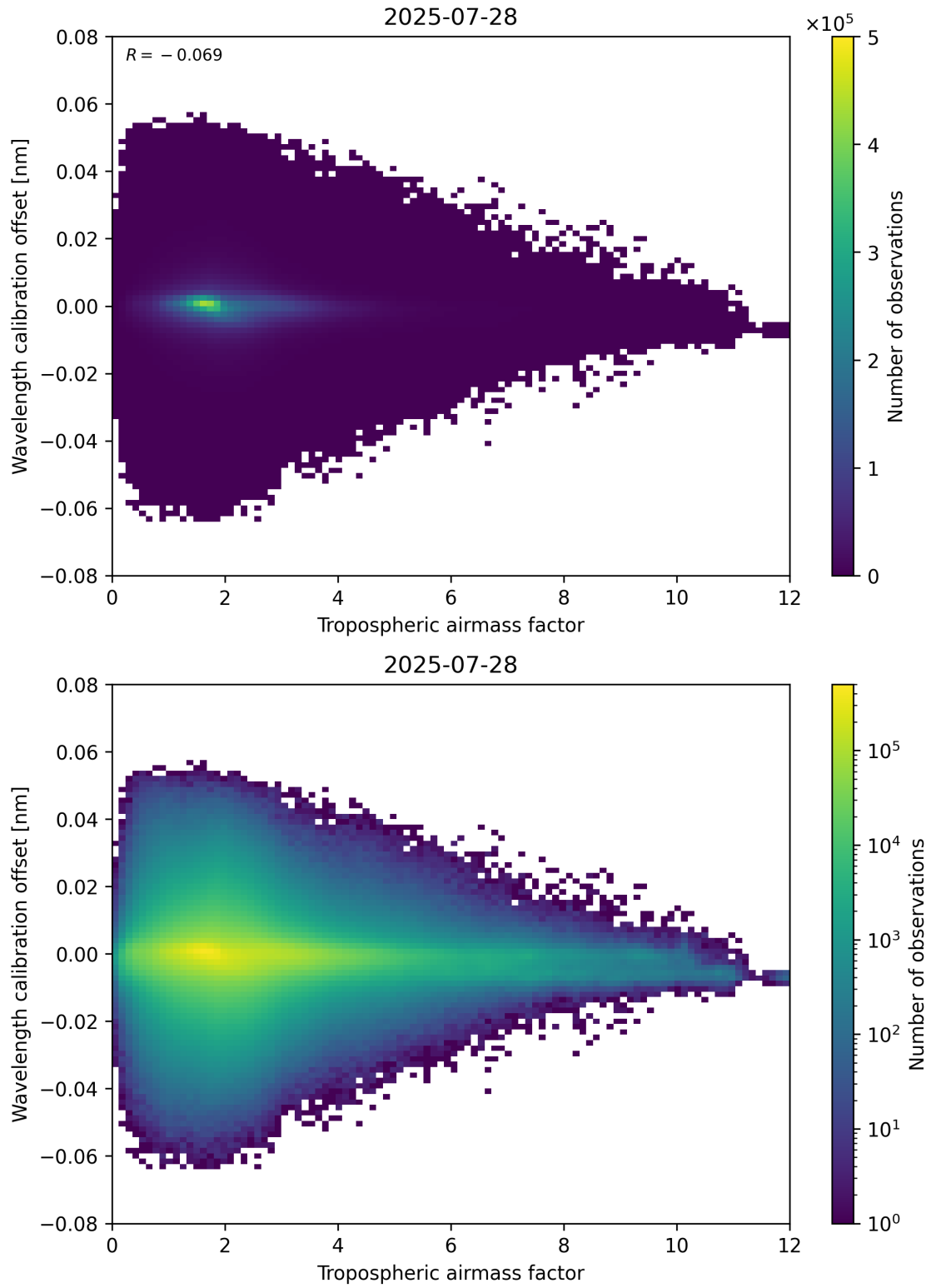
Figure 80: Scatter density plot of “Tropospheric air mass factor” against “Wavelength calibration offset” for 2025-07-27 to 2025-07-29.
