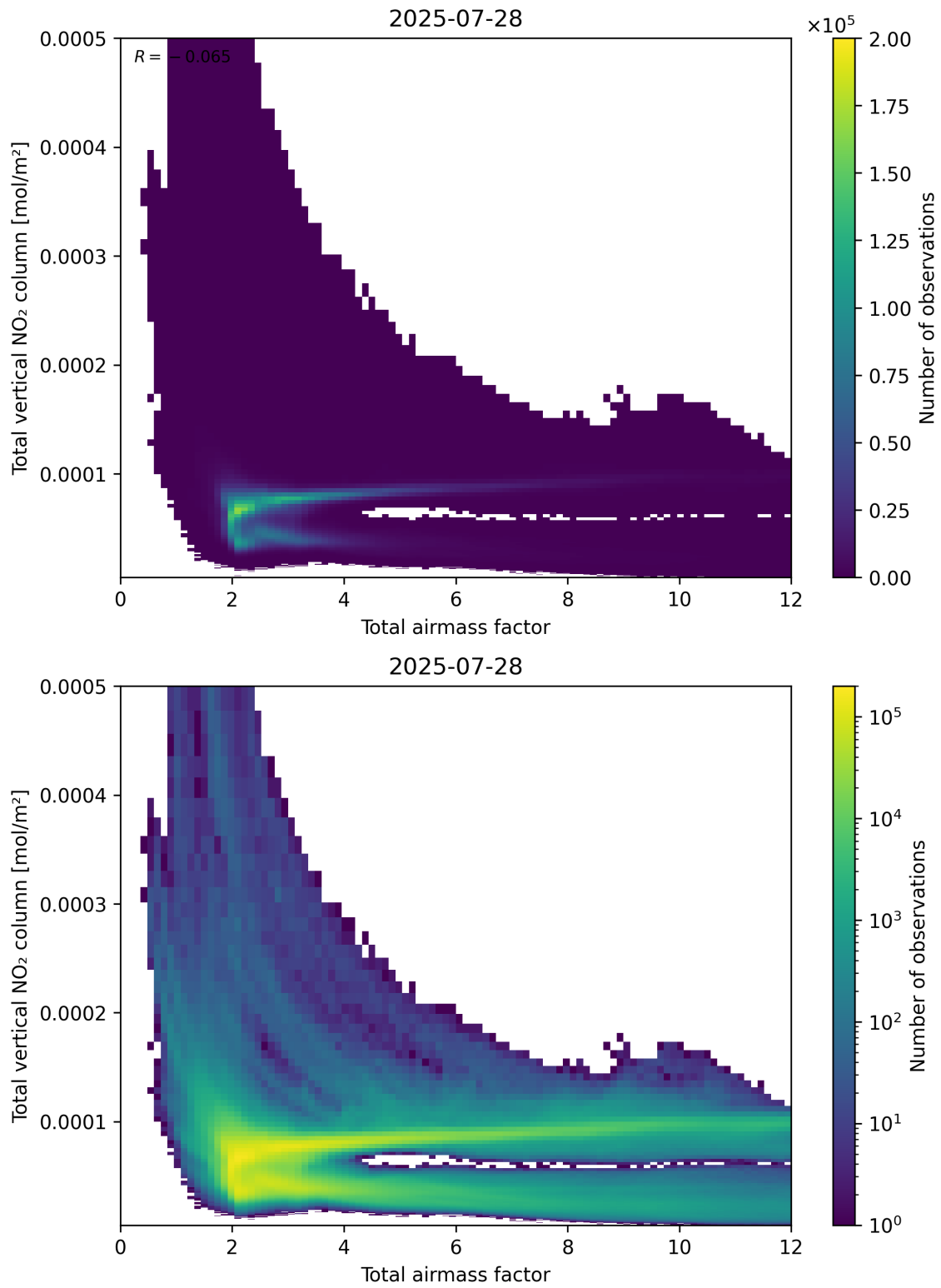
Figure 67: Scatter density plot of “Total airmass factor” against “Total vertical NO 2 column” for 2025-07-27 to 2025-07-29.
