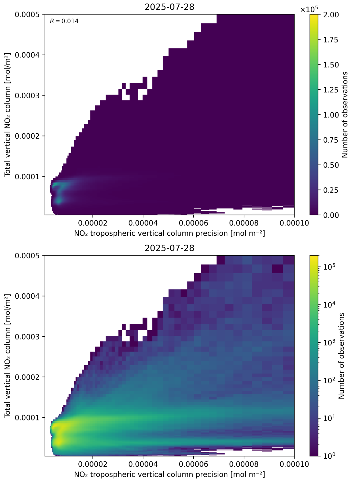
Figure 138: Scatter density plot of “NO 2 tropospheric vertical column precision” against “Total vertical NO 2 column” for 2025-07-27 to 2025-07-29.
