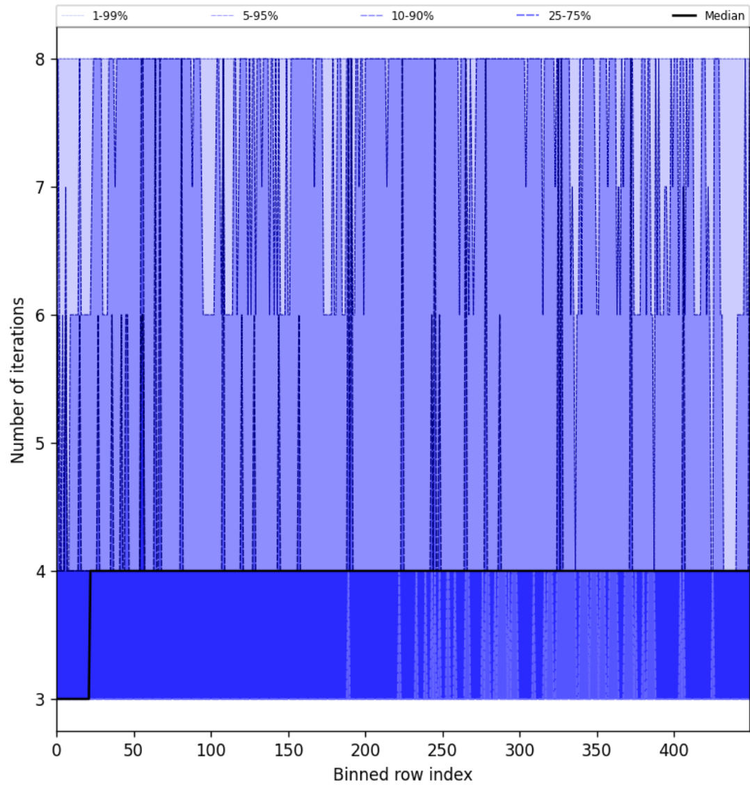
Figure 51: Along track statistics of “Number of iterations” for 2025-07-27 to 2025-07-29
