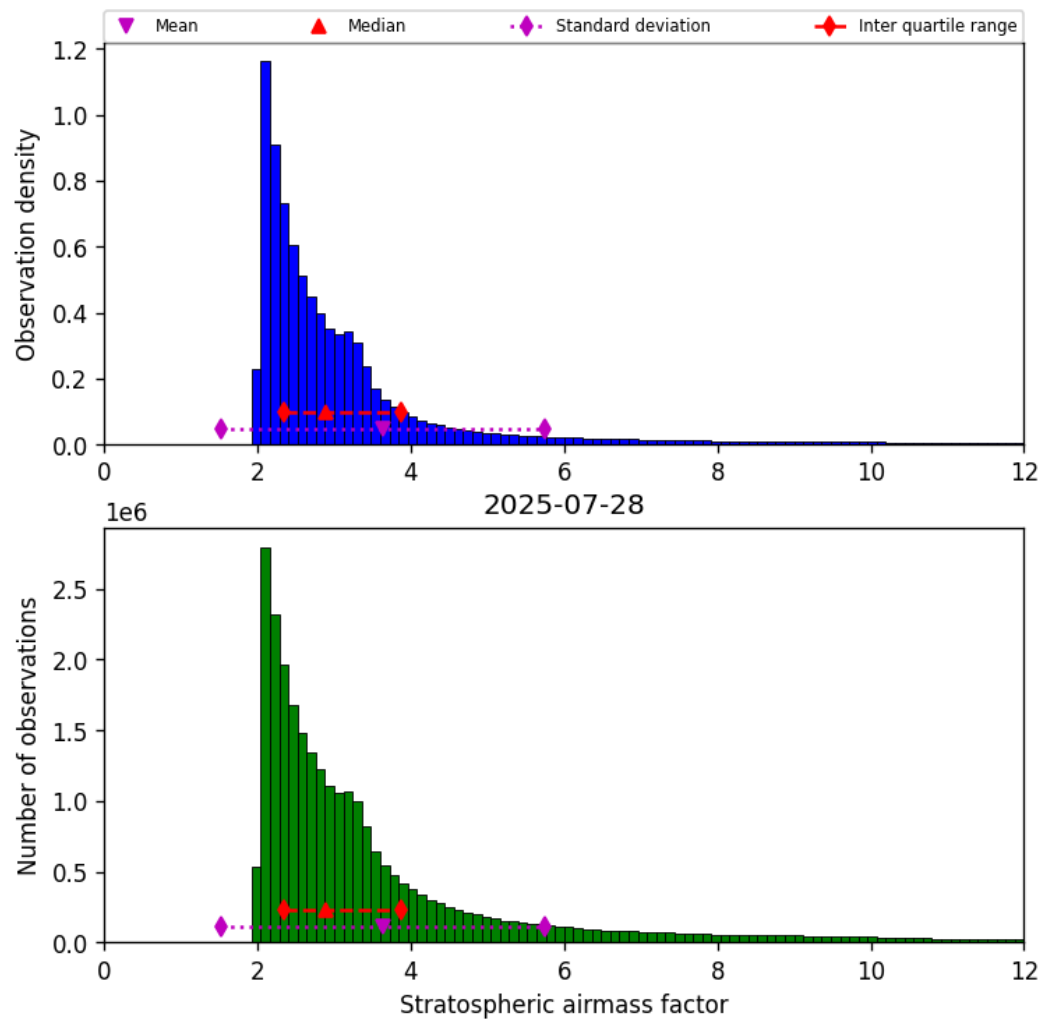
Figure 44: Histogram of “Stratospheric airmass factor” for 2025-07-27 to 2025-07-29
