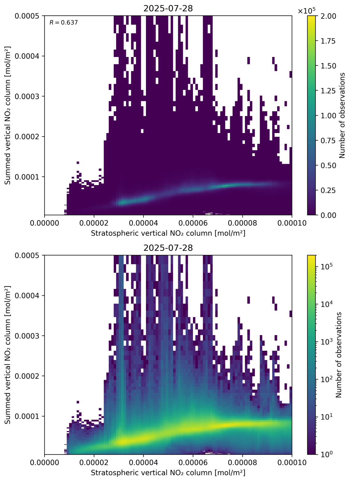
Figure 98: Scatter density plot of “Stratospheric vertical NO 2 column” against “Summed vertical NO 2 column” for 2025-07-27 to 2025-07-29.
