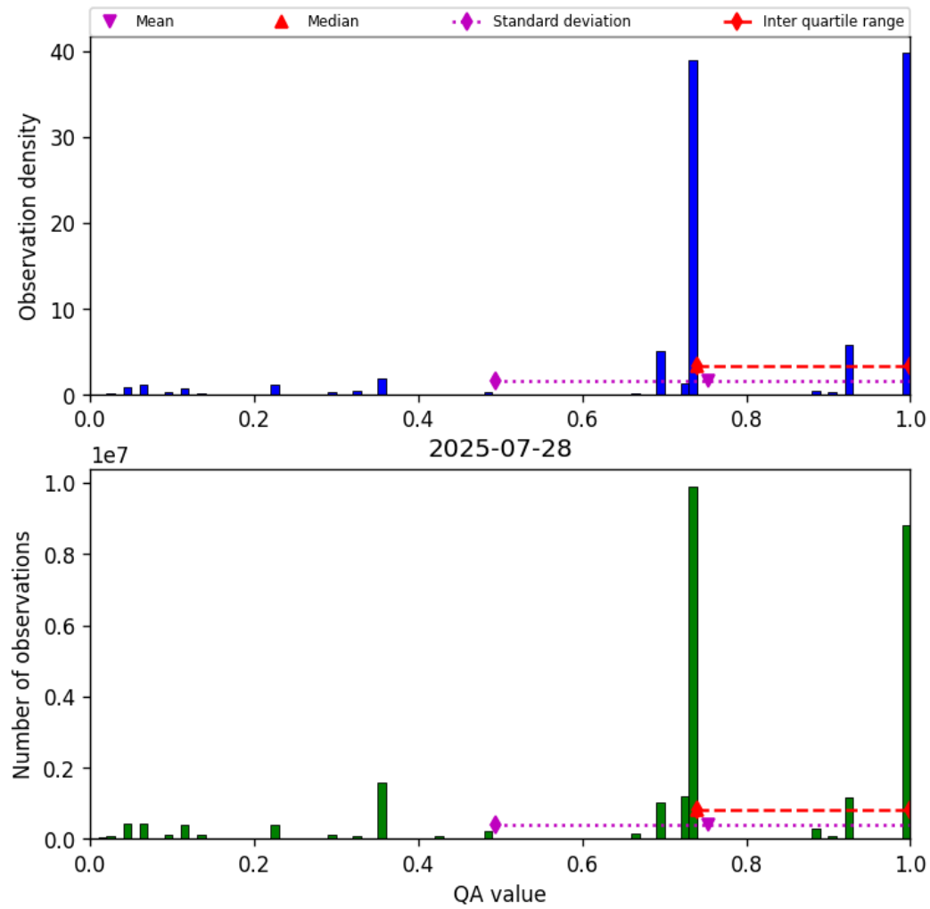
Figure 28: Histogram of “QA value” for 2025-07-27 to 2025-07-29
