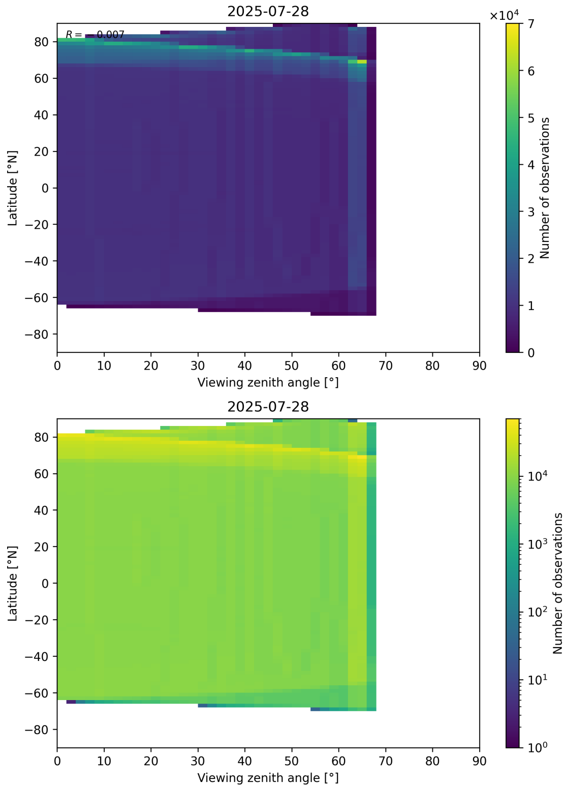
Figure 163: Scatter density plot of “Viewing zenith angle” against “Latitude” for 2025-07-27 to 2025-07-29.
