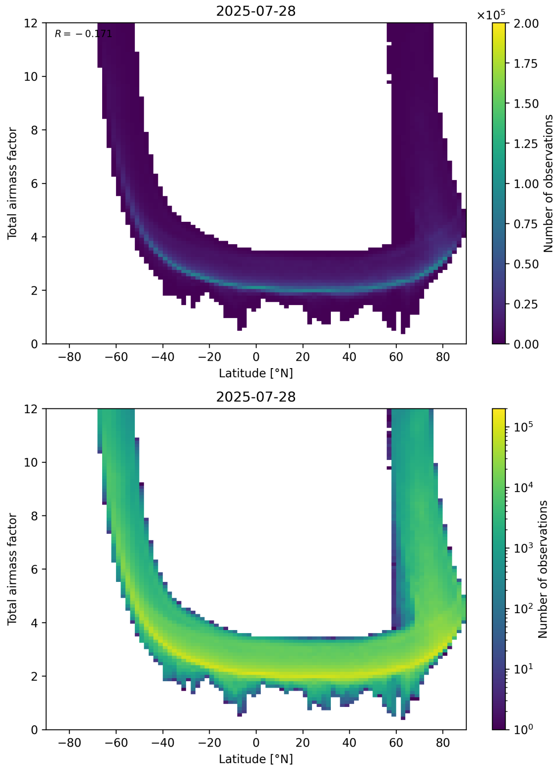
Figure 84: Scatter density plot of “Latitude” against “Total airmass factor” for 2025-07-27 to 2025-07-29.
