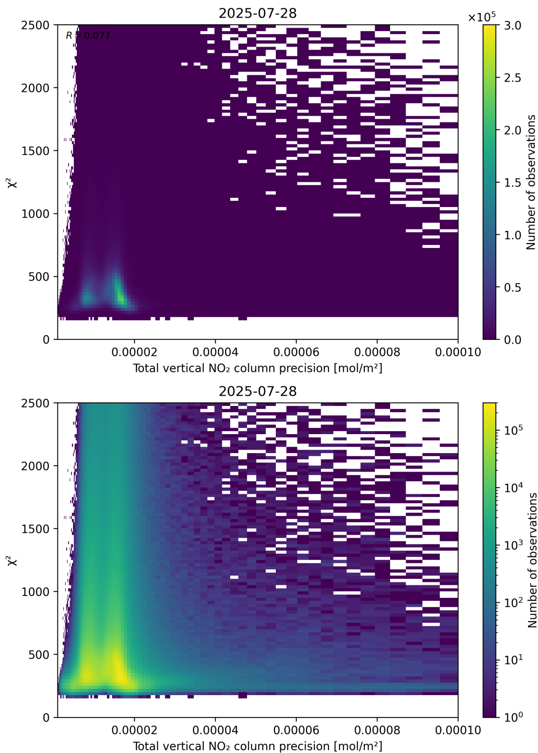
Figure 116: Scatter density plot of “Total vertical NO 2 column precision” against “ \chi^2 ” for 2025-07-27 to 2025-07-29.
