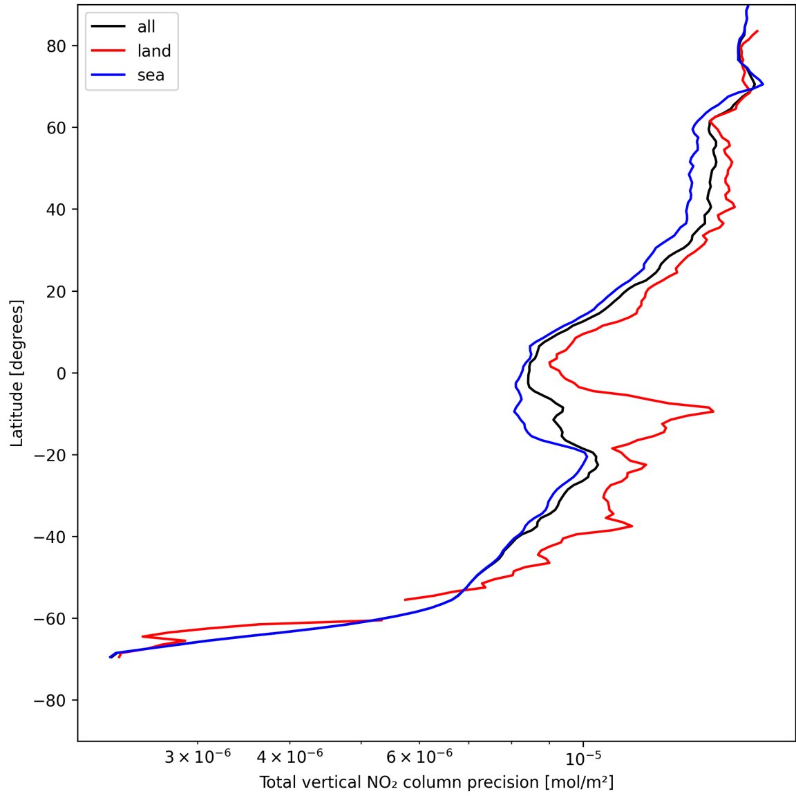
Figure 22: Zonal average of “Total vertical NO 2 column precision” for 2025-07-31 to 2025-08-02.
