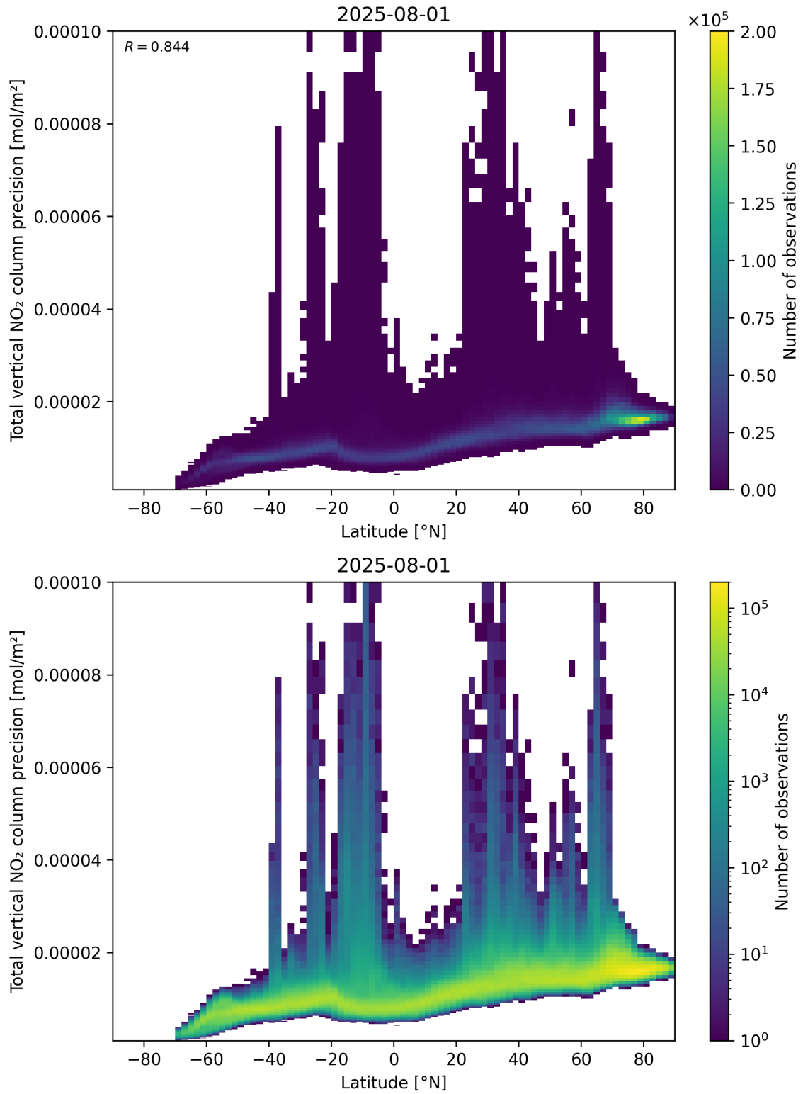
Figure 91: Scatter density plot of “Latitude” against “Total vertical NO 2 column precision” for 2025-07-31 to 2025-08-02.
