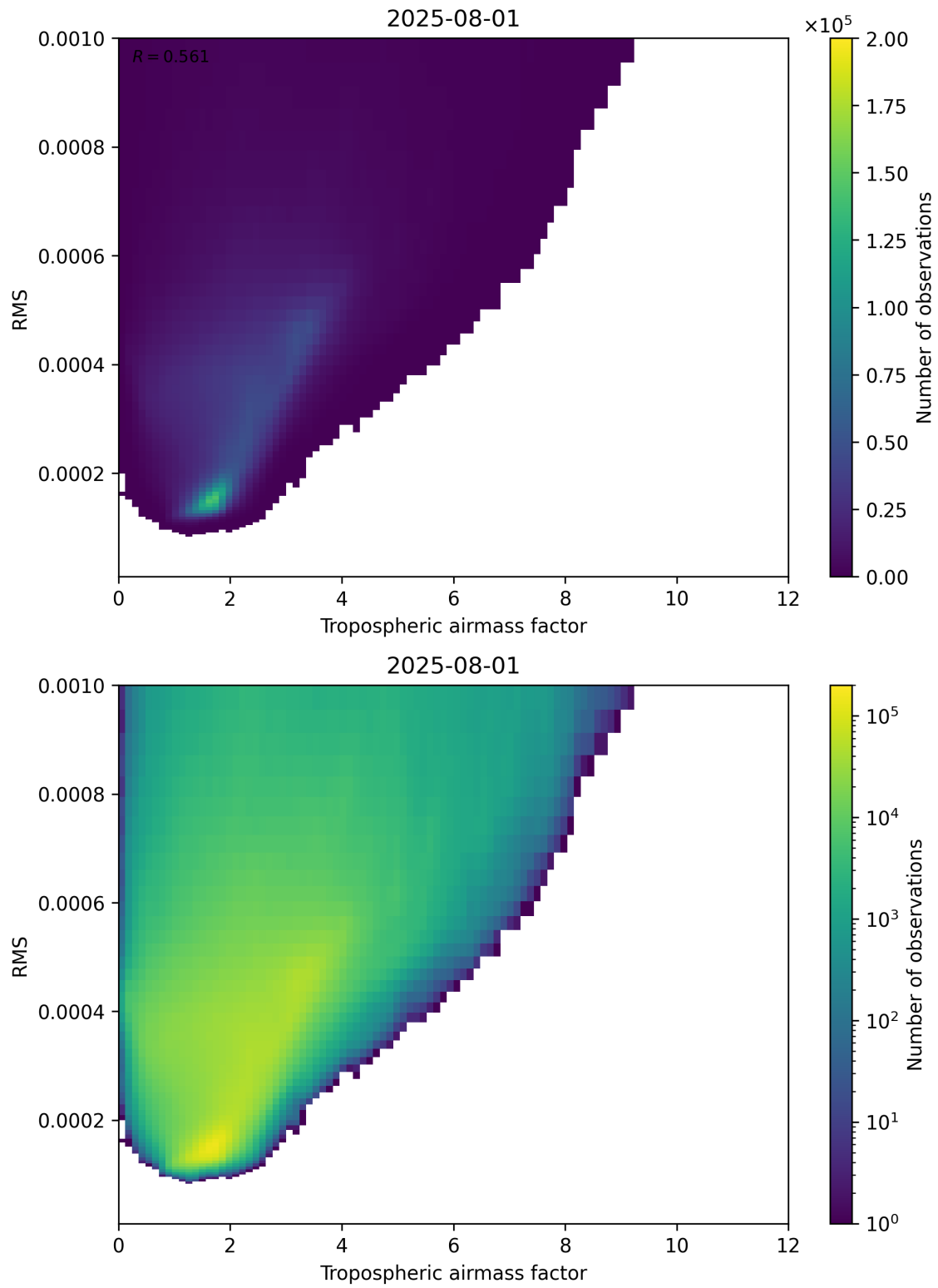
Figure 79: Scatter density plot of “Tropospheric airmass factor” against “RMS” for 2025-07-31 to 2025-08-02.
