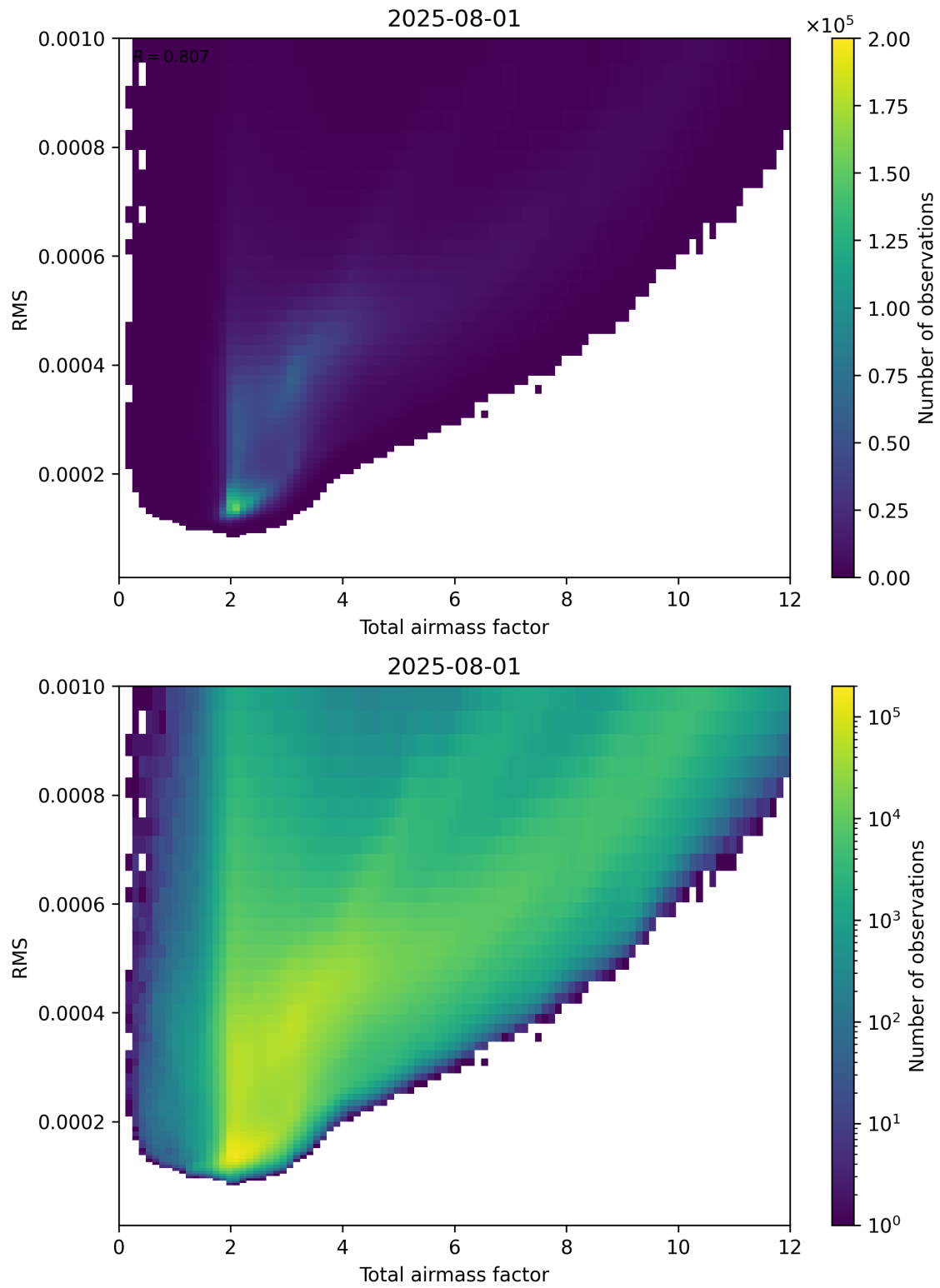
Figure 69: Scatter density plot of “Total airmass factor” against “RMS” for 2025-07-31 to 2025-08-02.
