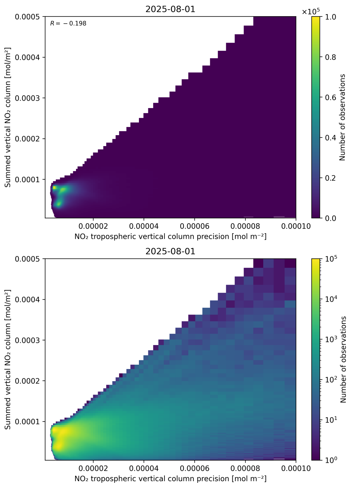
Figure 136: Scatter density plot of “NO 2 tropospheric vertical column precision” against “Summed vertical NO 2 column” for 2025-07-31 to 2025-08-02.
