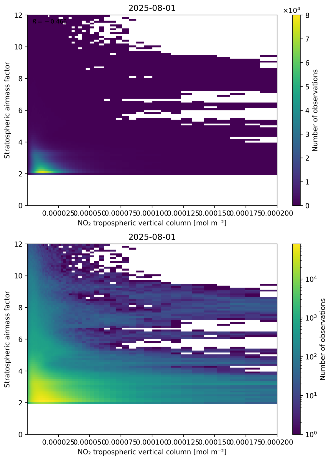
Figure 121: Scatter density plot of “NO 2 tropospheric vertical column” against “Stratospheric air mass factor” for 2025-07-31 to 2025-08-02.
