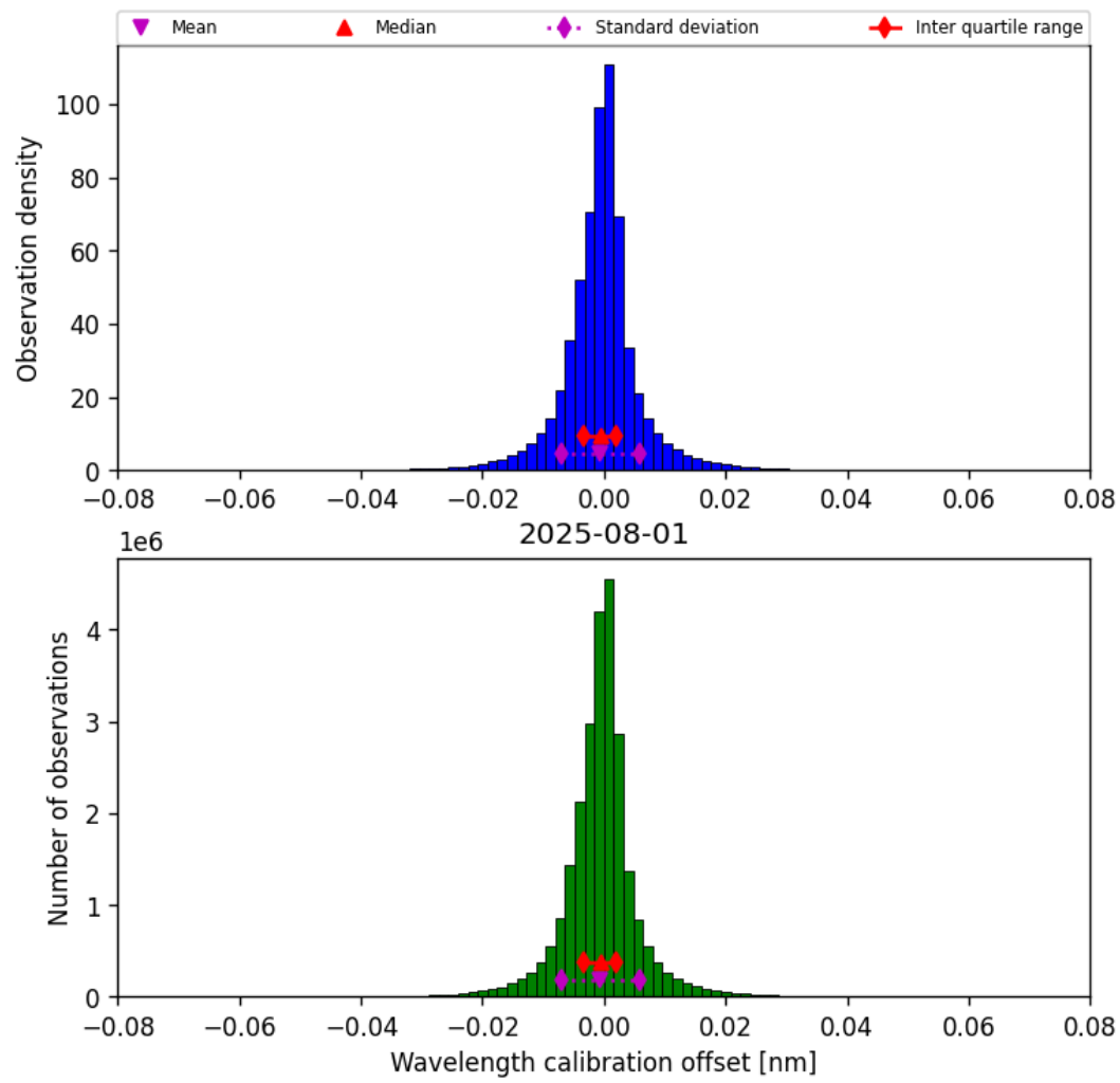
Figure 35: Histogram of “Wavelength calibration offset” for 2025-07-31 to 2025-08-02
