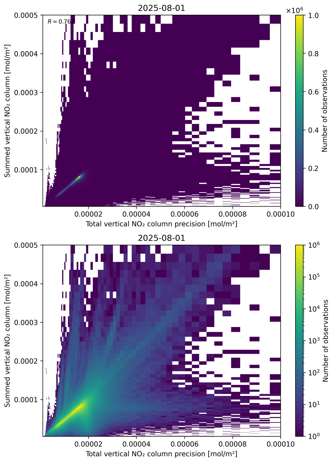
Figure 117: Scatter density plot of “Total vertical NO 2 column precision” against “Summed vertical NO 2 column” for 2025-07-31 to 2025-08-02.
