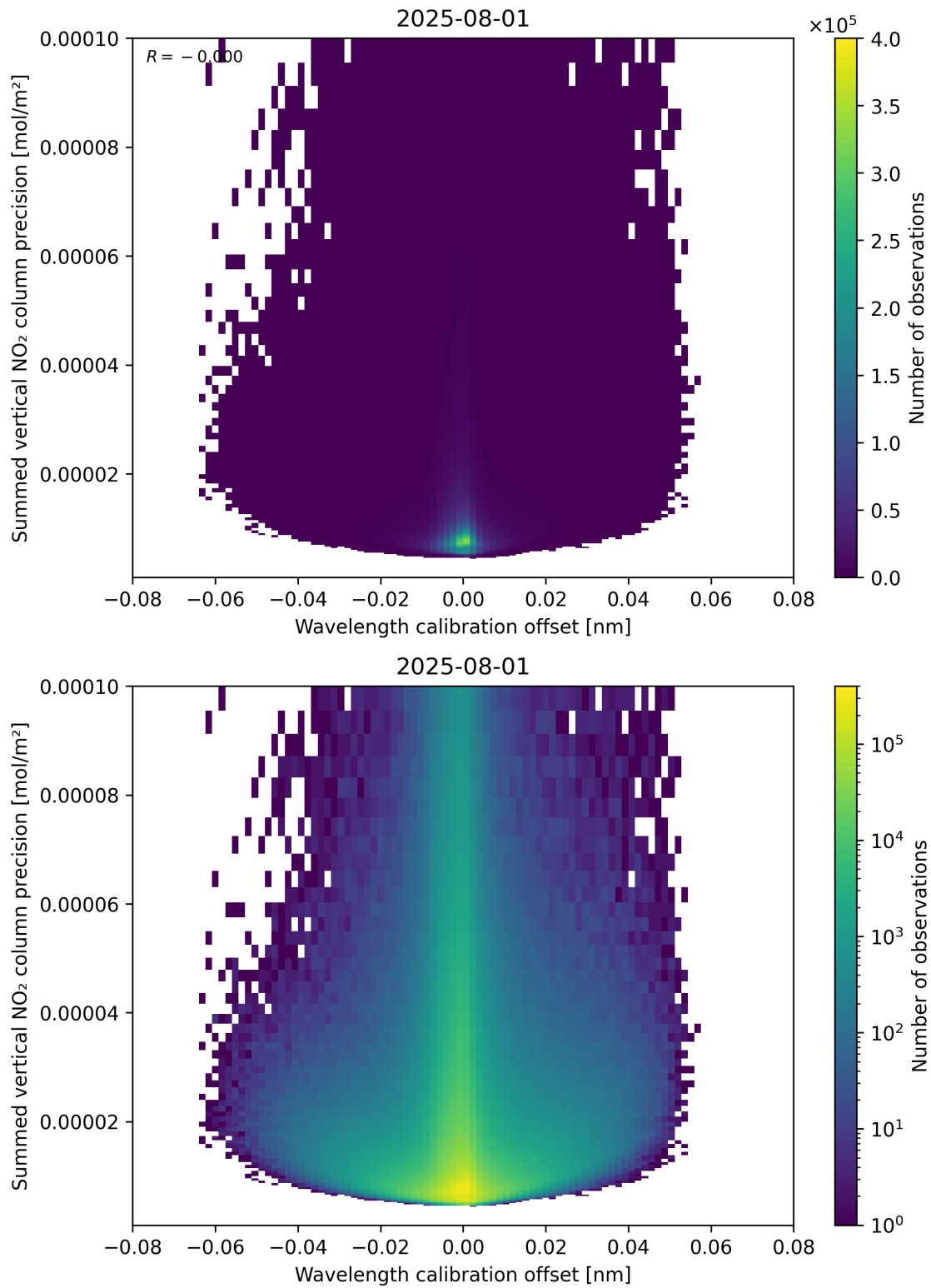
Figure 178: Scatter density plot of “Wavelength calibration offset” against “Summed vertical NO 2 column precision” for 2025-07-31 to 2025-08-02.
