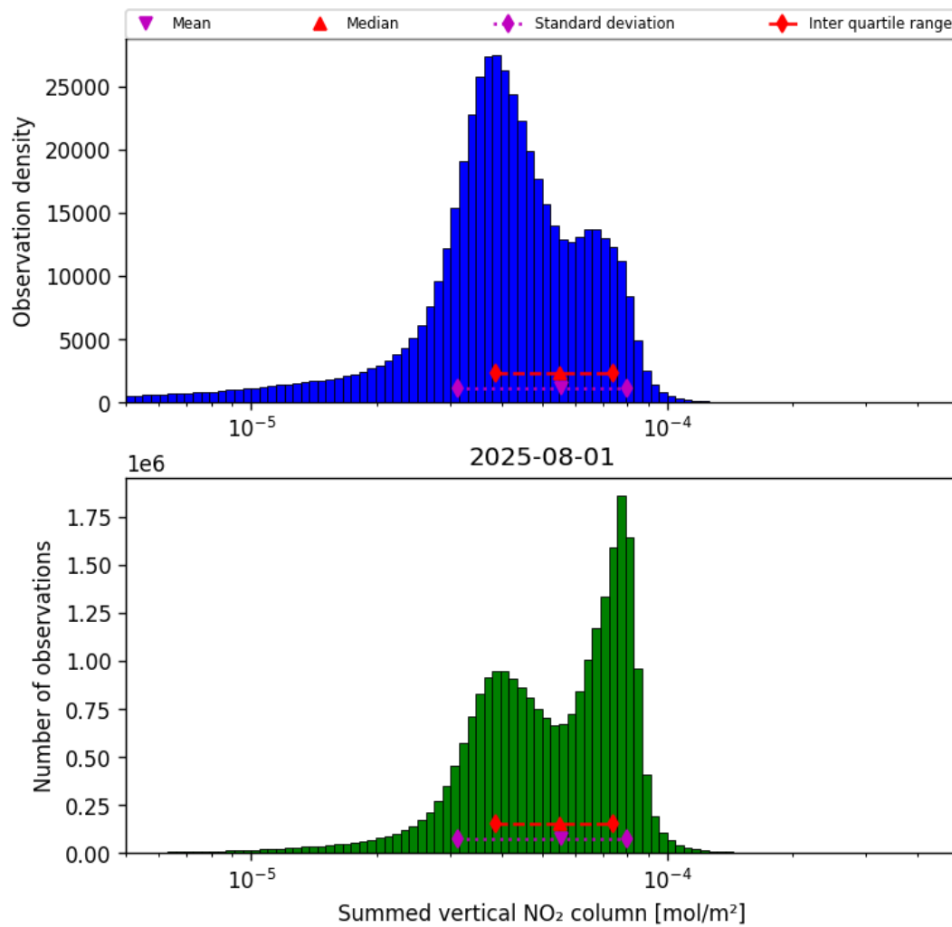
Figure 40: Histogram of “Summed vertical NO 2 column” for 2025-07-31 to 2025-08-02
