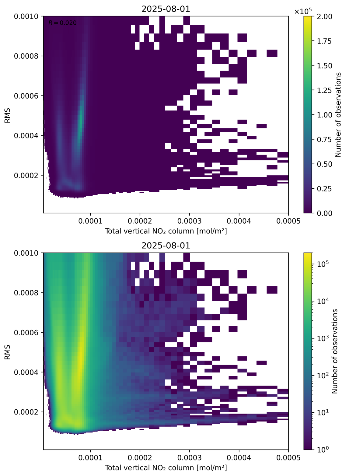
Figure 120: Scatter density plot of “Total vertical NO 2 column” against “RMS” for 2025-07-31 to 2025-08-02.
