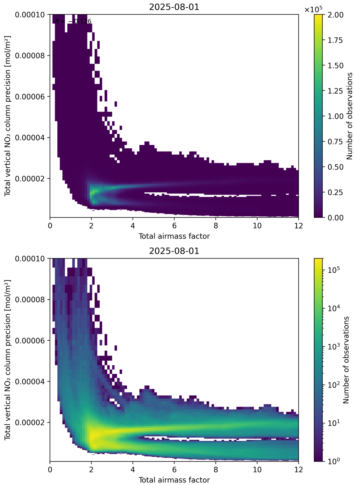
Figure 68: Scatter density plot of “Total airmass factor” against “Total vertical NO 2 column precision” for 2025-07-31 to 2025-08-02.
