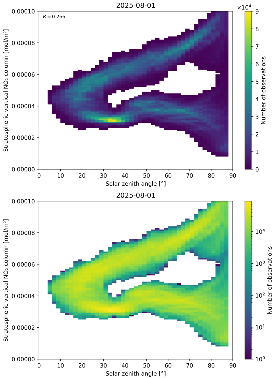
Figure 150: Scatter density plot of “Solar zenith angle” against “Stratospheric vertical NO 2 column” for 2025-07-31 to 2025-08-02.
