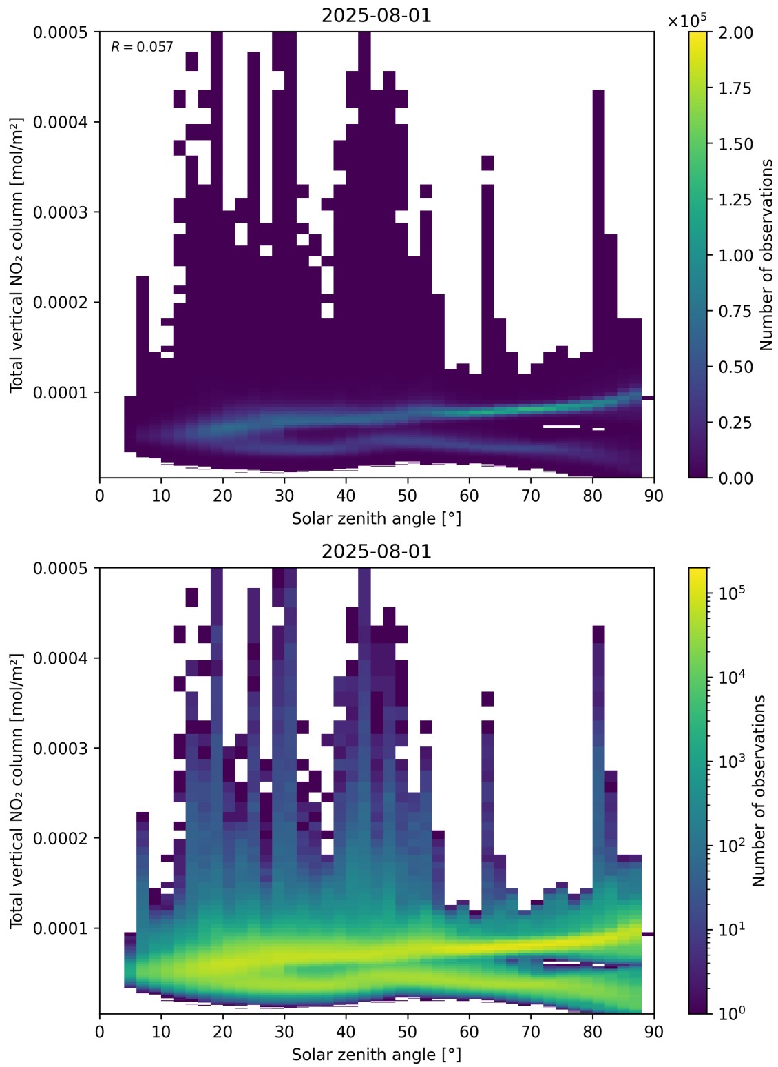
Figure 153: Scatter density plot of “Solar zenith angle” against “Total vertical NO 2 column” for 2025-07-31 to 2025-08-02.
