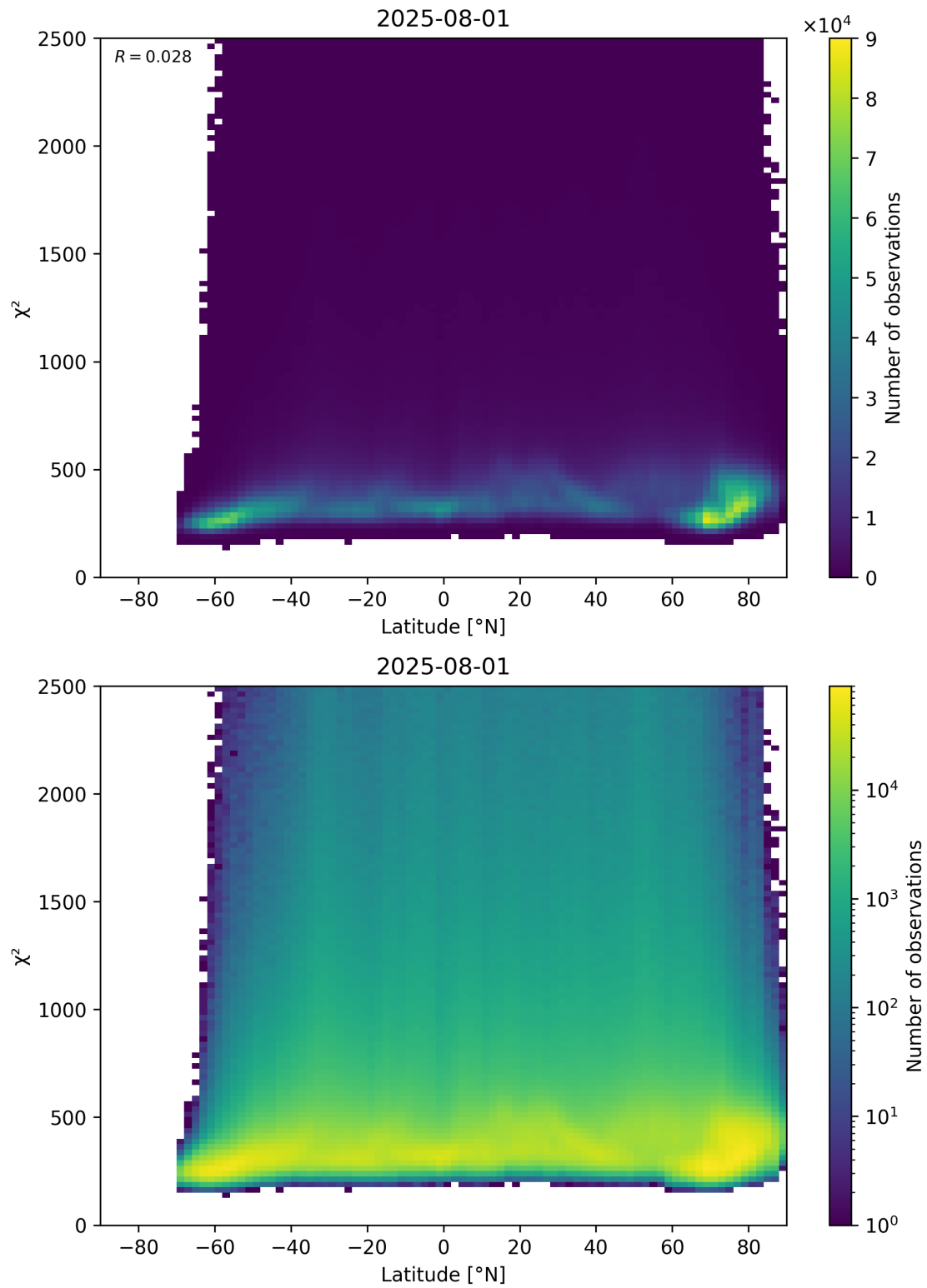
Figure 86: Scatter density plot of “Latitude” against “ \chi^2 ” for 2025-07-31 to 2025-08-02.
