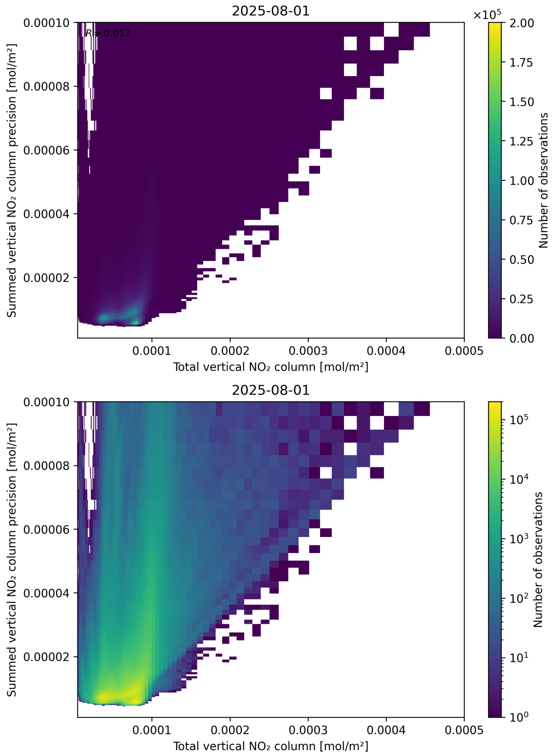
Figure 113: Scatter density plot of “Total vertical NO 2 column” against “Summed vertical NO 2 column precision” for 2025-07-31 to 2025-08-02.
