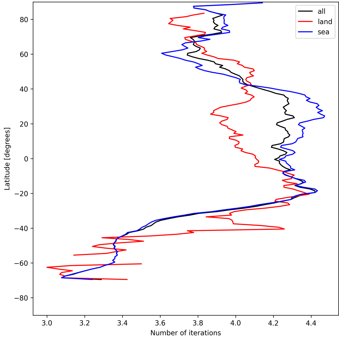
Figure 17: Zonal average of “Number of iterations” for 2025-07-31 to 2025-08-02.
