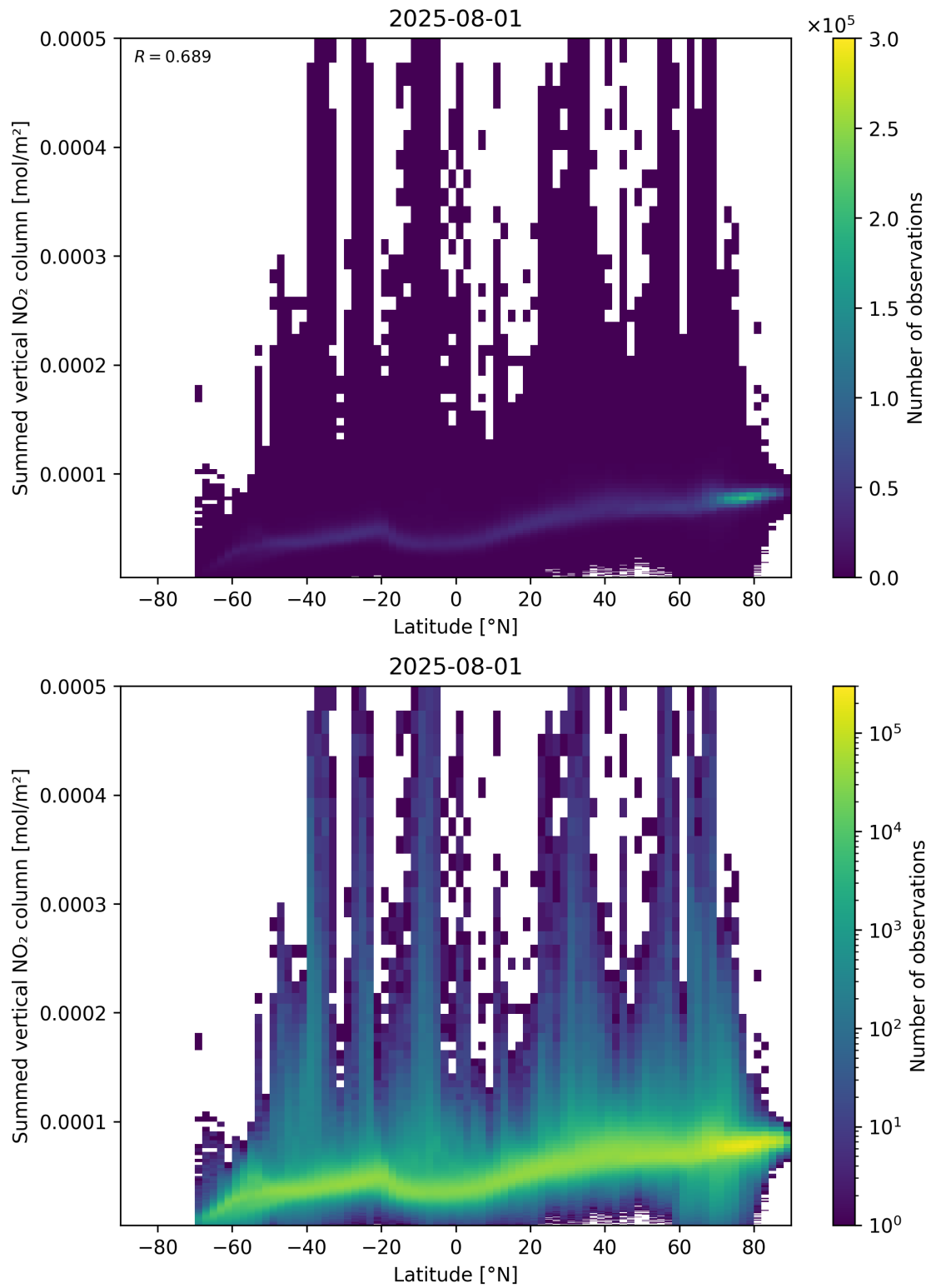
Figure 88: Scatter density plot of “Latitude” against “Summed vertical NO 2 column” for 2025-07-31 to 2025-08-02.
