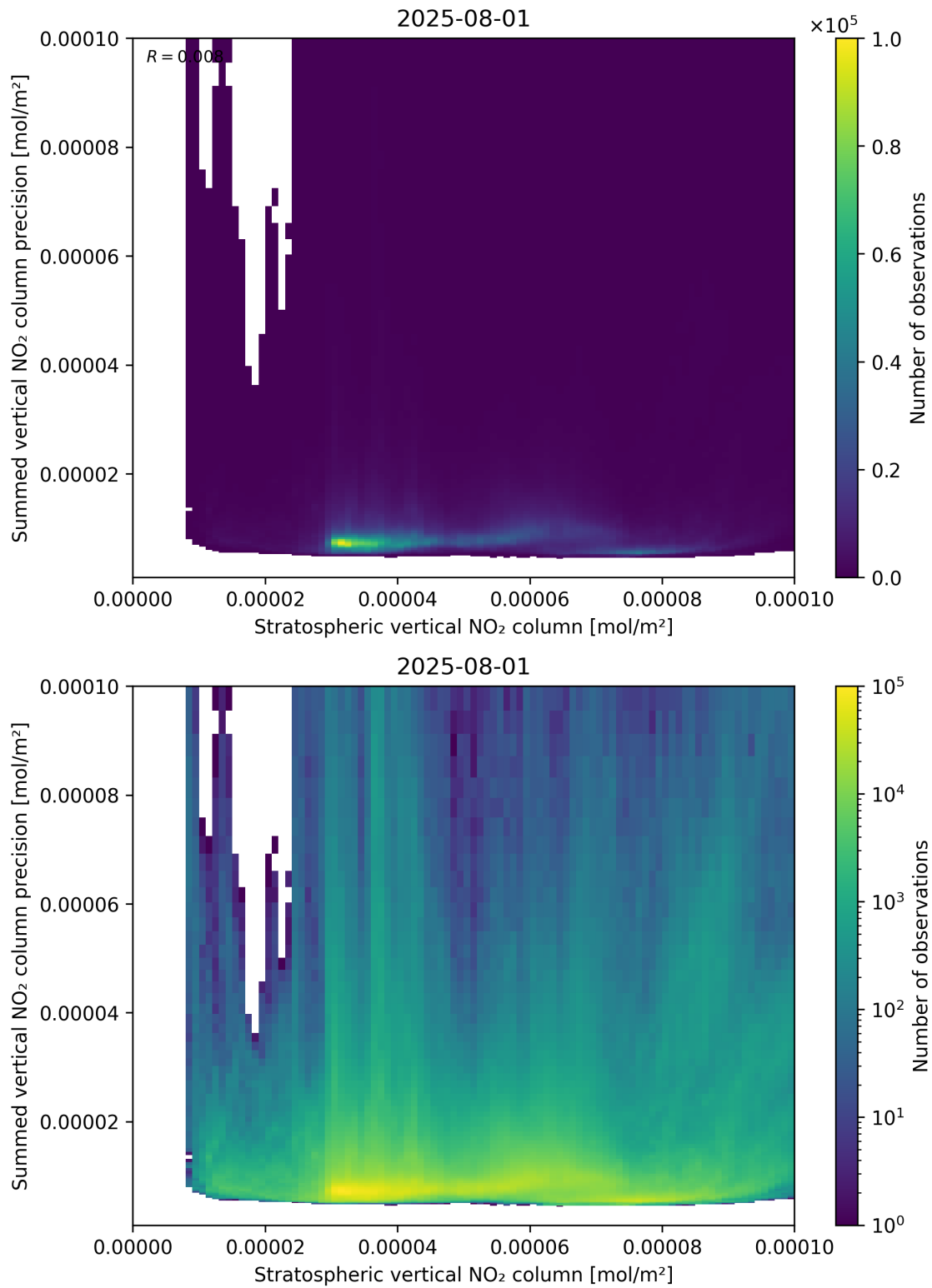
Figure 99: Scatter density plot of “Stratospheric vertical NO 2 column” against “Summed vertical NO 2 column precision” for 2025-07-31 to 2025-08-02.
