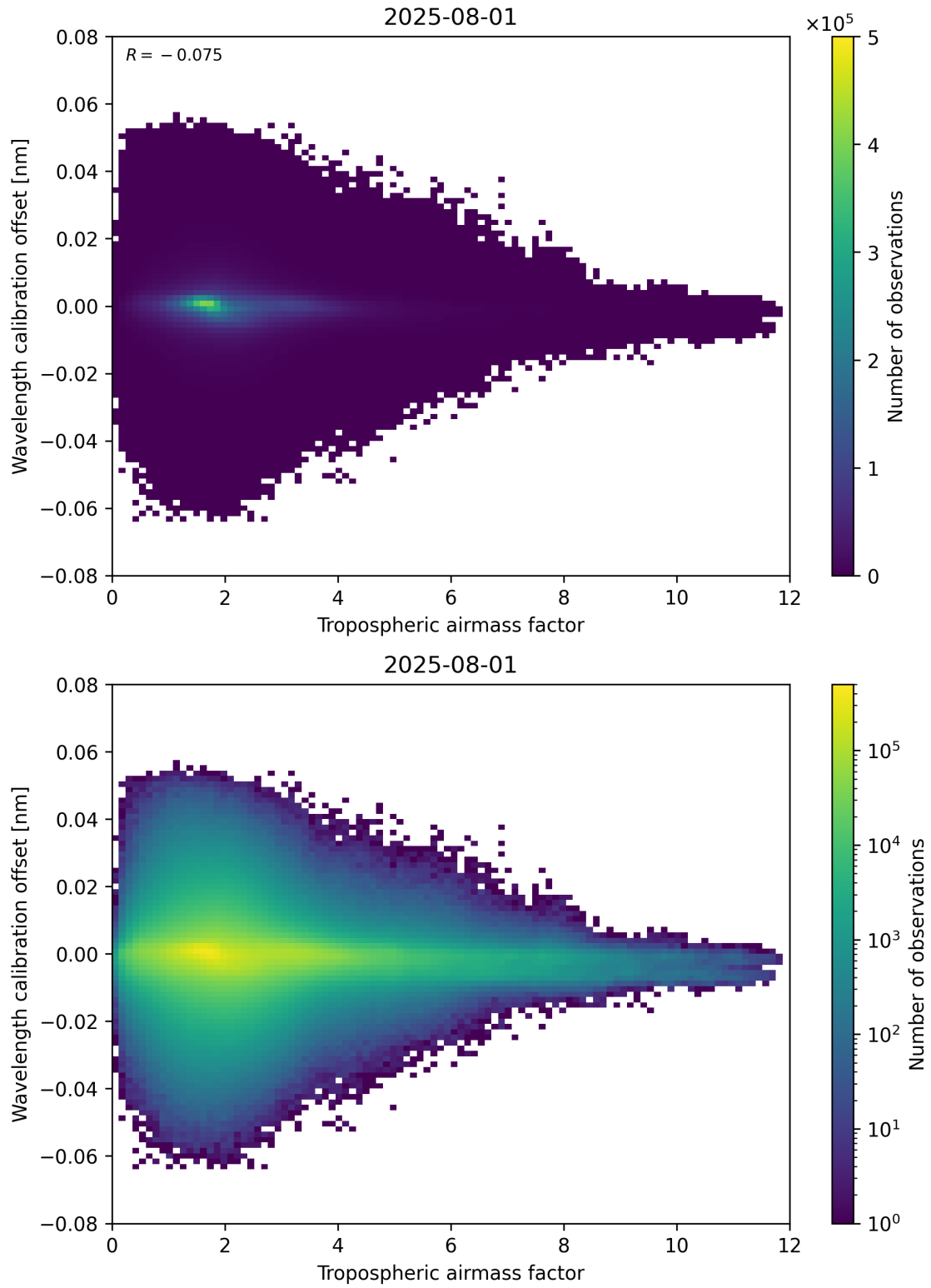
Figure 80: Scatter density plot of “Tropospheric airmass factor” against “Wavelength calibration offset” for 2025-07-31 to 2025-08-02.
