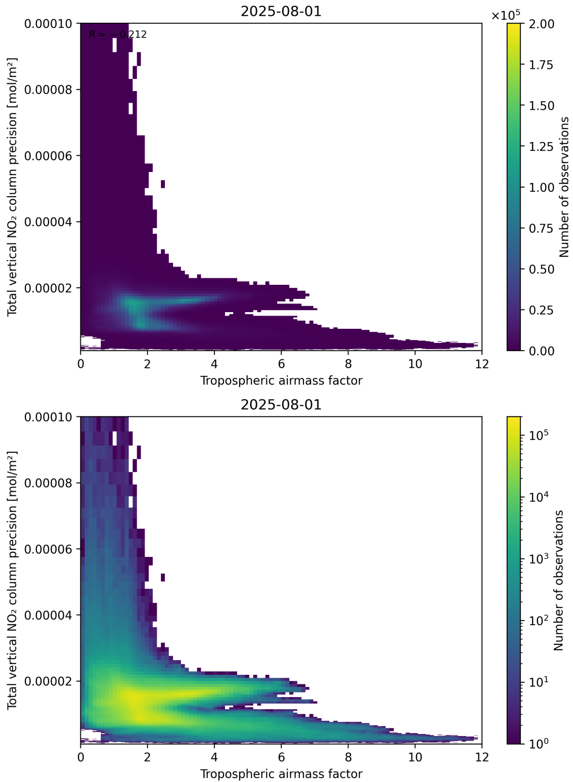
Figure 78: Scatter density plot of “Tropospheric air mass factor” against “Total vertical NO 2 column precision” for 2025-07-31 to 2025-08-02.
