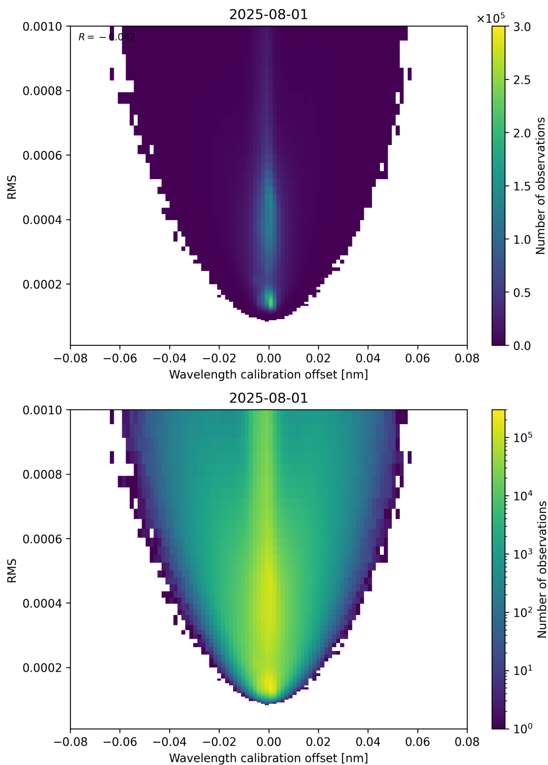
Figure 181: Scatter density plot of “Wavelength calibration offset” against “RMS” for 2025-07-31 to 2025-08-02.
