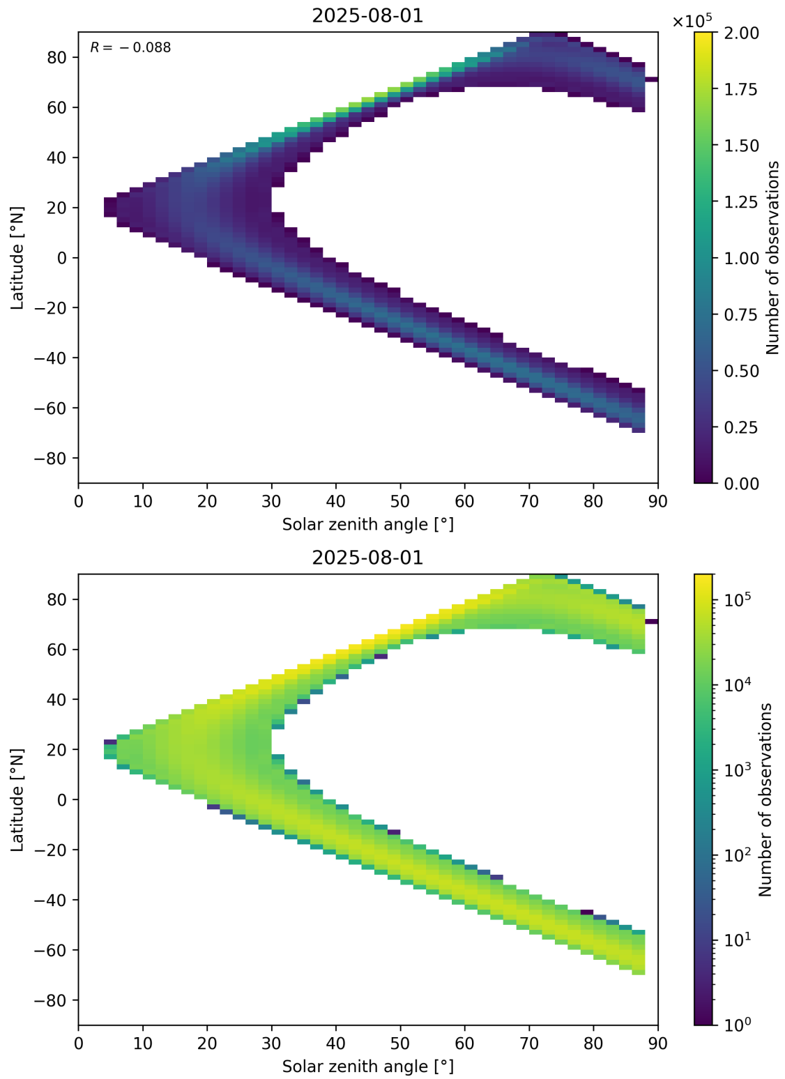
Figure 149: Scatter density plot of “Solar zenith angle” against “Latitude” for 2025-07-31 to 2025-08-02.
