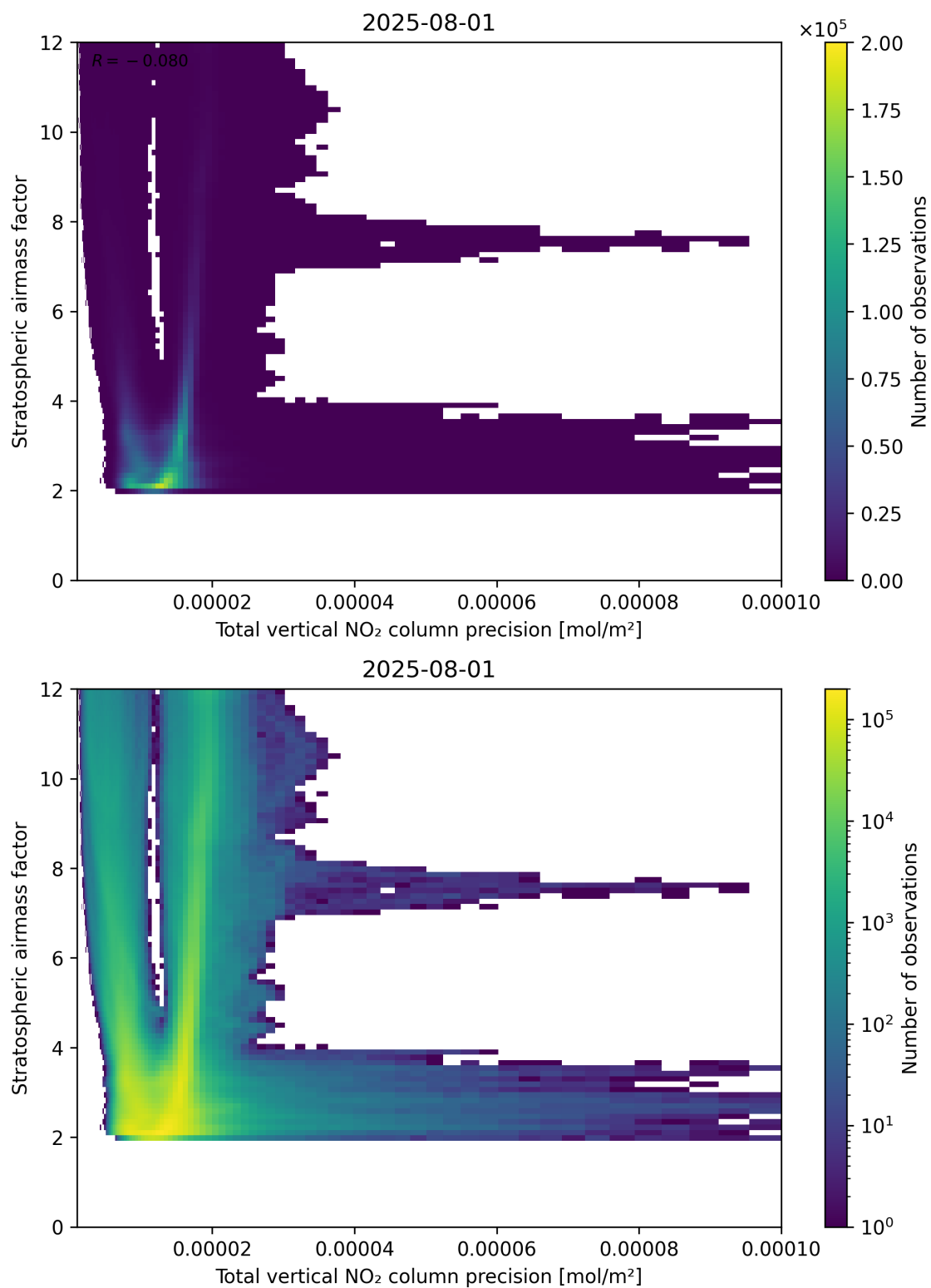
Figure 115: Scatter density plot of “Total vertical NO 2 column precision” against “Stratospheric air mass factor” for 2025-07-31 to 2025-08-02.
