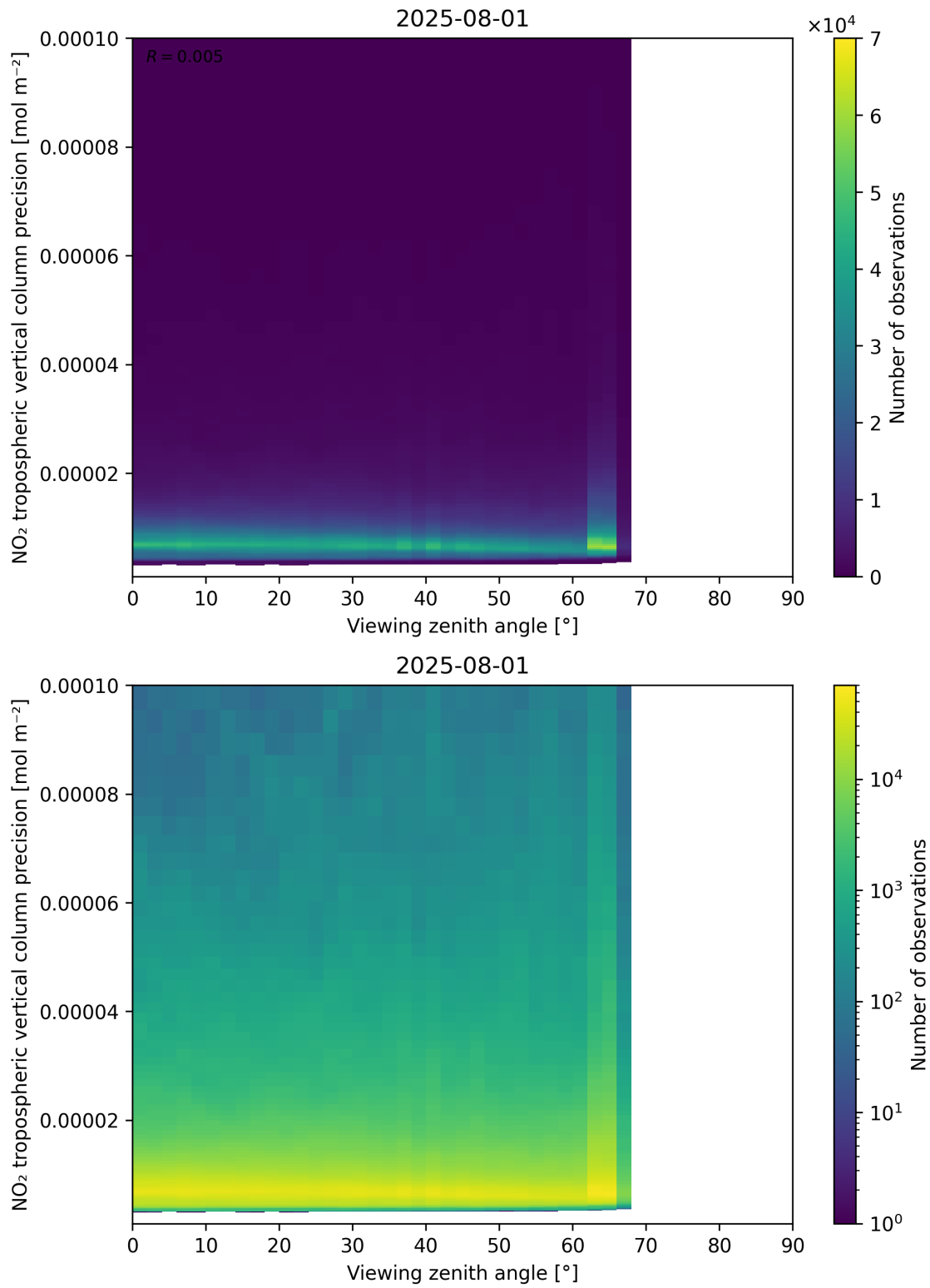
Figure 170: Scatter density plot of “Viewing zenith angle” against “NO 2 tropospheric vertical column precision” for 2025-07-31 to 2025-08-02.
