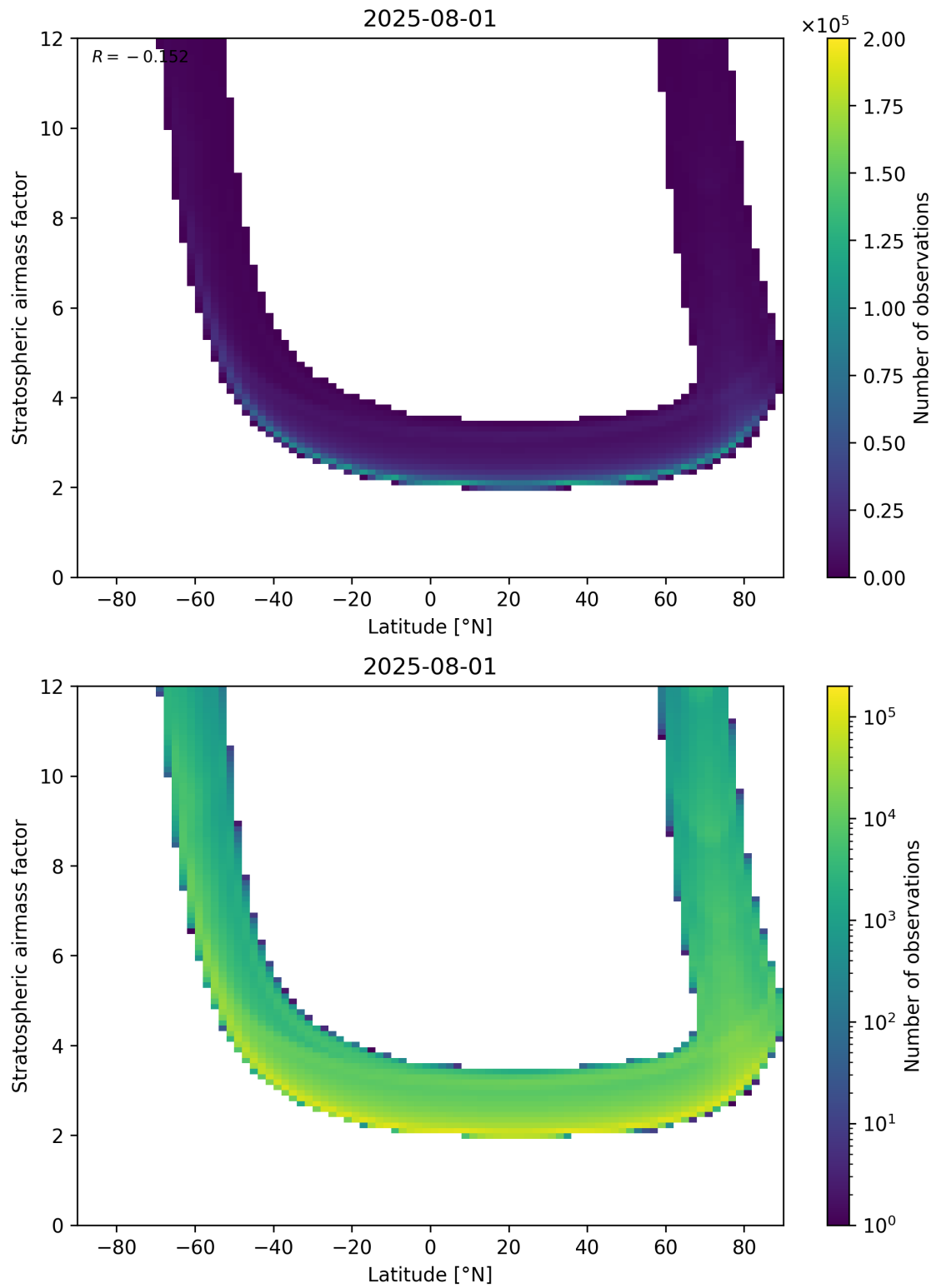
Figure 83: Scatter density plot of “Latitude” against “Stratospheric air mass factor” for 2025-07-31 to 2025-08-02.
