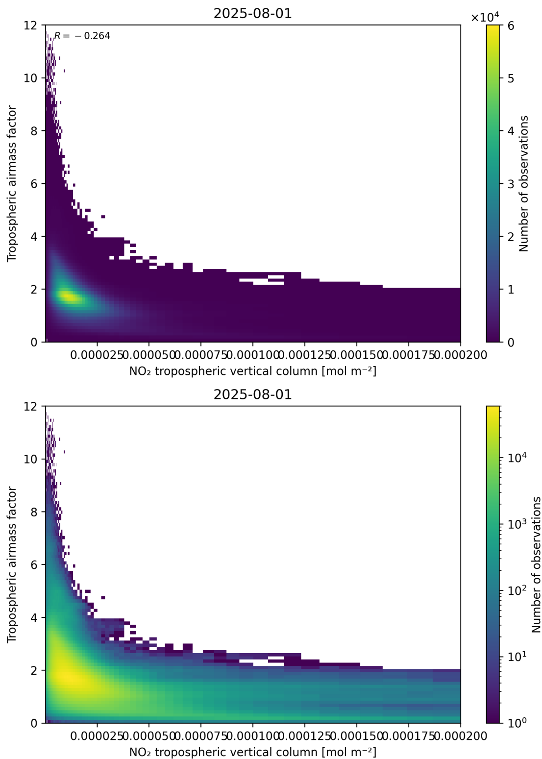
Figure 123: Scatter density plot of “NO 2 tropospheric vertical column” against “Tropospheric air mass factor” for 2025-07-31 to 2025-08-02.
