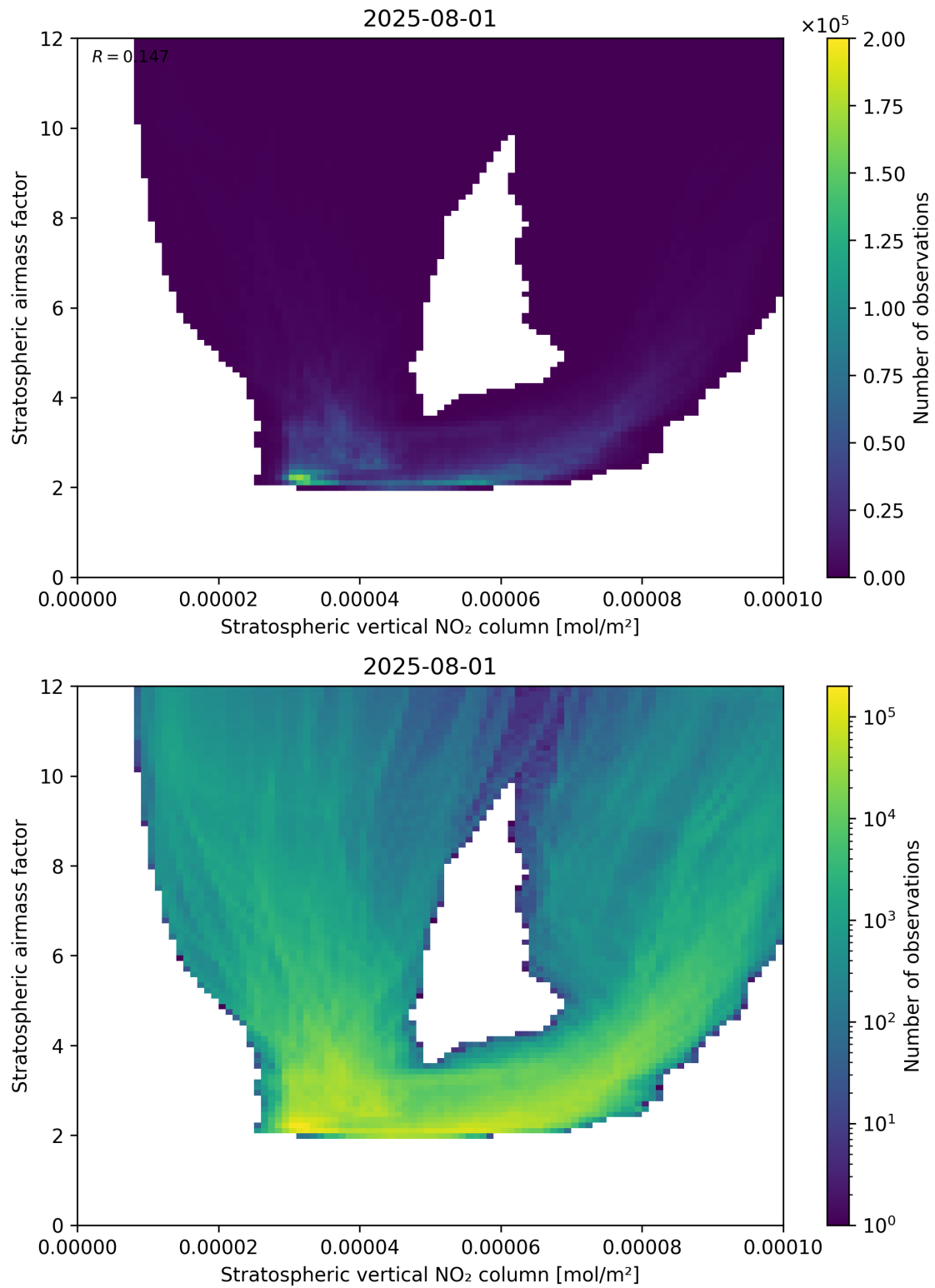
Figure 96: Scatter density plot of “Stratospheric vertical NO 2 column” against “Stratospheric airmass factor” for 2025-07-31 to 2025-08-02.
