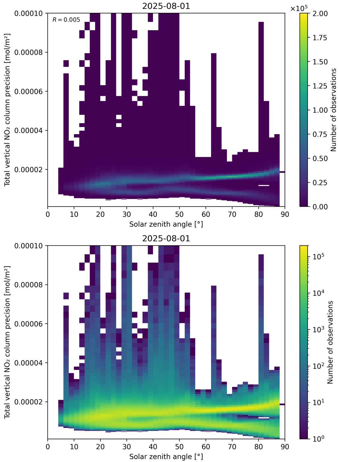
Figure 154: Scatter density plot of “Solar zenith angle” against “Total vertical NO 2 column precision” for 2025-07-31 to 2025-08-02.
