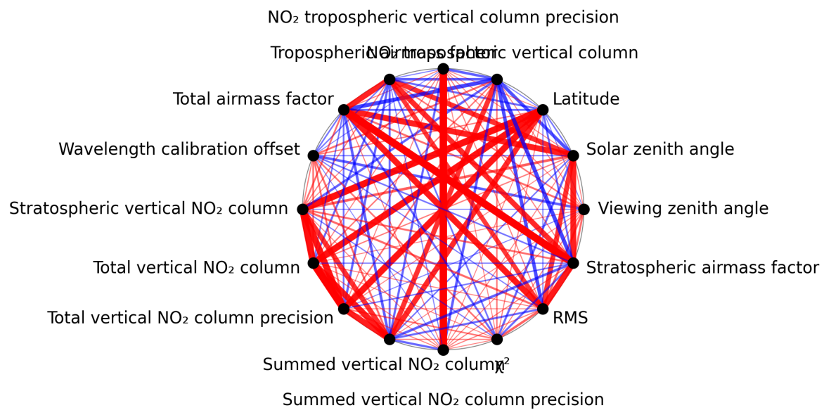
Figure 1: Map of correlation graph for 2025-07-31 to 2025-08-02.
