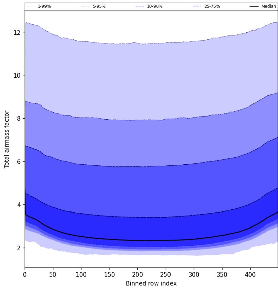
Figure 49: Along track statistics of “Total airmass factor” for 2025-07-31 to 2025-08-02
