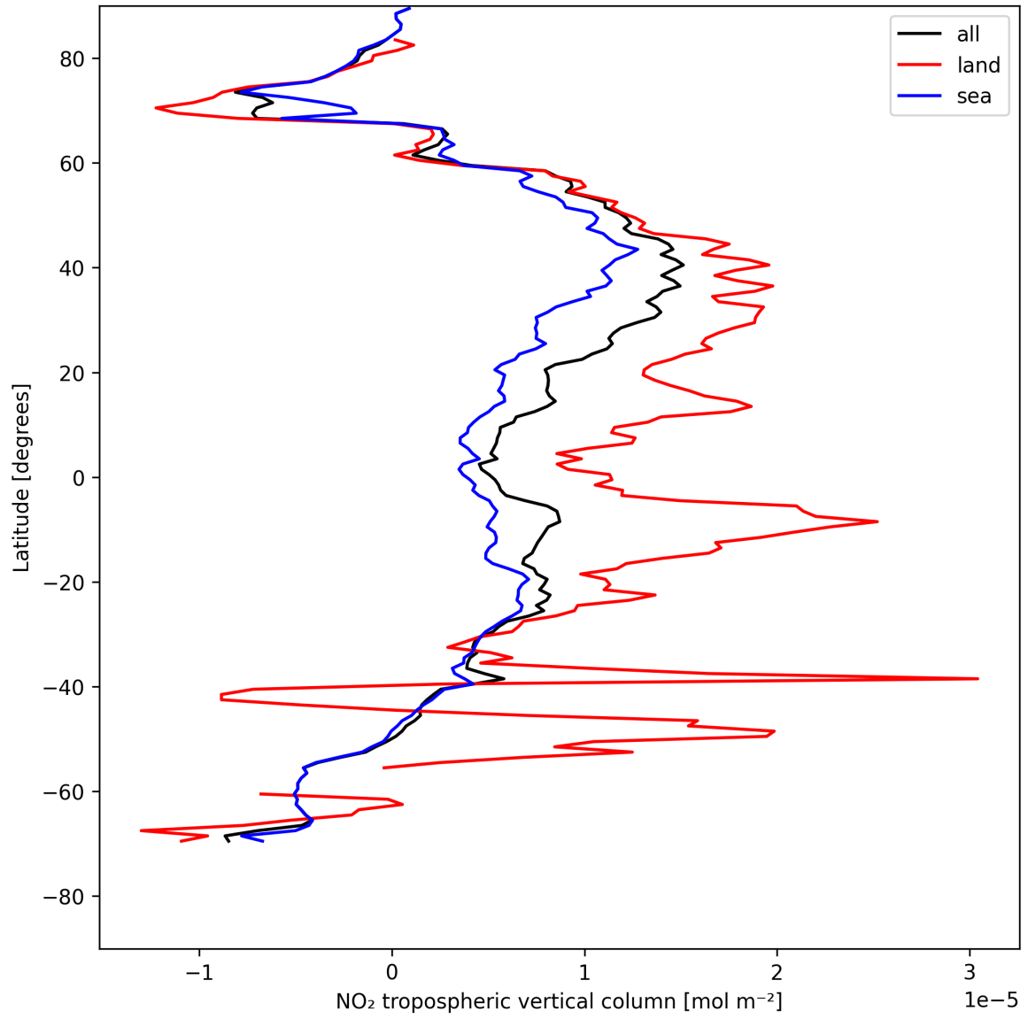
Figure 12: Zonal average of “NO 2 tropospheric vertical column” for 2025-07-31 to 2025-08-02.
