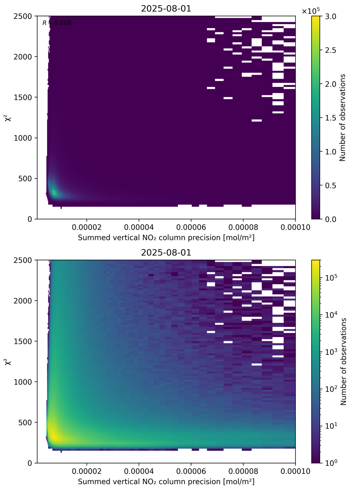
Figure 107: Scatter density plot of “Summed vertical NO 2 column precision” against “ \chi^2 ” for 2025-07-31 to 2025-08-02.
