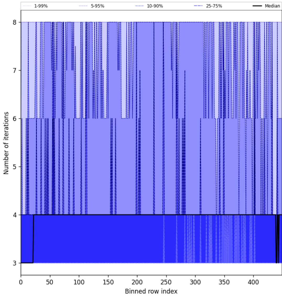
Figure 51: Along track statistics of “Number of iterations” for 2025-07-31 to 2025-08-02
