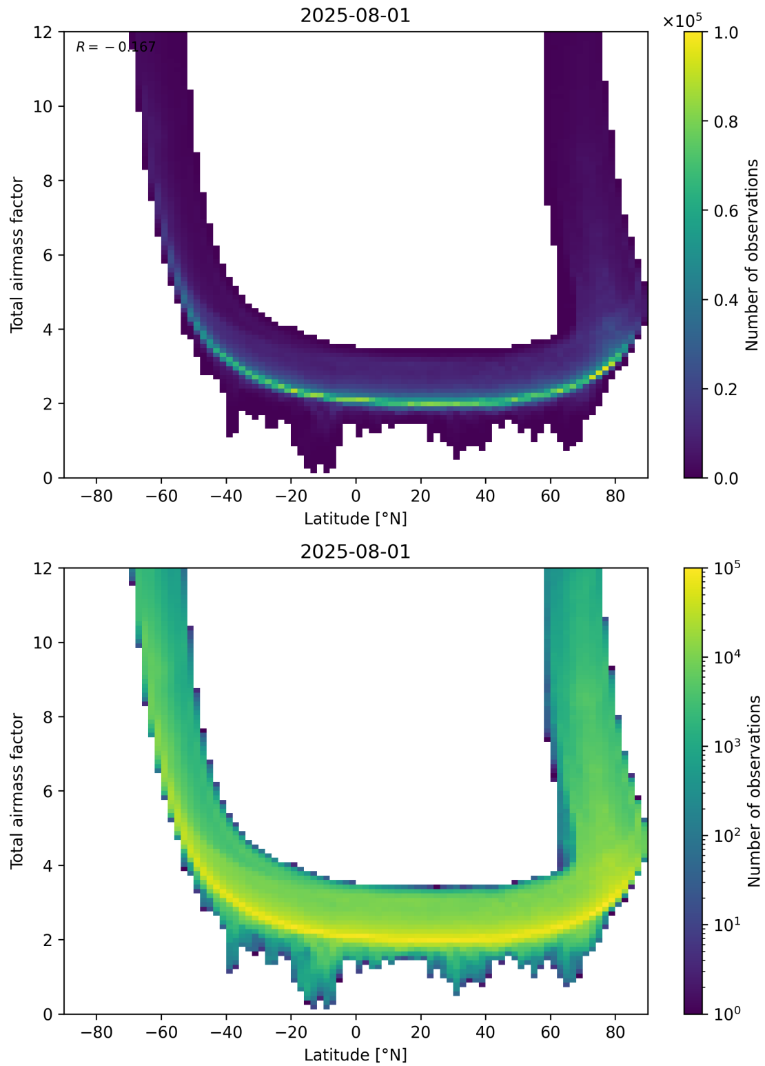
Figure 84: Scatter density plot of “Latitude” against “Total airmass factor” for 2025-07-31 to 2025-08-02.
