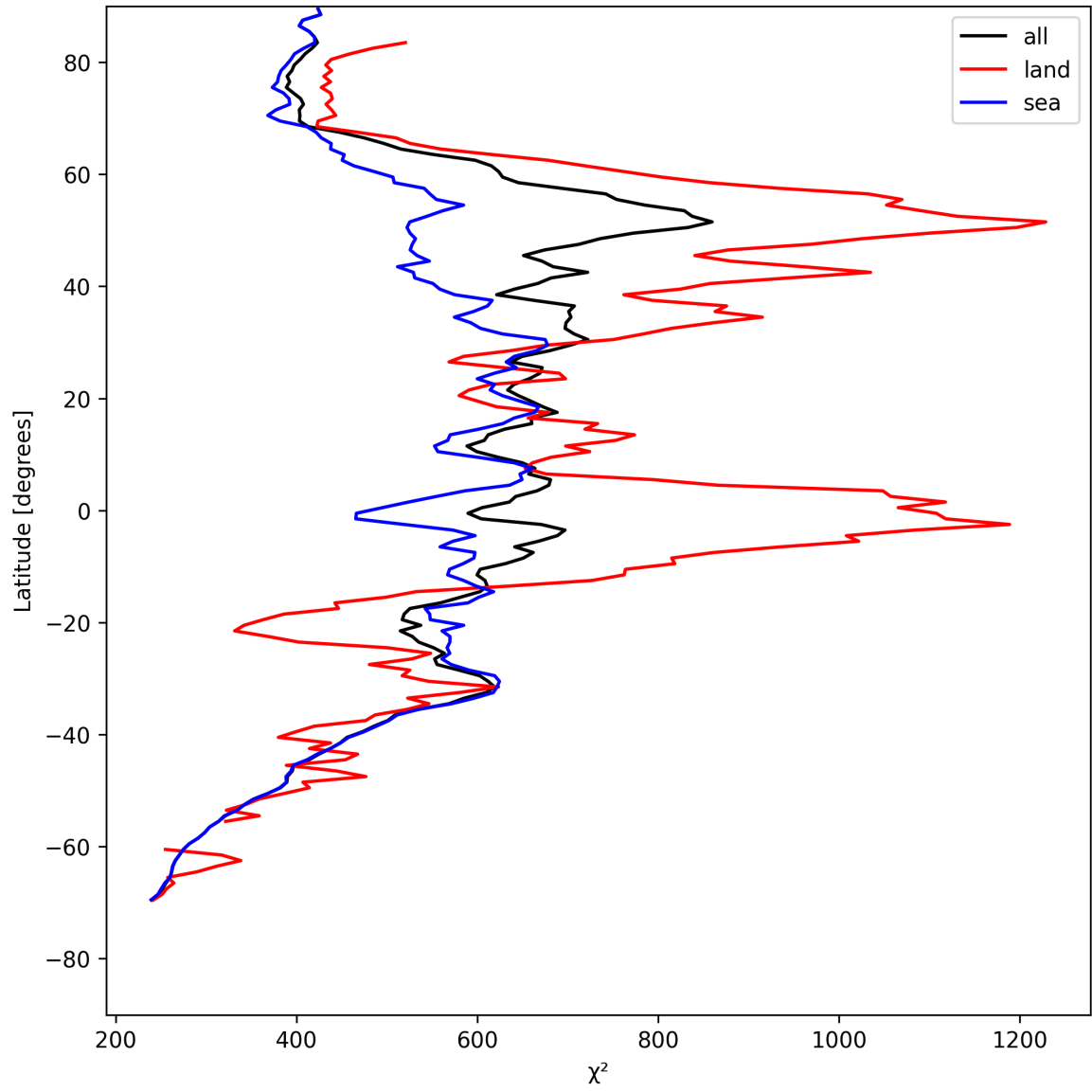
Figure 25: Zonal average of “ \chi^2 ” for 2025-07-31 to 2025-08-02.
