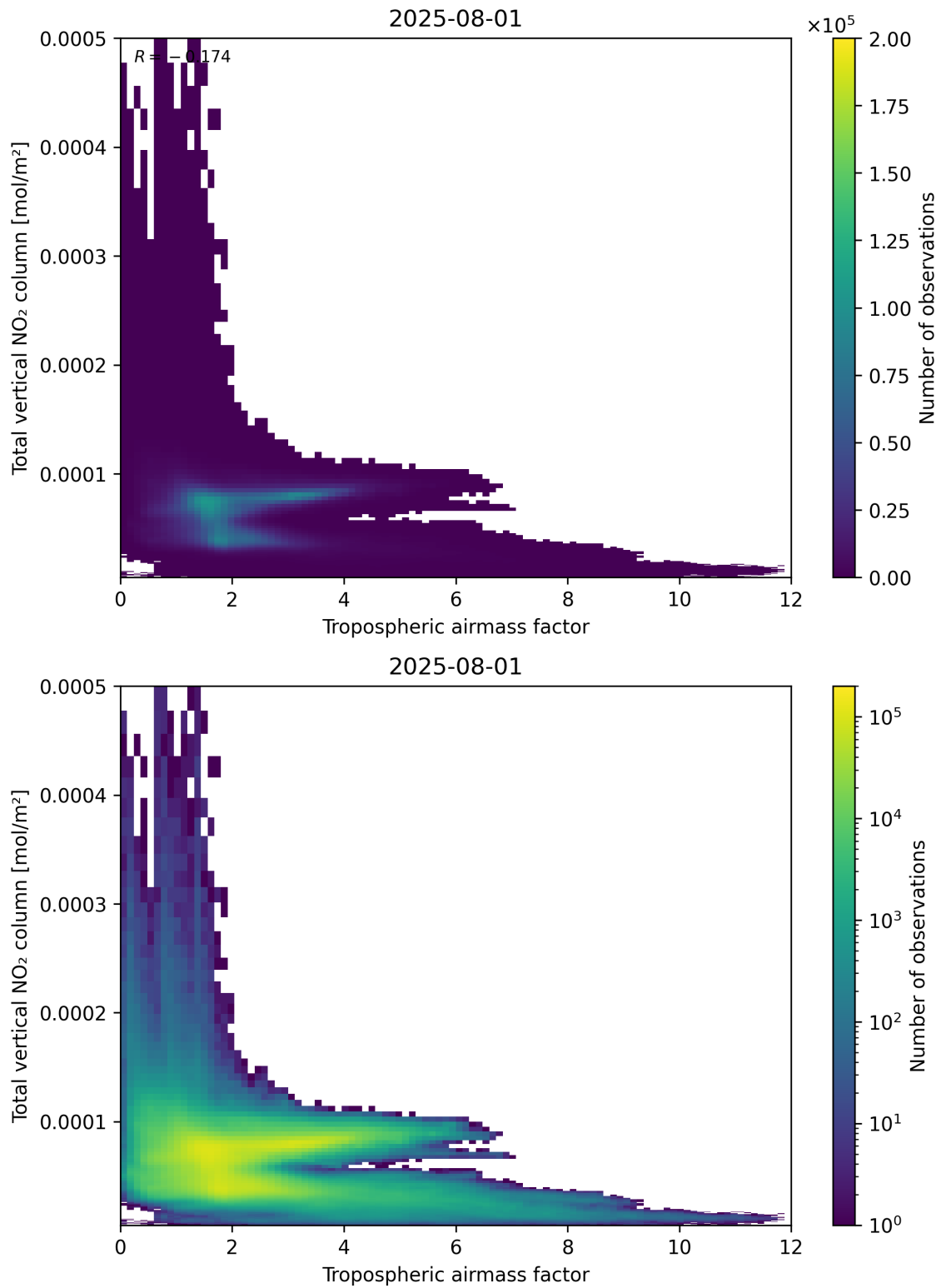
Figure 77: Scatter density plot of “Tropospheric airmass factor” against “Total vertical NO 2 column” for 2025-07-31 to 2025-08-02.
