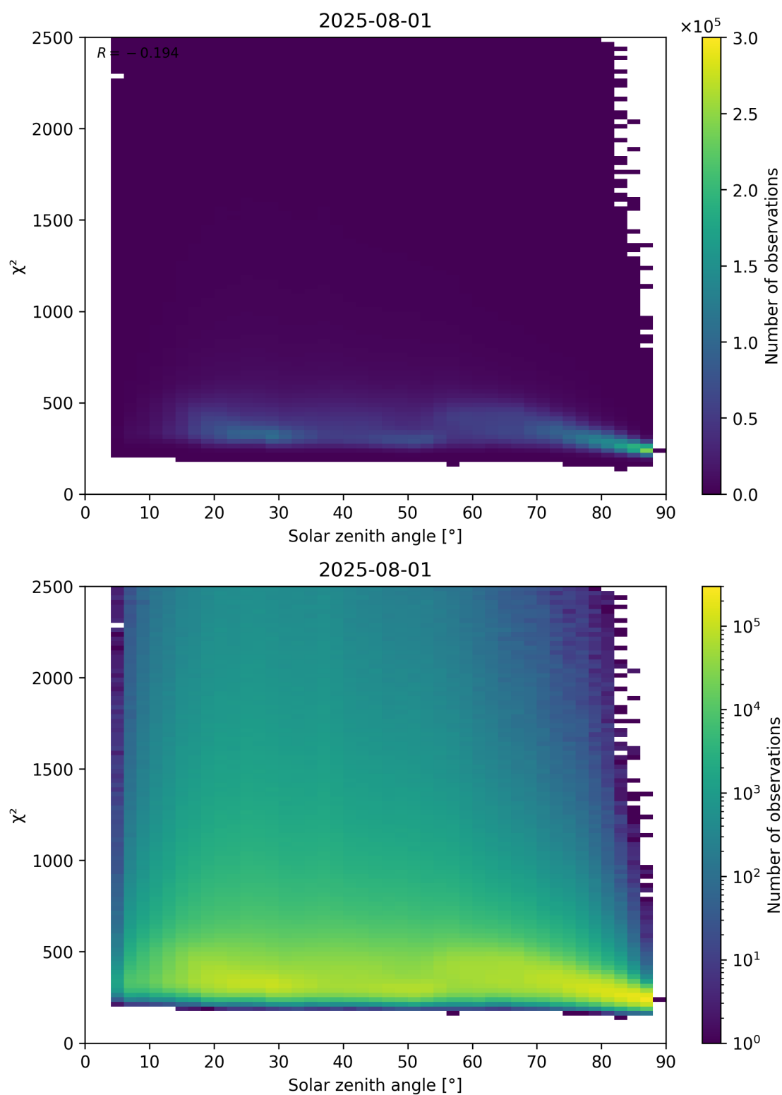
Figure 148: Scatter density plot of “Solar zenith angle” against “ \chi^2 ” for 2025-07-31 to 2025-08-02.
