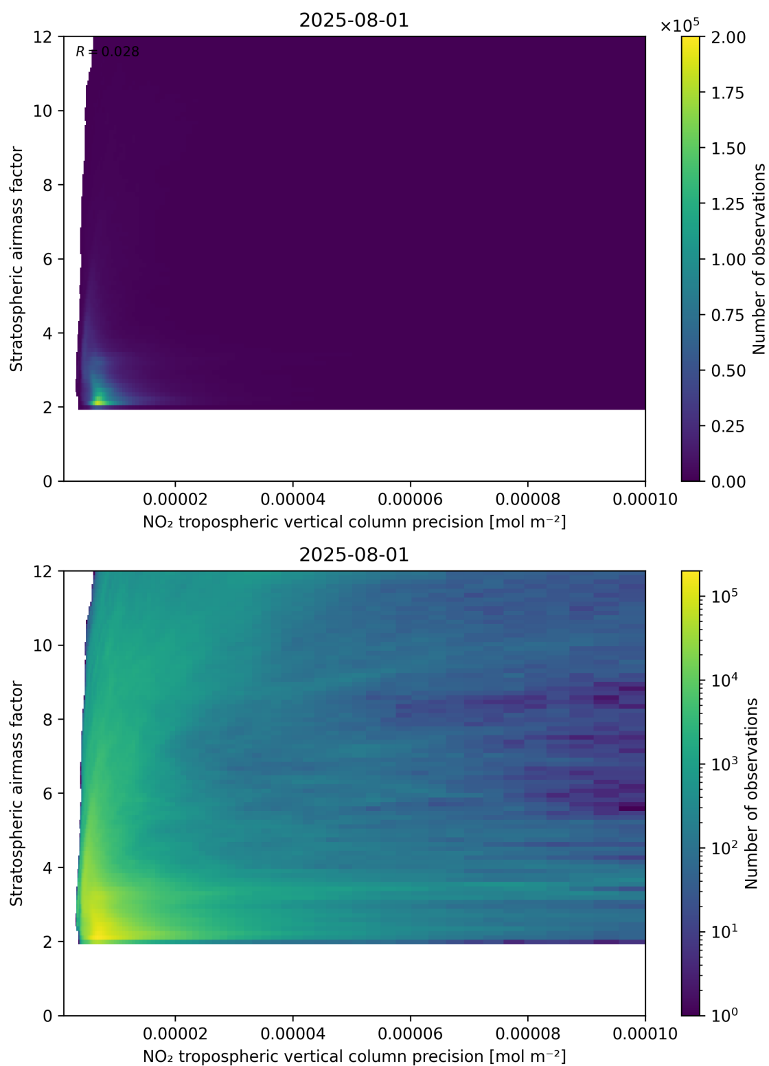
Figure 131: Scatter density plot of “NO 2 tropospheric vertical column precision” against “Stratospheric airmass factor” for 2025-07-31 to 2025-08-02.
