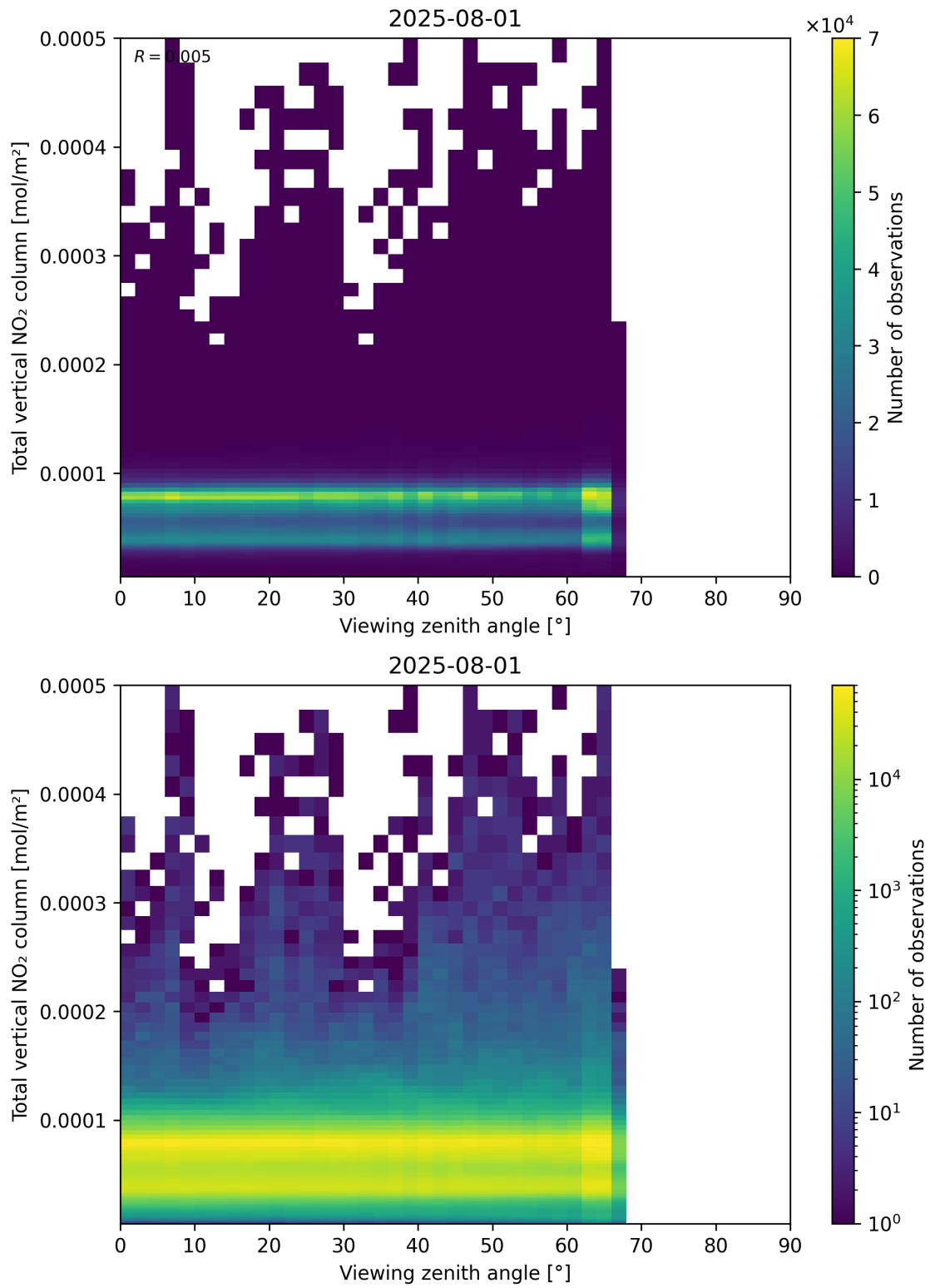
Figure 167: Scatter density plot of “Viewing zenith angle” against “Total vertical NO 2 column” for 2025-07-31 to 2025-08-02.
