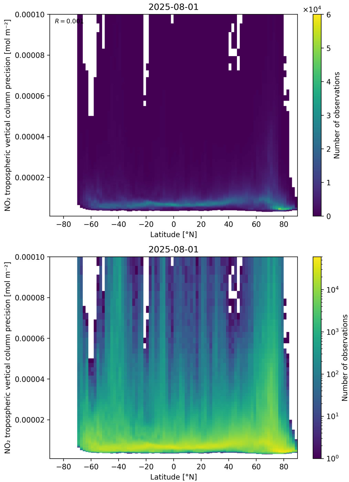
Figure 93: Scatter density plot of “Latitude” against “NO 2 tropospheric vertical column precision” for 2025-07-31 to 2025-08-02.
