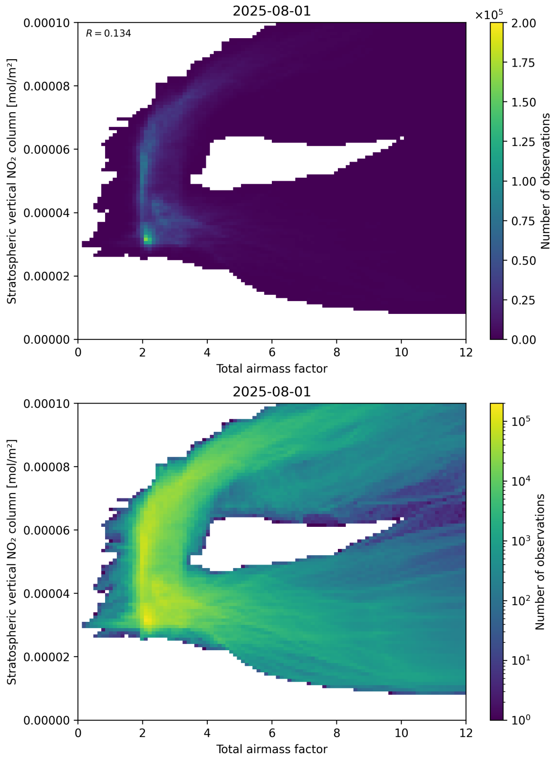
Figure 64: Scatter density plot of “Total airmass factor” against “Stratospheric vertical \text{NO}_2 column” for 2025-07-31 to 2025-08-02.
