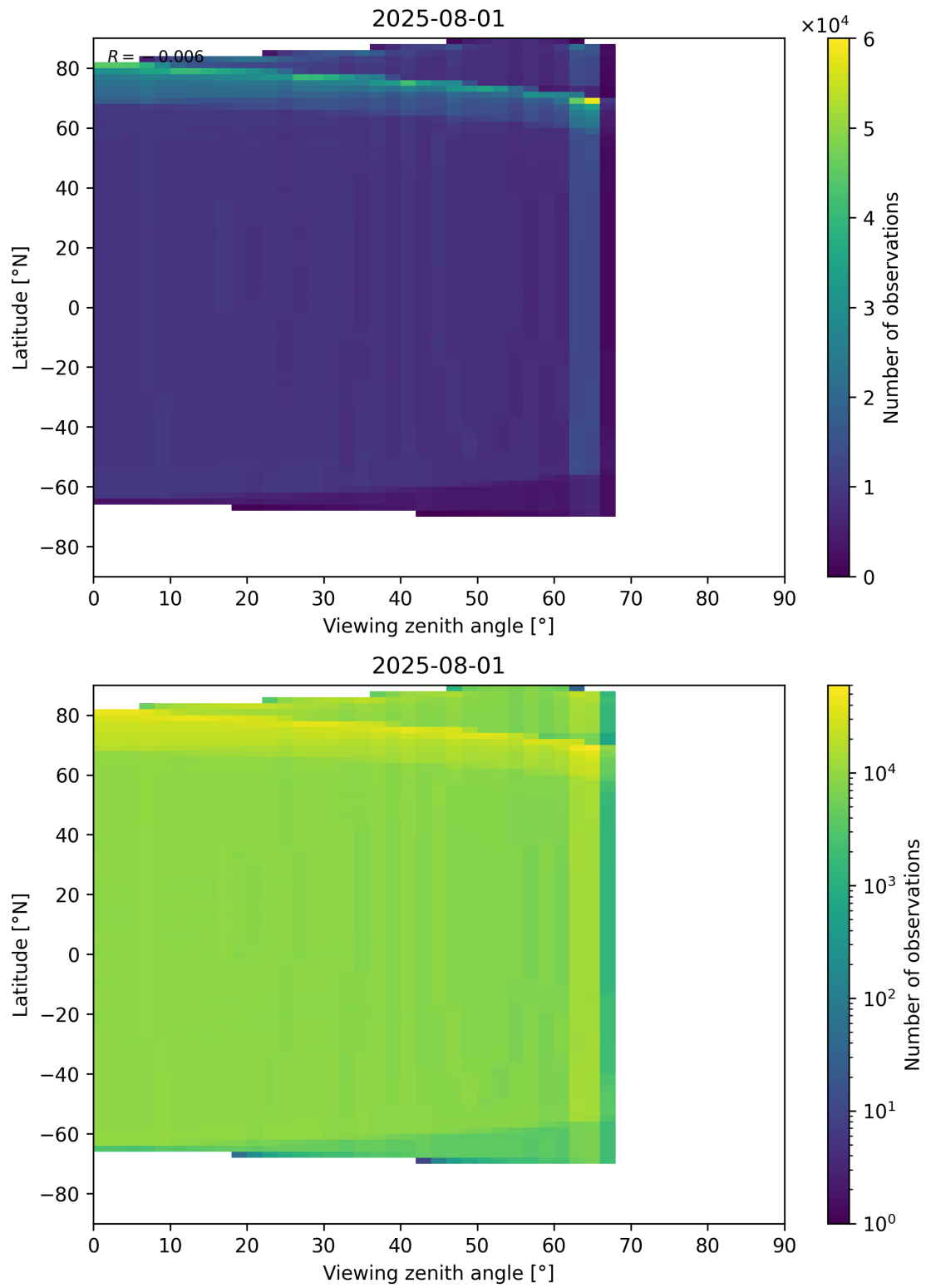
Figure 163: Scatter density plot of “Viewing zenith angle” against “Latitude” for 2025-07-31 to 2025-08-02.
