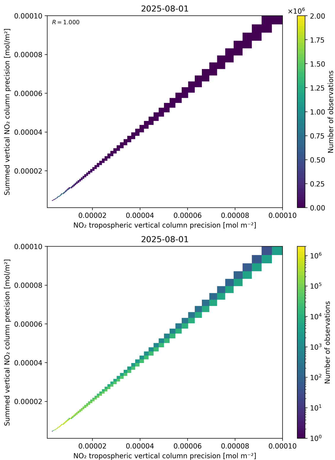
Figure 137: Scatter density plot of “NO 2 tropospheric vertical column precision” against “Summed vertical NO 2 column precision” for 2025-07-31 to 2025-08-02.
