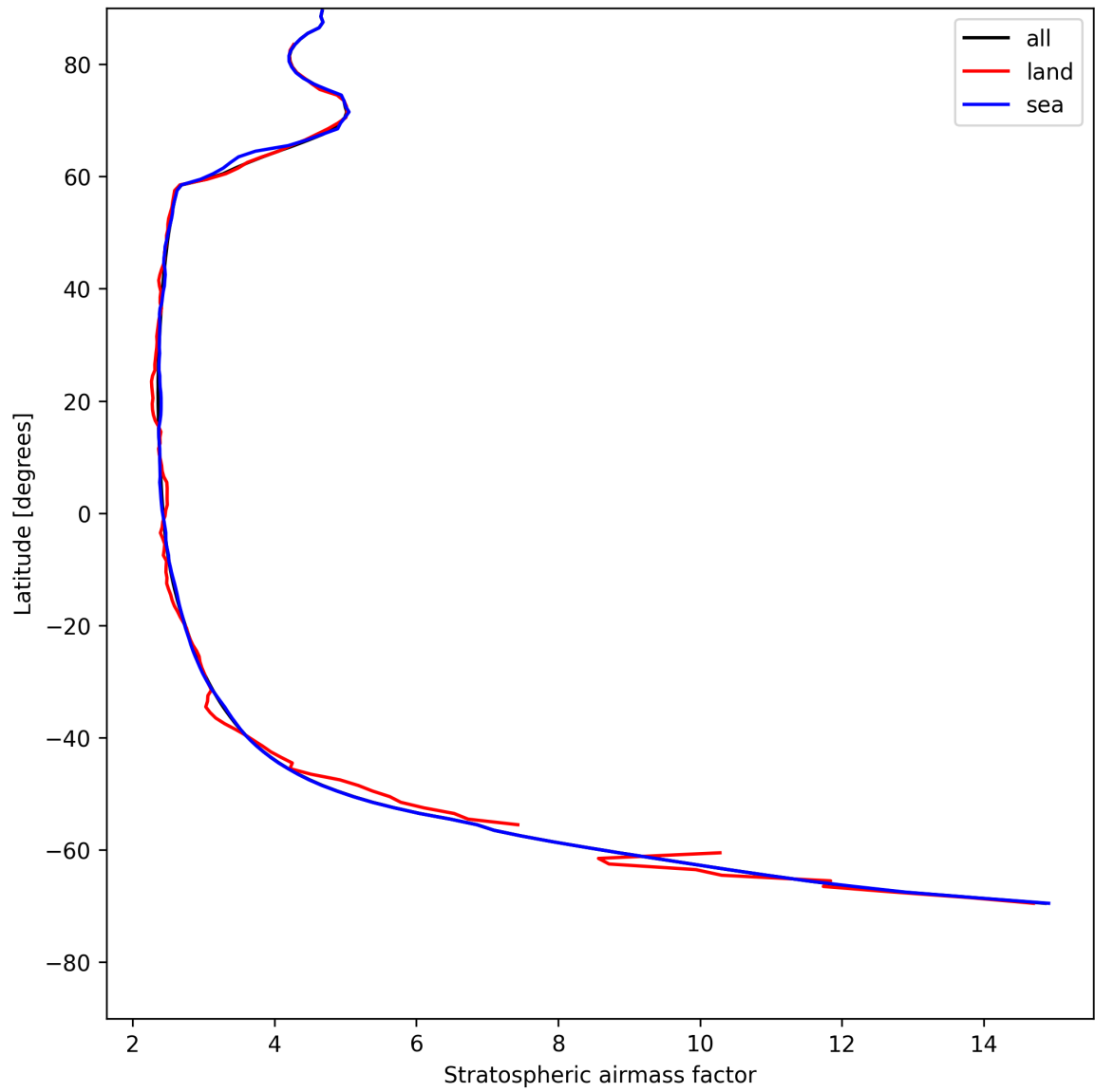
Figure 27: Zonal average of “Stratospheric airmass factor” for 2025-07-31 to 2025-08-02.
