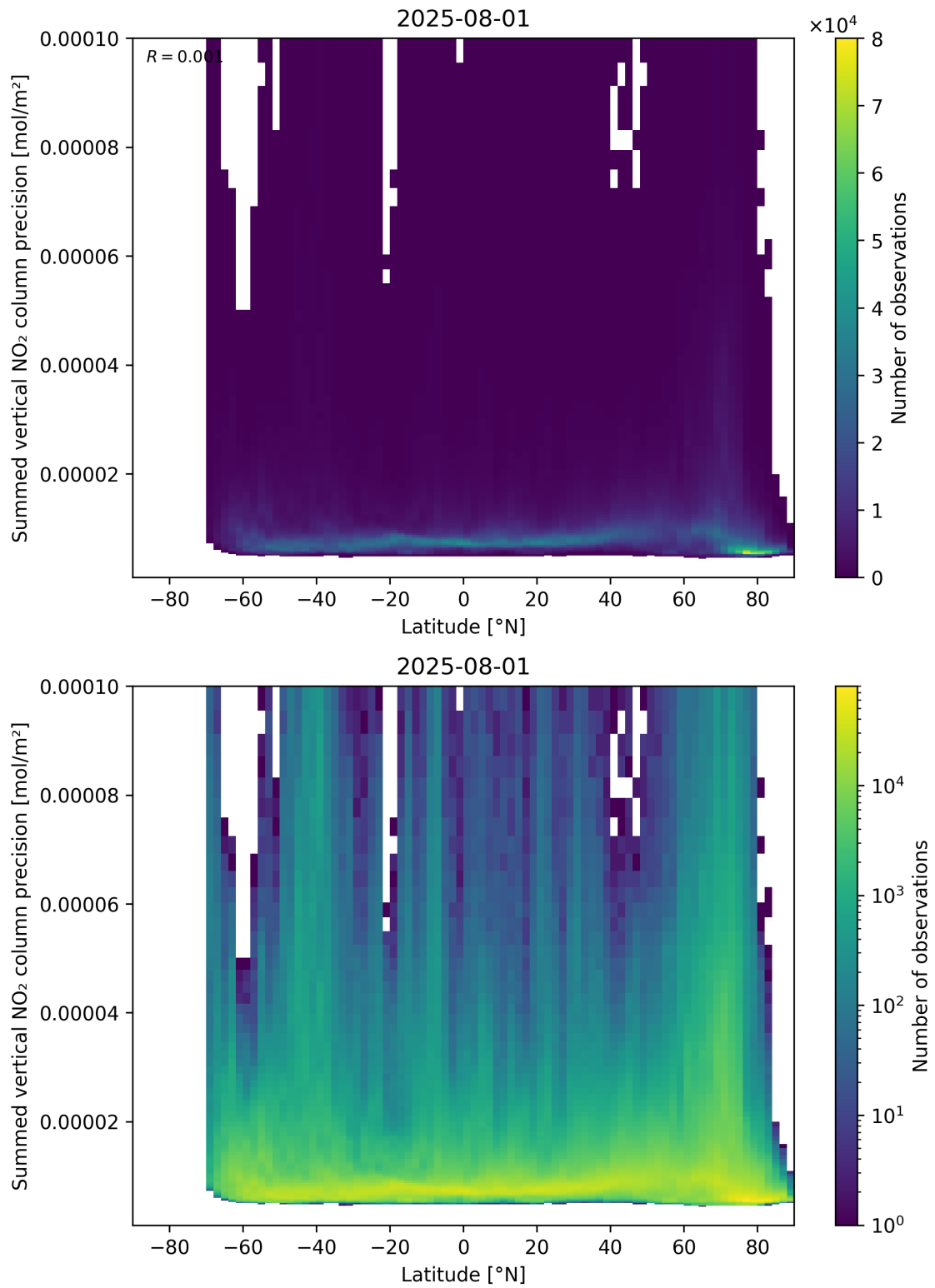
Figure 89: Scatter density plot of “Latitude” against “Summed vertical NO 2 column precision” for 2025-07-31 to 2025-08-02.
