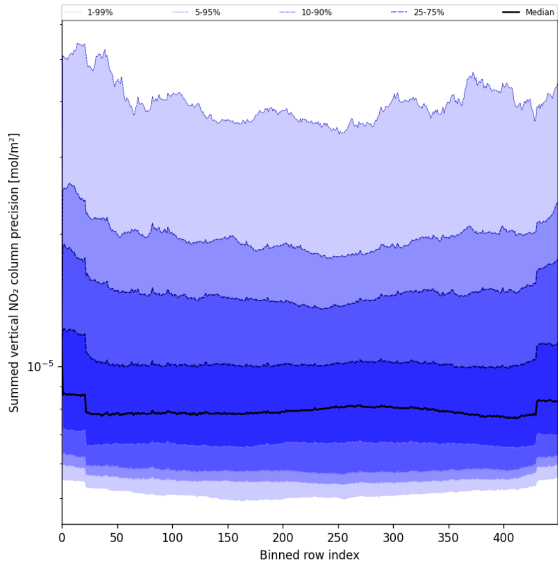
Figure 58: Along track statistics of “Summed vertical NO 2 column precision” for 2025-07-31 to 2025-08-02
