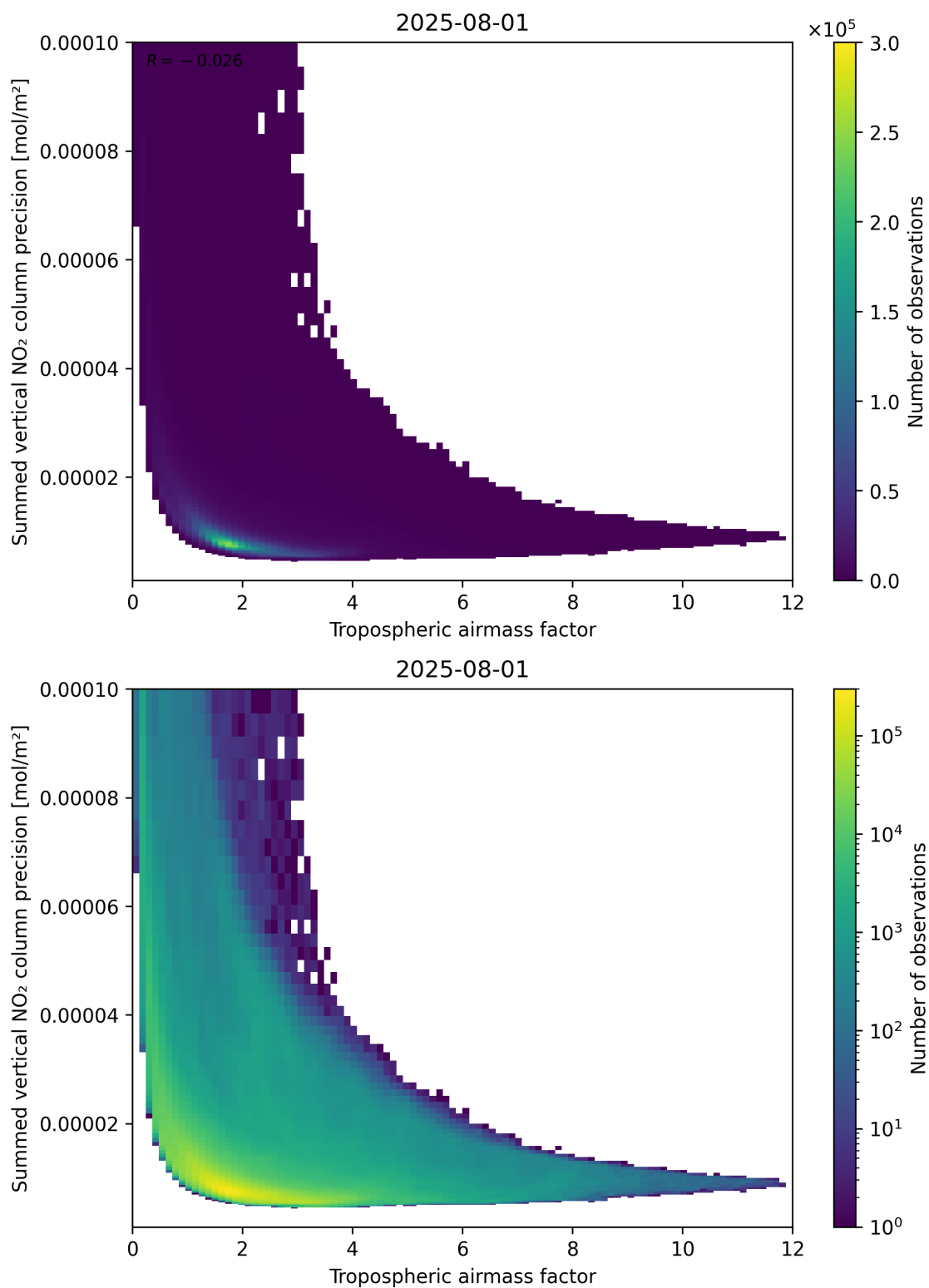
Figure 76: Scatter density plot of “Tropospheric air mass factor” against “Summed vertical NO 2 column precision” for 2025-07-31 to 2025-08-02.
