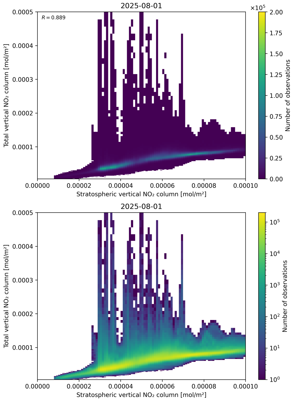
Figure 100: Scatter density plot of “Stratospheric vertical NO 2 column” against “Total vertical NO 2 column” for 2025-07-31 to 2025-08-02.
