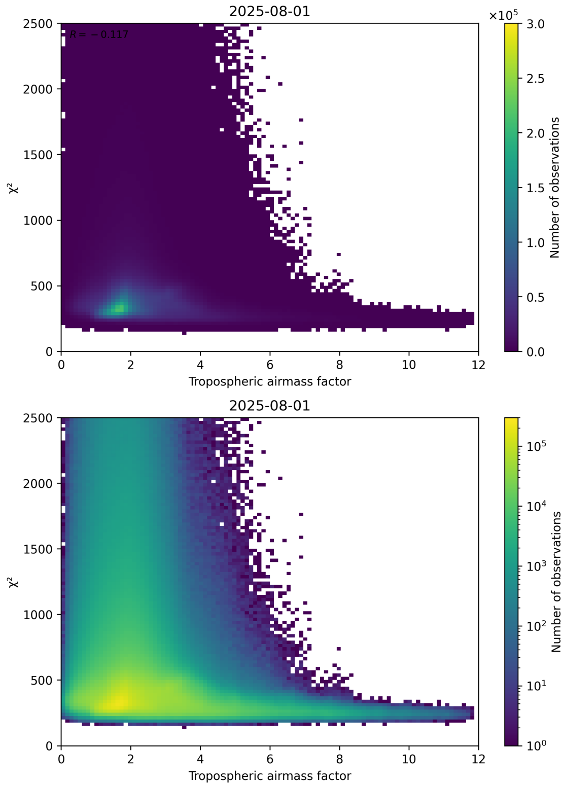
Figure 73: Scatter density plot of “Tropospheric airmass factor” against “ \chi^2 ” for 2025-07-31 to 2025-08-02.
