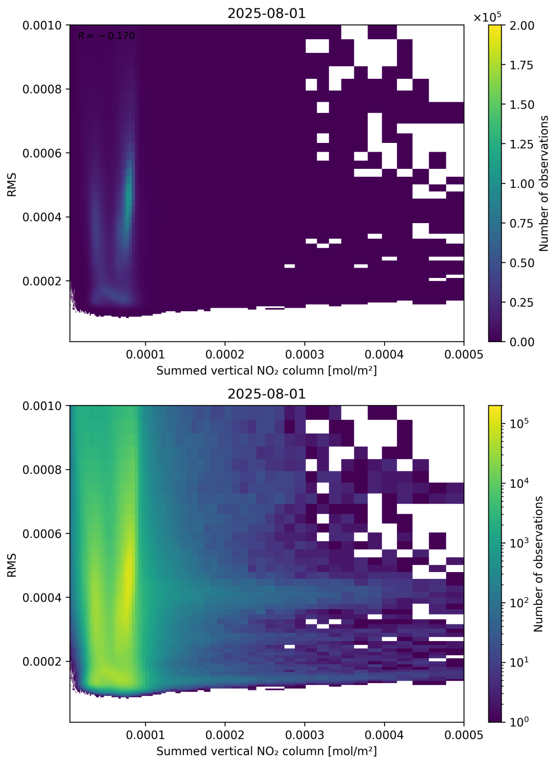
Figure 109: Scatter density plot of “Summed vertical NO 2 column” against “RMS” for 2025-07-31 to 2025-08-02.
