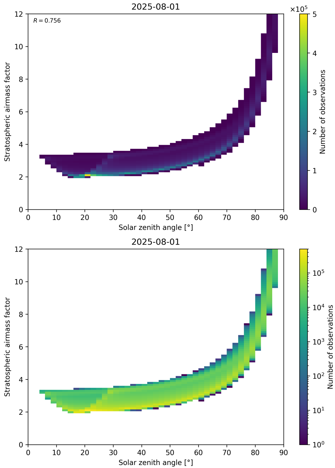
Figure 145: Scatter density plot of “Solar zenith angle” against “Stratospheric airmass factor” for 2025-07-31 to 2025-08-02.
