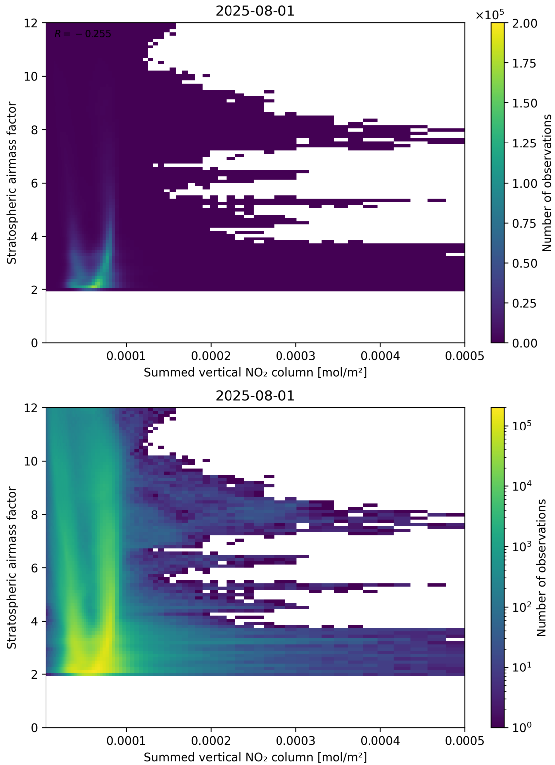
Figure 103: Scatter density plot of “Summed vertical NO 2 column” against “Stratospheric airmass factor” for 2025-07-31 to 2025-08-02.
