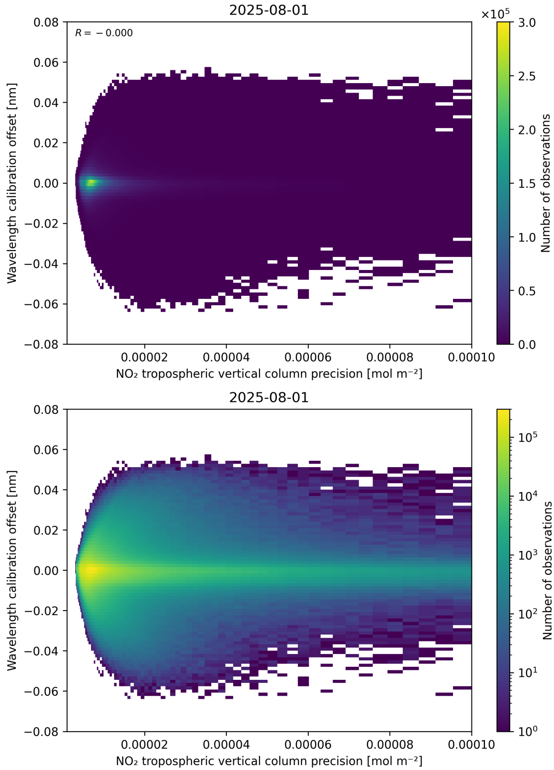
Figure 141: Scatter density plot of “NO 2 tropospheric vertical column precision” against “Wavelength calibration offset” for 2025-07-31 to 2025-08-02.
