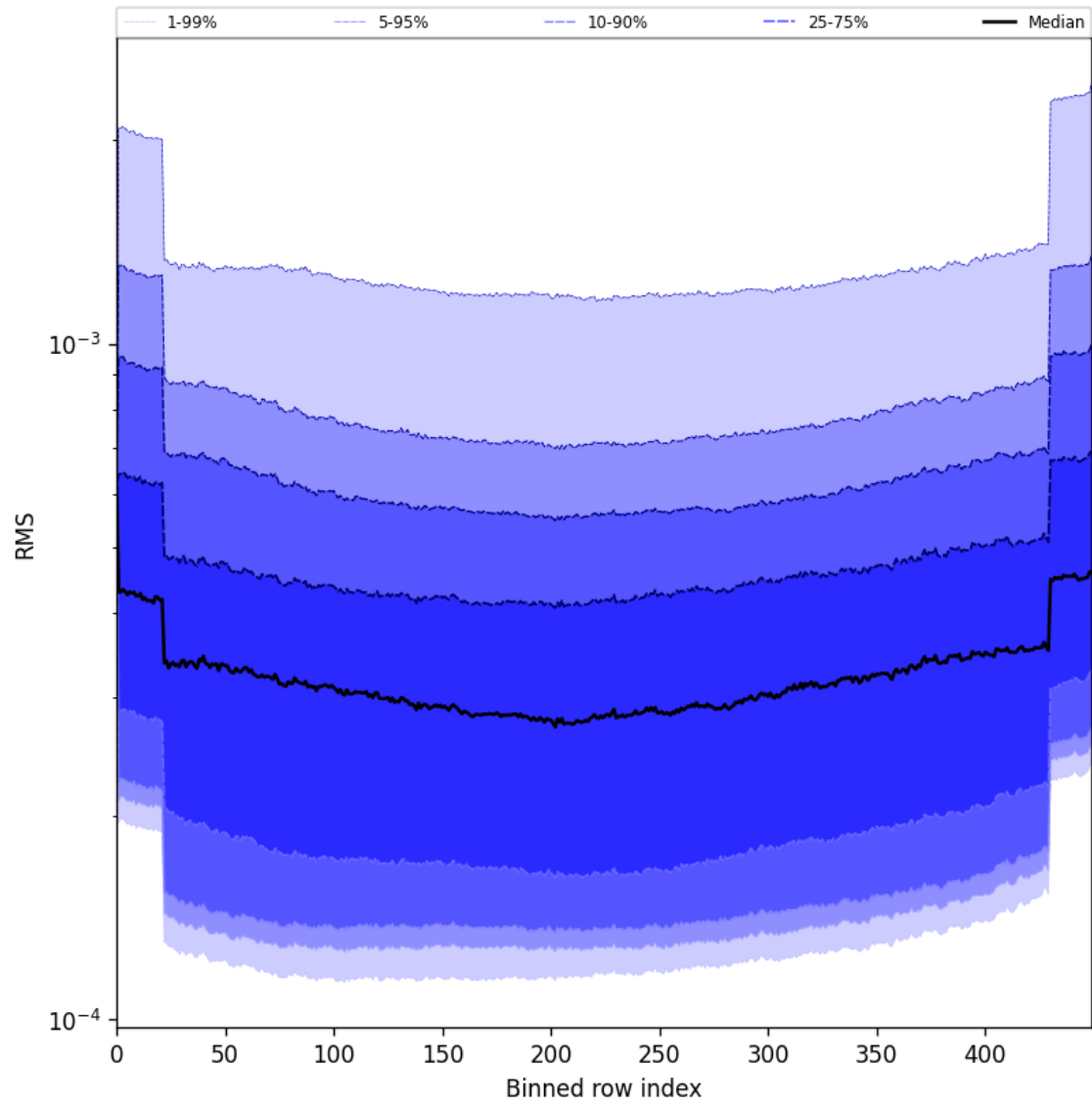
Figure 60: Along track statistics of “RMS” for 2025-07-31 to 2025-08-02
