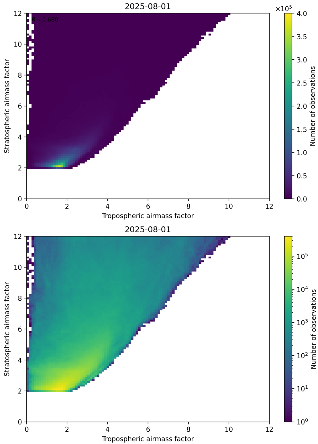
Figure 71: Scatter density plot of “Tropospheric airmass factor” against “Stratospheric airmass factor” for 2025-07-31 to 2025-08-02.
