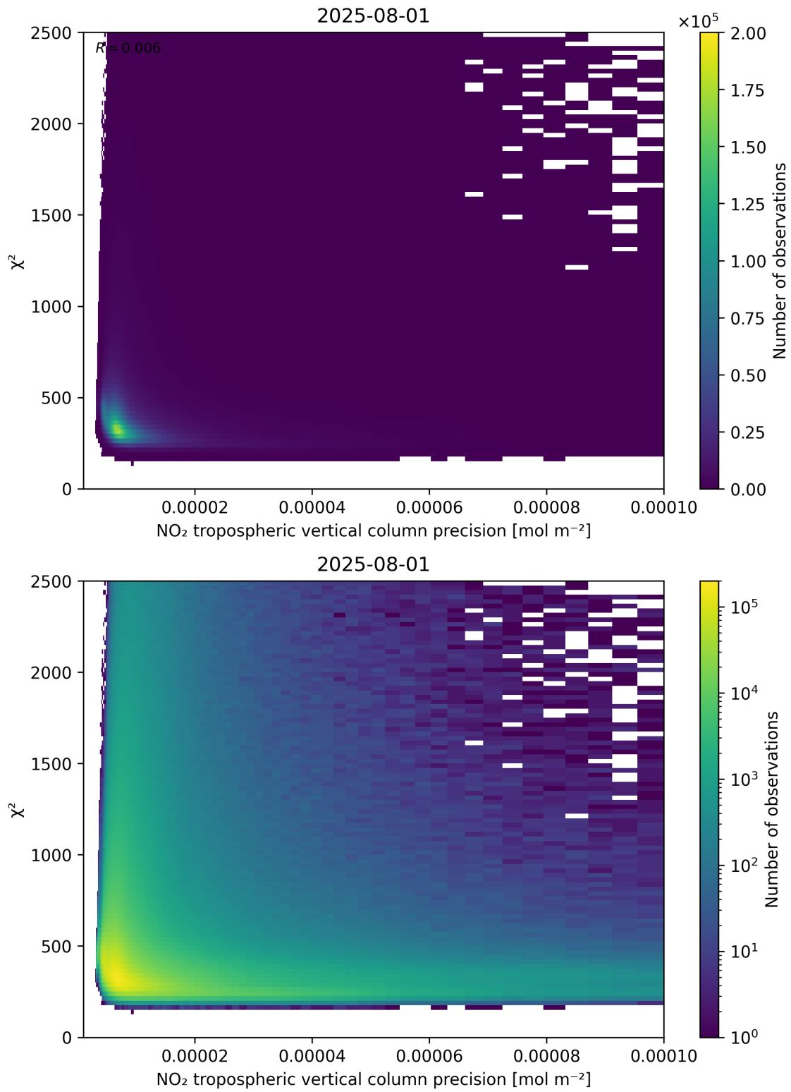
Figure 134: Scatter density plot of “NO 2 tropospheric vertical column precision” against “ \chi^2 ” for 2025-07-31 to 2025-08-02.
