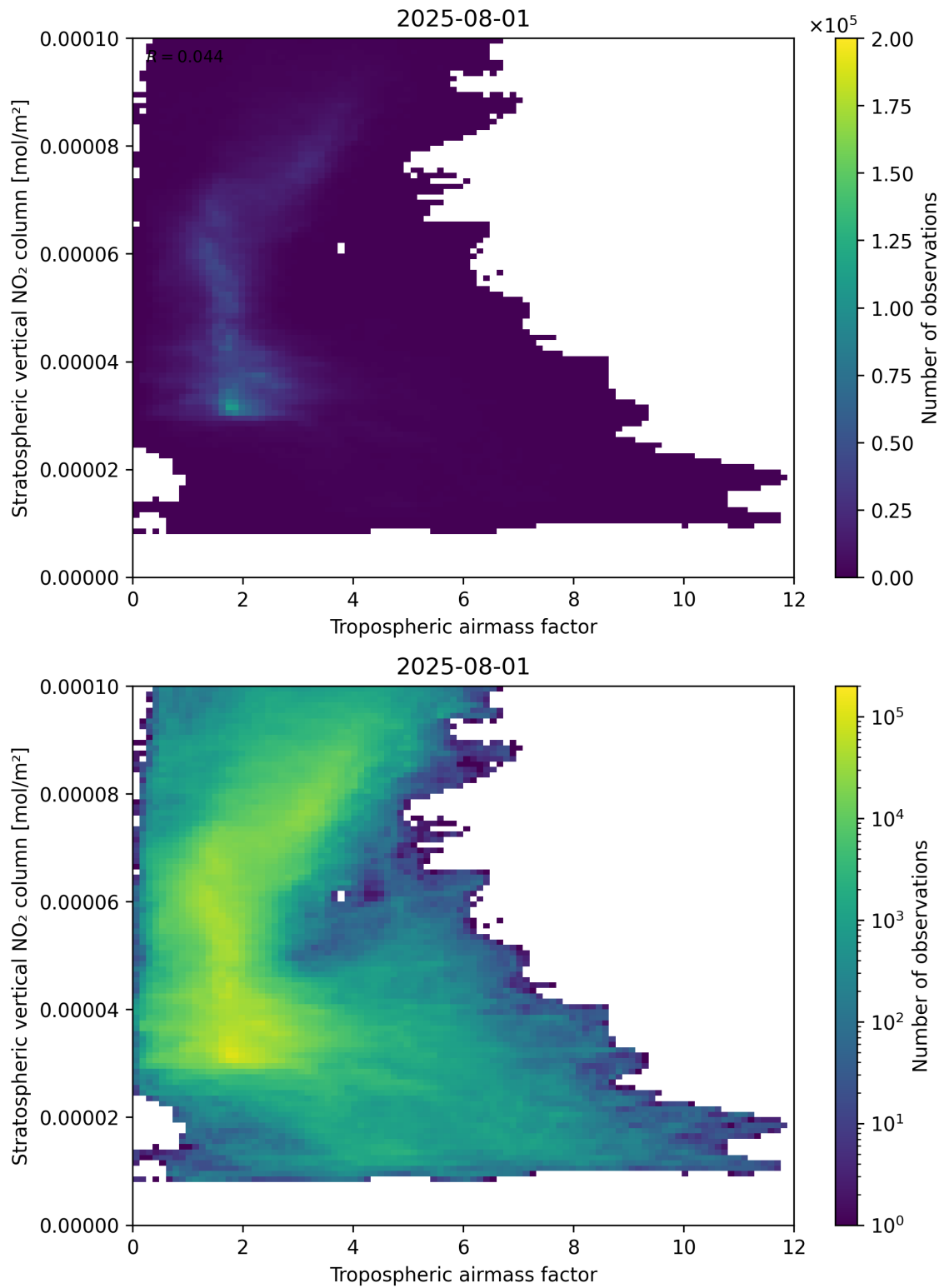
Figure 74: Scatter density plot of “Tropospheric airmass factor” against “Stratospheric vertical NO 2 column” for 2025-07-31 to 2025-08-02.
