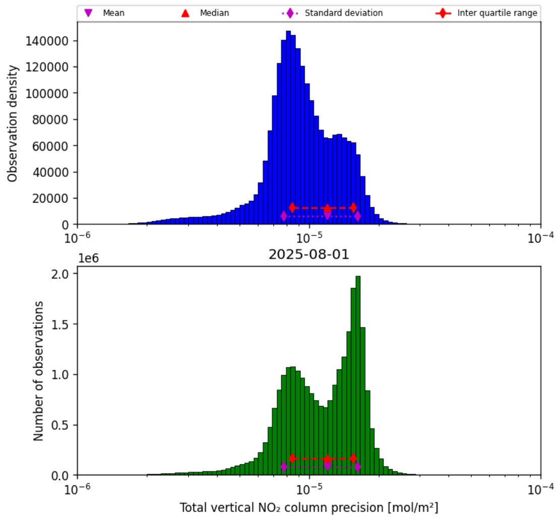
Figure 39: Histogram of “Total vertical NO 2 column precision” for 2025-07-31 to 2025-08-02
