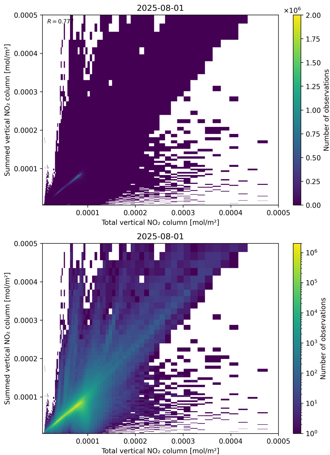
Figure 112: Scatter density plot of “Total vertical NO 2 column” against “Summed vertical NO 2 column” for 2025-07-31 to 2025-08-02.
