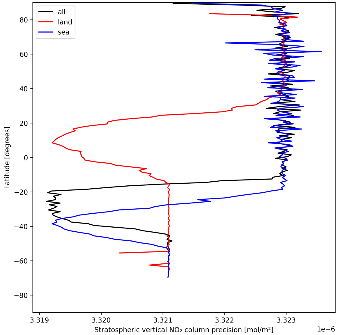
Figure 20: Zonal average of “Stratospheric vertical NO 2 column precision” for 2025-07-31 to 2025-08-02.
