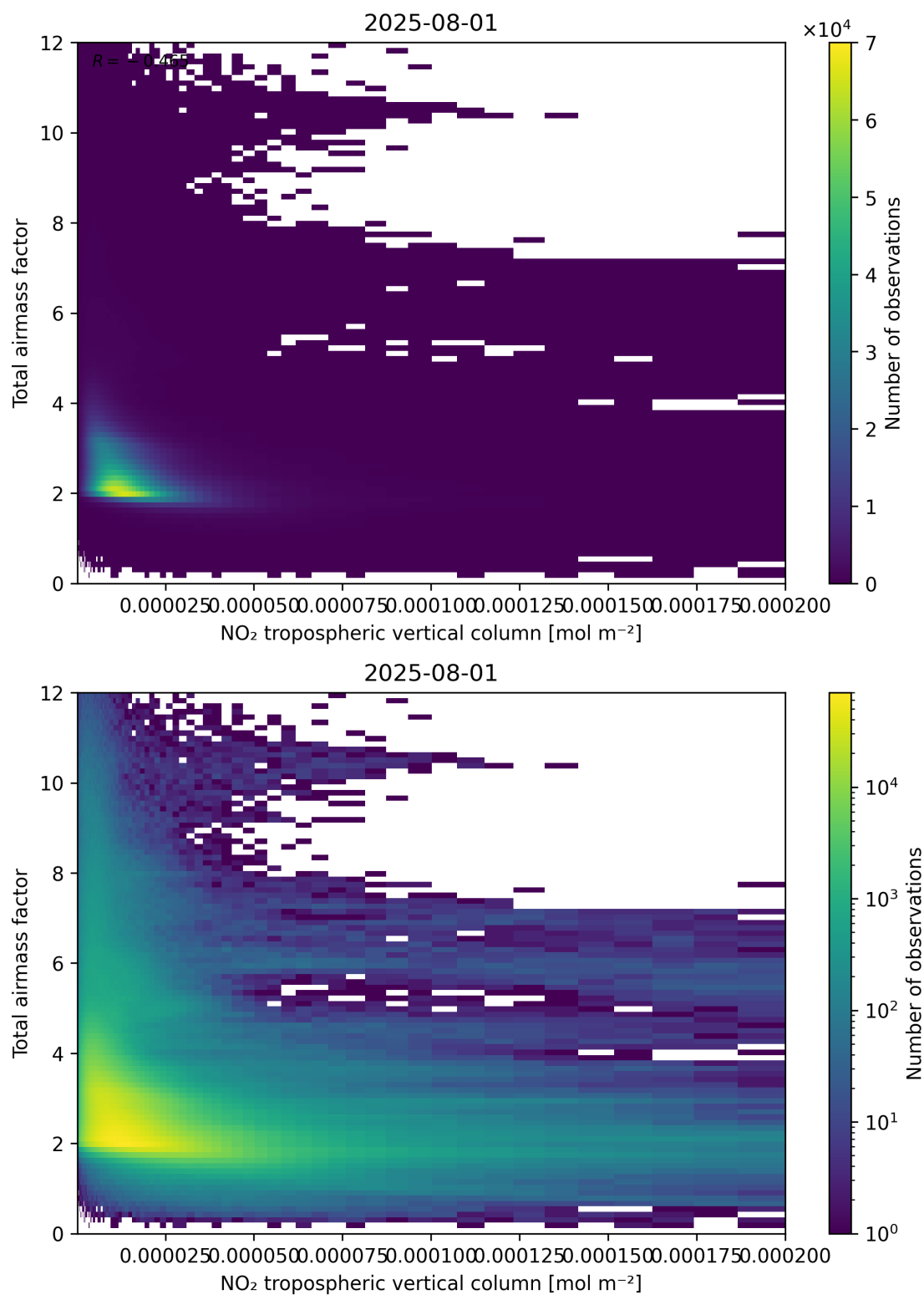
Figure 122: Scatter density plot of “NO 2 tropospheric vertical column” against “Total air mass factor” for 2025-07-31 to 2025-08-02.
