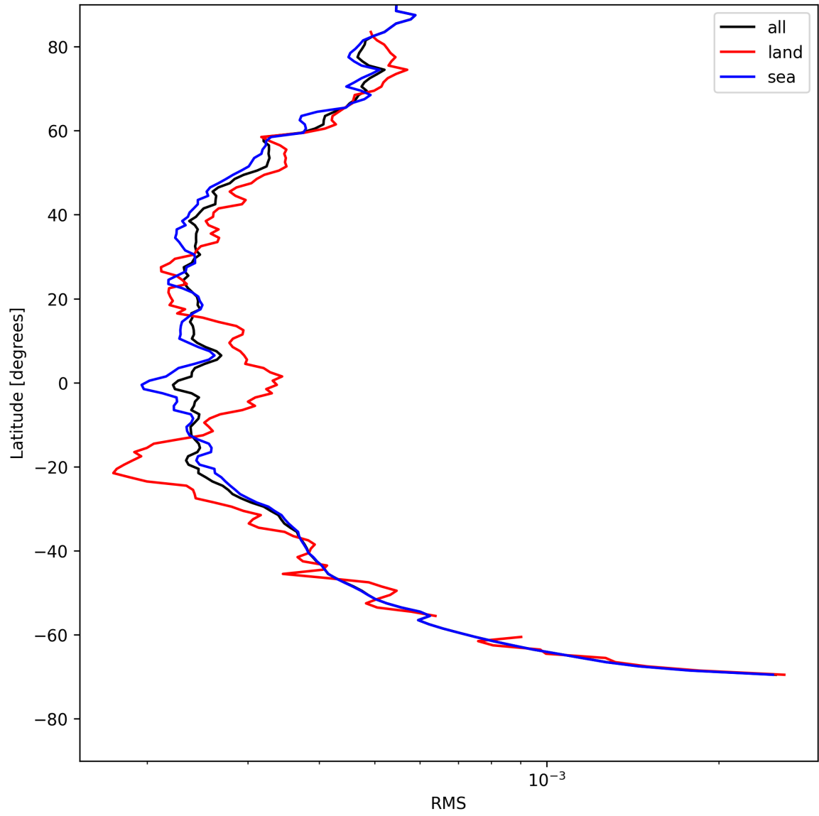
Figure 26: Zonal average of “RMS” for 2025-07-31 to 2025-08-02.
