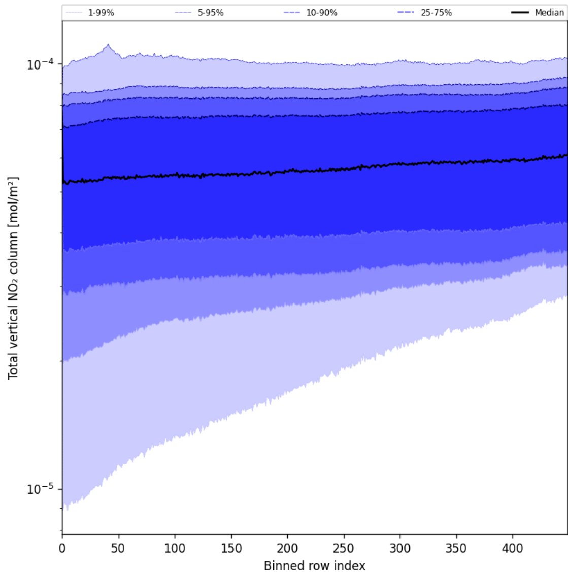
Figure 55: Along track statistics of “Total vertical NO 2 column” for 2025-07-31 to 2025-08-02
