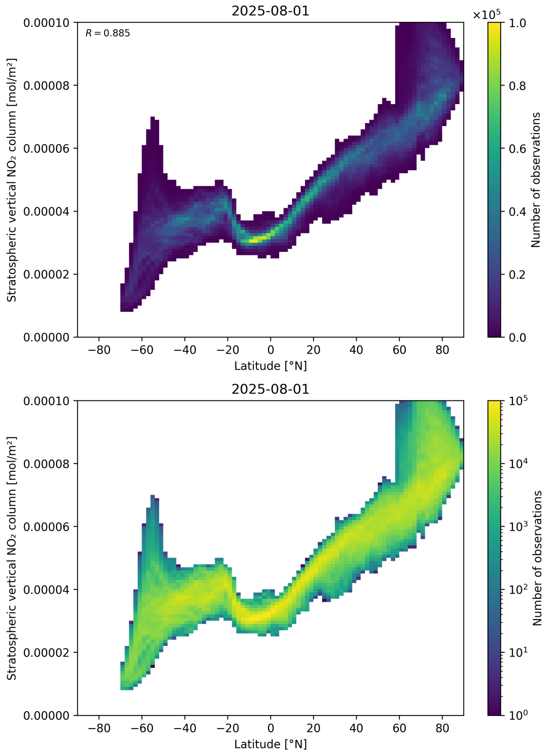
Figure 87: Scatter density plot of “Latitude” against “Stratospheric vertical NO 2 column” for 2025-07-31 to 2025-08-02.
