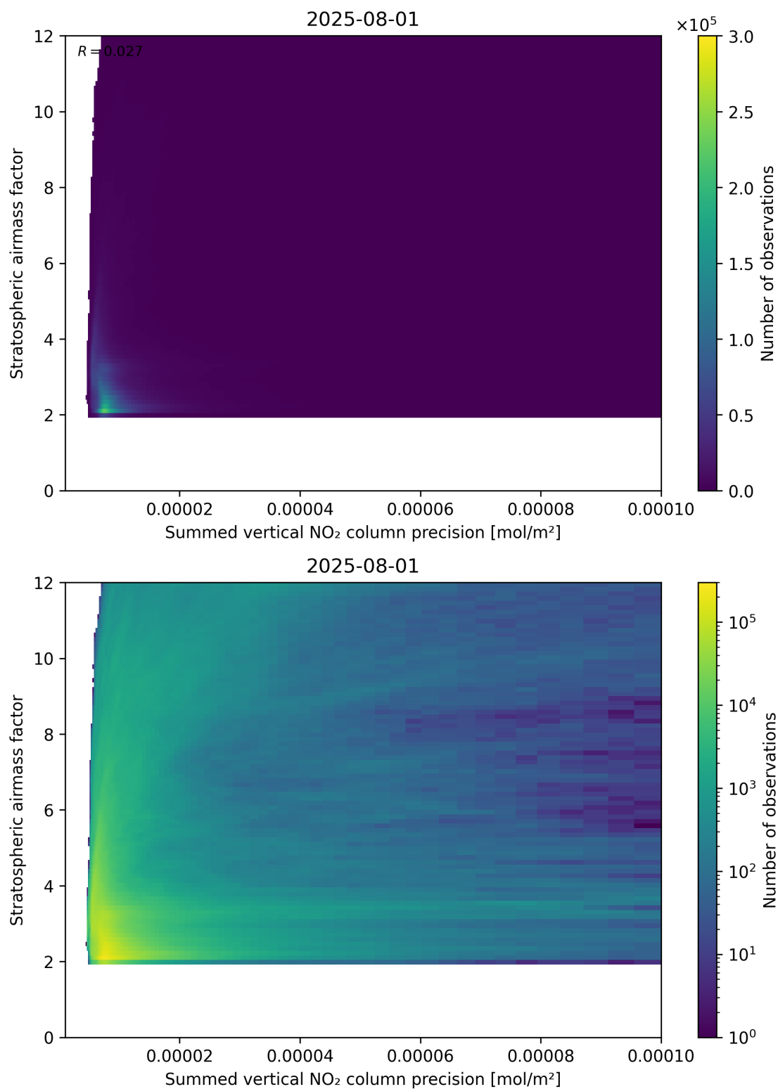
Figure 106: Scatter density plot of “Summed vertical NO 2 column precision” against “Stratospheric airmass factor” for 2025-07-31 to 2025-08-02.
