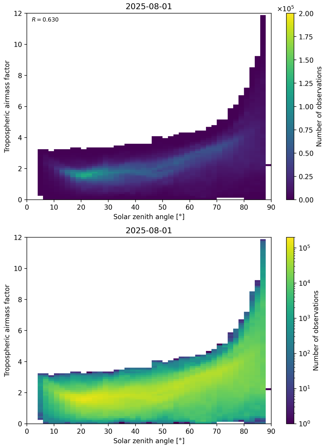
Figure 147: Scatter density plot of “Solar zenith angle” against “Tropospheric airmass factor” for 2025-07-31 to 2025-08-02.
