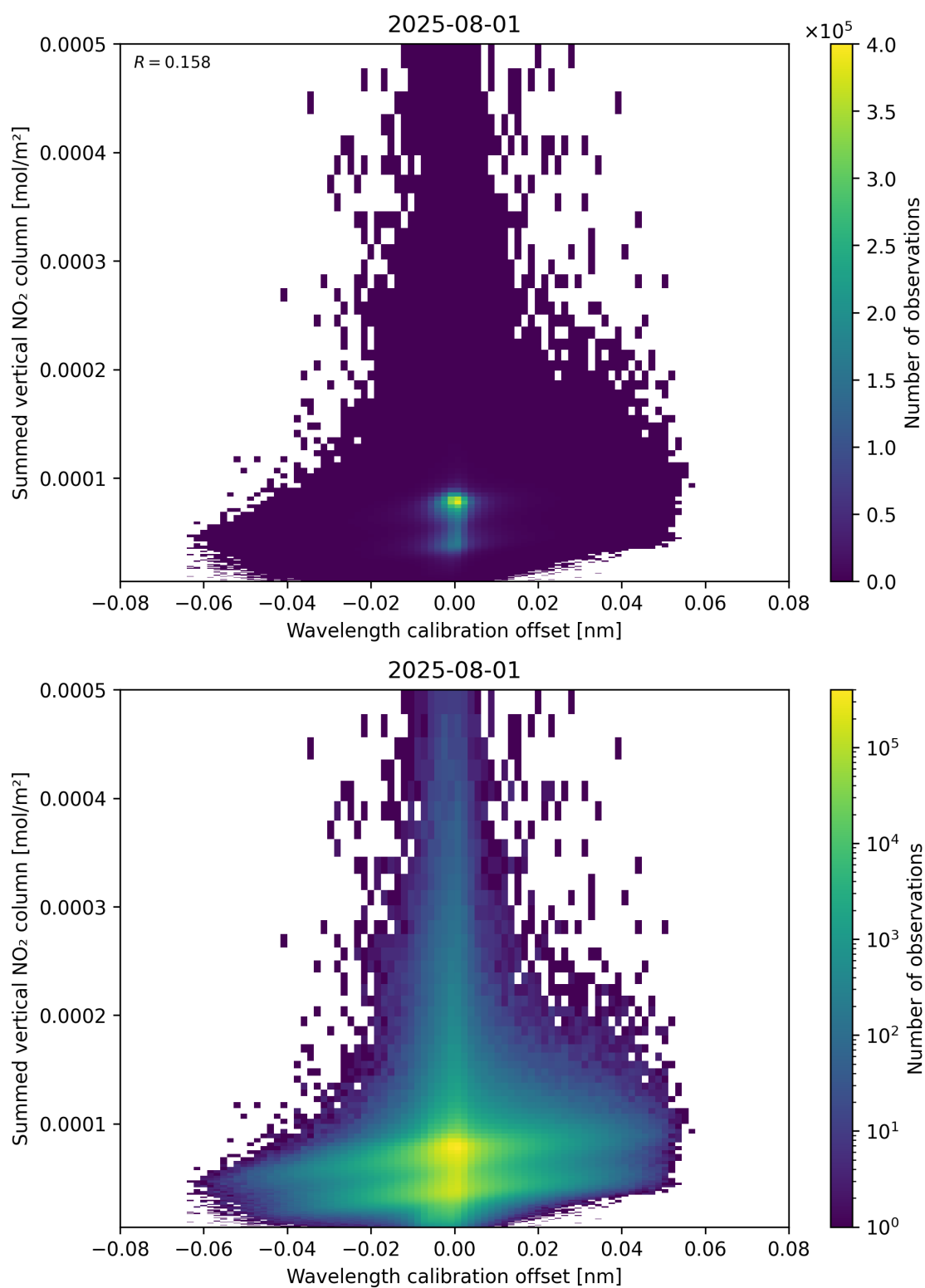
Figure 177: Scatter density plot of “Wavelength calibration offset” against “Summed vertical NO 2 column” for 2025-07-31 to 2025-08-02.
