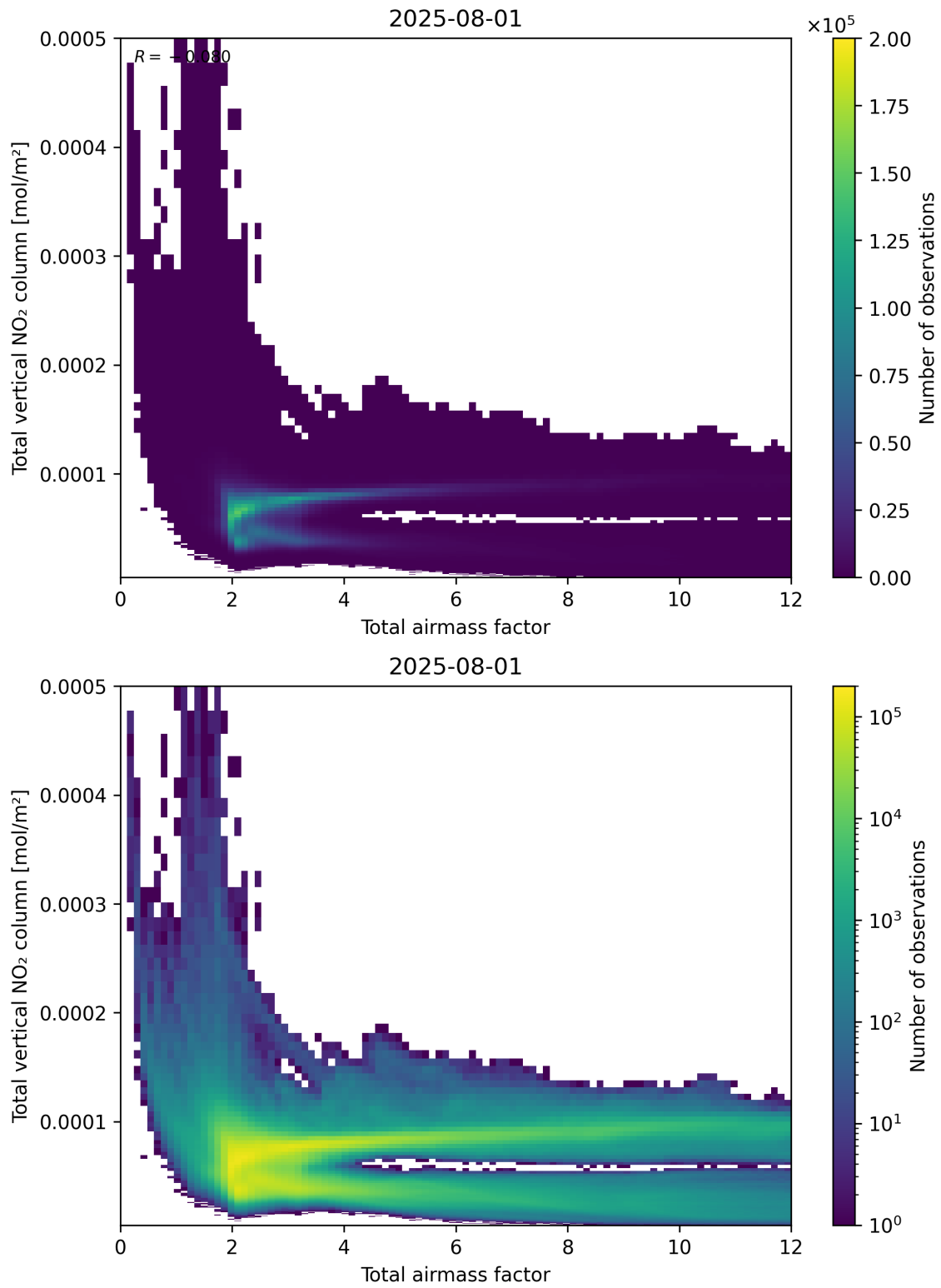
Figure 67: Scatter density plot of “Total airmass factor” against “Total vertical NO 2 column” for 2025-07-31 to 2025-08-02.
