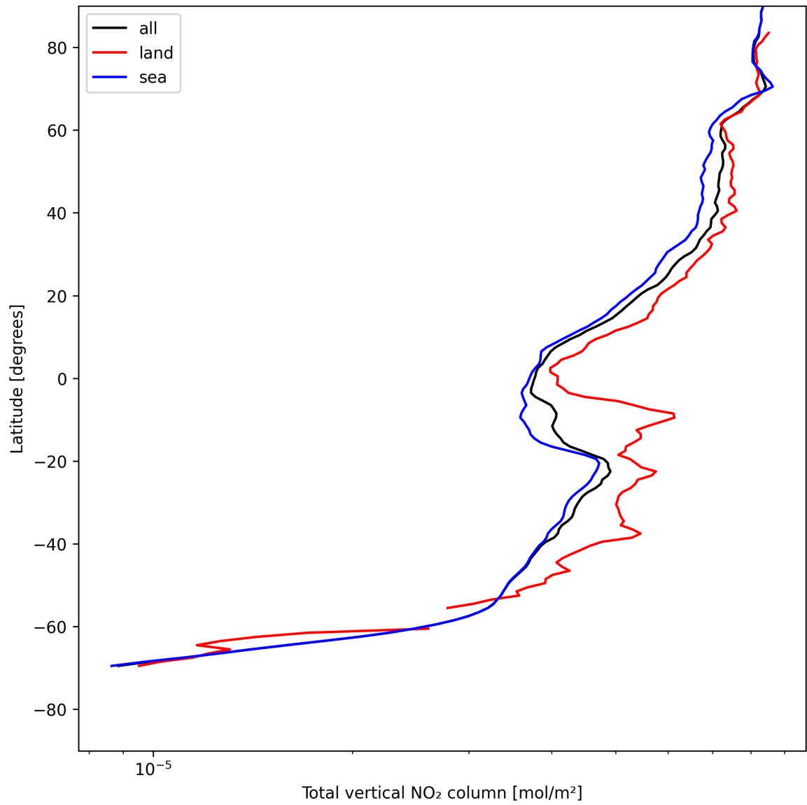
Figure 21: Zonal average of “Total vertical NO 2 column” for 2025-07-31 to 2025-08-02.
