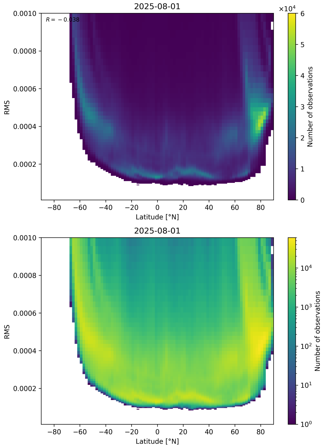
Figure 94: Scatter density plot of “Latitude” against “RMS” for 2025-07-31 to 2025-08-02.
