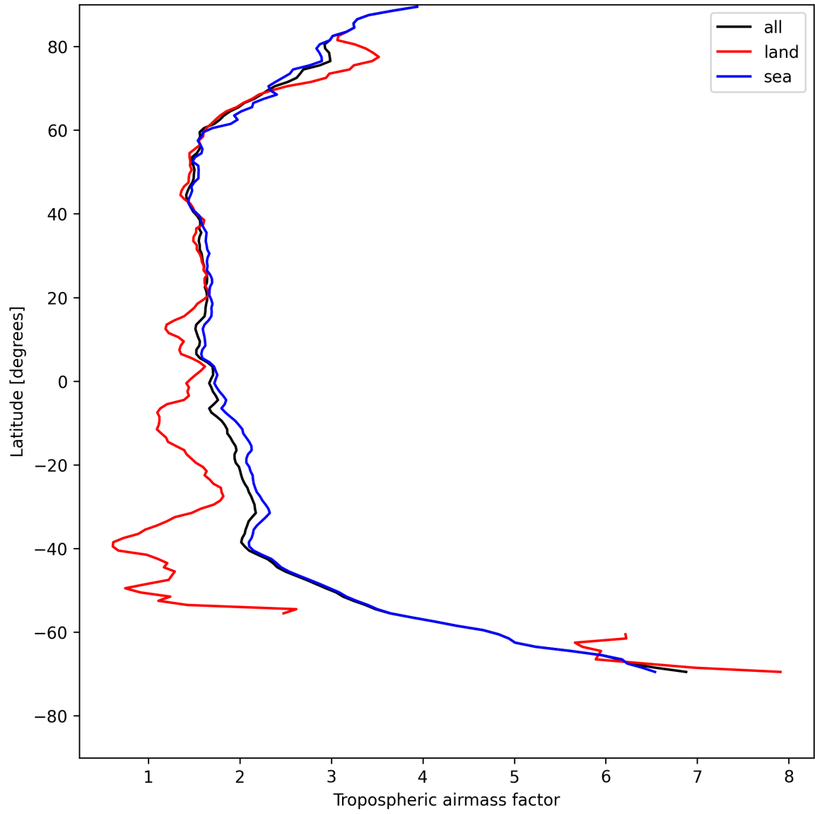
Figure 14: Zonal average of “Tropospheric air mass factor” for 2025-07-31 to 2025-08-02.
