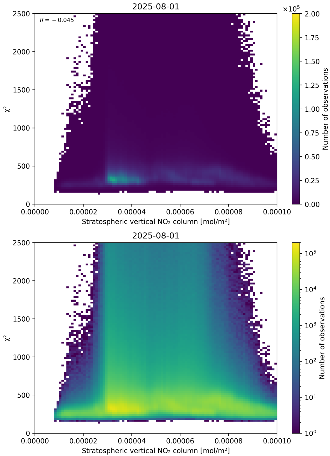
Figure 97: Scatter density plot of “Stratospheric vertical NO 2 column” against “ \chi^2 ” for 2025-07-31 to 2025-08-02.
