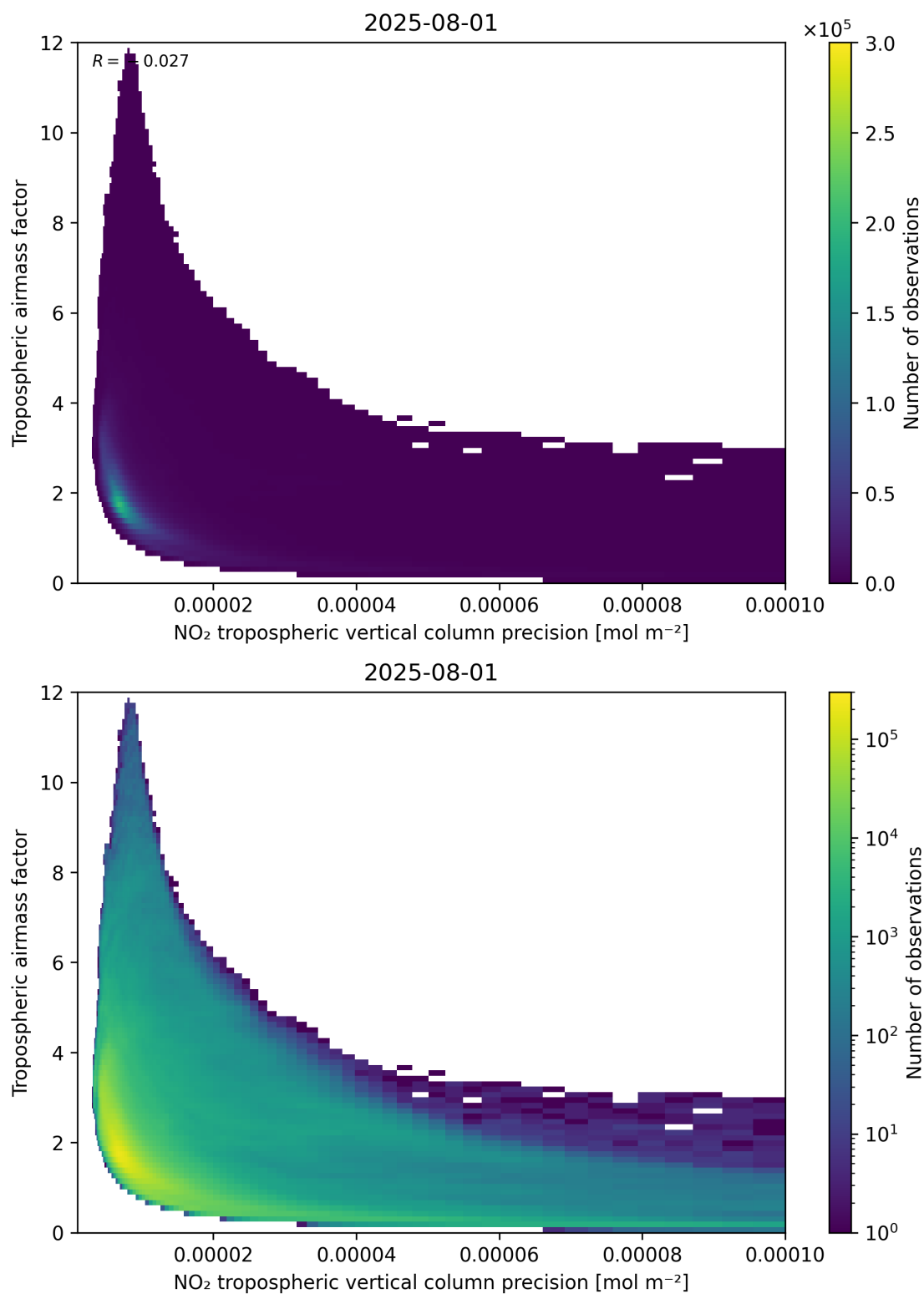
Figure 133: Scatter density plot of “NO 2 tropospheric vertical column precision” against “Tropospheric airmass factor” for 2025-07-31 to 2025-08-02.
