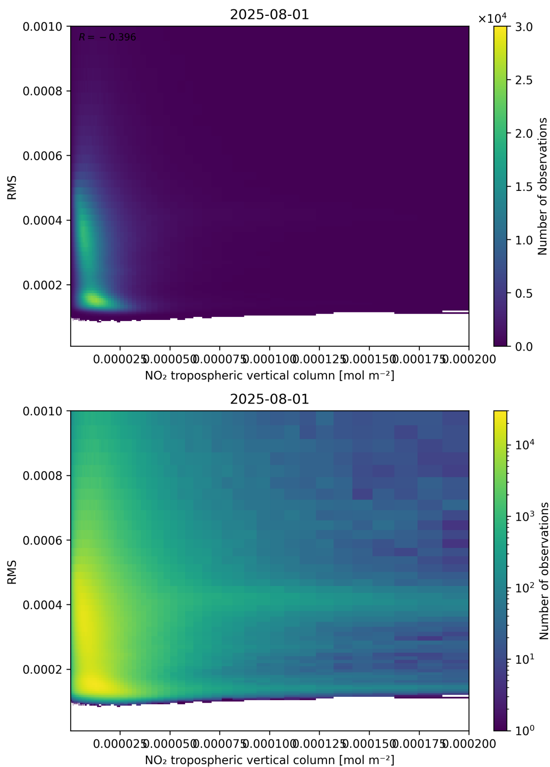
Figure 142: Scatter density plot of “NO 2 tropospheric vertical column” against “RMS” for 2025-07-31 to 2025-08-02.
