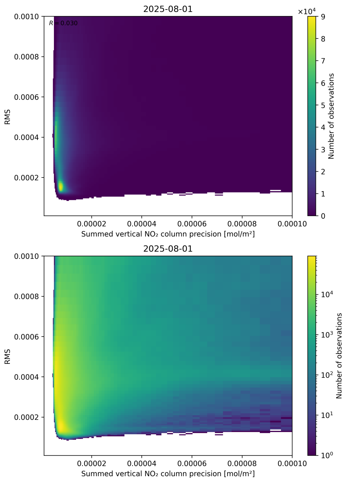
Figure 108: Scatter density plot of “Summed vertical NO 2 column precision” against “RMS” for 2025-07-31 to 2025-08-02.
