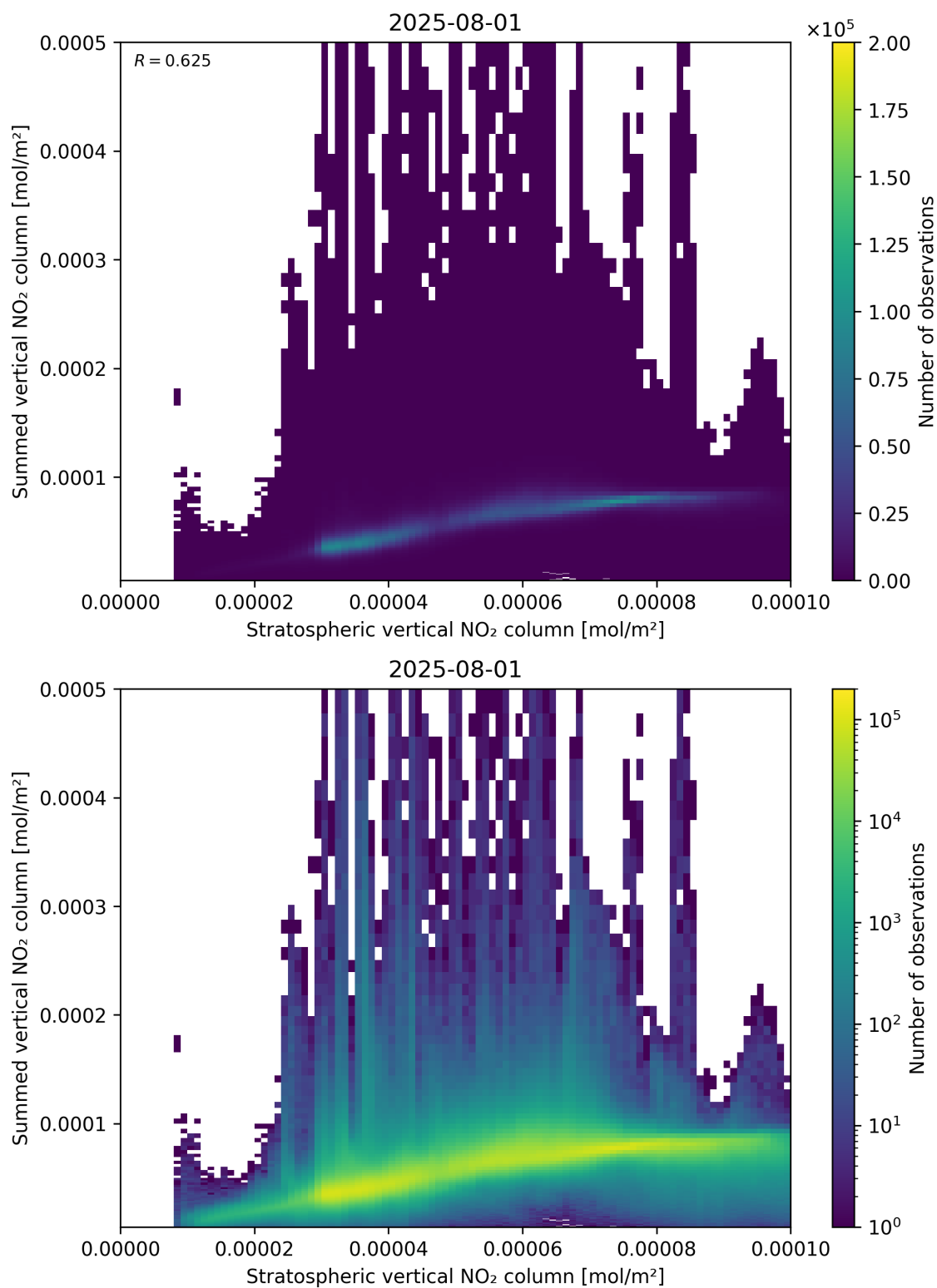
Figure 98: Scatter density plot of “Stratospheric vertical NO 2 column” against “Summed vertical NO 2 column” for 2025-07-31 to 2025-08-02.
