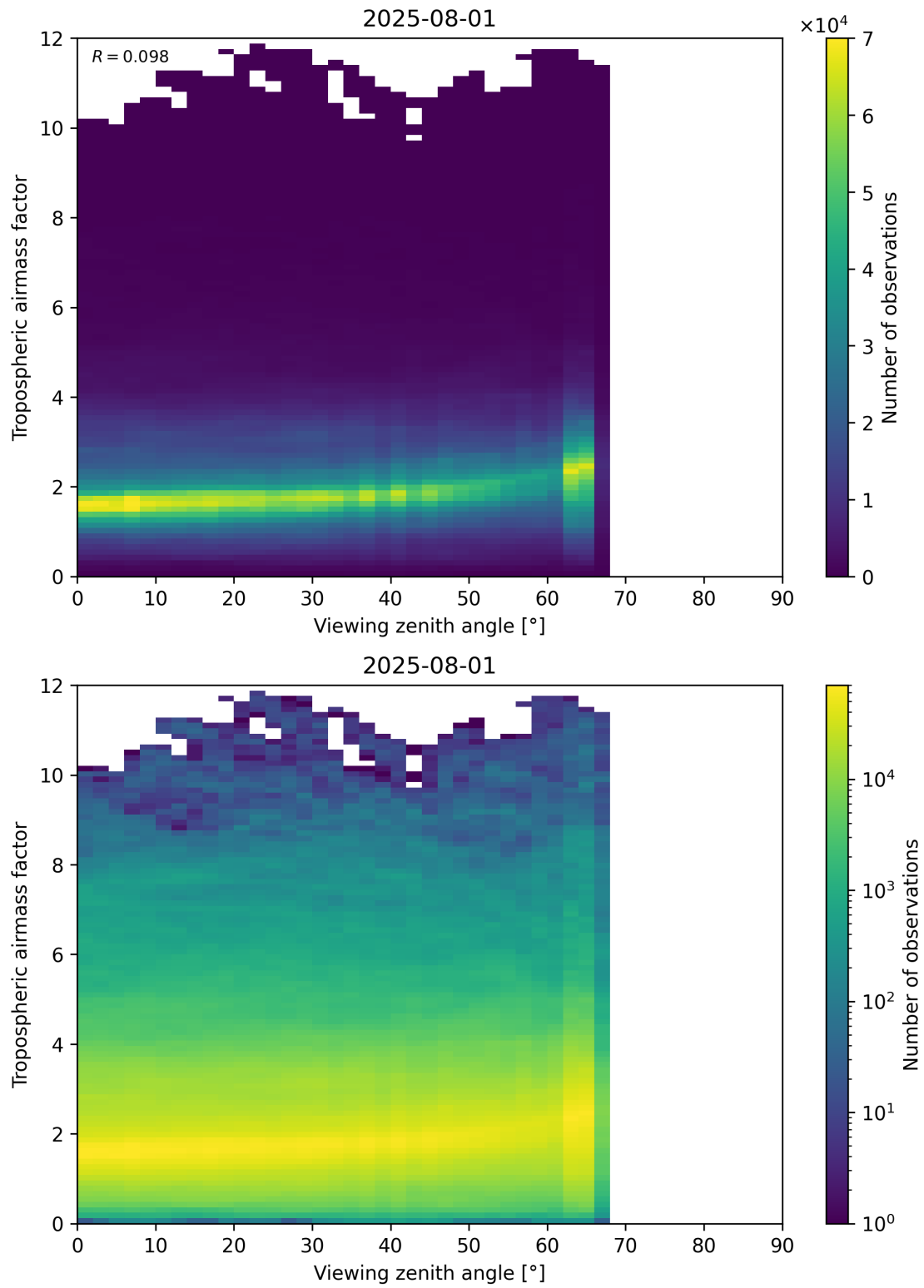
Figure 161: Scatter density plot of “Viewing zenith angle” against “Tropospheric airmass factor” for 2025-07-31 to 2025-08-02.
