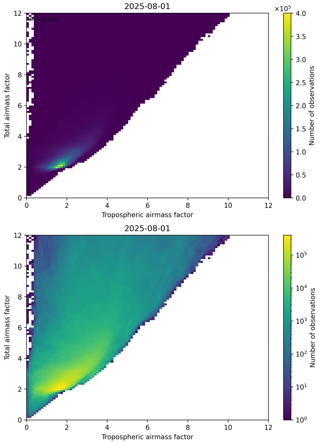
Figure 72: Scatter density plot of “Tropospheric airmass factor” against “Total airmass factor” for 2025-07-31 to 2025-08-02.
