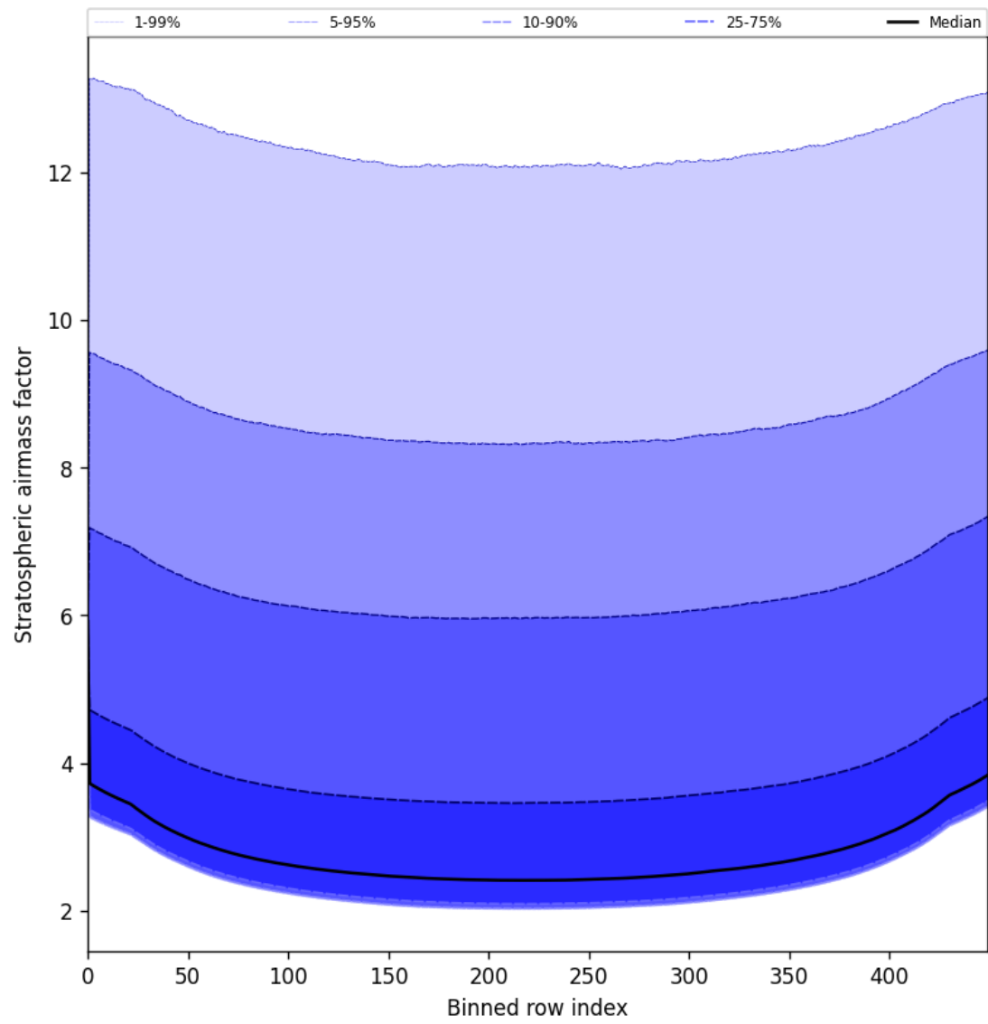
Figure 61: Along track statistics of “Stratospheric airmass factor” for 2025-07-31 to 2025-08-02
