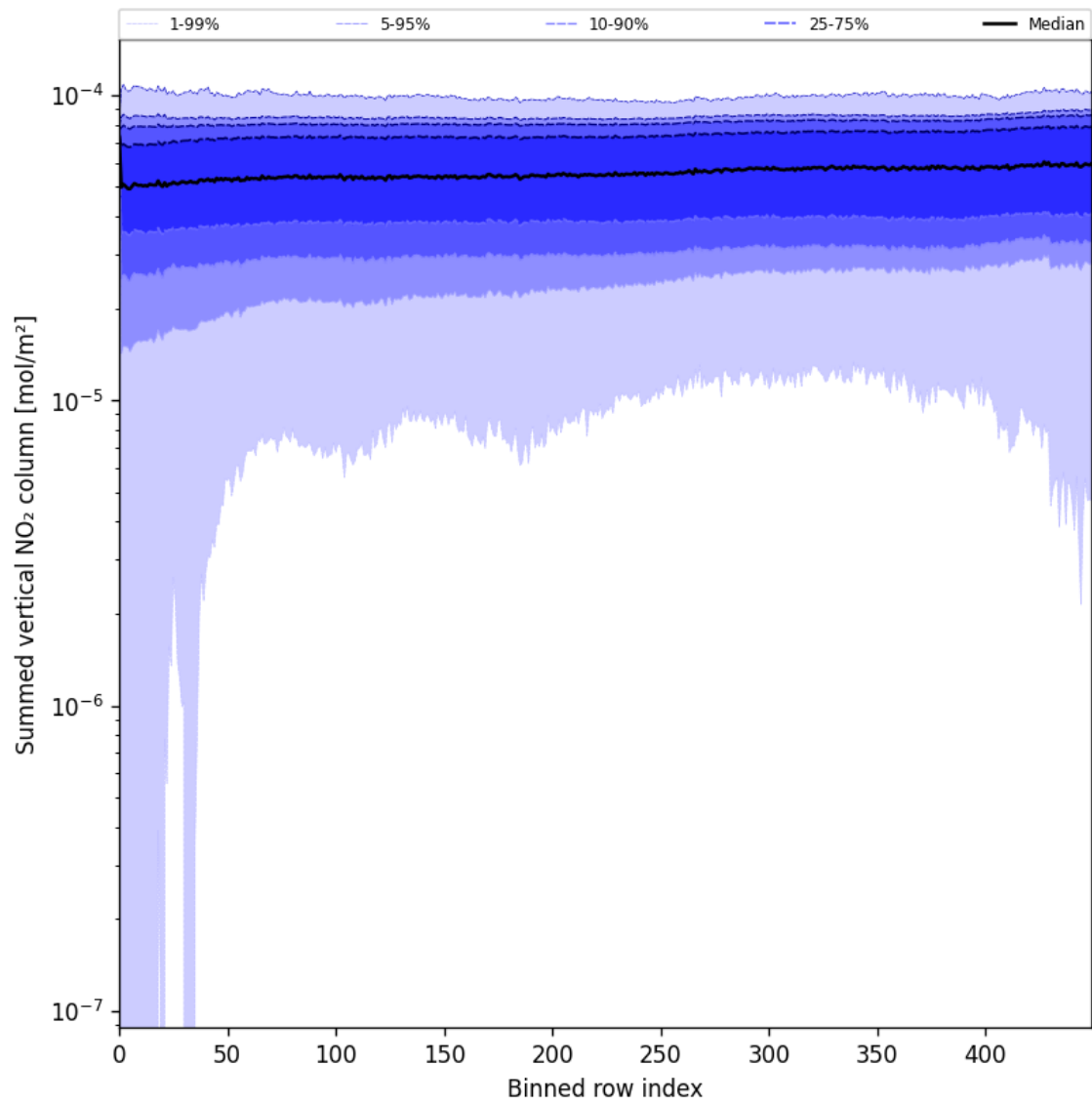
Figure 57: Along track statistics of “Summed vertical NO 2 column” for 2025-07-31 to 2025-08-02
