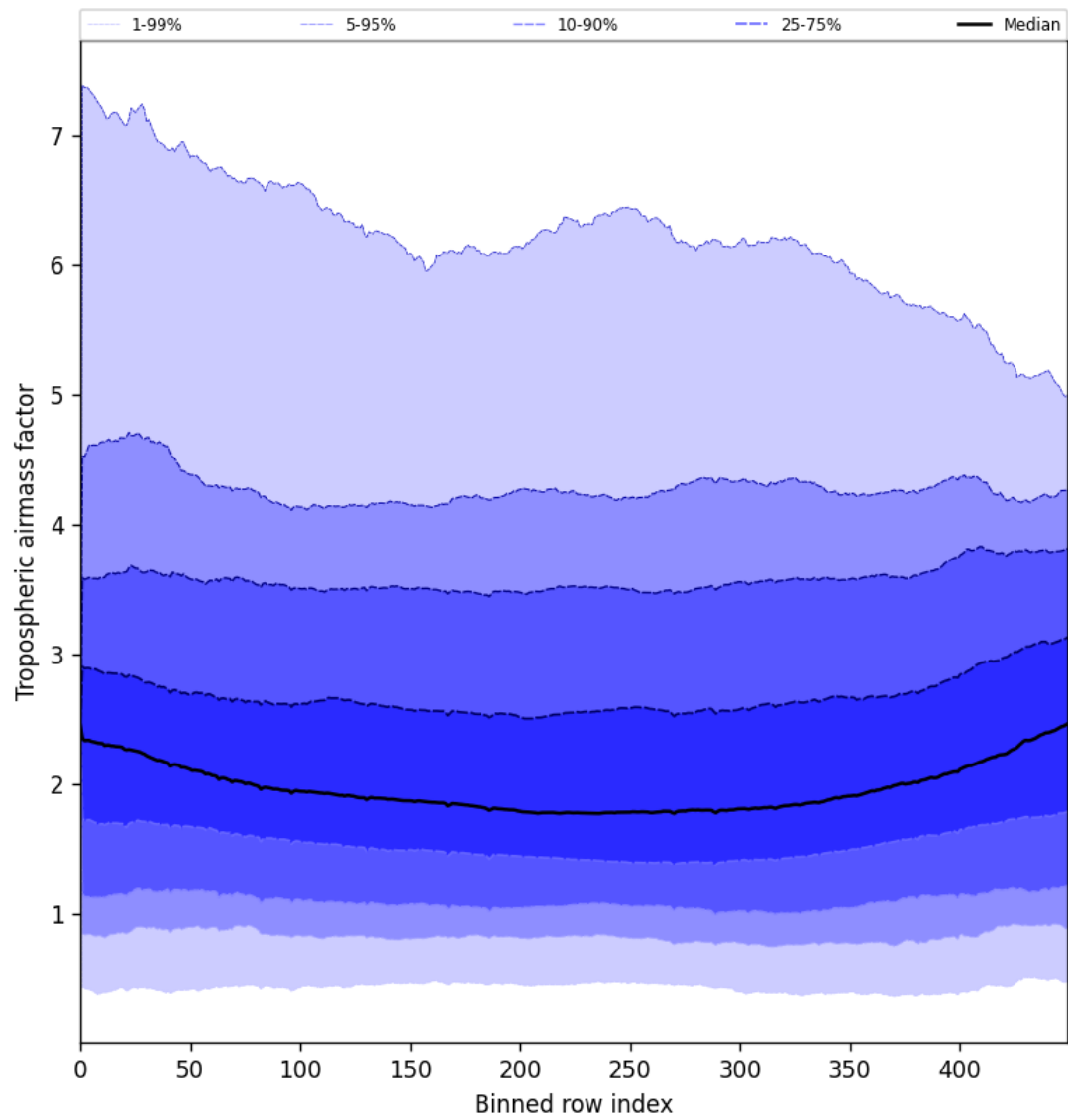
Figure 48: Along track statistics of “Tropospheric airmass factor” for 2025-07-31 to 2025-08-02
