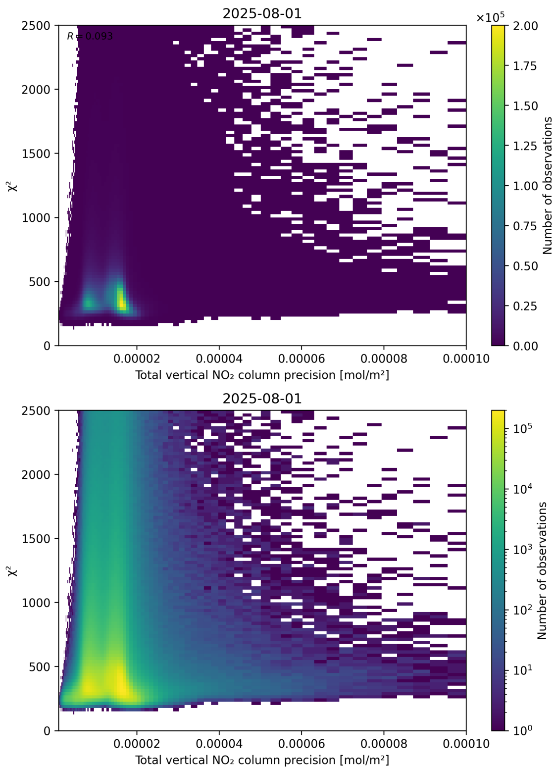
Figure 116: Scatter density plot of “Total vertical NO 2 column precision” against “ \chi^2 ” for 2025-07-31 to 2025-08-02.
