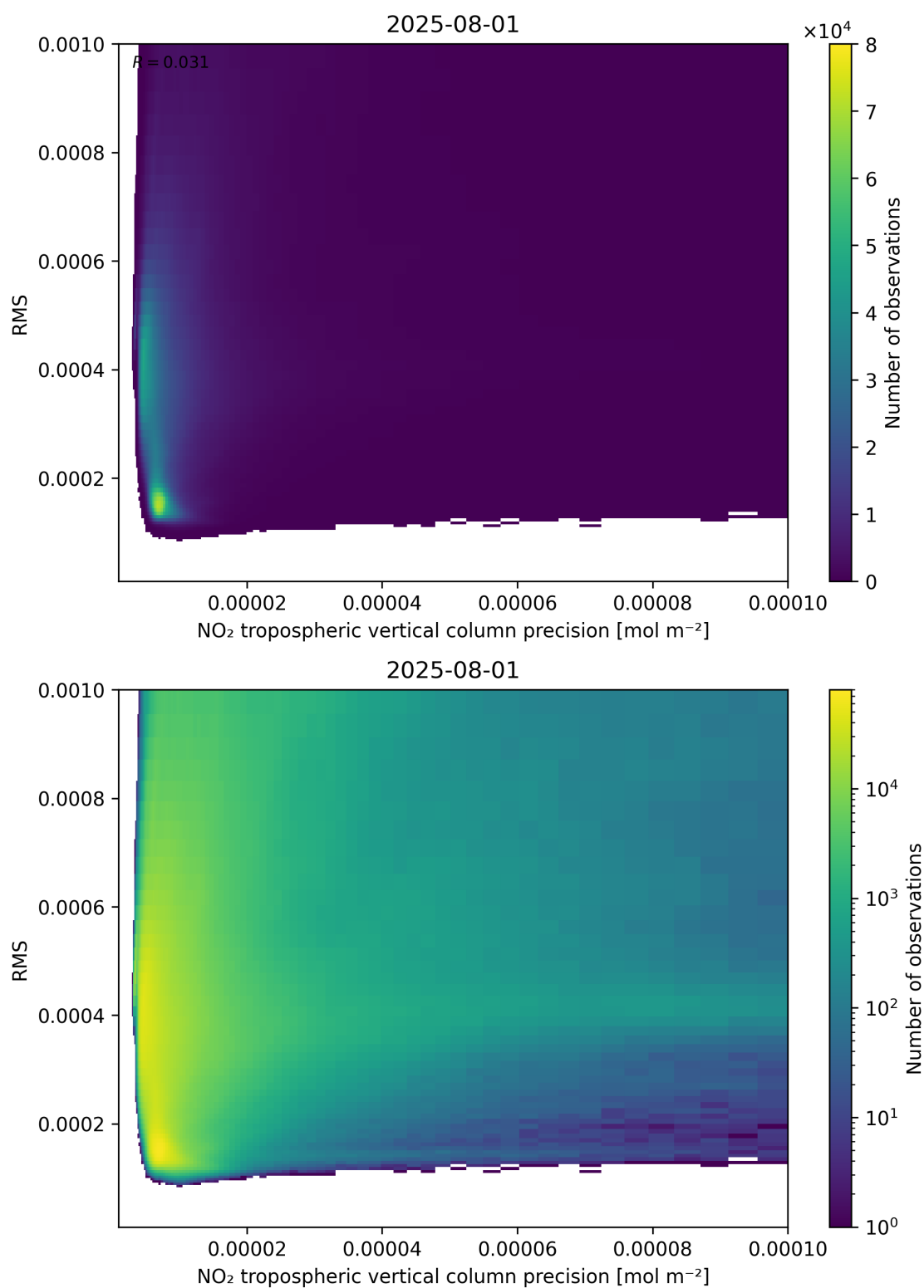
Figure 140: Scatter density plot of “NO 2 tropospheric vertical column precision” against “RMS” for 2025-07-31 to 2025-08-02.
