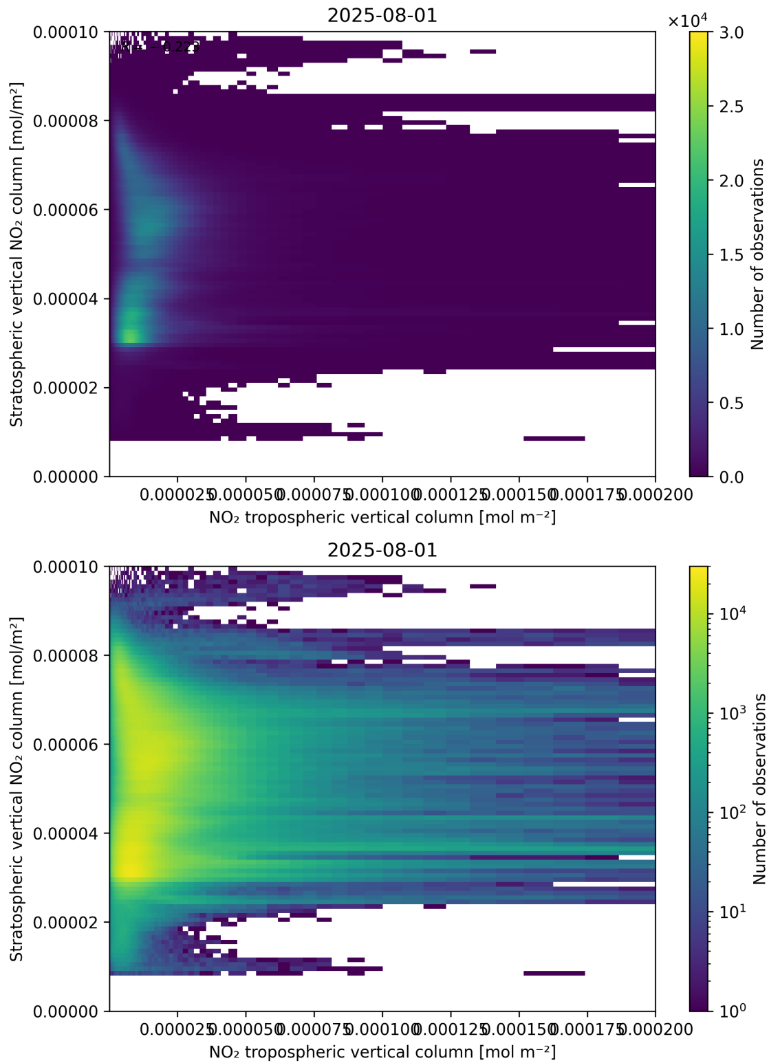
Figure 125: Scatter density plot of “NO 2 tropospheric vertical column” against “Stratospheric vertical NO 2 column” for 2025-07-31 to 2025-08-02.
