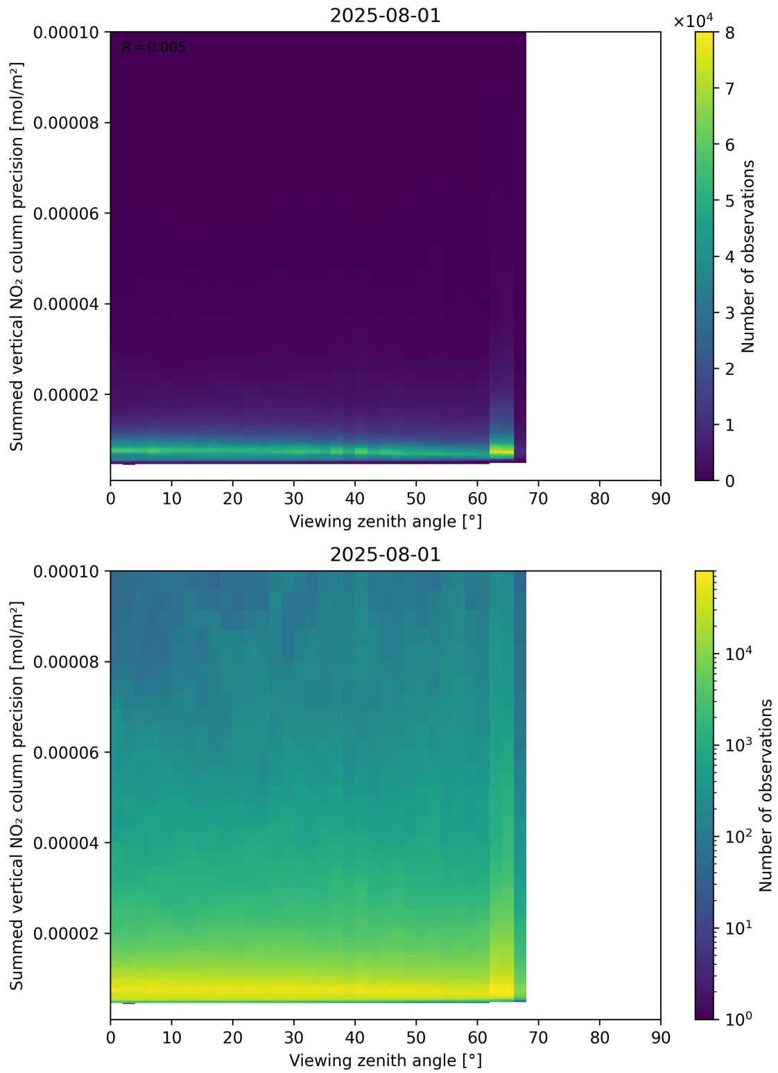
Figure 166: Scatter density plot of “Viewing zenith angle” against “Summed vertical NO 2 column precision” for 2025-07-31 to 2025-08-02.
