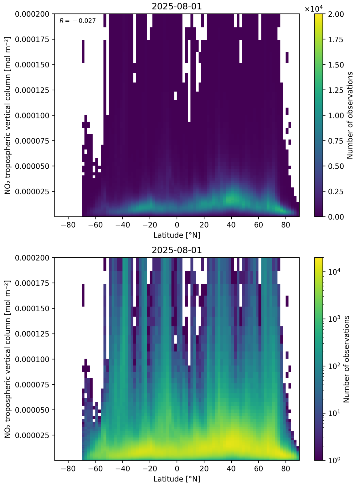
Figure 92: Scatter density plot of “Latitude” against “NO 2 tropospheric vertical column” for 2025-07-31 to 2025-08-02.
