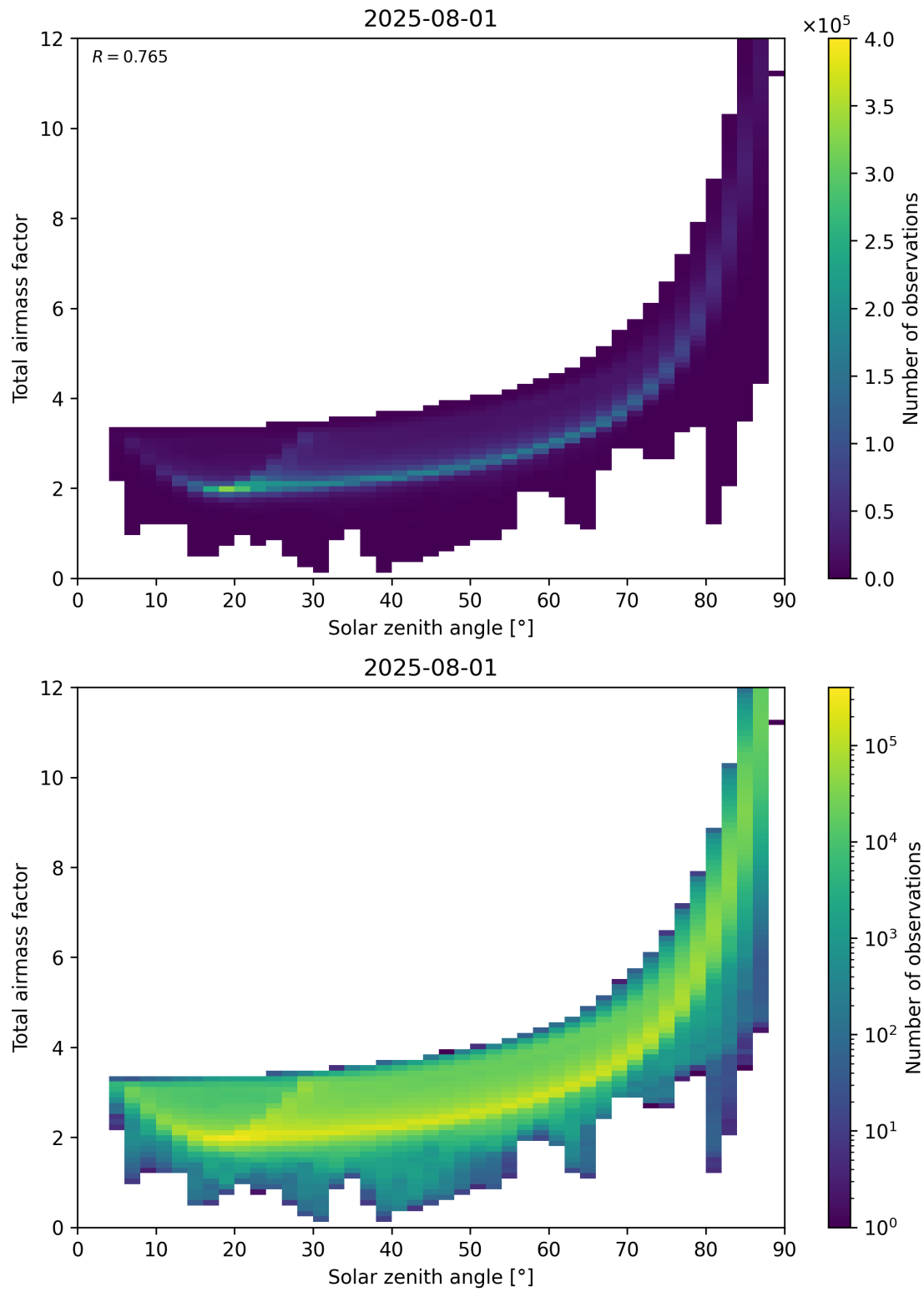
Figure 146: Scatter density plot of “Solar zenith angle” against “Total airmass factor” for 2025-07-31 to 2025-08-02.
