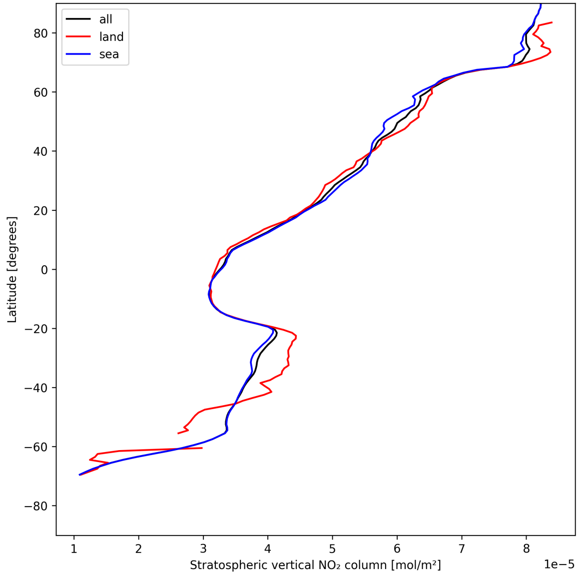
Figure 19: Zonal average of “Stratospheric vertical NO 2 column” for 2025-07-31 to 2025-08-02.
