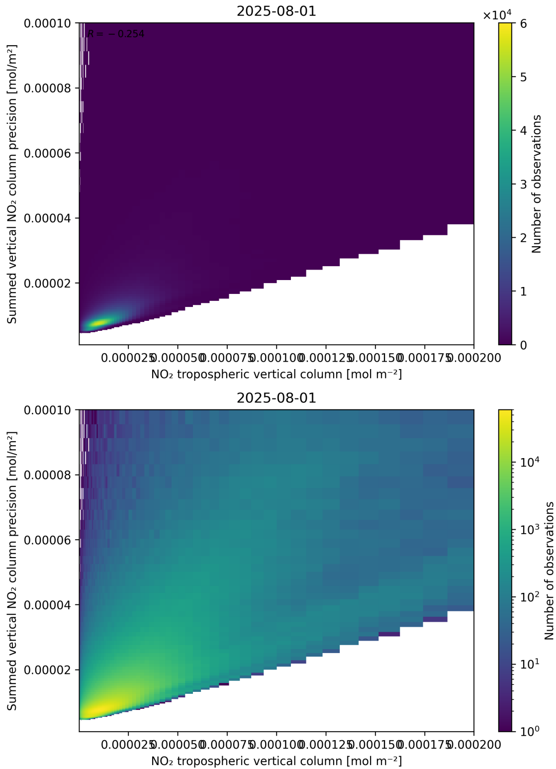
Figure 127: Scatter density plot of “NO 2 tropospheric vertical column” against “Summed vertical NO 2 column precision” for 2025-07-31 to 2025-08-02.
