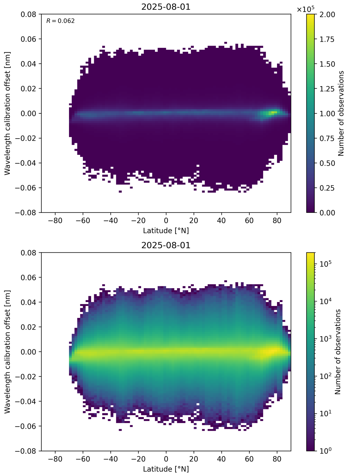
Figure 95: Scatter density plot of “Latitude” against “Wavelength calibration offset” for 2025-07-31 to 2025-08-02.
