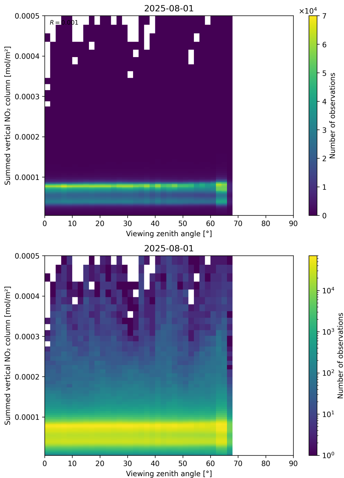
Figure 165: Scatter density plot of “Viewing zenith angle” against “Summed vertical NO 2 column” for 2025-07-31 to 2025-08-02.
