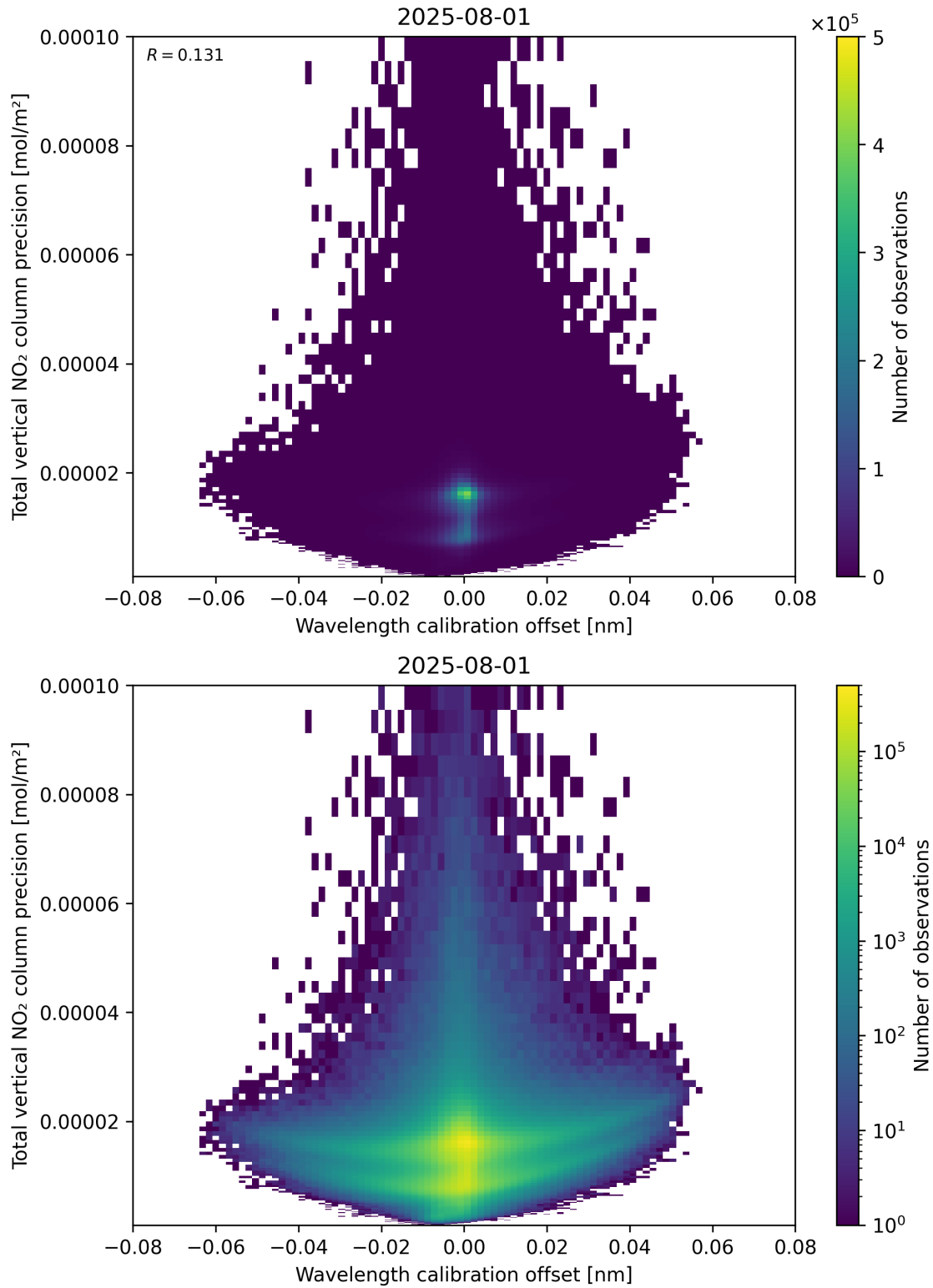
Figure 180: Scatter density plot of “Wavelength calibration offset” against “Total vertical NO 2 column precision” for 2025-07-31 to 2025-08-02.
