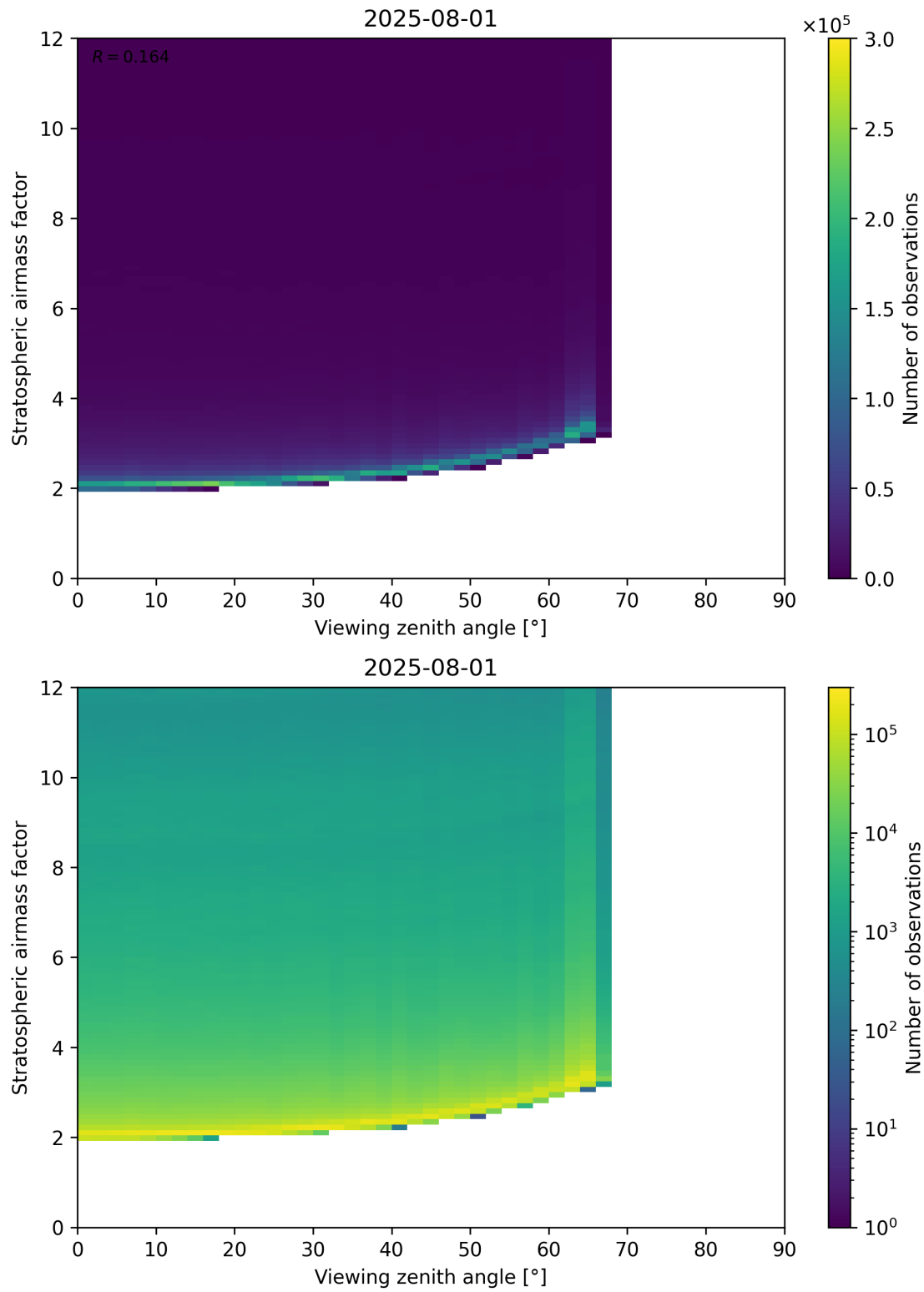
Figure 159: Scatter density plot of “Viewing zenith angle” against “Stratospheric airmass factor” for 2025-07-31 to 2025-08-02.
