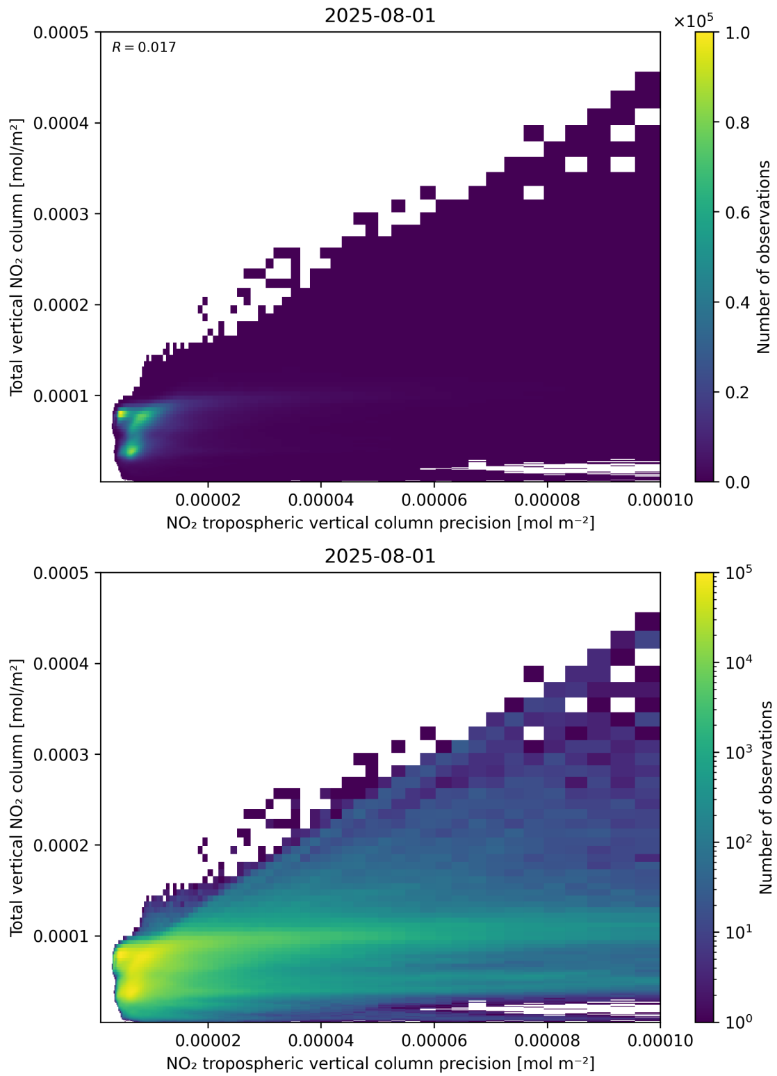
Figure 138: Scatter density plot of “NO 2 tropospheric vertical column precision” against “Total vertical NO 2 column” for 2025-07-31 to 2025-08-02.
