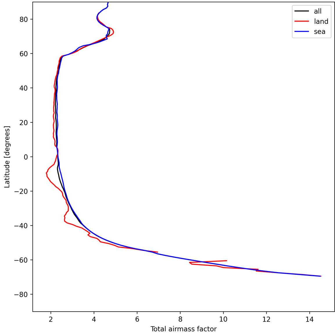
Figure 15: Zonal average of “Total airmass factor” for 2025-07-31 to 2025-08-02.
