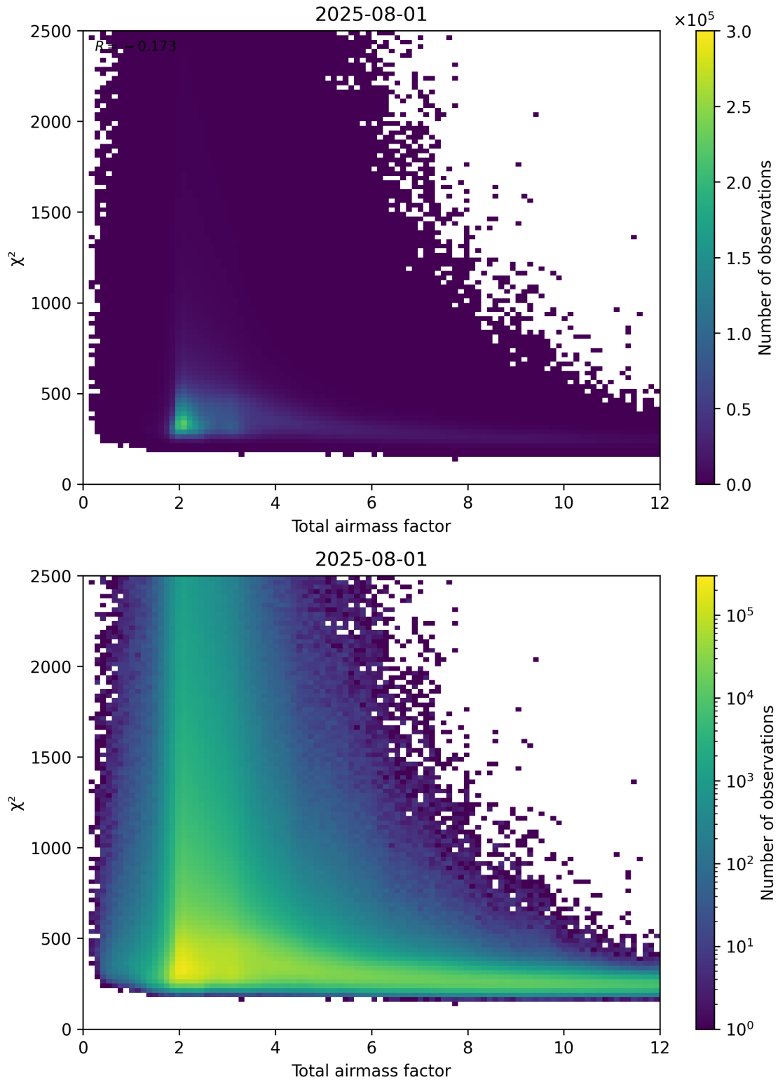
Figure 63: Scatter density plot of “Total airmass factor” against “ \chi^2 ” for 2025-07-31 to 2025-08-02.
