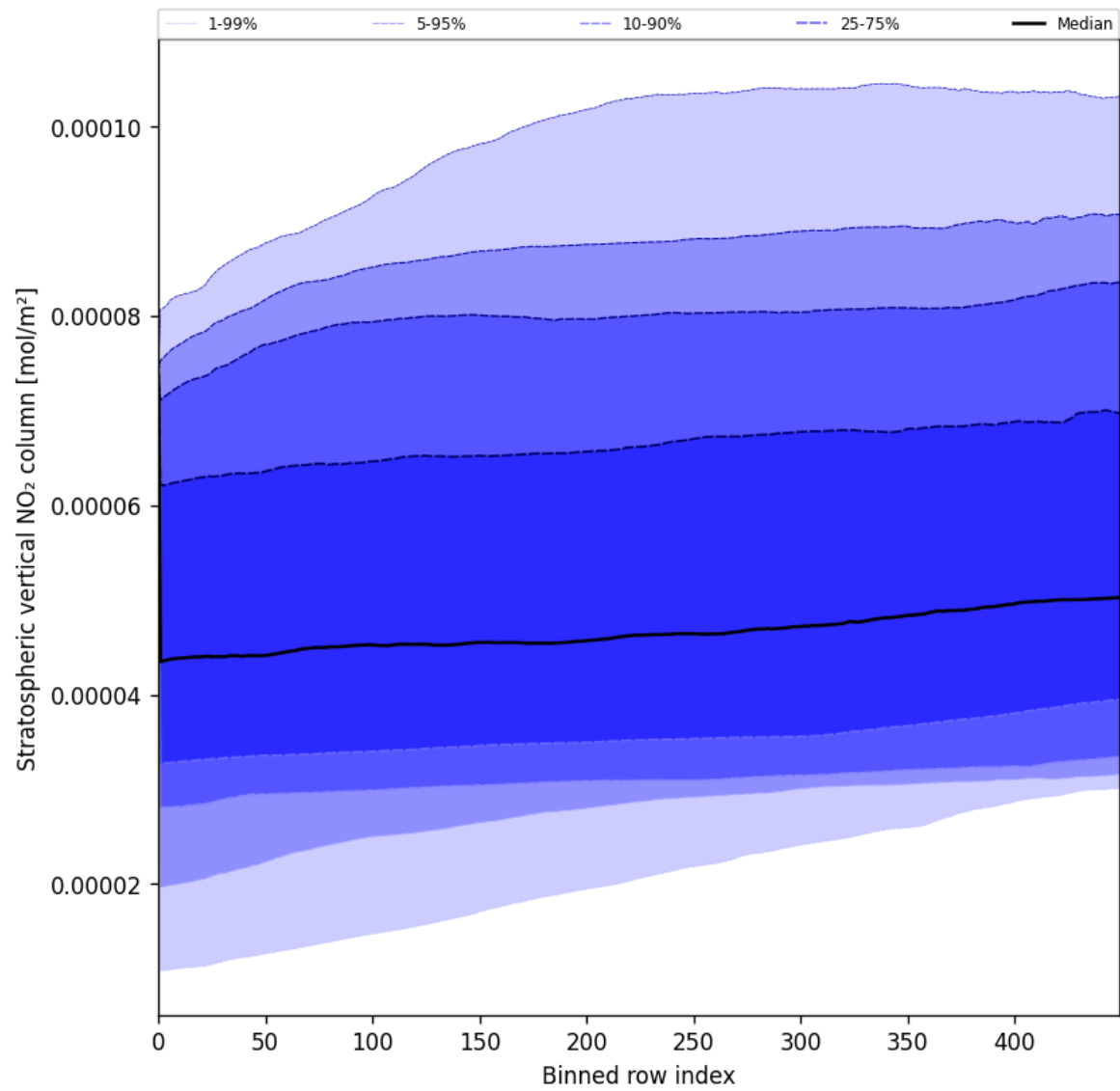
Figure 53: Along track statistics of “Stratospheric vertical NO 2 column” for 2025-07-31 to 2025-08-02
