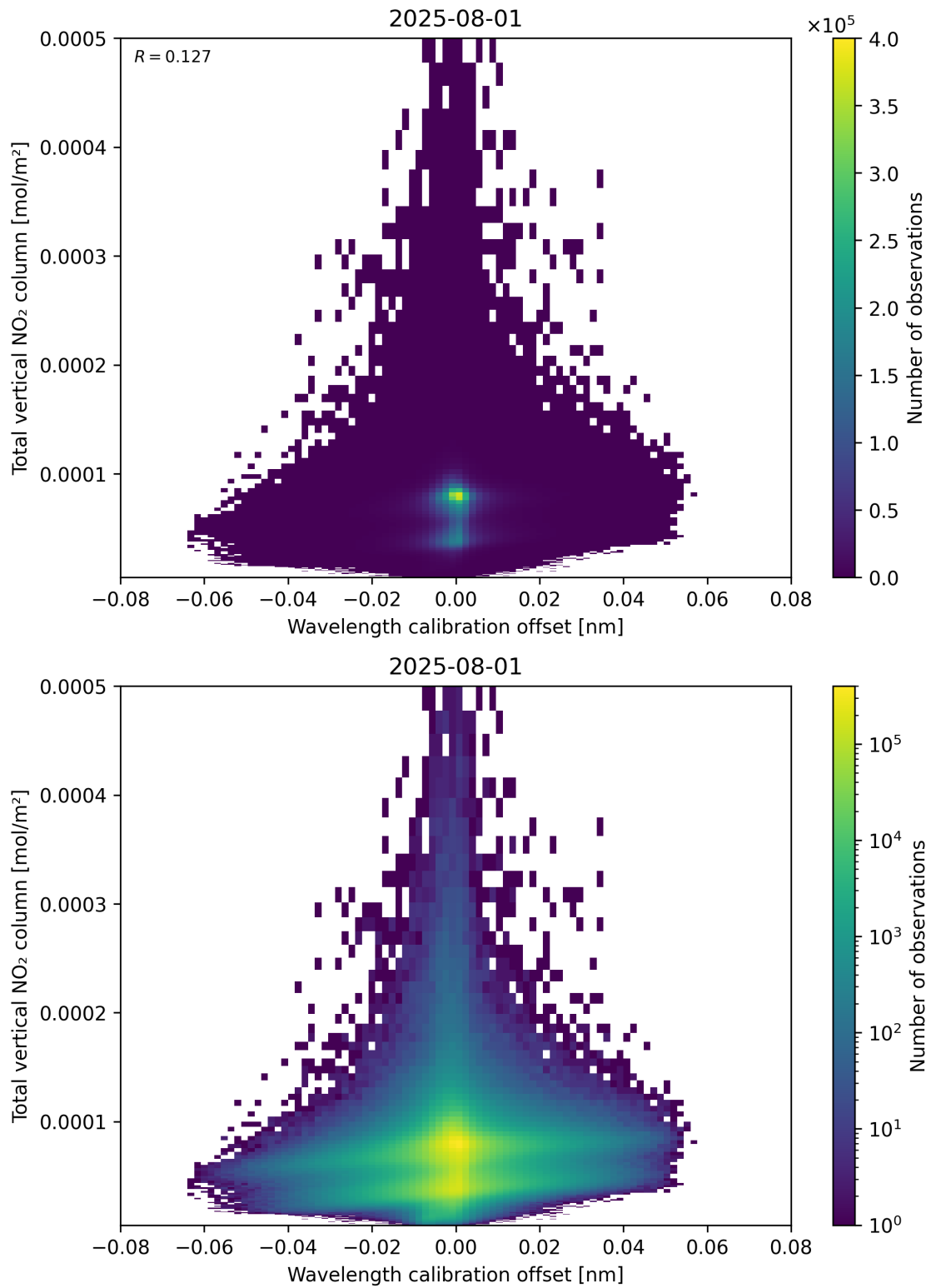
Figure 179: Scatter density plot of “Wavelength calibration offset” against “Total vertical NO 2 column” for 2025-07-31 to 2025-08-02.
