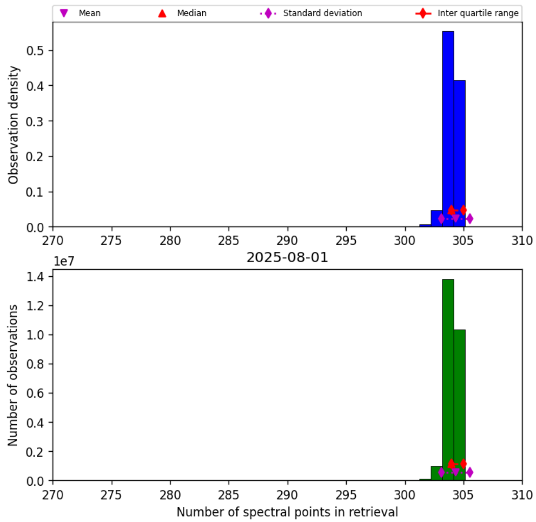
Figure 33: Histogram of “Number of spectral points in retrieval” for 2025-07-31 to 2025-08-02
