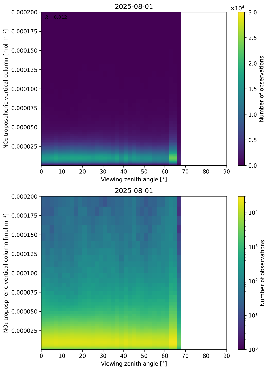
Figure 169: Scatter density plot of “Viewing zenith angle” against “NO 2 tropospheric vertical column” for 2025-07-31 to 2025-08-02.
