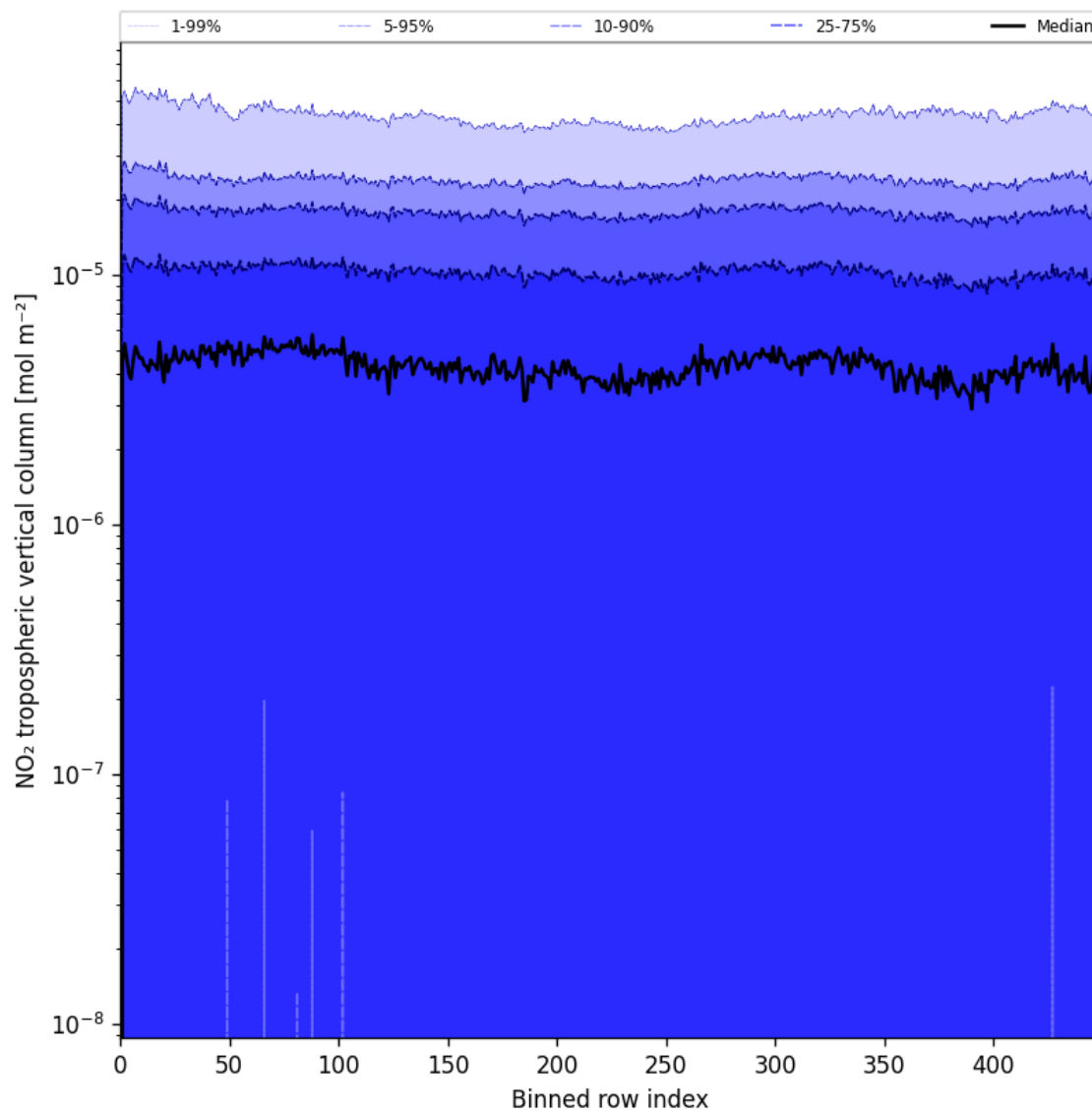
Figure 46: Along track statistics of “NO 2 tropospheric vertical column” for 2025-07-31 to 2025-08-02
