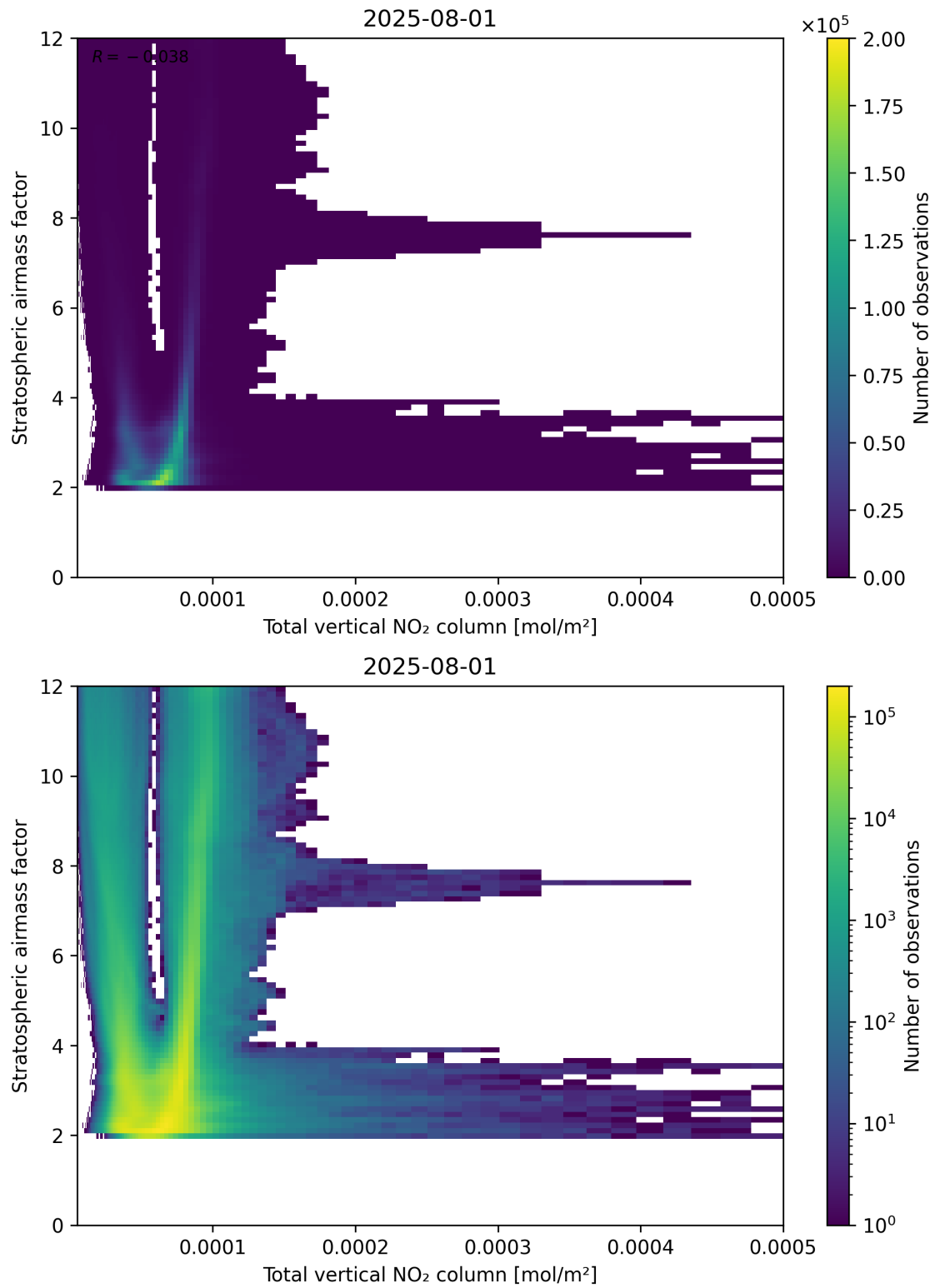
Figure 110: Scatter density plot of “Total vertical NO 2 column” against “Stratospheric airmass factor” for 2025-07-31 to 2025-08-02.
