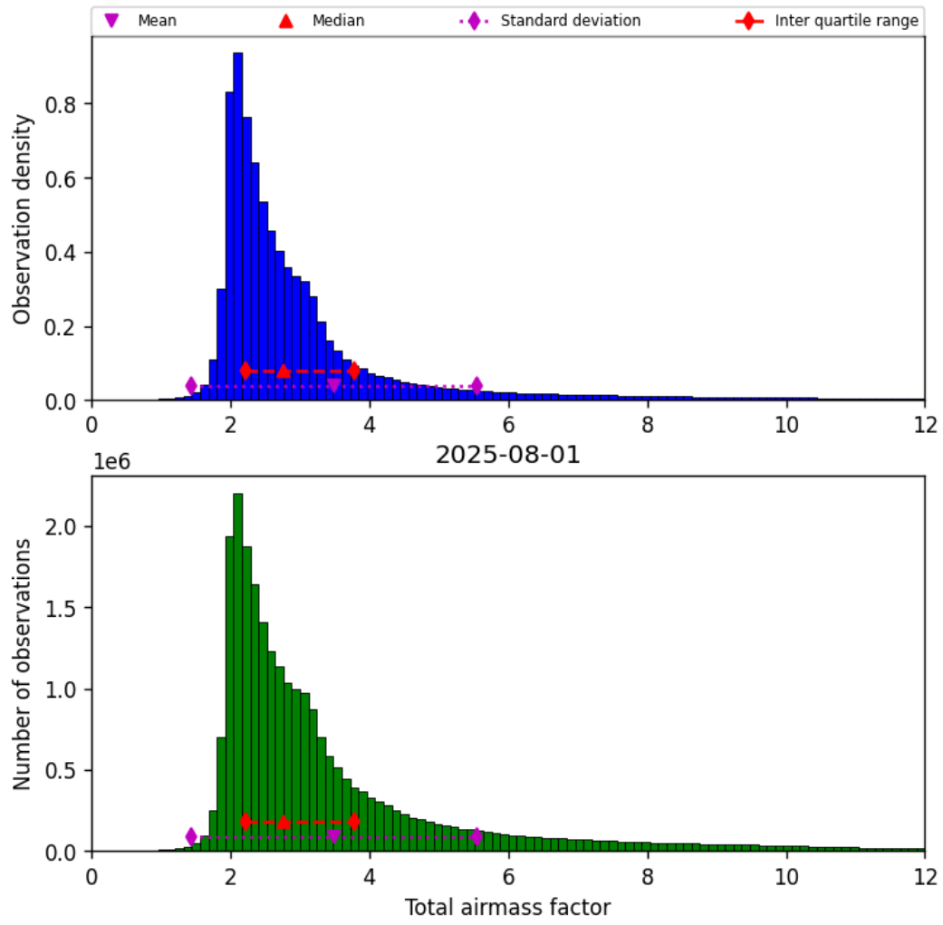
Figure 32: Histogram of “Total airmass factor” for 2025-07-31 to 2025-08-02
