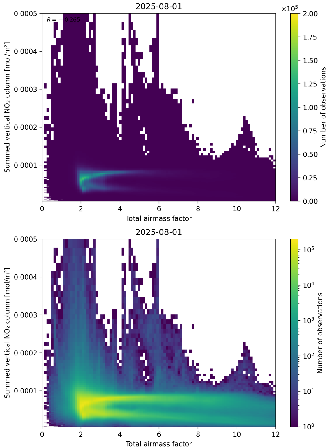
Figure 65: Scatter density plot of “Total airmass factor” against “Summed vertical NO 2 column” for 2025-07-31 to 2025-08-02.
