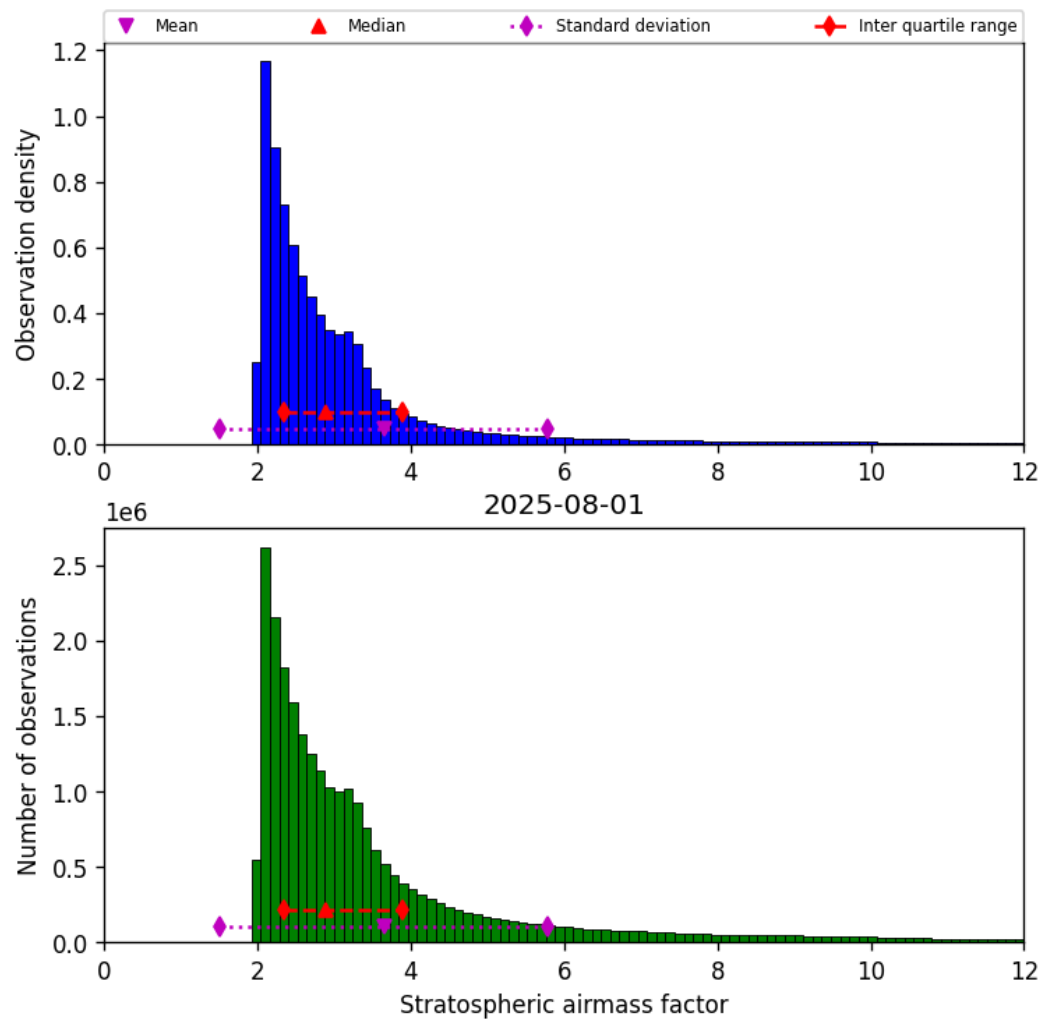
Figure 44: Histogram of “Stratospheric airmass factor” for 2025-07-31 to 2025-08-02
