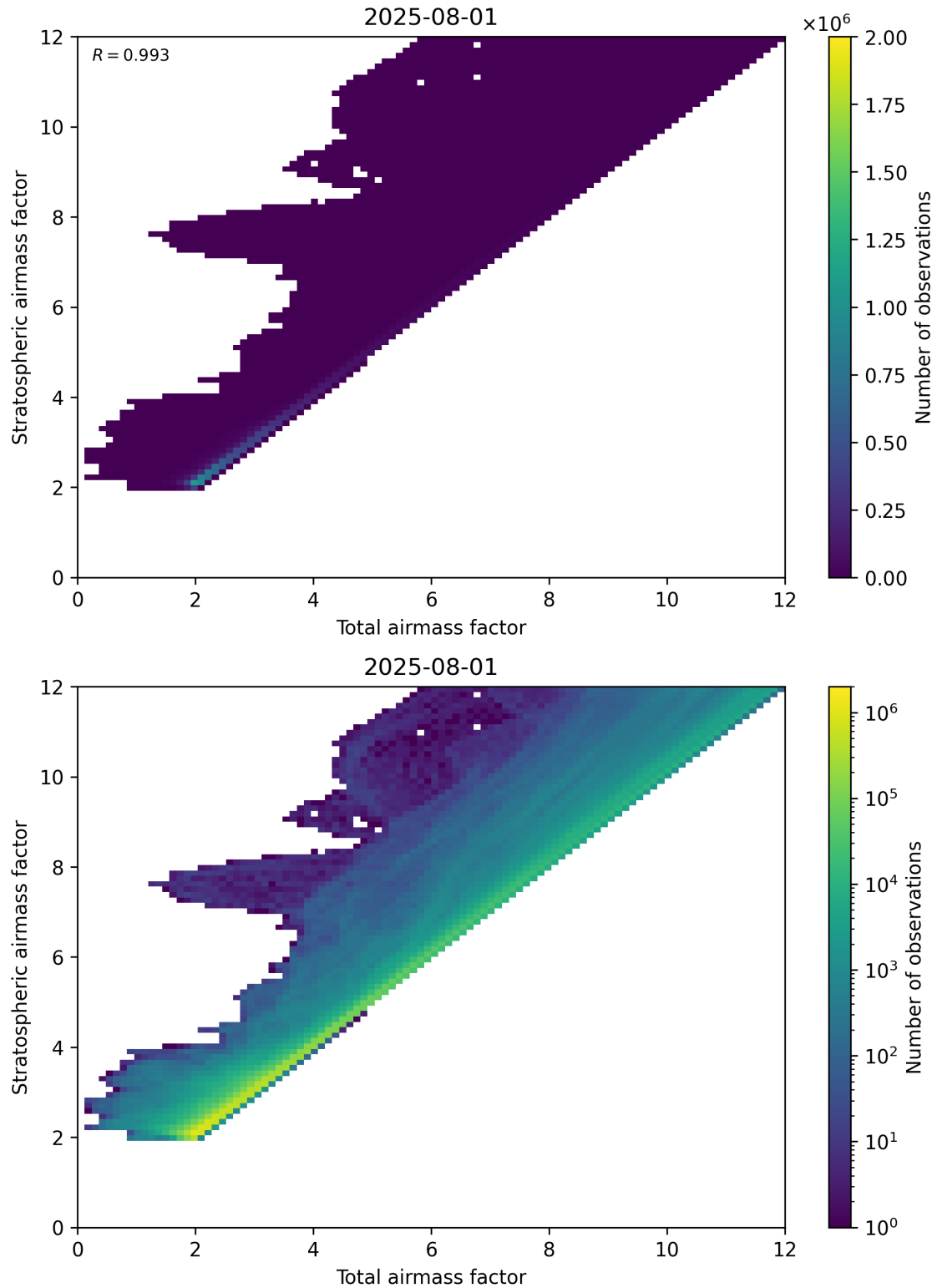
Figure 62: Scatter density plot of “Total airmass factor” against “Stratospheric airmass factor” for 2025-07-31 to 2025-08-02.
