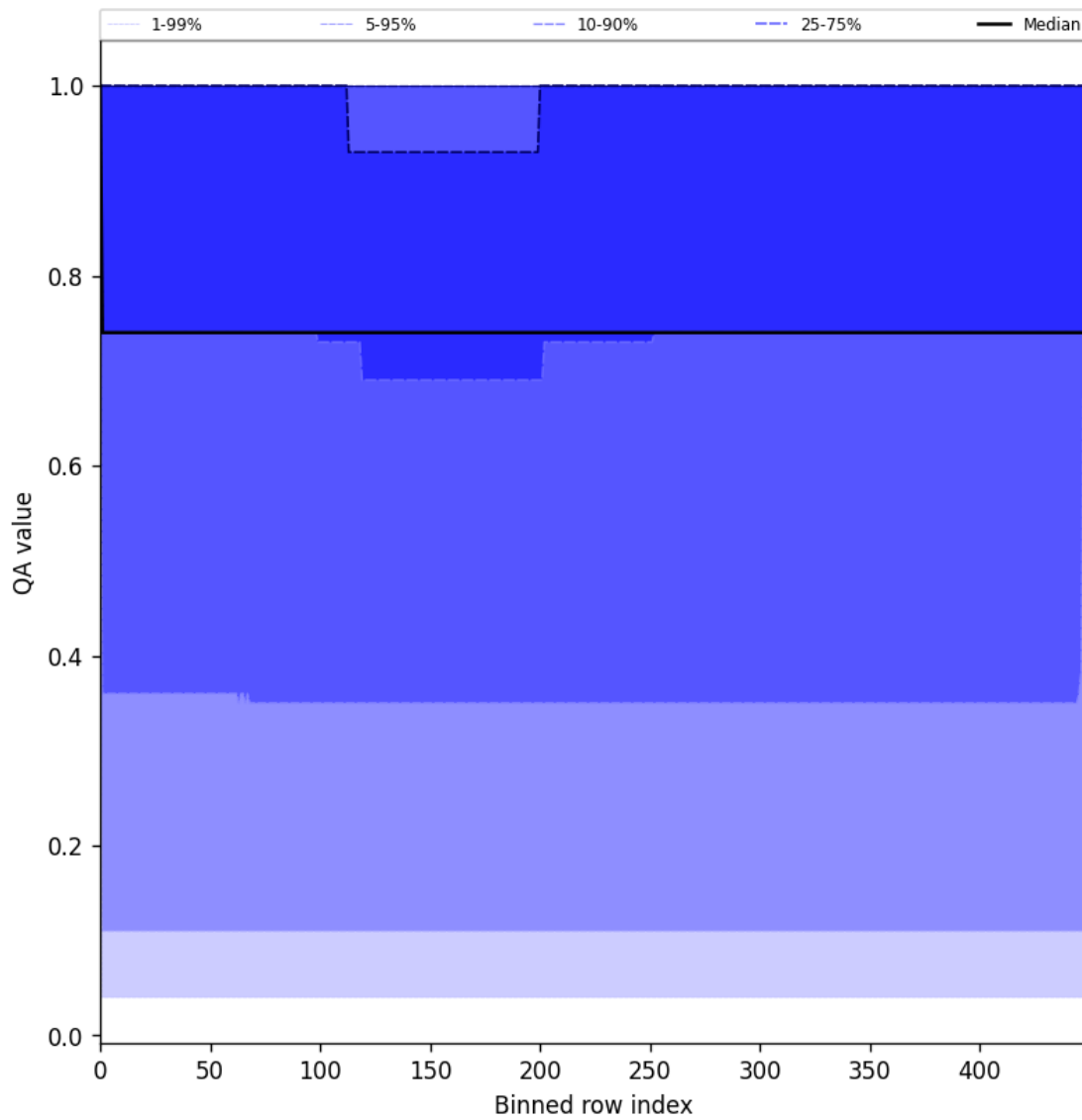
Figure 45: Along track statistics of “QA value” for 2025-07-31 to 2025-08-02
