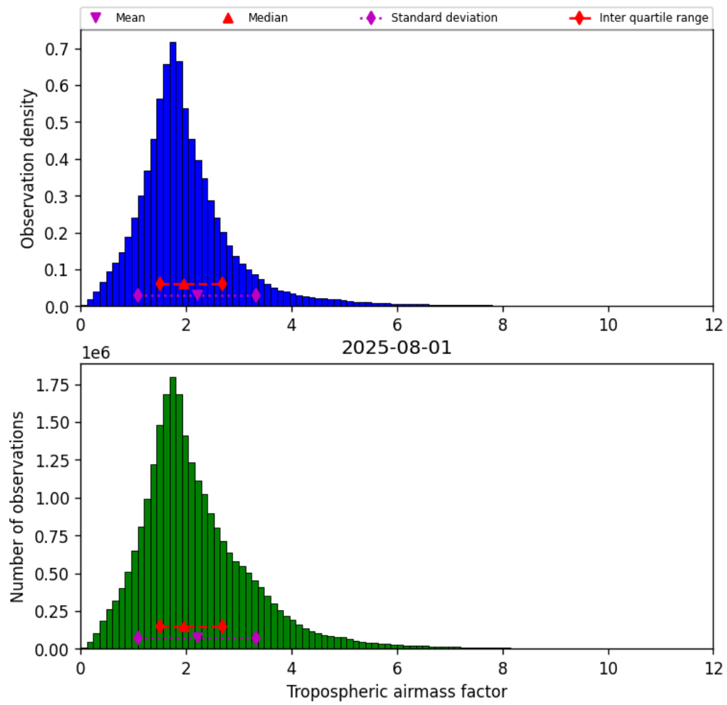
Figure 31: Histogram of “Tropospheric airmass factor” for 2025-07-31 to 2025-08-02
