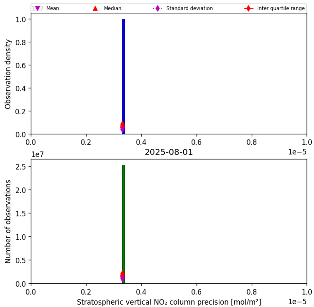
Figure 37: Histogram of “Stratospheric vertical NO 2 column precision” for 2025-07-31 to 2025-08-02
