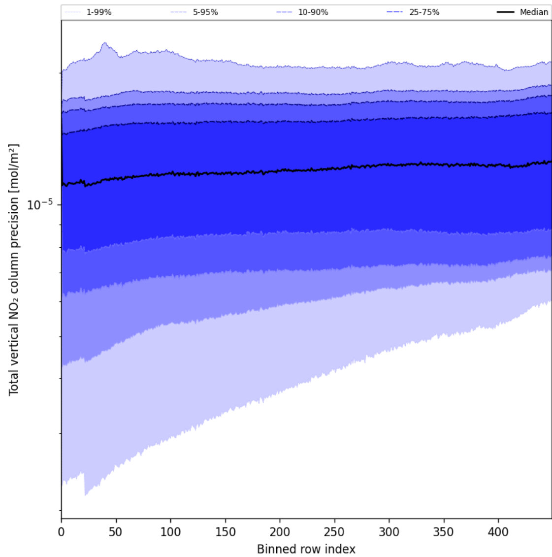
Figure 56: Along track statistics of “Total vertical NO 2 column precision” for 2025-07-31 to 2025-08-02
