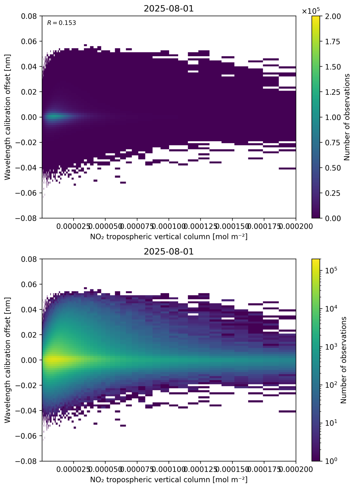
Figure 143: Scatter density plot of “NO 2 tropospheric vertical column” against “Wavelength calibration offset” for 2025-07-31 to 2025-08-02.
