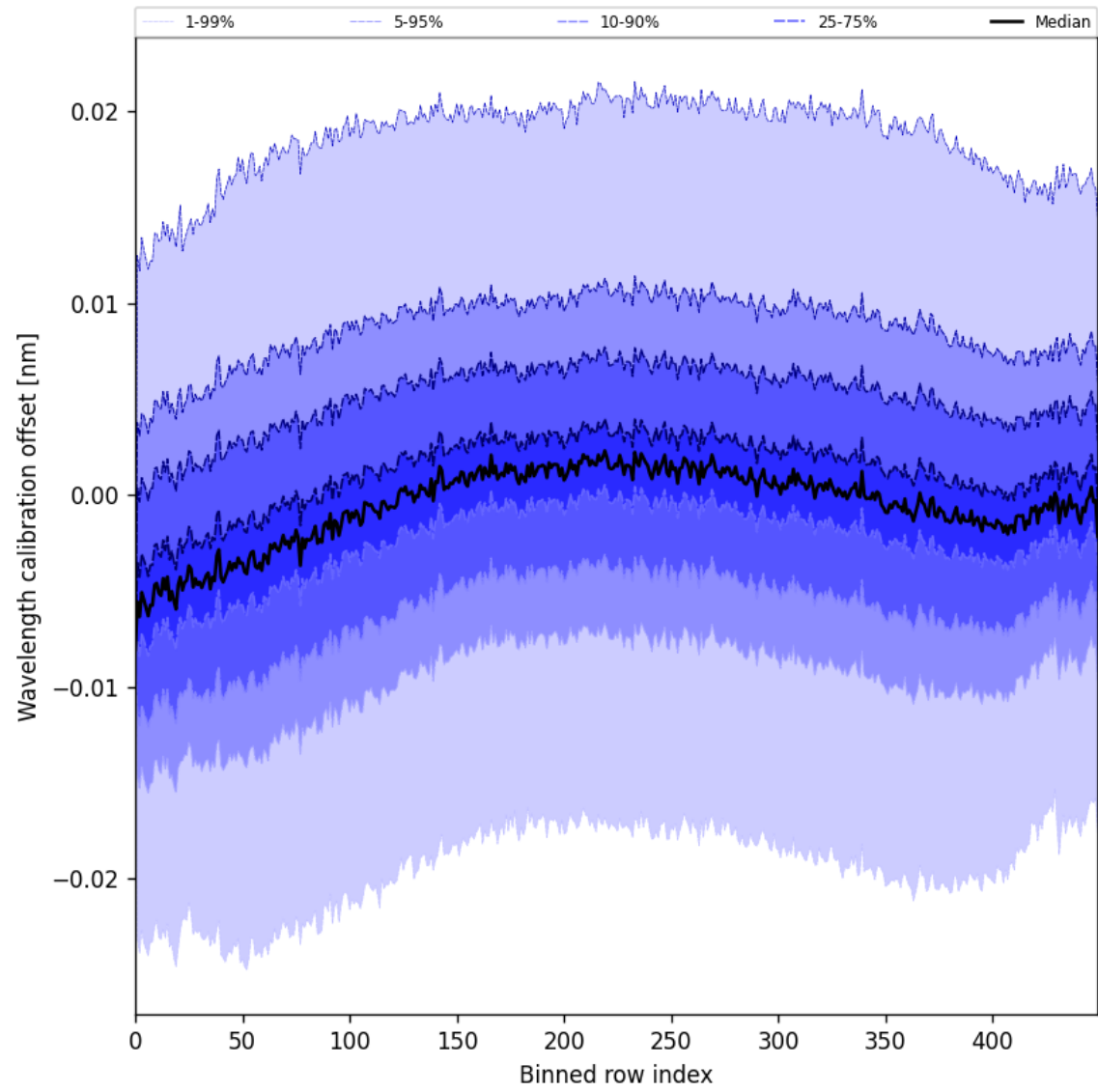
Figure 52: Along track statistics of “Wavelength calibration offset” for 2025-07-31 to 2025-08-02
