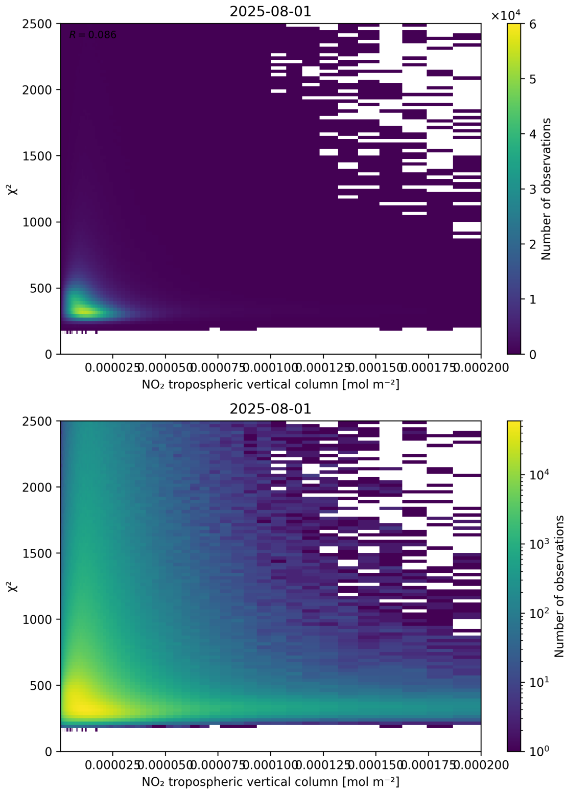
Figure 124: Scatter density plot of “NO 2 tropospheric vertical column” against “ \chi^2 ” for 2025-07-31 to 2025-08-02.
