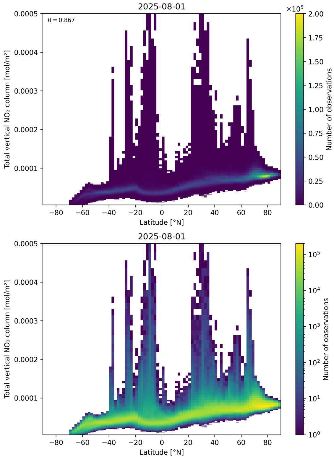
Figure 90: Scatter density plot of “Latitude” against “Total vertical NO 2 column” for 2025-07-31 to 2025-08-02.
