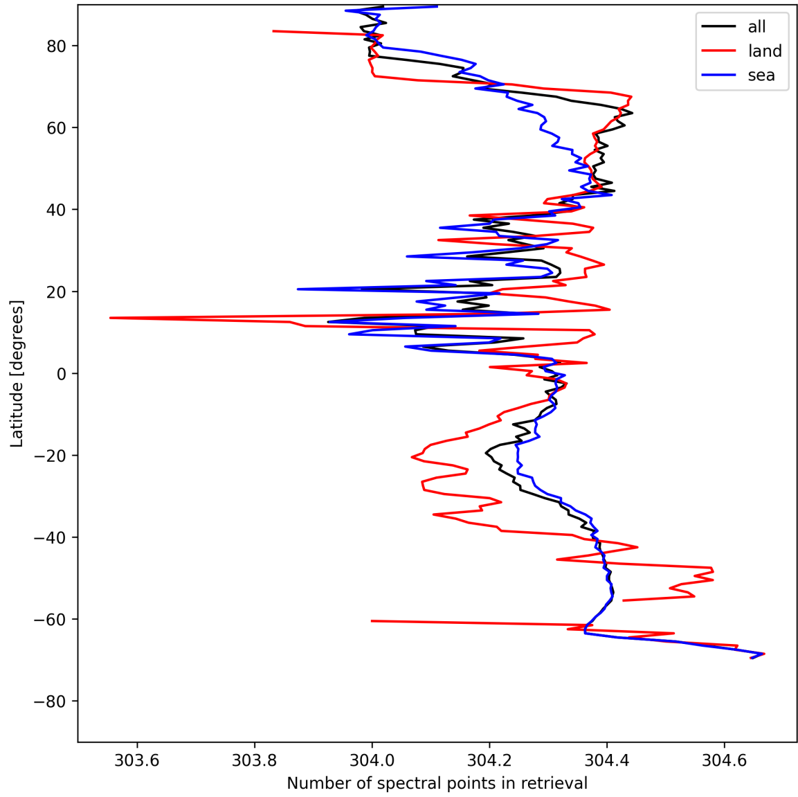
Figure 16: Zonal average of “Number of spectral points in retrieval” for 2025-07-31 to 2025-08-02.
