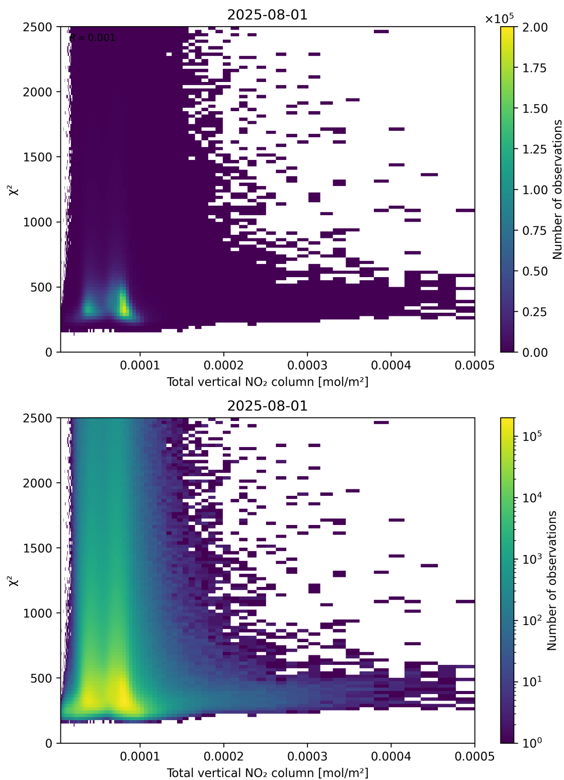
Figure 111: Scatter density plot of “Total vertical NO 2 column” against “ \chi^2 ” for 2025-07-31 to 2025-08-02.
