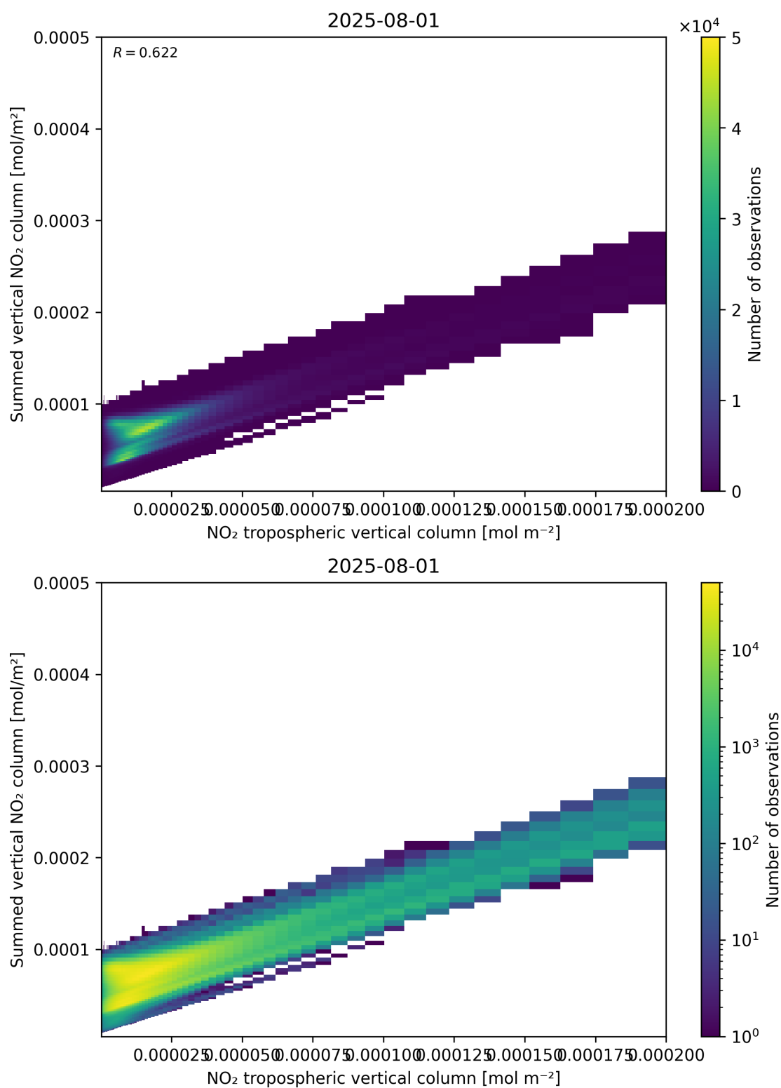
Figure 126: Scatter density plot of “NO 2 tropospheric vertical column” against “Summed vertical NO 2 column” for 2025-07-31 to 2025-08-02.
