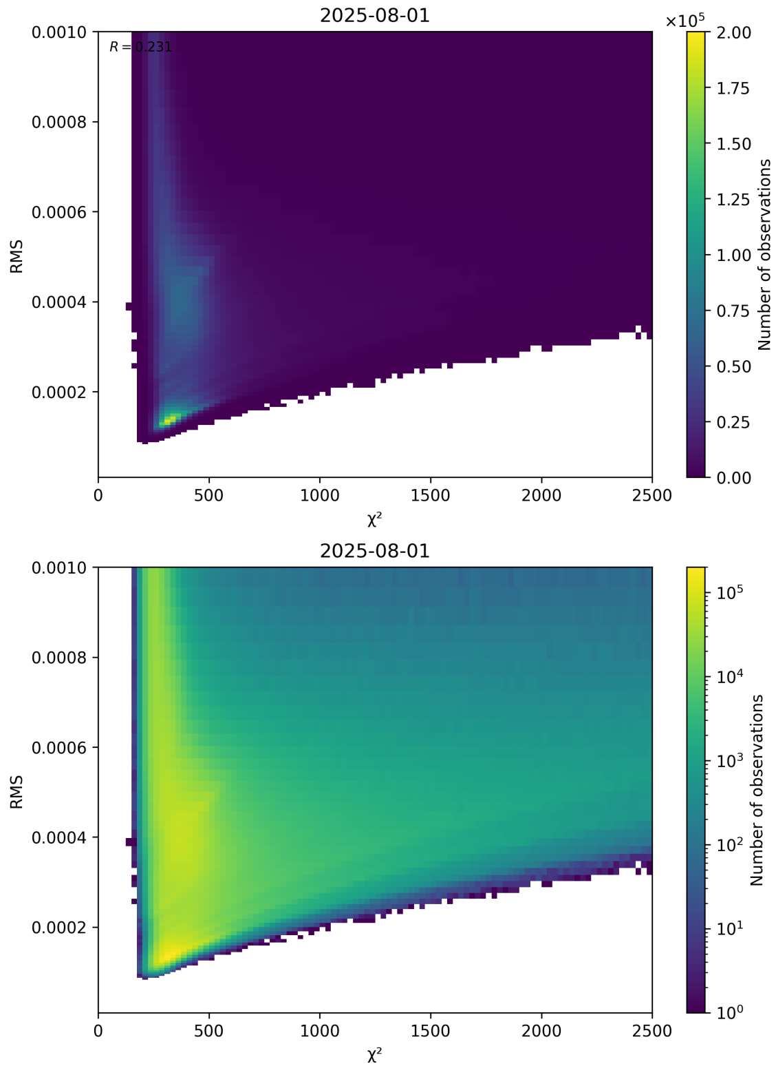
Figure 82: Scatter density plot of “ \chi^2 ” against “RMS” for 2025-07-31 to 2025-08-02.
