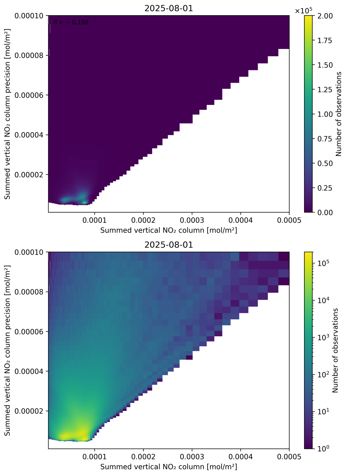
Figure 105: Scatter density plot of “Summed vertical NO 2 column” against “Summed vertical NO 2 column precision” for 2025-07-31 to 2025-08-02.
