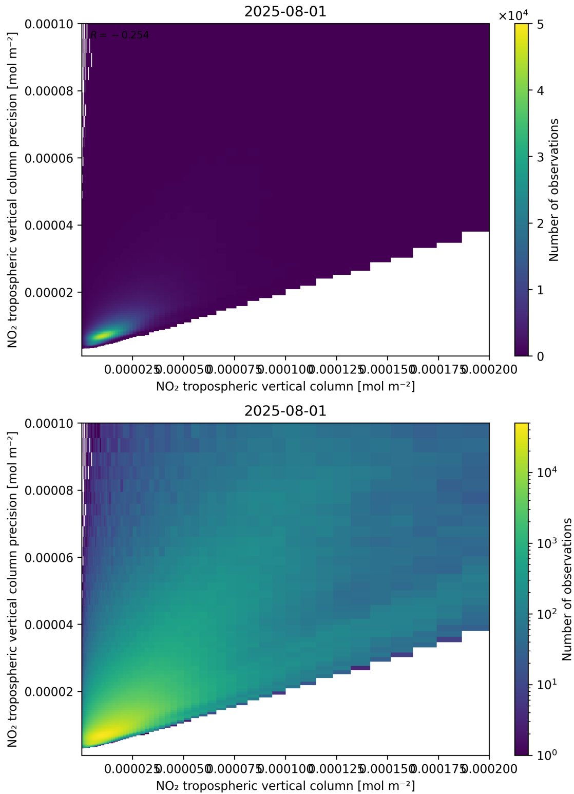
Figure 130: Scatter density plot of “NO 2 tropospheric vertical column” against “NO 2 tropospheric vertical column precision” for 2025-07-31 to 2025-08-02.
