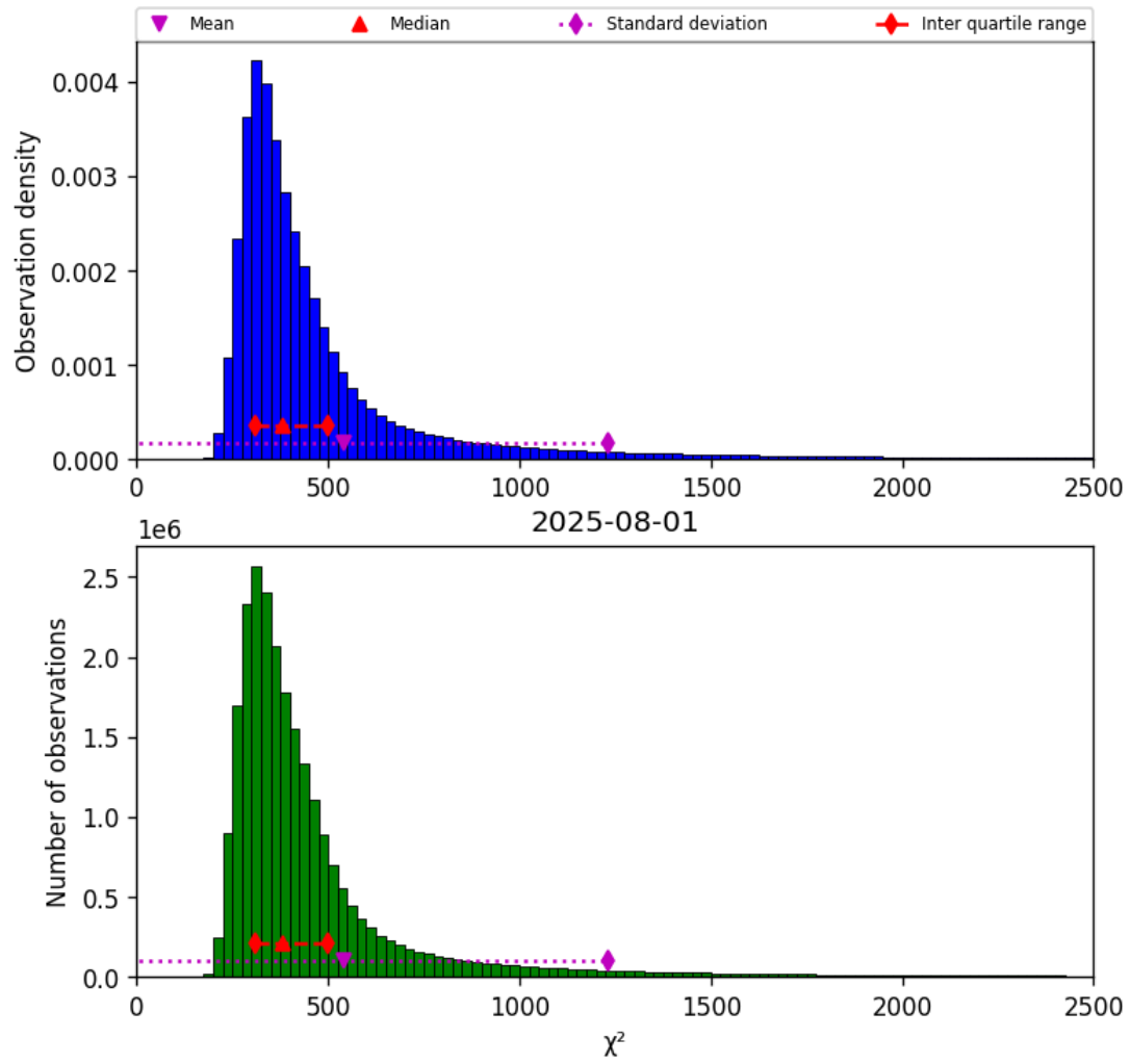
Figure 42: Histogram of “ \chi^2 ” for 2025-07-31 to 2025-08-02
