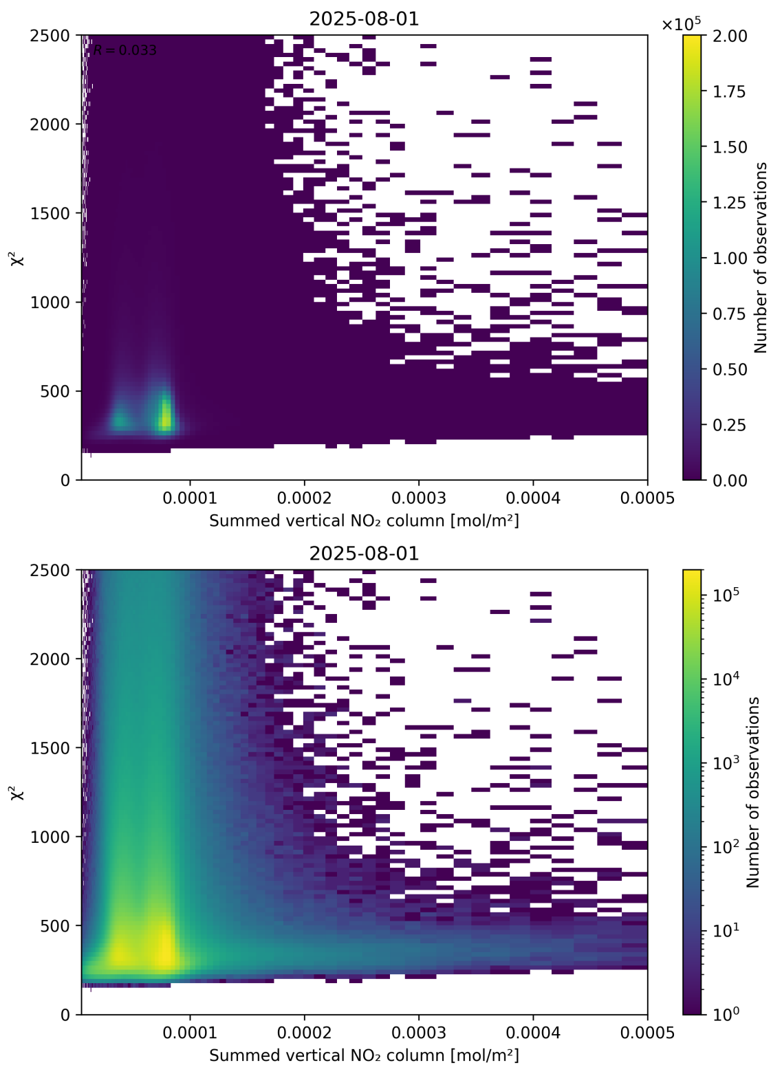
Figure 104: Scatter density plot of “Summed vertical NO 2 column” against “ \chi^2 ” for 2025-07-31 to 2025-08-02.
