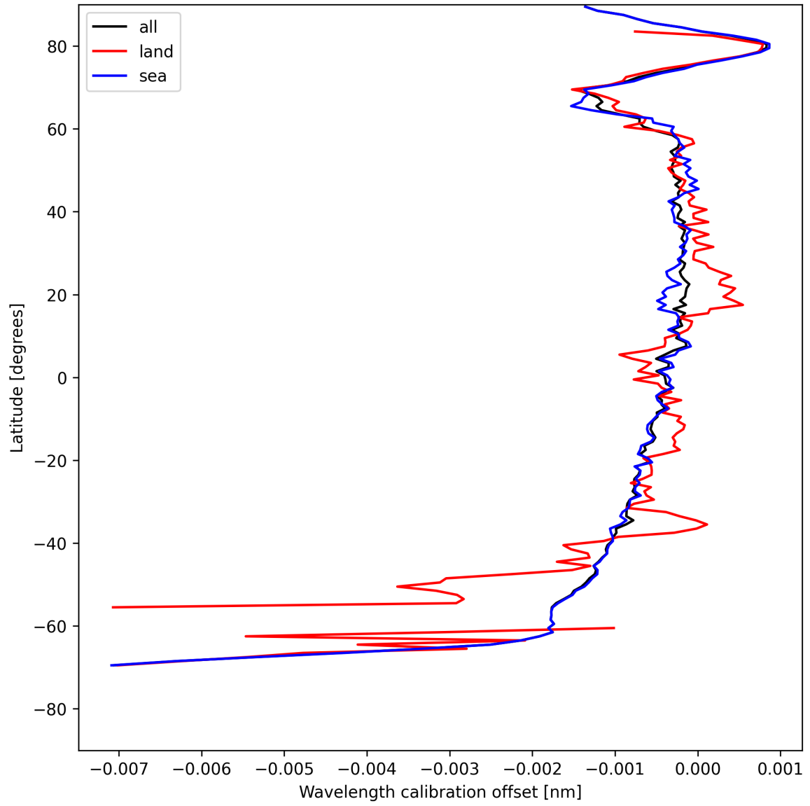
Figure 18: Zonal average of “Wavelength calibration offset” for 2025-07-31 to 2025-08-02.
