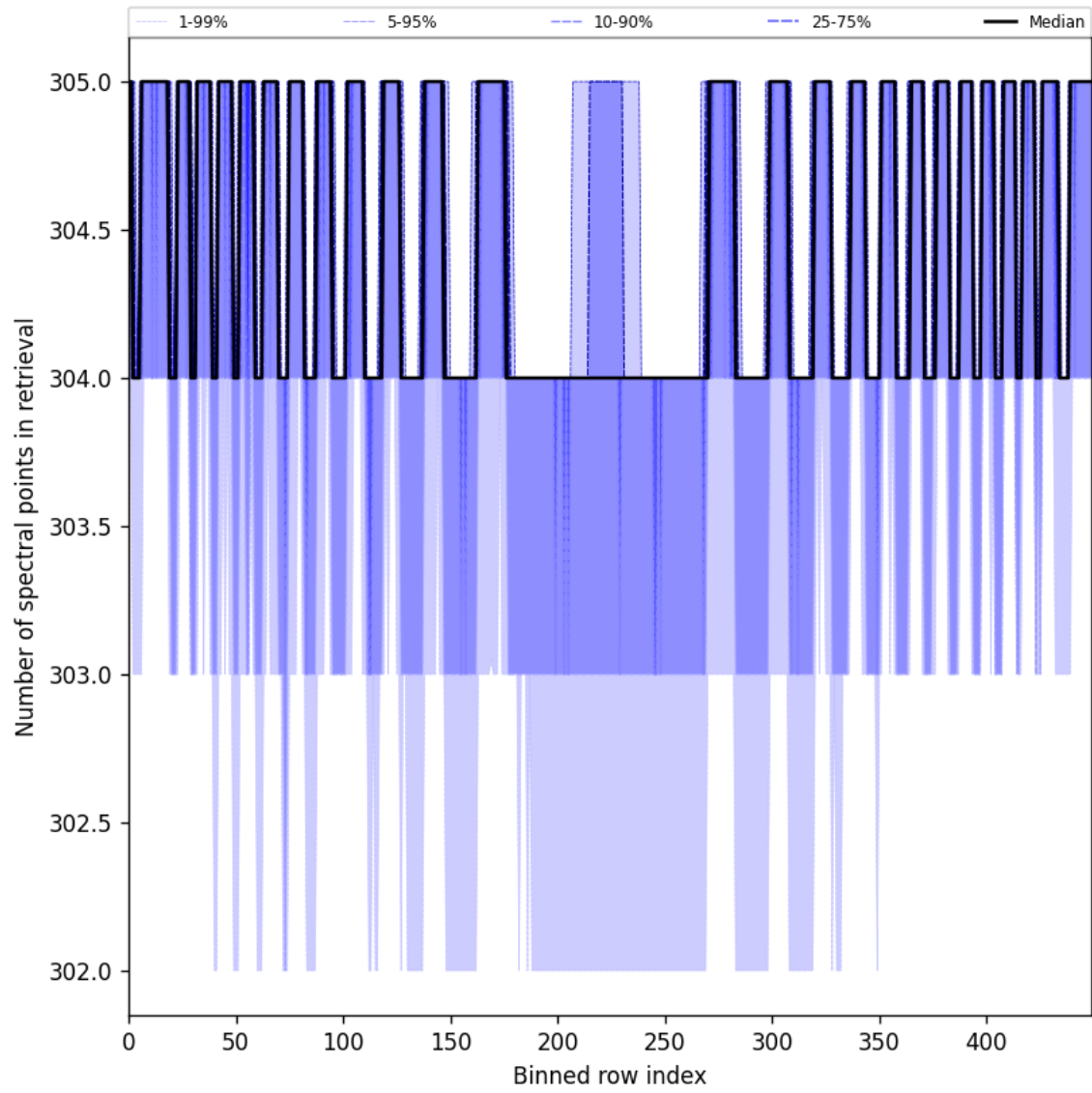
Figure 50: Along track statistics of “Number of spectral points in retrieval” for 2025-07-31 to 2025-08-02
