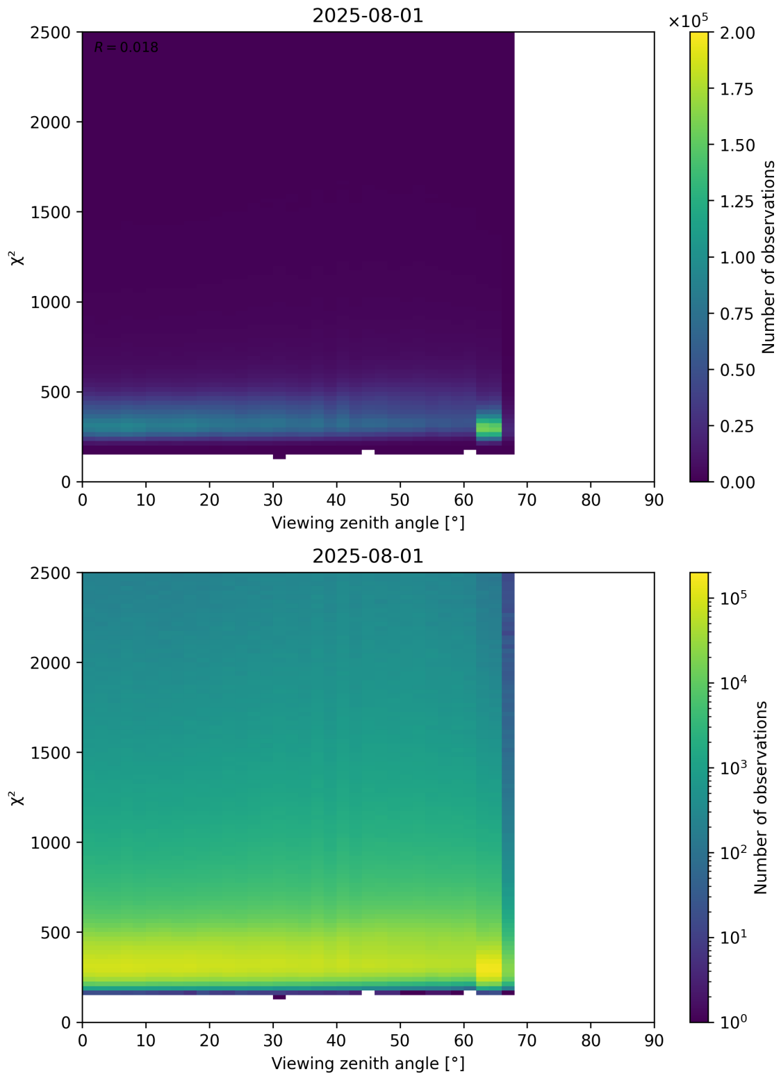
Figure 162: Scatter density plot of “Viewing zenith angle” against “ \chi^2 ” for 2025-07-31 to 2025-08-02.
