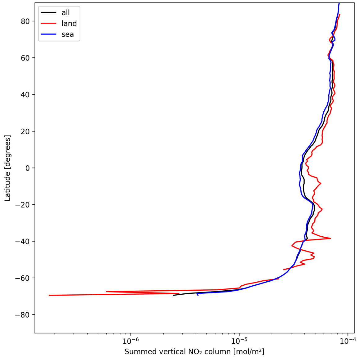
Figure 23: Zonal average of “Summed vertical NO 2 column” for 2025-07-31 to 2025-08-02.
