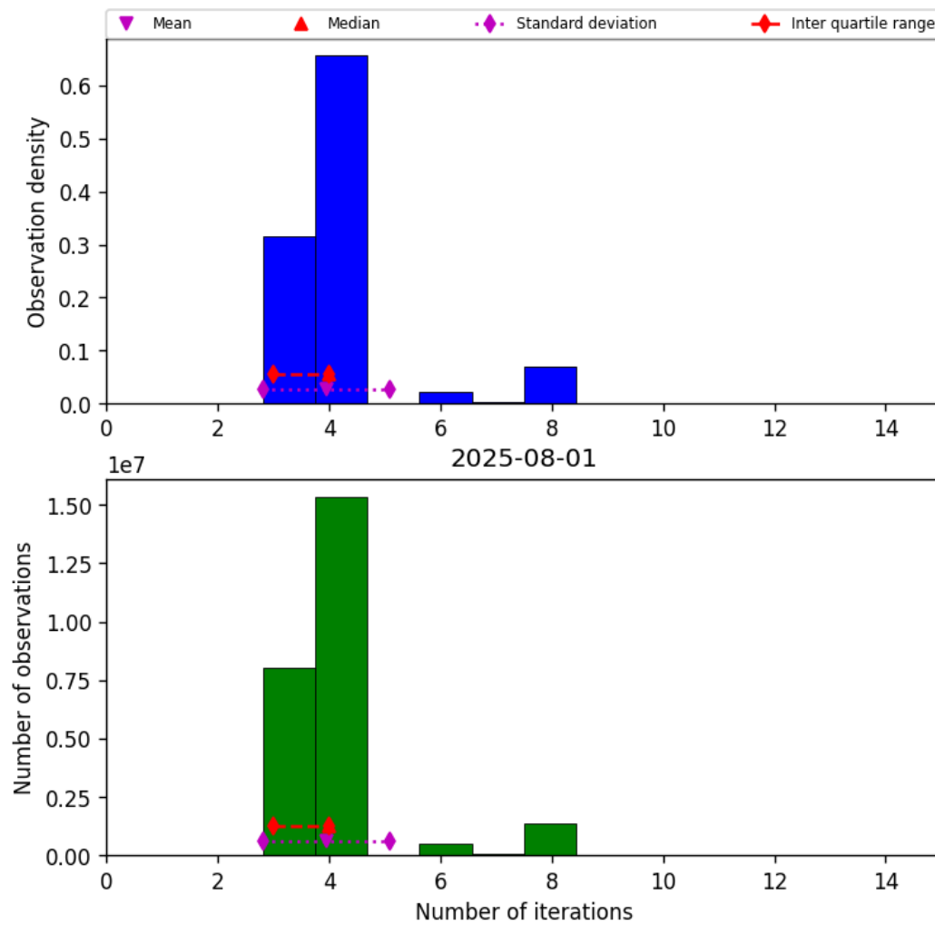
Figure 34: Histogram of “Number of iterations” for 2025-07-31 to 2025-08-02
