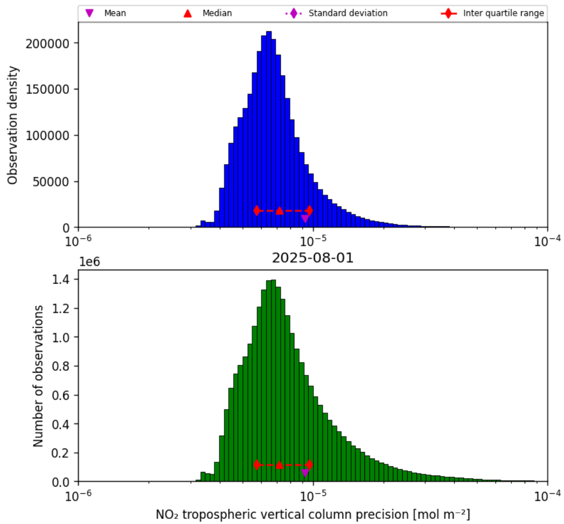
Figure 30: Histogram of “NO 2 tropospheric vertical column precision” for 2025-07-31 to 2025-08-02
