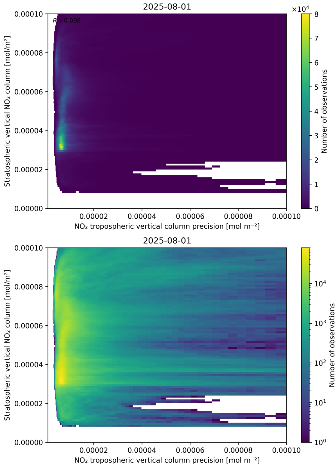
Figure 135: Scatter density plot of “NO 2 tropospheric vertical column precision” against “Stratospheric vertical NO 2 column” for 2025-07-31 to 2025-08-02.
