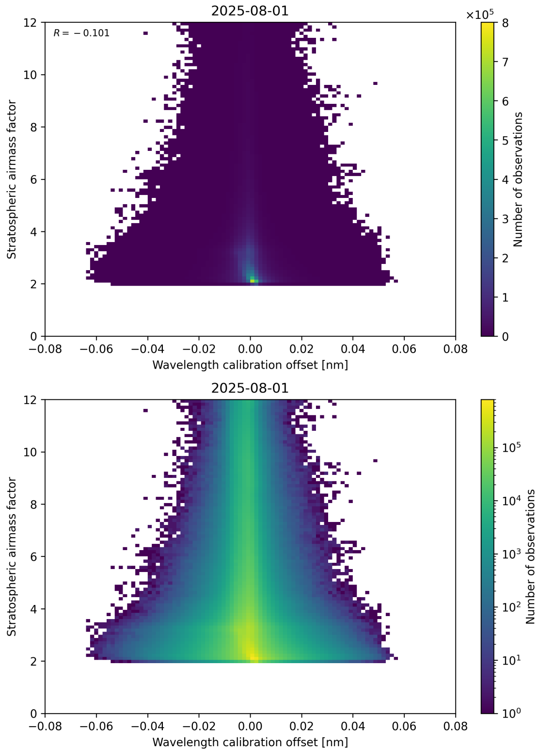
Figure 174: Scatter density plot of “Wavelength calibration offset” against “Stratospheric airmass factor” for 2025-07-31 to 2025-08-02.
