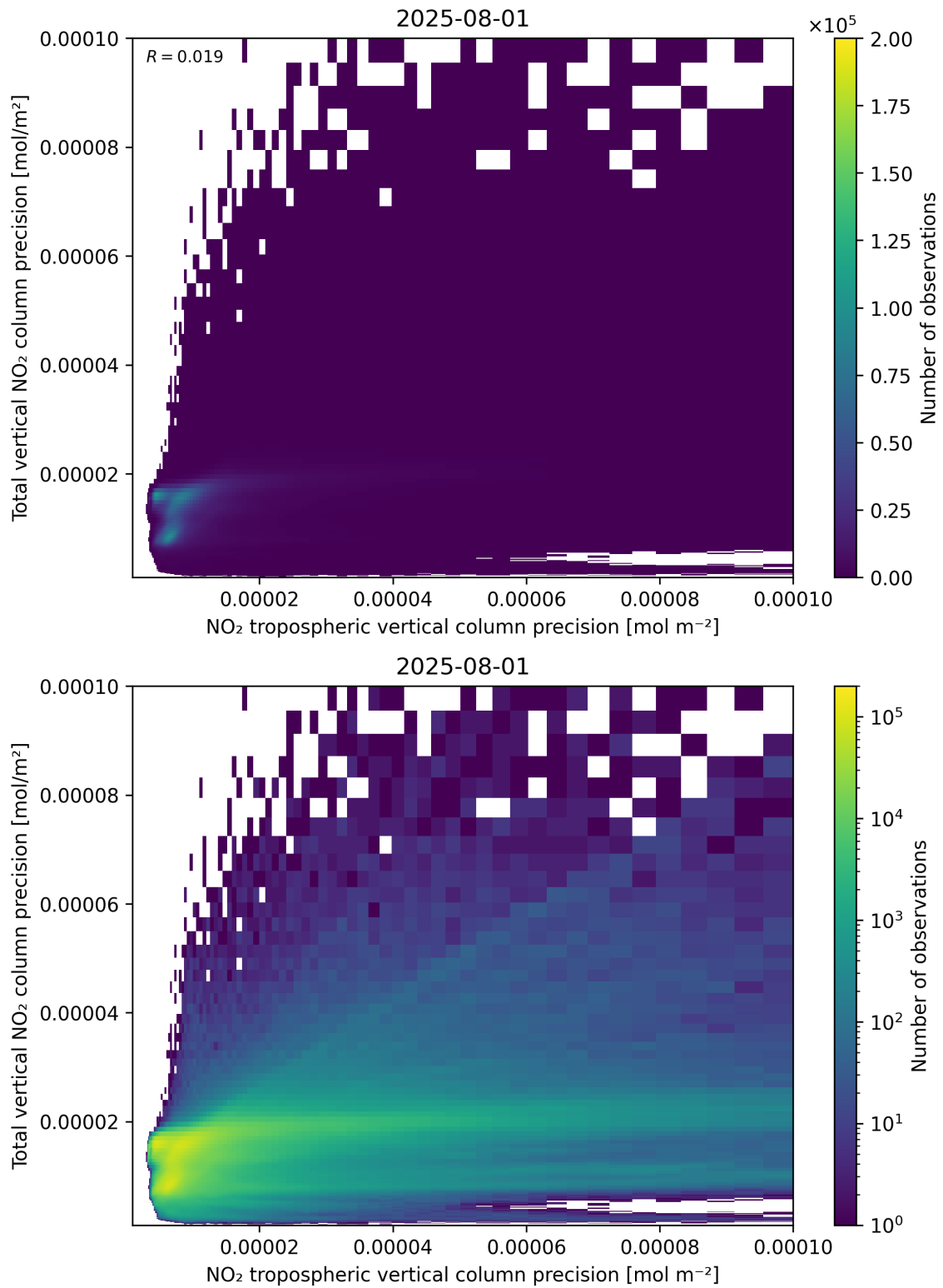
Figure 139: Scatter density plot of “NO 2 tropospheric vertical column precision” against “Total vertical NO 2 column precision” for 2025-07-31 to 2025-08-02.
