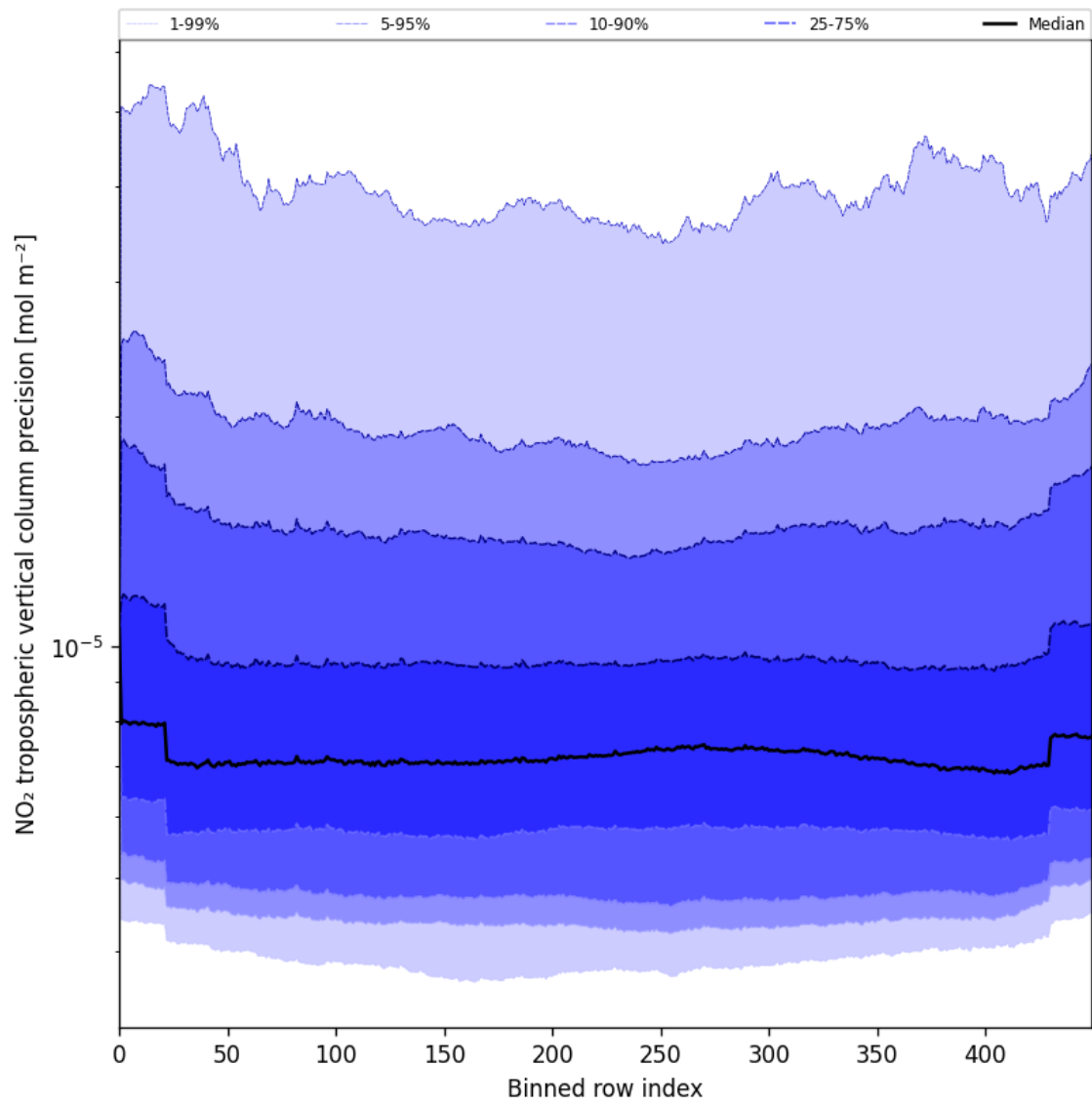
Figure 47: Along track statistics of “NO 2 tropospheric vertical column precision” for 2025-07-31 to 2025-08-02
