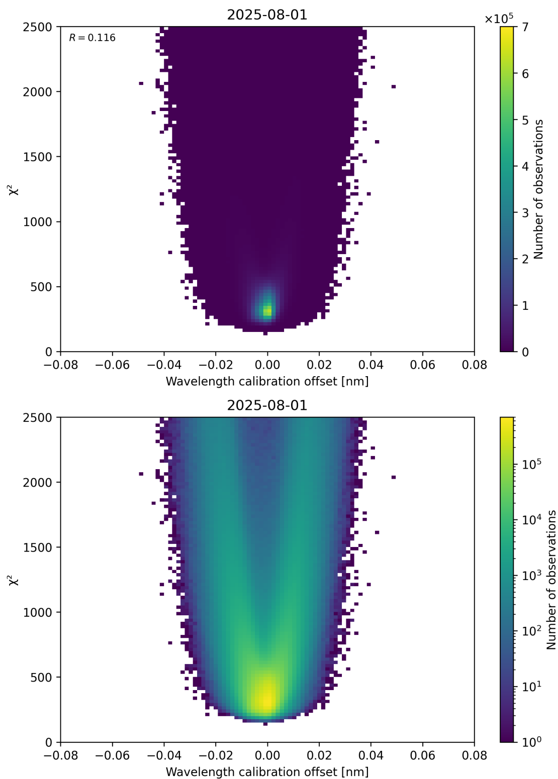
Figure 175: Scatter density plot of “Wavelength calibration offset” against “ \chi^2 ” for 2025-07-31 to 2025-08-02.
