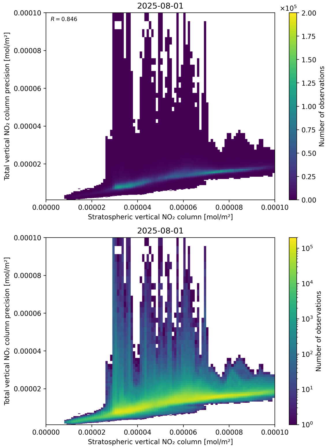
Figure 101: Scatter density plot of “Stratospheric vertical NO 2 column” against “Total vertical NO 2 column precision” for 2025-07-31 to 2025-08-02.
