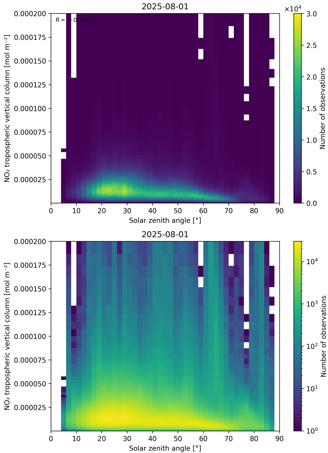
Figure 155: Scatter density plot of “Solar zenith angle” against “NO 2 tropospheric vertical column” for 2025-07-31 to 2025-08-02.
