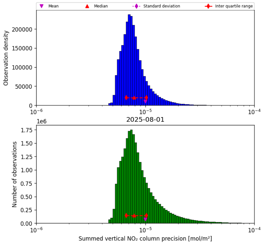
Figure 41: Histogram of "Summed vertical NO 2 column precision" for 2025-07-31 to 2025-08-02
