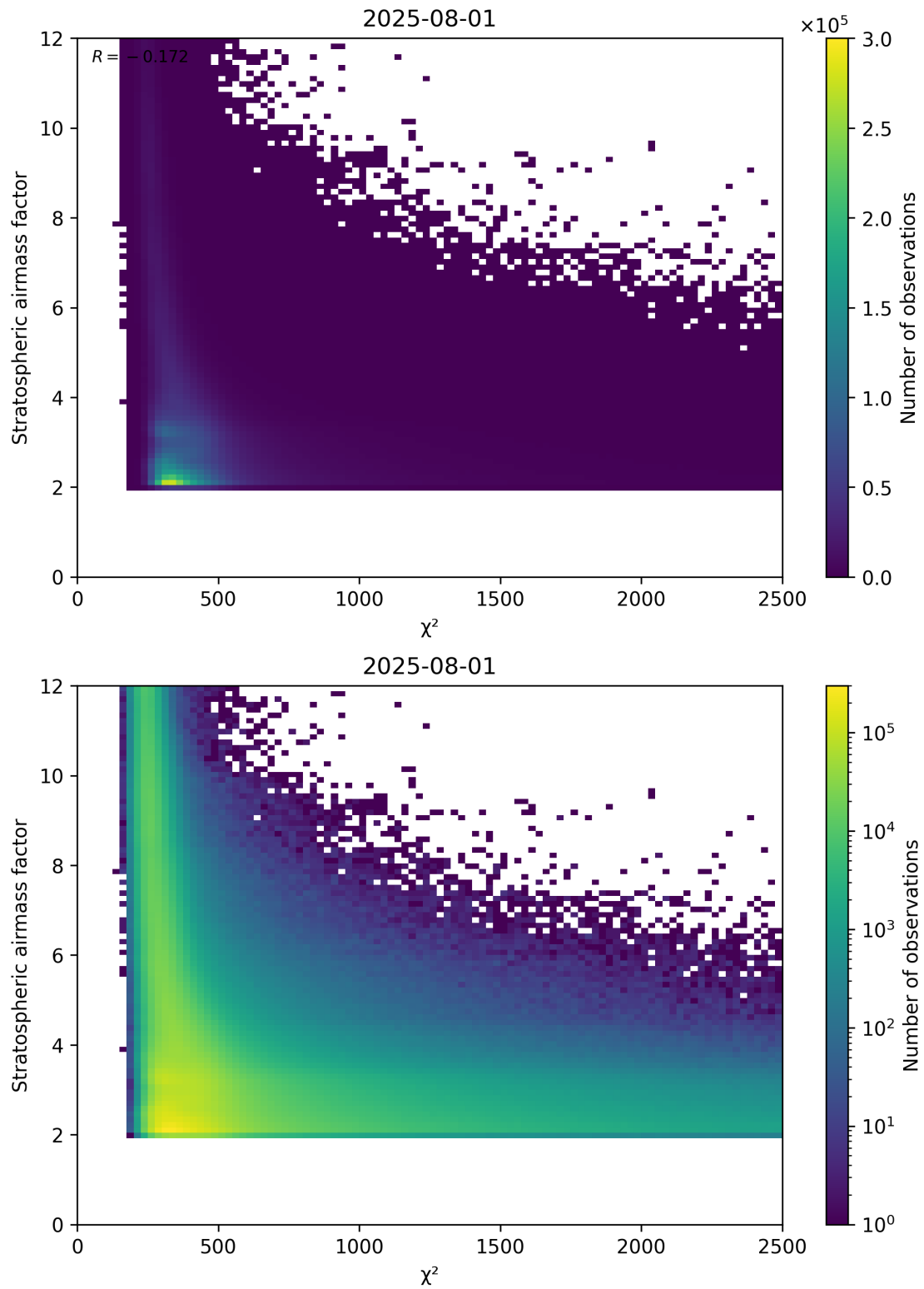
Figure 81: Scatter density plot of “ \chi^2 ” against “Stratospheric airmass factor” for 2025-07-31 to 2025-08-02.
