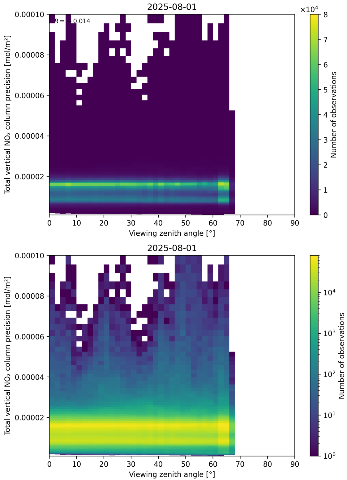
Figure 168: Scatter density plot of “Viewing zenith angle” against “Total vertical NO 2 column precision” for 2025-07-31 to 2025-08-02.
