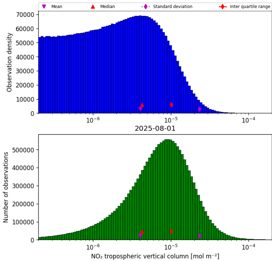
Figure 29: Histogram of “NO 2 tropospheric vertical column” for 2025-07-31 to 2025-08-02
