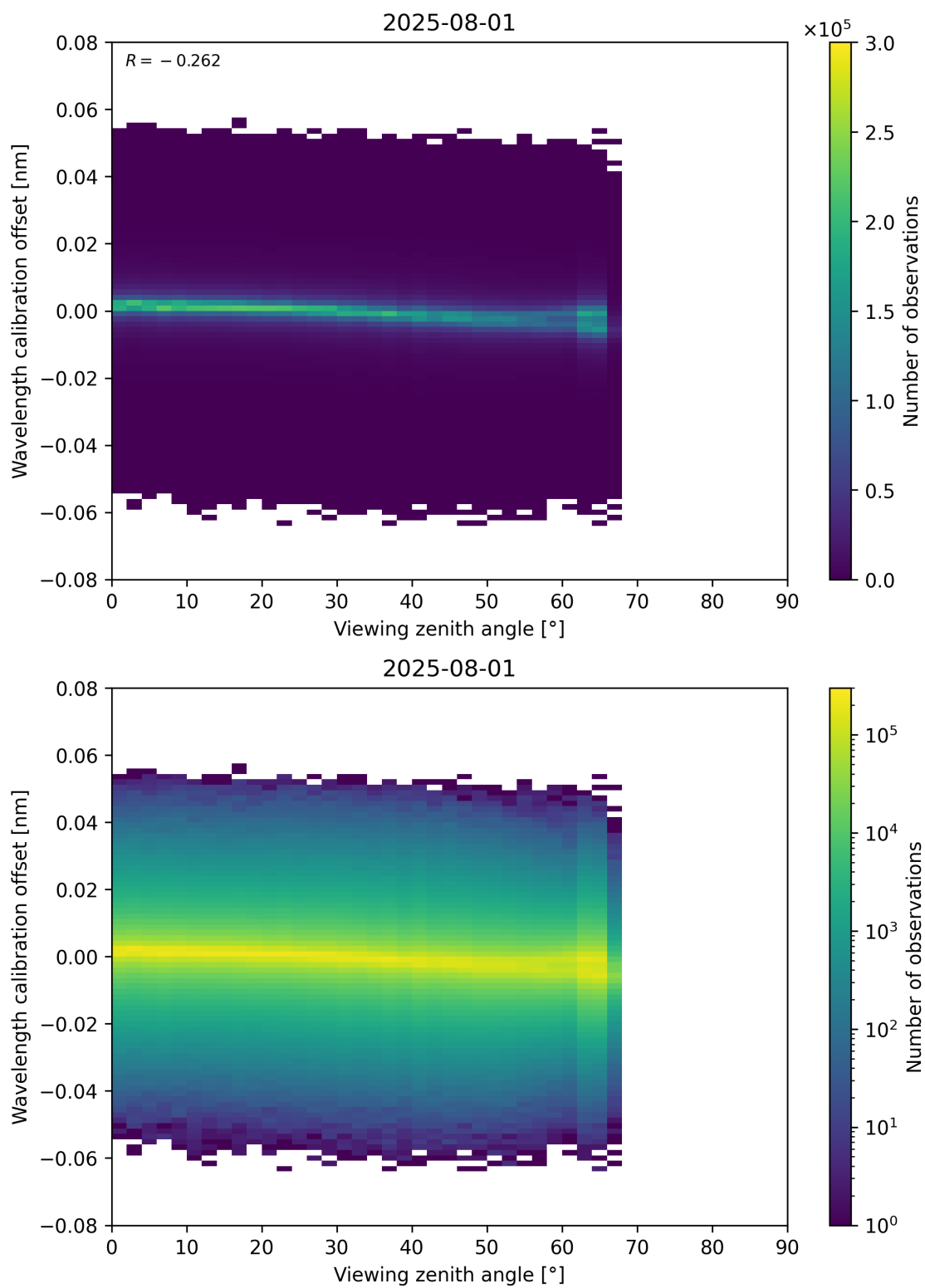
Figure 173: Scatter density plot of “Viewing zenith angle” against “Wavelength calibration offset” for 2025-07-31 to 2025-08-02.
