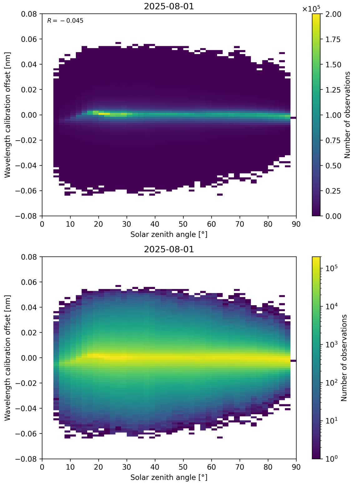
Figure 158: Scatter density plot of “Solar zenith angle” against “Wavelength calibration offset” for 2025-07-31 to 2025-08-02.
