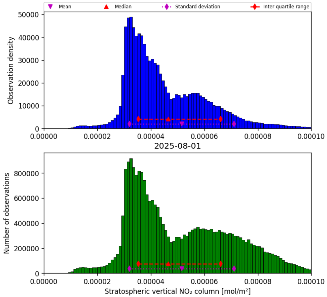
Figure 36: Histogram of “Stratospheric vertical NO 2 column” for 2025-07-31 to 2025-08-02
