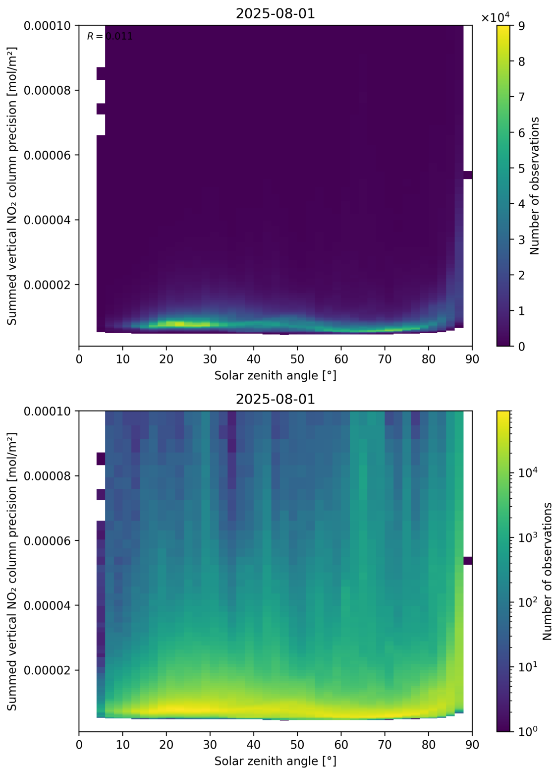
Figure 152: Scatter density plot of “Solar zenith angle” against “Summed vertical NO 2 column precision” for 2025-07-31 to 2025-08-02.
