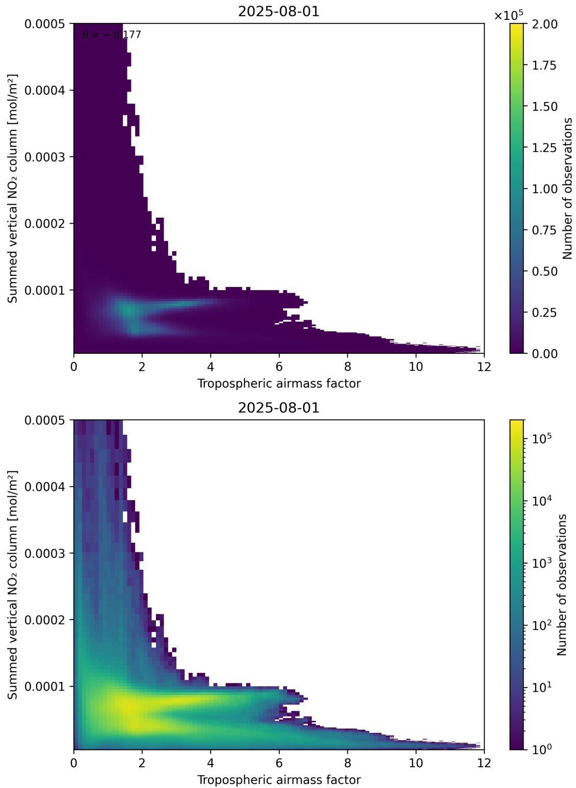
Figure 75: Scatter density plot of “Tropospheric airmass factor” against “Summed vertical NO 2 column” for 2025-07-31 to 2025-08-02.
