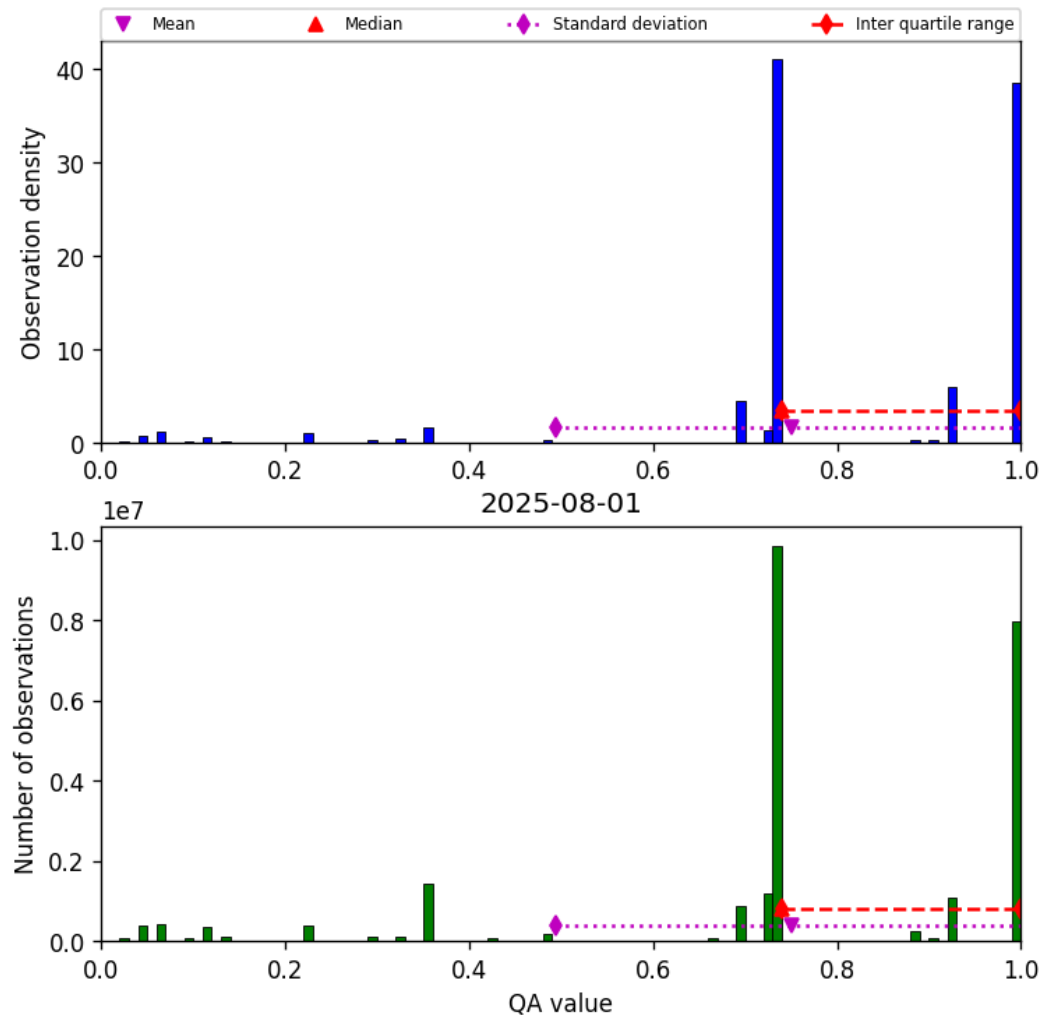
Figure 28: Histogram of “QA value” for 2025-07-31 to 2025-08-02
