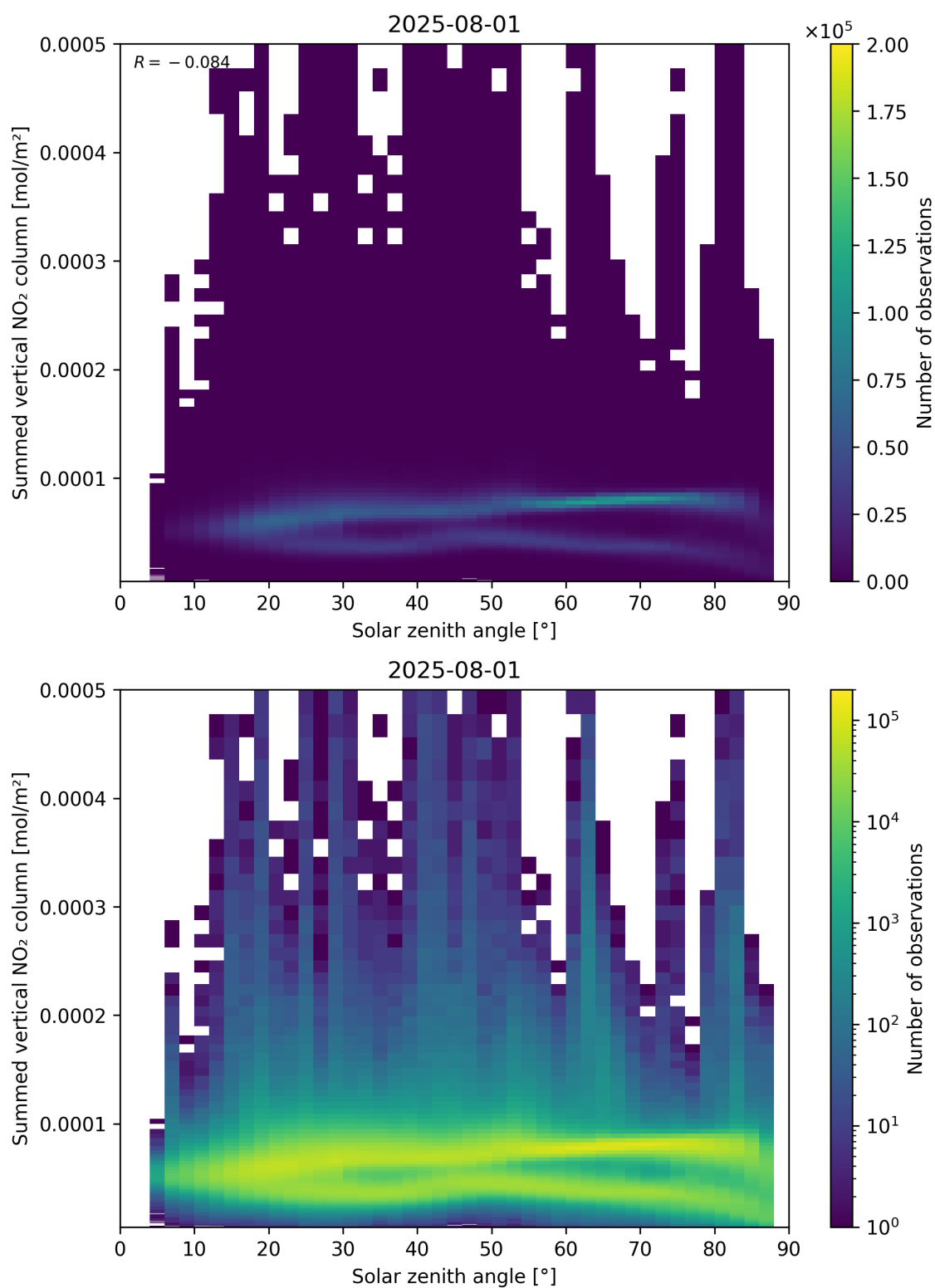
Figure 151: Scatter density plot of “Solar zenith angle” against “Summed vertical NO 2 column” for 2025-07-31 to 2025-08-02.
