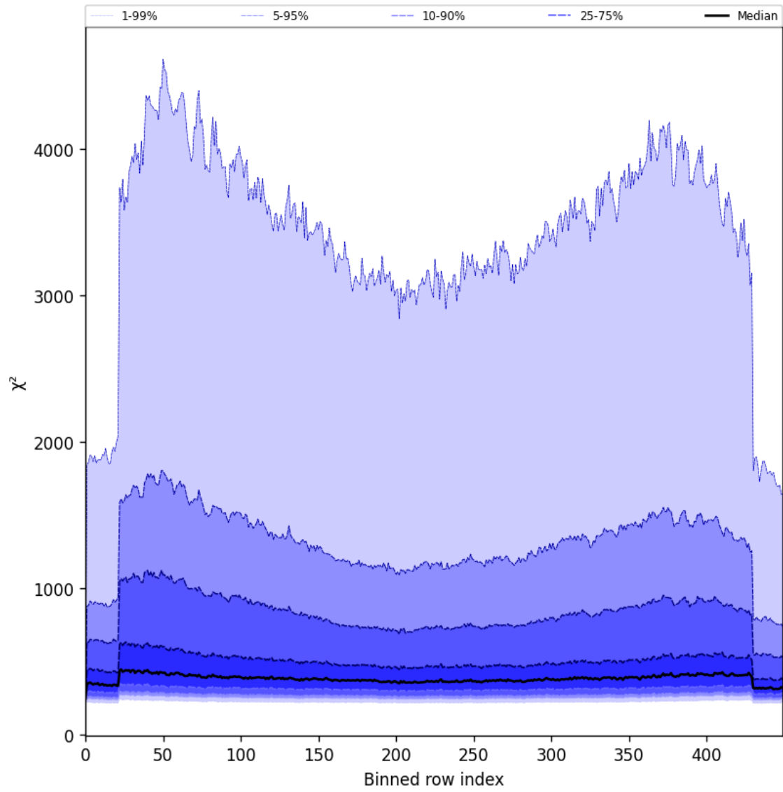
Figure 59: Along track statistics of “ \chi^2 ” for 2025-07-31 to 2025-08-02
