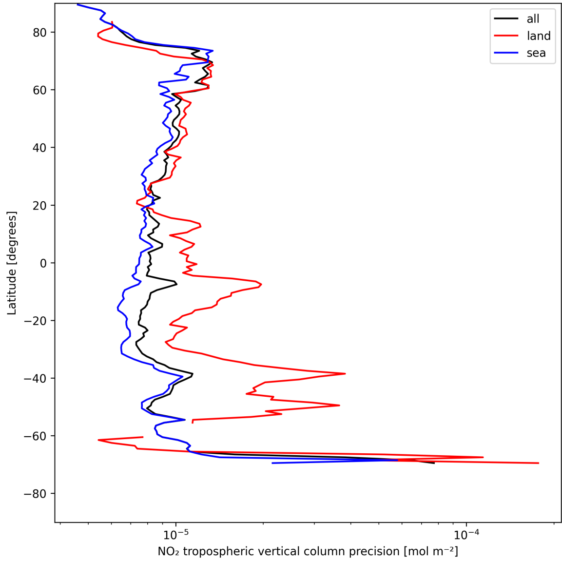
Figure 13: Zonal average of "NO 2 tropospheric vertical column precision" for 2025-07-31 to 2025-08-02.
