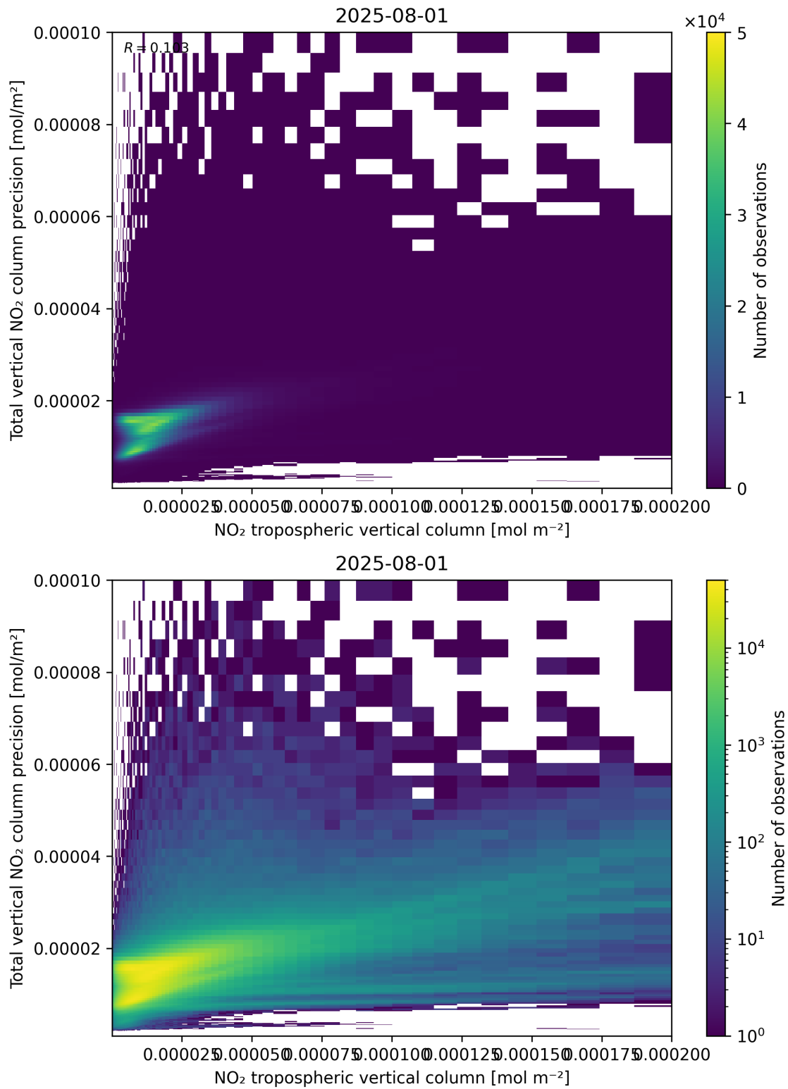
Figure 129: Scatter density plot of “NO 2 tropospheric vertical column” against “Total vertical NO 2 column precision” for 2025-07-31 to 2025-08-02.
