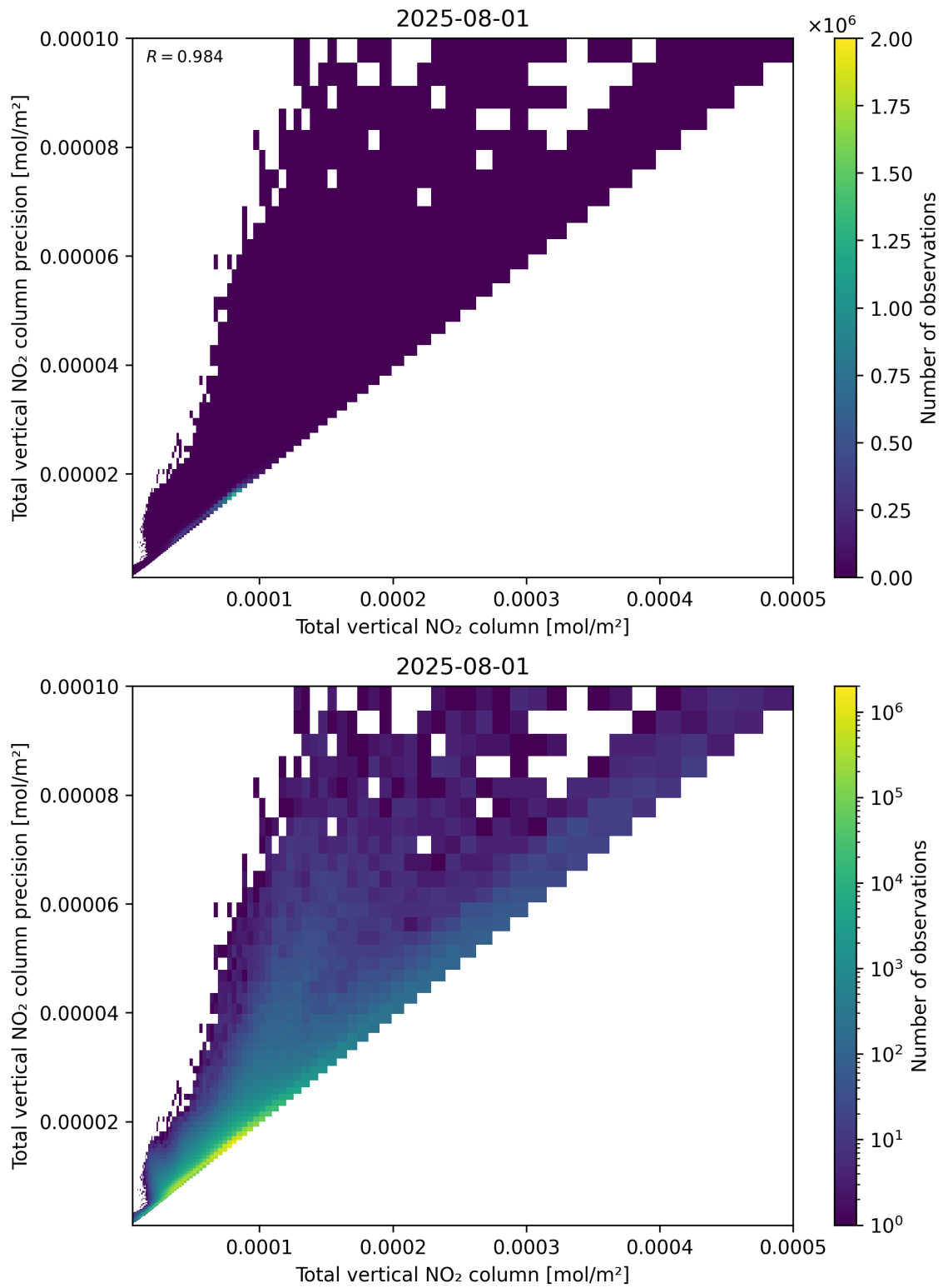
Figure 114: Scatter density plot of “Total vertical NO 2 column” against “Total vertical NO 2 column precision” for 2025-07-31 to 2025-08-02.
