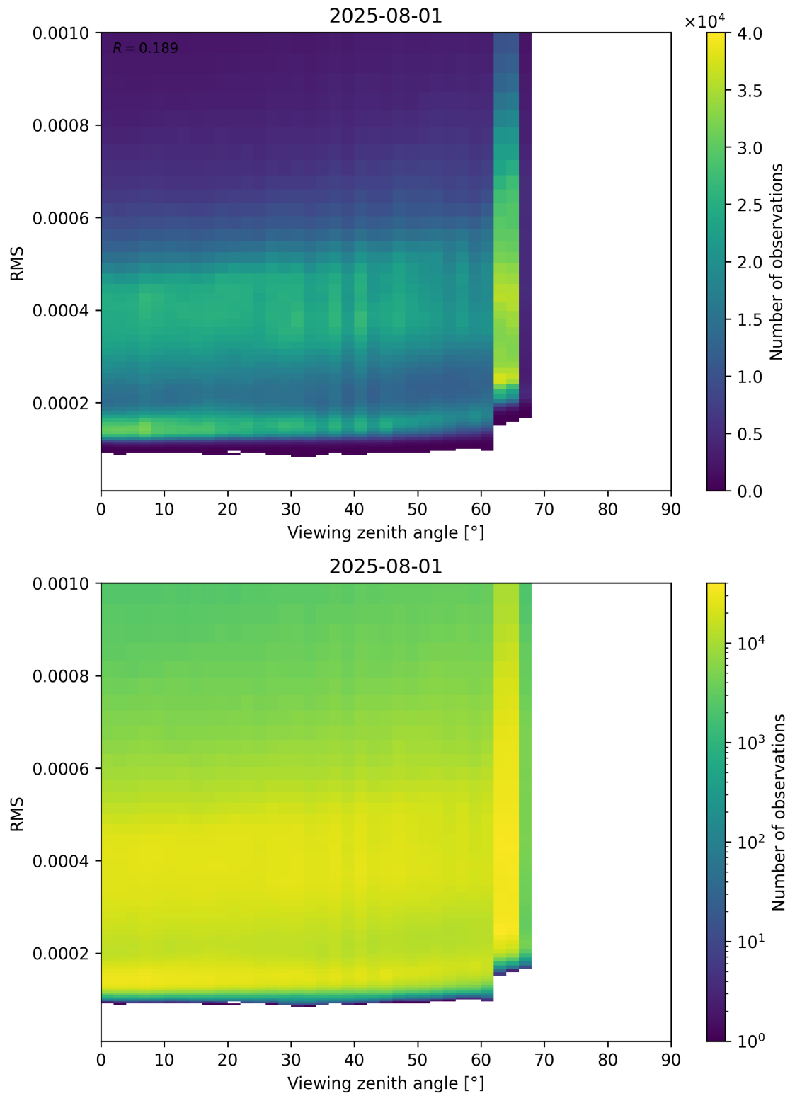
Figure 171: Scatter density plot of “Viewing zenith angle” against “RMS” for 2025-07-31 to 2025-08-02.
