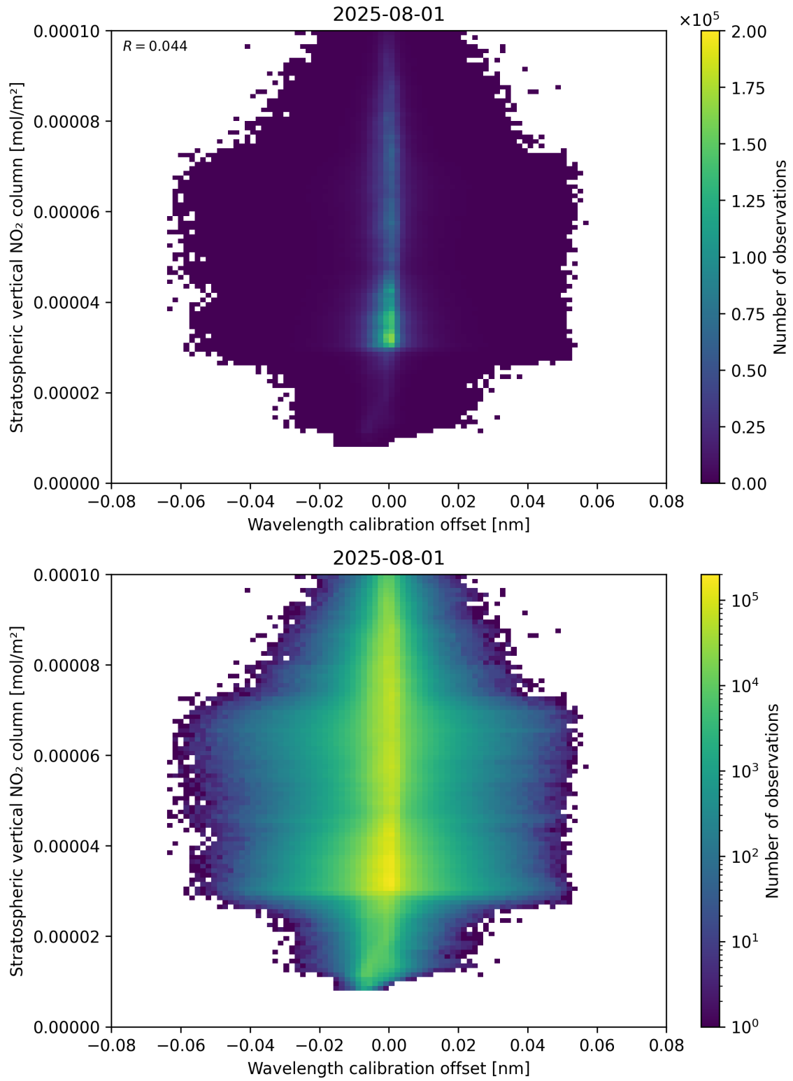
Figure 176: Scatter density plot of “Wavelength calibration offset” against “Stratospheric vertical NO 2 column” for 2025-07-31 to 2025-08-02.
