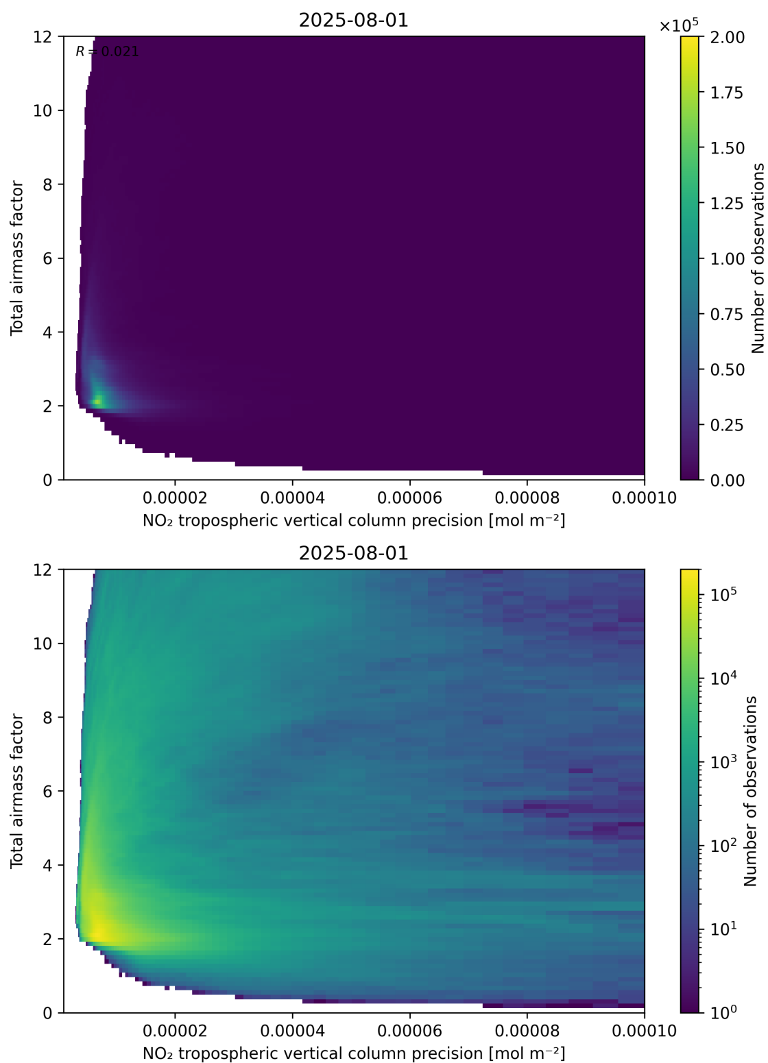
Figure 132: Scatter density plot of “NO 2 tropospheric vertical column precision” against “Total air mass factor” for 2025-07-31 to 2025-08-02.
