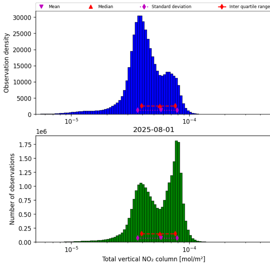
Figure 38: Histogram of “Total vertical NO 2 column” for 2025-07-31 to 2025-08-02
