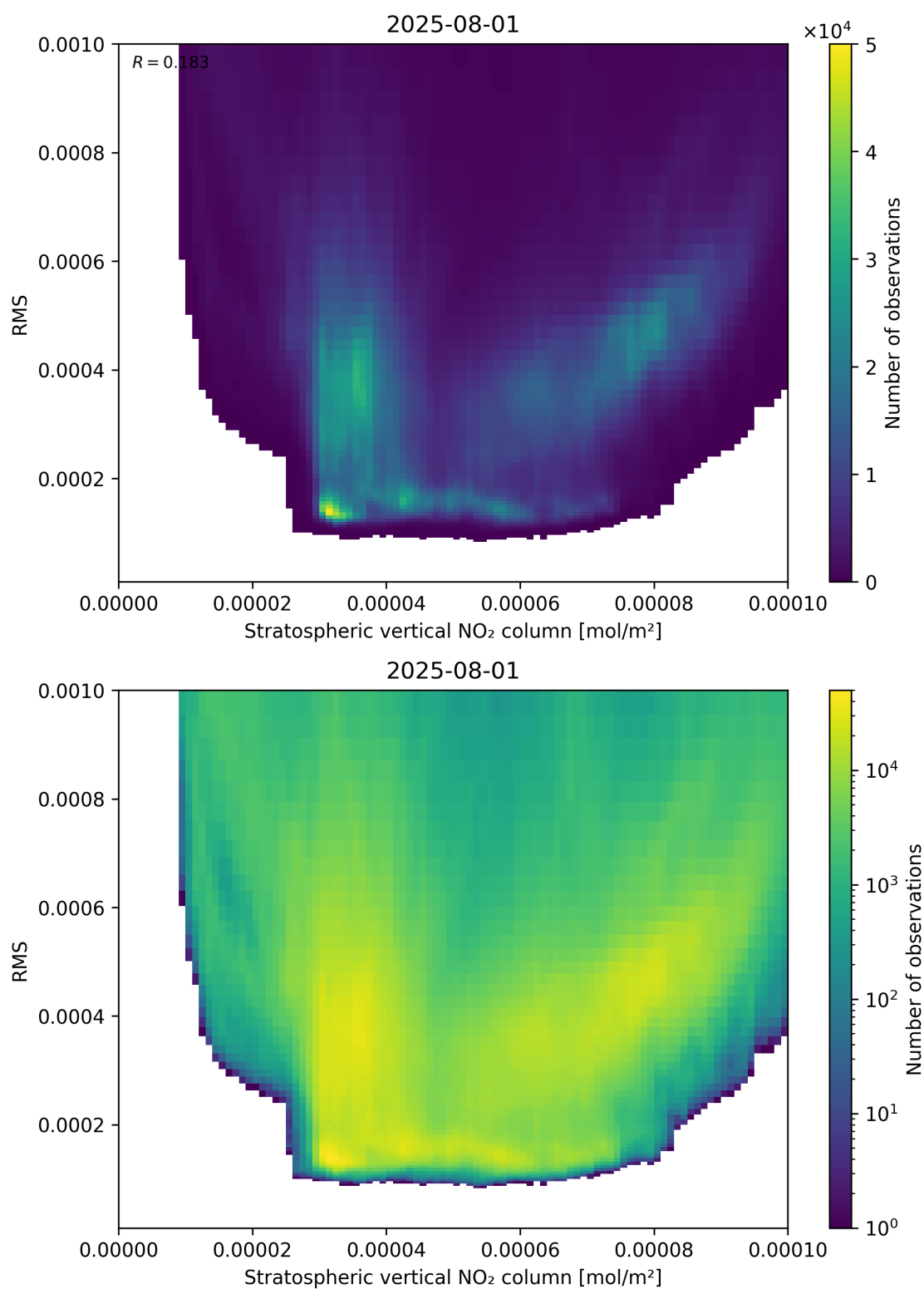
Figure 102: Scatter density plot of “Stratospheric vertical NO 2 column” against “RMS” for 2025-07-31 to 2025-08-02.
