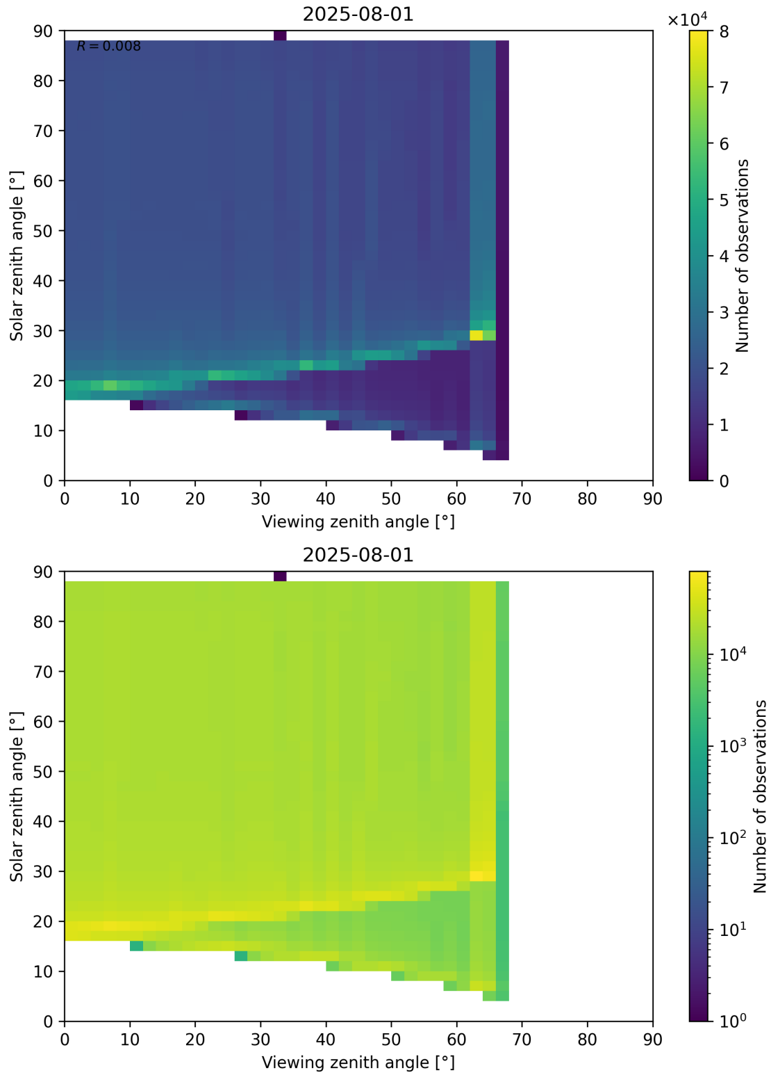
Figure 172: Scatter density plot of “Viewing zenith angle” against “Solar zenith angle” for 2025-07-31 to 2025-08-02.
