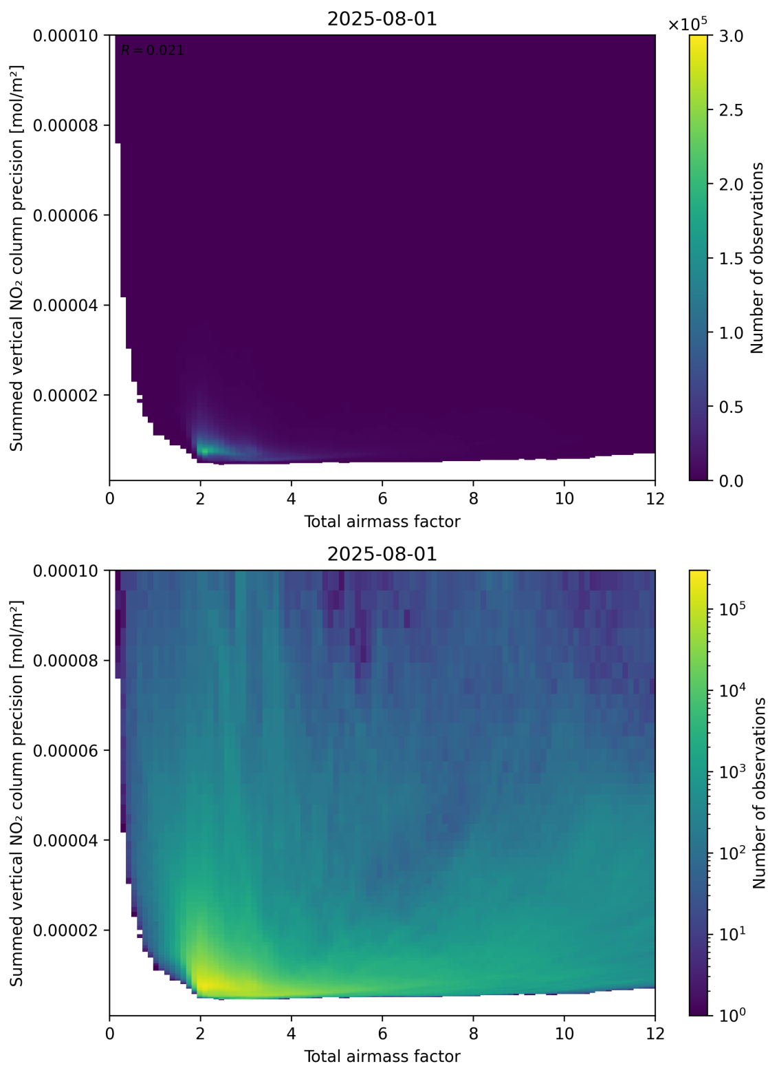
Figure 66: Scatter density plot of “Total airmass factor” against “Summed vertical NO 2 column precision” for 2025-07-31 to 2025-08-02.
