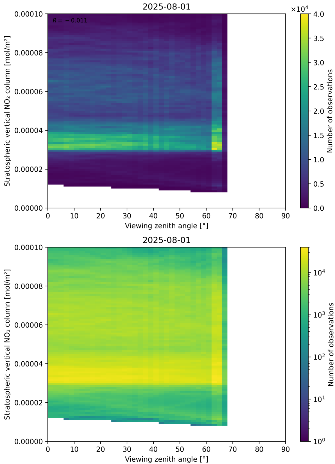
Figure 164: Scatter density plot of “Viewing zenith angle” against “Stratospheric vertical NO 2 column” for 2025-07-31 to 2025-08-02.
