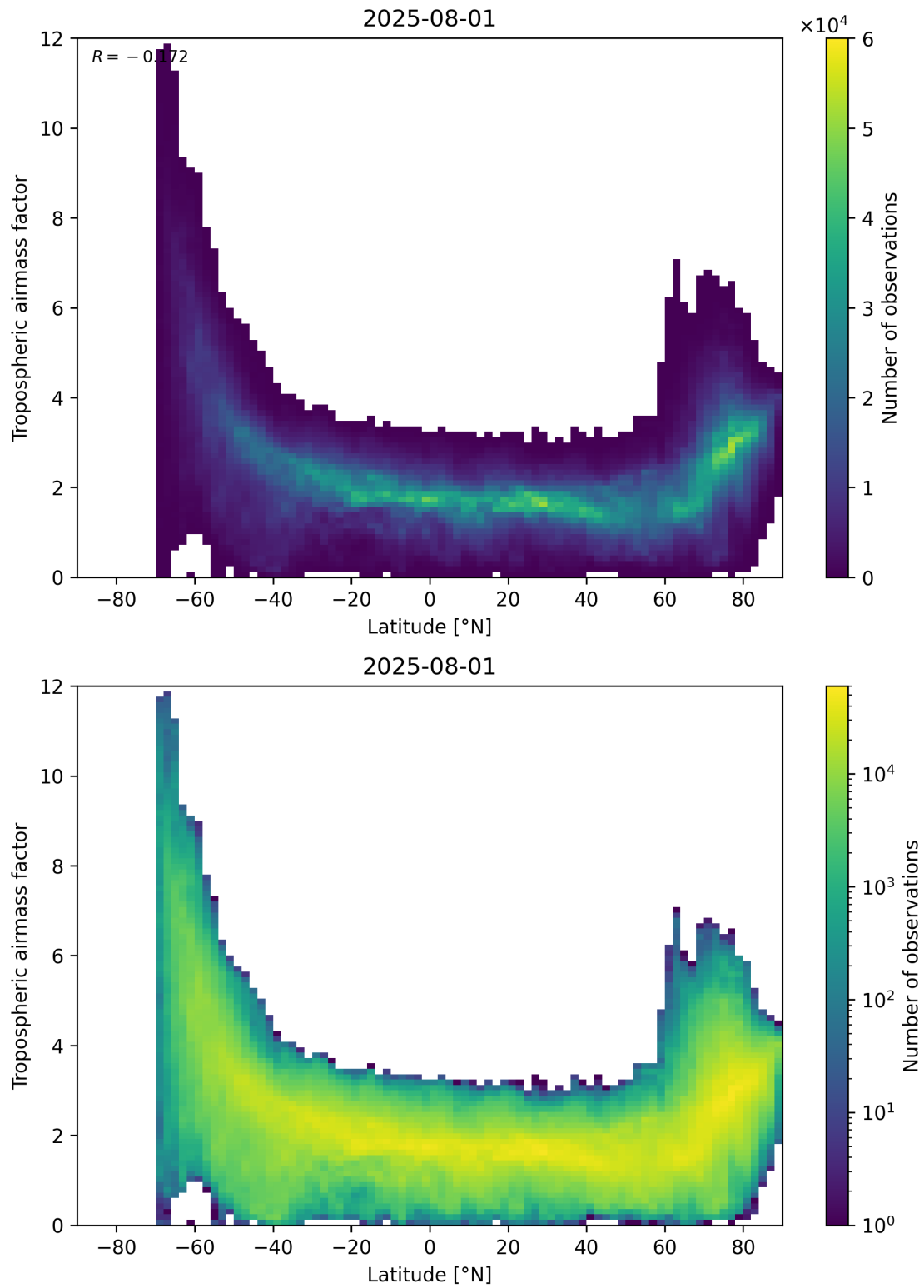
Figure 85: Scatter density plot of “Latitude” against “Tropospheric air mass factor” for 2025-07-31 to 2025-08-02.
