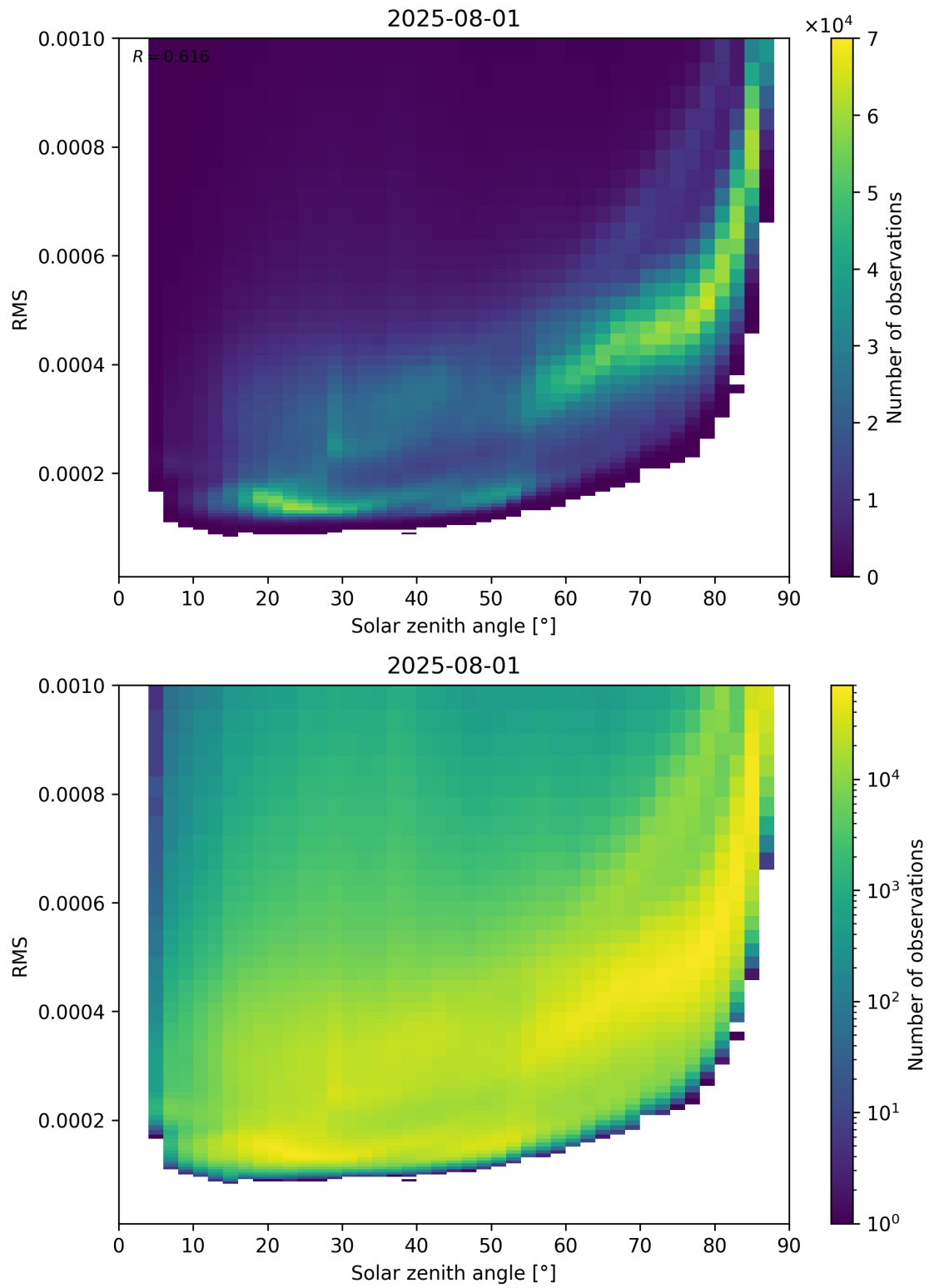
Figure 157: Scatter density plot of “Solar zenith angle” against “RMS” for 2025-07-31 to 2025-08-02.
