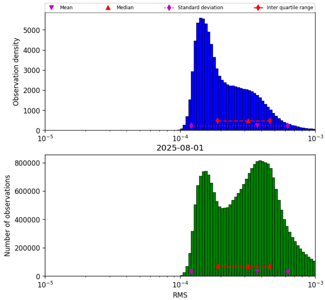
Figure 43: Histogram of “RMS” for 2025-07-31 to 2025-08-02
