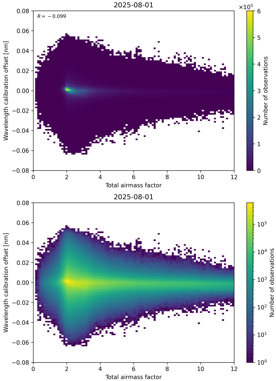
Figure 70: Scatter density plot of “Total airmass factor” against “Wavelength calibration offset” for 2025-07-31 to 2025-08-02.
