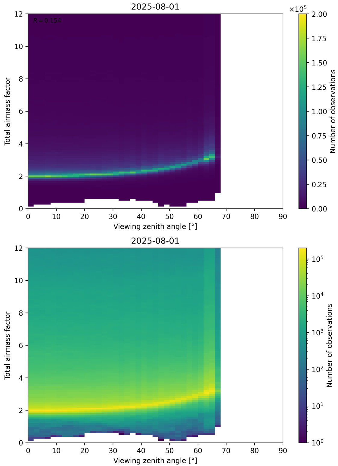
Figure 160: Scatter density plot of “Viewing zenith angle” against “Total airmass factor” for 2025-07-31 to 2025-08-02.
