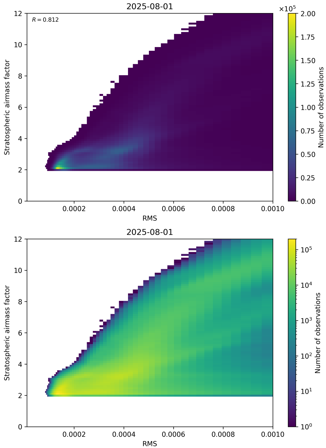
Figure 144: Scatter density plot of “RMS” against “Stratospheric airmass factor” for 2025-07-31 to 2025-08-02.
