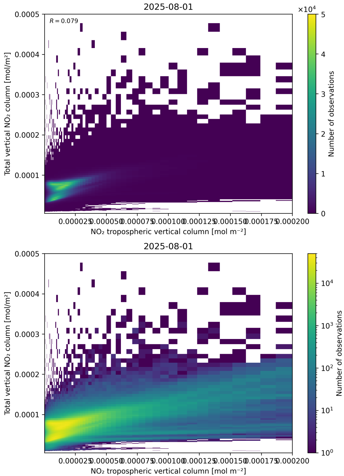
Figure 128: Scatter density plot of “NO 2 tropospheric vertical column” against “Total vertical NO 2 column” for 2025-07-31 to 2025-08-02.
