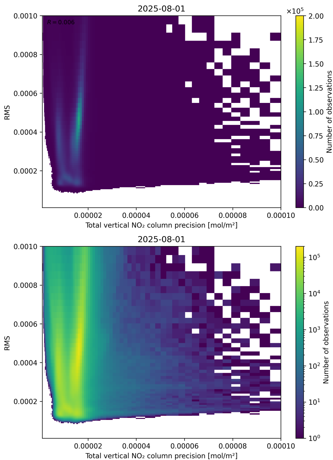
Figure 119: Scatter density plot of “Total vertical NO 2 column precision” against “RMS” for 2025-07-31 to 2025-08-02.
