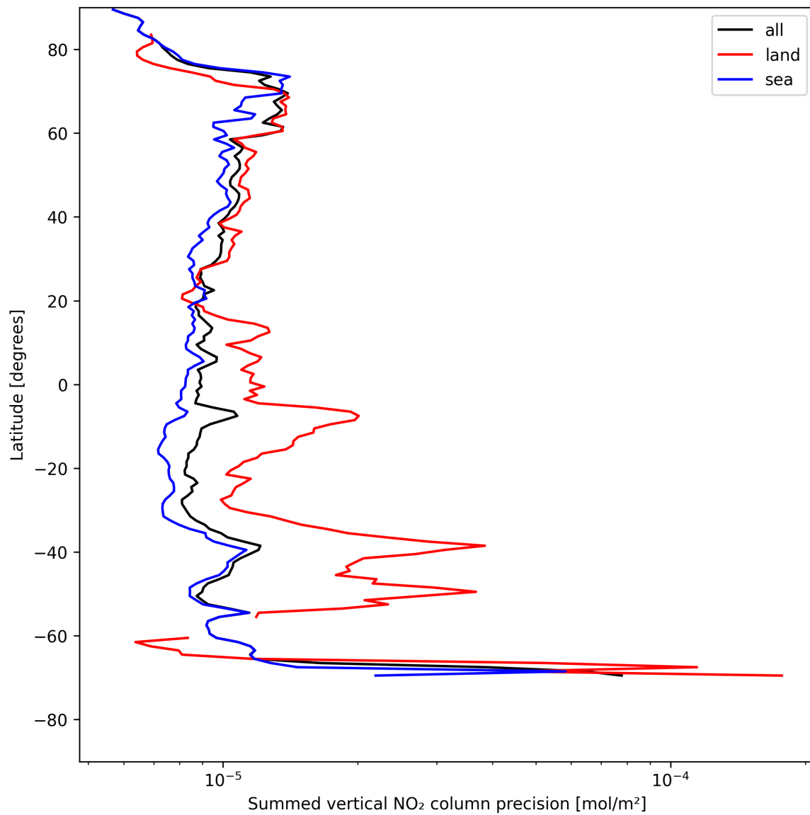
Figure 24: Zonal average of “Summed vertical NO 2 column precision” for 2025-07-31 to 2025-08-02.
