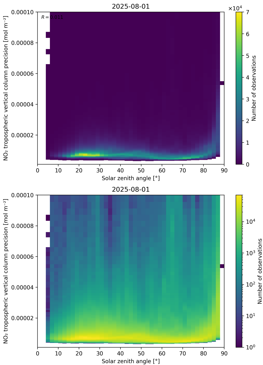
Figure 156: Scatter density plot of “Solar zenith angle” against “NO 2 tropospheric vertical column precision” for 2025-07-31 to 2025-08-02.
