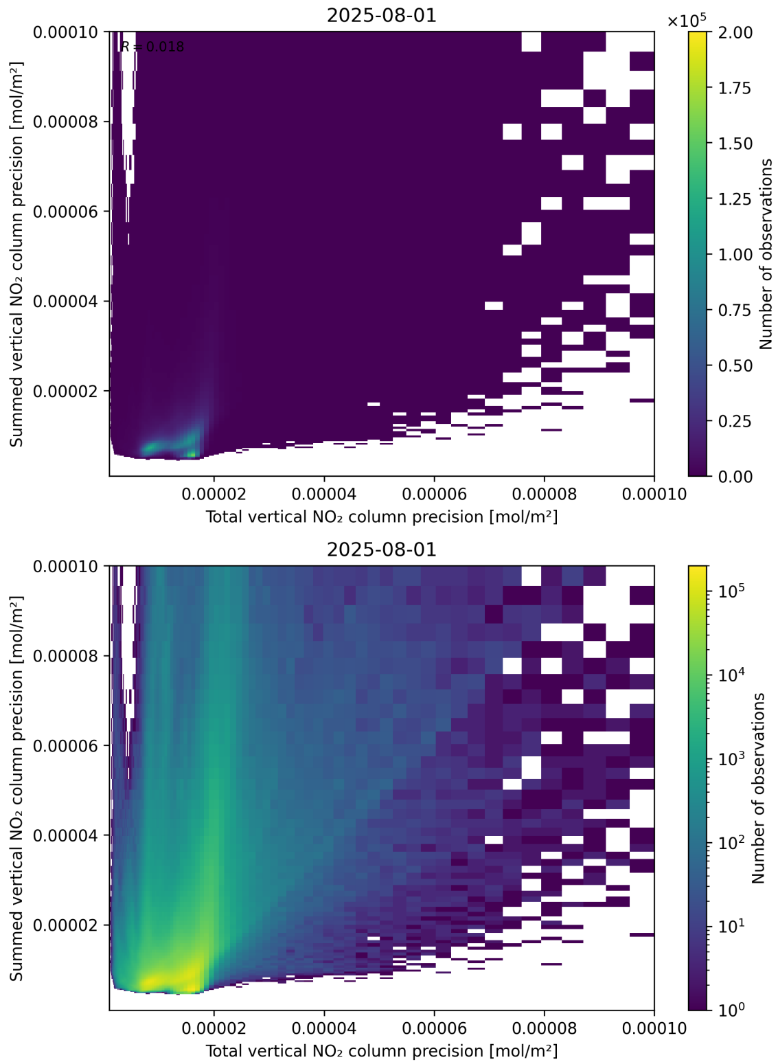
Figure 118: Scatter density plot of “Total vertical NO 2 column precision” against “Summed vertical NO 2 column precision” for 2025-07-31 to 2025-08-02.
