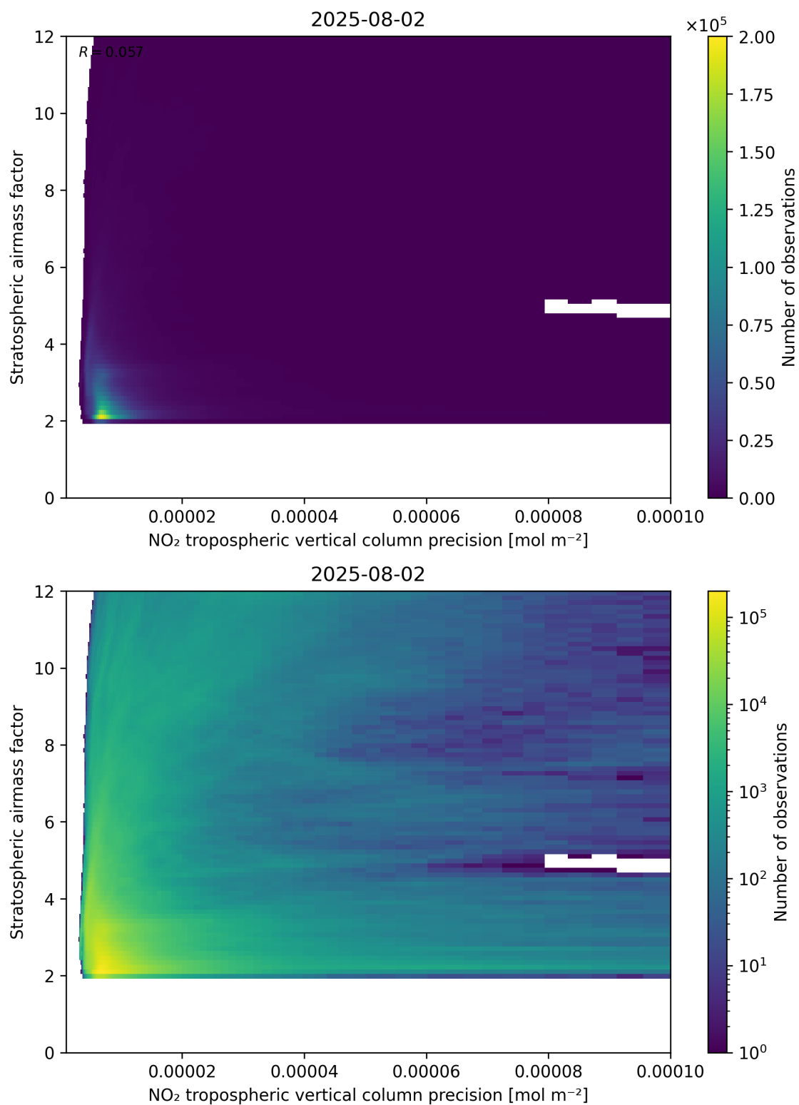
Figure 131: Scatter density plot of “NO 2 tropospheric vertical column precision” against “Stratospheric airmass factor” for 2025-08-01 to 2025-08-03.
