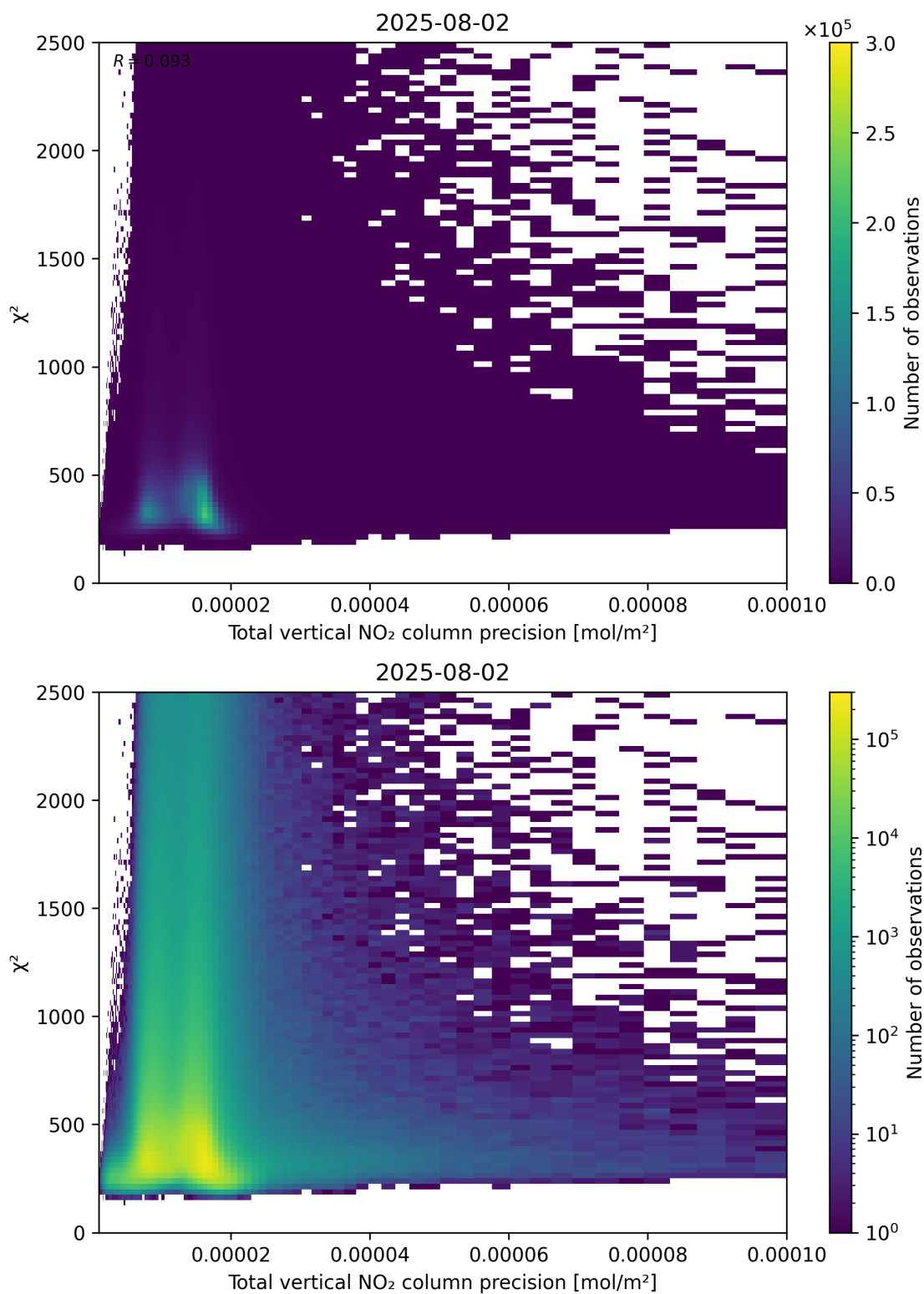
Figure 116: Scatter density plot of “Total vertical NO 2 column precision” against “ \chi^2 ” for 2025-08-01 to 2025-08-03.
