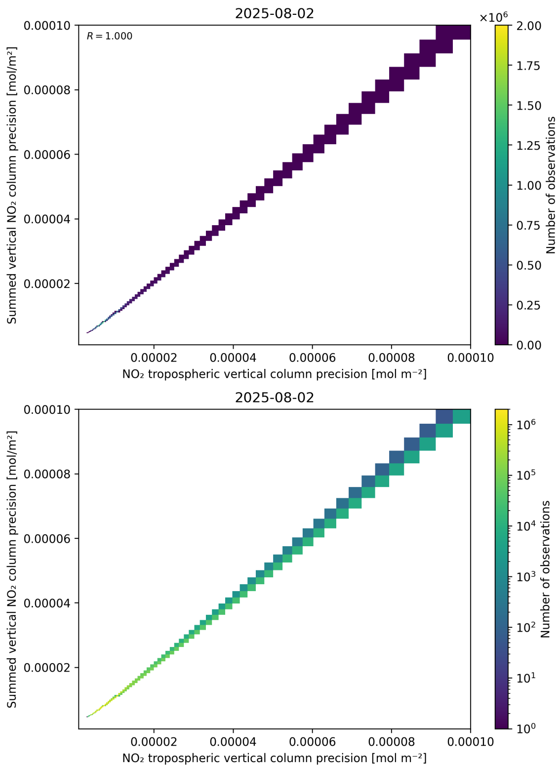
Figure 137: Scatter density plot of “NO 2 tropospheric vertical column precision” against “Summed vertical NO 2 column precision” for 2025-08-01 to 2025-08-03.
