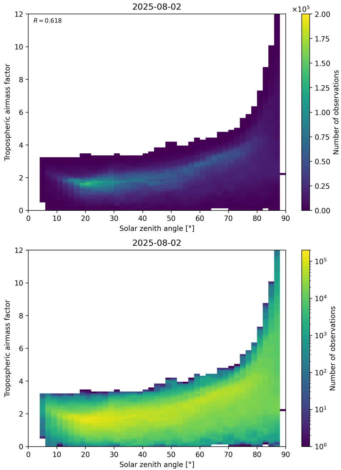
Figure 147: Scatter density plot of “Solar zenith angle” against “Tropospheric airmass factor” for 2025-08-01 to 2025-08-03.
