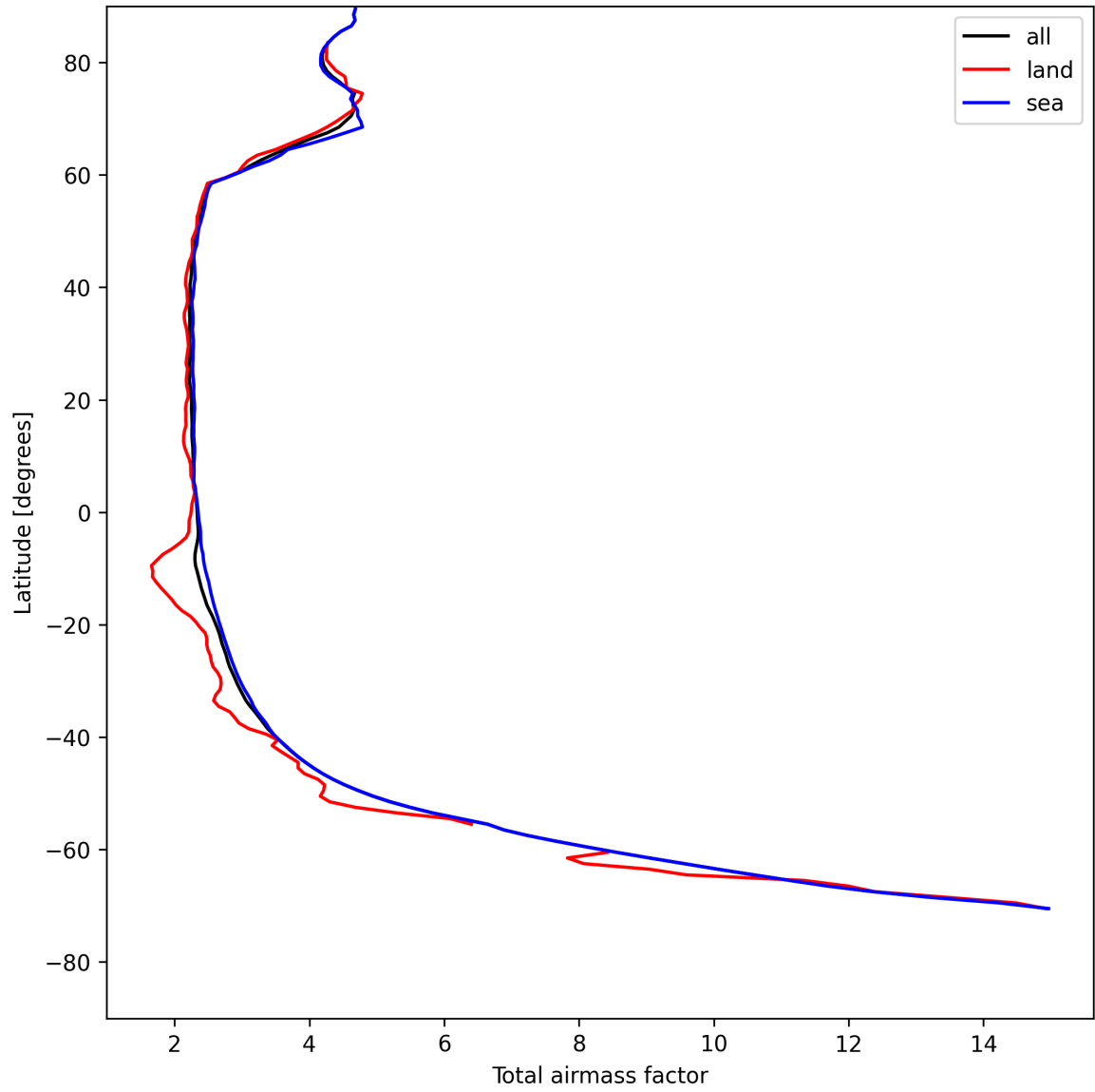
Figure 15: Zonal average of “Total airmass factor” for 2025-08-01 to 2025-08-03.
