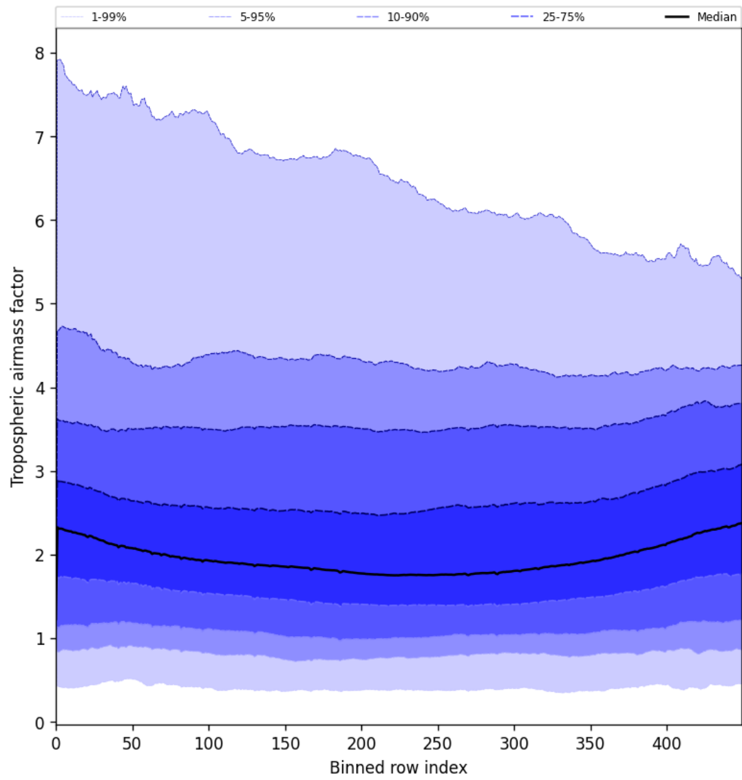
Figure 48: Along track statistics of “Tropospheric airmass factor” for 2025-08-01 to 2025-08-03
