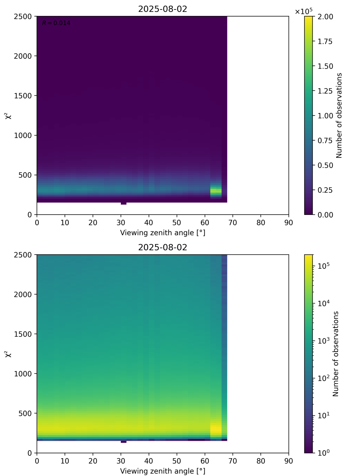
Figure 162: Scatter density plot of “Viewing zenith angle” against “ \chi^2 ” for 2025-08-01 to 2025-08-03.
