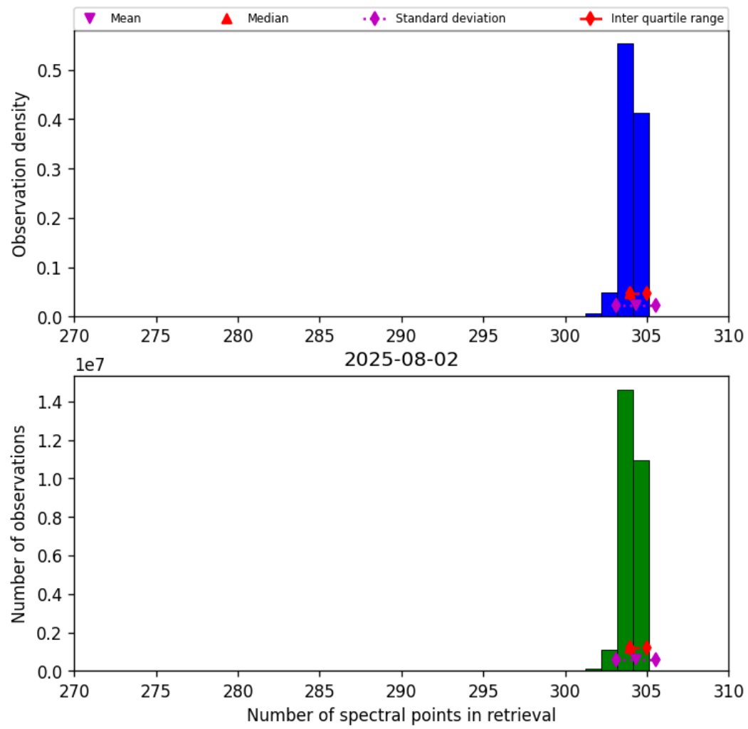
Figure 33: Histogram of “Number of spectral points in retrieval” for 2025-08-01 to 2025-08-03
