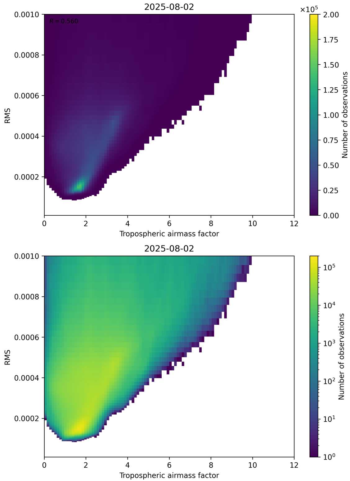
Figure 79: Scatter density plot of “Tropospheric airmass factor” against “RMS” for 2025-08-01 to 2025-08-03.
