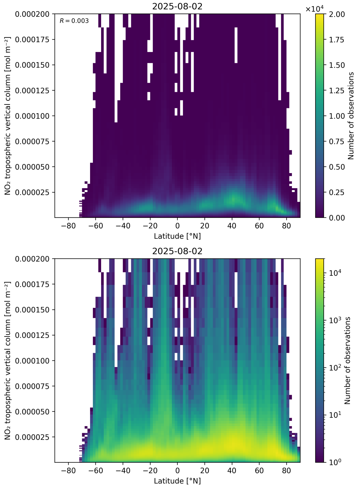
Figure 92: Scatter density plot of “Latitude” against “NO 2 tropospheric vertical column” for 2025-08-01 to 2025-08-03.
