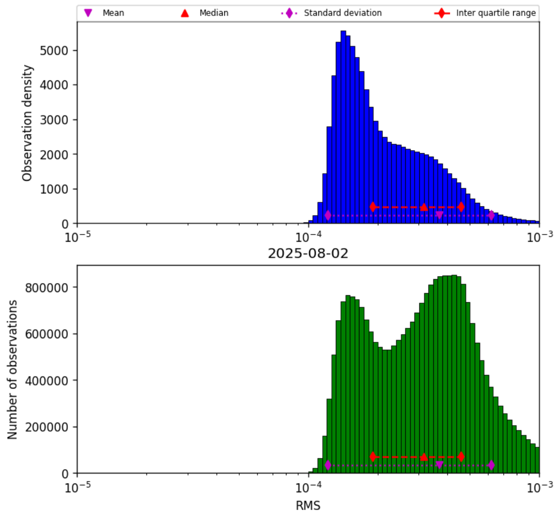
Figure 43: Histogram of “RMS” for 2025-08-01 to 2025-08-03
