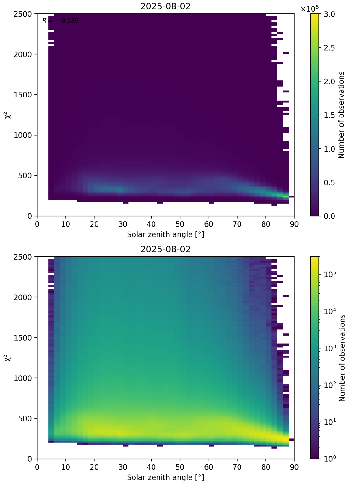
Figure 148: Scatter density plot of “Solar zenith angle” against “ \chi^2 ” for 2025-08-01 to 2025-08-03.
