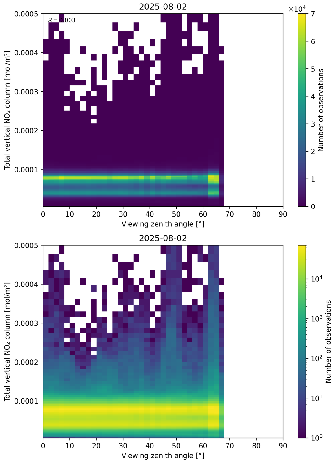
Figure 167: Scatter density plot of “Viewing zenith angle” against “Total vertical NO 2 column” for 2025-08-01 to 2025-08-03.
