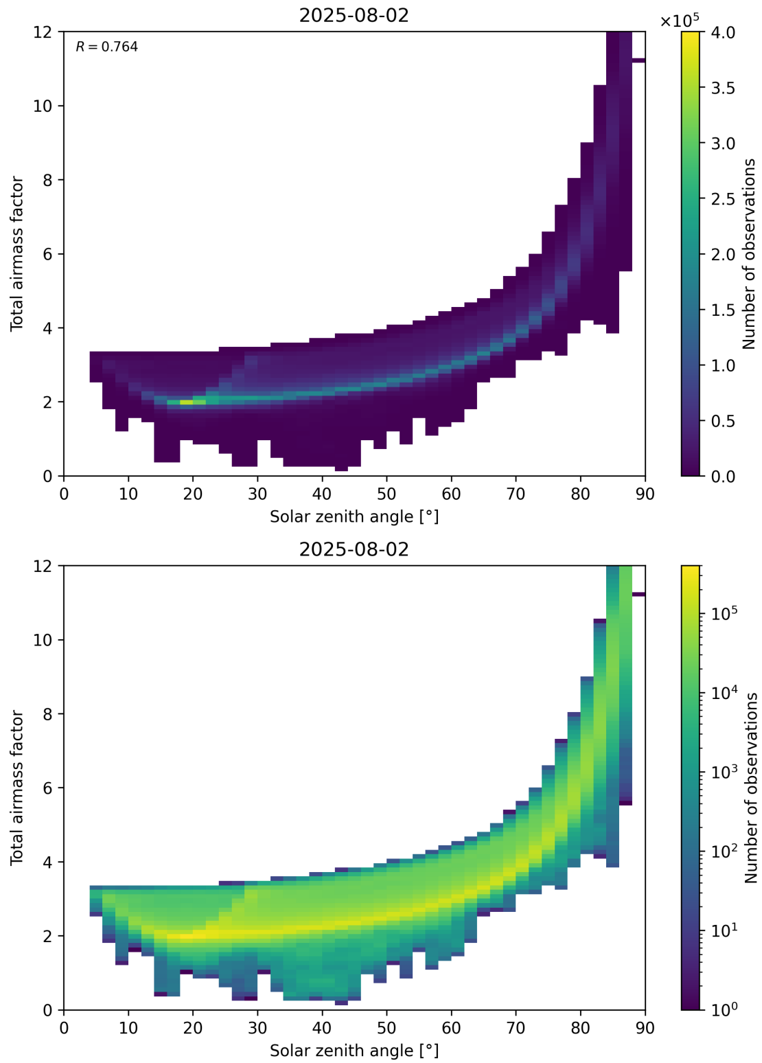
Figure 146: Scatter density plot of “Solar zenith angle” against “Total air mass factor” for 2025-08-01 to 2025-08-03.
