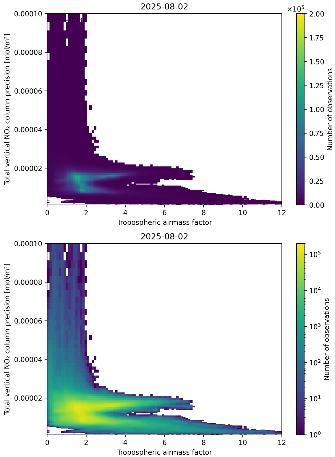
Figure 78: Scatter density plot of “Tropospheric air mass factor” against “Total vertical NO 2 column precision” for 2025-08-01 to 2025-08-03.
