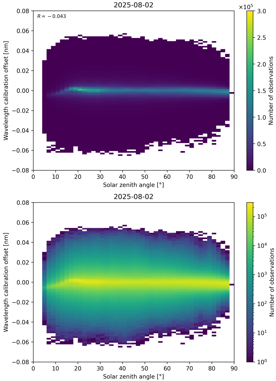
Figure 158: Scatter density plot of “Solar zenith angle” against “Wavelength calibration offset” for 2025-08-01 to 2025-08-03.
