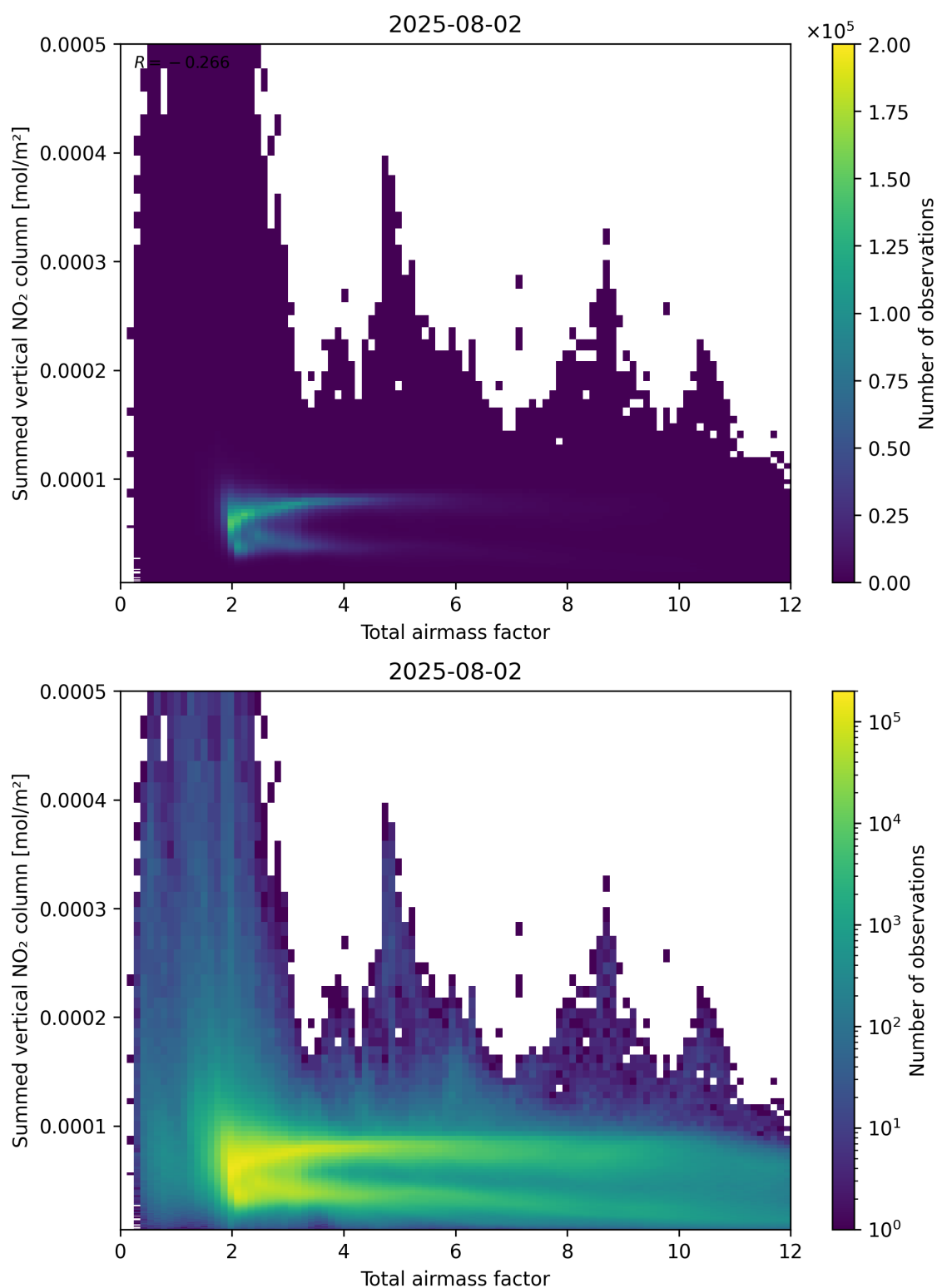
Figure 65: Scatter density plot of “Total airmass factor” against “Summed vertical NO 2 column” for 2025-08-01 to 2025-08-03.
