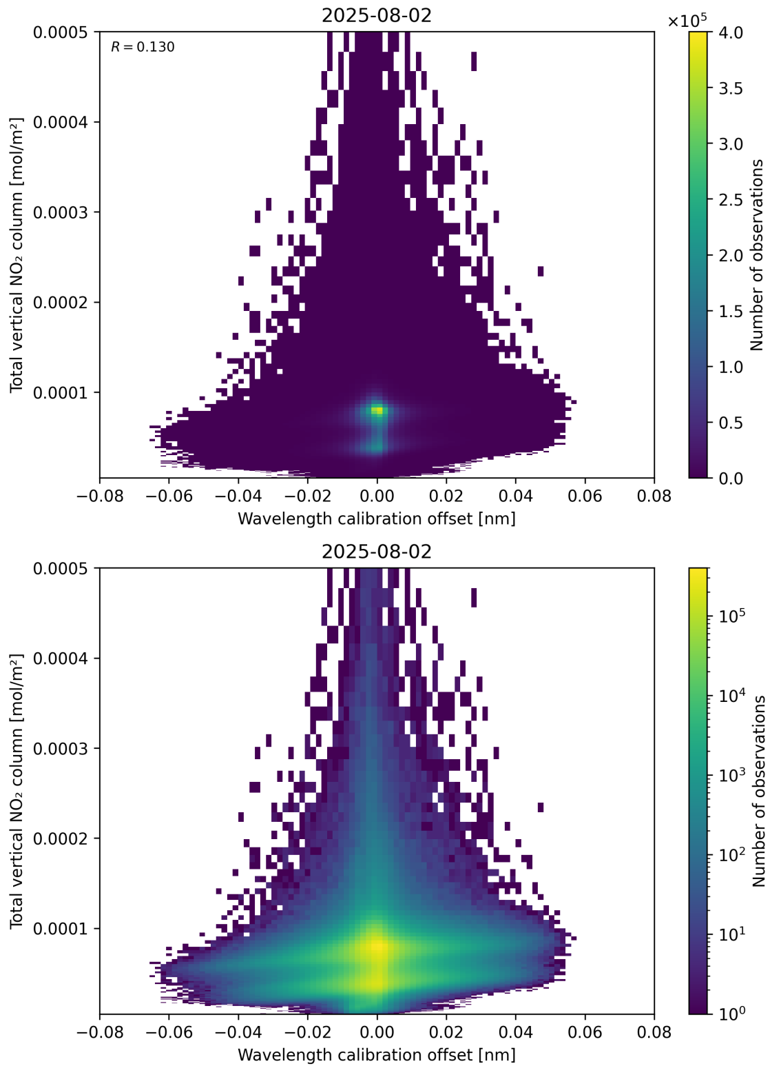
Figure 179: Scatter density plot of “Wavelength calibration offset” against “Total vertical NO 2 column” for 2025-08-01 to 2025-08-03.
