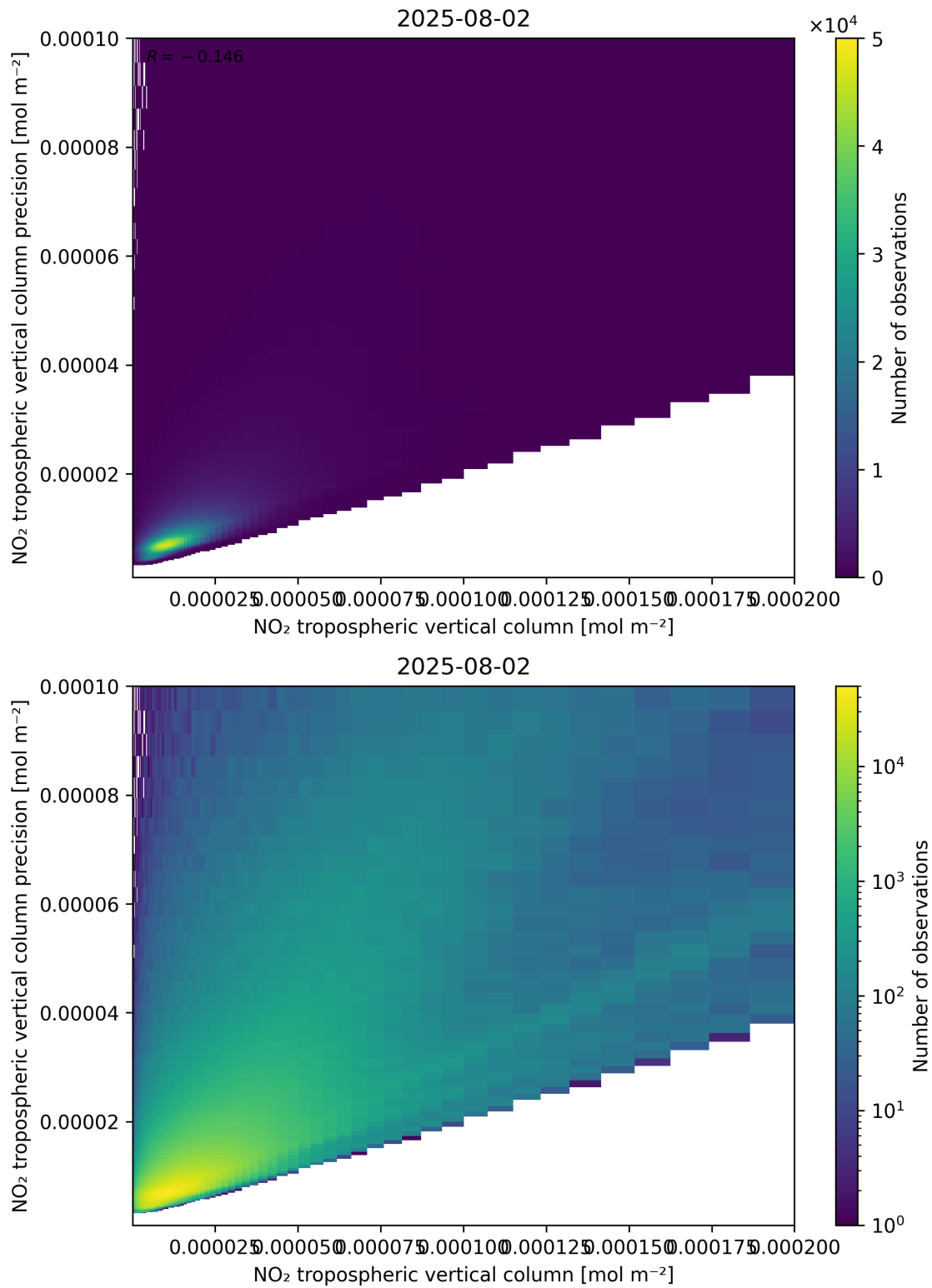
Figure 130: Scatter density plot of “NO 2 tropospheric vertical column” against “NO 2 tropospheric vertical column precision” for 2025-08-01 to 2025-08-03.
