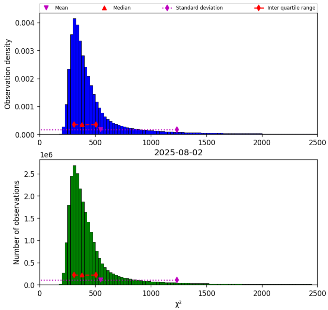
Figure 42: Histogram of “ \chi^2 ” for 2025-08-01 to 2025-08-03
