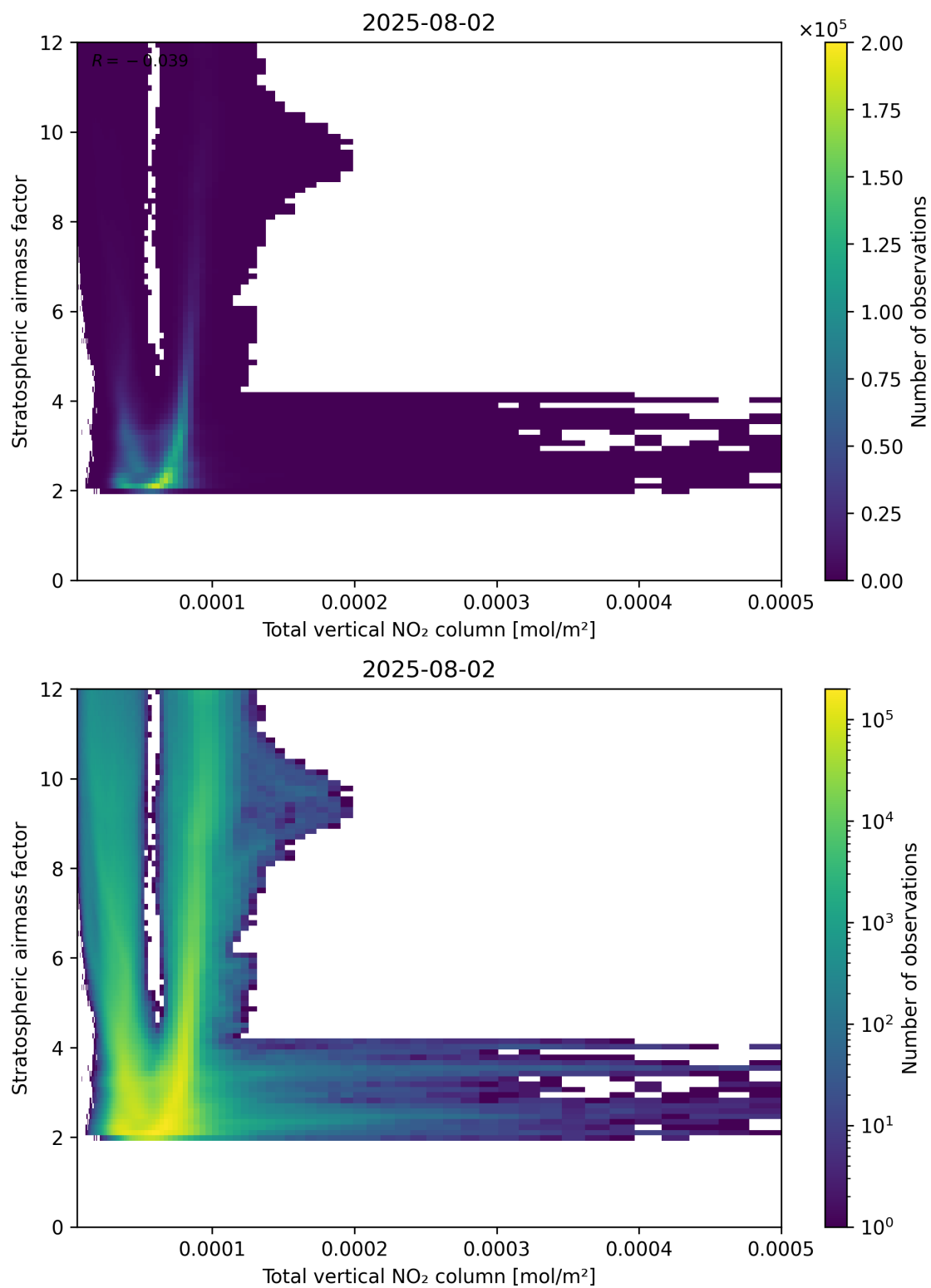
Figure 110: Scatter density plot of “Total vertical NO 2 column” against “Stratospheric airmass factor” for 2025-08-01 to 2025-08-03.
