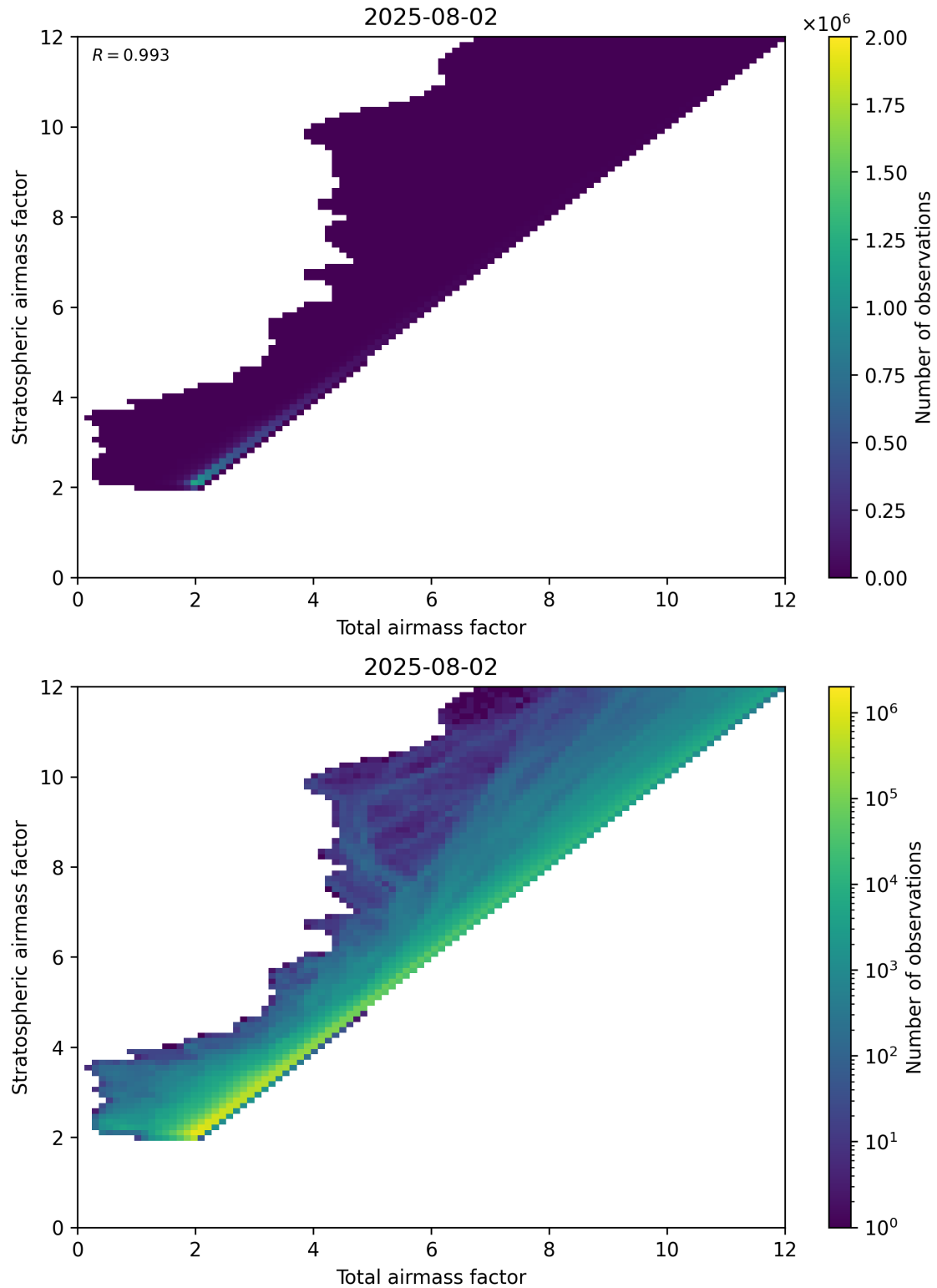
Figure 62: Scatter density plot of “Total airmass factor” against “Stratospheric airmass factor” for 2025-08-01 to 2025-08-03.
