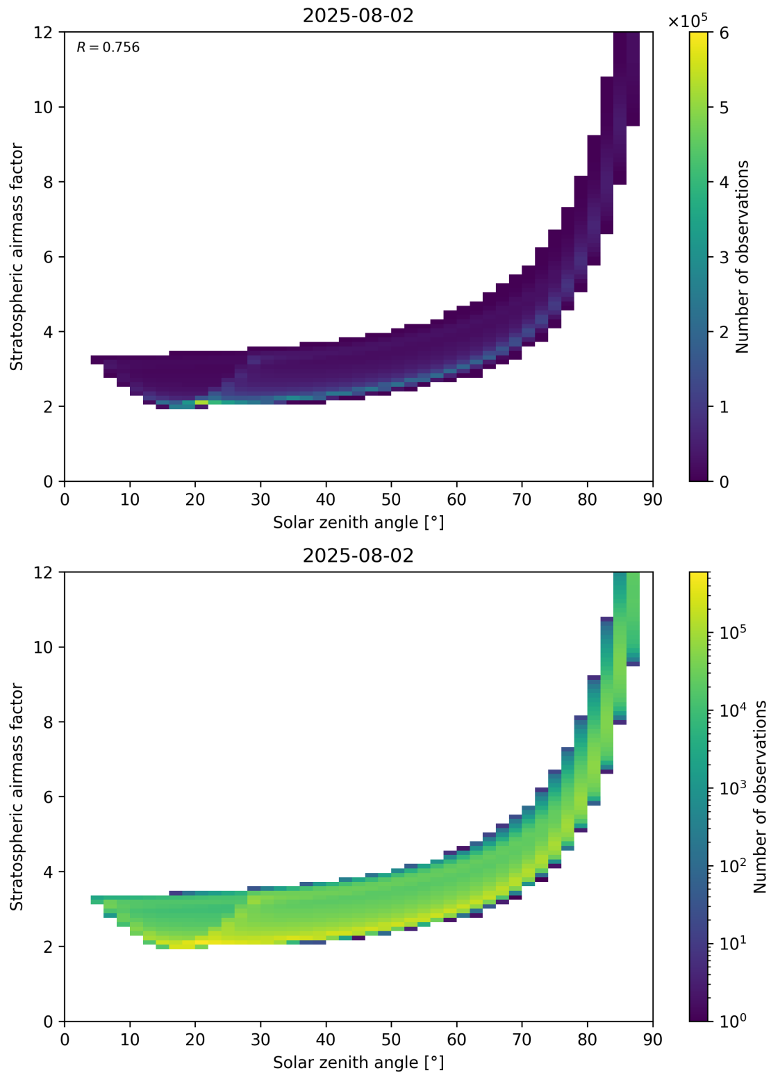
Figure 145: Scatter density plot of “Solar zenith angle” against “Stratospheric airmass factor” for 2025-08-01 to 2025-08-03.
