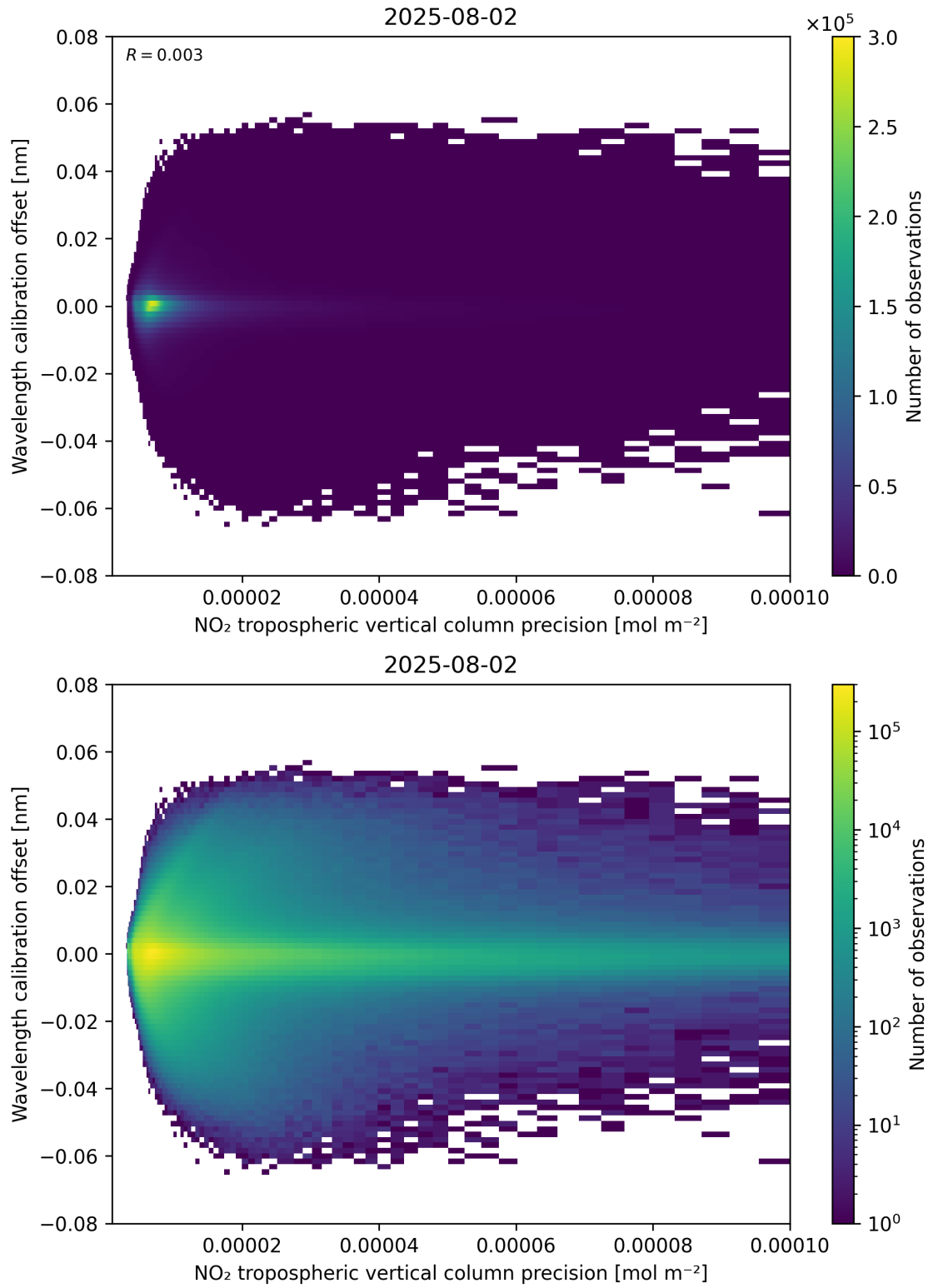
Figure 141: Scatter density plot of “NO 2 tropospheric vertical column precision” against “Wavelength calibration offset” for 2025-08-01 to 2025-08-03.
