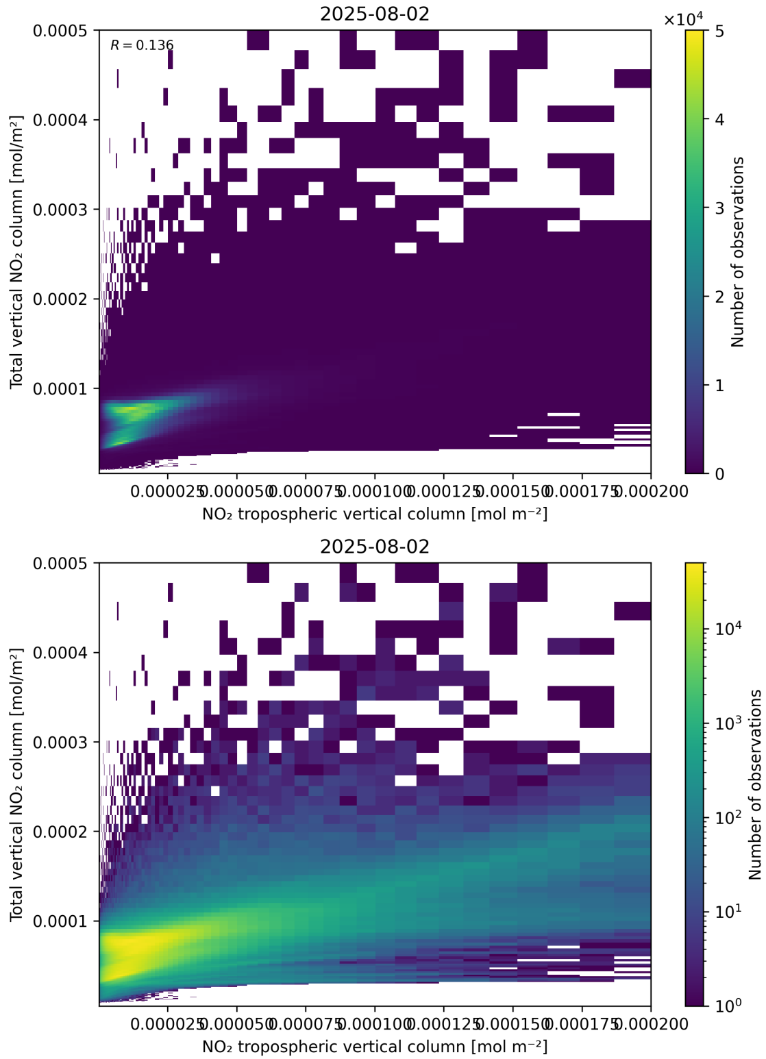
Figure 128: Scatter density plot of “NO 2 tropospheric vertical column” against “Total vertical NO 2 column” for 2025-08-01 to 2025-08-03.
