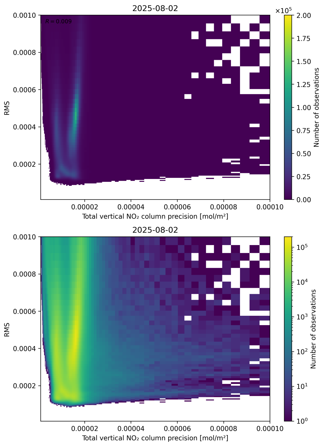
Figure 119: Scatter density plot of “Total vertical NO 2 column precision” against “RMS” for 2025-08-01 to 2025-08-03.
