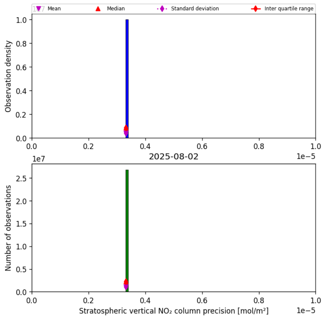
Figure 37: Histogram of “Stratospheric vertical NO 2 column precision” for 2025-08-01 to 2025-08-03
