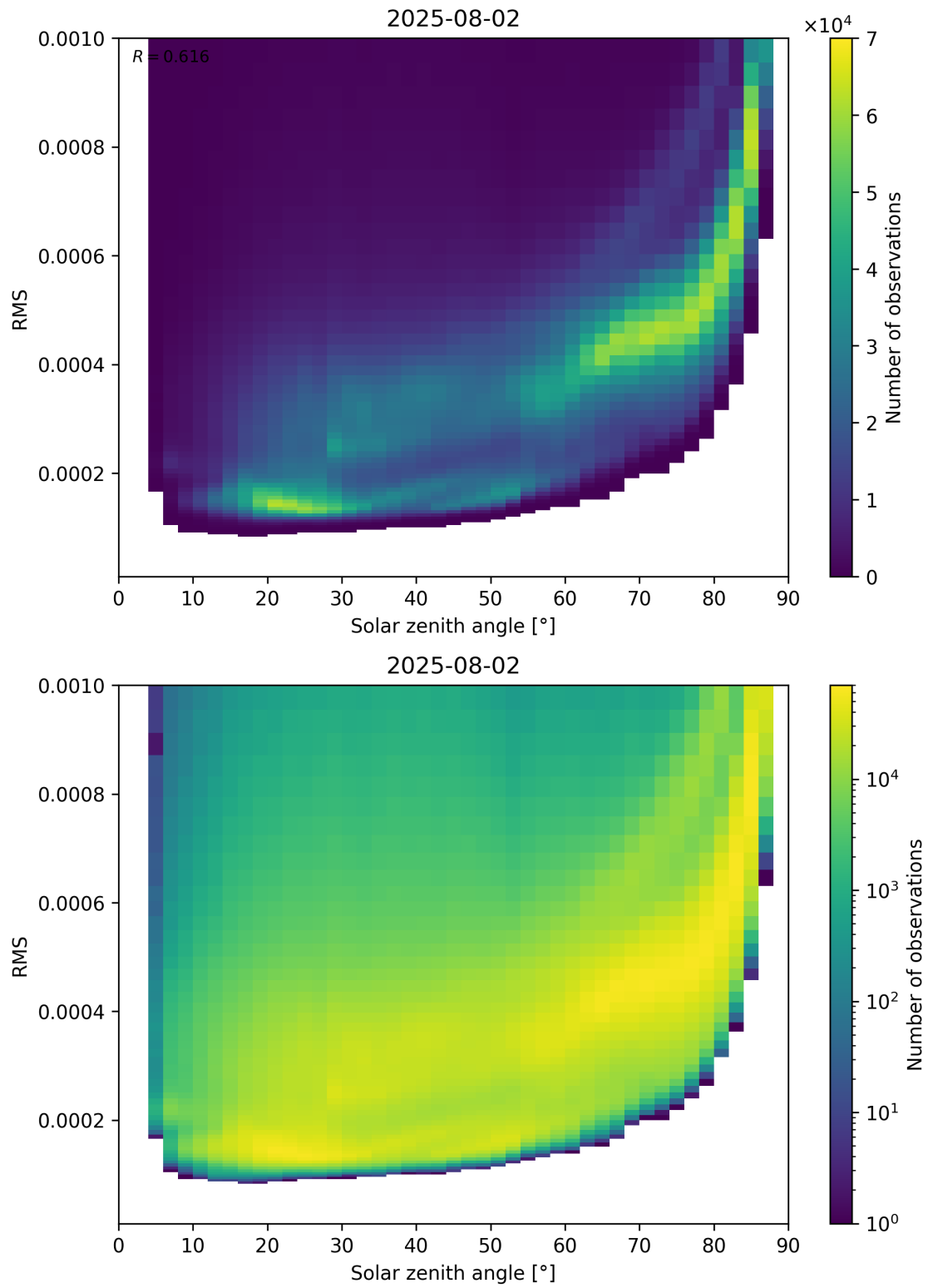
Figure 157: Scatter density plot of “Solar zenith angle” against “RMS” for 2025-08-01 to 2025-08-03.
