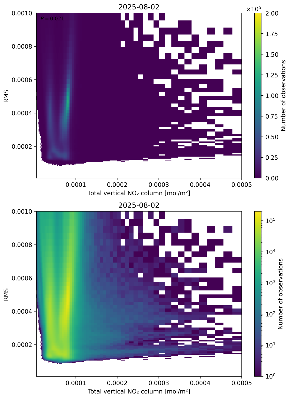
Figure 120: Scatter density plot of “Total vertical NO 2 column” against “RMS” for 2025-08-01 to 2025-08-03.
