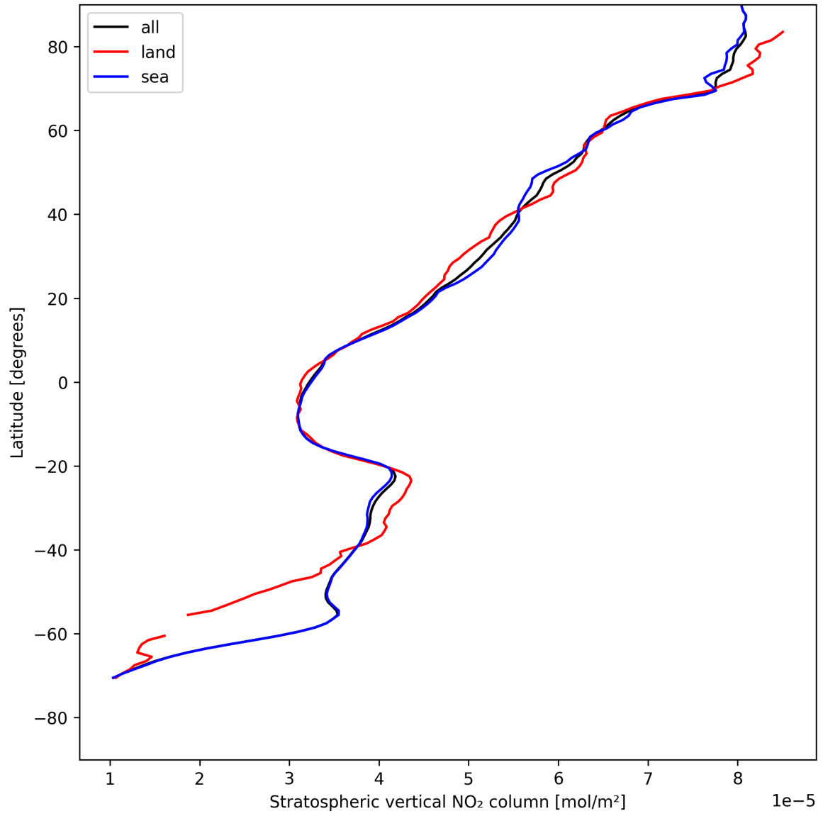
Figure 19: Zonal average of “Stratospheric vertical NO 2 column” for 2025-08-01 to 2025-08-03.
