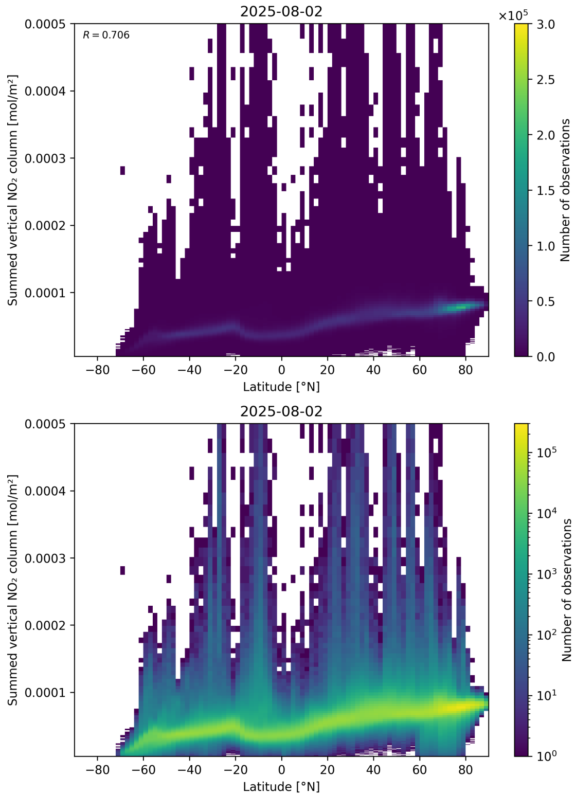
Figure 88: Scatter density plot of “Latitude” against “Summed vertical NO 2 column” for 2025-08-01 to 2025-08-03.
