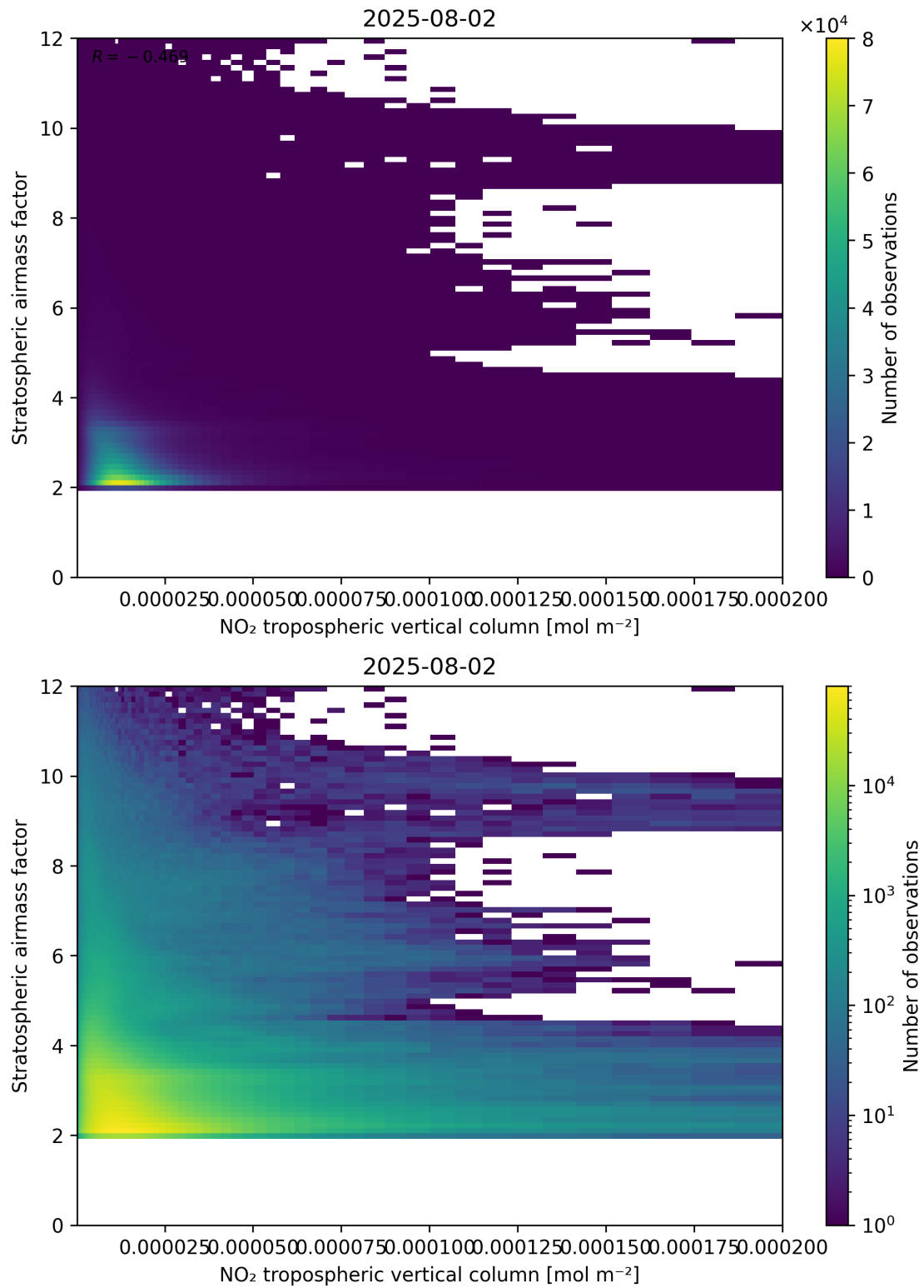
Figure 121: Scatter density plot of “NO 2 tropospheric vertical column” against “Stratospheric air mass factor” for 2025-08-01 to 2025-08-03.
