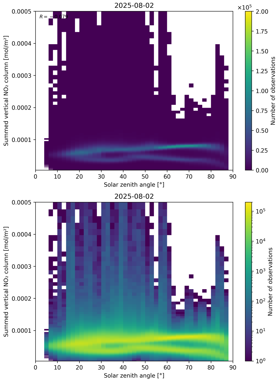
Figure 151: Scatter density plot of “Solar zenith angle” against “Summed vertical NO 2 column” for 2025-08-01 to 2025-08-03.
