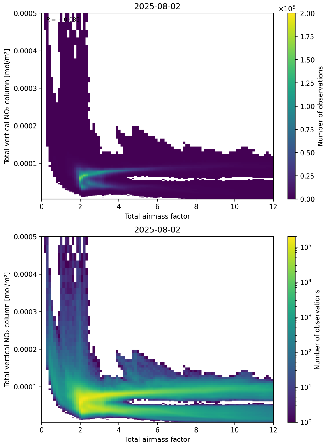
Figure 67: Scatter density plot of “Total airmass factor” against “Total vertical NO 2 column” for 2025-08-01 to 2025-08-03.
