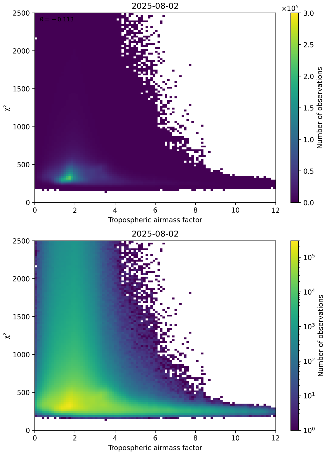
Figure 73: Scatter density plot of “Tropospheric airmass factor” against “ \chi^2 ” for 2025-08-01 to 2025-08-03.
