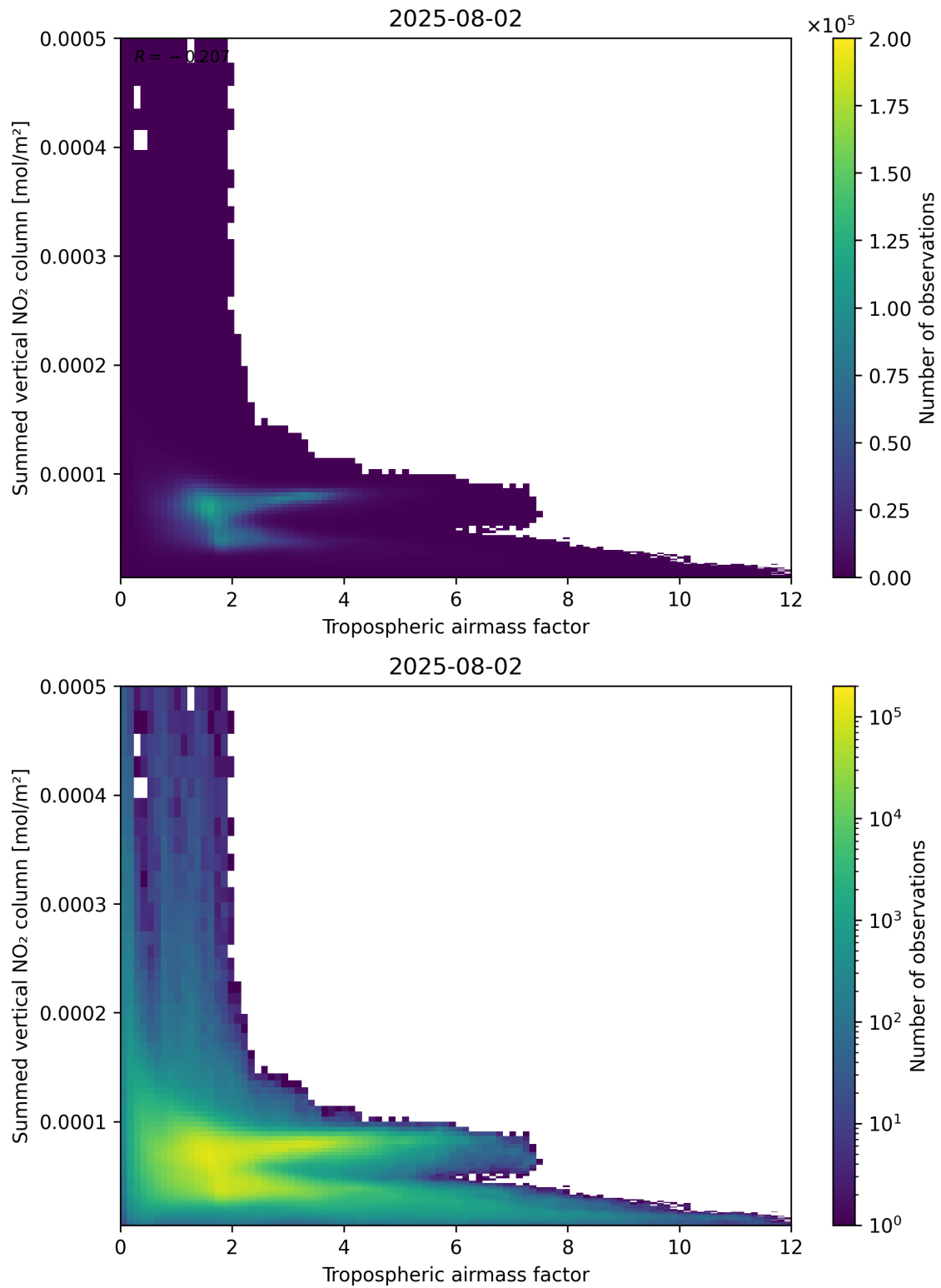
Figure 75: Scatter density plot of “Tropospheric airmass factor” against “Summed vertical NO 2 column” for 2025-08-01 to 2025-08-03.
