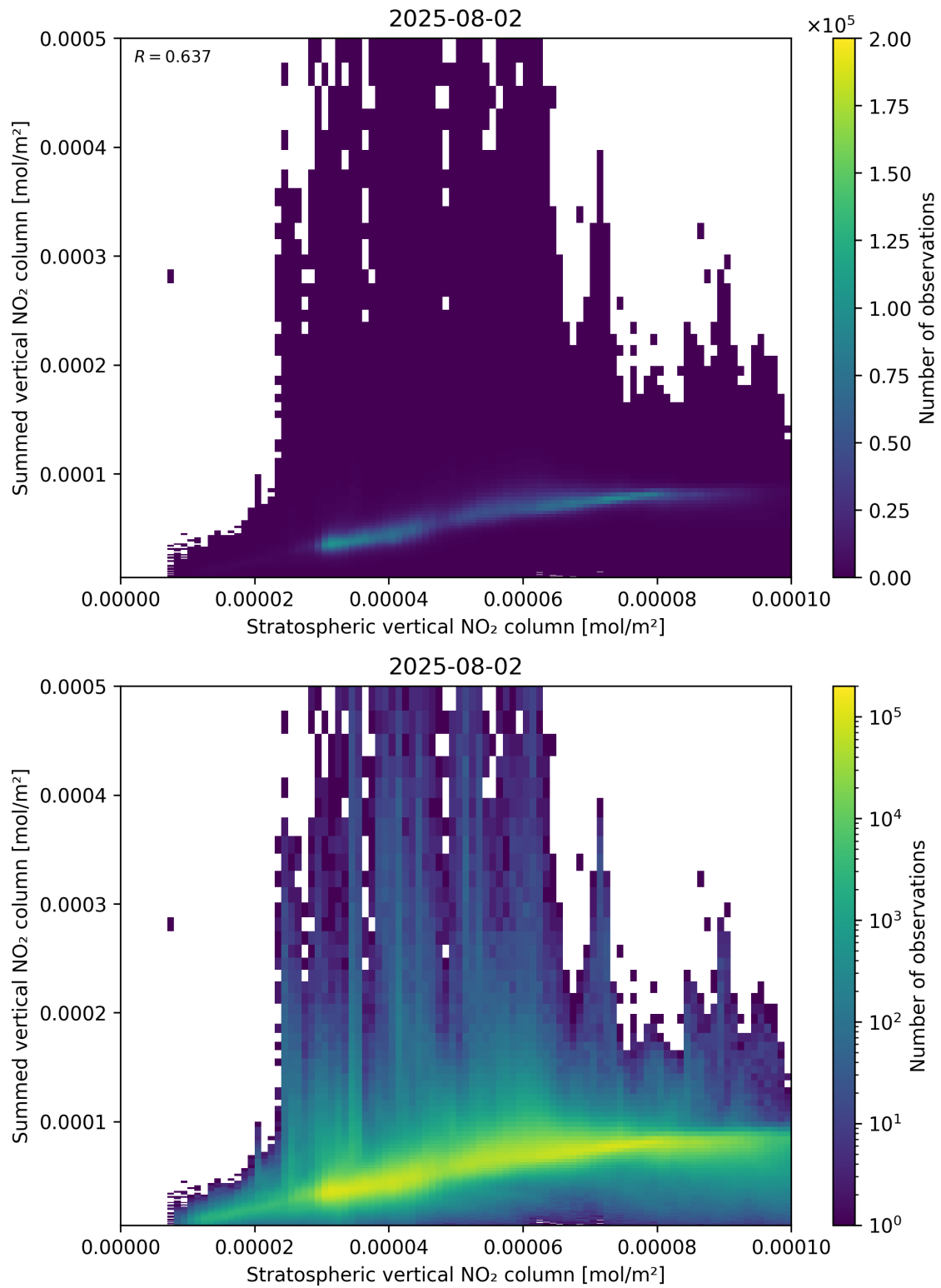
Figure 98: Scatter density plot of “Stratospheric vertical NO 2 column” against “Summed vertical NO 2 column” for 2025-08-01 to 2025-08-03.
