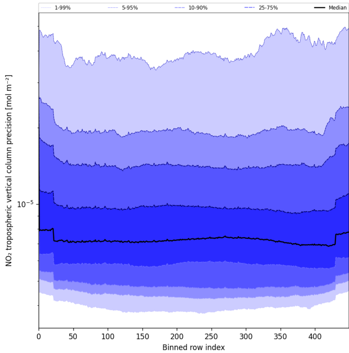
Figure 47: Along track statistics of “NO 2 tropospheric vertical column precision” for 2025-08-01 to 2025-08-03
