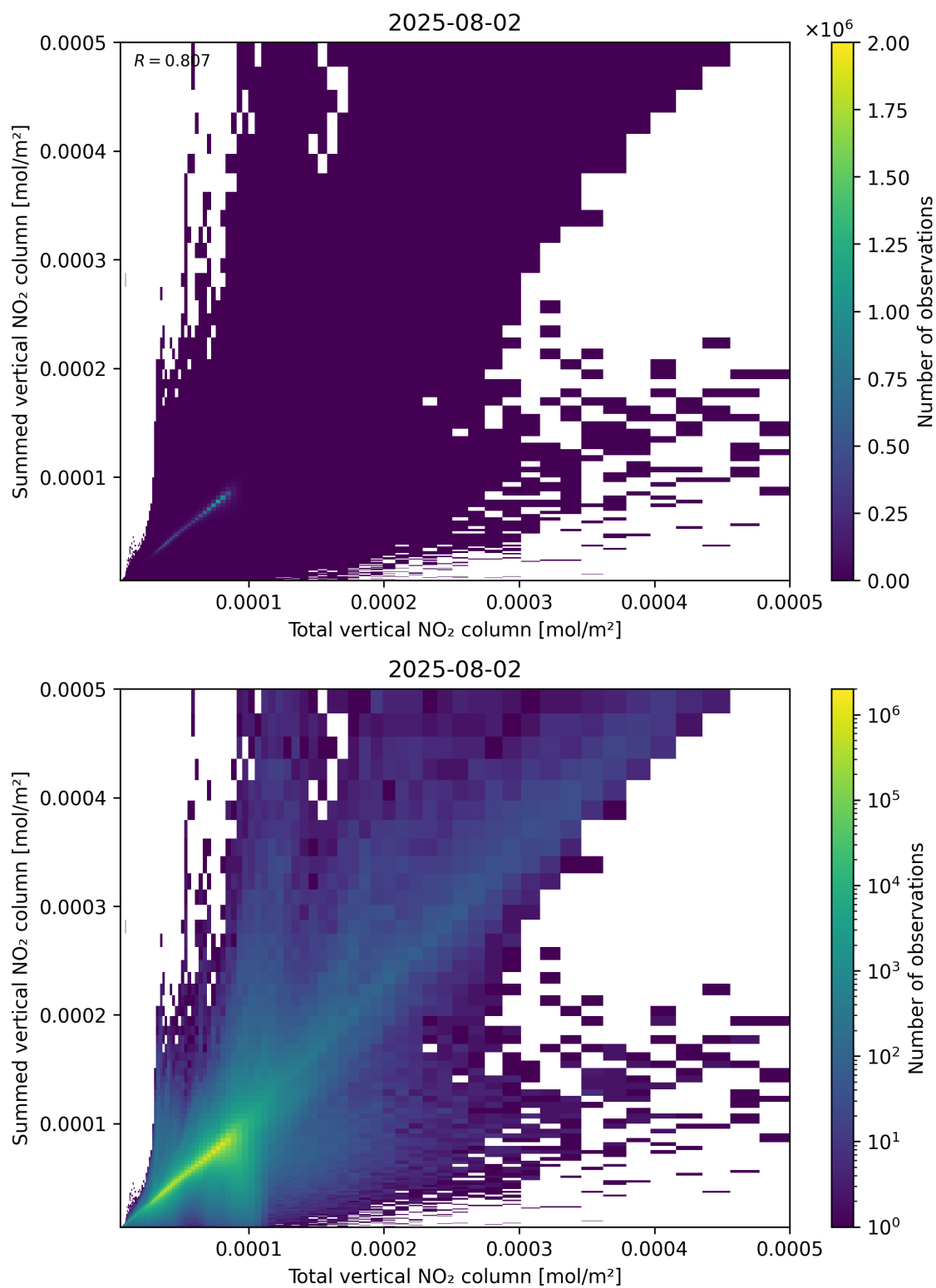
Figure 112: Scatter density plot of “Total vertical NO 2 column” against “Summed vertical NO 2 column” for 2025-08-01 to 2025-08-03.
