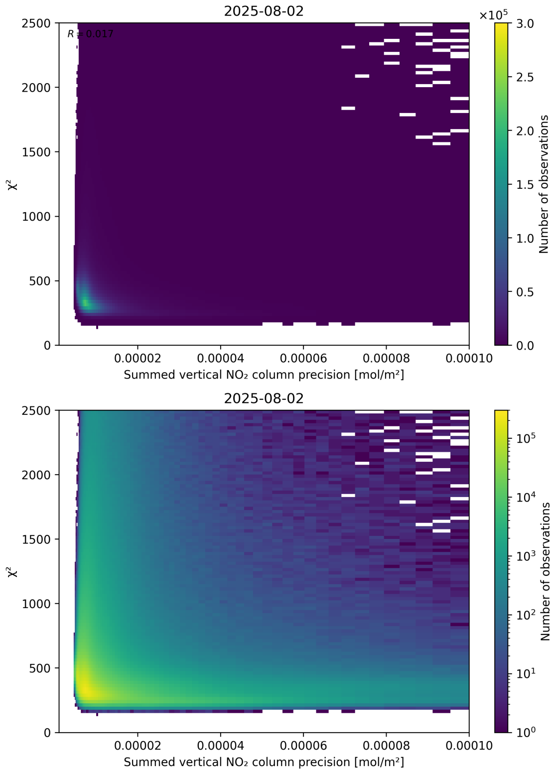
Figure 107: Scatter density plot of “Summed vertical NO 2 column precision” against “ \chi^2 ” for 2025-08-01 to 2025-08-03.
