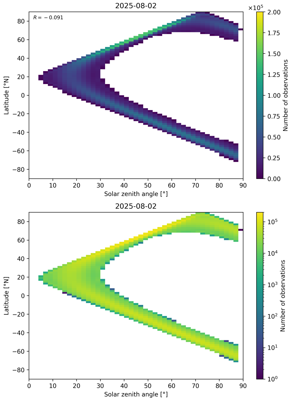
Figure 149: Scatter density plot of “Solar zenith angle” against “Latitude” for 2025-08-01 to 2025-08-03.
