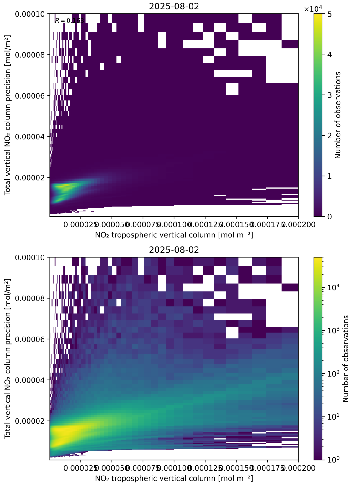
Figure 129: Scatter density plot of “NO 2 tropospheric vertical column” against “Total vertical NO 2 column precision” for 2025-08-01 to 2025-08-03.
