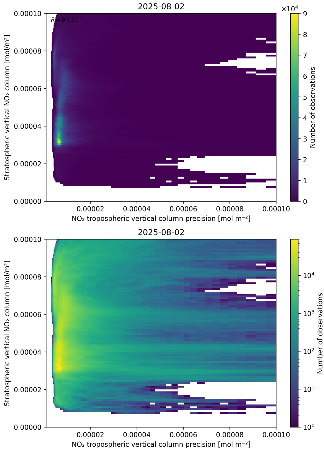
Figure 135: Scatter density plot of “NO 2 tropospheric vertical column precision” against “Stratospheric vertical NO 2 column” for 2025-08-01 to 2025-08-03.
