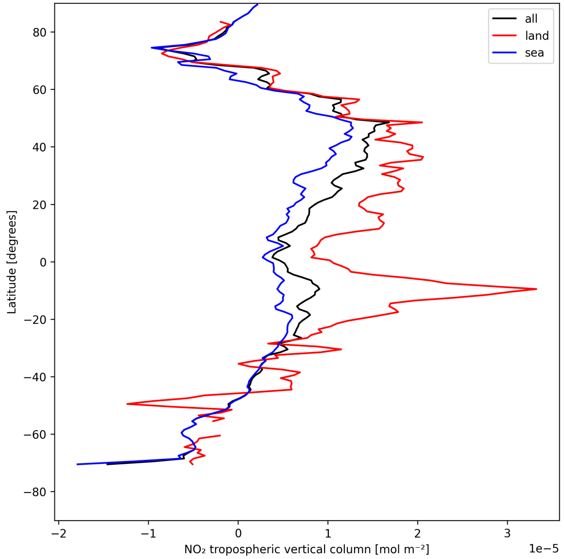
Figure 12: Zonal average of “NO 2 tropospheric vertical column” for 2025-08-01 to 2025-08-03.
