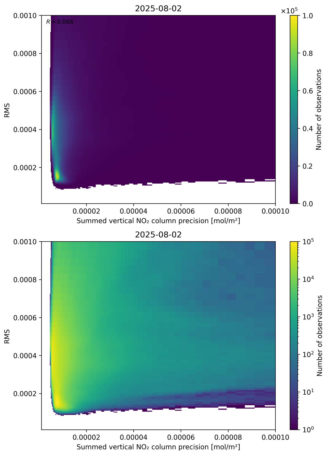
Figure 108: Scatter density plot of “Summed vertical NO 2 column precision” against “RMS” for 2025-08-01 to 2025-08-03.
