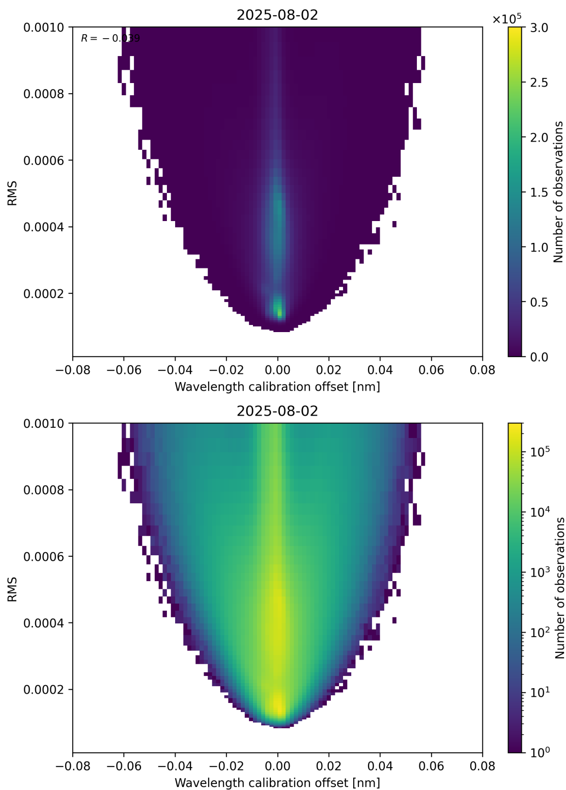
Figure 181: Scatter density plot of “Wavelength calibration offset” against “RMS” for 2025-08-01 to 2025-08-03.
