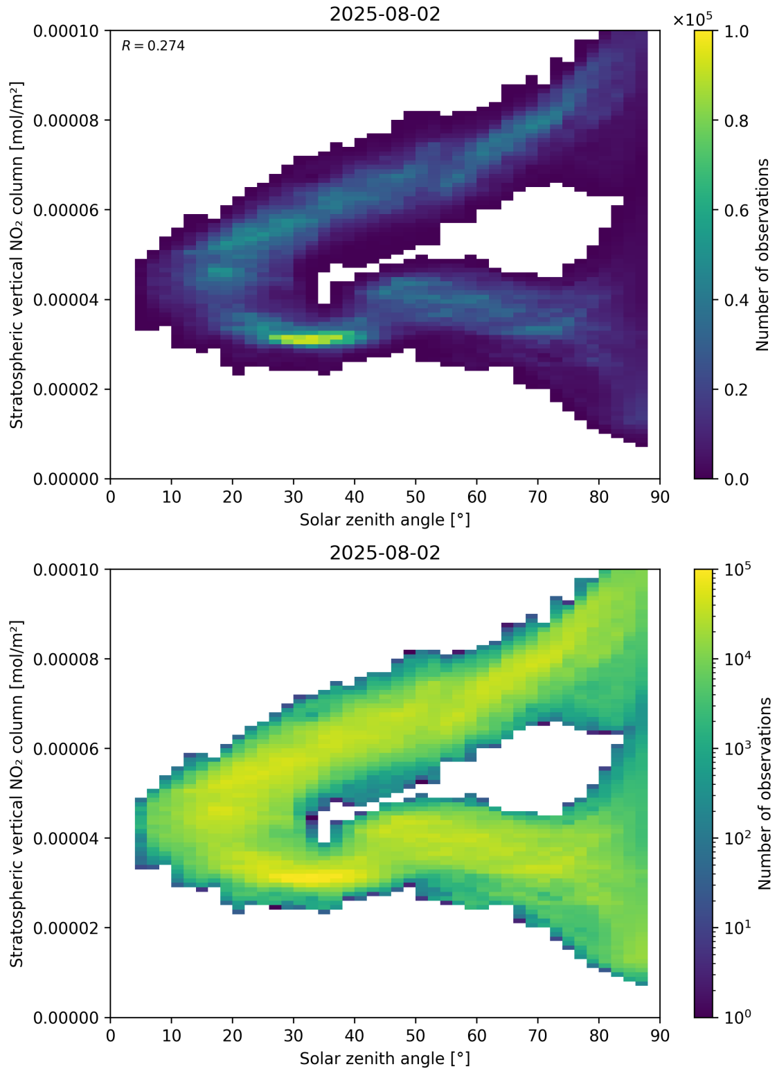
Figure 150: Scatter density plot of “Solar zenith angle” against “Stratospheric vertical NO 2 column” for 2025-08-01 to 2025-08-03.
