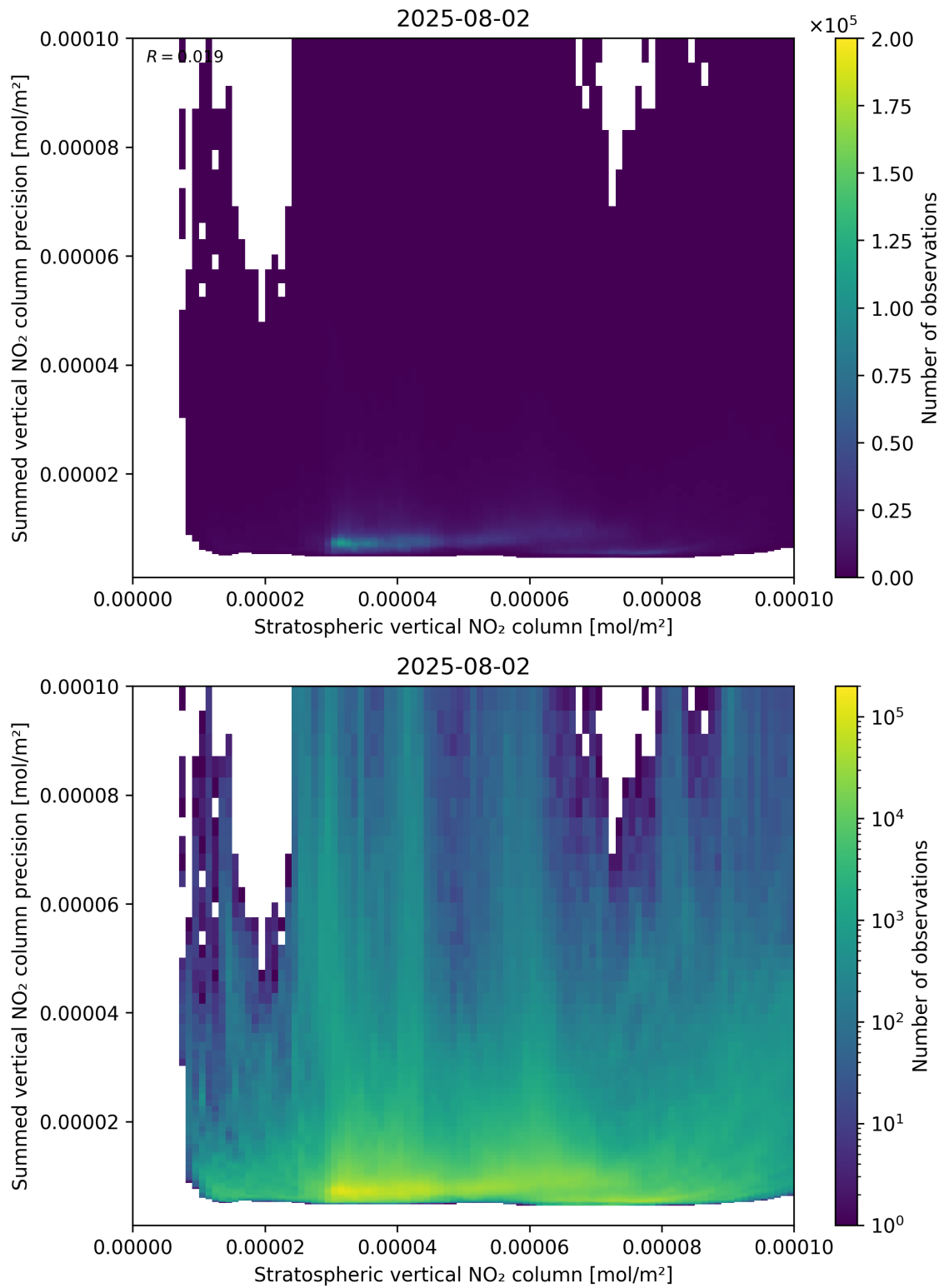
Figure 99: Scatter density plot of “Stratospheric vertical NO 2 column” against “Summed vertical NO 2 column precision” for 2025-08-01 to 2025-08-03.
