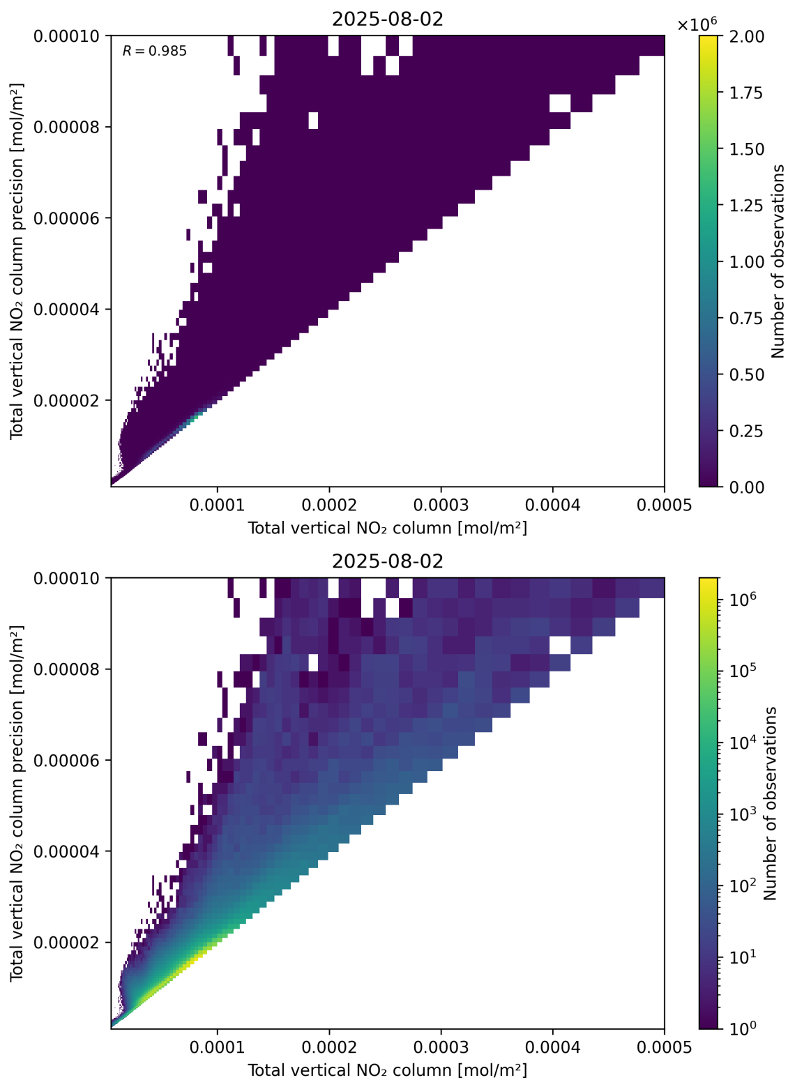
Figure 114: Scatter density plot of “Total vertical NO 2 column” against “Total vertical NO 2 column precision” for 2025-08-01 to 2025-08-03.
