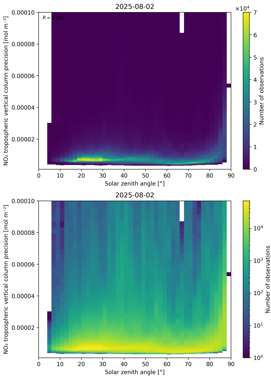
Figure 156: Scatter density plot of “Solar zenith angle” against “NO 2 tropospheric vertical column precision” for 2025-08-01 to 2025-08-03.
