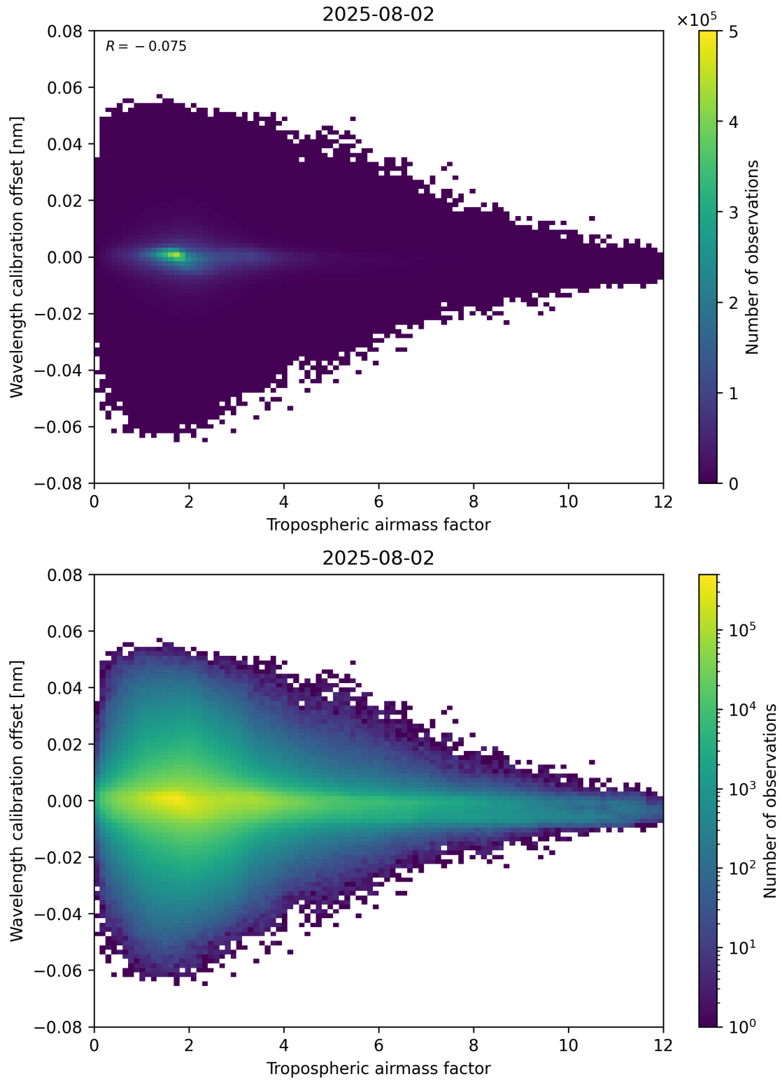
Figure 80: Scatter density plot of “Tropospheric airmass factor” against “Wavelength calibration offset” for 2025-08-01 to 2025-08-03.
