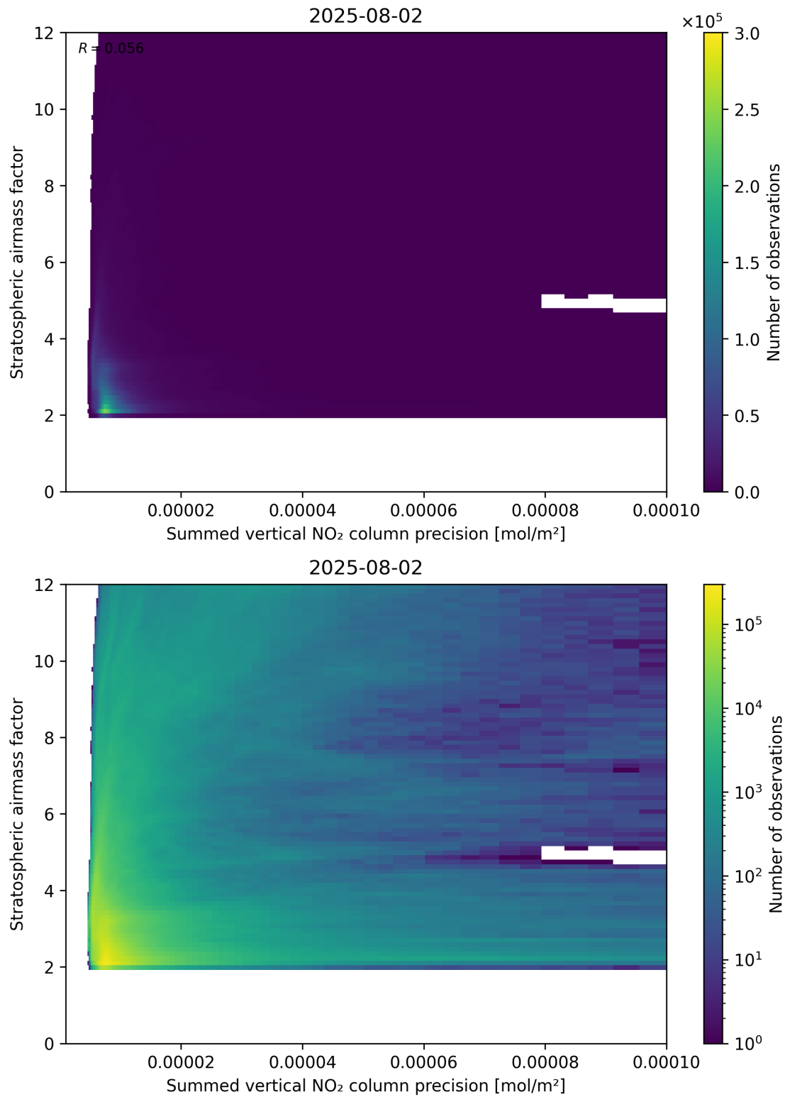
Figure 106: Scatter density plot of “Summed vertical NO 2 column precision” against “Stratospheric airmass factor” for 2025-08-01 to 2025-08-03.
