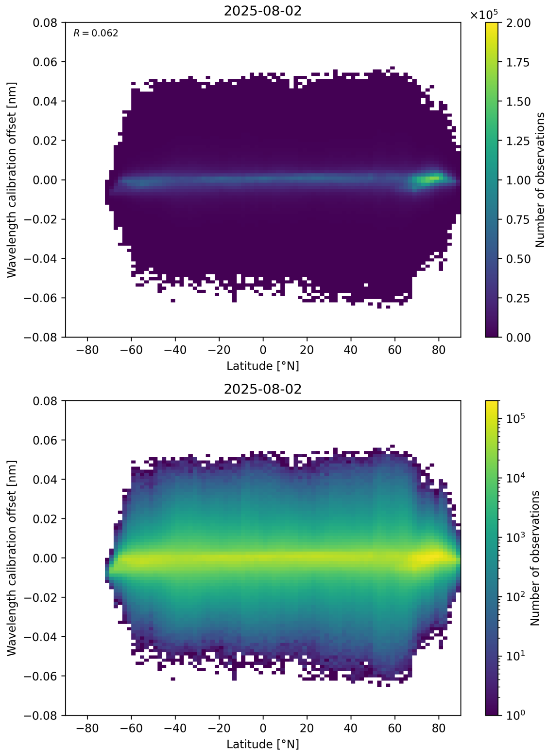
Figure 95: Scatter density plot of “Latitude” against “Wavelength calibration offset” for 2025-08-01 to 2025-08-03.
