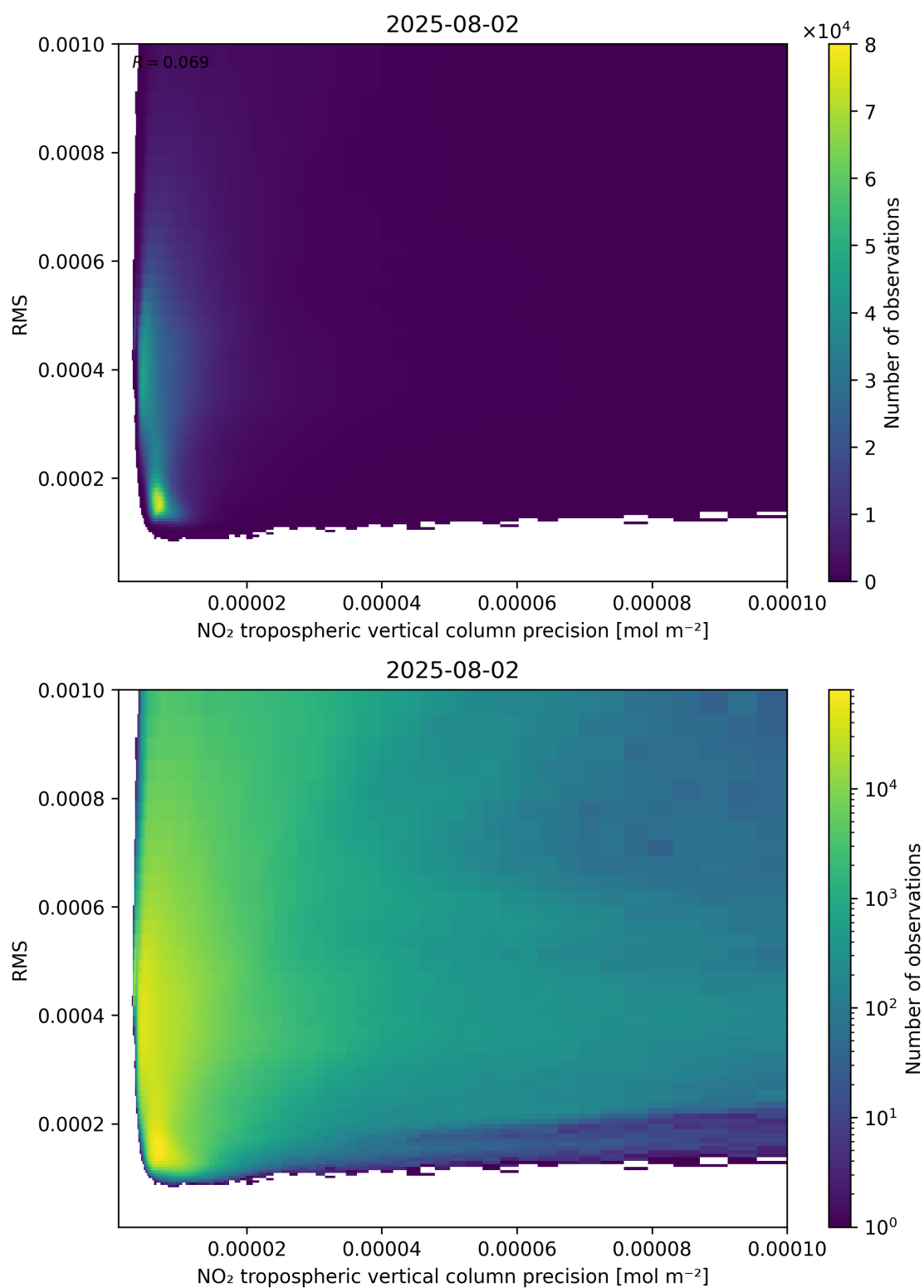
Figure 140: Scatter density plot of “NO 2 tropospheric vertical column precision” against “RMS” for 2025-08-01 to 2025-08-03.
