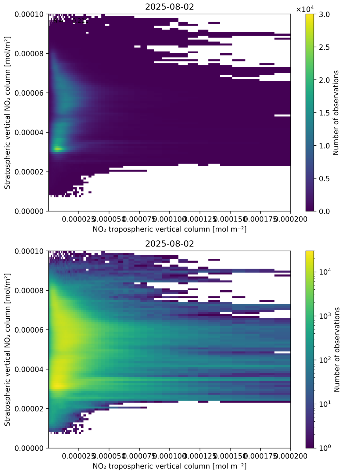
Figure 125: Scatter density plot of “NO 2 tropospheric vertical column” against “Stratospheric vertical NO 2 column” for 2025-08-01 to 2025-08-03.
