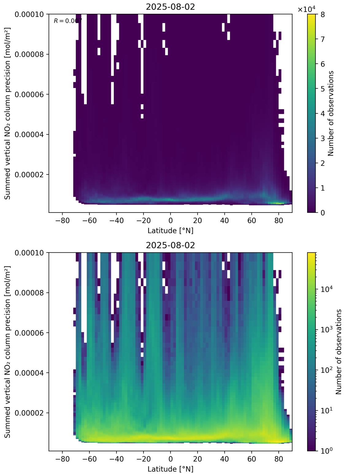
Figure 89: Scatter density plot of “Latitude” against “Summed vertical NO 2 column precision” for 2025-08-01 to 2025-08-03.
