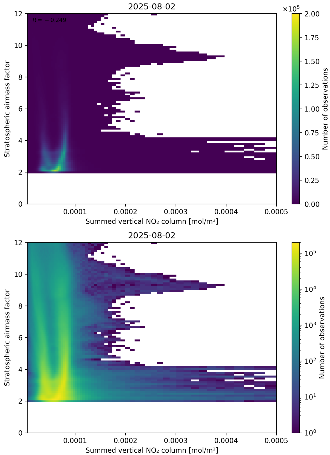
Figure 103: Scatter density plot of “Summed vertical NO 2 column” against “Stratospheric air mass factor” for 2025-08-01 to 2025-08-03.
