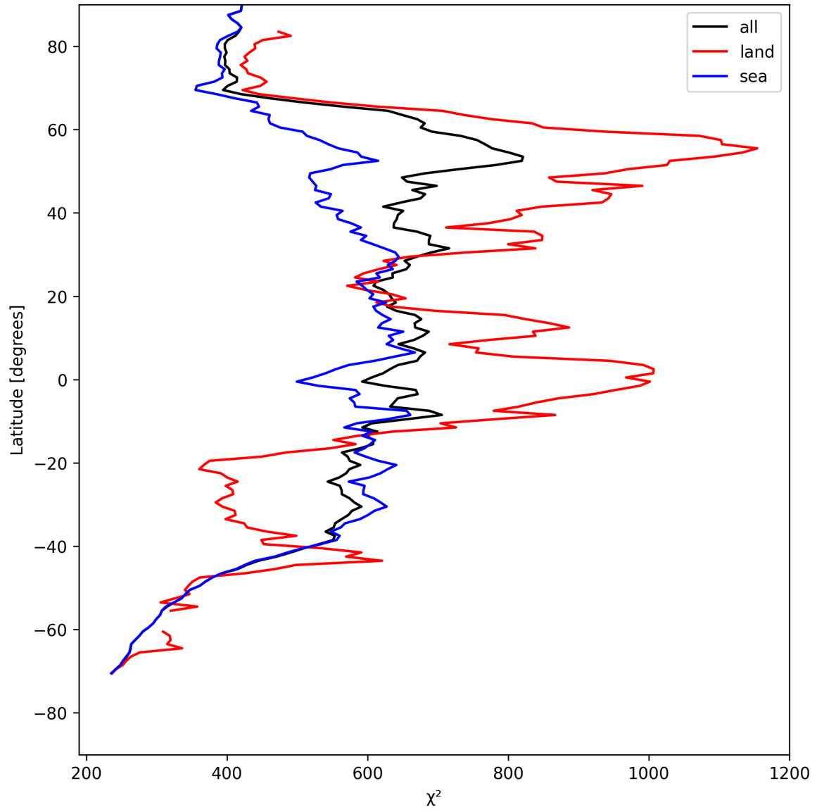
Figure 25: Zonal average of “ \chi^2 ” for 2025-08-01 to 2025-08-03.
