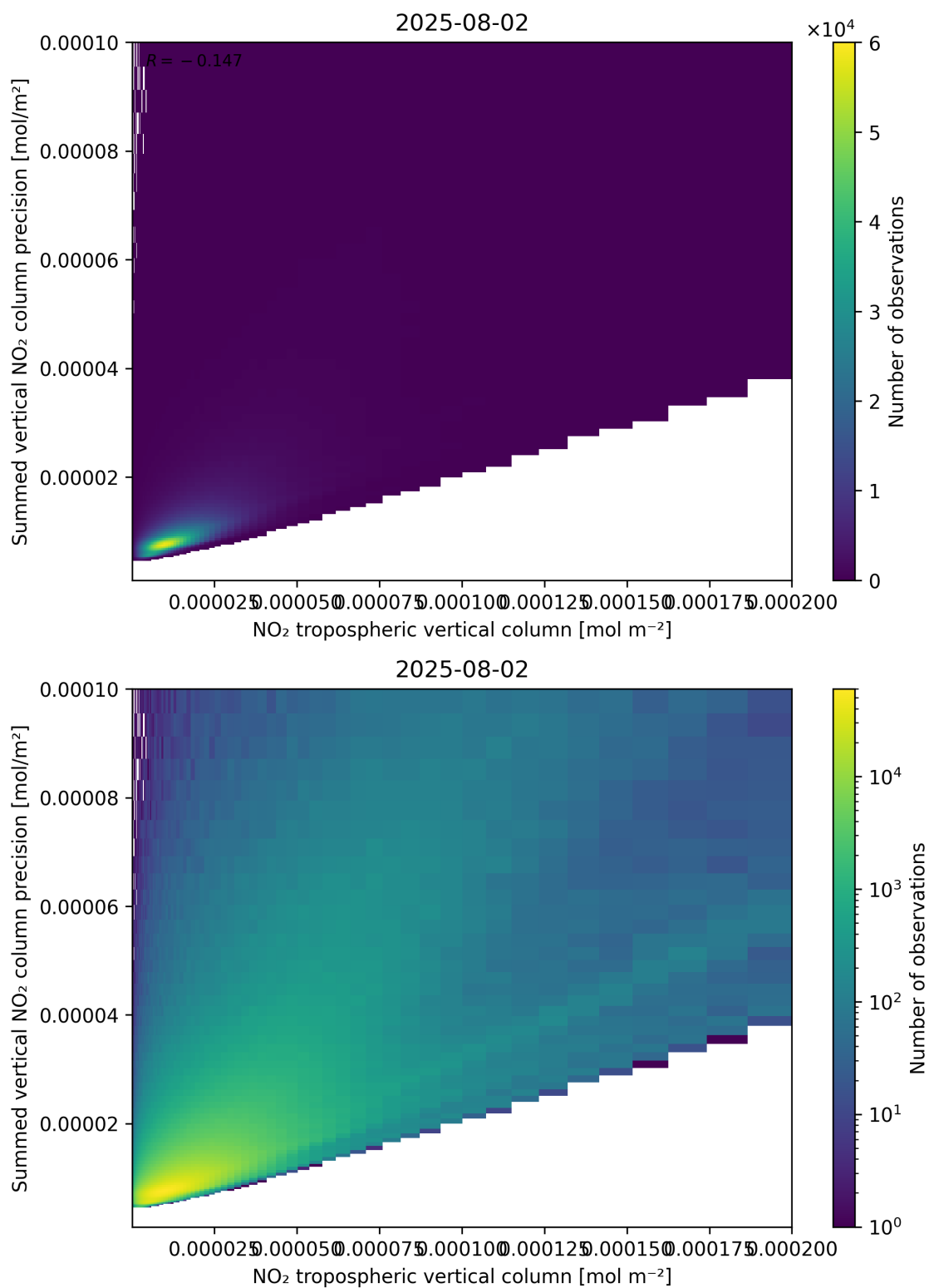
Figure 127: Scatter density plot of “NO 2 tropospheric vertical column” against “Summed vertical NO 2 column precision” for 2025-08-01 to 2025-08-03.
