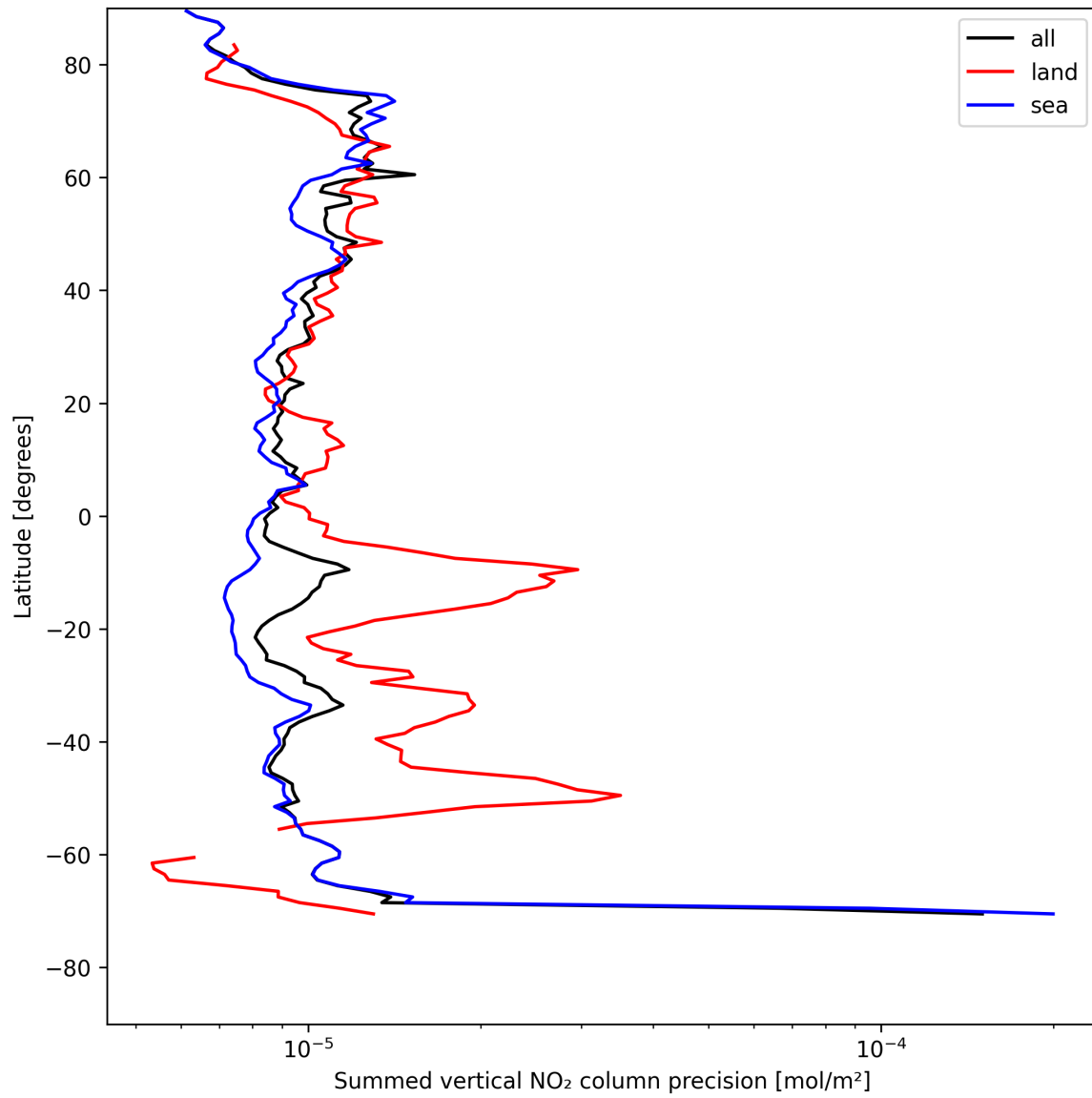
Figure 24: Zonal average of “Summed vertical NO 2 column precision” for 2025-08-01 to 2025-08-03.
