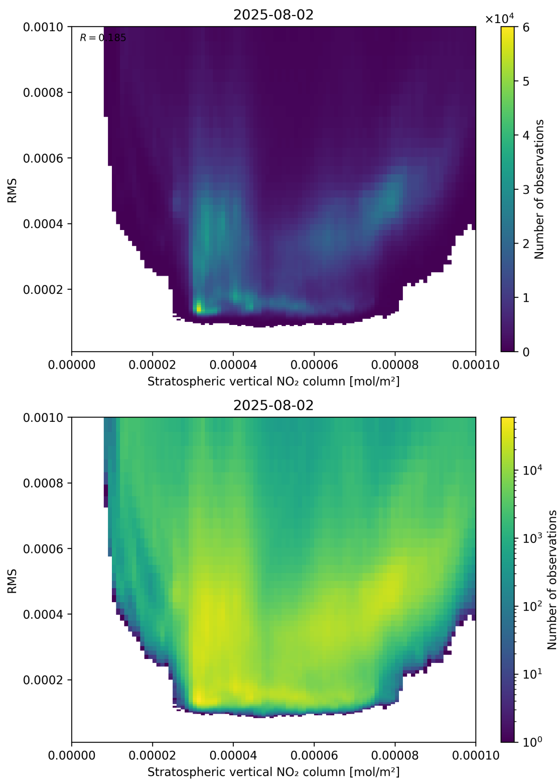
Figure 102: Scatter density plot of “Stratospheric vertical NO 2 column” against “RMS” for 2025-08-01 to 2025-08-03.
