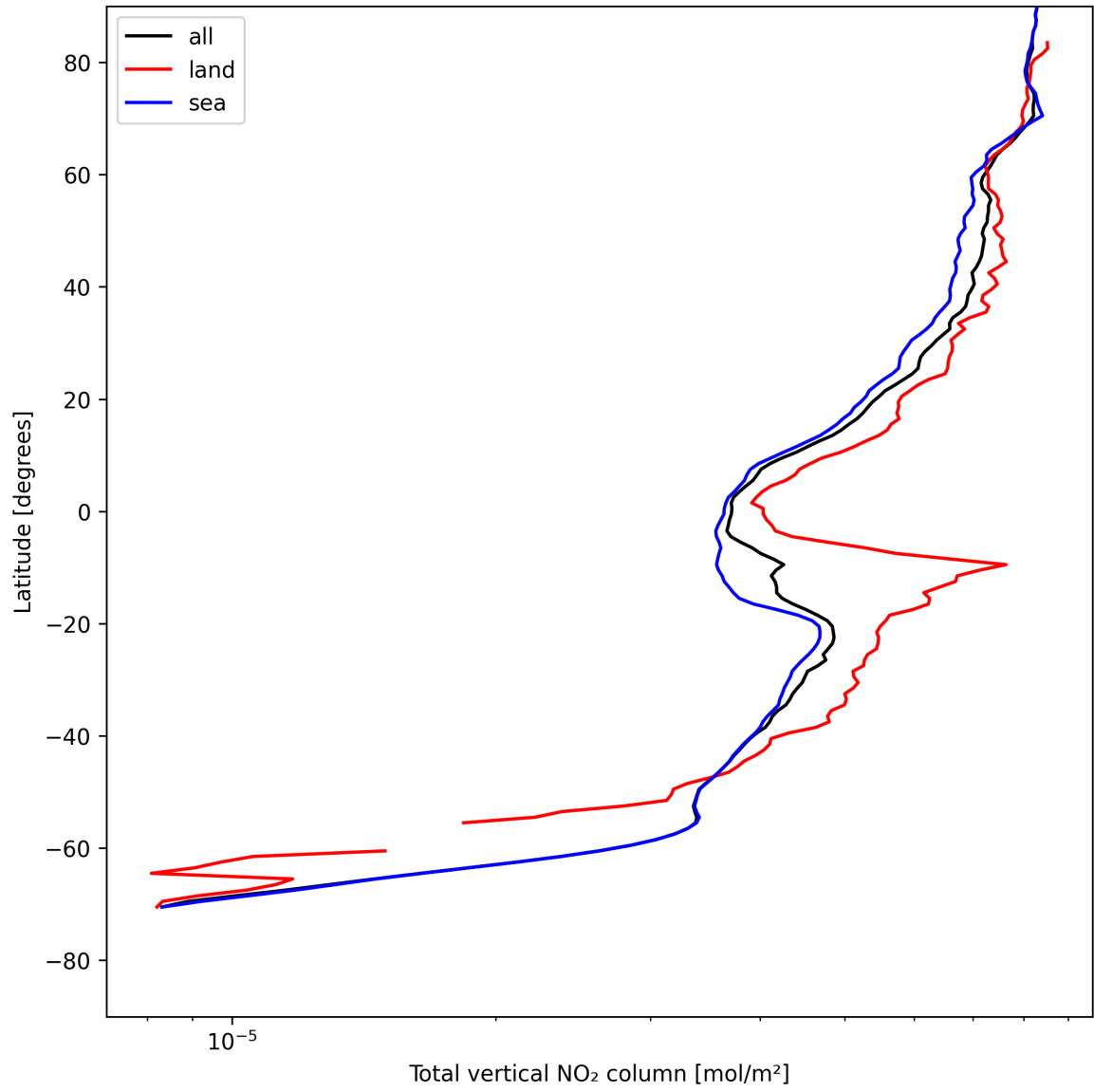
Figure 21: Zonal average of “Total vertical NO 2 column” for 2025-08-01 to 2025-08-03.
