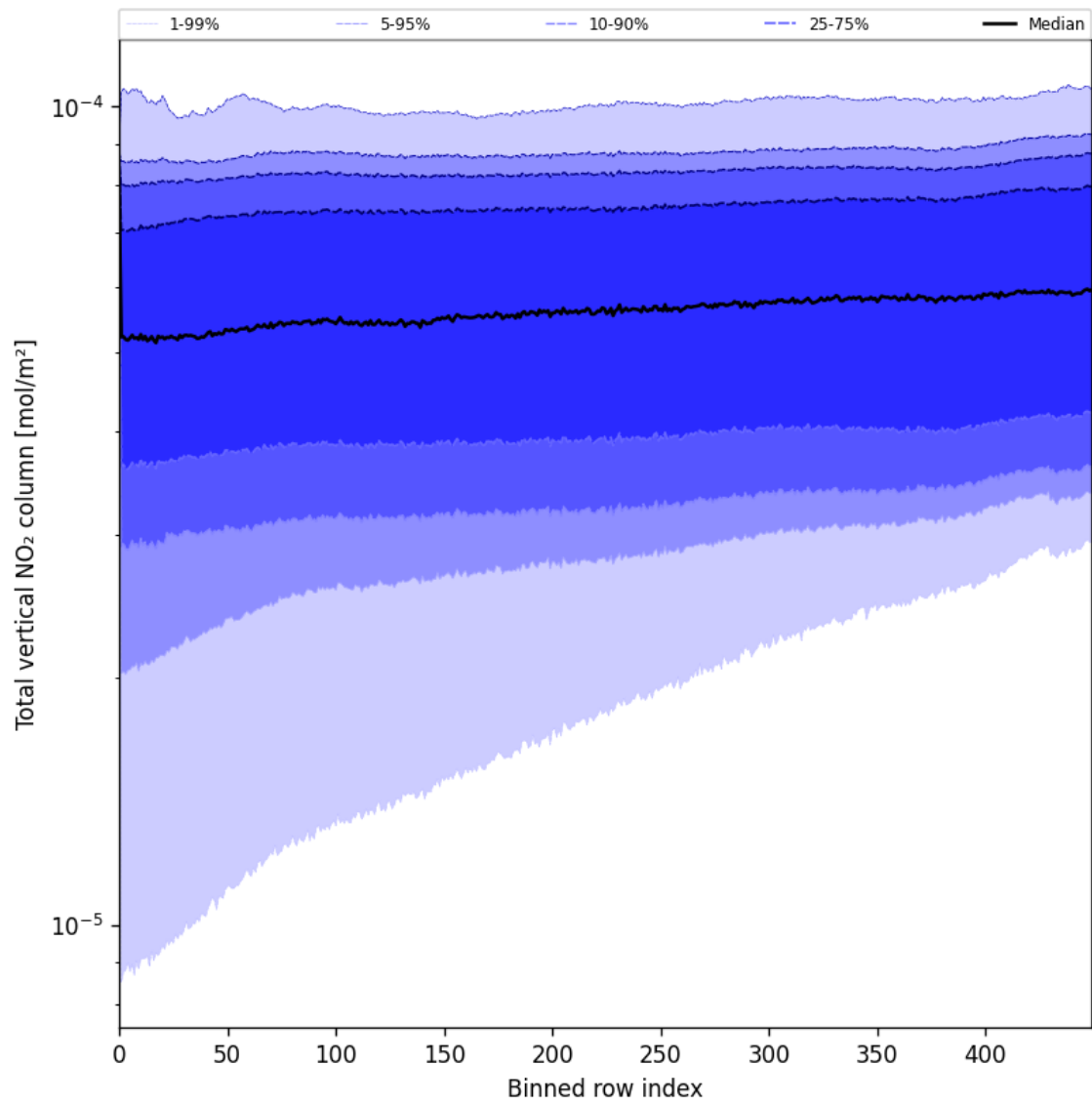
Figure 55: Along track statistics of “Total vertical NO 2 column” for 2025-08-01 to 2025-08-03
