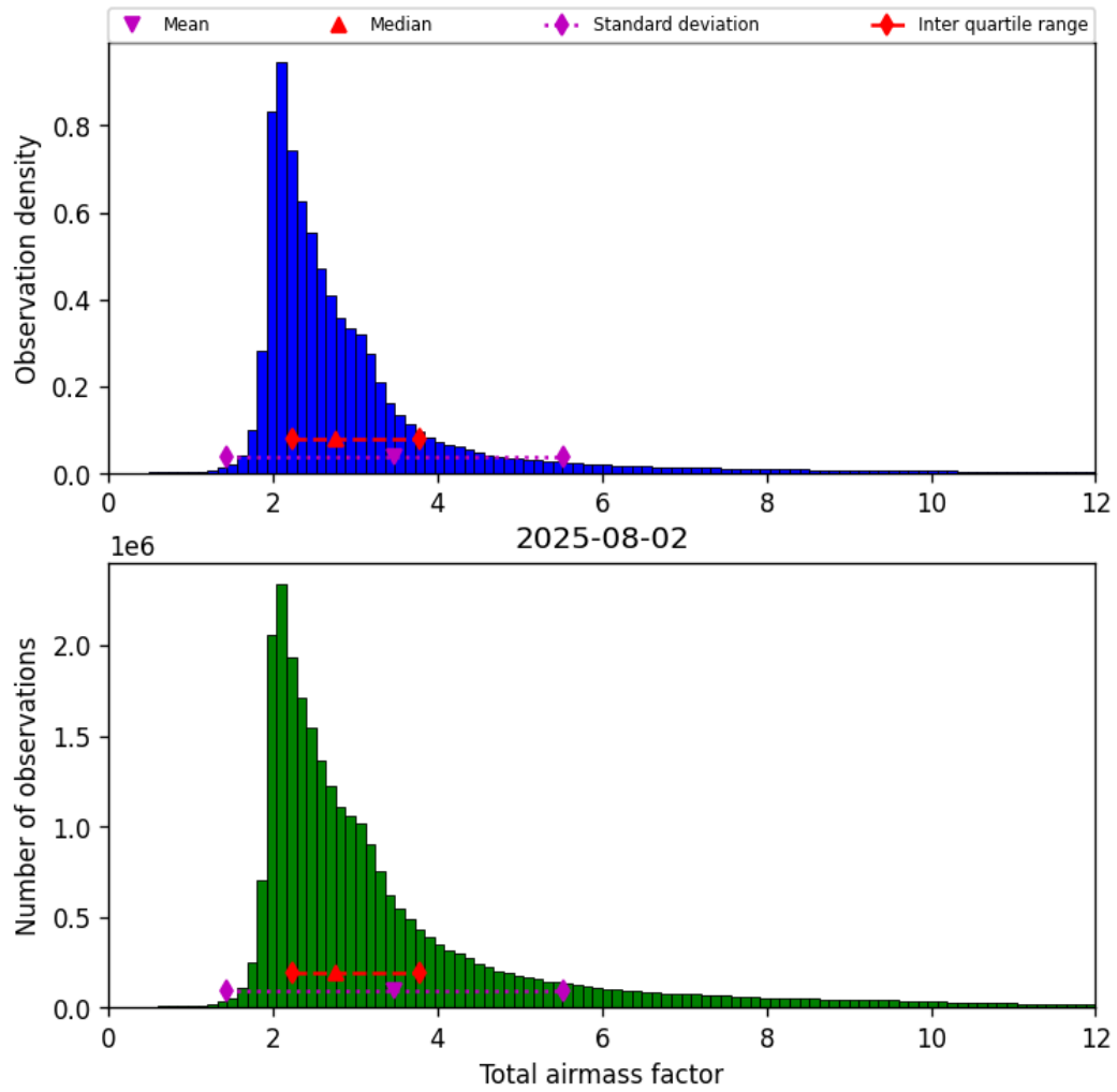
Figure 32: Histogram of “Total airmass factor” for 2025-08-01 to 2025-08-03
