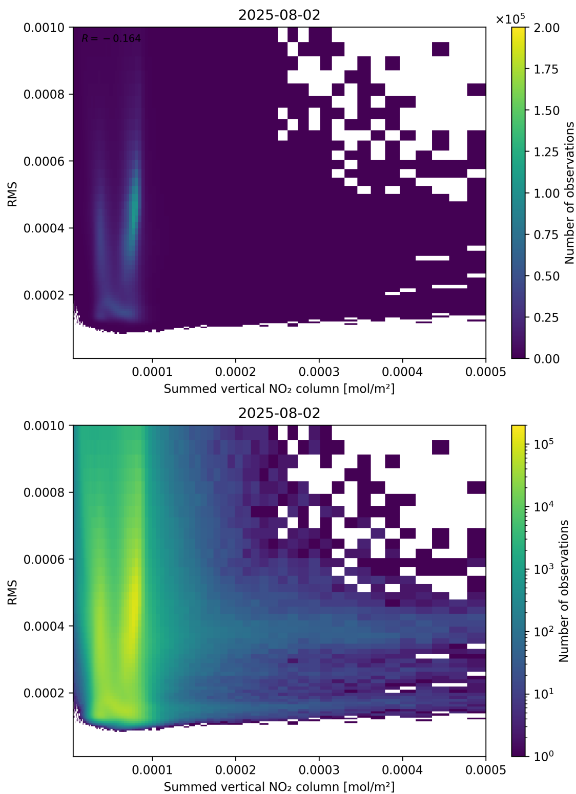
Figure 109: Scatter density plot of “Summed vertical NO 2 column” against “RMS” for 2025-08-01 to 2025-08-03.
