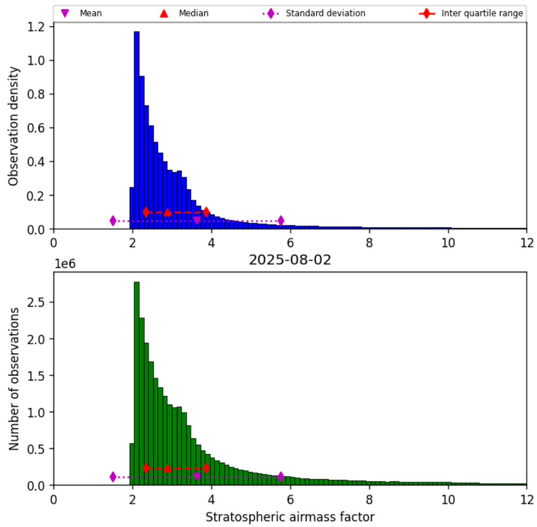
Figure 44: Histogram of “Stratospheric airmass factor” for 2025-08-01 to 2025-08-03
