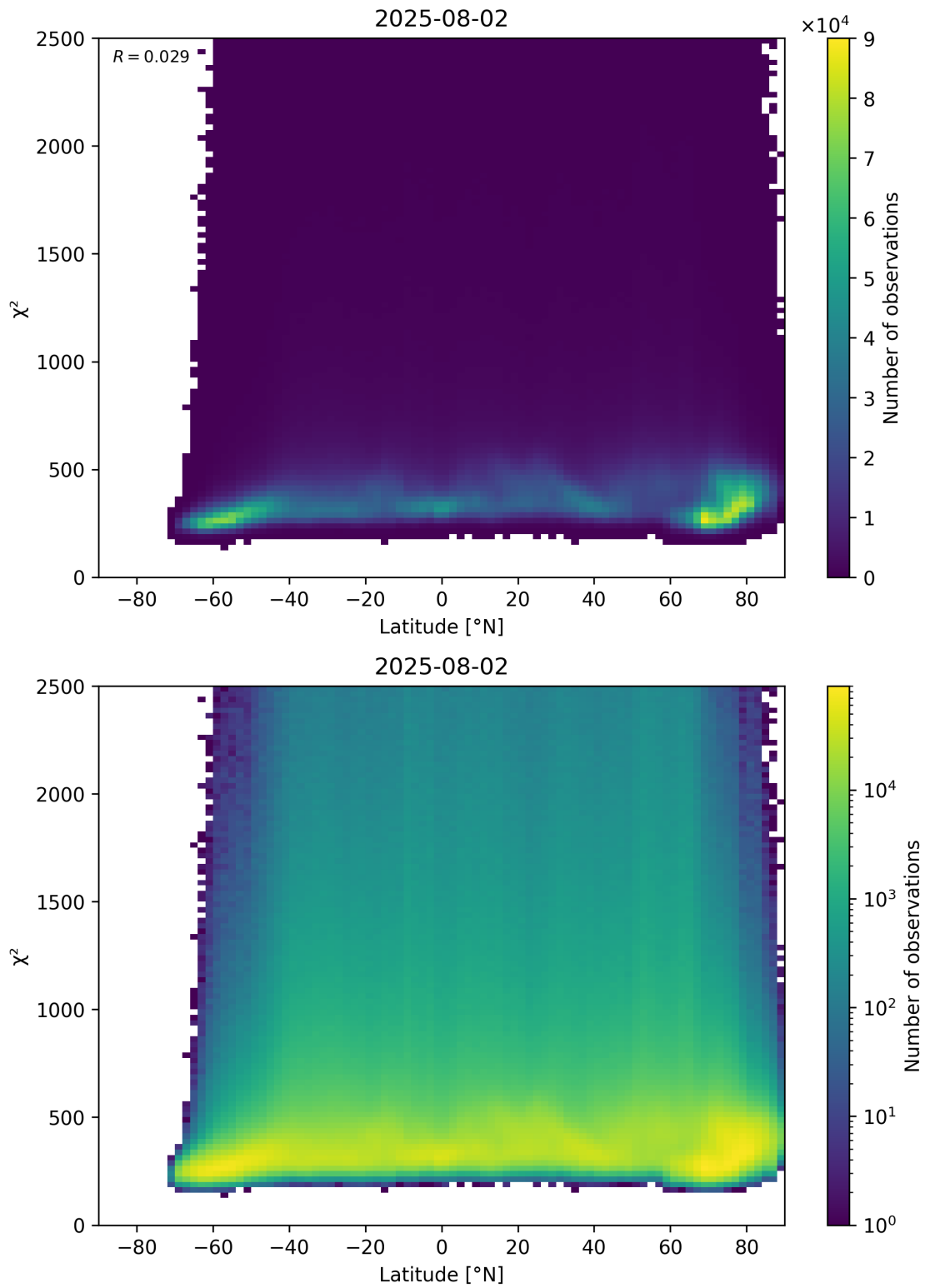
Figure 86: Scatter density plot of “Latitude” against “ \chi^2 ” for 2025-08-01 to 2025-08-03.
