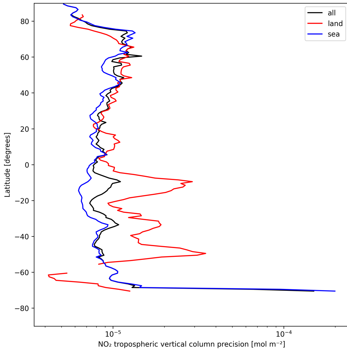
Figure 13: Zonal average of “NO 2 tropospheric vertical column precision” for 2025-08-01 to 2025-08-03.
