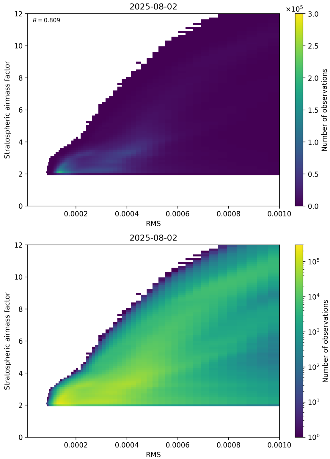
Figure 144: Scatter density plot of “RMS” against “Stratospheric airmass factor” for 2025-08-01 to 2025-08-03.
