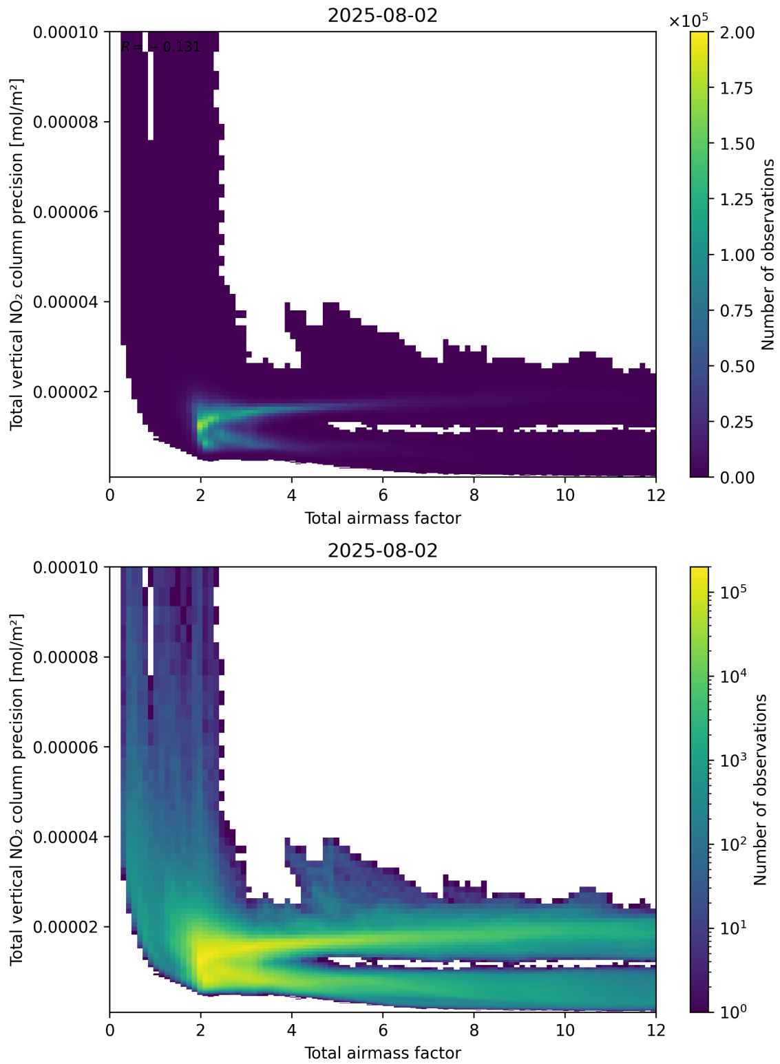
Figure 68: Scatter density plot of “Total airmass factor” against “Total vertical NO 2 column precision” for 2025-08-01 to 2025-08-03.
