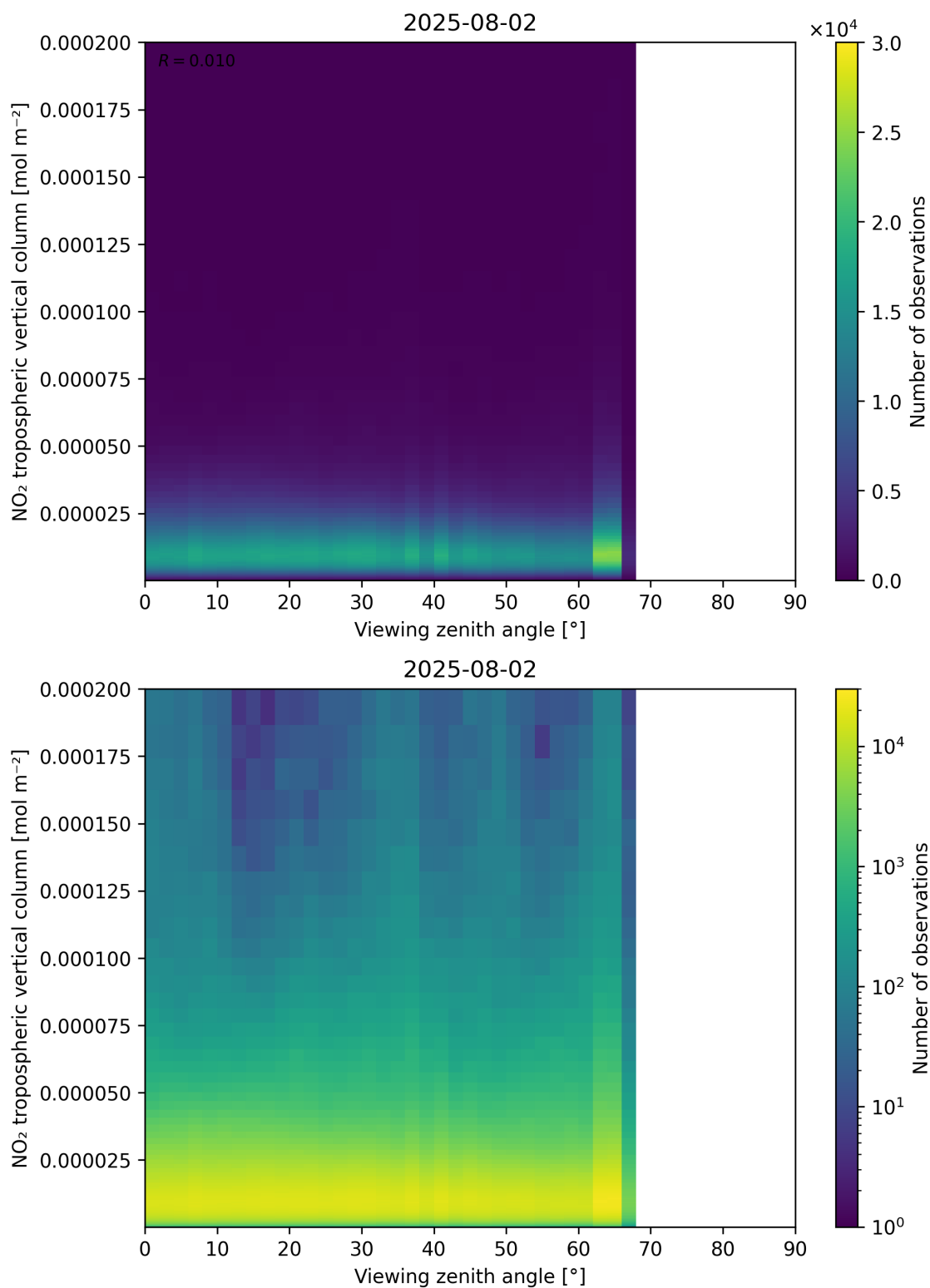
Figure 169: Scatter density plot of “Viewing zenith angle” against “NO 2 tropospheric vertical column” for 2025-08-01 to 2025-08-03.
