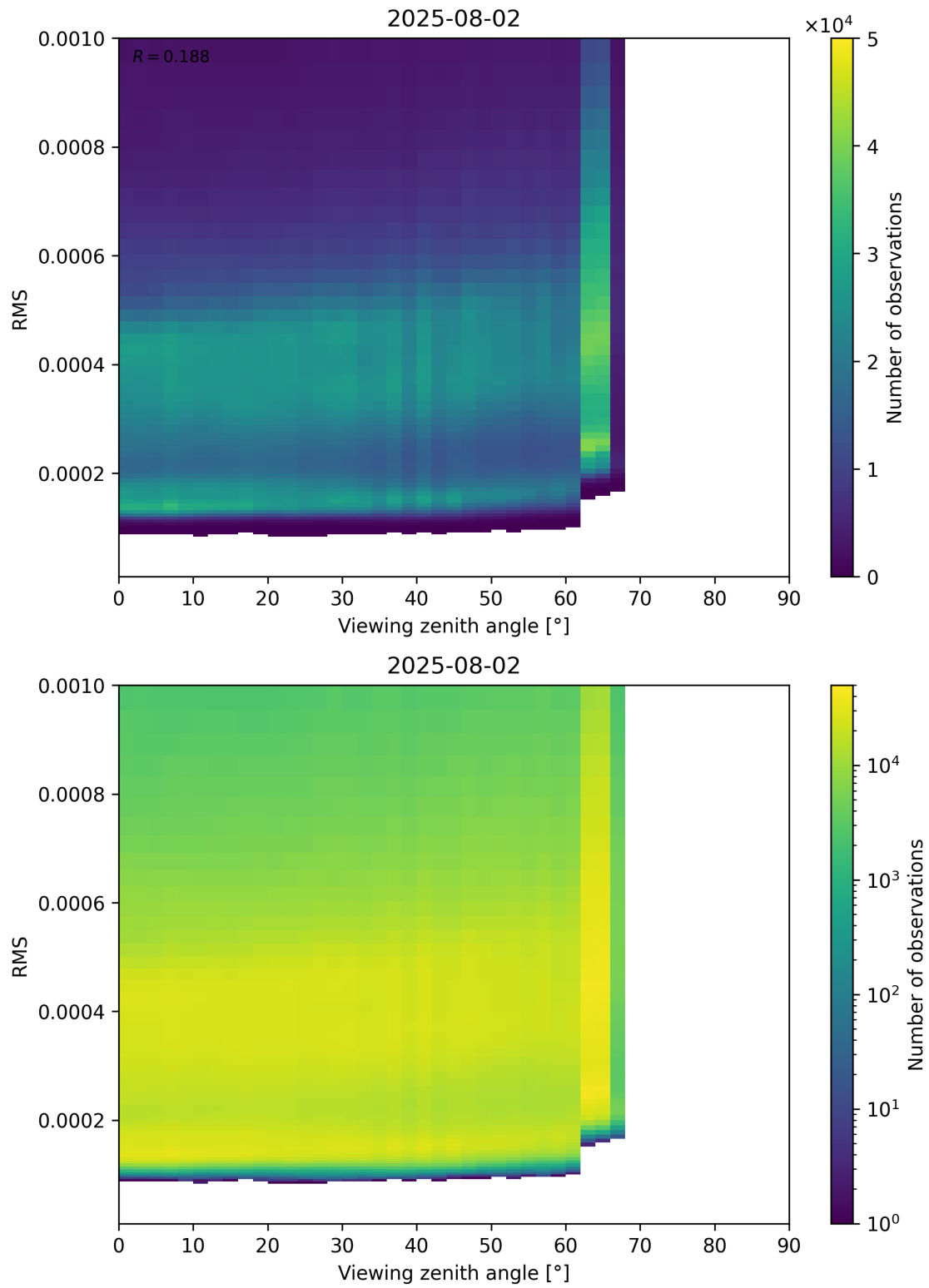
Figure 171: Scatter density plot of “Viewing zenith angle” against “RMS” for 2025-08-01 to 2025-08-03.
