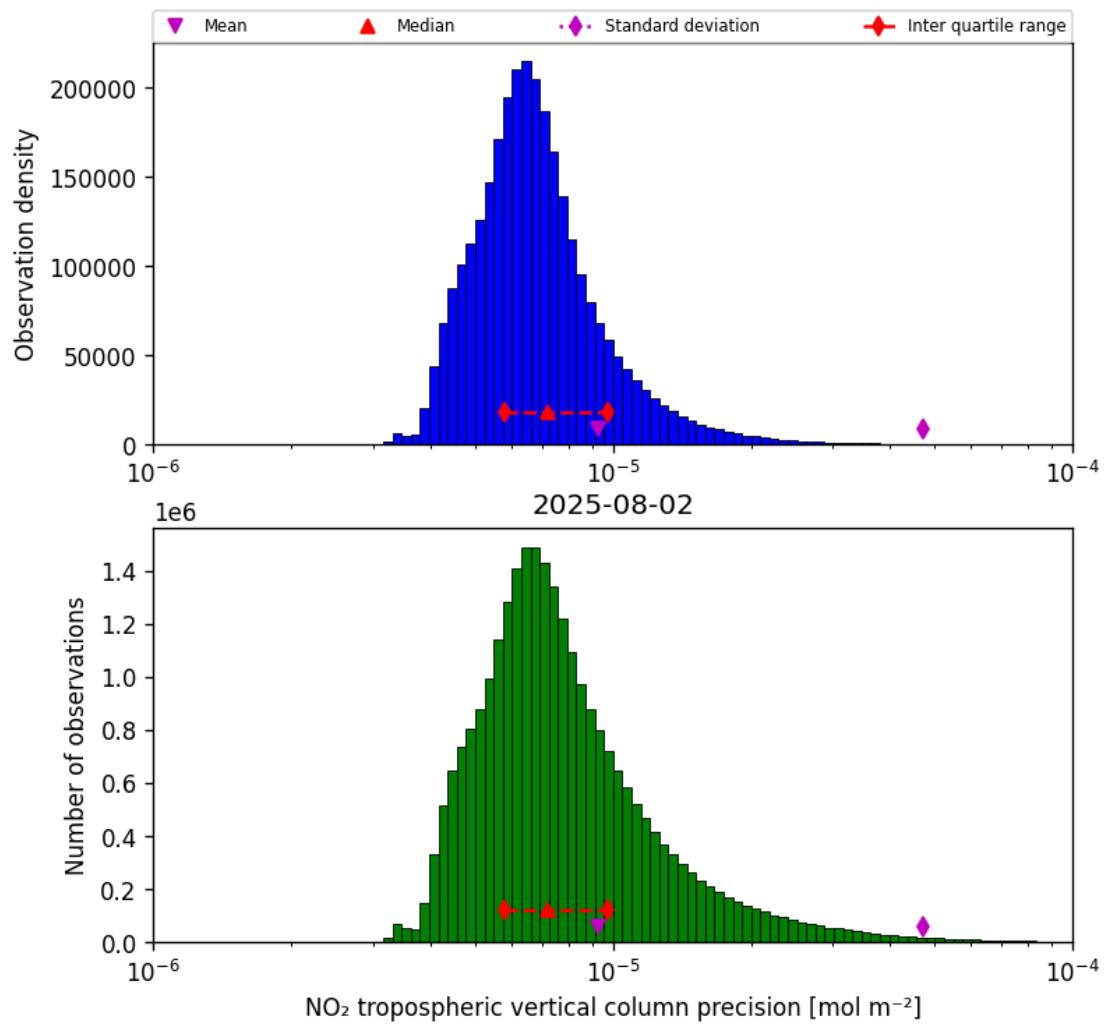
Figure 30: Histogram of “NO 2 tropospheric vertical column precision” for 2025-08-01 to 2025-08-03
