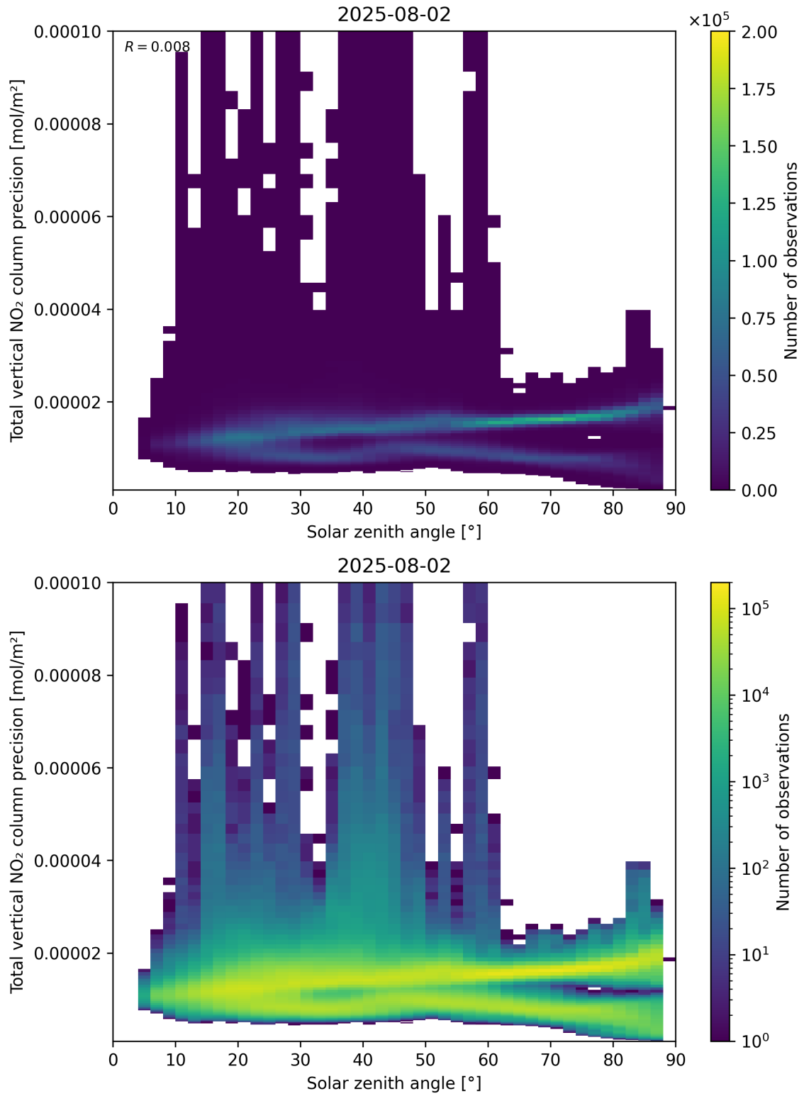
Figure 154: Scatter density plot of “Solar zenith angle” against “Total vertical NO 2 column precision” for 2025-08-01 to 2025-08-03.
