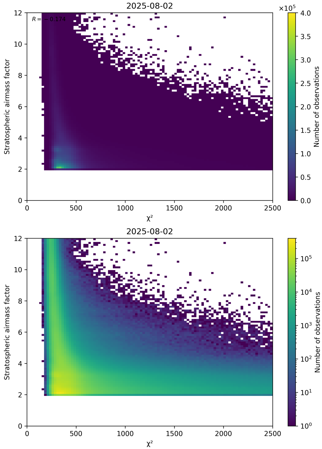
Figure 81: Scatter density plot of “ \chi^2 ” against “Stratospheric airmass factor” for 2025-08-01 to 2025-08-03.
