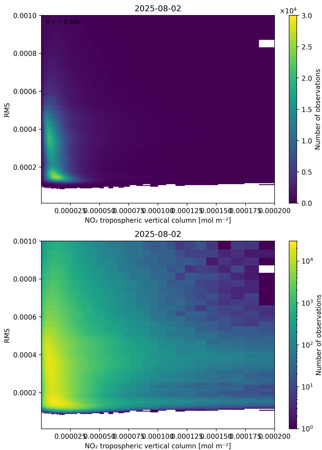
Figure 142: Scatter density plot of “NO 2 tropospheric vertical column” against “RMS” for 2025-08-01 to 2025-08-03.
