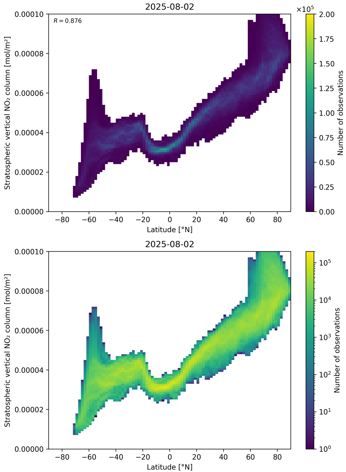
Figure 87: Scatter density plot of “Latitude” against “Stratospheric vertical NO 2 column” for 2025-08-01 to 2025-08-03.
