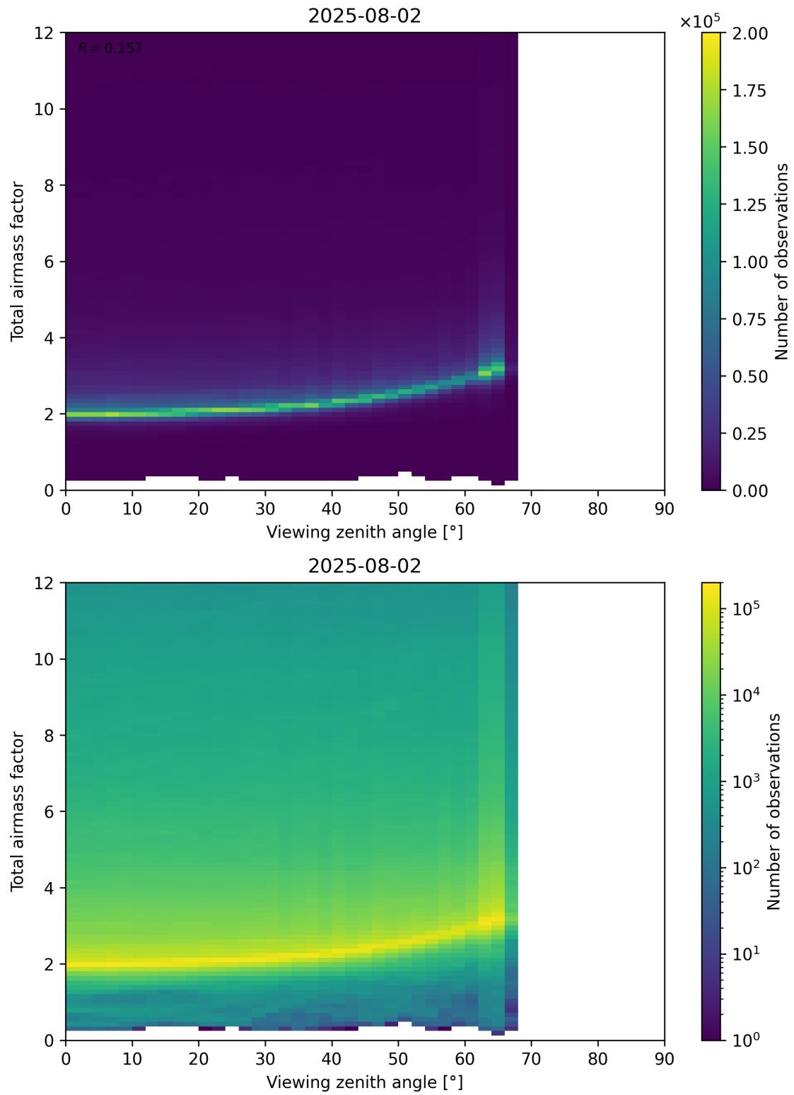
Figure 160: Scatter density plot of “Viewing zenith angle” against “Total airmass factor” for 2025-08-01 to 2025-08-03.
