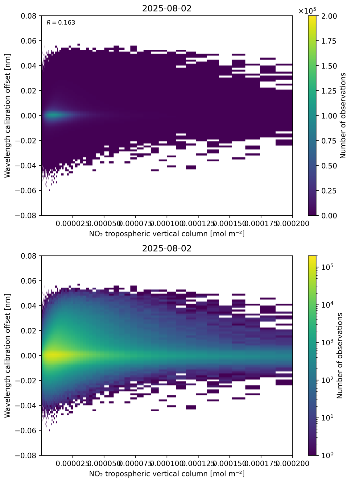
Figure 143: Scatter density plot of “NO 2 tropospheric vertical column” against “Wavelength calibration offset” for 2025-08-01 to 2025-08-03.
