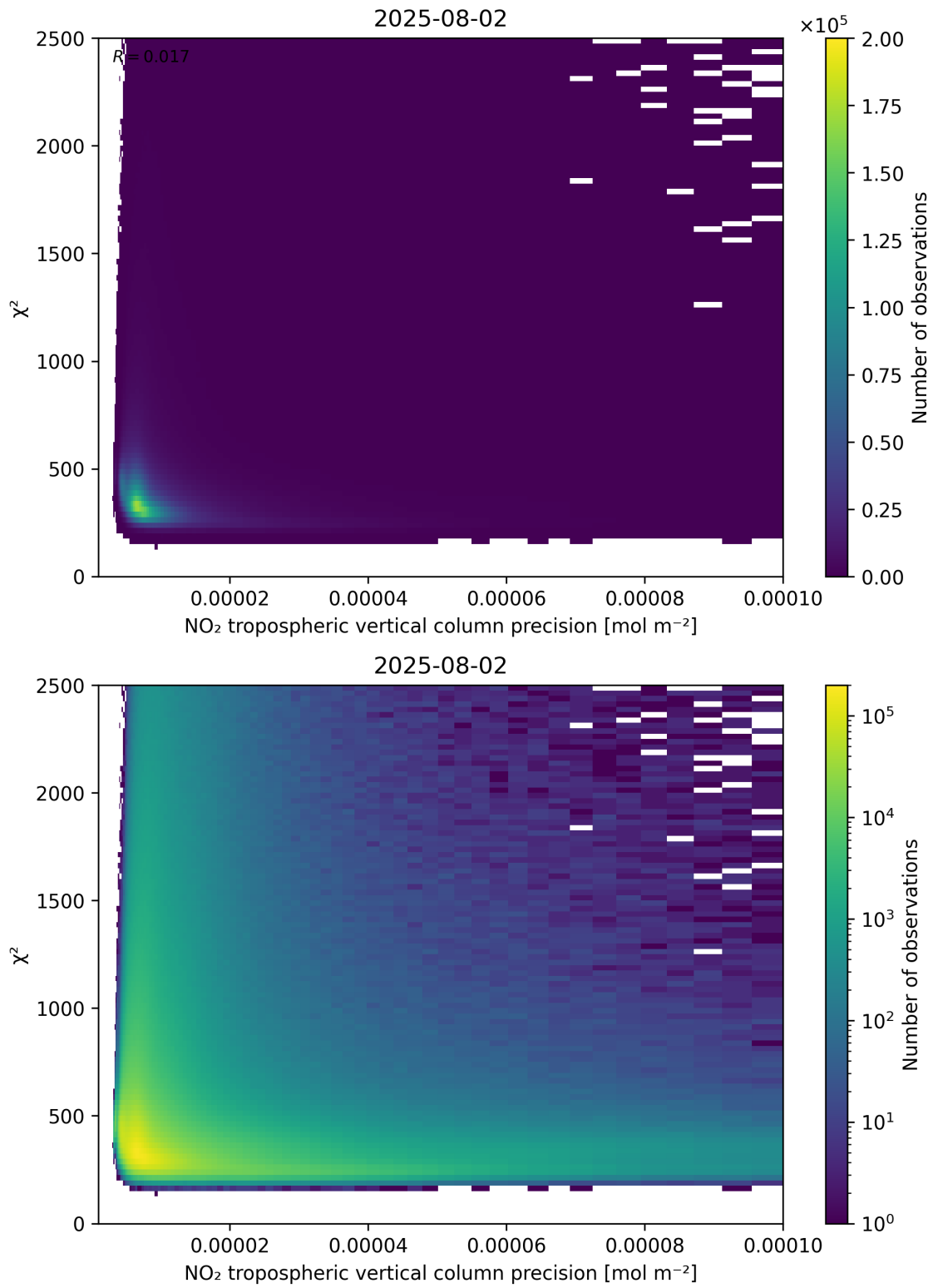
Figure 134: Scatter density plot of “NO 2 tropospheric vertical column precision” against “ \chi^2 ” for 2025-08-01 to 2025-08-03.
