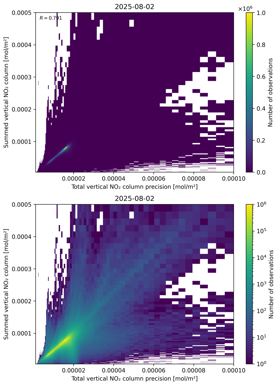
Figure 117: Scatter density plot of “Total vertical NO 2 column precision” against “Summed vertical NO 2 column” for 2025-08-01 to 2025-08-03.
