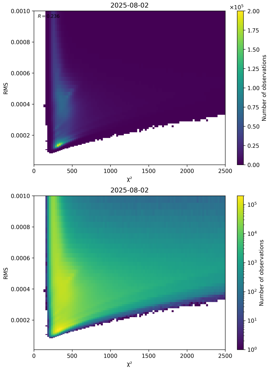
Figure 82: Scatter density plot of “ \chi^2 ” against “RMS” for 2025-08-01 to 2025-08-03.
