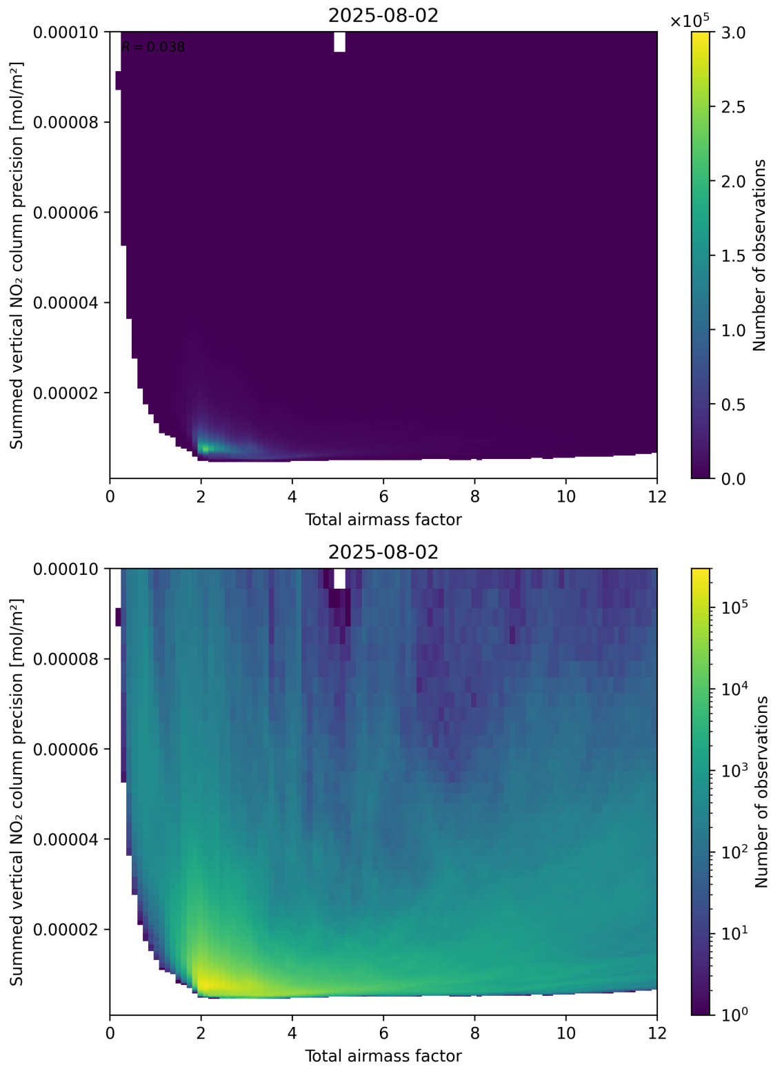
Figure 66: Scatter density plot of “Total airmass factor” against “Summed vertical NO 2 column precision” for 2025-08-01 to 2025-08-03.
