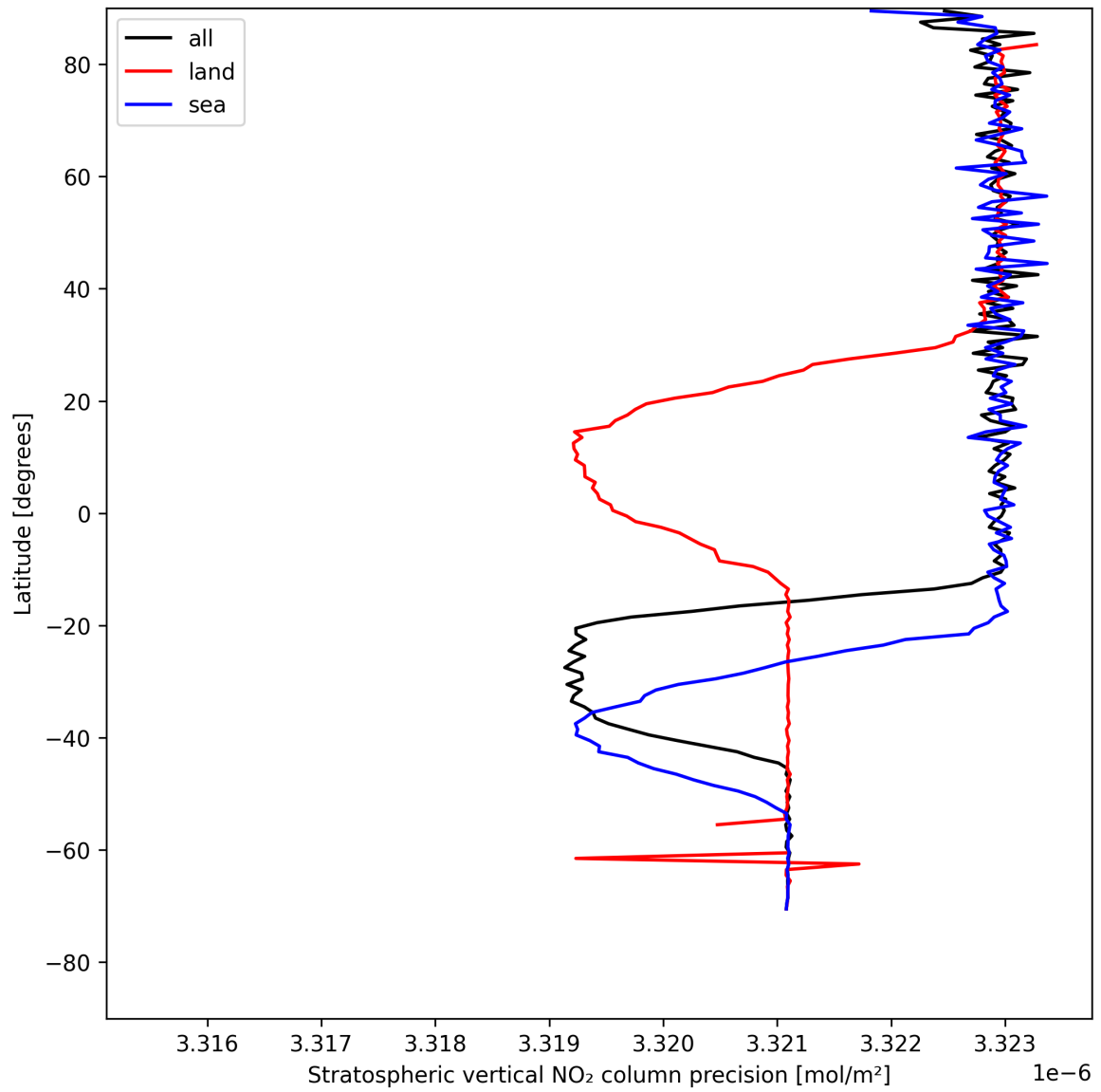
Figure 20: Zonal average of “Stratospheric vertical NO 2 column precision” for 2025-08-01 to 2025-08-03.
