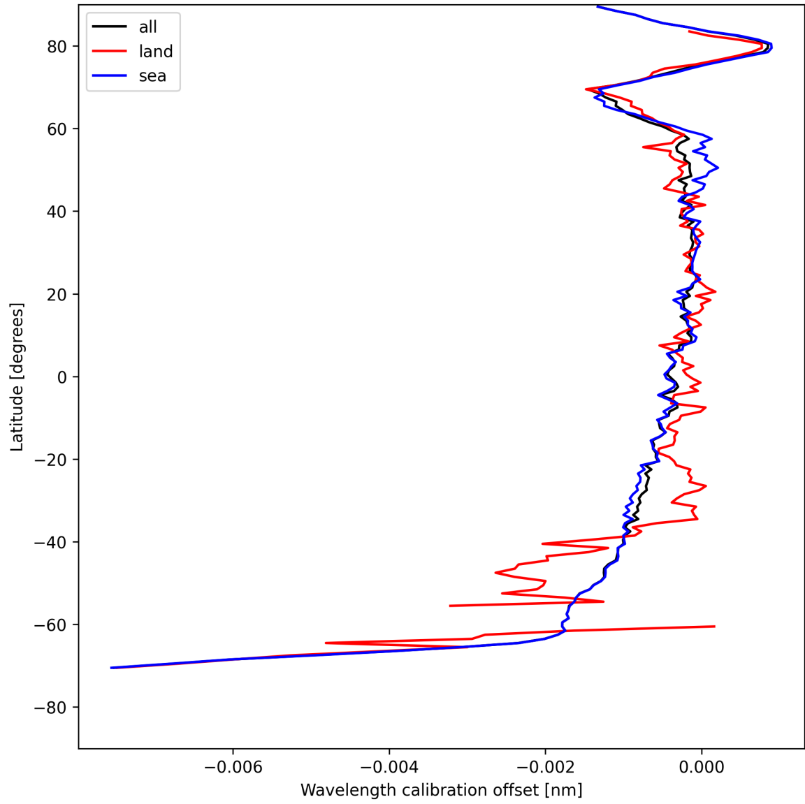
Figure 18: Zonal average of “Wavelength calibration offset” for 2025-08-01 to 2025-08-03.
