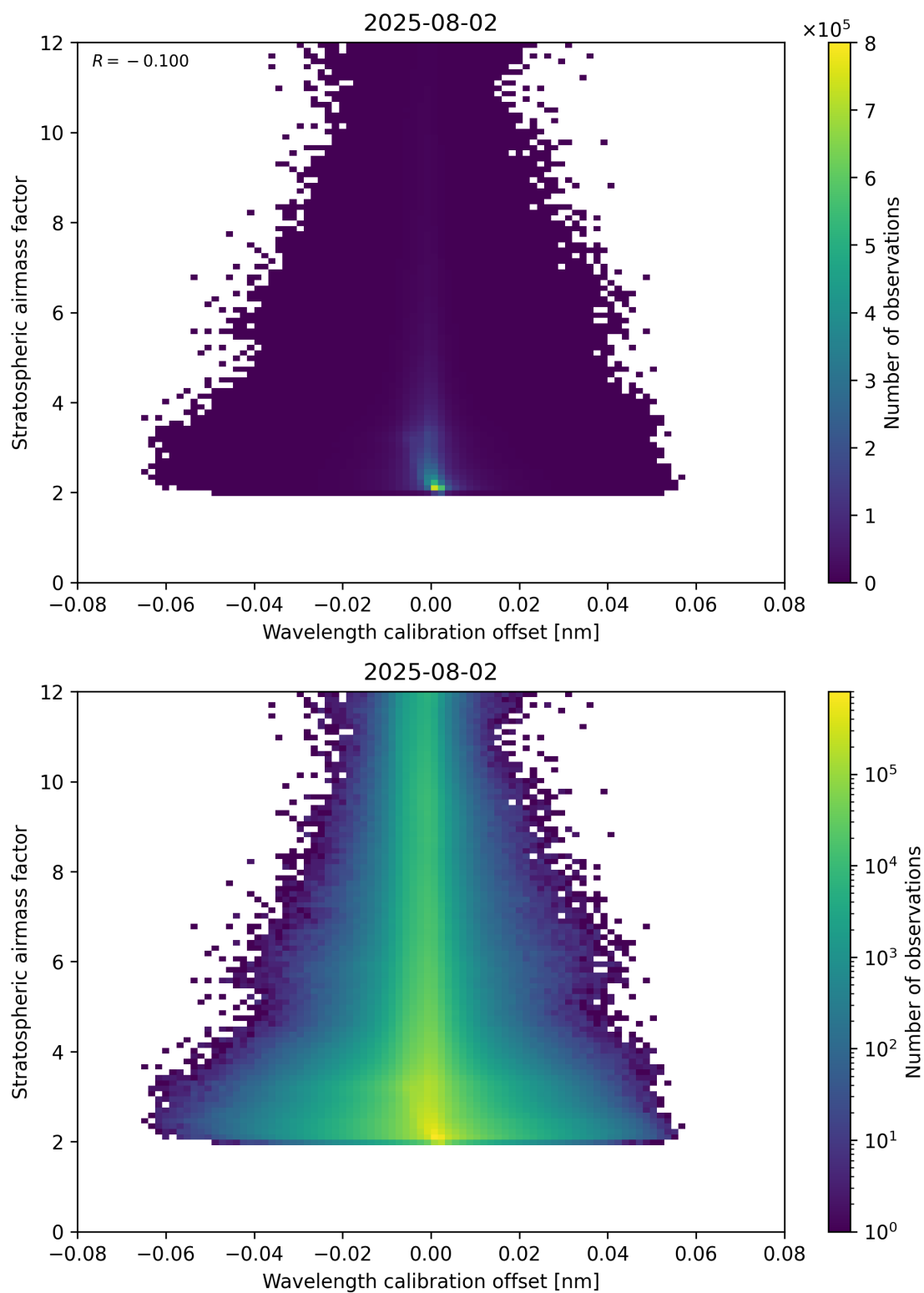
Figure 174: Scatter density plot of “Wavelength calibration offset” against “Stratospheric airmass factor” for 2025-08-01 to 2025-08-03.
