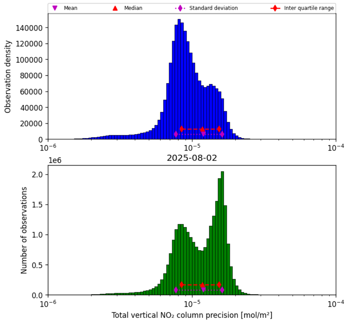
Figure 39: Histogram of “Total vertical NO 2 column precision” for 2025-08-01 to 2025-08-03
