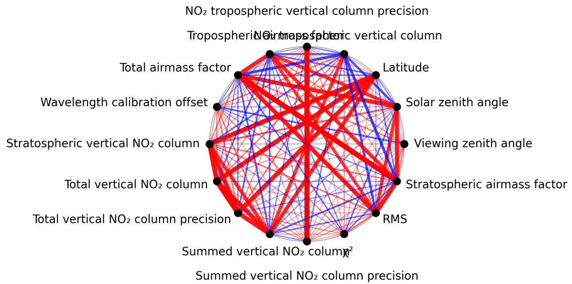
Figure 1: Map of correlation graph for 2025-08-01 to 2025-08-03.
