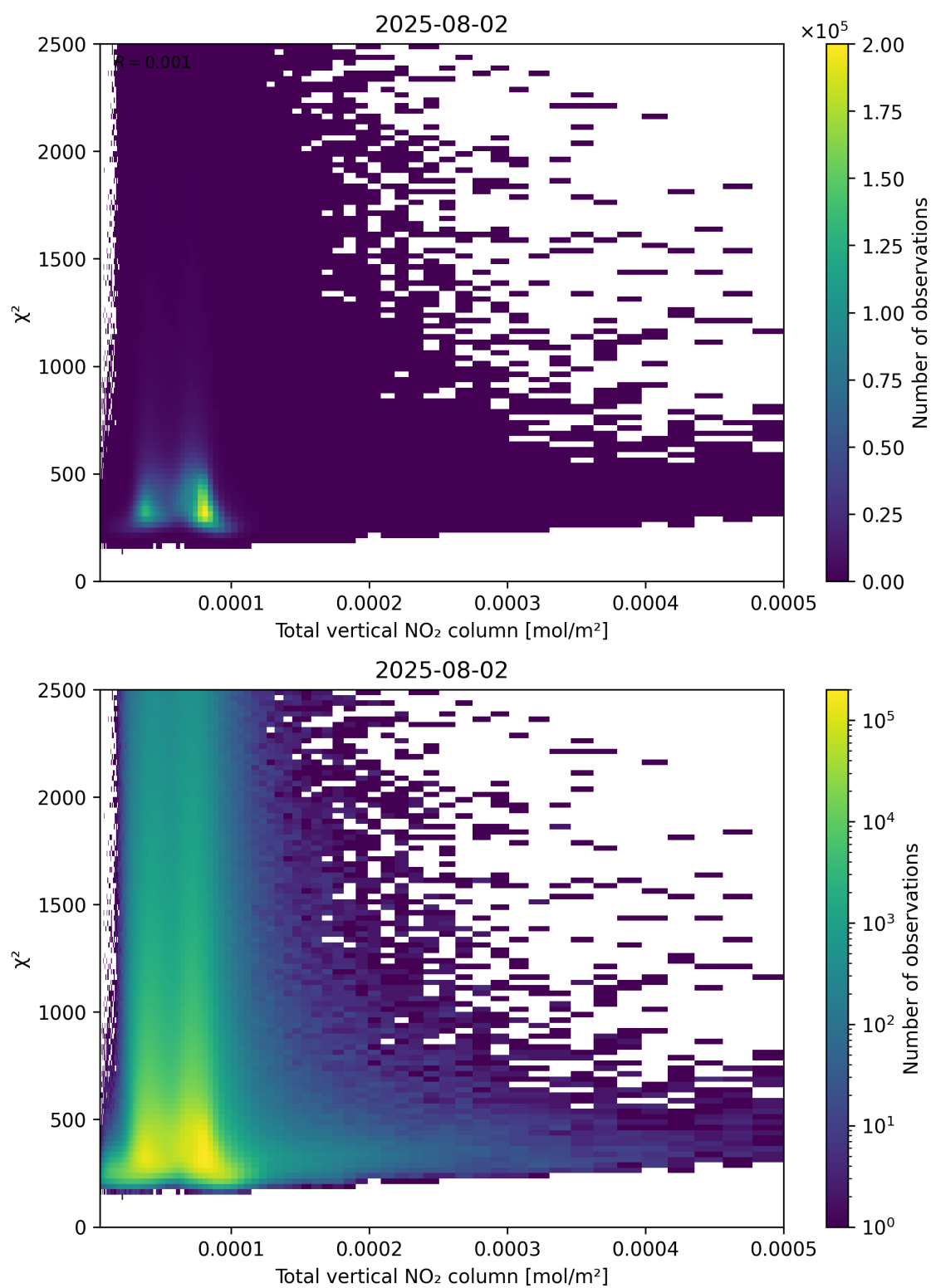
Figure 111: Scatter density plot of “Total vertical NO 2 column” against “ \chi^2 ” for 2025-08-01 to 2025-08-03.
