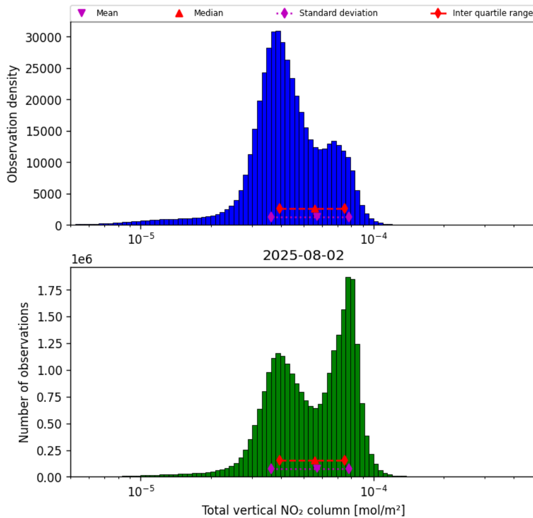
Figure 38: Histogram of “Total vertical NO 2 column” for 2025-08-01 to 2025-08-03
