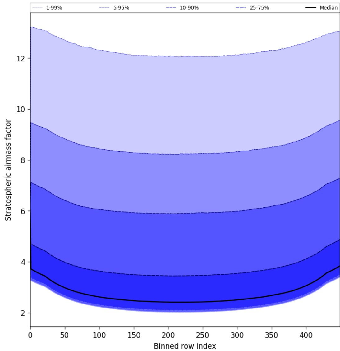
Figure 61: Along track statistics of “Stratospheric airmass factor” for 2025-08-01 to 2025-08-03
