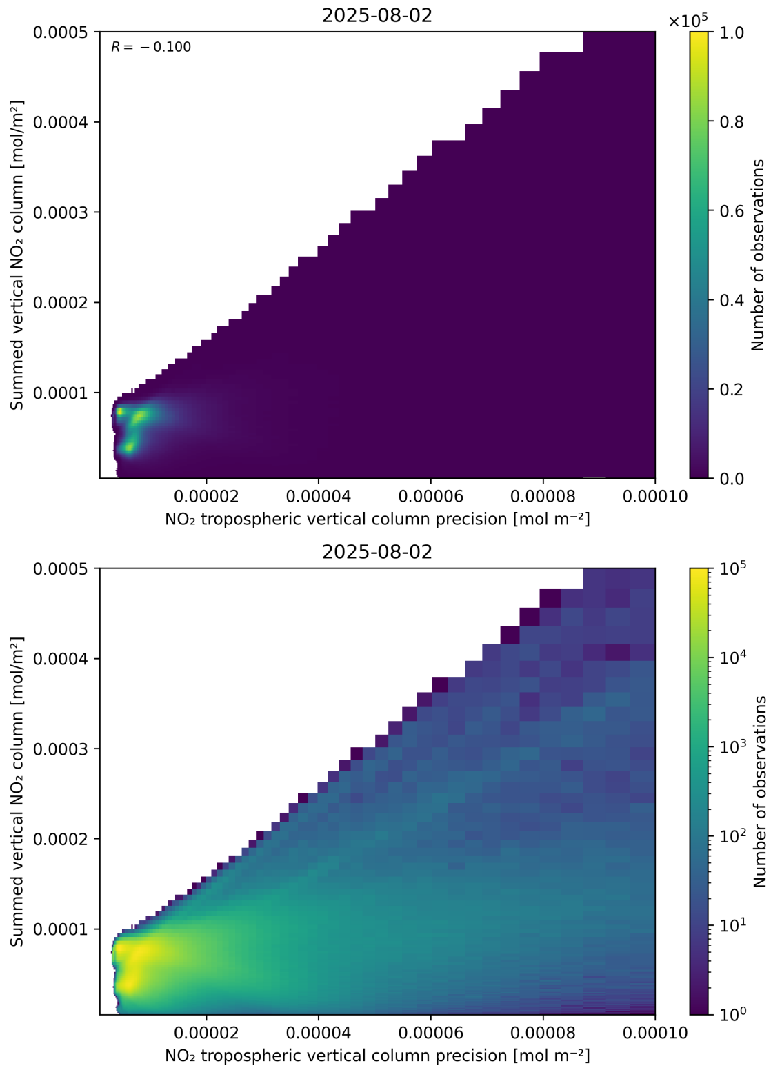
Figure 136: Scatter density plot of “NO 2 tropospheric vertical column precision” against “Summed vertical NO 2 column” for 2025-08-01 to 2025-08-03.
