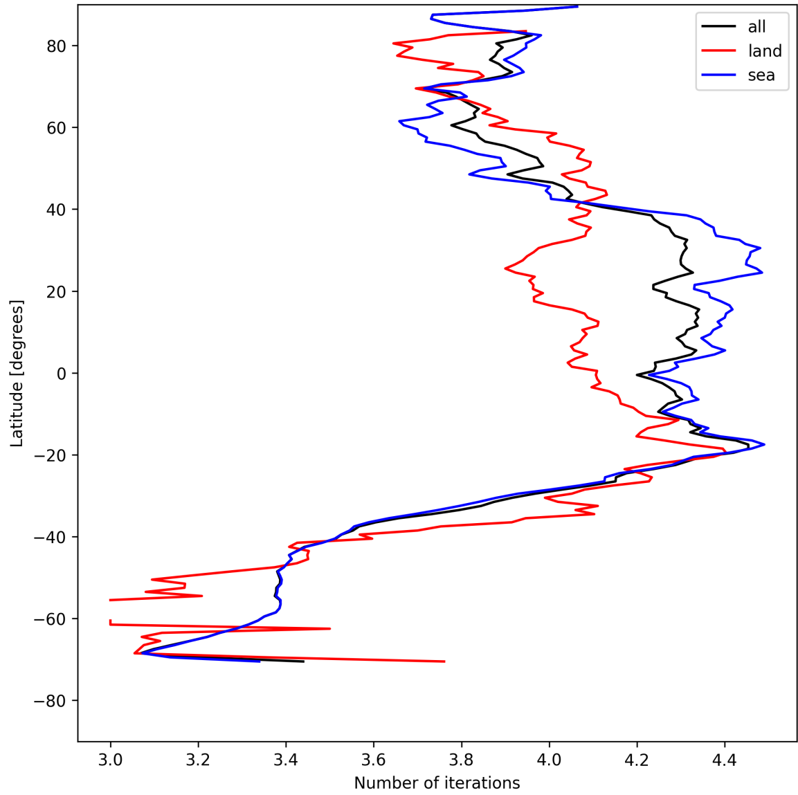
Figure 17: Zonal average of “Number of iterations” for 2025-08-01 to 2025-08-03.
