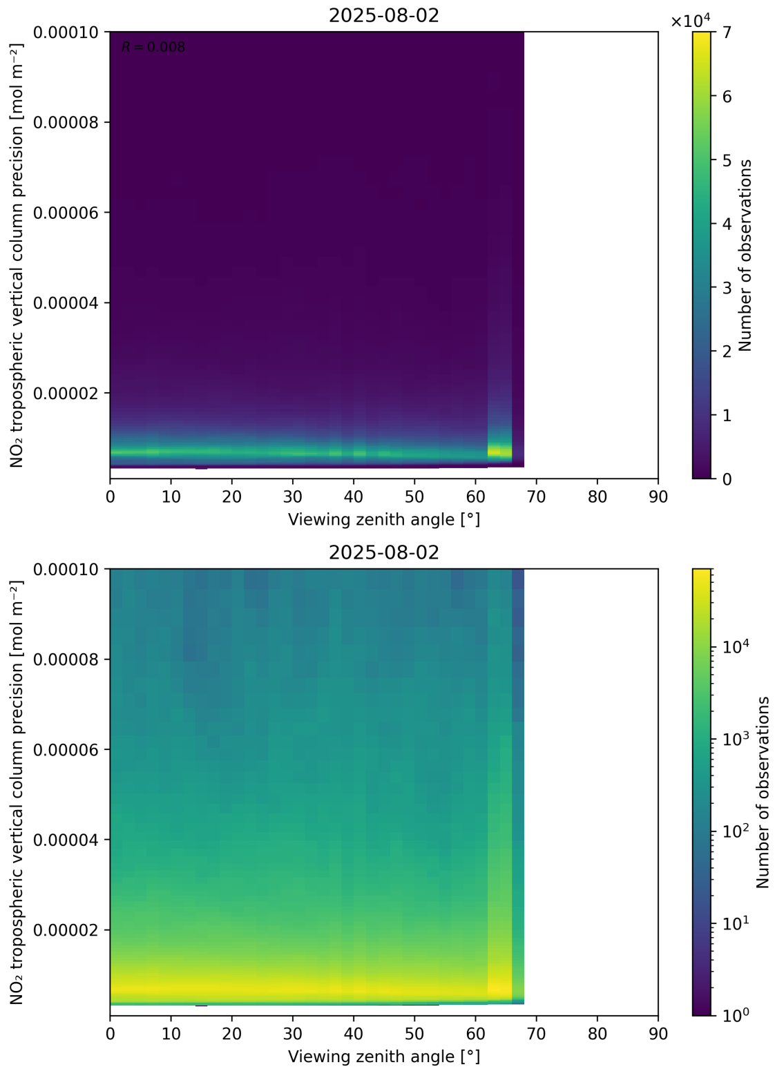
Figure 170: Scatter density plot of “Viewing zenith angle” against “NO 2 tropospheric vertical column precision” for 2025-08-01 to 2025-08-03.
