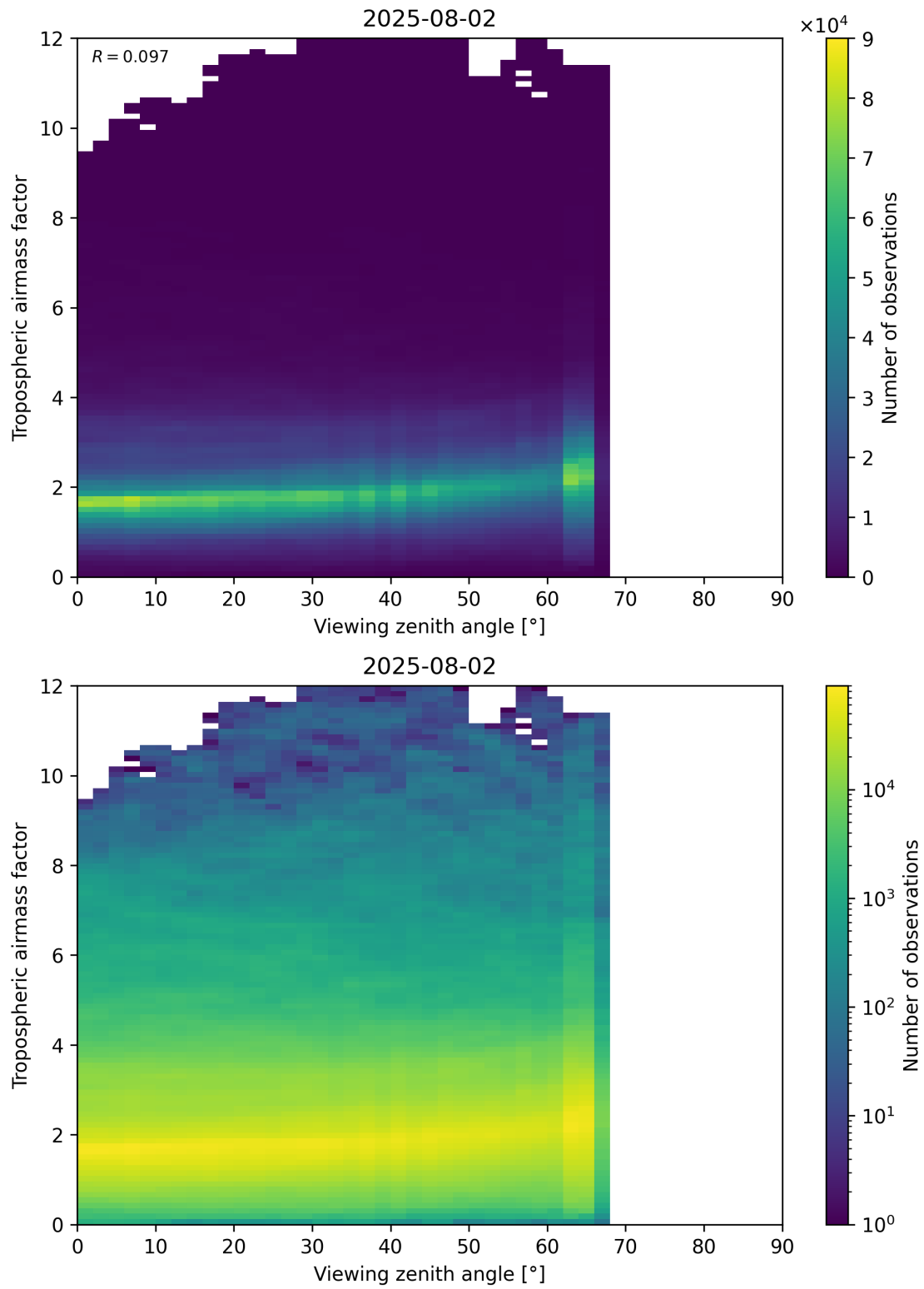
Figure 161: Scatter density plot of “Viewing zenith angle” against “Tropospheric airmass factor” for 2025-08-01 to 2025-08-03.
