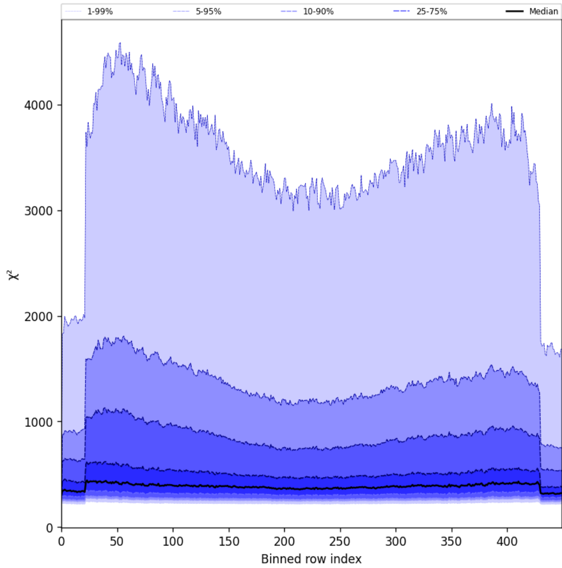
Figure 59: Along track statistics of “ \chi^2 ” for 2025-08-01 to 2025-08-03
