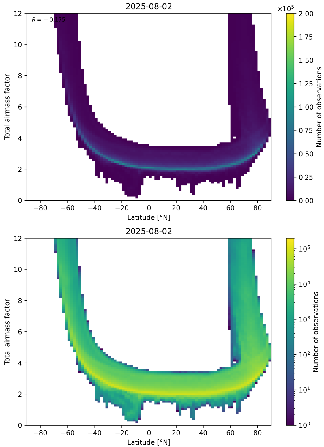
Figure 84: Scatter density plot of “Latitude” against “Total airmass factor” for 2025-08-01 to 2025-08-03.
