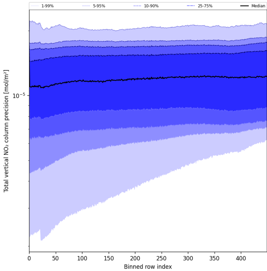
Figure 56: Along track statistics of “Total vertical NO 2 column precision” for 2025-08-01 to 2025-08-03
