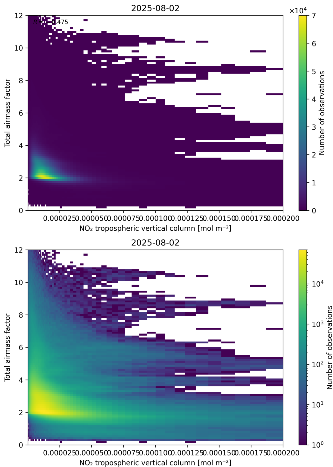
Figure 122: Scatter density plot of “NO 2 tropospheric vertical column” against “Total air mass factor” for 2025-08-01 to 2025-08-03.
