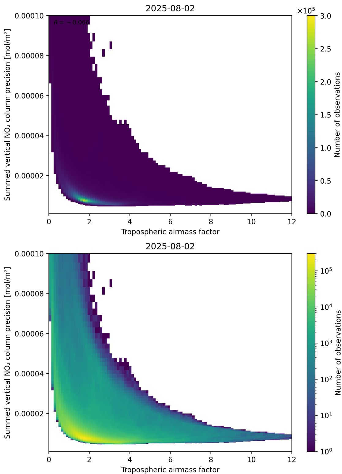
Figure 76: Scatter density plot of “Tropospheric airmass factor” against “Summed vertical NO 2 column precision” for 2025-08-01 to 2025-08-03.
