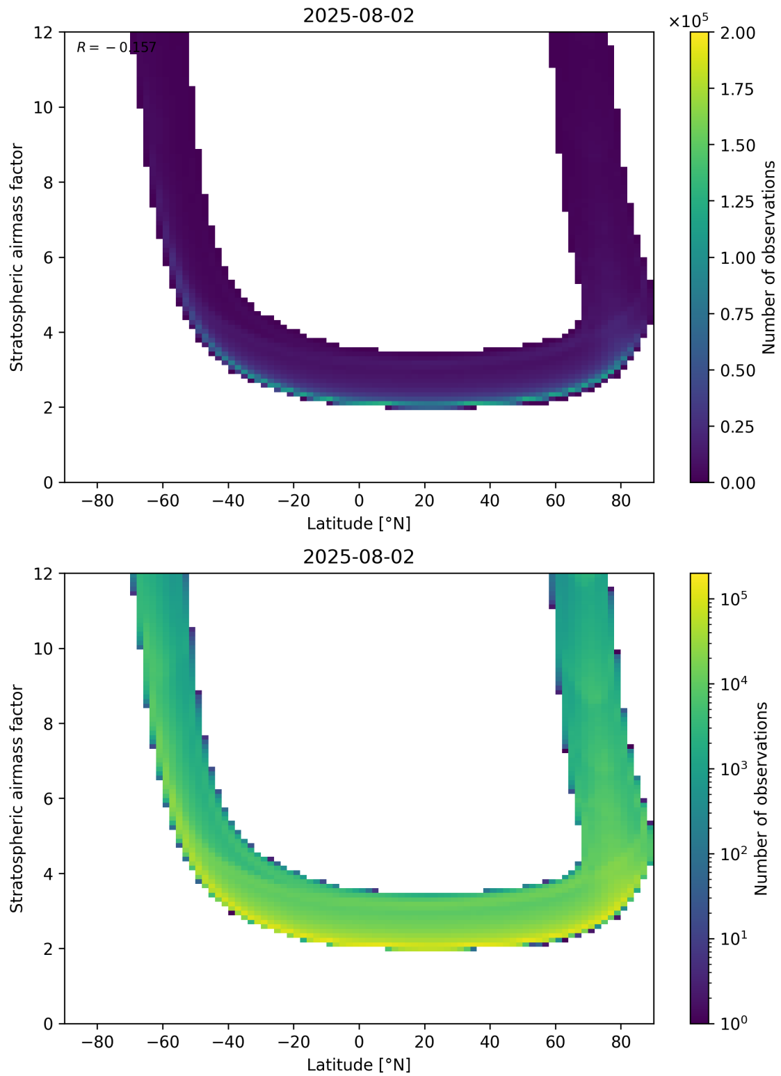
Figure 83: Scatter density plot of “Latitude” against “Stratospheric air mass factor” for 2025-08-01 to 2025-08-03.
