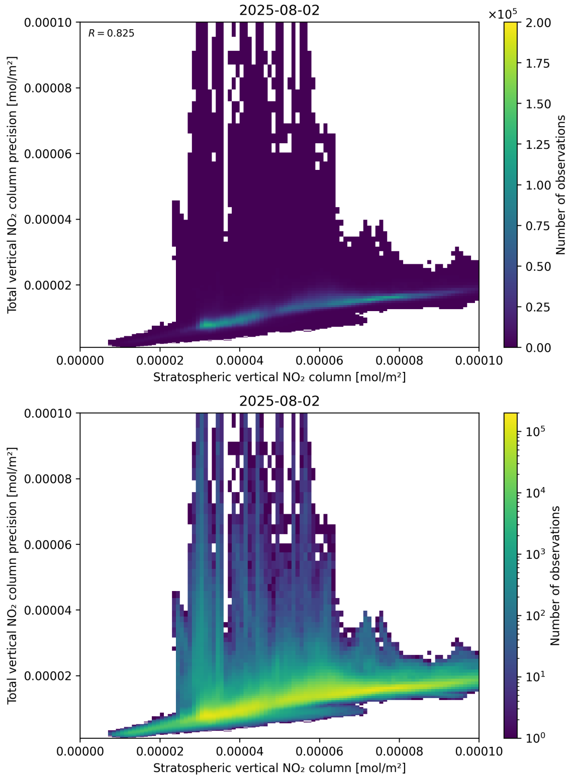
Figure 101: Scatter density plot of “Stratospheric vertical NO 2 column” against “Total vertical NO 2 column precision” for 2025-08-01 to 2025-08-03.
