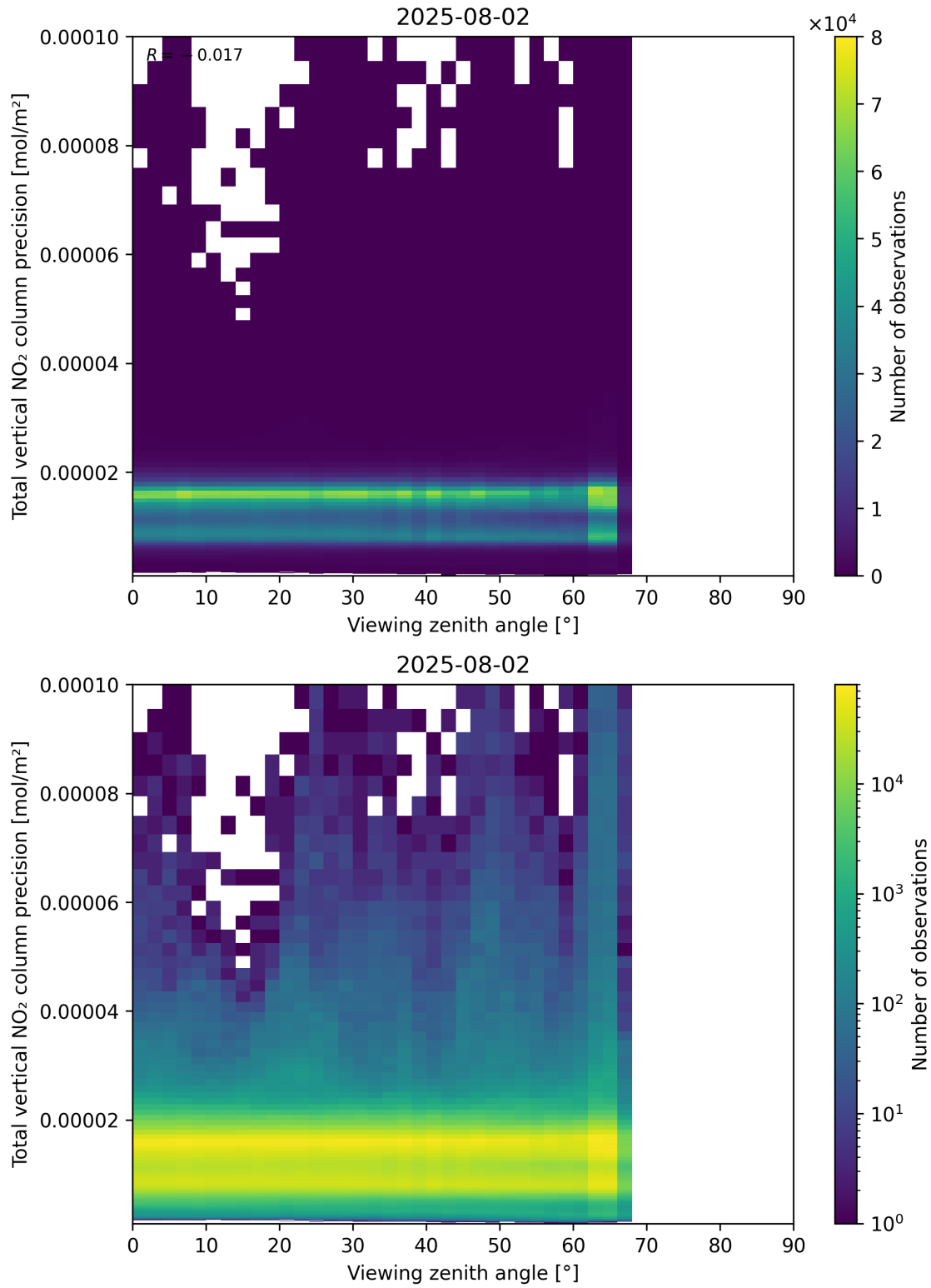
Figure 168: Scatter density plot of “Viewing zenith angle” against “Total vertical NO 2 column precision” for 2025-08-01 to 2025-08-03.
