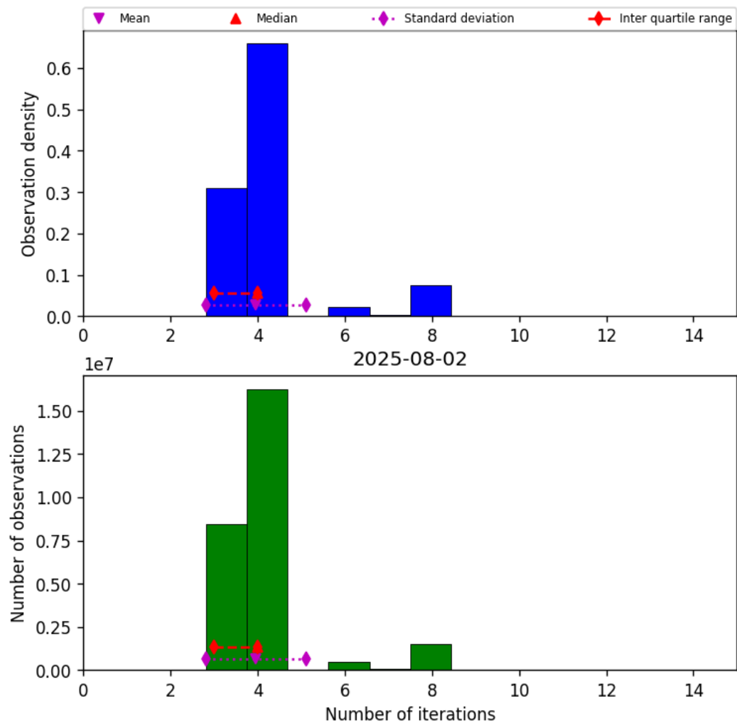
Figure 34: Histogram of “Number of iterations” for 2025-08-01 to 2025-08-03
