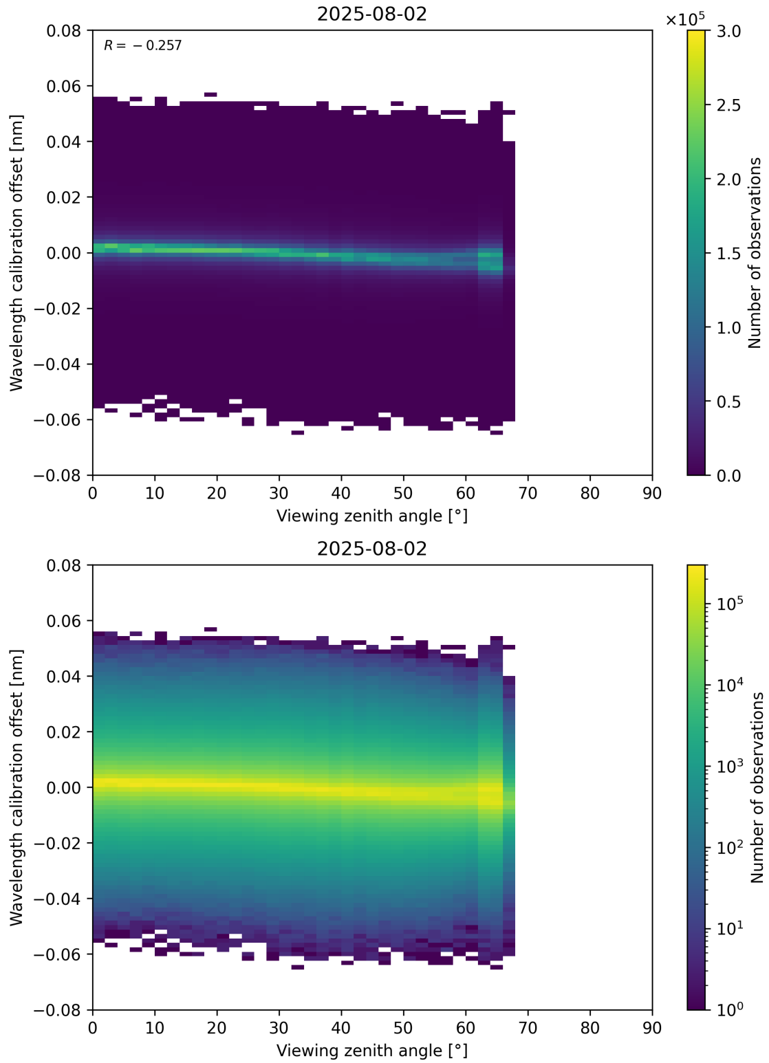
Figure 173: Scatter density plot of “Viewing zenith angle” against “Wavelength calibration offset” for 2025-08-01 to 2025-08-03.
