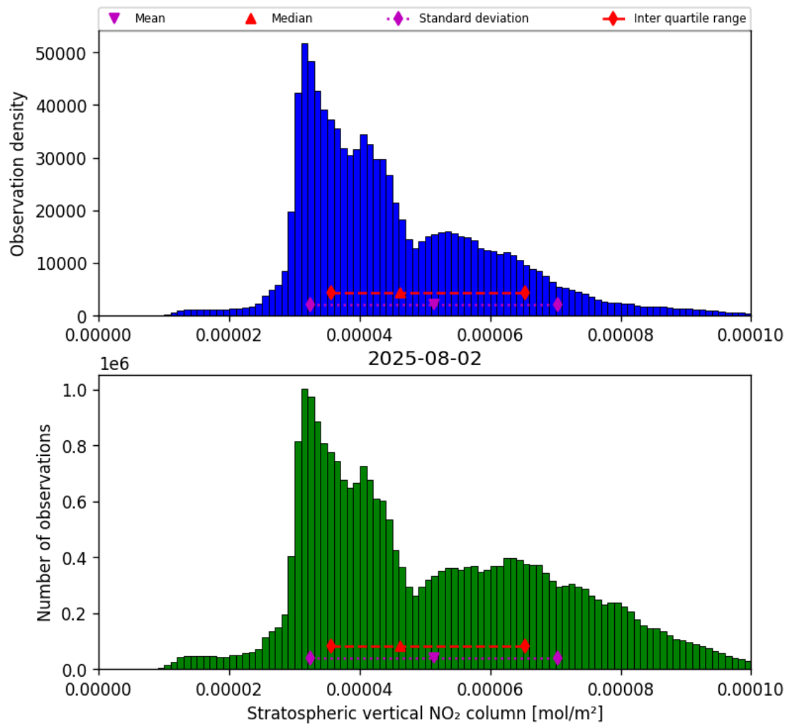
Figure 36: Histogram of “Stratospheric vertical NO 2 column” for 2025-08-01 to 2025-08-03
