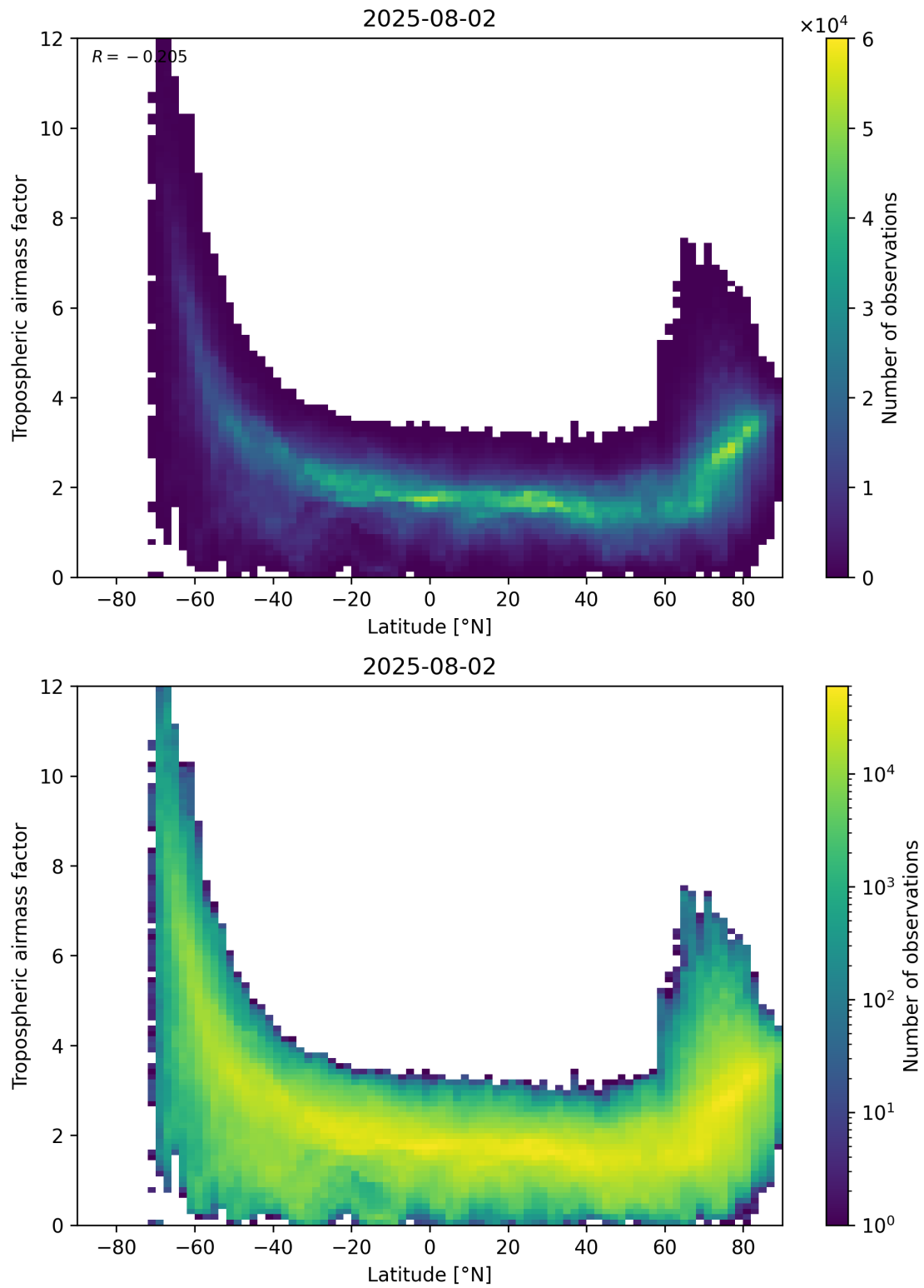
Figure 85: Scatter density plot of “Latitude” against “Tropospheric air mass factor” for 2025-08-01 to 2025-08-03.
