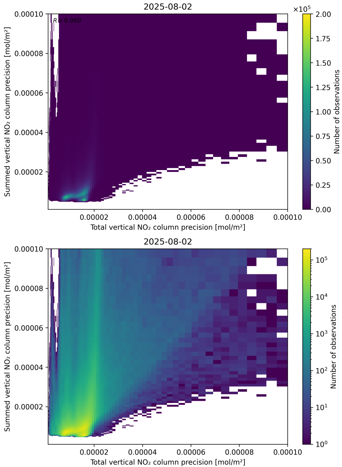
Figure 118: Scatter density plot of “Total vertical NO 2 column precision” against “Summed vertical NO 2 column precision” for 2025-08-01 to 2025-08-03.
