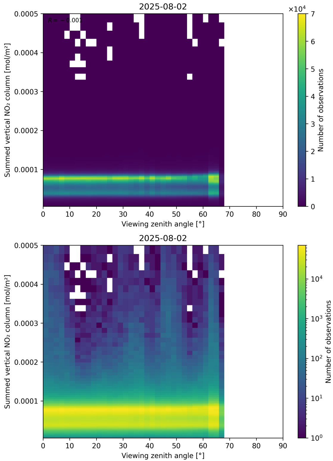
Figure 165: Scatter density plot of “Viewing zenith angle” against “Summed vertical NO 2 column” for 2025-08-01 to 2025-08-03.
