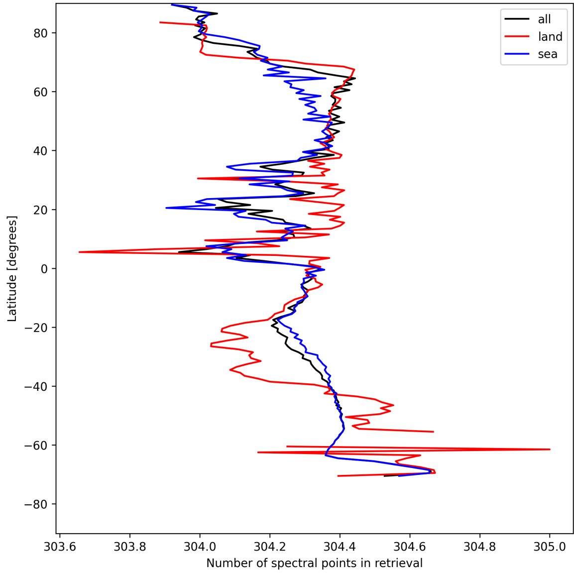
Figure 16: Zonal average of “Number of spectral points in retrieval” for 2025-08-01 to 2025-08-03.
