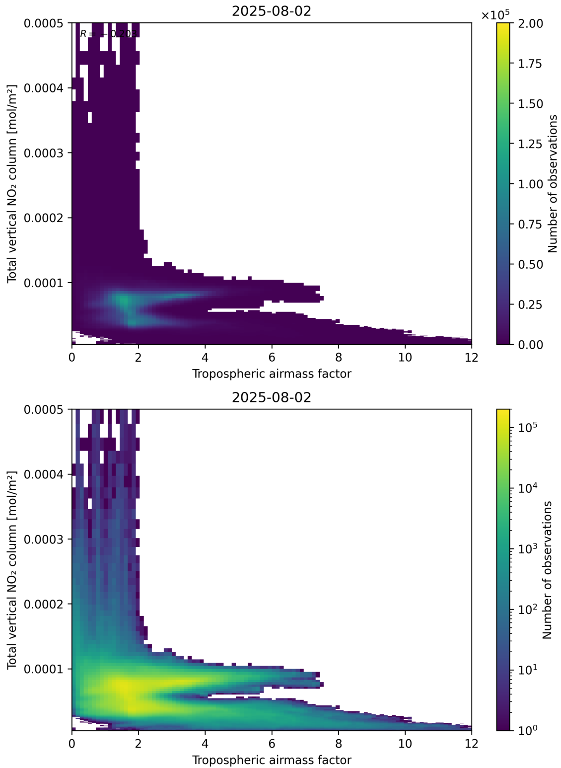
Figure 77: Scatter density plot of “Tropospheric airmass factor” against “Total vertical NO 2 column” for 2025-08-01 to 2025-08-03.
