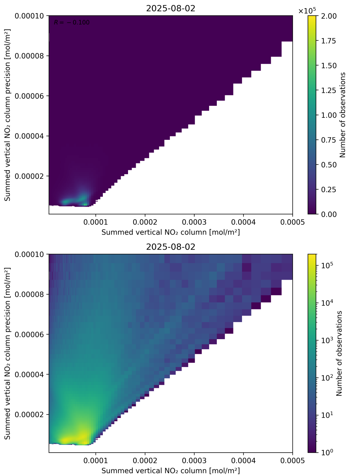
Figure 105: Scatter density plot of “Summed vertical NO 2 column” against “Summed vertical NO 2 column precision” for 2025-08-01 to 2025-08-03.
