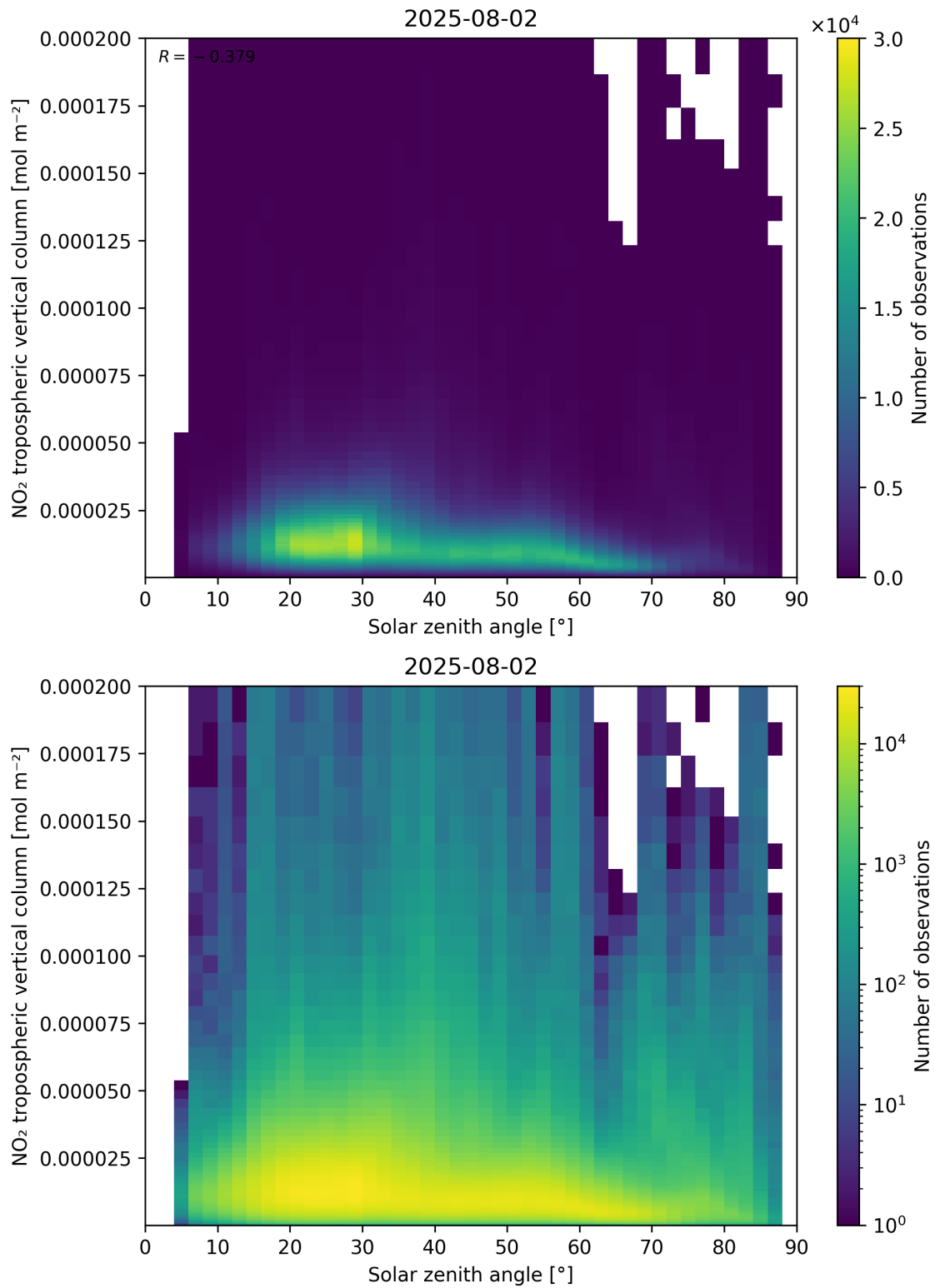
Figure 155: Scatter density plot of “Solar zenith angle” against “NO 2 tropospheric vertical column” for 2025-08-01 to 2025-08-03.
