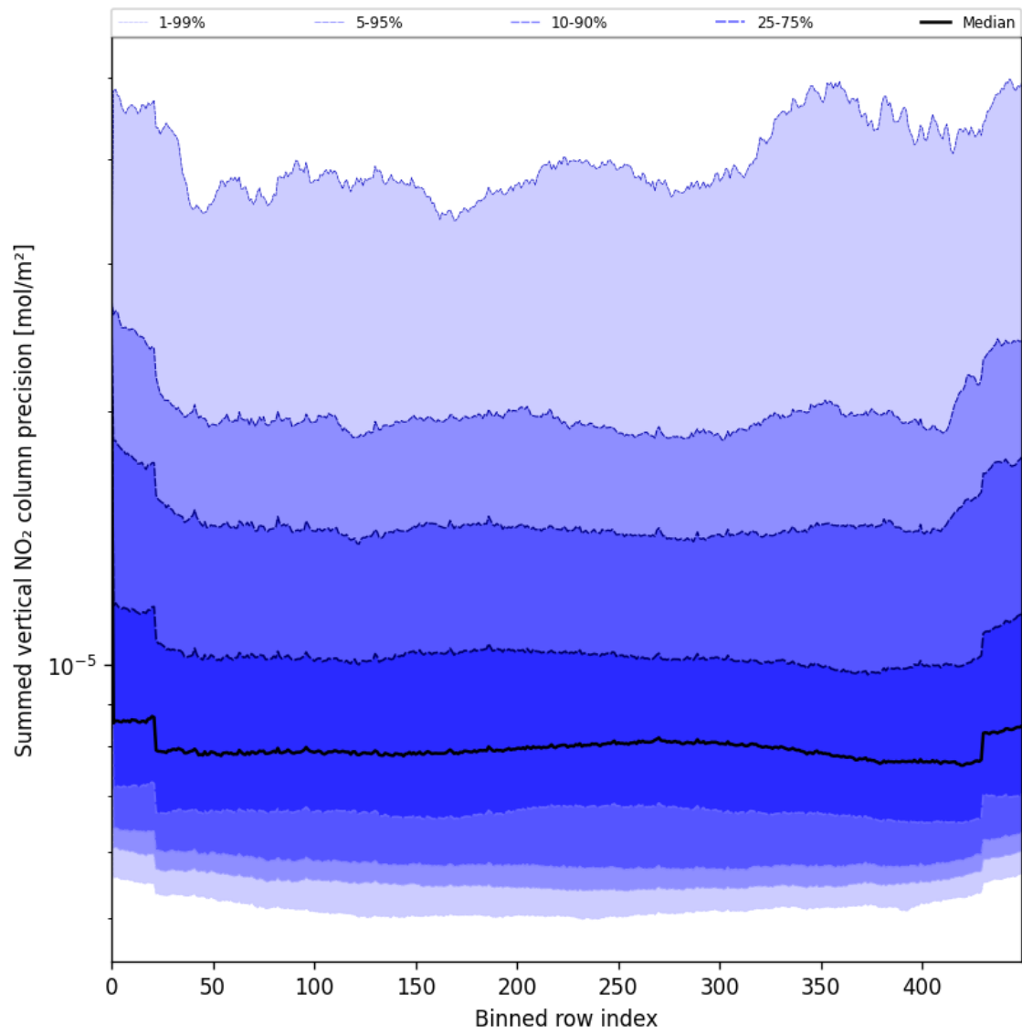
Figure 58: Along track statistics of “Summed vertical NO 2 column precision” for 2025-08-01 to 2025-08-03
