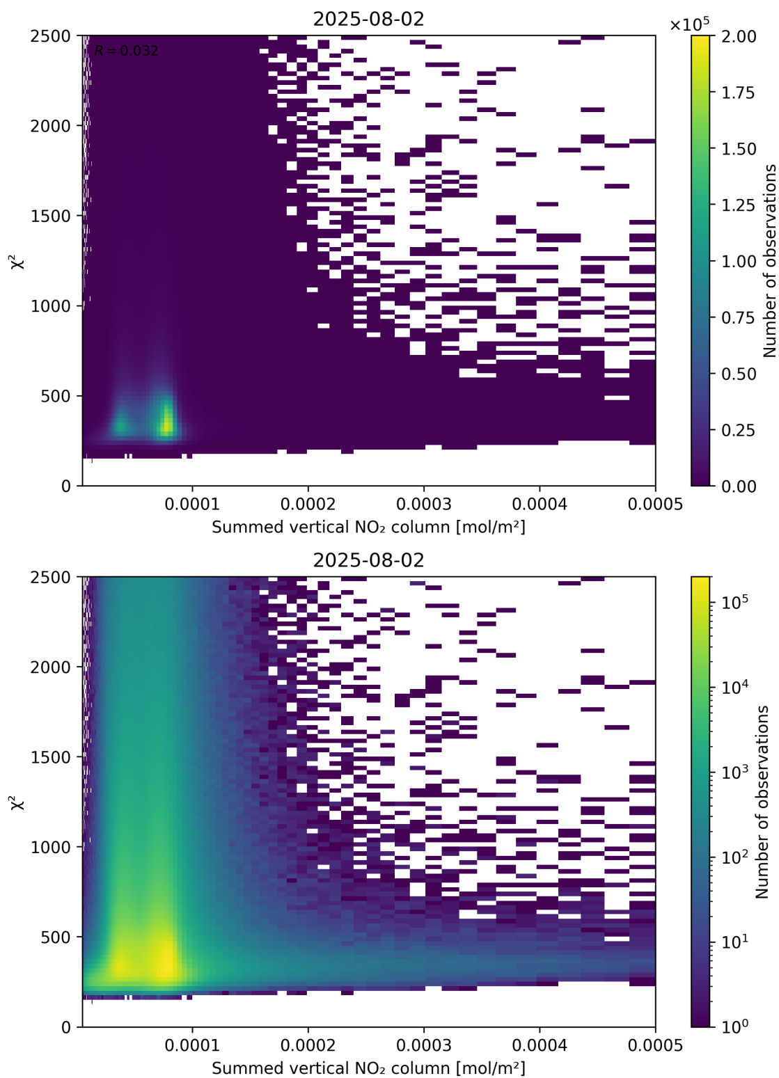
Figure 104: Scatter density plot of “Summed vertical NO 2 column” against “ \chi^2 ” for 2025-08-01 to 2025-08-03.
