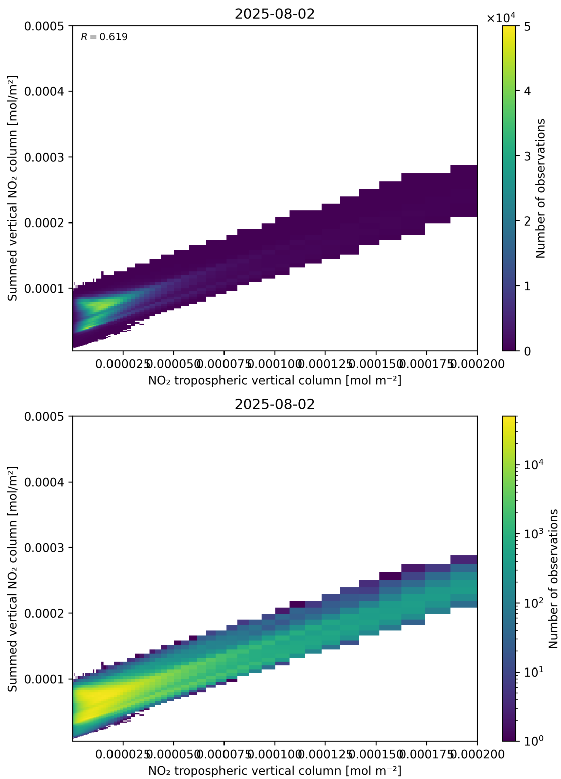
Figure 126: Scatter density plot of “NO 2 tropospheric vertical column” against “Summed vertical NO 2 column” for 2025-08-01 to 2025-08-03.
