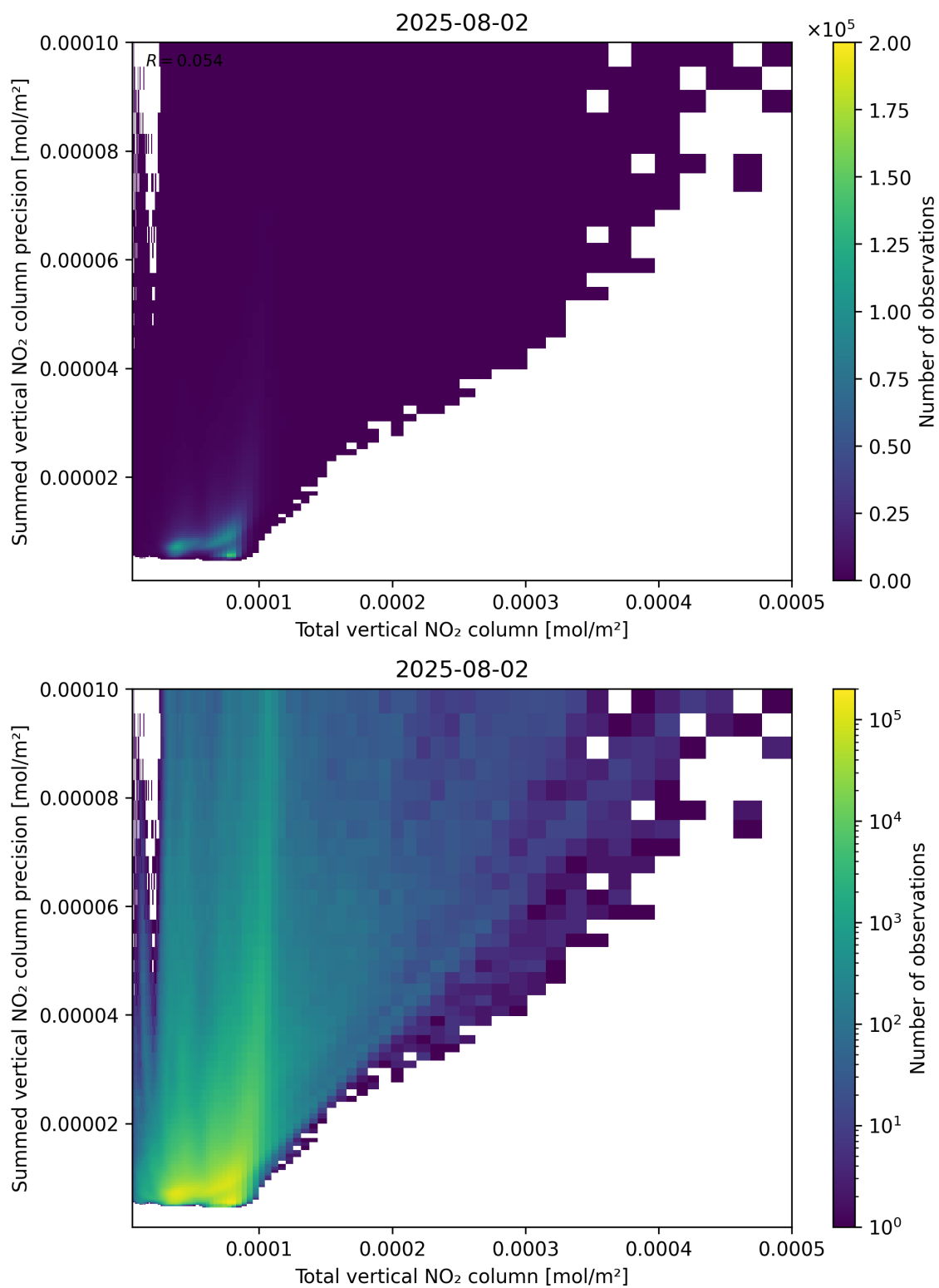
Figure 113: Scatter density plot of “Total vertical NO 2 column” against “Summed vertical NO 2 column precision” for 2025-08-01 to 2025-08-03.
