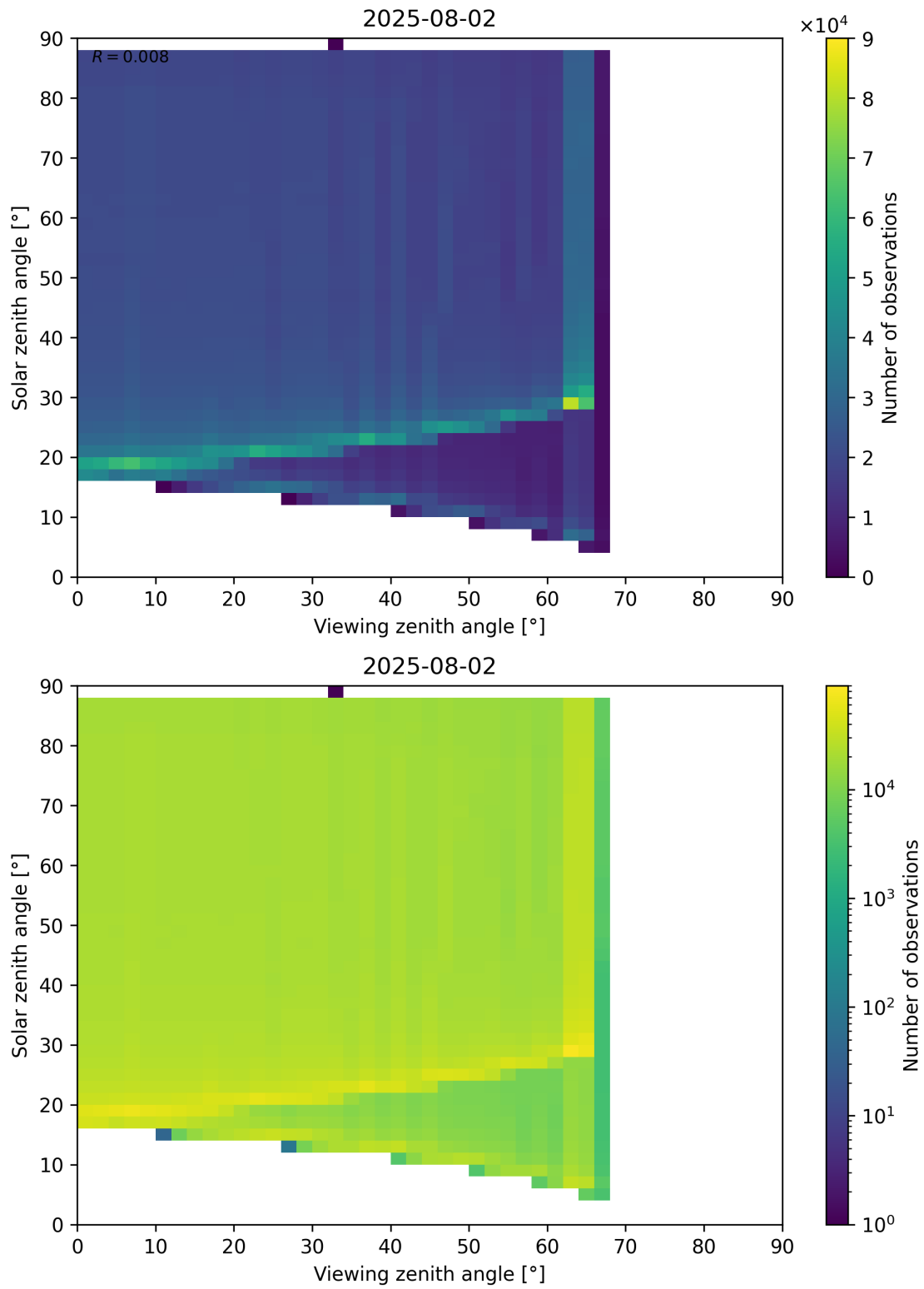
Figure 172: Scatter density plot of “Viewing zenith angle” against “Solar zenith angle” for 2025-08-01 to 2025-08-03.
