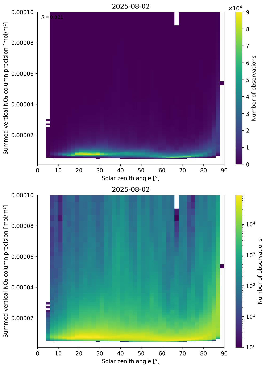
Figure 152: Scatter density plot of “Solar zenith angle” against “Summed vertical NO 2 column precision” for 2025-08-01 to 2025-08-03.
