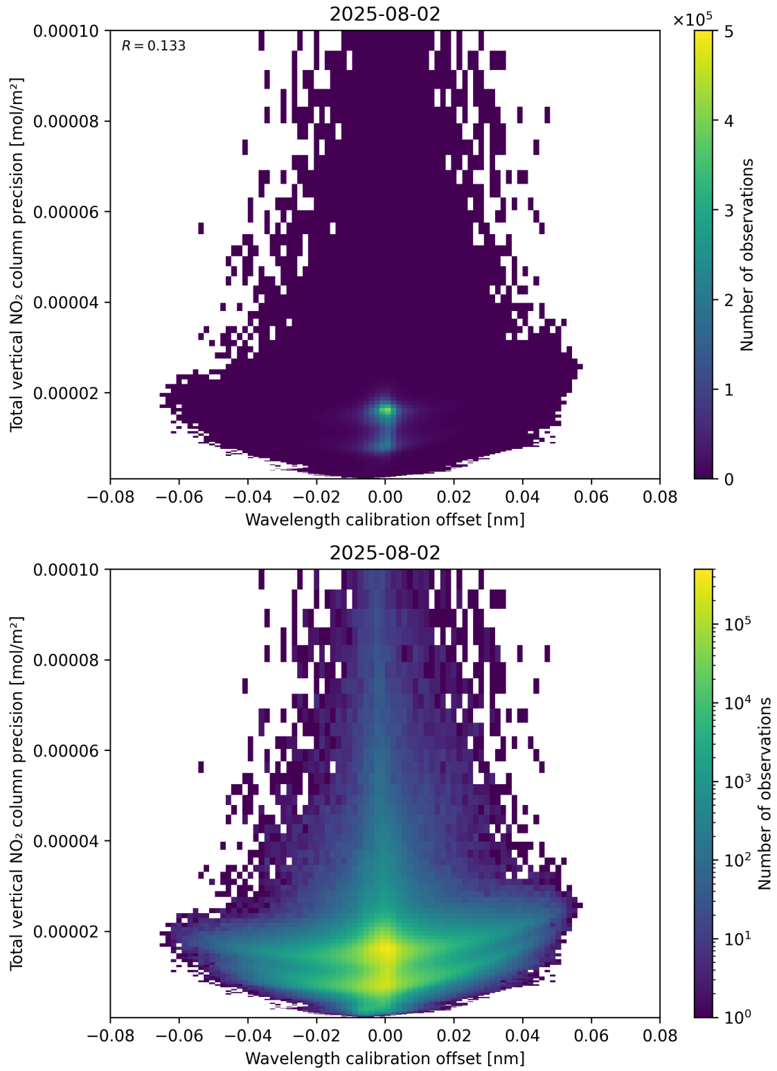
Figure 180: Scatter density plot of “Wavelength calibration offset” against “Total vertical NO 2 column precision” for 2025-08-01 to 2025-08-03.
