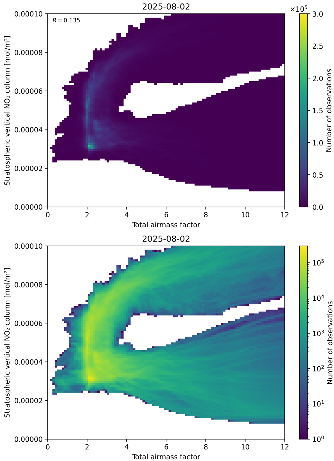
Figure 64: Scatter density plot of “Total airmass factor” against “Stratospheric vertical NO 2 column” for 2025-08-01 to 2025-08-03.
