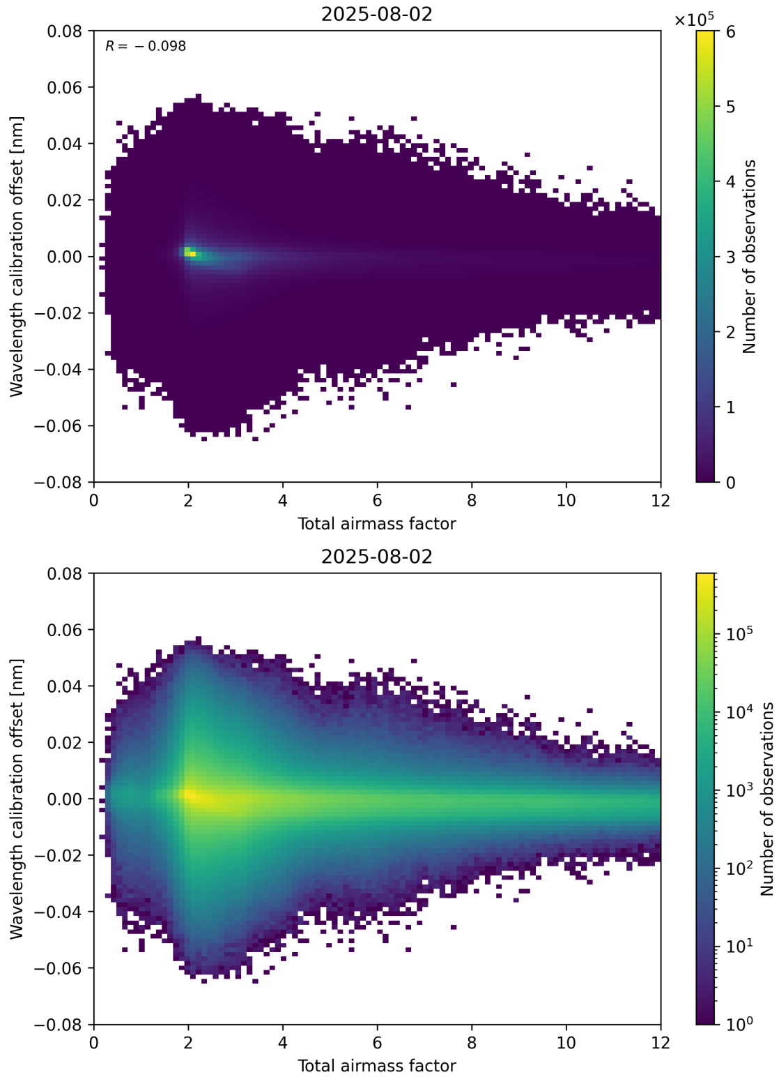
Figure 70: Scatter density plot of “Total airmass factor” against “Wavelength calibration offset” for 2025-08-01 to 2025-08-03.
