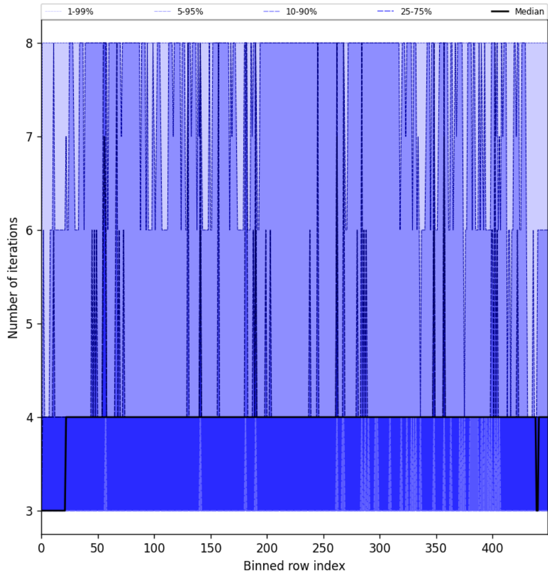
Figure 51: Along track statistics of “Number of iterations” for 2025-08-01 to 2025-08-03
