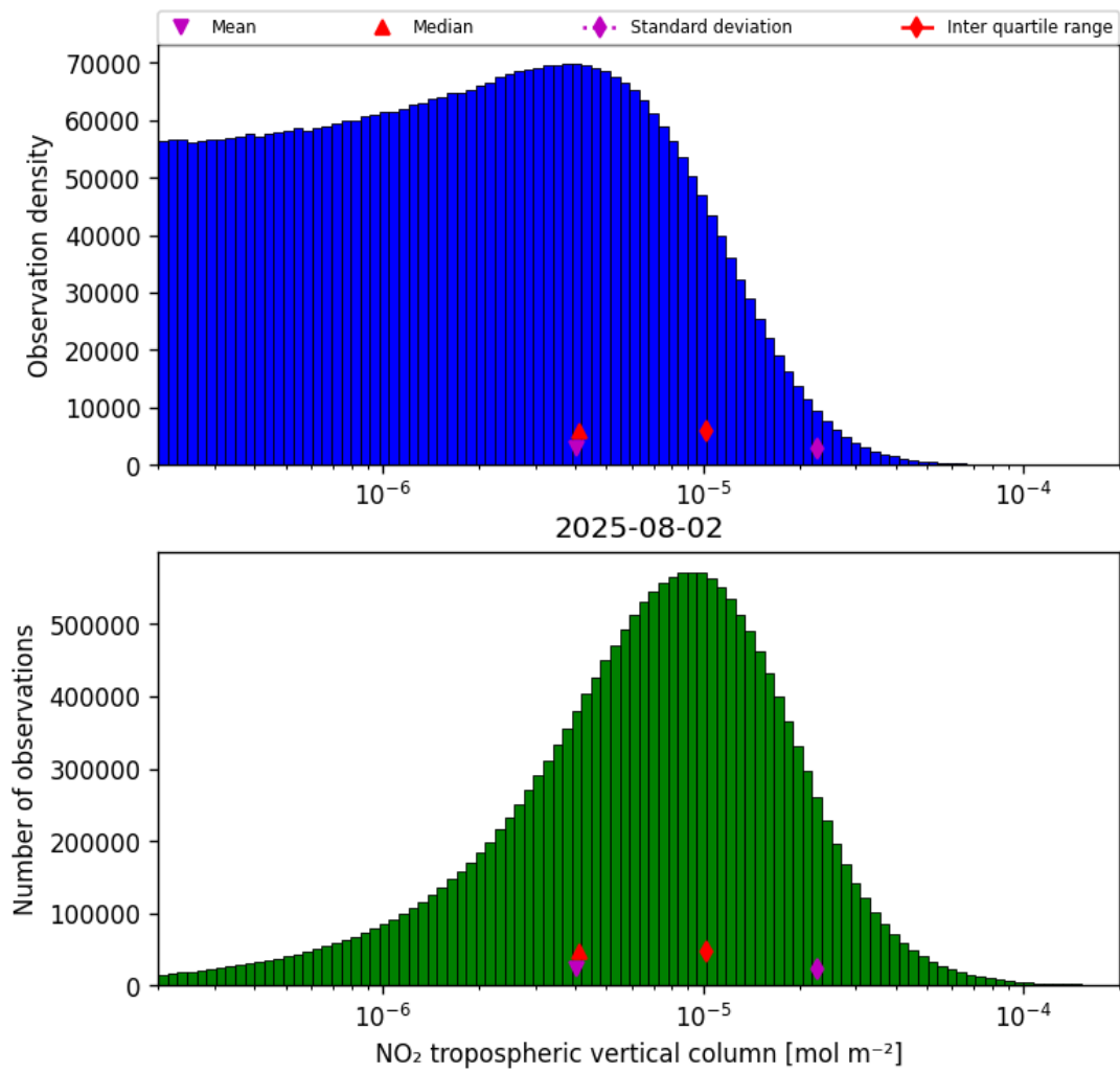
Figure 29: Histogram of “NO 2 tropospheric vertical column” for 2025-08-01 to 2025-08-03
