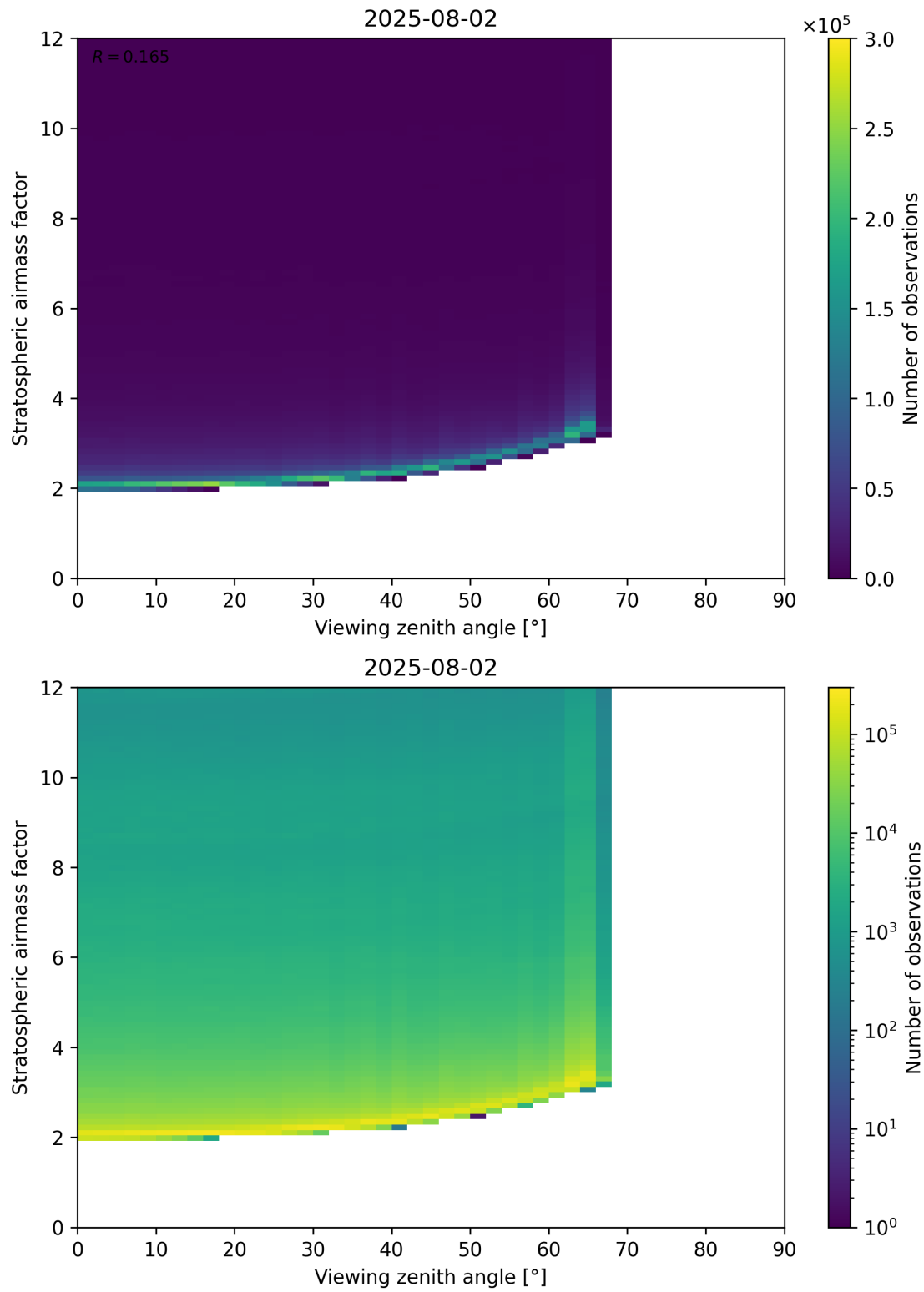
Figure 159: Scatter density plot of “Viewing zenith angle” against “Stratospheric airmass factor” for 2025-08-01 to 2025-08-03.
