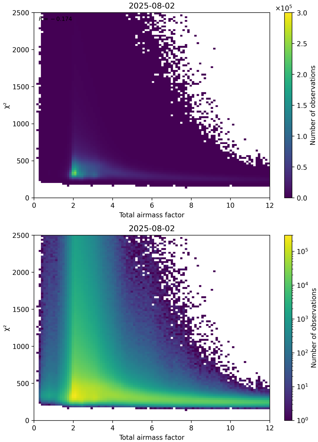
Figure 63: Scatter density plot of “Total airmass factor” against “ \chi^2 ” for 2025-08-01 to 2025-08-03.
