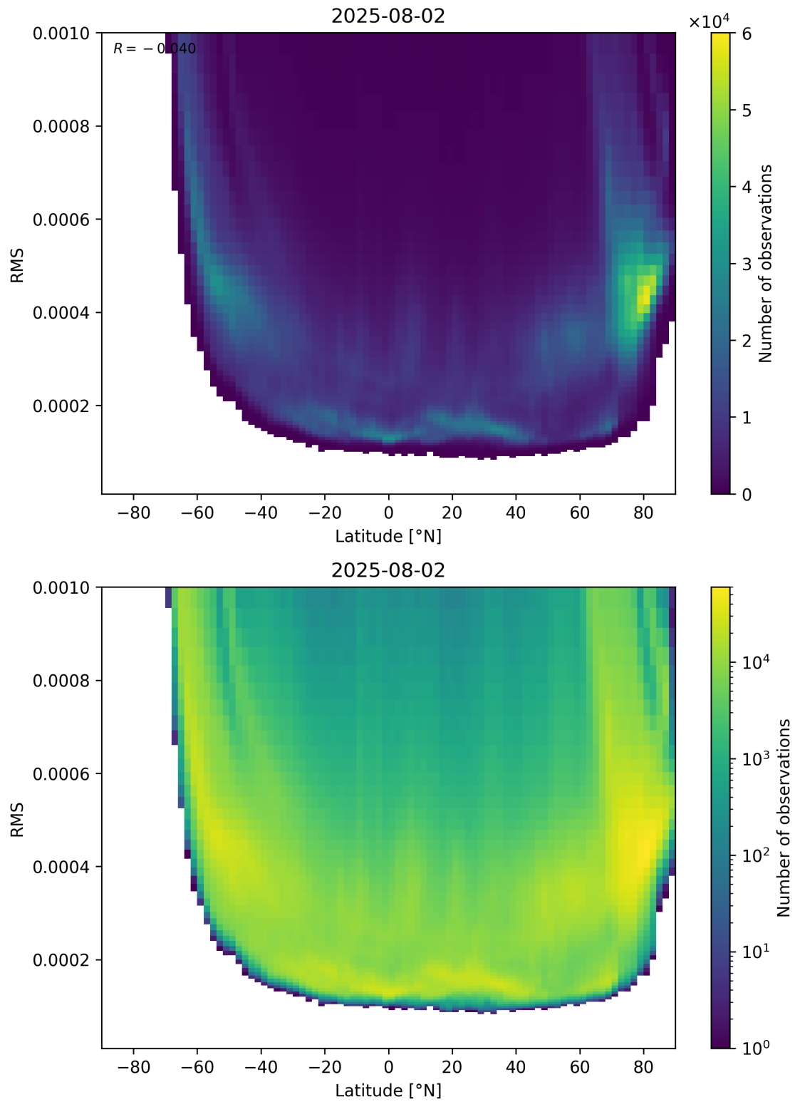
Figure 94: Scatter density plot of “Latitude” against “RMS” for 2025-08-01 to 2025-08-03.
