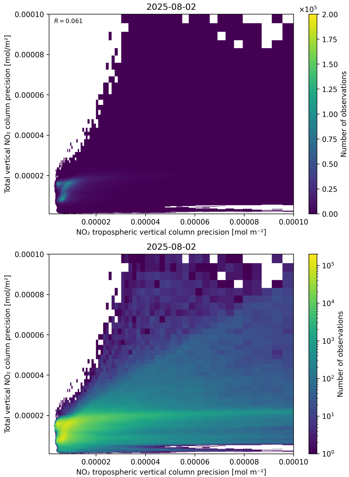
Figure 139: Scatter density plot of “NO 2 tropospheric vertical column precision” against “Total vertical NO 2 column precision” for 2025-08-01 to 2025-08-03.
