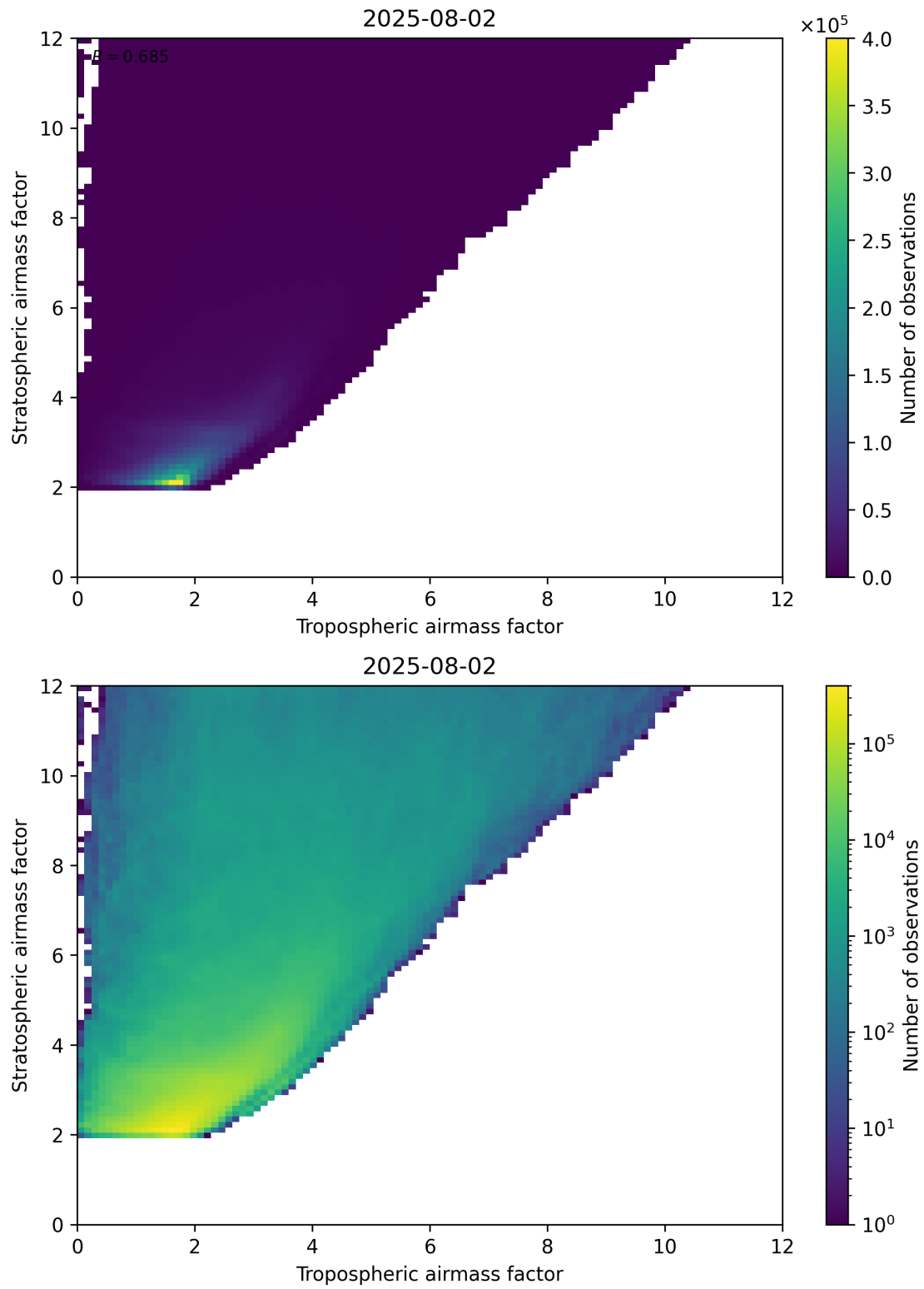
Figure 71: Scatter density plot of “Tropospheric airmass factor” against “Stratospheric airmass factor” for 2025-08-01 to 2025-08-03.
