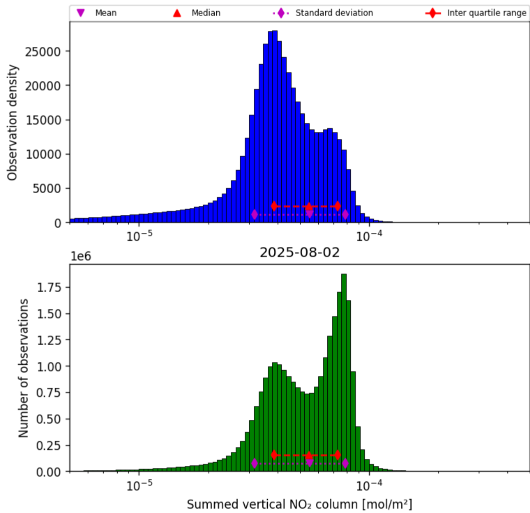
Figure 40: Histogram of “Summed vertical NO 2 column” for 2025-08-01 to 2025-08-03
