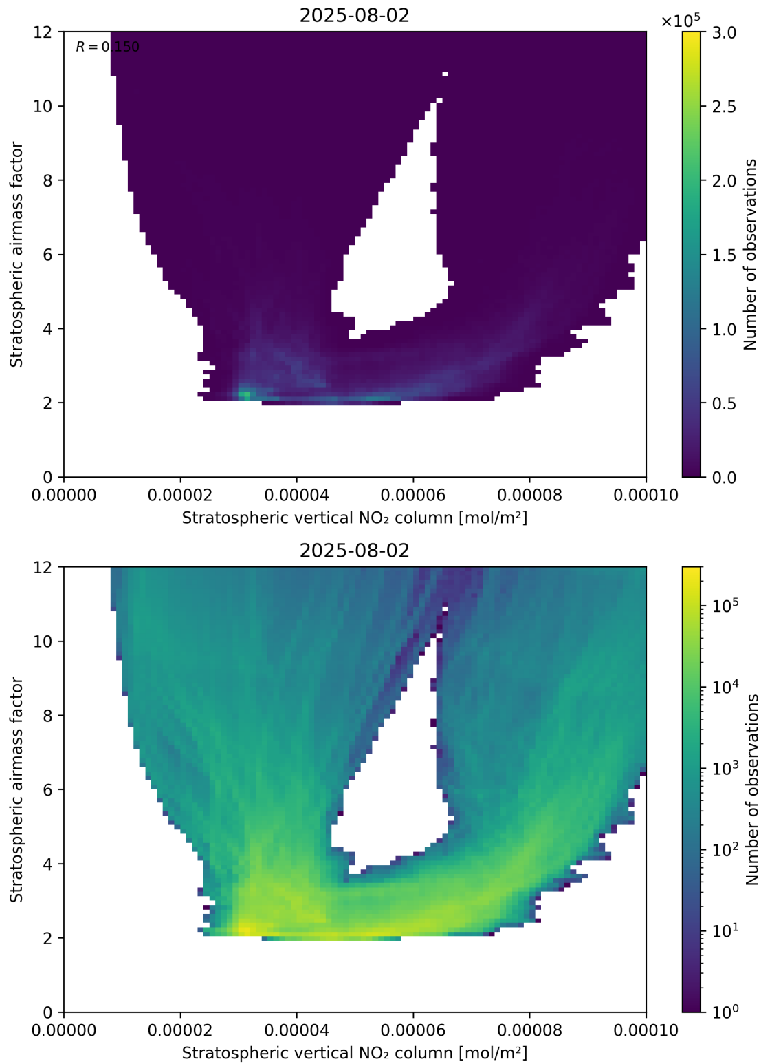
Figure 96: Scatter density plot of “Stratospheric vertical NO 2 column” against “Stratospheric airmass factor” for 2025-08-01 to 2025-08-03.
