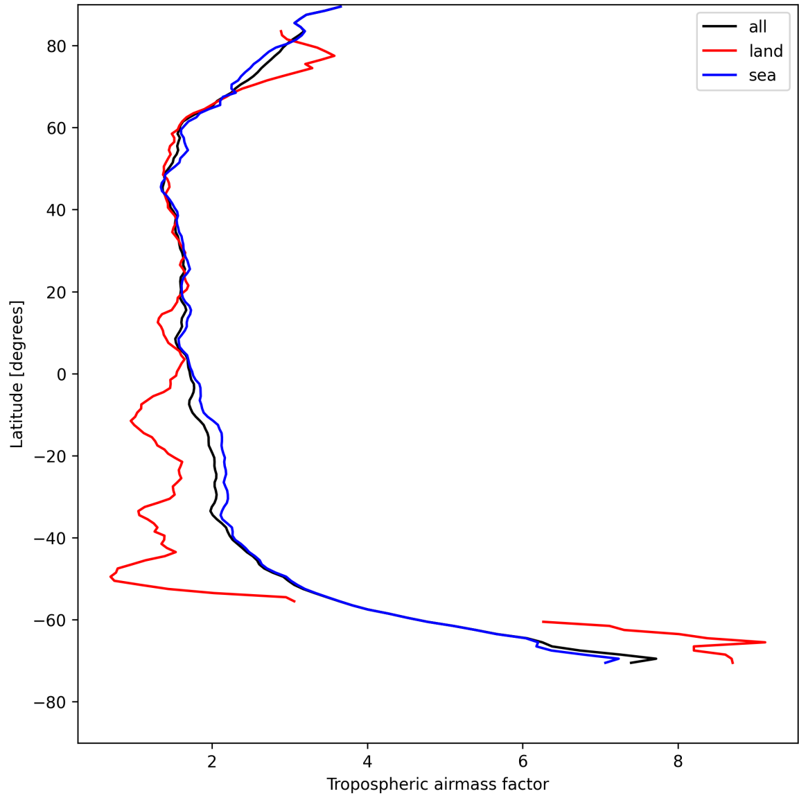
Figure 14: Zonal average of “Tropospheric airmass factor” for 2025-08-01 to 2025-08-03.
