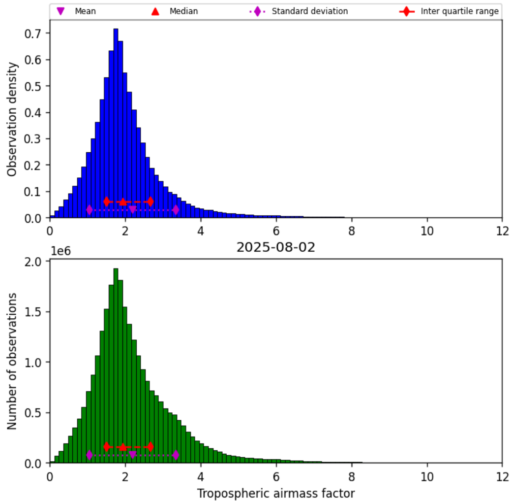
Figure 31: Histogram of “Tropospheric airmass factor” for 2025-08-01 to 2025-08-03
