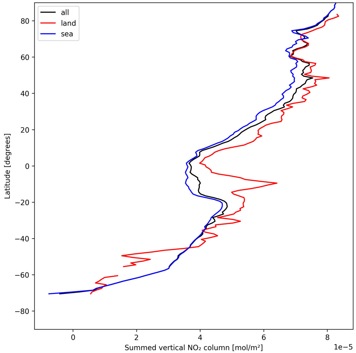
Figure 23: Zonal average of “Summed vertical NO 2 column” for 2025-08-01 to 2025-08-03.
