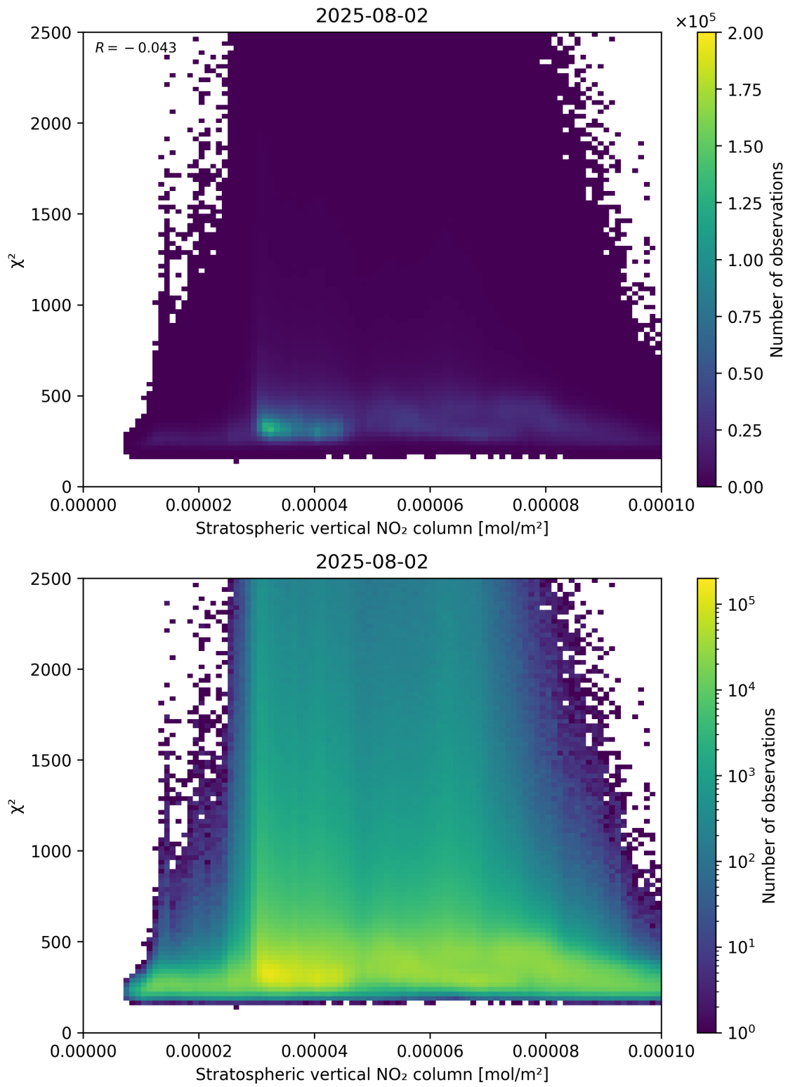
Figure 97: Scatter density plot of “Stratospheric vertical NO 2 column” against “ \chi^2 ” for 2025-08-01 to 2025-08-03.
