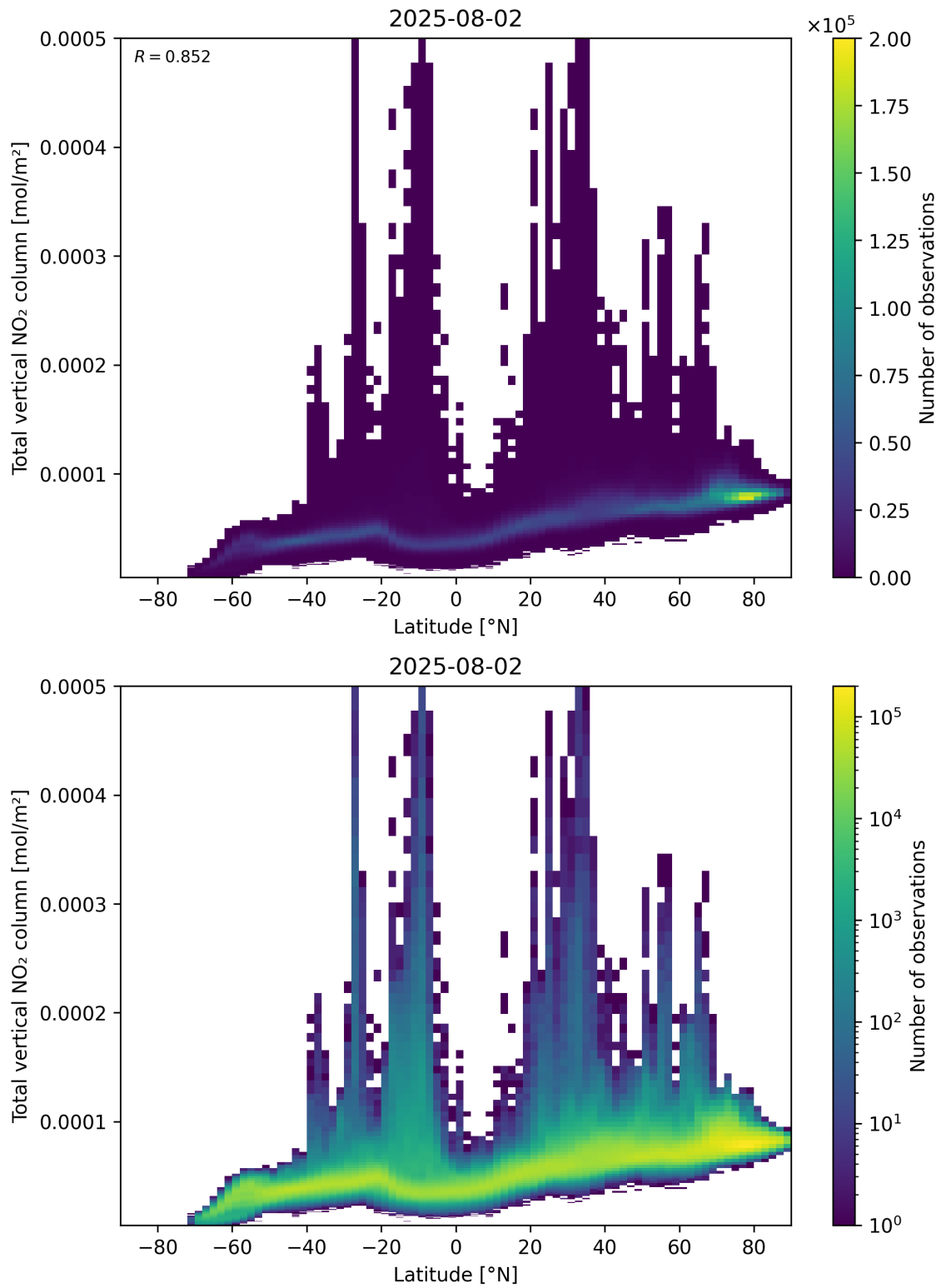
Figure 90: Scatter density plot of “Latitude” against “Total vertical NO 2 column” for 2025-08-01 to 2025-08-03.
