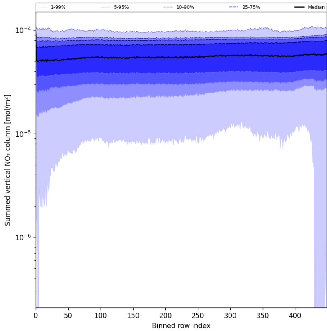
Figure 57: Along track statistics of “Summed vertical NO 2 column” for 2025-08-01 to 2025-08-03
