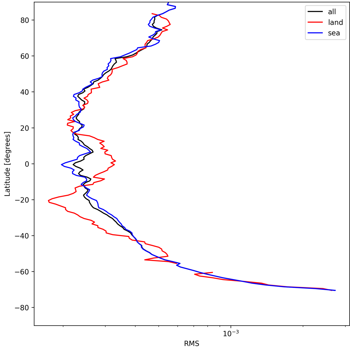
Figure 26: Zonal average of “RMS” for 2025-08-01 to 2025-08-03.
