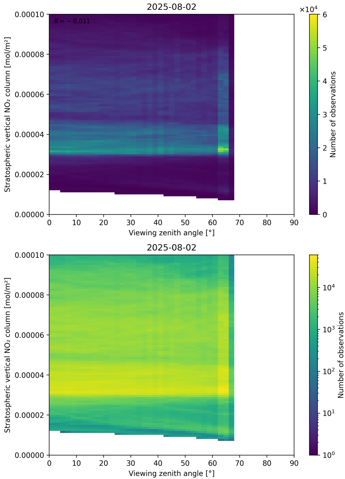
Figure 164: Scatter density plot of “Viewing zenith angle” against “Stratospheric vertical NO 2 column” for 2025-08-01 to 2025-08-03.
