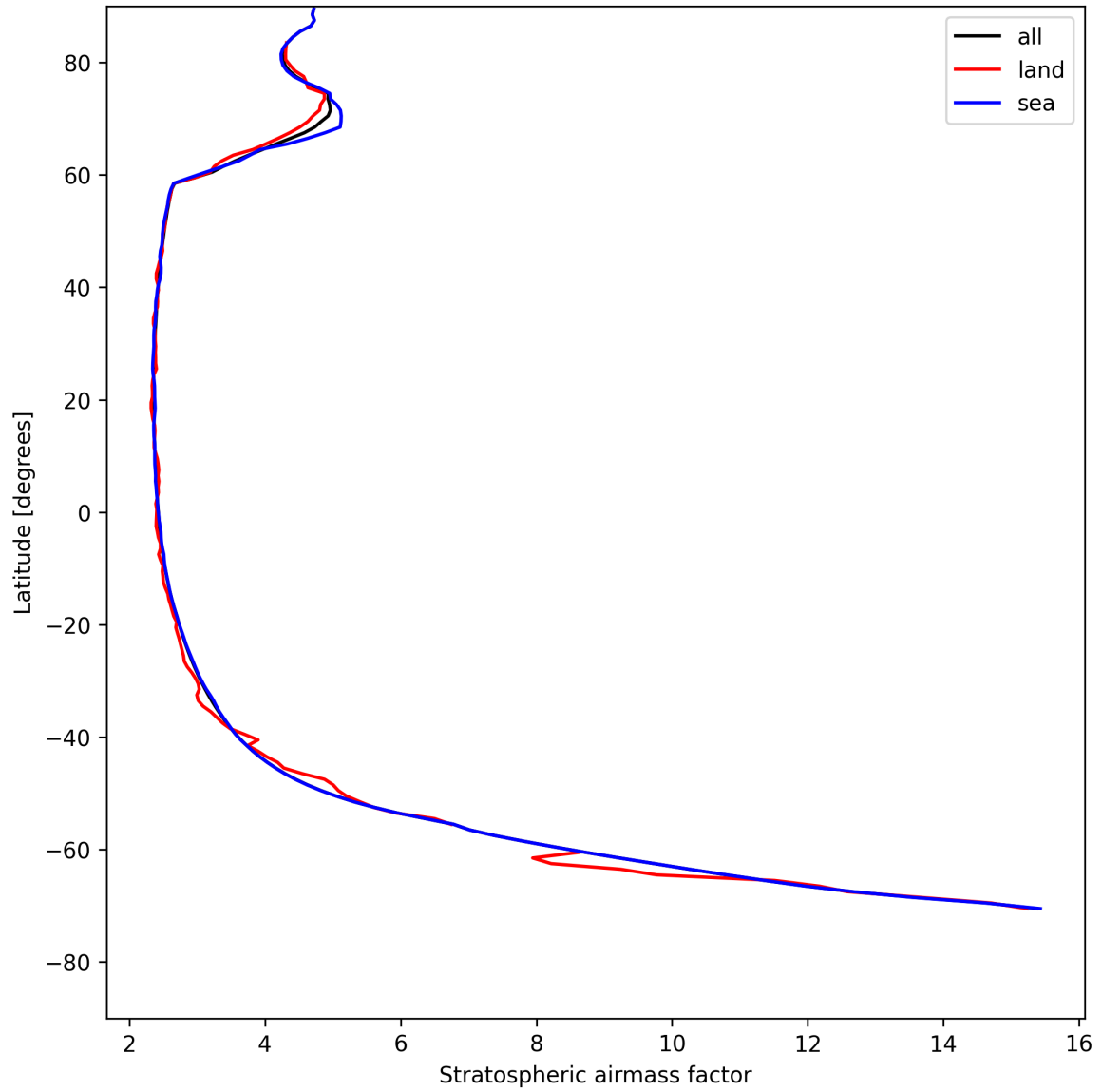
Figure 27: Zonal average of “Stratospheric airmass factor” for 2025-08-01 to 2025-08-03.
