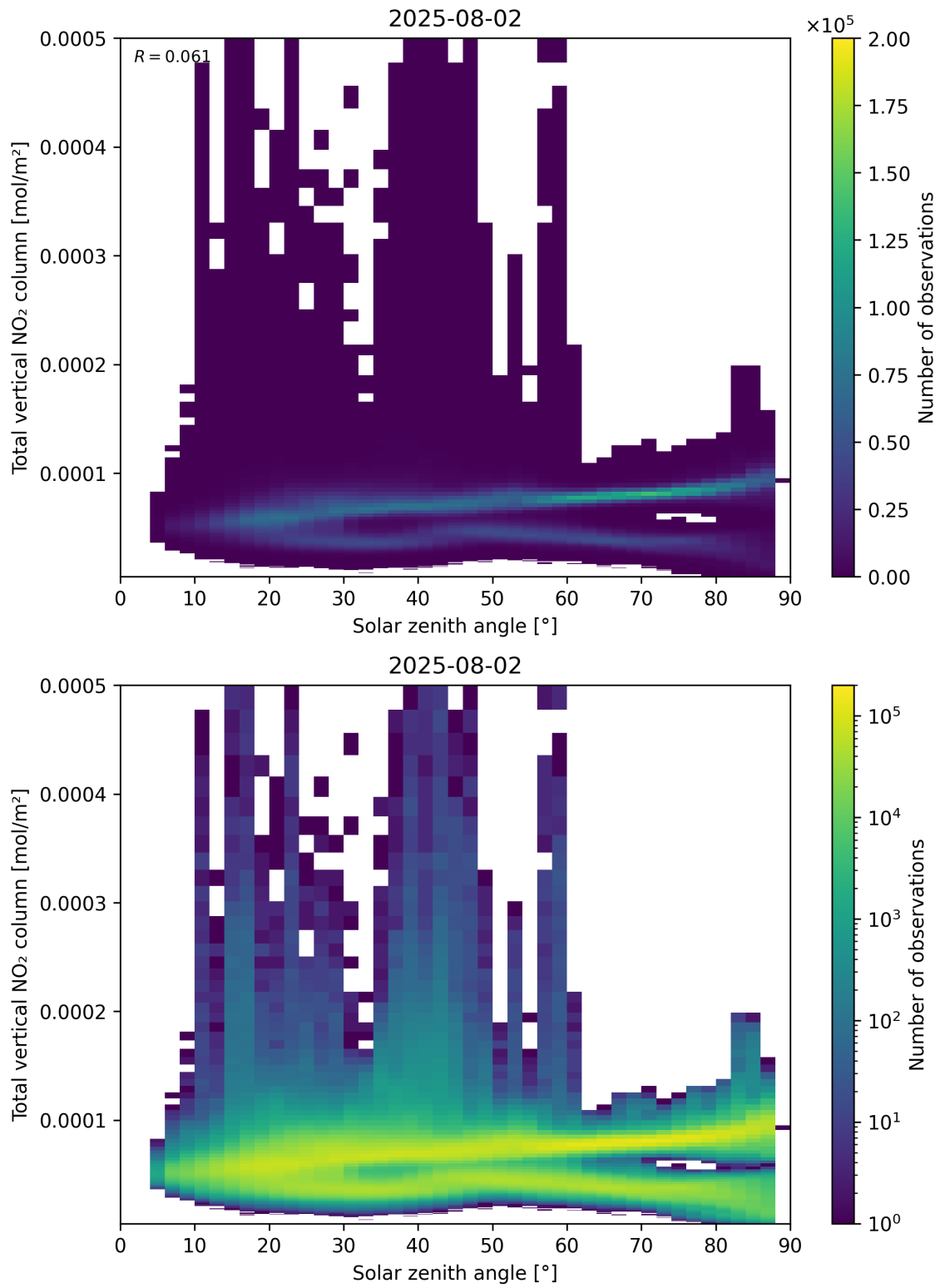
Figure 153: Scatter density plot of “Solar zenith angle” against “Total vertical NO 2 column” for 2025-08-01 to 2025-08-03.
