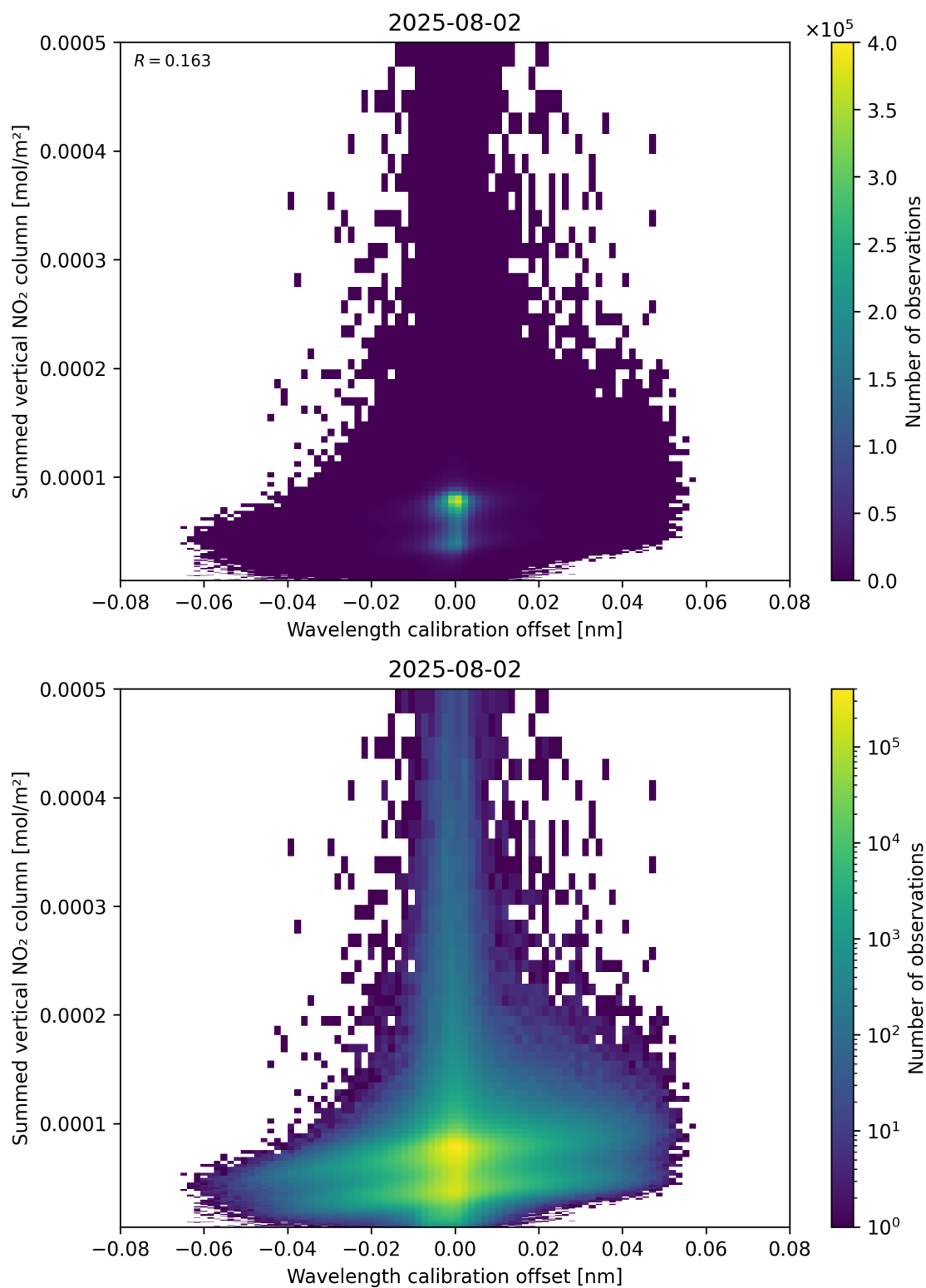
Figure 177: Scatter density plot of “Wavelength calibration offset” against “Summed vertical NO 2 column” for 2025-08-01 to 2025-08-03.
