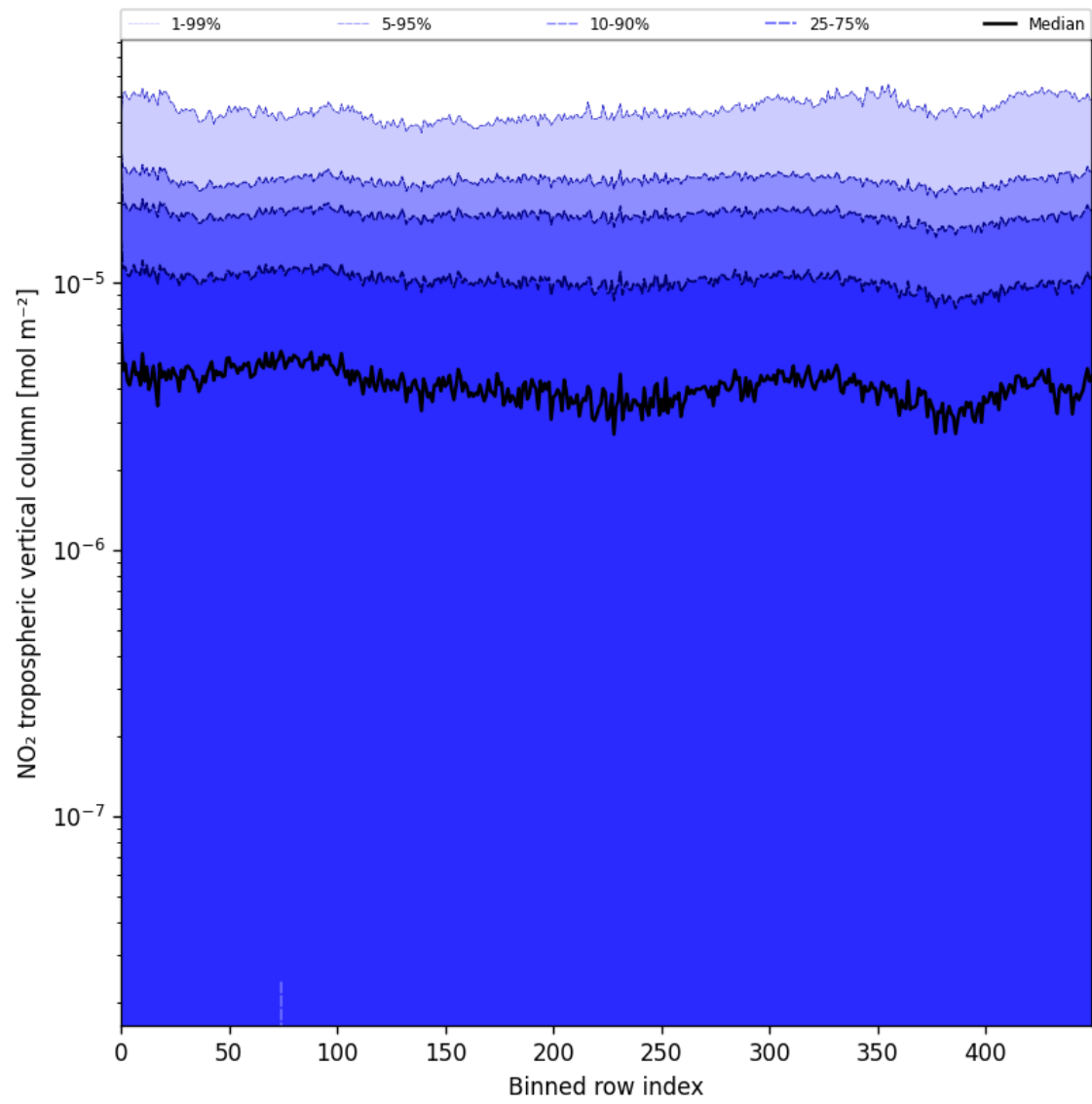
Figure 46: Along track statistics of “NO 2 tropospheric vertical column” for 2025-08-01 to 2025-08-03
