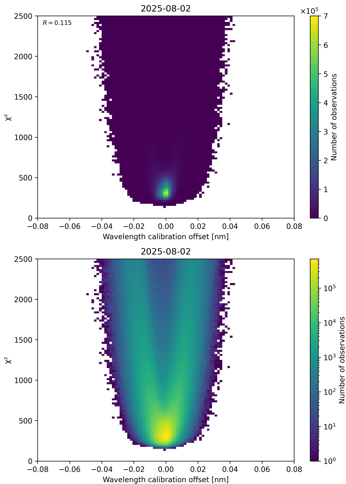
Figure 175: Scatter density plot of “Wavelength calibration offset” against “ \chi^2 ” for 2025-08-01 to 2025-08-03.
