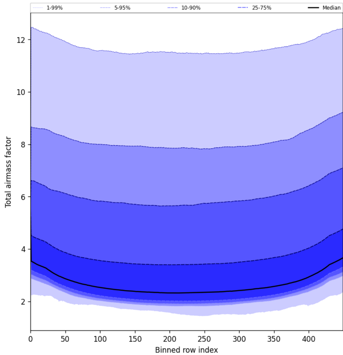
Figure 49: Along track statistics of “Total airmass factor” for 2025-08-01 to 2025-08-03
