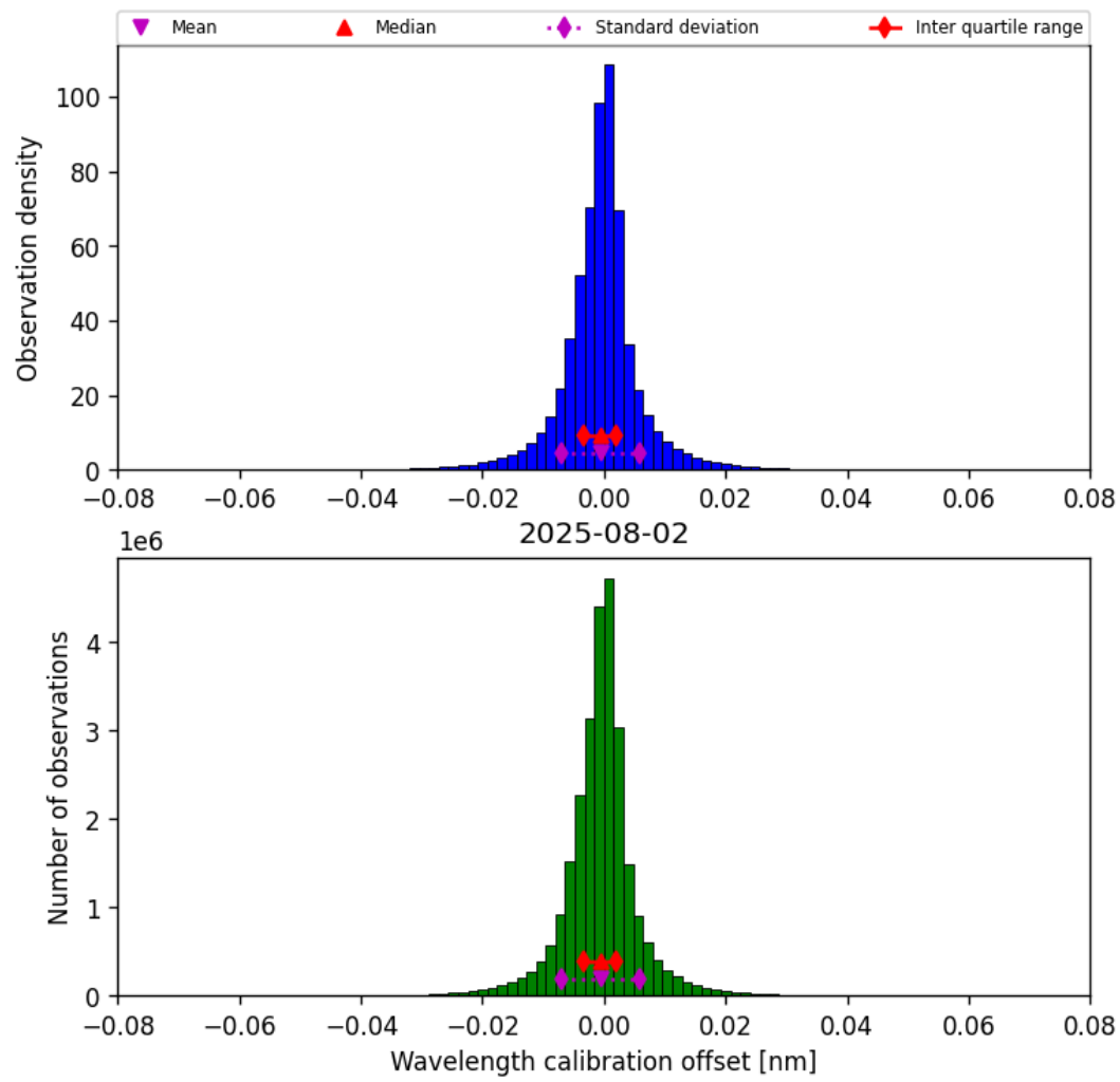
Figure 35: Histogram of “Wavelength calibration offset” for 2025-08-01 to 2025-08-03
