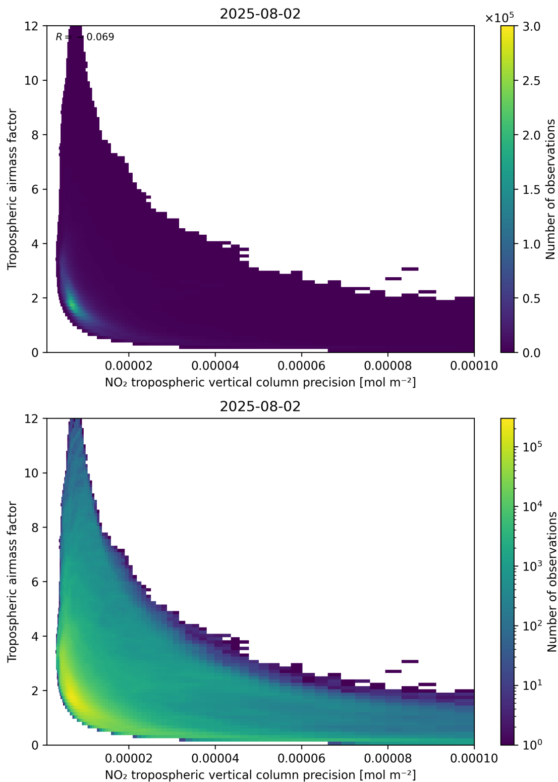
Figure 133: Scatter density plot of “NO 2 tropospheric vertical column precision” against “Tropospheric airmass factor” for 2025-08-01 to 2025-08-03.
