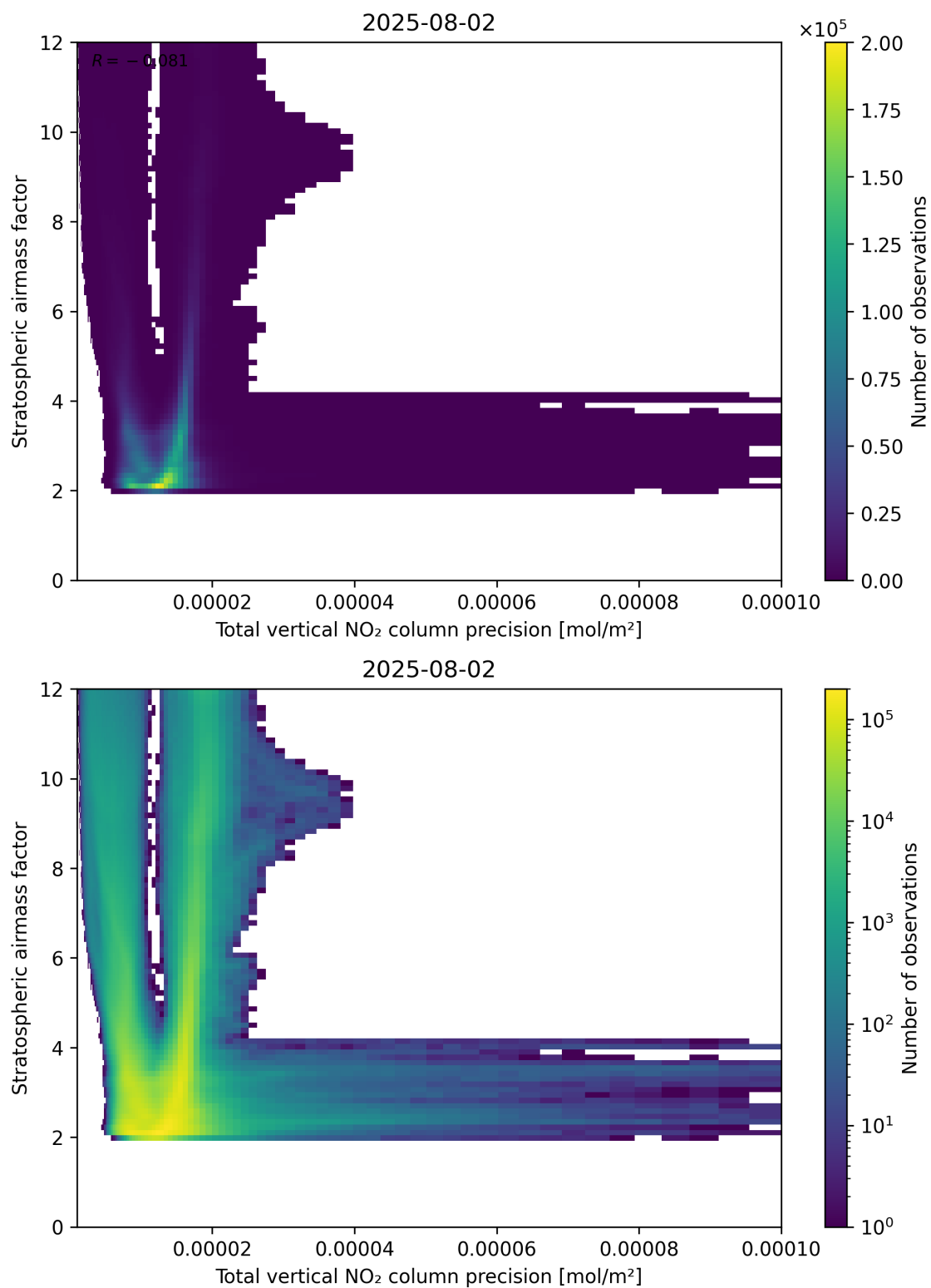
Figure 115: Scatter density plot of “Total vertical NO 2 column precision” against “Stratospheric air mass factor” for 2025-08-01 to 2025-08-03.
