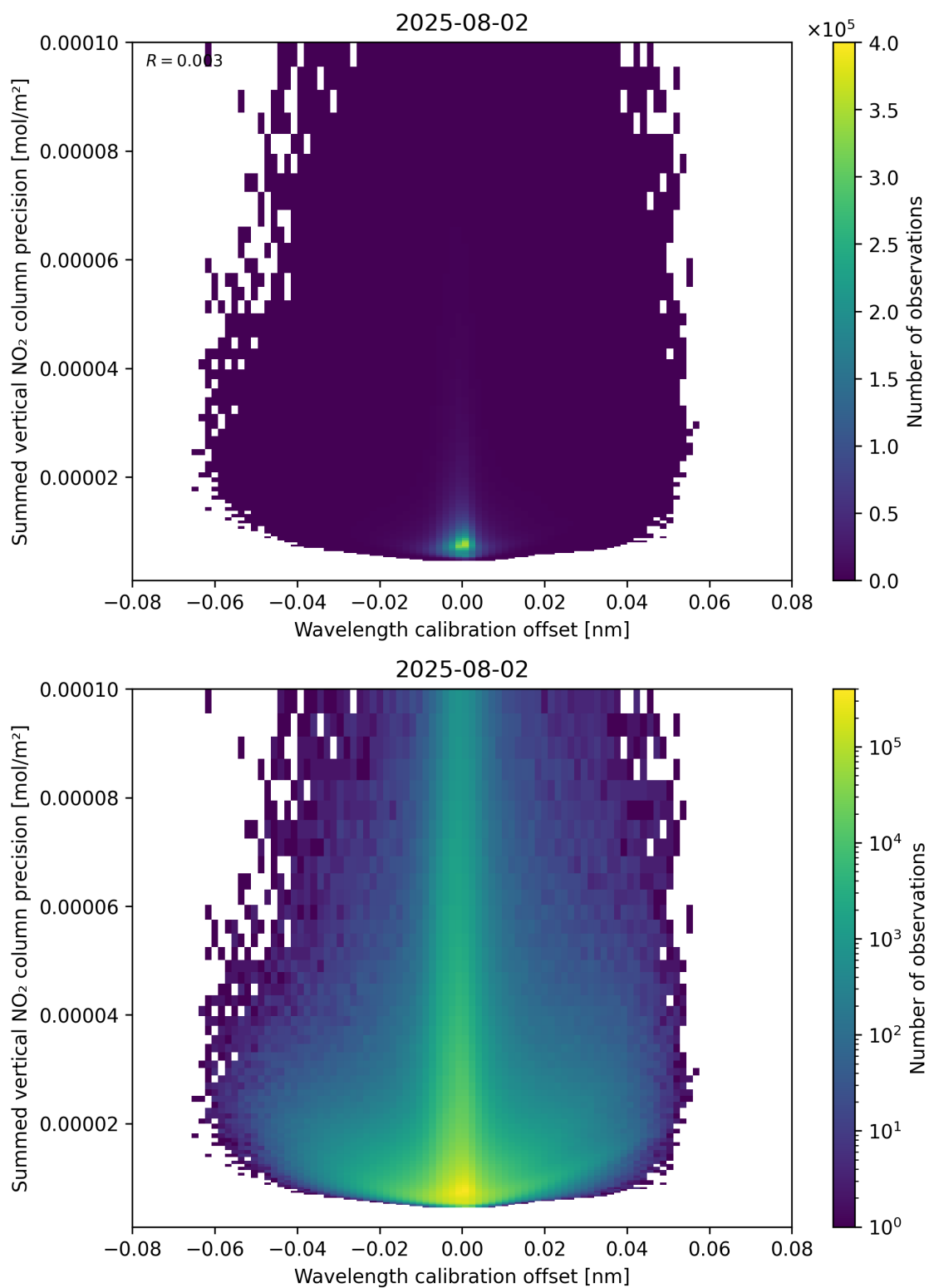
Figure 178: Scatter density plot of “Wavelength calibration offset” against “Summed vertical NO 2 column precision” for 2025-08-01 to 2025-08-03.
