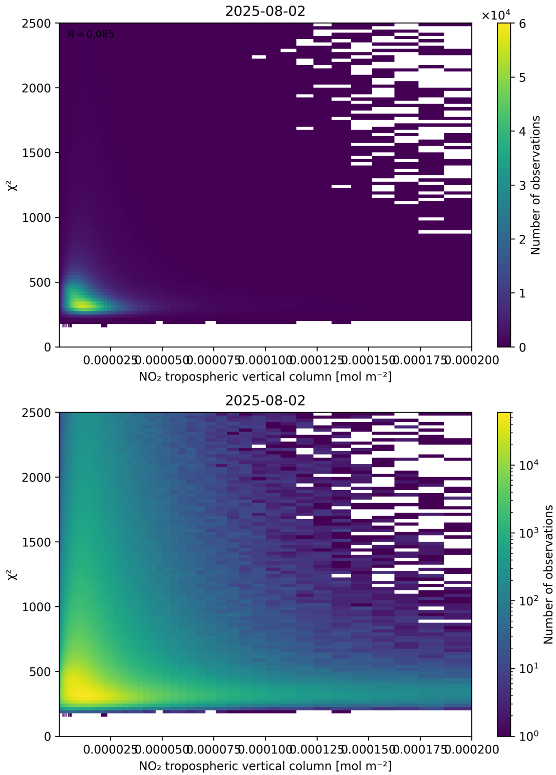
Figure 124: Scatter density plot of “NO 2 tropospheric vertical column” against “ \chi^2 ” for 2025-08-01 to 2025-08-03.
