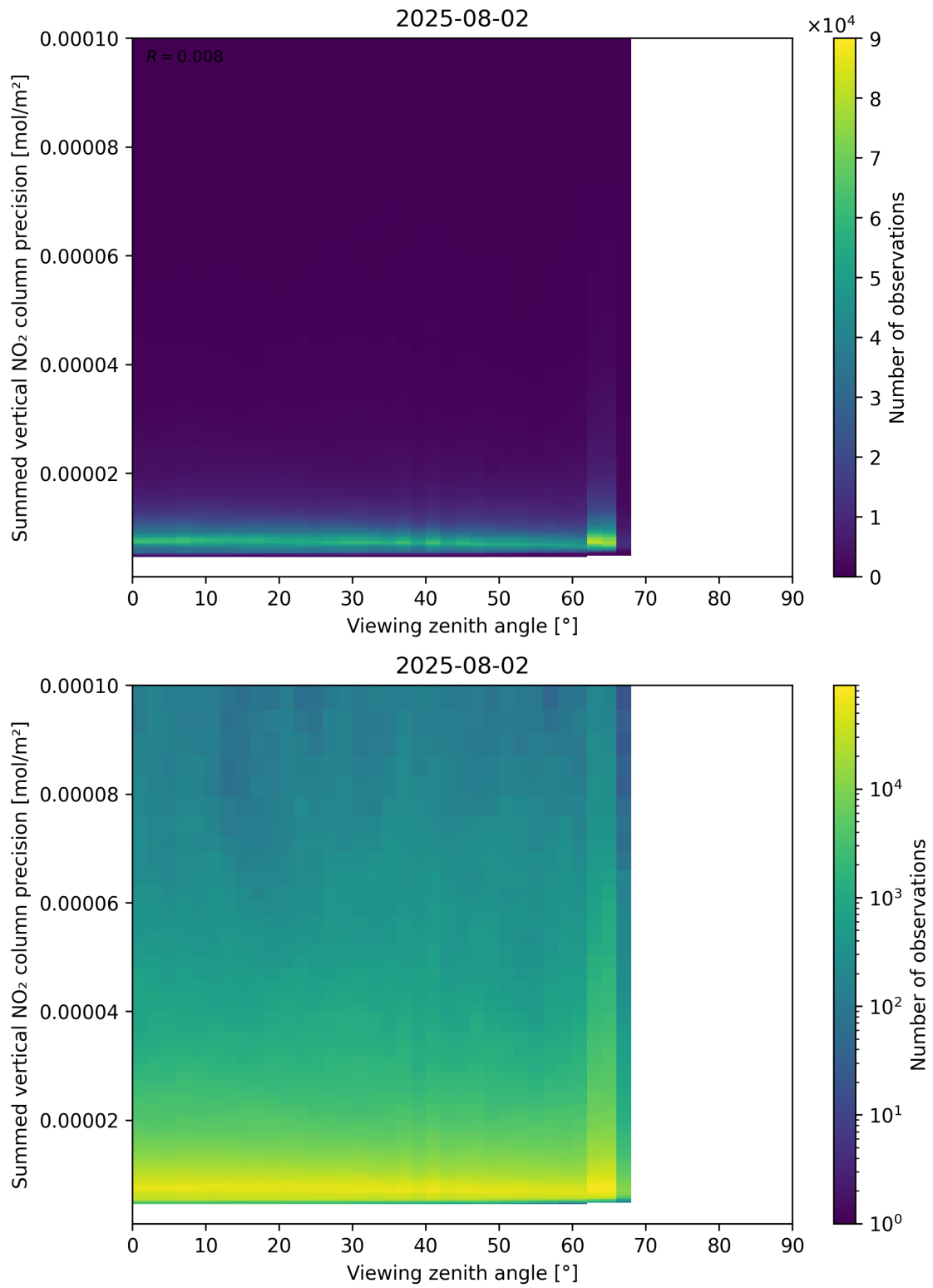
Figure 166: Scatter density plot of “Viewing zenith angle” against “Summed vertical NO 2 column precision” for 2025-08-01 to 2025-08-03.
