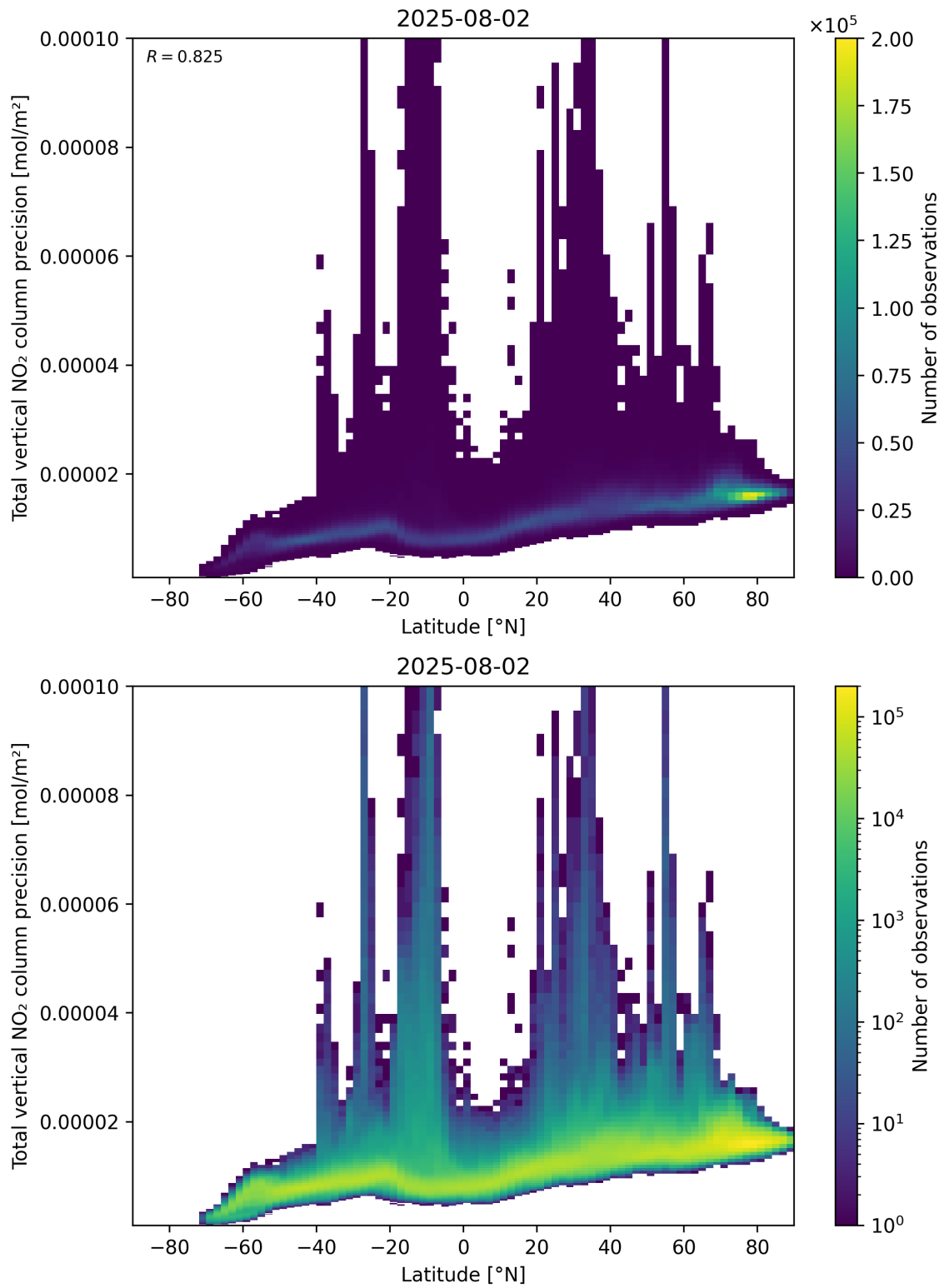
Figure 91: Scatter density plot of “Latitude” against “Total vertical NO 2 column precision” for 2025-08-01 to 2025-08-03.
