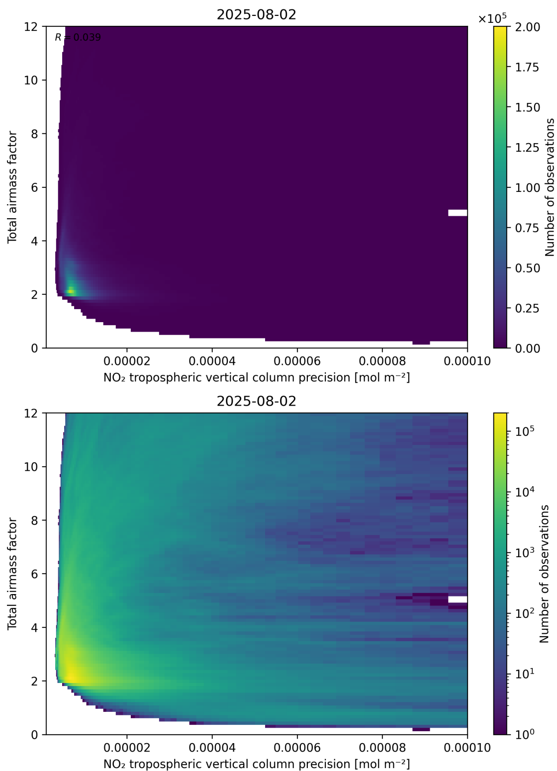
Figure 132: Scatter density plot of “NO 2 tropospheric vertical column precision” against “Total air mass factor” for 2025-08-01 to 2025-08-03.
