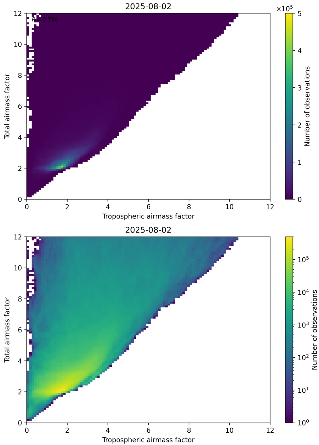
Figure 72: Scatter density plot of “Tropospheric airmass factor” against “Total airmass factor” for 2025-08-01 to 2025-08-03.
