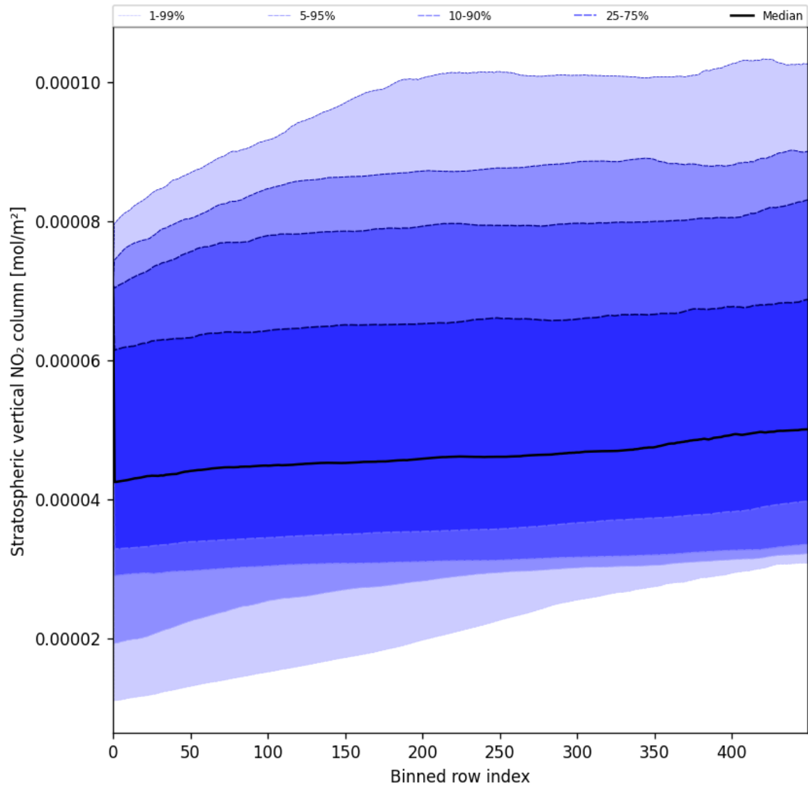
Figure 53: Along track statistics of “Stratospheric vertical NO 2 column” for 2025-08-01 to 2025-08-03
