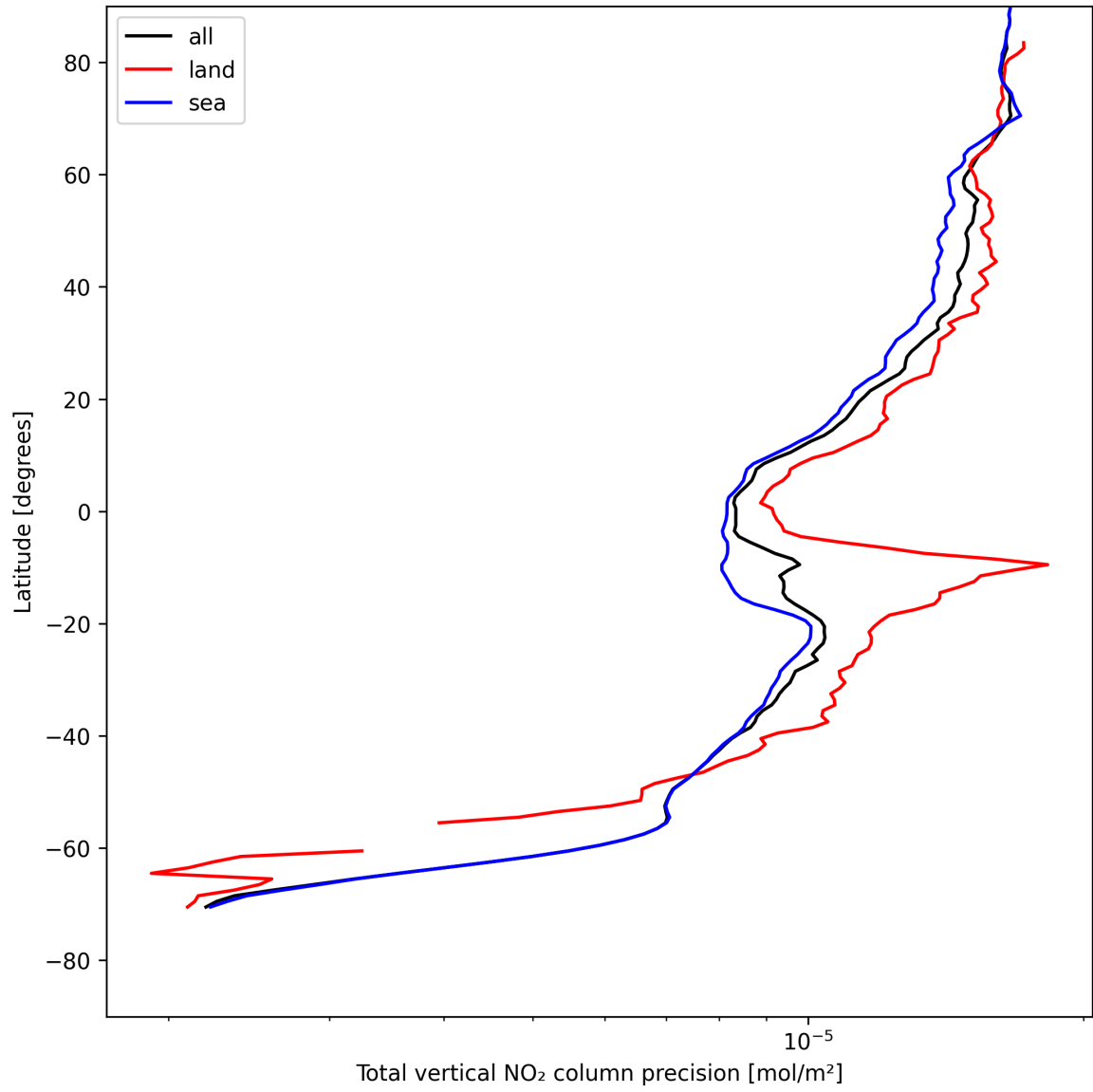
Figure 22: Zonal average of “Total vertical NO 2 column precision” for 2025-08-01 to 2025-08-03.
