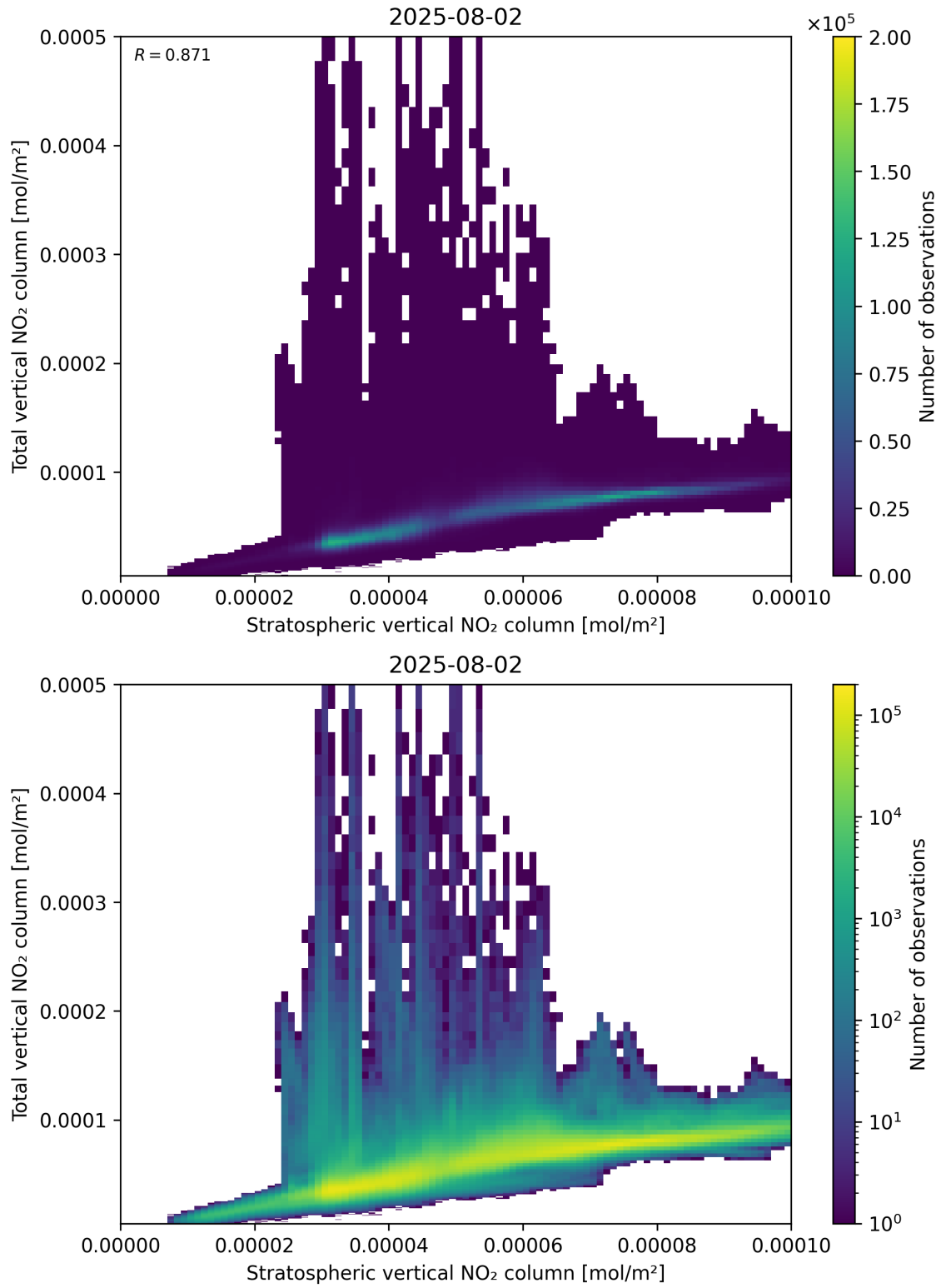
Figure 100: Scatter density plot of “Stratospheric vertical NO 2 column” against “Total vertical NO 2 column” for 2025-08-01 to 2025-08-03.
