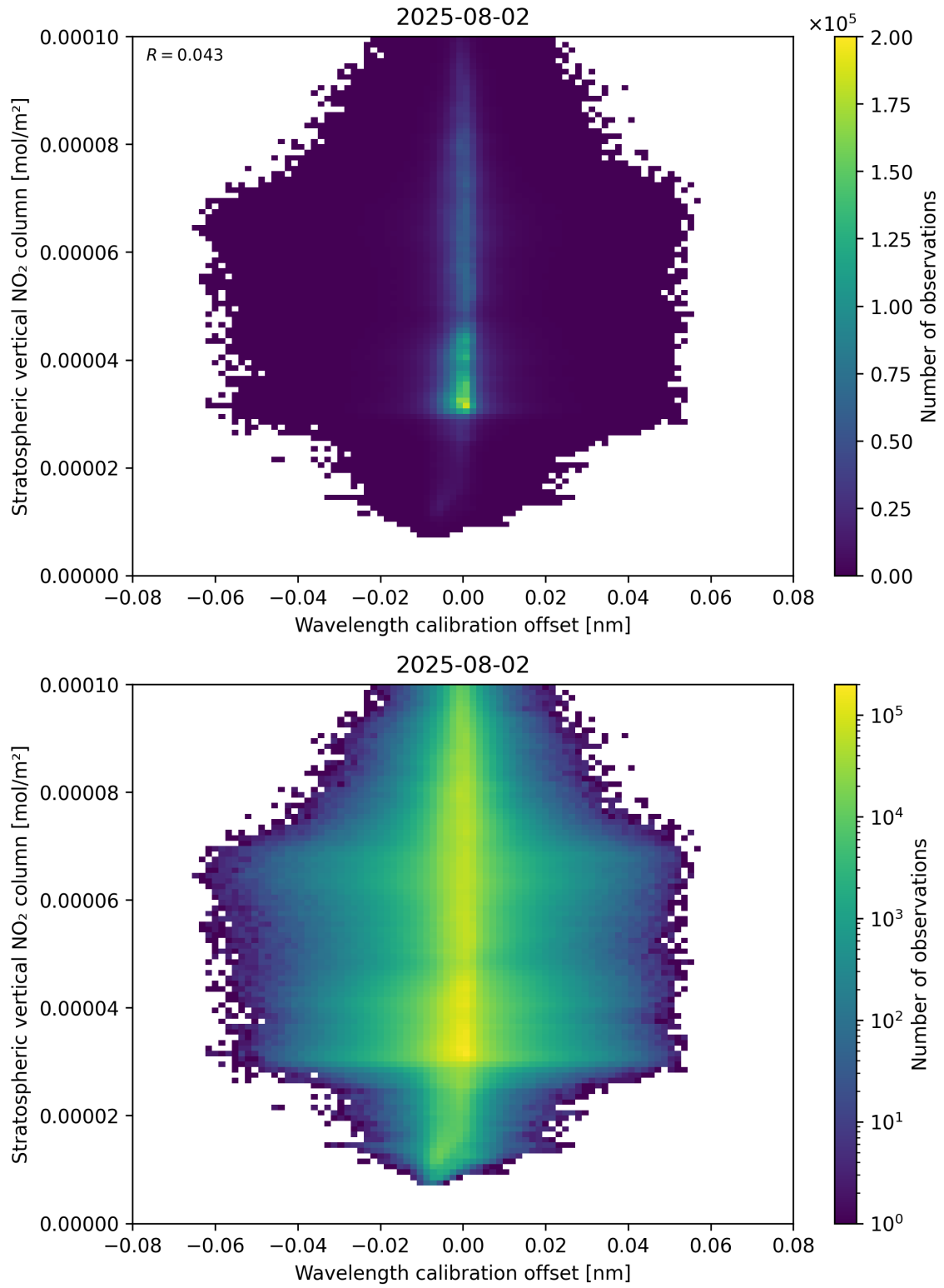
Figure 176: Scatter density plot of “Wavelength calibration offset” against “Stratospheric vertical NO 2 column” for 2025-08-01 to 2025-08-03.
