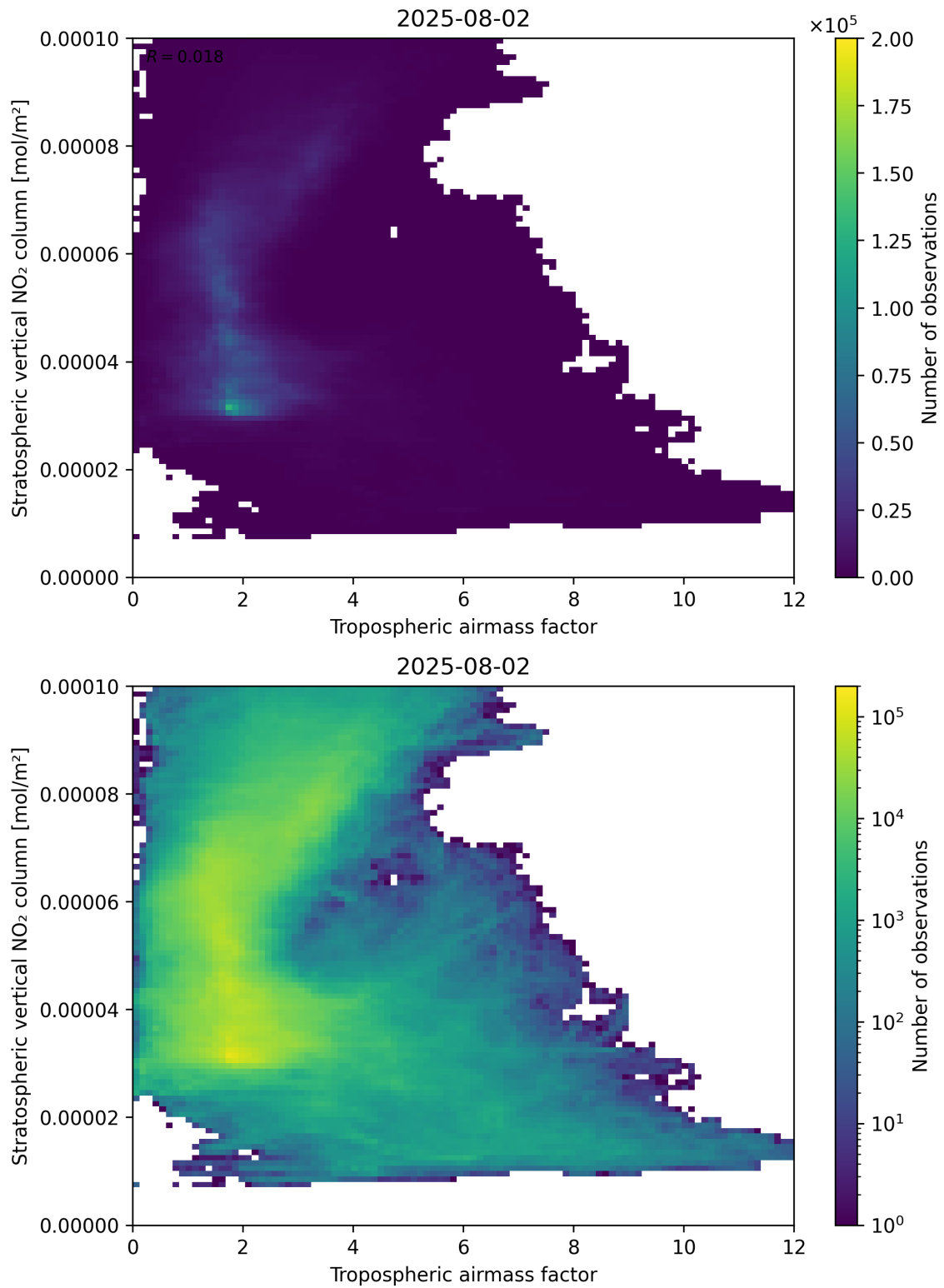
Figure 74: Scatter density plot of “Tropospheric air mass factor” against “Stratospheric vertical NO 2 column” for 2025-08-01 to 2025-08-03.
