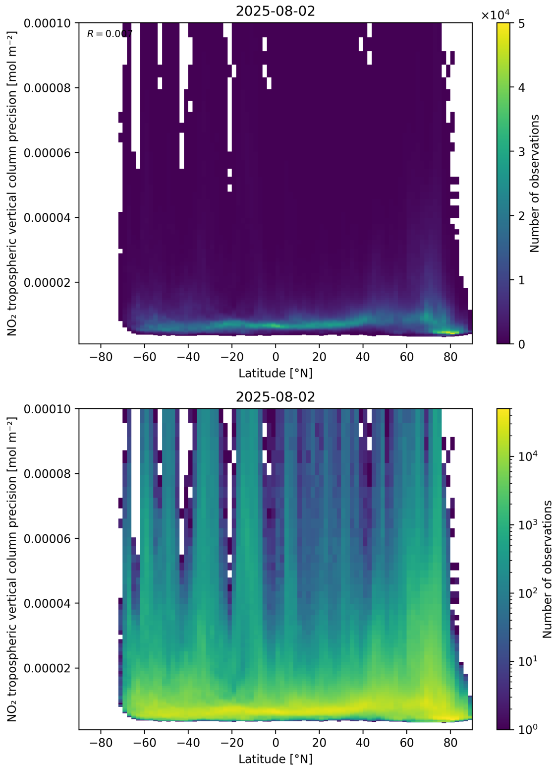
Figure 93: Scatter density plot of “Latitude” against “NO 2 tropospheric vertical column precision” for 2025-08-01 to 2025-08-03.
