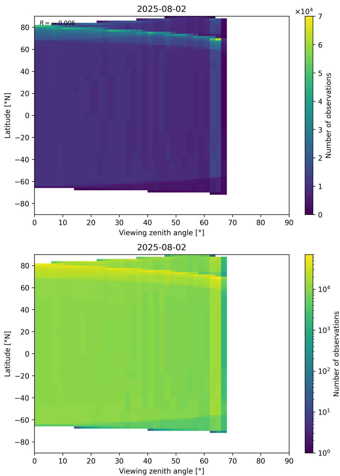
Figure 163: Scatter density plot of “Viewing zenith angle” against “Latitude” for 2025-08-01 to 2025-08-03.
