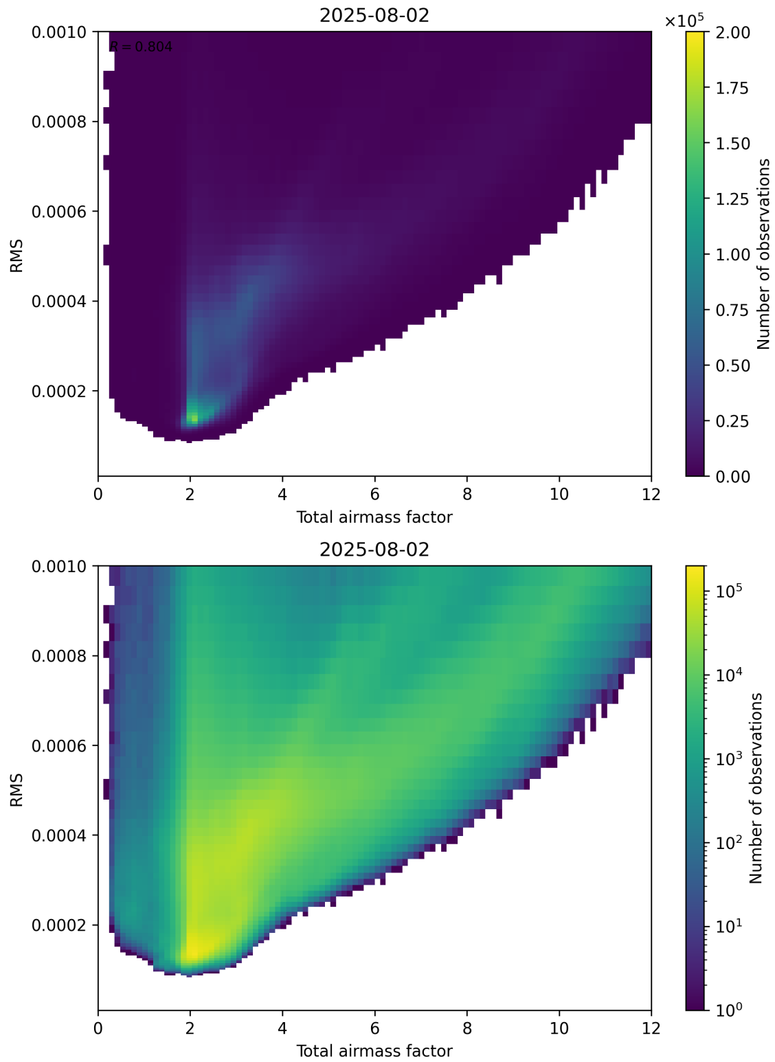
Figure 69: Scatter density plot of “Total airmass factor” against “RMS” for 2025-08-01 to 2025-08-03.
