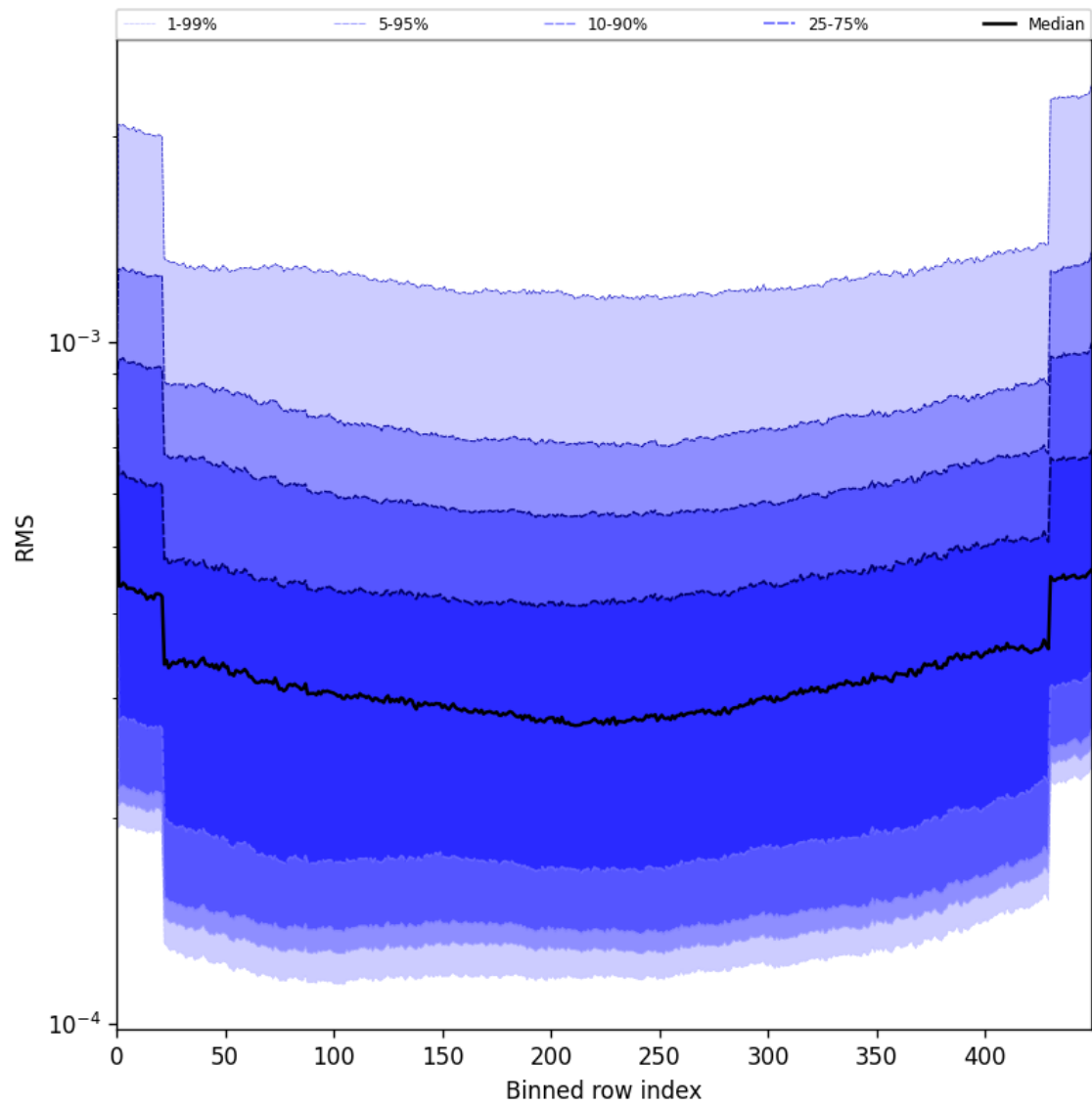
Figure 60: Along track statistics of “RMS” for 2025-08-01 to 2025-08-03
