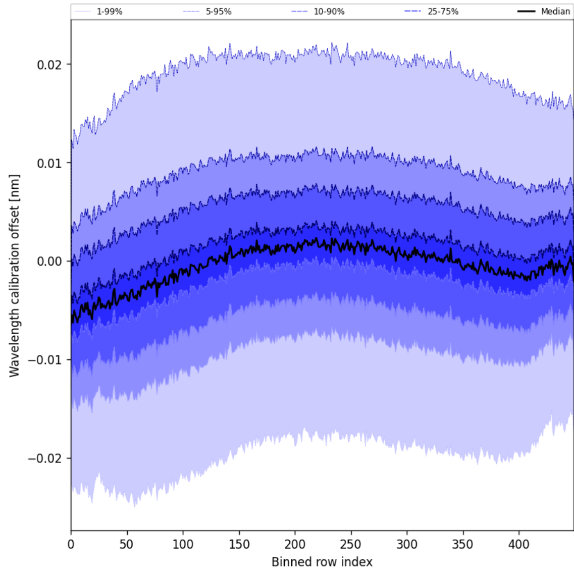
Figure 52: Along track statistics of “Wavelength calibration offset” for 2025-08-01 to 2025-08-03
