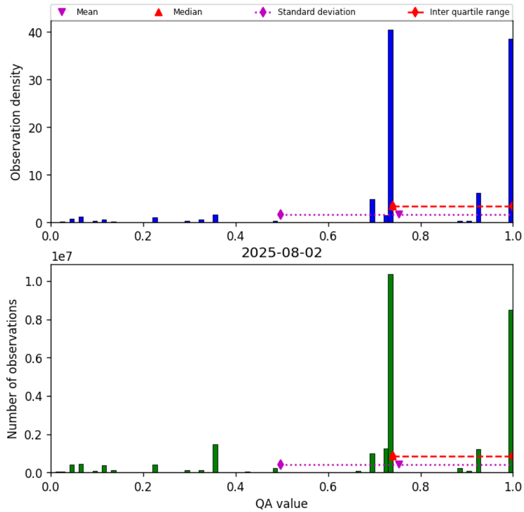
Figure 28: Histogram of “QA value” for 2025-08-01 to 2025-08-03
