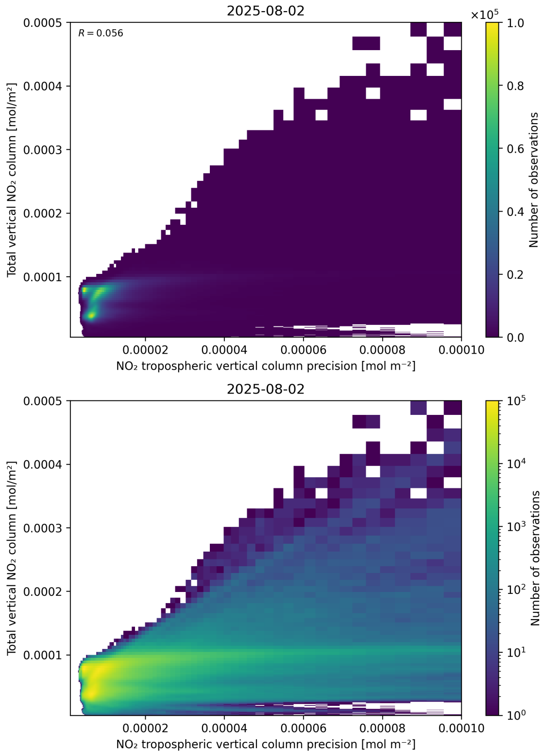
Figure 138: Scatter density plot of “NO 2 tropospheric vertical column precision” against “Total vertical NO 2 column” for 2025-08-01 to 2025-08-03.
