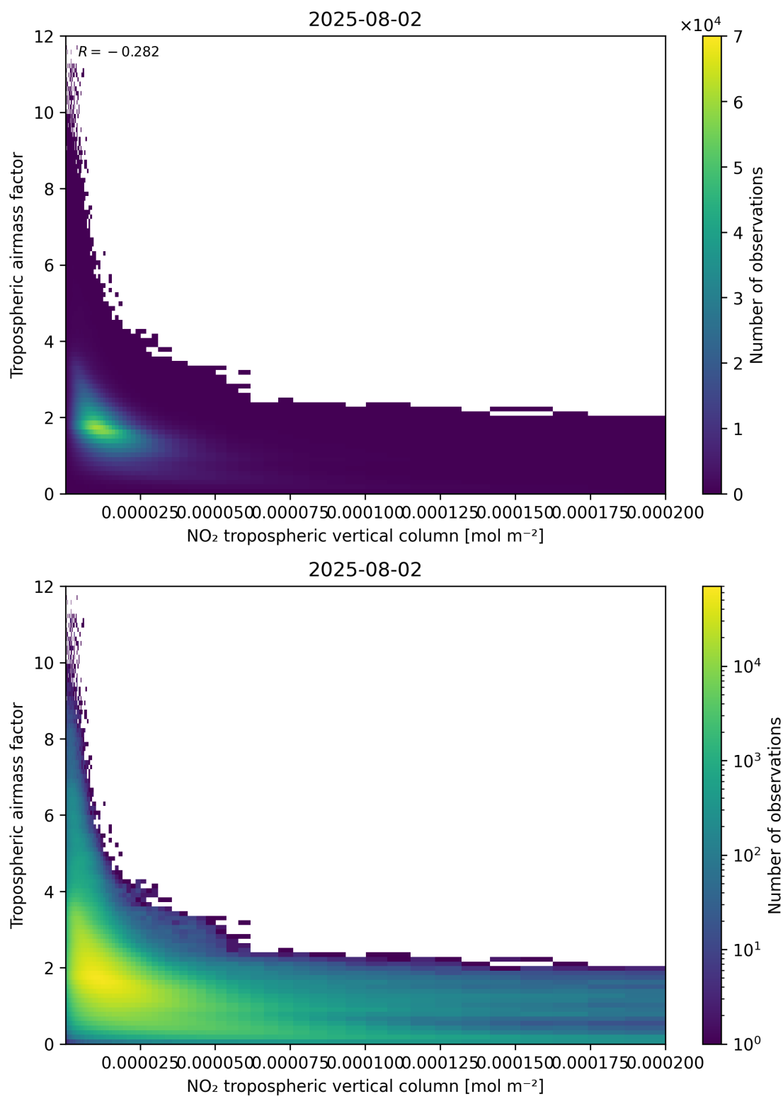
Figure 123: Scatter density plot of “NO 2 tropospheric vertical column” against “Tropospheric air mass factor” for 2025-08-01 to 2025-08-03.
