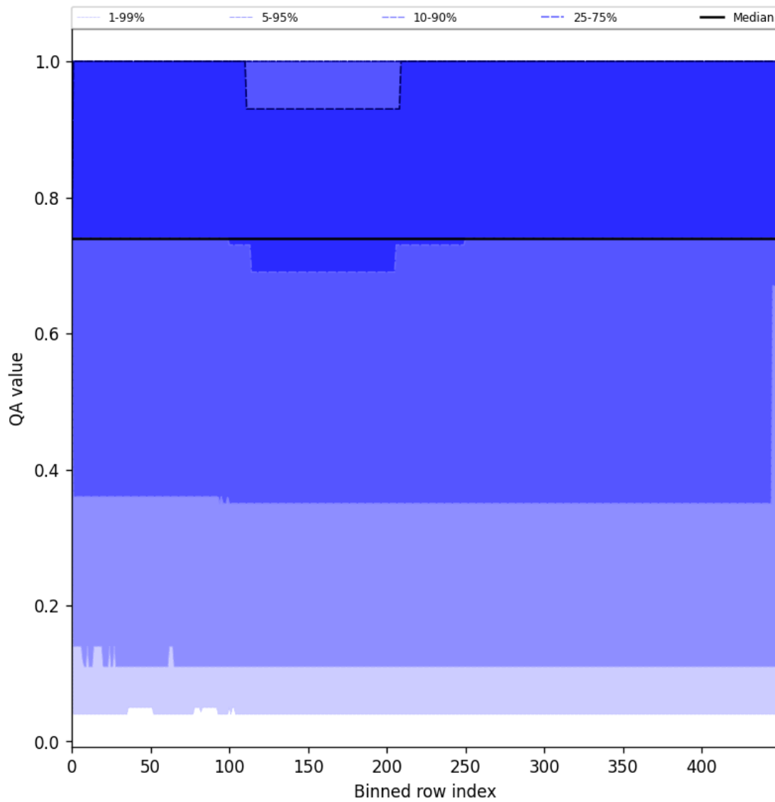
Figure 45: Along track statistics of “QA value” for 2025-08-01 to 2025-08-03
