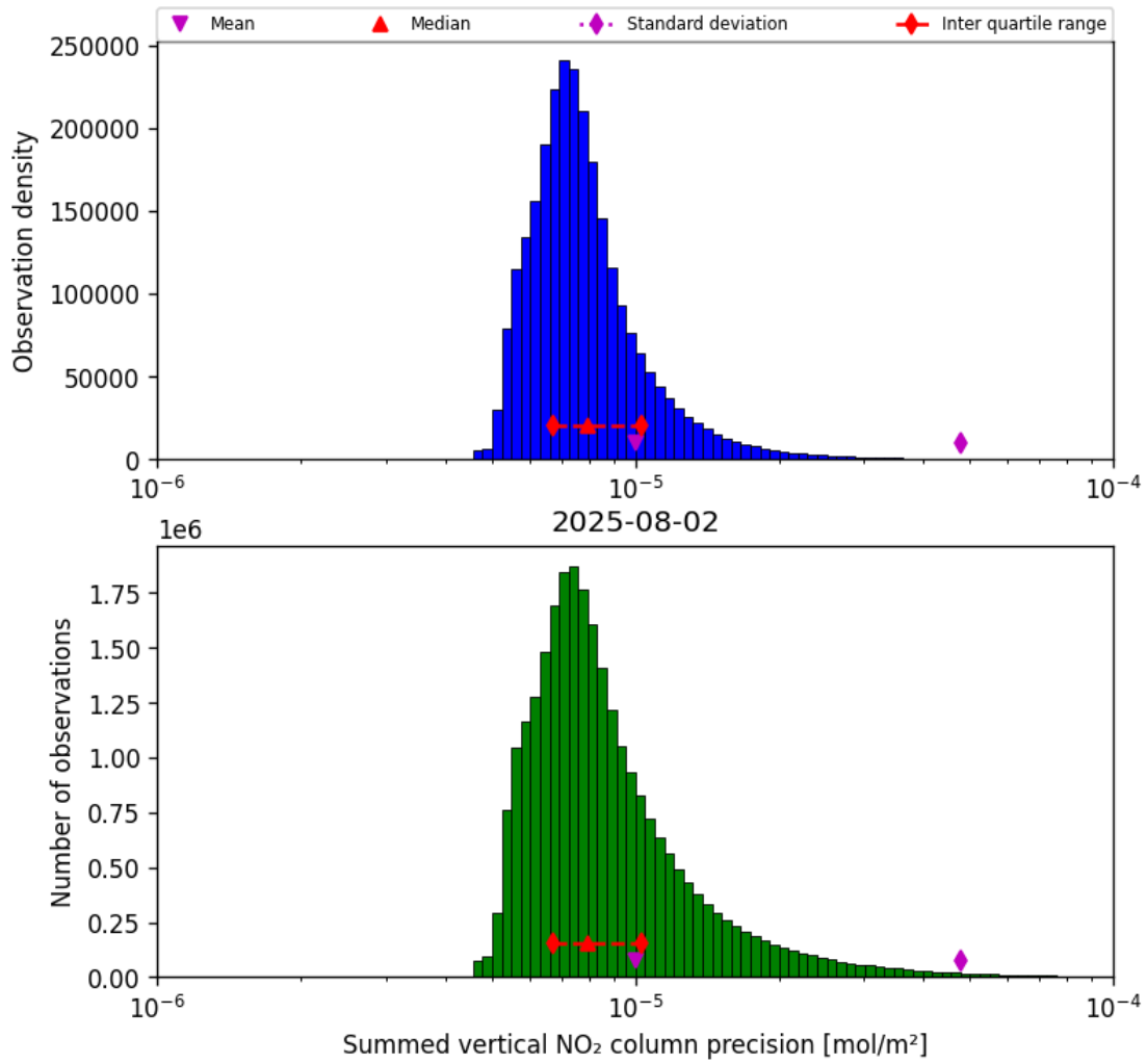
Figure 41: Histogram of “Summed vertical NO 2 column precision” for 2025-08-01 to 2025-08-03
