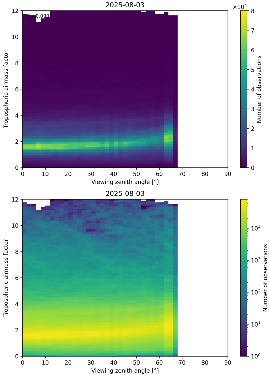
Figure 161: Scatter density plot of “Viewing zenith angle” against “Tropospheric airmass factor” for 2025-08-03 to 2025-08-04.
