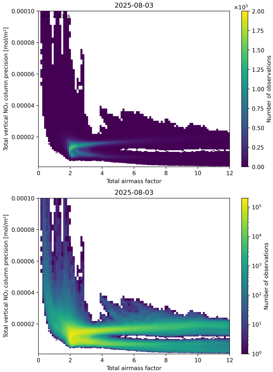
Figure 68: Scatter density plot of “Total airmass factor” against “Total vertical NO 2 column precision” for 2025-08-03 to 2025-08-04.
