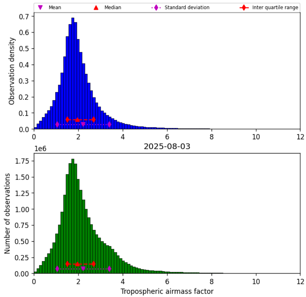
Figure 31: Histogram of “Tropospheric airmass factor” for 2025-08-03 to 2025-08-04
