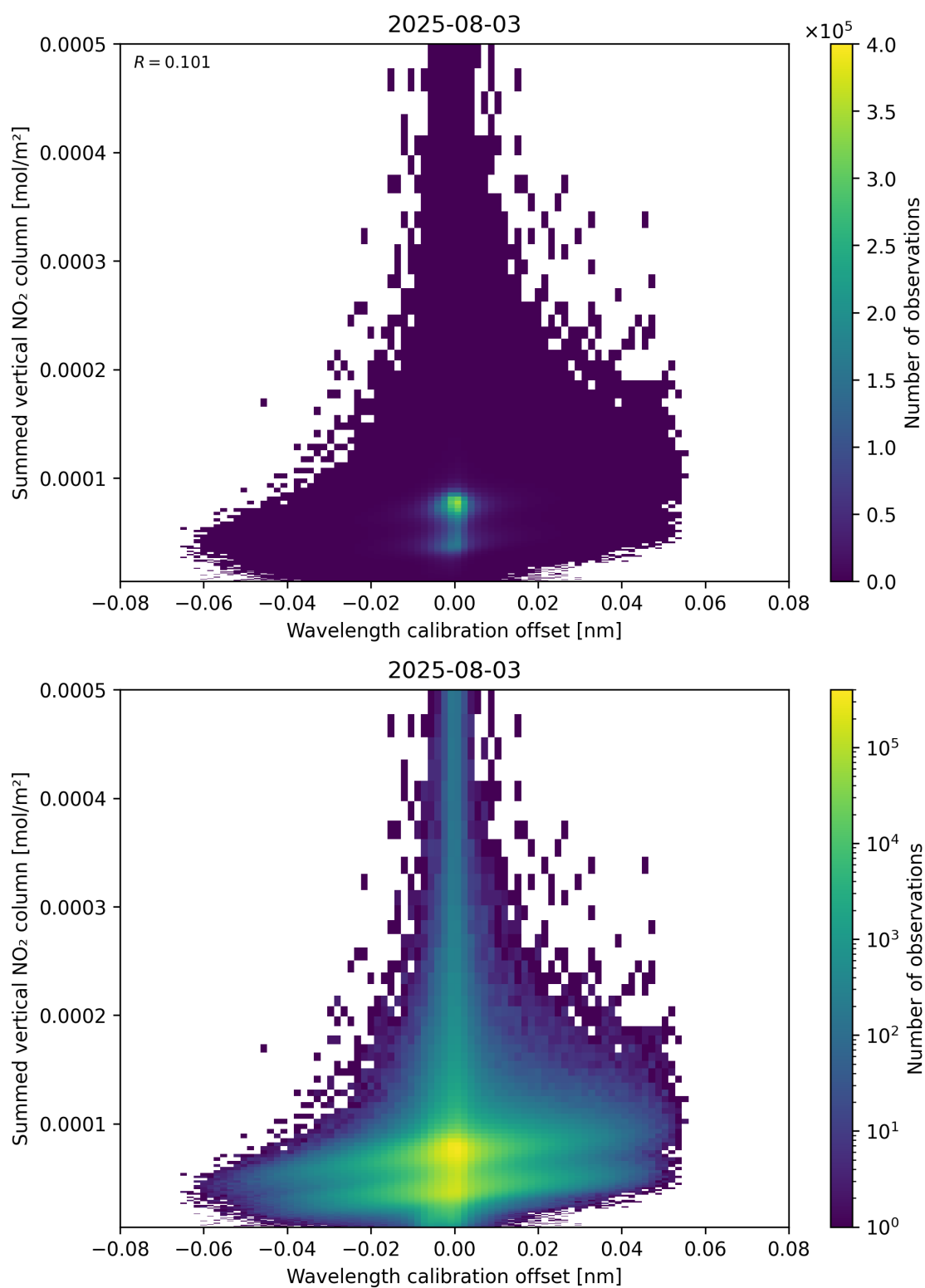
Figure 177: Scatter density plot of “Wavelength calibration offset” against “Summed vertical NO 2 column” for 2025-08-03 to 2025-08-04.
