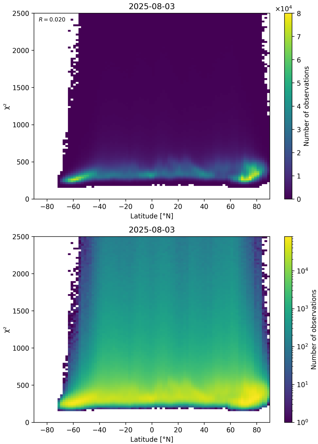
Figure 86: Scatter density plot of “Latitude” against “ \chi^2 ” for 2025-08-03 to 2025-08-04.
