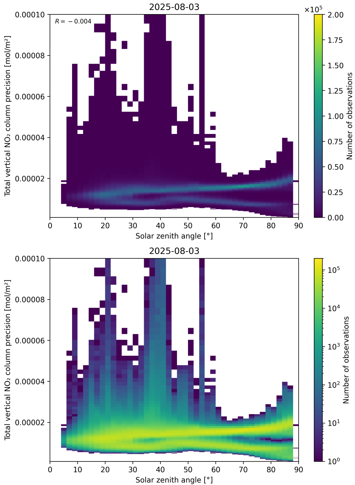
Figure 154: Scatter density plot of “Solar zenith angle” against “Total vertical NO 2 column precision” for 2025-08-03 to 2025-08-04.
