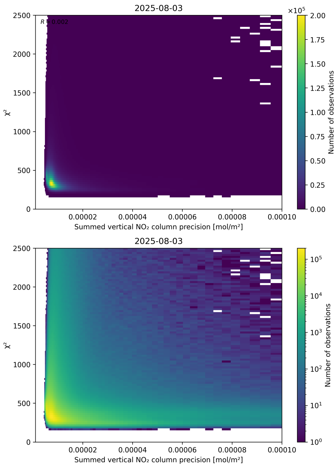
Figure 107: Scatter density plot of “Summed vertical NO 2 column precision” against “ \chi^2 ” for 2025-08-03 to 2025-08-04.
