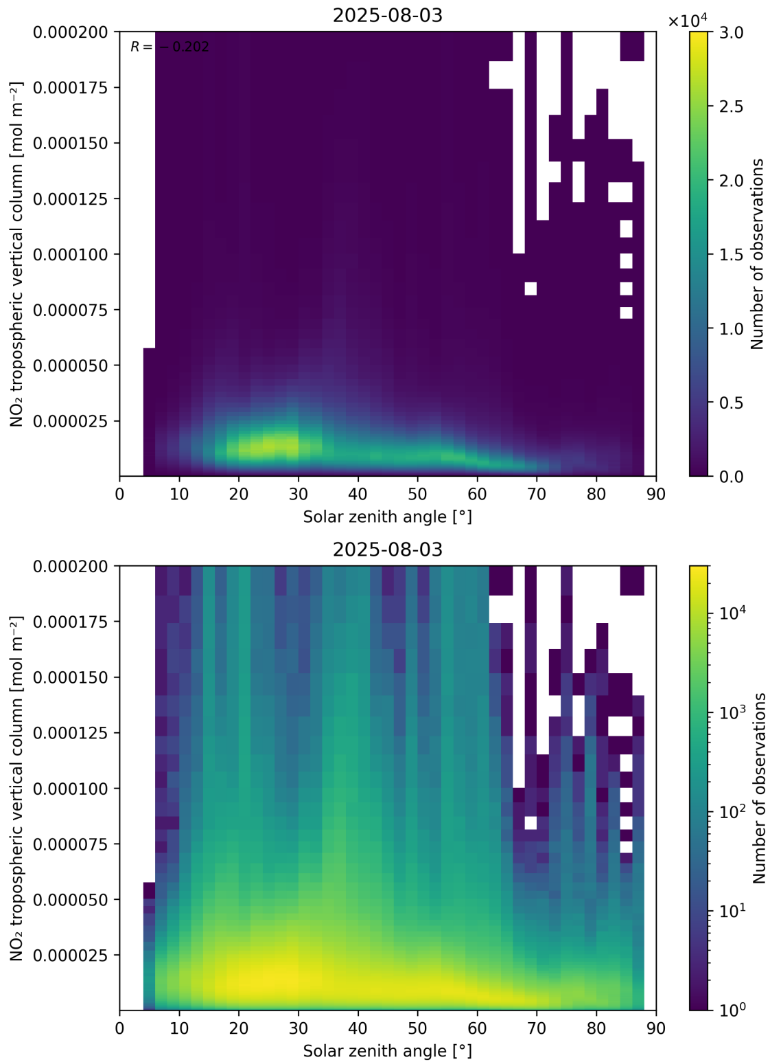
Figure 155: Scatter density plot of “Solar zenith angle” against “NO 2 tropospheric vertical column” for 2025-08-03 to 2025-08-04.
