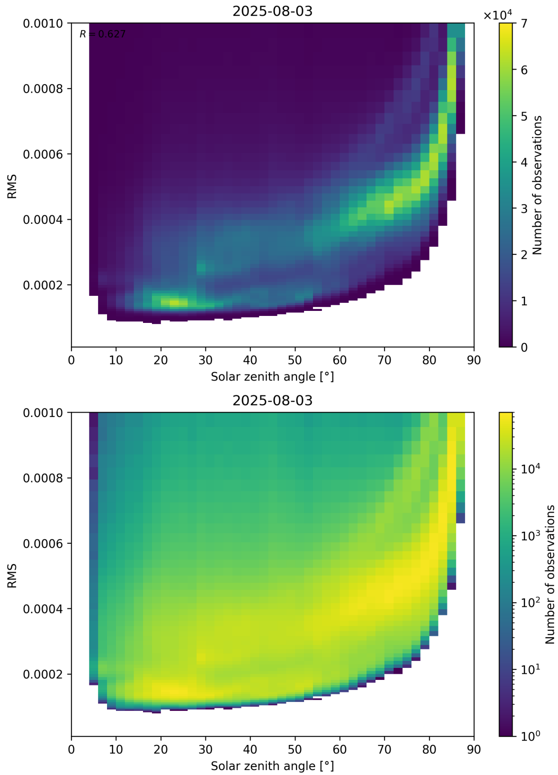
Figure 157: Scatter density plot of “Solar zenith angle” against “RMS” for 2025-08-03 to 2025-08-04.
