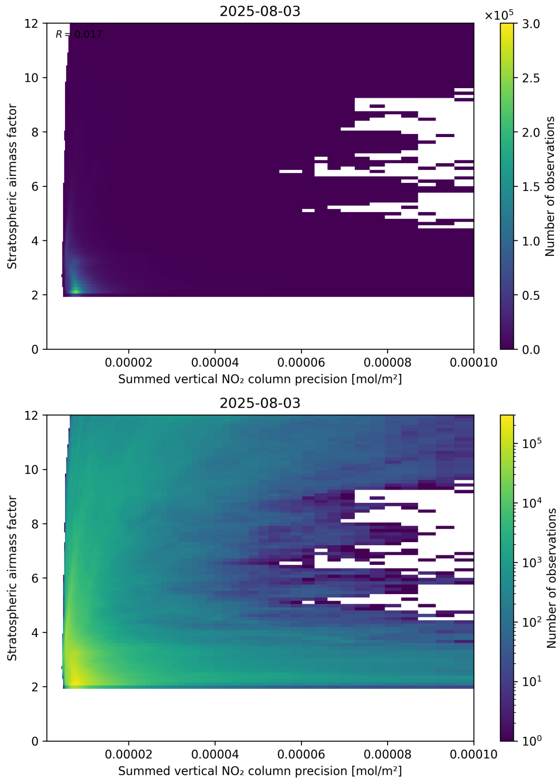
Figure 106: Scatter density plot of “Summed vertical NO 2 column precision” against “Stratospheric airmass factor” for 2025-08-03 to 2025-08-04.
