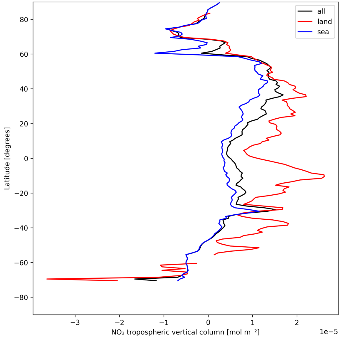
Figure 12: Zonal average of “NO 2 tropospheric vertical column” for 2025-08-03 to 2025-08-04.
