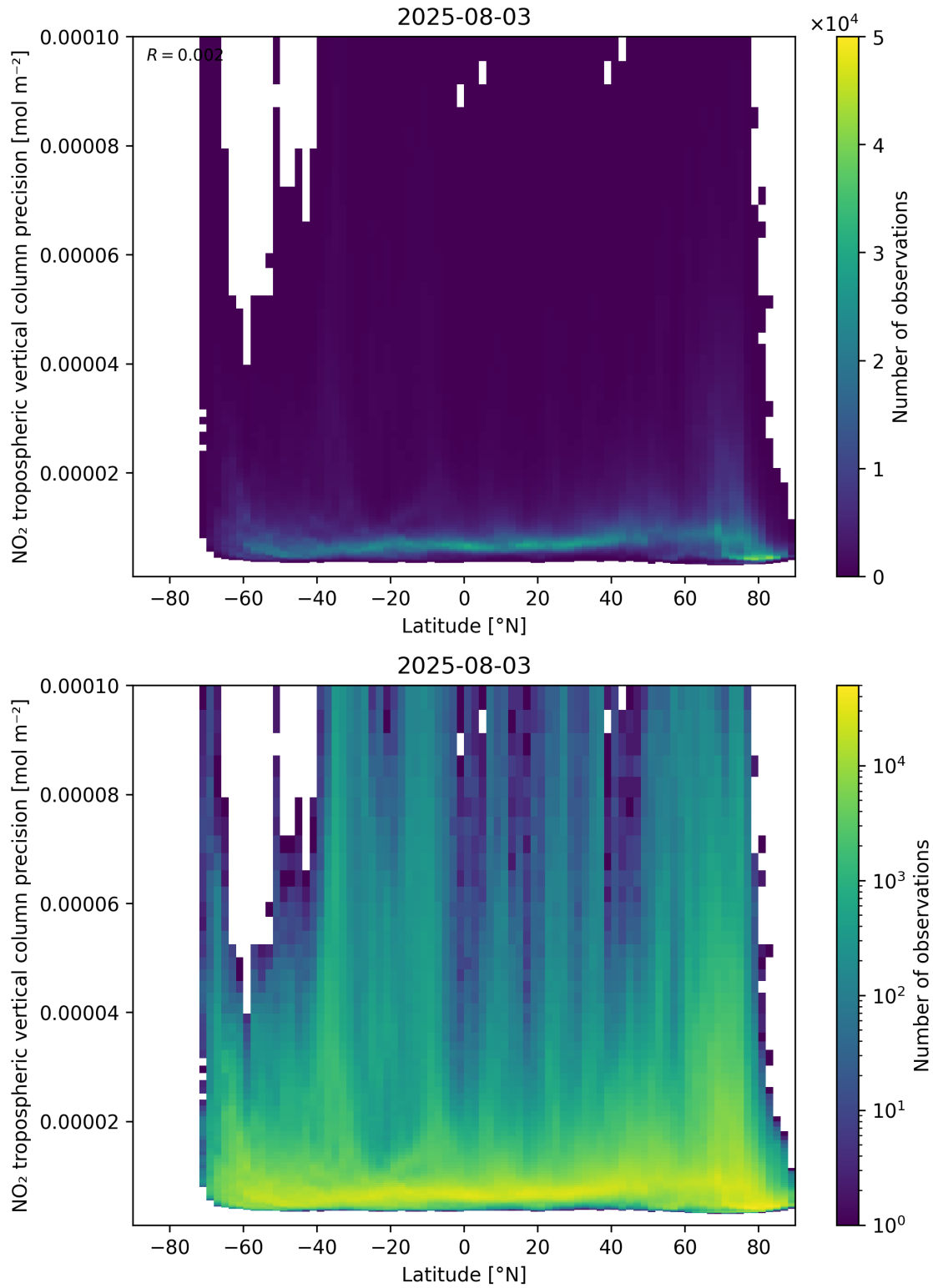
Figure 93: Scatter density plot of “Latitude” against “NO 2 tropospheric vertical column precision” for 2025-08-03 to 2025-08-04.
