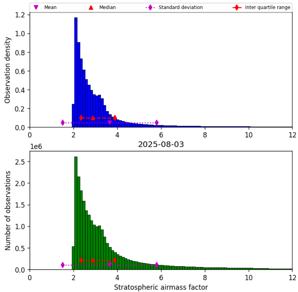
Figure 44: Histogram of “Stratospheric airmass factor” for 2025-08-03 to 2025-08-04
