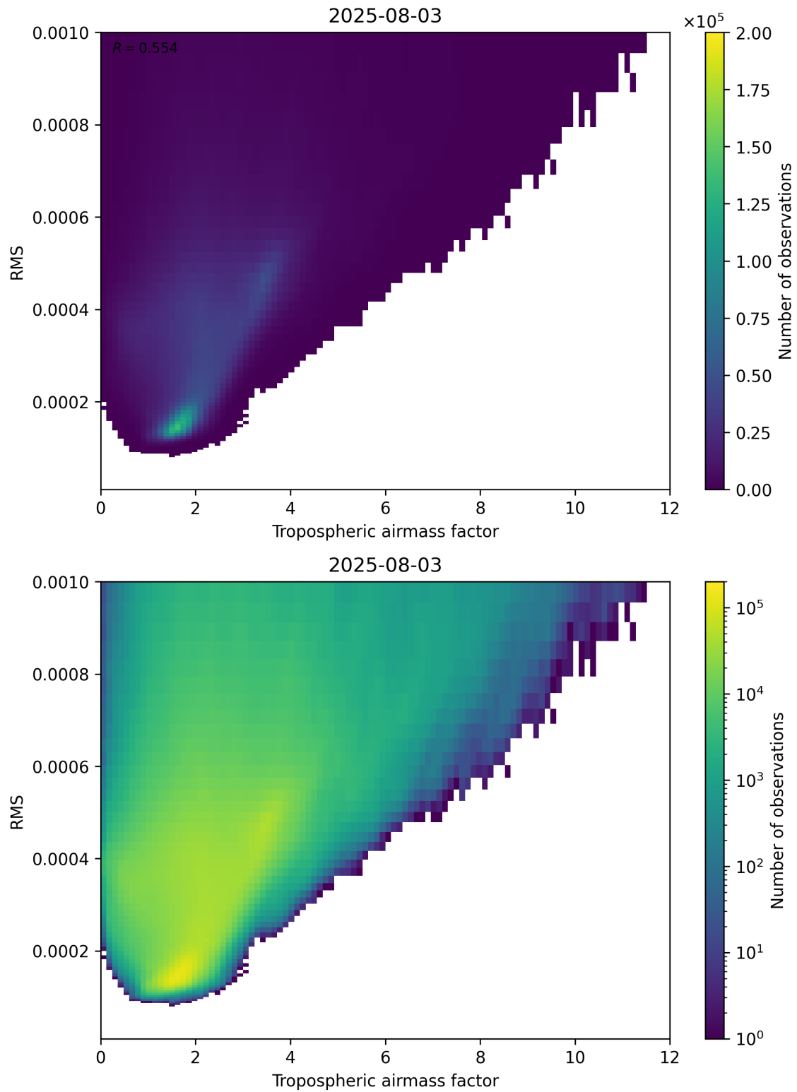
Figure 79: Scatter density plot of “Tropospheric airmass factor” against “RMS” for 2025-08-03 to 2025-08-04.
