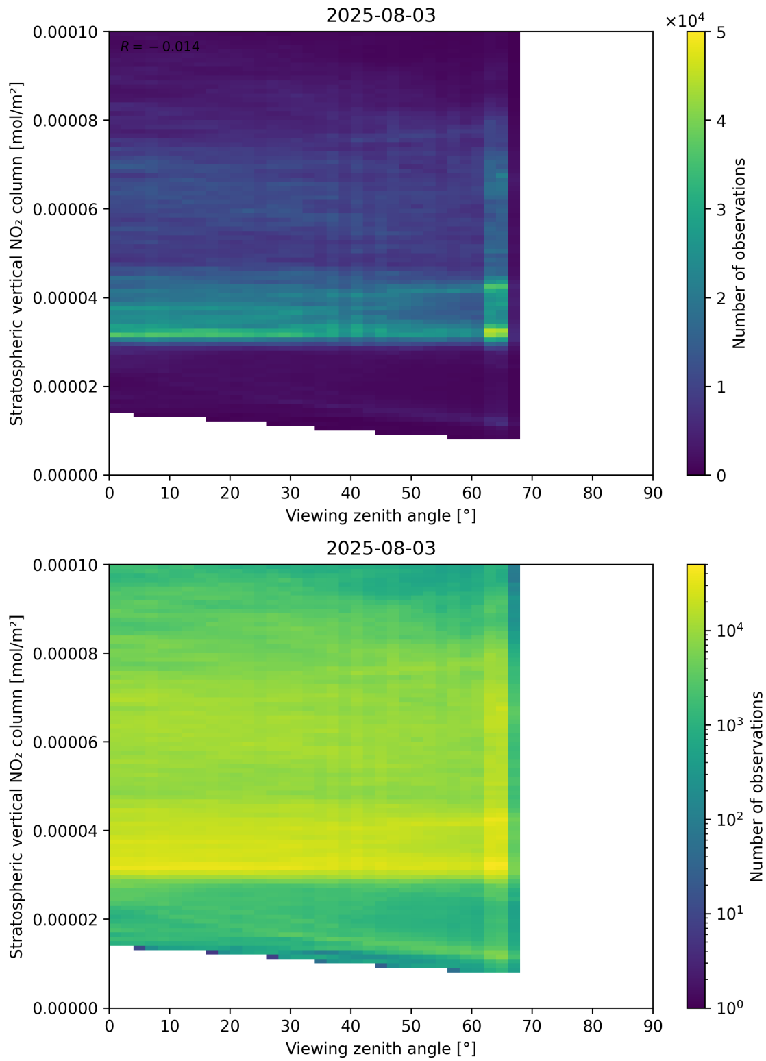
Figure 164: Scatter density plot of “Viewing zenith angle” against “Stratospheric vertical NO 2 column” for 2025-08-03 to 2025-08-04.
