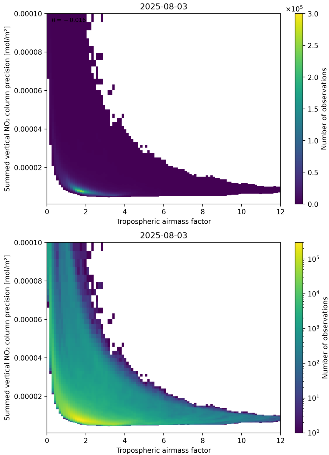
Figure 76: Scatter density plot of “Tropospheric airmass factor” against “Summed vertical NO 2 column precision” for 2025-08-03 to 2025-08-04.
