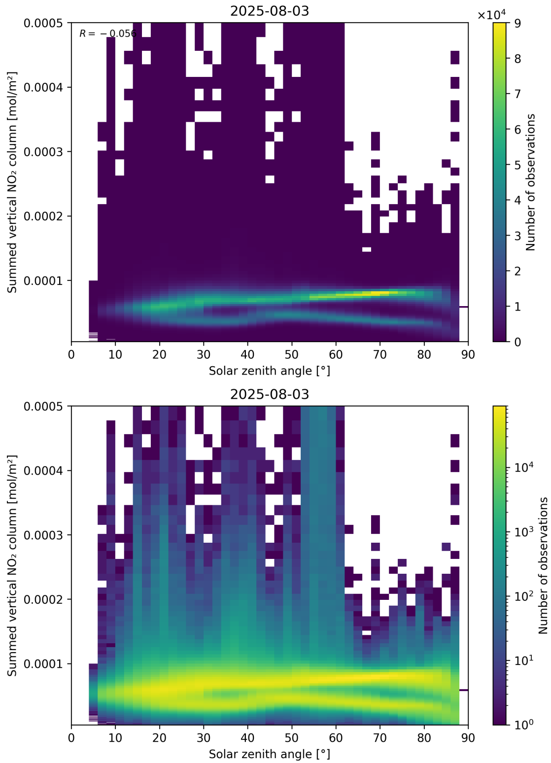
Figure 151: Scatter density plot of “Solar zenith angle” against “Summed vertical NO 2 column” for 2025-08-03 to 2025-08-04.
