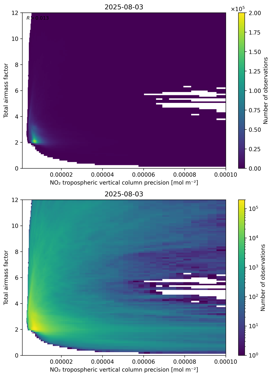
Figure 132: Scatter density plot of “NO 2 tropospheric vertical column precision” against “Total air mass factor” for 2025-08-03 to 2025-08-04.
