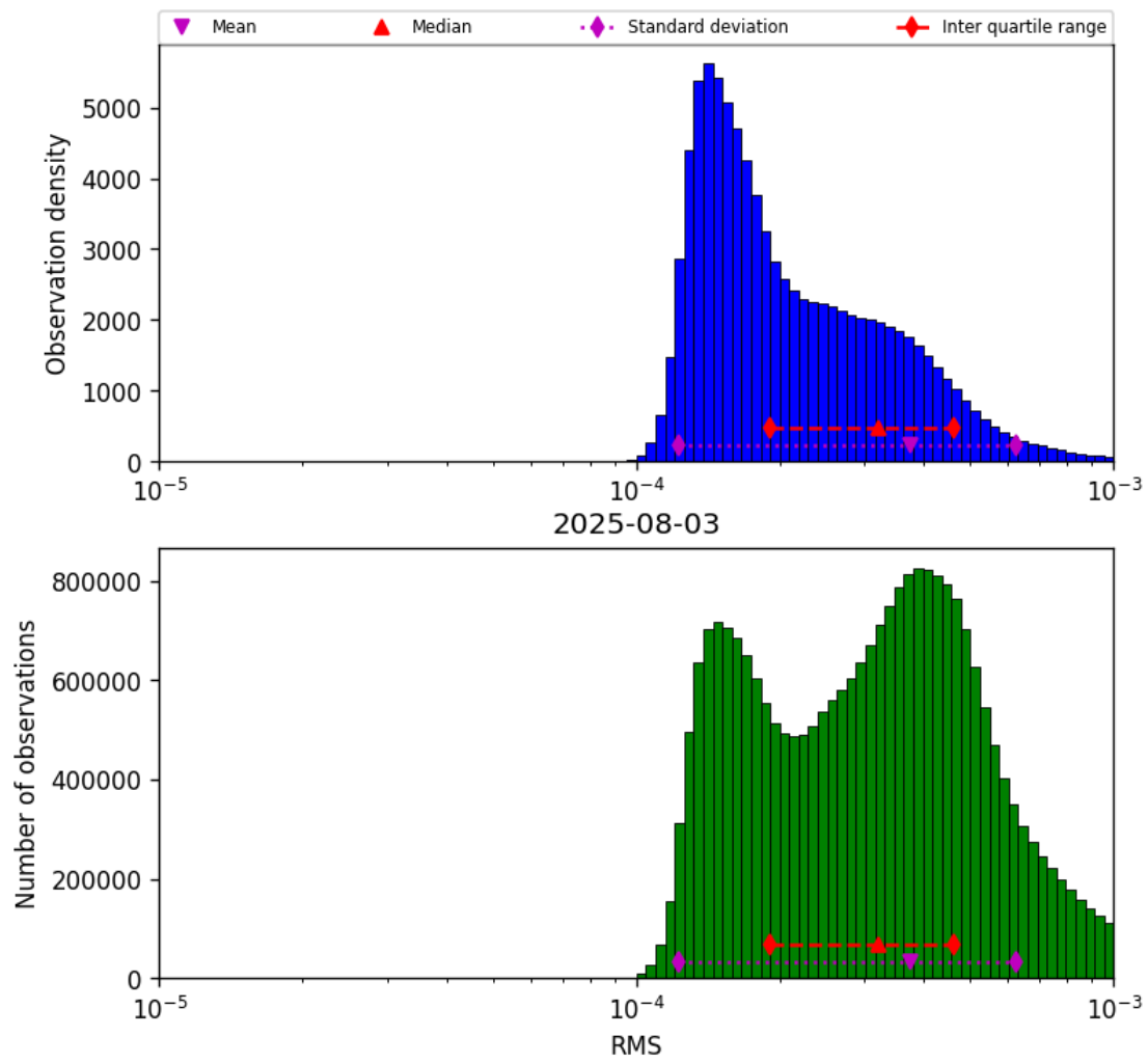
Figure 43: Histogram of “RMS” for 2025-08-03 to 2025-08-04
