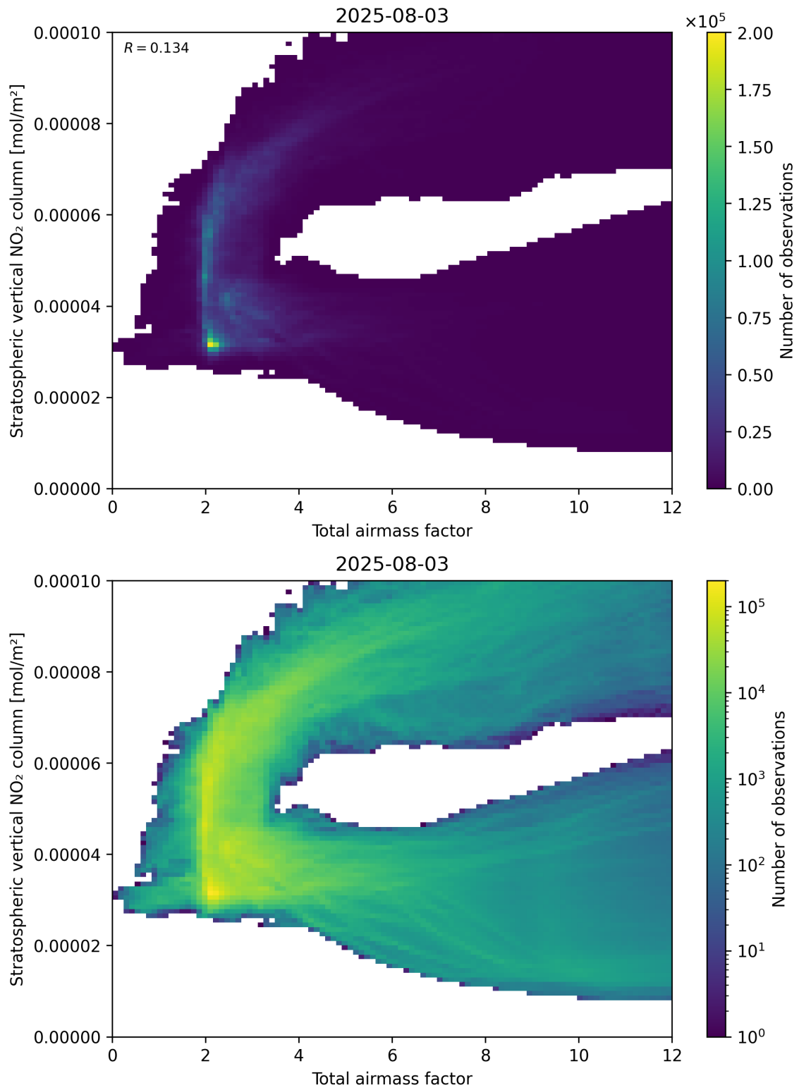
Figure 64: Scatter density plot of “Total airmass factor” against “Stratospheric vertical NO 2 column” for 2025-08-03 to 2025-08-04.
