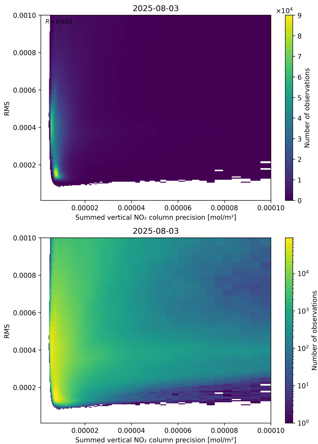
Figure 108: Scatter density plot of “Summed vertical NO 2 column precision” against “RMS” for 2025-08-03 to 2025-08-04.
