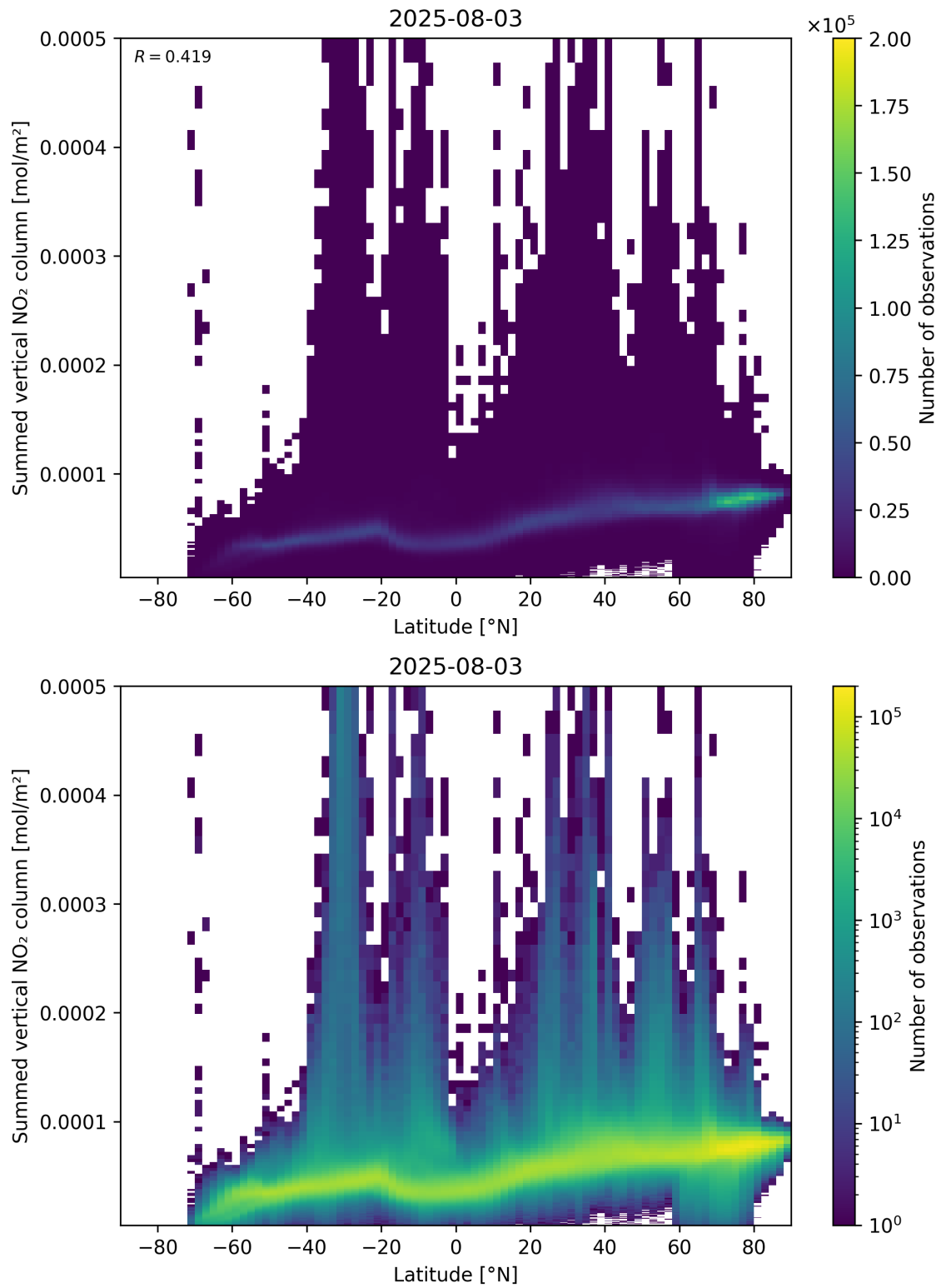
Figure 88: Scatter density plot of “Latitude” against “Summed vertical NO 2 column” for 2025-08-03 to 2025-08-04.
