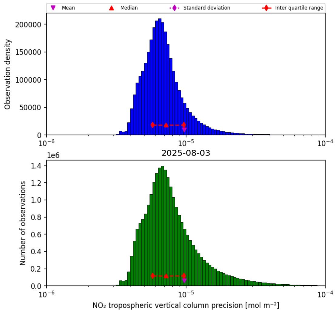
Figure 30: Histogram of “NO 2 tropospheric vertical column precision” for 2025-08-03 to 2025-08-04
