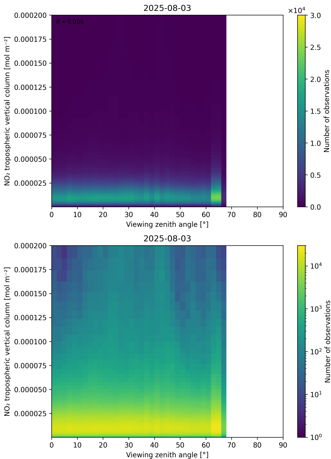
Figure 169: Scatter density plot of “Viewing zenith angle” against “NO 2 tropospheric vertical column” for 2025-08-03 to 2025-08-04.
