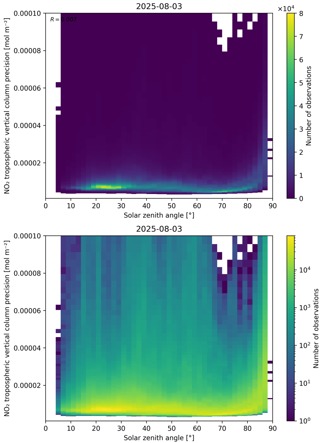
Figure 156: Scatter density plot of “Solar zenith angle” against “NO 2 tropospheric vertical column precision” for 2025-08-03 to 2025-08-04.
