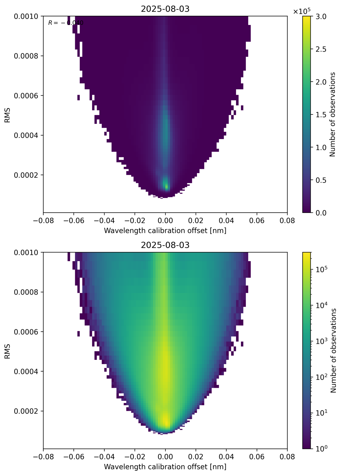
Figure 181: Scatter density plot of “Wavelength calibration offset” against “RMS” for 2025-08-03 to 2025-08-04.
