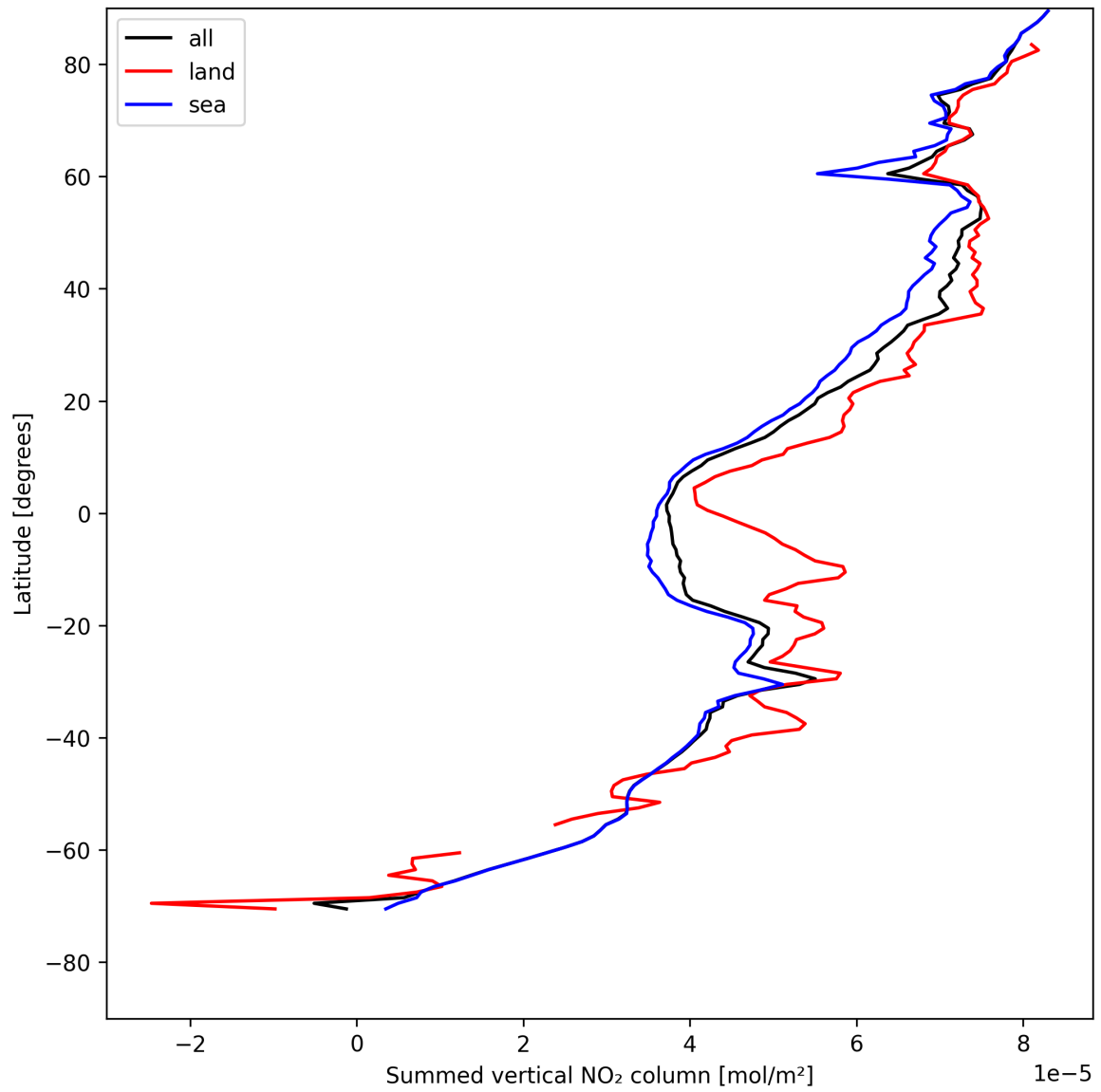
Figure 23: Zonal average of “Summed vertical NO 2 column” for 2025-08-03 to 2025-08-04.
