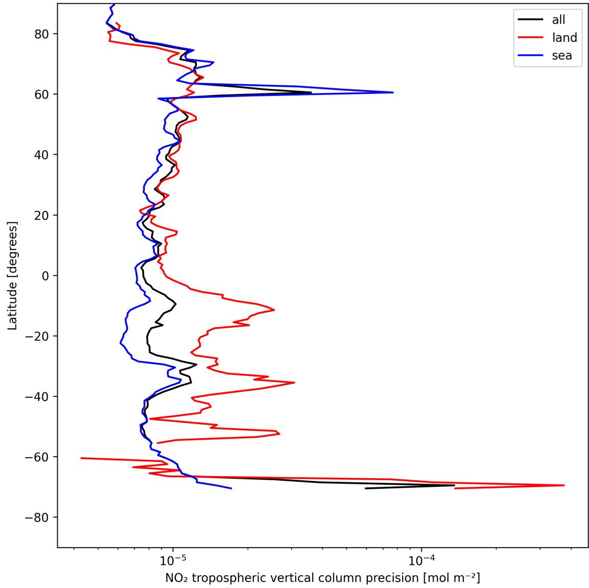
Figure 13: Zonal average of “NO 2 tropospheric vertical column precision” for 2025-08-03 to 2025-08-04.
