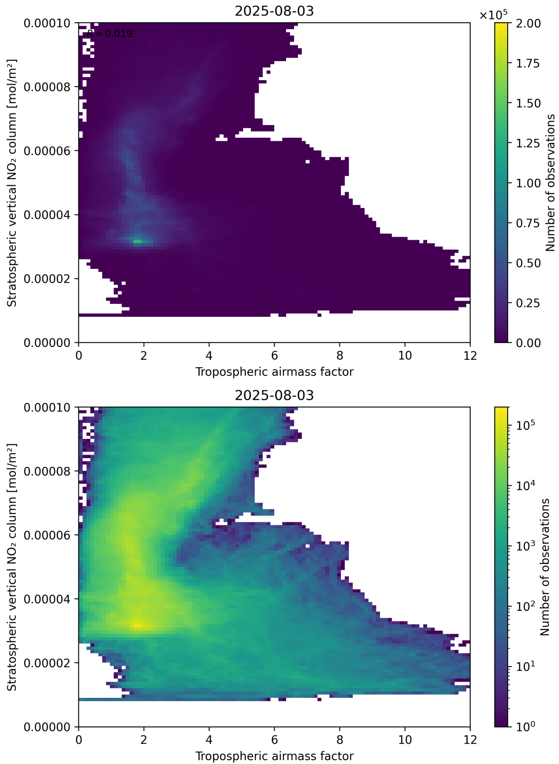
Figure 74: Scatter density plot of “Tropospheric air mass factor” against “Stratospheric vertical NO 2 column” for 2025-08-03 to 2025-08-04.
