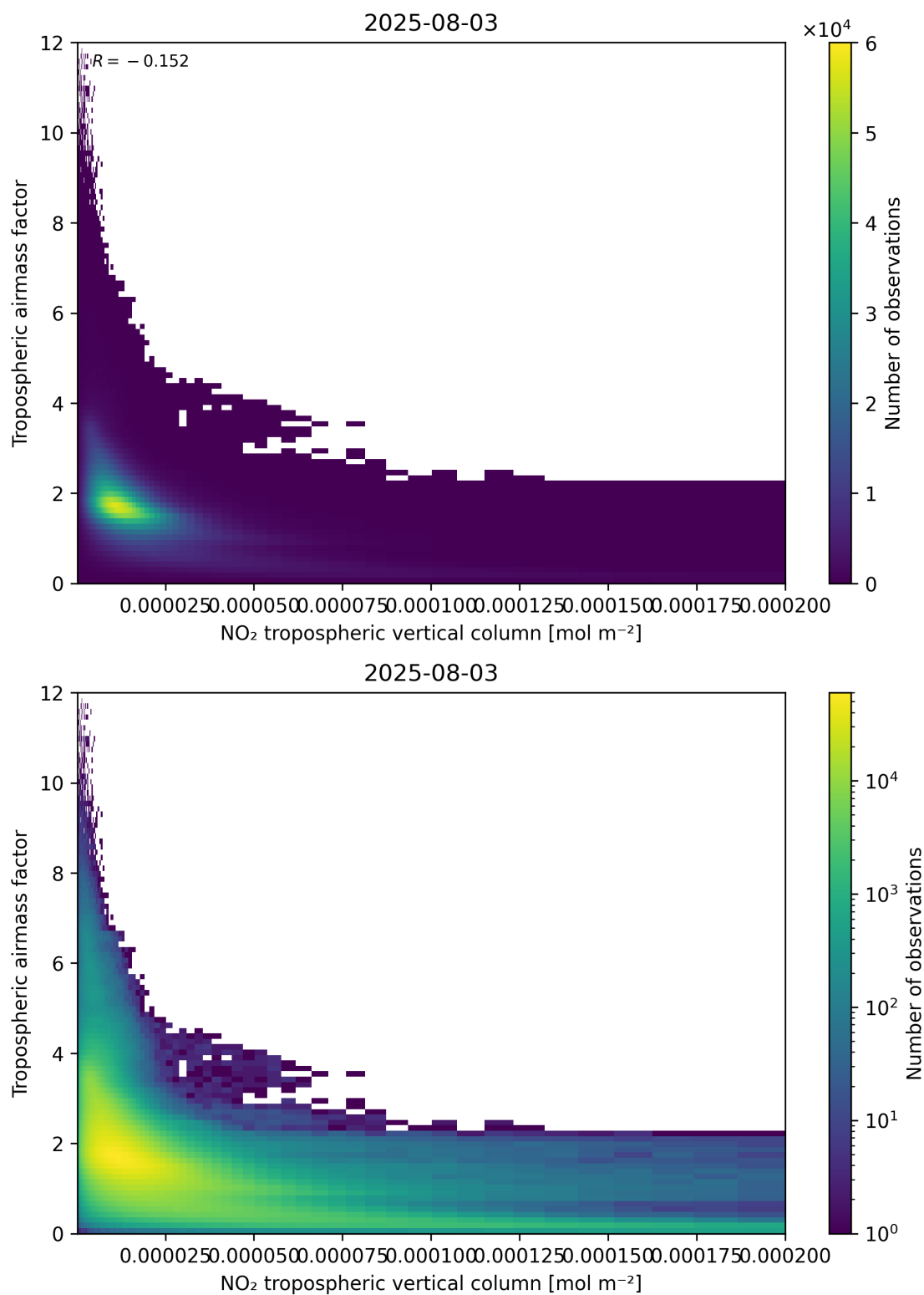
Figure 123: Scatter density plot of “NO 2 tropospheric vertical column” against “Tropospheric air mass factor” for 2025-08-03 to 2025-08-04.
