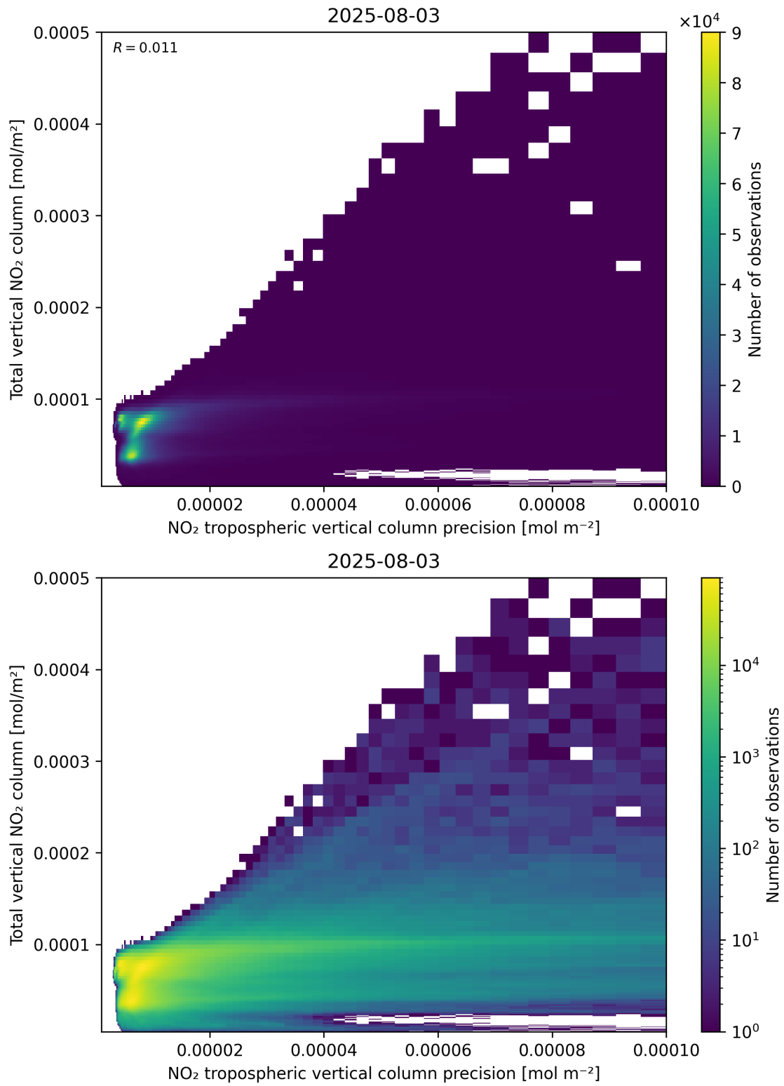
Figure 138: Scatter density plot of “NO 2 tropospheric vertical column precision” against “Total vertical NO 2 column” for 2025-08-03 to 2025-08-04.
