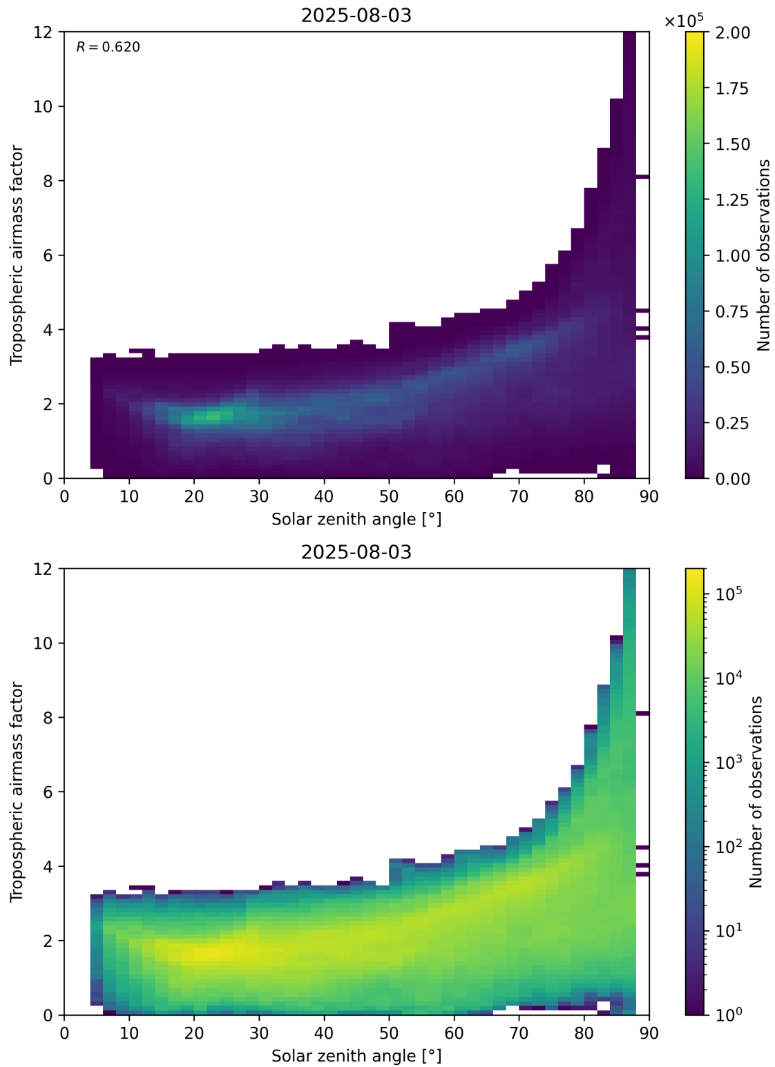
Figure 147: Scatter density plot of “Solar zenith angle” against “Tropospheric airmass factor” for 2025-08-03 to 2025-08-04.
