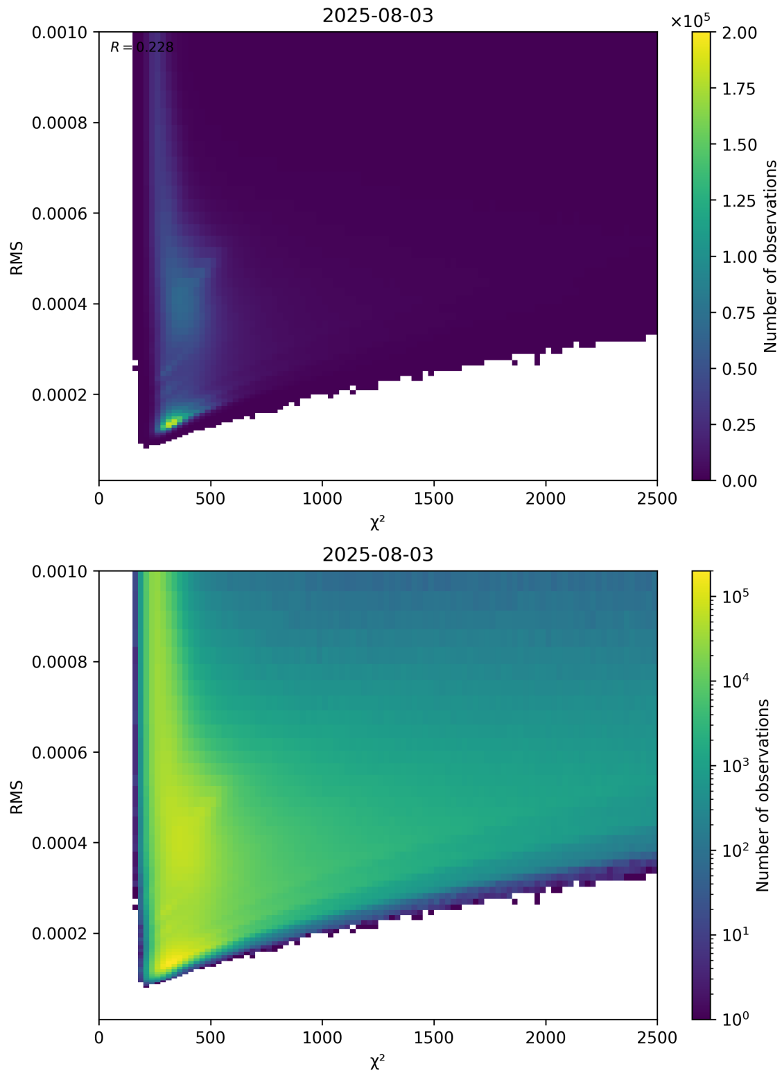
Figure 82: Scatter density plot of “ \chi^2 ” against “RMS” for 2025-08-03 to 2025-08-04.
