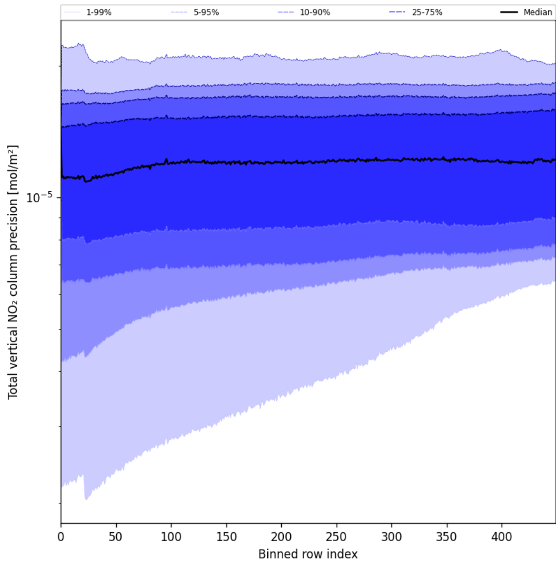
Figure 56: Along track statistics of “Total vertical NO 2 column precision” for 2025-08-03 to 2025-08-04
