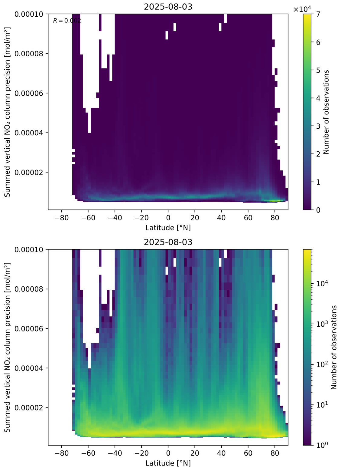
Figure 89: Scatter density plot of “Latitude” against “Summed vertical NO 2 column precision” for 2025-08-03 to 2025-08-04.
