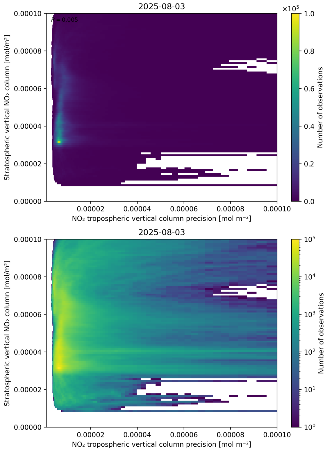
Figure 135: Scatter density plot of “NO 2 tropospheric vertical column precision” against “Stratospheric vertical NO 2 column” for 2025-08-03 to 2025-08-04.
