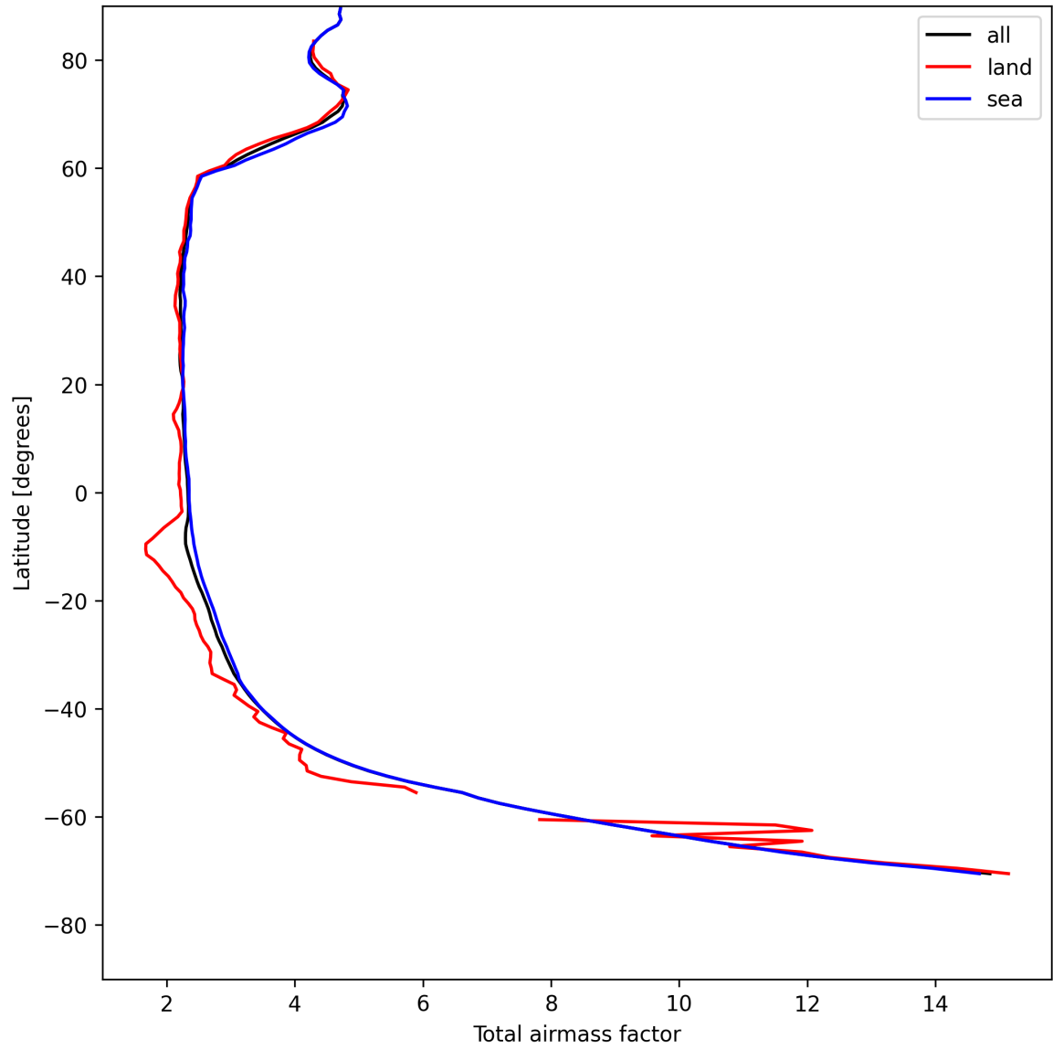
Figure 15: Zonal average of “Total airmass factor” for 2025-08-03 to 2025-08-04.
