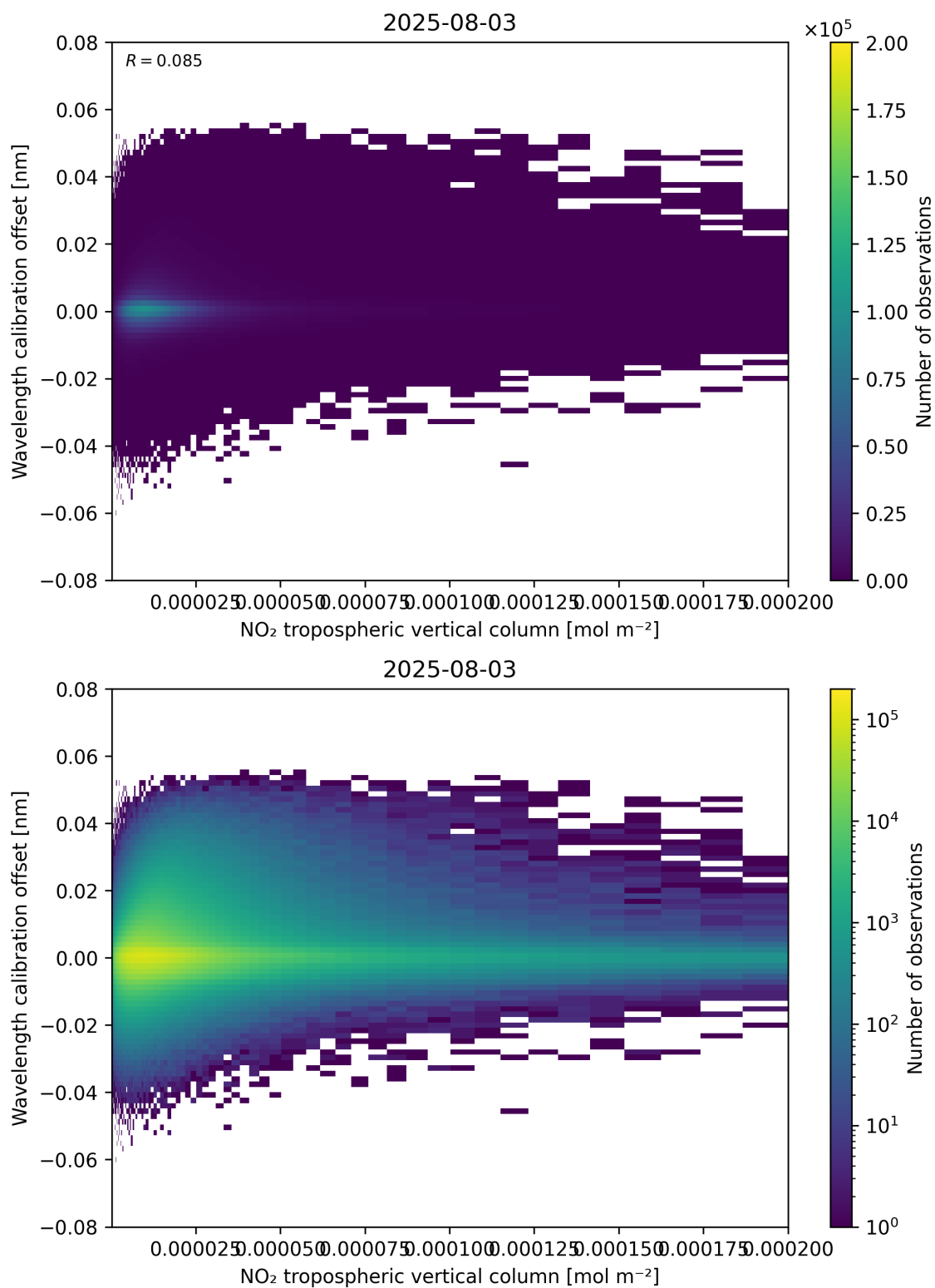
Figure 143: Scatter density plot of “NO 2 tropospheric vertical column” against “Wavelength calibration offset” for 2025-08-03 to 2025-08-04.
