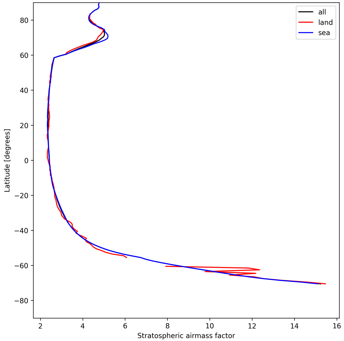
Figure 27: Zonal average of “Stratospheric airmass factor” for 2025-08-03 to 2025-08-04.
