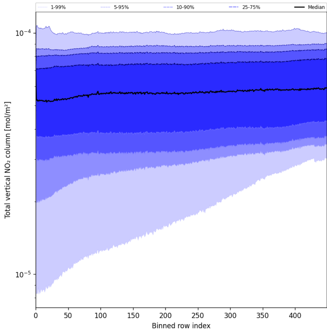
Figure 55: Along track statistics of “Total vertical NO 2 column” for 2025-08-03 to 2025-08-04
