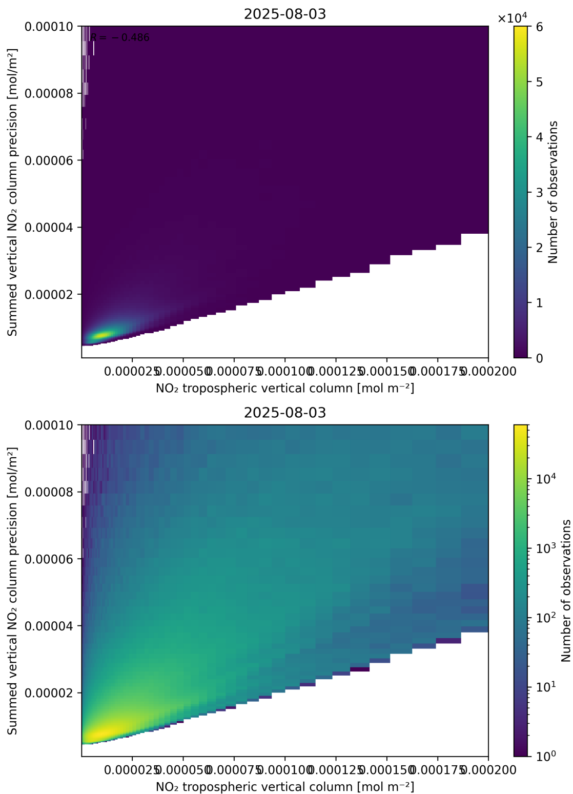
Figure 127: Scatter density plot of “NO 2 tropospheric vertical column” against “Summed vertical NO 2 column precision” for 2025-08-03 to 2025-08-04.
