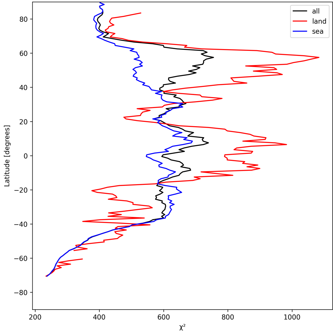
Figure 25: Zonal average of “ \chi^2 ” for 2025-08-03 to 2025-08-04.
