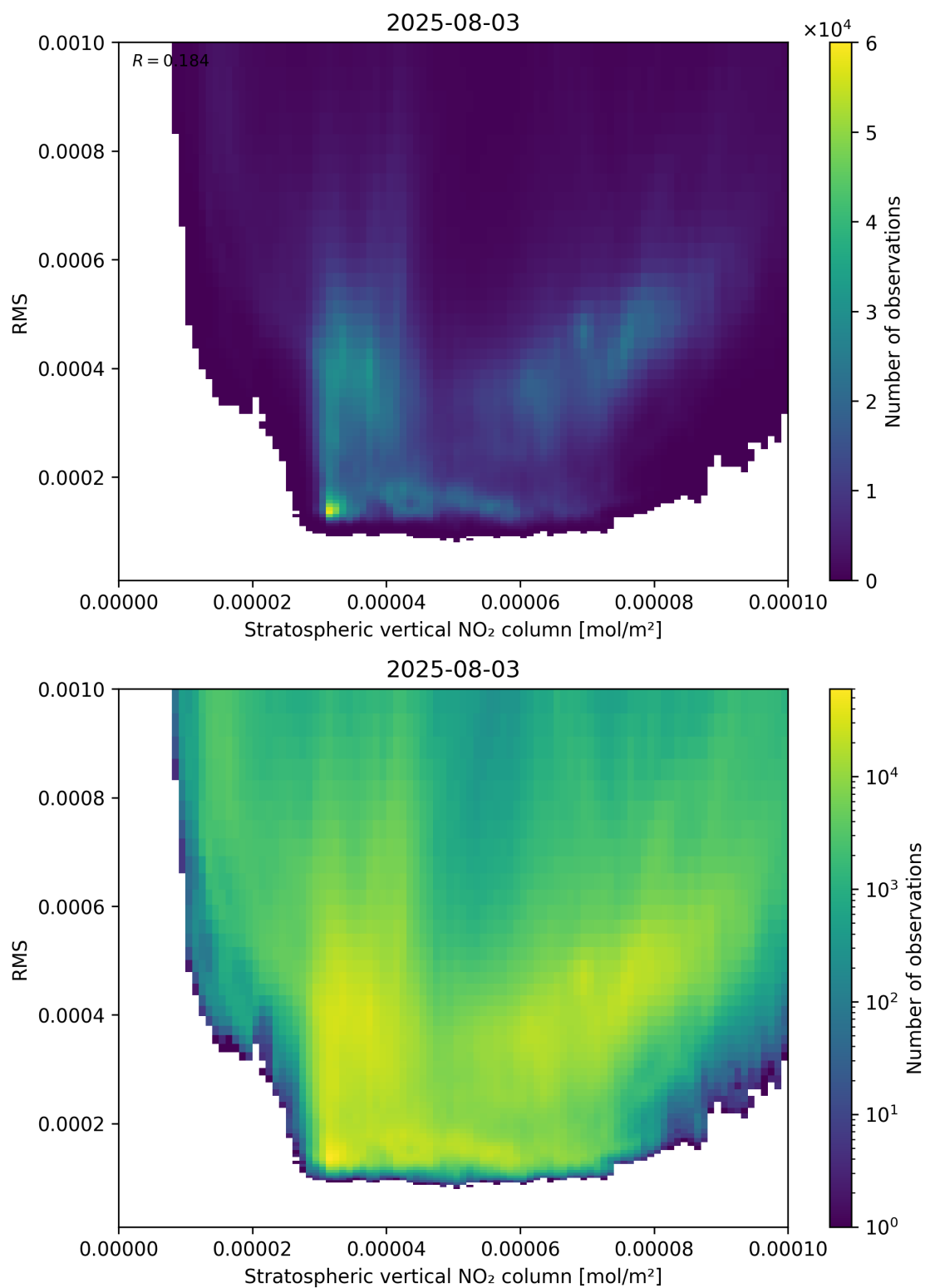
Figure 102: Scatter density plot of “Stratospheric vertical NO 2 column” against “RMS” for 2025-08-03 to 2025-08-04.
