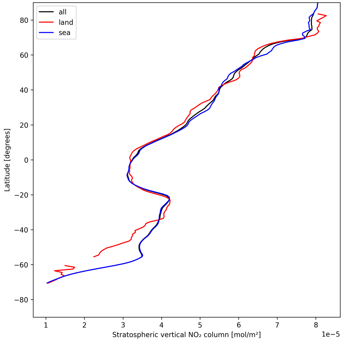
Figure 19: Zonal average of “Stratospheric vertical NO 2 column” for 2025-08-03 to 2025-08-04.
