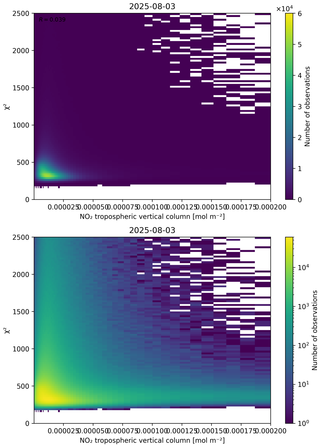
Figure 124: Scatter density plot of “NO 2 tropospheric vertical column” against “ \chi^2 ” for 2025-08-03 to 2025-08-04.
