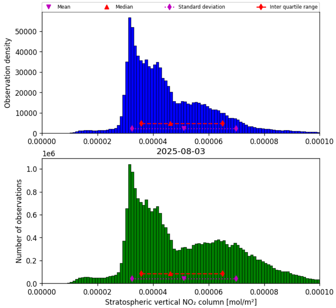
Figure 36: Histogram of “Stratospheric vertical NO 2 column” for 2025-08-03 to 2025-08-04
