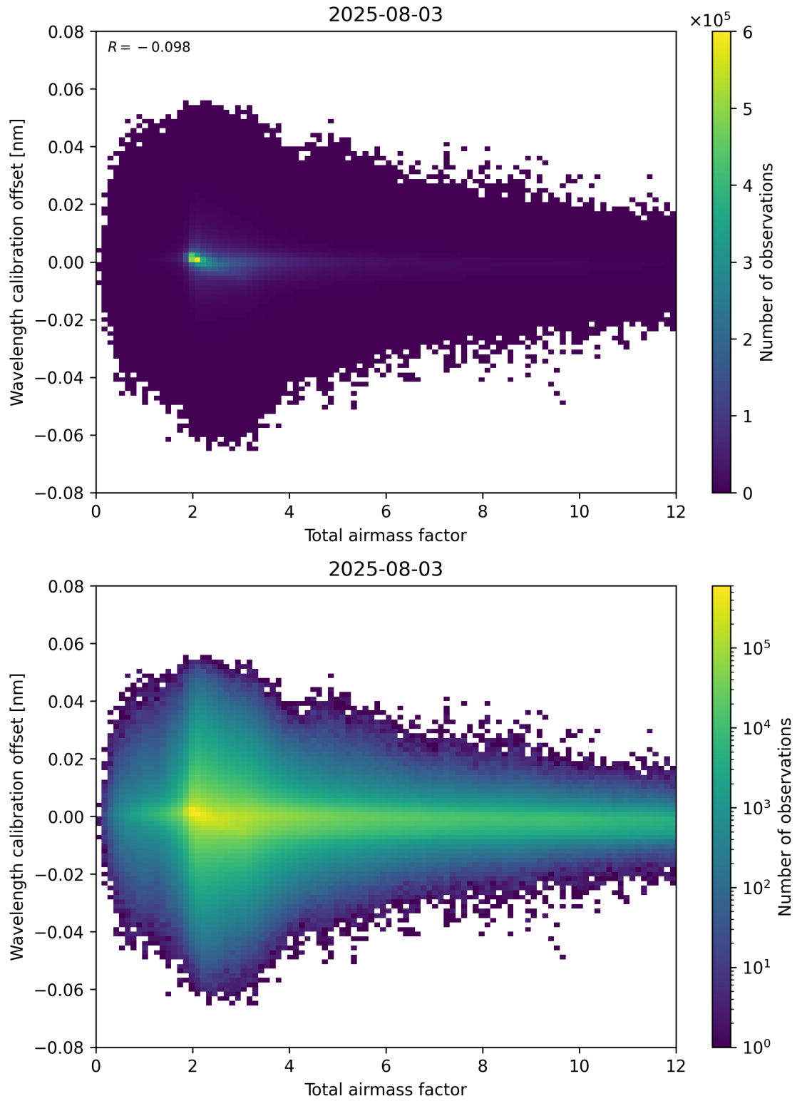
Figure 70: Scatter density plot of “Total airmass factor” against “Wavelength calibration offset” for 2025-08-03 to 2025-08-04.
