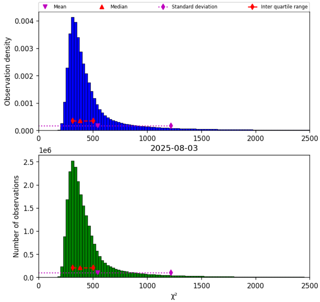
Figure 42: Histogram of “ \chi^2 ” for 2025-08-03 to 2025-08-04
