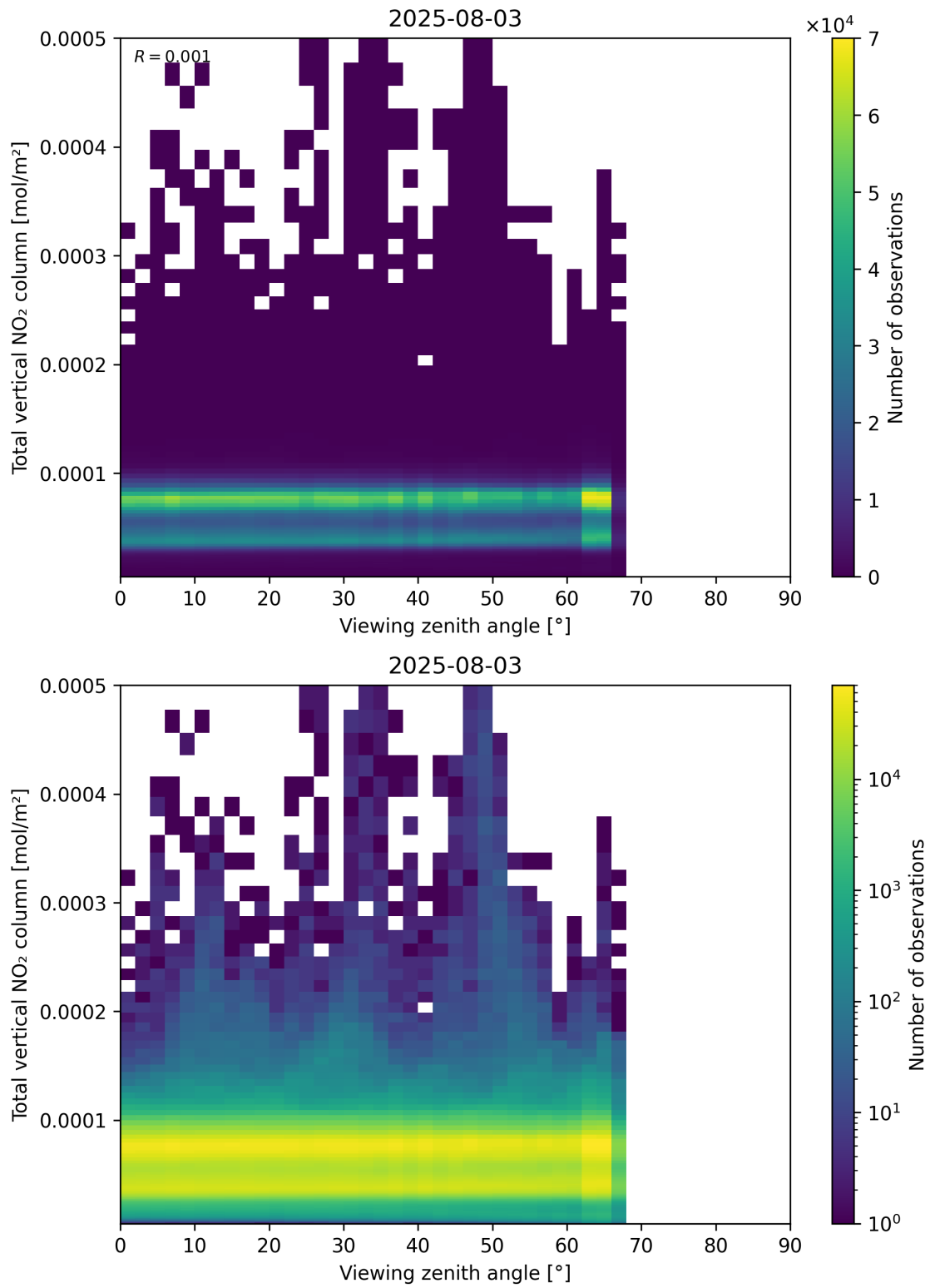
Figure 167: Scatter density plot of “Viewing zenith angle” against “Total vertical NO 2 column” for 2025-08-03 to 2025-08-04.
