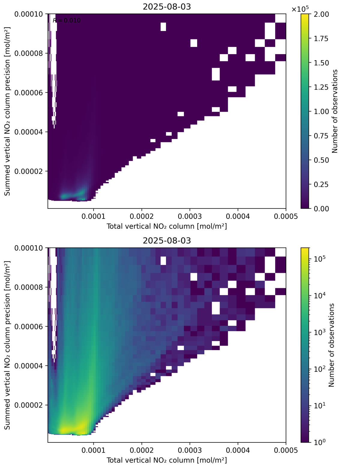
Figure 113: Scatter density plot of “Total vertical NO 2 column” against “Summed vertical NO 2 column precision” for 2025-08-03 to 2025-08-04.
