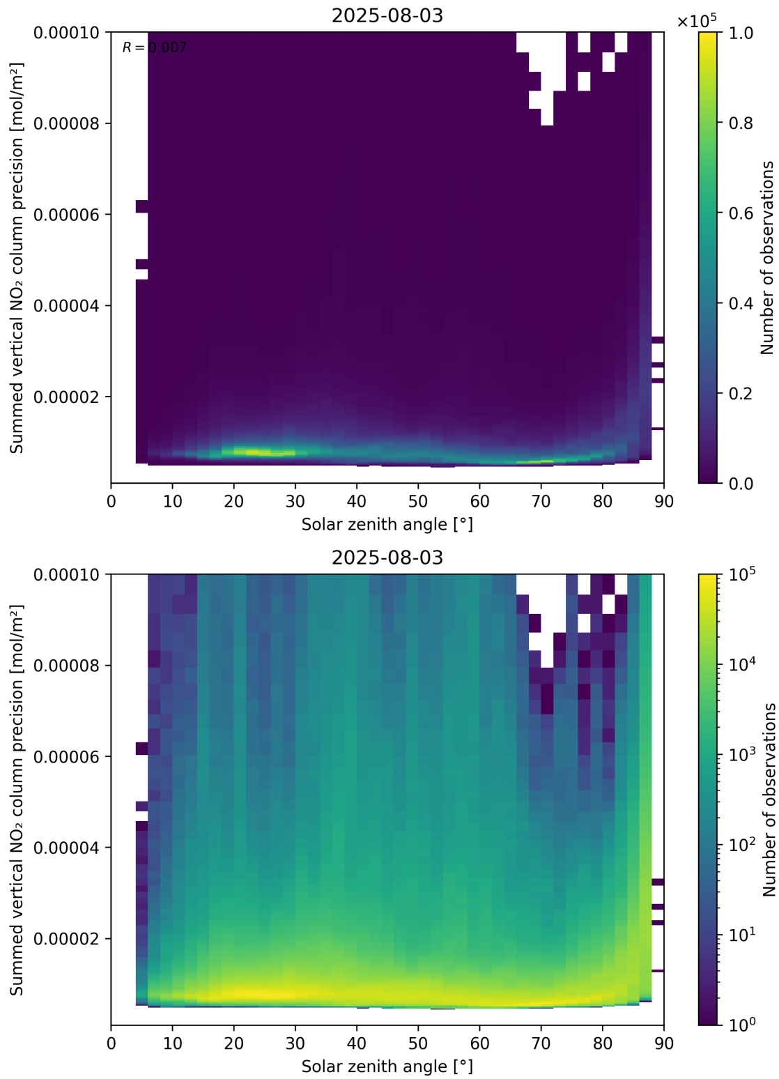
Figure 152: Scatter density plot of “Solar zenith angle” against “Summed vertical NO 2 column precision” for 2025-08-03 to 2025-08-04.
