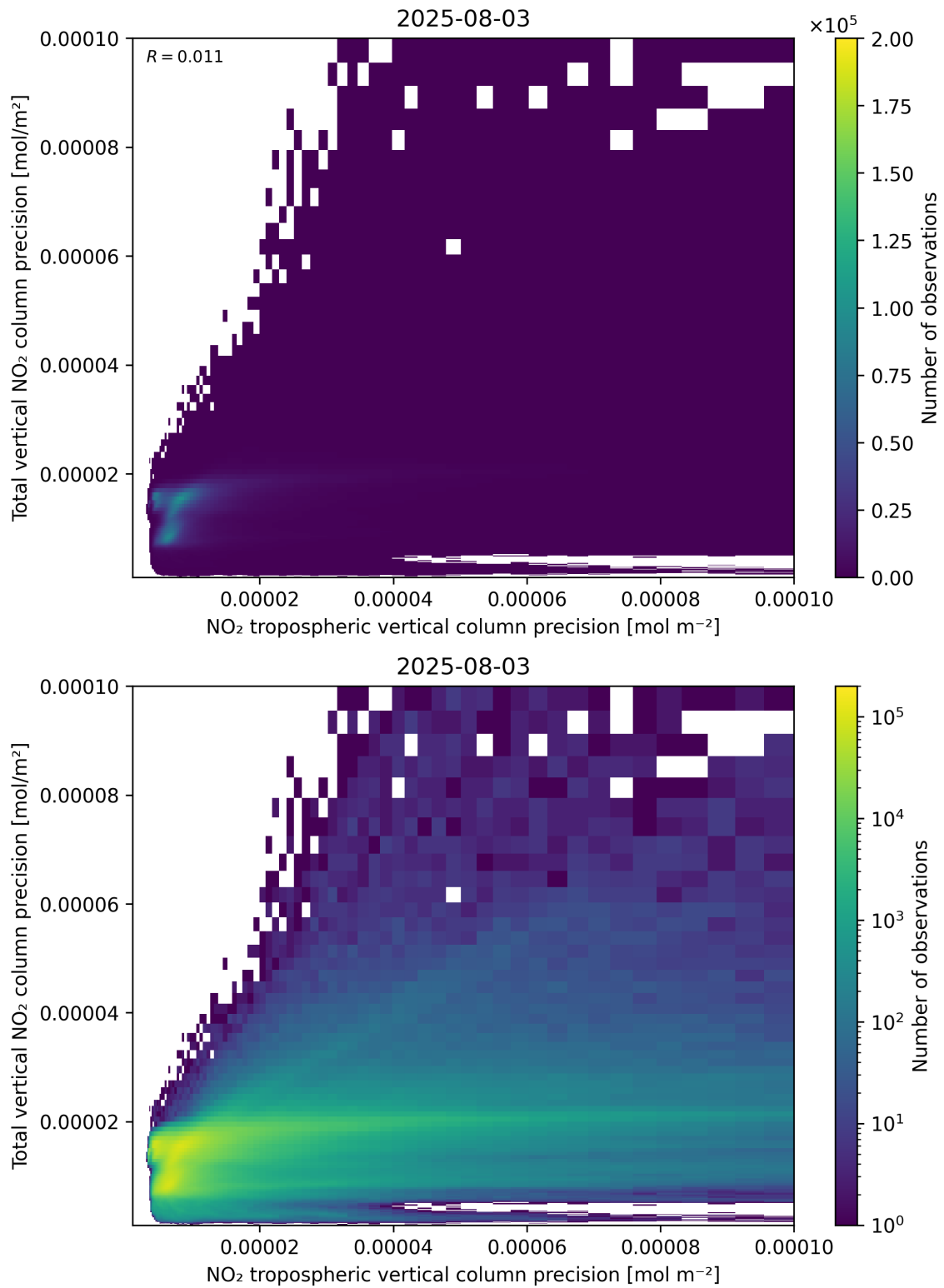
Figure 139: Scatter density plot of “NO 2 tropospheric vertical column precision” against “Total vertical NO 2 column precision” for 2025-08-03 to 2025-08-04.
