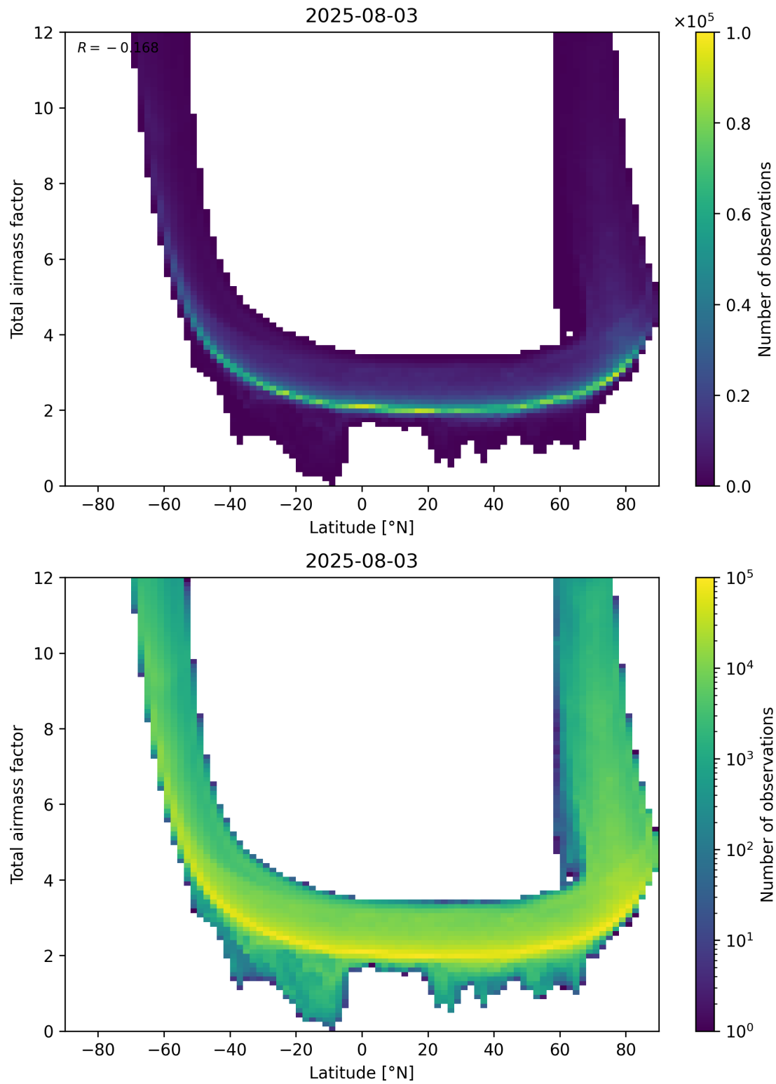
Figure 84: Scatter density plot of “Latitude” against “Total airmass factor” for 2025-08-03 to 2025-08-04.
