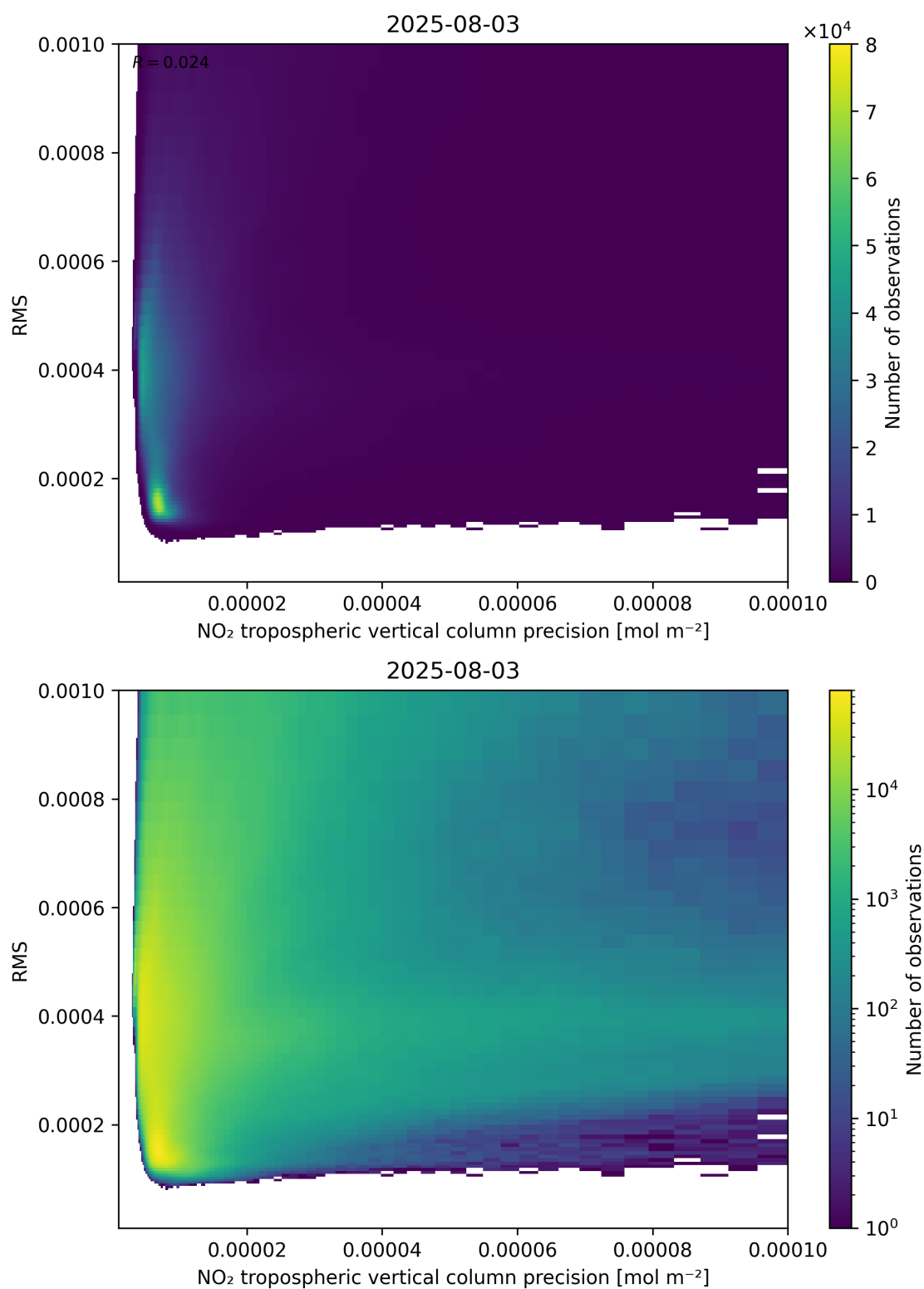
Figure 140: Scatter density plot of “NO 2 tropospheric vertical column precision” against “RMS” for 2025-08-03 to 2025-08-04.
