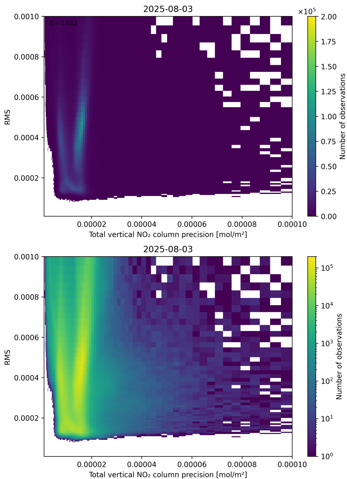
Figure 119: Scatter density plot of “Total vertical NO 2 column precision” against “RMS” for 2025-08-03 to 2025-08-04.
