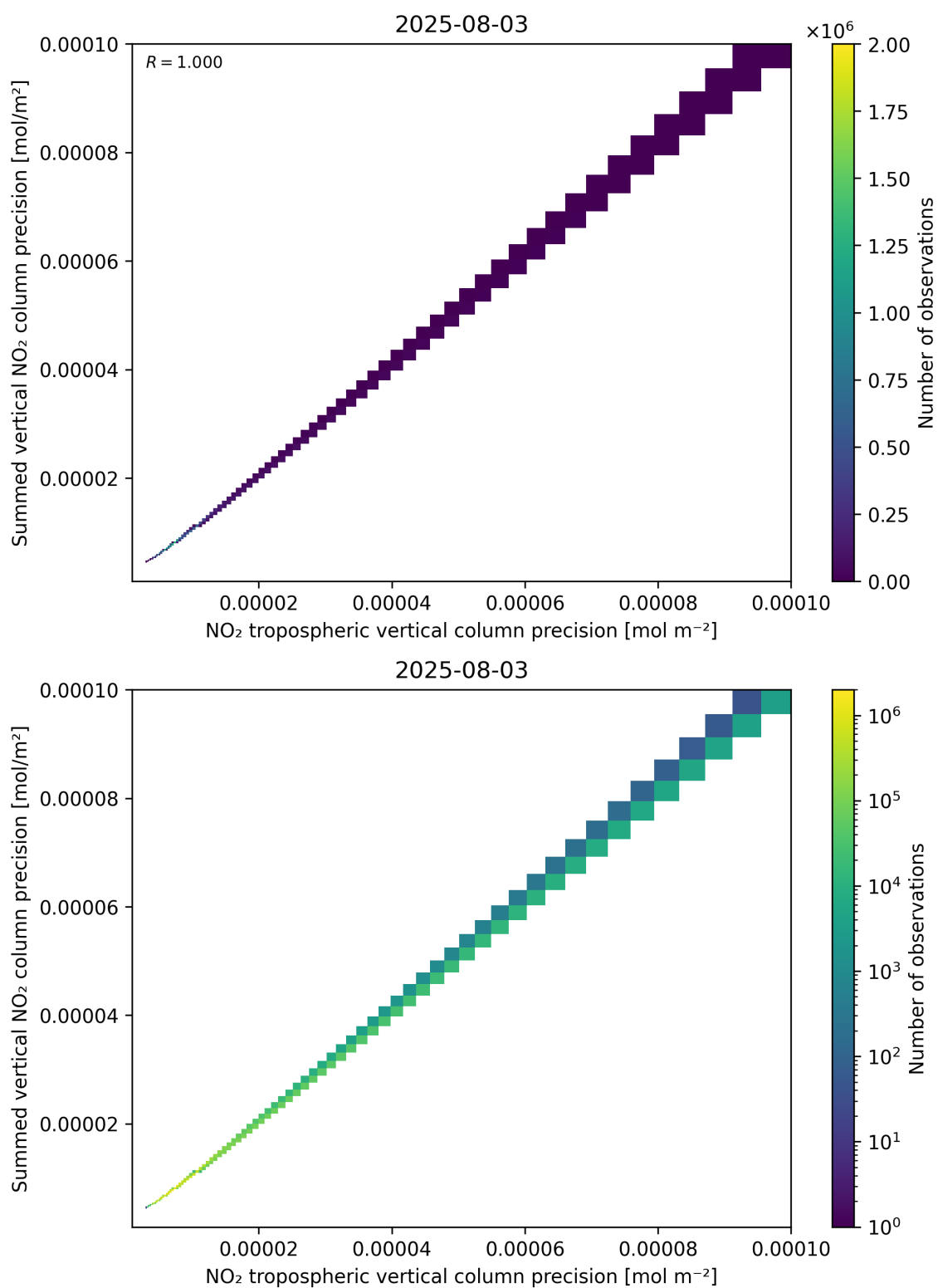
Figure 137: Scatter density plot of “NO 2 tropospheric vertical column precision” against “Summed vertical NO 2 column precision” for 2025-08-03 to 2025-08-04.
