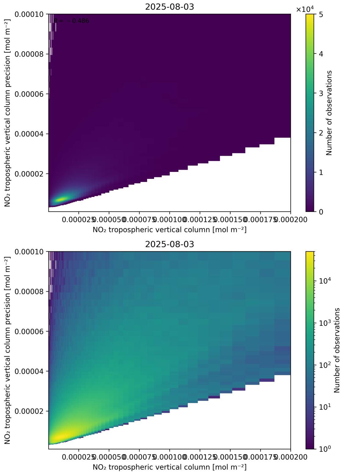
Figure 130: Scatter density plot of “NO 2 tropospheric vertical column” against “NO 2 tropospheric vertical column precision” for 2025-08-03 to 2025-08-04.
