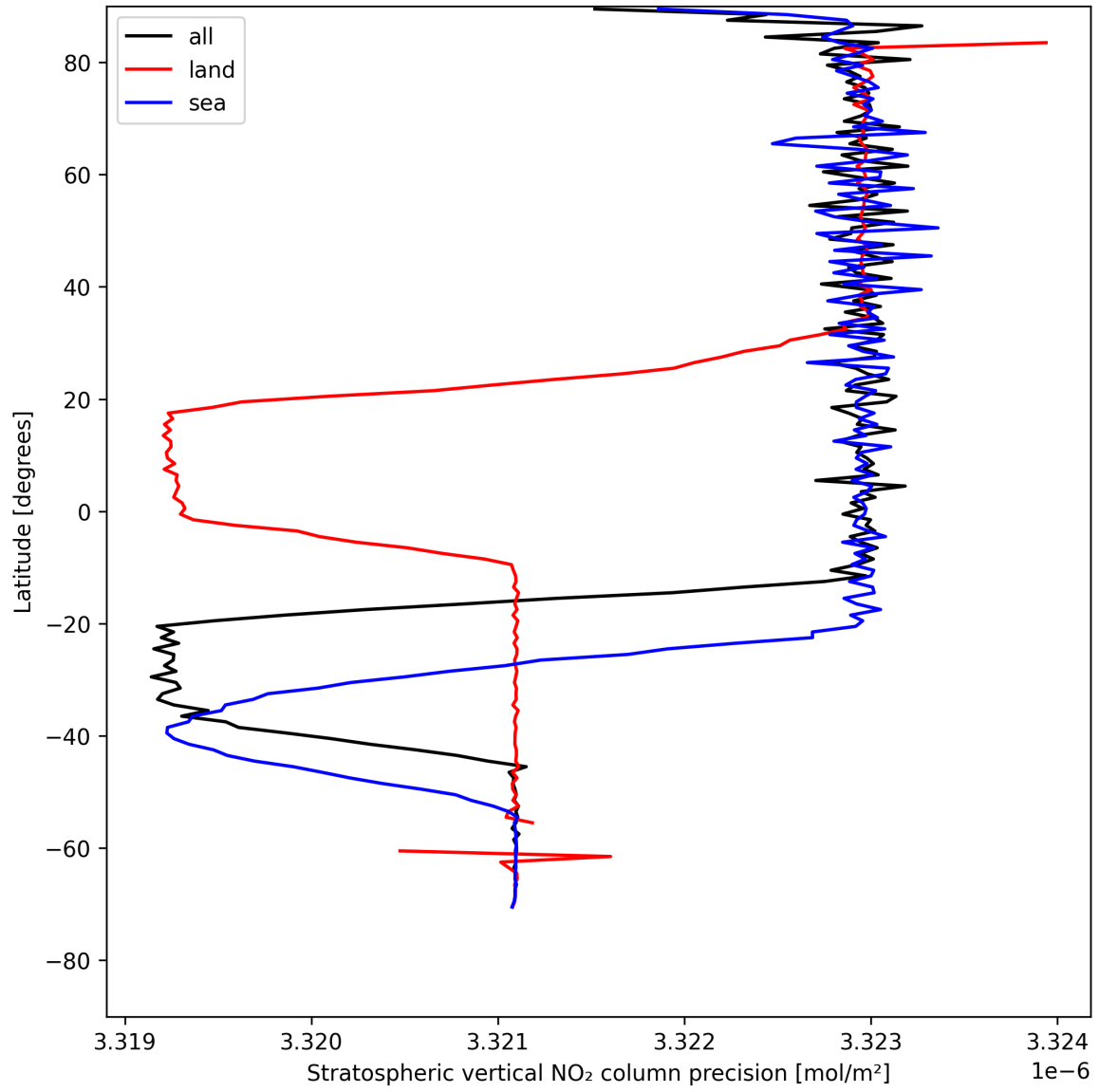
Figure 20: Zonal average of “Stratospheric vertical NO 2 column precision” for 2025-08-03 to 2025-08-04.
