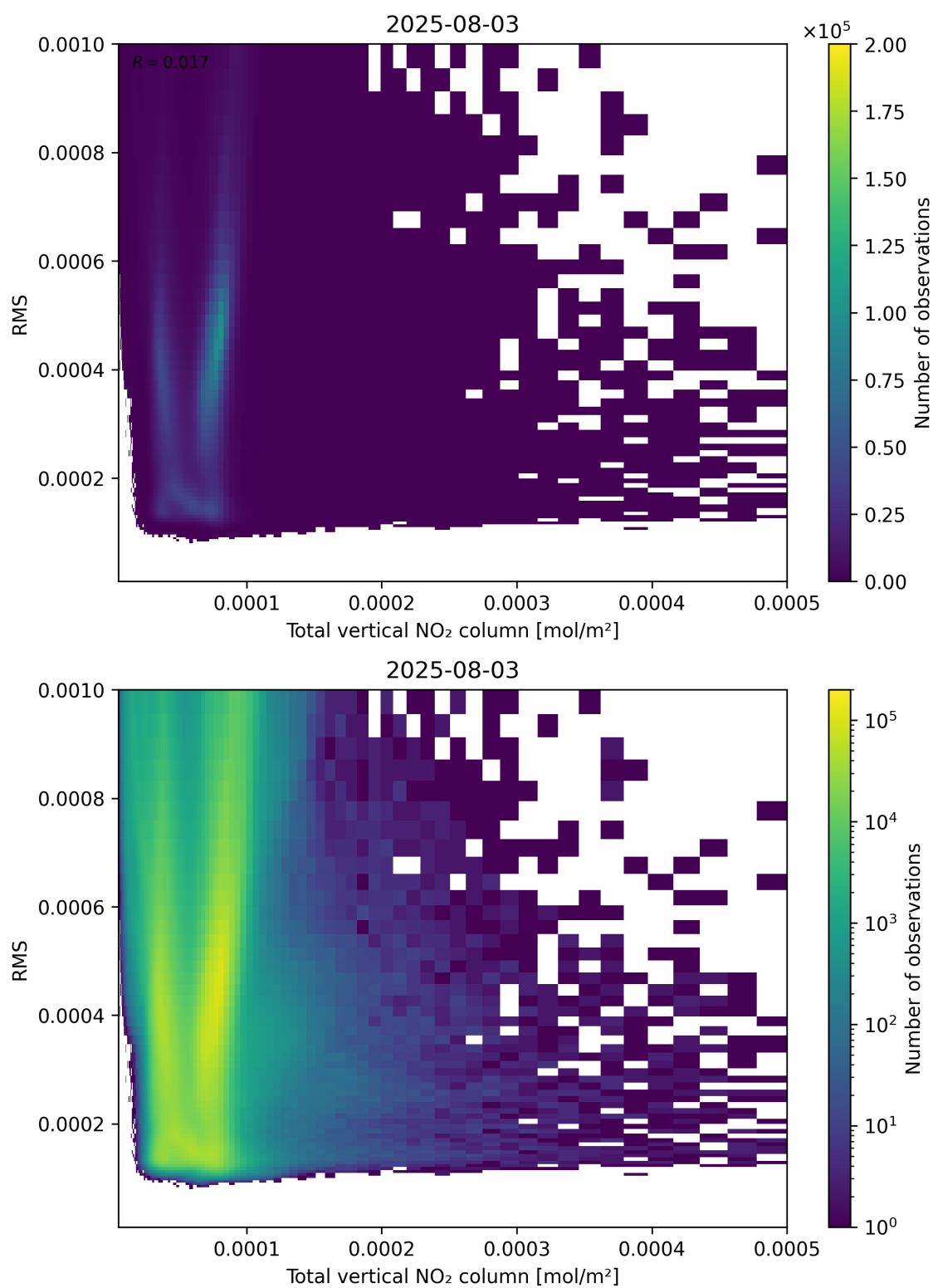
Figure 120: Scatter density plot of “Total vertical NO 2 column” against “RMS” for 2025-08-03 to 2025-08-04.
