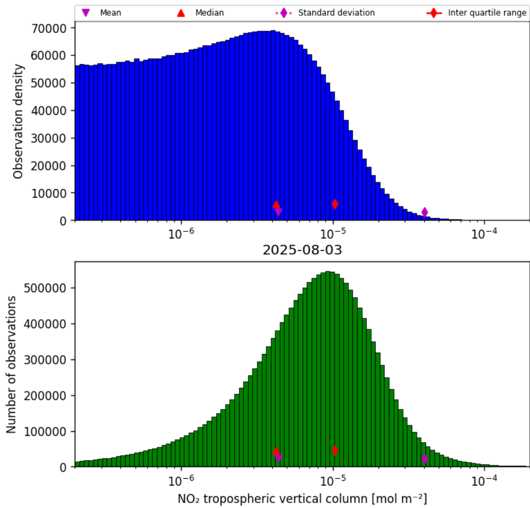
Figure 29: Histogram of “NO 2 tropospheric vertical column” for 2025-08-03 to 2025-08-04
