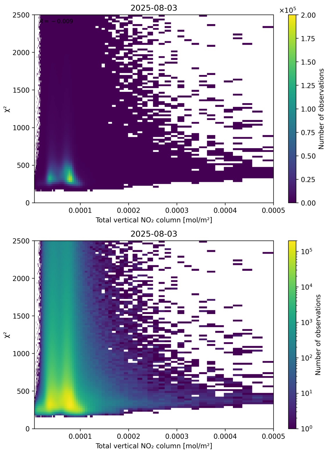
Figure 111: Scatter density plot of “Total vertical NO 2 column” against “ \chi^2 ” for 2025-08-03 to 2025-08-04.
