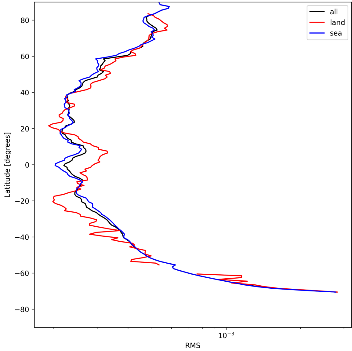
Figure 26: Zonal average of “RMS” for 2025-08-03 to 2025-08-04.
