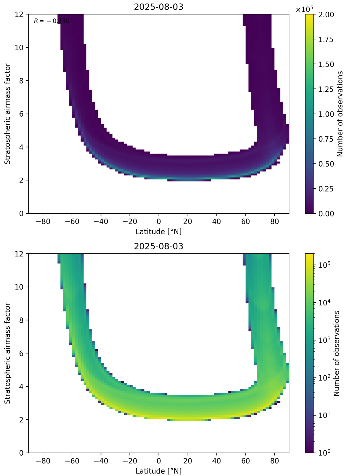
Figure 83: Scatter density plot of “Latitude” against “Stratospheric air mass factor” for 2025-08-03 to 2025-08-04.
