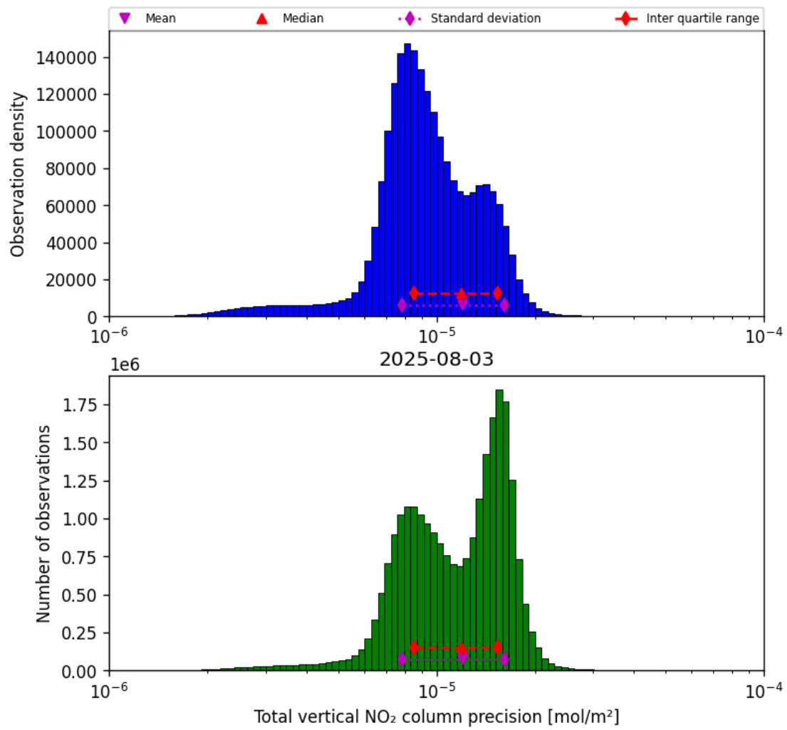
Figure 39: Histogram of “Total vertical NO 2 column precision” for 2025-08-03 to 2025-08-04
