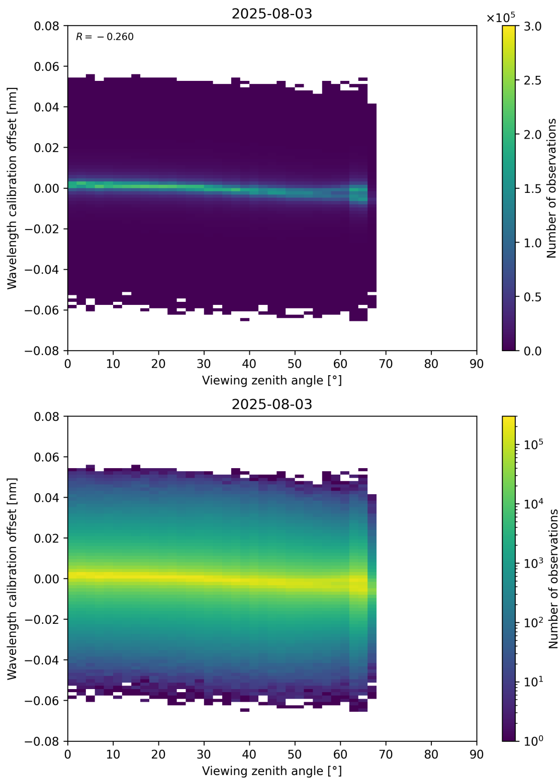
Figure 173: Scatter density plot of “Viewing zenith angle” against “Wavelength calibration offset” for 2025-08-03 to 2025-08-04.
