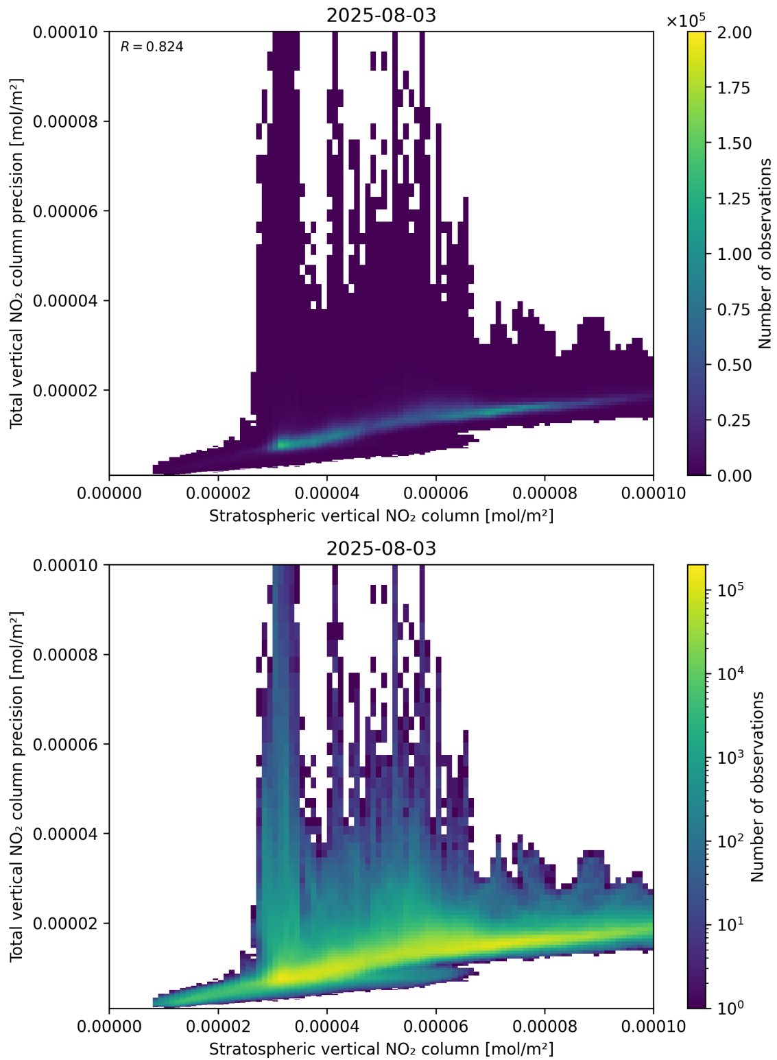
Figure 101: Scatter density plot of “Stratospheric vertical NO 2 column” against “Total vertical NO 2 column precision” for 2025-08-03 to 2025-08-04.
