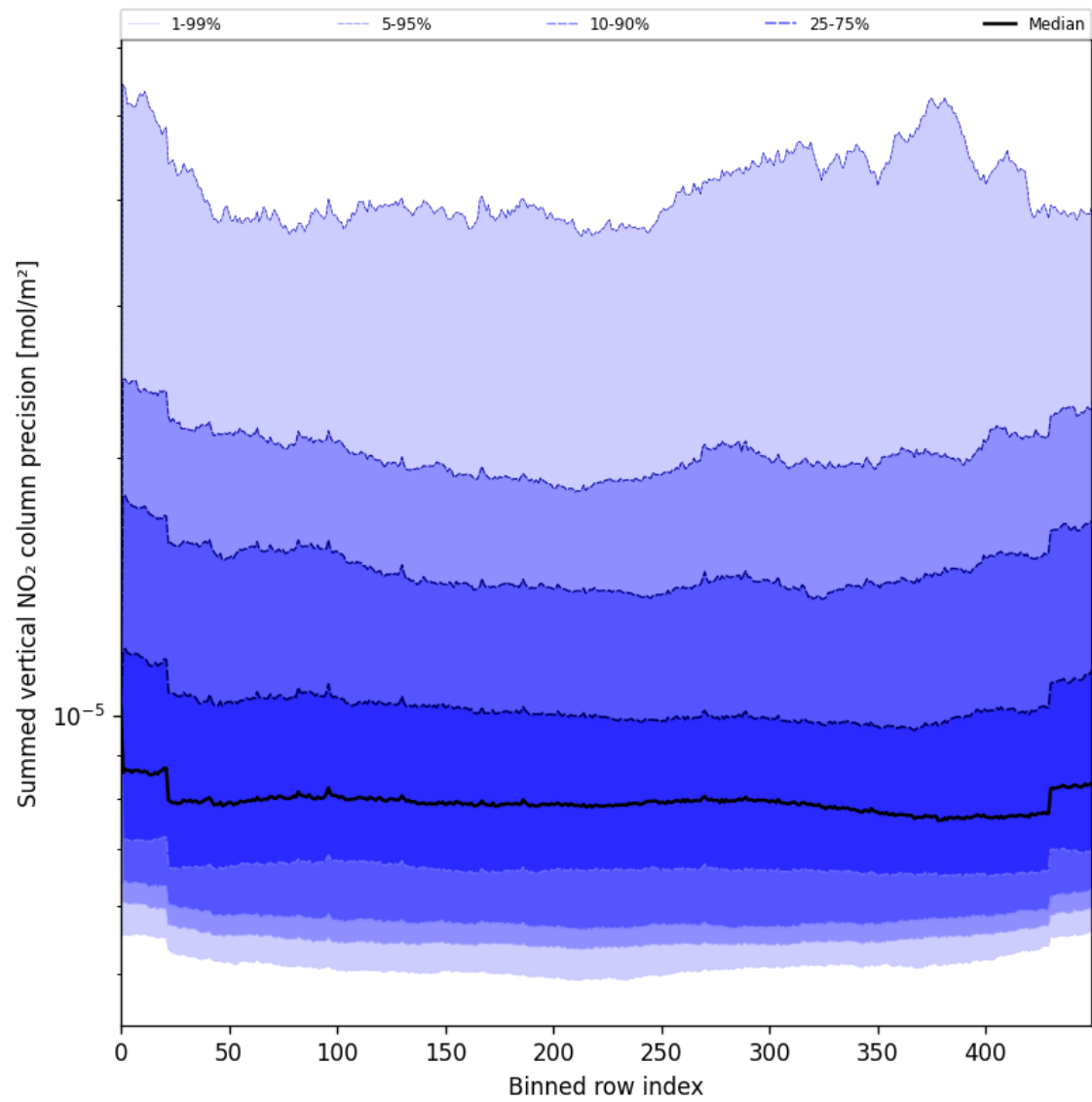
Figure 58: Along track statistics of “Summed vertical NO 2 column precision” for 2025-08-03 to 2025-08-04
