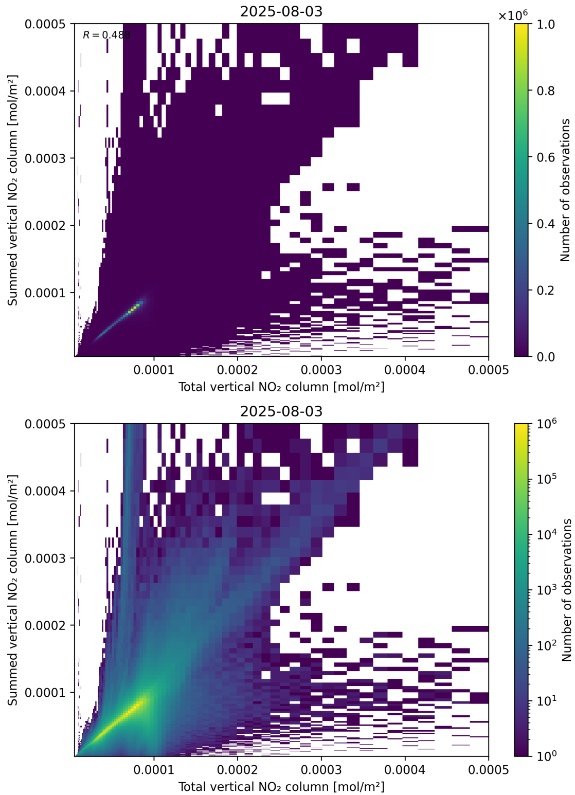
Figure 112: Scatter density plot of “Total vertical NO 2 column” against “Summed vertical NO 2 column” for 2025-08-03 to 2025-08-04.
