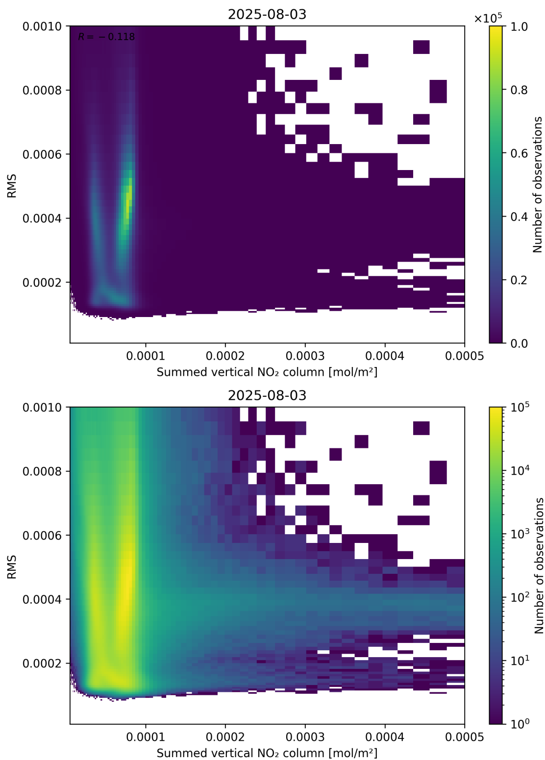
Figure 109: Scatter density plot of “Summed vertical NO 2 column” against “RMS” for 2025-08-03 to 2025-08-04.
