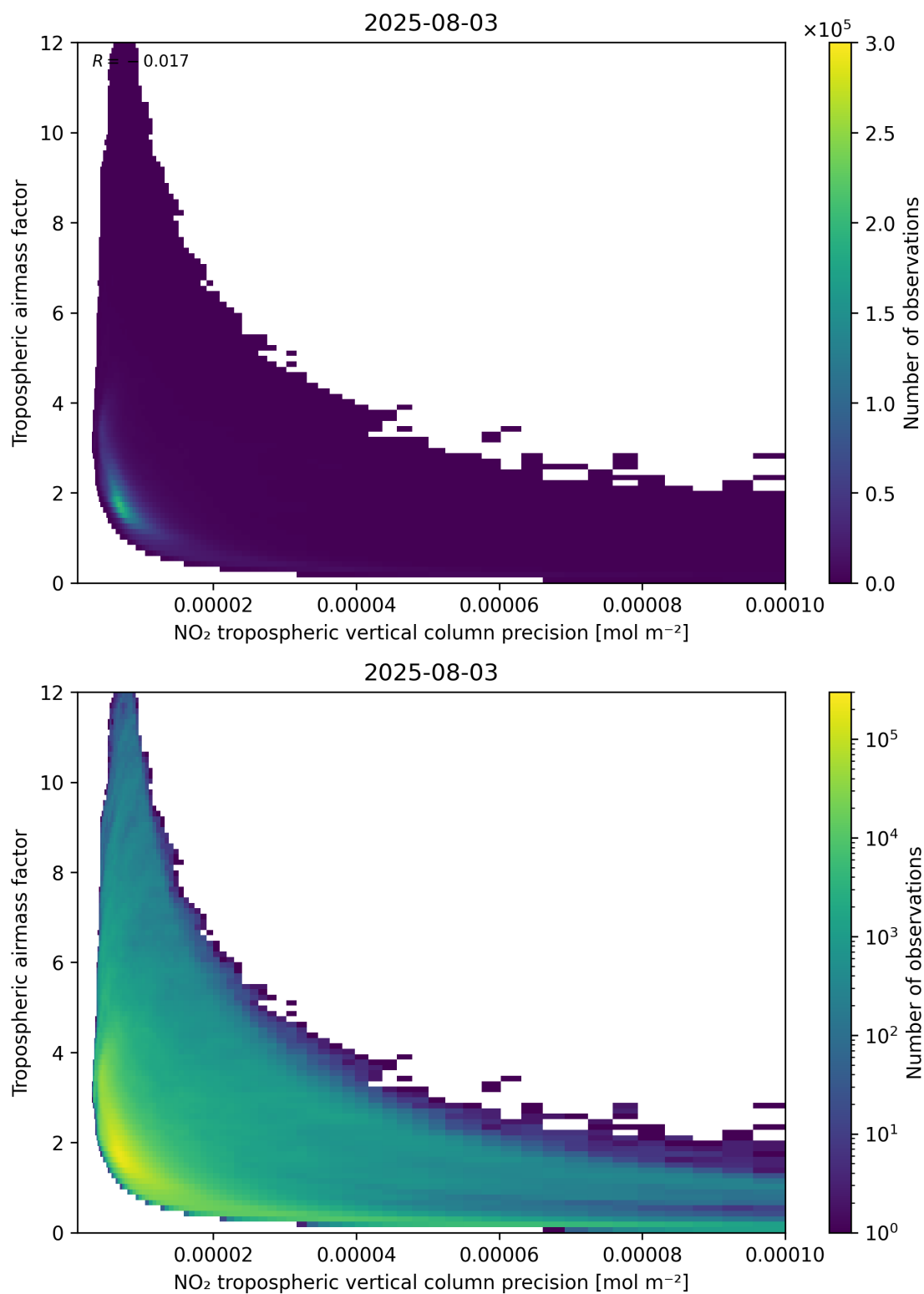
Figure 133: Scatter density plot of “NO 2 tropospheric vertical column precision” against “Tropospheric airmass factor” for 2025-08-03 to 2025-08-04.
