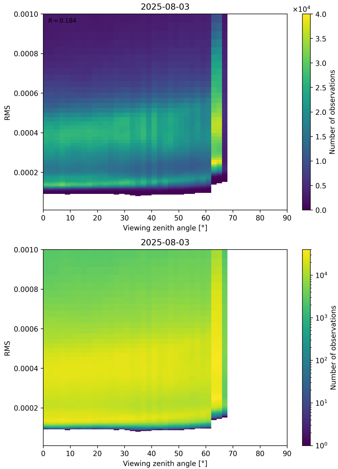
Figure 171: Scatter density plot of “Viewing zenith angle” against “RMS” for 2025-08-03 to 2025-08-04.
