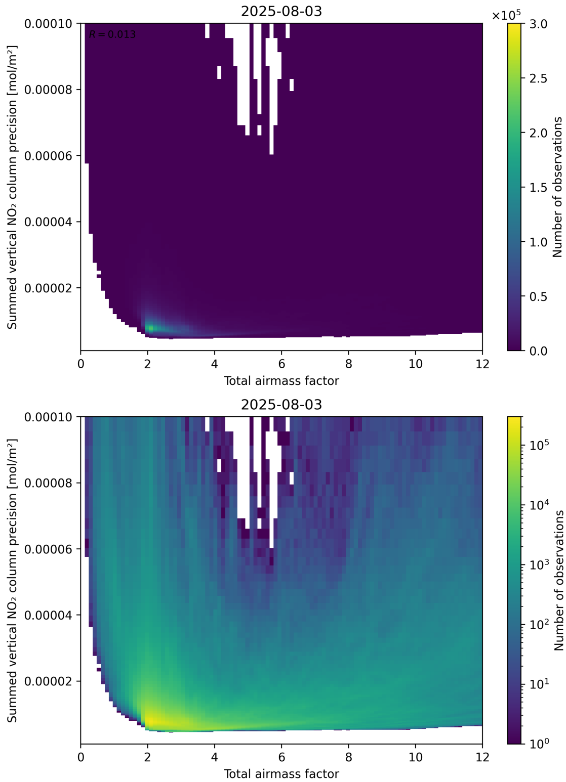
Figure 66: Scatter density plot of “Total airmass factor” against “Summed vertical NO 2 column precision” for 2025-08-03 to 2025-08-04.
