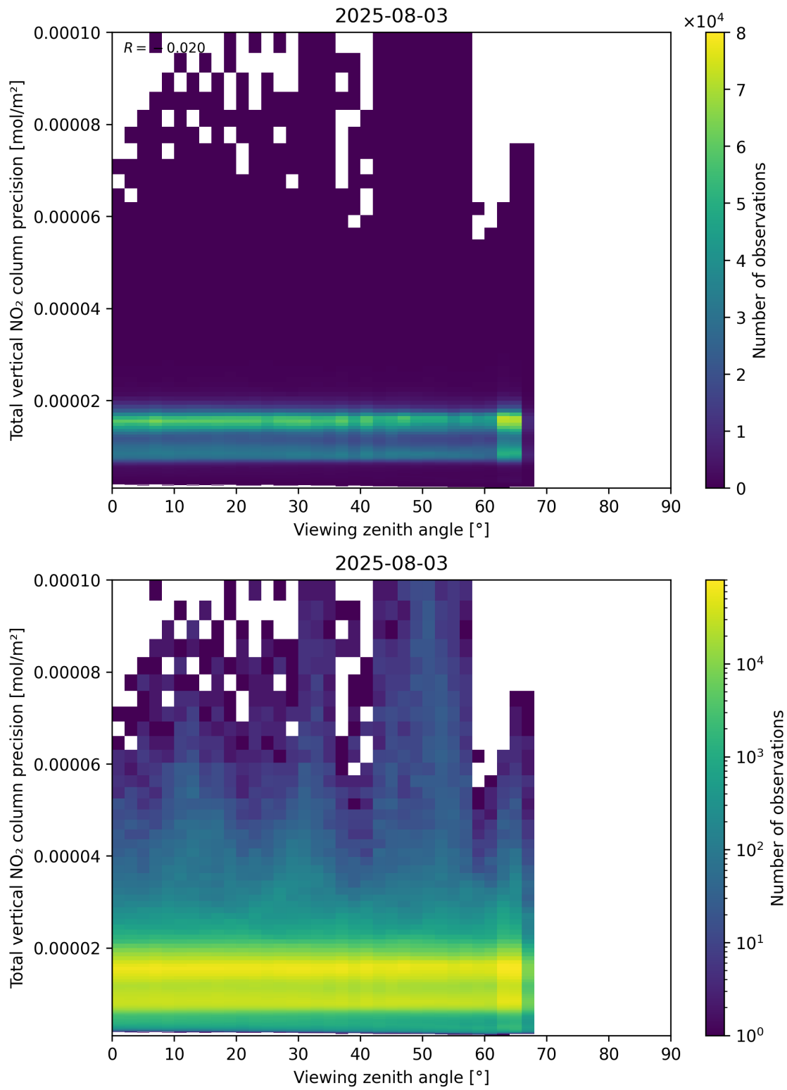
Figure 168: Scatter density plot of “Viewing zenith angle” against “Total vertical NO 2 column precision” for 2025-08-03 to 2025-08-04.
