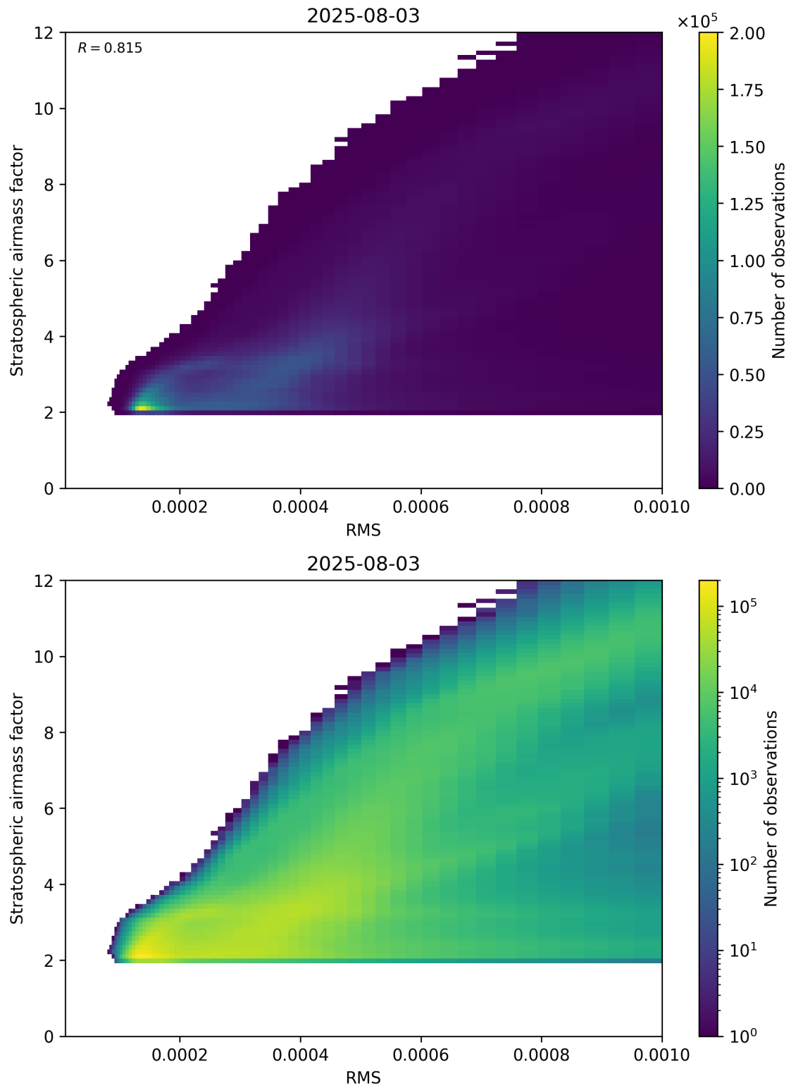
Figure 144: Scatter density plot of “RMS” against “Stratospheric airmass factor” for 2025-08-03 to 2025-08-04.
