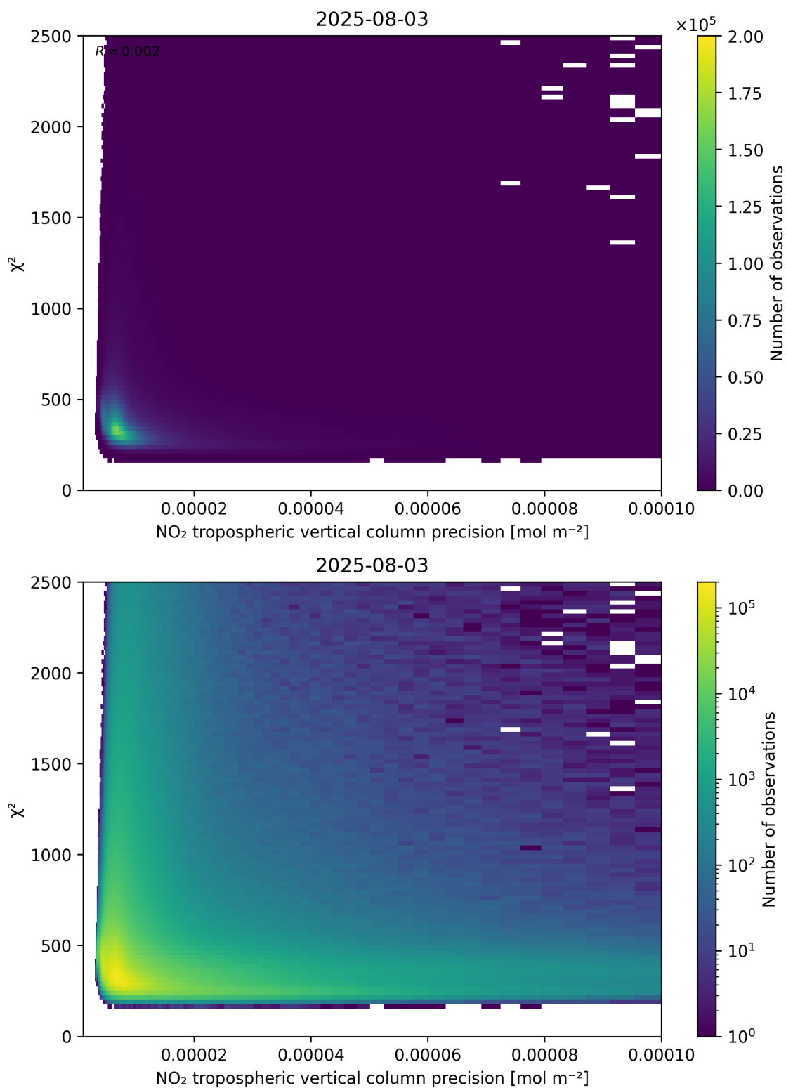
Figure 134: Scatter density plot of “NO 2 tropospheric vertical column precision” against “ \chi^2 ” for 2025-08-03 to 2025-08-04.
