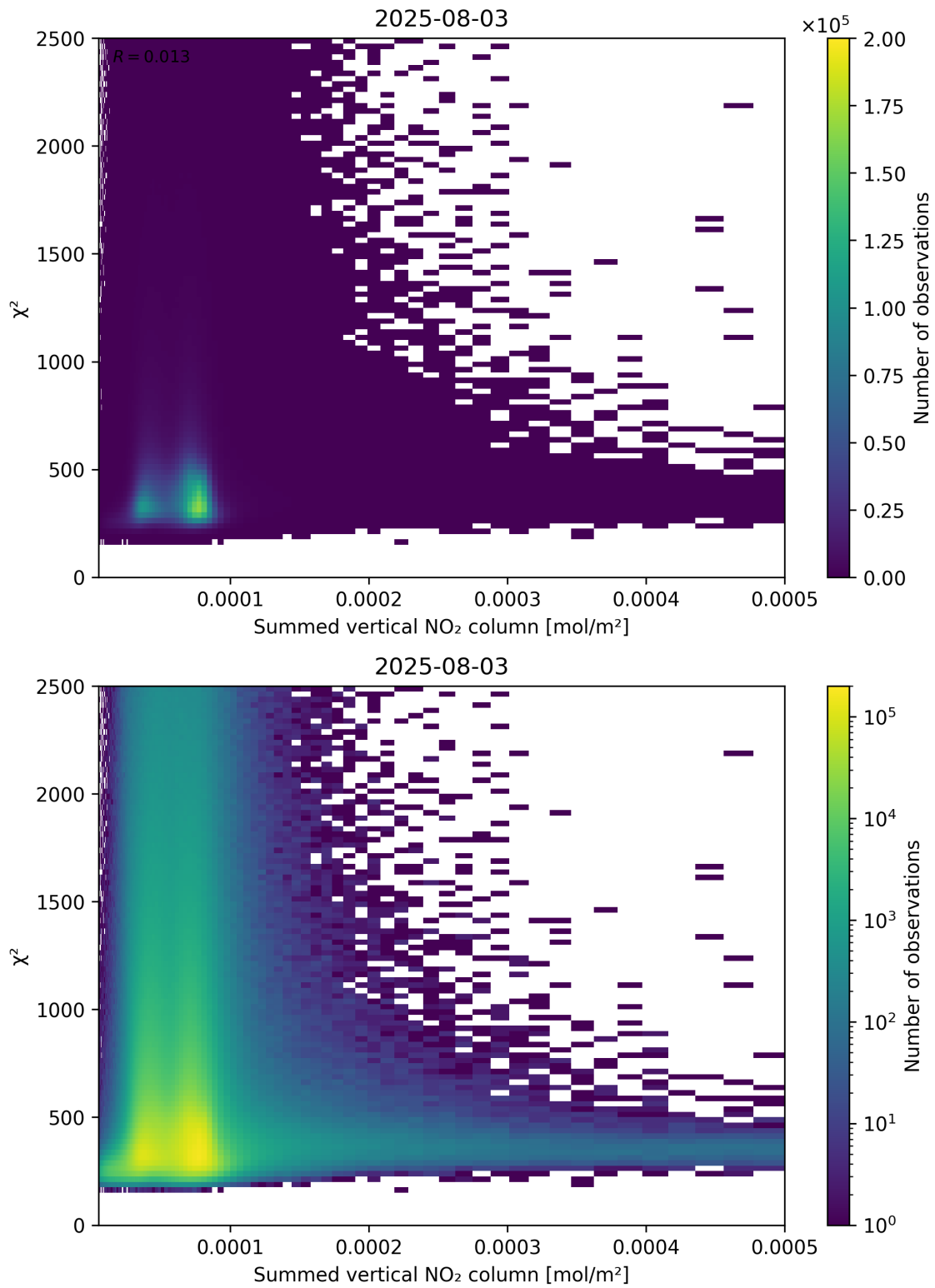
Figure 104: Scatter density plot of “Summed vertical NO 2 column” against “ \chi^2 ” for 2025-08-03 to 2025-08-04.
