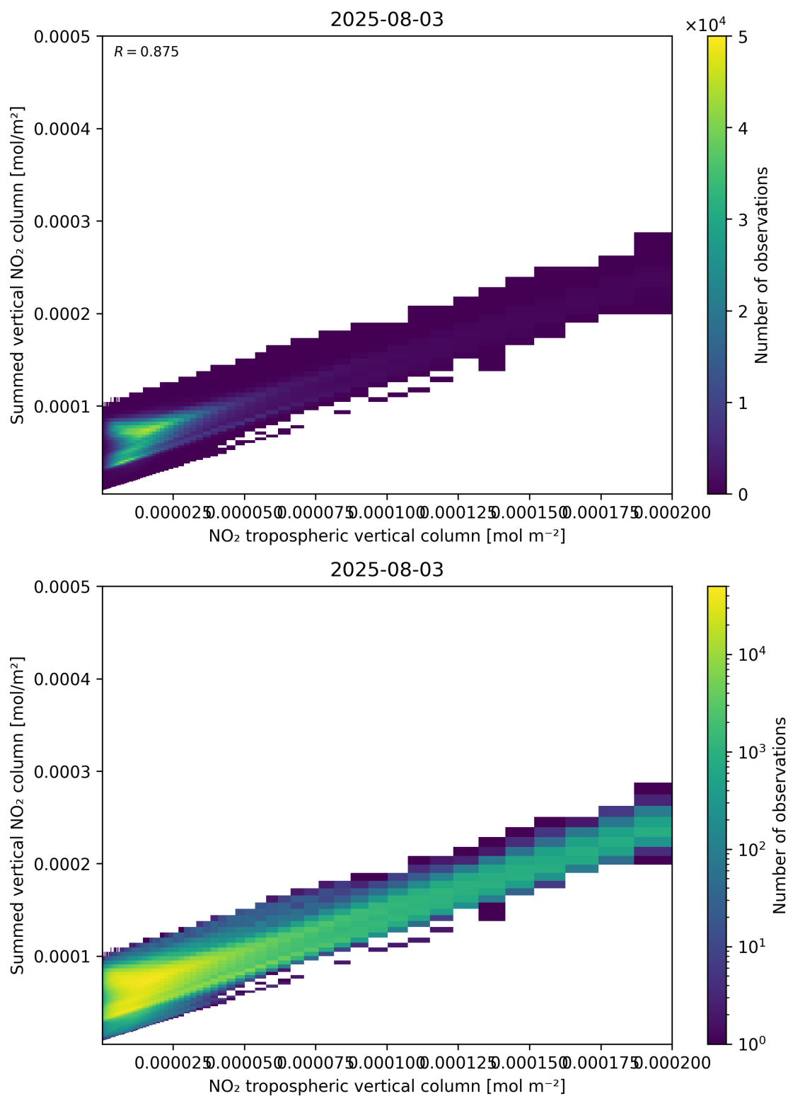
Figure 126: Scatter density plot of “NO 2 tropospheric vertical column” against “Summed vertical NO 2 column” for 2025-08-03 to 2025-08-04.
