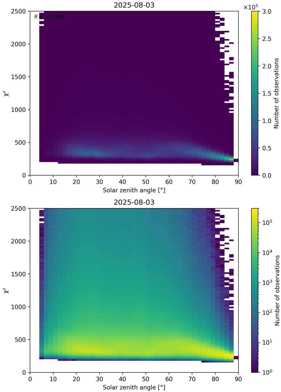
Figure 148: Scatter density plot of “Solar zenith angle” against “ \chi^2 ” for 2025-08-03 to 2025-08-04.
