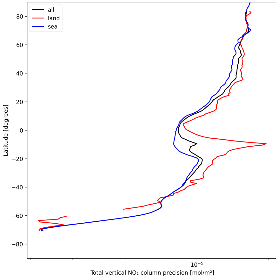
Figure 22: Zonal average of “Total vertical NO 2 column precision” for 2025-08-03 to 2025-08-04.
