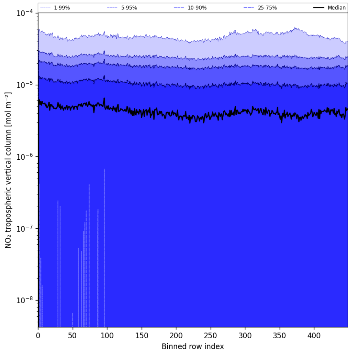
Figure 46: Along track statistics of “NO 2 tropospheric vertical column” for 2025-08-03 to 2025-08-04
