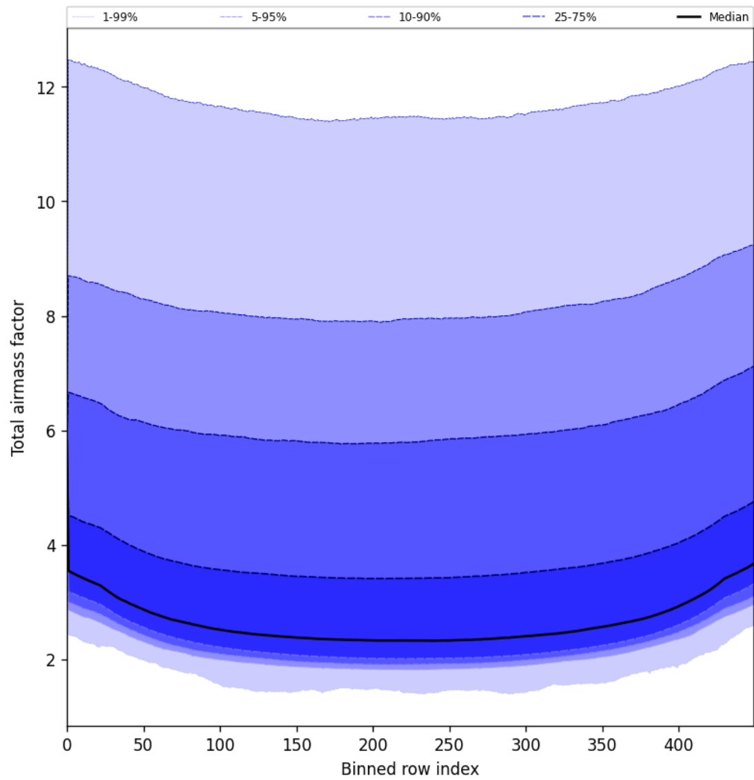
Figure 49: Along track statistics of “Total airmass factor” for 2025-08-03 to 2025-08-04
