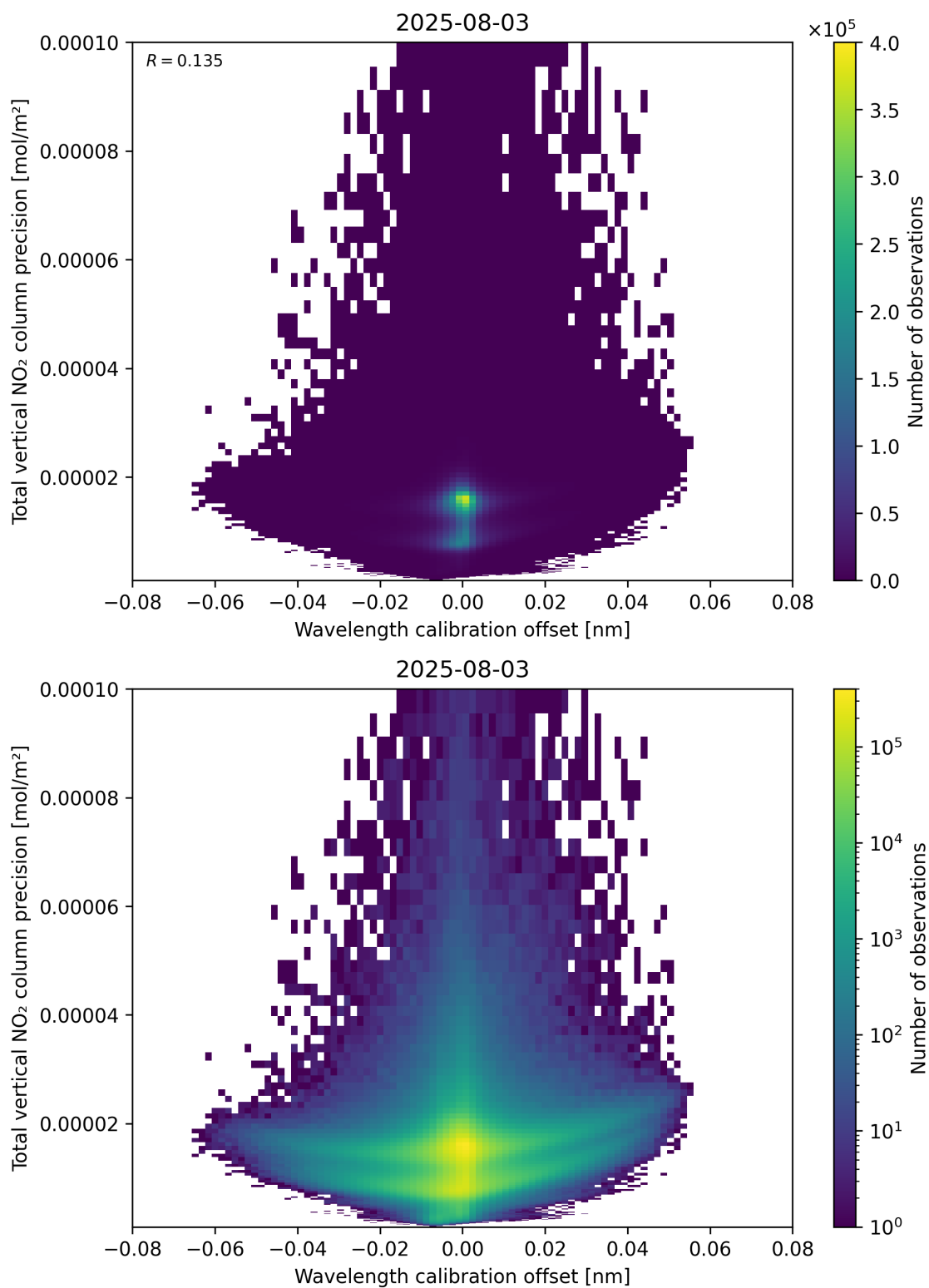
Figure 180: Scatter density plot of “Wavelength calibration offset” against “Total vertical NO 2 column precision” for 2025-08-03 to 2025-08-04.
