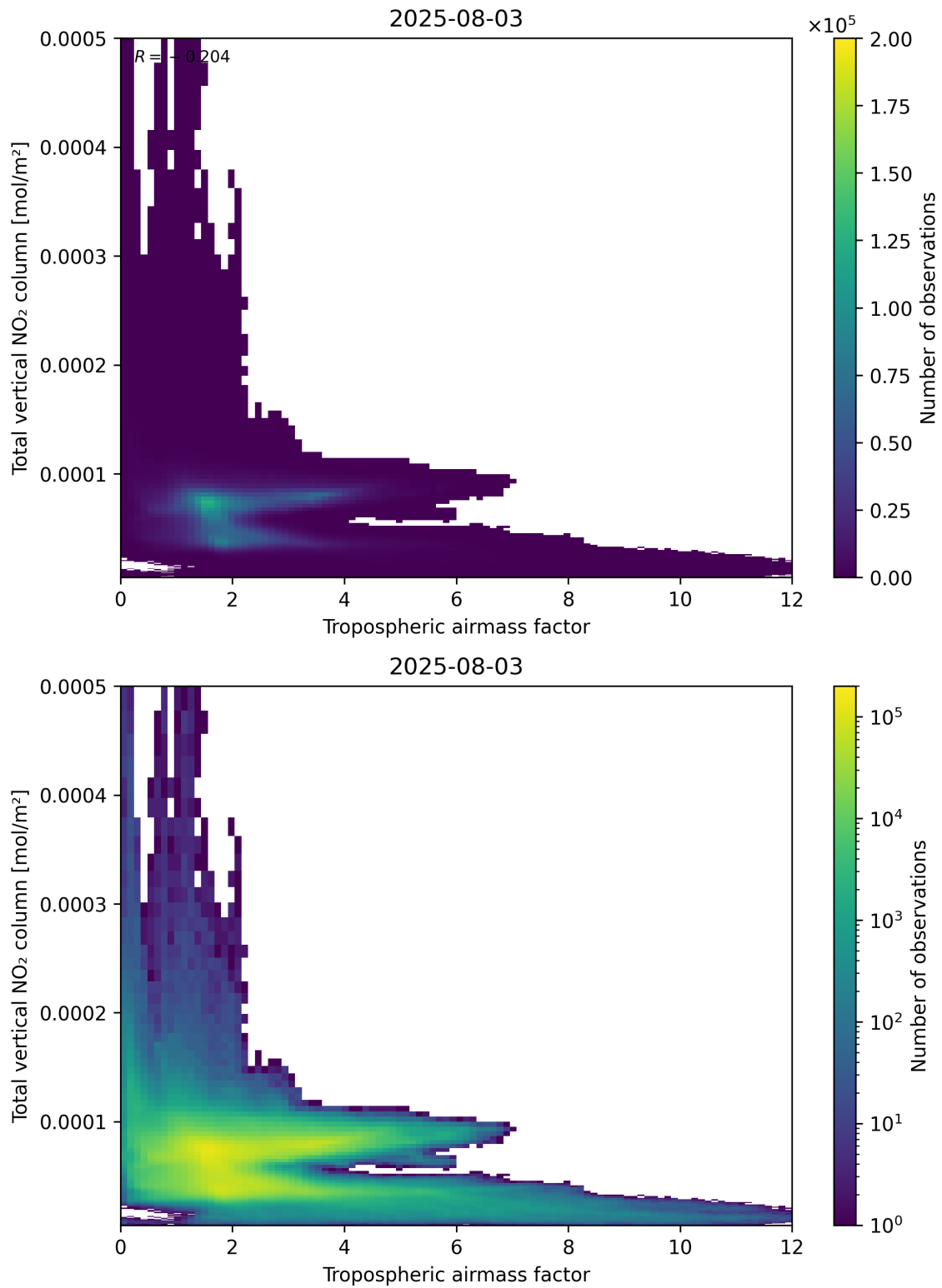
Figure 77: Scatter density plot of “Tropospheric airmass factor” against “Total vertical NO 2 column” for 2025-08-03 to 2025-08-04.
