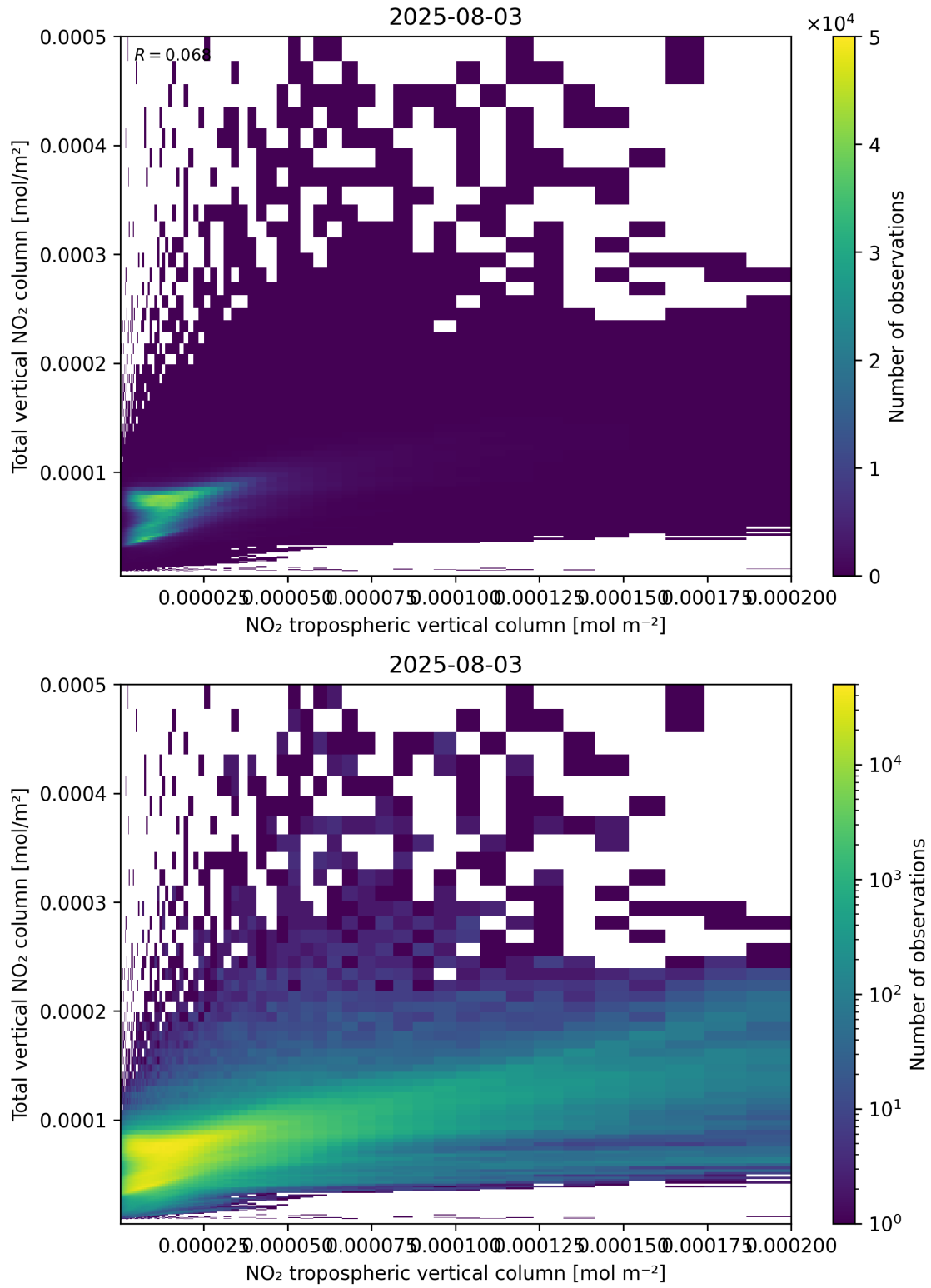
Figure 128: Scatter density plot of “NO 2 tropospheric vertical column” against “Total vertical NO 2 column” for 2025-08-03 to 2025-08-04.
