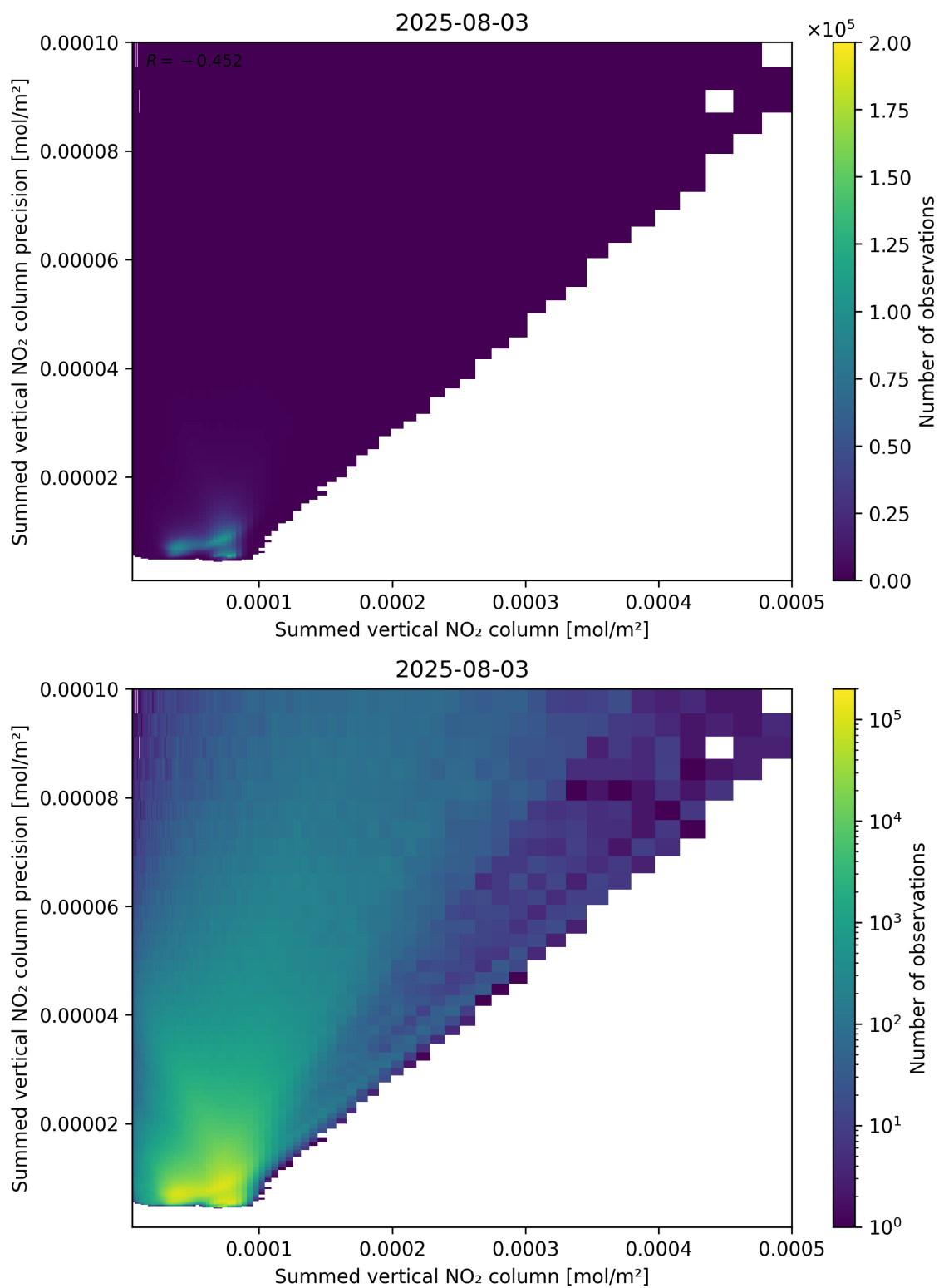
Figure 105: Scatter density plot of “Summed vertical NO 2 column” against “Summed vertical NO 2 column precision” for 2025-08-03 to 2025-08-04.
