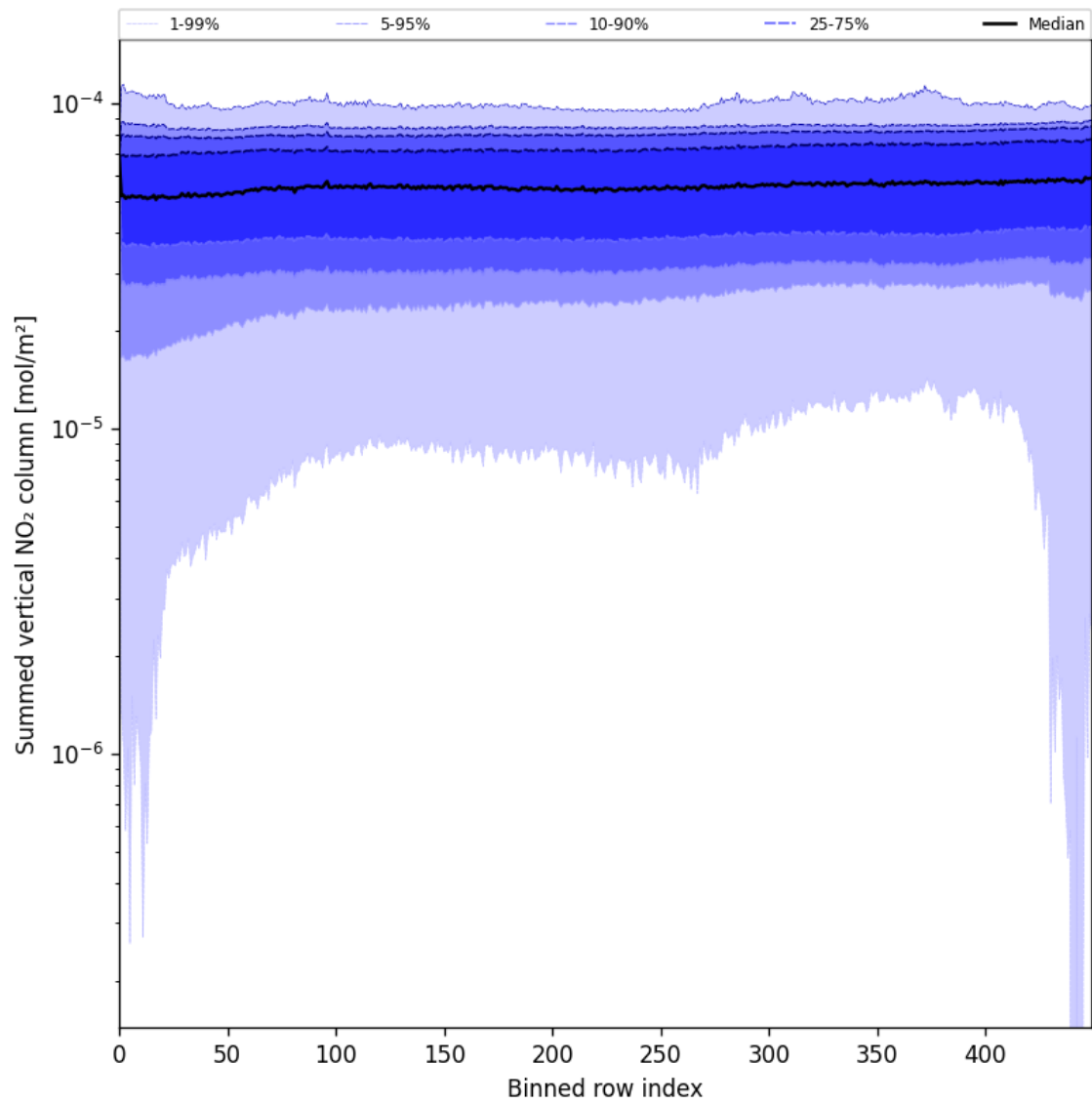
Figure 57: Along track statistics of “Summed vertical NO 2 column” for 2025-08-03 to 2025-08-04
