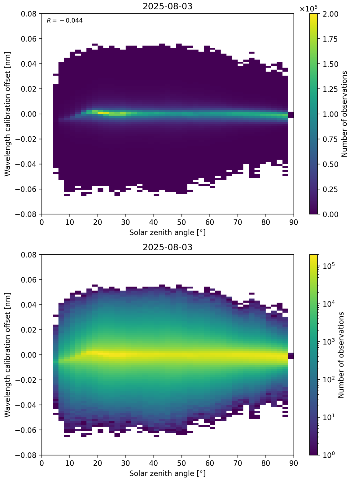
Figure 158: Scatter density plot of “Solar zenith angle” against “Wavelength calibration offset” for 2025-08-03 to 2025-08-04.
