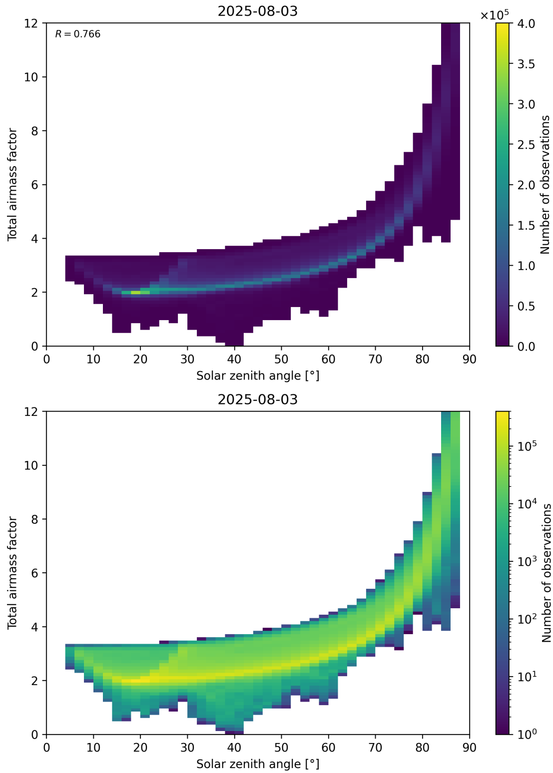
Figure 146: Scatter density plot of “Solar zenith angle” against “Total air mass factor” for 2025-08-03 to 2025-08-04.
