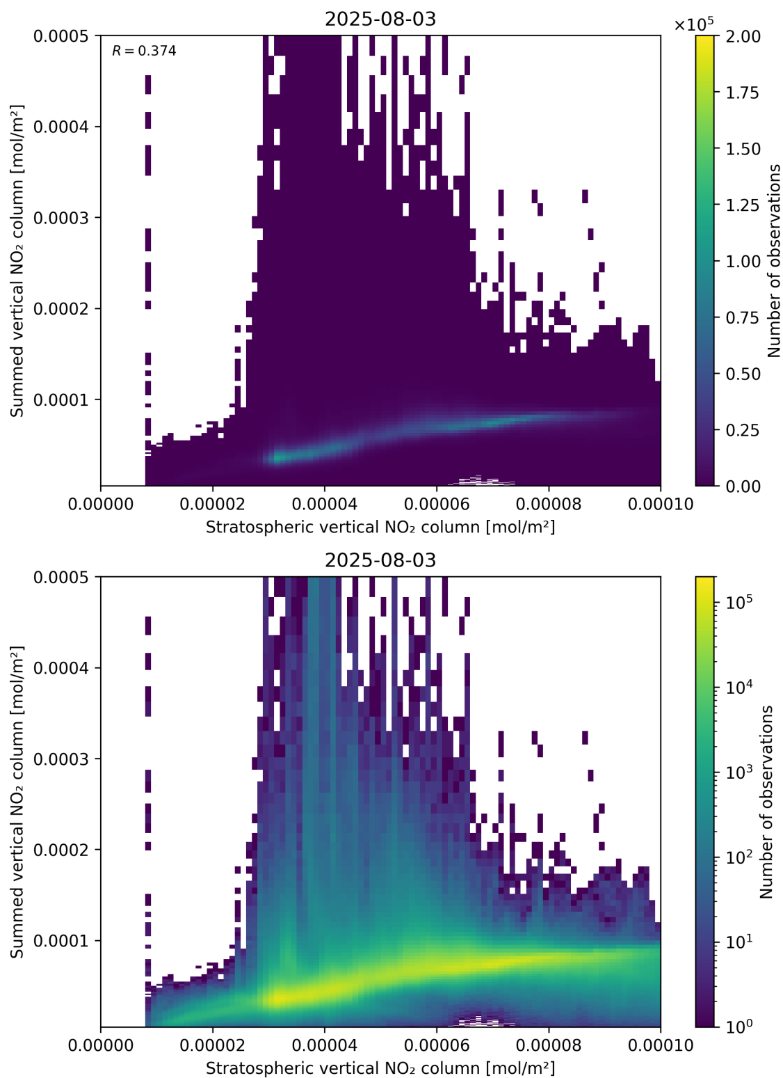
Figure 98: Scatter density plot of “Stratospheric vertical NO 2 column” against “Summed vertical NO 2 column” for 2025-08-03 to 2025-08-04.
