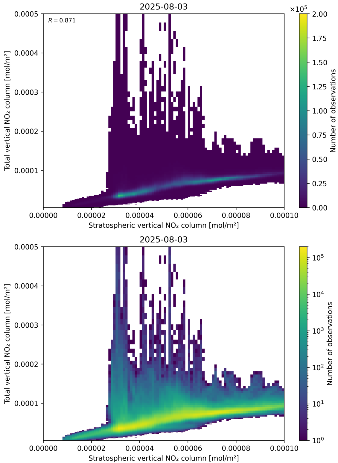
Figure 100: Scatter density plot of “Stratospheric vertical NO 2 column” against “Total vertical NO 2 column” for 2025-08-03 to 2025-08-04.
