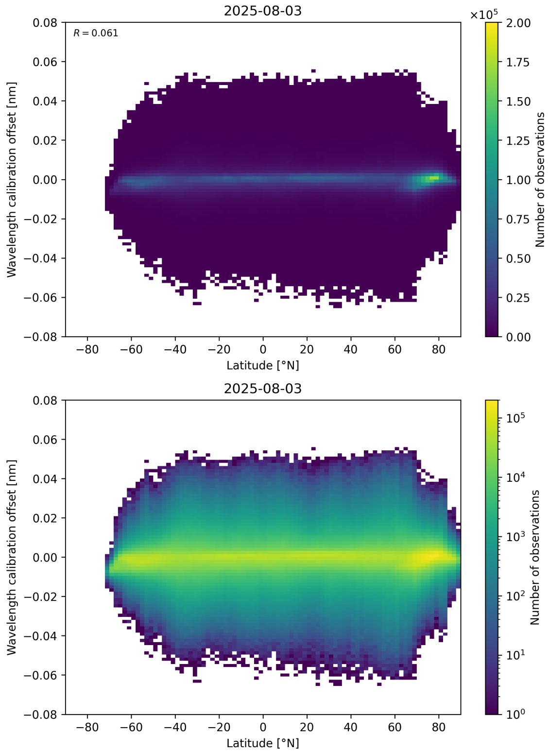
Figure 95: Scatter density plot of “Latitude” against “Wavelength calibration offset” for 2025-08-03 to 2025-08-04.
