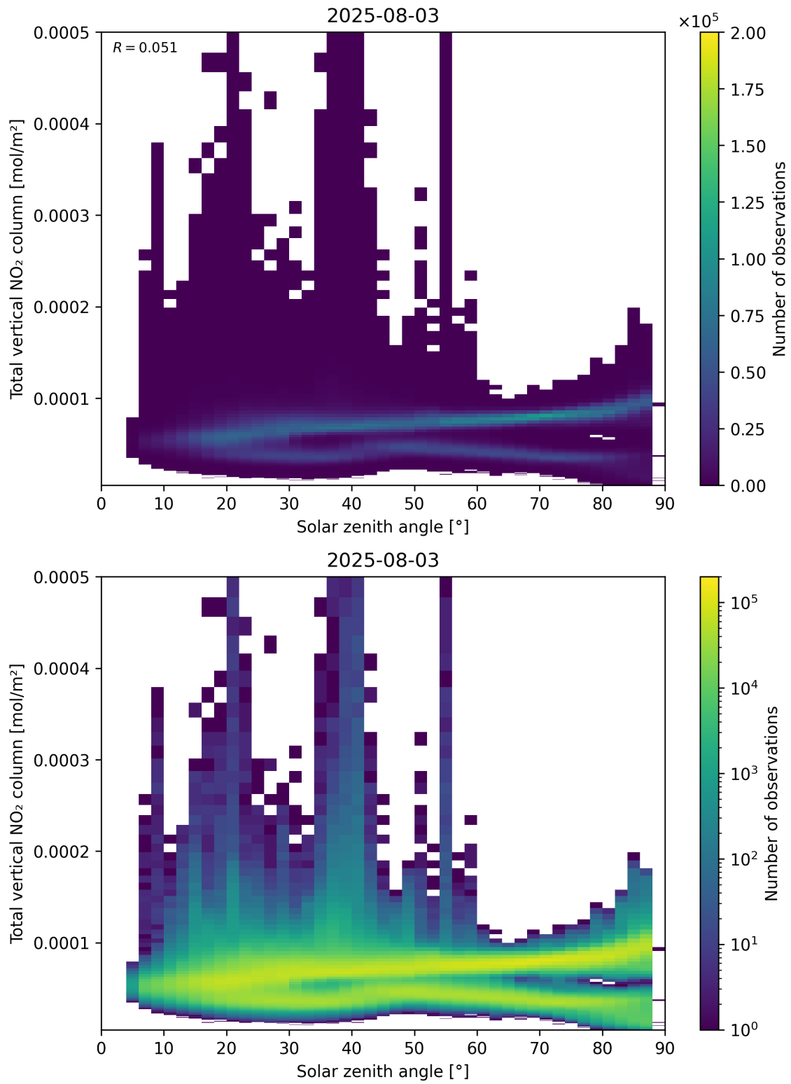
Figure 153: Scatter density plot of “Solar zenith angle” against “Total vertical \text{NO}_2 column” for 2025-08-03 to 2025-08-04.
