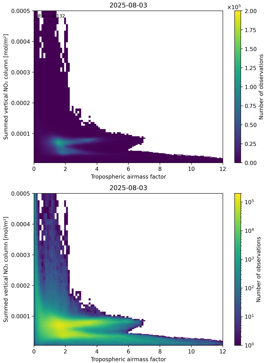
Figure 75: Scatter density plot of “Tropospheric air mass factor” against “Summed vertical NO 2 column” for 2025-08-03 to 2025-08-04.
