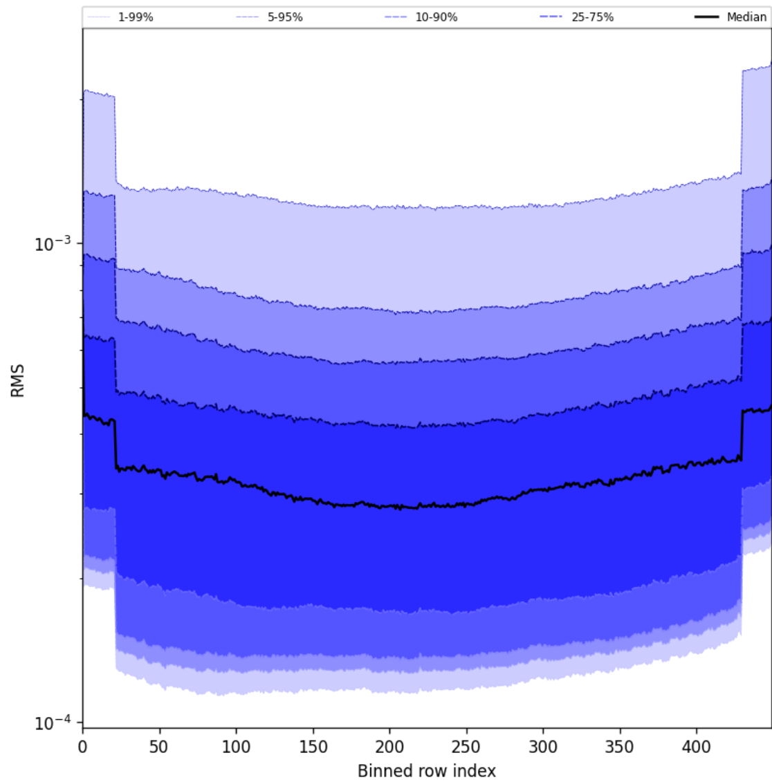
Figure 60: Along track statistics of “RMS” for 2025-08-03 to 2025-08-04
