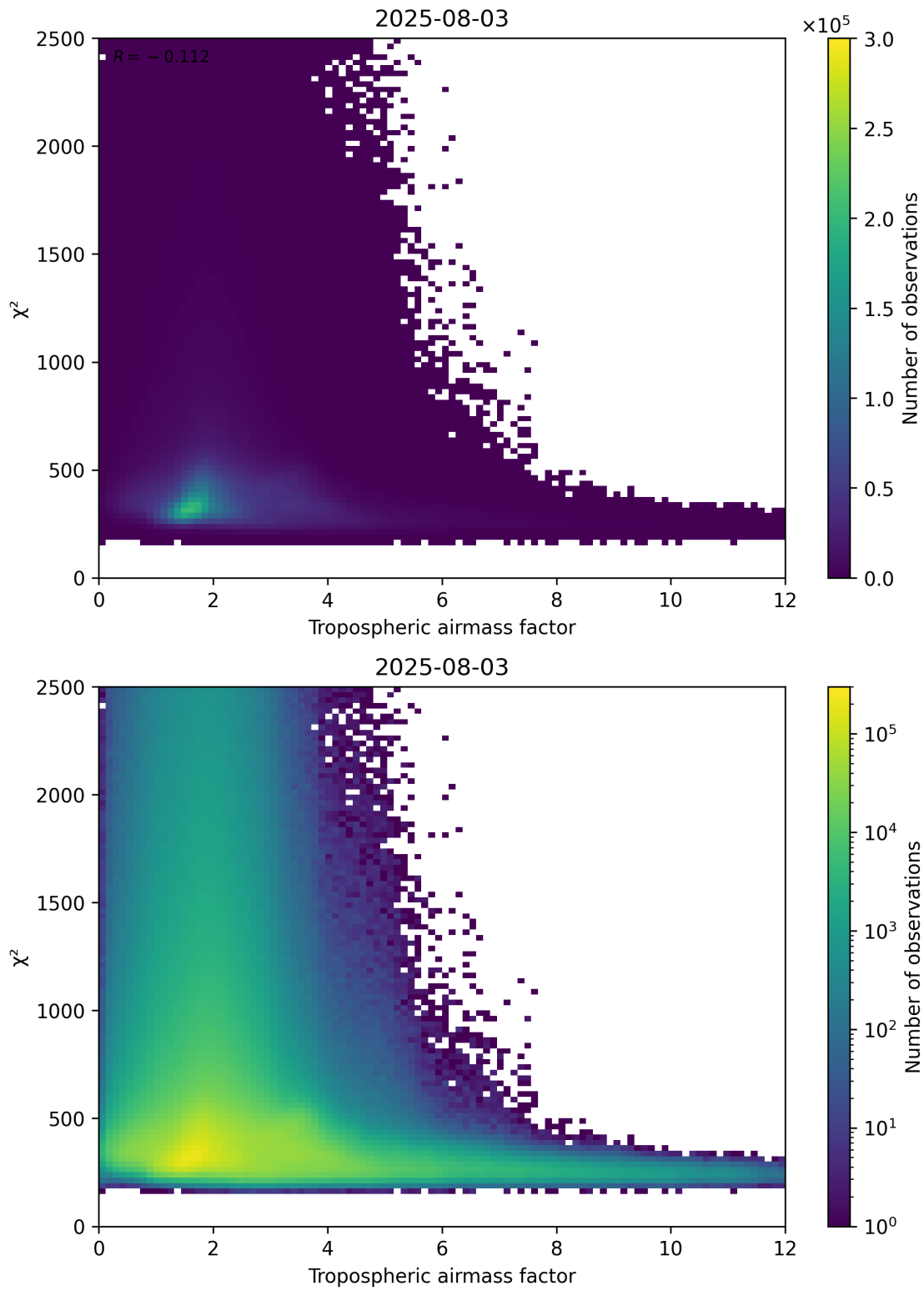
Figure 73: Scatter density plot of “Tropospheric airmass factor” against “ \chi^2 ” for 2025-08-03 to 2025-08-04.
