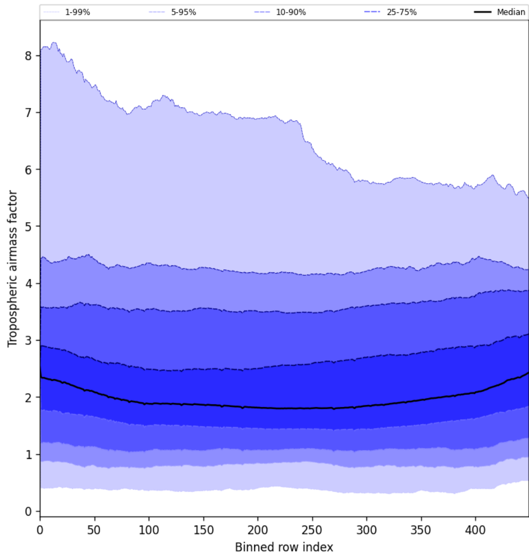
Figure 48: Along track statistics of “Tropospheric air mass factor” for 2025-08-03 to 2025-08-04
