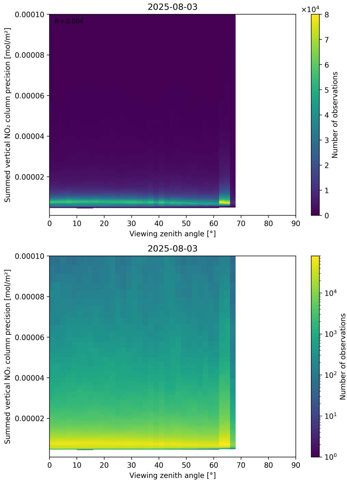
Figure 166: Scatter density plot of “Viewing zenith angle” against “Summed vertical NO 2 column precision” for 2025-08-03 to 2025-08-04.
