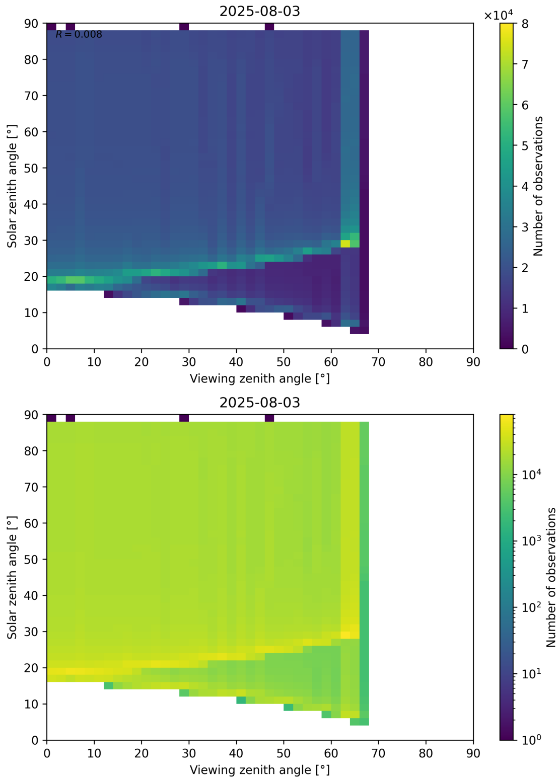
Figure 172: Scatter density plot of “Viewing zenith angle” against “Solar zenith angle” for 2025-08-03 to 2025-08-04.
