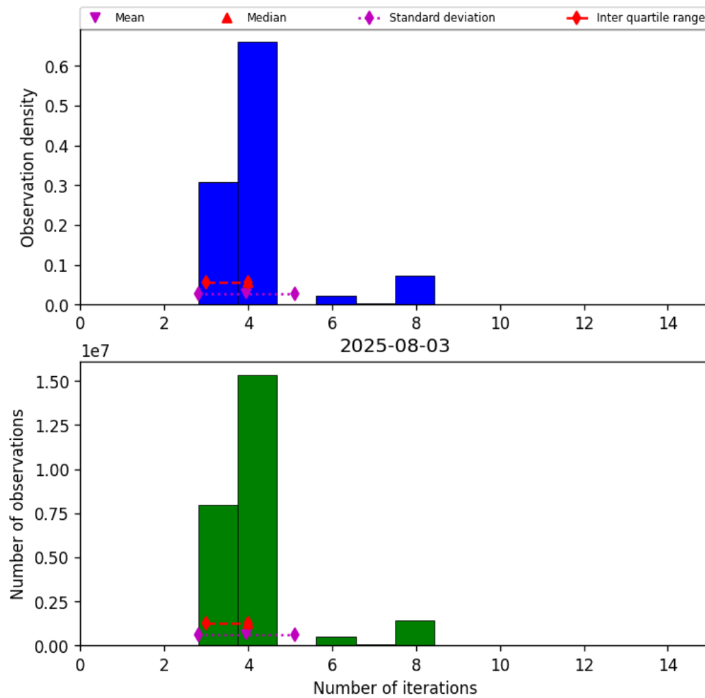
Figure 34: Histogram of “Number of iterations” for 2025-08-03 to 2025-08-04
