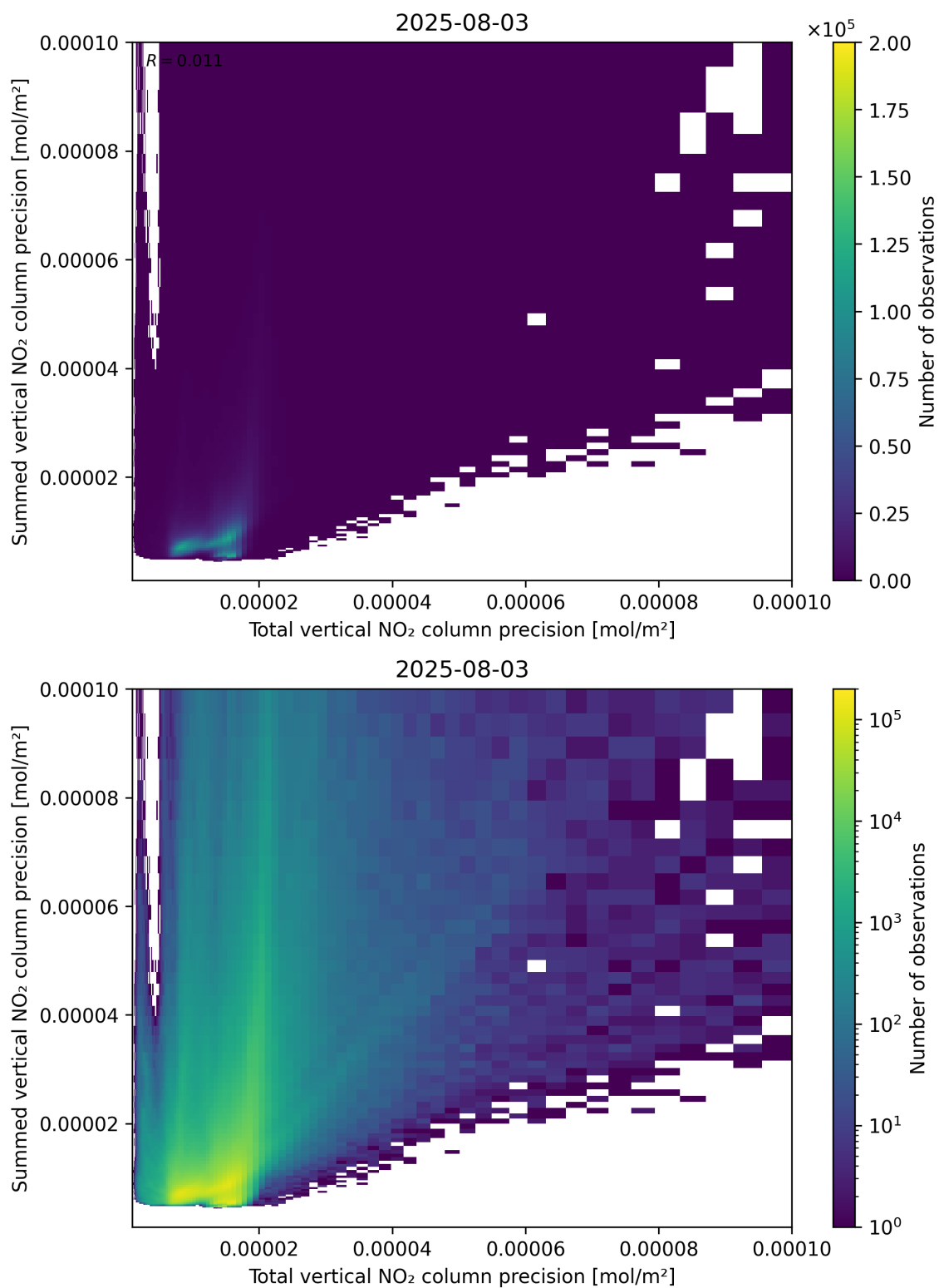
Figure 118: Scatter density plot of “Total vertical NO 2 column precision” against “Summed vertical NO 2 column precision” for 2025-08-03 to 2025-08-04.
