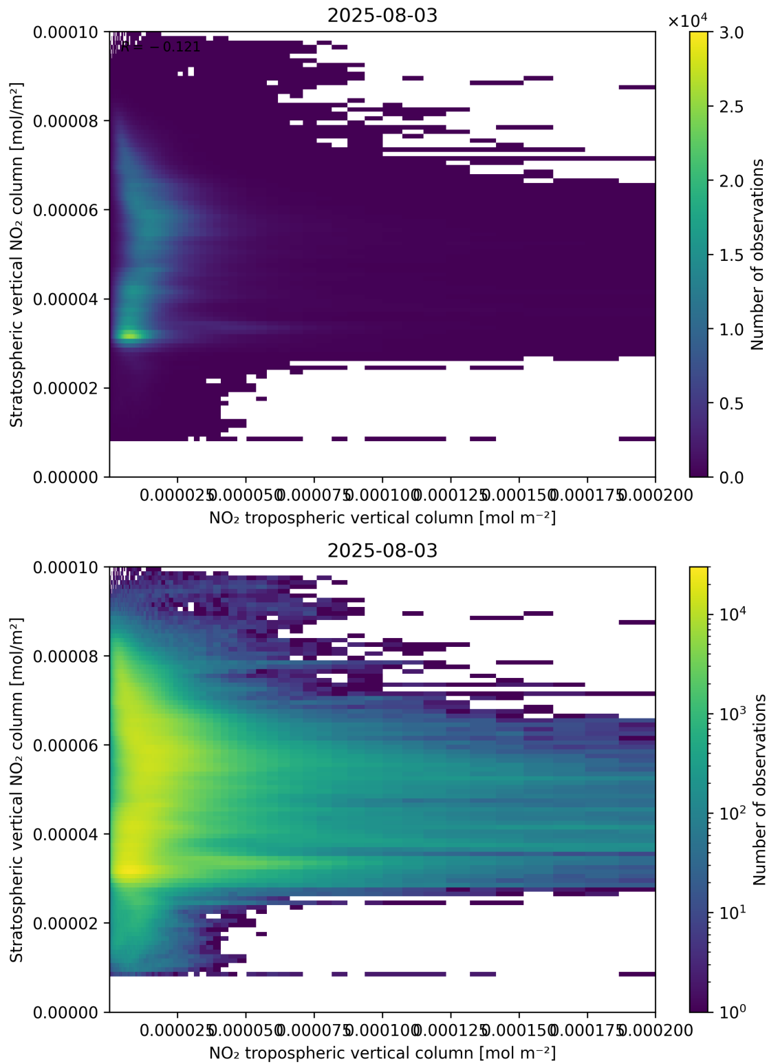
Figure 125: Scatter density plot of “NO 2 tropospheric vertical column” against “Stratospheric vertical NO 2 column” for 2025-08-03 to 2025-08-04.
