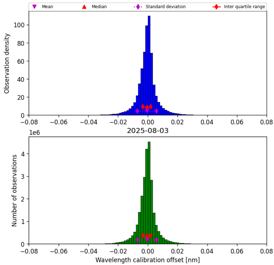
Figure 35: Histogram of “Wavelength calibration offset” for 2025-08-03 to 2025-08-04
