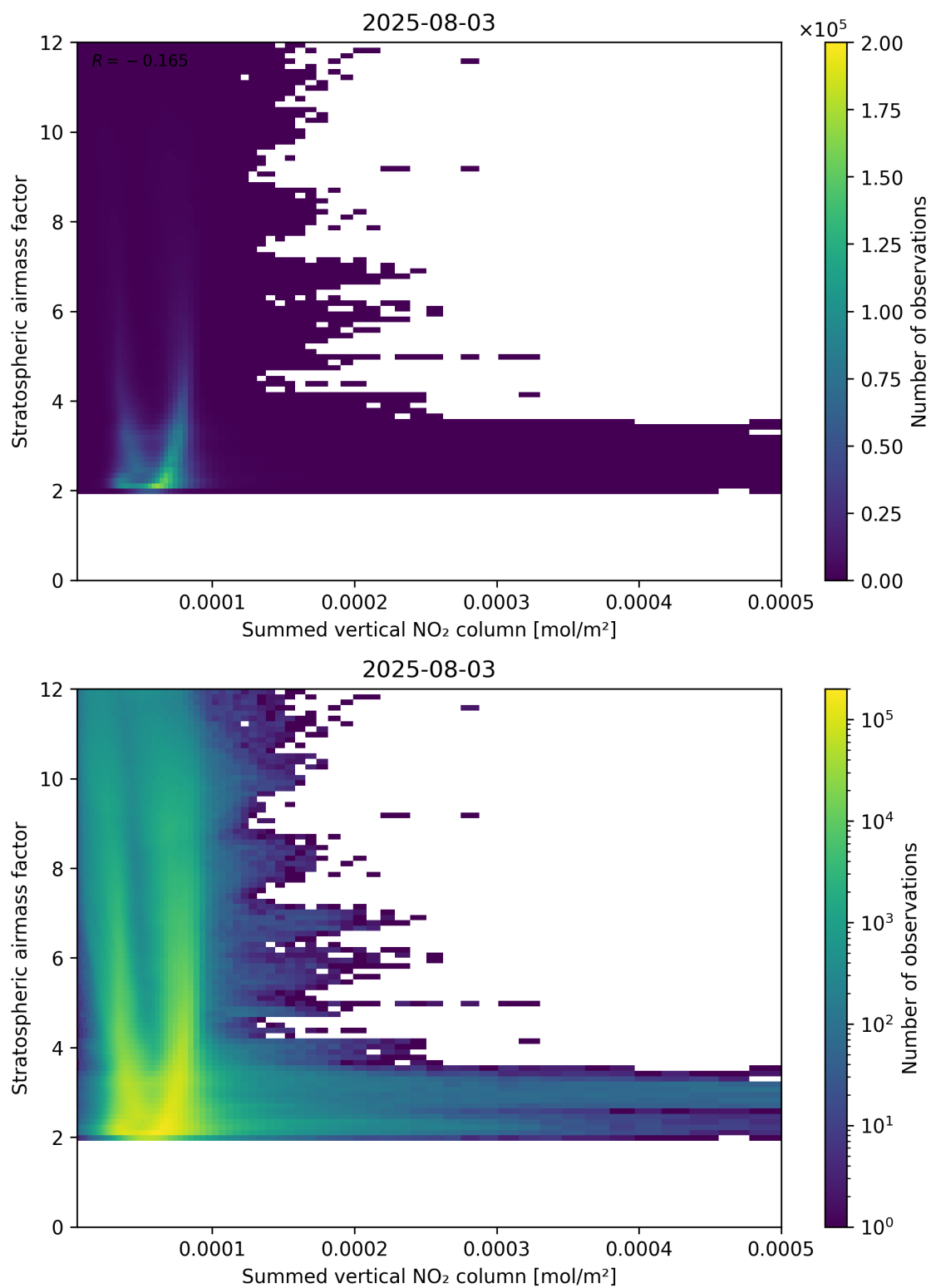
Figure 103: Scatter density plot of “Summed vertical NO 2 column” against “Stratospheric air mass factor” for 2025-08-03 to 2025-08-04.
