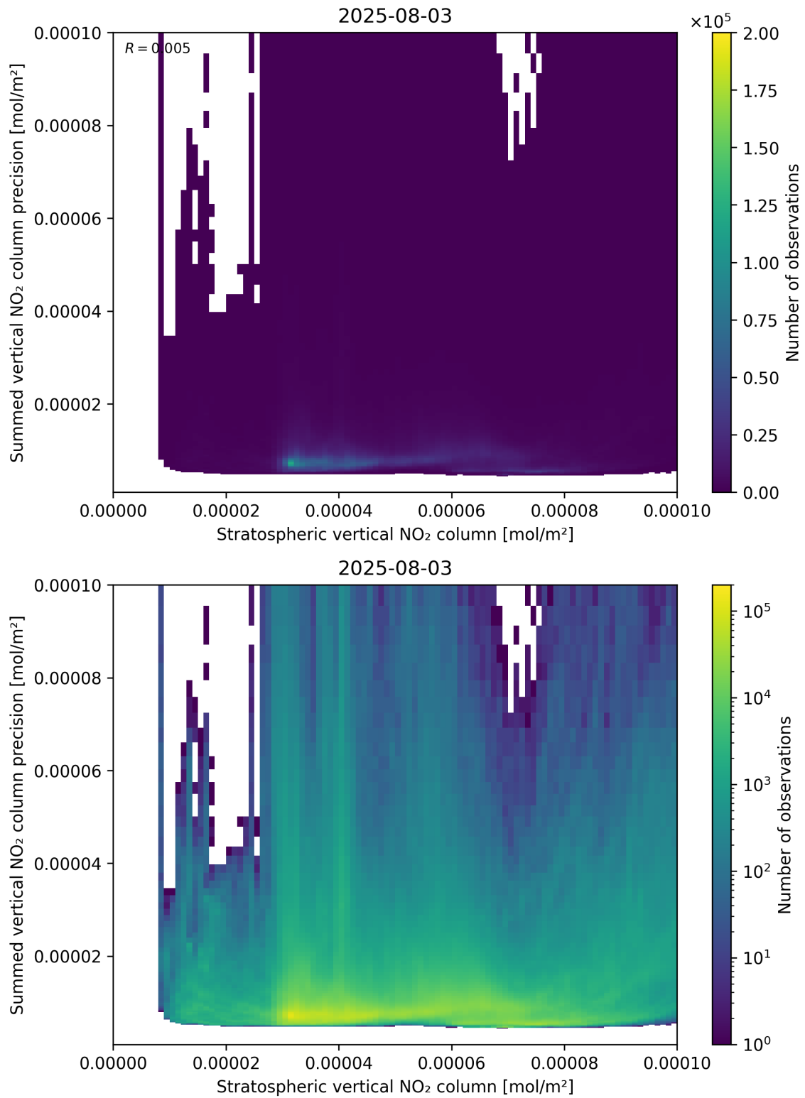
Figure 99: Scatter density plot of “Stratospheric vertical NO 2 column” against “Summed vertical NO 2 column precision” for 2025-08-03 to 2025-08-04.
