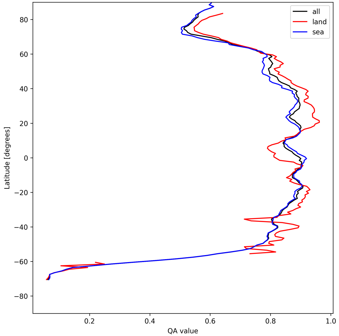
Figure 11: Zonal average of “QA value” for 2025-08-03 to 2025-08-04.
