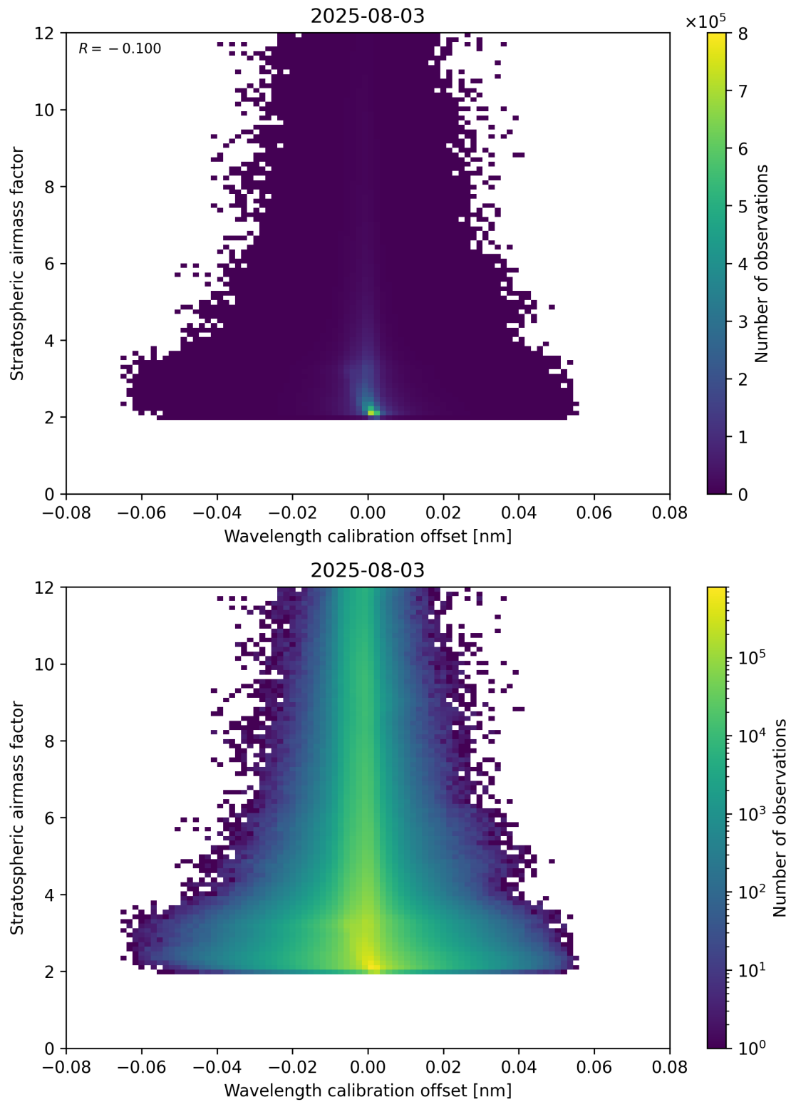
Figure 174: Scatter density plot of “Wavelength calibration offset” against “Stratospheric airmass factor” for 2025-08-03 to 2025-08-04.
