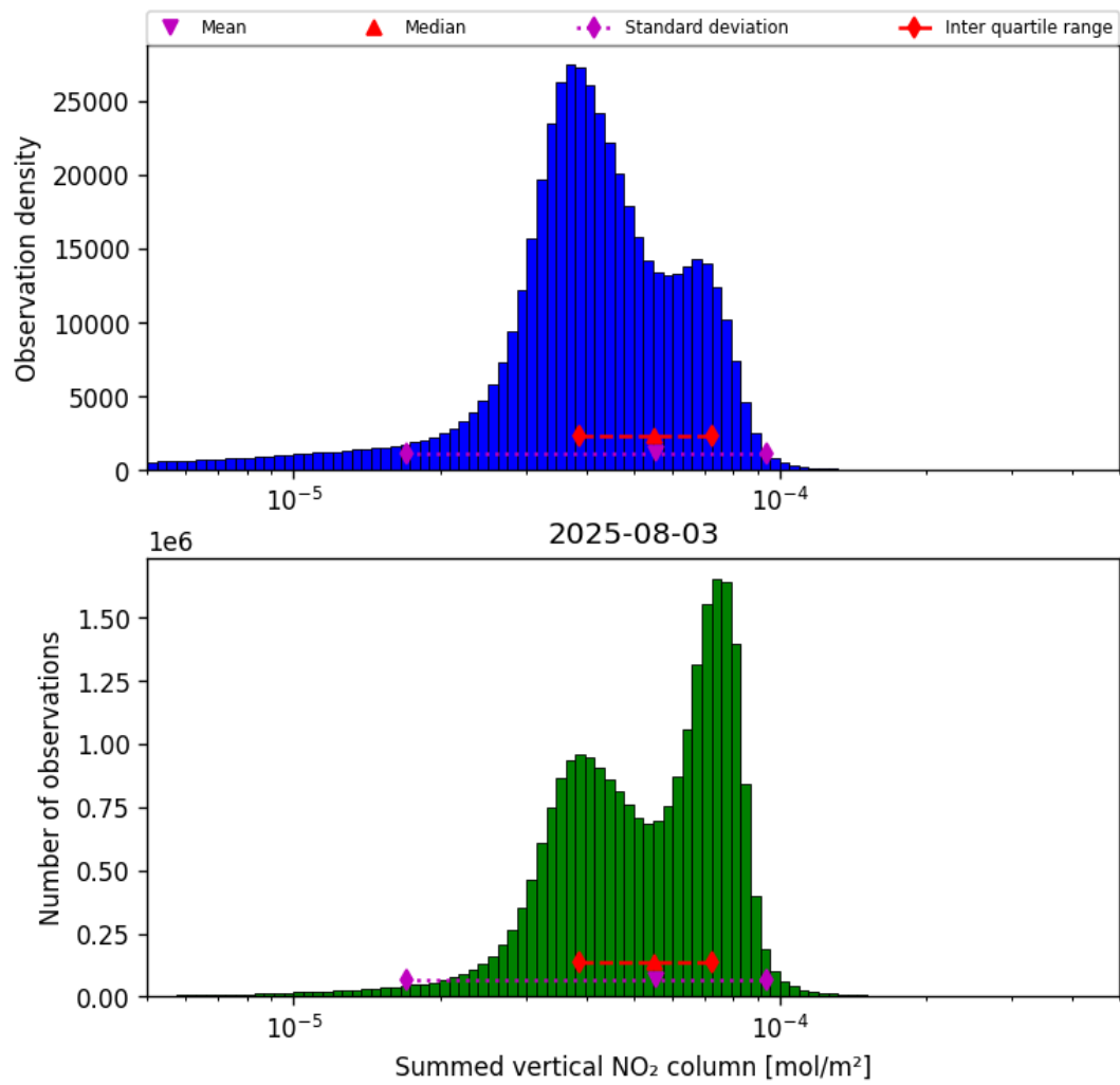
Figure 40: Histogram of “Summed vertical NO 2 column” for 2025-08-03 to 2025-08-04
