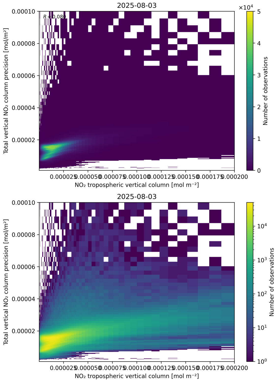
Figure 129: Scatter density plot of “NO 2 tropospheric vertical column” against “Total vertical NO 2 column precision” for 2025-08-03 to 2025-08-04.
