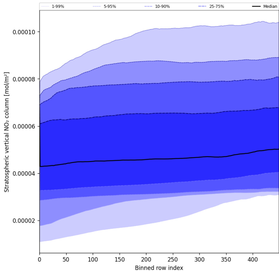
Figure 53: Along track statistics of “Stratospheric vertical NO 2 column” for 2025-08-03 to 2025-08-04
