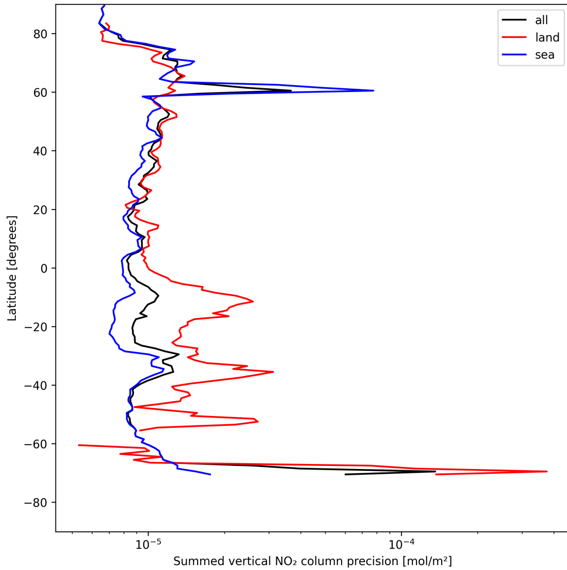
Figure 24: Zonal average of “Summed vertical NO 2 column precision” for 2025-08-03 to 2025-08-04.
