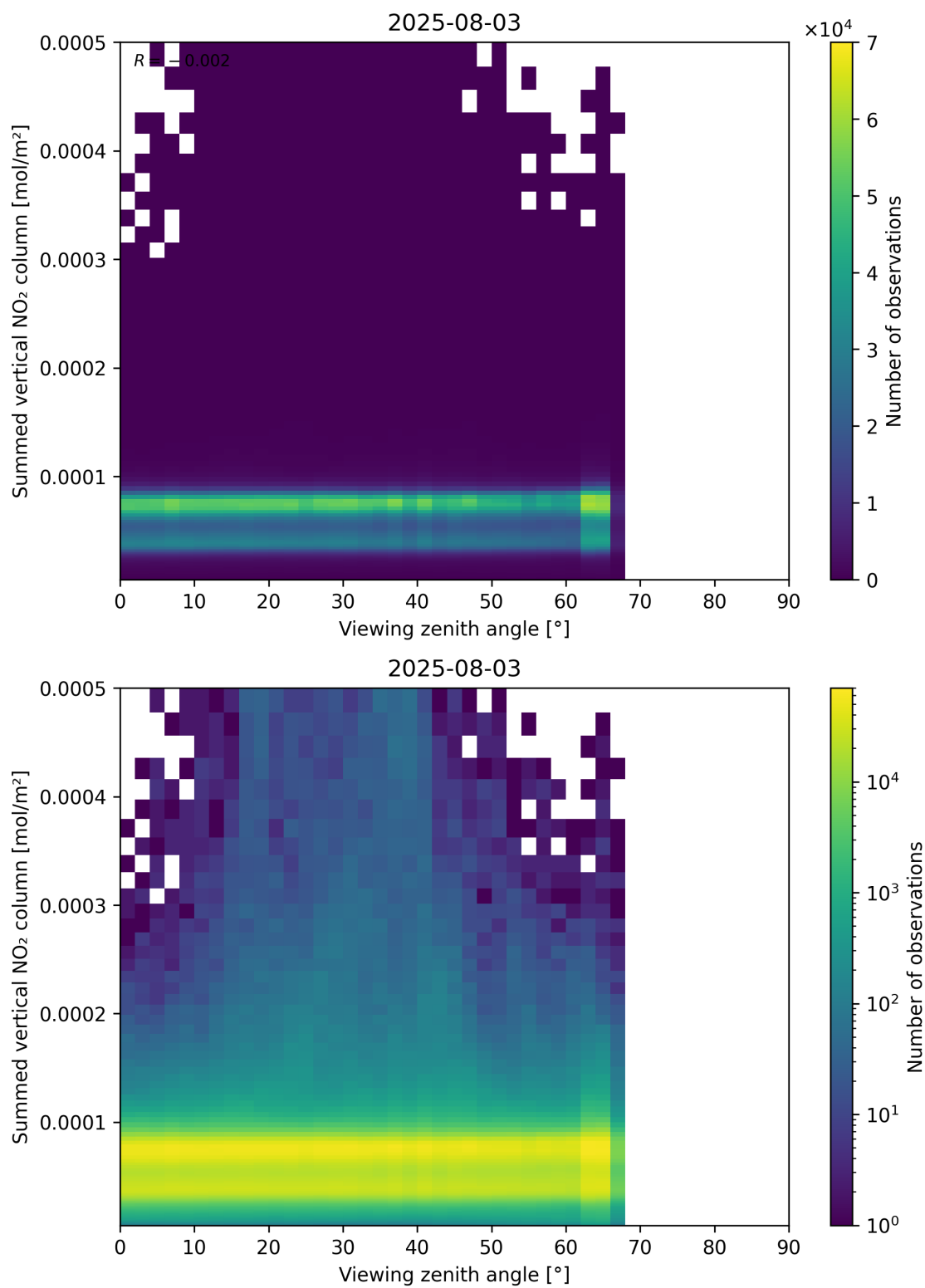
Figure 165: Scatter density plot of “Viewing zenith angle” against “Summed vertical NO 2 column” for 2025-08-03 to 2025-08-04.
