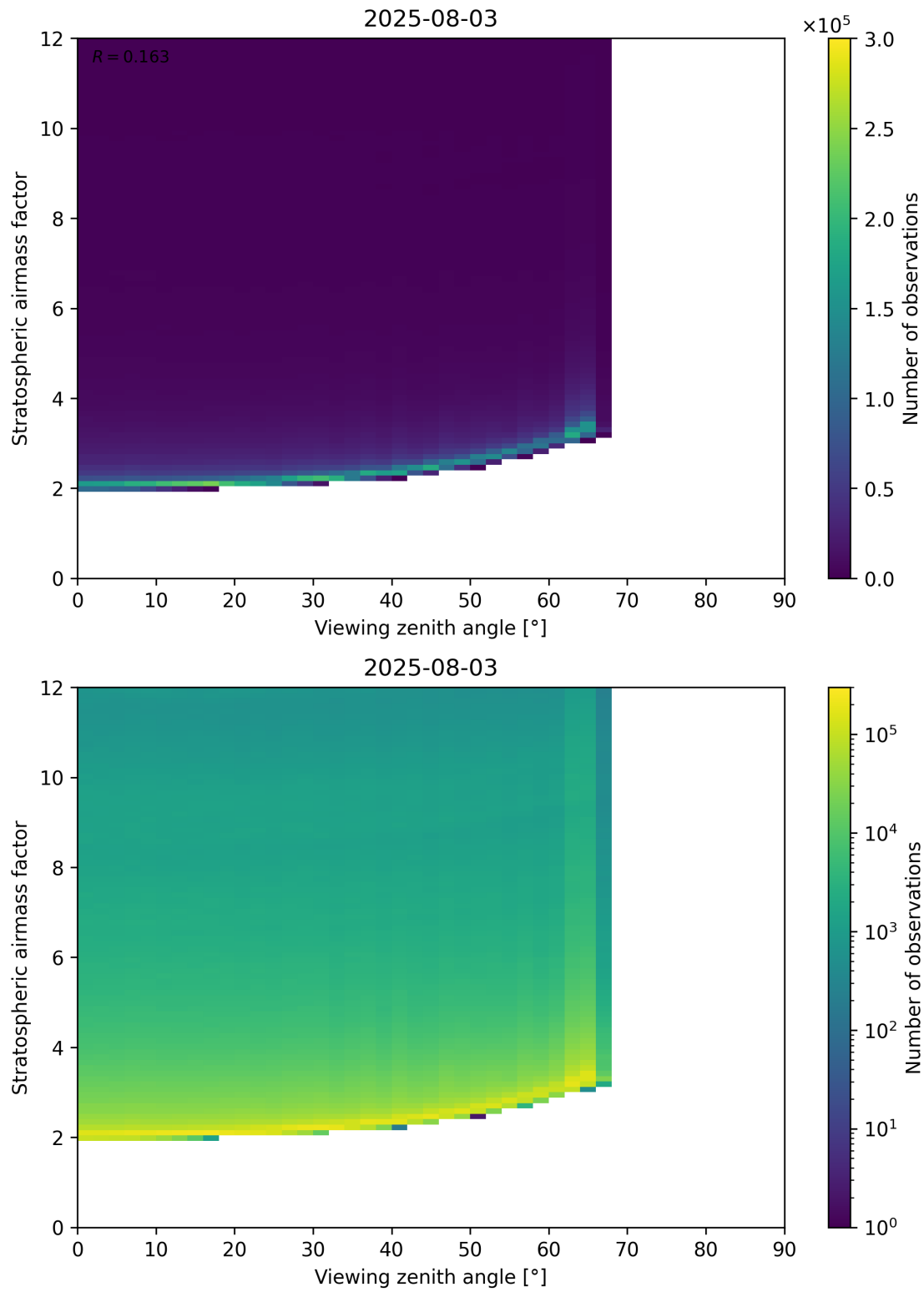
Figure 159: Scatter density plot of “Viewing zenith angle” against “Stratospheric airmass factor” for 2025-08-03 to 2025-08-04.
