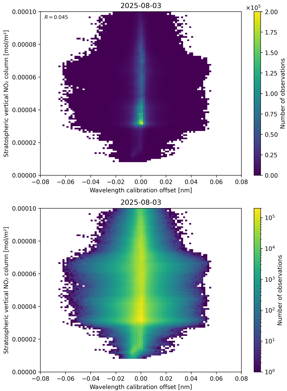
Figure 176: Scatter density plot of “Wavelength calibration offset” against “Stratospheric vertical NO 2 column” for 2025-08-03 to 2025-08-04.
