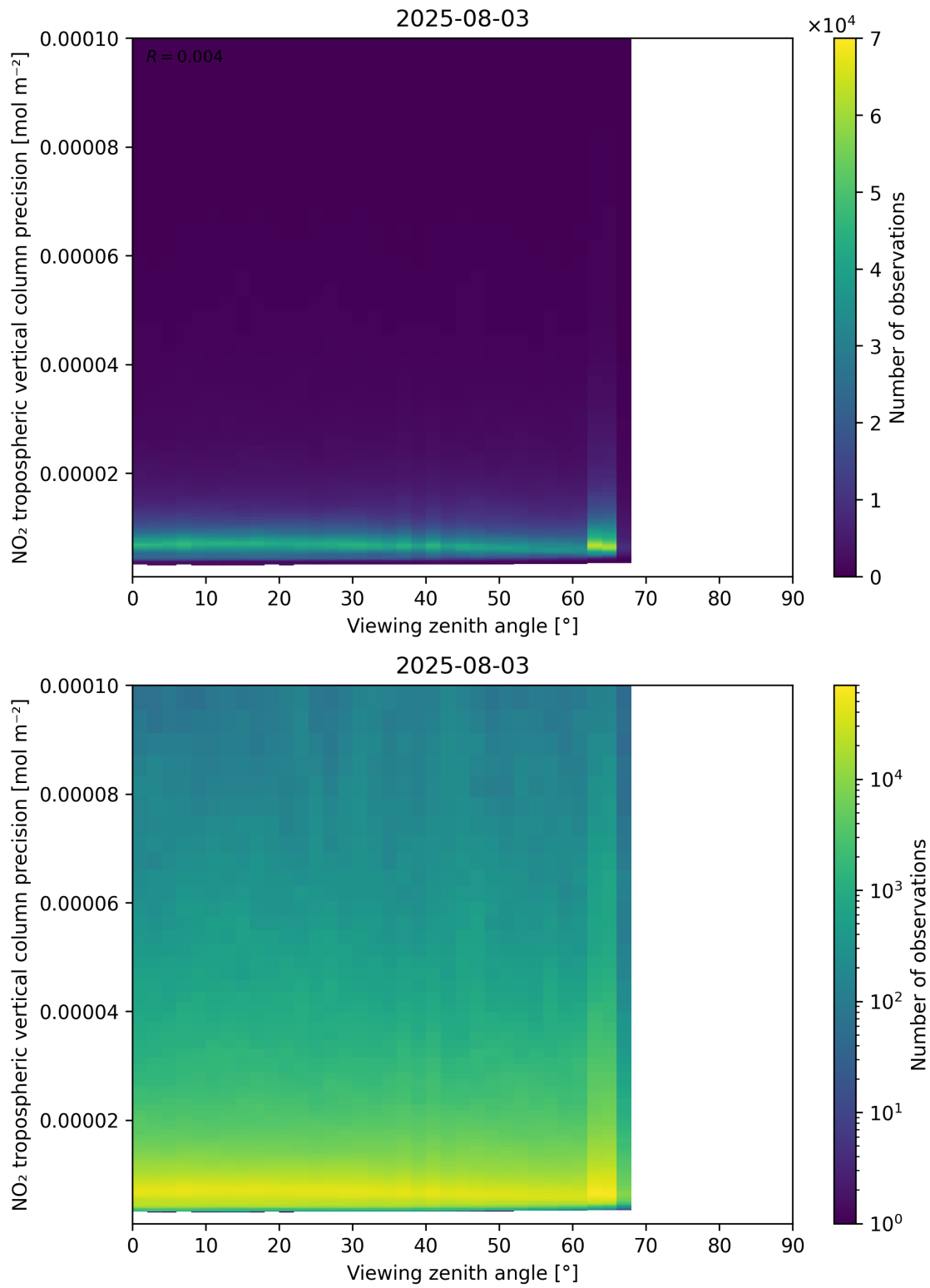
Figure 170: Scatter density plot of “Viewing zenith angle” against “NO 2 tropospheric vertical column precision” for 2025-08-03 to 2025-08-04.
