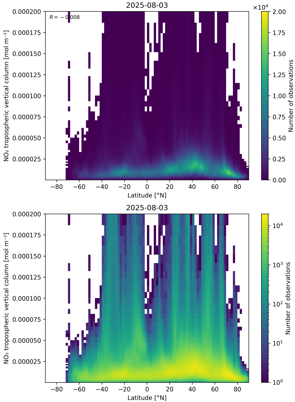
Figure 92: Scatter density plot of “Latitude” against “NO 2 tropospheric vertical column” for 2025-08-03 to 2025-08-04.
