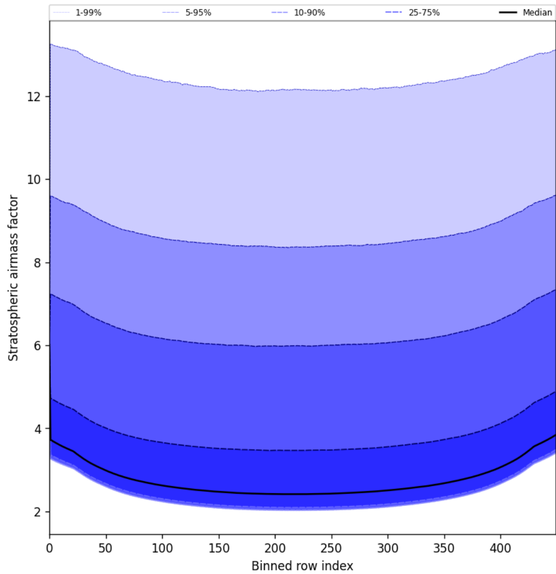
Figure 61: Along track statistics of “Stratospheric airmass factor” for 2025-08-03 to 2025-08-04
