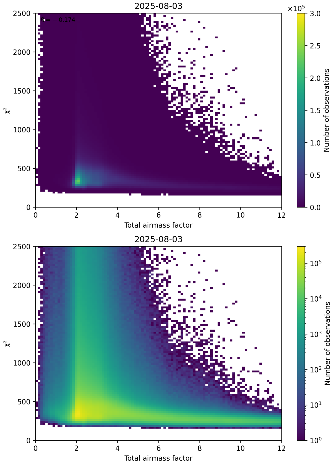
Figure 63: Scatter density plot of “Total airmass factor” against “ \chi^2 ” for 2025-08-03 to 2025-08-04.
