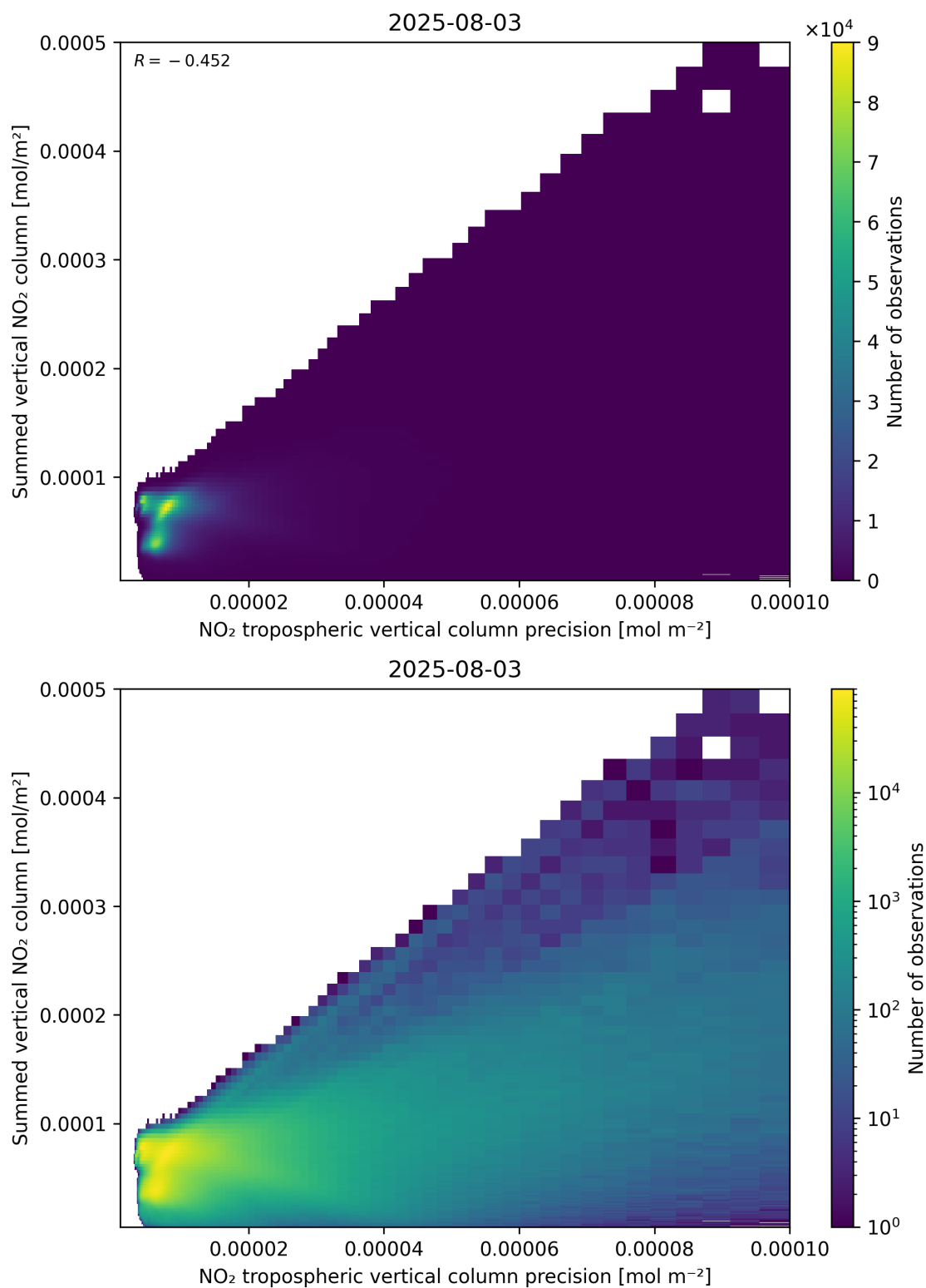
Figure 136: Scatter density plot of “NO 2 tropospheric vertical column precision” against “Summed vertical NO 2 column” for 2025-08-03 to 2025-08-04.
