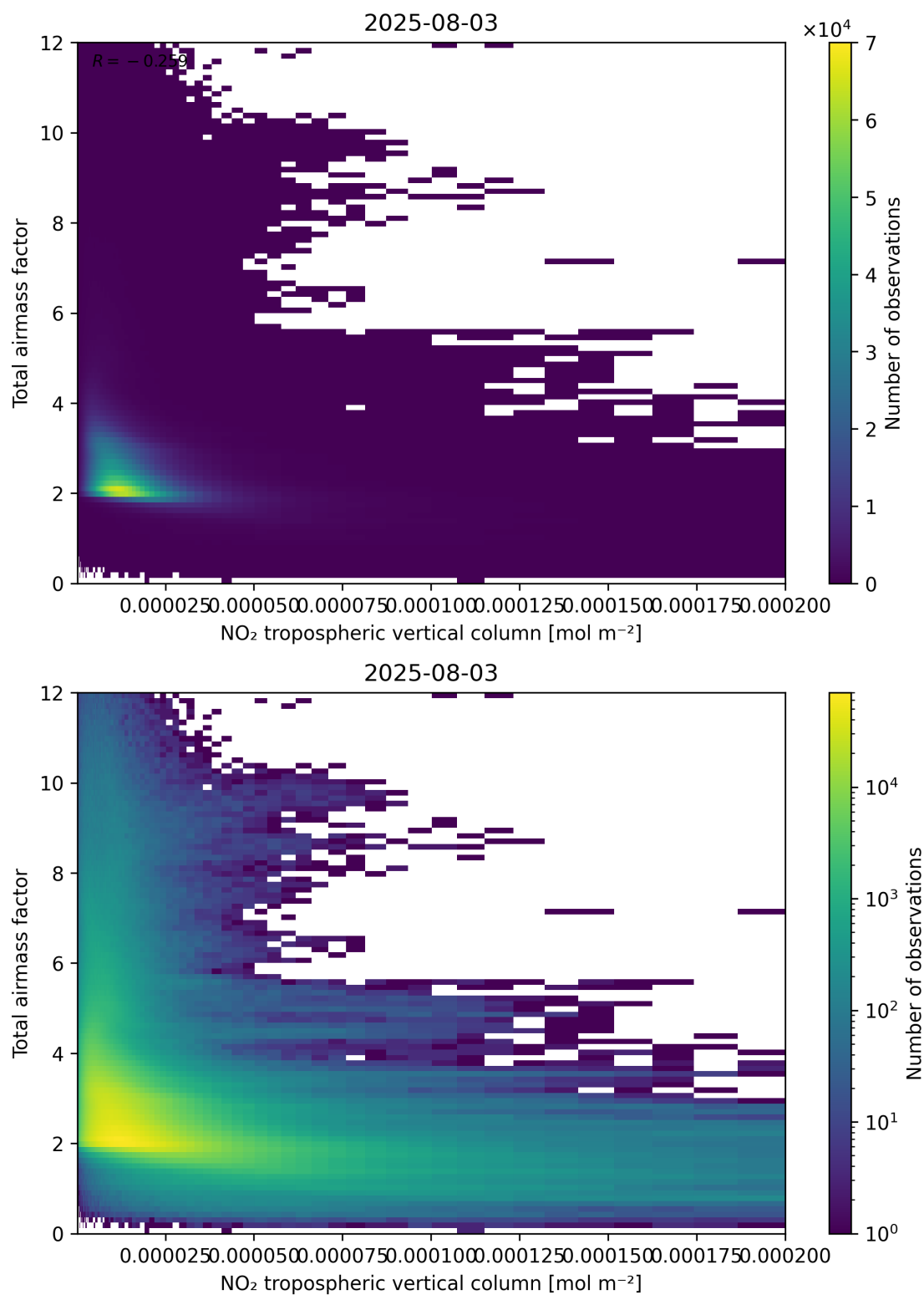
Figure 122: Scatter density plot of “NO 2 tropospheric vertical column” against “Total air mass factor” for 2025-08-03 to 2025-08-04.
