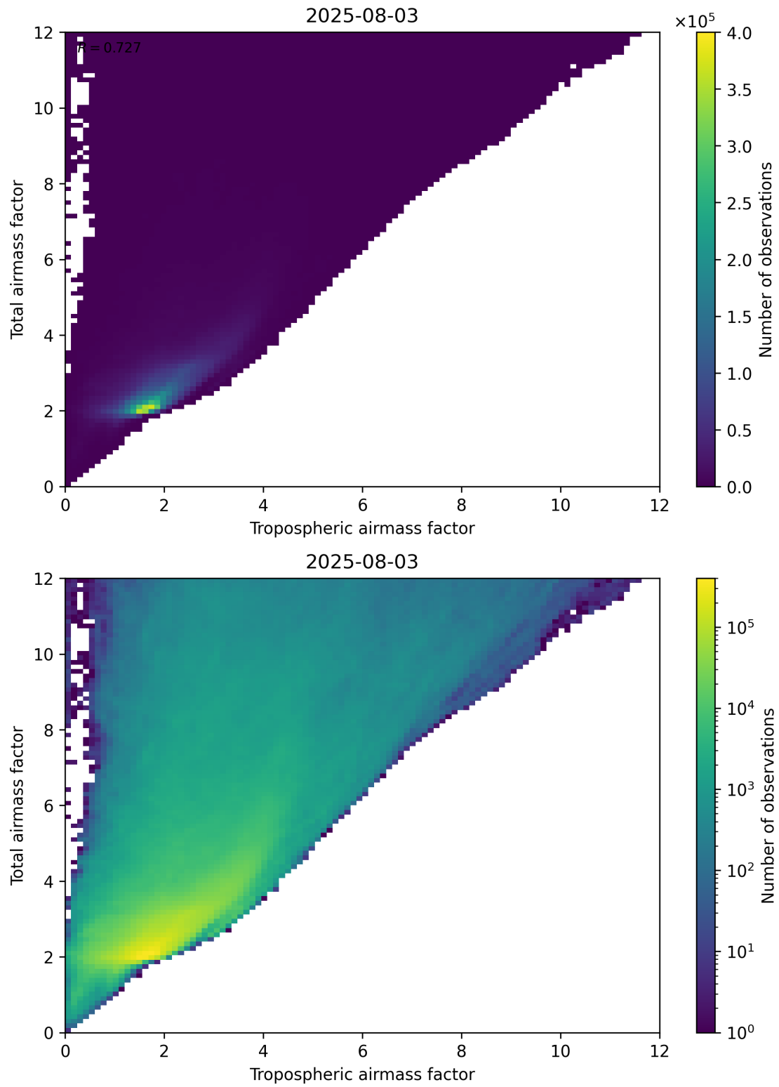
Figure 72: Scatter density plot of “Tropospheric airmass factor” against “Total airmass factor” for 2025-08-03 to 2025-08-04.
