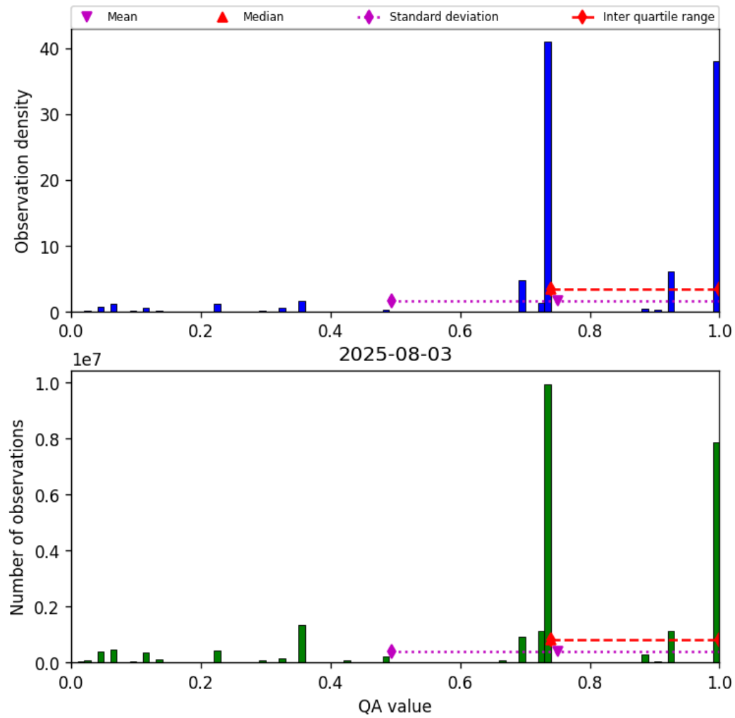
Figure 28: Histogram of “QA value” for 2025-08-03 to 2025-08-04
