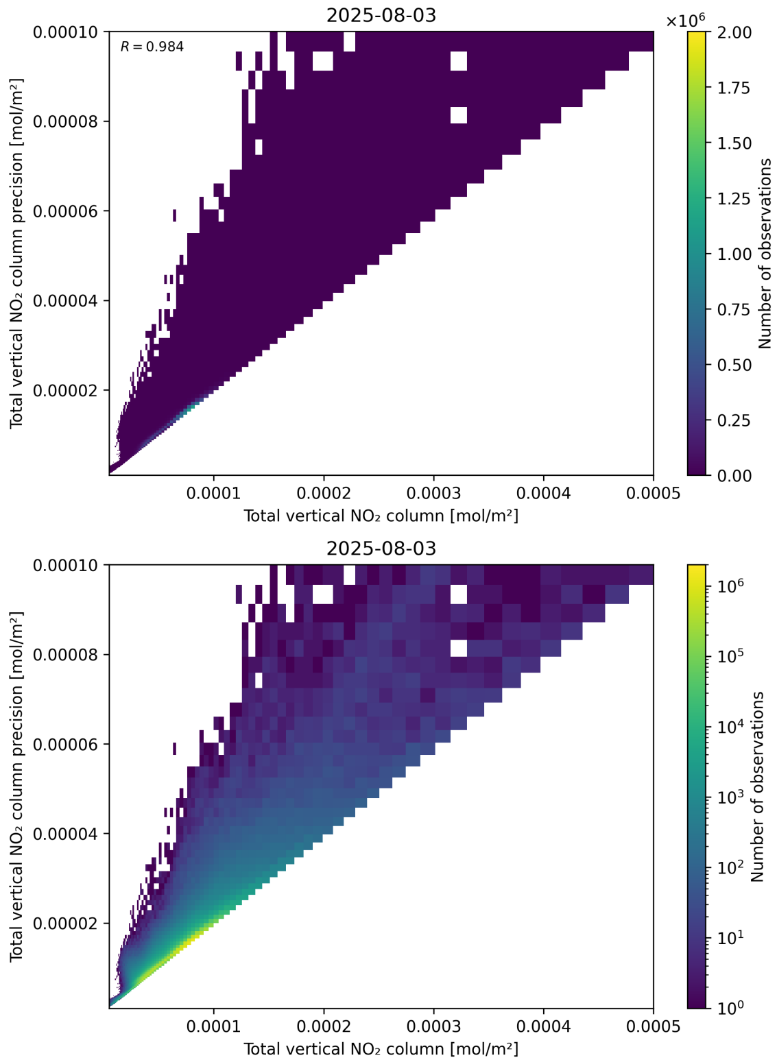
Figure 114: Scatter density plot of “Total vertical NO 2 column” against “Total vertical NO 2 column precision” for 2025-08-03 to 2025-08-04.
