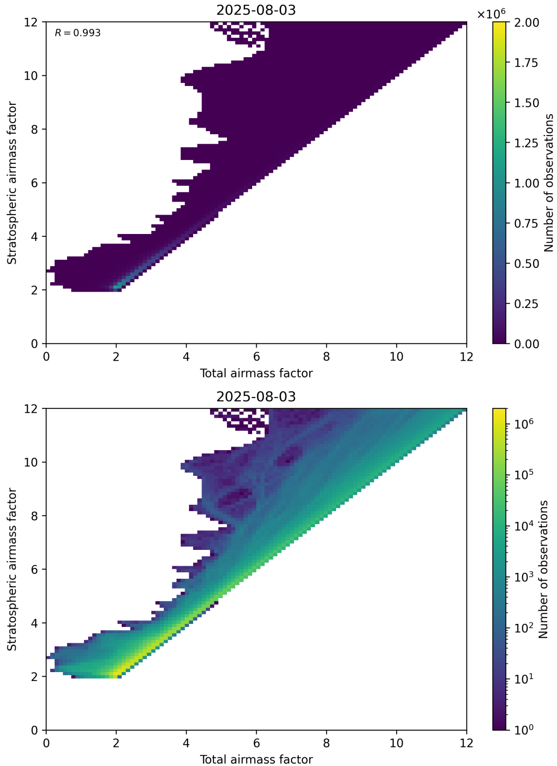
Figure 62: Scatter density plot of “Total airmass factor” against “Stratospheric airmass factor” for 2025-08-03 to 2025-08-04.
