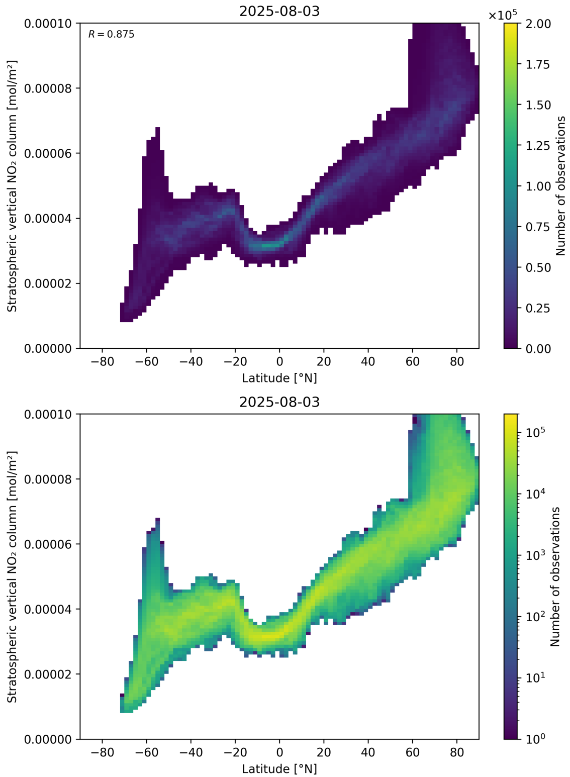
Figure 87: Scatter density plot of “Latitude” against “Stratospheric vertical NO 2 column” for 2025-08-03 to 2025-08-04.
