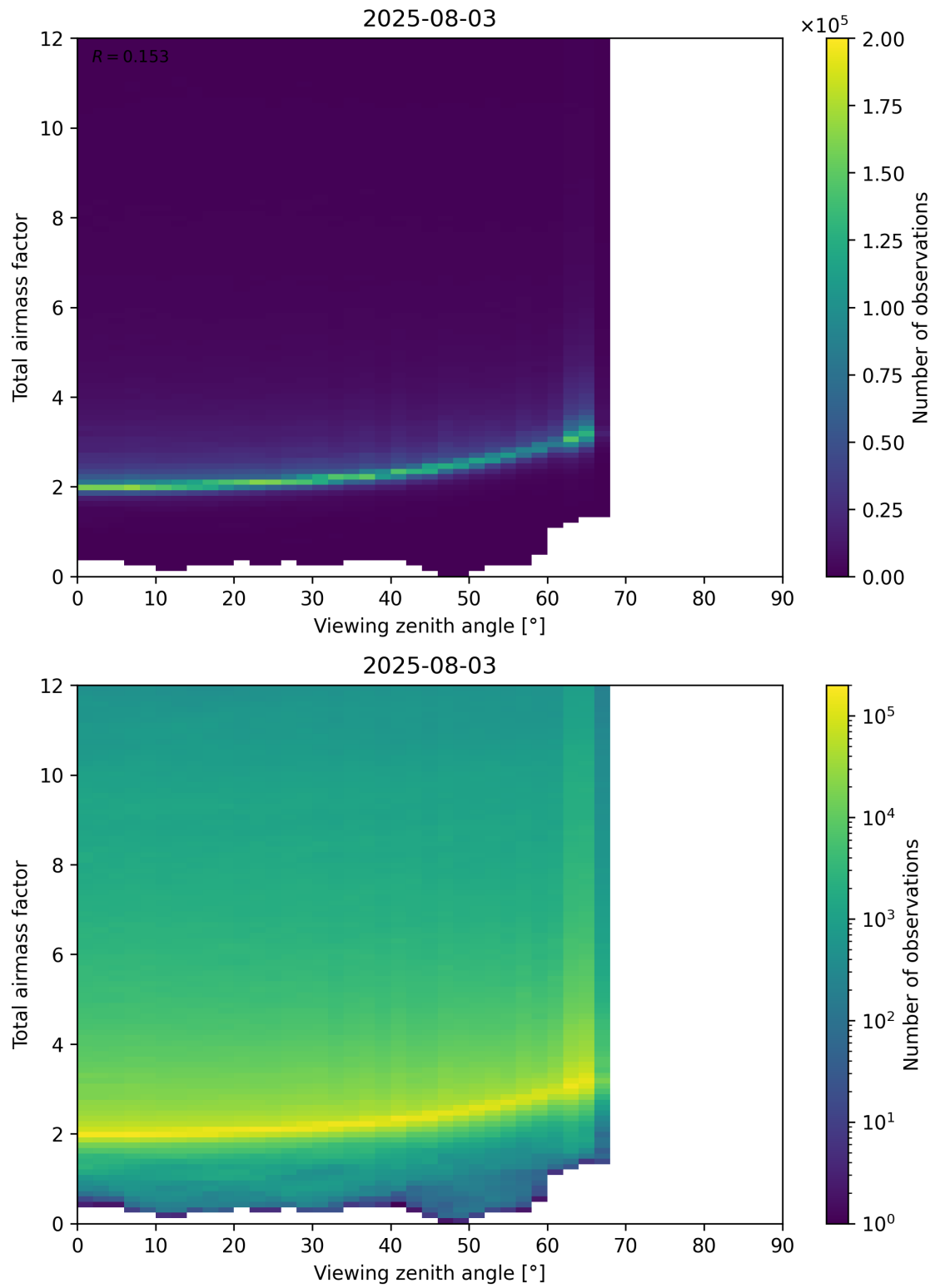
Figure 160: Scatter density plot of “Viewing zenith angle” against “Total airmass factor” for 2025-08-03 to 2025-08-04.
