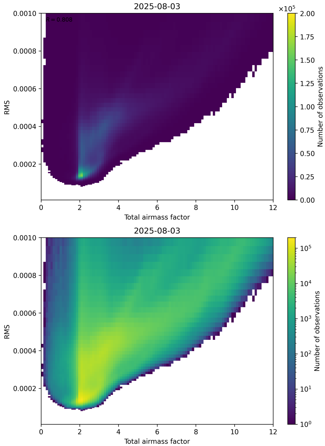
Figure 69: Scatter density plot of “Total airmass factor” against “RMS” for 2025-08-03 to 2025-08-04.
