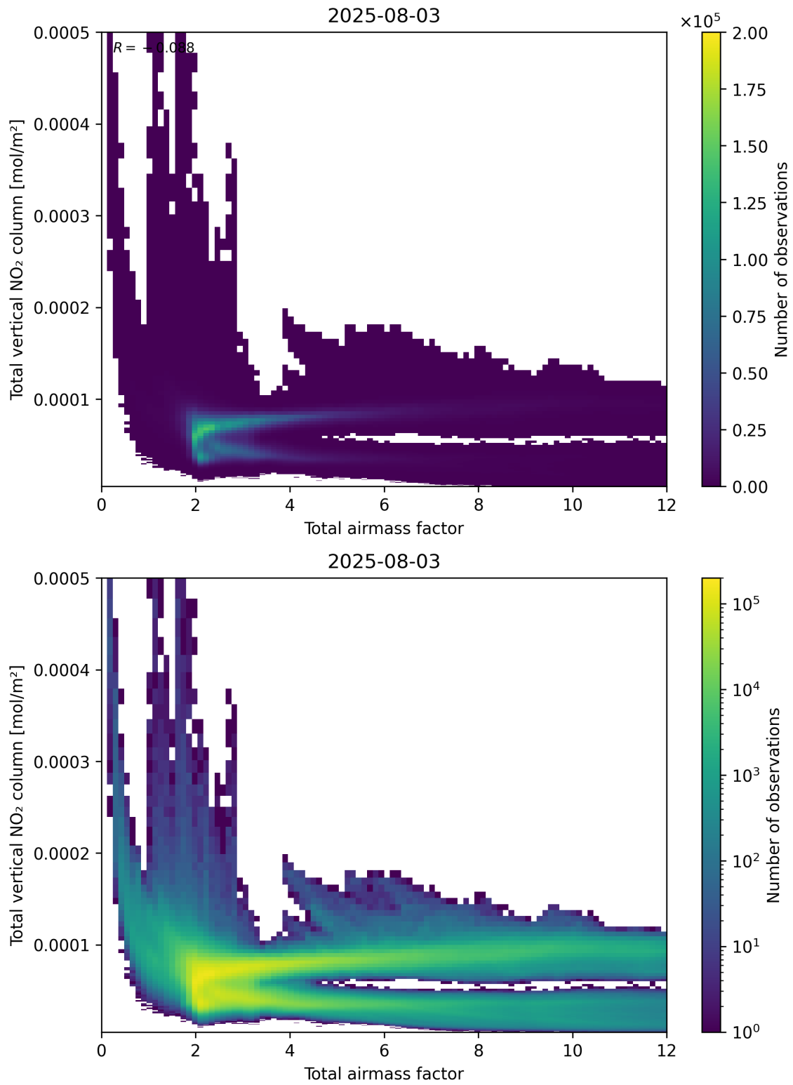
Figure 67: Scatter density plot of “Total airmass factor” against “Total vertical NO 2 column” for 2025-08-03 to 2025-08-04.
