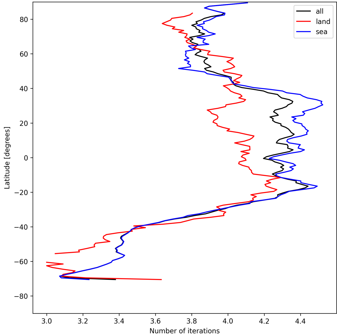
Figure 17: Zonal average of “Number of iterations” for 2025-08-03 to 2025-08-04.
