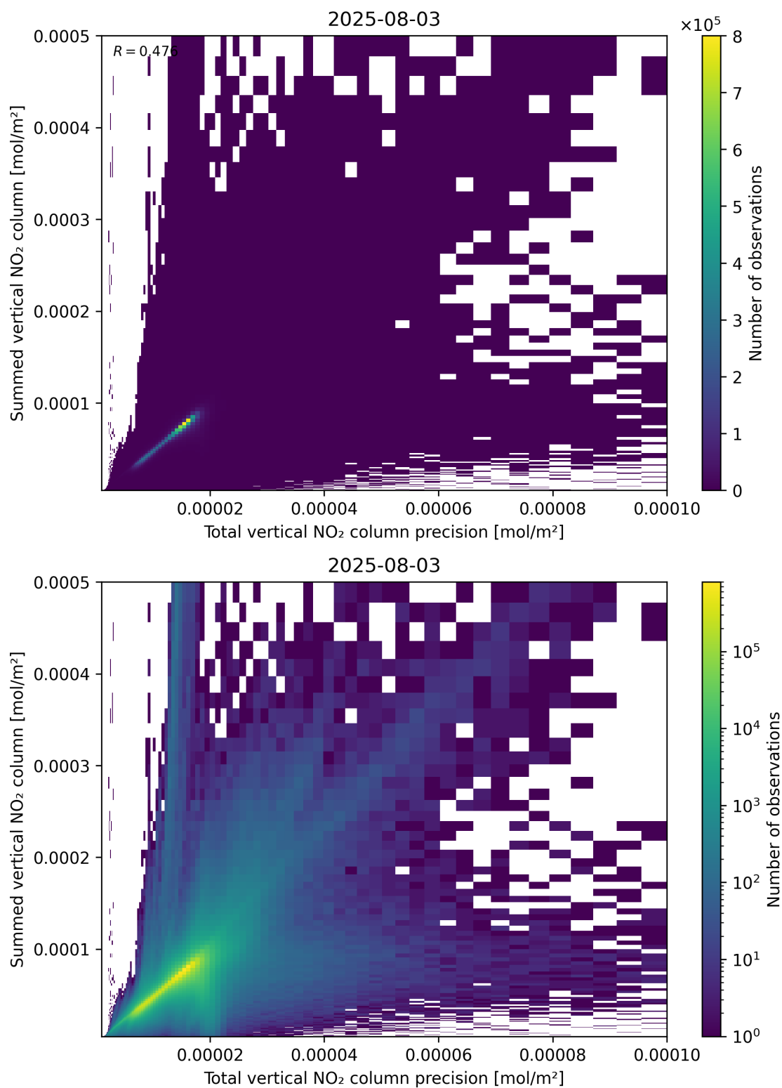
Figure 117: Scatter density plot of “Total vertical NO 2 column precision” against “Summed vertical NO 2 column” for 2025-08-03 to 2025-08-04.
