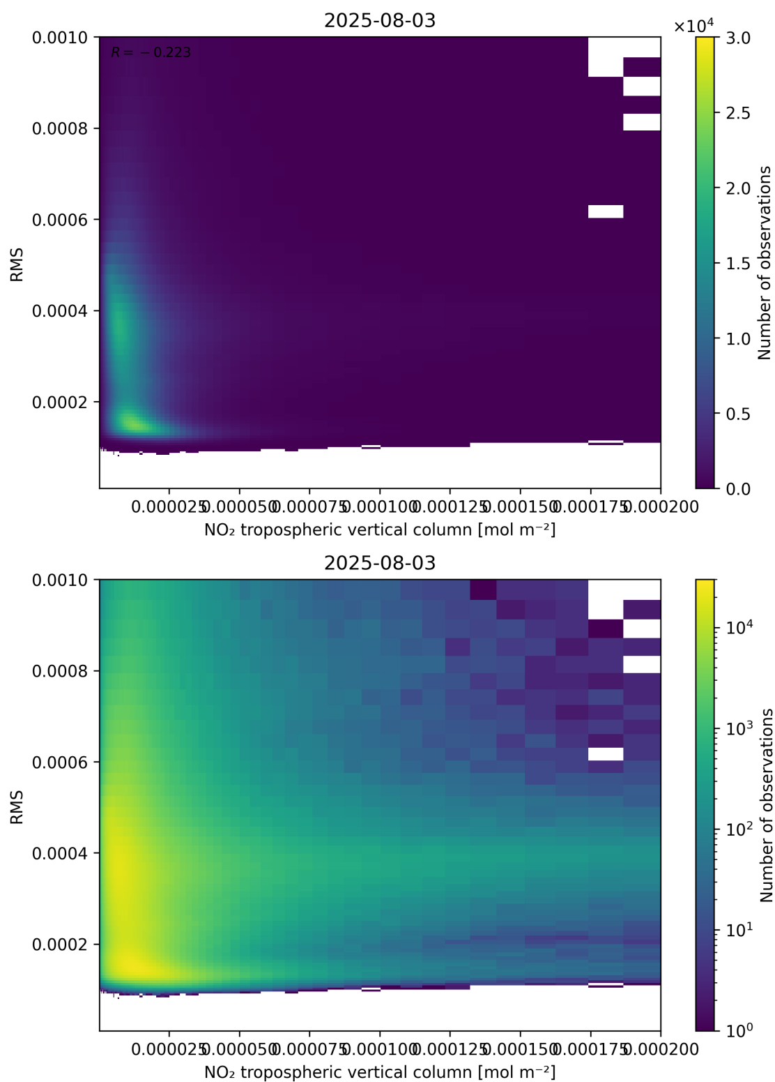
Figure 142: Scatter density plot of “NO 2 tropospheric vertical column” against “RMS” for 2025-08-03 to 2025-08-04.
