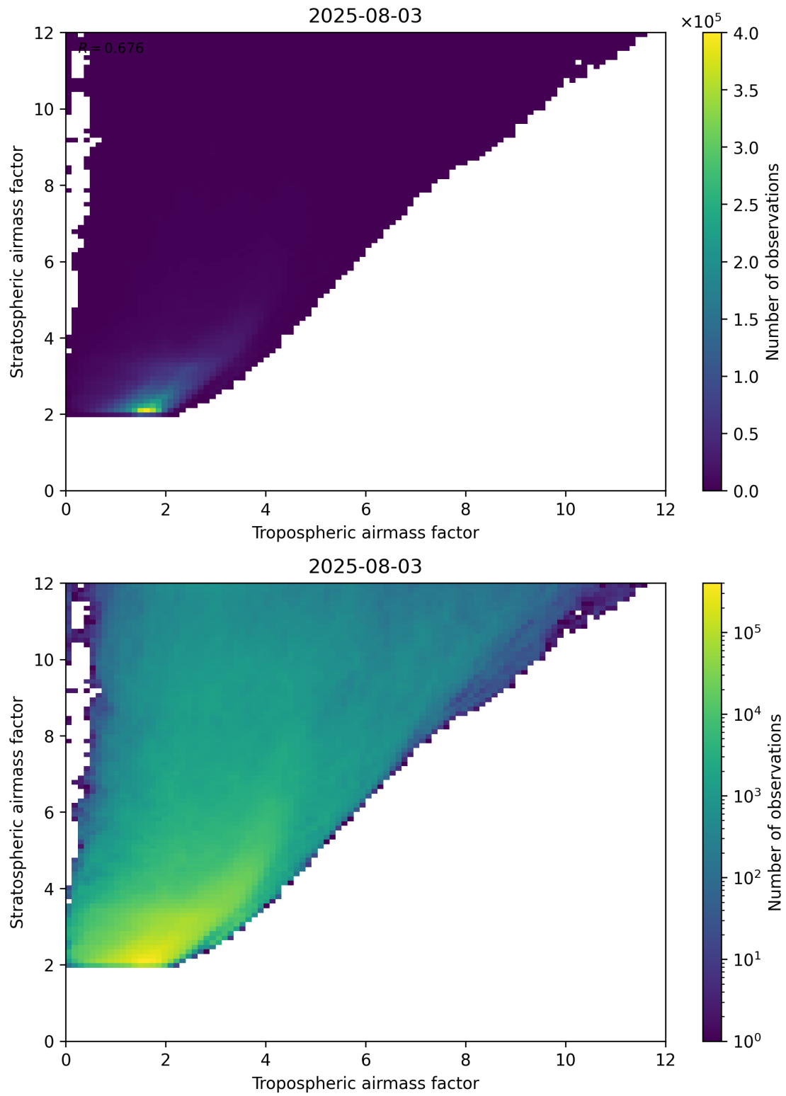
Figure 71: Scatter density plot of “Tropospheric airmass factor” against “Stratospheric airmass factor” for 2025-08-03 to 2025-08-04.
