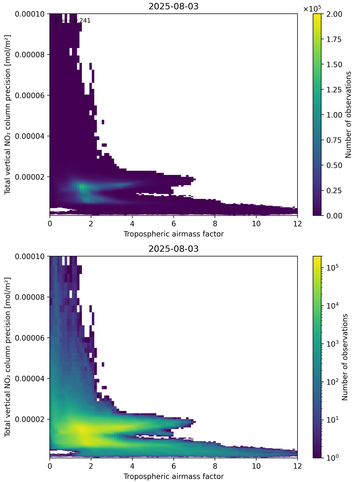
Figure 78: Scatter density plot of “Tropospheric air mass factor” against “Total vertical NO 2 column precision” for 2025-08-03 to 2025-08-04.
