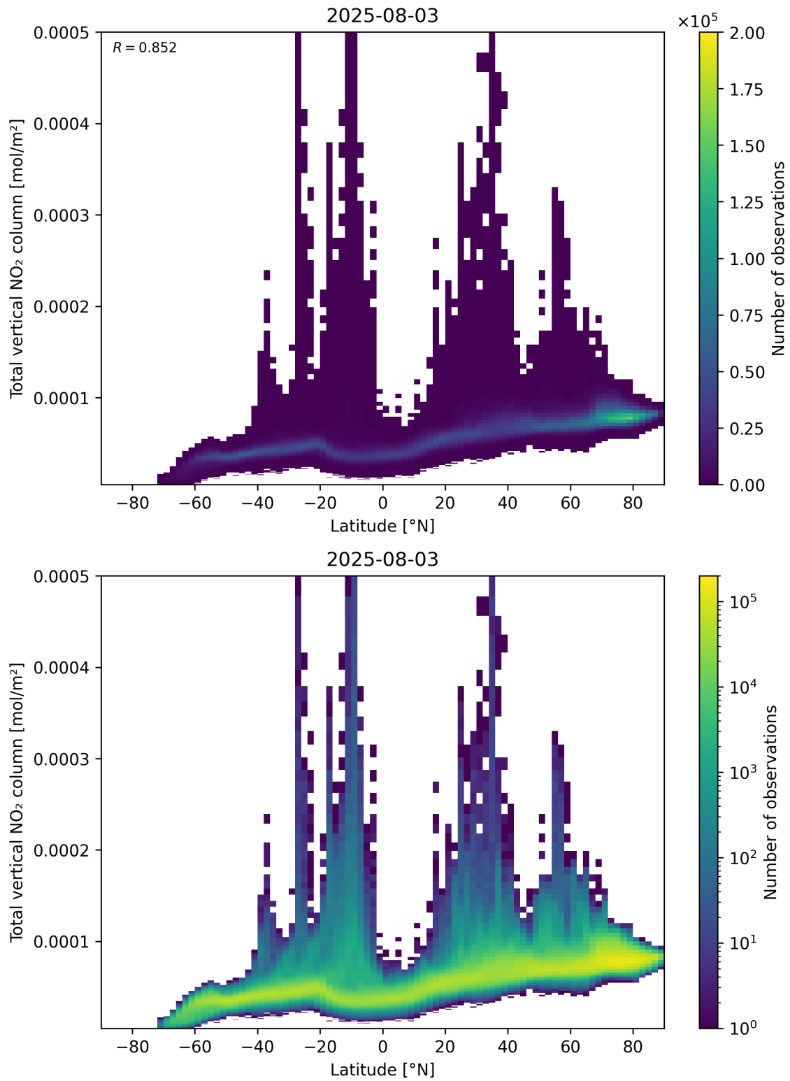
Figure 90: Scatter density plot of “Latitude” against “Total vertical NO 2 column” for 2025-08-03 to 2025-08-04.
