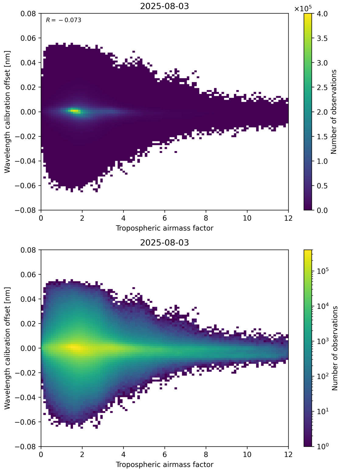
Figure 80: Scatter density plot of “Tropospheric airmass factor” against “Wavelength calibration offset” for 2025-08-03 to 2025-08-04.
