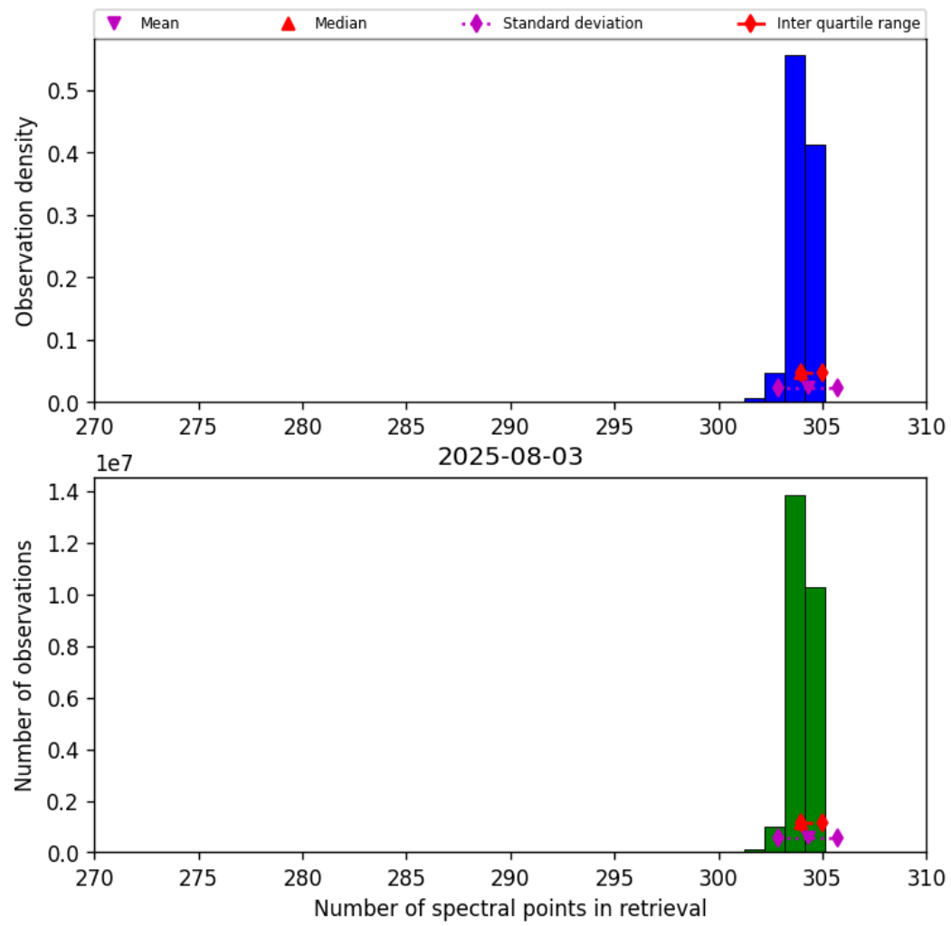
Figure 33: Histogram of “Number of spectral points in retrieval” for 2025-08-03 to 2025-08-04
