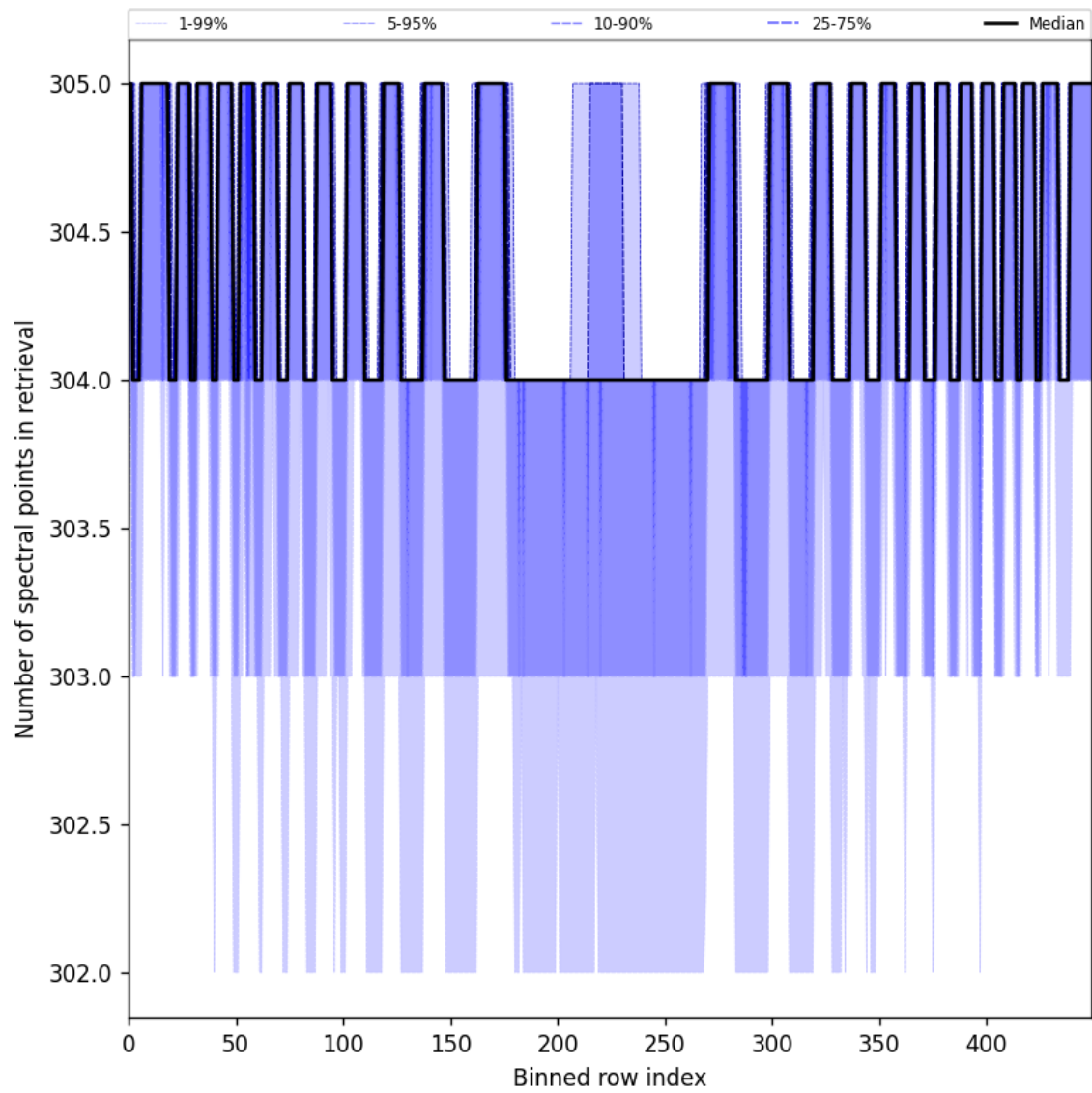
Figure 50: Along track statistics of “Number of spectral points in retrieval” for 2025-08-03 to 2025-08-04
