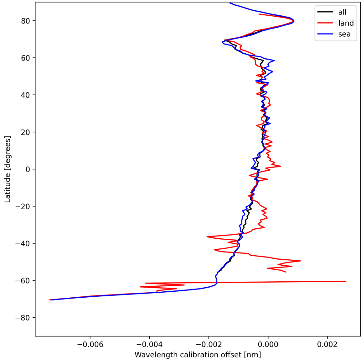
Figure 18: Zonal average of “Wavelength calibration offset” for 2025-08-03 to 2025-08-04.
