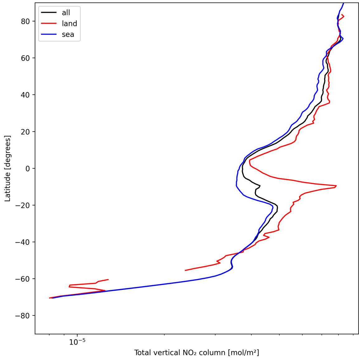
Figure 21: Zonal average of “Total vertical NO 2 column” for 2025-08-03 to 2025-08-04.
