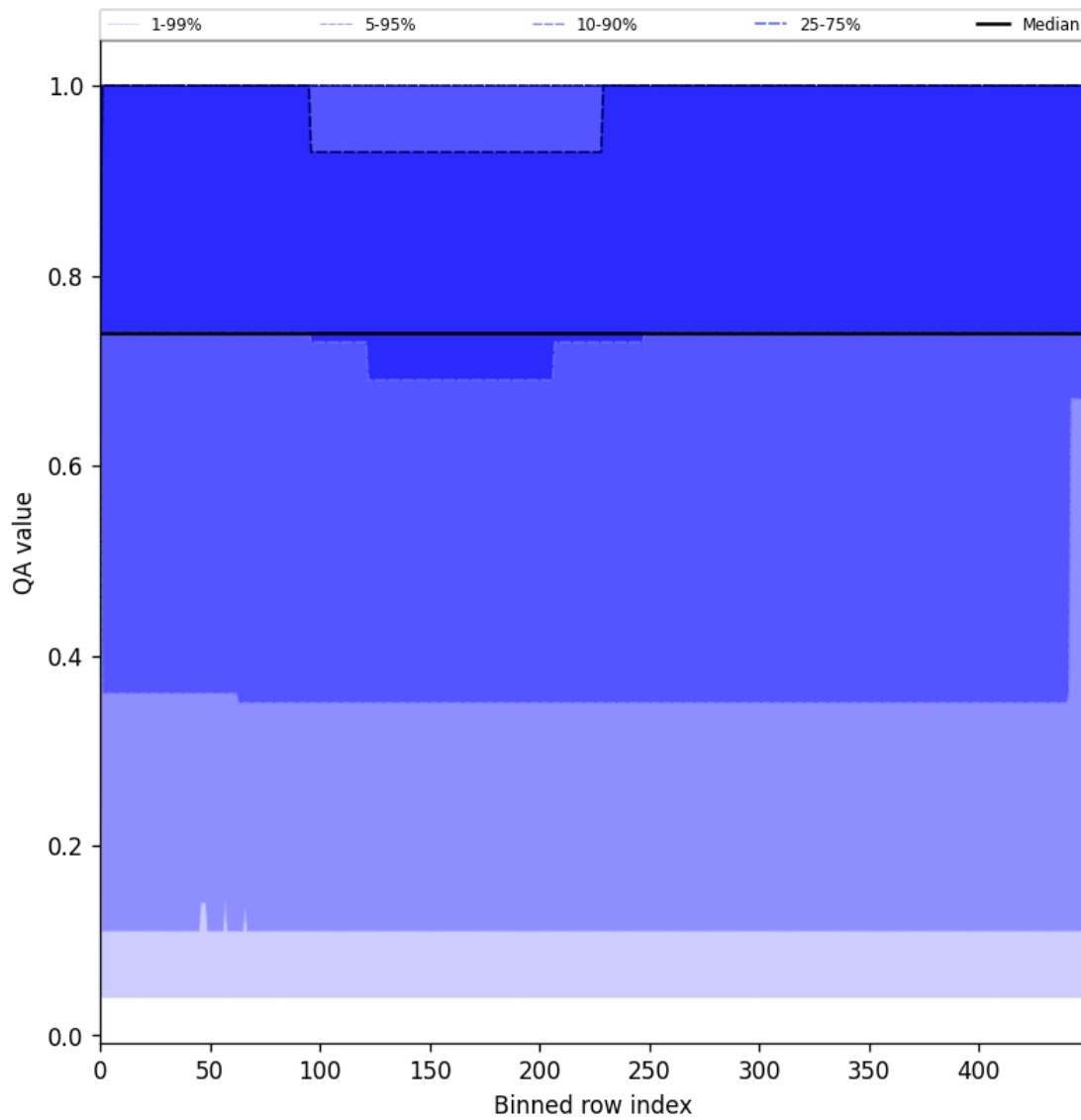
Figure 45: Along track statistics of “QA value” for 2025-08-03 to 2025-08-04
