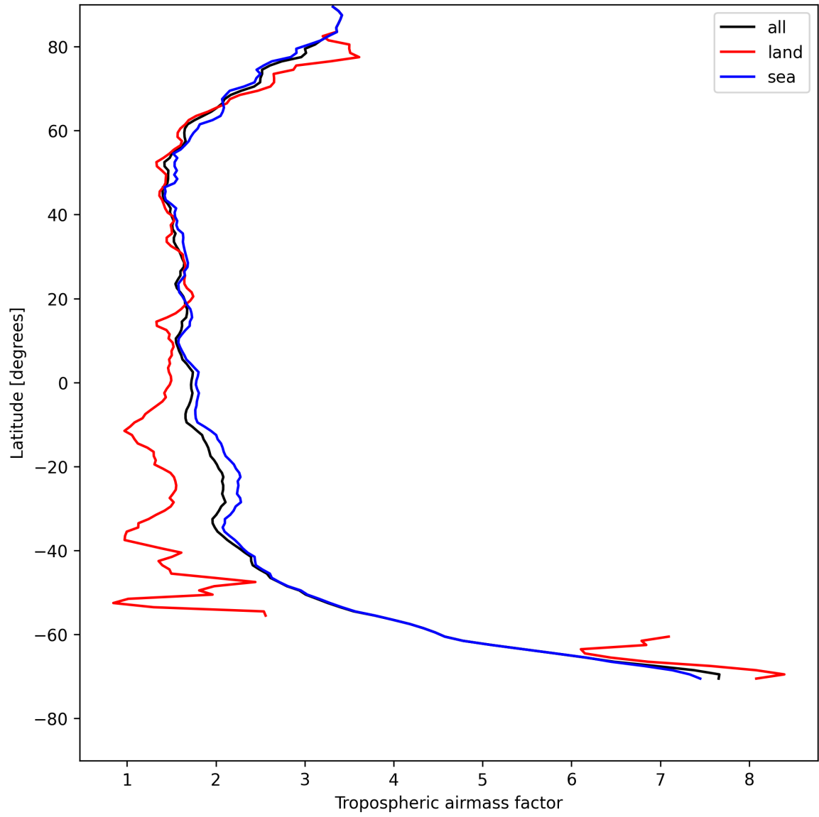
Figure 14: Zonal average of “Tropospheric airmass factor” for 2025-08-03 to 2025-08-04.
