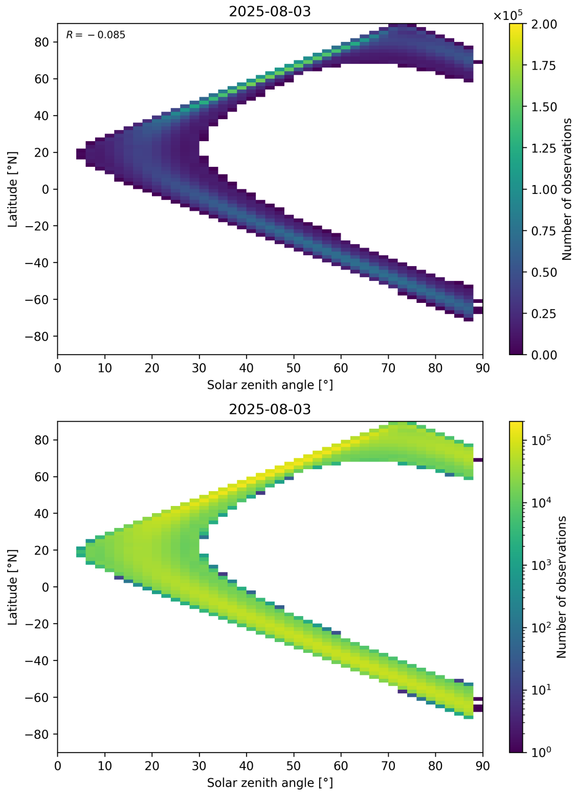
Figure 149: Scatter density plot of “Solar zenith angle” against “Latitude” for 2025-08-03 to 2025-08-04.
