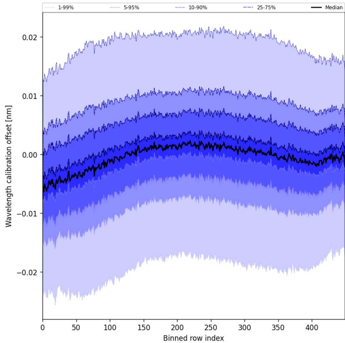
Figure 52: Along track statistics of “Wavelength calibration offset” for 2025-08-03 to 2025-08-04
