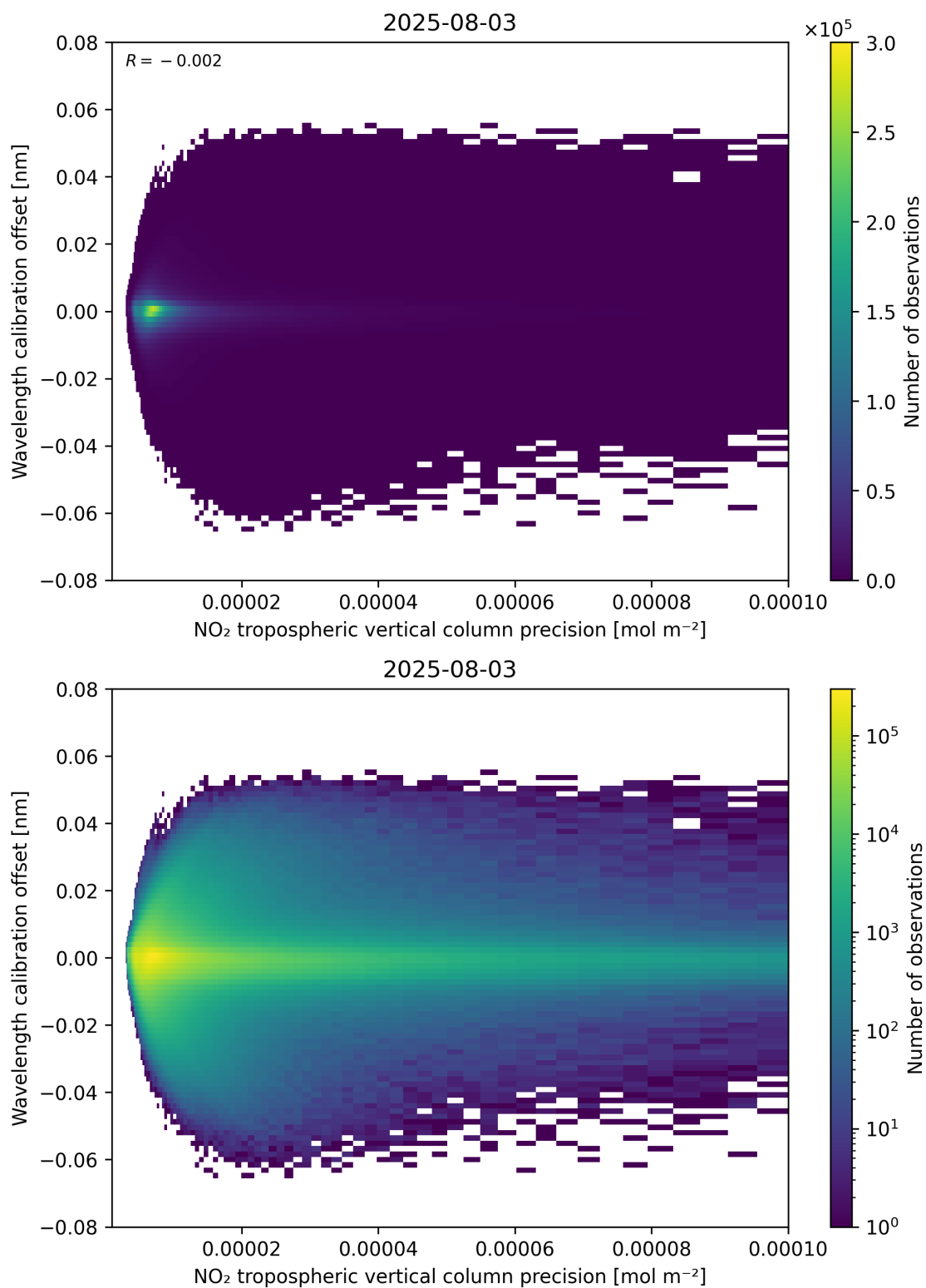
Figure 141: Scatter density plot of “NO 2 tropospheric vertical column precision” against “Wavelength calibration offset” for 2025-08-03 to 2025-08-04.
