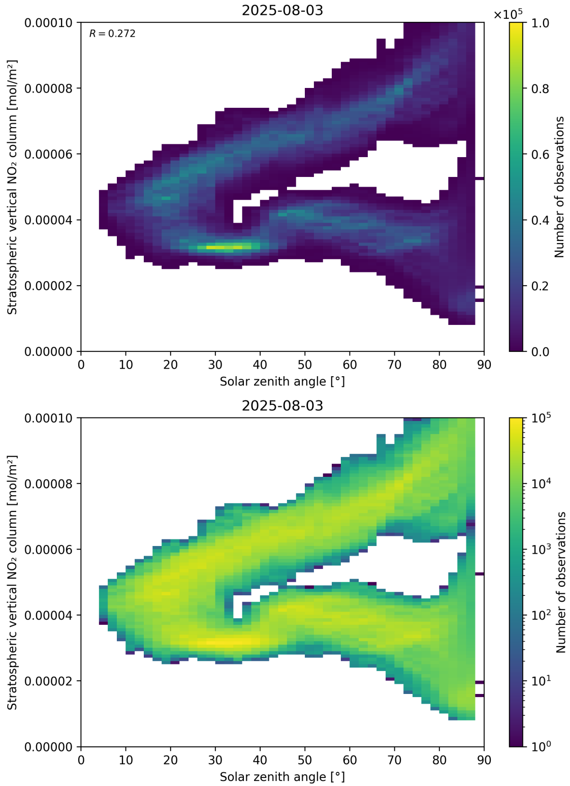
Figure 150: Scatter density plot of “Solar zenith angle” against “Stratospheric vertical NO 2 column” for 2025-08-03 to 2025-08-04.
