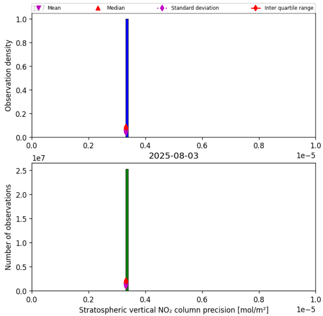
Figure 37: Histogram of “Stratospheric vertical NO 2 column precision” for 2025-08-03 to 2025-08-04
