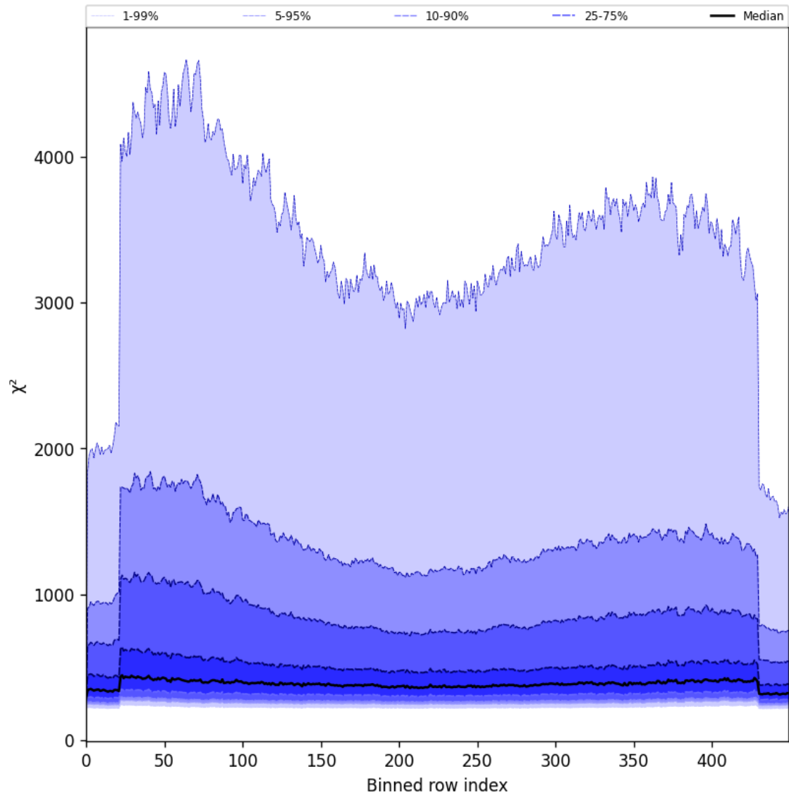
Figure 59: Along track statistics of “ \chi^2 ” for 2025-08-03 to 2025-08-04
