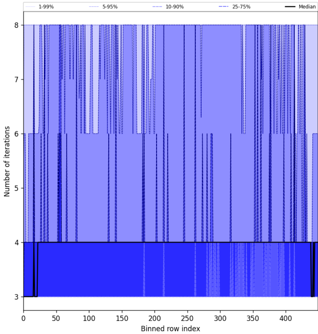
Figure 51: Along track statistics of “Number of iterations” for 2025-08-03 to 2025-08-04
