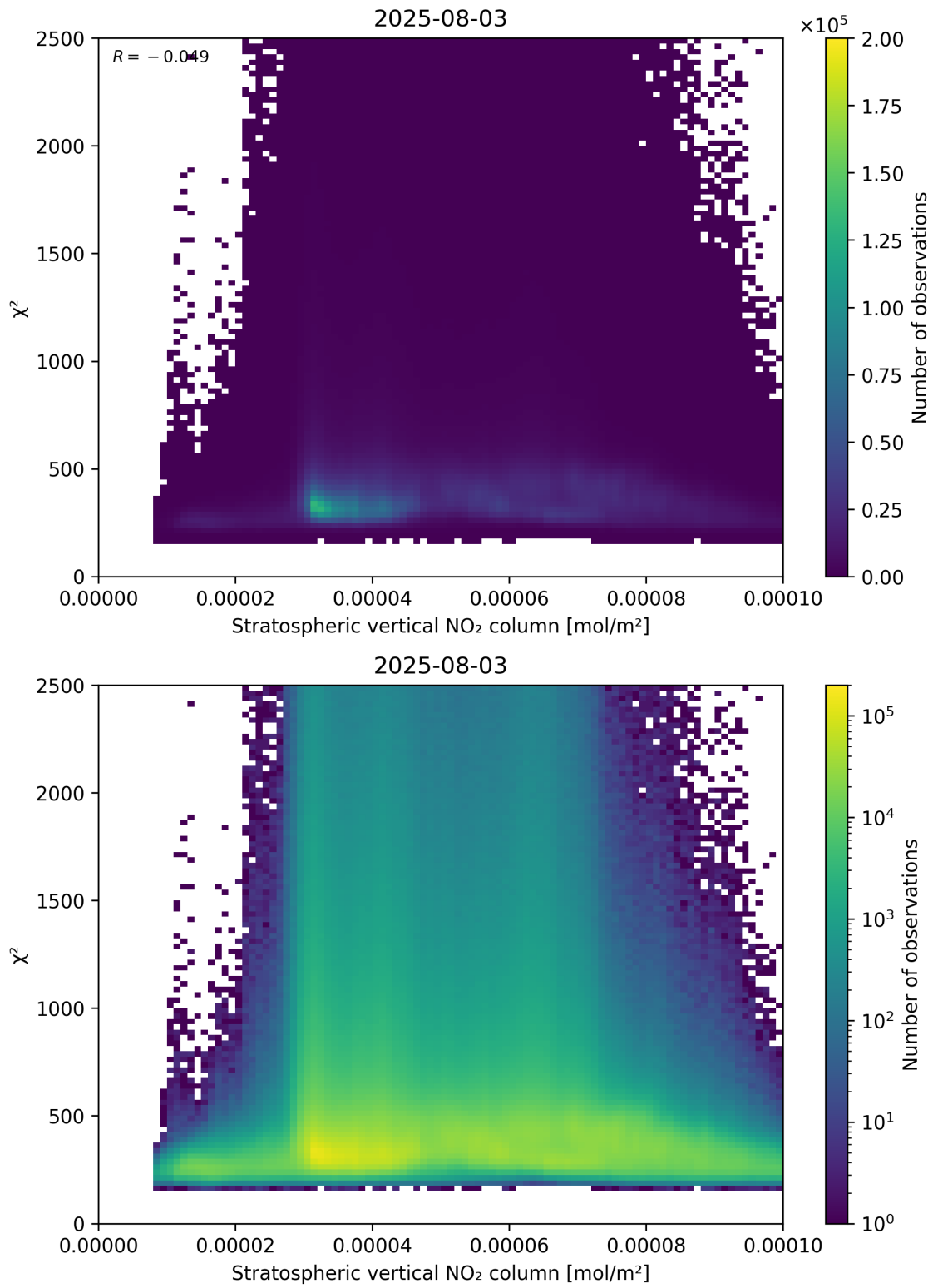
Figure 97: Scatter density plot of “Stratospheric vertical NO 2 column” against “ \chi^2 ” for 2025-08-03 to 2025-08-04.
