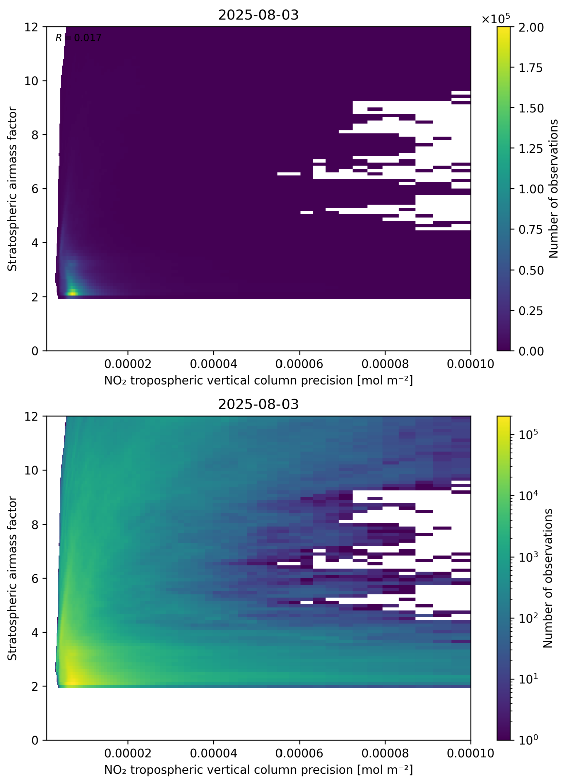
Figure 131: Scatter density plot of “NO 2 tropospheric vertical column precision” against “Stratospheric airmass factor” for 2025-08-03 to 2025-08-04.
