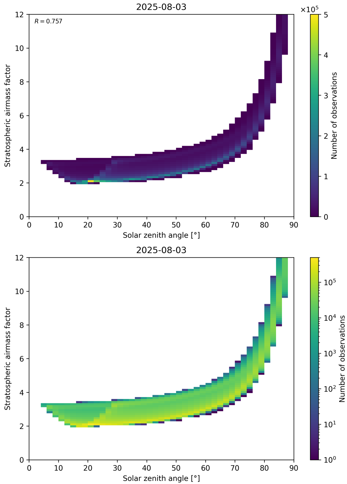
Figure 145: Scatter density plot of “Solar zenith angle” against “Stratospheric airmass factor” for 2025-08-03 to 2025-08-04.
