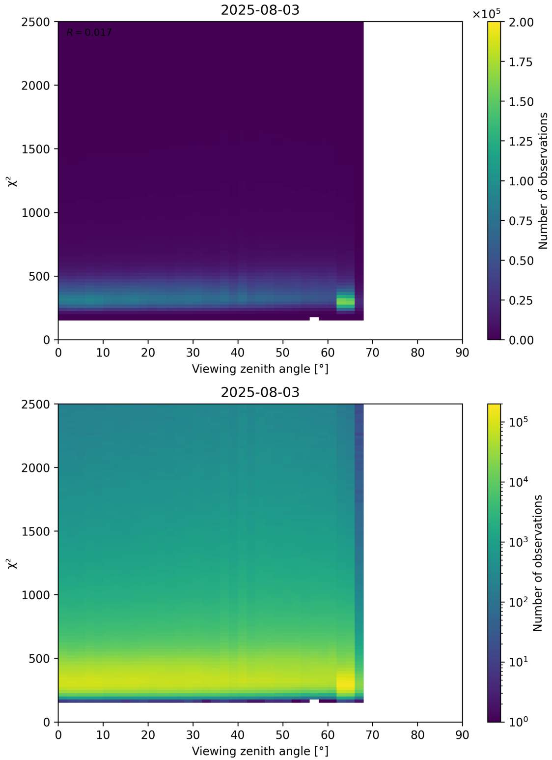
Figure 162: Scatter density plot of “Viewing zenith angle” against “ \chi^2 ” for 2025-08-03 to 2025-08-04.
