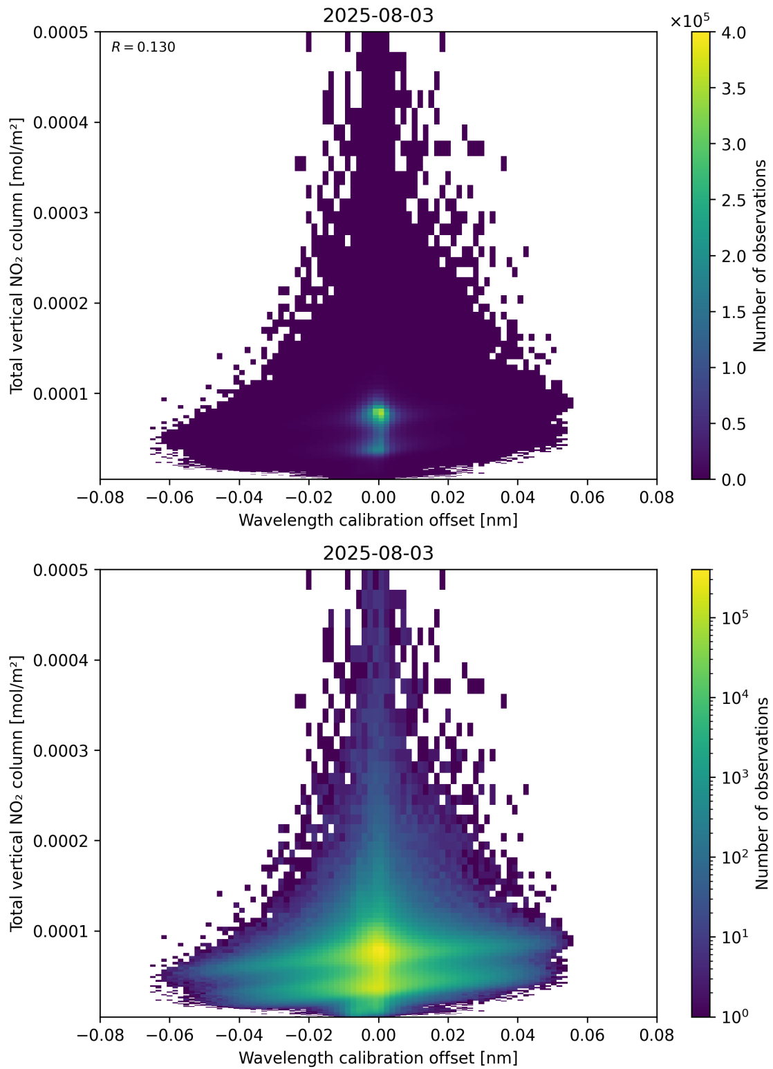
Figure 179: Scatter density plot of “Wavelength calibration offset” against “Total vertical NO 2 column” for 2025-08-03 to 2025-08-04.
