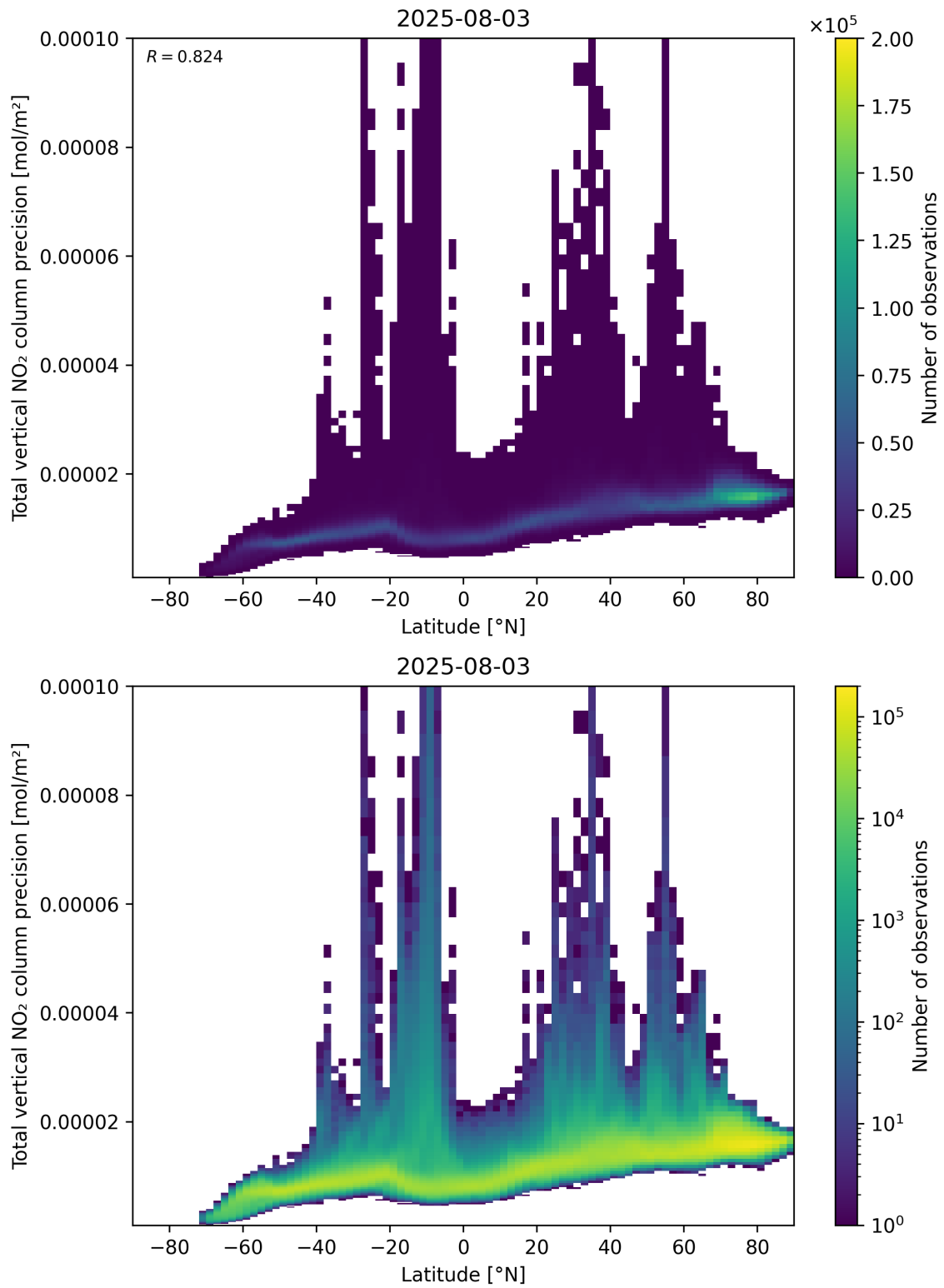
Figure 91: Scatter density plot of “Latitude” against “Total vertical NO 2 column precision” for 2025-08-03 to 2025-08-04.
