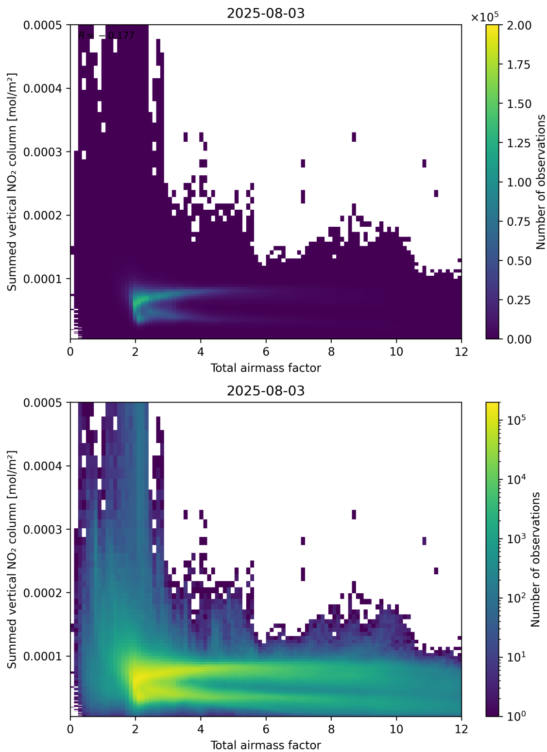
Figure 65: Scatter density plot of “Total airmass factor” against “Summed vertical NO 2 column” for 2025-08-03 to 2025-08-04.
