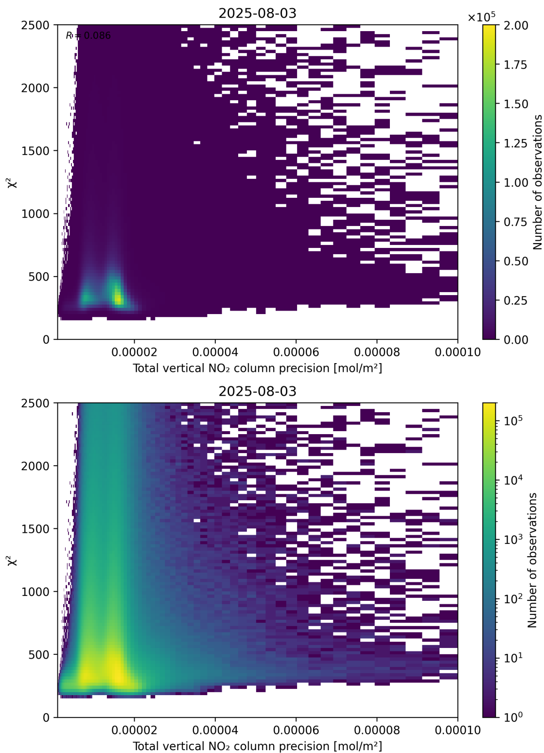
Figure 116: Scatter density plot of “Total vertical NO 2 column precision” against “ \chi^2 ” for 2025-08-03 to 2025-08-04.
