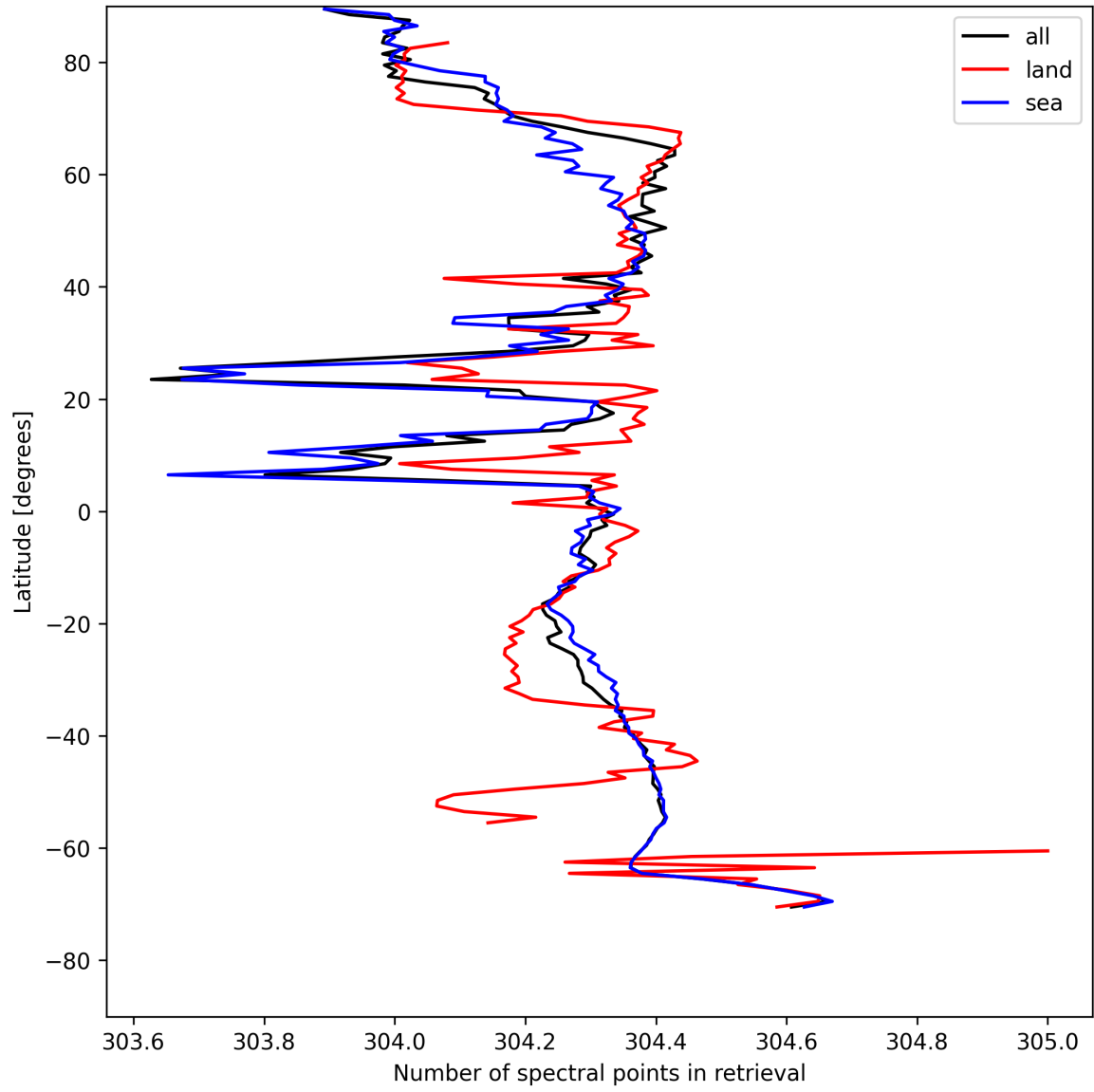
Figure 16: Zonal average of “Number of spectral points in retrieval” for 2025-08-03 to 2025-08-04.
