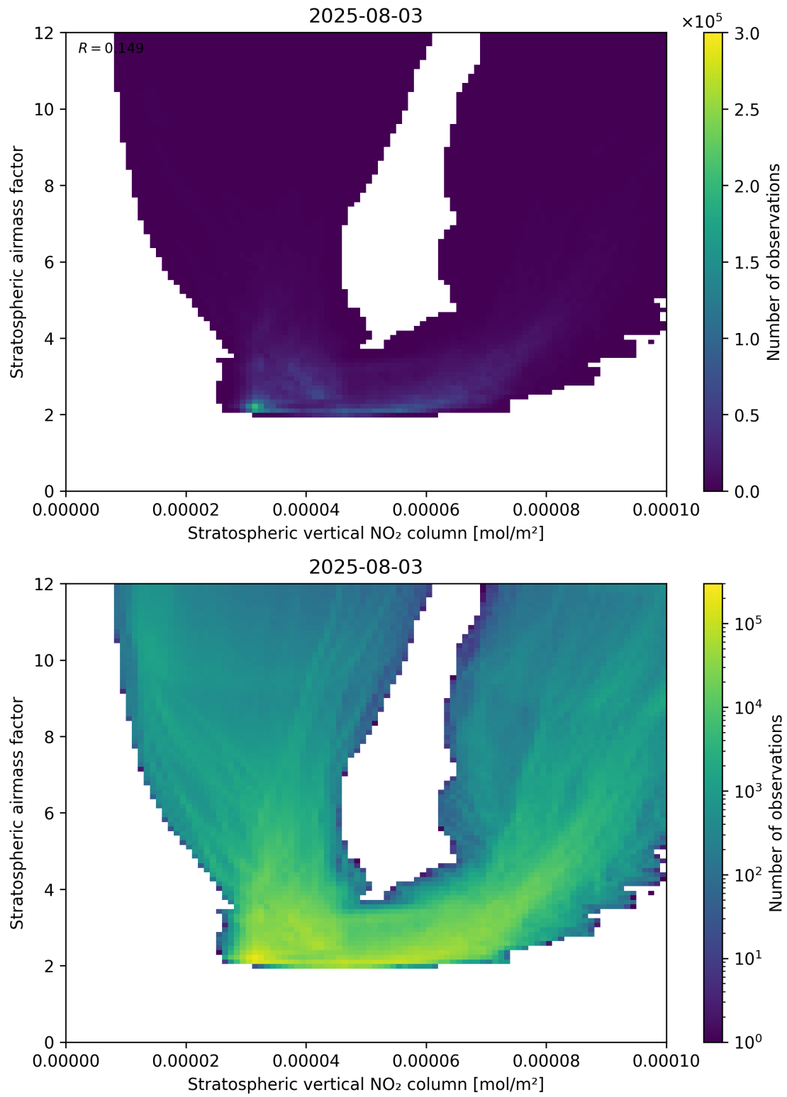
Figure 96: Scatter density plot of “Stratospheric vertical NO 2 column” against “Stratospheric airmass factor” for 2025-08-03 to 2025-08-04.
