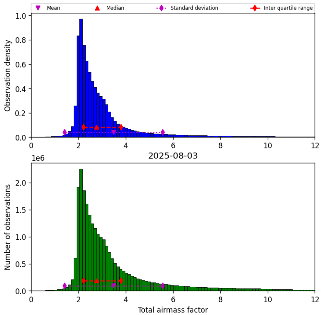
Figure 32: Histogram of “Total airmass factor” for 2025-08-03 to 2025-08-04
