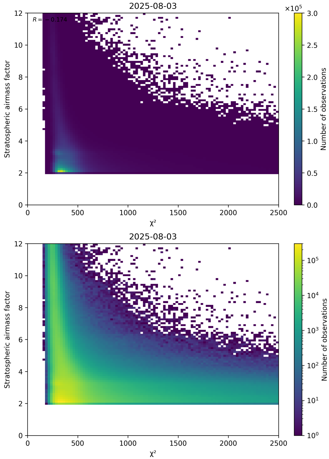
Figure 81: Scatter density plot of “ \chi^2 ” against “Stratospheric airmass factor” for 2025-08-03 to 2025-08-04.
