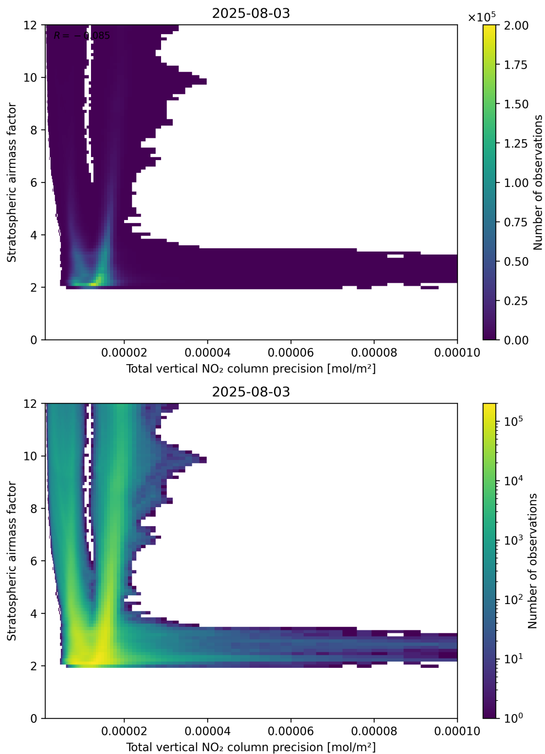
Figure 115: Scatter density plot of “Total vertical NO 2 column precision” against “Stratospheric airmass factor” for 2025-08-03 to 2025-08-04.
