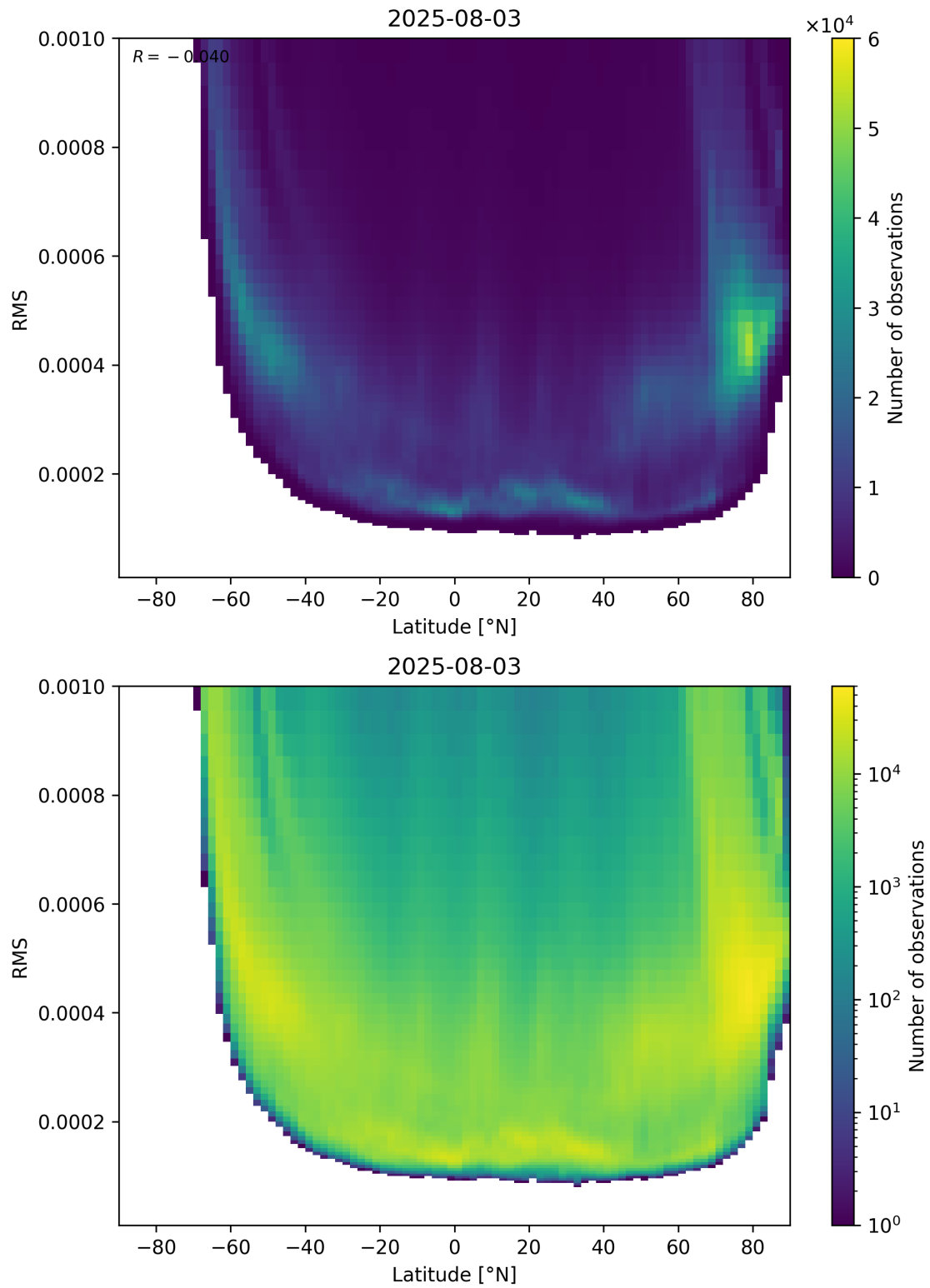
Figure 94: Scatter density plot of “Latitude” against “RMS” for 2025-08-03 to 2025-08-04.
