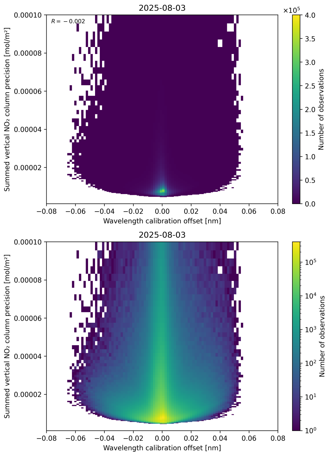
Figure 178: Scatter density plot of “Wavelength calibration offset” against “Summed vertical NO 2 column precision” for 2025-08-03 to 2025-08-04.
