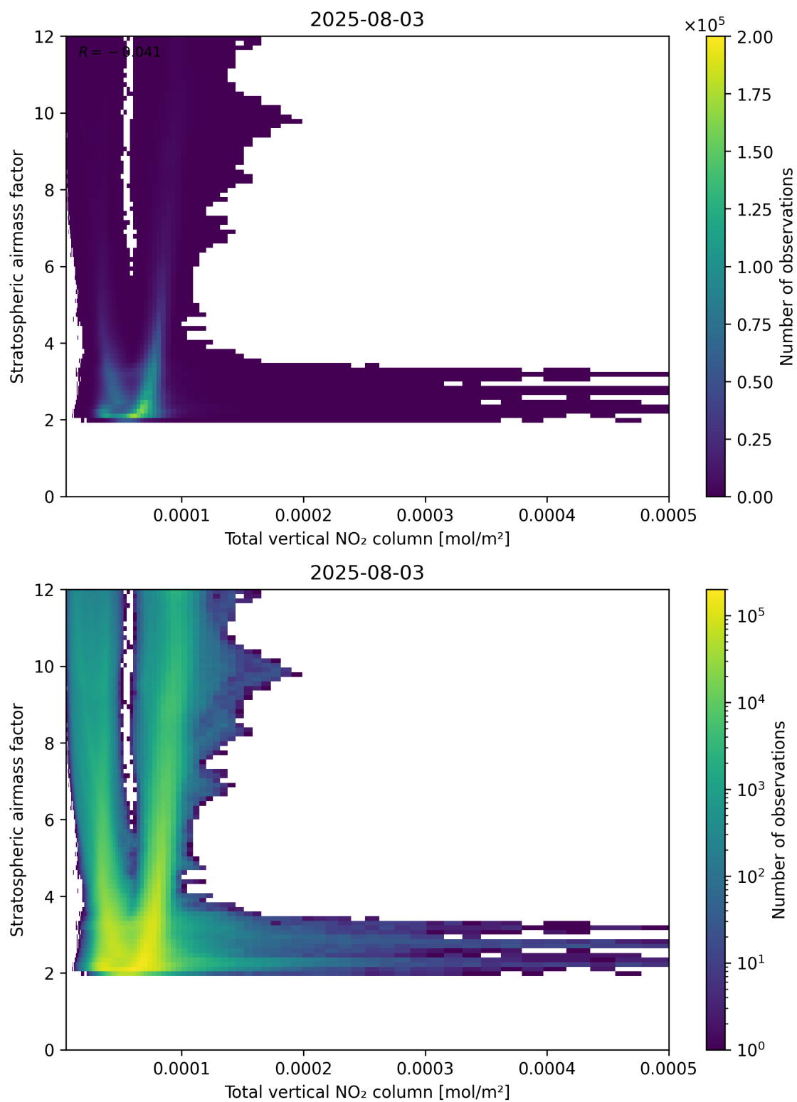
Figure 110: Scatter density plot of “Total vertical NO 2 column” against “Stratospheric airmass factor” for 2025-08-03 to 2025-08-04.
