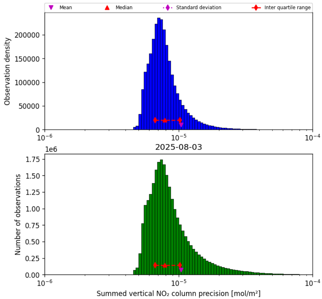
Figure 41: Histogram of “Summed vertical NO 2 column precision” for 2025-08-03 to 2025-08-04
