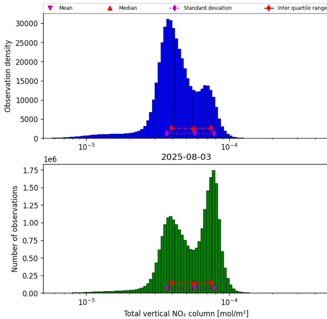
Figure 38: Histogram of “Total vertical NO 2 column” for 2025-08-03 to 2025-08-04
