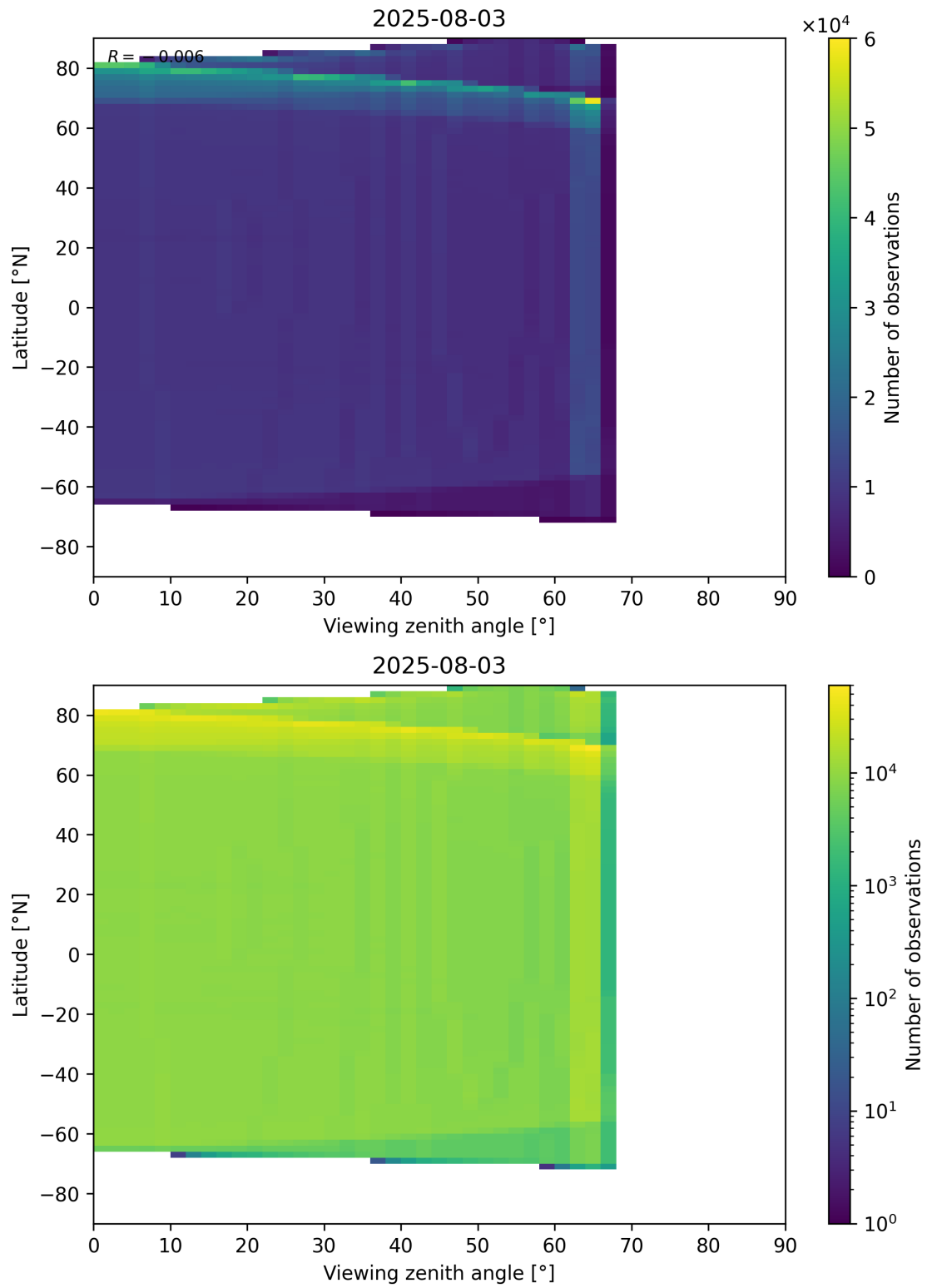
Figure 163: Scatter density plot of “Viewing zenith angle” against “Latitude” for 2025-08-03 to 2025-08-04.
