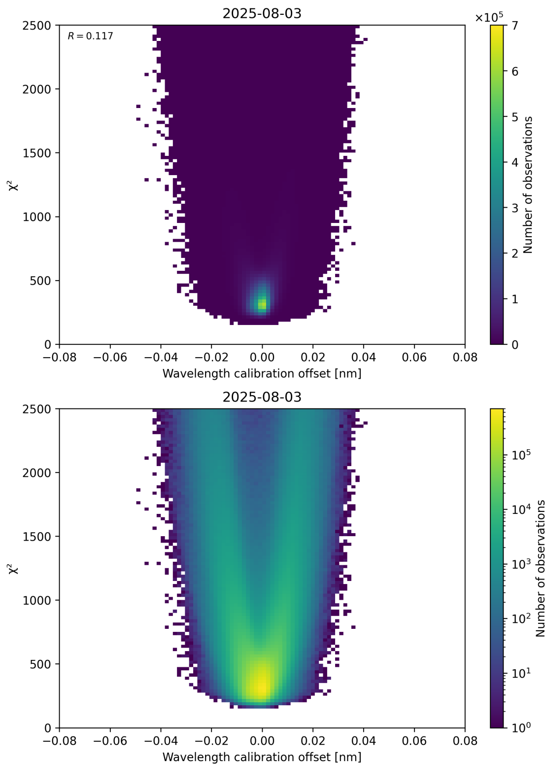
Figure 175: Scatter density plot of “Wavelength calibration offset” against “ \chi^2 ” for 2025-08-03 to 2025-08-04.
