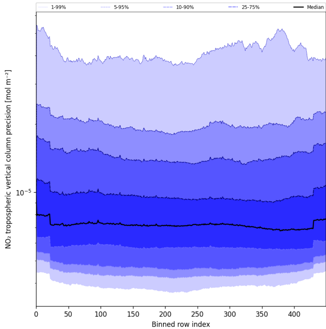
Figure 47: Along track statistics of “NO 2 tropospheric vertical column precision” for 2025-08-03 to 2025-08-04
