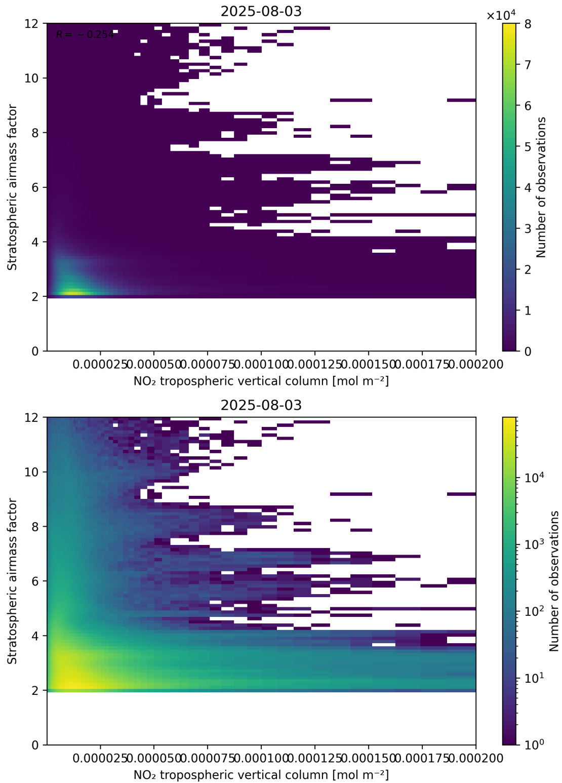
Figure 121: Scatter density plot of “NO 2 tropospheric vertical column” against “Stratospheric air mass factor” for 2025-08-03 to 2025-08-04.
