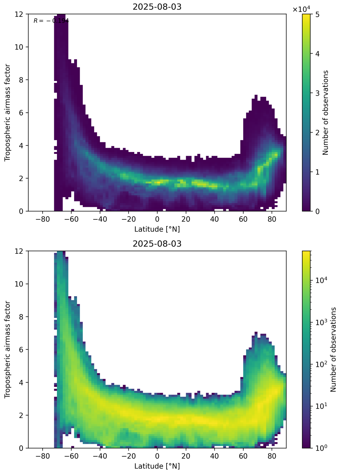
Figure 85: Scatter density plot of “Latitude” against “Tropospheric air mass factor” for 2025-08-03 to 2025-08-04.
