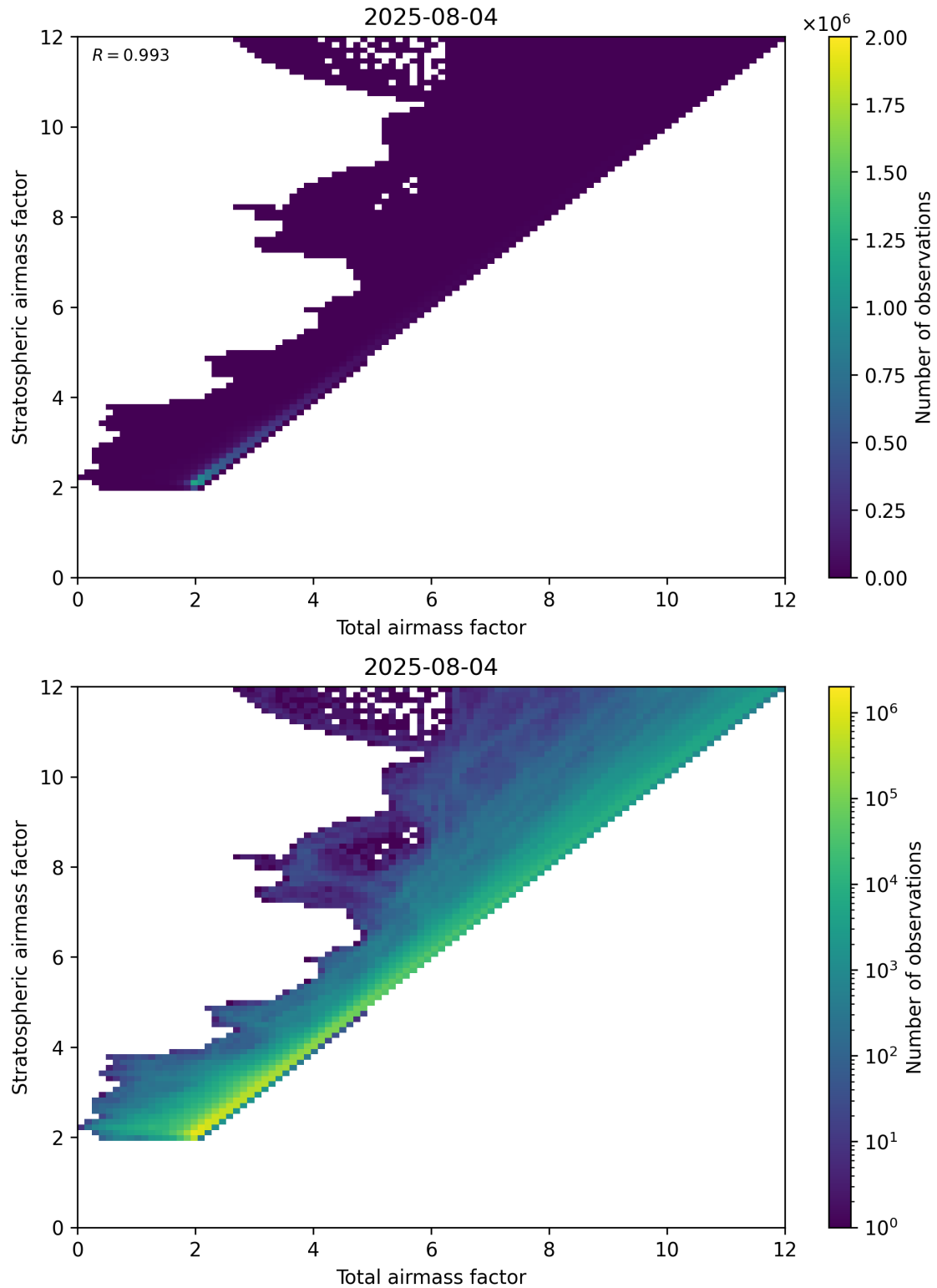
Figure 62: Scatter density plot of “Total airmass factor” against “Stratospheric airmass factor” for 2025-08-04 to 2025-08-05.
