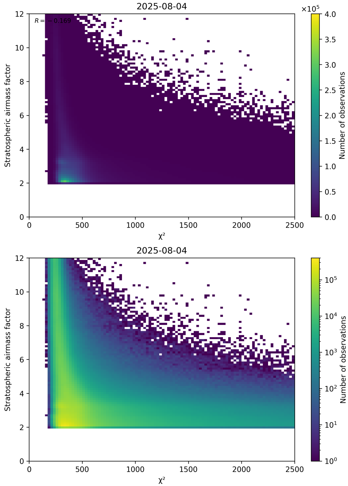
Figure 81: Scatter density plot of “ \chi^2 ” against “Stratospheric airmass factor” for 2025-08-04 to 2025-08-05.
