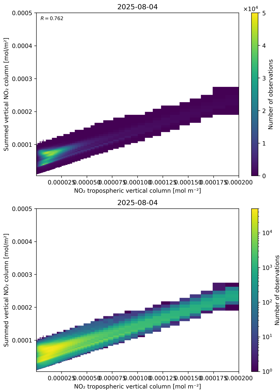
Figure 126: Scatter density plot of “NO 2 tropospheric vertical column” against “Summed vertical NO 2 column” for 2025-08-04 to 2025-08-05.
