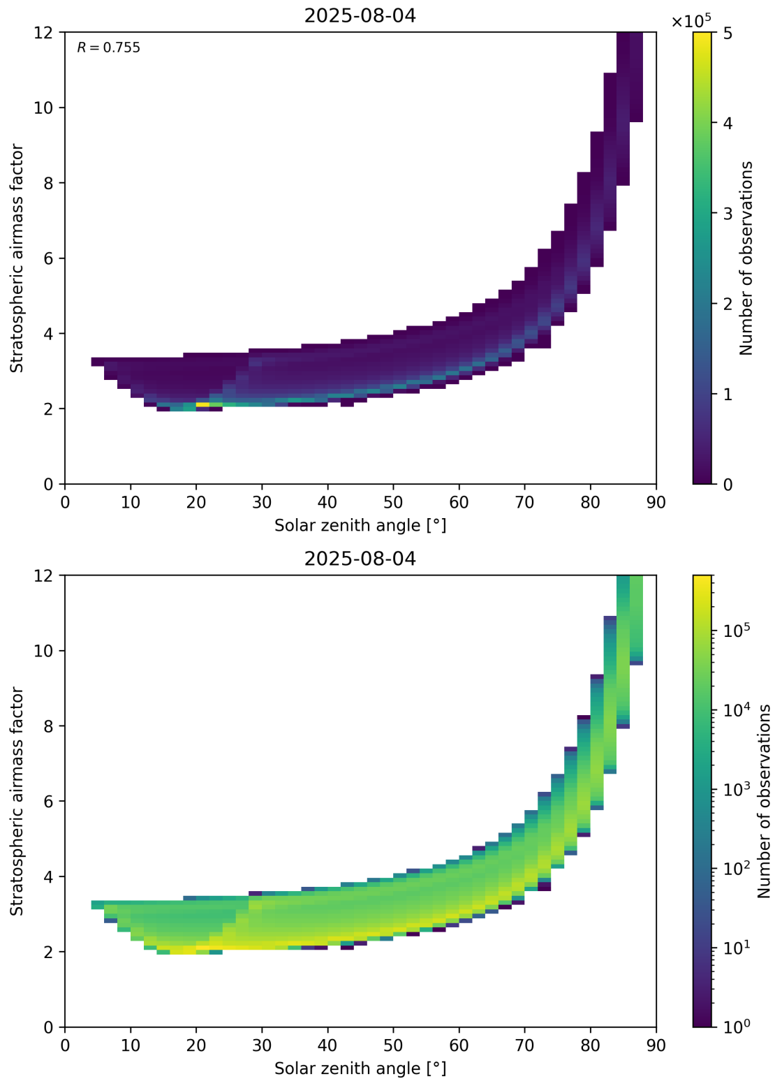
Figure 145: Scatter density plot of “Solar zenith angle” against “Stratospheric airmass factor” for 2025-08-04 to 2025-08-05.
