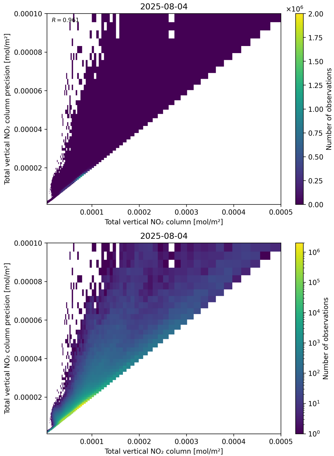
Figure 114: Scatter density plot of “Total vertical NO 2 column” against “Total vertical NO 2 column precision” for 2025-08-04 to 2025-08-05.
