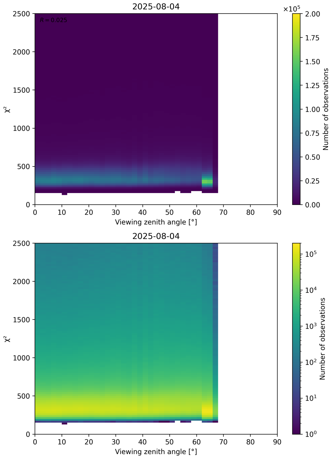
Figure 162: Scatter density plot of “Viewing zenith angle” against “ \chi^2 ” for 2025-08-04 to 2025-08-05.
