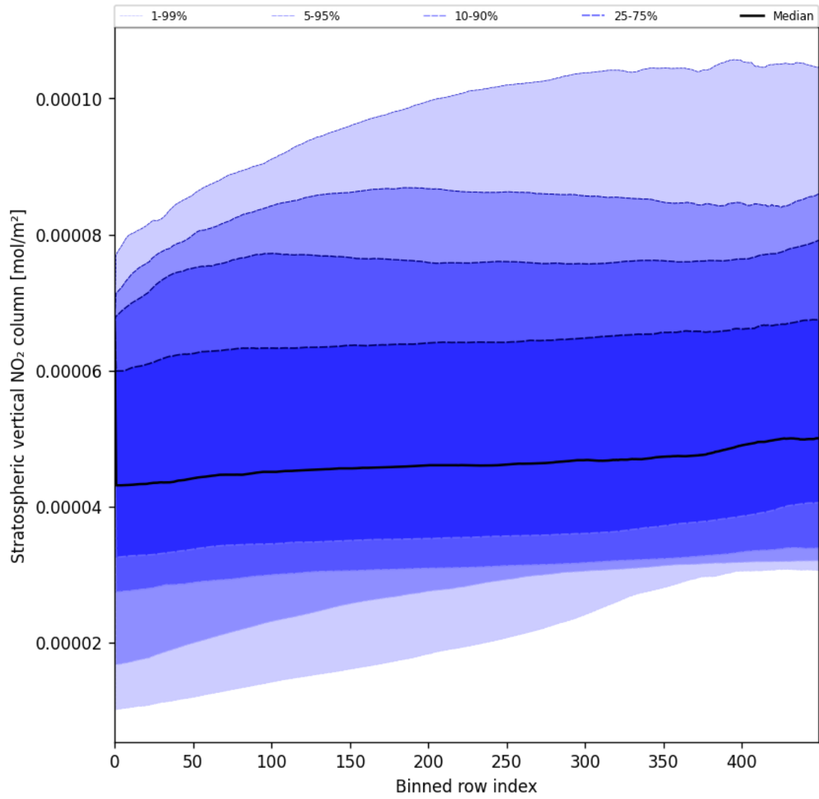
Figure 53: Along track statistics of “Stratospheric vertical NO 2 column” for 2025-08-04 to 2025-08-05
