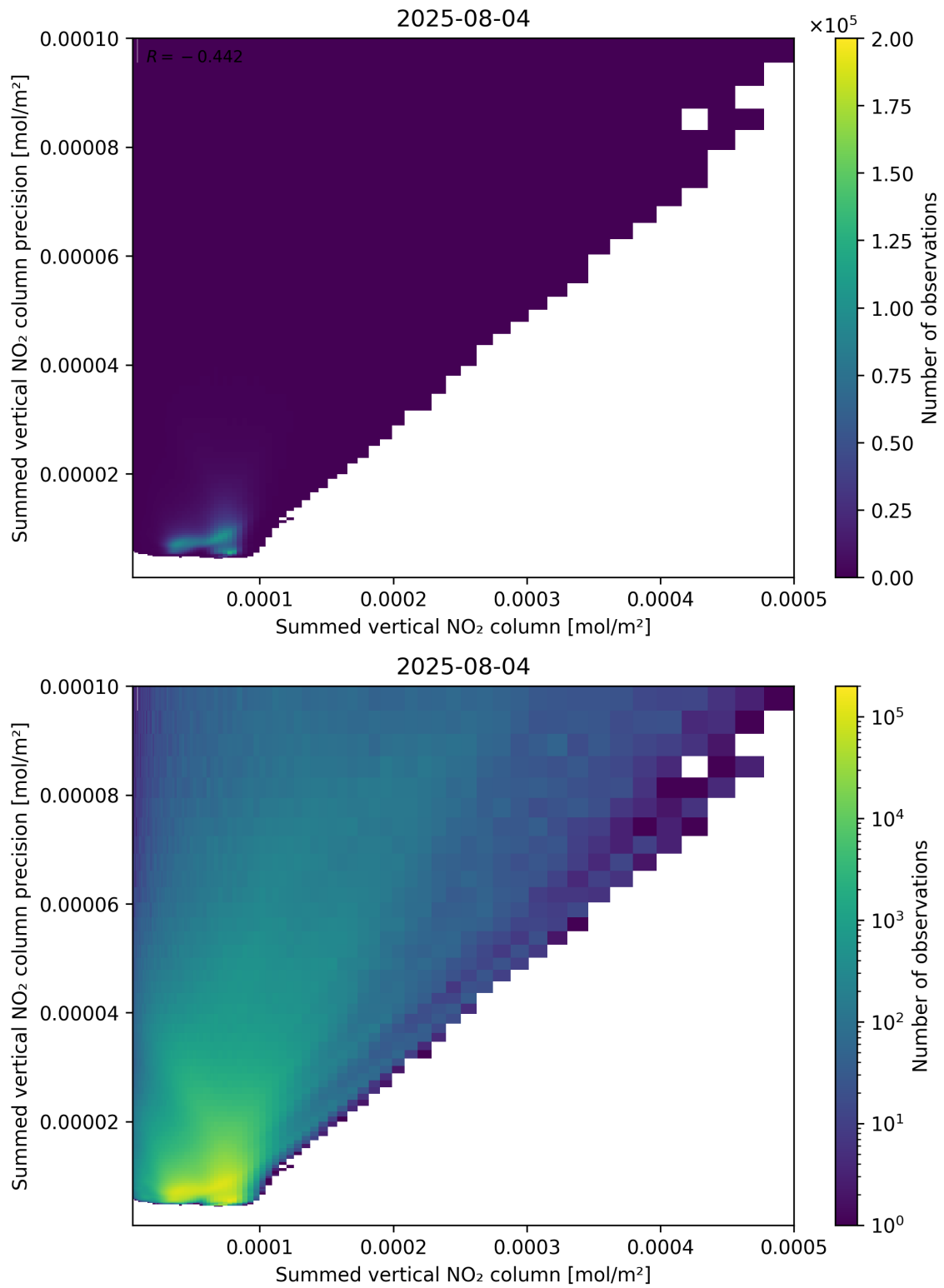
Figure 105: Scatter density plot of “Summed vertical NO 2 column” against “Summed vertical NO 2 column precision” for 2025-08-04 to 2025-08-05.
