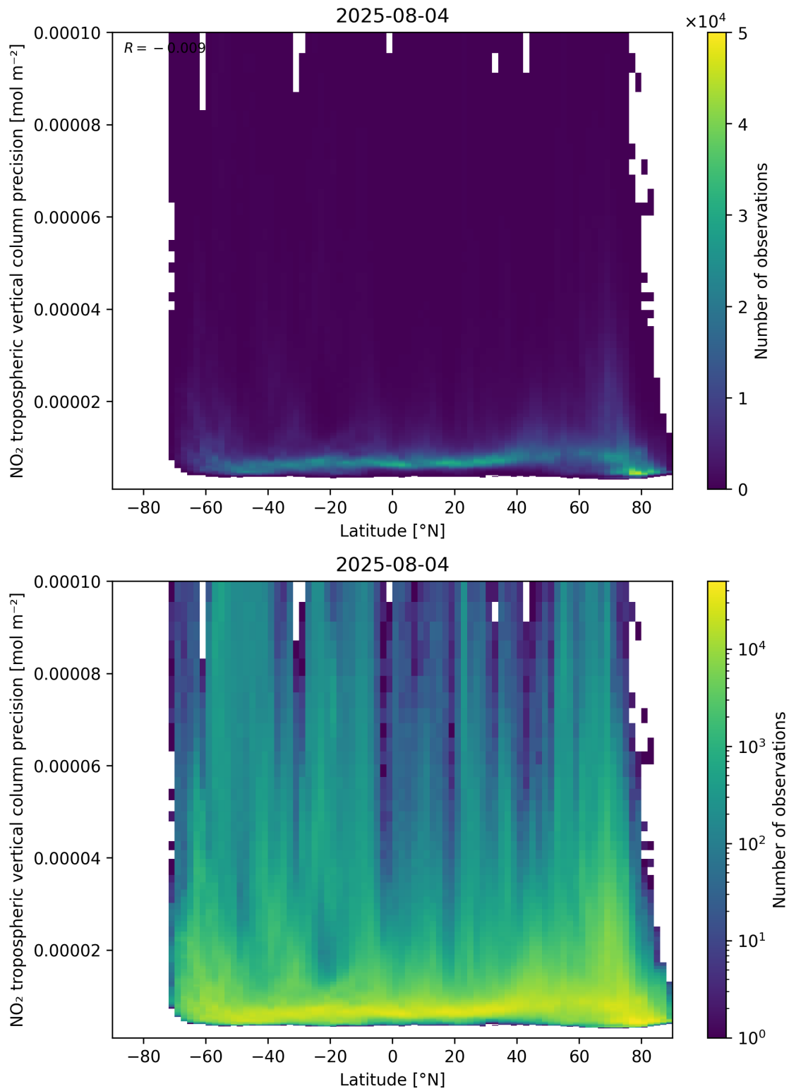
Figure 93: Scatter density plot of “Latitude” against “NO 2 tropospheric vertical column precision” for 2025-08-04 to 2025-08-05.
