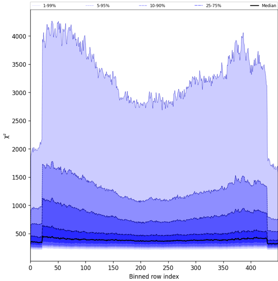
Figure 59: Along track statistics of “ \chi^2 ” for 2025-08-04 to 2025-08-05
