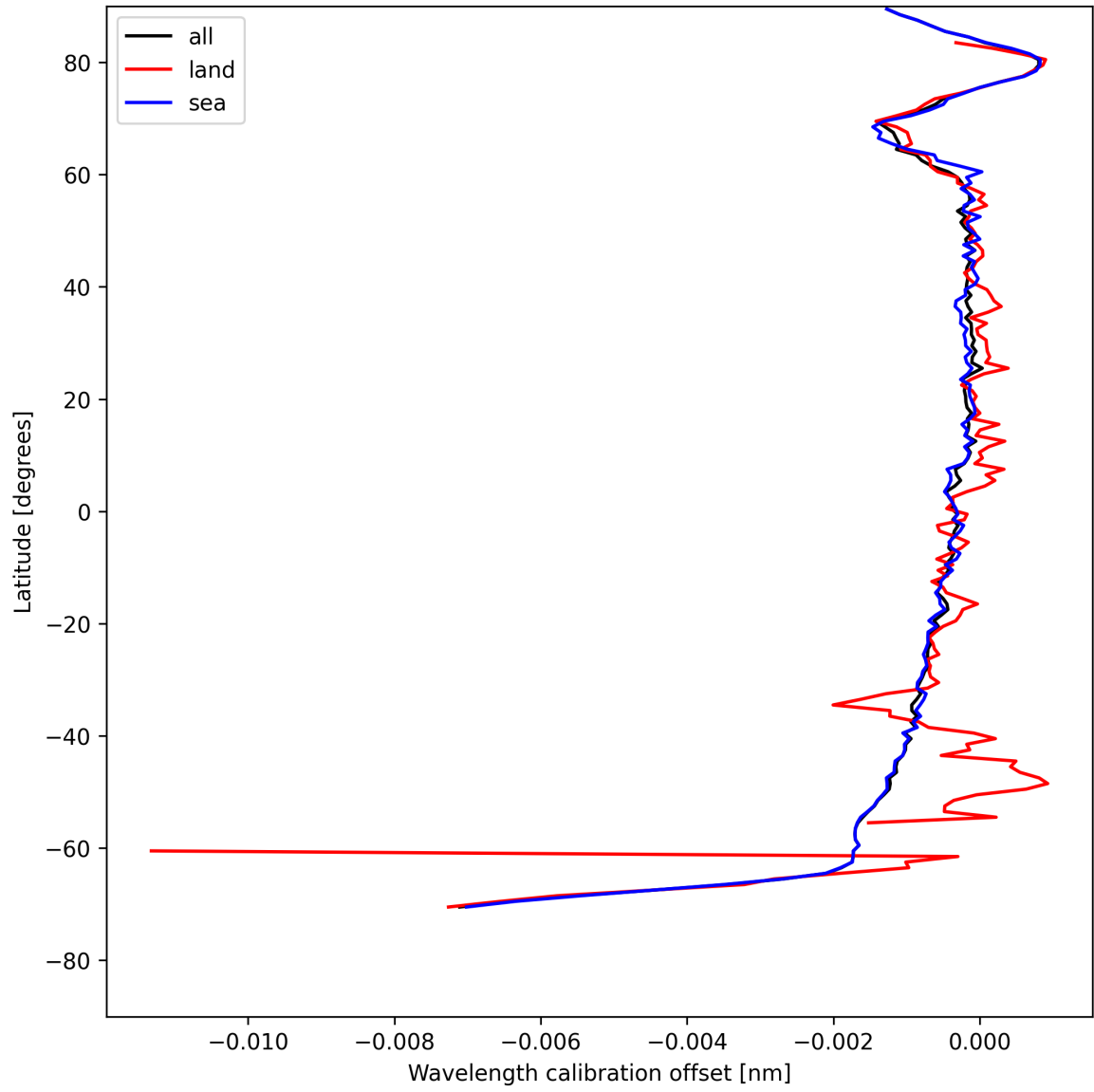
Figure 18: Zonal average of “Wavelength calibration offset” for 2025-08-04 to 2025-08-05.
