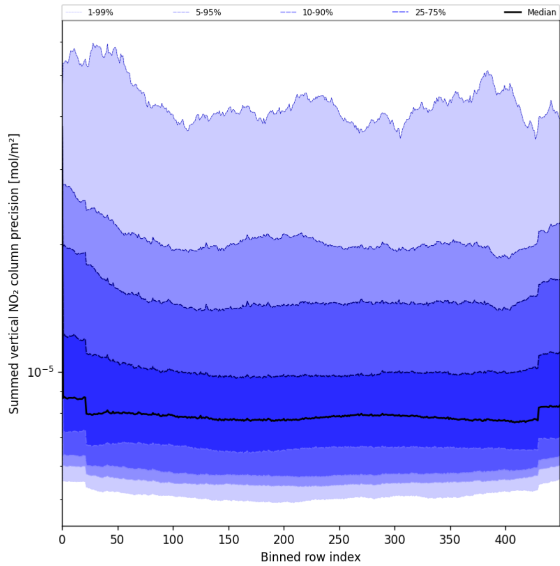
Figure 58: Along track statistics of “Summed vertical NO 2 column precision” for 2025-08-04 to 2025-08-05
