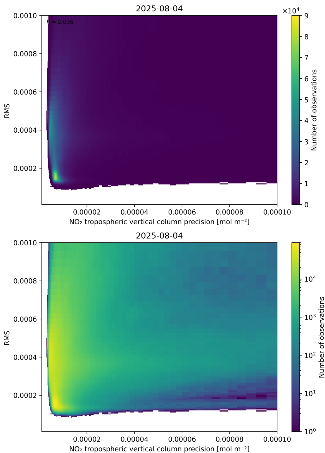
Figure 140: Scatter density plot of “NO 2 tropospheric vertical column precision” against “RMS” for 2025-08-04 to 2025-08-05.
