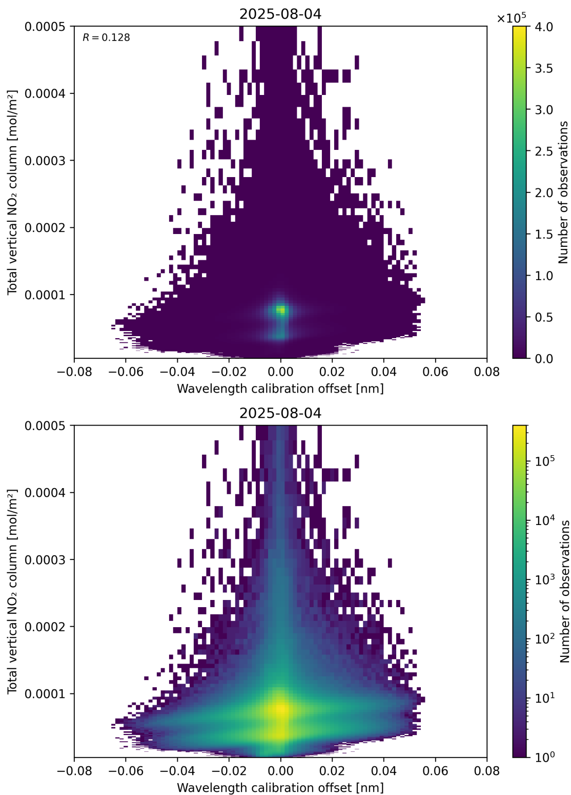
Figure 179: Scatter density plot of “Wavelength calibration offset” against “Total vertical NO 2 column” for 2025-08-04 to 2025-08-05.
