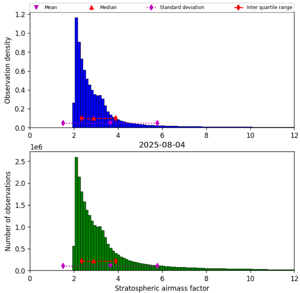
Figure 44: Histogram of “Stratospheric airmass factor” for 2025-08-04 to 2025-08-05
