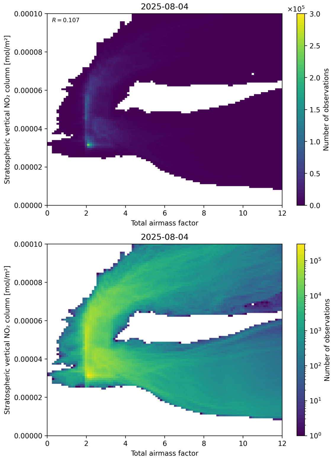
Figure 64: Scatter density plot of “Total airmass factor” against “Stratospheric vertical NO 2 column” for 2025-08-04 to 2025-08-05.
