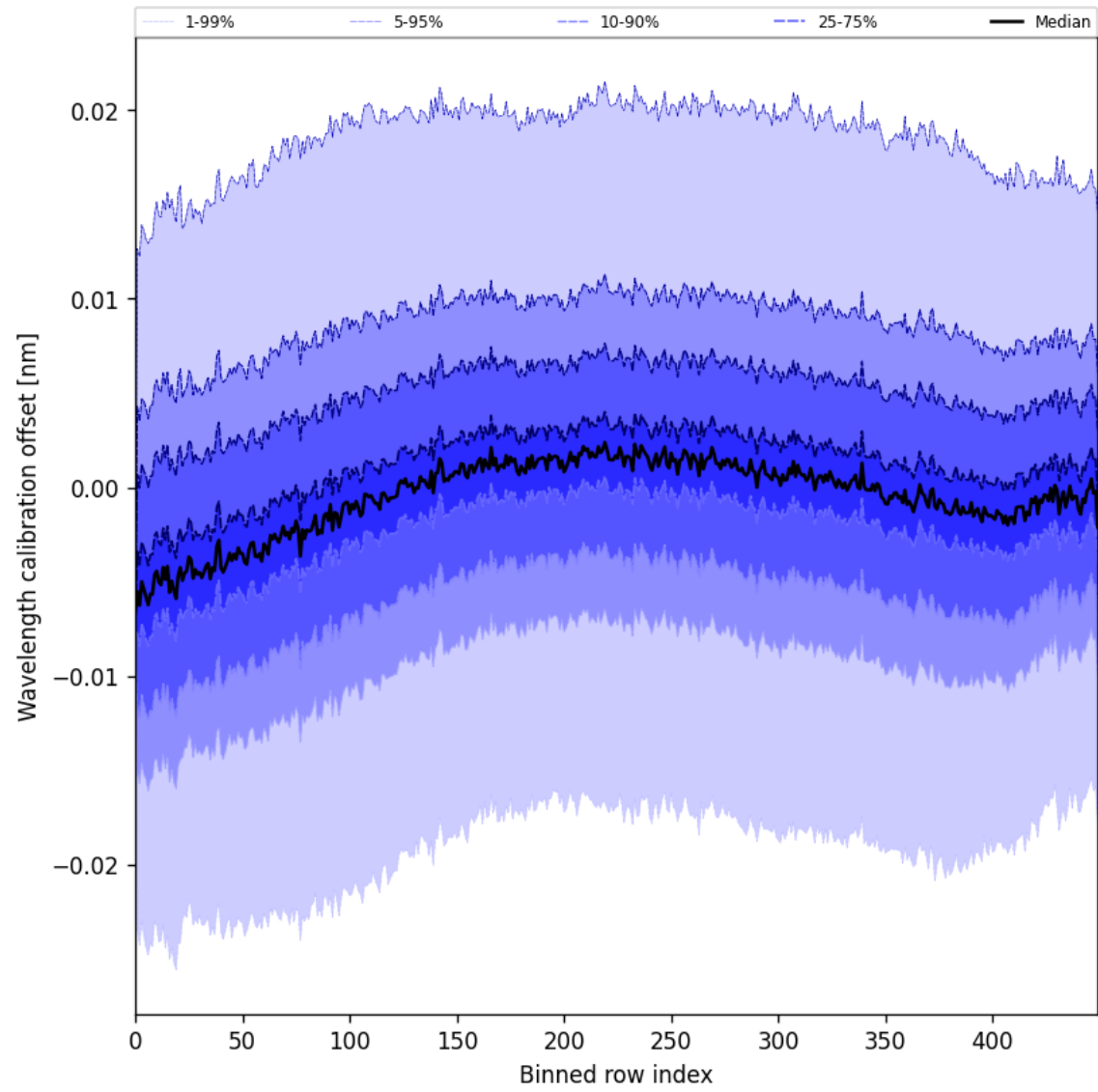
Figure 52: Along track statistics of “Wavelength calibration offset” for 2025-08-04 to 2025-08-05
