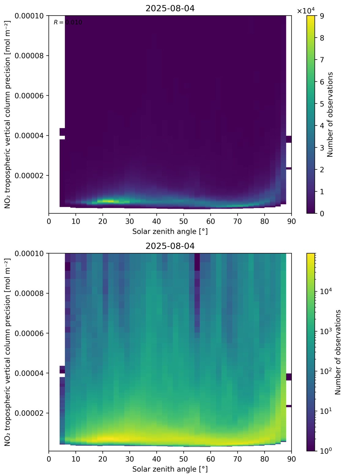
Figure 156: Scatter density plot of “Solar zenith angle” against “NO 2 tropospheric vertical column precision” for 2025-08-04 to 2025-08-05.
