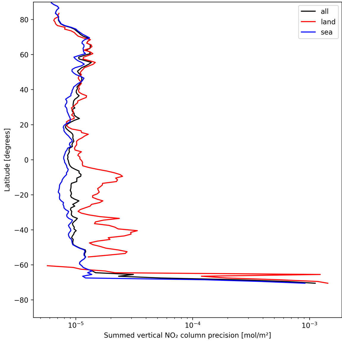
Figure 24: Zonal average of “Summed vertical NO 2 column precision” for 2025-08-04 to 2025-08-05.
