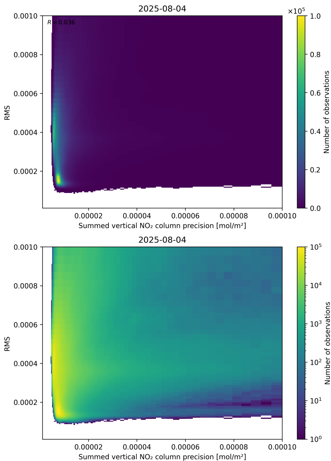
Figure 108: Scatter density plot of “Summed vertical NO 2 column precision” against “RMS” for 2025-08-04 to 2025-08-05.
