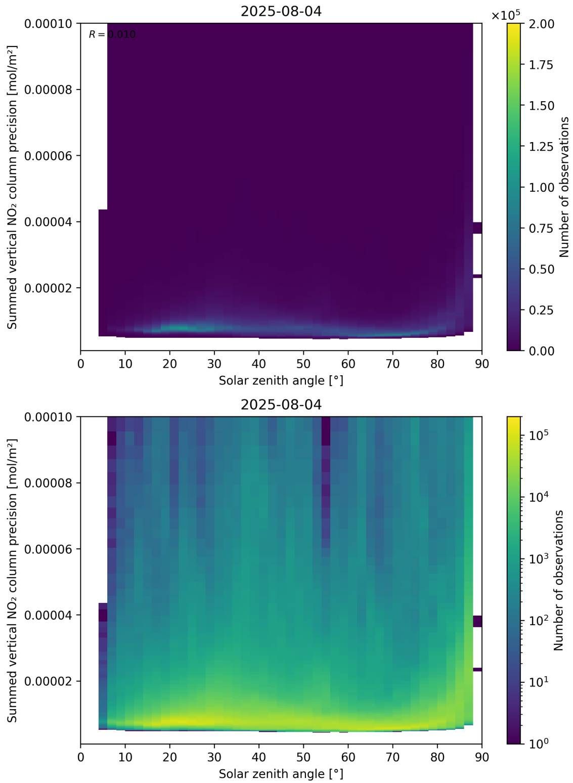
Figure 152: Scatter density plot of “Solar zenith angle” against “Summed vertical NO 2 column precision” for 2025-08-04 to 2025-08-05.
