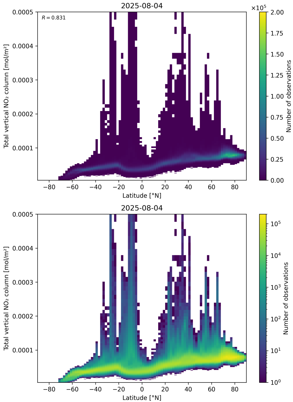
Figure 90: Scatter density plot of “Latitude” against “Total vertical NO 2 column” for 2025-08-04 to 2025-08-05.
