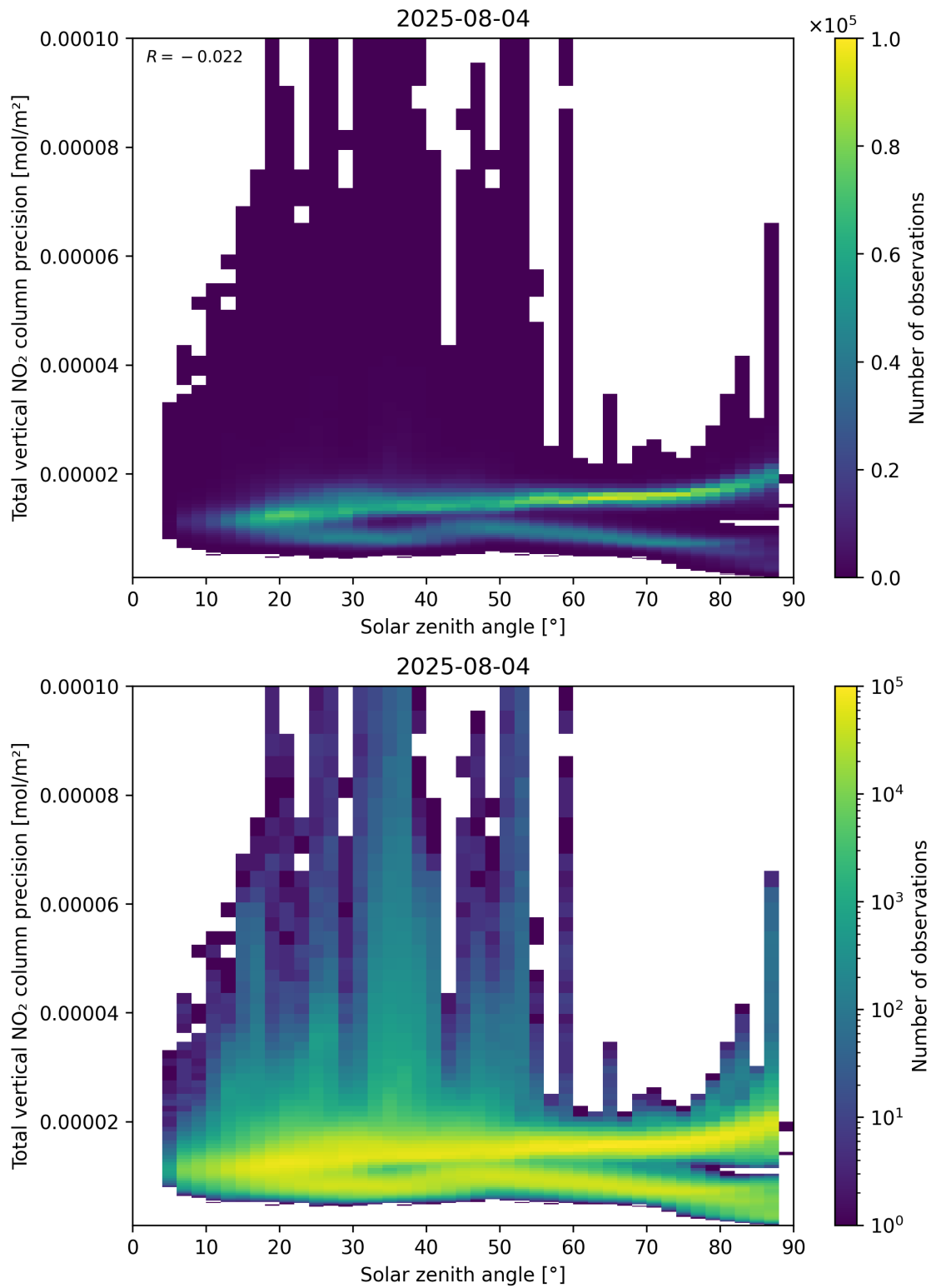
Figure 154: Scatter density plot of “Solar zenith angle” against “Total vertical NO 2 column precision” for 2025-08-04 to 2025-08-05.
