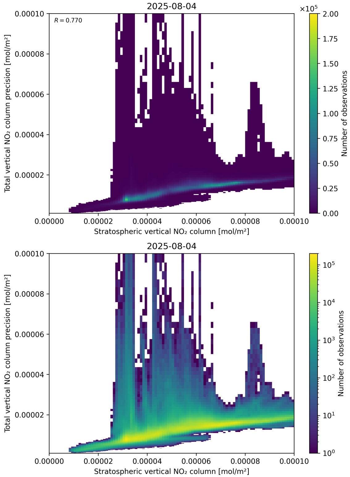
Figure 101: Scatter density plot of “Stratospheric vertical NO 2 column” against “Total vertical NO 2 column precision” for 2025-08-04 to 2025-08-05.
