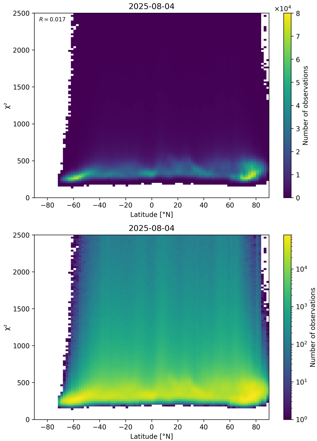
Figure 86: Scatter density plot of “Latitude” against “ \chi^2 ” for 2025-08-04 to 2025-08-05.
