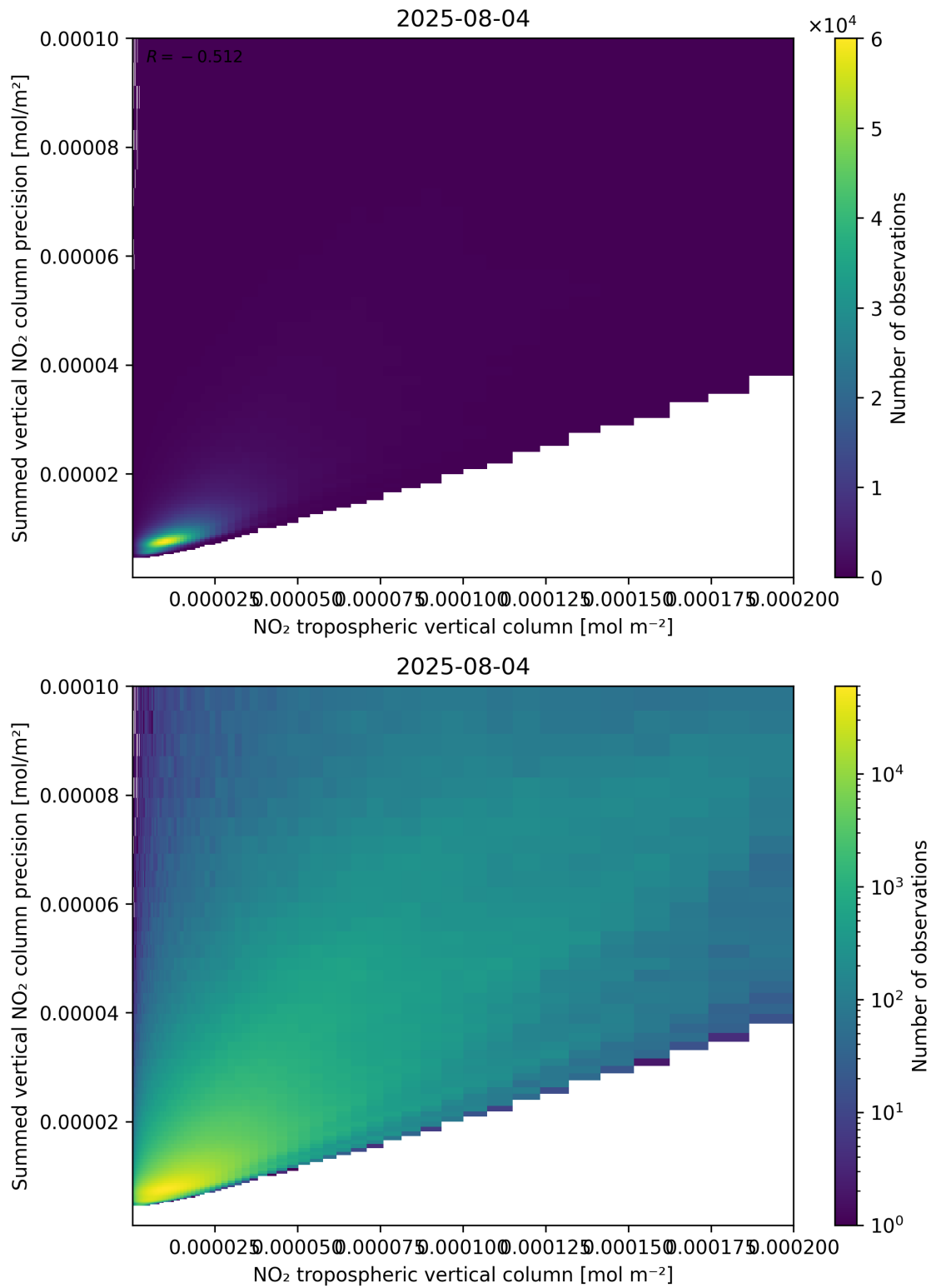
Figure 127: Scatter density plot of “NO 2 tropospheric vertical column” against “Summed vertical NO 2 column precision” for 2025-08-04 to 2025-08-05.
