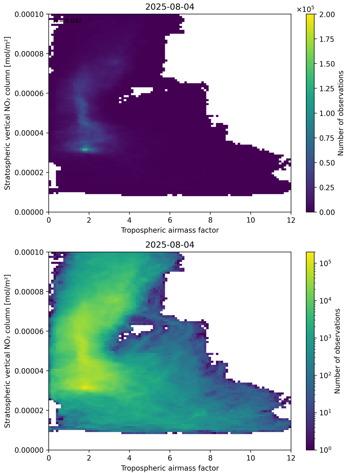
Figure 74: Scatter density plot of “Tropospheric air mass factor” against “Stratospheric vertical NO 2 column” for 2025-08-04 to 2025-08-05.
