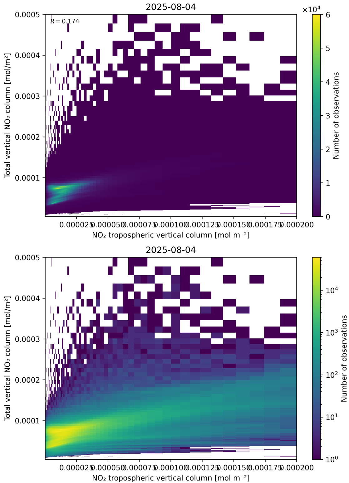
Figure 128: Scatter density plot of “NO 2 tropospheric vertical column” against “Total vertical NO 2 column” for 2025-08-04 to 2025-08-05.
