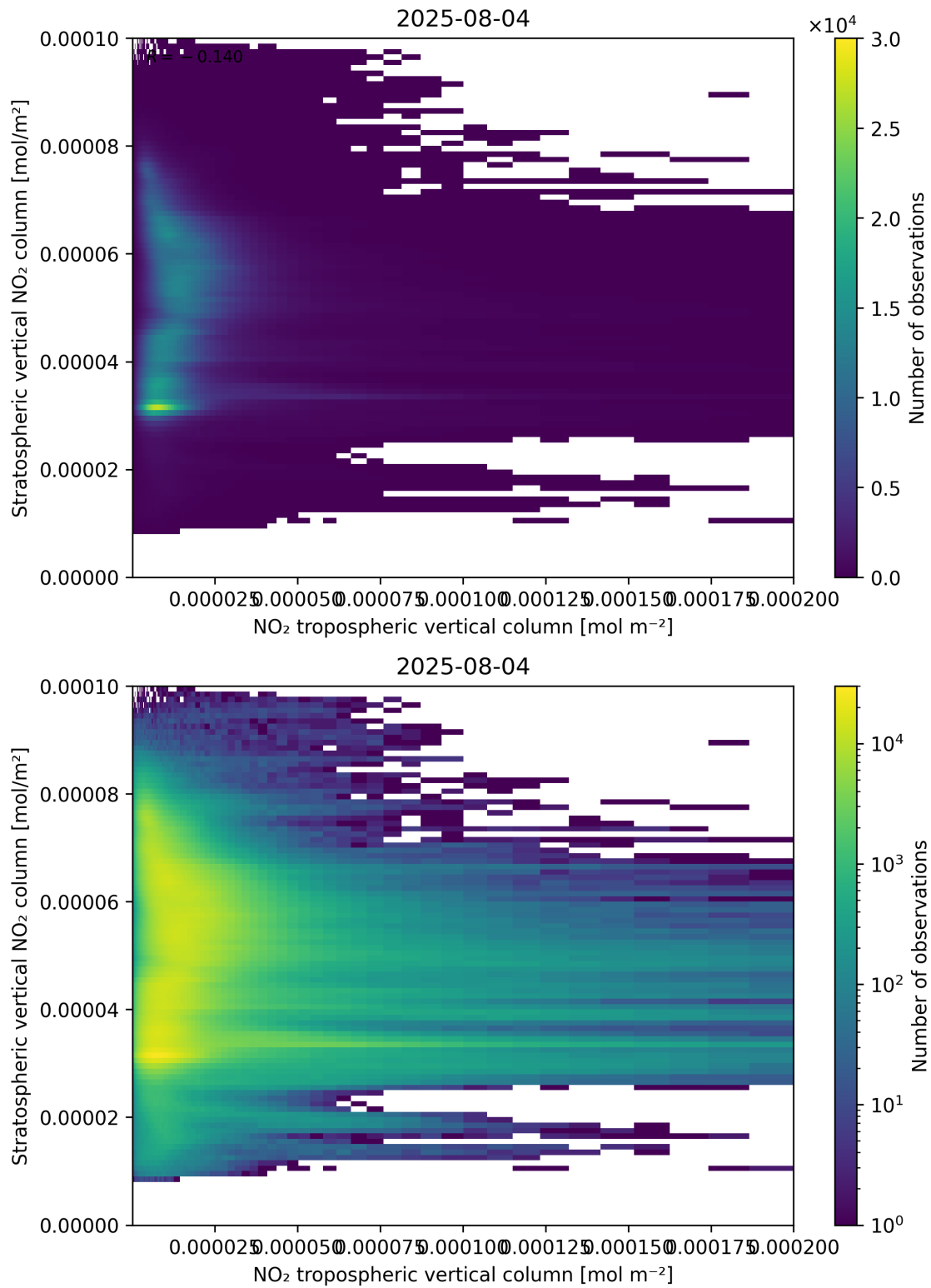
Figure 125: Scatter density plot of “NO 2 tropospheric vertical column” against “Stratospheric vertical NO 2 column” for 2025-08-04 to 2025-08-05.
