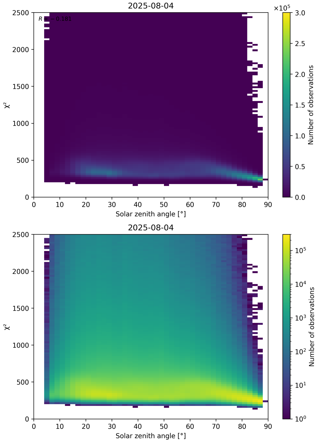
Figure 148: Scatter density plot of “Solar zenith angle” against “ \chi^2 ” for 2025-08-04 to 2025-08-05.
