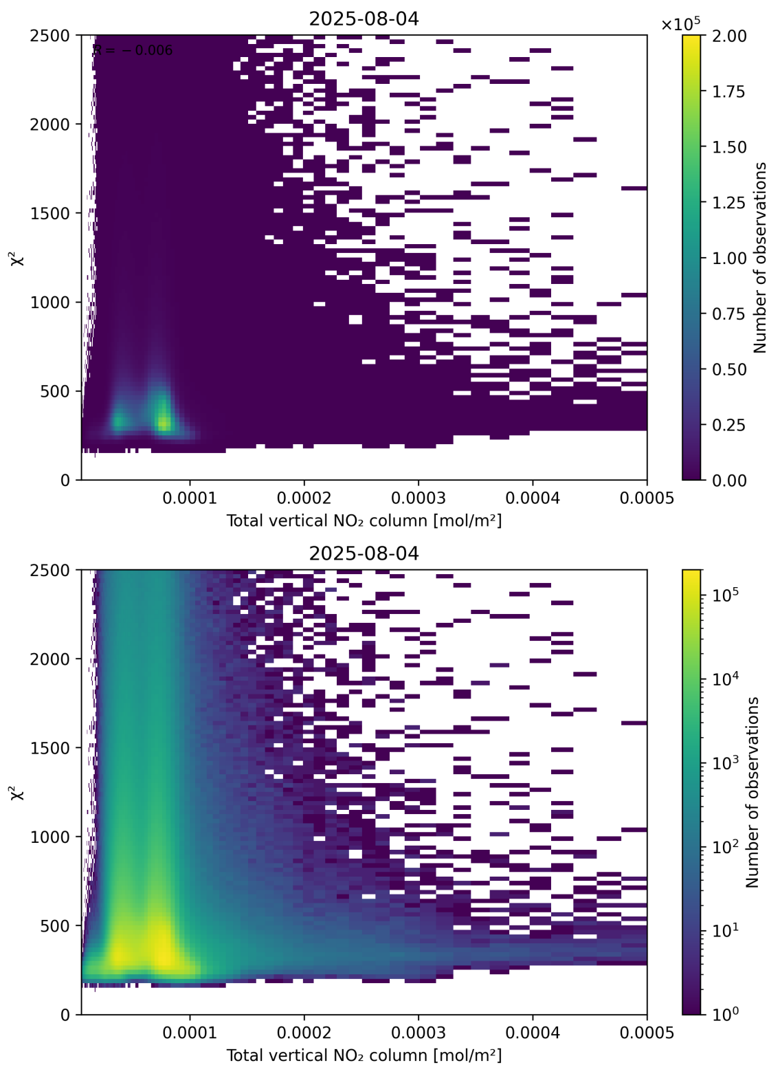
Figure 111: Scatter density plot of “Total vertical NO 2 column” against “ \chi^2 ” for 2025-08-04 to 2025-08-05.
