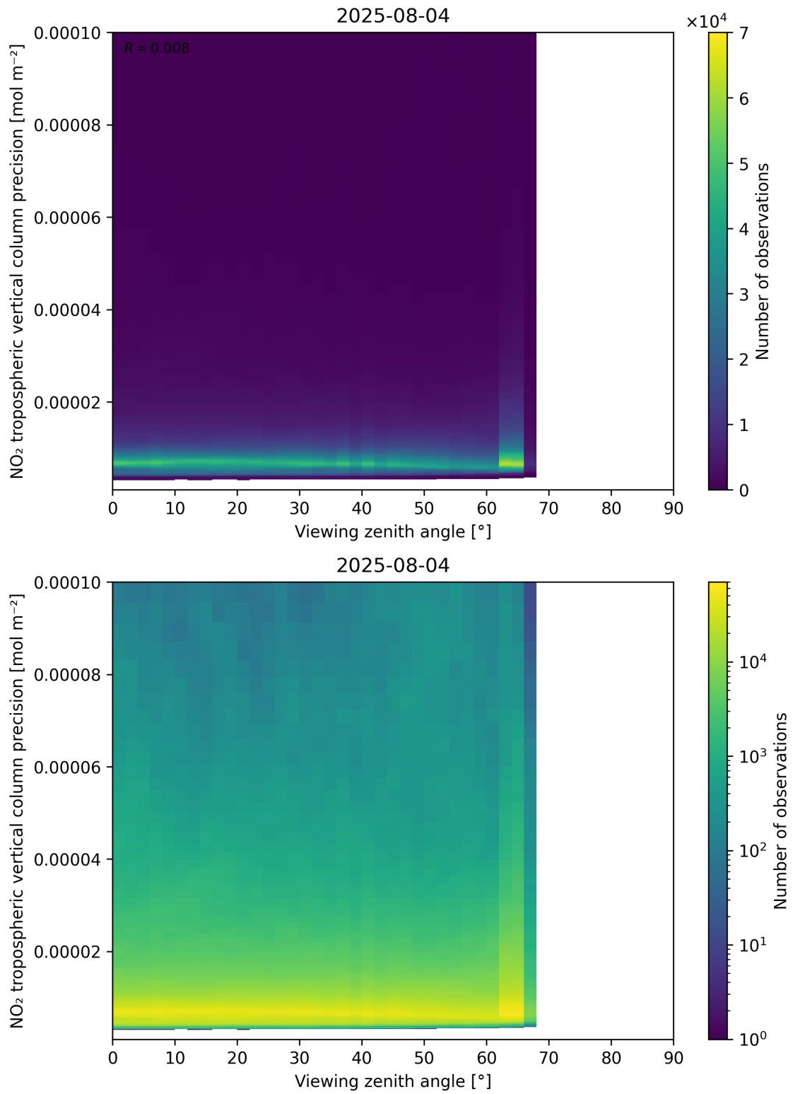
Figure 170: Scatter density plot of “Viewing zenith angle” against “NO 2 tropospheric vertical column precision” for 2025-08-04 to 2025-08-05.
