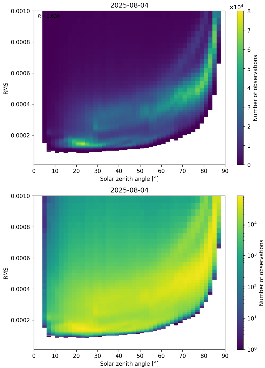
Figure 157: Scatter density plot of “Solar zenith angle” against “RMS” for 2025-08-04 to 2025-08-05.
