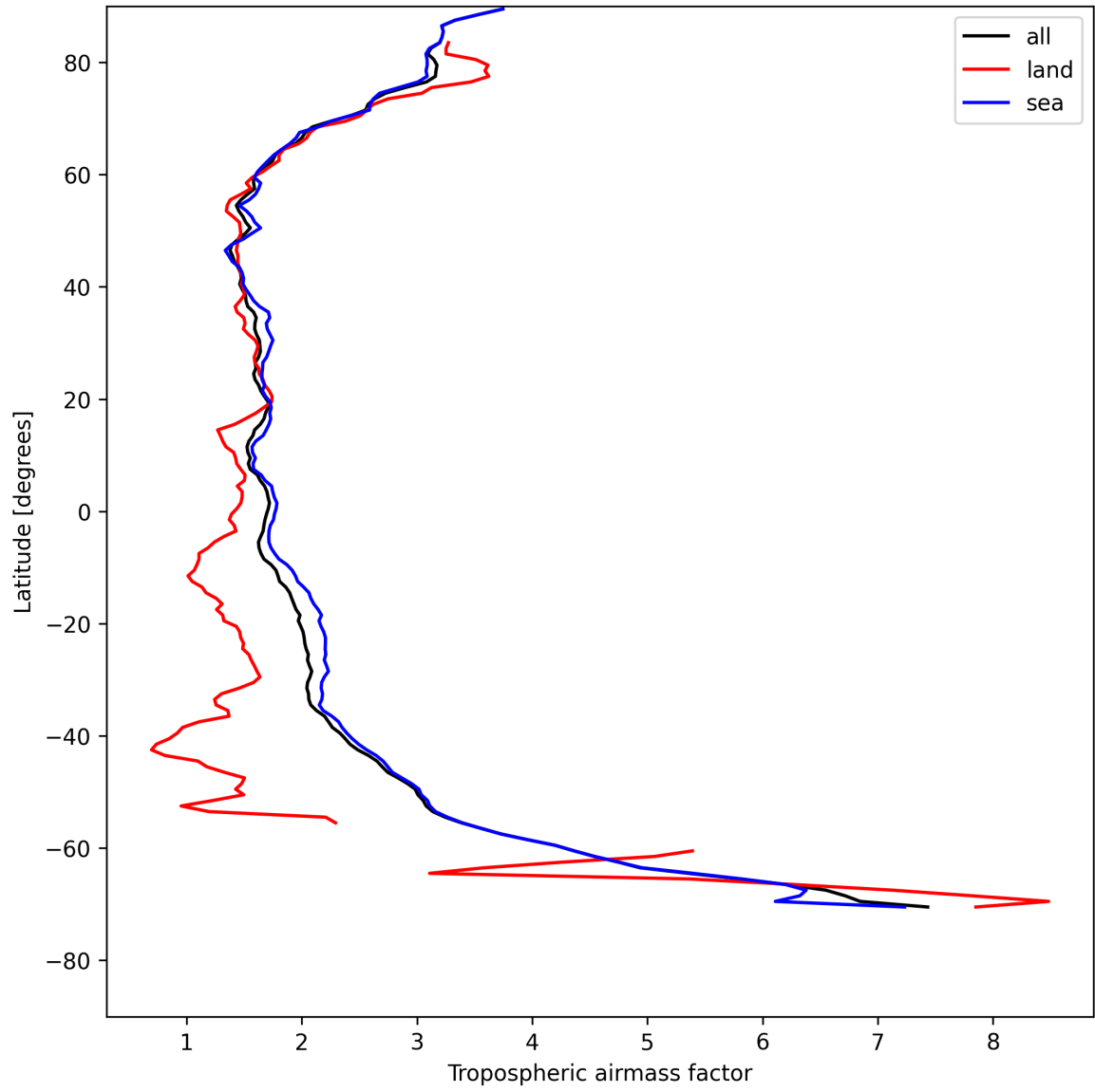
Figure 14: Zonal average of “Tropospheric airmass factor” for 2025-08-04 to 2025-08-05.
