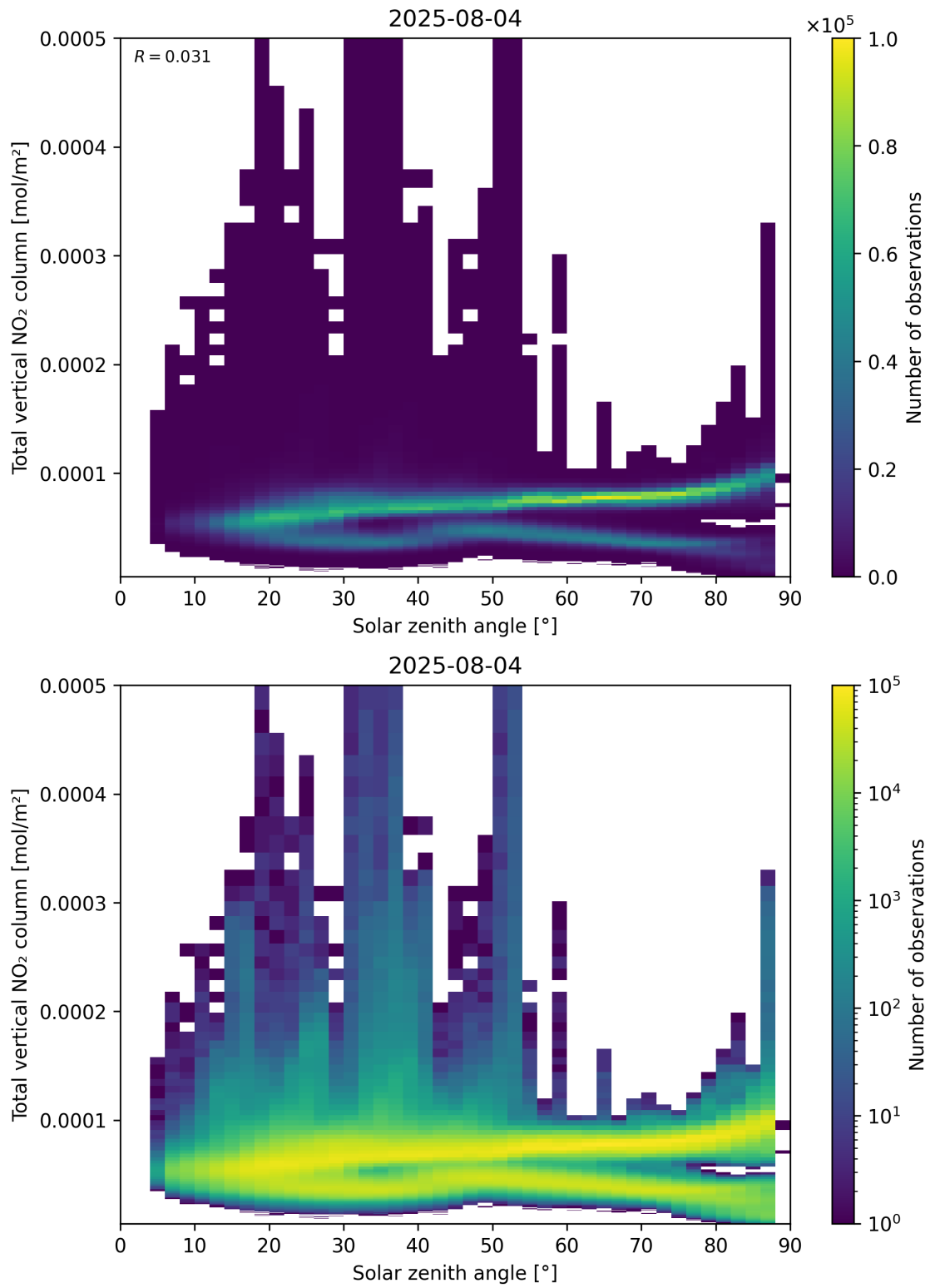
Figure 153: Scatter density plot of “Solar zenith angle” against “Total vertical NO 2 column” for 2025-08-04 to 2025-08-05.
