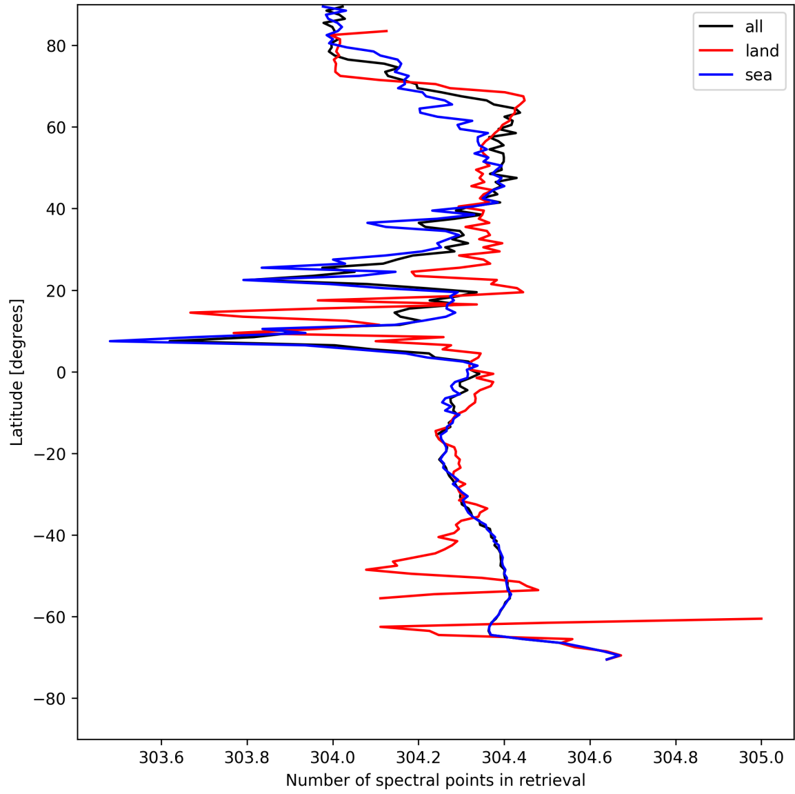
Figure 16: Zonal average of “Number of spectral points in retrieval” for 2025-08-04 to 2025-08-05.
