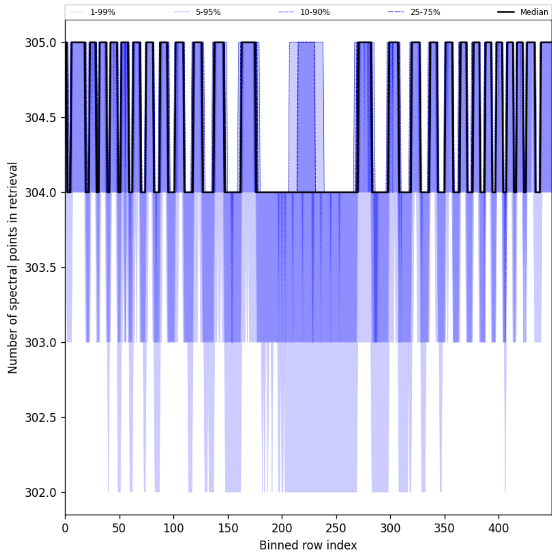
Figure 50: Along track statistics of “Number of spectral points in retrieval” for 2025-08-04 to 2025-08-05
