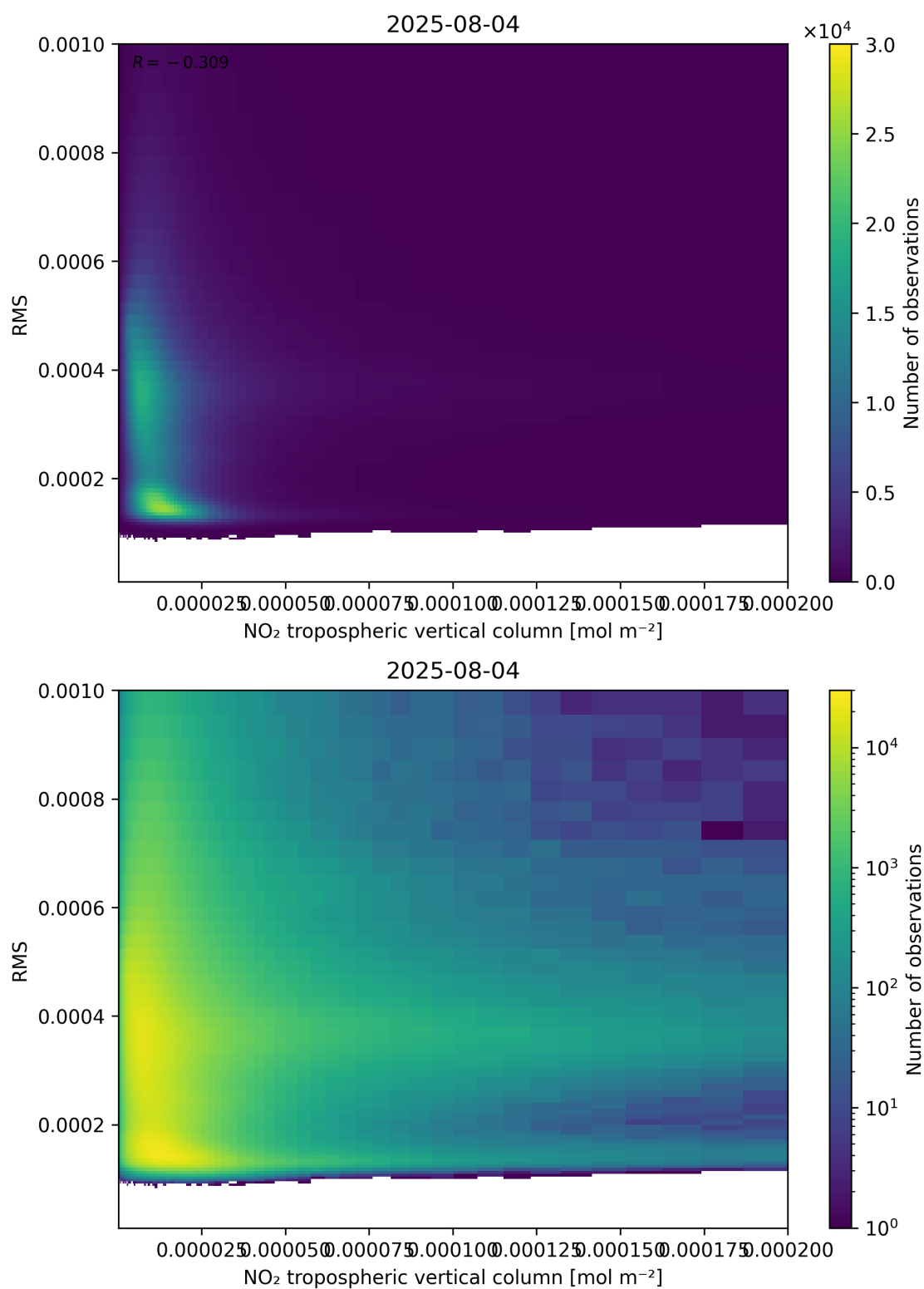
Figure 142: Scatter density plot of “NO 2 tropospheric vertical column” against “RMS” for 2025-08-04 to 2025-08-05.
