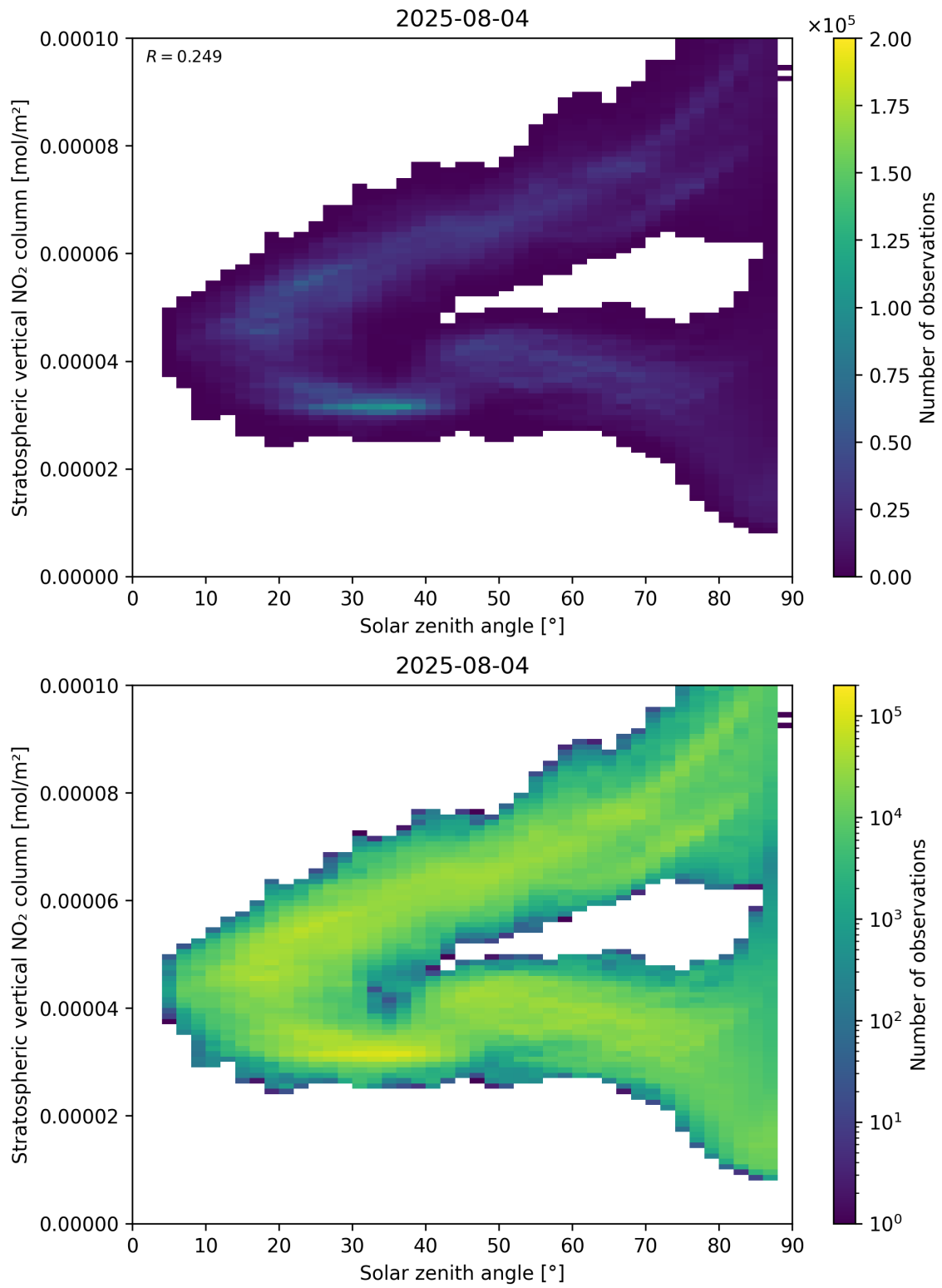
Figure 150: Scatter density plot of “Solar zenith angle” against “Stratospheric vertical NO 2 column” for 2025-08-04 to 2025-08-05.
