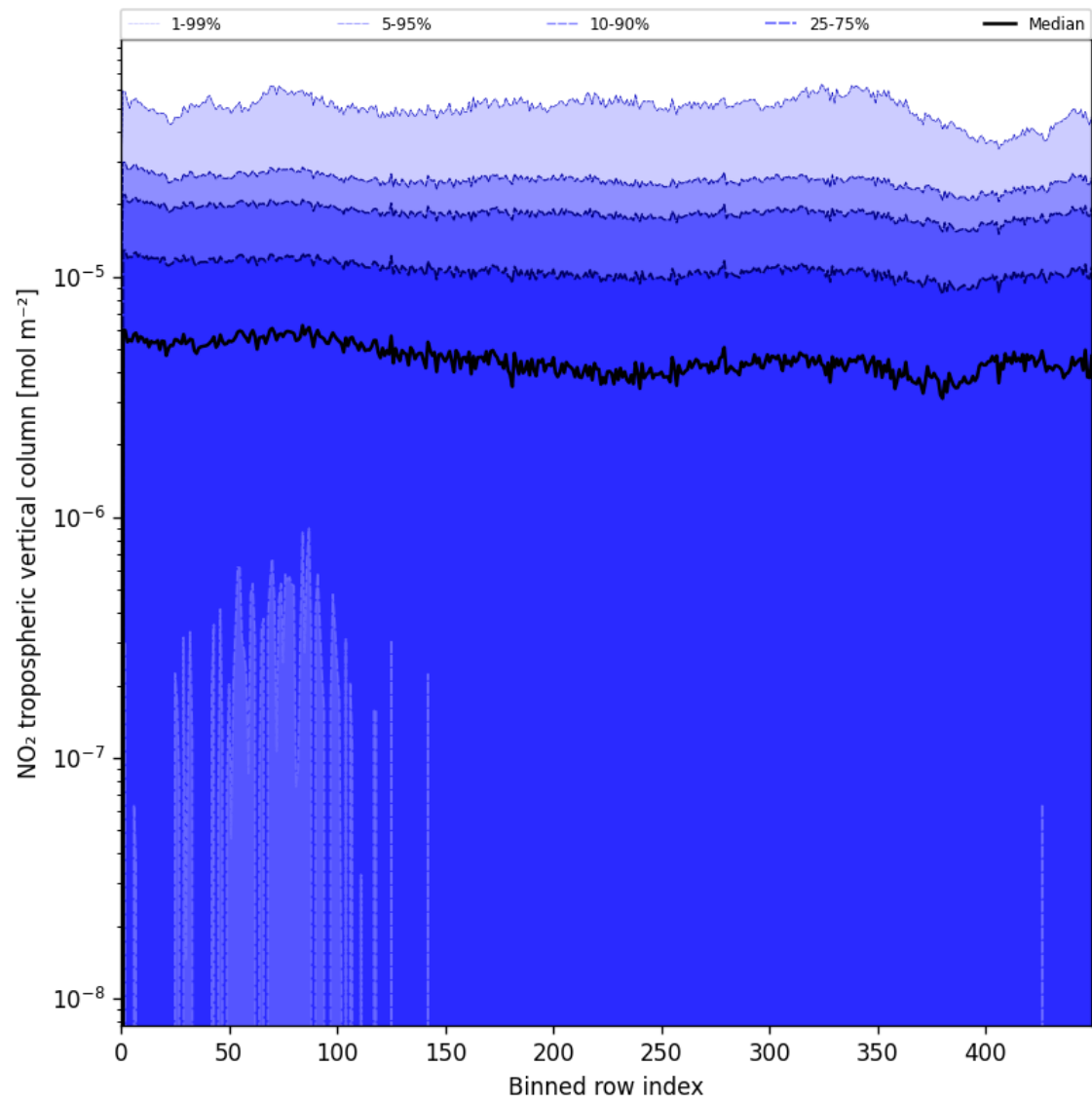
Figure 46: Along track statistics of “NO 2 tropospheric vertical column” for 2025-08-04 to 2025-08-05
