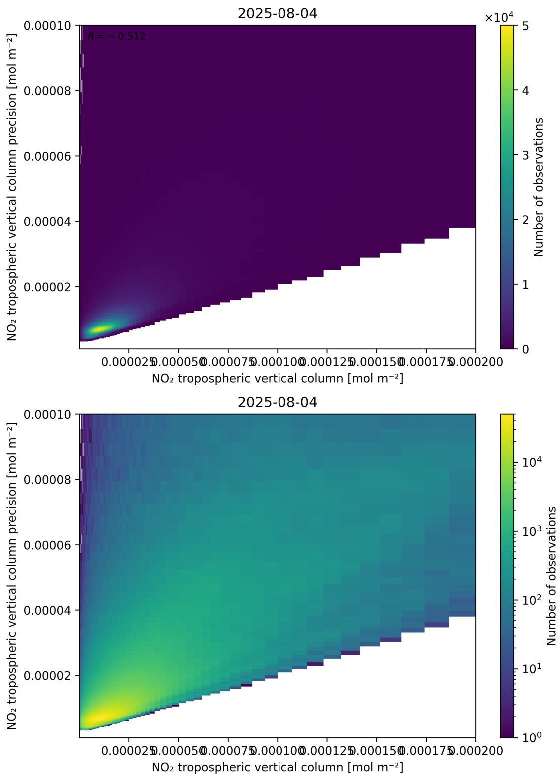
Figure 130: Scatter density plot of “NO 2 tropospheric vertical column” against “NO 2 tropospheric vertical column precision” for 2025-08-04 to 2025-08-05.
