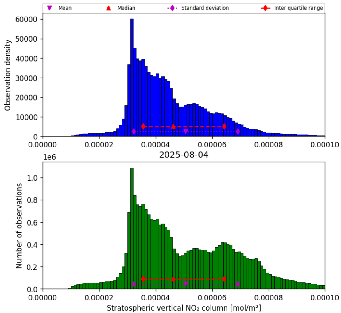
Figure 36: Histogram of “Stratospheric vertical NO 2 column” for 2025-08-04 to 2025-08-05
