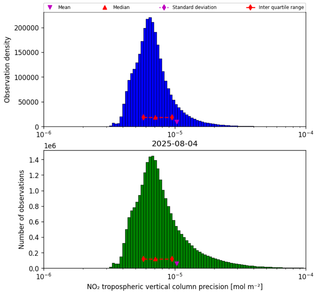
Figure 30: Histogram of “NO 2 tropospheric vertical column precision” for 2025-08-04 to 2025-08-05
