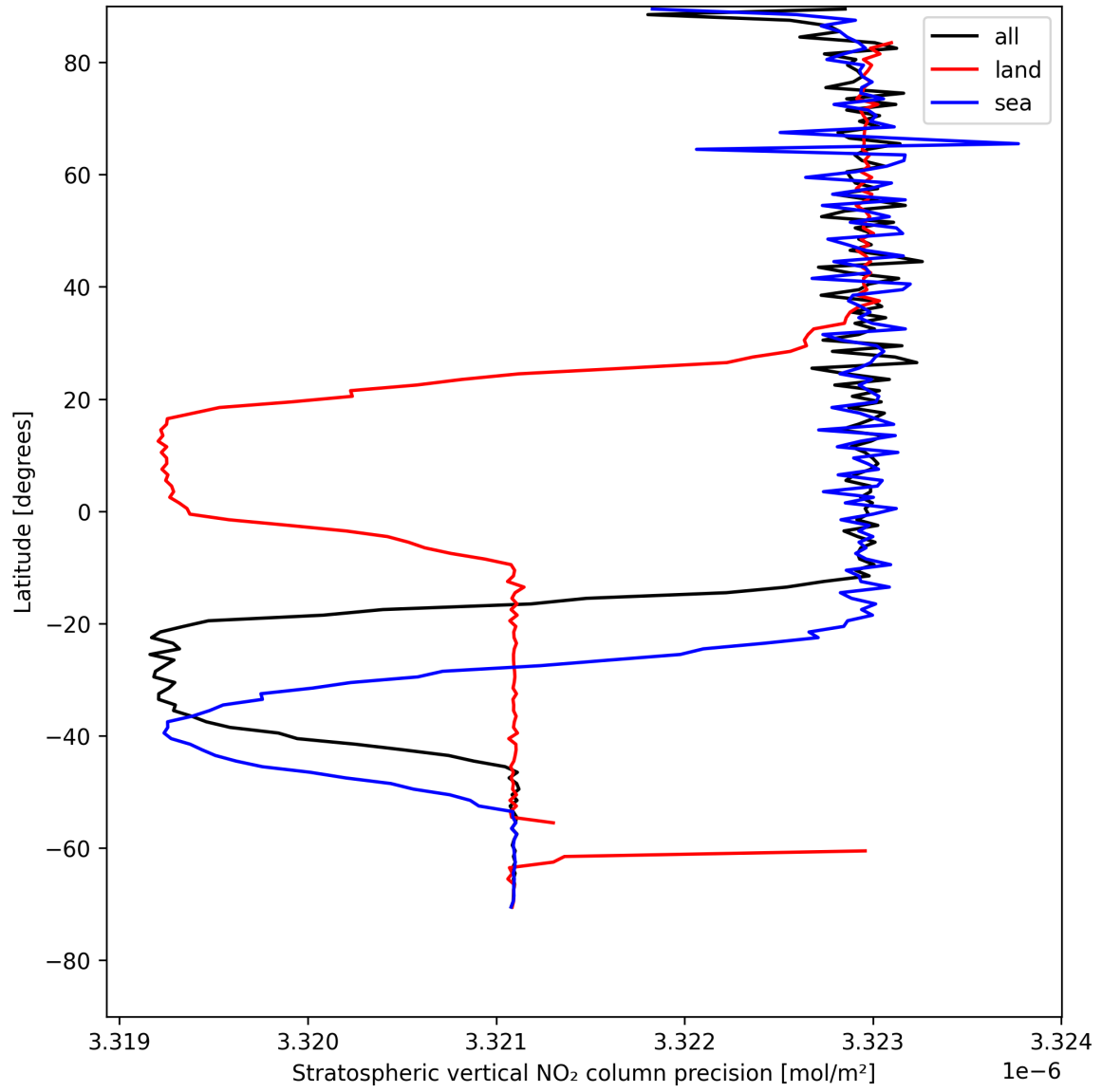
Figure 20: Zonal average of “Stratospheric vertical NO 2 column precision” for 2025-08-04 to 2025-08-05.
