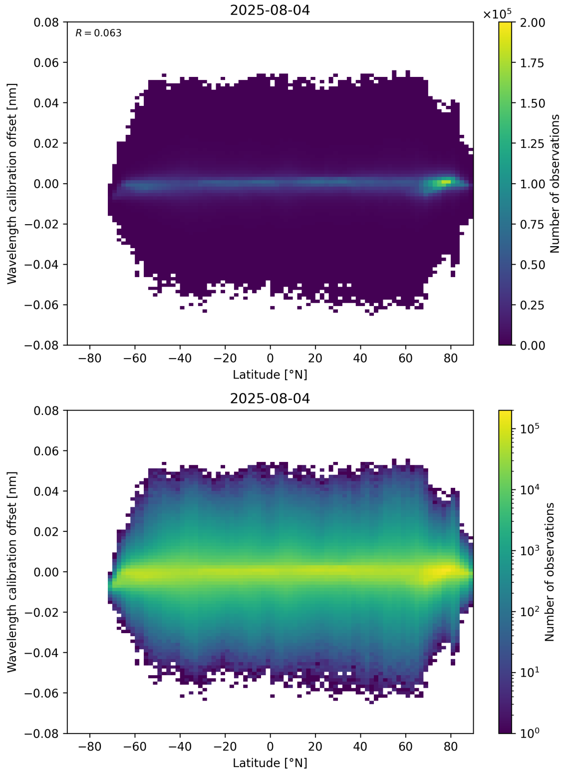
Figure 95: Scatter density plot of “Latitude” against “Wavelength calibration offset” for 2025-08-04 to 2025-08-05.
