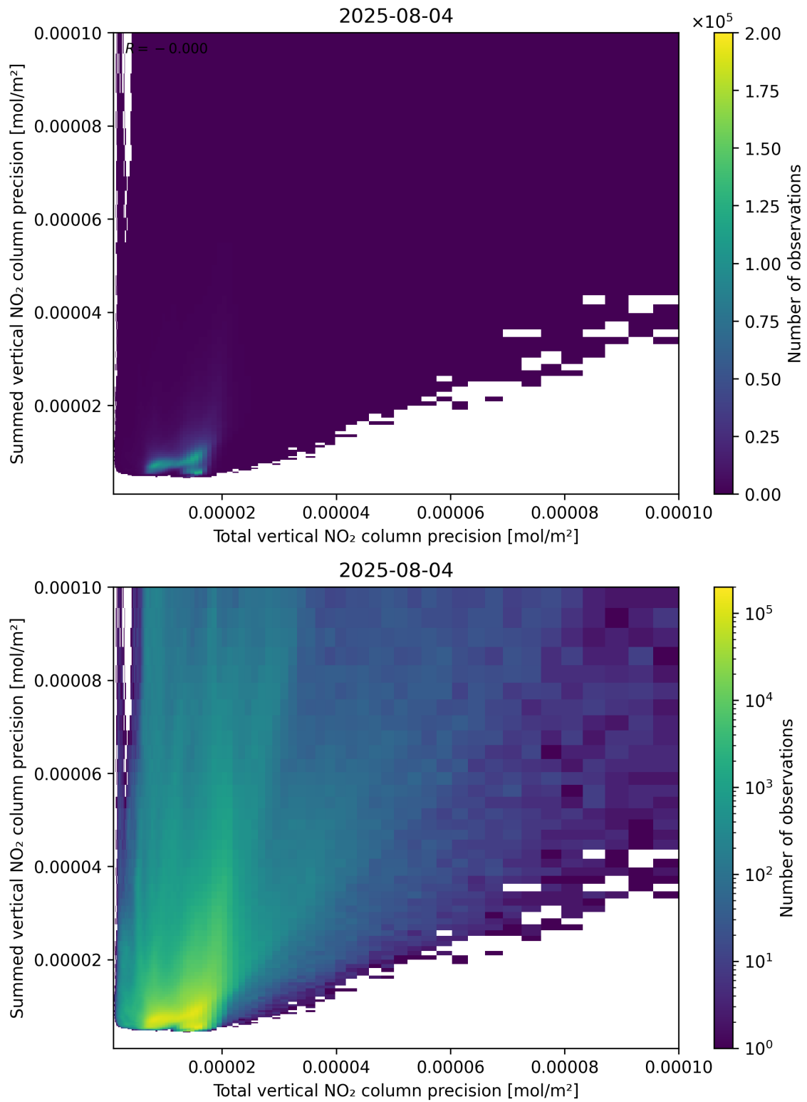
Figure 118: Scatter density plot of “Total vertical NO 2 column precision” against “Summed vertical NO 2 column precision” for 2025-08-04 to 2025-08-05.
