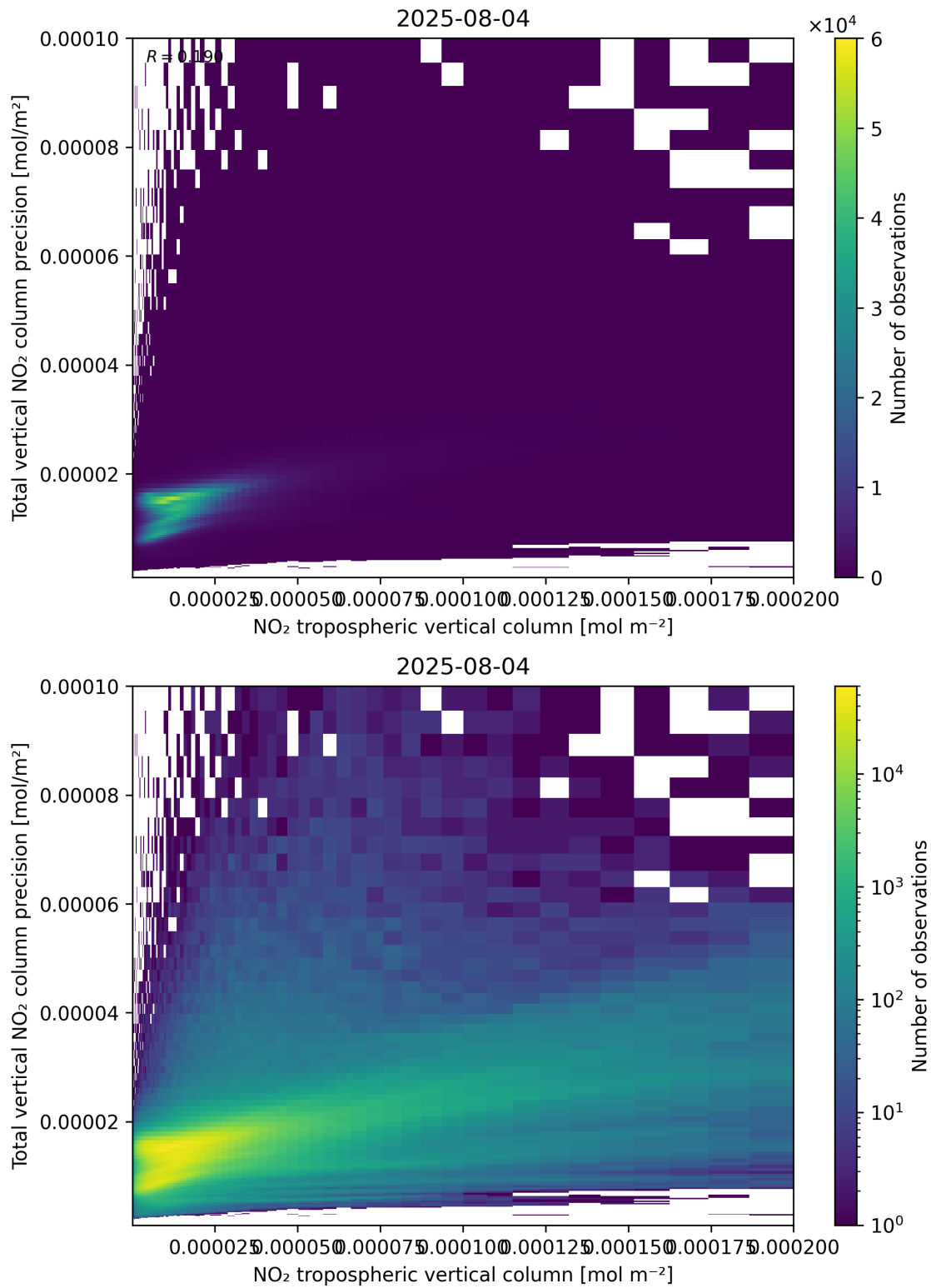
Figure 129: Scatter density plot of “NO 2 tropospheric vertical column” against “Total vertical NO 2 column precision” for 2025-08-04 to 2025-08-05.
