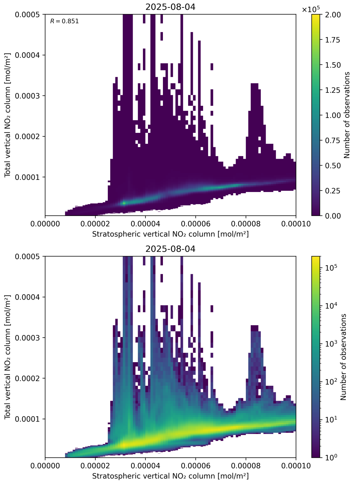
Figure 100: Scatter density plot of “Stratospheric vertical NO 2 column” against “Total vertical NO 2 column” for 2025-08-04 to 2025-08-05.
