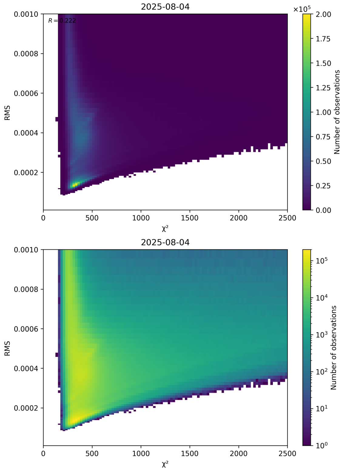
Figure 82: Scatter density plot of “ \chi^2 ” against “RMS” for 2025-08-04 to 2025-08-05.
