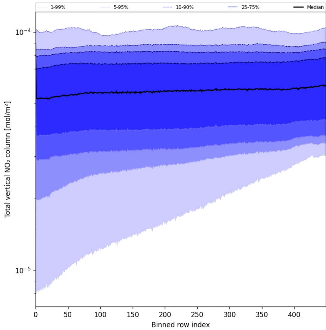
Figure 55: Along track statistics of “Total vertical NO 2 column” for 2025-08-04 to 2025-08-05
