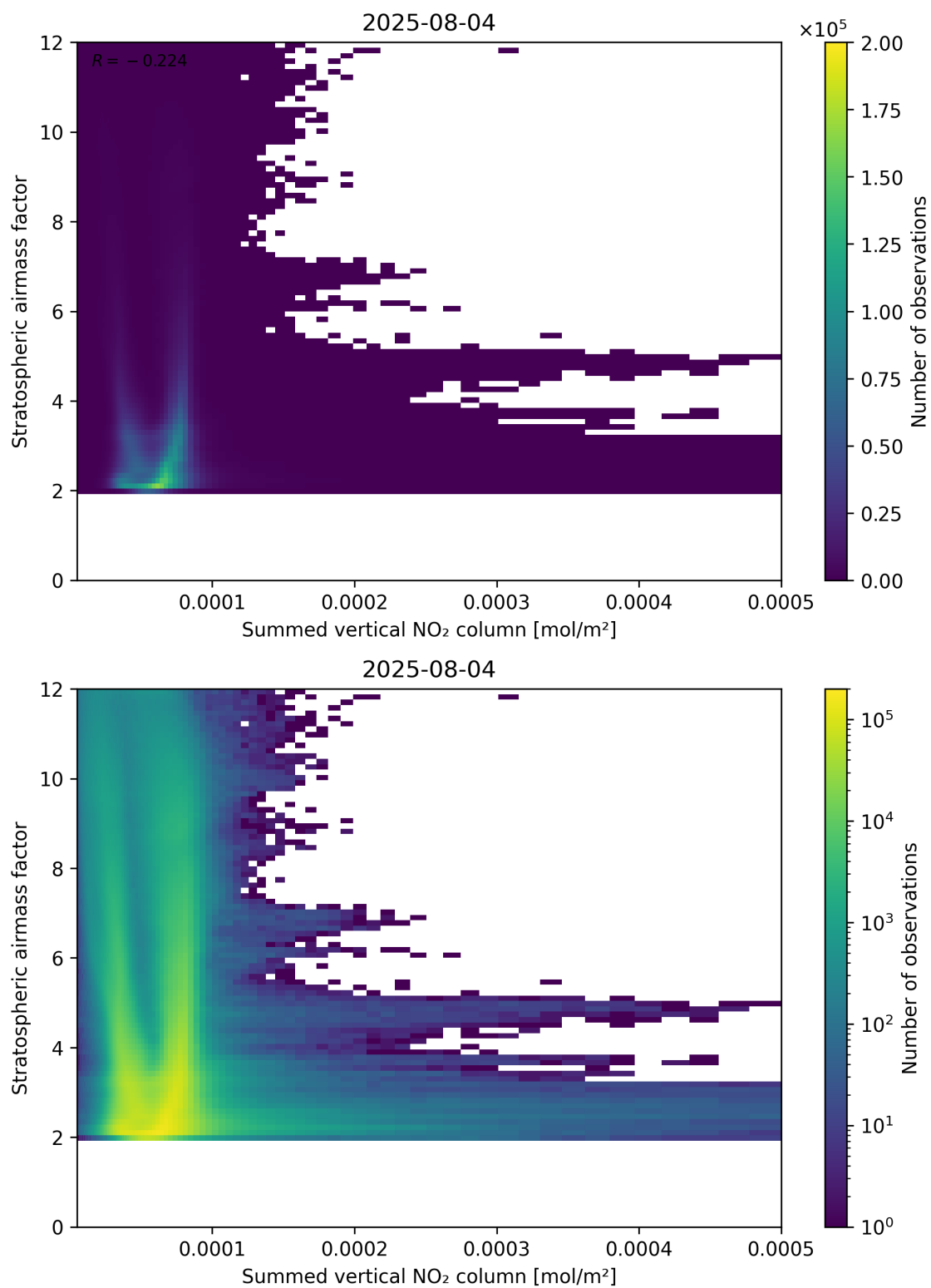
Figure 103: Scatter density plot of “Summed vertical NO 2 column” against “Stratospheric airmass factor” for 2025-08-04 to 2025-08-05.
