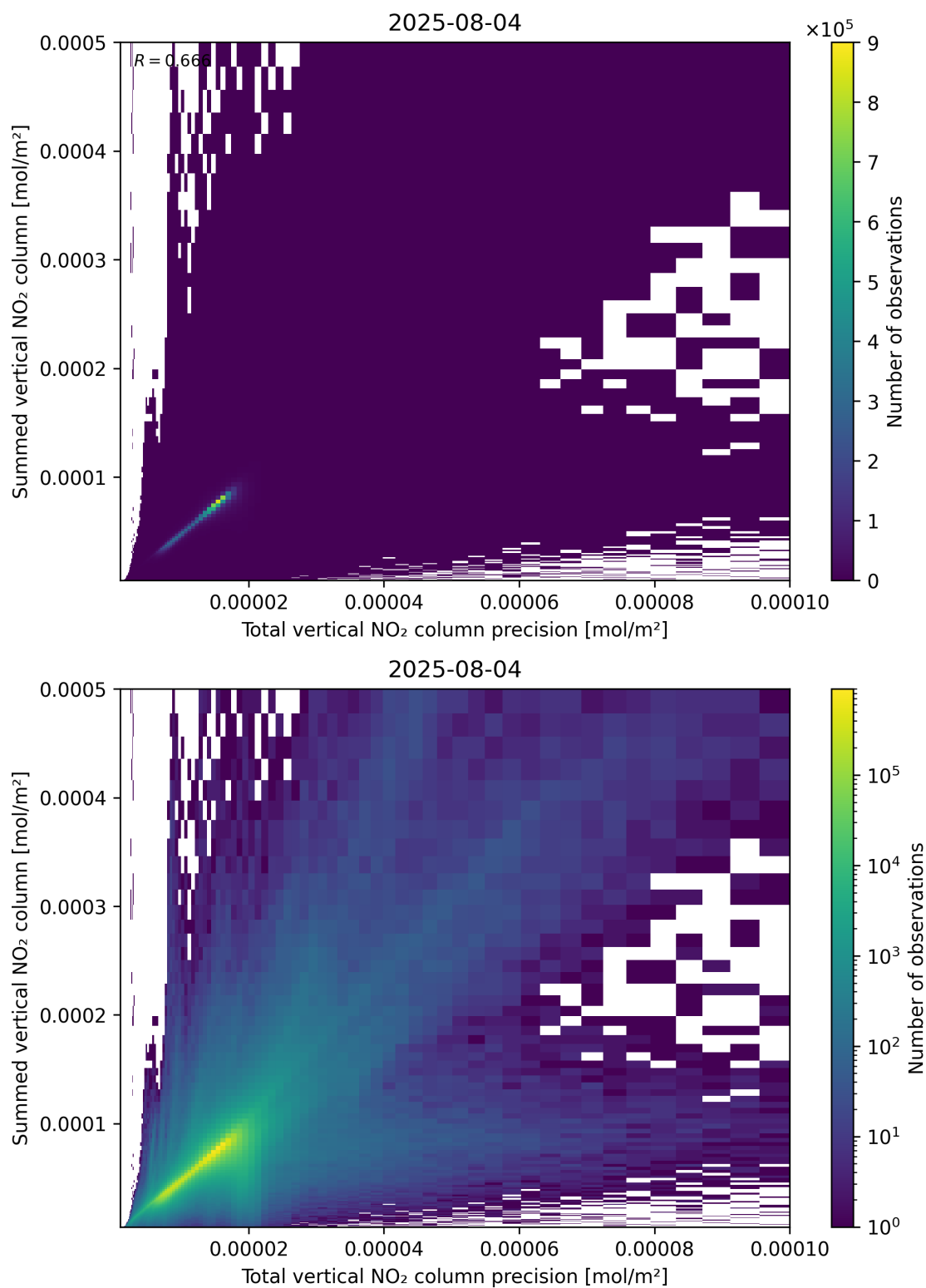
Figure 117: Scatter density plot of “Total vertical NO 2 column precision” against “Summed vertical NO 2 column” for 2025-08-04 to 2025-08-05.
