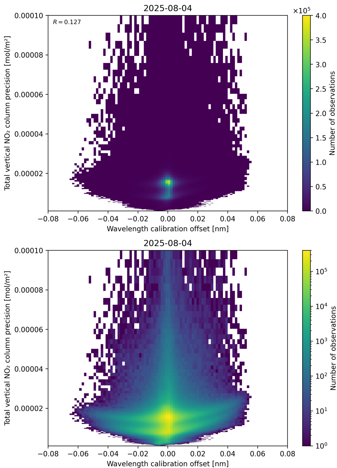
Figure 180: Scatter density plot of “Wavelength calibration offset” against “Total vertical NO 2 column precision” for 2025-08-04 to 2025-08-05.
