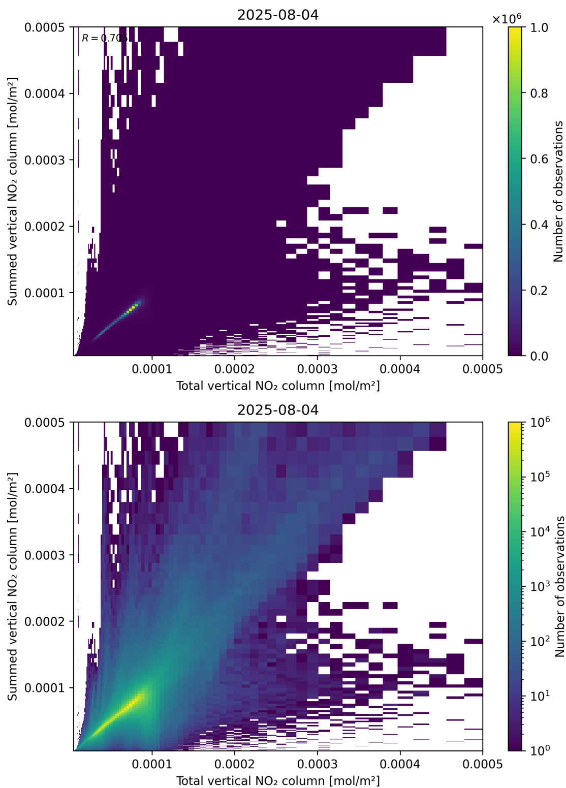
Figure 112: Scatter density plot of “Total vertical NO 2 column” against “Summed vertical NO 2 column” for 2025-08-04 to 2025-08-05.
