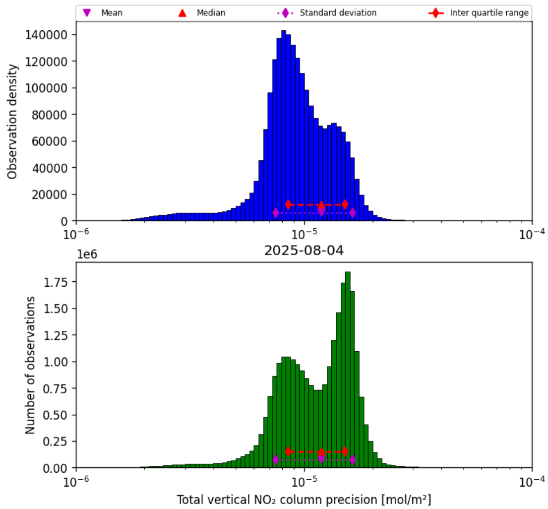
Figure 39: Histogram of “Total vertical NO 2 column precision” for 2025-08-04 to 2025-08-05
