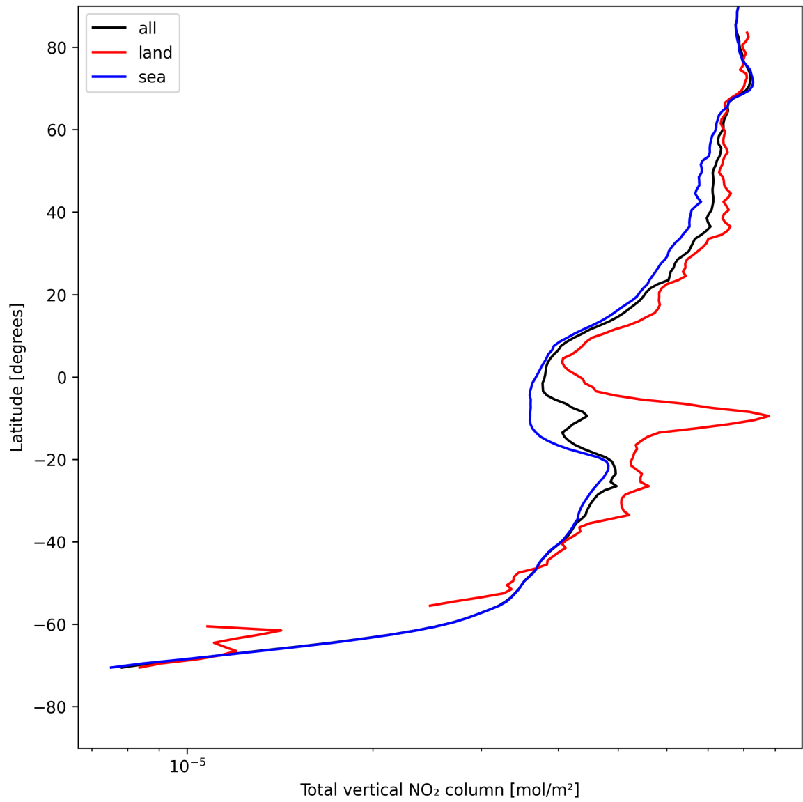
Figure 21: Zonal average of “Total vertical NO 2 column” for 2025-08-04 to 2025-08-05.
