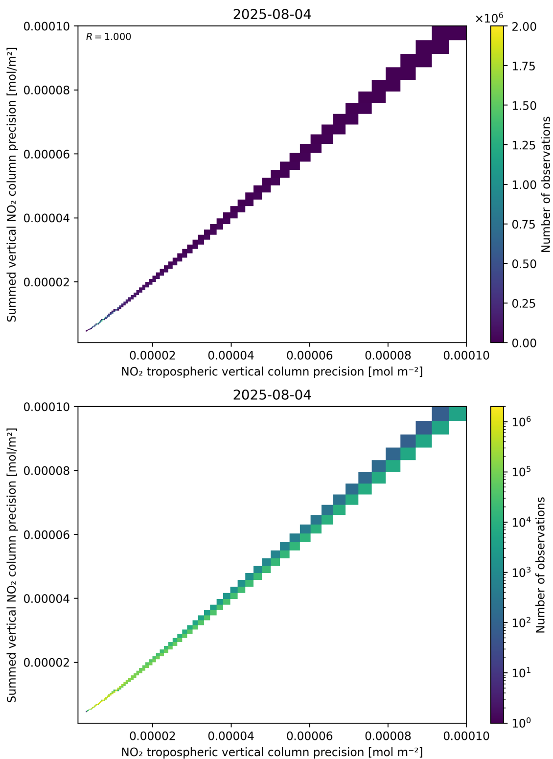
Figure 137: Scatter density plot of “NO 2 tropospheric vertical column precision” against “Summed vertical NO 2 column precision” for 2025-08-04 to 2025-08-05.
