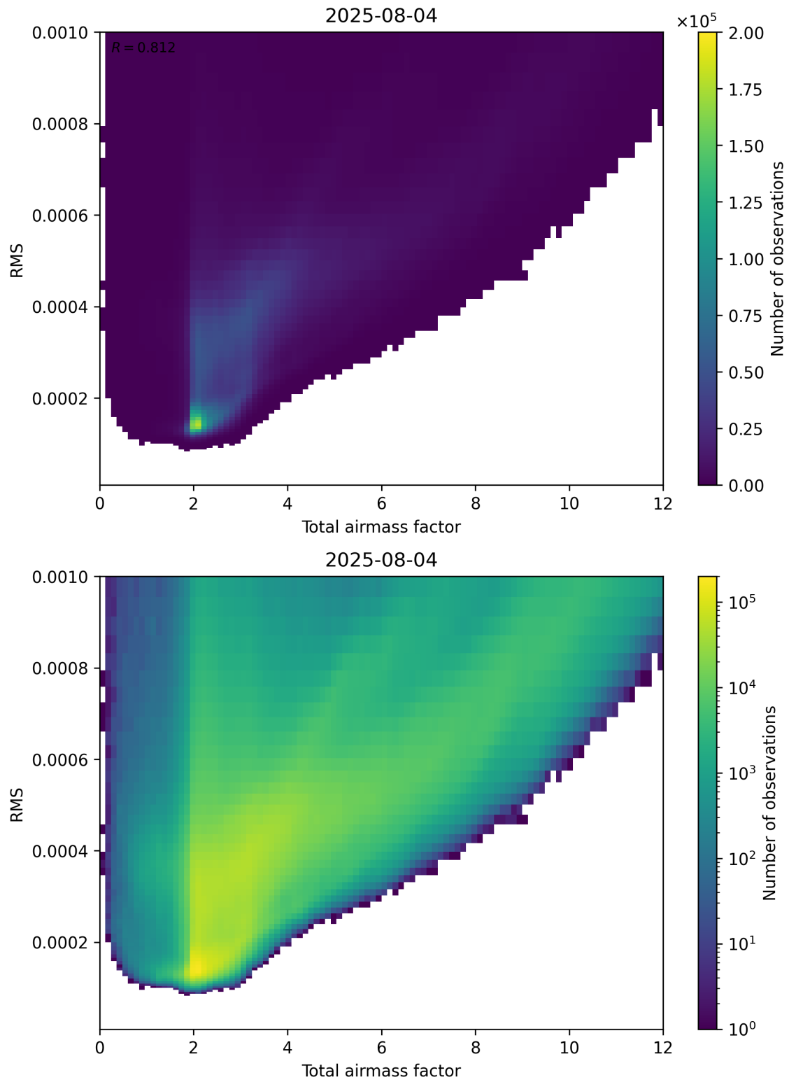
Figure 69: Scatter density plot of “Total airmass factor” against “RMS” for 2025-08-04 to 2025-08-05.
