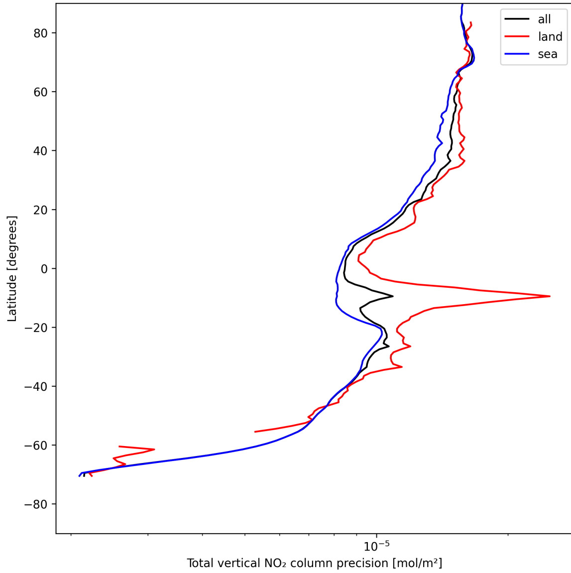
Figure 22: Zonal average of “Total vertical NO 2 column precision” for 2025-08-04 to 2025-08-05.
