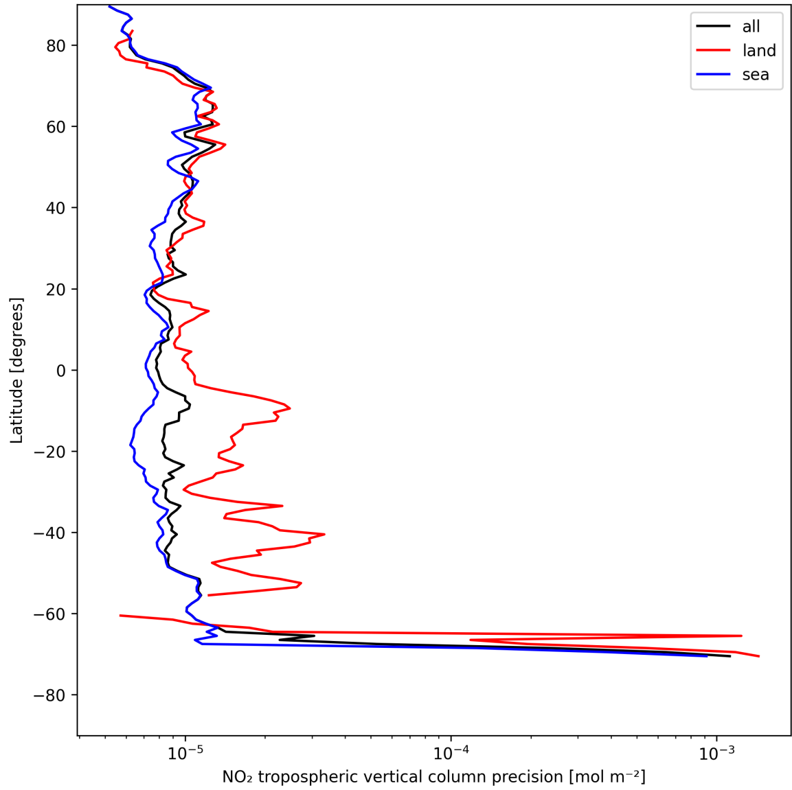
Figure 13: Zonal average of “NO 2 tropospheric vertical column precision” for 2025-08-04 to 2025-08-05.
