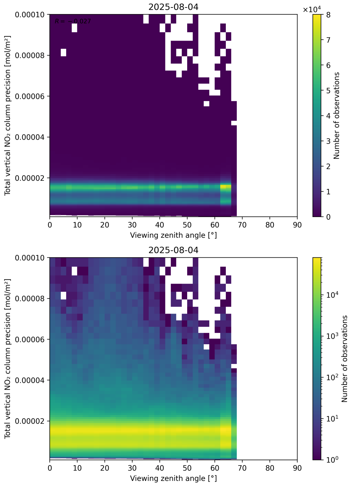
Figure 168: Scatter density plot of “Viewing zenith angle” against “Total vertical NO 2 column precision” for 2025-08-04 to 2025-08-05.
