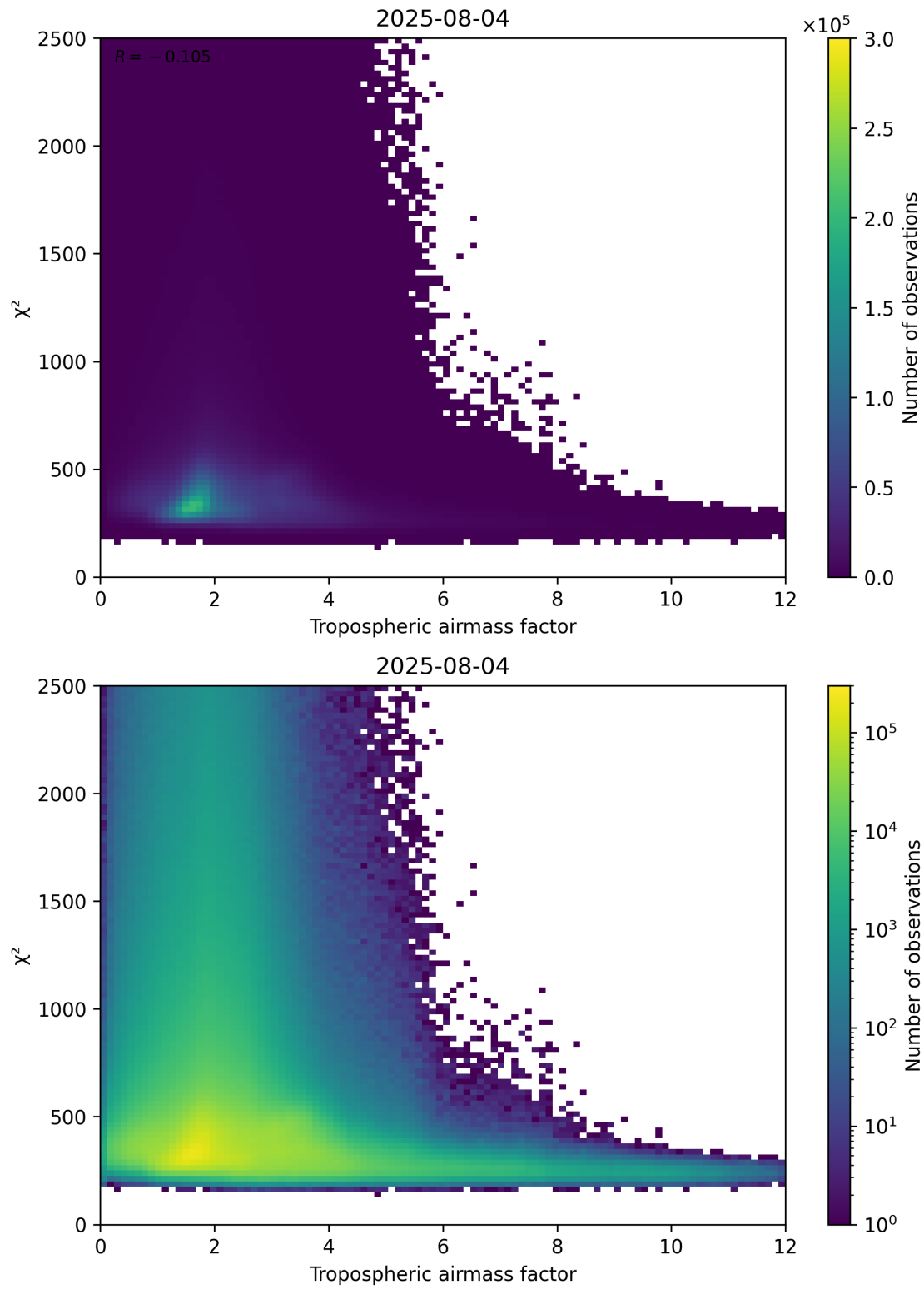
Figure 73: Scatter density plot of “Tropospheric airmass factor” against “ \chi^2 ” for 2025-08-04 to 2025-08-05.
