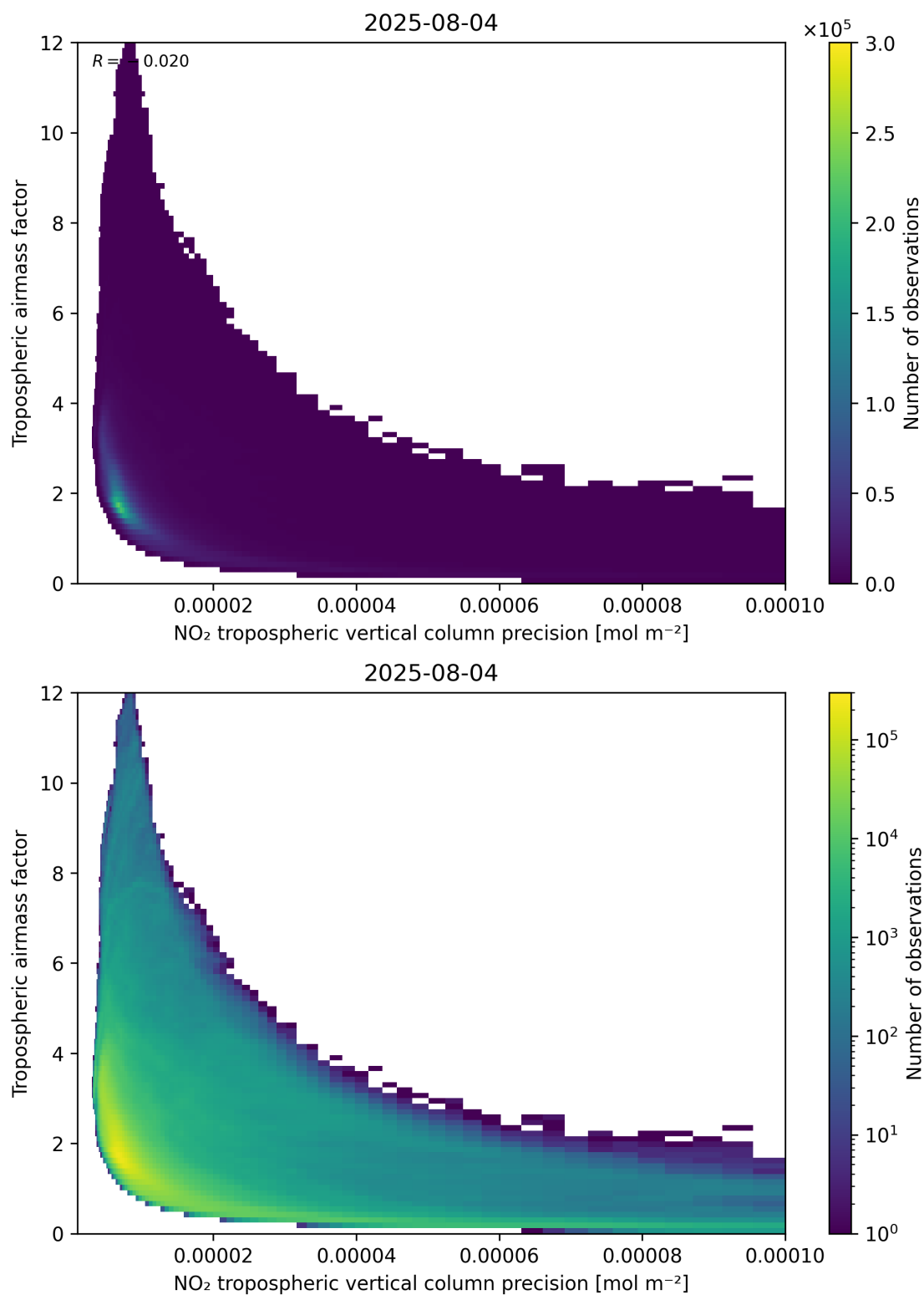
Figure 133: Scatter density plot of “NO 2 tropospheric vertical column precision” against “Tropospheric air mass factor” for 2025-08-04 to 2025-08-05.
