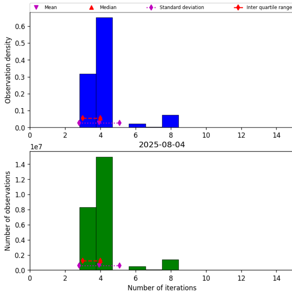
Figure 34: Histogram of “Number of iterations” for 2025-08-04 to 2025-08-05
