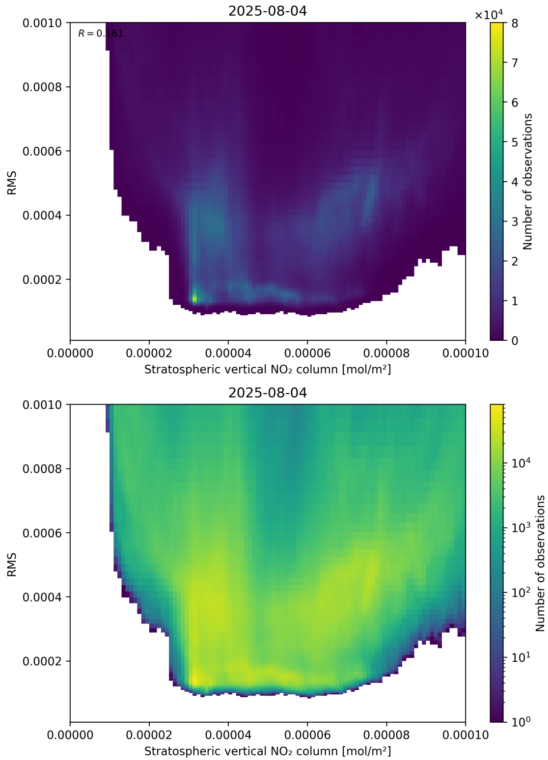
Figure 102: Scatter density plot of “Stratospheric vertical NO 2 column” against “RMS” for 2025-08-04 to 2025-08-05.
