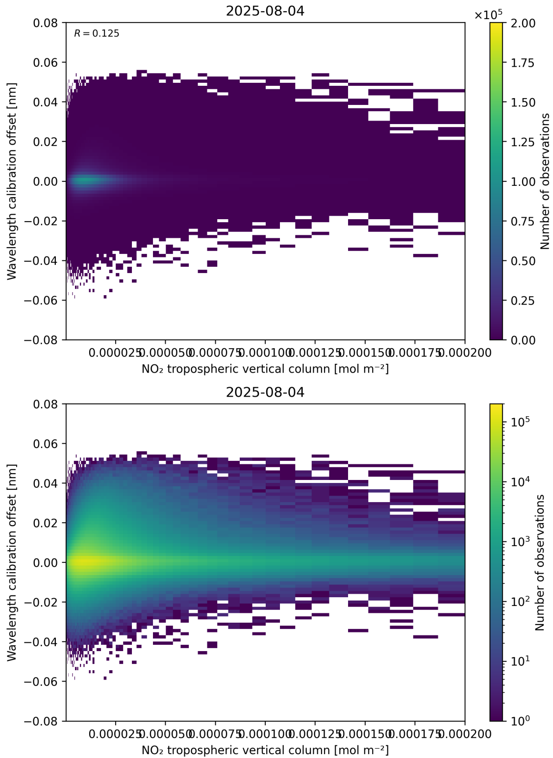
Figure 143: Scatter density plot of “NO 2 tropospheric vertical column” against “Wavelength calibration offset” for 2025-08-04 to 2025-08-05.
