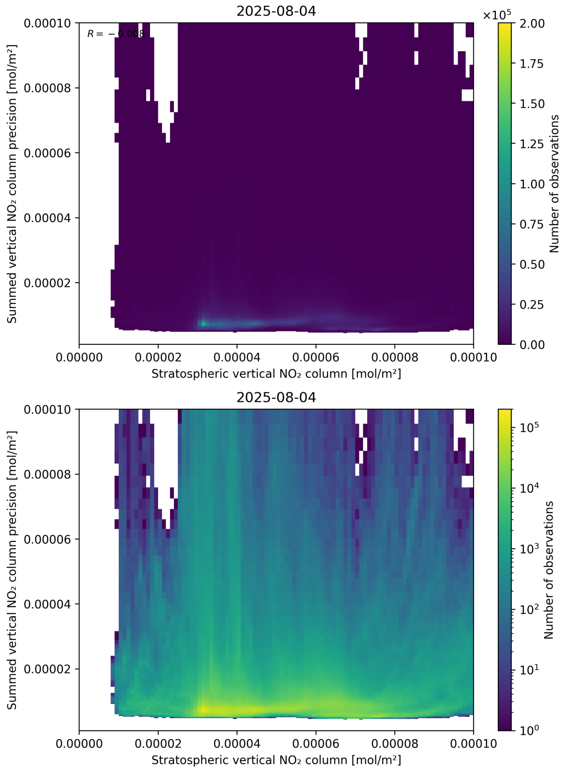
Figure 99: Scatter density plot of “Stratospheric vertical NO 2 column” against “Summed vertical NO 2 column precision” for 2025-08-04 to 2025-08-05.
