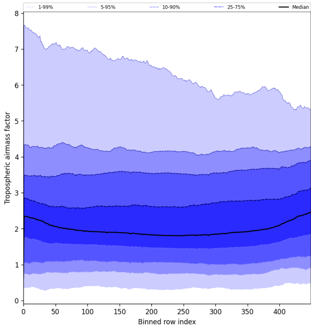
Figure 48: Along track statistics of “Tropospheric airmass factor” for 2025-08-04 to 2025-08-05
