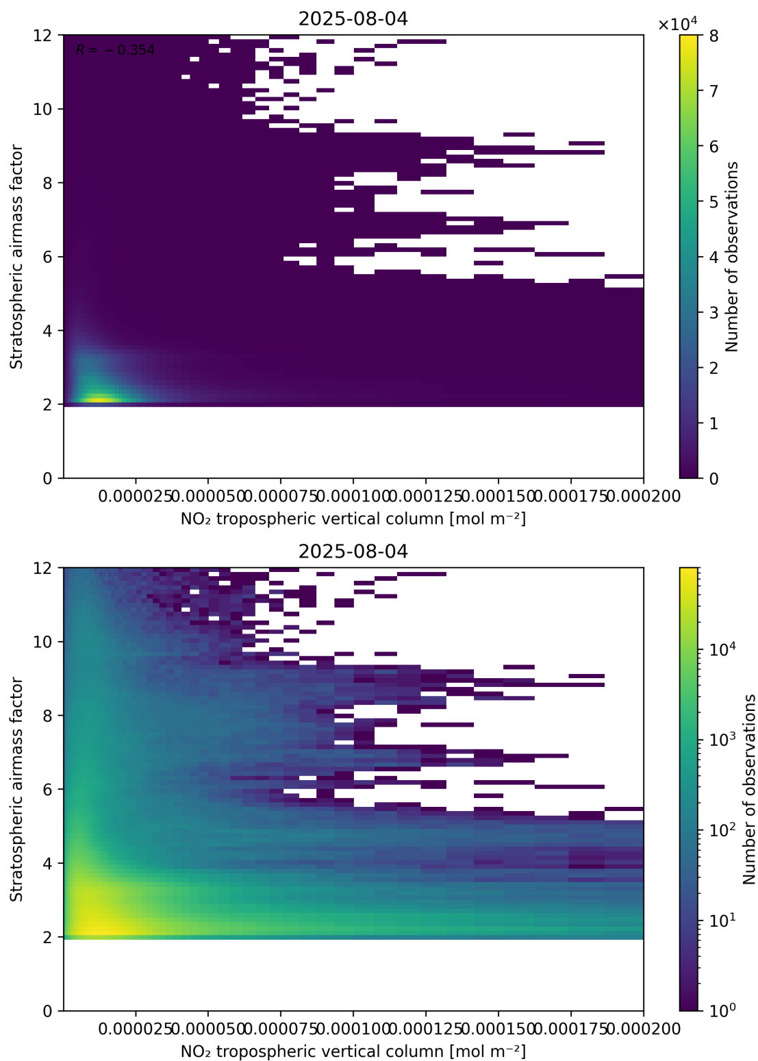
Figure 121: Scatter density plot of “NO 2 tropospheric vertical column” against “Stratospheric air mass factor” for 2025-08-04 to 2025-08-05.
