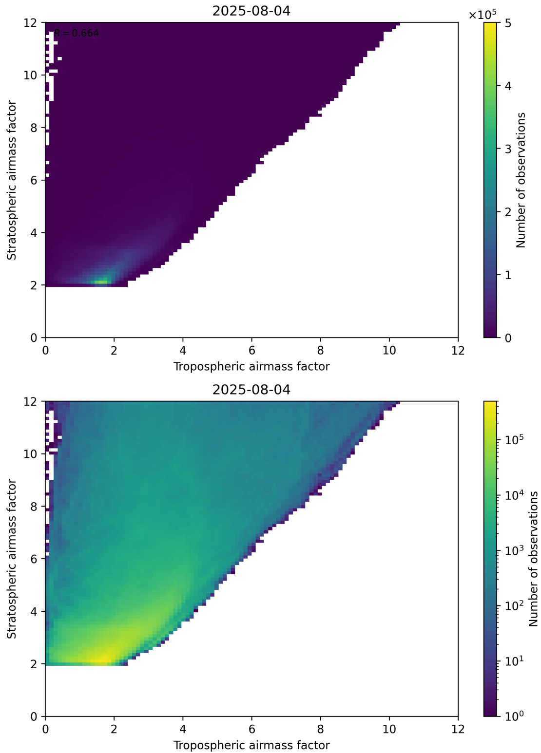
Figure 71: Scatter density plot of “Tropospheric airmass factor” against “Stratospheric airmass factor” for 2025-08-04 to 2025-08-05.
