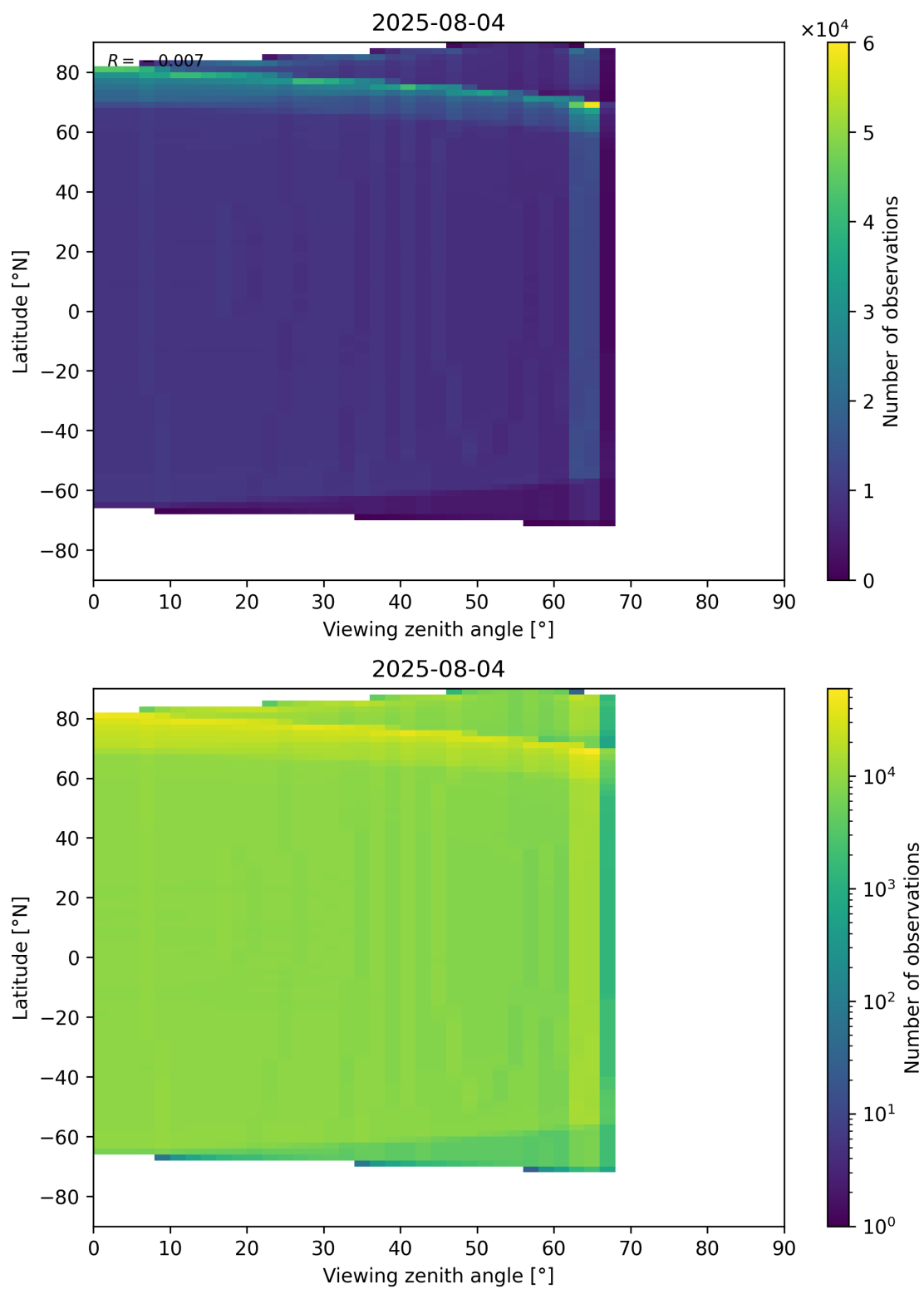
Figure 163: Scatter density plot of “Viewing zenith angle” against “Latitude” for 2025-08-04 to 2025-08-05.
