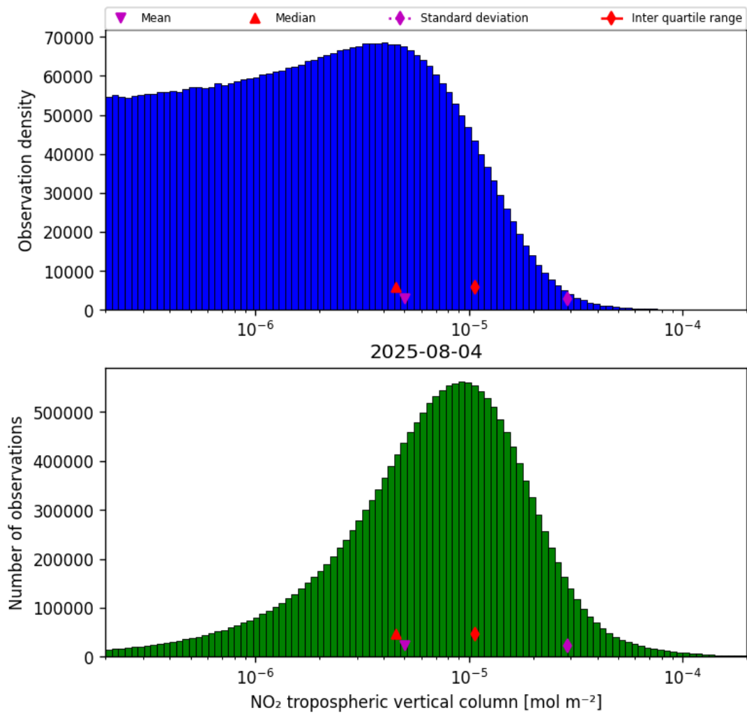
Figure 29: Histogram of “NO 2 tropospheric vertical column” for 2025-08-04 to 2025-08-05
