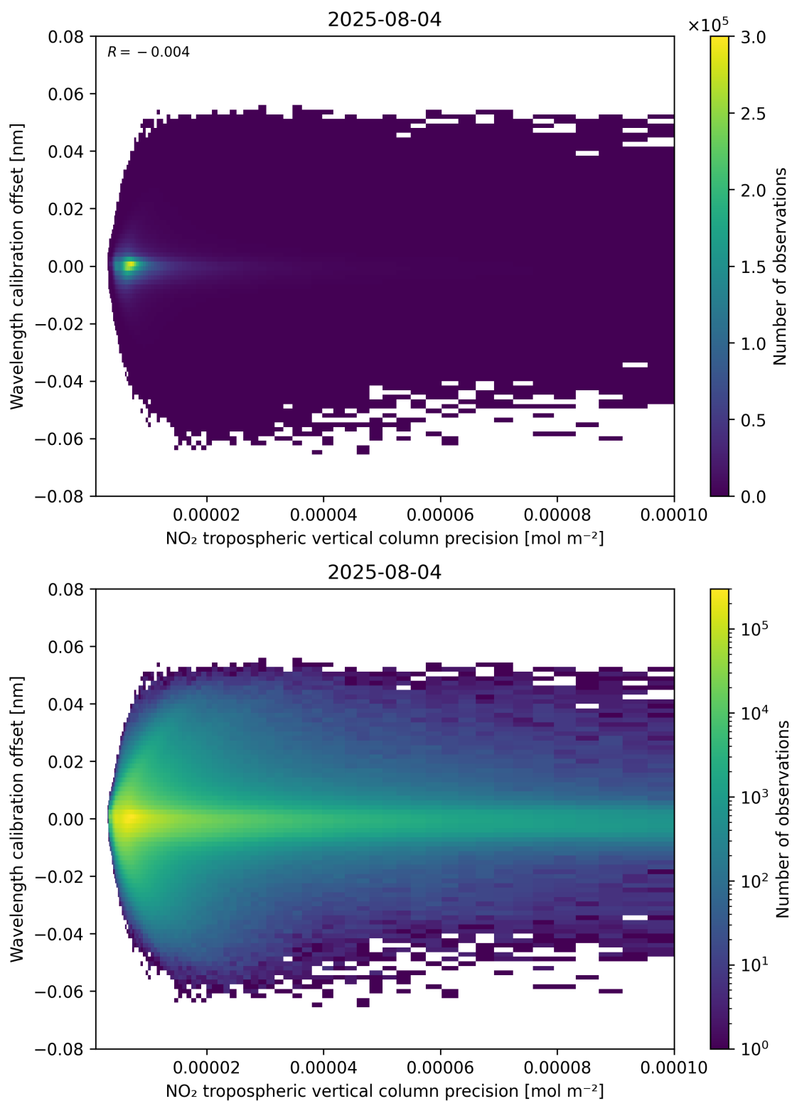
Figure 141: Scatter density plot of “NO 2 tropospheric vertical column precision” against “Wavelength calibration offset” for 2025-08-04 to 2025-08-05.
