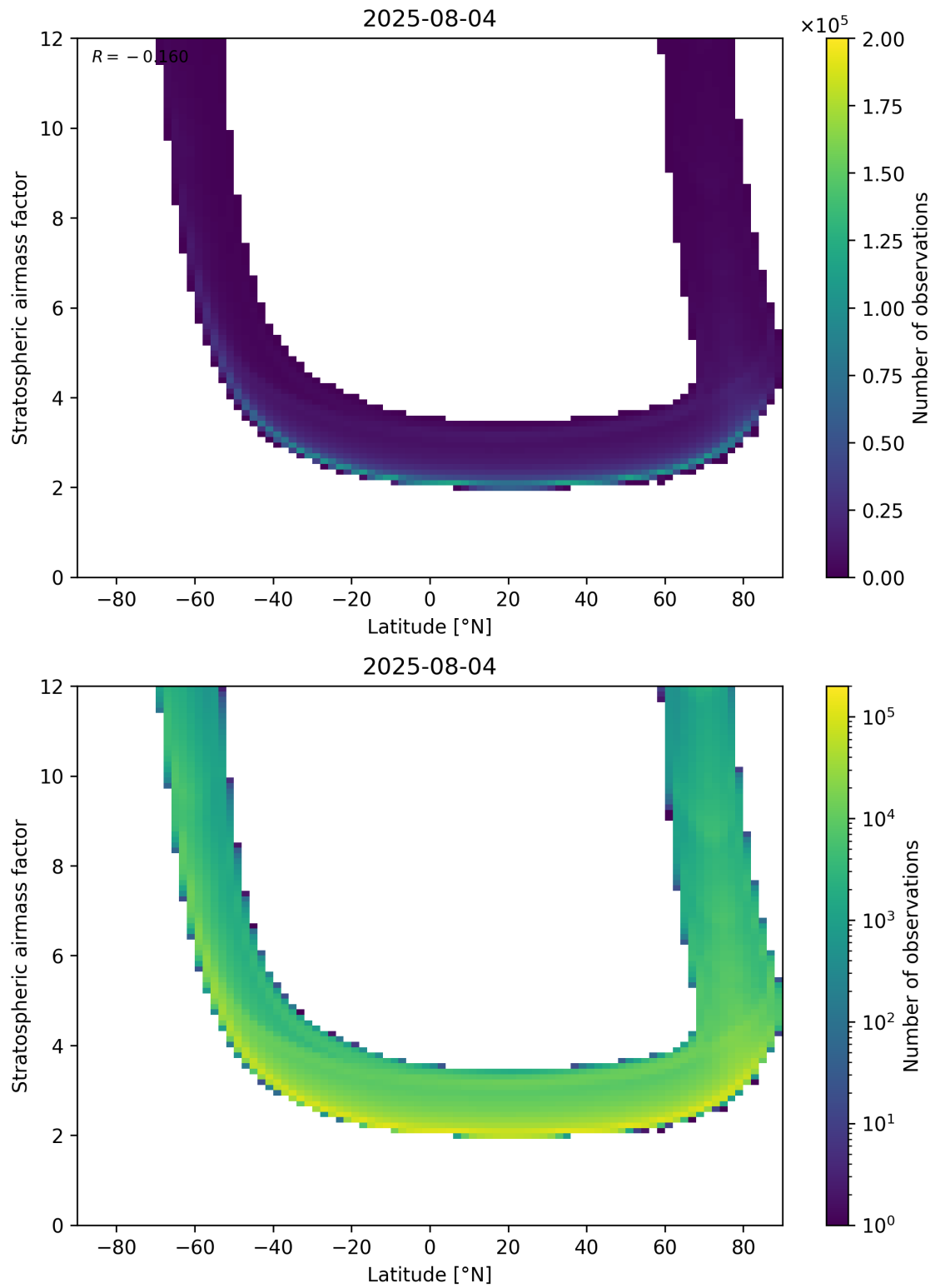
Figure 83: Scatter density plot of “Latitude” against “Stratospheric air mass factor” for 2025-08-04 to 2025-08-05.
