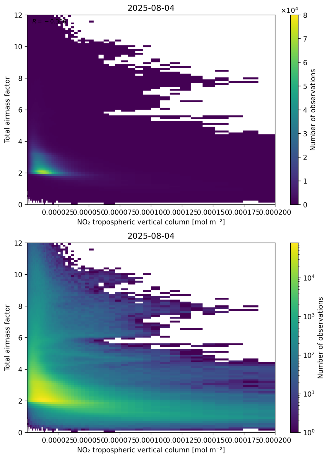
Figure 122: Scatter density plot of “NO 2 tropospheric vertical column” against “Total air mass factor” for 2025-08-04 to 2025-08-05.
