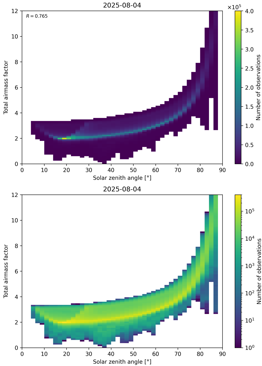
Figure 146: Scatter density plot of “Solar zenith angle” against “Total air mass factor” for 2025-08-04 to 2025-08-05.
