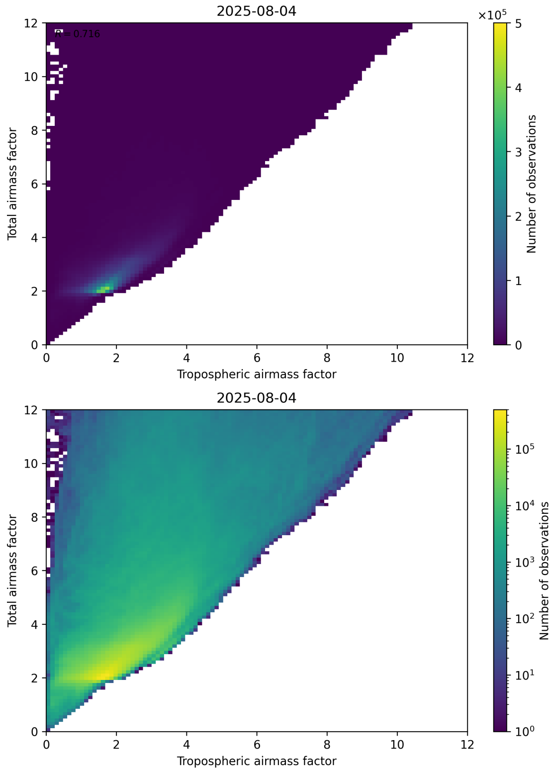
Figure 72: Scatter density plot of “Tropospheric airmass factor” against “Total airmass factor” for 2025-08-04 to 2025-08-05.
