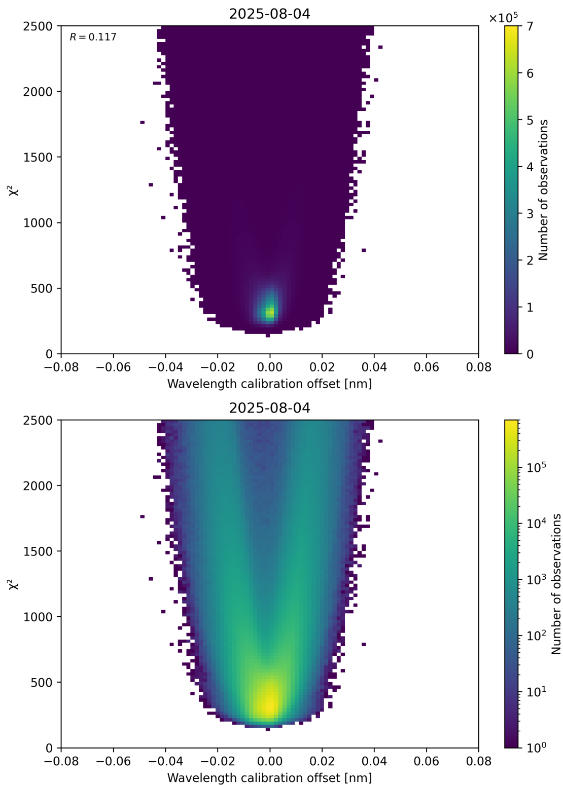
Figure 175: Scatter density plot of “Wavelength calibration offset” against “ \chi^2 ” for 2025-08-04 to 2025-08-05.
