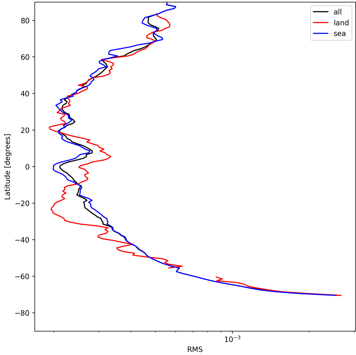
Figure 26: Zonal average of “RMS” for 2025-08-04 to 2025-08-05.
