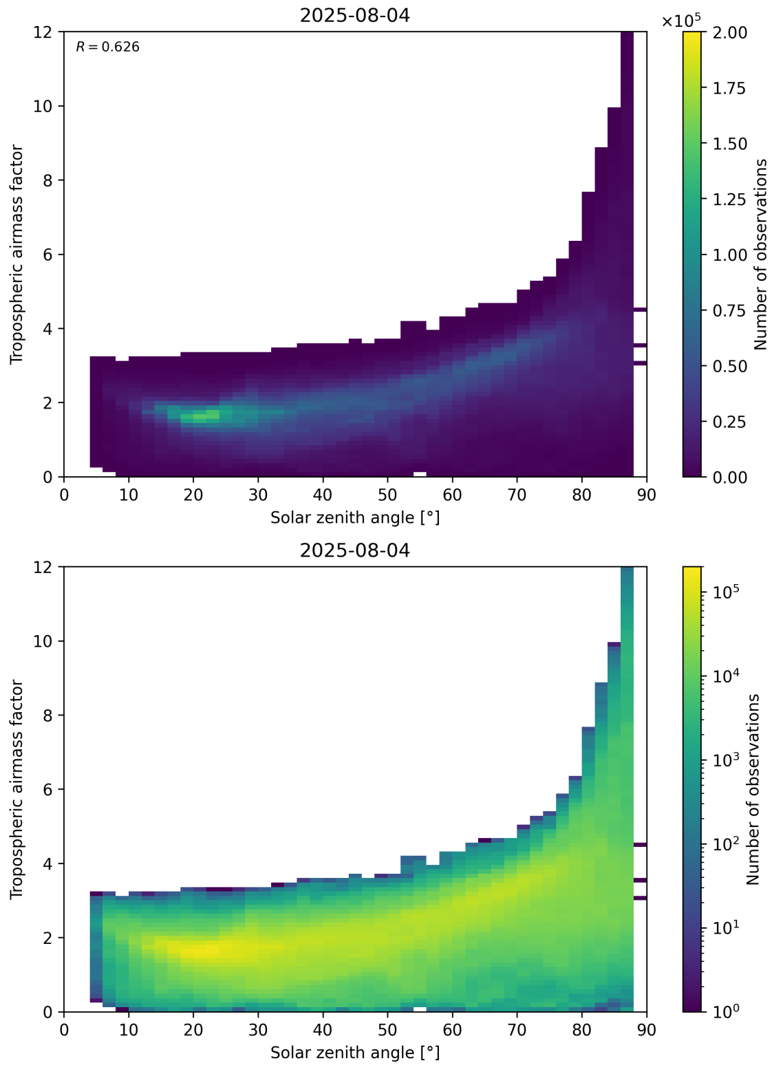
Figure 147: Scatter density plot of “Solar zenith angle” against “Tropospheric airmass factor” for 2025-08-04 to 2025-08-05.
