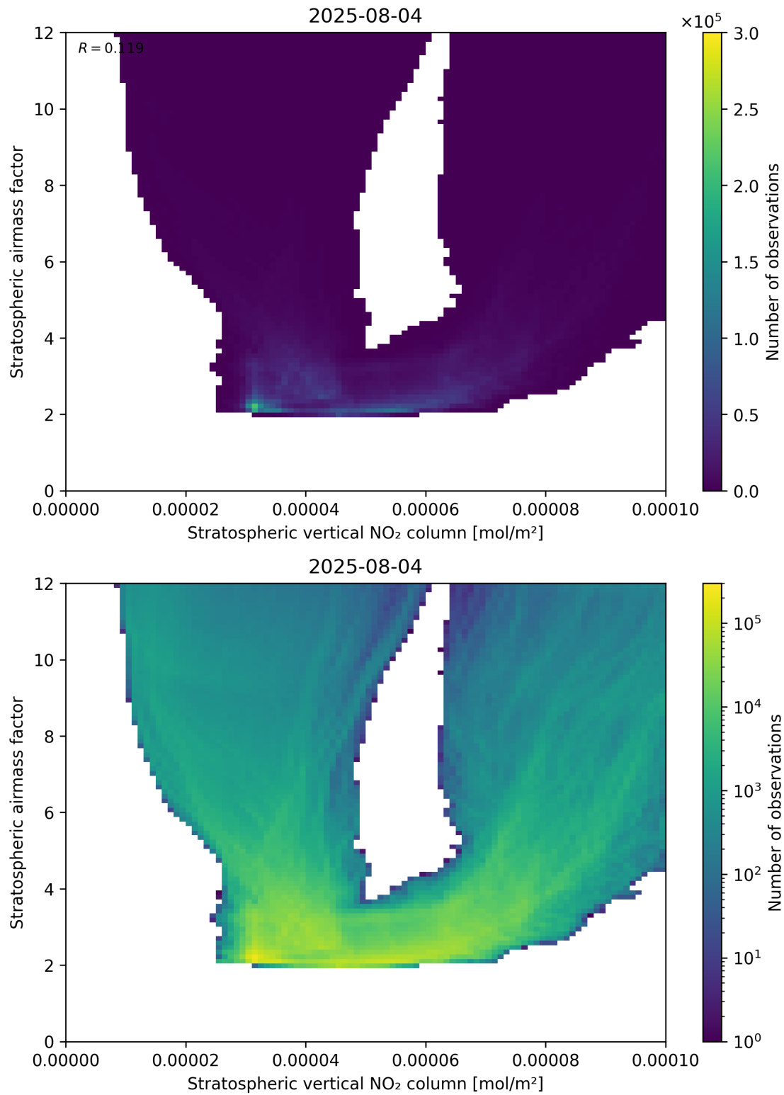
Figure 96: Scatter density plot of “Stratospheric vertical NO 2 column” against “Stratospheric airmass factor” for 2025-08-04 to 2025-08-05.
