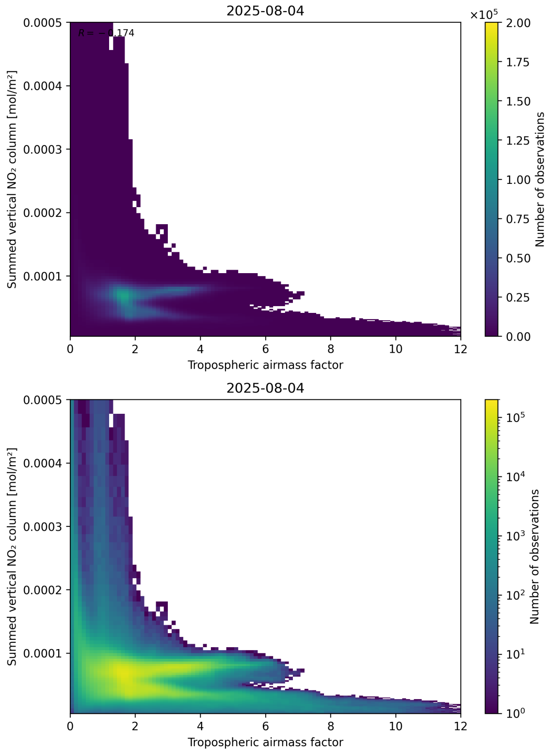
Figure 75: Scatter density plot of “Tropospheric air mass factor” against “Summed vertical NO 2 column” for 2025-08-04 to 2025-08-05.
