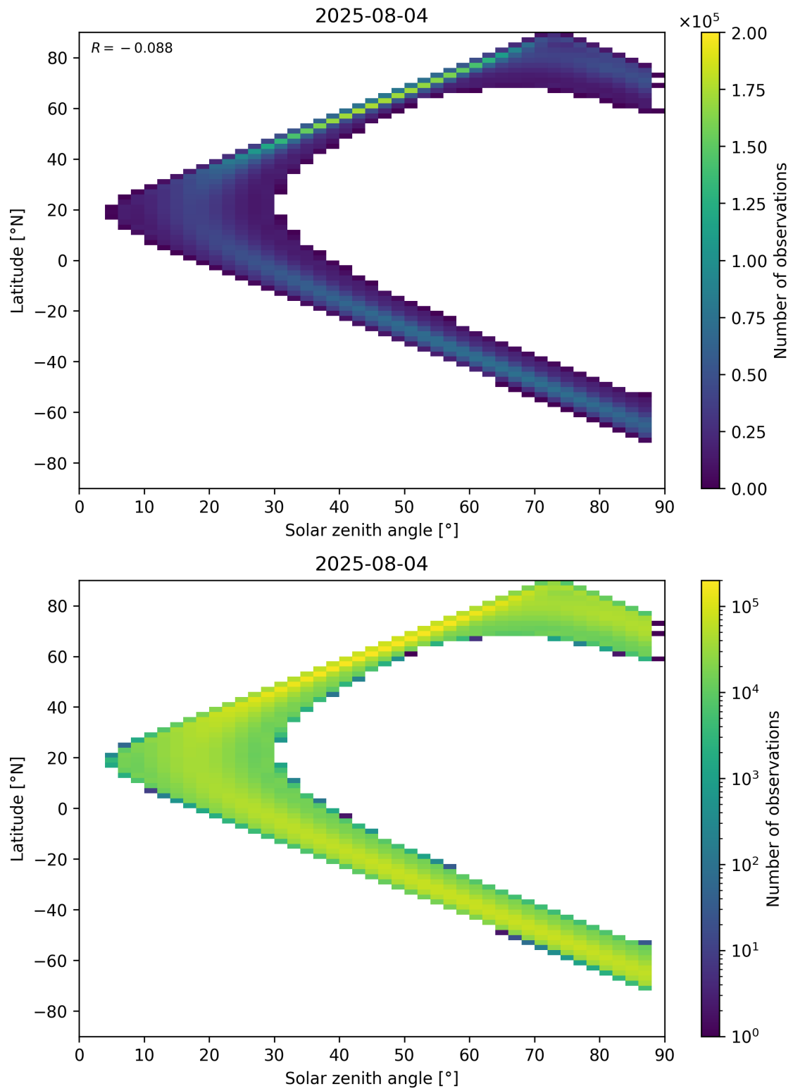
Figure 149: Scatter density plot of “Solar zenith angle” against “Latitude” for 2025-08-04 to 2025-08-05.
