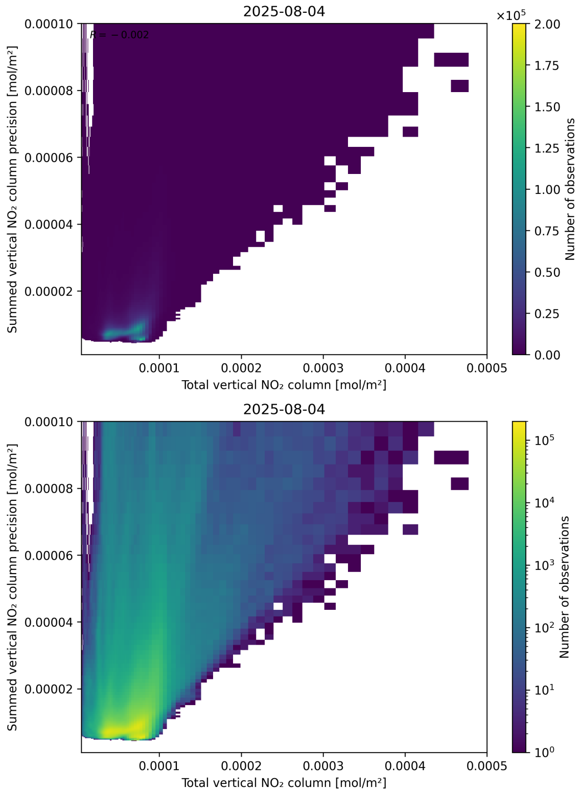
Figure 113: Scatter density plot of “Total vertical NO 2 column” against “Summed vertical NO 2 column precision” for 2025-08-04 to 2025-08-05.
