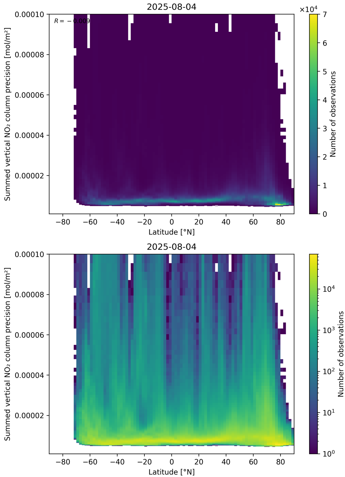
Figure 89: Scatter density plot of “Latitude” against “Summed vertical NO 2 column precision” for 2025-08-04 to 2025-08-05.
