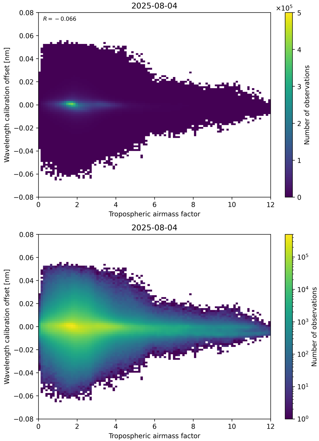
Figure 80: Scatter density plot of “Tropospheric airmass factor” against “Wavelength calibration offset” for 2025-08-04 to 2025-08-05.
