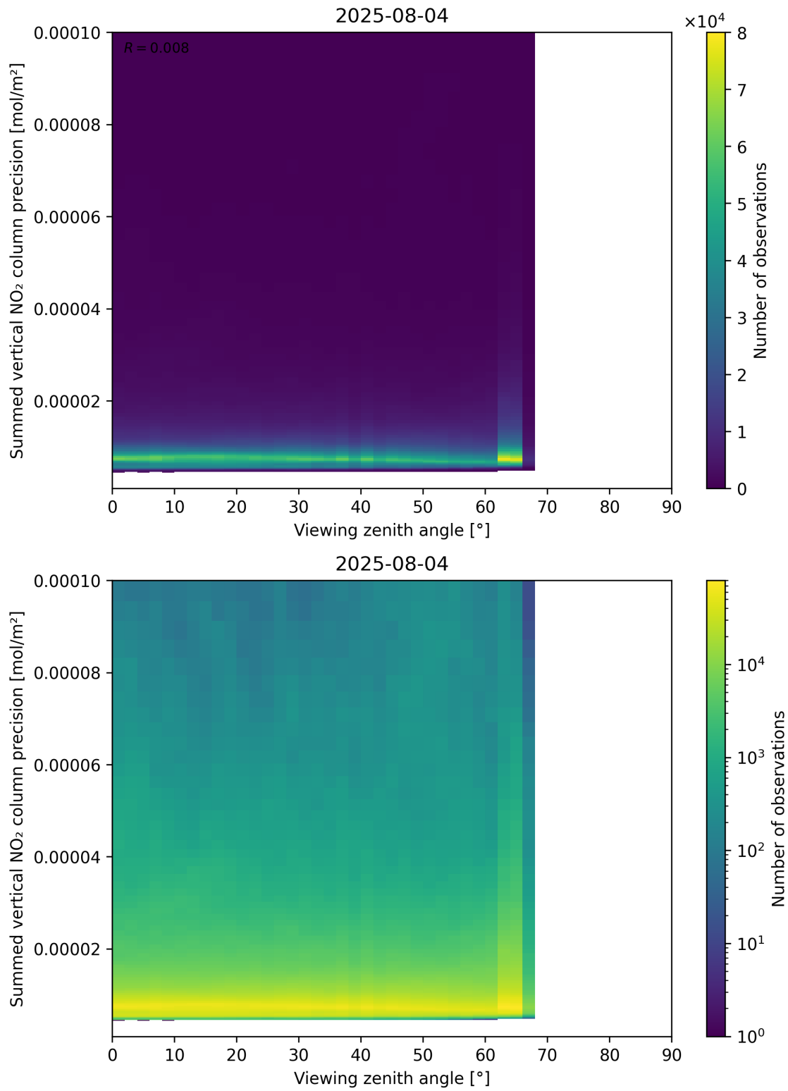
Figure 166: Scatter density plot of “Viewing zenith angle” against “Summed vertical NO 2 column precision” for 2025-08-04 to 2025-08-05.
