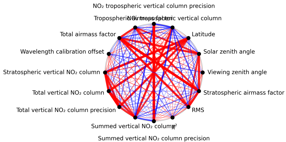
Figure 1: Map of correlation graph for 2025-08-04 to 2025-08-05.
