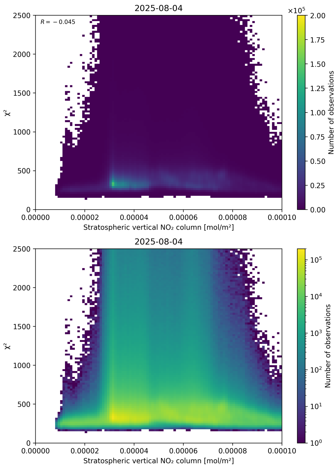
Figure 97: Scatter density plot of “Stratospheric vertical NO 2 column” against “ \chi^2 ” for 2025-08-04 to 2025-08-05.
