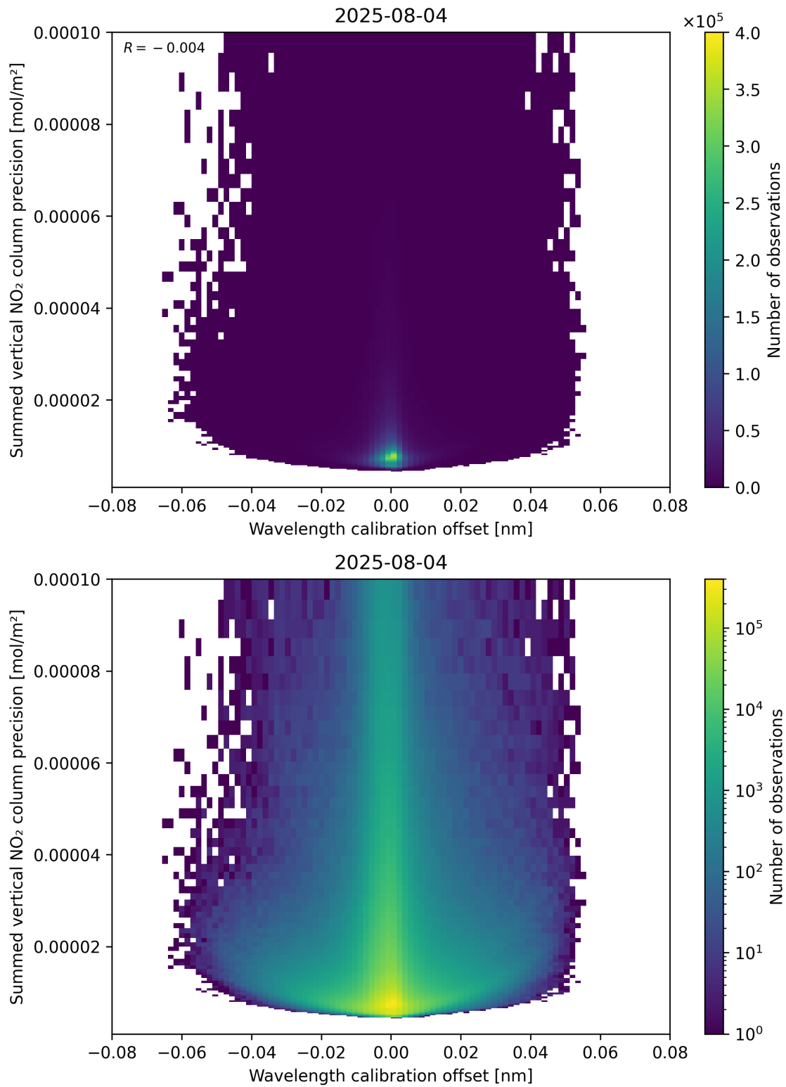
Figure 178: Scatter density plot of “Wavelength calibration offset” against “Summed vertical NO 2 column precision” for 2025-08-04 to 2025-08-05.
