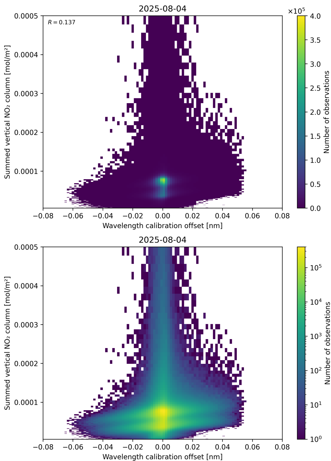
Figure 177: Scatter density plot of “Wavelength calibration offset” against “Summed vertical NO 2 column” for 2025-08-04 to 2025-08-05.
