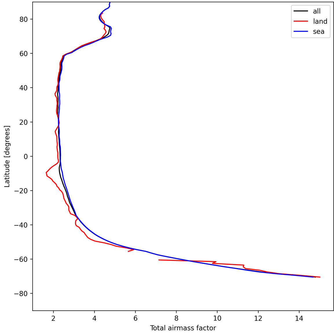
Figure 15: Zonal average of “Total airmass factor” for 2025-08-04 to 2025-08-05.
