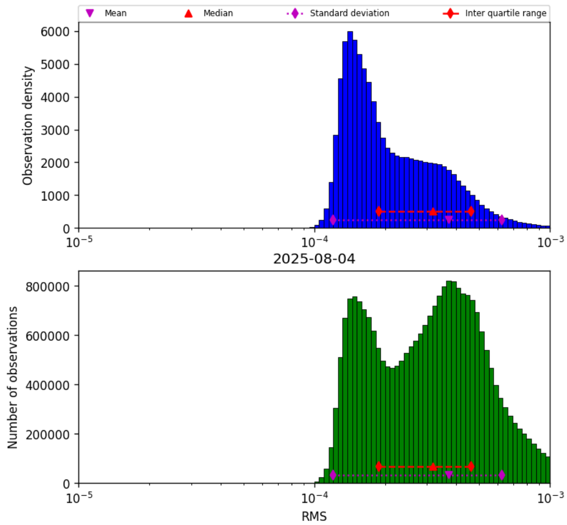
Figure 43: Histogram of “RMS” for 2025-08-04 to 2025-08-05
