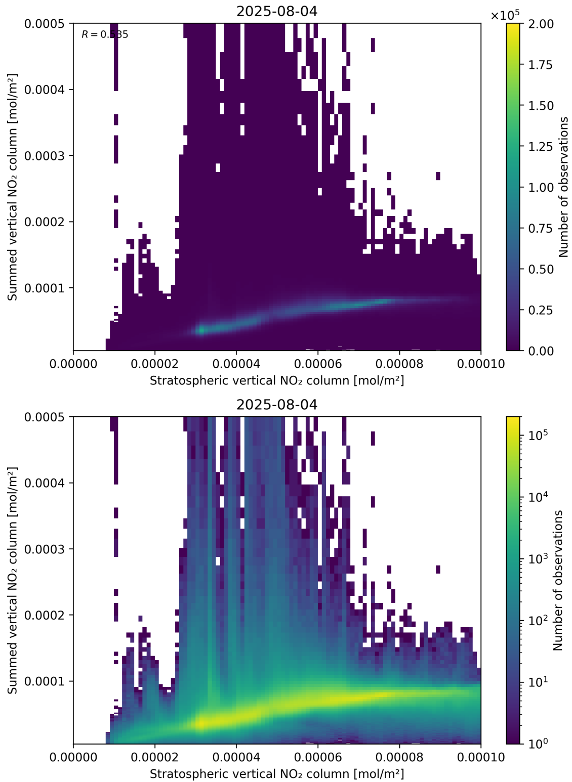
Figure 98: Scatter density plot of “Stratospheric vertical NO 2 column” against “Summed vertical NO 2 column” for 2025-08-04 to 2025-08-05.
