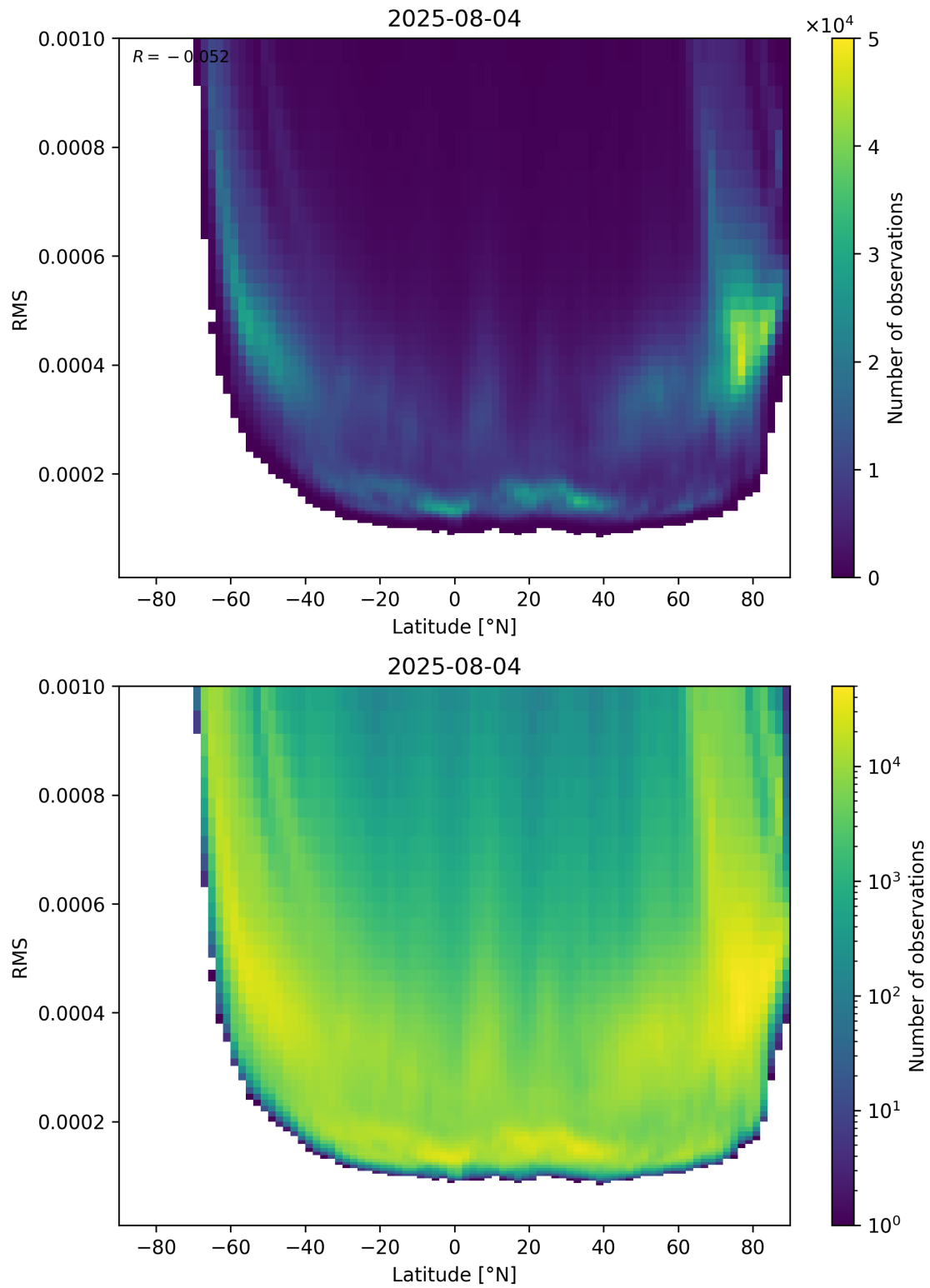
Figure 94: Scatter density plot of “Latitude” against “RMS” for 2025-08-04 to 2025-08-05.
