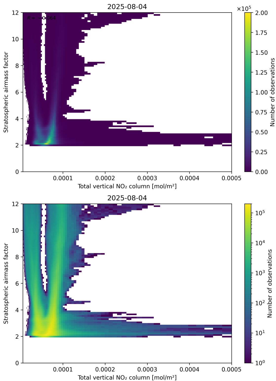
Figure 110: Scatter density plot of “Total vertical NO 2 column” against “Stratospheric airmass factor” for 2025-08-04 to 2025-08-05.
