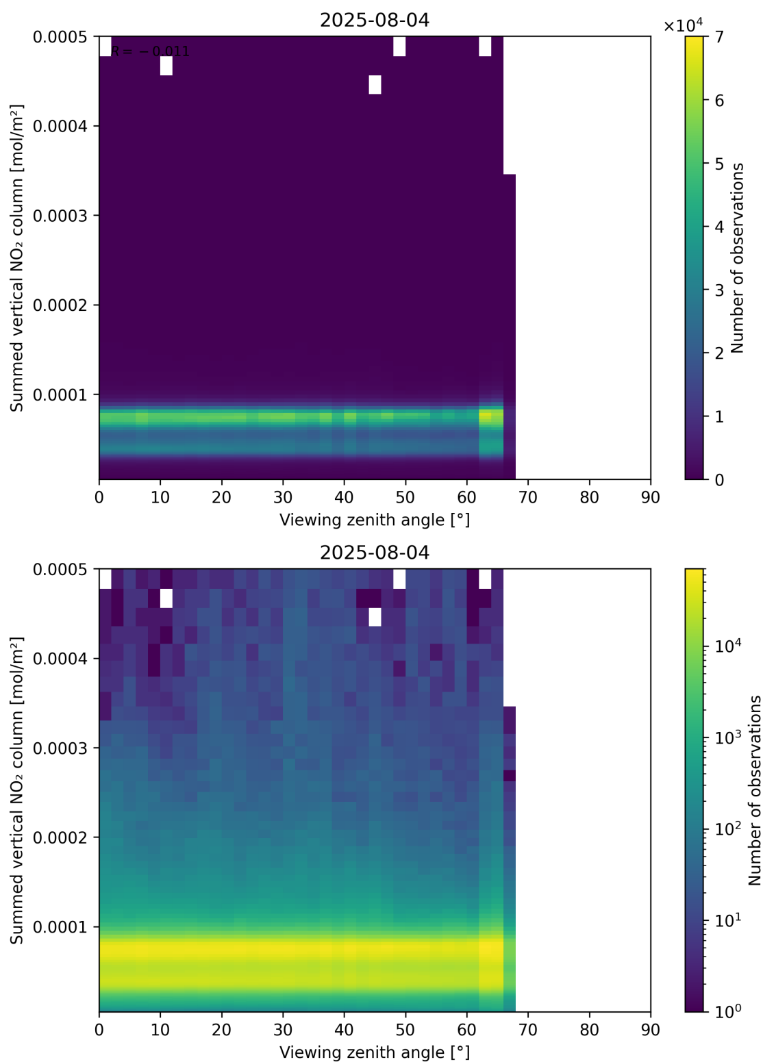
Figure 165: Scatter density plot of “Viewing zenith angle” against “Summed vertical NO 2 column” for 2025-08-04 to 2025-08-05.
