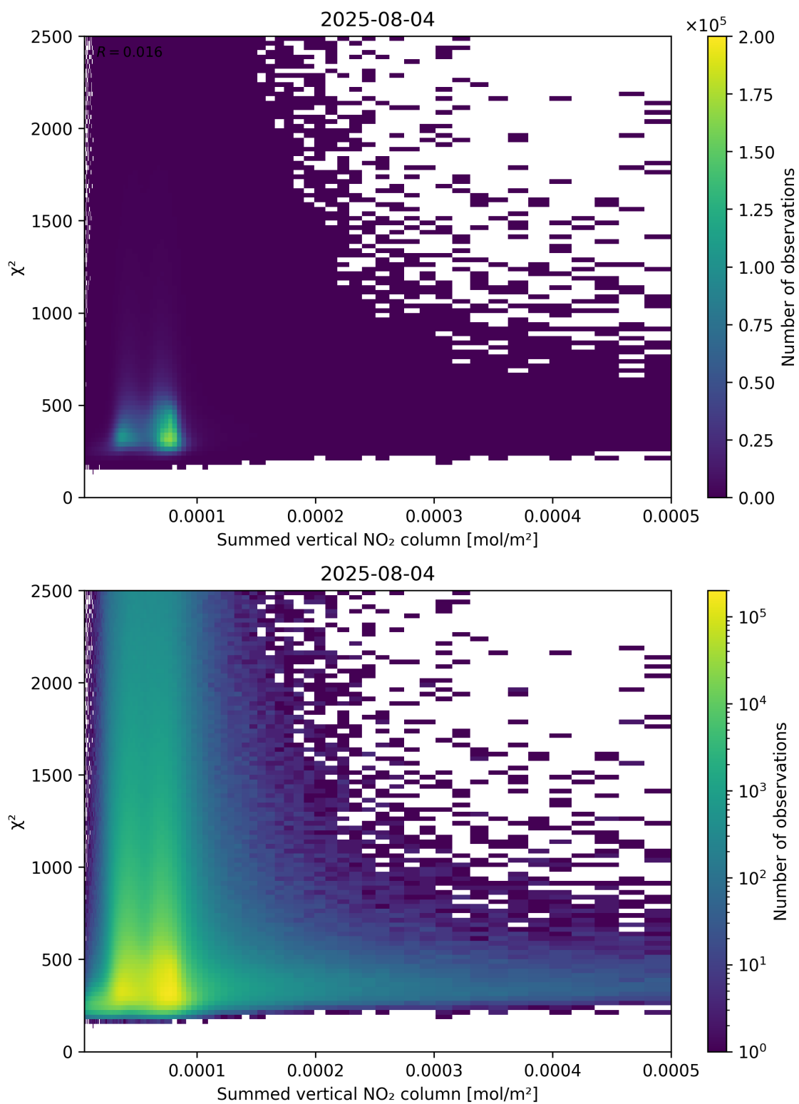
Figure 104: Scatter density plot of “Summed vertical NO 2 column” against “ \chi^2 ” for 2025-08-04 to 2025-08-05.
