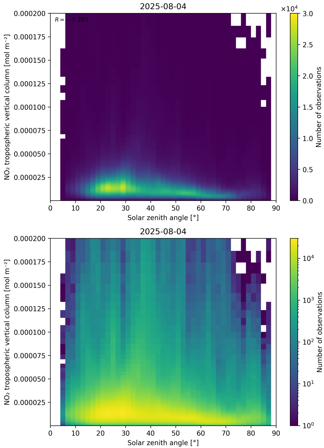
Figure 155: Scatter density plot of “Solar zenith angle” against “NO 2 tropospheric vertical column” for 2025-08-04 to 2025-08-05.
