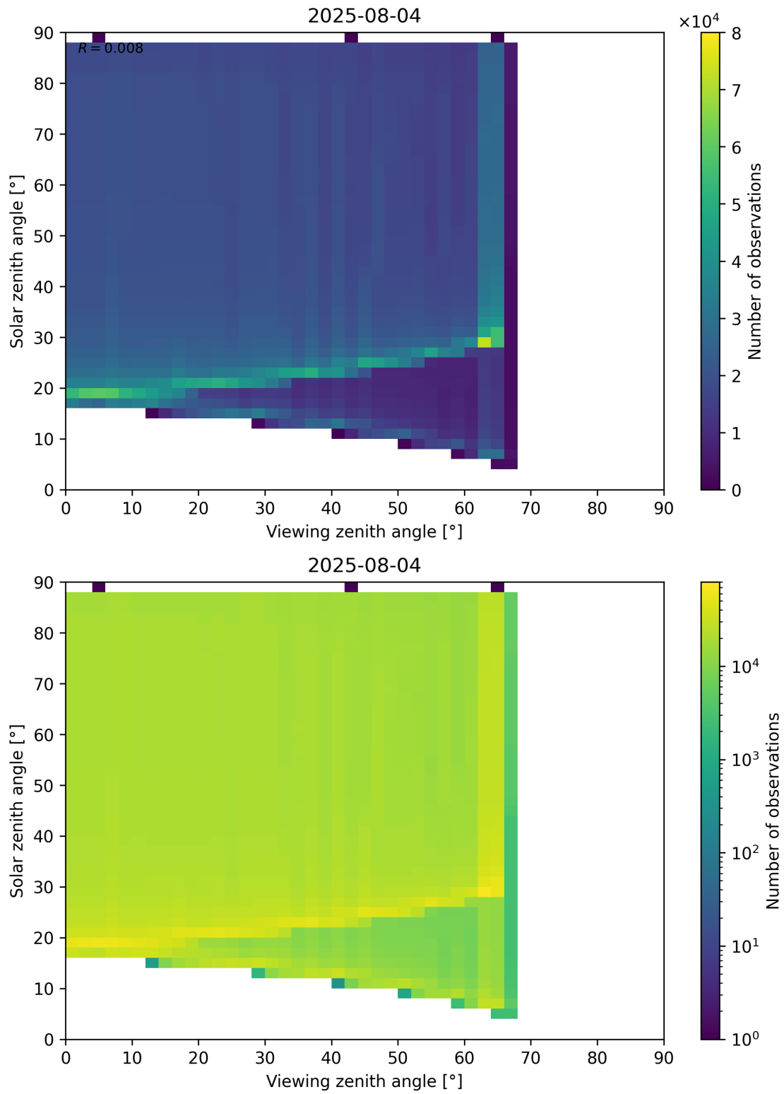
Figure 172: Scatter density plot of “Viewing zenith angle” against “Solar zenith angle” for 2025-08-04 to 2025-08-05.
