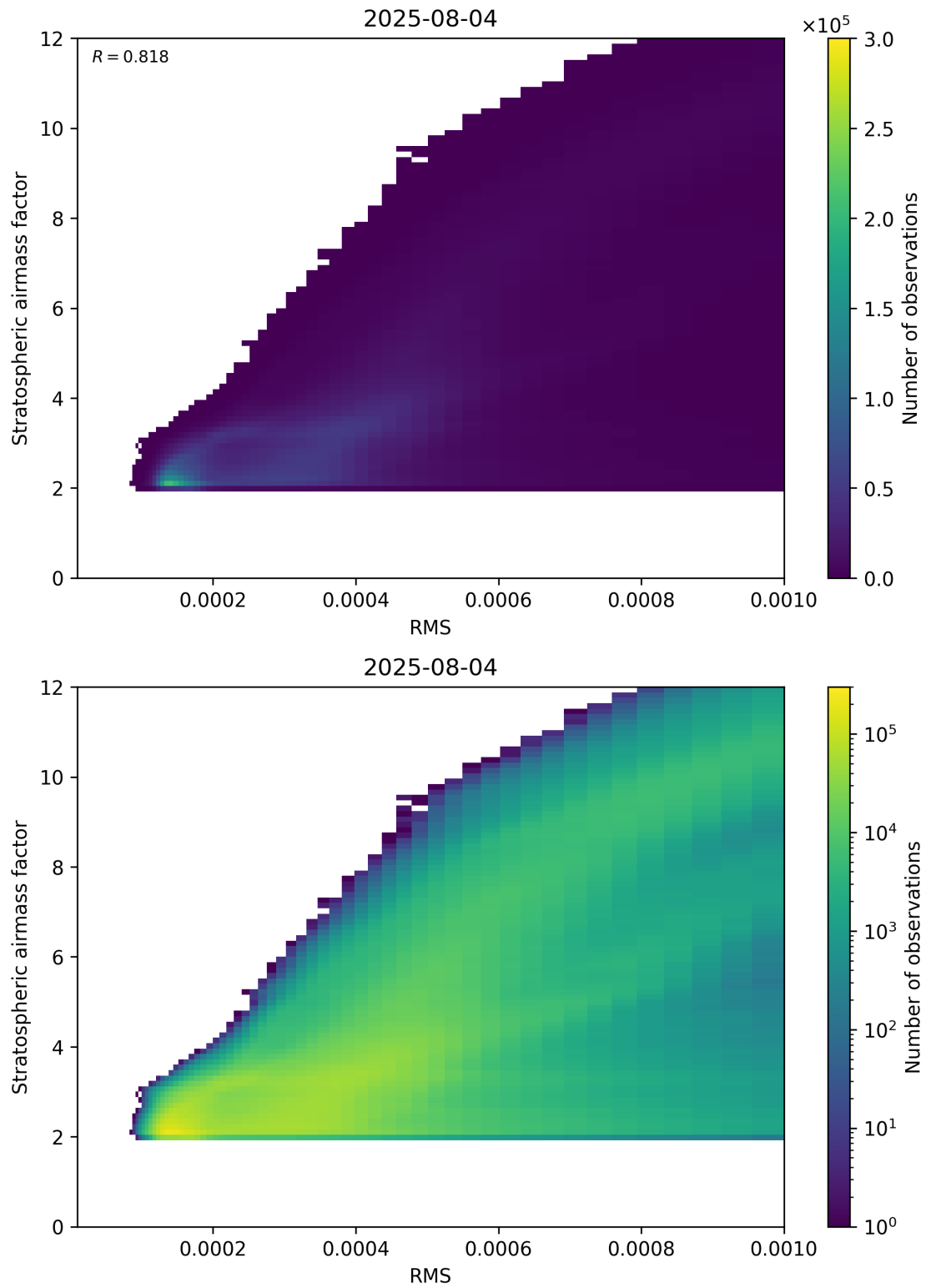
Figure 144: Scatter density plot of “RMS” against “Stratospheric airmass factor” for 2025-08-04 to 2025-08-05.
