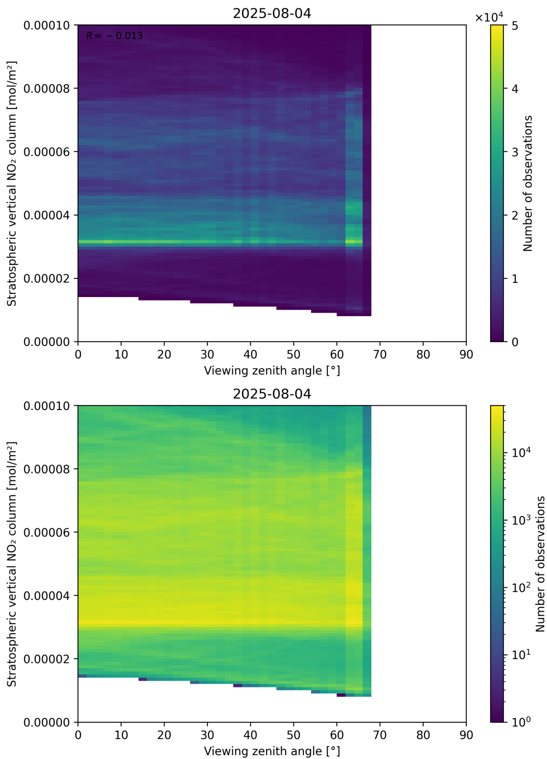
Figure 164: Scatter density plot of “Viewing zenith angle” against “Stratospheric vertical NO 2 column” for 2025-08-04 to 2025-08-05.
