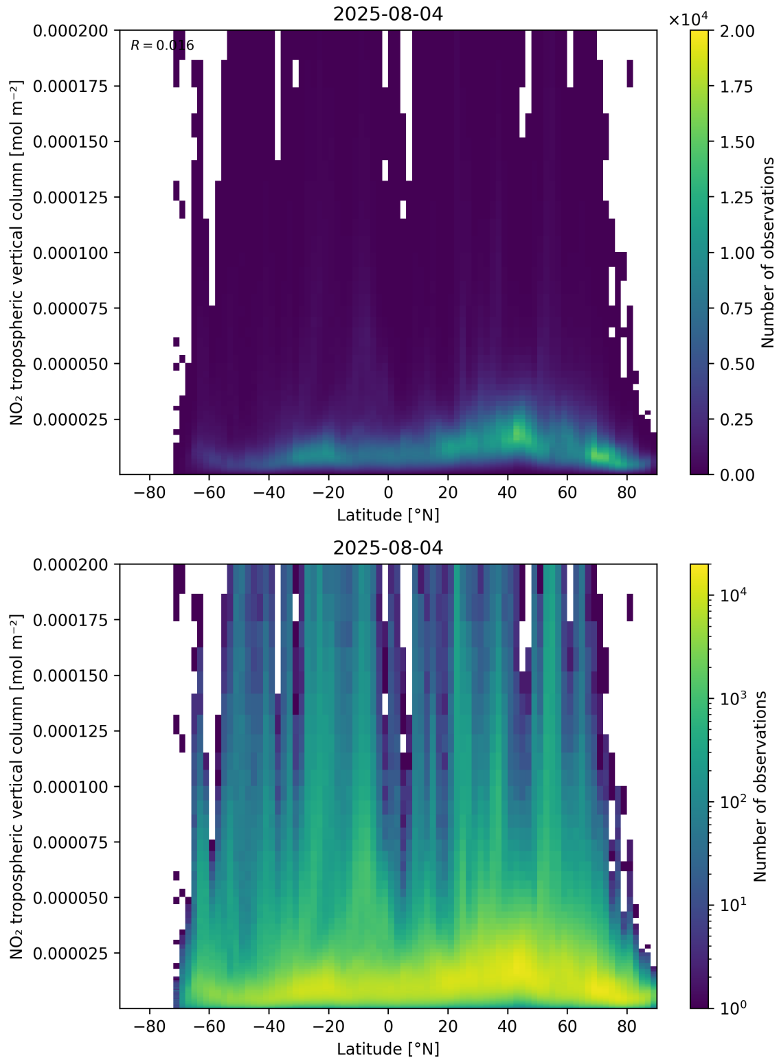
Figure 92: Scatter density plot of “Latitude” against “NO 2 tropospheric vertical column” for 2025-08-04 to 2025-08-05.
