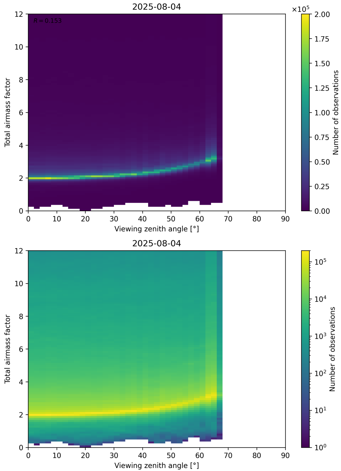
Figure 160: Scatter density plot of “Viewing zenith angle” against “Total airmass factor” for 2025-08-04 to 2025-08-05.
