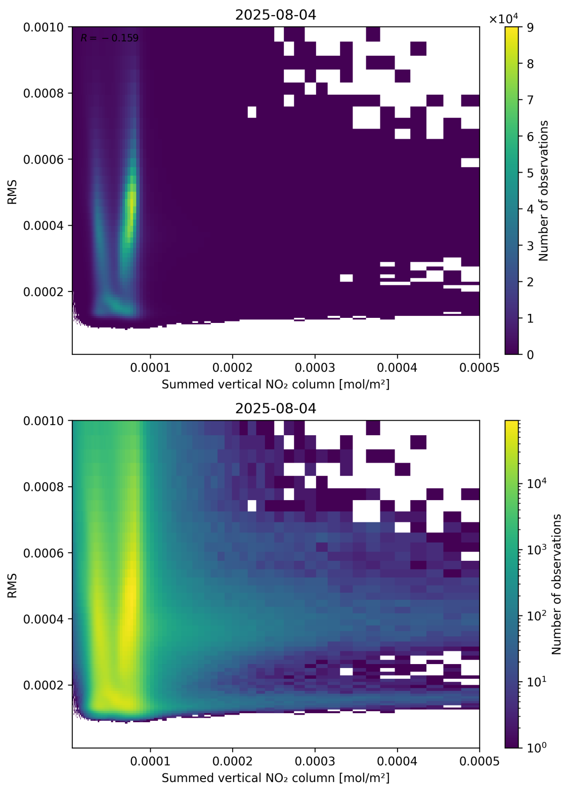
Figure 109: Scatter density plot of “Summed vertical NO 2 column” against “RMS” for 2025-08-04 to 2025-08-05.
