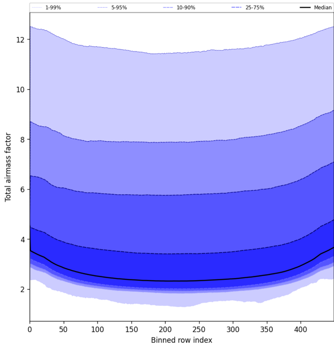
Figure 49: Along track statistics of “Total airmass factor” for 2025-08-04 to 2025-08-05
