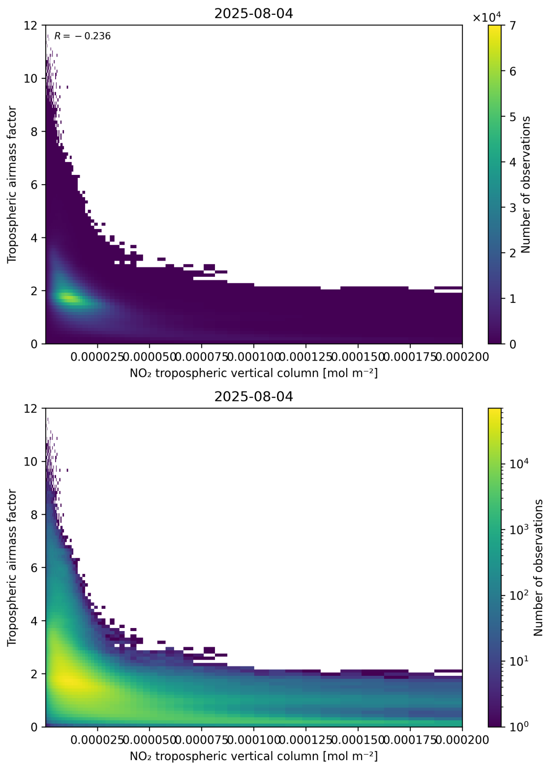
Figure 123: Scatter density plot of “NO 2 tropospheric vertical column” against “Tropospheric air mass factor” for 2025-08-04 to 2025-08-05.
