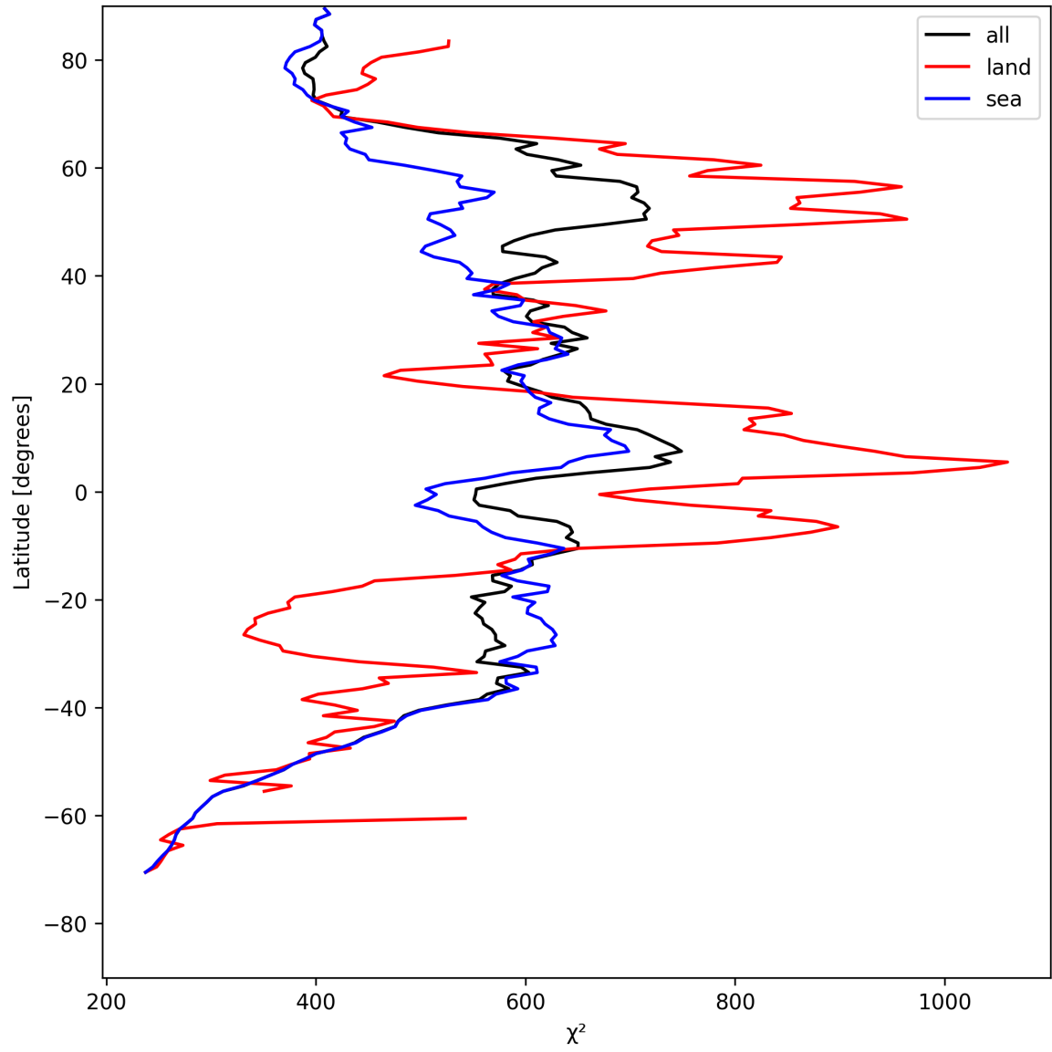
Figure 25: Zonal average of “ \chi^2 ” for 2025-08-04 to 2025-08-05.
