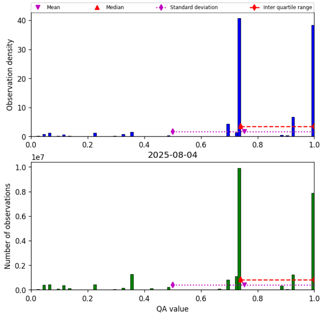
Figure 28: Histogram of “QA value” for 2025-08-04 to 2025-08-05
