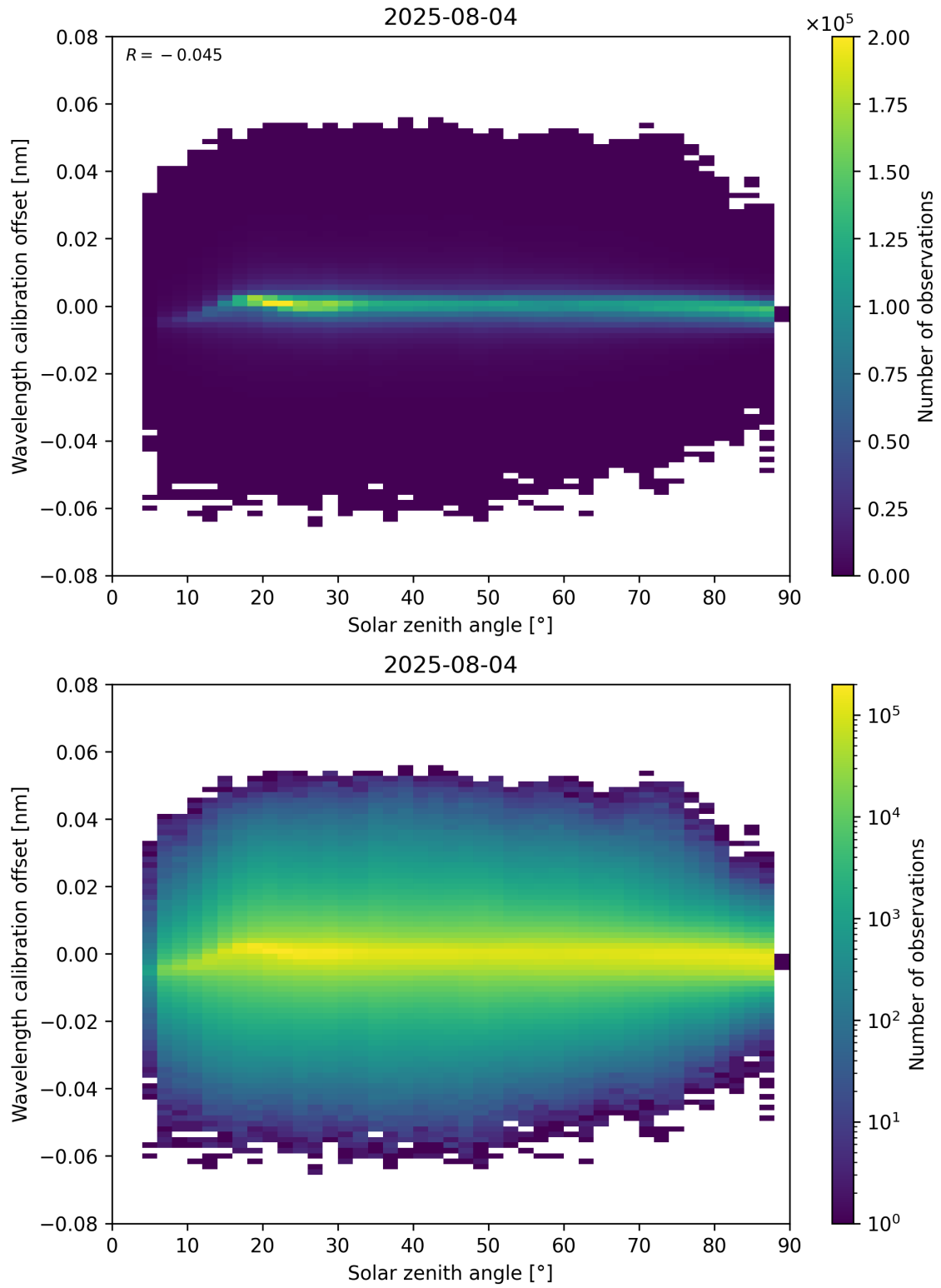
Figure 158: Scatter density plot of “Solar zenith angle” against “Wavelength calibration offset” for 2025-08-04 to 2025-08-05.
