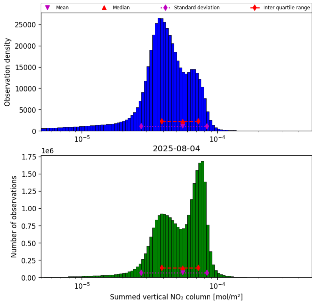
Figure 40: Histogram of “Summed vertical NO 2 column” for 2025-08-04 to 2025-08-05
