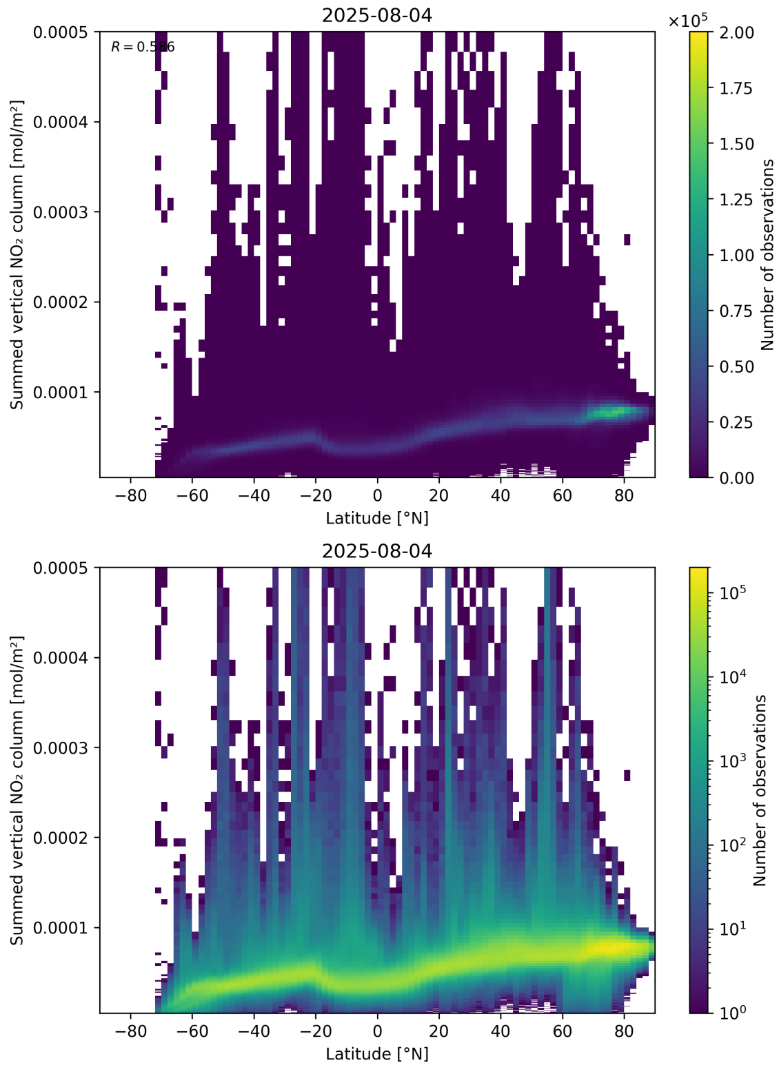
Figure 88: Scatter density plot of “Latitude” against “Summed vertical NO 2 column” for 2025-08-04 to 2025-08-05.
