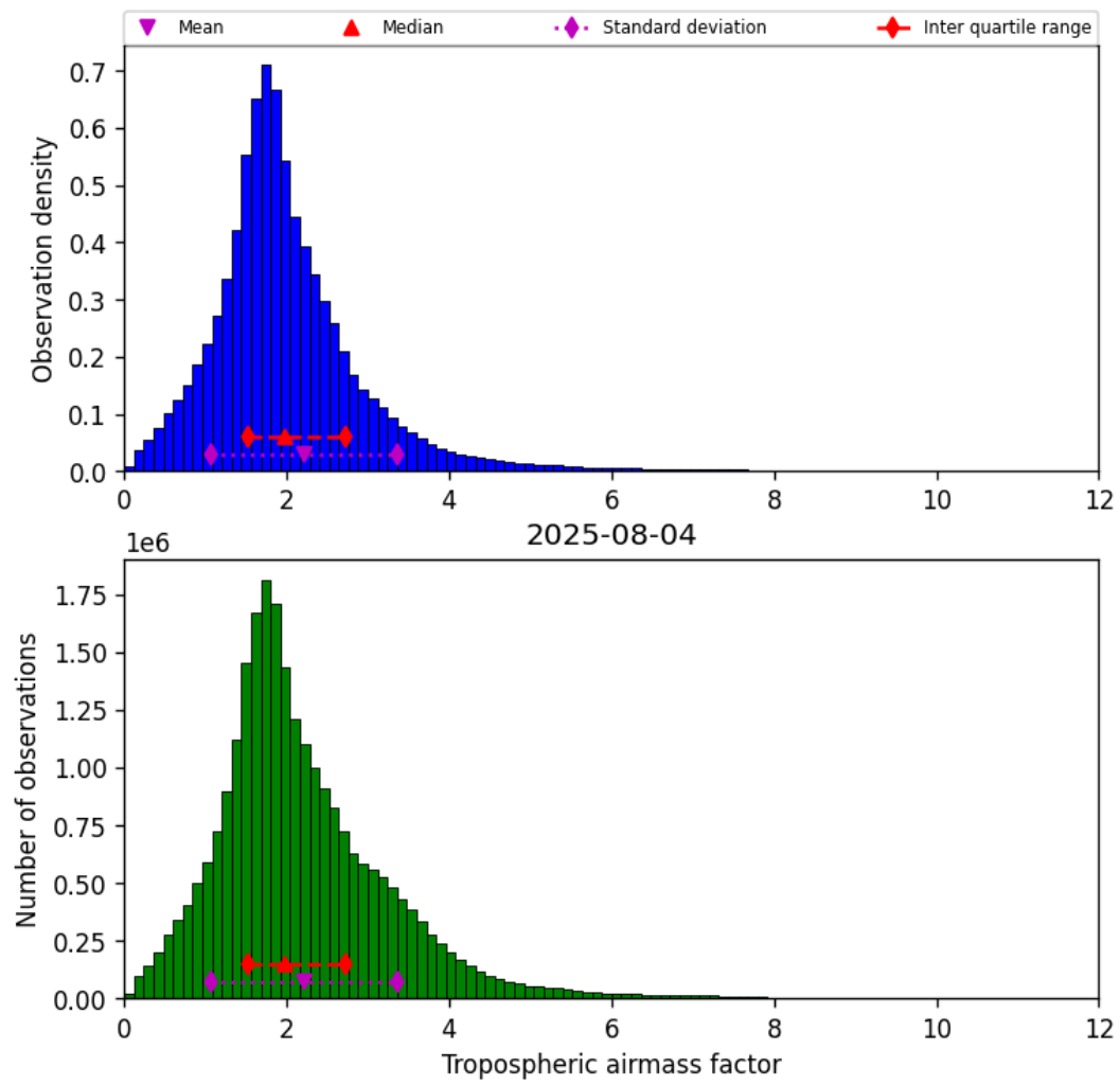
Figure 31: Histogram of “Tropospheric airmass factor” for 2025-08-04 to 2025-08-05
