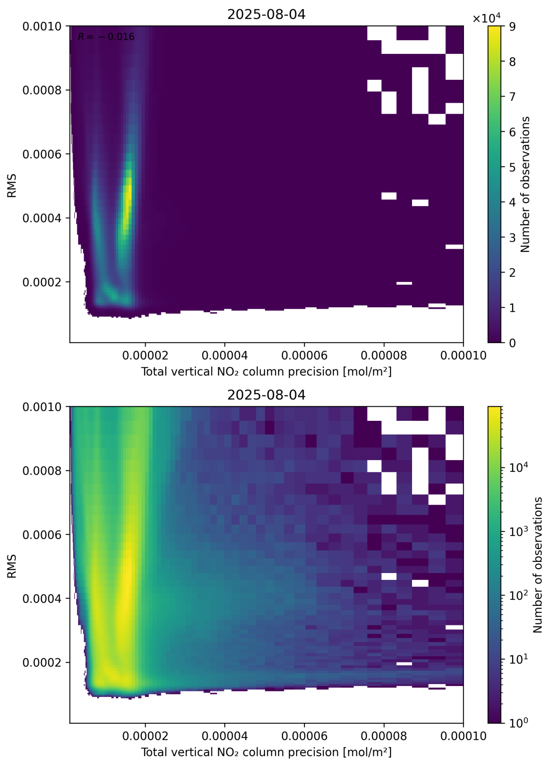
Figure 119: Scatter density plot of “Total vertical NO 2 column precision” against “RMS” for 2025-08-04 to 2025-08-05.
