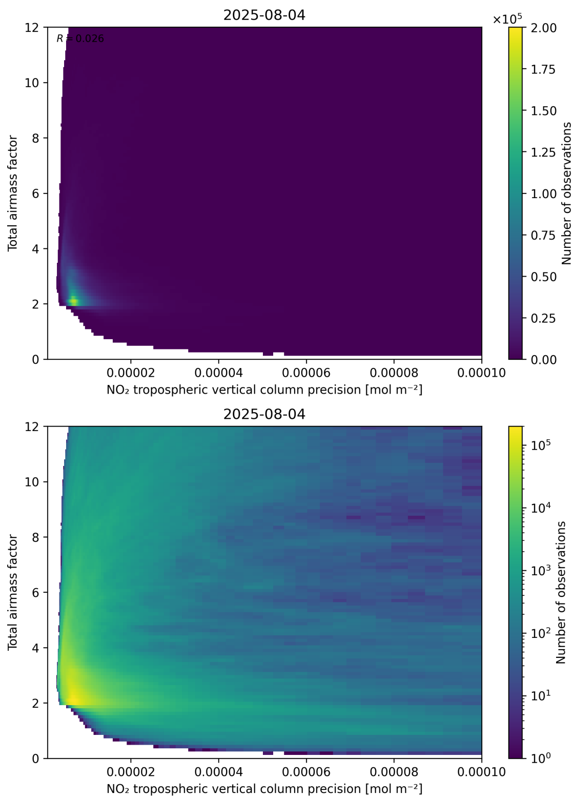
Figure 132: Scatter density plot of “NO 2 tropospheric vertical column precision” against “Total air mass factor” for 2025-08-04 to 2025-08-05.
