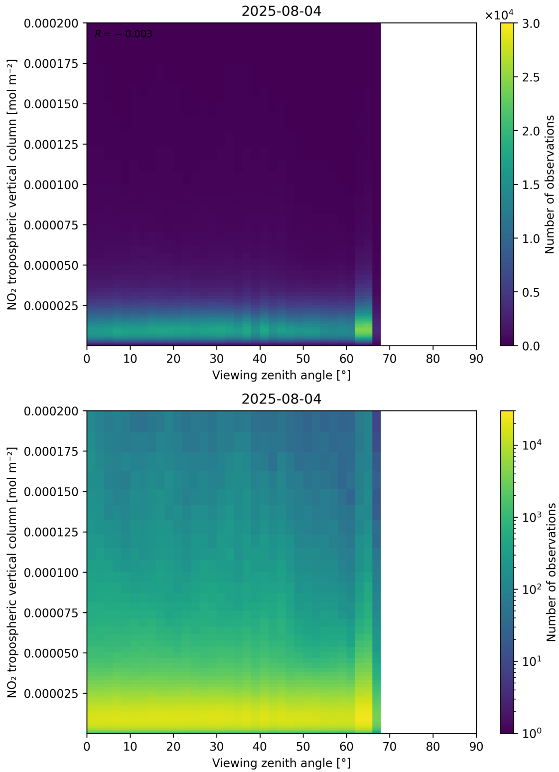
Figure 169: Scatter density plot of “Viewing zenith angle” against “NO 2 tropospheric vertical column” for 2025-08-04 to 2025-08-05.
