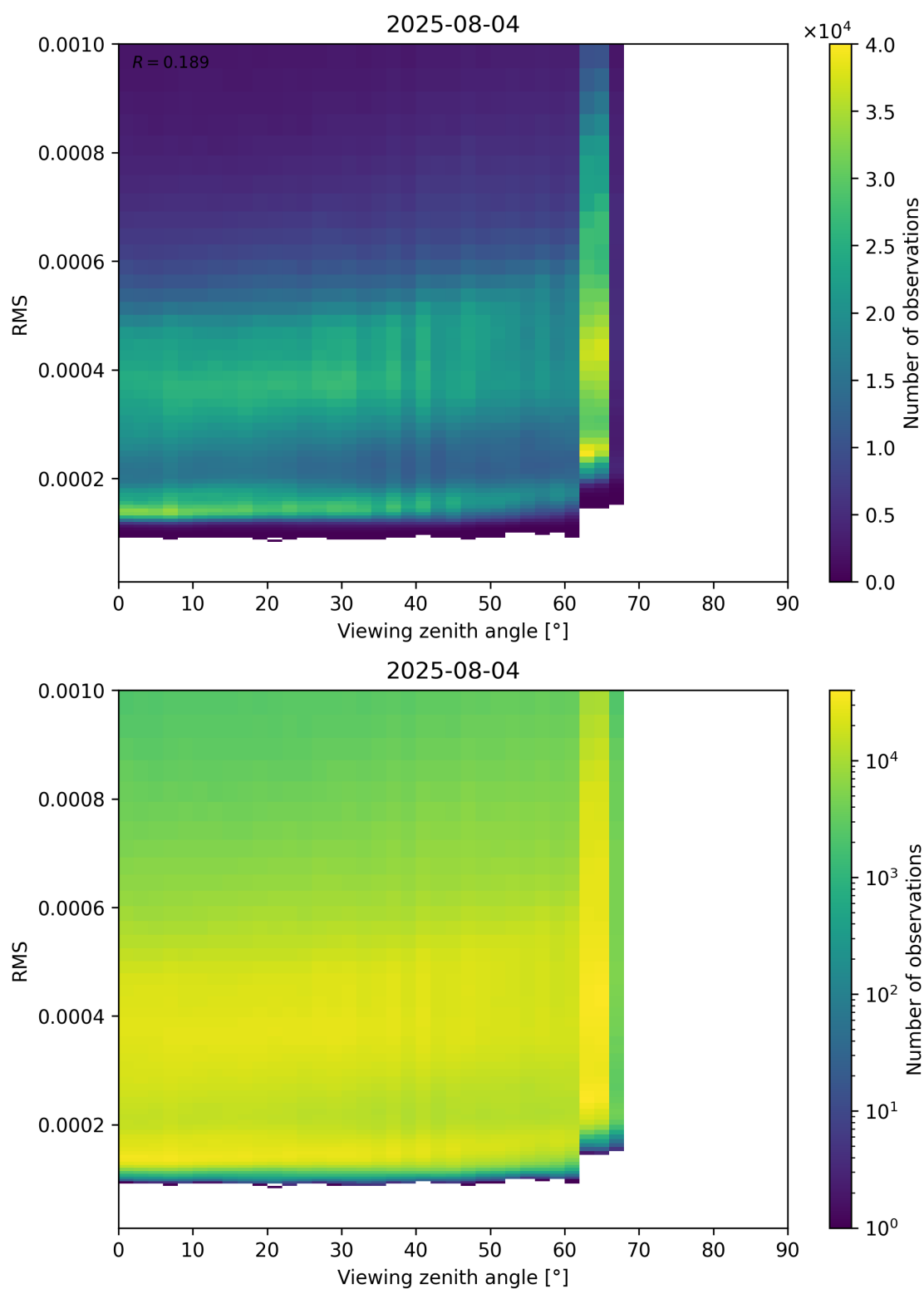
Figure 171: Scatter density plot of “Viewing zenith angle” against “RMS” for 2025-08-04 to 2025-08-05.
