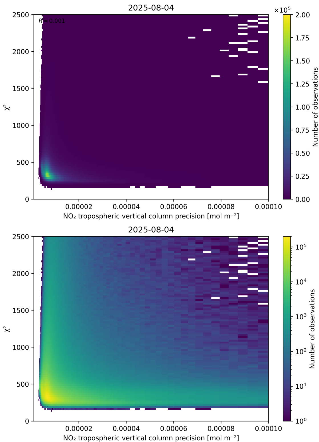
Figure 134: Scatter density plot of “NO 2 tropospheric vertical column precision” against “ \chi^2 ” for 2025-08-04 to 2025-08-05.
