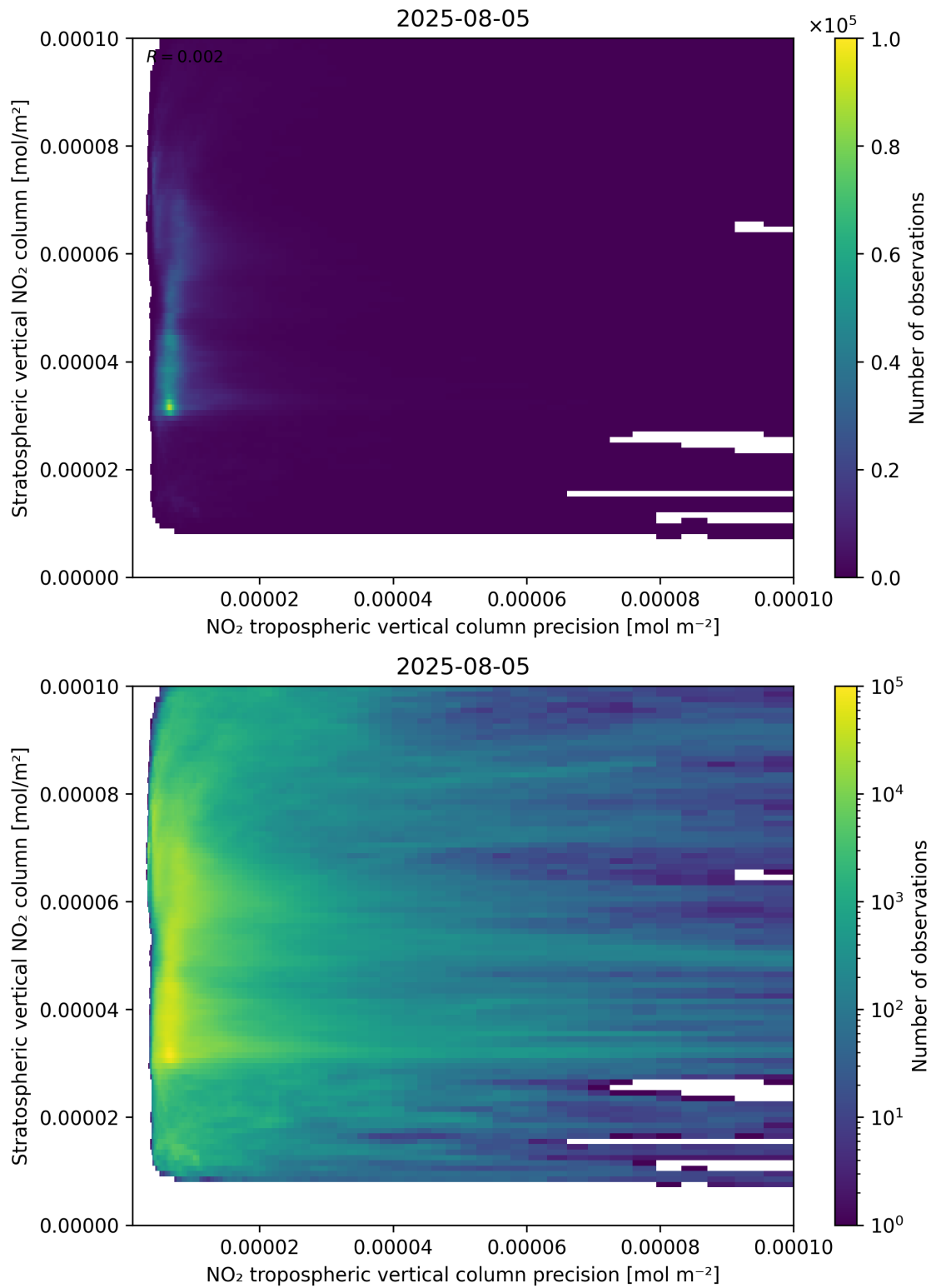
Figure 135: Scatter density plot of “NO 2 tropospheric vertical column precision” against “Stratospheric vertical NO 2 column” for 2025-08-04 to 2025-08-06.
