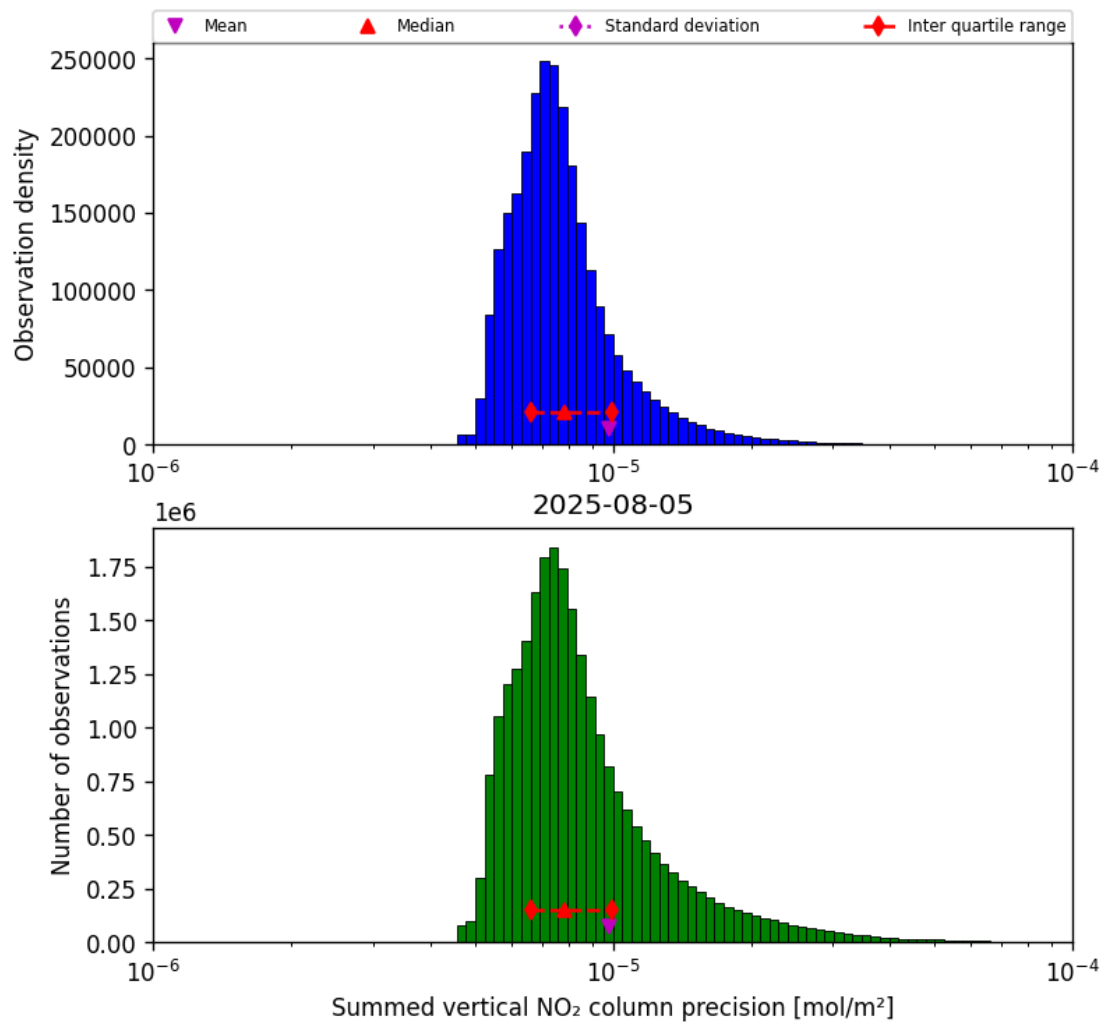
Figure 41: Histogram of "Summed vertical NO 2 column precision" for 2025-08-04 to 2025-08-06
