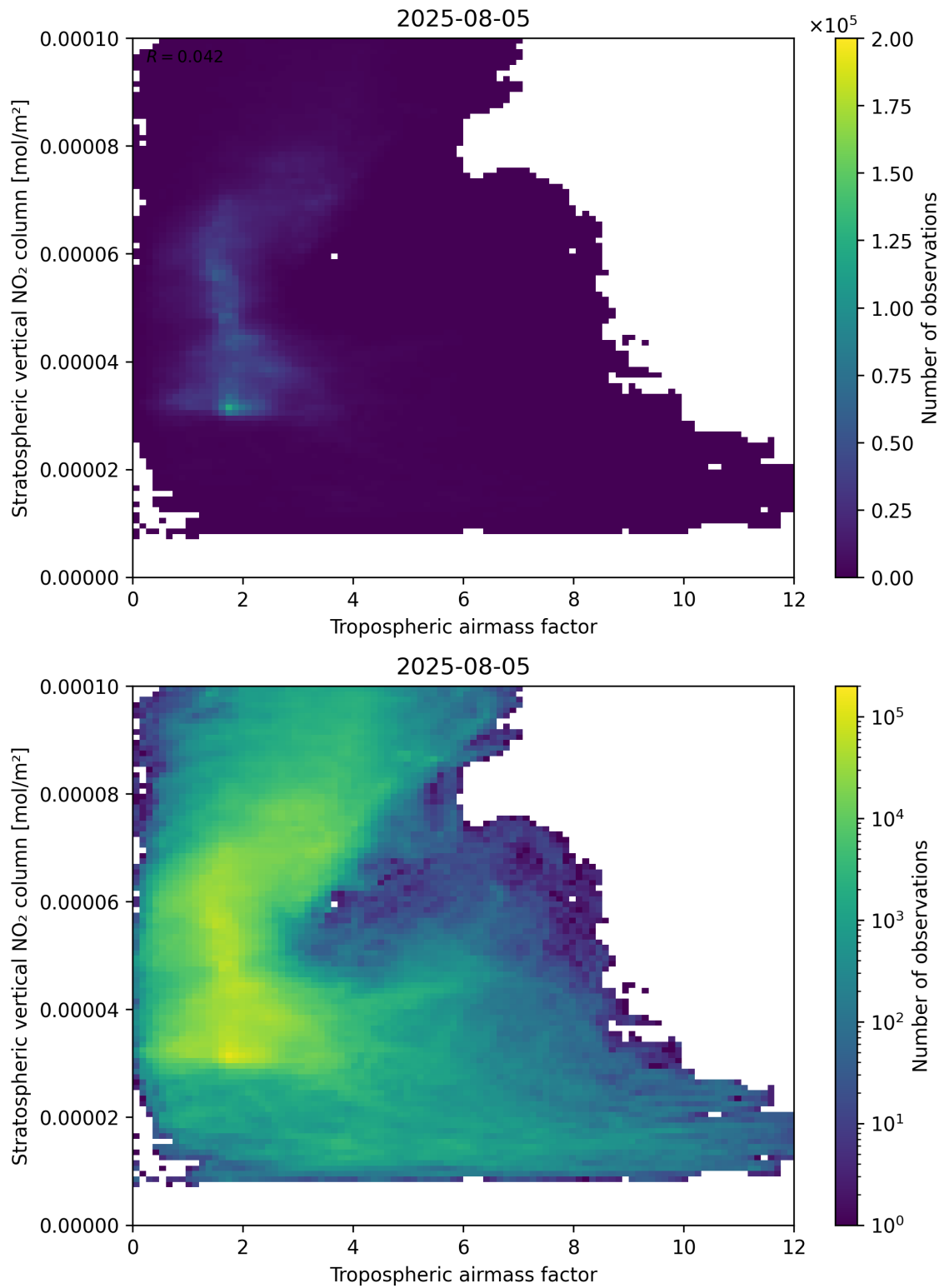
Figure 74: Scatter density plot of “Tropospheric air mass factor” against “Stratospheric vertical NO 2 column” for 2025-08-04 to 2025-08-06.
