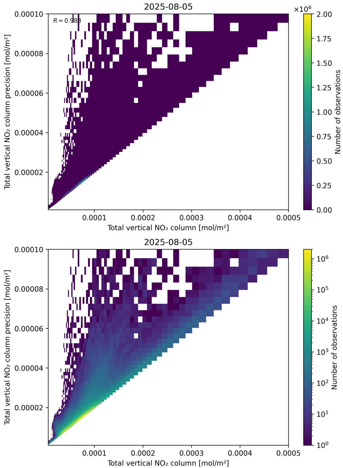
Figure 114: Scatter density plot of “Total vertical NO 2 column” against “Total vertical NO 2 column precision” for 2025-08-04 to 2025-08-06.
