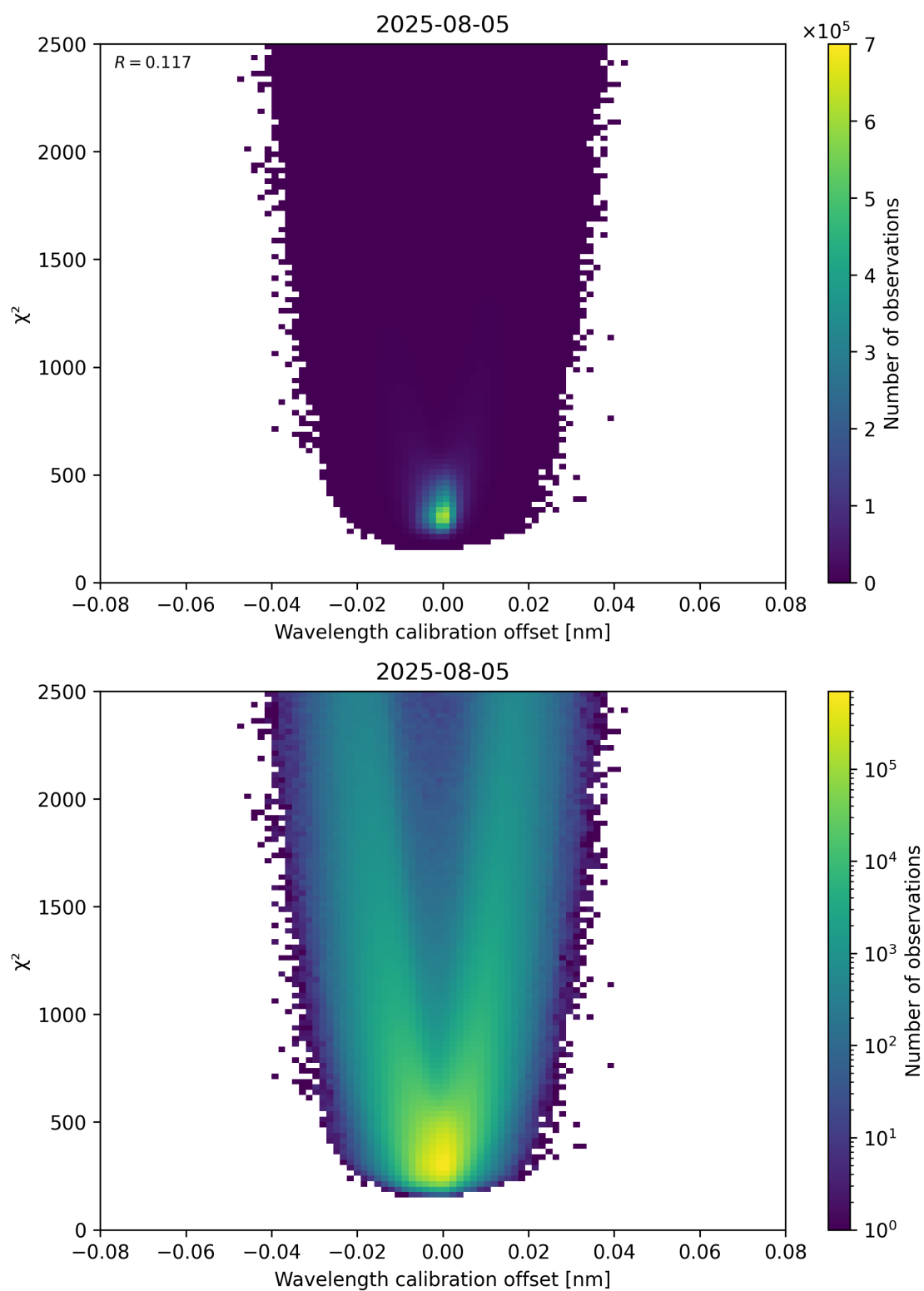
Figure 175: Scatter density plot of “Wavelength calibration offset” against “ \chi^2 ” for 2025-08-04 to 2025-08-06.
