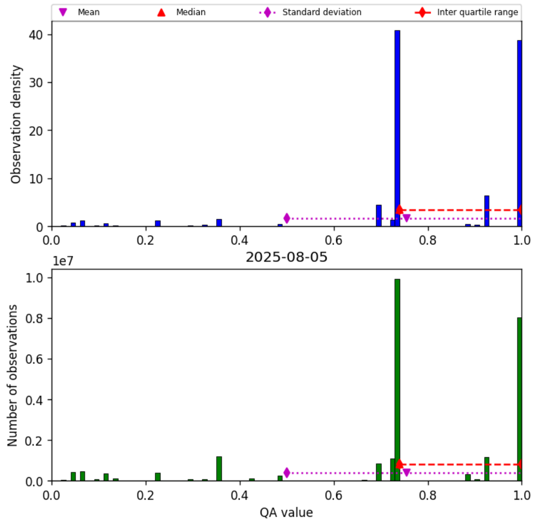
Figure 28: Histogram of “QA value” for 2025-08-04 to 2025-08-06
