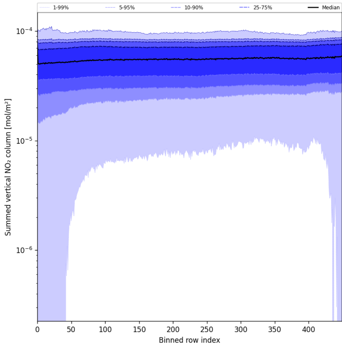
Figure 57: Along track statistics of “Summed vertical NO 2 column” for 2025-08-04 to 2025-08-06
