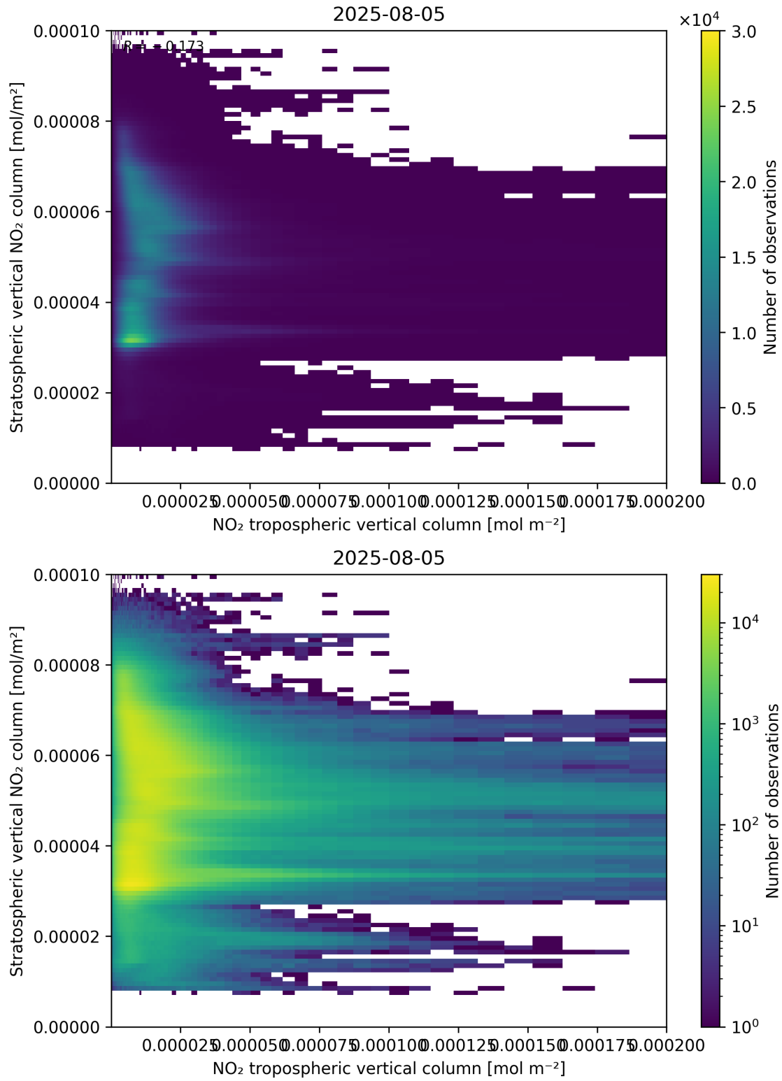
Figure 125: Scatter density plot of “NO 2 tropospheric vertical column” against “Stratospheric vertical NO 2 column” for 2025-08-04 to 2025-08-06.
