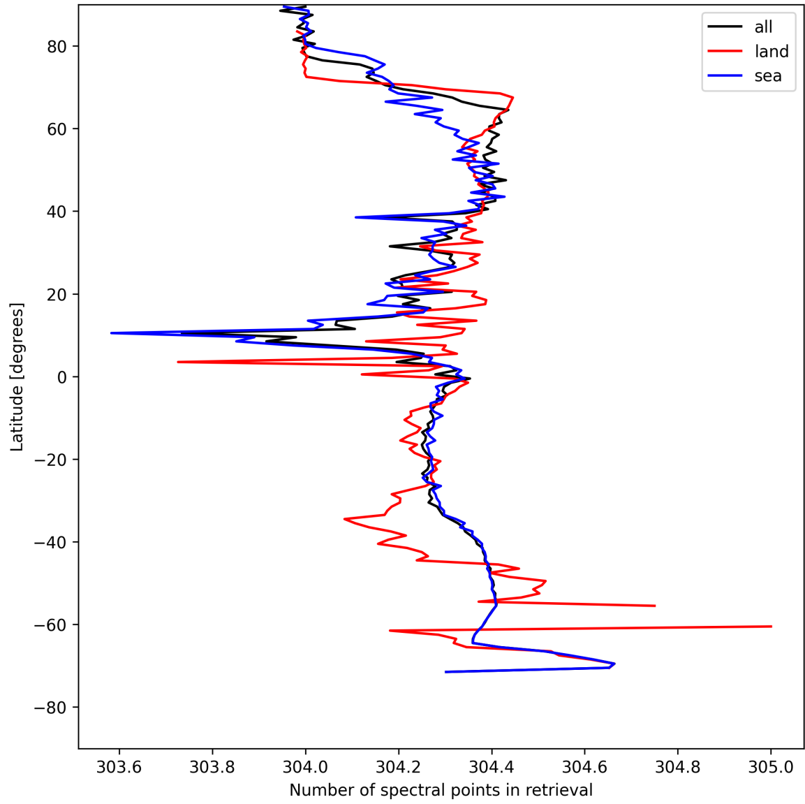
Figure 16: Zonal average of “Number of spectral points in retrieval” for 2025-08-04 to 2025-08-06.
