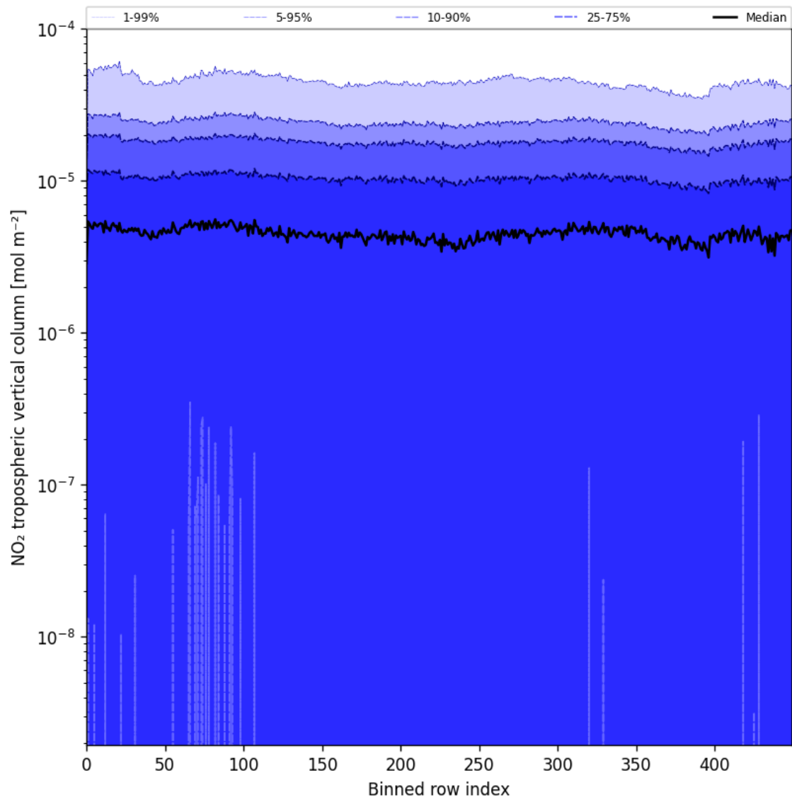
Figure 46: Along track statistics of “NO 2 tropospheric vertical column” for 2025-08-04 to 2025-08-06
