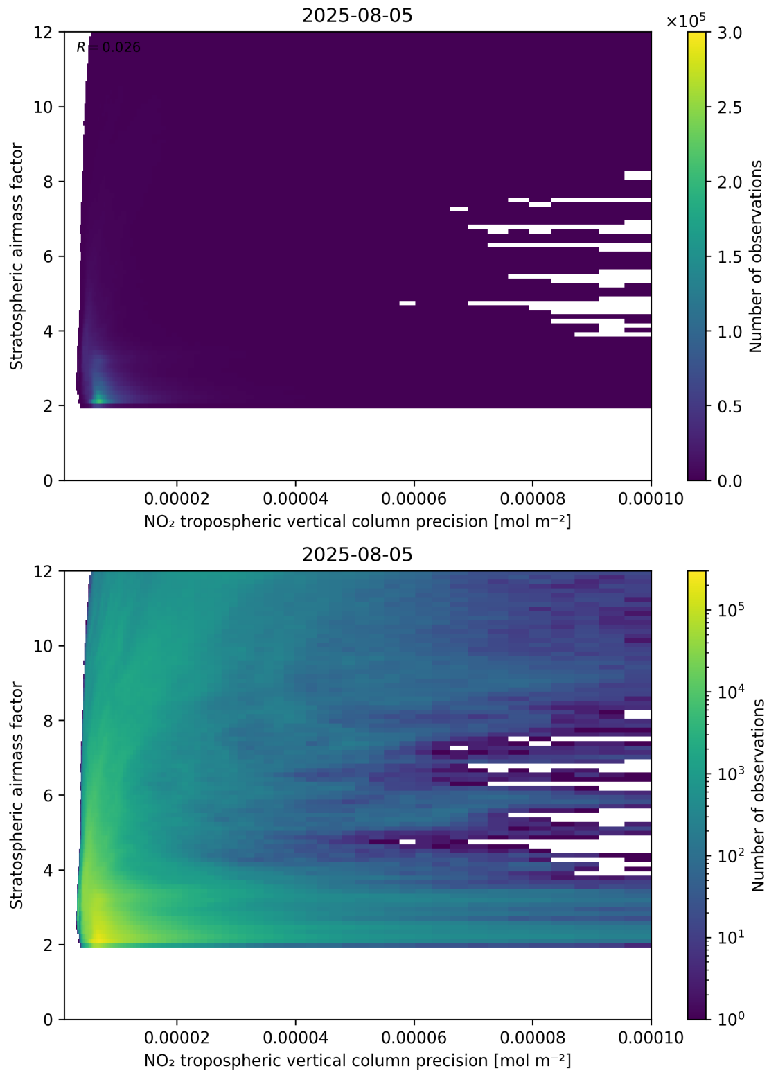
Figure 131: Scatter density plot of “NO 2 tropospheric vertical column precision” against “Stratospheric airmass factor” for 2025-08-04 to 2025-08-06.
