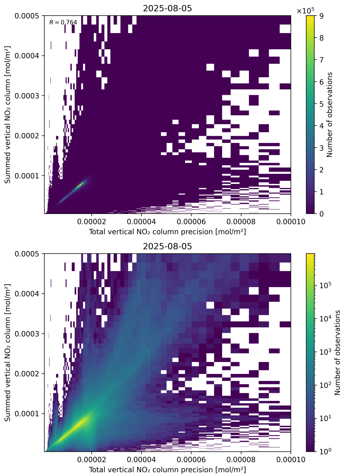
Figure 117: Scatter density plot of “Total vertical NO 2 column precision” against “Summed vertical NO 2 column” for 2025-08-04 to 2025-08-06.
