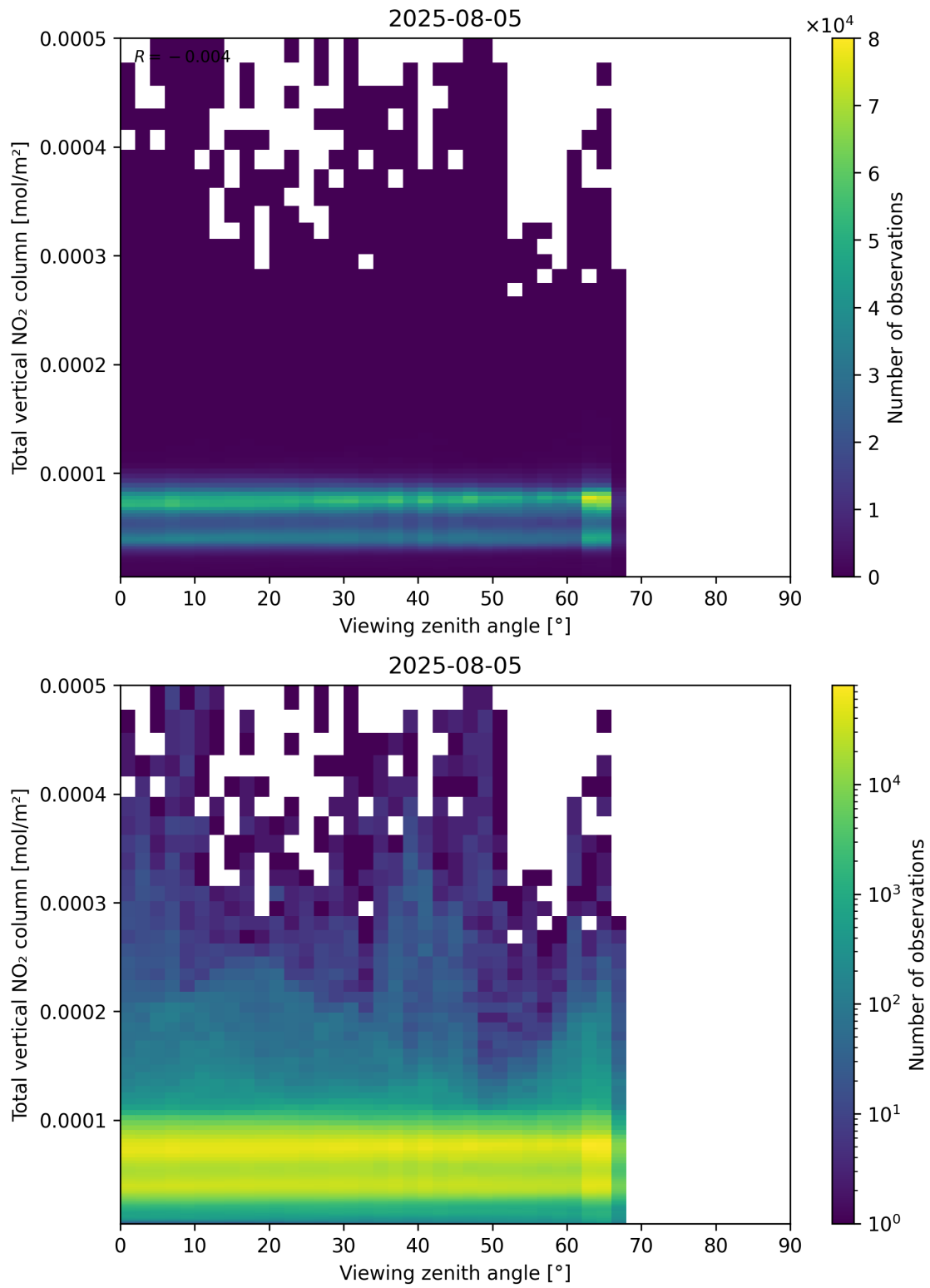
Figure 167: Scatter density plot of “Viewing zenith angle” against “Total vertical NO 2 column” for 2025-08-04 to 2025-08-06.
