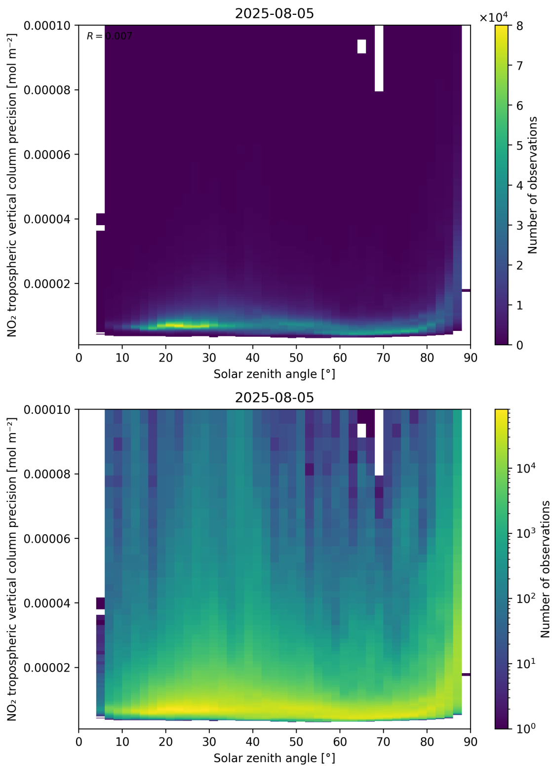
Figure 156: Scatter density plot of “Solar zenith angle” against “NO 2 tropospheric vertical column precision” for 2025-08-04 to 2025-08-06.
