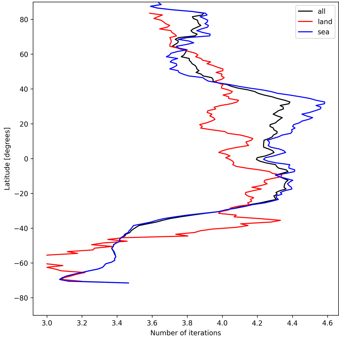
Figure 17: Zonal average of “Number of iterations” for 2025-08-04 to 2025-08-06.
