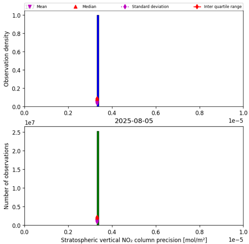
Figure 37: Histogram of “Stratospheric vertical NO 2 column precision” for 2025-08-04 to 2025-08-06
