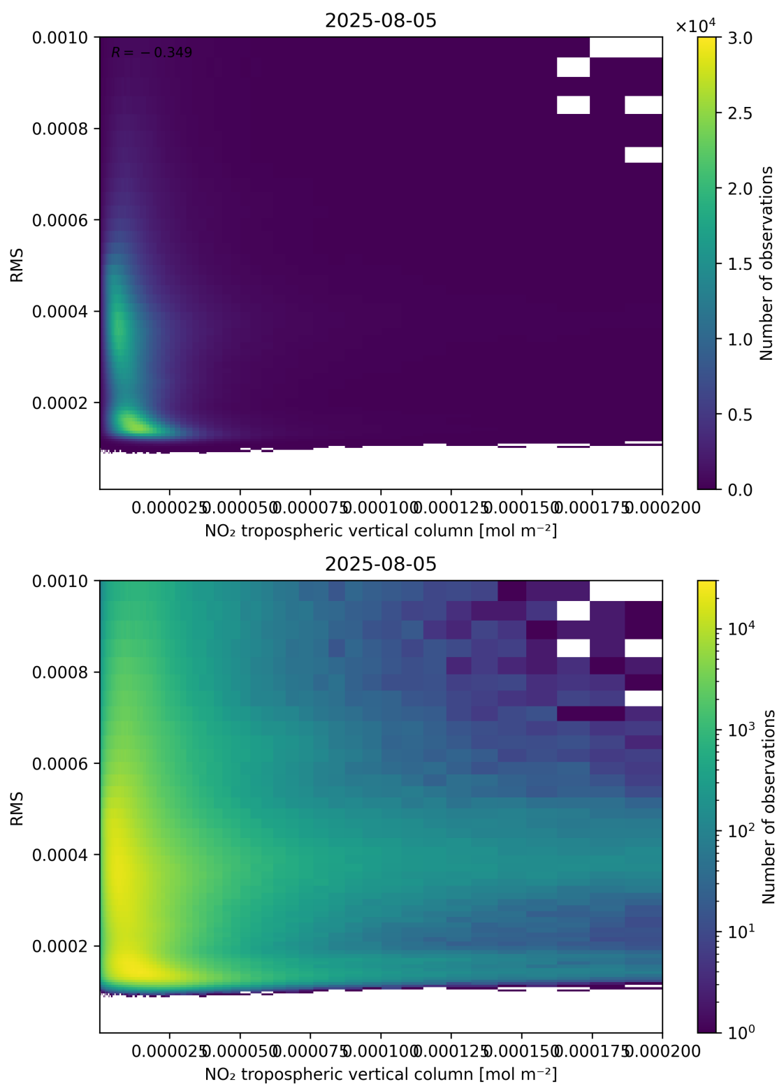
Figure 142: Scatter density plot of “NO 2 tropospheric vertical column” against “RMS” for 2025-08-04 to 2025-08-06.
