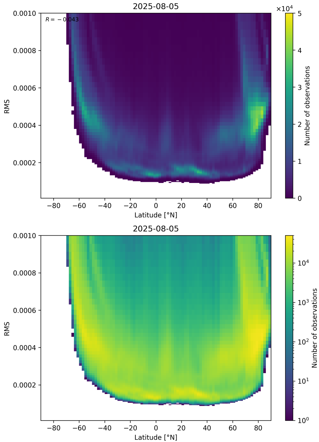
Figure 94: Scatter density plot of “Latitude” against “RMS” for 2025-08-04 to 2025-08-06.
