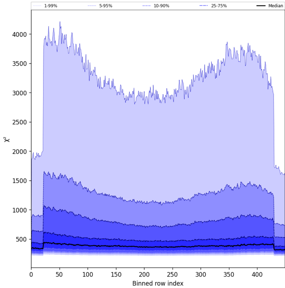
Figure 59: Along track statistics of “ \chi^2 ” for 2025-08-04 to 2025-08-06
