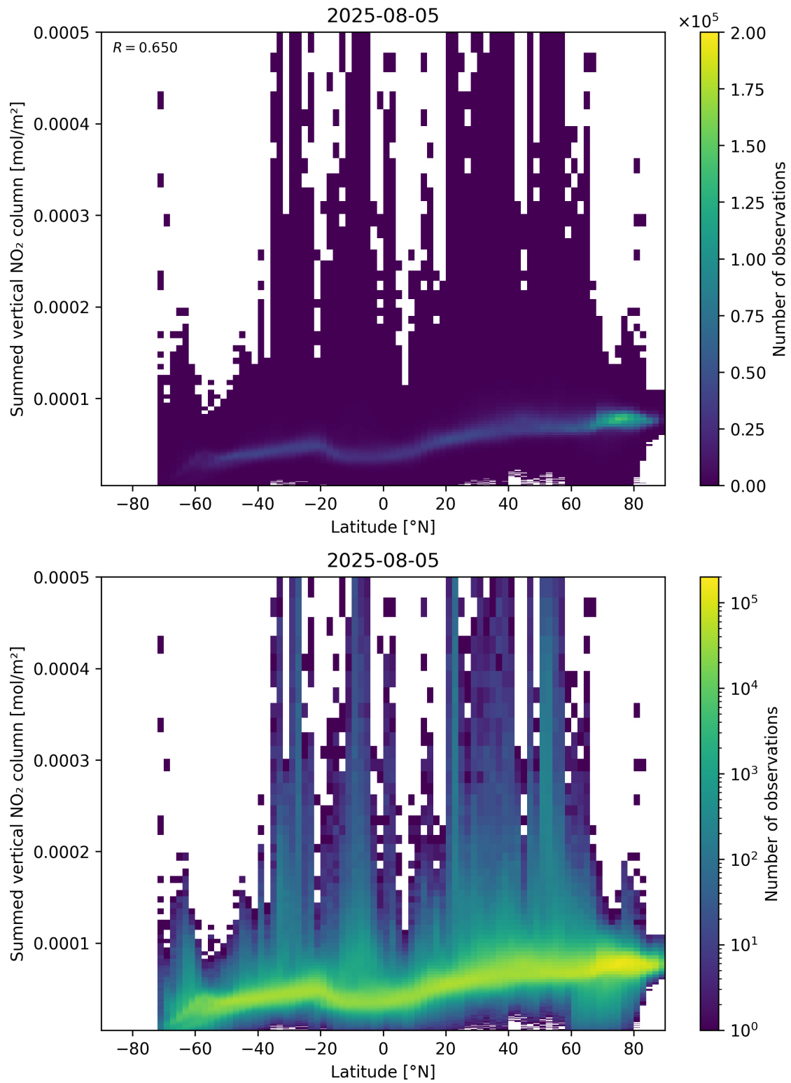
Figure 88: Scatter density plot of “Latitude” against “Summed vertical NO 2 column” for 2025-08-04 to 2025-08-06.
