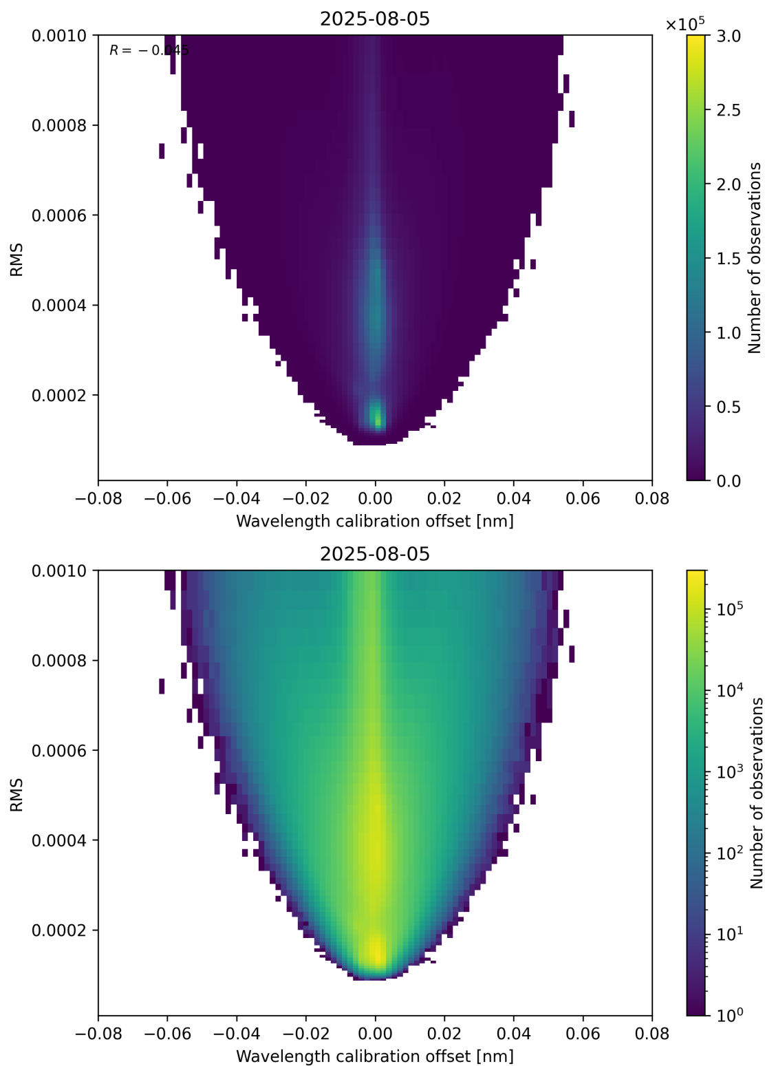
Figure 181: Scatter density plot of “Wavelength calibration offset” against “RMS” for 2025-08-04 to 2025-08-06.
