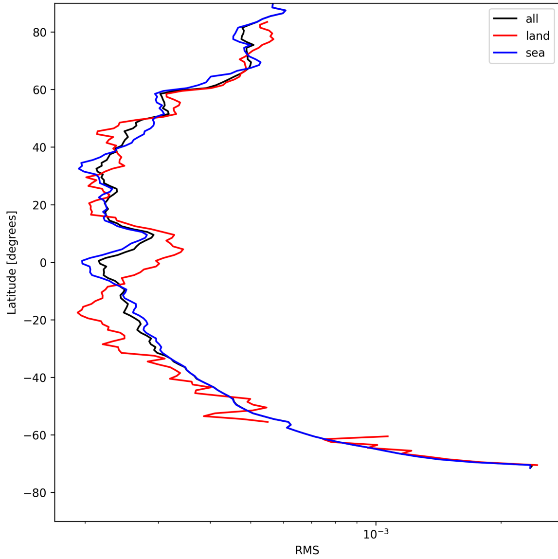
Figure 26: Zonal average of “RMS” for 2025-08-04 to 2025-08-06.
