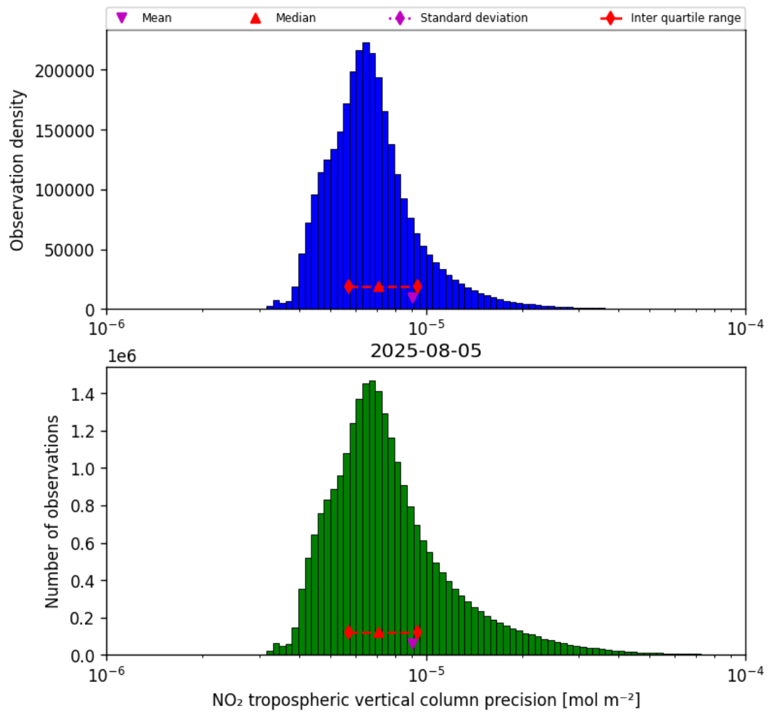
Figure 30: Histogram of “NO 2 tropospheric vertical column precision” for 2025-08-04 to 2025-08-06
