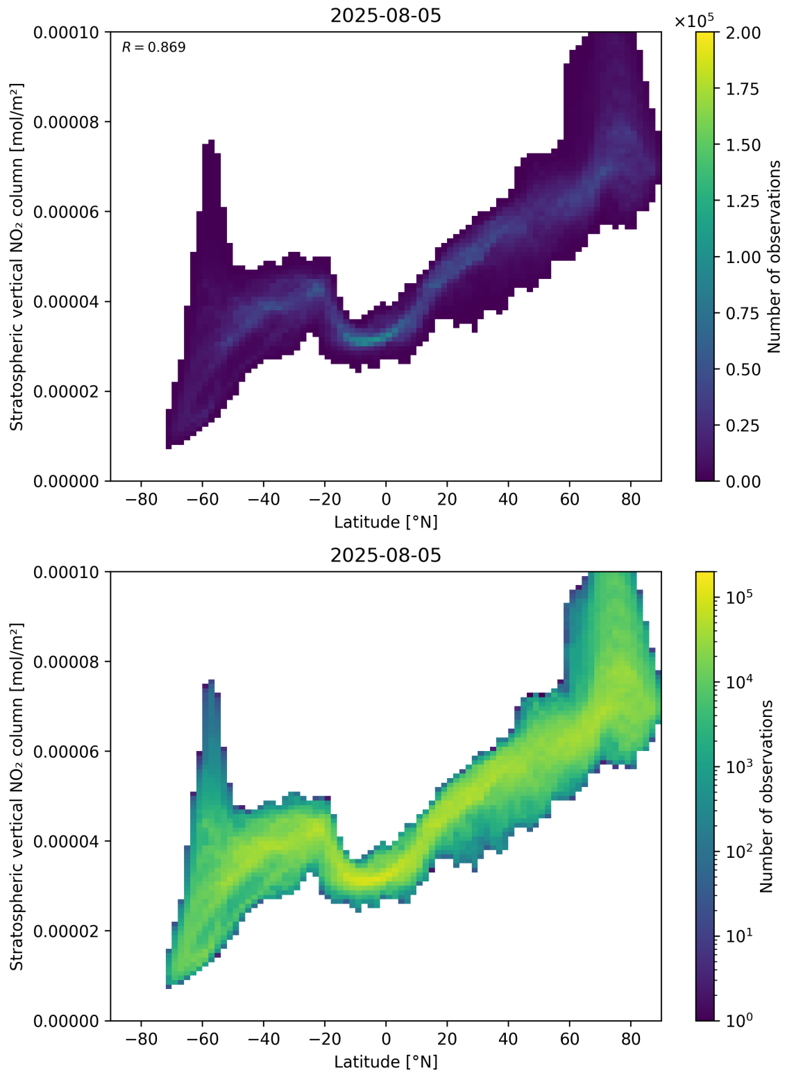
Figure 87: Scatter density plot of “Latitude” against “Stratospheric vertical NO 2 column” for 2025-08-04 to 2025-08-06.
