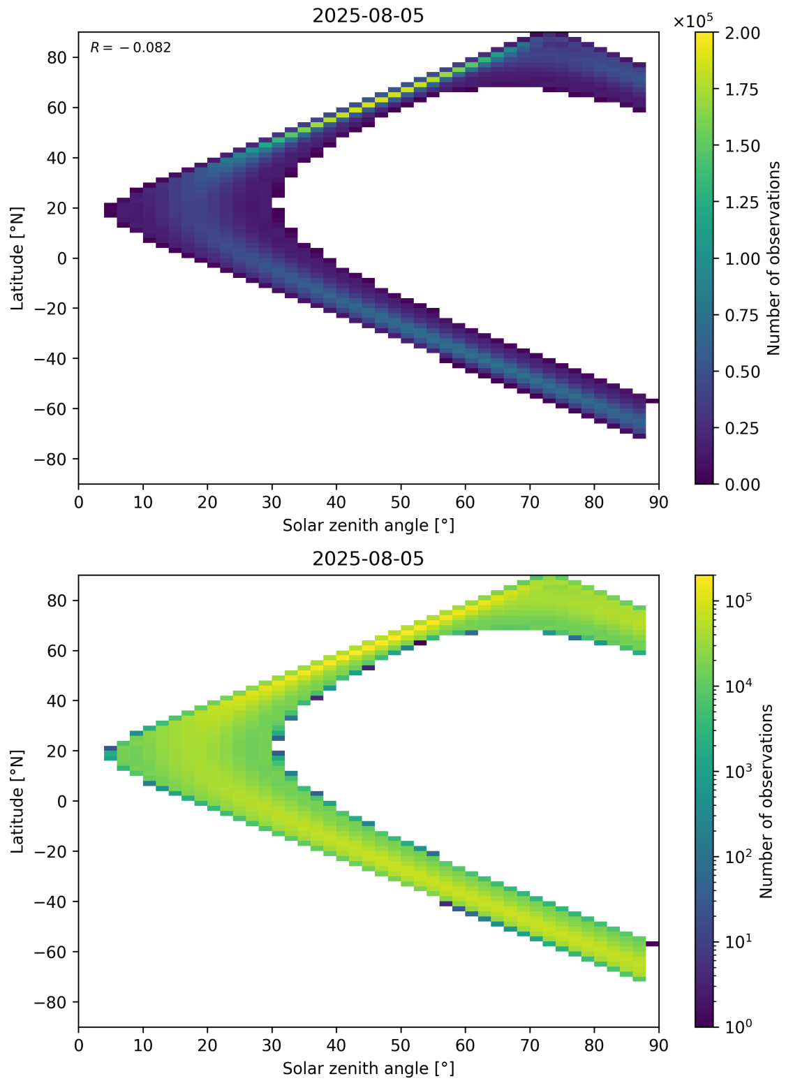
Figure 149: Scatter density plot of “Solar zenith angle” against “Latitude” for 2025-08-04 to 2025-08-06.
