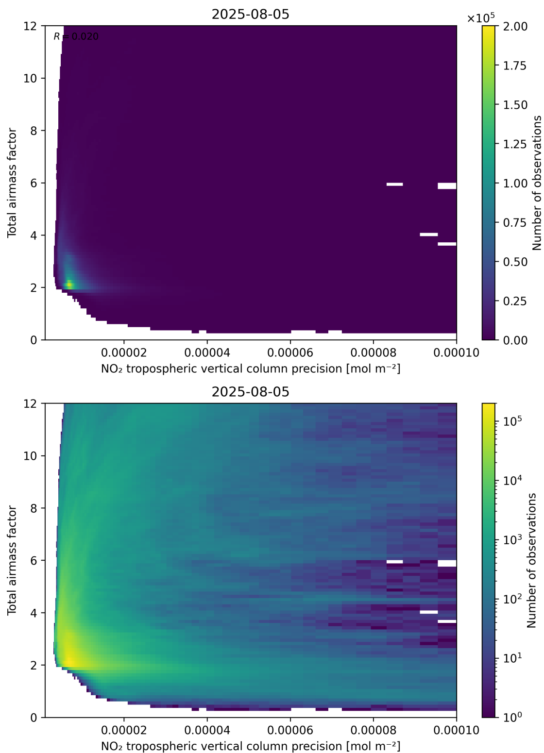
Figure 132: Scatter density plot of “NO 2 tropospheric vertical column precision” against “Total air mass factor” for 2025-08-04 to 2025-08-06.
