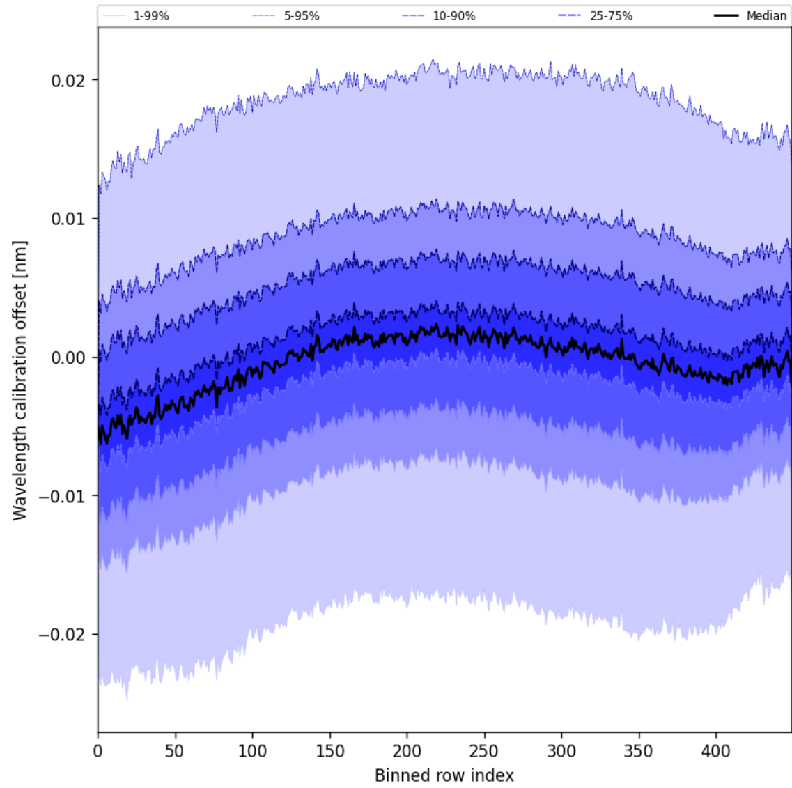
Figure 52: Along track statistics of “Wavelength calibration offset” for 2025-08-04 to 2025-08-06
