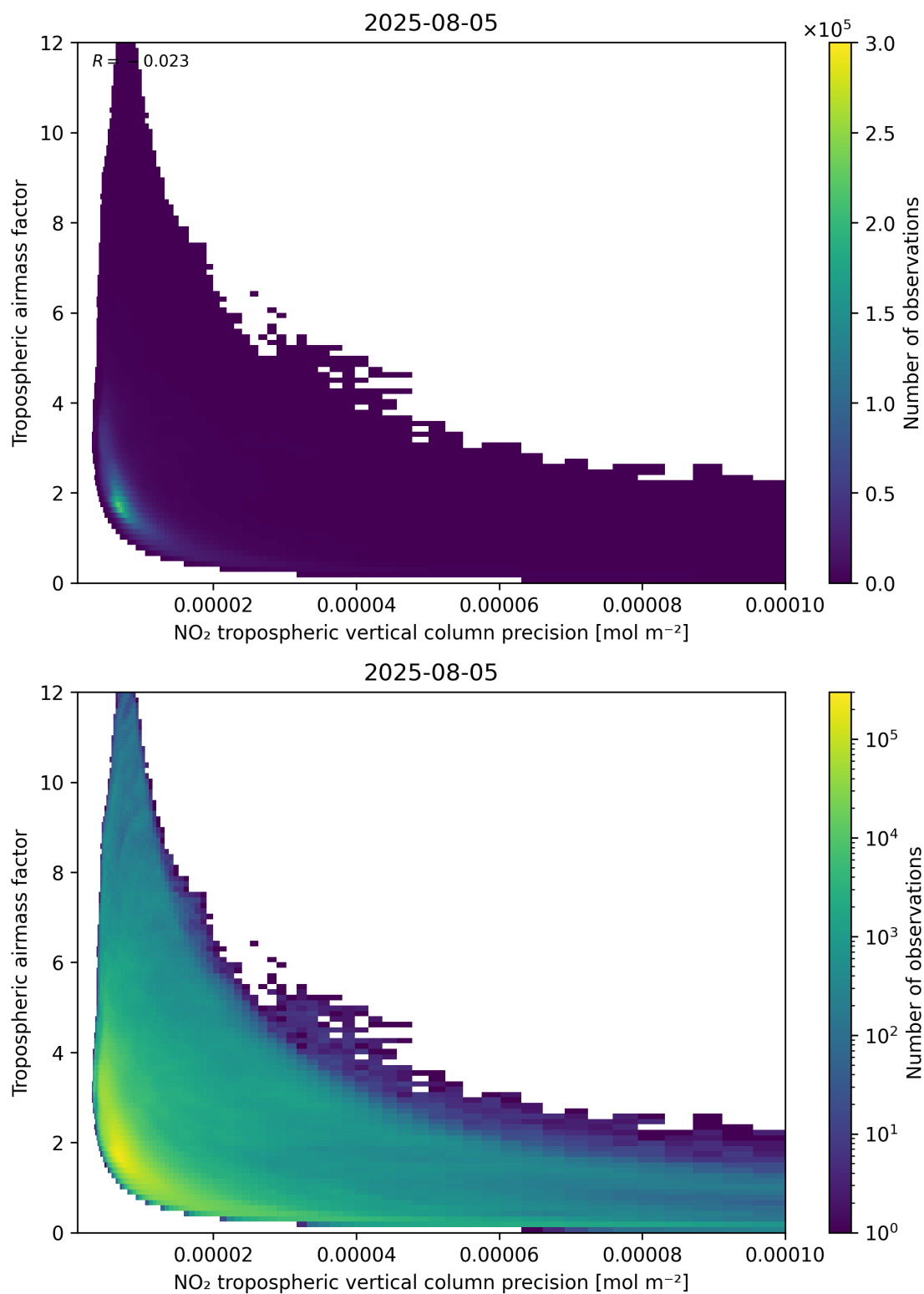
Figure 133: Scatter density plot of “NO 2 tropospheric vertical column precision” against “Tropospheric air mass factor” for 2025-08-04 to 2025-08-06.
