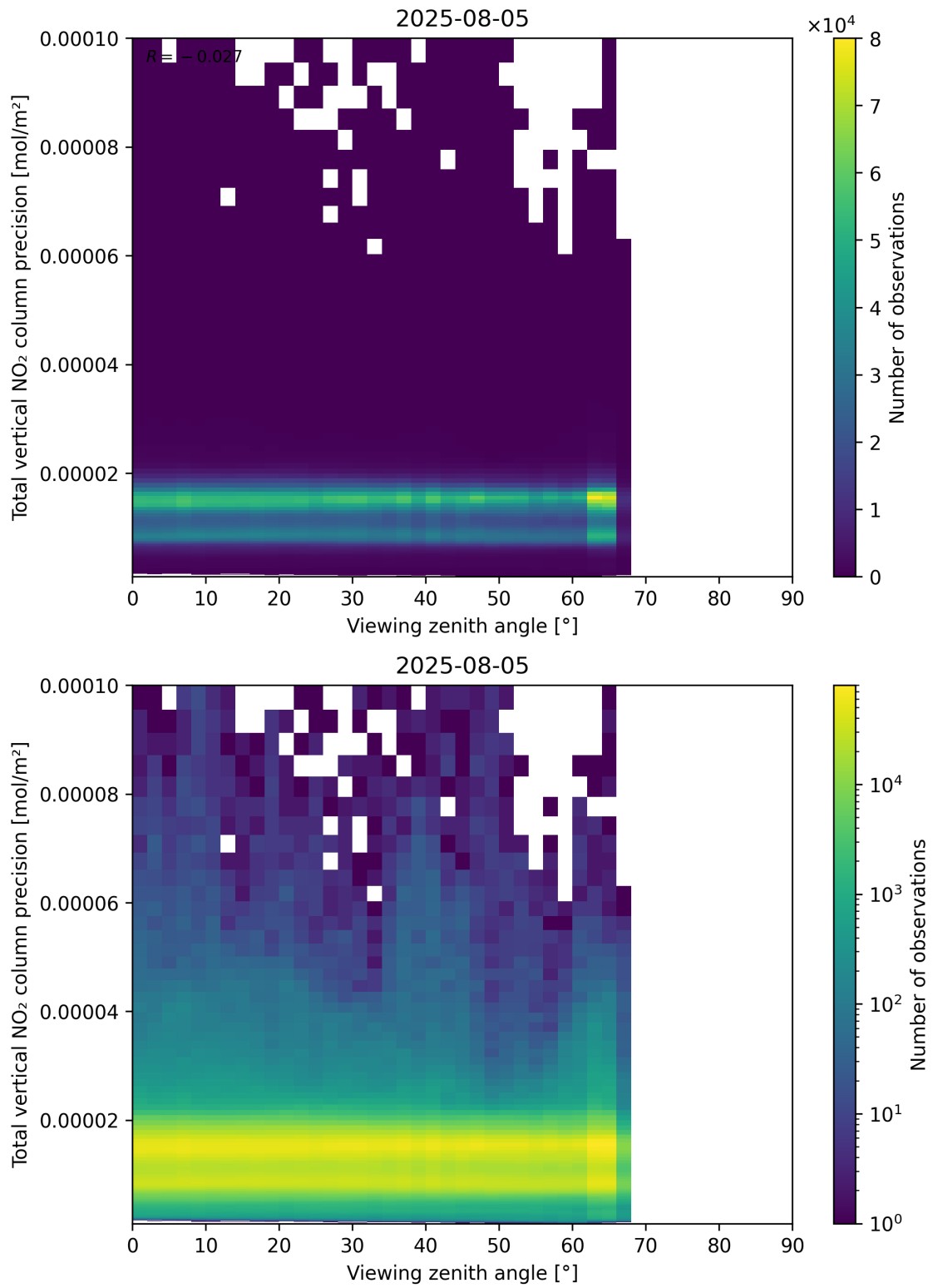
Figure 168: Scatter density plot of “Viewing zenith angle” against “Total vertical NO 2 column precision” for 2025-08-04 to 2025-08-06.
