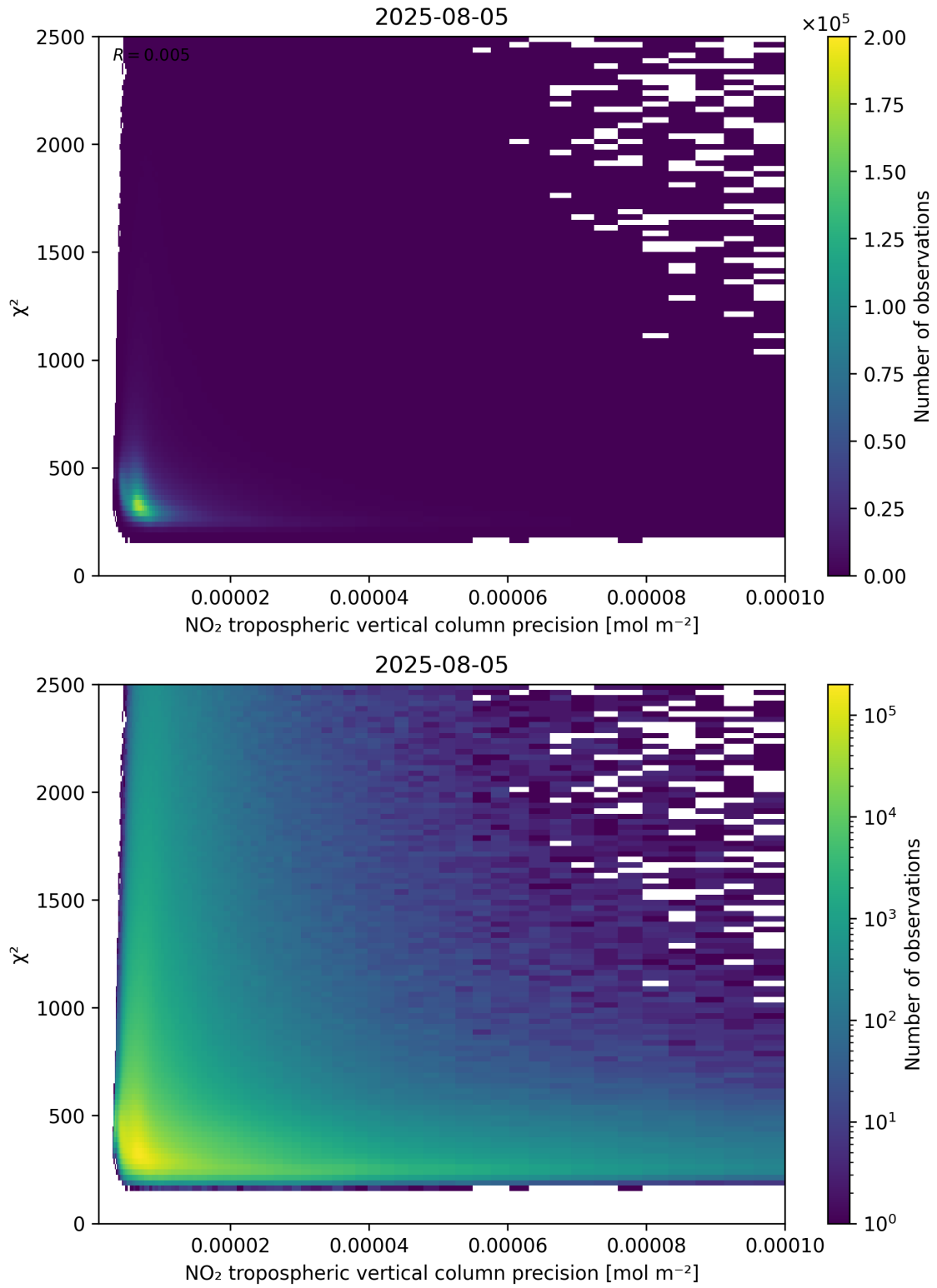
Figure 134: Scatter density plot of “NO 2 tropospheric vertical column precision” against “ \chi^2 ” for 2025-08-04 to 2025-08-06.
