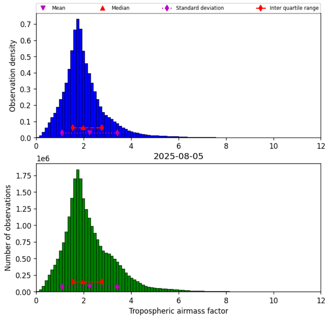
Figure 31: Histogram of “Tropospheric airmass factor” for 2025-08-04 to 2025-08-06
