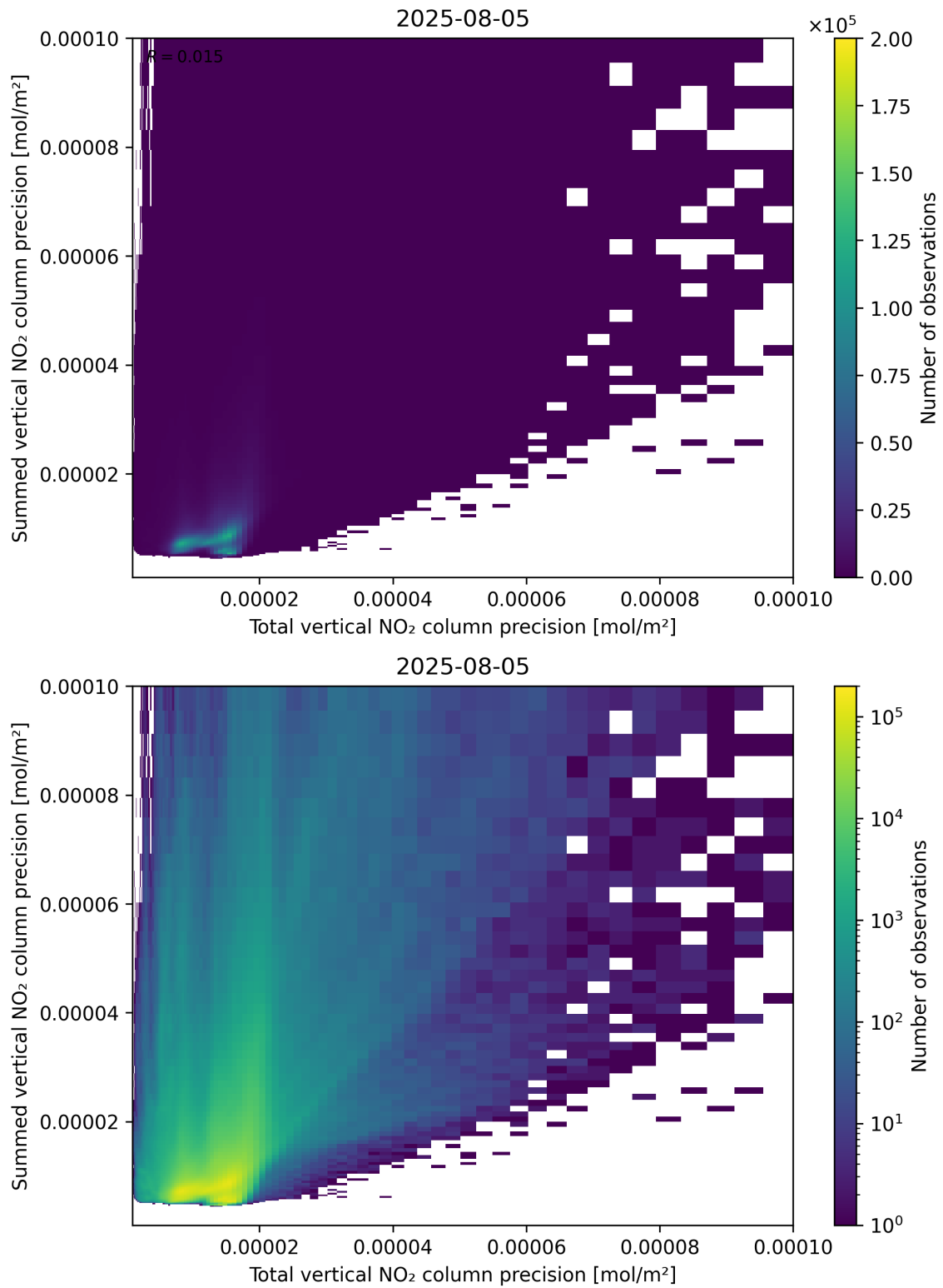
Figure 118: Scatter density plot of “Total vertical NO 2 column precision” against “Summed vertical NO 2 column precision” for 2025-08-04 to 2025-08-06.
