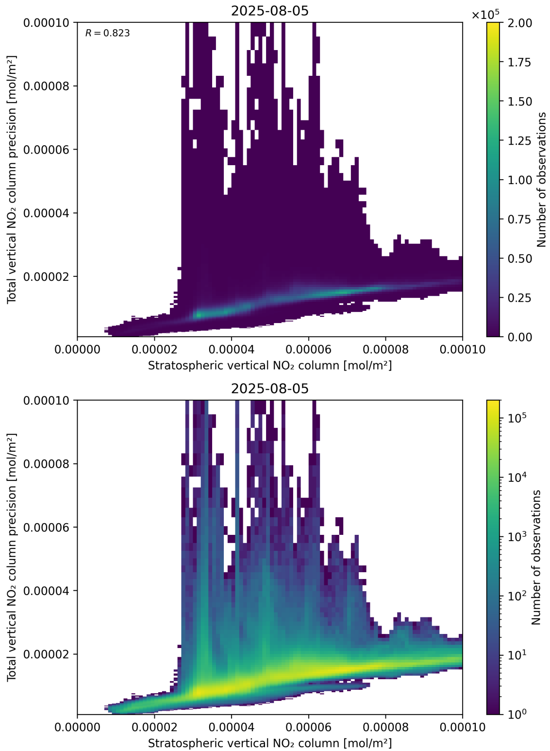
Figure 101: Scatter density plot of “Stratospheric vertical NO 2 column” against “Total vertical NO 2 column precision” for 2025-08-04 to 2025-08-06.
