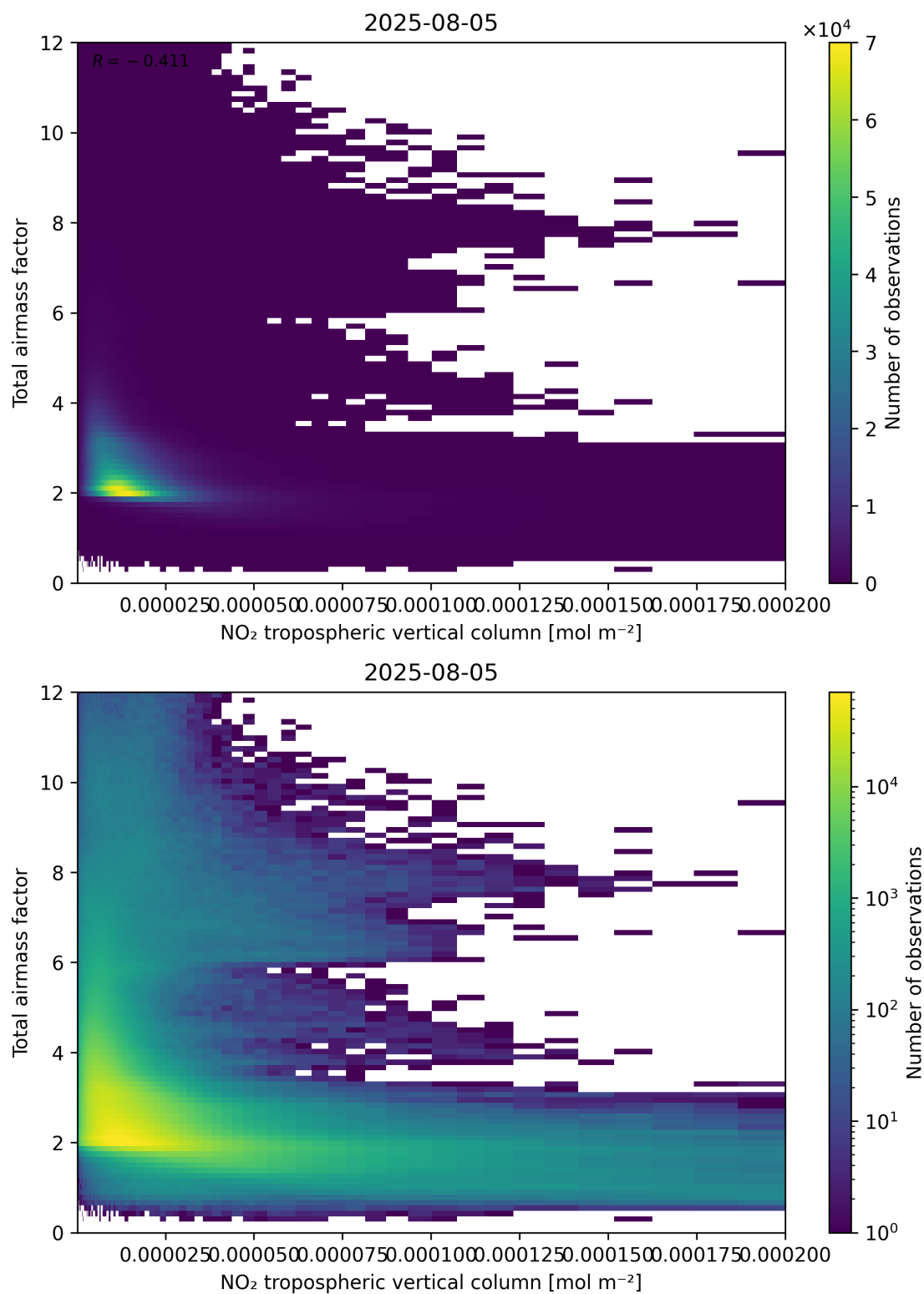
Figure 122: Scatter density plot of “NO 2 tropospheric vertical column” against “Total air mass factor” for 2025-08-04 to 2025-08-06.
