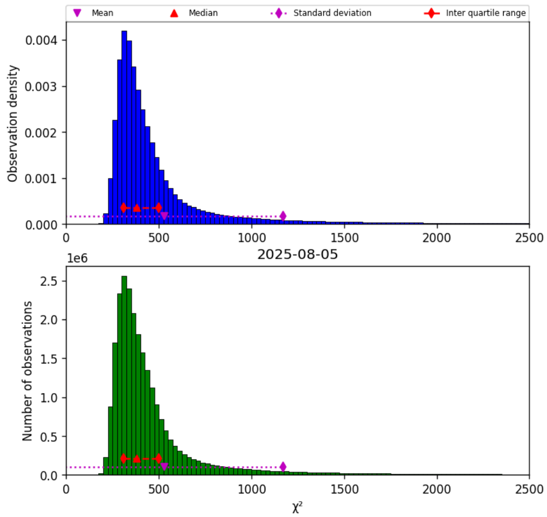
Figure 42: Histogram of “ \chi^2 ” for 2025-08-04 to 2025-08-06
