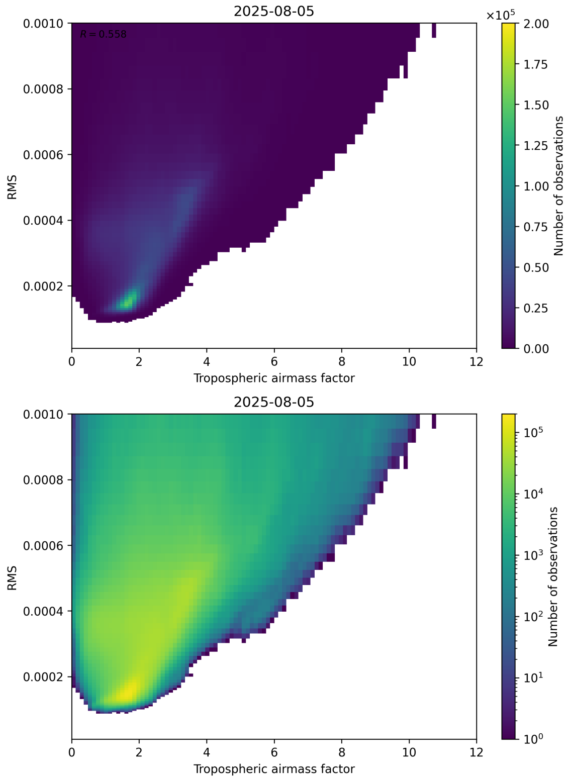
Figure 79: Scatter density plot of “Tropospheric airmass factor” against “RMS” for 2025-08-04 to 2025-08-06.
