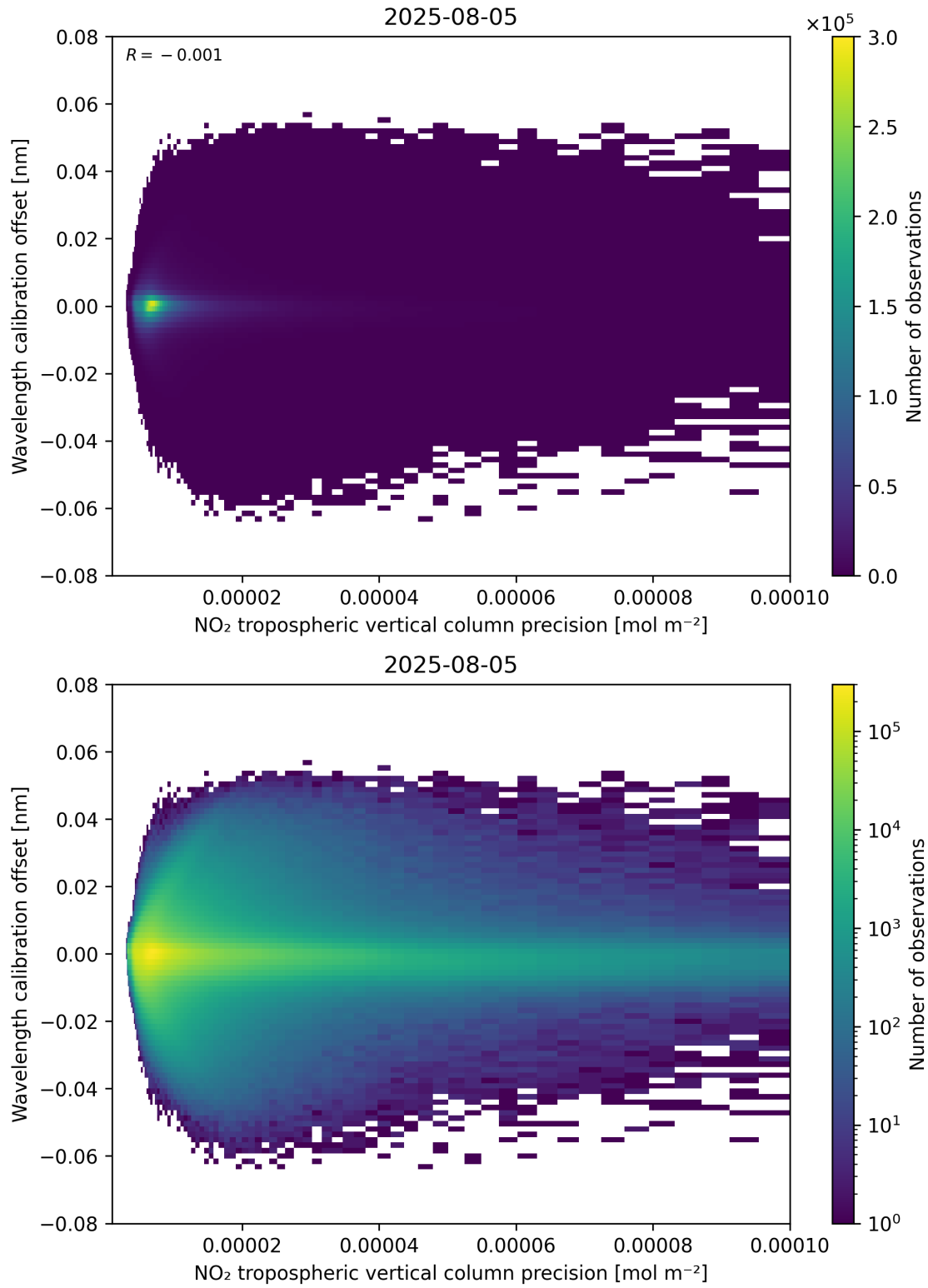
Figure 141: Scatter density plot of “NO 2 tropospheric vertical column precision” against “Wavelength calibration offset” for 2025-08-04 to 2025-08-06.
