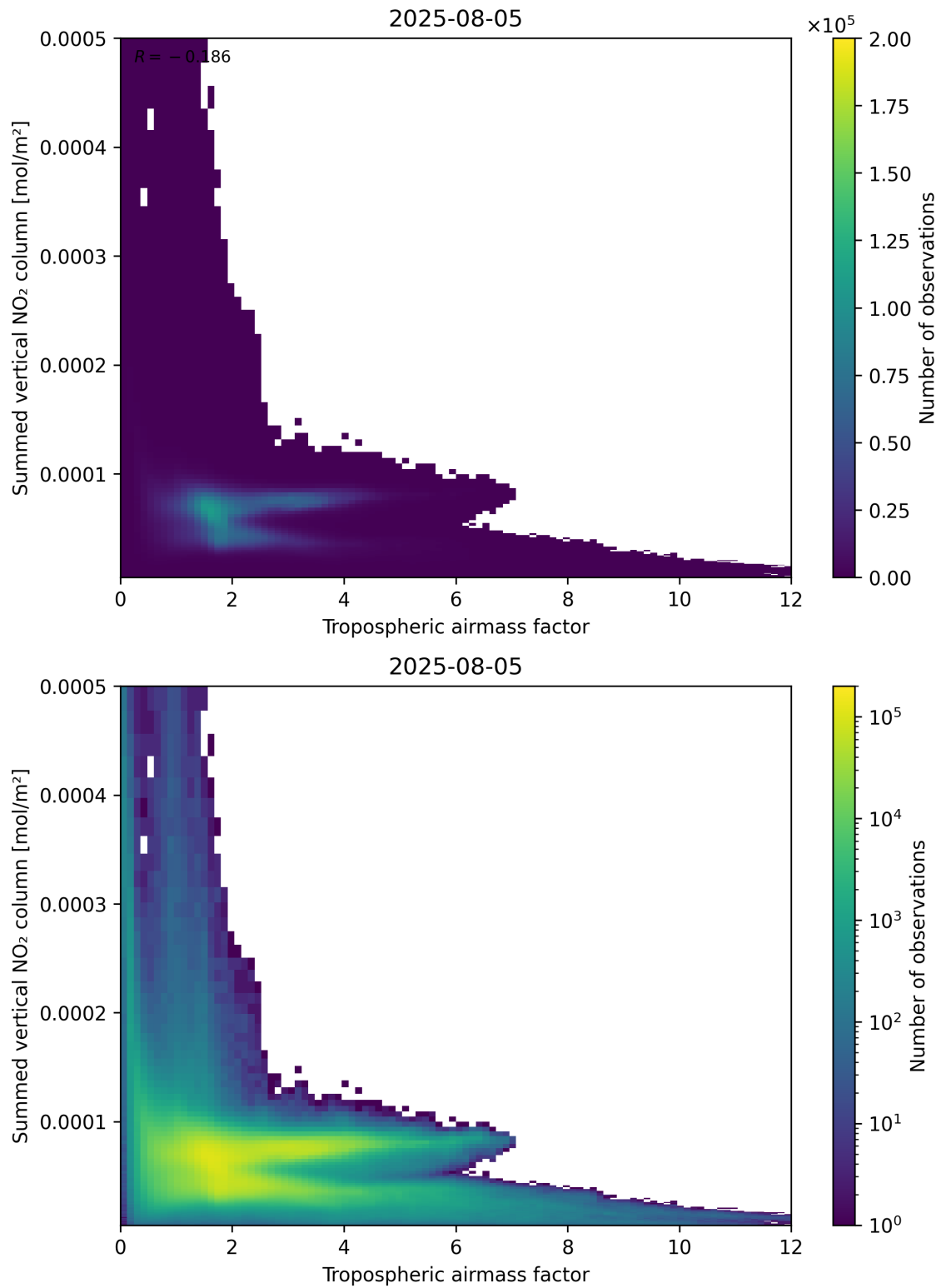
Figure 75: Scatter density plot of “Tropospheric airmass factor” against “Summed vertical NO 2 column” for 2025-08-04 to 2025-08-06.
