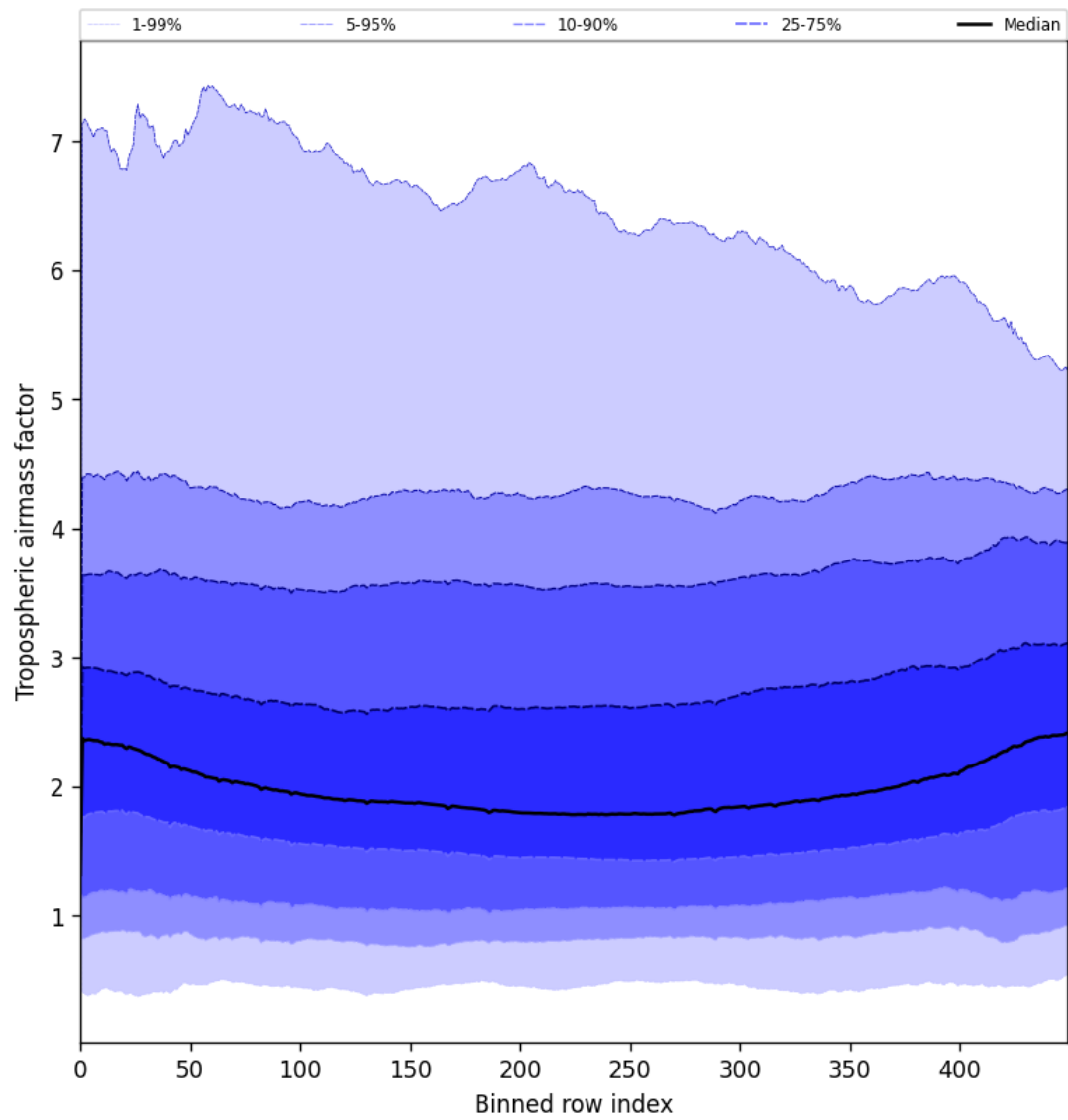
Figure 48: Along track statistics of “Tropospheric air mass factor” for 2025-08-04 to 2025-08-06
