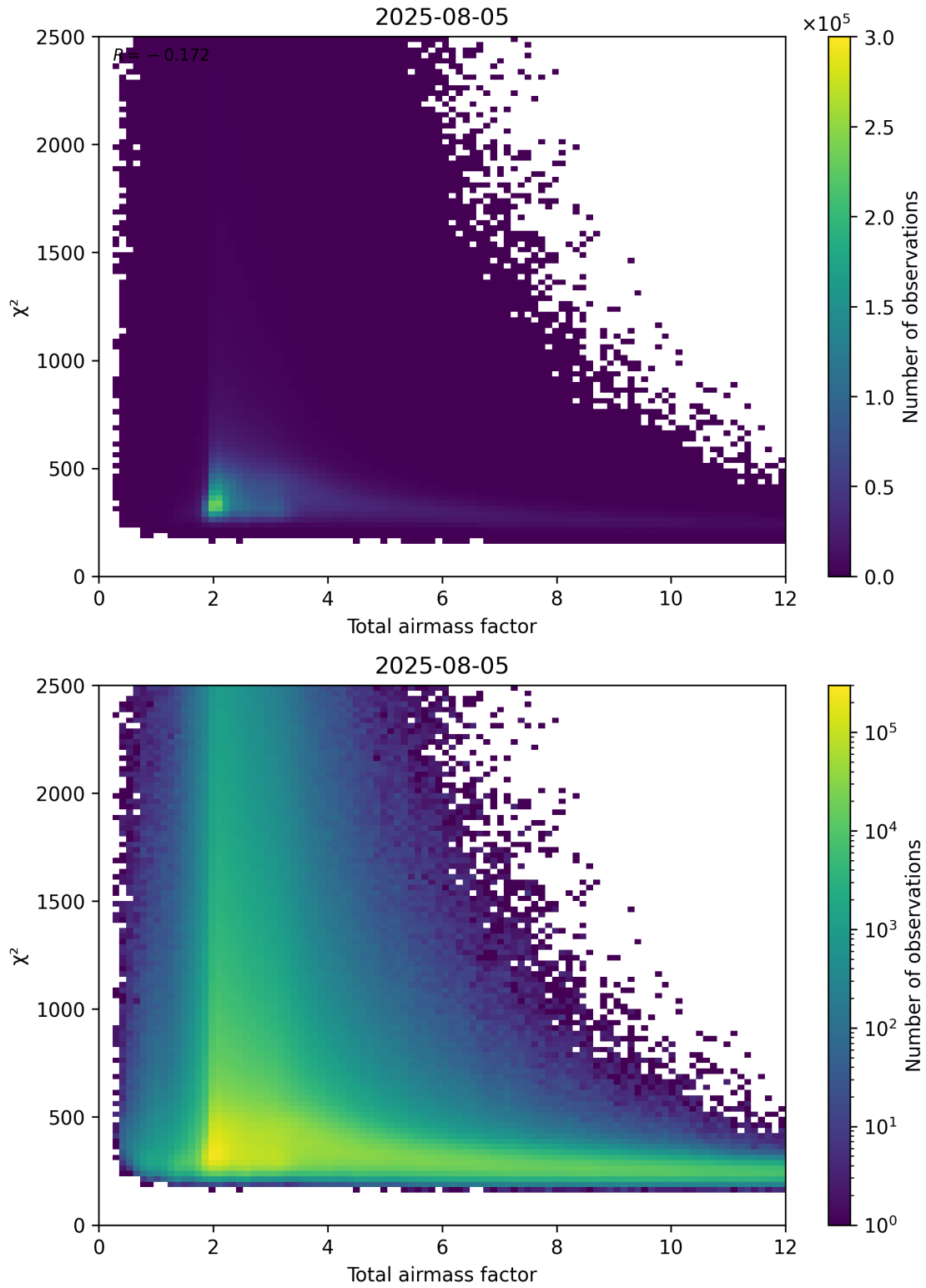
Figure 63: Scatter density plot of “Total airmass factor” against “ \chi^2 ” for 2025-08-04 to 2025-08-06.
