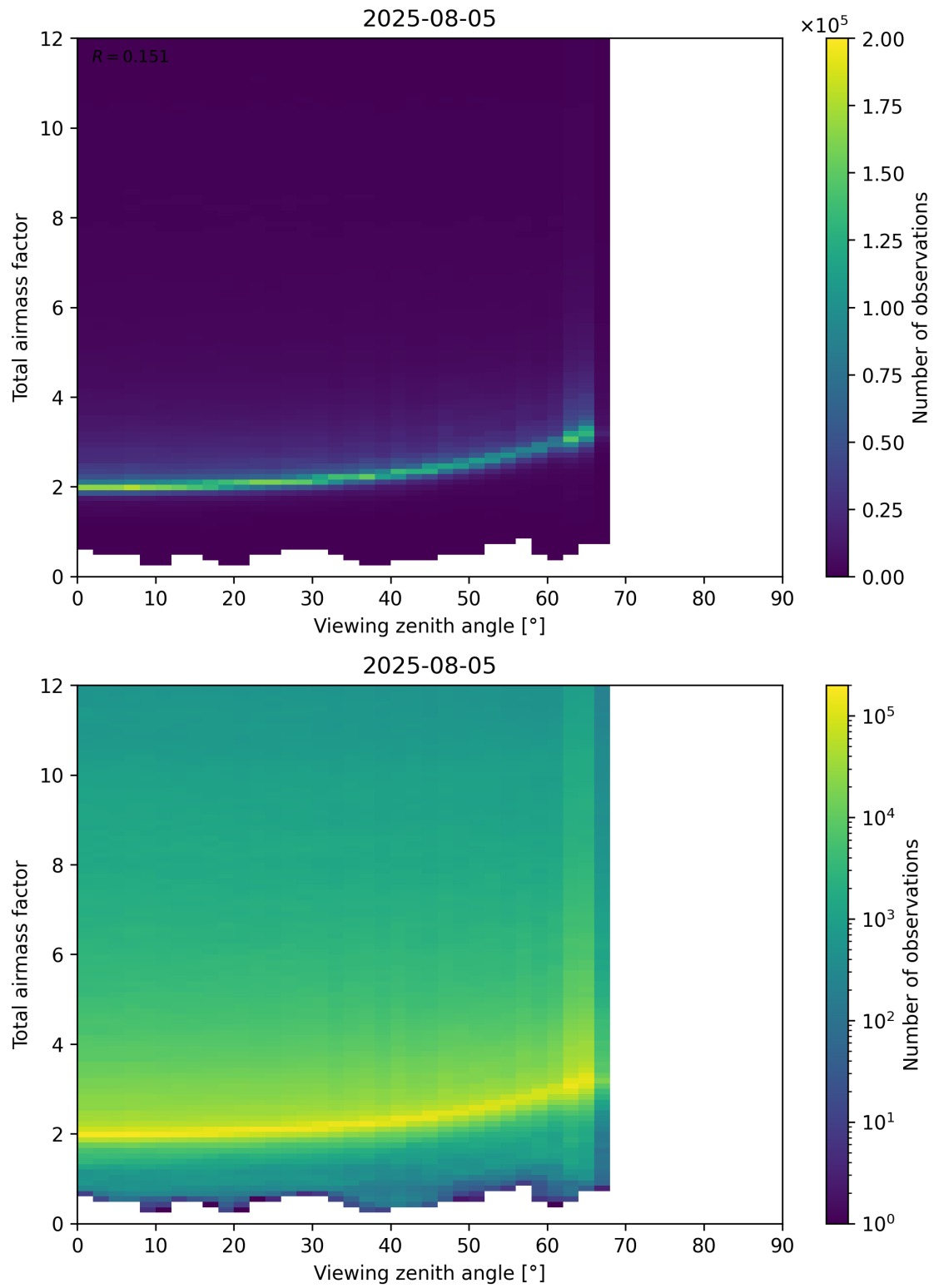
Figure 160: Scatter density plot of “Viewing zenith angle” against “Total airmass factor” for 2025-08-04 to 2025-08-06.
