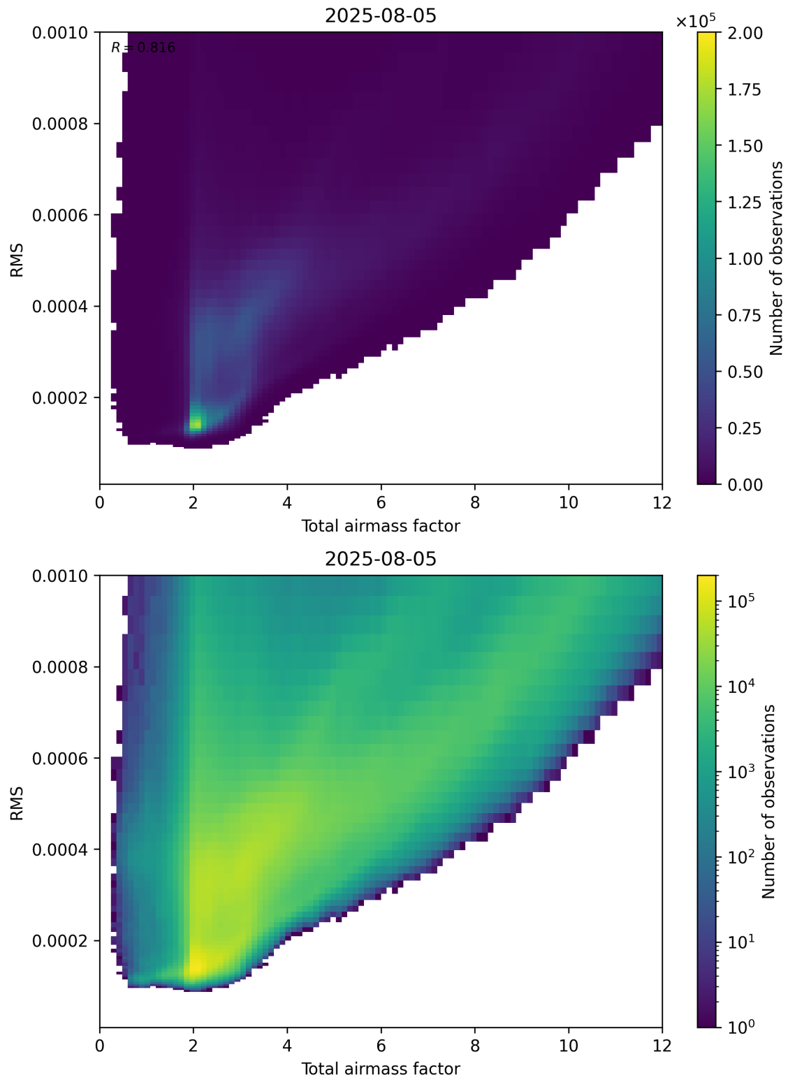
Figure 69: Scatter density plot of “Total airmass factor” against “RMS” for 2025-08-04 to 2025-08-06.
