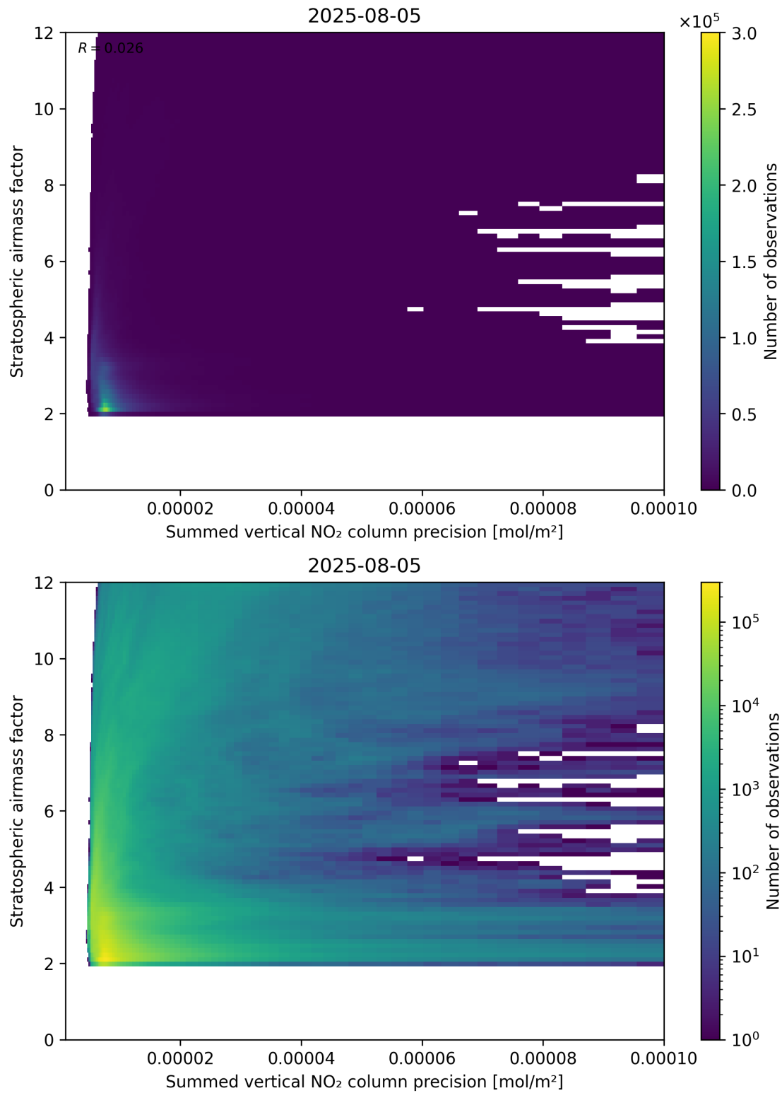
Figure 106: Scatter density plot of “Summed vertical NO 2 column precision” against “Stratospheric airmass factor” for 2025-08-04 to 2025-08-06.
