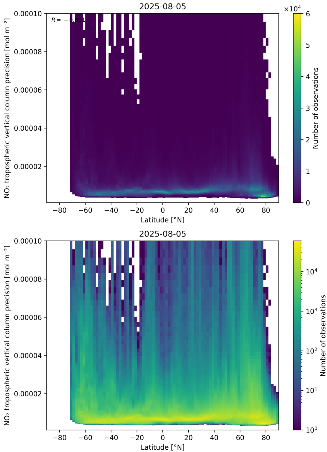
Figure 93: Scatter density plot of “Latitude” against “NO 2 tropospheric vertical column precision” for 2025-08-04 to 2025-08-06.
