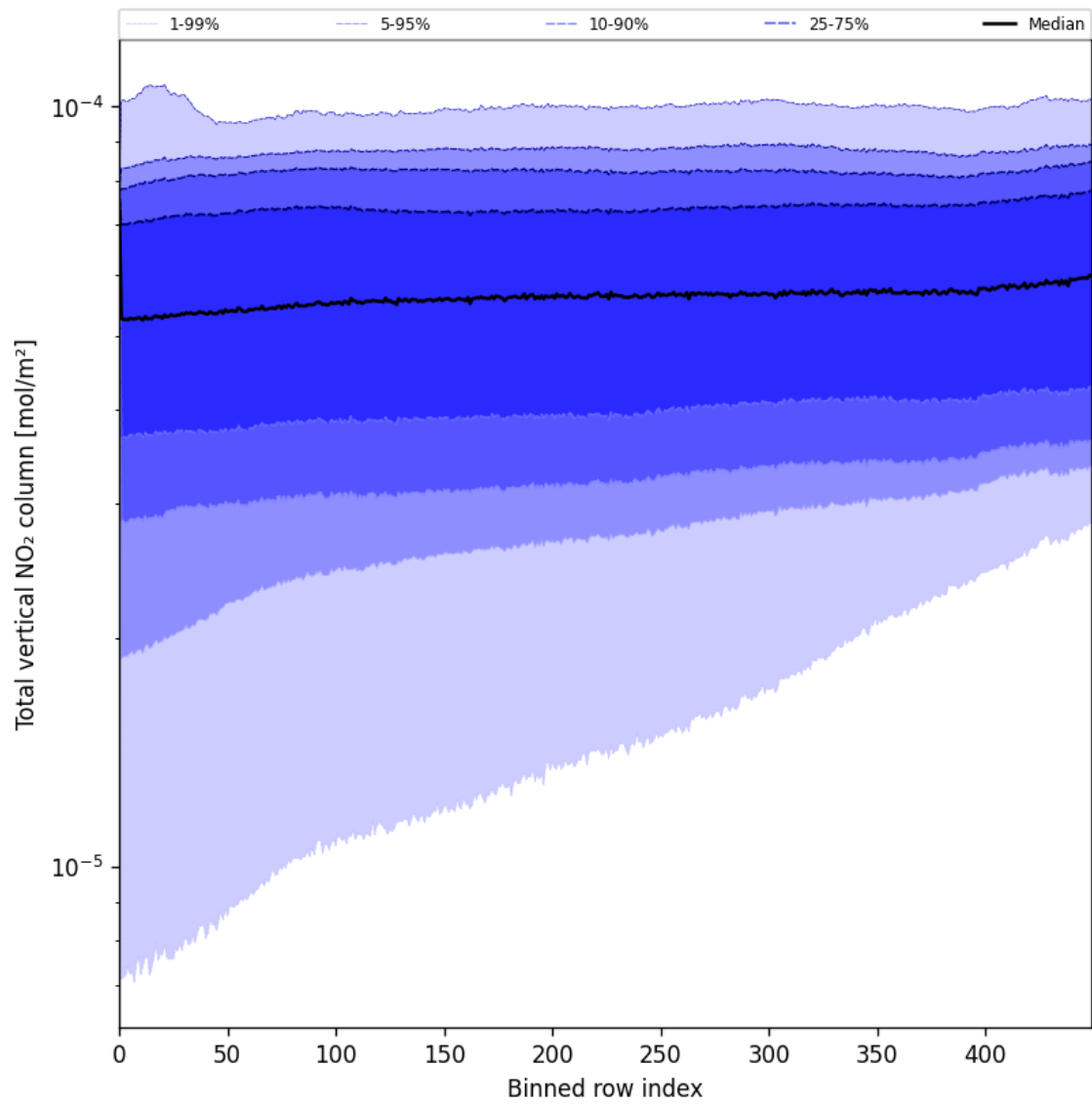
Figure 55: Along track statistics of “Total vertical NO 2 column” for 2025-08-04 to 2025-08-06
