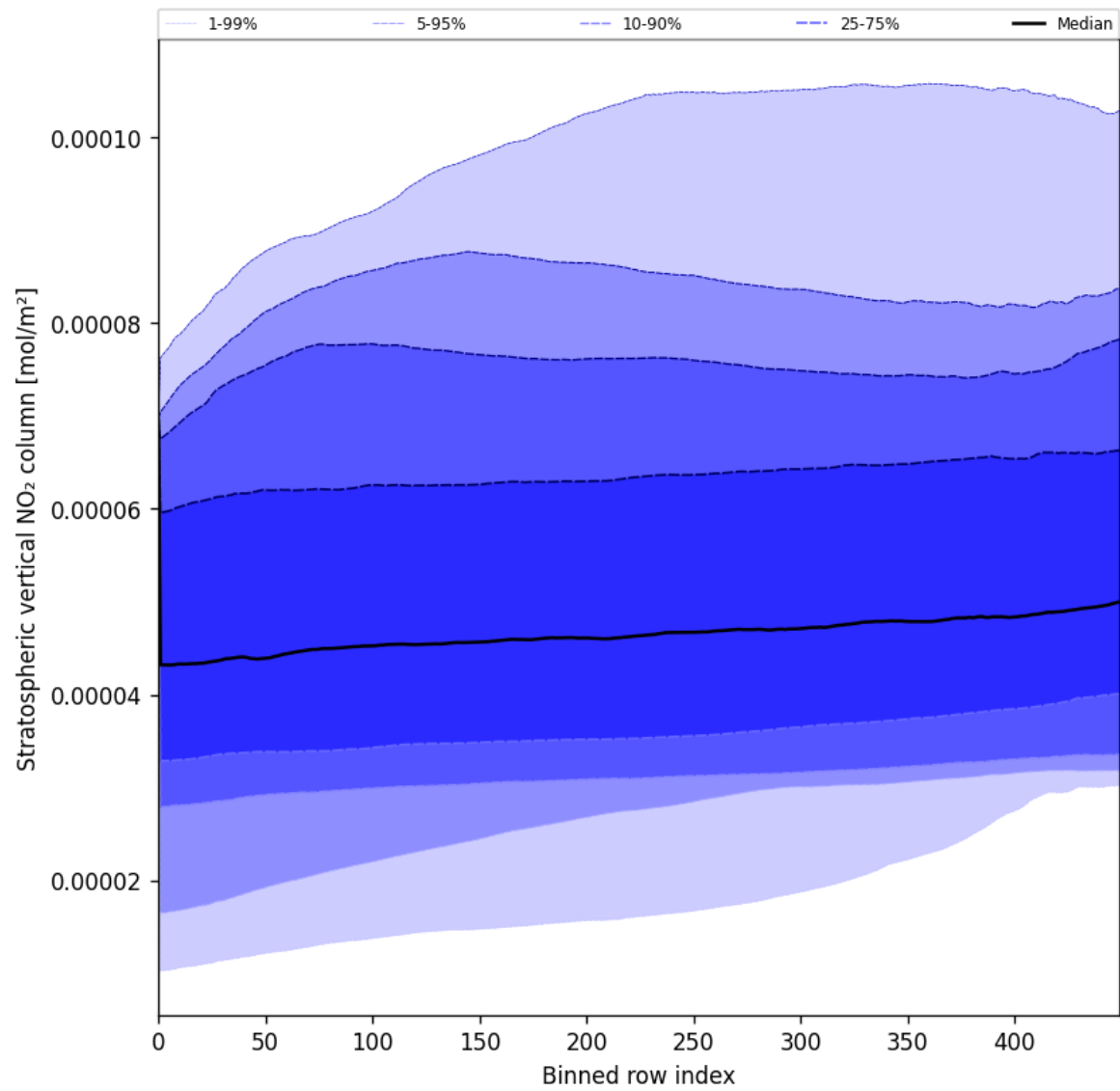
Figure 53: Along track statistics of “Stratospheric vertical NO 2 column” for 2025-08-04 to 2025-08-06
