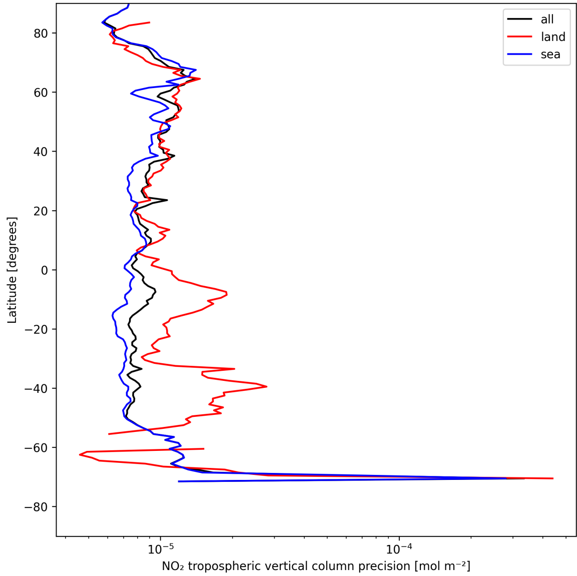
Figure 13: Zonal average of “NO 2 tropospheric vertical column precision” for 2025-08-04 to 2025-08-06.
