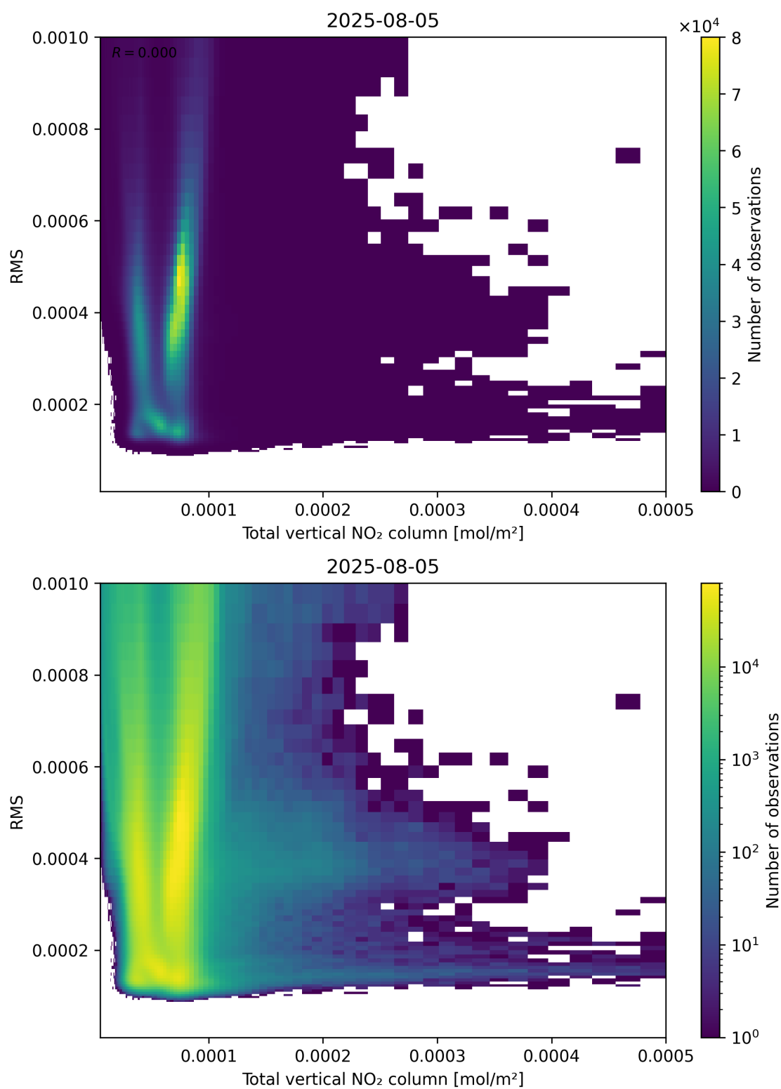
Figure 120: Scatter density plot of “Total vertical NO 2 column” against “RMS” for 2025-08-04 to 2025-08-06.
