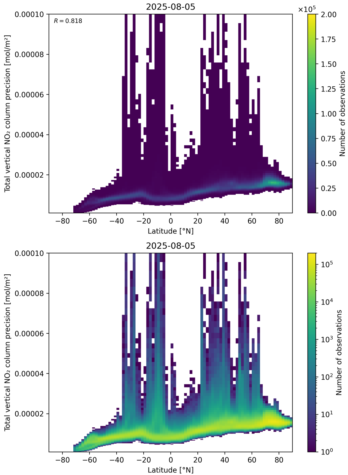
Figure 91: Scatter density plot of “Latitude” against “Total vertical NO 2 column precision” for 2025-08-04 to 2025-08-06.
