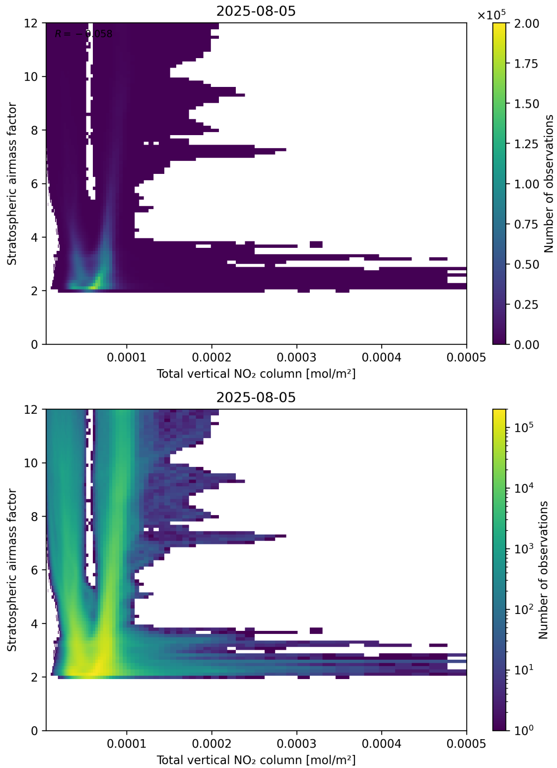
Figure 110: Scatter density plot of “Total vertical NO 2 column” against “Stratospheric airmass factor” for 2025-08-04 to 2025-08-06.
