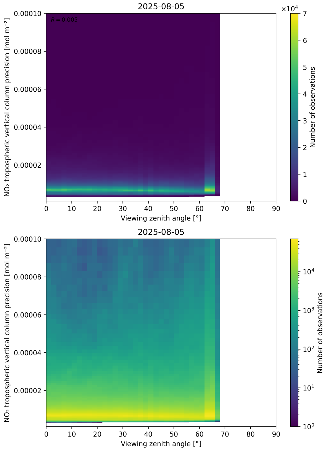
Figure 170: Scatter density plot of “Viewing zenith angle” against “NO 2 tropospheric vertical column precision” for 2025-08-04 to 2025-08-06.
