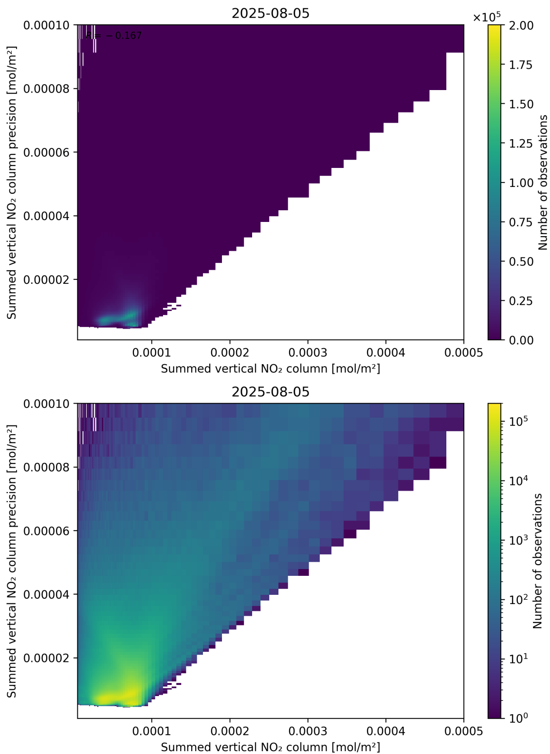
Figure 105: Scatter density plot of “Summed vertical NO 2 column” against “Summed vertical NO 2 column precision” for 2025-08-04 to 2025-08-06.
