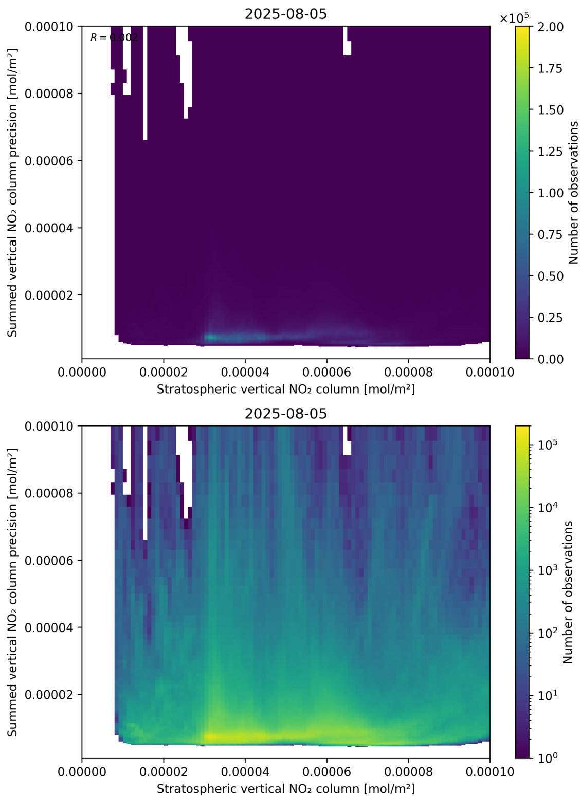
Figure 99: Scatter density plot of “Stratospheric vertical NO 2 column” against “Summed vertical NO 2 column precision” for 2025-08-04 to 2025-08-06.
