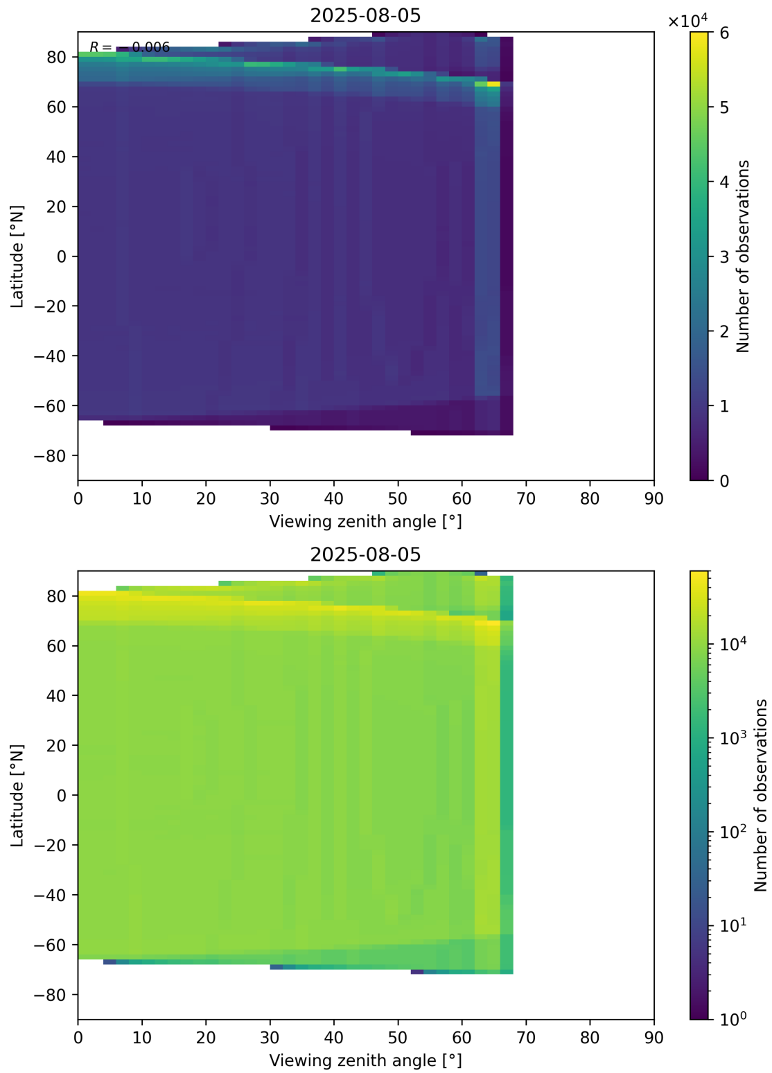
Figure 163: Scatter density plot of “Viewing zenith angle” against “Latitude” for 2025-08-04 to 2025-08-06.
