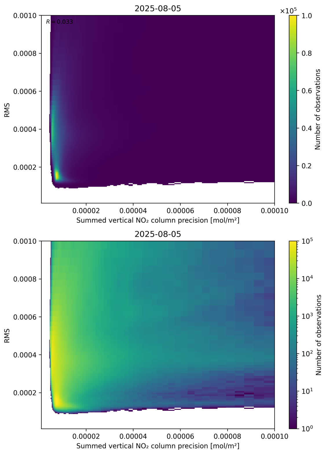
Figure 108: Scatter density plot of “Summed vertical NO 2 column precision” against “RMS” for 2025-08-04 to 2025-08-06.
