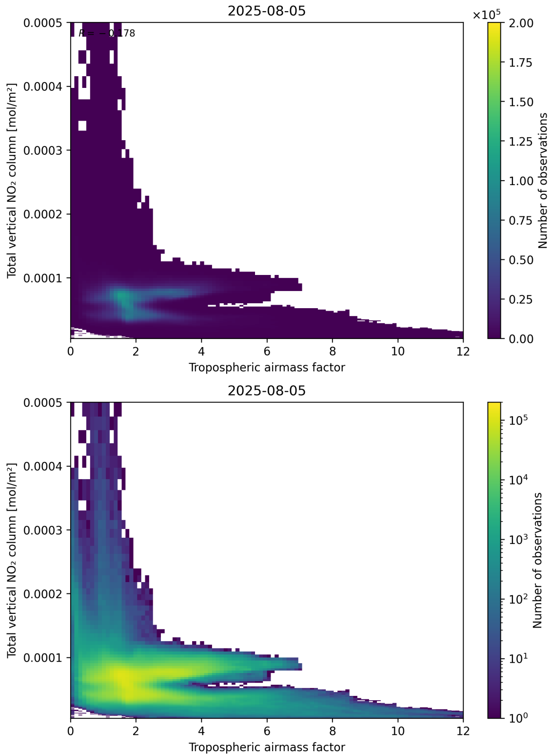
Figure 77: Scatter density plot of “Tropospheric airmass factor” against “Total vertical NO 2 column” for 2025-08-04 to 2025-08-06.
