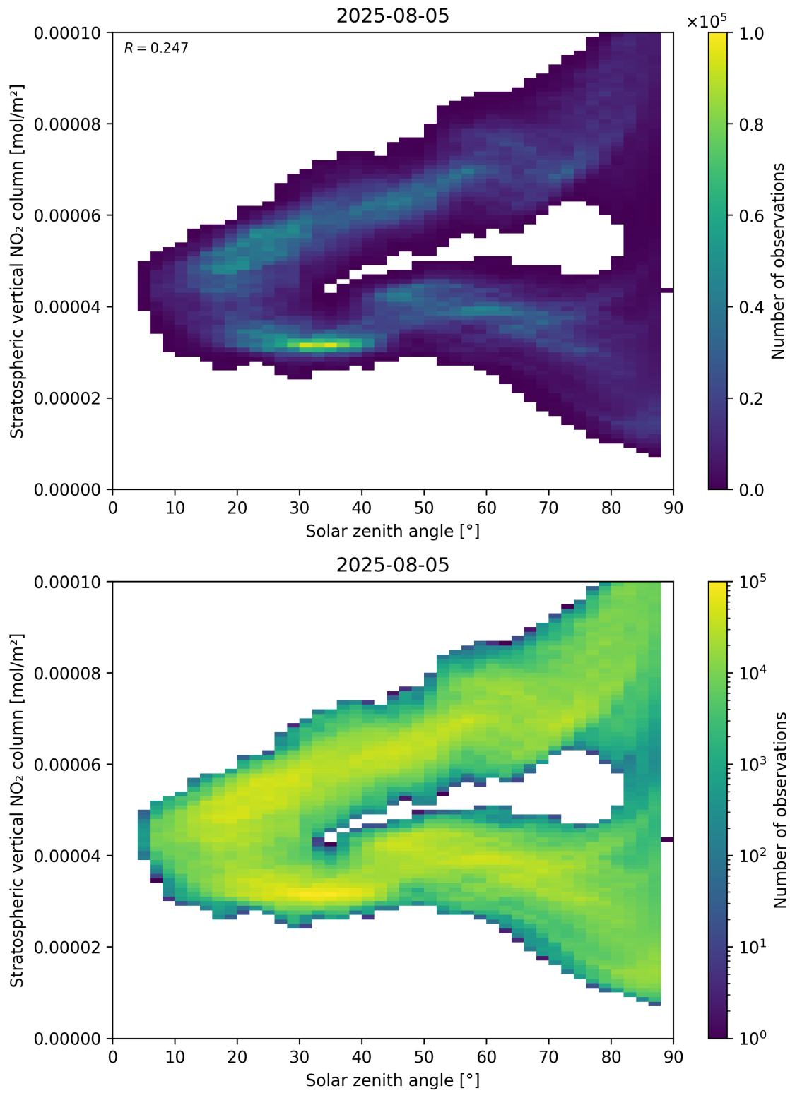
Figure 150: Scatter density plot of “Solar zenith angle” against “Stratospheric vertical NO 2 column” for 2025-08-04 to 2025-08-06.
