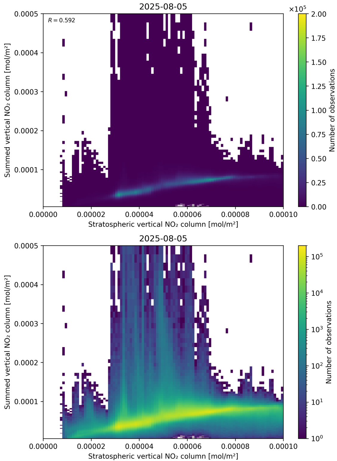
Figure 98: Scatter density plot of “Stratospheric vertical NO 2 column” against “Summed vertical NO 2 column” for 2025-08-04 to 2025-08-06.
