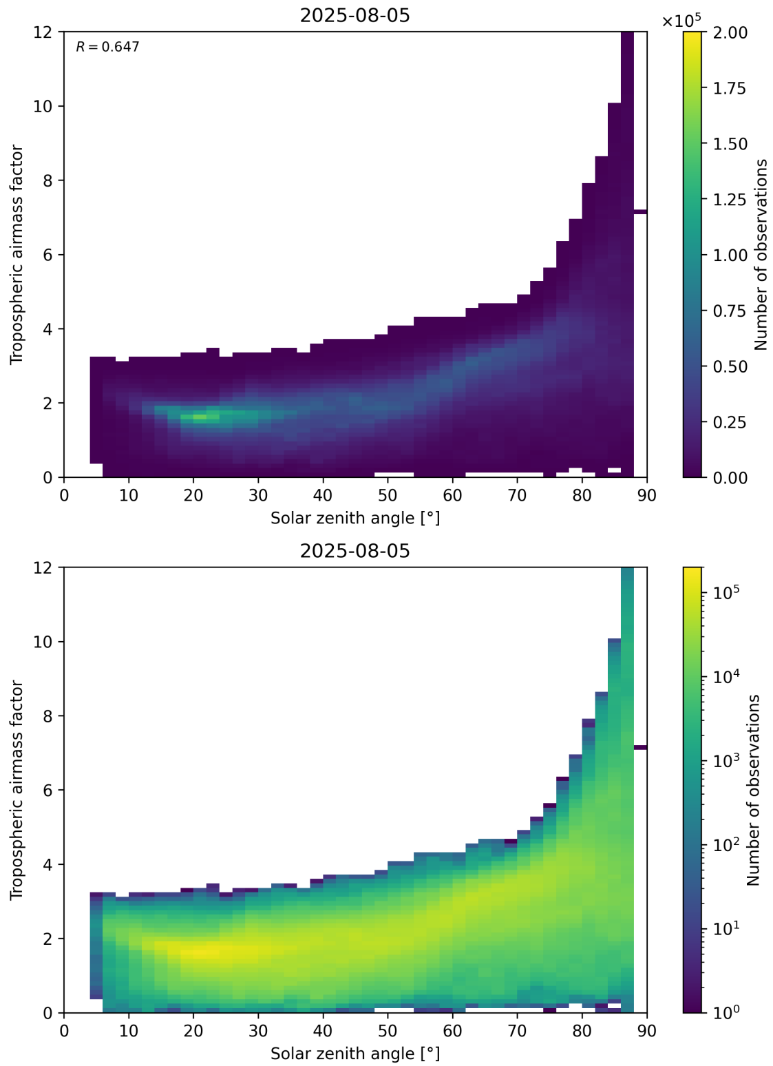
Figure 147: Scatter density plot of “Solar zenith angle” against “Tropospheric airmass factor” for 2025-08-04 to 2025-08-06.
