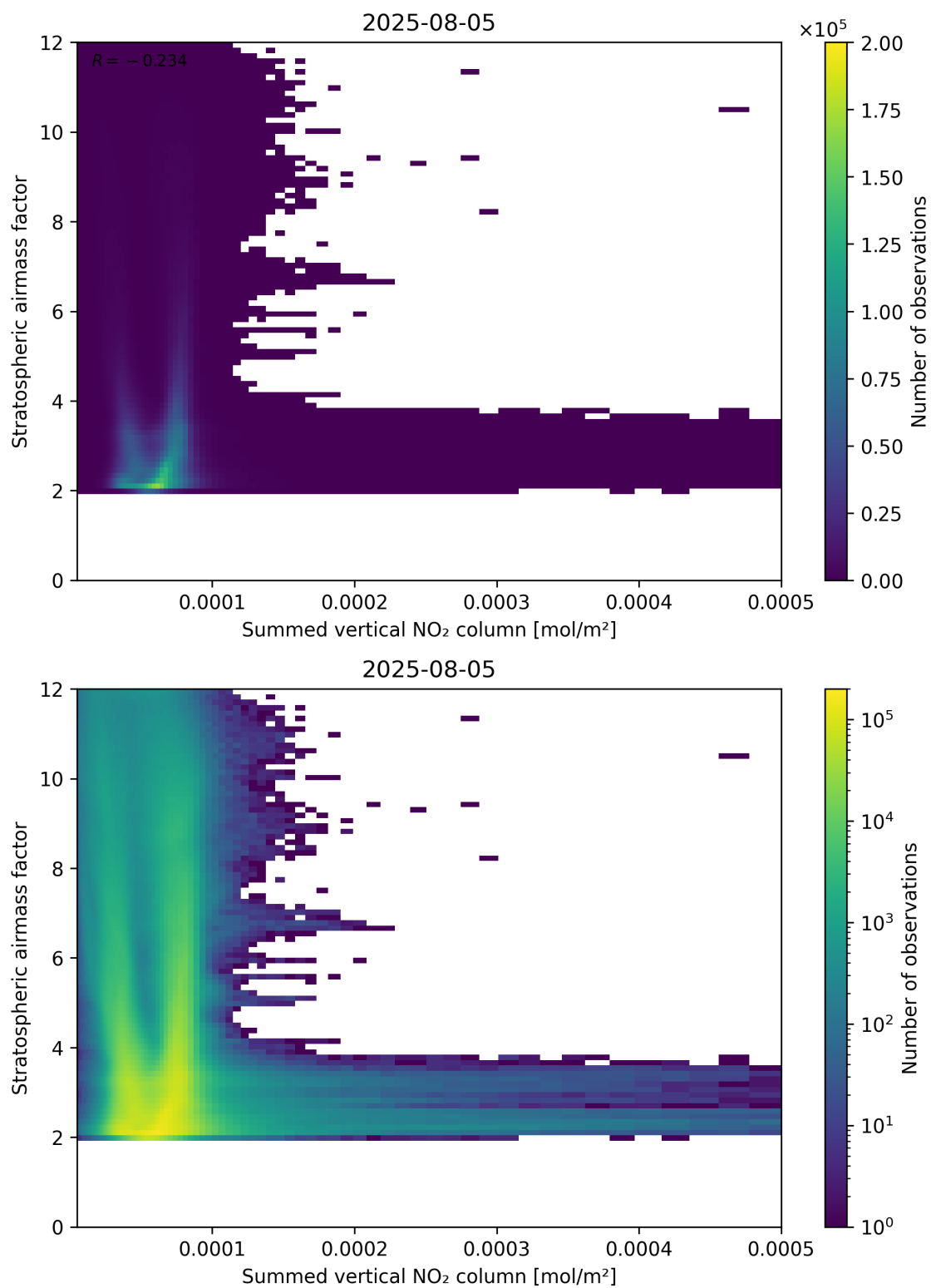
Figure 103: Scatter density plot of “Summed vertical NO 2 column” against “Stratospheric airmass factor” for 2025-08-04 to 2025-08-06.
