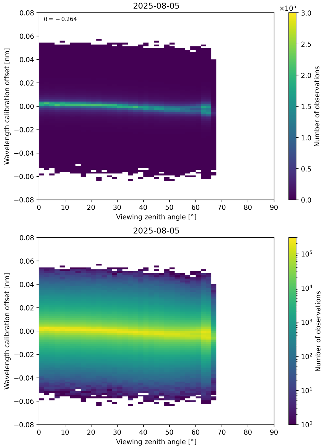
Figure 173: Scatter density plot of “Viewing zenith angle” against “Wavelength calibration offset” for 2025-08-04 to 2025-08-06.
