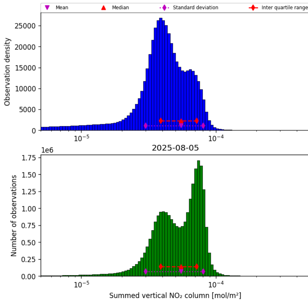
Figure 40: Histogram of “Summed vertical NO 2 column” for 2025-08-04 to 2025-08-06
