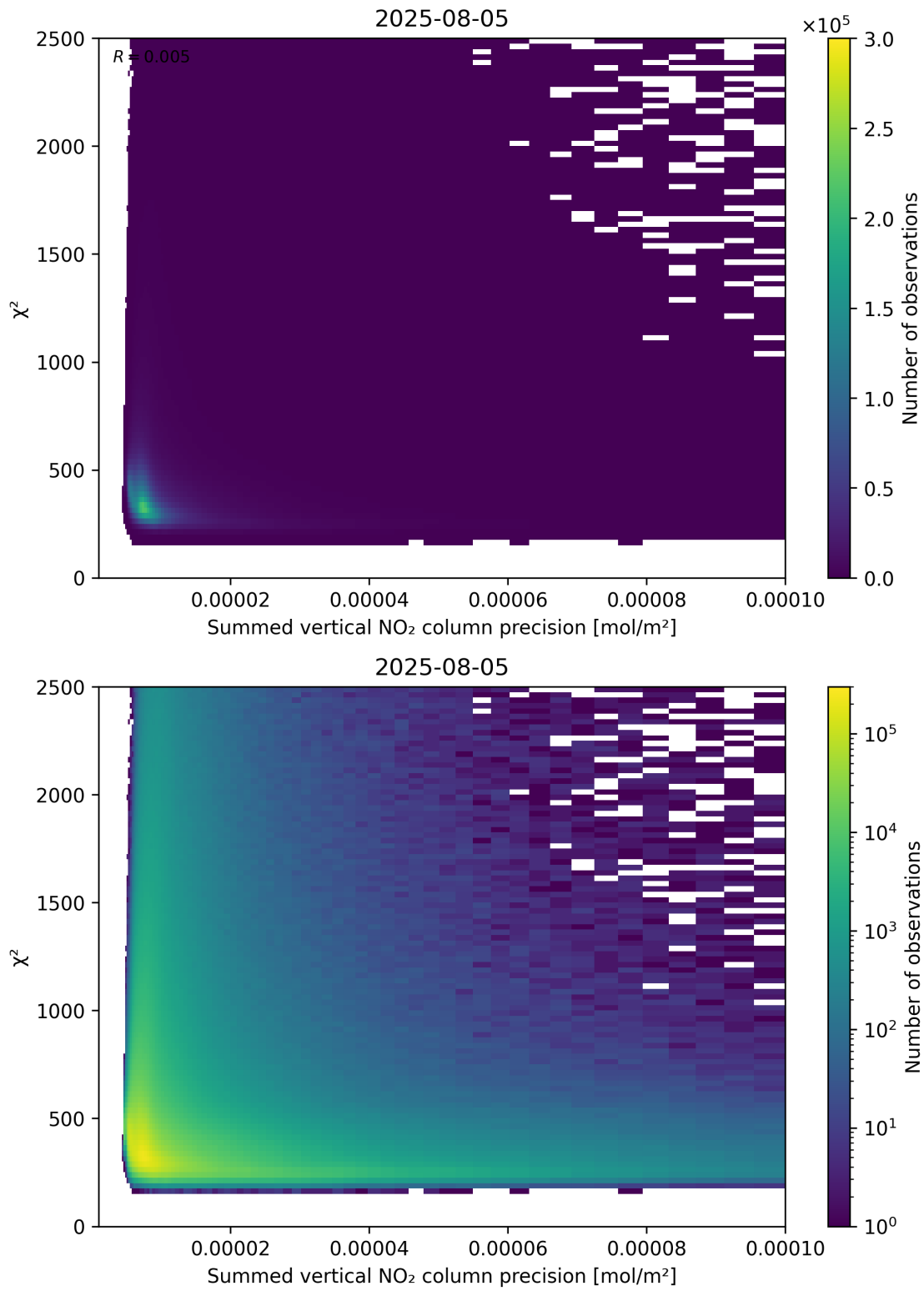
Figure 107: Scatter density plot of “Summed vertical NO 2 column precision” against “ \chi^2 ” for 2025-08-04 to 2025-08-06.
