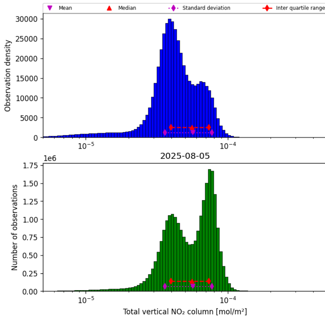
Figure 38: Histogram of “Total vertical NO 2 column” for 2025-08-04 to 2025-08-06
