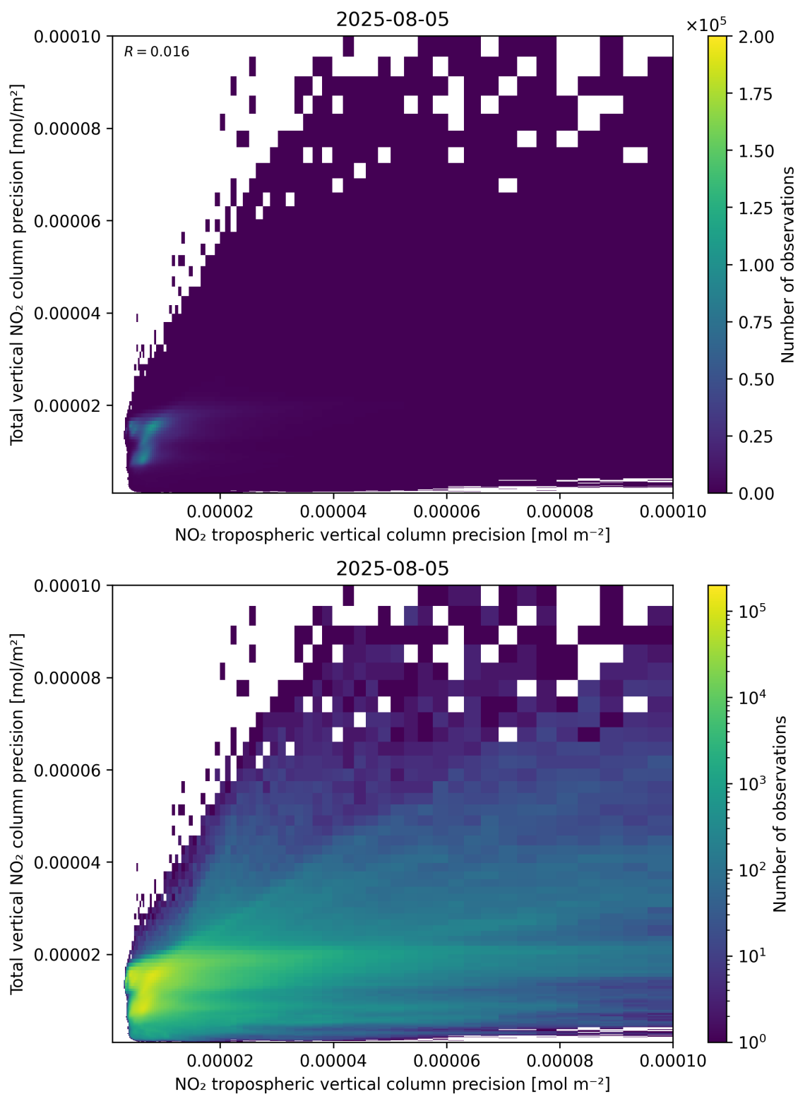
Figure 139: Scatter density plot of “NO 2 tropospheric vertical column precision” against “Total vertical NO 2 column precision” for 2025-08-04 to 2025-08-06.
