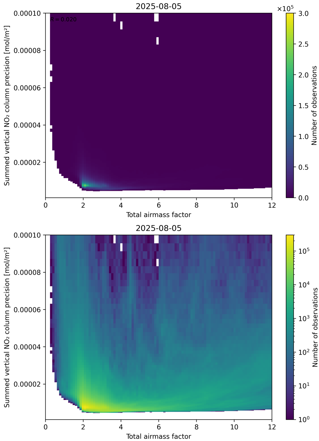
Figure 66: Scatter density plot of “Total airmass factor” against “Summed vertical NO 2 column precision” for 2025-08-04 to 2025-08-06.
