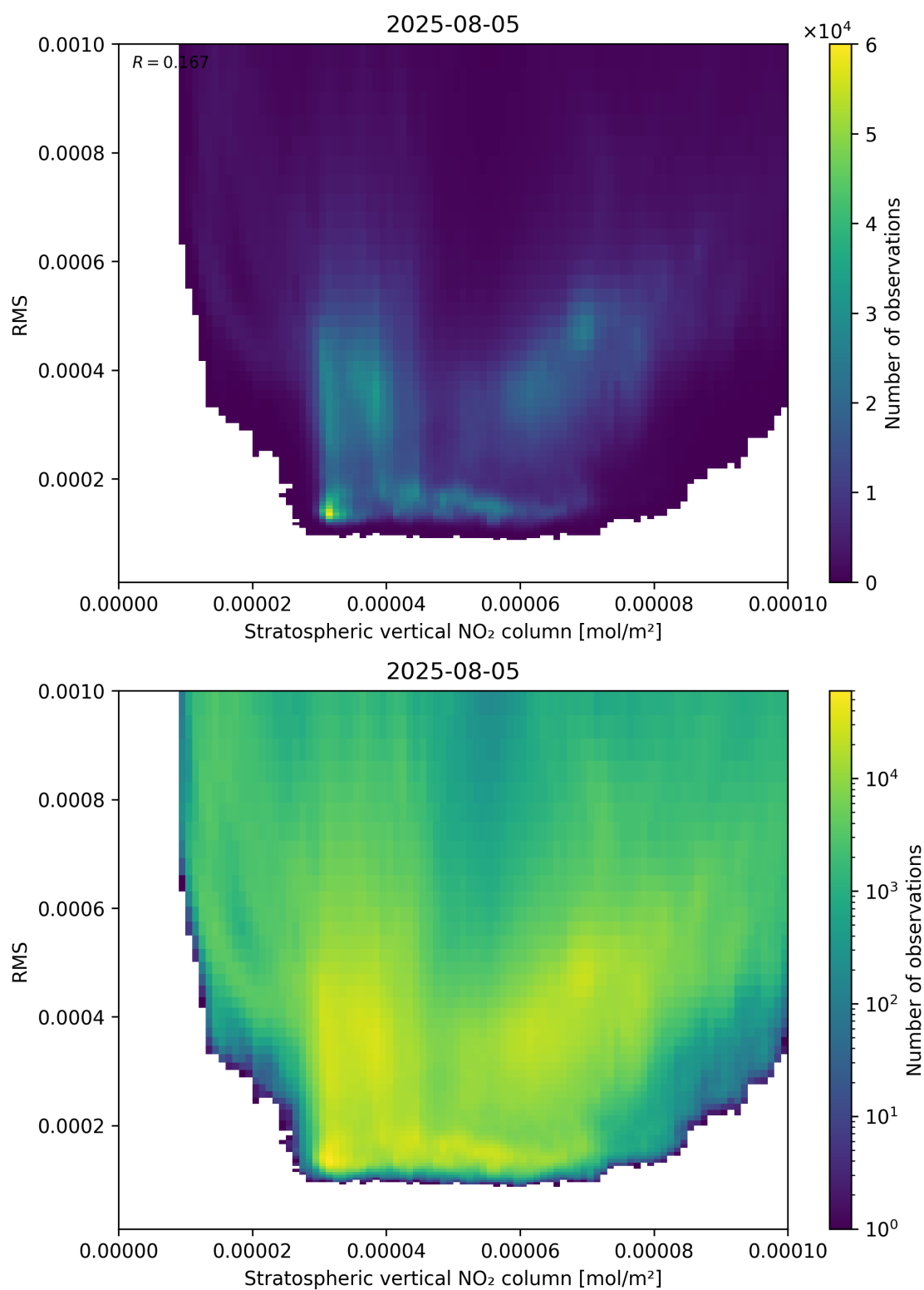
Figure 102: Scatter density plot of “Stratospheric vertical NO 2 column” against “RMS” for 2025-08-04 to 2025-08-06.
