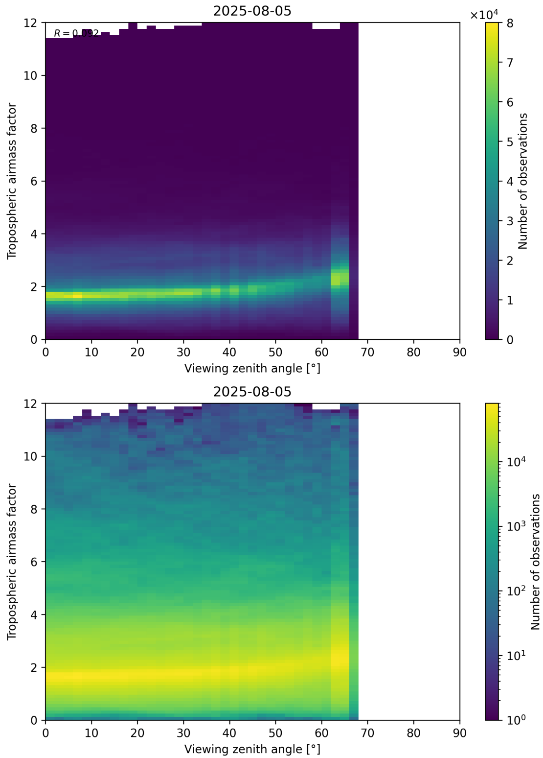
Figure 161: Scatter density plot of “Viewing zenith angle” against “Tropospheric airmass factor” for 2025-08-04 to 2025-08-06.
