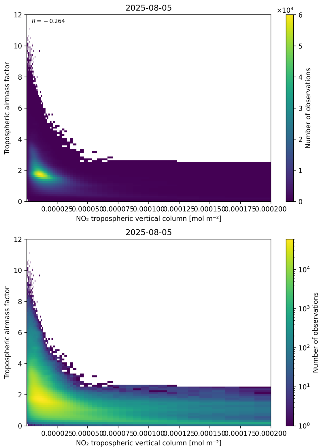
Figure 123: Scatter density plot of “NO 2 tropospheric vertical column” against “Tropospheric air mass factor” for 2025-08-04 to 2025-08-06.
