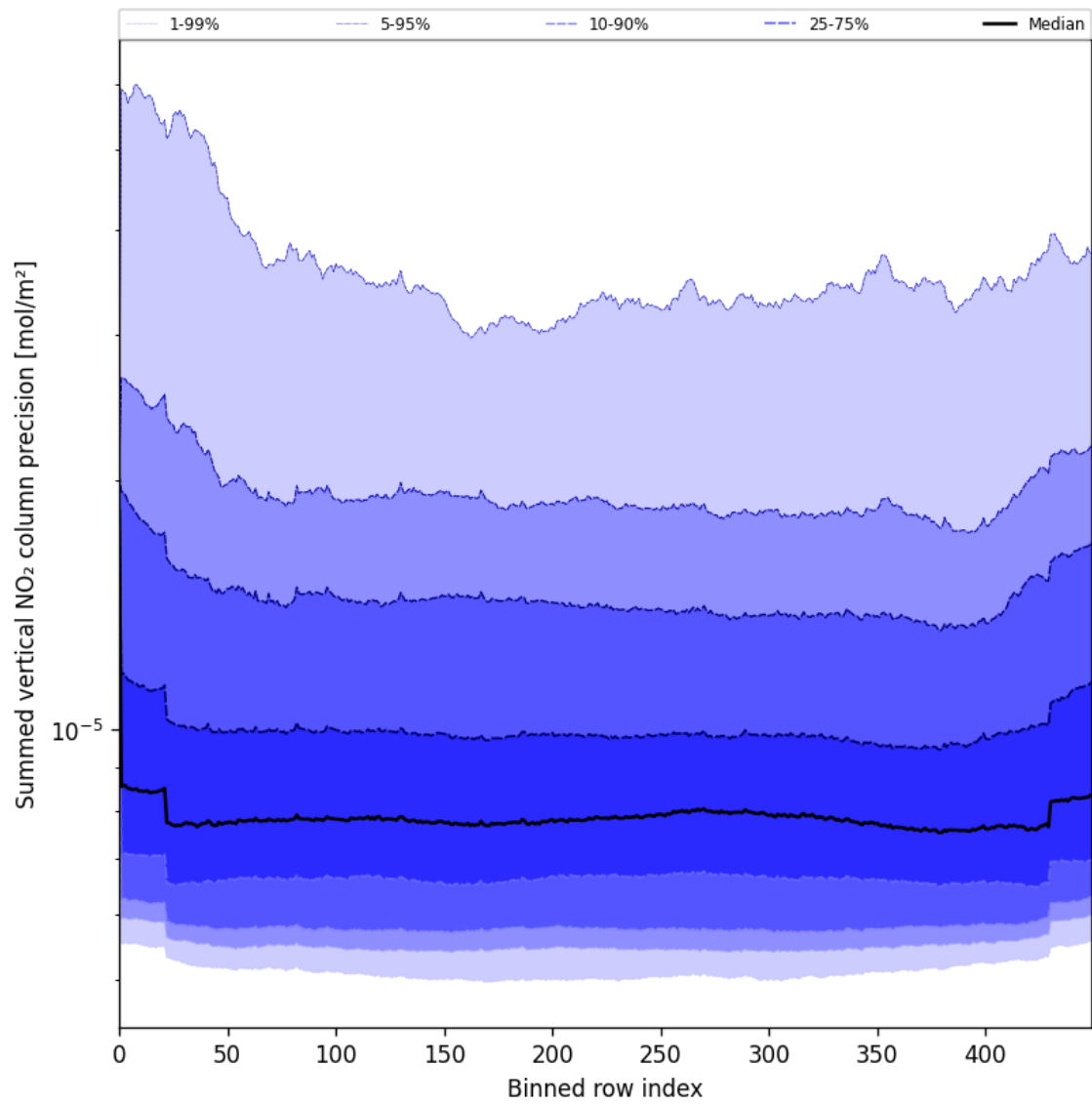
Figure 58: Along track statistics of “Summed vertical NO 2 column precision” for 2025-08-04 to 2025-08-06
