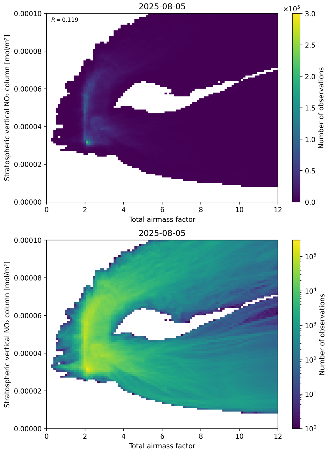
Figure 64: Scatter density plot of “Total airmass factor” against “Stratospheric vertical \text{NO}_2 column” for 2025-08-04 to 2025-08-06.
