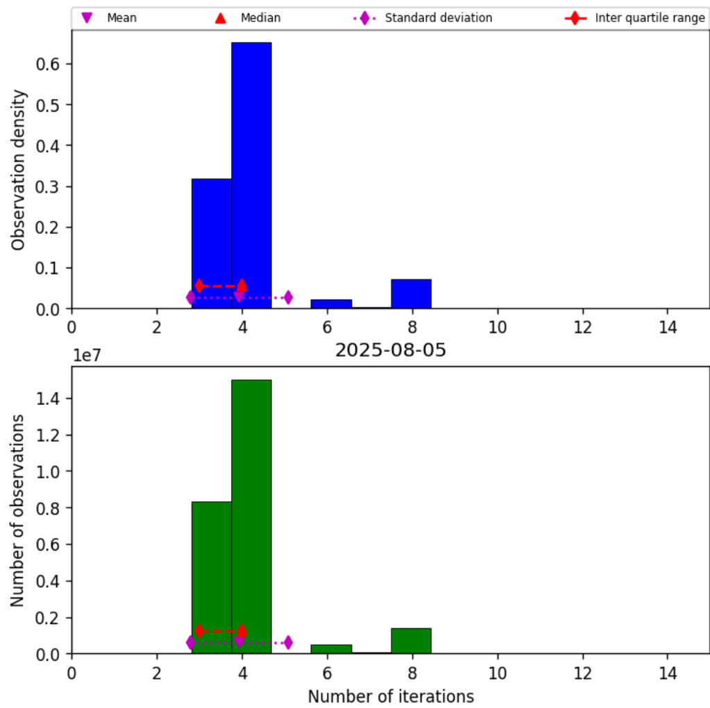
Figure 34: Histogram of “Number of iterations” for 2025-08-04 to 2025-08-06
