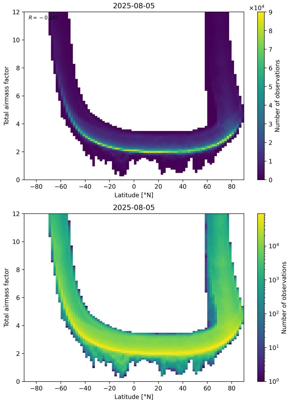
Figure 84: Scatter density plot of “Latitude” against “Total airmass factor” for 2025-08-04 to 2025-08-06.
