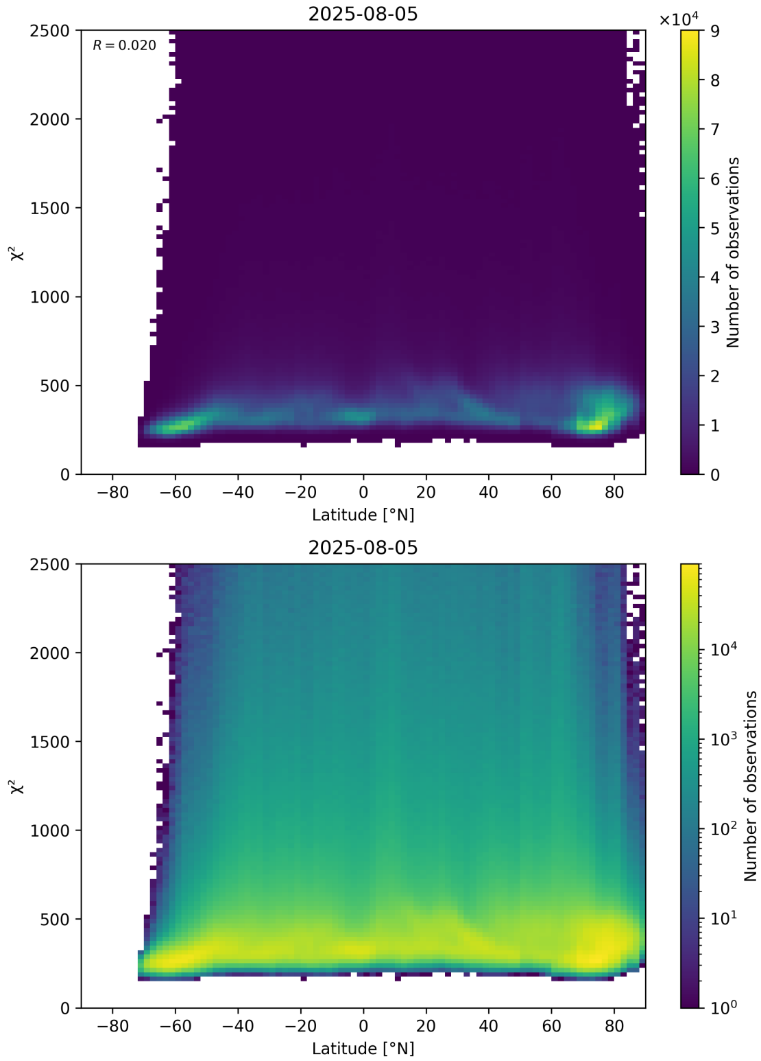
Figure 86: Scatter density plot of “Latitude” against “ \chi^2 ” for 2025-08-04 to 2025-08-06.
