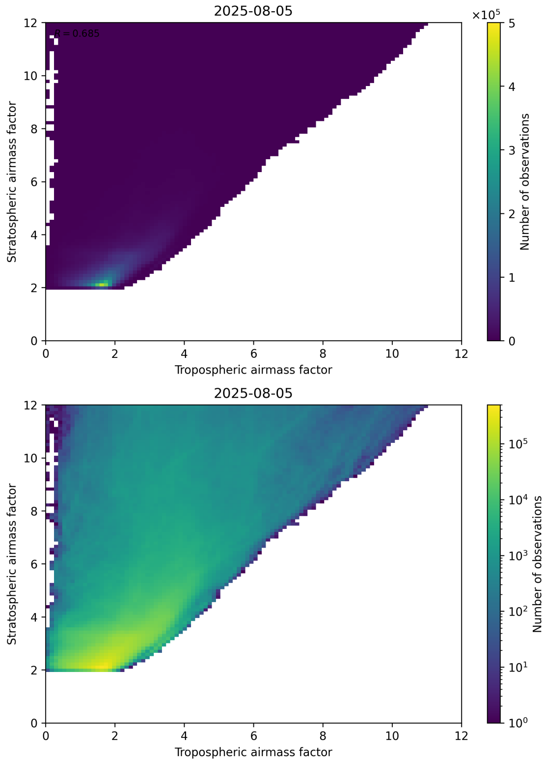
Figure 71: Scatter density plot of “Tropospheric airmass factor” against “Stratospheric airmass factor” for 2025-08-04 to 2025-08-06.
