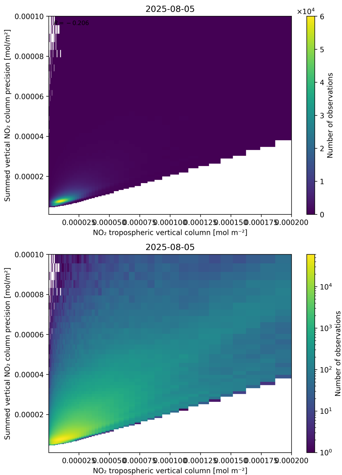
Figure 127: Scatter density plot of “NO 2 tropospheric vertical column” against “Summed vertical NO 2 column precision” for 2025-08-04 to 2025-08-06.
