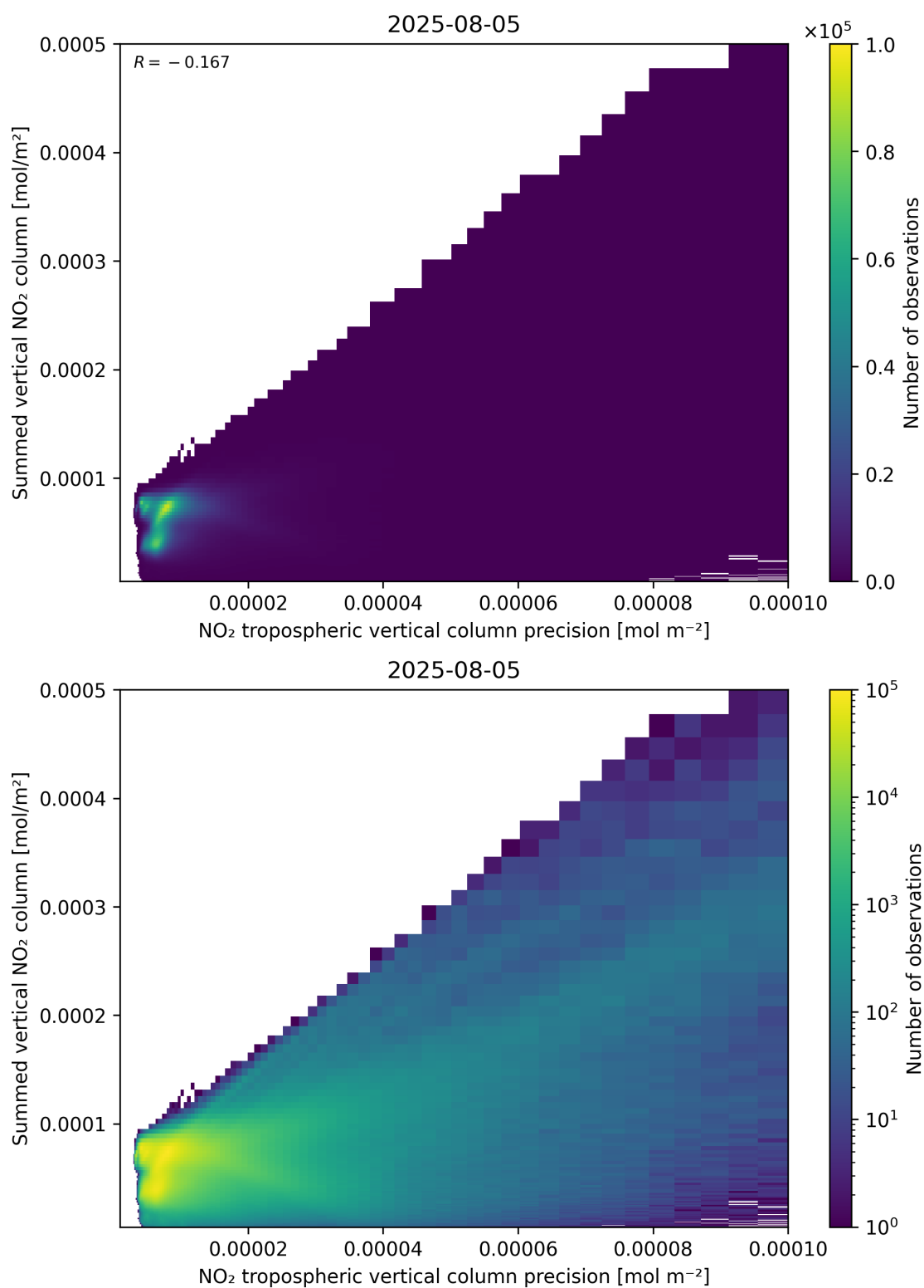
Figure 136: Scatter density plot of “NO 2 tropospheric vertical column precision” against “Summed vertical NO 2 column” for 2025-08-04 to 2025-08-06.
