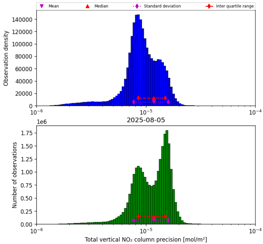
Figure 39: Histogram of “Total vertical NO 2 column precision” for 2025-08-04 to 2025-08-06
