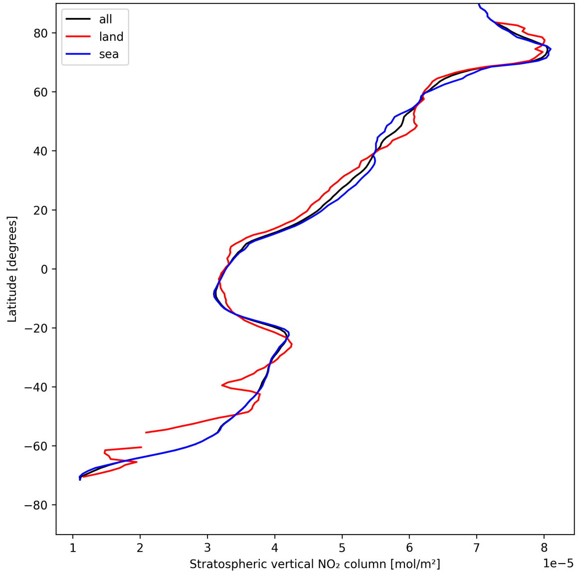
Figure 19: Zonal average of “Stratospheric vertical NO 2 column” for 2025-08-04 to 2025-08-06.
