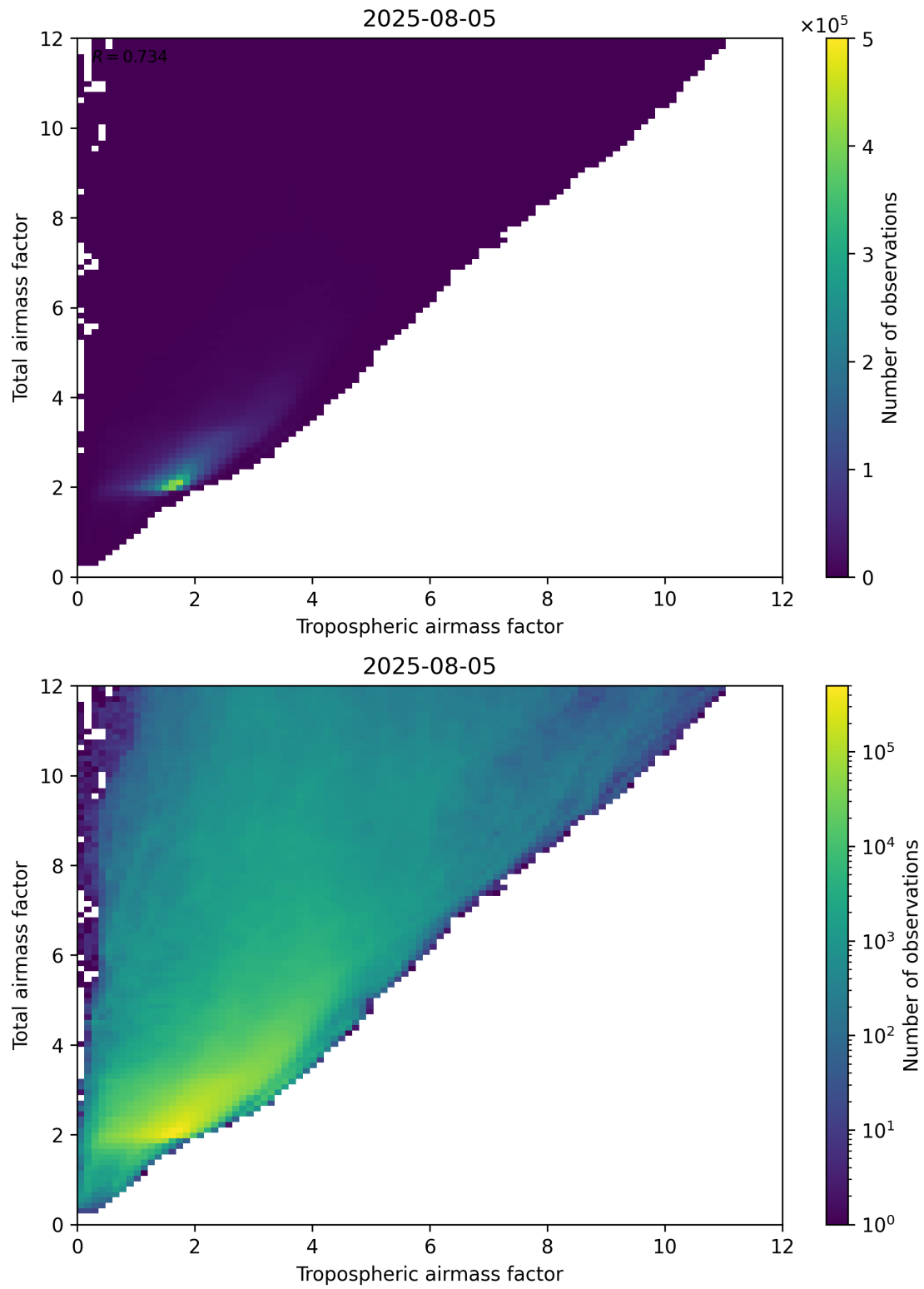
Figure 72: Scatter density plot of “Tropospheric airmass factor” against “Total airmass factor” for 2025-08-04 to 2025-08-06.
