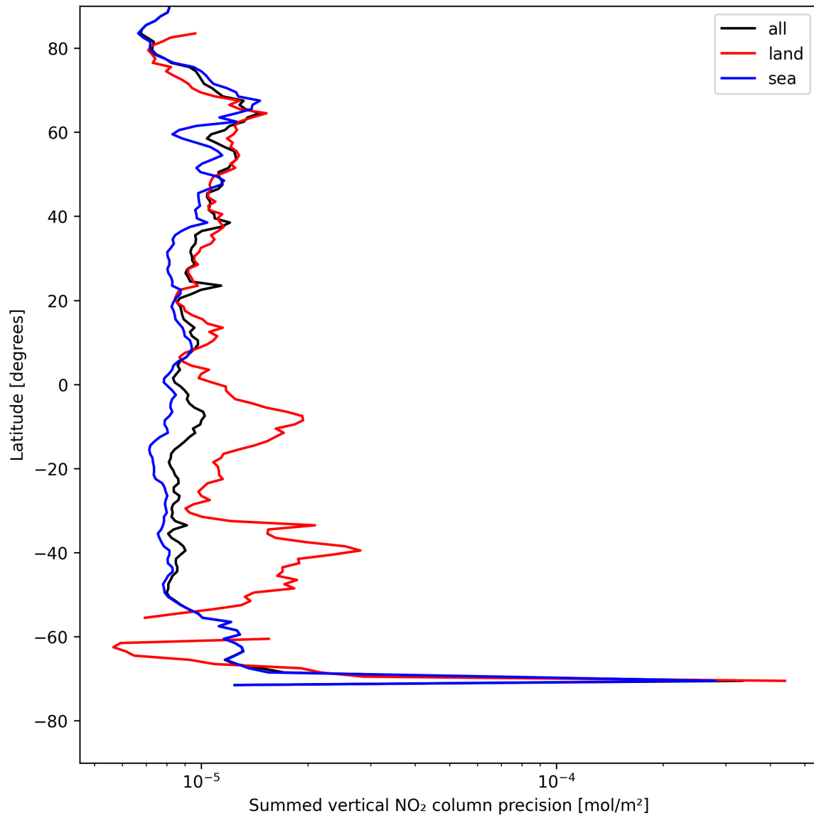
Figure 24: Zonal average of “Summed vertical NO 2 column precision” for 2025-08-04 to 2025-08-06.
