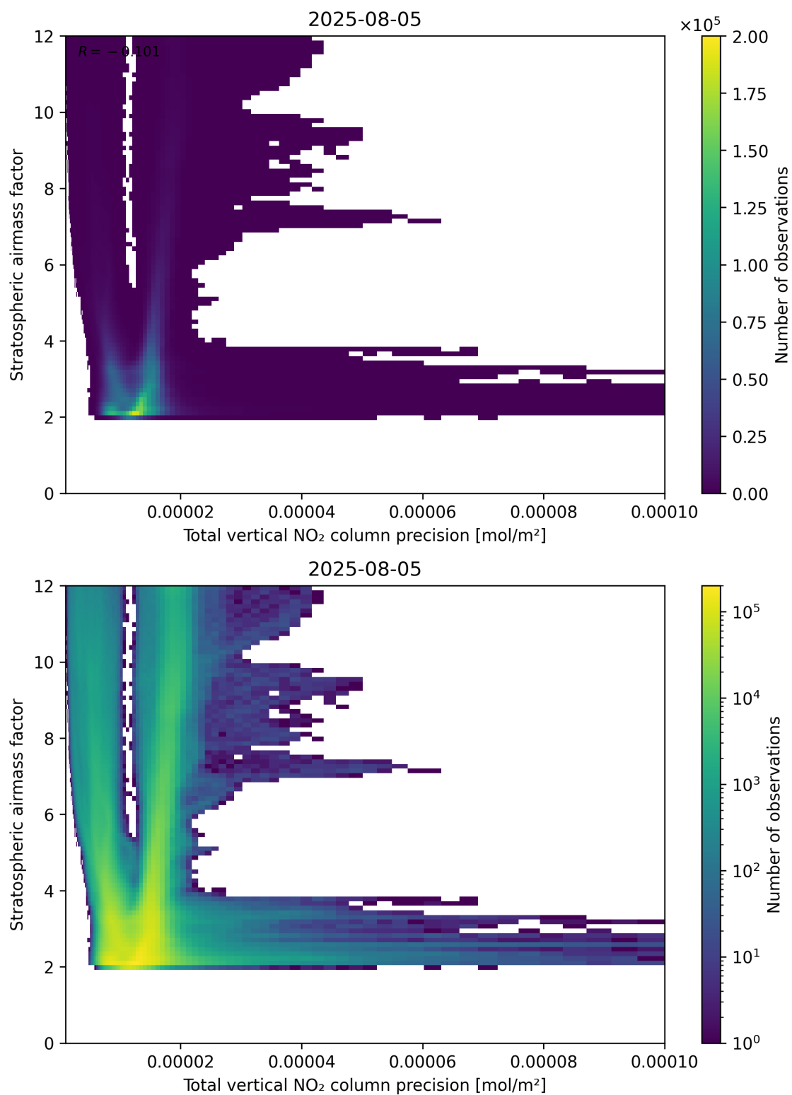
Figure 115: Scatter density plot of “Total vertical NO 2 column precision” against “Stratospheric air mass factor” for 2025-08-04 to 2025-08-06.
