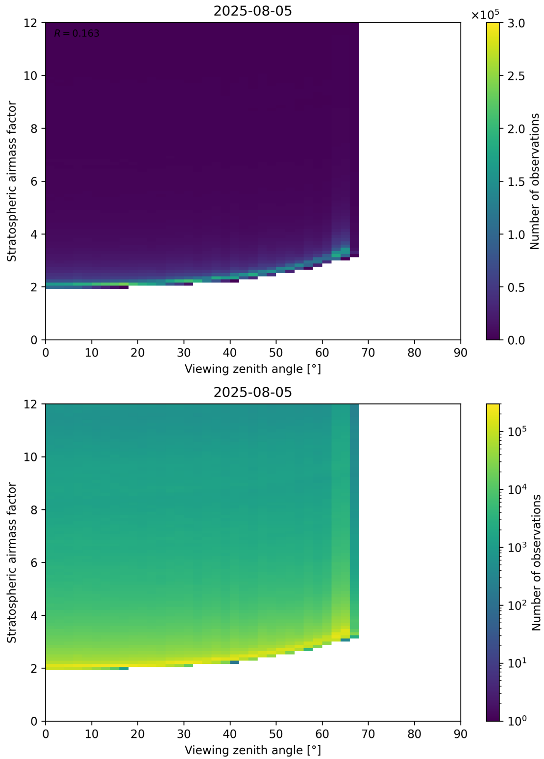
Figure 159: Scatter density plot of “Viewing zenith angle” against “Stratospheric airmass factor” for 2025-08-04 to 2025-08-06.
