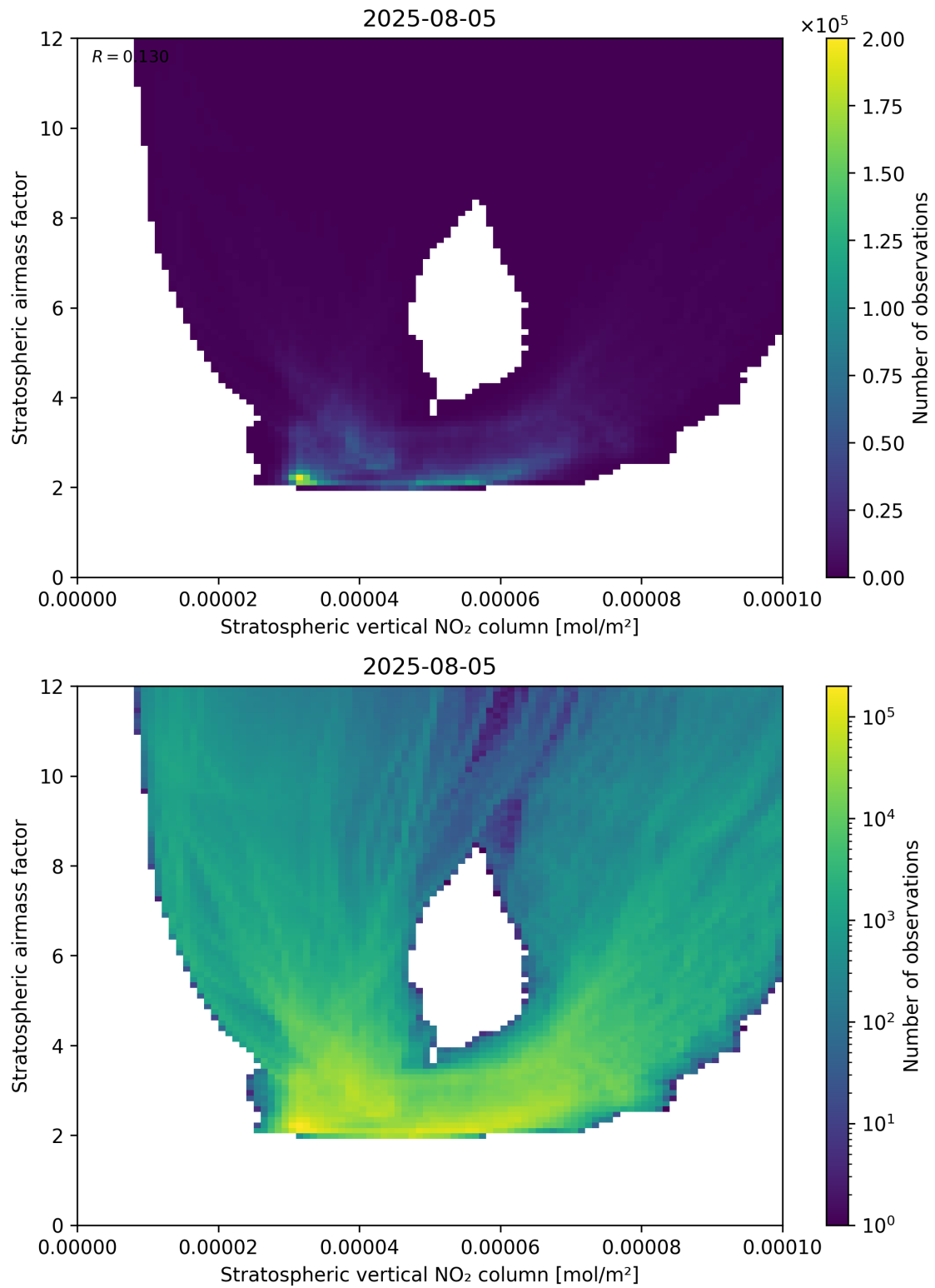
Figure 96: Scatter density plot of “Stratospheric vertical NO 2 column” against “Stratospheric airmass factor” for 2025-08-04 to 2025-08-06.
