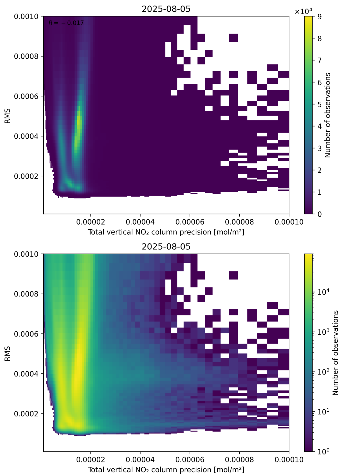
Figure 119: Scatter density plot of “Total vertical NO 2 column precision” against “RMS” for 2025-08-04 to 2025-08-06.
