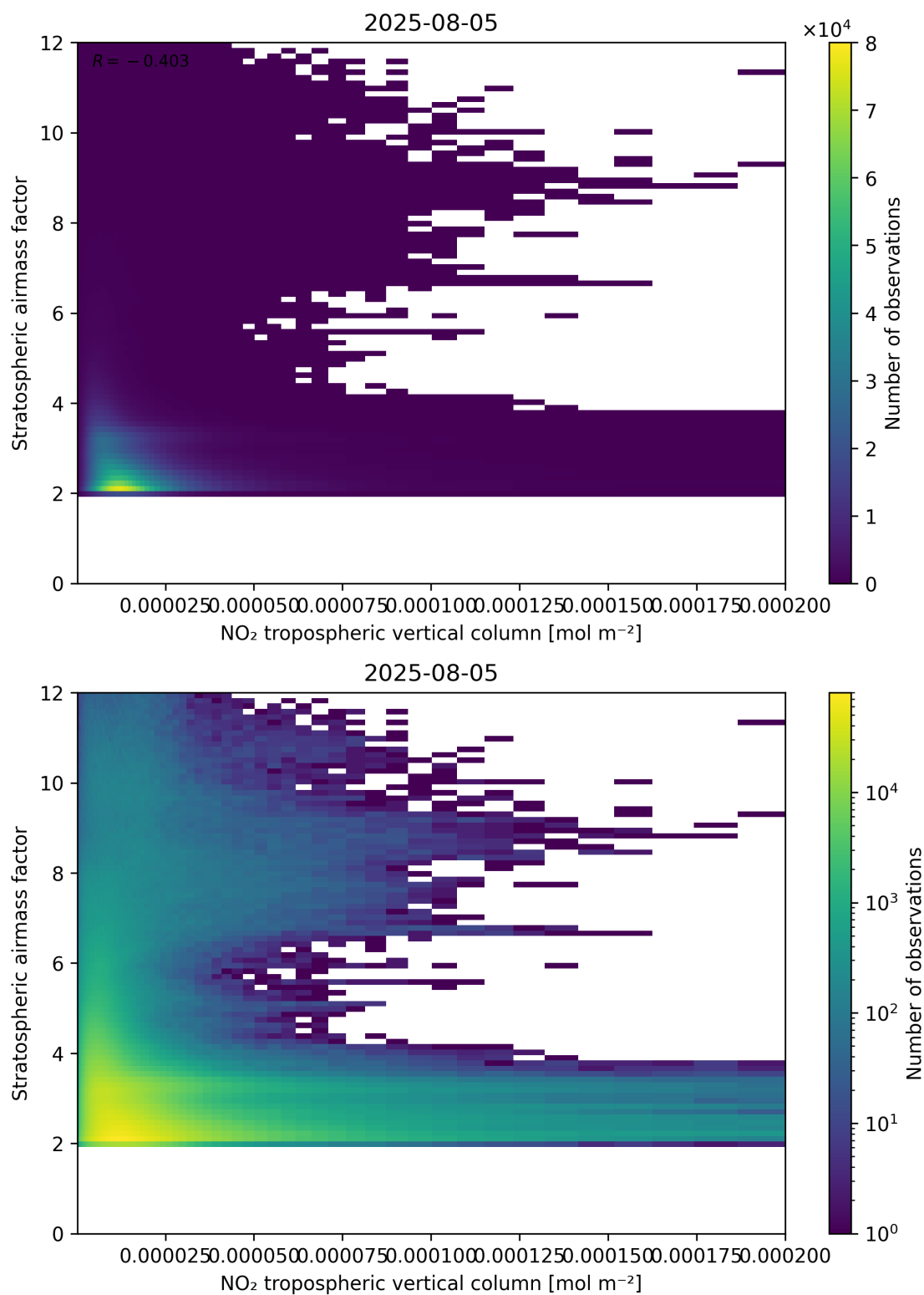
Figure 121: Scatter density plot of “NO 2 tropospheric vertical column” against “Stratospheric air mass factor” for 2025-08-04 to 2025-08-06.
