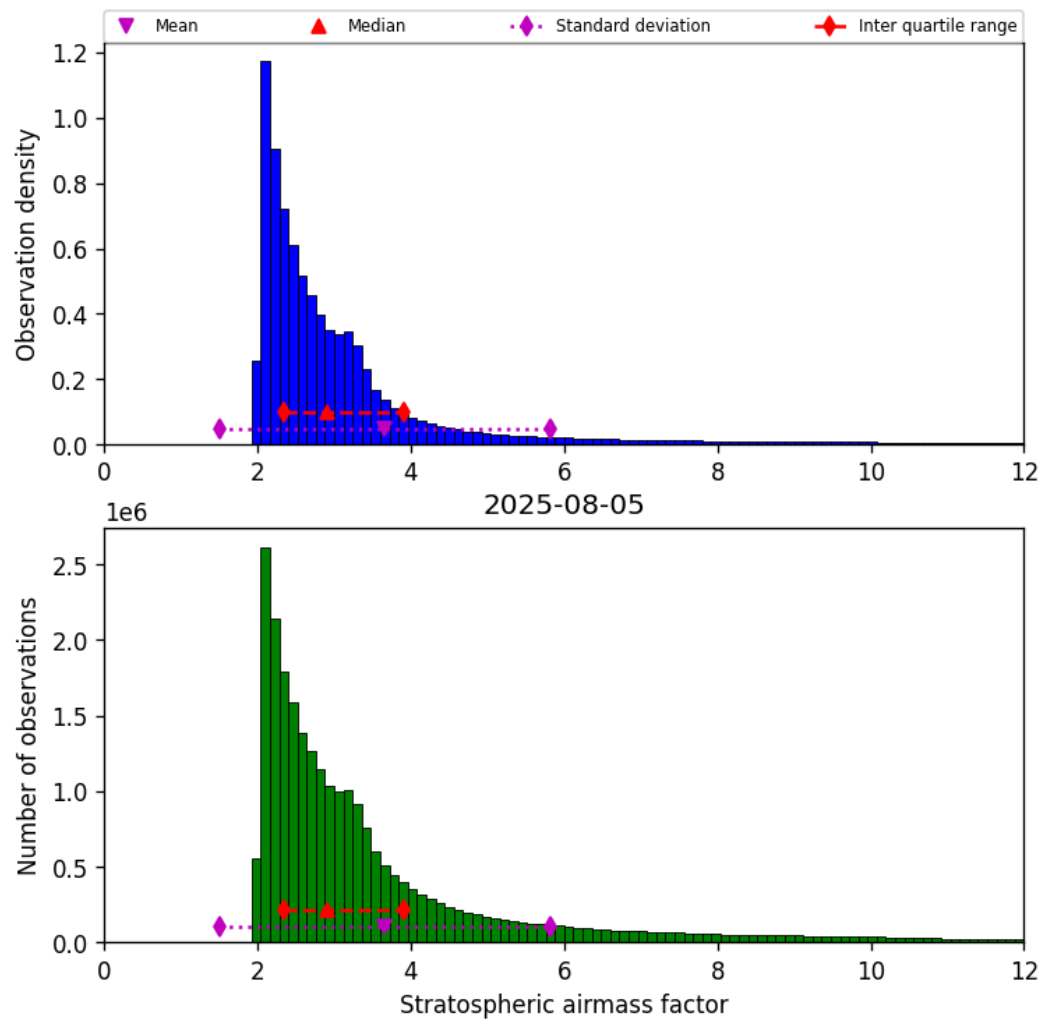
Figure 44: Histogram of “Stratospheric airmass factor” for 2025-08-04 to 2025-08-06
