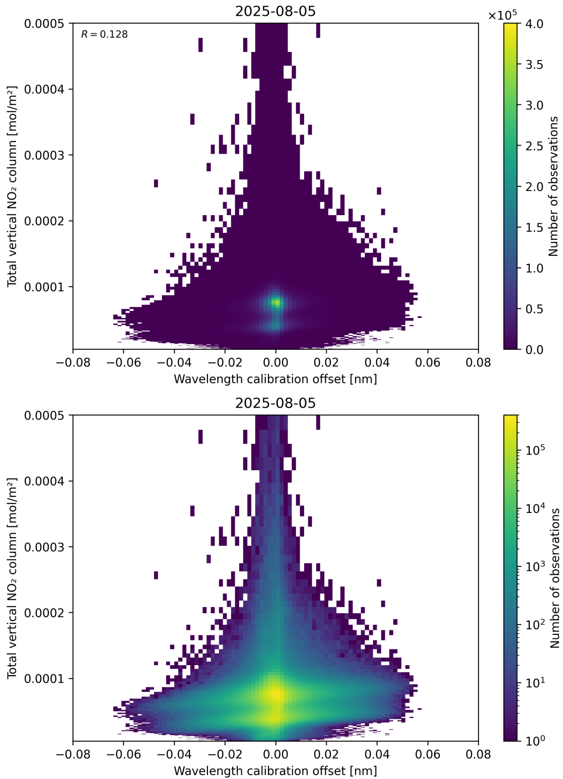
Figure 179: Scatter density plot of “Wavelength calibration offset” against “Total vertical NO 2 column” for 2025-08-04 to 2025-08-06.
