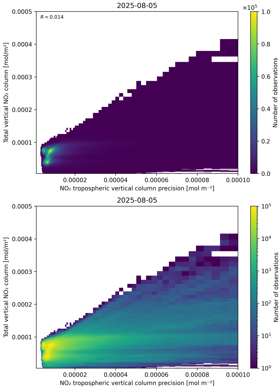
Figure 138: Scatter density plot of “NO 2 tropospheric vertical column precision” against “Total vertical NO 2 column” for 2025-08-04 to 2025-08-06.
