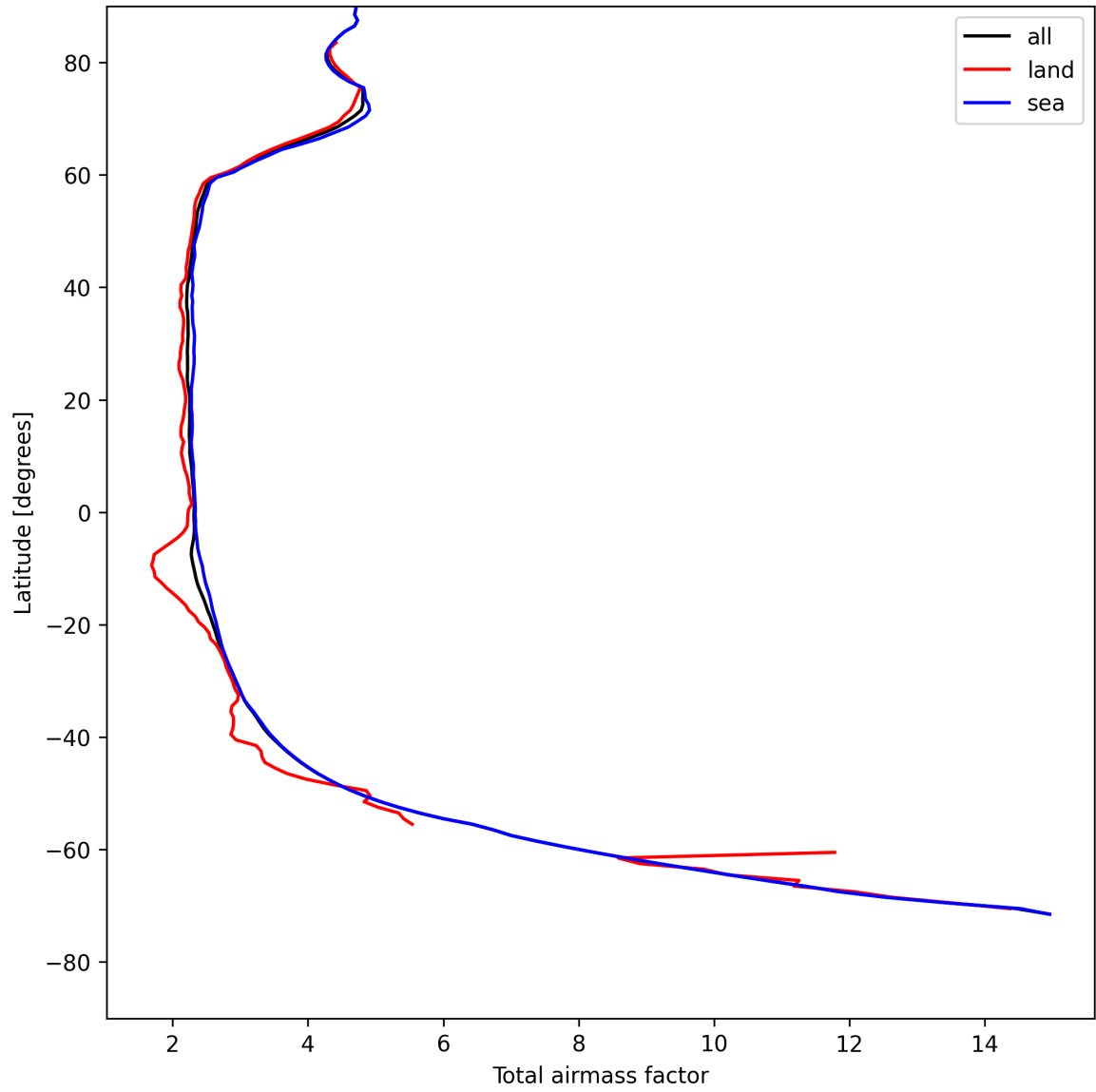
Figure 15: Zonal average of “Total airmass factor” for 2025-08-04 to 2025-08-06.
