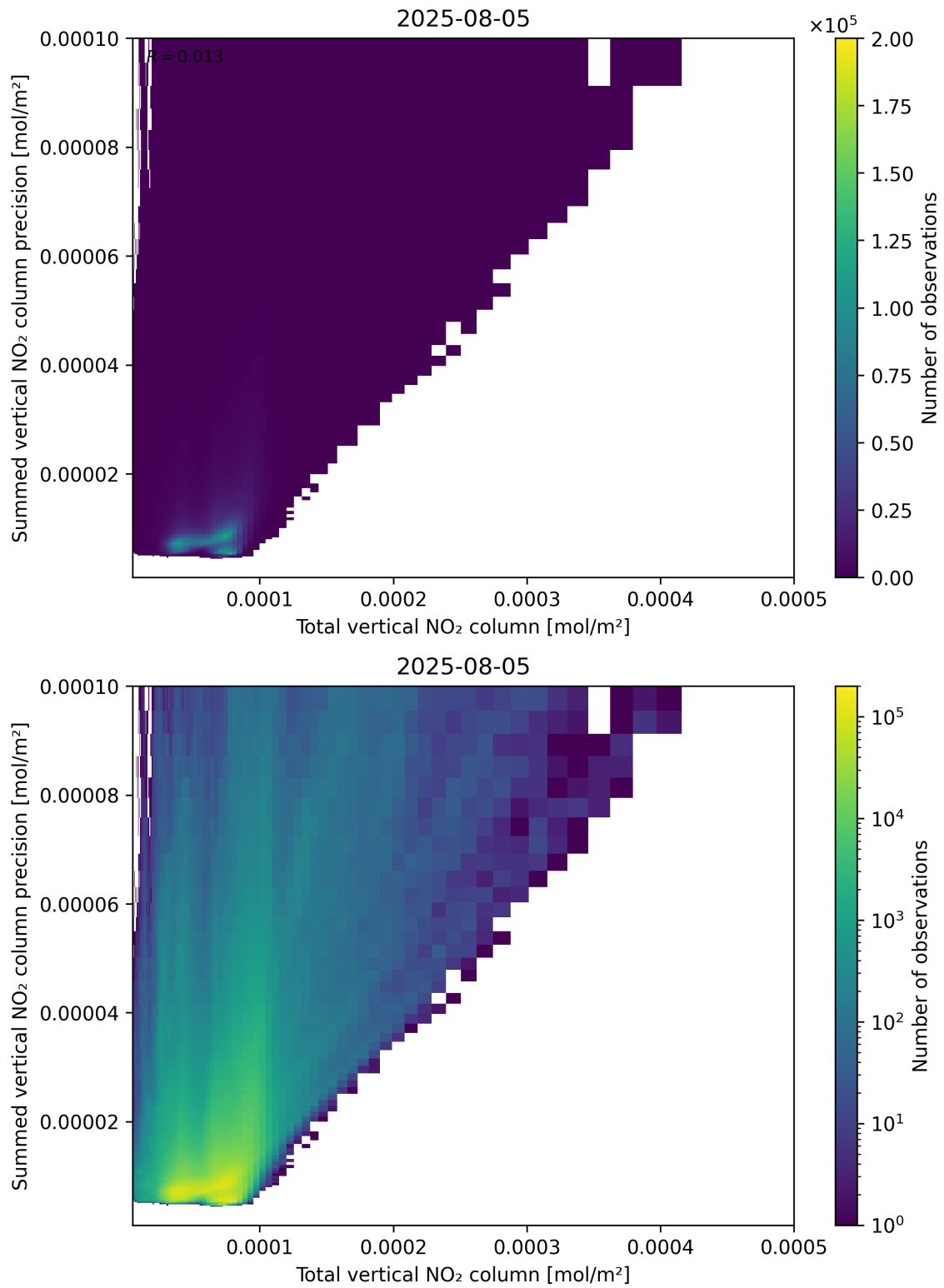
Figure 113: Scatter density plot of “Total vertical NO 2 column” against “Summed vertical NO 2 column precision” for 2025-08-04 to 2025-08-06.
