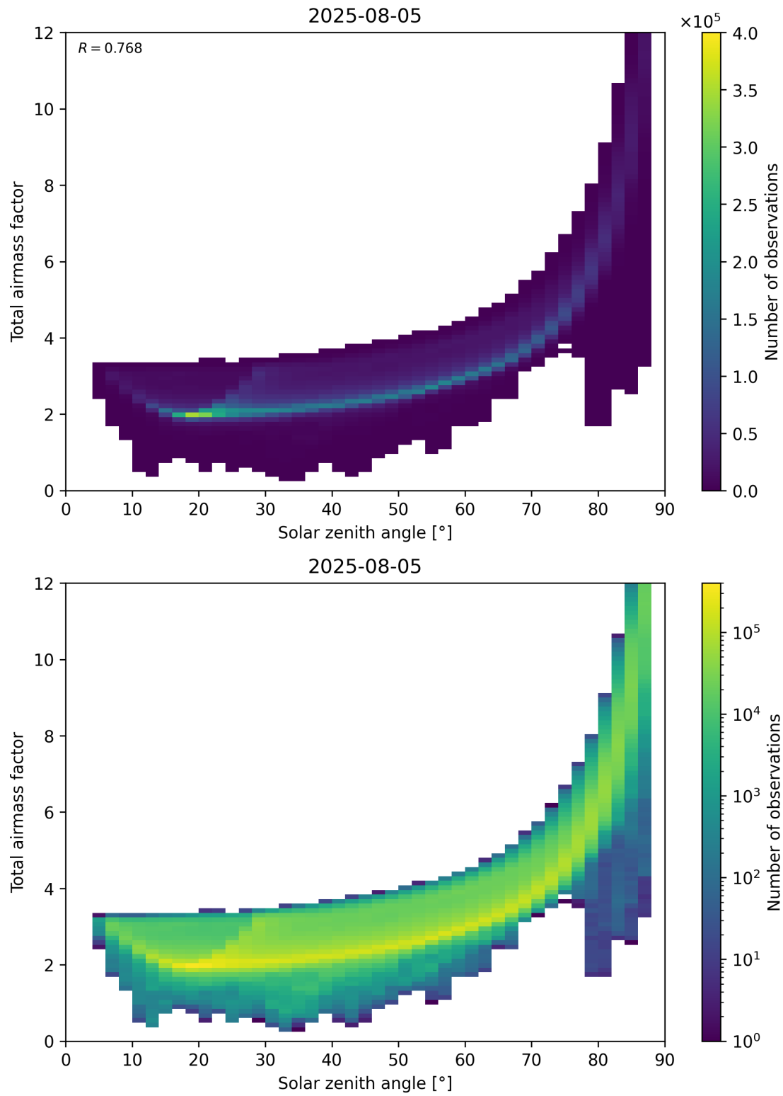
Figure 146: Scatter density plot of “Solar zenith angle” against “Total air mass factor” for 2025-08-04 to 2025-08-06.
