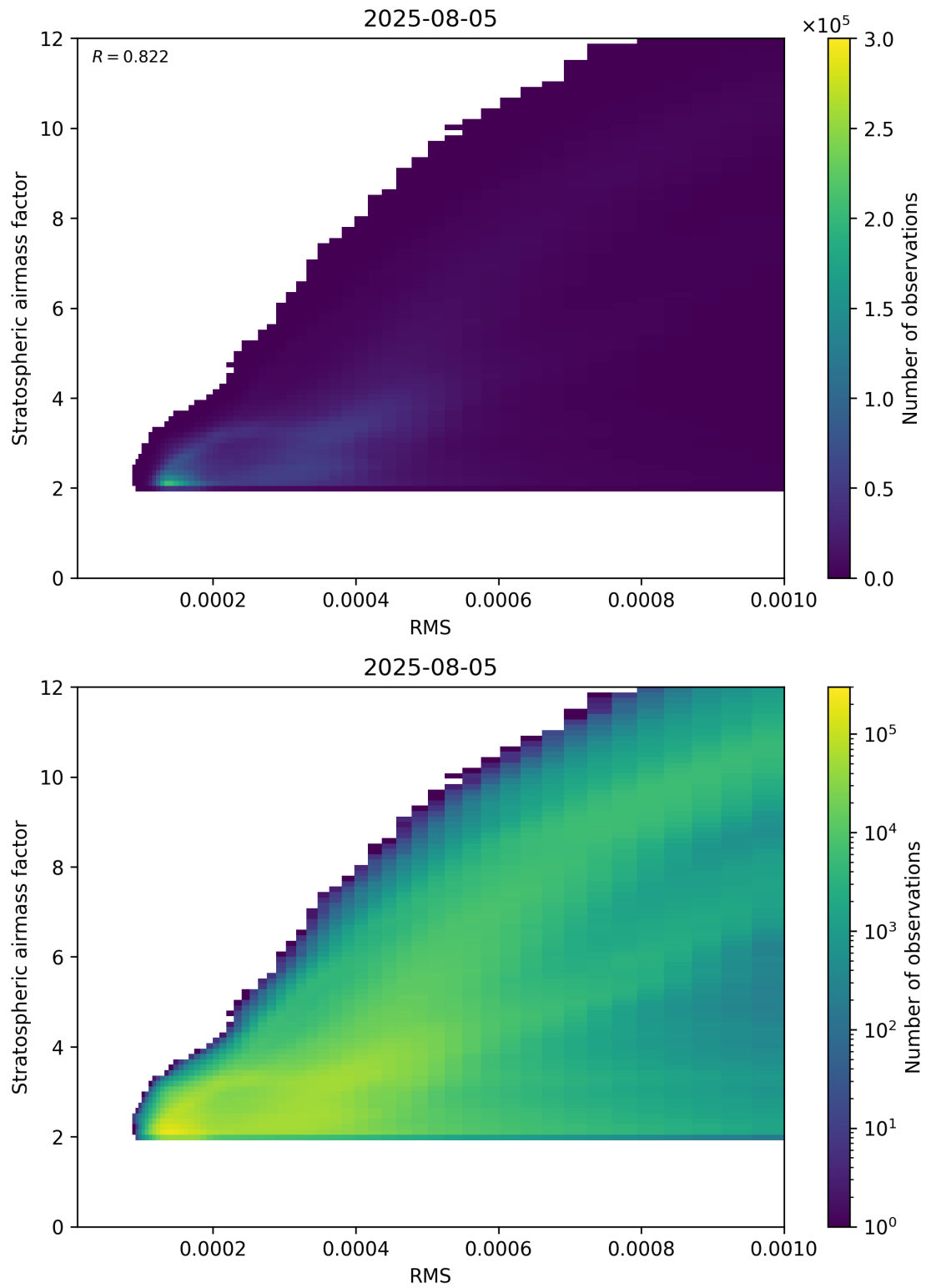
Figure 144: Scatter density plot of “RMS” against “Stratospheric airmass factor” for 2025-08-04 to 2025-08-06.
