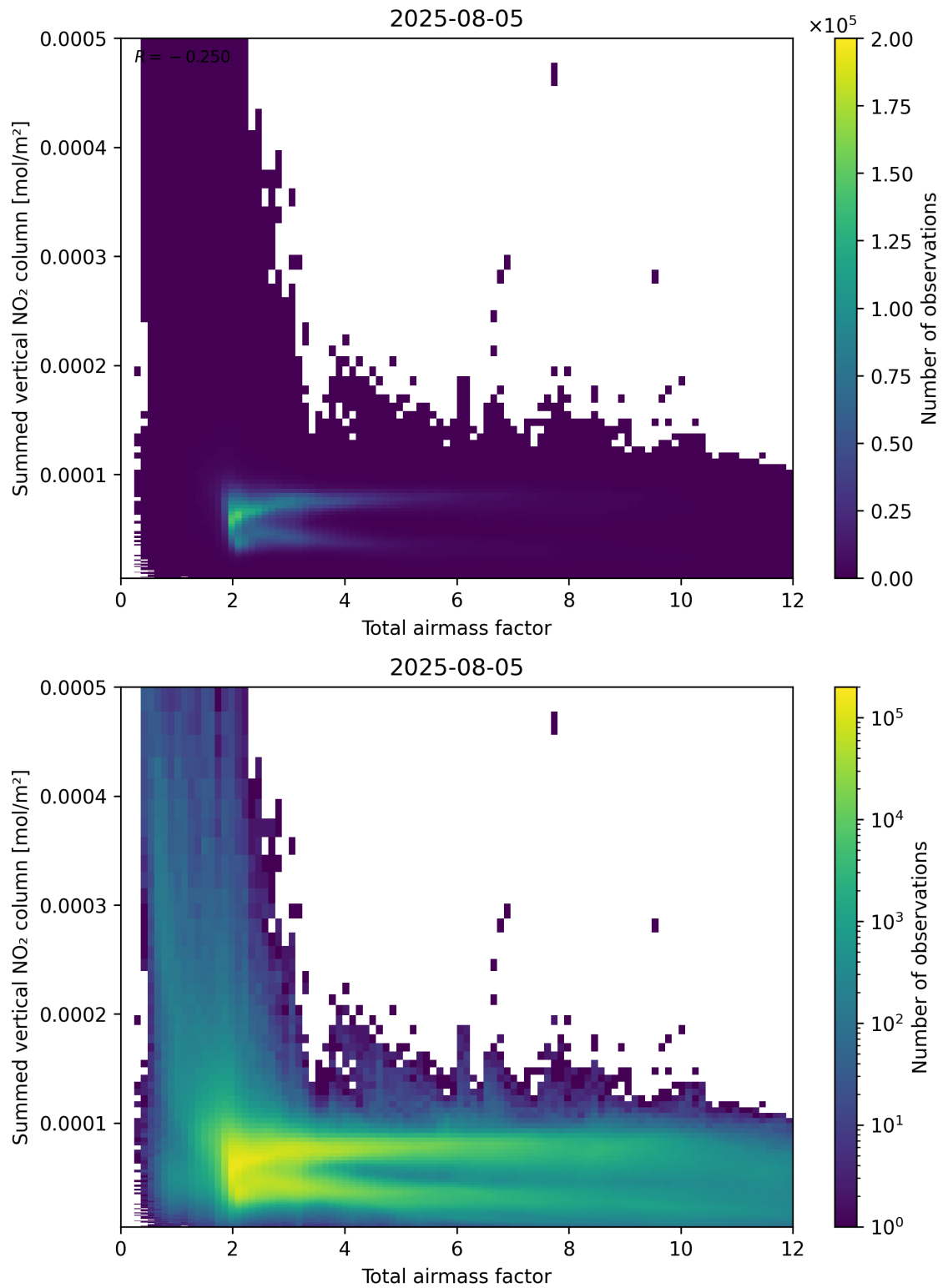
Figure 65: Scatter density plot of “Total airmass factor” against “Summed vertical NO 2 column” for 2025-08-04 to 2025-08-06.
