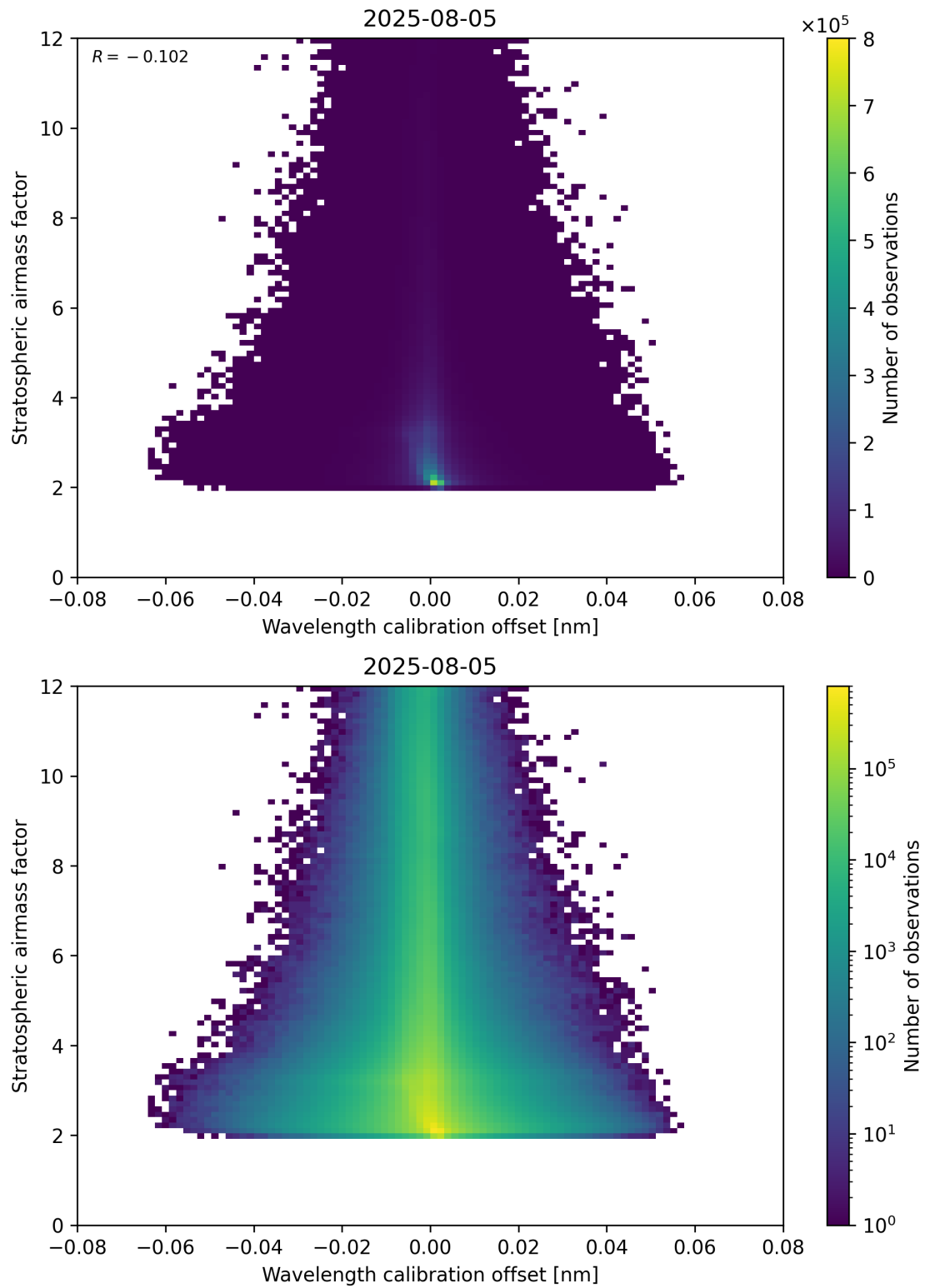
Figure 174: Scatter density plot of “Wavelength calibration offset” against “Stratospheric airmass factor” for 2025-08-04 to 2025-08-06.
