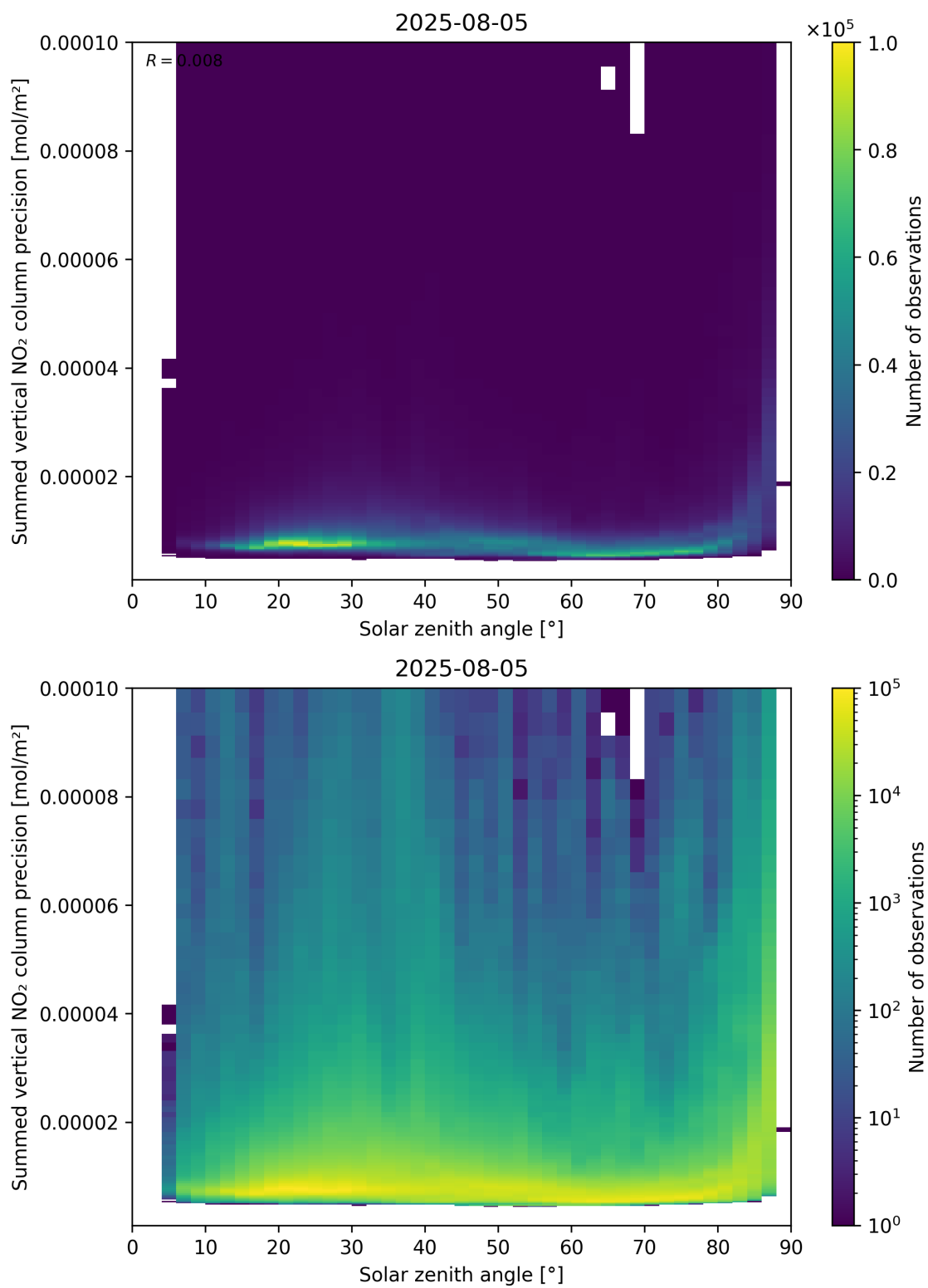
Figure 152: Scatter density plot of “Solar zenith angle” against “Summed vertical NO 2 column precision” for 2025-08-04 to 2025-08-06.
