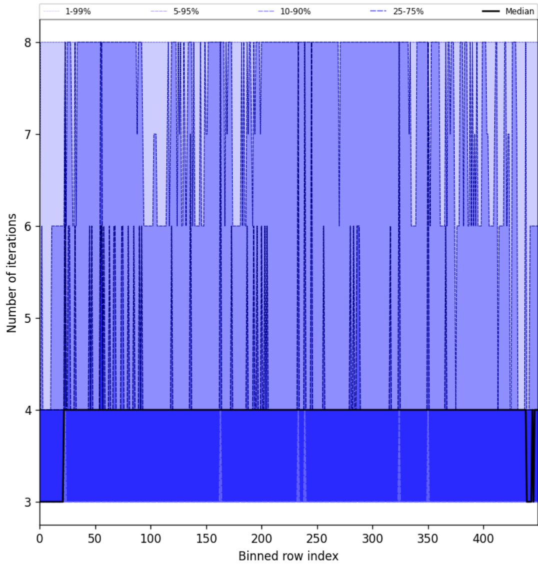
Figure 51: Along track statistics of “Number of iterations” for 2025-08-04 to 2025-08-06
