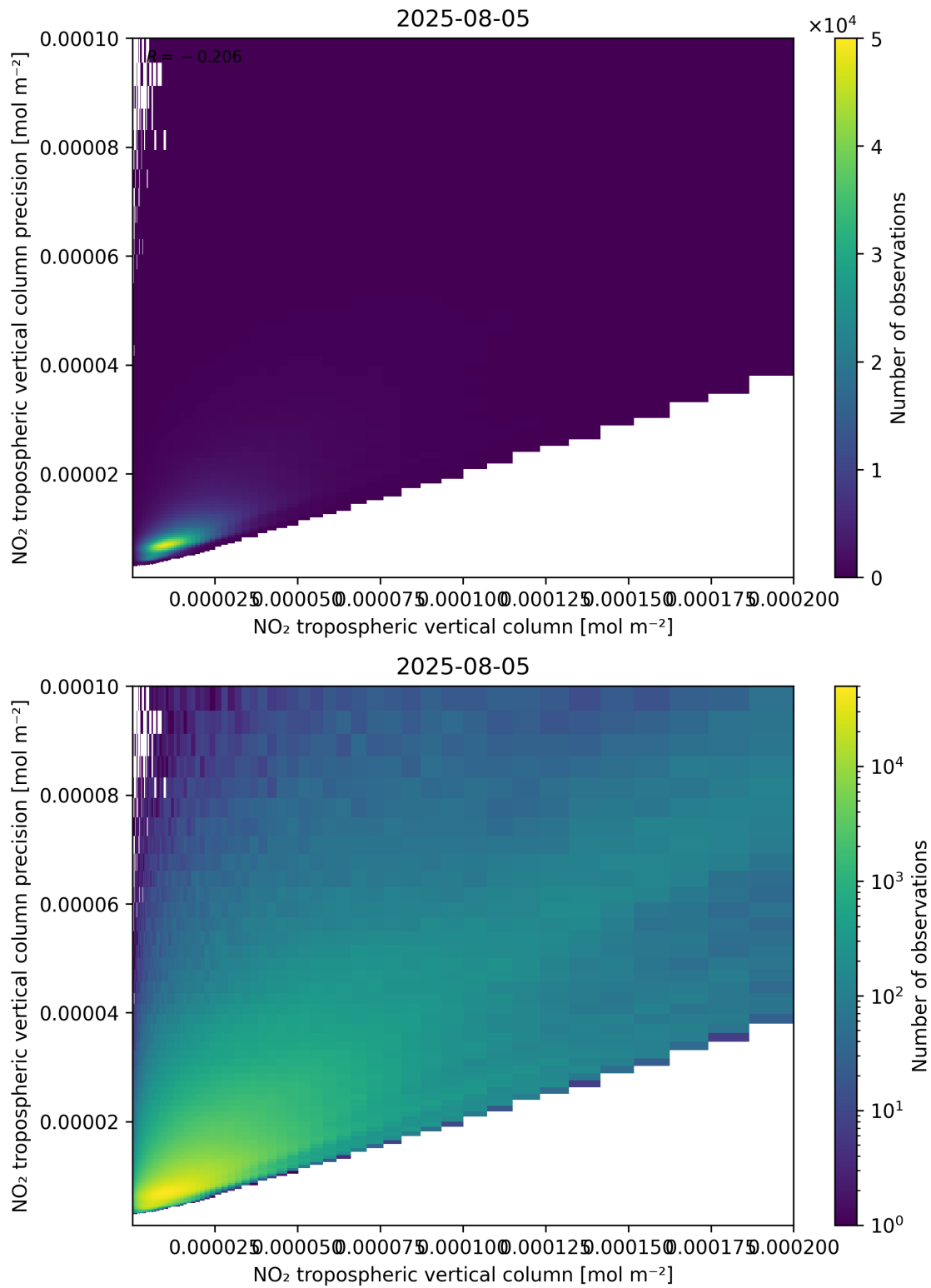
Figure 130: Scatter density plot of “NO 2 tropospheric vertical column” against “NO 2 tropospheric vertical column precision” for 2025-08-04 to 2025-08-06.
