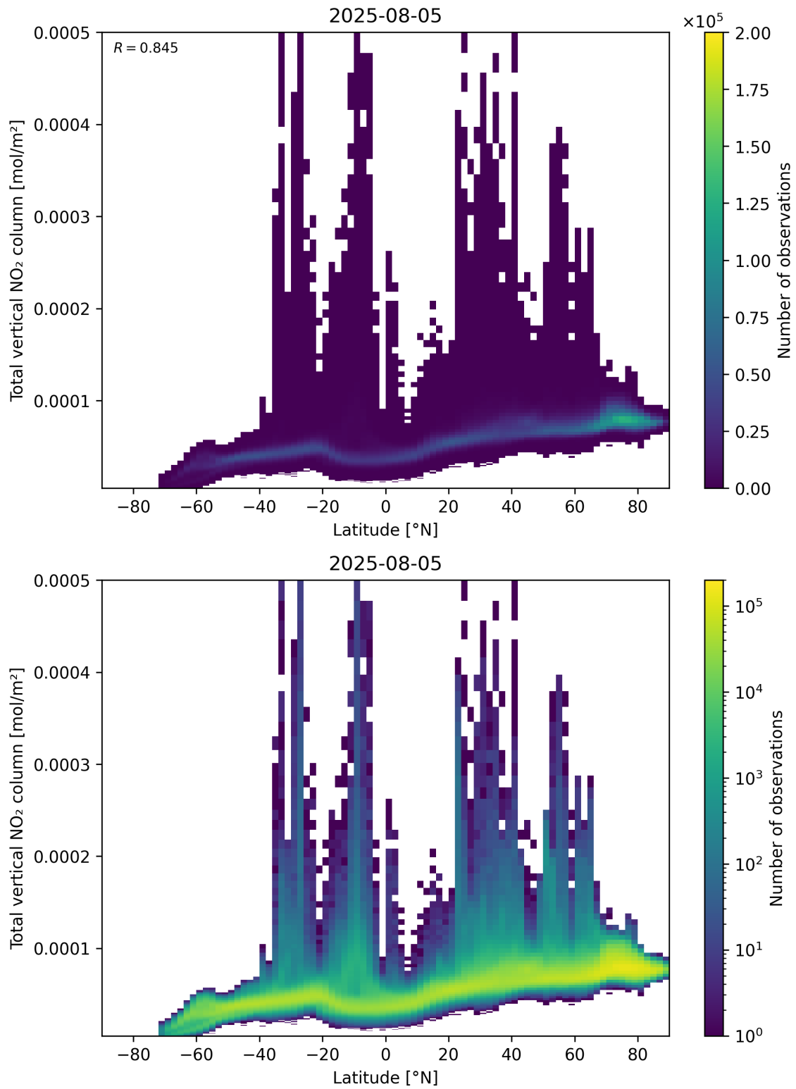
Figure 90: Scatter density plot of “Latitude” against “Total vertical NO 2 column” for 2025-08-04 to 2025-08-06.
