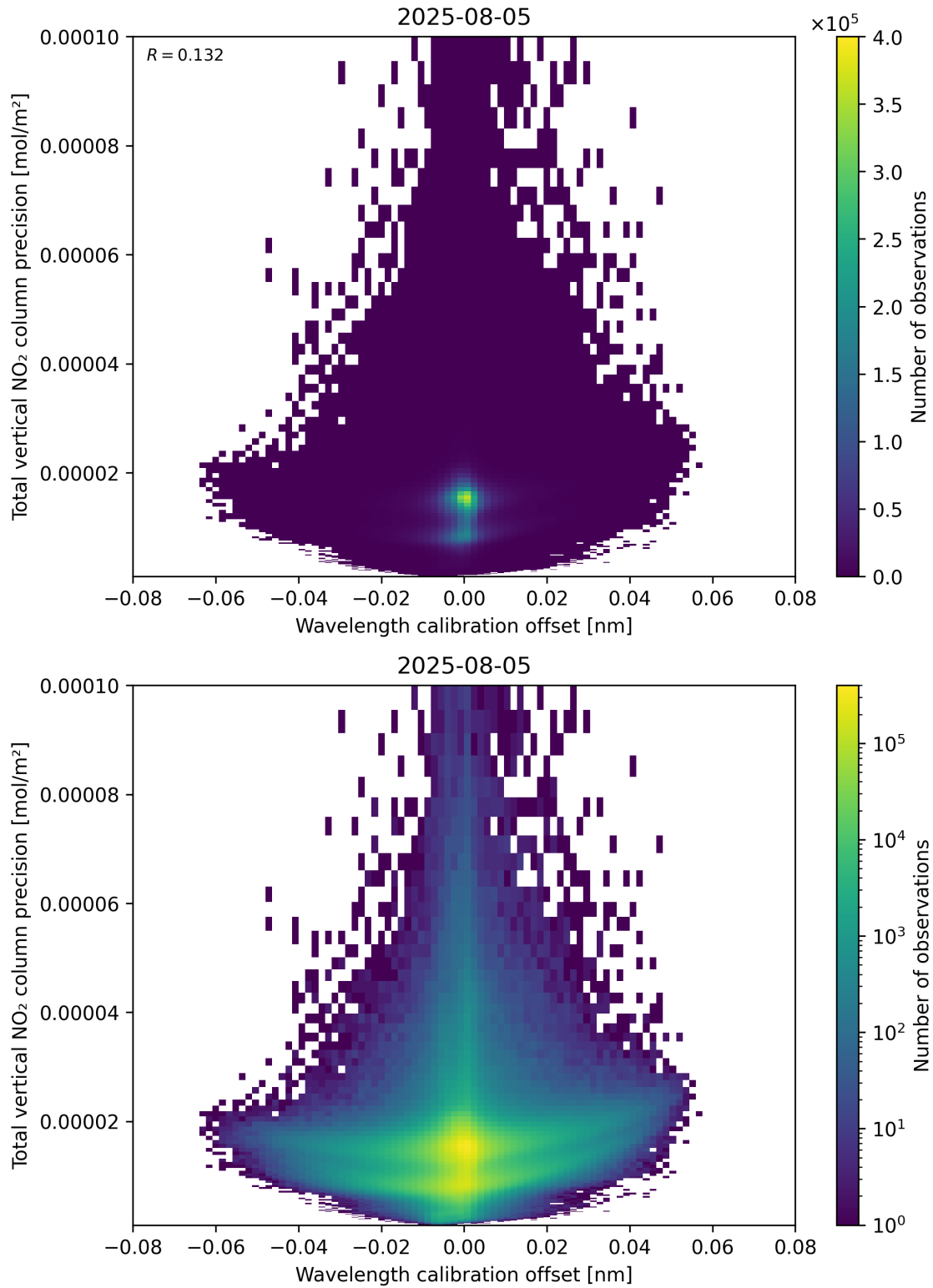
Figure 180: Scatter density plot of “Wavelength calibration offset” against “Total vertical NO 2 column precision” for 2025-08-04 to 2025-08-06.
