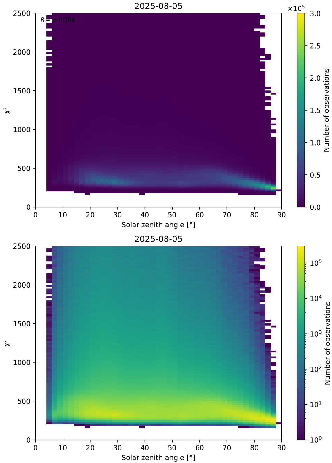
Figure 148: Scatter density plot of “Solar zenith angle” against “ \chi^2 ” for 2025-08-04 to 2025-08-06.
