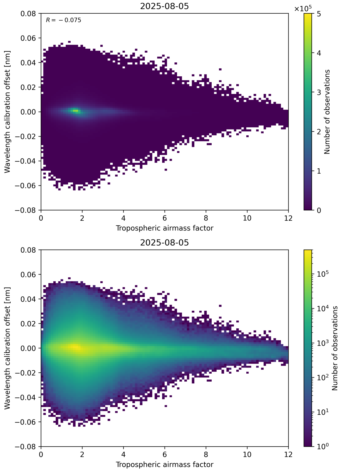
Figure 80: Scatter density plot of “Tropospheric airmass factor” against “Wavelength calibration offset” for 2025-08-04 to 2025-08-06.
