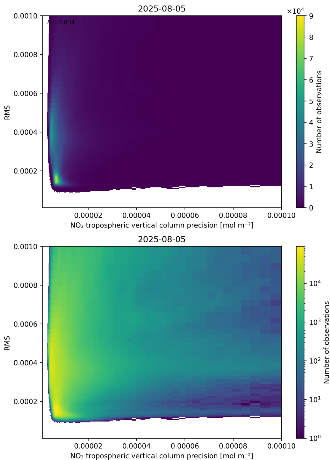
Figure 140: Scatter density plot of “NO 2 tropospheric vertical column precision” against “RMS” for 2025-08-04 to 2025-08-06.
