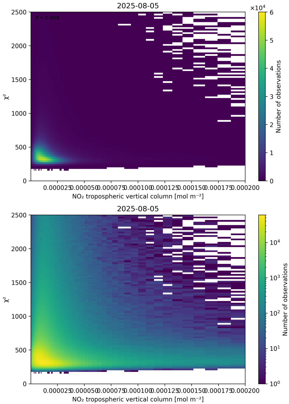
Figure 124: Scatter density plot of “NO 2 tropospheric vertical column” against “ \chi^2 ” for 2025-08-04 to 2025-08-06.
