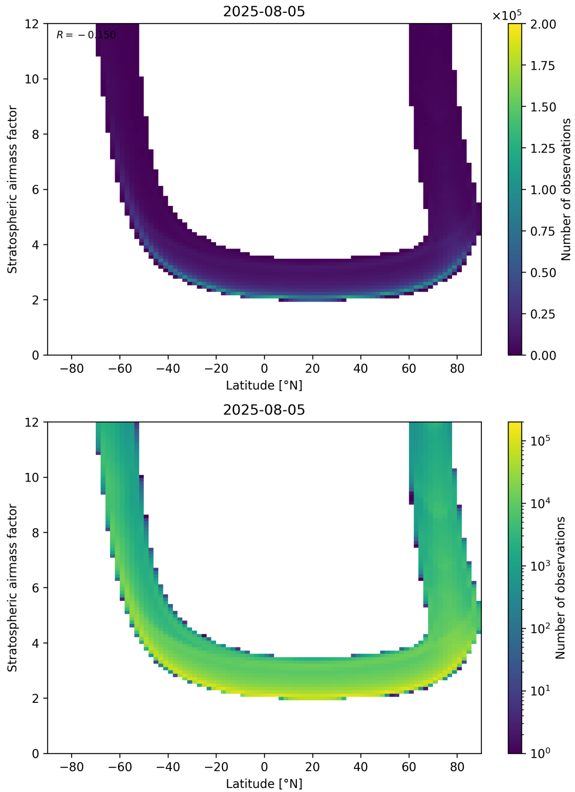
Figure 83: Scatter density plot of “Latitude” against “Stratospheric air mass factor” for 2025-08-04 to 2025-08-06.
