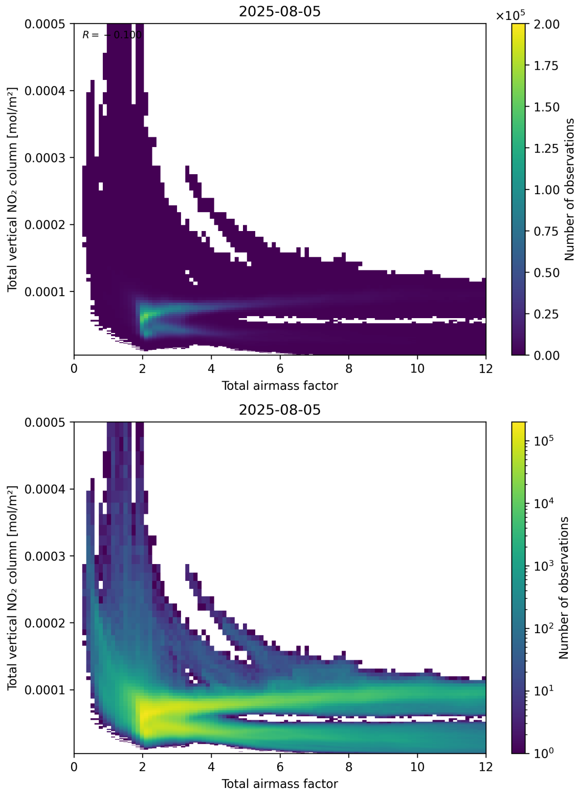
Figure 67: Scatter density plot of “Total airmass factor” against “Total vertical NO 2 column” for 2025-08-04 to 2025-08-06.
