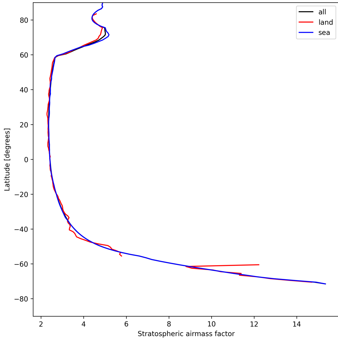
Figure 27: Zonal average of “Stratospheric airmass factor” for 2025-08-04 to 2025-08-06.
