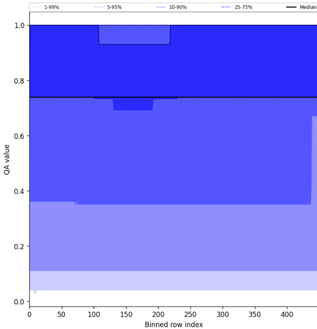
Figure 45: Along track statistics of “QA value” for 2025-08-04 to 2025-08-06
