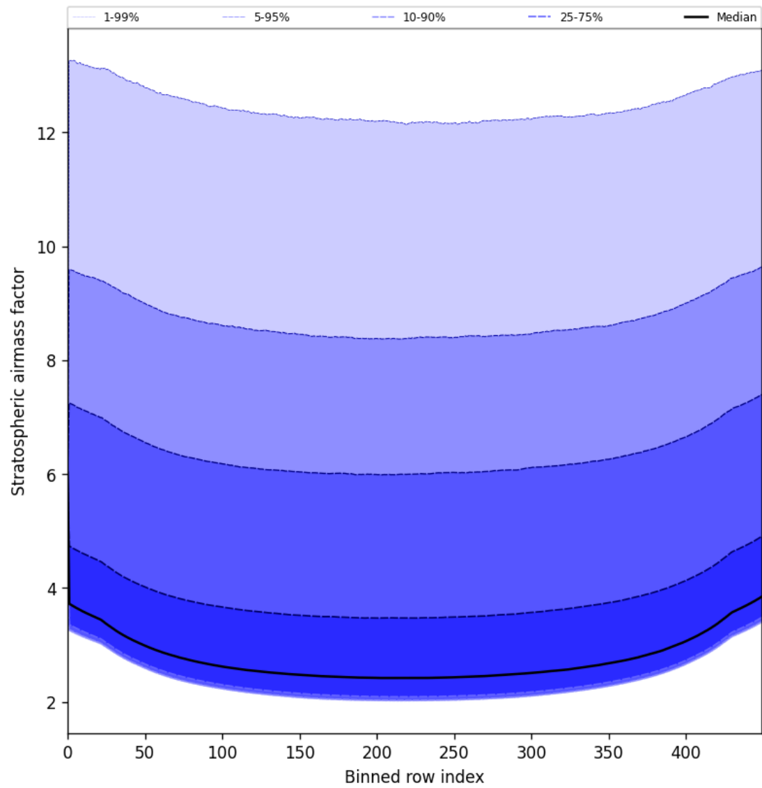
Figure 61: Along track statistics of “Stratospheric airmass factor” for 2025-08-04 to 2025-08-06
