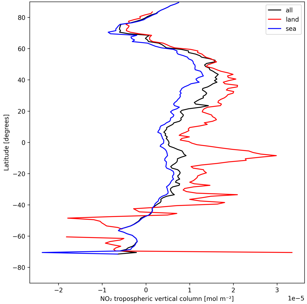
Figure 12: Zonal average of “NO 2 tropospheric vertical column” for 2025-08-04 to 2025-08-06.
