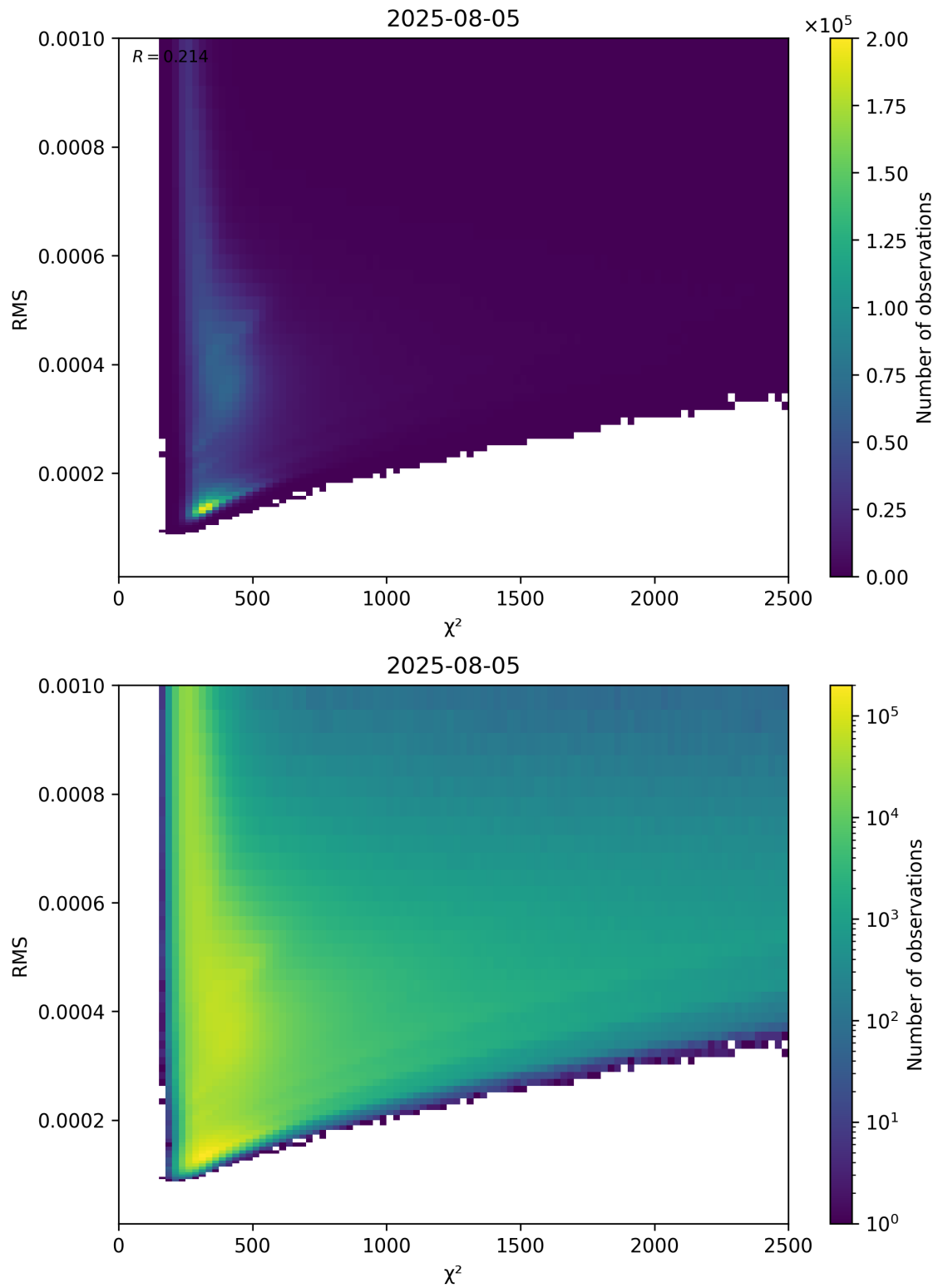
Figure 82: Scatter density plot of “ \chi^2 ” against “RMS” for 2025-08-04 to 2025-08-06.
