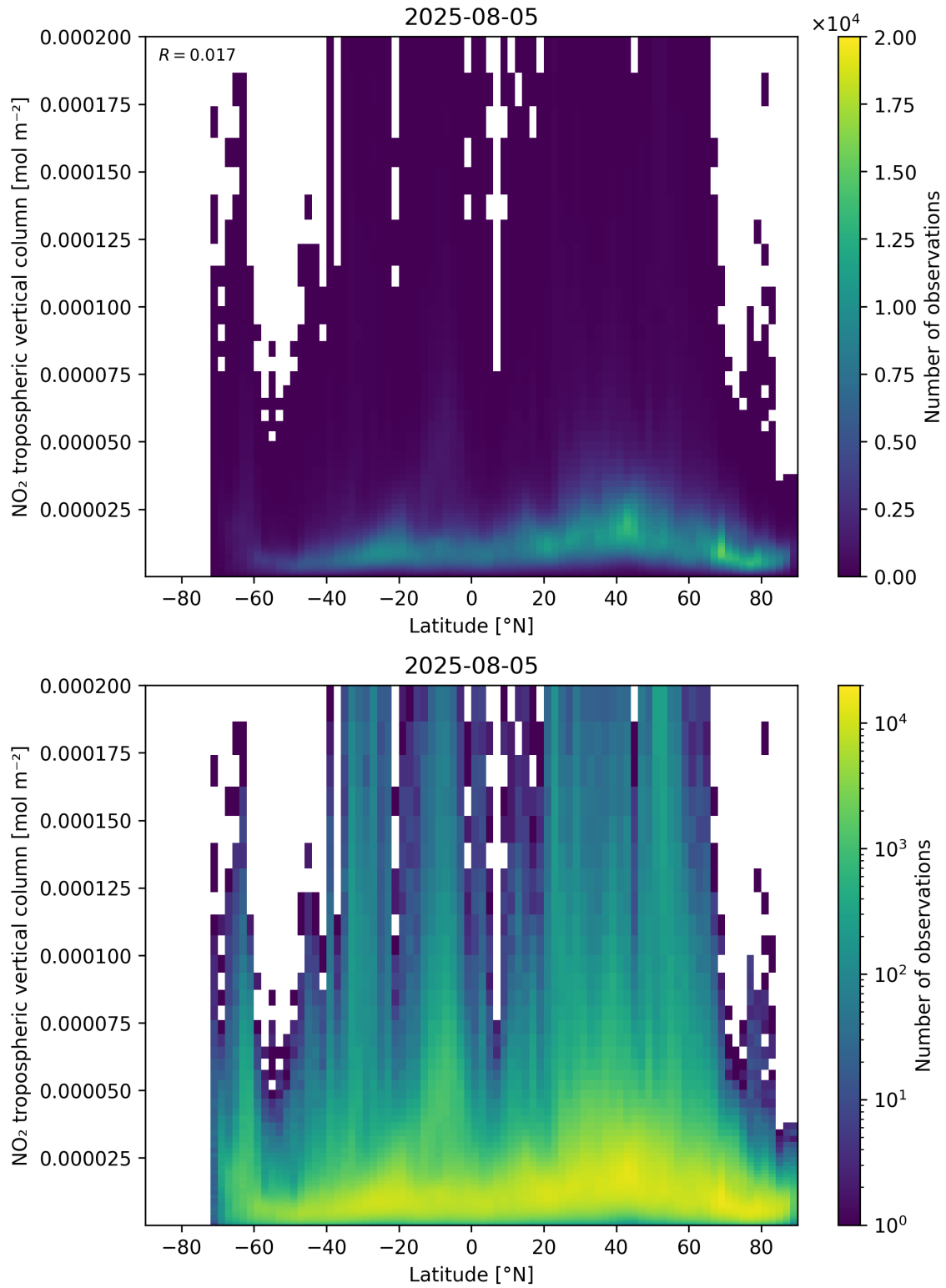
Figure 92: Scatter density plot of “Latitude” against “NO 2 tropospheric vertical column” for 2025-08-04 to 2025-08-06.
