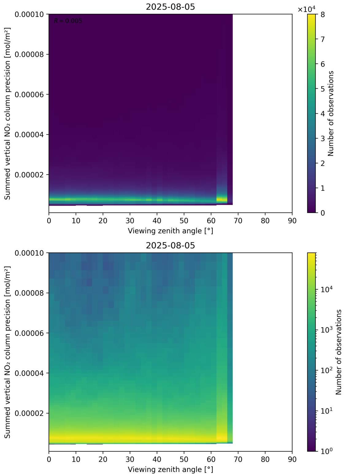
Figure 166: Scatter density plot of “Viewing zenith angle” against “Summed vertical NO 2 column precision” for 2025-08-04 to 2025-08-06.
