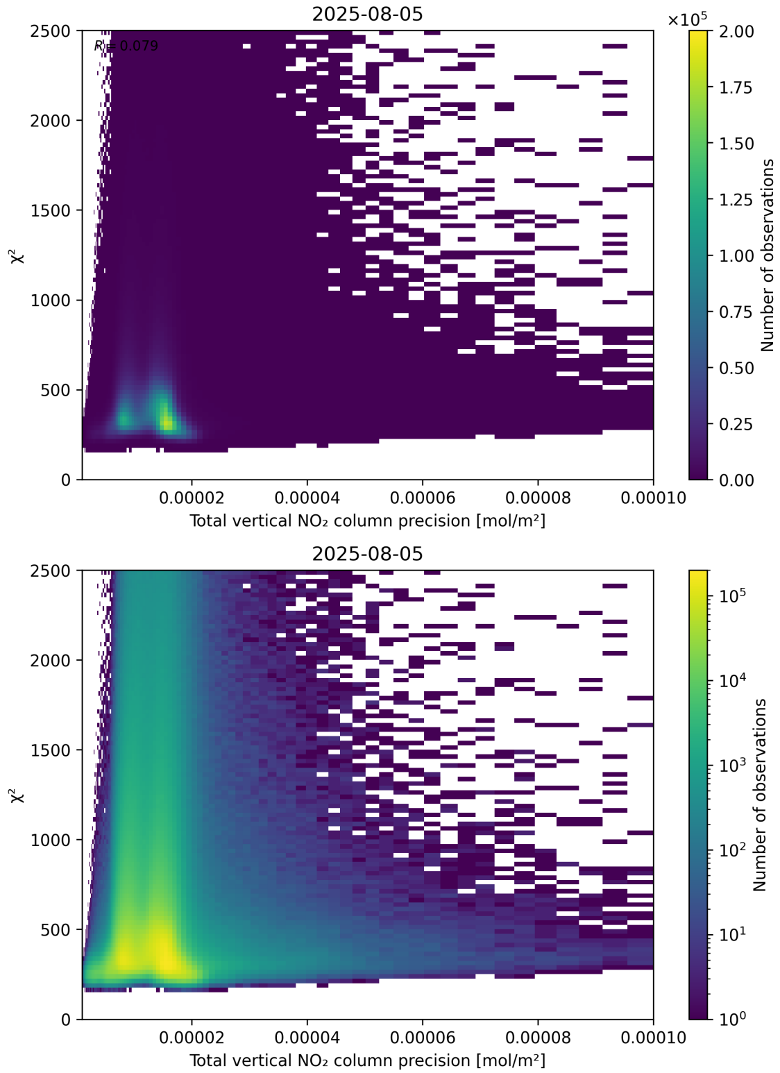
Figure 116: Scatter density plot of “Total vertical NO 2 column precision” against “ \chi^2 ” for 2025-08-04 to 2025-08-06.
