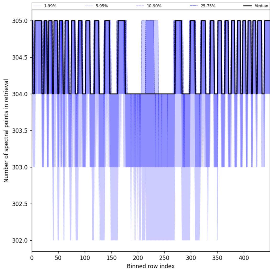
Figure 50: Along track statistics of “Number of spectral points in retrieval” for 2025-08-04 to 2025-08-06
