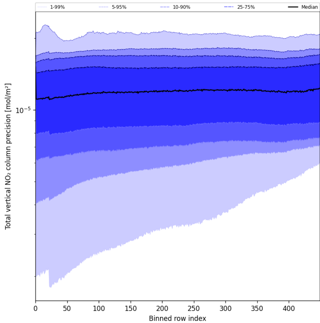
Figure 56: Along track statistics of “Total vertical NO 2 column precision” for 2025-08-04 to 2025-08-06
