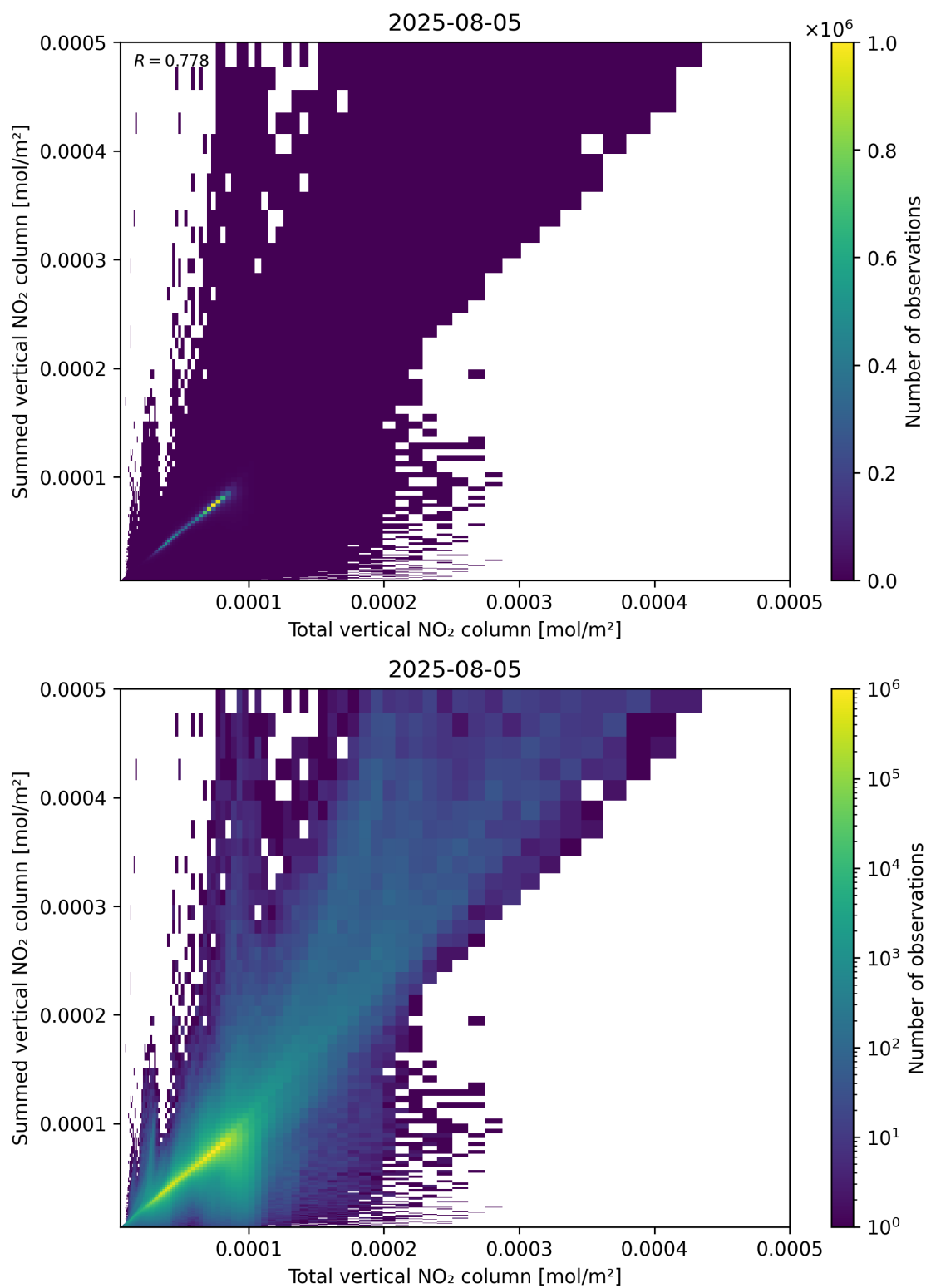
Figure 112: Scatter density plot of “Total vertical NO 2 column” against “Summed vertical NO 2 column” for 2025-08-04 to 2025-08-06.
