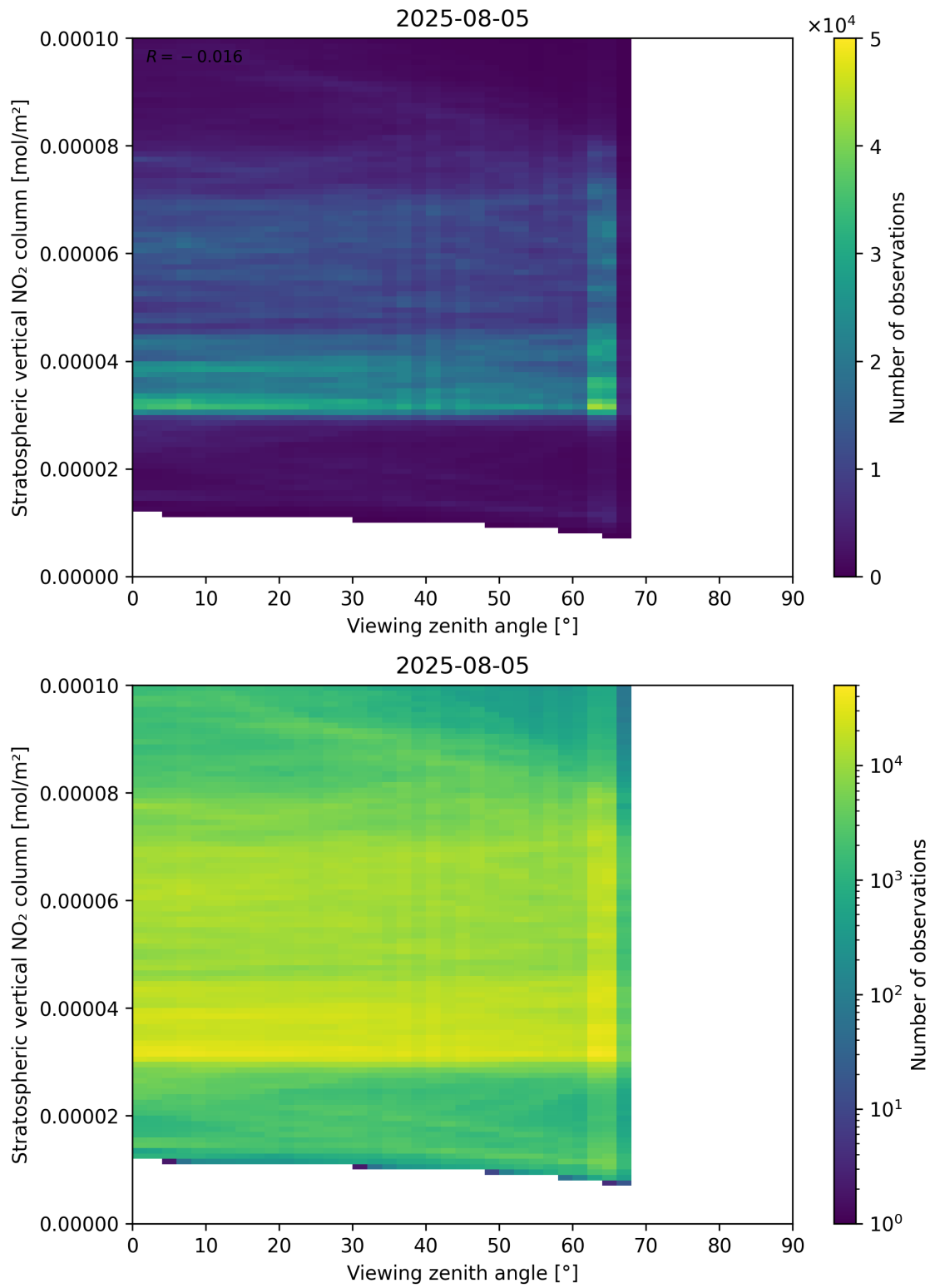
Figure 164: Scatter density plot of “Viewing zenith angle” against “Stratospheric vertical NO 2 column” for 2025-08-04 to 2025-08-06.
