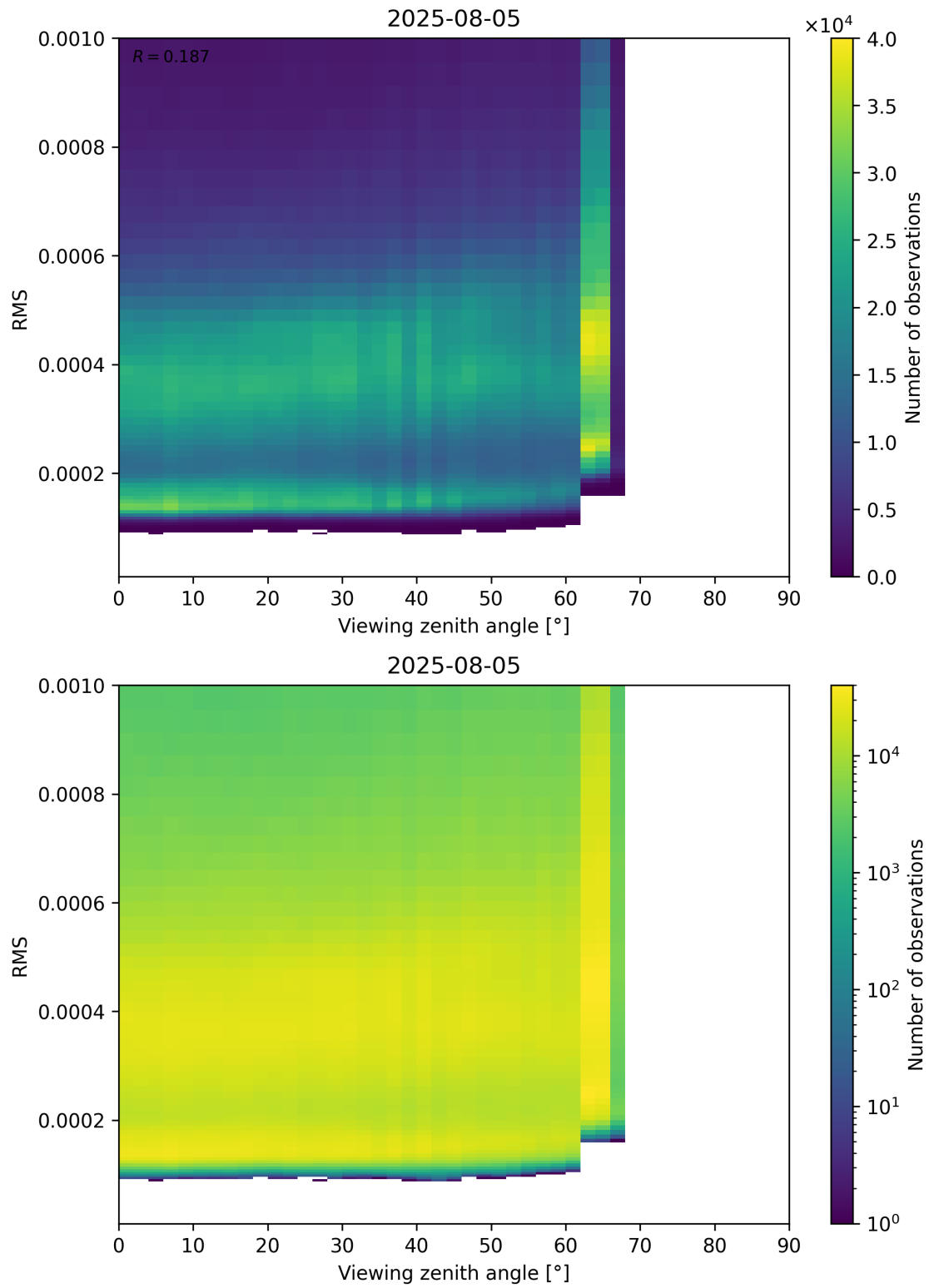
Figure 171: Scatter density plot of “Viewing zenith angle” against “RMS” for 2025-08-04 to 2025-08-06.
