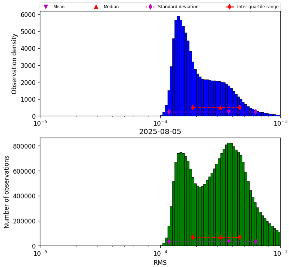
Figure 43: Histogram of “RMS” for 2025-08-04 to 2025-08-06
