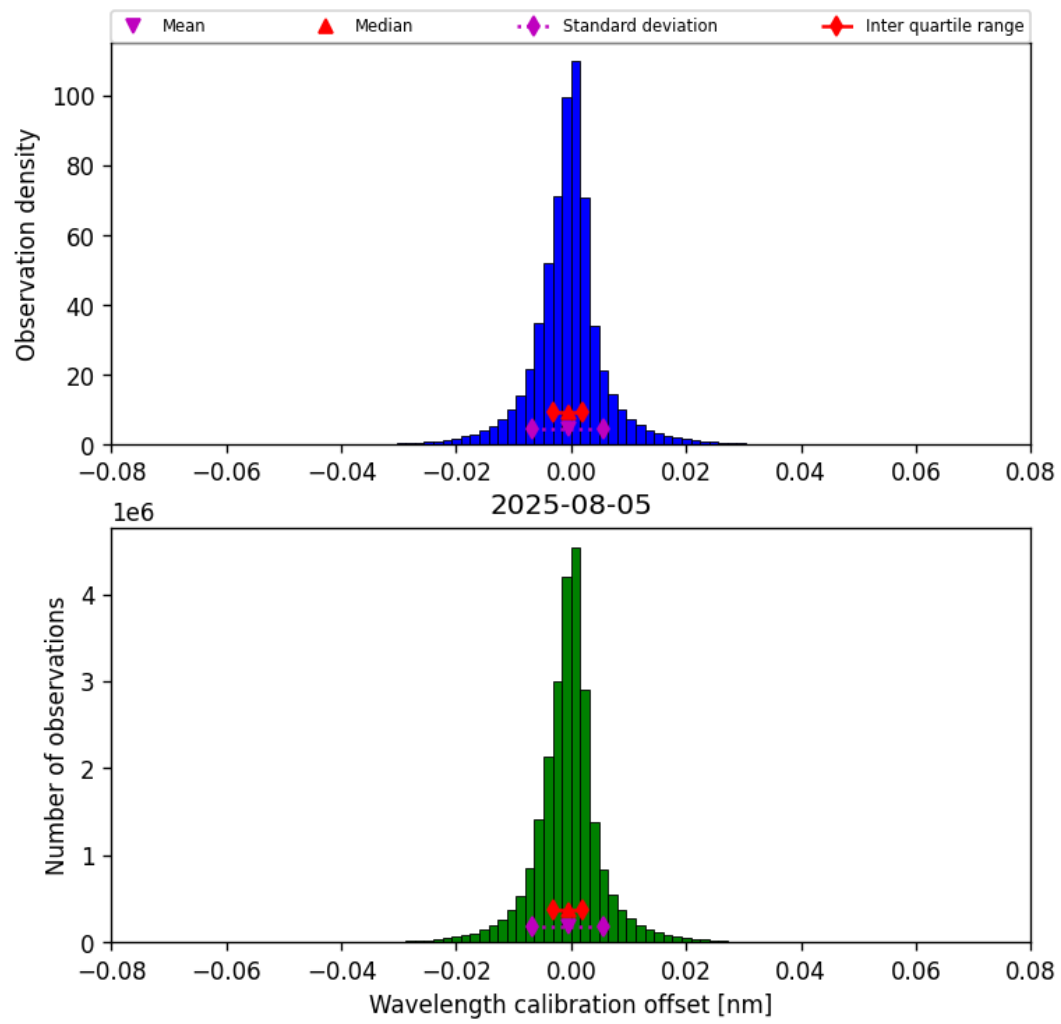
Figure 35: Histogram of “Wavelength calibration offset” for 2025-08-04 to 2025-08-06
