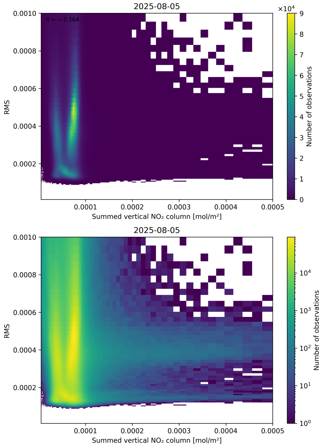
Figure 109: Scatter density plot of “Summed vertical NO 2 column” against “RMS” for 2025-08-04 to 2025-08-06.
