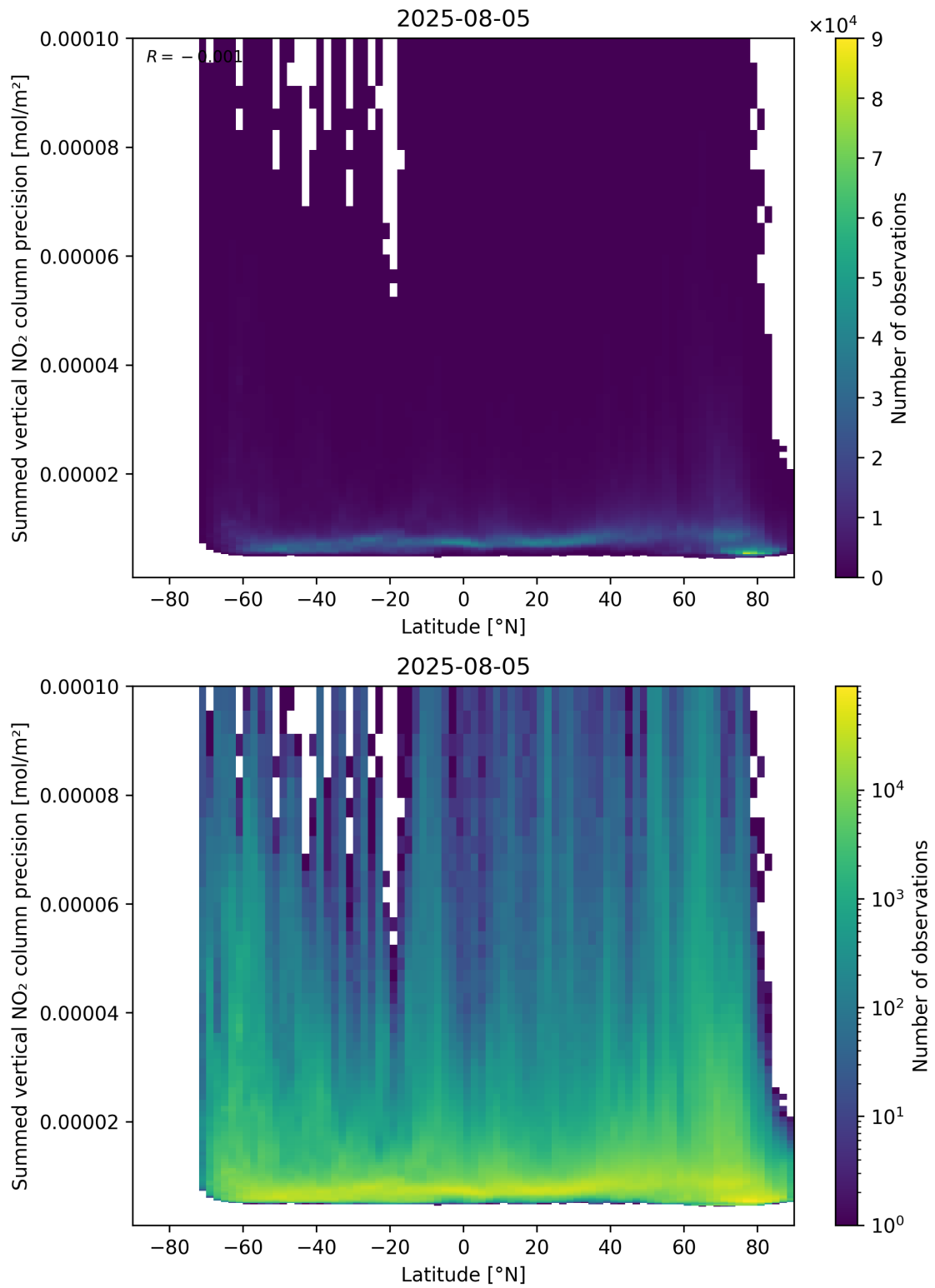
Figure 89: Scatter density plot of “Latitude” against “Summed vertical NO 2 column precision” for 2025-08-04 to 2025-08-06.
