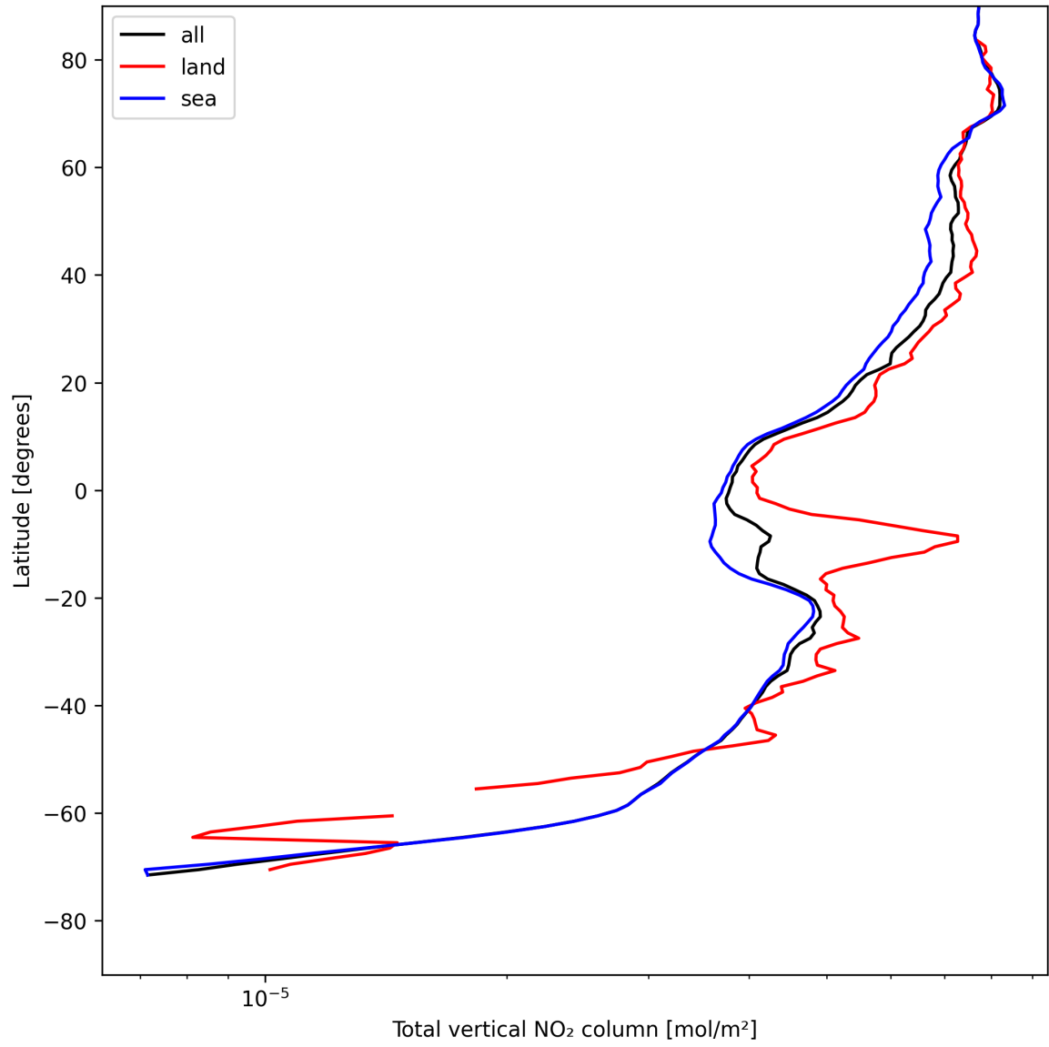
Figure 21: Zonal average of “Total vertical NO 2 column” for 2025-08-04 to 2025-08-06.
