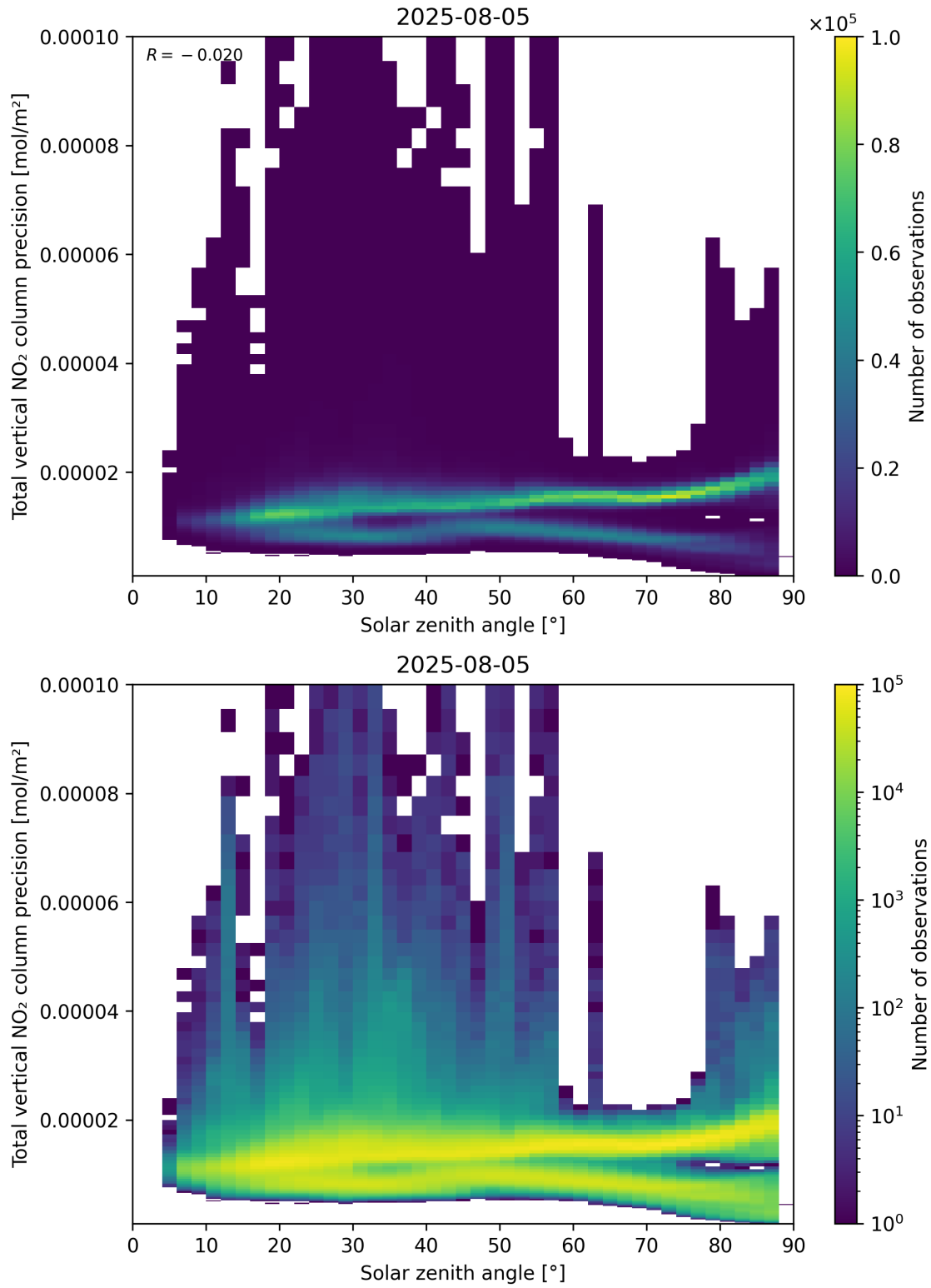
Figure 154: Scatter density plot of “Solar zenith angle” against “Total vertical NO 2 column precision” for 2025-08-04 to 2025-08-06.
