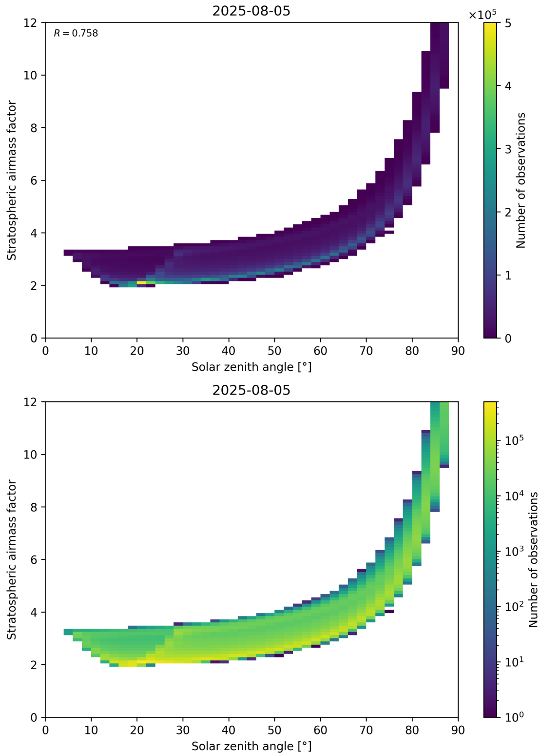
Figure 145: Scatter density plot of “Solar zenith angle” against “Stratospheric airmass factor” for 2025-08-04 to 2025-08-06.
