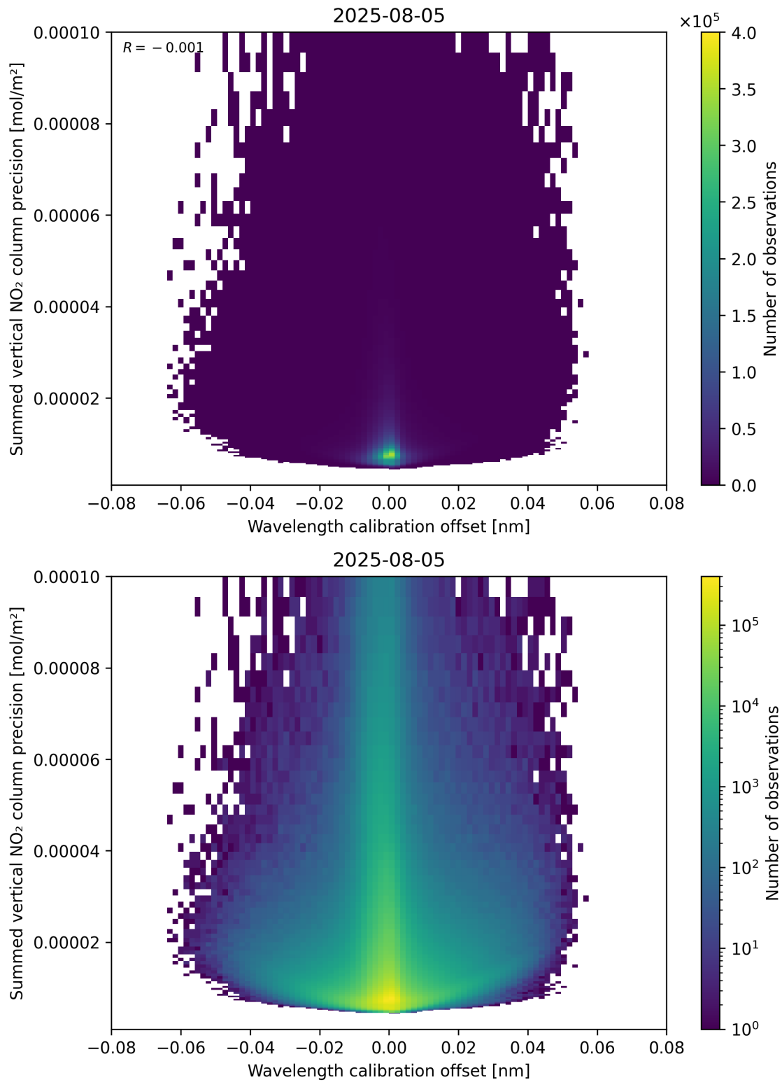
Figure 178: Scatter density plot of “Wavelength calibration offset” against “Summed vertical NO 2 column precision” for 2025-08-04 to 2025-08-06.
