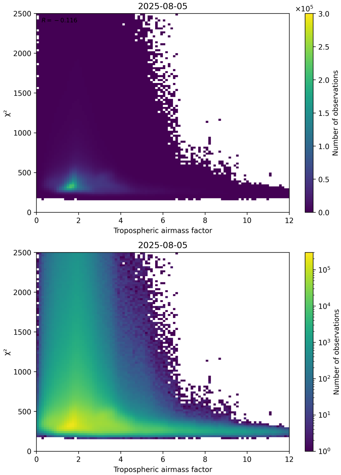
Figure 73: Scatter density plot of “Tropospheric airmass factor” against “ \chi^2 ” for 2025-08-04 to 2025-08-06.
