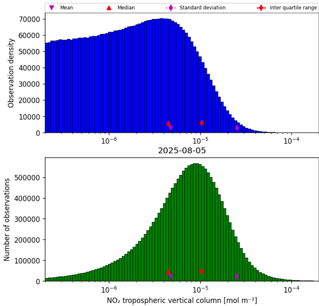
Figure 29: Histogram of “NO 2 tropospheric vertical column” for 2025-08-04 to 2025-08-06
