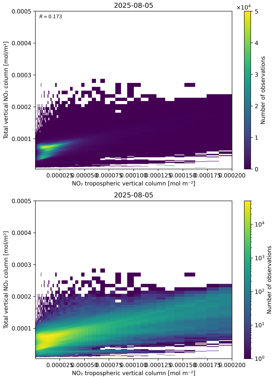
Figure 128: Scatter density plot of “NO 2 tropospheric vertical column” against “Total vertical NO 2 column” for 2025-08-04 to 2025-08-06.
