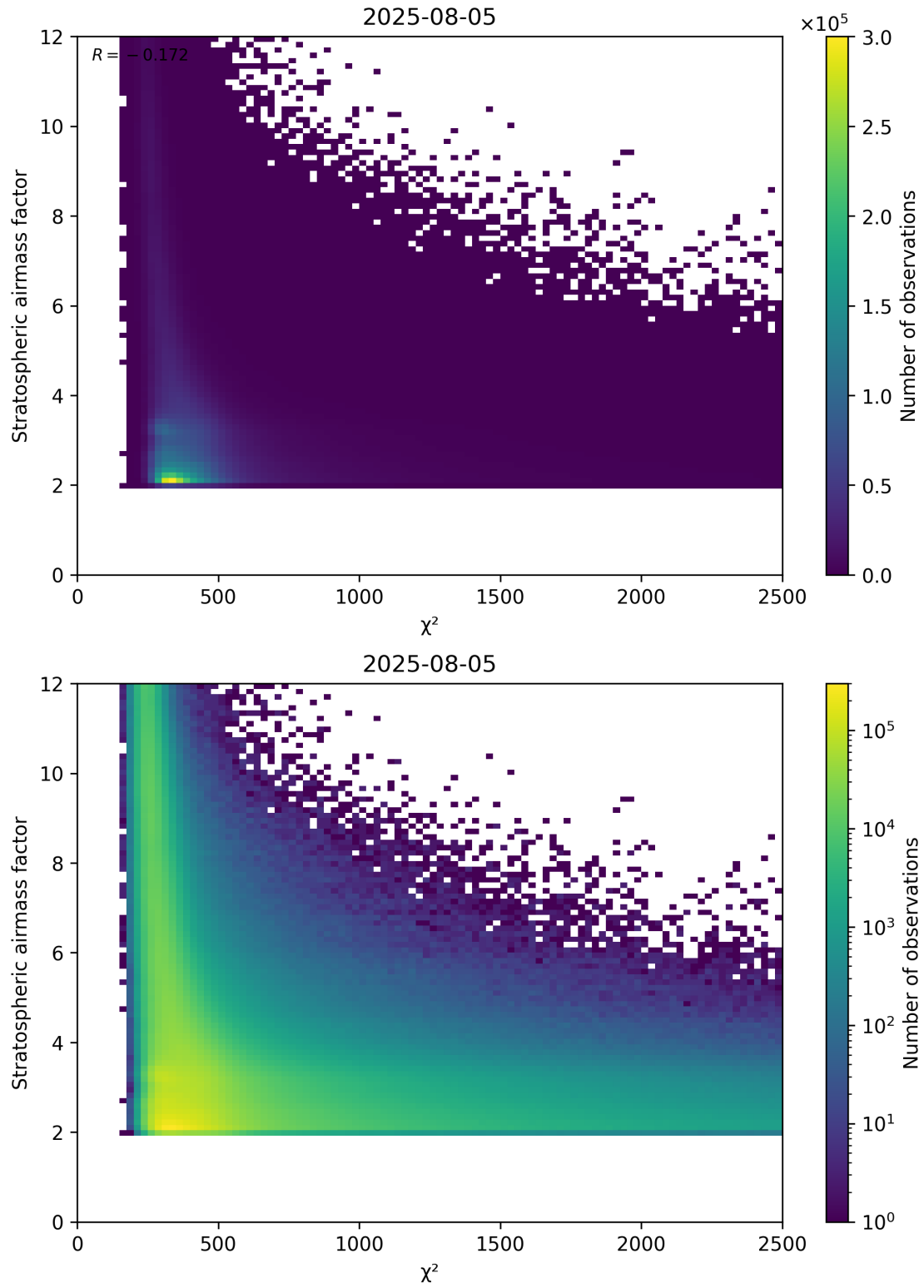
Figure 81: Scatter density plot of “ \chi^2 ” against “Stratospheric airmass factor” for 2025-08-04 to 2025-08-06.
