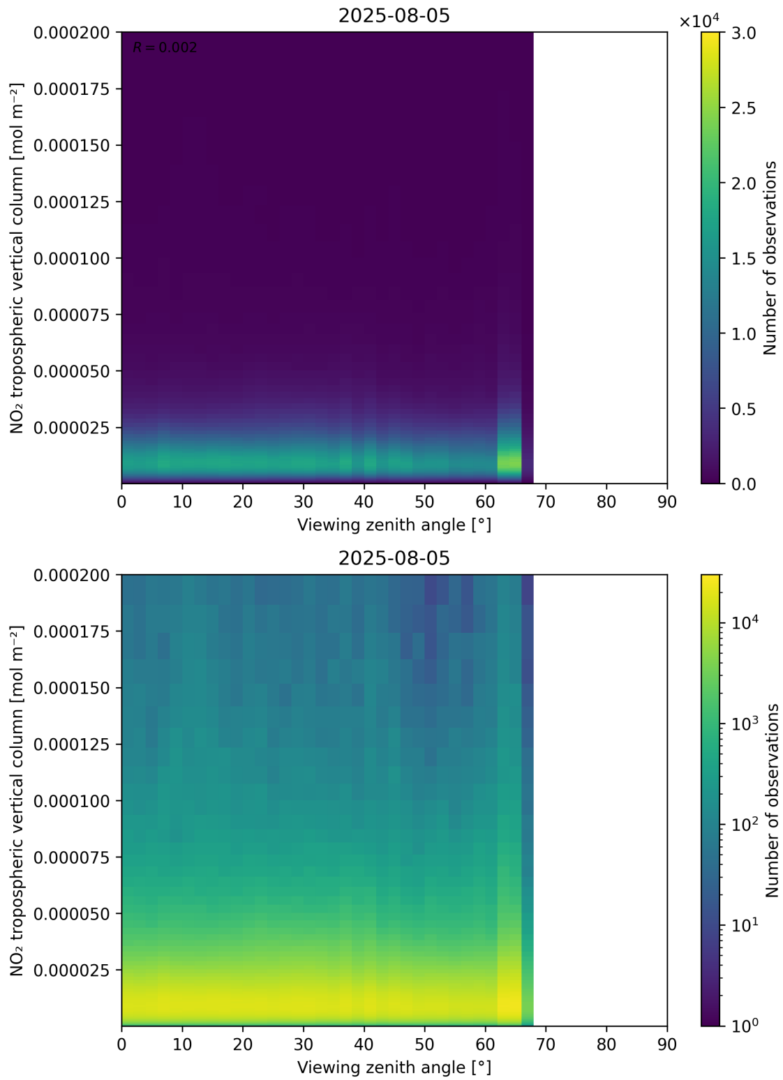
Figure 169: Scatter density plot of “Viewing zenith angle” against “NO 2 tropospheric vertical column” for 2025-08-04 to 2025-08-06.
