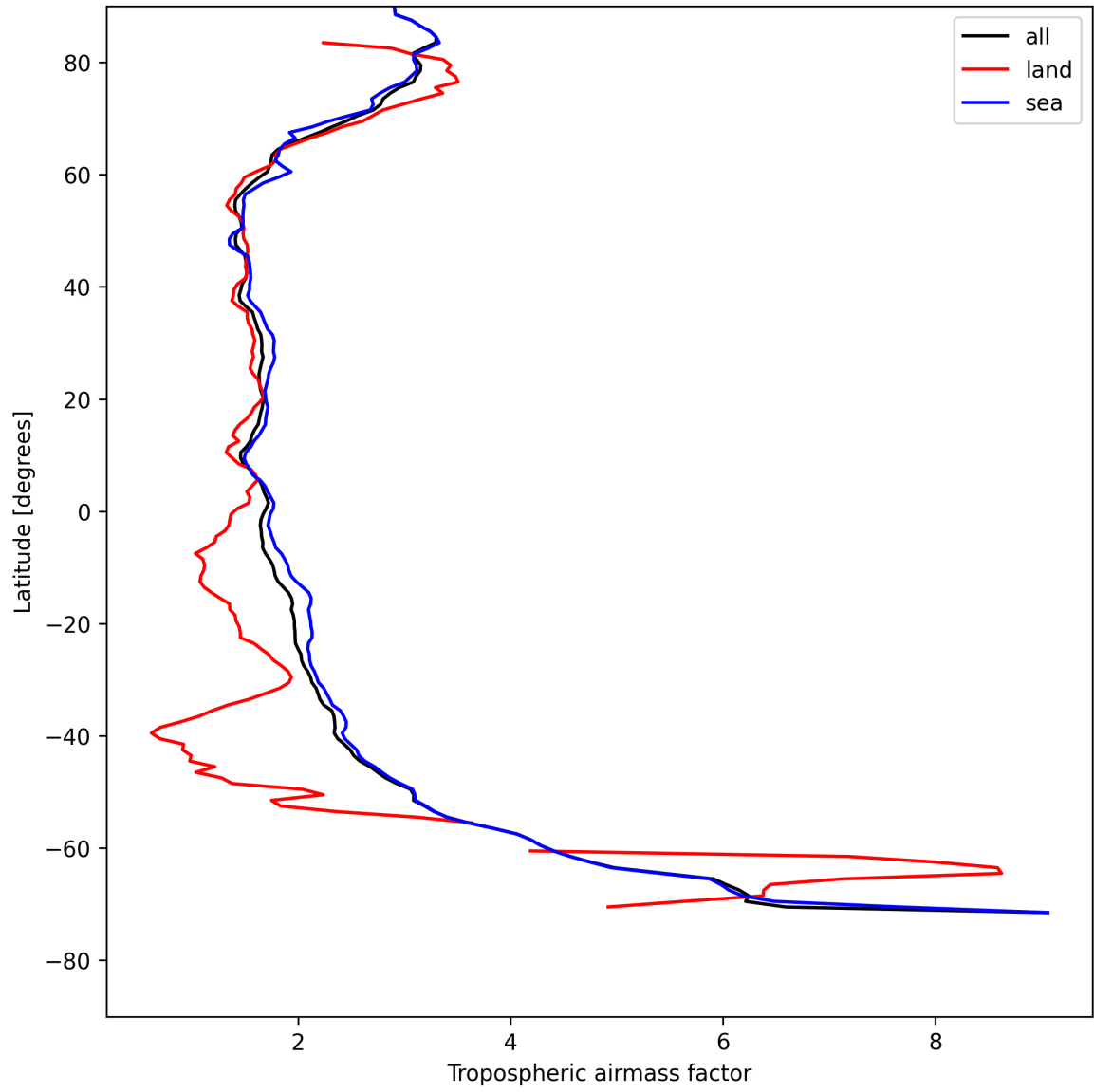
Figure 14: Zonal average of “Tropospheric airmass factor” for 2025-08-04 to 2025-08-06.
