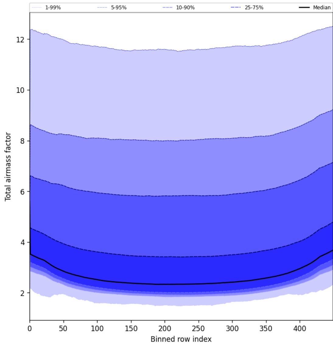
Figure 49: Along track statistics of “Total airmass factor” for 2025-08-04 to 2025-08-06
