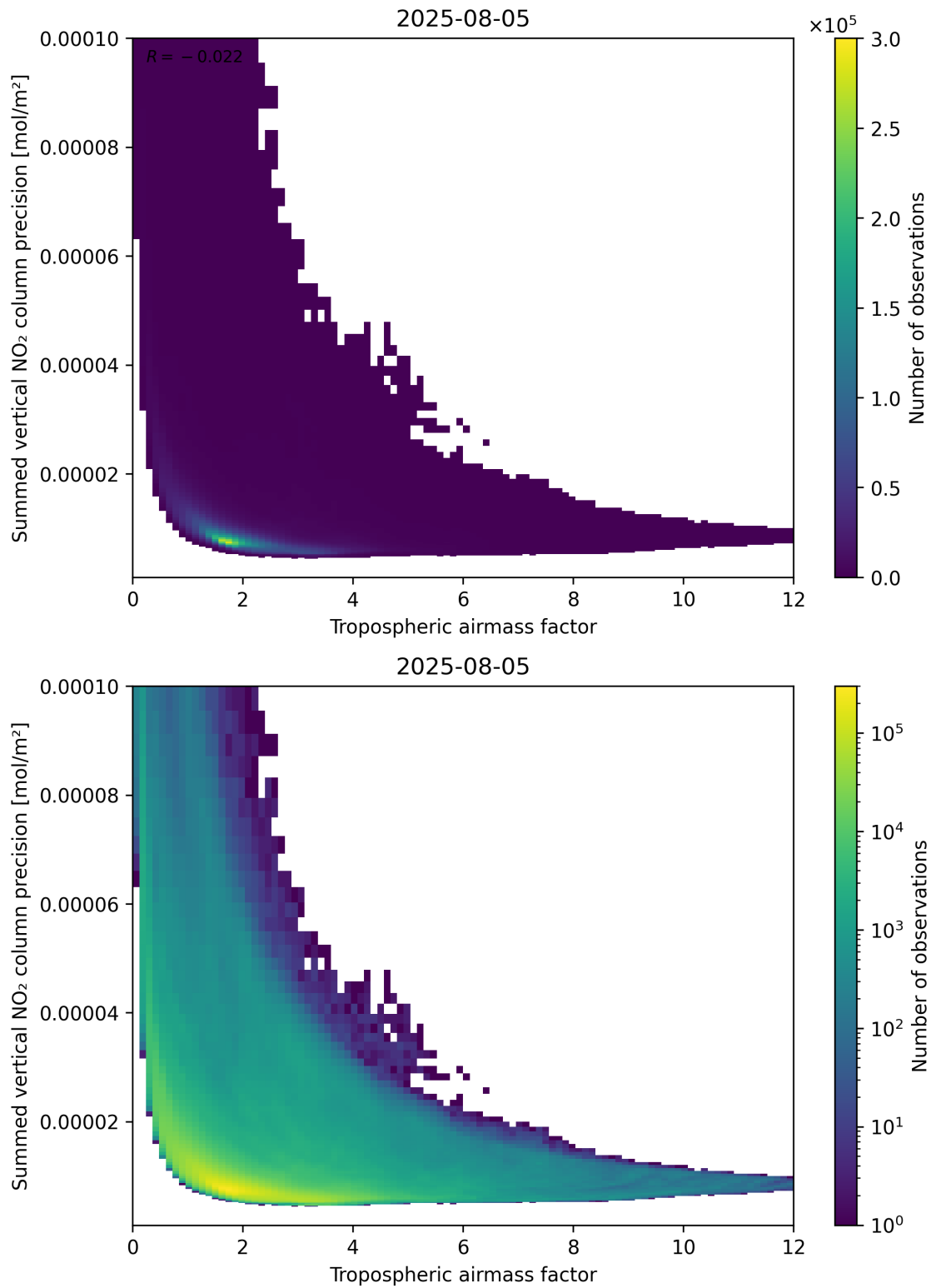
Figure 76: Scatter density plot of “Tropospheric air mass factor” against “Summed vertical NO 2 column precision” for 2025-08-04 to 2025-08-06.
