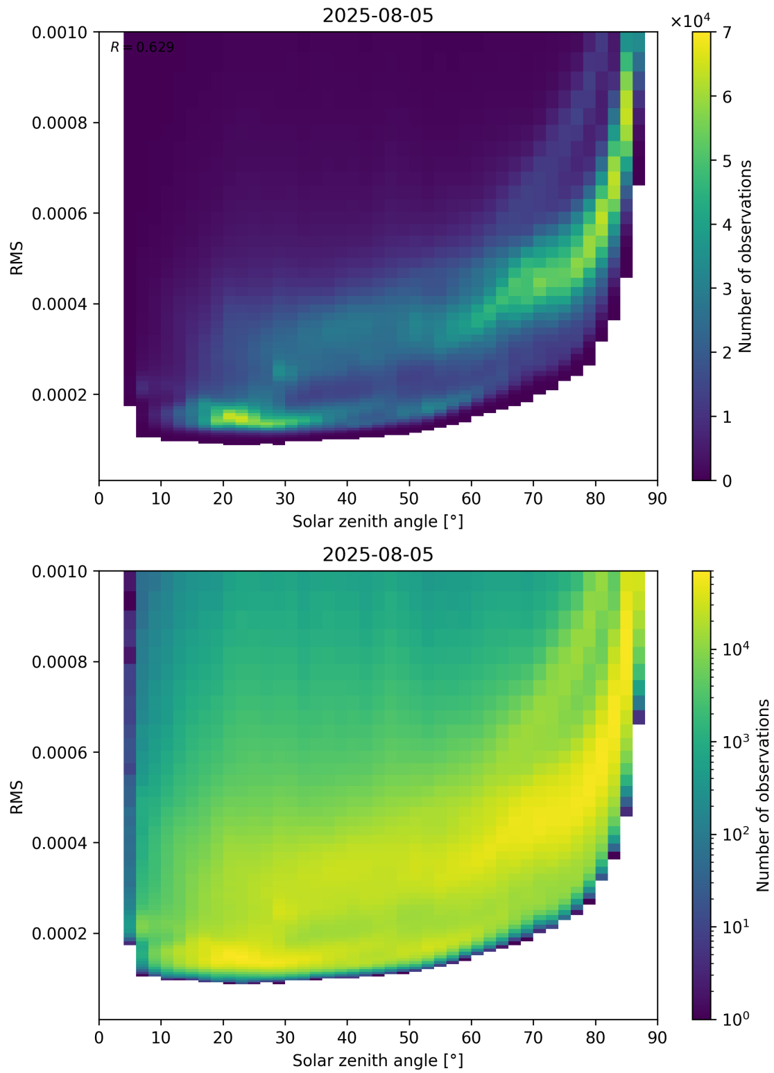
Figure 157: Scatter density plot of “Solar zenith angle” against “RMS” for 2025-08-04 to 2025-08-06.
