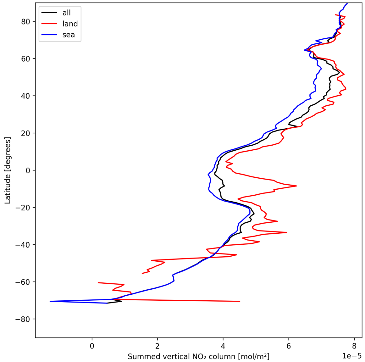
Figure 23: Zonal average of “Summed vertical NO 2 column” for 2025-08-04 to 2025-08-06.
