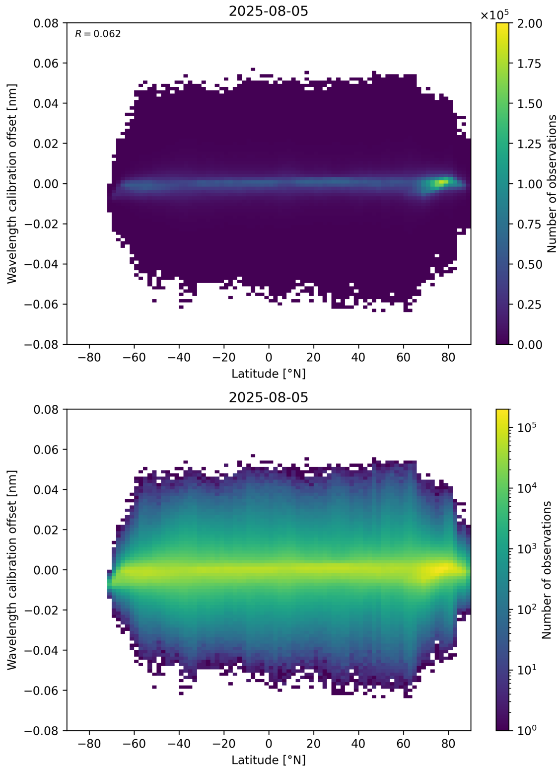
Figure 95: Scatter density plot of “Latitude” against “Wavelength calibration offset” for 2025-08-04 to 2025-08-06.
