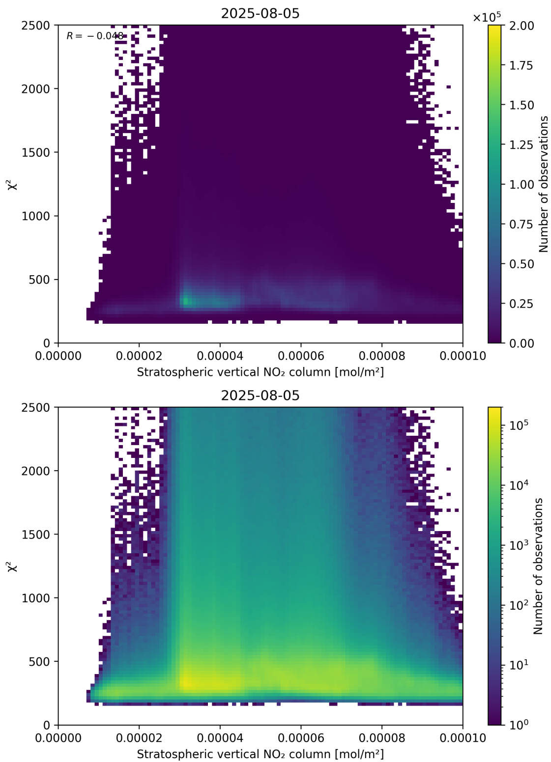
Figure 97: Scatter density plot of “Stratospheric vertical NO 2 column” against “ \chi^2 ” for 2025-08-04 to 2025-08-06.
