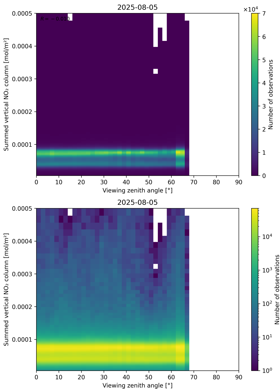
Figure 165: Scatter density plot of “Viewing zenith angle” against “Summed vertical NO 2 column” for 2025-08-04 to 2025-08-06.
