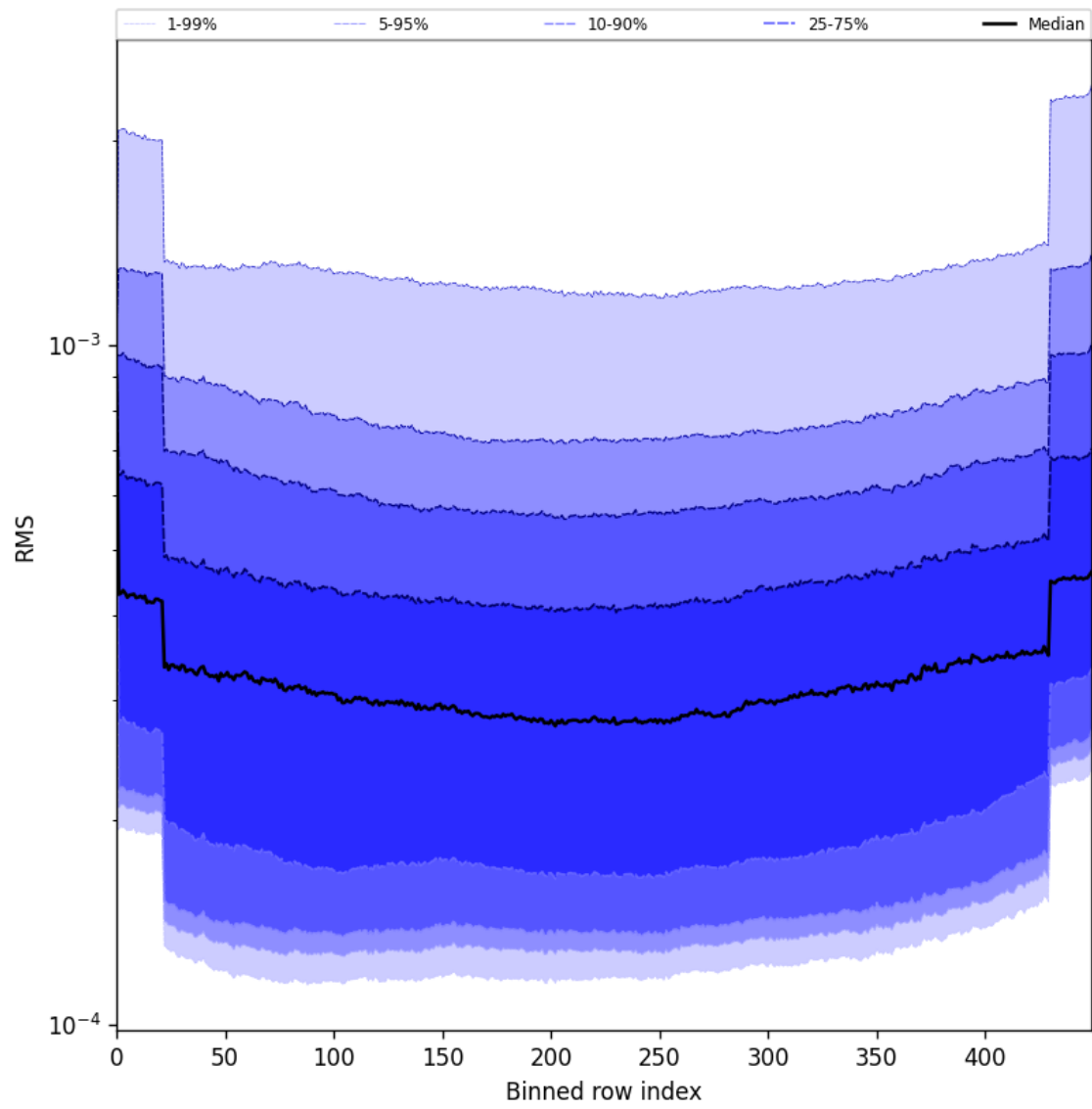
Figure 60: Along track statistics of “RMS” for 2025-08-04 to 2025-08-06
