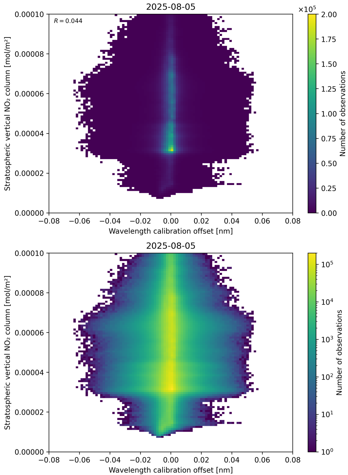
Figure 176: Scatter density plot of “Wavelength calibration offset” against “Stratospheric vertical NO 2 column” for 2025-08-04 to 2025-08-06.
