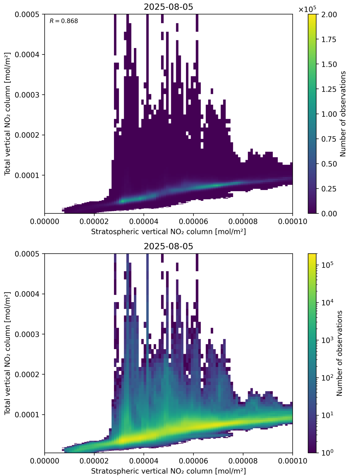
Figure 100: Scatter density plot of “Stratospheric vertical NO 2 column” against “Total vertical NO 2 column” for 2025-08-04 to 2025-08-06.
