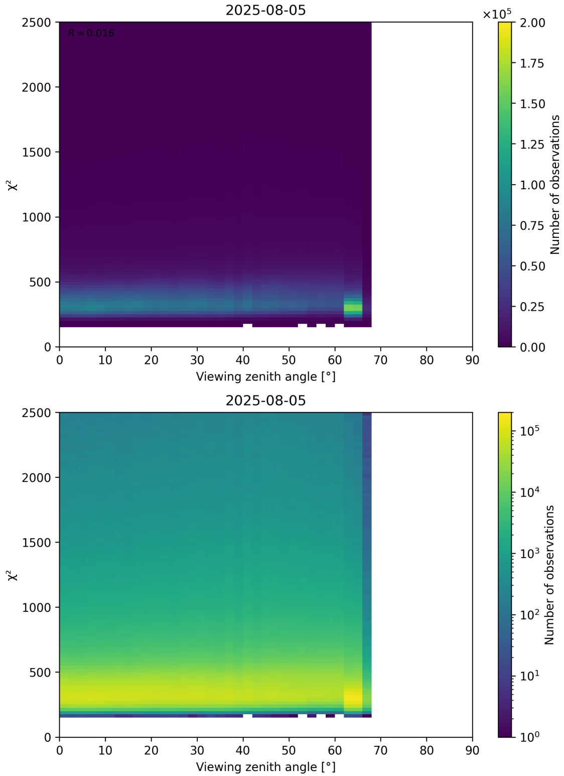
Figure 162: Scatter density plot of “Viewing zenith angle” against “ \chi^2 ” for 2025-08-04 to 2025-08-06.
