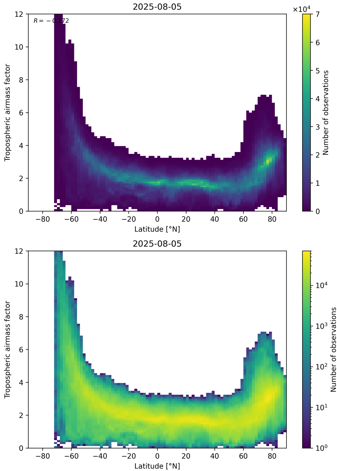
Figure 85: Scatter density plot of “Latitude” against “Tropospheric air mass factor” for 2025-08-04 to 2025-08-06.
