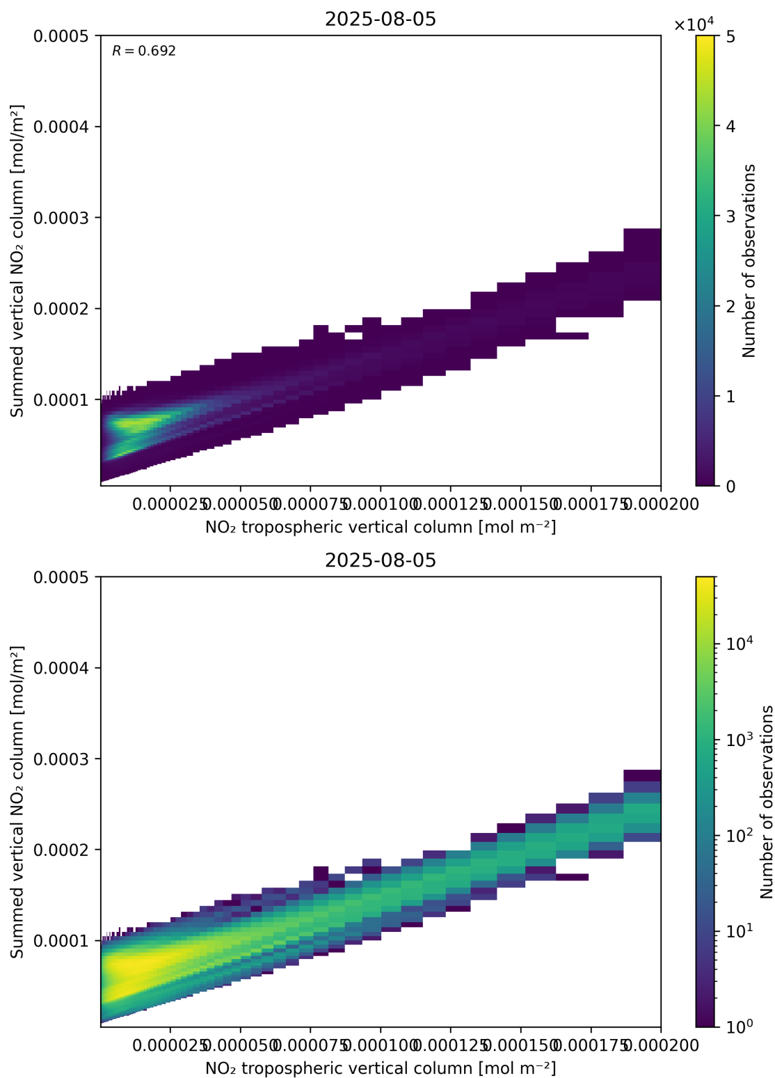
Figure 126: Scatter density plot of “NO 2 tropospheric vertical column” against “Summed vertical NO 2 column” for 2025-08-04 to 2025-08-06.
