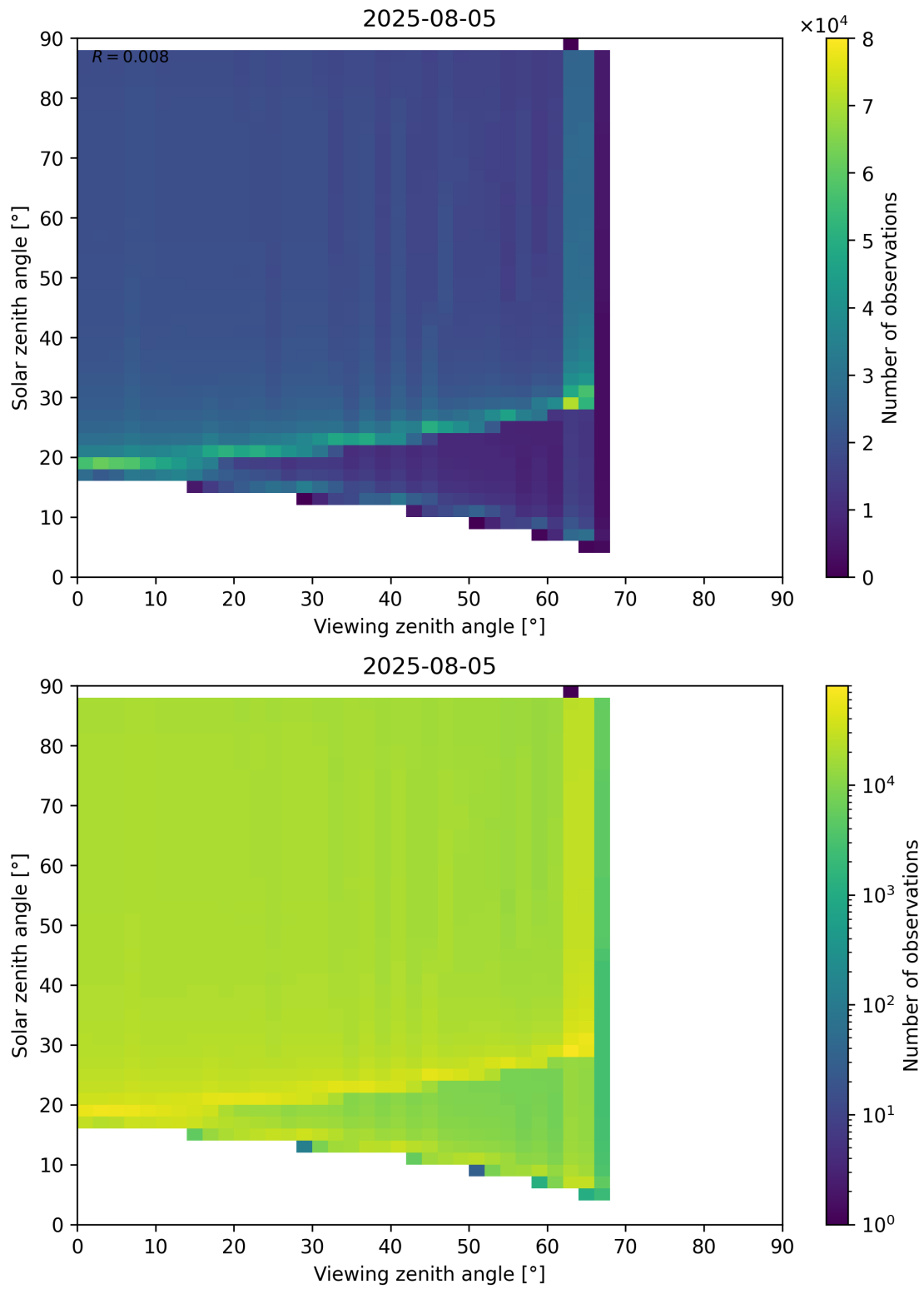
Figure 172: Scatter density plot of “Viewing zenith angle” against “Solar zenith angle” for 2025-08-04 to 2025-08-06.
