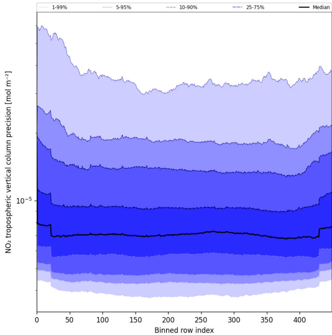
Figure 47: Along track statistics of “NO 2 tropospheric vertical column precision” for 2025-08-04 to 2025-08-06
