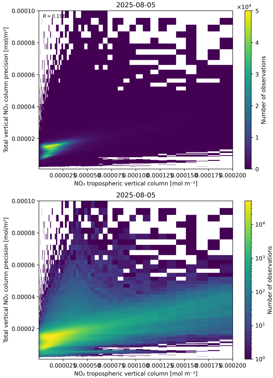
Figure 129: Scatter density plot of “NO 2 tropospheric vertical column” against “Total vertical NO 2 column precision” for 2025-08-04 to 2025-08-06.
