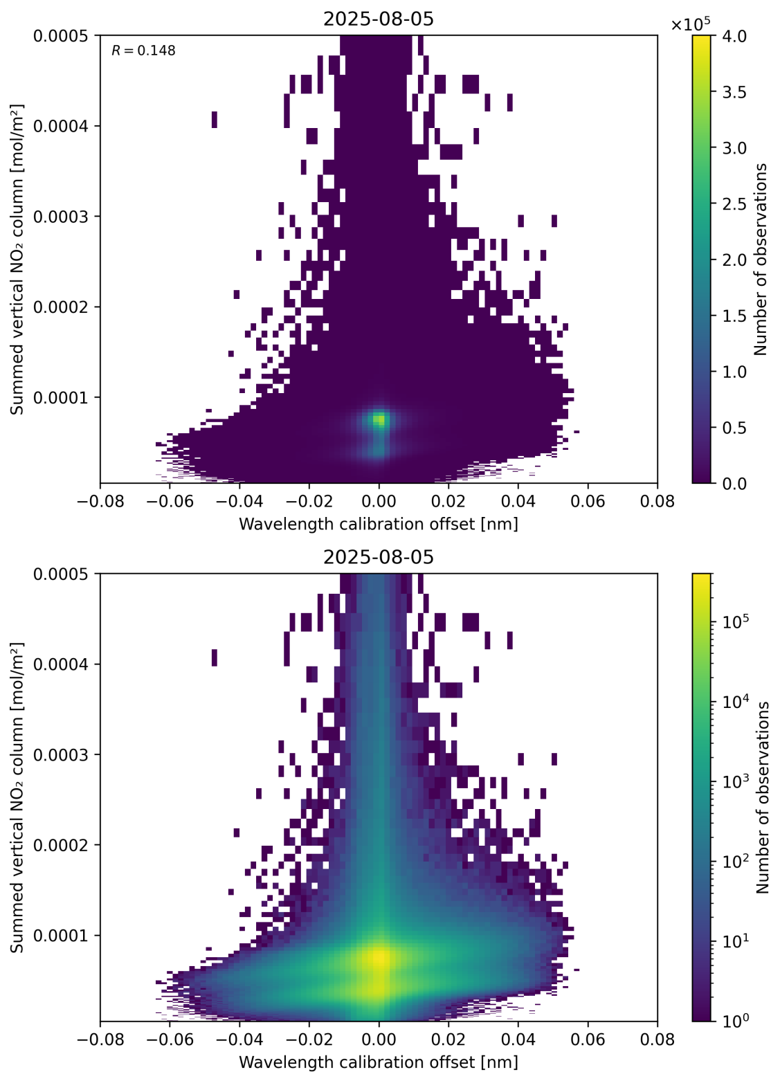
Figure 177: Scatter density plot of “Wavelength calibration offset” against “Summed vertical NO 2 column” for 2025-08-04 to 2025-08-06.
