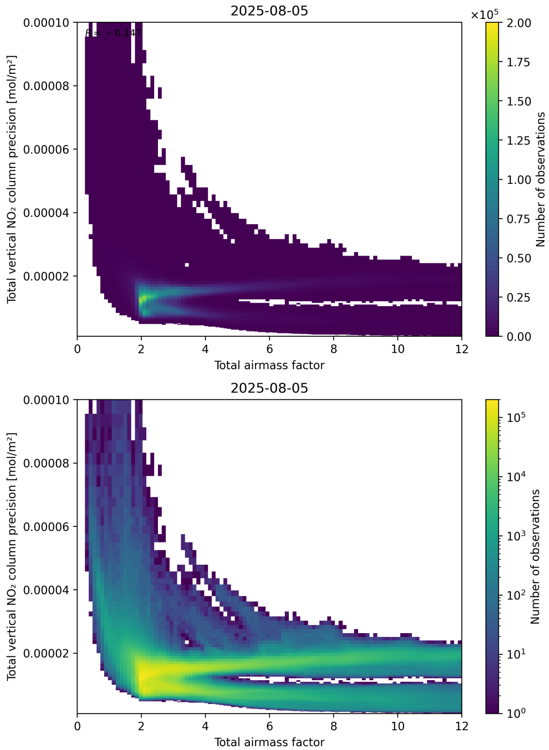
Figure 68: Scatter density plot of “Total airmass factor” against “Total vertical NO 2 column precision” for 2025-08-04 to 2025-08-06.
