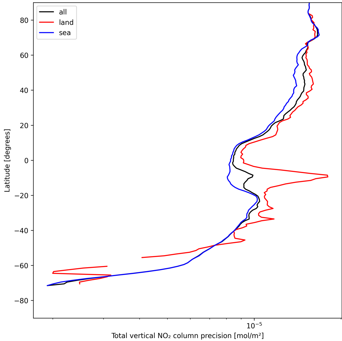
Figure 22: Zonal average of “Total vertical NO 2 column precision” for 2025-08-04 to 2025-08-06.
