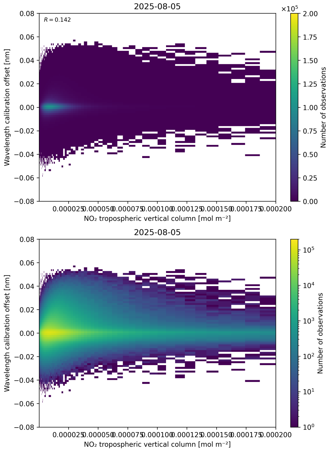
Figure 143: Scatter density plot of “NO 2 tropospheric vertical column” against “Wavelength calibration offset” for 2025-08-04 to 2025-08-06.
