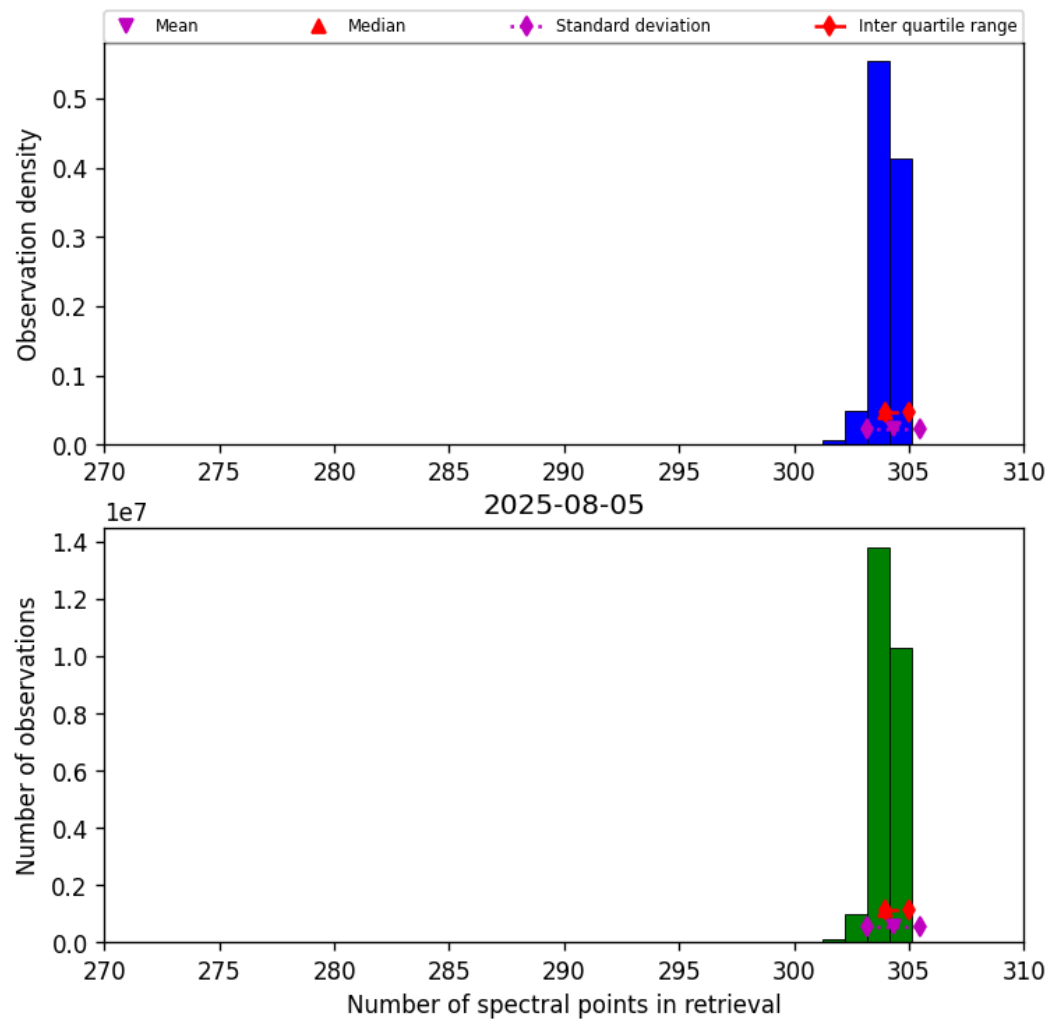
Figure 33: Histogram of “Number of spectral points in retrieval” for 2025-08-04 to 2025-08-06
