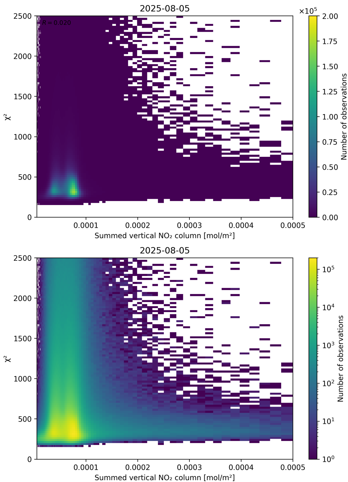
Figure 104: Scatter density plot of “Summed vertical NO 2 column” against “ \chi^2 ” for 2025-08-04 to 2025-08-06.
