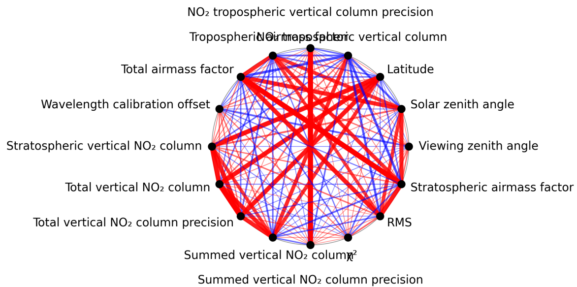
Figure 1: Map of correlation graph for 2025-08-04 to 2025-08-06.
