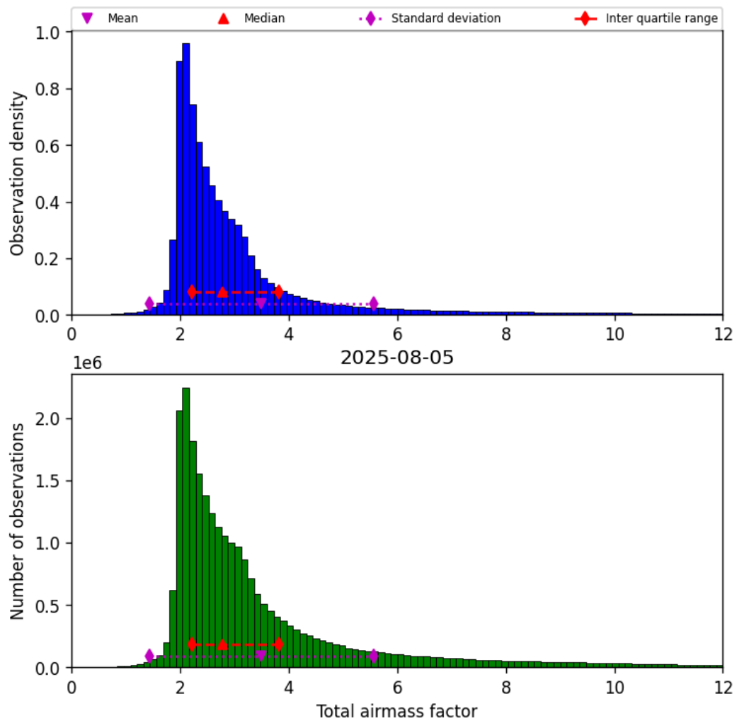
Figure 32: Histogram of “Total airmass factor” for 2025-08-04 to 2025-08-06
