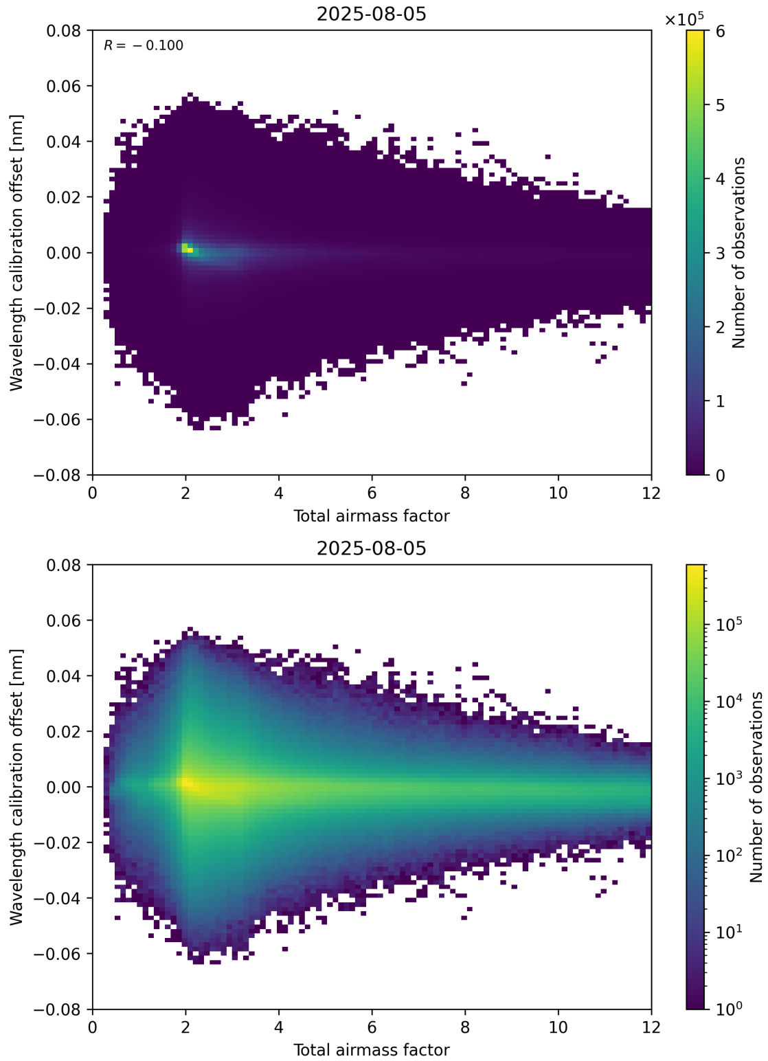
Figure 70: Scatter density plot of “Total airmass factor” against “Wavelength calibration offset” for 2025-08-04 to 2025-08-06.
