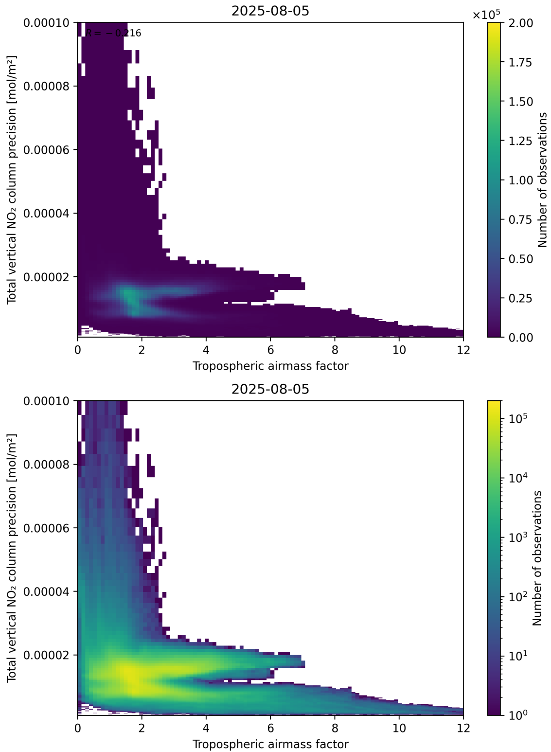
Figure 78: Scatter density plot of “Tropospheric air mass factor” against “Total vertical NO 2 column precision” for 2025-08-04 to 2025-08-06.
