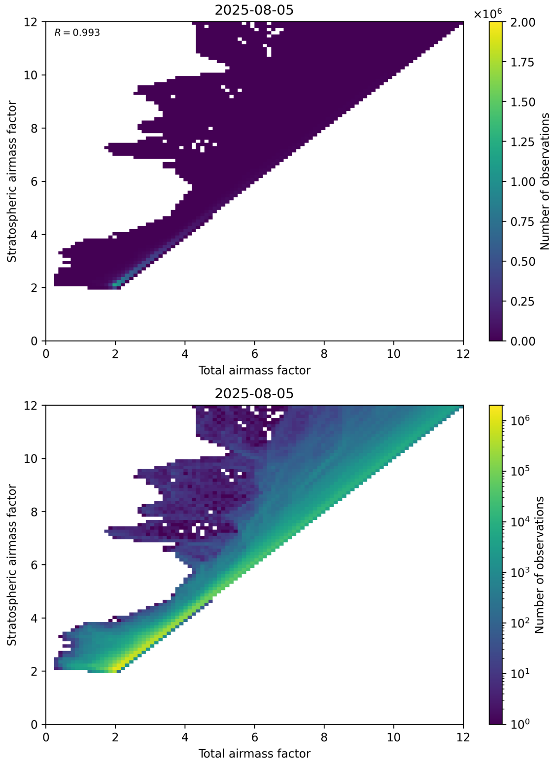
Figure 62: Scatter density plot of “Total airmass factor” against “Stratospheric airmass factor” for 2025-08-04 to 2025-08-06.
