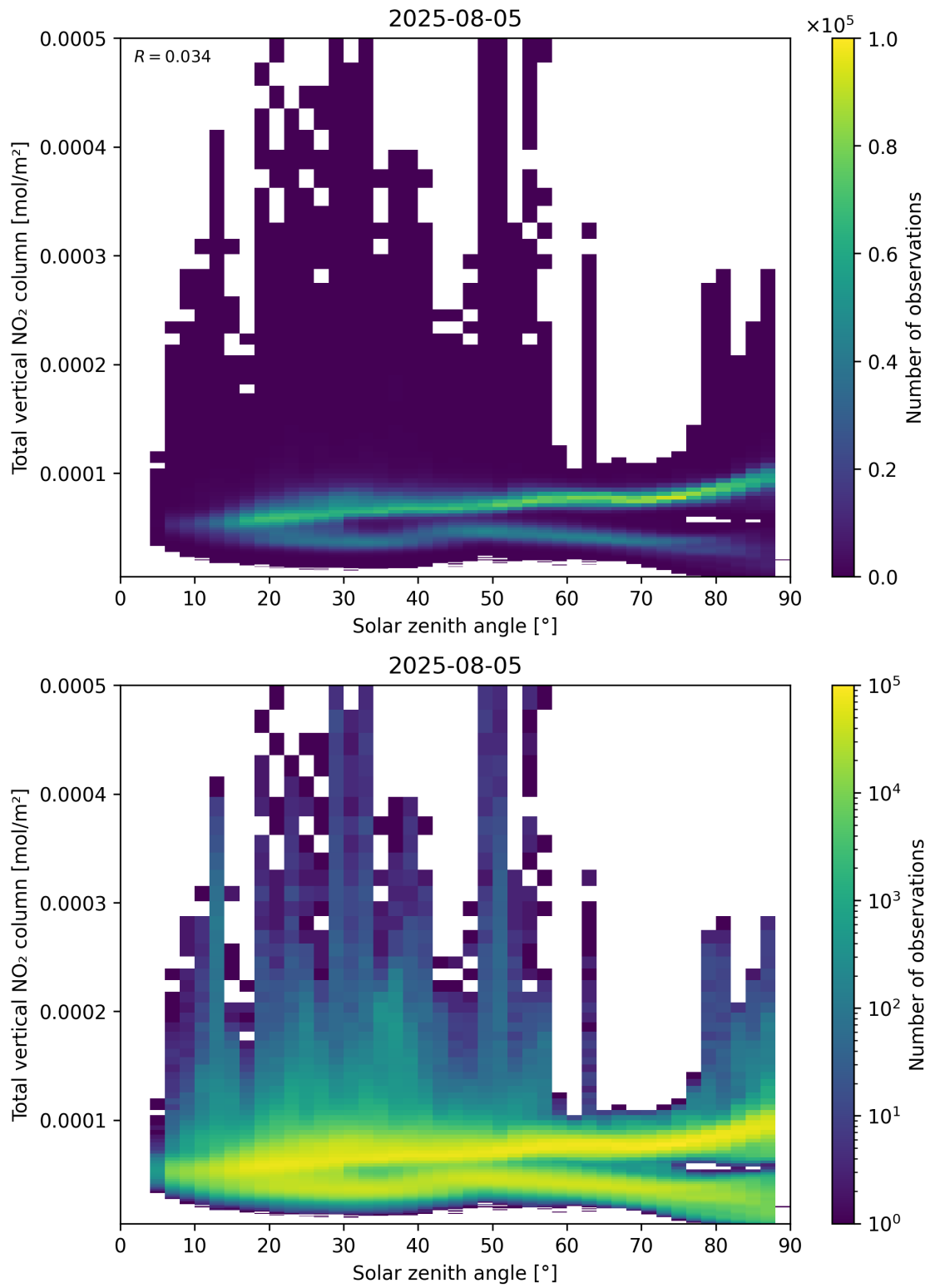
Figure 153: Scatter density plot of “Solar zenith angle” against “Total vertical NO 2 column” for 2025-08-04 to 2025-08-06.
