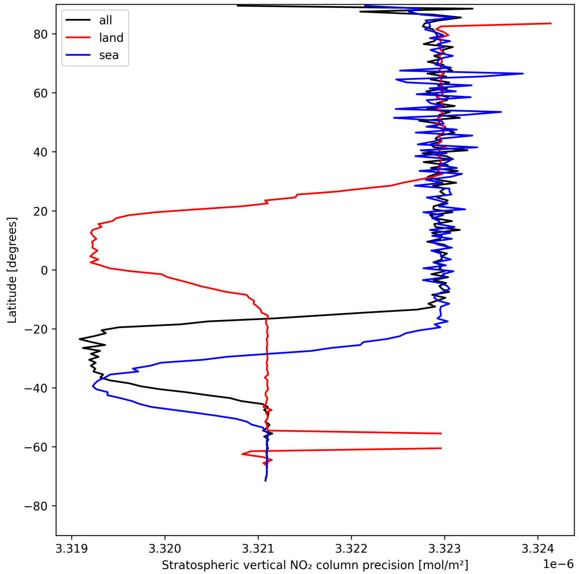
Figure 20: Zonal average of “Stratospheric vertical NO 2 column precision” for 2025-08-04 to 2025-08-06.
