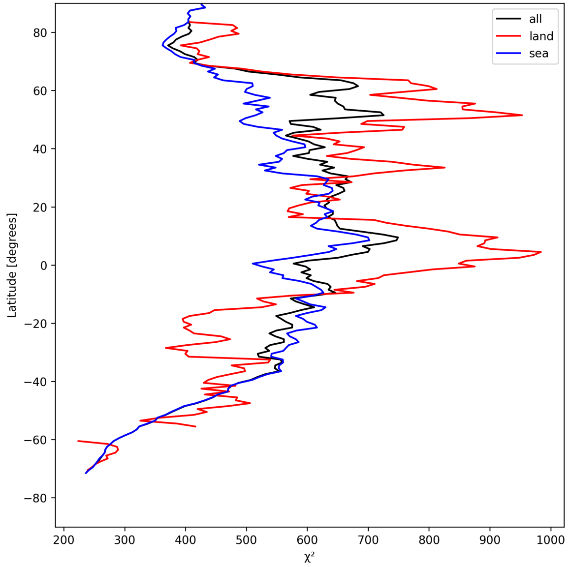
Figure 25: Zonal average of “ \chi^2 ” for 2025-08-04 to 2025-08-06.
