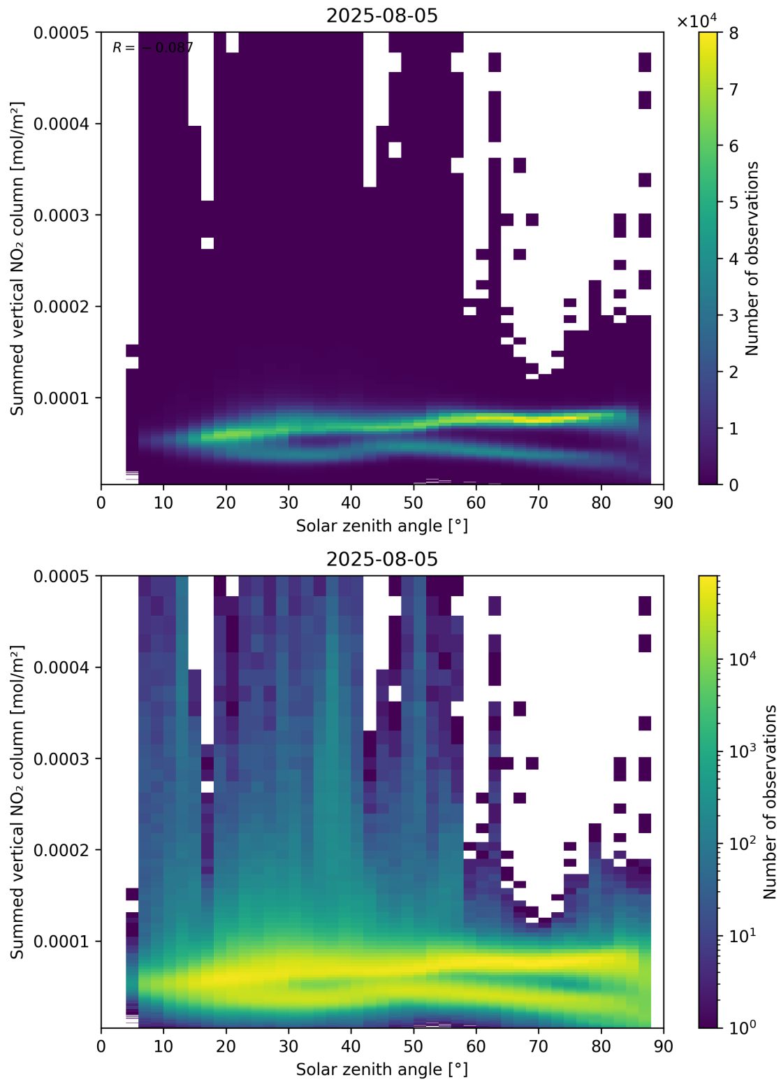
Figure 151: Scatter density plot of “Solar zenith angle” against “Summed vertical NO 2 column” for 2025-08-04 to 2025-08-06.
