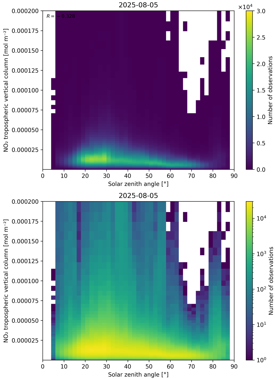
Figure 155: Scatter density plot of “Solar zenith angle” against “NO 2 tropospheric vertical column” for 2025-08-04 to 2025-08-06.
