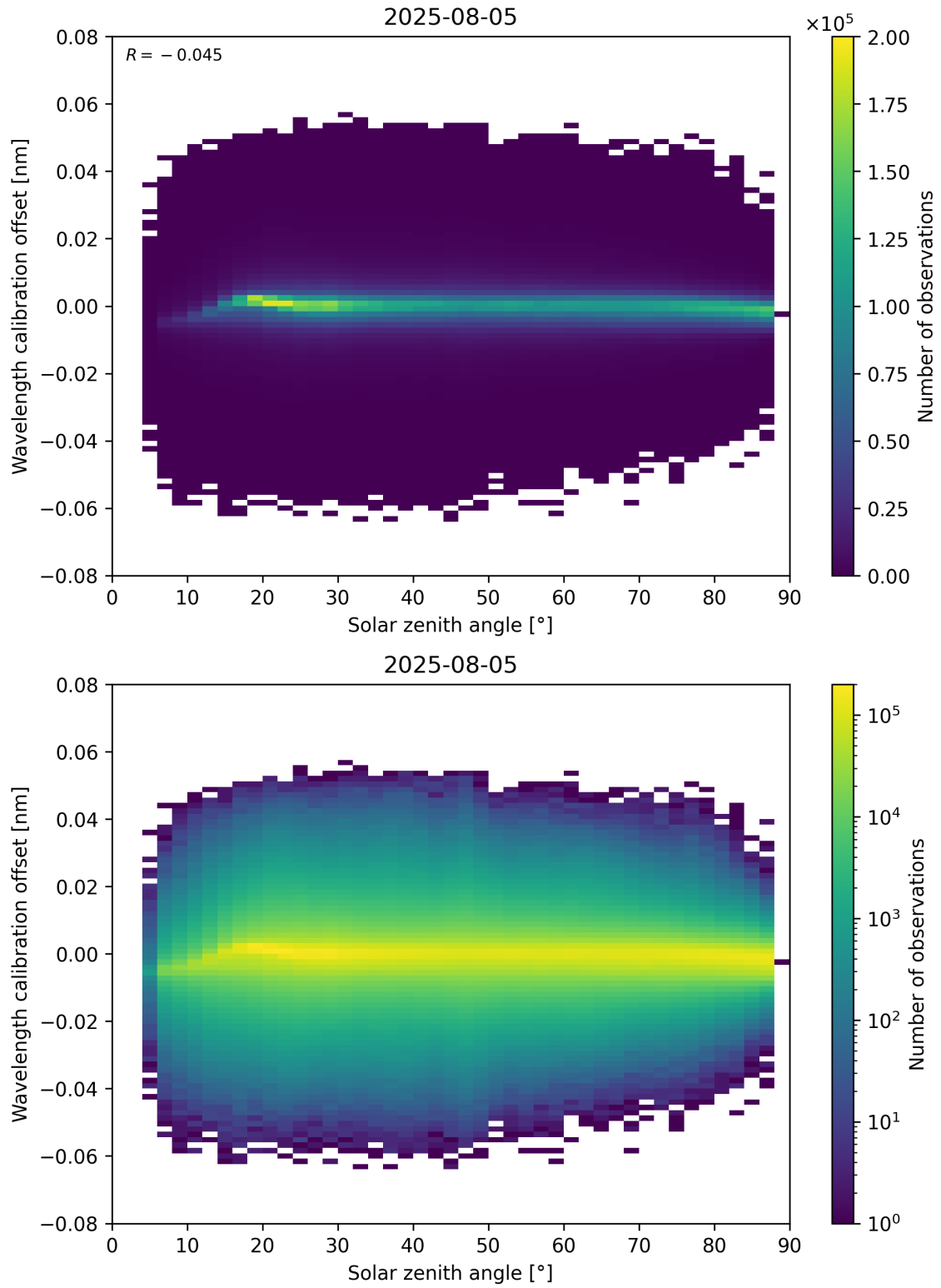
Figure 158: Scatter density plot of “Solar zenith angle” against “Wavelength calibration offset” for 2025-08-04 to 2025-08-06.
