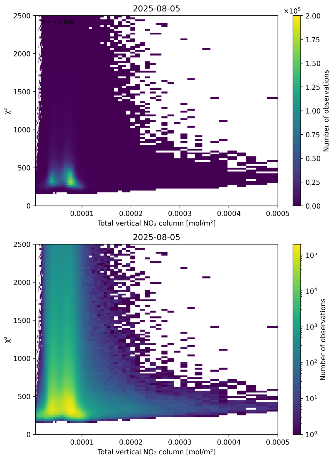
Figure 111: Scatter density plot of “Total vertical NO 2 column” against “ \chi^2 ” for 2025-08-04 to 2025-08-06.
