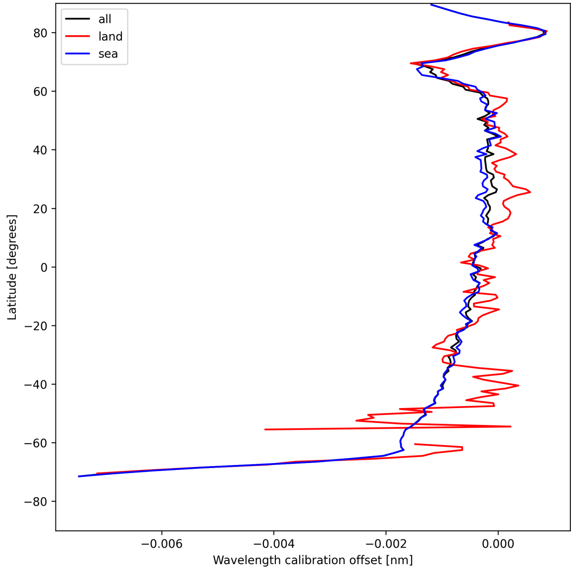
Figure 18: Zonal average of “Wavelength calibration offset” for 2025-08-04 to 2025-08-06.
