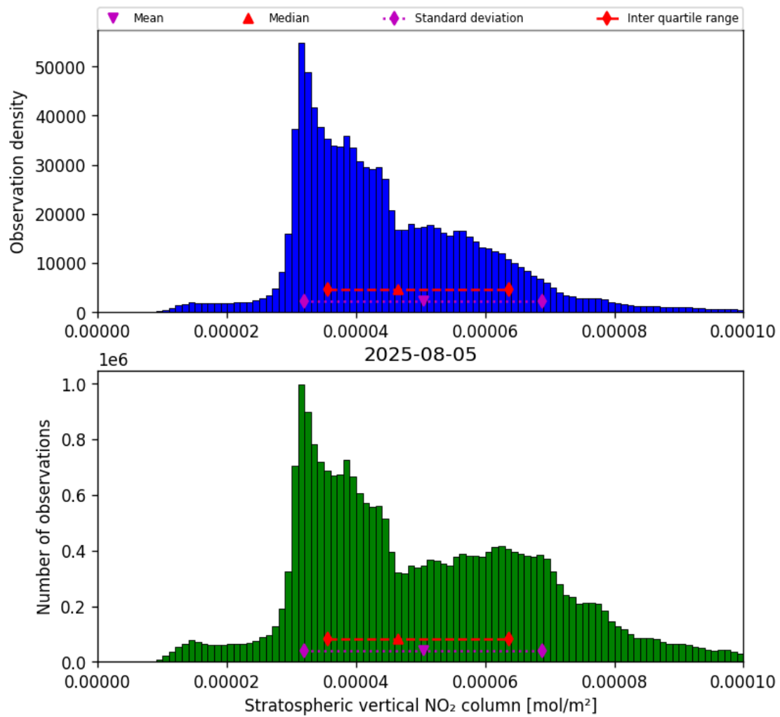
Figure 36: Histogram of “Stratospheric vertical NO 2 column” for 2025-08-04 to 2025-08-06
