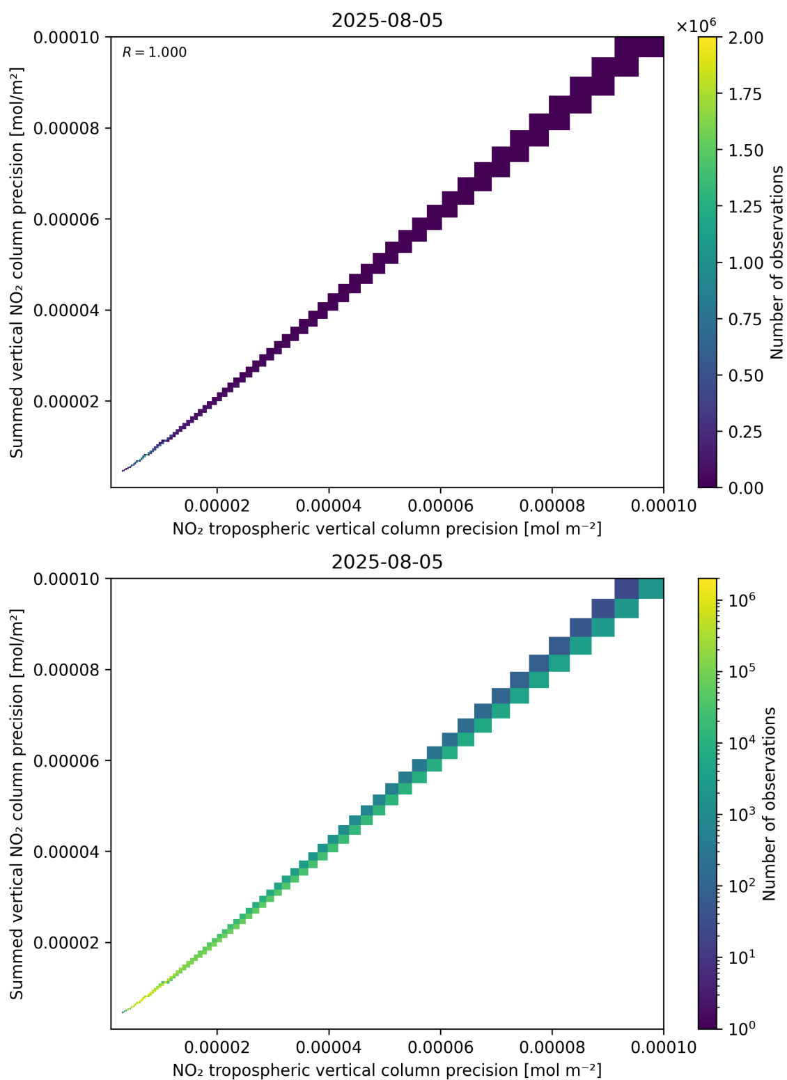
Figure 137: Scatter density plot of “NO 2 tropospheric vertical column precision” against “Summed vertical NO 2 column precision” for 2025-08-04 to 2025-08-06.
