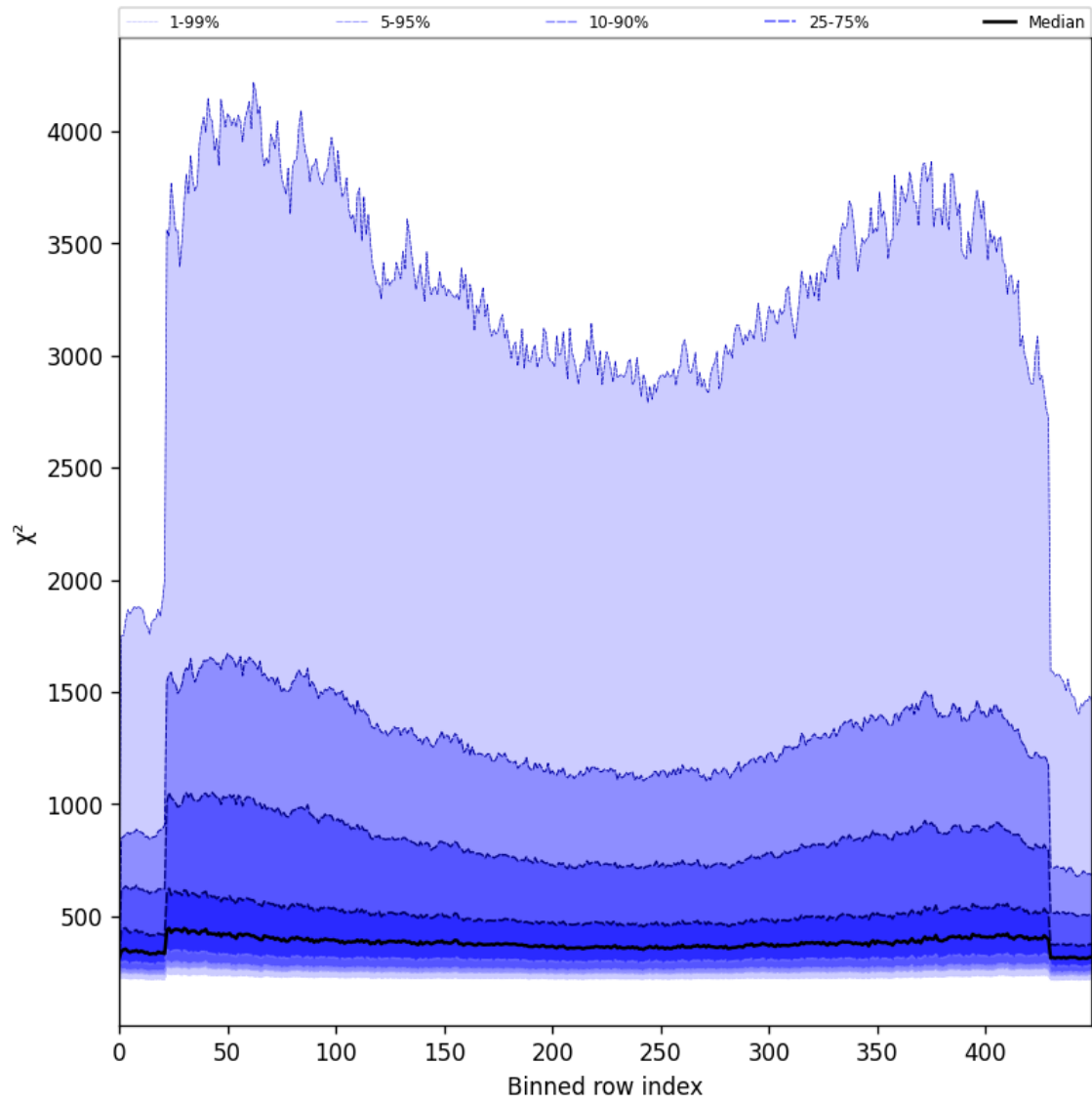
Figure 59: Along track statistics of “ \chi^2 ” for 2025-08-05 to 2025-08-07
