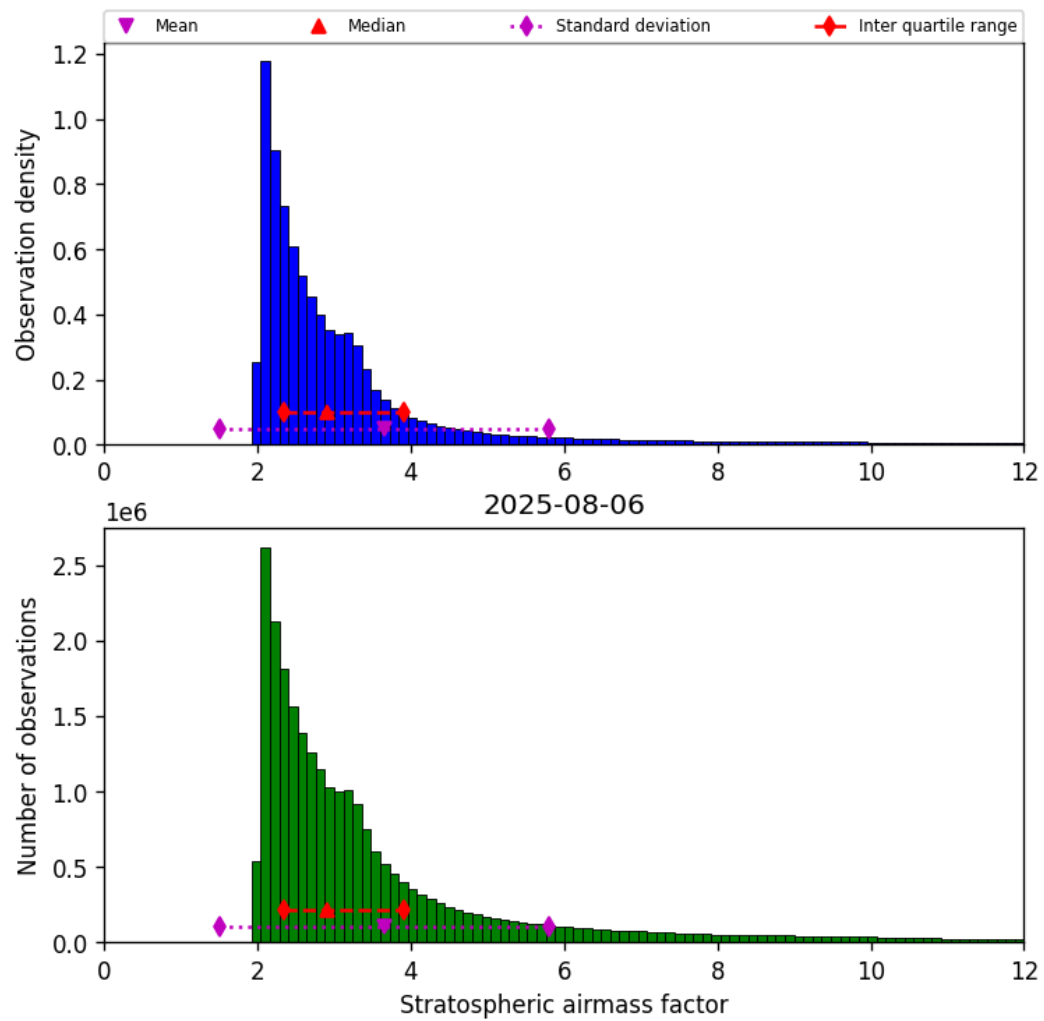
Figure 44: Histogram of “Stratospheric airmass factor” for 2025-08-05 to 2025-08-07
