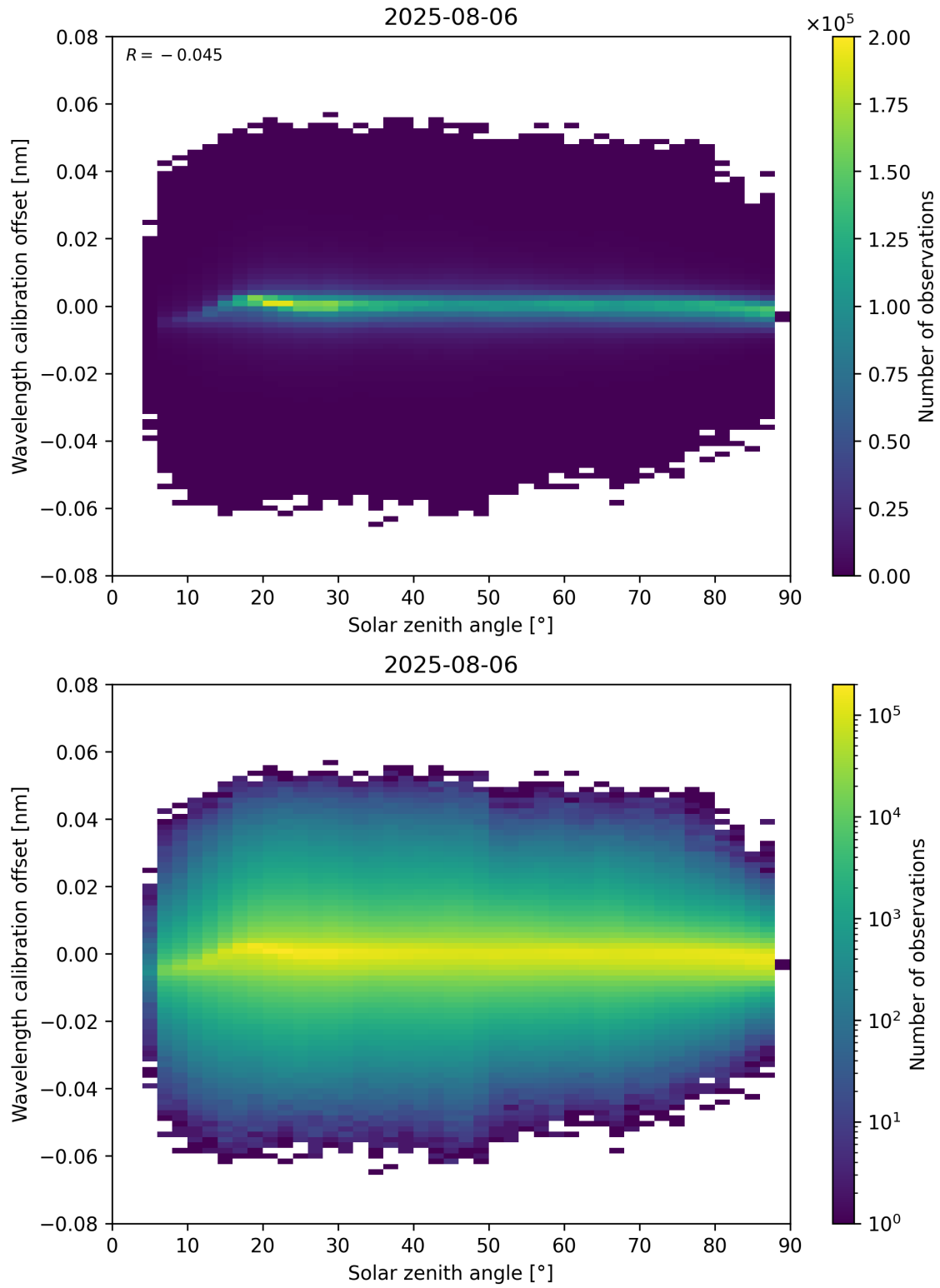
Figure 158: Scatter density plot of “Solar zenith angle” against “Wavelength calibration offset” for 2025-08-05 to 2025-08-07.
