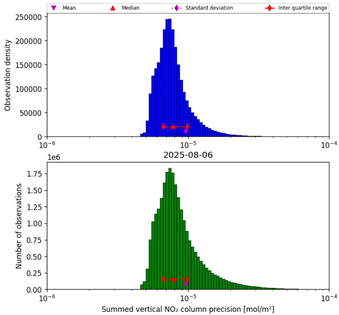
Figure 41: Histogram of "Summed vertical NO 2 column precision" for 2025-08-05 to 2025-08-07
