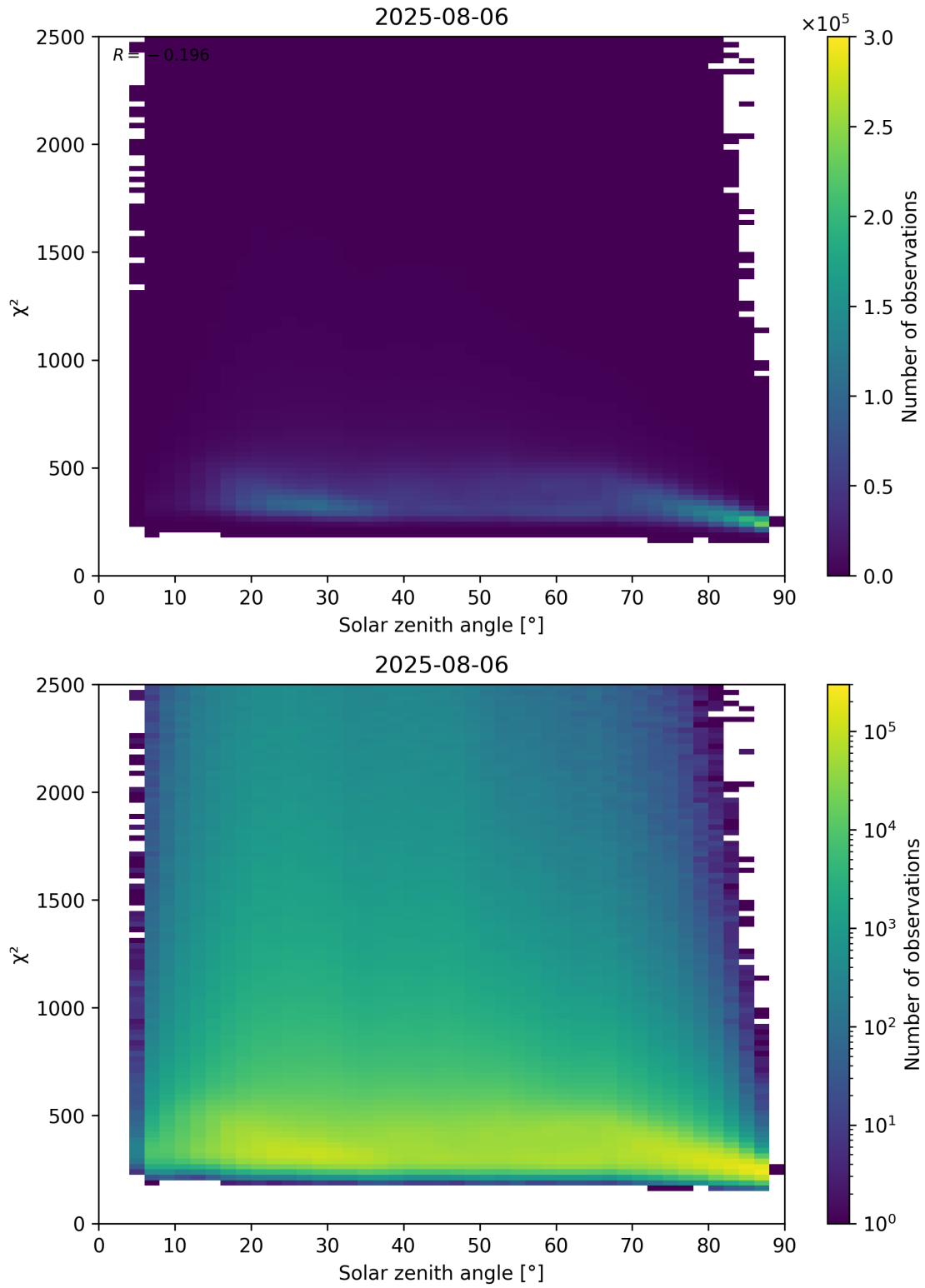
Figure 148: Scatter density plot of “Solar zenith angle” against “ \chi^2 ” for 2025-08-05 to 2025-08-07.
