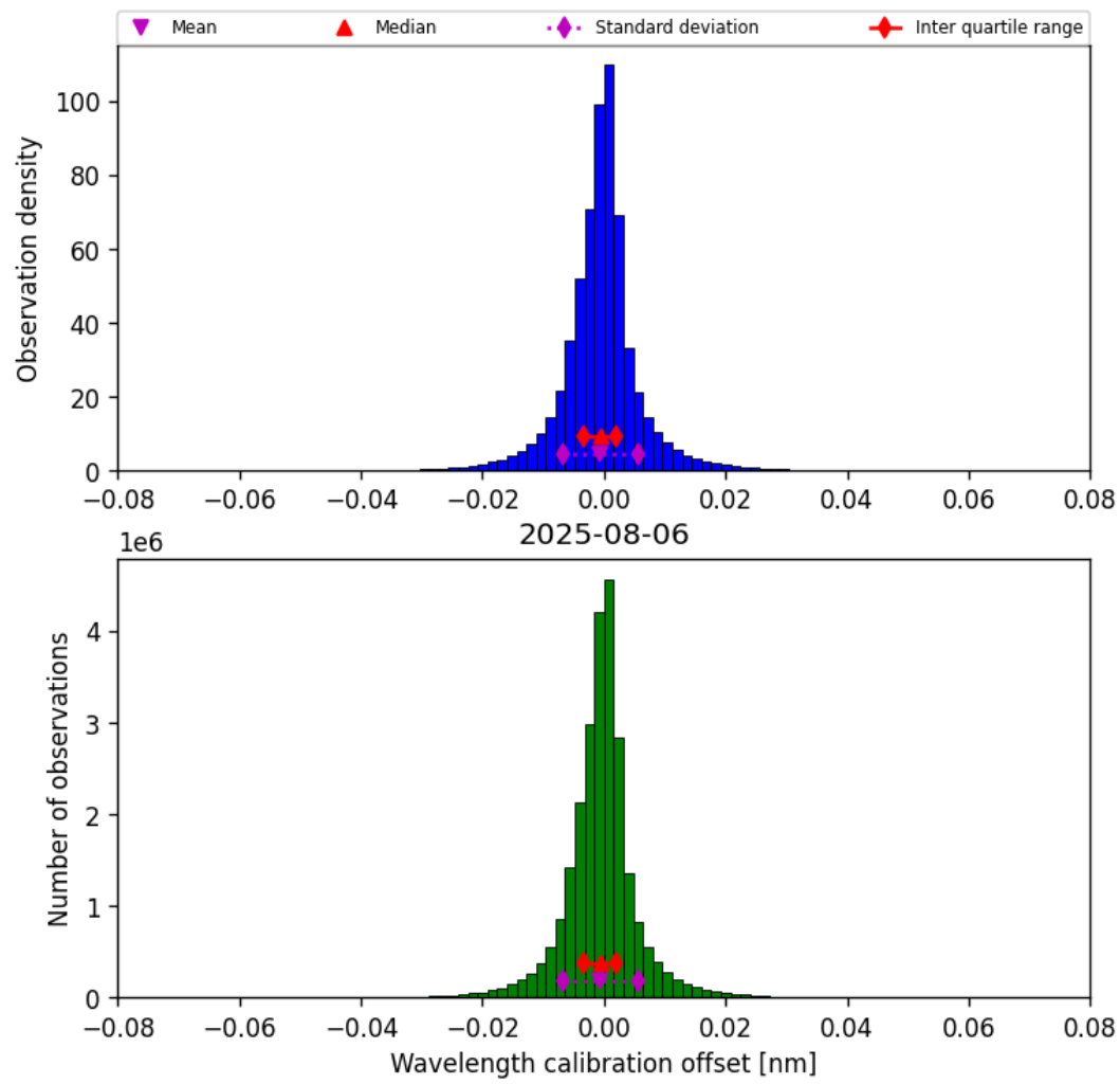
Figure 35: Histogram of “Wavelength calibration offset” for 2025-08-05 to 2025-08-07
