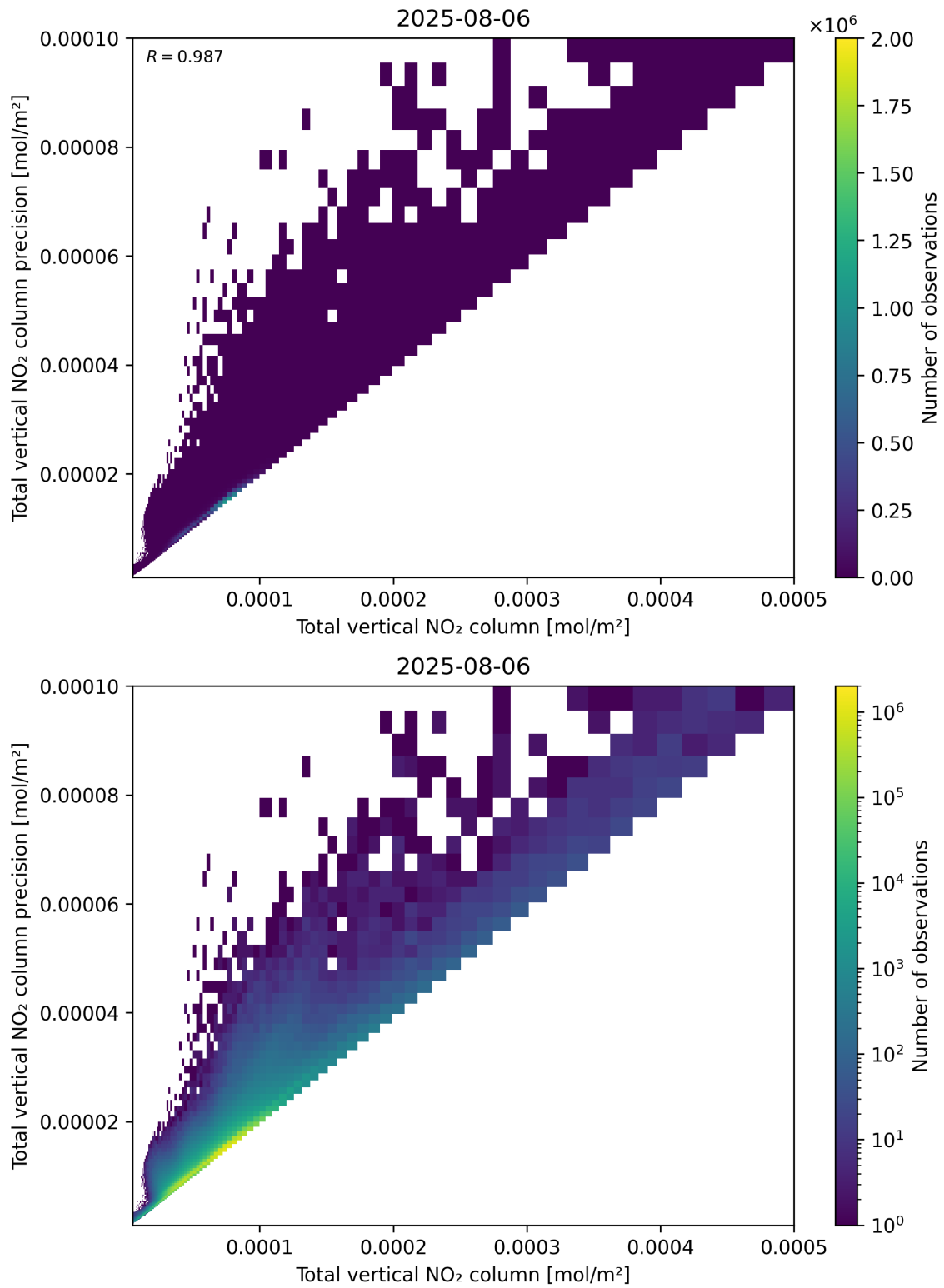
Figure 114: Scatter density plot of “Total vertical NO 2 column” against “Total vertical NO 2 column precision” for 2025-08-05 to 2025-08-07.
