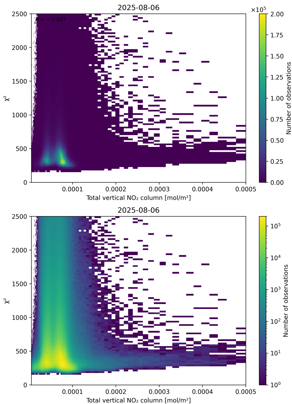
Figure 111: Scatter density plot of “Total vertical NO 2 column” against “ \chi^2 ” for 2025-08-05 to 2025-08-07.
