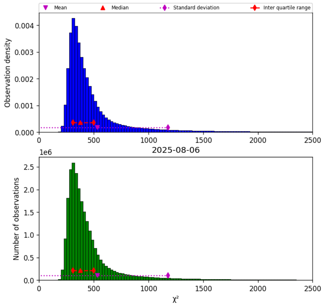
Figure 42: Histogram of “ \chi^2 ” for 2025-08-05 to 2025-08-07
