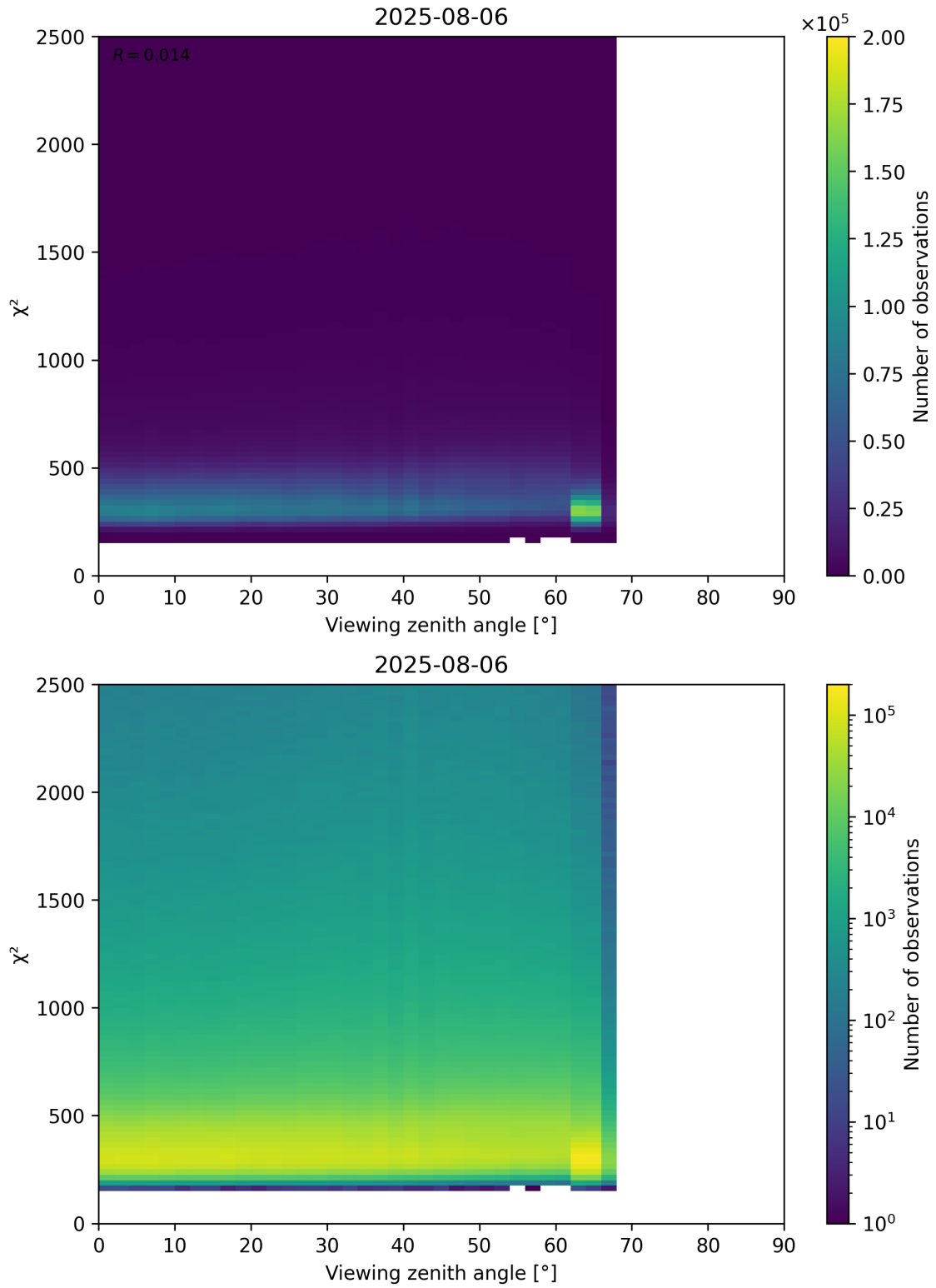
Figure 162: Scatter density plot of “Viewing zenith angle” against “ \chi^2 ” for 2025-08-05 to 2025-08-07.
