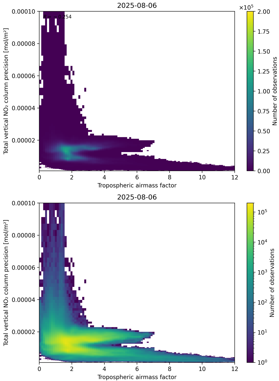
Figure 78: Scatter density plot of “Tropospheric air mass factor” against “Total vertical NO 2 column precision” for 2025-08-05 to 2025-08-07.
