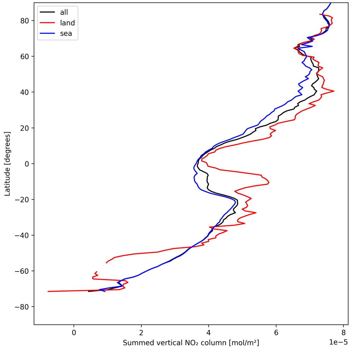
Figure 23: Zonal average of “Summed vertical NO 2 column” for 2025-08-05 to 2025-08-07.
