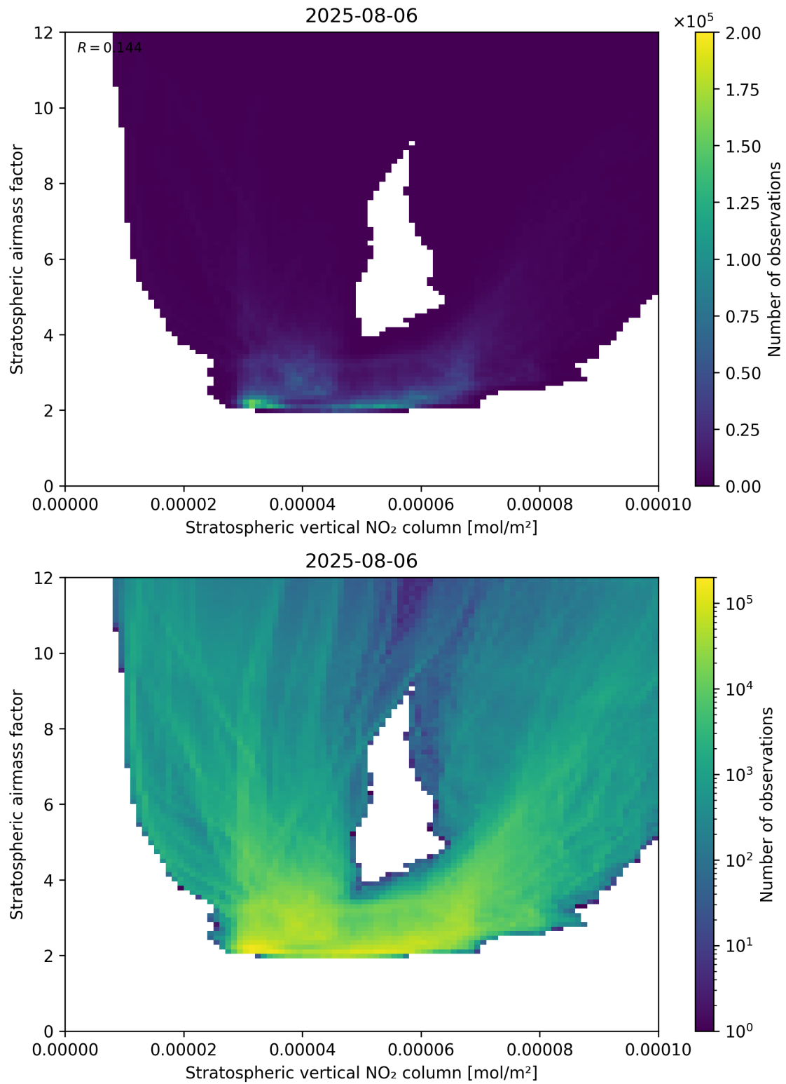
Figure 96: Scatter density plot of “Stratospheric vertical NO 2 column” against “Stratospheric airmass factor” for 2025-08-05 to 2025-08-07.
