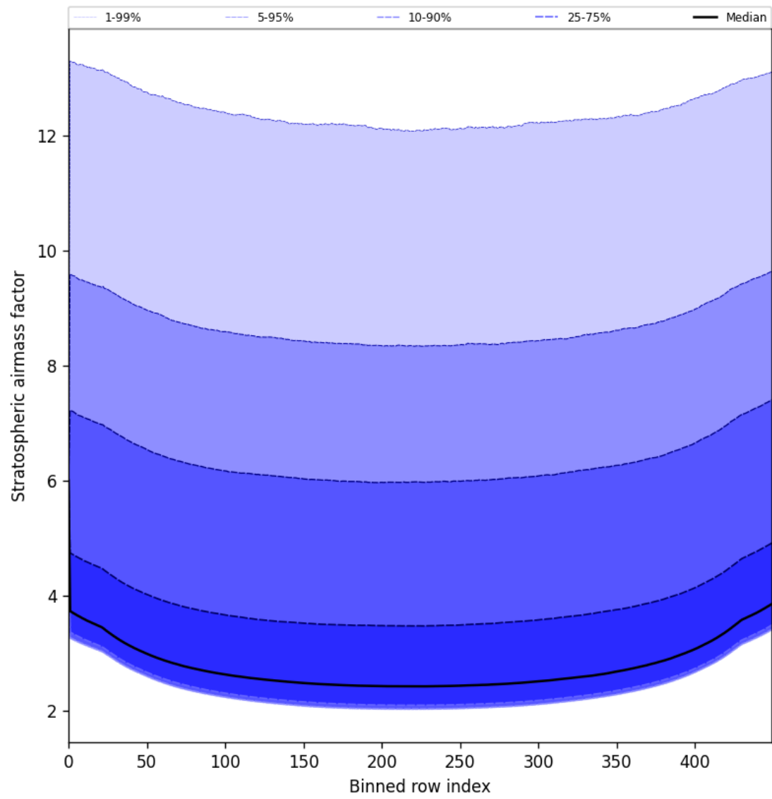
Figure 61: Along track statistics of “Stratospheric airmass factor” for 2025-08-05 to 2025-08-07
