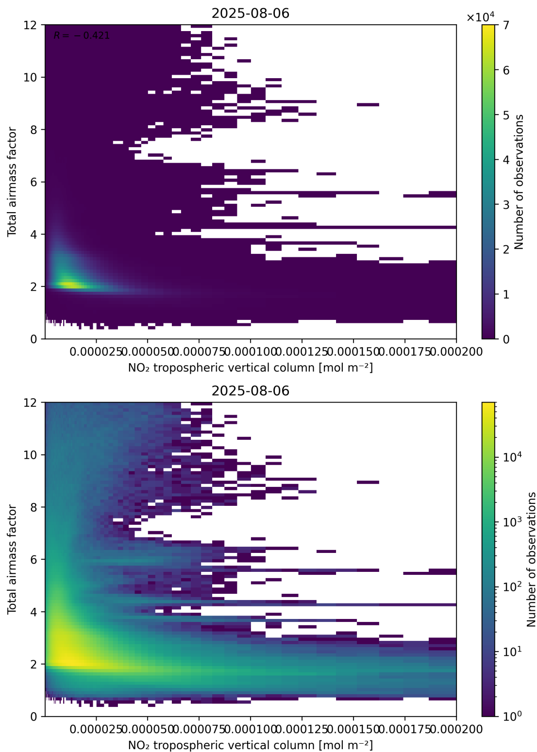
Figure 122: Scatter density plot of “NO 2 tropospheric vertical column” against “Total air mass factor” for 2025-08-05 to 2025-08-07.
