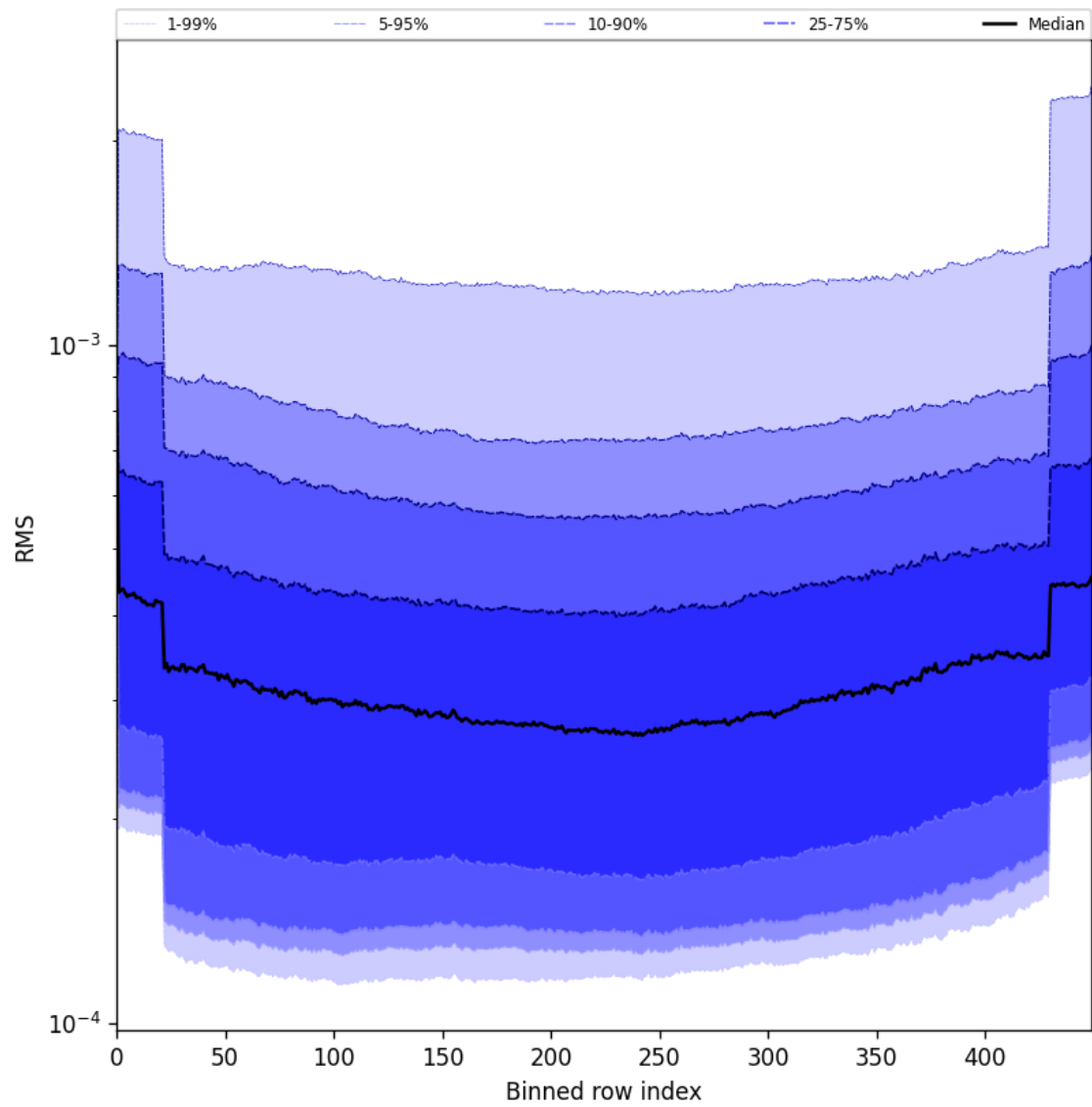
Figure 60: Along track statistics of “RMS” for 2025-08-05 to 2025-08-07
