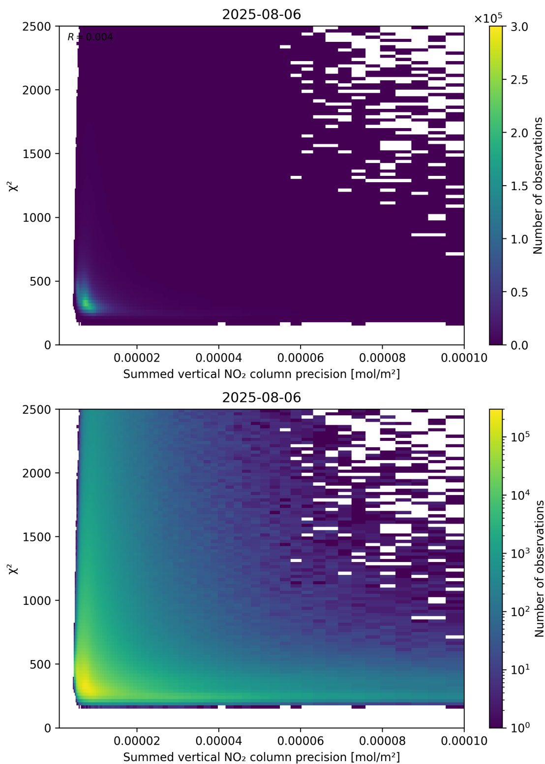
Figure 107: Scatter density plot of “Summed vertical NO 2 column precision” against “ \chi^2 ” for 2025-08-05 to 2025-08-07.
