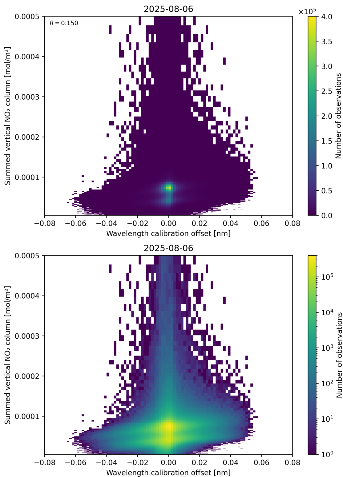
Figure 177: Scatter density plot of “Wavelength calibration offset” against “Summed vertical NO 2 column” for 2025-08-05 to 2025-08-07.
