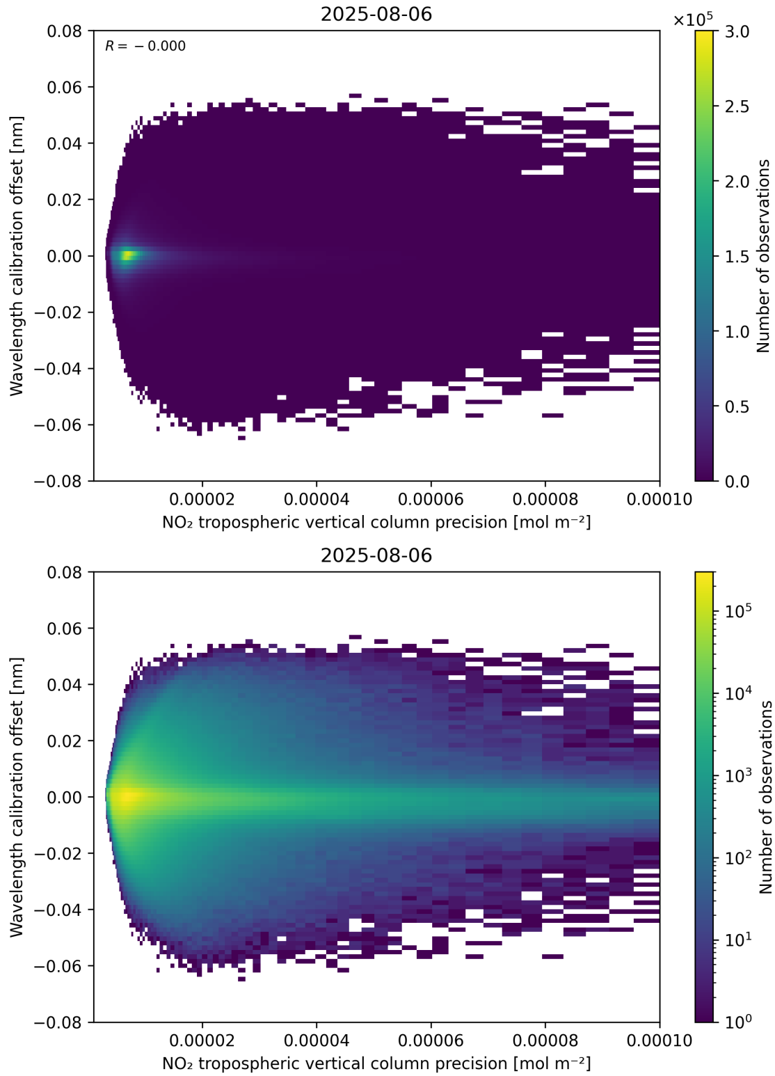
Figure 141: Scatter density plot of “NO 2 tropospheric vertical column precision” against “Wavelength calibration offset” for 2025-08-05 to 2025-08-07.
