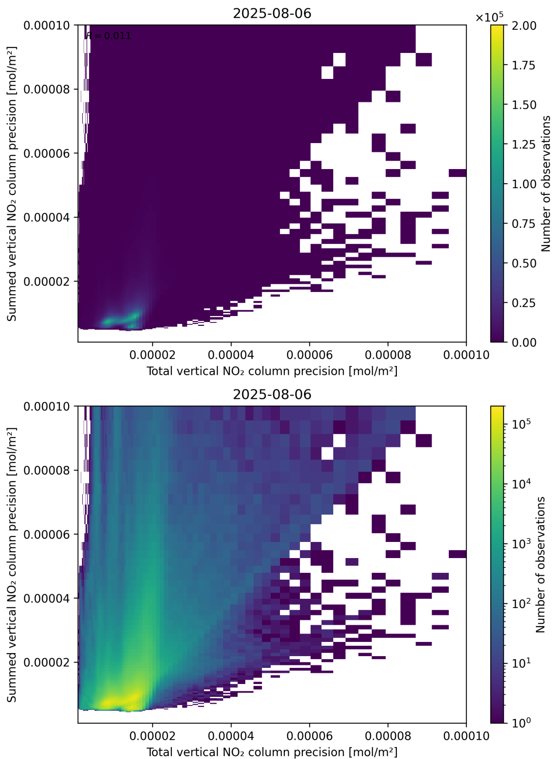
Figure 118: Scatter density plot of “Total vertical NO 2 column precision” against “Summed vertical NO 2 column precision” for 2025-08-05 to 2025-08-07.
