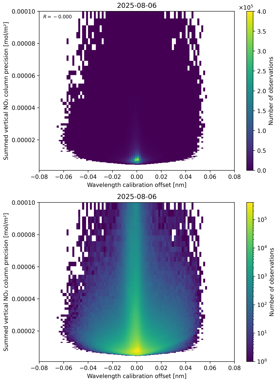
Figure 178: Scatter density plot of “Wavelength calibration offset” against “Summed vertical NO 2 column precision” for 2025-08-05 to 2025-08-07.
