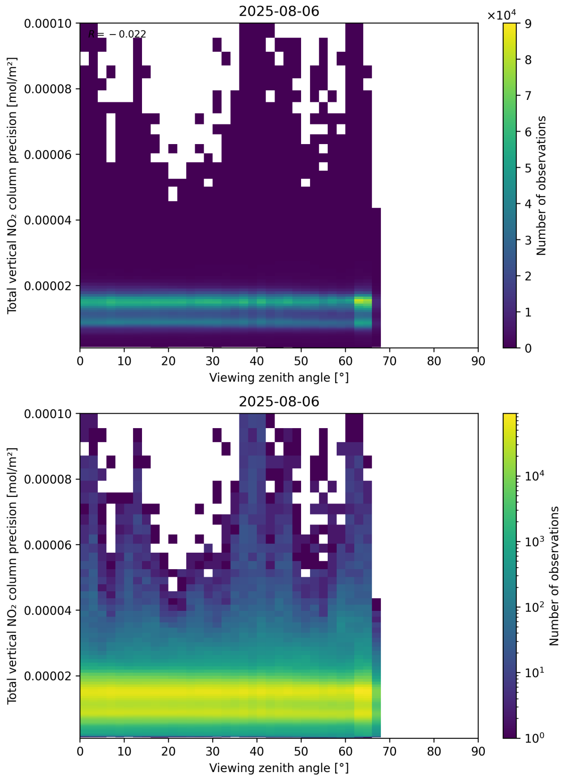
Figure 168: Scatter density plot of “Viewing zenith angle” against “Total vertical NO 2 column precision” for 2025-08-05 to 2025-08-07.
