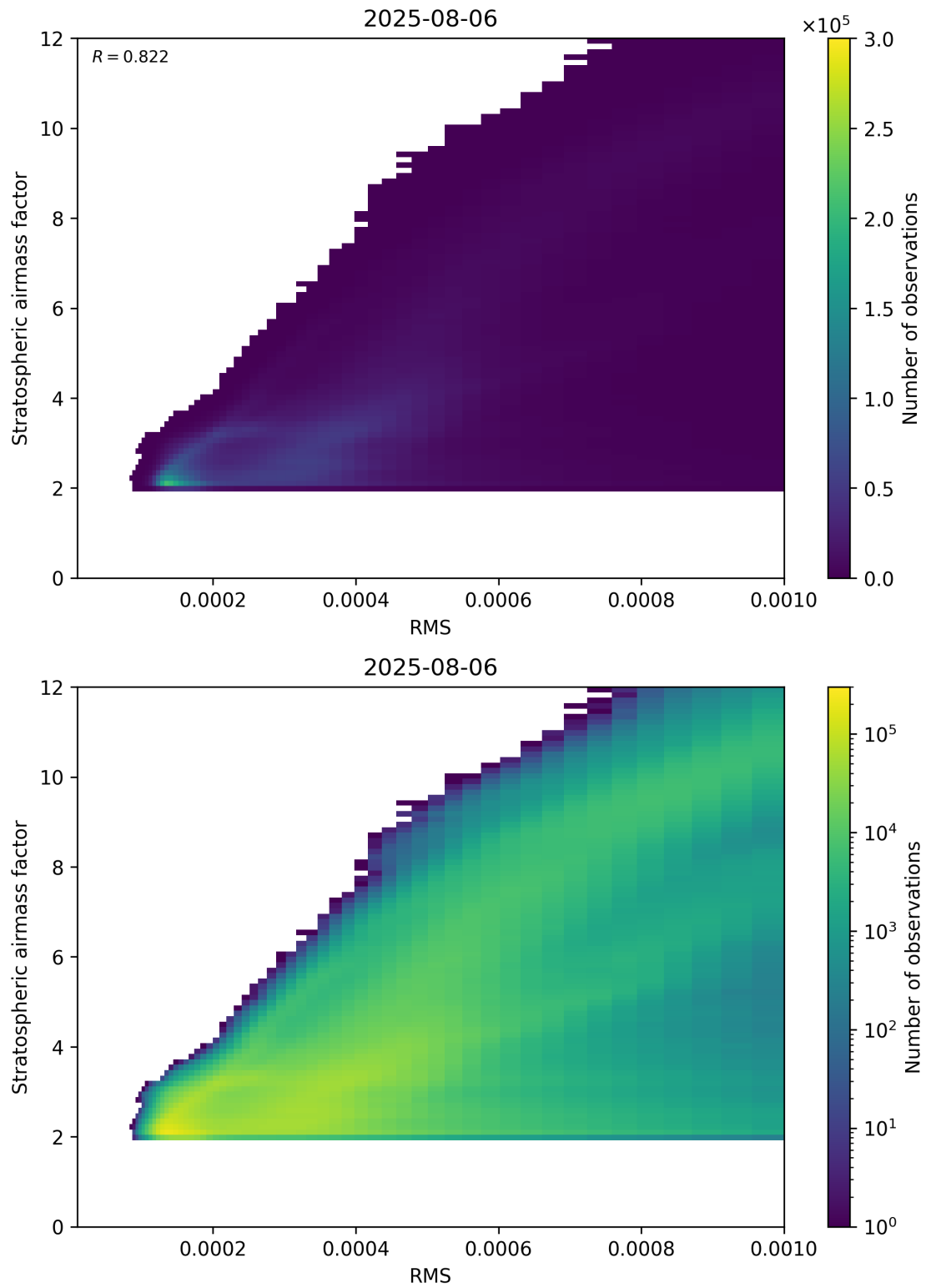
Figure 144: Scatter density plot of “RMS” against “Stratospheric airmass factor” for 2025-08-05 to 2025-08-07.
