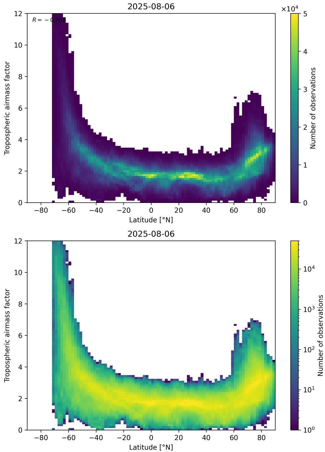
Figure 85: Scatter density plot of “Latitude” against “Tropospheric air mass factor” for 2025-08-05 to 2025-08-07.
