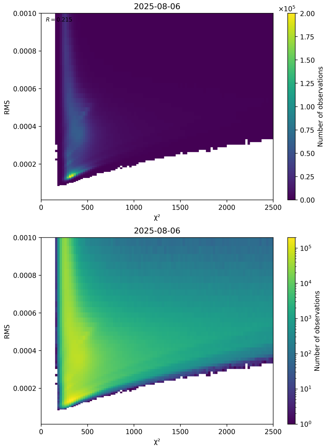
Figure 82: Scatter density plot of “ \chi^2 ” against “RMS” for 2025-08-05 to 2025-08-07.
