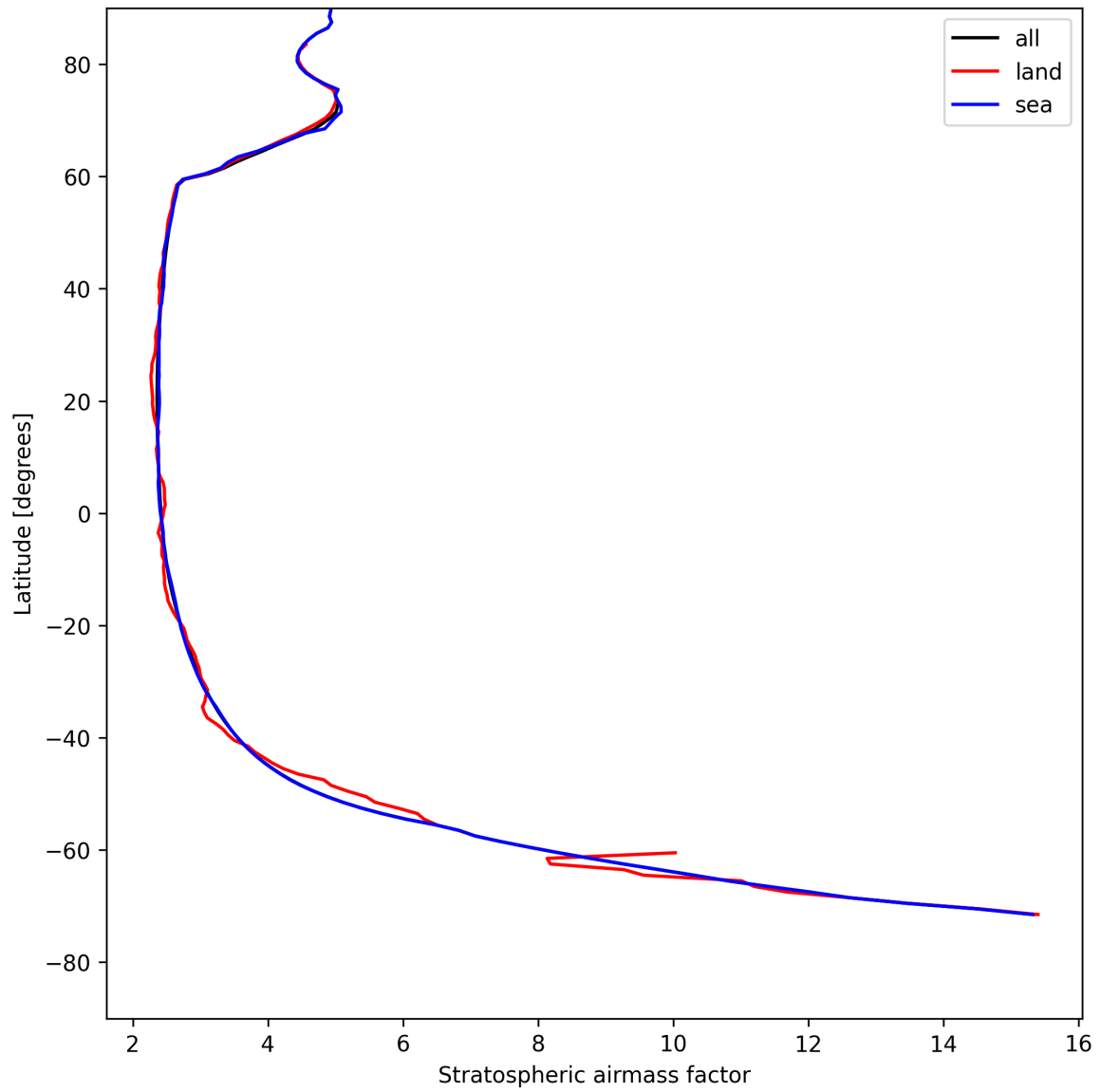
Figure 27: Zonal average of “Stratospheric airmass factor” for 2025-08-05 to 2025-08-07.
