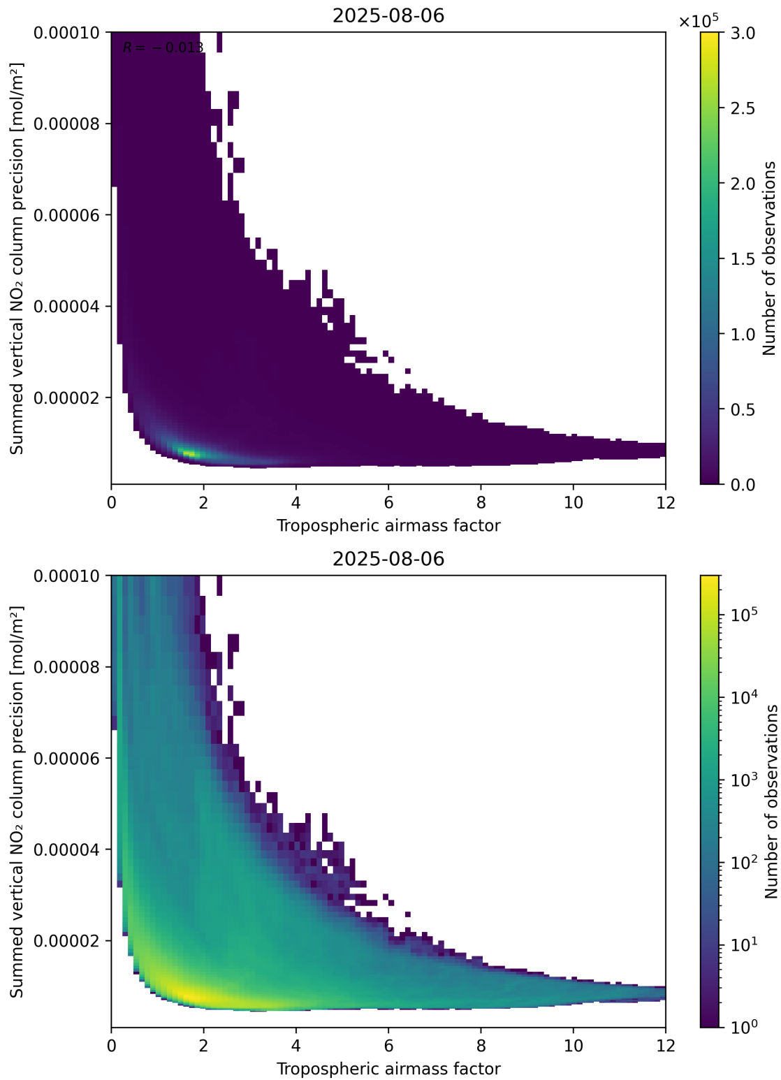
Figure 76: Scatter density plot of “Tropospheric air mass factor” against “Summed vertical NO 2 column precision” for 2025-08-05 to 2025-08-07.
