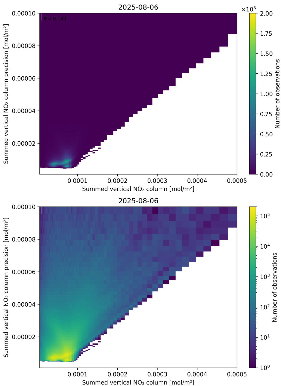
Figure 105: Scatter density plot of “Summed vertical NO 2 column” against “Summed vertical NO 2 column precision” for 2025-08-05 to 2025-08-07.
