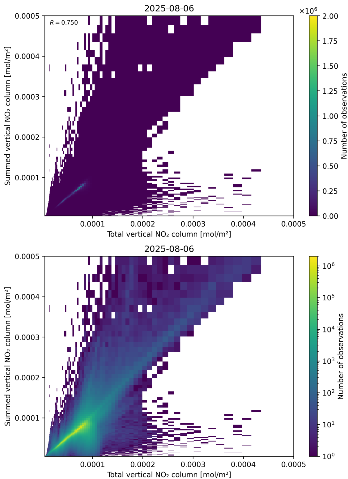
Figure 112: Scatter density plot of “Total vertical NO 2 column” against “Summed vertical NO 2 column” for 2025-08-05 to 2025-08-07.
