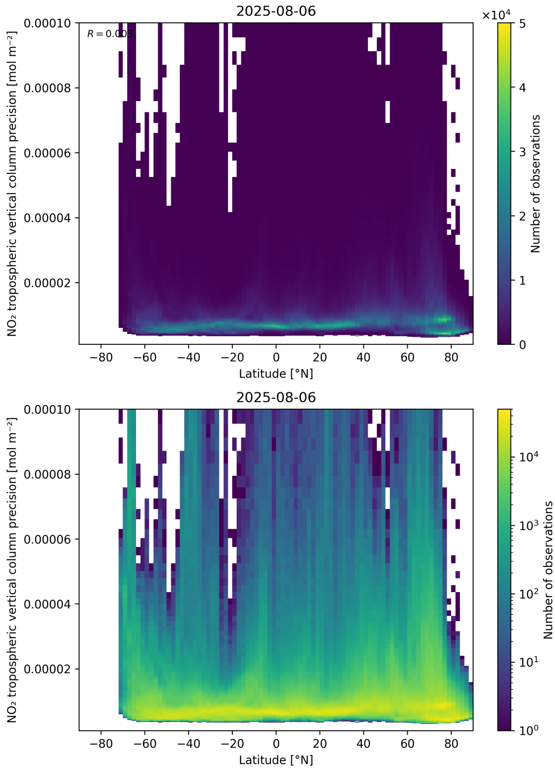
Figure 93: Scatter density plot of “Latitude” against “NO 2 tropospheric vertical column precision” for 2025-08-05 to 2025-08-07.
