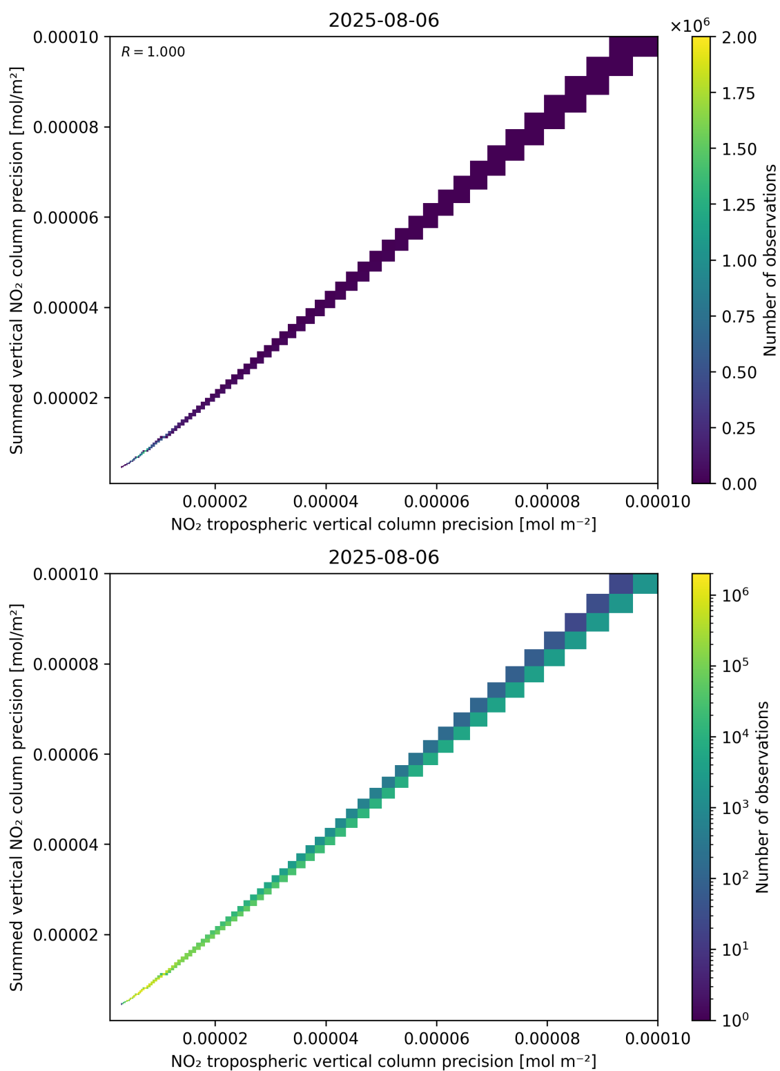
Figure 137: Scatter density plot of “NO 2 tropospheric vertical column precision” against “Summed vertical NO 2 column precision” for 2025-08-05 to 2025-08-07.
