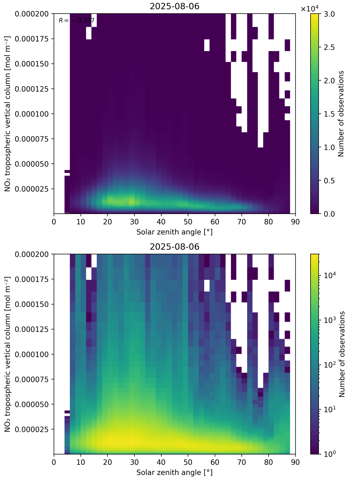
Figure 155: Scatter density plot of “Solar zenith angle” against “NO 2 tropospheric vertical column” for 2025-08-05 to 2025-08-07.
