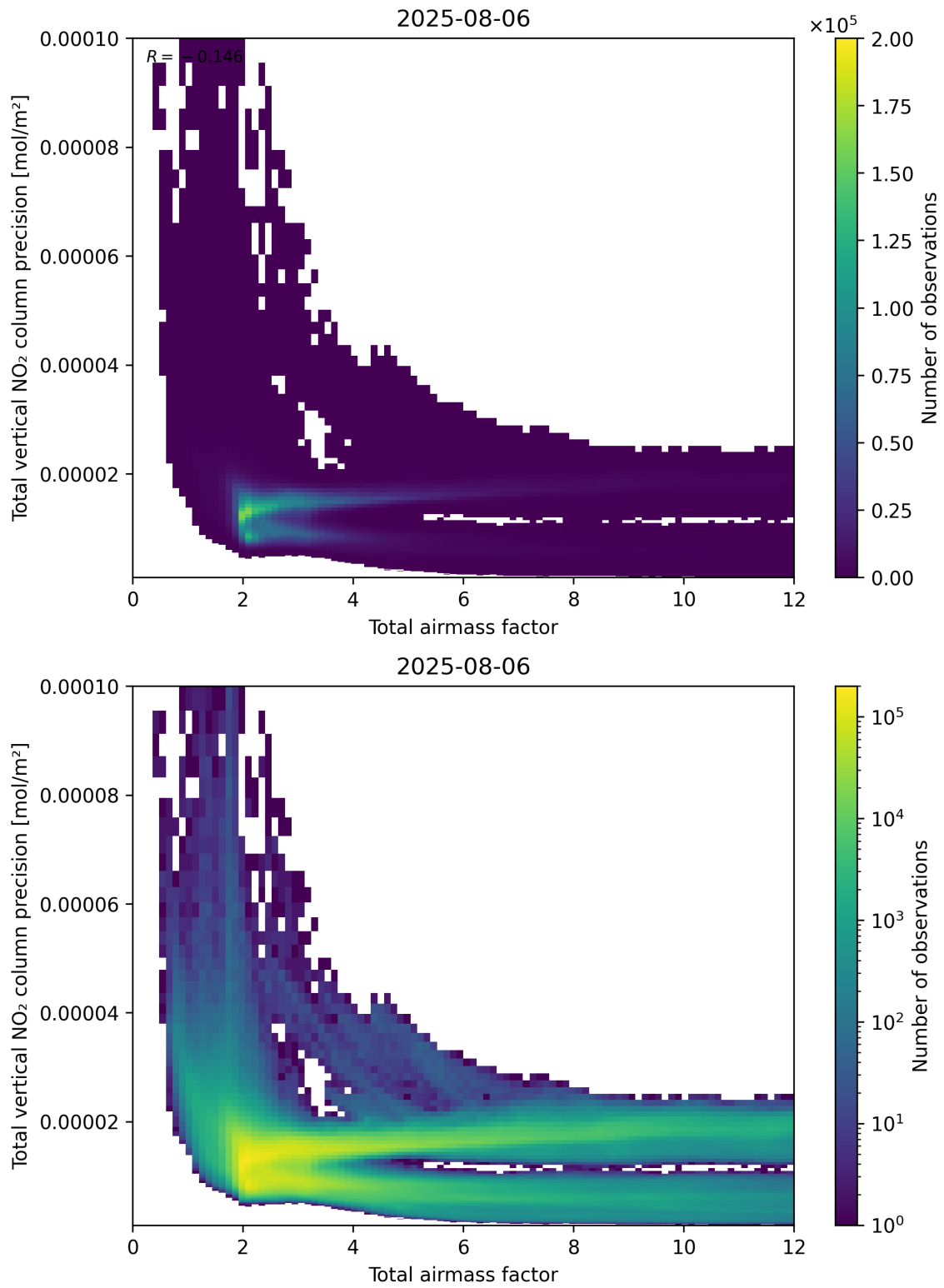
Figure 68: Scatter density plot of “Total airmass factor” against “Total vertical NO 2 column precision” for 2025-08-05 to 2025-08-07.
