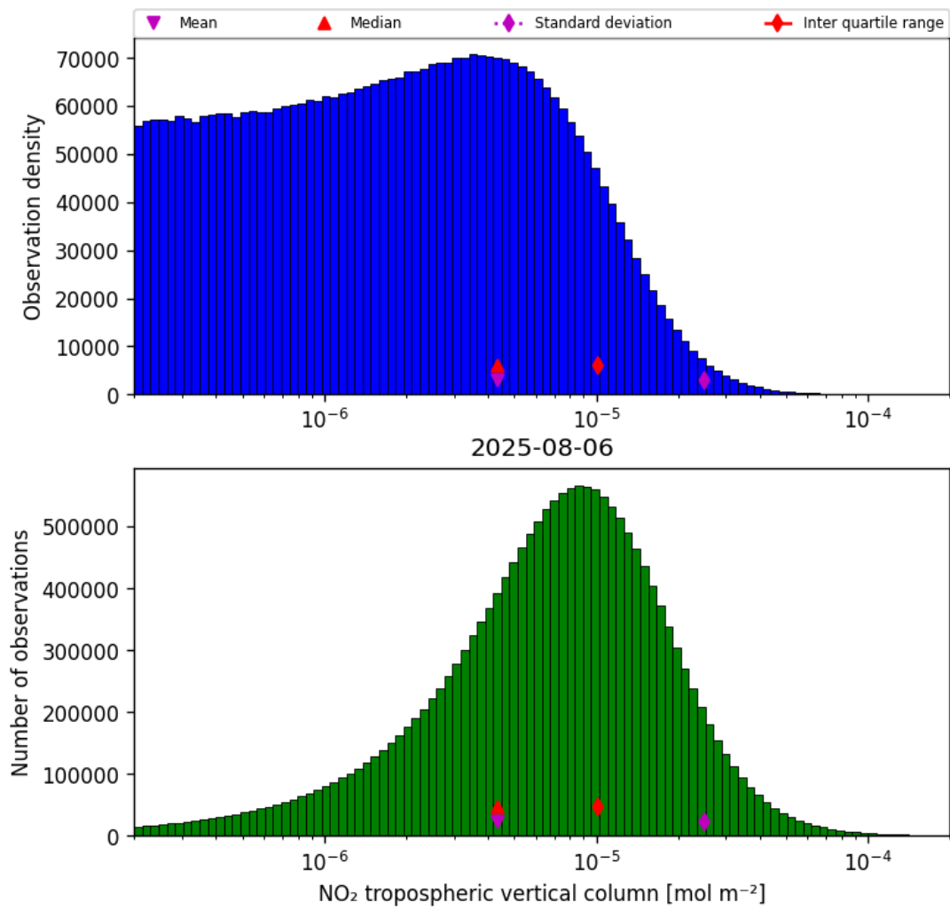
Figure 29: Histogram of “NO 2 tropospheric vertical column” for 2025-08-05 to 2025-08-07
