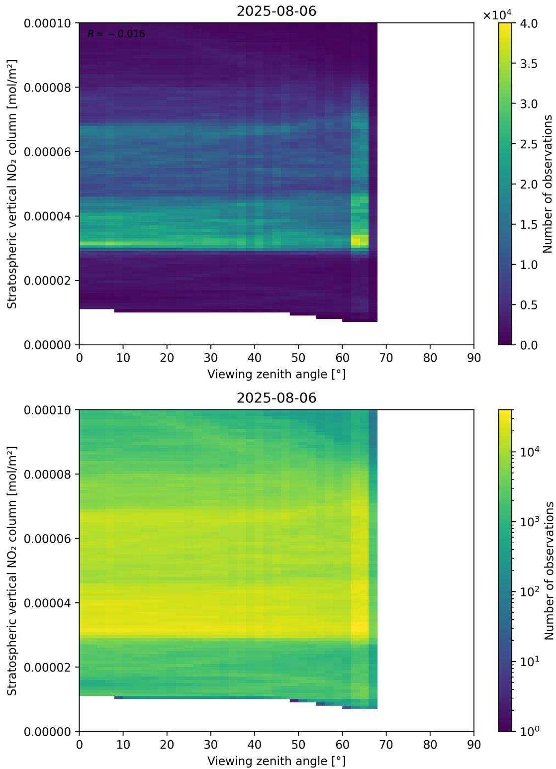
Figure 164: Scatter density plot of “Viewing zenith angle” against “Stratospheric vertical NO 2 column” for 2025-08-05 to 2025-08-07.
