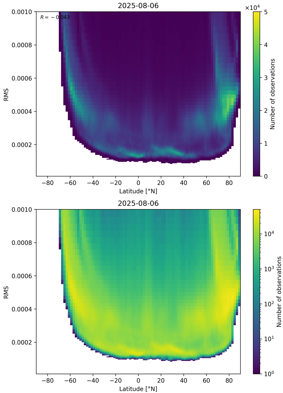
Figure 94: Scatter density plot of “Latitude” against “RMS” for 2025-08-05 to 2025-08-07.
