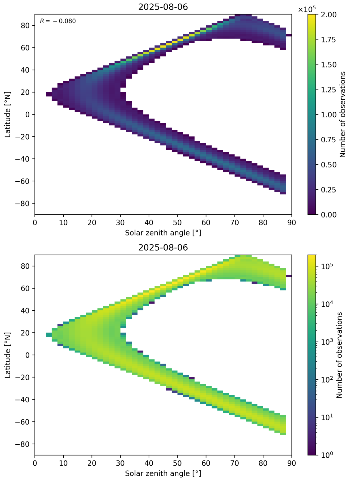
Figure 149: Scatter density plot of “Solar zenith angle” against “Latitude” for 2025-08-05 to 2025-08-07.
