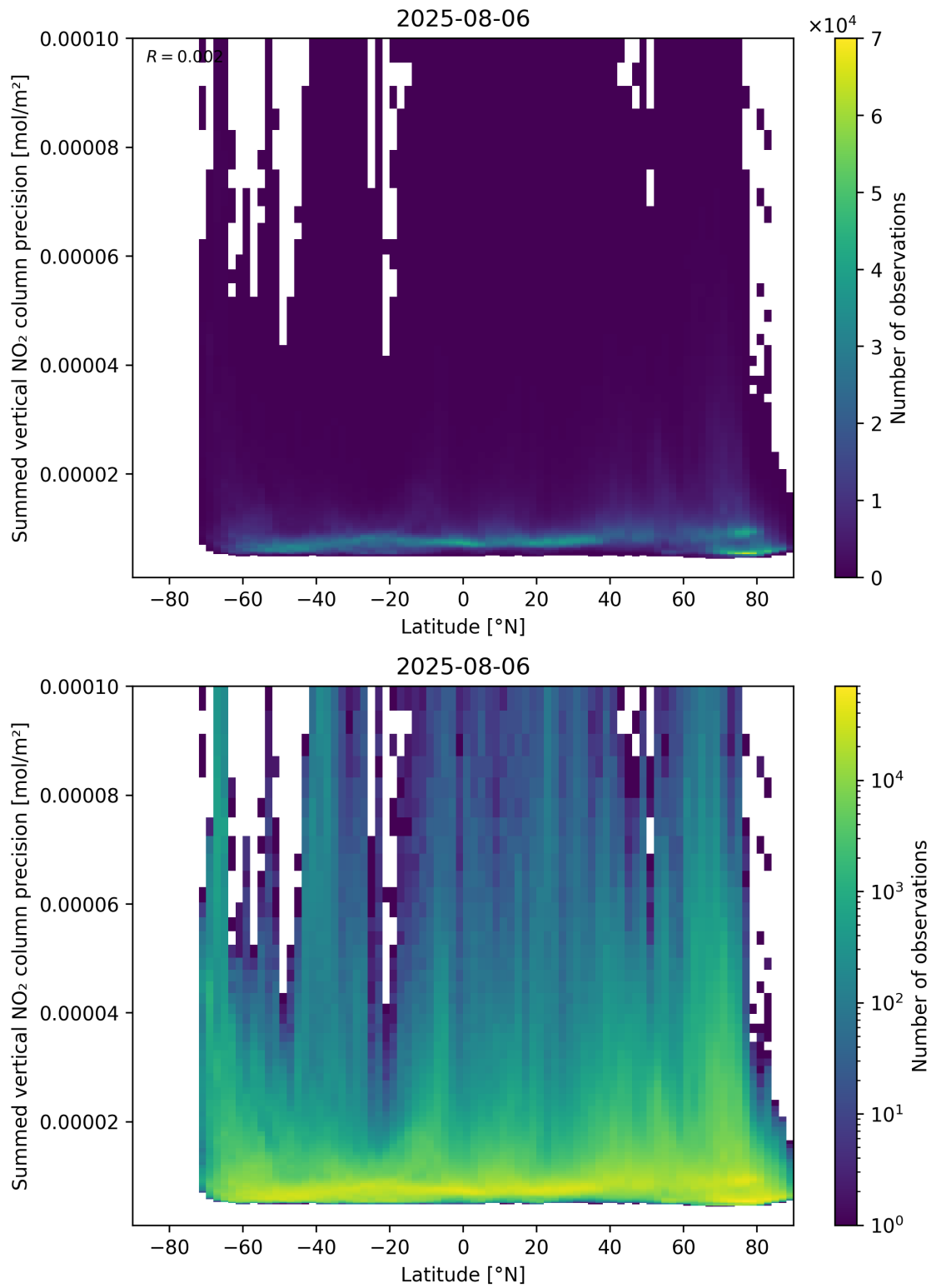
Figure 89: Scatter density plot of “Latitude” against “Summed vertical NO 2 column precision” for 2025-08-05 to 2025-08-07.
