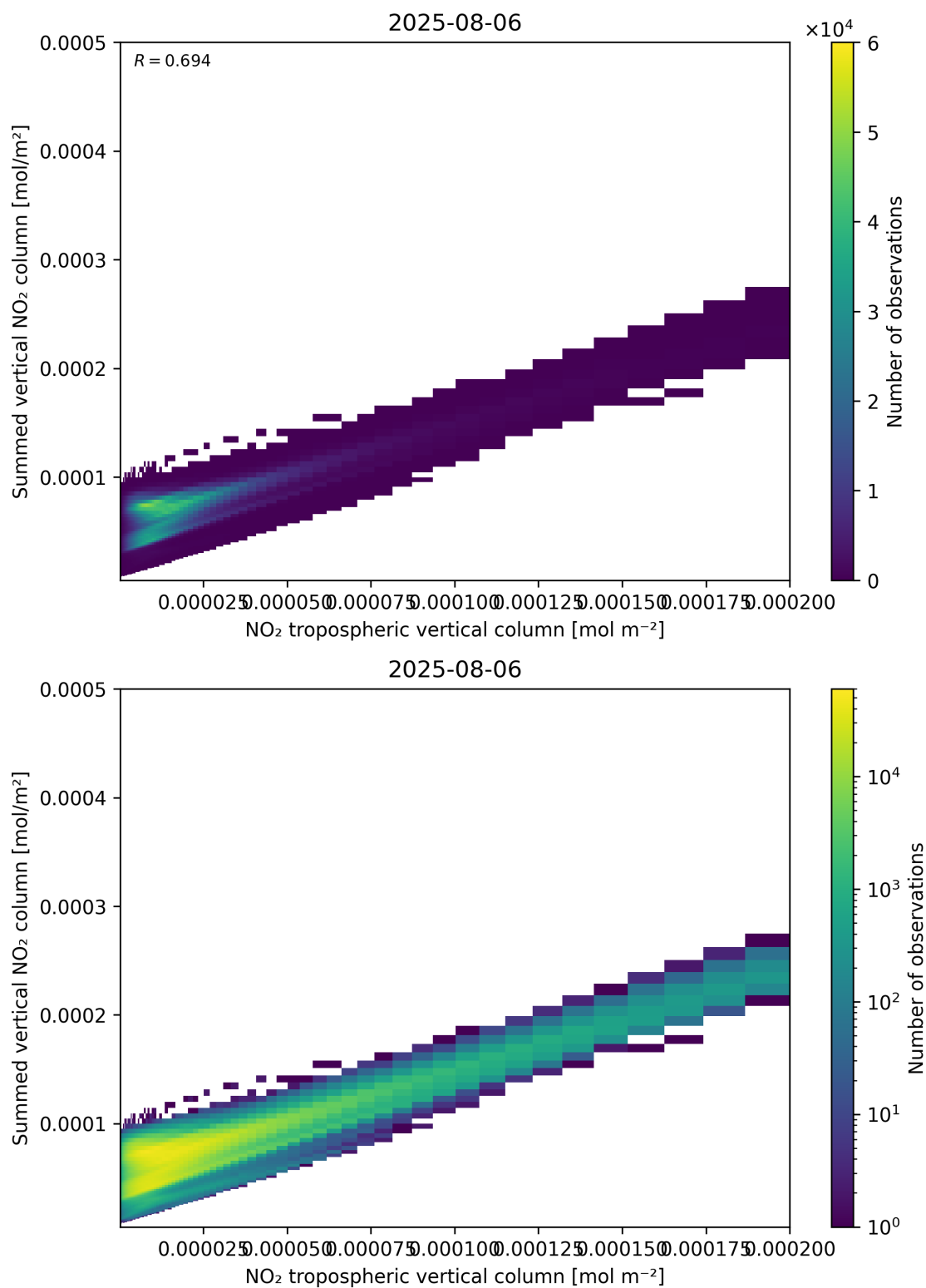
Figure 126: Scatter density plot of “NO 2 tropospheric vertical column” against “Summed vertical NO 2 column” for 2025-08-05 to 2025-08-07.
