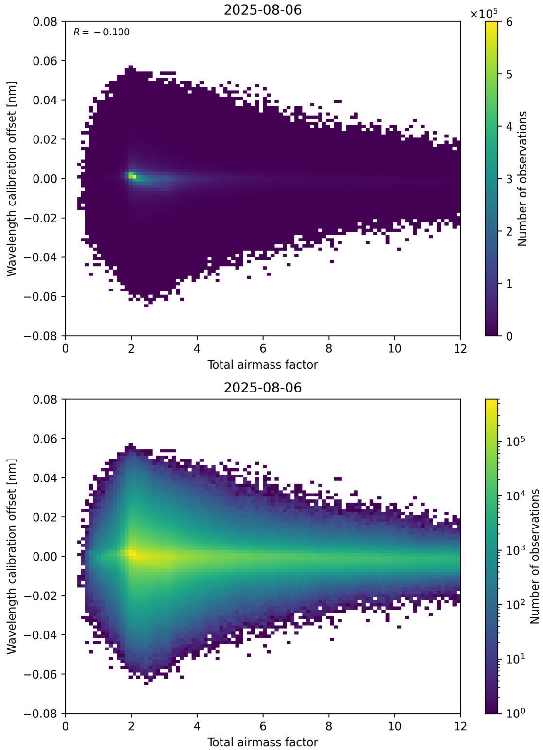
Figure 70: Scatter density plot of “Total airmass factor” against “Wavelength calibration offset” for 2025-08-05 to 2025-08-07.
