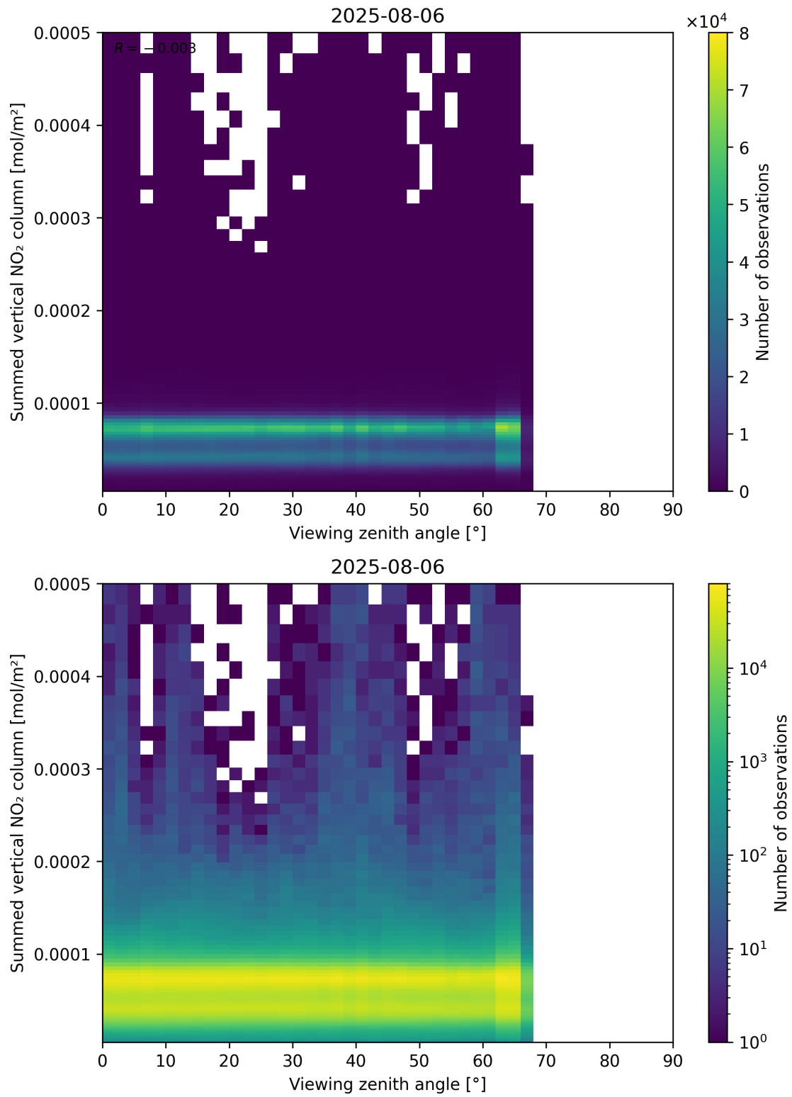
Figure 165: Scatter density plot of “Viewing zenith angle” against “Summed vertical NO 2 column” for 2025-08-05 to 2025-08-07.
