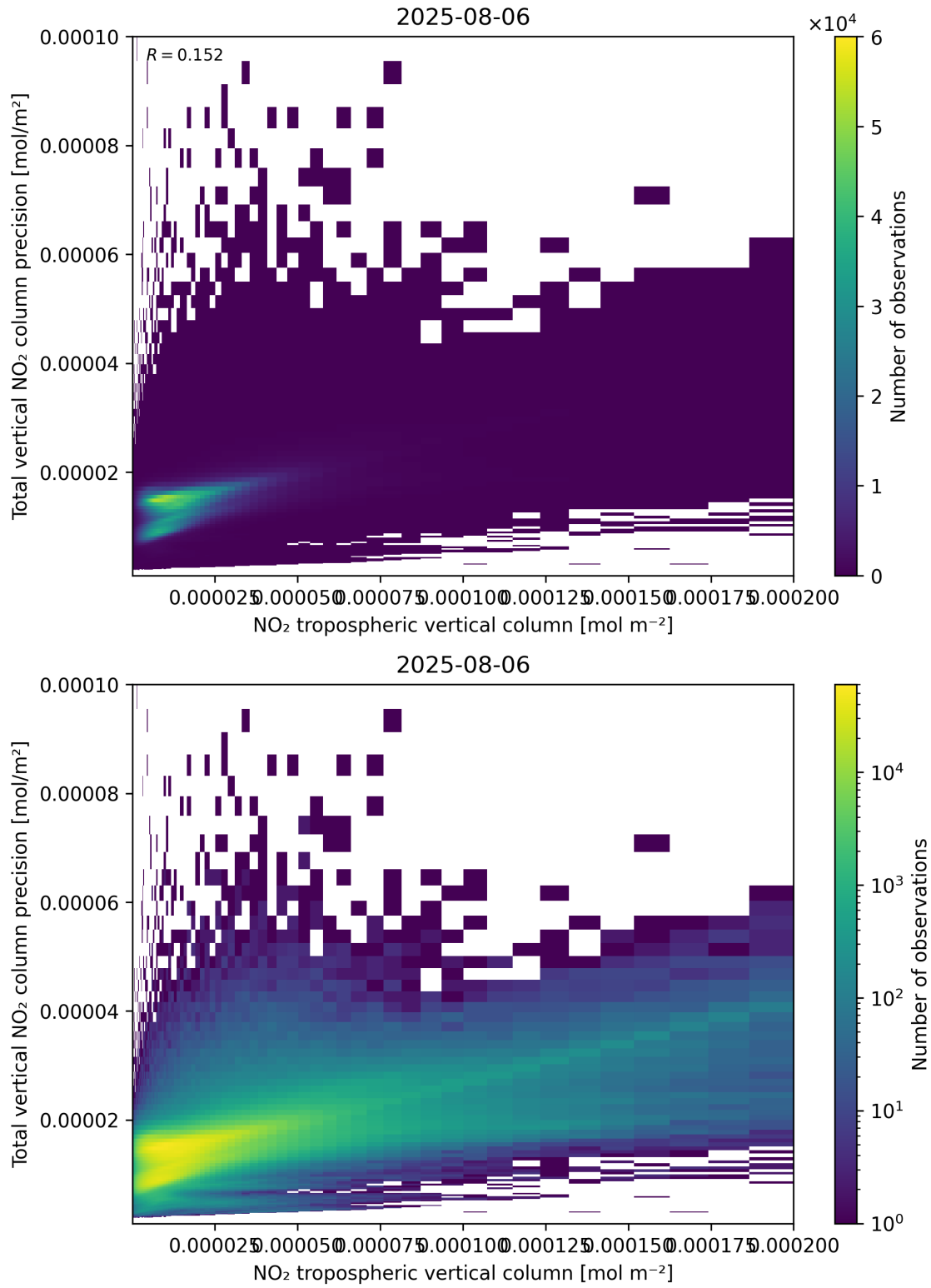
Figure 129: Scatter density plot of “NO 2 tropospheric vertical column” against “Total vertical NO 2 column precision” for 2025-08-05 to 2025-08-07.
