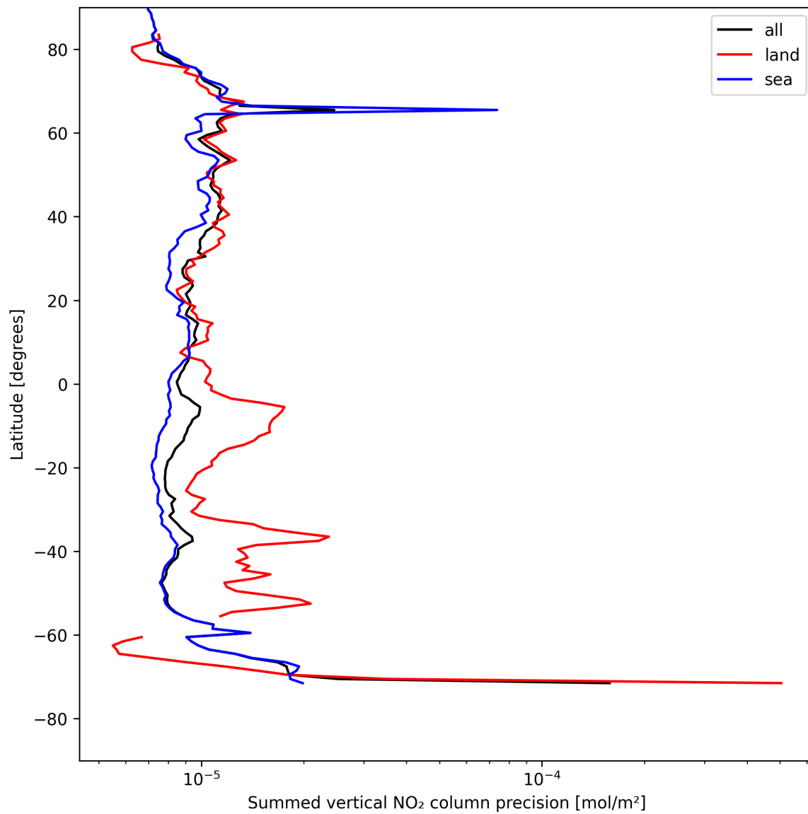
Figure 24: Zonal average of “Summed vertical NO 2 column precision” for 2025-08-05 to 2025-08-07.
