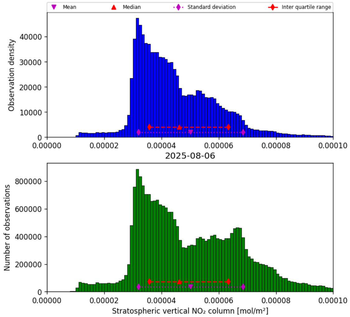
Figure 36: Histogram of “Stratospheric vertical NO 2 column” for 2025-08-05 to 2025-08-07
