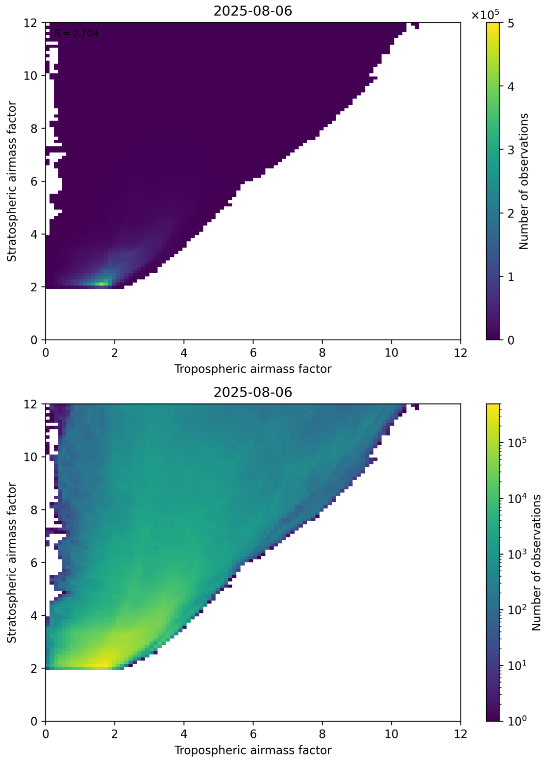
Figure 71: Scatter density plot of “Tropospheric airmass factor” against “Stratospheric airmass factor” for 2025-08-05 to 2025-08-07.
