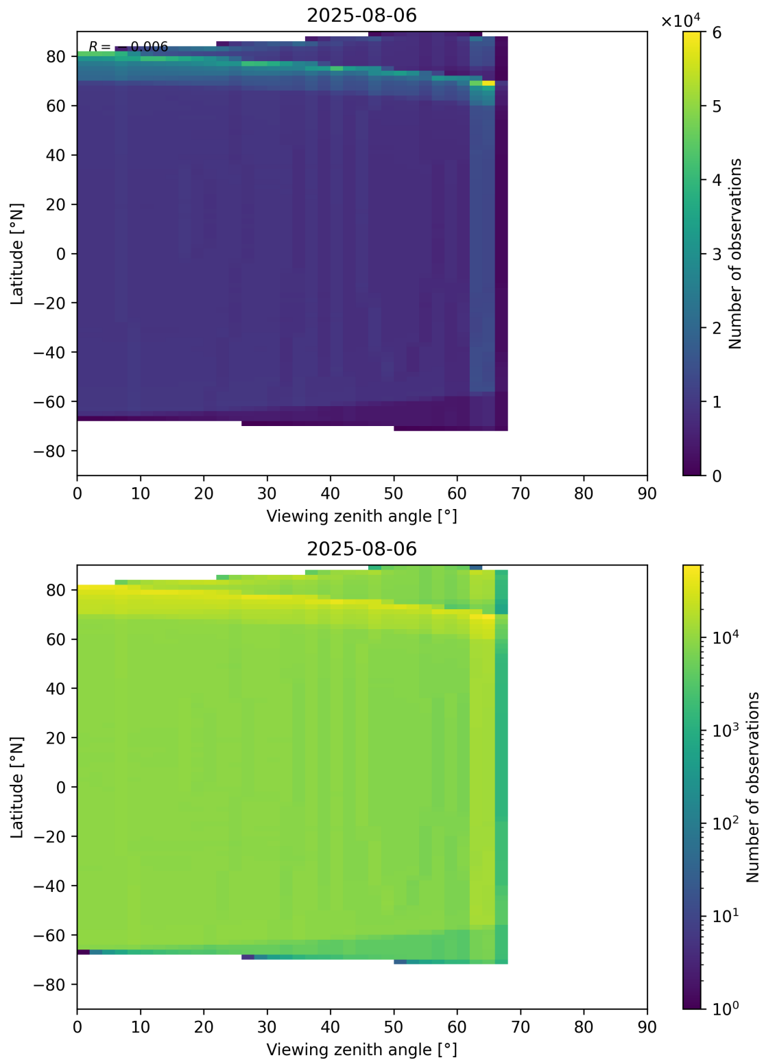
Figure 163: Scatter density plot of “Viewing zenith angle” against “Latitude” for 2025-08-05 to 2025-08-07.
