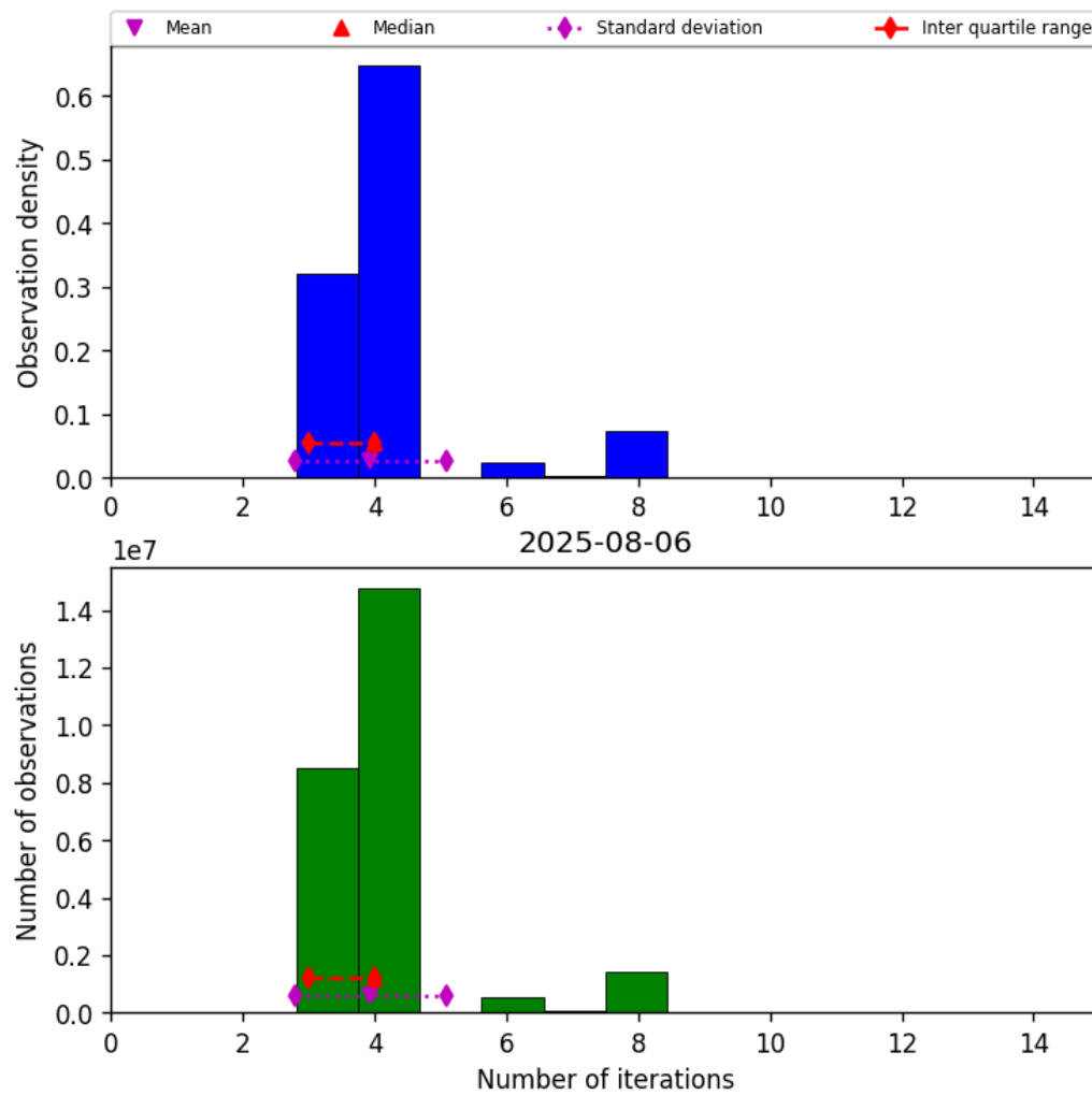
Figure 34: Histogram of “Number of iterations” for 2025-08-05 to 2025-08-07
