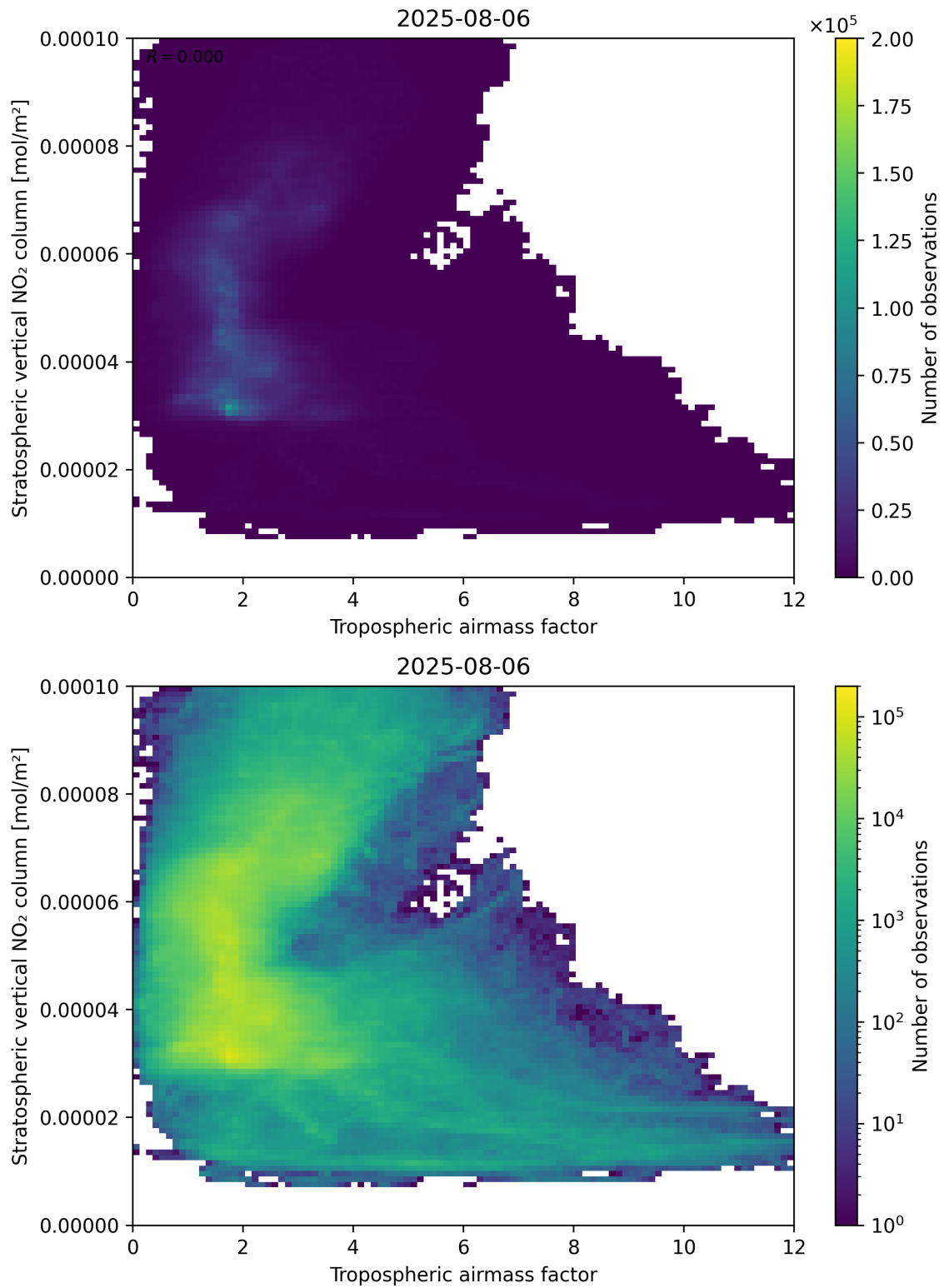
Figure 74: Scatter density plot of “Tropospheric air mass factor” against “Stratospheric vertical NO 2 column” for 2025-08-05 to 2025-08-07.
