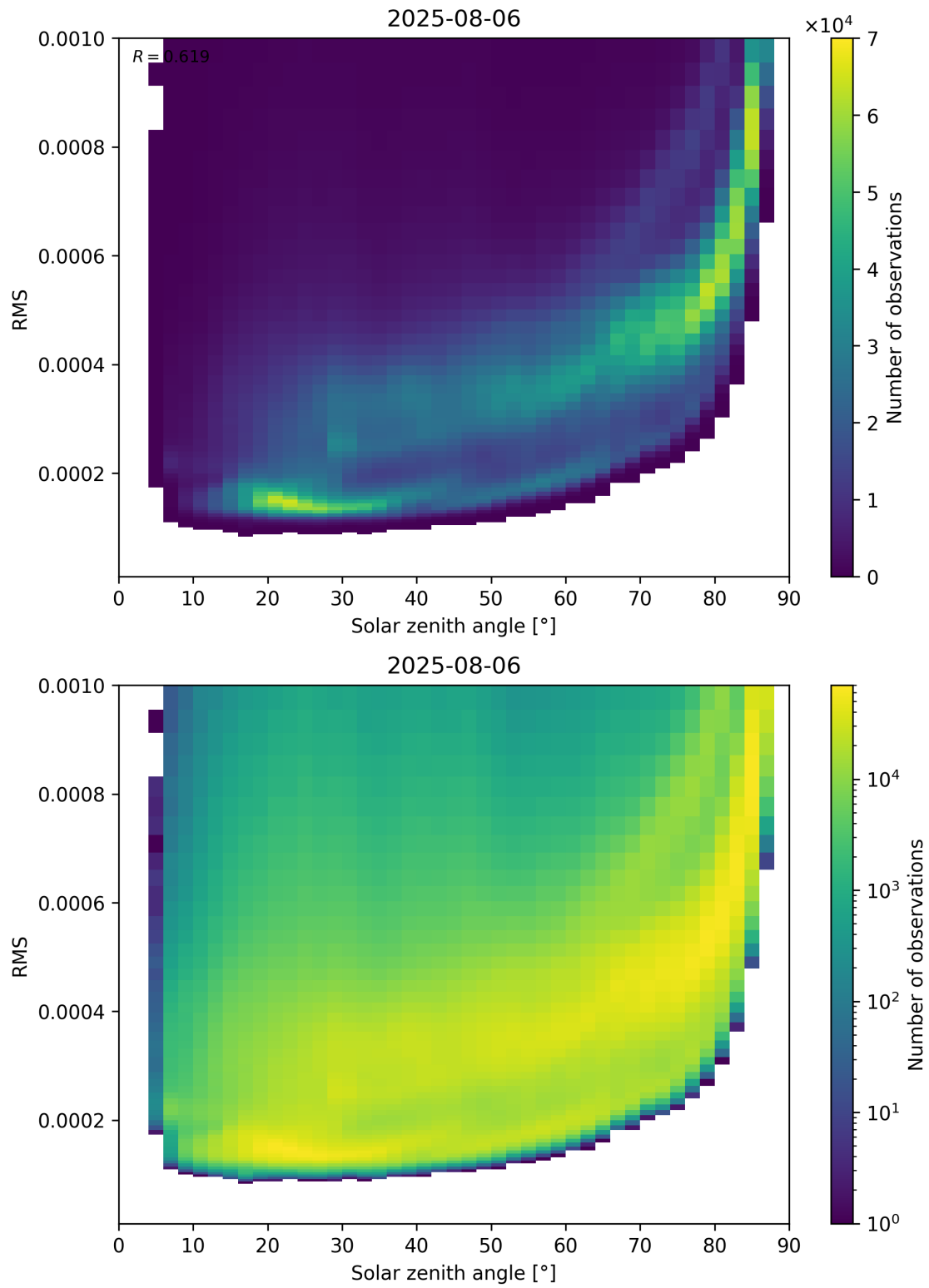
Figure 157: Scatter density plot of “Solar zenith angle” against “RMS” for 2025-08-05 to 2025-08-07.
