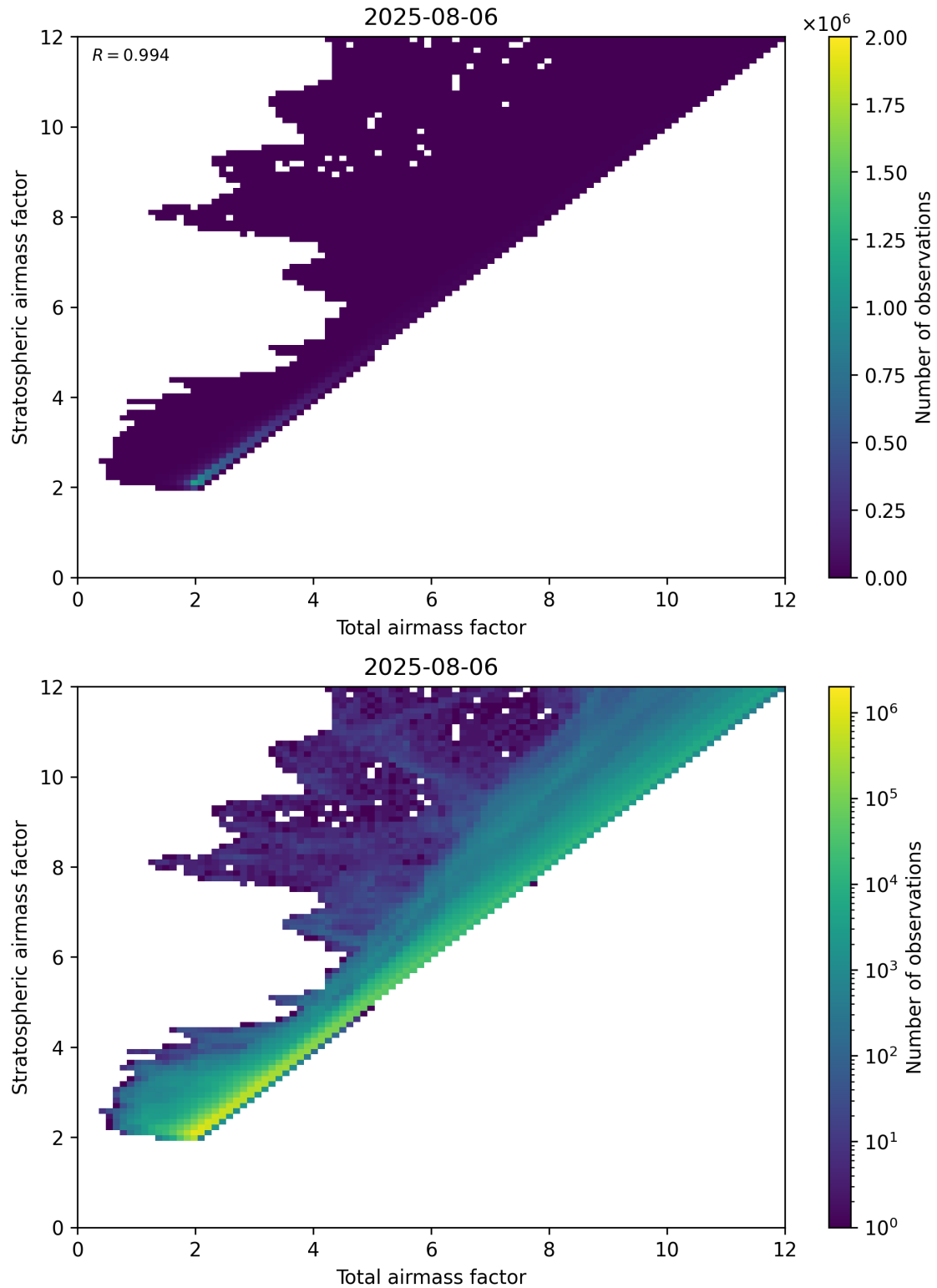
Figure 62: Scatter density plot of “Total airmass factor” against “Stratospheric airmass factor” for 2025-08-05 to 2025-08-07.
