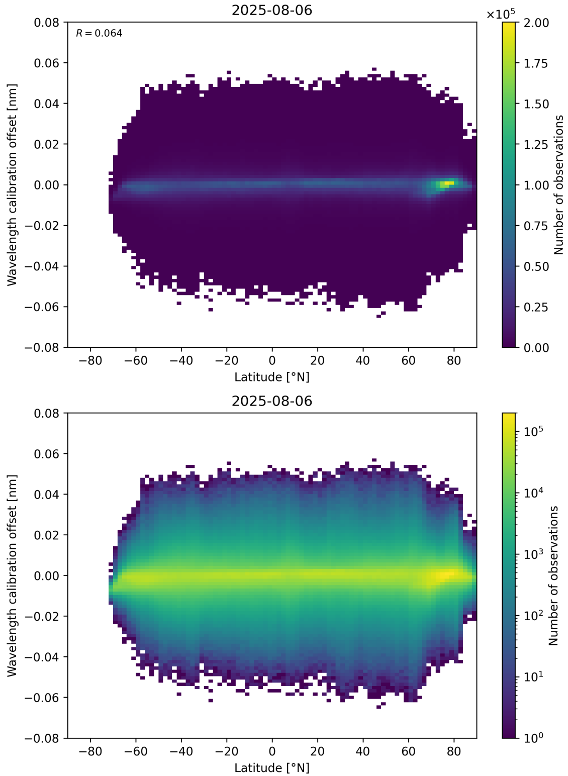
Figure 95: Scatter density plot of “Latitude” against “Wavelength calibration offset” for 2025-08-05 to 2025-08-07.
