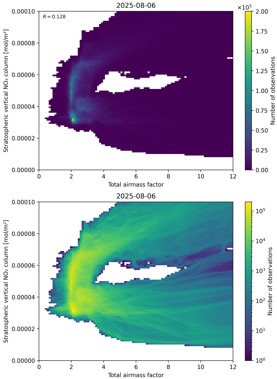
Figure 64: Scatter density plot of “Total airmass factor” against “Stratospheric vertical NO 2 column” for 2025-08-05 to 2025-08-07.
