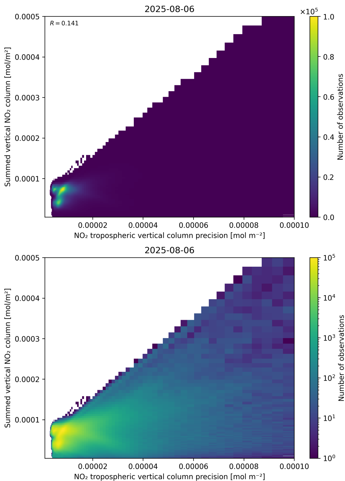
Figure 136: Scatter density plot of “NO 2 tropospheric vertical column precision” against “Summed vertical NO 2 column” for 2025-08-05 to 2025-08-07.
