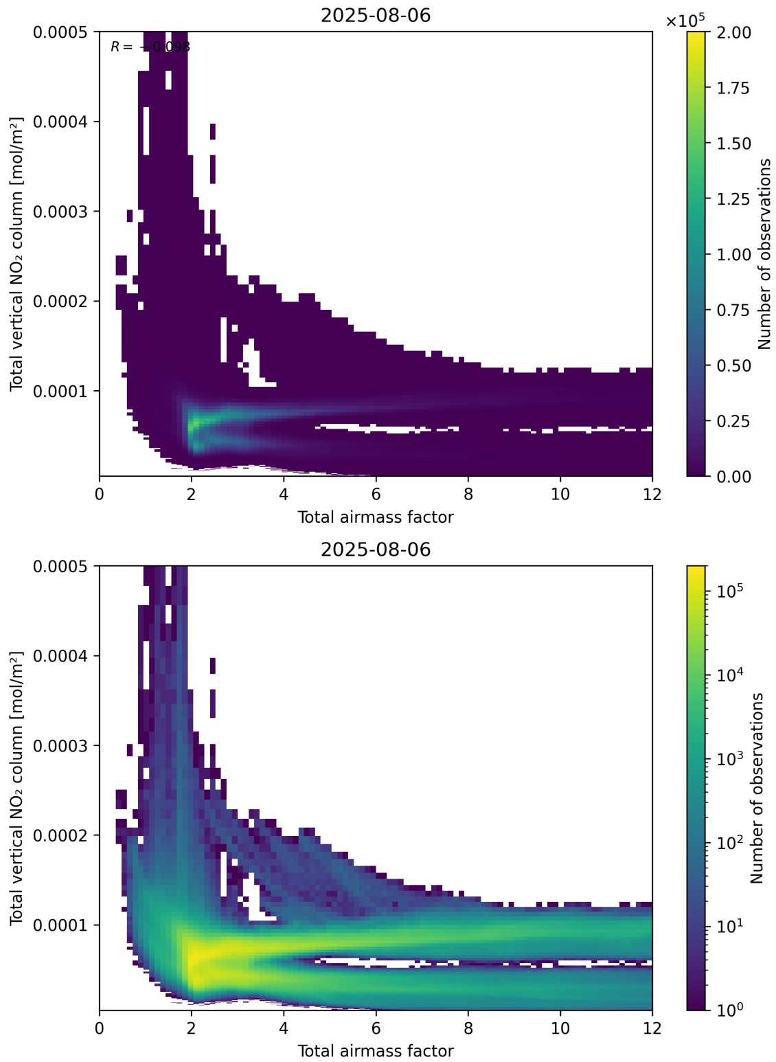
Figure 67: Scatter density plot of “Total airmass factor” against “Total vertical NO 2 column” for 2025-08-05 to 2025-08-07.
