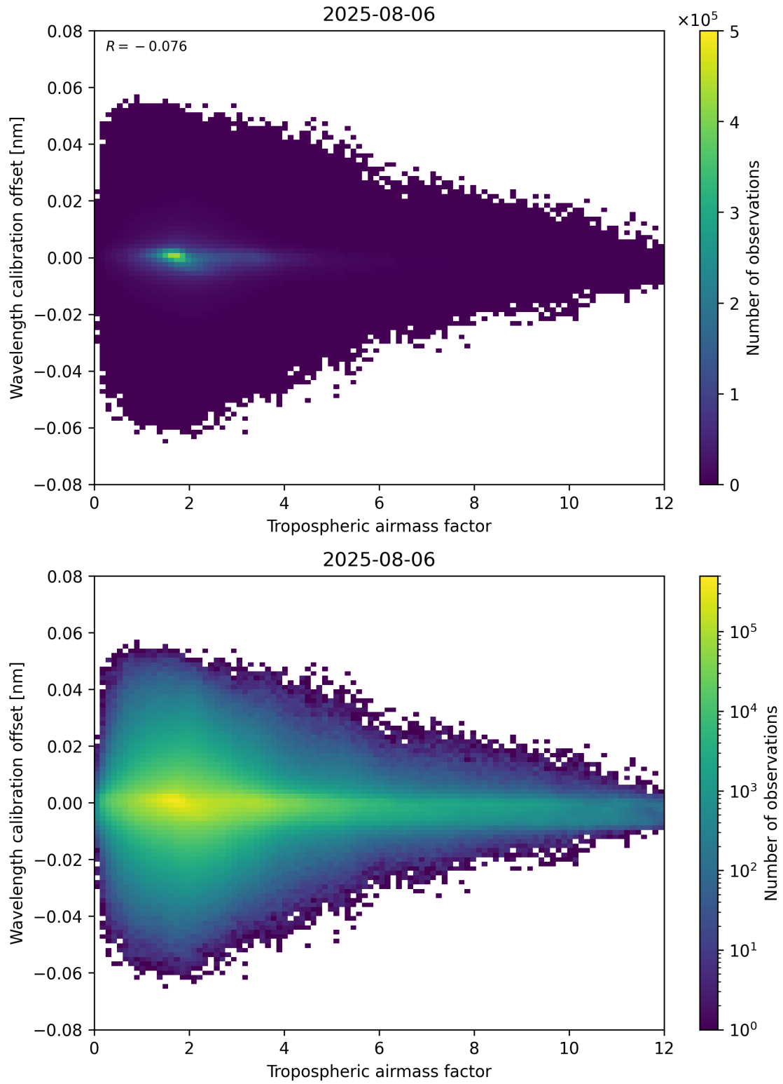
Figure 80: Scatter density plot of “Tropospheric airmass factor” against “Wavelength calibration offset” for 2025-08-05 to 2025-08-07.
