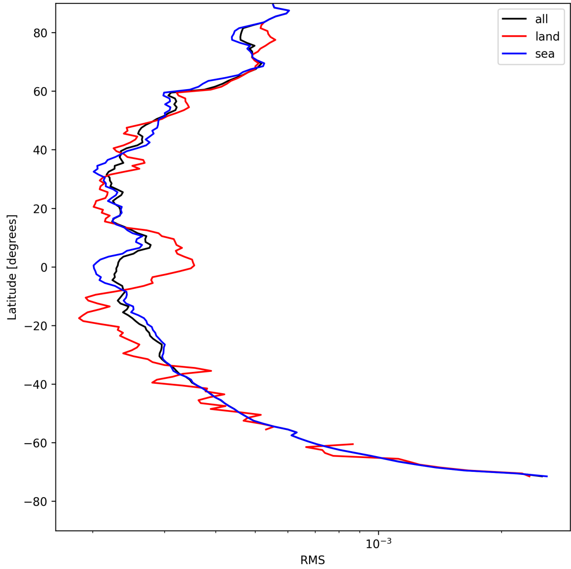
Figure 26: Zonal average of “RMS” for 2025-08-05 to 2025-08-07.
