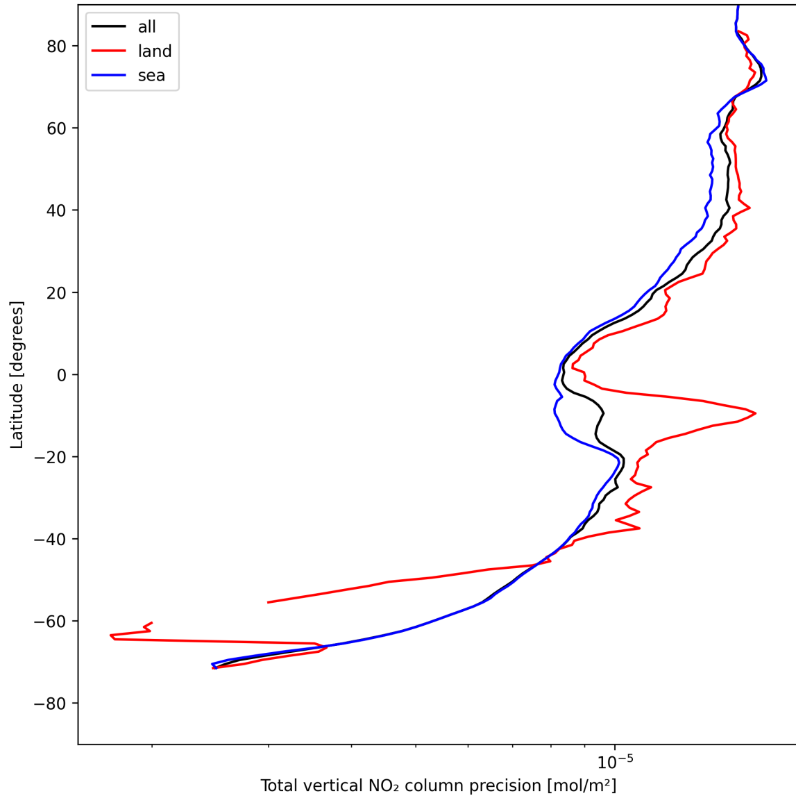
Figure 22: Zonal average of “Total vertical NO 2 column precision” for 2025-08-05 to 2025-08-07.
