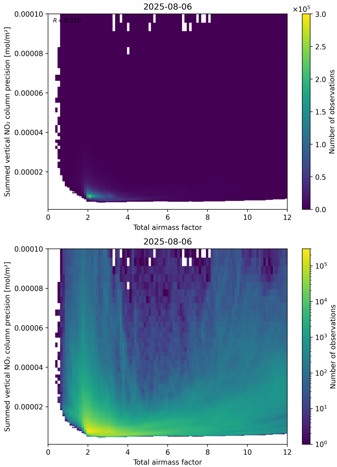
Figure 66: Scatter density plot of “Total airmass factor” against “Summed vertical NO 2 column precision” for 2025-08-05 to 2025-08-07.
