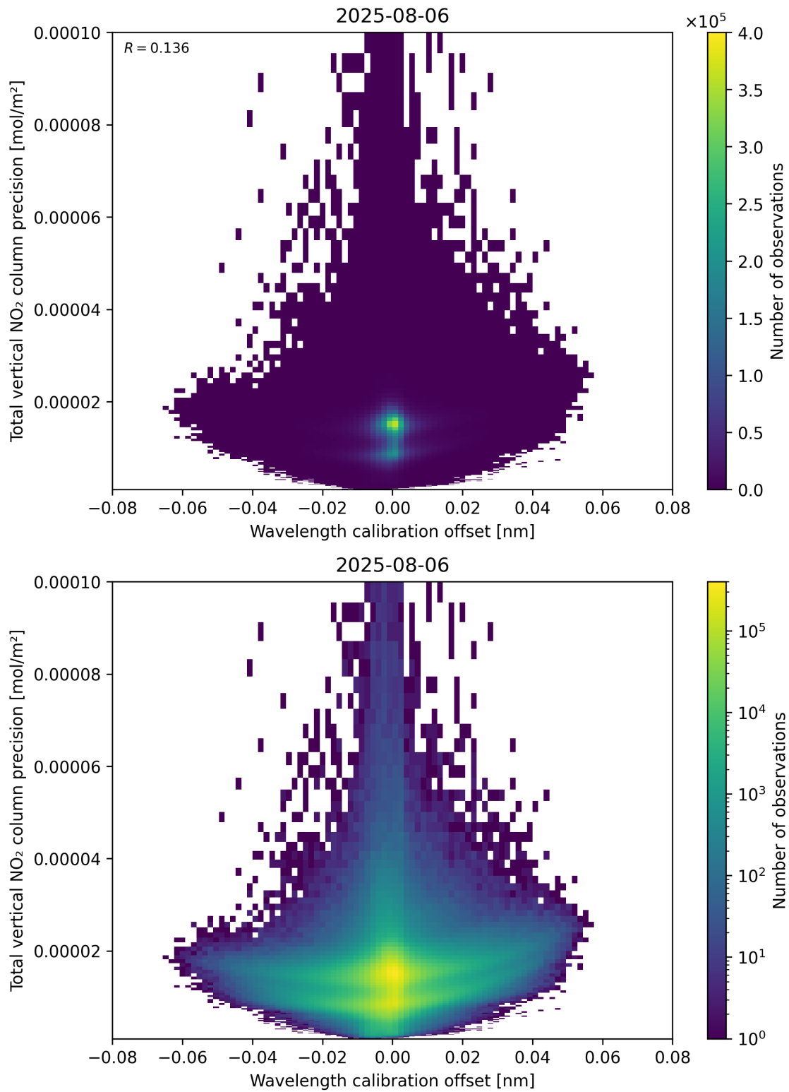
Figure 180: Scatter density plot of “Wavelength calibration offset” against “Total vertical NO 2 column precision” for 2025-08-05 to 2025-08-07.
