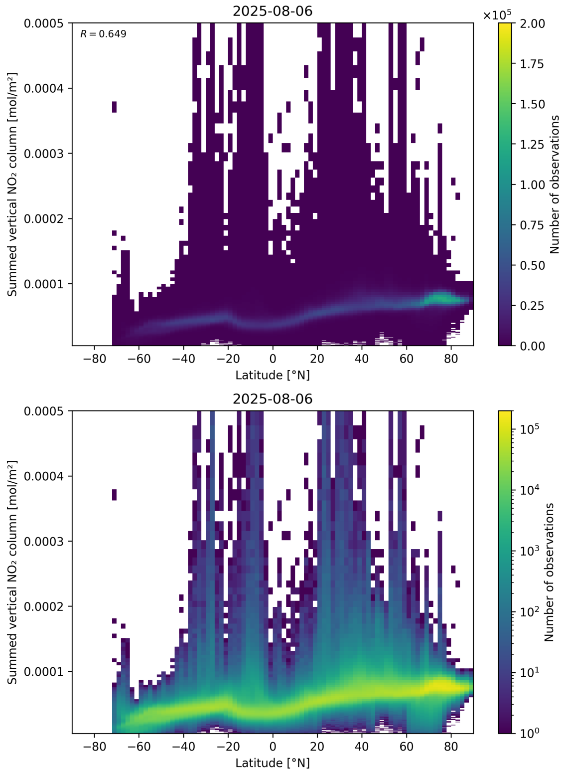
Figure 88: Scatter density plot of “Latitude” against “Summed vertical NO 2 column” for 2025-08-05 to 2025-08-07.
