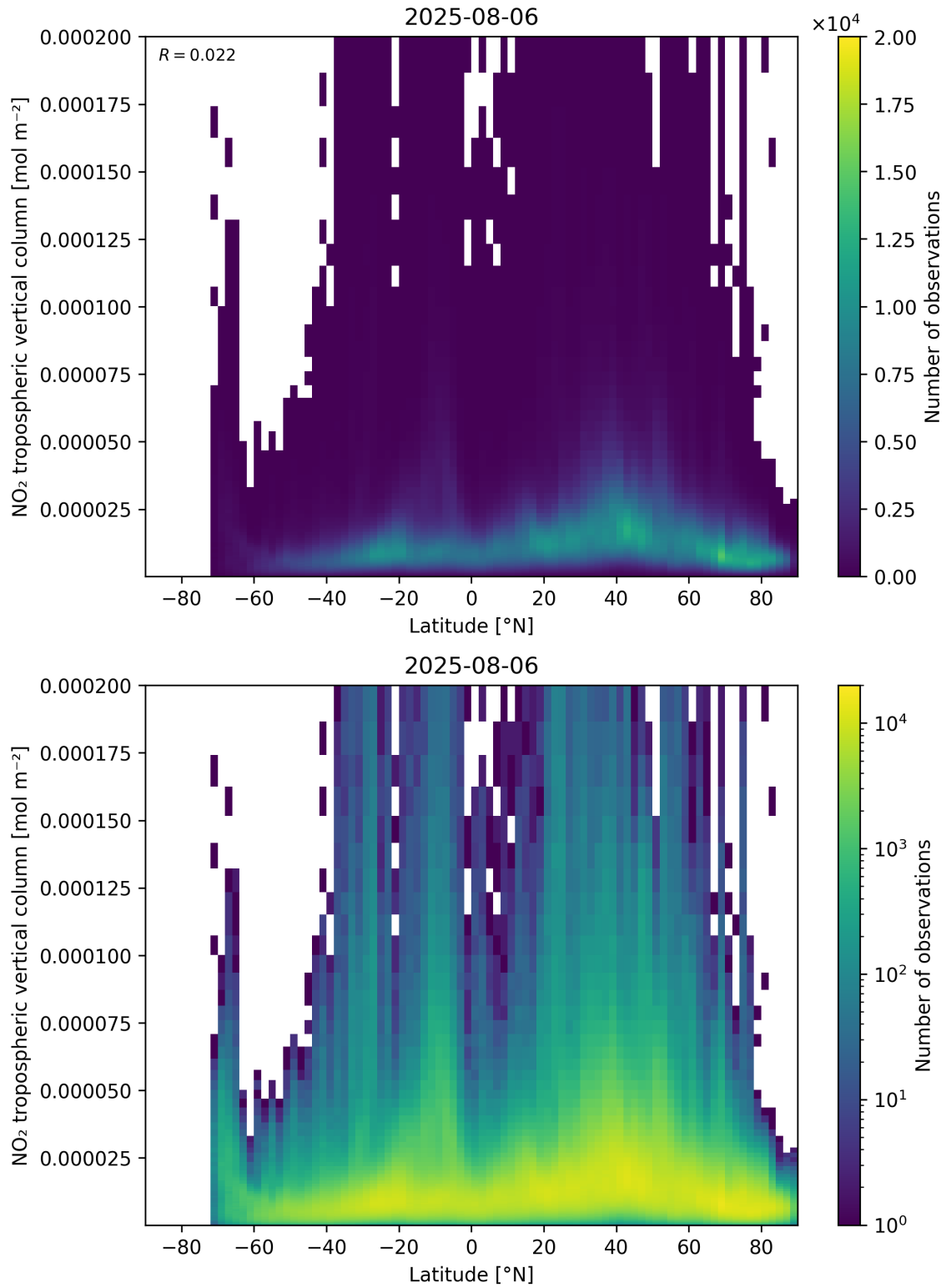
Figure 92: Scatter density plot of “Latitude” against “NO 2 tropospheric vertical column” for 2025-08-05 to 2025-08-07.
