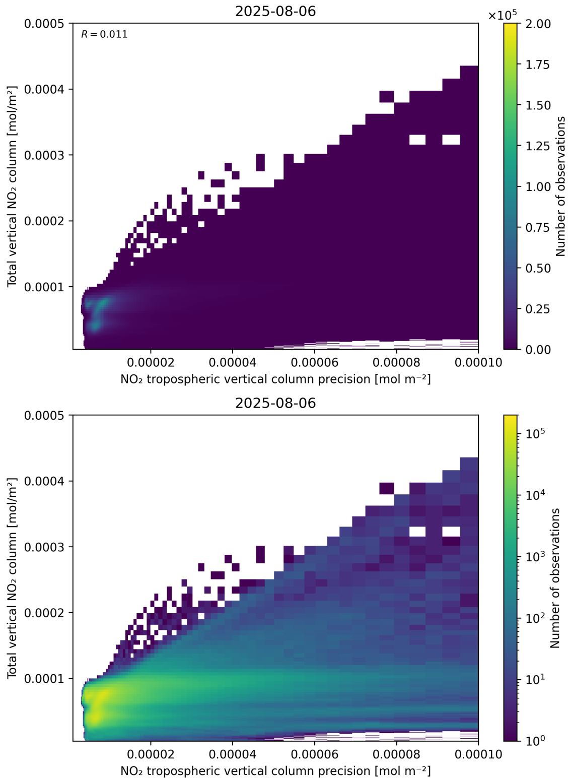
Figure 138: Scatter density plot of “NO 2 tropospheric vertical column precision” against “Total vertical NO 2 column” for 2025-08-05 to 2025-08-07.
