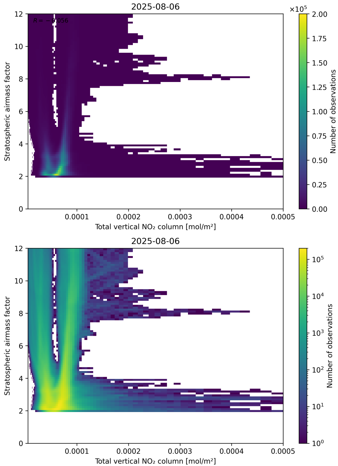
Figure 110: Scatter density plot of “Total vertical NO 2 column” against “Stratospheric airmass factor” for 2025-08-05 to 2025-08-07.
