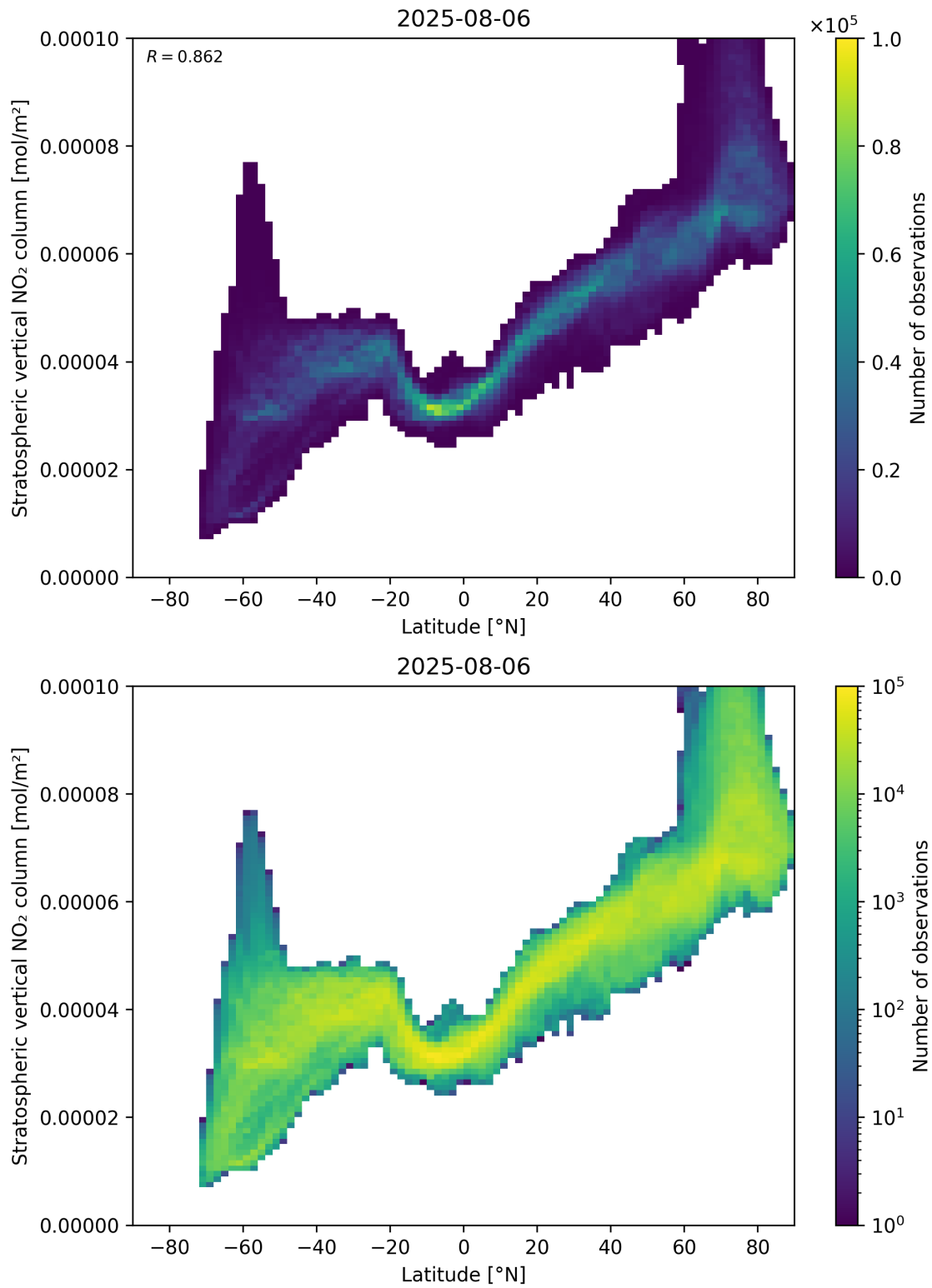
Figure 87: Scatter density plot of “Latitude” against “Stratospheric vertical NO 2 column” for 2025-08-05 to 2025-08-07.
