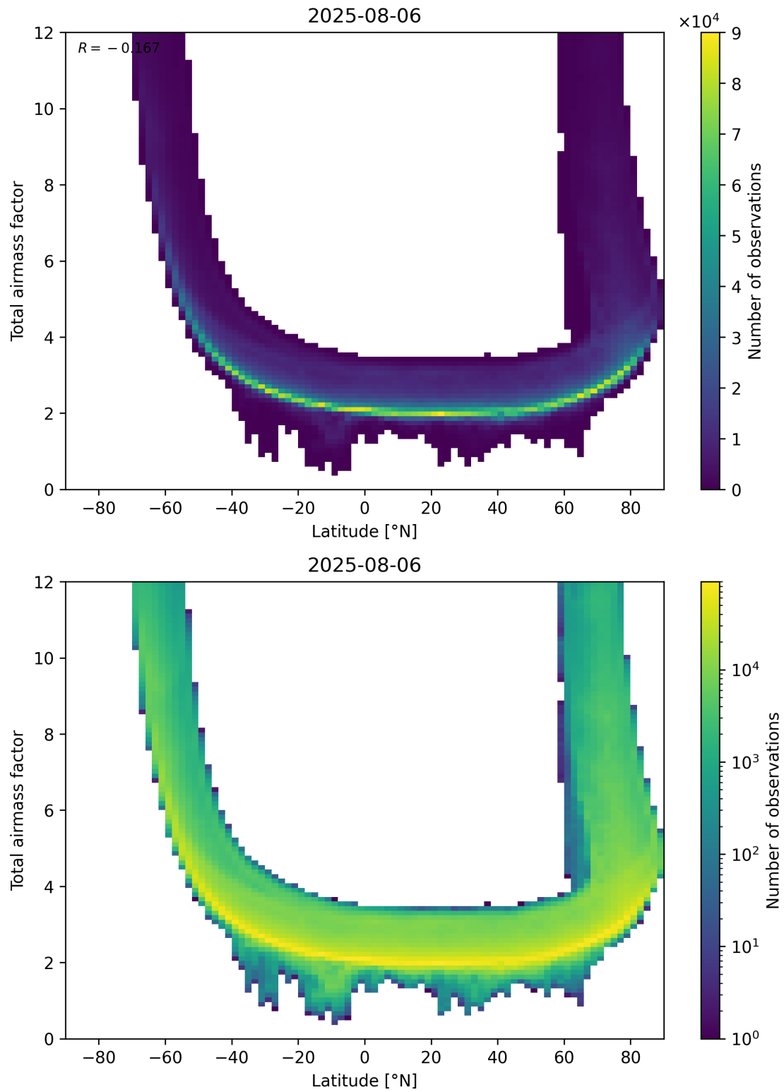
Figure 84: Scatter density plot of “Latitude” against “Total airmass factor” for 2025-08-05 to 2025-08-07.
