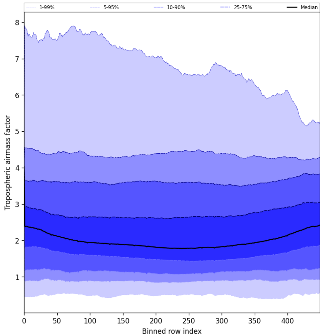
Figure 48: Along track statistics of “Tropospheric airmass factor” for 2025-08-05 to 2025-08-07
