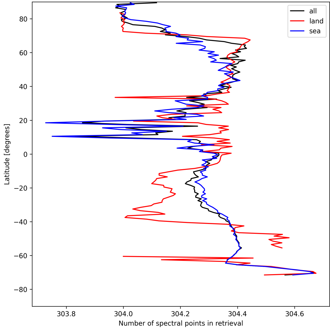
Figure 16: Zonal average of “Number of spectral points in retrieval” for 2025-08-05 to 2025-08-07.
