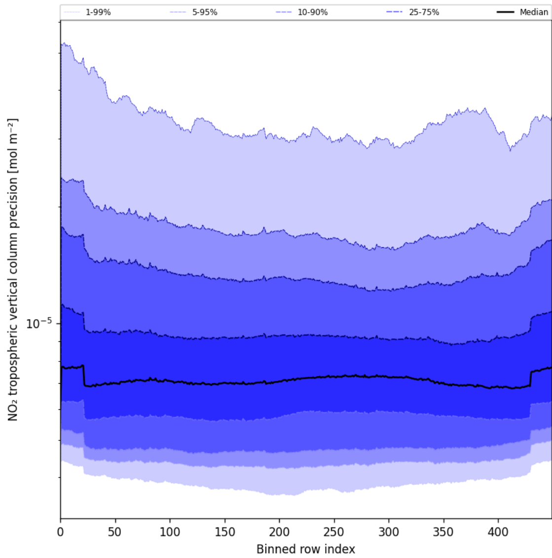
Figure 47: Along track statistics of “NO 2 tropospheric vertical column precision” for 2025-08-05 to 2025-08-07
