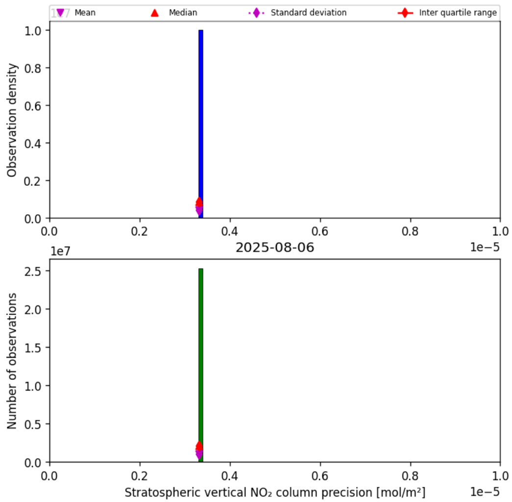
Figure 37: Histogram of “Stratospheric vertical NO 2 column precision” for 2025-08-05 to 2025-08-07
