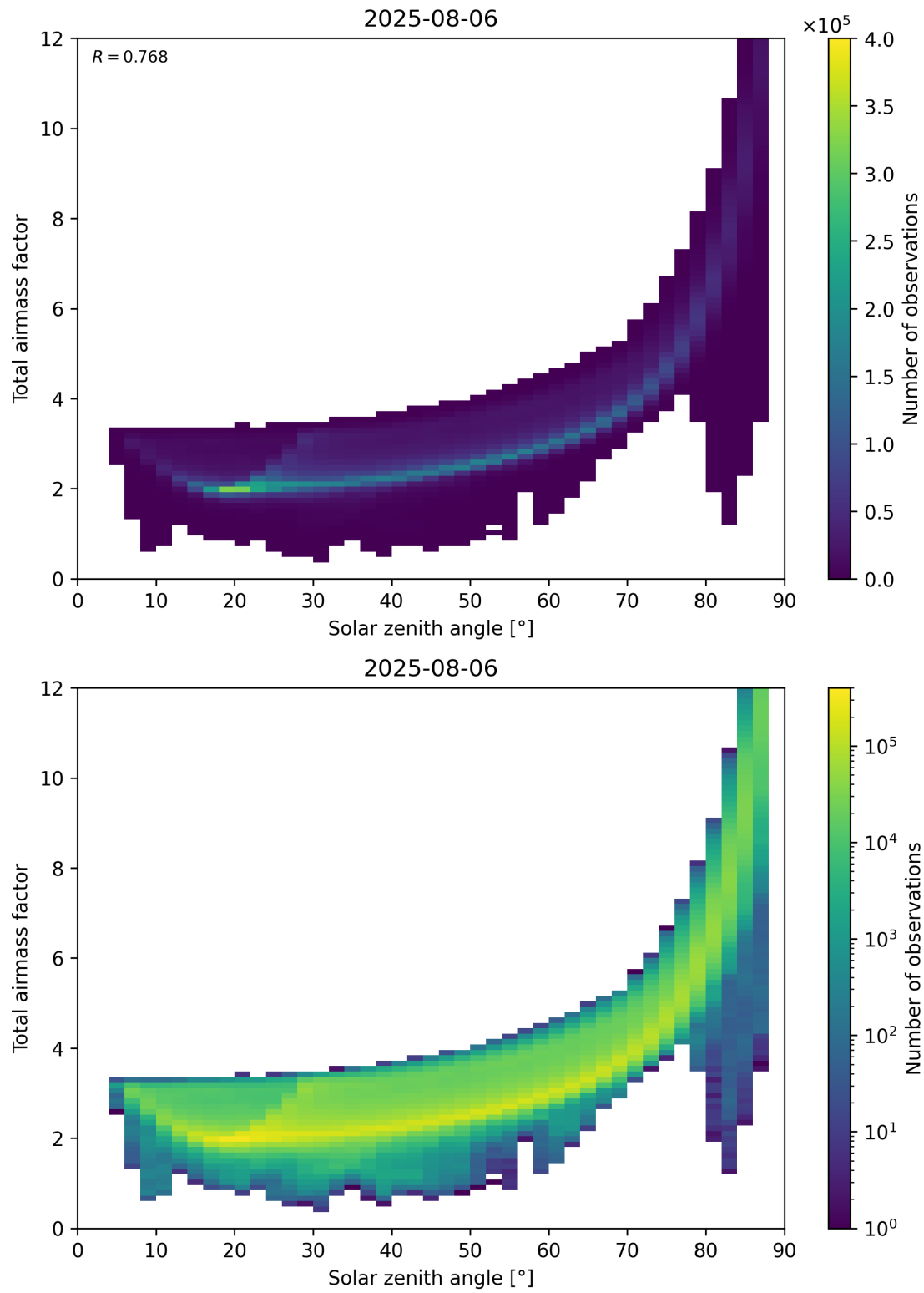
Figure 146: Scatter density plot of “Solar zenith angle” against “Total airmass factor” for 2025-08-05 to 2025-08-07.
