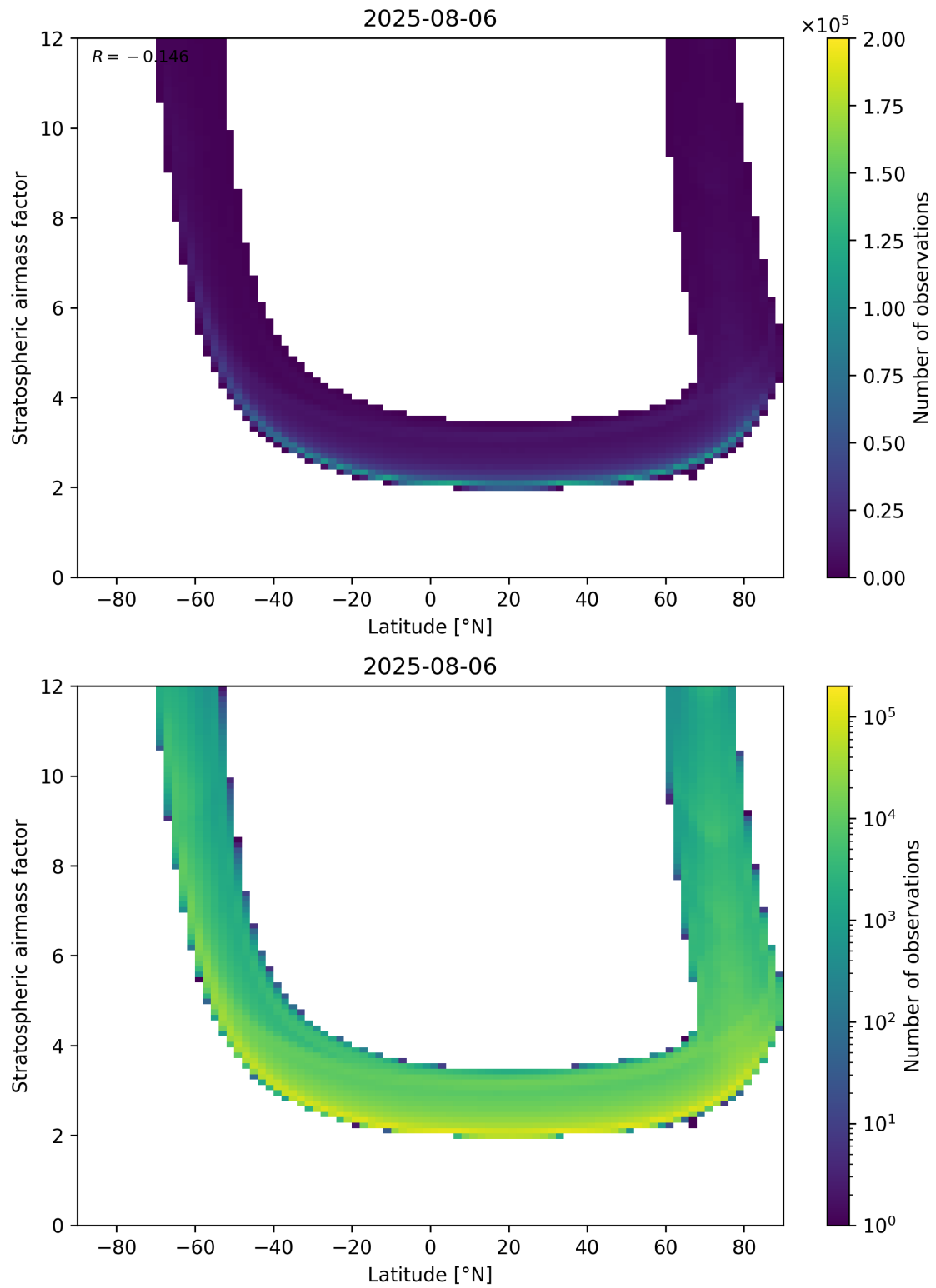
Figure 83: Scatter density plot of “Latitude” against “Stratospheric air mass factor” for 2025-08-05 to 2025-08-07.
