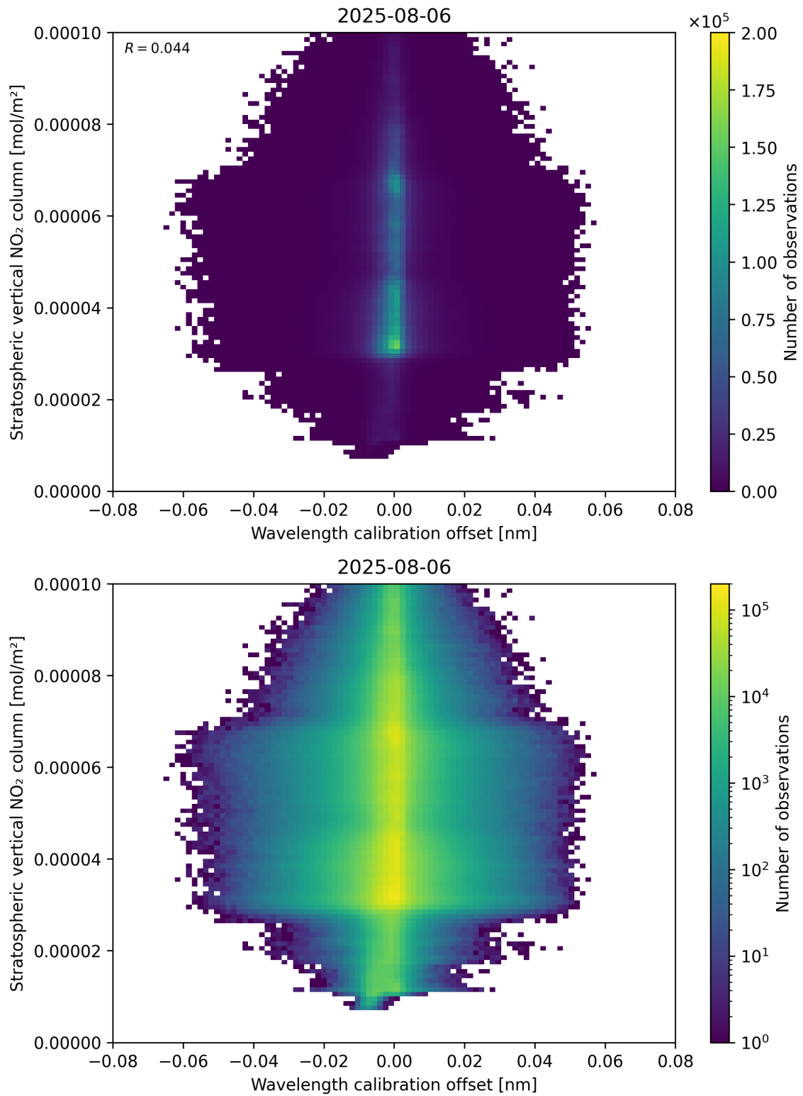
Figure 176: Scatter density plot of “Wavelength calibration offset” against “Stratospheric vertical NO 2 column” for 2025-08-05 to 2025-08-07.
