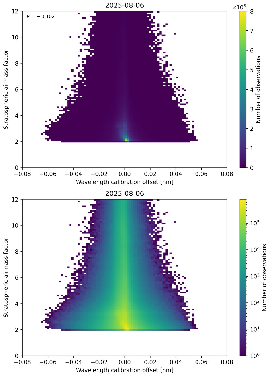
Figure 174: Scatter density plot of “Wavelength calibration offset” against “Stratospheric air mass factor” for 2025-08-05 to 2025-08-07.
