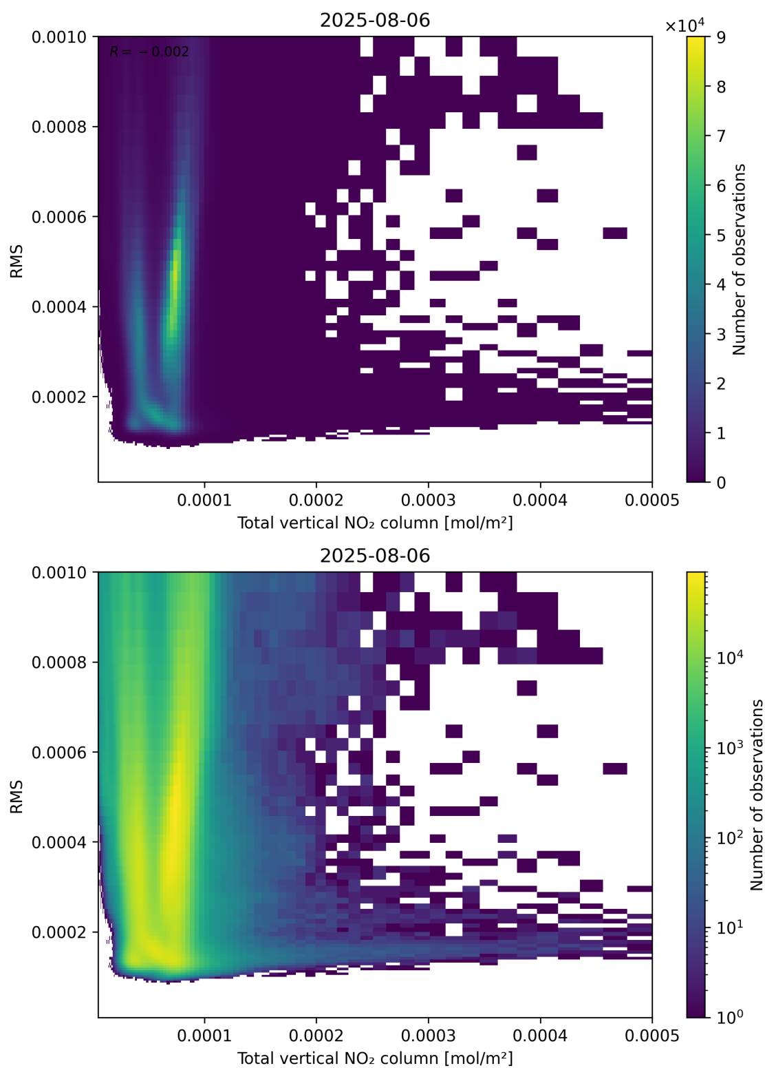
Figure 120: Scatter density plot of “Total vertical NO 2 column” against “RMS” for 2025-08-05 to 2025-08-07.
