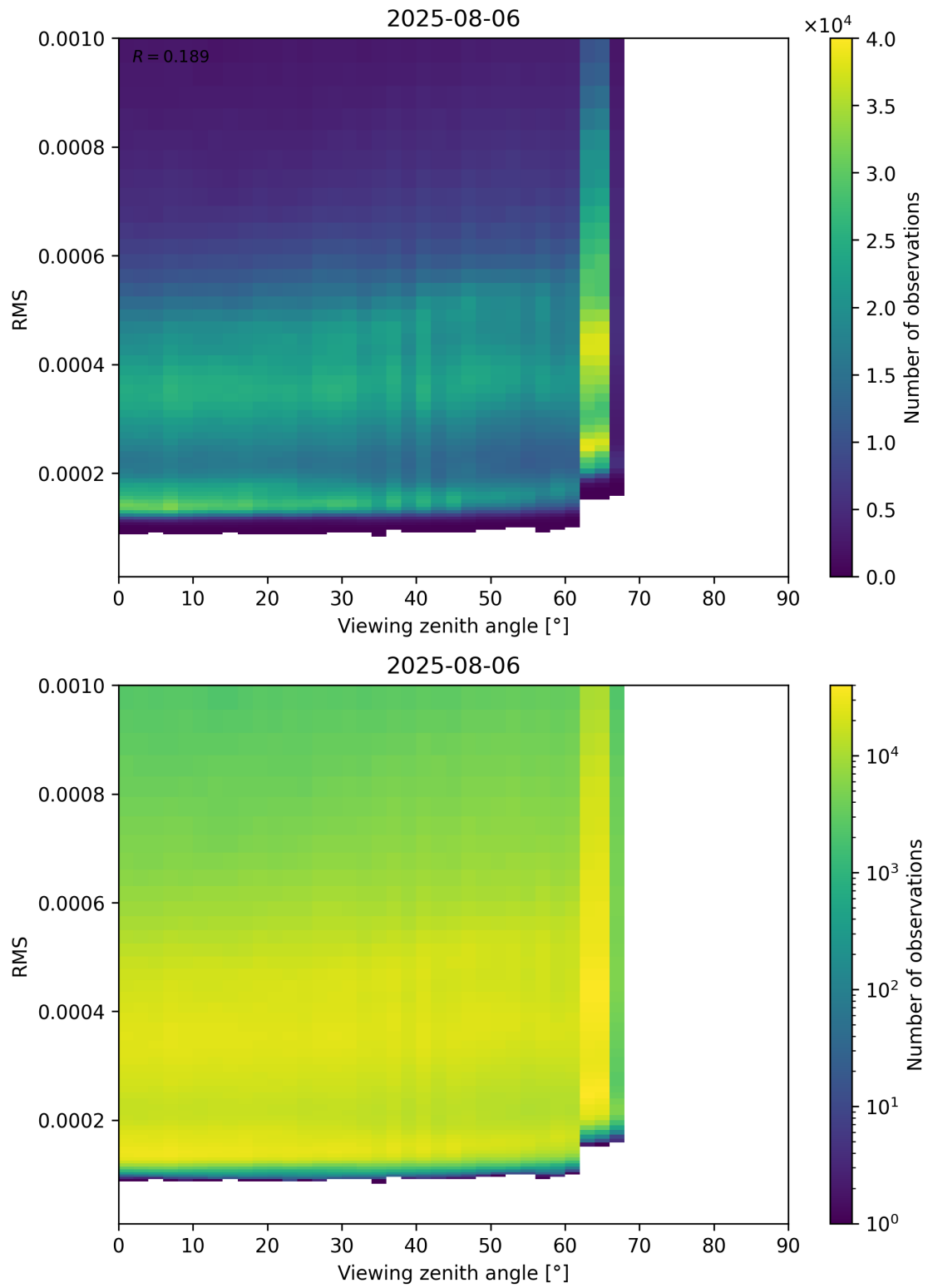
Figure 171: Scatter density plot of “Viewing zenith angle” against “RMS” for 2025-08-05 to 2025-08-07.
