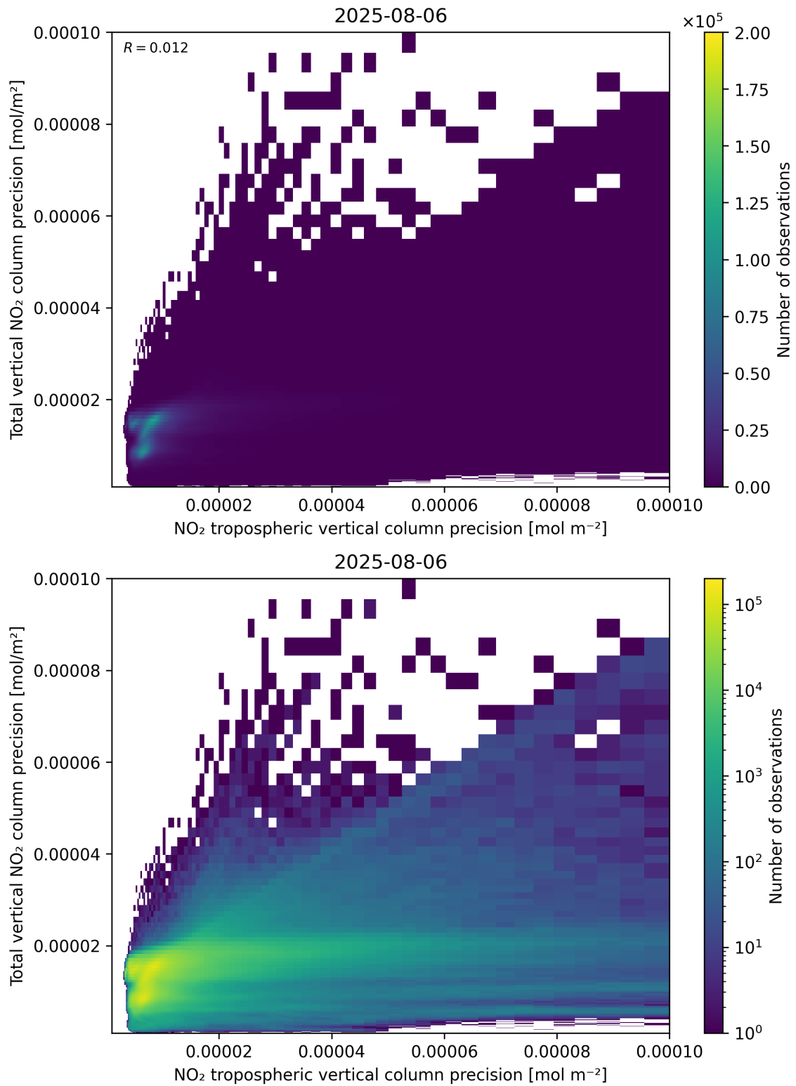
Figure 139: Scatter density plot of “NO 2 tropospheric vertical column precision” against “Total vertical NO 2 column precision” for 2025-08-05 to 2025-08-07.
