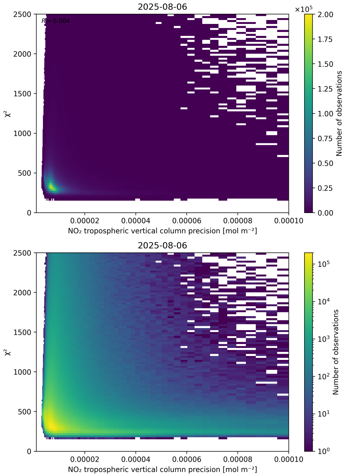
Figure 134: Scatter density plot of “NO 2 tropospheric vertical column precision” against “ \chi^2 ” for 2025-08-05 to 2025-08-07.
