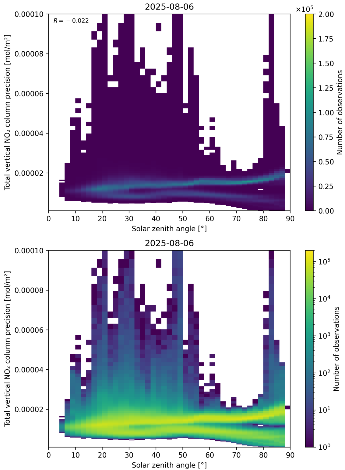
Figure 154: Scatter density plot of “Solar zenith angle” against “Total vertical NO 2 column precision” for 2025-08-05 to 2025-08-07.
