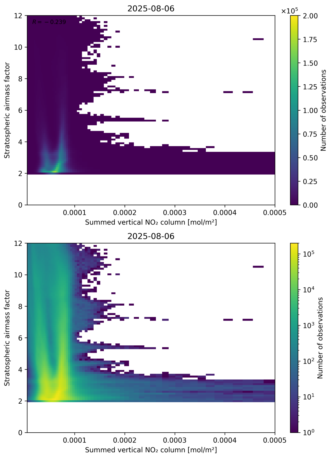
Figure 103: Scatter density plot of “Summed vertical NO 2 column” against “Stratospheric air mass factor” for 2025-08-05 to 2025-08-07.
