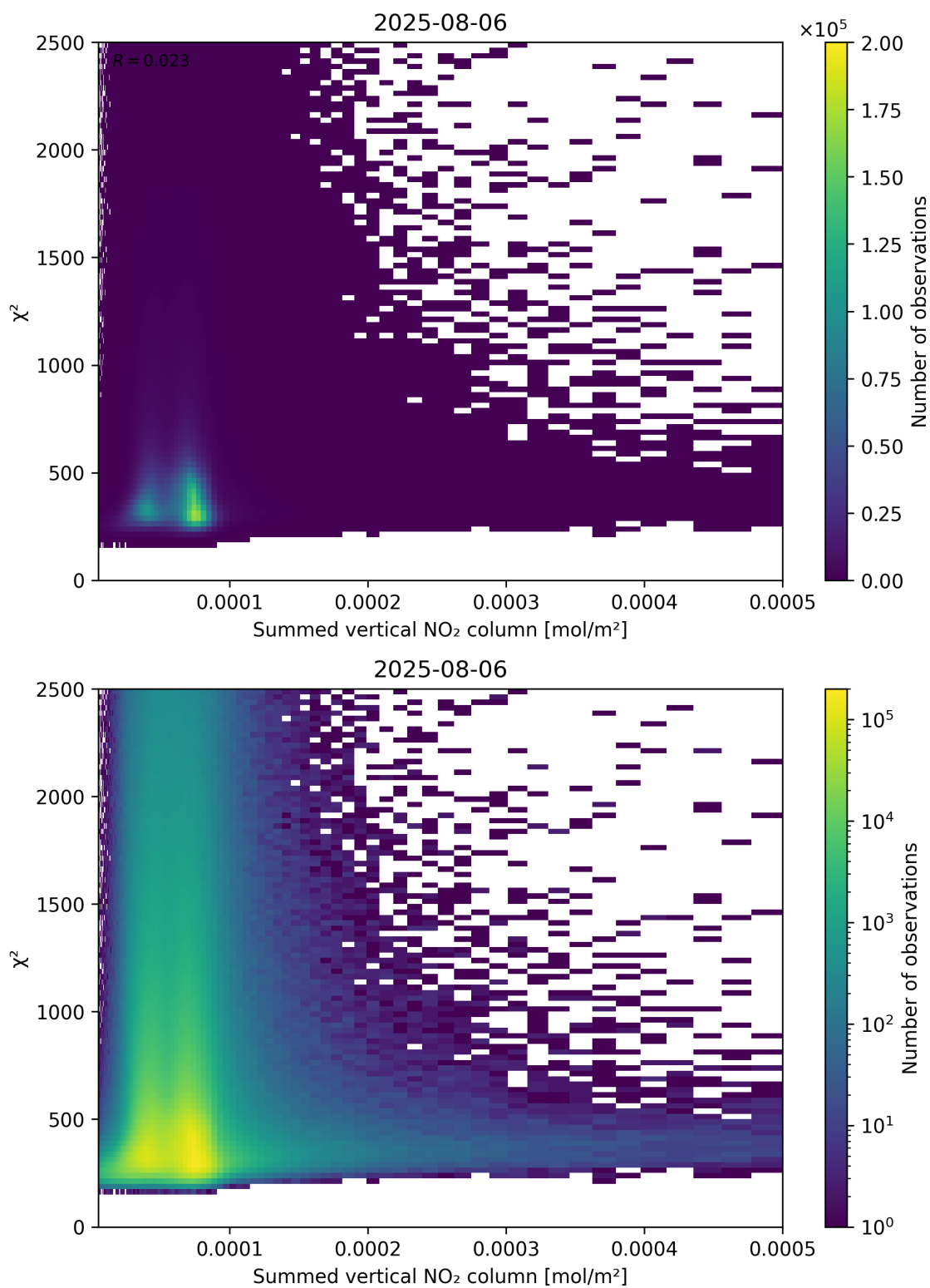
Figure 104: Scatter density plot of “Summed vertical NO 2 column” against “ \chi^2 ” for 2025-08-05 to 2025-08-07.
