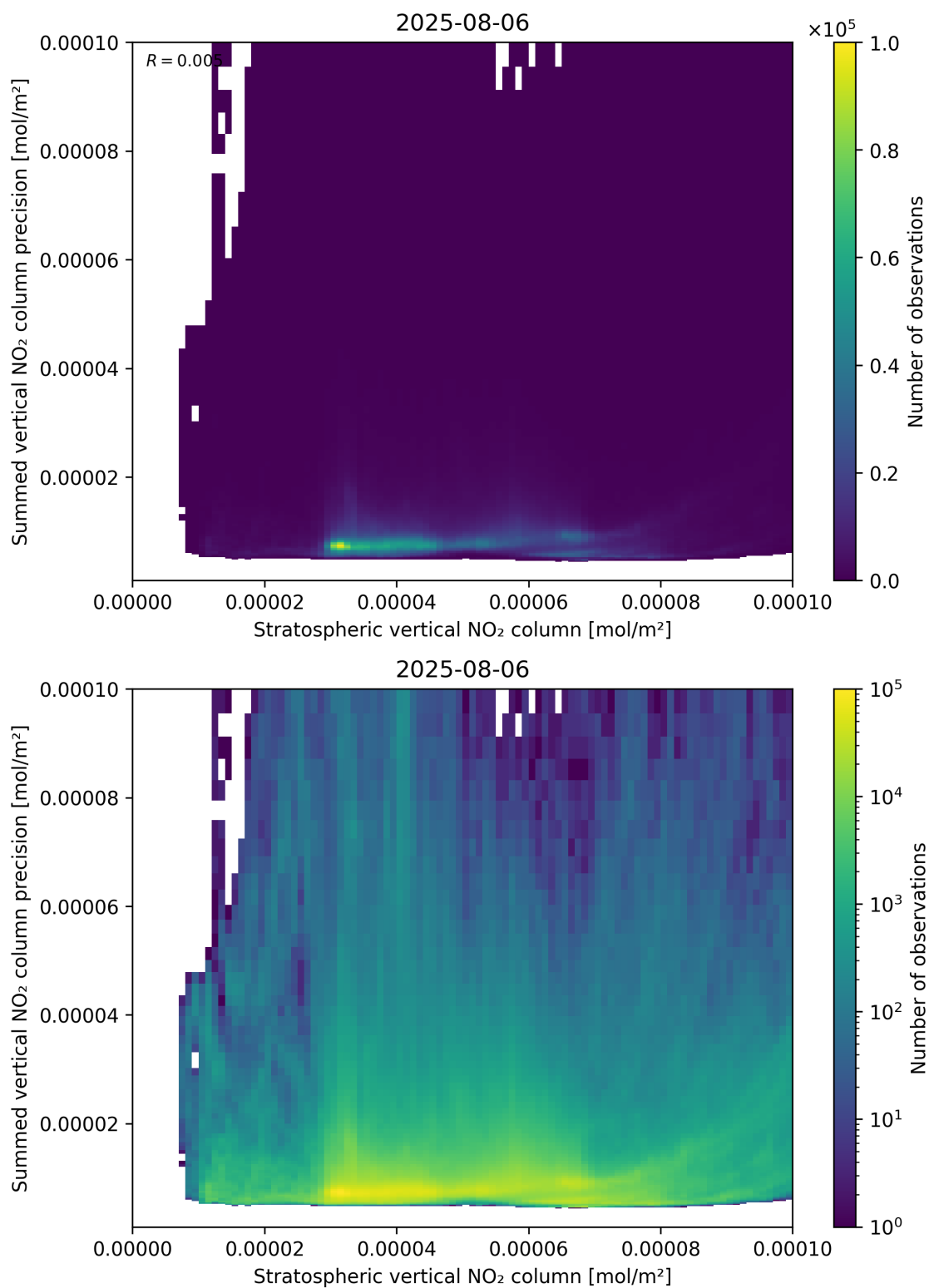
Figure 99: Scatter density plot of “Stratospheric vertical NO 2 column” against “Summed vertical NO 2 column precision” for 2025-08-05 to 2025-08-07.
