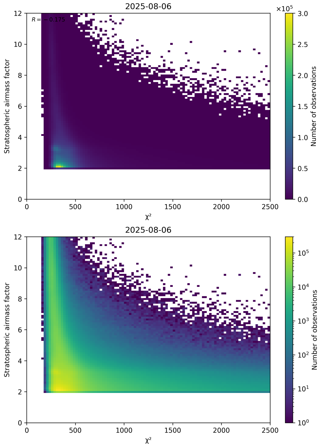
Figure 81: Scatter density plot of “ \chi^2 ” against “Stratospheric airmass factor” for 2025-08-05 to 2025-08-07.
