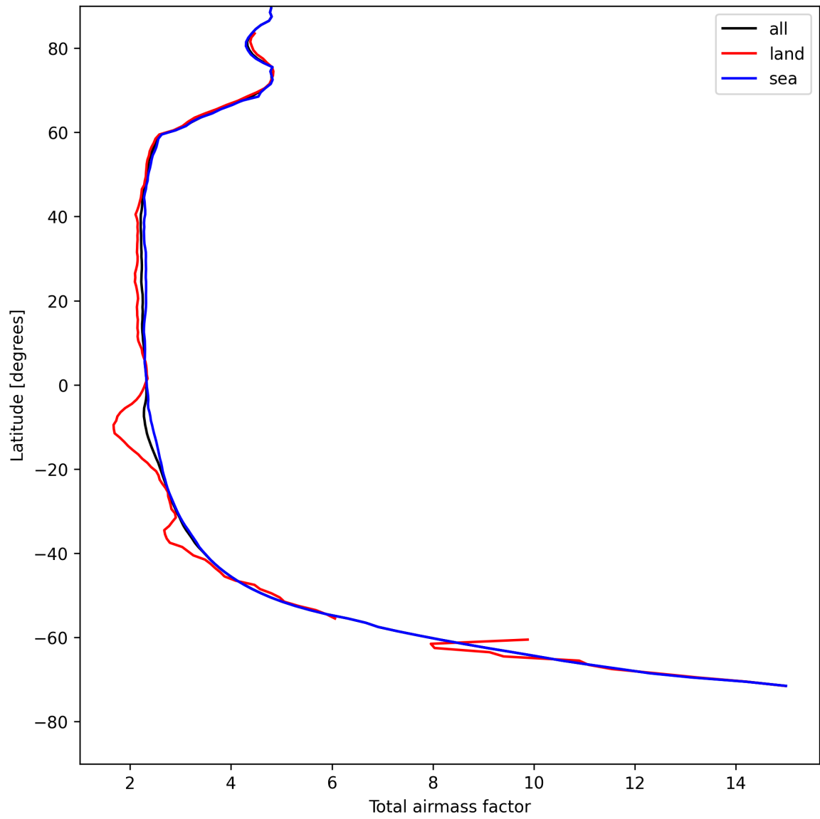
Figure 15: Zonal average of “Total airmass factor” for 2025-08-05 to 2025-08-07.
