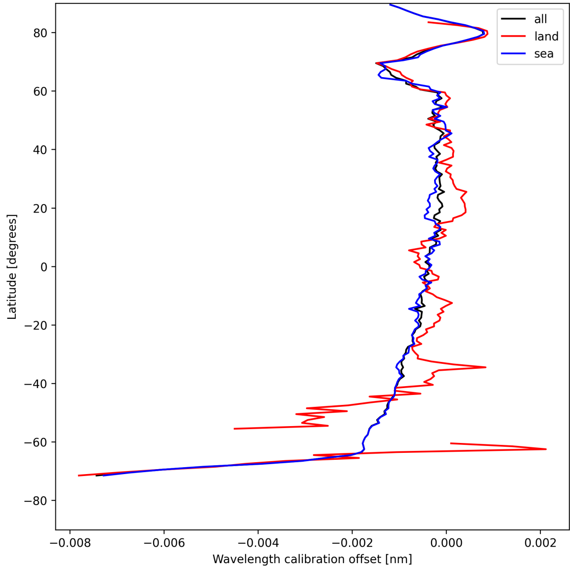
Figure 18: Zonal average of “Wavelength calibration offset” for 2025-08-05 to 2025-08-07.
