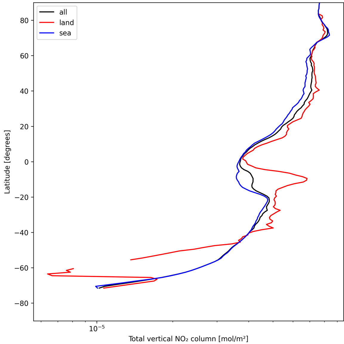
Figure 21: Zonal average of “Total vertical NO 2 column” for 2025-08-05 to 2025-08-07.
