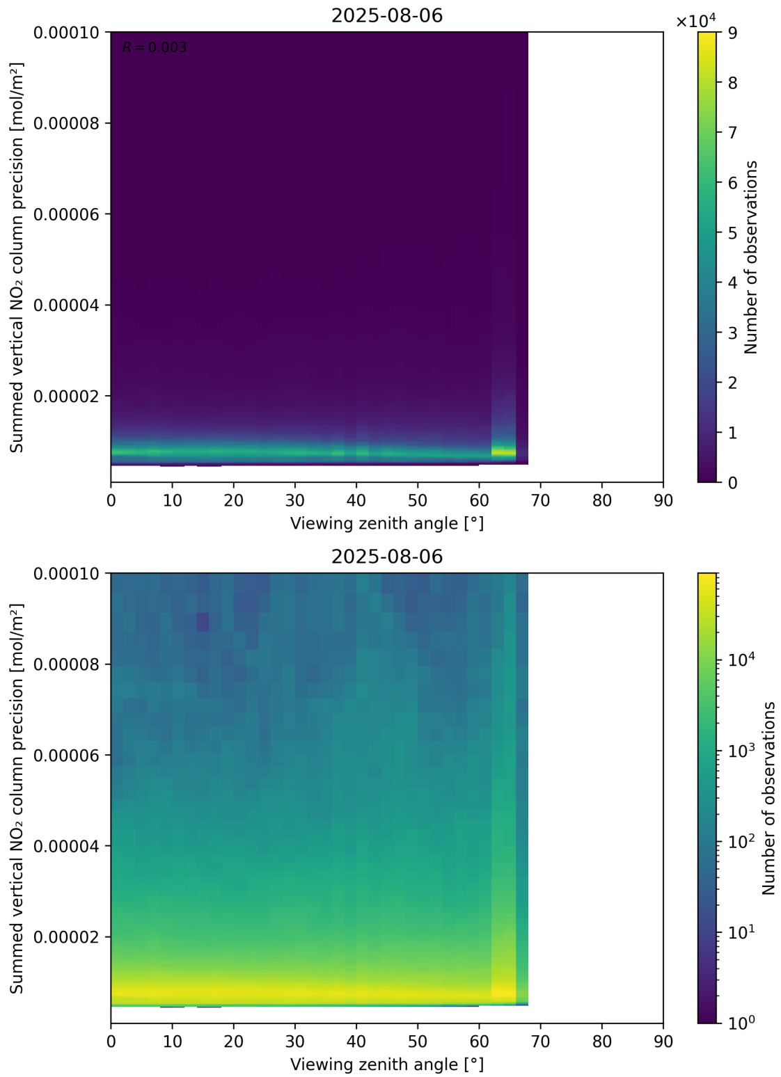
Figure 166: Scatter density plot of “Viewing zenith angle” against “Summed vertical NO 2 column precision” for 2025-08-05 to 2025-08-07.
