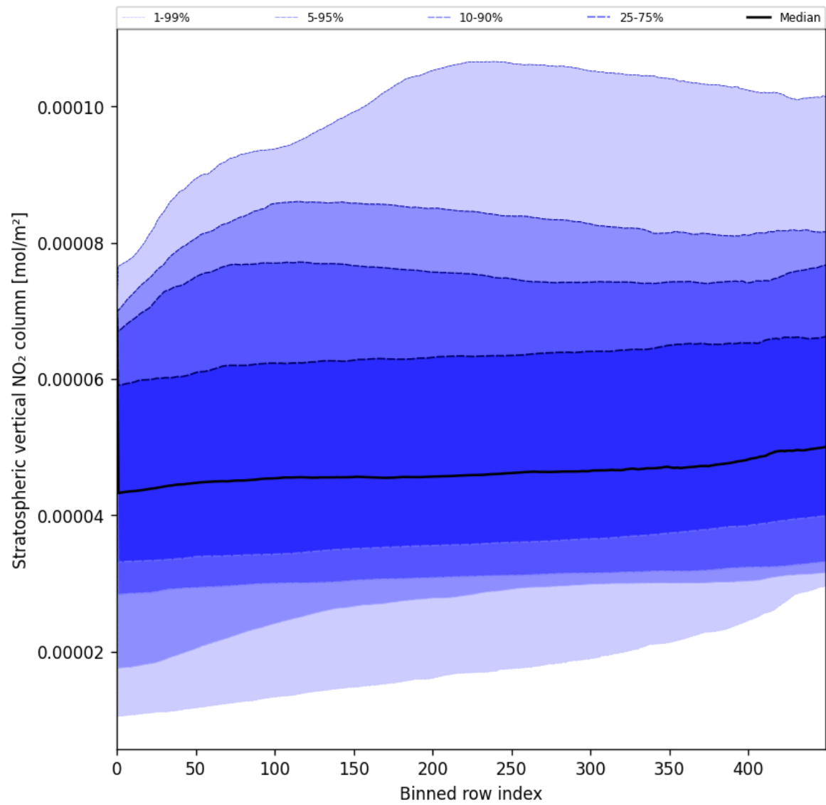
Figure 53: Along track statistics of “Stratospheric vertical NO 2 column” for 2025-08-05 to 2025-08-07
