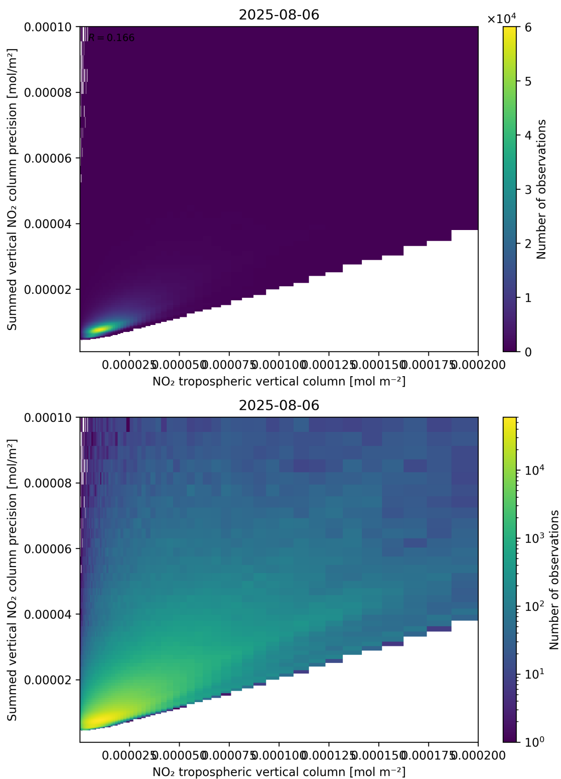
Figure 127: Scatter density plot of “NO 2 tropospheric vertical column” against “Summed vertical NO 2 column precision” for 2025-08-05 to 2025-08-07.
