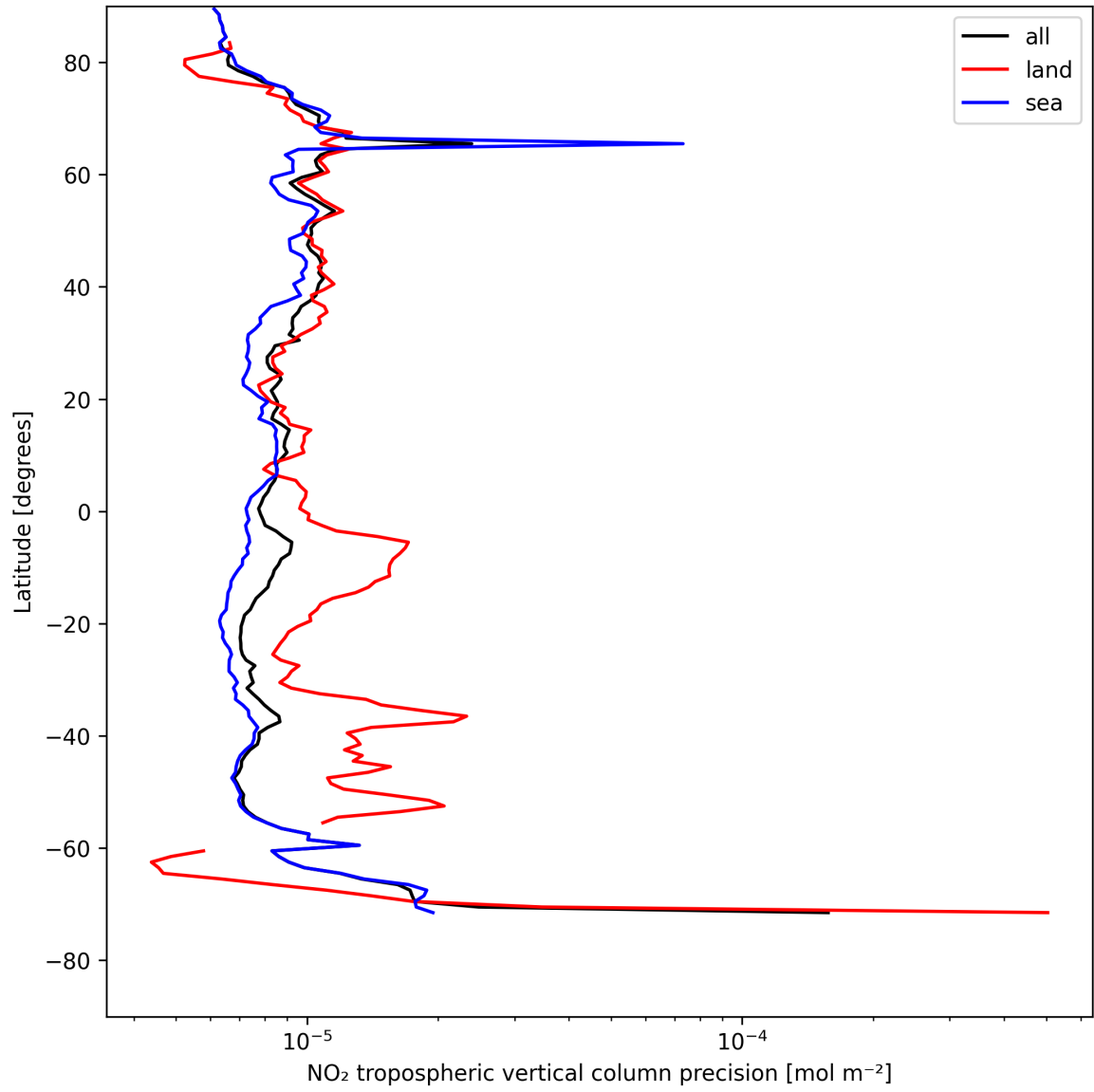
Figure 13: Zonal average of “NO 2 tropospheric vertical column precision” for 2025-08-05 to 2025-08-07.
