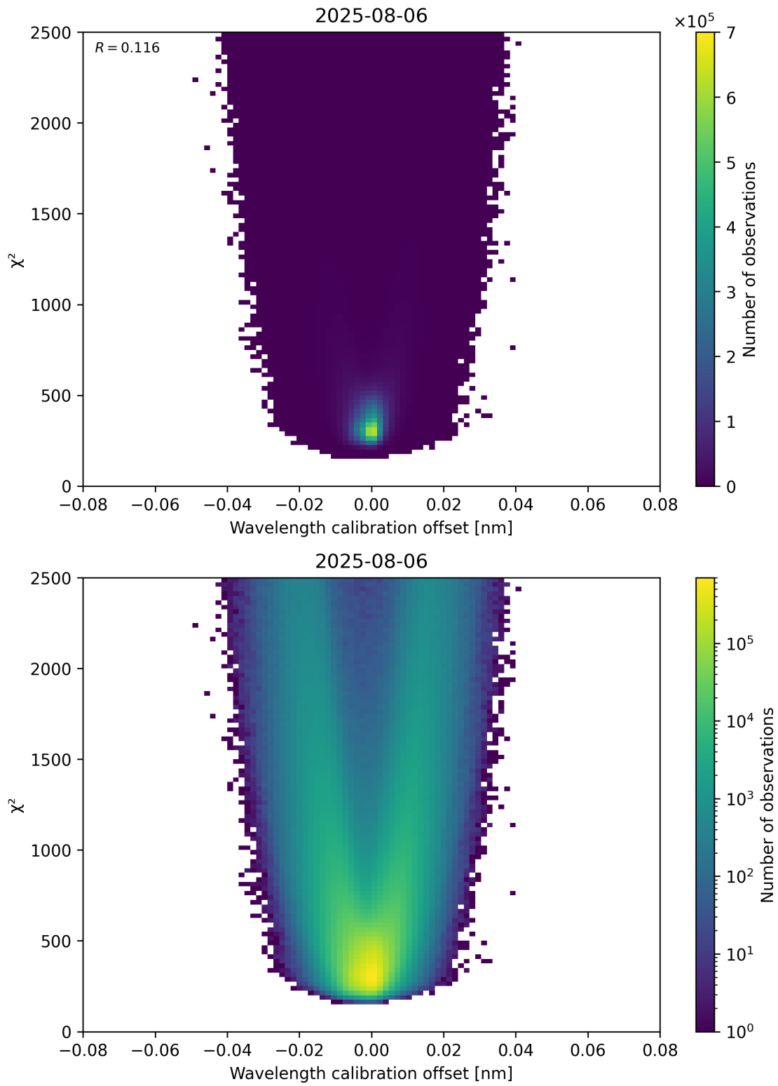
Figure 175: Scatter density plot of “Wavelength calibration offset” against “ \chi^2 ” for 2025-08-05 to 2025-08-07.
