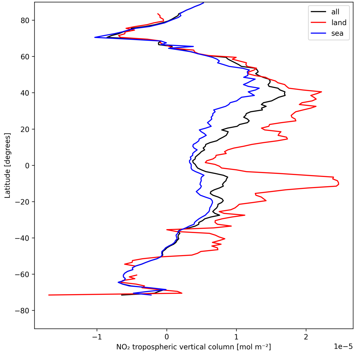
Figure 12: Zonal average of “NO 2 tropospheric vertical column” for 2025-08-05 to 2025-08-07.
