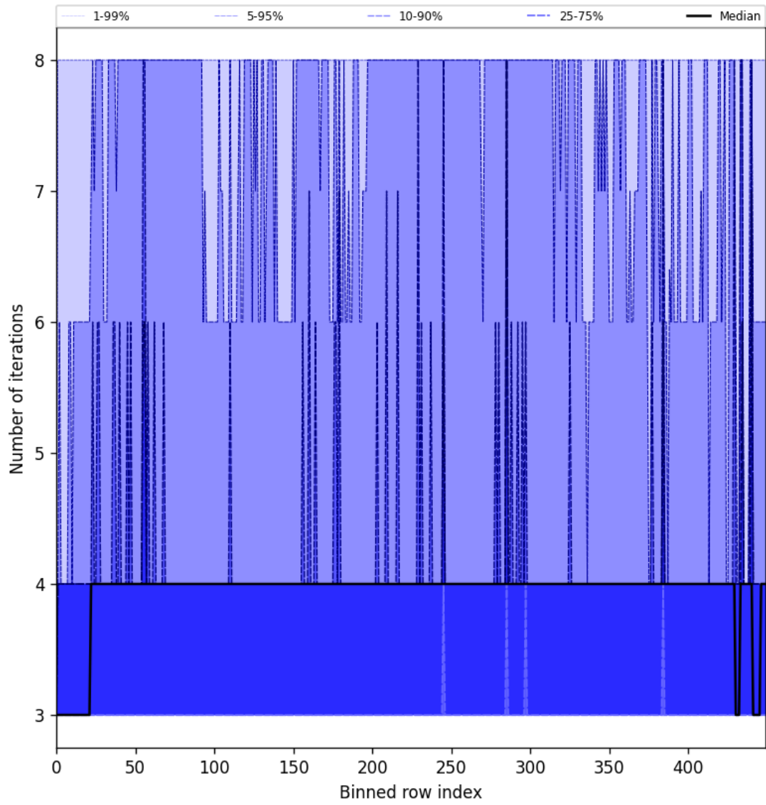
Figure 51: Along track statistics of “Number of iterations” for 2025-08-05 to 2025-08-07
