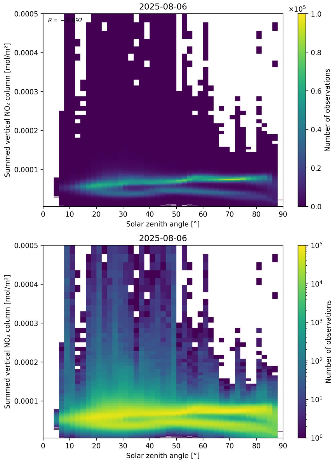
Figure 151: Scatter density plot of “Solar zenith angle” against “Summed vertical NO 2 column” for 2025-08-05 to 2025-08-07.
