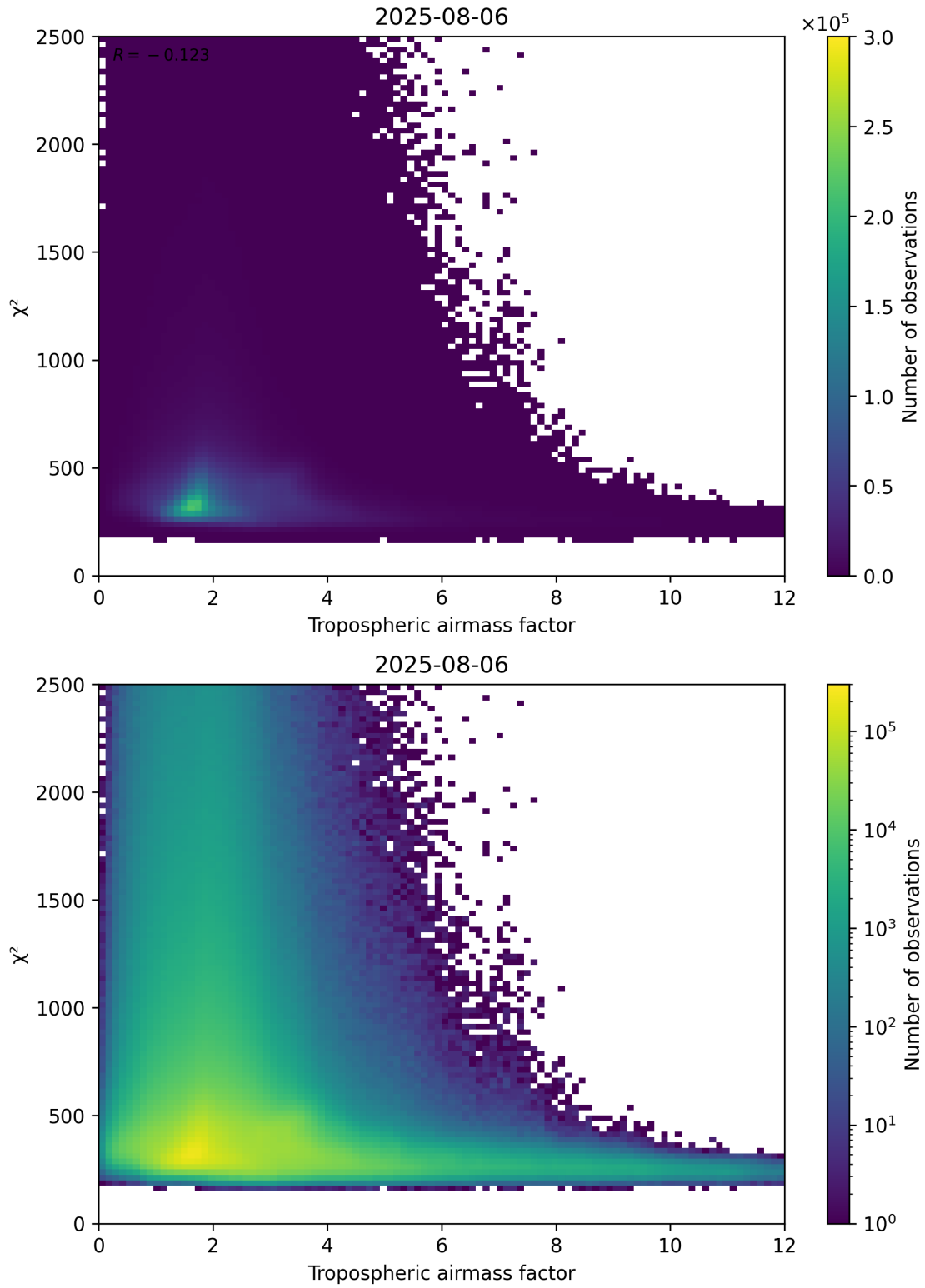
Figure 73: Scatter density plot of “Tropospheric airmass factor” against “ \chi^2 ” for 2025-08-05 to 2025-08-07.
