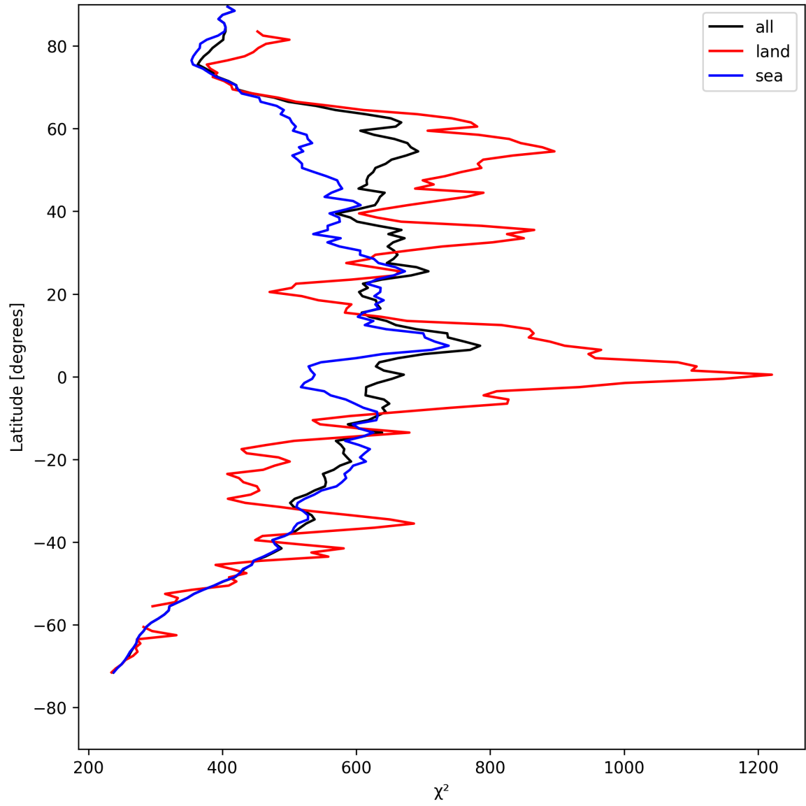
Figure 25: Zonal average of “ \chi^2 ” for 2025-08-05 to 2025-08-07.
