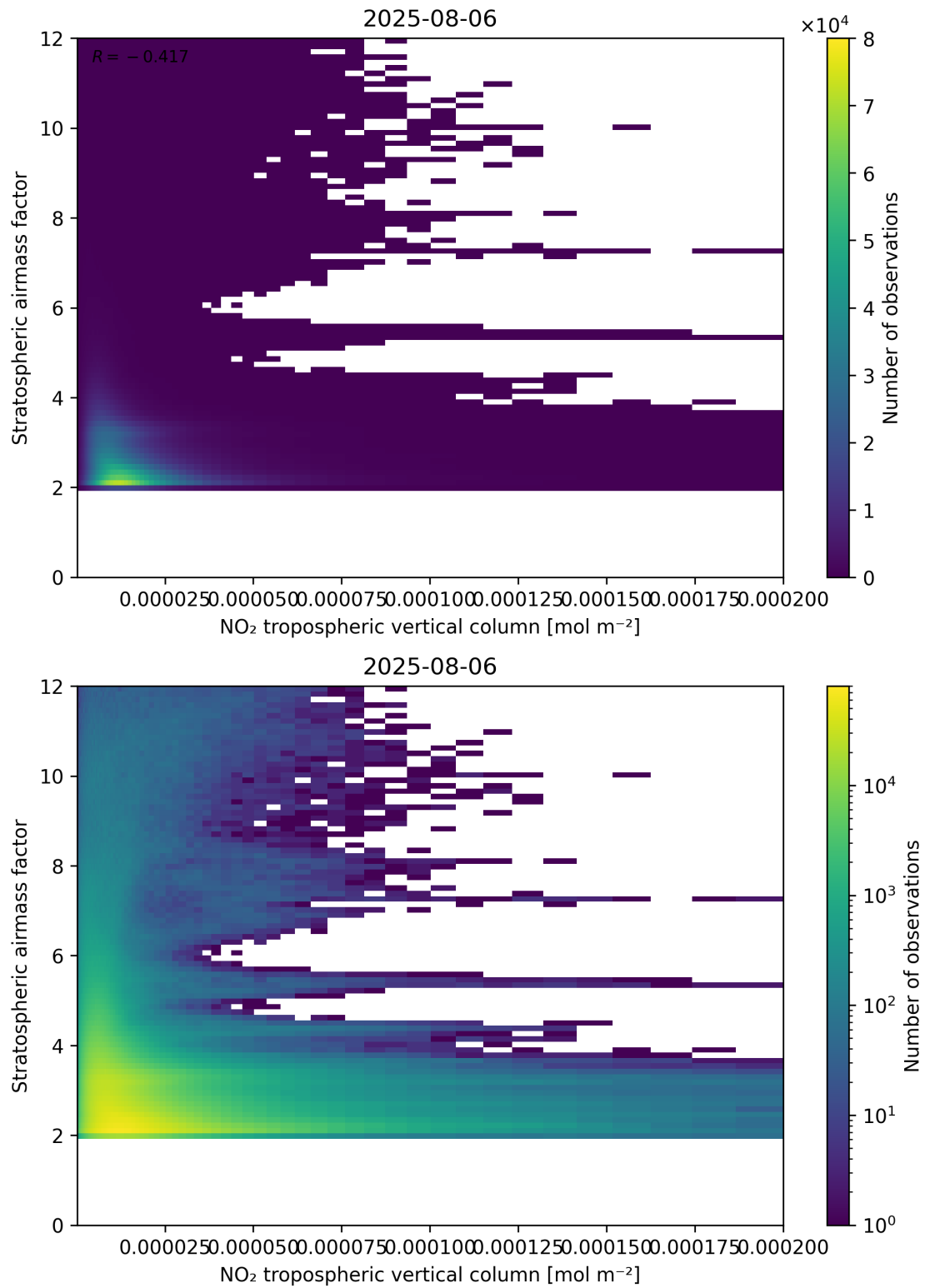
Figure 121: Scatter density plot of “NO 2 tropospheric vertical column” against “Stratospheric air mass factor” for 2025-08-05 to 2025-08-07.
