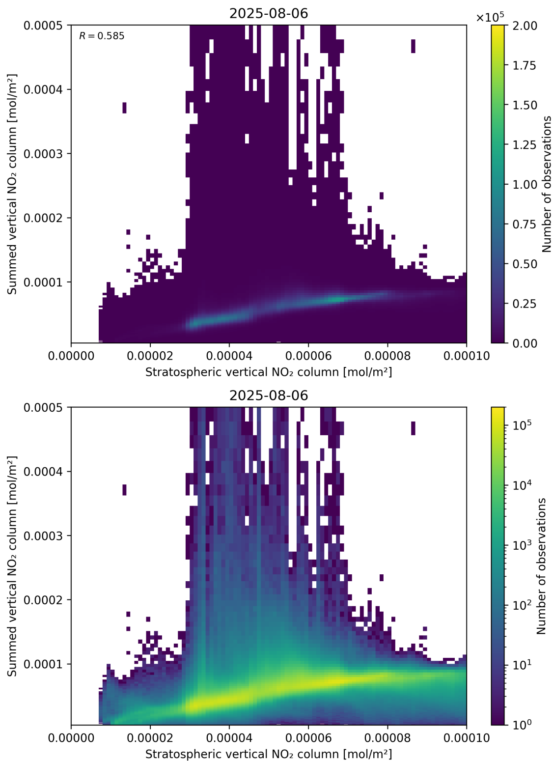
Figure 98: Scatter density plot of “Stratospheric vertical NO 2 column” against “Summed vertical NO 2 column” for 2025-08-05 to 2025-08-07.
