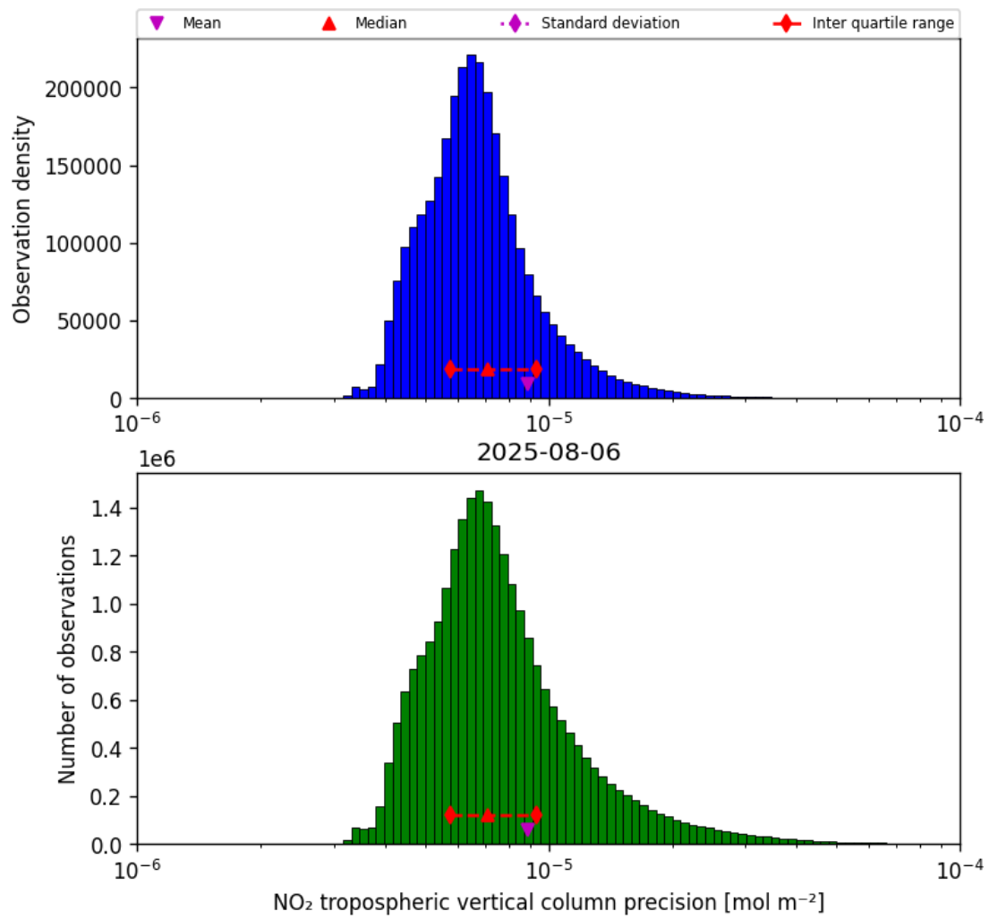
Figure 30: Histogram of “NO 2 tropospheric vertical column precision” for 2025-08-05 to 2025-08-07
