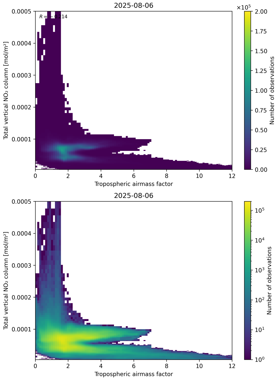
Figure 77: Scatter density plot of “Tropospheric airmass factor” against “Total vertical NO 2 column” for 2025-08-05 to 2025-08-07.
