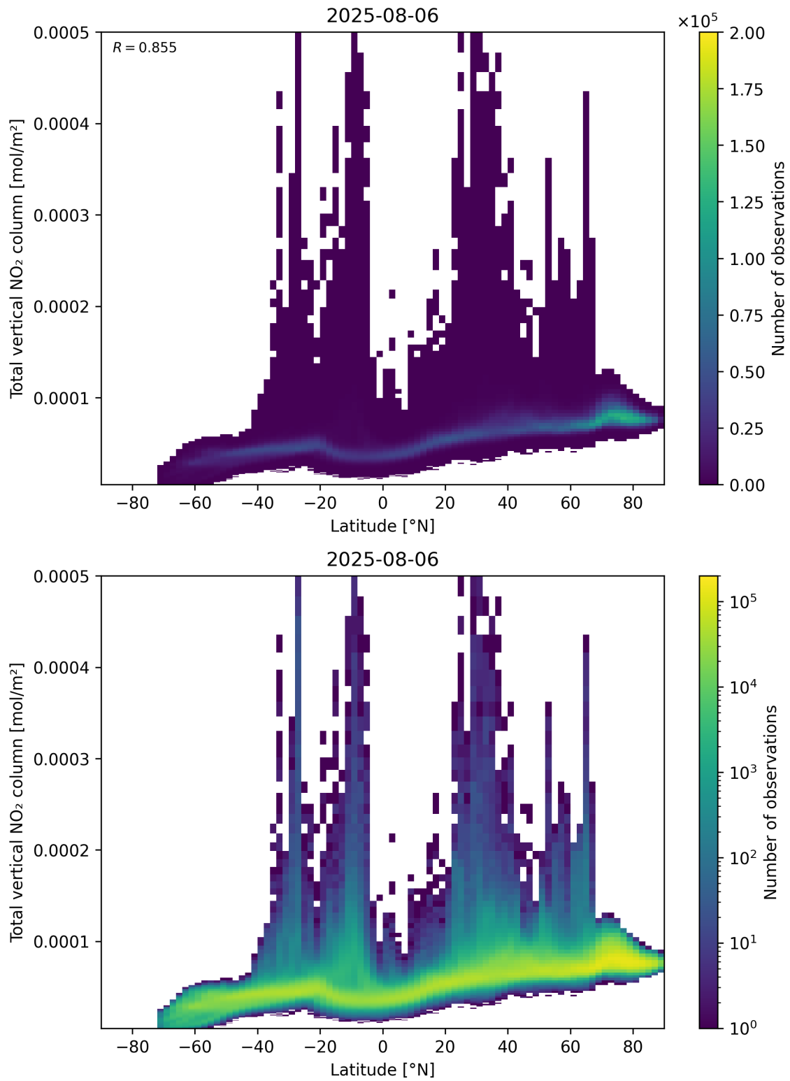
Figure 90: Scatter density plot of “Latitude” against “Total vertical NO 2 column” for 2025-08-05 to 2025-08-07.
