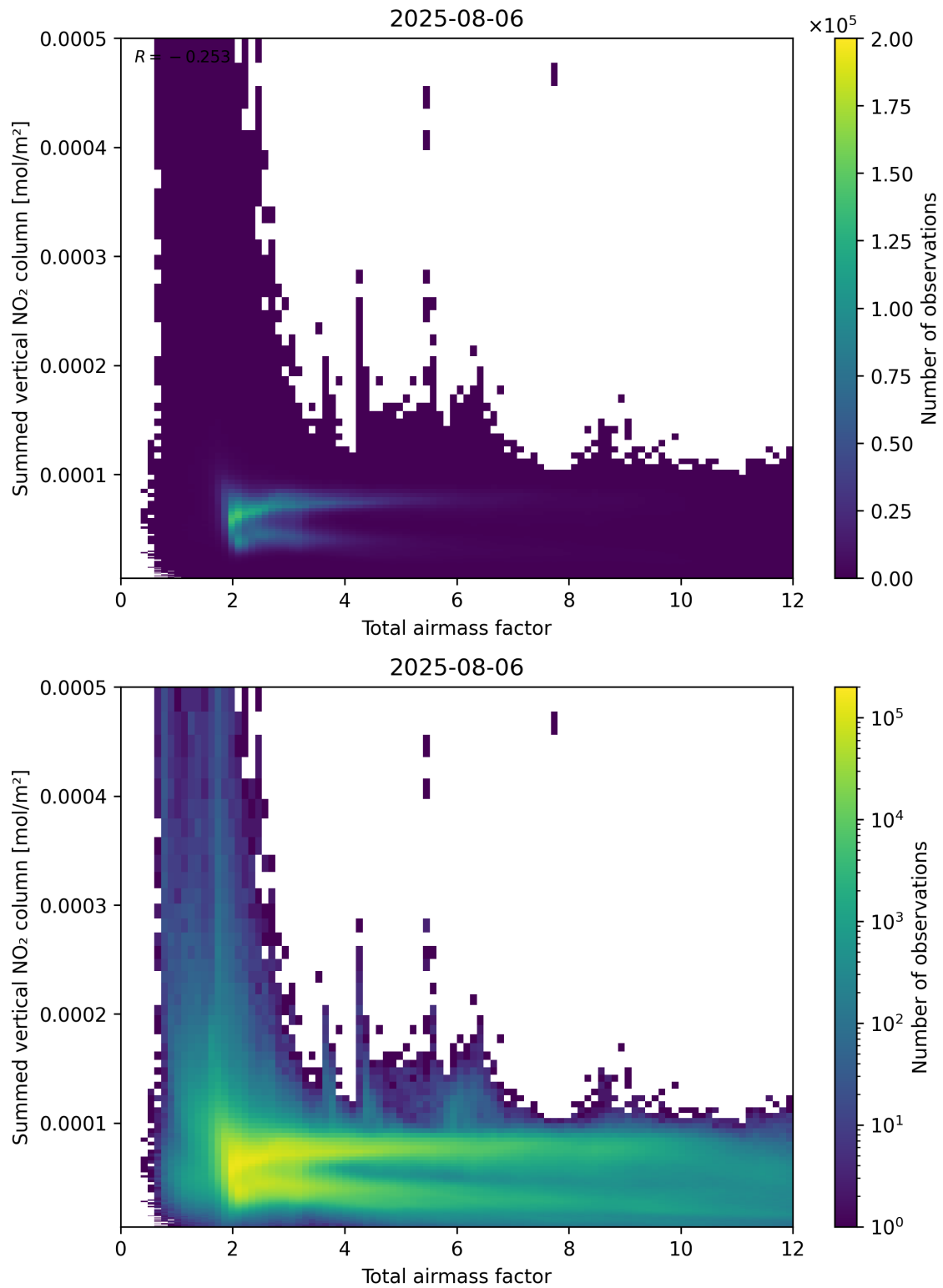
Figure 65: Scatter density plot of “Total airmass factor” against “Summed vertical NO 2 column” for 2025-08-05 to 2025-08-07.
