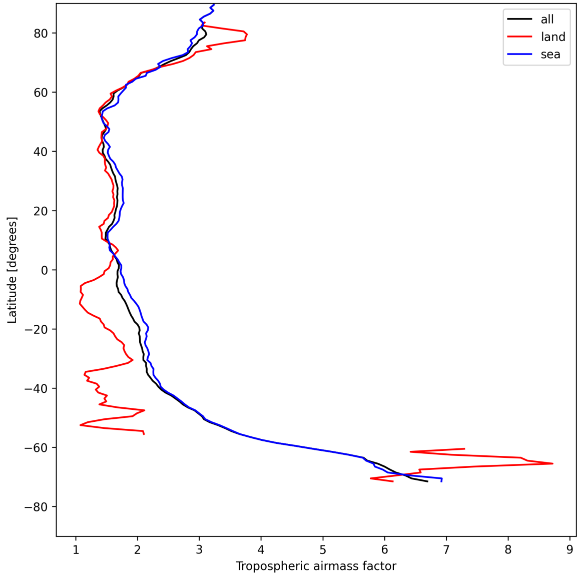
Figure 14: Zonal average of “Tropospheric airmass factor” for 2025-08-05 to 2025-08-07.
