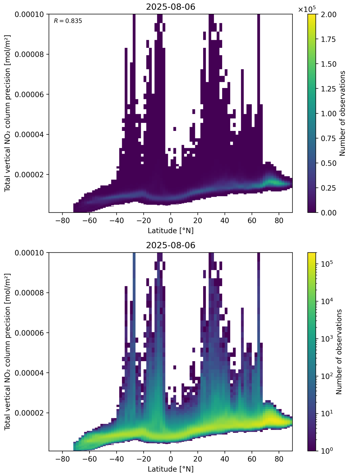
Figure 91: Scatter density plot of “Latitude” against “Total vertical NO 2 column precision” for 2025-08-05 to 2025-08-07.
