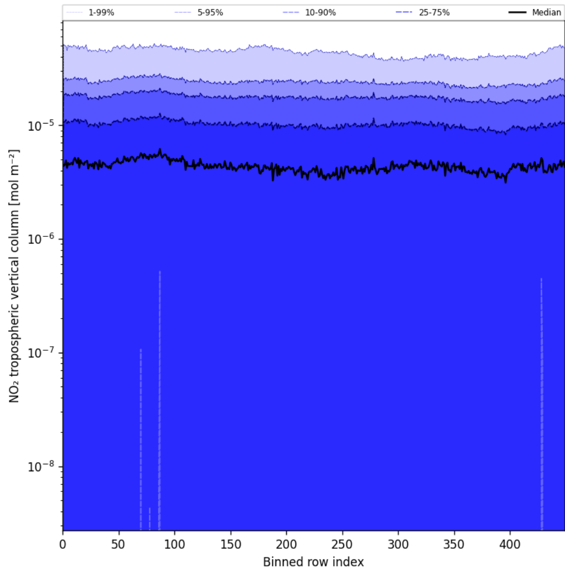
Figure 46: Along track statistics of “NO 2 tropospheric vertical column” for 2025-08-05 to 2025-08-07
