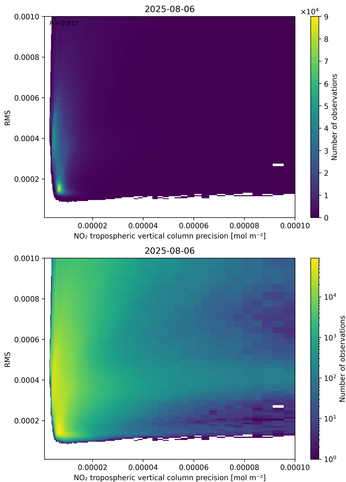
Figure 140: Scatter density plot of “NO 2 tropospheric vertical column precision” against “RMS” for 2025-08-05 to 2025-08-07.
