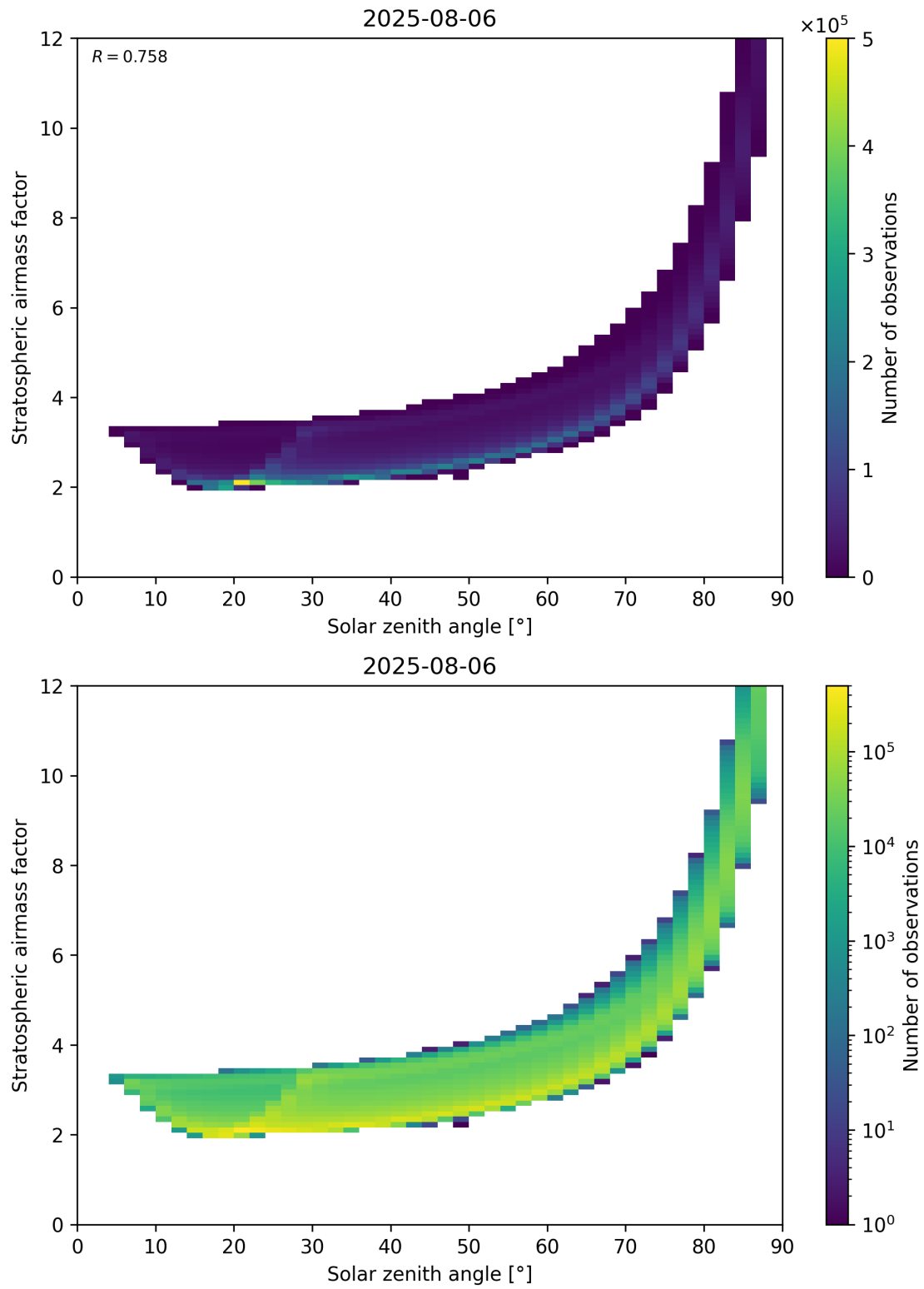
Figure 145: Scatter density plot of “Solar zenith angle” against “Stratospheric airmass factor” for 2025-08-05 to 2025-08-07.
