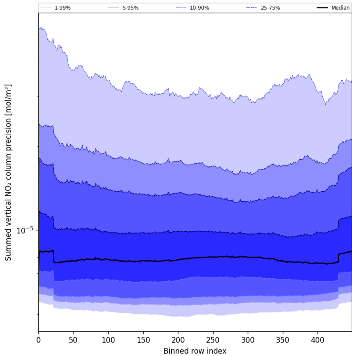
Figure 58: Along track statistics of “Summed vertical NO 2 column precision” for 2025-08-05 to 2025-08-07
