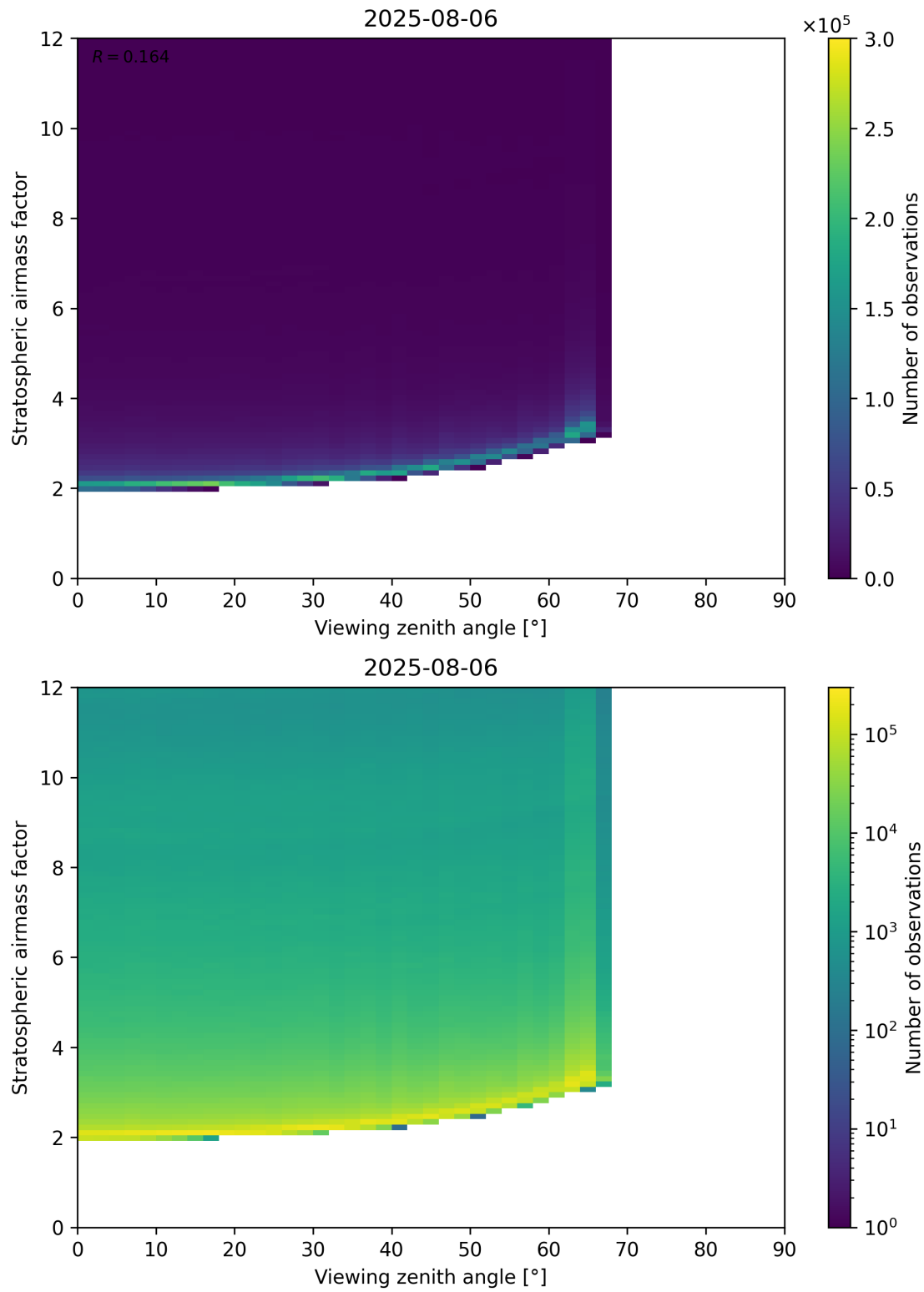
Figure 159: Scatter density plot of “Viewing zenith angle” against “Stratospheric airmass factor” for 2025-08-05 to 2025-08-07.
