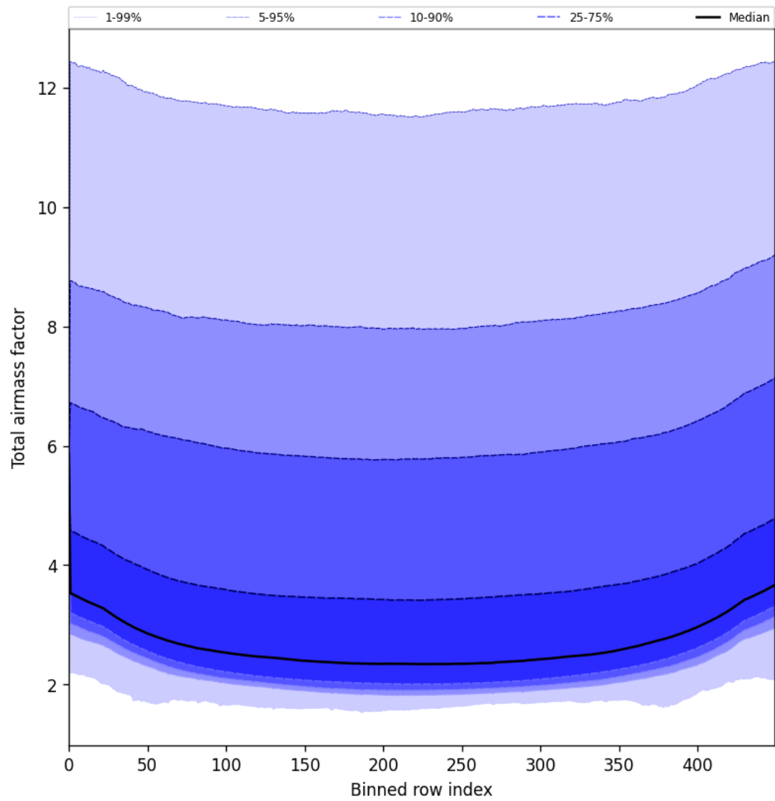
Figure 49: Along track statistics of “Total airmass factor” for 2025-08-05 to 2025-08-07
