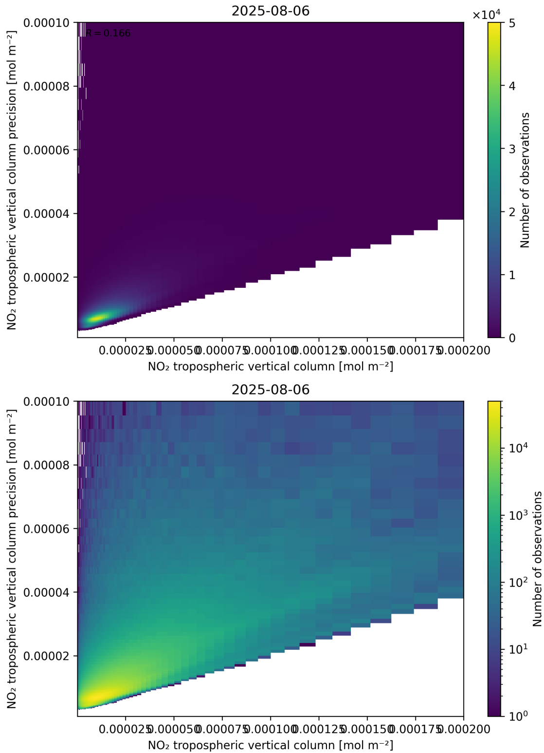
Figure 130: Scatter density plot of “NO 2 tropospheric vertical column” against “NO 2 tropospheric vertical column precision” for 2025-08-05 to 2025-08-07.
