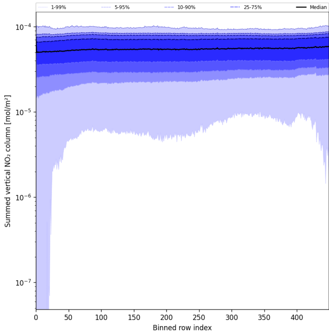
Figure 57: Along track statistics of “Summed vertical NO 2 column” for 2025-08-05 to 2025-08-07
