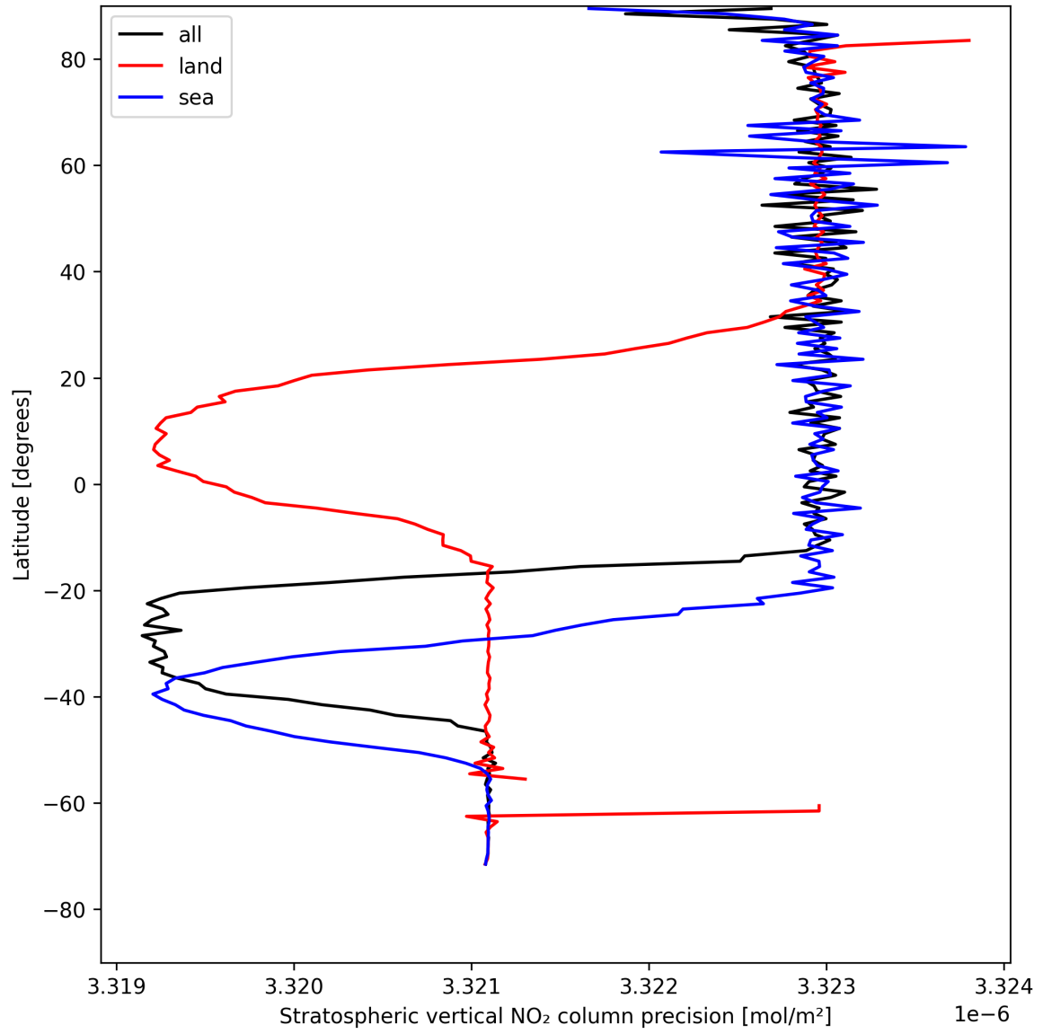
Figure 20: Zonal average of “Stratospheric vertical NO 2 column precision” for 2025-08-05 to 2025-08-07.
