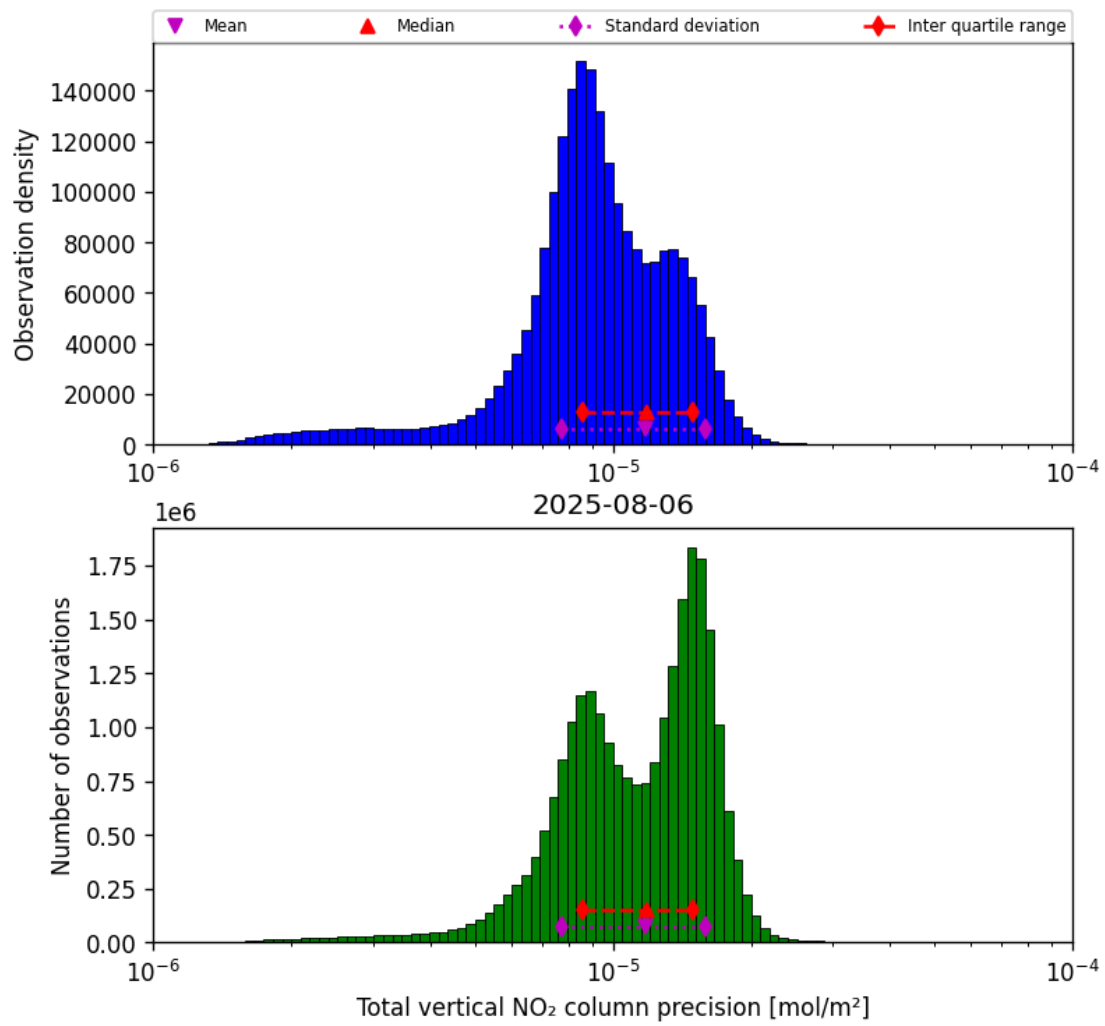
Figure 39: Histogram of “Total vertical NO 2 column precision” for 2025-08-05 to 2025-08-07
