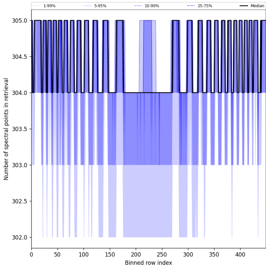
Figure 50: Along track statistics of “Number of spectral points in retrieval” for 2025-08-05 to 2025-08-07
