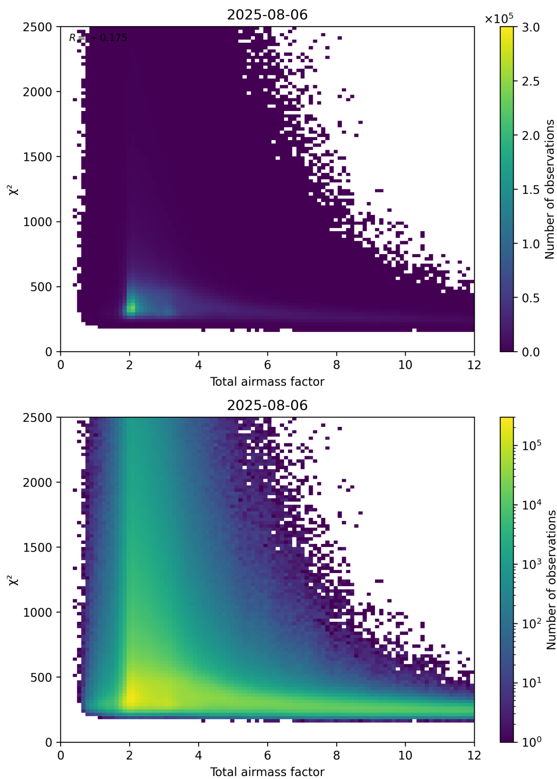
Figure 63: Scatter density plot of “Total airmass factor” against “ \chi^2 ” for 2025-08-05 to 2025-08-07.
