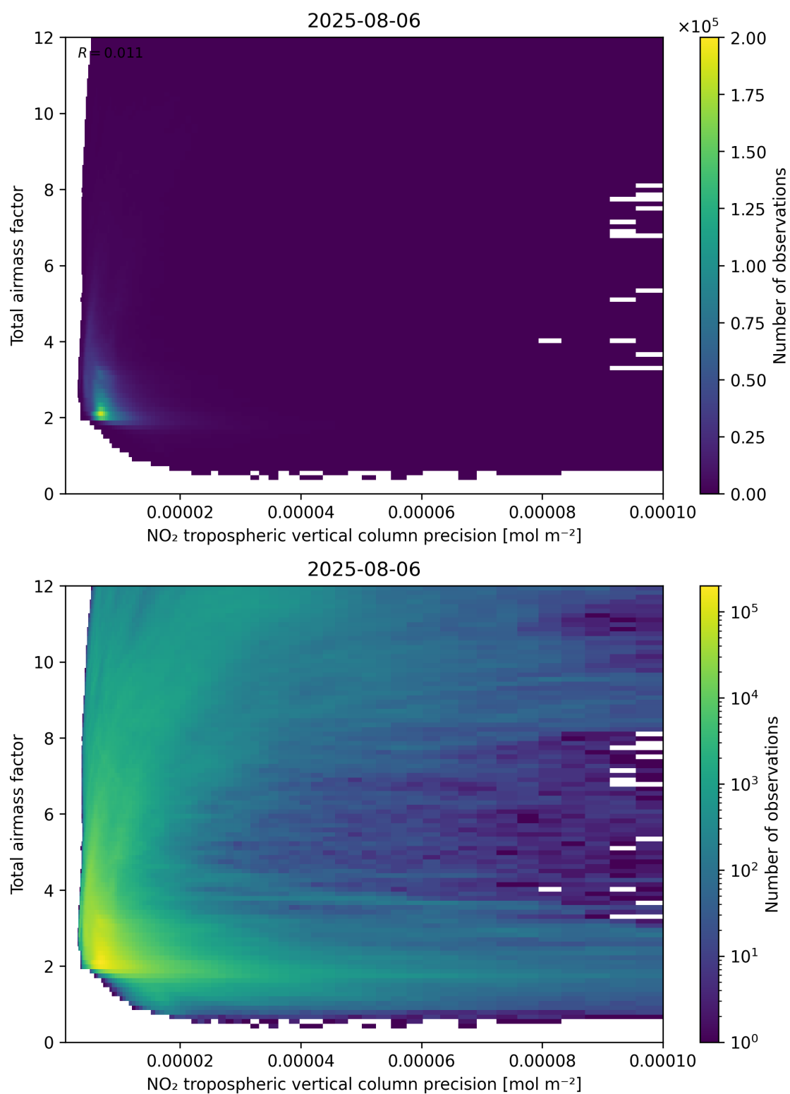
Figure 132: Scatter density plot of “NO 2 tropospheric vertical column precision” against “Total air mass factor” for 2025-08-05 to 2025-08-07.
