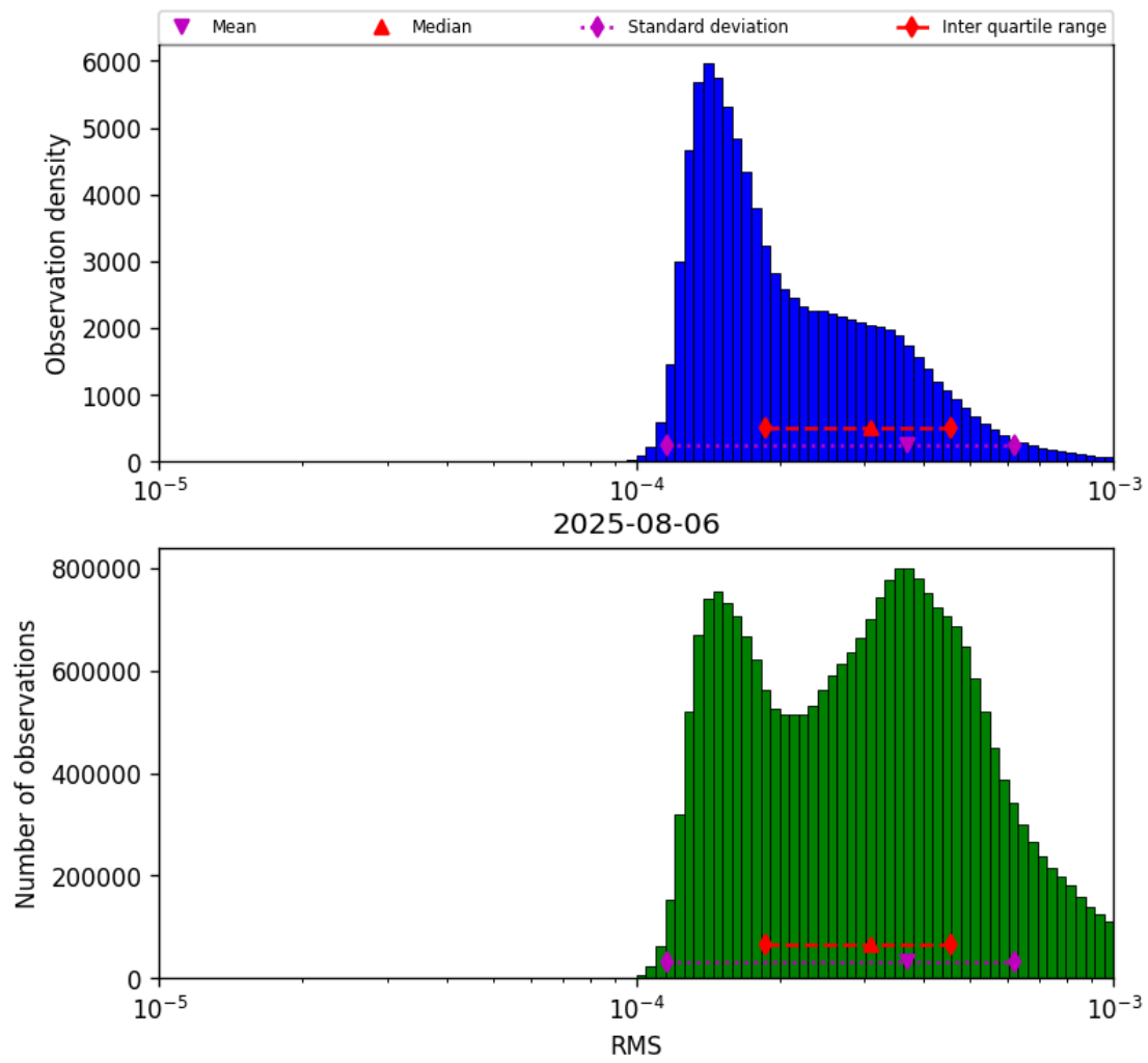
Figure 43: Histogram of “RMS” for 2025-08-05 to 2025-08-07
