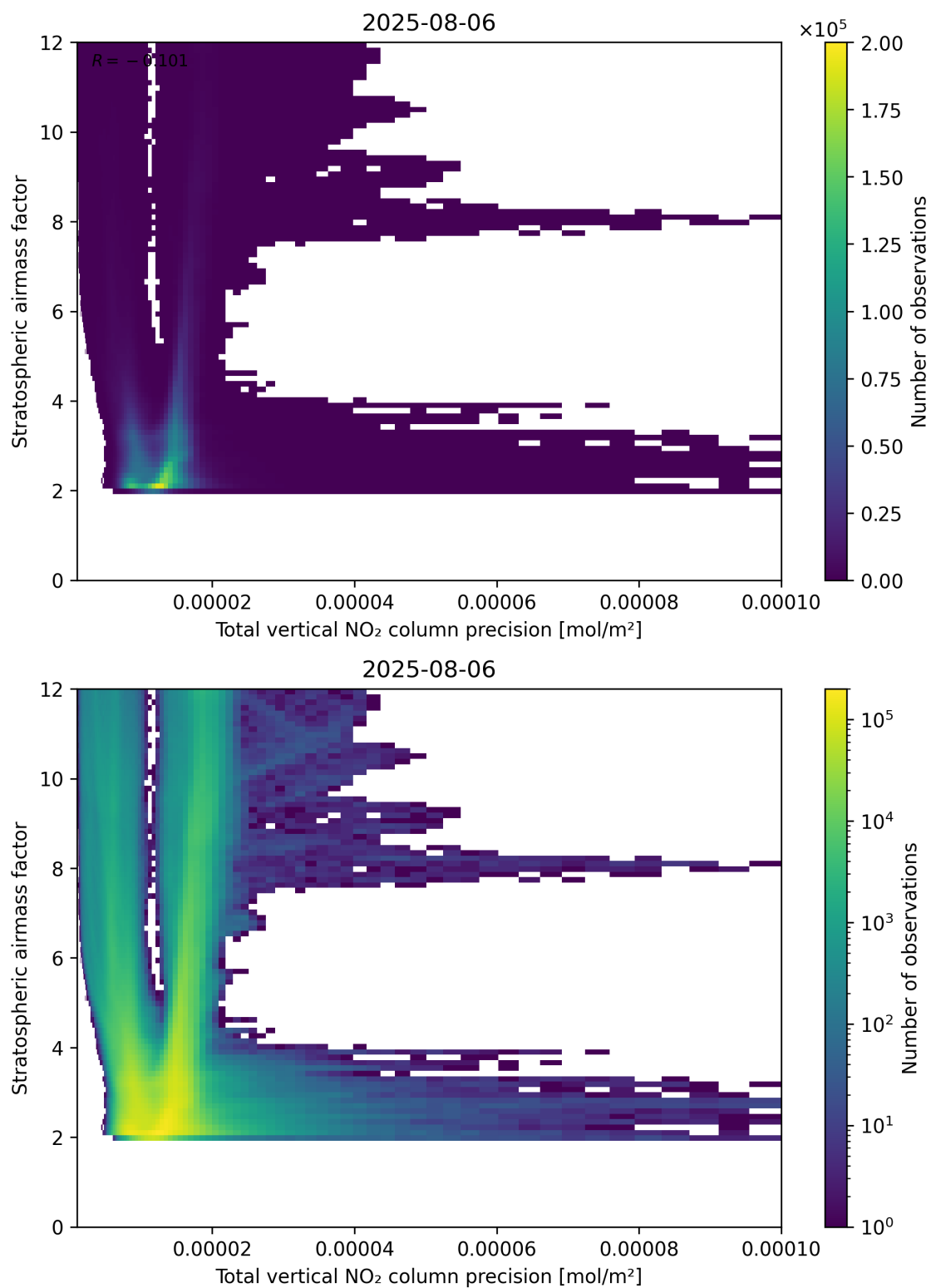
Figure 115: Scatter density plot of “Total vertical NO 2 column precision” against “Stratospheric air mass factor” for 2025-08-05 to 2025-08-07.
