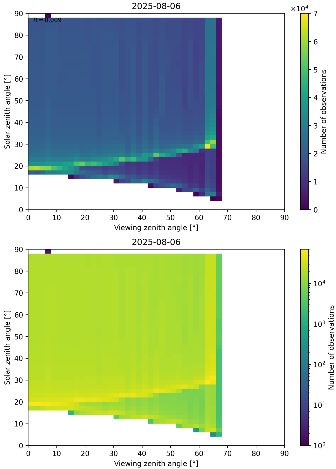
Figure 172: Scatter density plot of “Viewing zenith angle” against “Solar zenith angle” for 2025-08-05 to 2025-08-07.
