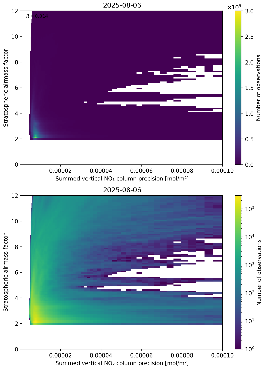
Figure 106: Scatter density plot of “Summed vertical NO 2 column precision” against “Stratospheric airmass factor” for 2025-08-05 to 2025-08-07.
