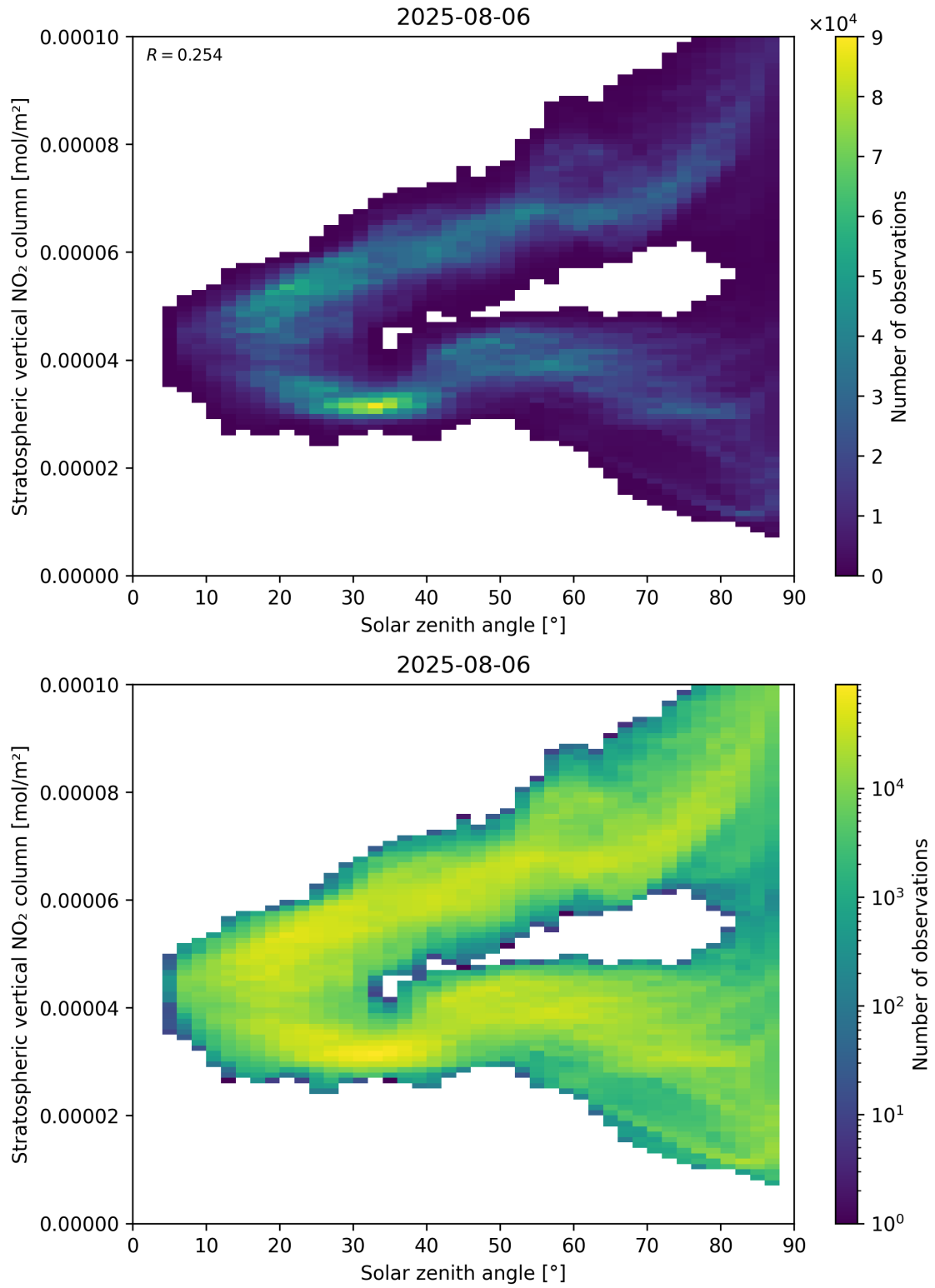
Figure 150: Scatter density plot of “Solar zenith angle” against “Stratospheric vertical NO 2 column” for 2025-08-05 to 2025-08-07.
