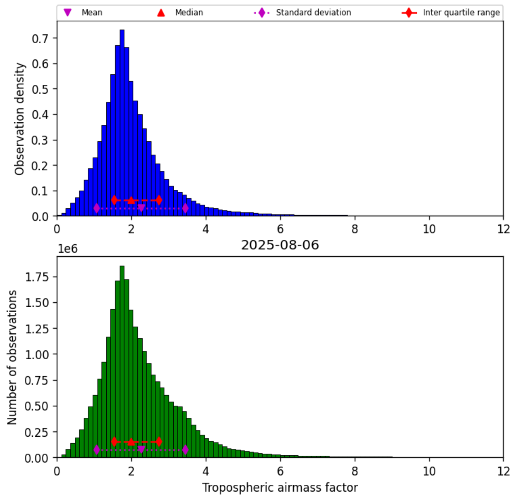
Figure 31: Histogram of “Tropospheric airmass factor” for 2025-08-05 to 2025-08-07
