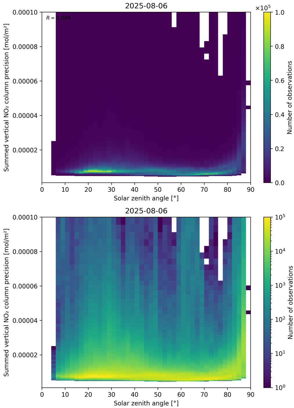
Figure 152: Scatter density plot of “Solar zenith angle” against “Summed vertical NO 2 column precision” for 2025-08-05 to 2025-08-07.
