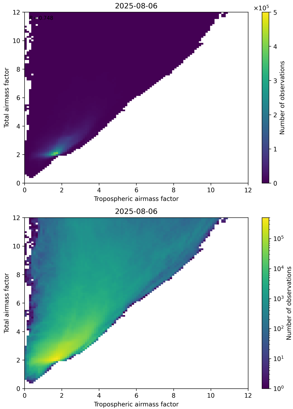
Figure 72: Scatter density plot of “Tropospheric airmass factor” against “Total airmass factor” for 2025-08-05 to 2025-08-07.
