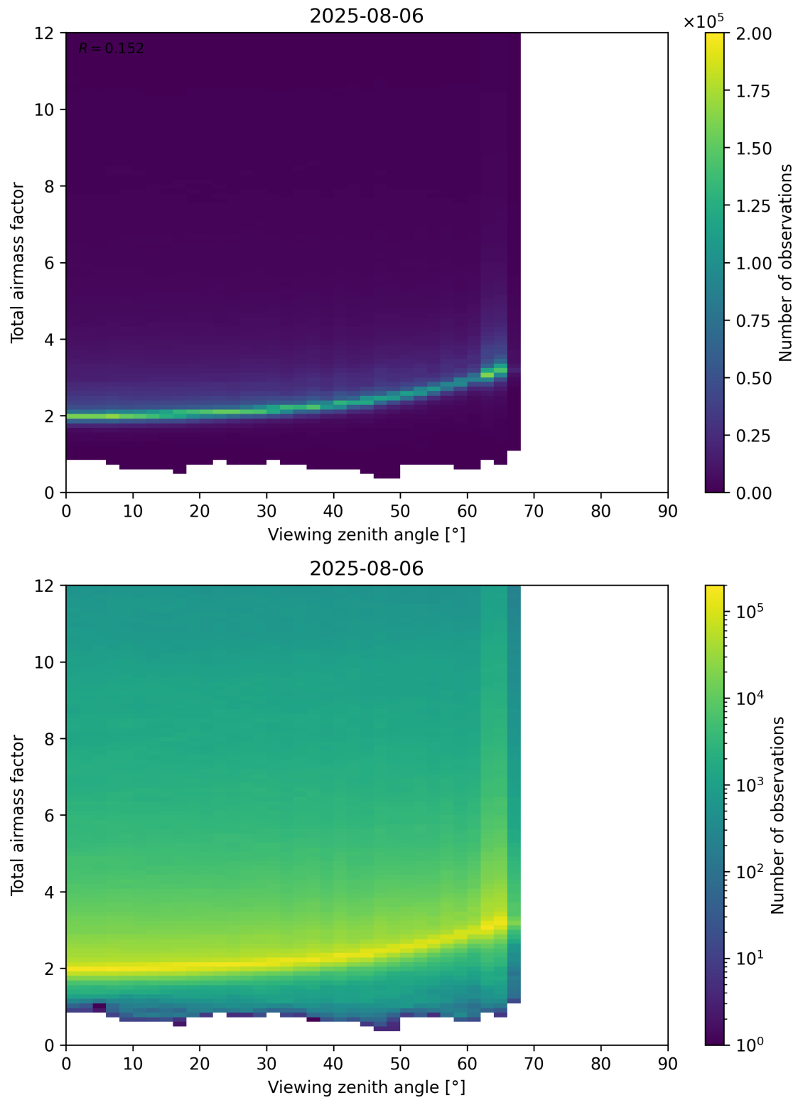
Figure 160: Scatter density plot of “Viewing zenith angle” against “Total airmass factor” for 2025-08-05 to 2025-08-07.
