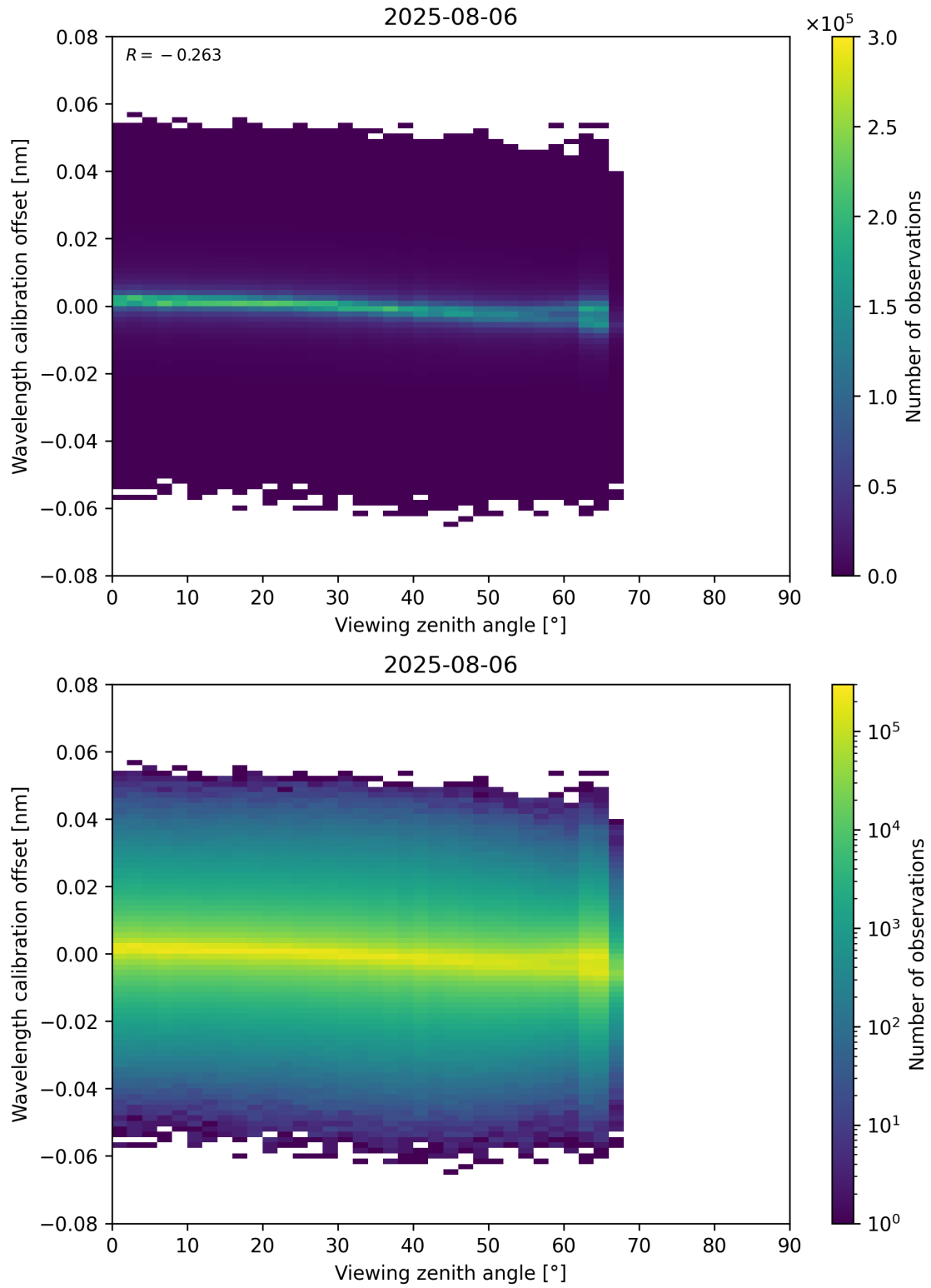
Figure 173: Scatter density plot of “Viewing zenith angle” against “Wavelength calibration offset” for 2025-08-05 to 2025-08-07.
