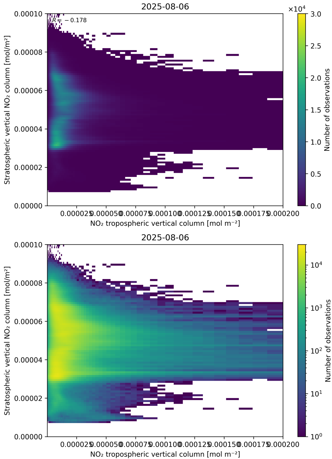
Figure 125: Scatter density plot of “NO 2 tropospheric vertical column” against “Stratospheric vertical NO 2 column” for 2025-08-05 to 2025-08-07.
