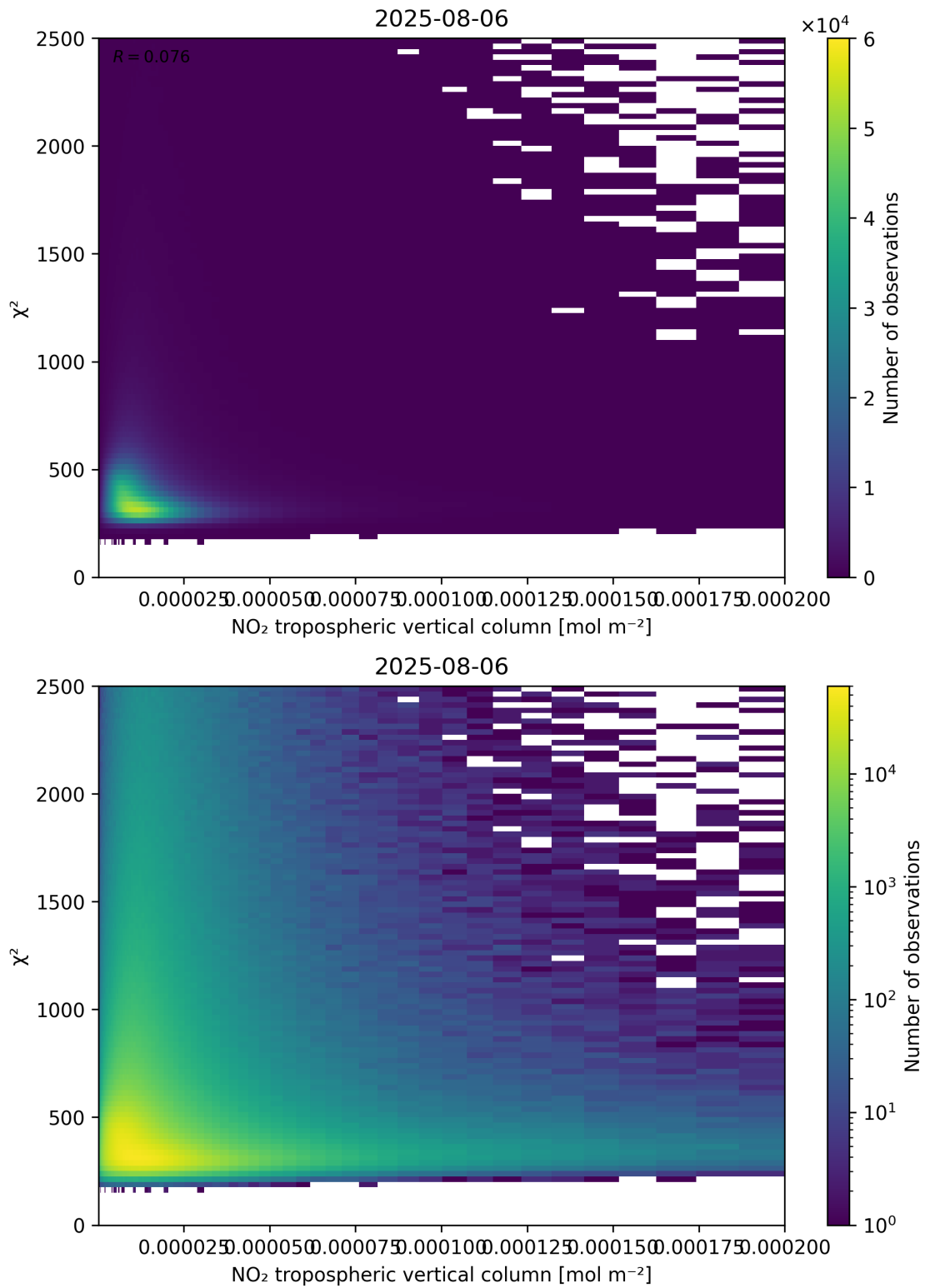
Figure 124: Scatter density plot of “NO 2 tropospheric vertical column” against “ \chi^2 ” for 2025-08-05 to 2025-08-07.
