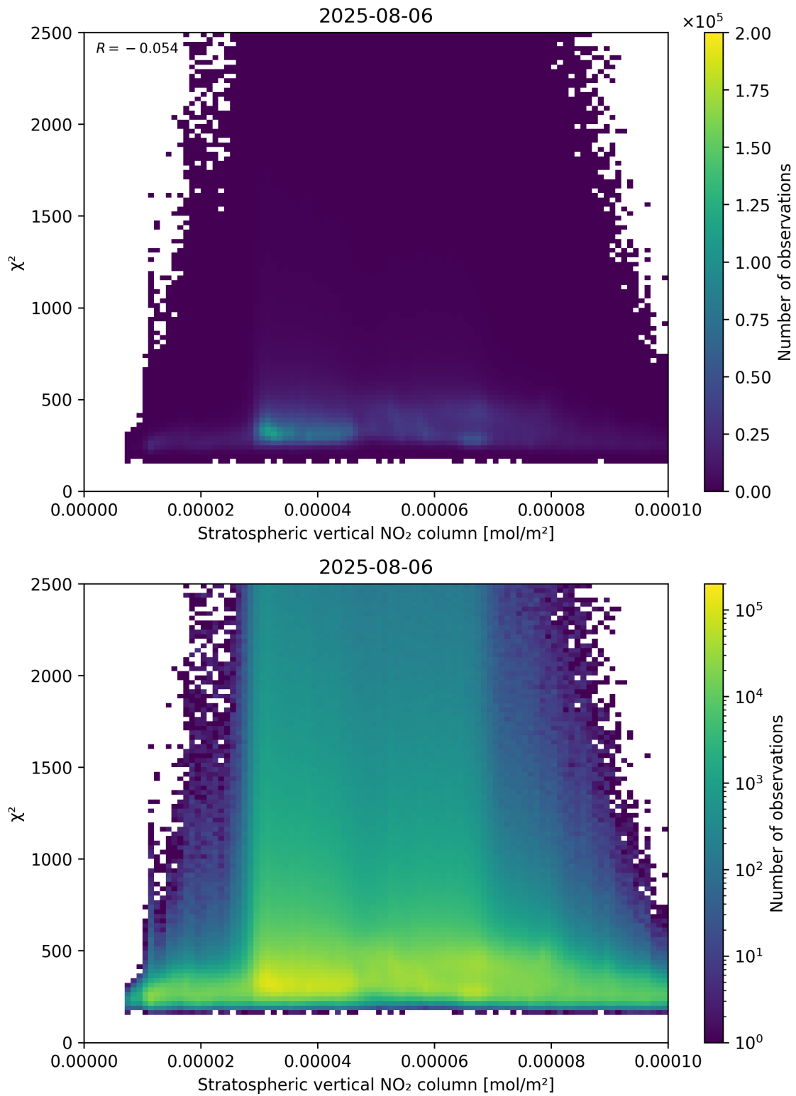
Figure 97: Scatter density plot of “Stratospheric vertical NO 2 column” against “ \chi^2 ” for 2025-08-05 to 2025-08-07.
