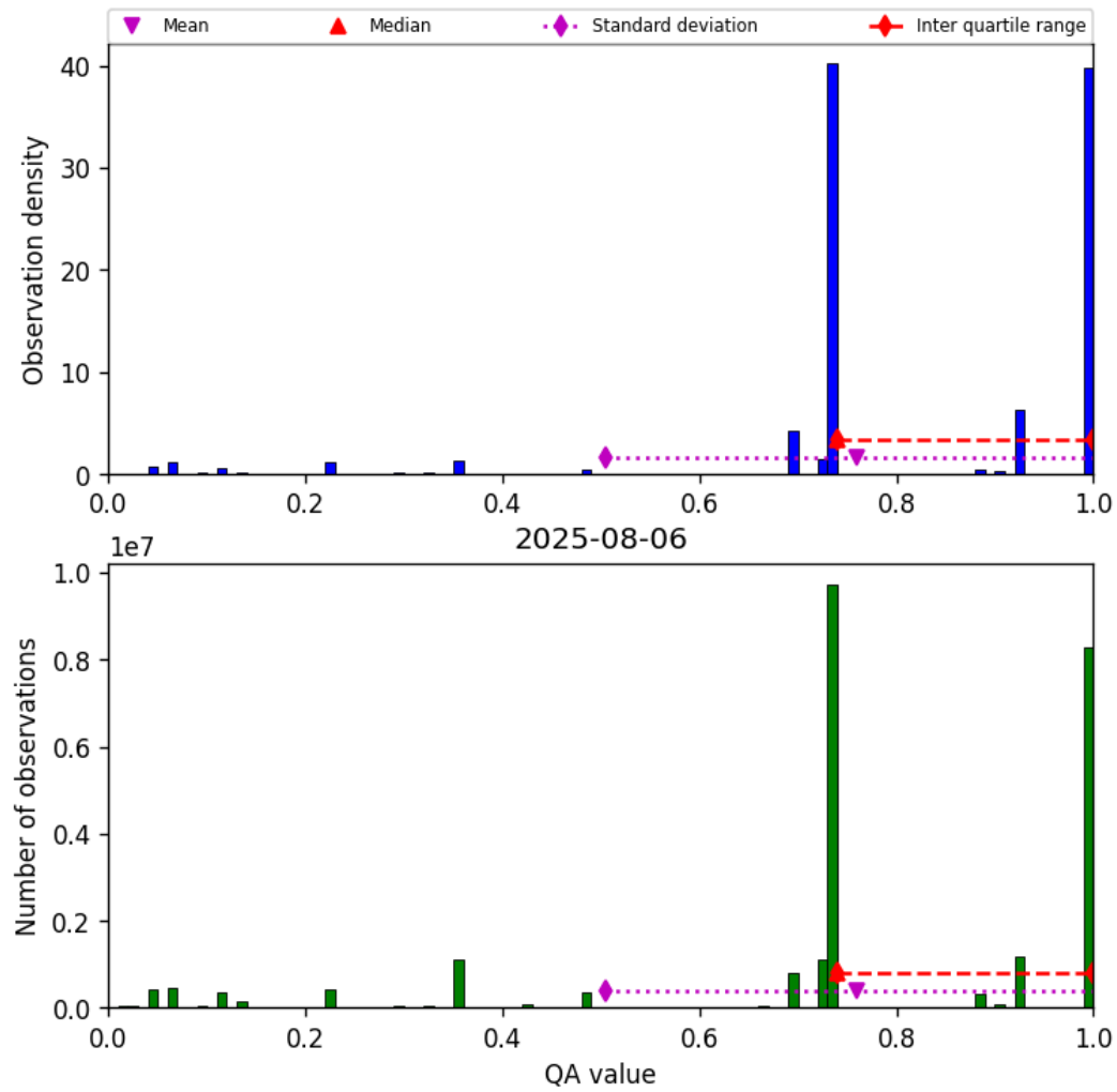
Figure 28: Histogram of “QA value” for 2025-08-05 to 2025-08-07
