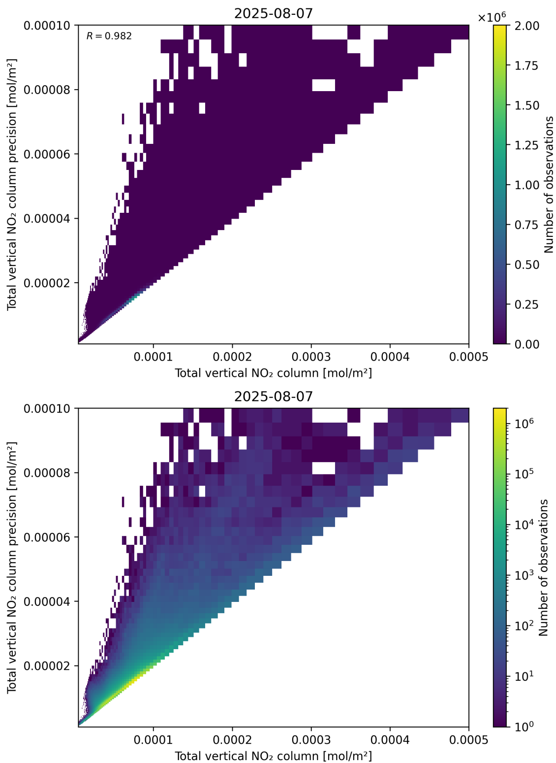
Figure 114: Scatter density plot of “Total vertical NO 2 column” against “Total vertical NO 2 column precision” for 2025-08-06 to 2025-08-08.
