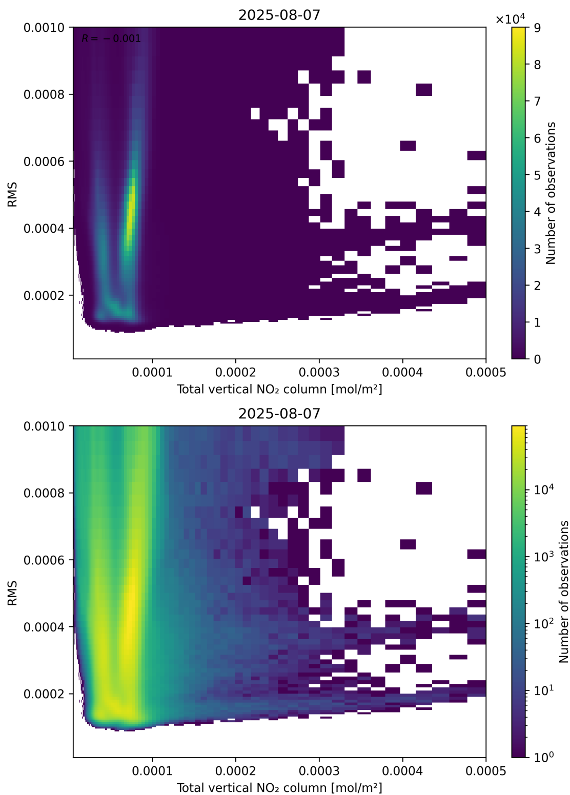
Figure 120: Scatter density plot of “Total vertical NO 2 column” against “RMS” for 2025-08-06 to 2025-08-08.
