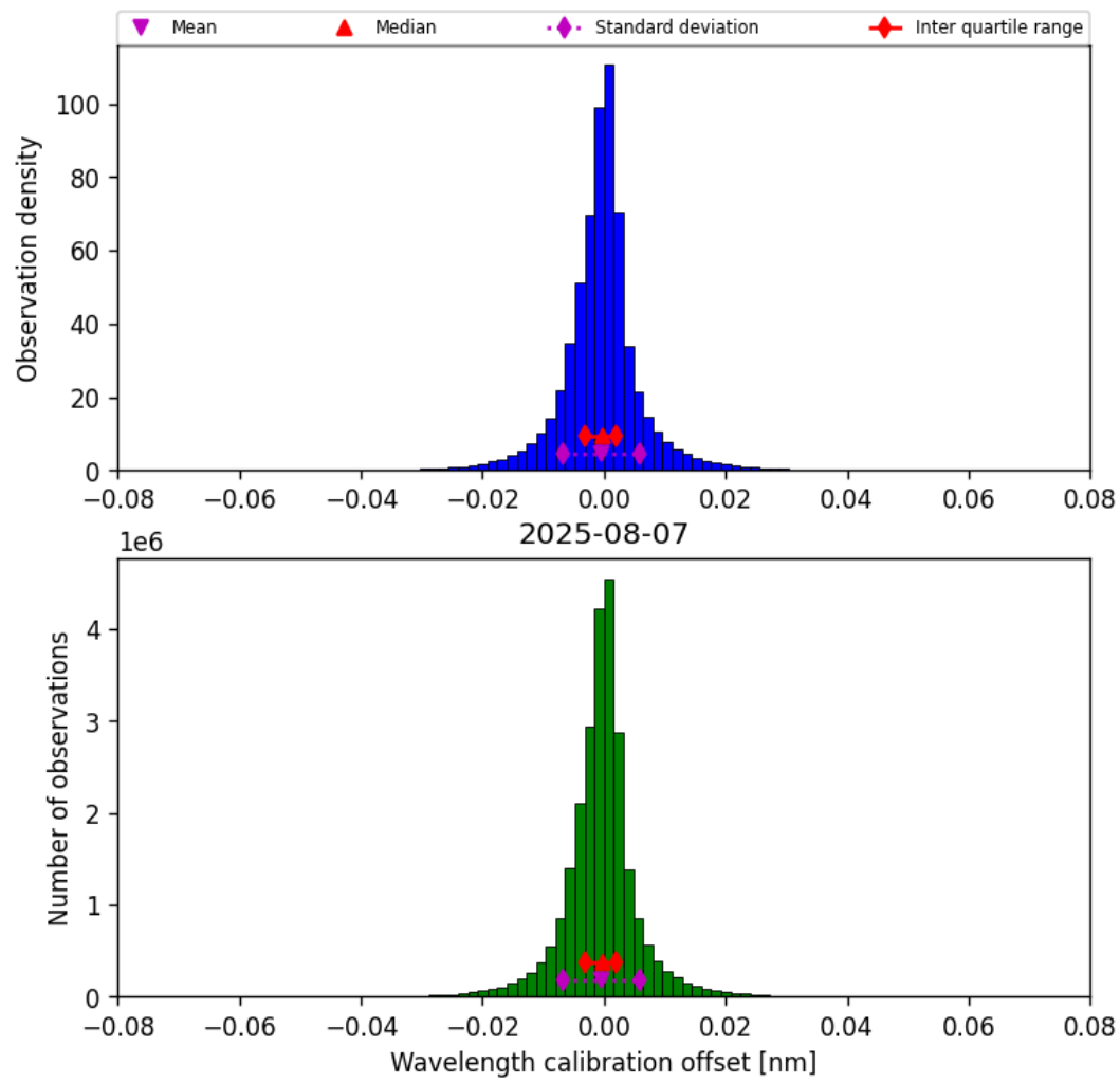
Figure 35: Histogram of “Wavelength calibration offset” for 2025-08-06 to 2025-08-08
