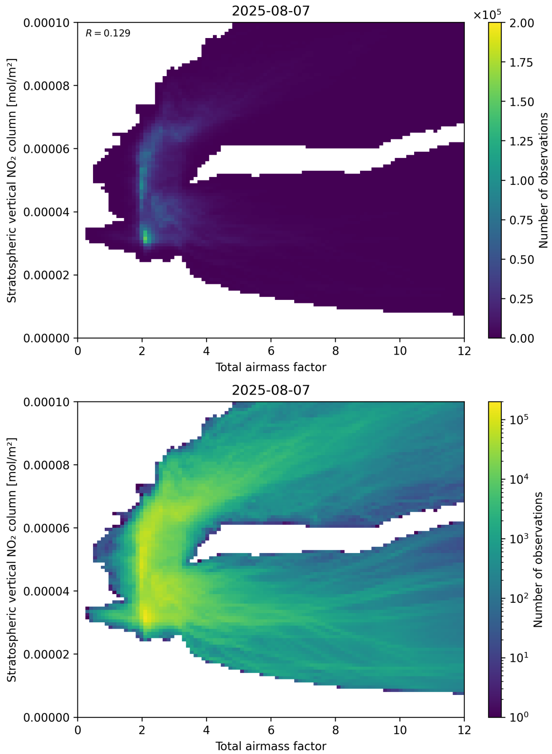
Figure 64: Scatter density plot of “Total airmass factor” against “Stratospheric vertical NO 2 column” for 2025-08-06 to 2025-08-08.
