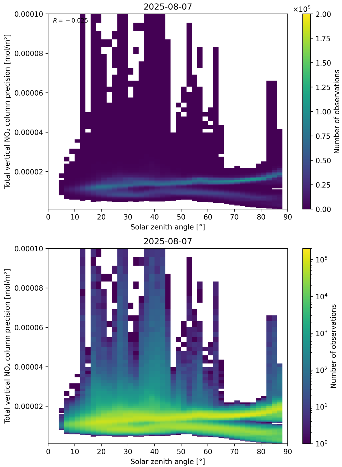
Figure 154: Scatter density plot of “Solar zenith angle” against “Total vertical NO 2 column precision” for 2025-08-06 to 2025-08-08.
