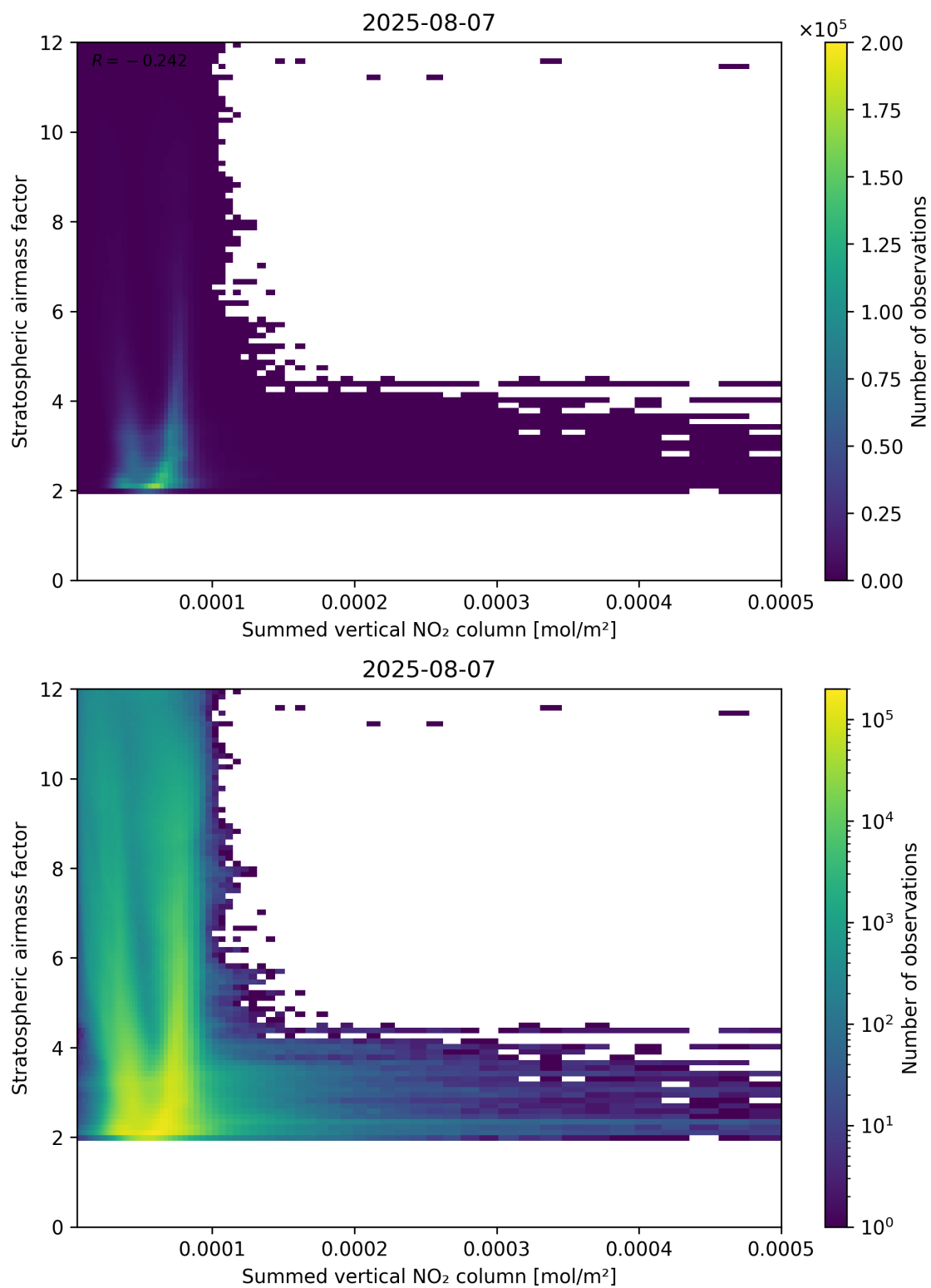
Figure 103: Scatter density plot of “Summed vertical NO 2 column” against “Stratospheric air mass factor” for 2025-08-06 to 2025-08-08.
