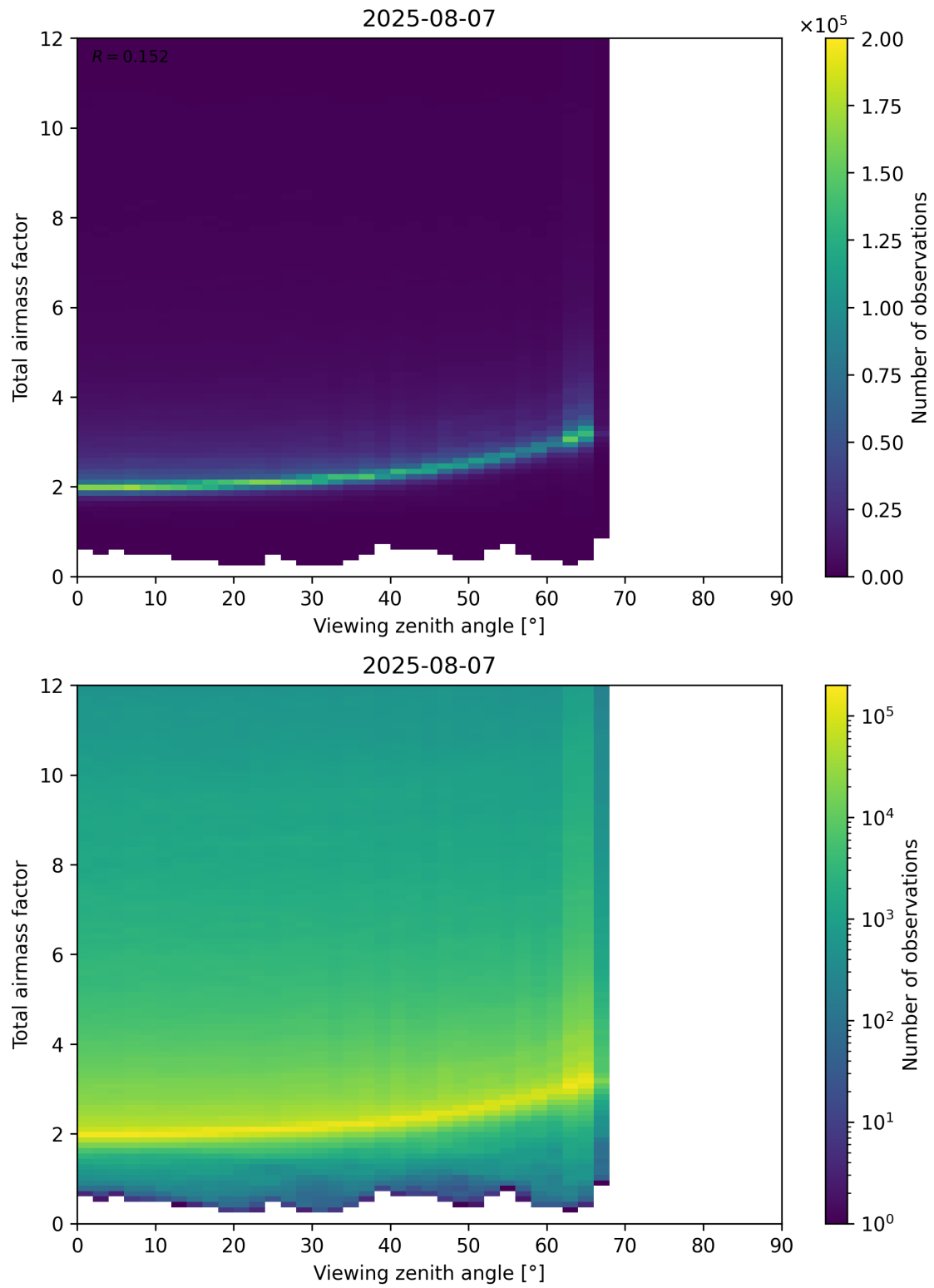
Figure 160: Scatter density plot of “Viewing zenith angle” against “Total airmass factor” for 2025-08-06 to 2025-08-08.
