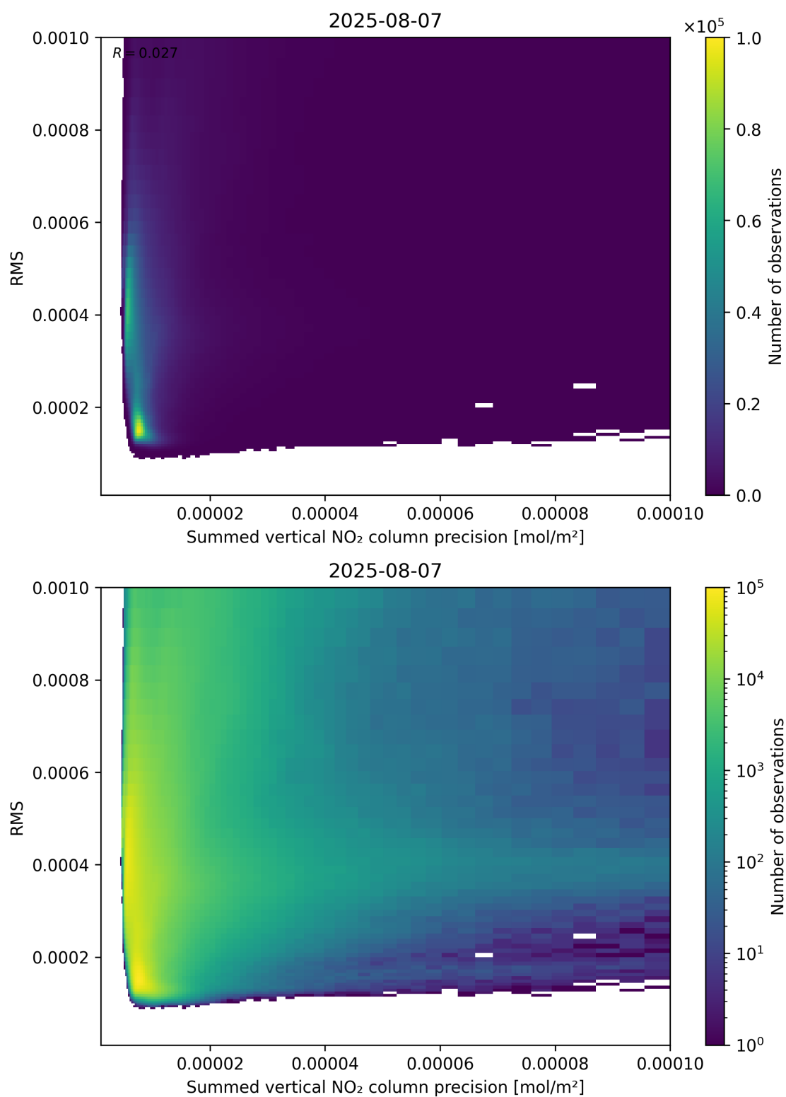
Figure 108: Scatter density plot of “Summed vertical NO 2 column precision” against “RMS” for 2025-08-06 to 2025-08-08.
