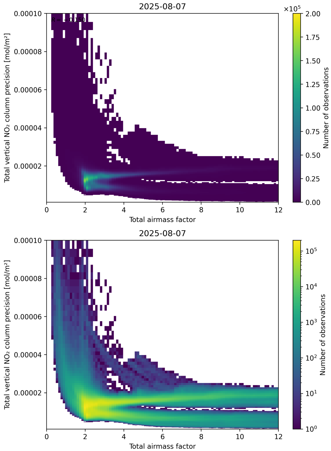
Figure 68: Scatter density plot of “Total airmass factor” against “Total vertical NO 2 column precision” for 2025-08-06 to 2025-08-08.
