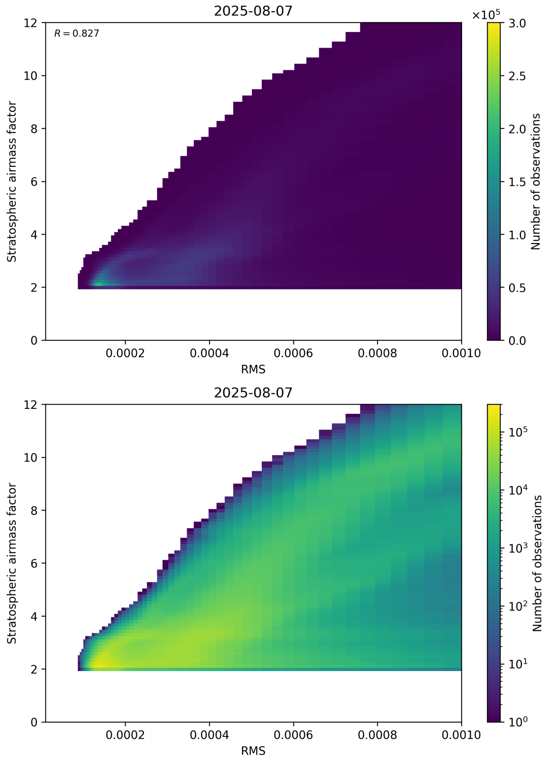
Figure 144: Scatter density plot of “RMS” against “Stratospheric airmass factor” for 2025-08-06 to 2025-08-08.
