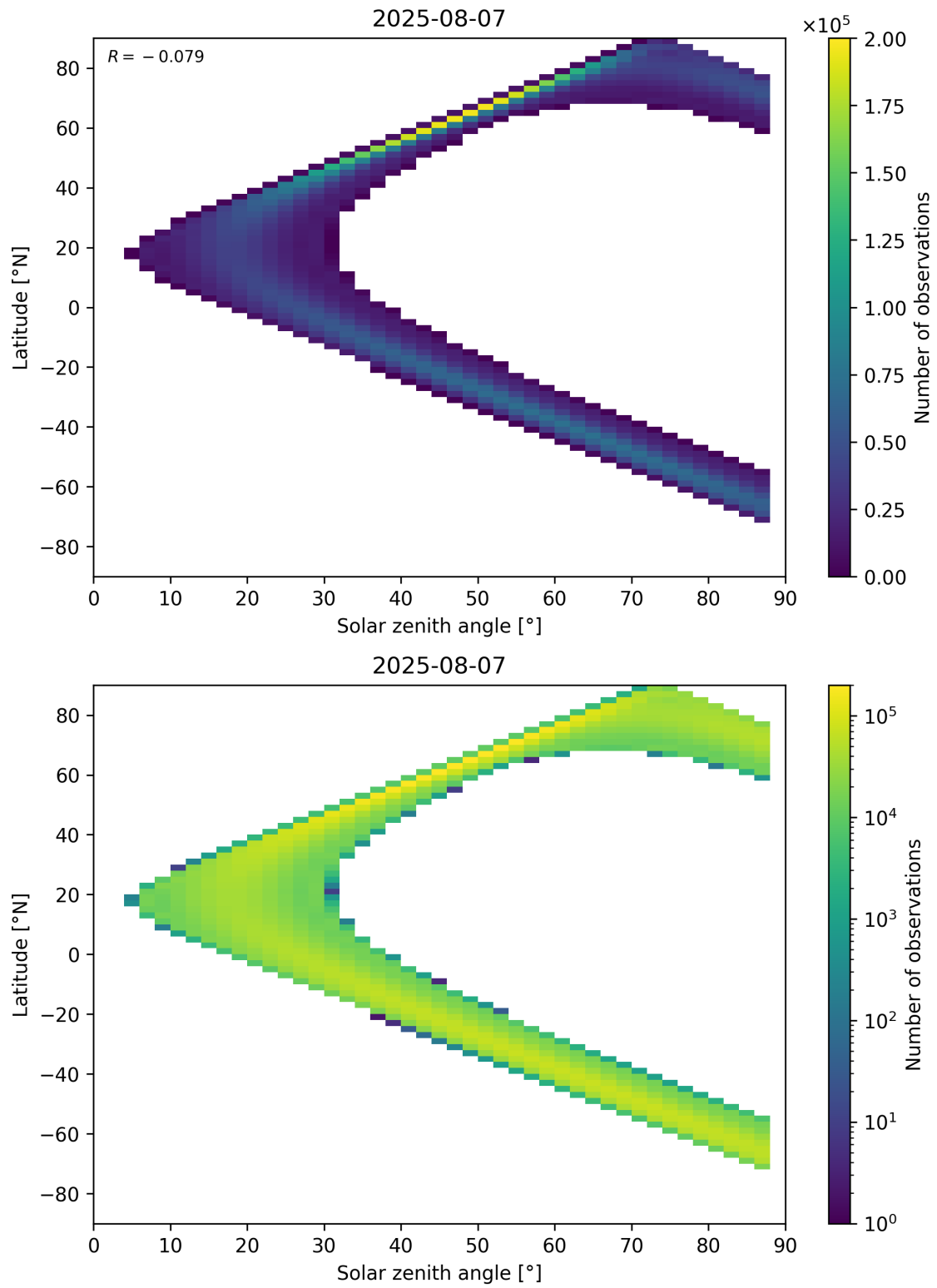
Figure 149: Scatter density plot of “Solar zenith angle” against “Latitude” for 2025-08-06 to 2025-08-08.
