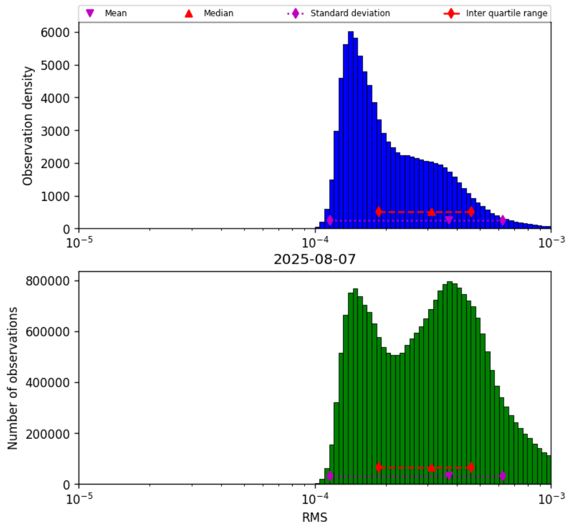
Figure 43: Histogram of “RMS” for 2025-08-06 to 2025-08-08
