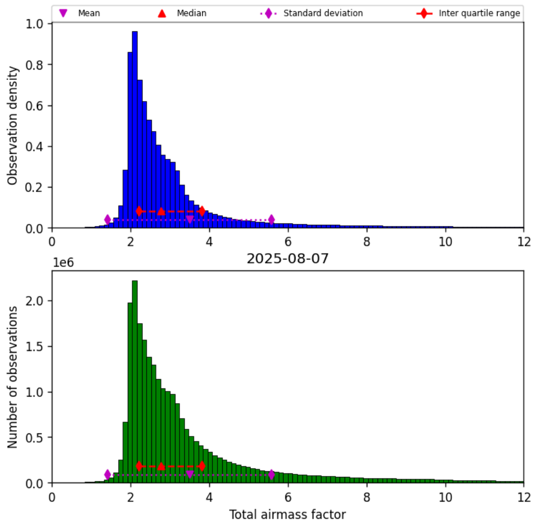
Figure 32: Histogram of “Total airmass factor” for 2025-08-06 to 2025-08-08
