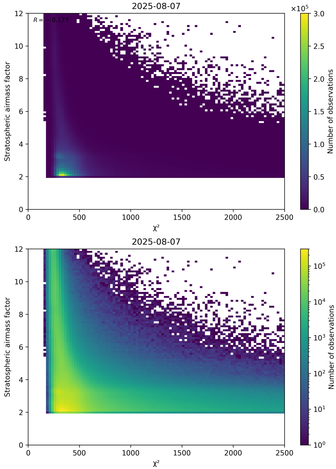
Figure 81: Scatter density plot of “ \chi^2 ” against “Stratospheric airmass factor” for 2025-08-06 to 2025-08-08.
