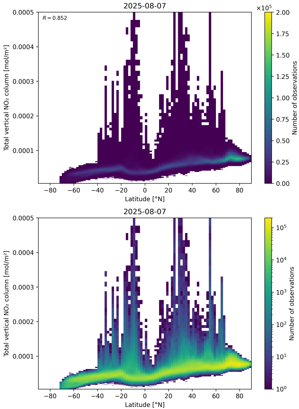
Figure 90: Scatter density plot of “Latitude” against “Total vertical NO 2 column” for 2025-08-06 to 2025-08-08.
