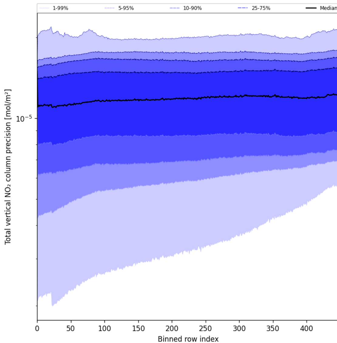
Figure 56: Along track statistics of “Total vertical NO 2 column precision” for 2025-08-06 to 2025-08-08
