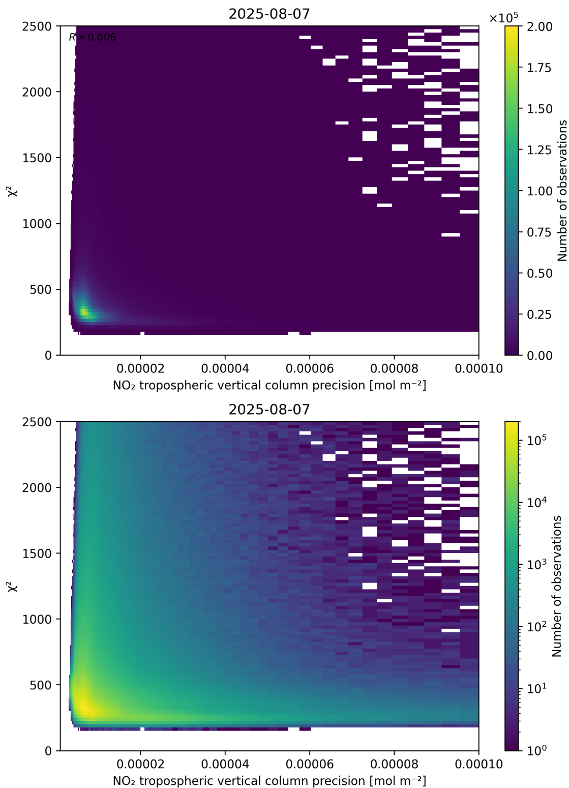
Figure 134: Scatter density plot of “NO 2 tropospheric vertical column precision” against “ \chi^2 ” for 2025-08-06 to 2025-08-08.
