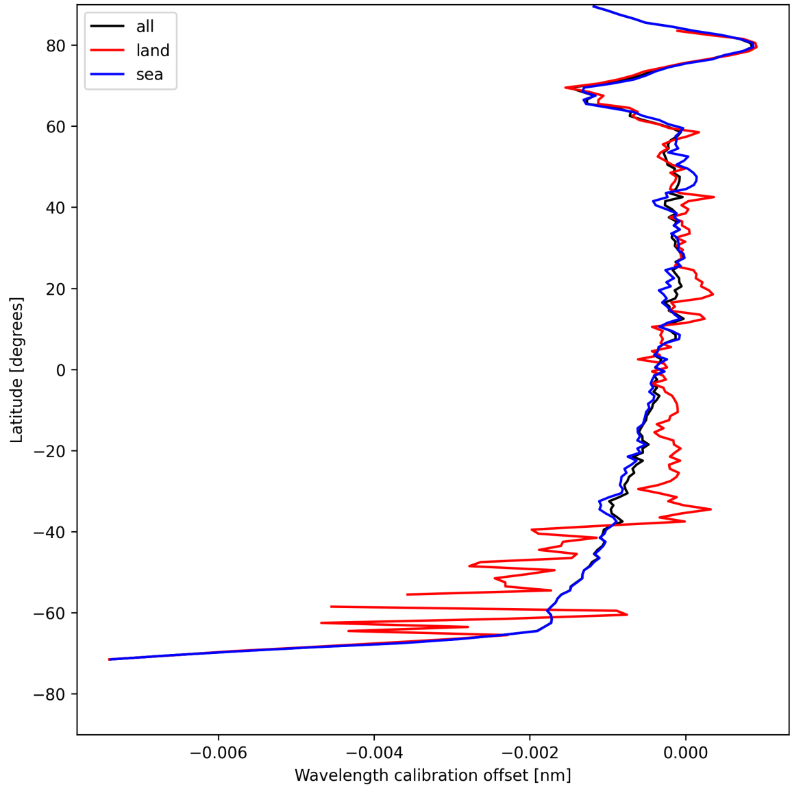
Figure 18: Zonal average of “Wavelength calibration offset” for 2025-08-06 to 2025-08-08.
