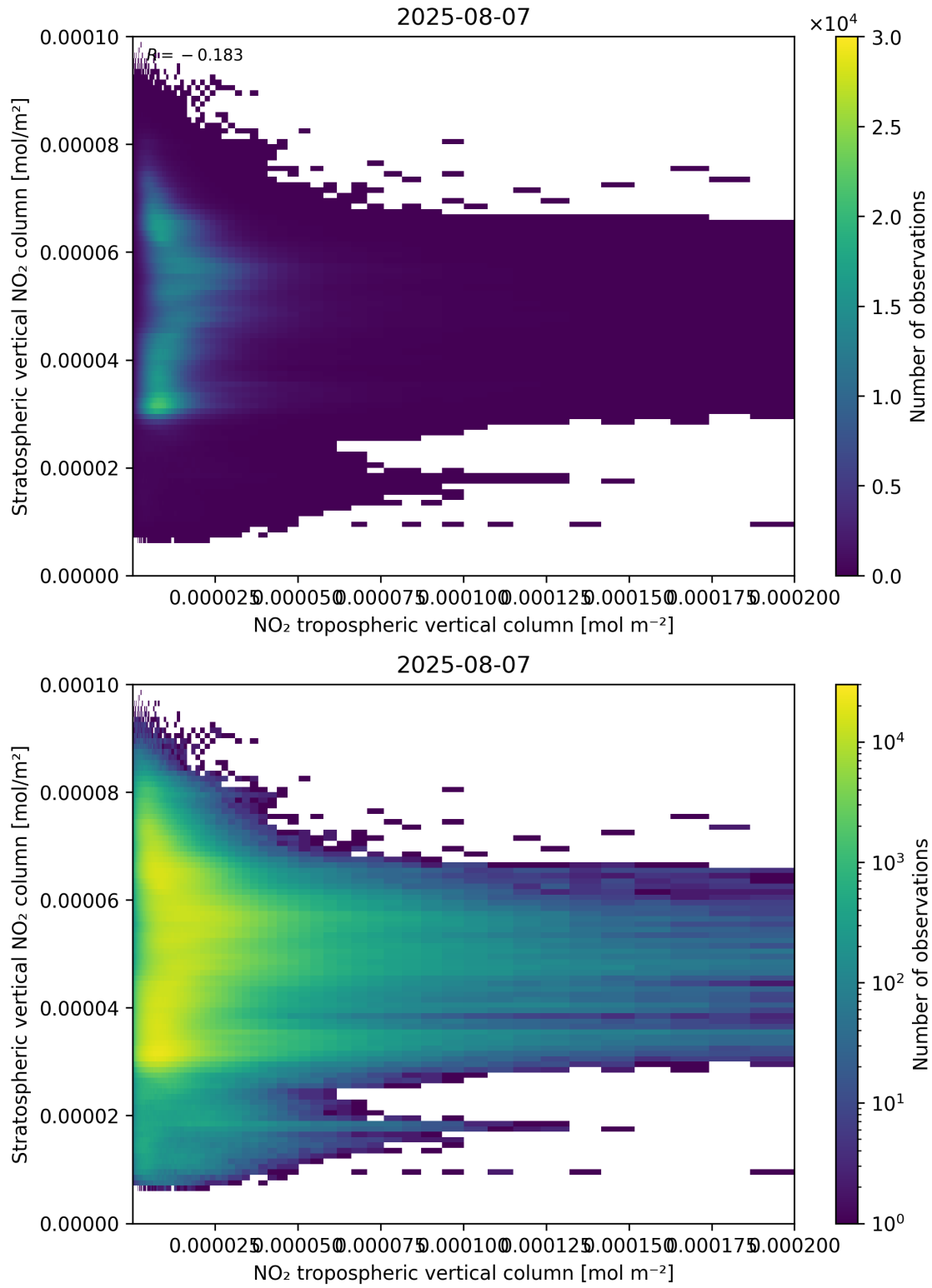
Figure 125: Scatter density plot of “NO 2 tropospheric vertical column” against “Stratospheric vertical NO 2 column” for 2025-08-06 to 2025-08-08.
