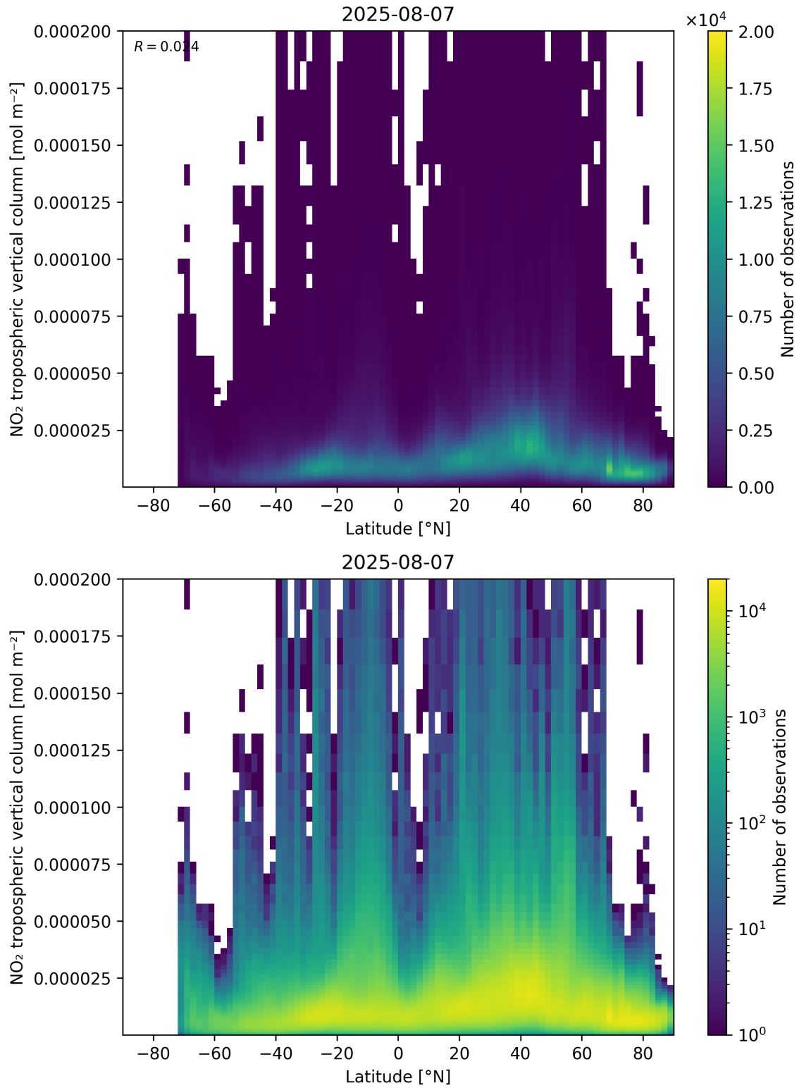
Figure 92: Scatter density plot of “Latitude” against “NO 2 tropospheric vertical column” for 2025-08-06 to 2025-08-08.
