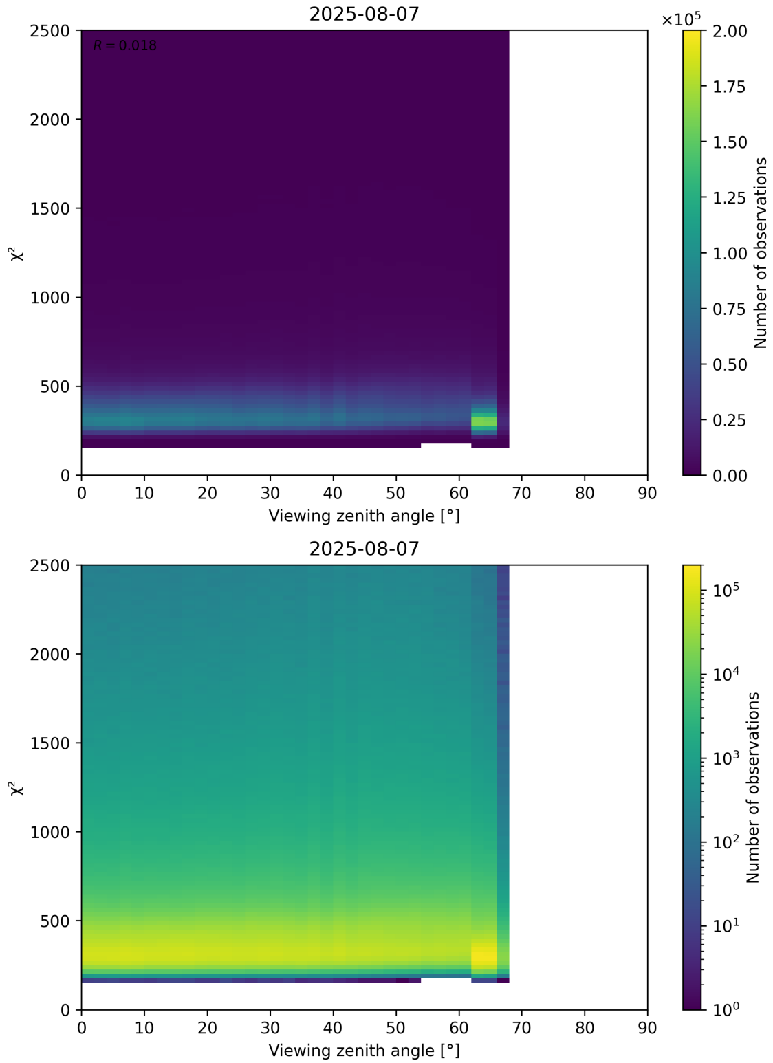
Figure 162: Scatter density plot of “Viewing zenith angle” against “ \chi^2 ” for 2025-08-06 to 2025-08-08.
