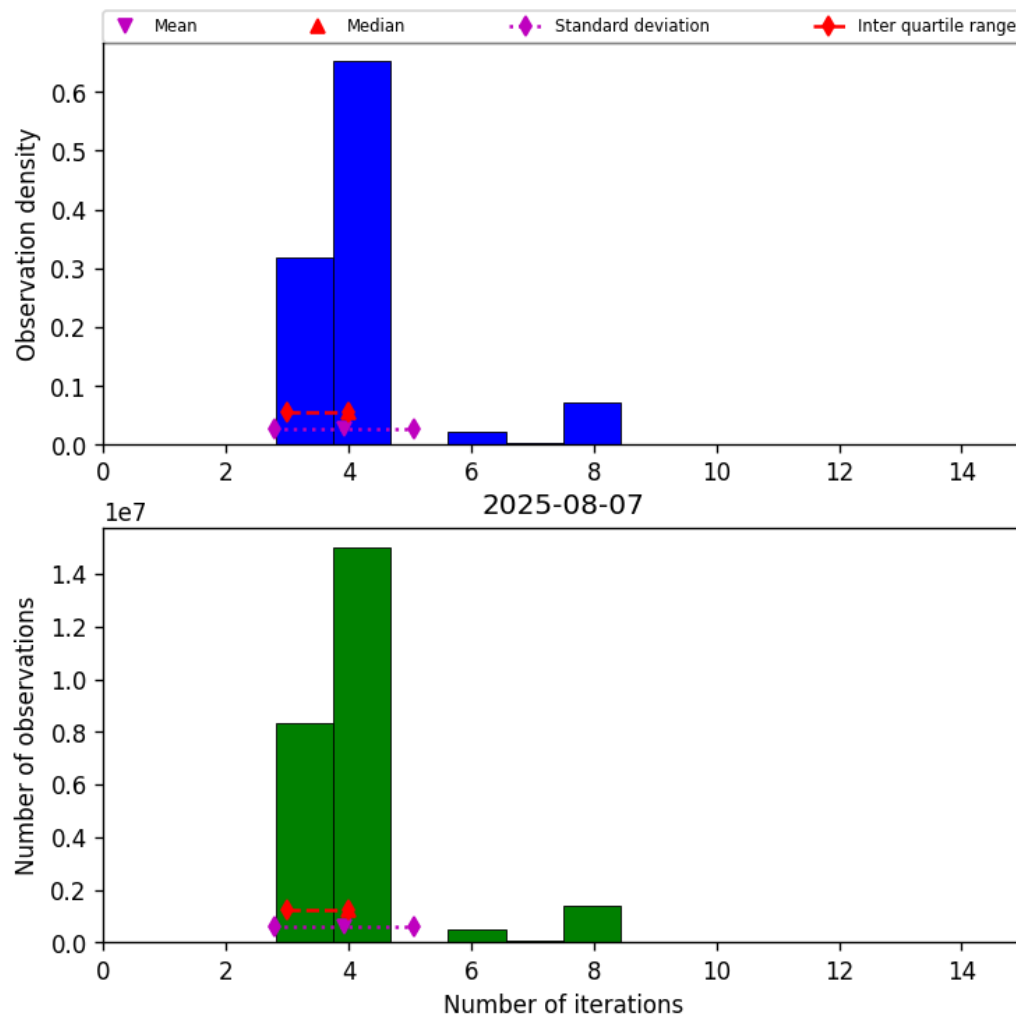
Figure 34: Histogram of “Number of iterations” for 2025-08-06 to 2025-08-08
