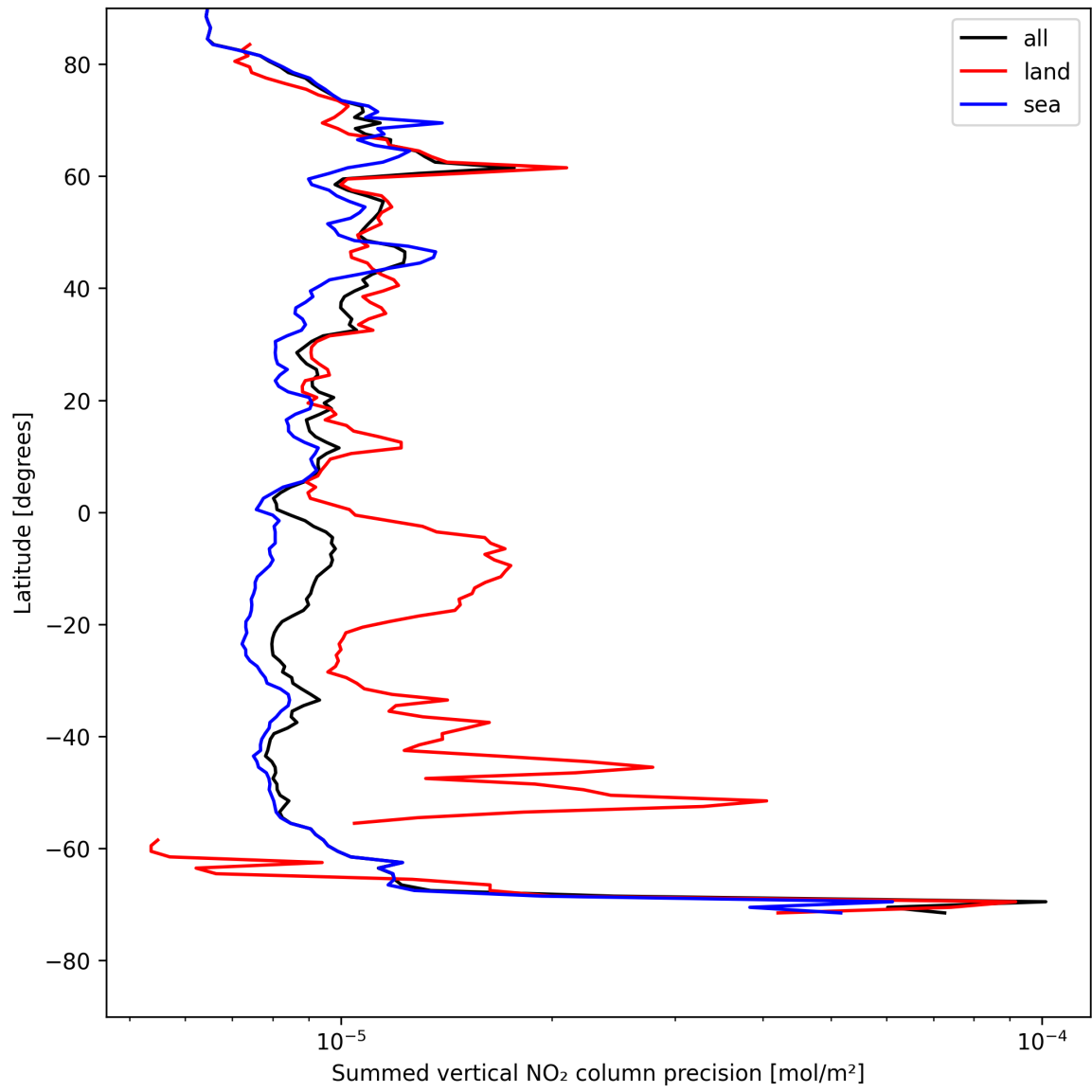
Figure 24: Zonal average of “Summed vertical NO 2 column precision” for 2025-08-06 to 2025-08-08.
