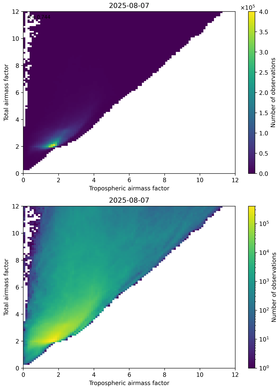
Figure 72: Scatter density plot of “Tropospheric airmass factor” against “Total airmass factor” for 2025-08-06 to 2025-08-08.
