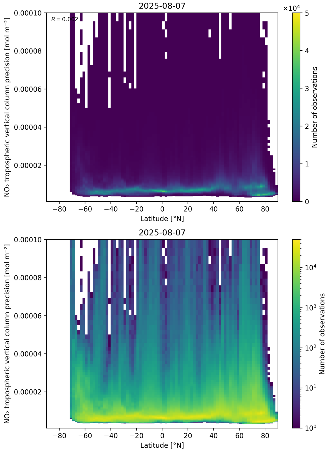
Figure 93: Scatter density plot of “Latitude” against “NO 2 tropospheric vertical column precision” for 2025-08-06 to 2025-08-08.
