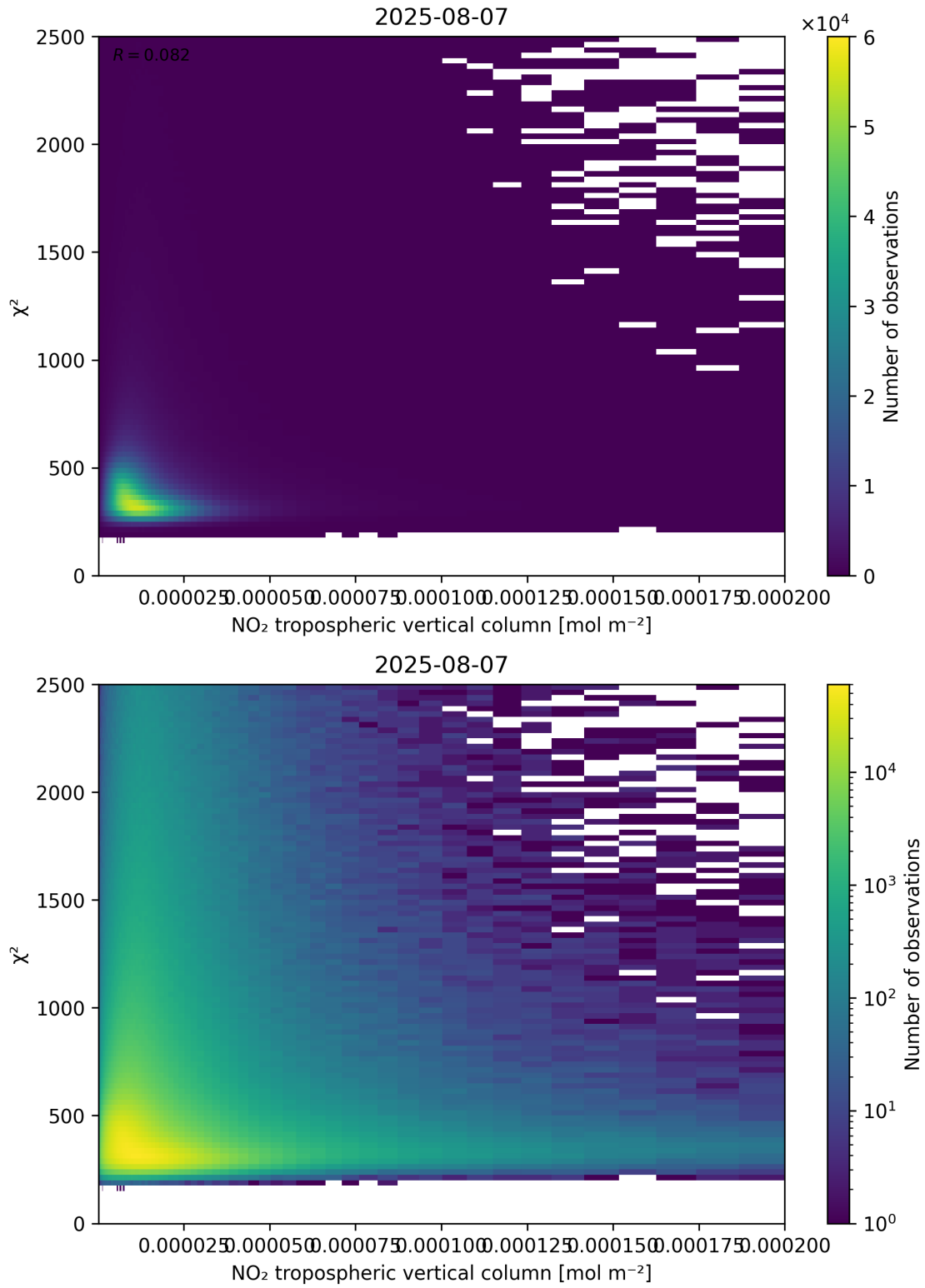
Figure 124: Scatter density plot of “NO 2 tropospheric vertical column” against “ \chi^2 ” for 2025-08-06 to 2025-08-08.
