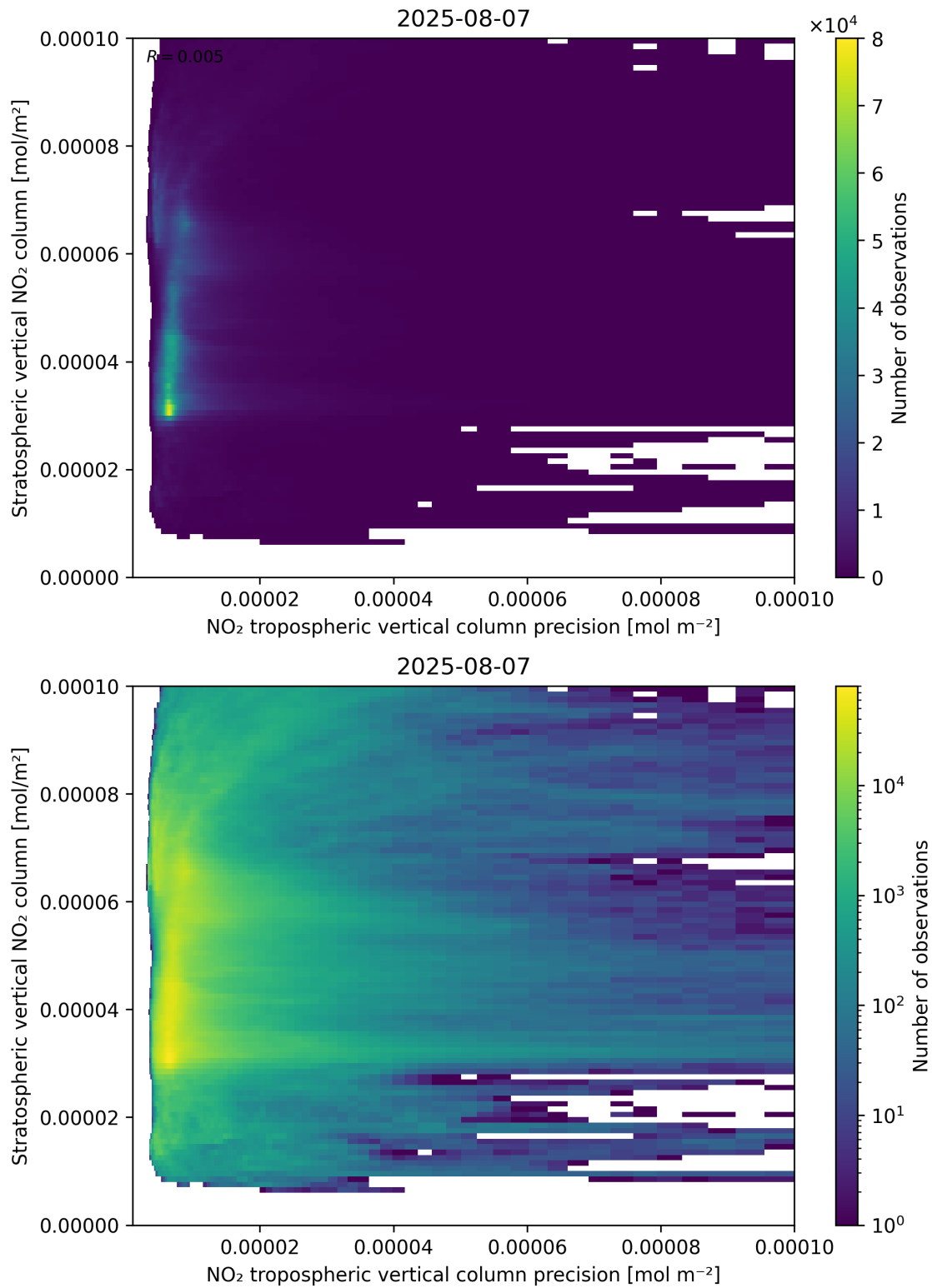
Figure 135: Scatter density plot of “NO 2 tropospheric vertical column precision” against “Stratospheric vertical NO 2 column” for 2025-08-06 to 2025-08-08.
