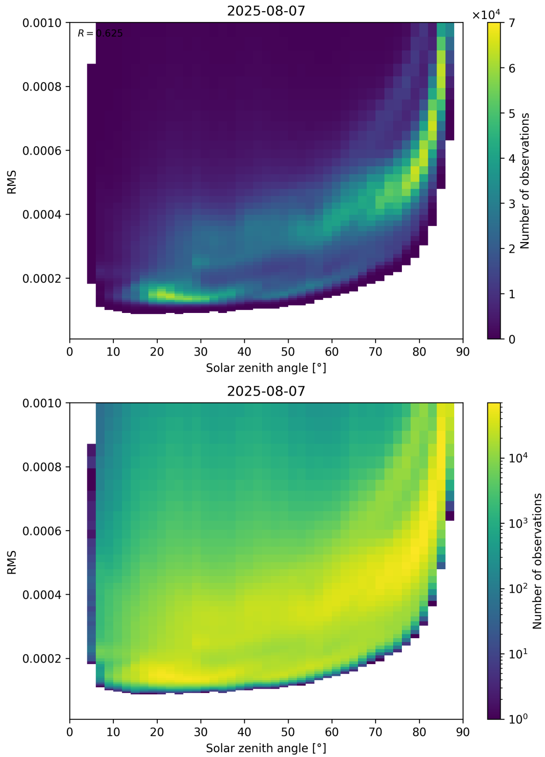
Figure 157: Scatter density plot of “Solar zenith angle” against “RMS” for 2025-08-06 to 2025-08-08.
