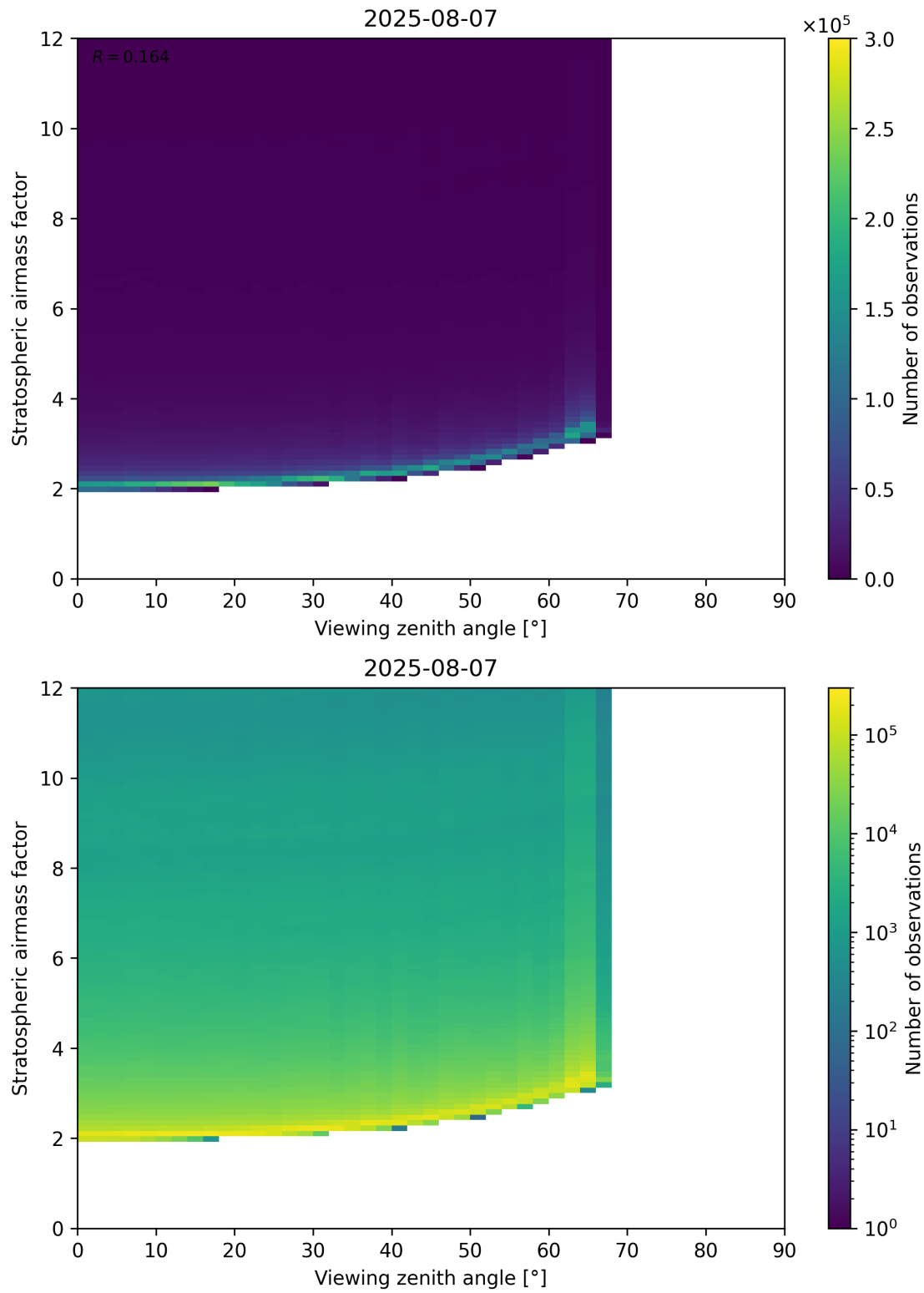
Figure 159: Scatter density plot of “Viewing zenith angle” against “Stratospheric airmass factor” for 2025-08-06 to 2025-08-08.
