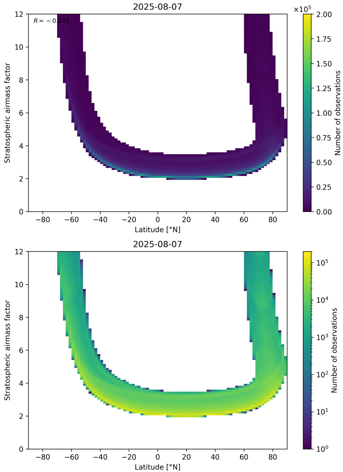
Figure 83: Scatter density plot of “Latitude” against “Stratospheric air mass factor” for 2025-08-06 to 2025-08-08.
