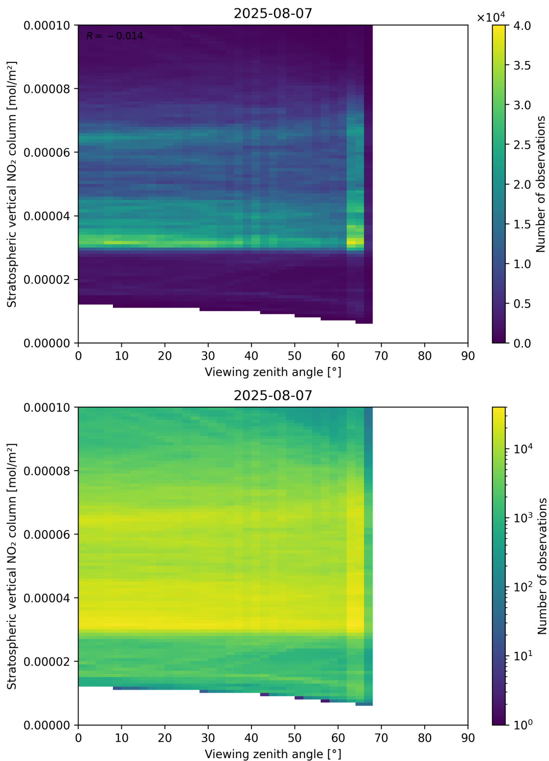
Figure 164: Scatter density plot of “Viewing zenith angle” against “Stratospheric vertical NO 2 column” for 2025-08-06 to 2025-08-08.
