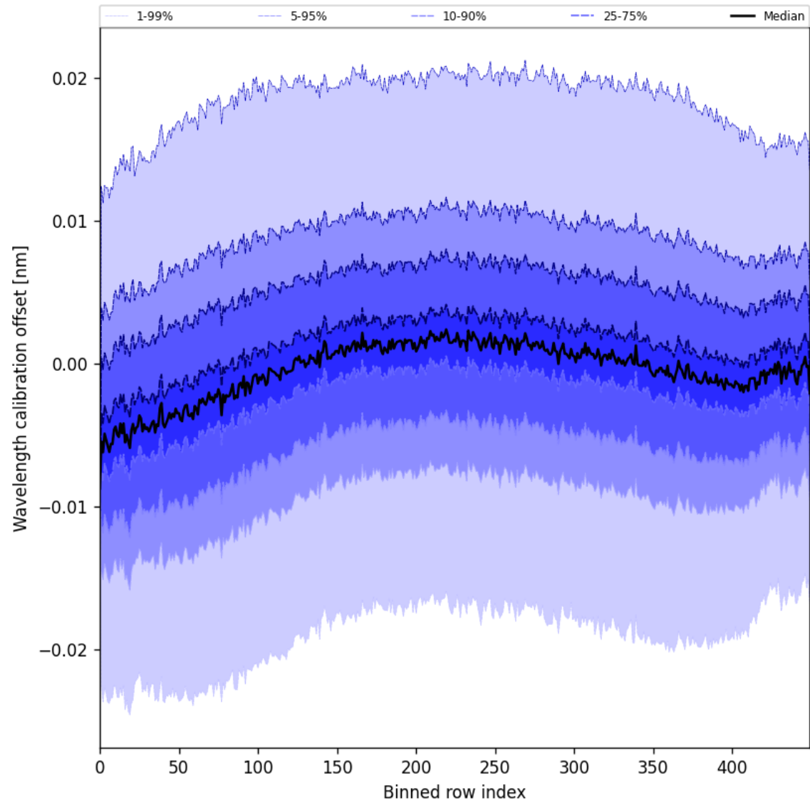
Figure 52: Along track statistics of “Wavelength calibration offset” for 2025-08-06 to 2025-08-08
