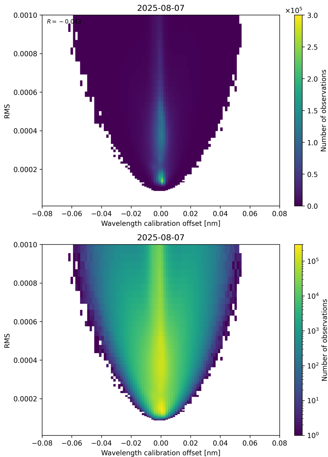
Figure 181: Scatter density plot of “Wavelength calibration offset” against “RMS” for 2025-08-06 to 2025-08-08.
