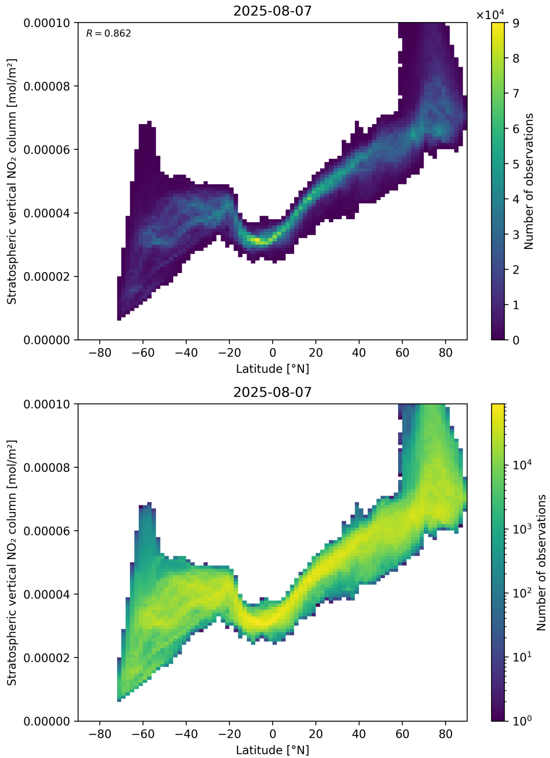
Figure 87: Scatter density plot of “Latitude” against “Stratospheric vertical NO 2 column” for 2025-08-06 to 2025-08-08.
