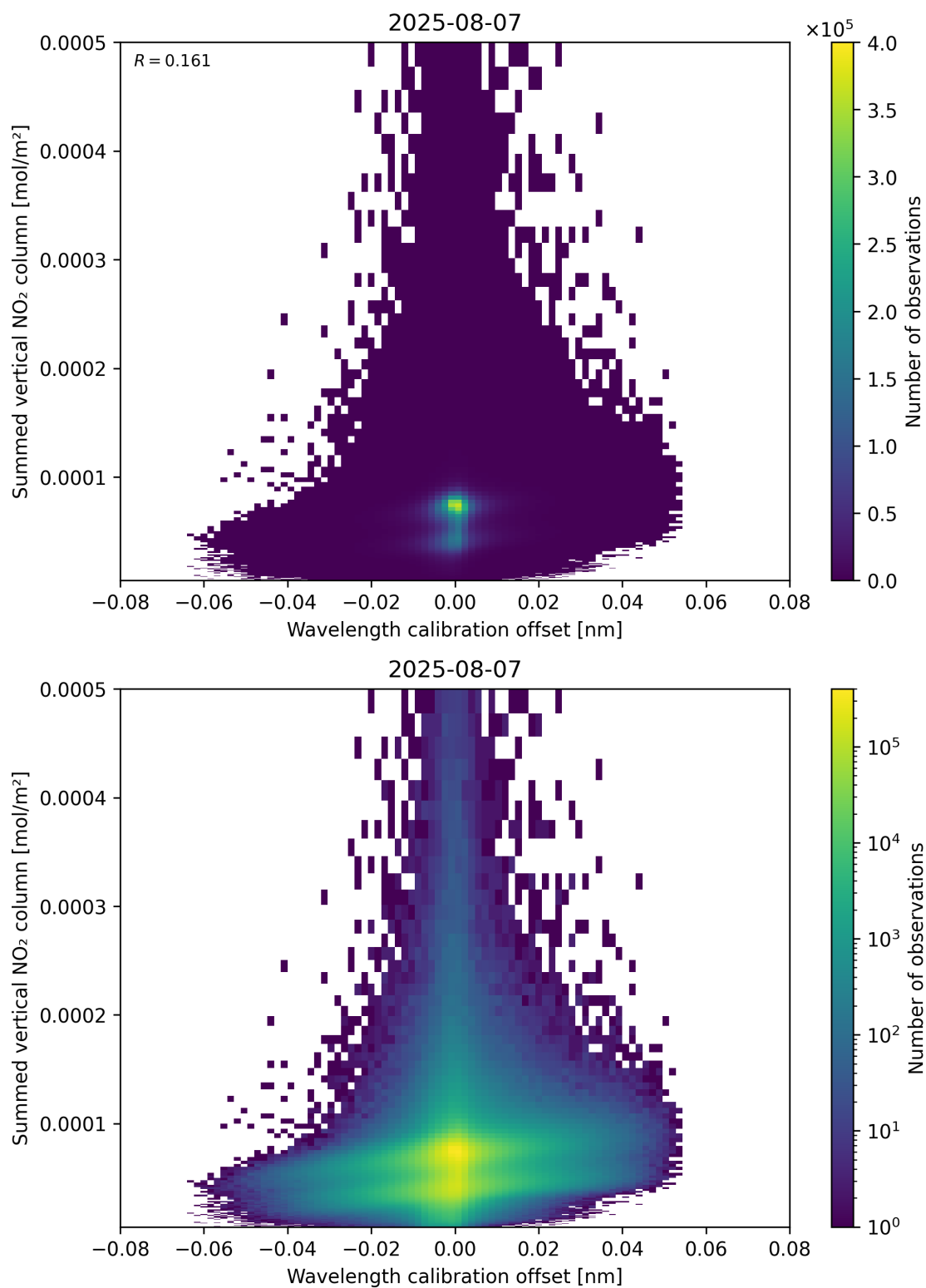
Figure 177: Scatter density plot of “Wavelength calibration offset” against “Summed vertical NO 2 column” for 2025-08-06 to 2025-08-08.
