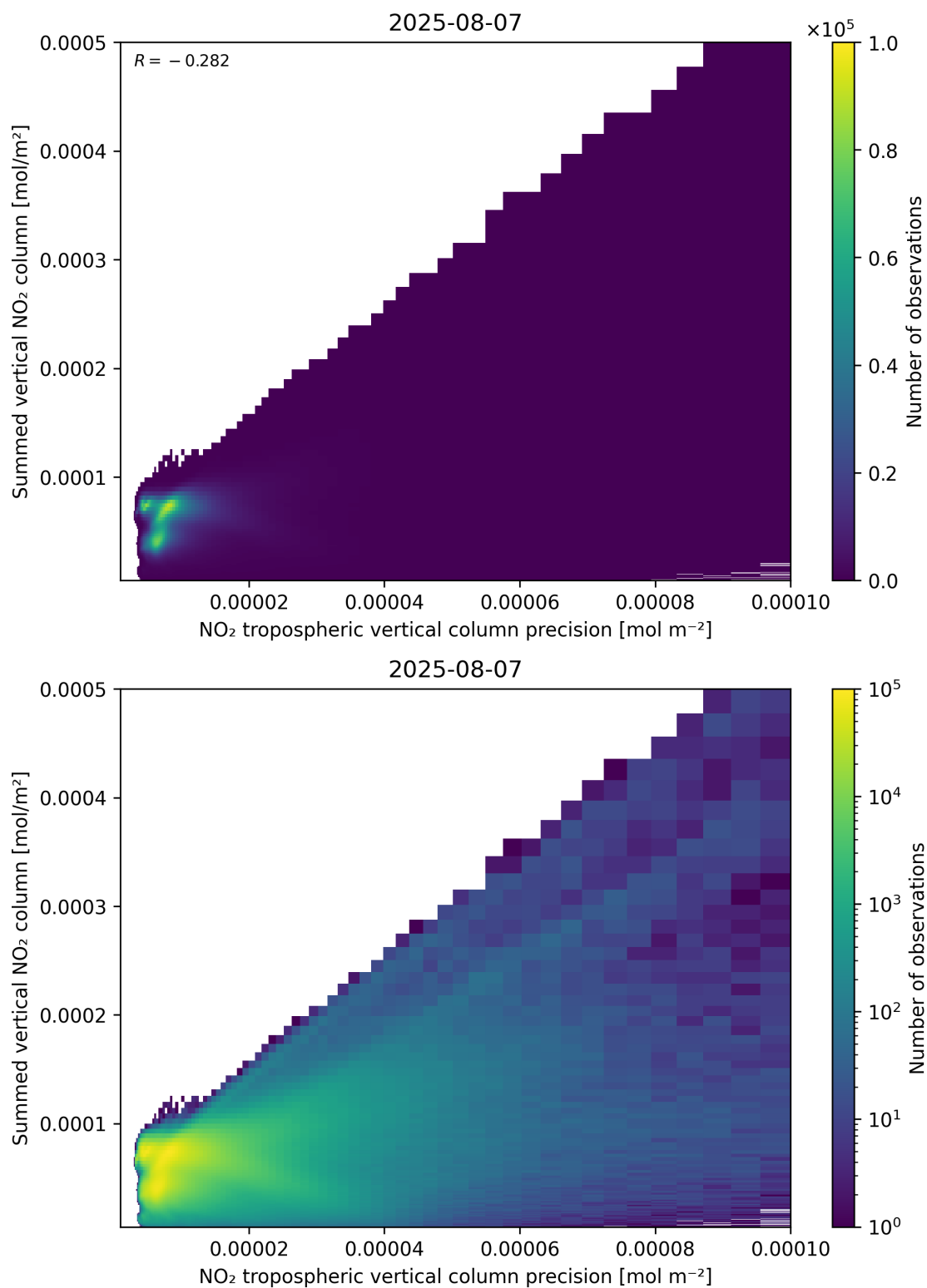
Figure 136: Scatter density plot of “NO 2 tropospheric vertical column precision” against “Summed vertical NO 2 column” for 2025-08-06 to 2025-08-08.
