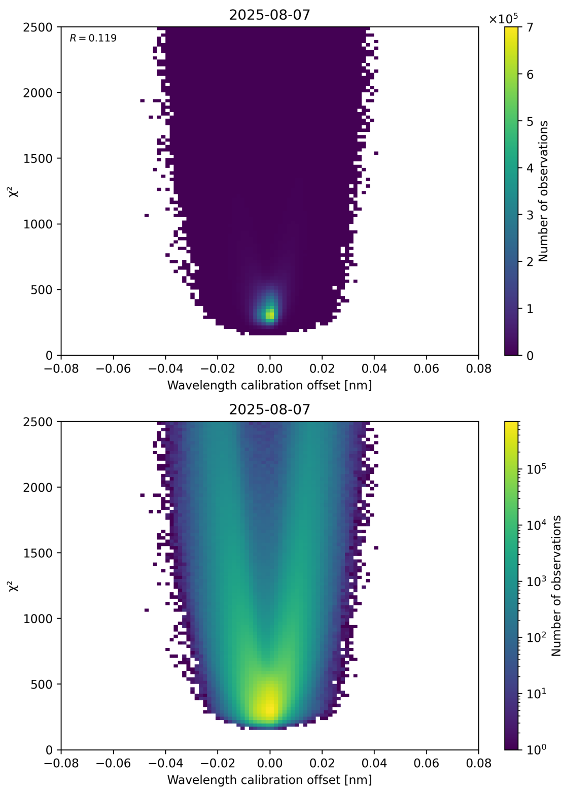
Figure 175: Scatter density plot of “Wavelength calibration offset” against “ \chi^2 ” for 2025-08-06 to 2025-08-08.
