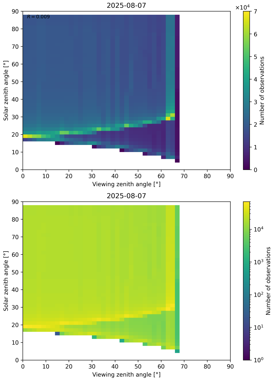
Figure 172: Scatter density plot of “Viewing zenith angle” against “Solar zenith angle” for 2025-08-06 to 2025-08-08.
