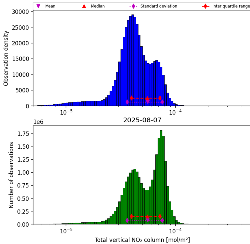
Figure 38: Histogram of “Total vertical NO 2 column” for 2025-08-06 to 2025-08-08
