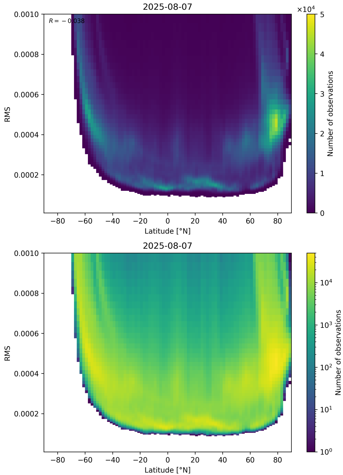
Figure 94: Scatter density plot of “Latitude” against “RMS” for 2025-08-06 to 2025-08-08.
