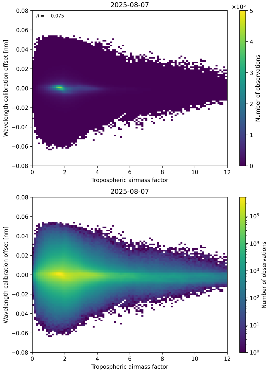
Figure 80: Scatter density plot of “Tropospheric airmass factor” against “Wavelength calibration offset” for 2025-08-06 to 2025-08-08.
