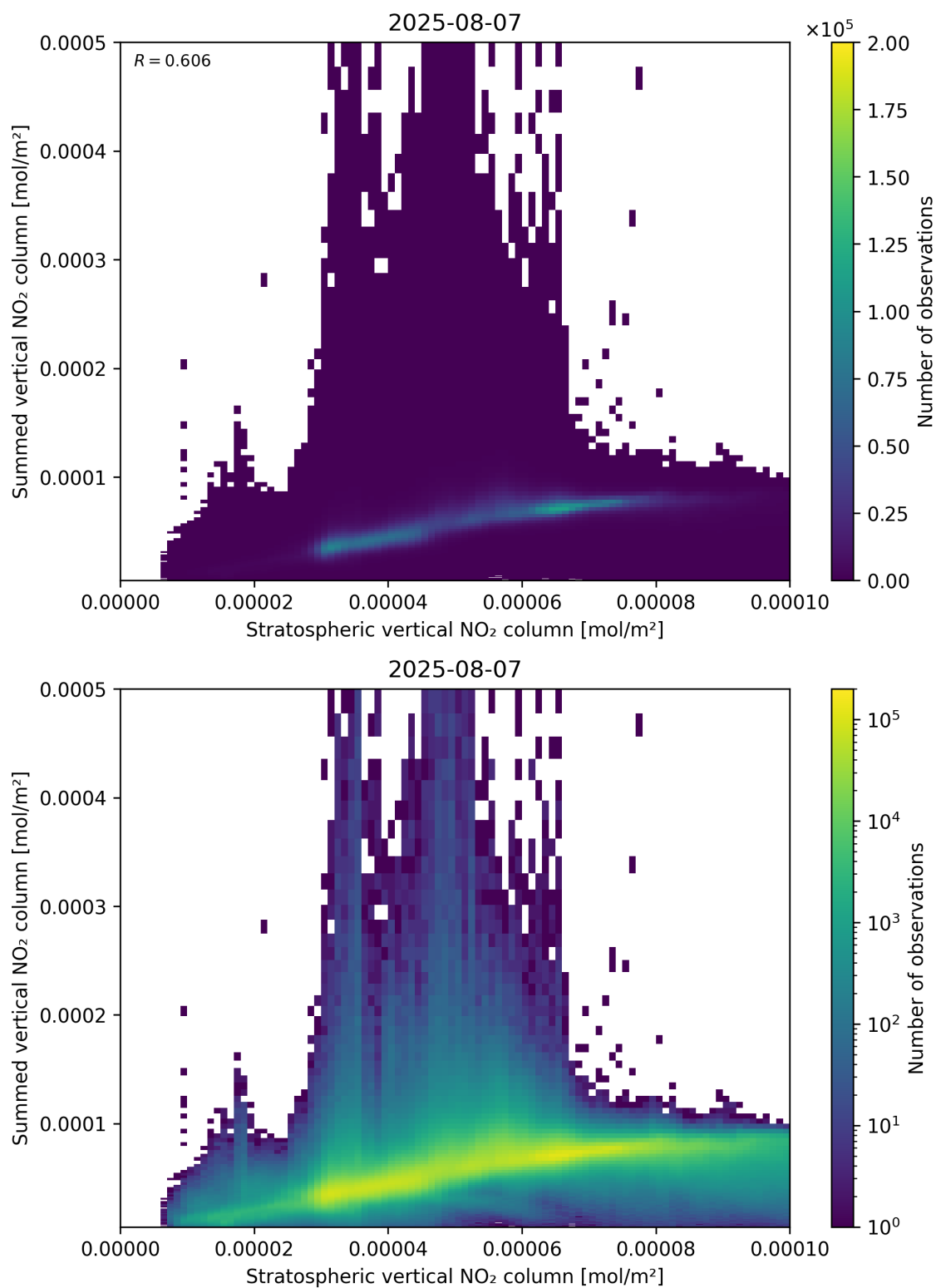
Figure 98: Scatter density plot of “Stratospheric vertical NO 2 column” against “Summed vertical NO 2 column” for 2025-08-06 to 2025-08-08.
