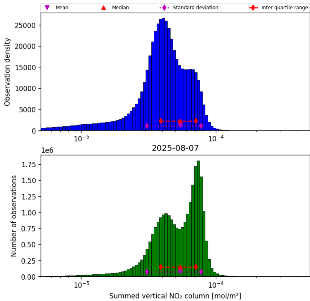
Figure 40: Histogram of “Summed vertical NO 2 column” for 2025-08-06 to 2025-08-08
