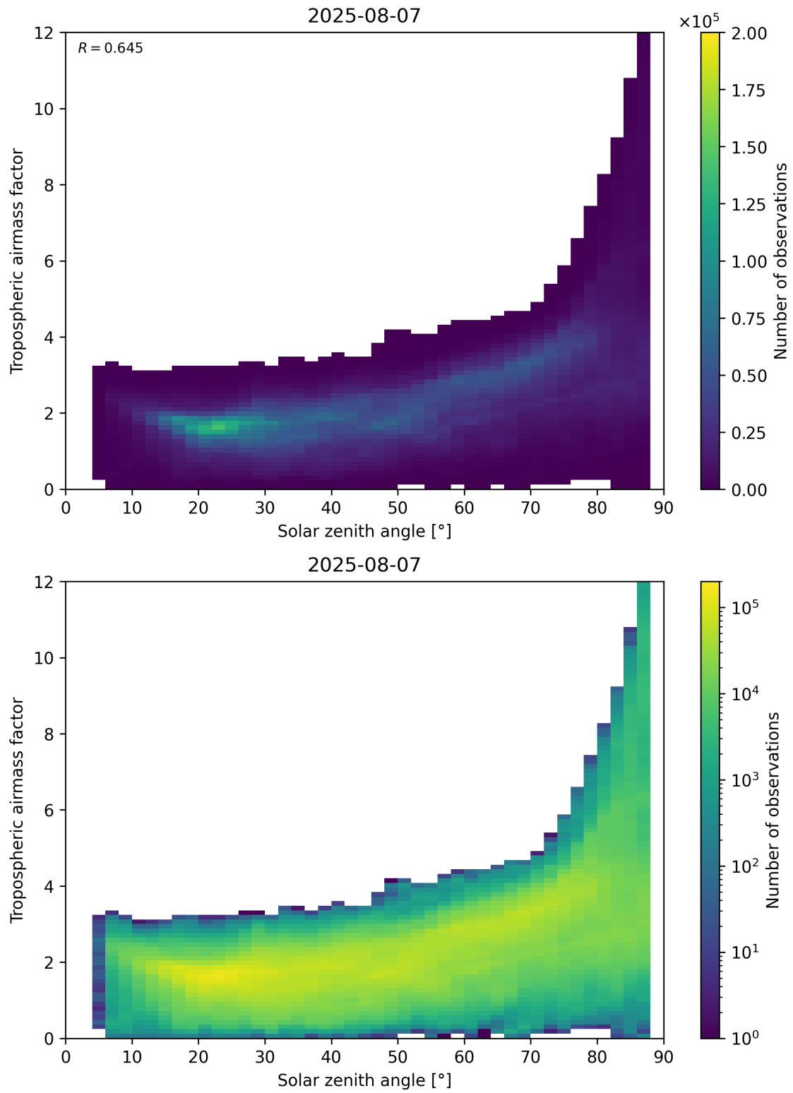
Figure 147: Scatter density plot of “Solar zenith angle” against “Tropospheric airmass factor” for 2025-08-06 to 2025-08-08.
