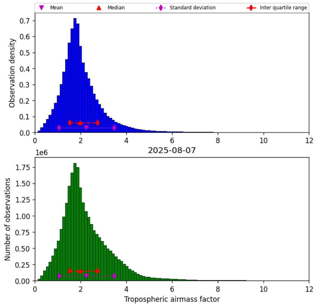
Figure 31: Histogram of “Tropospheric airmass factor” for 2025-08-06 to 2025-08-08
