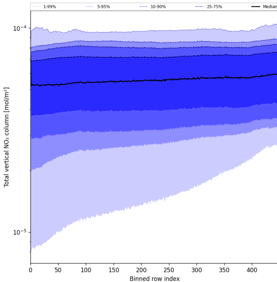
Figure 55: Along track statistics of “Total vertical NO 2 column” for 2025-08-06 to 2025-08-08
