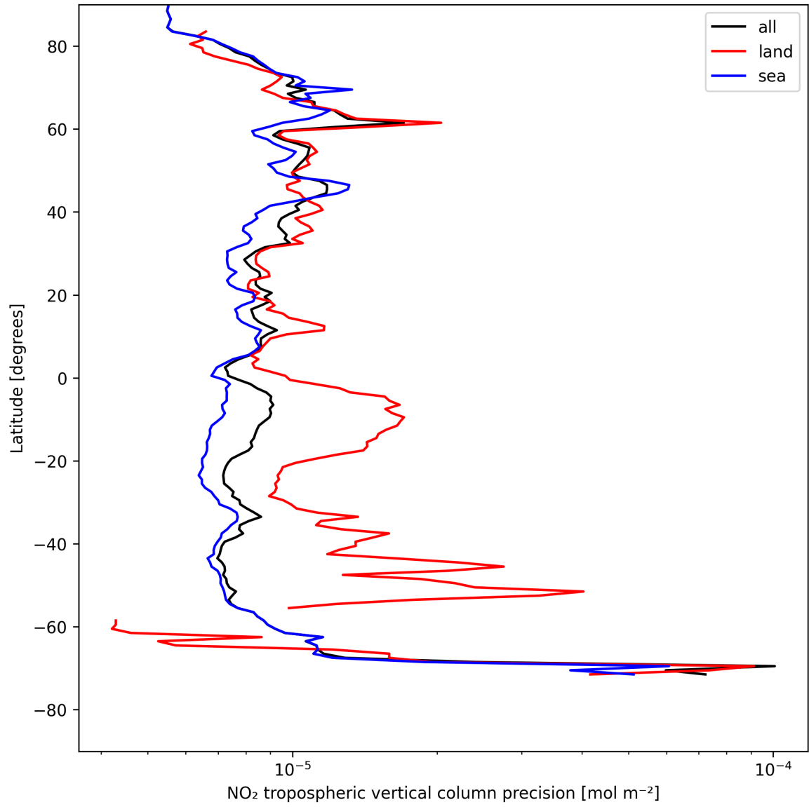
Figure 13: Zonal average of “NO 2 tropospheric vertical column precision” for 2025-08-06 to 2025-08-08.
