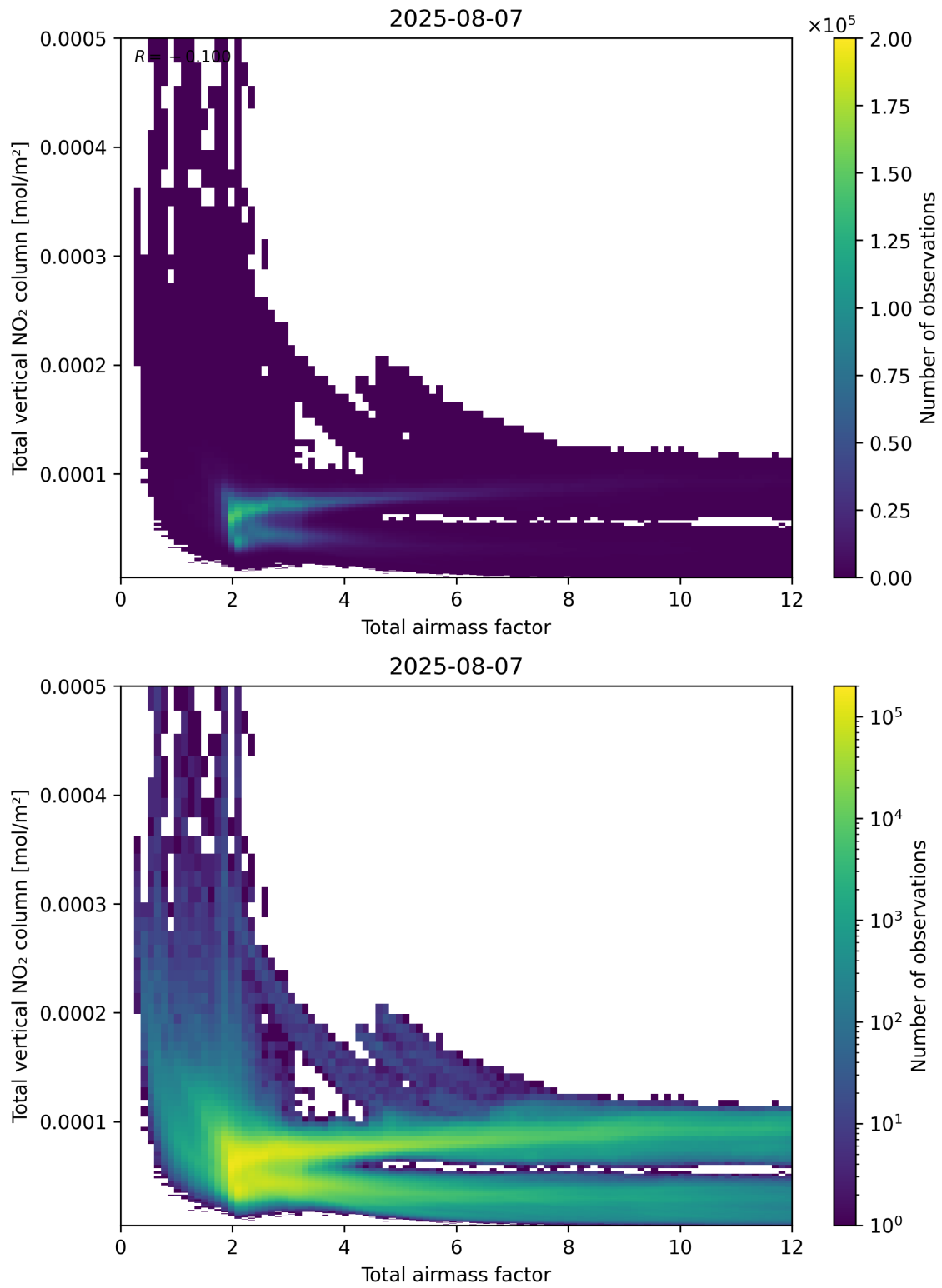
Figure 67: Scatter density plot of “Total airmass factor” against “Total vertical NO 2 column” for 2025-08-06 to 2025-08-08.
