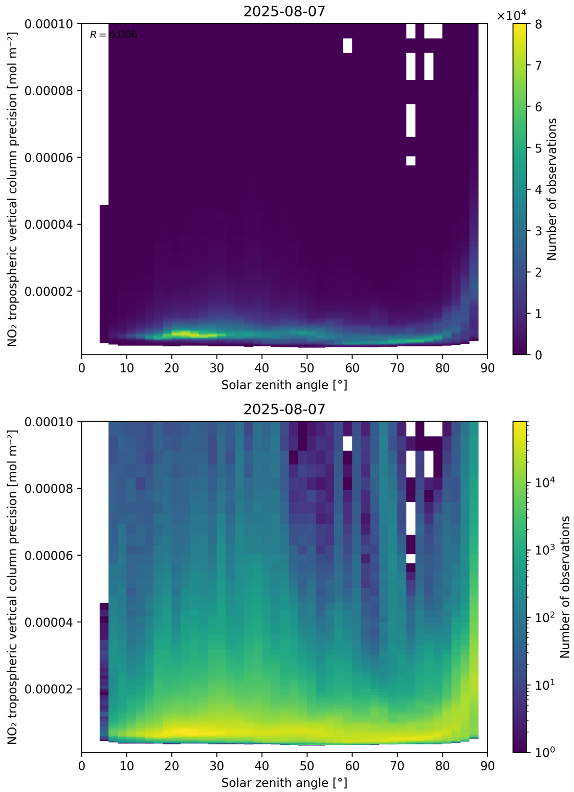
Figure 156: Scatter density plot of “Solar zenith angle” against “NO 2 tropospheric vertical column precision” for 2025-08-06 to 2025-08-08.
