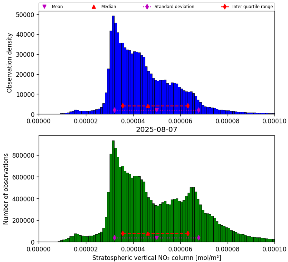
Figure 36: Histogram of “Stratospheric vertical NO 2 column” for 2025-08-06 to 2025-08-08
