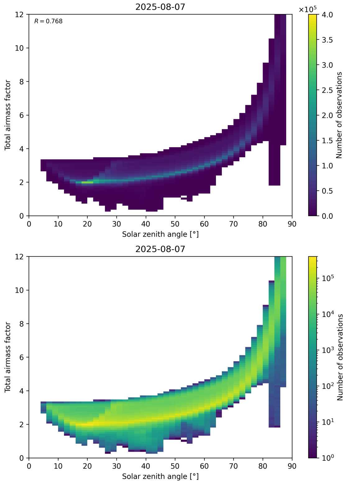
Figure 146: Scatter density plot of “Solar zenith angle” against “Total airmass factor” for 2025-08-06 to 2025-08-08.
