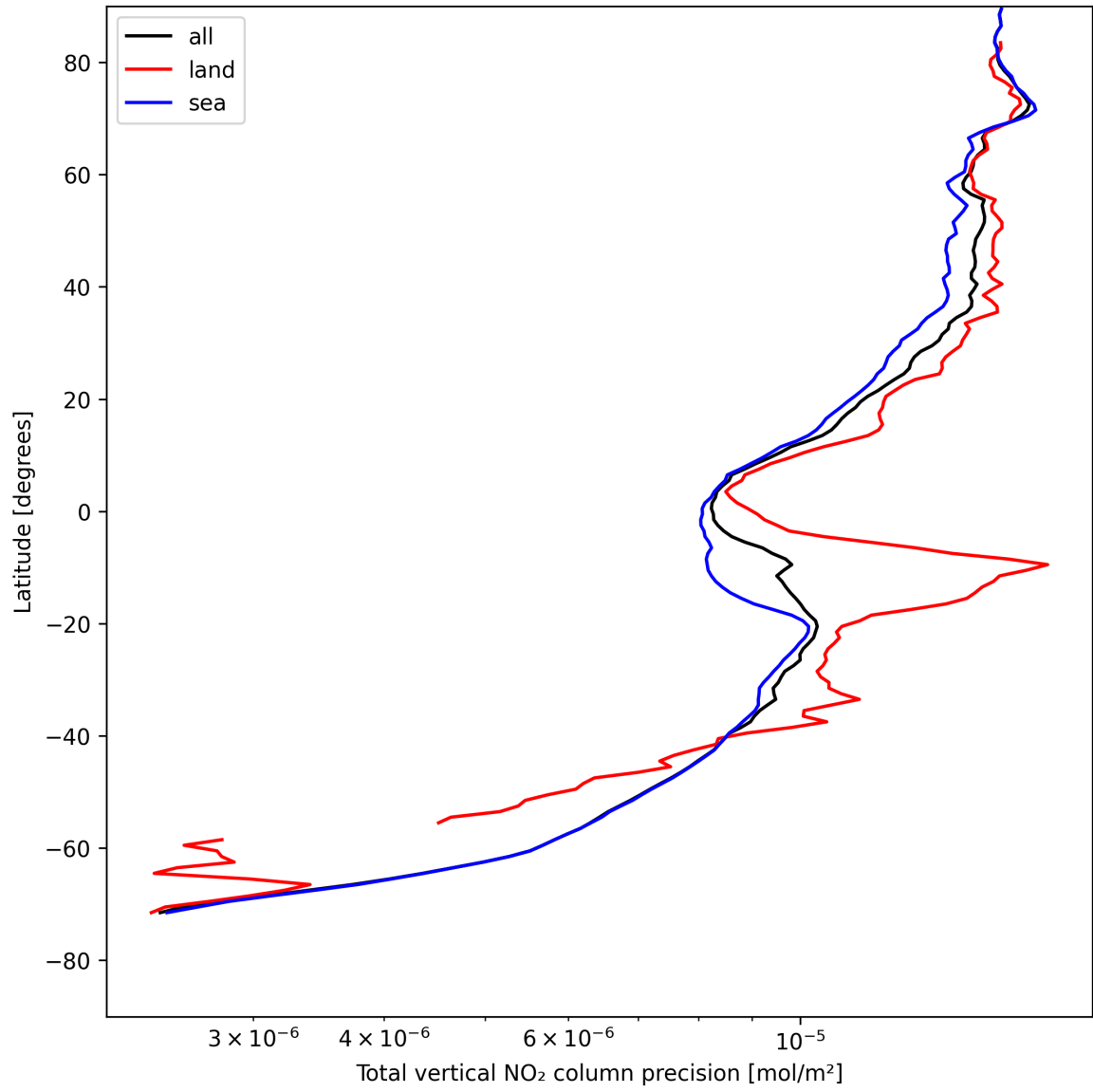
Figure 22: Zonal average of “Total vertical NO 2 column precision” for 2025-08-06 to 2025-08-08.
