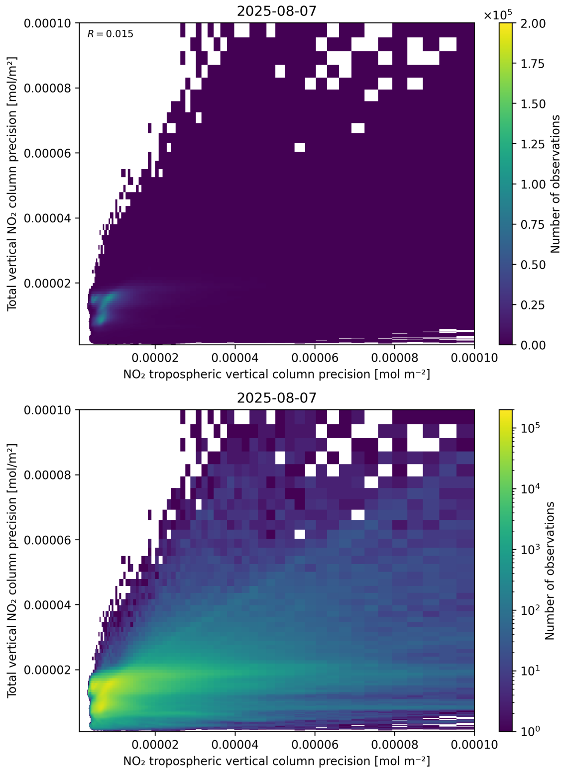
Figure 139: Scatter density plot of “NO 2 tropospheric vertical column precision” against “Total vertical NO 2 column precision” for 2025-08-06 to 2025-08-08.
