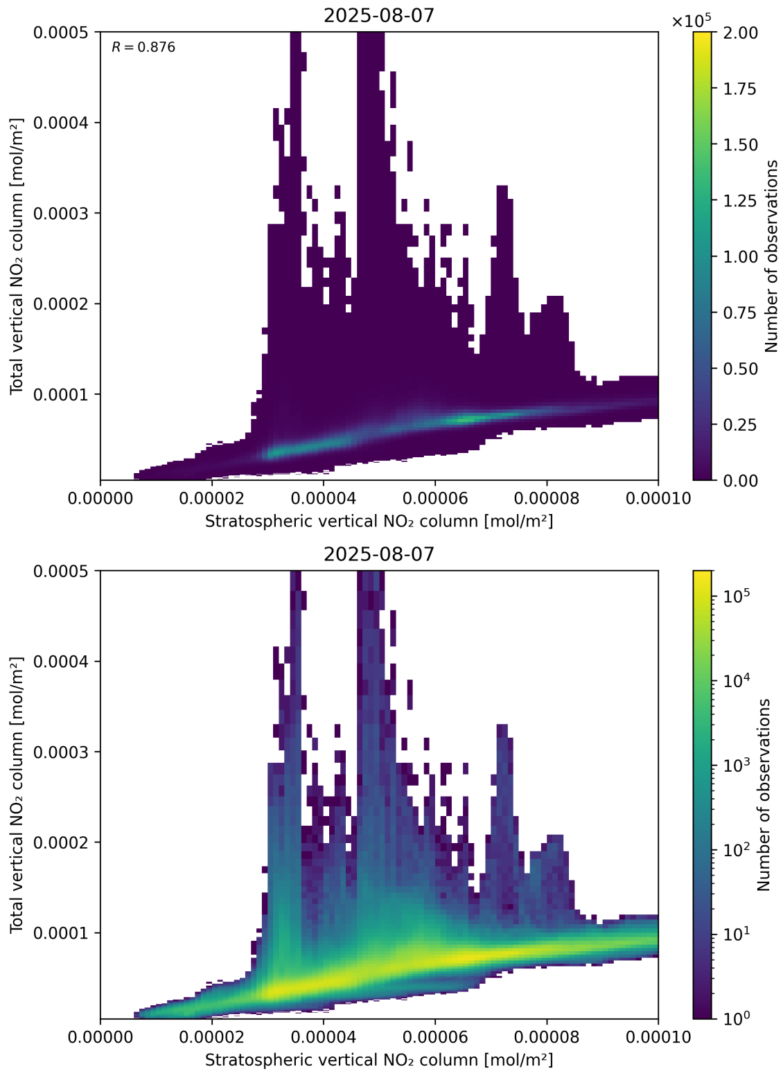
Figure 100: Scatter density plot of “Stratospheric vertical NO 2 column” against “Total vertical NO 2 column” for 2025-08-06 to 2025-08-08.
