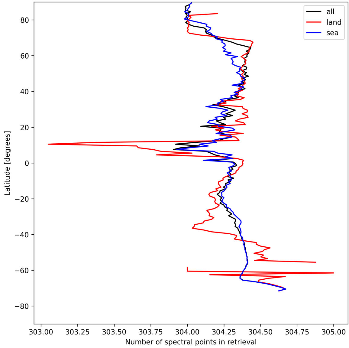
Figure 16: Zonal average of “Number of spectral points in retrieval” for 2025-08-06 to 2025-08-08.
