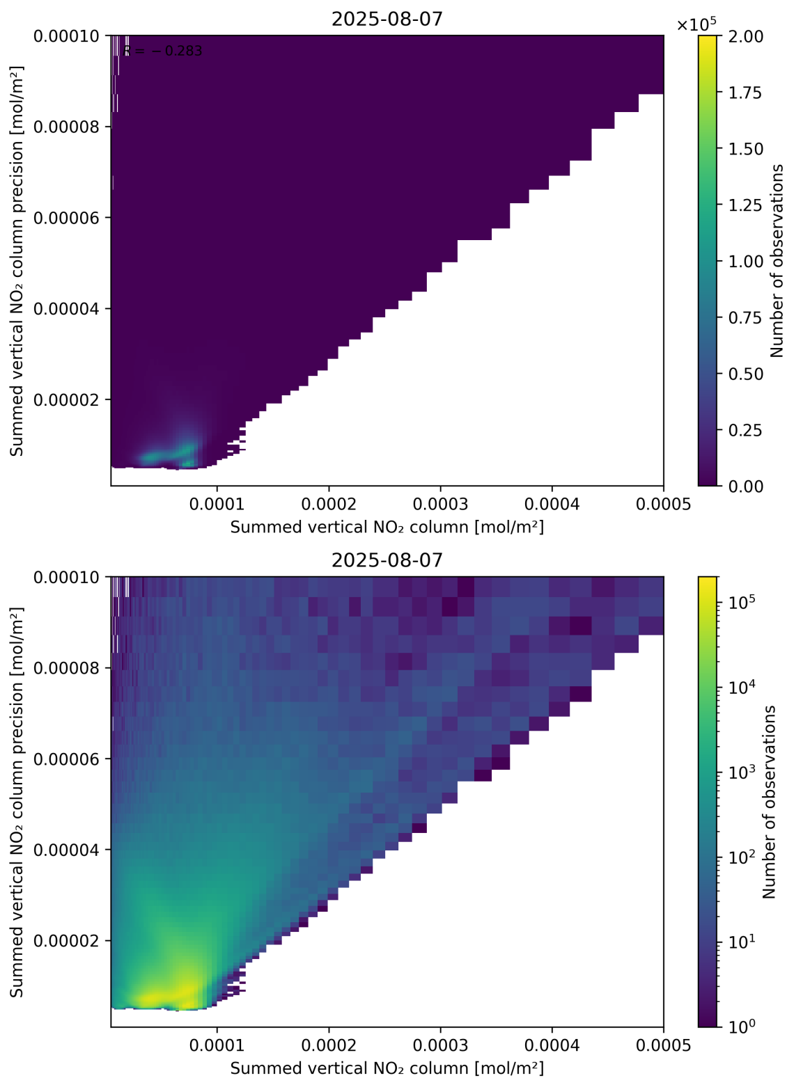
Figure 105: Scatter density plot of “Summed vertical NO 2 column” against “Summed vertical NO 2 column precision” for 2025-08-06 to 2025-08-08.
