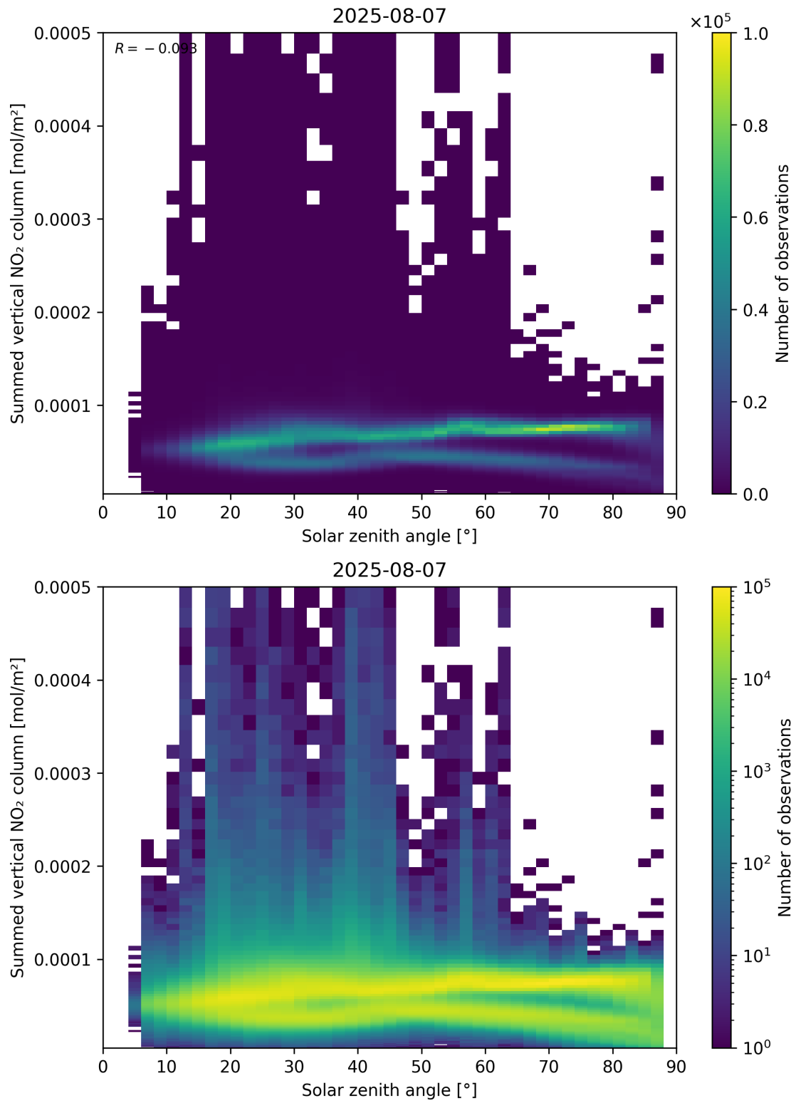
Figure 151: Scatter density plot of “Solar zenith angle” against “Summed vertical NO 2 column” for 2025-08-06 to 2025-08-08.
