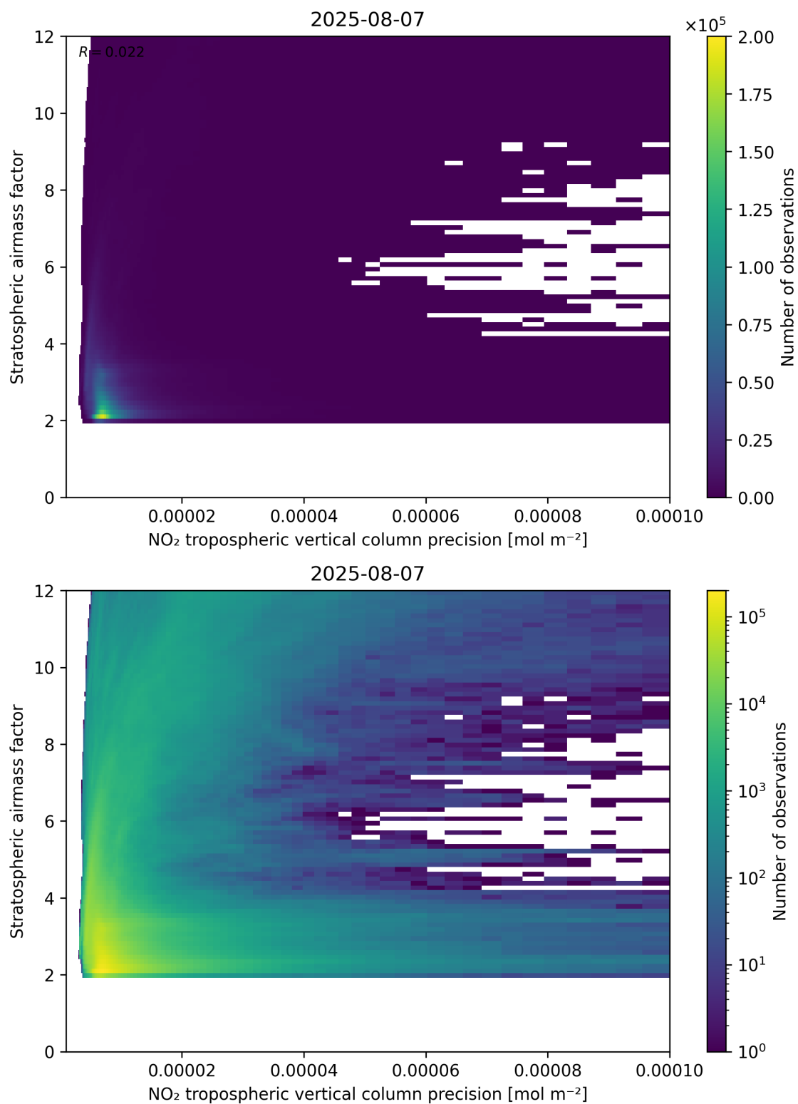
Figure 131: Scatter density plot of “NO 2 tropospheric vertical column precision” against “Stratospheric airmass factor” for 2025-08-06 to 2025-08-08.
