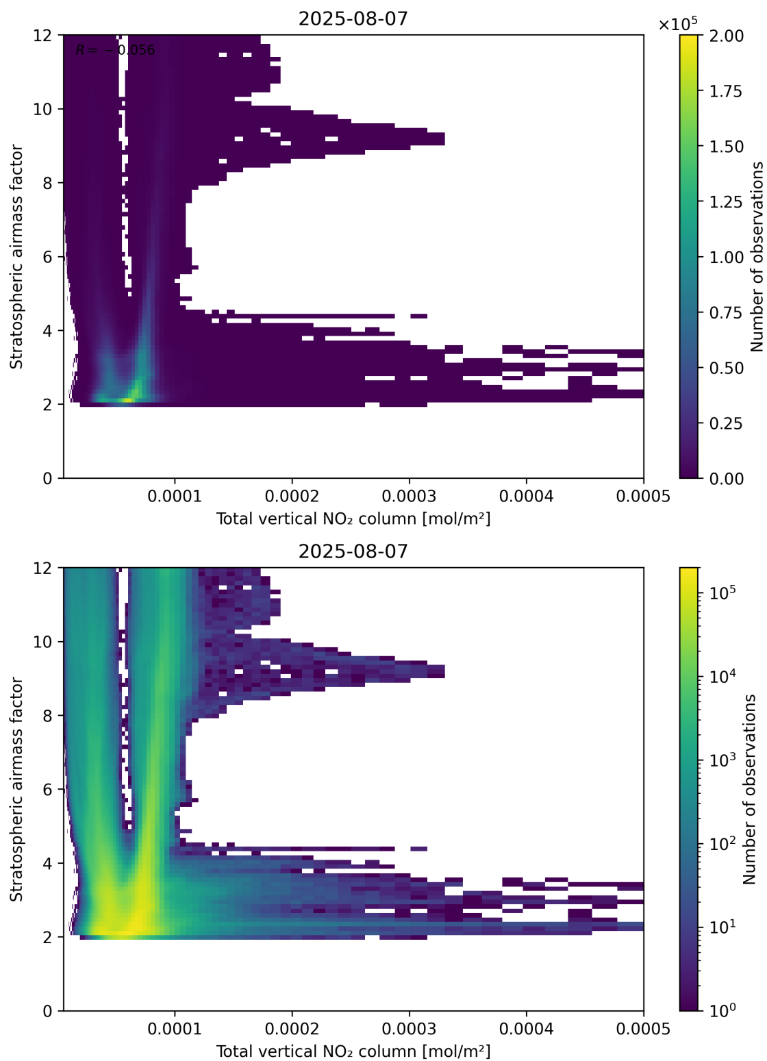
Figure 110: Scatter density plot of “Total vertical NO 2 column” against “Stratospheric air mass factor” for 2025-08-06 to 2025-08-08.
