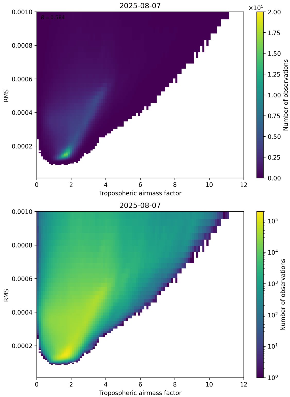
Figure 79: Scatter density plot of “Tropospheric airmass factor” against “RMS” for 2025-08-06 to 2025-08-08.
