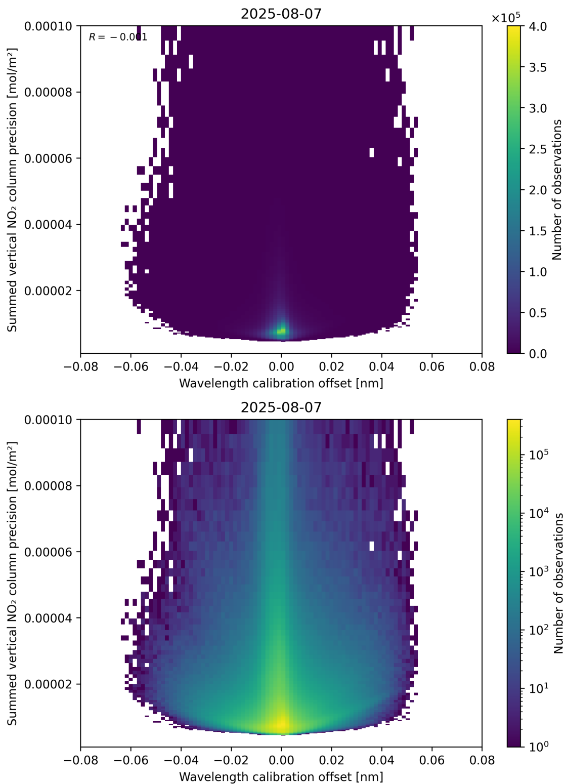
Figure 178: Scatter density plot of “Wavelength calibration offset” against “Summed vertical NO 2 column precision” for 2025-08-06 to 2025-08-08.
