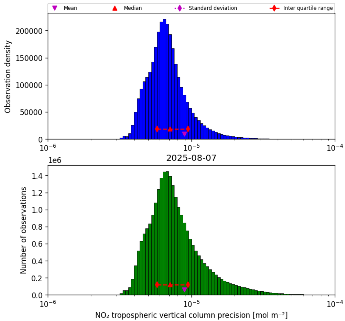
Figure 30: Histogram of “NO 2 tropospheric vertical column precision” for 2025-08-06 to 2025-08-08
