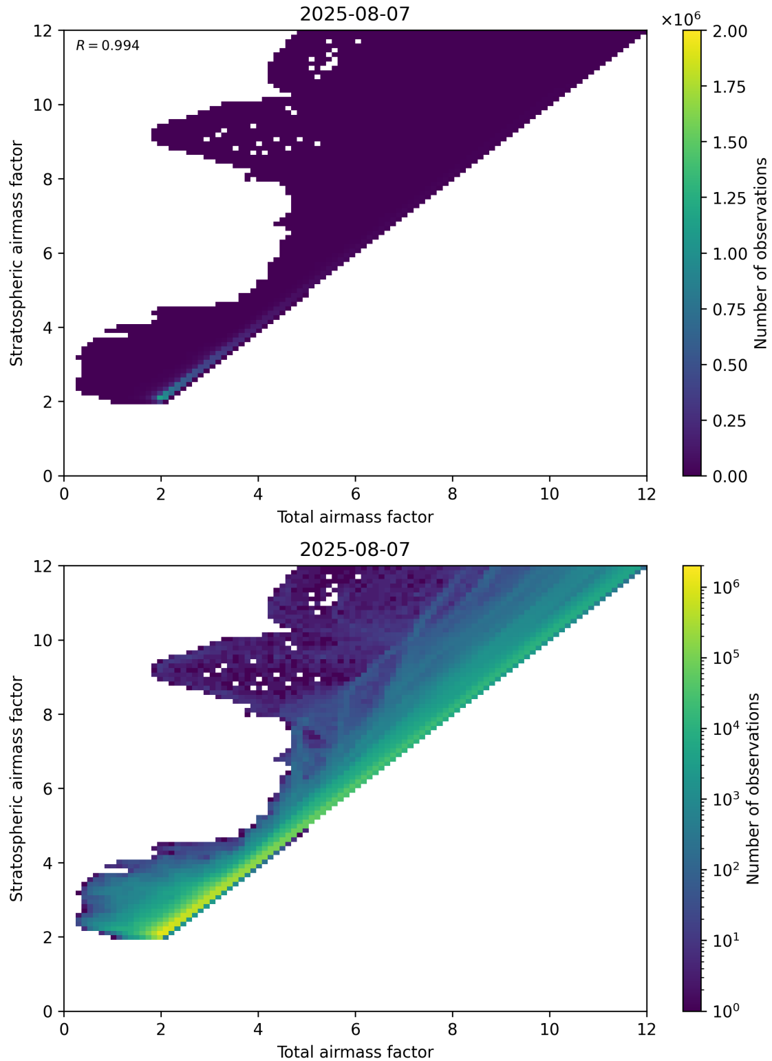
Figure 62: Scatter density plot of “Total airmass factor” against “Stratospheric airmass factor” for 2025-08-06 to 2025-08-08.
