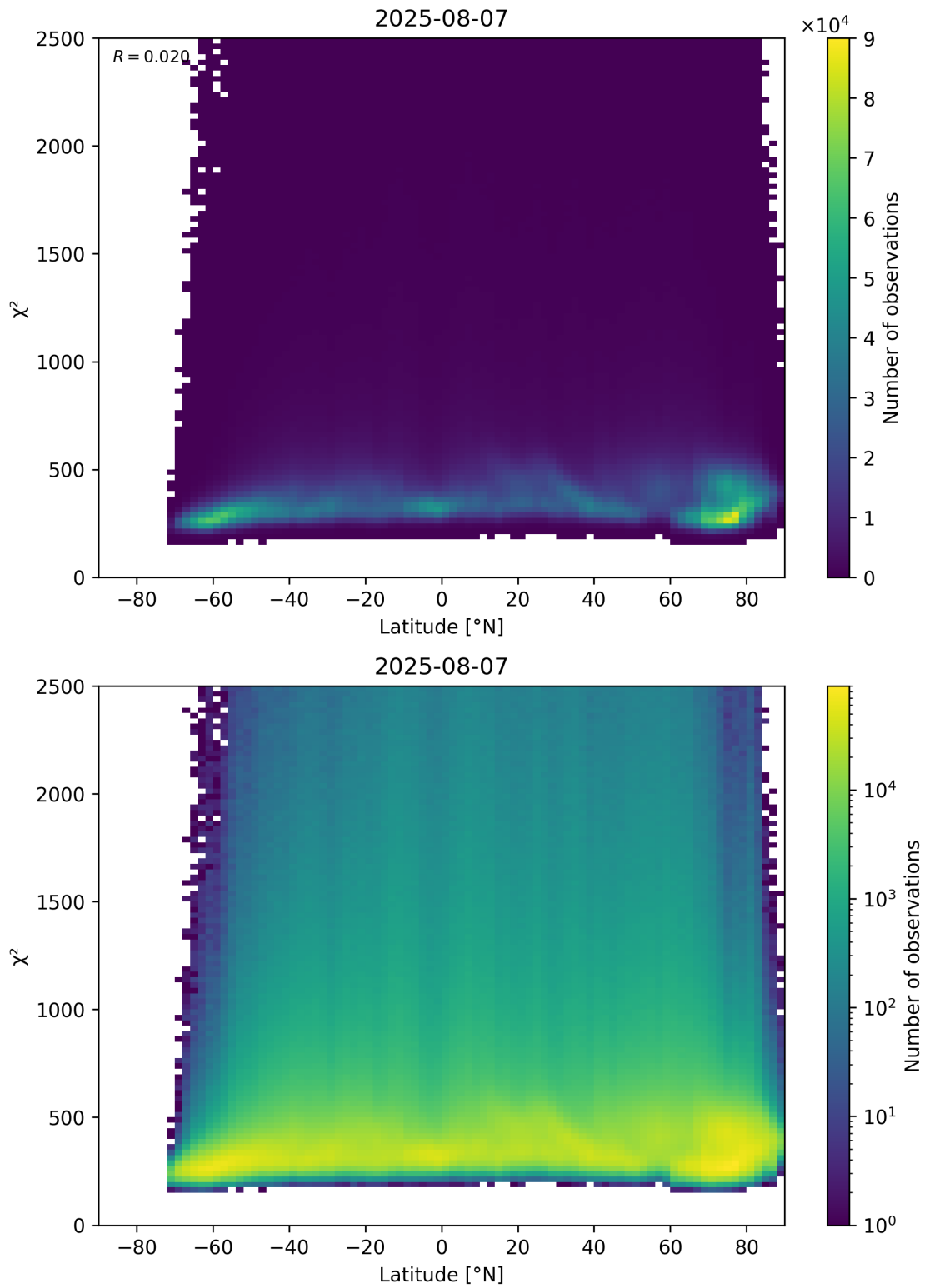
Figure 86: Scatter density plot of “Latitude” against “ \chi^2 ” for 2025-08-06 to 2025-08-08.
