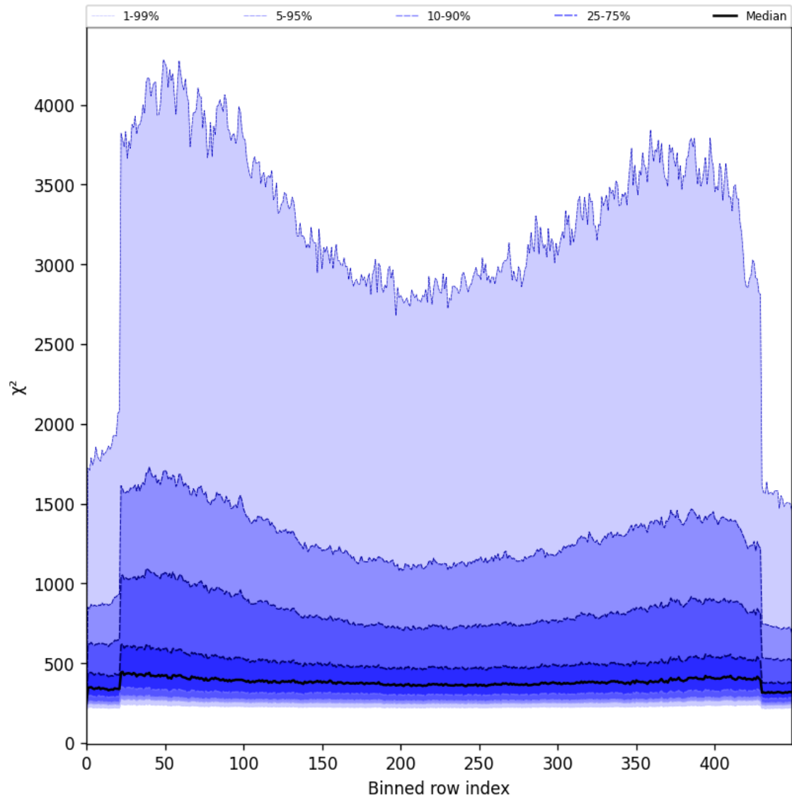
Figure 59: Along track statistics of “ \chi^2 ” for 2025-08-06 to 2025-08-08
