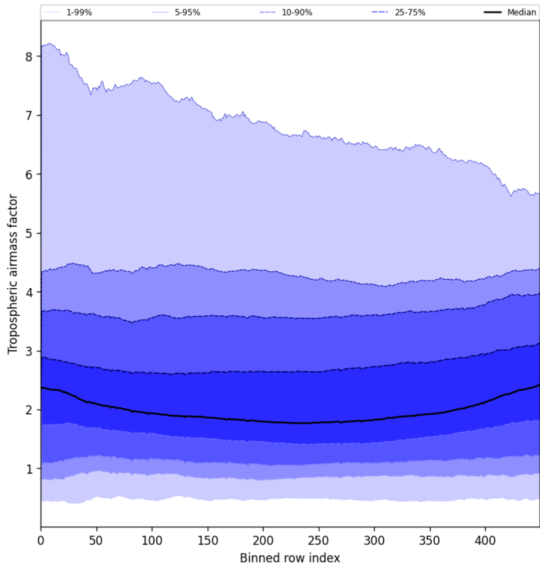
Figure 48: Along track statistics of “Tropospheric air mass factor” for 2025-08-06 to 2025-08-08
