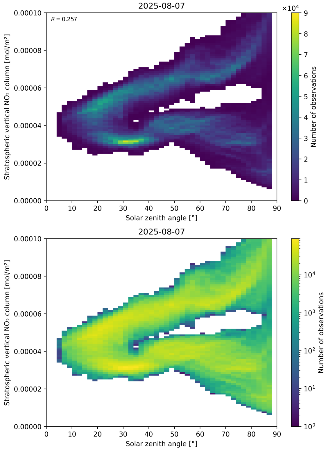
Figure 150: Scatter density plot of “Solar zenith angle” against “Stratospheric vertical NO 2 column” for 2025-08-06 to 2025-08-08.
