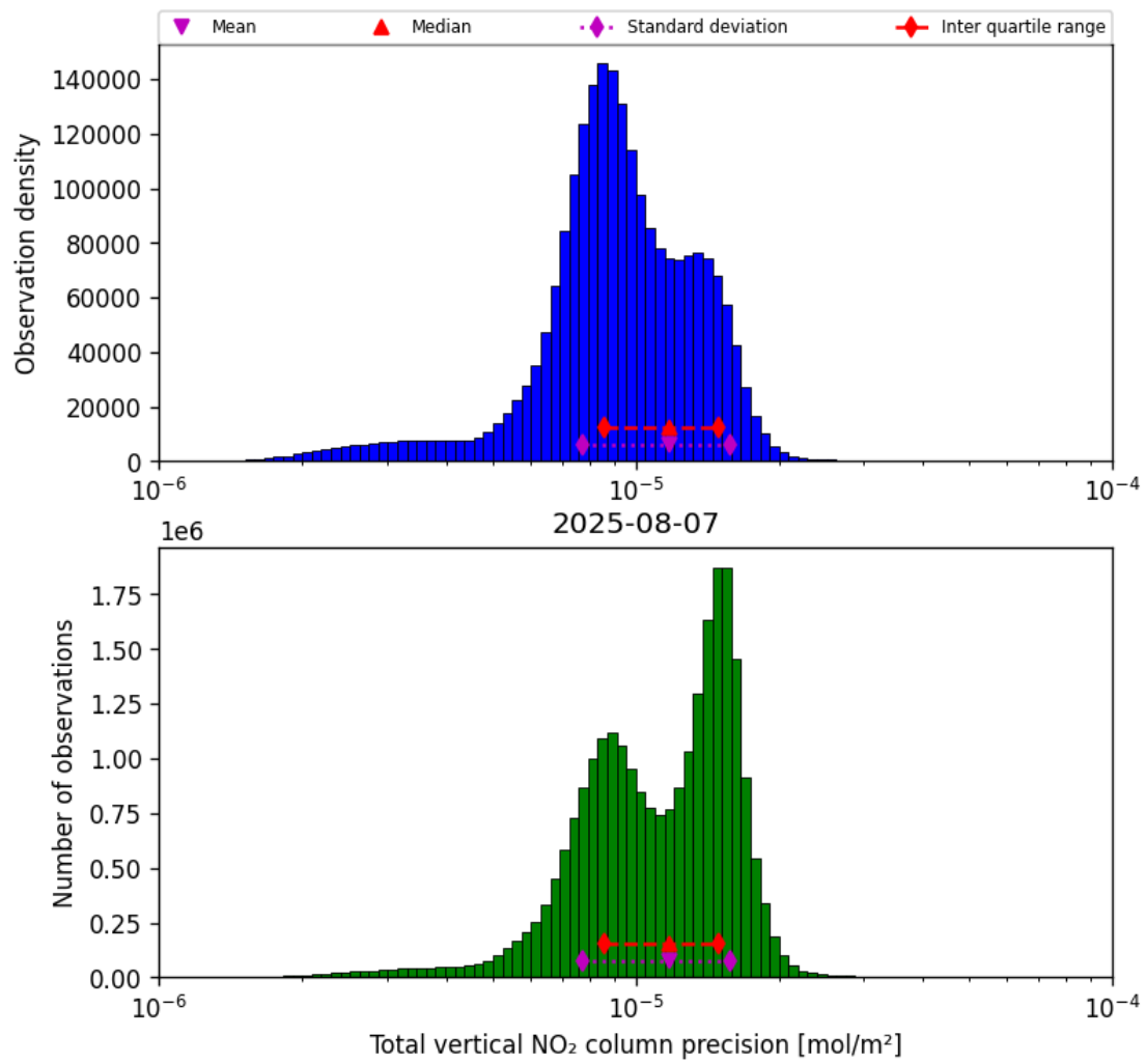
Figure 39: Histogram of “Total vertical NO 2 column precision” for 2025-08-06 to 2025-08-08
