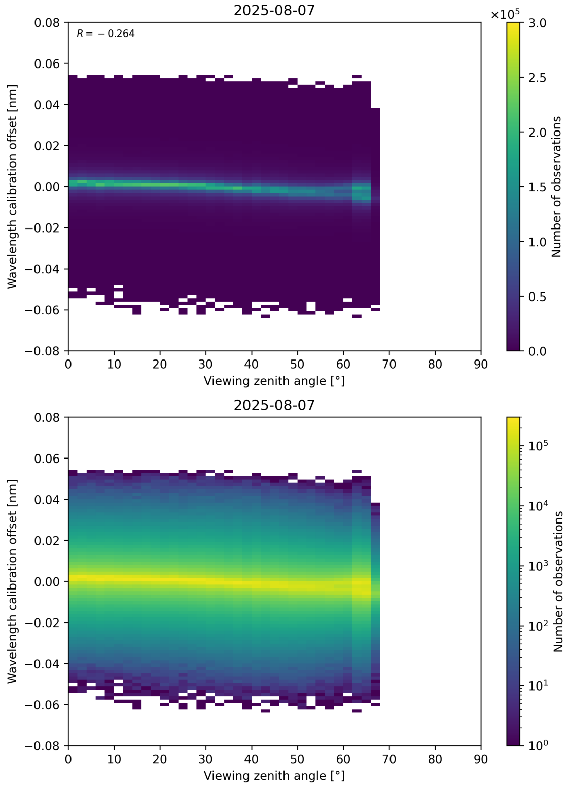
Figure 173: Scatter density plot of “Viewing zenith angle” against “Wavelength calibration offset” for 2025-08-06 to 2025-08-08.
