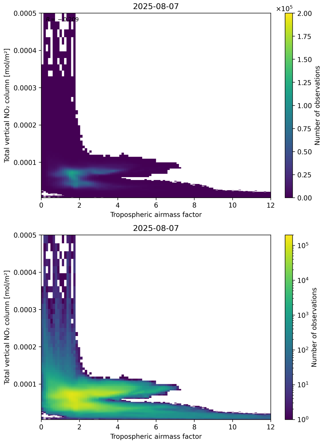
Figure 77: Scatter density plot of “Tropospheric airmass factor” against “Total vertical NO 2 column” for 2025-08-06 to 2025-08-08.
