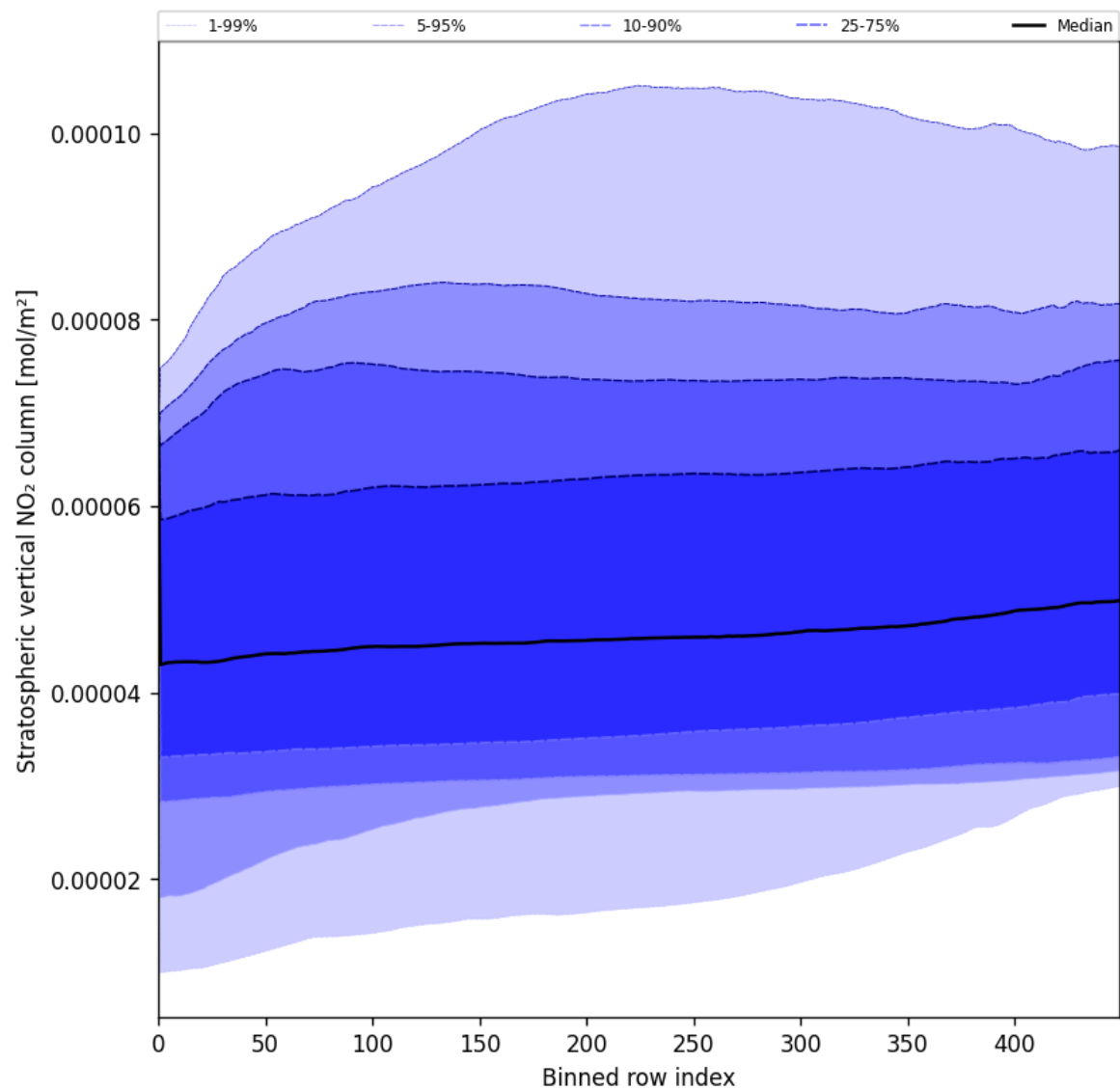
Figure 53: Along track statistics of “Stratospheric vertical NO 2 column” for 2025-08-06 to 2025-08-08
