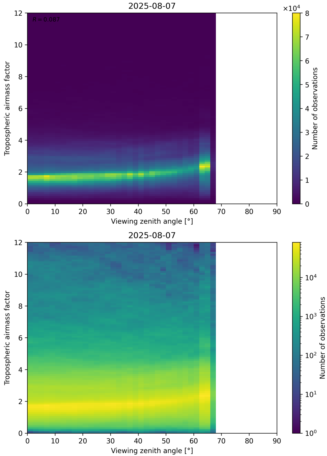
Figure 161: Scatter density plot of “Viewing zenith angle” against “Tropospheric airmass factor” for 2025-08-06 to 2025-08-08.
