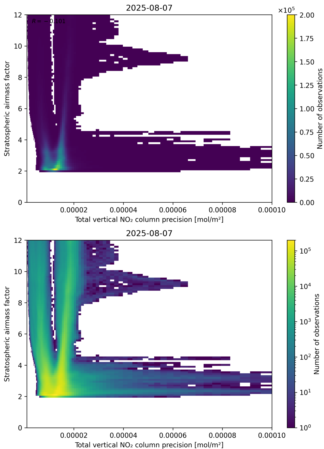
Figure 115: Scatter density plot of “Total vertical NO 2 column precision” against “Stratospheric air mass factor” for 2025-08-06 to 2025-08-08.
