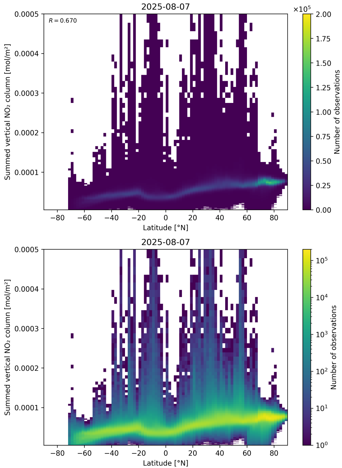
Figure 88: Scatter density plot of “Latitude” against “Summed vertical NO 2 column” for 2025-08-06 to 2025-08-08.
