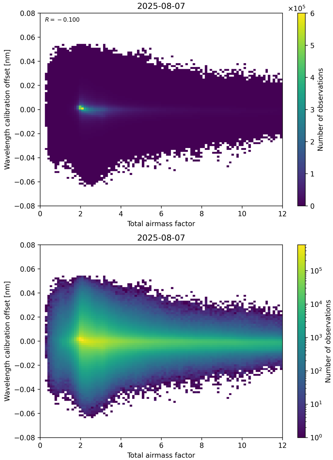
Figure 70: Scatter density plot of “Total airmass factor” against “Wavelength calibration offset” for 2025-08-06 to 2025-08-08.
