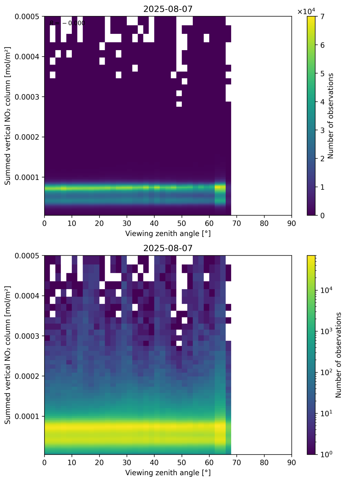
Figure 165: Scatter density plot of “Viewing zenith angle” against “Summed vertical NO 2 column” for 2025-08-06 to 2025-08-08.
