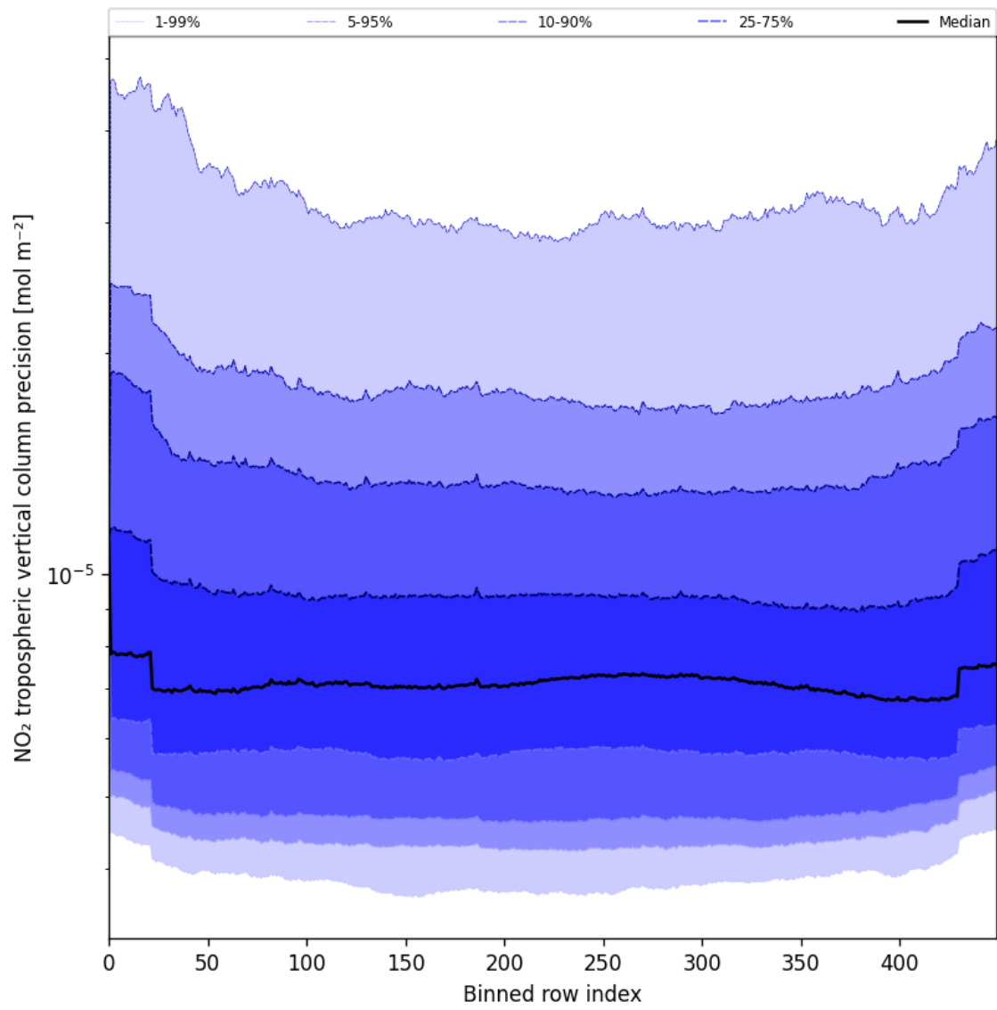
Figure 47: Along track statistics of “NO 2 tropospheric vertical column precision” for 2025-08-06 to 2025-08-08
