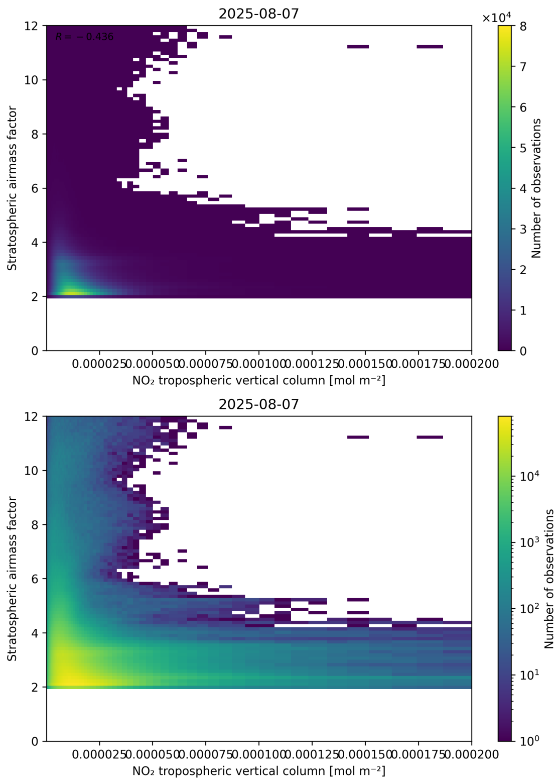
Figure 121: Scatter density plot of “NO 2 tropospheric vertical column” against “Stratospheric air mass factor” for 2025-08-06 to 2025-08-08.
