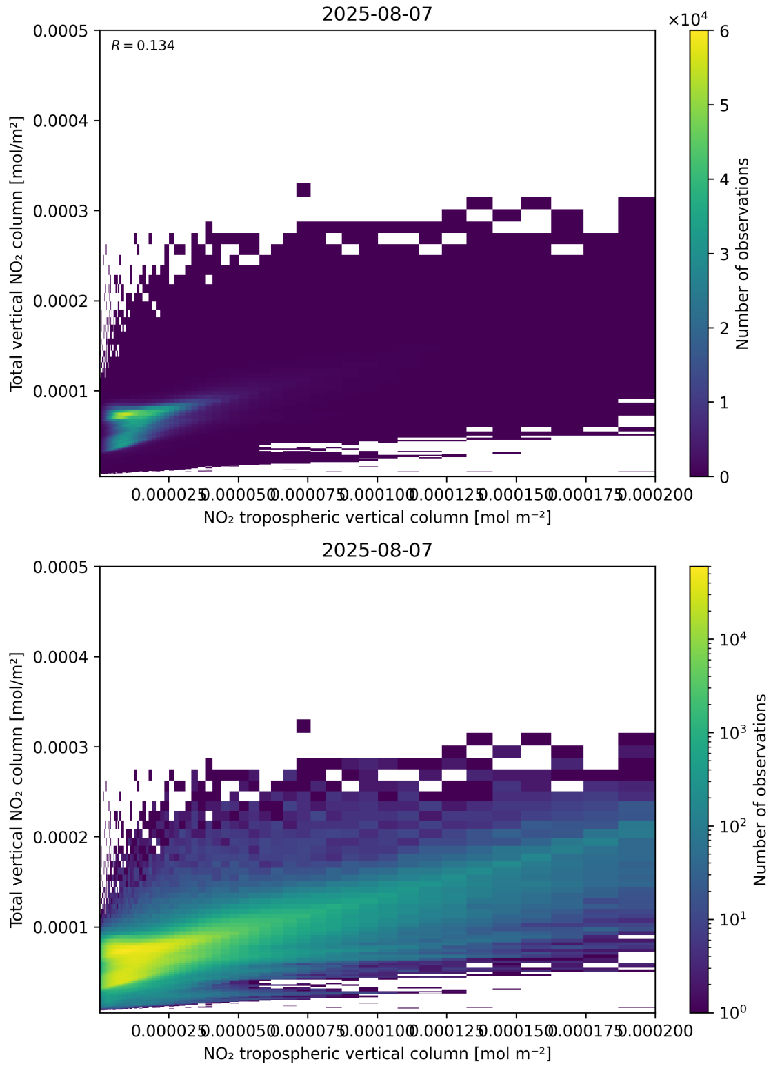
Figure 128: Scatter density plot of “NO 2 tropospheric vertical column” against “Total vertical NO 2 column” for 2025-08-06 to 2025-08-08.
