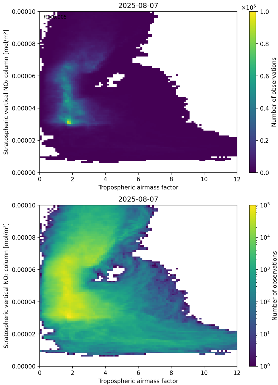
Figure 74: Scatter density plot of “Tropospheric air mass factor” against “Stratospheric vertical NO 2 column” for 2025-08-06 to 2025-08-08.
