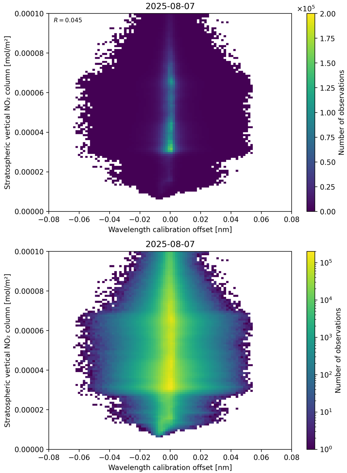
Figure 176: Scatter density plot of “Wavelength calibration offset” against “Stratospheric vertical NO 2 column” for 2025-08-06 to 2025-08-08.
