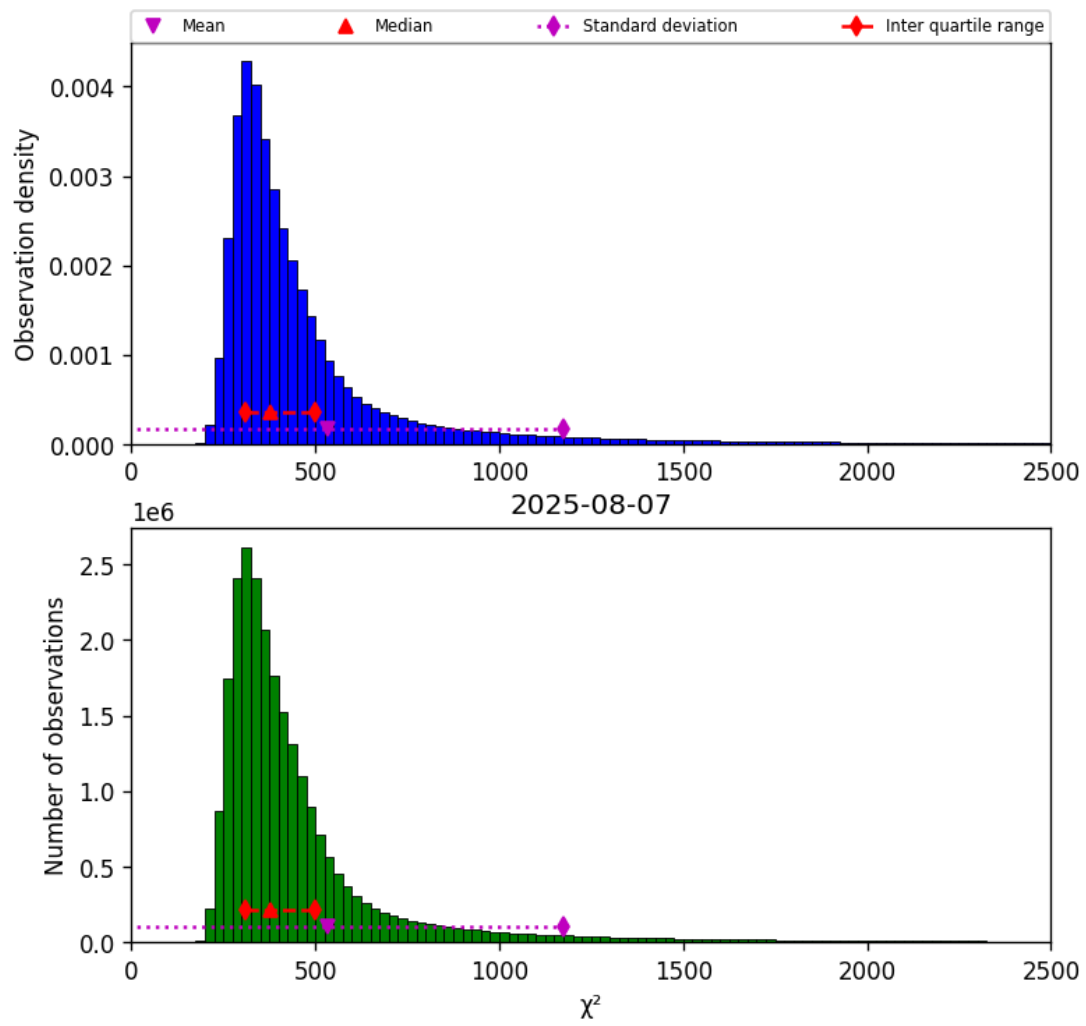
Figure 42: Histogram of “ \chi^2 ” for 2025-08-06 to 2025-08-08
