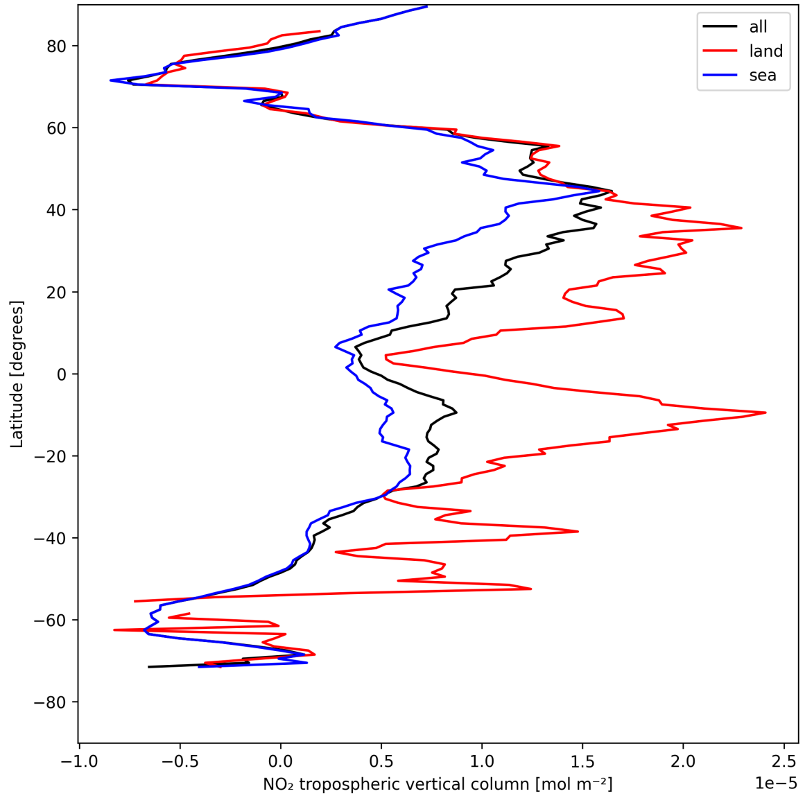
Figure 12: Zonal average of “NO 2 tropospheric vertical column” for 2025-08-06 to 2025-08-08.
