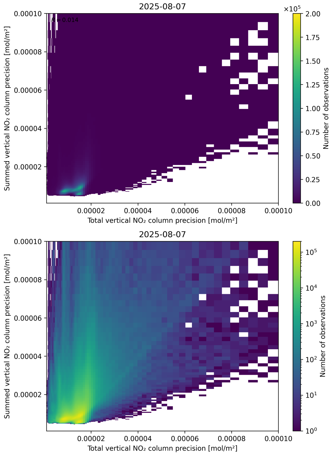
Figure 118: Scatter density plot of “Total vertical NO 2 column precision” against “Summed vertical NO 2 column precision” for 2025-08-06 to 2025-08-08.
