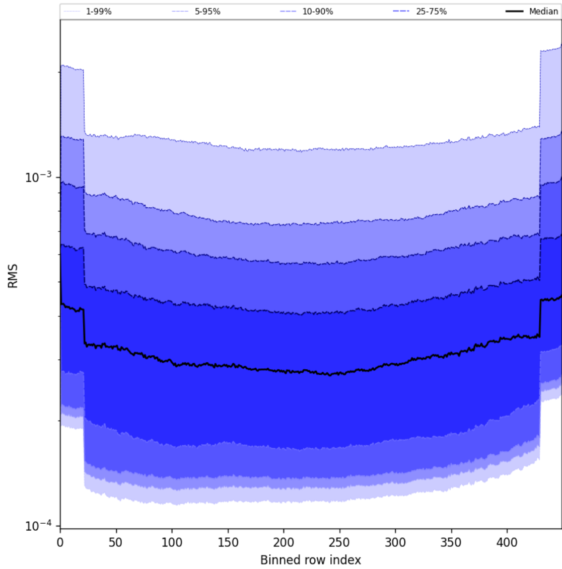
Figure 60: Along track statistics of “RMS” for 2025-08-06 to 2025-08-08
