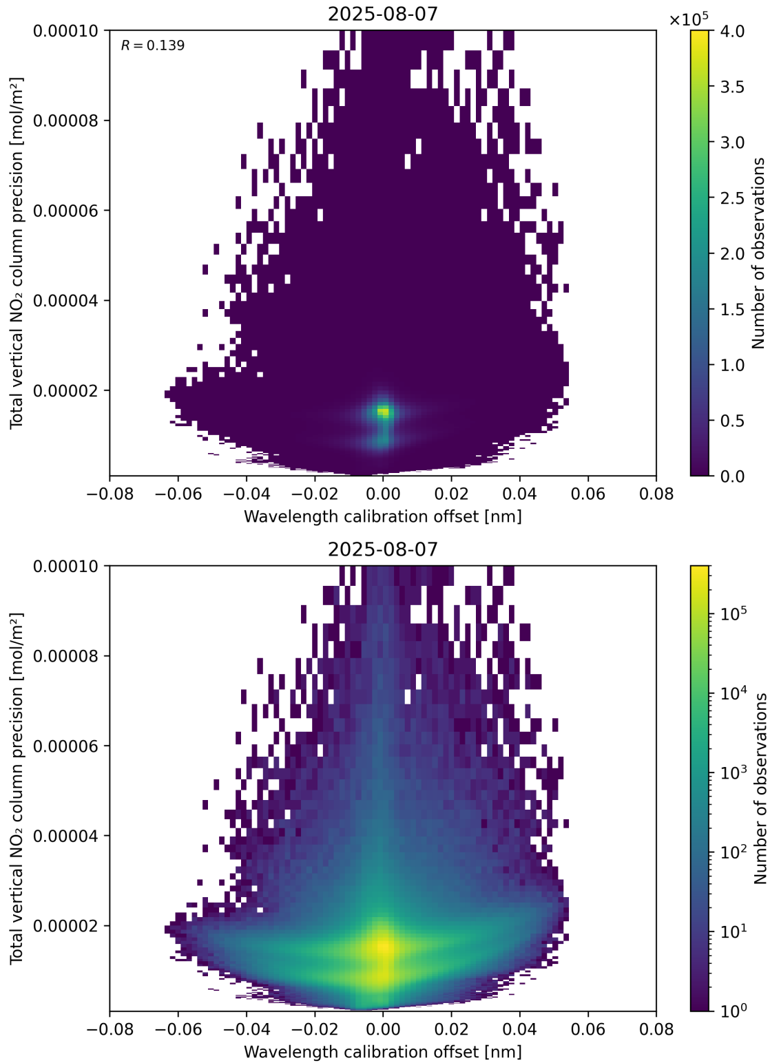
Figure 180: Scatter density plot of “Wavelength calibration offset” against “Total vertical NO 2 column precision” for 2025-08-06 to 2025-08-08.
