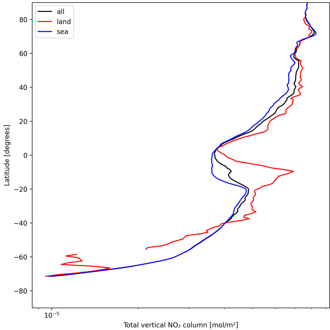
Figure 21: Zonal average of “Total vertical NO 2 column” for 2025-08-06 to 2025-08-08.
