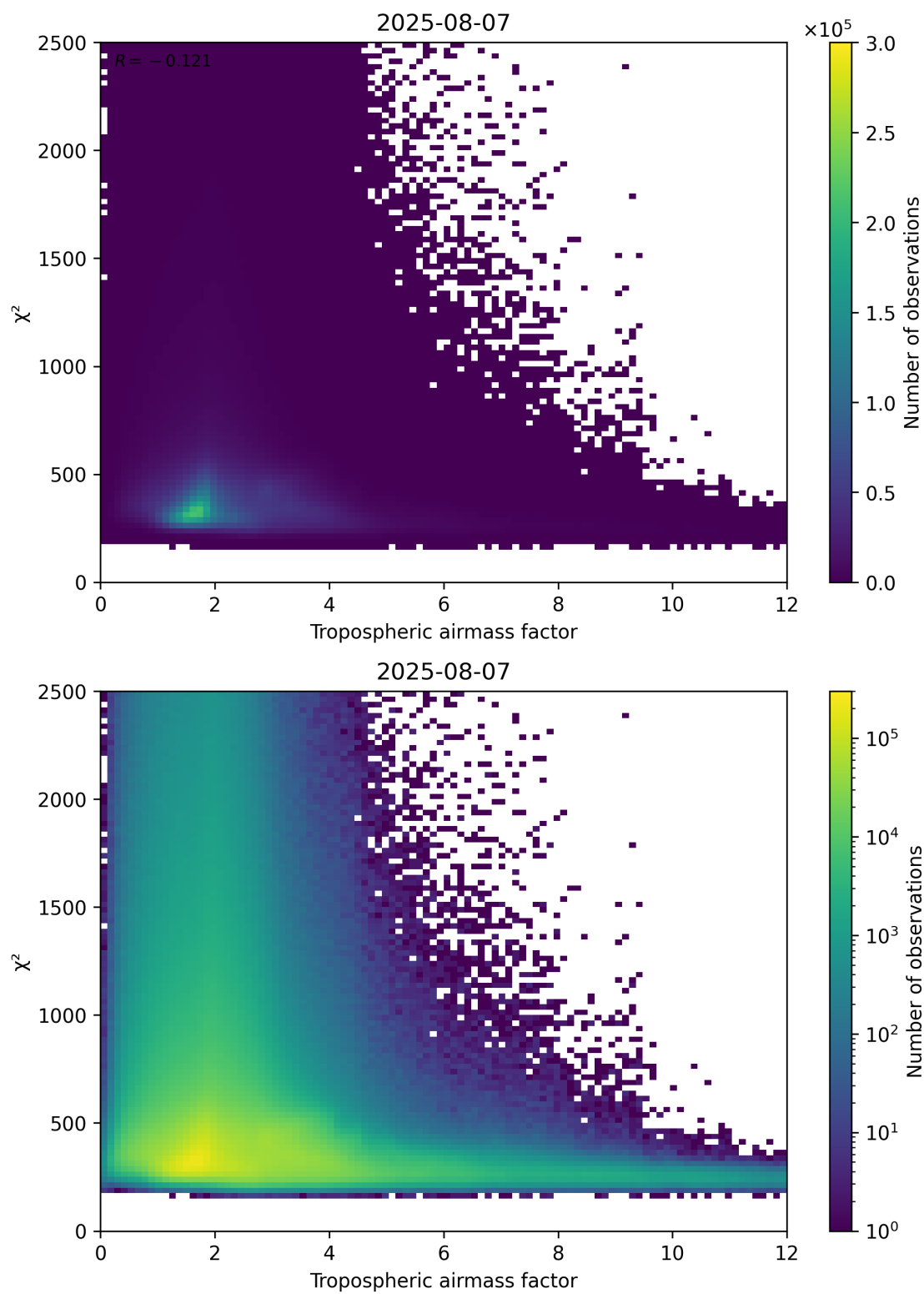
Figure 73: Scatter density plot of “Tropospheric airmass factor” against “ \chi^2 ” for 2025-08-06 to 2025-08-08.
