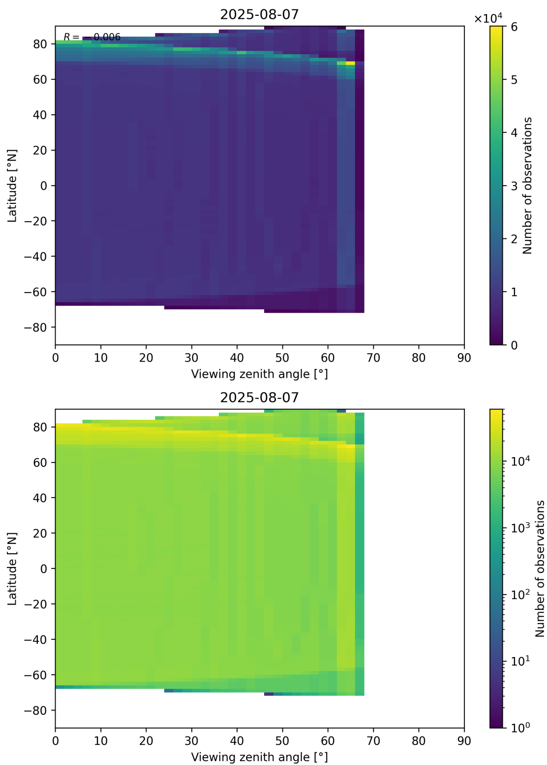
Figure 163: Scatter density plot of “Viewing zenith angle” against “Latitude” for 2025-08-06 to 2025-08-08.
