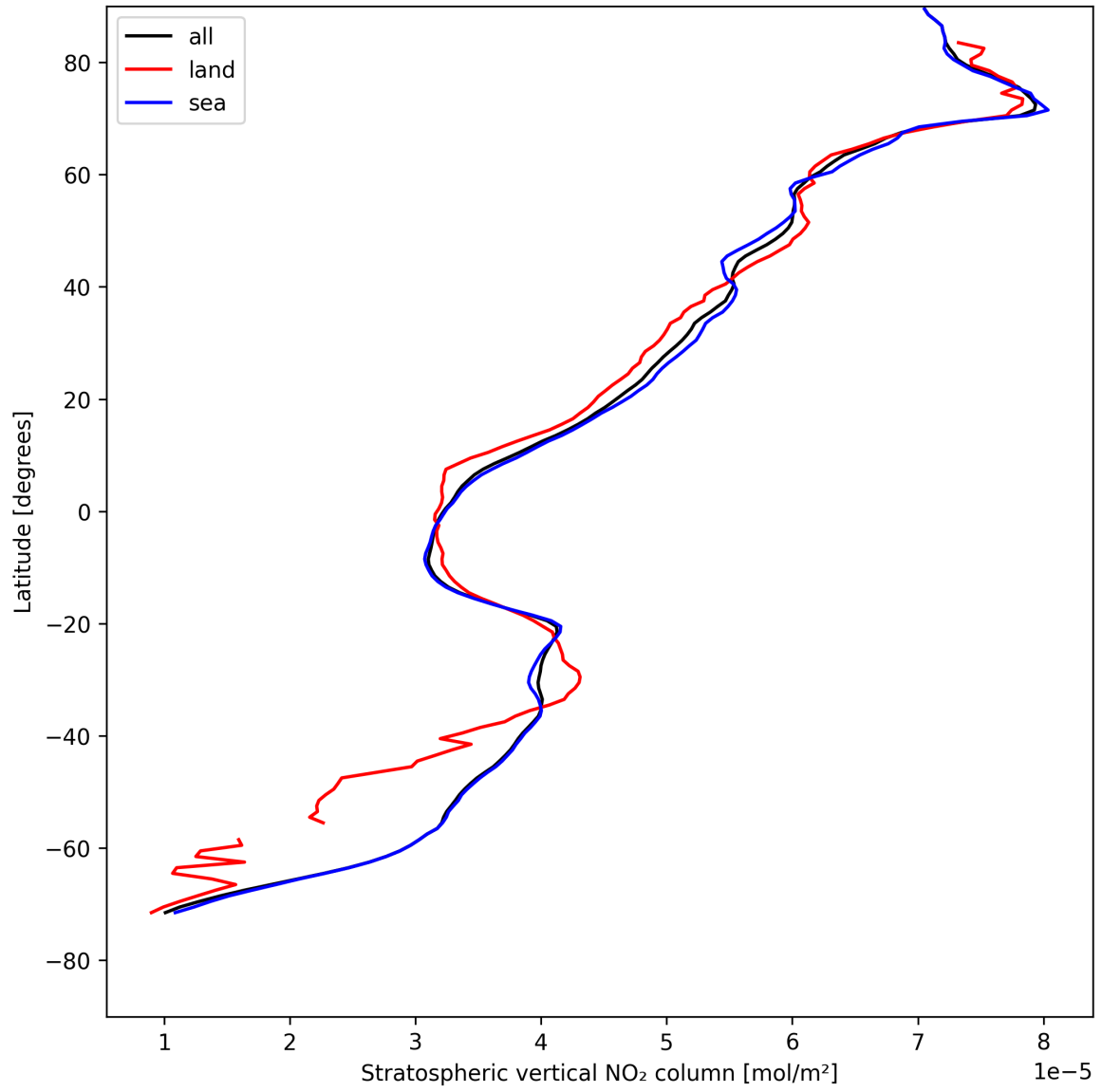
Figure 19: Zonal average of “Stratospheric vertical NO 2 column” for 2025-08-06 to 2025-08-08.
