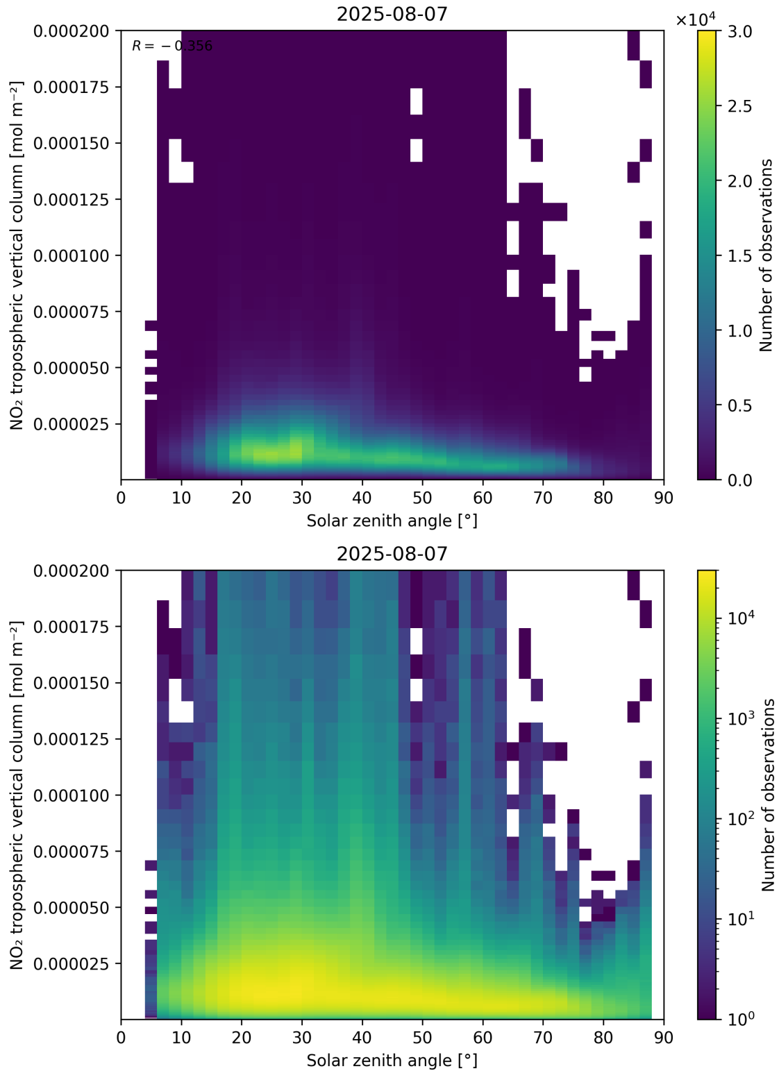
Figure 155: Scatter density plot of “Solar zenith angle” against “NO 2 tropospheric vertical column” for 2025-08-06 to 2025-08-08.
