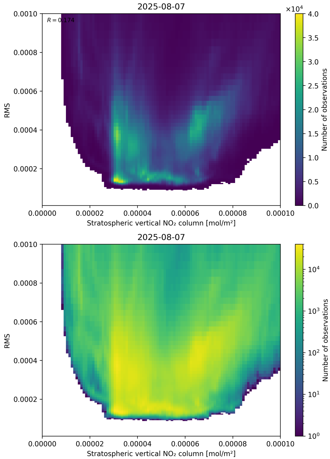
Figure 102: Scatter density plot of “Stratospheric vertical NO 2 column” against “RMS” for 2025-08-06 to 2025-08-08.
