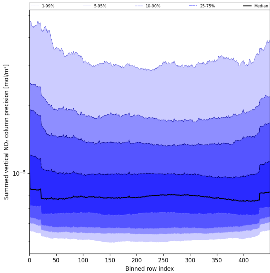
Figure 58: Along track statistics of “Summed vertical NO 2 column precision” for 2025-08-06 to 2025-08-08
