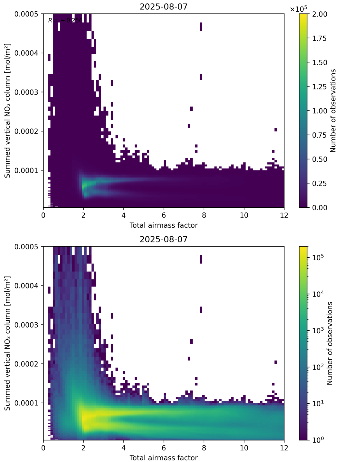
Figure 65: Scatter density plot of “Total airmass factor” against “Summed vertical NO 2 column” for 2025-08-06 to 2025-08-08.
