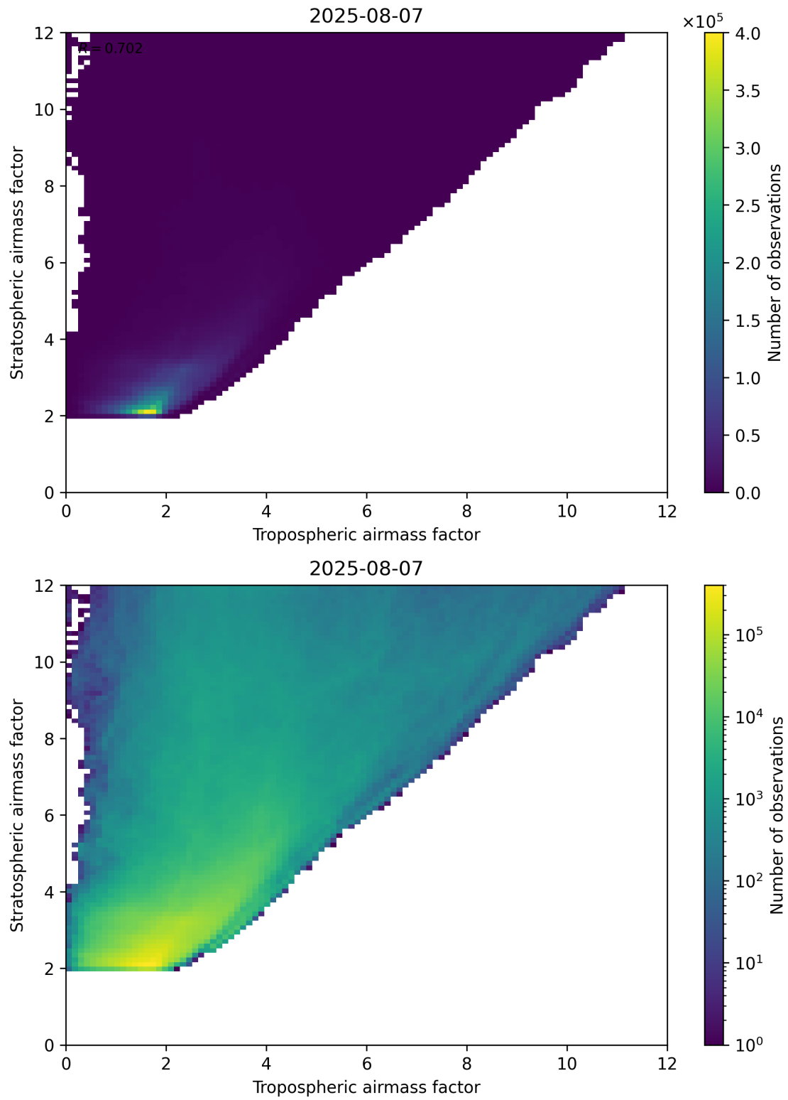
Figure 71: Scatter density plot of “Tropospheric airmass factor” against “Stratospheric airmass factor” for 2025-08-06 to 2025-08-08.
