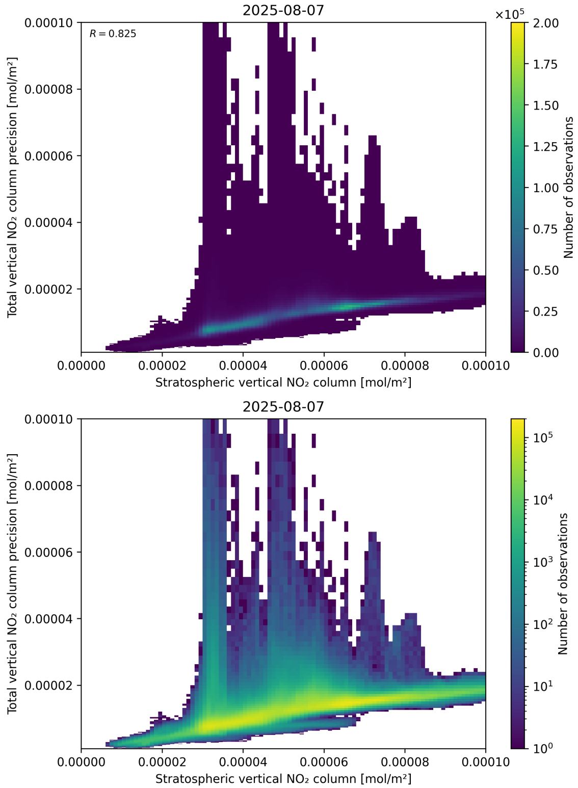
Figure 101: Scatter density plot of “Stratospheric vertical NO 2 column” against “Total vertical NO 2 column precision” for 2025-08-06 to 2025-08-08.
