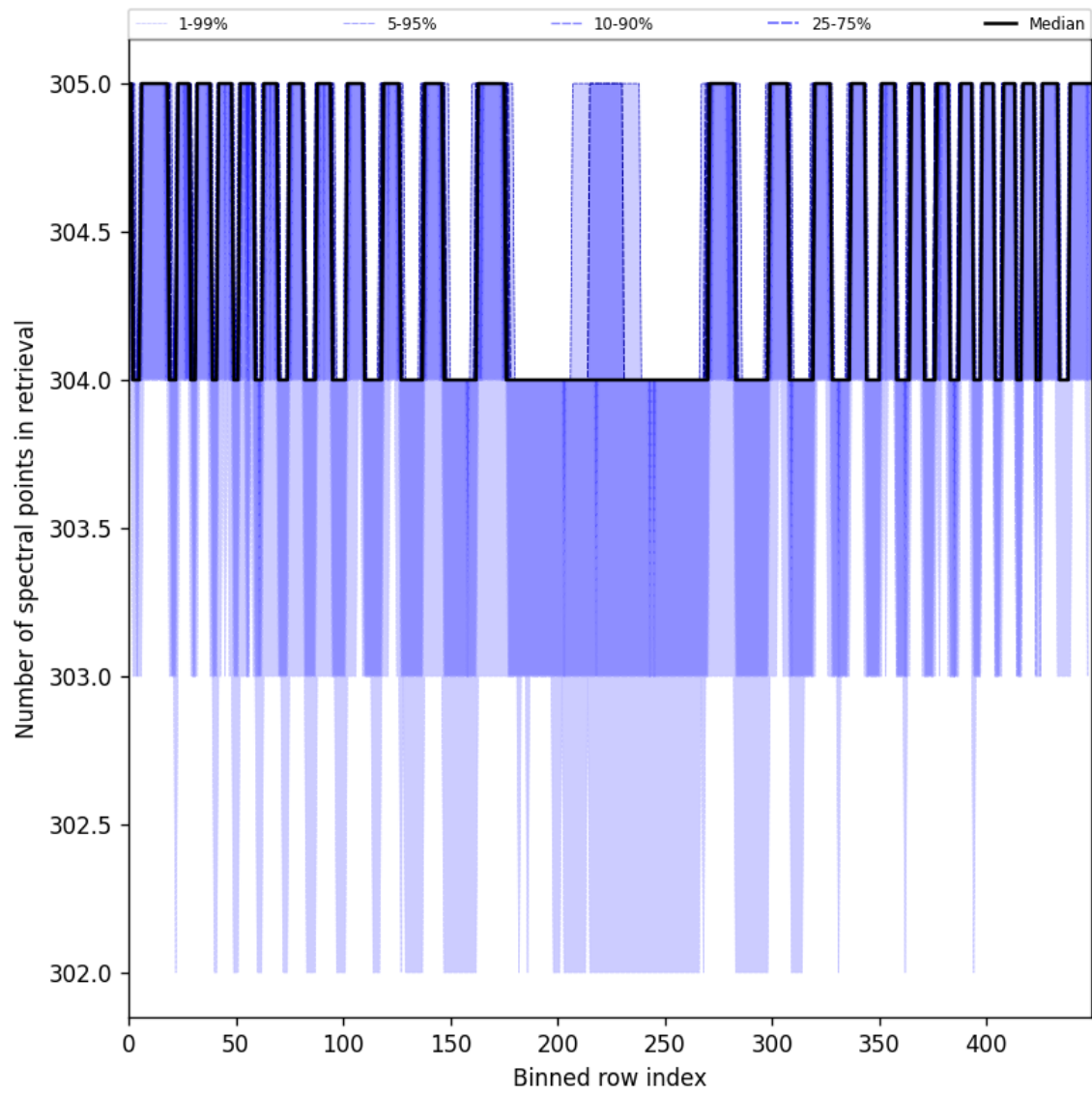
Figure 50: Along track statistics of “Number of spectral points in retrieval” for 2025-08-06 to 2025-08-08
