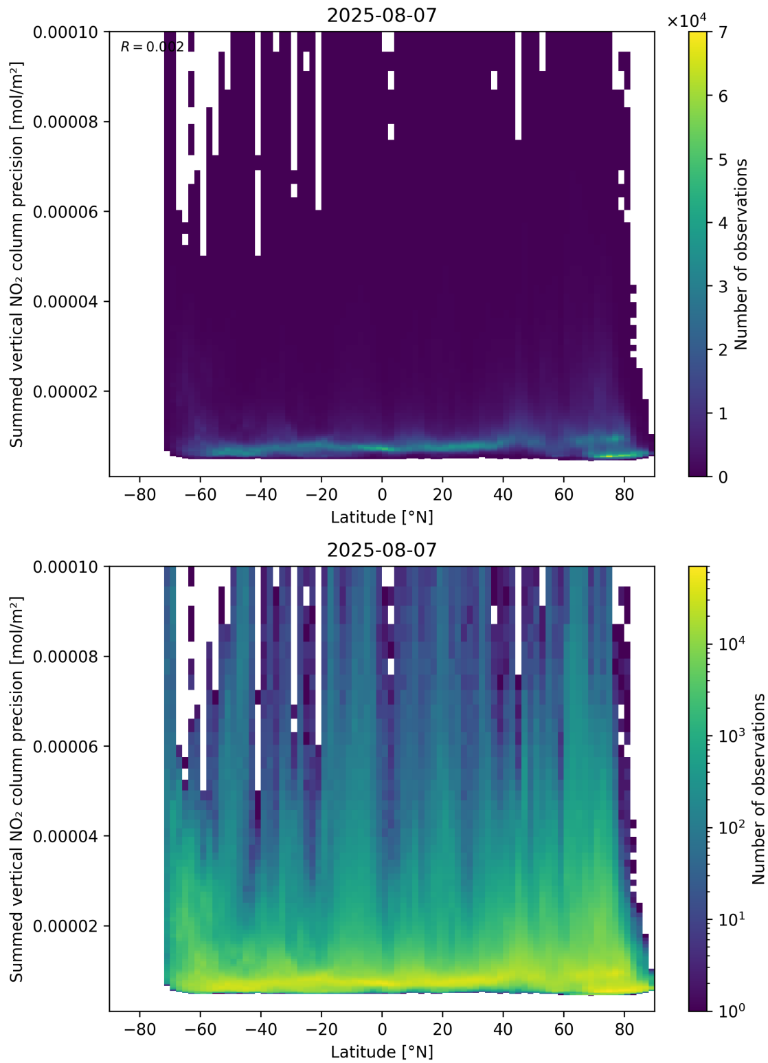
Figure 89: Scatter density plot of “Latitude” against “Summed vertical NO 2 column precision” for 2025-08-06 to 2025-08-08.
