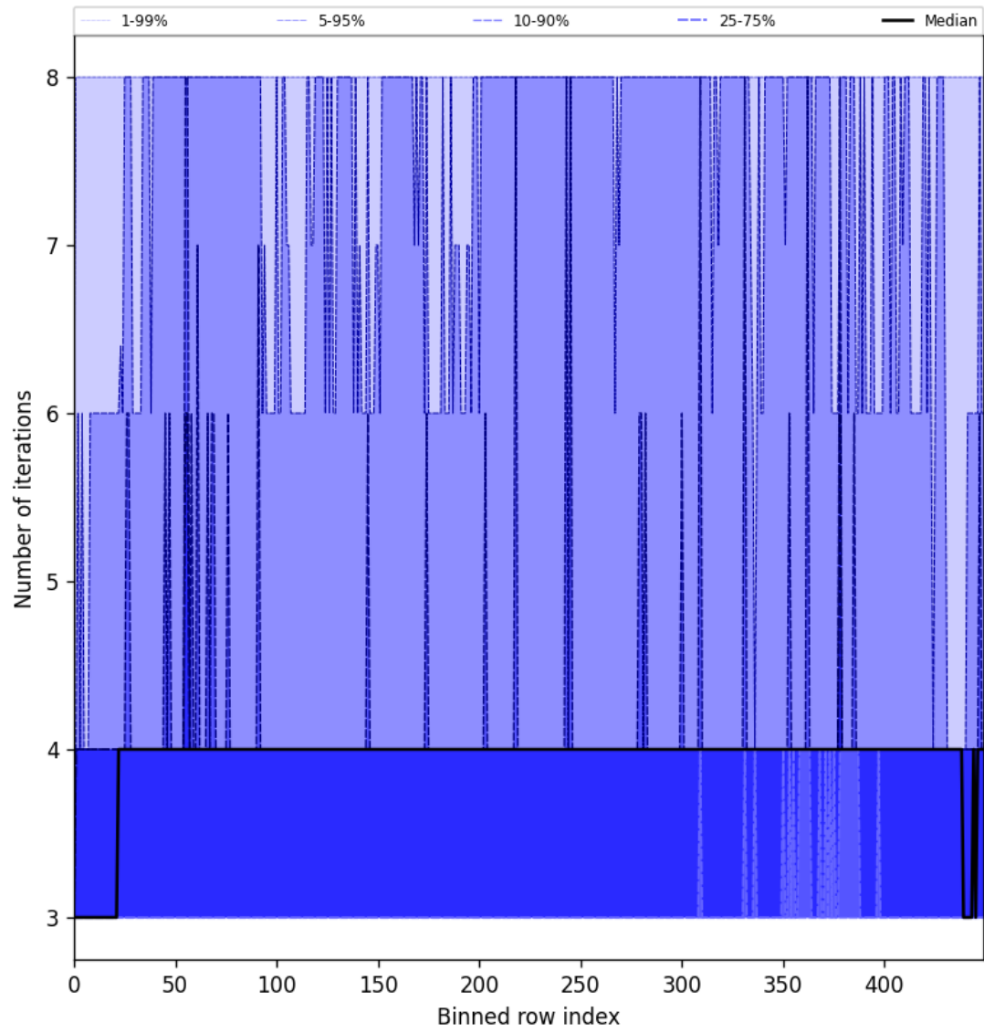
Figure 51: Along track statistics of “Number of iterations” for 2025-08-06 to 2025-08-08
