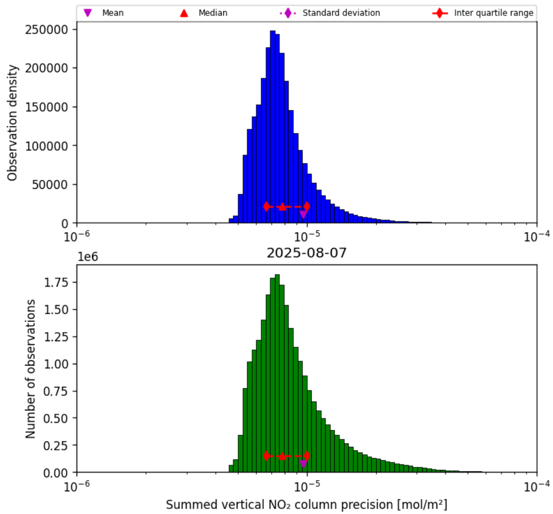
Figure 41: Histogram of “Summed vertical NO 2 column precision” for 2025-08-06 to 2025-08-08
