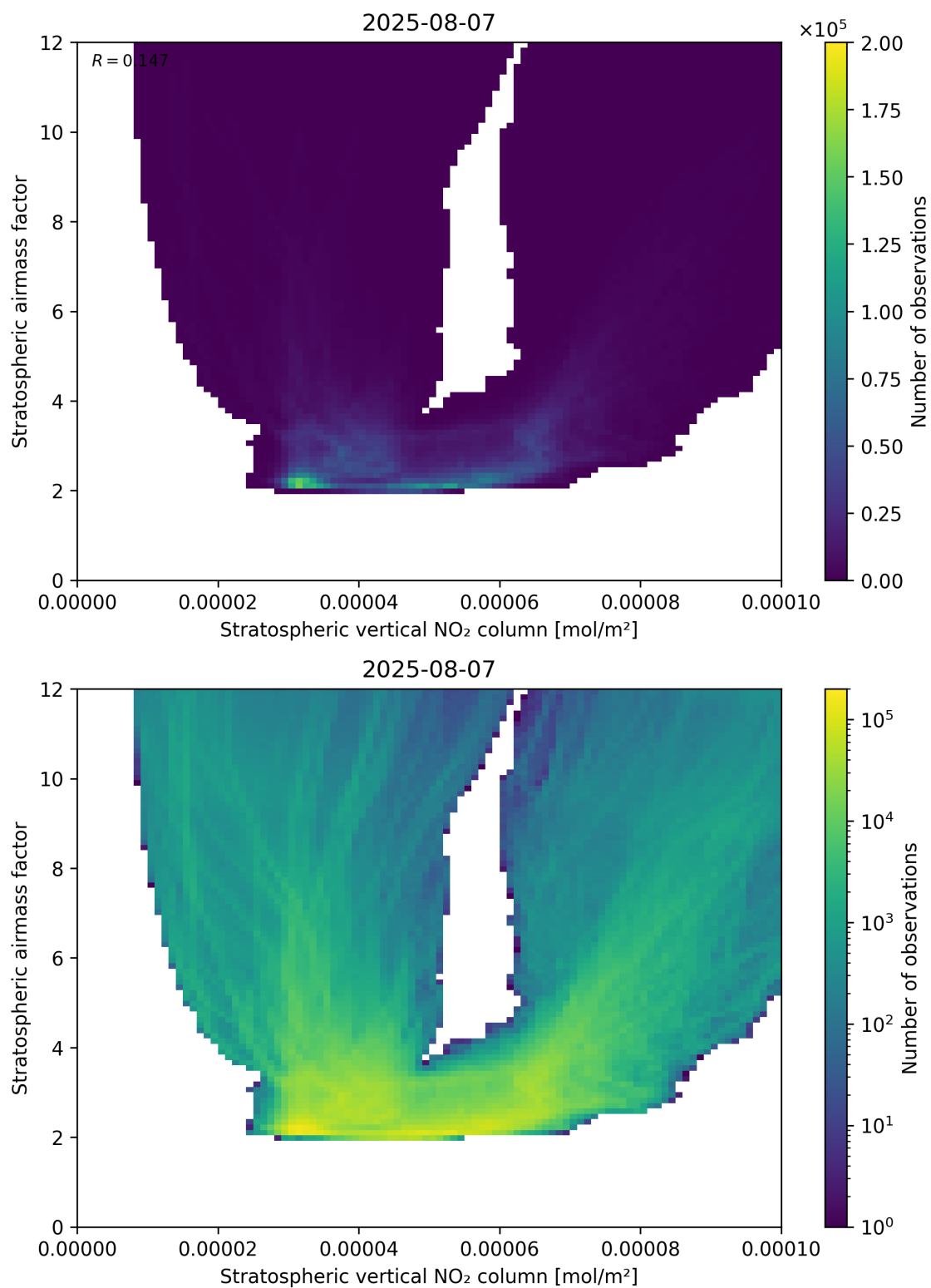
Figure 96: Scatter density plot of “Stratospheric vertical NO 2 column” against “Stratospheric airmass factor” for 2025-08-06 to 2025-08-08.
