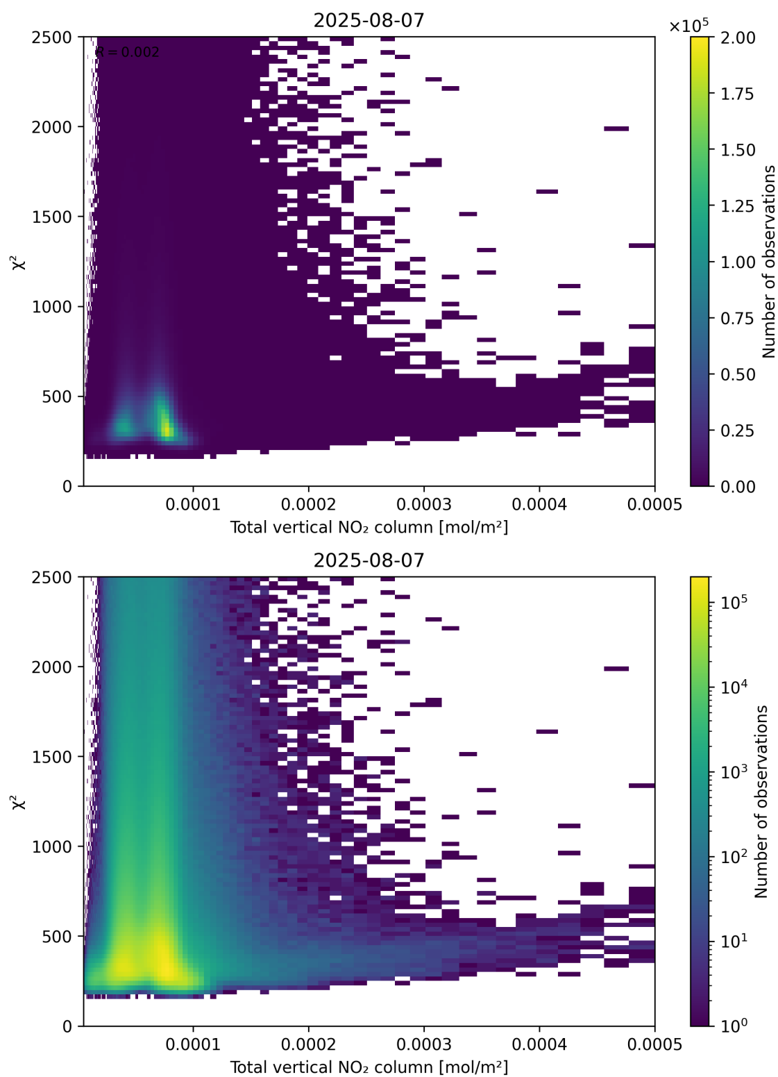
Figure 111: Scatter density plot of “Total vertical NO 2 column” against “ \chi^2 ” for 2025-08-06 to 2025-08-08.
