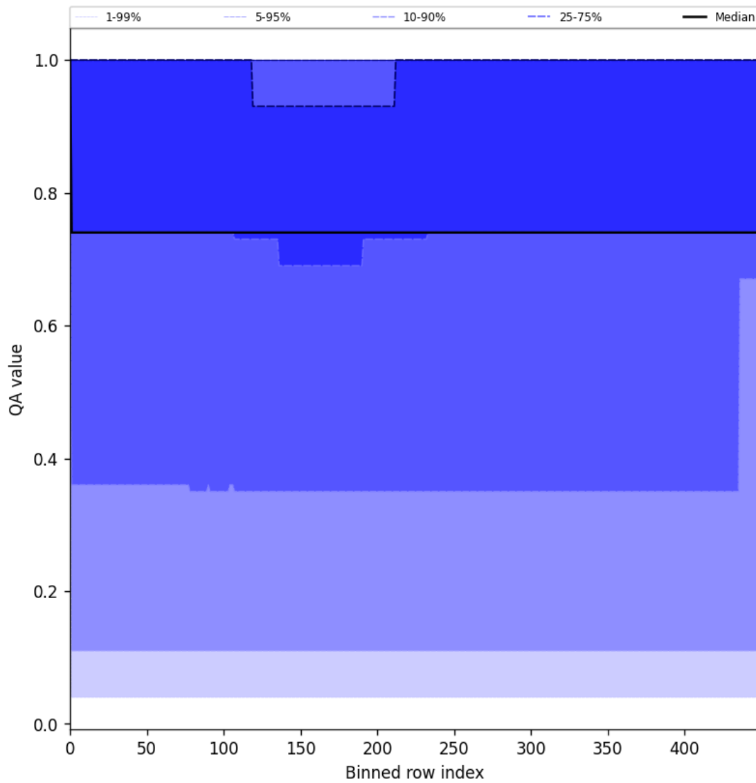
Figure 45: Along track statistics of “QA value” for 2025-08-06 to 2025-08-08
