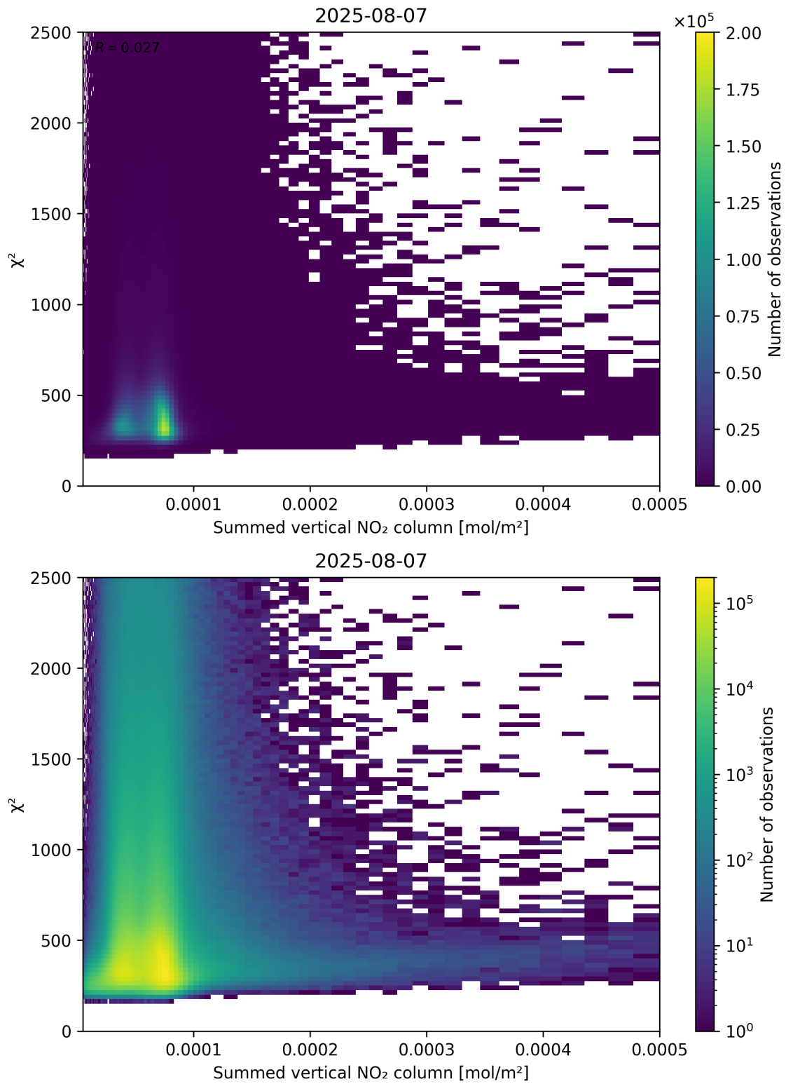
Figure 104: Scatter density plot of “Summed vertical NO 2 column” against “ \chi^2 ” for 2025-08-06 to 2025-08-08.
