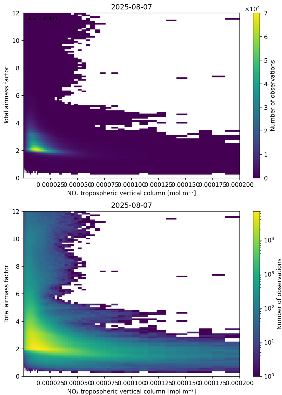
Figure 122: Scatter density plot of “NO 2 tropospheric vertical column” against “Total air mass factor” for 2025-08-06 to 2025-08-08.
