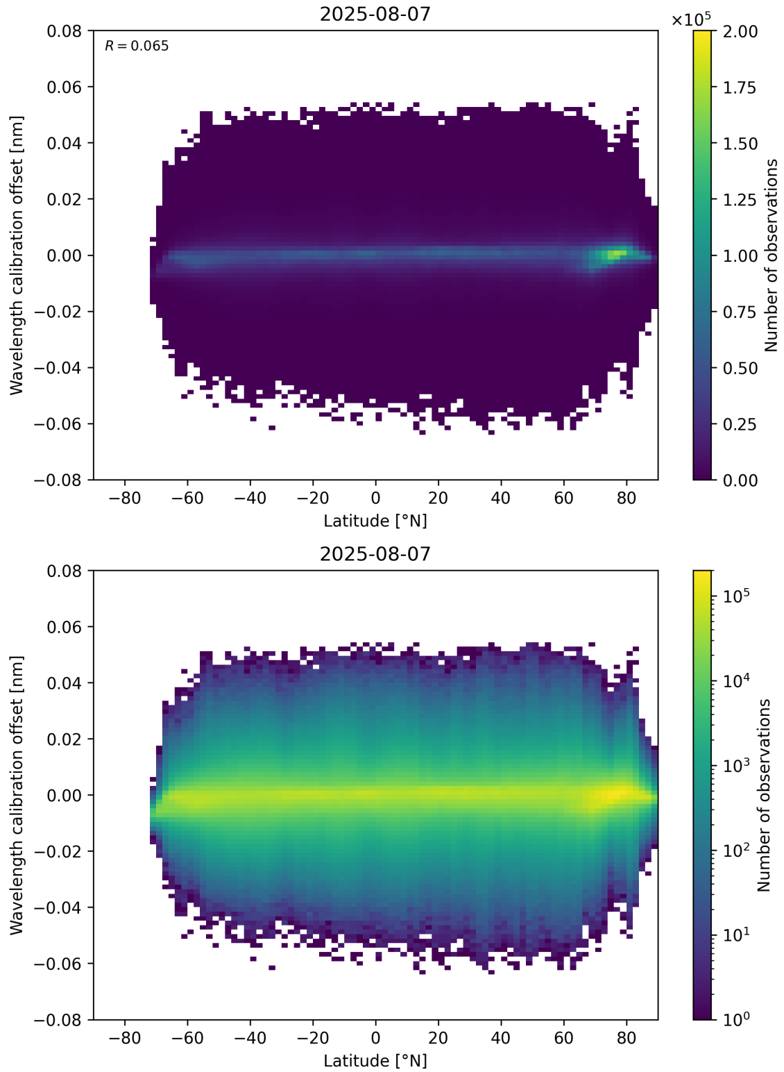
Figure 95: Scatter density plot of “Latitude” against “Wavelength calibration offset” for 2025-08-06 to 2025-08-08.
