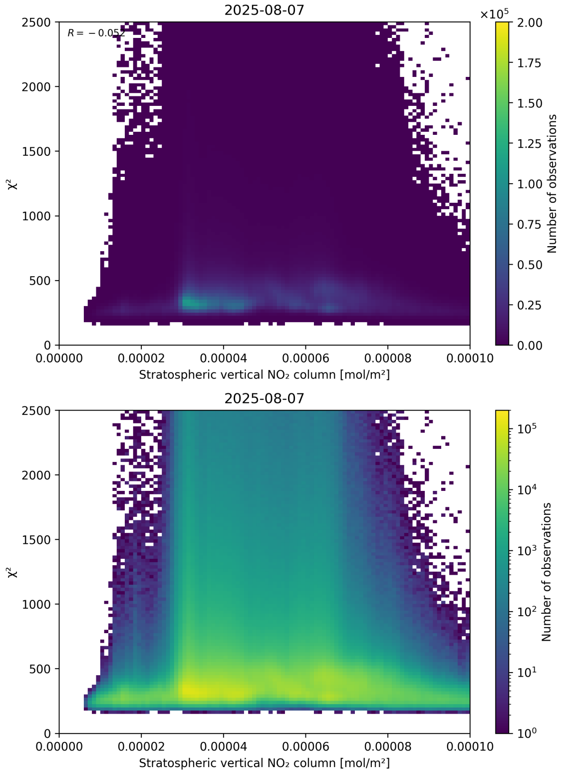
Figure 97: Scatter density plot of “Stratospheric vertical NO 2 column” against “ \chi^2 ” for 2025-08-06 to 2025-08-08.
