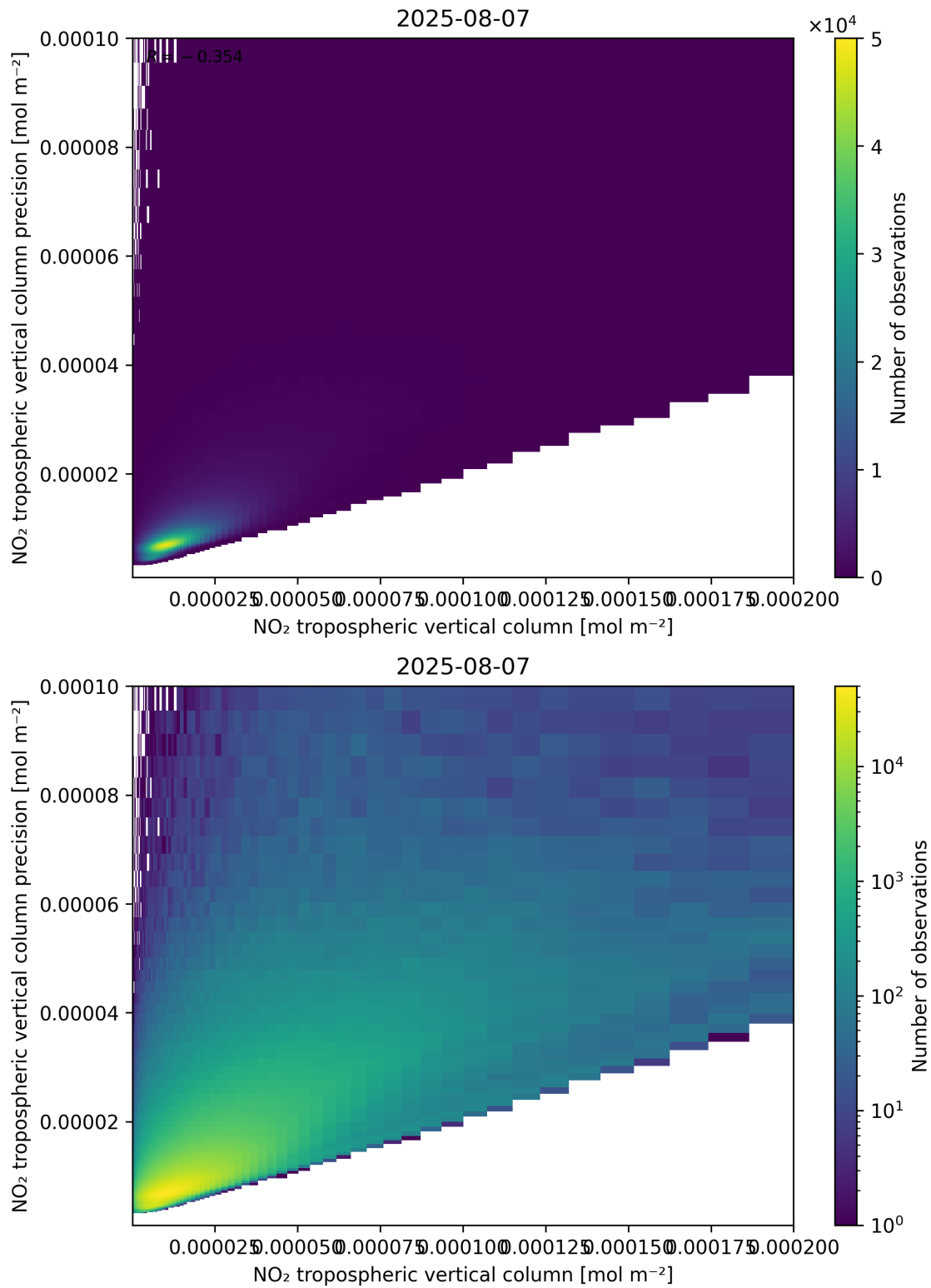
Figure 130: Scatter density plot of “NO 2 tropospheric vertical column” against “NO 2 tropospheric vertical column precision” for 2025-08-06 to 2025-08-08.
