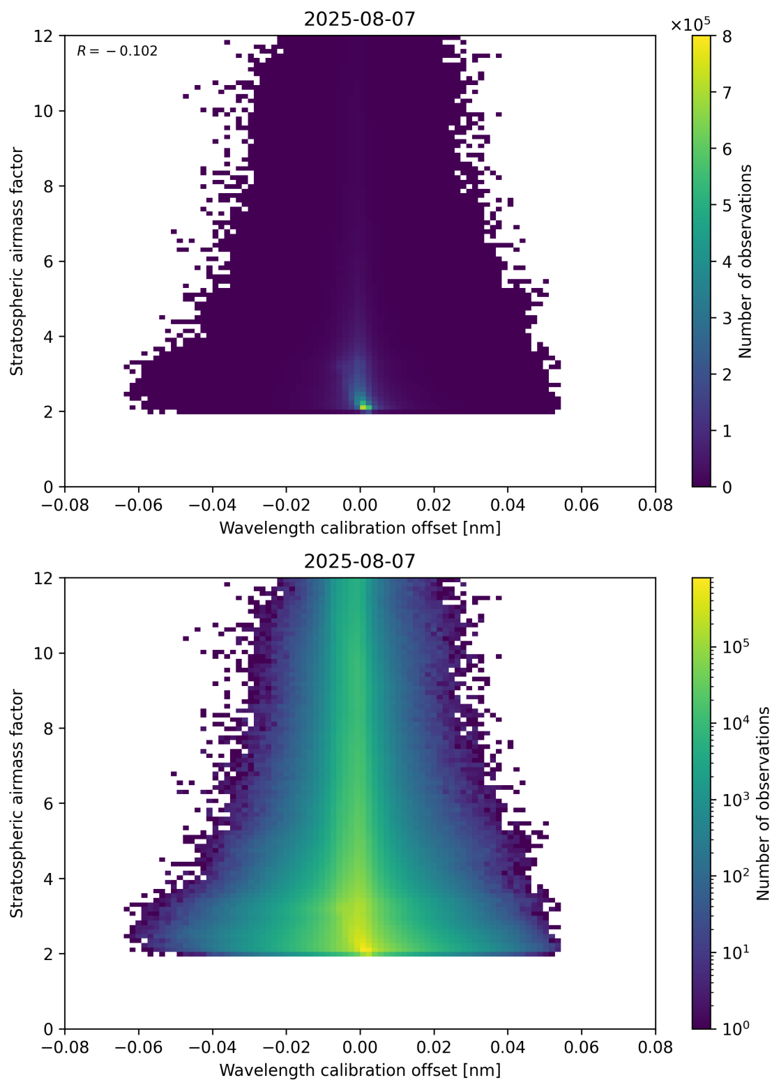
Figure 174: Scatter density plot of “Wavelength calibration offset” against “Stratospheric airmass factor” for 2025-08-06 to 2025-08-08.
