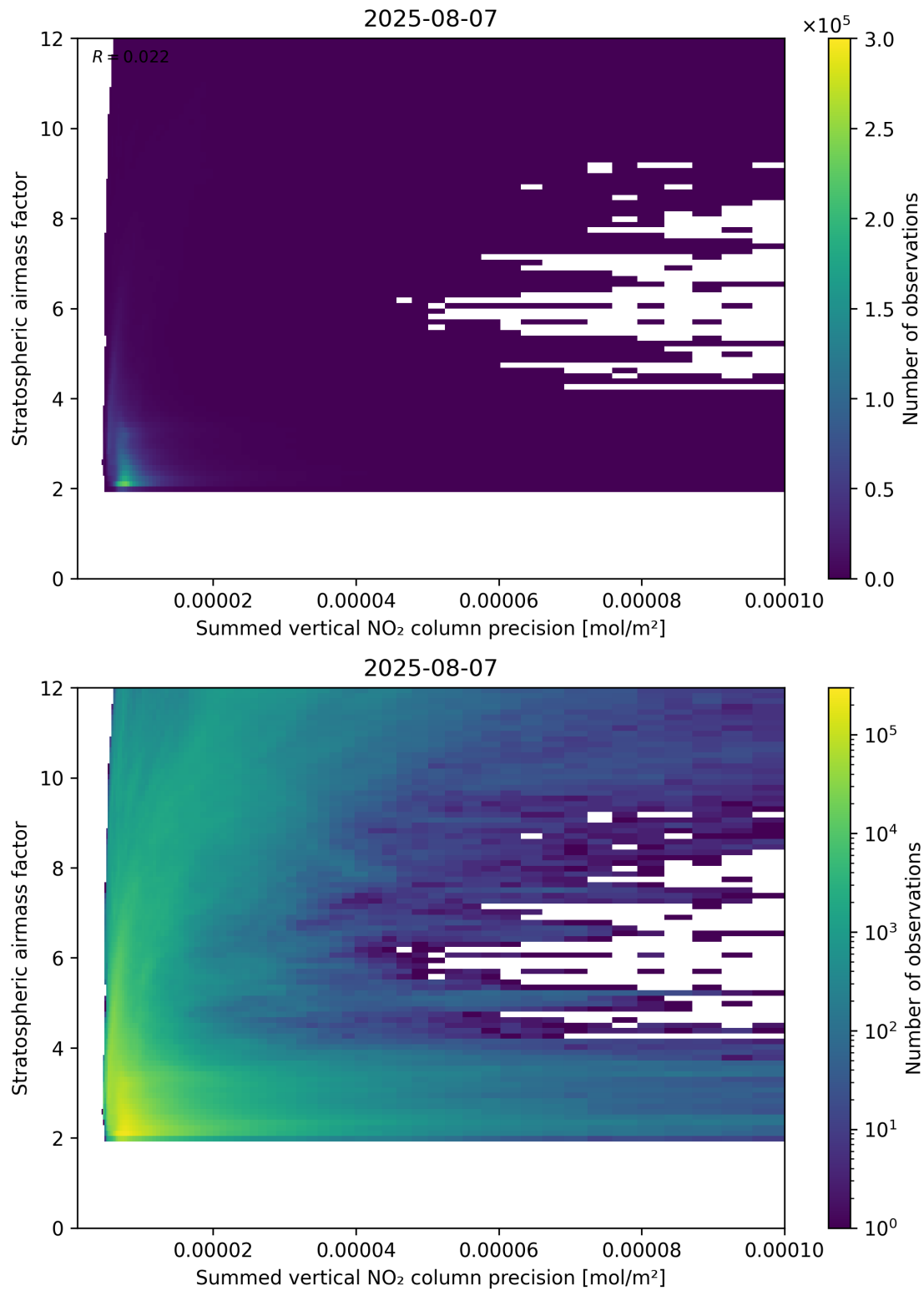
Figure 106: Scatter density plot of “Summed vertical NO 2 column precision” against “Stratospheric airmass factor” for 2025-08-06 to 2025-08-08.
