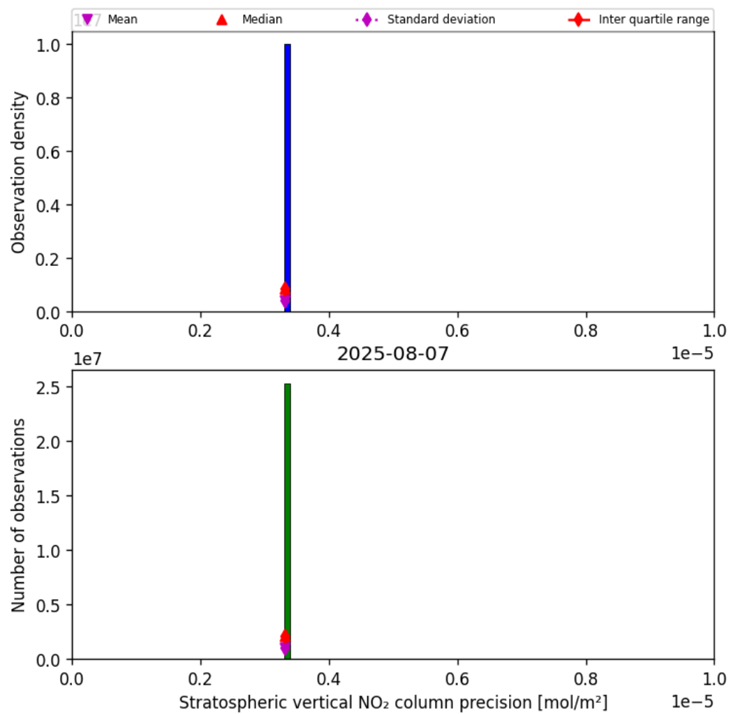
Figure 37: Histogram of “Stratospheric vertical NO 2 column precision” for 2025-08-06 to 2025-08-08
