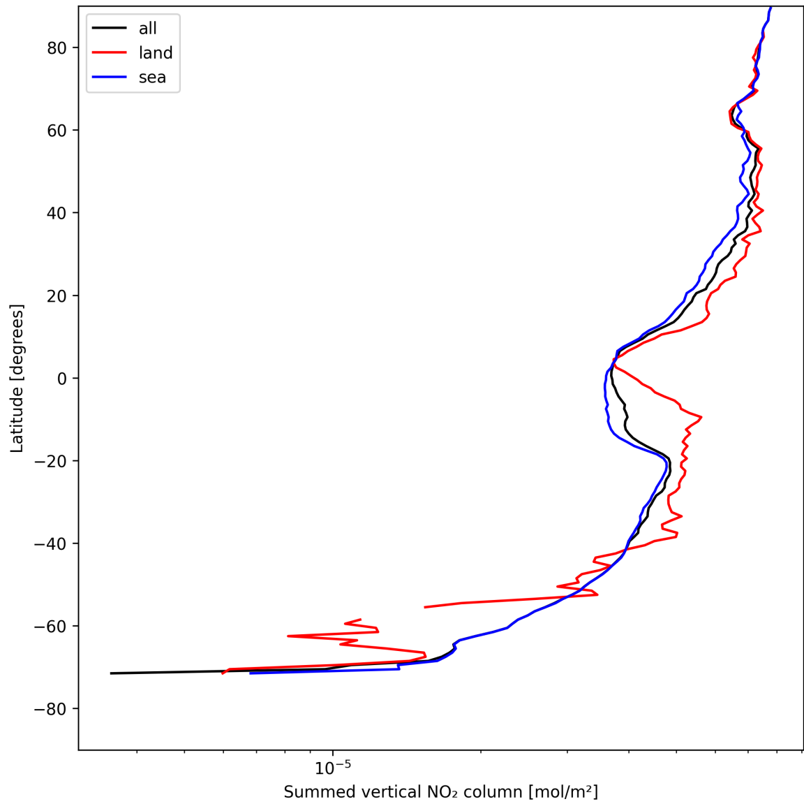
Figure 23: Zonal average of “Summed vertical NO 2 column” for 2025-08-06 to 2025-08-08.
