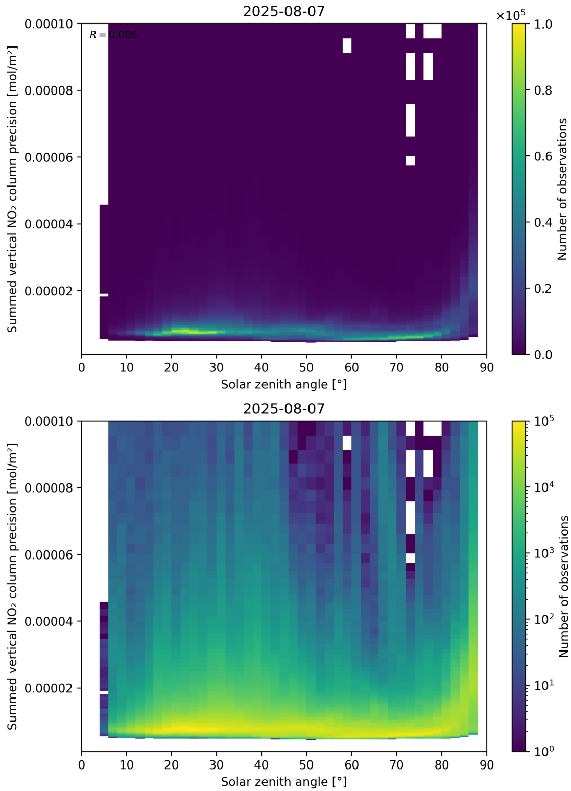
Figure 152: Scatter density plot of “Solar zenith angle” against “Summed vertical NO 2 column precision” for 2025-08-06 to 2025-08-08.
