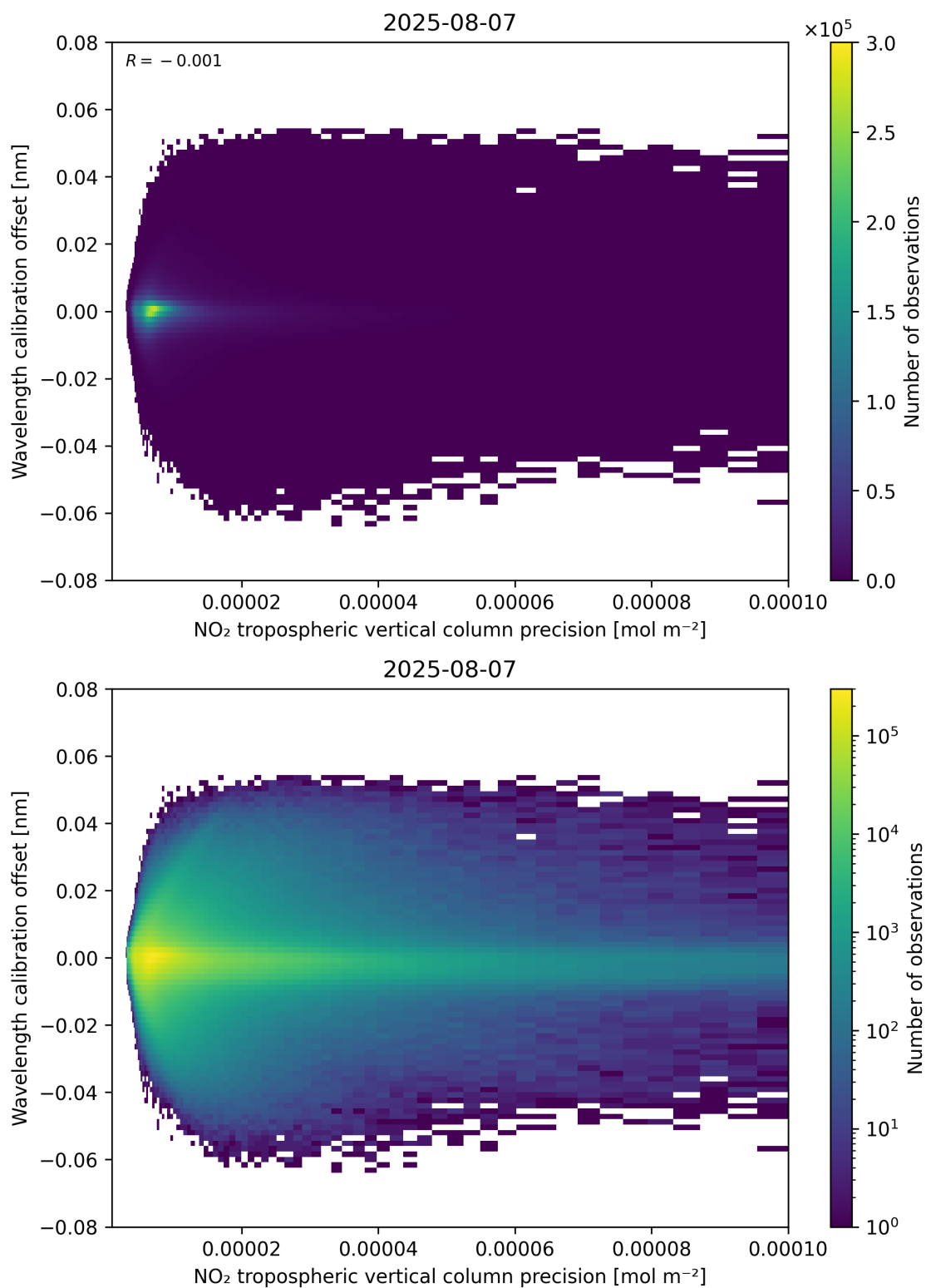
Figure 141: Scatter density plot of “NO 2 tropospheric vertical column precision” against “Wavelength calibration offset” for 2025-08-06 to 2025-08-08.
