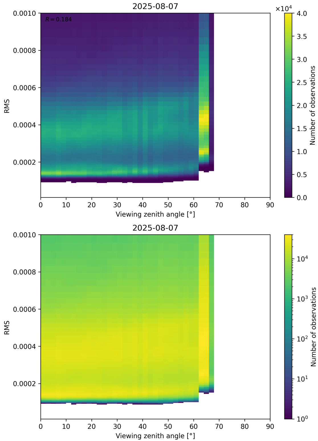
Figure 171: Scatter density plot of “Viewing zenith angle” against “RMS” for 2025-08-06 to 2025-08-08.
