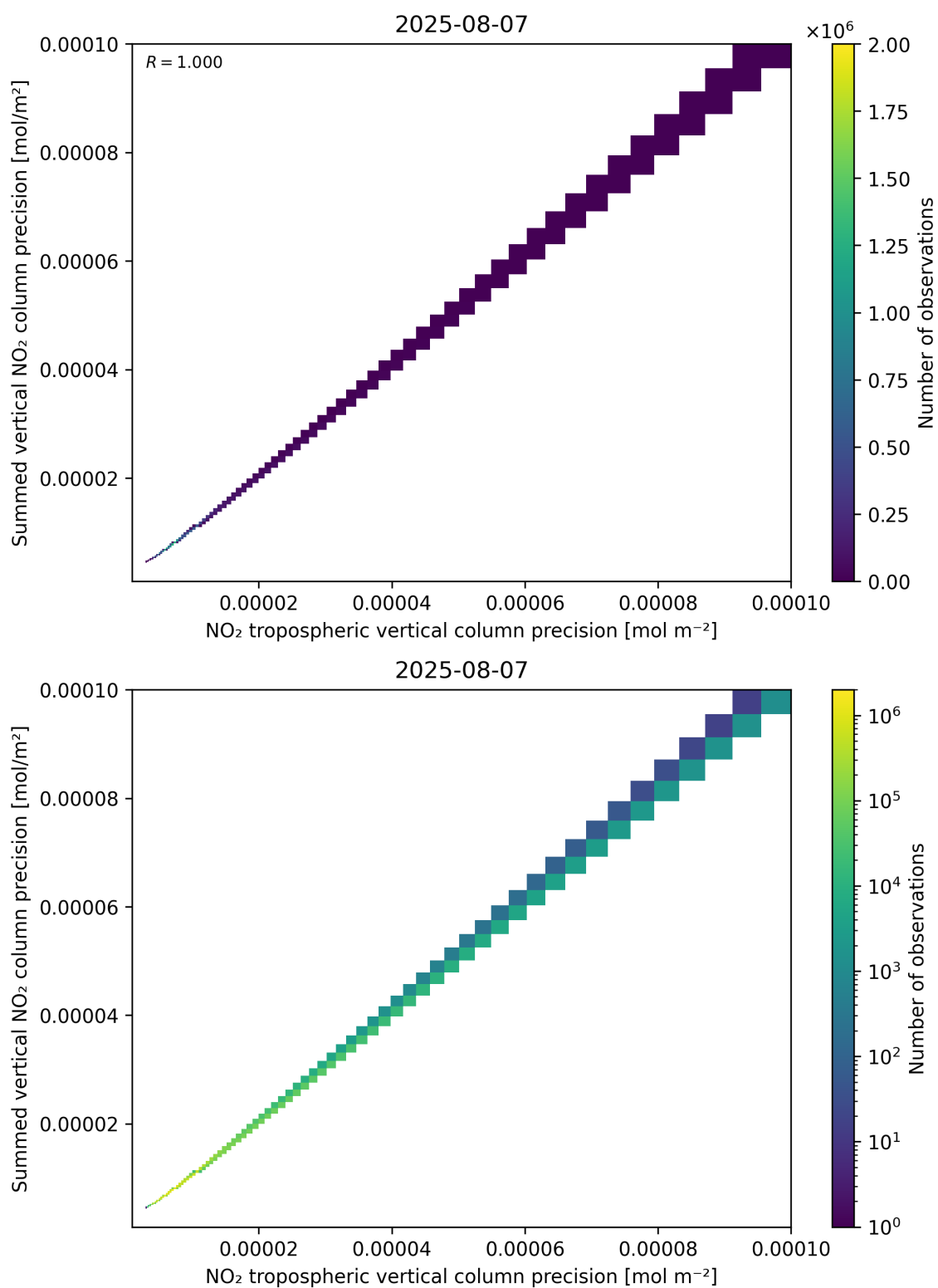
Figure 137: Scatter density plot of “NO 2 tropospheric vertical column precision” against “Summed vertical NO 2 column precision” for 2025-08-06 to 2025-08-08.
