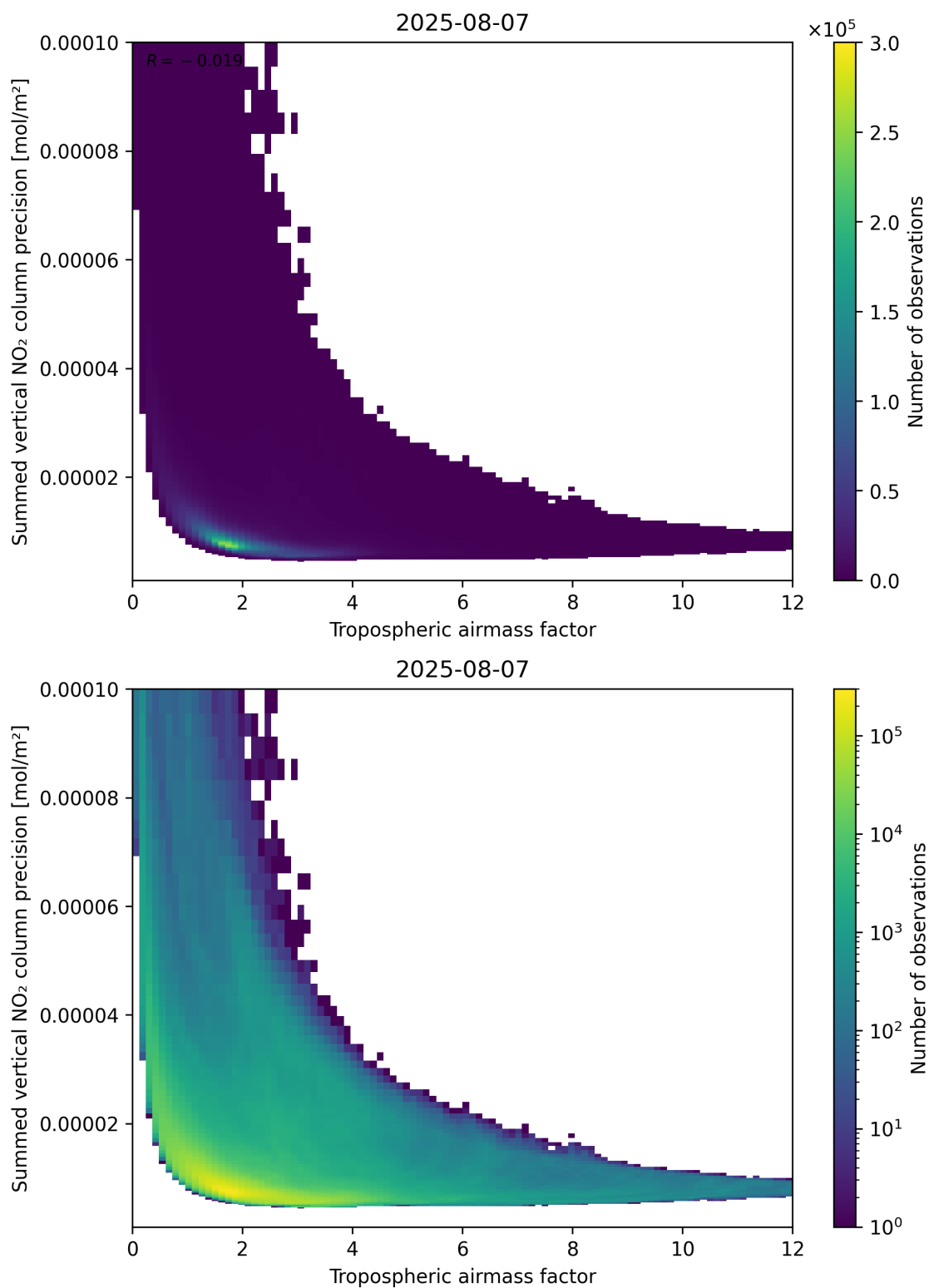
Figure 76: Scatter density plot of “Tropospheric air mass factor” against “Summed vertical NO 2 column precision” for 2025-08-06 to 2025-08-08.
