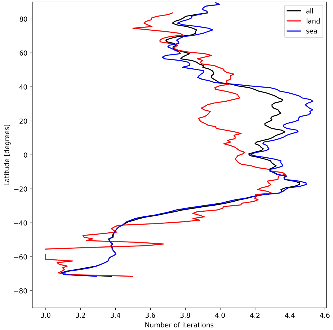
Figure 17: Zonal average of “Number of iterations” for 2025-08-06 to 2025-08-08.
