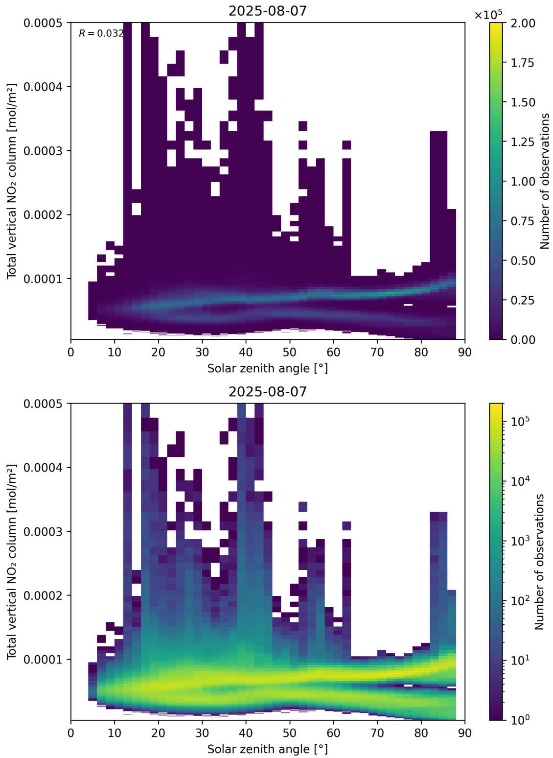
Figure 153: Scatter density plot of “Solar zenith angle” against “Total vertical NO 2 column” for 2025-08-06 to 2025-08-08.
