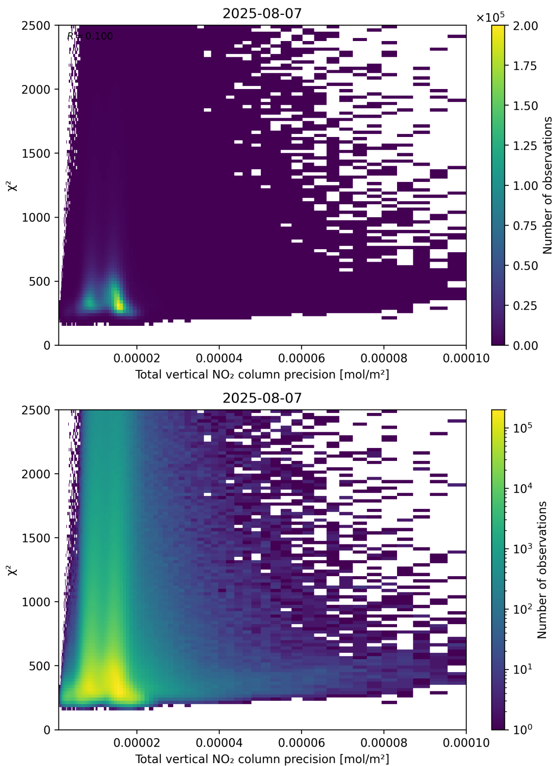
Figure 116: Scatter density plot of “Total vertical NO 2 column precision” against “ \chi^2 ” for 2025-08-06 to 2025-08-08.
