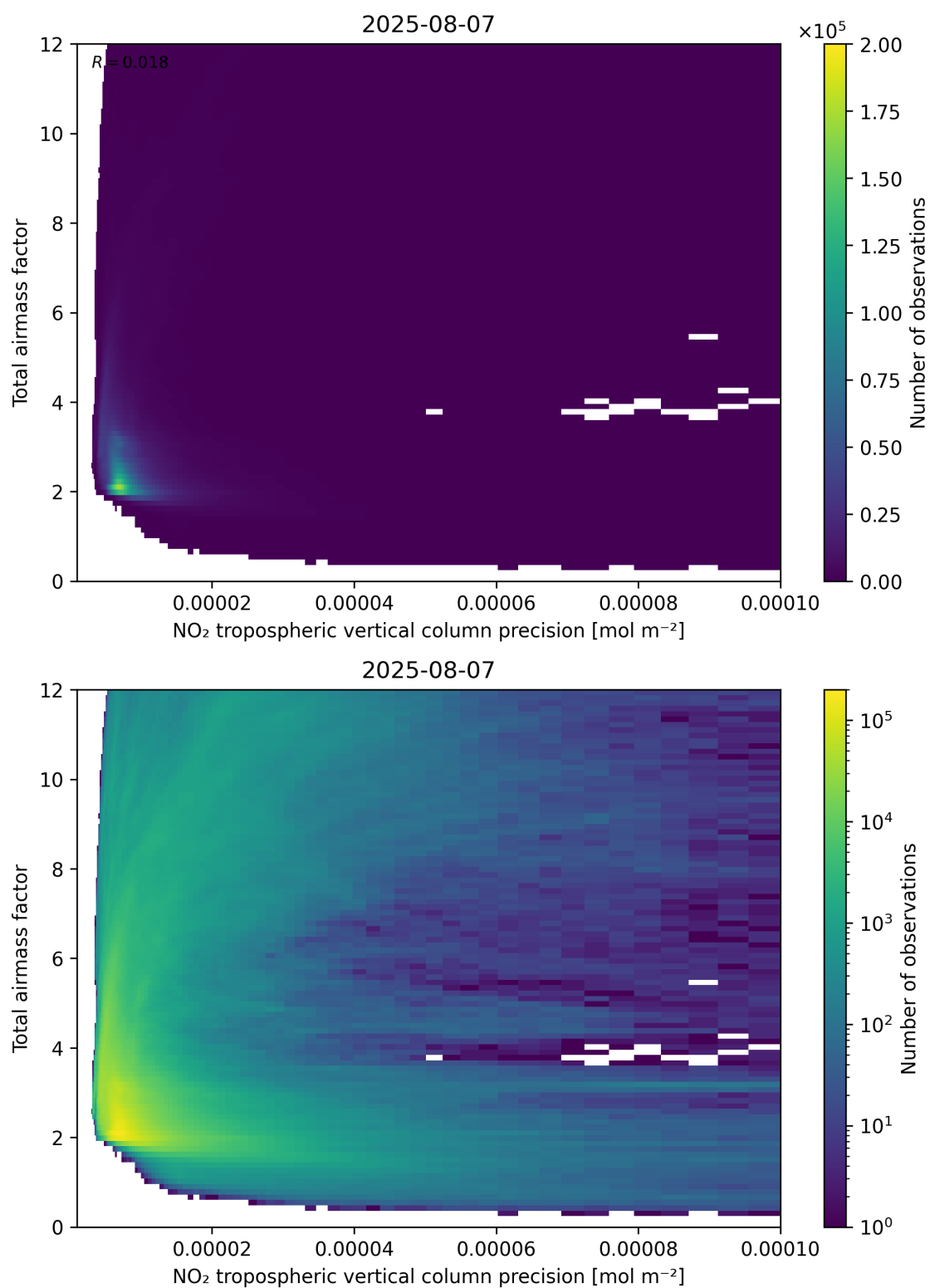
Figure 132: Scatter density plot of “NO 2 tropospheric vertical column precision” against “Total air mass factor” for 2025-08-06 to 2025-08-08.
