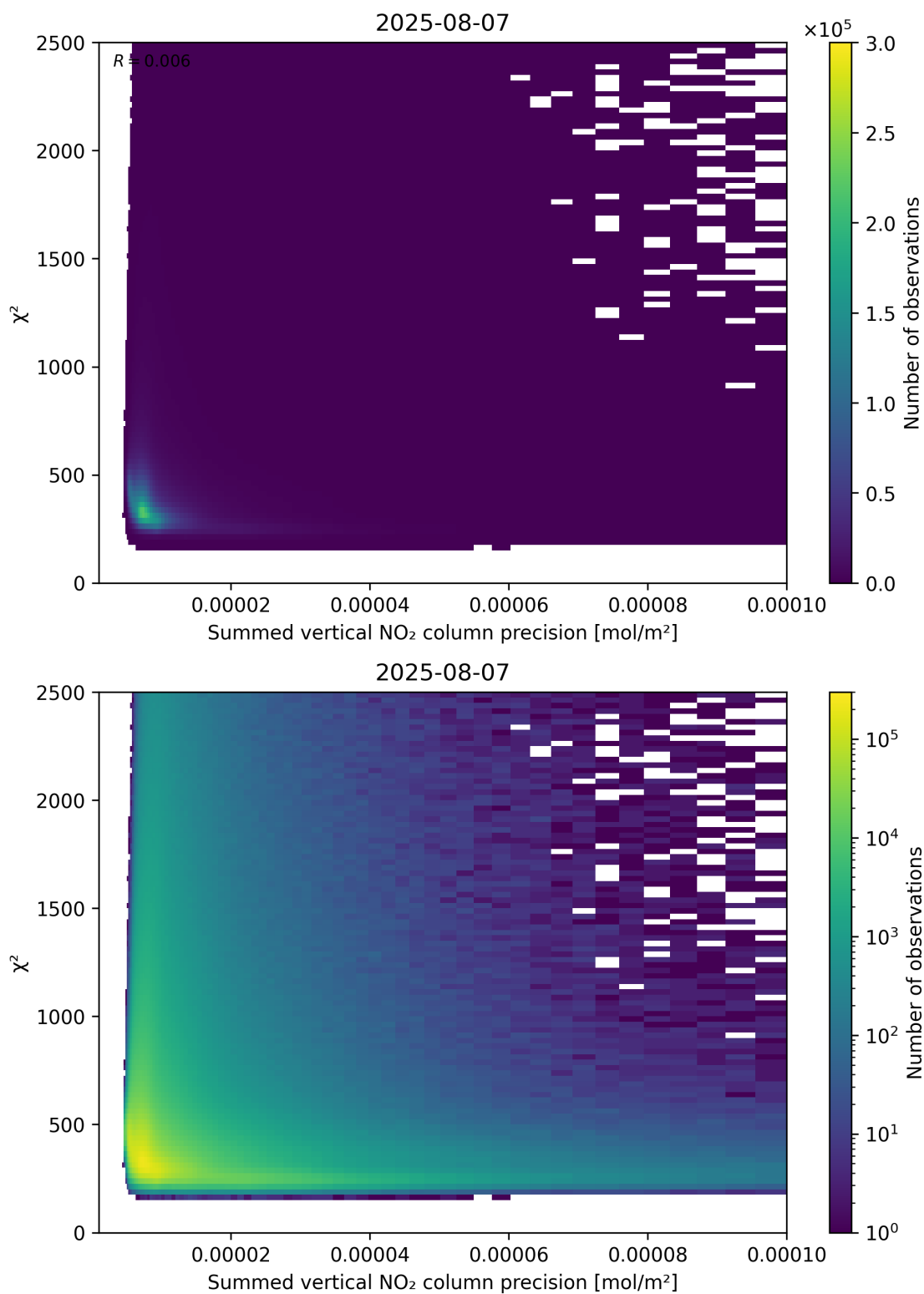
Figure 107: Scatter density plot of “Summed vertical NO 2 column precision” against “ \chi^2 ” for 2025-08-06 to 2025-08-08.
