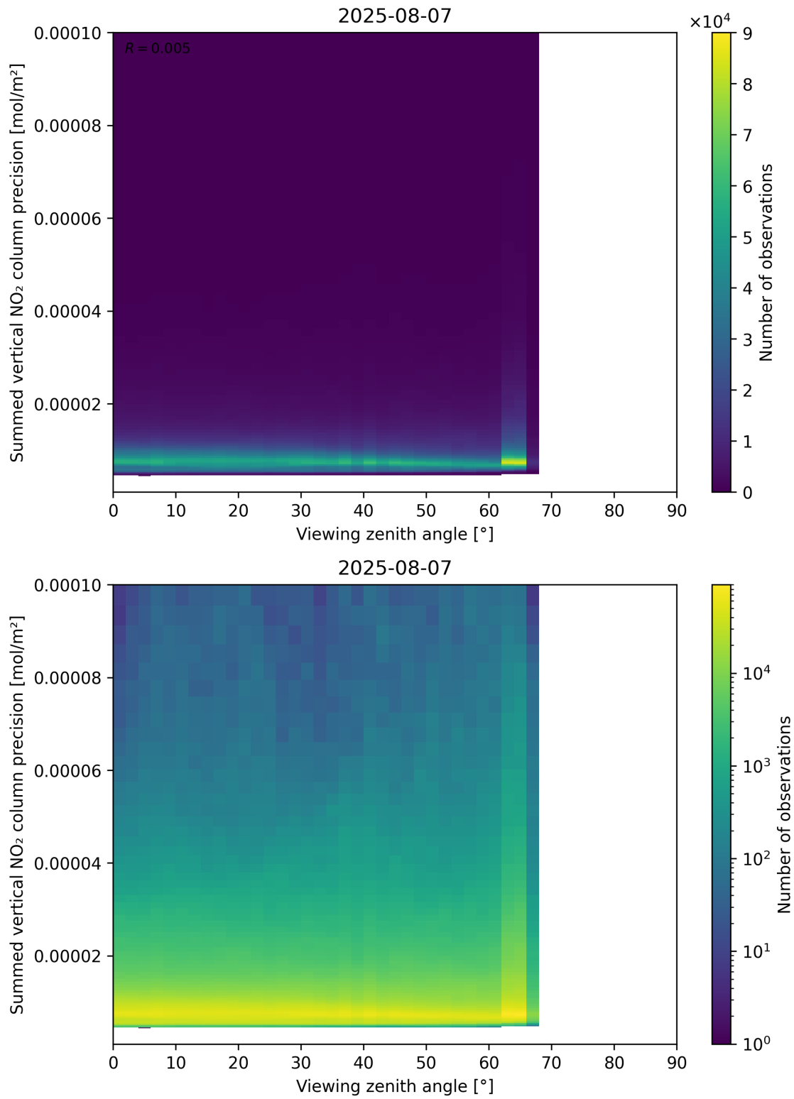
Figure 166: Scatter density plot of “Viewing zenith angle” against “Summed vertical NO 2 column precision” for 2025-08-06 to 2025-08-08.
