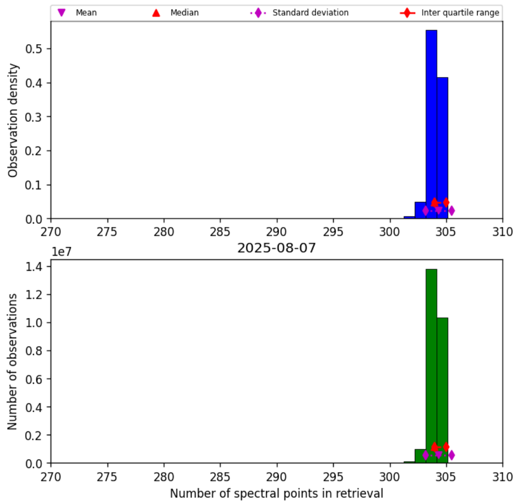
Figure 33: Histogram of “Number of spectral points in retrieval” for 2025-08-06 to 2025-08-08
