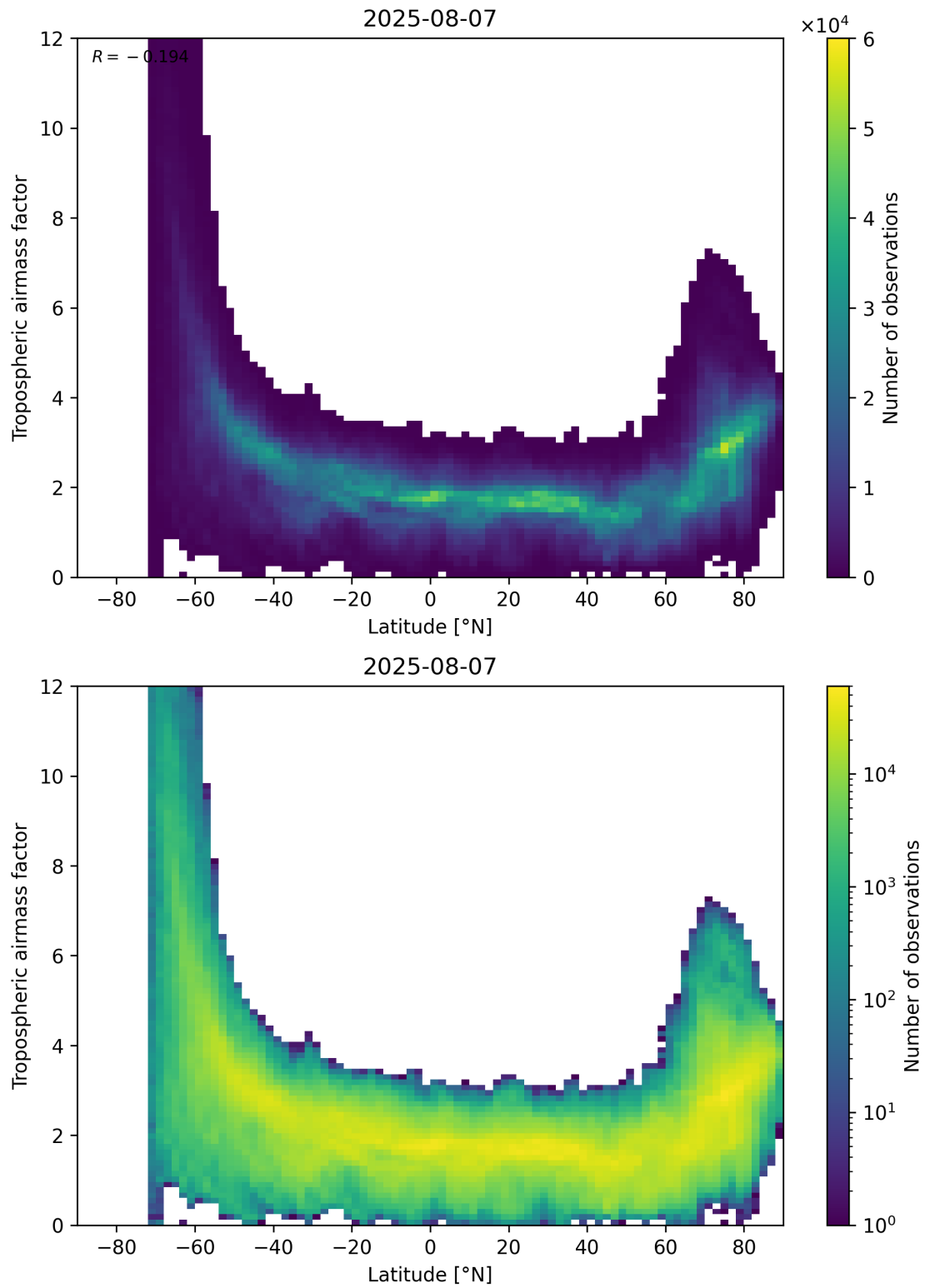
Figure 85: Scatter density plot of “Latitude” against “Tropospheric air mass factor” for 2025-08-06 to 2025-08-08.
