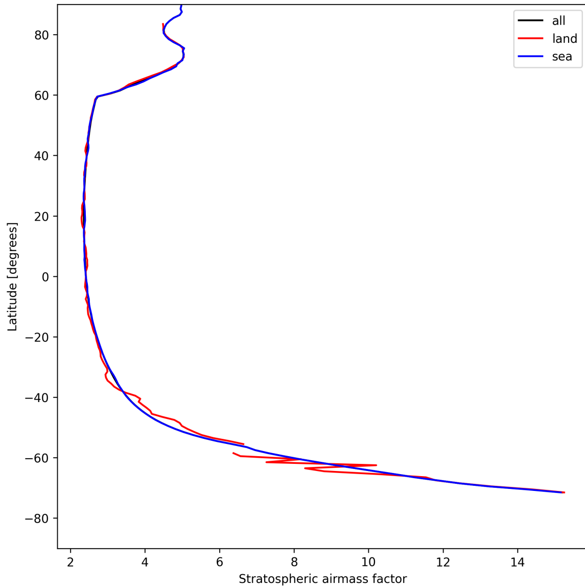
Figure 27: Zonal average of “Stratospheric airmass factor” for 2025-08-06 to 2025-08-08.
