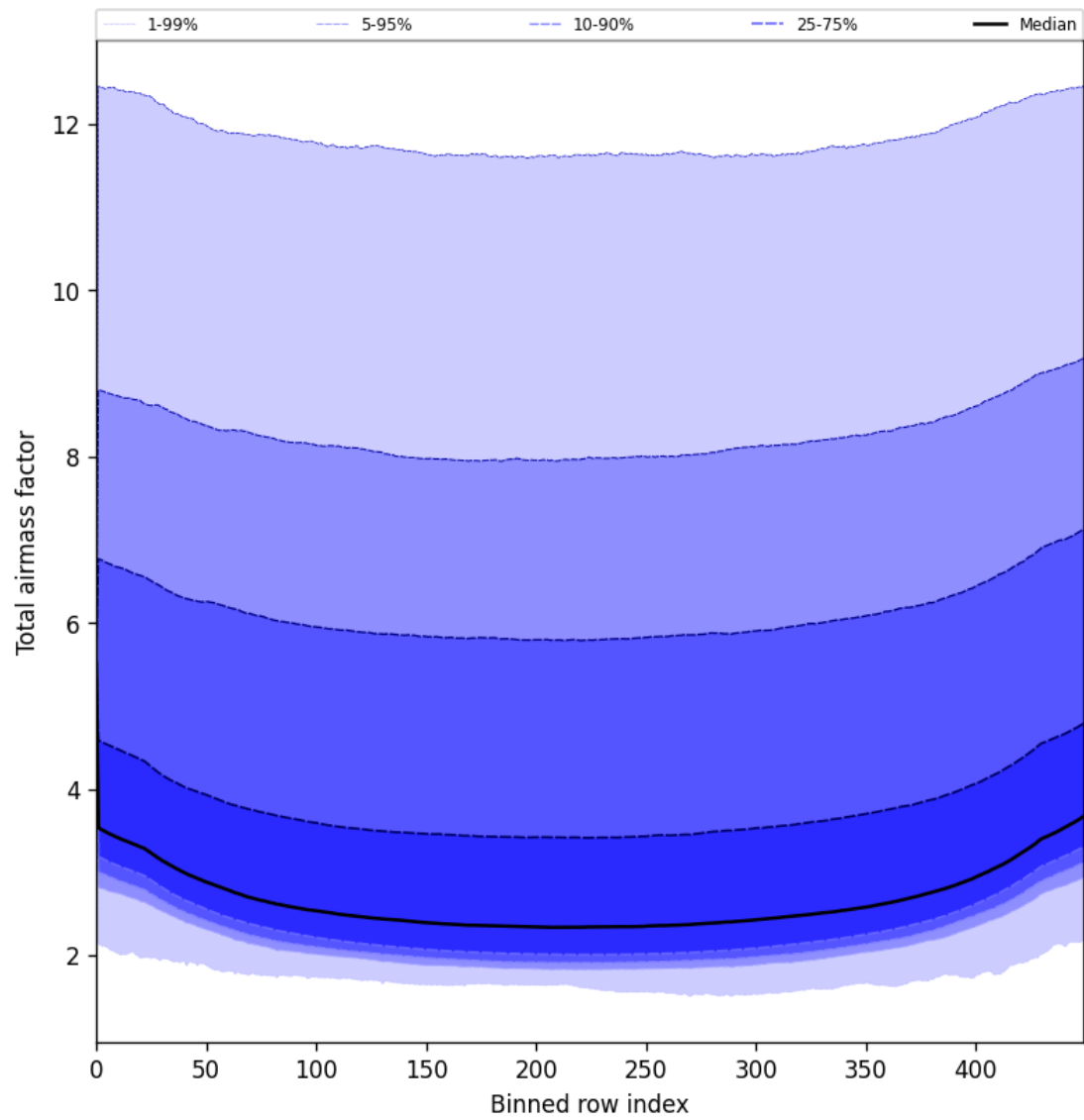
Figure 49: Along track statistics of “Total airmass factor” for 2025-08-06 to 2025-08-08
