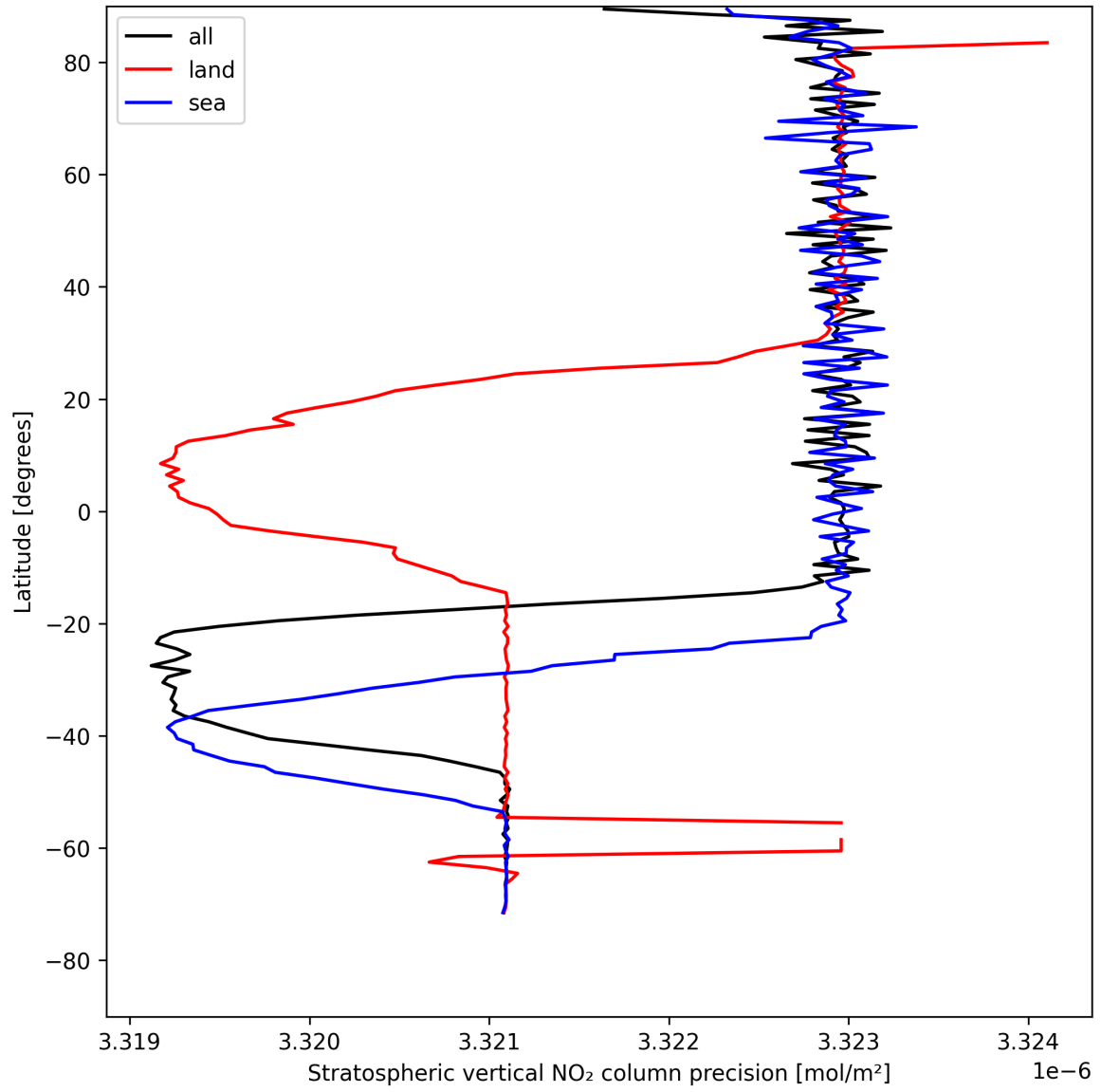
Figure 20: Zonal average of “Stratospheric vertical NO 2 column precision” for 2025-08-06 to 2025-08-08.
