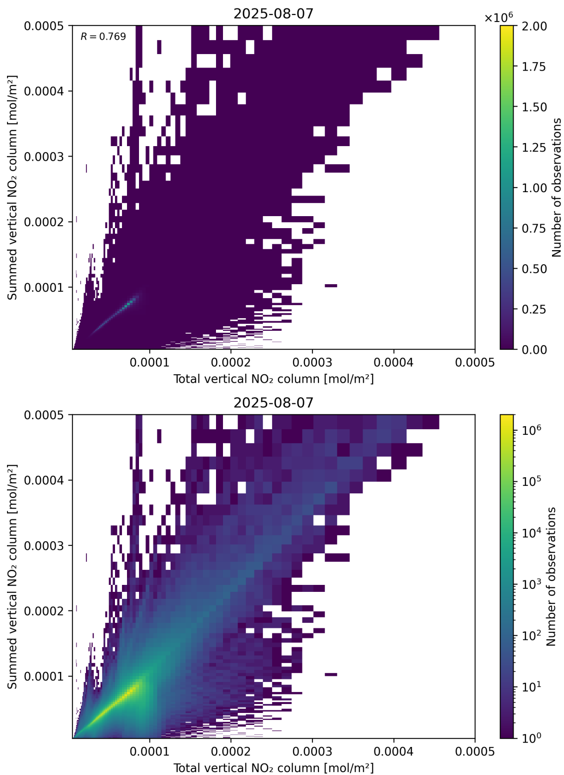
Figure 112: Scatter density plot of “Total vertical NO 2 column” against “Summed vertical NO 2 column” for 2025-08-06 to 2025-08-08.
