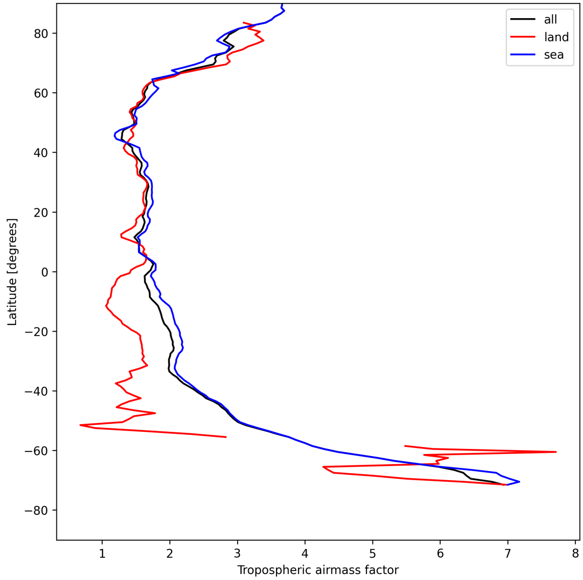
Figure 14: Zonal average of “Tropospheric airmass factor” for 2025-08-06 to 2025-08-08.
