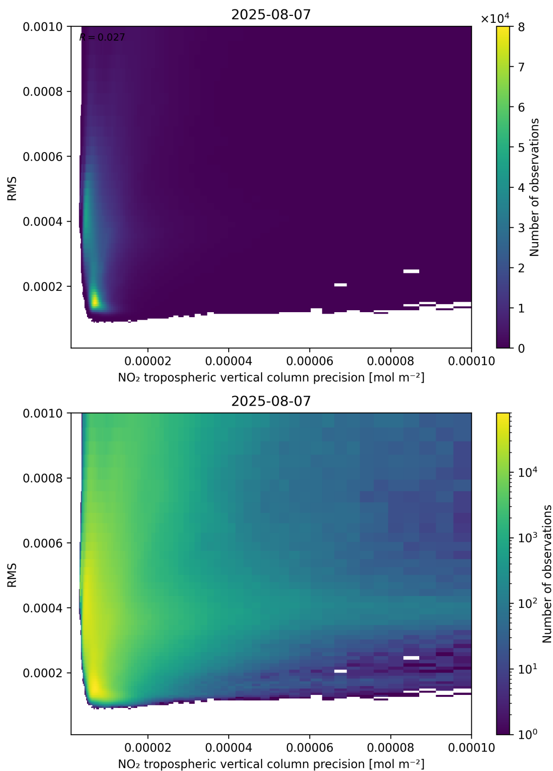
Figure 140: Scatter density plot of “NO 2 tropospheric vertical column precision” against “RMS” for 2025-08-06 to 2025-08-08.
