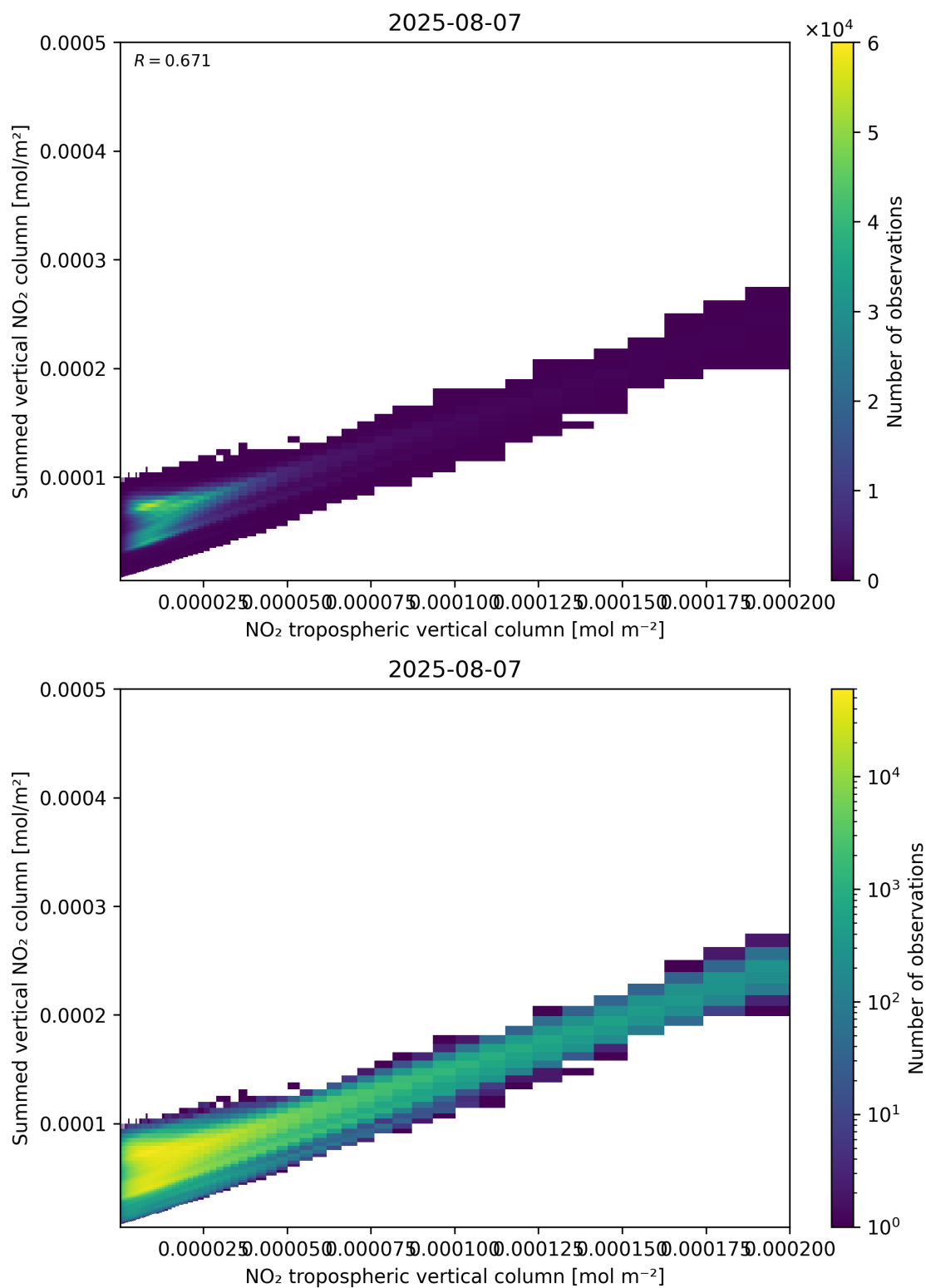
Figure 126: Scatter density plot of “NO 2 tropospheric vertical column” against “Summed vertical NO 2 column” for 2025-08-06 to 2025-08-08.
