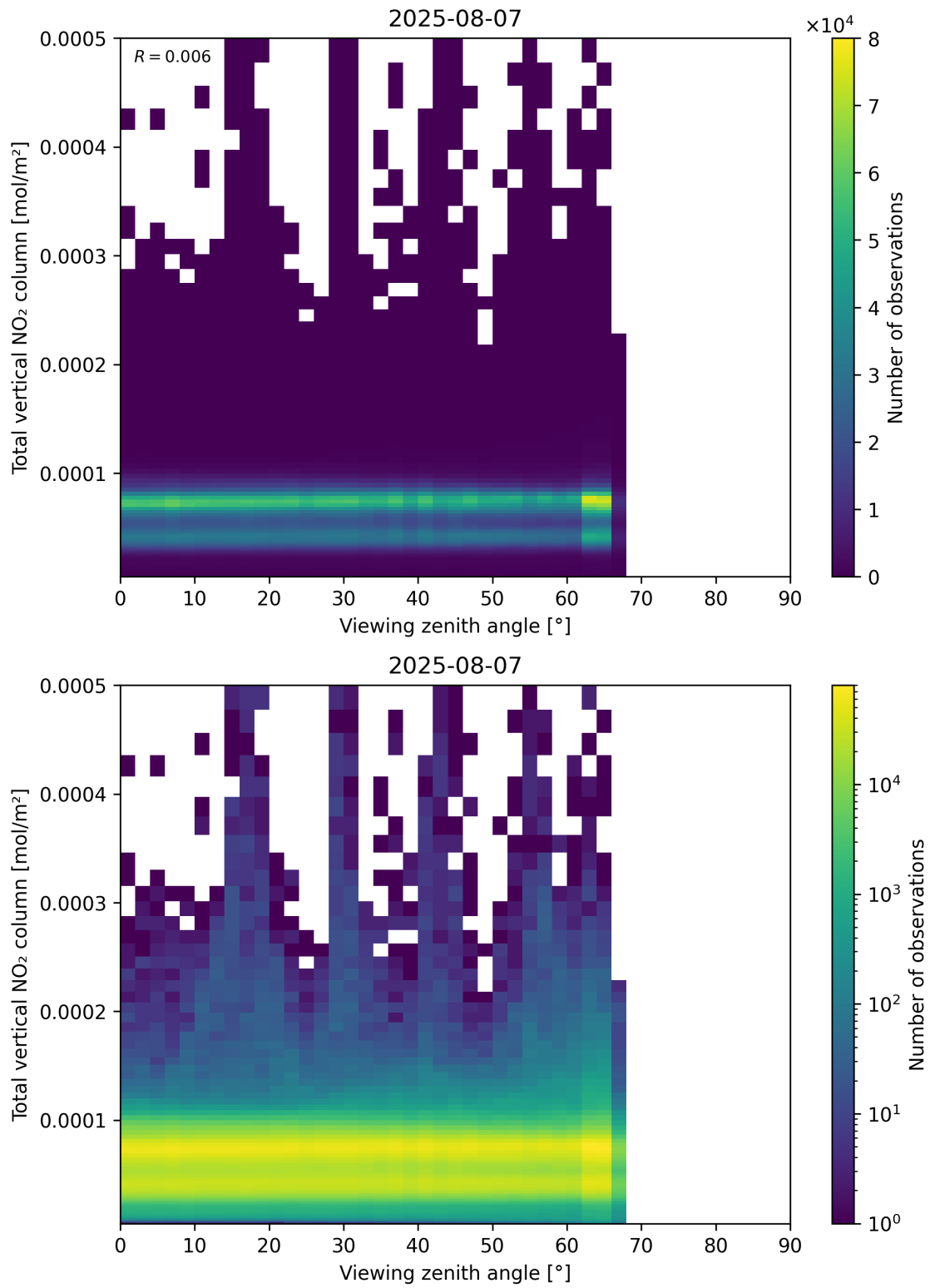
Figure 167: Scatter density plot of “Viewing zenith angle” against “Total vertical NO 2 column” for 2025-08-06 to 2025-08-08.
