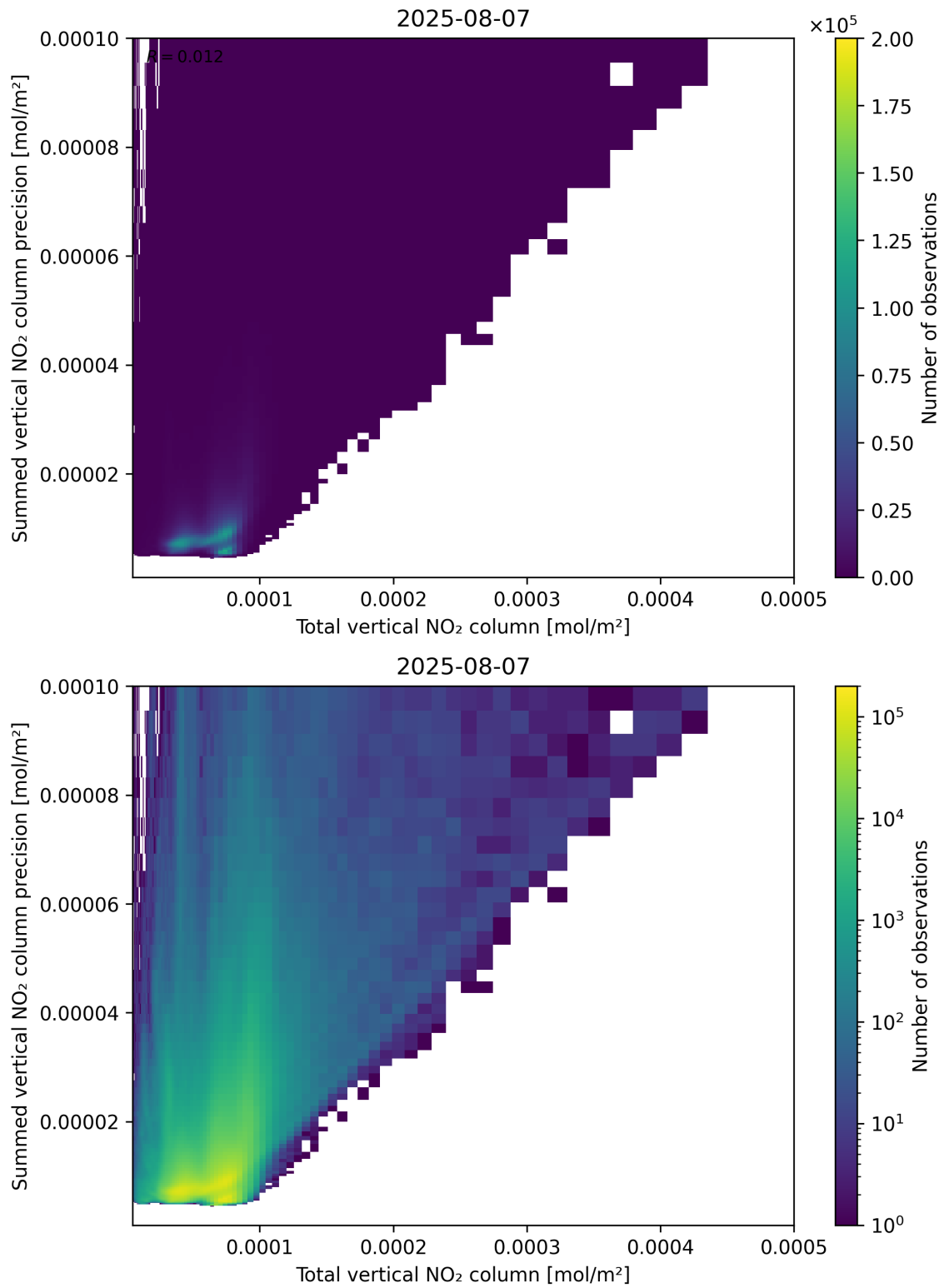
Figure 113: Scatter density plot of “Total vertical NO 2 column” against “Summed vertical NO 2 column precision” for 2025-08-06 to 2025-08-08.
