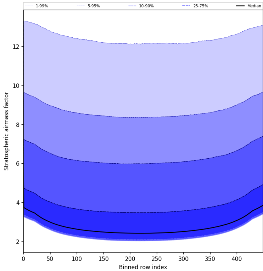
Figure 61: Along track statistics of “Stratospheric airmass factor” for 2025-08-06 to 2025-08-08
