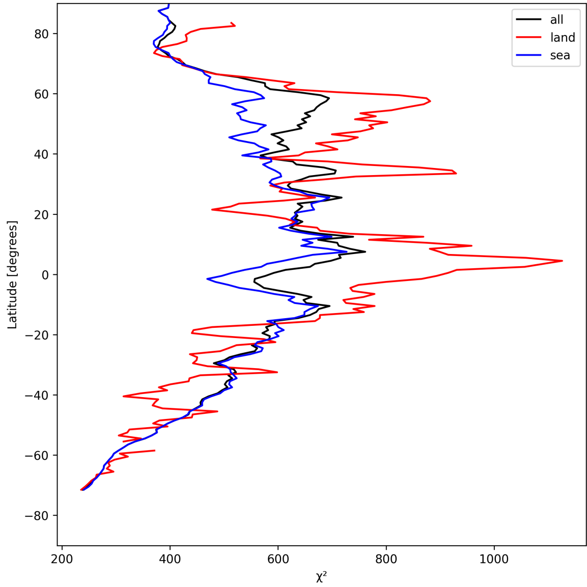
Figure 25: Zonal average of “ \chi^2 ” for 2025-08-06 to 2025-08-08.
