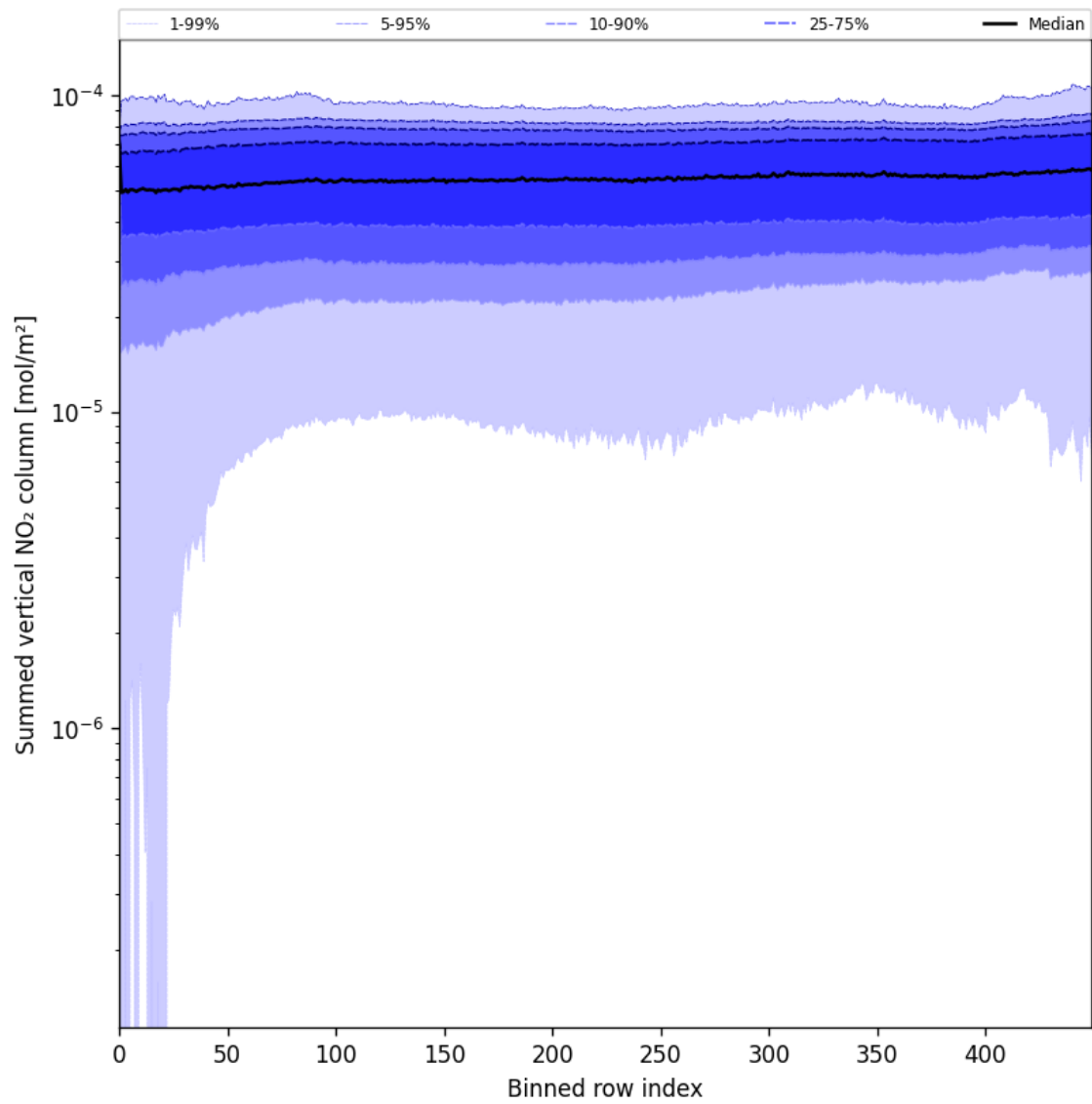
Figure 57: Along track statistics of “Summed vertical NO 2 column” for 2025-08-06 to 2025-08-08
