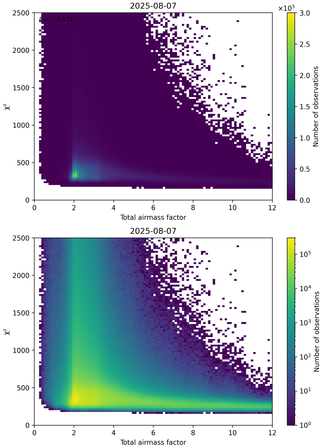
Figure 63: Scatter density plot of “Total airmass factor” against “ \chi^2 ” for 2025-08-06 to 2025-08-08.
