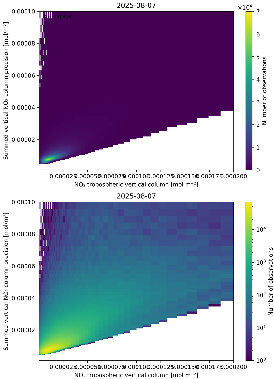
Figure 127: Scatter density plot of “NO 2 tropospheric vertical column” against “Summed vertical NO 2 column precision” for 2025-08-06 to 2025-08-08.
