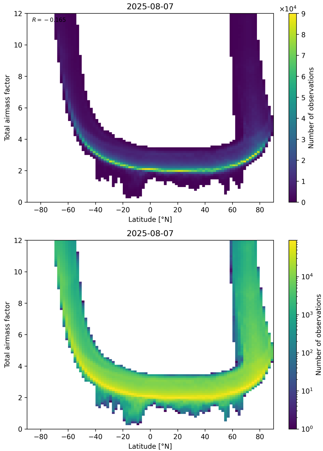
Figure 84: Scatter density plot of “Latitude” against “Total airmass factor” for 2025-08-06 to 2025-08-08.
