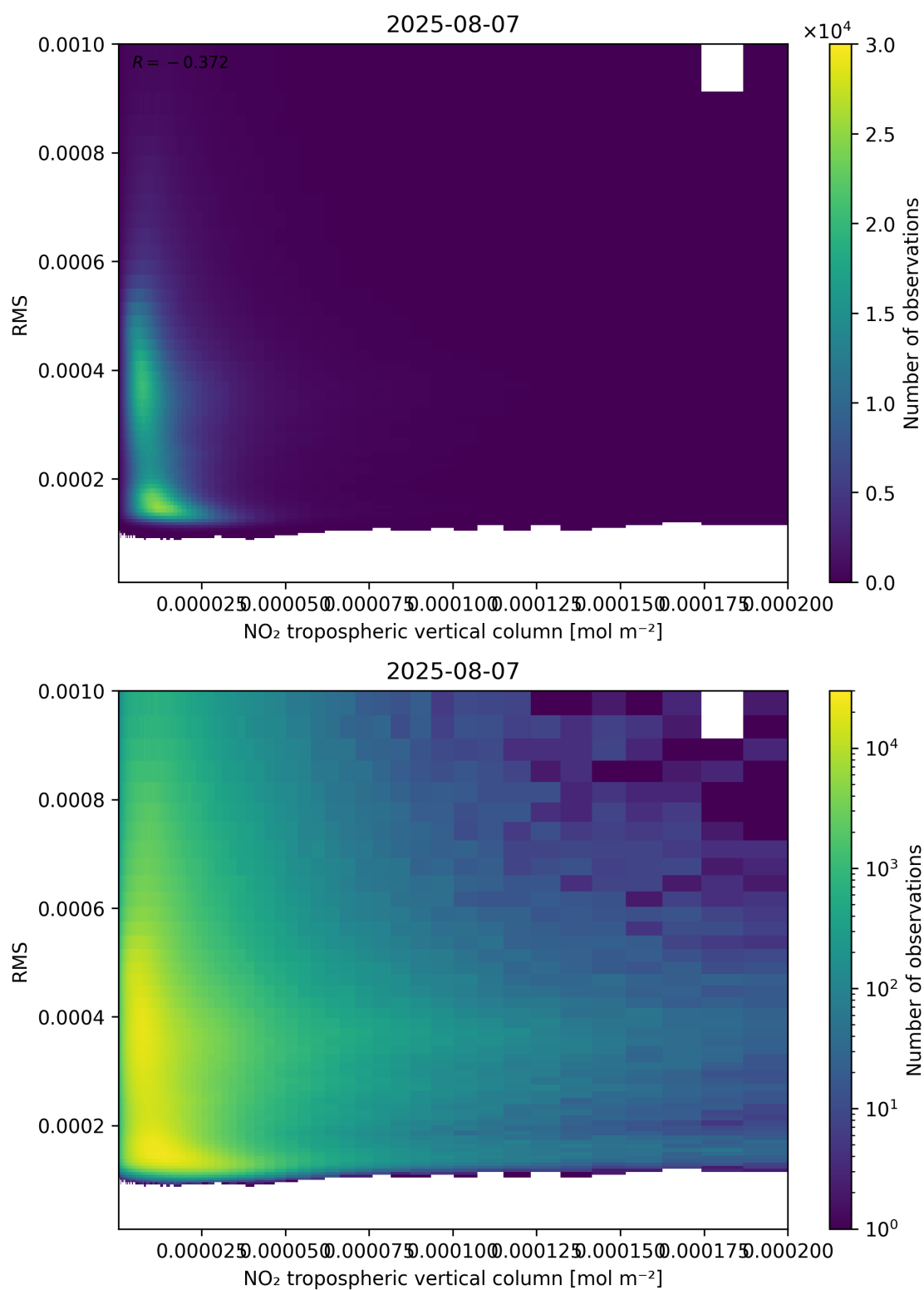
Figure 142: Scatter density plot of “NO 2 tropospheric vertical column” against “RMS” for 2025-08-06 to 2025-08-08.
