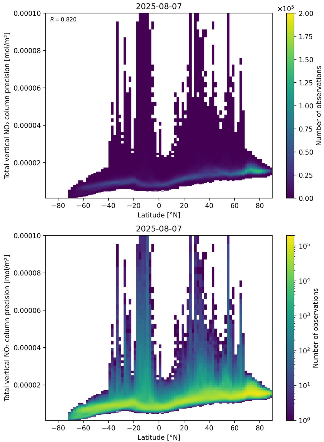
Figure 91: Scatter density plot of “Latitude” against “Total vertical NO 2 column precision” for 2025-08-06 to 2025-08-08.
