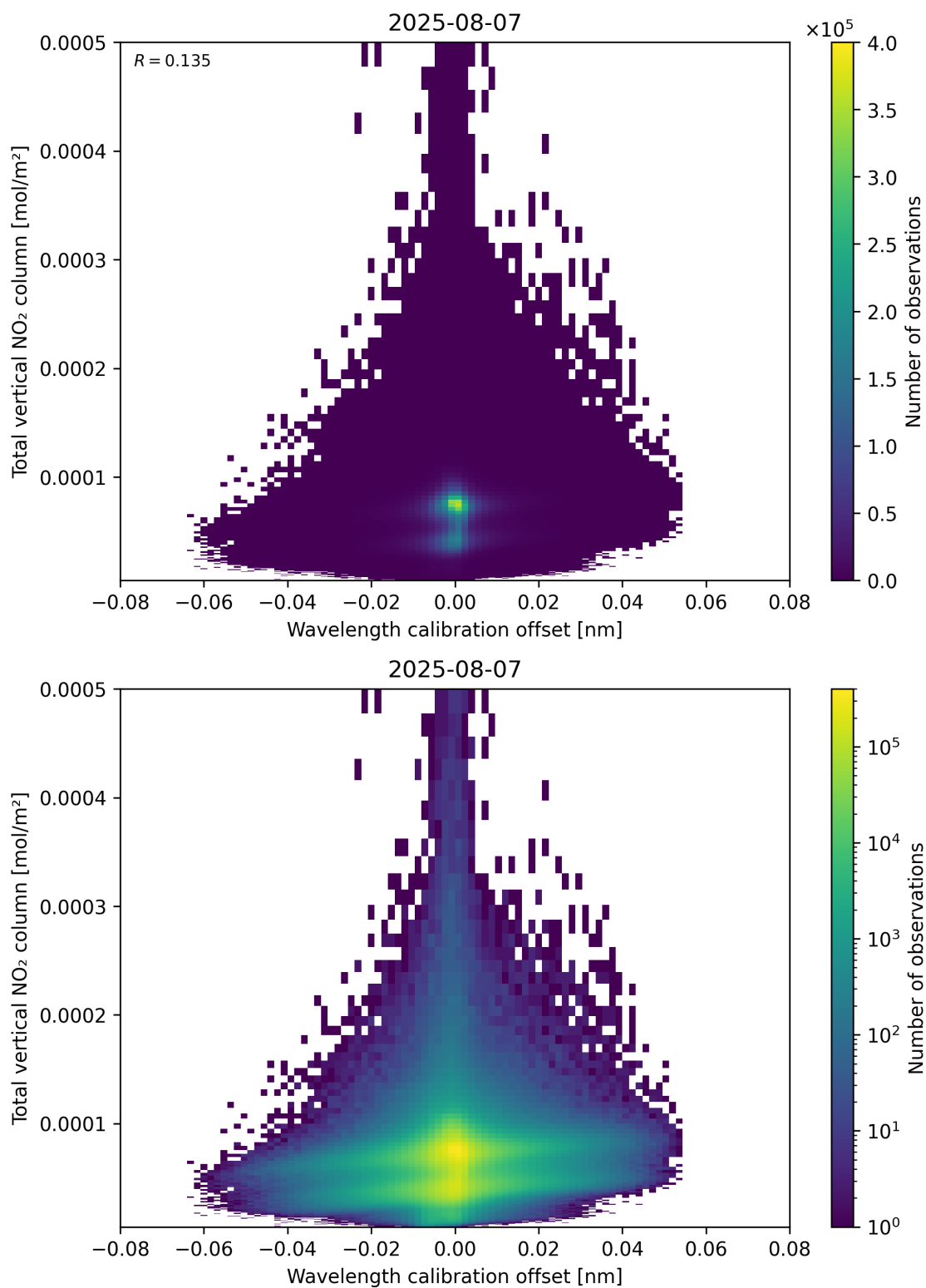
Figure 179: Scatter density plot of “Wavelength calibration offset” against “Total vertical NO 2 column” for 2025-08-06 to 2025-08-08.
