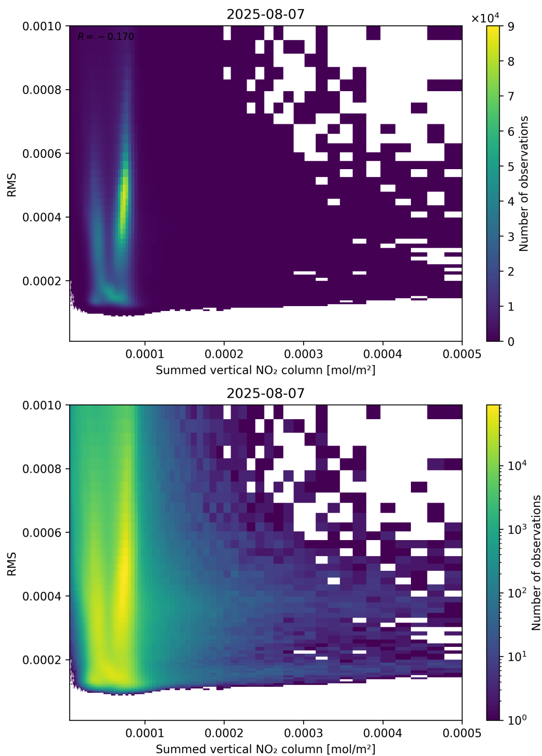
Figure 109: Scatter density plot of “Summed vertical NO 2 column” against “RMS” for 2025-08-06 to 2025-08-08.
