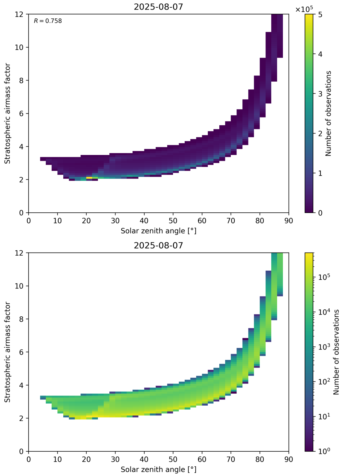
Figure 145: Scatter density plot of “Solar zenith angle” against “Stratospheric airmass factor” for 2025-08-06 to 2025-08-08.
