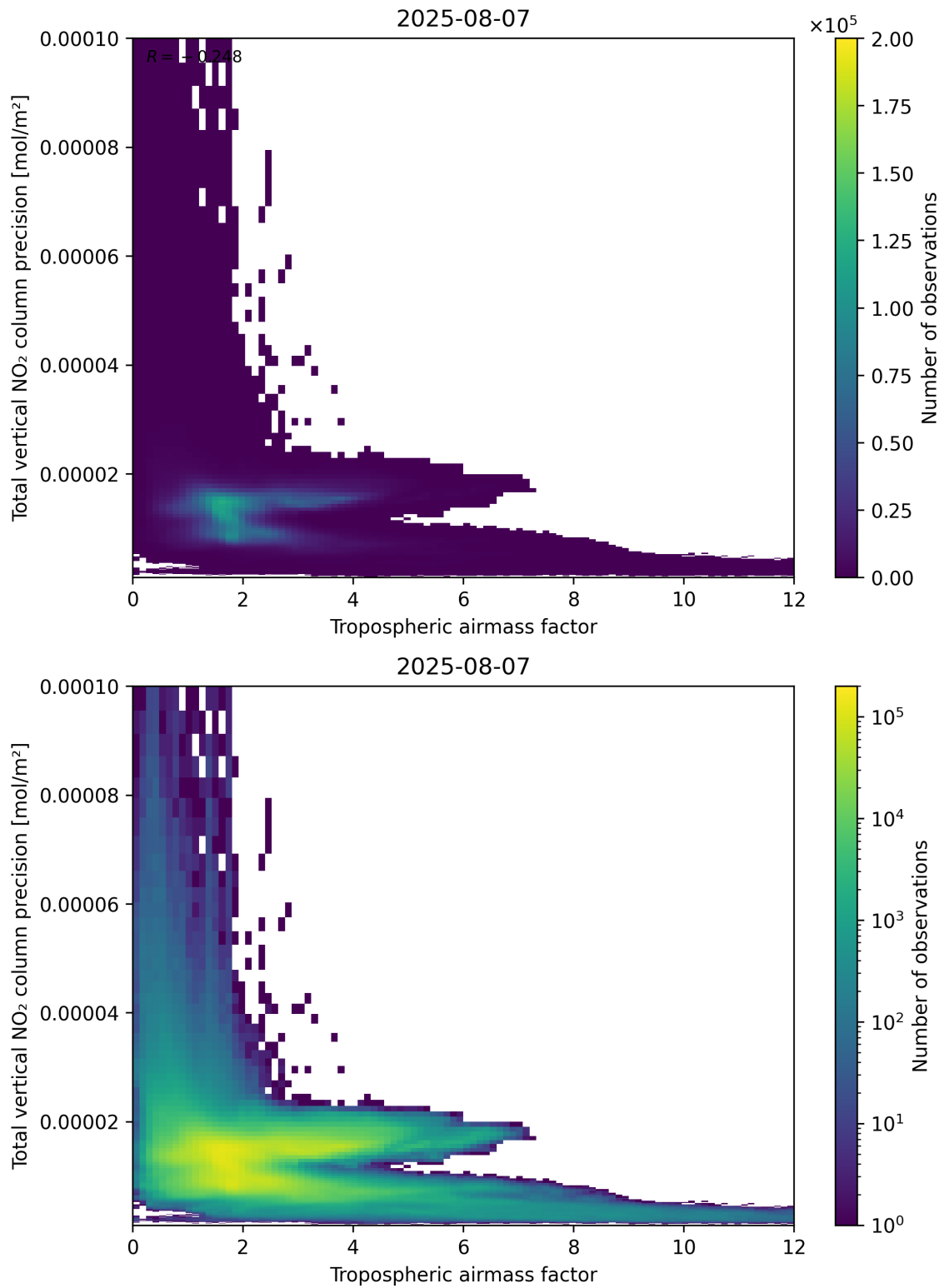
Figure 78: Scatter density plot of “Tropospheric air mass factor” against “Total vertical NO 2 column precision” for 2025-08-06 to 2025-08-08.
