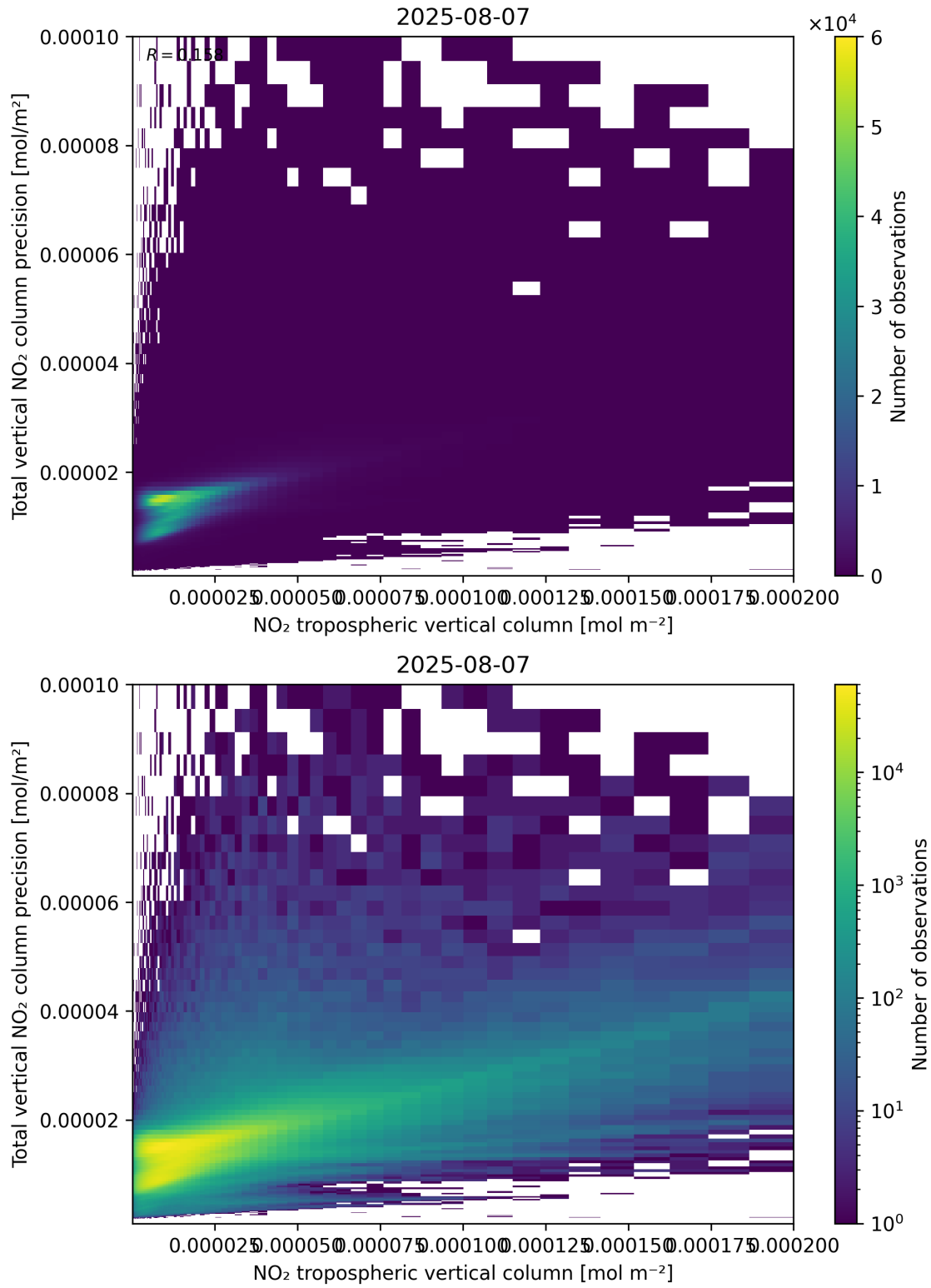
Figure 129: Scatter density plot of “NO 2 tropospheric vertical column” against “Total vertical NO 2 column precision” for 2025-08-06 to 2025-08-08.
