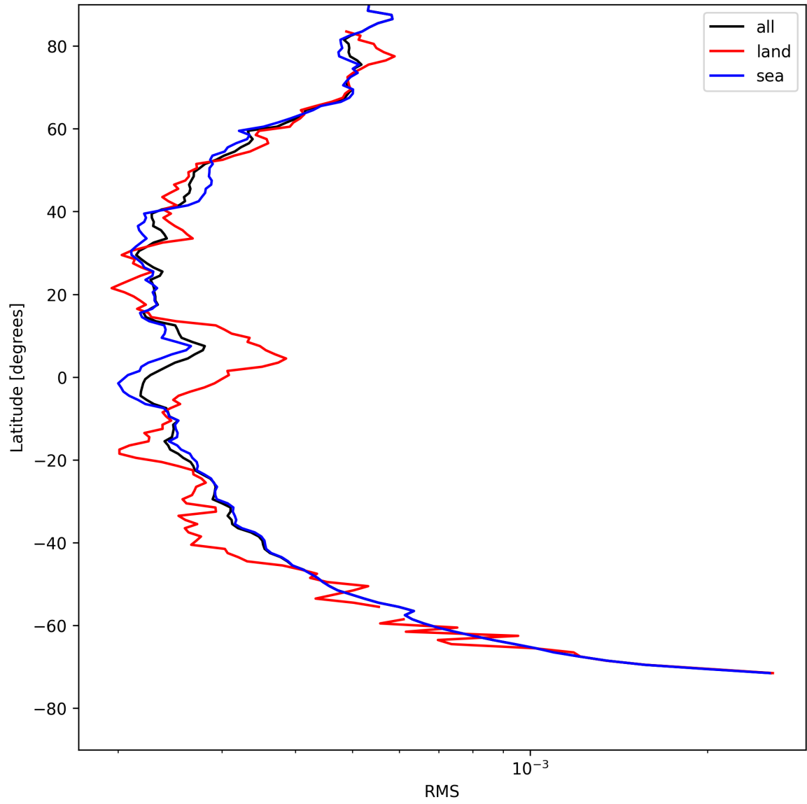
Figure 26: Zonal average of “RMS” for 2025-08-06 to 2025-08-08.
