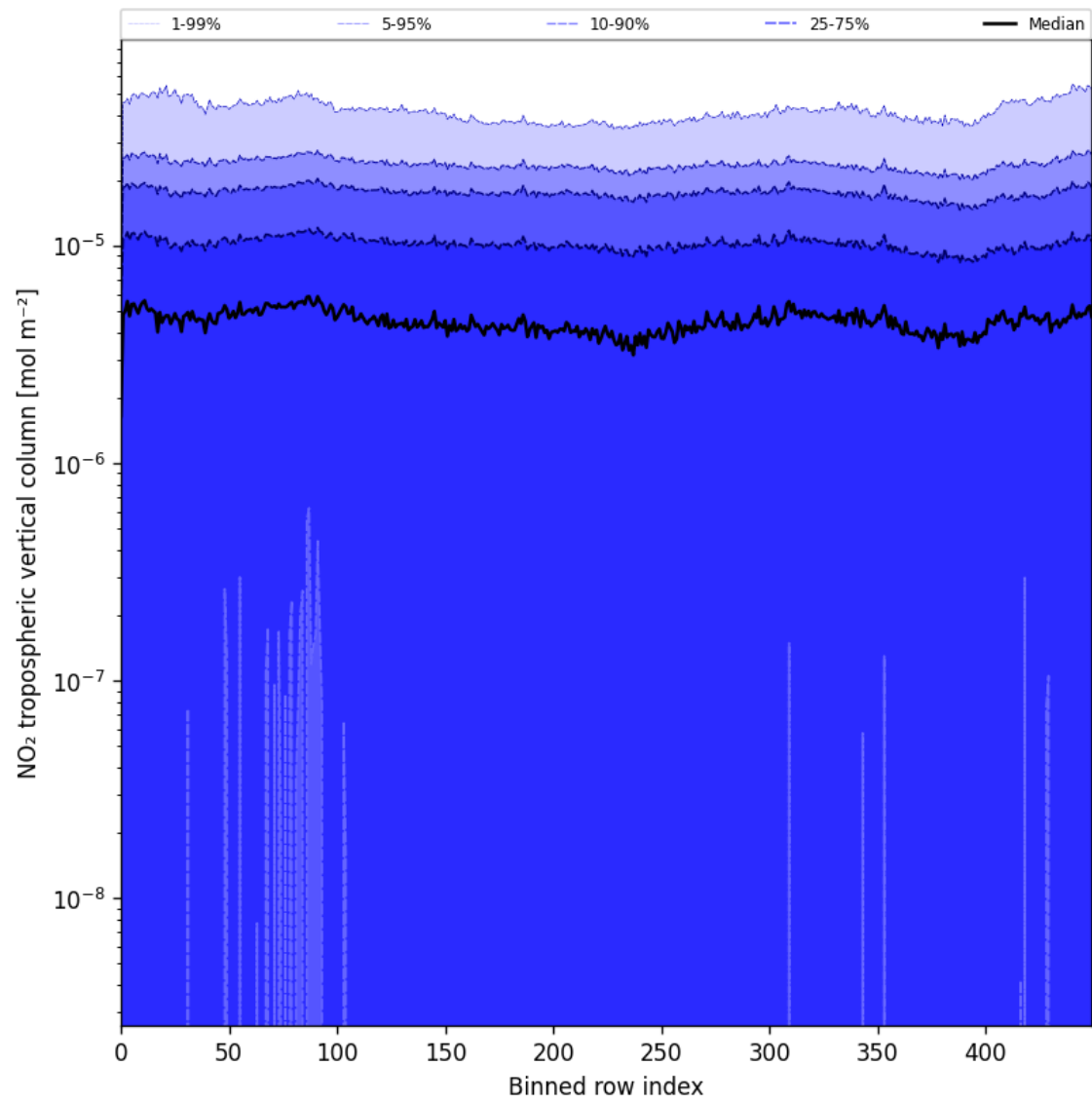
Figure 46: Along track statistics of “NO 2 tropospheric vertical column” for 2025-08-06 to 2025-08-08
