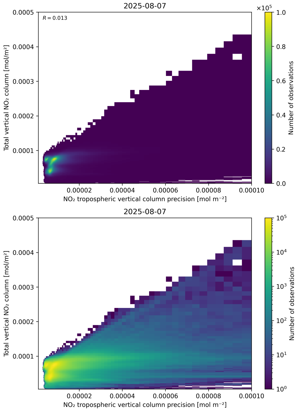
Figure 138: Scatter density plot of “NO 2 tropospheric vertical column precision” against “Total vertical NO 2 column” for 2025-08-06 to 2025-08-08.
