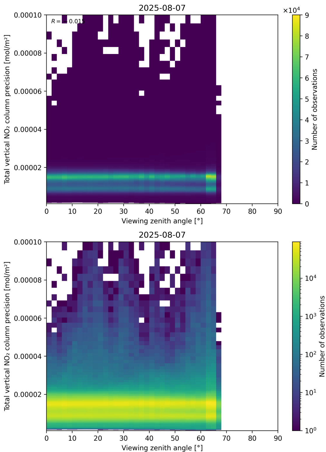
Figure 168: Scatter density plot of “Viewing zenith angle” against “Total vertical NO 2 column precision” for 2025-08-06 to 2025-08-08.
