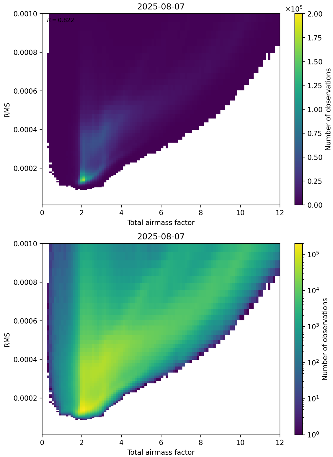
Figure 69: Scatter density plot of “Total airmass factor” against “RMS” for 2025-08-06 to 2025-08-08.
