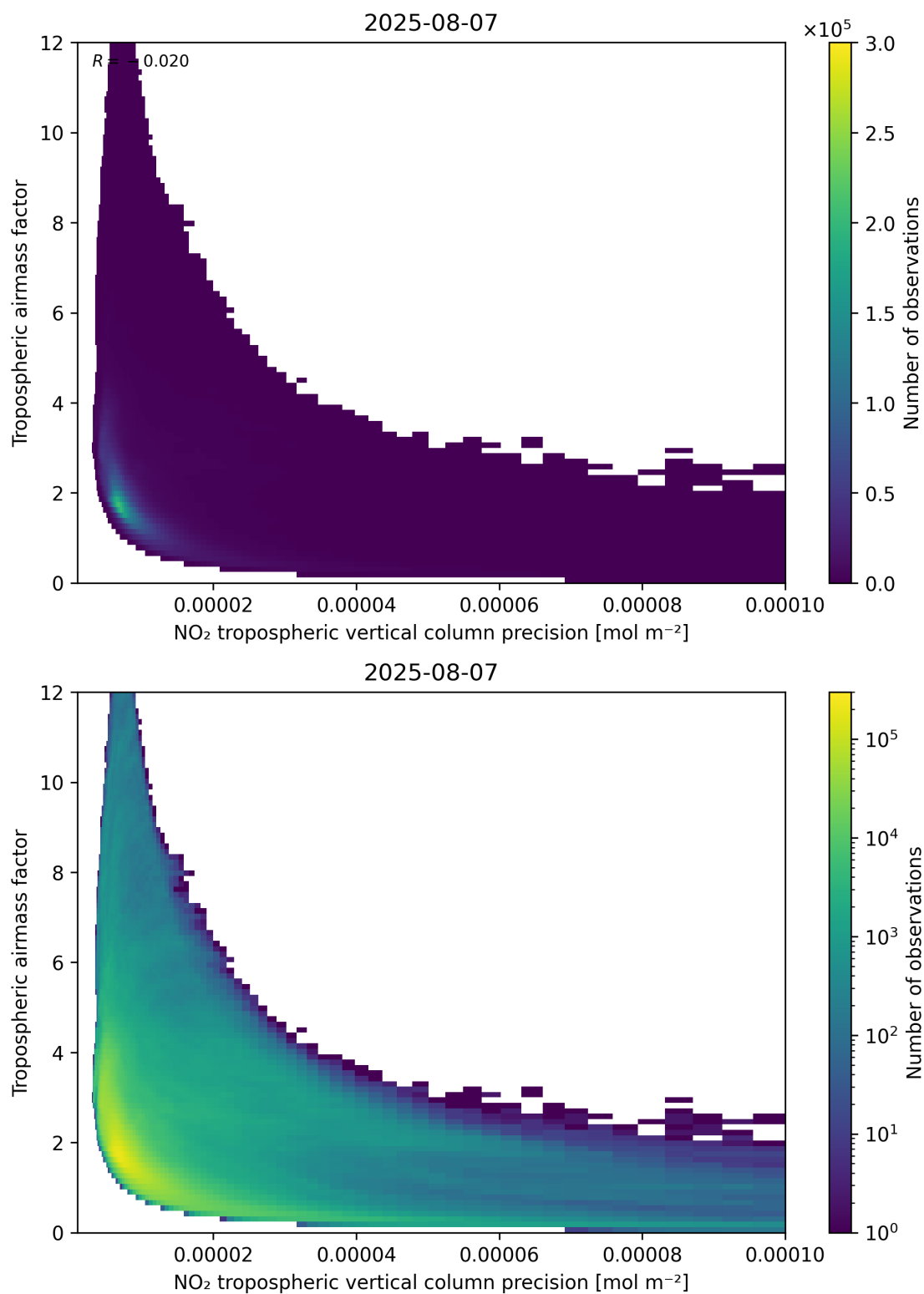
Figure 133: Scatter density plot of “NO 2 tropospheric vertical column precision” against “Tropospheric air mass factor” for 2025-08-06 to 2025-08-08.
