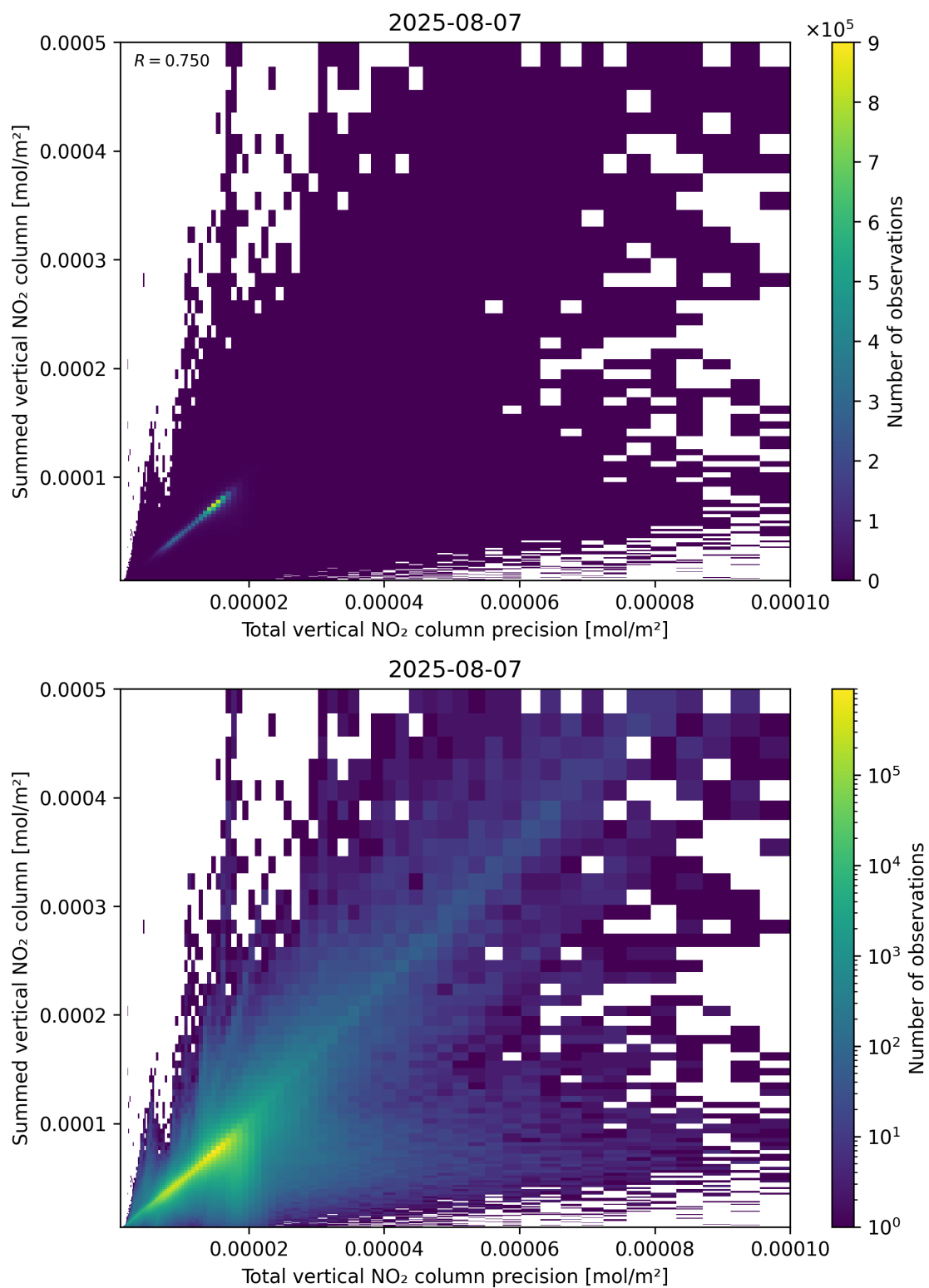
Figure 117: Scatter density plot of “Total vertical NO 2 column precision” against “Summed vertical NO 2 column” for 2025-08-06 to 2025-08-08.
