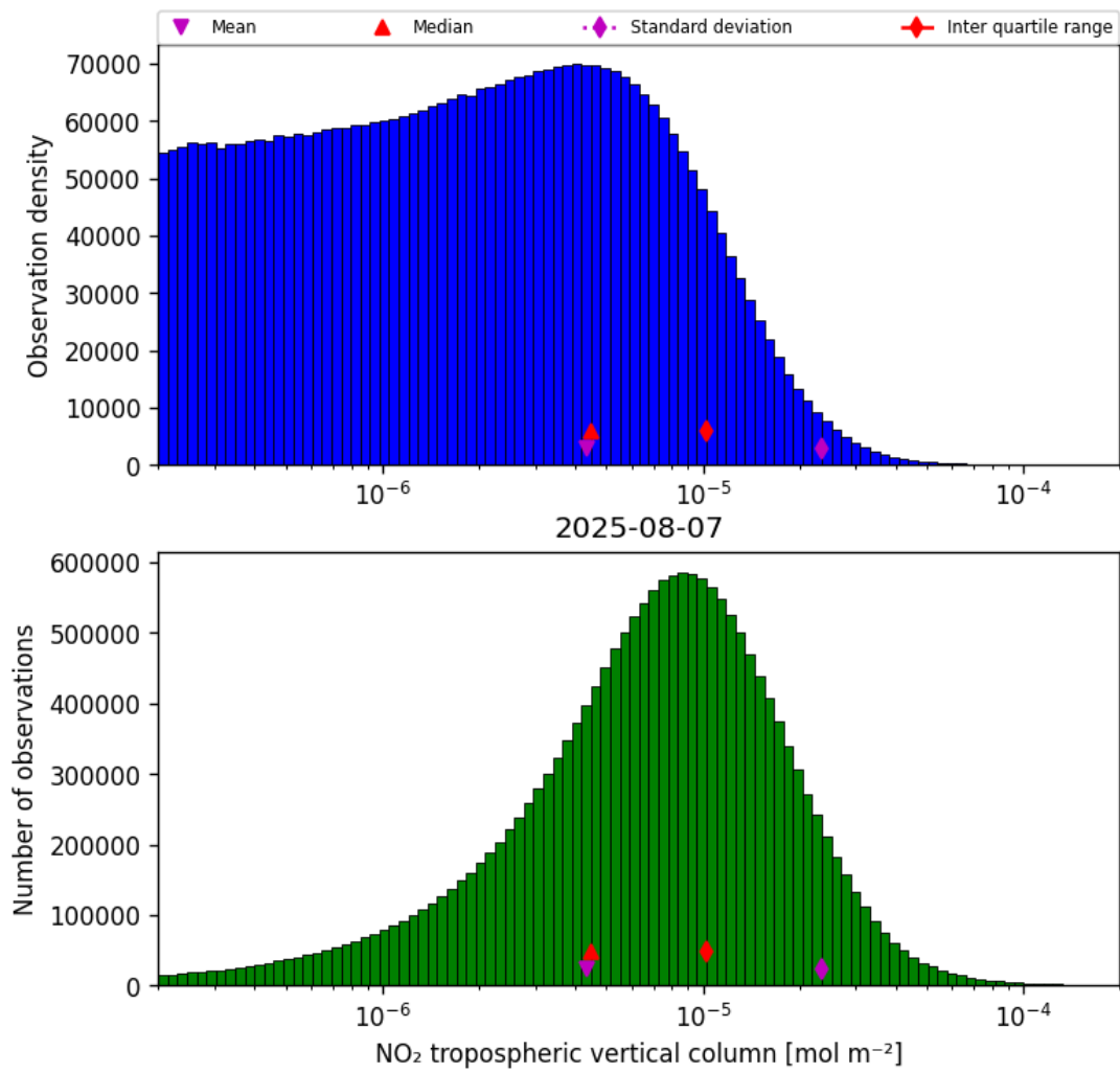
Figure 29: Histogram of “NO 2 tropospheric vertical column” for 2025-08-06 to 2025-08-08
