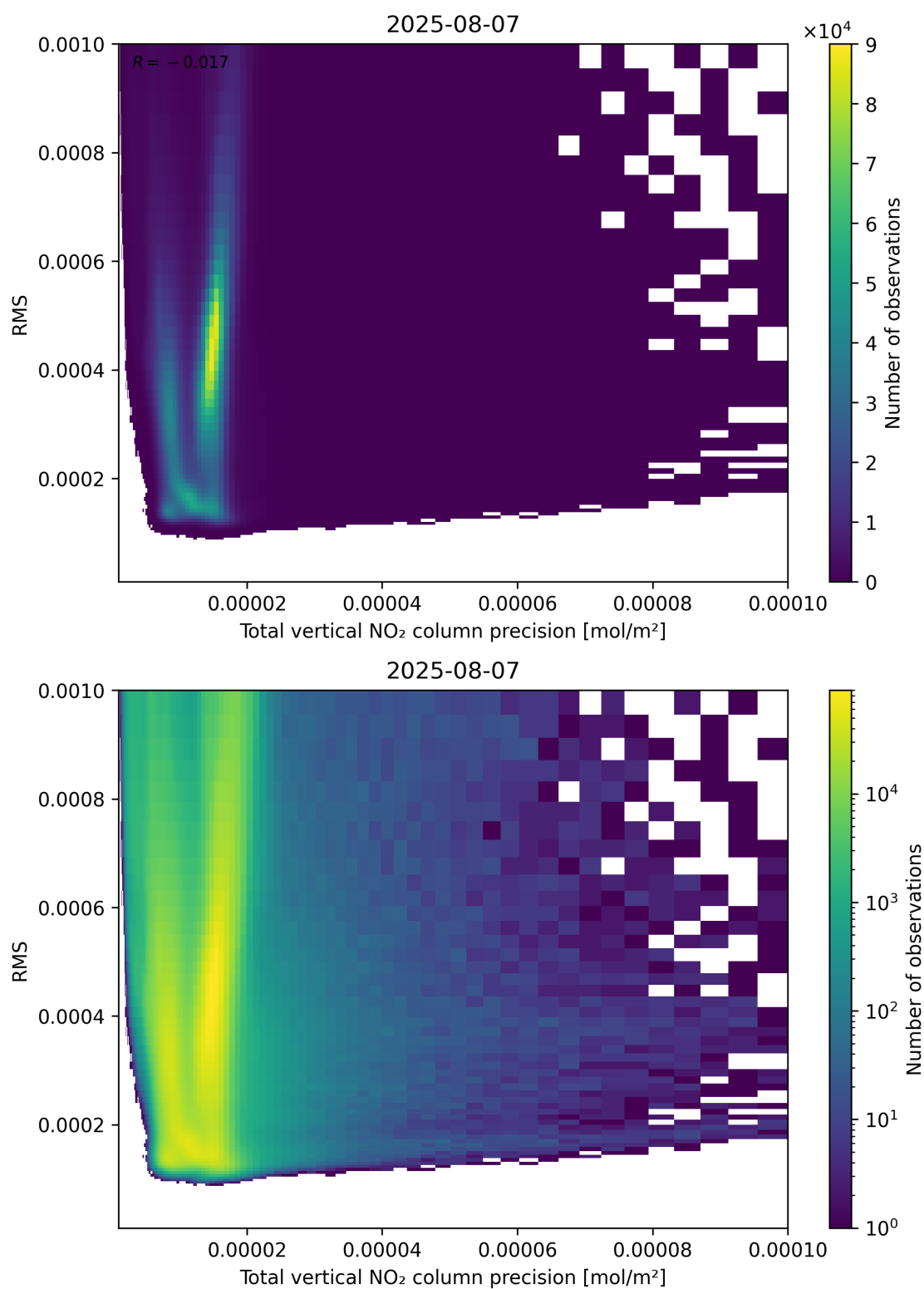
Figure 119: Scatter density plot of “Total vertical NO 2 column precision” against “RMS” for 2025-08-06 to 2025-08-08.
