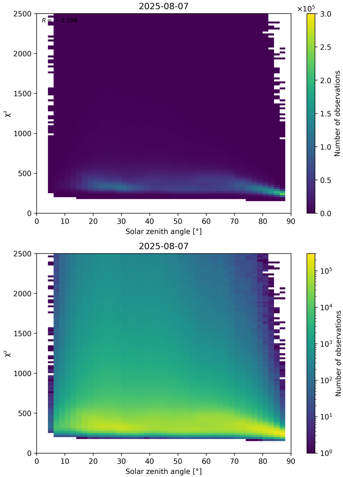
Figure 148: Scatter density plot of “Solar zenith angle” against “ \chi^2 ” for 2025-08-06 to 2025-08-08.
