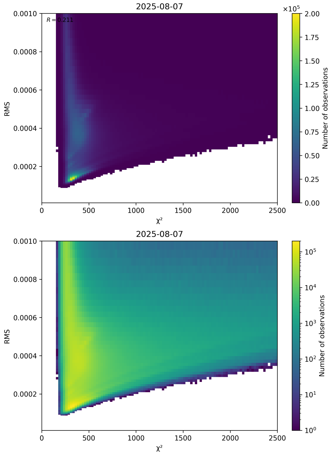
Figure 82: Scatter density plot of “ \chi^2 ” against “RMS” for 2025-08-06 to 2025-08-08.
