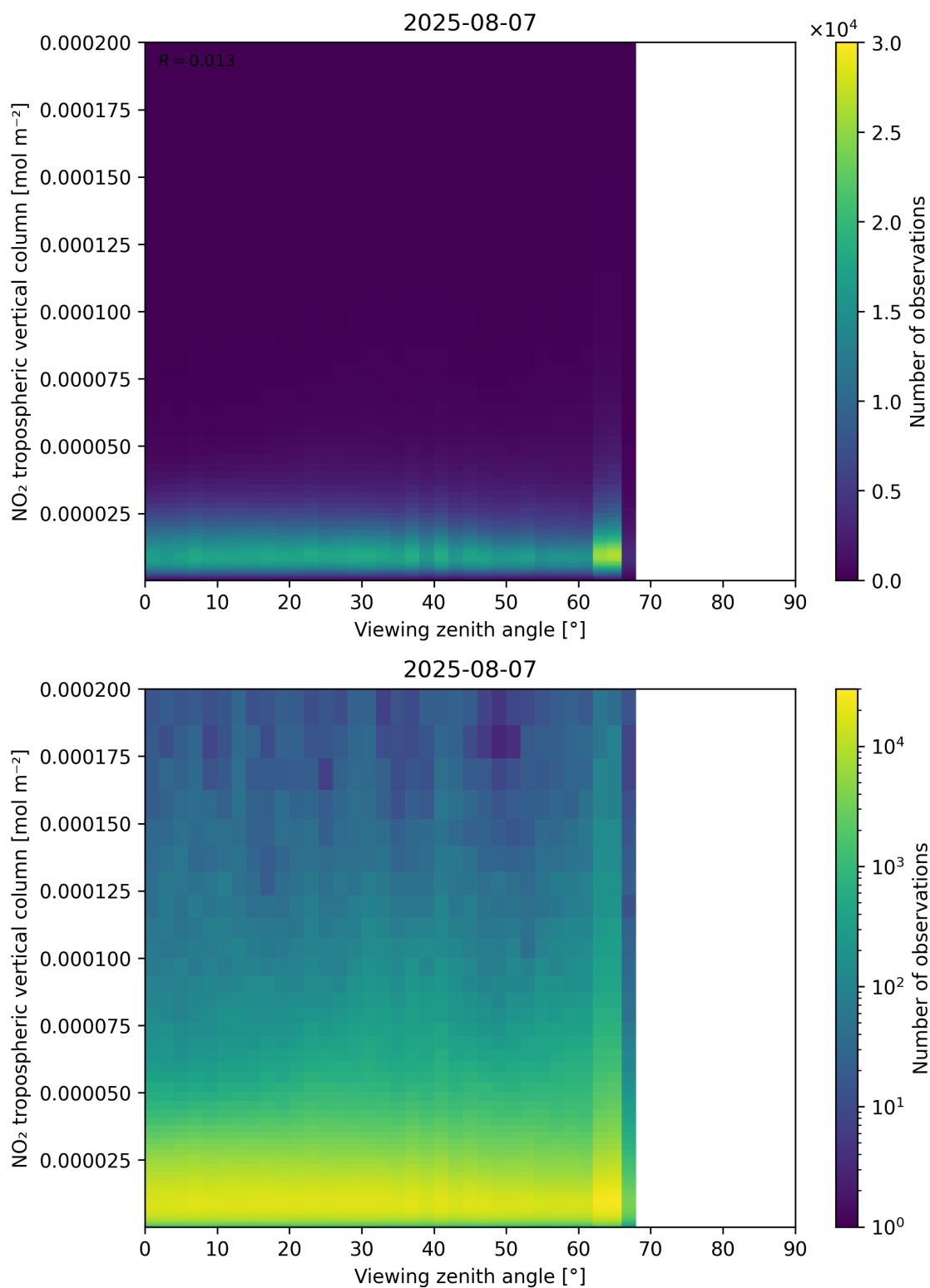
Figure 169: Scatter density plot of “Viewing zenith angle” against “NO 2 tropospheric vertical column” for 2025-08-06 to 2025-08-08.
