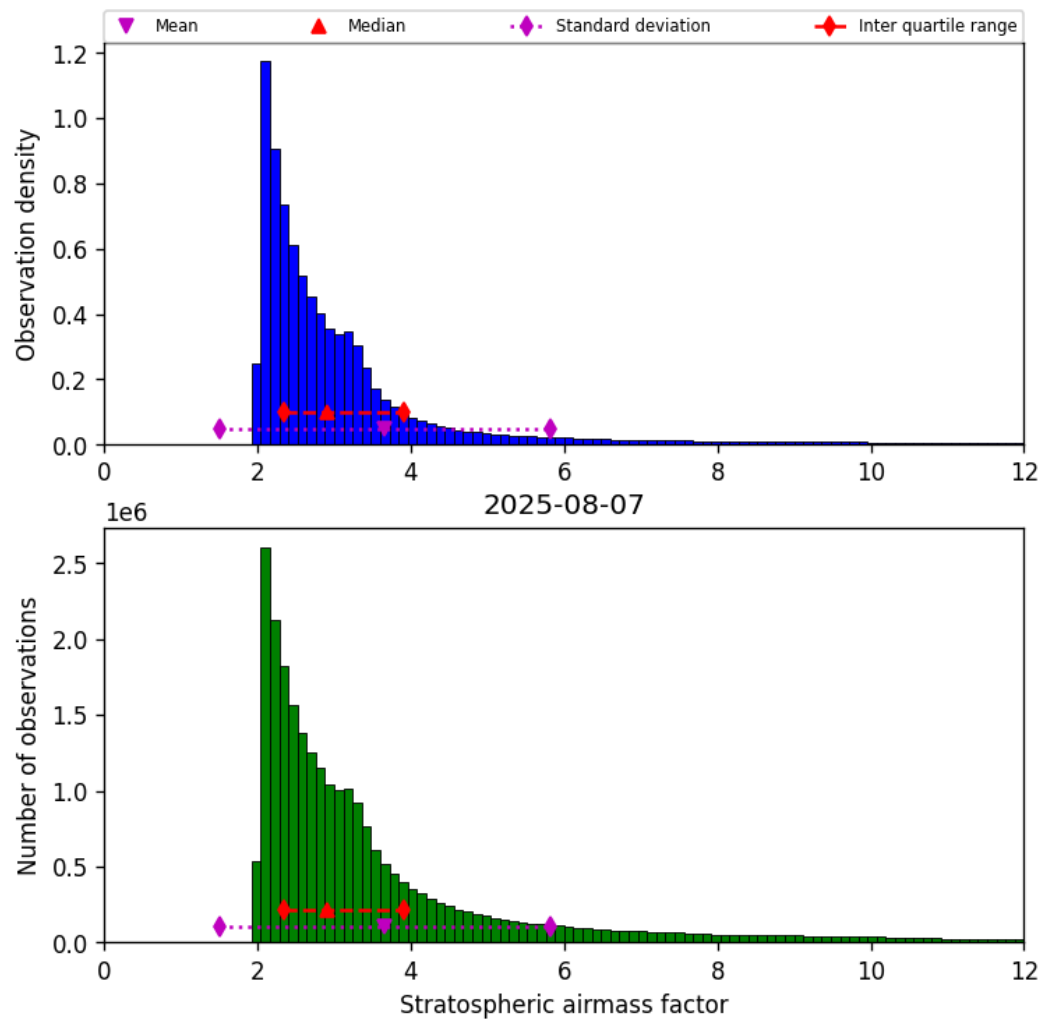
Figure 44: Histogram of “Stratospheric airmass factor” for 2025-08-06 to 2025-08-08
