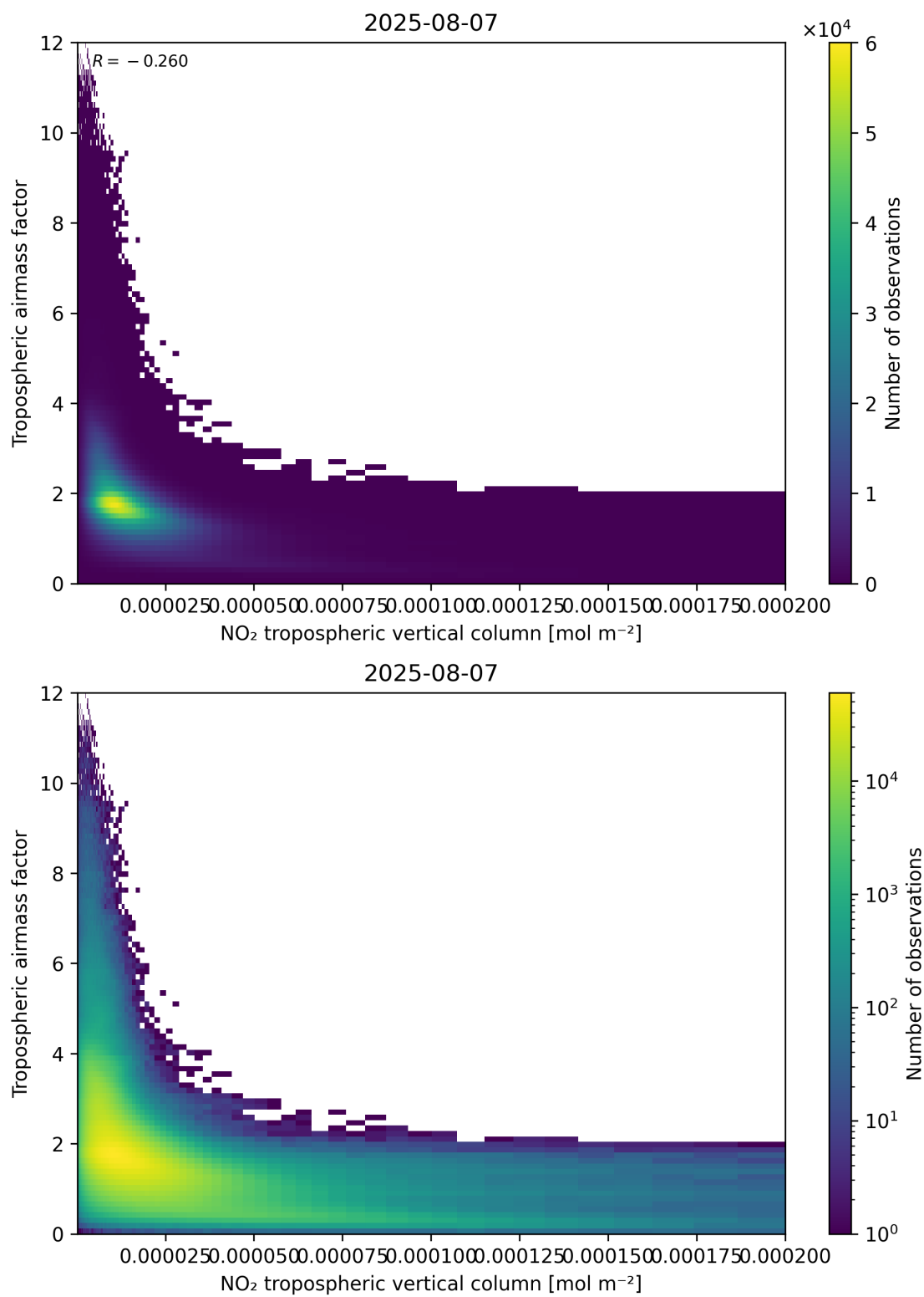
Figure 123: Scatter density plot of “NO 2 tropospheric vertical column” against “Tropospheric air mass factor” for 2025-08-06 to 2025-08-08.
