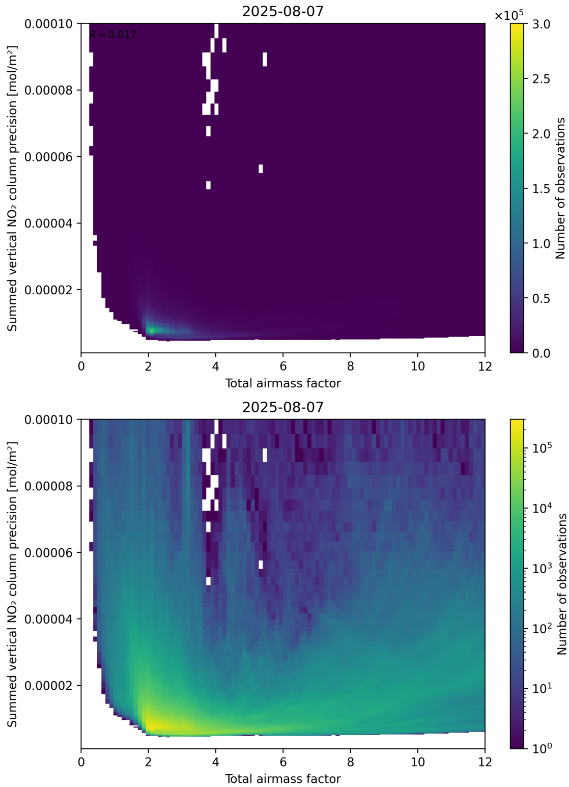
Figure 66: Scatter density plot of “Total airmass factor” against “Summed vertical NO 2 column precision” for 2025-08-06 to 2025-08-08.
