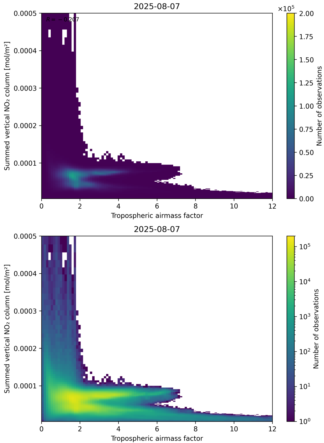
Figure 75: Scatter density plot of “Tropospheric air mass factor” against “Summed vertical NO 2 column” for 2025-08-06 to 2025-08-08.
