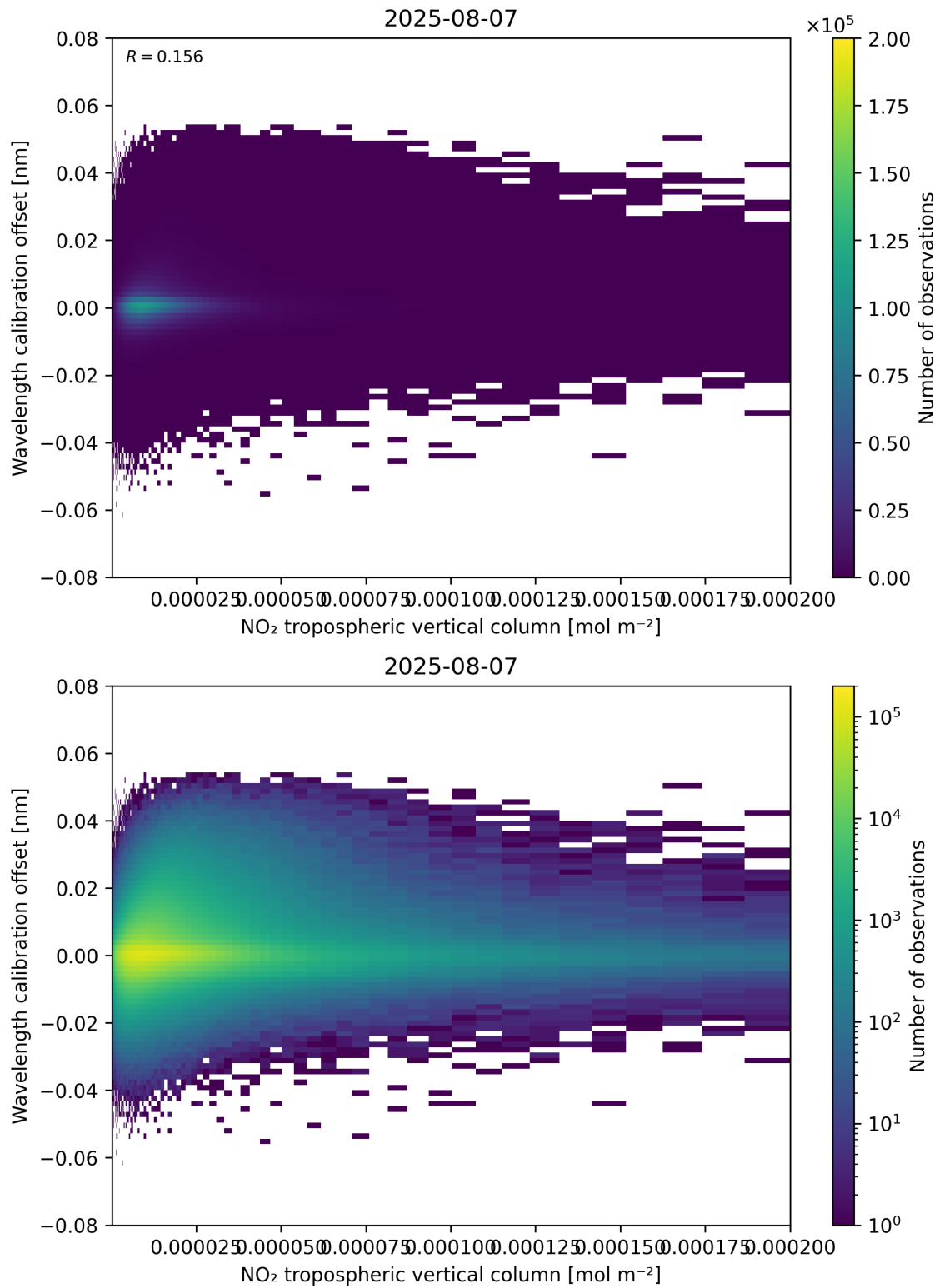
Figure 143: Scatter density plot of “NO 2 tropospheric vertical column” against “Wavelength calibration offset” for 2025-08-06 to 2025-08-08.
