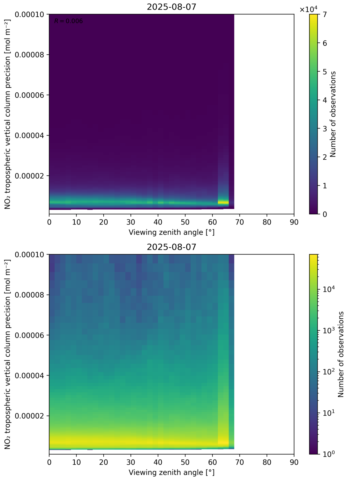
Figure 170: Scatter density plot of “Viewing zenith angle” against “NO 2 tropospheric vertical column precision” for 2025-08-06 to 2025-08-08.
