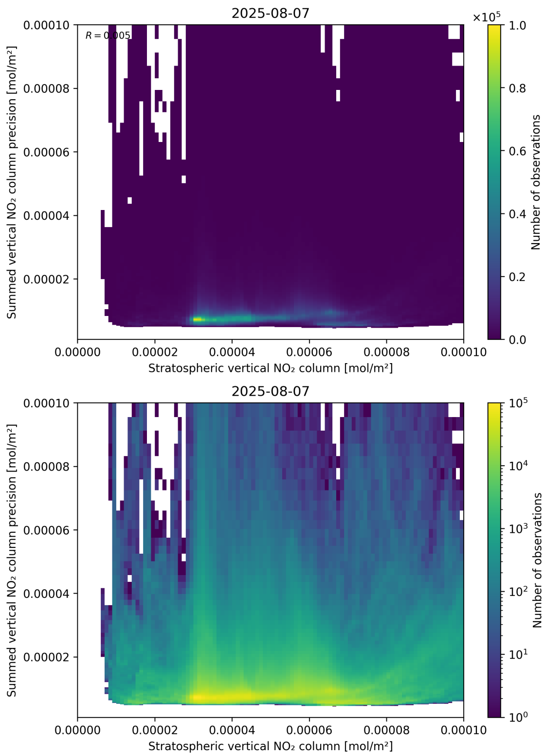
Figure 99: Scatter density plot of “Stratospheric vertical NO 2 column” against “Summed vertical NO 2 column precision” for 2025-08-06 to 2025-08-08.
