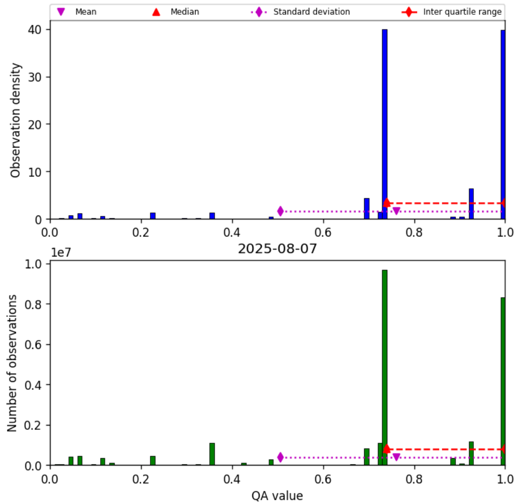
Figure 28: Histogram of “QA value” for 2025-08-06 to 2025-08-08
