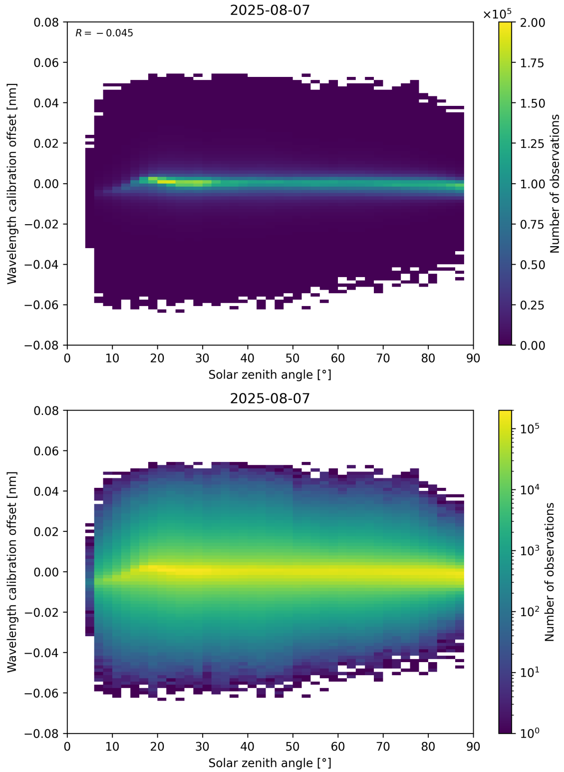
Figure 158: Scatter density plot of “Solar zenith angle” against “Wavelength calibration offset” for 2025-08-06 to 2025-08-08.
