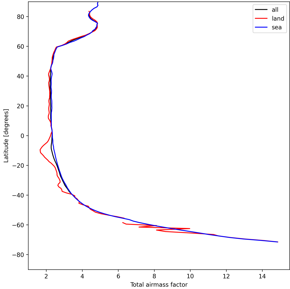
Figure 15: Zonal average of “Total airmass factor” for 2025-08-06 to 2025-08-08.
