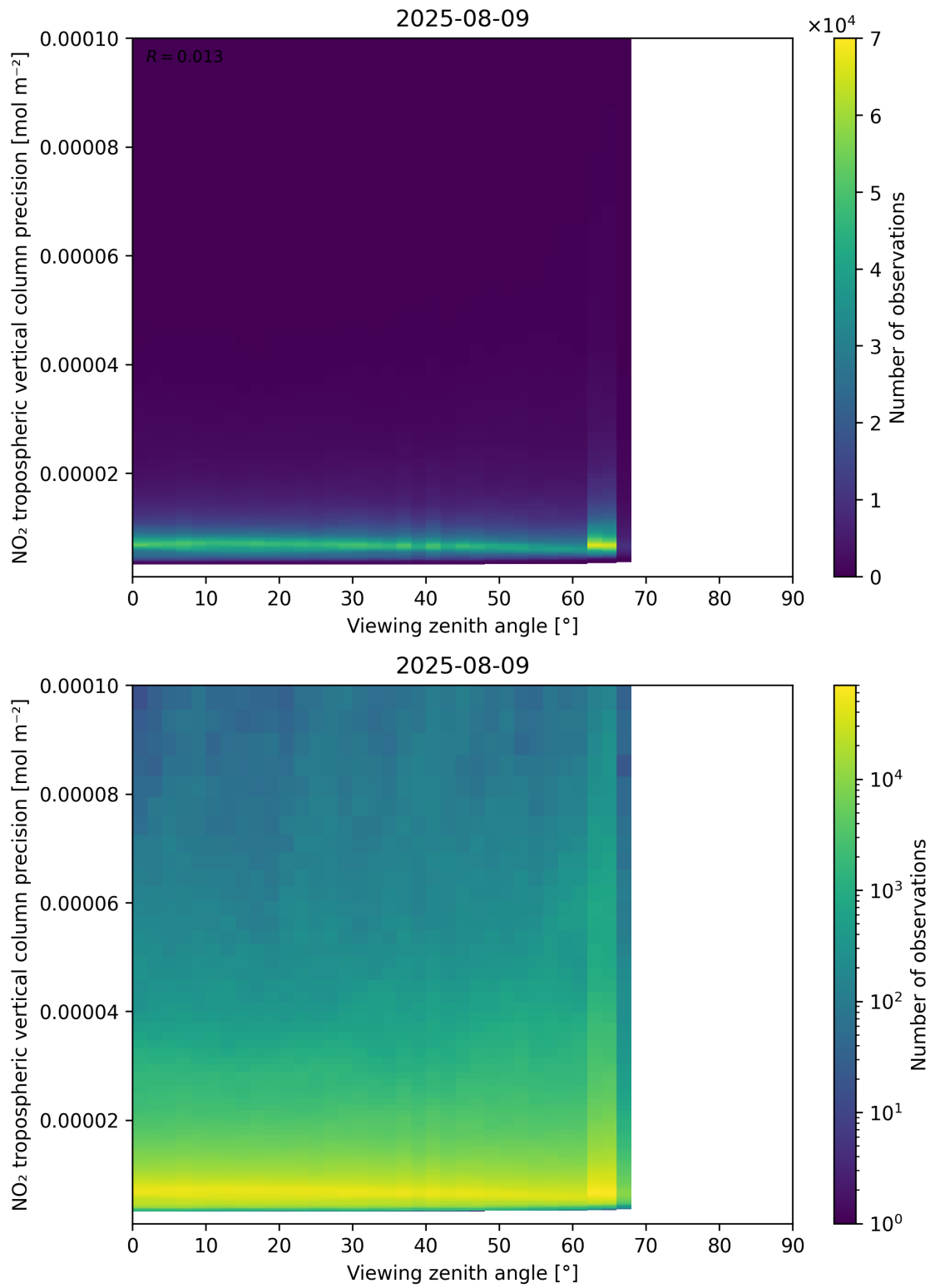
Figure 170: Scatter density plot of “Viewing zenith angle” against “NO 2 tropospheric vertical column precision” for 2025-08-09 to 2025-08-10.
