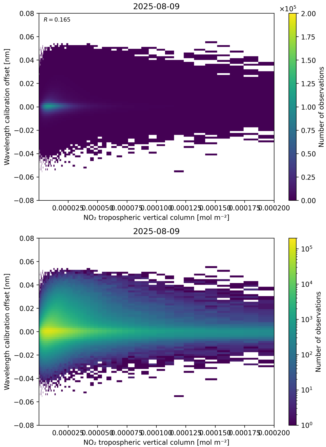
Figure 143: Scatter density plot of “NO 2 tropospheric vertical column” against “Wavelength calibration offset” for 2025-08-09 to 2025-08-10.
