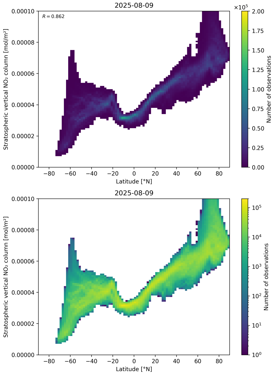
Figure 87: Scatter density plot of “Latitude” against “Stratospheric vertical NO 2 column” for 2025-08-09 to 2025-08-10.
