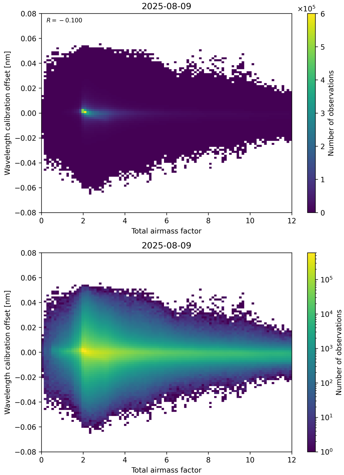
Figure 70: Scatter density plot of “Total airmass factor” against “Wavelength calibration offset” for 2025-08-09 to 2025-08-10.
