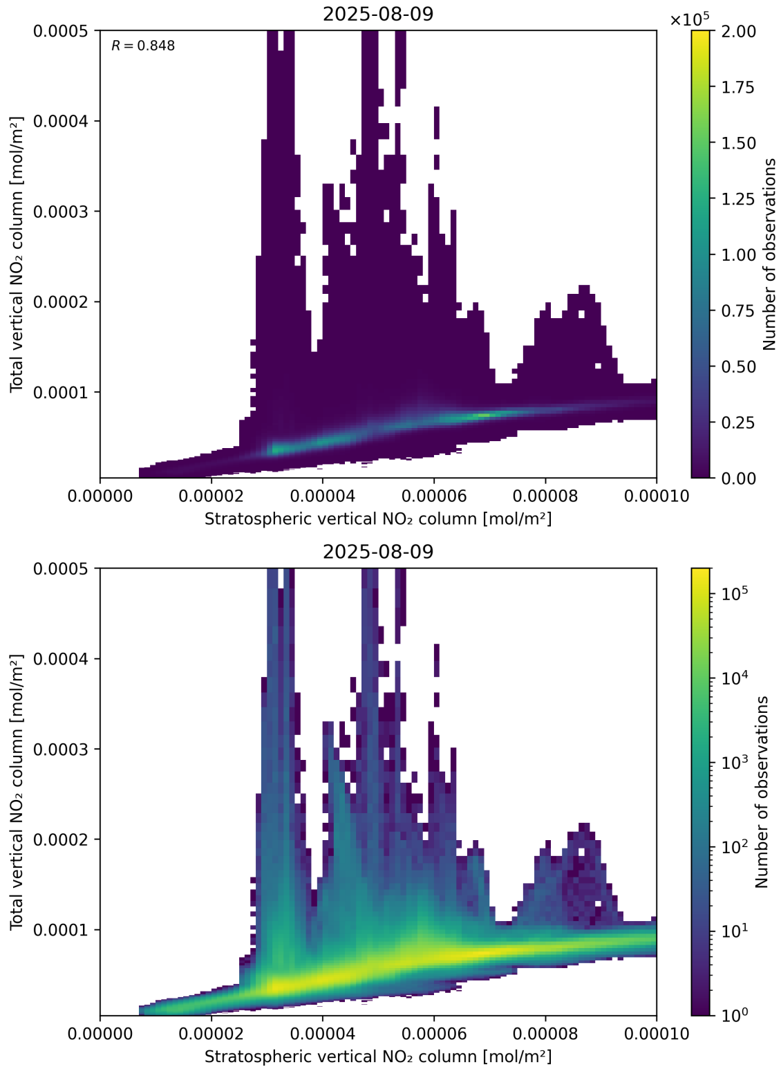
Figure 100: Scatter density plot of “Stratospheric vertical NO 2 column” against “Total vertical NO 2 column” for 2025-08-09 to 2025-08-10.
