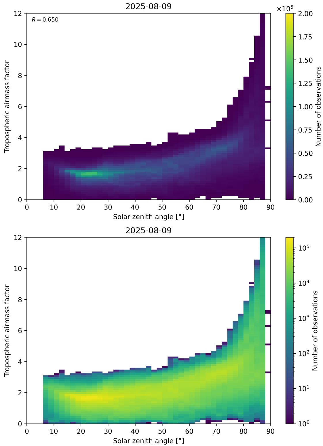
Figure 147: Scatter density plot of “Solar zenith angle” against “Tropospheric airmass factor” for 2025-08-09 to 2025-08-10.
