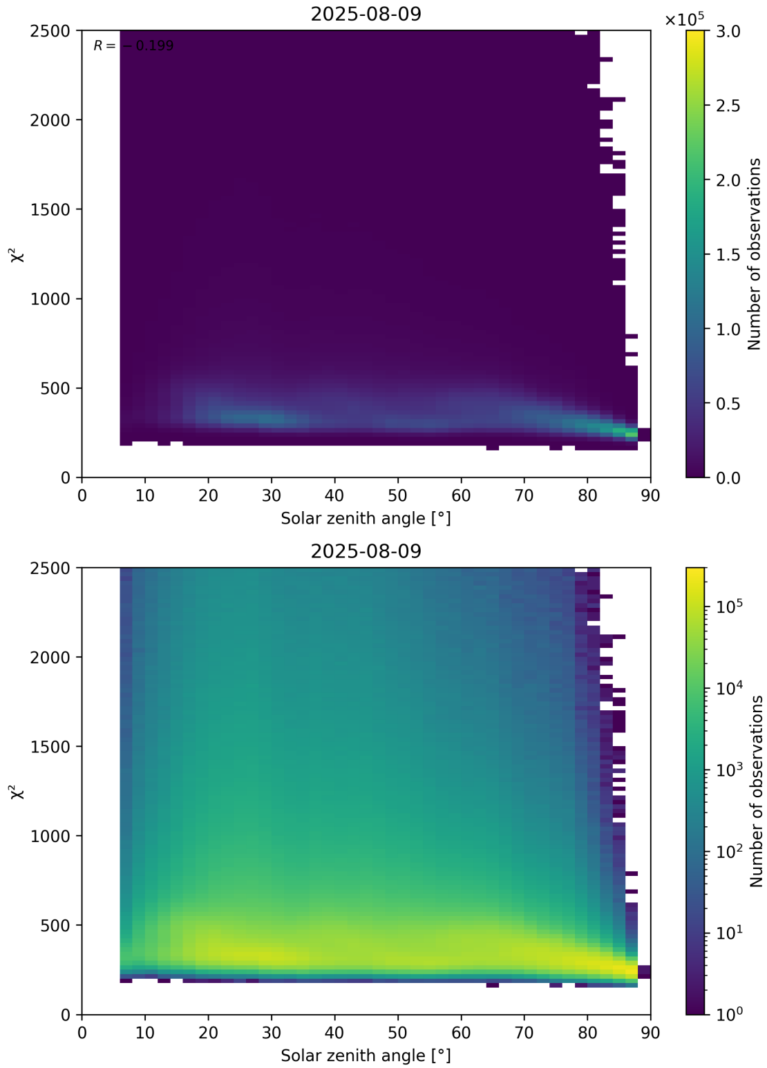
Figure 148: Scatter density plot of “Solar zenith angle” against “ \chi^2 ” for 2025-08-09 to 2025-08-10.
