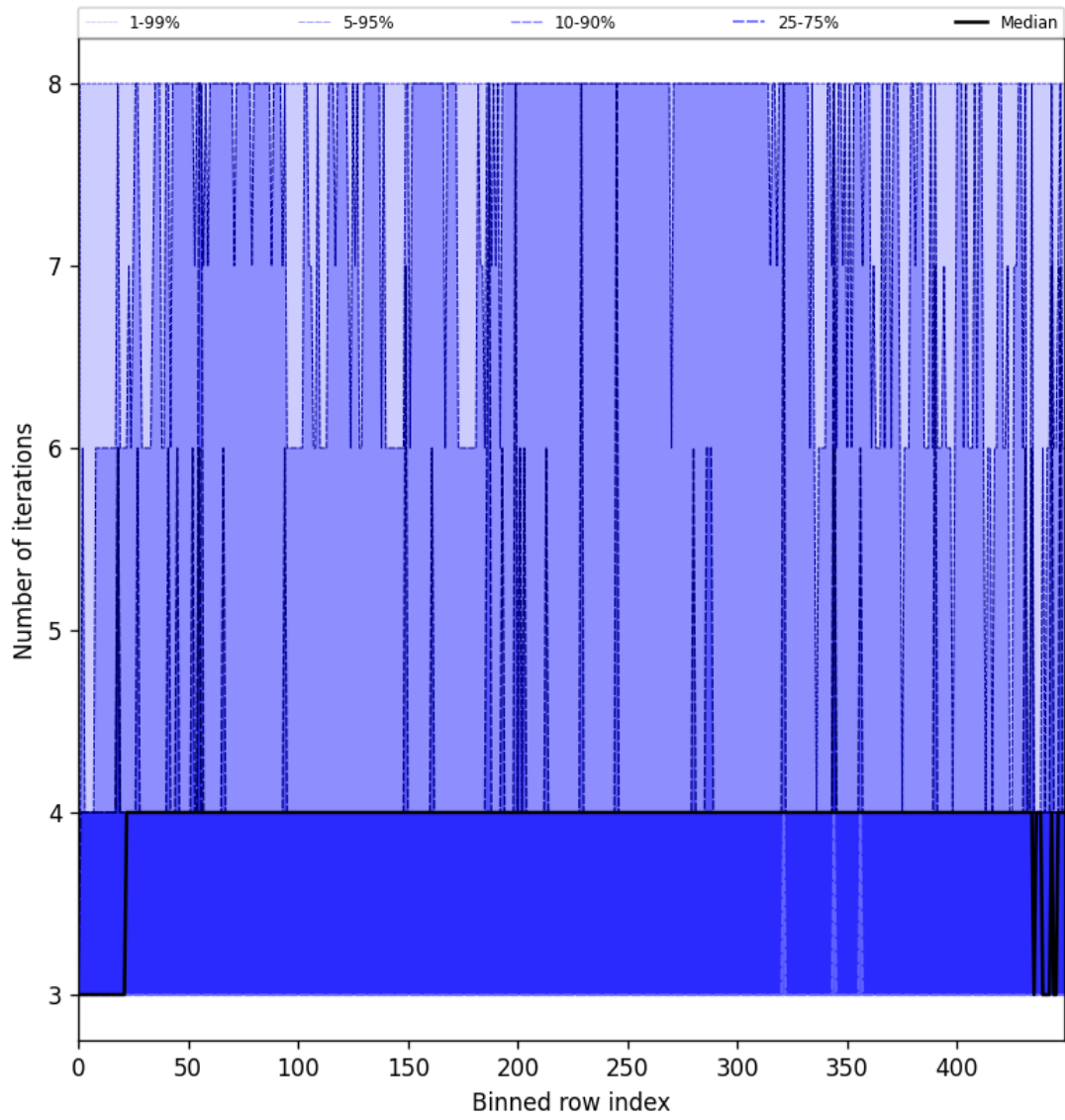
Figure 51: Along track statistics of “Number of iterations” for 2025-08-09 to 2025-08-10
