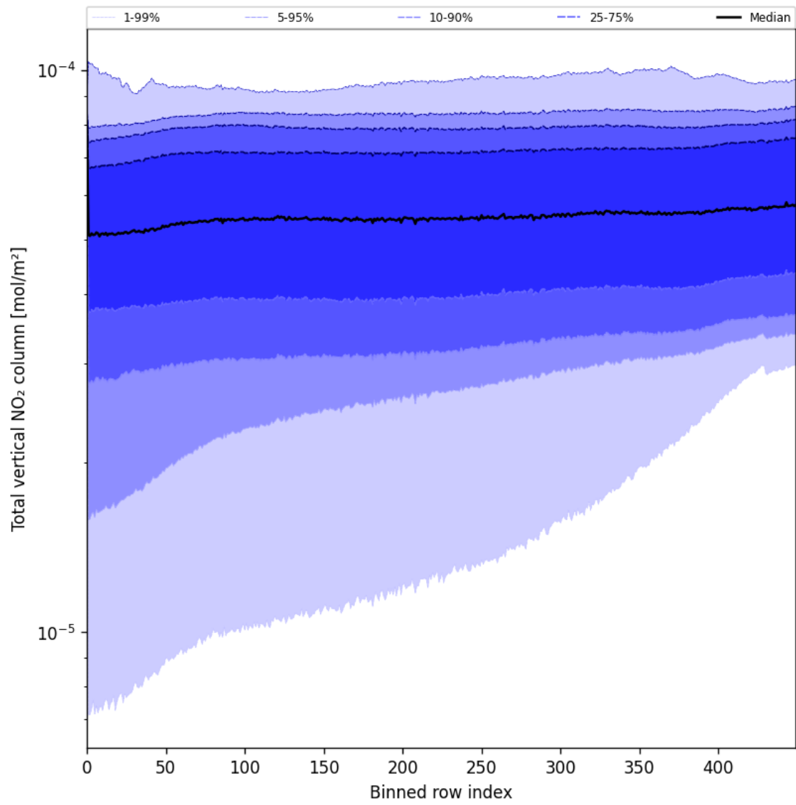
Figure 55: Along track statistics of “Total vertical NO 2 column” for 2025-08-09 to 2025-08-10
