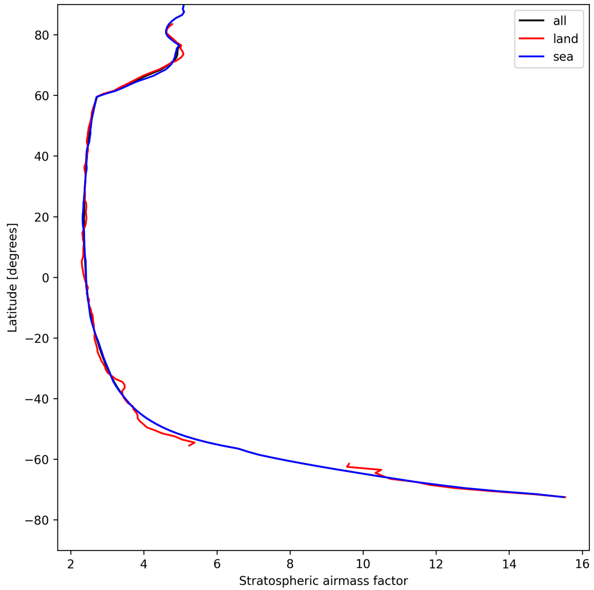
Figure 27: Zonal average of “Stratospheric airmass factor” for 2025-08-09 to 2025-08-10.
