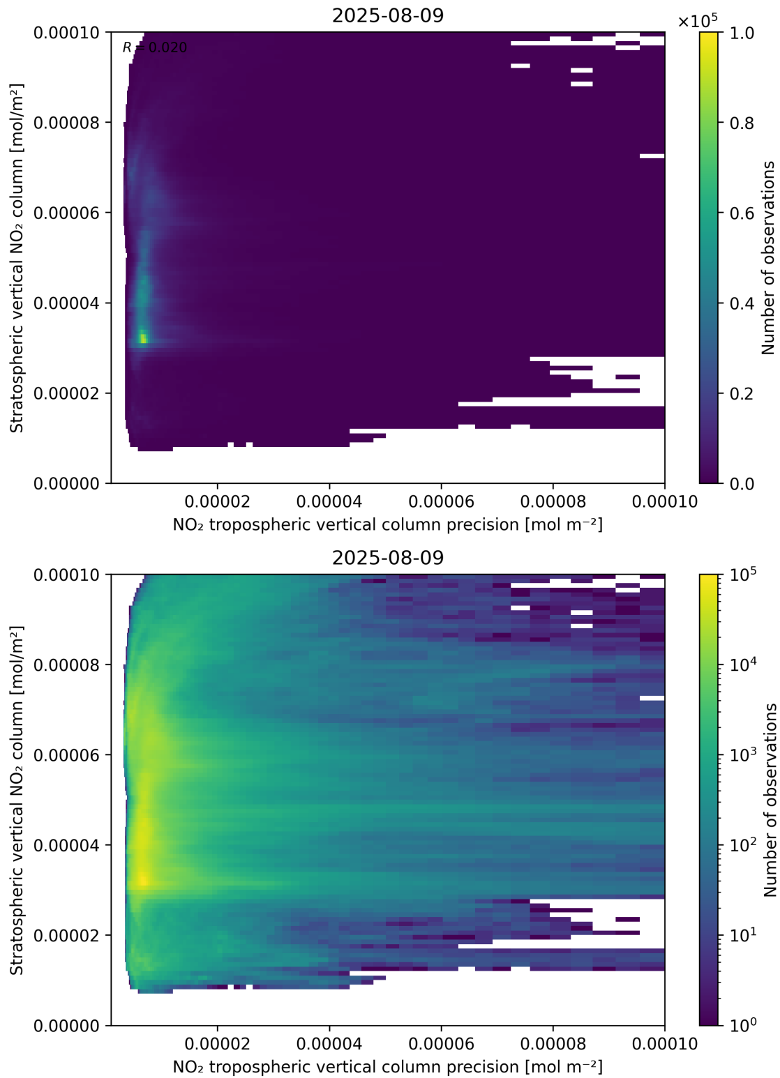
Figure 135: Scatter density plot of “NO 2 tropospheric vertical column precision” against “Stratospheric vertical NO 2 column” for 2025-08-09 to 2025-08-10.
