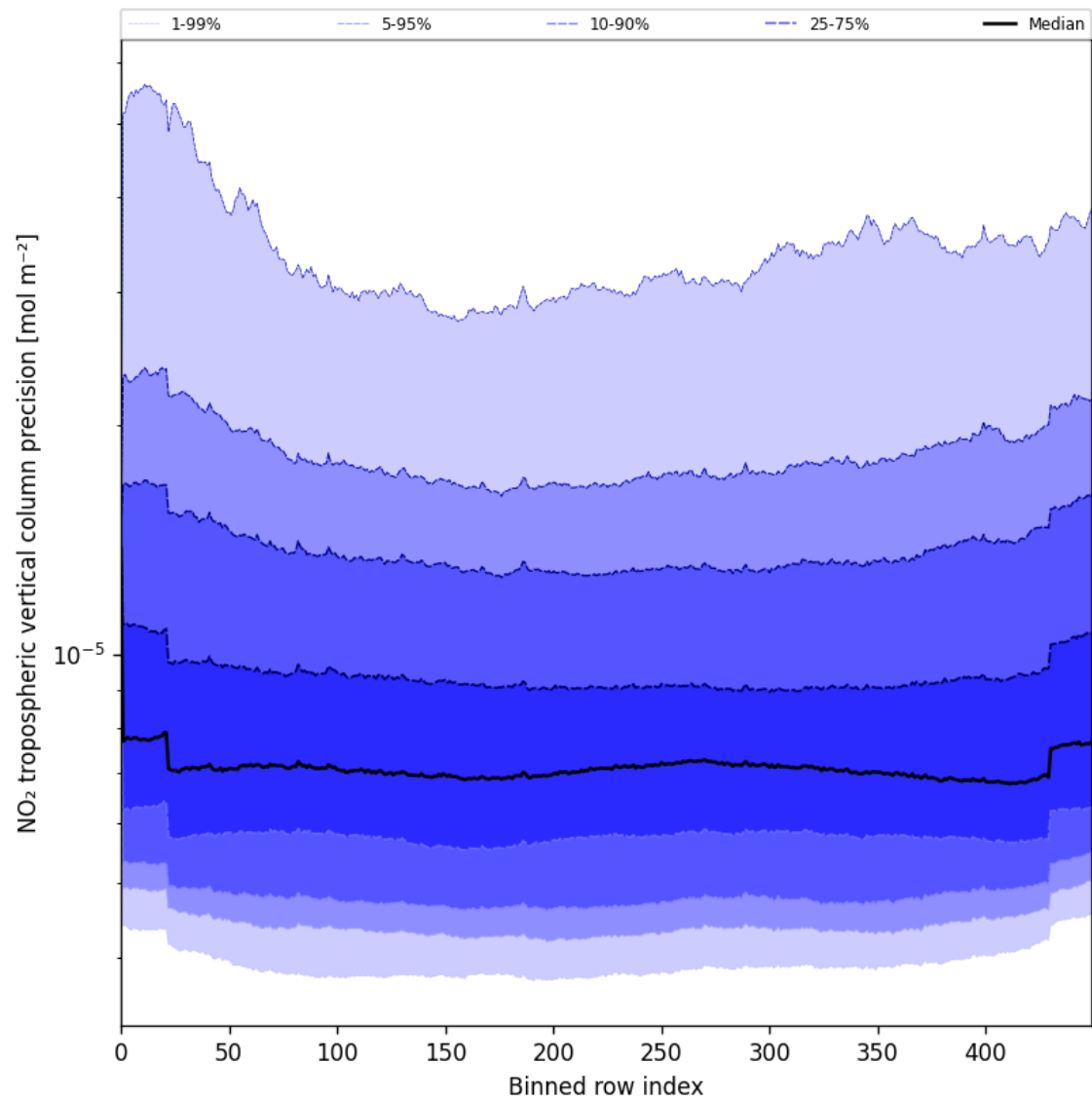
Figure 47: Along track statistics of “NO 2 tropospheric vertical column precision” for 2025-08-09 to 2025-08-10
