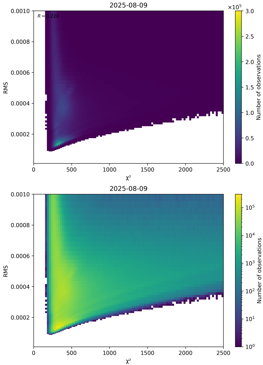
Figure 82: Scatter density plot of “ \chi^2 ” against “RMS” for 2025-08-09 to 2025-08-10.
