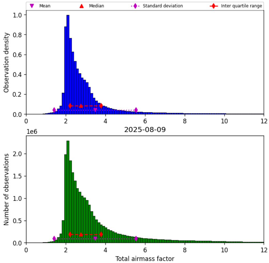
Figure 32: Histogram of “Total airmass factor” for 2025-08-09 to 2025-08-10
