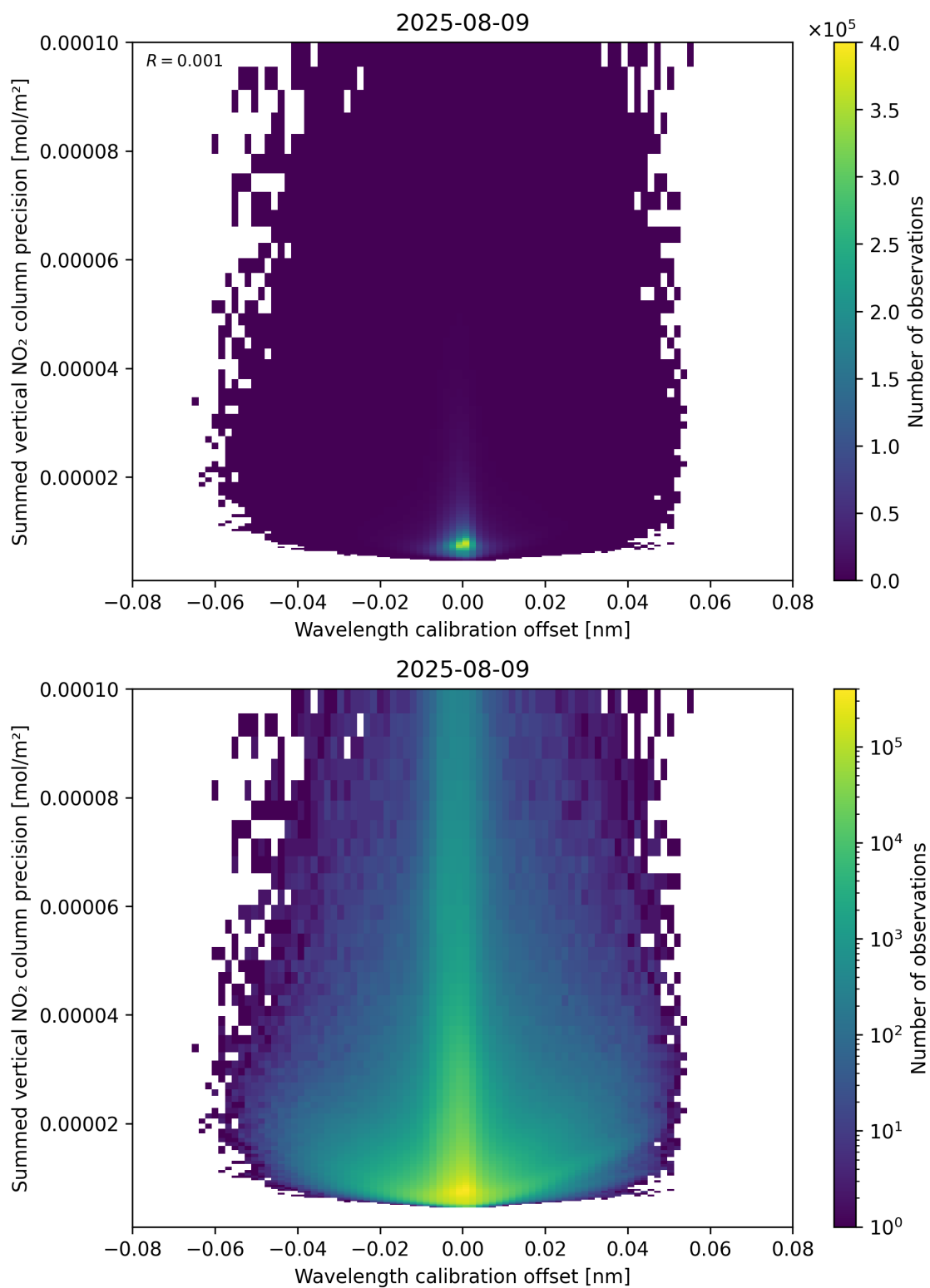
Figure 178: Scatter density plot of “Wavelength calibration offset” against “Summed vertical NO 2 column precision” for 2025-08-09 to 2025-08-10.
