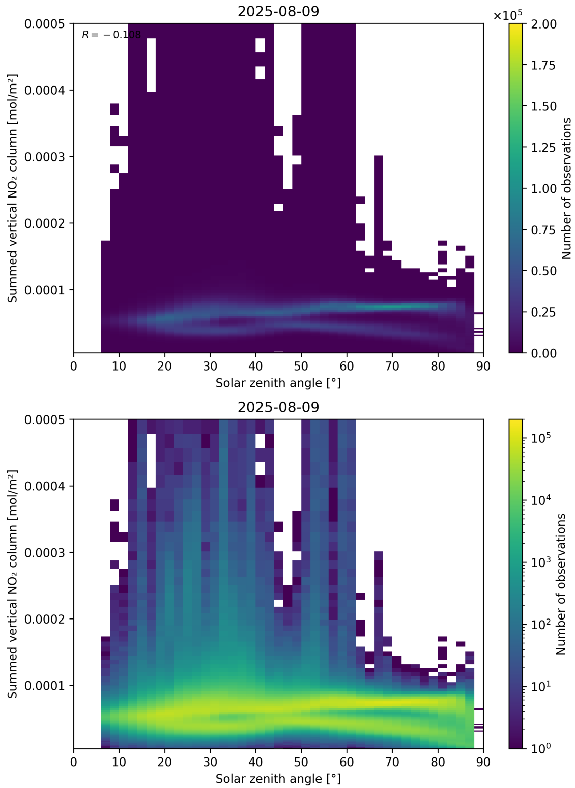
Figure 151: Scatter density plot of “Solar zenith angle” against “Summed vertical NO 2 column” for 2025-08-09 to 2025-08-10.
