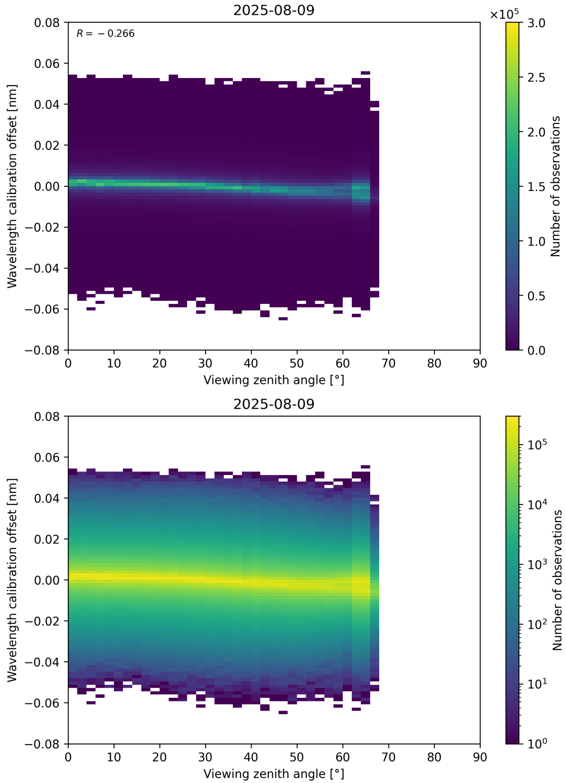
Figure 173: Scatter density plot of “Viewing zenith angle” against “Wavelength calibration offset” for 2025-08-09 to 2025-08-10.
