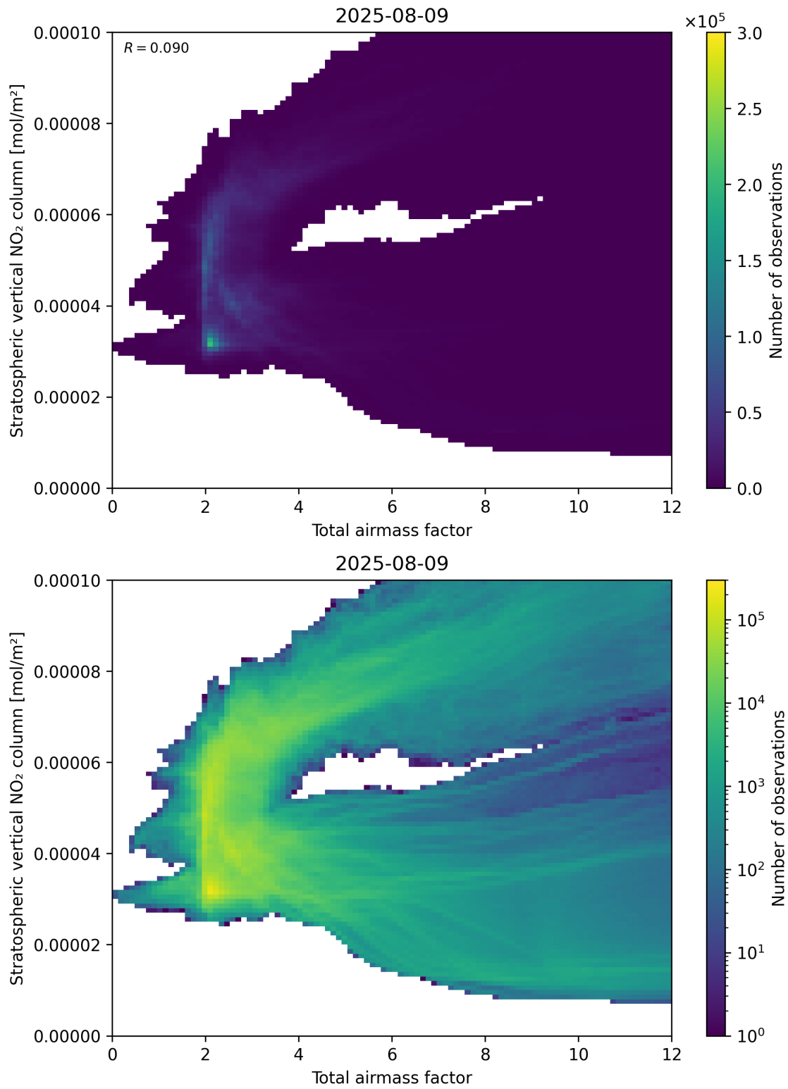
Figure 64: Scatter density plot of “Total airmass factor” against “Stratospheric vertical \text{NO}_2 column” for 2025-08-09 to 2025-08-10.
