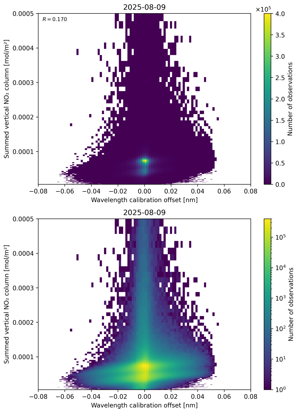
Figure 177: Scatter density plot of “Wavelength calibration offset” against “Summed vertical NO 2 column” for 2025-08-09 to 2025-08-10.
