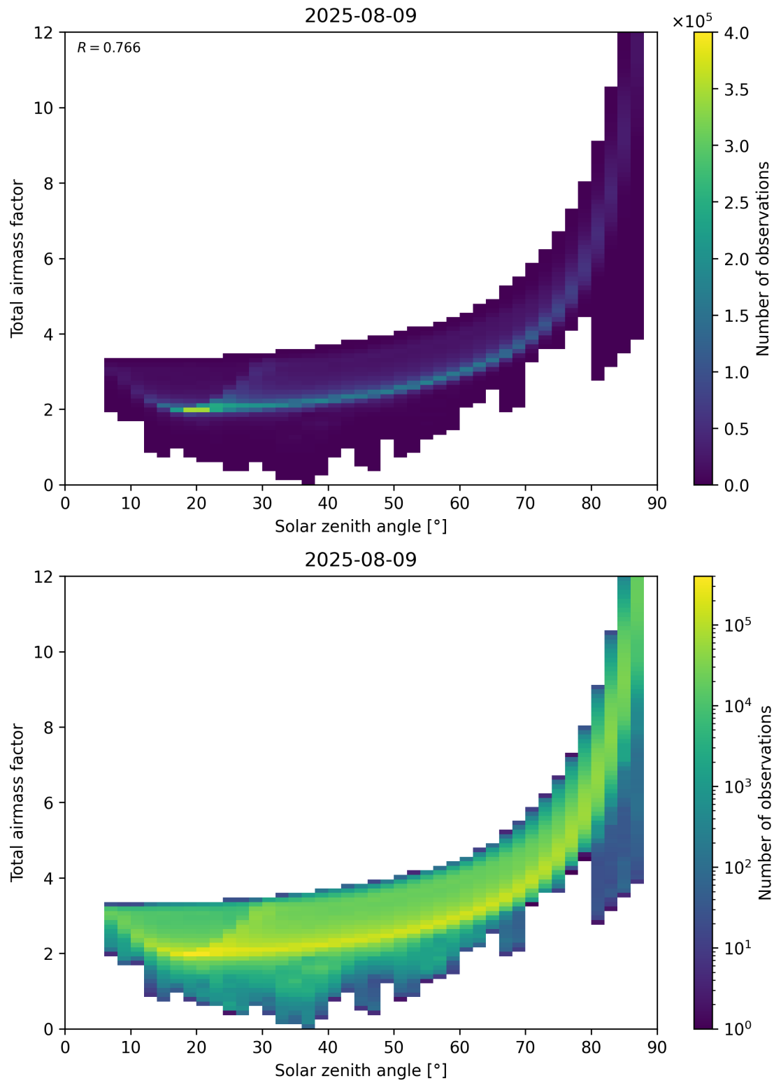
Figure 146: Scatter density plot of “Solar zenith angle” against “Total air mass factor” for 2025-08-09 to 2025-08-10.
