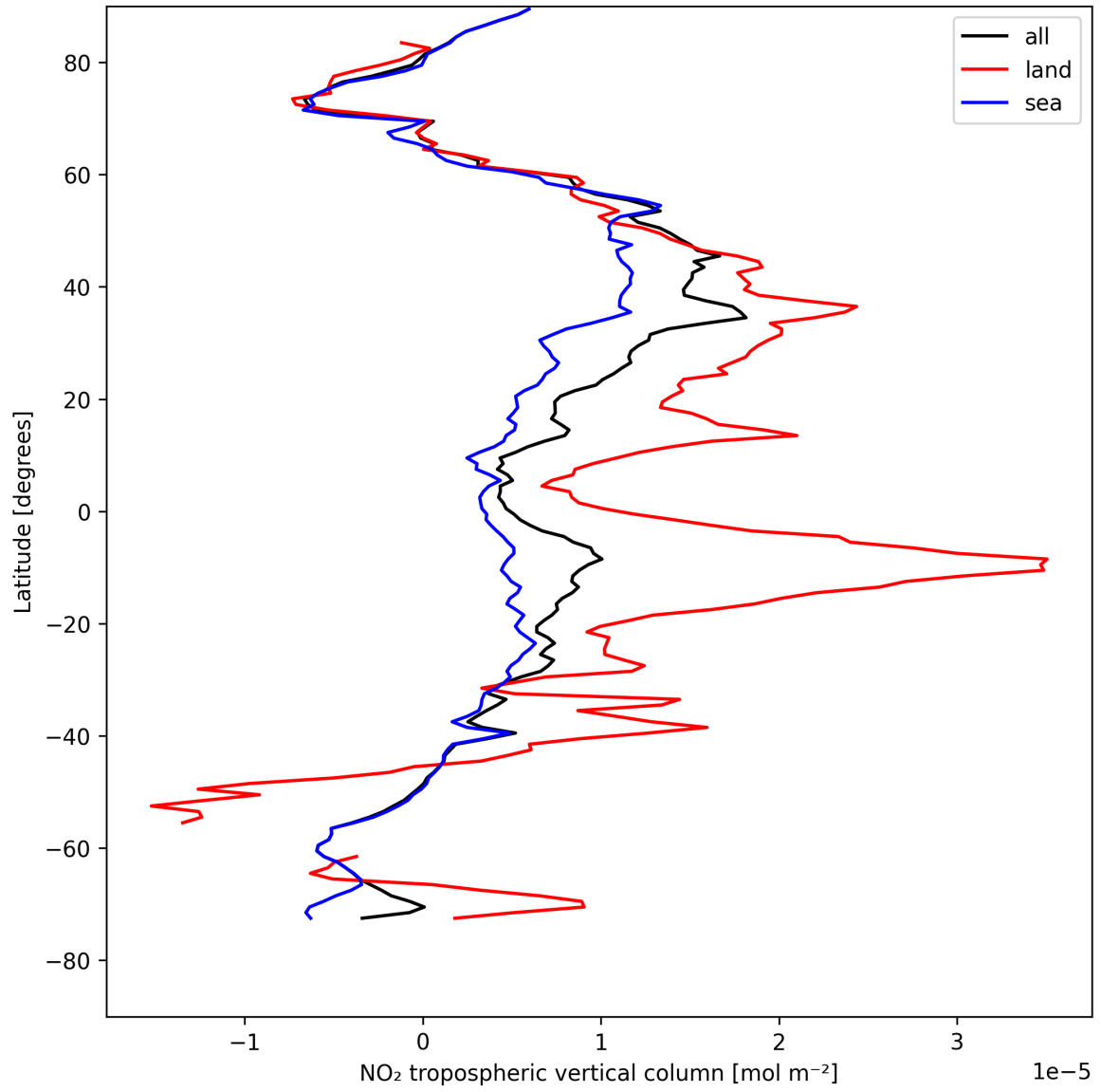
Figure 12: Zonal average of “NO 2 tropospheric vertical column” for 2025-08-09 to 2025-08-10.
