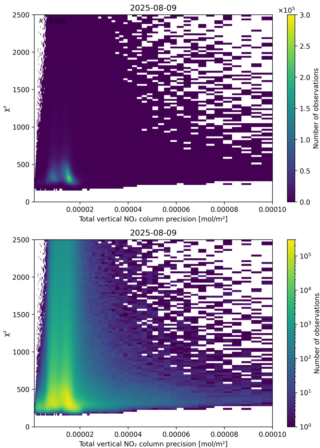
Figure 116: Scatter density plot of “Total vertical NO 2 column precision” against “ \chi^2 ” for 2025-08-09 to 2025-08-10.
