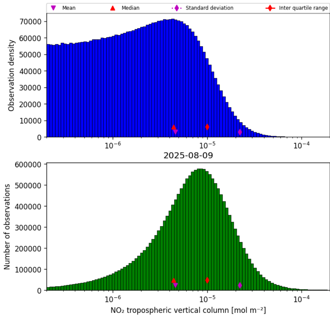
Figure 29: Histogram of “NO 2 tropospheric vertical column” for 2025-08-09 to 2025-08-10
