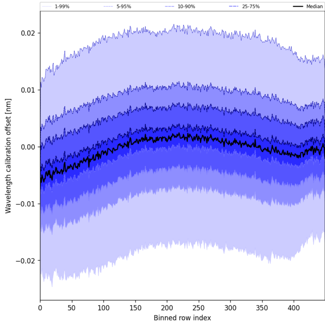
Figure 52: Along track statistics of “Wavelength calibration offset” for 2025-08-09 to 2025-08-10
