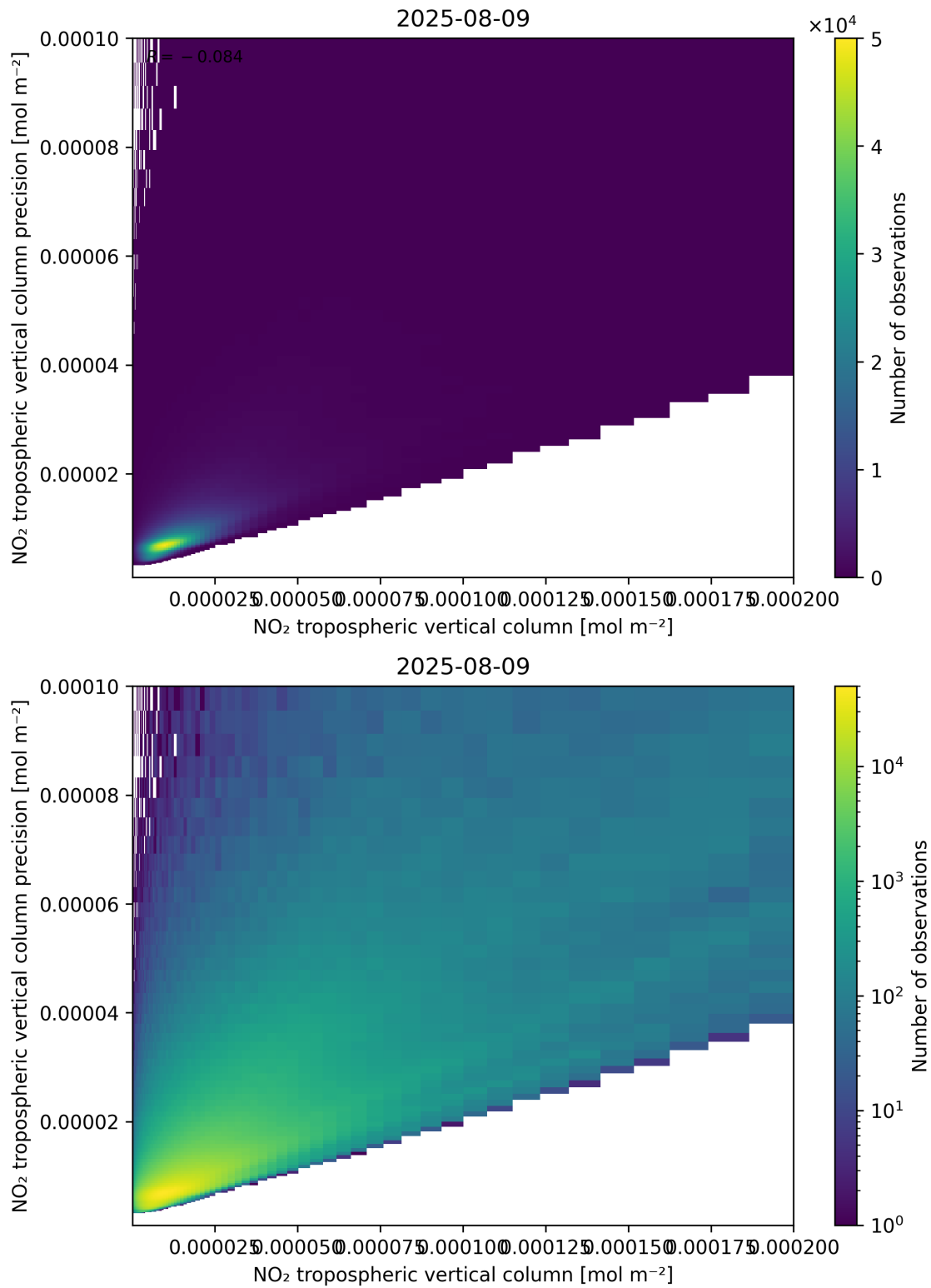
Figure 130: Scatter density plot of “NO 2 tropospheric vertical column” against “NO 2 tropospheric vertical column precision” for 2025-08-09 to 2025-08-10.
