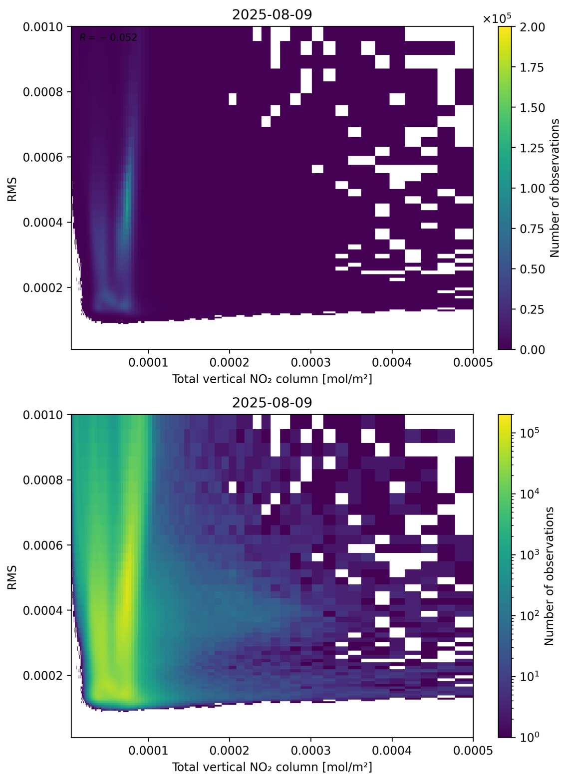
Figure 120: Scatter density plot of “Total vertical NO 2 column” against “RMS” for 2025-08-09 to 2025-08-10.
