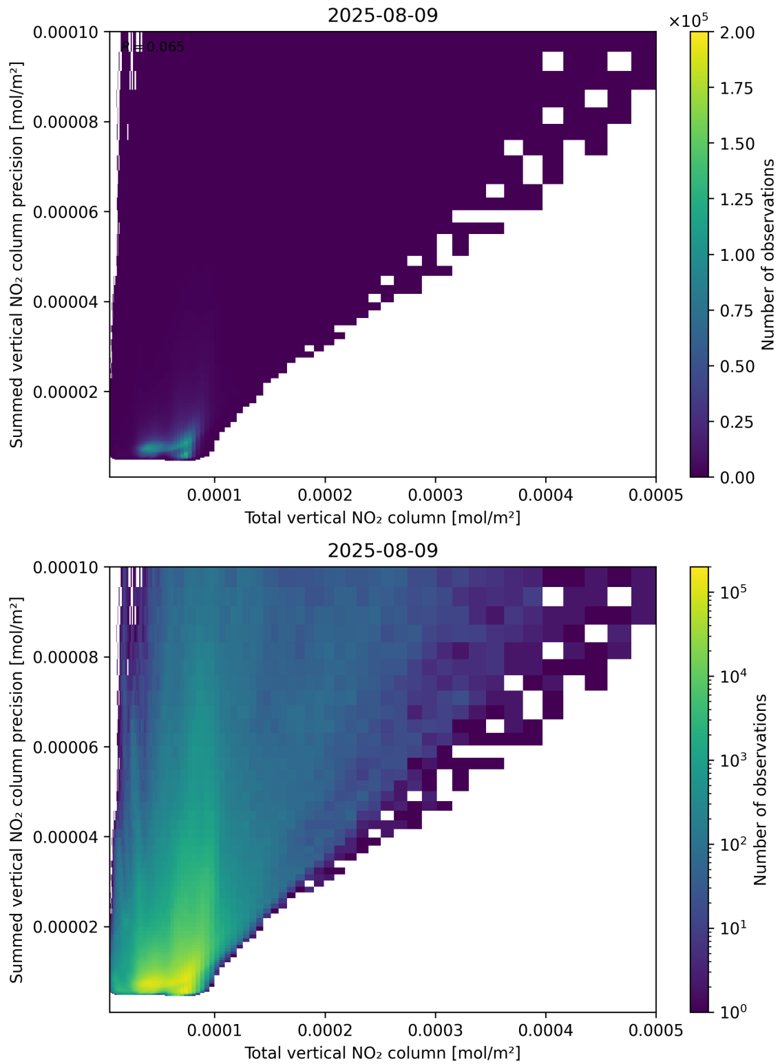
Figure 113: Scatter density plot of “Total vertical NO 2 column” against “Summed vertical NO 2 column precision” for 2025-08-09 to 2025-08-10.
