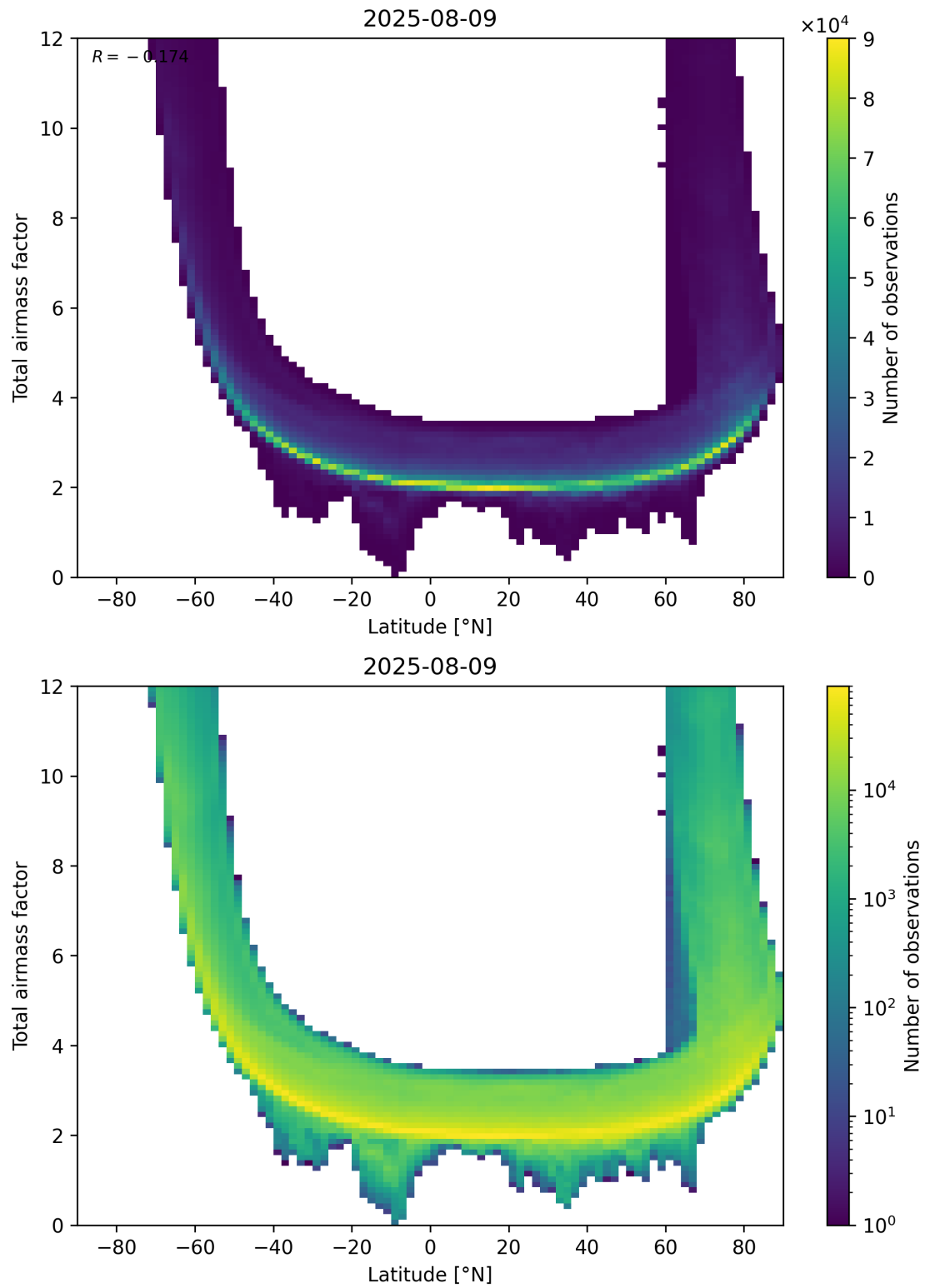
Figure 84: Scatter density plot of “Latitude” against “Total airmass factor” for 2025-08-09 to 2025-08-10.
