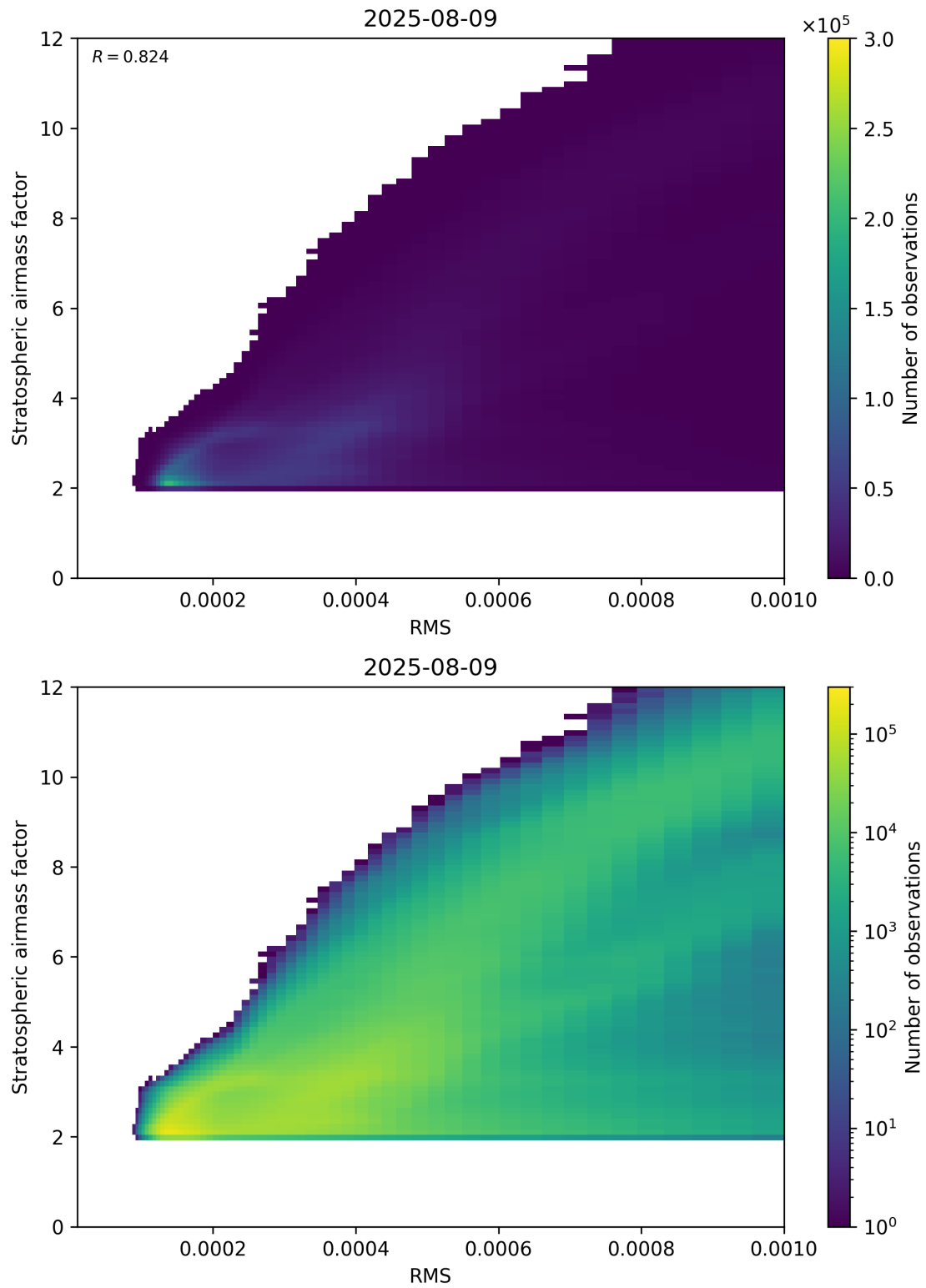
Figure 144: Scatter density plot of “RMS” against “Stratospheric airmass factor” for 2025-08-09 to 2025-08-10.
