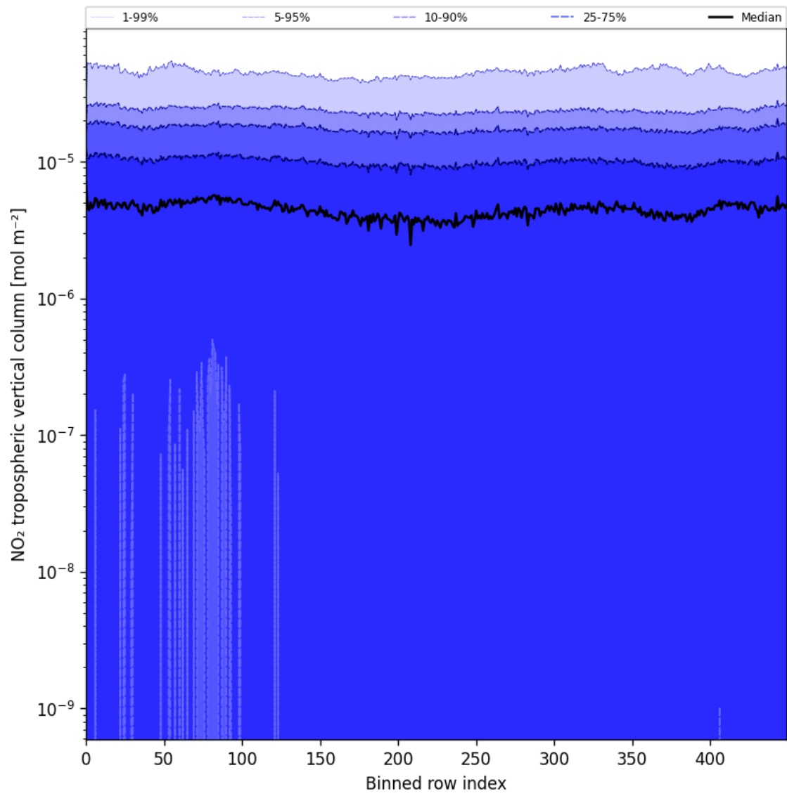
Figure 46: Along track statistics of “NO 2 tropospheric vertical column” for 2025-08-09 to 2025-08-10
