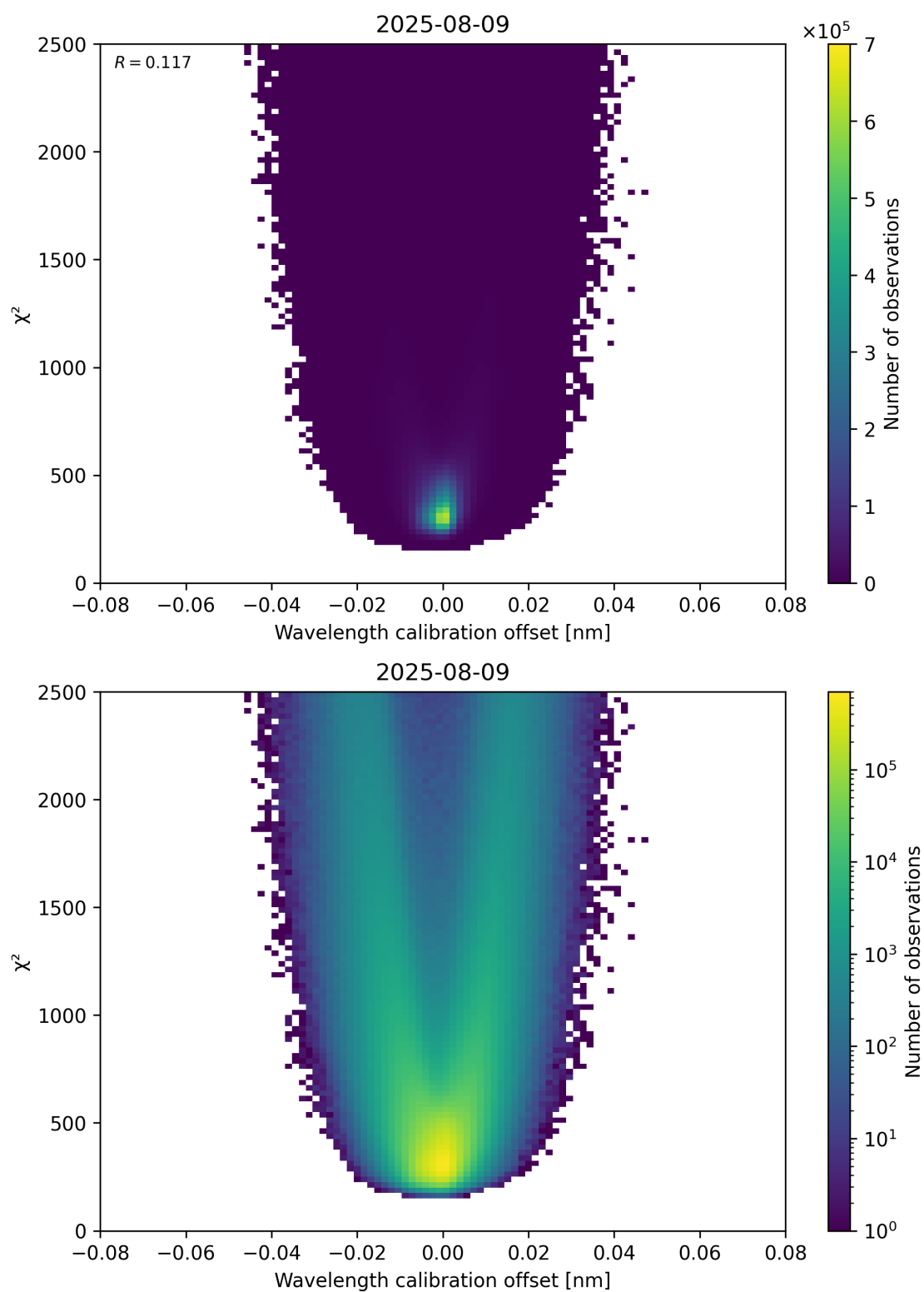
Figure 175: Scatter density plot of “Wavelength calibration offset” against “ \chi^2 ” for 2025-08-09 to 2025-08-10.
