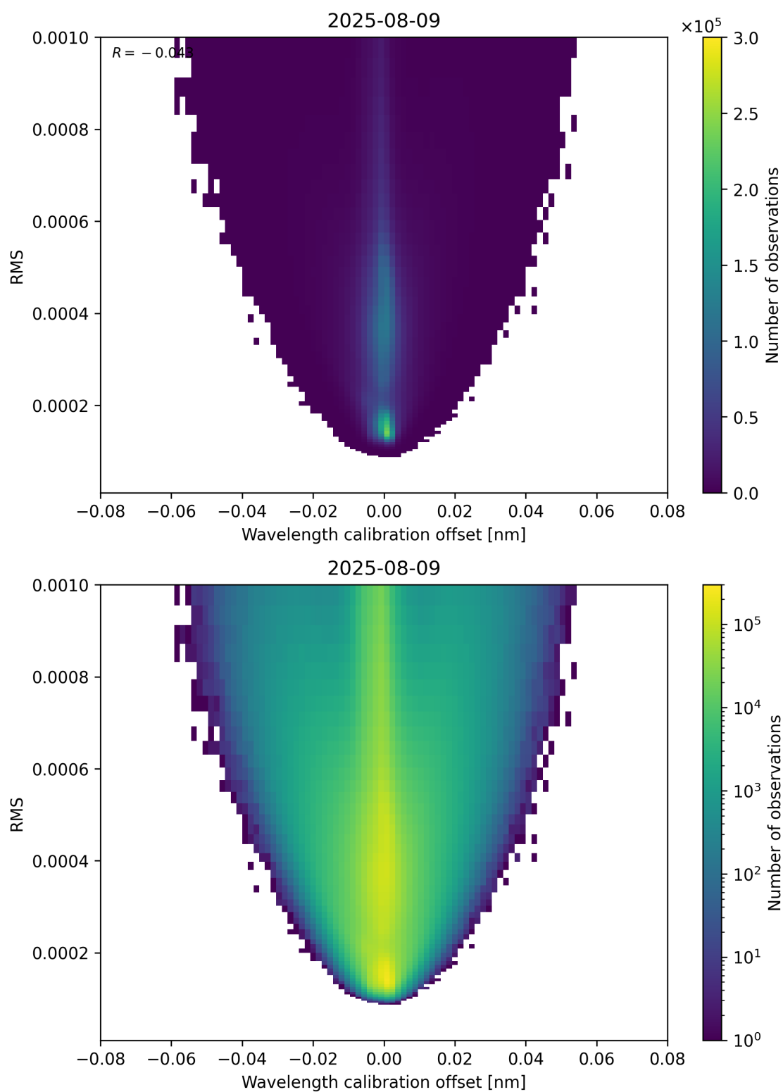
Figure 181: Scatter density plot of “Wavelength calibration offset” against “RMS” for 2025-08-09 to 2025-08-10.
