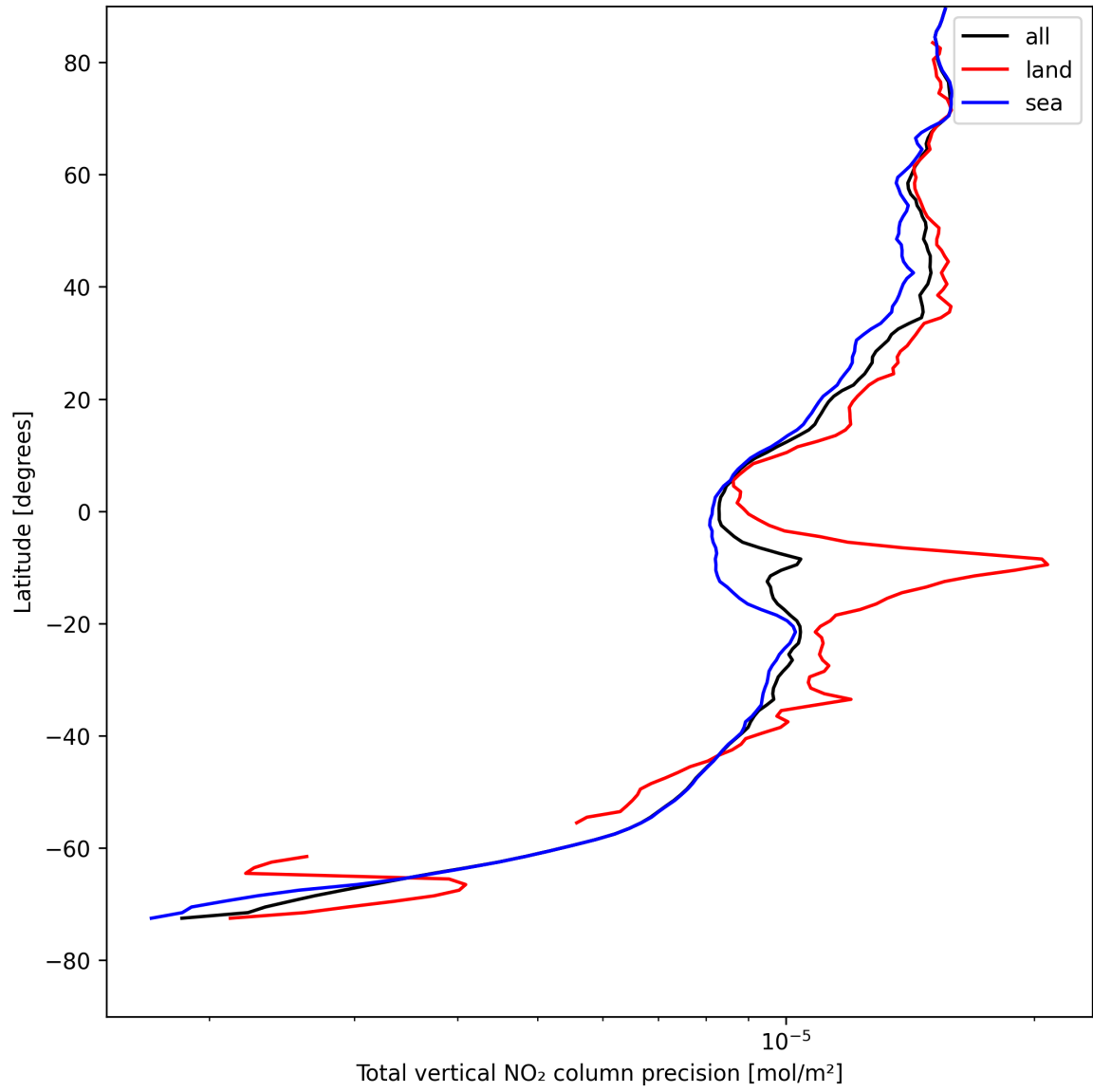
Figure 22: Zonal average of “Total vertical NO 2 column precision” for 2025-08-09 to 2025-08-10.
