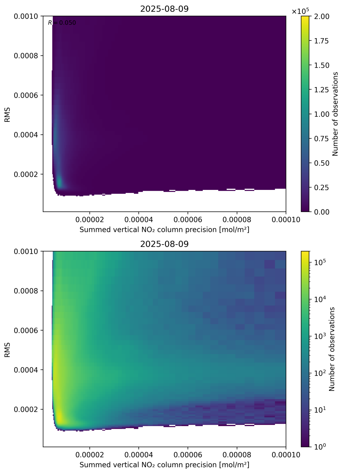
Figure 108: Scatter density plot of “Summed vertical NO 2 column precision” against “RMS” for 2025-08-09 to 2025-08-10.
