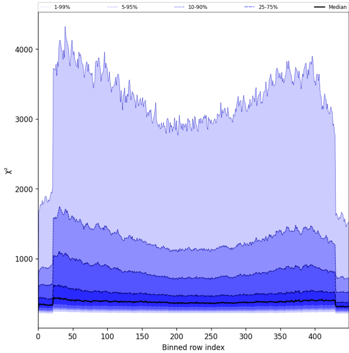
Figure 59: Along track statistics of “ \chi^2 ” for 2025-08-09 to 2025-08-10
