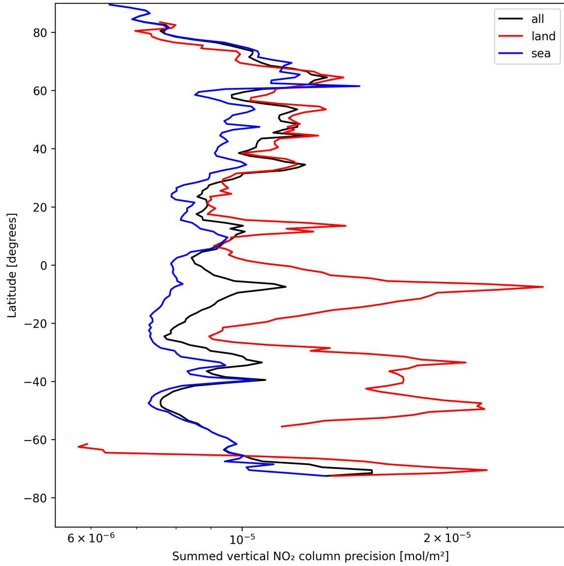
Figure 24: Zonal average of “Summed vertical NO 2 column precision” for 2025-08-09 to 2025-08-10.
