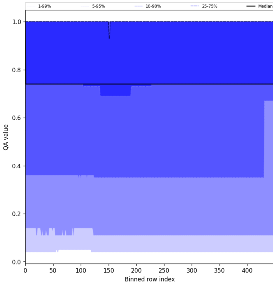
Figure 45: Along track statistics of “QA value” for 2025-08-09 to 2025-08-10
