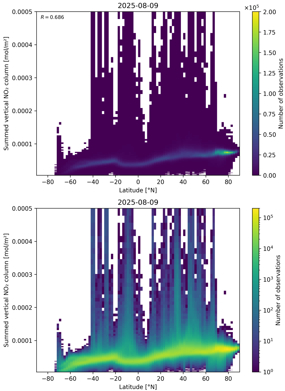
Figure 88: Scatter density plot of “Latitude” against “Summed vertical NO 2 column” for 2025-08-09 to 2025-08-10.
