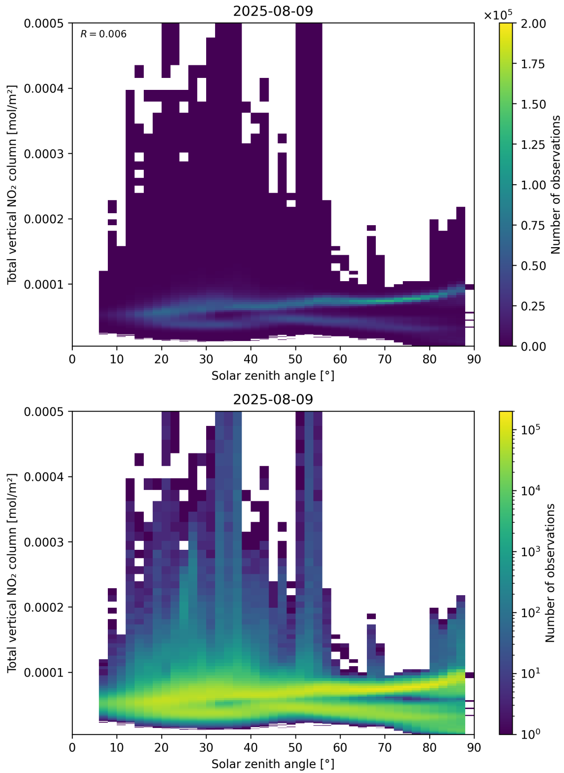
Figure 153: Scatter density plot of “Solar zenith angle” against “Total vertical NO 2 column” for 2025-08-09 to 2025-08-10.
