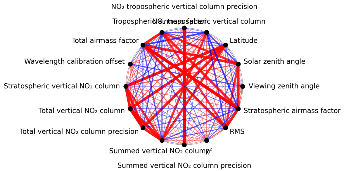
Figure 1: Map of correlation graph for 2025-08-09 to 2025-08-10.
