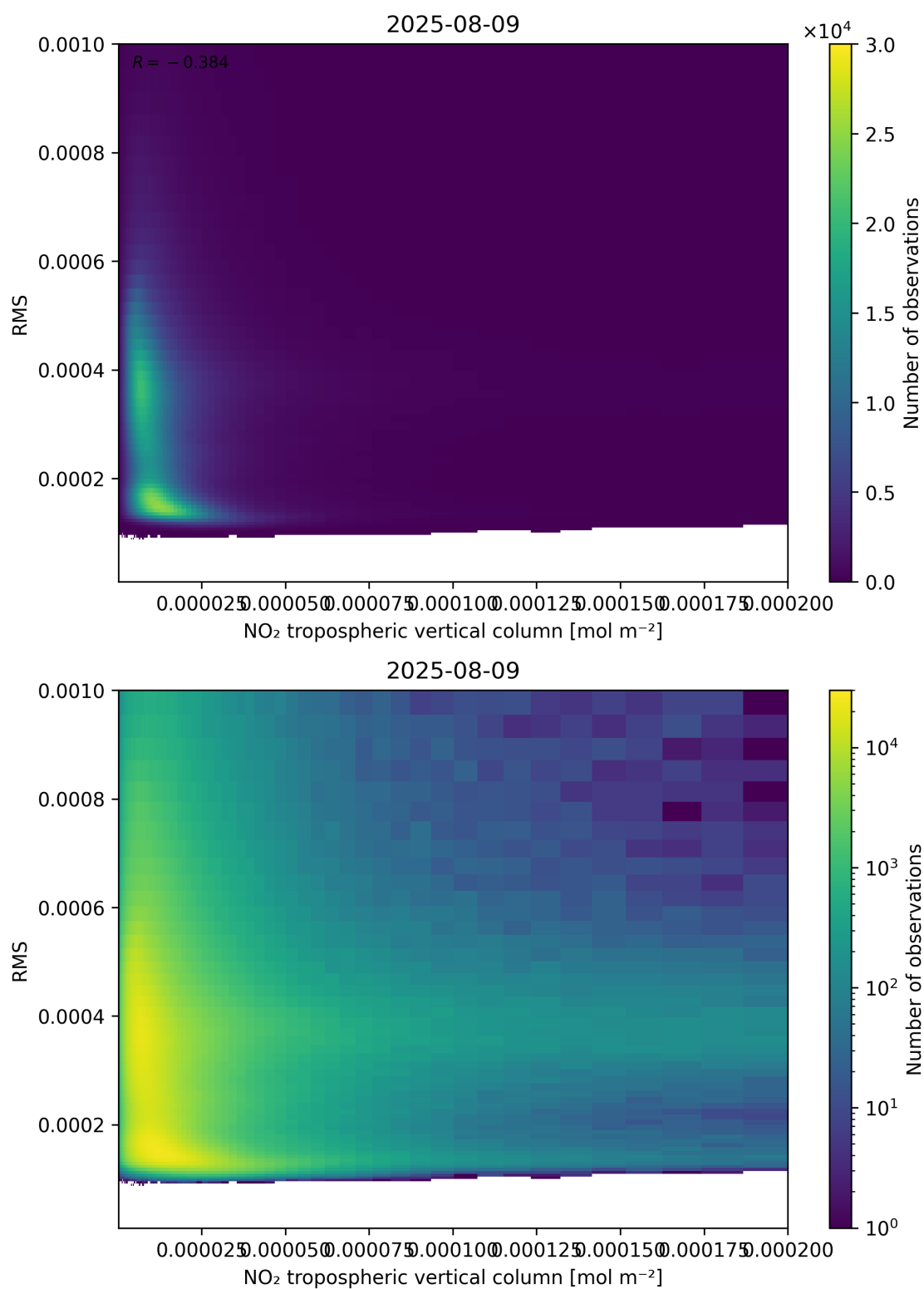
Figure 142: Scatter density plot of “NO 2 tropospheric vertical column” against “RMS” for 2025-08-09 to 2025-08-10.
