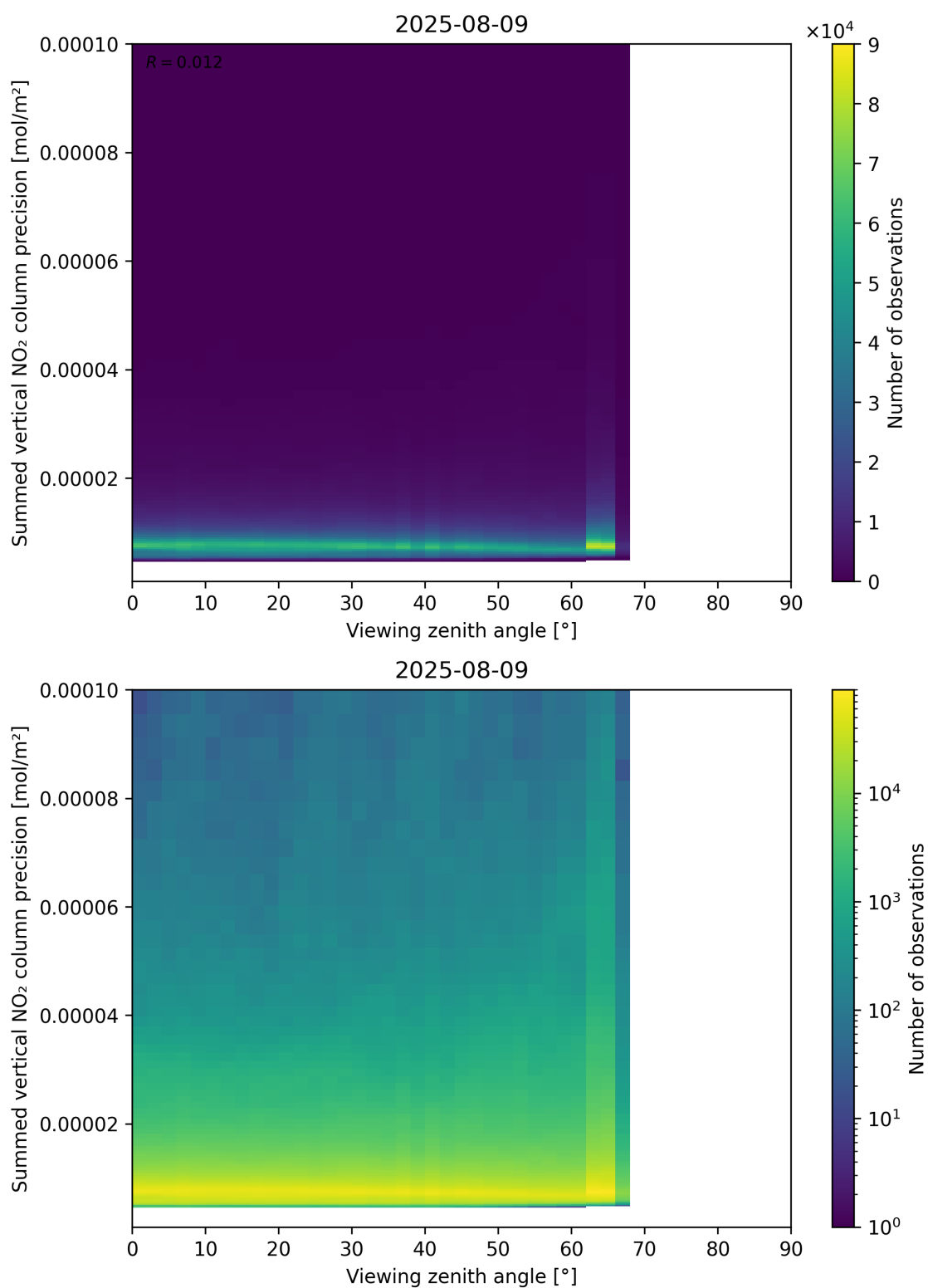
Figure 166: Scatter density plot of “Viewing zenith angle” against “Summed vertical NO 2 column precision” for 2025-08-09 to 2025-08-10.
