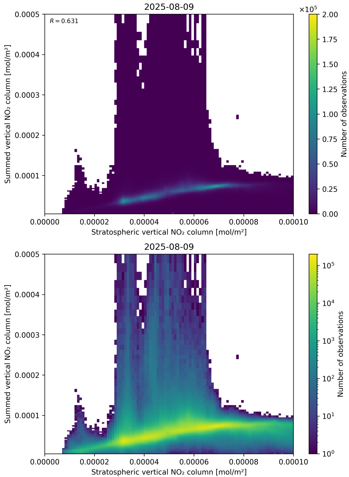
Figure 98: Scatter density plot of “Stratospheric vertical NO 2 column” against “Summed vertical NO 2 column” for 2025-08-09 to 2025-08-10.
