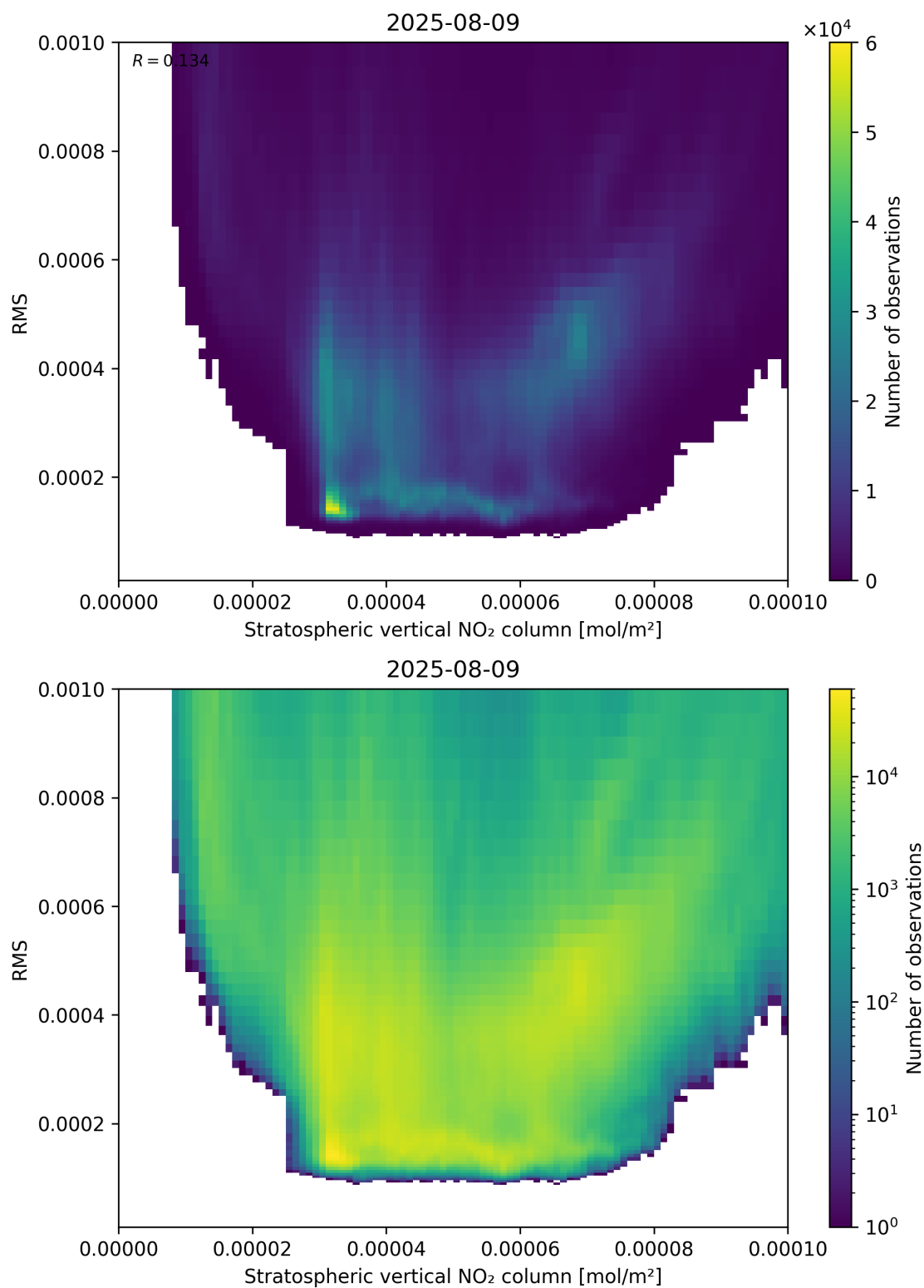
Figure 102: Scatter density plot of “Stratospheric vertical NO 2 column” against “RMS” for 2025-08-09 to 2025-08-10.
