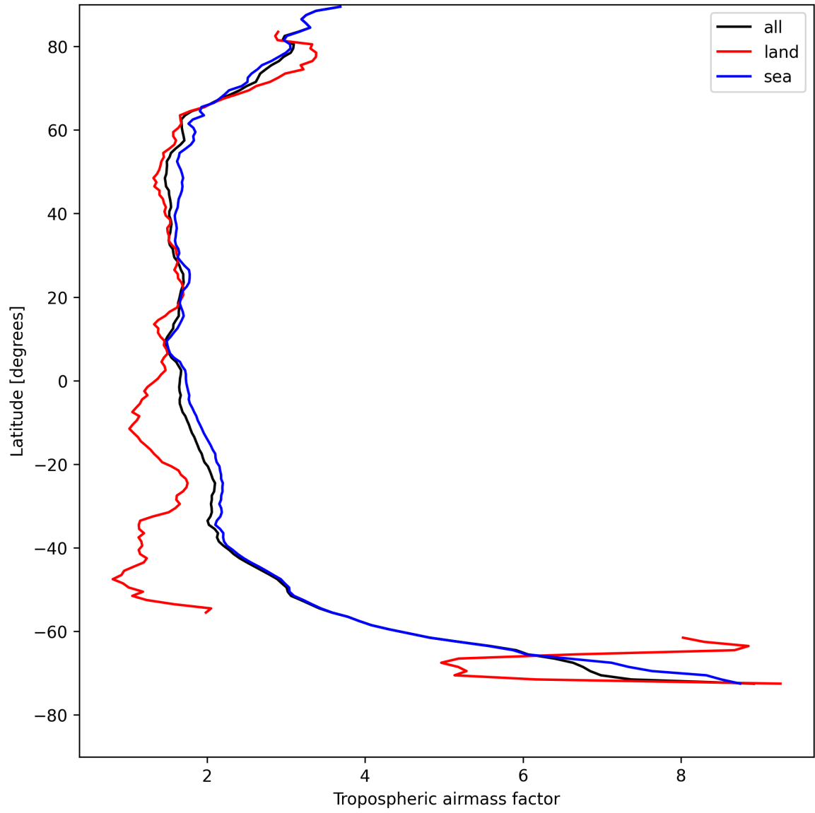
Figure 14: Zonal average of “Tropospheric airmass factor” for 2025-08-09 to 2025-08-10.
