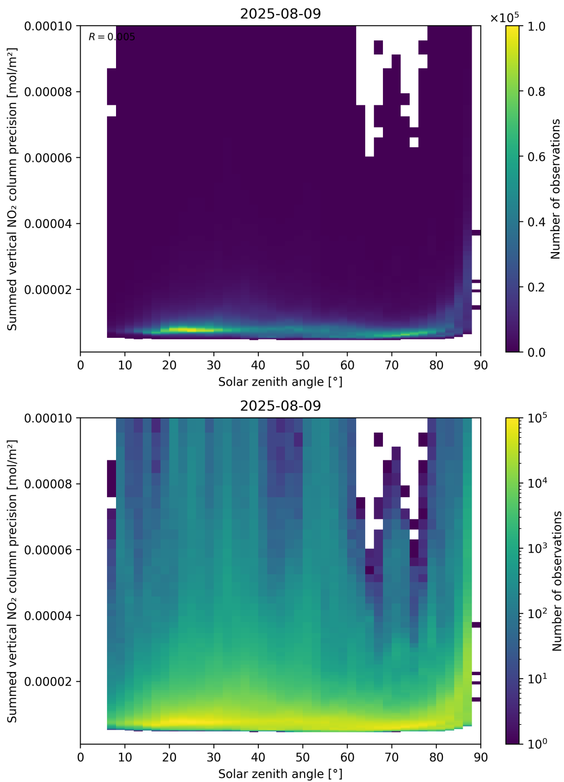
Figure 152: Scatter density plot of “Solar zenith angle” against “Summed vertical NO 2 column precision” for 2025-08-09 to 2025-08-10.
