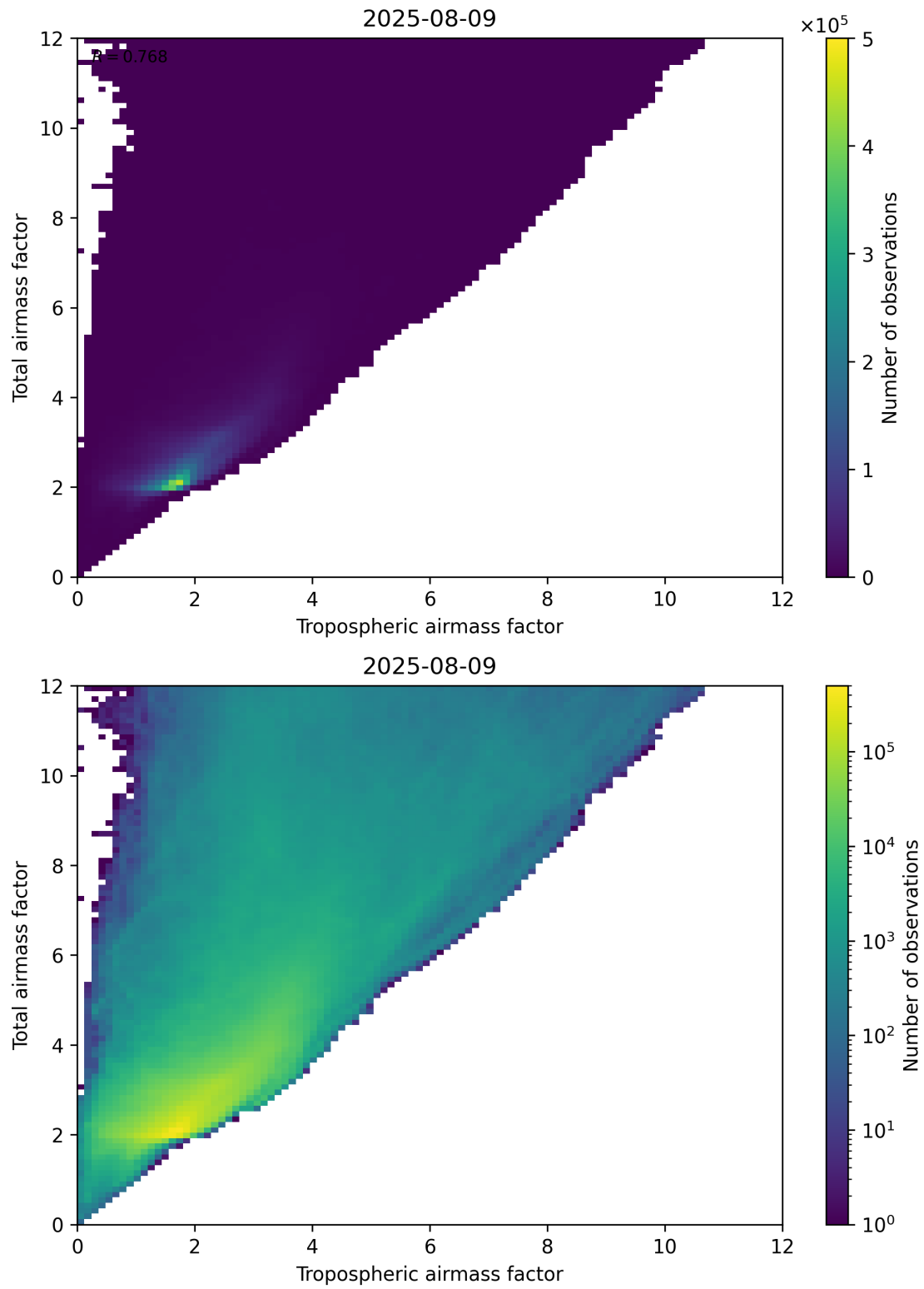
Figure 72: Scatter density plot of “Tropospheric airmass factor” against “Total airmass factor” for 2025-08-09 to 2025-08-10.
