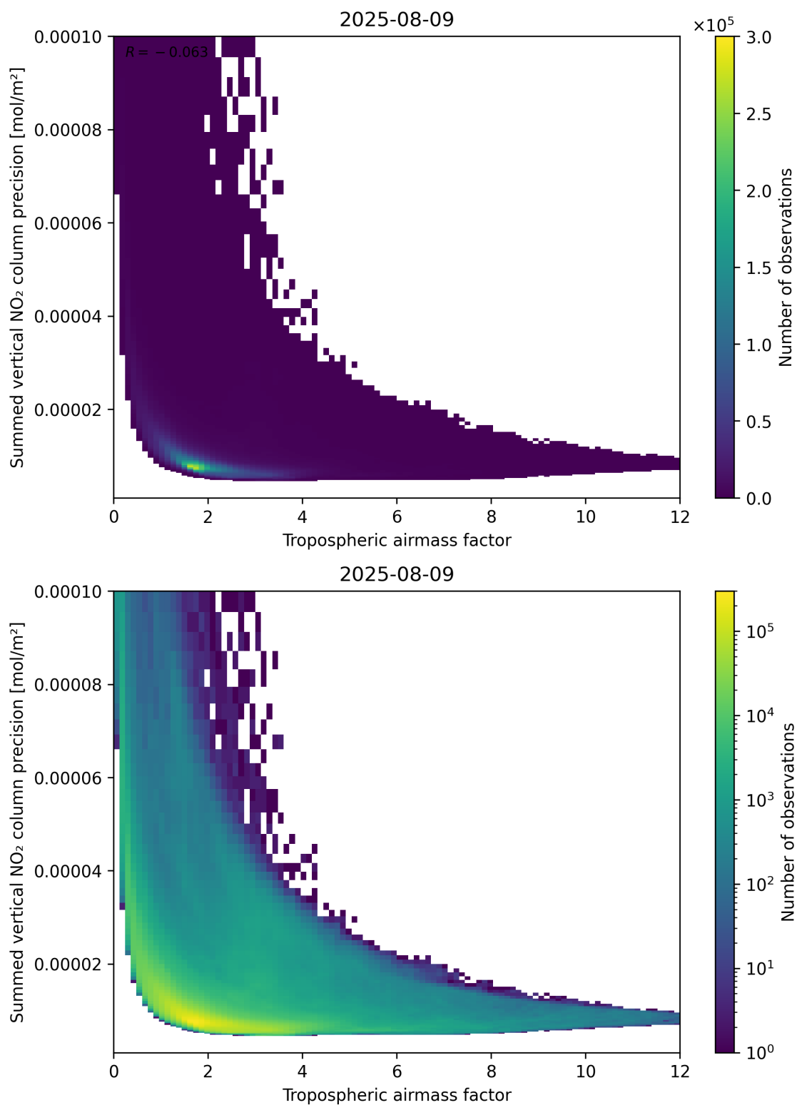
Figure 76: Scatter density plot of “Tropospheric air mass factor” against “Summed vertical NO 2 column precision” for 2025-08-09 to 2025-08-10.
