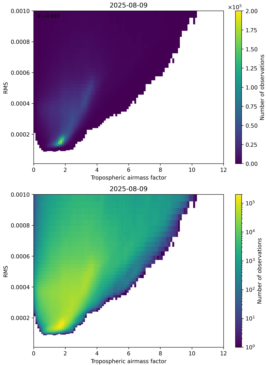
Figure 79: Scatter density plot of “Tropospheric airmass factor” against “RMS” for 2025-08-09 to 2025-08-10.
