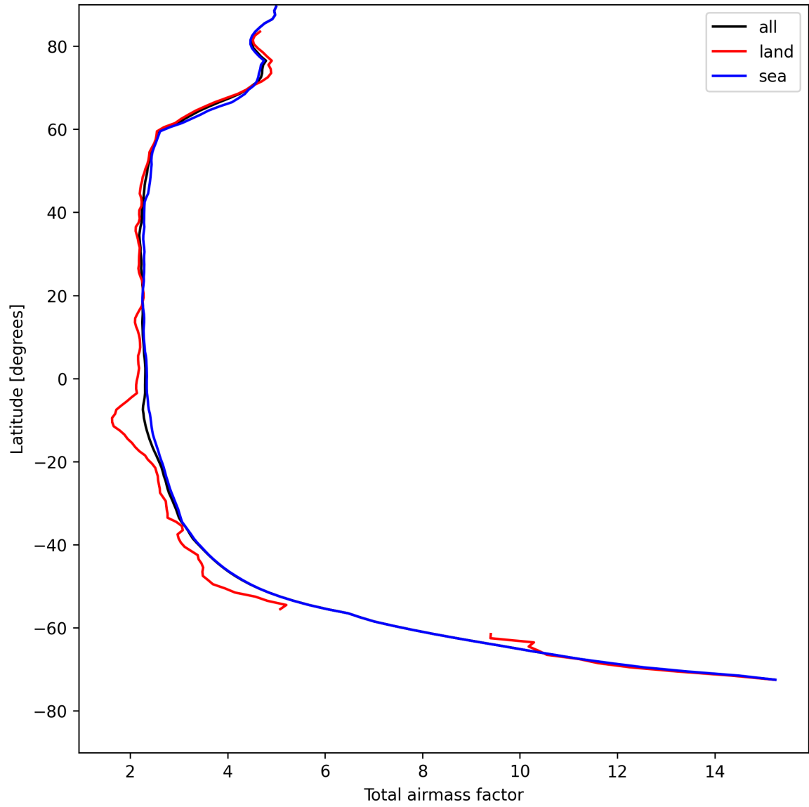
Figure 15: Zonal average of “Total airmass factor” for 2025-08-09 to 2025-08-10.
