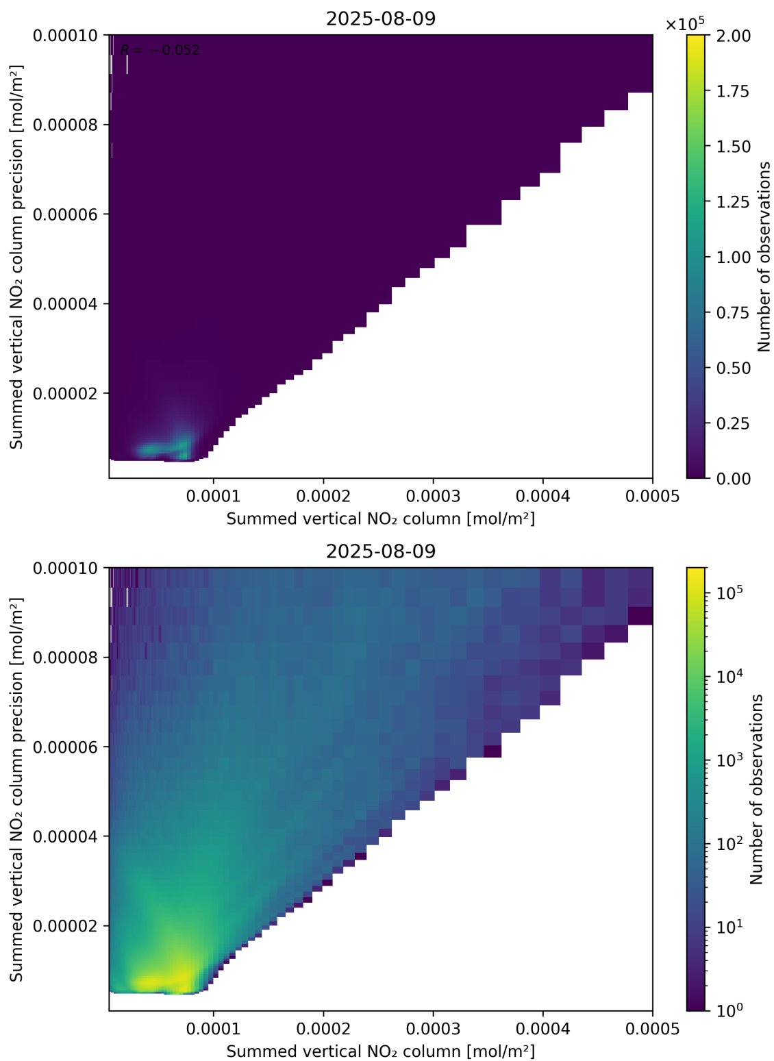
Figure 105: Scatter density plot of “Summed vertical NO 2 column” against “Summed vertical NO 2 column precision” for 2025-08-09 to 2025-08-10.
