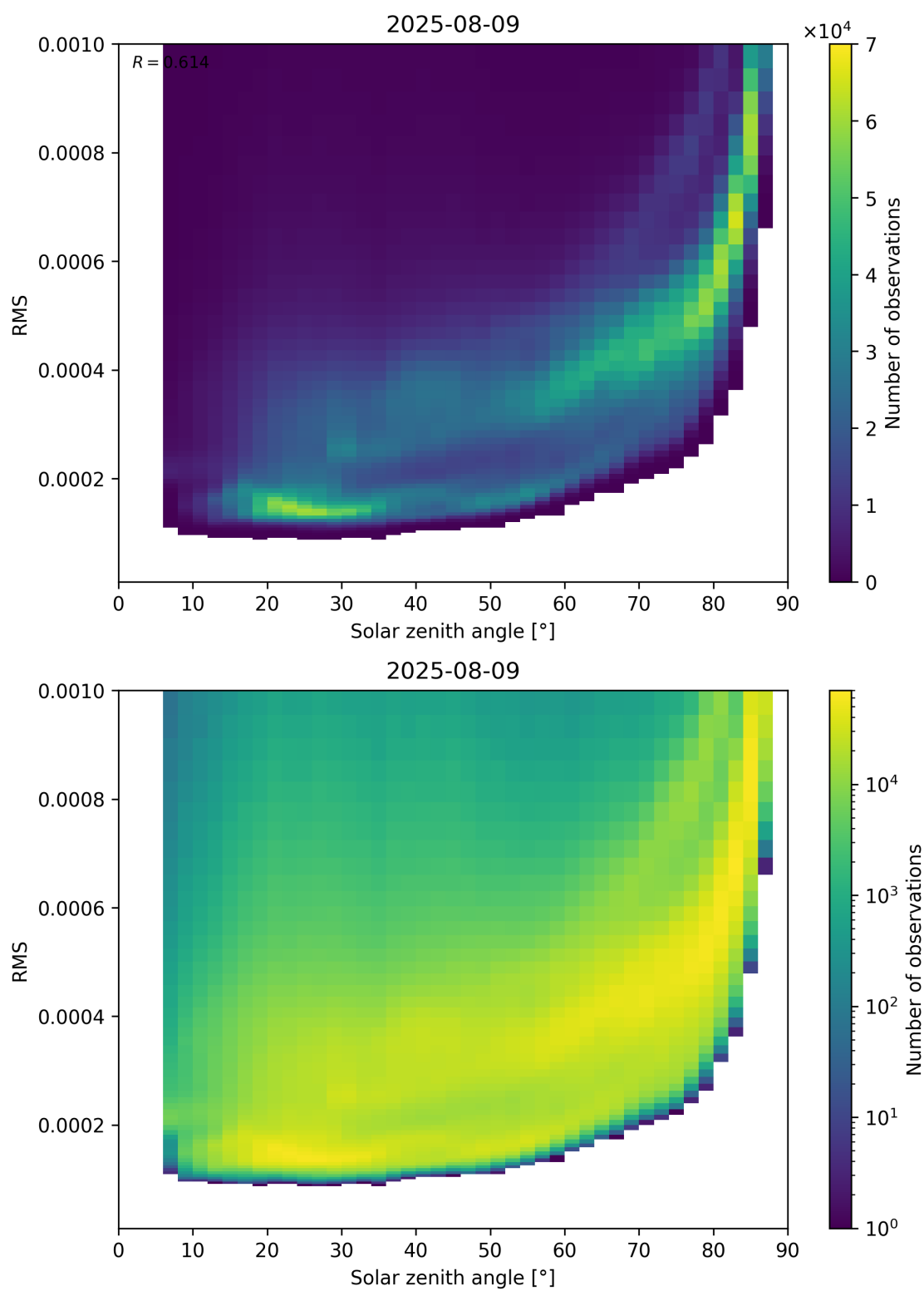
Figure 157: Scatter density plot of “Solar zenith angle” against “RMS” for 2025-08-09 to 2025-08-10.
