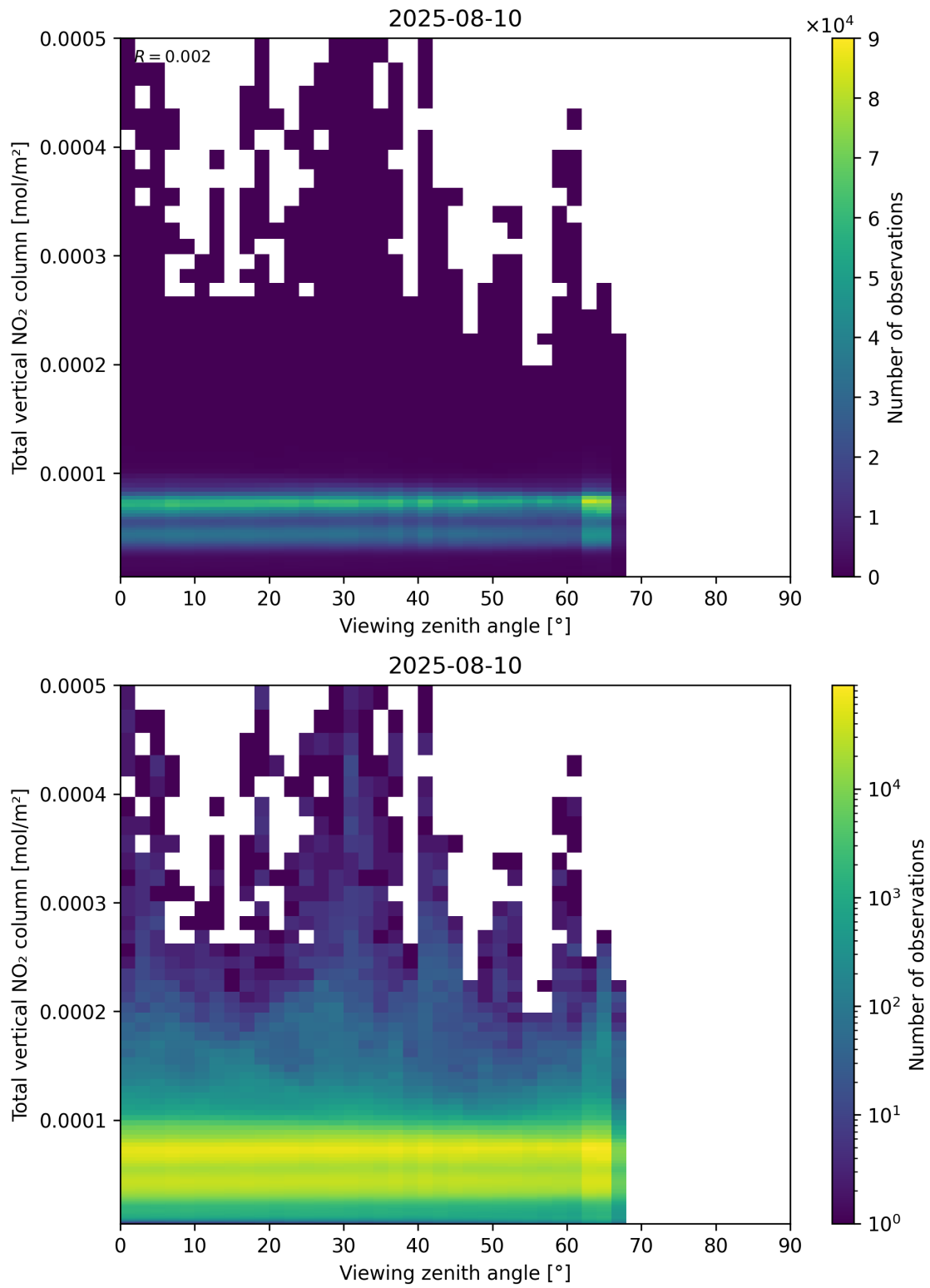
Figure 167: Scatter density plot of “Viewing zenith angle” against “Total vertical NO 2 column” for 2025-08-09 to 2025-08-11.
