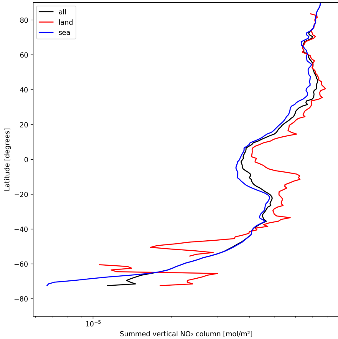
Figure 23: Zonal average of “Summed vertical NO 2 column” for 2025-08-09 to 2025-08-11.
