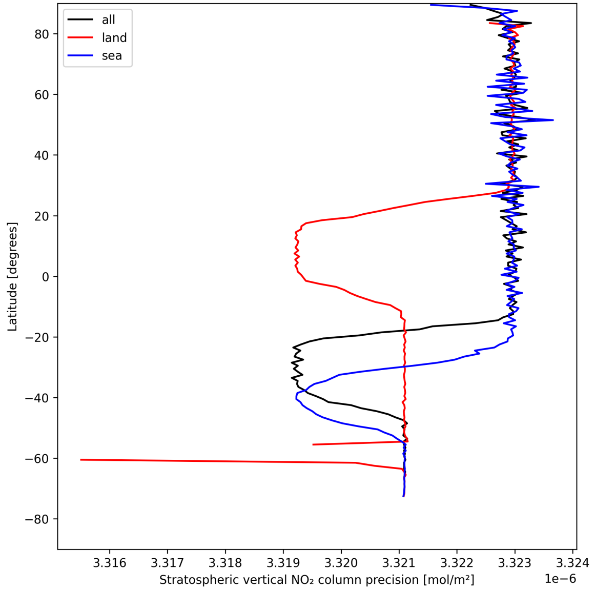
Figure 20: Zonal average of “Stratospheric vertical NO 2 column precision” for 2025-08-09 to 2025-08-11.
