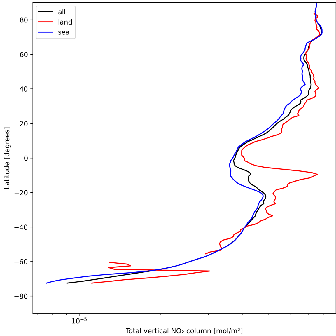
Figure 21: Zonal average of “Total vertical NO 2 column” for 2025-08-09 to 2025-08-11.
