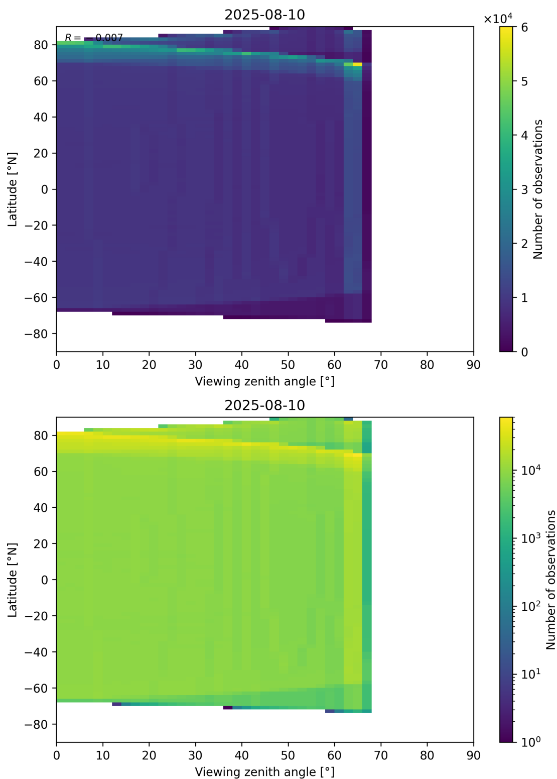
Figure 163: Scatter density plot of “Viewing zenith angle” against “Latitude” for 2025-08-09 to 2025-08-11.
