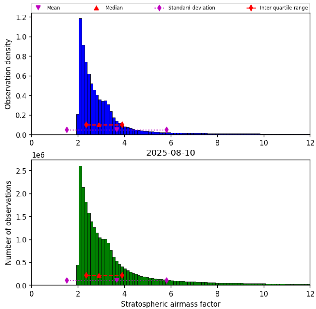
Figure 44: Histogram of “Stratospheric airmass factor” for 2025-08-09 to 2025-08-11
