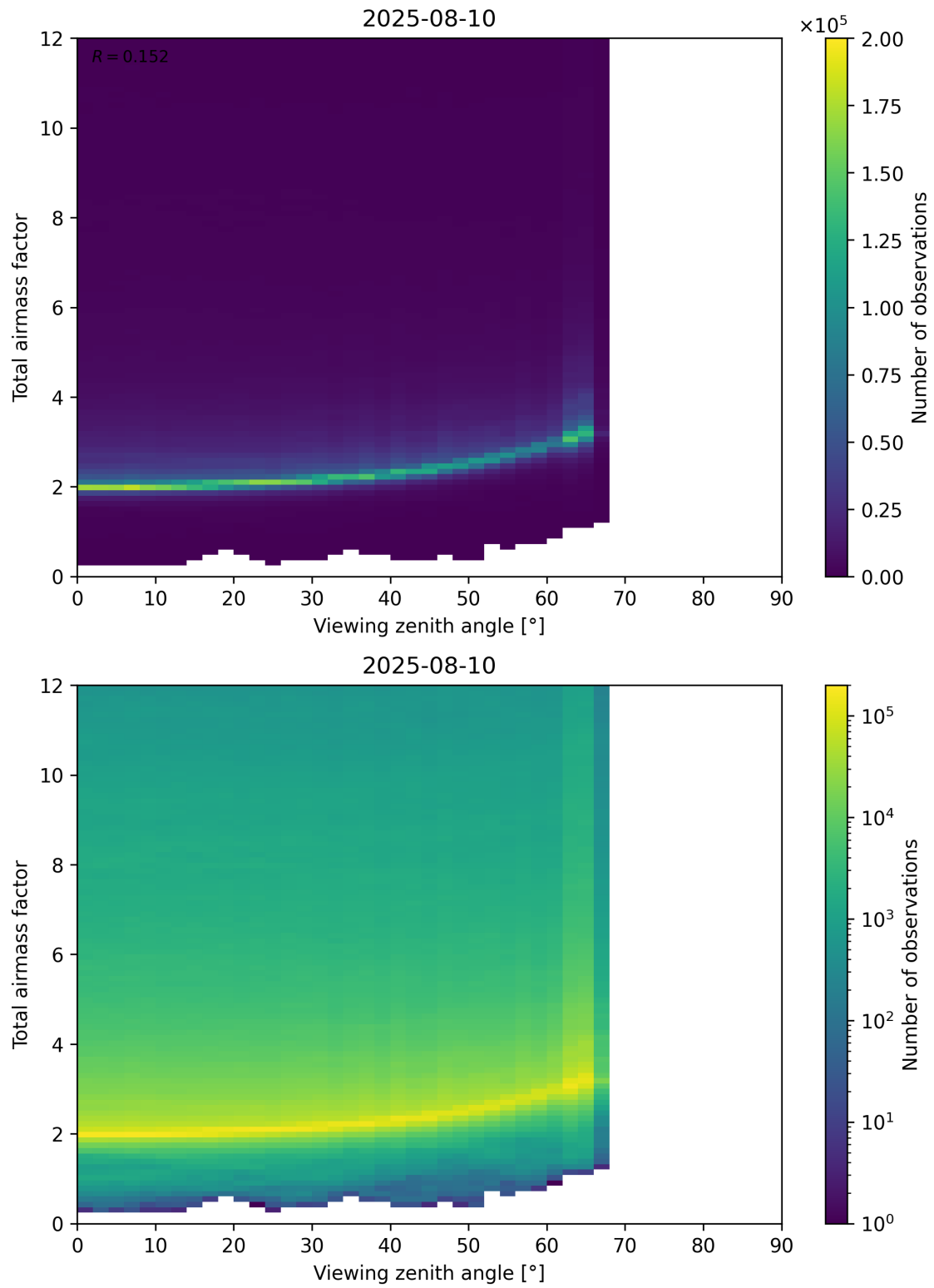
Figure 160: Scatter density plot of “Viewing zenith angle” against “Total airmass factor” for 2025-08-09 to 2025-08-11.
