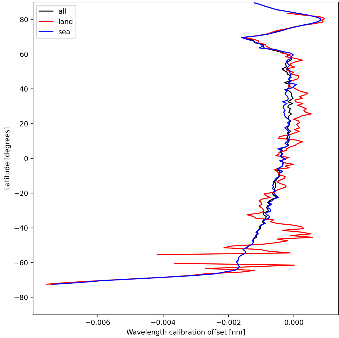
Figure 18: Zonal average of “Wavelength calibration offset” for 2025-08-09 to 2025-08-11.
