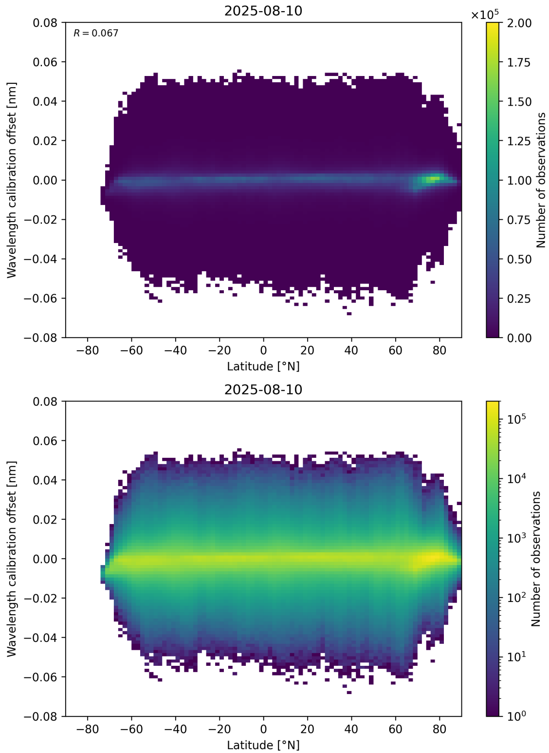
Figure 95: Scatter density plot of “Latitude” against “Wavelength calibration offset” for 2025-08-09 to 2025-08-11.
