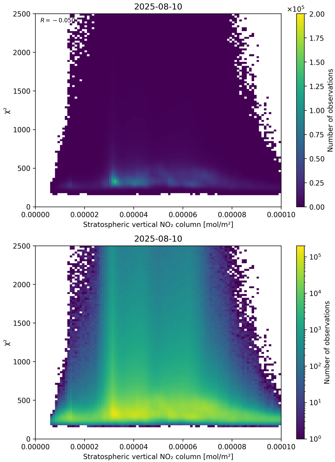
Figure 97: Scatter density plot of “Stratospheric vertical NO 2 column” against “ \chi^2 ” for 2025-08-09 to 2025-08-11.
