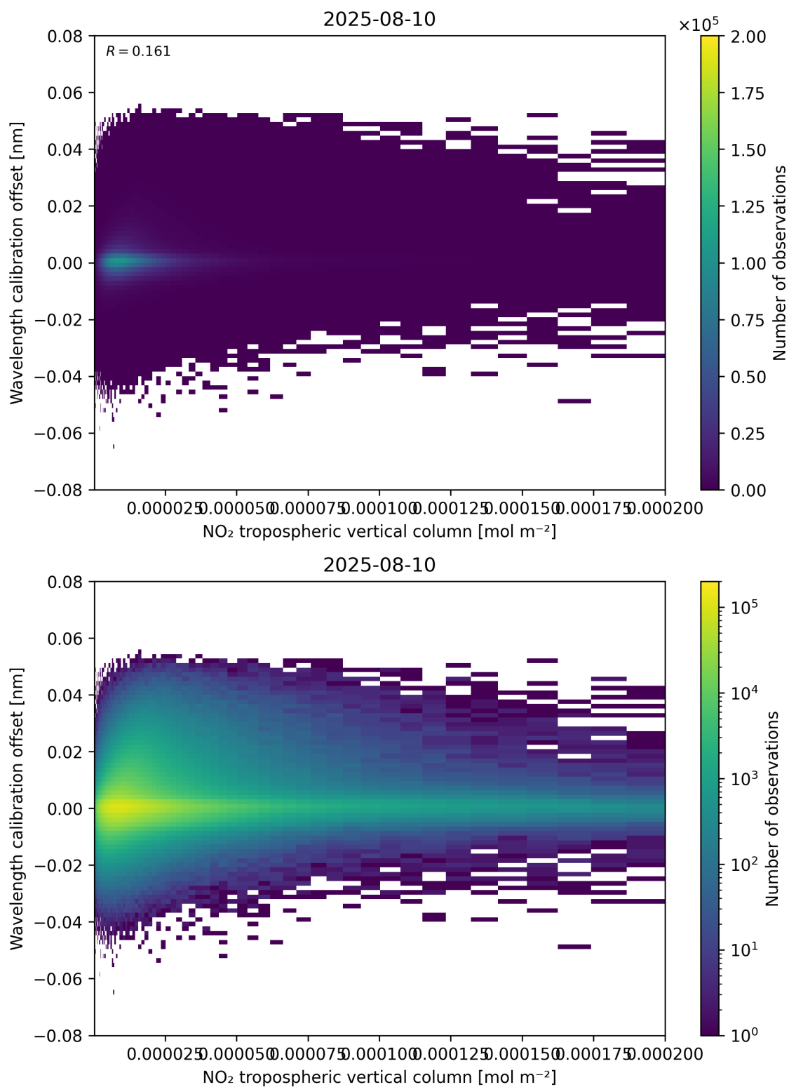
Figure 143: Scatter density plot of “NO 2 tropospheric vertical column” against “Wavelength calibration offset” for 2025-08-09 to 2025-08-11.
