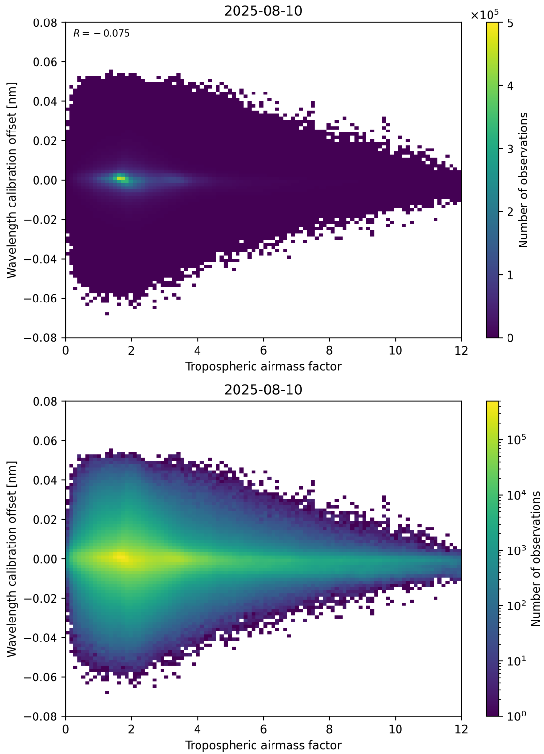
Figure 80: Scatter density plot of “Tropospheric airmass factor” against “Wavelength calibration offset” for 2025-08-09 to 2025-08-11.
