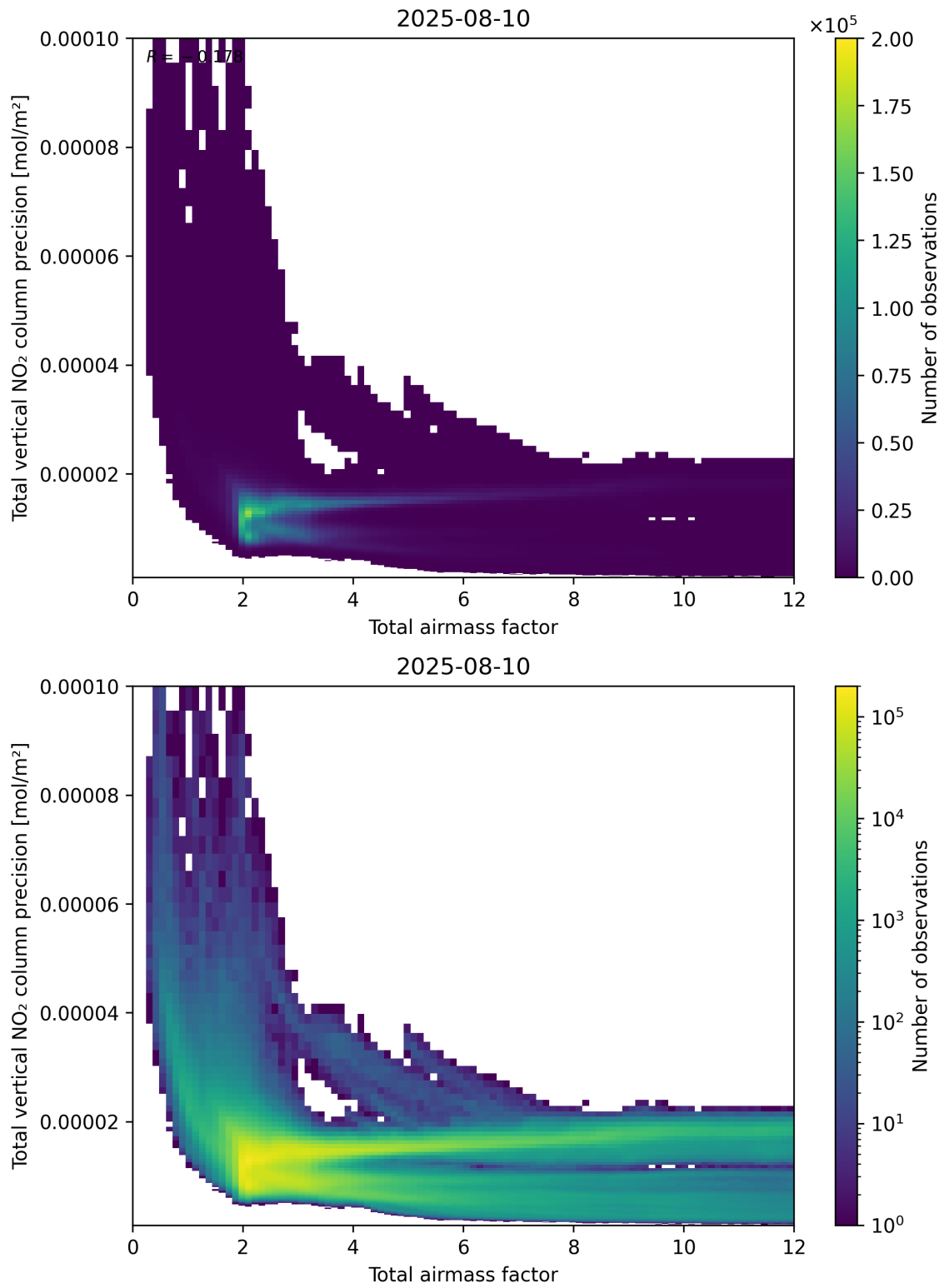
Figure 68: Scatter density plot of “Total airmass factor” against “Total vertical NO 2 column precision” for 2025-08-09 to 2025-08-11.
