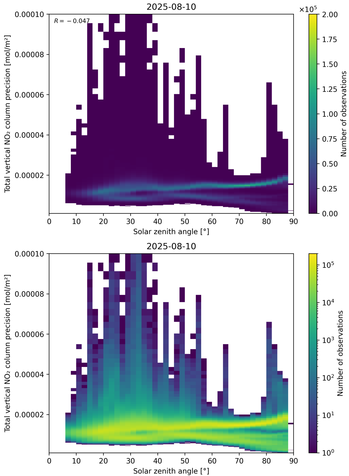
Figure 154: Scatter density plot of “Solar zenith angle” against “Total vertical NO 2 column precision” for 2025-08-09 to 2025-08-11.
