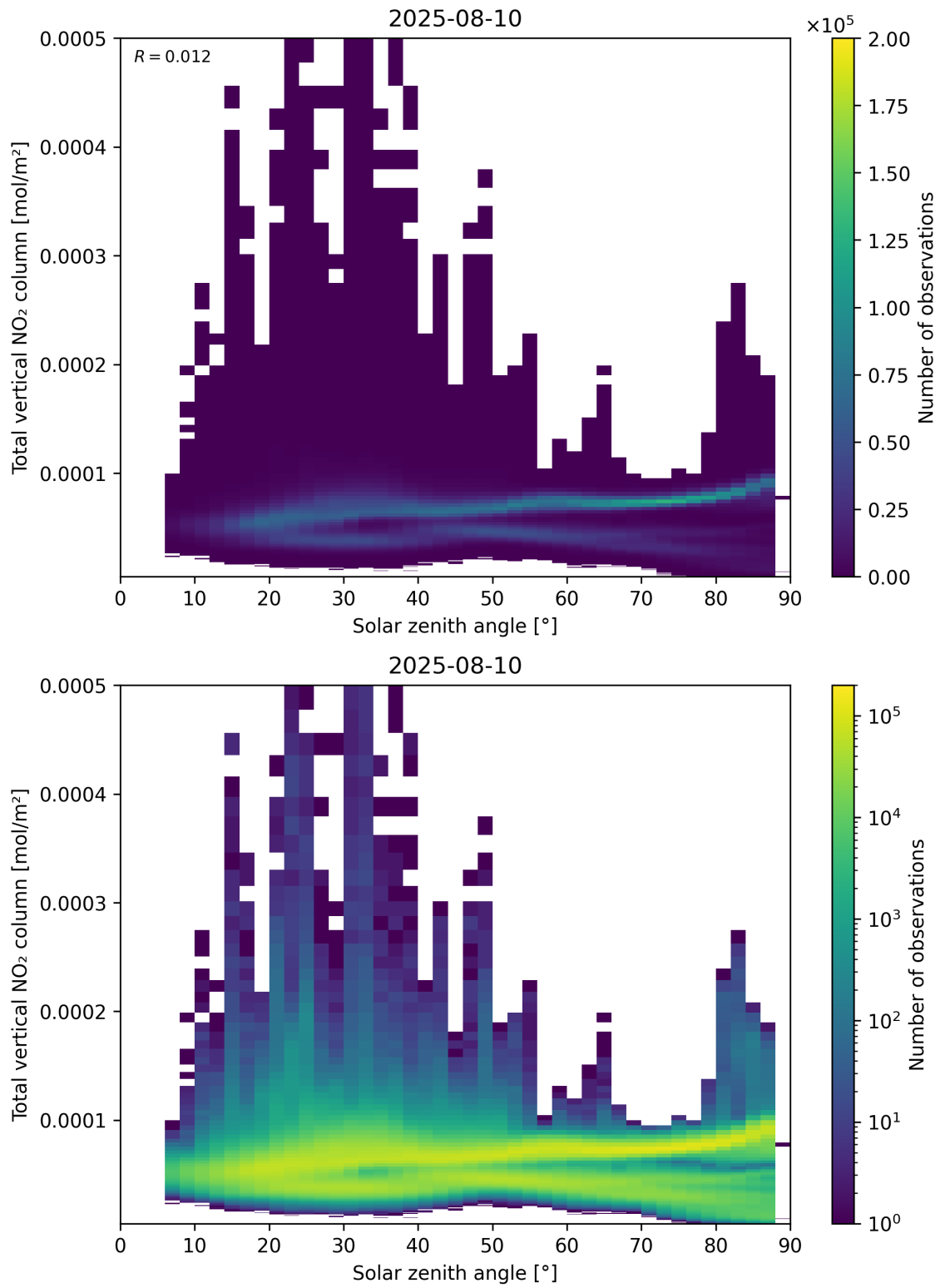
Figure 153: Scatter density plot of “Solar zenith angle” against “Total vertical NO 2 column” for 2025-08-09 to 2025-08-11.
