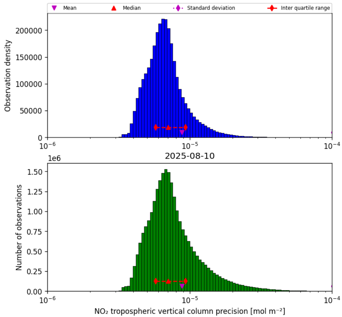
Figure 30: Histogram of “NO 2 tropospheric vertical column precision” for 2025-08-09 to 2025-08-11
