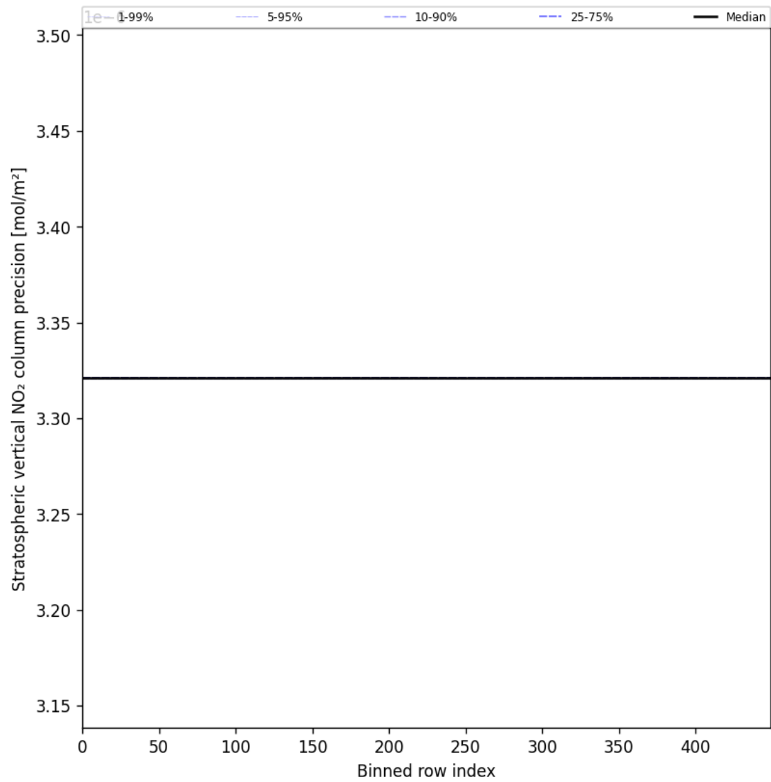
Figure 54: Along track statistics of “Stratospheric vertical NO 2 column precision” for 2025-08-09 to 2025-08-11
