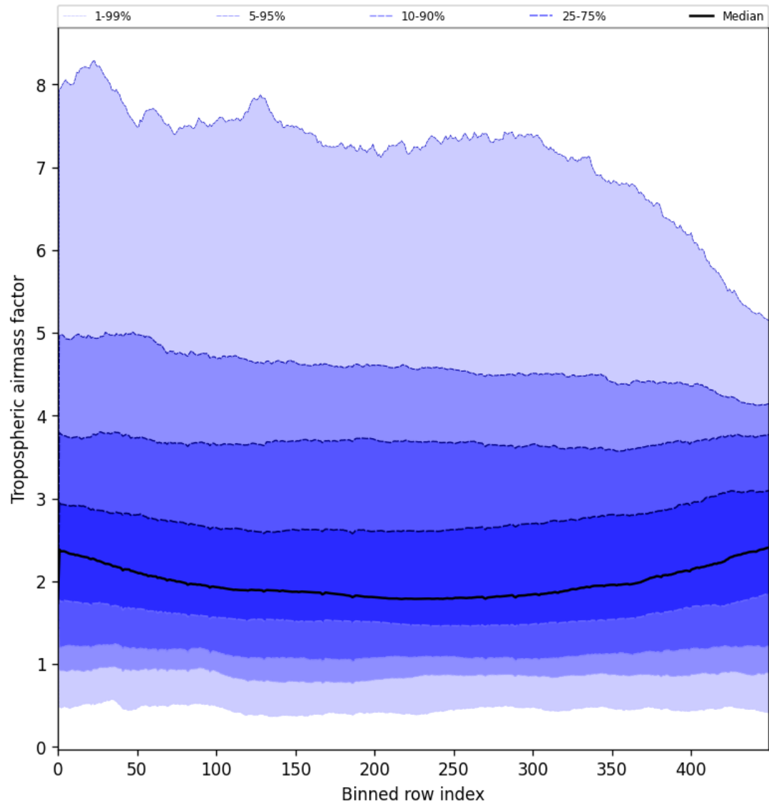
Figure 48: Along track statistics of “Tropospheric airmass factor” for 2025-08-09 to 2025-08-11
