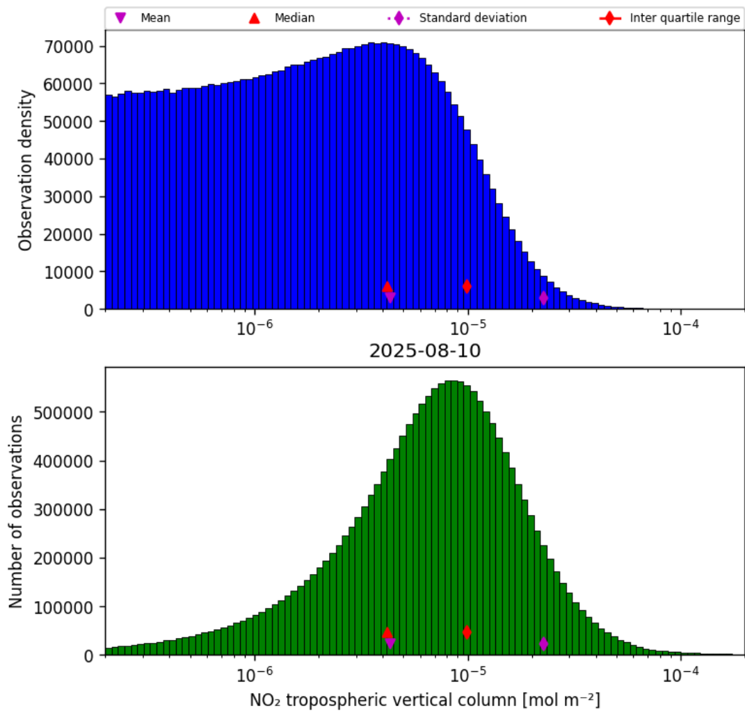
Figure 29: Histogram of “NO 2 tropospheric vertical column” for 2025-08-09 to 2025-08-11
