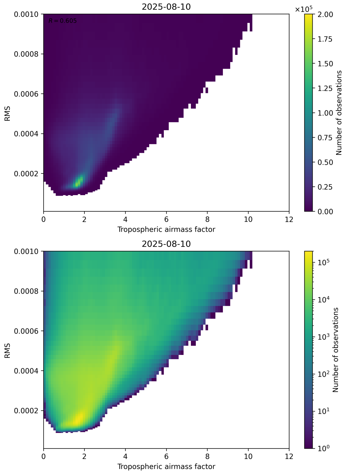
Figure 79: Scatter density plot of “Tropospheric airmass factor” against “RMS” for 2025-08-09 to 2025-08-11.
