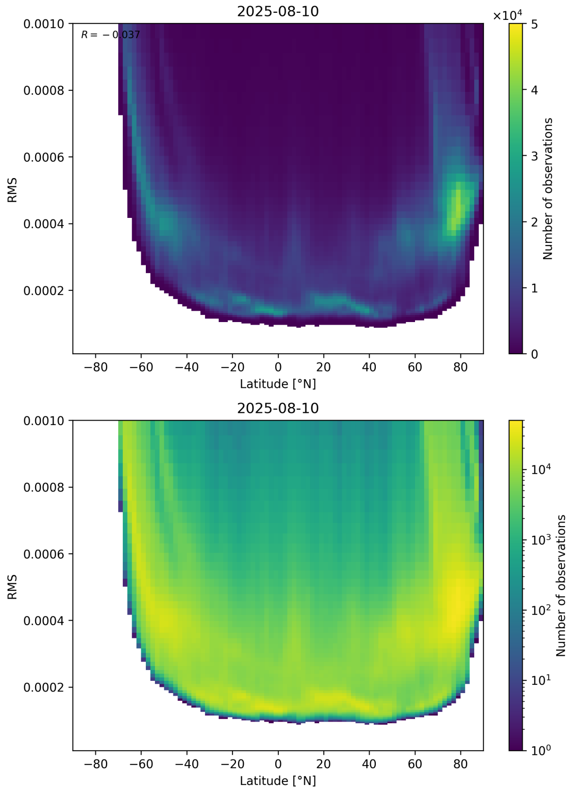
Figure 94: Scatter density plot of “Latitude” against “RMS” for 2025-08-09 to 2025-08-11.
