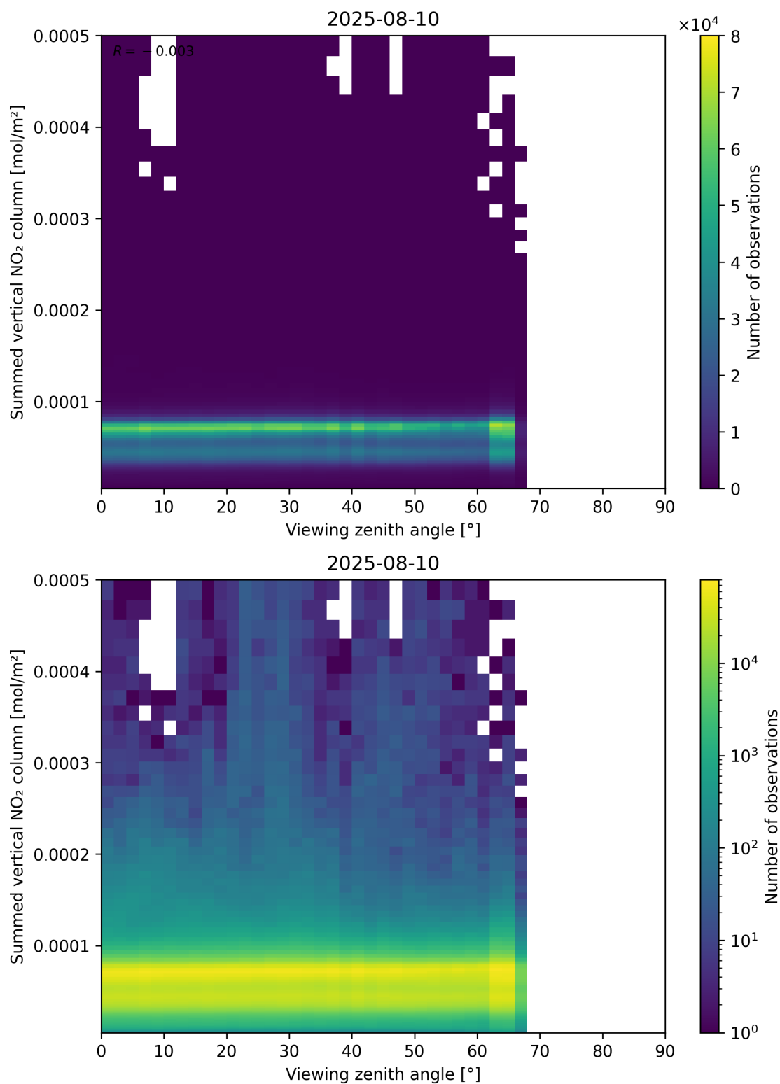
Figure 165: Scatter density plot of “Viewing zenith angle” against “Summed vertical NO 2 column” for 2025-08-09 to 2025-08-11.
