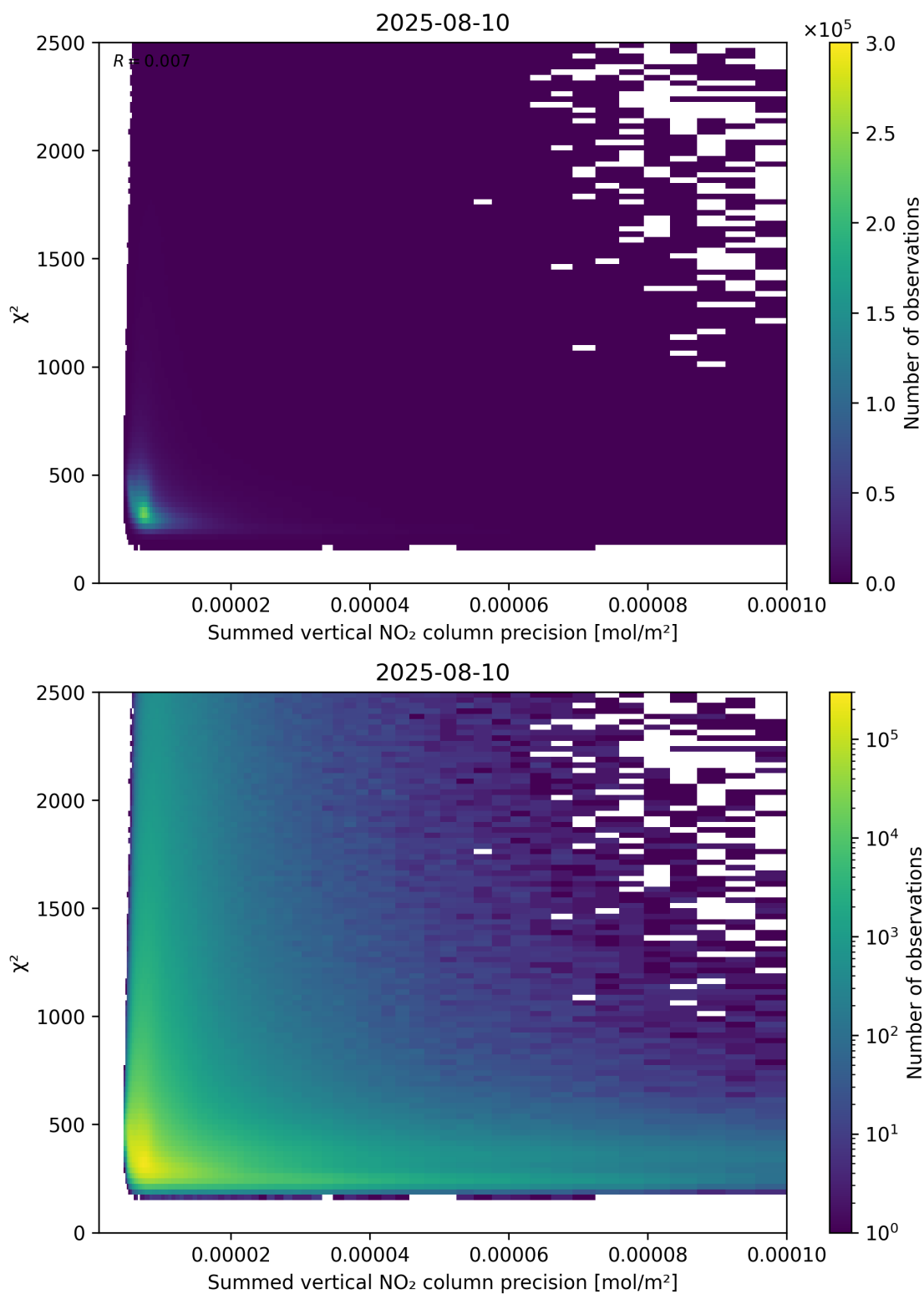
Figure 107: Scatter density plot of “Summed vertical NO 2 column precision” against “ \chi^2 ” for 2025-08-09 to 2025-08-11.
