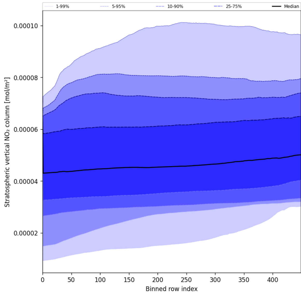
Figure 53: Along track statistics of “Stratospheric vertical NO 2 column” for 2025-08-09 to 2025-08-11
