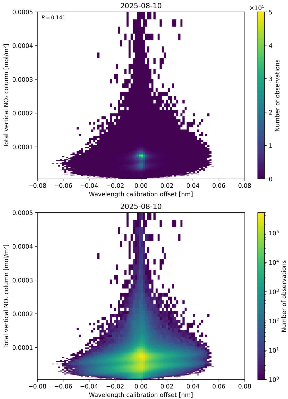
Figure 179: Scatter density plot of “Wavelength calibration offset” against “Total vertical NO 2 column” for 2025-08-09 to 2025-08-11.
