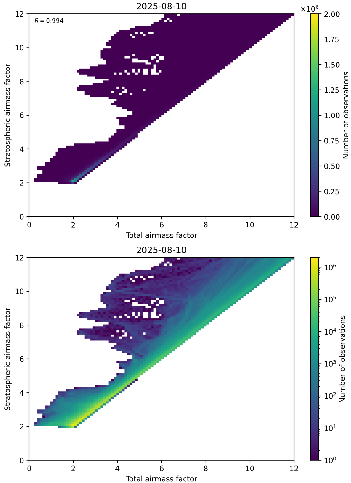
Figure 62: Scatter density plot of “Total airmass factor” against “Stratospheric airmass factor” for 2025-08-09 to 2025-08-11.
