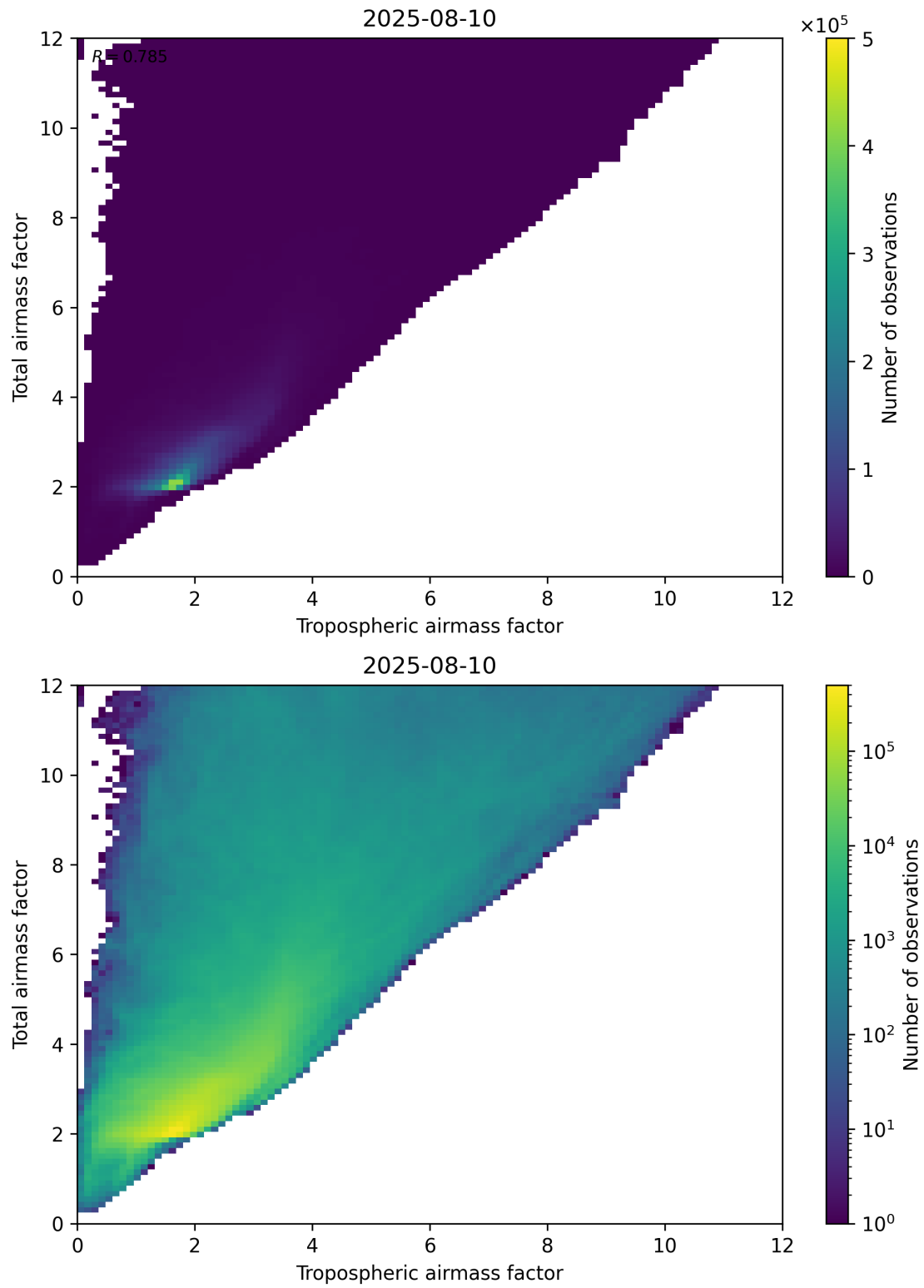
Figure 72: Scatter density plot of “Tropospheric airmass factor” against “Total airmass factor” for 2025-08-09 to 2025-08-11.
