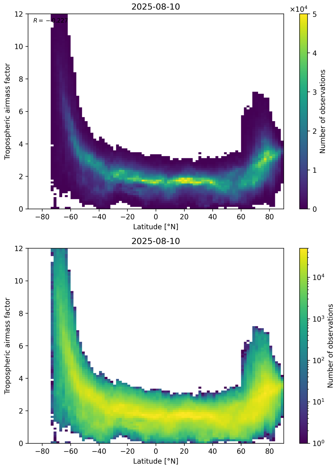
Figure 85: Scatter density plot of “Latitude” against “Tropospheric air mass factor” for 2025-08-09 to 2025-08-11.
