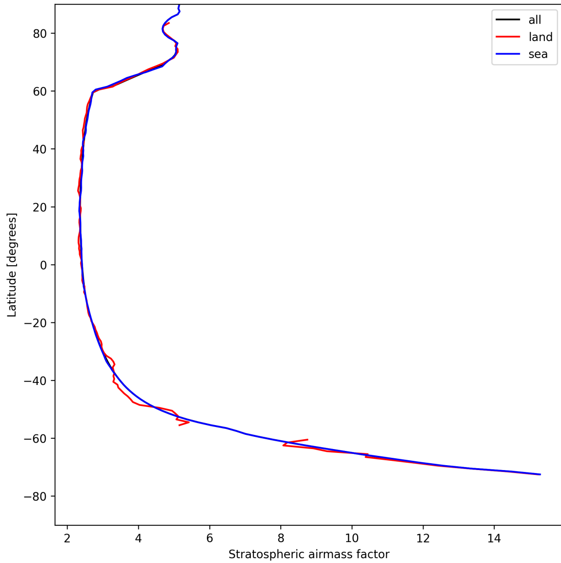
Figure 27: Zonal average of “Stratospheric airmass factor” for 2025-08-09 to 2025-08-11.
