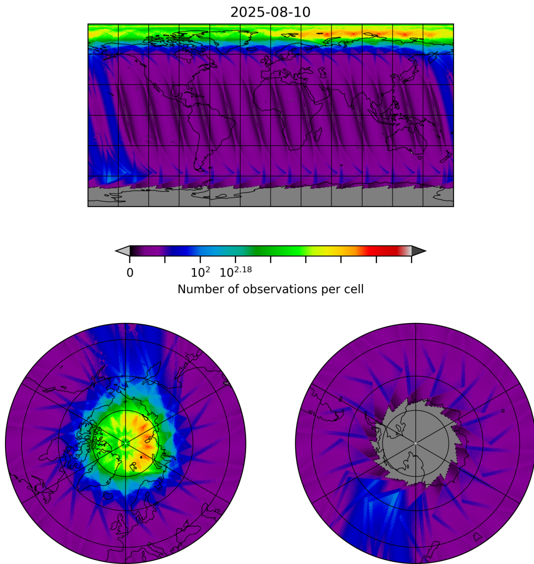
Figure 10: Map of the number of observations for 2025-08-09 to 2025-08-11
