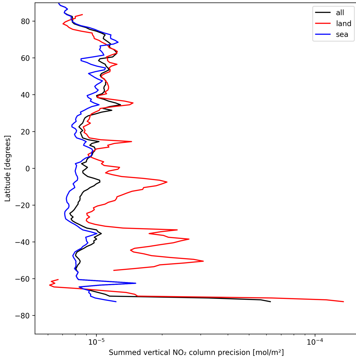
Figure 24: Zonal average of “Summed vertical NO 2 column precision” for 2025-08-09 to 2025-08-11.
