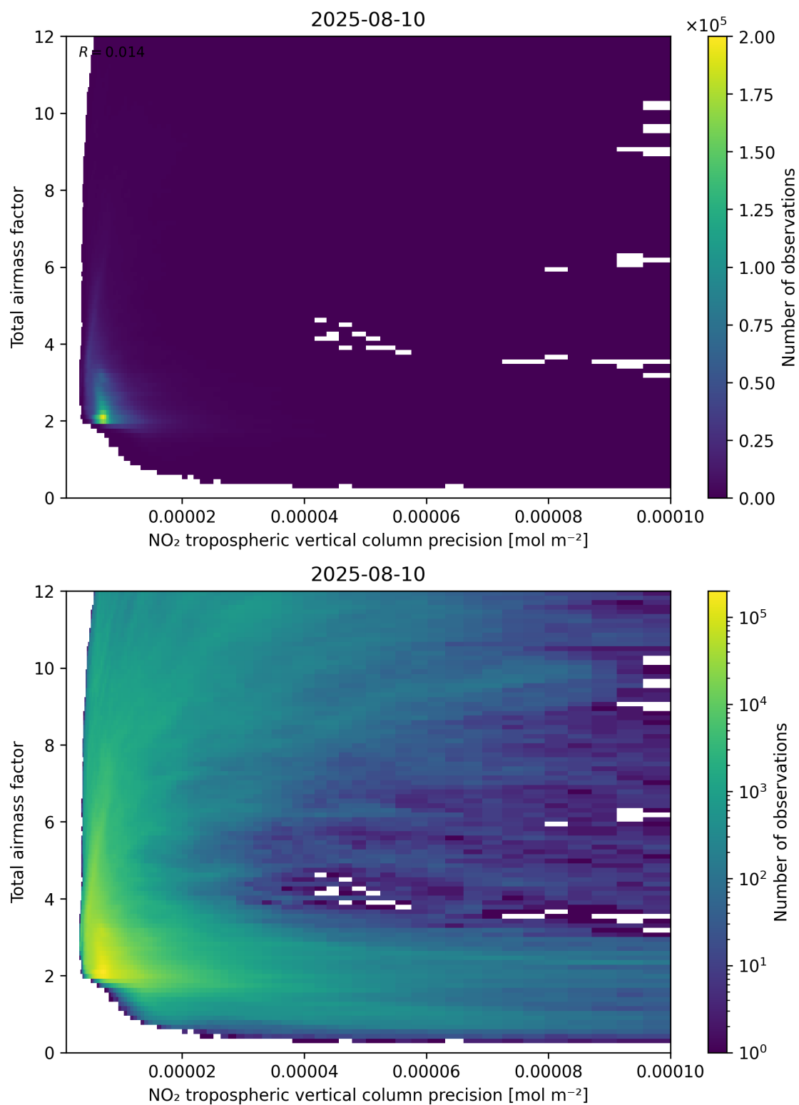
Figure 132: Scatter density plot of “NO 2 tropospheric vertical column precision” against “Total air mass factor” for 2025-08-09 to 2025-08-11.
