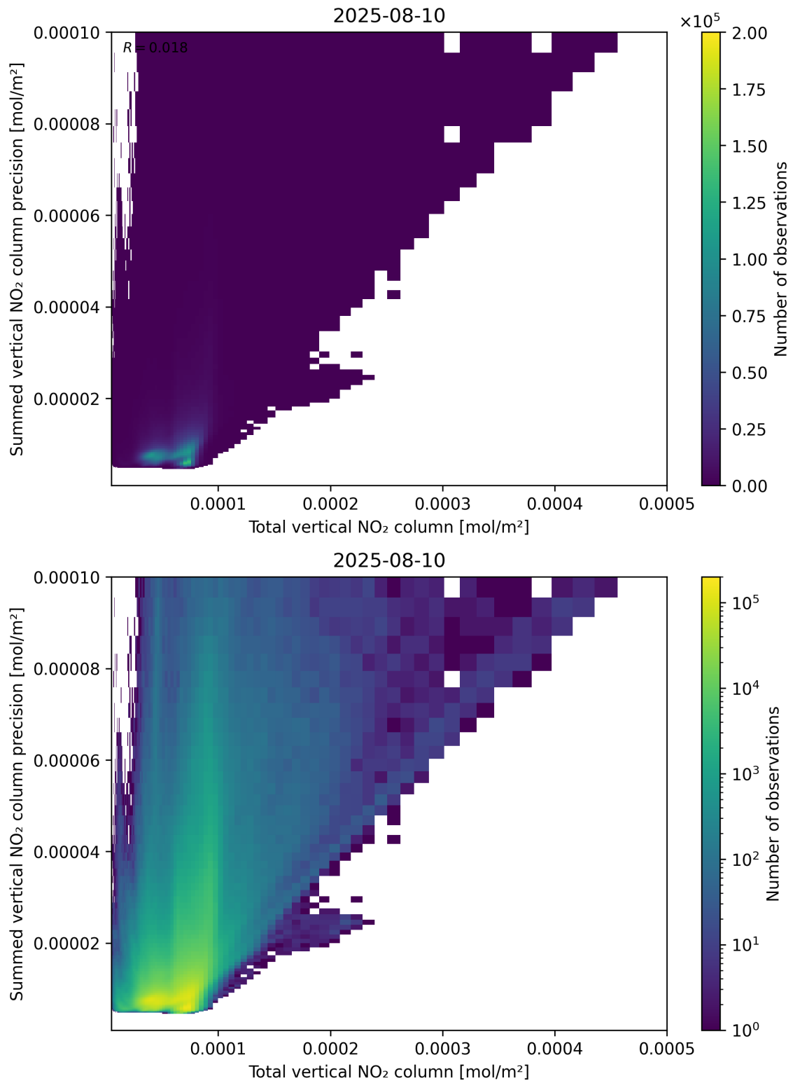
Figure 113: Scatter density plot of “Total vertical NO 2 column” against “Summed vertical NO 2 column precision” for 2025-08-09 to 2025-08-11.
