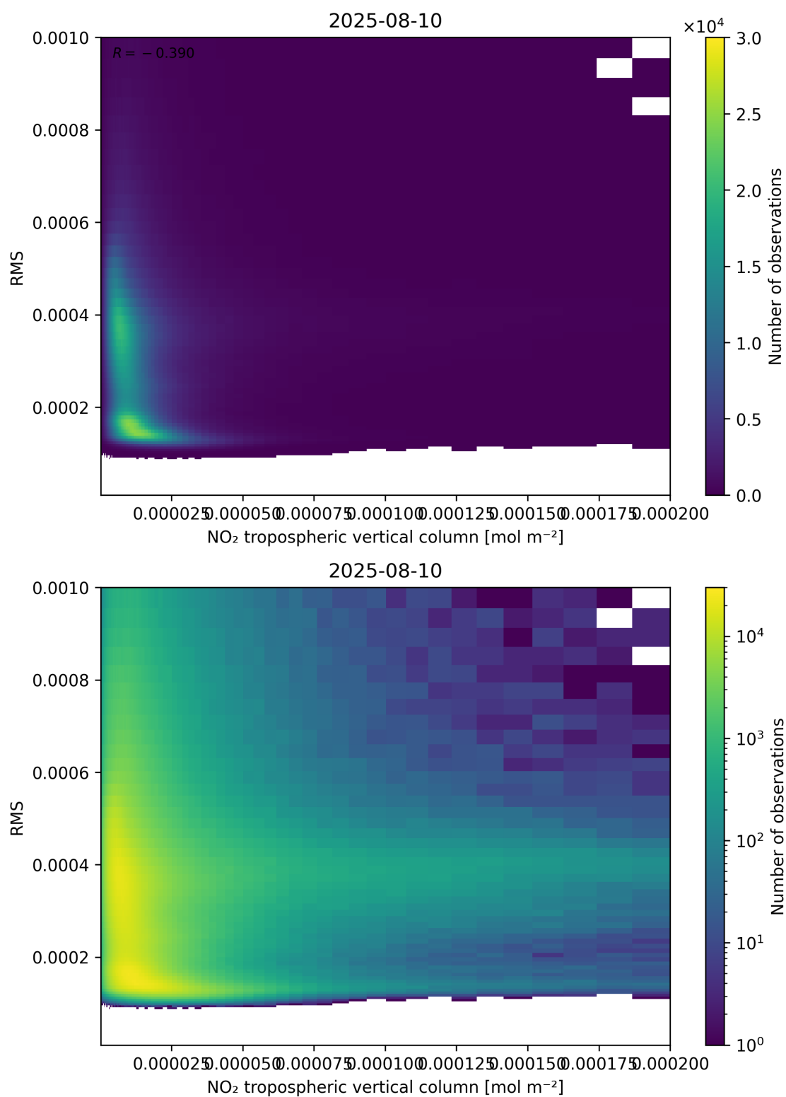
Figure 142: Scatter density plot of “NO 2 tropospheric vertical column” against “RMS” for 2025-08-09 to 2025-08-11.
