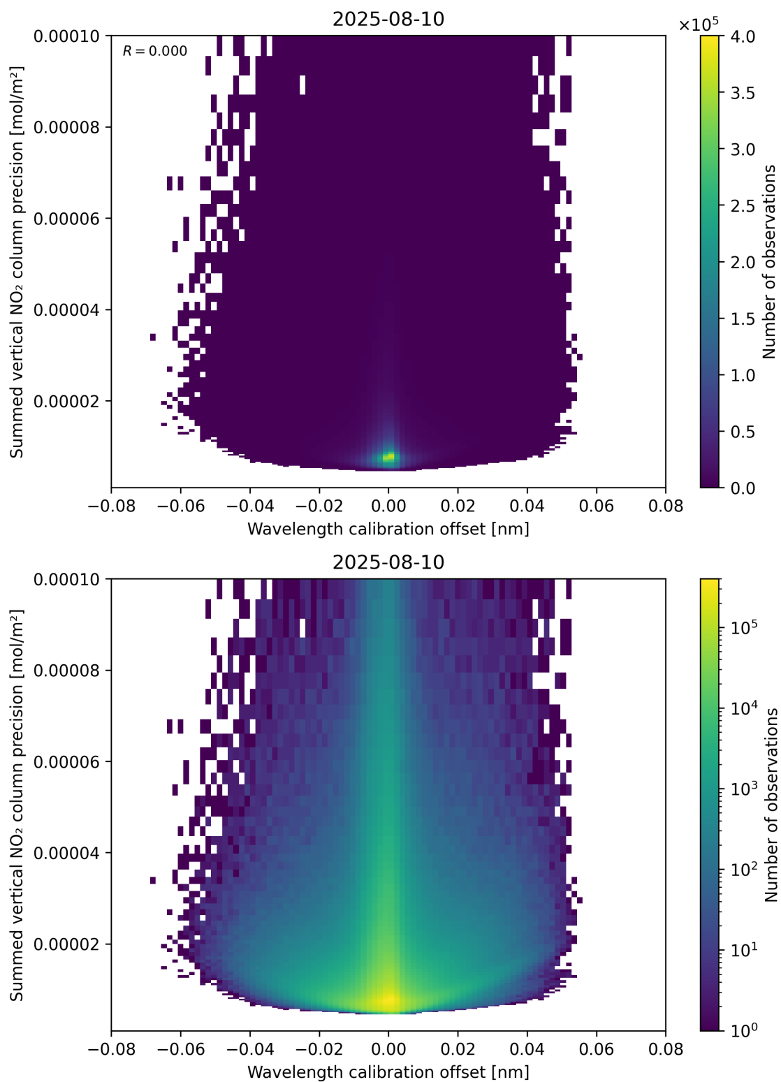
Figure 178: Scatter density plot of “Wavelength calibration offset” against “Summed vertical NO 2 column precision” for 2025-08-09 to 2025-08-11.
