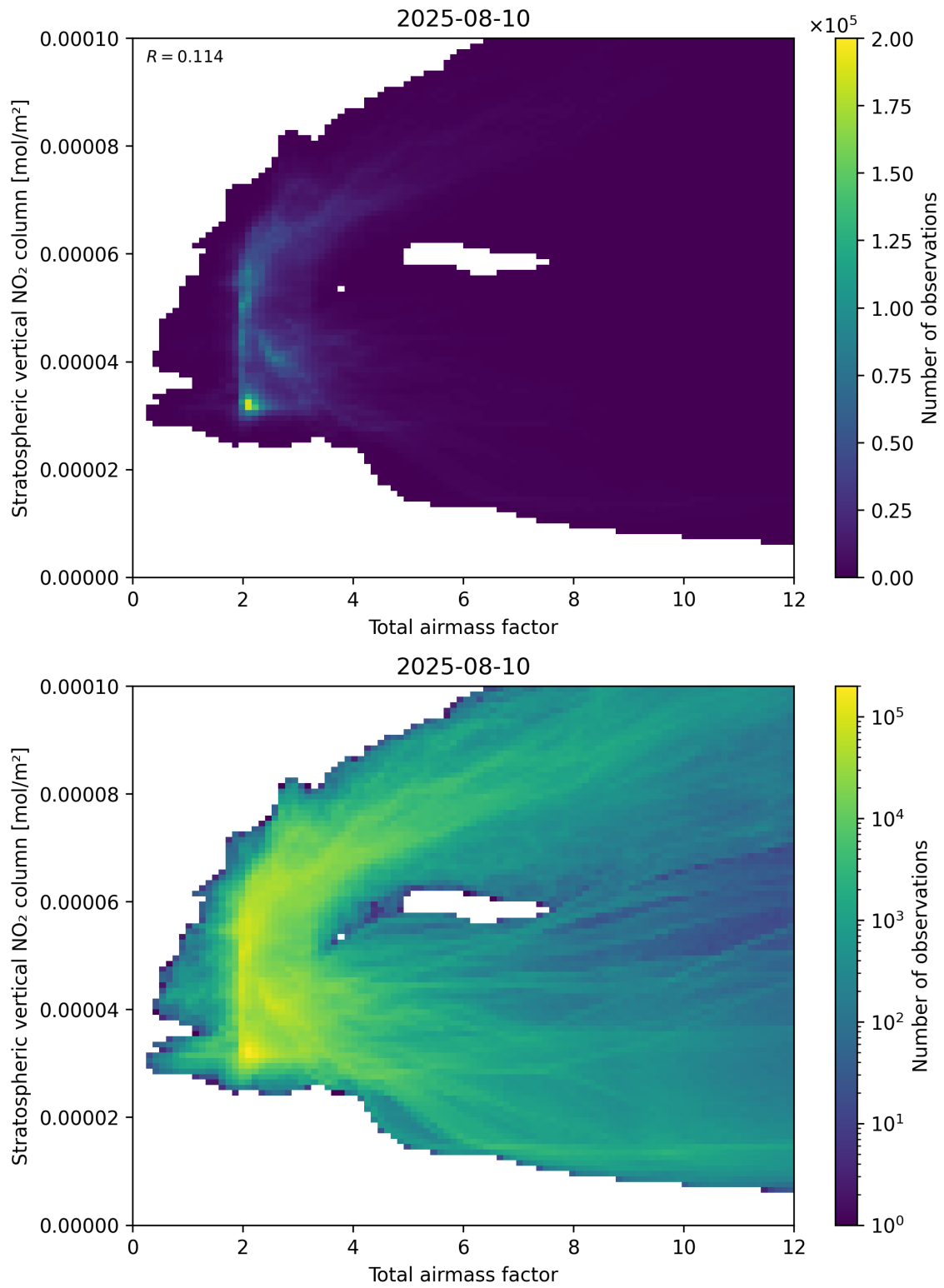
Figure 64: Scatter density plot of “Total airmass factor” against “Stratospheric vertical NO 2 column” for 2025-08-09 to 2025-08-11.
