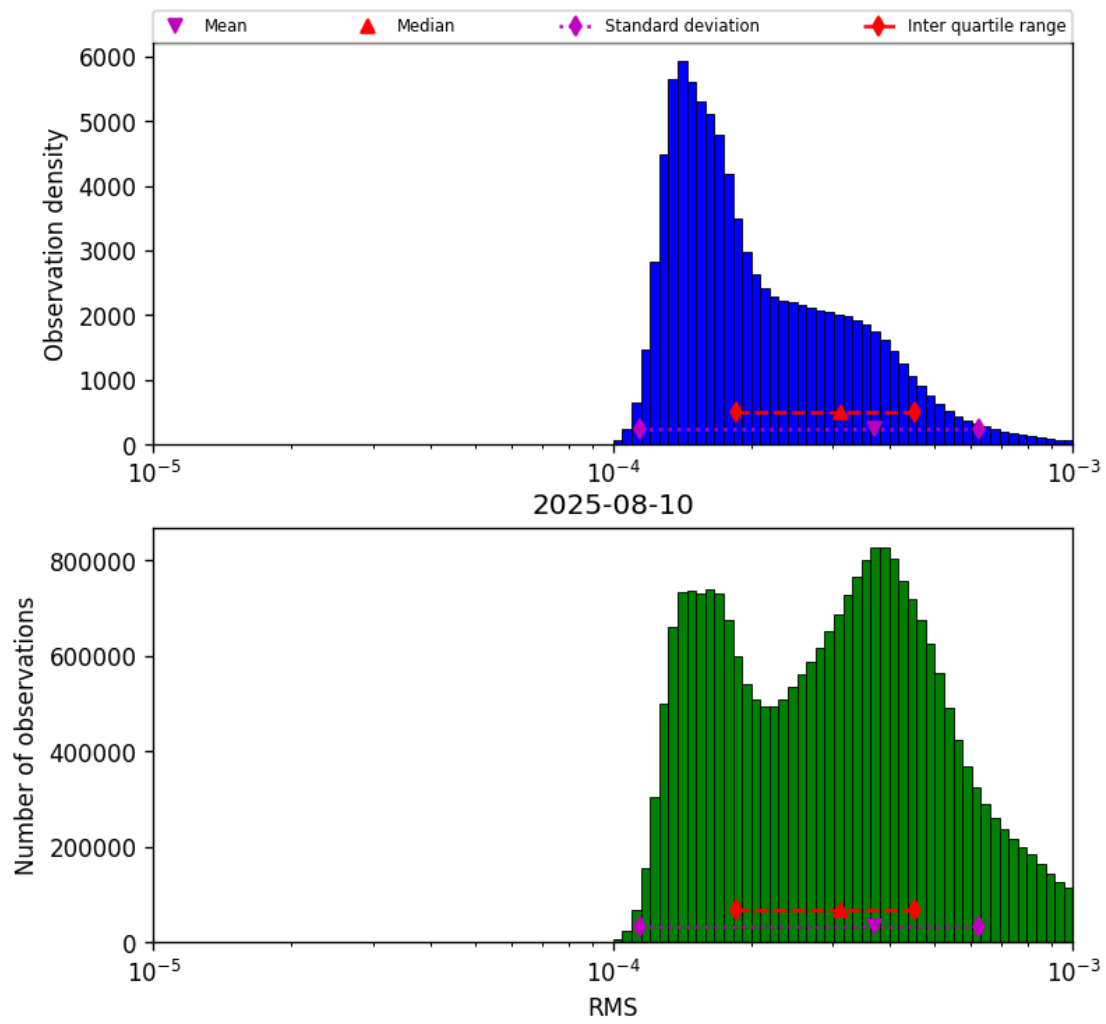
Figure 43: Histogram of “RMS” for 2025-08-09 to 2025-08-11
