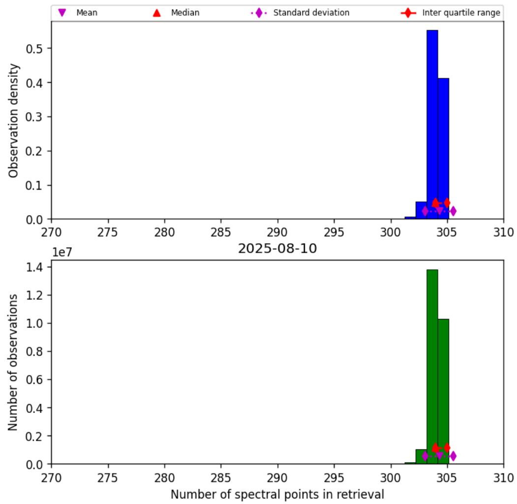
Figure 33: Histogram of “Number of spectral points in retrieval” for 2025-08-09 to 2025-08-11
