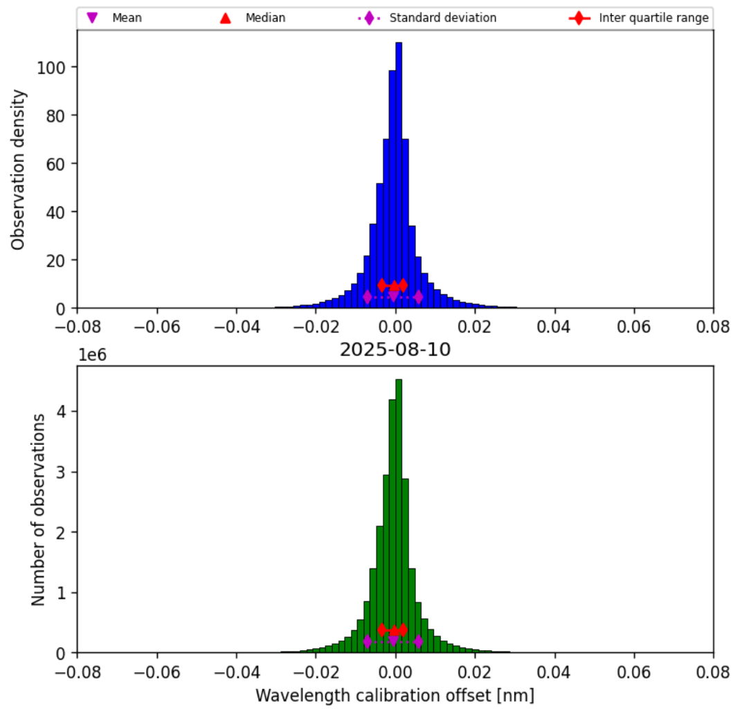
Figure 35: Histogram of “Wavelength calibration offset” for 2025-08-09 to 2025-08-11
