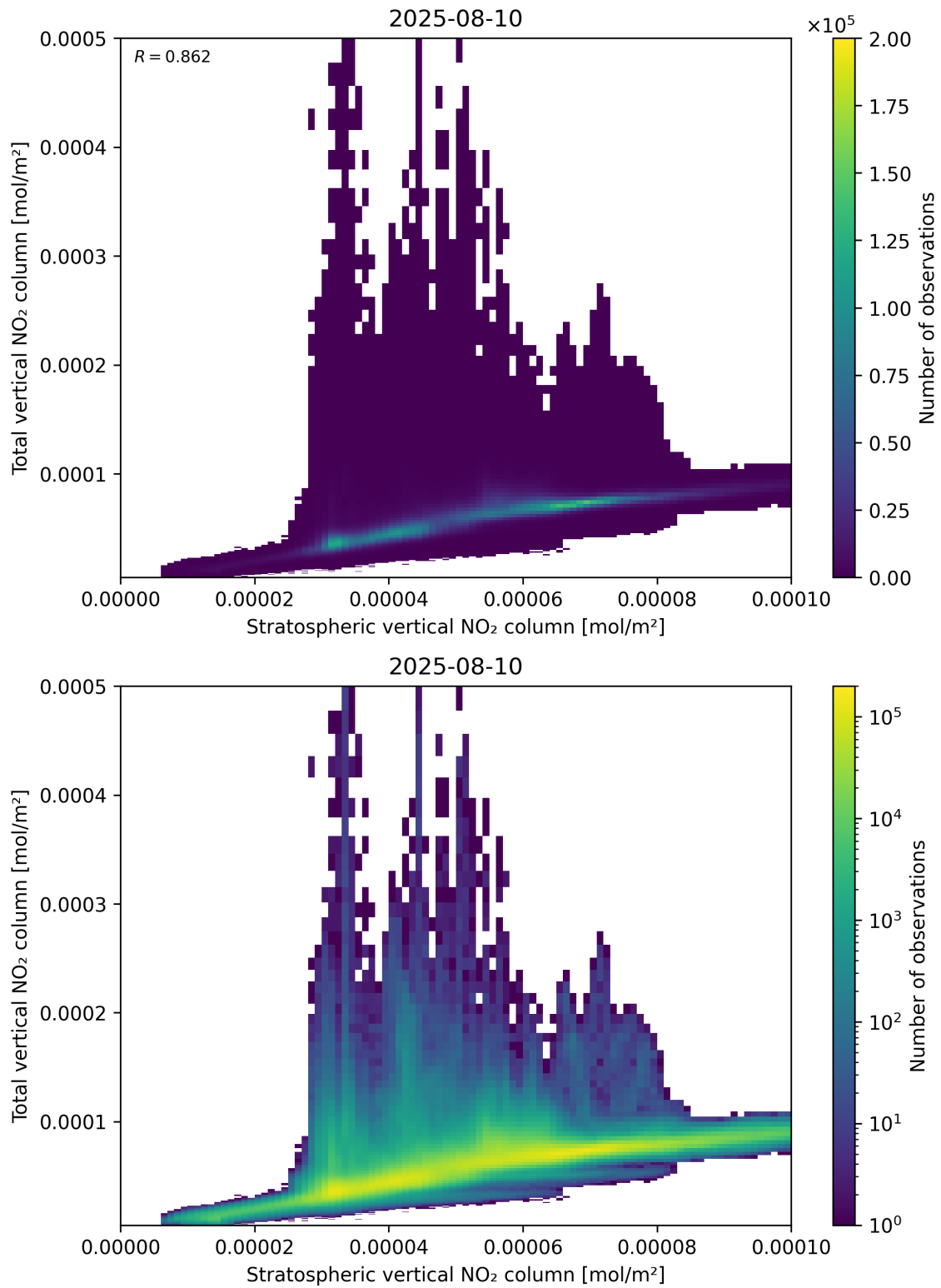
Figure 100: Scatter density plot of “Stratospheric vertical NO 2 column” against “Total vertical NO 2 column” for 2025-08-09 to 2025-08-11.
