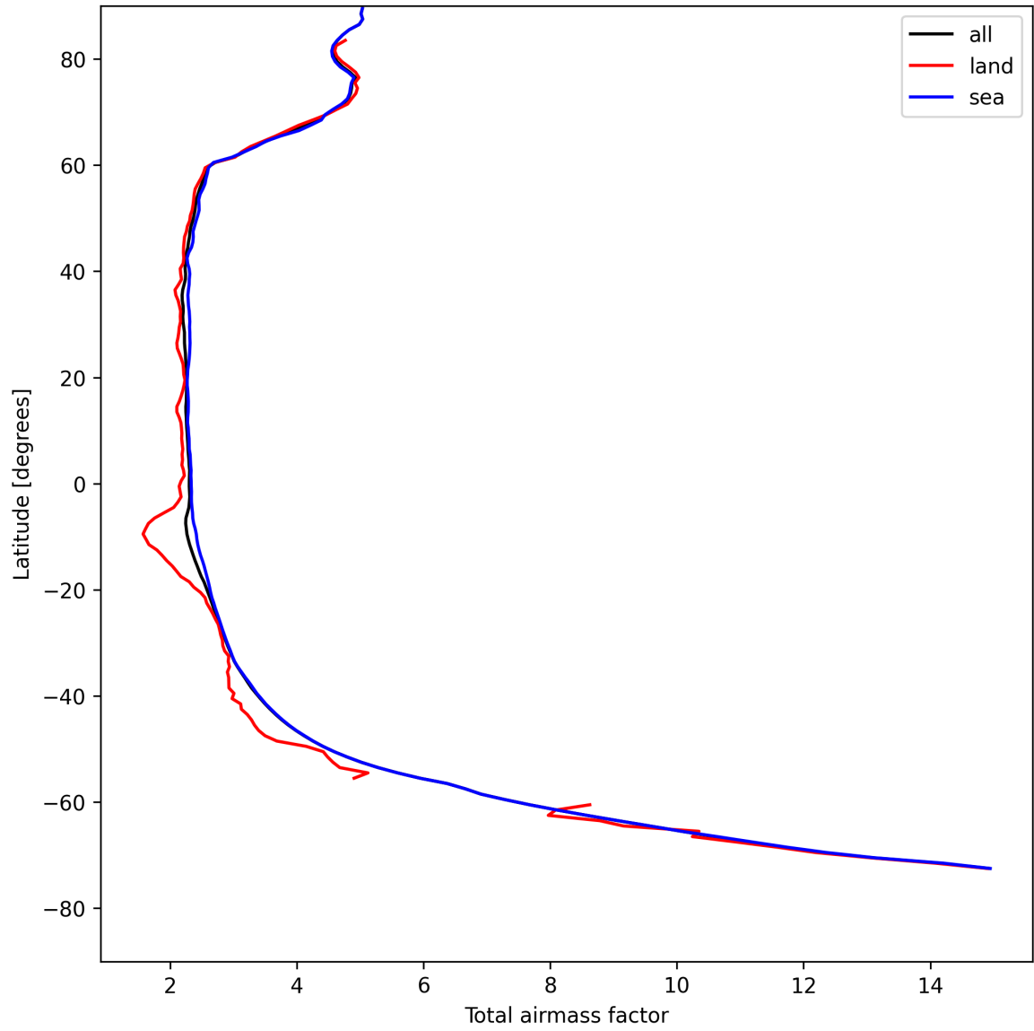
Figure 15: Zonal average of “Total airmass factor” for 2025-08-09 to 2025-08-11.
