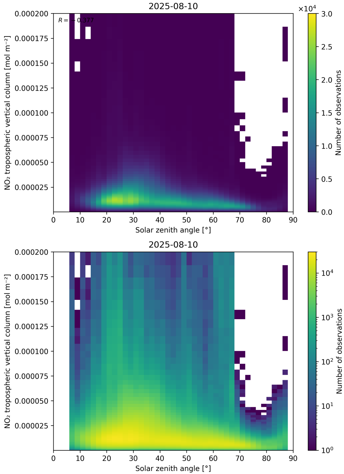
Figure 155: Scatter density plot of “Solar zenith angle” against “NO 2 tropospheric vertical column” for 2025-08-09 to 2025-08-11.
