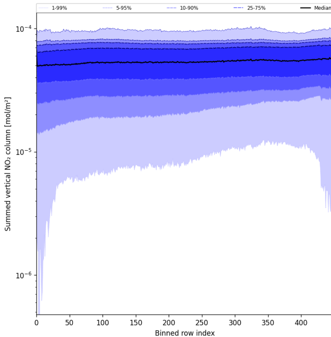
Figure 57: Along track statistics of “Summed vertical NO 2 column” for 2025-08-09 to 2025-08-11
