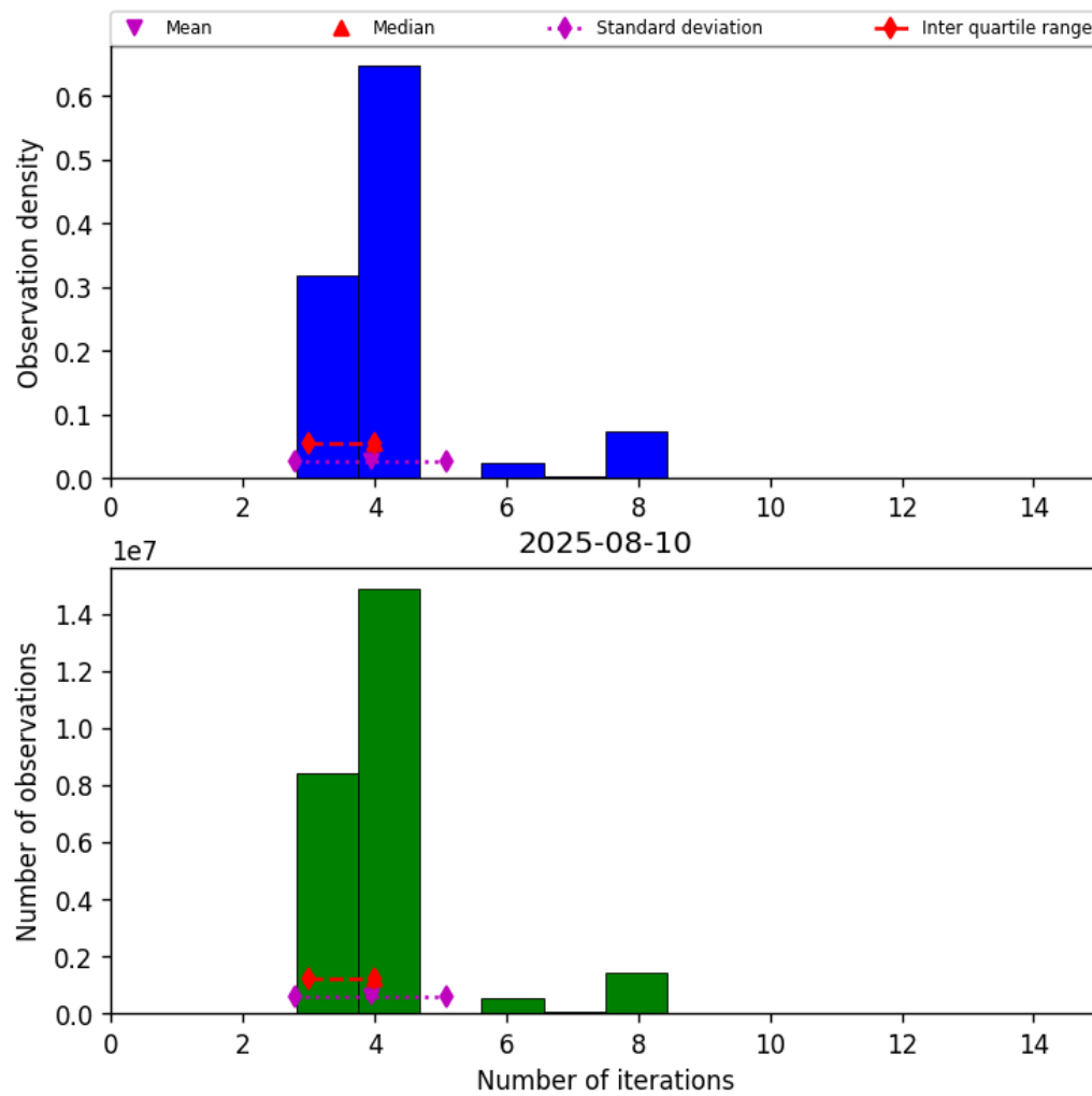
Figure 34: Histogram of “Number of iterations” for 2025-08-09 to 2025-08-11
