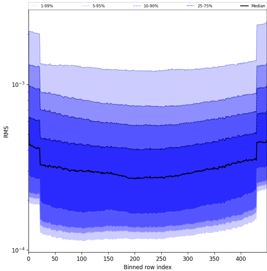
Figure 60: Along track statistics of “RMS” for 2025-08-09 to 2025-08-11
