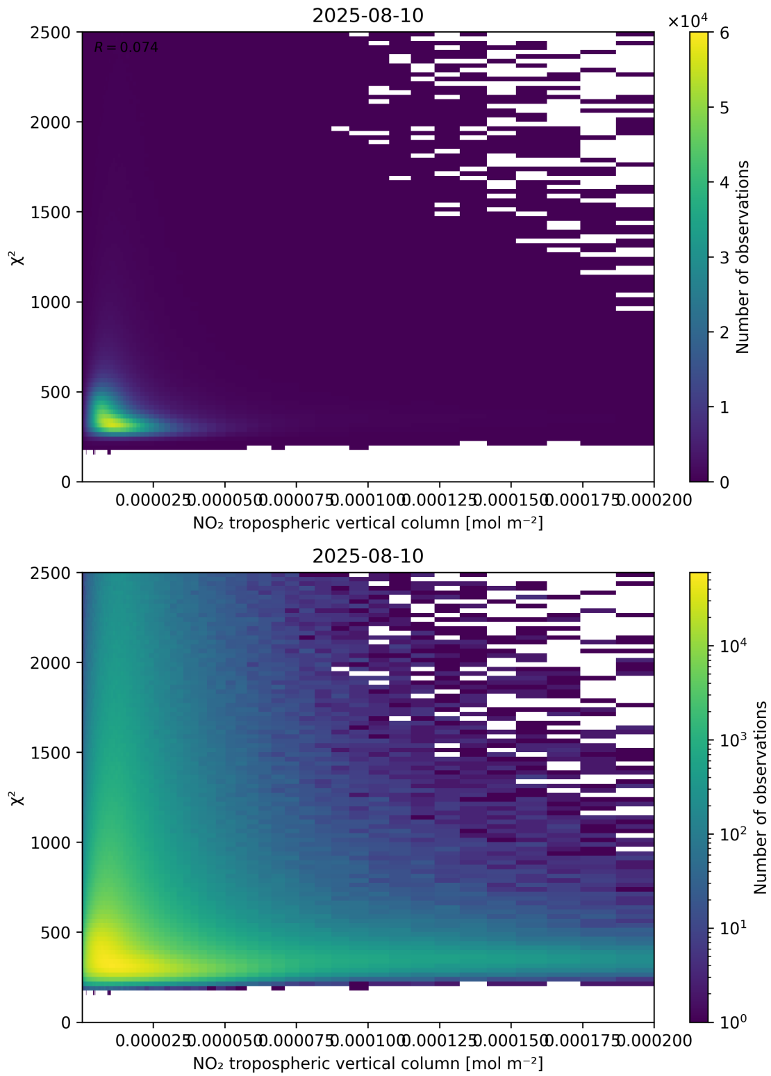
Figure 124: Scatter density plot of “NO 2 tropospheric vertical column” against “ \chi^2 ” for 2025-08-09 to 2025-08-11.
