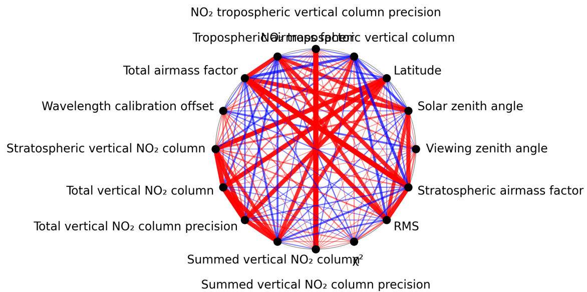
Figure 1: Map of correlation graph for 2025-08-09 to 2025-08-11.
