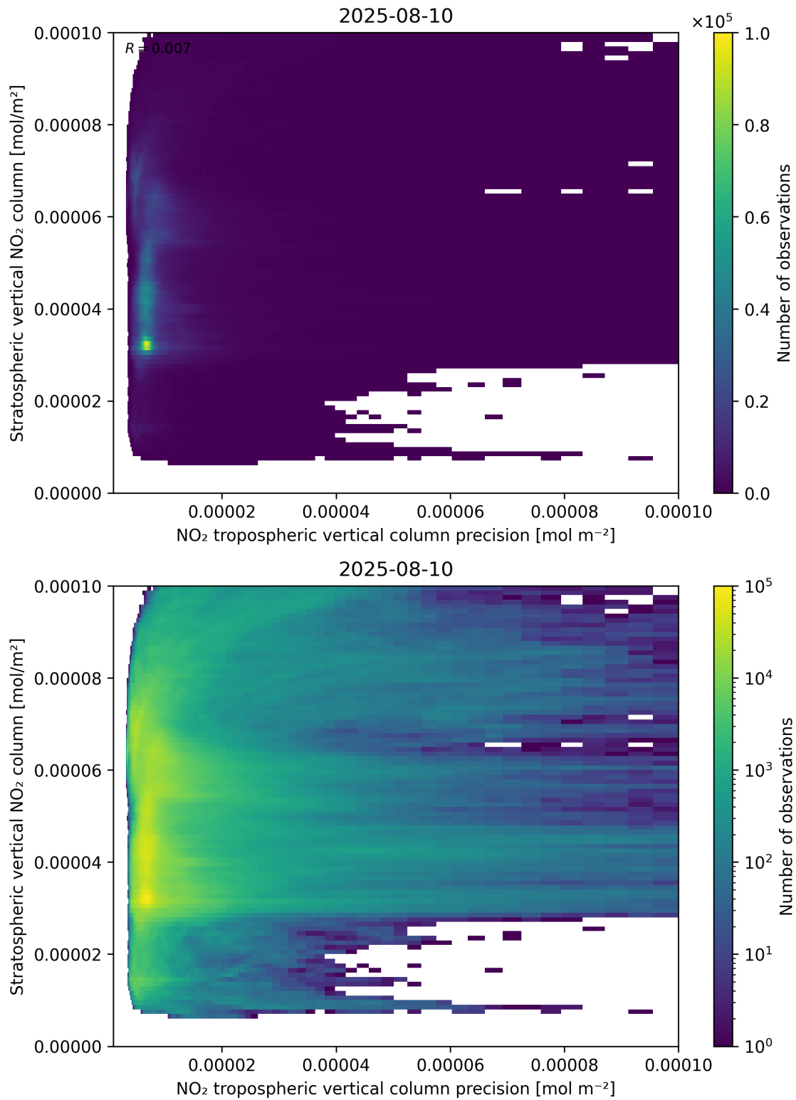
Figure 135: Scatter density plot of “NO 2 tropospheric vertical column precision” against “Stratospheric vertical NO 2 column” for 2025-08-09 to 2025-08-11.
