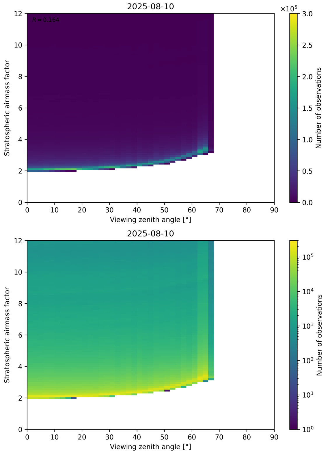
Figure 159: Scatter density plot of “Viewing zenith angle” against “Stratospheric airmass factor” for 2025-08-09 to 2025-08-11.
