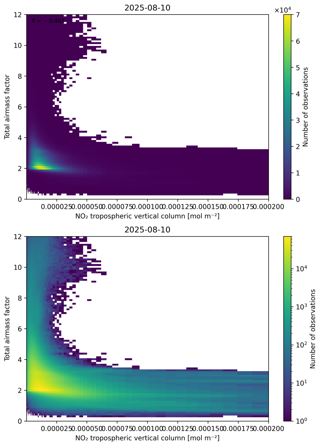
Figure 122: Scatter density plot of “NO 2 tropospheric vertical column” against “Total air mass factor” for 2025-08-09 to 2025-08-11.
