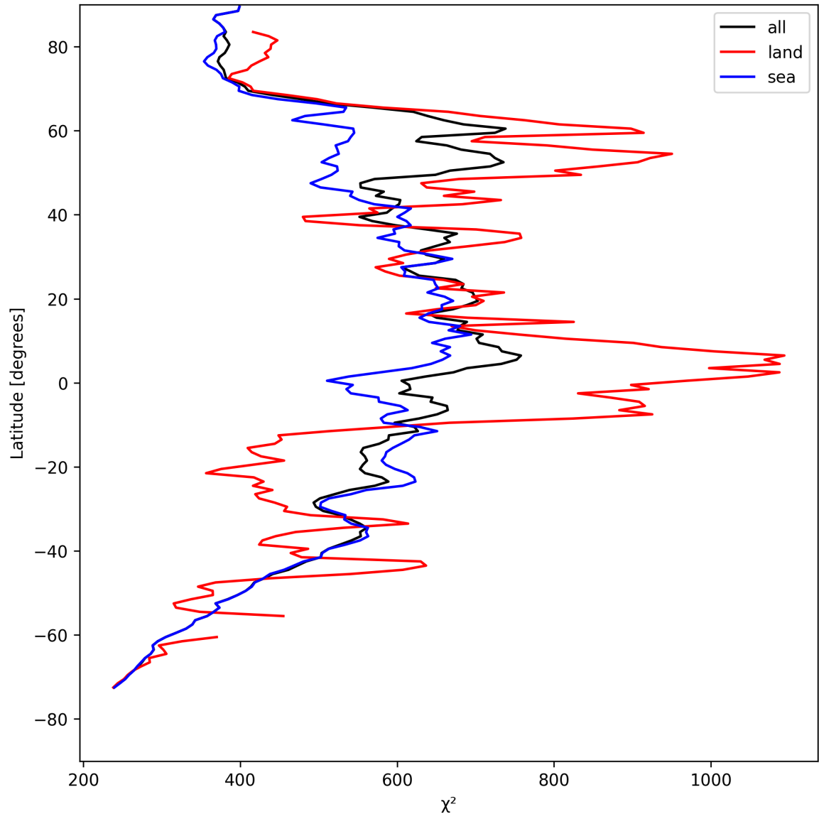
Figure 25: Zonal average of “ \chi^2 ” for 2025-08-09 to 2025-08-11.
