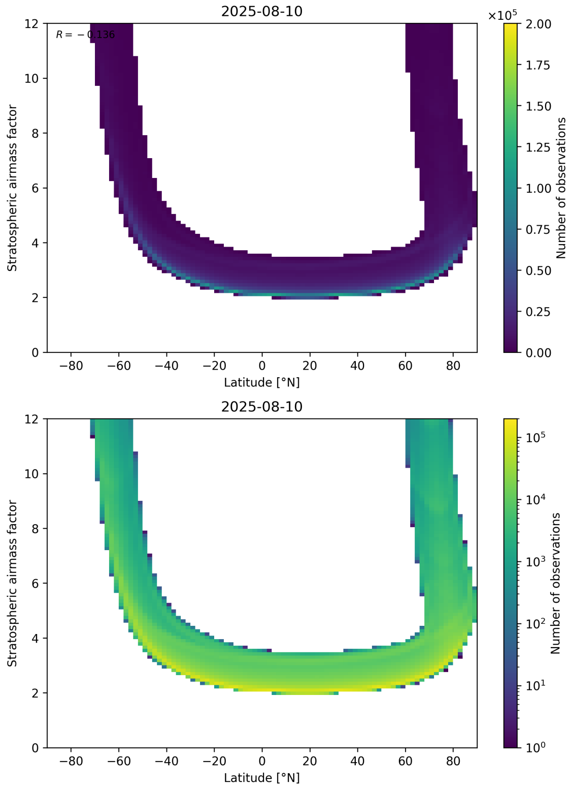
Figure 83: Scatter density plot of “Latitude” against “Stratospheric air mass factor” for 2025-08-09 to 2025-08-11.
