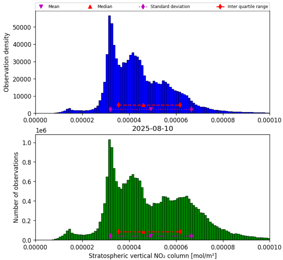
Figure 36: Histogram of “Stratospheric vertical NO 2 column” for 2025-08-09 to 2025-08-11
