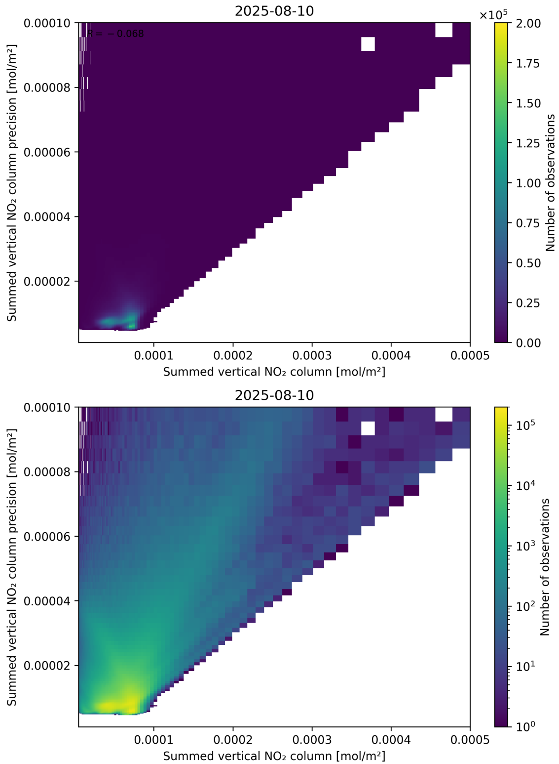
Figure 105: Scatter density plot of “Summed vertical NO 2 column” against “Summed vertical NO 2 column precision” for 2025-08-09 to 2025-08-11.
