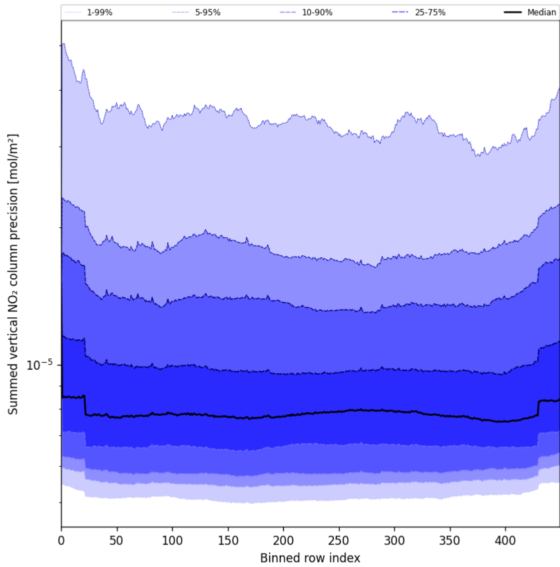
Figure 58: Along track statistics of “Summed vertical NO 2 column precision” for 2025-08-09 to 2025-08-11
