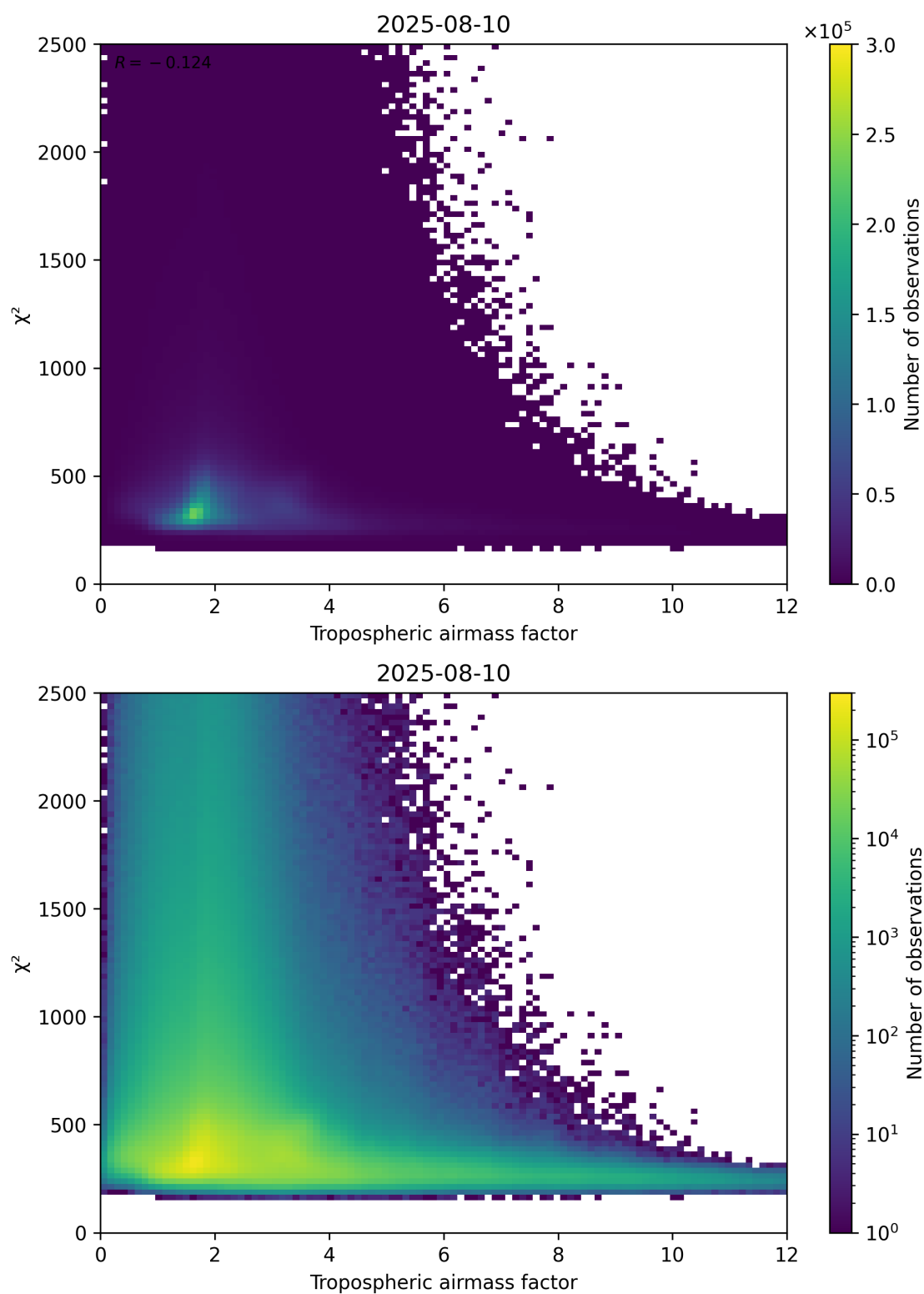
Figure 73: Scatter density plot of “Tropospheric airmass factor” against “ \chi^2 ” for 2025-08-09 to 2025-08-11.
