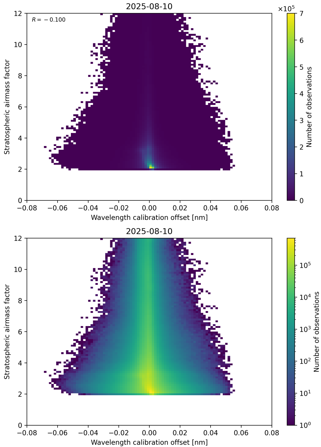
Figure 174: Scatter density plot of “Wavelength calibration offset” against “Stratospheric airmass factor” for 2025-08-09 to 2025-08-11.
