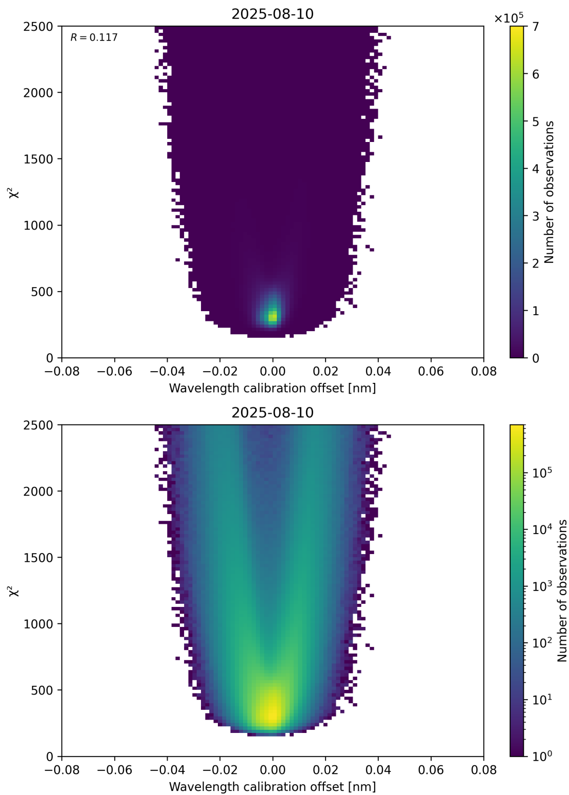
Figure 175: Scatter density plot of “Wavelength calibration offset” against “ \chi^2 ” for 2025-08-09 to 2025-08-11.
