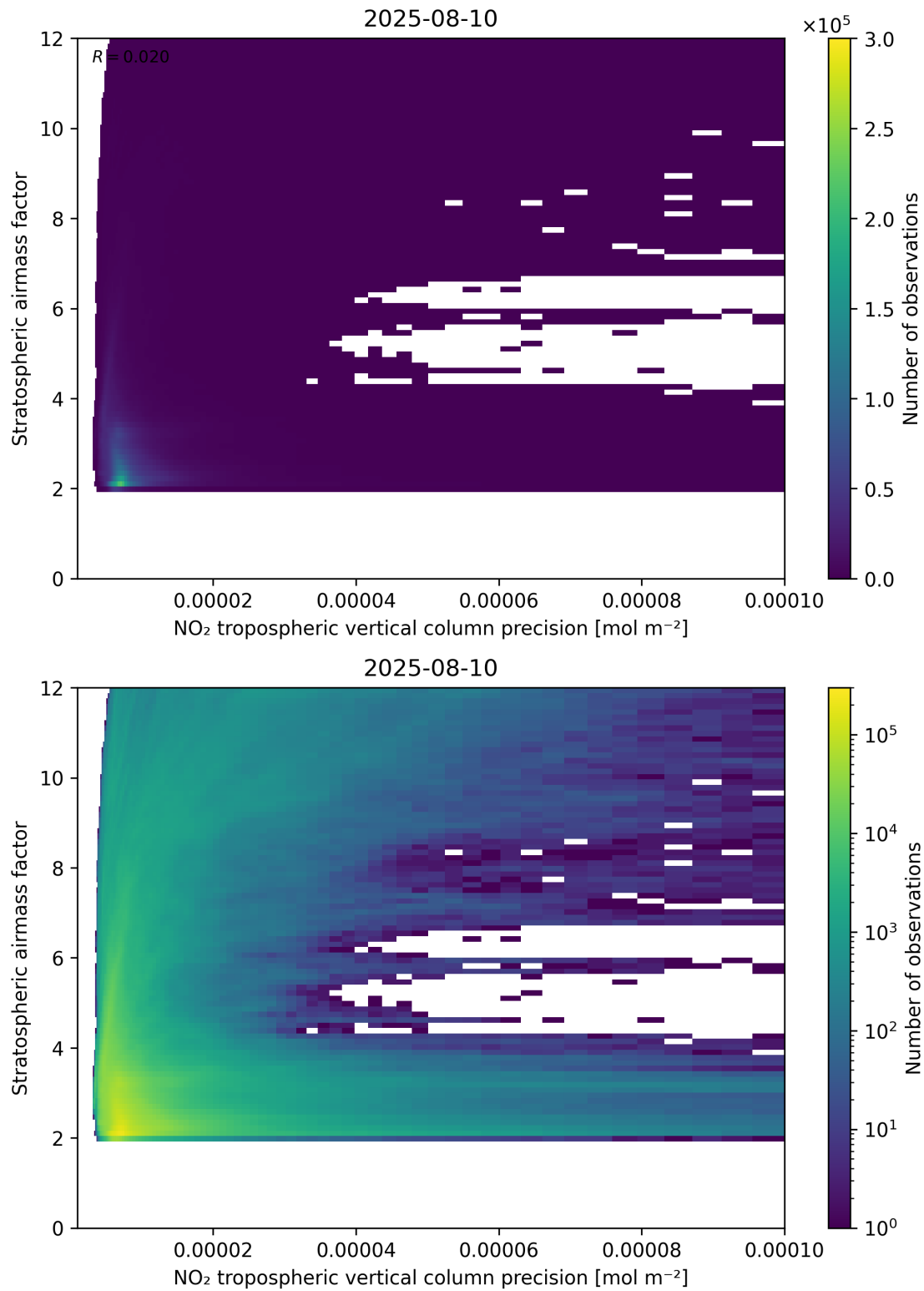
Figure 131: Scatter density plot of “NO 2 tropospheric vertical column precision” against “Stratospheric airmass factor” for 2025-08-09 to 2025-08-11.
