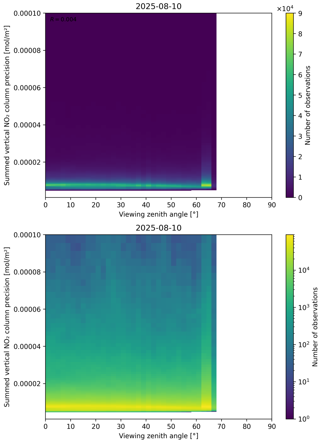
Figure 166: Scatter density plot of “Viewing zenith angle” against “Summed vertical NO 2 column precision” for 2025-08-09 to 2025-08-11.
