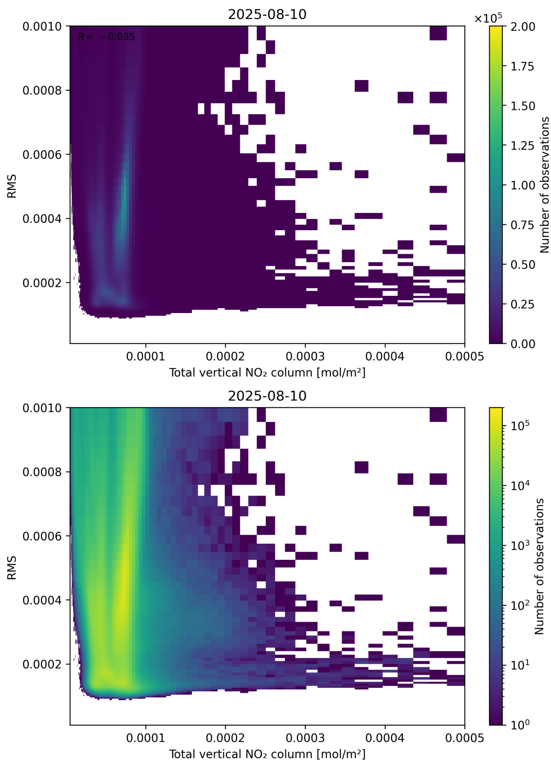
Figure 120: Scatter density plot of “Total vertical NO 2 column” against “RMS” for 2025-08-09 to 2025-08-11.
