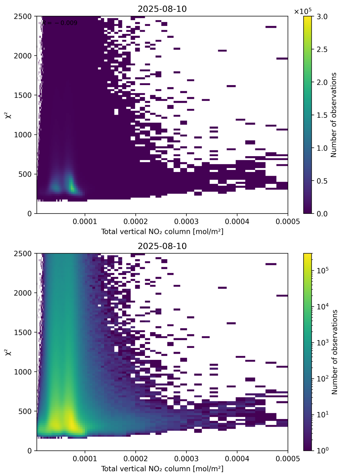
Figure 111: Scatter density plot of “Total vertical NO 2 column” against “ \chi^2 ” for 2025-08-09 to 2025-08-11.
