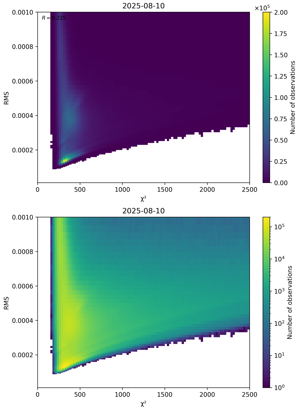
Figure 82: Scatter density plot of “ \chi^2 ” against “RMS” for 2025-08-09 to 2025-08-11.
