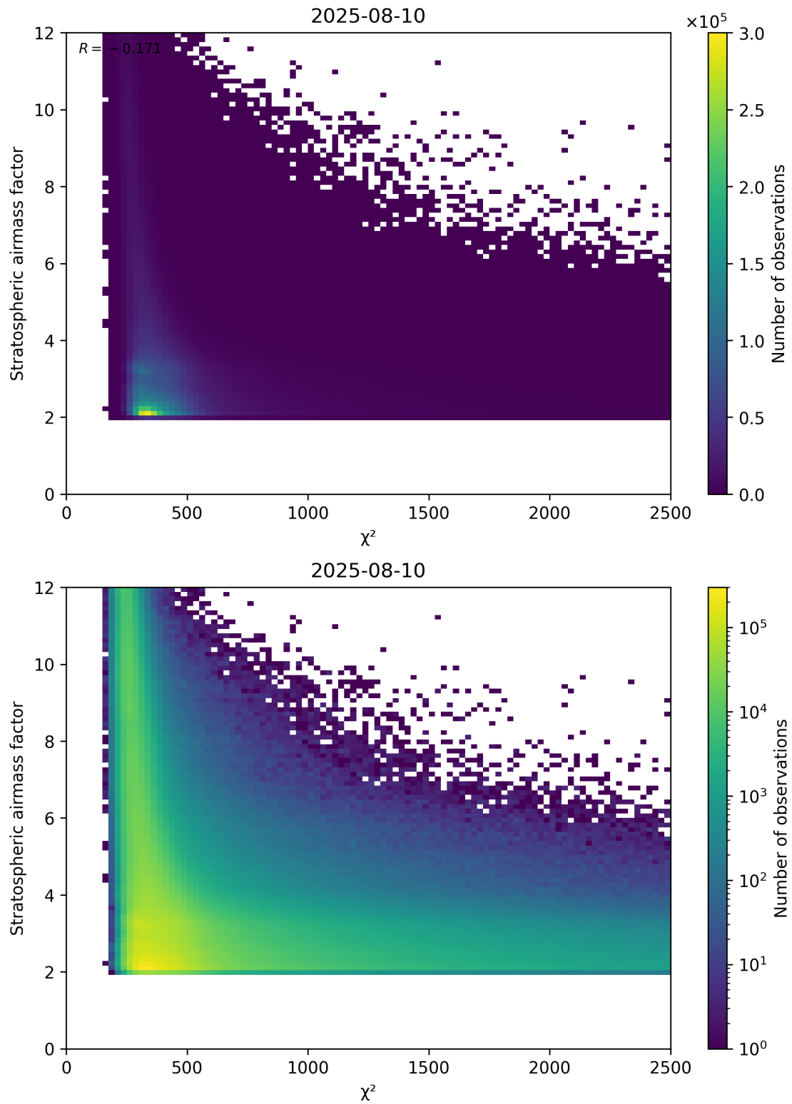
Figure 81: Scatter density plot of “ \chi^2 ” against “Stratospheric airmass factor” for 2025-08-09 to 2025-08-11.
