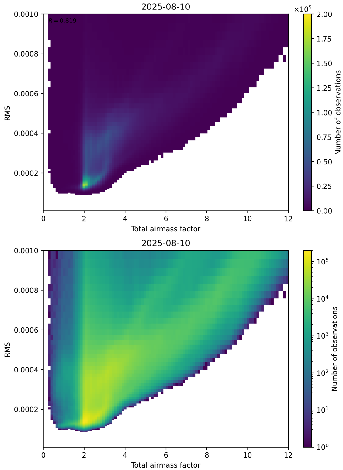
Figure 69: Scatter density plot of “Total airmass factor” against “RMS” for 2025-08-09 to 2025-08-11.
