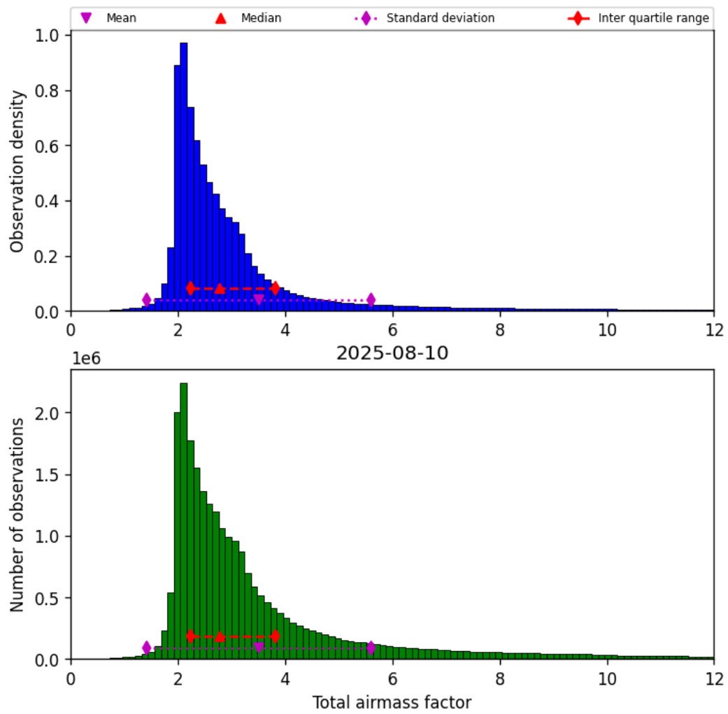
Figure 32: Histogram of “Total airmass factor” for 2025-08-09 to 2025-08-11
