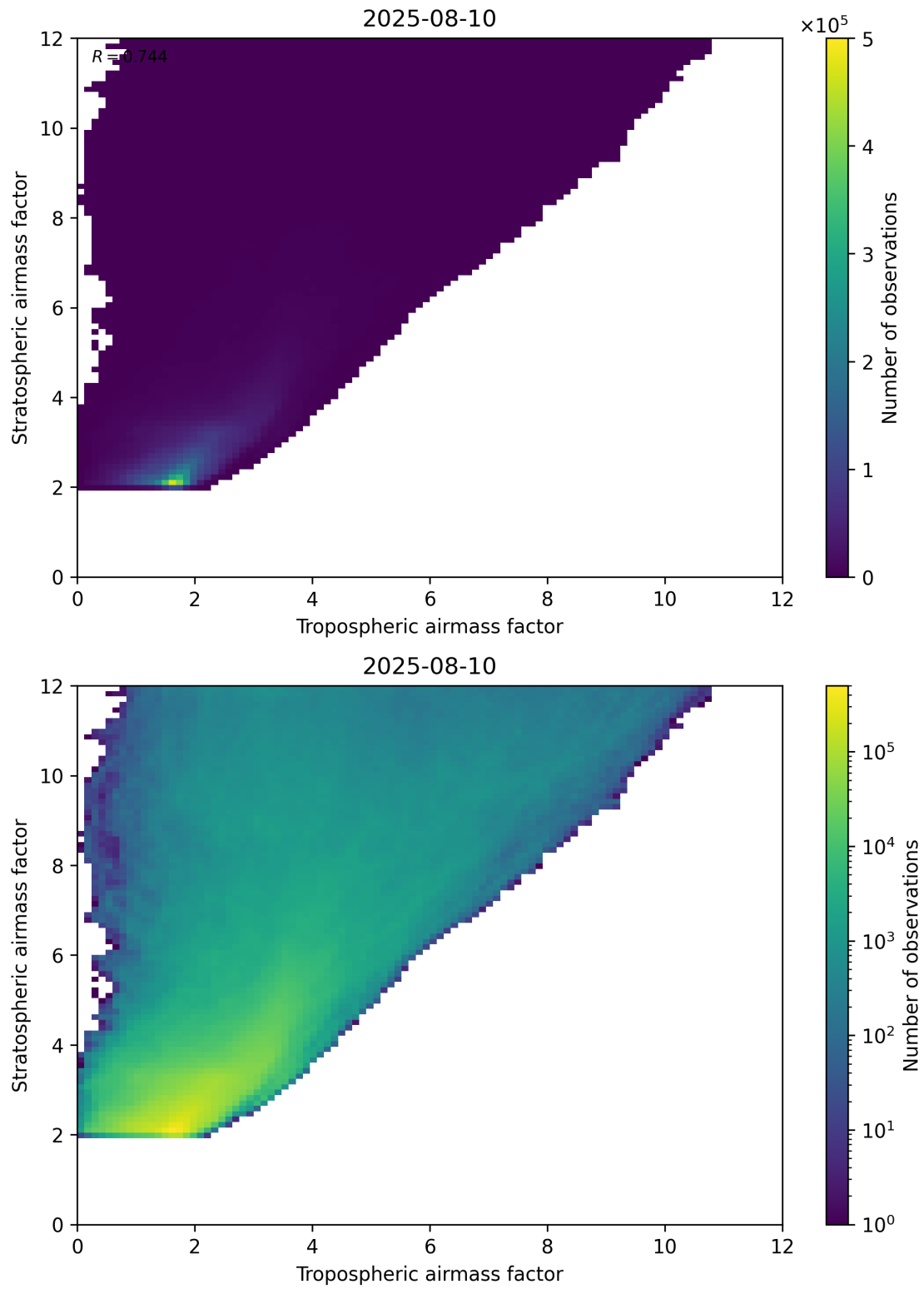
Figure 71: Scatter density plot of “Tropospheric airmass factor” against “Stratospheric airmass factor” for 2025-08-09 to 2025-08-11.
