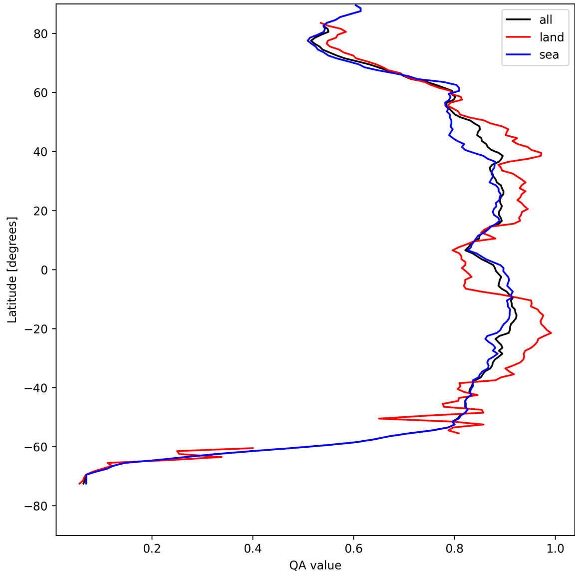
Figure 11: Zonal average of “QA value” for 2025-08-09 to 2025-08-11.
