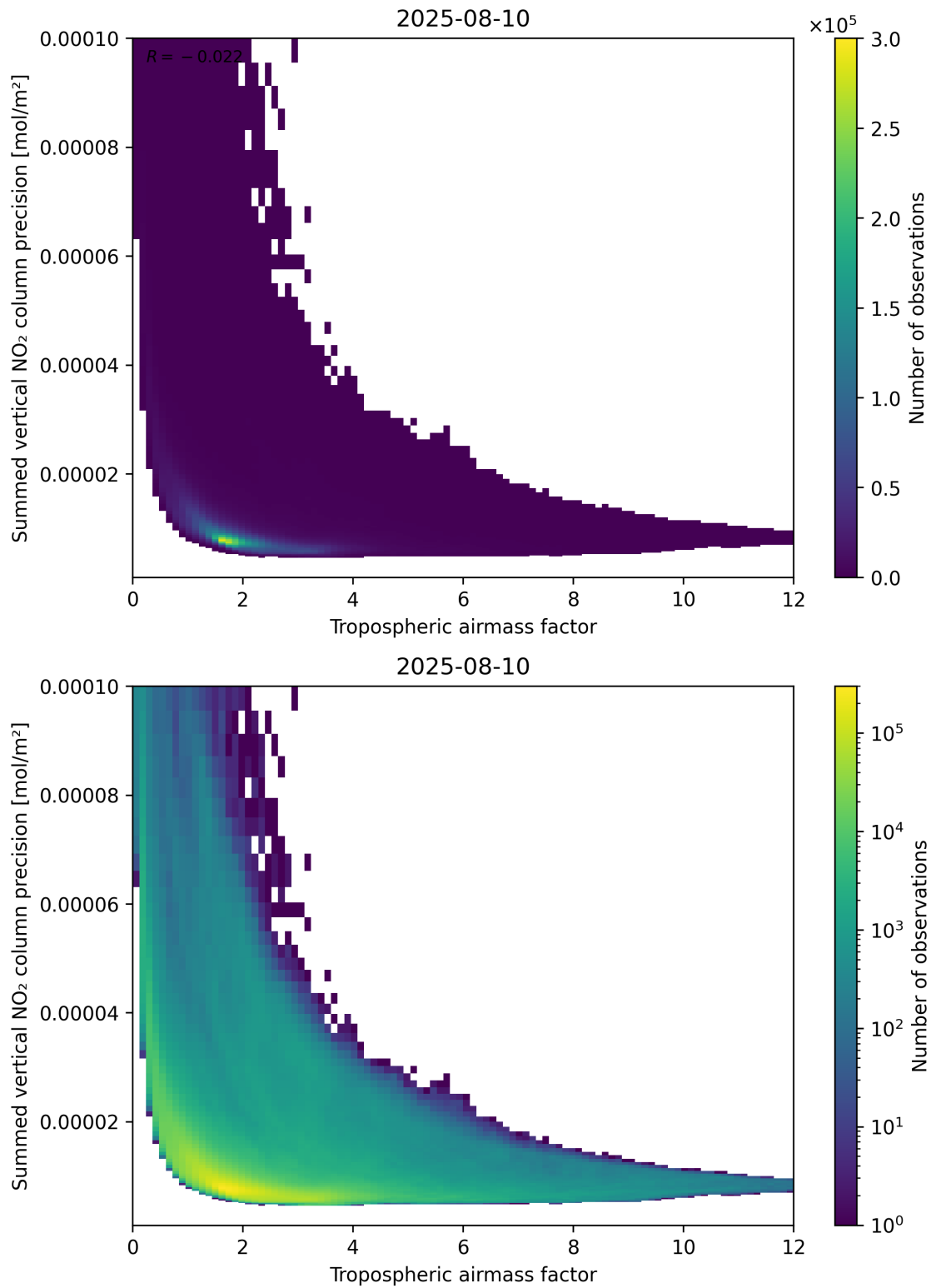
Figure 76: Scatter density plot of “Tropospheric air mass factor” against “Summed vertical NO 2 column precision” for 2025-08-09 to 2025-08-11.
