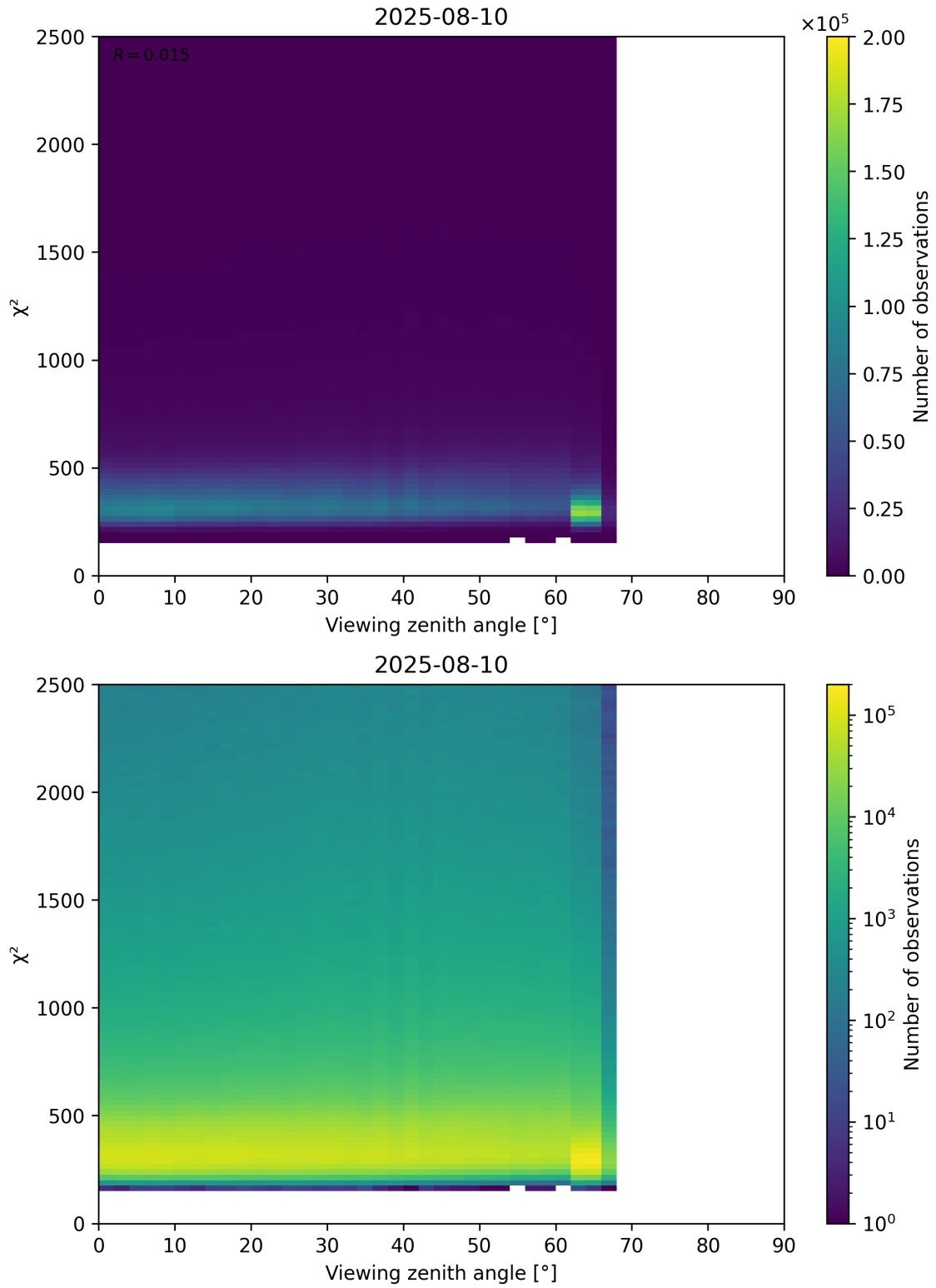
Figure 162: Scatter density plot of “Viewing zenith angle” against “ \chi^2 ” for 2025-08-09 to 2025-08-11.
