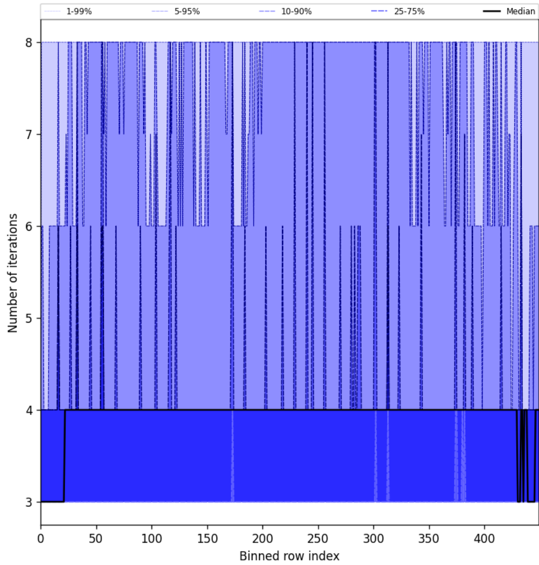
Figure 51: Along track statistics of “Number of iterations” for 2025-08-09 to 2025-08-11
