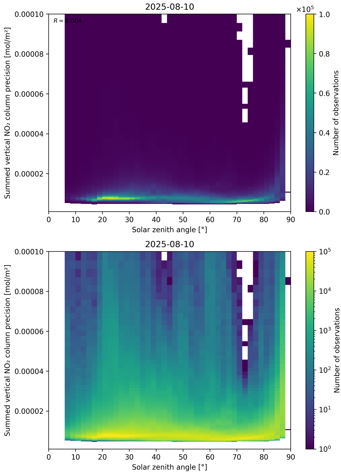
Figure 152: Scatter density plot of “Solar zenith angle” against “Summed vertical NO 2 column precision” for 2025-08-09 to 2025-08-11.
