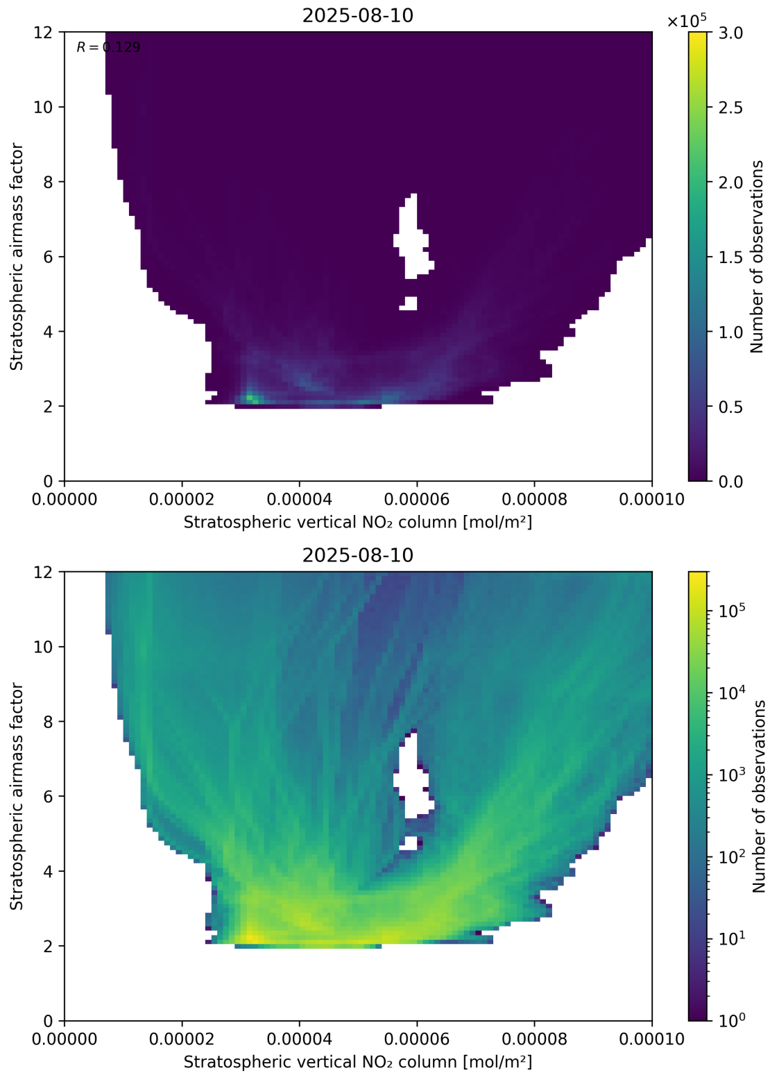
Figure 96: Scatter density plot of “Stratospheric vertical NO 2 column” against “Stratospheric airmass factor” for 2025-08-09 to 2025-08-11.
