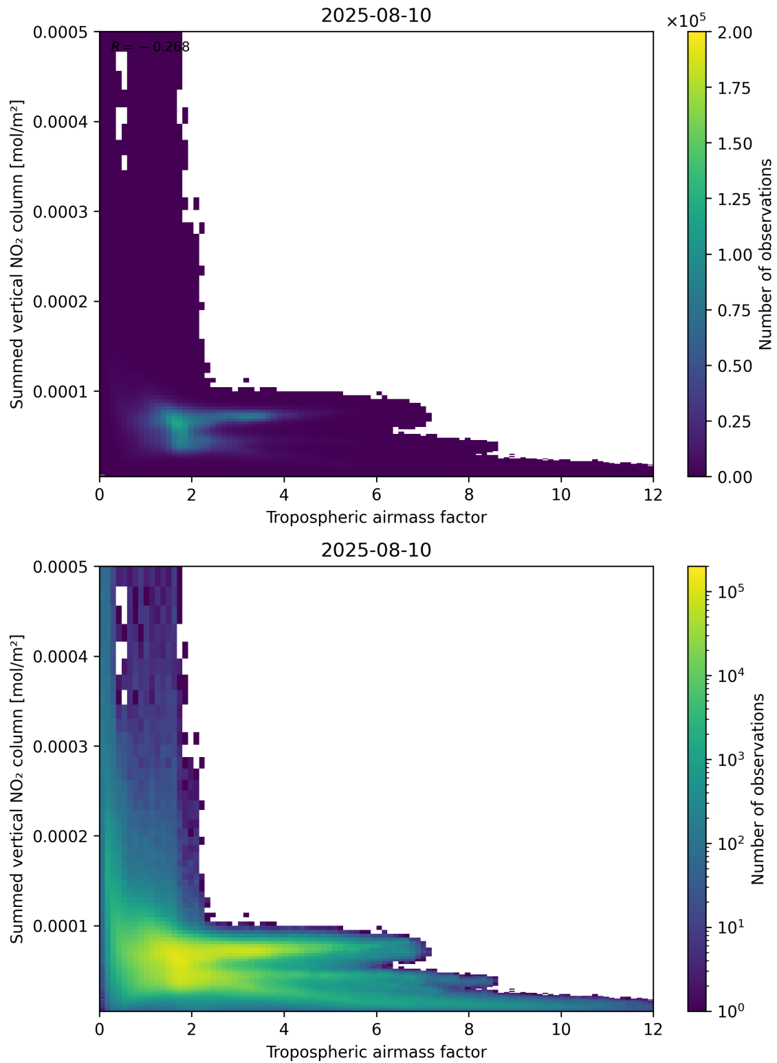
Figure 75: Scatter density plot of “Tropospheric air mass factor” against “Summed vertical NO 2 column” for 2025-08-09 to 2025-08-11.
