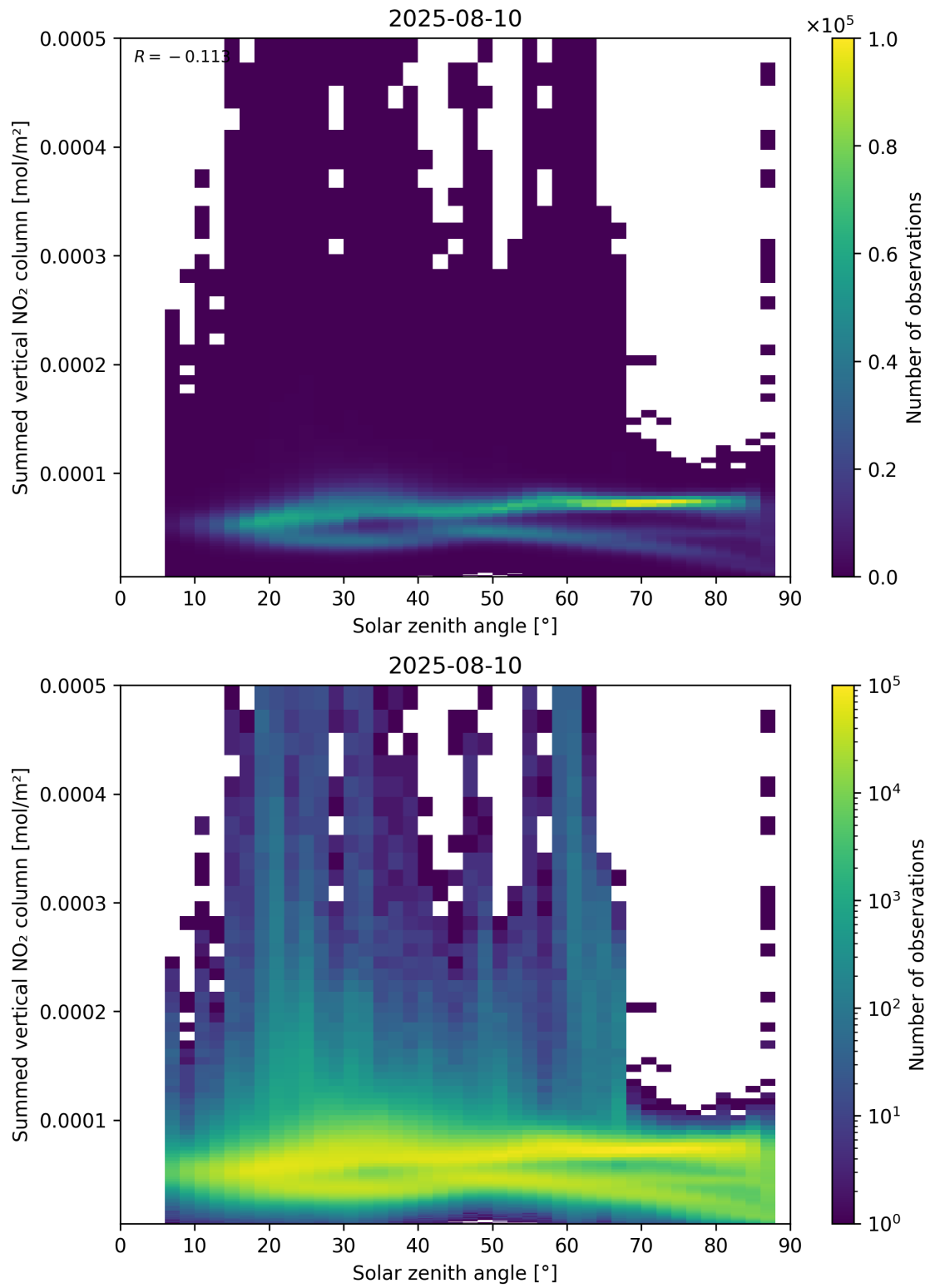
Figure 151: Scatter density plot of “Solar zenith angle” against “Summed vertical NO 2 column” for 2025-08-09 to 2025-08-11.
