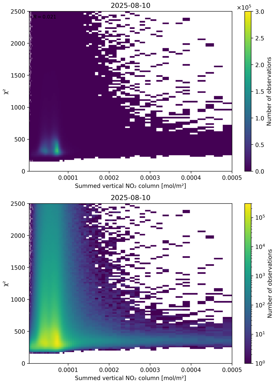
Figure 104: Scatter density plot of “Summed vertical NO 2 column” against “ \chi^2 ” for 2025-08-09 to 2025-08-11.
