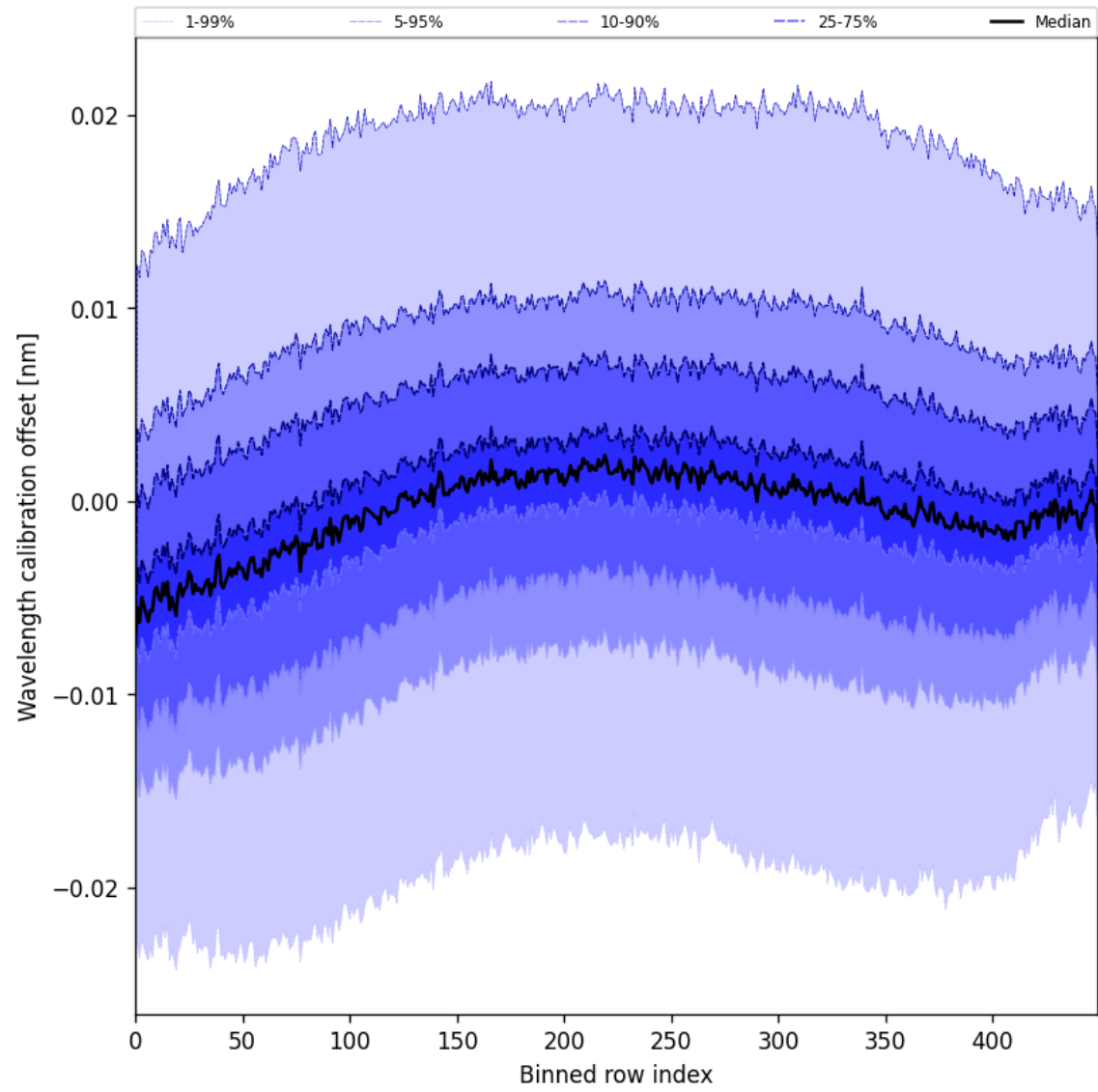
Figure 52: Along track statistics of “Wavelength calibration offset” for 2025-08-09 to 2025-08-11
