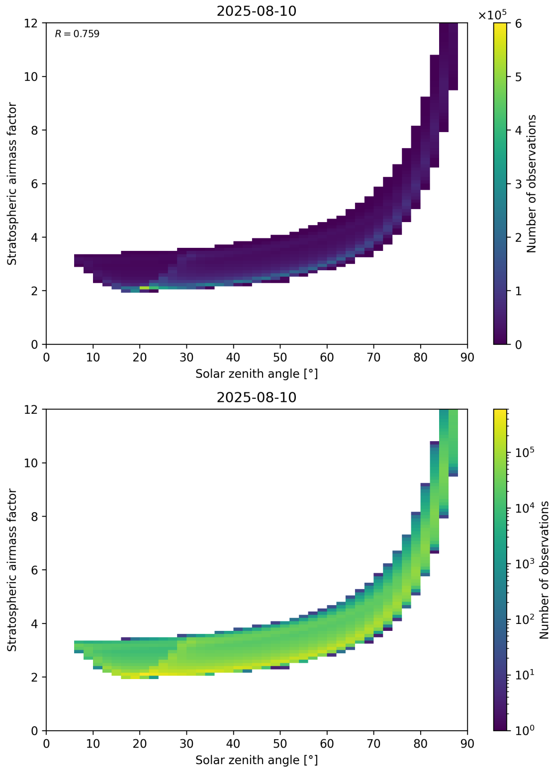
Figure 145: Scatter density plot of “Solar zenith angle” against “Stratospheric airmass factor” for 2025-08-09 to 2025-08-11.
