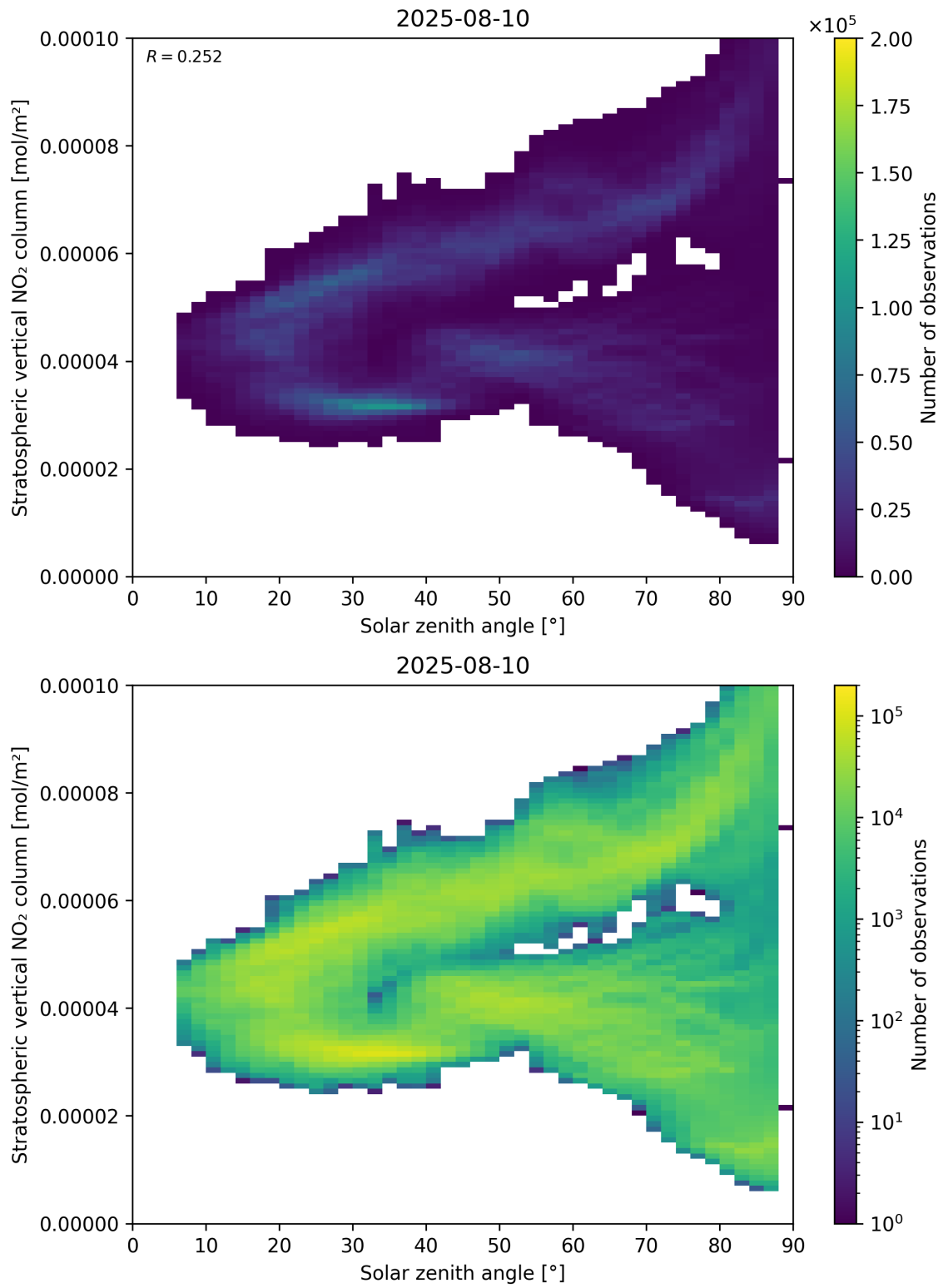
Figure 150: Scatter density plot of “Solar zenith angle” against “Stratospheric vertical NO 2 column” for 2025-08-09 to 2025-08-11.
