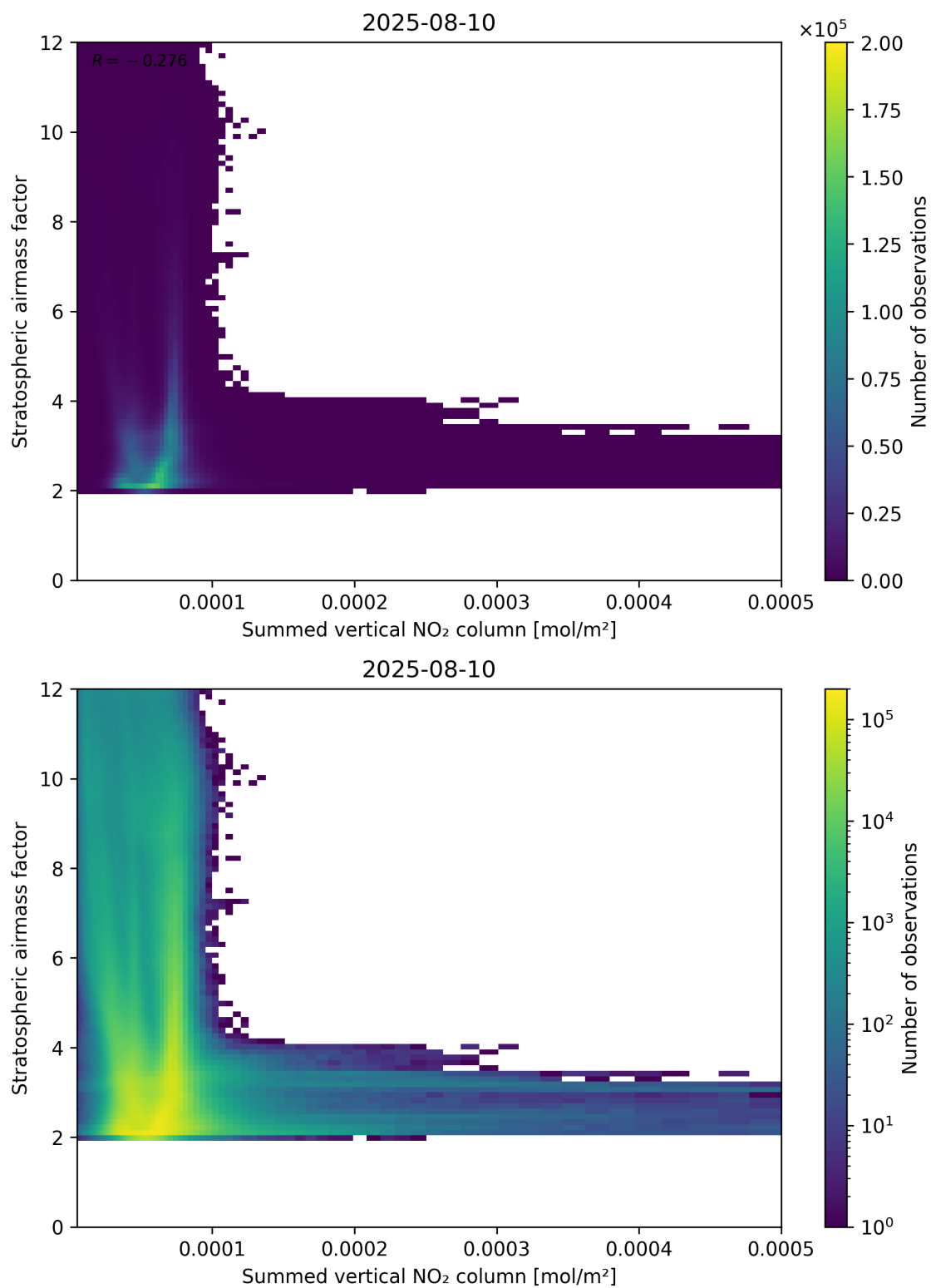
Figure 103: Scatter density plot of “Summed vertical NO 2 column” against “Stratospheric airmass factor” for 2025-08-09 to 2025-08-11.
