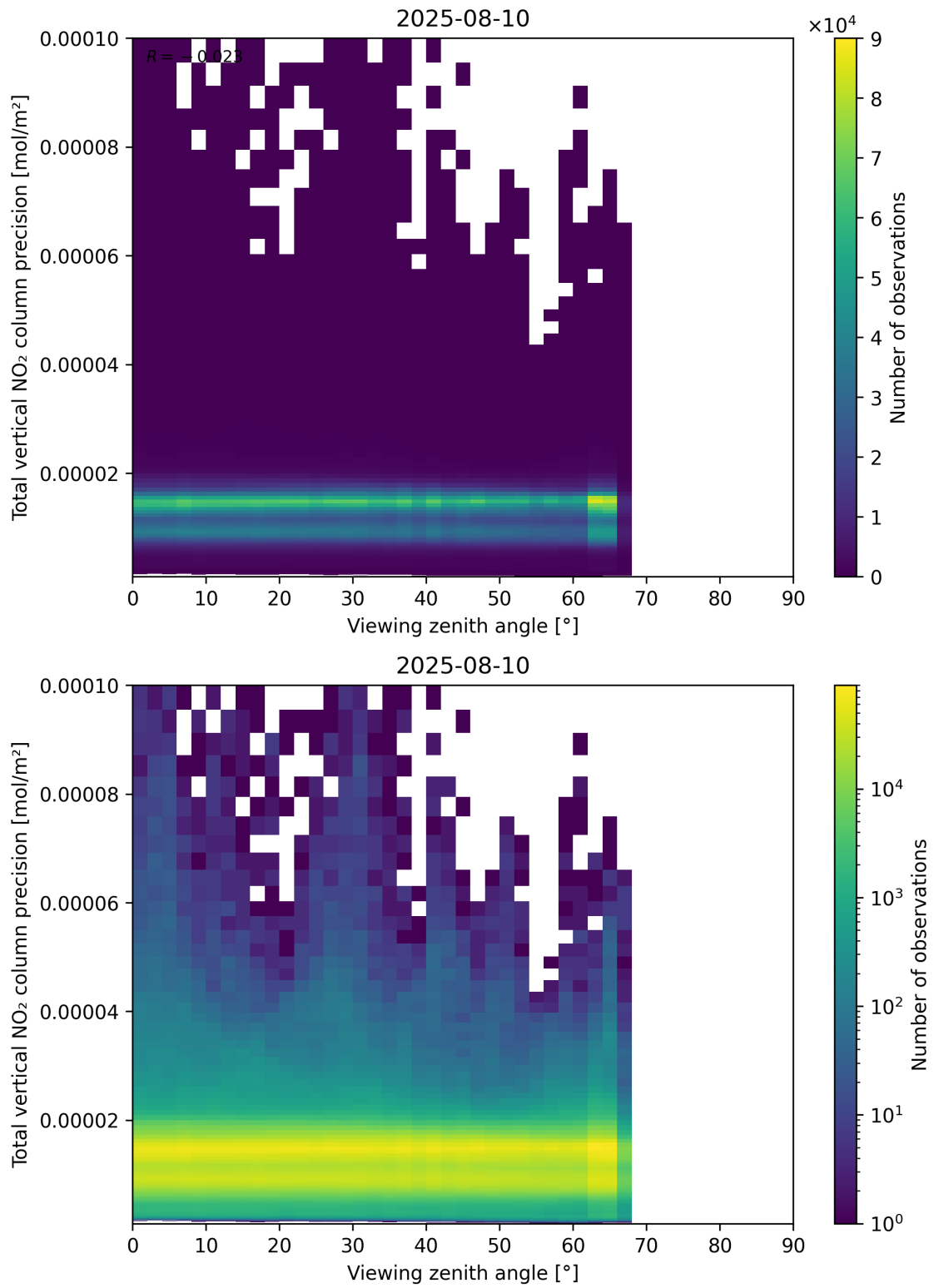
Figure 168: Scatter density plot of “Viewing zenith angle” against “Total vertical NO 2 column precision” for 2025-08-09 to 2025-08-11.
