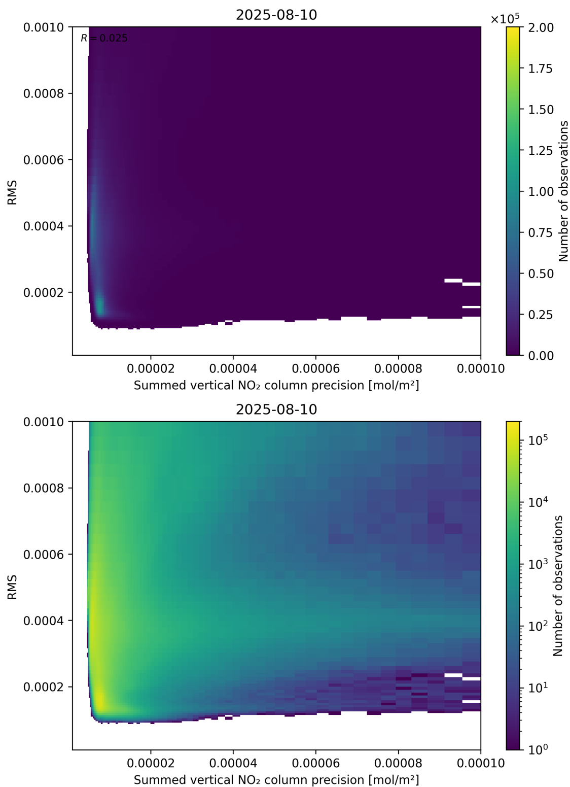
Figure 108: Scatter density plot of “Summed vertical NO 2 column precision” against “RMS” for 2025-08-09 to 2025-08-11.
