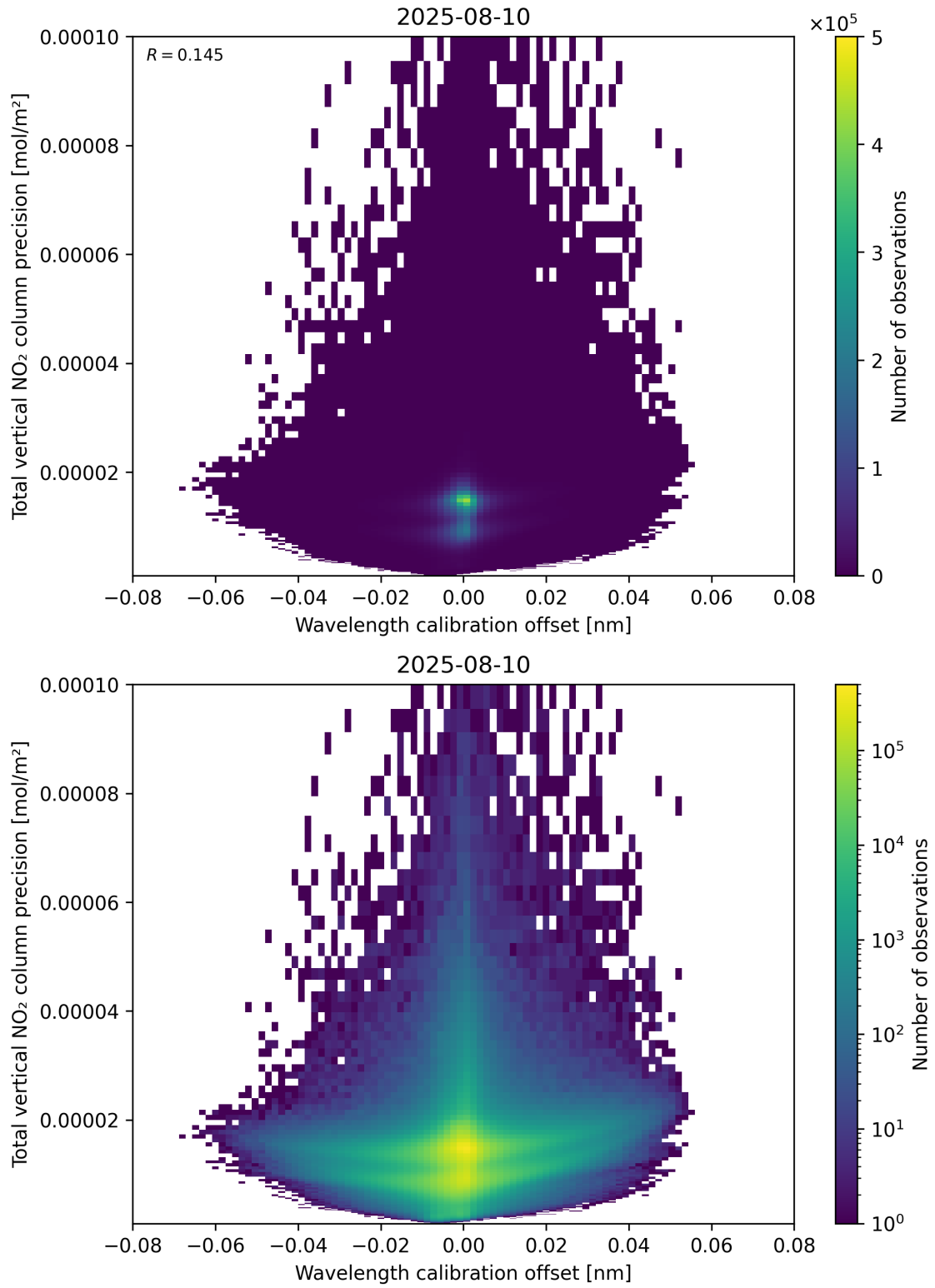
Figure 180: Scatter density plot of “Wavelength calibration offset” against “Total vertical NO 2 column precision” for 2025-08-09 to 2025-08-11.
