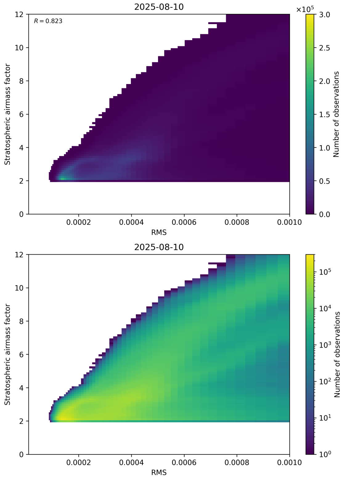
Figure 144: Scatter density plot of “RMS” against “Stratospheric airmass factor” for 2025-08-09 to 2025-08-11.
