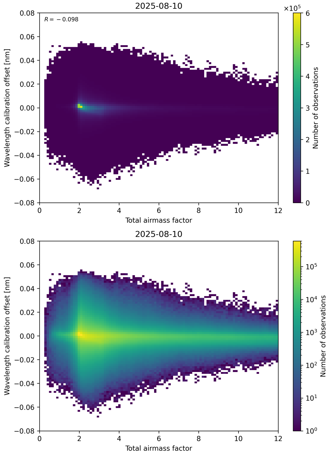
Figure 70: Scatter density plot of “Total airmass factor” against “Wavelength calibration offset” for 2025-08-09 to 2025-08-11.
