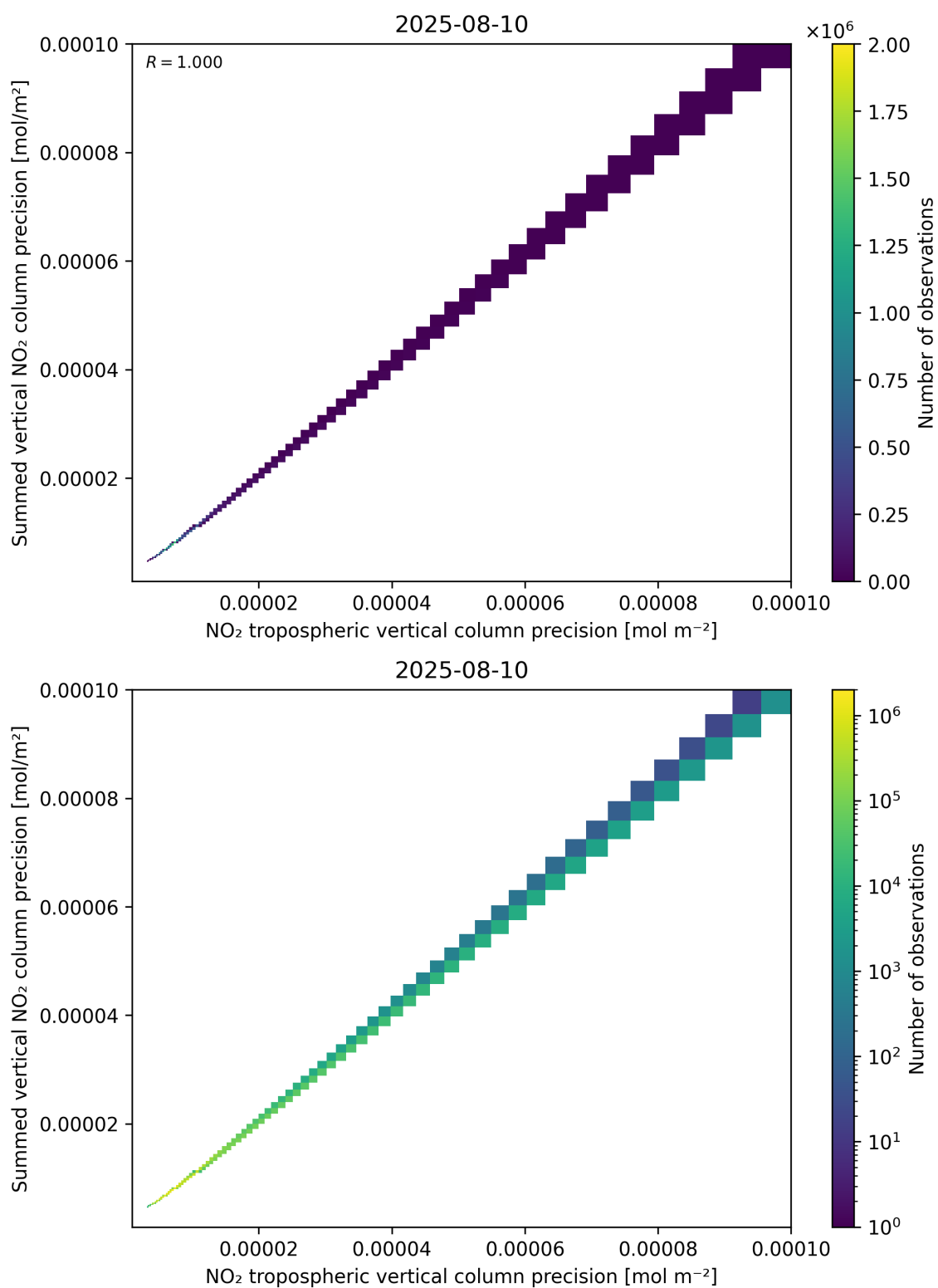
Figure 137: Scatter density plot of “NO 2 tropospheric vertical column precision” against “Summed vertical NO 2 column precision” for 2025-08-09 to 2025-08-11.
