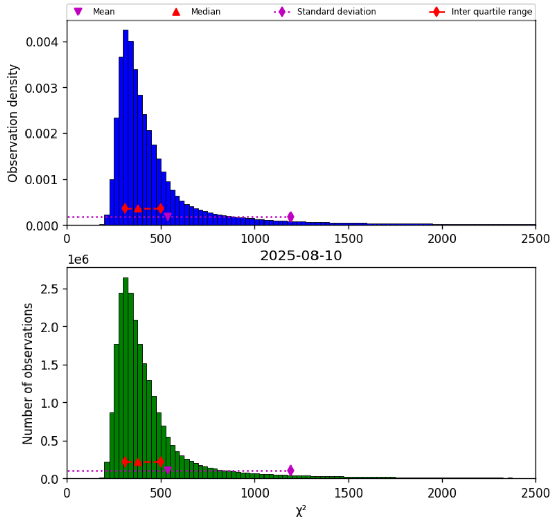
Figure 42: Histogram of “ \chi^2 ” for 2025-08-09 to 2025-08-11
