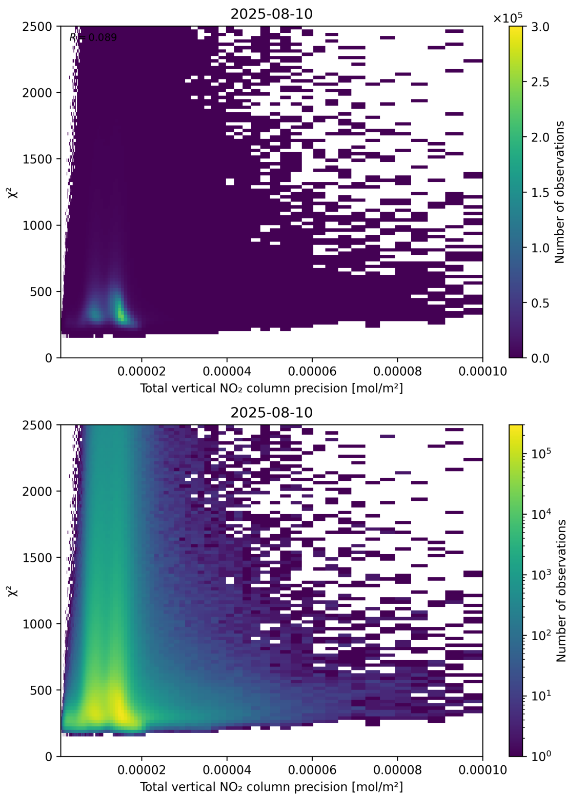
Figure 116: Scatter density plot of “Total vertical NO 2 column precision” against “ \chi^2 ” for 2025-08-09 to 2025-08-11.
