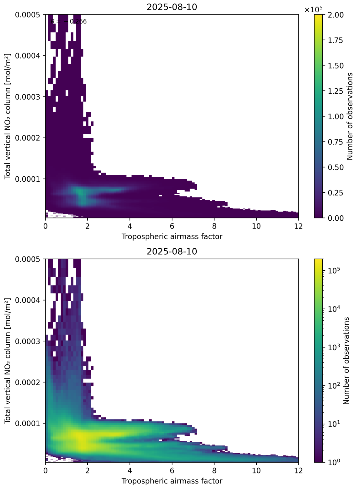
Figure 77: Scatter density plot of “Tropospheric airmass factor” against “Total vertical \text{NO}_2 column” for 2025-08-09 to 2025-08-11.
