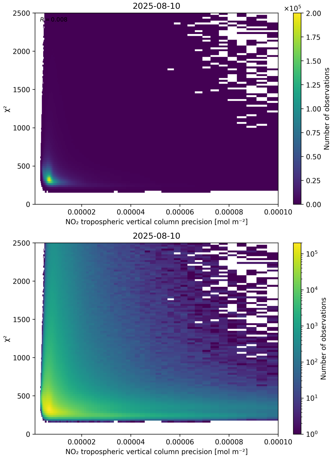
Figure 134: Scatter density plot of “NO 2 tropospheric vertical column precision” against “ \chi^2 ” for 2025-08-09 to 2025-08-11.
