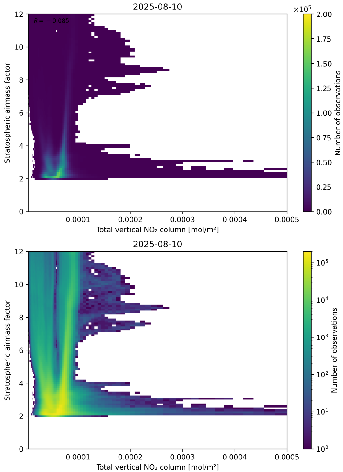
Figure 110: Scatter density plot of “Total vertical NO 2 column” against “Stratospheric airmass factor” for 2025-08-09 to 2025-08-11.
