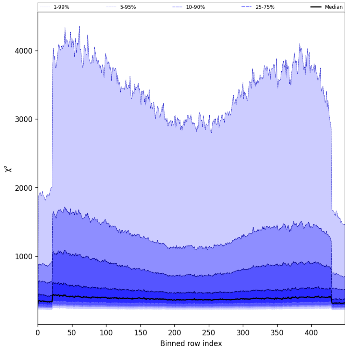
Figure 59: Along track statistics of “ \chi^2 ” for 2025-08-09 to 2025-08-11
