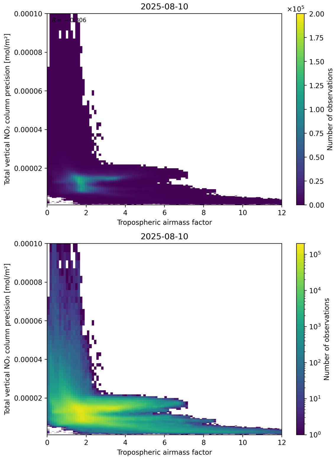
Figure 78: Scatter density plot of “Tropospheric airmass factor” against “Total vertical NO 2 column precision” for 2025-08-09 to 2025-08-11.
