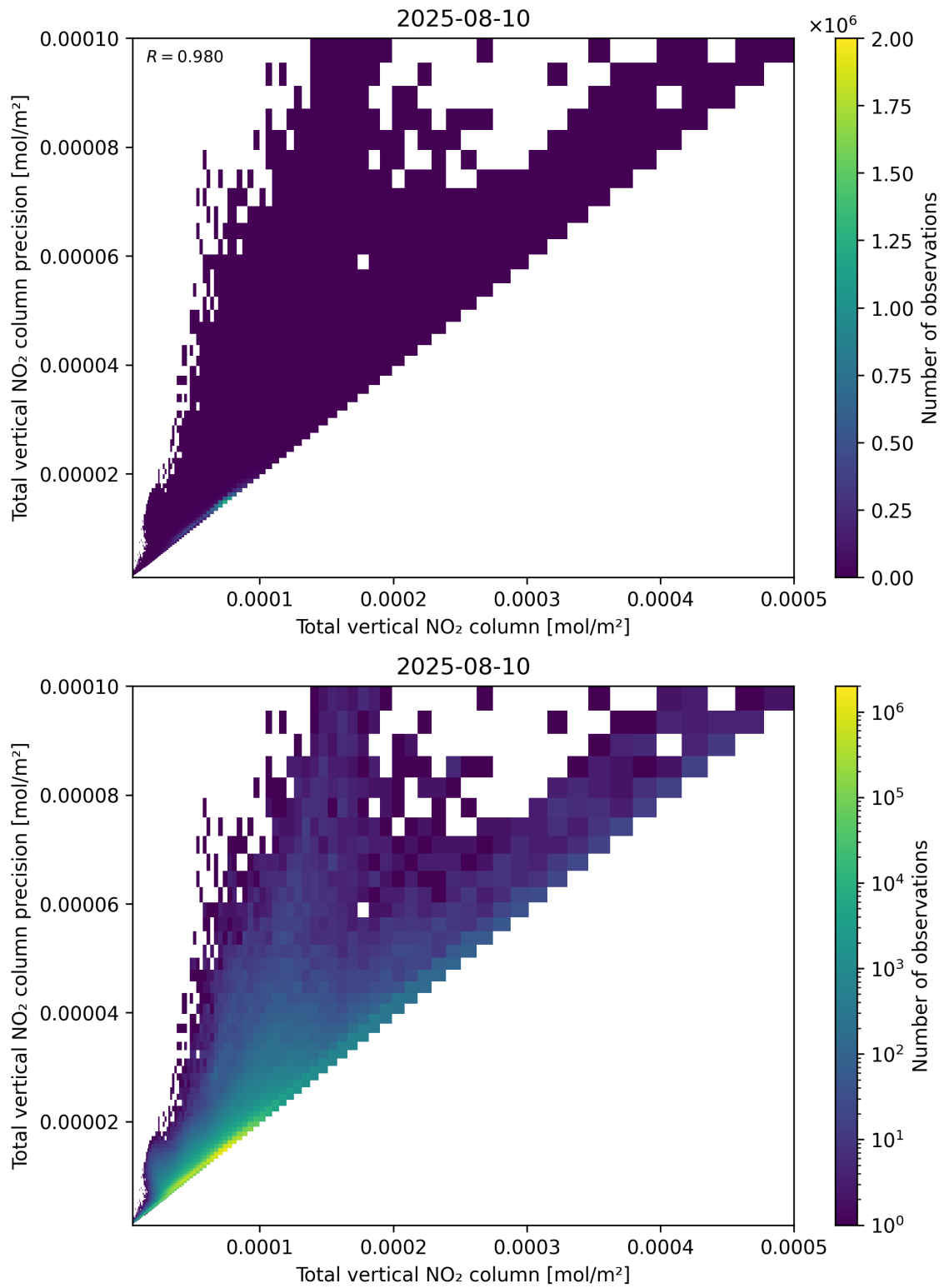
Figure 114: Scatter density plot of “Total vertical NO 2 column” against “Total vertical NO 2 column precision” for 2025-08-09 to 2025-08-11.
