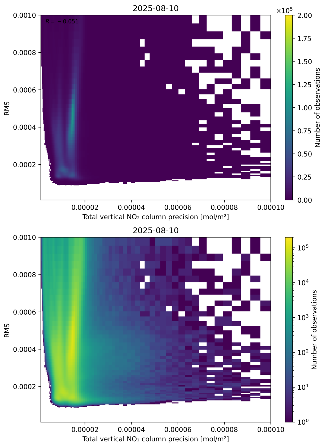
Figure 119: Scatter density plot of “Total vertical NO 2 column precision” against “RMS” for 2025-08-09 to 2025-08-11.
