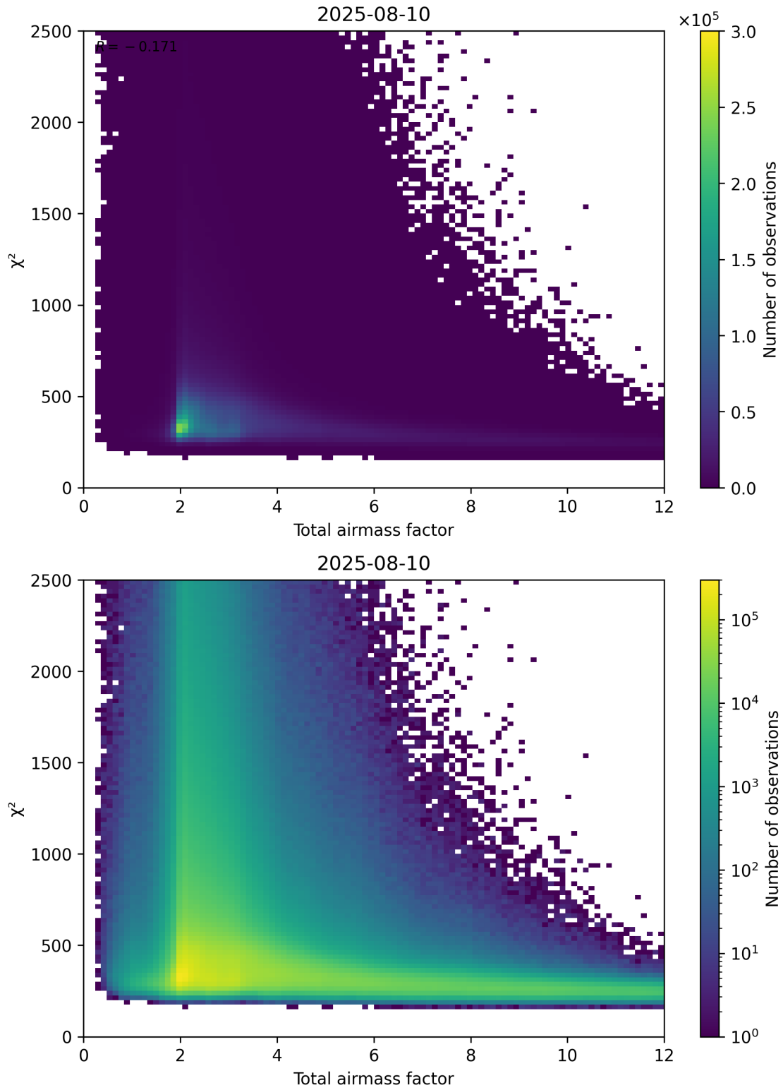
Figure 63: Scatter density plot of “Total airmass factor” against “ \chi^2 ” for 2025-08-09 to 2025-08-11.
