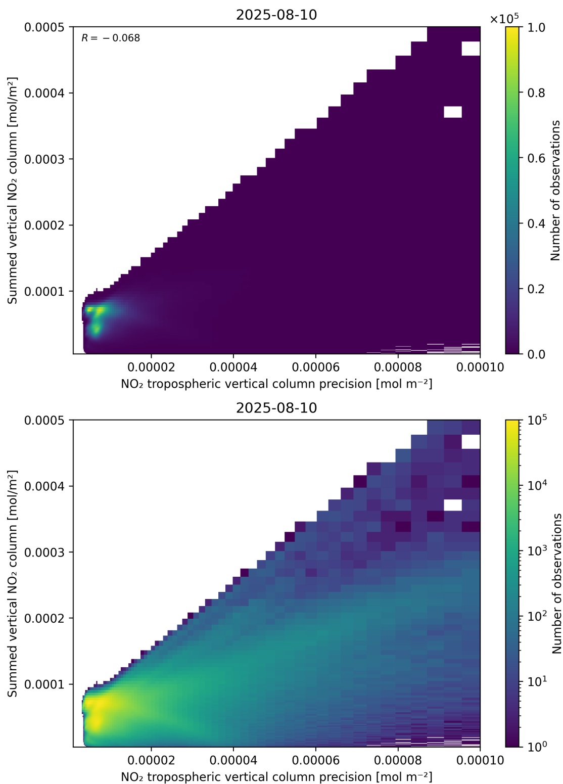
Figure 136: Scatter density plot of “NO 2 tropospheric vertical column precision” against “Summed vertical NO 2 column” for 2025-08-09 to 2025-08-11.
