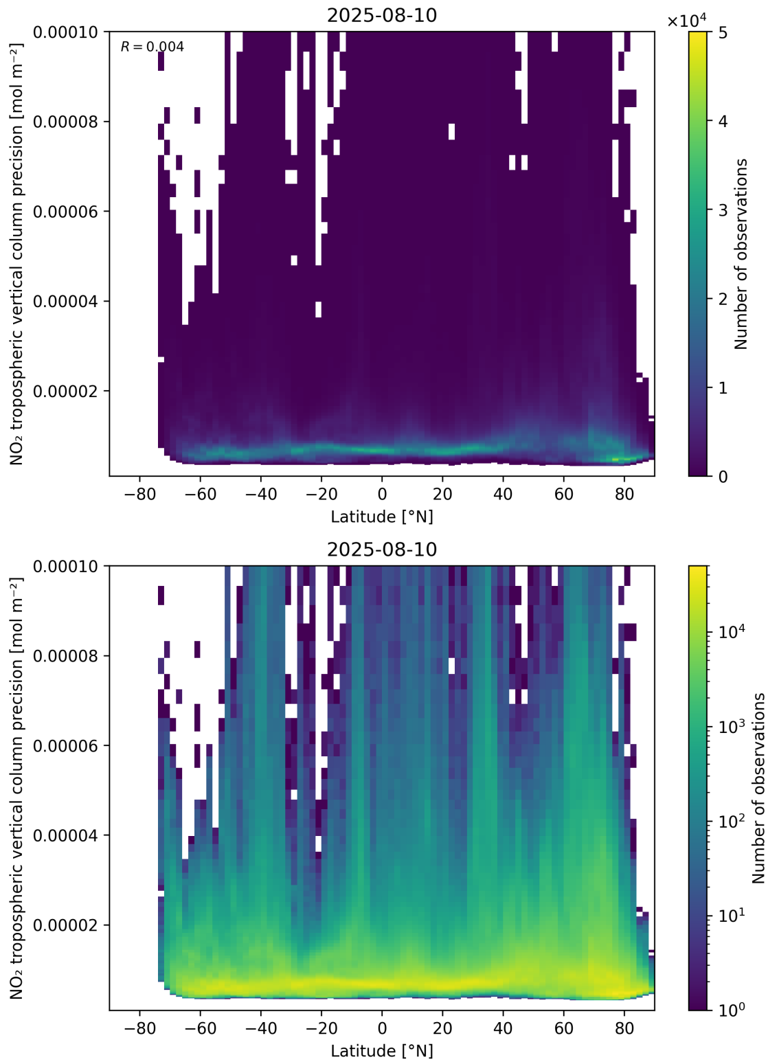
Figure 93: Scatter density plot of “Latitude” against “NO 2 tropospheric vertical column precision” for 2025-08-09 to 2025-08-11.
