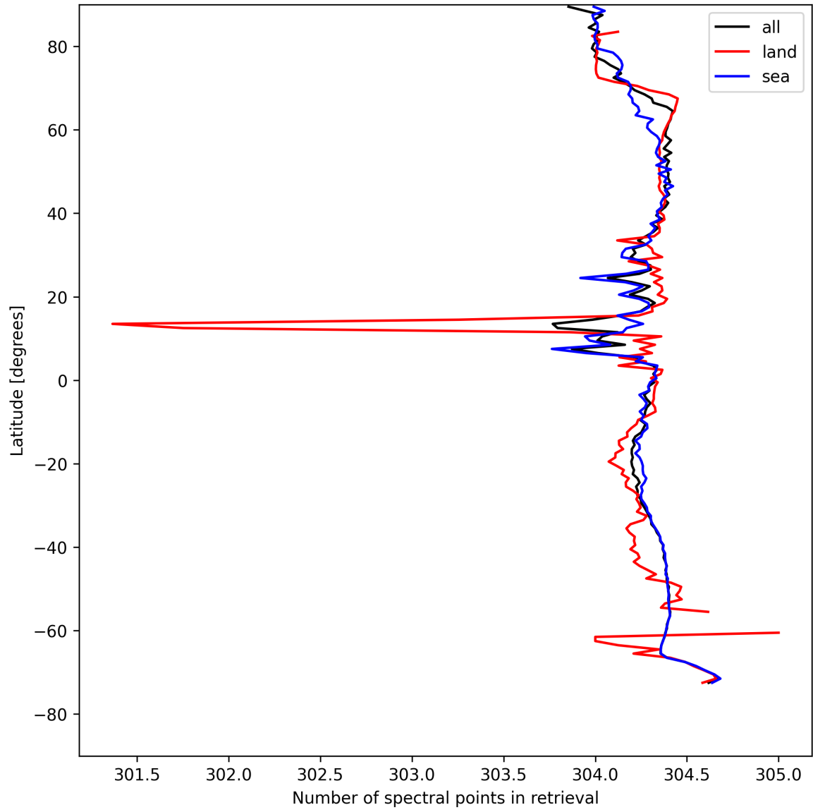
Figure 16: Zonal average of “Number of spectral points in retrieval” for 2025-08-09 to 2025-08-11.
