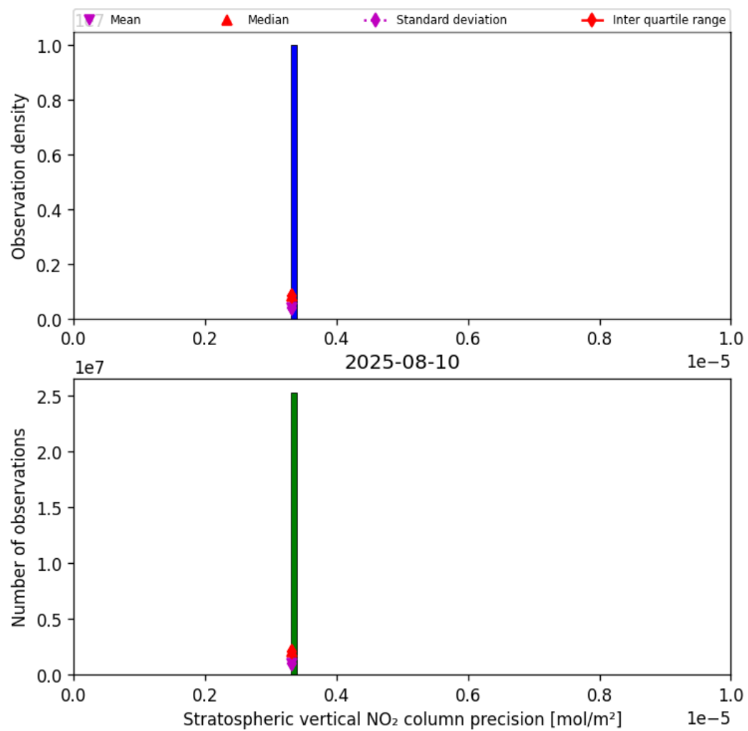
Figure 37: Histogram of “Stratospheric vertical NO 2 column precision” for 2025-08-09 to 2025-08-11
