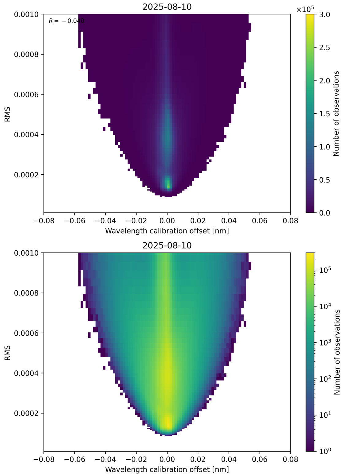
Figure 181: Scatter density plot of “Wavelength calibration offset” against “RMS” for 2025-08-09 to 2025-08-11.
