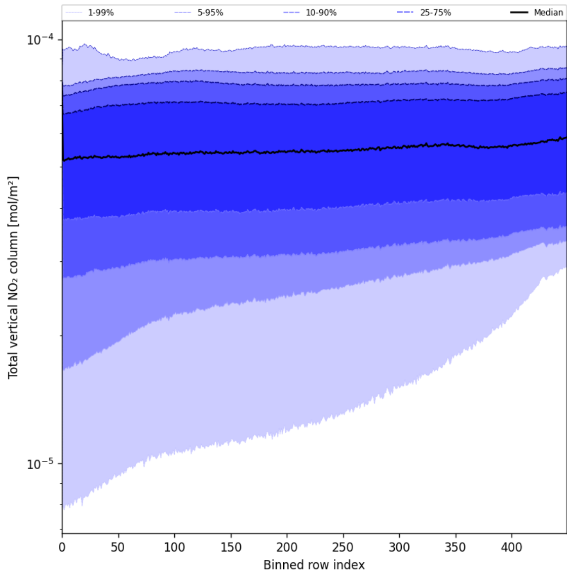
Figure 55: Along track statistics of “Total vertical NO 2 column” for 2025-08-09 to 2025-08-11
