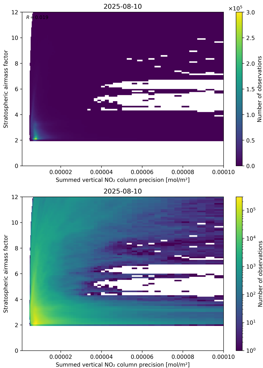
Figure 106: Scatter density plot of “Summed vertical NO 2 column precision” against “Stratospheric airmass factor” for 2025-08-09 to 2025-08-11.
