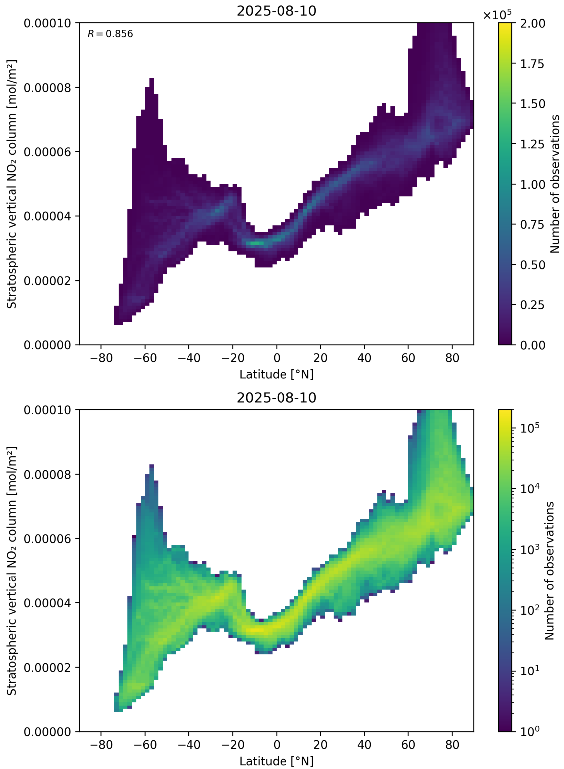
Figure 87: Scatter density plot of “Latitude” against “Stratospheric vertical \text{NO}_2 column” for 2025-08-09 to 2025-08-11.
