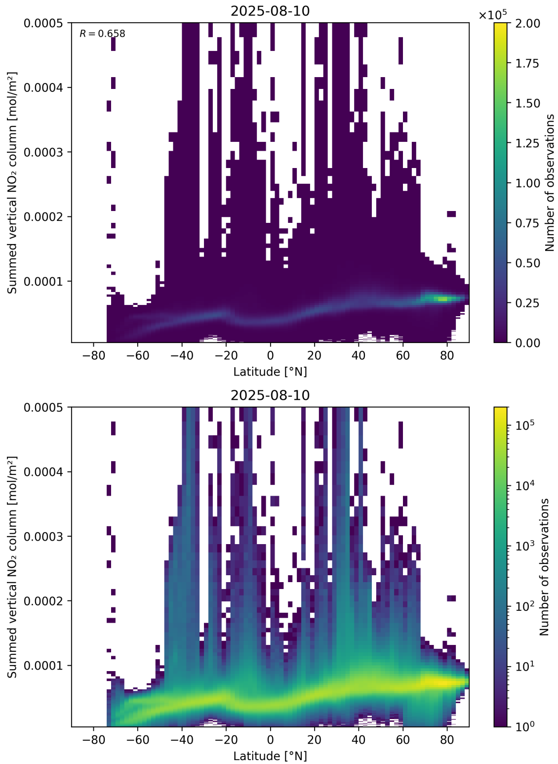
Figure 88: Scatter density plot of “Latitude” against “Summed vertical NO 2 column” for 2025-08-09 to 2025-08-11.
