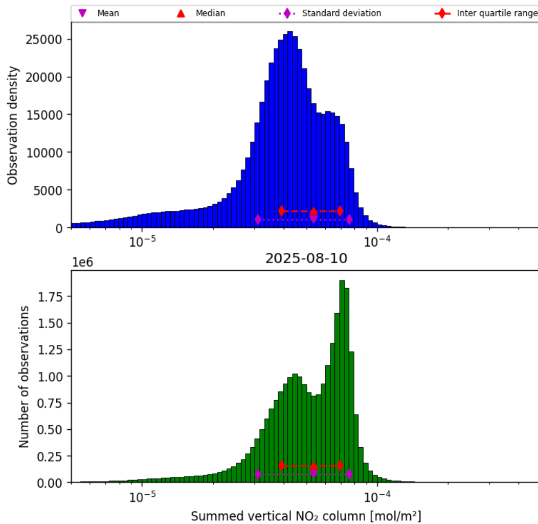
Figure 40: Histogram of “Summed vertical NO 2 column” for 2025-08-09 to 2025-08-11
