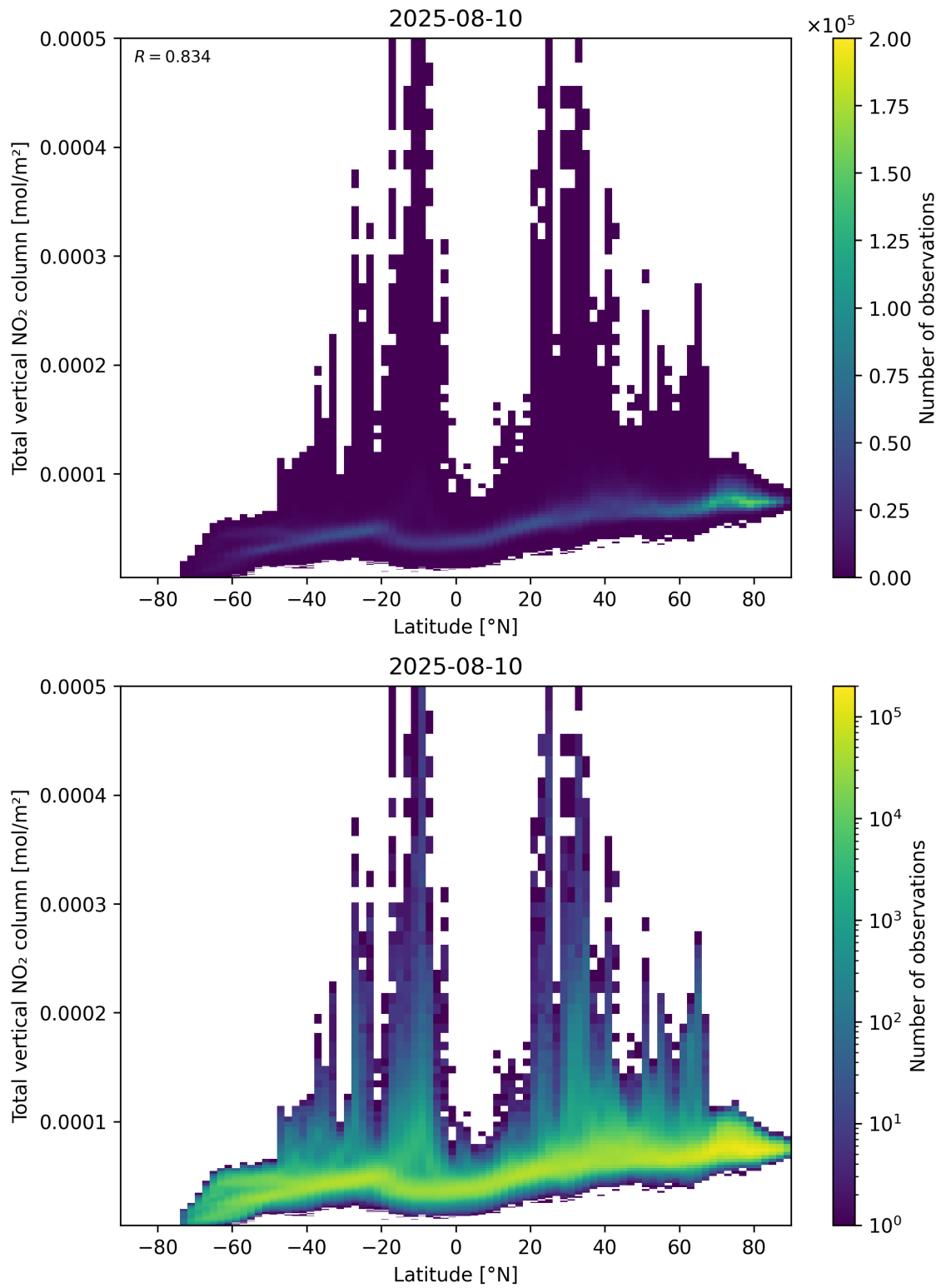
Figure 90: Scatter density plot of “Latitude” against “Total vertical NO 2 column” for 2025-08-09 to 2025-08-11.
