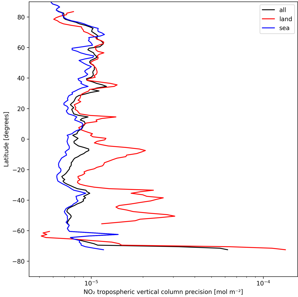
Figure 13: Zonal average of “NO 2 tropospheric vertical column precision” for 2025-08-09 to 2025-08-11.
