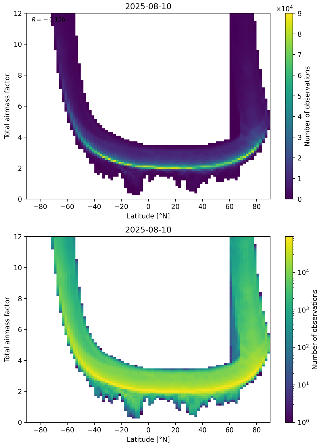
Figure 84: Scatter density plot of “Latitude” against “Total airmass factor” for 2025-08-09 to 2025-08-11.
