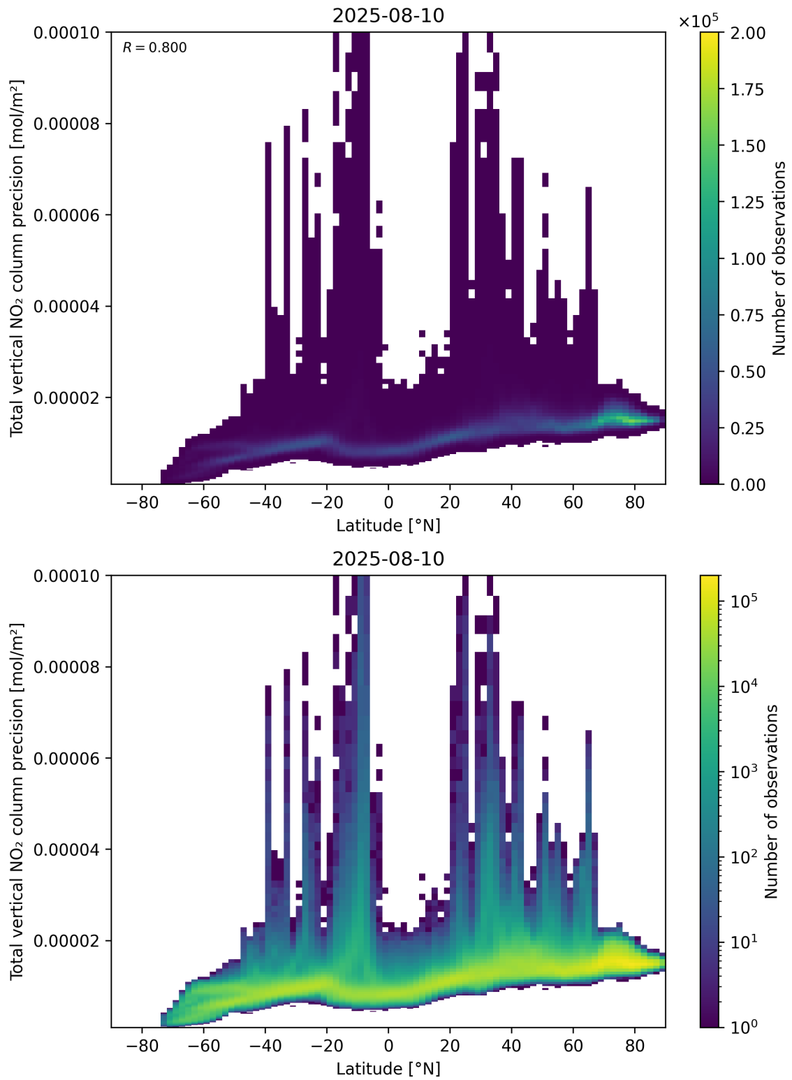
Figure 91: Scatter density plot of “Latitude” against “Total vertical NO 2 column precision” for 2025-08-09 to 2025-08-11.
