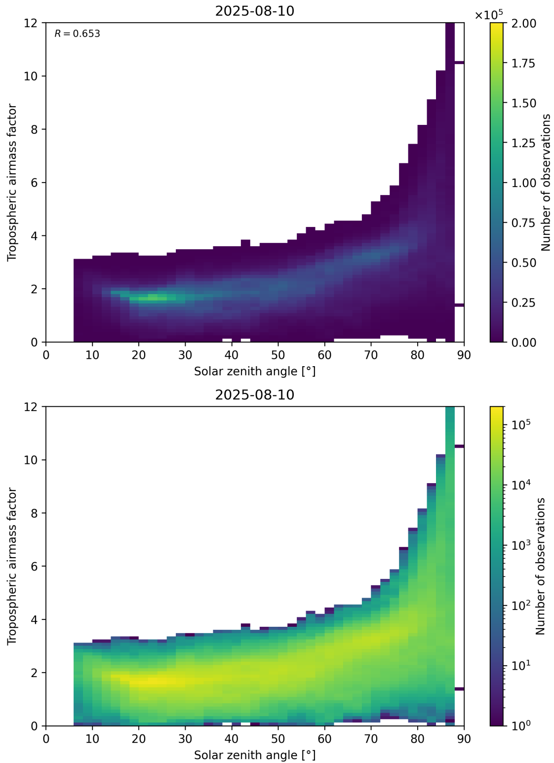
Figure 147: Scatter density plot of “Solar zenith angle” against “Tropospheric airmass factor” for 2025-08-09 to 2025-08-11.
