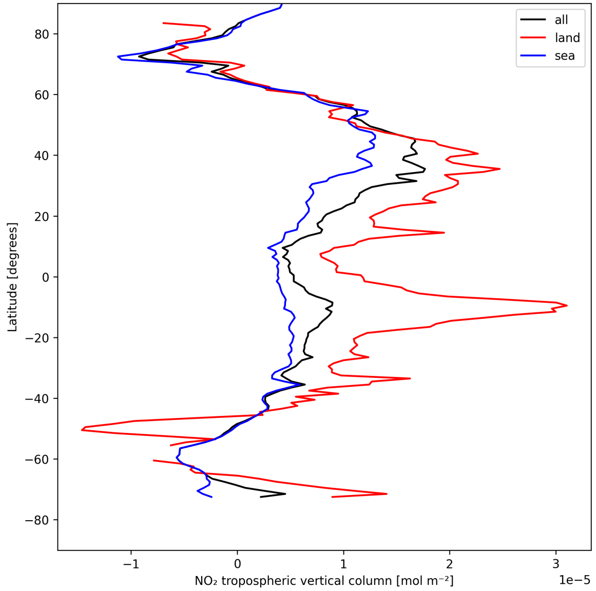
Figure 12: Zonal average of “NO 2 tropospheric vertical column” for 2025-08-09 to 2025-08-11.
