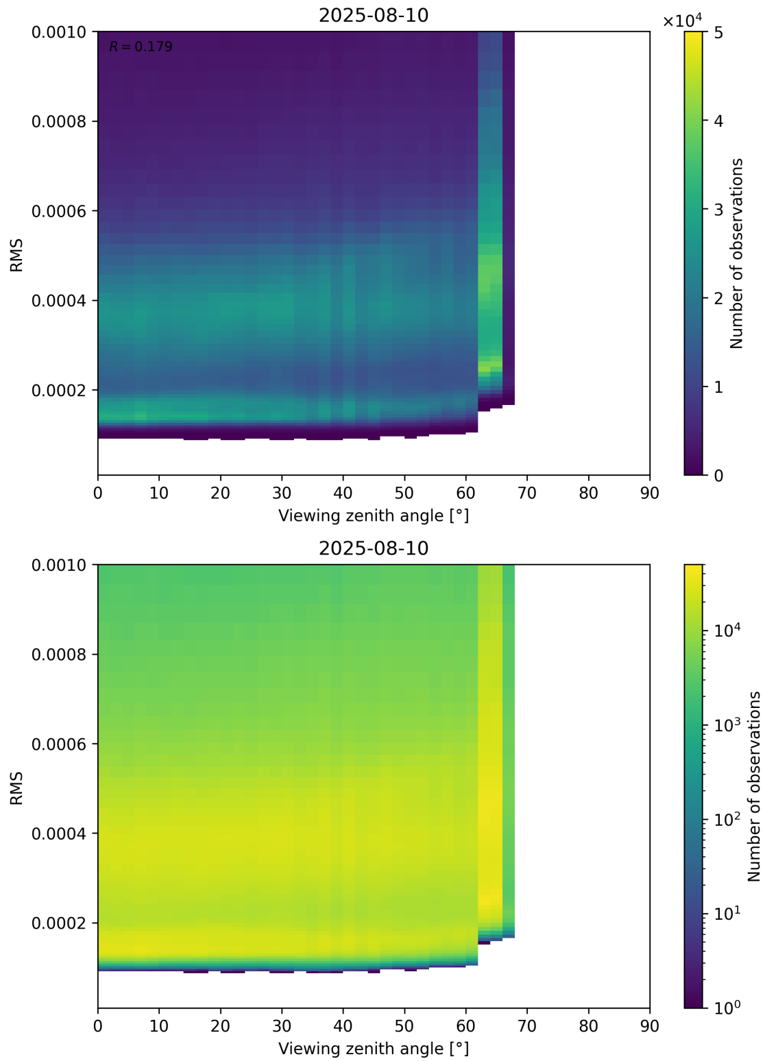
Figure 171: Scatter density plot of “Viewing zenith angle” against “RMS” for 2025-08-09 to 2025-08-11.
