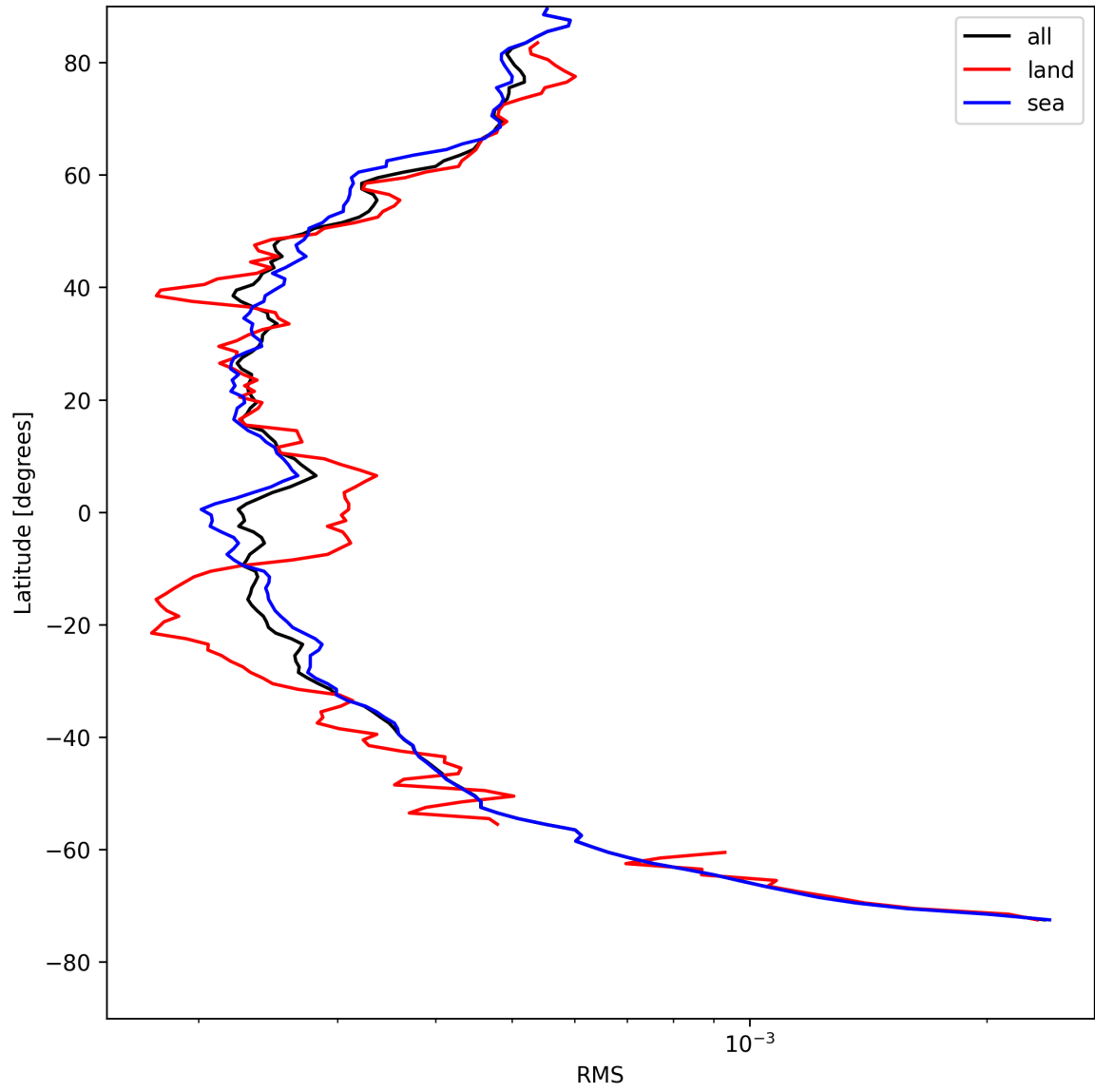
Figure 26: Zonal average of “RMS” for 2025-08-09 to 2025-08-11.
