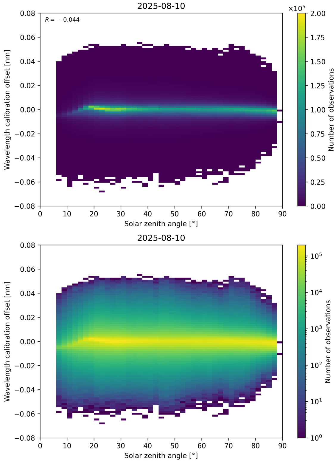
Figure 158: Scatter density plot of “Solar zenith angle” against “Wavelength calibration offset” for 2025-08-09 to 2025-08-11.
