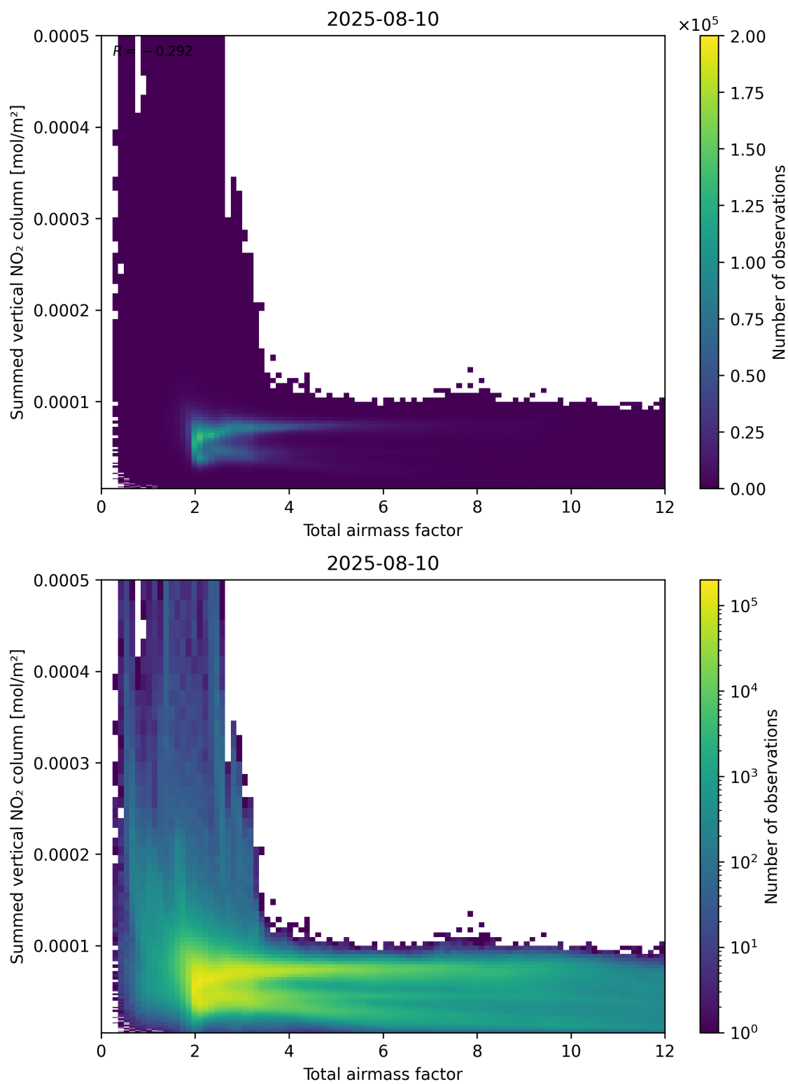
Figure 65: Scatter density plot of “Total airmass factor” against “Summed vertical NO 2 column” for 2025-08-09 to 2025-08-11.
