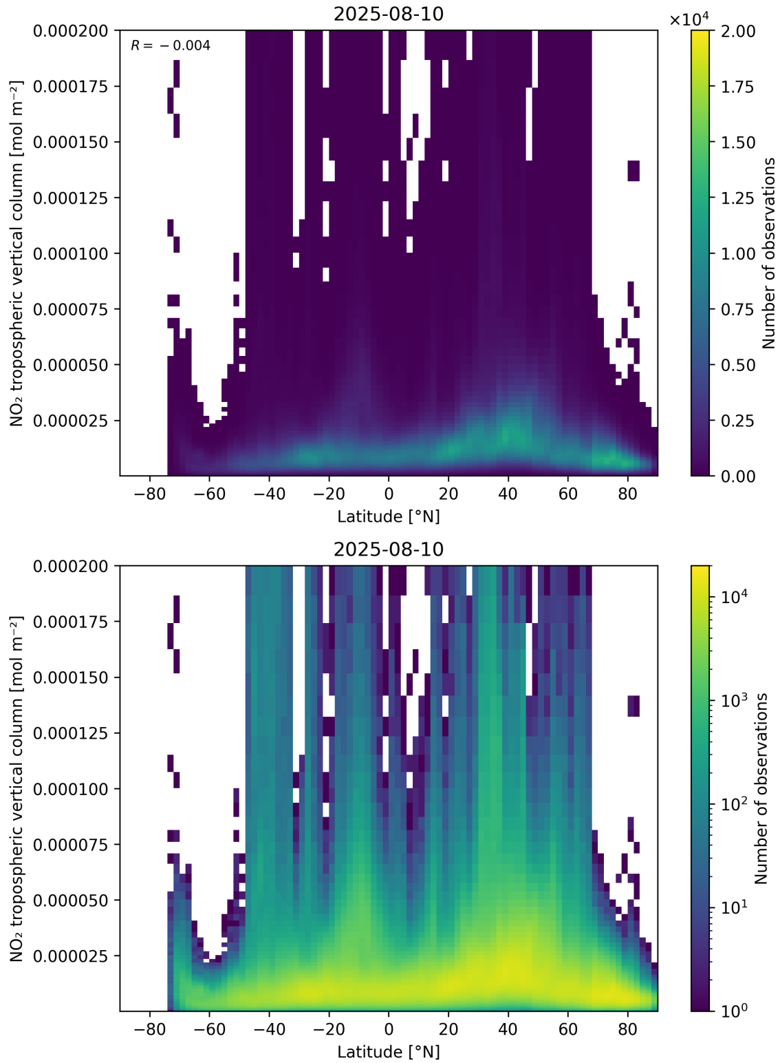
Figure 92: Scatter density plot of “Latitude” against “NO 2 tropospheric vertical column” for 2025-08-09 to 2025-08-11.
