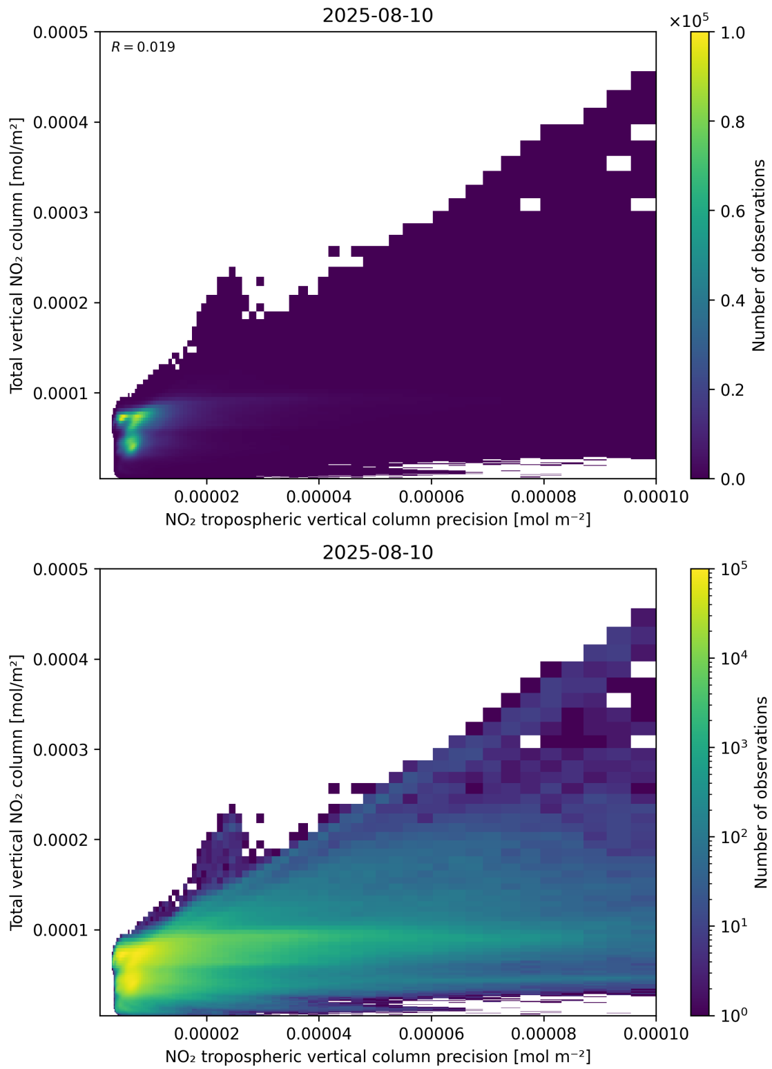
Figure 138: Scatter density plot of “NO 2 tropospheric vertical column precision” against “Total vertical NO 2 column” for 2025-08-09 to 2025-08-11.
