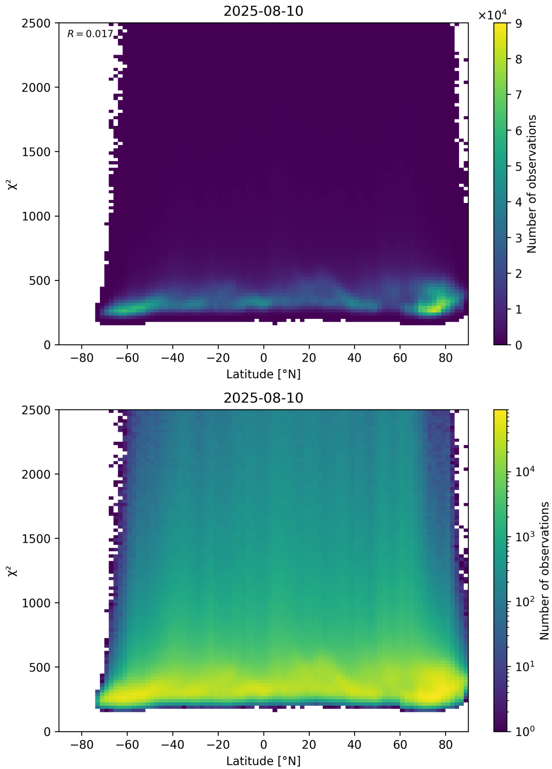
Figure 86: Scatter density plot of “Latitude” against “ \chi^2 ” for 2025-08-09 to 2025-08-11.
