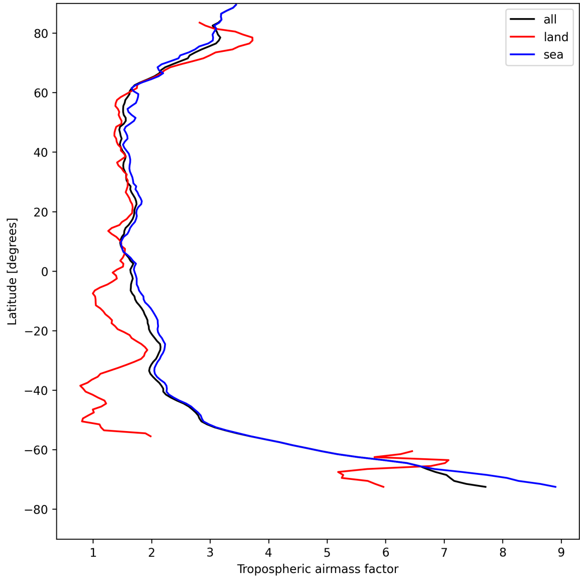
Figure 14: Zonal average of “Tropospheric air mass factor” for 2025-08-09 to 2025-08-11.
