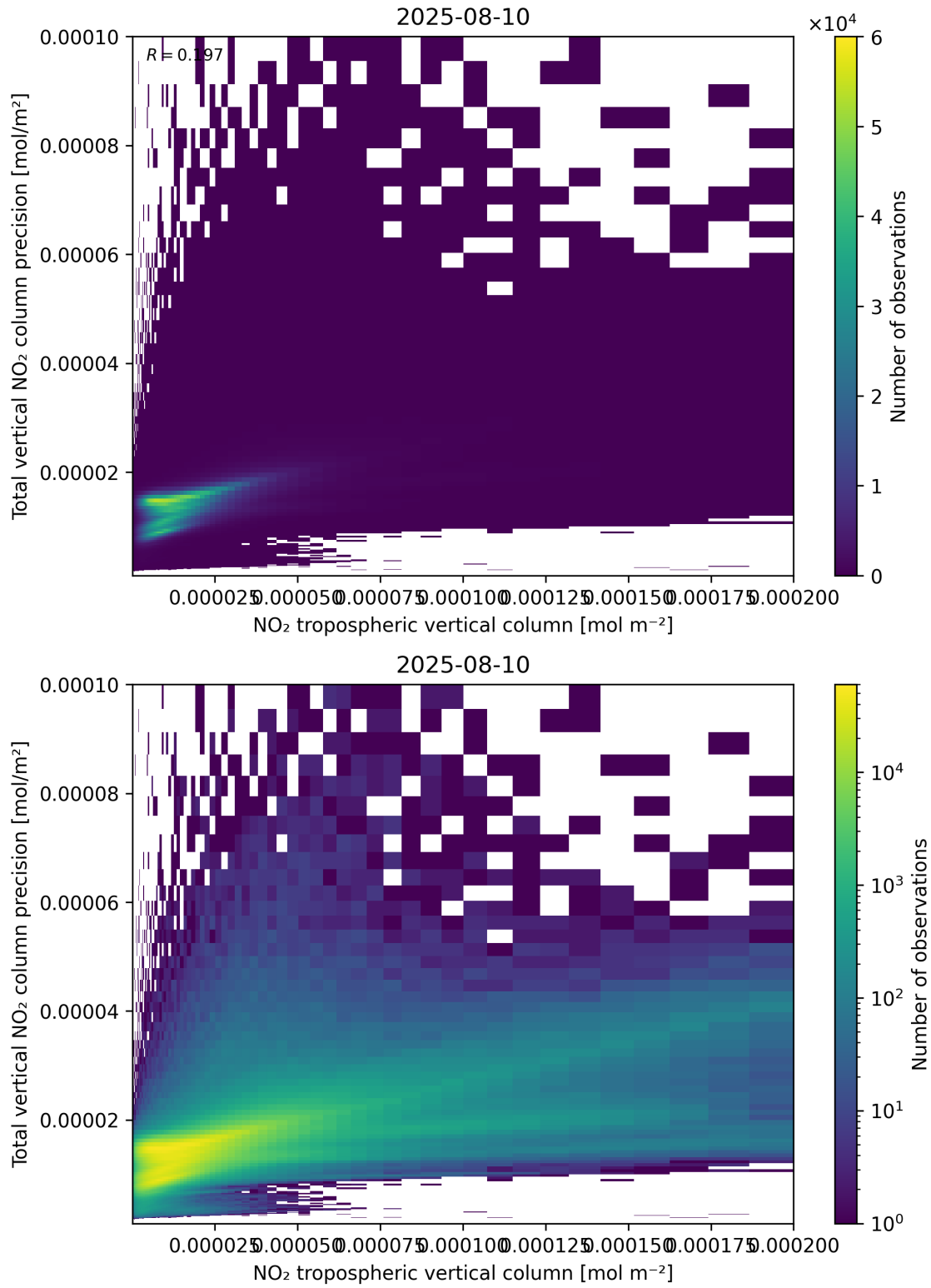
Figure 129: Scatter density plot of “NO 2 tropospheric vertical column” against “Total vertical NO 2 column precision” for 2025-08-09 to 2025-08-11.
