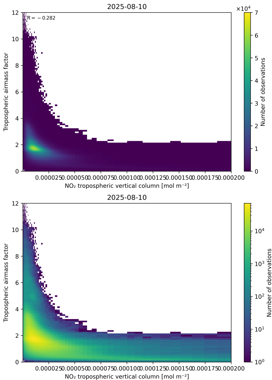
Figure 123: Scatter density plot of “NO 2 tropospheric vertical column” against “Tropospheric air mass factor” for 2025-08-09 to 2025-08-11.
