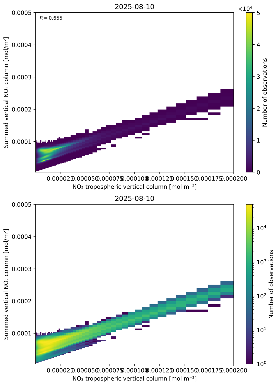
Figure 126: Scatter density plot of “NO 2 tropospheric vertical column” against “Summed vertical NO 2 column” for 2025-08-09 to 2025-08-11.
