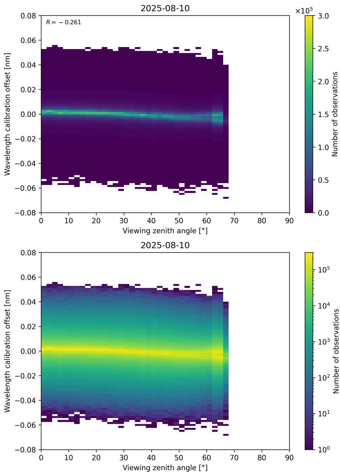
Figure 173: Scatter density plot of “Viewing zenith angle” against “Wavelength calibration offset” for 2025-08-09 to 2025-08-11.
