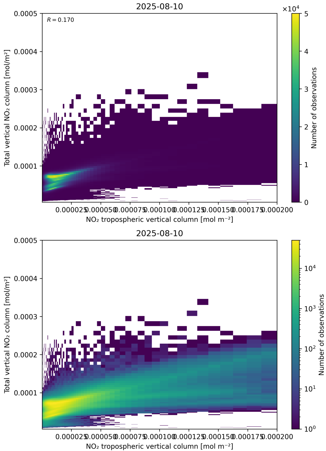
Figure 128: Scatter density plot of “NO 2 tropospheric vertical column” against “Total vertical NO 2 column” for 2025-08-09 to 2025-08-11.
