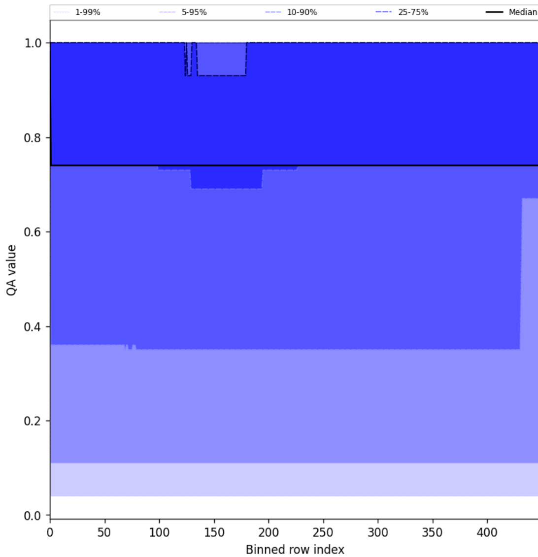
Figure 45: Along track statistics of “QA value” for 2025-08-09 to 2025-08-11
