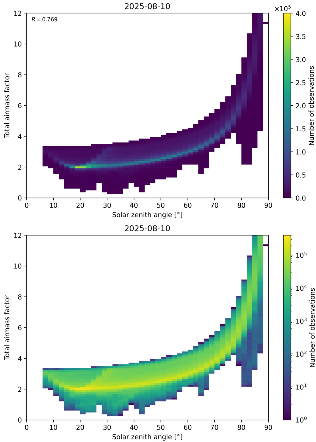
Figure 146: Scatter density plot of “Solar zenith angle” against “Total air mass factor” for 2025-08-09 to 2025-08-11.
