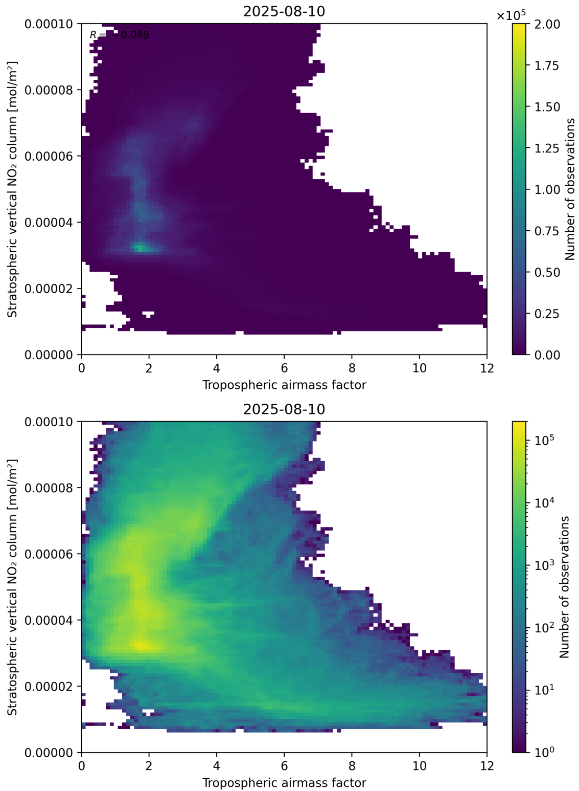
Figure 74: Scatter density plot of “Tropospheric air mass factor” against “Stratospheric vertical NO 2 column” for 2025-08-09 to 2025-08-11.
