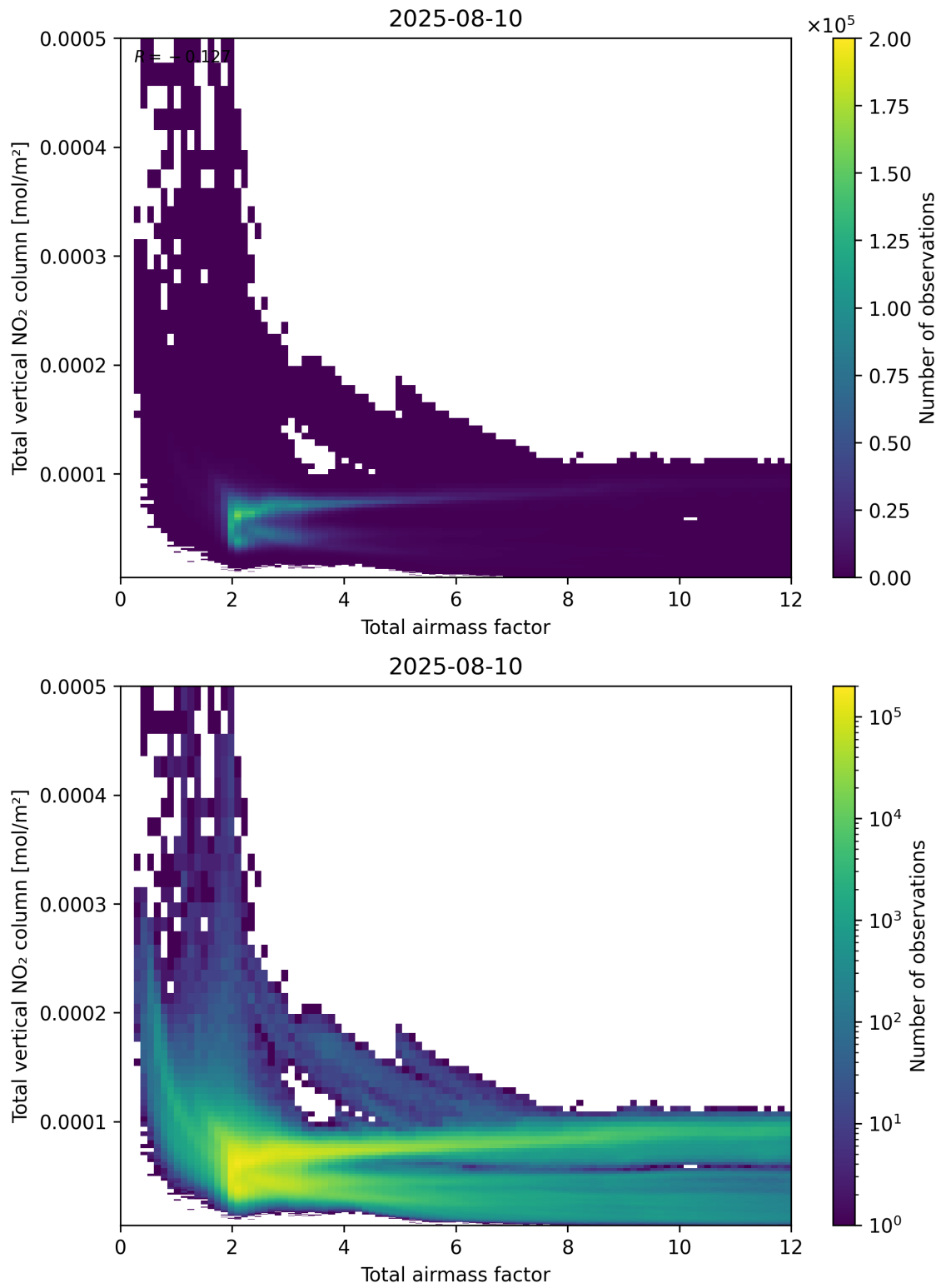
Figure 67: Scatter density plot of “Total airmass factor” against “Total vertical NO 2 column” for 2025-08-09 to 2025-08-11.
