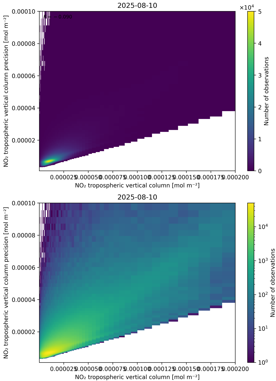
Figure 130: Scatter density plot of “NO 2 tropospheric vertical column” against “NO 2 tropospheric vertical column precision” for 2025-08-09 to 2025-08-11.
