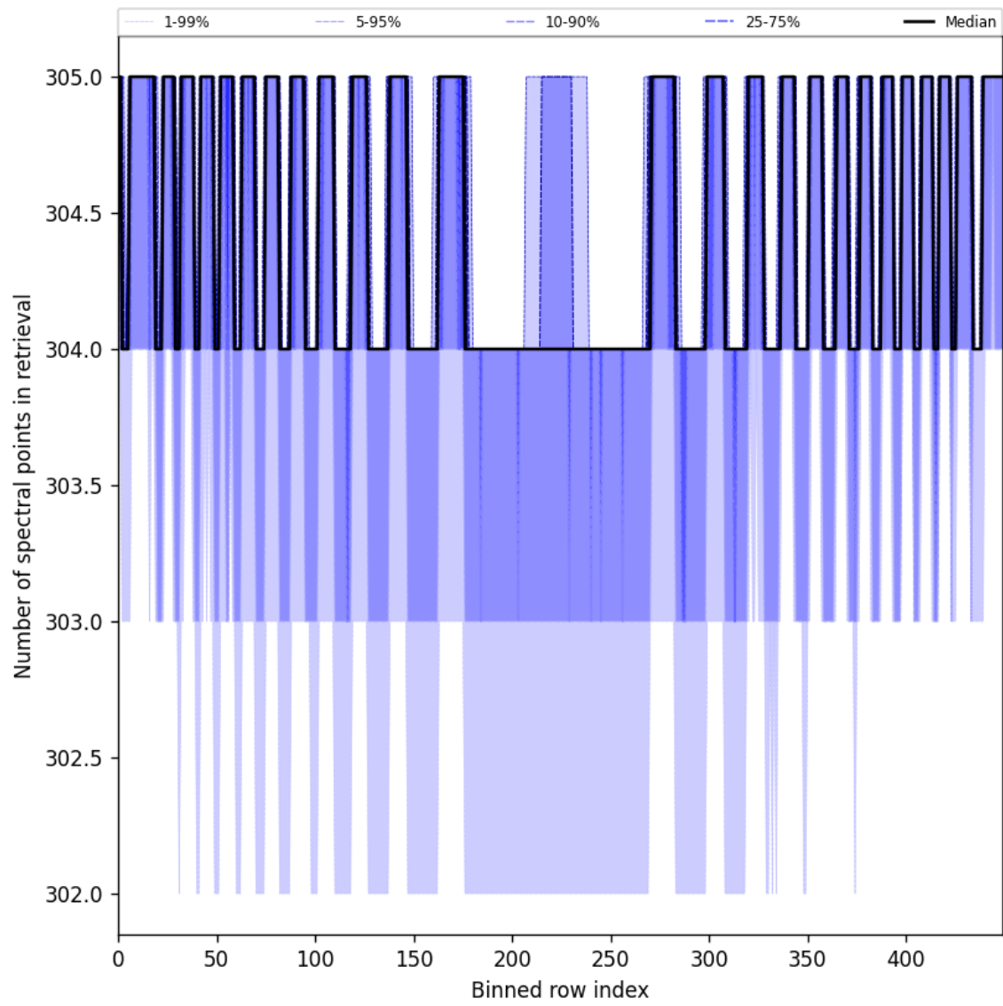
Figure 50: Along track statistics of “Number of spectral points in retrieval” for 2025-08-09 to 2025-08-11
