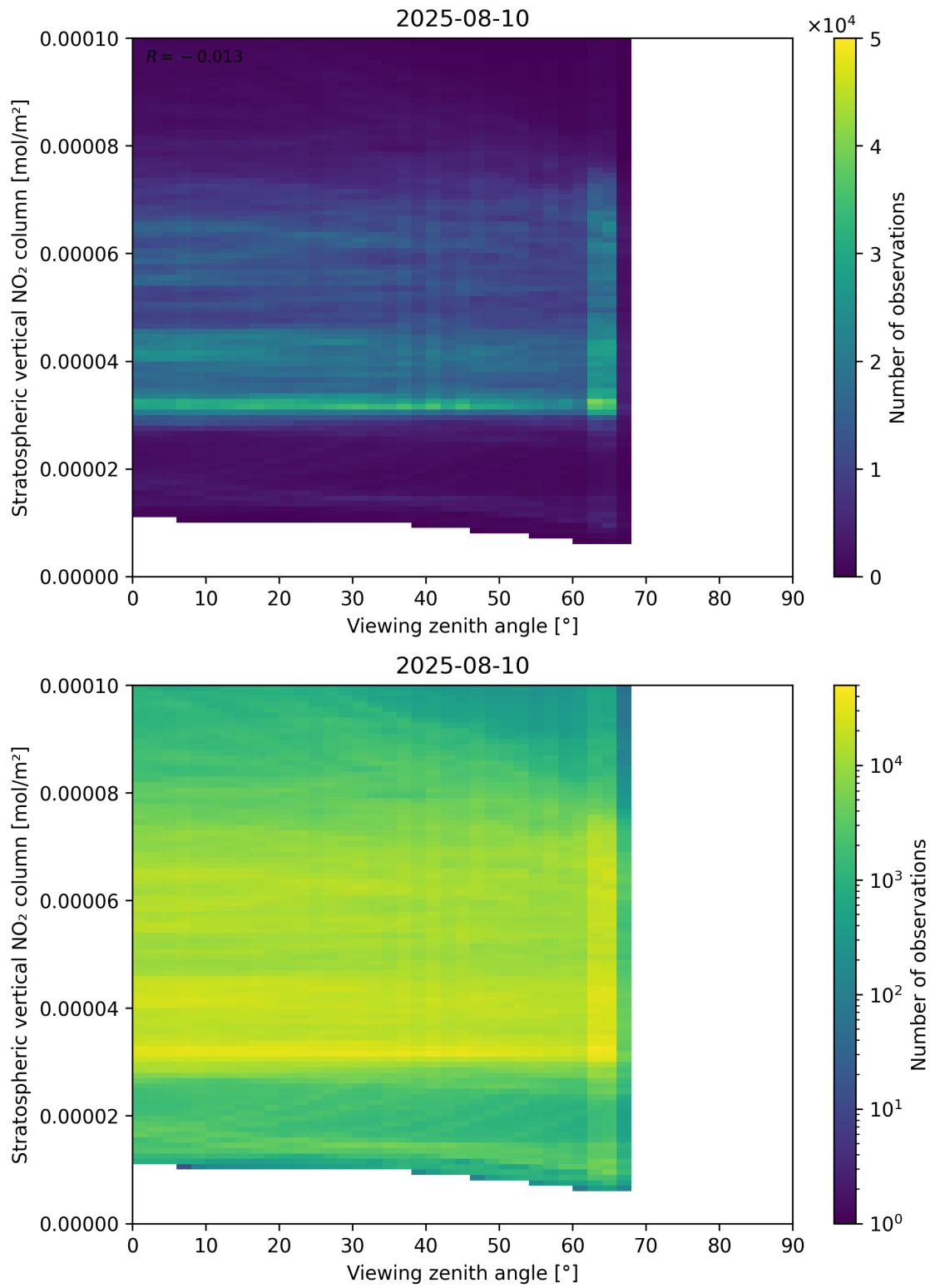
Figure 164: Scatter density plot of “Viewing zenith angle” against “Stratospheric vertical NO 2 column” for 2025-08-09 to 2025-08-11.
