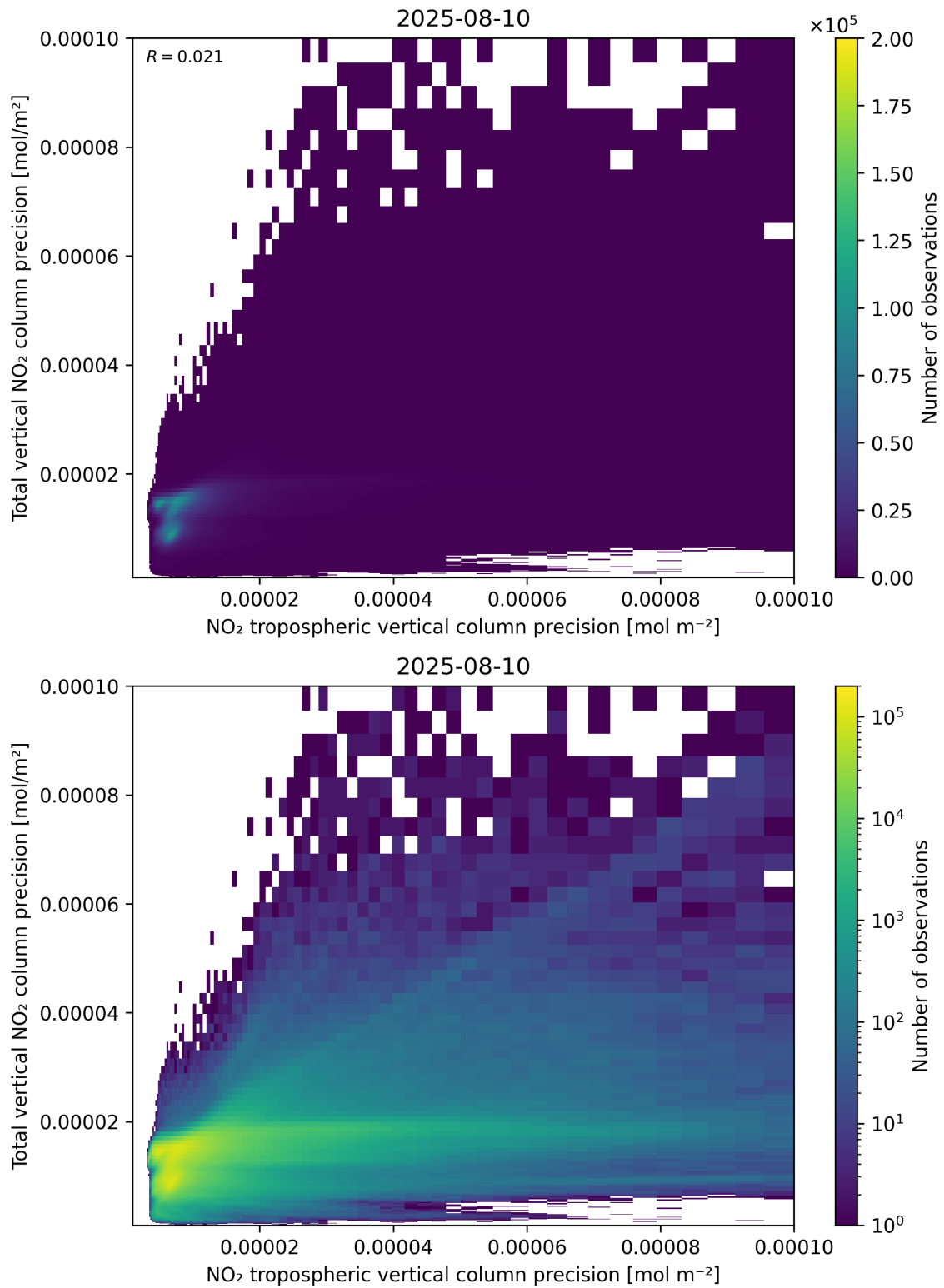
Figure 139: Scatter density plot of “NO 2 tropospheric vertical column precision” against “Total vertical NO 2 column precision” for 2025-08-09 to 2025-08-11.
