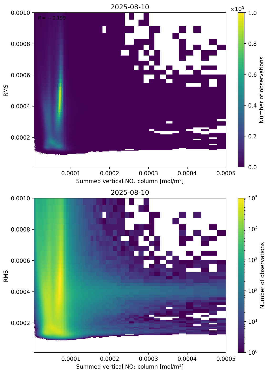
Figure 109: Scatter density plot of “Summed vertical NO 2 column” against “RMS” for 2025-08-09 to 2025-08-11.
