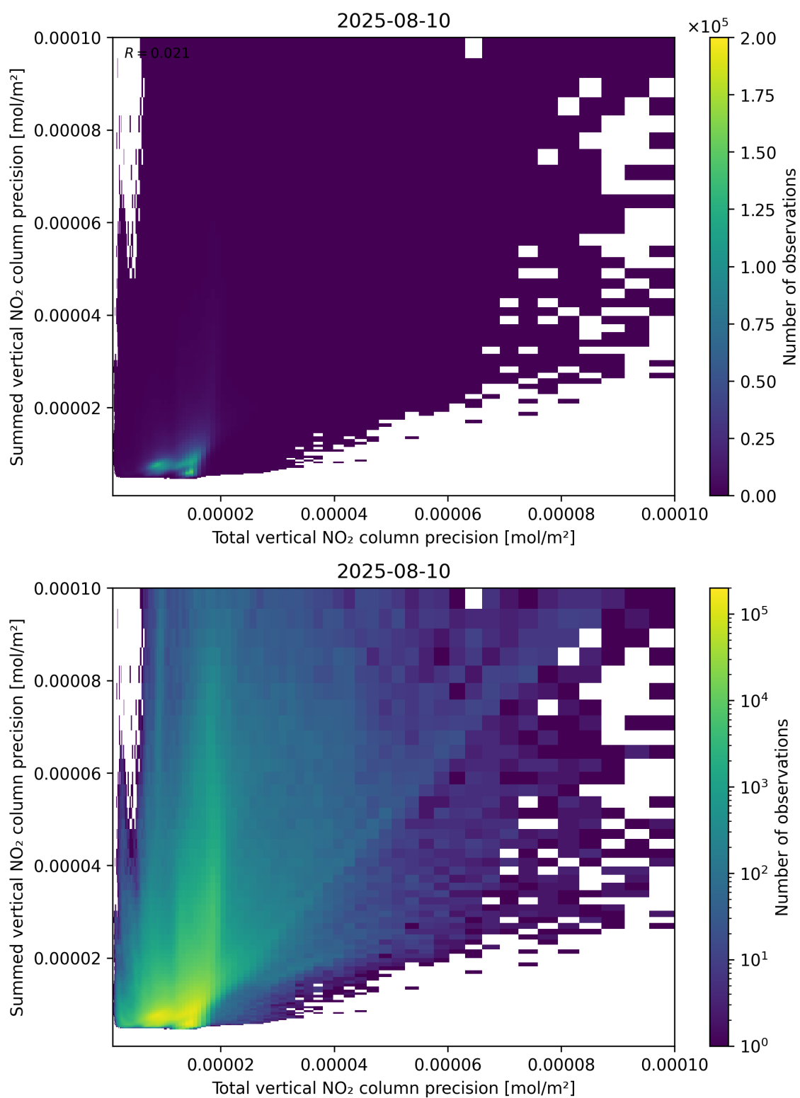
Figure 118: Scatter density plot of “Total vertical NO 2 column precision” against “Summed vertical NO 2 column precision” for 2025-08-09 to 2025-08-11.
