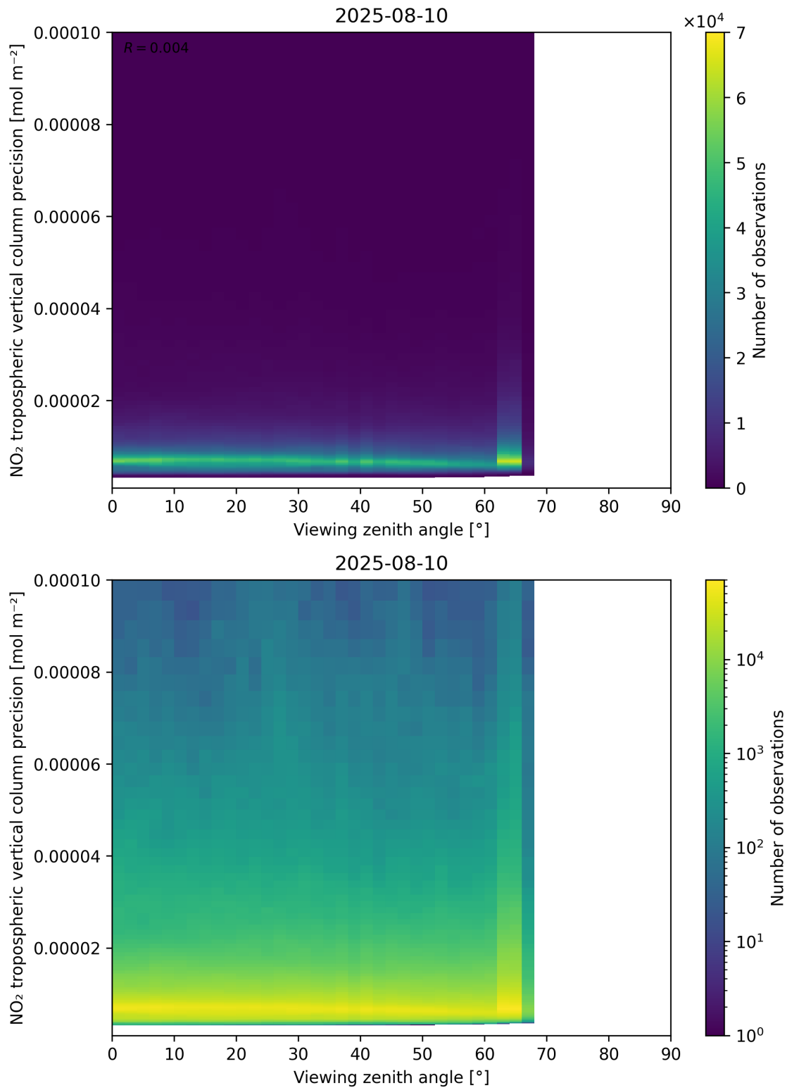
Figure 170: Scatter density plot of “Viewing zenith angle” against “NO 2 tropospheric vertical column precision” for 2025-08-09 to 2025-08-11.
