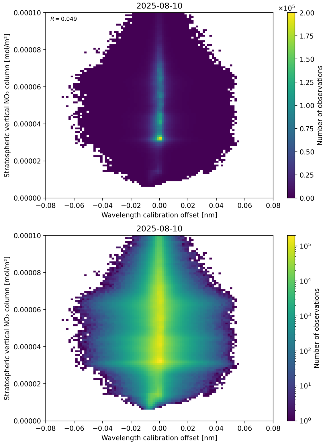
Figure 176: Scatter density plot of “Wavelength calibration offset” against “Stratospheric vertical NO 2 column” for 2025-08-09 to 2025-08-11.
