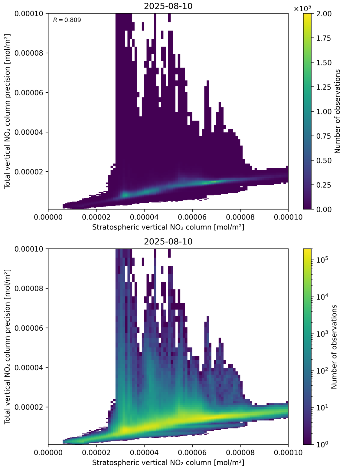
Figure 101: Scatter density plot of “Stratospheric vertical NO 2 column” against “Total vertical NO 2 column precision” for 2025-08-09 to 2025-08-11.
