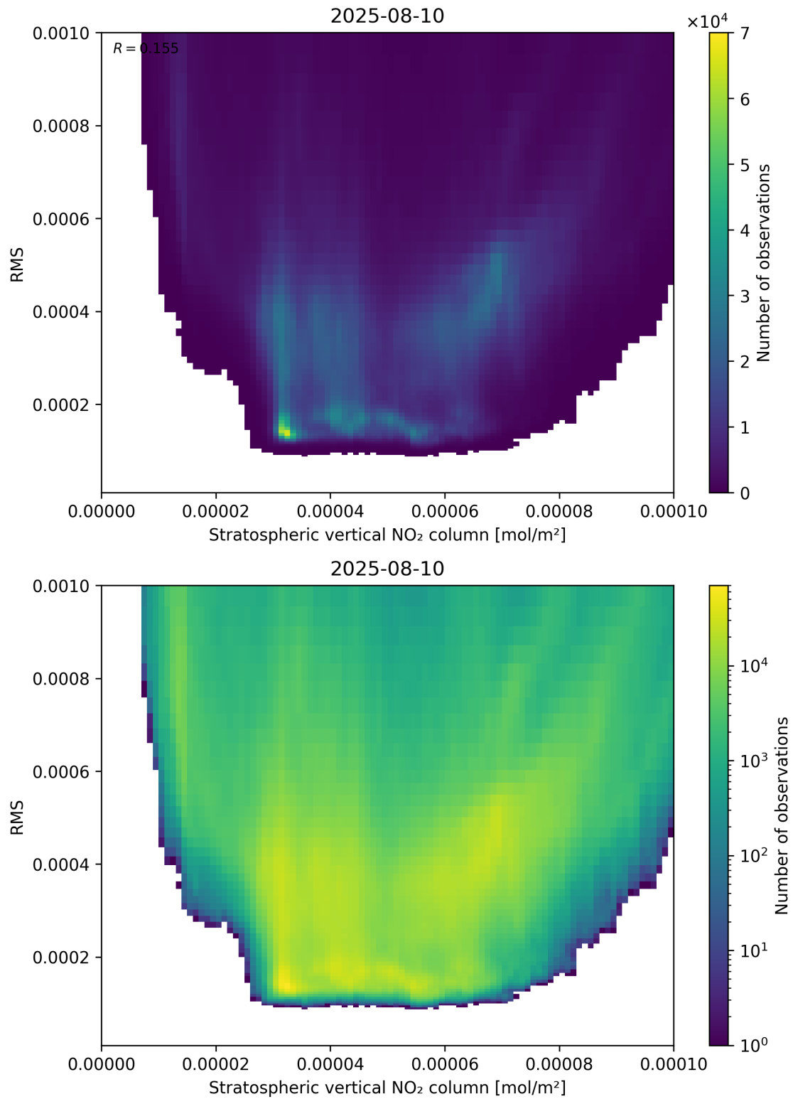
Figure 102: Scatter density plot of “Stratospheric vertical NO 2 column” against “RMS” for 2025-08-09 to 2025-08-11.
