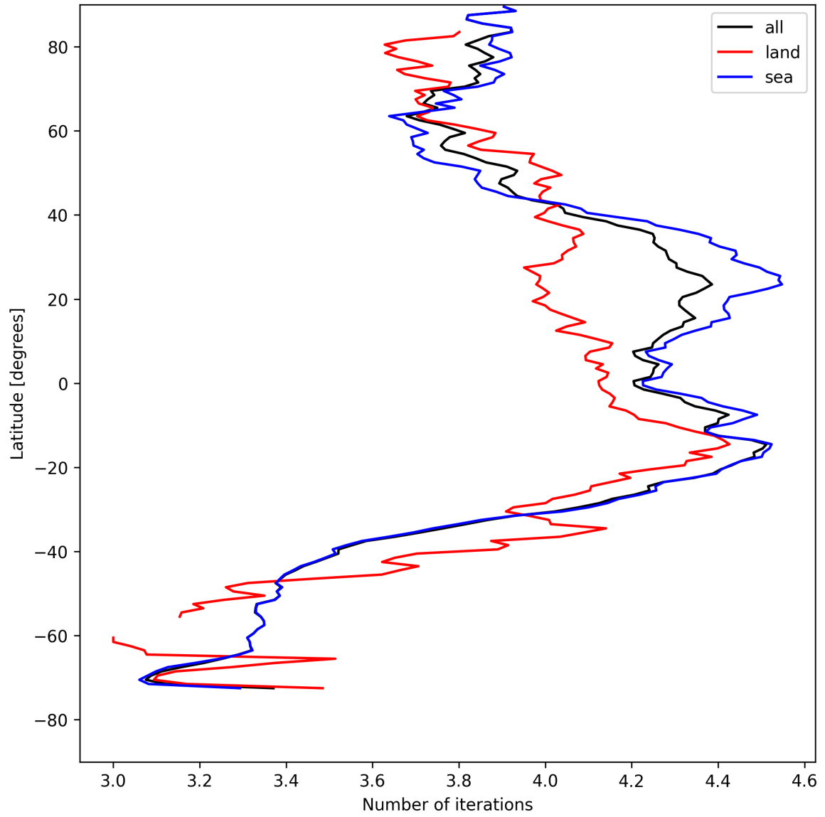
Figure 17: Zonal average of “Number of iterations” for 2025-08-09 to 2025-08-11.
