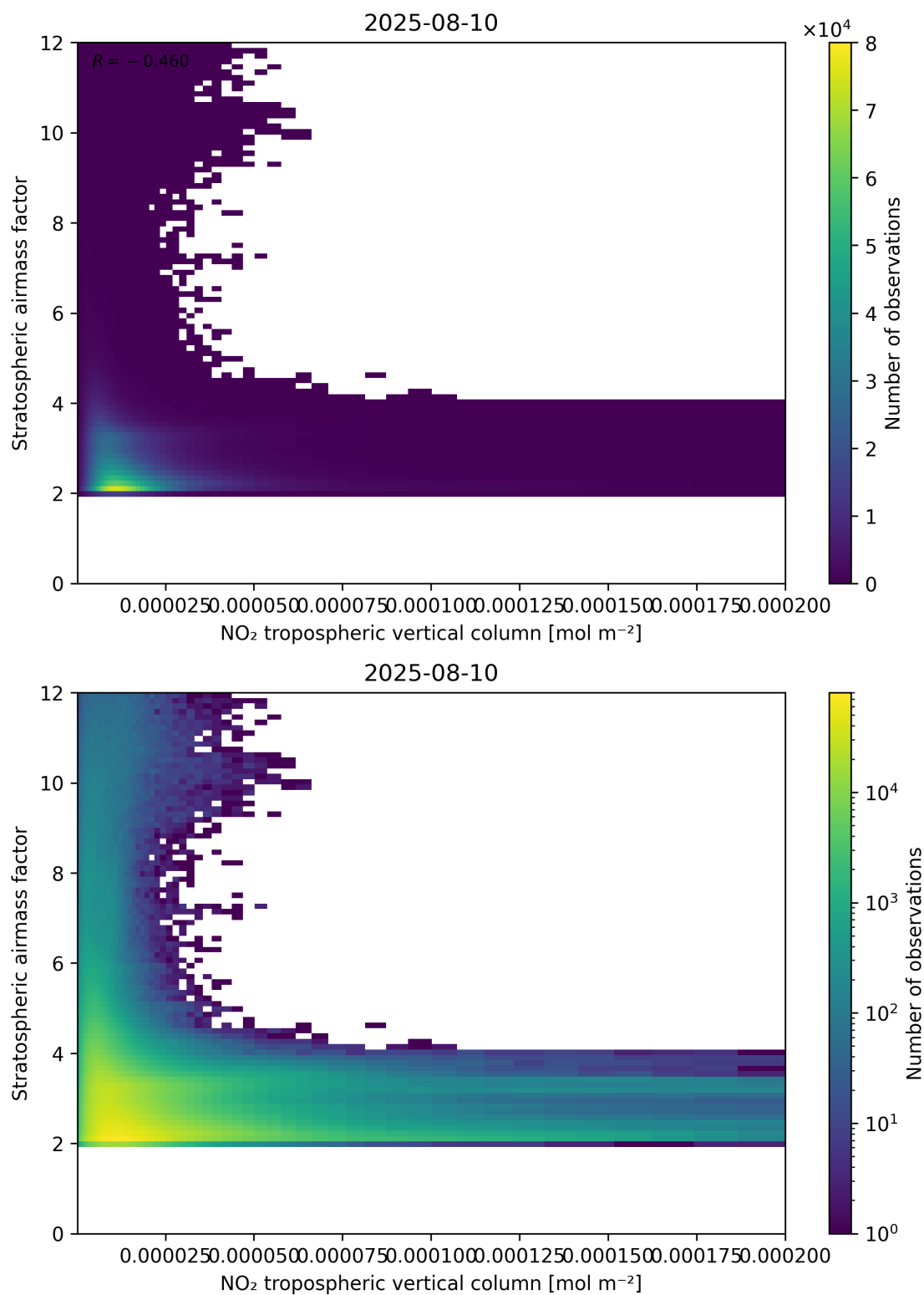
Figure 121: Scatter density plot of “NO 2 tropospheric vertical column” against “Stratospheric airmass factor” for 2025-08-09 to 2025-08-11.
