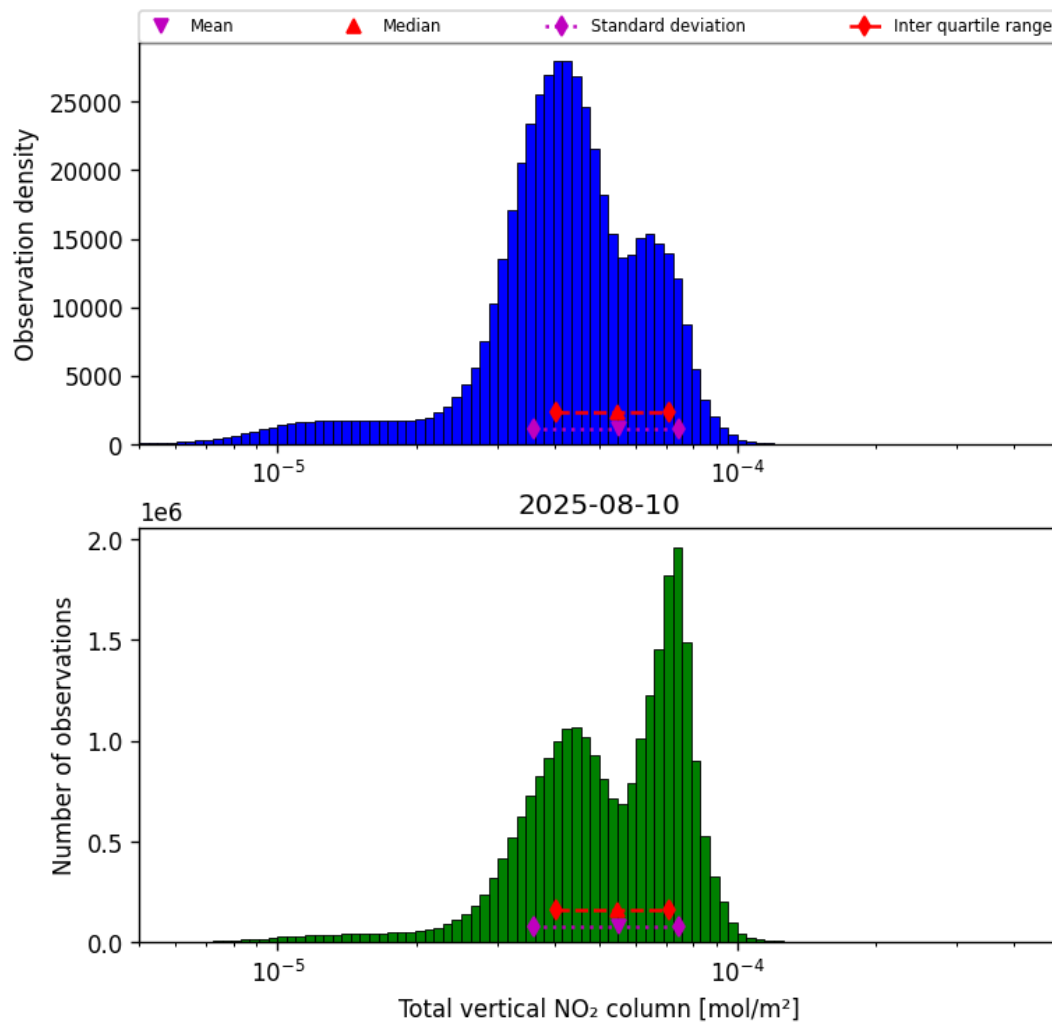
Figure 38: Histogram of “Total vertical NO 2 column” for 2025-08-09 to 2025-08-11
