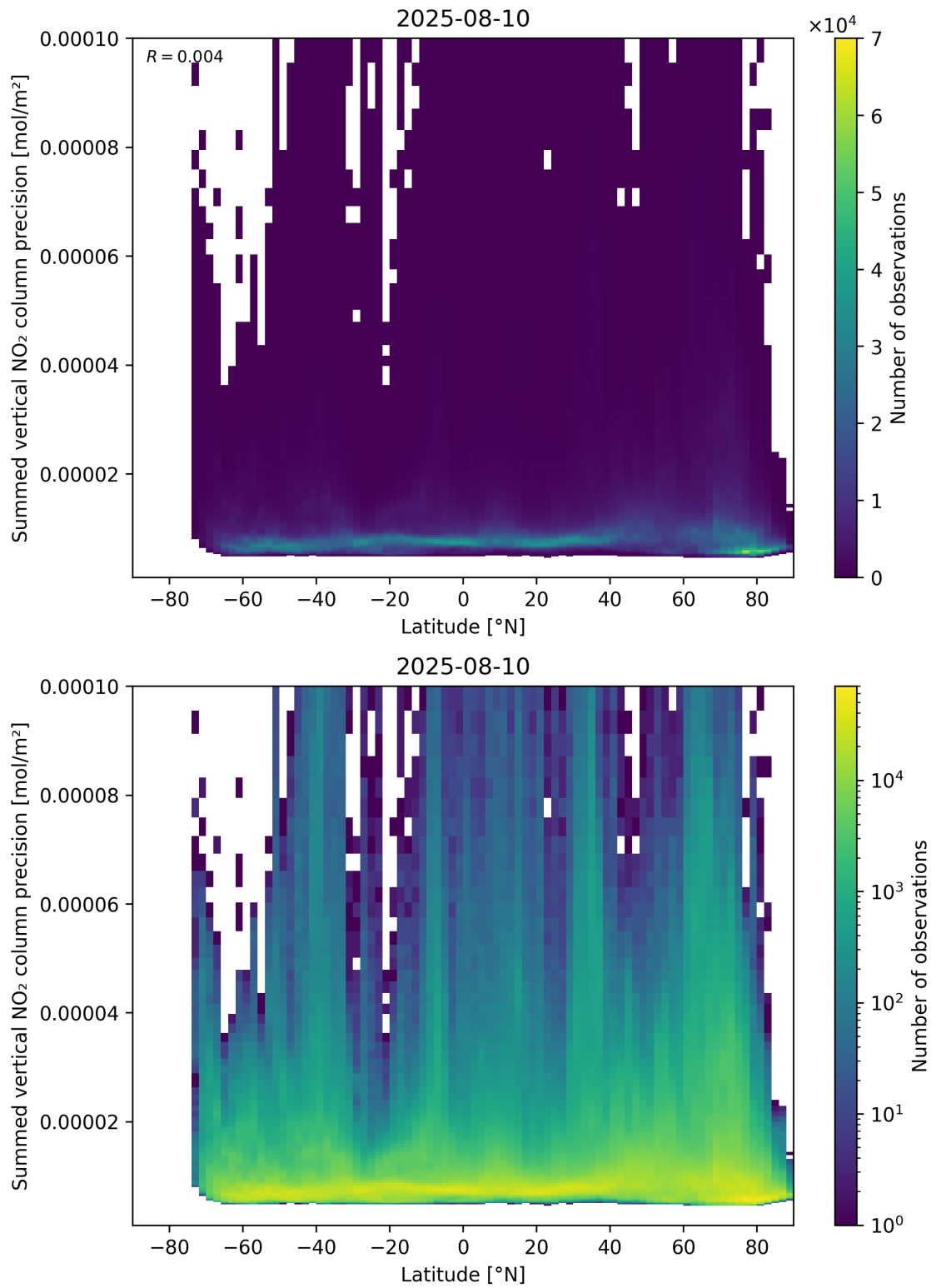
Figure 89: Scatter density plot of “Latitude” against “Summed vertical NO 2 column precision” for 2025-08-09 to 2025-08-11.
