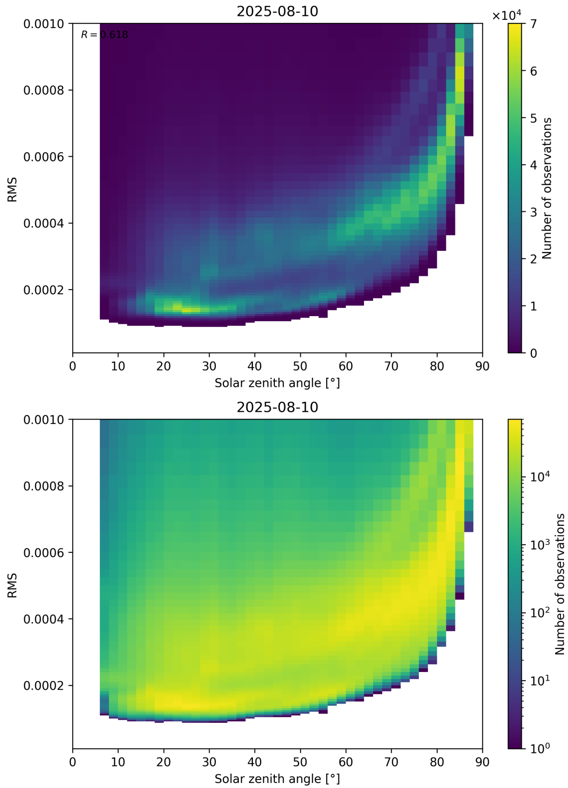
Figure 157: Scatter density plot of “Solar zenith angle” against “RMS” for 2025-08-09 to 2025-08-11.
