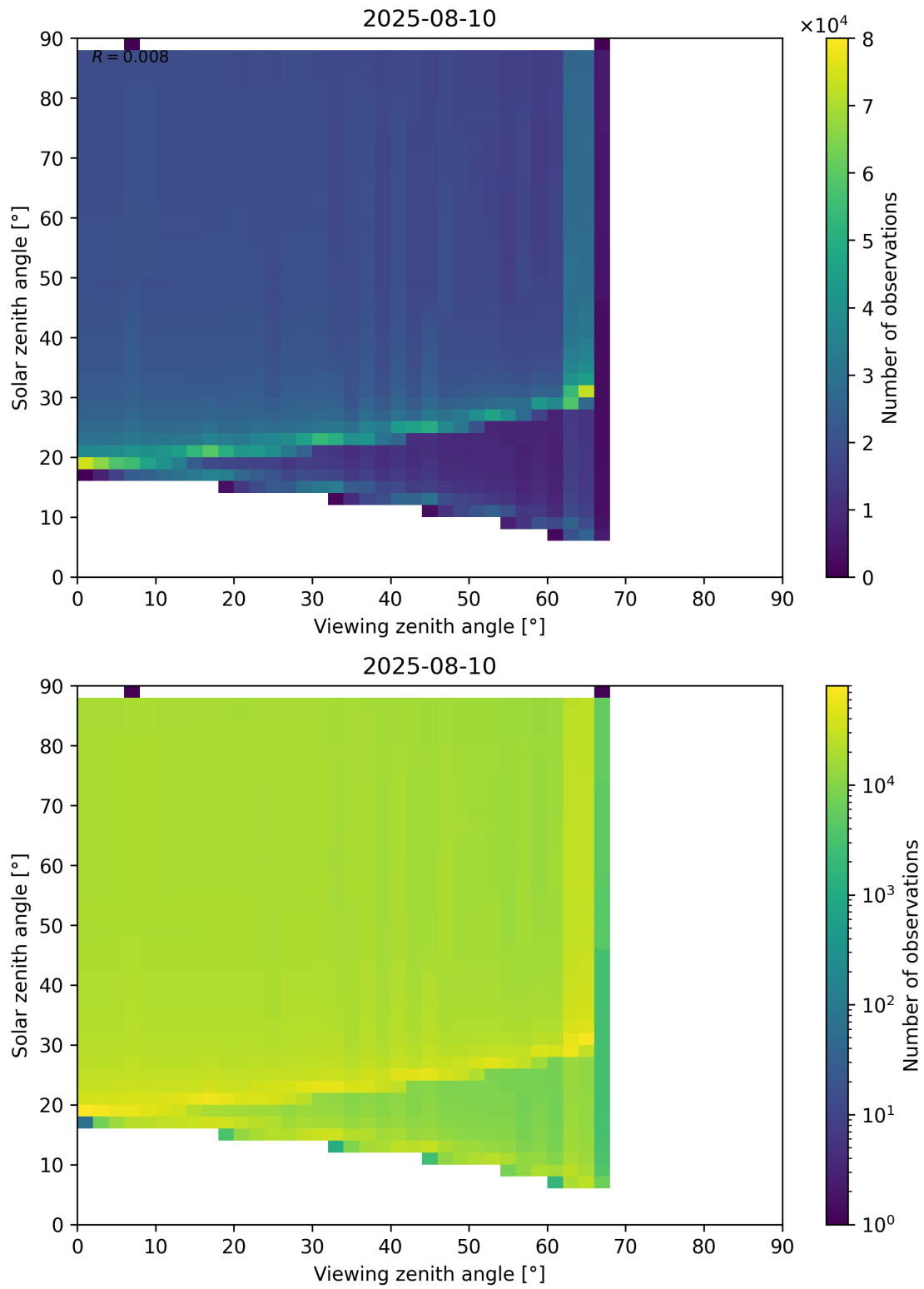
Figure 172: Scatter density plot of “Viewing zenith angle” against “Solar zenith angle” for 2025-08-09 to 2025-08-11.
