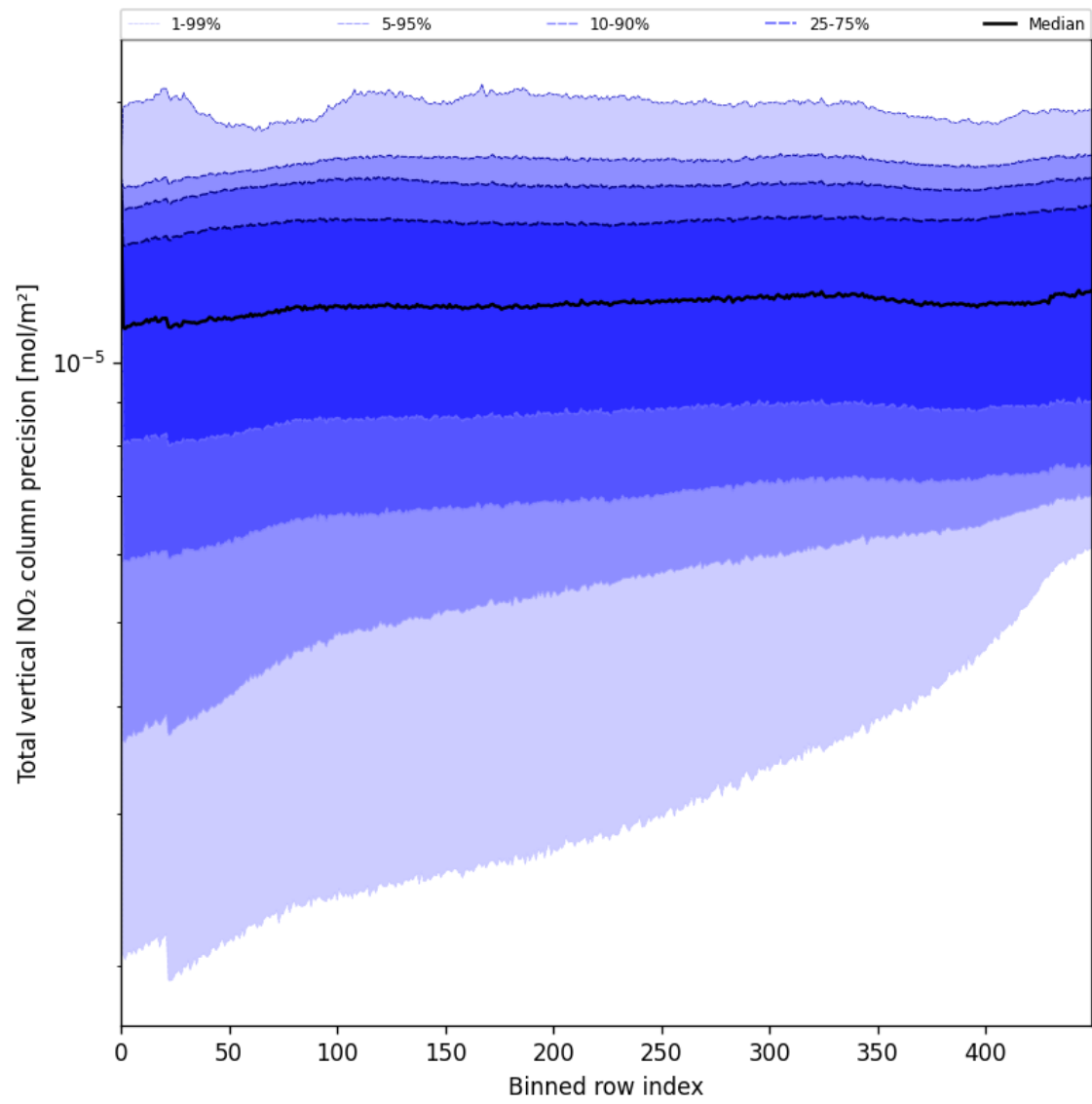
Figure 56: Along track statistics of “Total vertical NO 2 column precision” for 2025-08-09 to 2025-08-11
