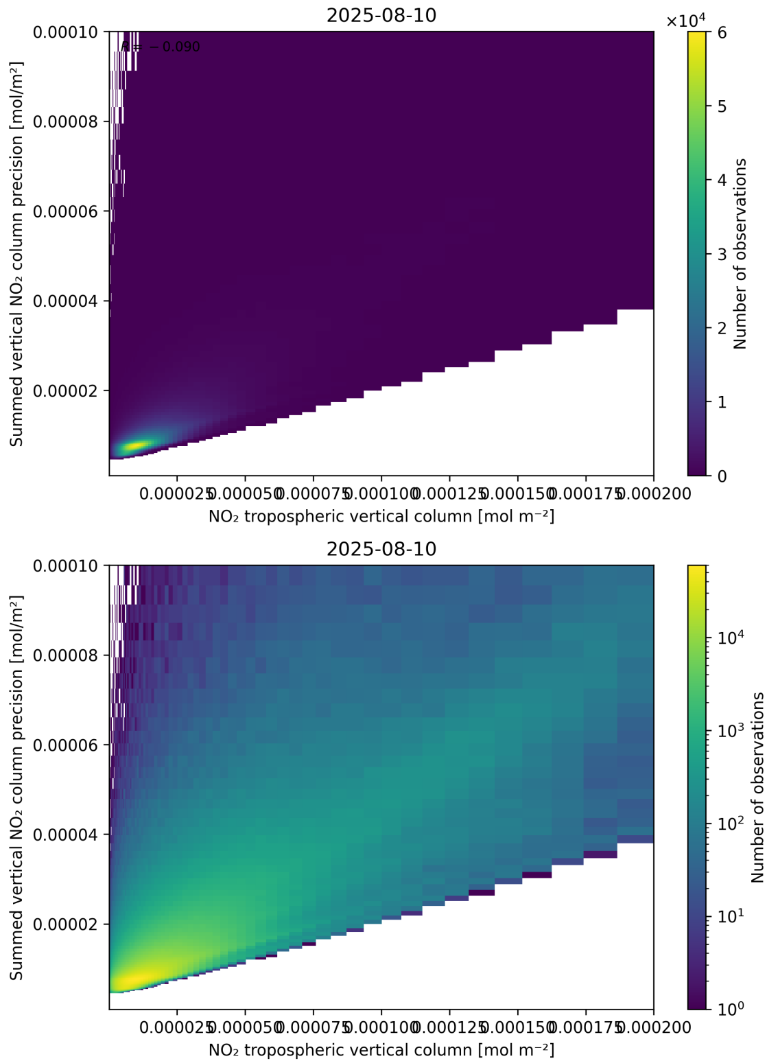
Figure 127: Scatter density plot of “NO 2 tropospheric vertical column” against “Summed vertical NO 2 column precision” for 2025-08-09 to 2025-08-11.
