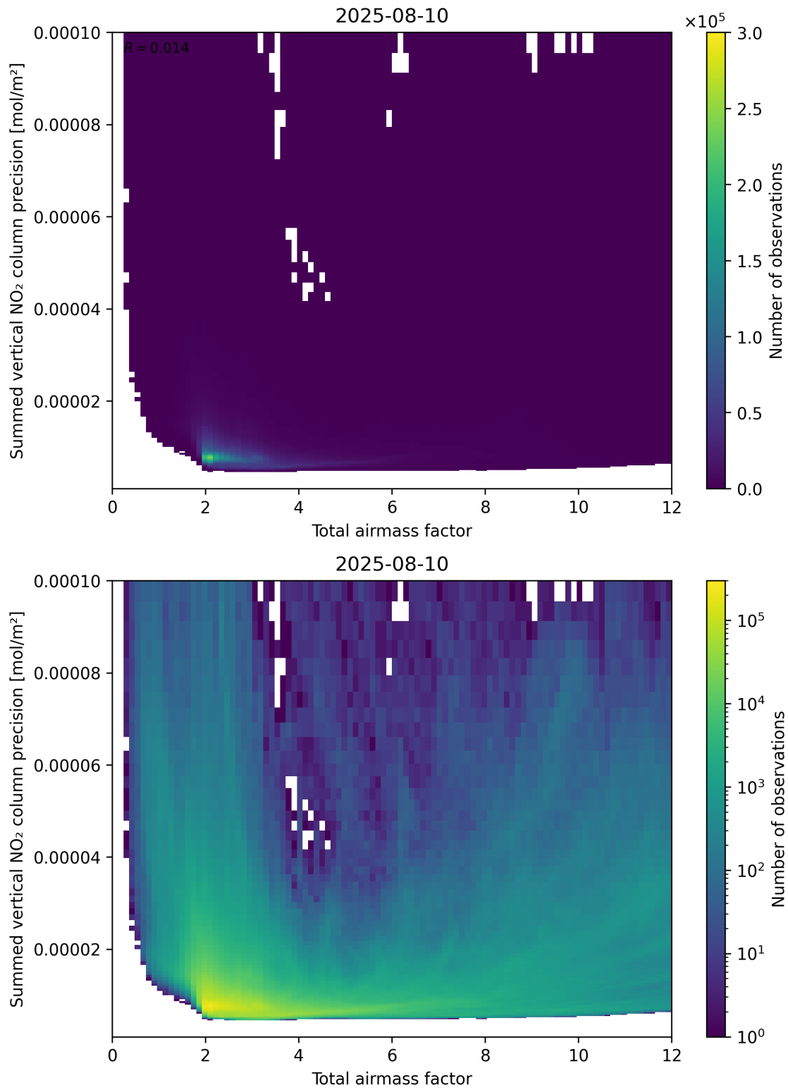
Figure 66: Scatter density plot of “Total airmass factor” against “Summed vertical NO 2 column precision” for 2025-08-09 to 2025-08-11.
