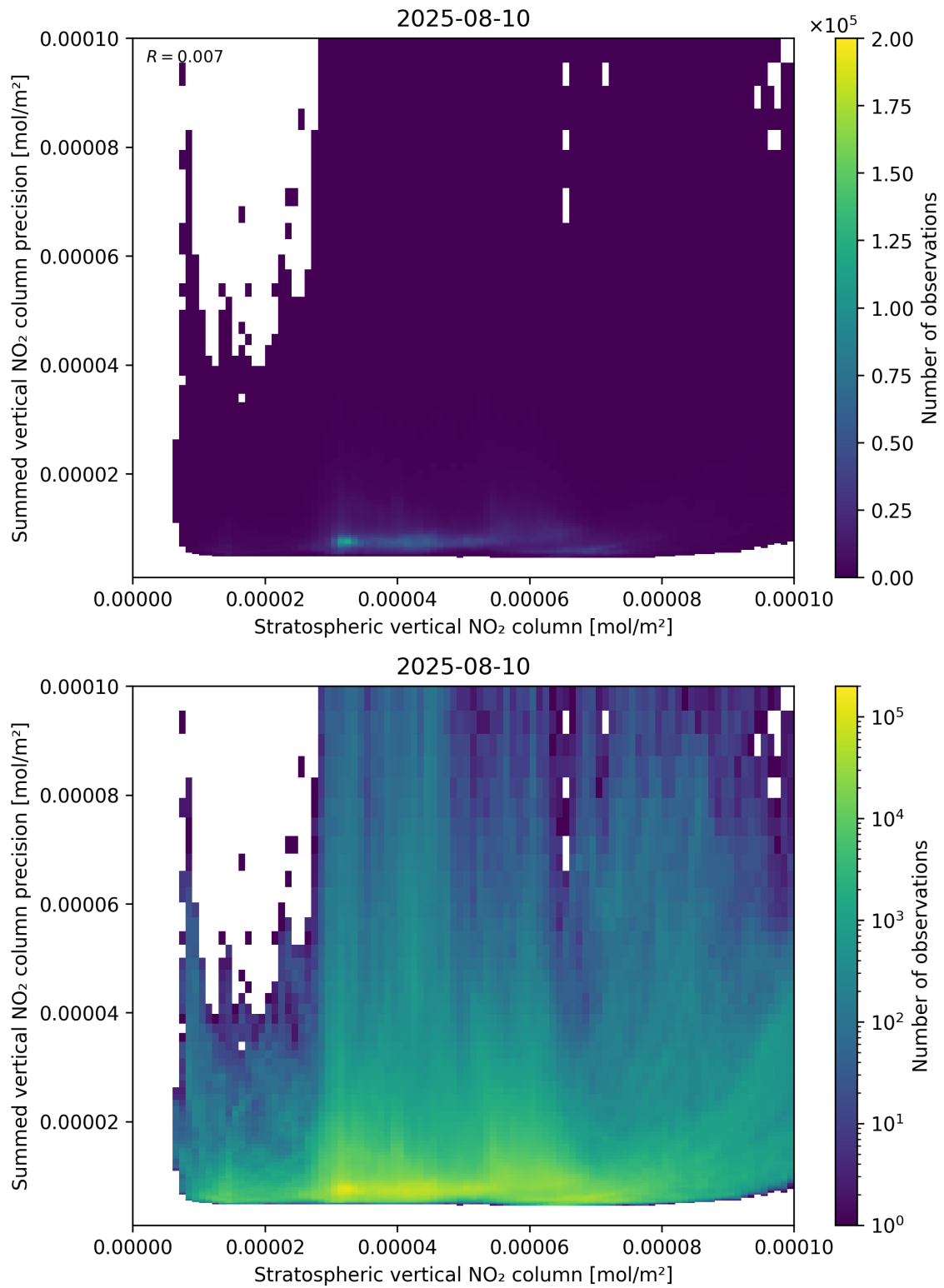
Figure 99: Scatter density plot of “Stratospheric vertical NO 2 column” against “Summed vertical NO 2 column precision” for 2025-08-09 to 2025-08-11.
