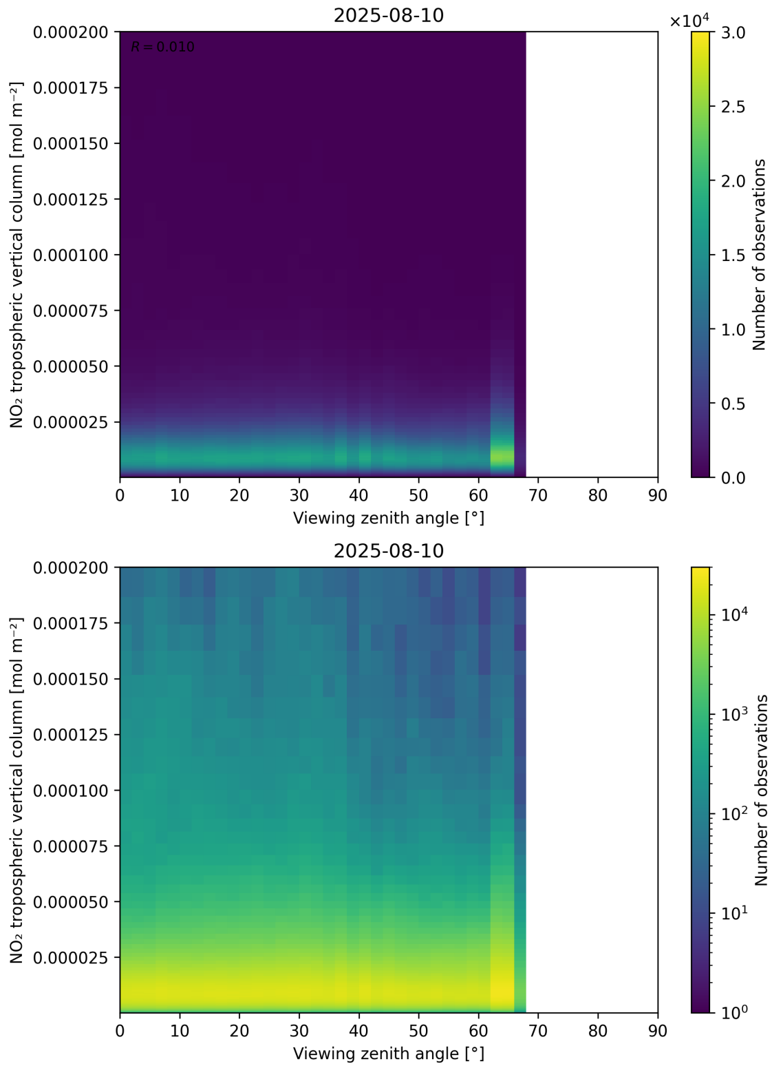
Figure 169: Scatter density plot of “Viewing zenith angle” against “NO 2 tropospheric vertical column” for 2025-08-09 to 2025-08-11.
