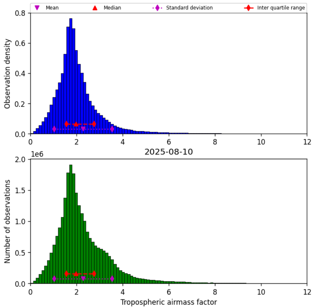
Figure 31: Histogram of “Tropospheric airmass factor” for 2025-08-09 to 2025-08-11
