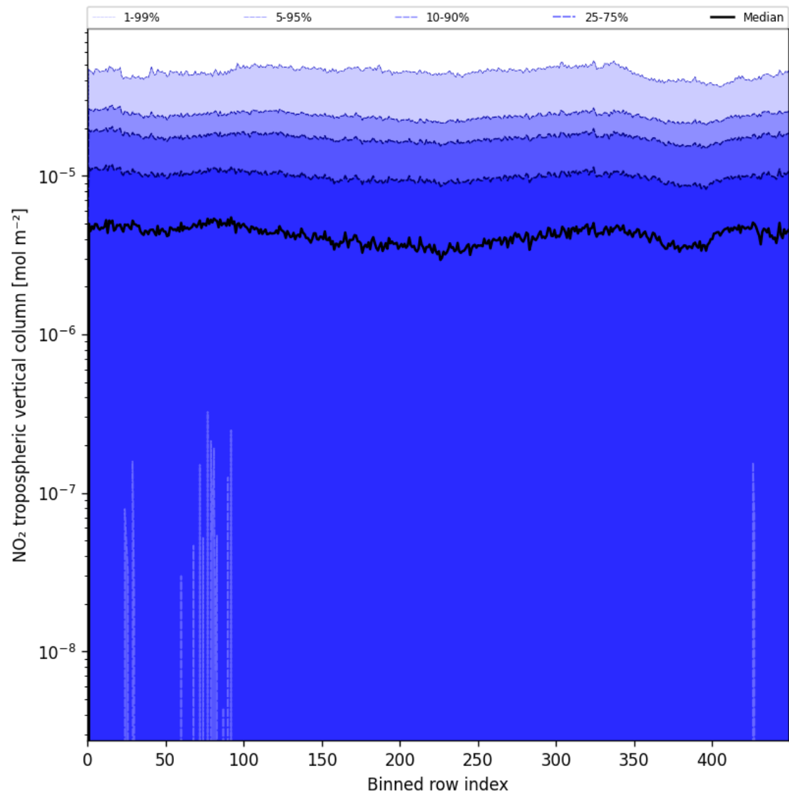
Figure 46: Along track statistics of “NO 2 tropospheric vertical column” for 2025-08-09 to 2025-08-11
