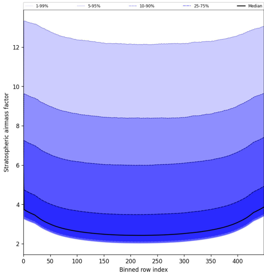
Figure 61: Along track statistics of “Stratospheric airmass factor” for 2025-08-09 to 2025-08-11
