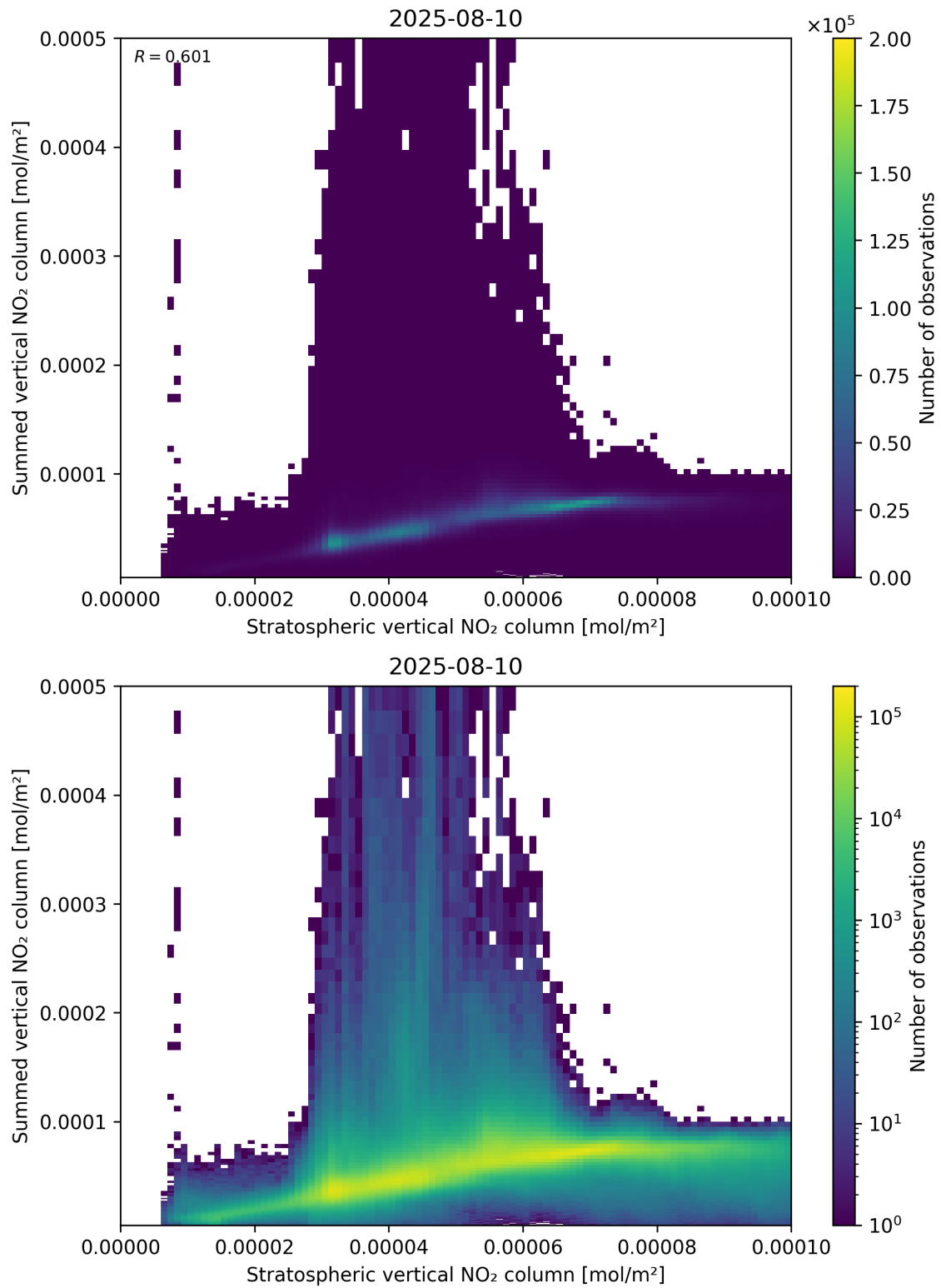
Figure 98: Scatter density plot of “Stratospheric vertical NO 2 column” against “Summed vertical NO 2 column” for 2025-08-09 to 2025-08-11.
