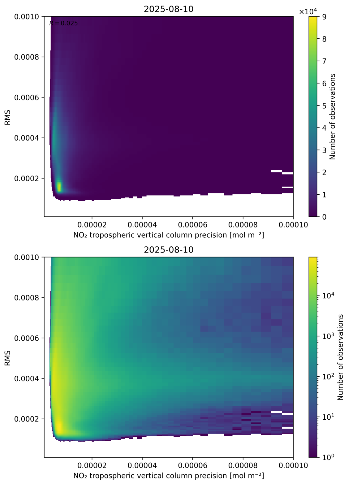
Figure 140: Scatter density plot of “NO 2 tropospheric vertical column precision” against “RMS” for 2025-08-09 to 2025-08-11.
