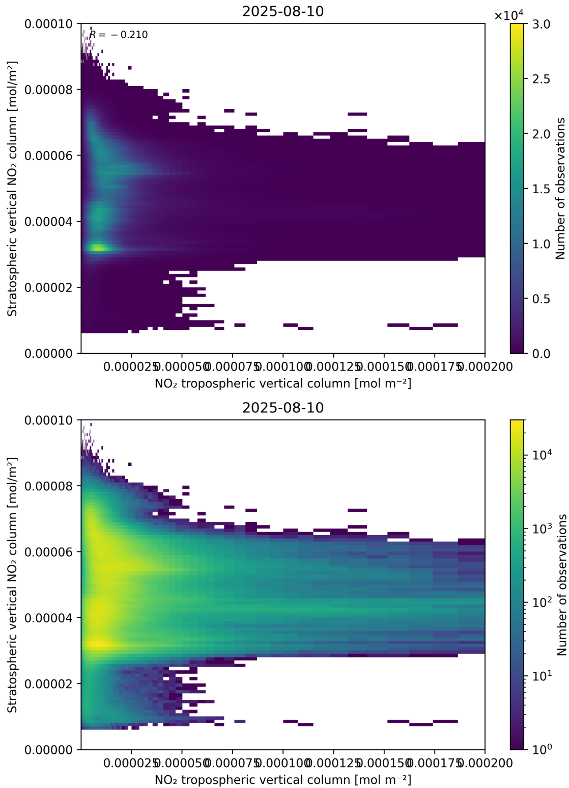
Figure 125: Scatter density plot of “NO 2 tropospheric vertical column” against “Stratospheric vertical NO 2 column” for 2025-08-09 to 2025-08-11.
