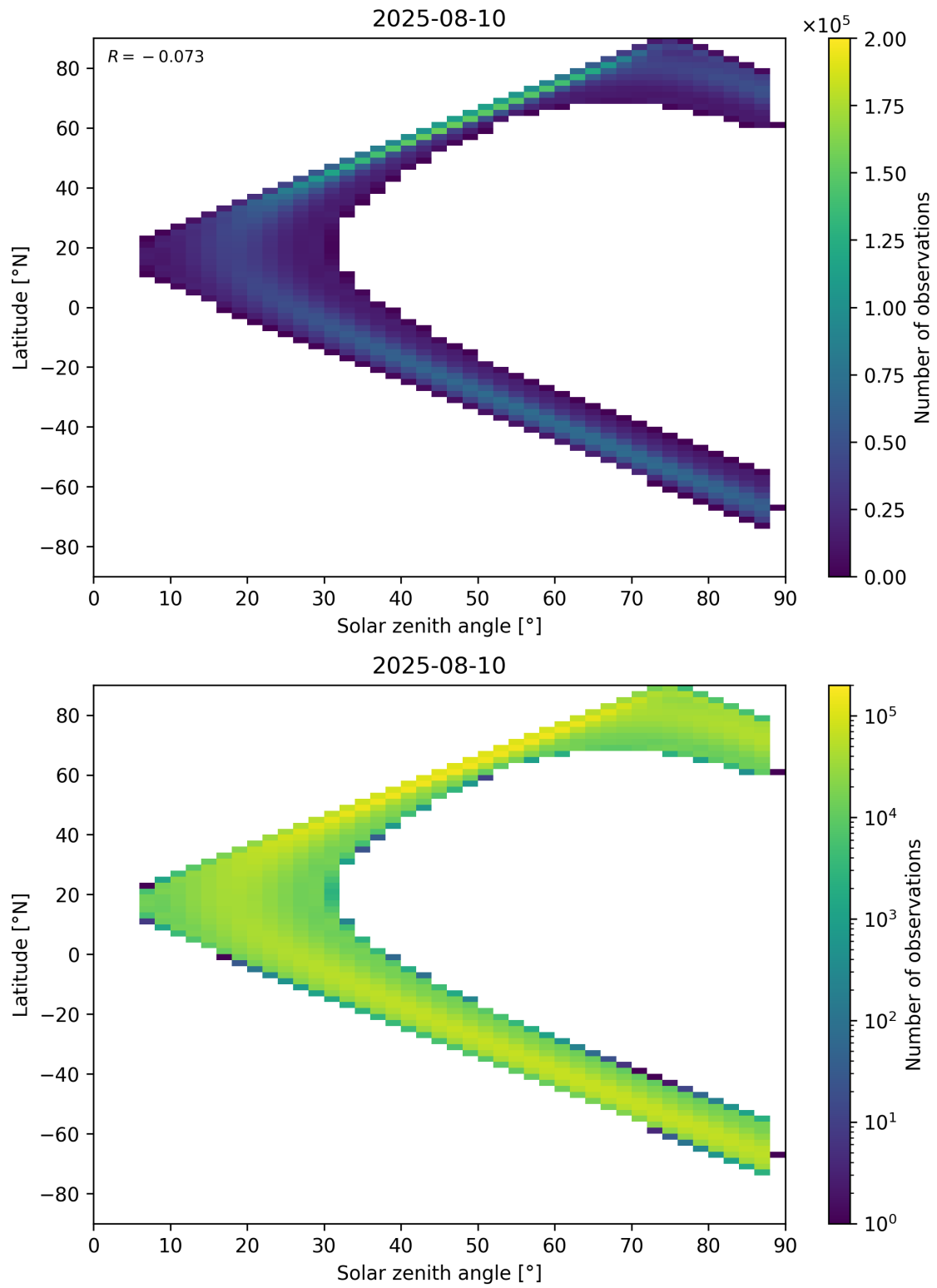
Figure 149: Scatter density plot of “Solar zenith angle” against “Latitude” for 2025-08-09 to 2025-08-11.
