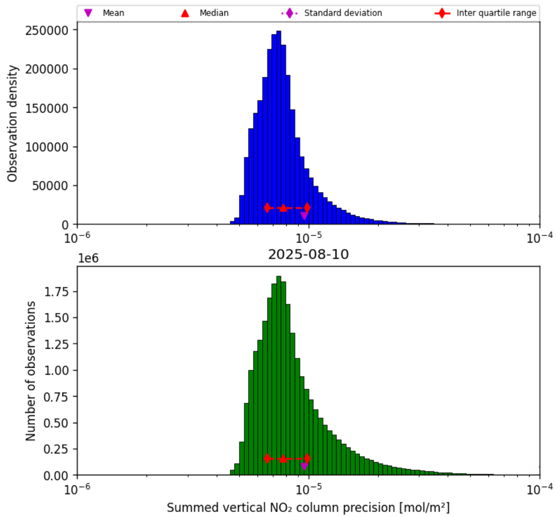
Figure 41: Histogram of "Summed vertical NO 2 column precision" for 2025-08-09 to 2025-08-11
