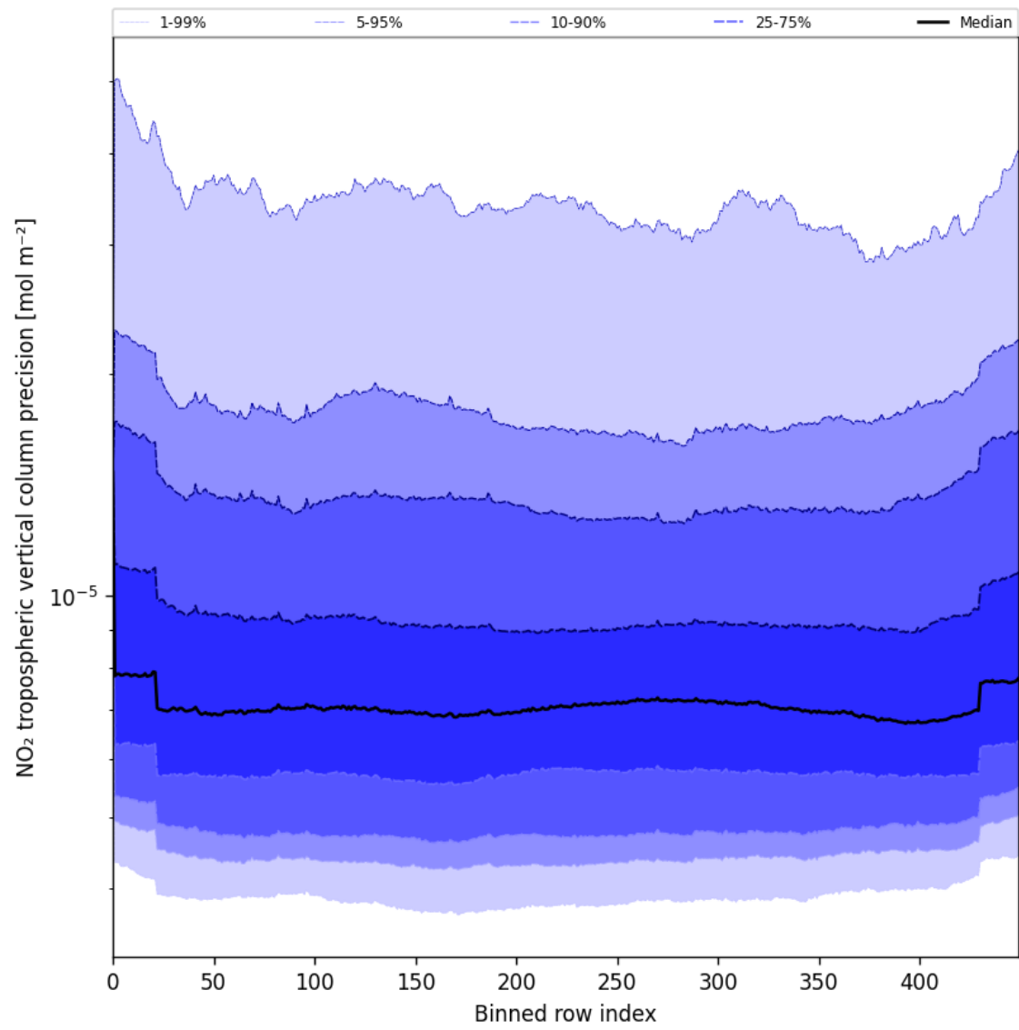
Figure 47: Along track statistics of “NO 2 tropospheric vertical column precision” for 2025-08-09 to 2025-08-11
