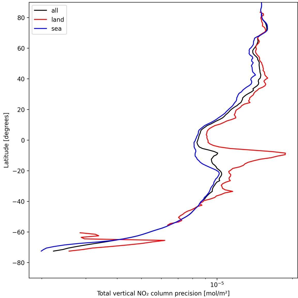
Figure 22: Zonal average of “Total vertical NO 2 column precision” for 2025-08-09 to 2025-08-11.
