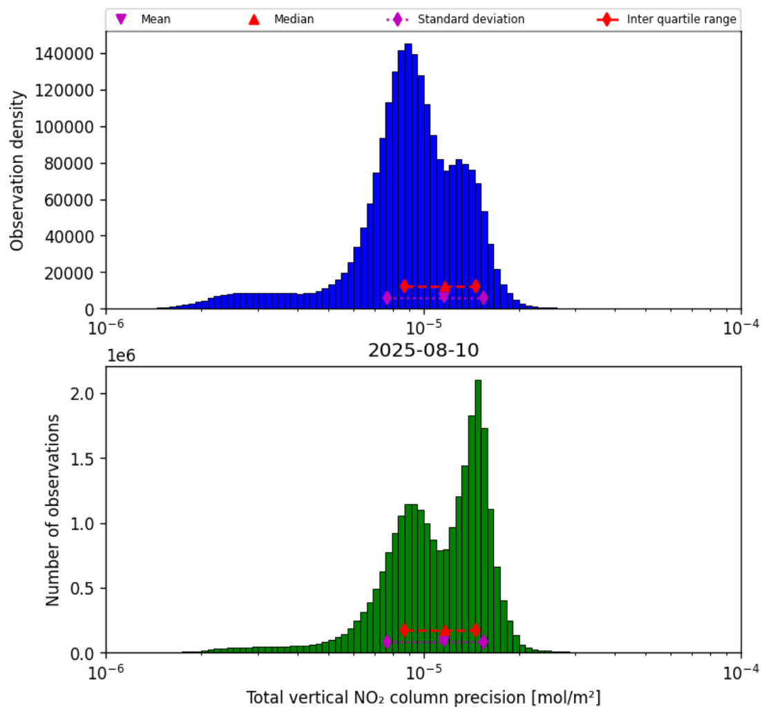
Figure 39: Histogram of “Total vertical NO 2 column precision” for 2025-08-09 to 2025-08-11
