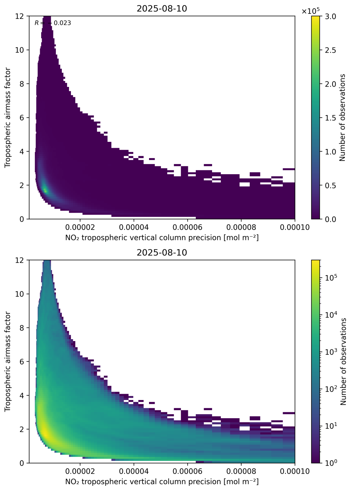
Figure 133: Scatter density plot of “NO 2 tropospheric vertical column precision” against “Tropospheric airmass factor” for 2025-08-09 to 2025-08-11.
