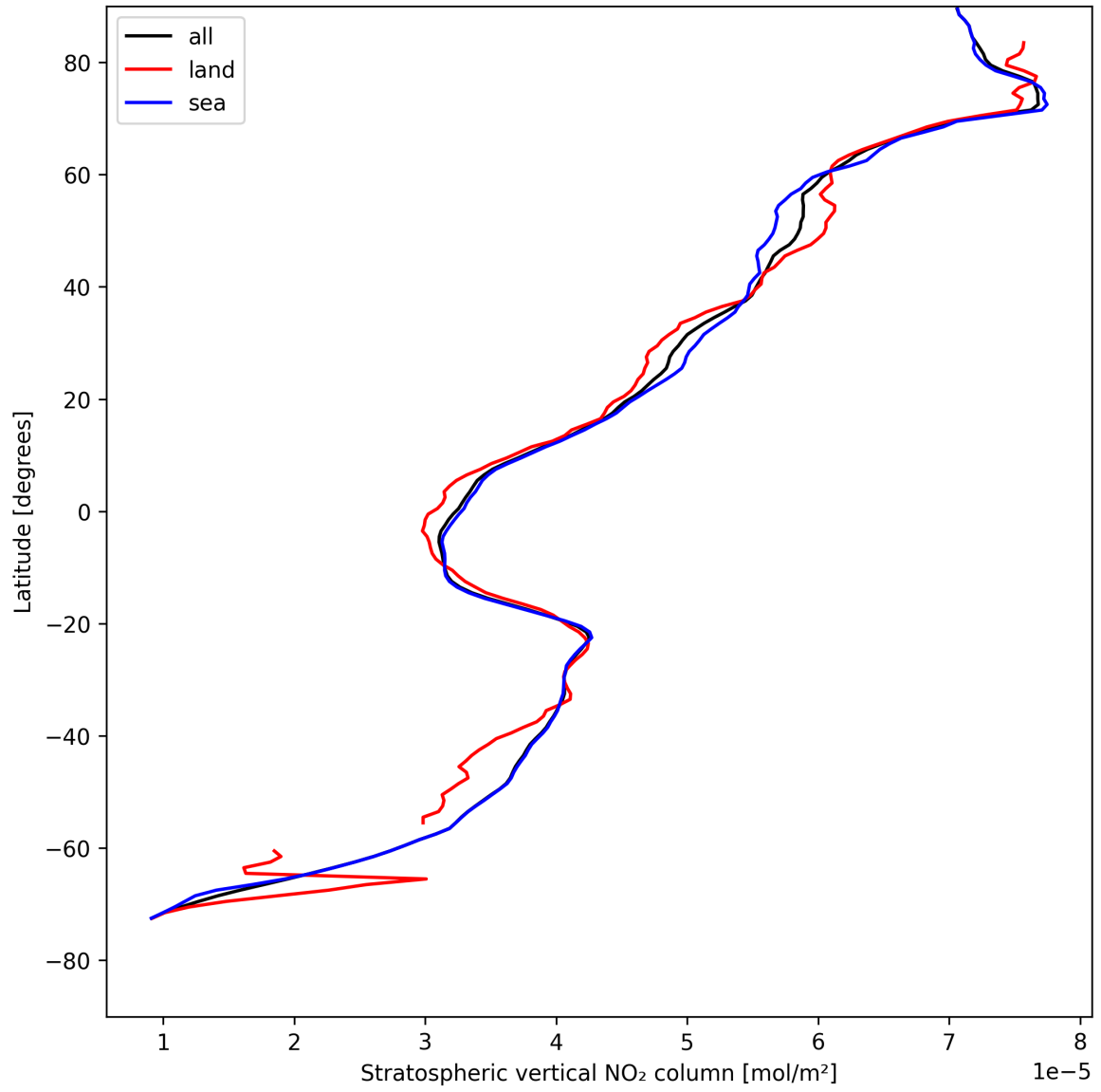
Figure 19: Zonal average of “Stratospheric vertical NO 2 column” for 2025-08-09 to 2025-08-11.
