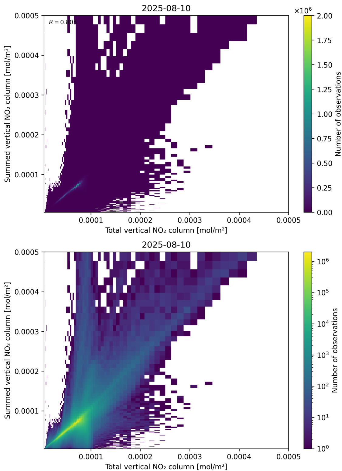
Figure 112: Scatter density plot of “Total vertical NO 2 column” against “Summed vertical NO 2 column” for 2025-08-09 to 2025-08-11.
