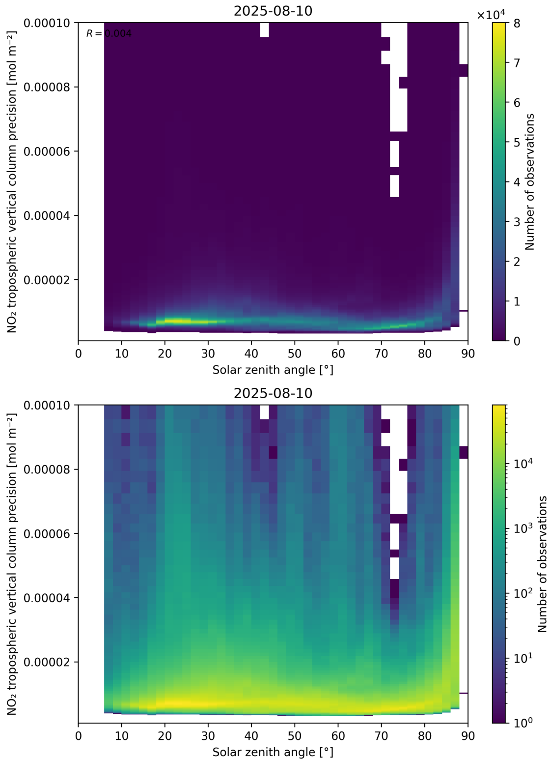
Figure 156: Scatter density plot of “Solar zenith angle” against “NO 2 tropospheric vertical column precision” for 2025-08-09 to 2025-08-11.
