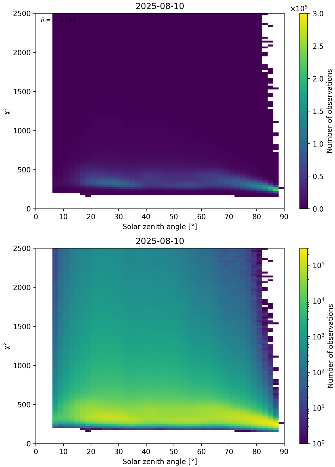
Figure 148: Scatter density plot of “Solar zenith angle” against “ \chi^2 ” for 2025-08-09 to 2025-08-11.
