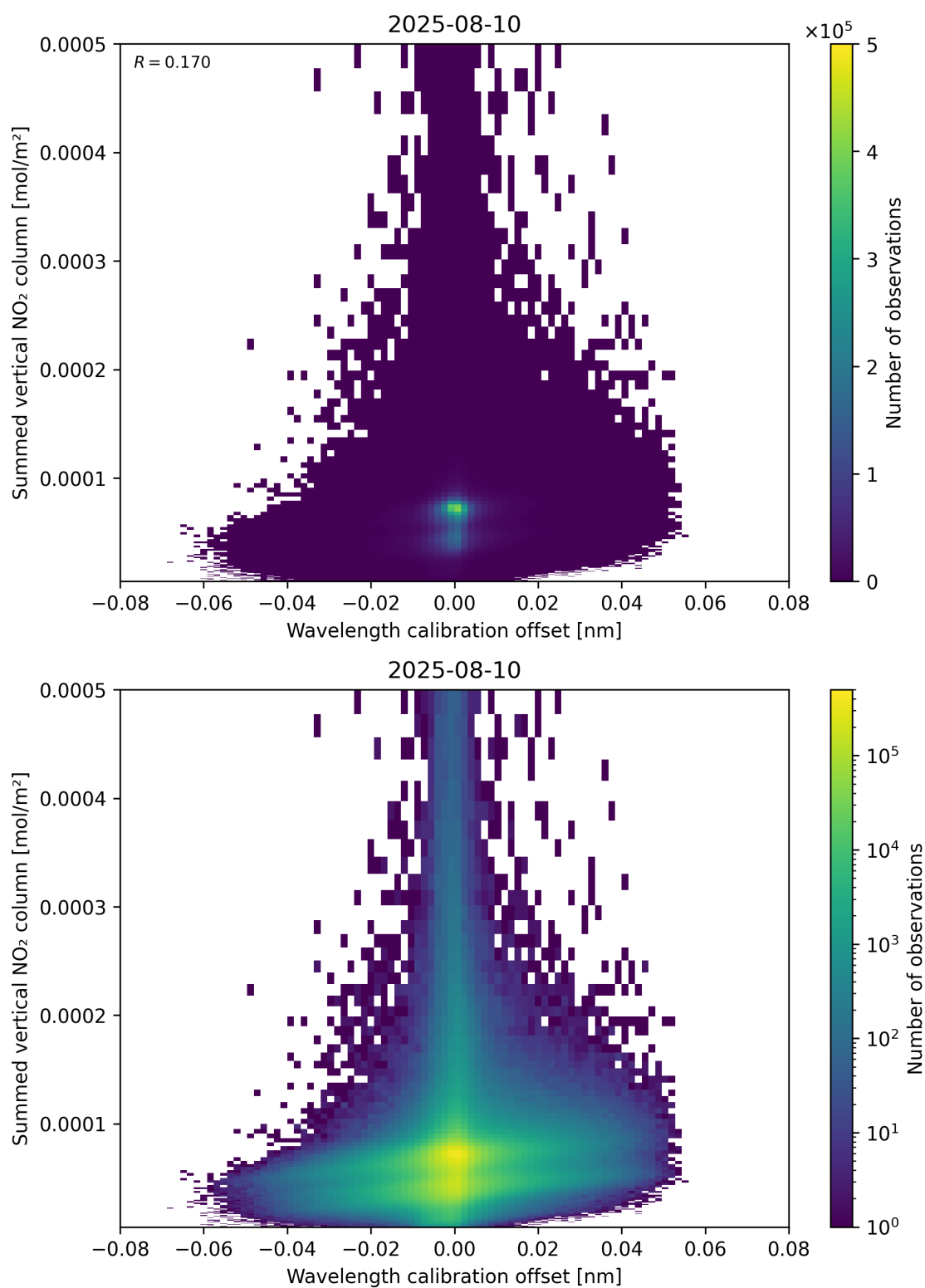
Figure 177: Scatter density plot of “Wavelength calibration offset” against “Summed vertical NO 2 column” for 2025-08-09 to 2025-08-11.
