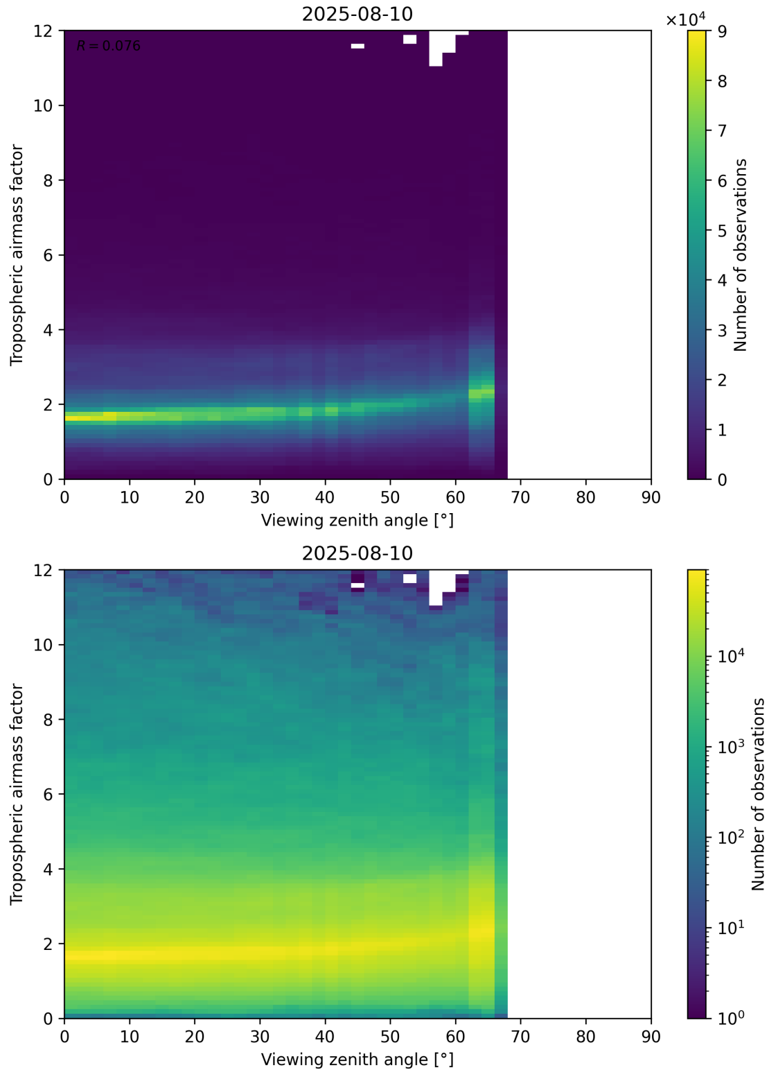
Figure 161: Scatter density plot of “Viewing zenith angle” against “Tropospheric airmass factor” for 2025-08-09 to 2025-08-11.
