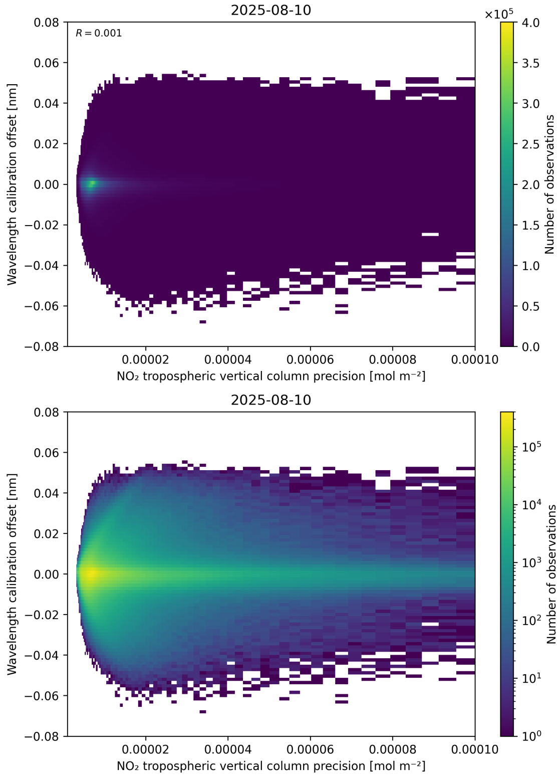
Figure 141: Scatter density plot of “NO 2 tropospheric vertical column precision” against “Wavelength calibration offset” for 2025-08-09 to 2025-08-11.
