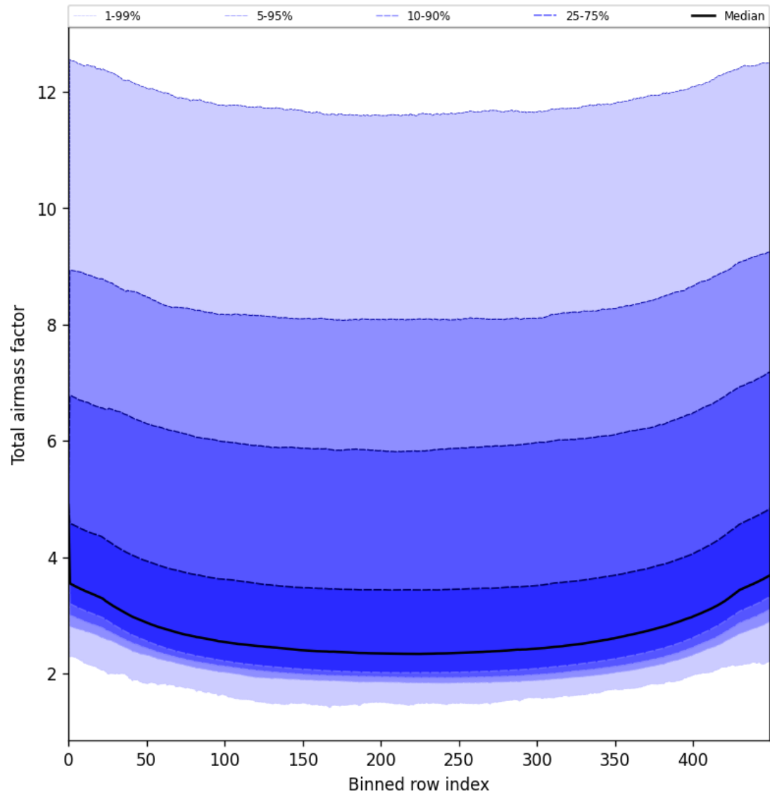
Figure 49: Along track statistics of “Total airmass factor” for 2025-08-09 to 2025-08-11
