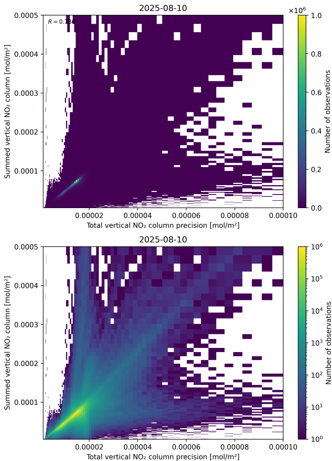
Figure 117: Scatter density plot of “Total vertical NO 2 column precision” against “Summed vertical NO 2 column” for 2025-08-09 to 2025-08-11.
