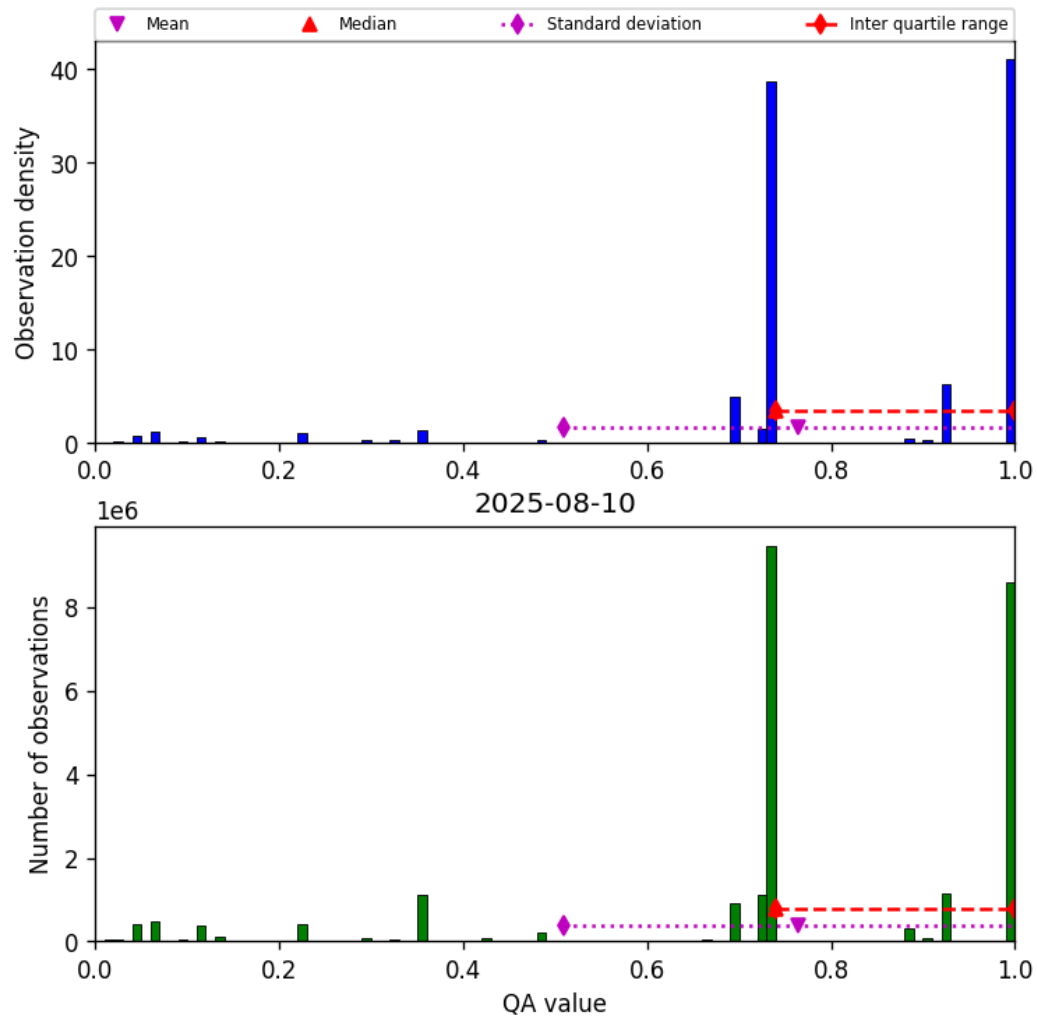
Figure 28: Histogram of “QA value” for 2025-08-09 to 2025-08-11
