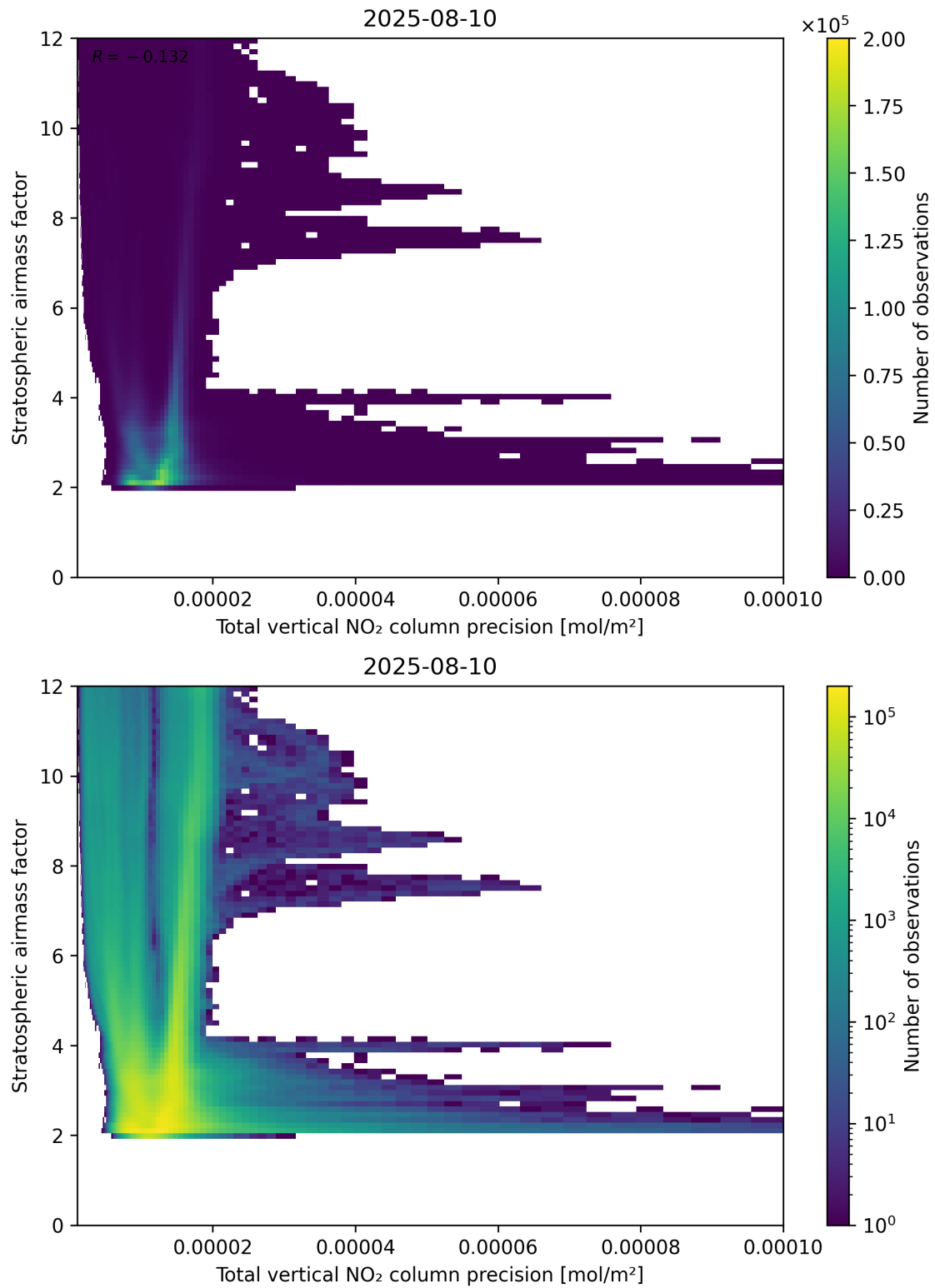
Figure 115: Scatter density plot of “Total vertical NO 2 column precision” against “Stratospheric air mass factor” for 2025-08-09 to 2025-08-11.
