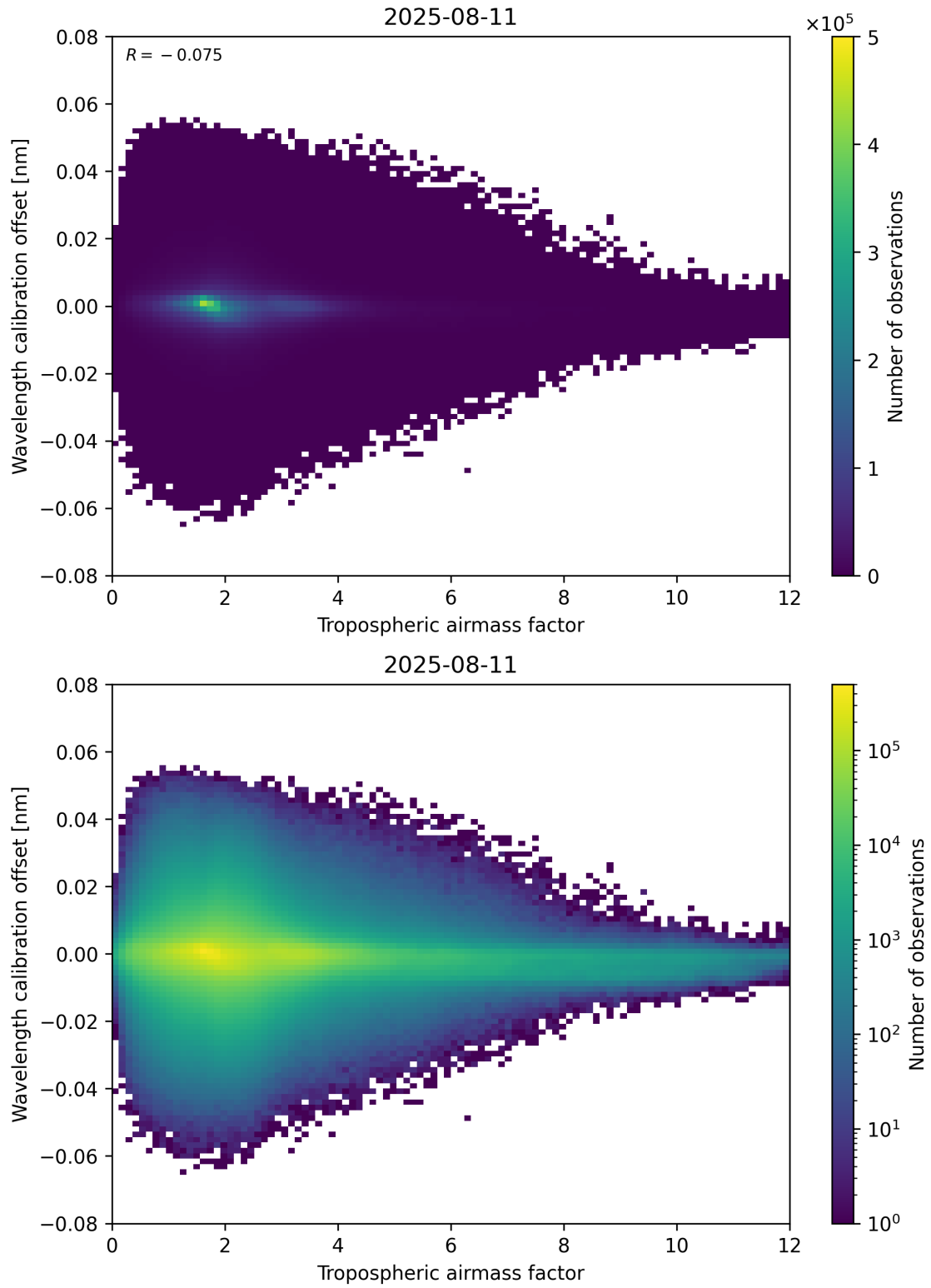
Figure 80: Scatter density plot of “Tropospheric airmass factor” against “Wavelength calibration offset” for 2025-08-10 to 2025-08-12.
