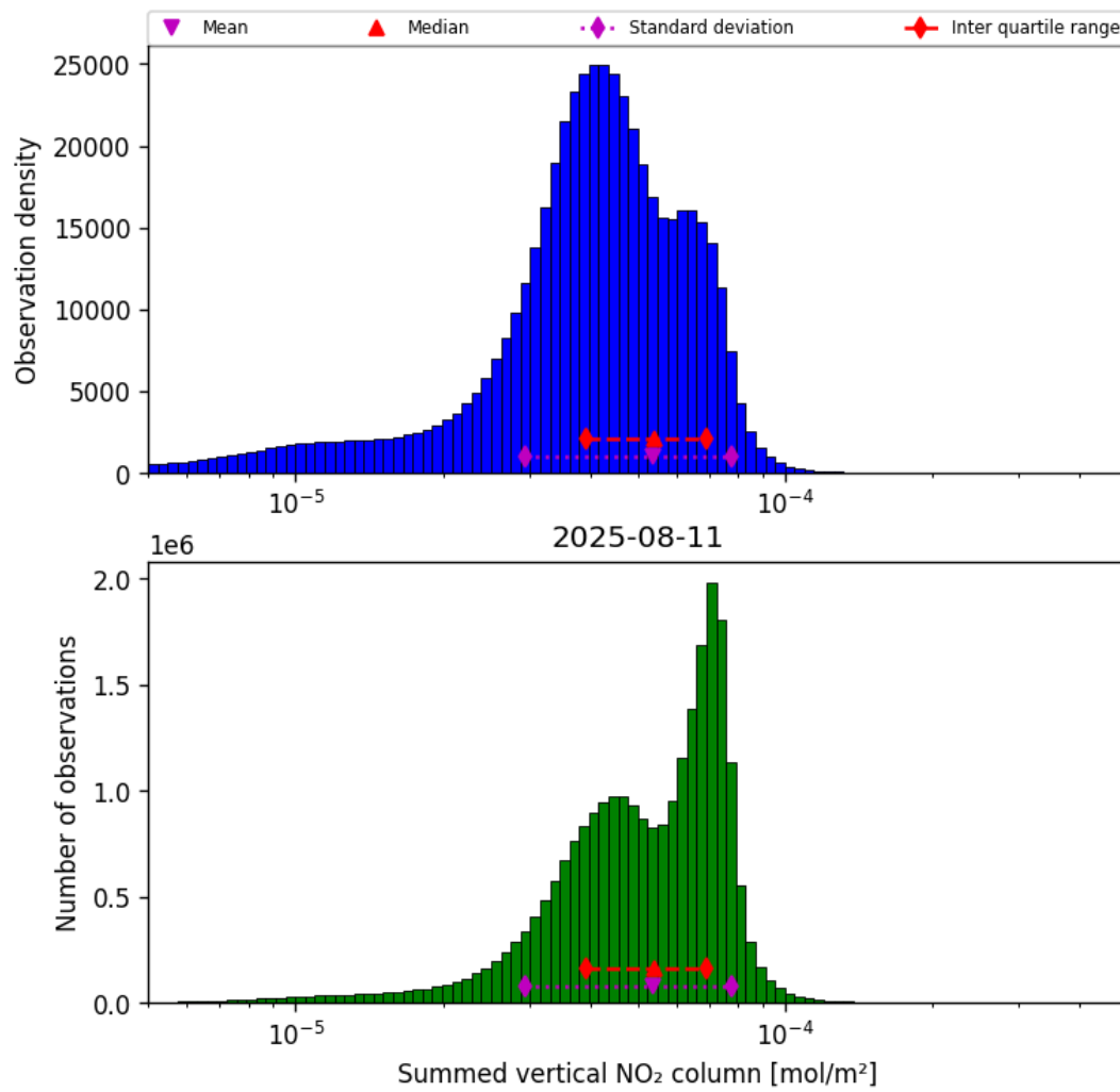
Figure 40: Histogram of “Summed vertical NO 2 column” for 2025-08-10 to 2025-08-12
