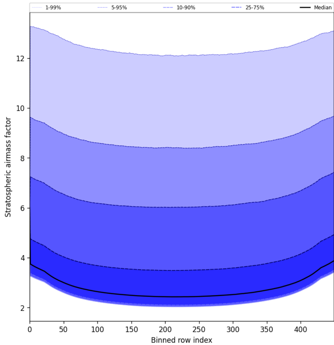
Figure 61: Along track statistics of “Stratospheric airmass factor” for 2025-08-10 to 2025-08-12
