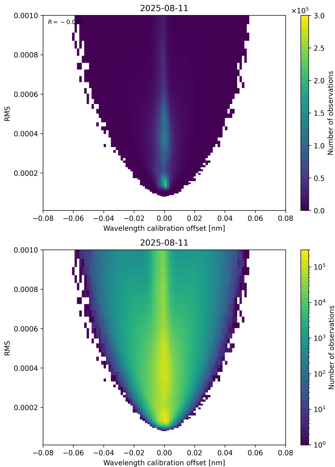
Figure 181: Scatter density plot of “Wavelength calibration offset” against “RMS” for 2025-08-10 to 2025-08-12.
