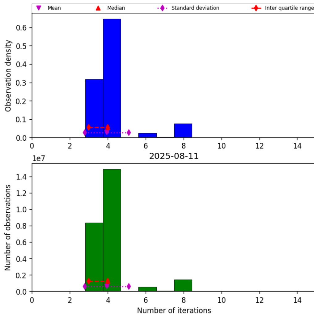
Figure 34: Histogram of “Number of iterations” for 2025-08-10 to 2025-08-12
