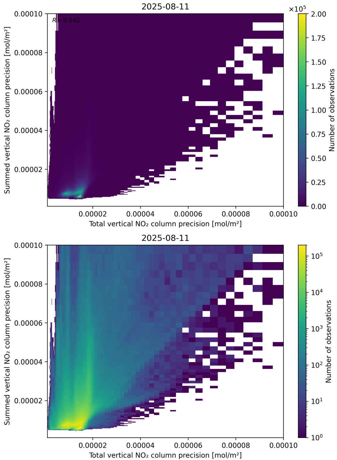
Figure 118: Scatter density plot of “Total vertical NO 2 column precision” against “Summed vertical NO 2 column precision” for 2025-08-10 to 2025-08-12.
