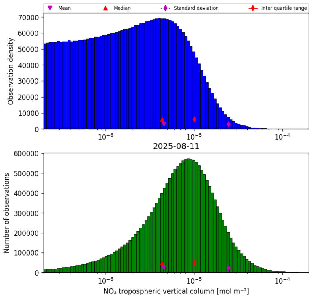
Figure 29: Histogram of “ \text{NO}_2 tropospheric vertical column” for 2025-08-10 to 2025-08-12
