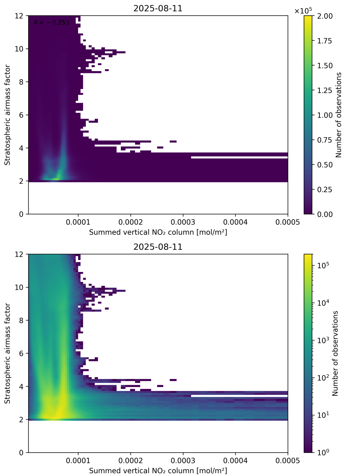
Figure 103: Scatter density plot of “Summed vertical NO 2 column” against “Stratospheric airmass factor” for 2025-08-10 to 2025-08-12.
