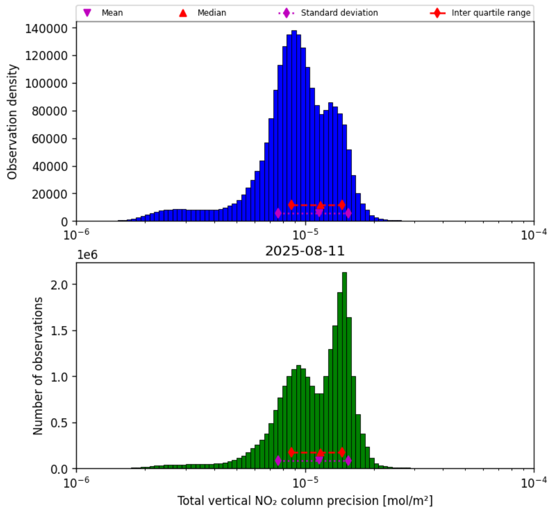
Figure 39: Histogram of “Total vertical NO 2 column precision” for 2025-08-10 to 2025-08-12
