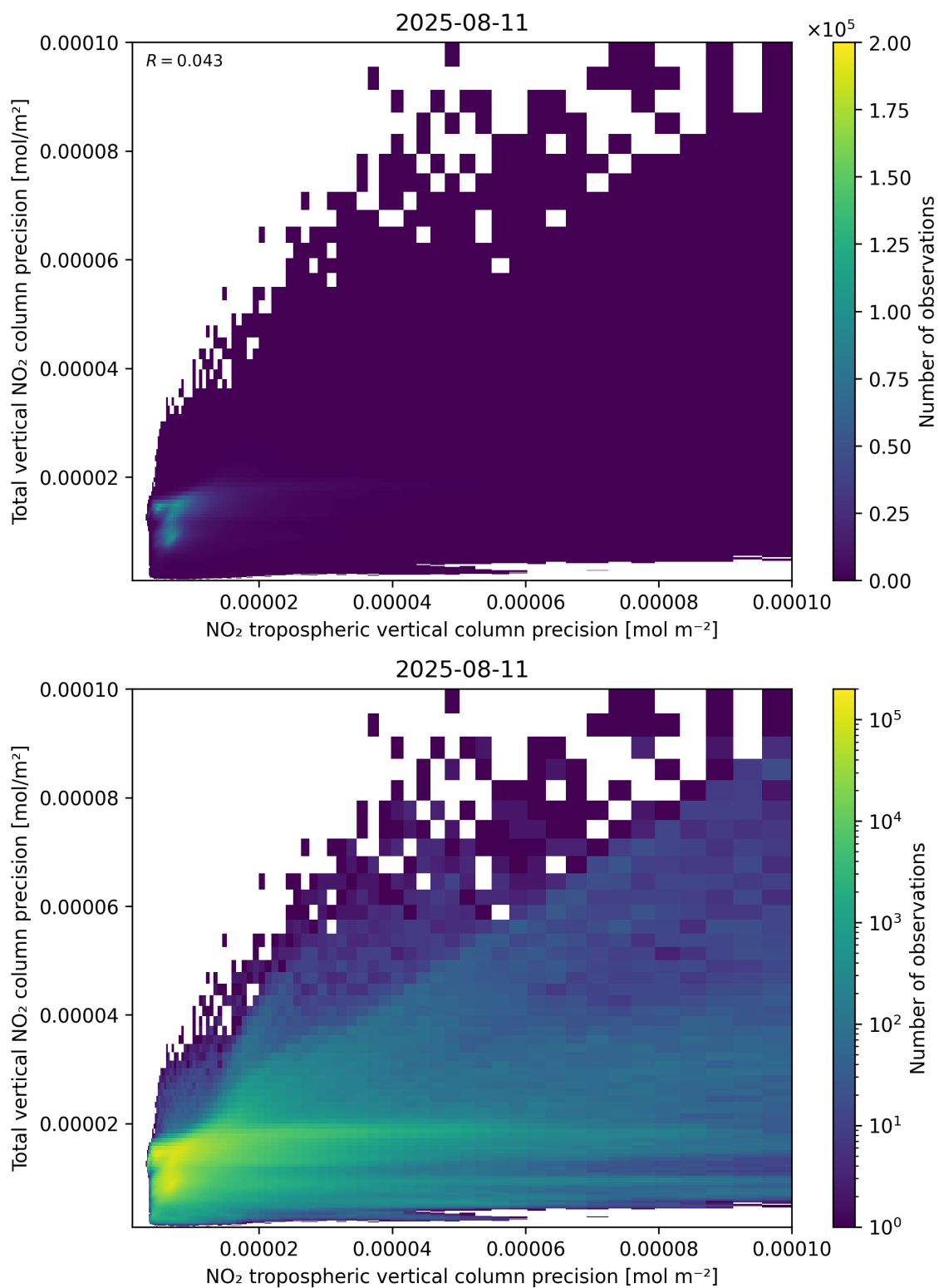
Figure 139: Scatter density plot of “NO 2 tropospheric vertical column precision” against “Total vertical NO 2 column precision” for 2025-08-10 to 2025-08-12.
