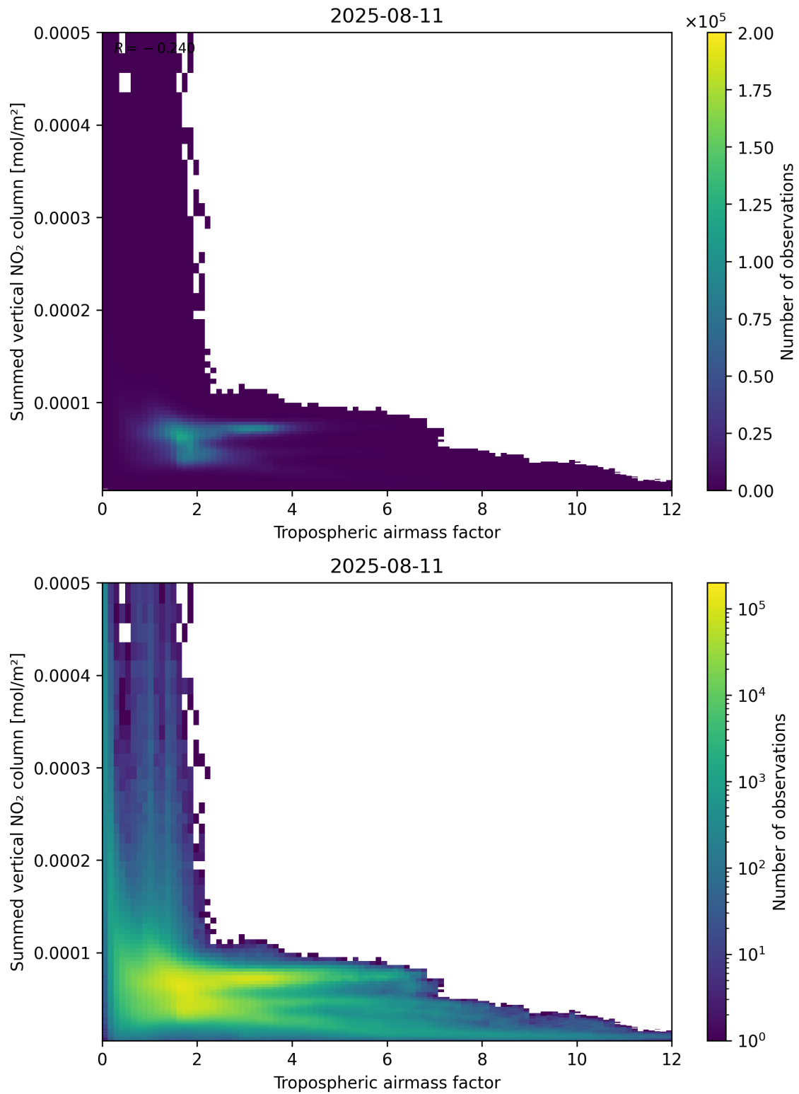
Figure 75: Scatter density plot of “Tropospheric air mass factor” against “Summed vertical NO 2 column” for 2025-08-10 to 2025-08-12.
