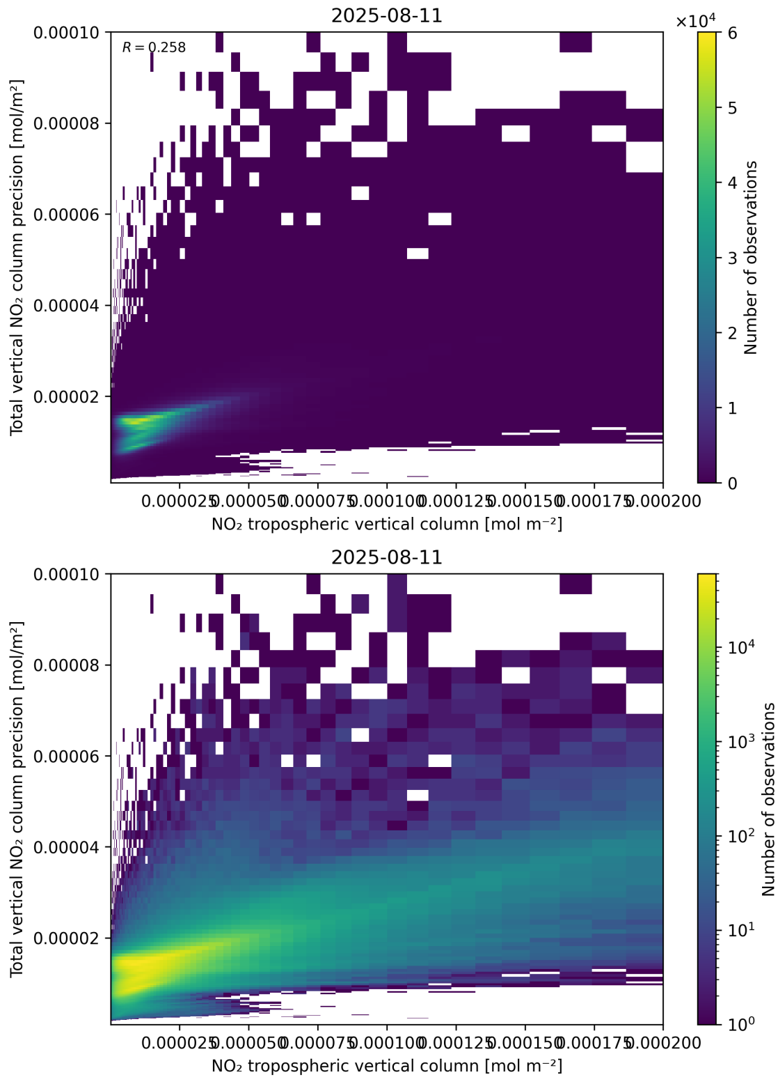
Figure 129: Scatter density plot of “NO 2 tropospheric vertical column” against “Total vertical NO 2 column precision” for 2025-08-10 to 2025-08-12.
