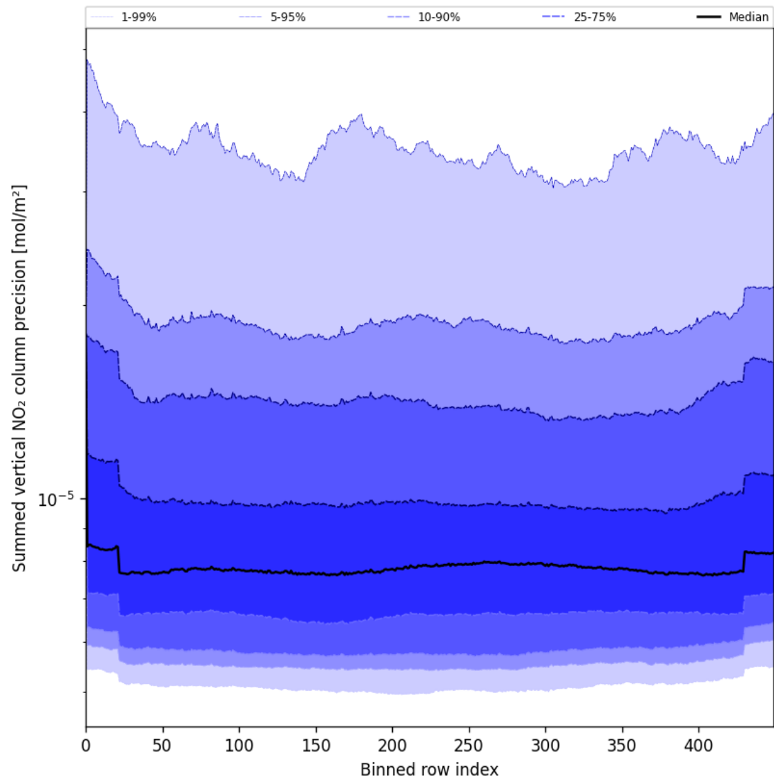
Figure 58: Along track statistics of “Summed vertical NO 2 column precision” for 2025-08-10 to 2025-08-12
