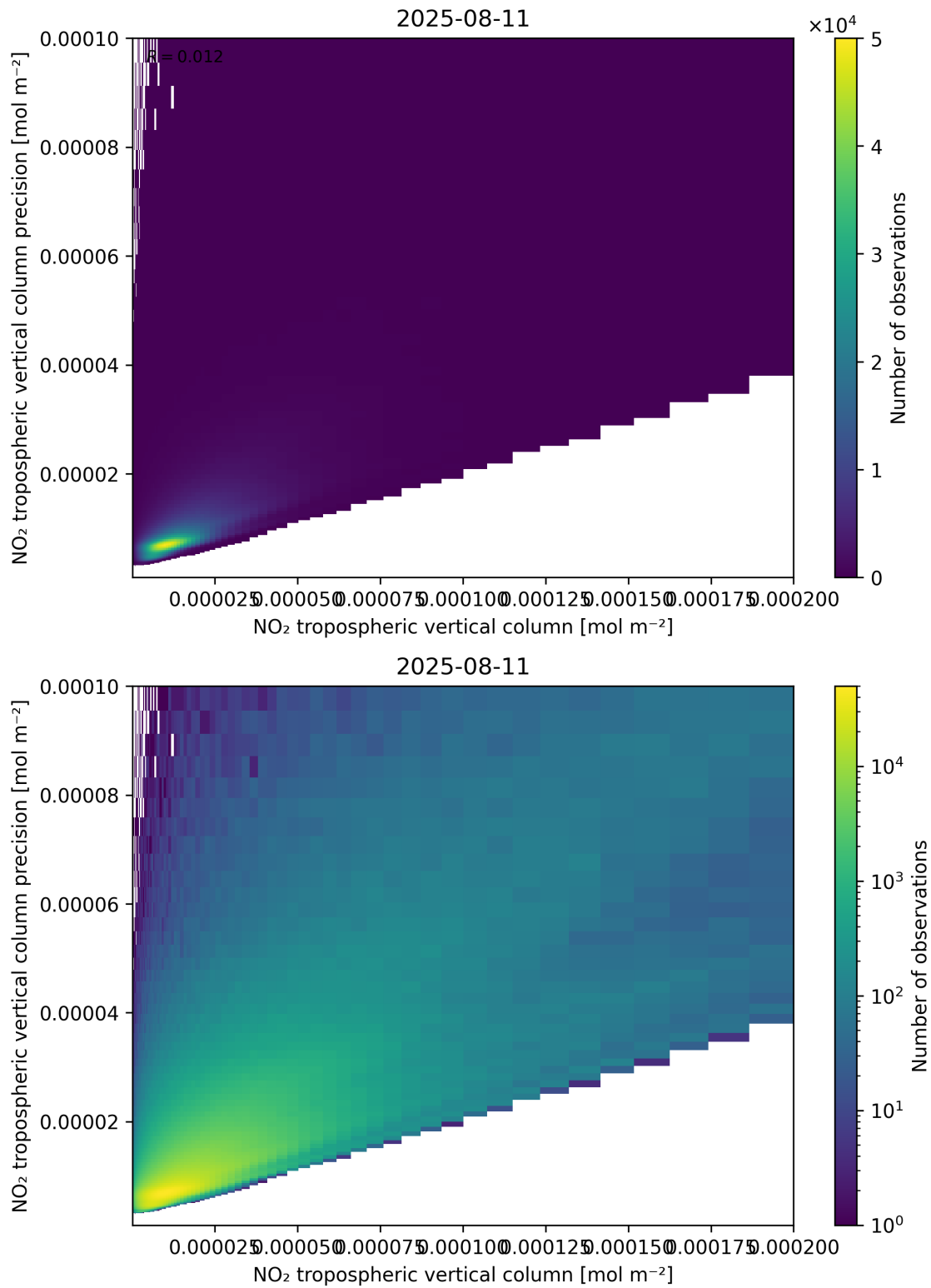
Figure 130: Scatter density plot of “NO 2 tropospheric vertical column” against “NO 2 tropospheric vertical column precision” for 2025-08-10 to 2025-08-12.
