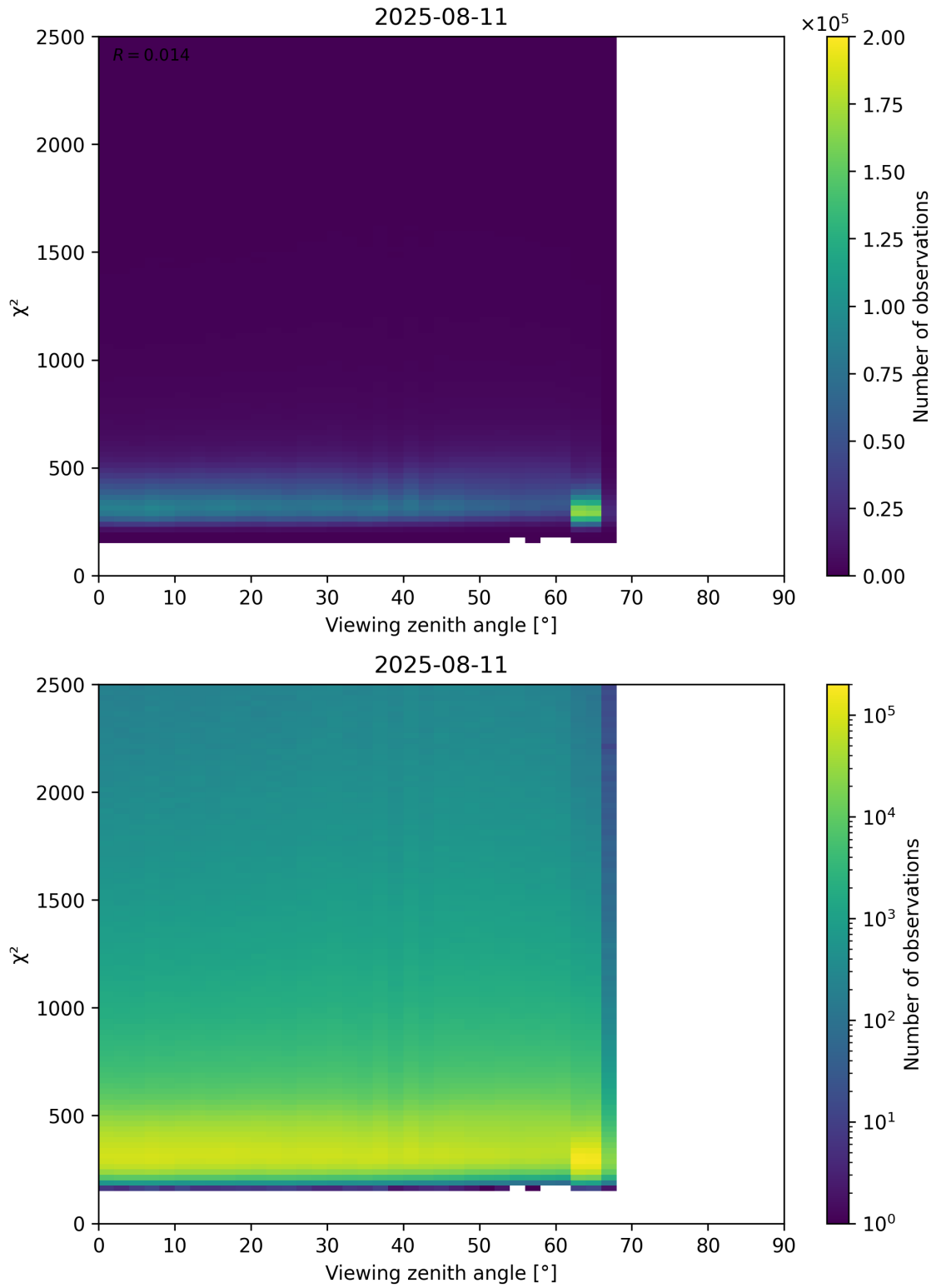
Figure 162: Scatter density plot of “Viewing zenith angle” against “ \chi^2 ” for 2025-08-10 to 2025-08-12.
