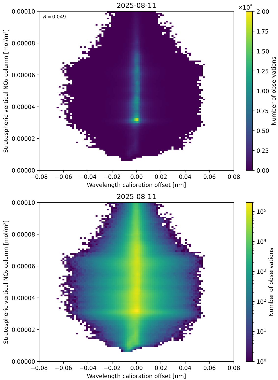
Figure 176: Scatter density plot of “Wavelength calibration offset” against “Stratospheric vertical NO 2 column” for 2025-08-10 to 2025-08-12.
