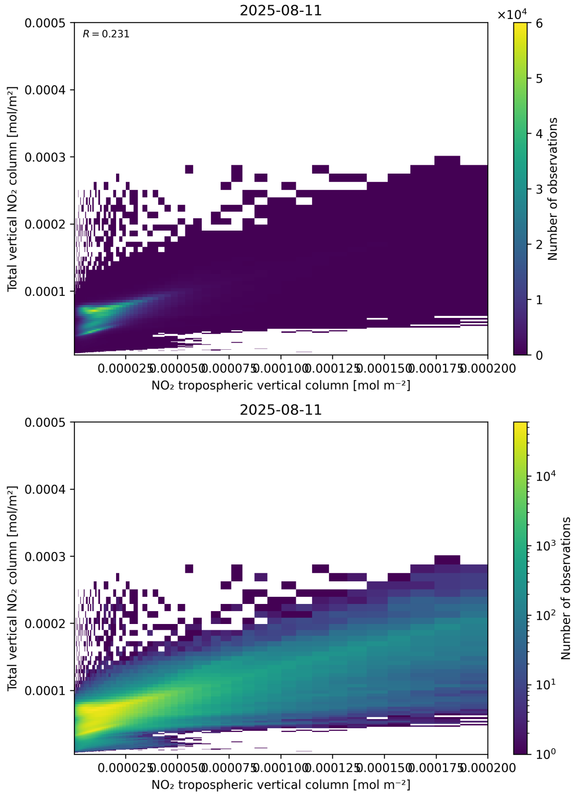
Figure 128: Scatter density plot of “NO 2 tropospheric vertical column” against “Total vertical NO 2 column” for 2025-08-10 to 2025-08-12.
