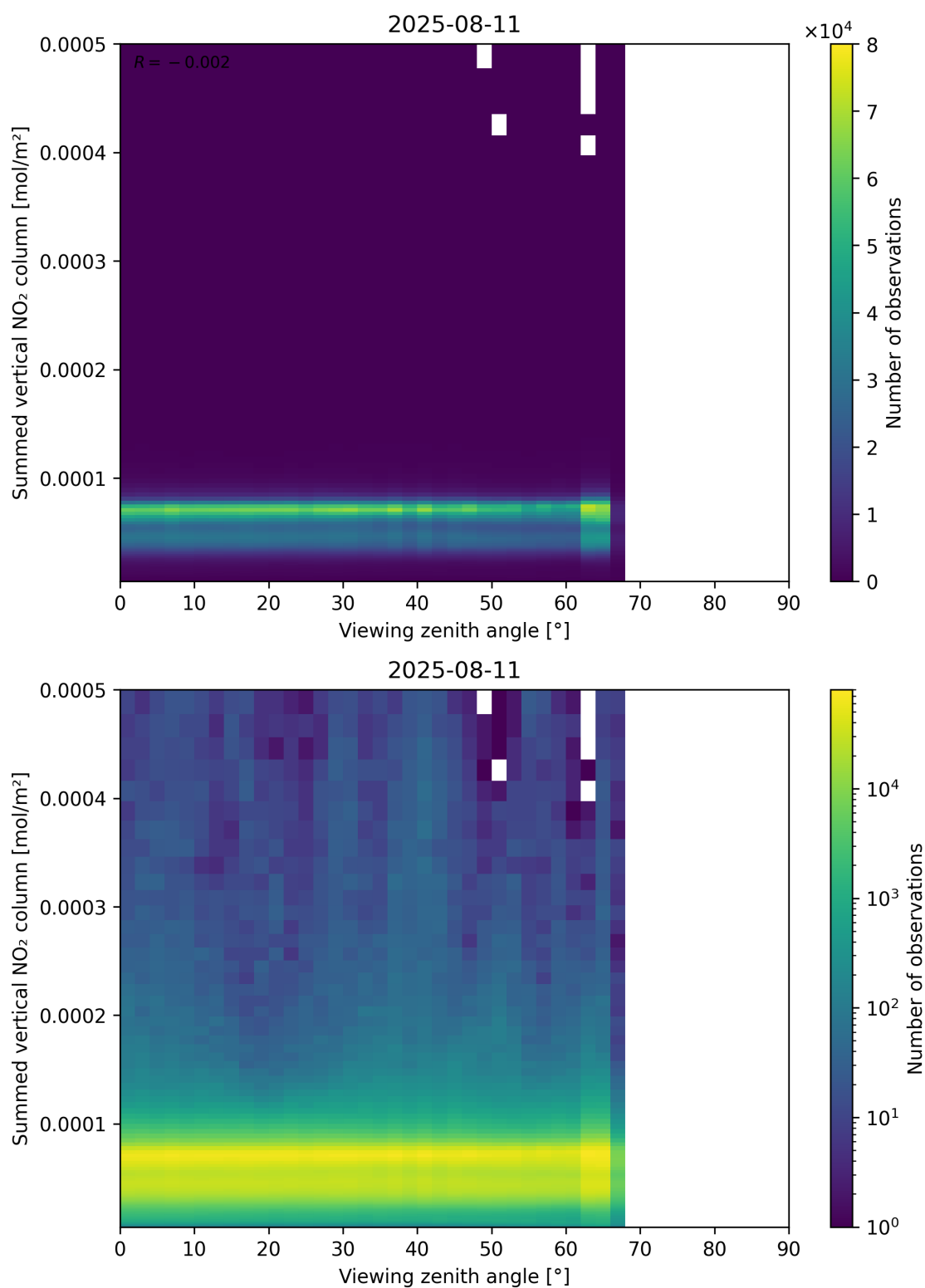
Figure 165: Scatter density plot of “Viewing zenith angle” against “Summed vertical NO 2 column” for 2025-08-10 to 2025-08-12.
