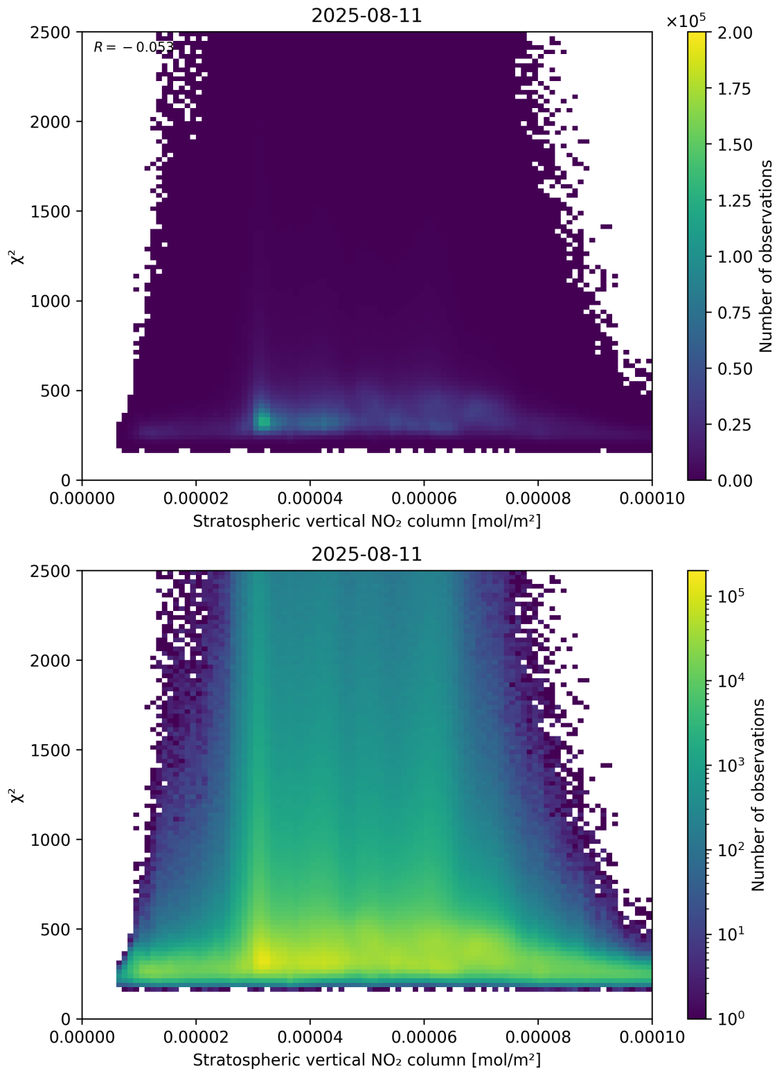
Figure 97: Scatter density plot of “Stratospheric vertical NO 2 column” against “ \chi^2 ” for 2025-08-10 to 2025-08-12.
