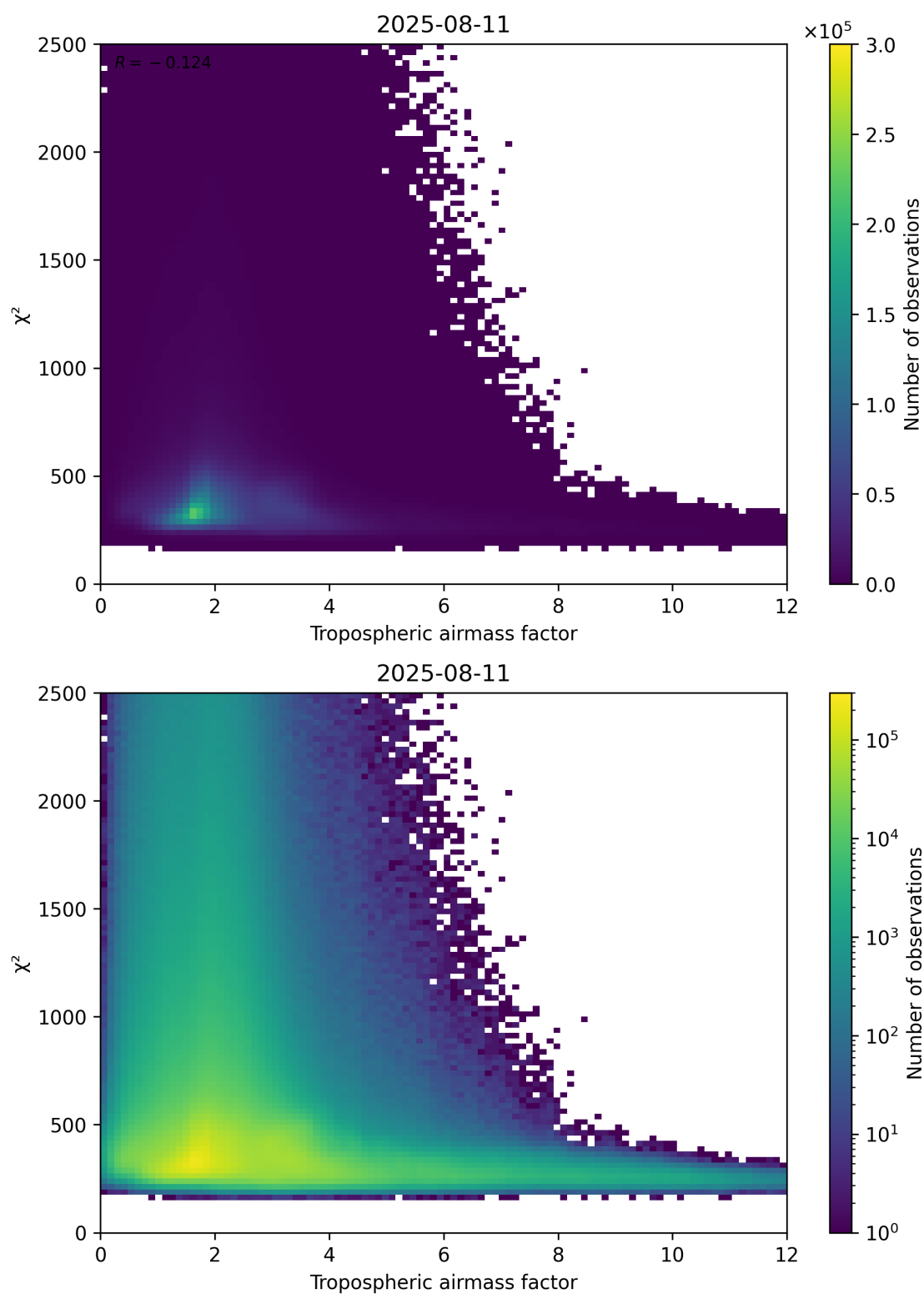
Figure 73: Scatter density plot of “Tropospheric airmass factor” against “ \chi^2 ” for 2025-08-10 to 2025-08-12.
