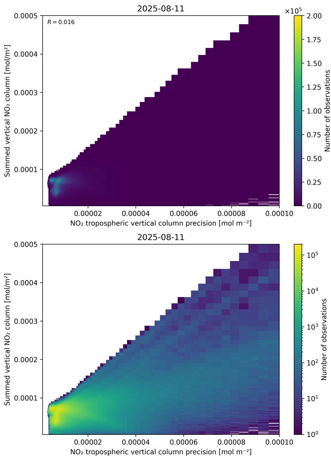
Figure 136: Scatter density plot of “NO 2 tropospheric vertical column precision” against “Summed vertical NO 2 column” for 2025-08-10 to 2025-08-12.
