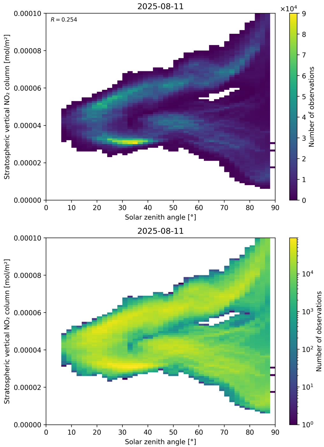
Figure 150: Scatter density plot of “Solar zenith angle” against “Stratospheric vertical NO 2 column” for 2025-08-10 to 2025-08-12.
