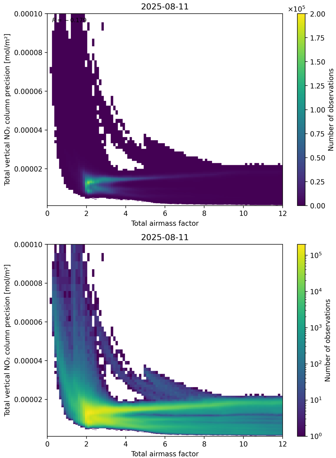
Figure 68: Scatter density plot of “Total airmass factor” against “Total vertical NO 2 column precision” for 2025-08-10 to 2025-08-12.
