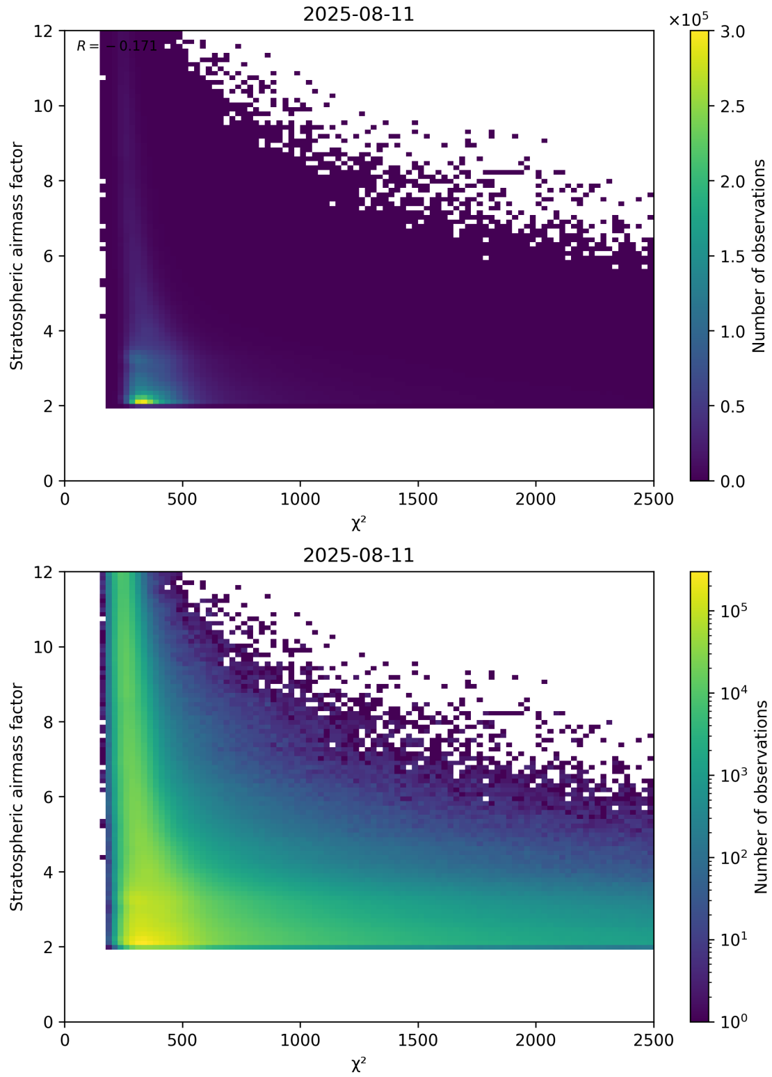
Figure 81: Scatter density plot of “ \chi^2 ” against “Stratospheric airmass factor” for 2025-08-10 to 2025-08-12.
