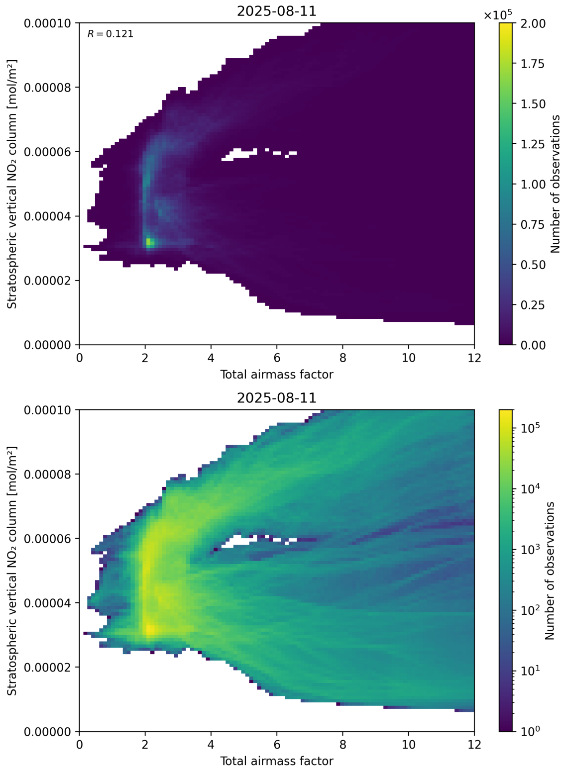
Figure 64: Scatter density plot of “Total airmass factor” against “Stratospheric vertical \text{NO}_2 column” for 2025-08-10 to 2025-08-12.
