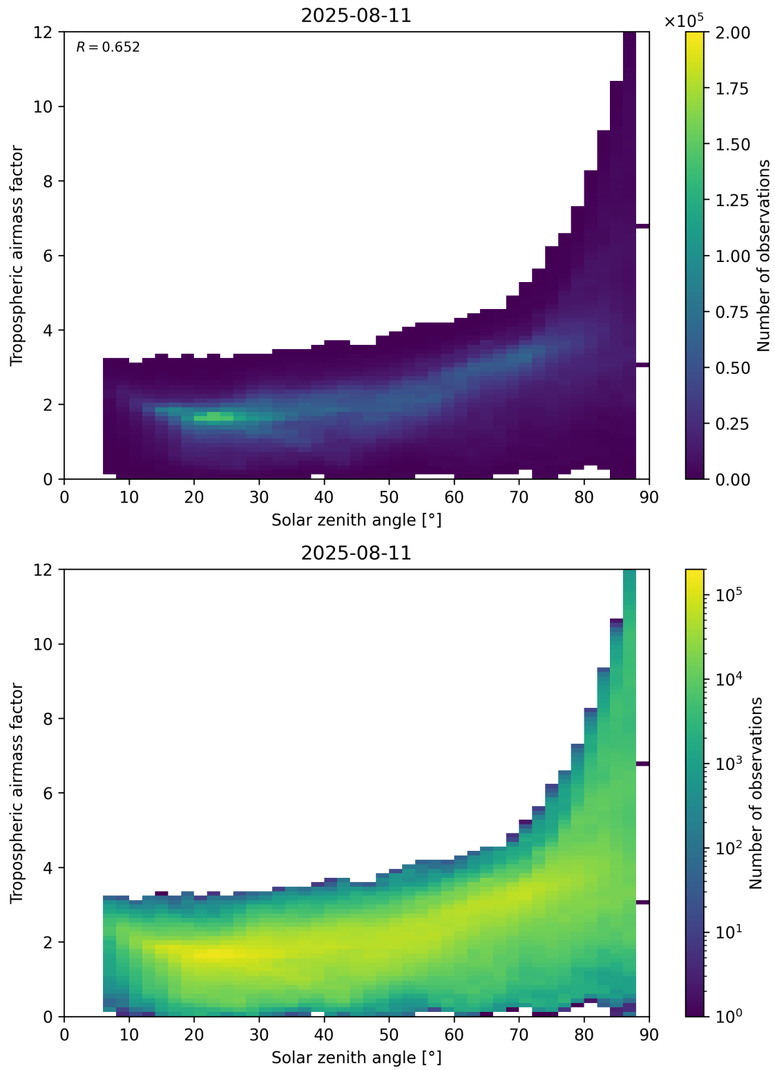
Figure 147: Scatter density plot of “Solar zenith angle” against “Tropospheric airmass factor” for 2025-08-10 to 2025-08-12.
