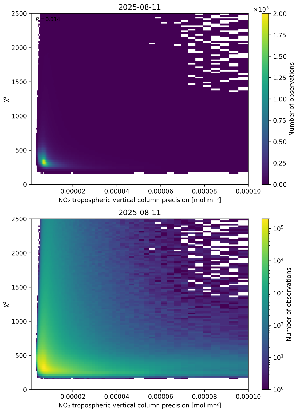
Figure 134: Scatter density plot of “NO 2 tropospheric vertical column precision” against “ \chi^2 ” for 2025-08-10 to 2025-08-12.
