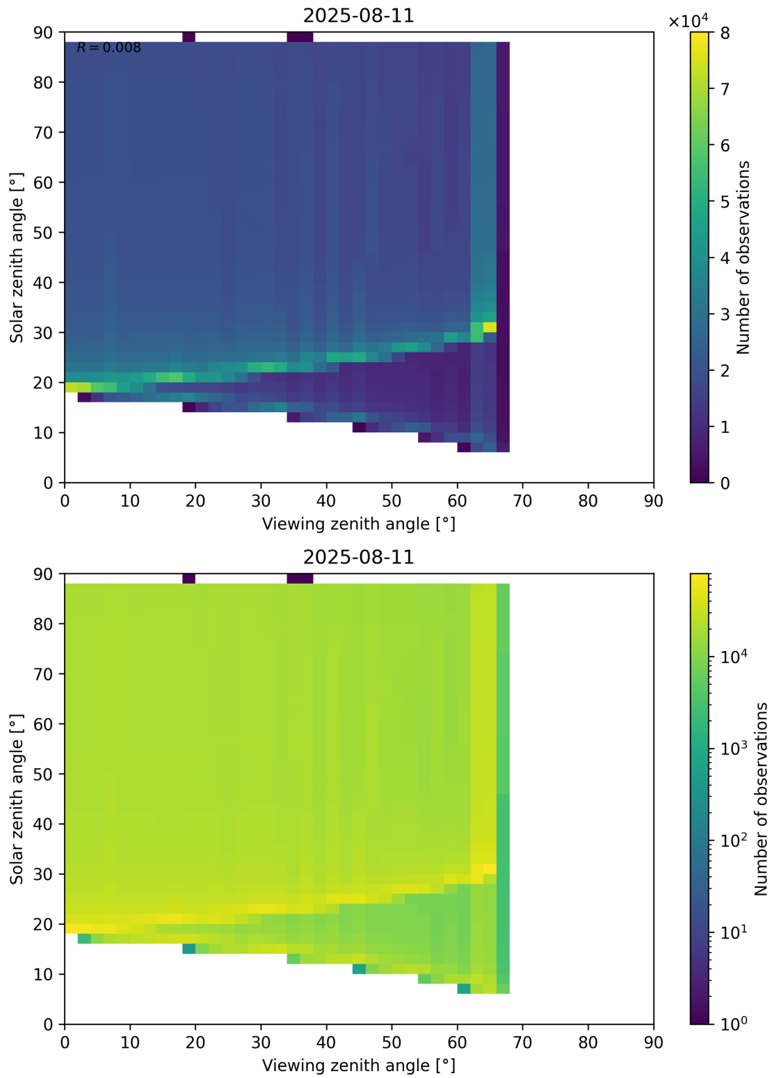
Figure 172: Scatter density plot of “Viewing zenith angle” against “Solar zenith angle” for 2025-08-10 to 2025-08-12.
