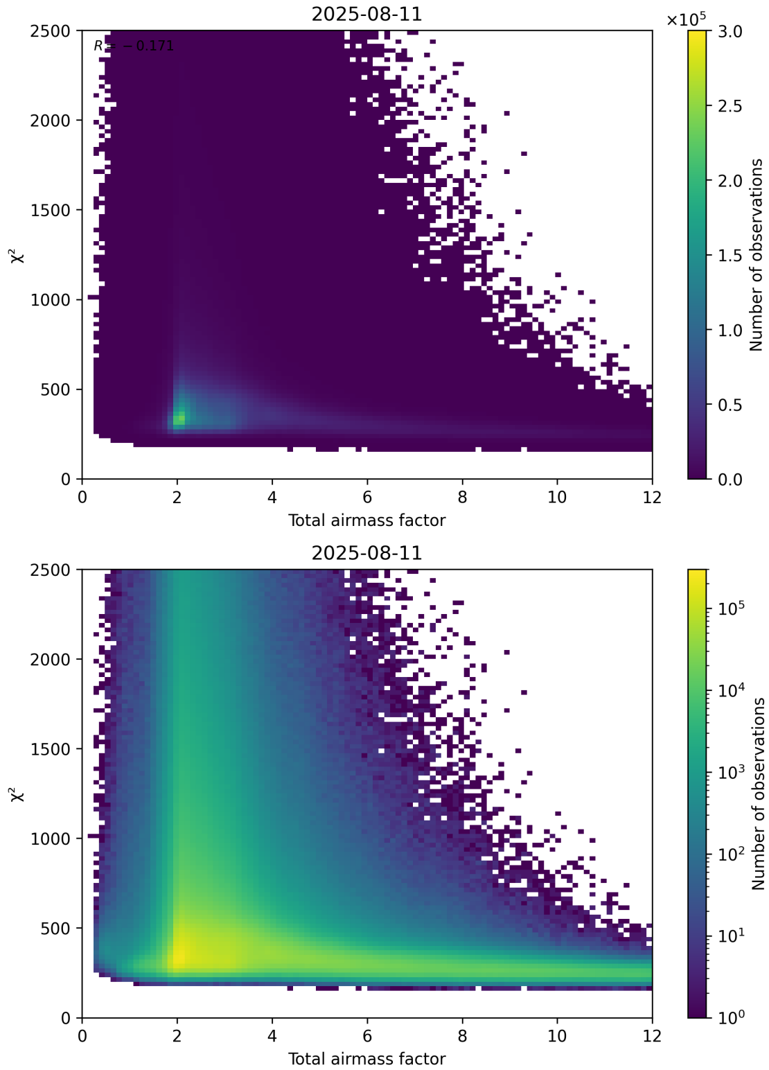
Figure 63: Scatter density plot of “Total airmass factor” against “ \chi^2 ” for 2025-08-10 to 2025-08-12.
