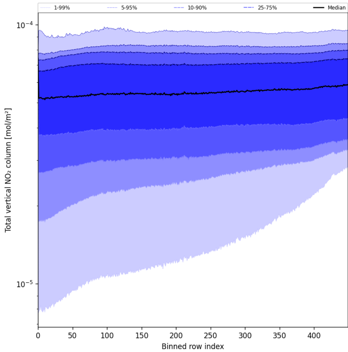
Figure 55: Along track statistics of “Total vertical NO 2 column” for 2025-08-10 to 2025-08-12
