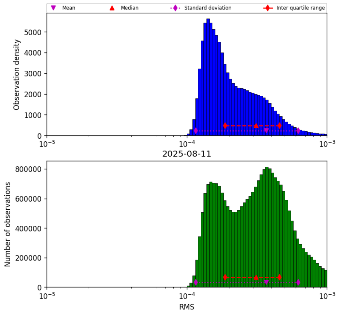
Figure 43: Histogram of “RMS” for 2025-08-10 to 2025-08-12
