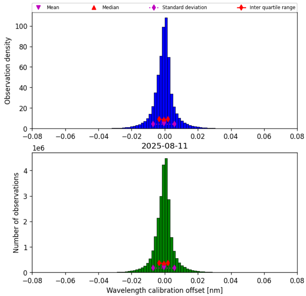
Figure 35: Histogram of “Wavelength calibration offset” for 2025-08-10 to 2025-08-12
