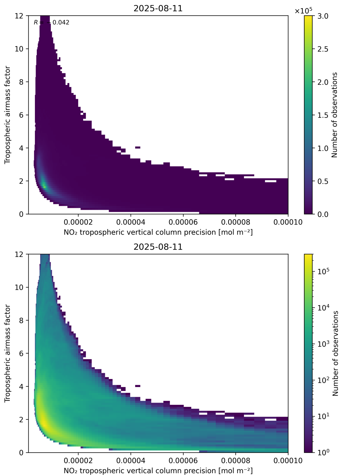
Figure 133: Scatter density plot of “NO 2 tropospheric vertical column precision” against “Tropospheric air mass factor” for 2025-08-10 to 2025-08-12.
