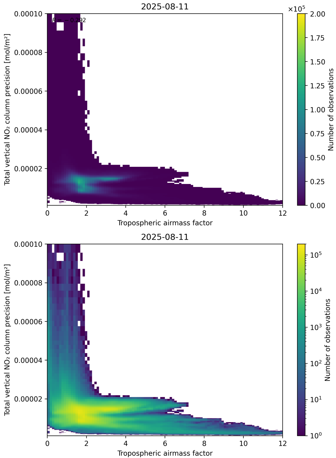
Figure 78: Scatter density plot of “Tropospheric air mass factor” against “Total vertical NO 2 column precision” for 2025-08-10 to 2025-08-12.
