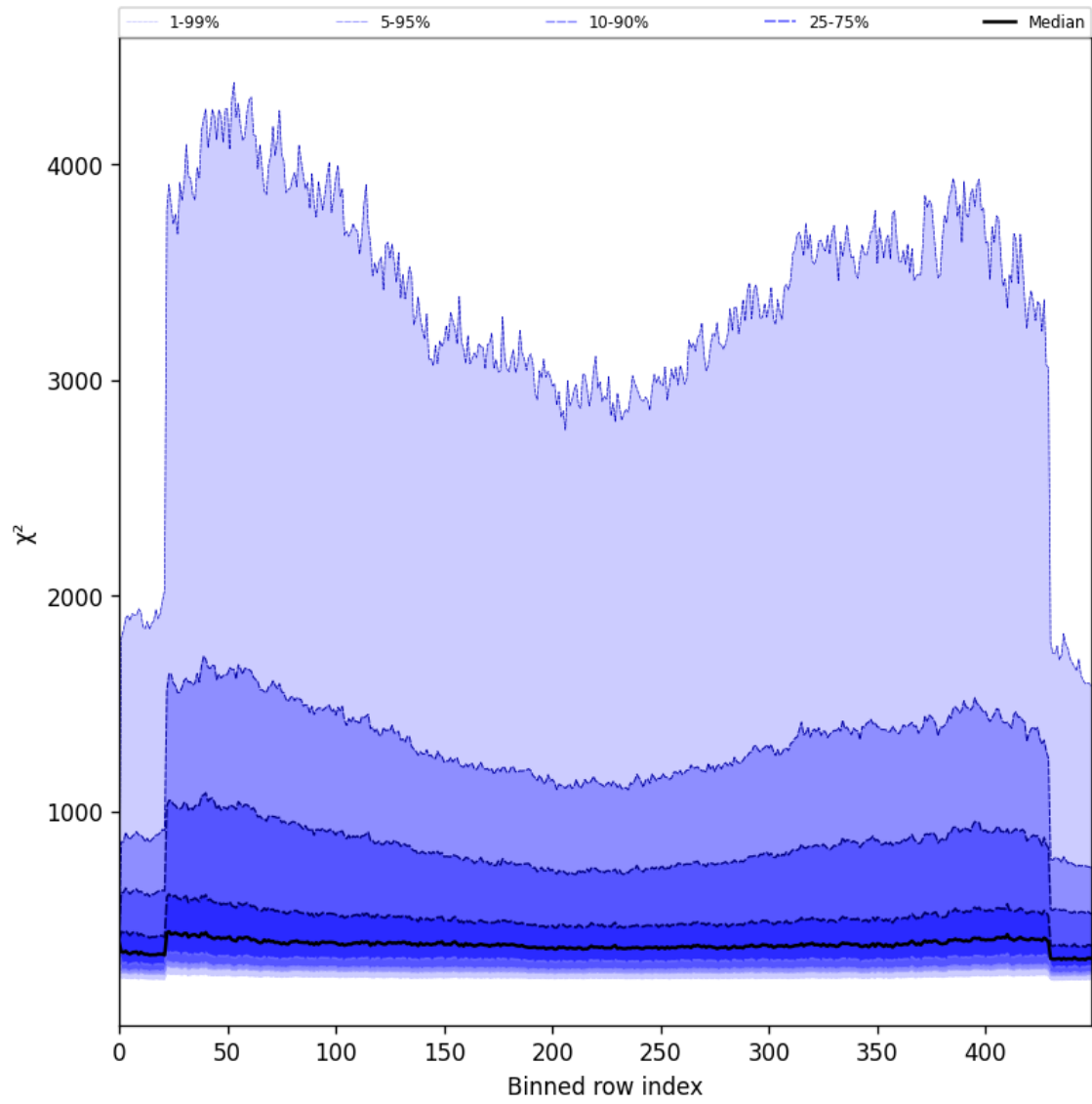
Figure 59: Along track statistics of “ \chi^2 ” for 2025-08-10 to 2025-08-12
