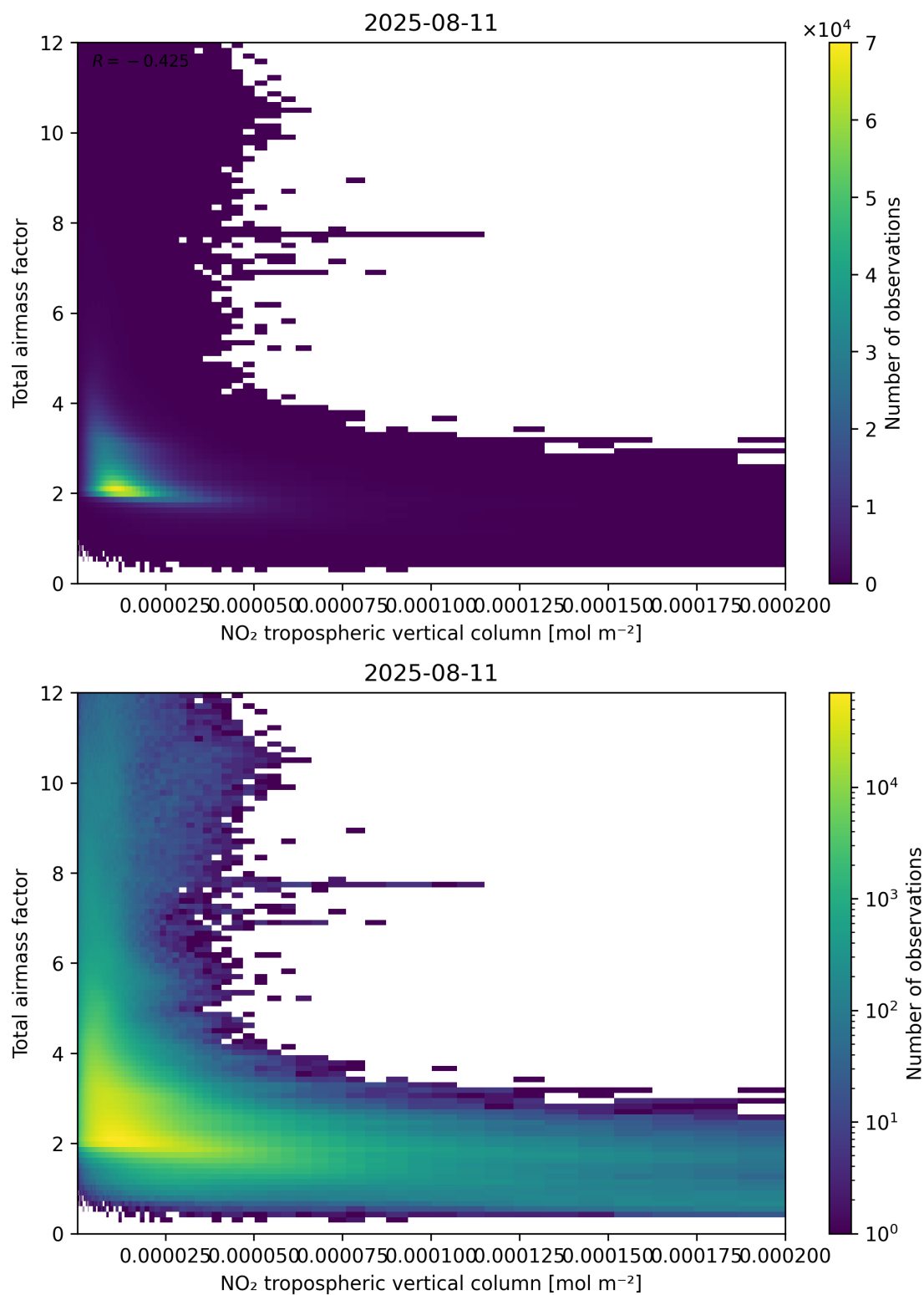
Figure 122: Scatter density plot of “NO 2 tropospheric vertical column” against “Total air mass factor” for 2025-08-10 to 2025-08-12.
