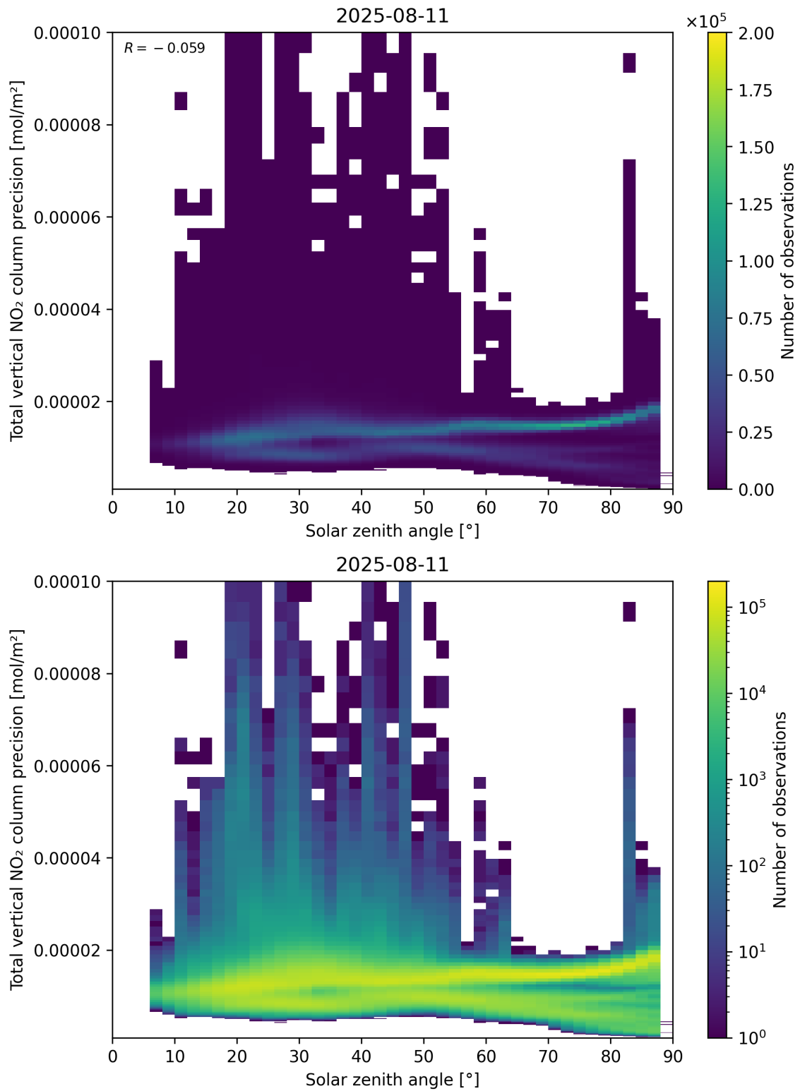
Figure 154: Scatter density plot of “Solar zenith angle” against “Total vertical NO 2 column precision” for 2025-08-10 to 2025-08-12.
