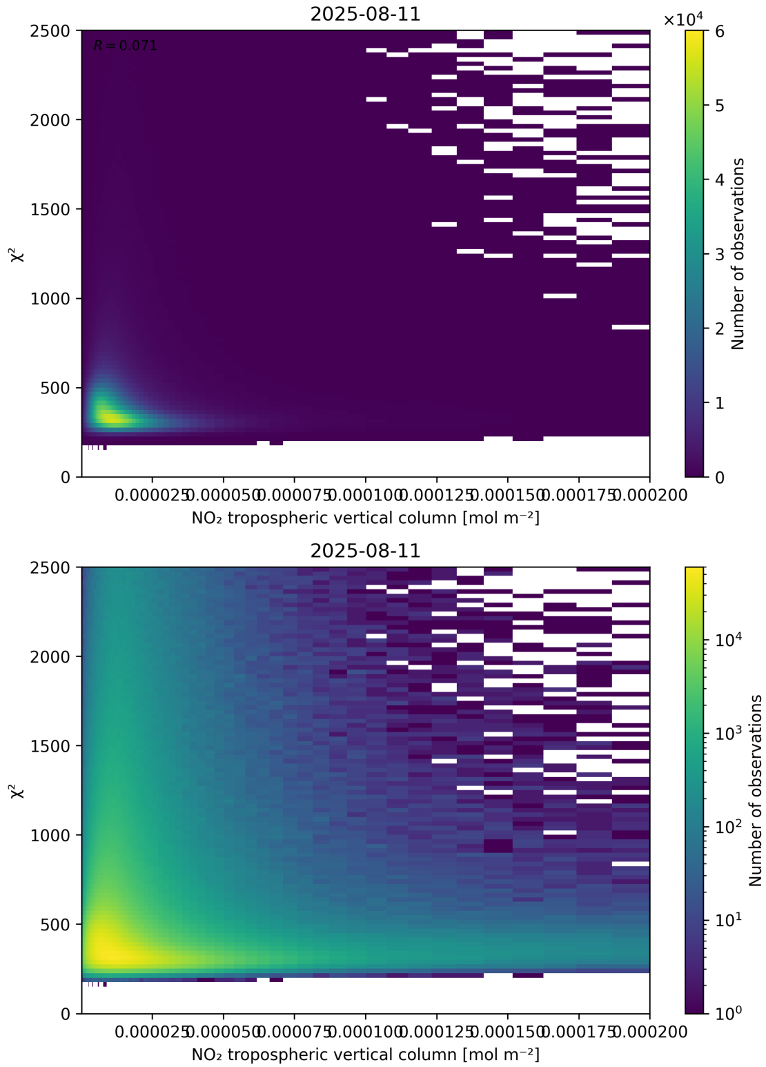
Figure 124: Scatter density plot of “NO 2 tropospheric vertical column” against “ \chi^2 ” for 2025-08-10 to 2025-08-12.
