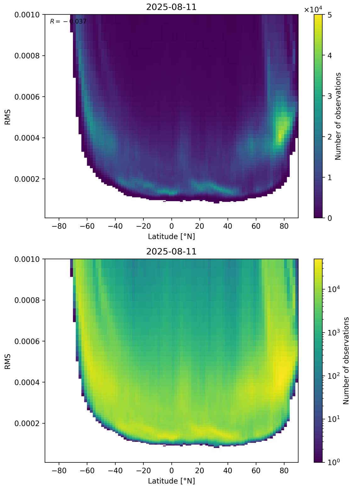
Figure 94: Scatter density plot of “Latitude” against “RMS” for 2025-08-10 to 2025-08-12.
