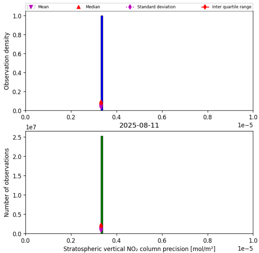
Figure 37: Histogram of “Stratospheric vertical NO 2 column precision” for 2025-08-10 to 2025-08-12
