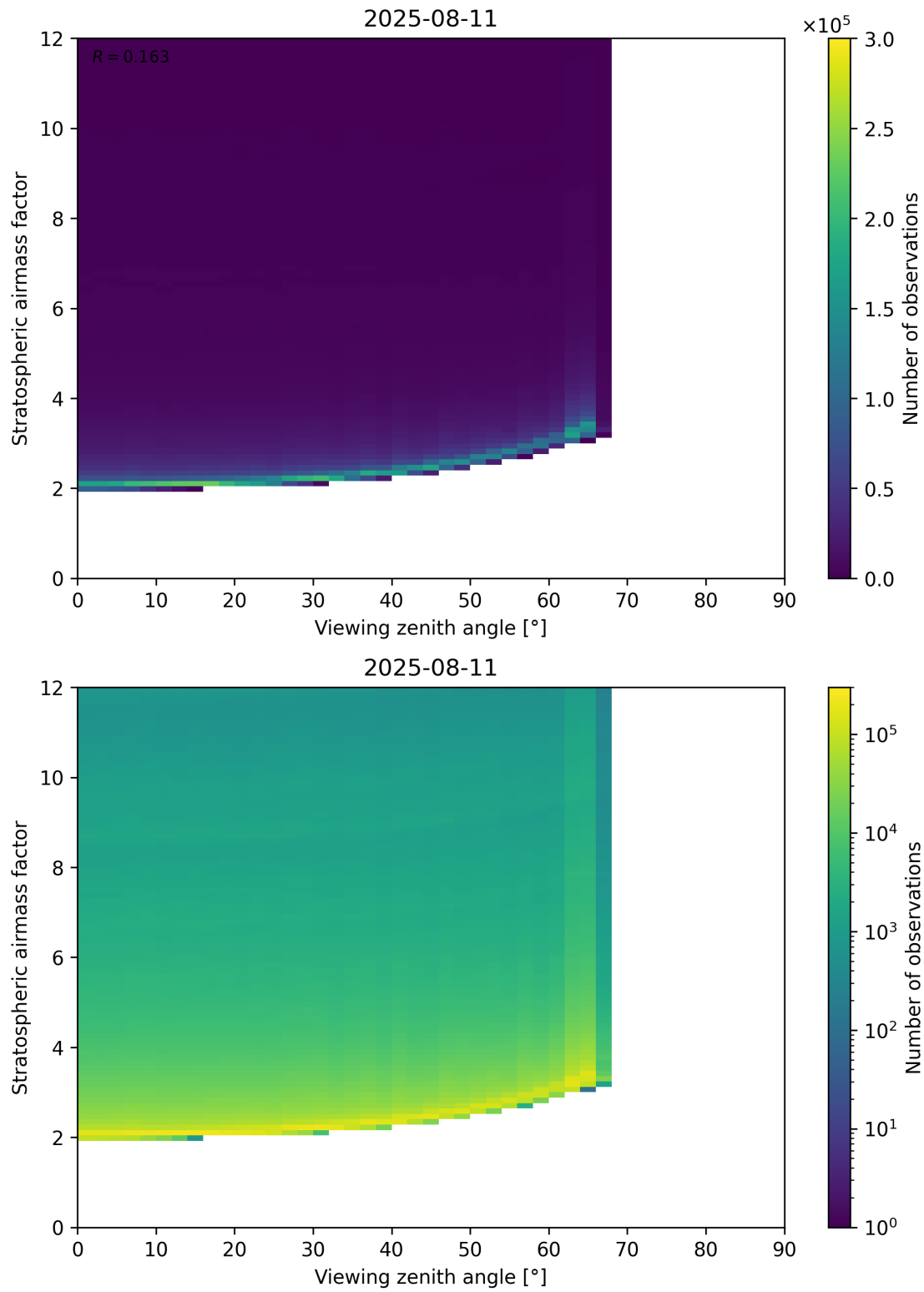
Figure 159: Scatter density plot of “Viewing zenith angle” against “Stratospheric airmass factor” for 2025-08-10 to 2025-08-12.
