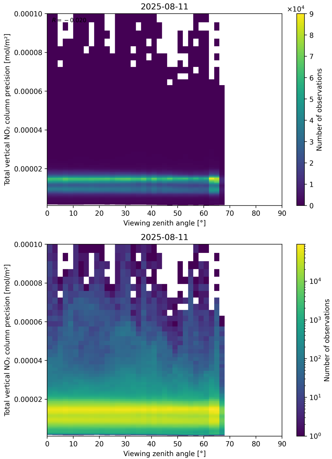
Figure 168: Scatter density plot of “Viewing zenith angle” against “Total vertical NO 2 column precision” for 2025-08-10 to 2025-08-12.
