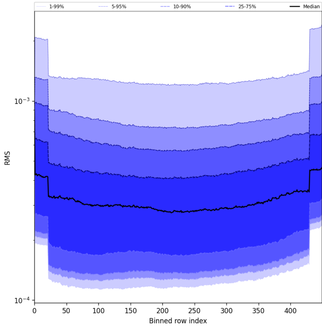
Figure 60: Along track statistics of “RMS” for 2025-08-10 to 2025-08-12
