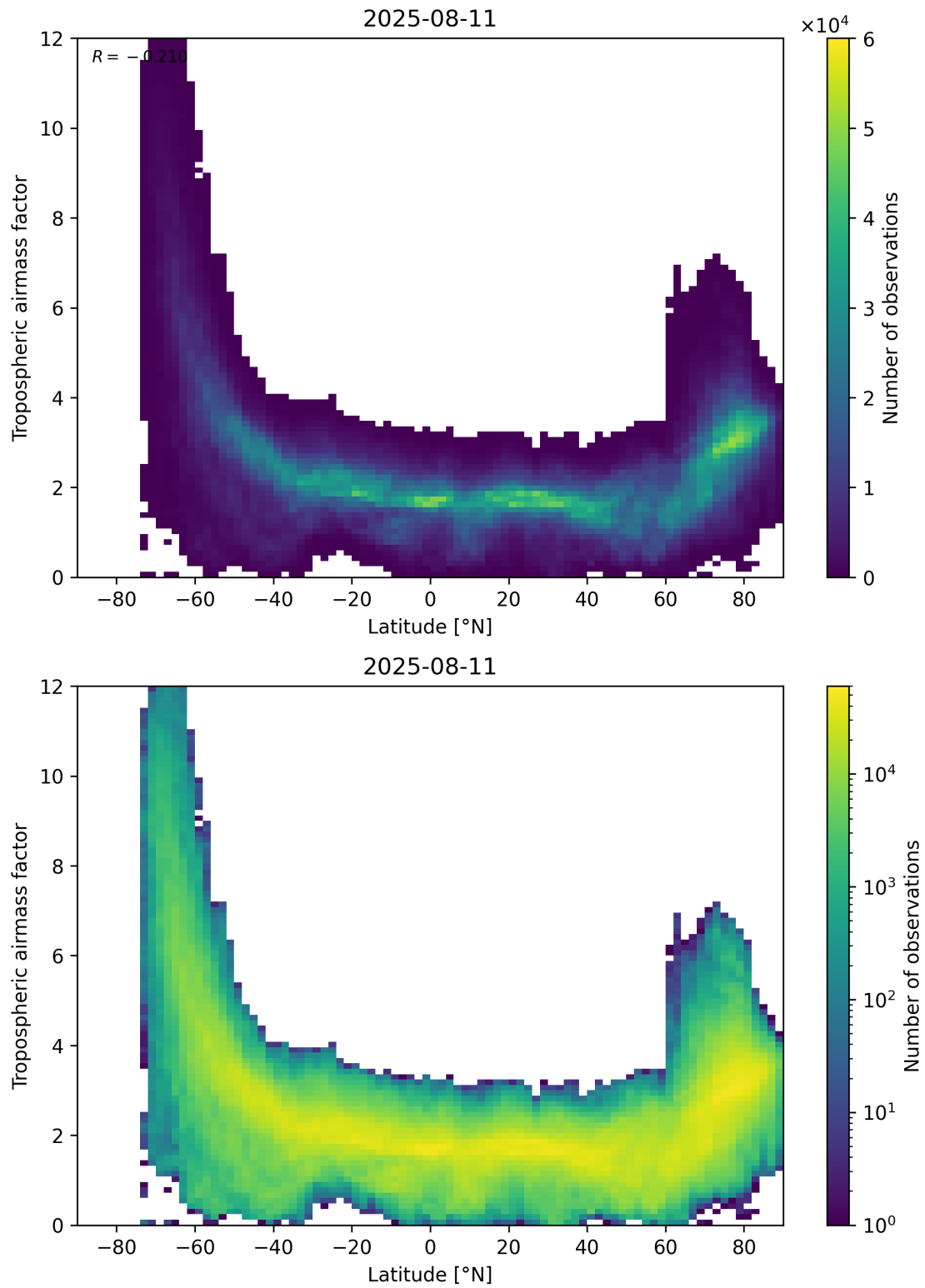
Figure 85: Scatter density plot of “Latitude” against “Tropospheric air mass factor” for 2025-08-10 to 2025-08-12.
