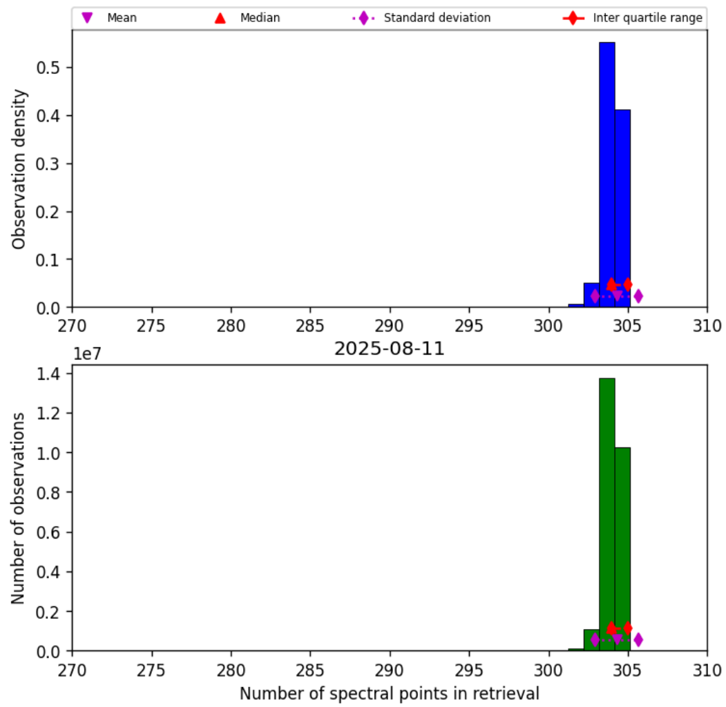
Figure 33: Histogram of “Number of spectral points in retrieval” for 2025-08-10 to 2025-08-12
