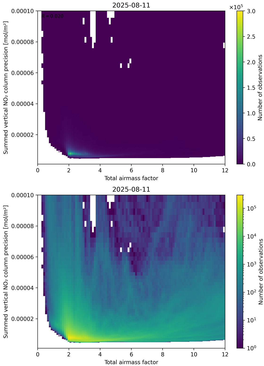
Figure 66: Scatter density plot of “Total airmass factor” against “Summed vertical NO 2 column precision” for 2025-08-10 to 2025-08-12.
