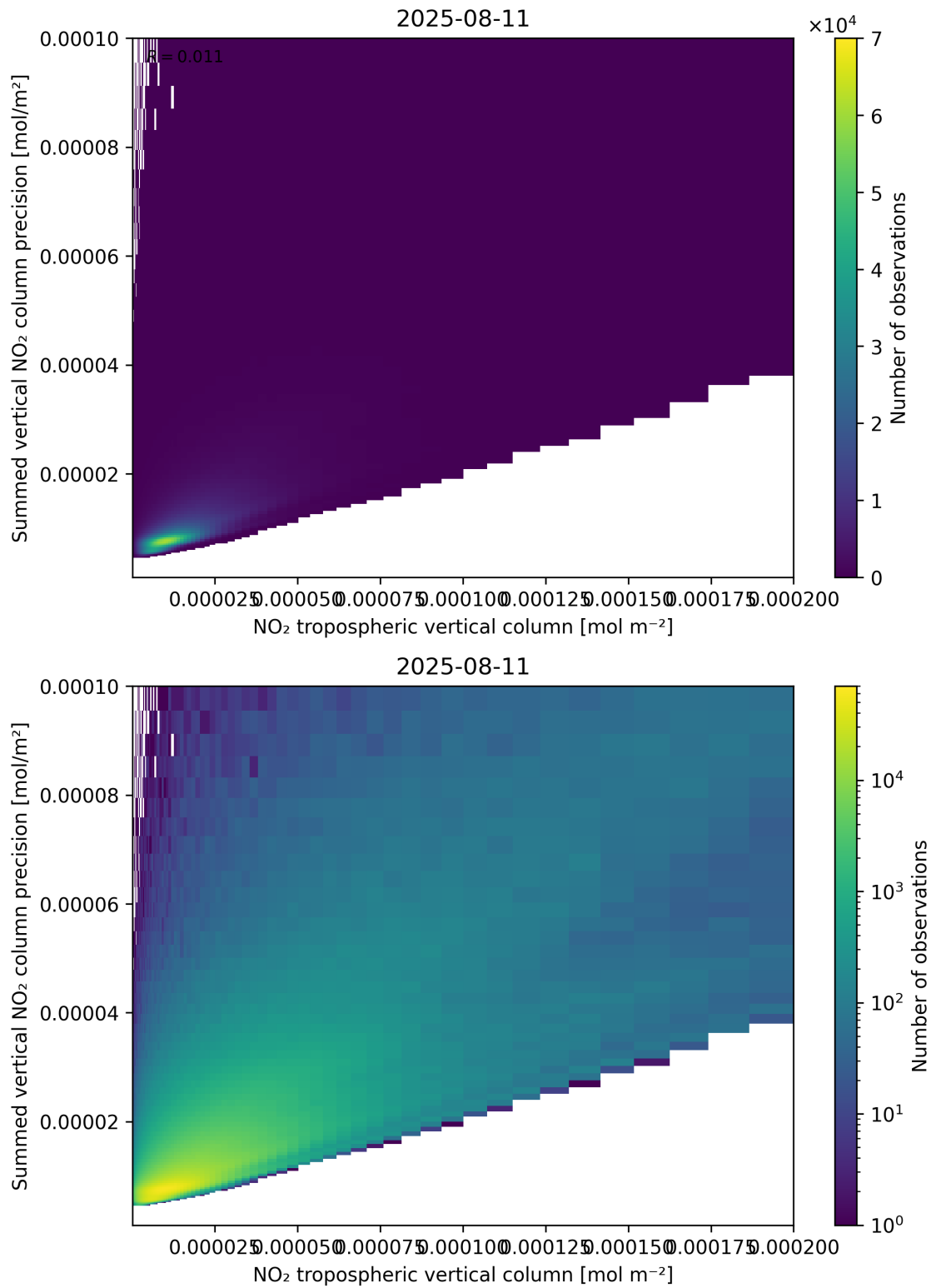
Figure 127: Scatter density plot of “NO 2 tropospheric vertical column” against “Summed vertical NO 2 column precision” for 2025-08-10 to 2025-08-12.
