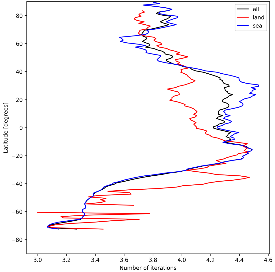
Figure 17: Zonal average of “Number of iterations” for 2025-08-10 to 2025-08-12.
