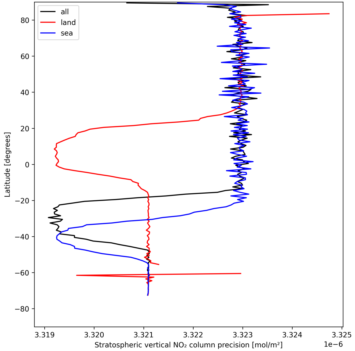
Figure 20: Zonal average of “Stratospheric vertical NO 2 column precision” for 2025-08-10 to 2025-08-12.
