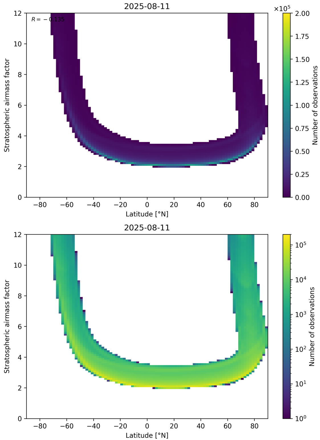
Figure 83: Scatter density plot of “Latitude” against “Stratospheric air mass factor” for 2025-08-10 to 2025-08-12.
