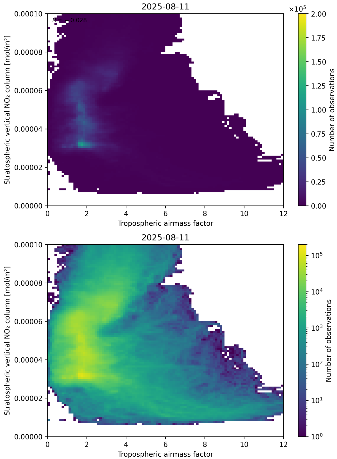
Figure 74: Scatter density plot of “Tropospheric airmass factor” against “Stratospheric vertical NO 2 column” for 2025-08-10 to 2025-08-12.
