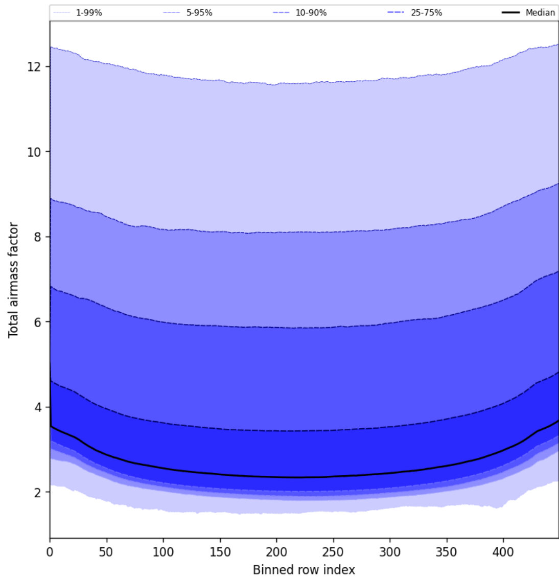
Figure 49: Along track statistics of “Total airmass factor” for 2025-08-10 to 2025-08-12
