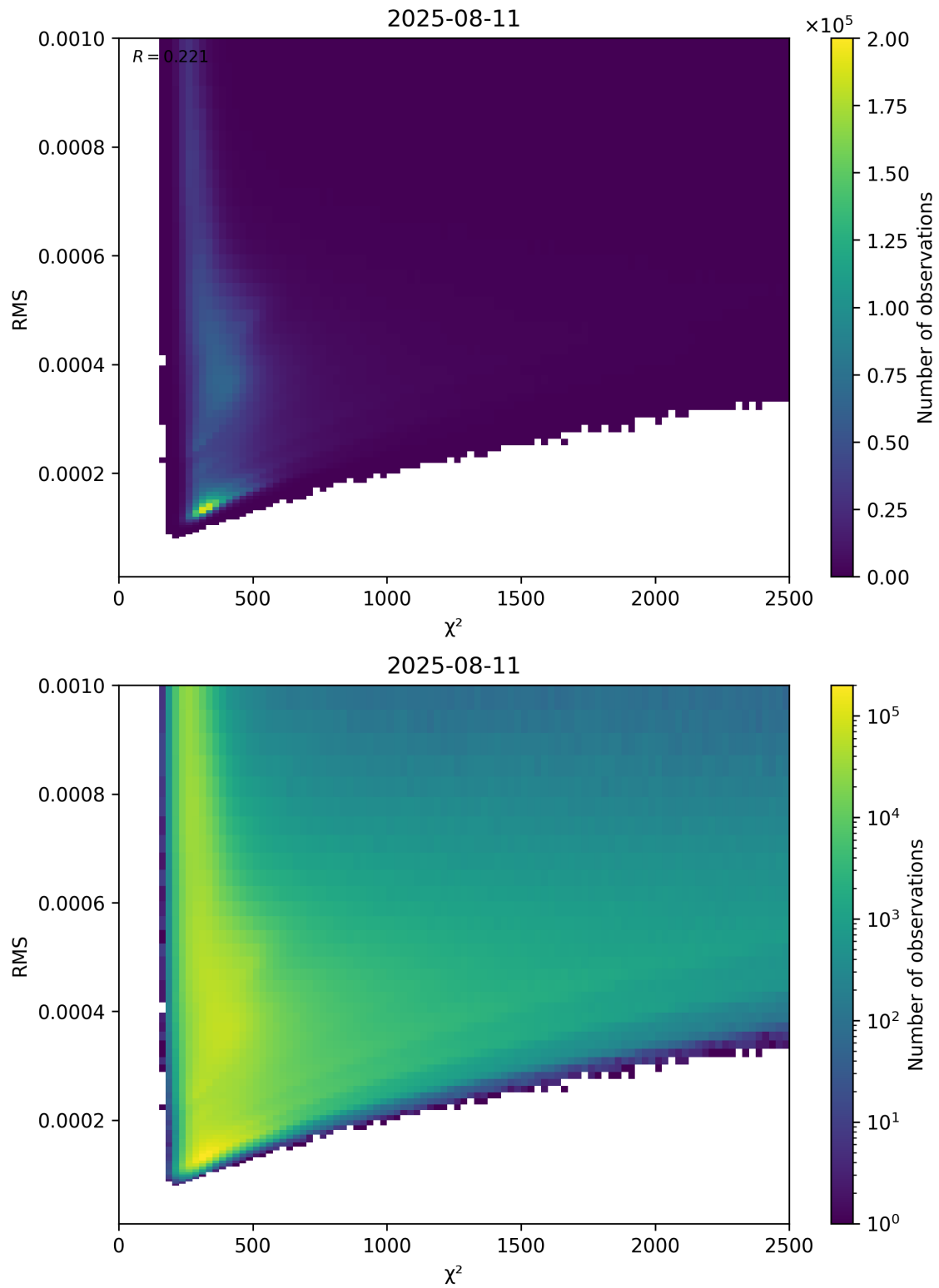
Figure 82: Scatter density plot of “ \chi^2 ” against “RMS” for 2025-08-10 to 2025-08-12.
