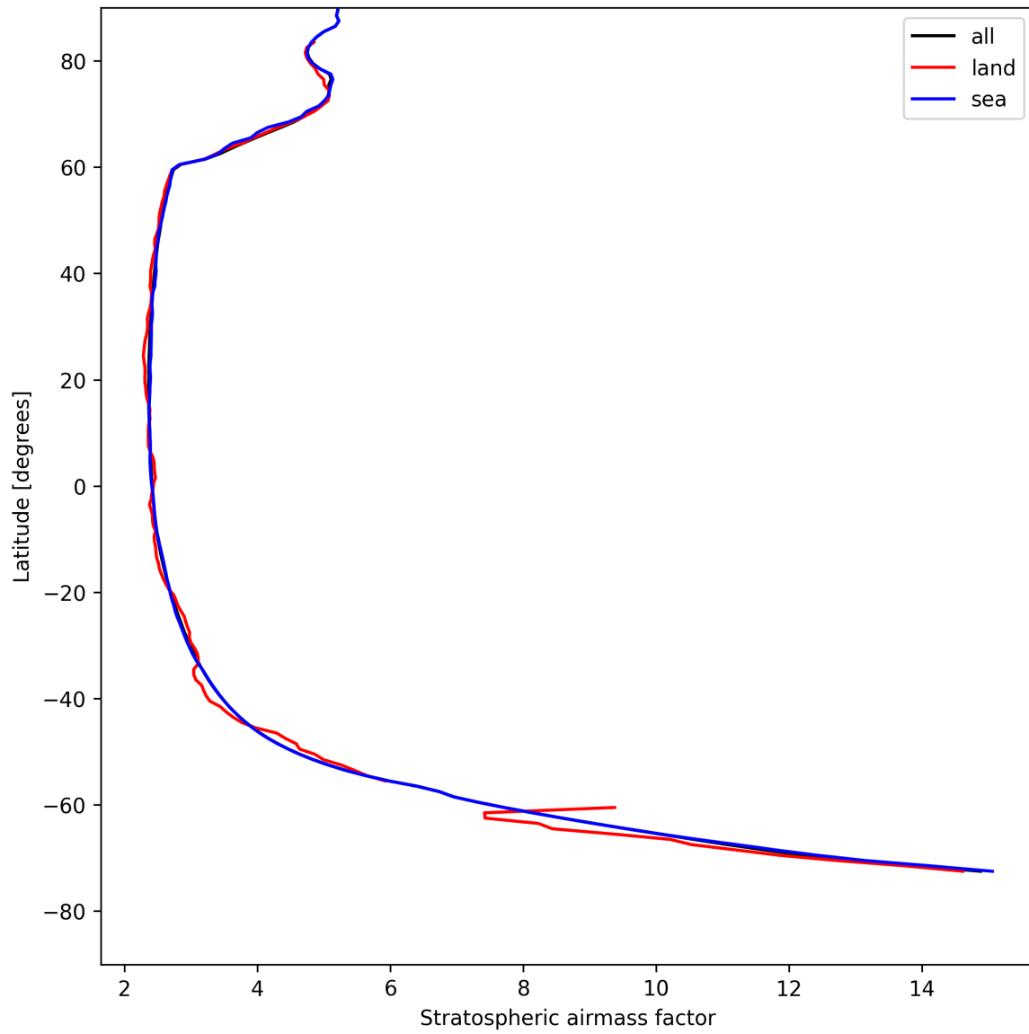
Figure 27: Zonal average of “Stratospheric air mass factor” for 2025-08-10 to 2025-08-12.
