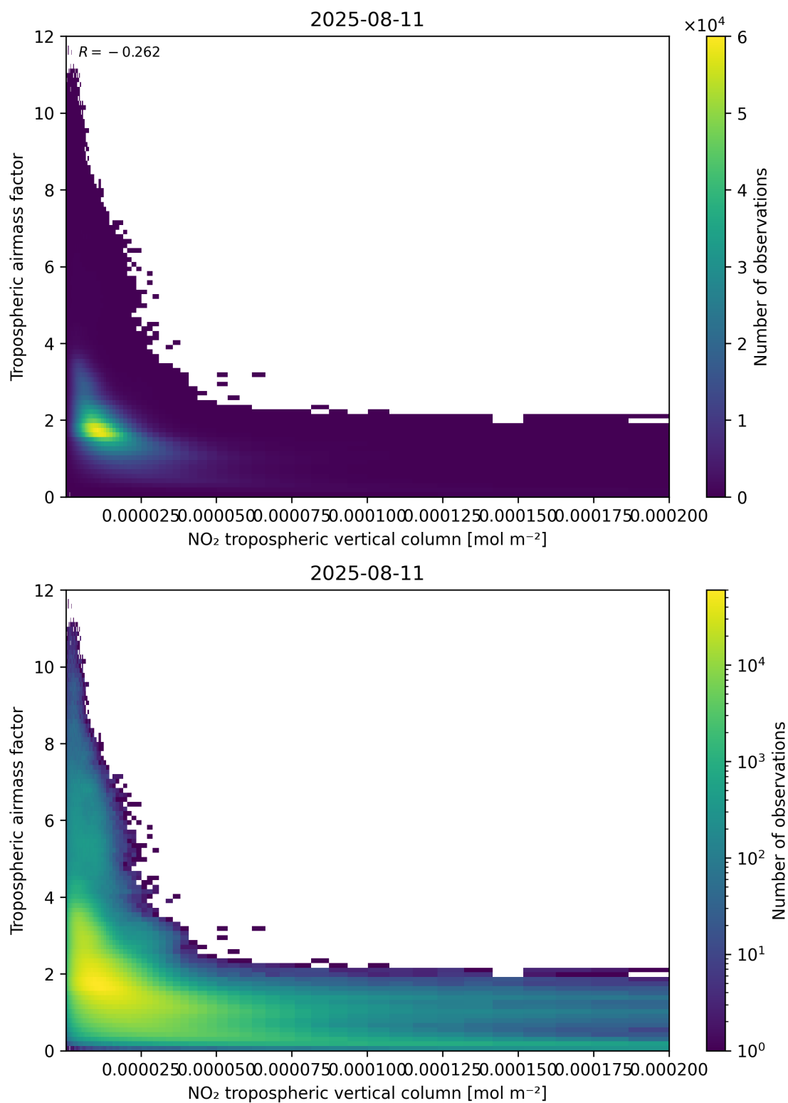
Figure 123: Scatter density plot of “NO 2 tropospheric vertical column” against “Tropospheric air mass factor” for 2025-08-10 to 2025-08-12.
