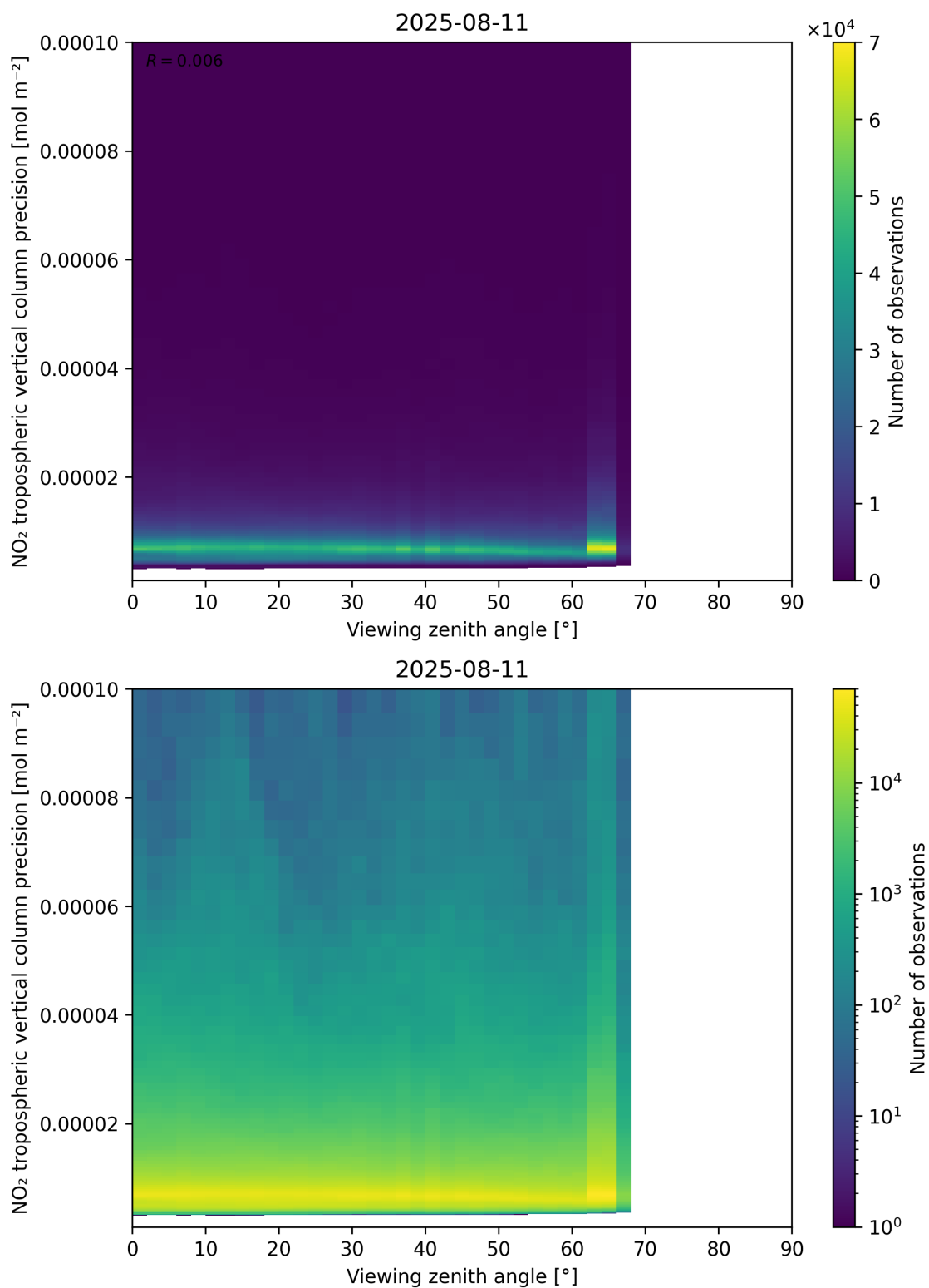
Figure 170: Scatter density plot of “Viewing zenith angle” against “NO 2 tropospheric vertical column precision” for 2025-08-10 to 2025-08-12.
