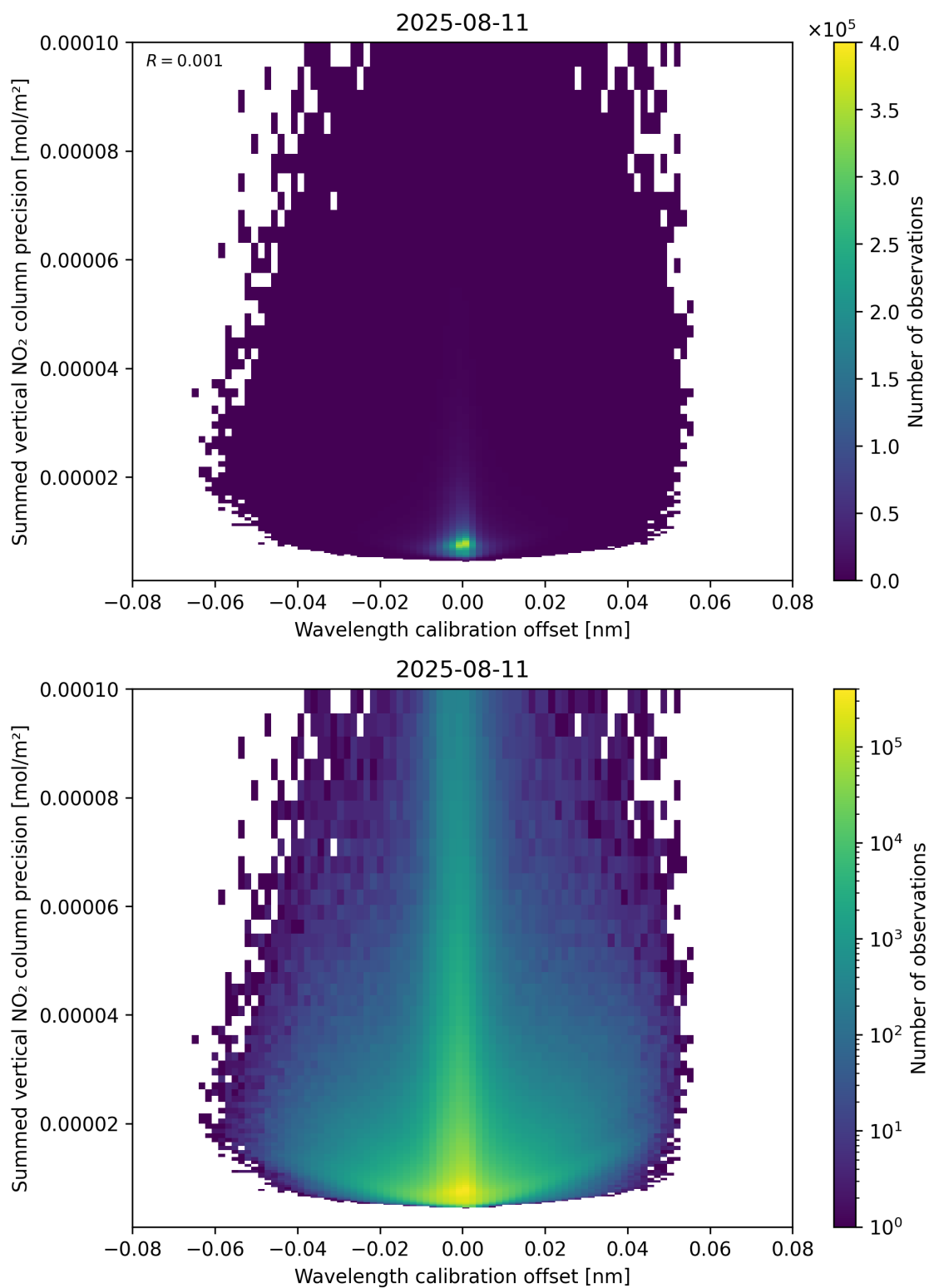
Figure 178: Scatter density plot of “Wavelength calibration offset” against “Summed vertical NO 2 column precision” for 2025-08-10 to 2025-08-12.
