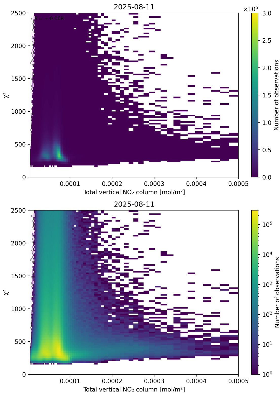
Figure 111: Scatter density plot of “Total vertical NO 2 column” against “ \chi^2 ” for 2025-08-10 to 2025-08-12.
