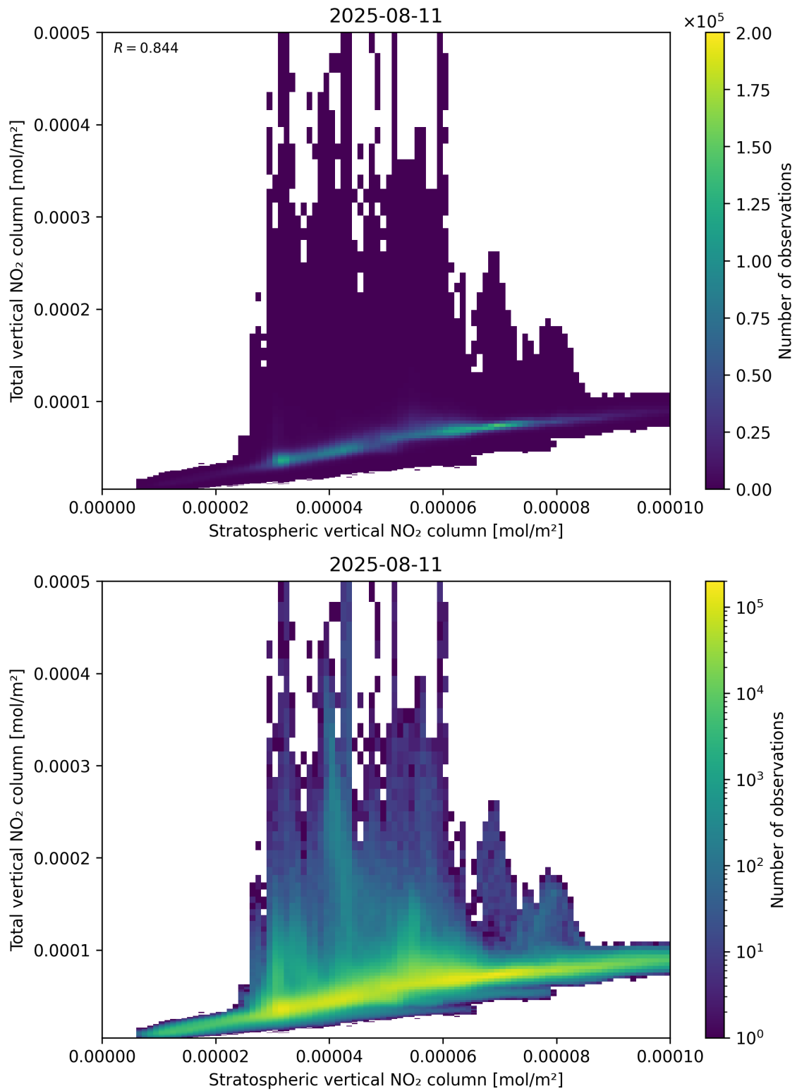
Figure 100: Scatter density plot of “Stratospheric vertical NO 2 column” against “Total vertical NO 2 column” for 2025-08-10 to 2025-08-12.
