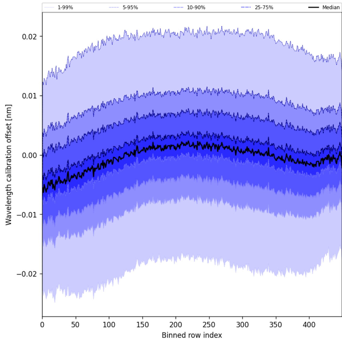
Figure 52: Along track statistics of “Wavelength calibration offset” for 2025-08-10 to 2025-08-12
