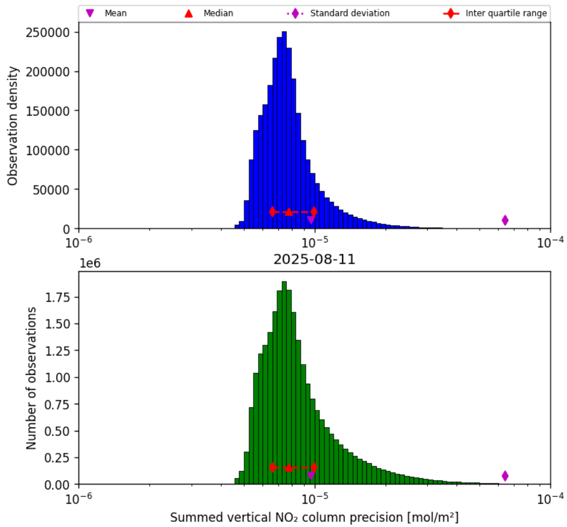
Figure 41: Histogram of “Summed vertical NO 2 column precision” for 2025-08-10 to 2025-08-12
