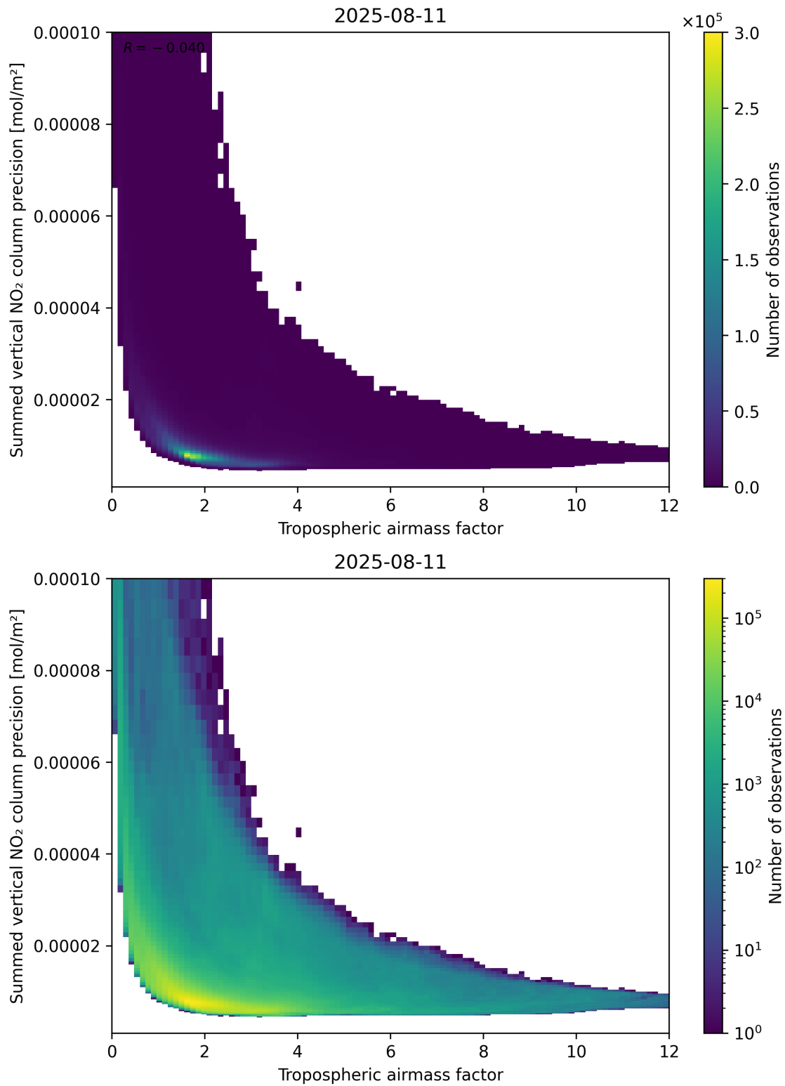
Figure 76: Scatter density plot of “Tropospheric air mass factor” against “Summed vertical NO 2 column precision” for 2025-08-10 to 2025-08-12.
