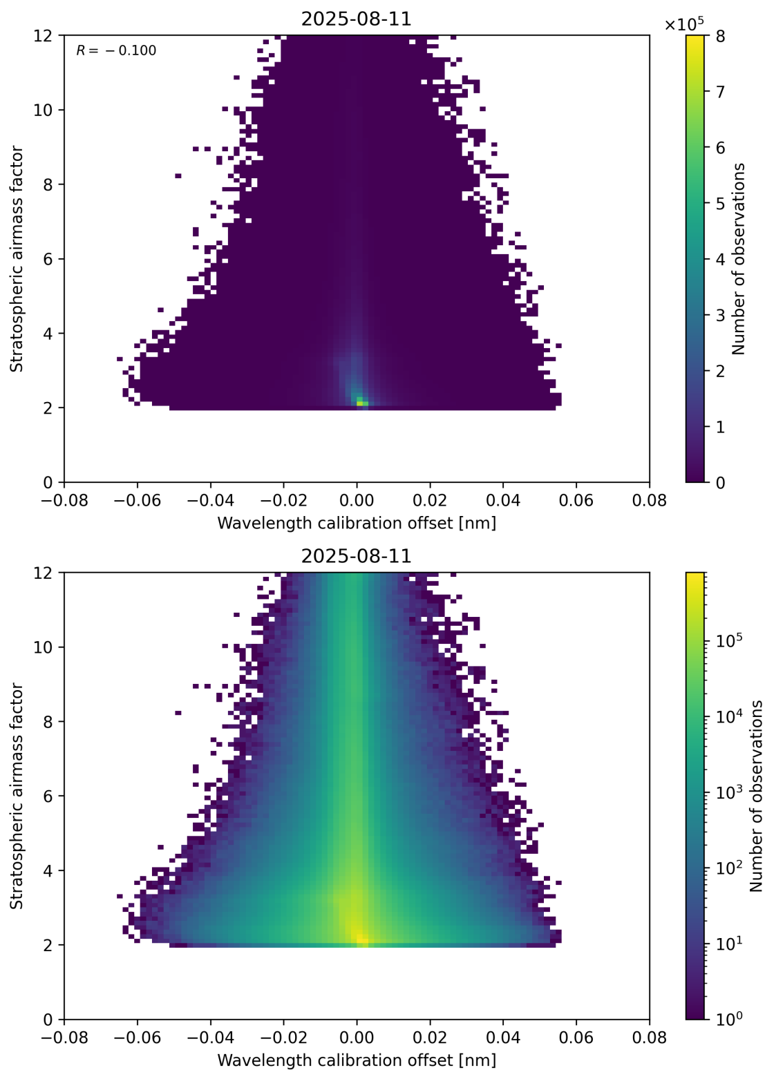
Figure 174: Scatter density plot of “Wavelength calibration offset” against “Stratospheric airmass factor” for 2025-08-10 to 2025-08-12.
