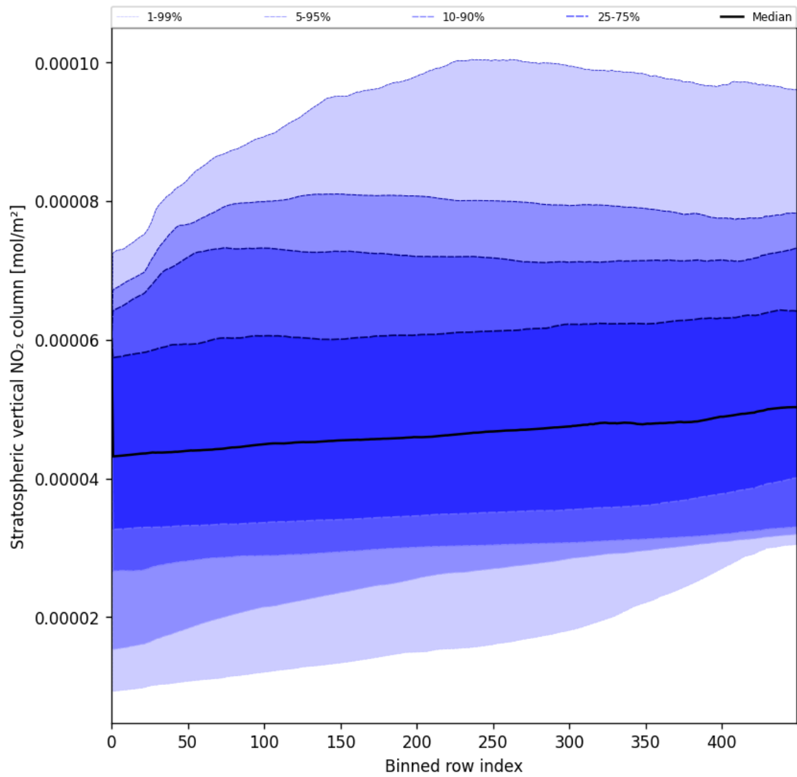
Figure 53: Along track statistics of “Stratospheric vertical NO 2 column” for 2025-08-10 to 2025-08-12
