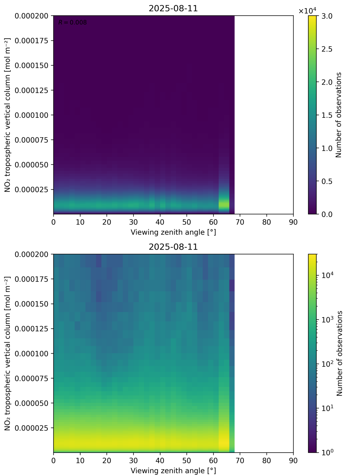
Figure 169: Scatter density plot of “Viewing zenith angle” against “NO 2 tropospheric vertical column” for 2025-08-10 to 2025-08-12.
