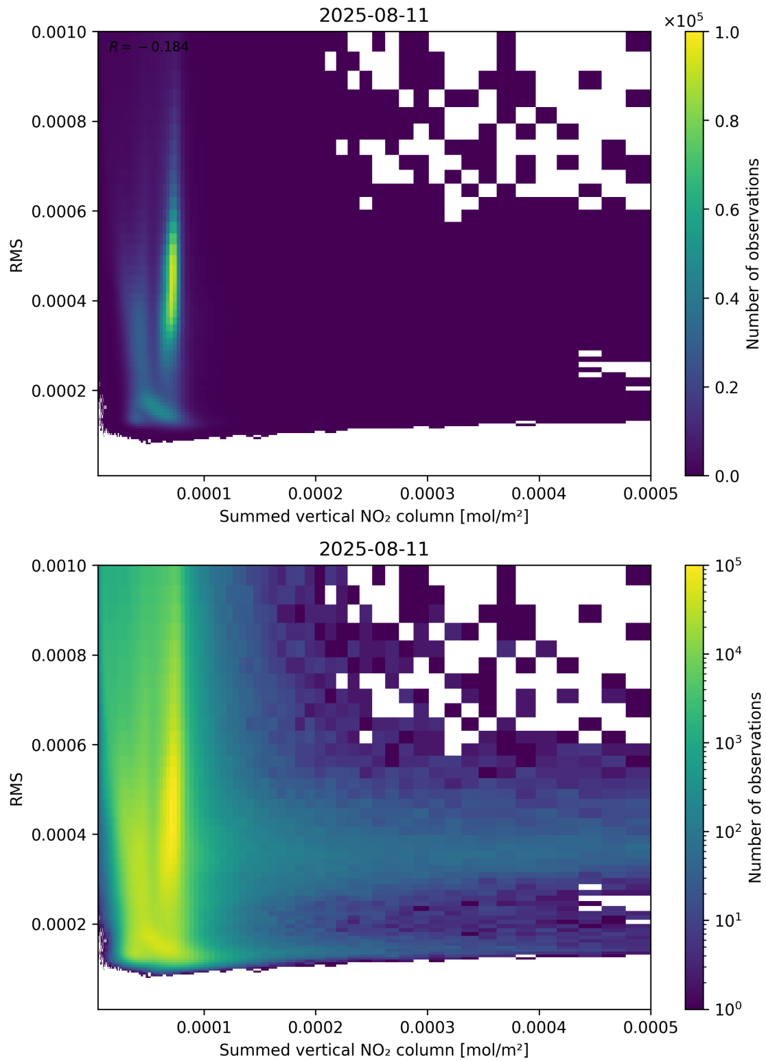
Figure 109: Scatter density plot of “Summed vertical NO 2 column” against “RMS” for 2025-08-10 to 2025-08-12.
