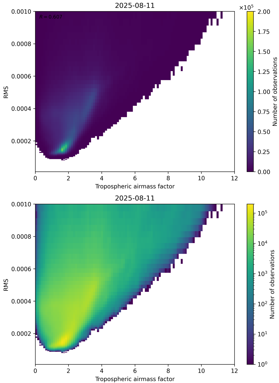
Figure 79: Scatter density plot of “Tropospheric airmass factor” against “RMS” for 2025-08-10 to 2025-08-12.
