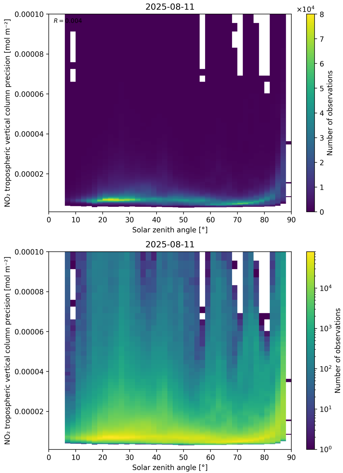
Figure 156: Scatter density plot of “Solar zenith angle” against “NO 2 tropospheric vertical column precision” for 2025-08-10 to 2025-08-12.
