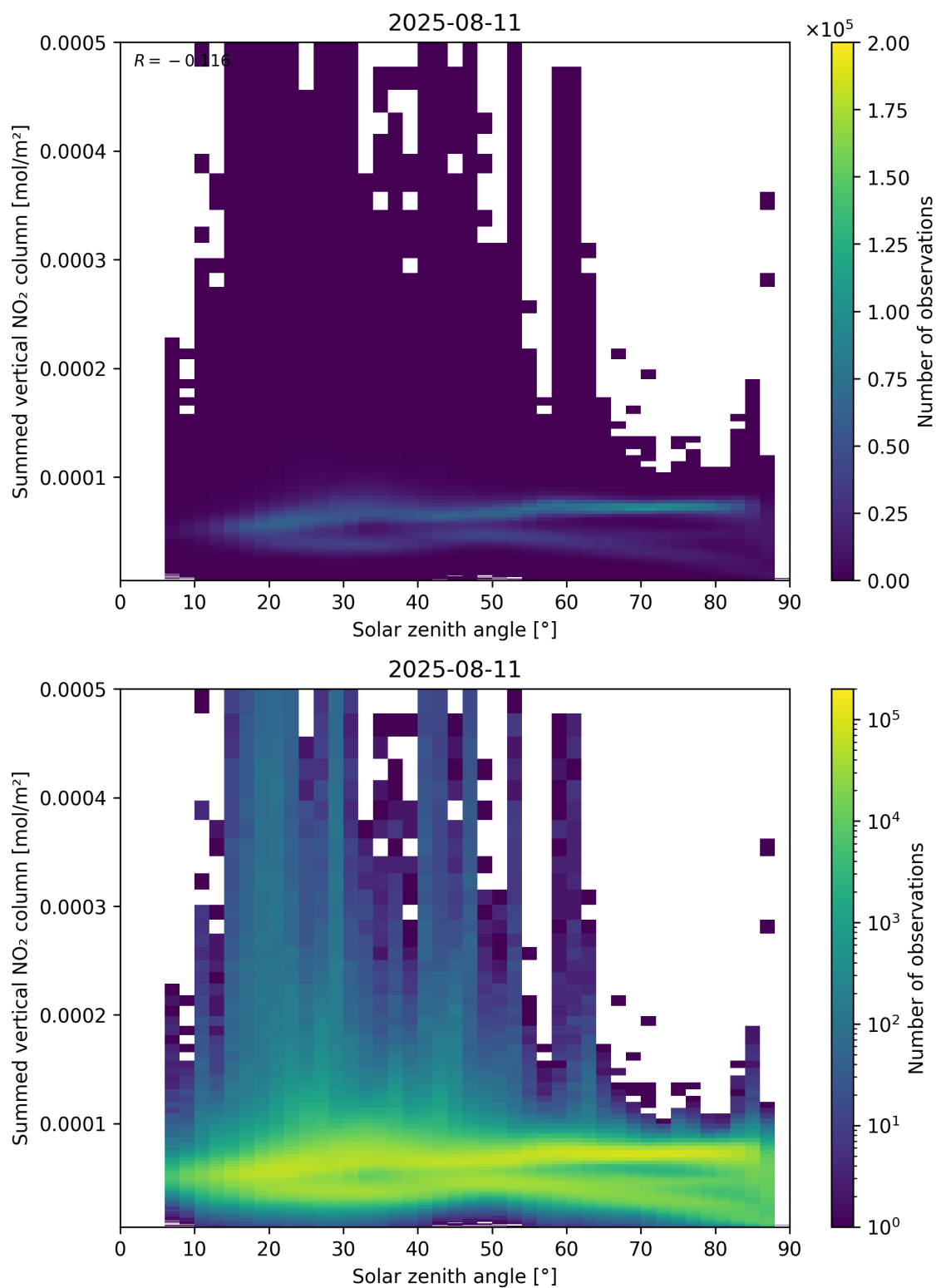
Figure 151: Scatter density plot of “Solar zenith angle” against “Summed vertical NO 2 column” for 2025-08-10 to 2025-08-12.
