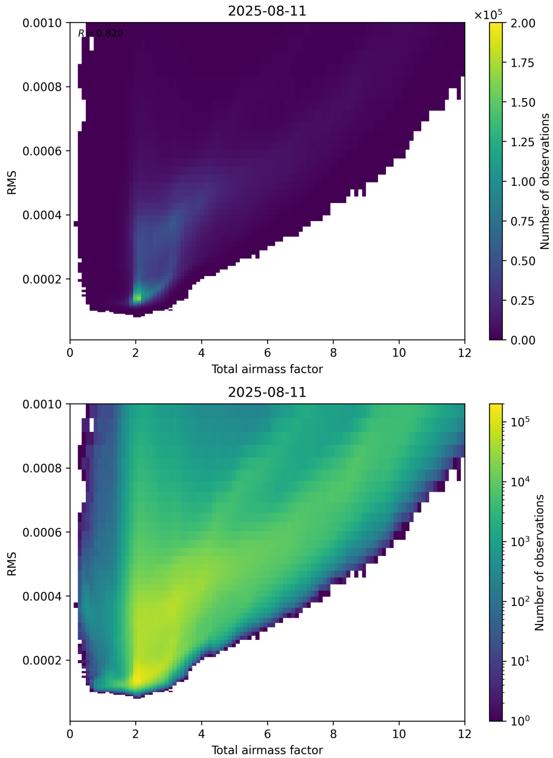
Figure 69: Scatter density plot of “Total airmass factor” against “RMS” for 2025-08-10 to 2025-08-12.
