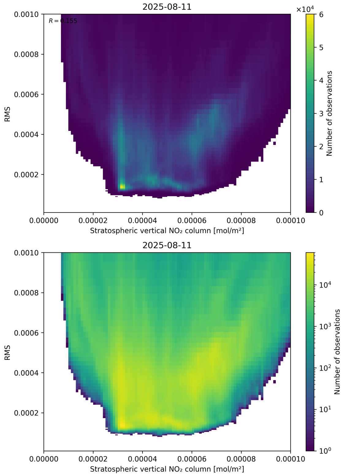
Figure 102: Scatter density plot of “Stratospheric vertical NO 2 column” against “RMS” for 2025-08-10 to 2025-08-12.
