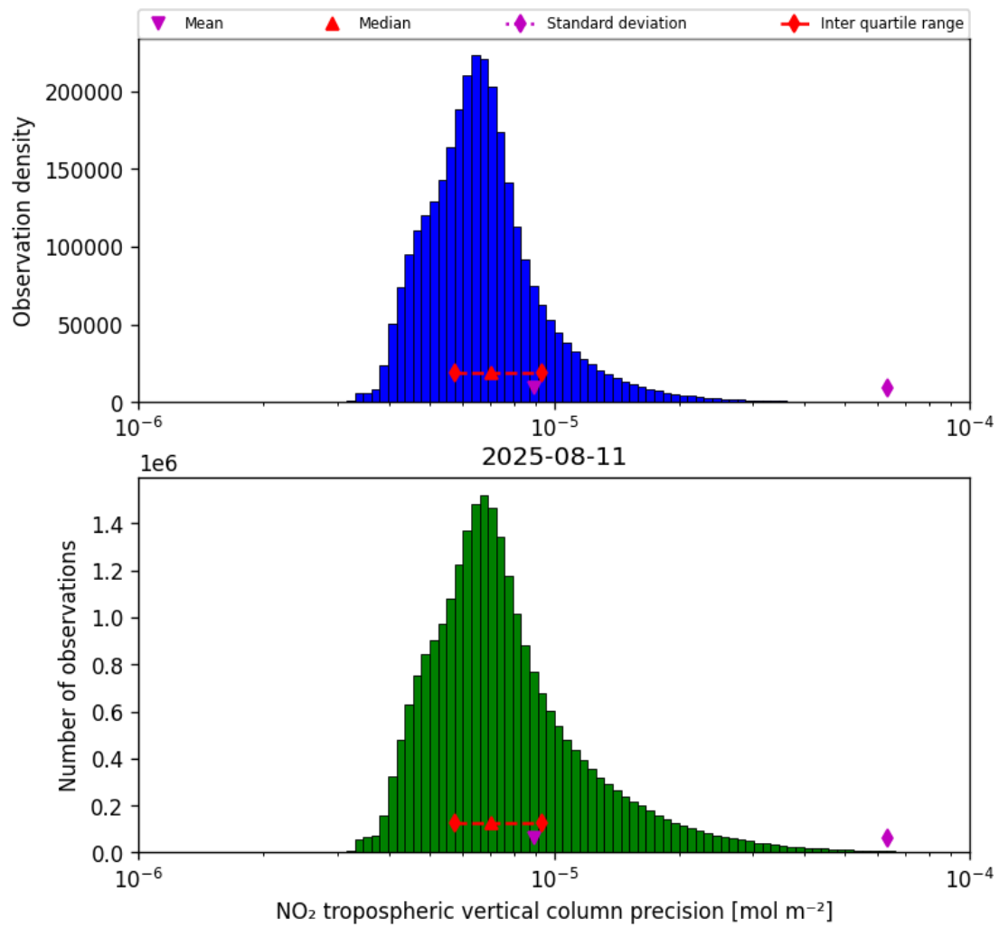
Figure 30: Histogram of “NO 2 tropospheric vertical column precision” for 2025-08-10 to 2025-08-12
