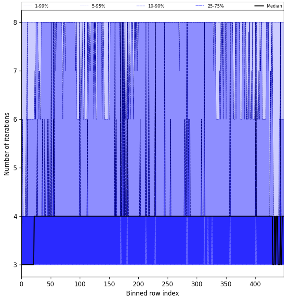
Figure 51: Along track statistics of “Number of iterations” for 2025-08-10 to 2025-08-12
