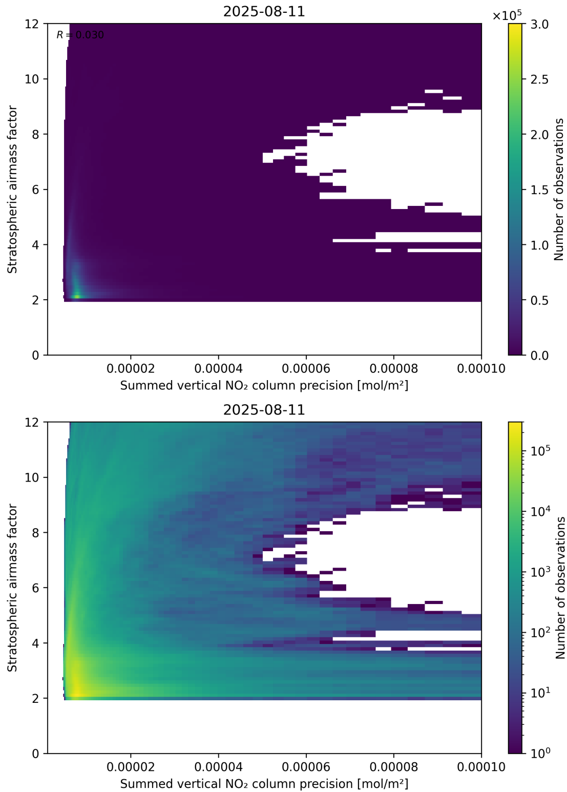
Figure 106: Scatter density plot of “Summed vertical NO 2 column precision” against “Stratospheric airmass factor” for 2025-08-10 to 2025-08-12.
