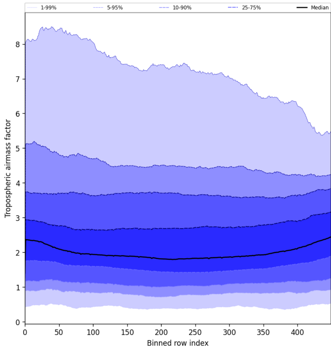
Figure 48: Along track statistics of “Tropospheric air mass factor” for 2025-08-10 to 2025-08-12
