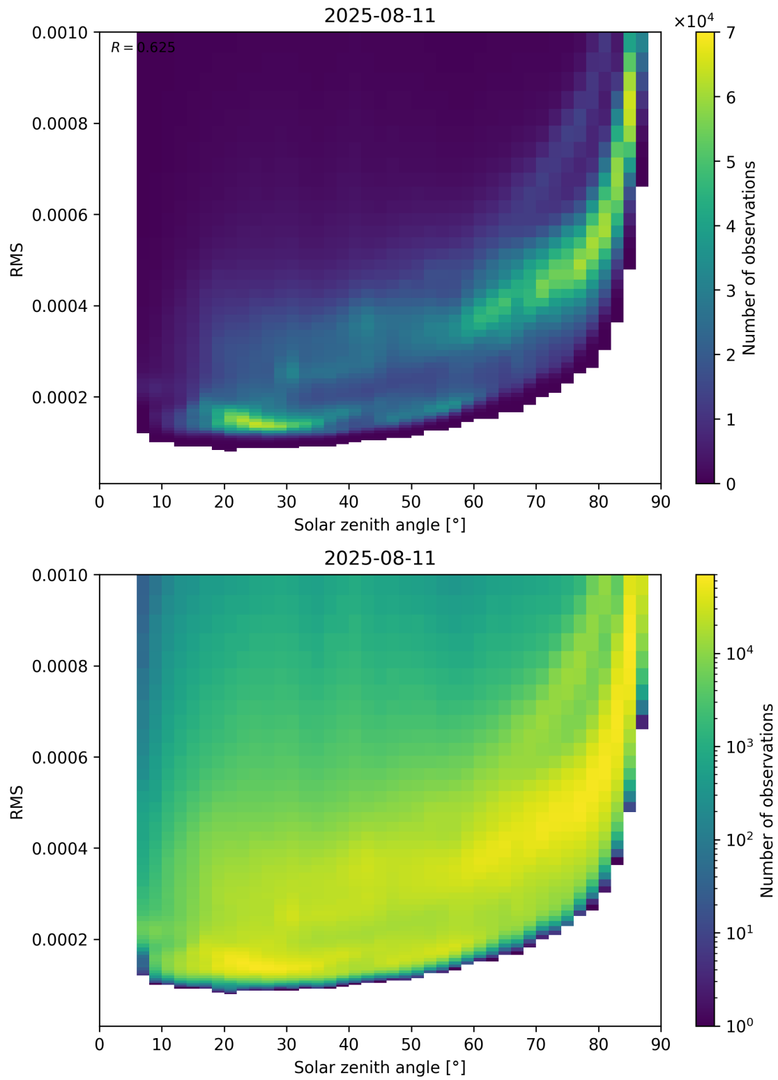
Figure 157: Scatter density plot of “Solar zenith angle” against “RMS” for 2025-08-10 to 2025-08-12.
