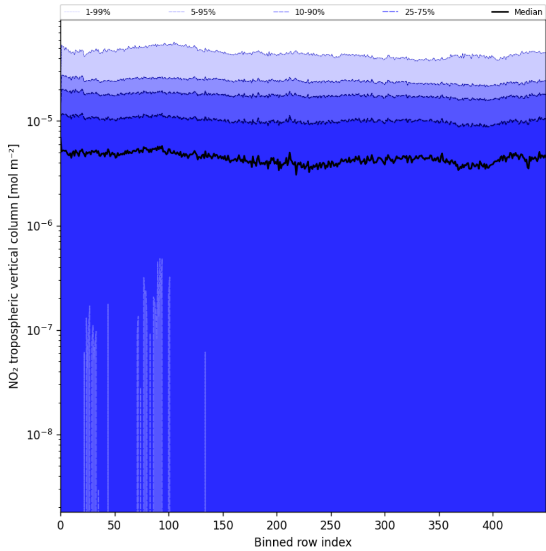
Figure 46: Along track statistics of “NO 2 tropospheric vertical column” for 2025-08-10 to 2025-08-12
