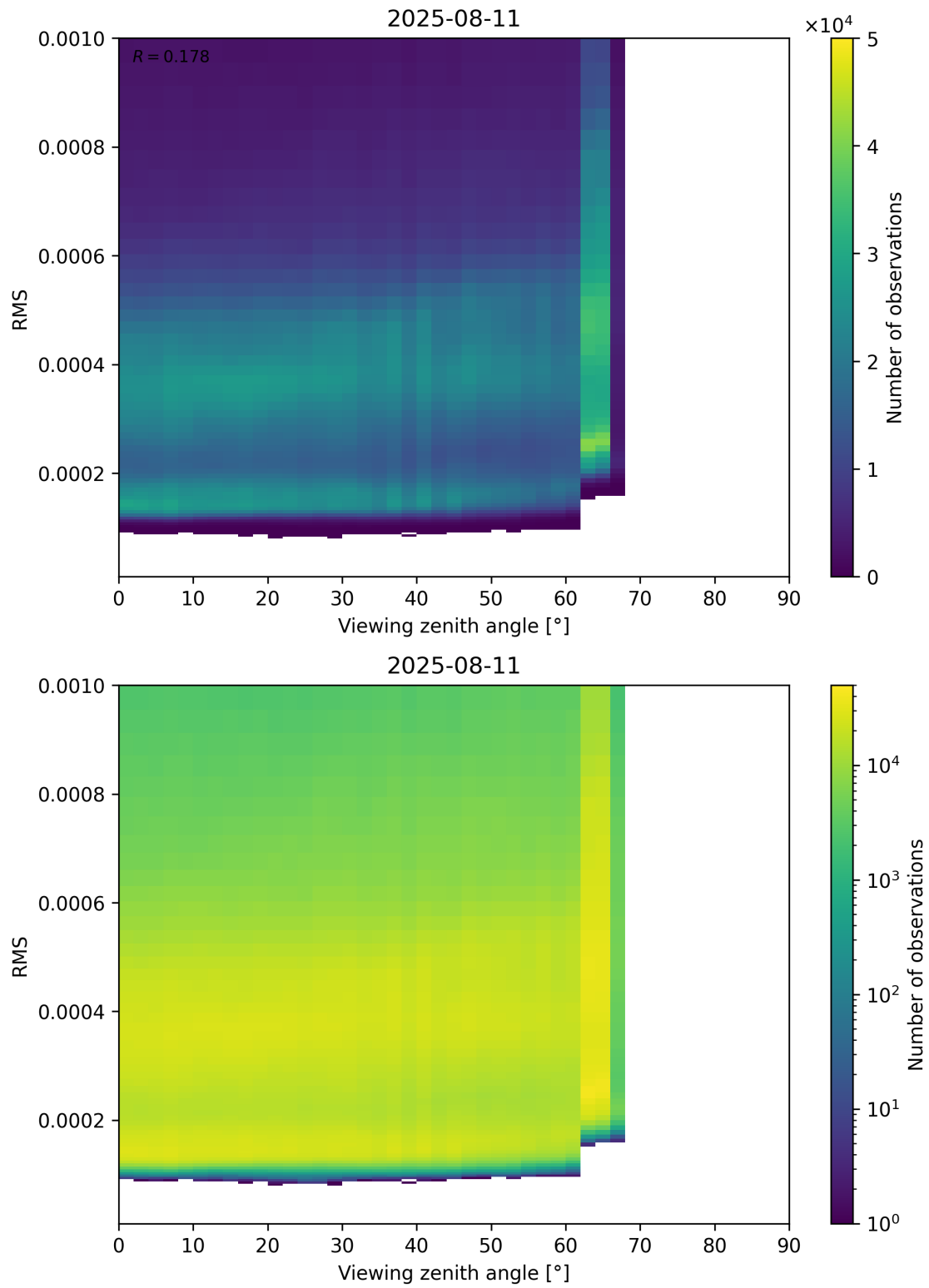
Figure 171: Scatter density plot of “Viewing zenith angle” against “RMS” for 2025-08-10 to 2025-08-12.
