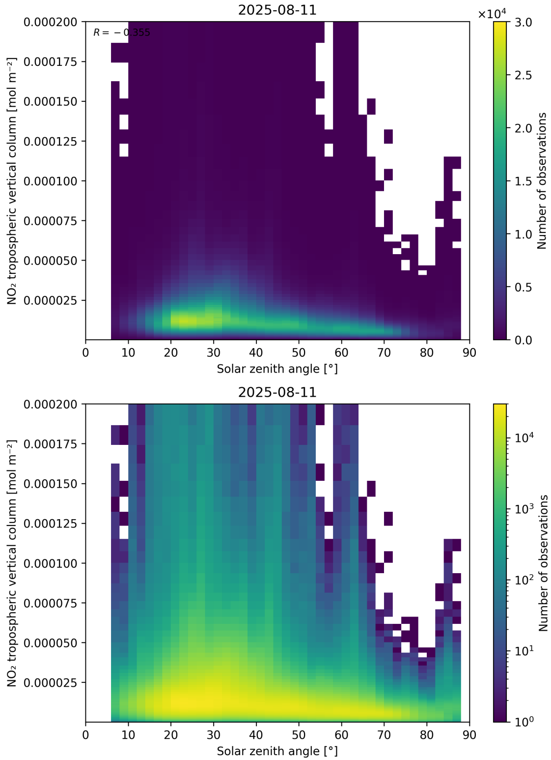
Figure 155: Scatter density plot of “Solar zenith angle” against “NO 2 tropospheric vertical column” for 2025-08-10 to 2025-08-12.
