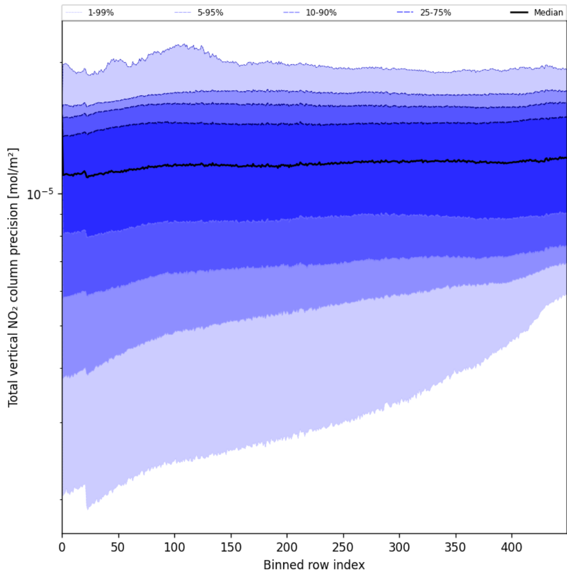
Figure 56: Along track statistics of “Total vertical NO 2 column precision” for 2025-08-10 to 2025-08-12
