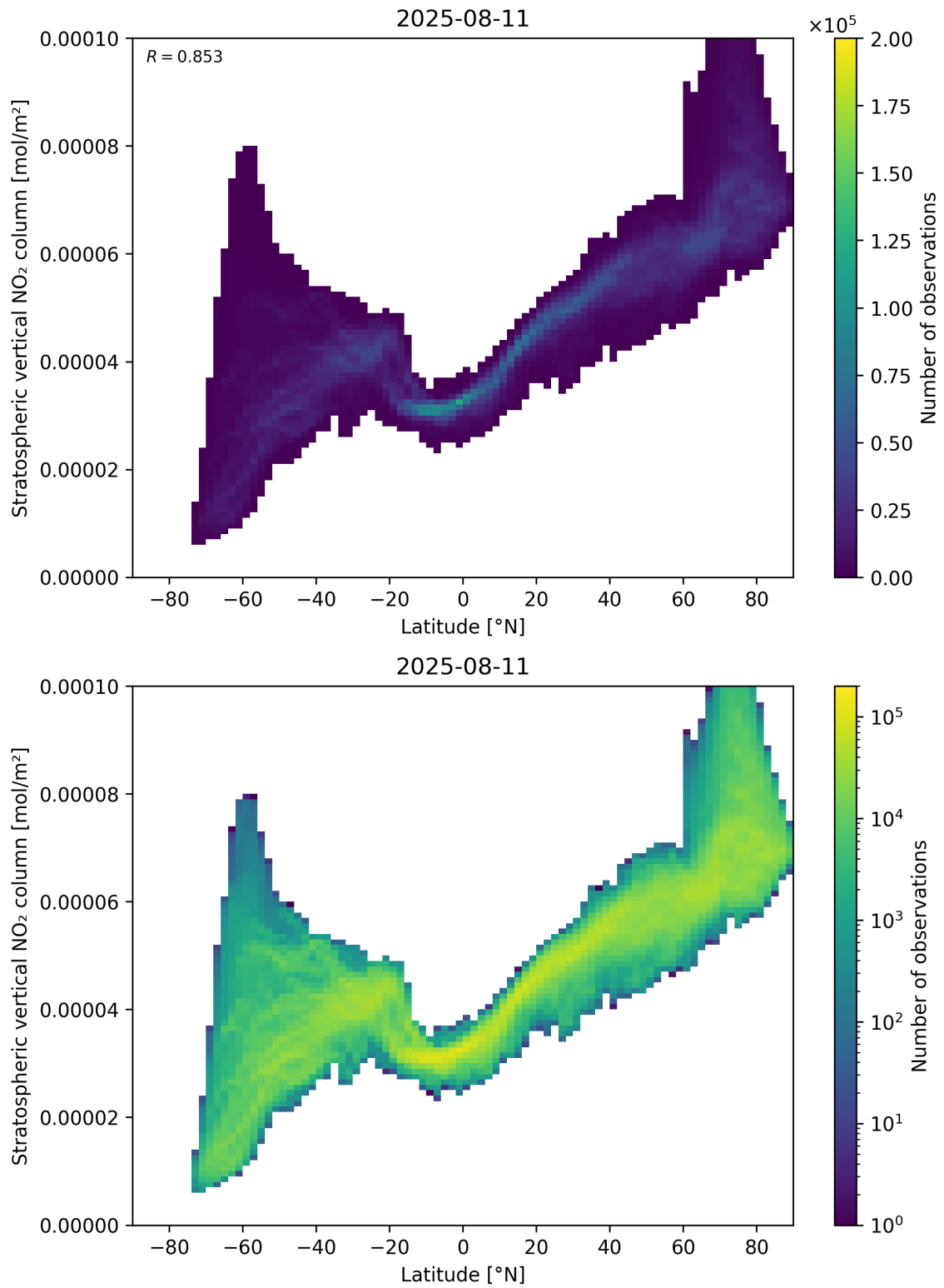
Figure 87: Scatter density plot of “Latitude” against “Stratospheric vertical NO 2 column” for 2025-08-10 to 2025-08-12.
