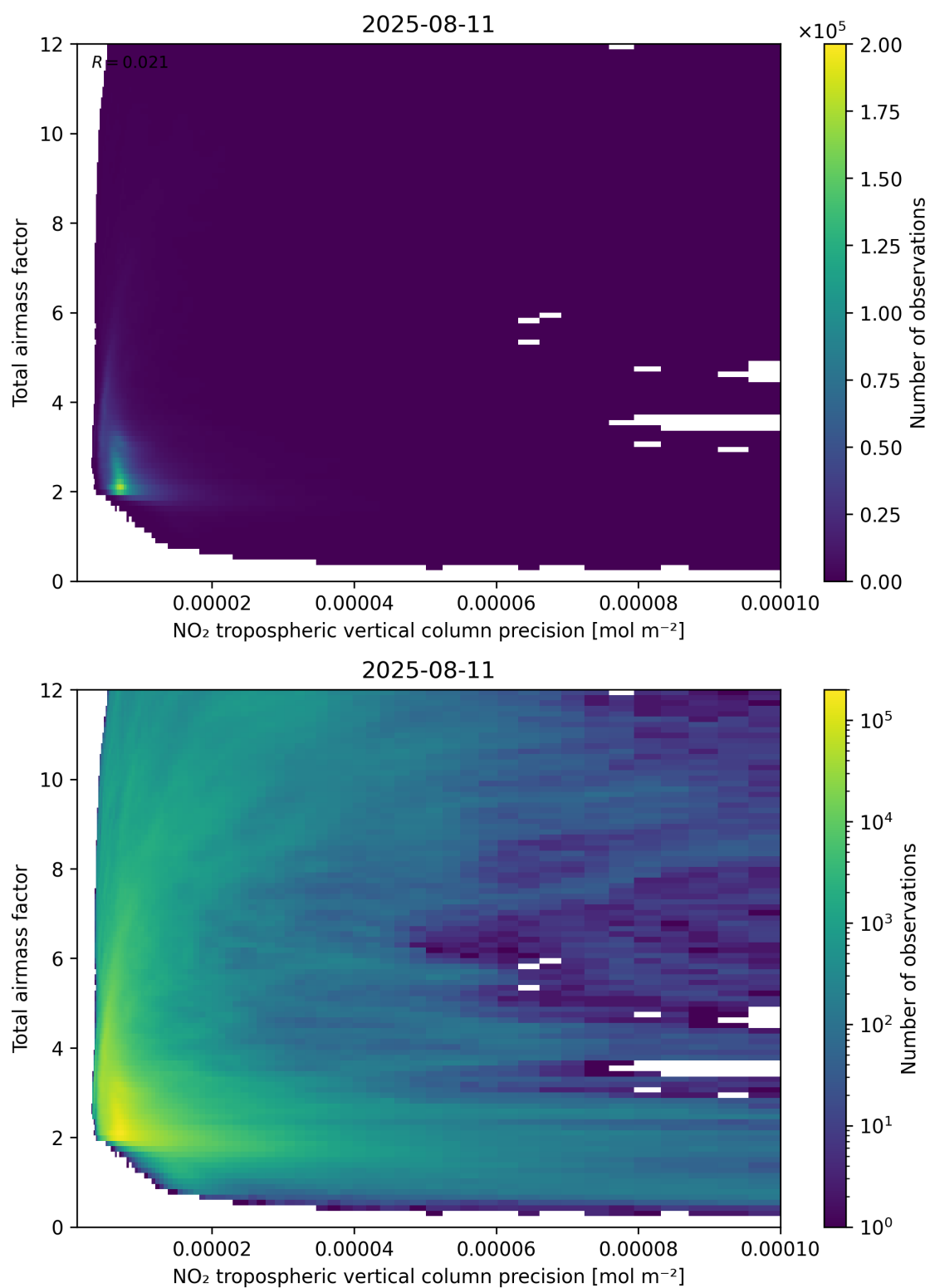
Figure 132: Scatter density plot of “NO 2 tropospheric vertical column precision” against “Total air mass factor” for 2025-08-10 to 2025-08-12.
