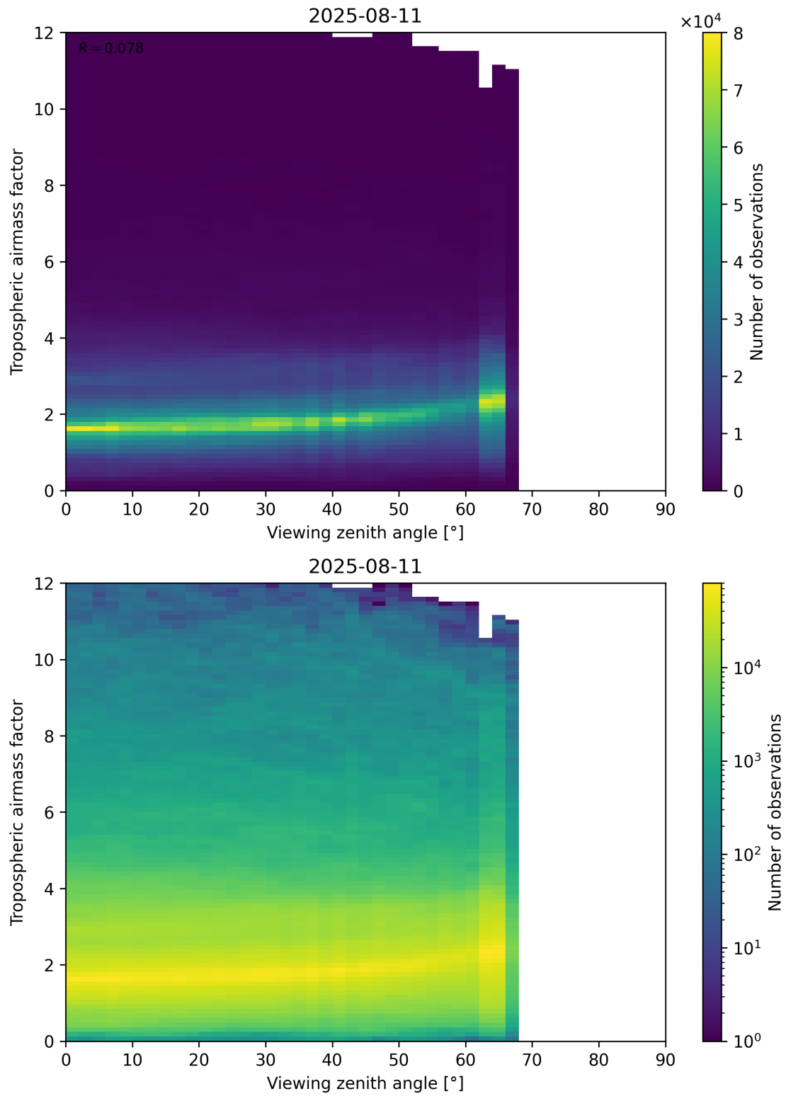
Figure 161: Scatter density plot of “Viewing zenith angle” against “Tropospheric airmass factor” for 2025-08-10 to 2025-08-12.
