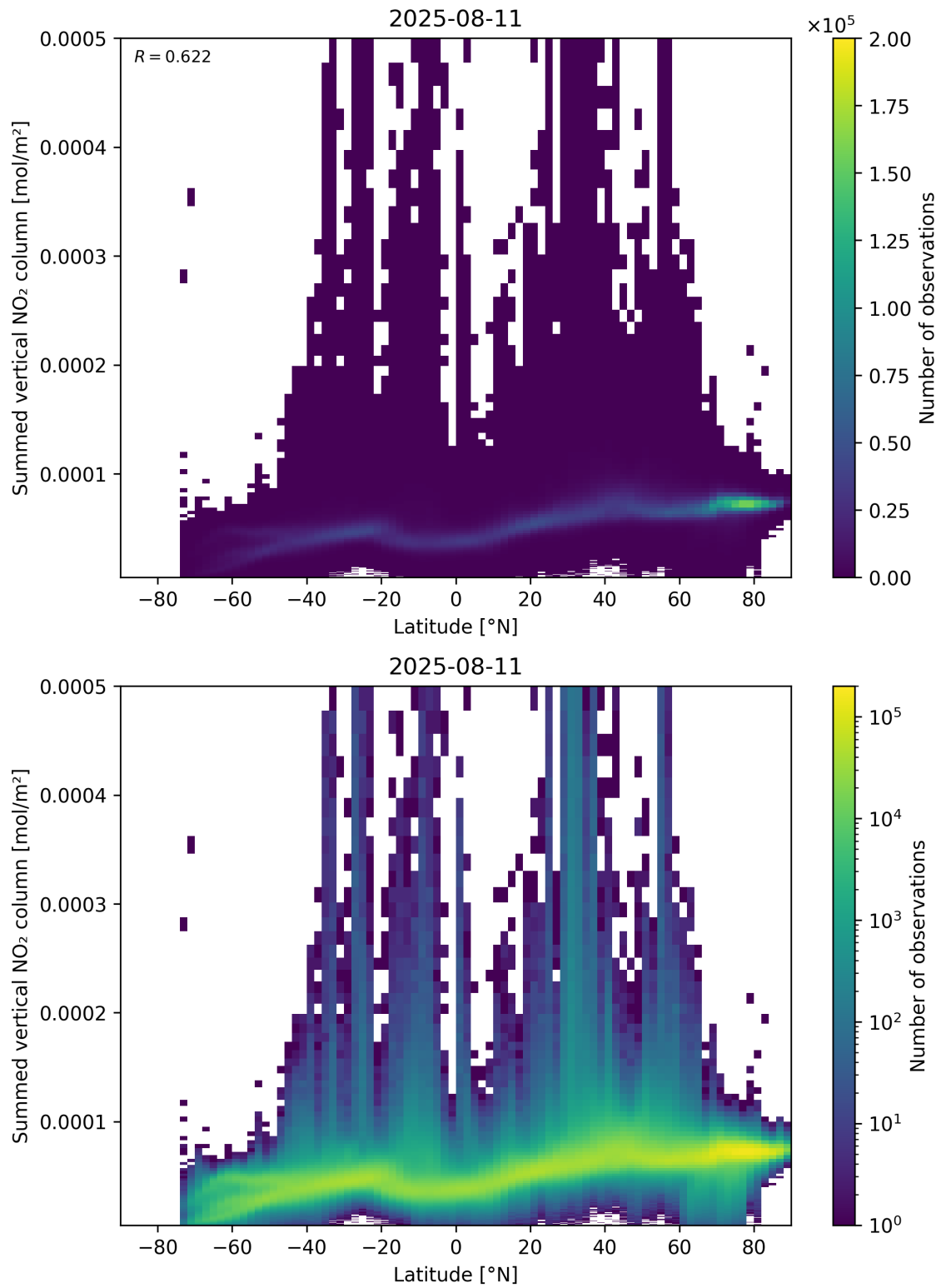
Figure 88: Scatter density plot of “Latitude” against “Summed vertical NO 2 column” for 2025-08-10 to 2025-08-12.
