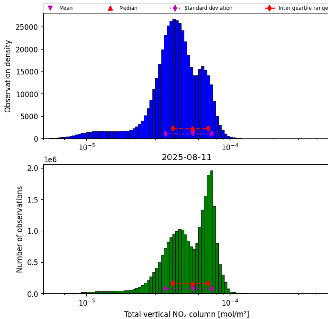
Figure 38: Histogram of “Total vertical NO 2 column” for 2025-08-10 to 2025-08-12
