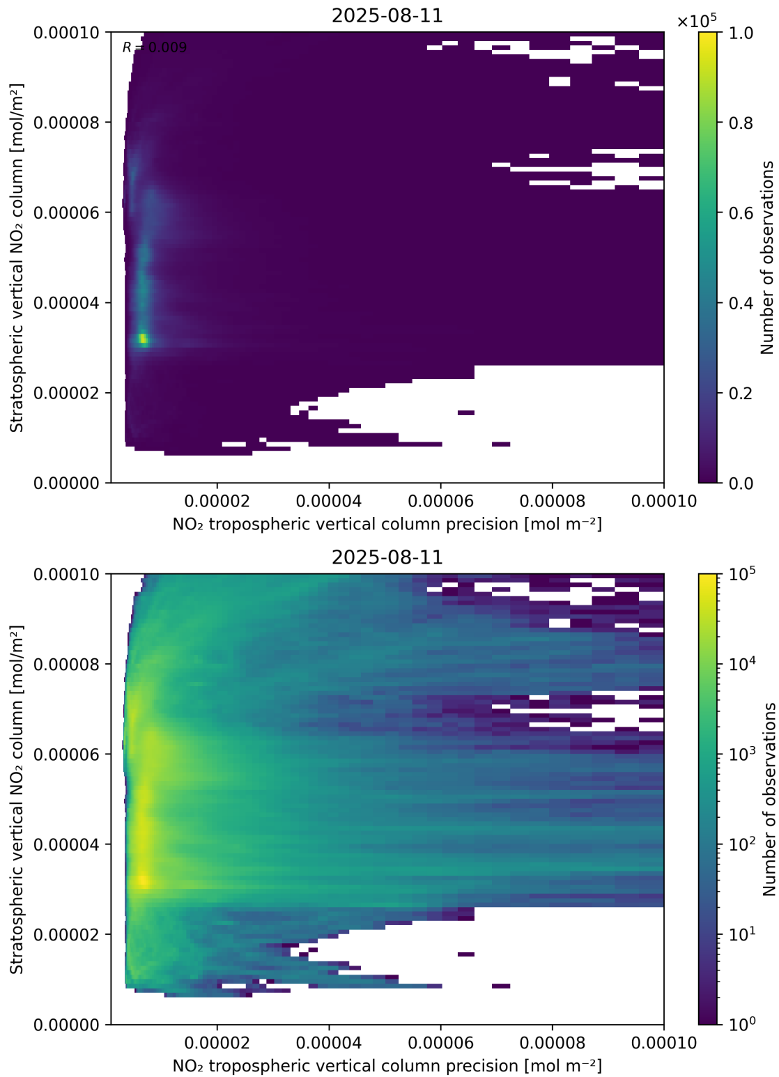
Figure 135: Scatter density plot of “NO 2 tropospheric vertical column precision” against “Stratospheric vertical NO 2 column” for 2025-08-10 to 2025-08-12.
