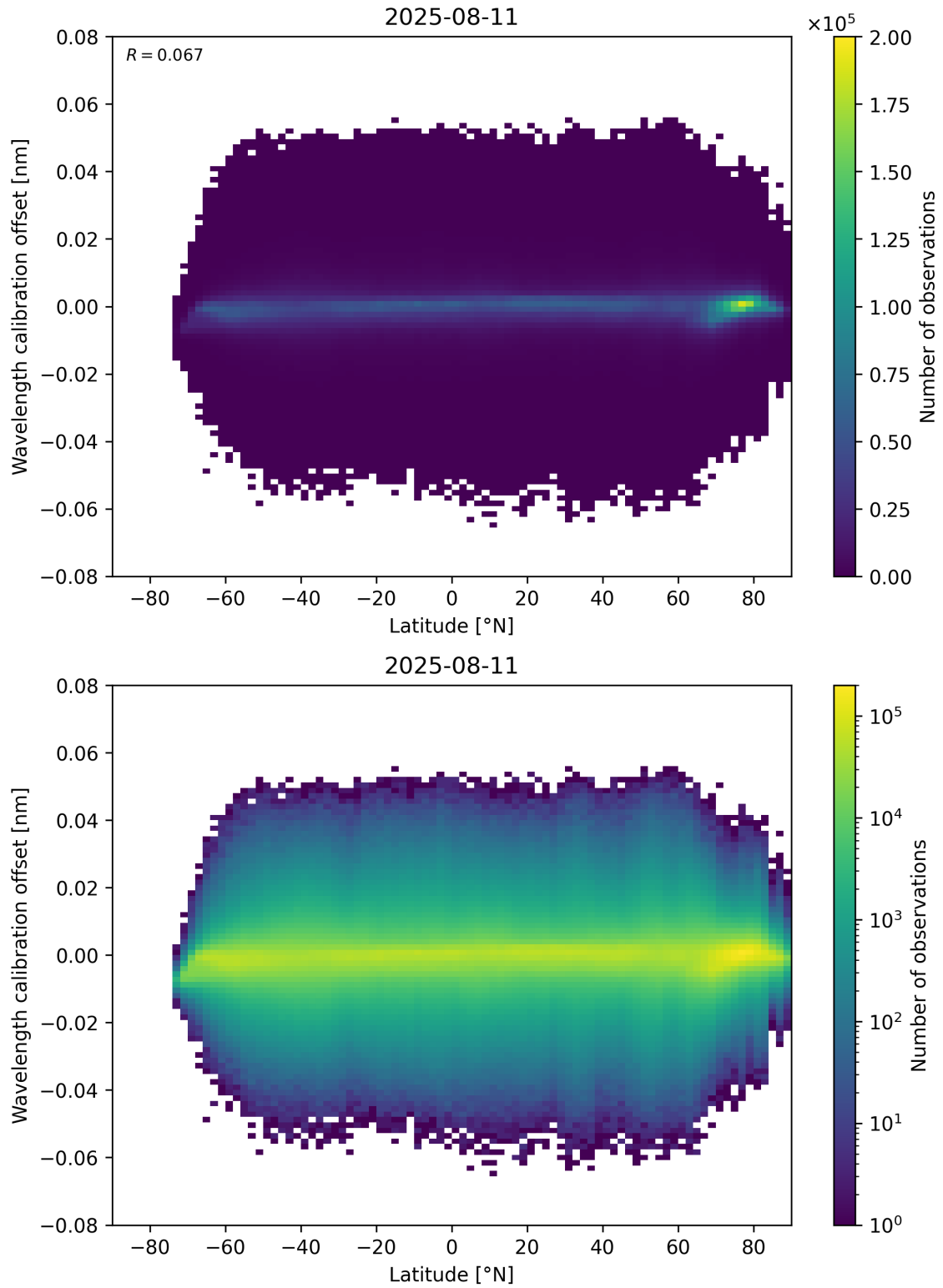
Figure 95: Scatter density plot of “Latitude” against “Wavelength calibration offset” for 2025-08-10 to 2025-08-12.
