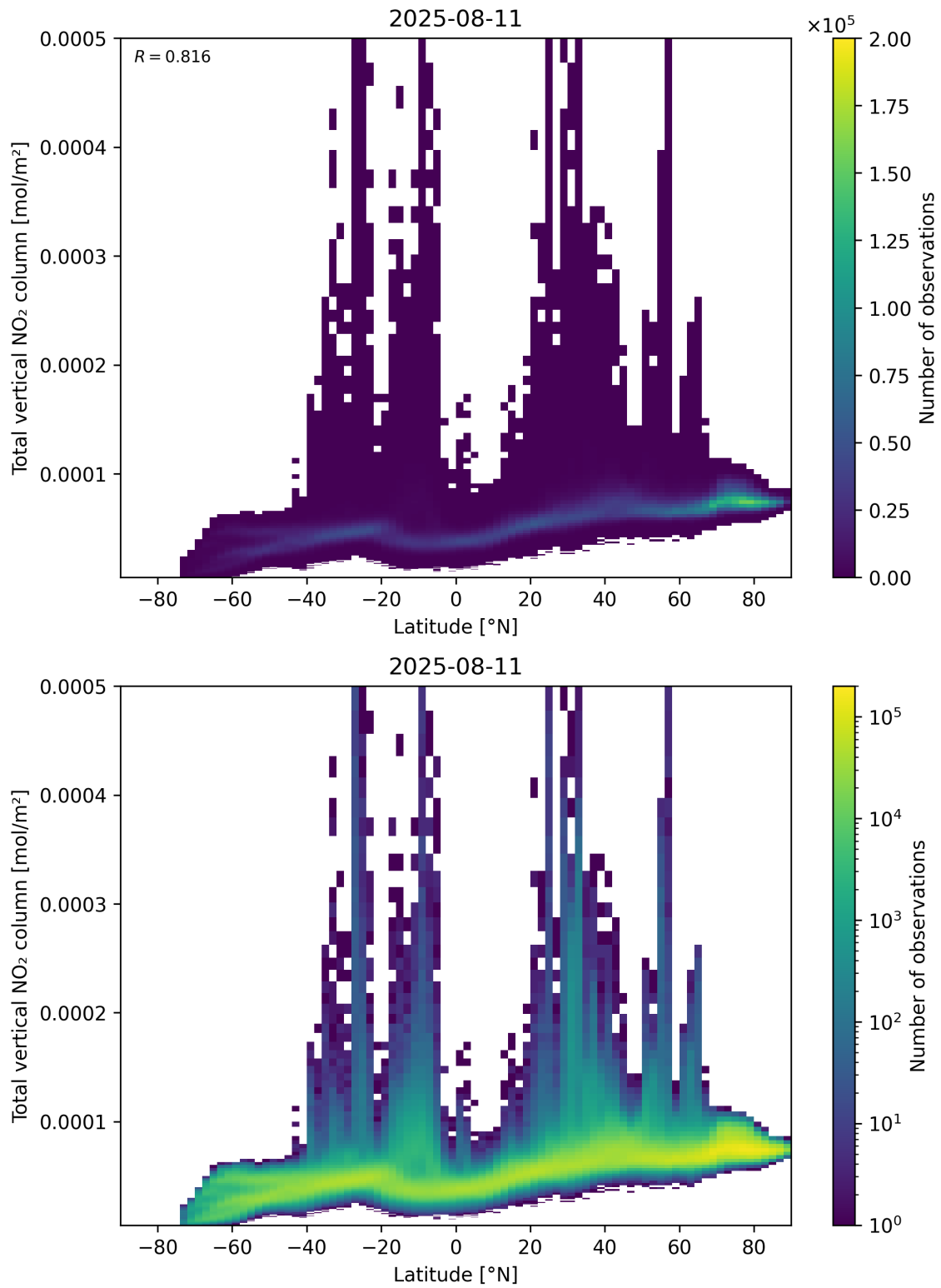
Figure 90: Scatter density plot of “Latitude” against “Total vertical NO 2 column” for 2025-08-10 to 2025-08-12.
