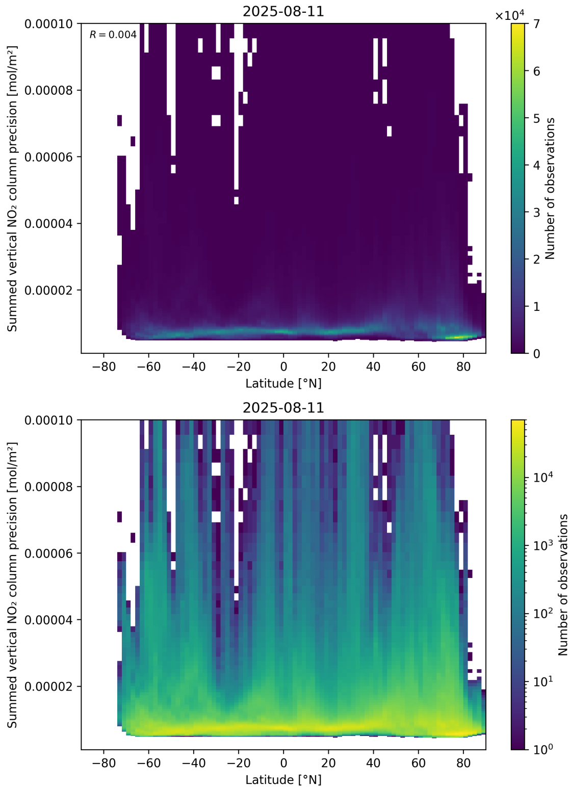
Figure 89: Scatter density plot of “Latitude” against “Summed vertical NO 2 column precision” for 2025-08-10 to 2025-08-12.
