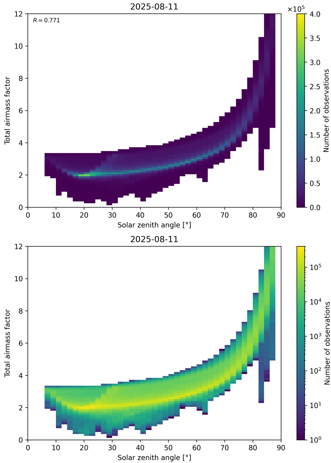
Figure 146: Scatter density plot of “Solar zenith angle” against “Total air mass factor” for 2025-08-10 to 2025-08-12.
