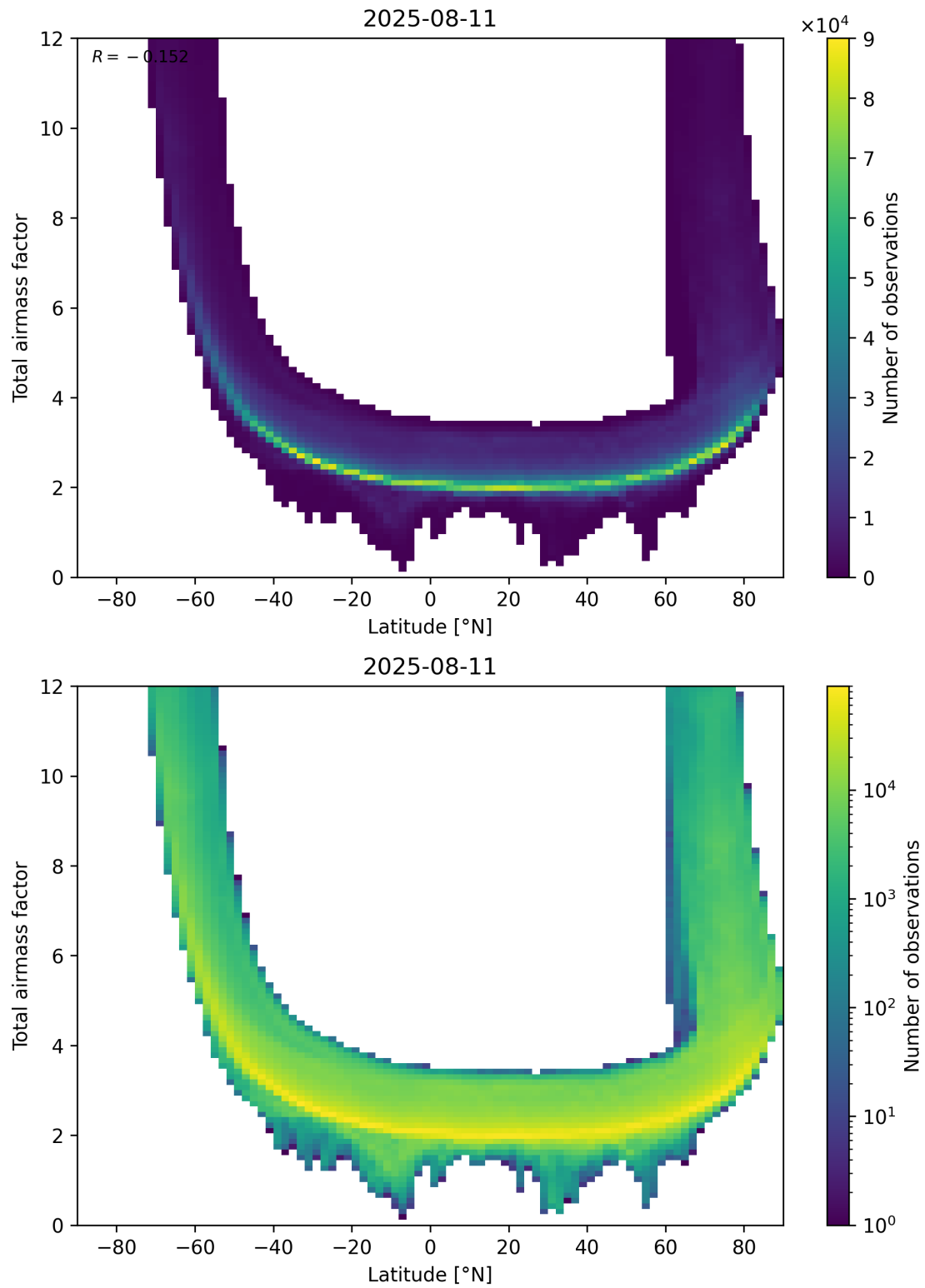
Figure 84: Scatter density plot of “Latitude” against “Total airmass factor” for 2025-08-10 to 2025-08-12.
