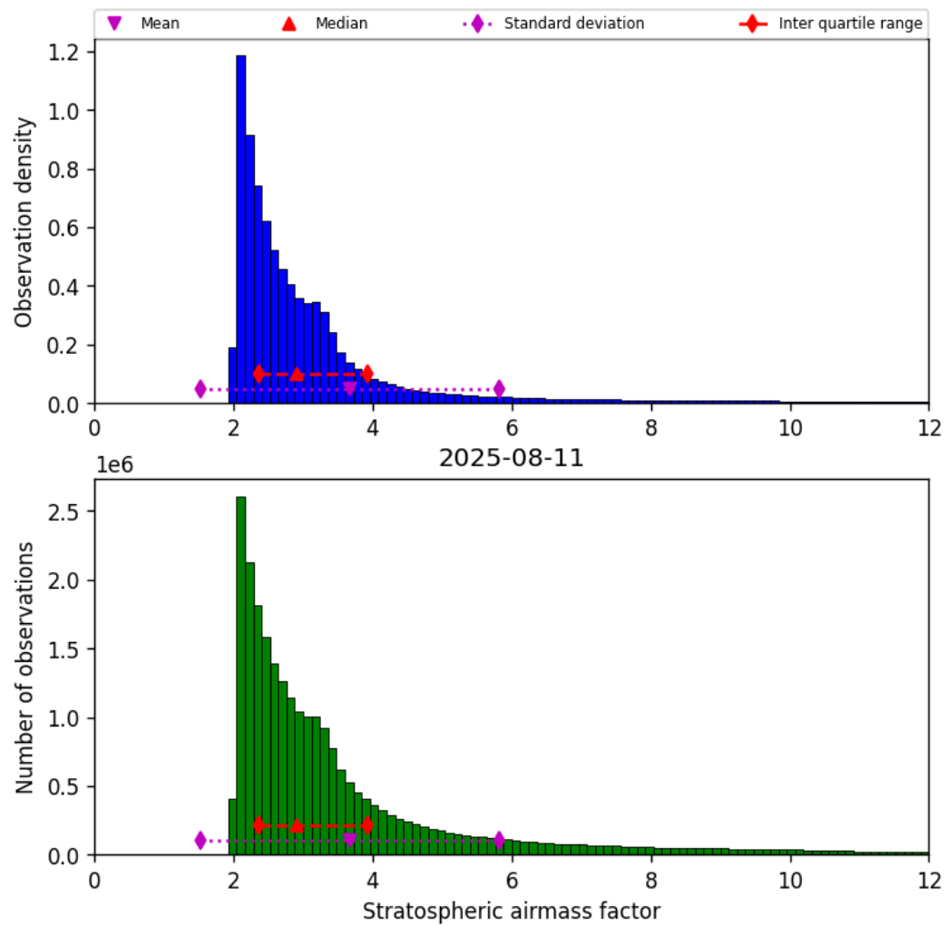
Figure 44: Histogram of “Stratospheric airmass factor” for 2025-08-10 to 2025-08-12
