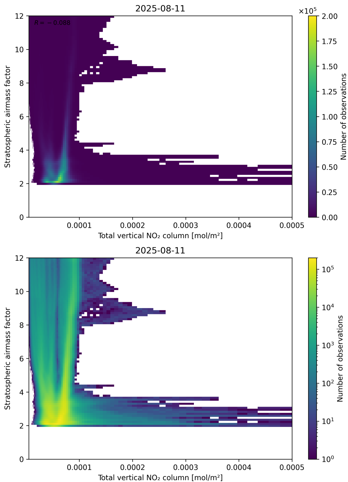
Figure 110: Scatter density plot of “Total vertical NO 2 column” against “Stratospheric airmass factor” for 2025-08-10 to 2025-08-12.
