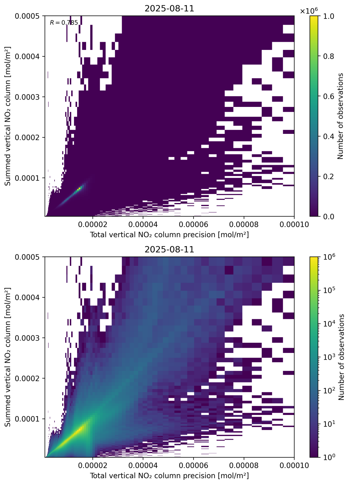
Figure 117: Scatter density plot of “Total vertical NO 2 column precision” against “Summed vertical NO 2 column” for 2025-08-10 to 2025-08-12.
