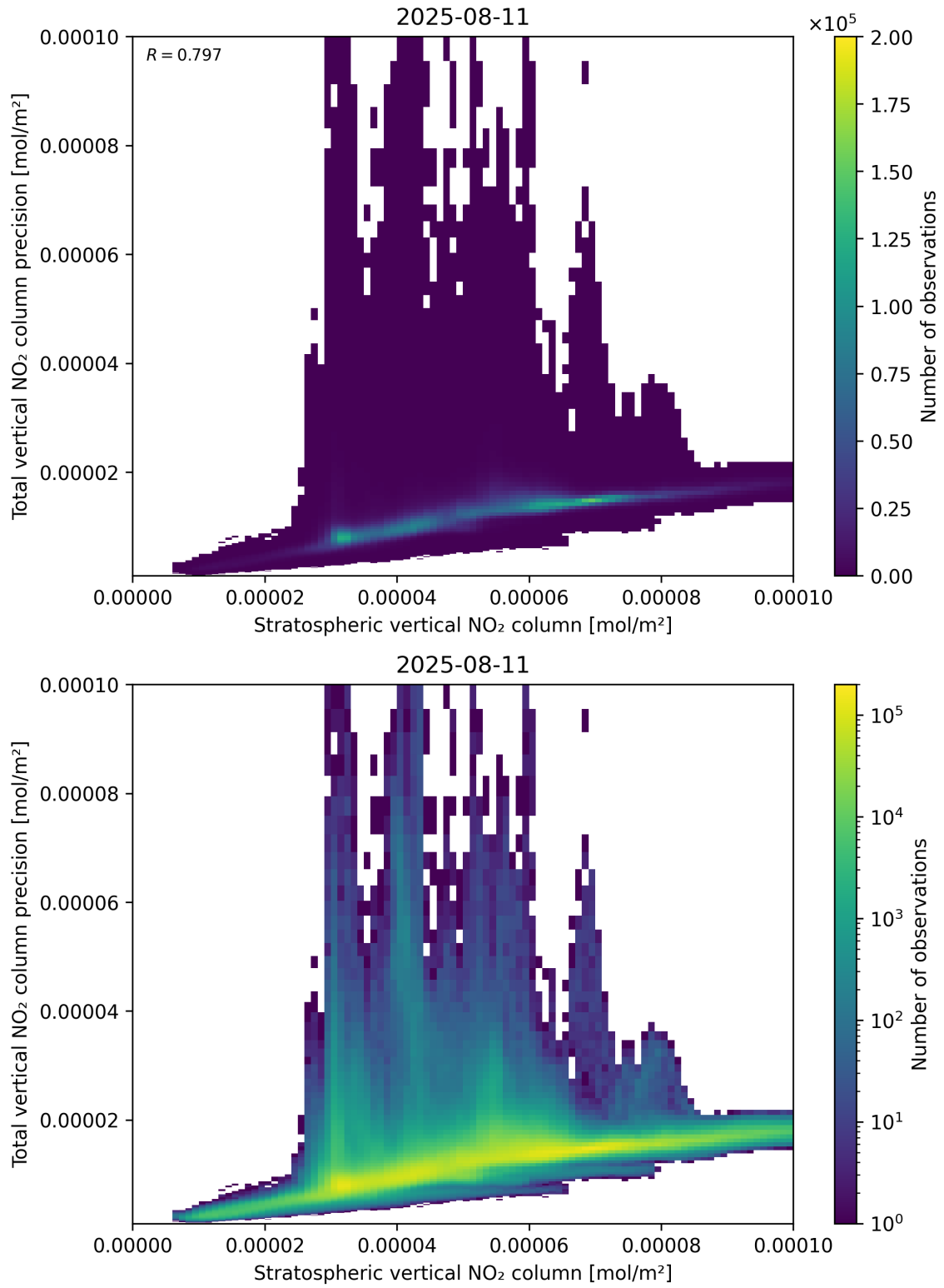
Figure 101: Scatter density plot of “Stratospheric vertical NO 2 column” against “Total vertical NO 2 column precision” for 2025-08-10 to 2025-08-12.
