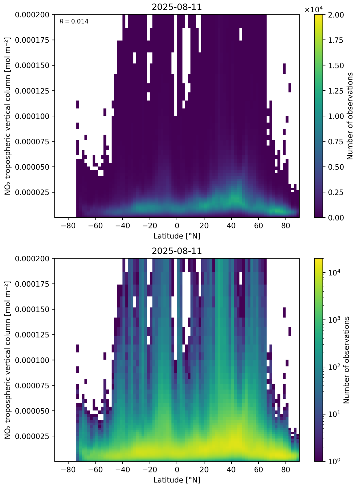
Figure 92: Scatter density plot of “Latitude” against “NO 2 tropospheric vertical column” for 2025-08-10 to 2025-08-12.
