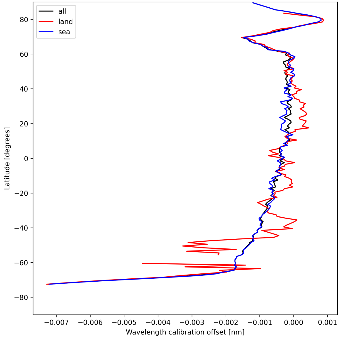
Figure 18: Zonal average of “Wavelength calibration offset” for 2025-08-10 to 2025-08-12.
