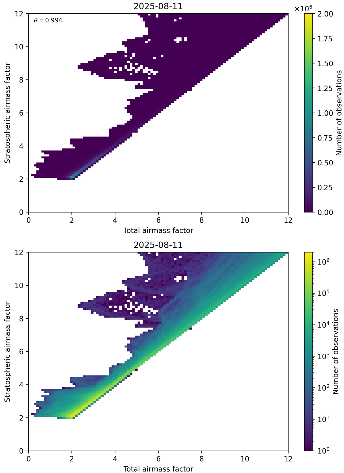
Figure 62: Scatter density plot of “Total airmass factor” against “Stratospheric airmass factor” for 2025-08-10 to 2025-08-12.
