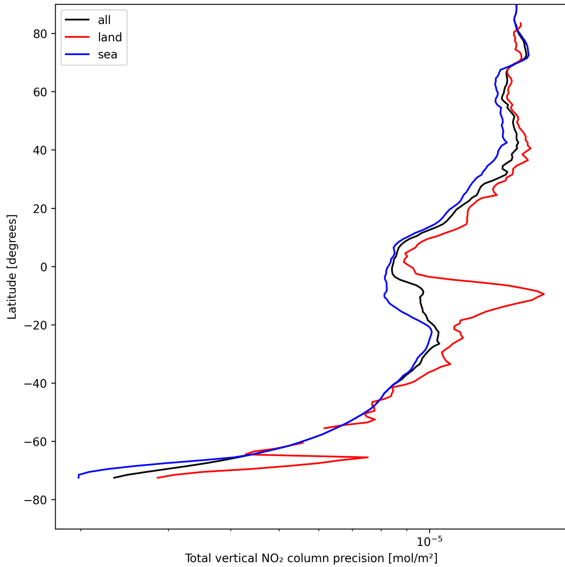
Figure 22: Zonal average of “Total vertical NO 2 column precision” for 2025-08-10 to 2025-08-12.
