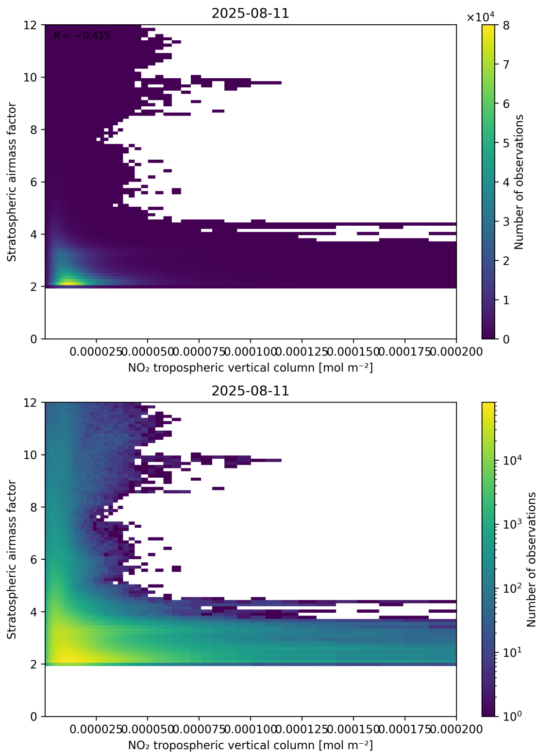
Figure 121: Scatter density plot of “NO 2 tropospheric vertical column” against “Stratospheric airmass factor” for 2025-08-10 to 2025-08-12.
