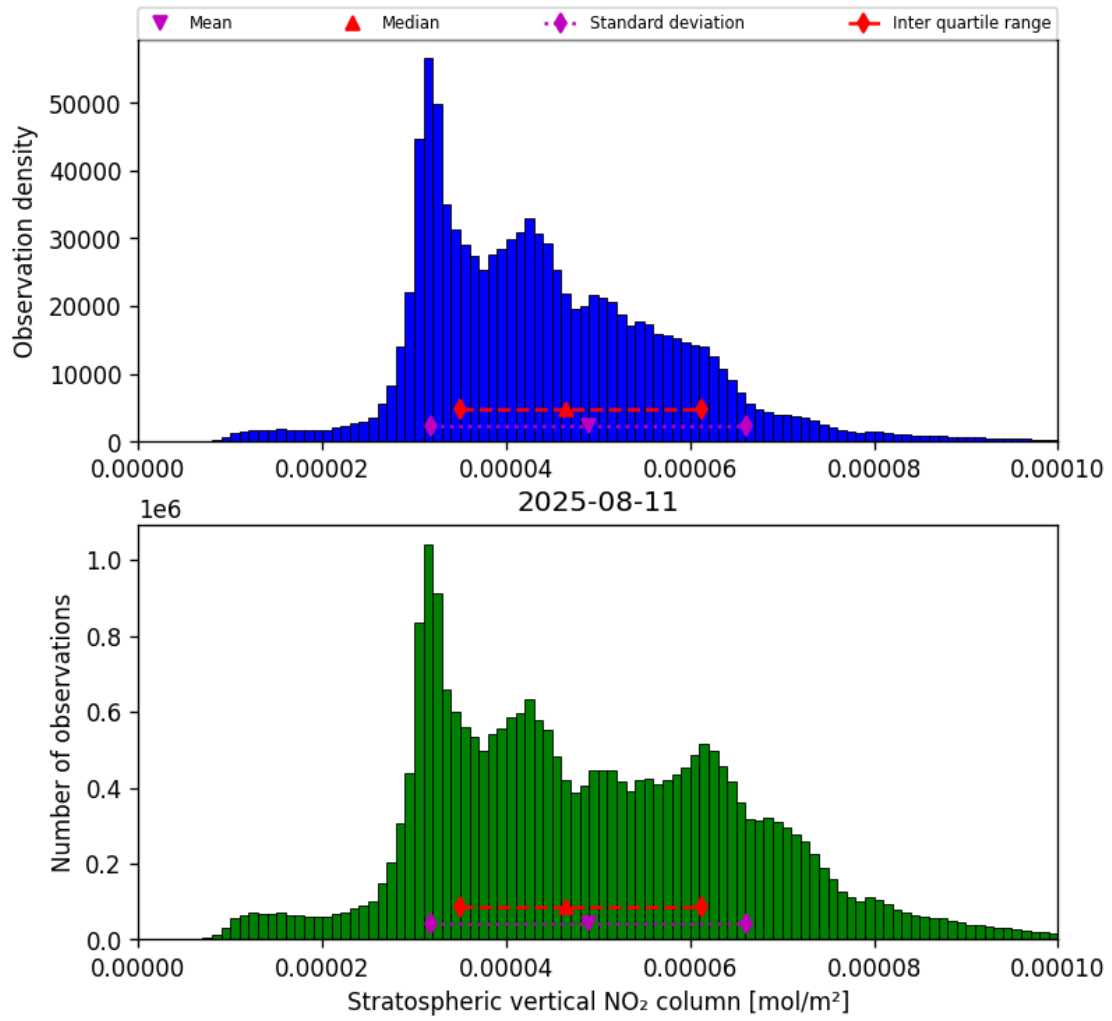
Figure 36: Histogram of “Stratospheric vertical NO 2 column” for 2025-08-10 to 2025-08-12
