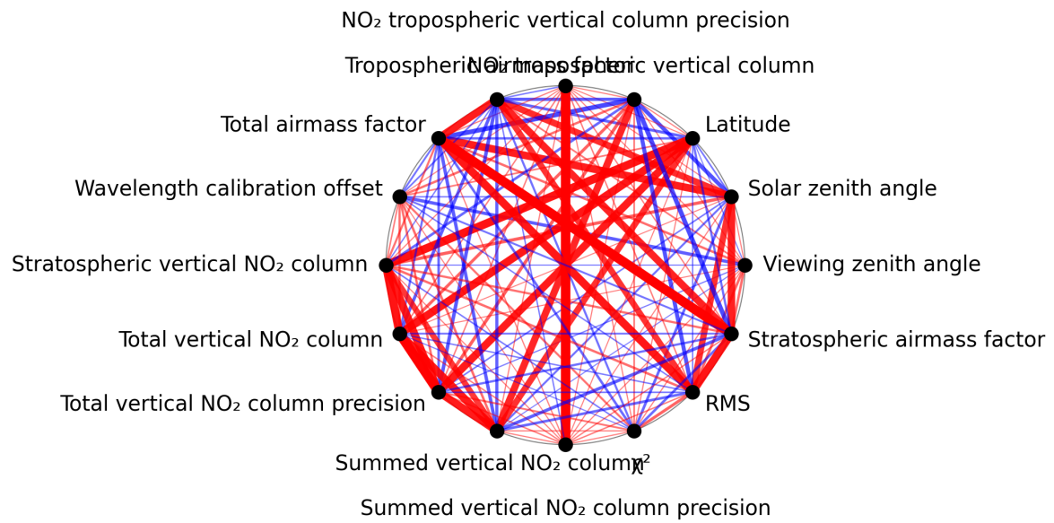
Figure 1: Map of correlation graph for 2025-08-10 to 2025-08-12.
