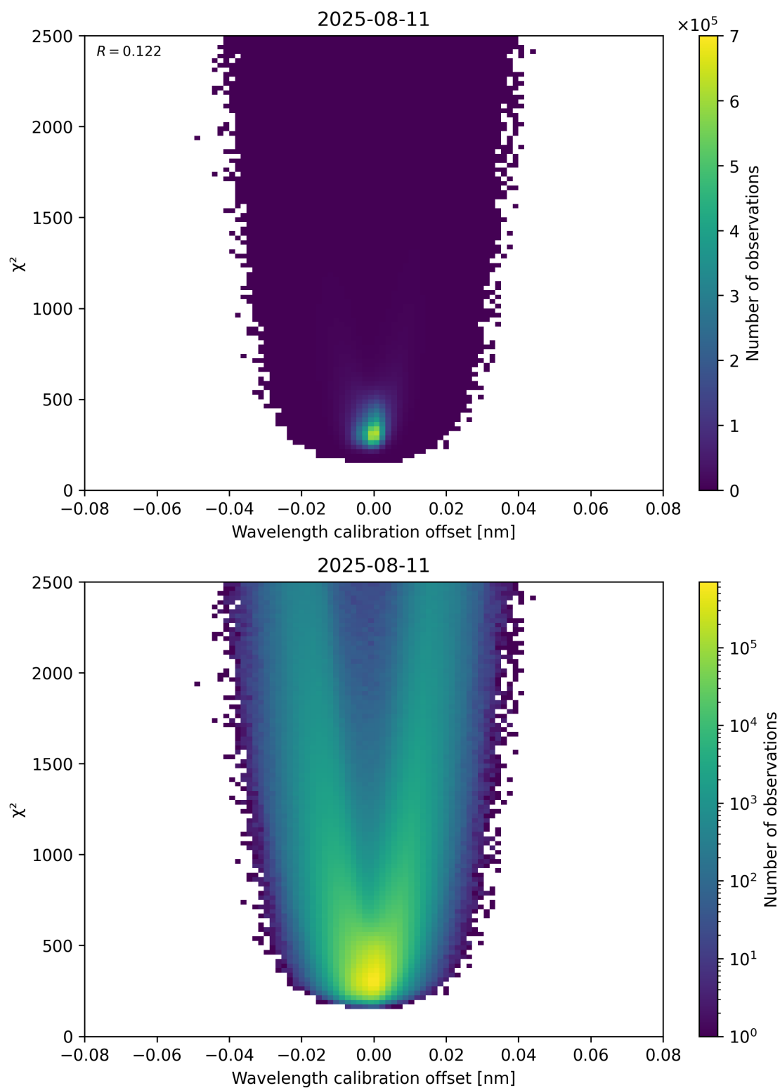
Figure 175: Scatter density plot of “Wavelength calibration offset” against “ \chi^2 ” for 2025-08-10 to 2025-08-12.
