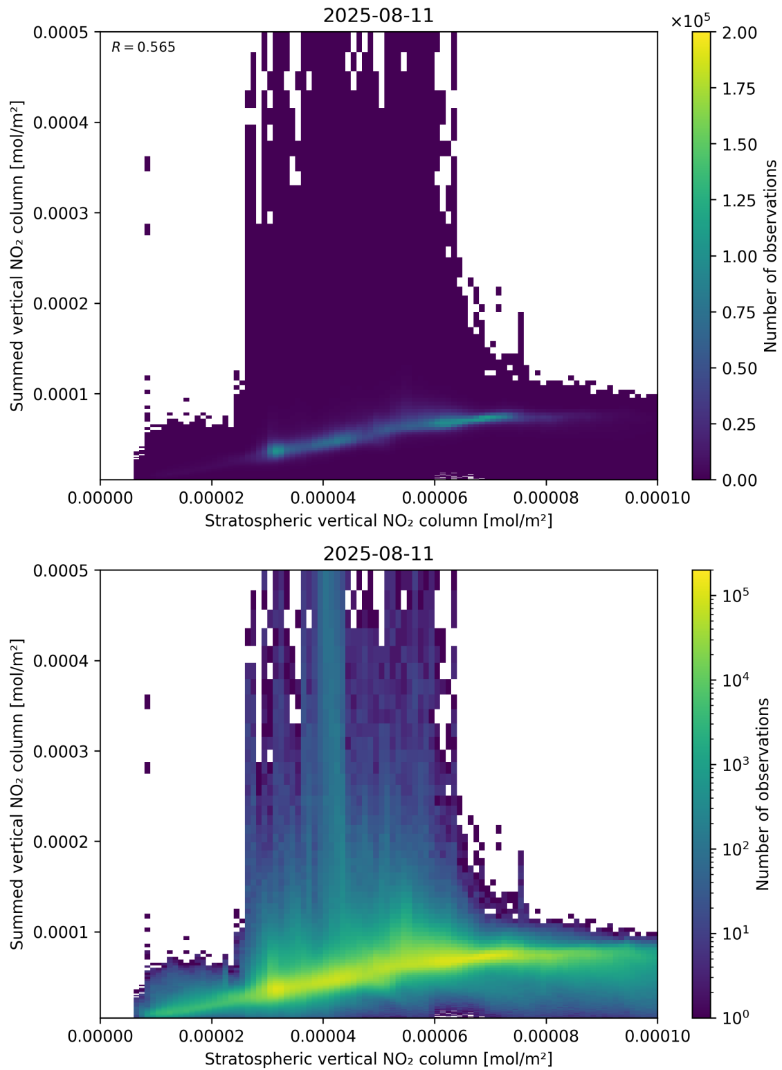
Figure 98: Scatter density plot of “Stratospheric vertical NO 2 column” against “Summed vertical NO 2 column” for 2025-08-10 to 2025-08-12.
