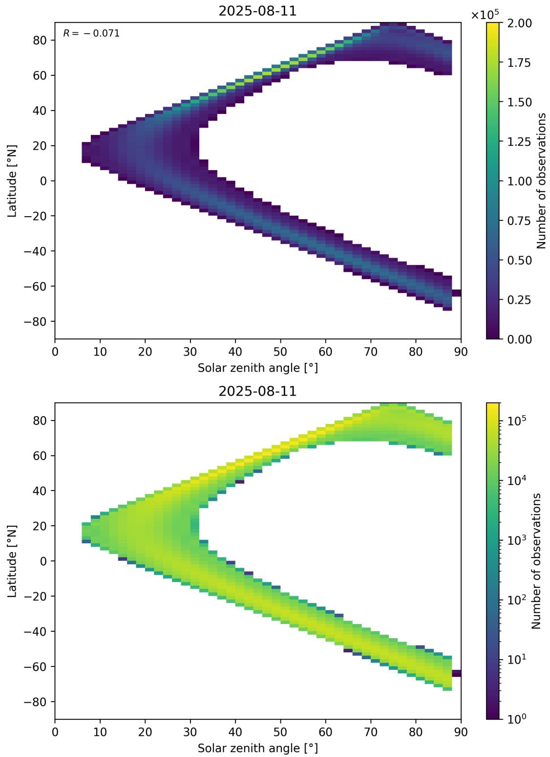
Figure 149: Scatter density plot of “Solar zenith angle” against “Latitude” for 2025-08-10 to 2025-08-12.
