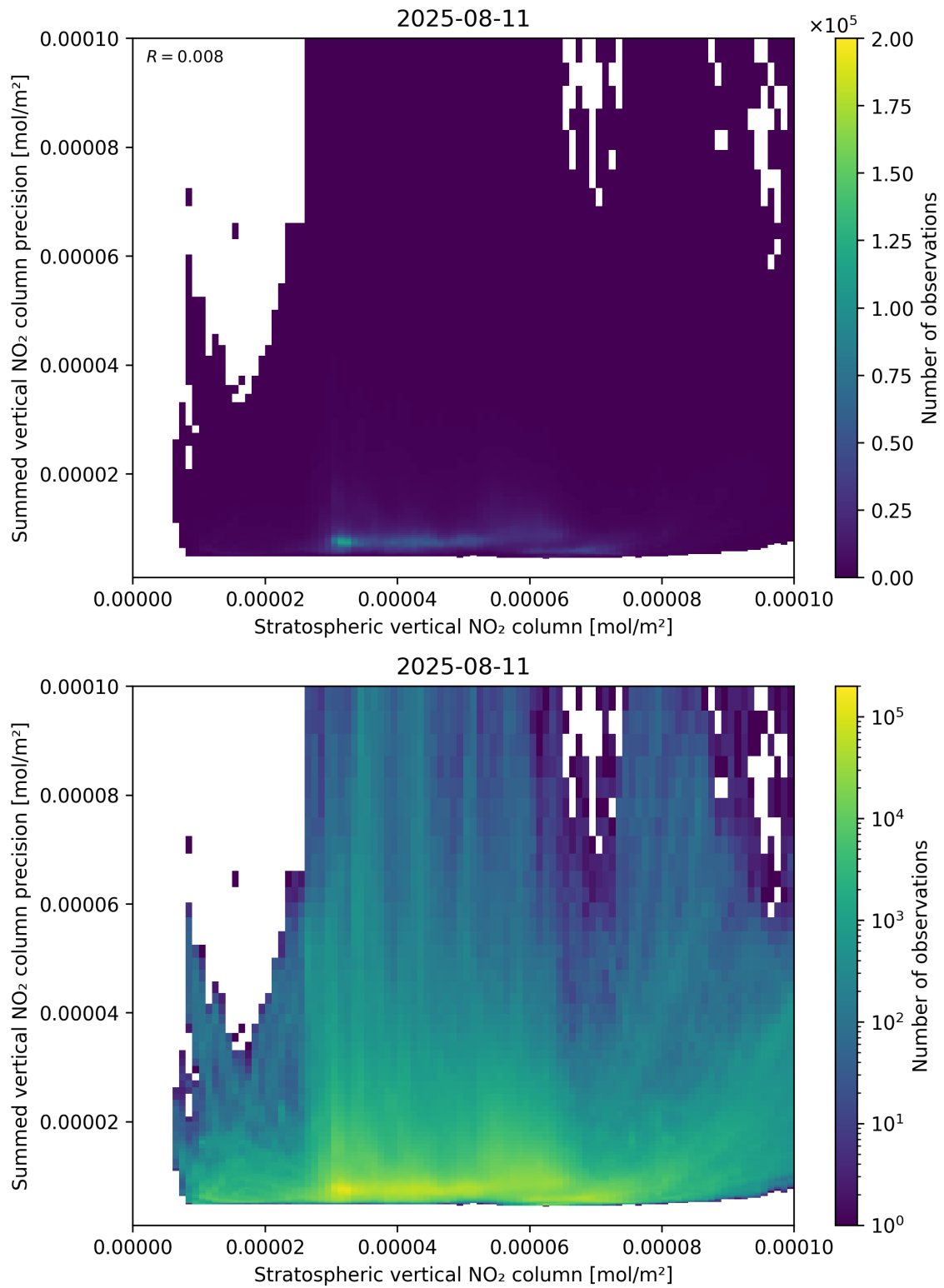
Figure 99: Scatter density plot of “Stratospheric vertical NO 2 column” against “Summed vertical NO 2 column precision” for 2025-08-10 to 2025-08-12.
