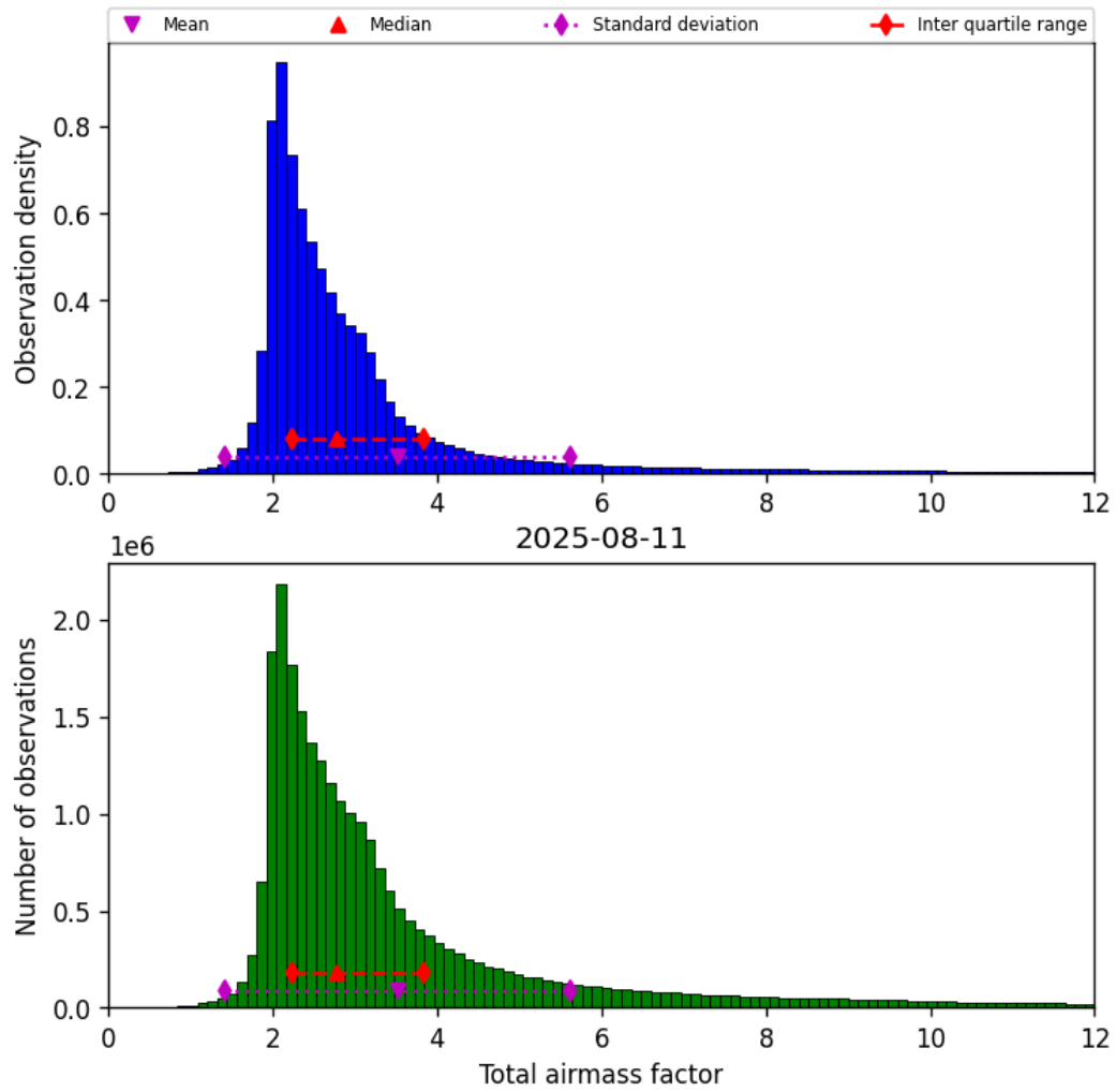
Figure 32: Histogram of “Total airmass factor” for 2025-08-10 to 2025-08-12
