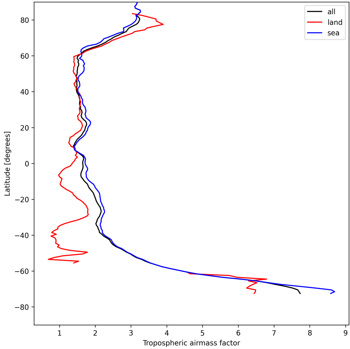
Figure 14: Zonal average of “Tropospheric airmass factor” for 2025-08-10 to 2025-08-12.
