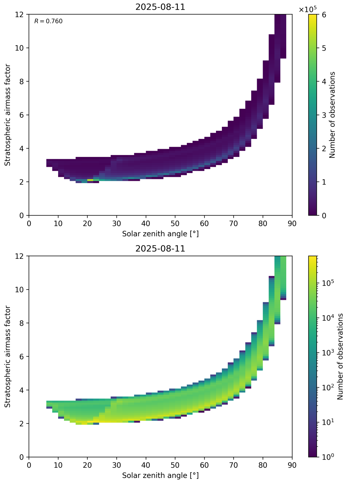
Figure 145: Scatter density plot of “Solar zenith angle” against “Stratospheric airmass factor” for 2025-08-10 to 2025-08-12.
