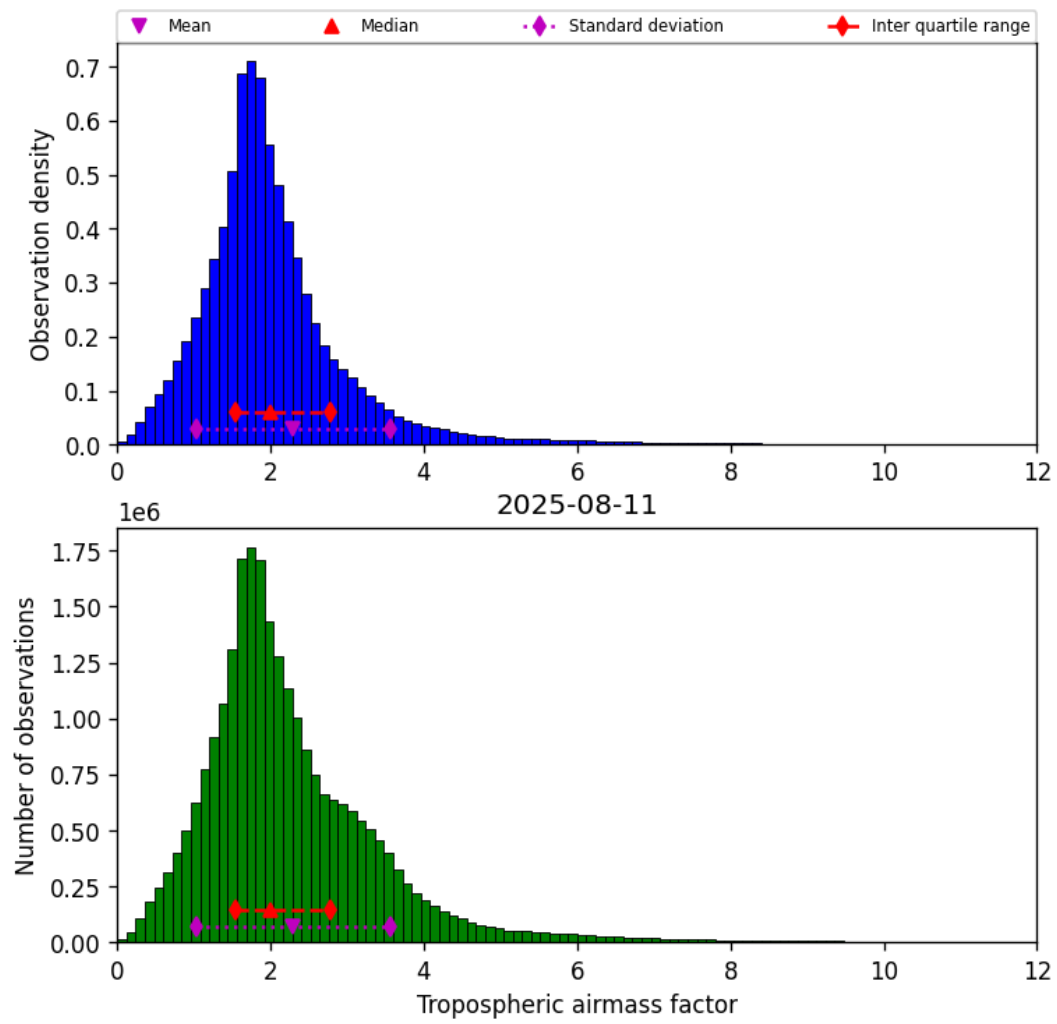
Figure 31: Histogram of “Tropospheric airmass factor” for 2025-08-10 to 2025-08-12
