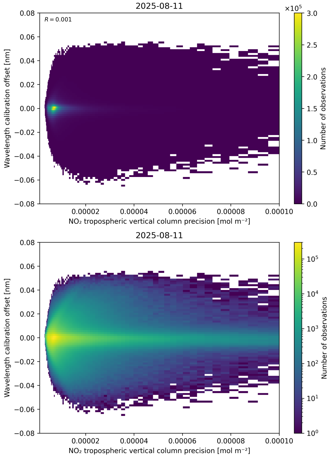
Figure 141: Scatter density plot of “NO 2 tropospheric vertical column precision” against “Wavelength calibration offset” for 2025-08-10 to 2025-08-12.
