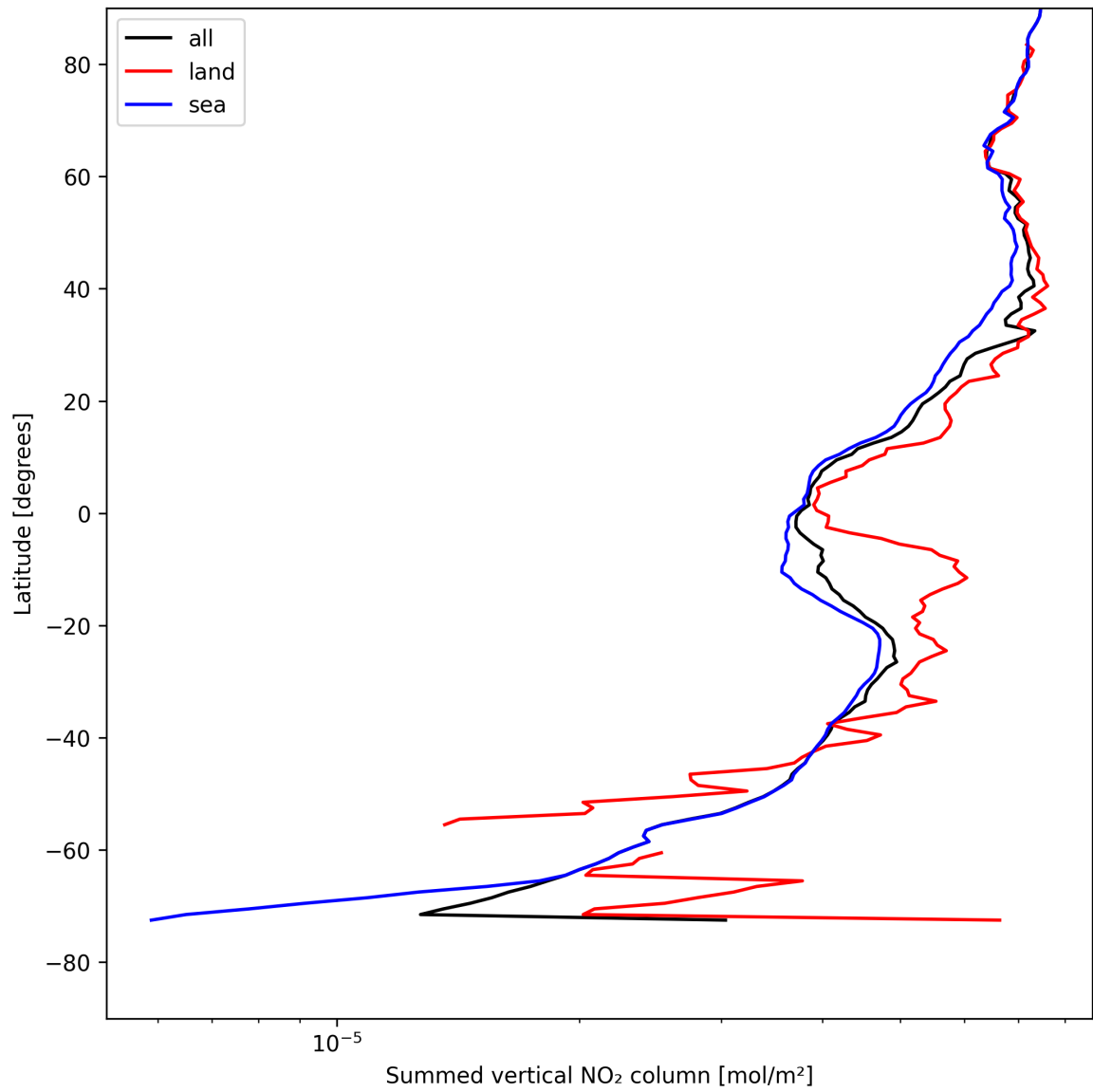
Figure 23: Zonal average of “Summed vertical NO 2 column” for 2025-08-10 to 2025-08-12.
