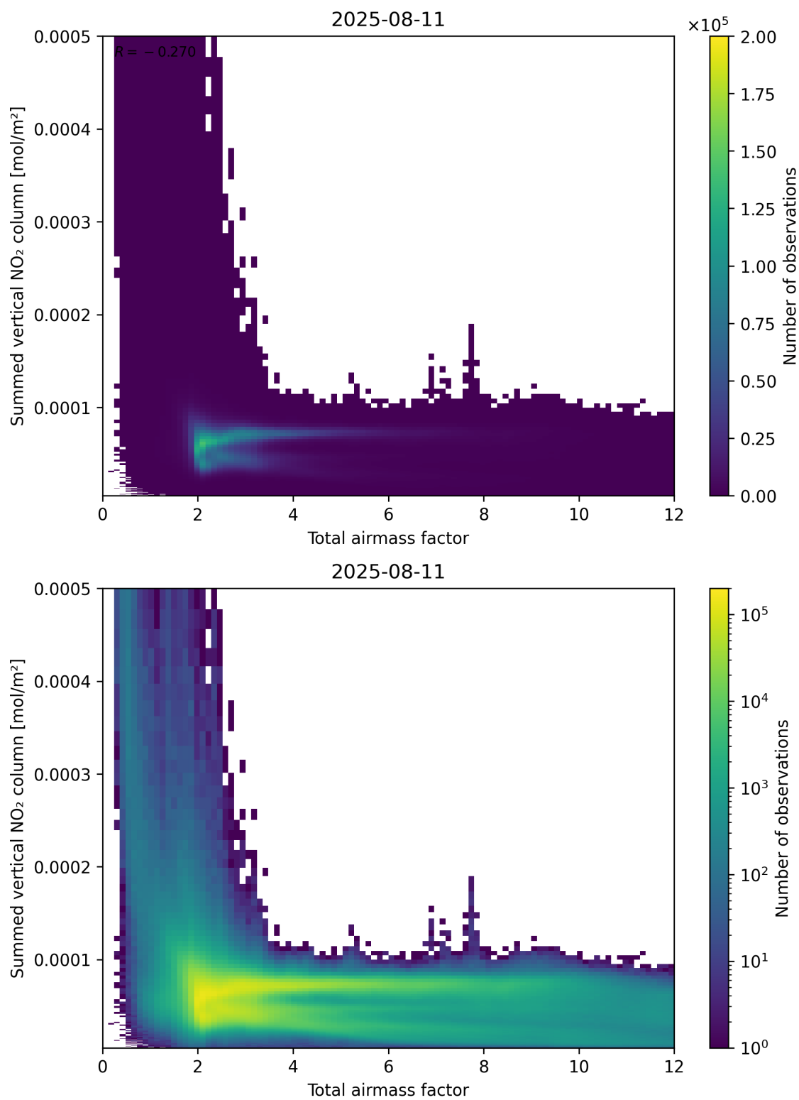
Figure 65: Scatter density plot of “Total airmass factor” against “Summed vertical NO 2 column” for 2025-08-10 to 2025-08-12.
