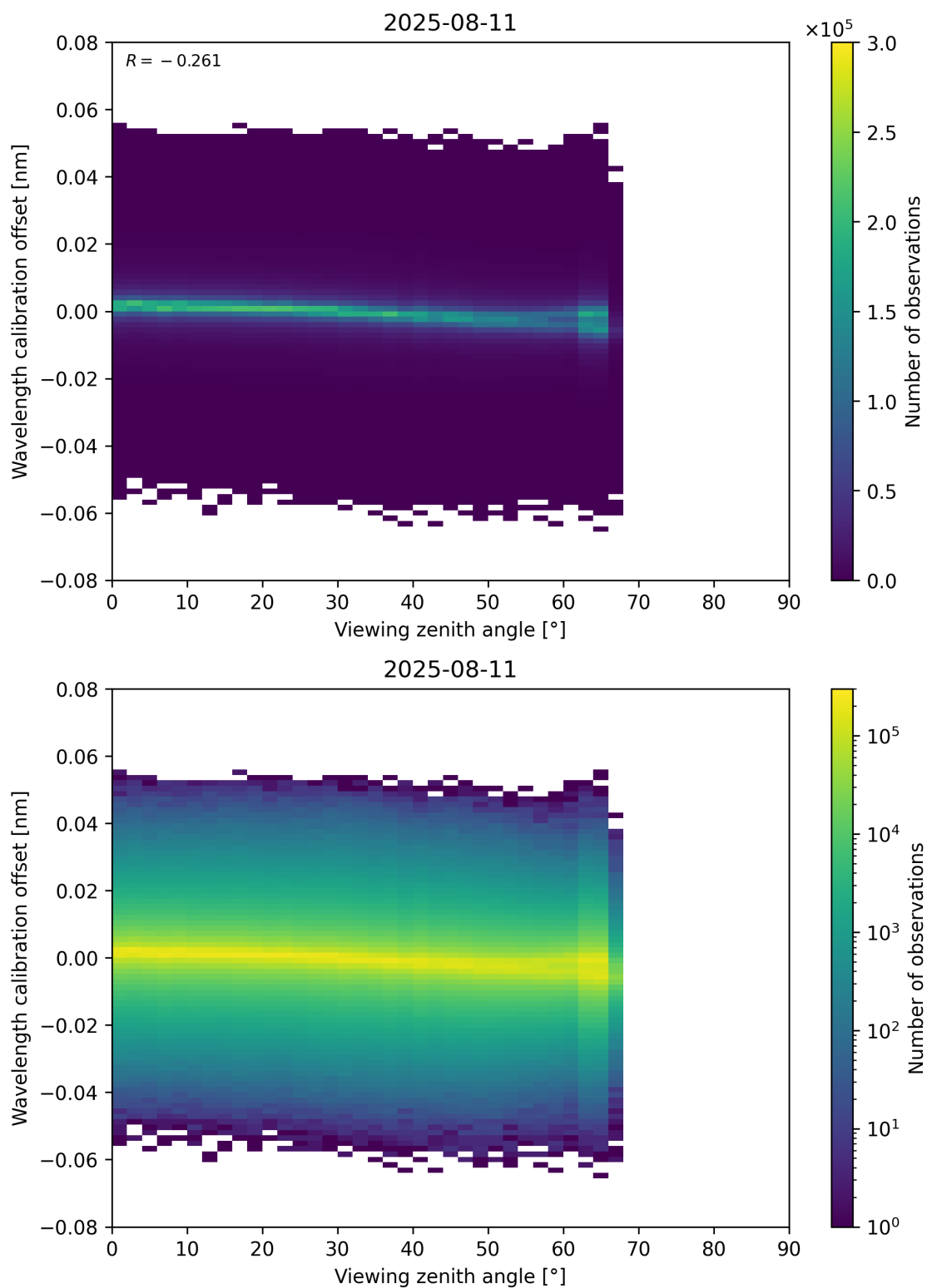
Figure 173: Scatter density plot of “Viewing zenith angle” against “Wavelength calibration offset” for 2025-08-10 to 2025-08-12.
