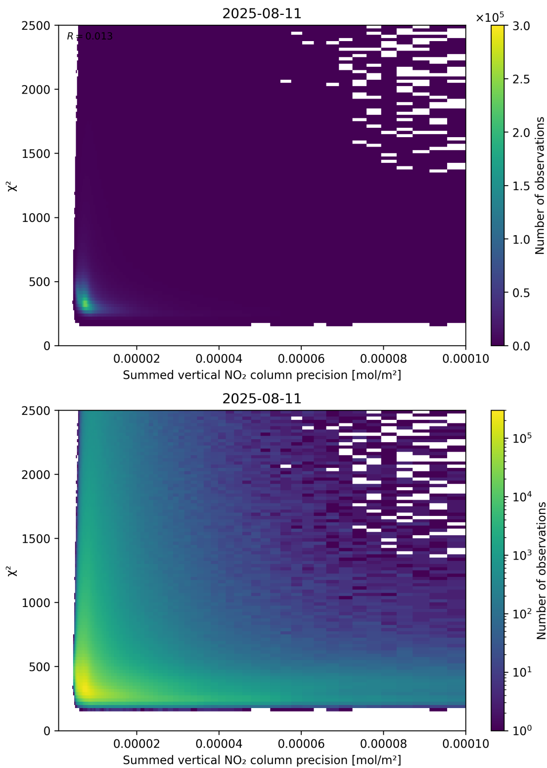
Figure 107: Scatter density plot of “Summed vertical NO 2 column precision” against “ \chi^2 ” for 2025-08-10 to 2025-08-12.
