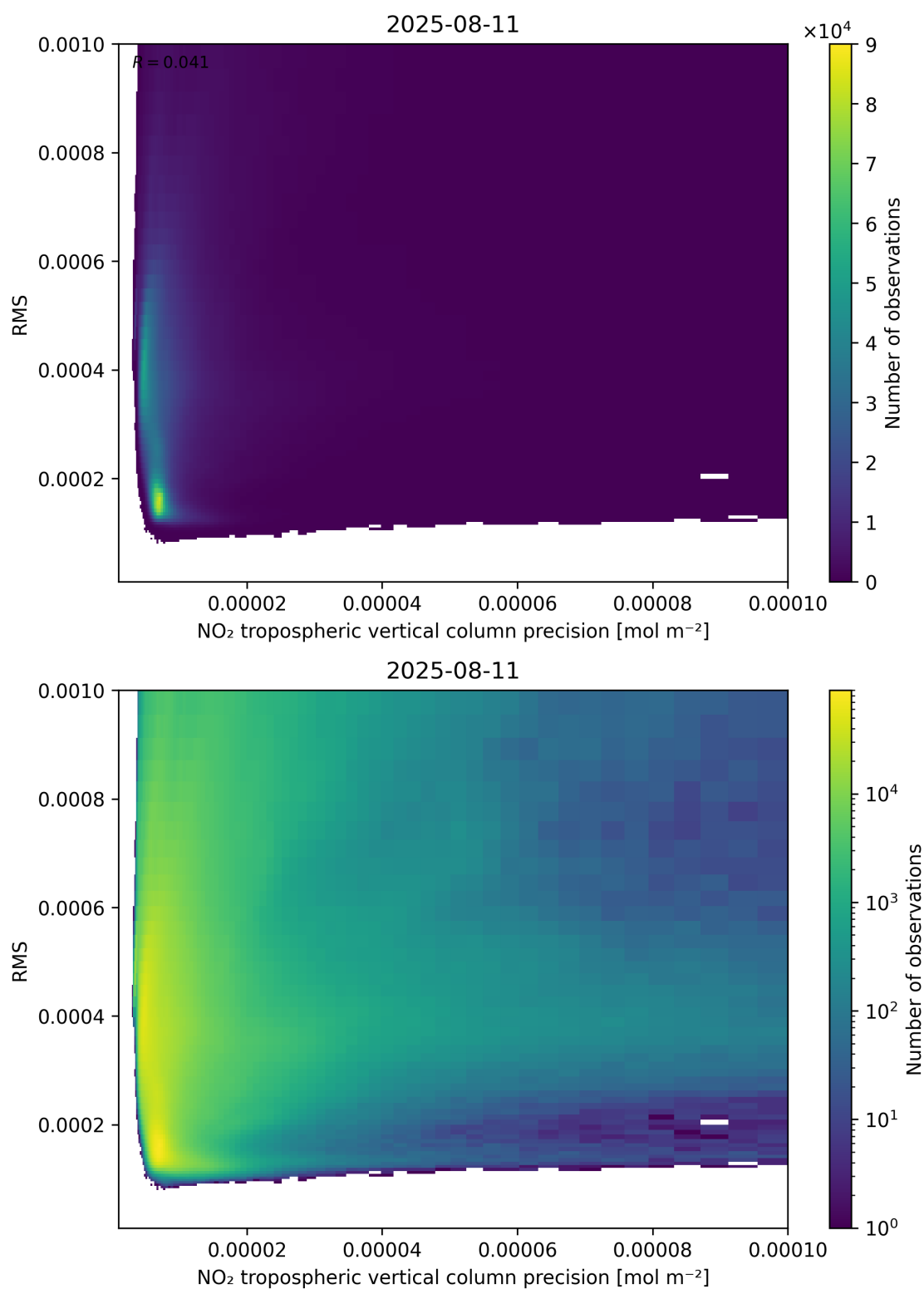
Figure 140: Scatter density plot of “NO 2 tropospheric vertical column precision” against “RMS” for 2025-08-10 to 2025-08-12.
