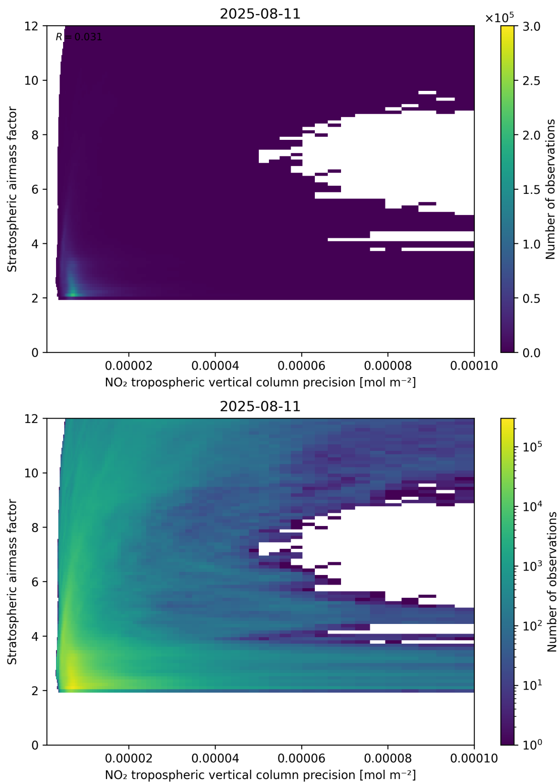
Figure 131: Scatter density plot of “NO 2 tropospheric vertical column precision” against “Stratospheric airmass factor” for 2025-08-10 to 2025-08-12.
