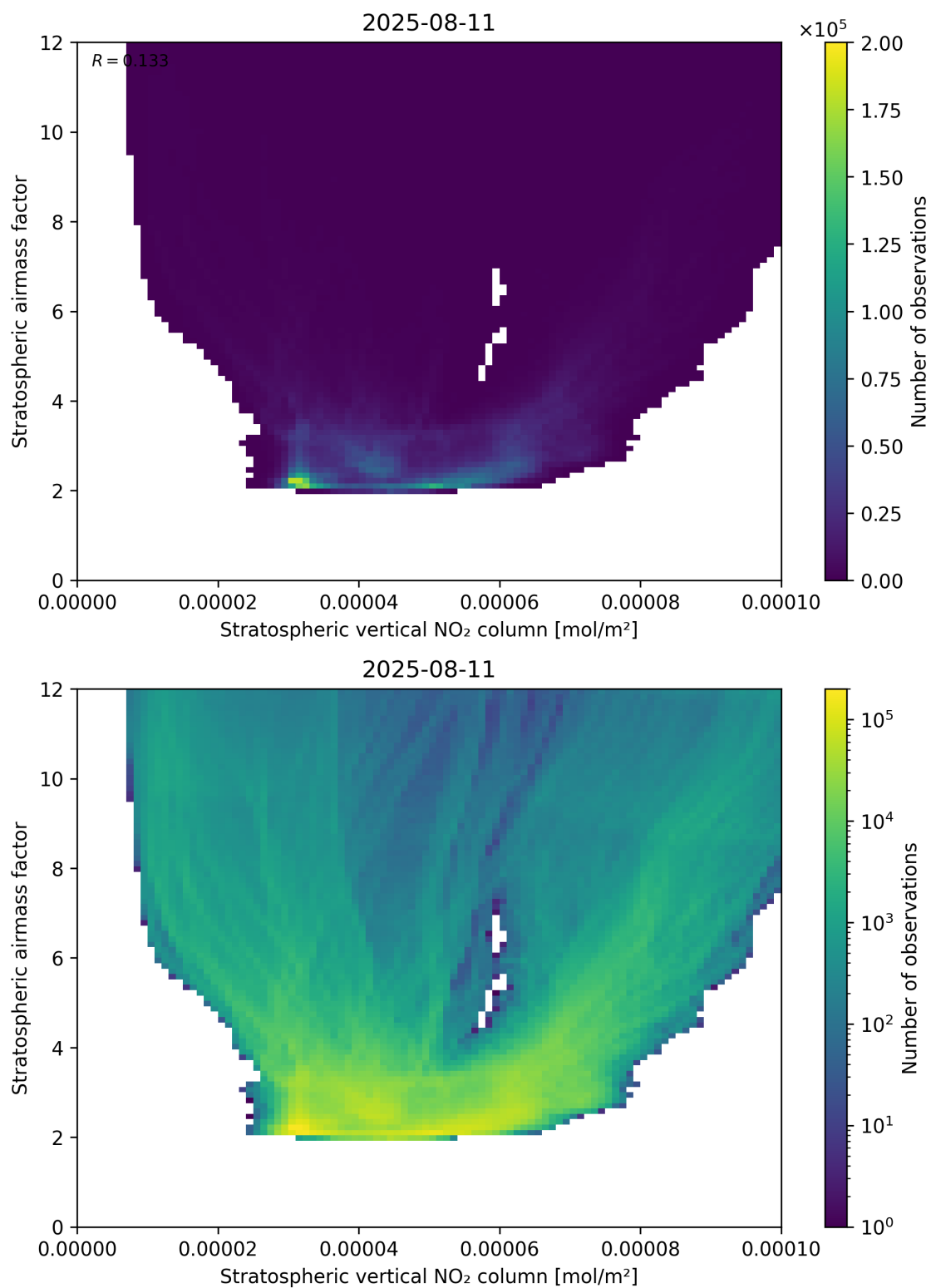
Figure 96: Scatter density plot of “Stratospheric vertical NO 2 column” against “Stratospheric airmass factor” for 2025-08-10 to 2025-08-12.
