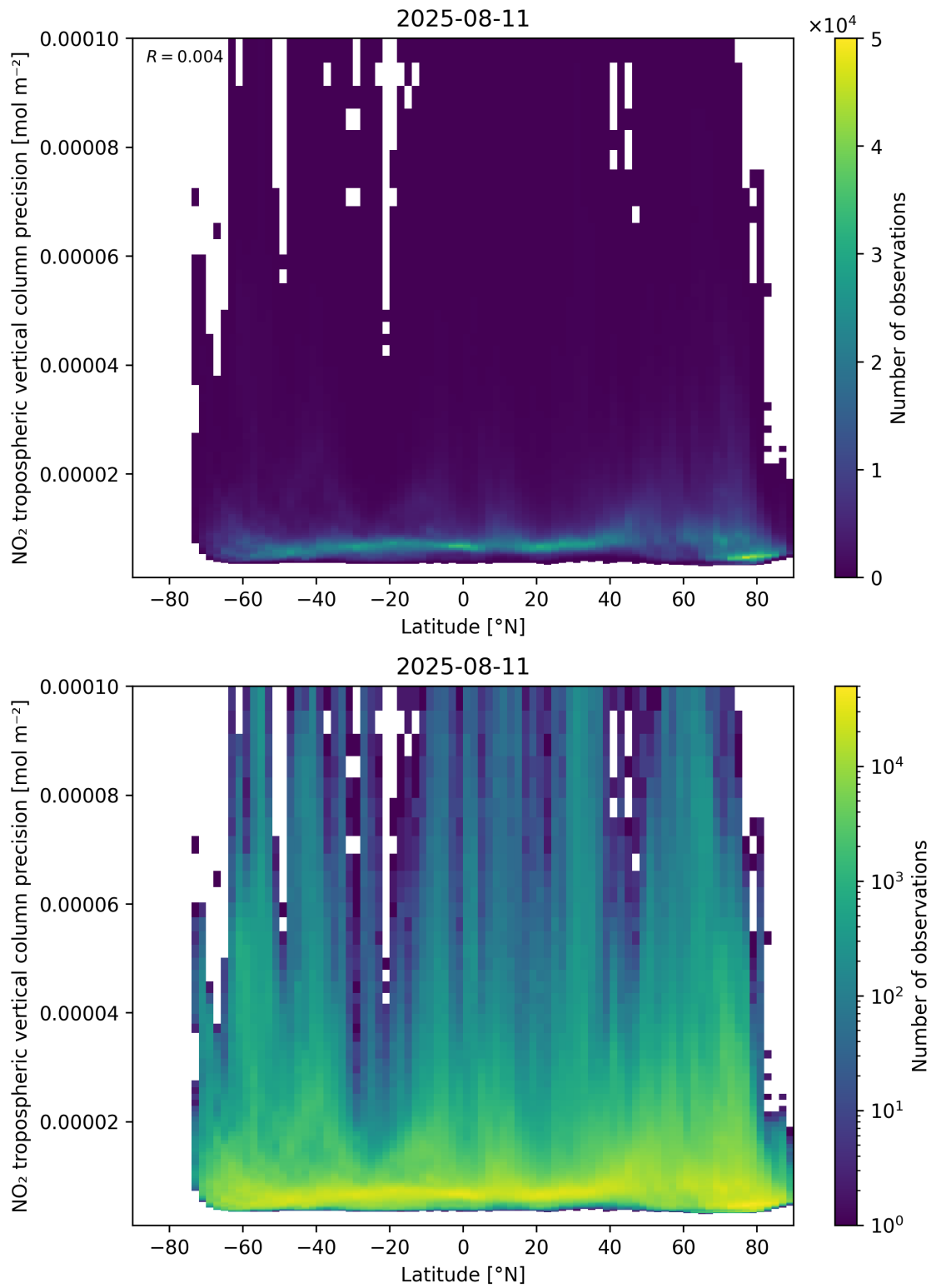
Figure 93: Scatter density plot of “Latitude” against “NO 2 tropospheric vertical column precision” for 2025-08-10 to 2025-08-12.
