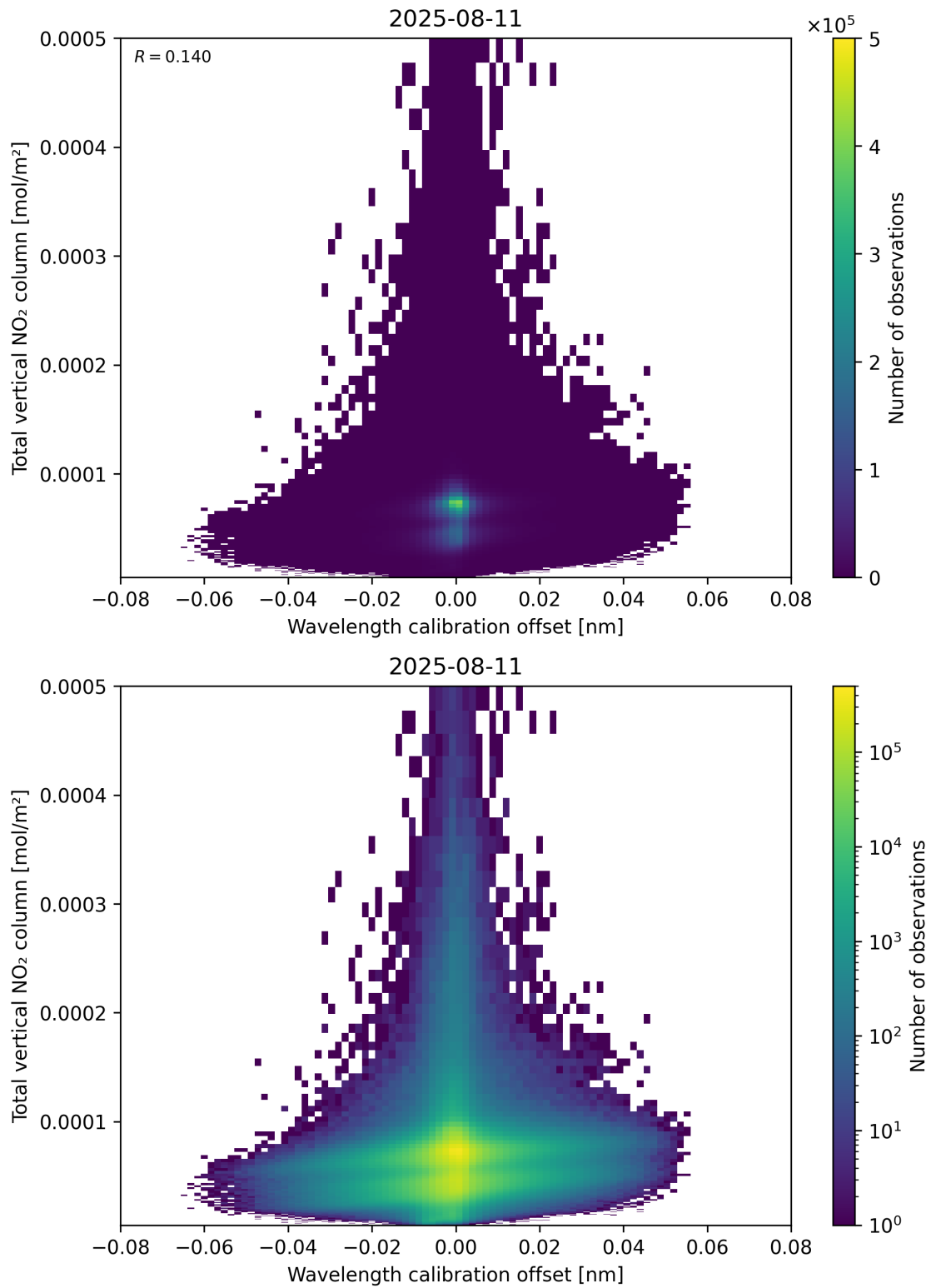
Figure 179: Scatter density plot of “Wavelength calibration offset” against “Total vertical NO 2 column” for 2025-08-10 to 2025-08-12.
