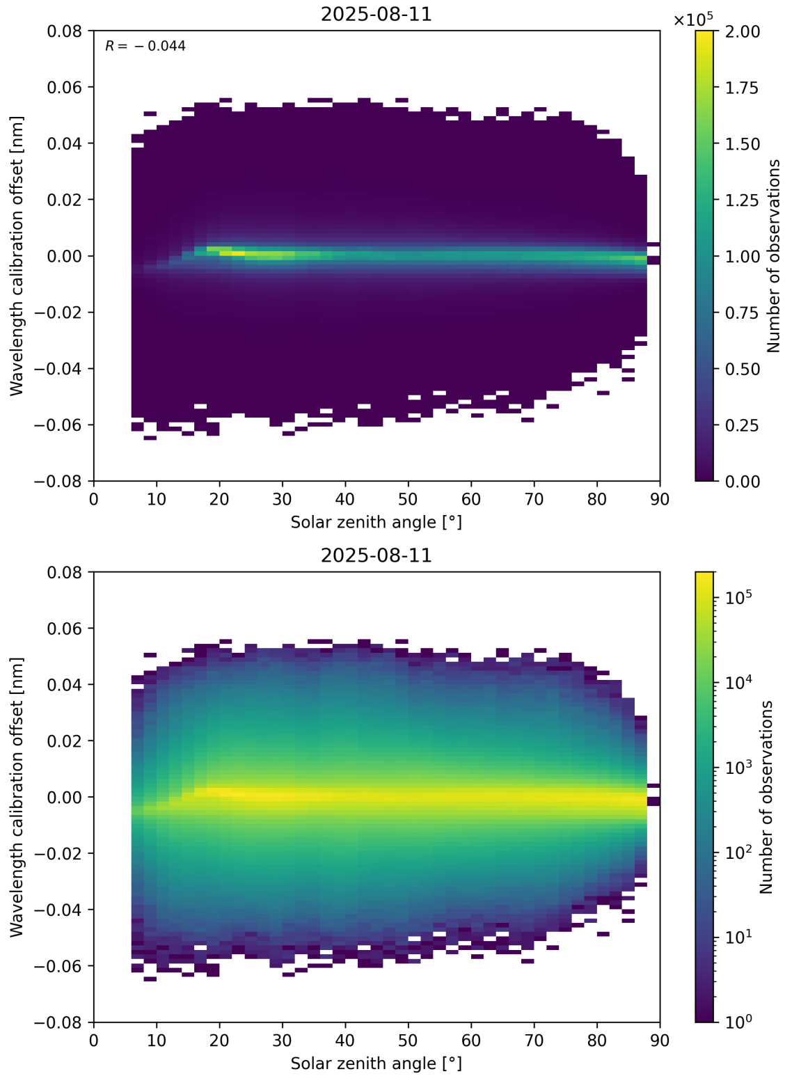
Figure 158: Scatter density plot of “Solar zenith angle” against “Wavelength calibration offset” for 2025-08-10 to 2025-08-12.
