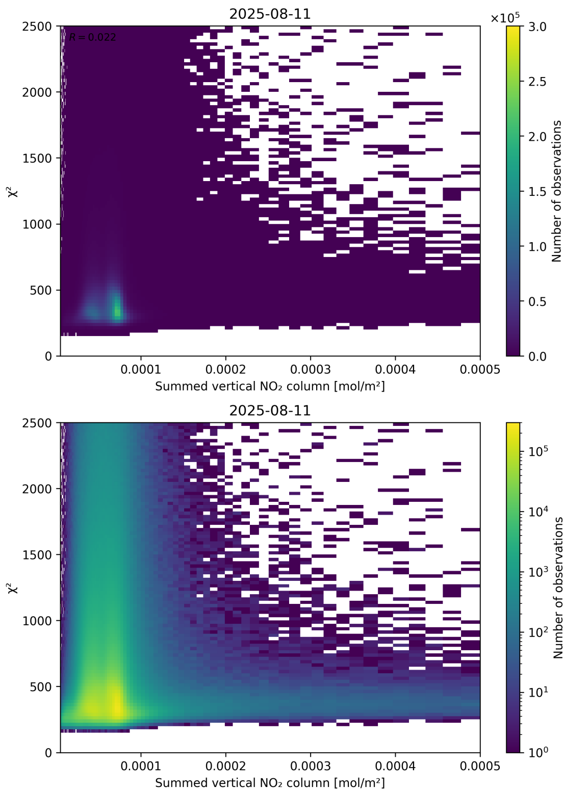
Figure 104: Scatter density plot of “Summed vertical NO 2 column” against “ \chi^2 ” for 2025-08-10 to 2025-08-12.
