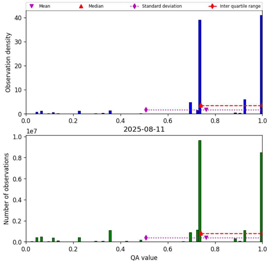
Figure 28: Histogram of “QA value” for 2025-08-10 to 2025-08-12
