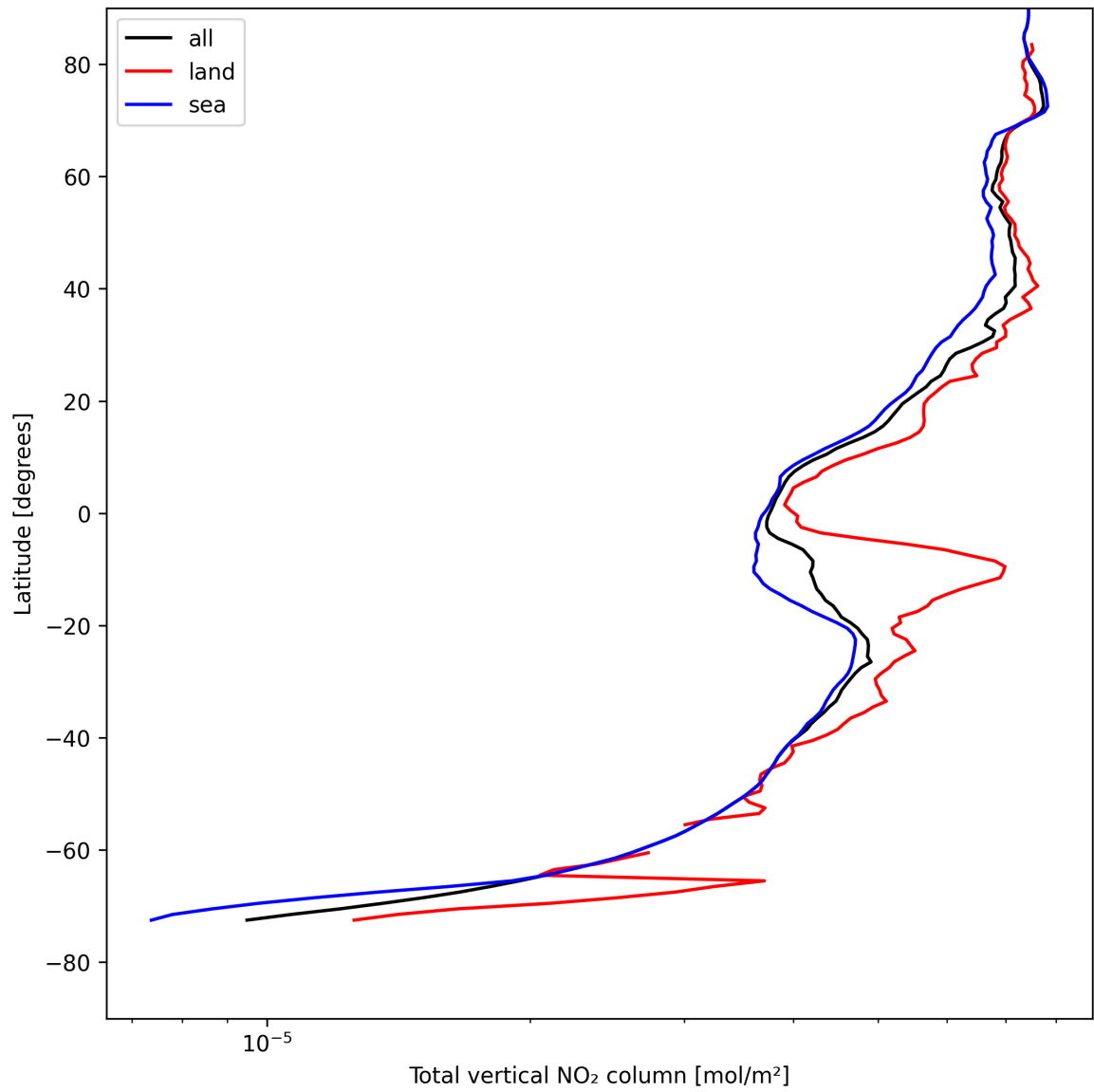
Figure 21: Zonal average of “Total vertical NO 2 column” for 2025-08-10 to 2025-08-12.
