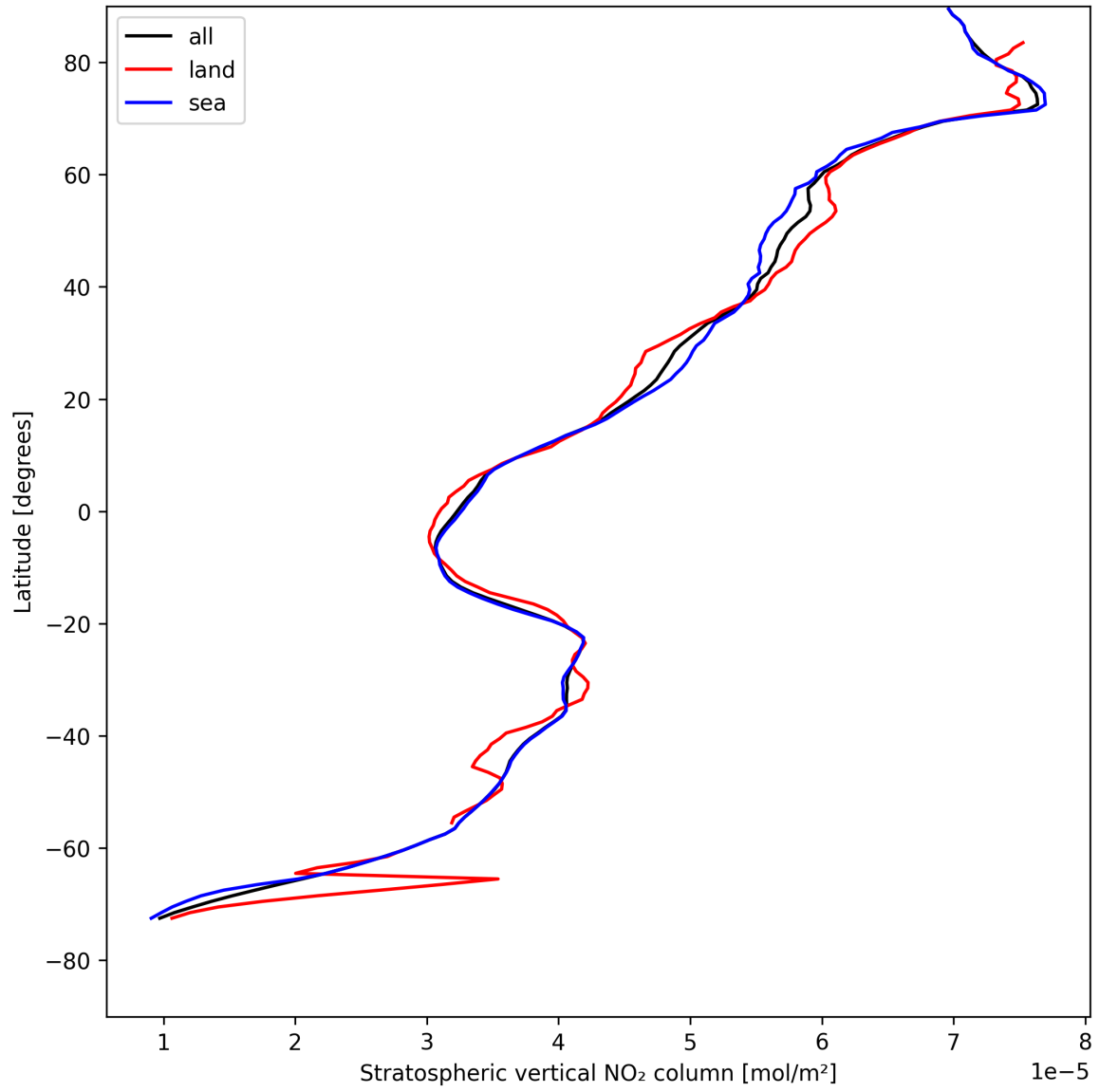
Figure 19: Zonal average of “Stratospheric vertical NO 2 column” for 2025-08-10 to 2025-08-12.
