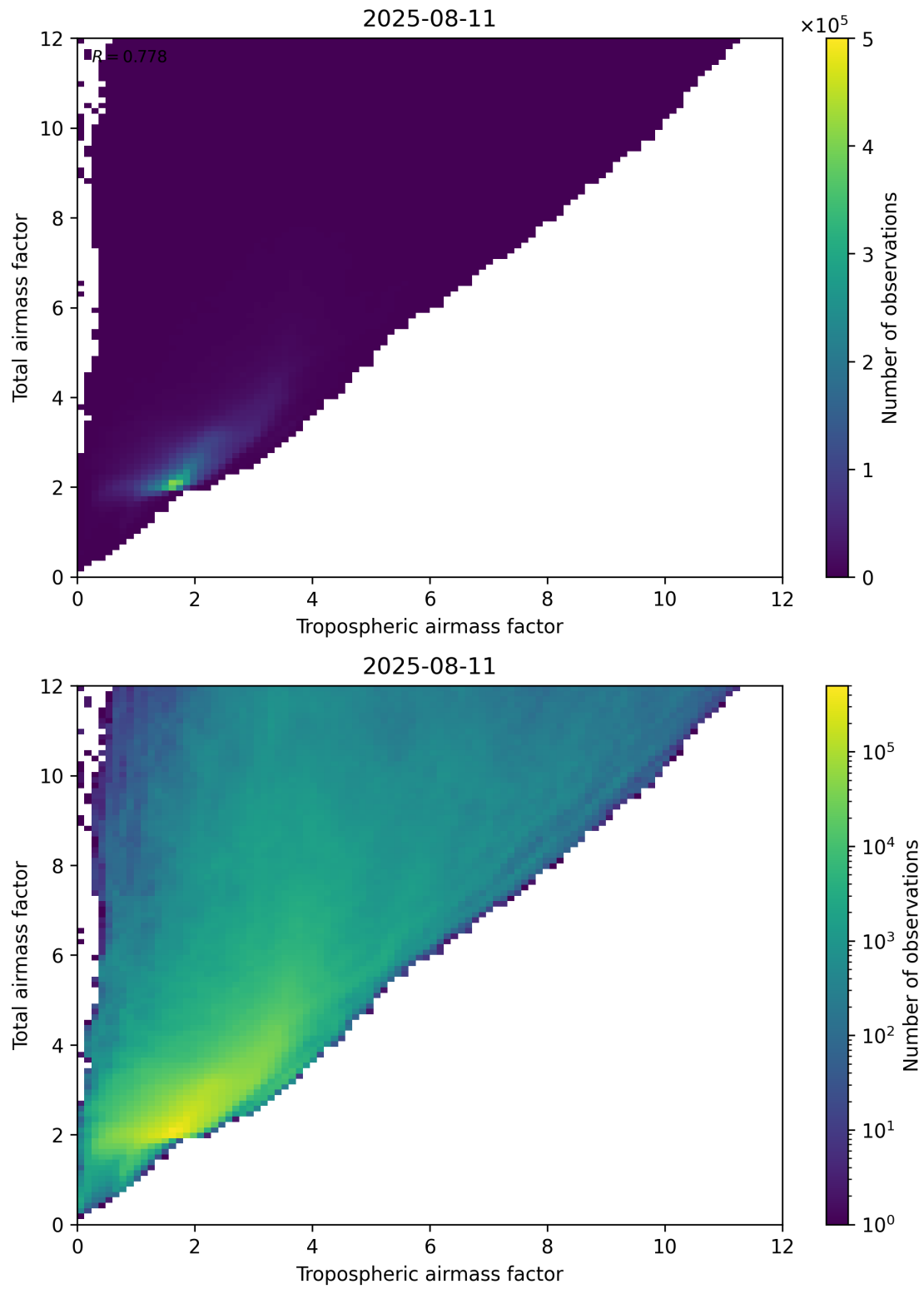
Figure 72: Scatter density plot of “Tropospheric airmass factor” against “Total airmass factor” for 2025-08-10 to 2025-08-12.
