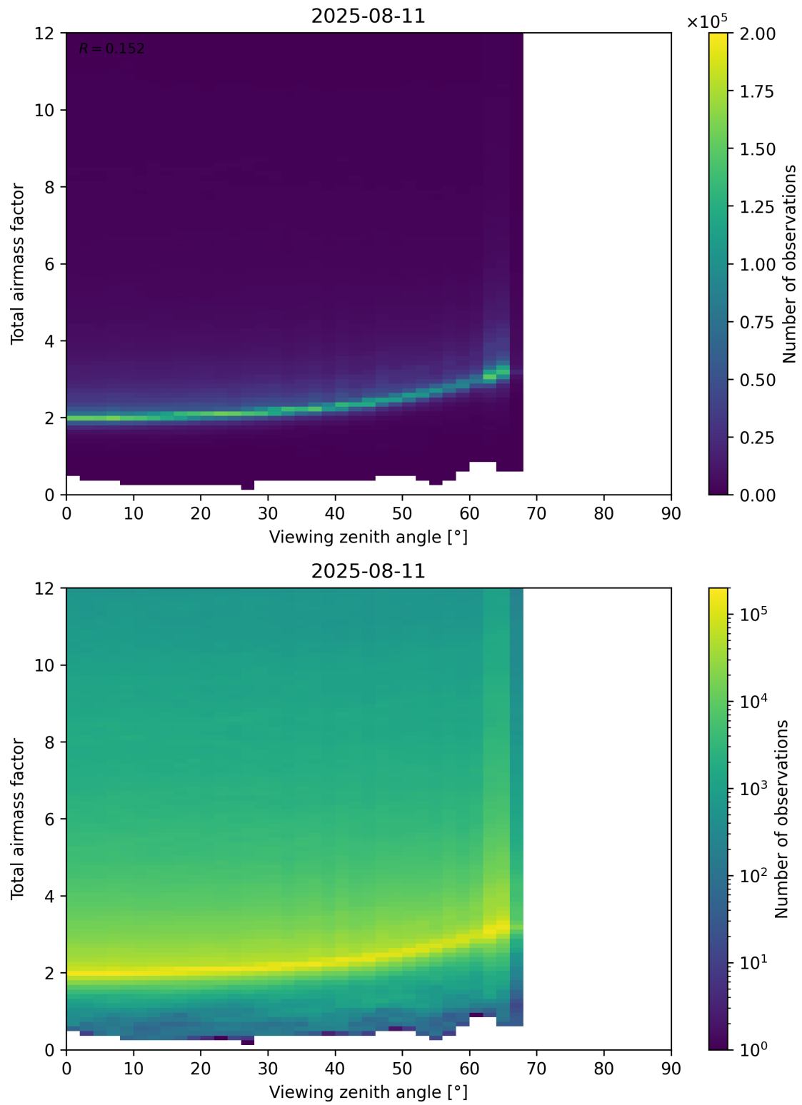
Figure 160: Scatter density plot of “Viewing zenith angle” against “Total airmass factor” for 2025-08-10 to 2025-08-12.
