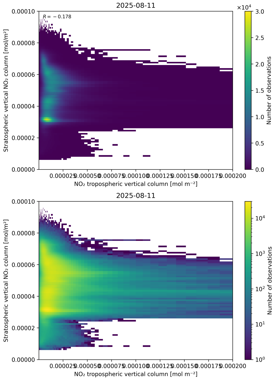
Figure 125: Scatter density plot of “NO 2 tropospheric vertical column” against “Stratospheric vertical NO 2 column” for 2025-08-10 to 2025-08-12.
