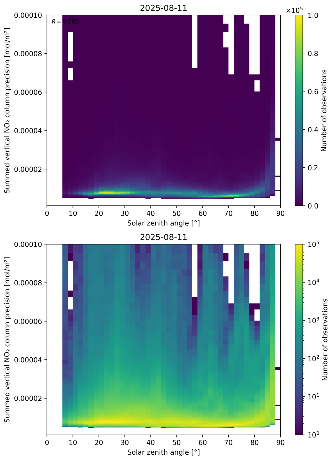
Figure 152: Scatter density plot of “Solar zenith angle” against “Summed vertical NO 2 column precision” for 2025-08-10 to 2025-08-12.
