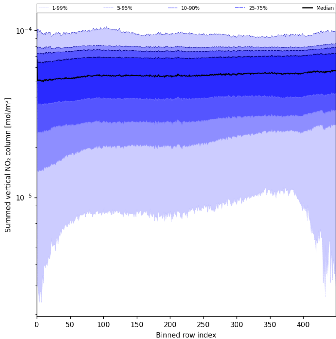
Figure 57: Along track statistics of “Summed vertical NO 2 column” for 2025-08-10 to 2025-08-12
