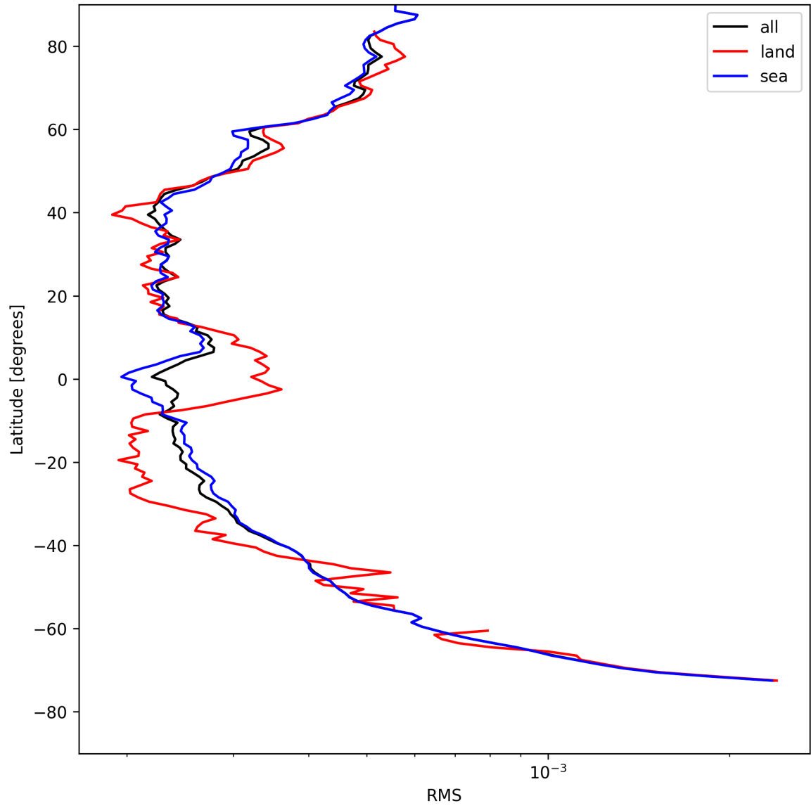
Figure 26: Zonal average of “RMS” for 2025-08-10 to 2025-08-12.
