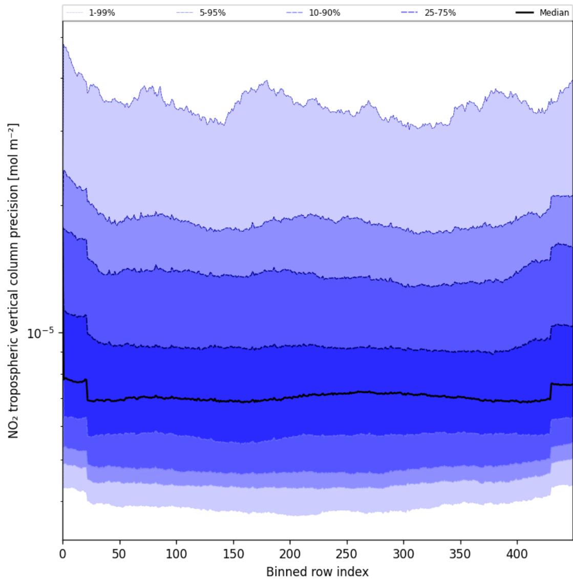
Figure 47: Along track statistics of “NO 2 tropospheric vertical column precision” for 2025-08-10 to 2025-08-12
