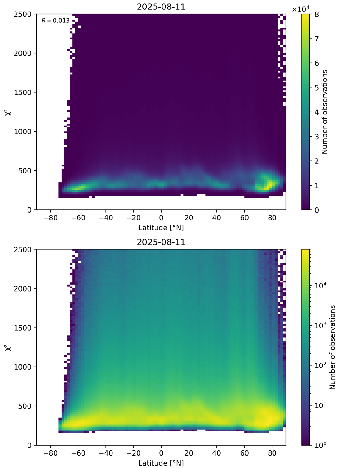
Figure 86: Scatter density plot of “Latitude” against “ \chi^2 ” for 2025-08-10 to 2025-08-12.
