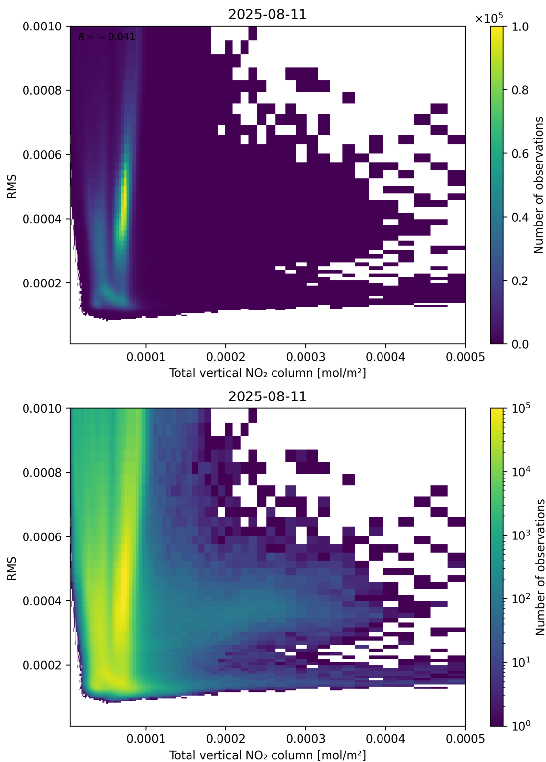
Figure 120: Scatter density plot of “Total vertical NO 2 column” against “RMS” for 2025-08-10 to 2025-08-12.
