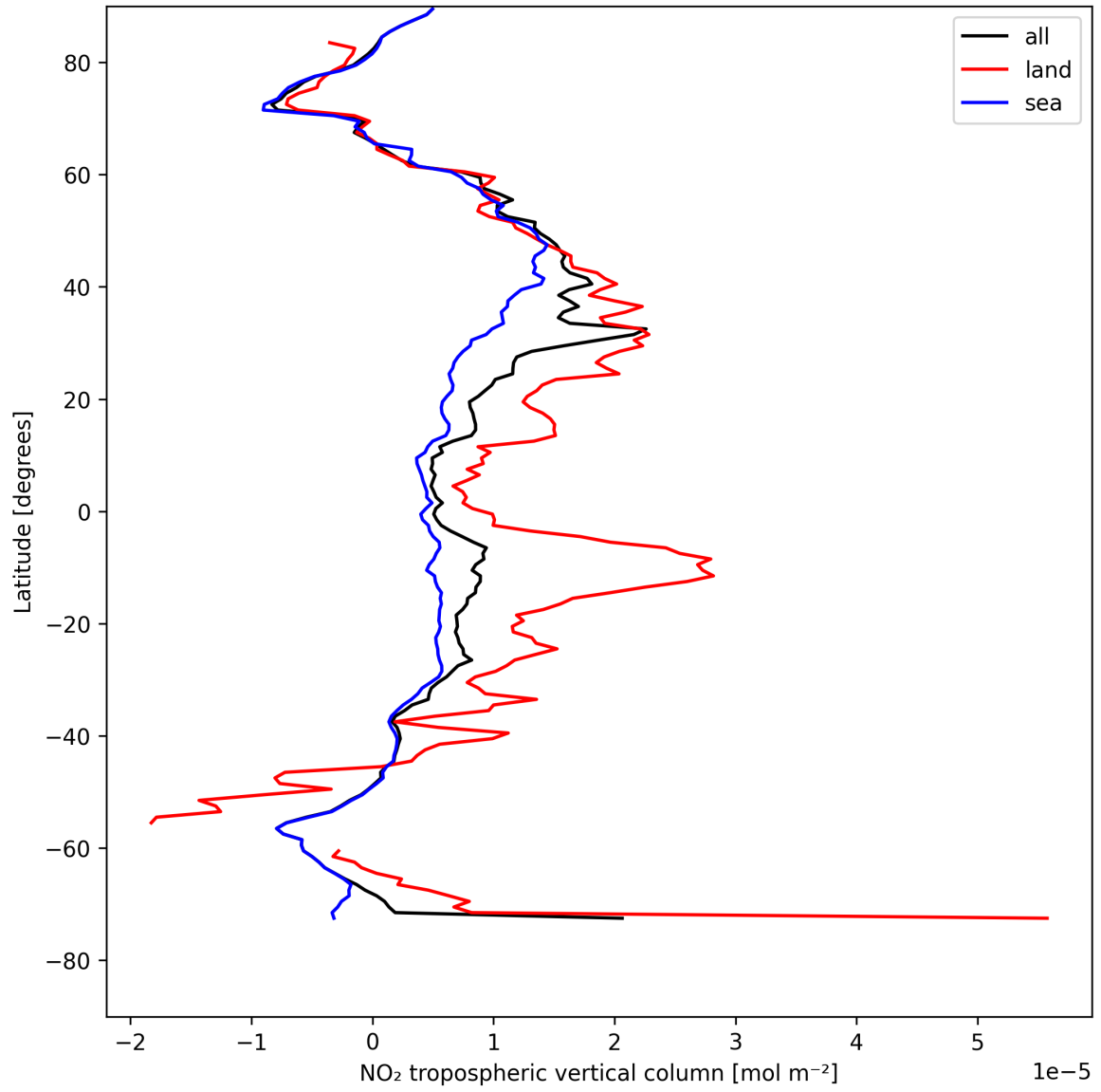
Figure 12: Zonal average of “NO 2 tropospheric vertical column” for 2025-08-10 to 2025-08-12.
