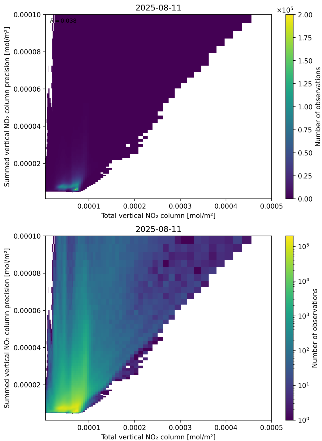
Figure 113: Scatter density plot of “Total vertical NO 2 column” against “Summed vertical NO 2 column precision” for 2025-08-10 to 2025-08-12.
