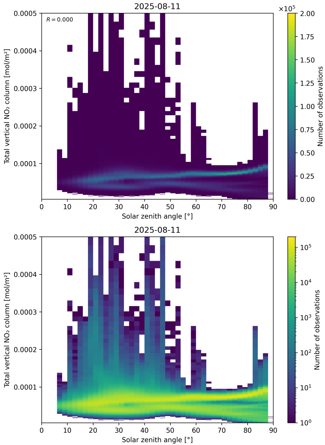
Figure 153: Scatter density plot of “Solar zenith angle” against “Total vertical NO 2 column” for 2025-08-10 to 2025-08-12.
