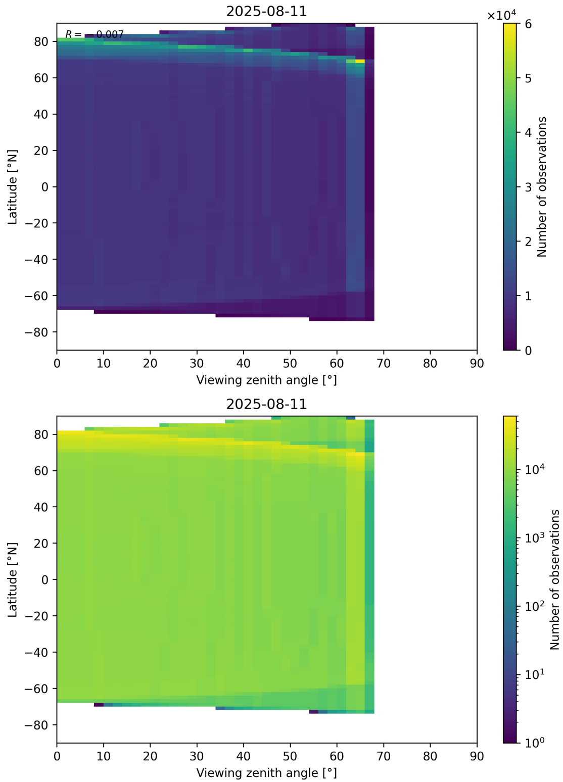
Figure 163: Scatter density plot of “Viewing zenith angle” against “Latitude” for 2025-08-10 to 2025-08-12.
