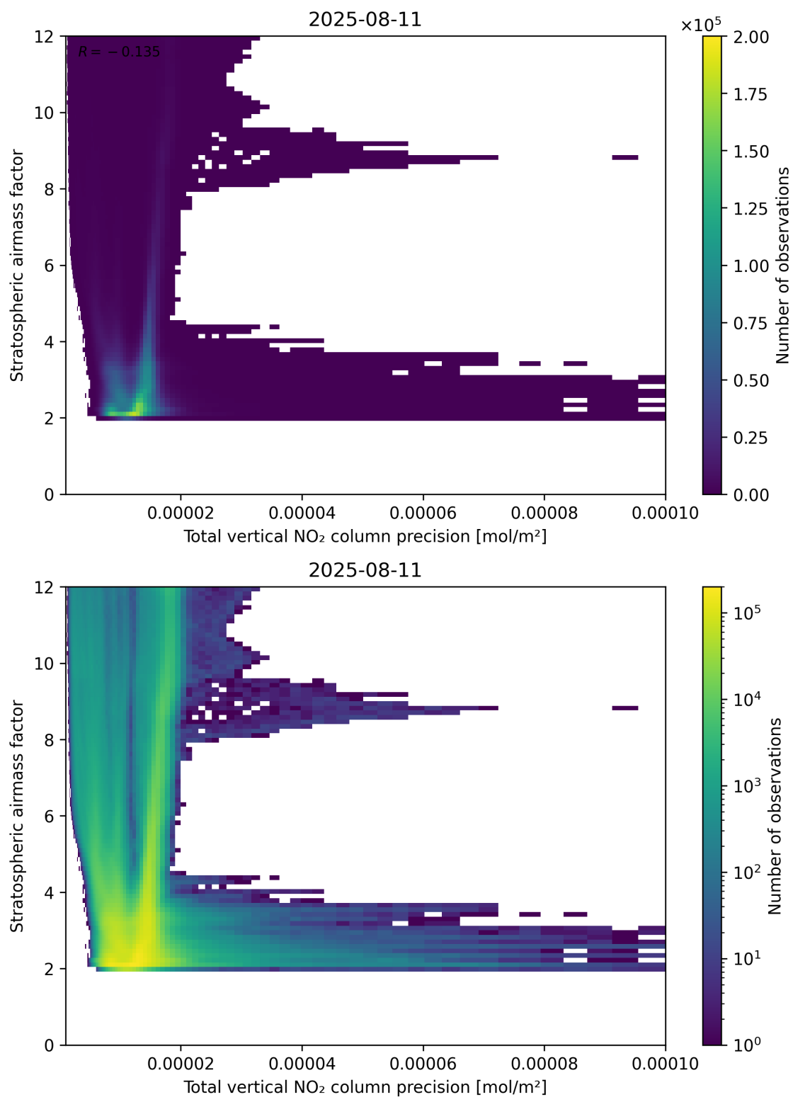
Figure 115: Scatter density plot of “Total vertical NO 2 column precision” against “Stratospheric air mass factor” for 2025-08-10 to 2025-08-12.
