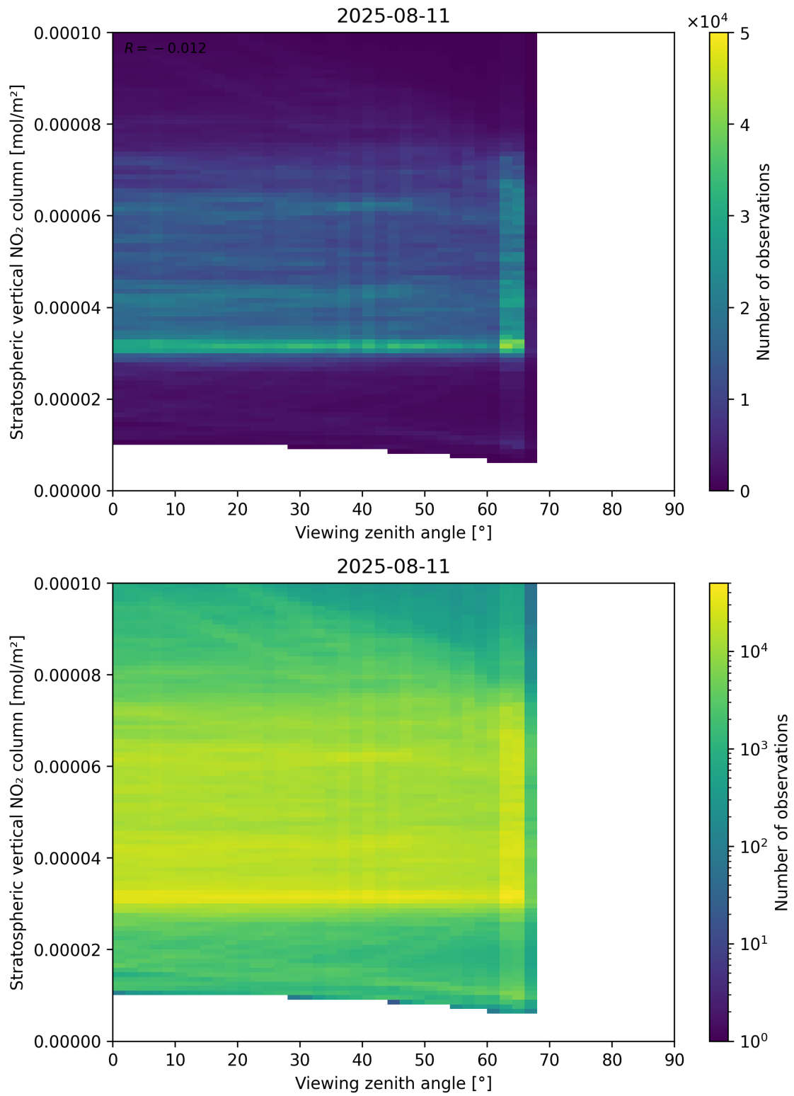
Figure 164: Scatter density plot of “Viewing zenith angle” against “Stratospheric vertical NO 2 column” for 2025-08-10 to 2025-08-12.
