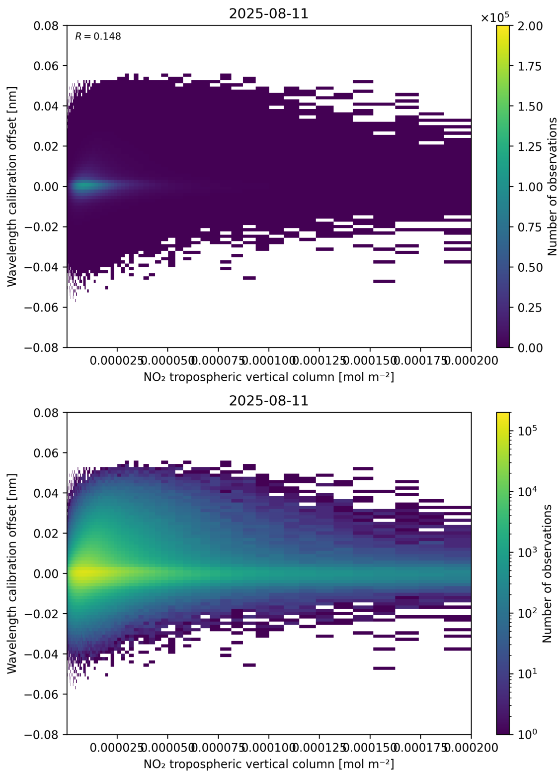
Figure 143: Scatter density plot of “NO 2 tropospheric vertical column” against “Wavelength calibration offset” for 2025-08-10 to 2025-08-12.
