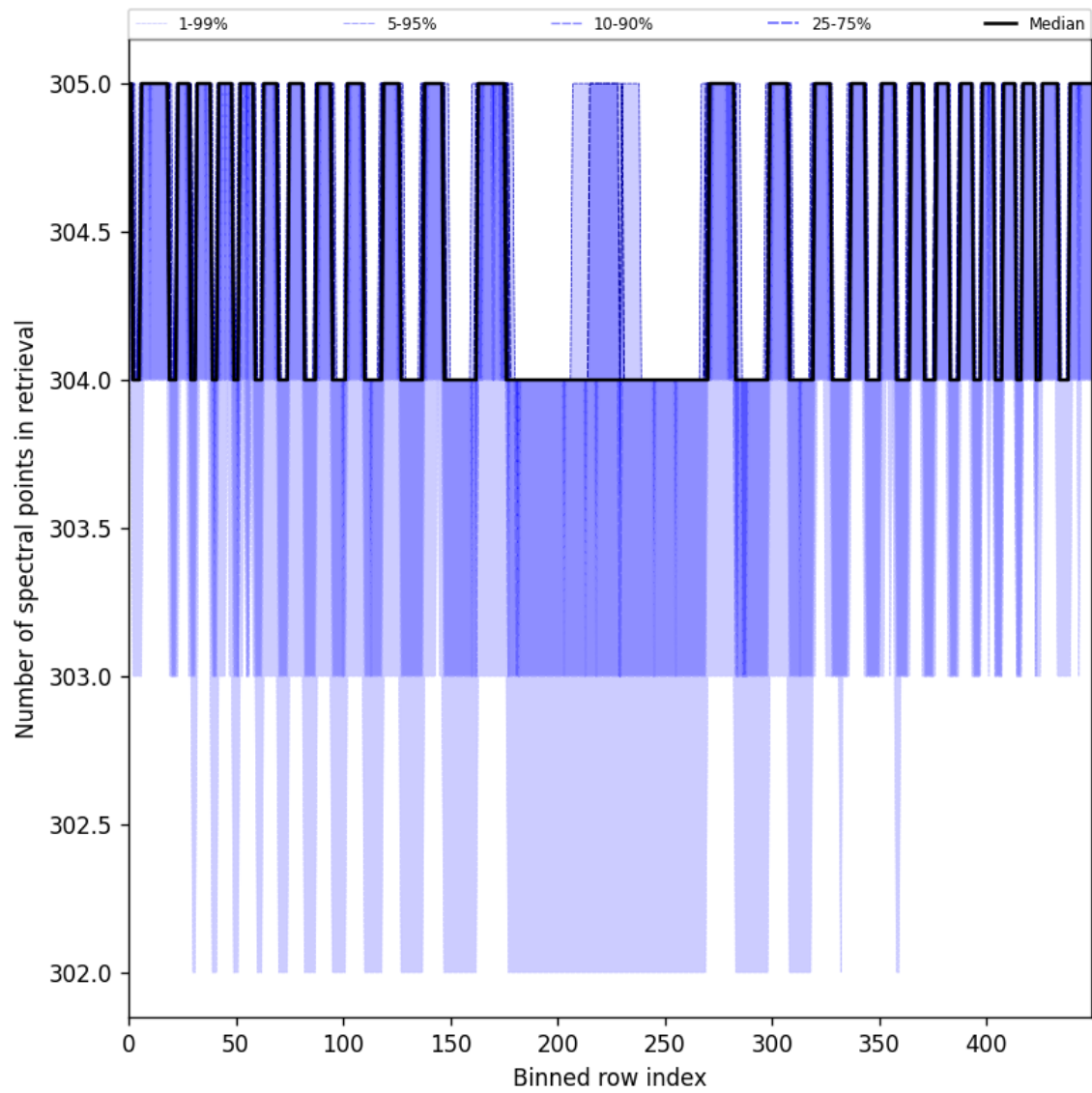
Figure 50: Along track statistics of “Number of spectral points in retrieval” for 2025-08-10 to 2025-08-12
