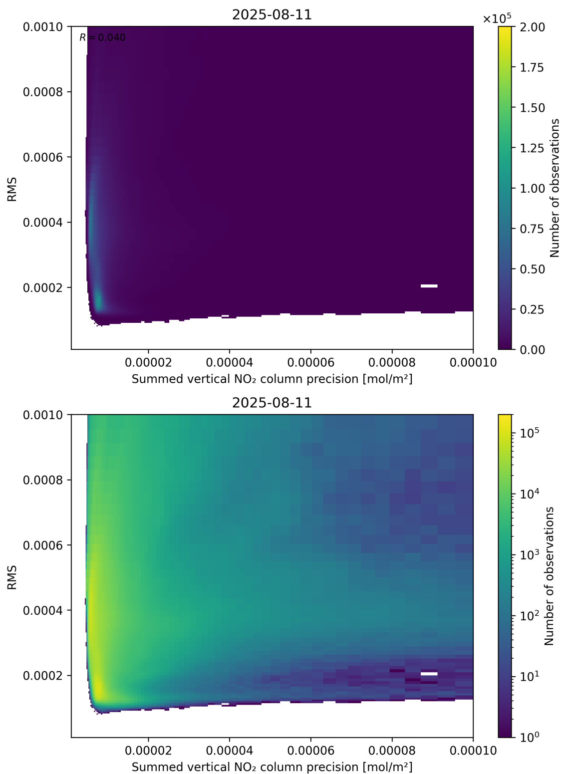
Figure 108: Scatter density plot of “Summed vertical NO 2 column precision” against “RMS” for 2025-08-10 to 2025-08-12.
