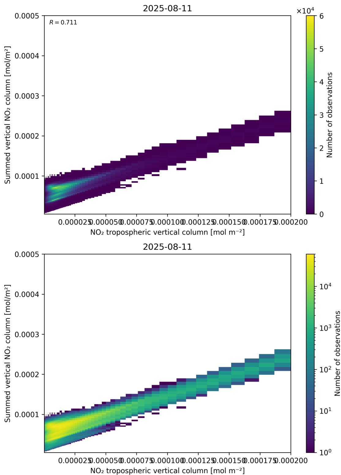
Figure 126: Scatter density plot of “NO 2 tropospheric vertical column” against “Summed vertical NO 2 column” for 2025-08-10 to 2025-08-12.
