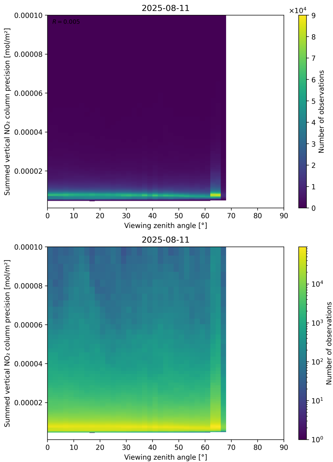
Figure 166: Scatter density plot of “Viewing zenith angle” against “Summed vertical NO 2 column precision” for 2025-08-10 to 2025-08-12.
