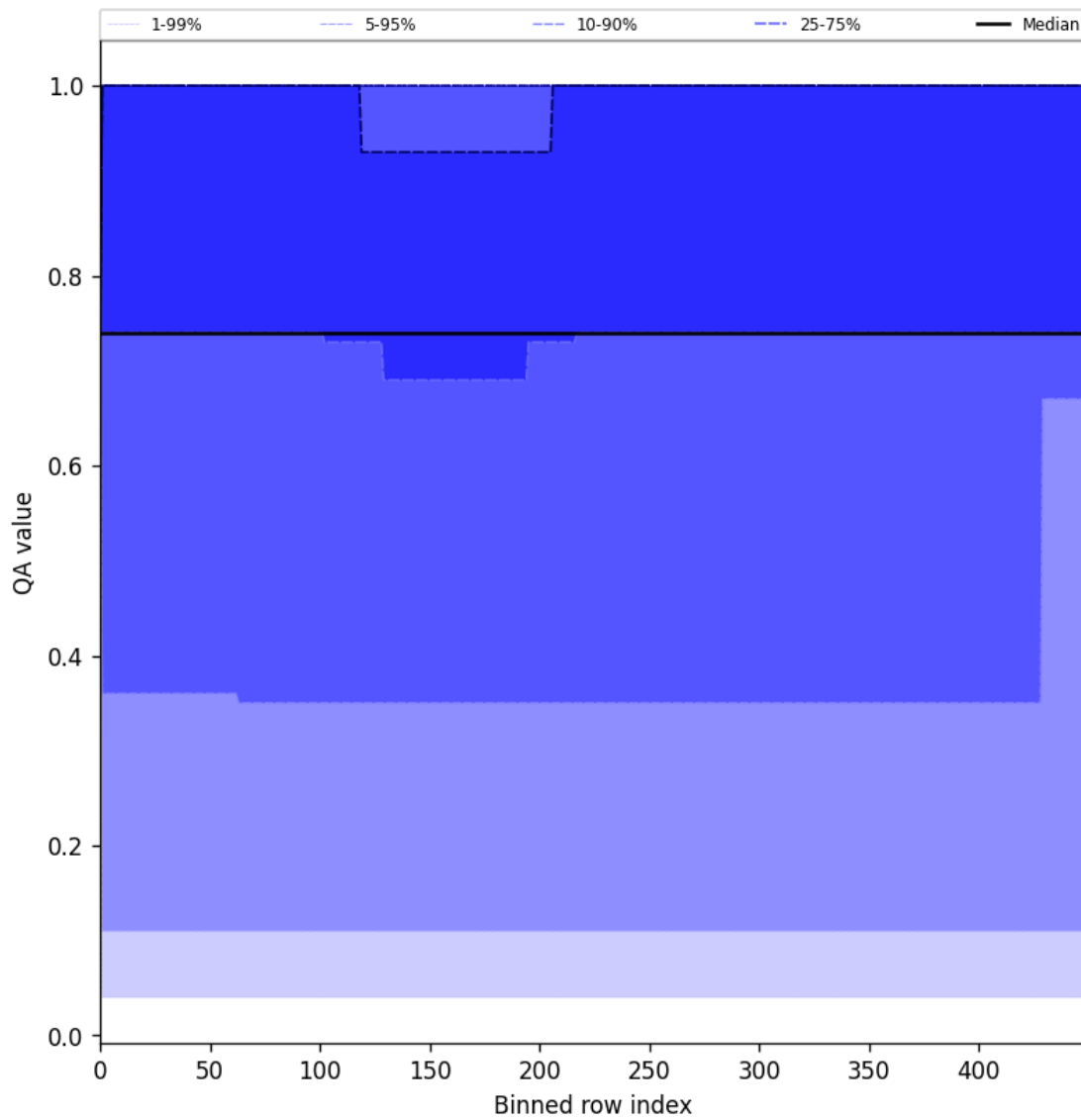
Figure 45: Along track statistics of “QA value” for 2025-08-10 to 2025-08-12
