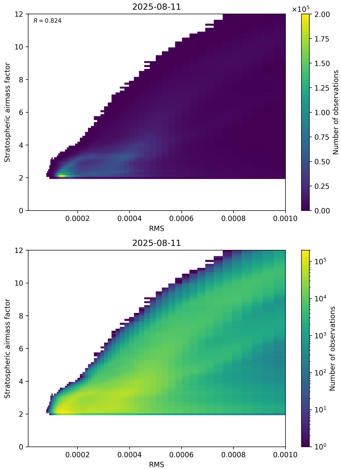
Figure 144: Scatter density plot of “RMS” against “Stratospheric airmass factor” for 2025-08-10 to 2025-08-12.
