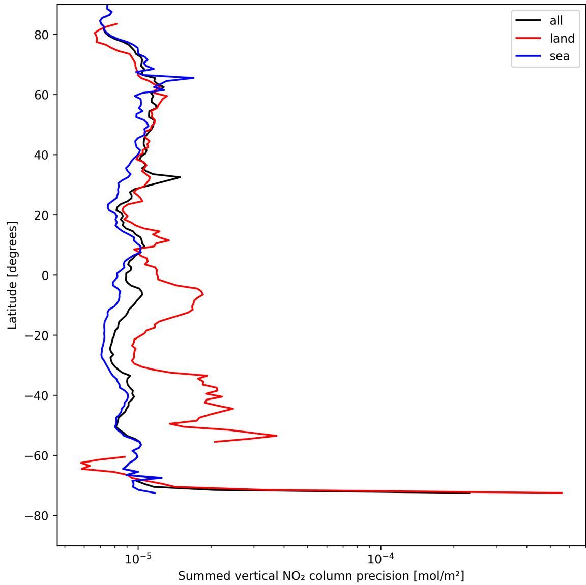
Figure 24: Zonal average of “Summed vertical NO 2 column precision” for 2025-08-10 to 2025-08-12.
