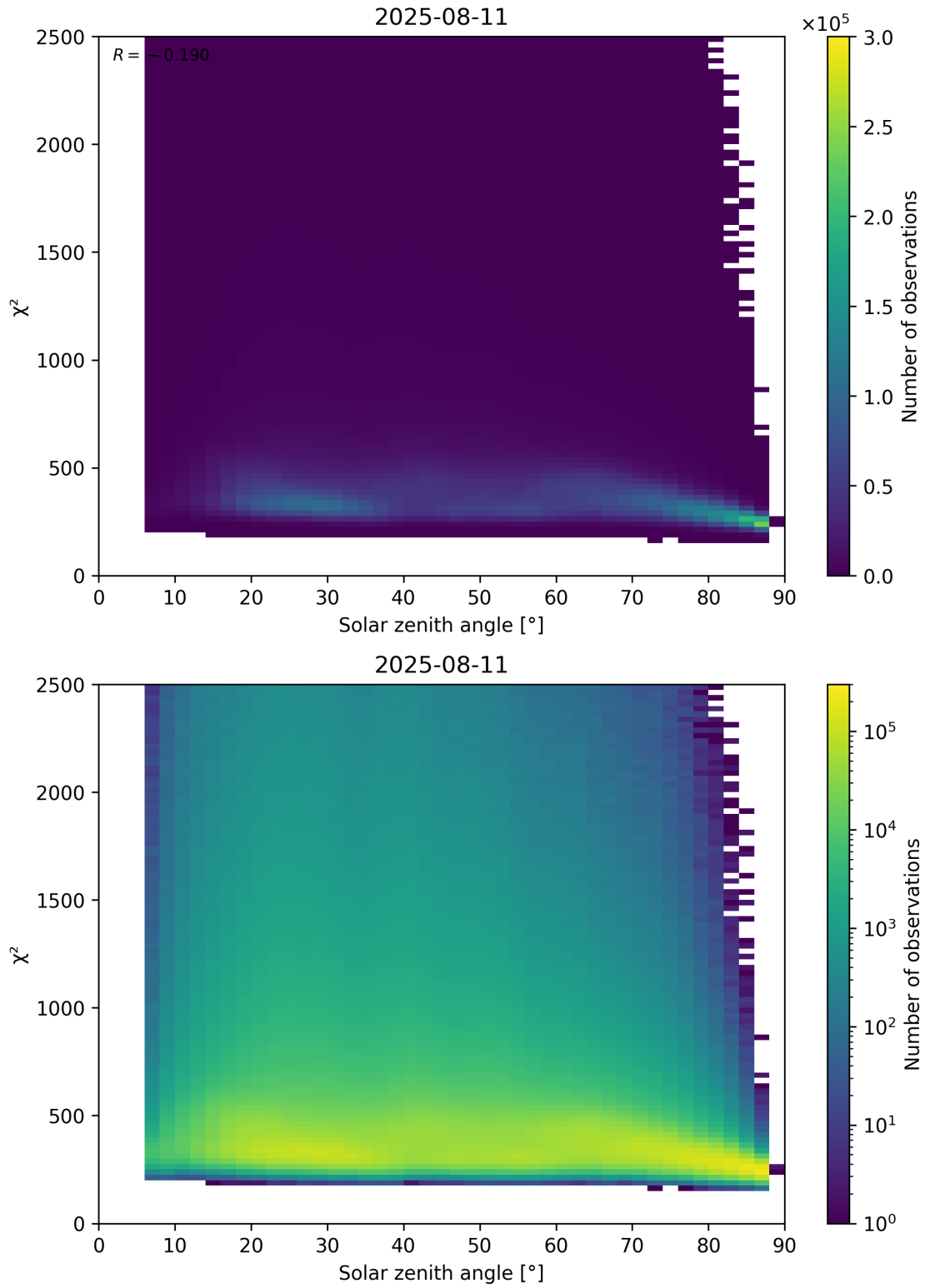
Figure 148: Scatter density plot of “Solar zenith angle” against “ \chi^2 ” for 2025-08-10 to 2025-08-12.
