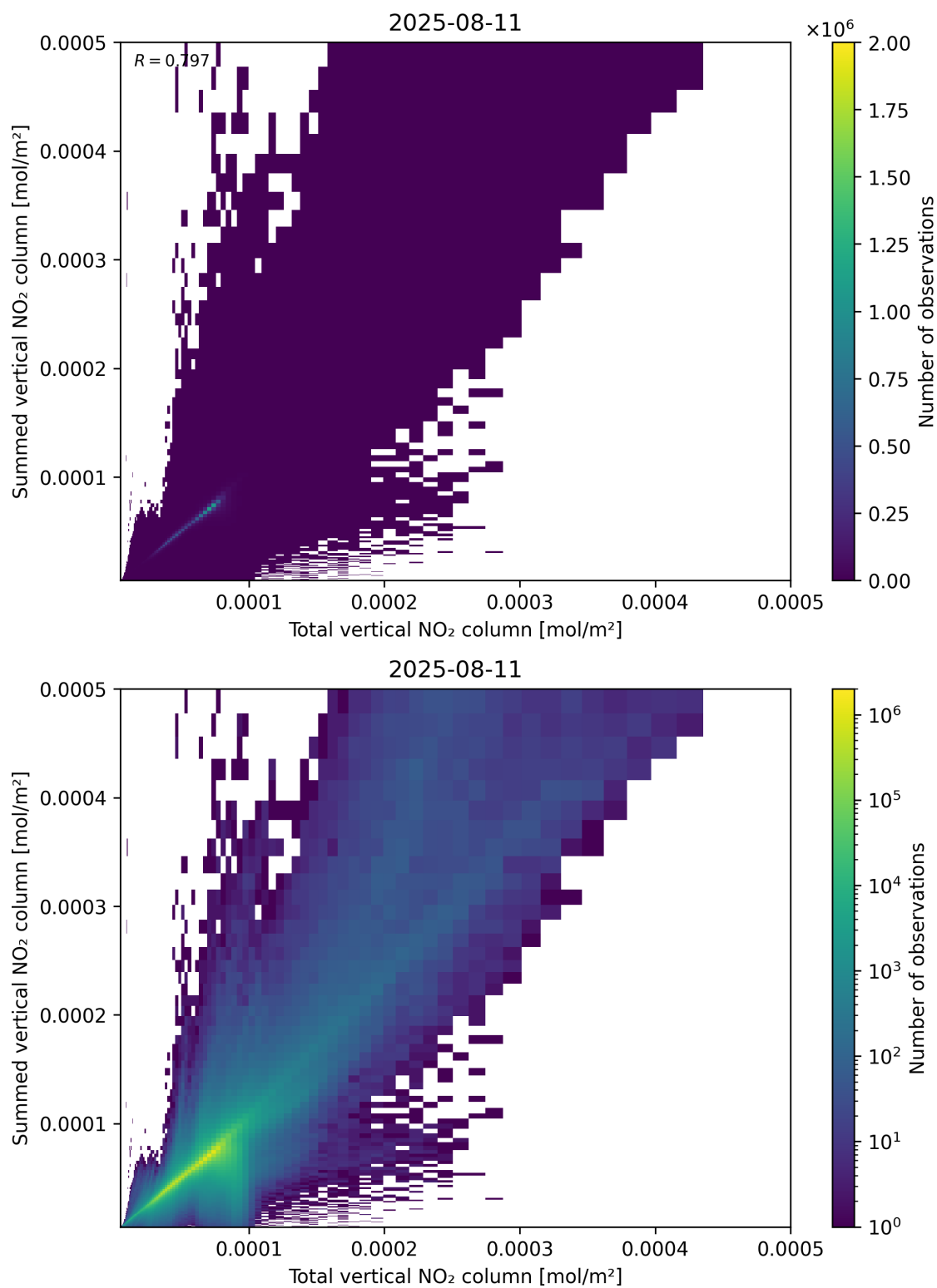
Figure 112: Scatter density plot of “Total vertical NO 2 column” against “Summed vertical NO 2 column” for 2025-08-10 to 2025-08-12.
