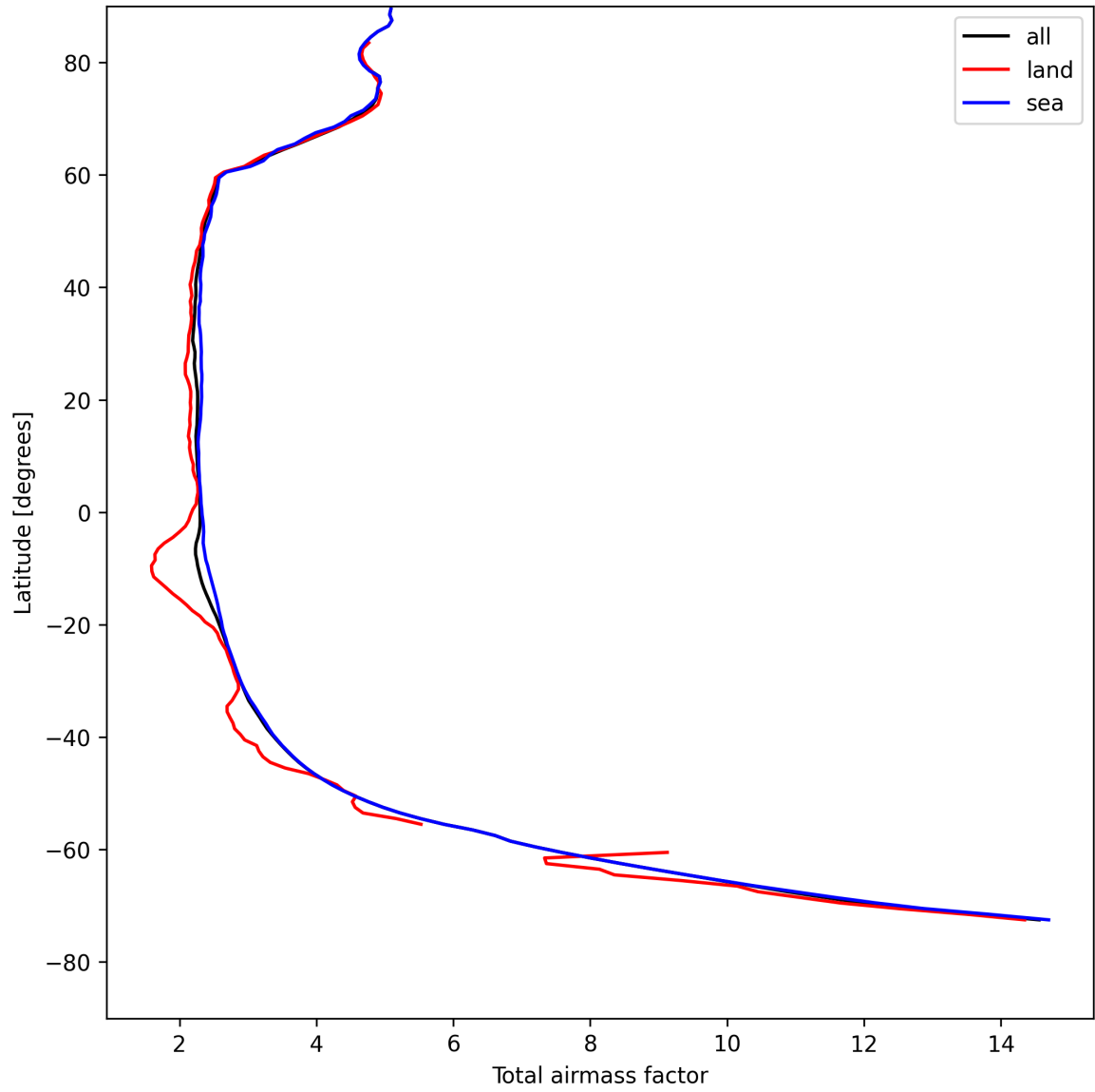
Figure 15: Zonal average of “Total airmass factor” for 2025-08-10 to 2025-08-12.
