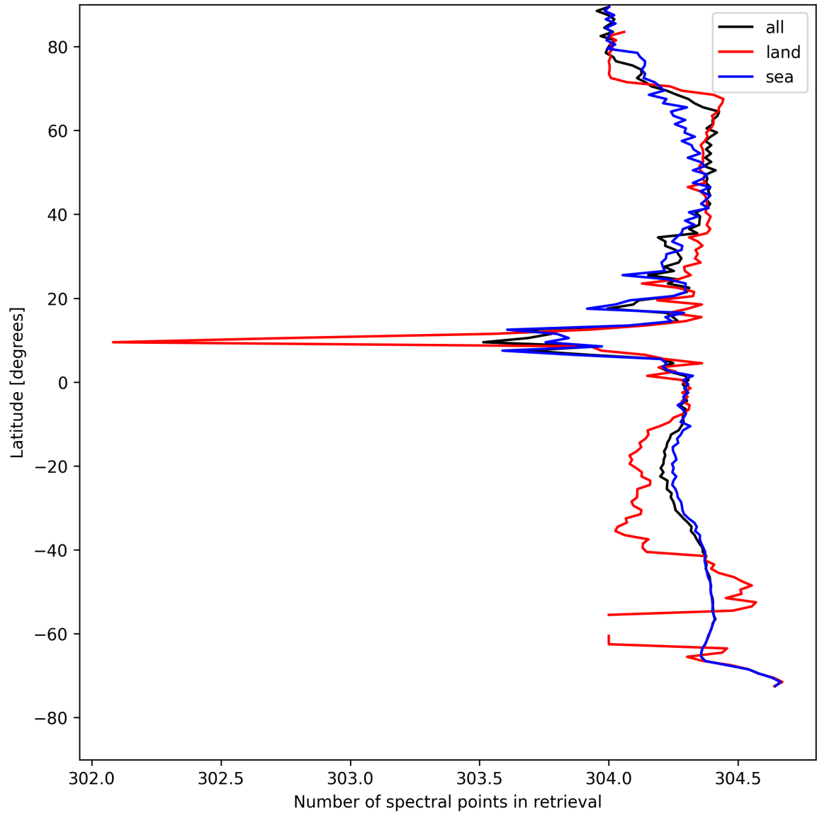
Figure 16: Zonal average of “Number of spectral points in retrieval” for 2025-08-10 to 2025-08-12.
