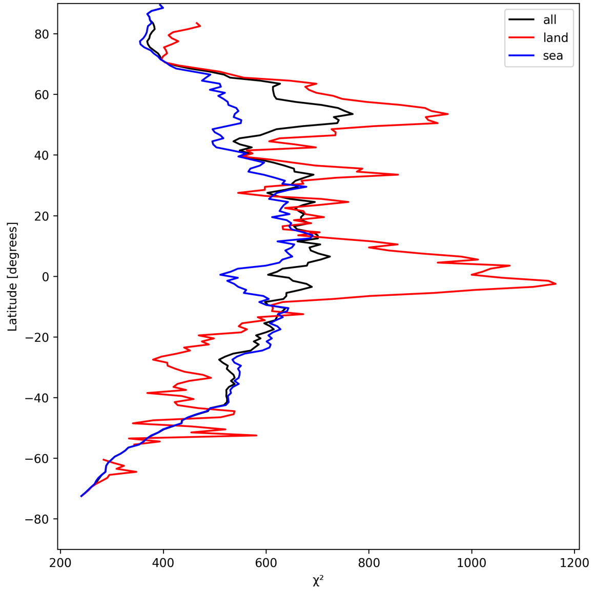
Figure 25: Zonal average of “ \chi^2 ” for 2025-08-10 to 2025-08-12.
