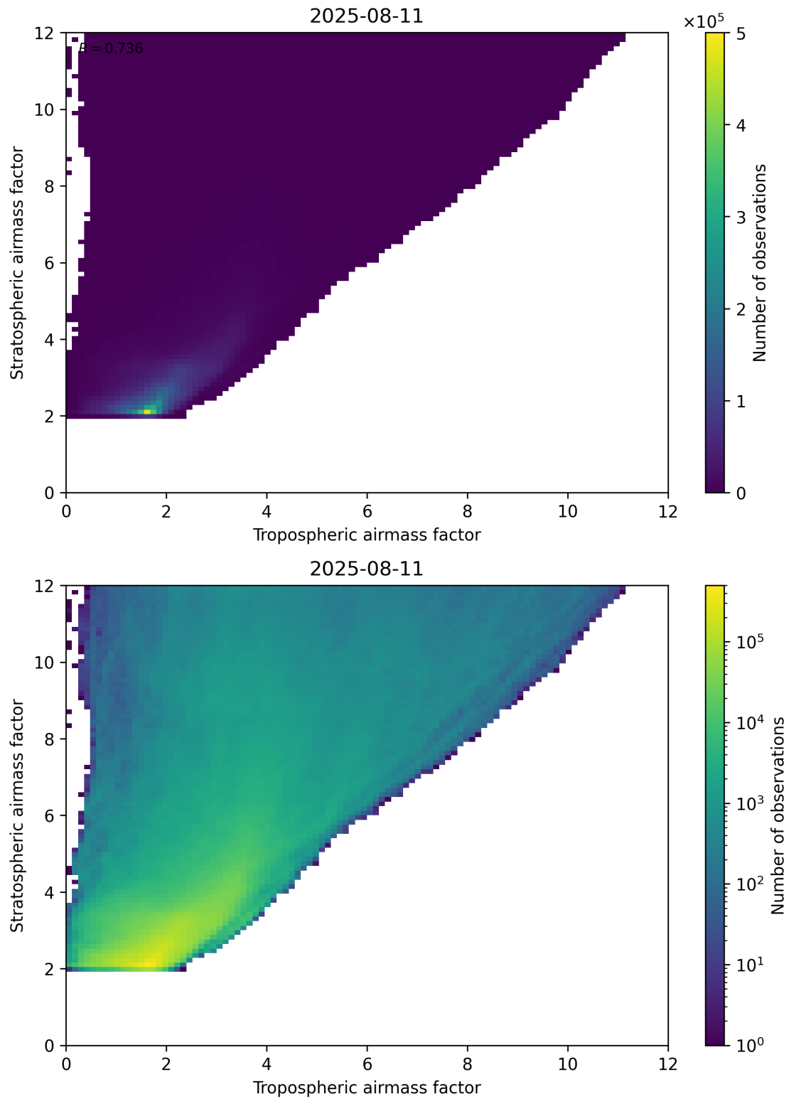
Figure 71: Scatter density plot of “Tropospheric airmass factor” against “Stratospheric airmass factor” for 2025-08-10 to 2025-08-12.
