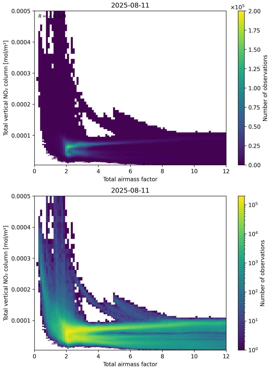
Figure 67: Scatter density plot of “Total airmass factor” against “Total vertical NO 2 column” for 2025-08-10 to 2025-08-12.
