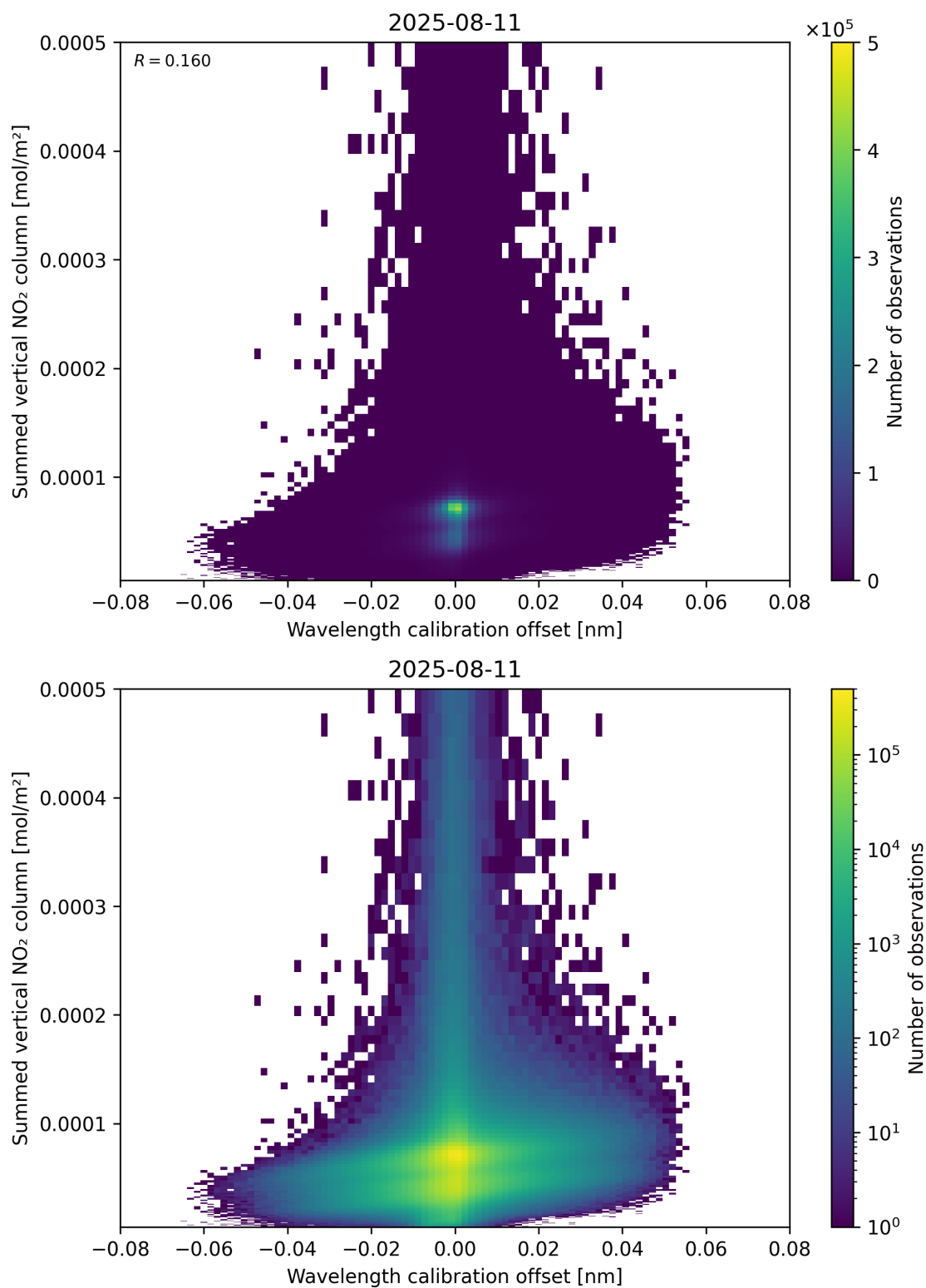
Figure 177: Scatter density plot of “Wavelength calibration offset” against “Summed vertical NO 2 column” for 2025-08-10 to 2025-08-12.
