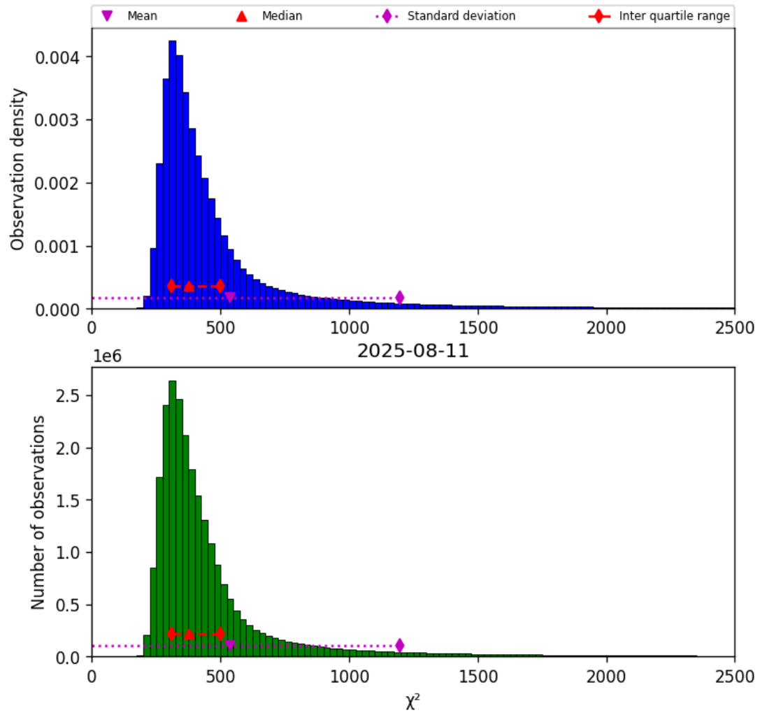
Figure 42: Histogram of “ \chi^2 ” for 2025-08-10 to 2025-08-12
