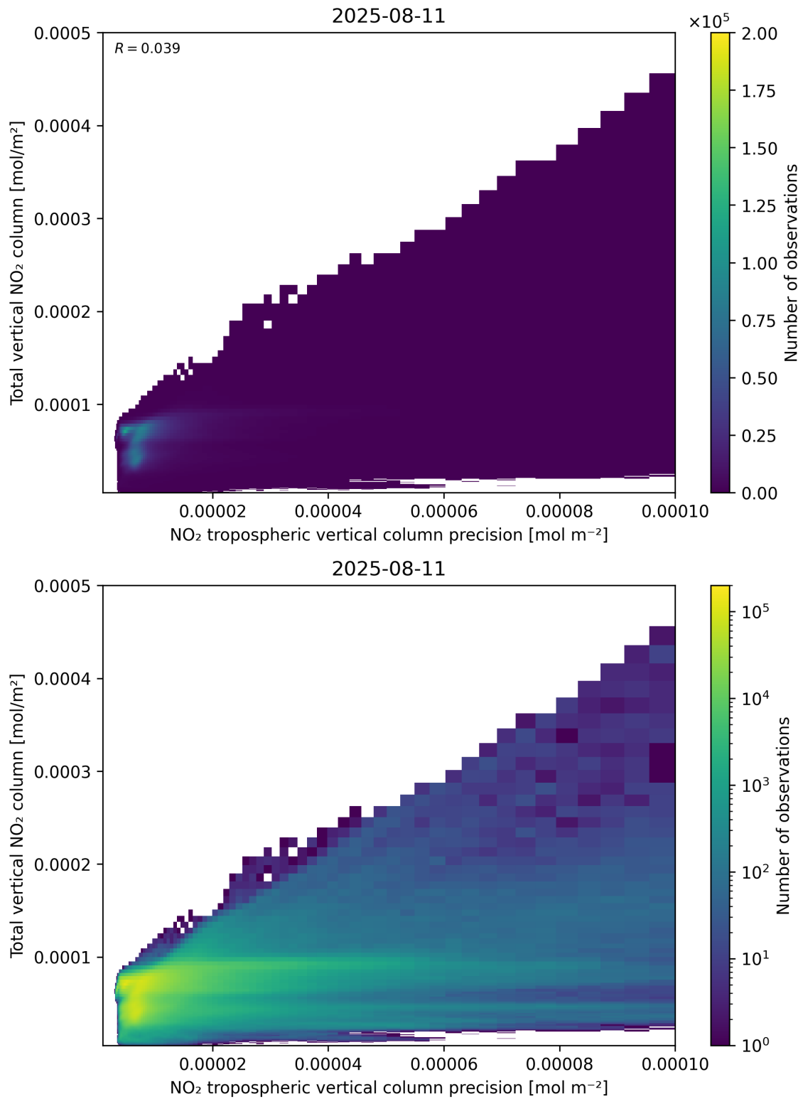
Figure 138: Scatter density plot of “NO 2 tropospheric vertical column precision” against “Total vertical NO 2 column” for 2025-08-10 to 2025-08-12.
