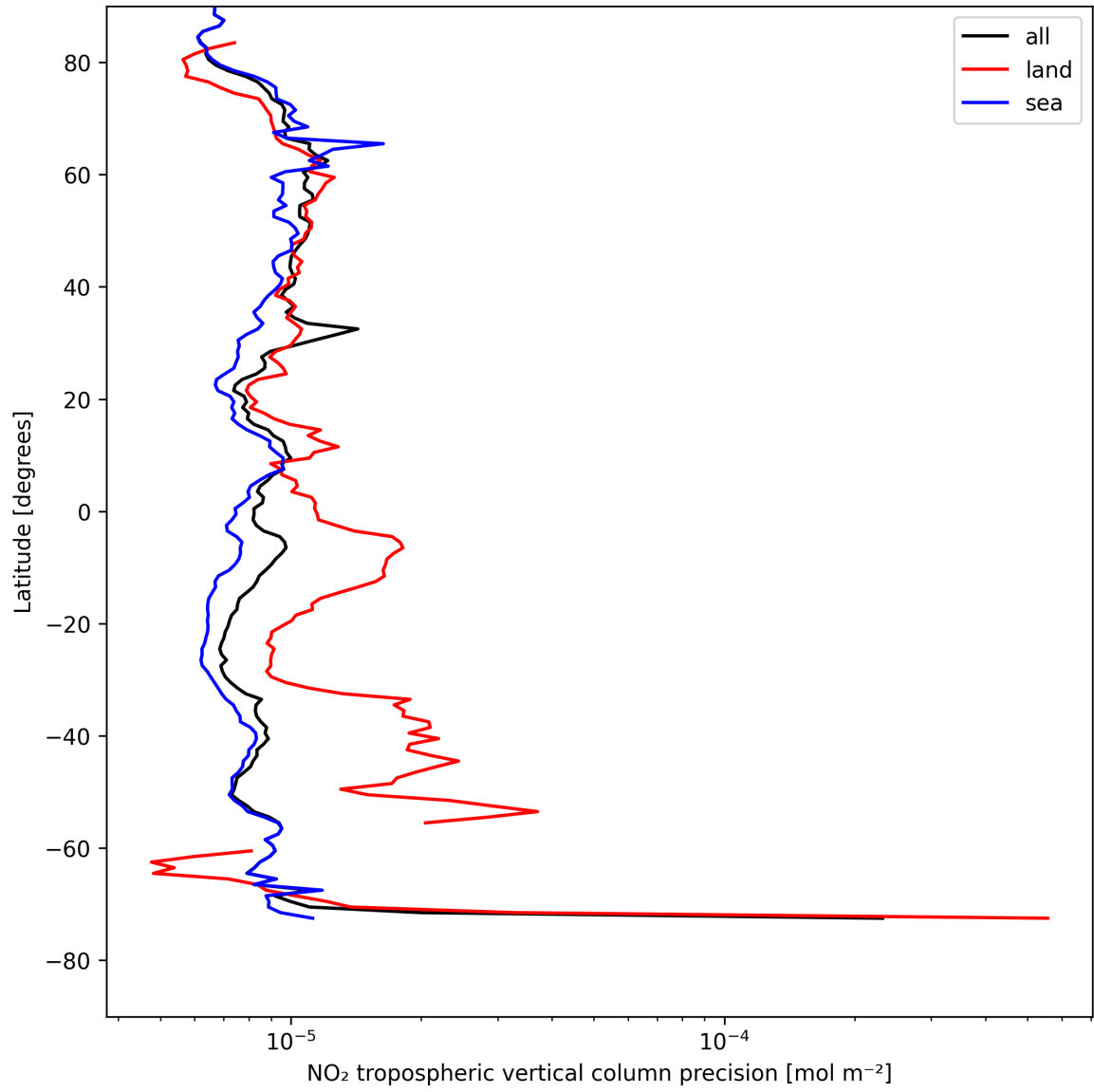
Figure 13: Zonal average of “NO 2 tropospheric vertical column precision” for 2025-08-10 to 2025-08-12.
