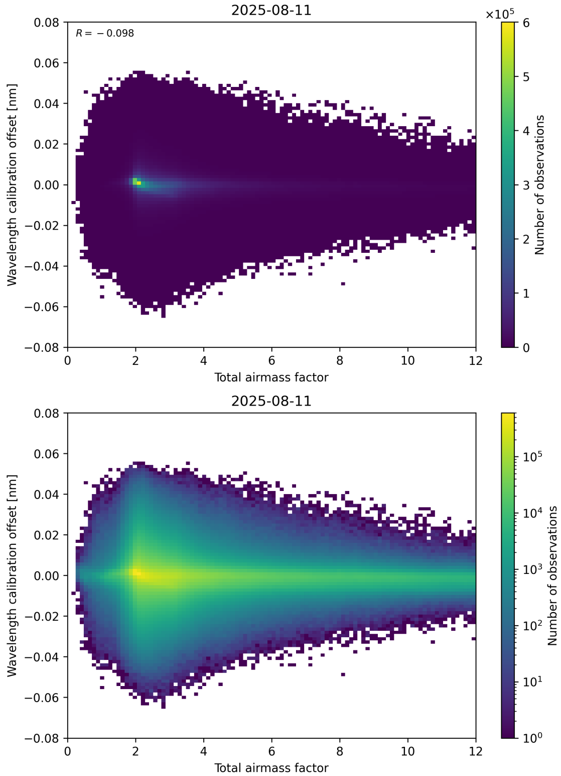
Figure 70: Scatter density plot of “Total airmass factor” against “Wavelength calibration offset” for 2025-08-10 to 2025-08-12.
