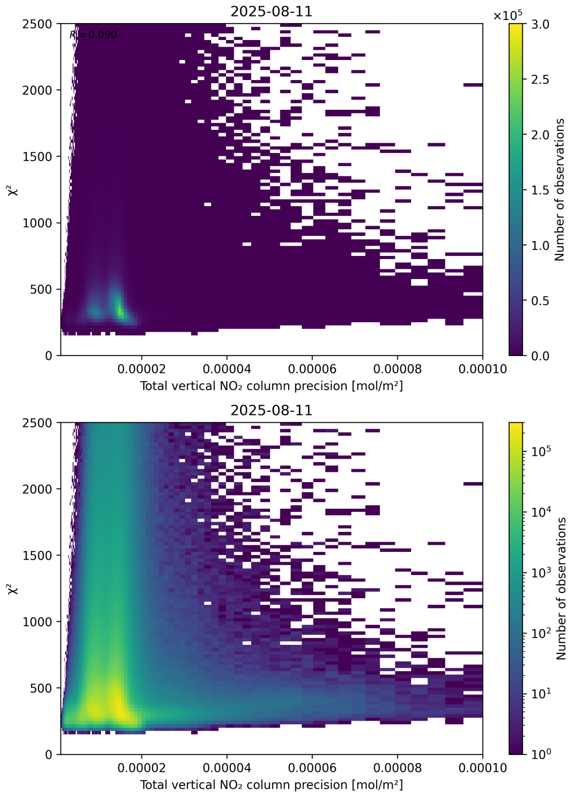
Figure 116: Scatter density plot of “Total vertical NO 2 column precision” against “ \chi^2 ” for 2025-08-10 to 2025-08-12.
