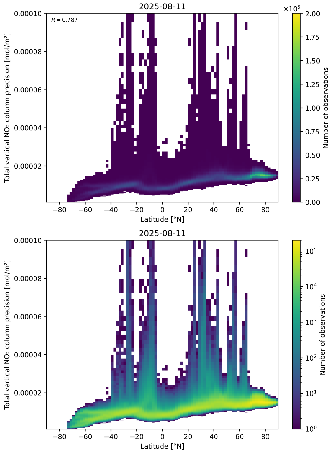
Figure 91: Scatter density plot of “Latitude” against “Total vertical NO 2 column precision” for 2025-08-10 to 2025-08-12.
