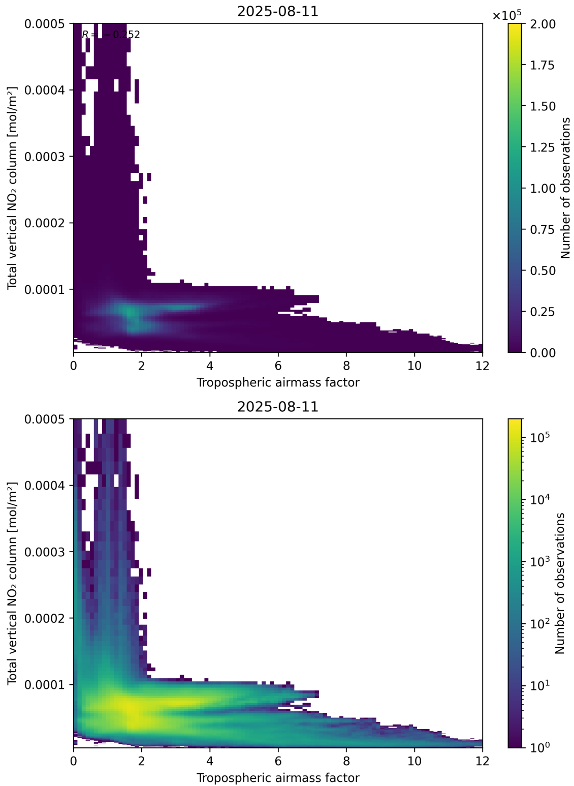
Figure 77: Scatter density plot of “Tropospheric airmass factor” against “Total vertical NO 2 column” for 2025-08-10 to 2025-08-12.
