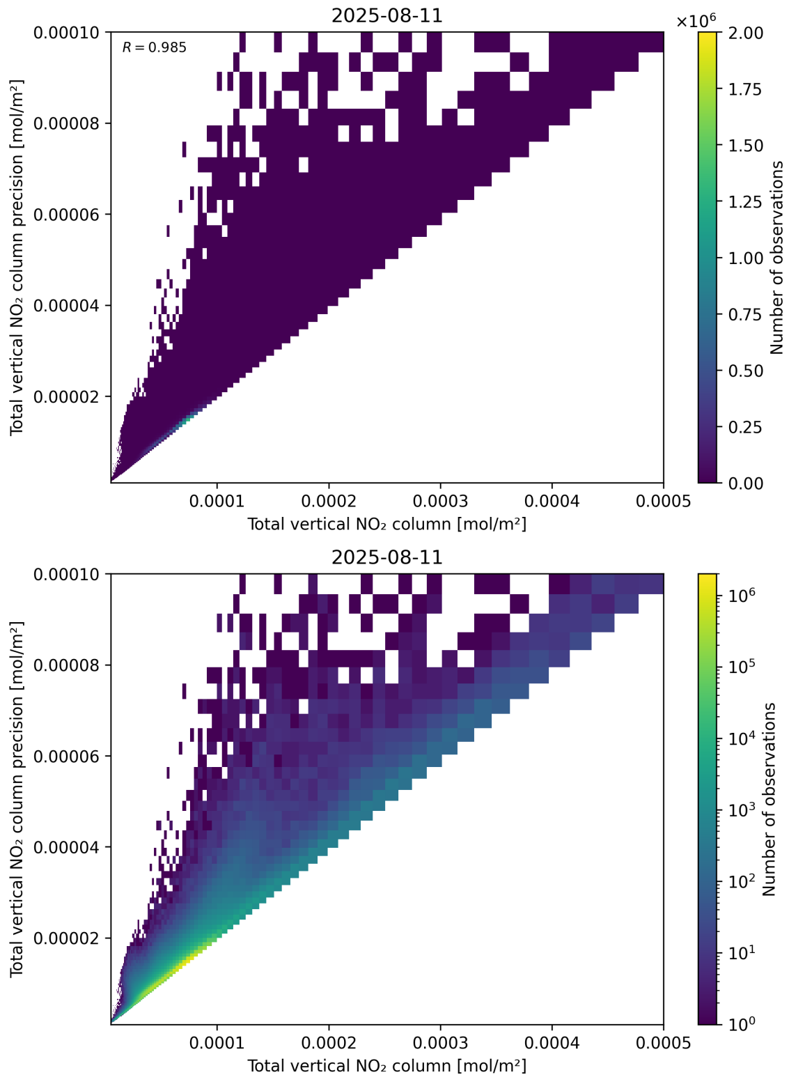
Figure 114: Scatter density plot of “Total vertical NO 2 column” against “Total vertical NO 2 column precision” for 2025-08-10 to 2025-08-12.
