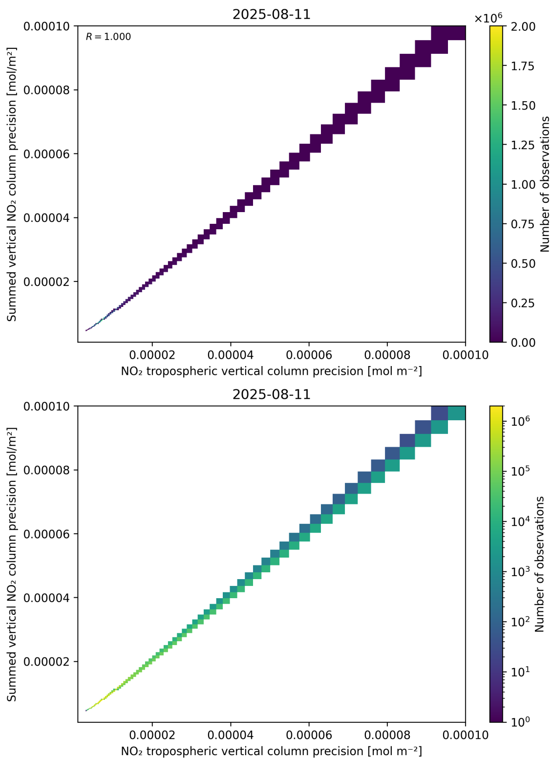
Figure 137: Scatter density plot of “NO 2 tropospheric vertical column precision” against “Summed vertical NO 2 column precision” for 2025-08-10 to 2025-08-12.
