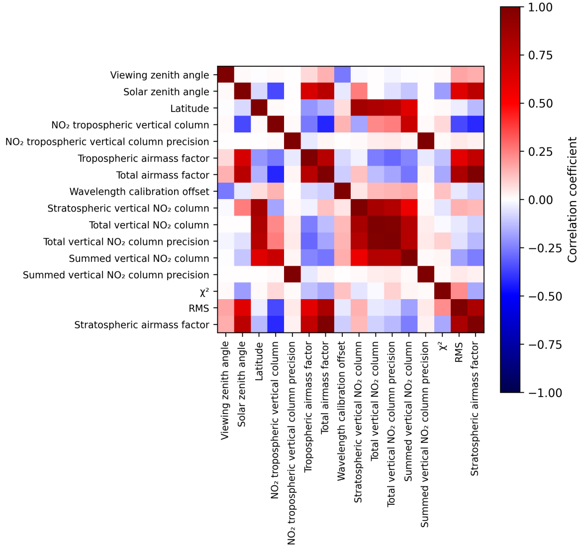
Figure 2: Map of correlation matrix for 2025-08-10 to 2025-08-12.
