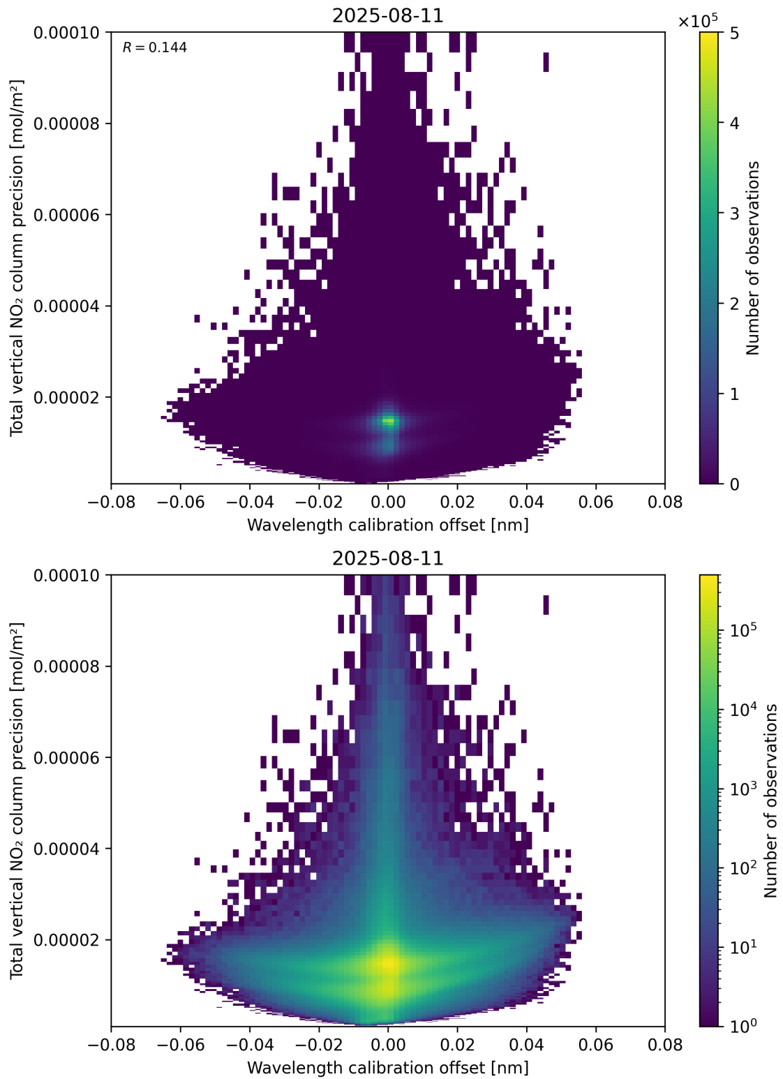
Figure 180: Scatter density plot of “Wavelength calibration offset” against “Total vertical NO 2 column precision” for 2025-08-10 to 2025-08-12.
