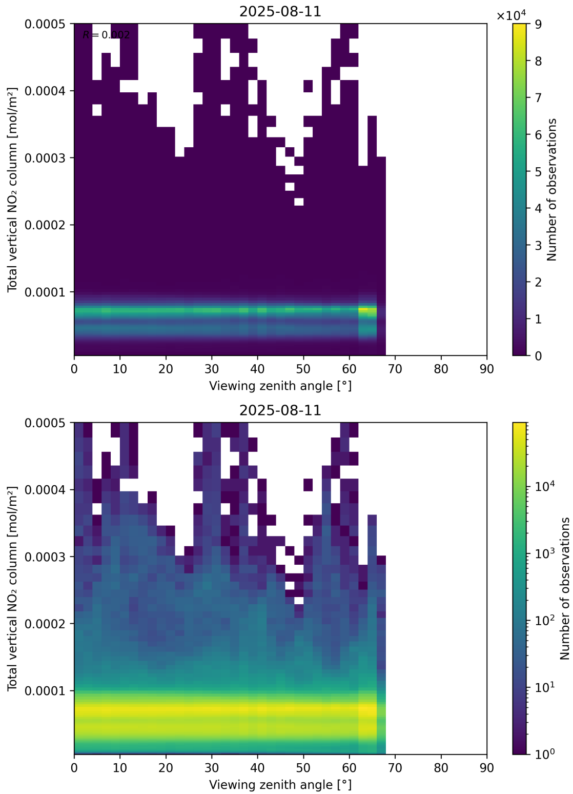
Figure 167: Scatter density plot of “Viewing zenith angle” against “Total vertical NO 2 column” for 2025-08-10 to 2025-08-12.
