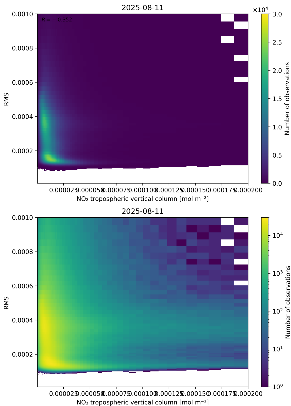
Figure 142: Scatter density plot of “NO 2 tropospheric vertical column” against “RMS” for 2025-08-10 to 2025-08-12.
