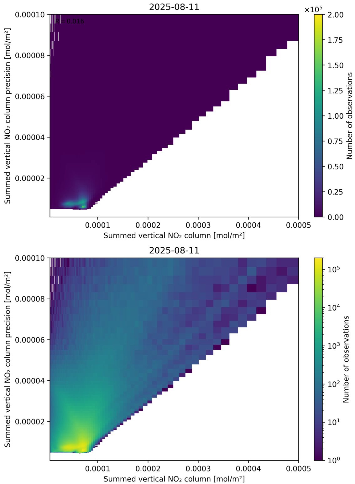
Figure 105: Scatter density plot of “Summed vertical NO 2 column” against “Summed vertical NO 2 column precision” for 2025-08-10 to 2025-08-12.
