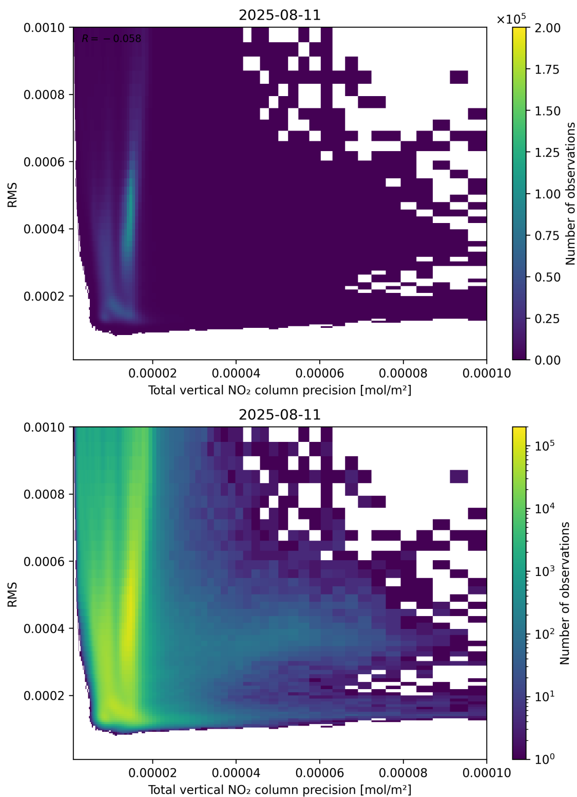
Figure 119: Scatter density plot of “Total vertical NO 2 column precision” against “RMS” for 2025-08-10 to 2025-08-12.
