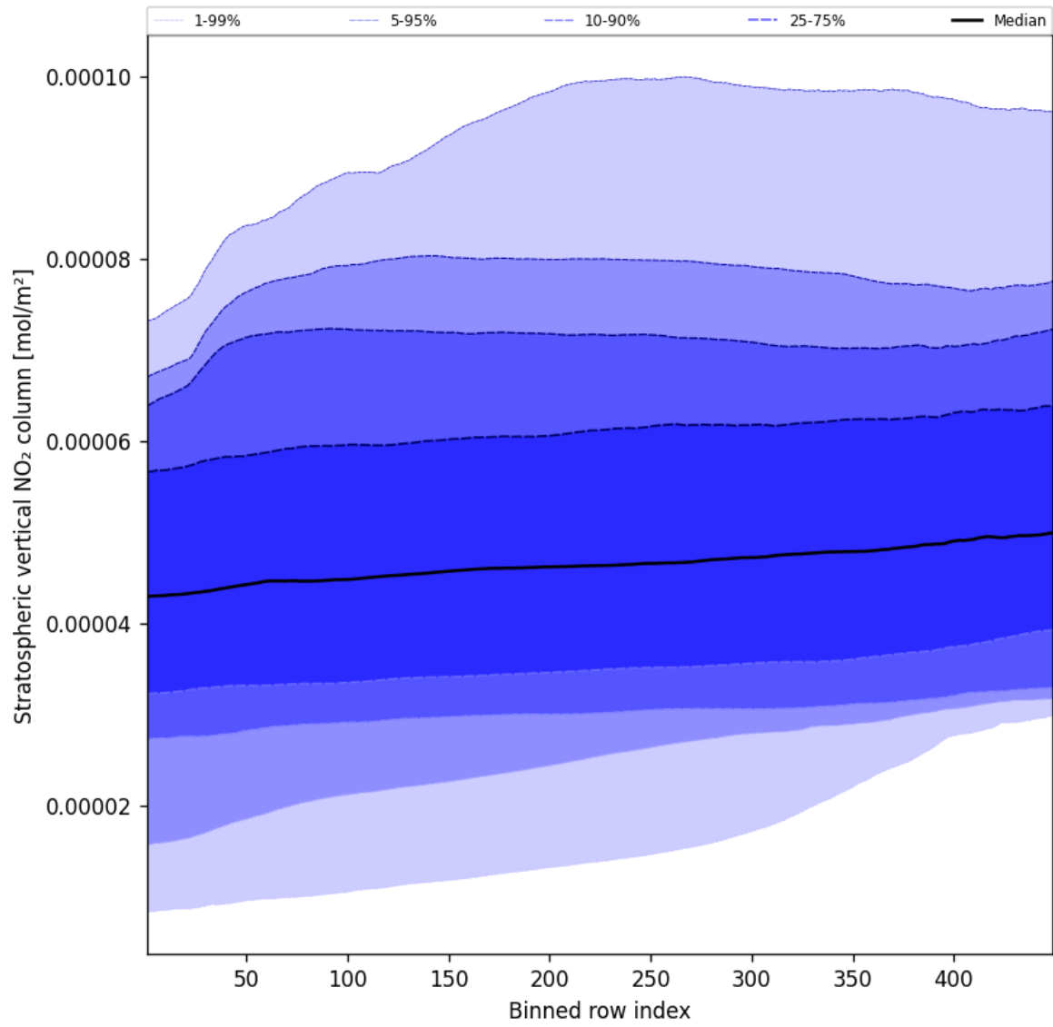
Figure 53: Along track statistics of “Stratospheric vertical NO 2 column” for 2025-08-11 to 2025-08-13
