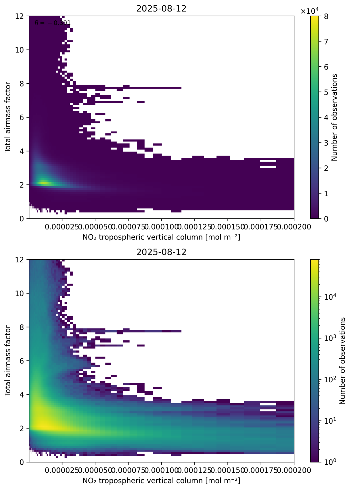
Figure 122: Scatter density plot of “NO 2 tropospheric vertical column” against “Total air mass factor” for 2025-08-11 to 2025-08-13.
