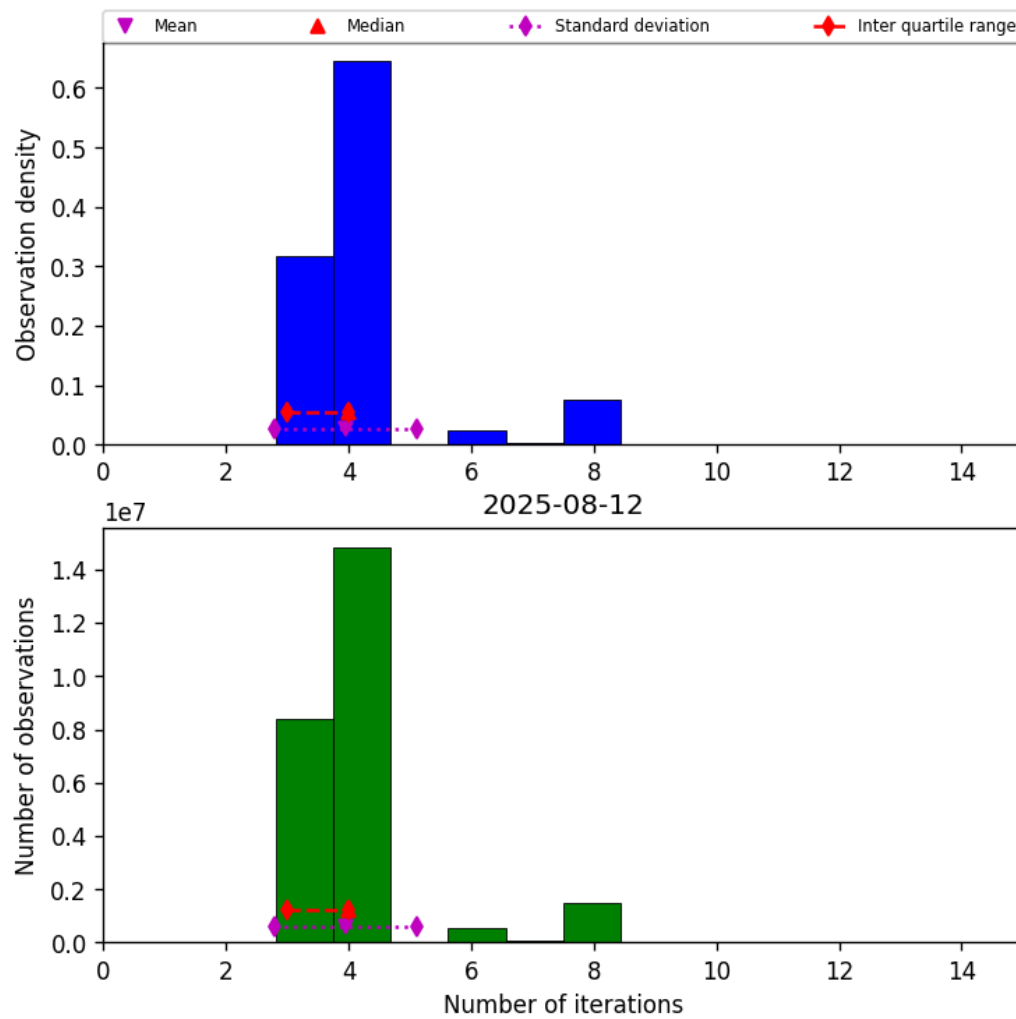
Figure 34: Histogram of “Number of iterations” for 2025-08-11 to 2025-08-13
