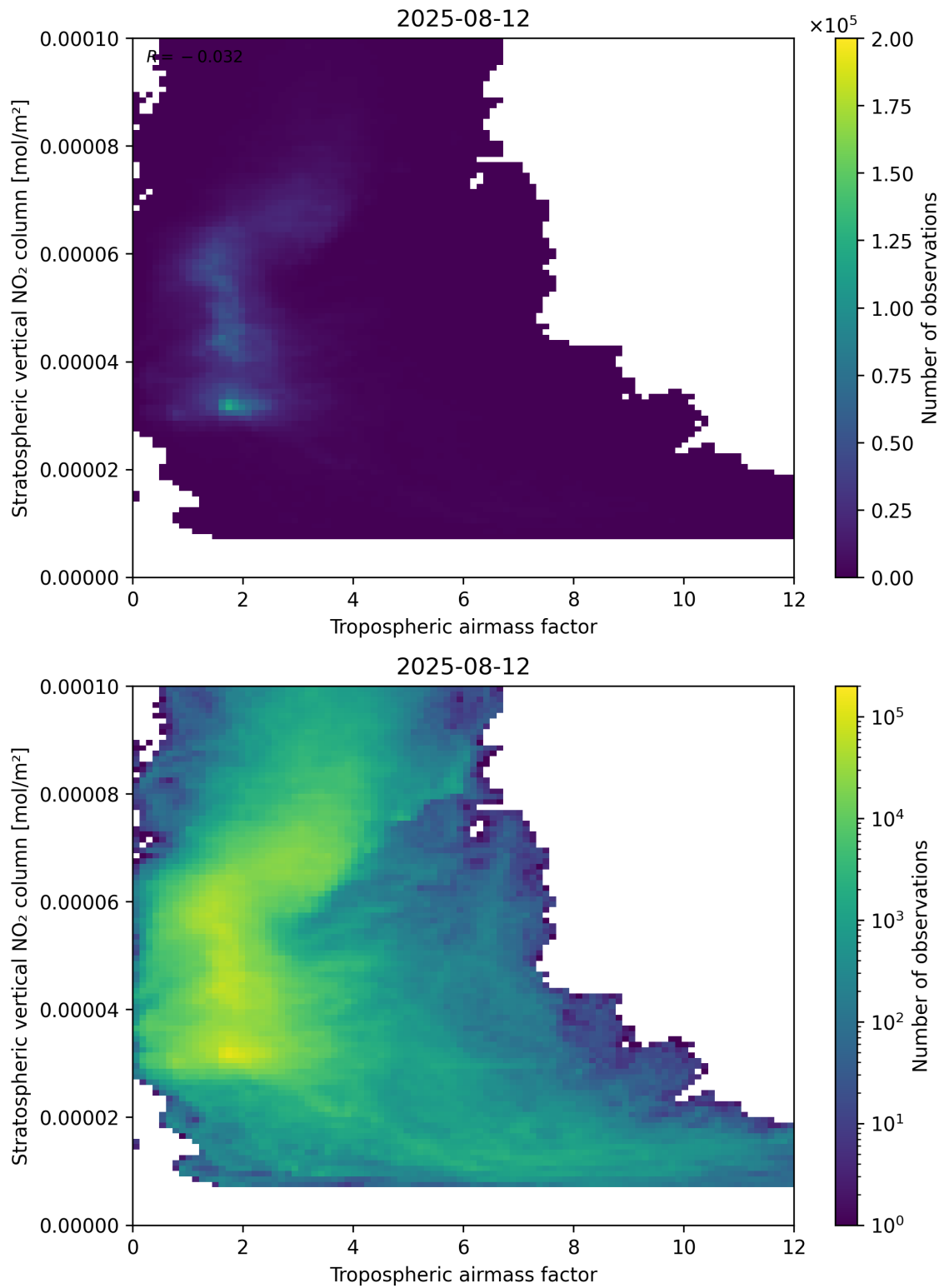
Figure 74: Scatter density plot of “Tropospheric air mass factor” against “Stratospheric vertical NO 2 column” for 2025-08-11 to 2025-08-13.
