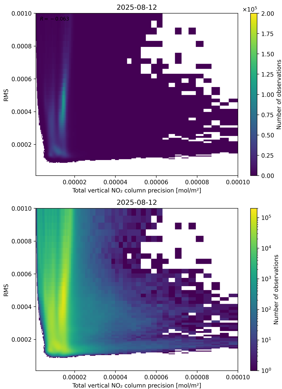
Figure 119: Scatter density plot of “Total vertical NO 2 column precision” against “RMS” for 2025-08-11 to 2025-08-13.
