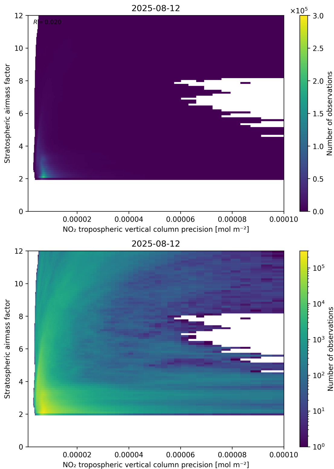
Figure 131: Scatter density plot of “NO 2 tropospheric vertical column precision” against “Stratospheric airmass factor” for 2025-08-11 to 2025-08-13.
