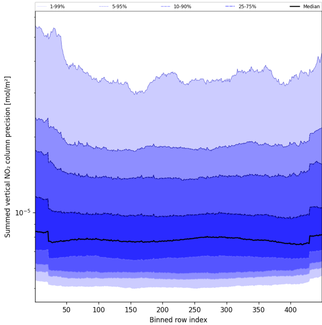
Figure 58: Along track statistics of “Summed vertical NO 2 column precision” for 2025-08-11 to 2025-08-13
