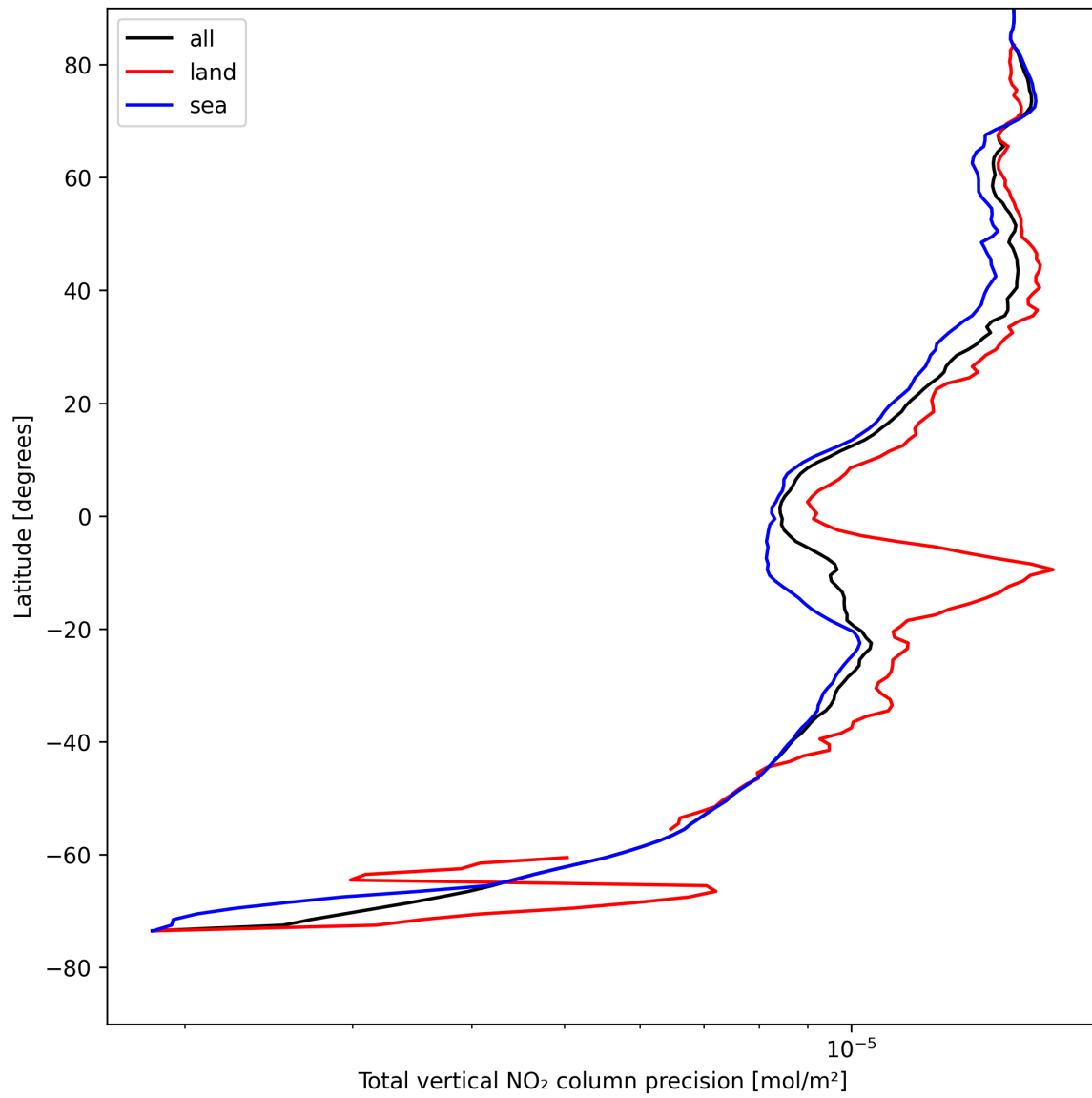
Figure 22: Zonal average of “Total vertical NO 2 column precision” for 2025-08-11 to 2025-08-13.
