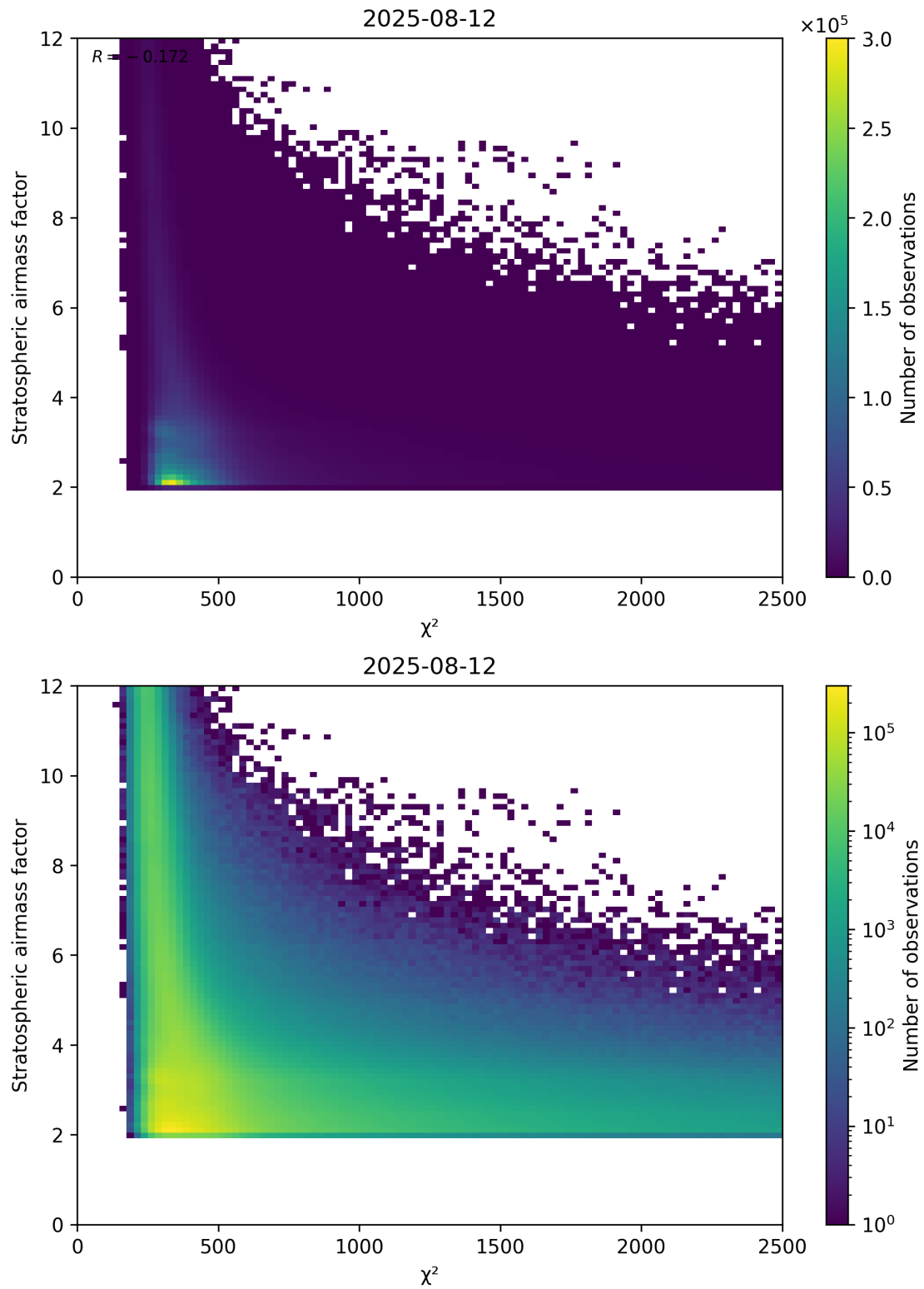
Figure 81: Scatter density plot of “ \chi^2 ” against “Stratospheric airmass factor” for 2025-08-11 to 2025-08-13.
