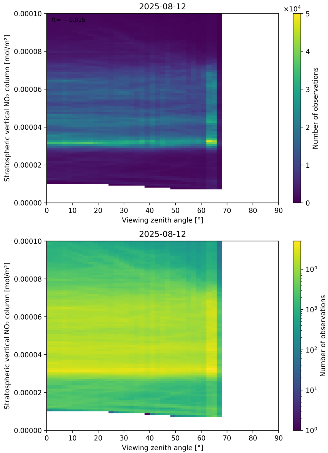
Figure 164: Scatter density plot of “Viewing zenith angle” against “Stratospheric vertical NO 2 column” for 2025-08-11 to 2025-08-13.
