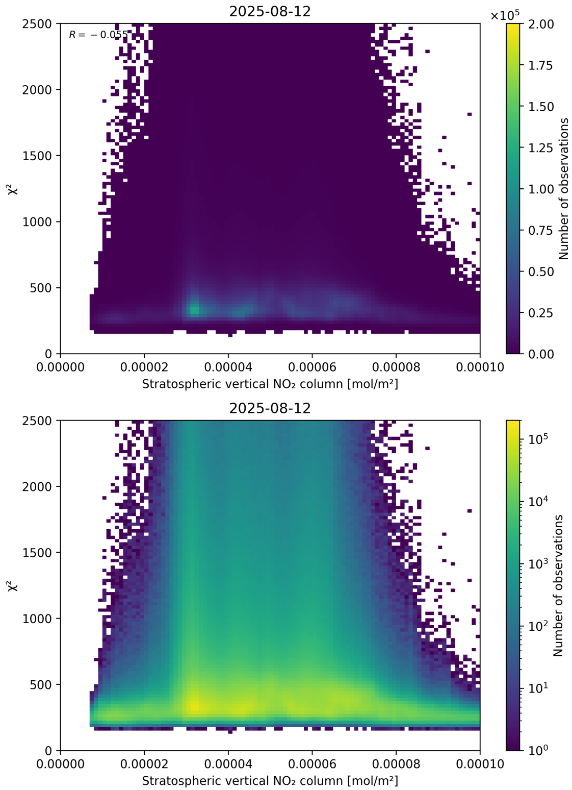
Figure 97: Scatter density plot of “Stratospheric vertical NO 2 column” against “ \chi^2 ” for 2025-08-11 to 2025-08-13.
