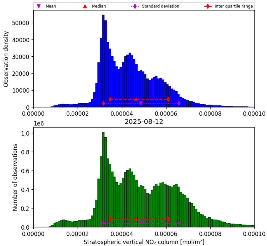
Figure 36: Histogram of “Stratospheric vertical NO 2 column” for 2025-08-11 to 2025-08-13
