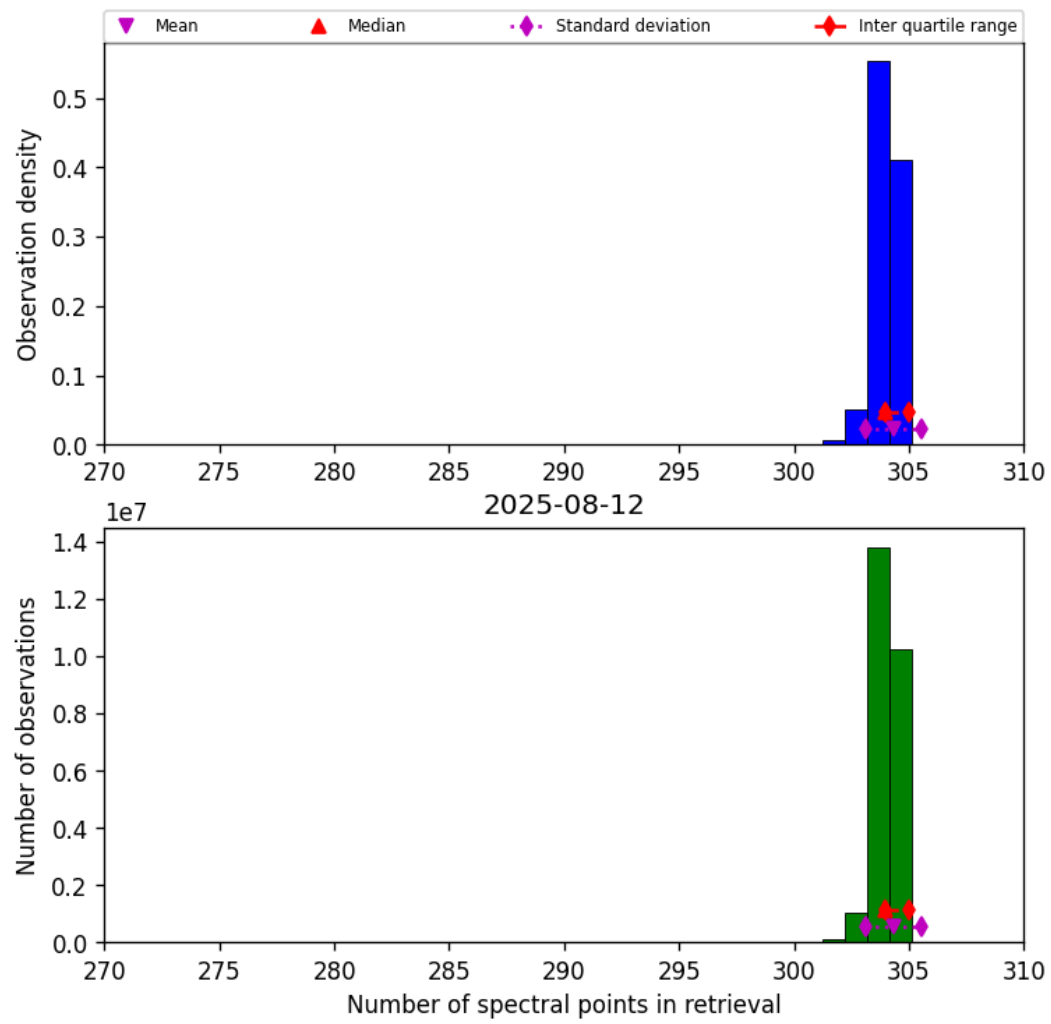
Figure 33: Histogram of “Number of spectral points in retrieval” for 2025-08-11 to 2025-08-13
