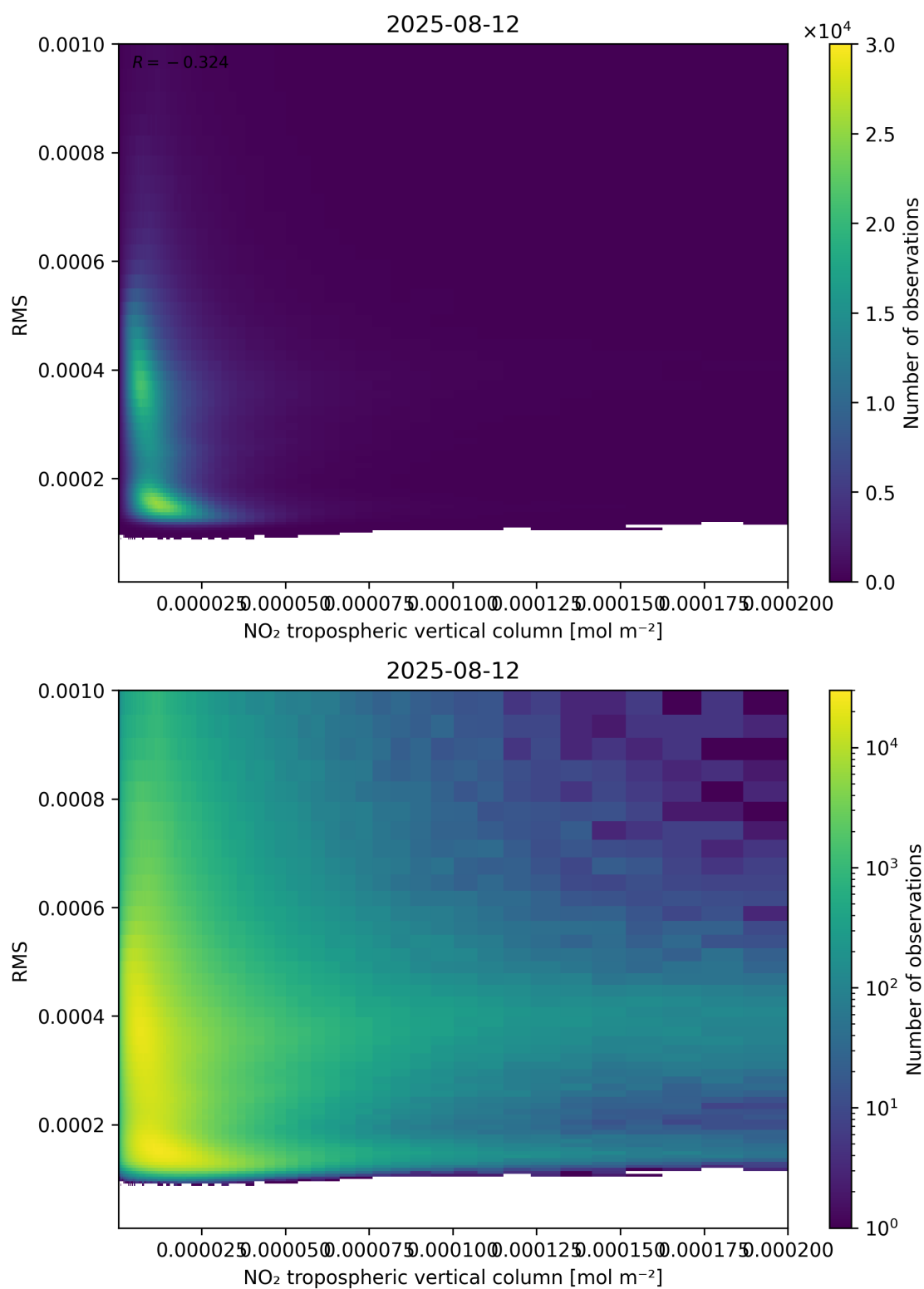
Figure 142: Scatter density plot of “NO 2 tropospheric vertical column” against “RMS” for 2025-08-11 to 2025-08-13.
