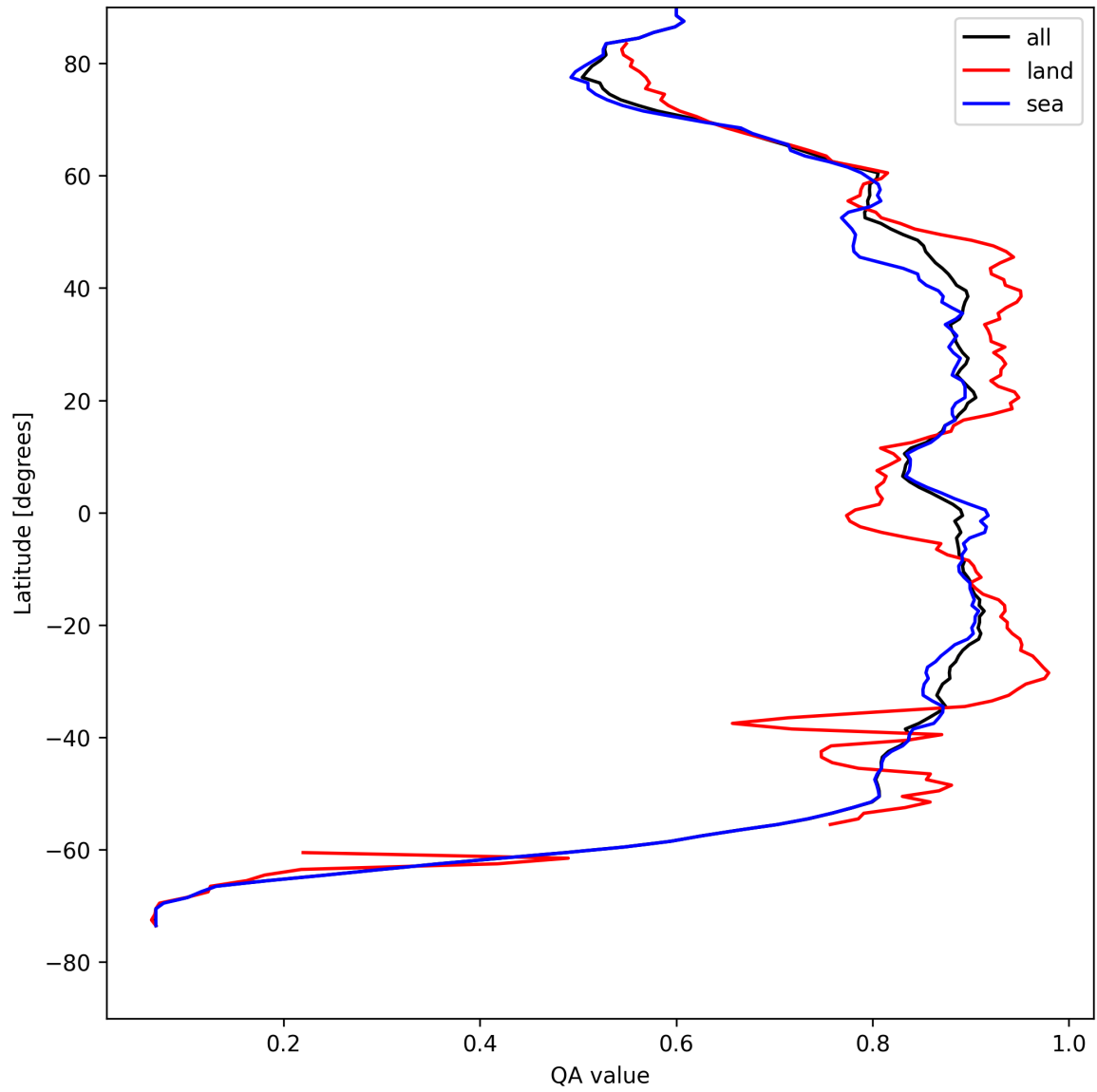
Figure 11: Zonal average of “QA value” for 2025-08-11 to 2025-08-13.
