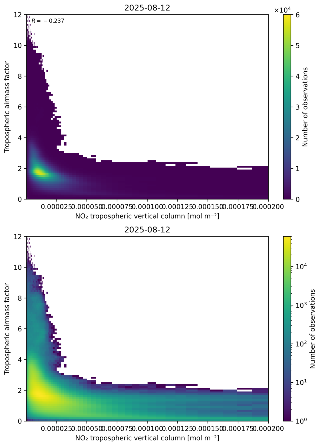
Figure 123: Scatter density plot of “NO 2 tropospheric vertical column” against “Tropospheric air mass factor” for 2025-08-11 to 2025-08-13.
