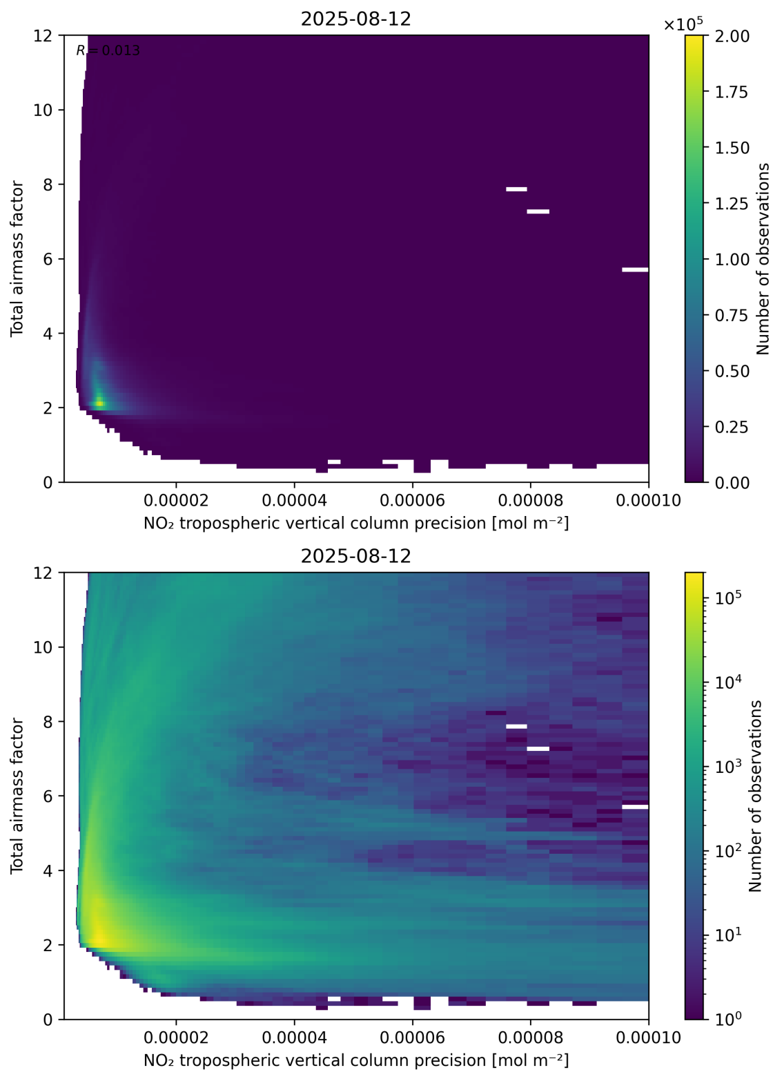
Figure 132: Scatter density plot of “NO 2 tropospheric vertical column precision” against “Total air mass factor” for 2025-08-11 to 2025-08-13.
