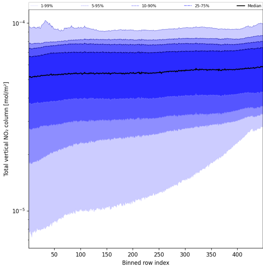
Figure 55: Along track statistics of “Total vertical NO 2 column” for 2025-08-11 to 2025-08-13
