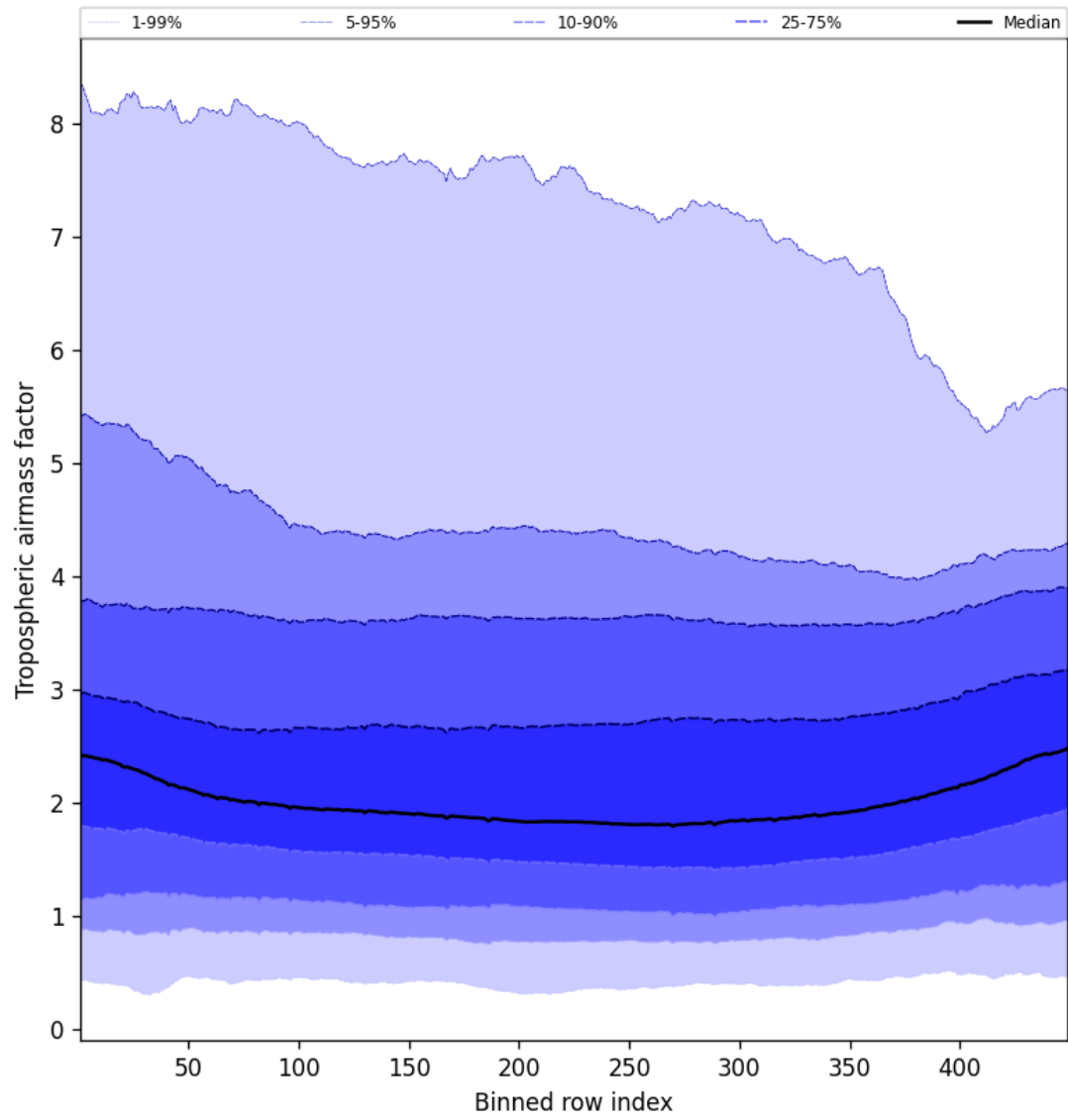
Figure 48: Along track statistics of “Tropospheric airmass factor” for 2025-08-11 to 2025-08-13
