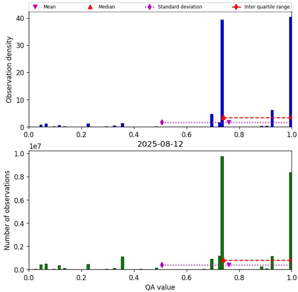
Figure 28: Histogram of “QA value” for 2025-08-11 to 2025-08-13
