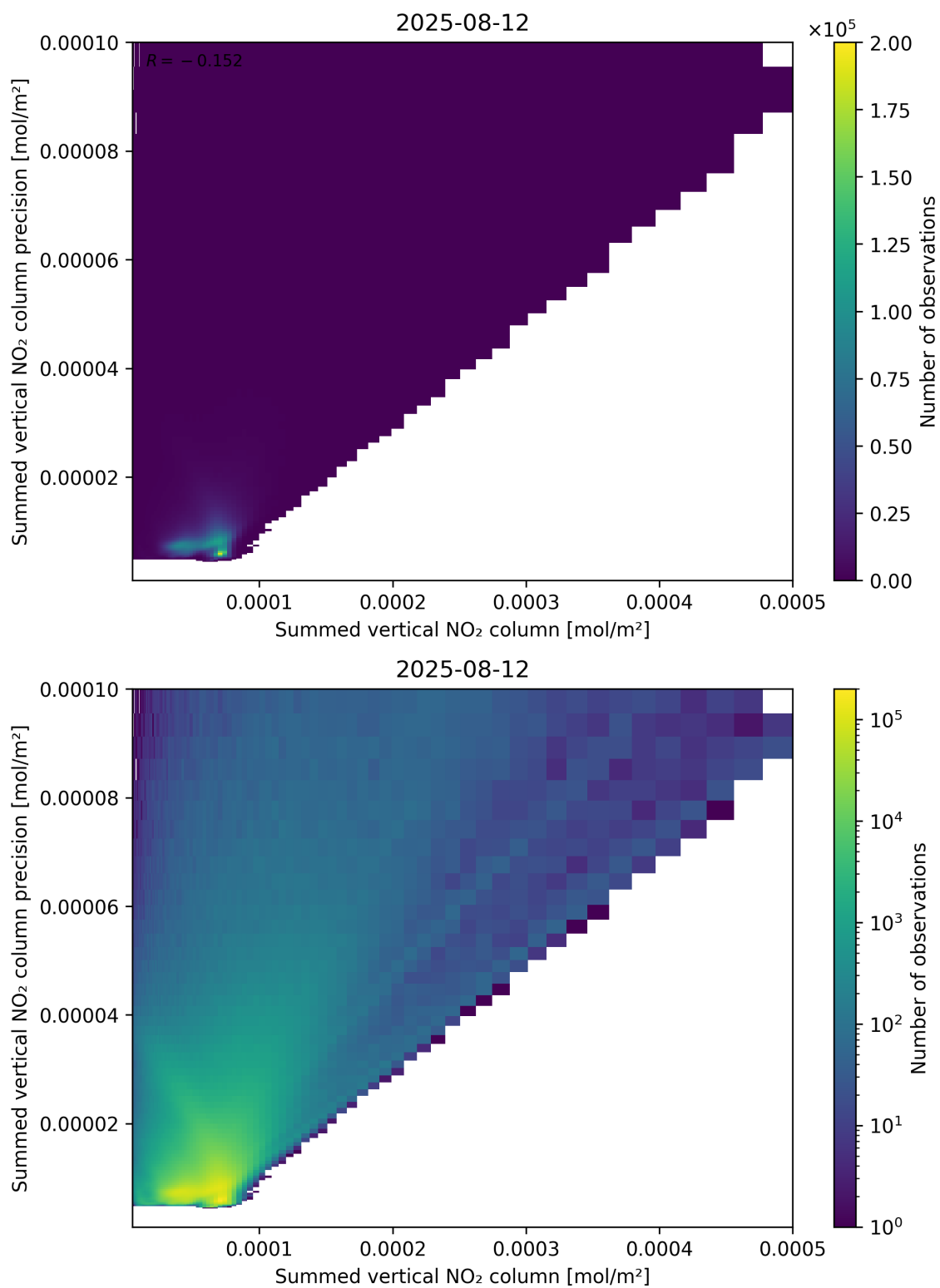
Figure 105: Scatter density plot of “Summed vertical NO 2 column” against “Summed vertical NO 2 column precision” for 2025-08-11 to 2025-08-13.
