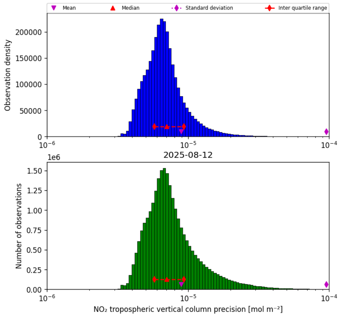
Figure 30: Histogram of “NO 2 tropospheric vertical column precision” for 2025-08-11 to 2025-08-13
