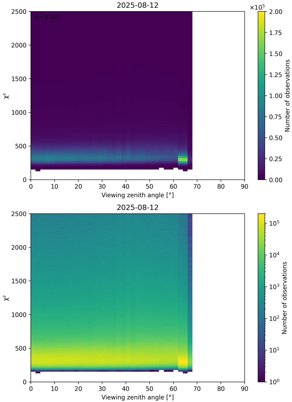
Figure 162: Scatter density plot of “Viewing zenith angle” against “ \chi^2 ” for 2025-08-11 to 2025-08-13.
