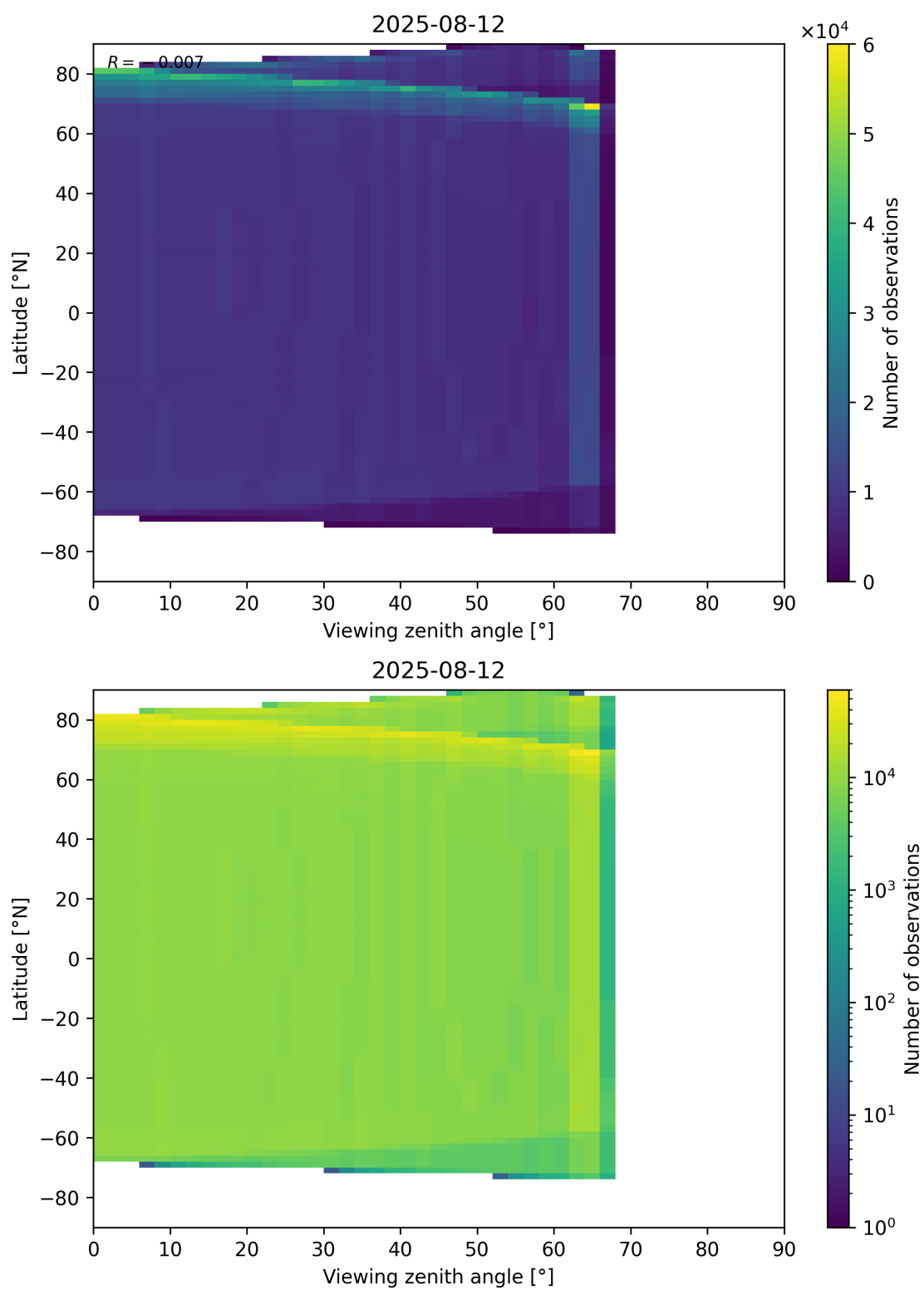
Figure 163: Scatter density plot of “Viewing zenith angle” against “Latitude” for 2025-08-11 to 2025-08-13.
