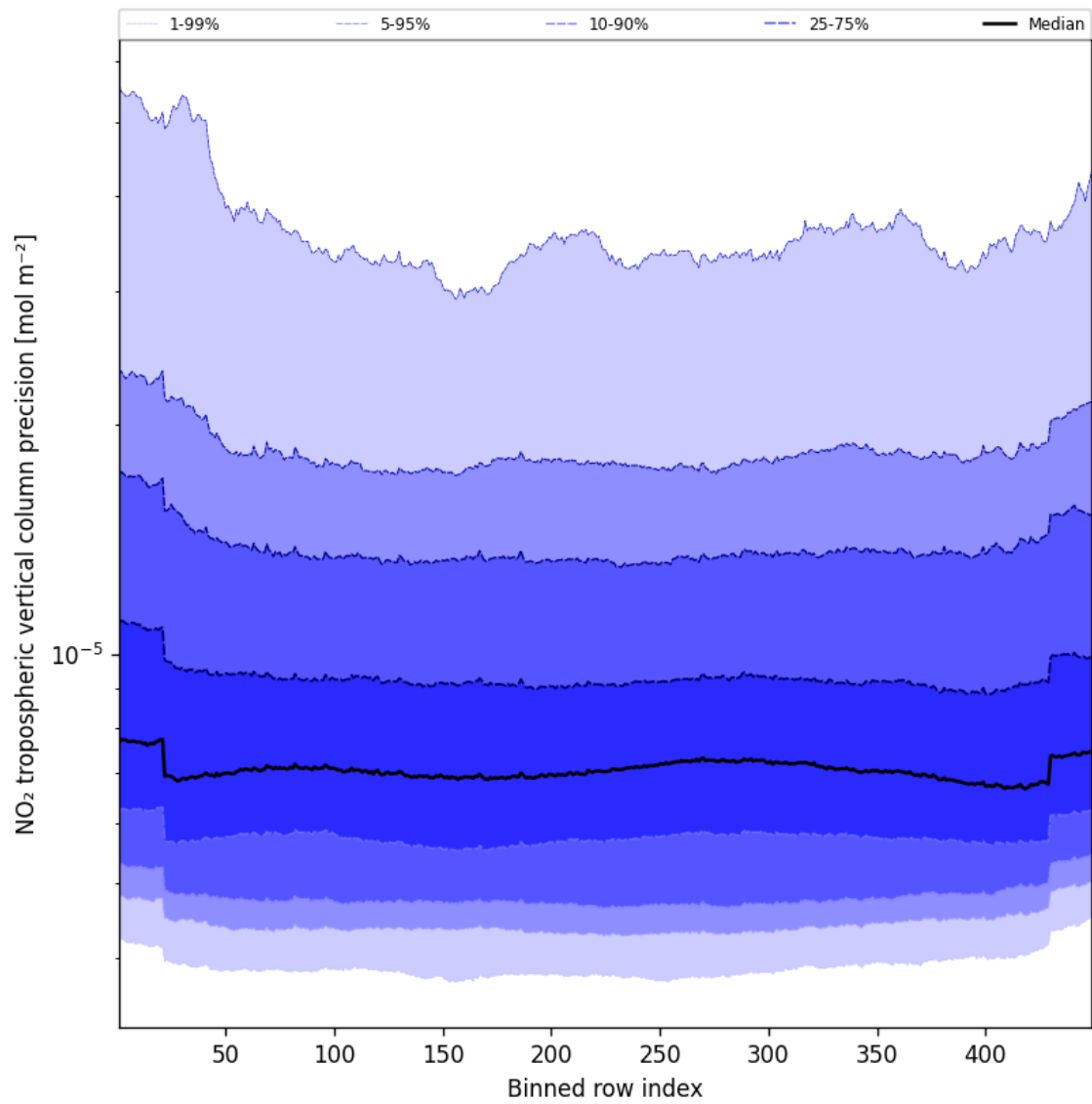
Figure 47: Along track statistics of “NO 2 tropospheric vertical column precision” for 2025-08-11 to 2025-08-13
