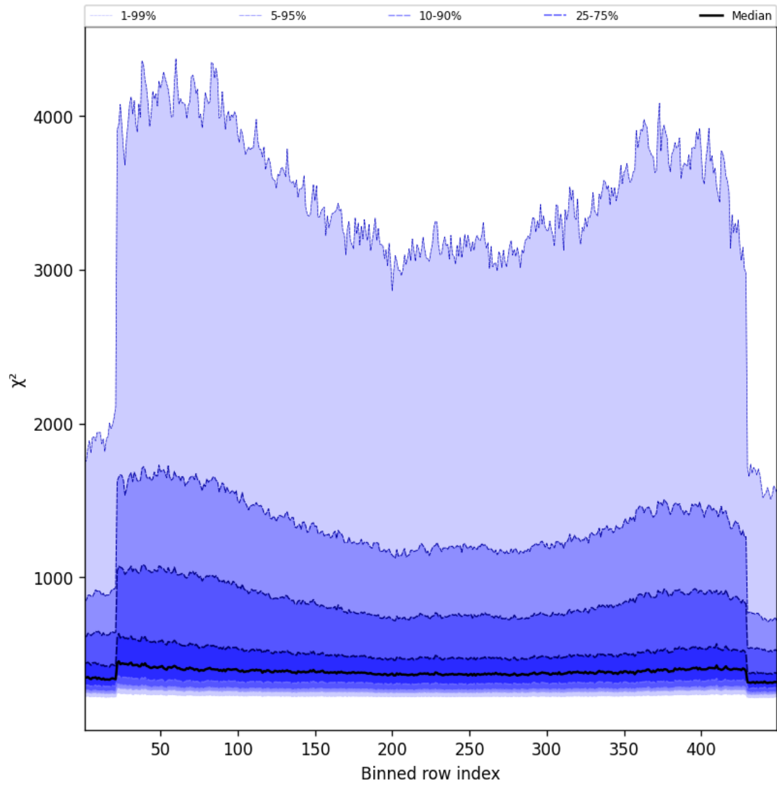
Figure 59: Along track statistics of “ \chi^2 ” for 2025-08-11 to 2025-08-13
