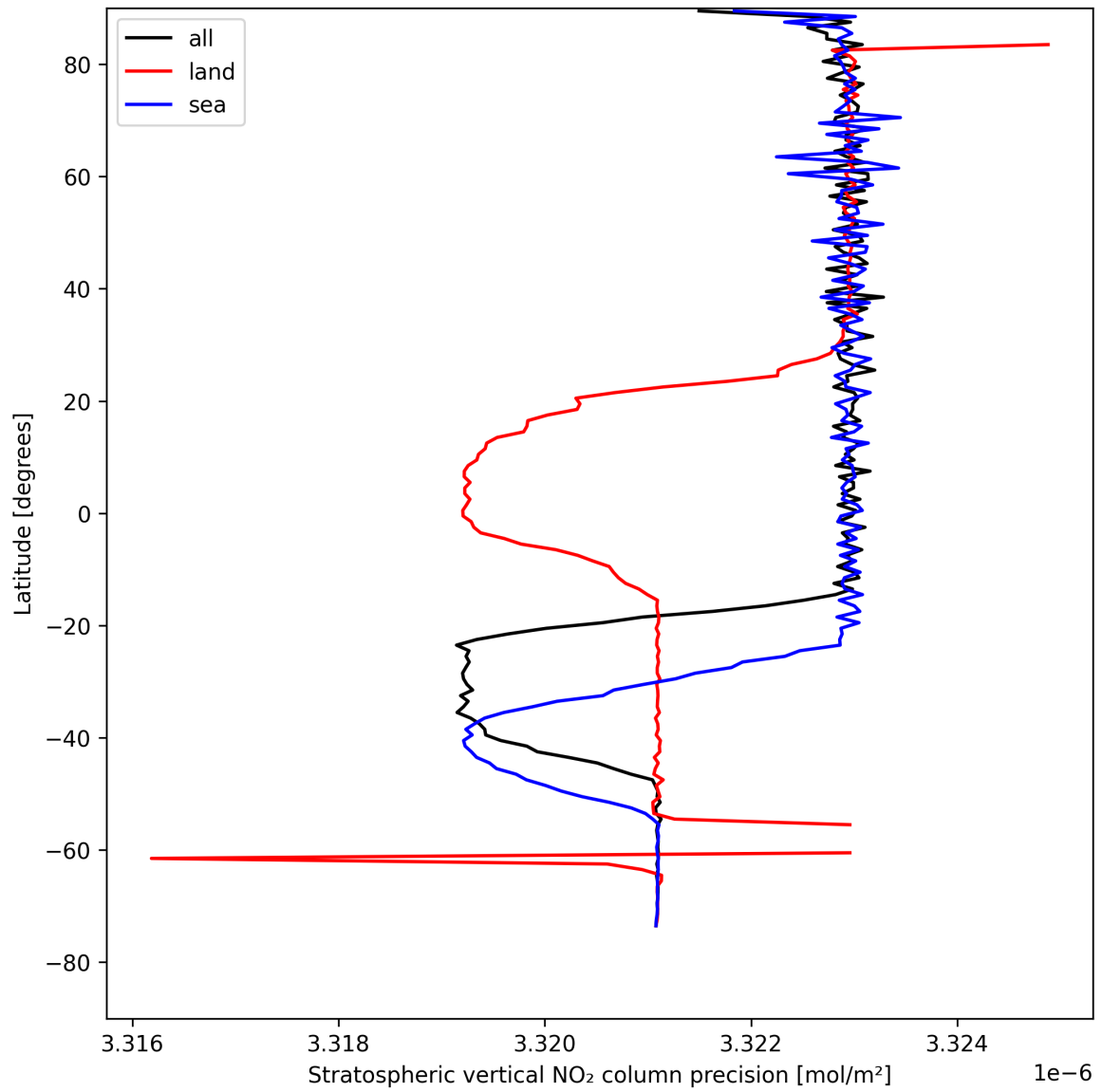
Figure 20: Zonal average of “Stratospheric vertical NO 2 column precision” for 2025-08-11 to 2025-08-13.
