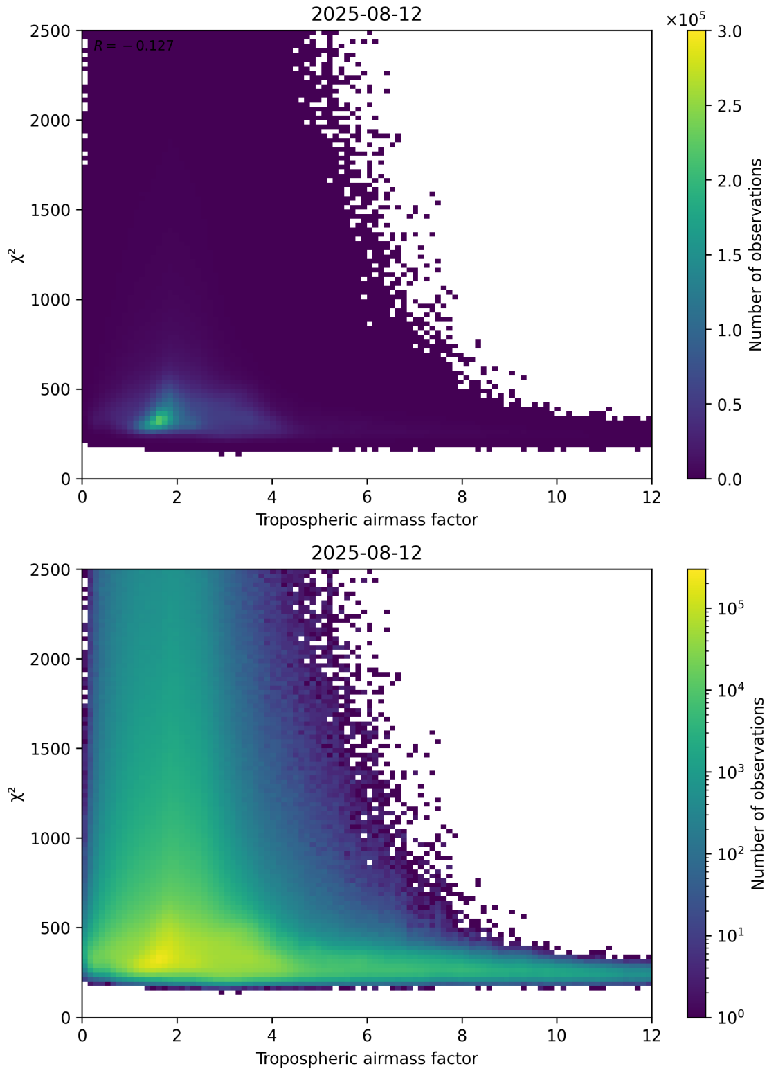
Figure 73: Scatter density plot of “Tropospheric airmass factor” against “ \chi^2 ” for 2025-08-11 to 2025-08-13.
