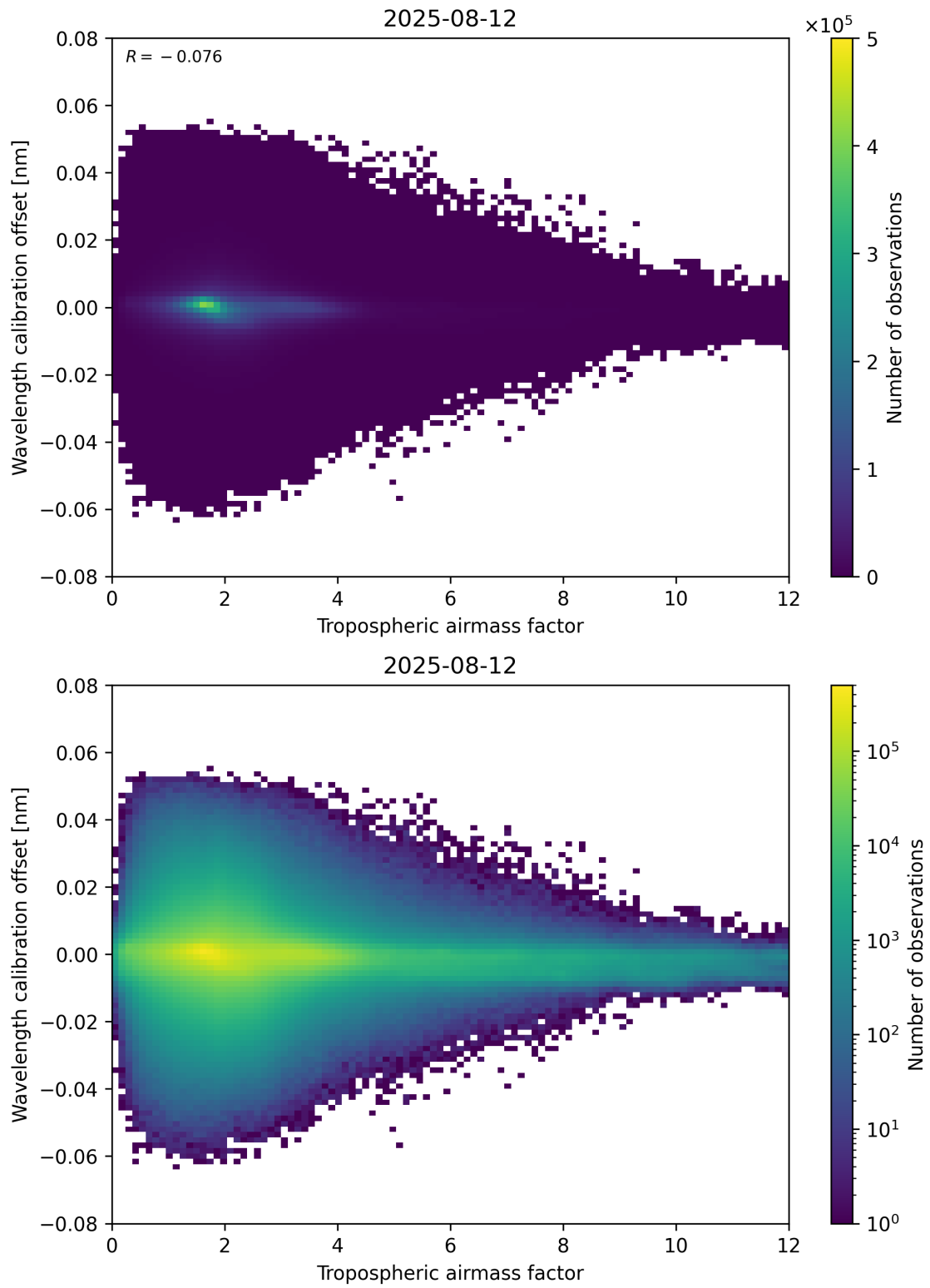
Figure 80: Scatter density plot of “Tropospheric air mass factor” against “Wavelength calibration offset” for 2025-08-11 to 2025-08-13.
