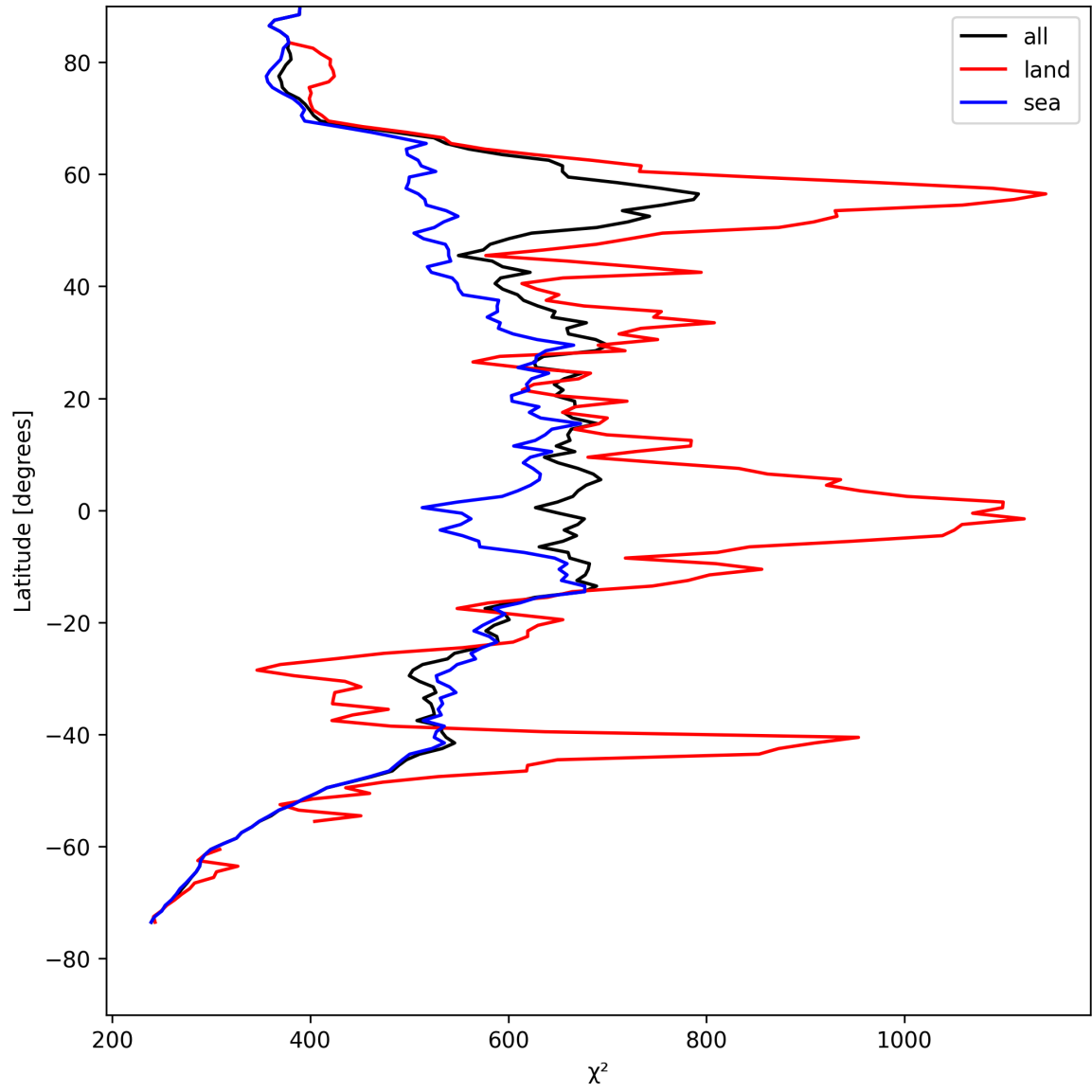
Figure 25: Zonal average of “ \chi^2 ” for 2025-08-11 to 2025-08-13.
