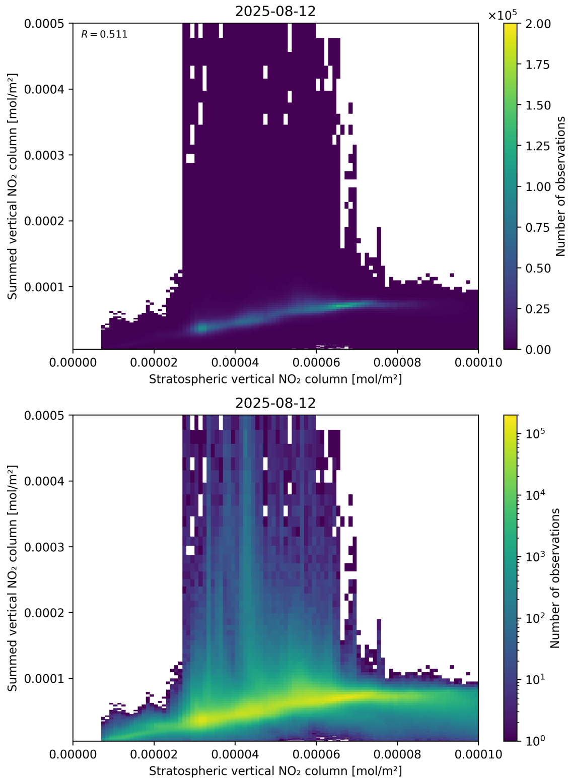
Figure 98: Scatter density plot of “Stratospheric vertical NO 2 column” against “Summed vertical NO 2 column” for 2025-08-11 to 2025-08-13.
