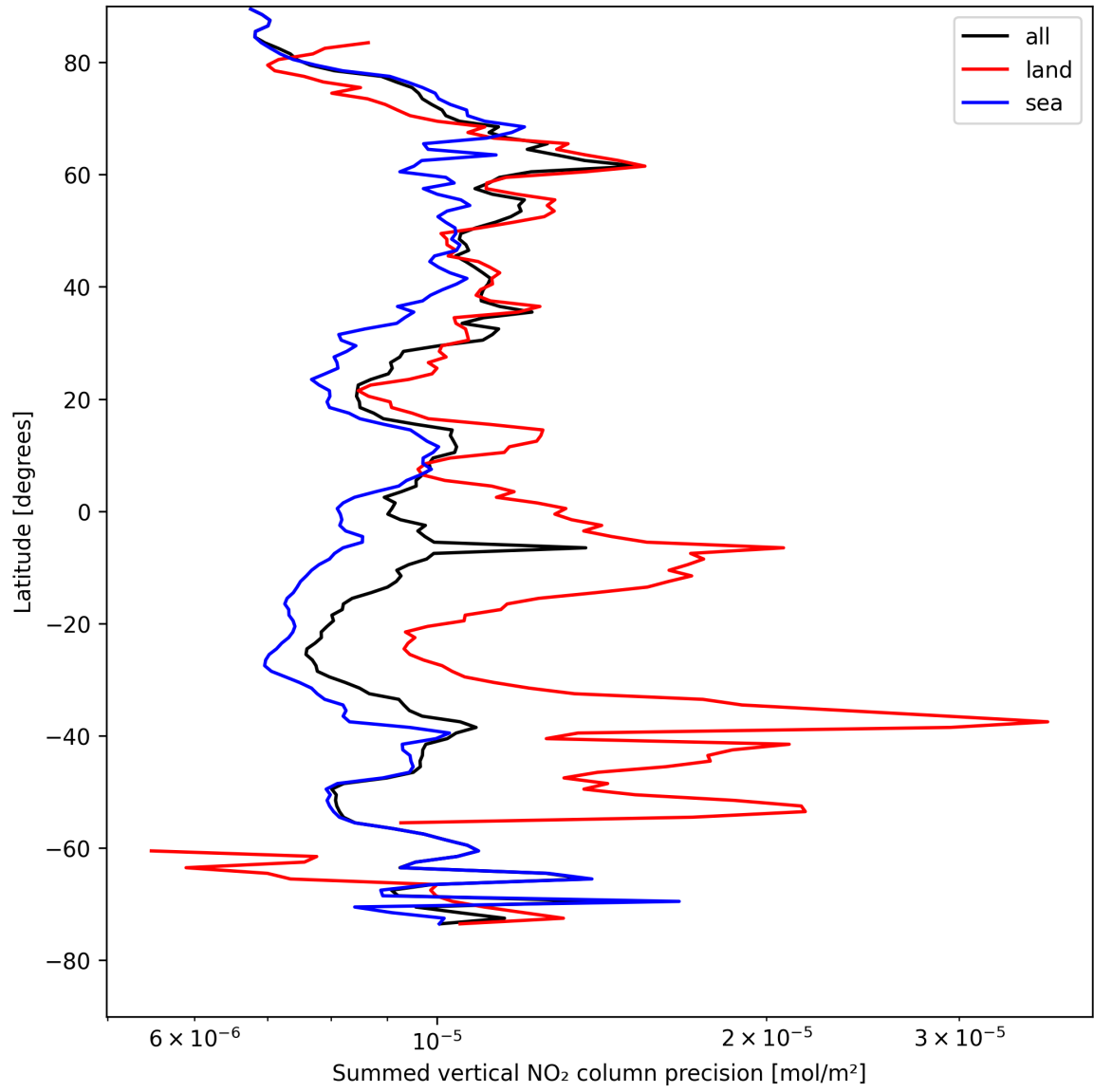
Figure 24: Zonal average of “Summed vertical NO 2 column precision” for 2025-08-11 to 2025-08-13.
