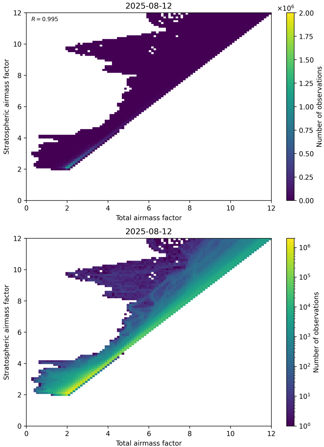
Figure 62: Scatter density plot of “Total airmass factor” against “Stratospheric airmass factor” for 2025-08-11 to 2025-08-13.
