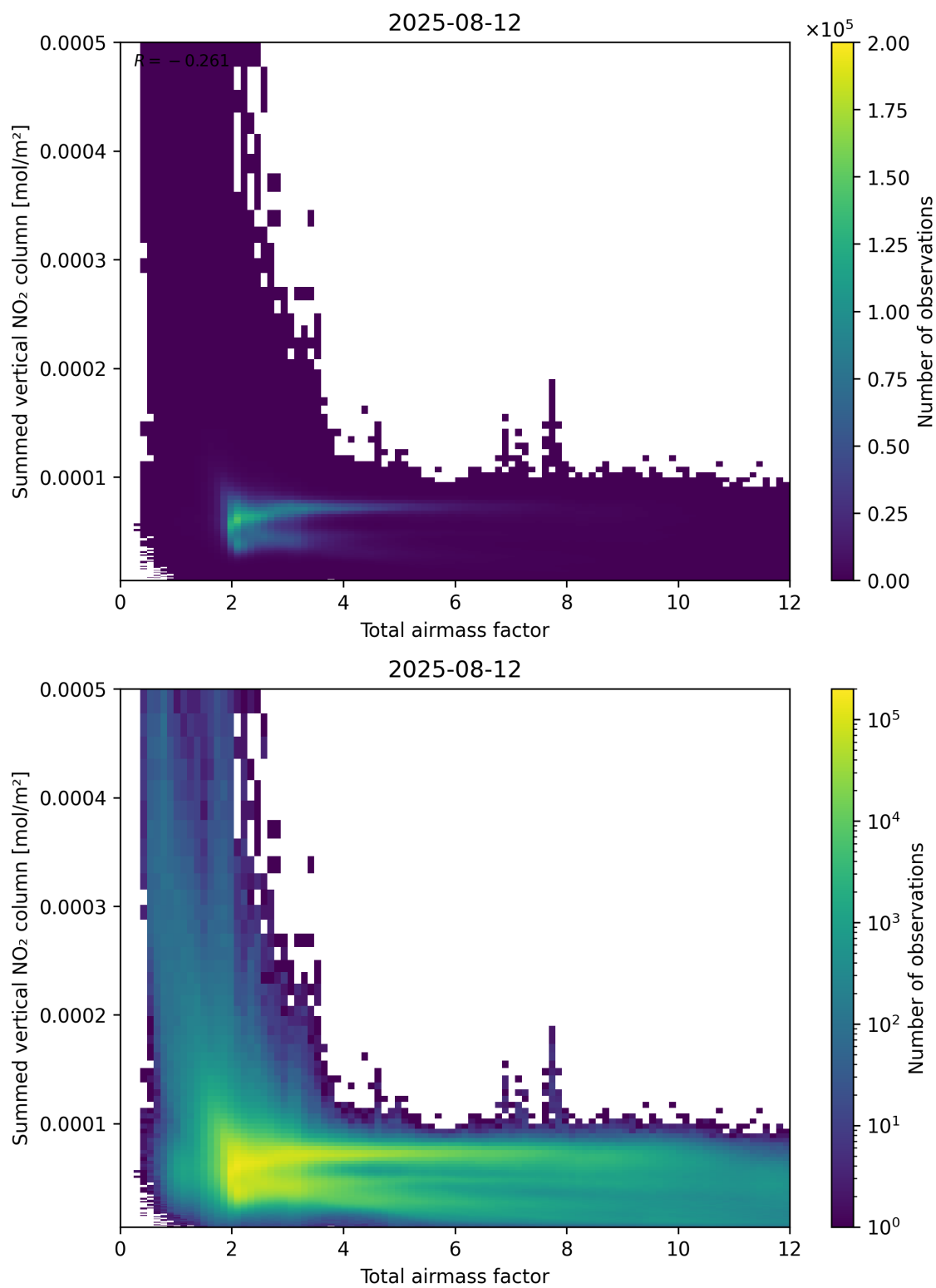
Figure 65: Scatter density plot of “Total airmass factor” against “Summed vertical NO 2 column” for 2025-08-11 to 2025-08-13.
