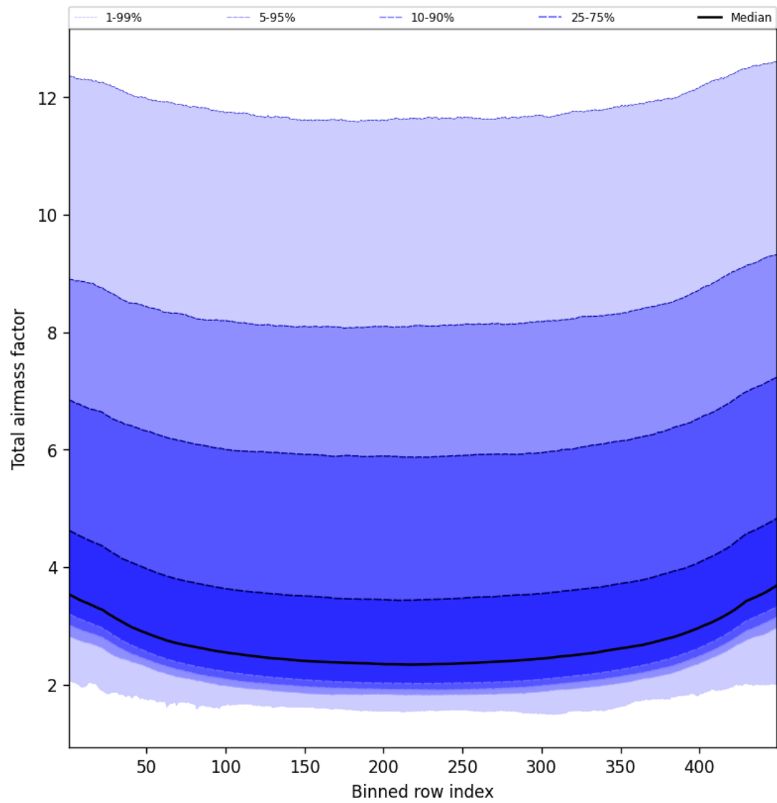
Figure 49: Along track statistics of “Total airmass factor” for 2025-08-11 to 2025-08-13
