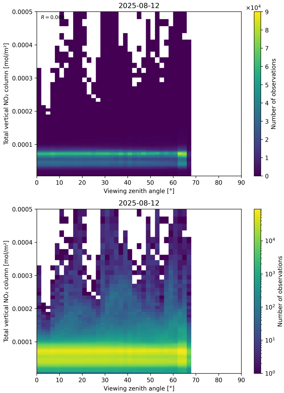
Figure 167: Scatter density plot of “Viewing zenith angle” against “Total vertical NO 2 column” for 2025-08-11 to 2025-08-13.
