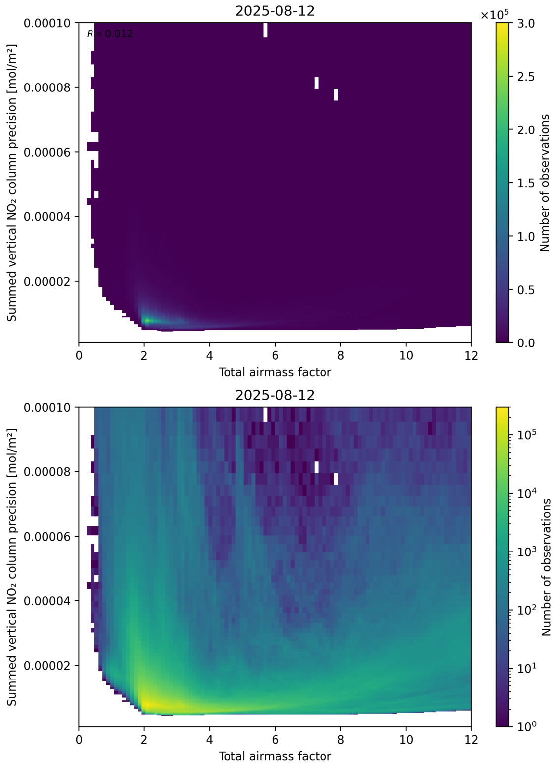
Figure 66: Scatter density plot of “Total airmass factor” against “Summed vertical NO 2 column precision” for 2025-08-11 to 2025-08-13.
