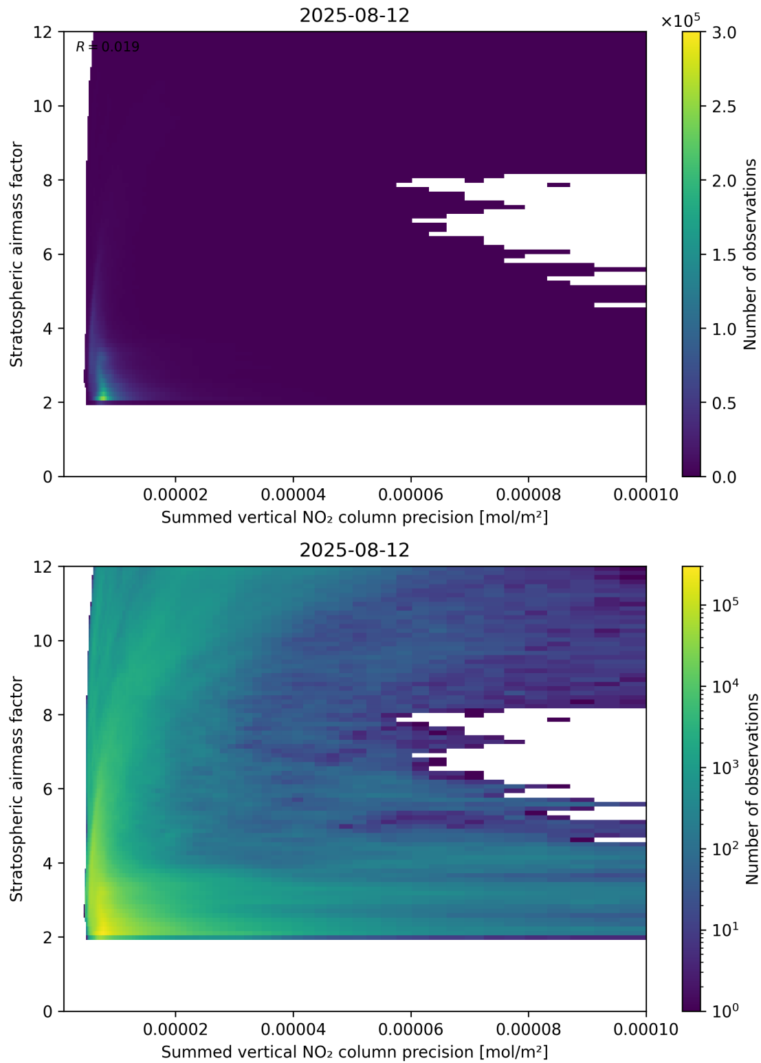
Figure 106: Scatter density plot of “Summed vertical NO 2 column precision” against “Stratospheric airmass factor” for 2025-08-11 to 2025-08-13.
