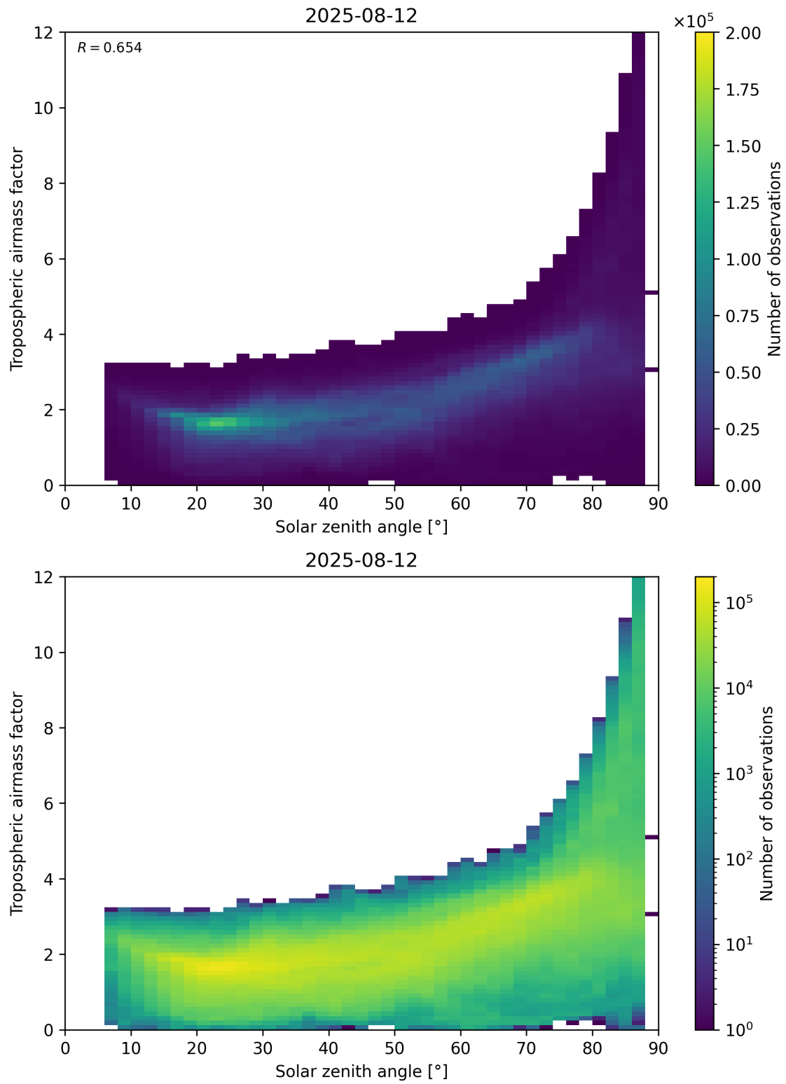
Figure 147: Scatter density plot of “Solar zenith angle” against “Tropospheric airmass factor” for 2025-08-11 to 2025-08-13.
