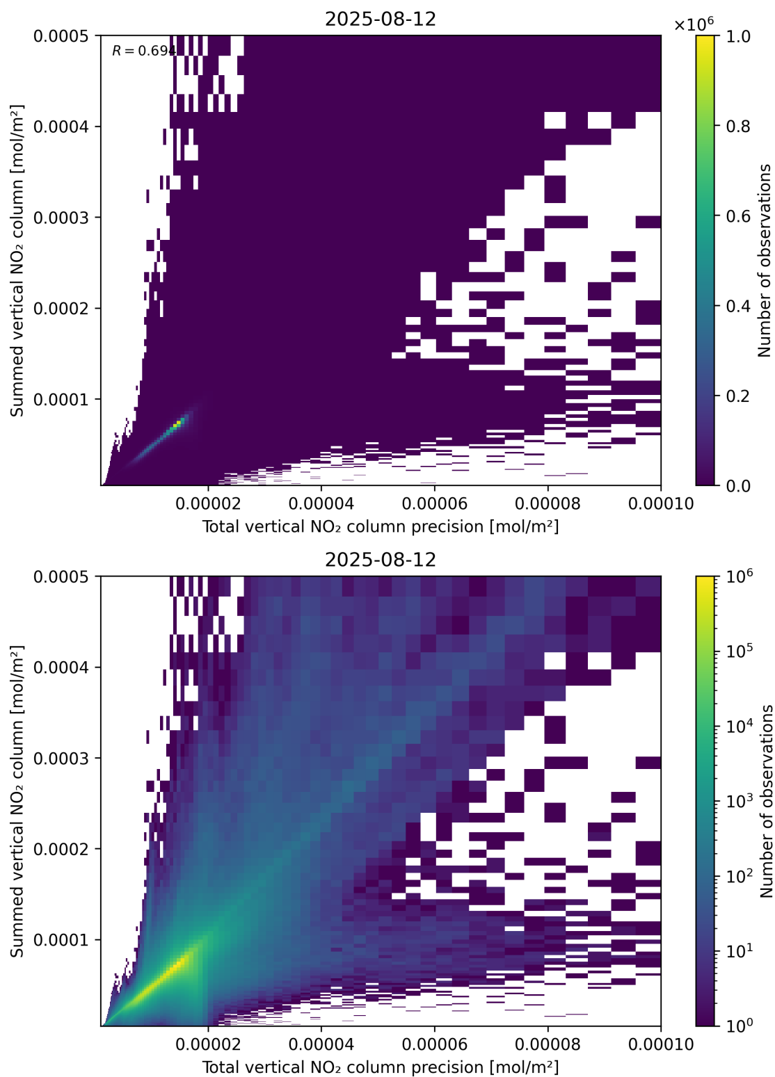
Figure 117: Scatter density plot of “Total vertical NO 2 column precision” against “Summed vertical NO 2 column” for 2025-08-11 to 2025-08-13.
