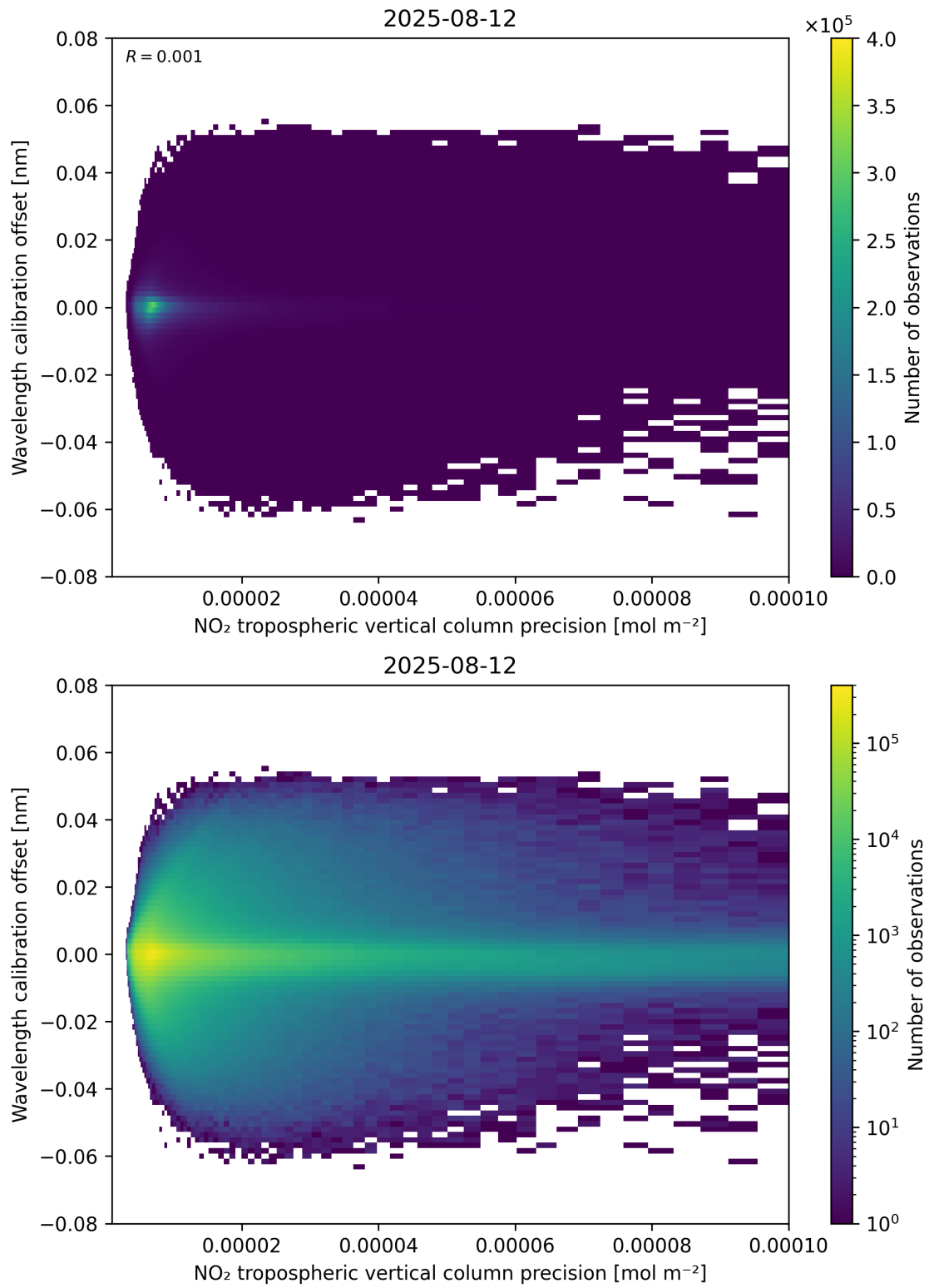
Figure 141: Scatter density plot of “NO 2 tropospheric vertical column precision” against “Wavelength calibration offset” for 2025-08-11 to 2025-08-13.
