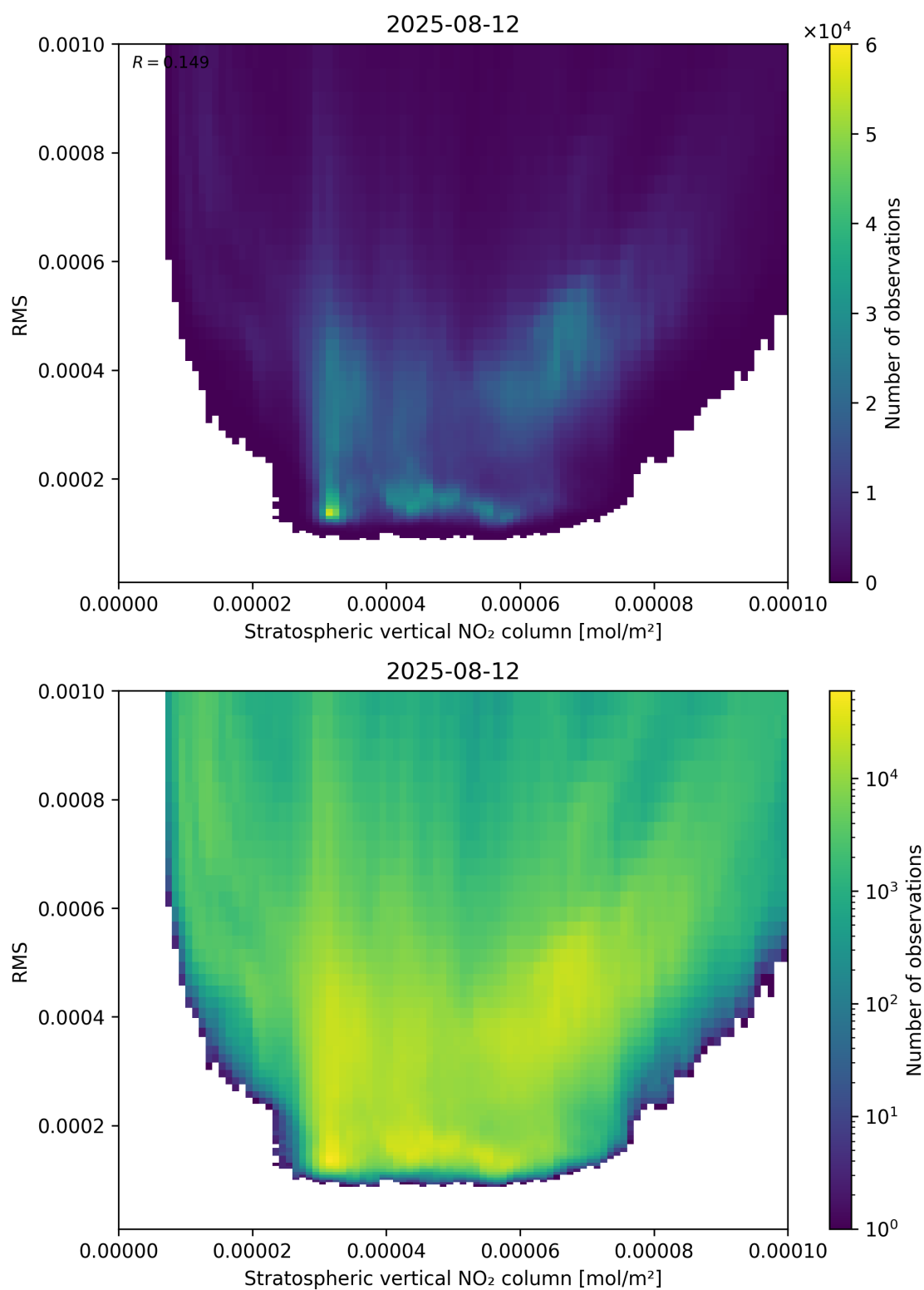
Figure 102: Scatter density plot of “Stratospheric vertical NO 2 column” against “RMS” for 2025-08-11 to 2025-08-13.
