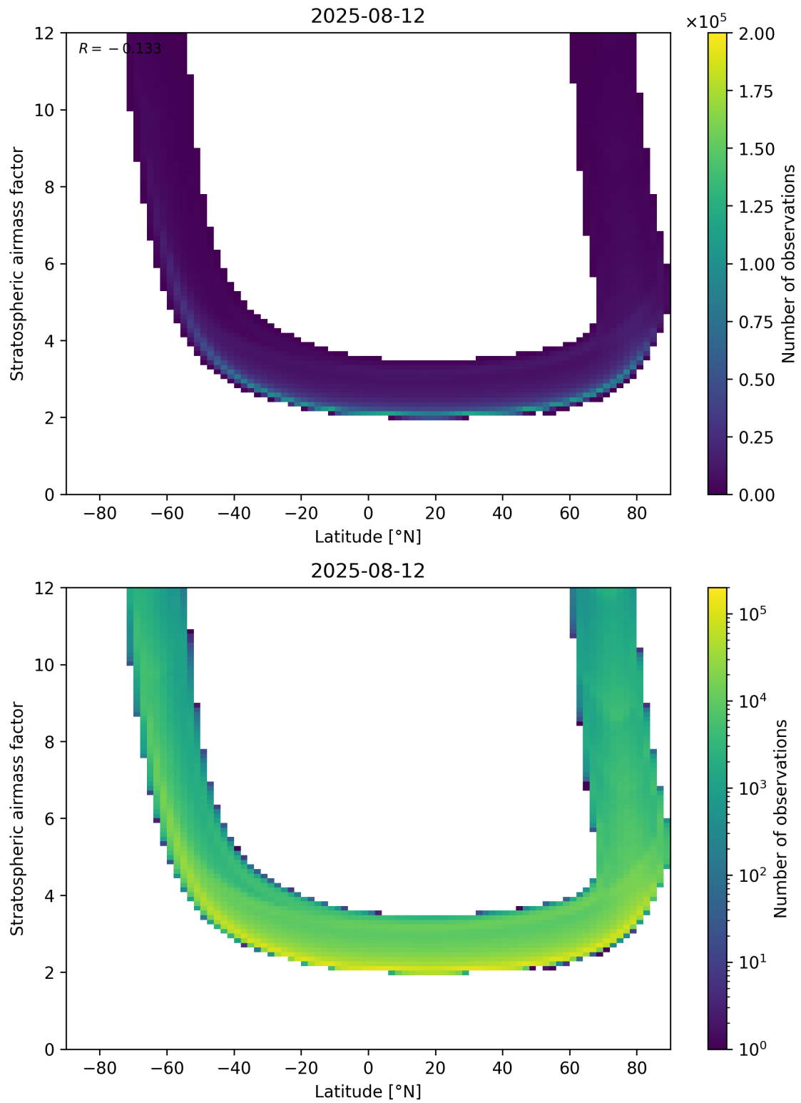
Figure 83: Scatter density plot of “Latitude” against “Stratospheric airmass factor” for 2025-08-11 to 2025-08-13.
