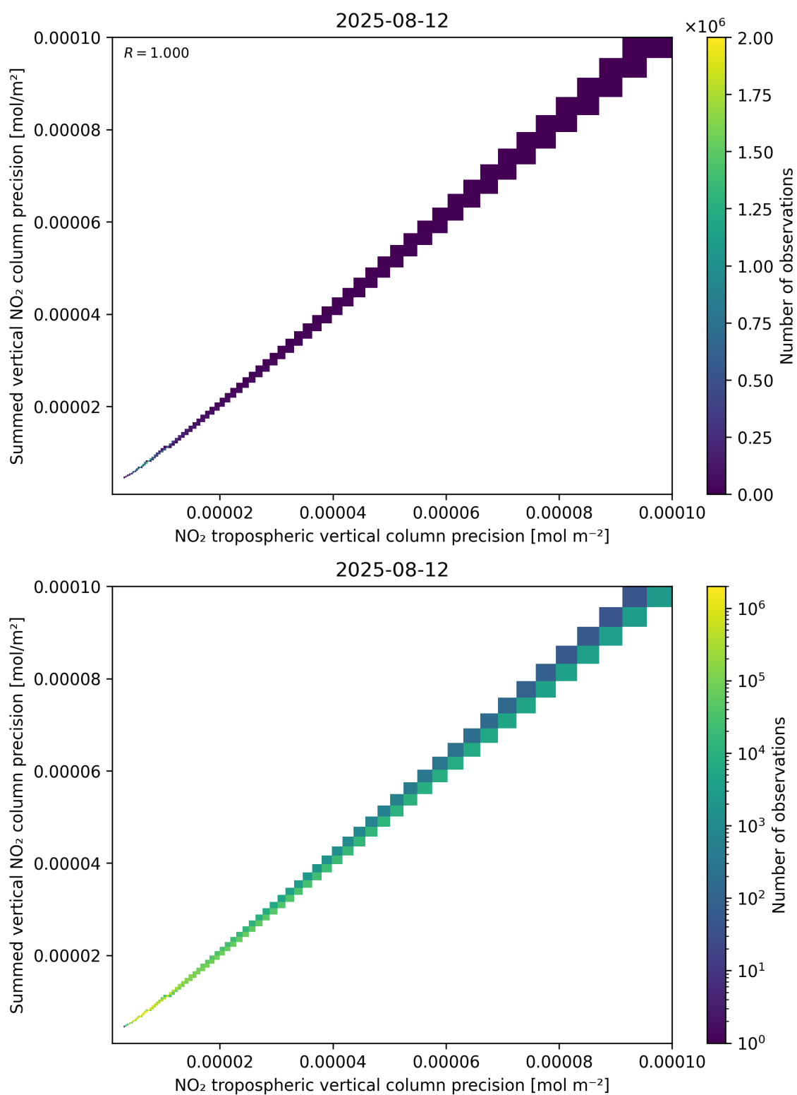
Figure 137: Scatter density plot of “NO 2 tropospheric vertical column precision” against “Summed vertical NO 2 column precision” for 2025-08-11 to 2025-08-13.
