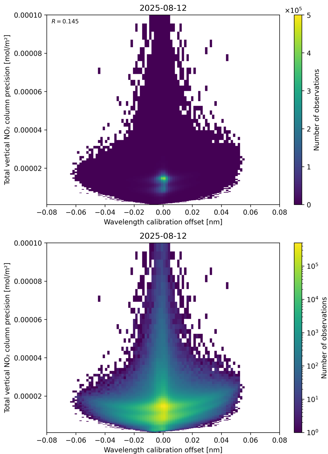
Figure 180: Scatter density plot of “Wavelength calibration offset” against “Total vertical NO 2 column precision” for 2025-08-11 to 2025-08-13.
