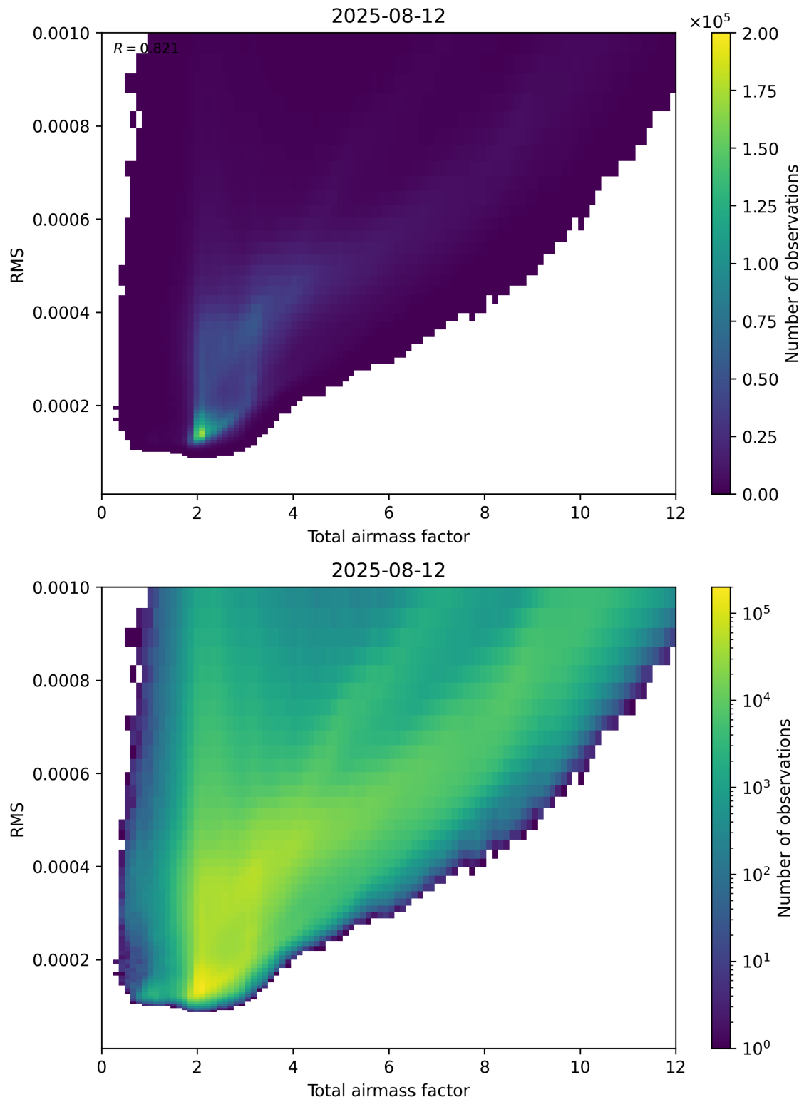
Figure 69: Scatter density plot of “Total airmass factor” against “RMS” for 2025-08-11 to 2025-08-13.
