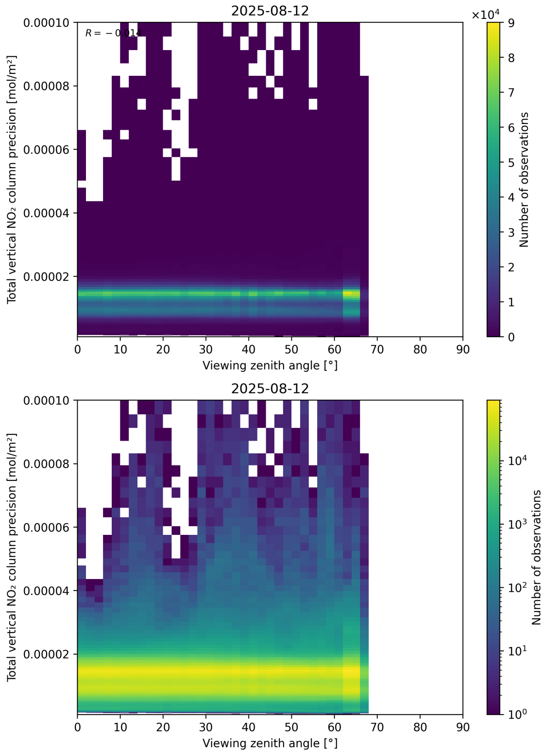
Figure 168: Scatter density plot of “Viewing zenith angle” against “Total vertical NO 2 column precision” for 2025-08-11 to 2025-08-13.
