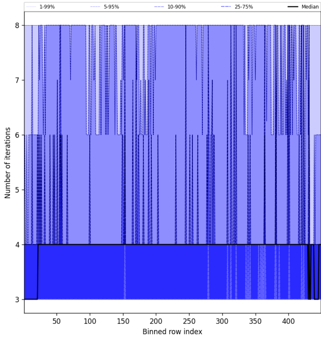
Figure 51: Along track statistics of “Number of iterations” for 2025-08-11 to 2025-08-13
