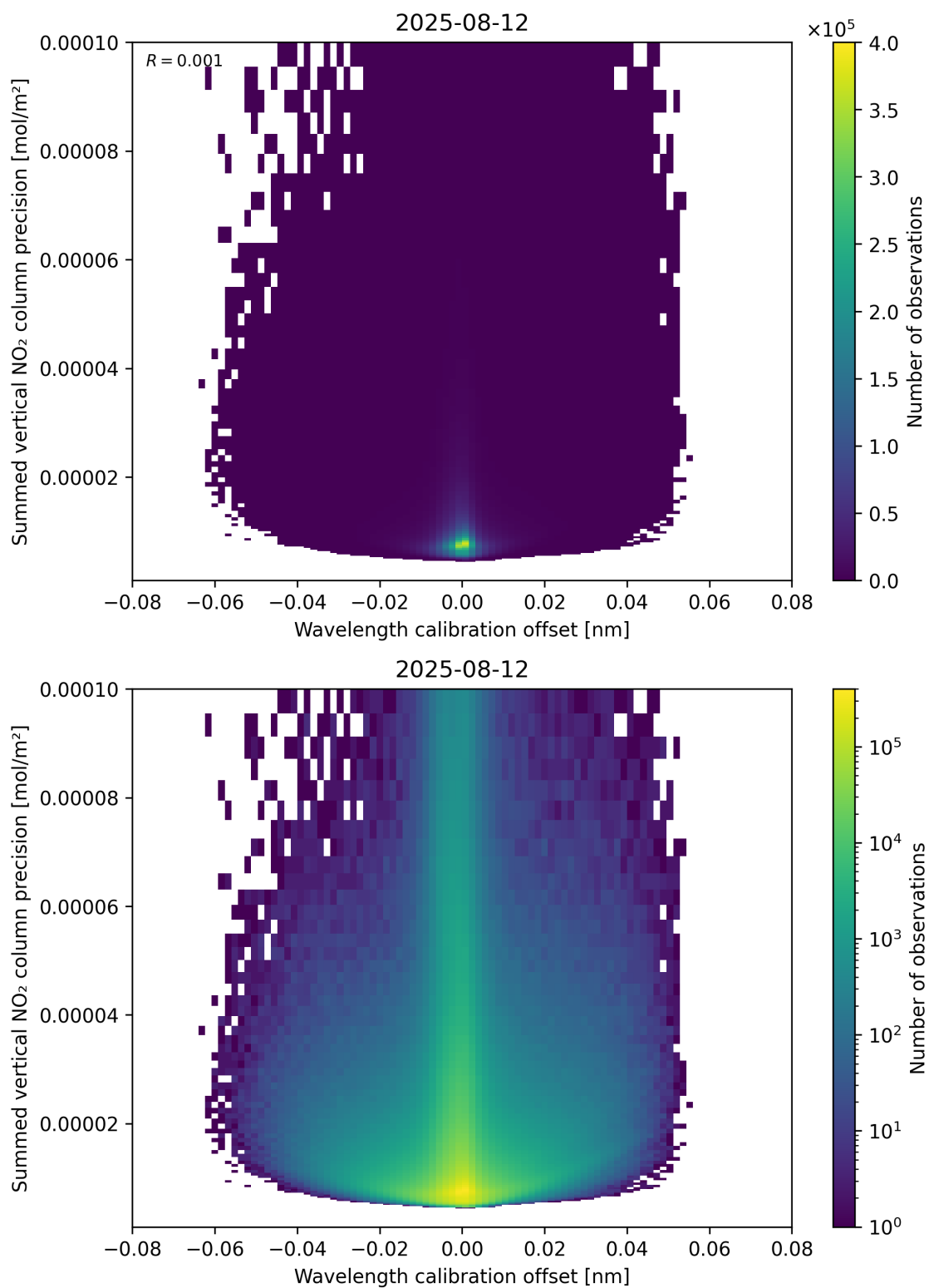
Figure 178: Scatter density plot of “Wavelength calibration offset” against “Summed vertical NO 2 column precision” for 2025-08-11 to 2025-08-13.
