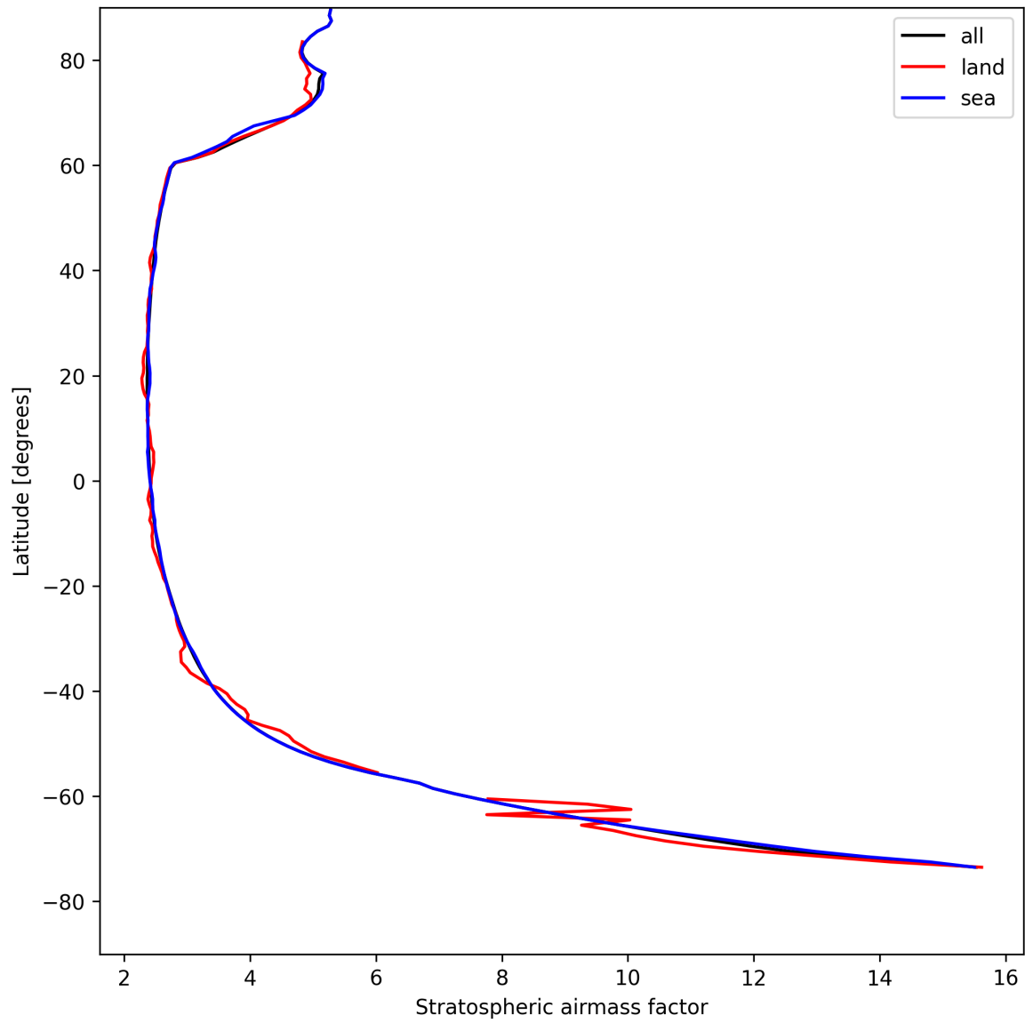
Figure 27: Zonal average of “Stratospheric airmass factor” for 2025-08-11 to 2025-08-13.
