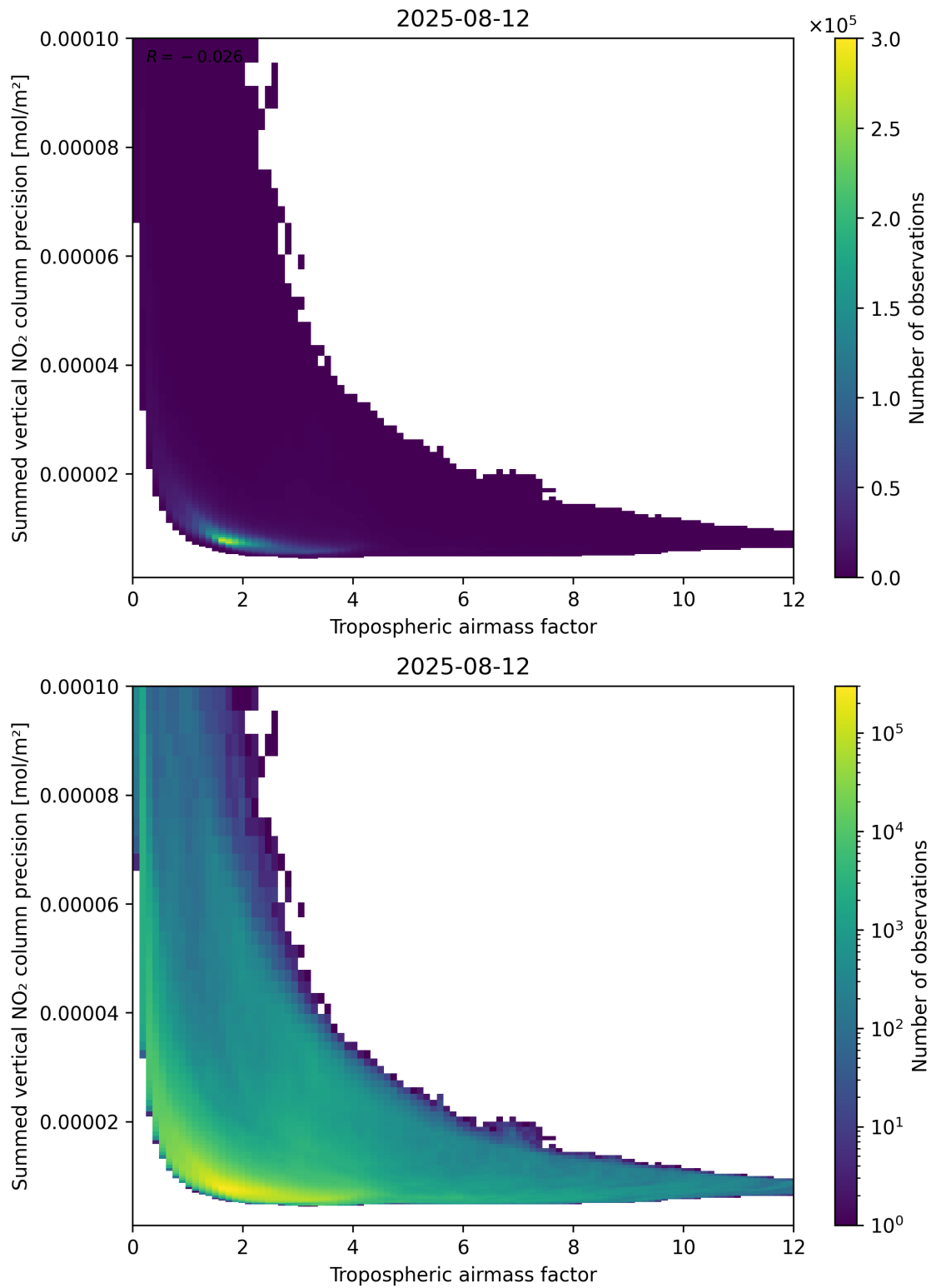
Figure 76: Scatter density plot of “Tropospheric air mass factor” against “Summed vertical NO 2 column precision” for 2025-08-11 to 2025-08-13.
