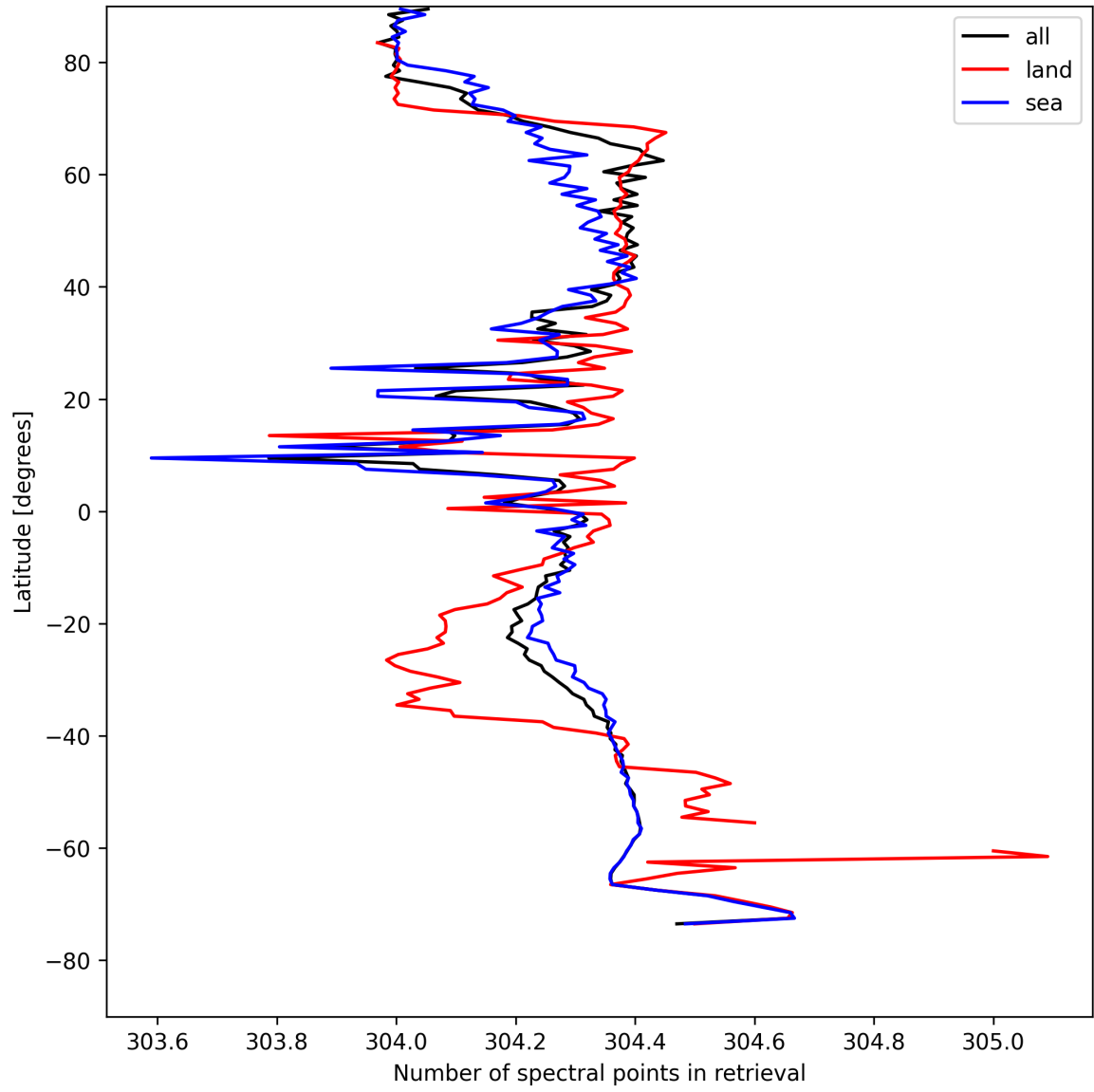
Figure 16: Zonal average of “Number of spectral points in retrieval” for 2025-08-11 to 2025-08-13.
