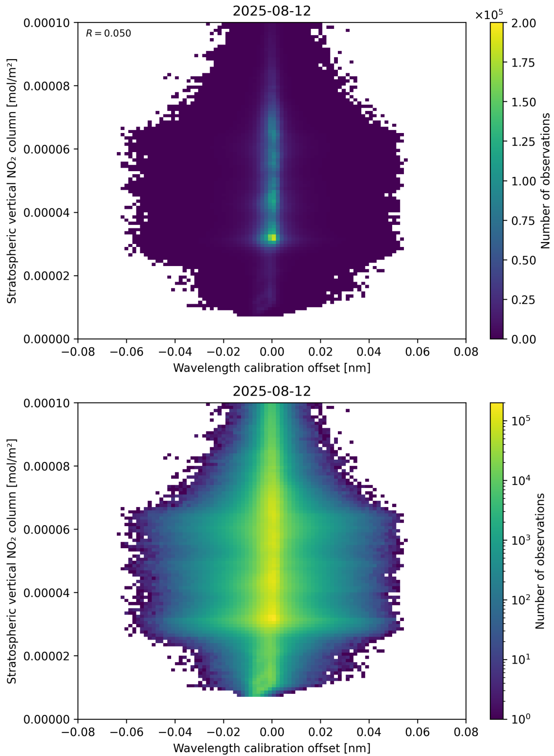
Figure 176: Scatter density plot of “Wavelength calibration offset” against “Stratospheric vertical NO 2 column” for 2025-08-11 to 2025-08-13.
