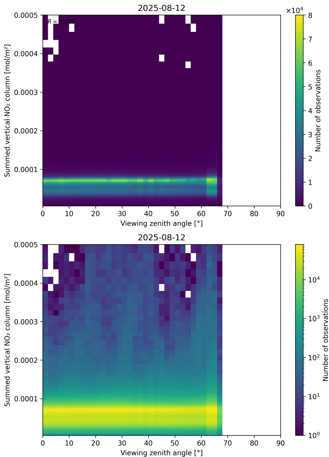
Figure 165: Scatter density plot of “Viewing zenith angle” against “Summed vertical NO 2 column” for 2025-08-11 to 2025-08-13.
