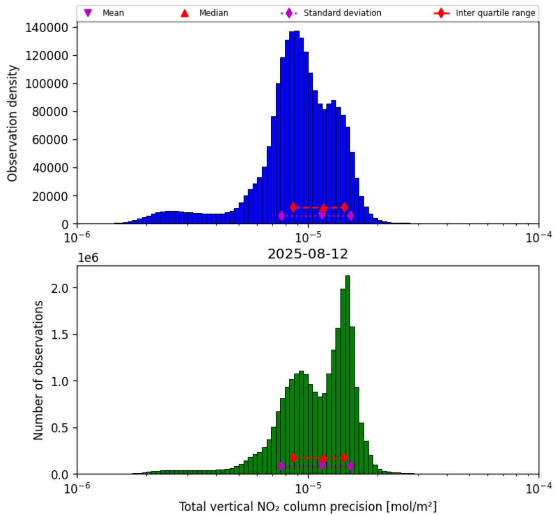
Figure 39: Histogram of “Total vertical NO 2 column precision” for 2025-08-11 to 2025-08-13
