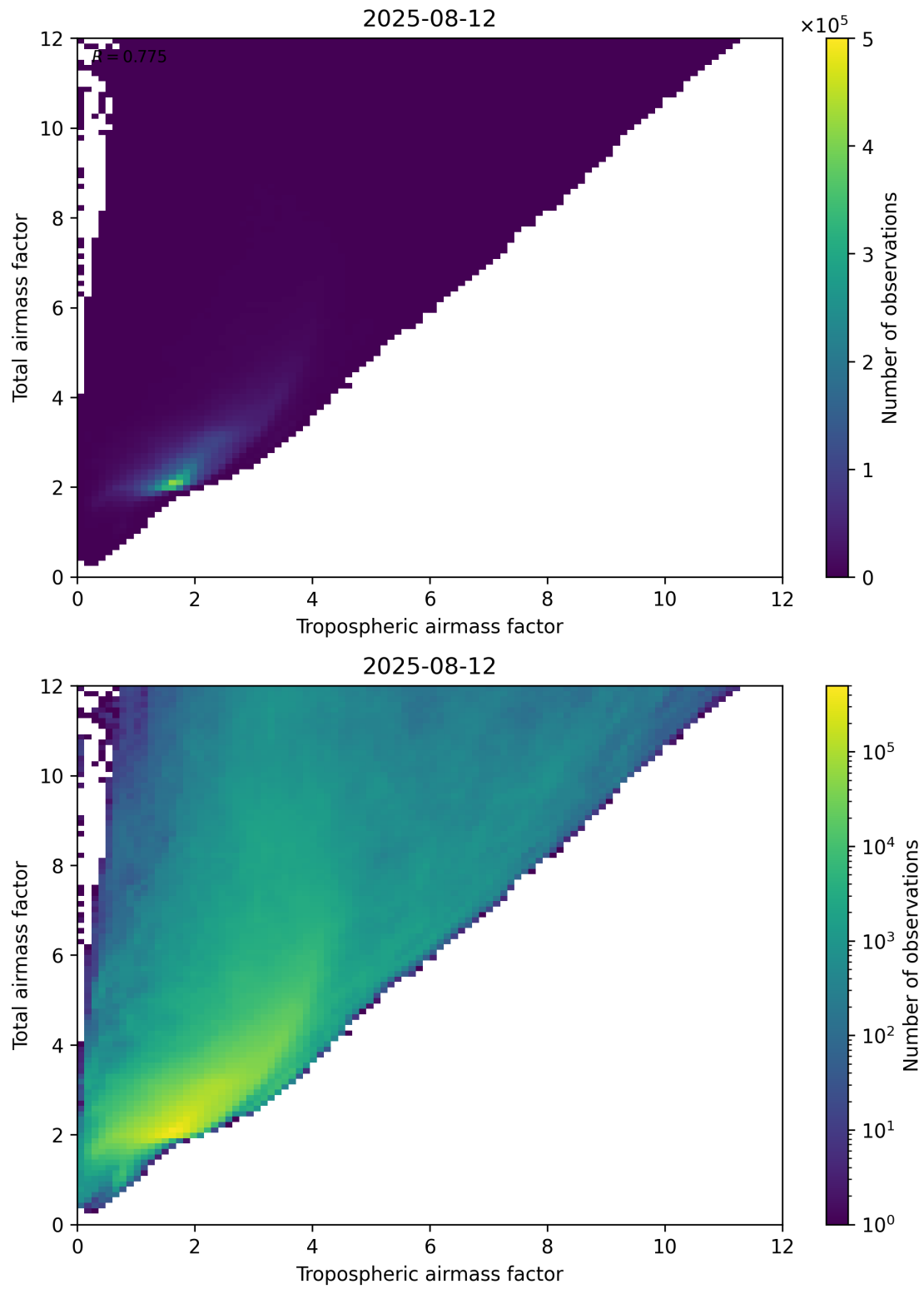
Figure 72: Scatter density plot of “Tropospheric airmass factor” against “Total airmass factor” for 2025-08-11 to 2025-08-13.
