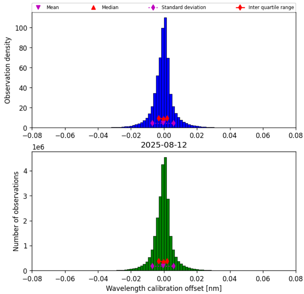
Figure 35: Histogram of “Wavelength calibration offset” for 2025-08-11 to 2025-08-13
