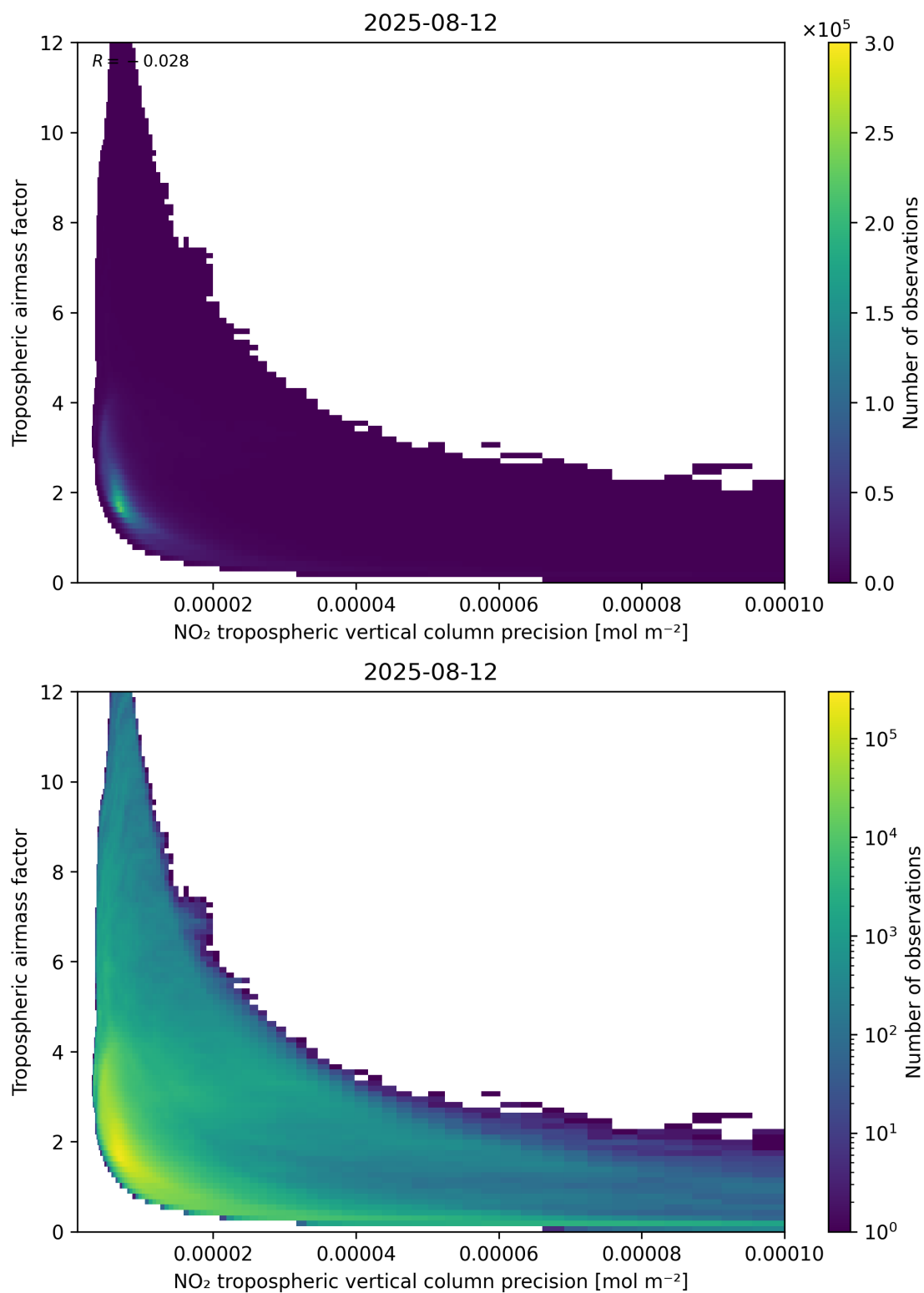
Figure 133: Scatter density plot of “NO 2 tropospheric vertical column precision” against “Tropospheric air mass factor” for 2025-08-11 to 2025-08-13.
