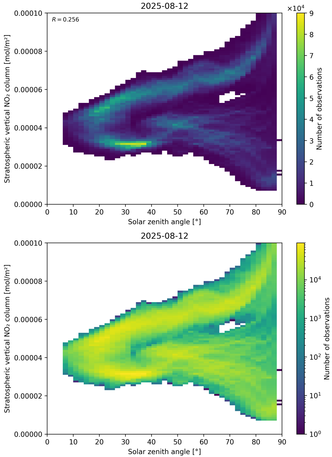
Figure 150: Scatter density plot of “Solar zenith angle” against “Stratospheric vertical NO 2 column” for 2025-08-11 to 2025-08-13.
