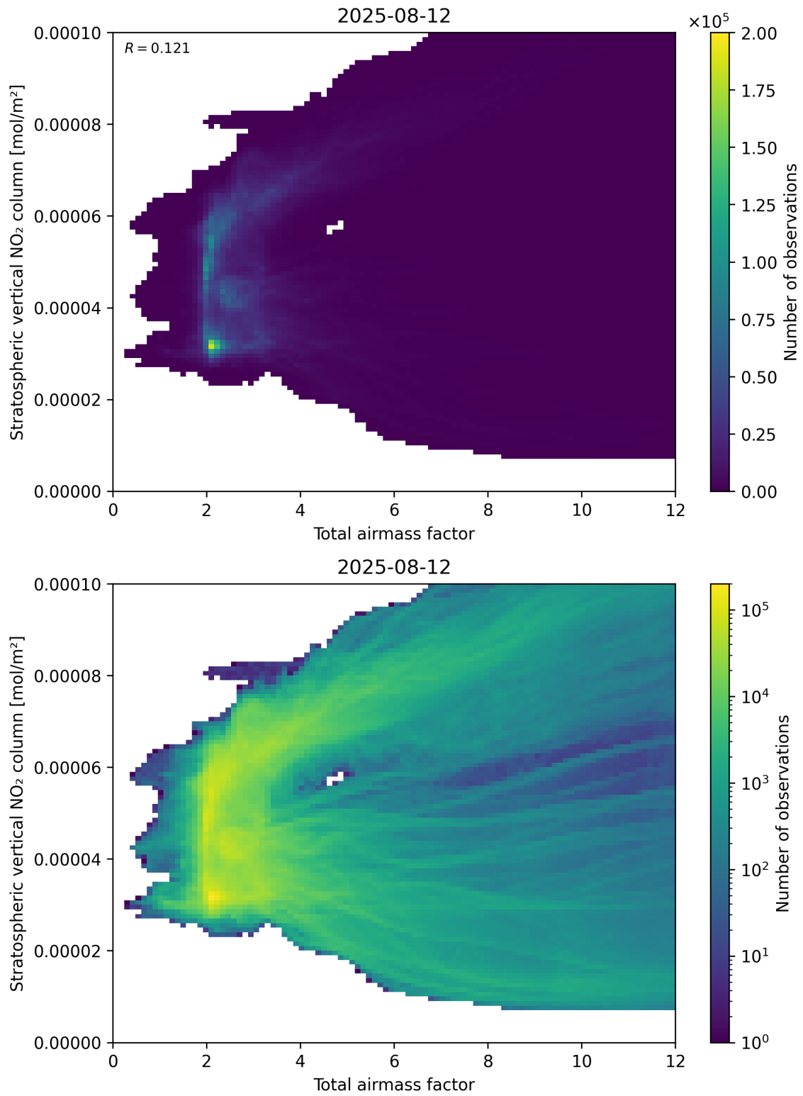
Figure 64: Scatter density plot of “Total airmass factor” against “Stratospheric vertical \text{NO}_2 column” for 2025-08-11 to 2025-08-13.
