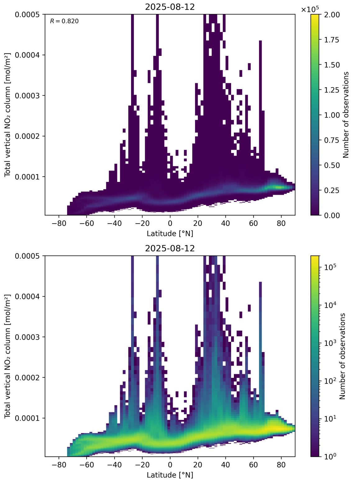
Figure 90: Scatter density plot of “Latitude” against “Total vertical NO 2 column” for 2025-08-11 to 2025-08-13.
