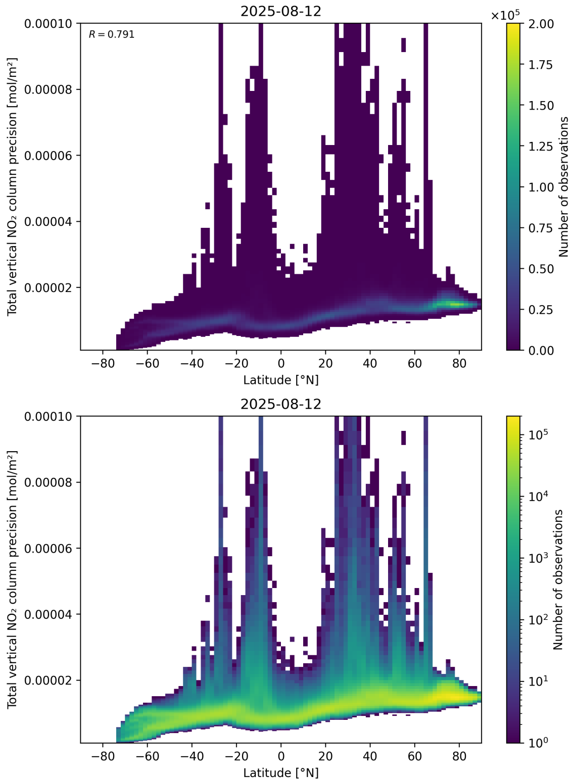
Figure 91: Scatter density plot of “Latitude” against “Total vertical NO 2 column precision” for 2025-08-11 to 2025-08-13.
