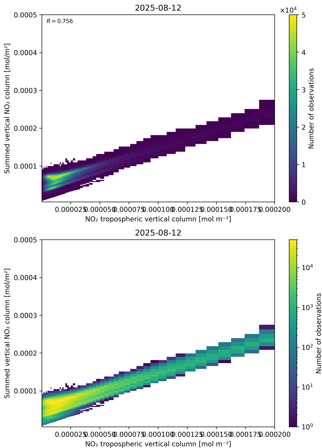
Figure 126: Scatter density plot of “NO 2 tropospheric vertical column” against “Summed vertical NO 2 column” for 2025-08-11 to 2025-08-13.
