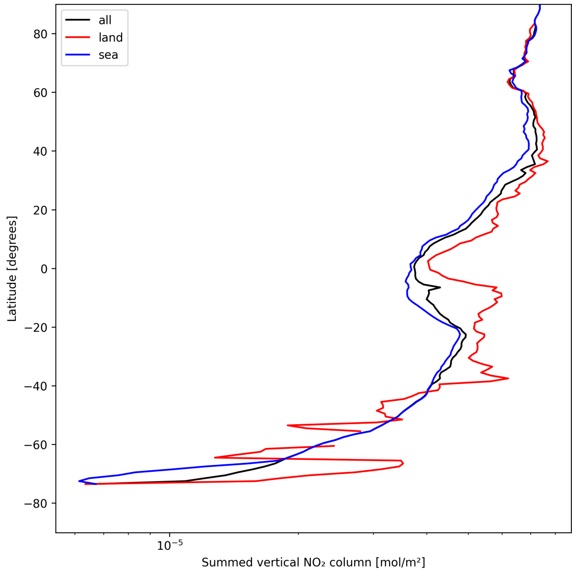
Figure 23: Zonal average of “Summed vertical NO 2 column” for 2025-08-11 to 2025-08-13.
