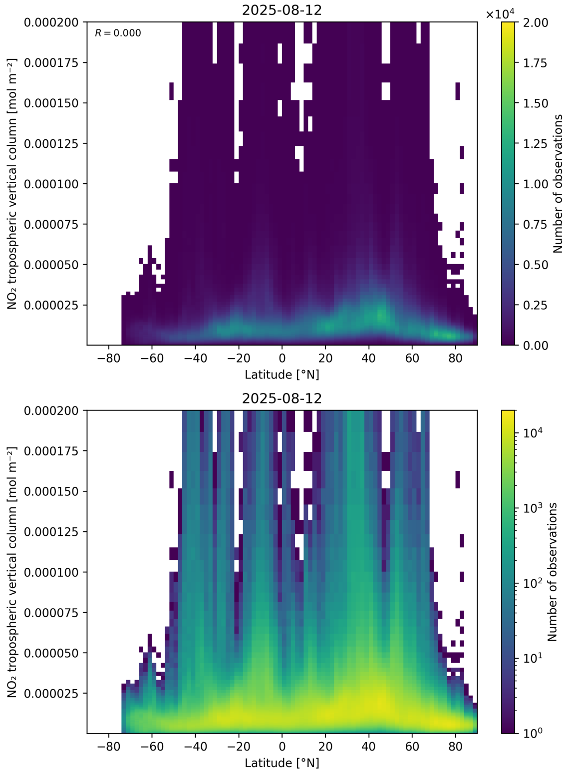
Figure 92: Scatter density plot of “Latitude” against “NO 2 tropospheric vertical column” for 2025-08-11 to 2025-08-13.
