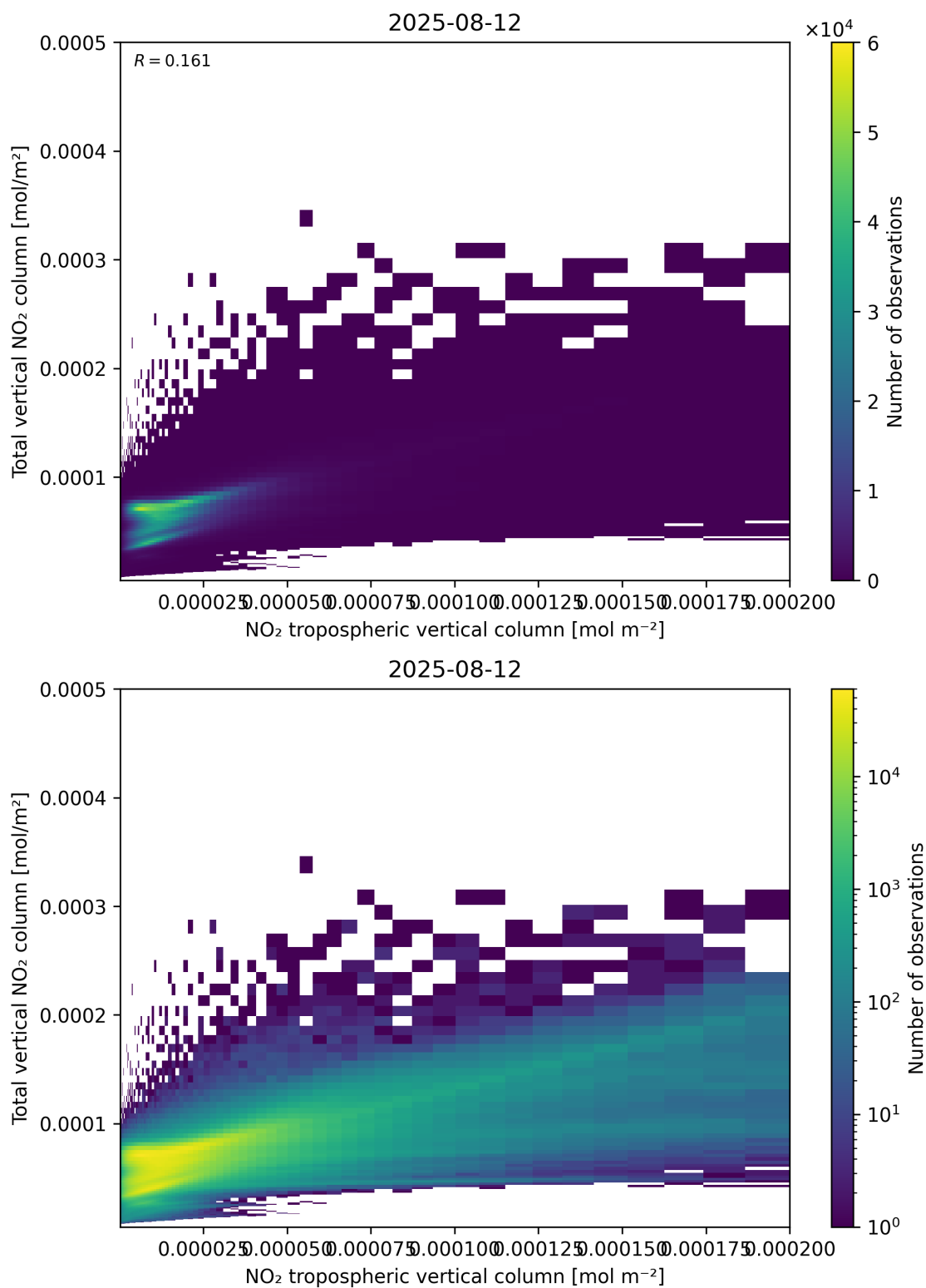
Figure 128: Scatter density plot of “NO 2 tropospheric vertical column” against “Total vertical NO 2 column” for 2025-08-11 to 2025-08-13.
