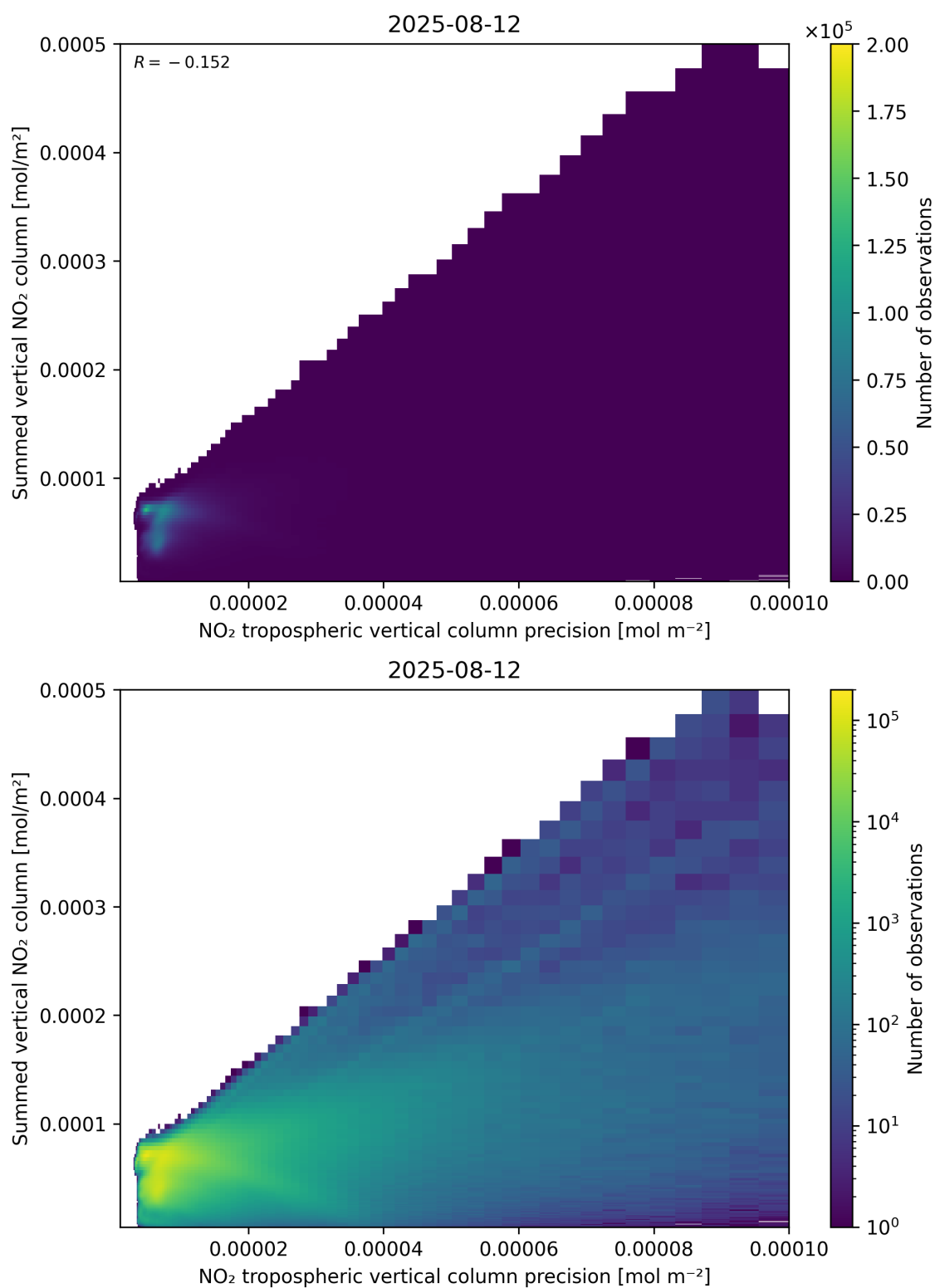
Figure 136: Scatter density plot of “NO 2 tropospheric vertical column precision” against “Summed vertical NO 2 column” for 2025-08-11 to 2025-08-13.
