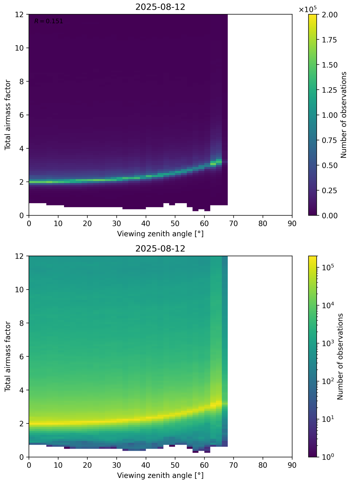
Figure 160: Scatter density plot of “Viewing zenith angle” against “Total airmass factor” for 2025-08-11 to 2025-08-13.
