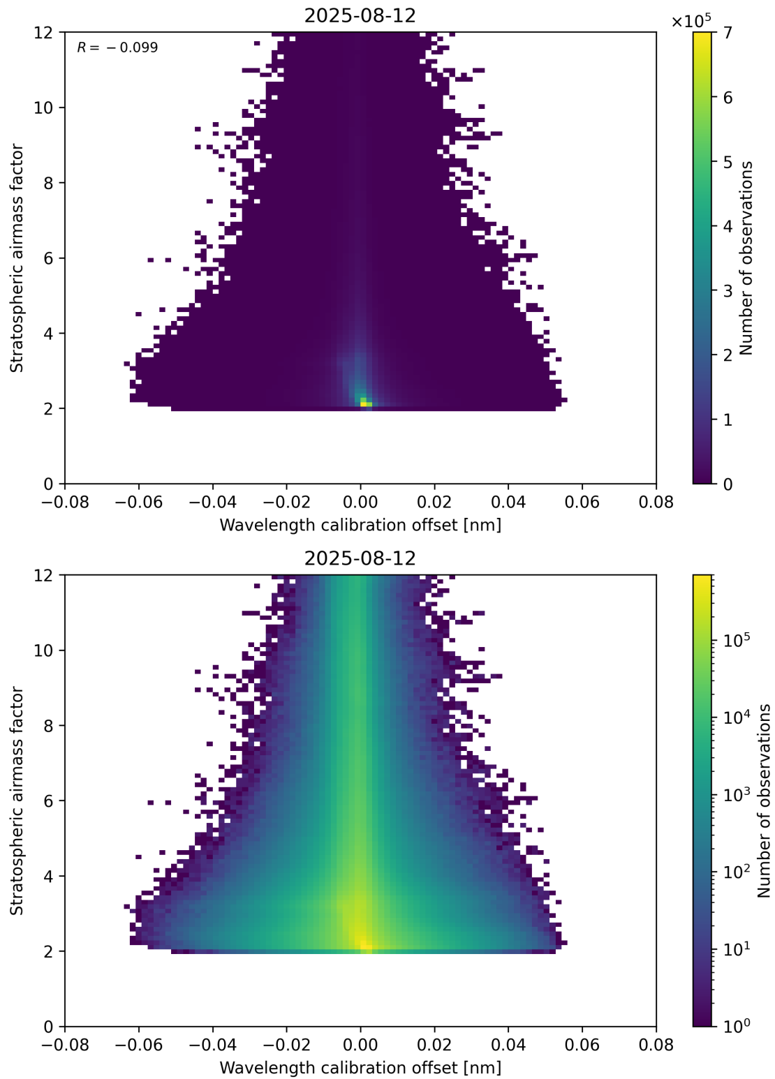
Figure 174: Scatter density plot of “Wavelength calibration offset” against “Stratospheric airmass factor” for 2025-08-11 to 2025-08-13.
