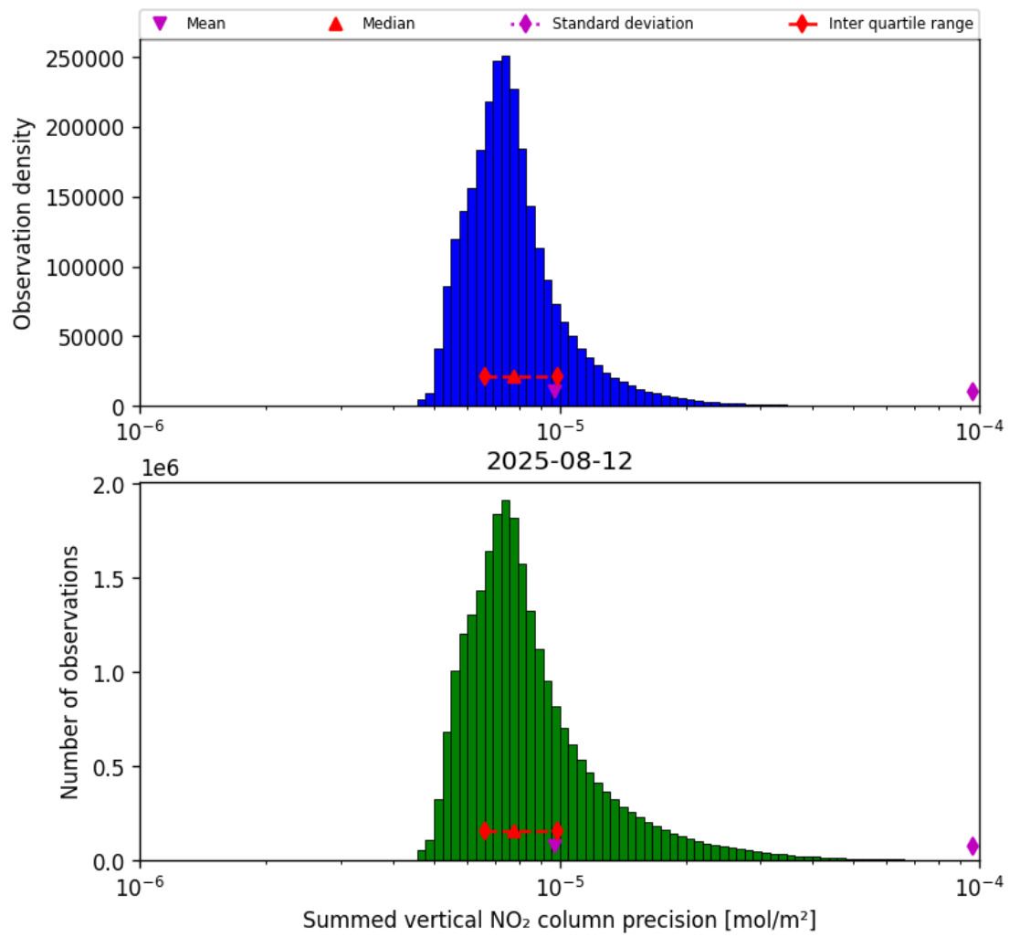
Figure 41: Histogram of "Summed vertical NO 2 column precision" for 2025-08-11 to 2025-08-13
