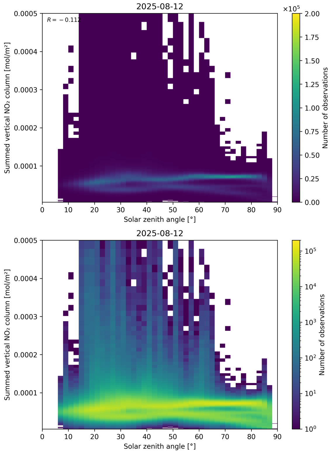
Figure 151: Scatter density plot of “Solar zenith angle” against “Summed vertical NO 2 column” for 2025-08-11 to 2025-08-13.
