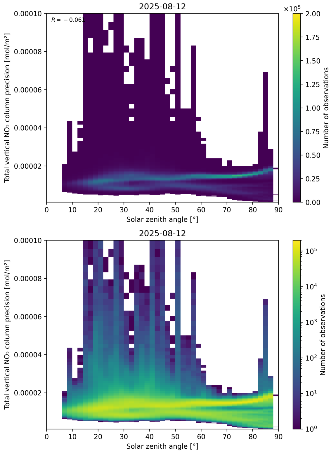
Figure 154: Scatter density plot of “Solar zenith angle” against “Total vertical NO 2 column precision” for 2025-08-11 to 2025-08-13.
