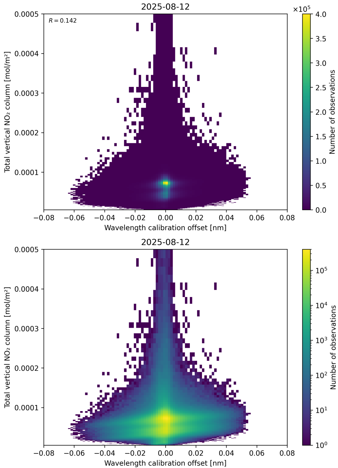
Figure 179: Scatter density plot of “Wavelength calibration offset” against “Total vertical NO 2 column” for 2025-08-11 to 2025-08-13.
