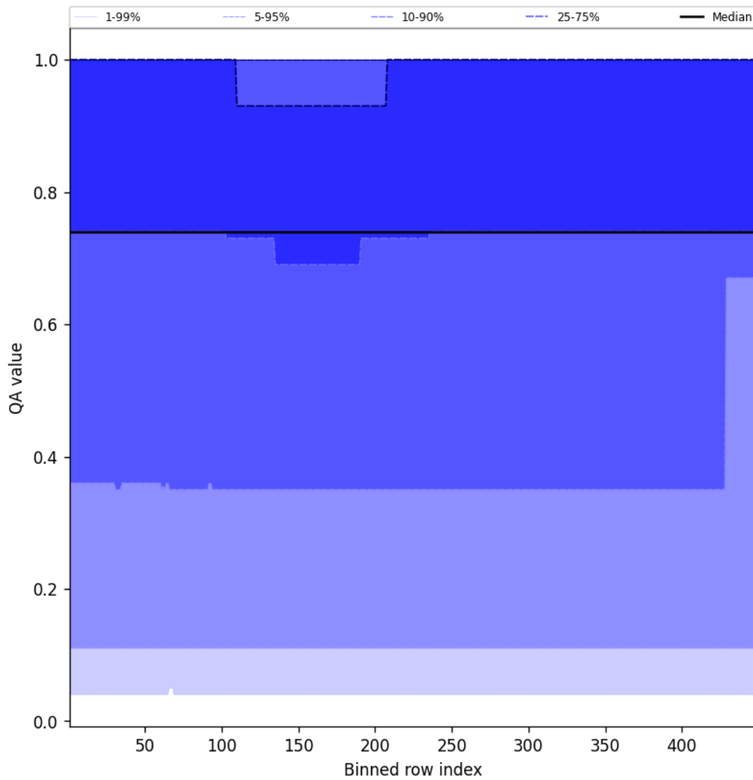
Figure 45: Along track statistics of “QA value” for 2025-08-11 to 2025-08-13
