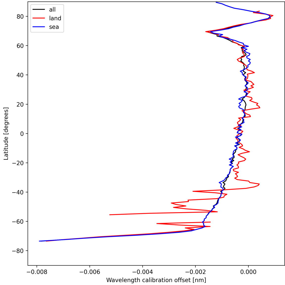
Figure 18: Zonal average of “Wavelength calibration offset” for 2025-08-11 to 2025-08-13.
