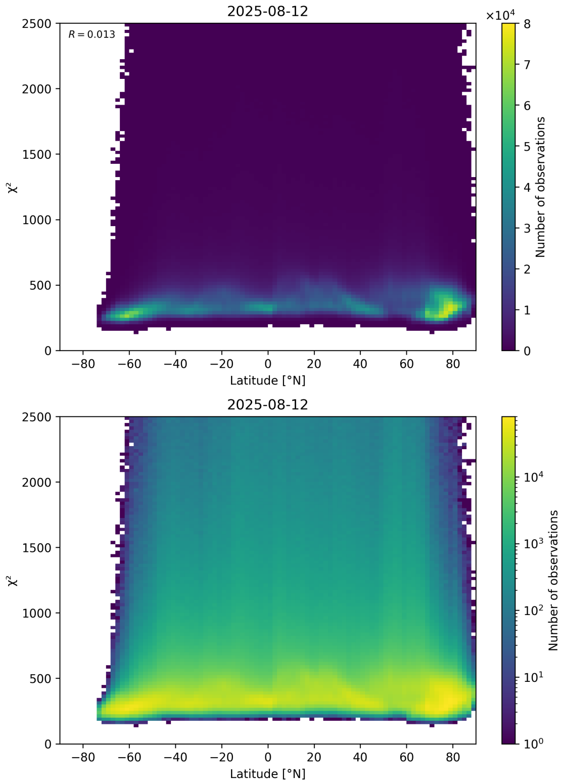
Figure 86: Scatter density plot of “Latitude” against “ \chi^2 ” for 2025-08-11 to 2025-08-13.
