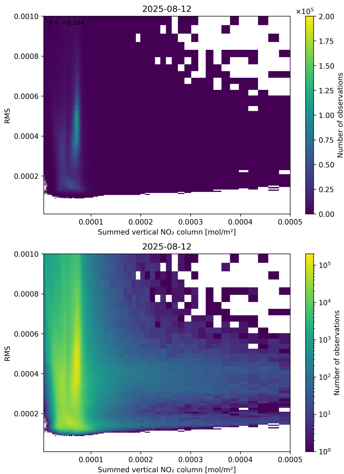
Figure 109: Scatter density plot of “Summed vertical NO 2 column” against “RMS” for 2025-08-11 to 2025-08-13.
