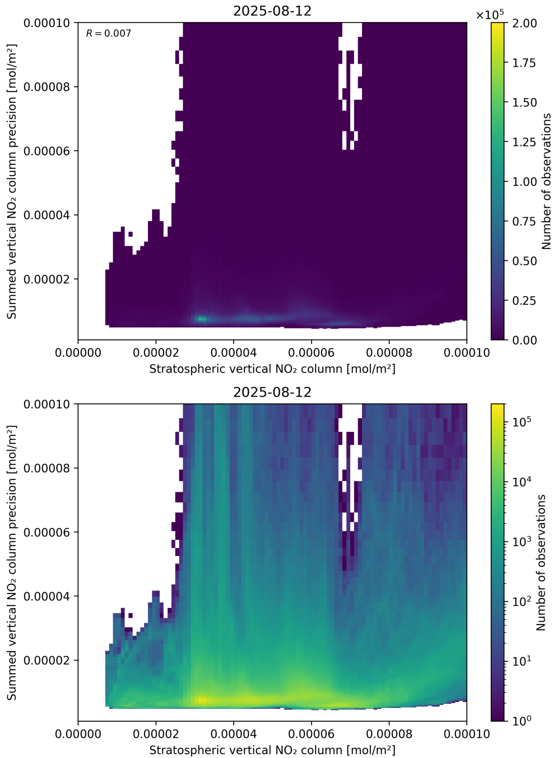
Figure 99: Scatter density plot of “Stratospheric vertical NO 2 column” against “Summed vertical NO 2 column precision” for 2025-08-11 to 2025-08-13.
