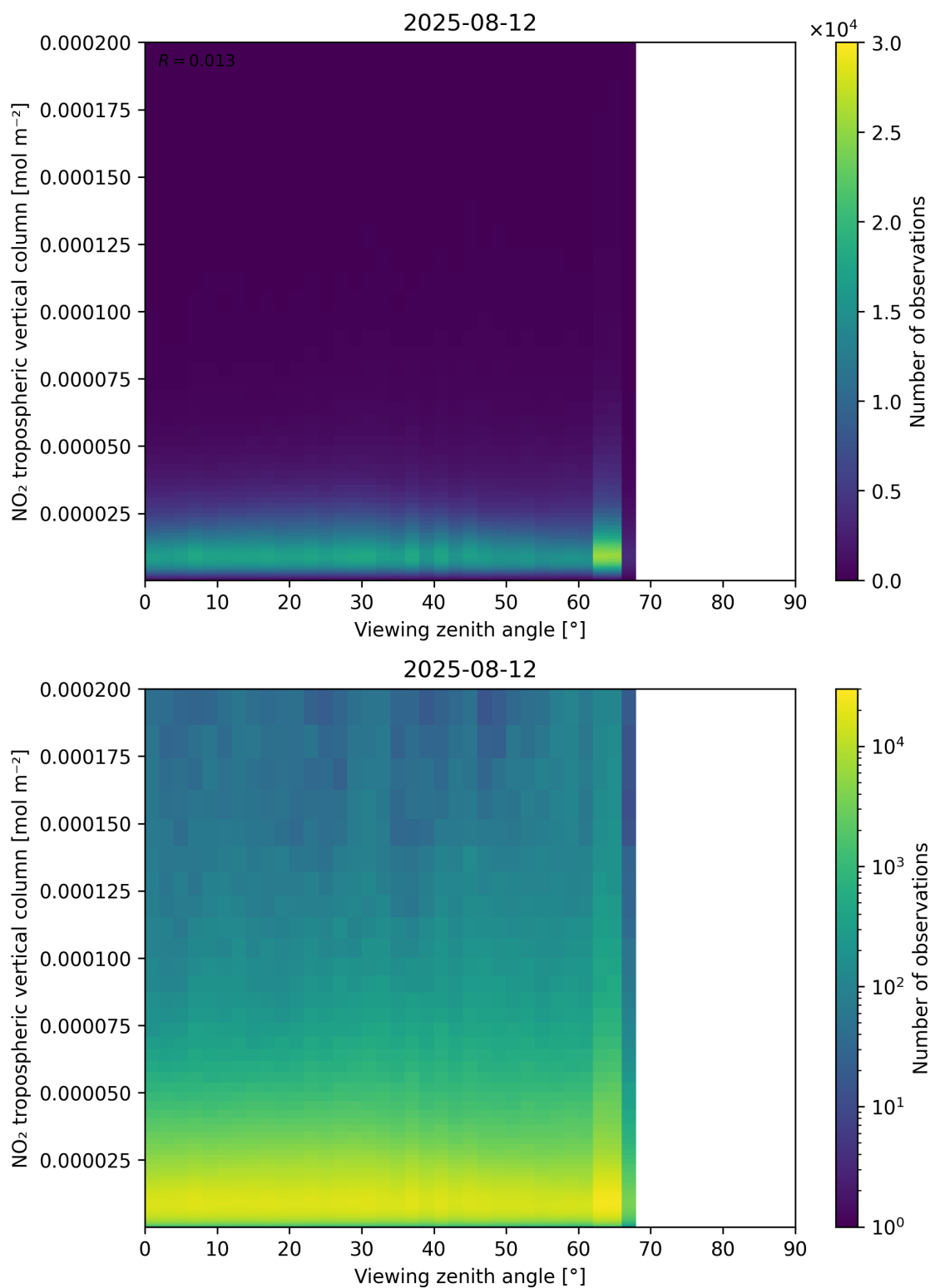
Figure 169: Scatter density plot of “Viewing zenith angle” against “NO 2 tropospheric vertical column” for 2025-08-11 to 2025-08-13.
