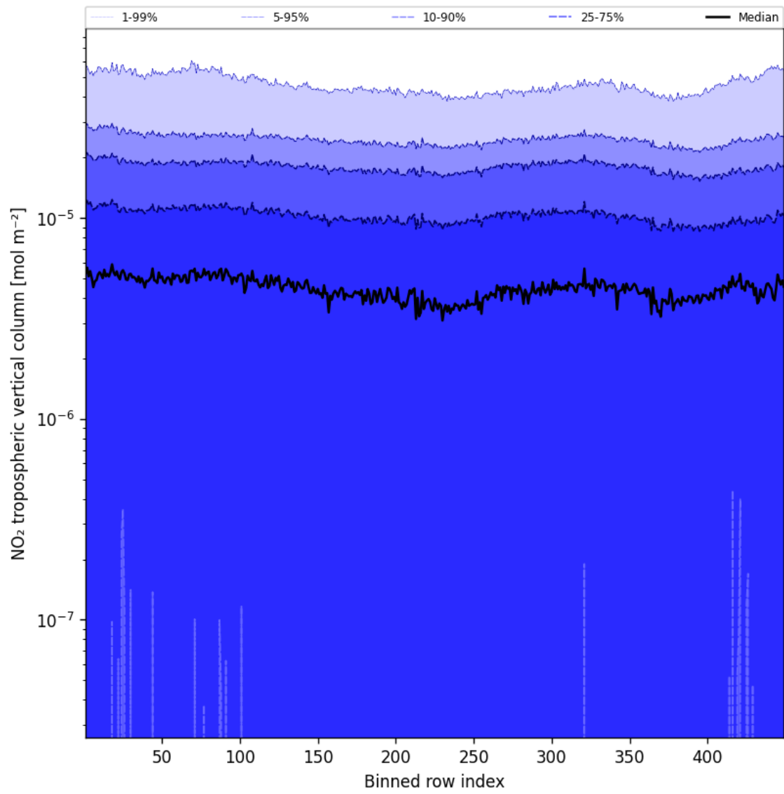
Figure 46: Along track statistics of “NO 2 tropospheric vertical column” for 2025-08-11 to 2025-08-13
