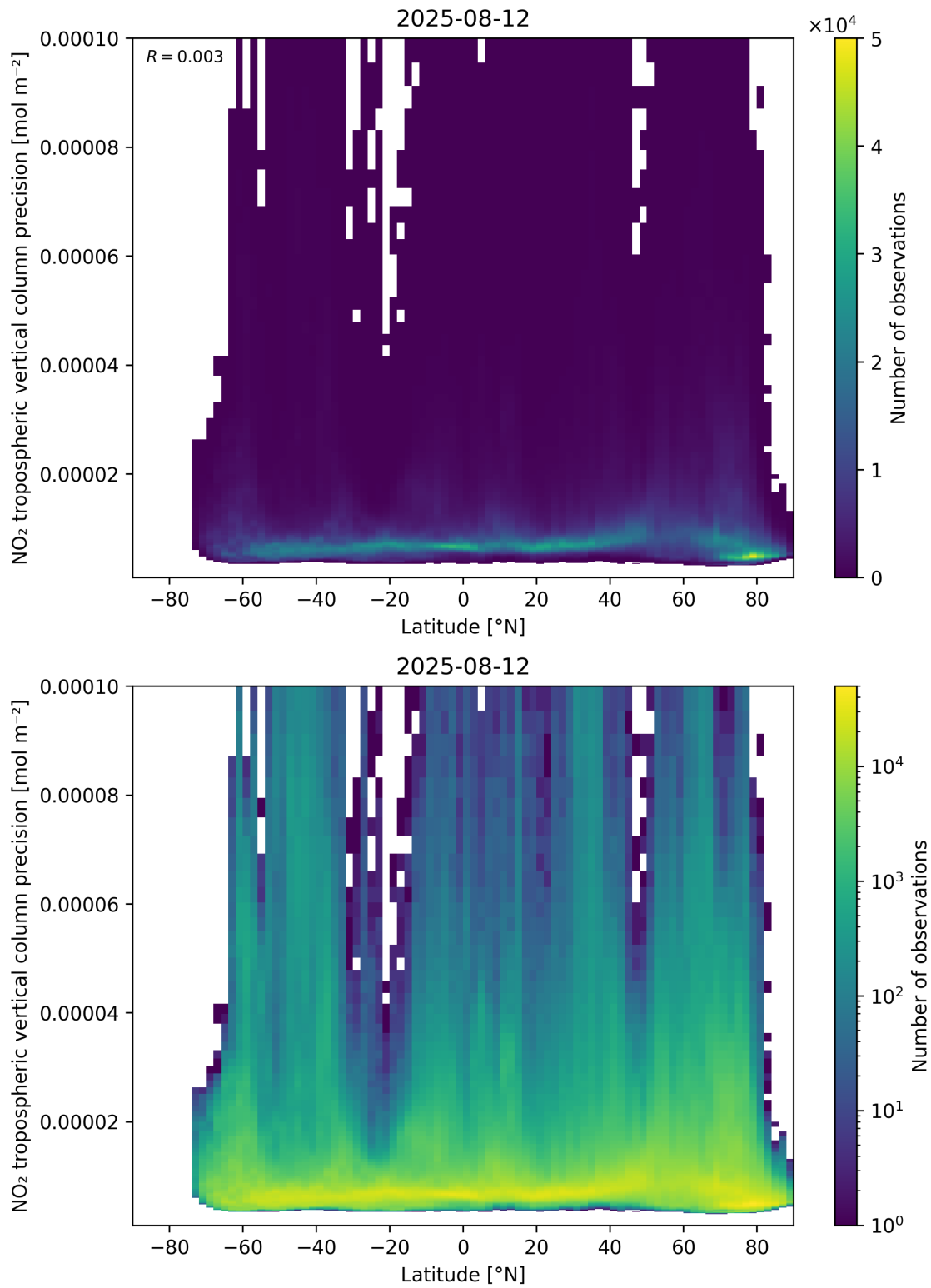
Figure 93: Scatter density plot of “Latitude” against “NO 2 tropospheric vertical column precision” for 2025-08-11 to 2025-08-13.
