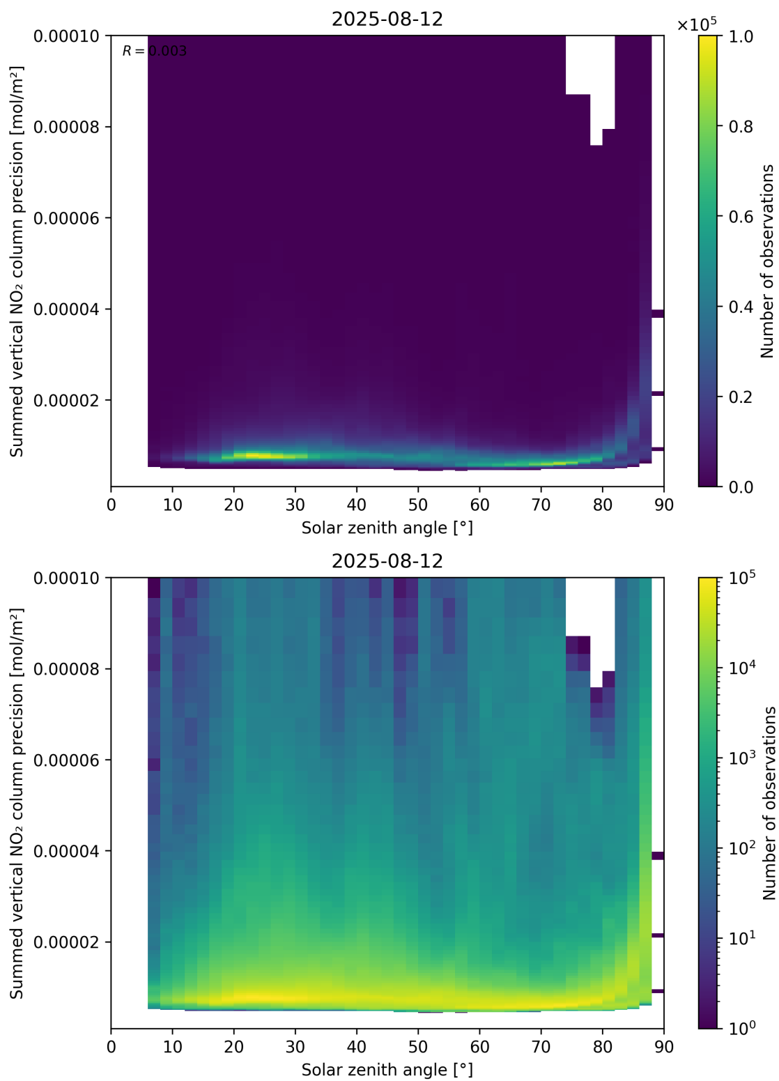
Figure 152: Scatter density plot of “Solar zenith angle” against “Summed vertical NO 2 column precision” for 2025-08-11 to 2025-08-13.
