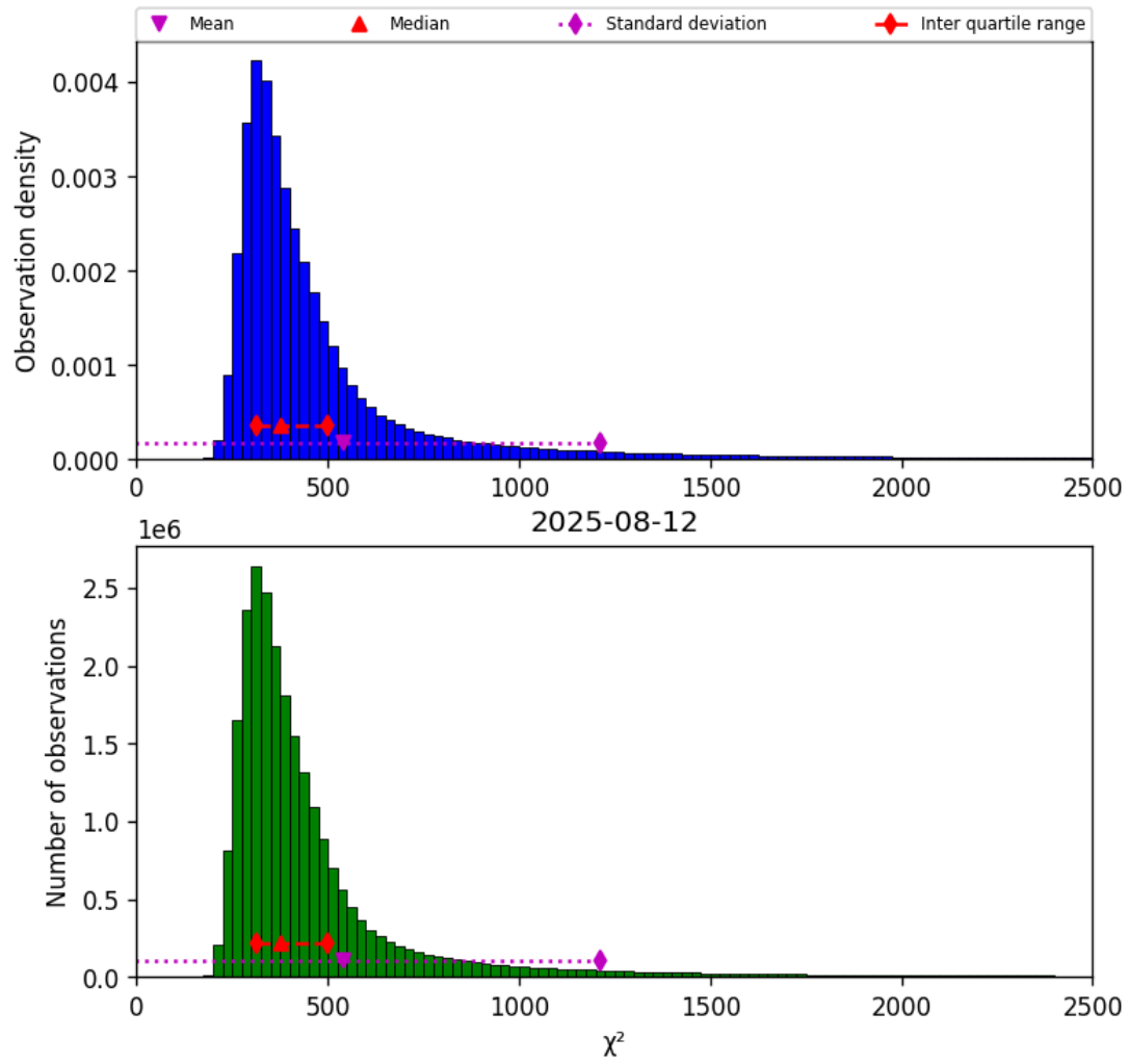
Figure 42: Histogram of “ \chi^2 ” for 2025-08-11 to 2025-08-13
