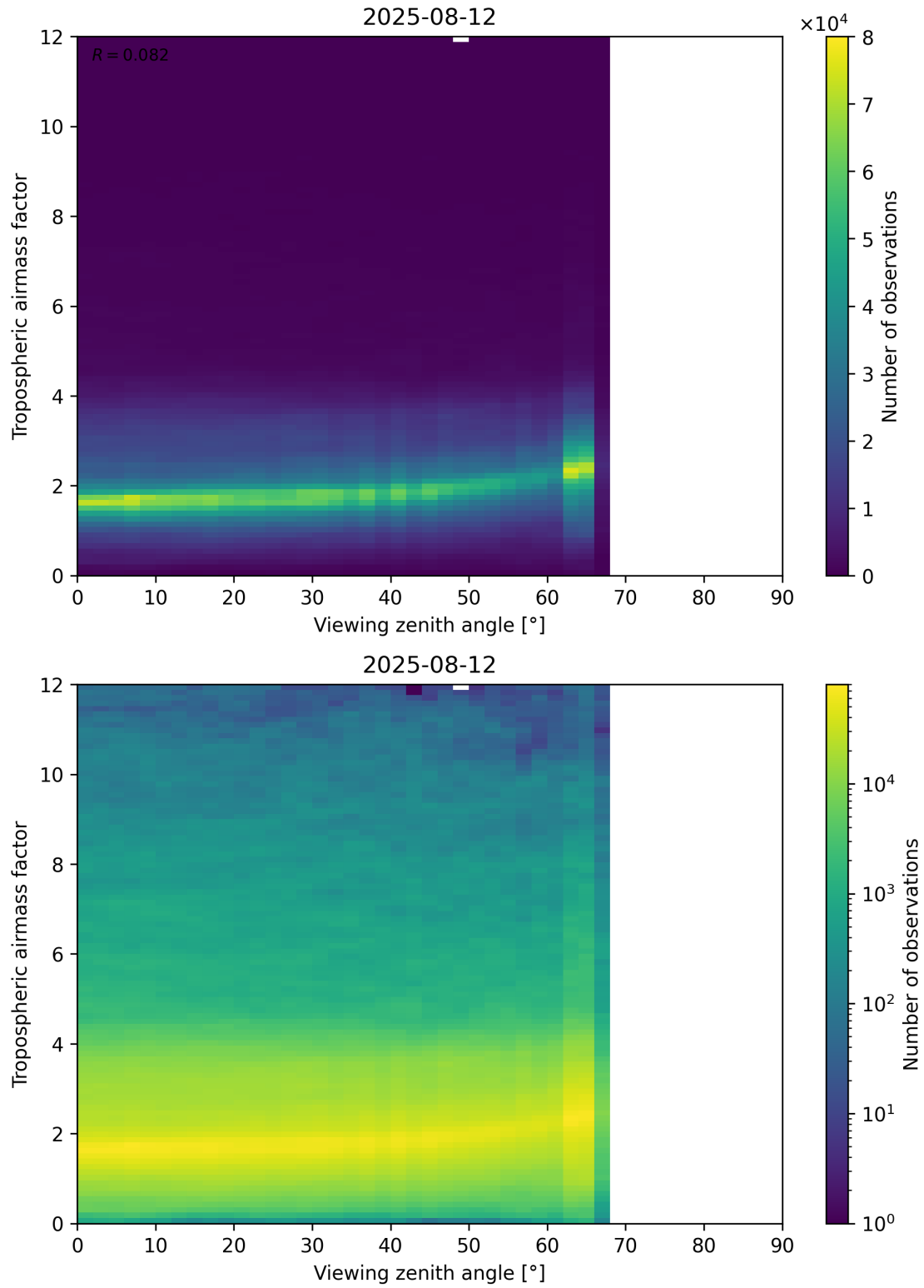
Figure 161: Scatter density plot of “Viewing zenith angle” against “Tropospheric airmass factor” for 2025-08-11 to 2025-08-13.
