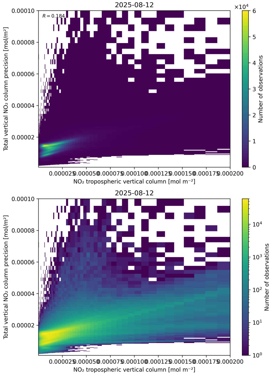
Figure 129: Scatter density plot of “NO 2 tropospheric vertical column” against “Total vertical NO 2 column precision” for 2025-08-11 to 2025-08-13.
