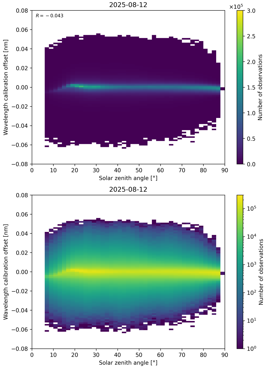
Figure 158: Scatter density plot of “Solar zenith angle” against “Wavelength calibration offset” for 2025-08-11 to 2025-08-13.
