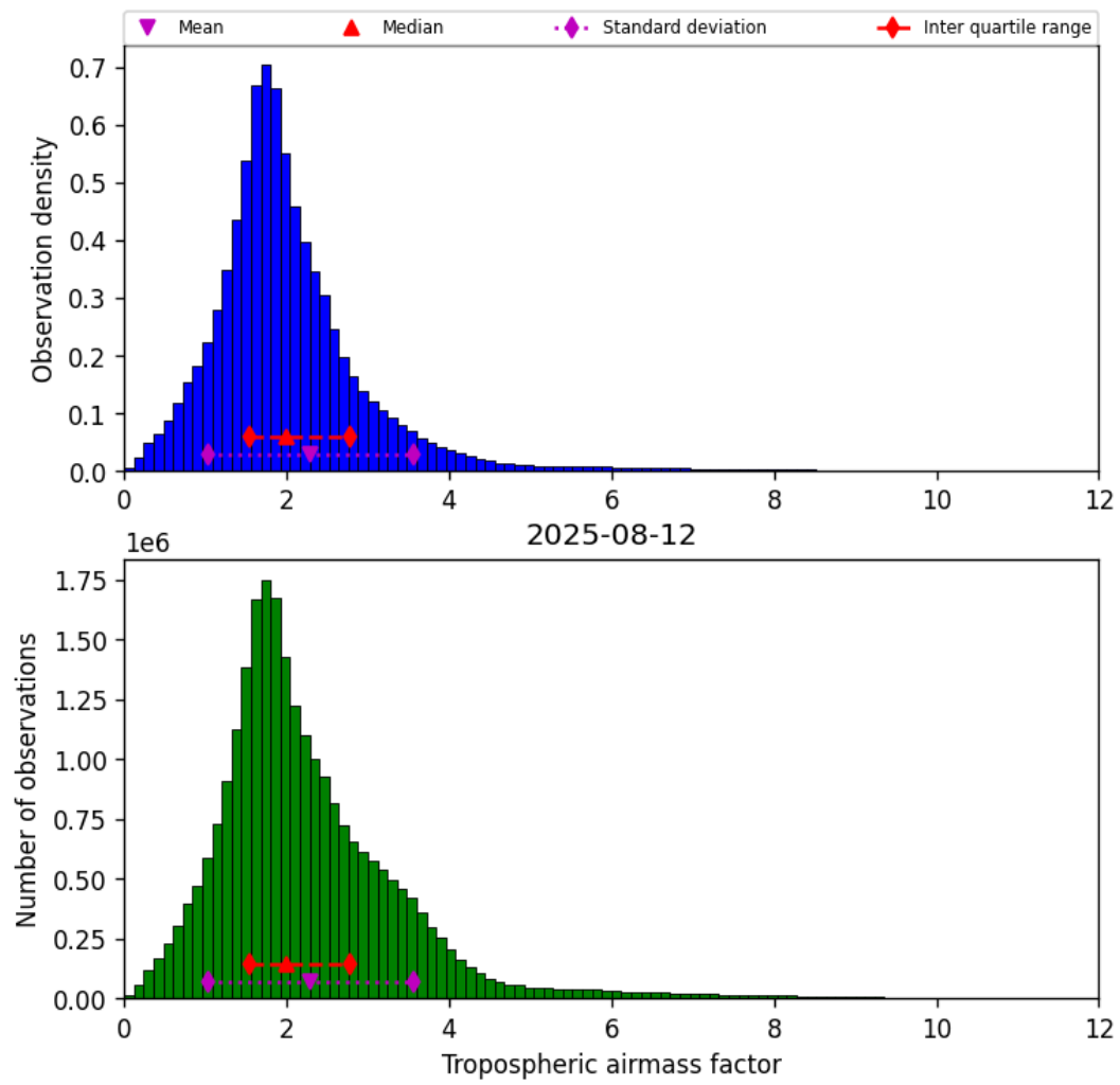
Figure 31: Histogram of “Tropospheric airmass factor” for 2025-08-11 to 2025-08-13
