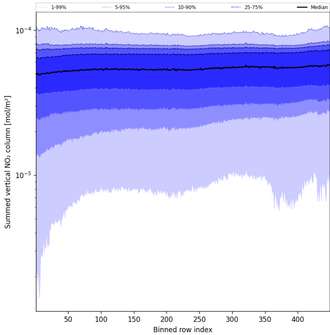
Figure 57: Along track statistics of “Summed vertical NO 2 column” for 2025-08-11 to 2025-08-13
