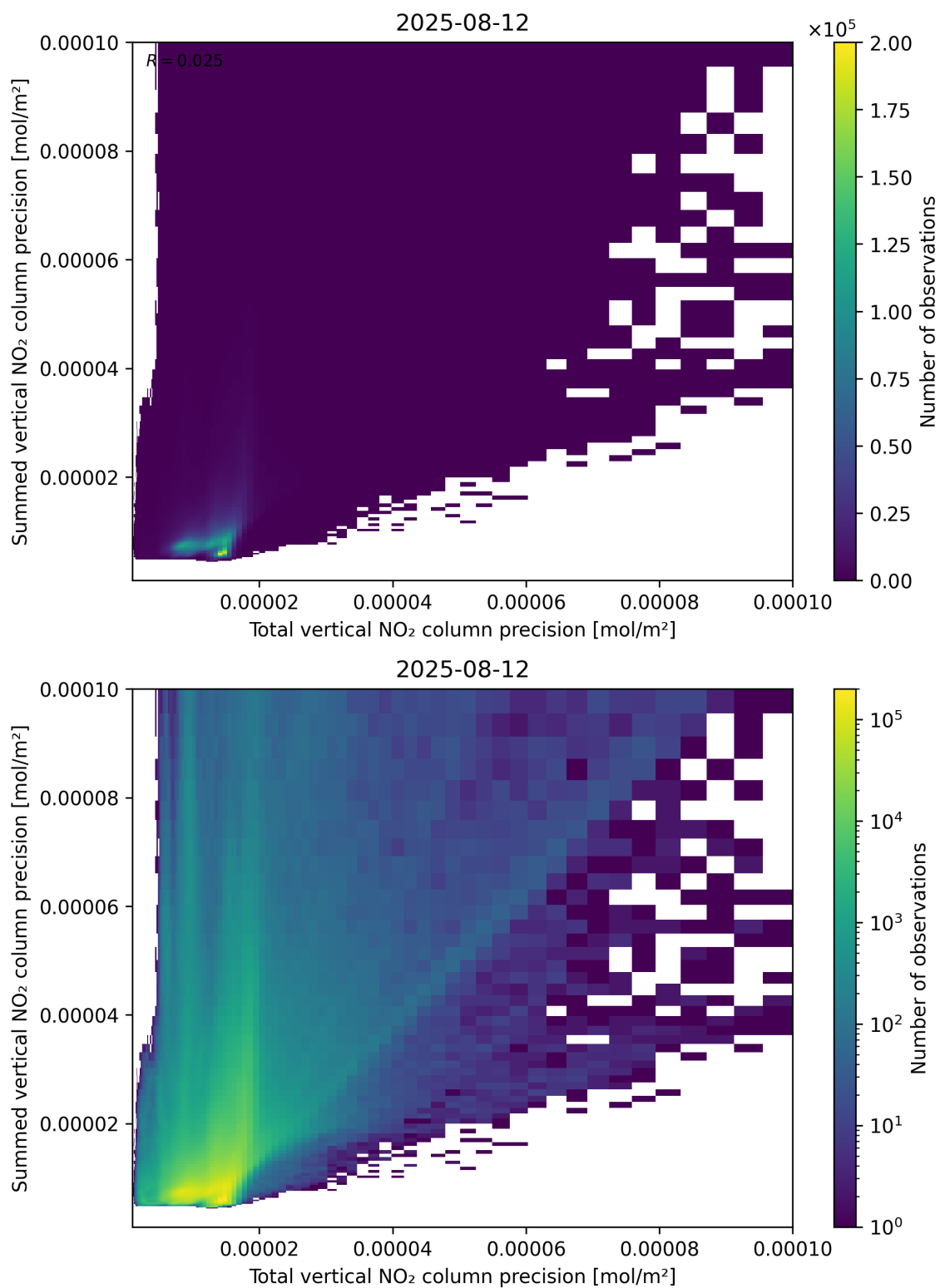
Figure 118: Scatter density plot of “Total vertical NO 2 column precision” against “Summed vertical NO 2 column precision” for 2025-08-11 to 2025-08-13.
