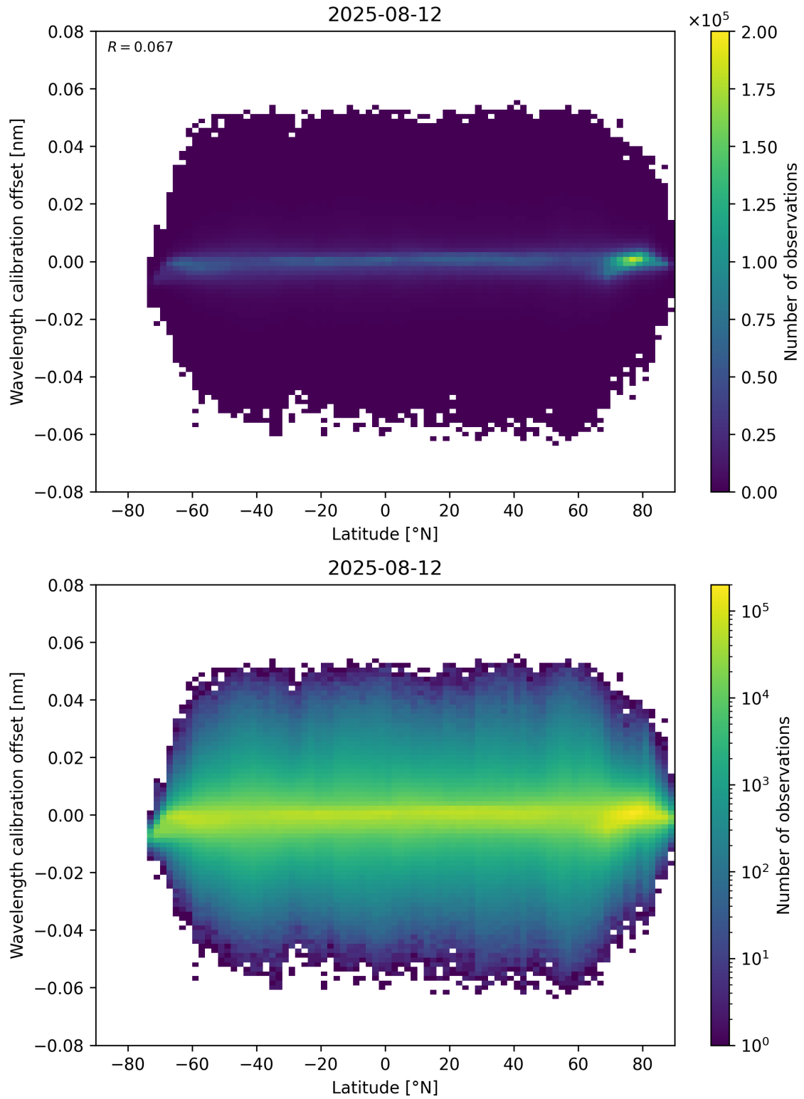
Figure 95: Scatter density plot of “Latitude” against “Wavelength calibration offset” for 2025-08-11 to 2025-08-13.
