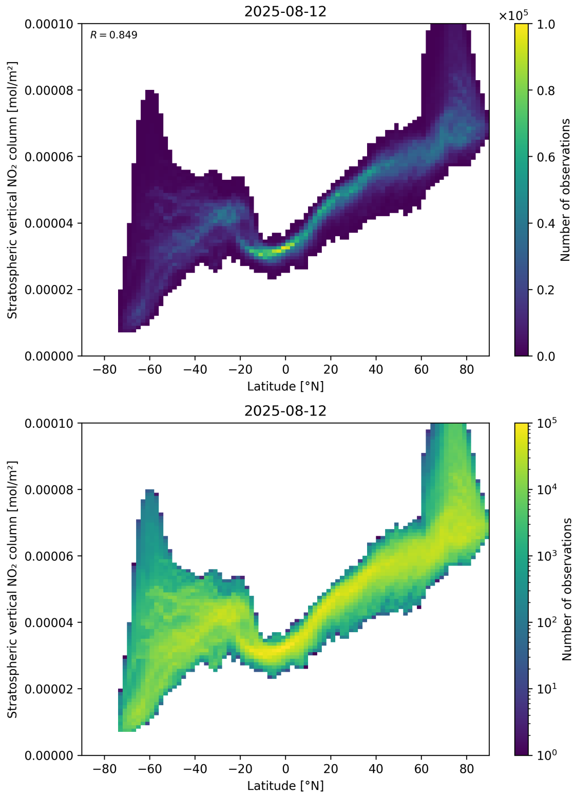
Figure 87: Scatter density plot of “Latitude” against “Stratospheric vertical NO 2 column” for 2025-08-11 to 2025-08-13.
