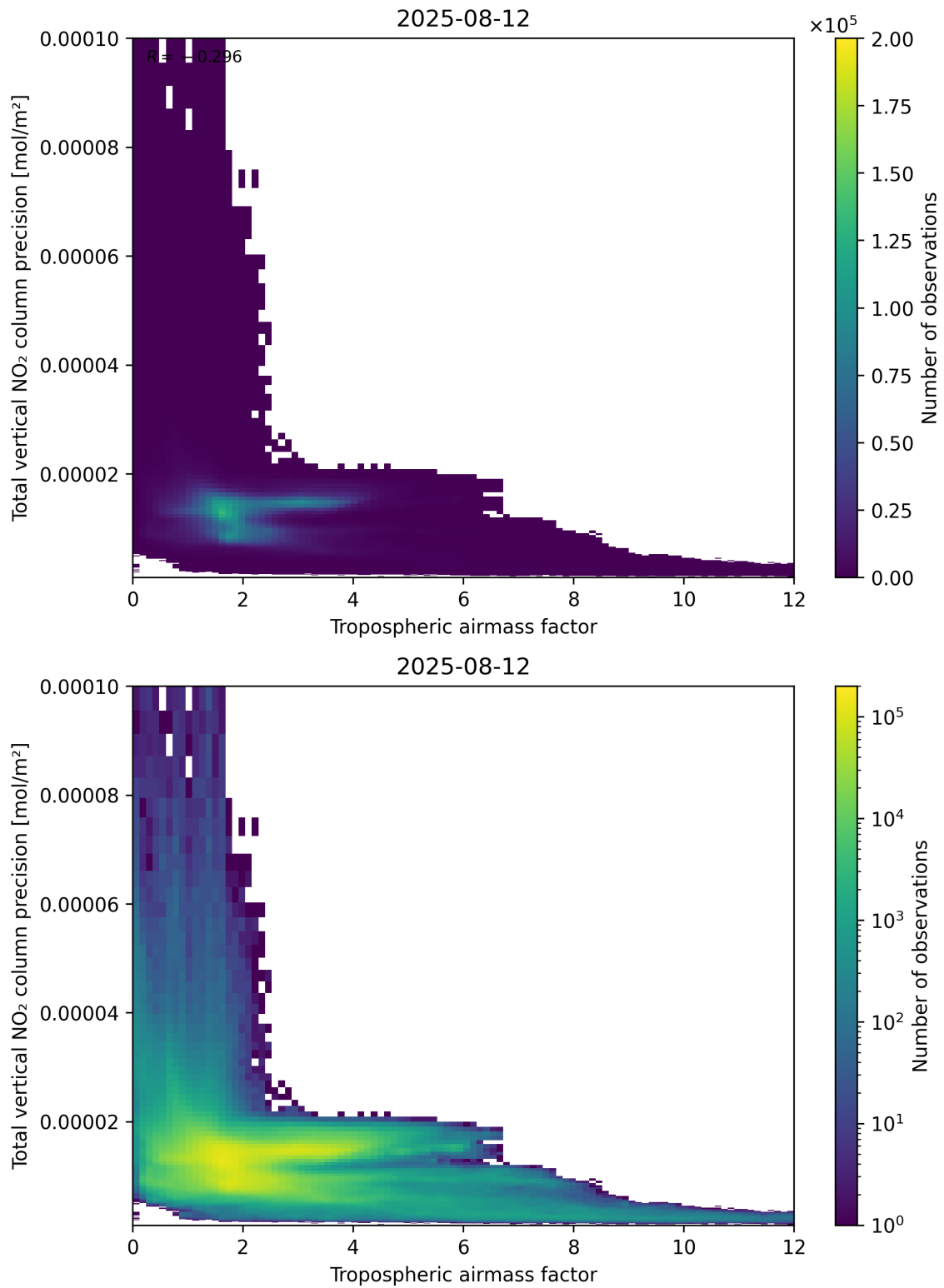
Figure 78: Scatter density plot of “Tropospheric airmass factor” against “Total vertical NO 2 column precision” for 2025-08-11 to 2025-08-13.
