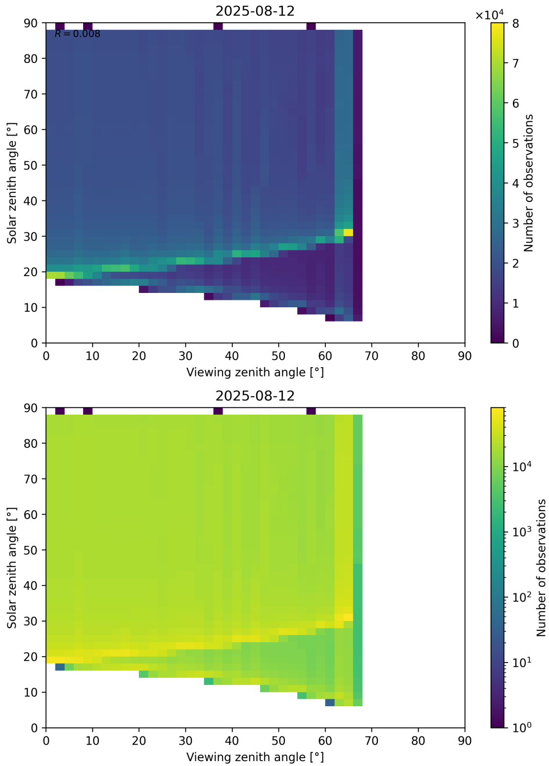
Figure 172: Scatter density plot of “Viewing zenith angle” against “Solar zenith angle” for 2025-08-11 to 2025-08-13.
