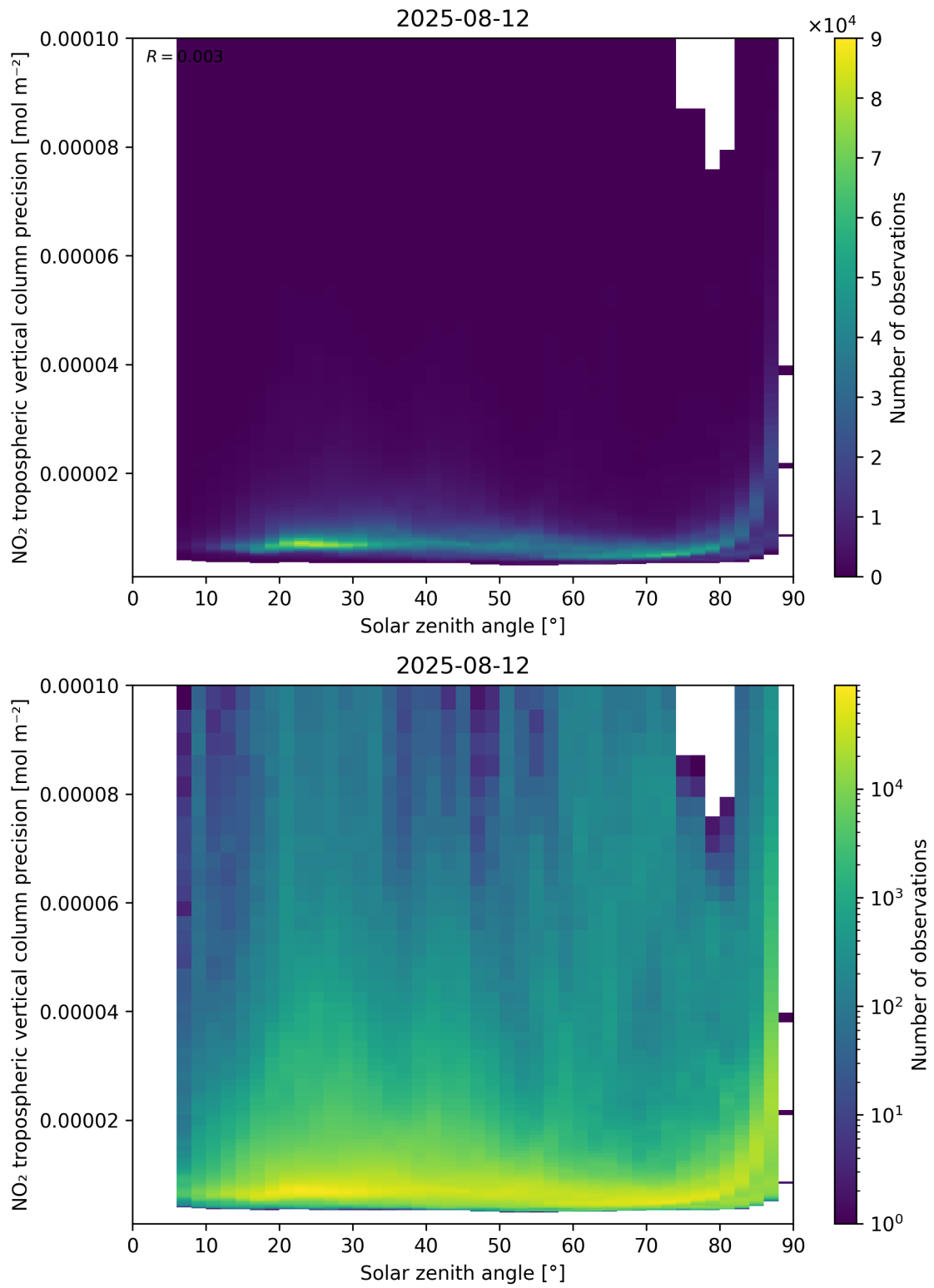
Figure 156: Scatter density plot of “Solar zenith angle” against “NO 2 tropospheric vertical column precision” for 2025-08-11 to 2025-08-13.
