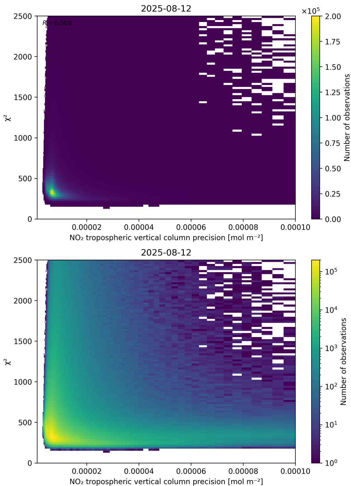
Figure 134: Scatter density plot of “NO 2 tropospheric vertical column precision” against “ \chi^2 ” for 2025-08-11 to 2025-08-13.
