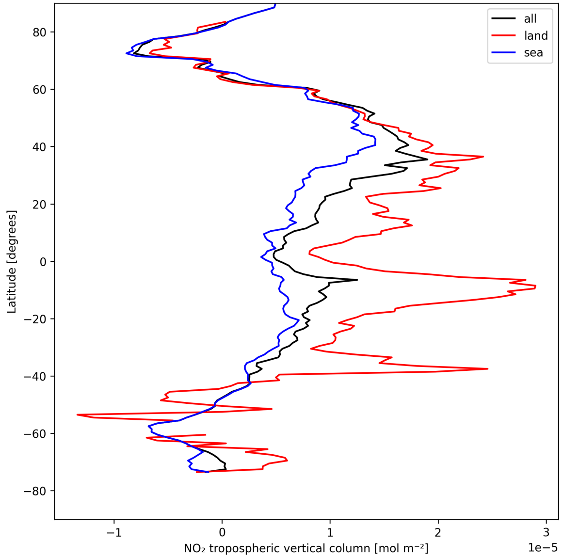
Figure 12: Zonal average of “NO 2 tropospheric vertical column” for 2025-08-11 to 2025-08-13.
