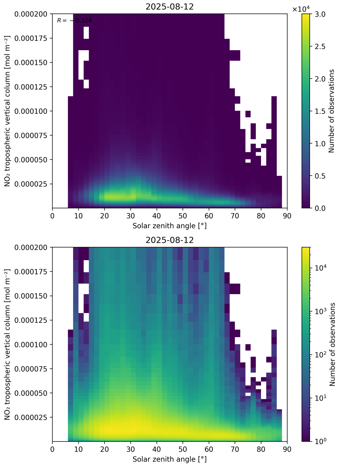
Figure 155: Scatter density plot of “Solar zenith angle” against “NO 2 tropospheric vertical column” for 2025-08-11 to 2025-08-13.
