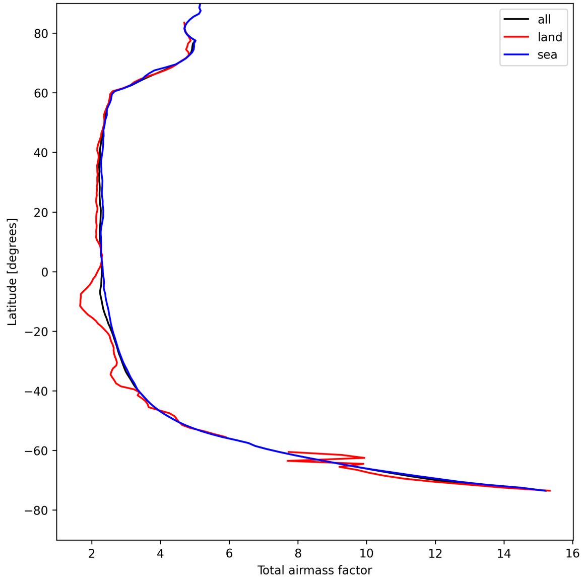
Figure 15: Zonal average of “Total airmass factor” for 2025-08-11 to 2025-08-13.
