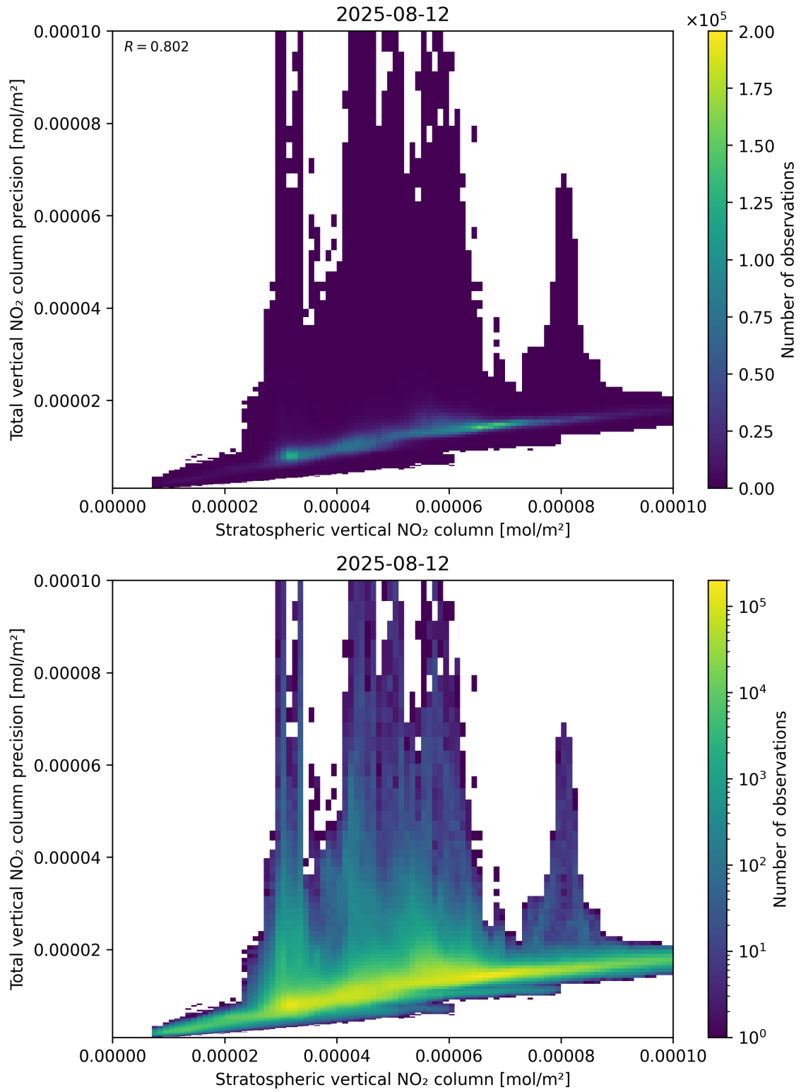
Figure 101: Scatter density plot of “Stratospheric vertical NO 2 column” against “Total vertical NO 2 column precision” for 2025-08-11 to 2025-08-13.
