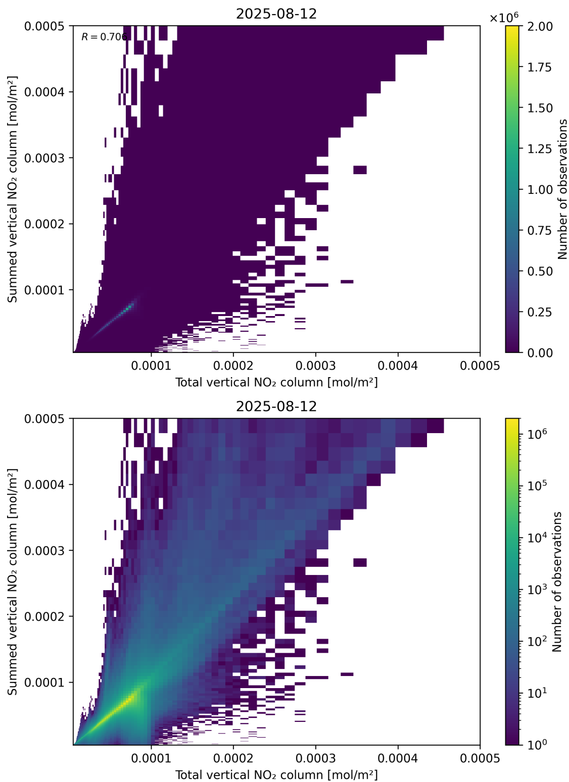
Figure 112: Scatter density plot of “Total vertical NO 2 column” against “Summed vertical NO 2 column” for 2025-08-11 to 2025-08-13.
