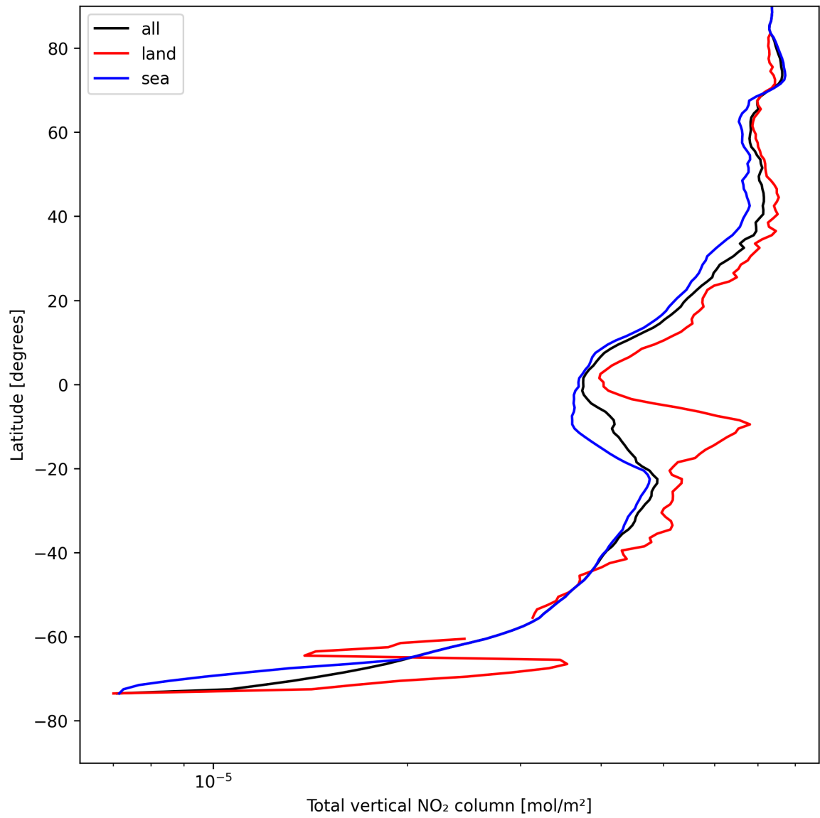
Figure 21: Zonal average of “Total vertical NO 2 column” for 2025-08-11 to 2025-08-13.
