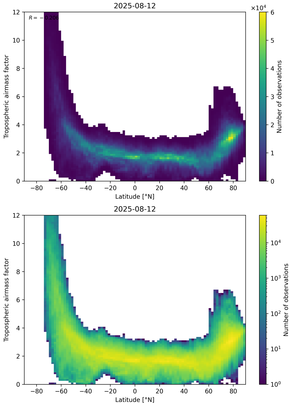
Figure 85: Scatter density plot of “Latitude” against “Tropospheric air mass factor” for 2025-08-11 to 2025-08-13.
