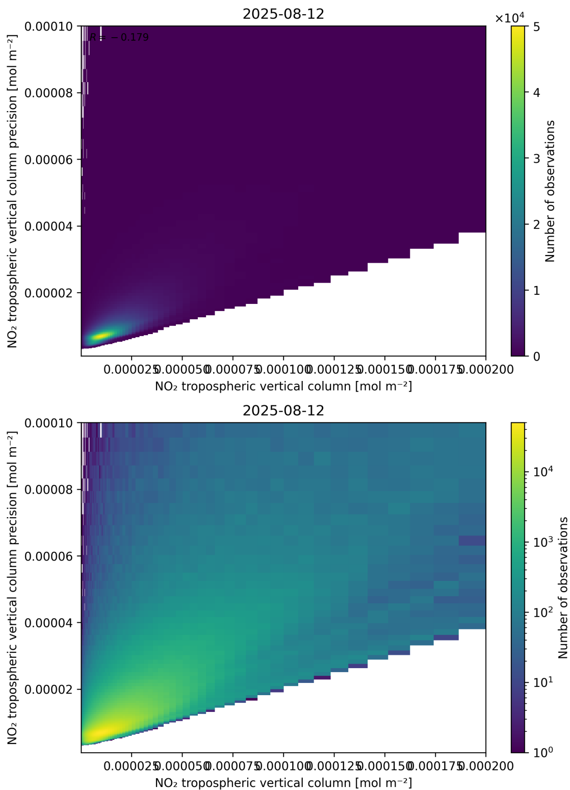
Figure 130: Scatter density plot of “NO 2 tropospheric vertical column” against “NO 2 tropospheric vertical column precision” for 2025-08-11 to 2025-08-13.
