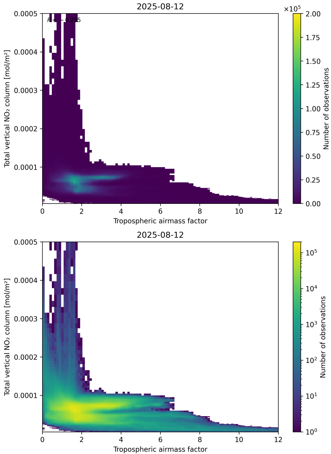
Figure 77: Scatter density plot of “Tropospheric airmass factor” against “Total vertical NO 2 column” for 2025-08-11 to 2025-08-13.
