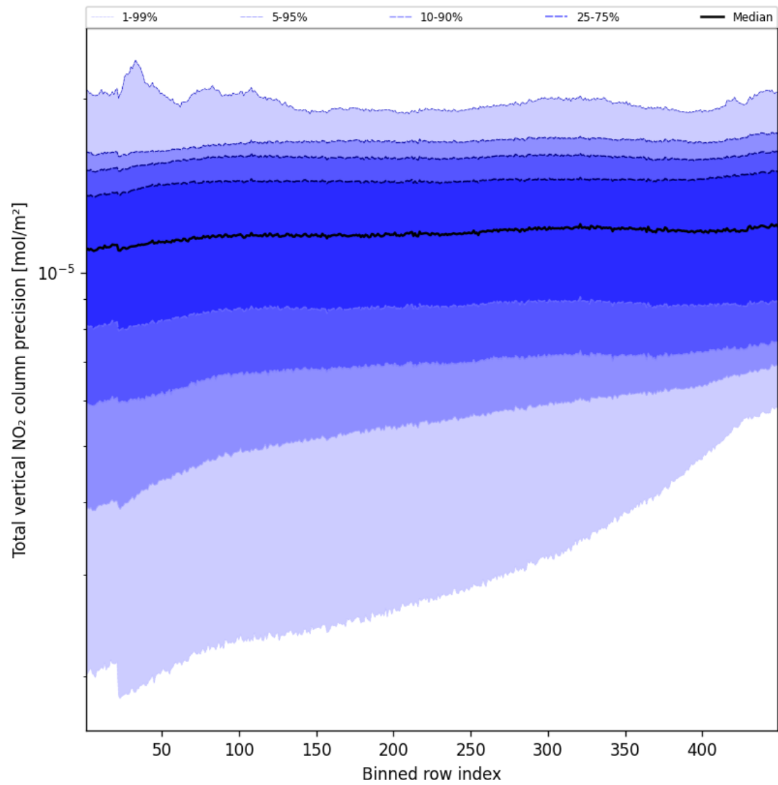
Figure 56: Along track statistics of “Total vertical NO 2 column precision” for 2025-08-11 to 2025-08-13
