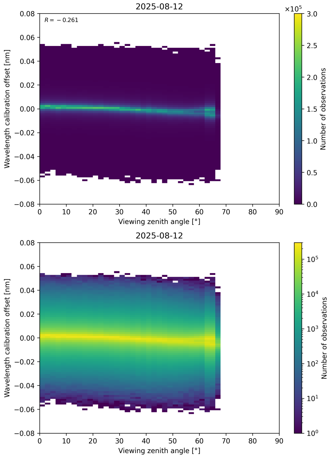
Figure 173: Scatter density plot of “Viewing zenith angle” against “Wavelength calibration offset” for 2025-08-11 to 2025-08-13.
