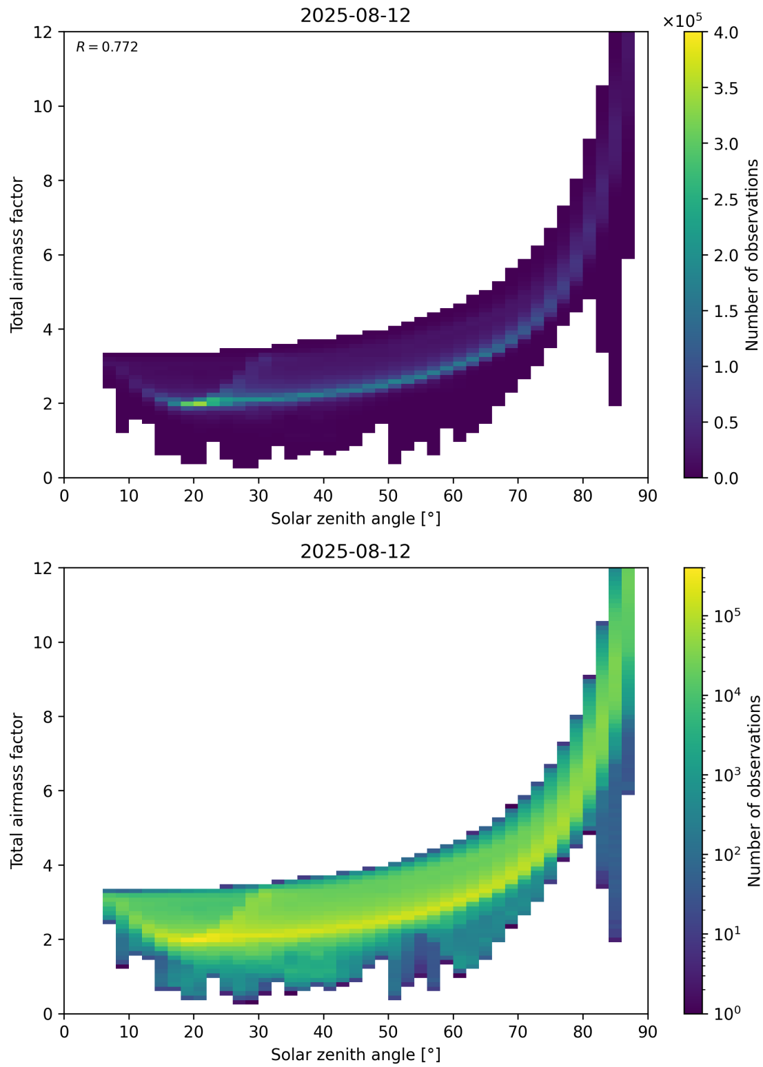
Figure 146: Scatter density plot of “Solar zenith angle” against “Total air mass factor” for 2025-08-11 to 2025-08-13.
