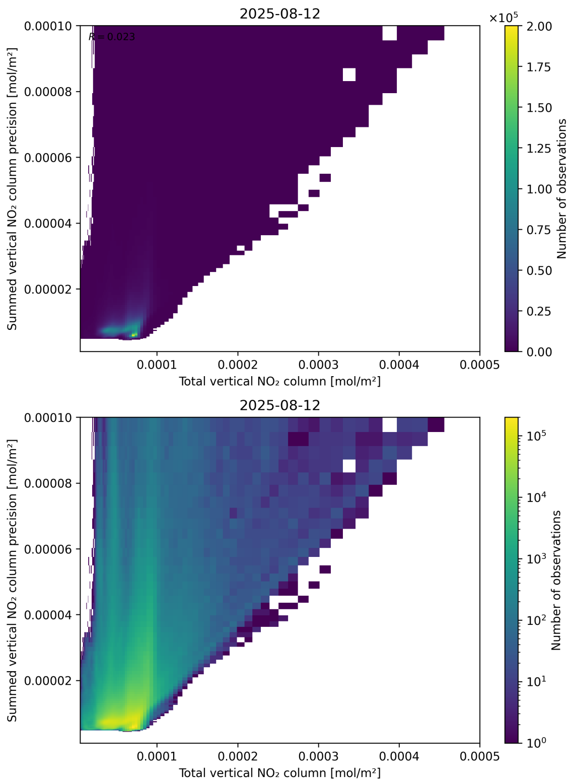
Figure 113: Scatter density plot of “Total vertical NO 2 column” against “Summed vertical NO 2 column precision” for 2025-08-11 to 2025-08-13.
