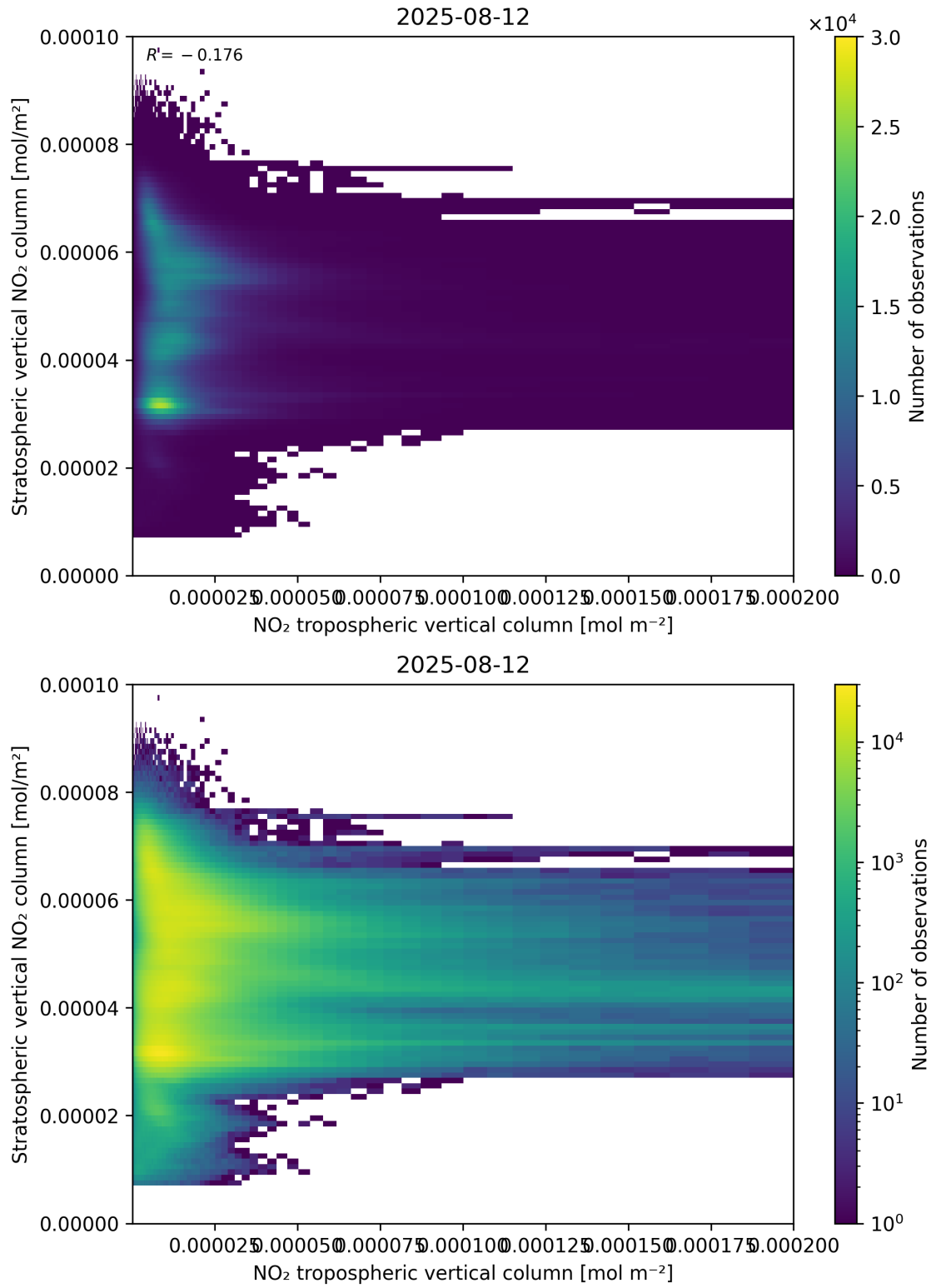
Figure 125: Scatter density plot of “NO 2 tropospheric vertical column” against “Stratospheric vertical NO 2 column” for 2025-08-11 to 2025-08-13.
