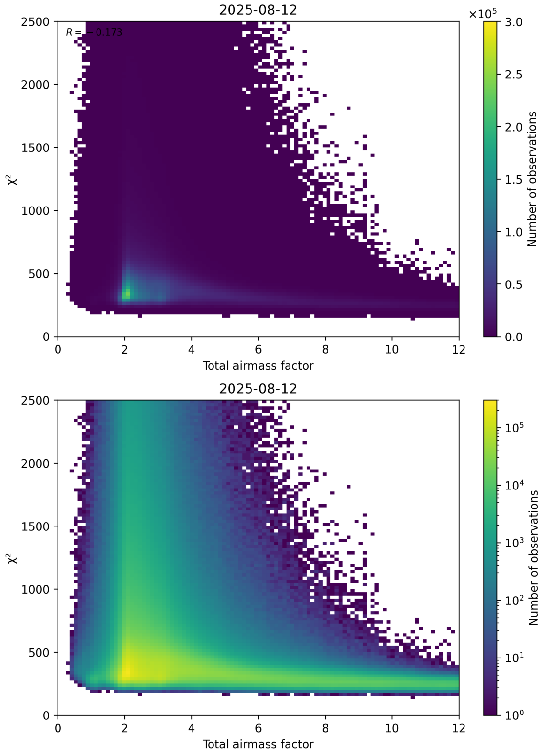
Figure 63: Scatter density plot of “Total airmass factor” against “ \chi^2 ” for 2025-08-11 to 2025-08-13.
