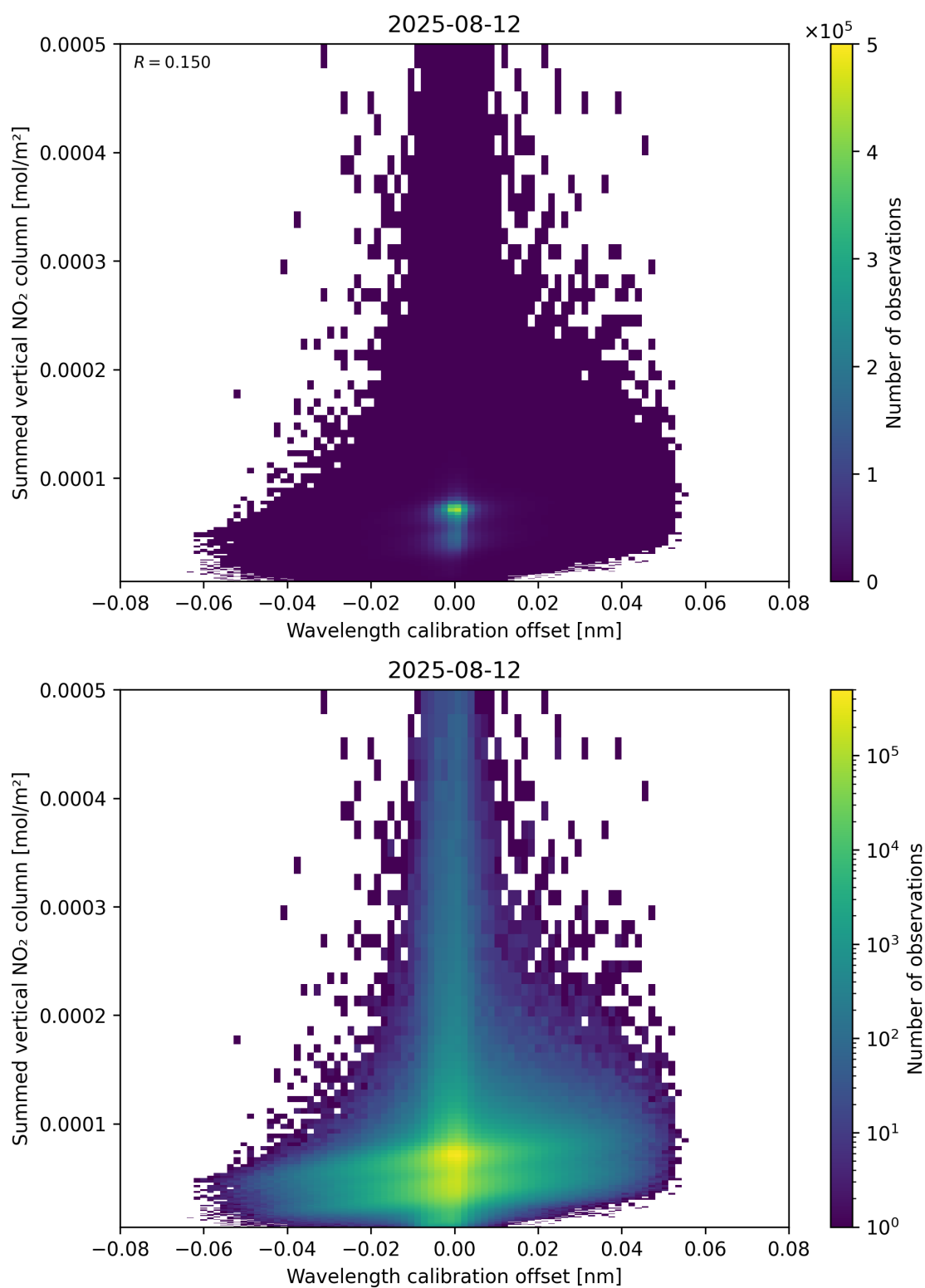
Figure 177: Scatter density plot of “Wavelength calibration offset” against “Summed vertical NO 2 column” for 2025-08-11 to 2025-08-13.
