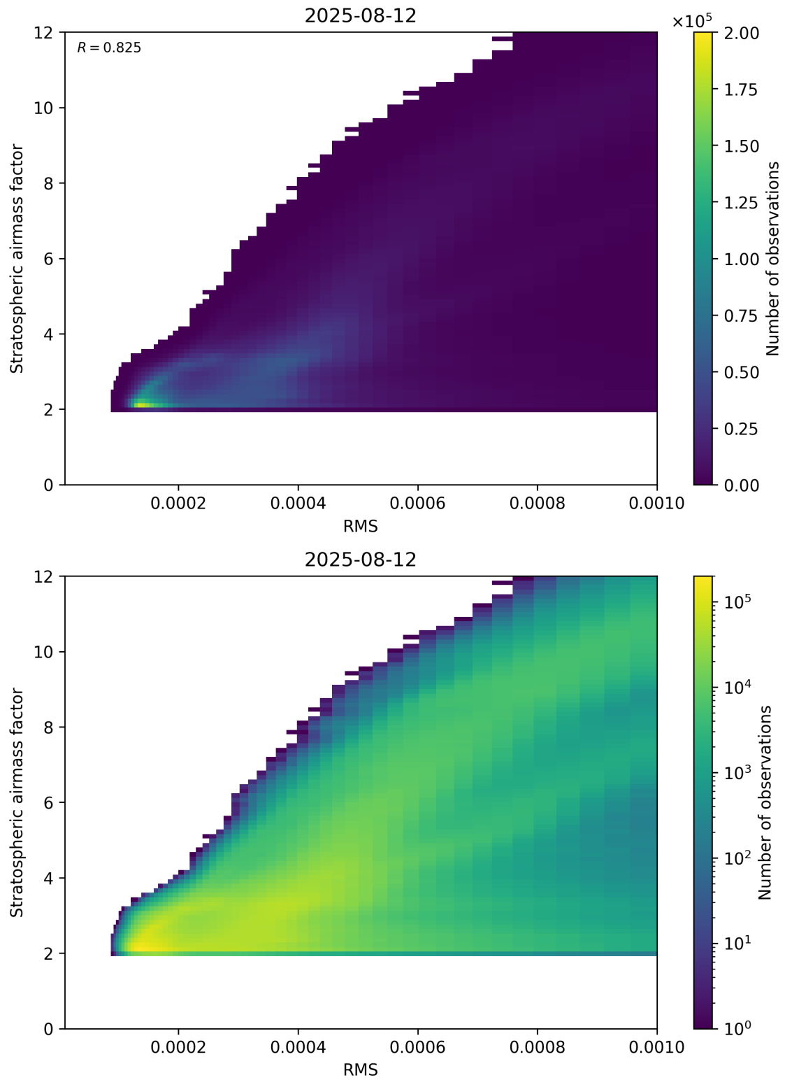
Figure 144: Scatter density plot of “RMS” against “Stratospheric airmass factor” for 2025-08-11 to 2025-08-13.
