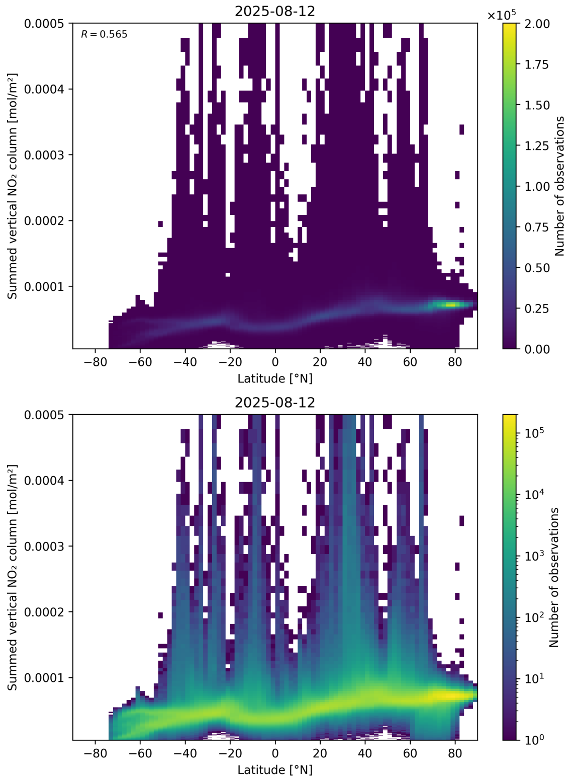
Figure 88: Scatter density plot of “Latitude” against “Summed vertical NO 2 column” for 2025-08-11 to 2025-08-13.
