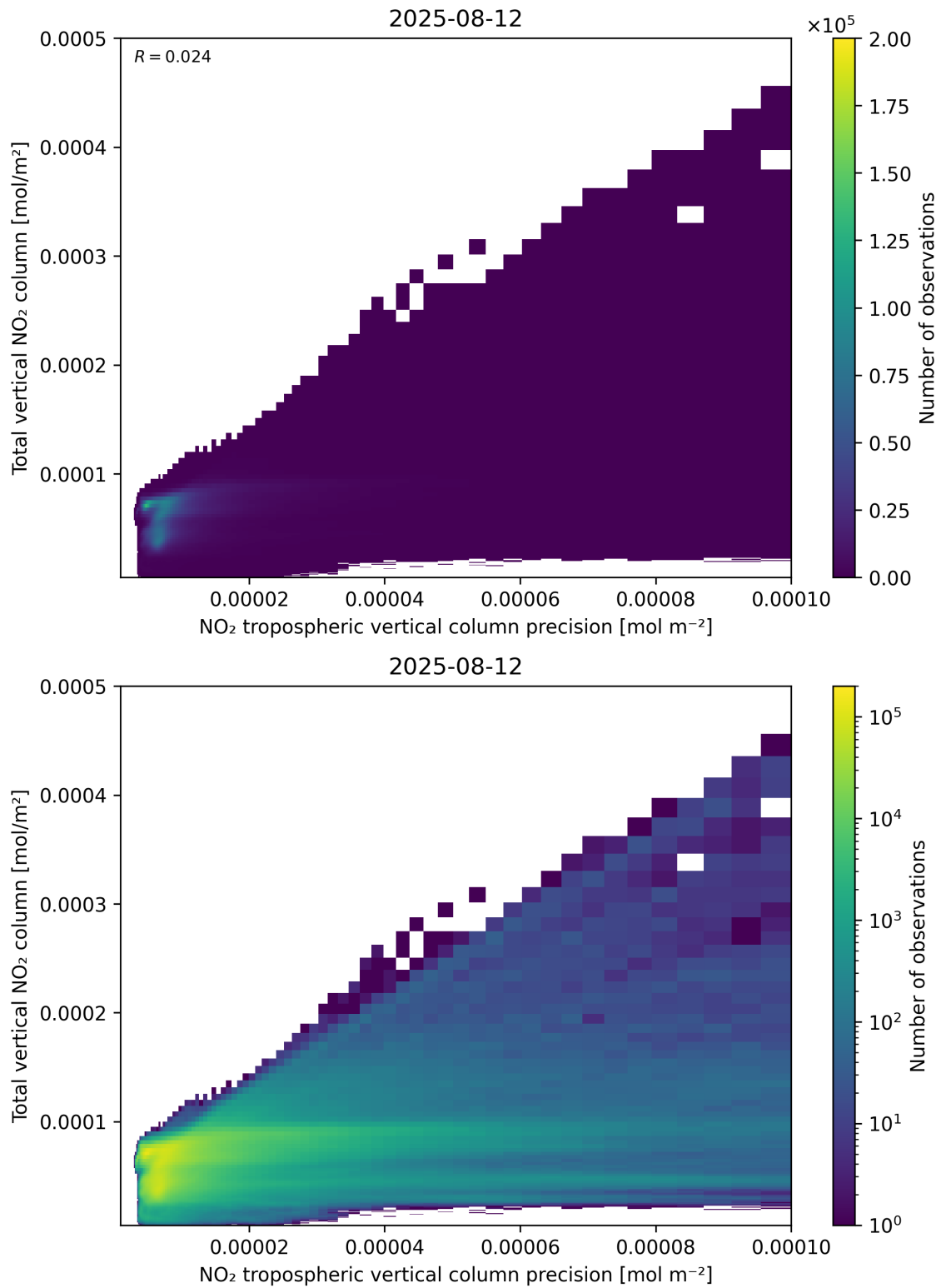
Figure 138: Scatter density plot of “NO 2 tropospheric vertical column precision” against “Total vertical NO 2 column” for 2025-08-11 to 2025-08-13.
