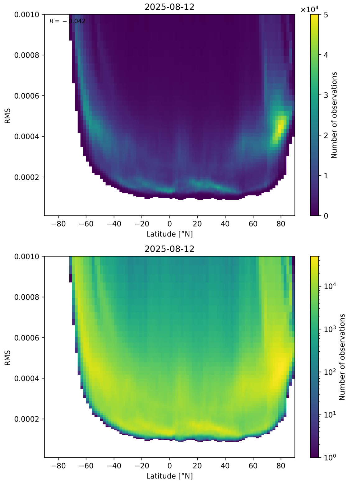
Figure 94: Scatter density plot of “Latitude” against “RMS” for 2025-08-11 to 2025-08-13.
