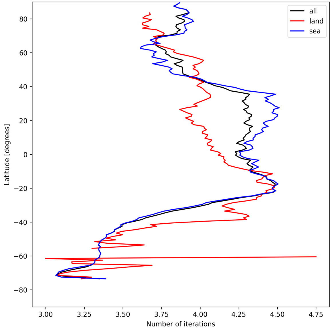
Figure 17: Zonal average of “Number of iterations” for 2025-08-11 to 2025-08-13.
