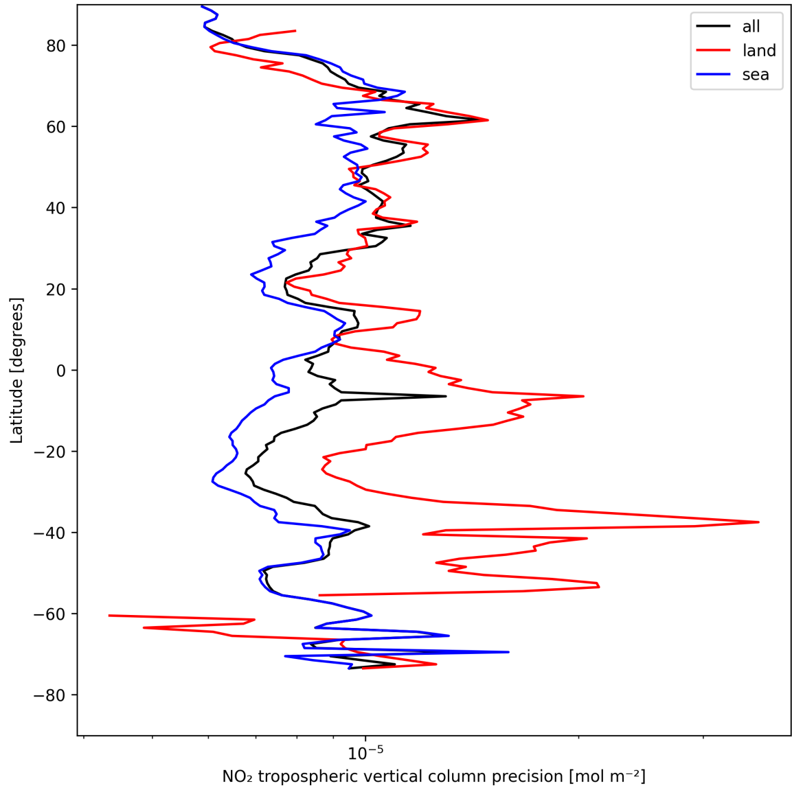
Figure 13: Zonal average of “NO 2 tropospheric vertical column precision” for 2025-08-11 to 2025-08-13.
