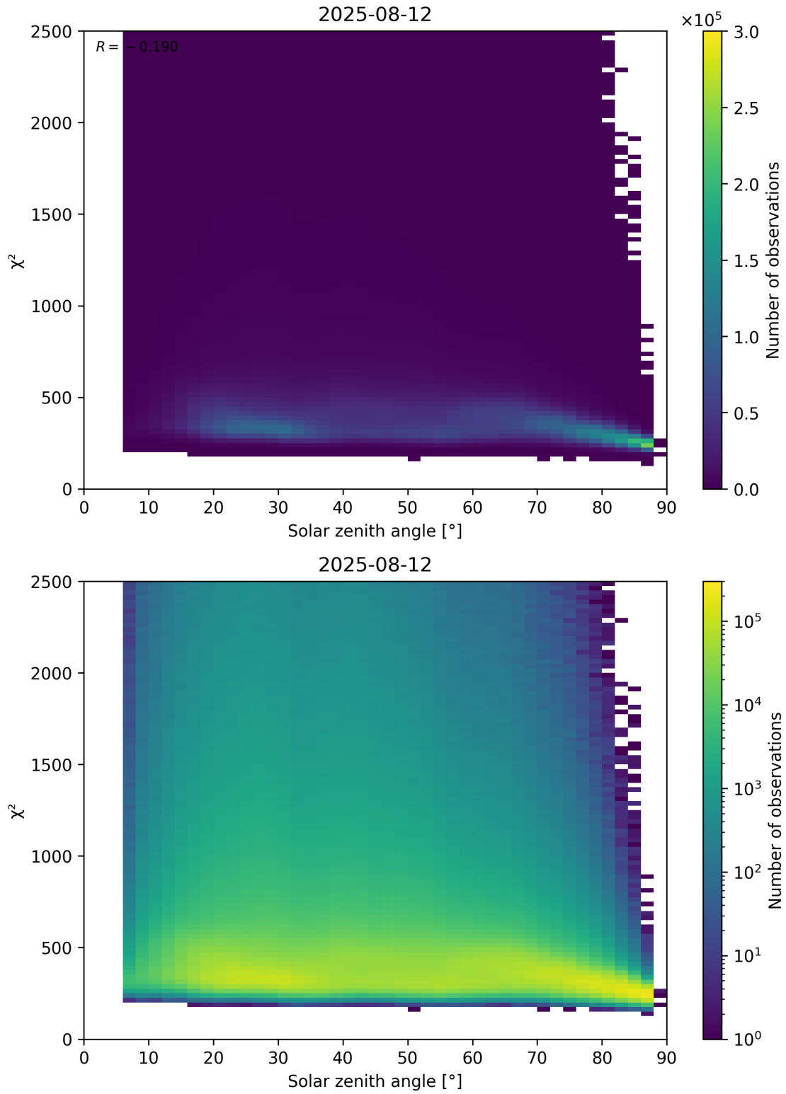
Figure 148: Scatter density plot of “Solar zenith angle” against “ \chi^2 ” for 2025-08-11 to 2025-08-13.
