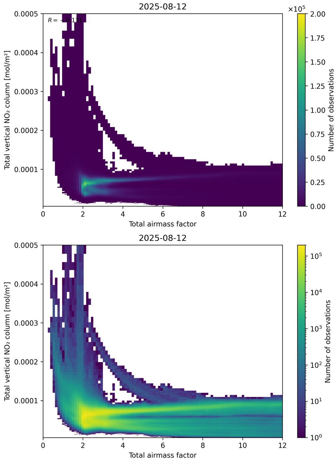
Figure 67: Scatter density plot of “Total airmass factor” against “Total vertical NO 2 column” for 2025-08-11 to 2025-08-13.
