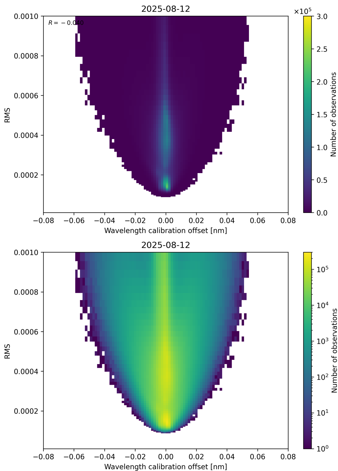
Figure 181: Scatter density plot of “Wavelength calibration offset” against “RMS” for 2025-08-11 to 2025-08-13.
