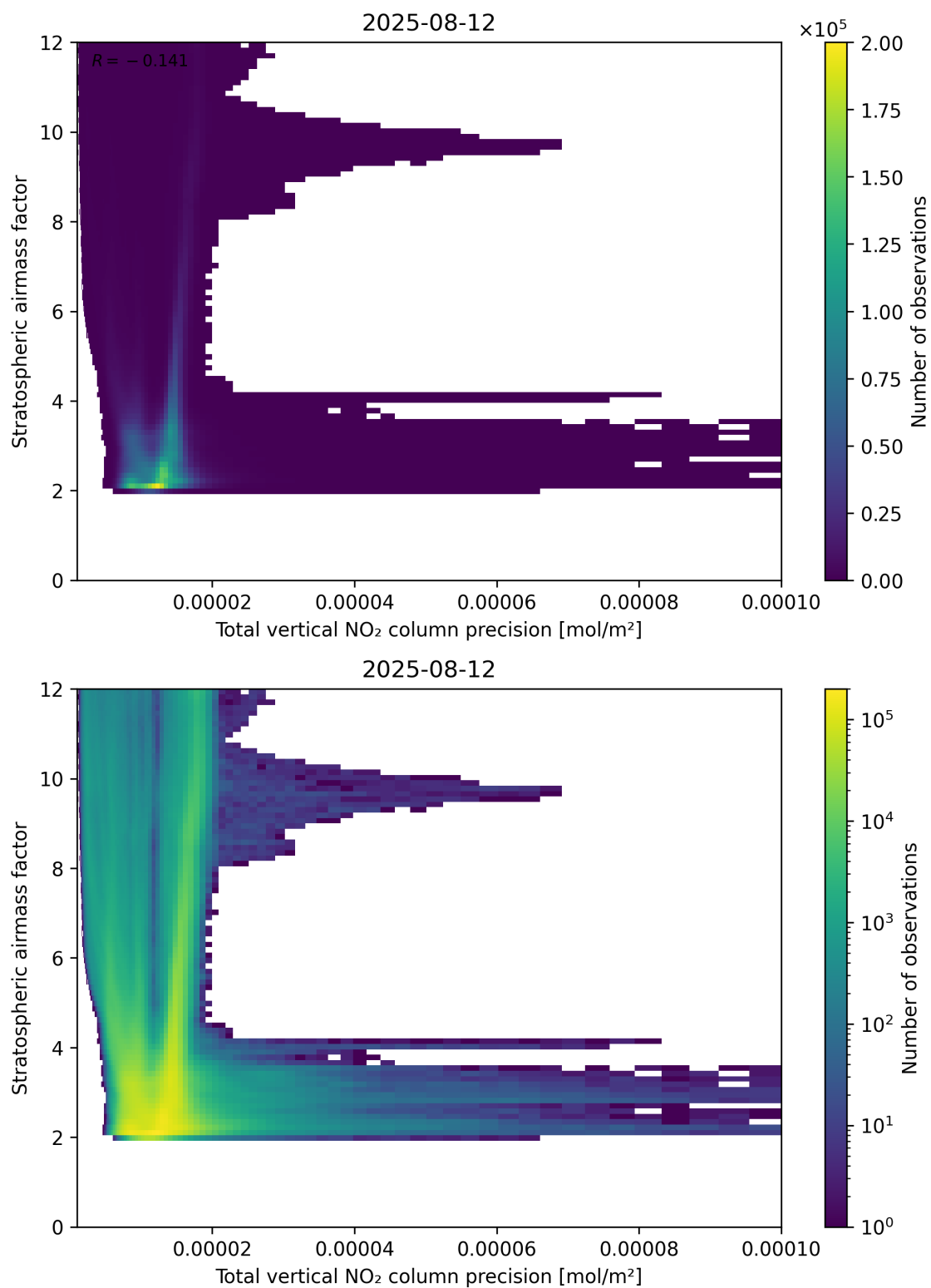
Figure 115: Scatter density plot of “Total vertical NO 2 column precision” against “Stratospheric airmass factor” for 2025-08-11 to 2025-08-13.
