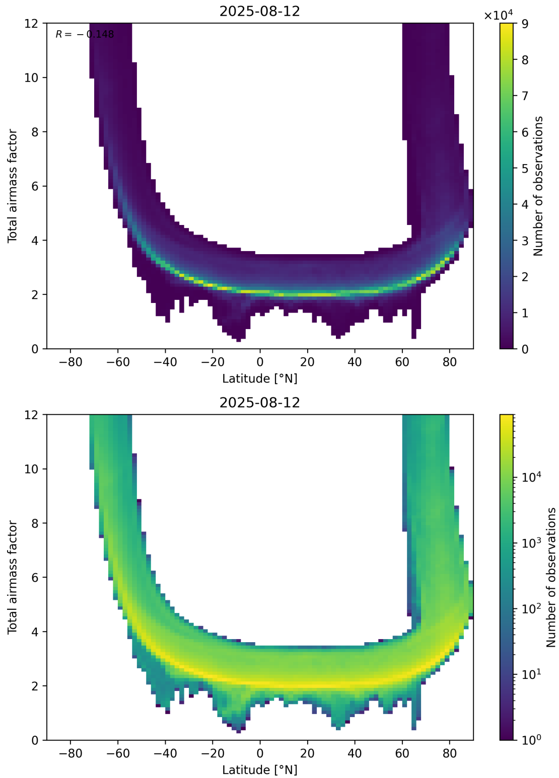
Figure 84: Scatter density plot of “Latitude” against “Total airmass factor” for 2025-08-11 to 2025-08-13.
