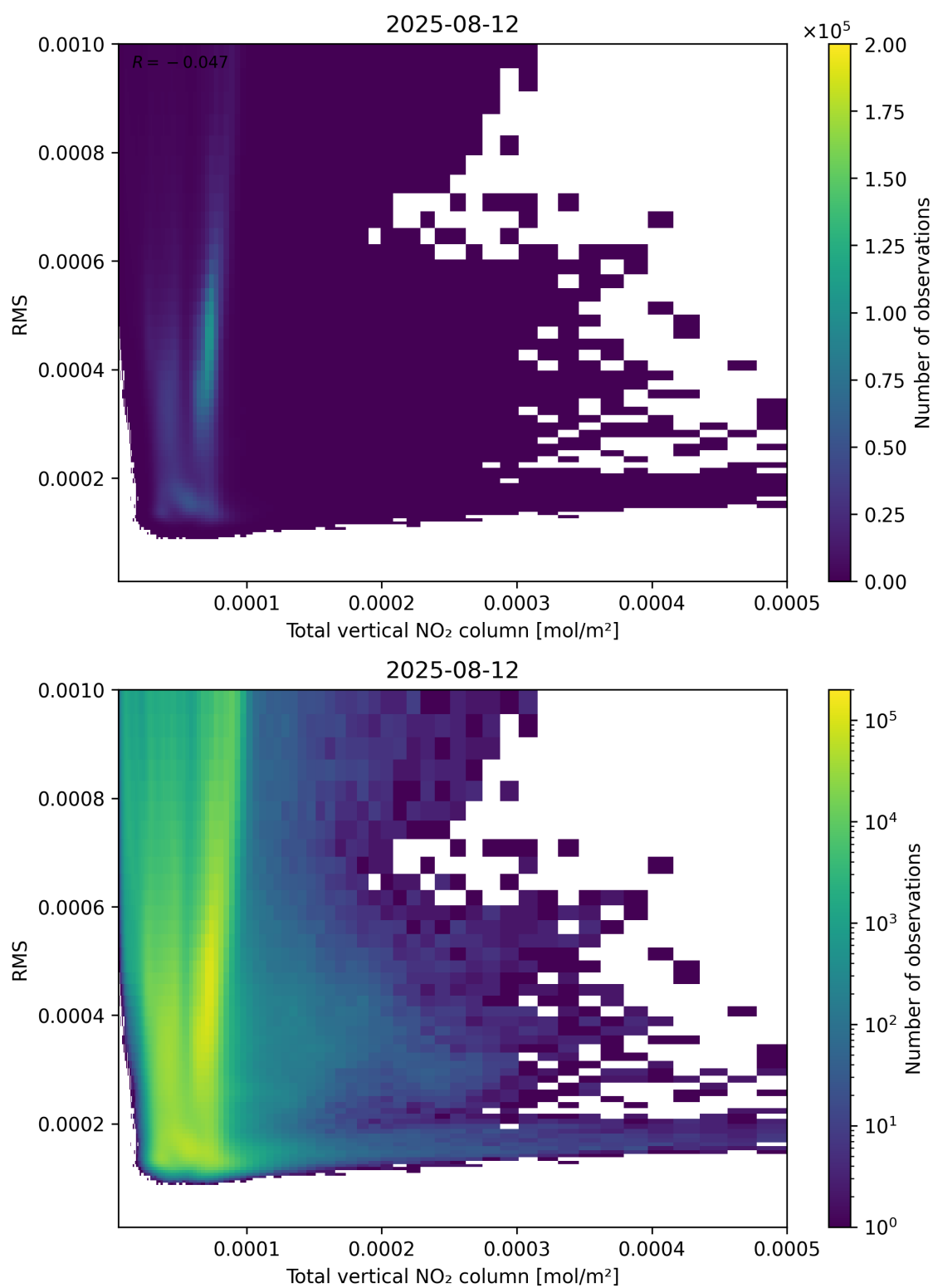
Figure 120: Scatter density plot of “Total vertical NO 2 column” against “RMS” for 2025-08-11 to 2025-08-13.
