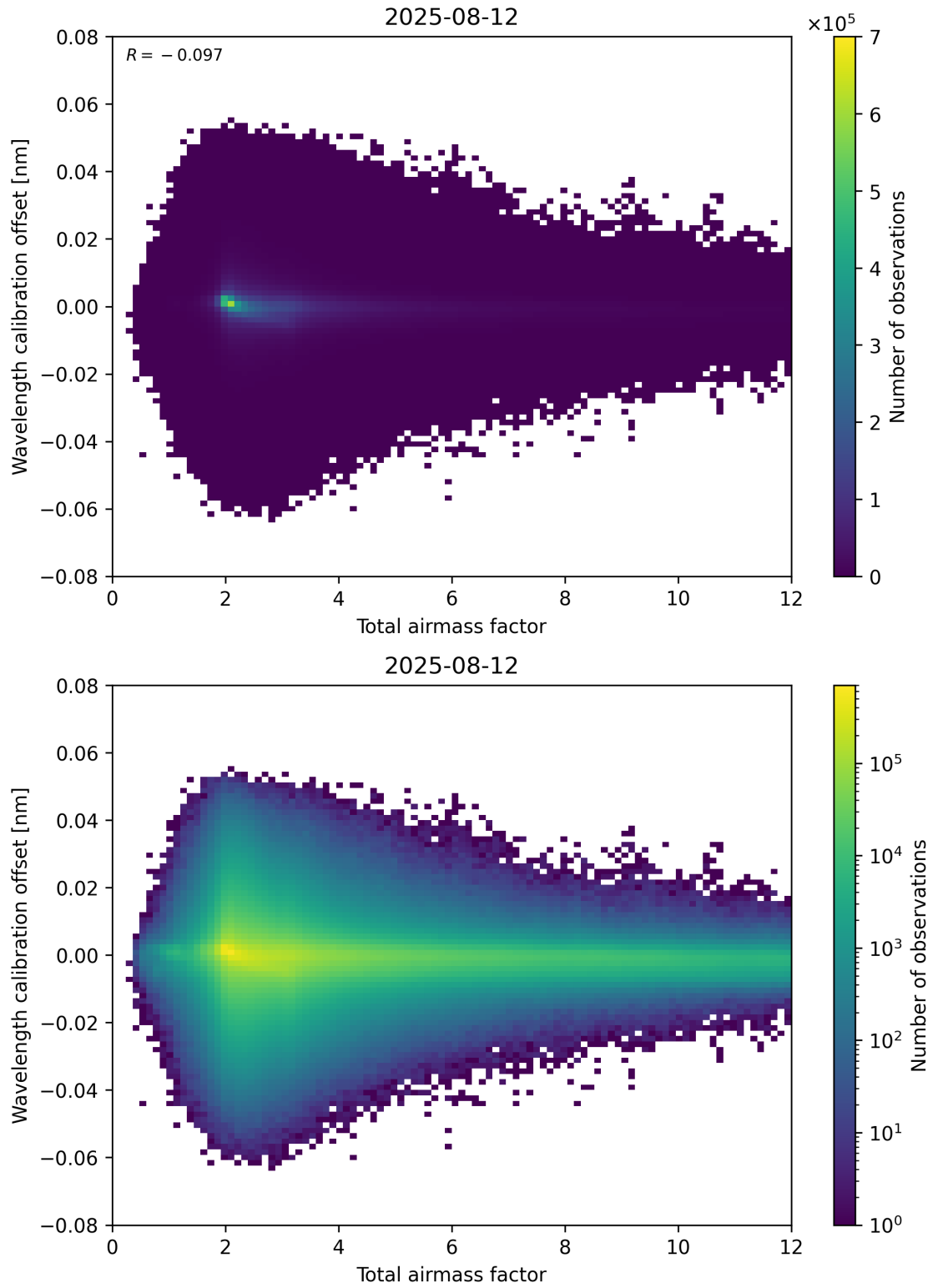
Figure 70: Scatter density plot of “Total airmass factor” against “Wavelength calibration offset” for 2025-08-11 to 2025-08-13.
