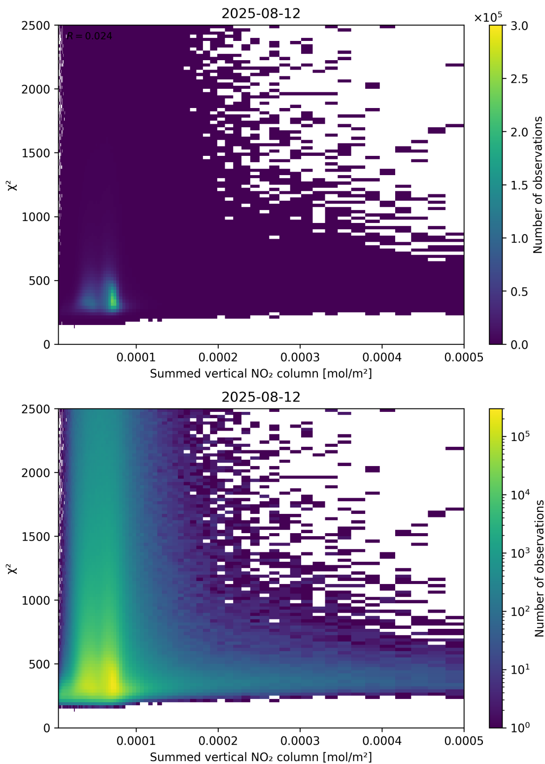
Figure 104: Scatter density plot of “Summed vertical NO 2 column” against “ \chi^2 ” for 2025-08-11 to 2025-08-13.
