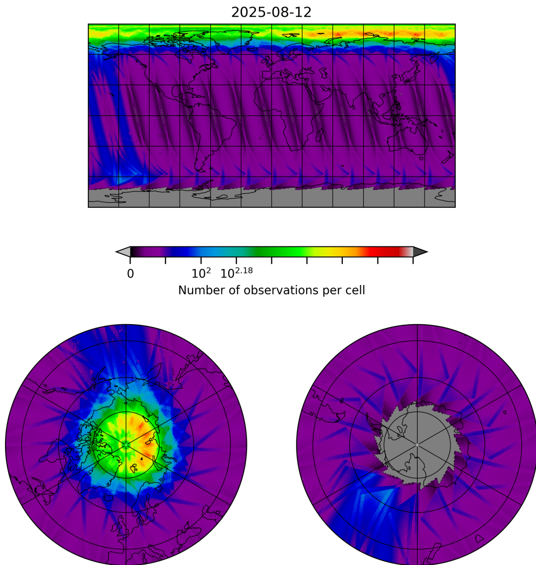
Figure 10: Map of the number of observations for 2025-08-11 to 2025-08-13
