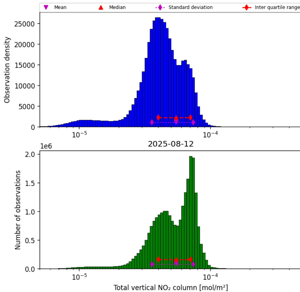
Figure 38: Histogram of “Total vertical NO 2 column” for 2025-08-11 to 2025-08-13
