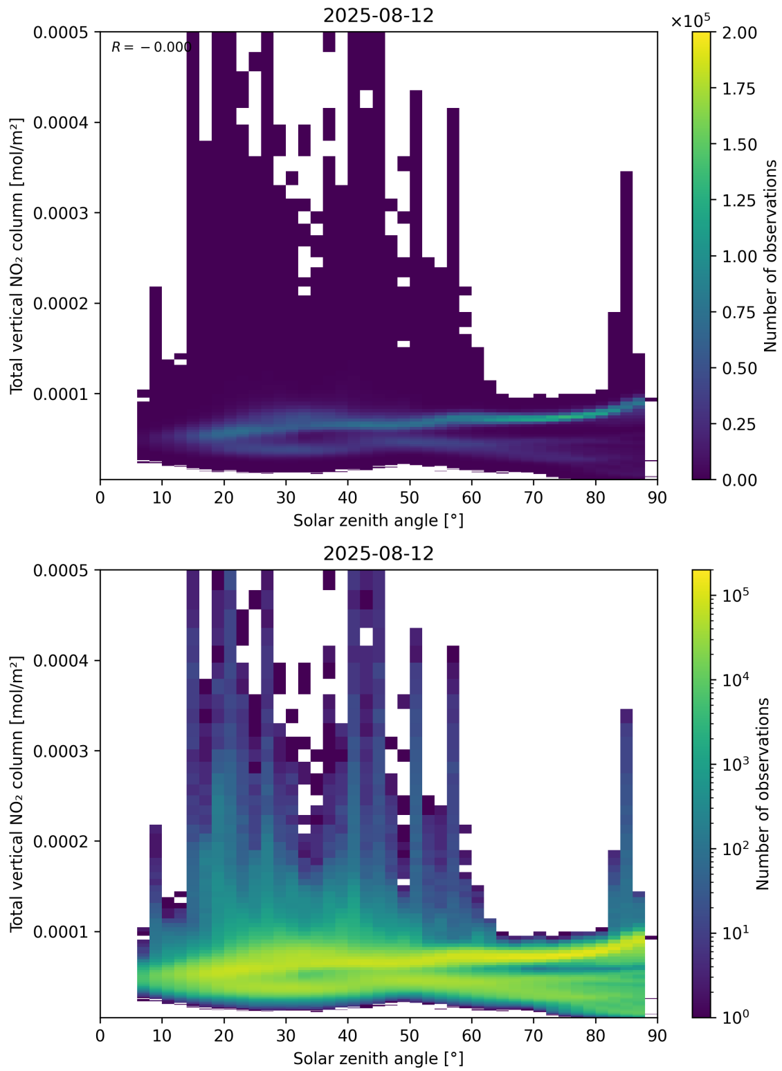
Figure 153: Scatter density plot of “Solar zenith angle” against “Total vertical NO 2 column” for 2025-08-11 to 2025-08-13.
