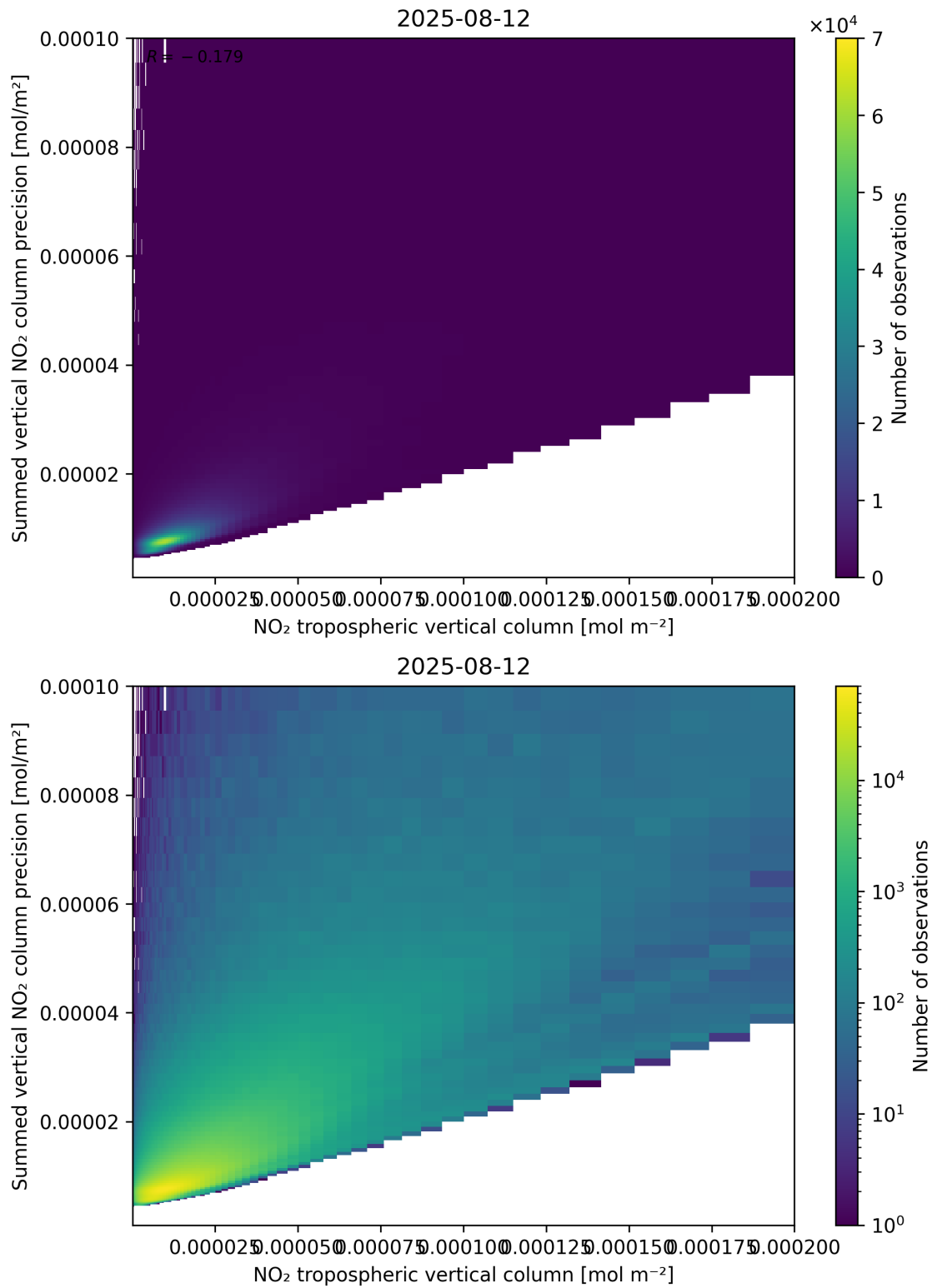
Figure 127: Scatter density plot of “NO 2 tropospheric vertical column” against “Summed vertical NO 2 column precision” for 2025-08-11 to 2025-08-13.
