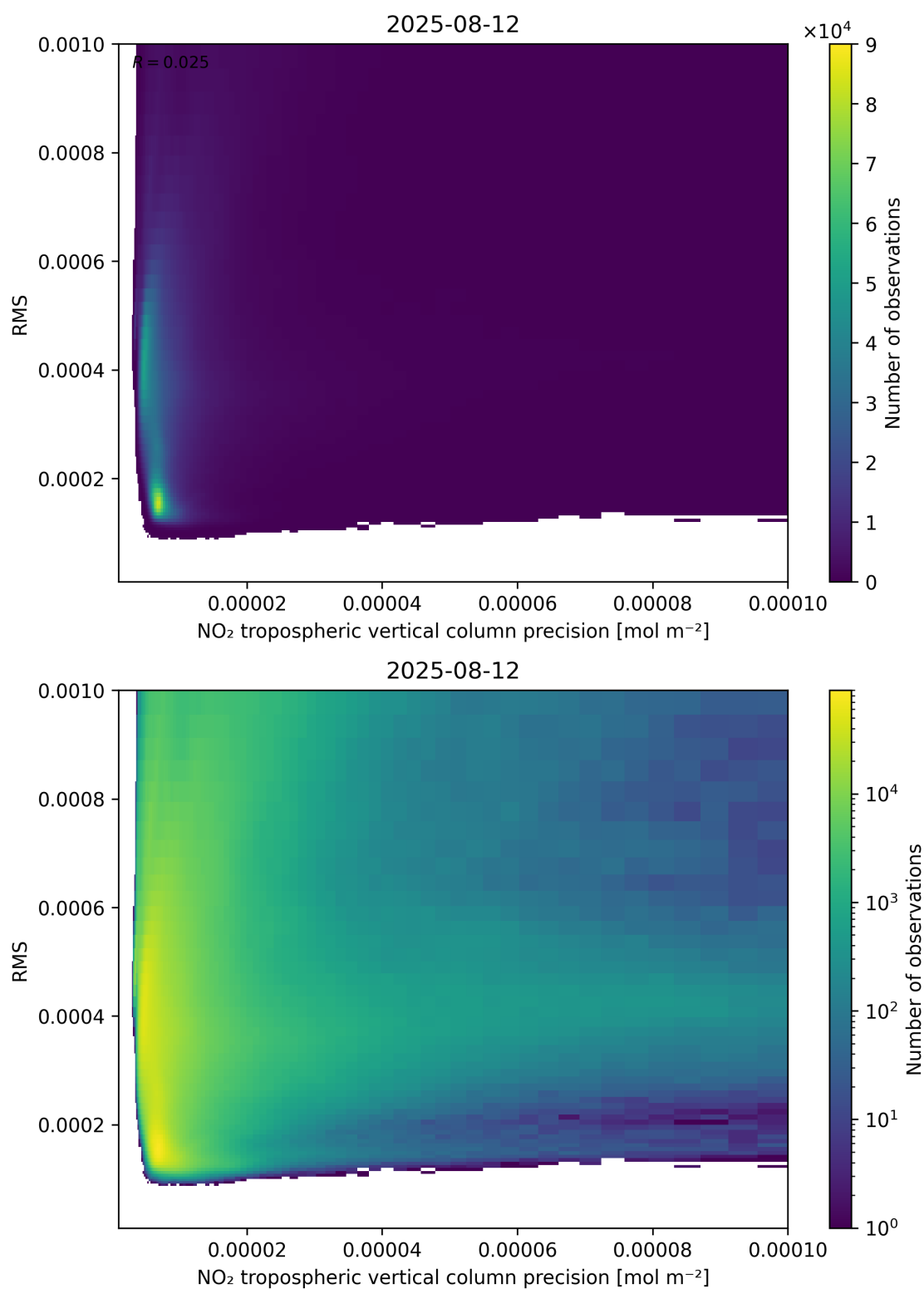
Figure 140: Scatter density plot of “NO 2 tropospheric vertical column precision” against “RMS” for 2025-08-11 to 2025-08-13.
