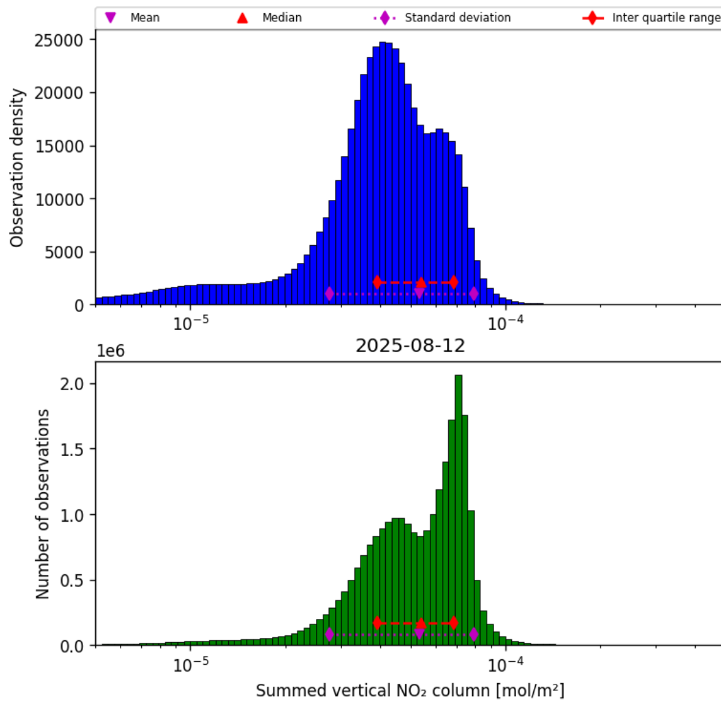
Figure 40: Histogram of “Summed vertical NO 2 column” for 2025-08-11 to 2025-08-13
