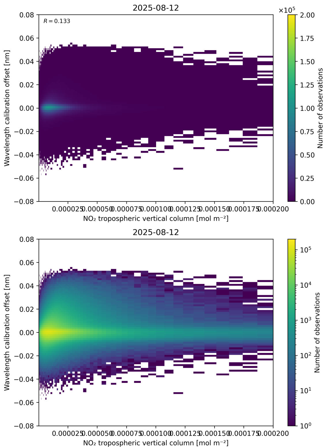
Figure 143: Scatter density plot of “NO 2 tropospheric vertical column” against “Wavelength calibration offset” for 2025-08-11 to 2025-08-13.
