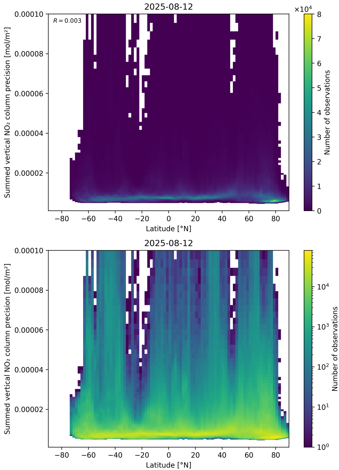
Figure 89: Scatter density plot of “Latitude” against “Summed vertical NO 2 column precision” for 2025-08-11 to 2025-08-13.
