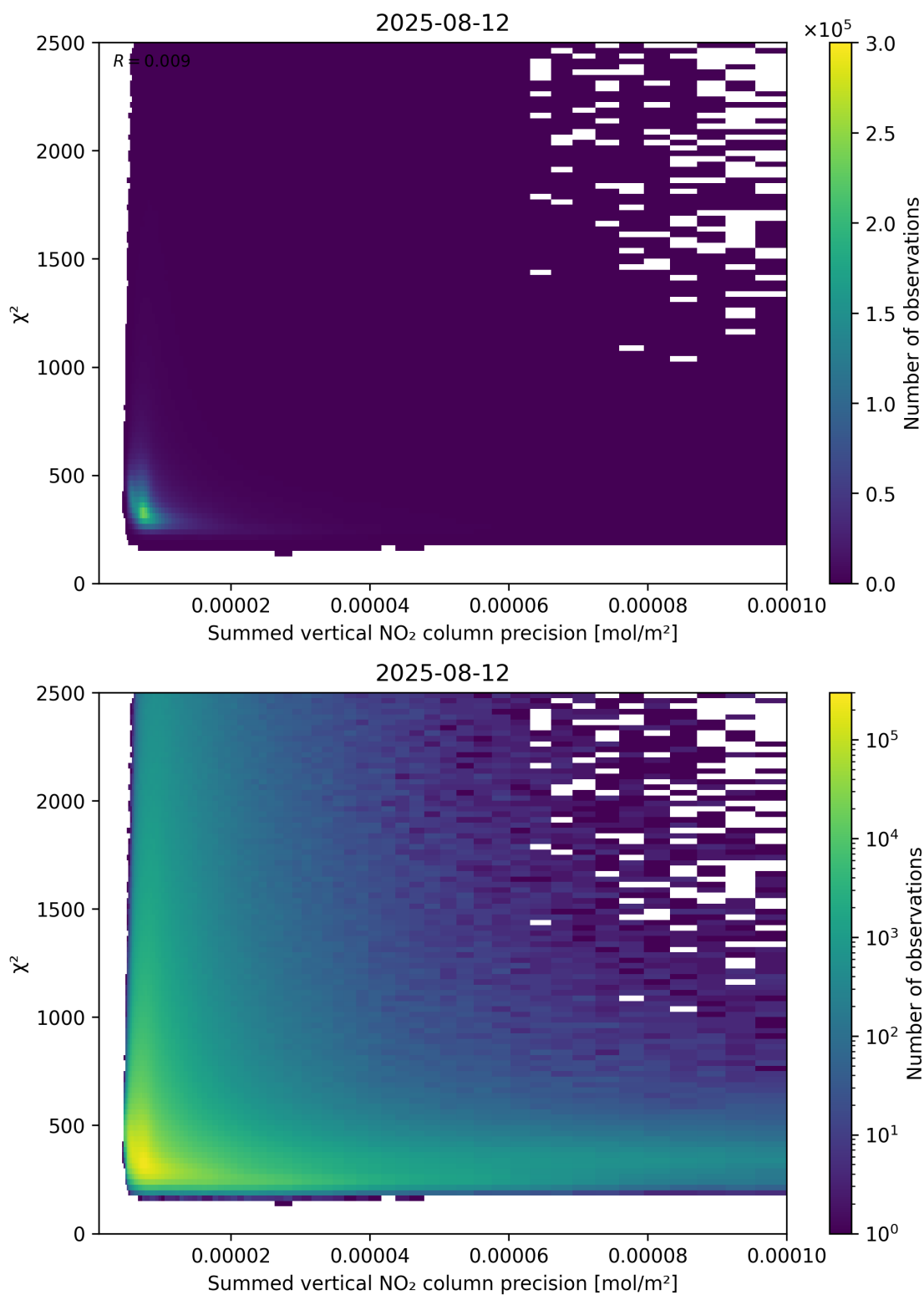
Figure 107: Scatter density plot of “Summed vertical NO 2 column precision” against “ \chi^2 ” for 2025-08-11 to 2025-08-13.
