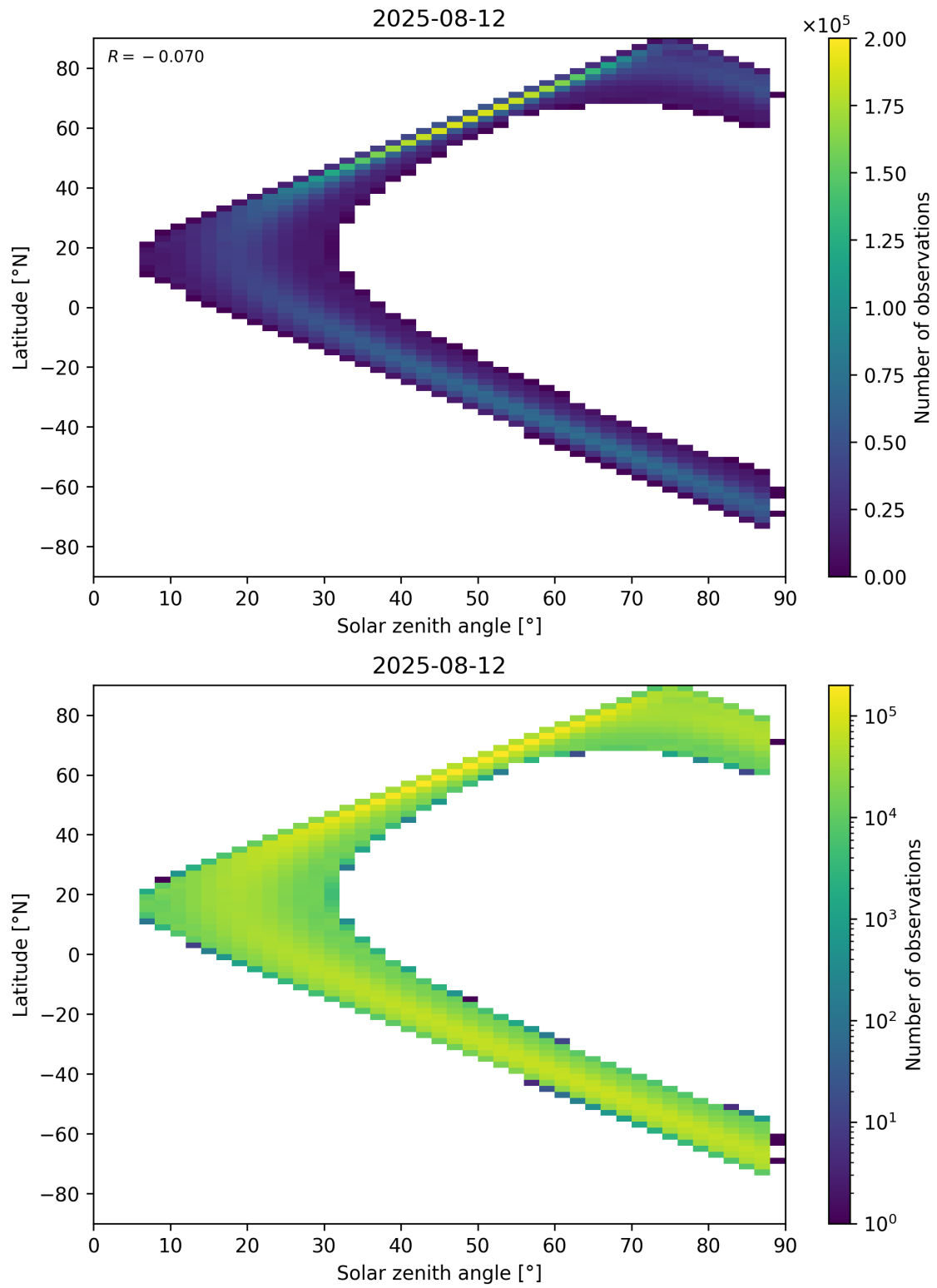
Figure 149: Scatter density plot of “Solar zenith angle” against “Latitude” for 2025-08-11 to 2025-08-13.
