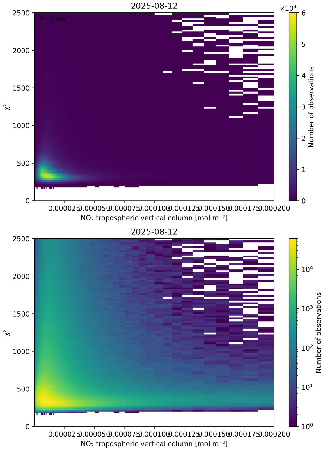
Figure 124: Scatter density plot of “NO 2 tropospheric vertical column” against “ \chi^2 ” for 2025-08-11 to 2025-08-13.
