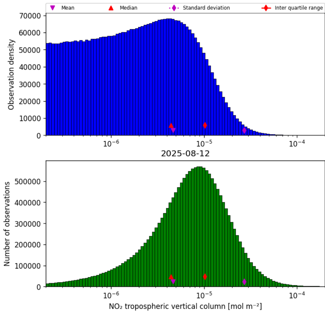
Figure 29: Histogram of “NO 2 tropospheric vertical column” for 2025-08-11 to 2025-08-13
