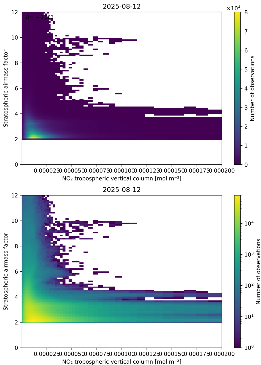
Figure 121: Scatter density plot of “NO 2 tropospheric vertical column” against “Stratospheric air mass factor” for 2025-08-11 to 2025-08-13.
