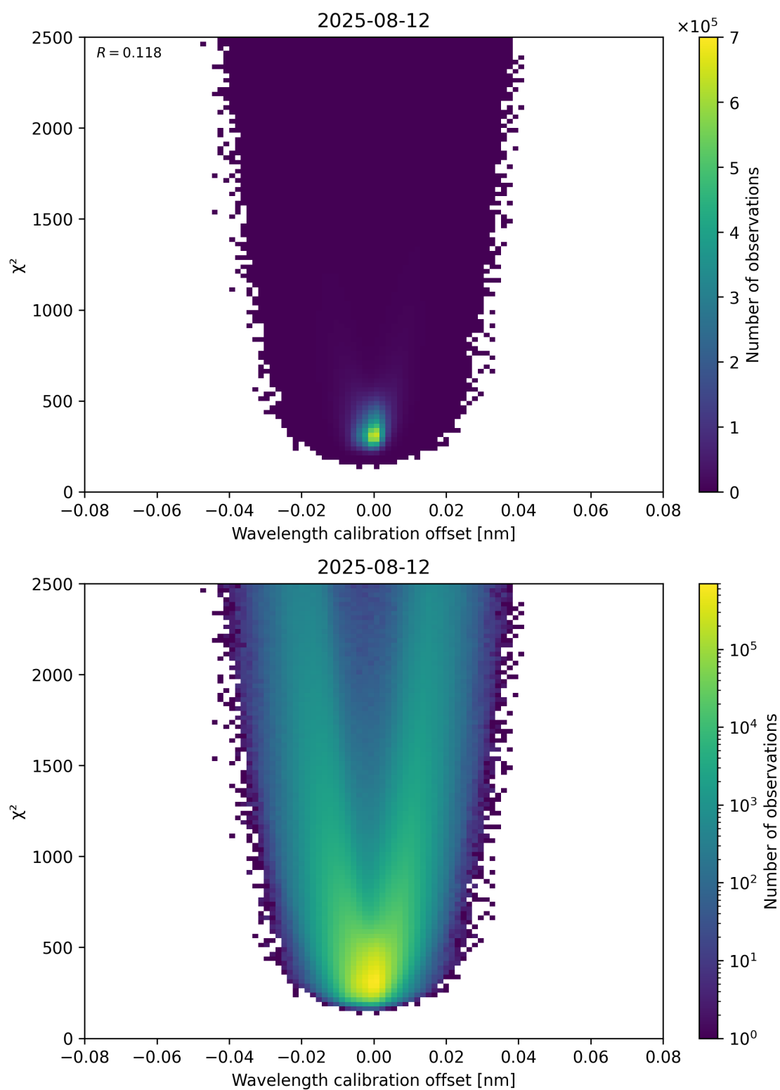
Figure 175: Scatter density plot of “Wavelength calibration offset” against “ \chi^2 ” for 2025-08-11 to 2025-08-13.
