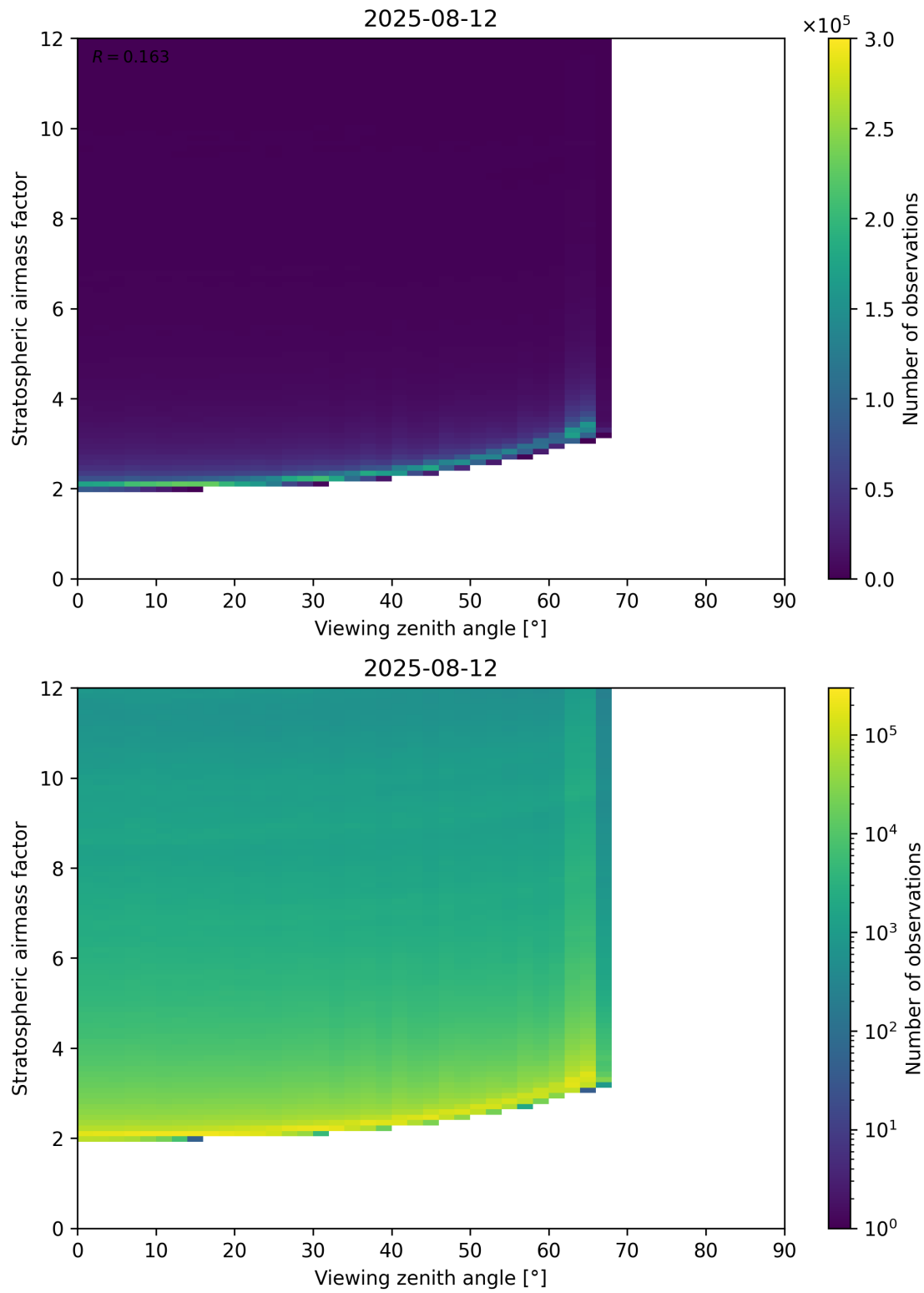
Figure 159: Scatter density plot of “Viewing zenith angle” against “Stratospheric airmass factor” for 2025-08-11 to 2025-08-13.
