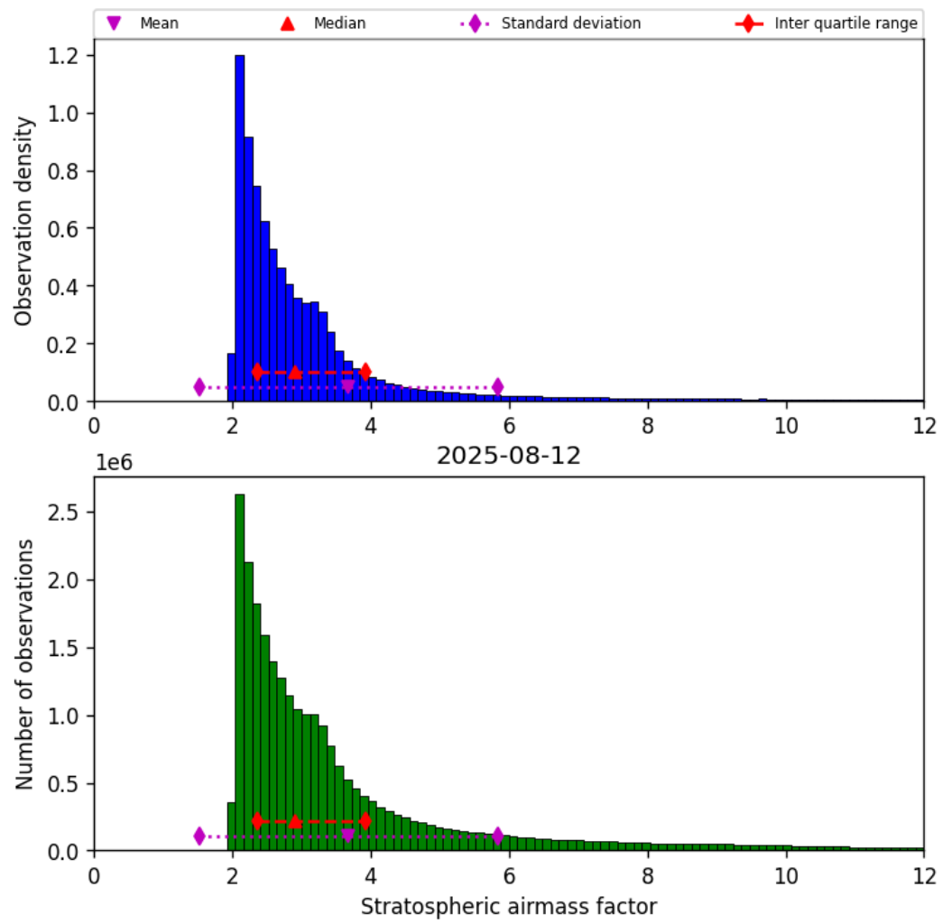
Figure 44: Histogram of “Stratospheric airmass factor” for 2025-08-11 to 2025-08-13
