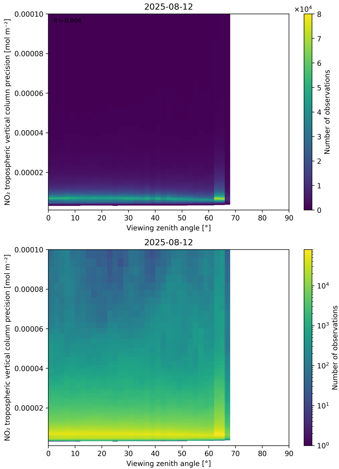
Figure 170: Scatter density plot of “Viewing zenith angle” against “NO 2 tropospheric vertical column precision” for 2025-08-11 to 2025-08-13.
