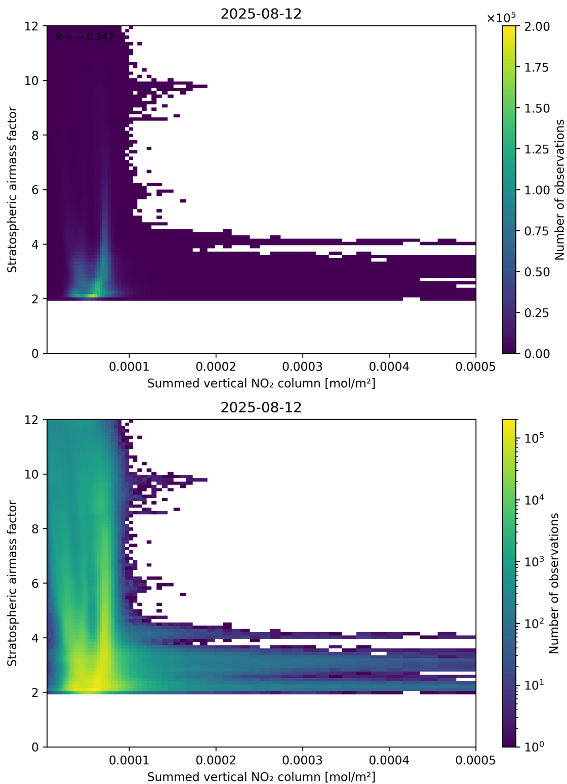
Figure 103: Scatter density plot of “Summed vertical NO 2 column” against “Stratospheric airmass factor” for 2025-08-11 to 2025-08-13.
