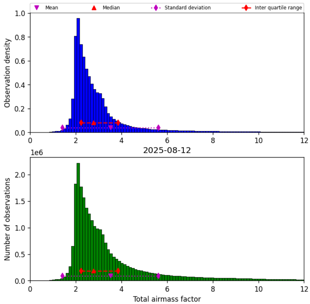
Figure 32: Histogram of “Total airmass factor” for 2025-08-11 to 2025-08-13
