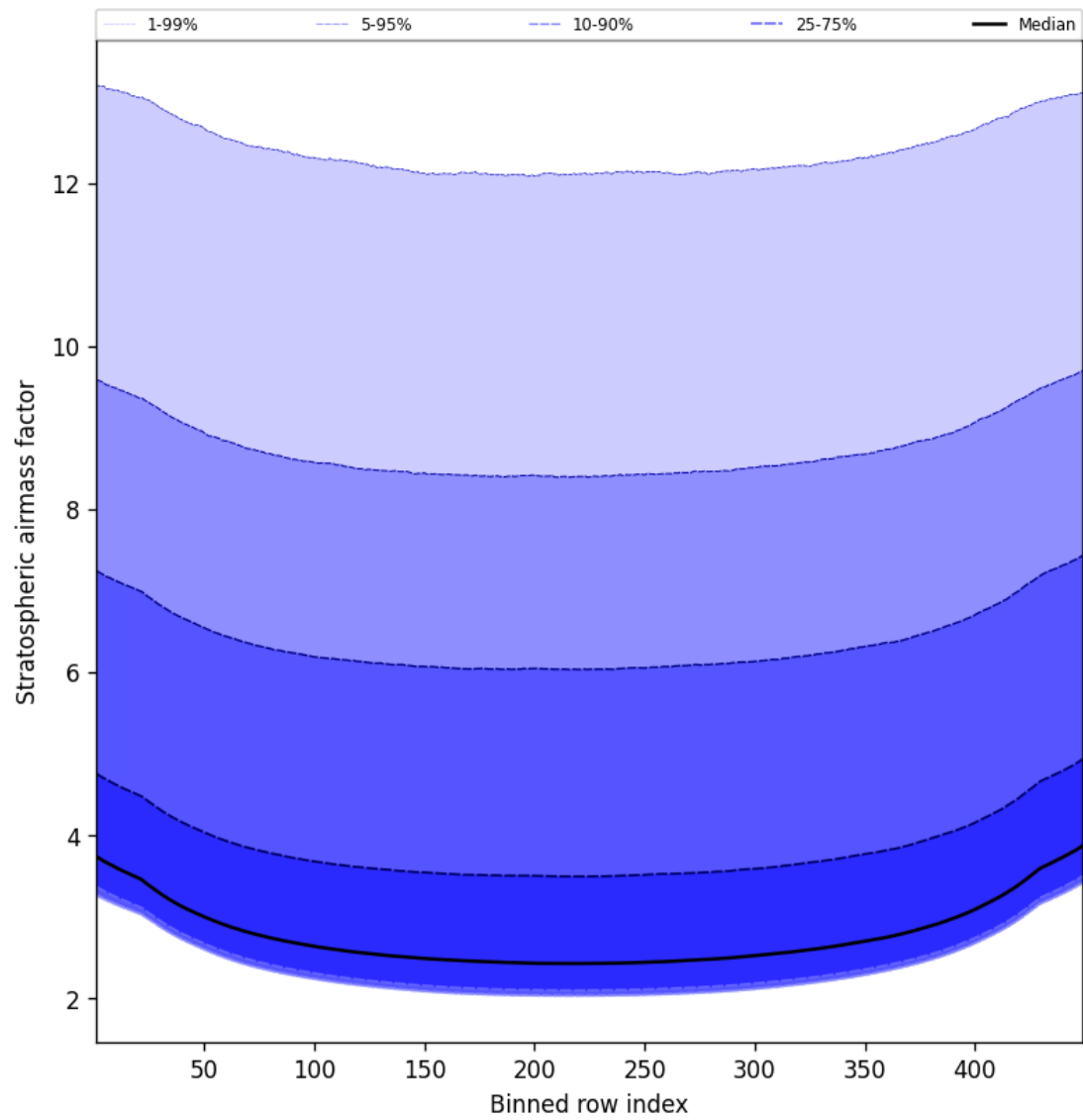
Figure 61: Along track statistics of “Stratospheric airmass factor” for 2025-08-11 to 2025-08-13
