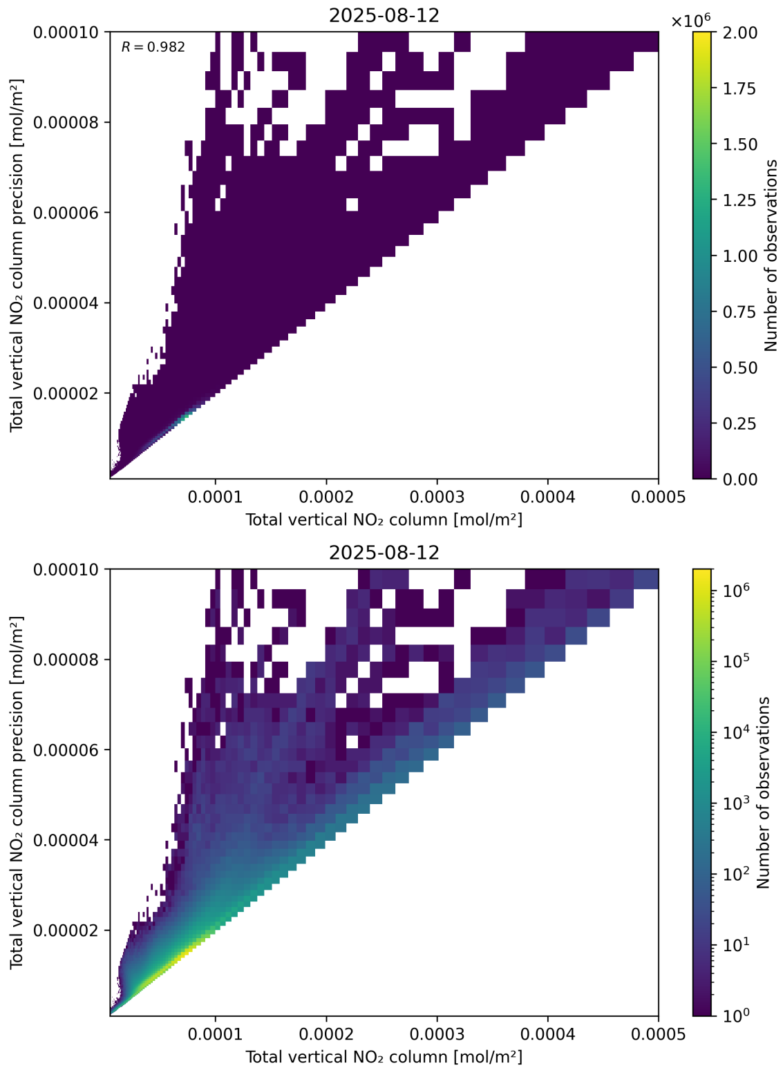
Figure 114: Scatter density plot of “Total vertical NO 2 column” against “Total vertical NO 2 column precision” for 2025-08-11 to 2025-08-13.
