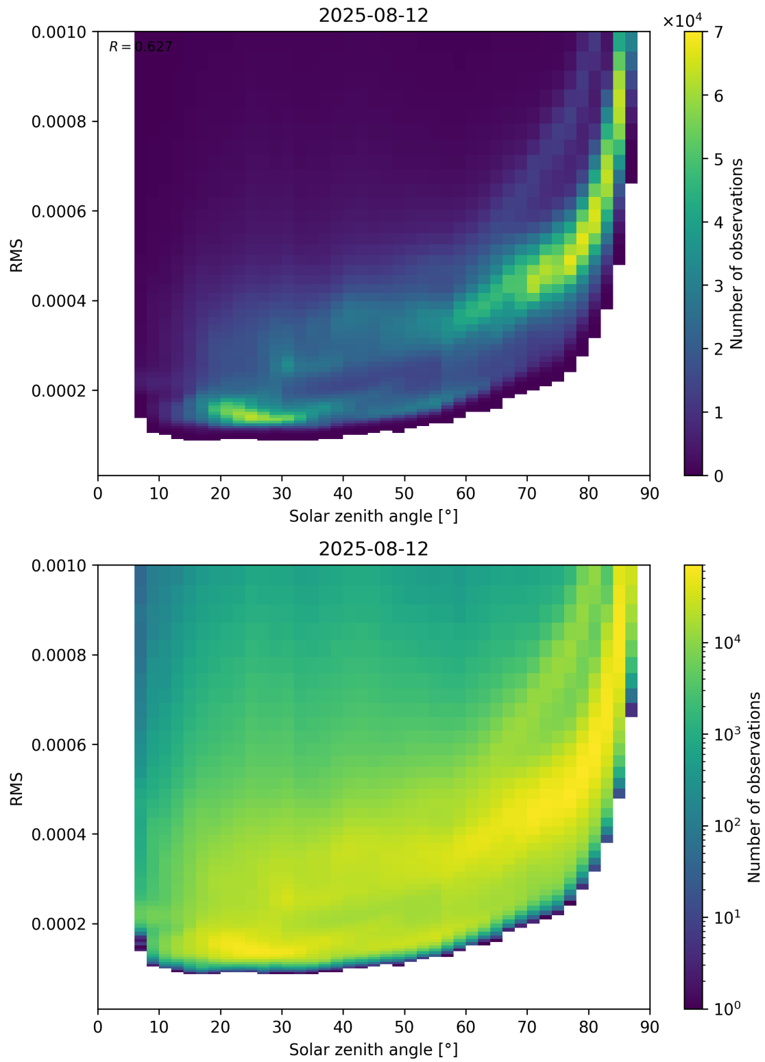
Figure 157: Scatter density plot of “Solar zenith angle” against “RMS” for 2025-08-11 to 2025-08-13.
