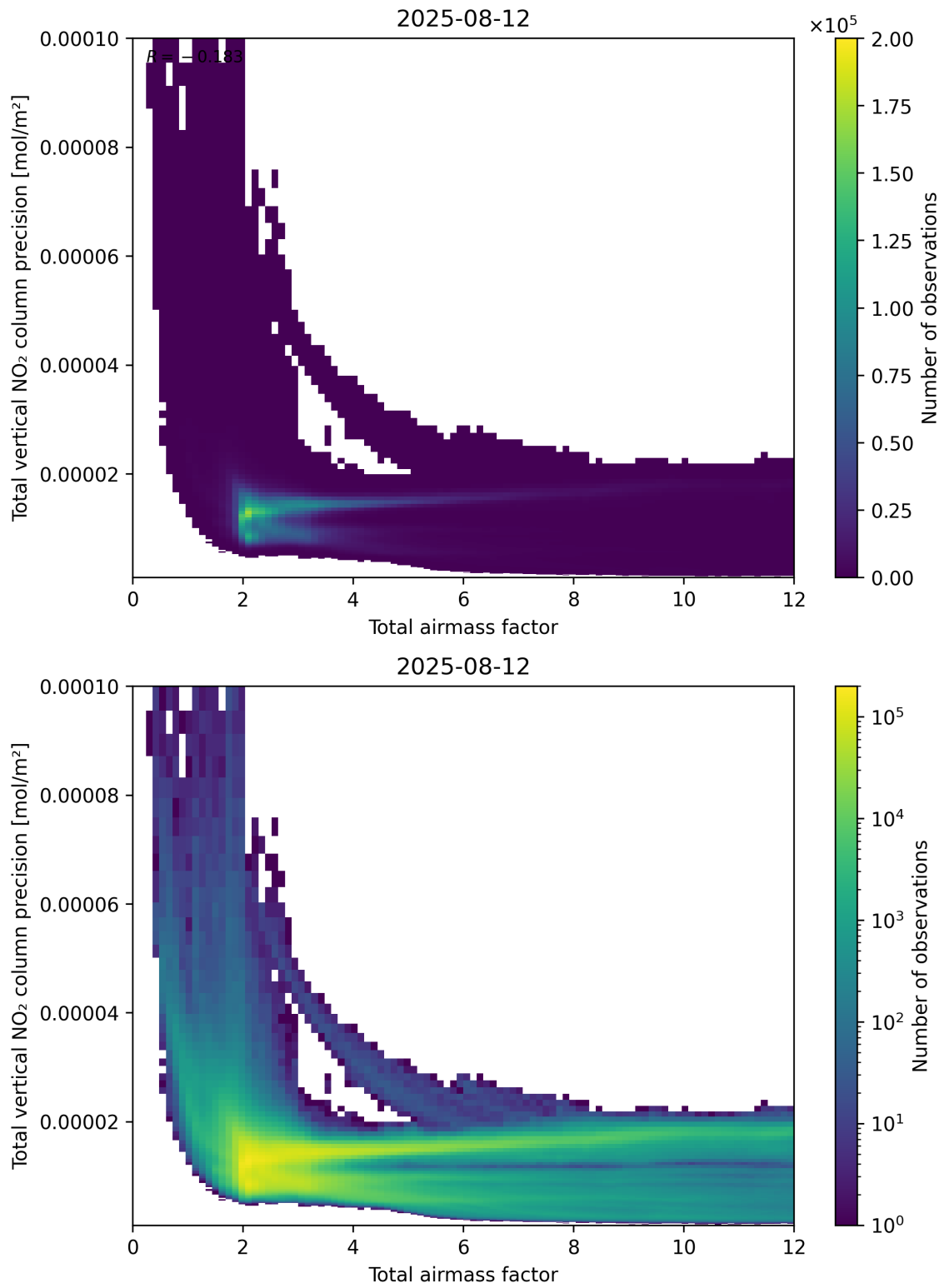
Figure 68: Scatter density plot of “Total airmass factor” against “Total vertical NO 2 column precision” for 2025-08-11 to 2025-08-13.
