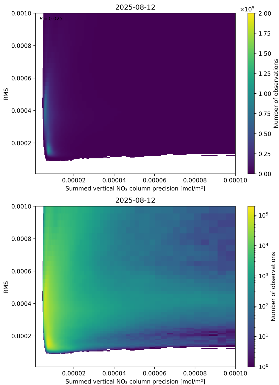
Figure 108: Scatter density plot of “Summed vertical NO 2 column precision” against “RMS” for 2025-08-11 to 2025-08-13.
