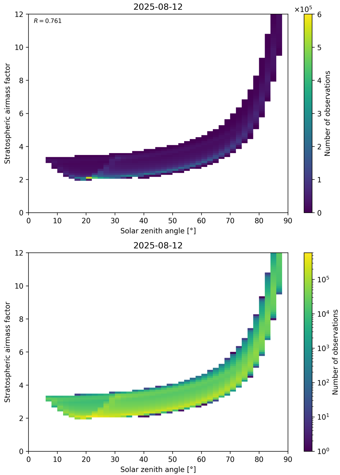
Figure 145: Scatter density plot of “Solar zenith angle” against “Stratospheric airmass factor” for 2025-08-11 to 2025-08-13.
