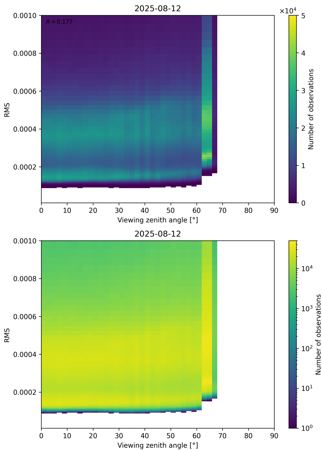
Figure 171: Scatter density plot of “Viewing zenith angle” against “RMS” for 2025-08-11 to 2025-08-13.
