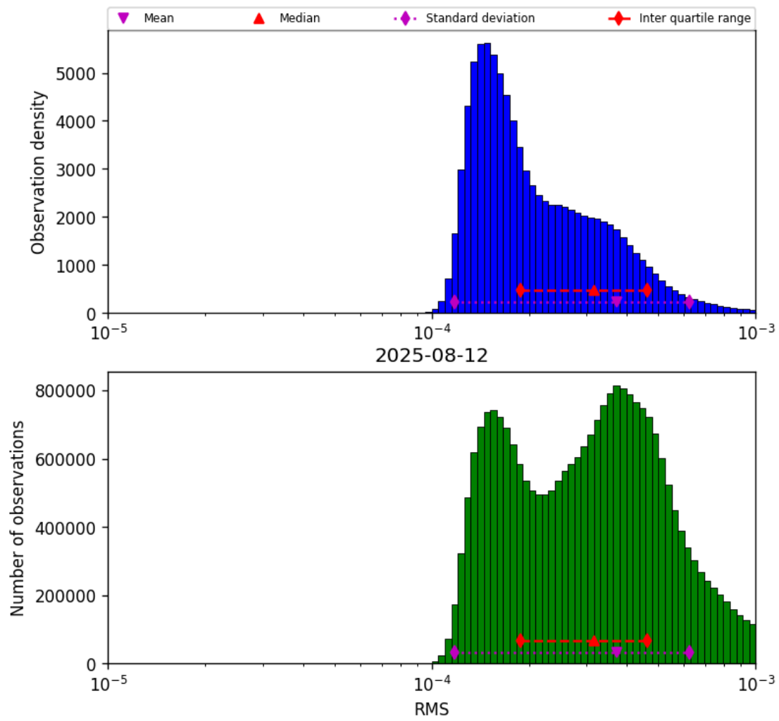
Figure 43: Histogram of “RMS” for 2025-08-11 to 2025-08-13
