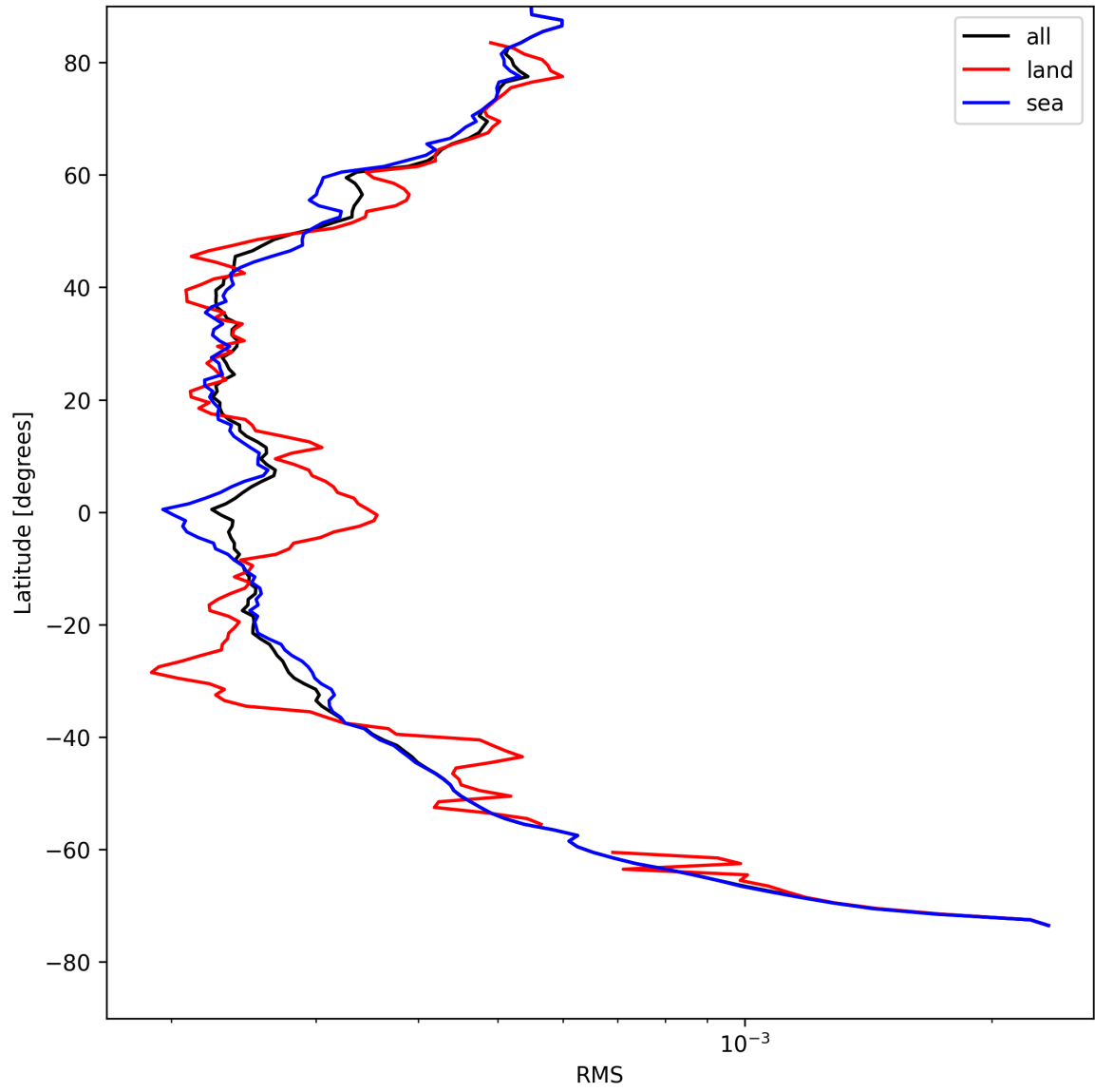
Figure 26: Zonal average of “RMS” for 2025-08-11 to 2025-08-13.
