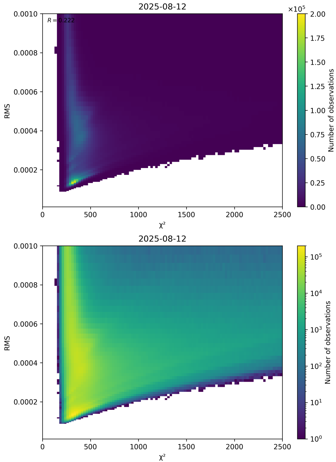
Figure 82: Scatter density plot of “ \chi^2 ” against “RMS” for 2025-08-11 to 2025-08-13.
