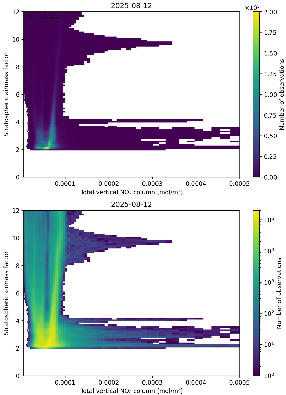
Figure 110: Scatter density plot of “Total vertical NO 2 column” against “Stratospheric airmass factor” for 2025-08-11 to 2025-08-13.
