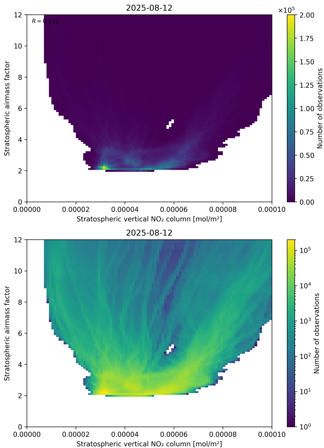
Figure 96: Scatter density plot of “Stratospheric vertical NO 2 column” against “Stratospheric airmass factor” for 2025-08-11 to 2025-08-13.
