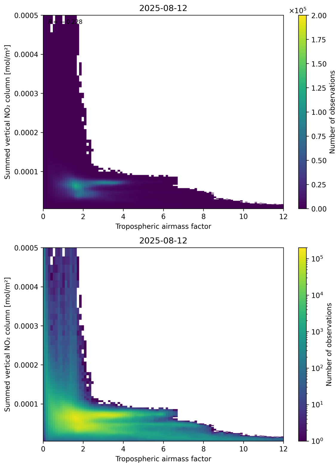
Figure 75: Scatter density plot of “Tropospheric airmass factor” against “Summed vertical NO 2 column” for 2025-08-11 to 2025-08-13.
