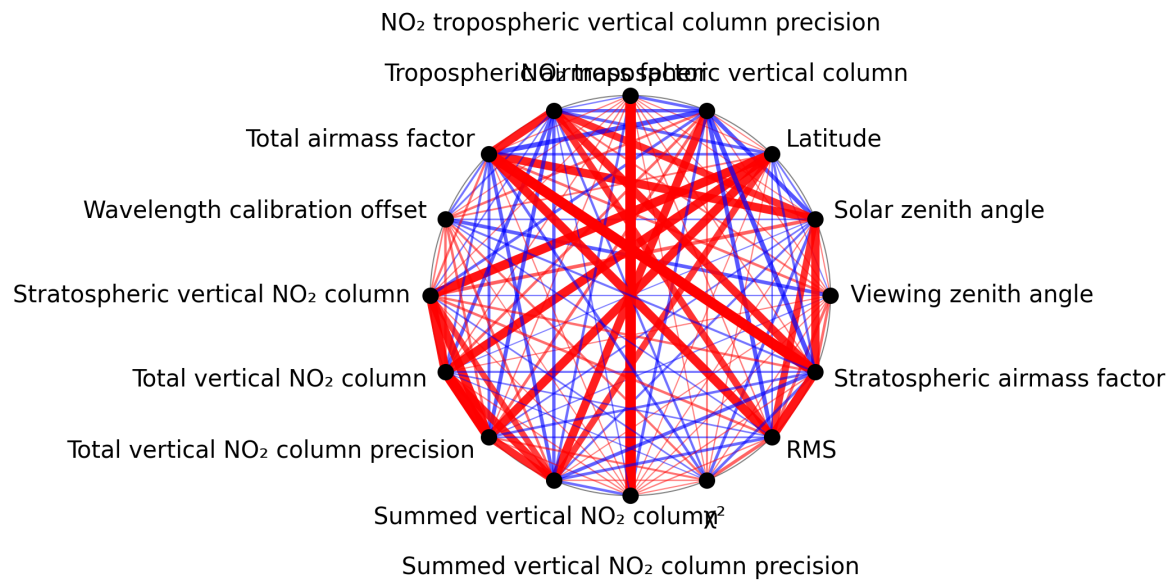
Figure 1: Map of correlation graph for 2025-08-11 to 2025-08-13.
