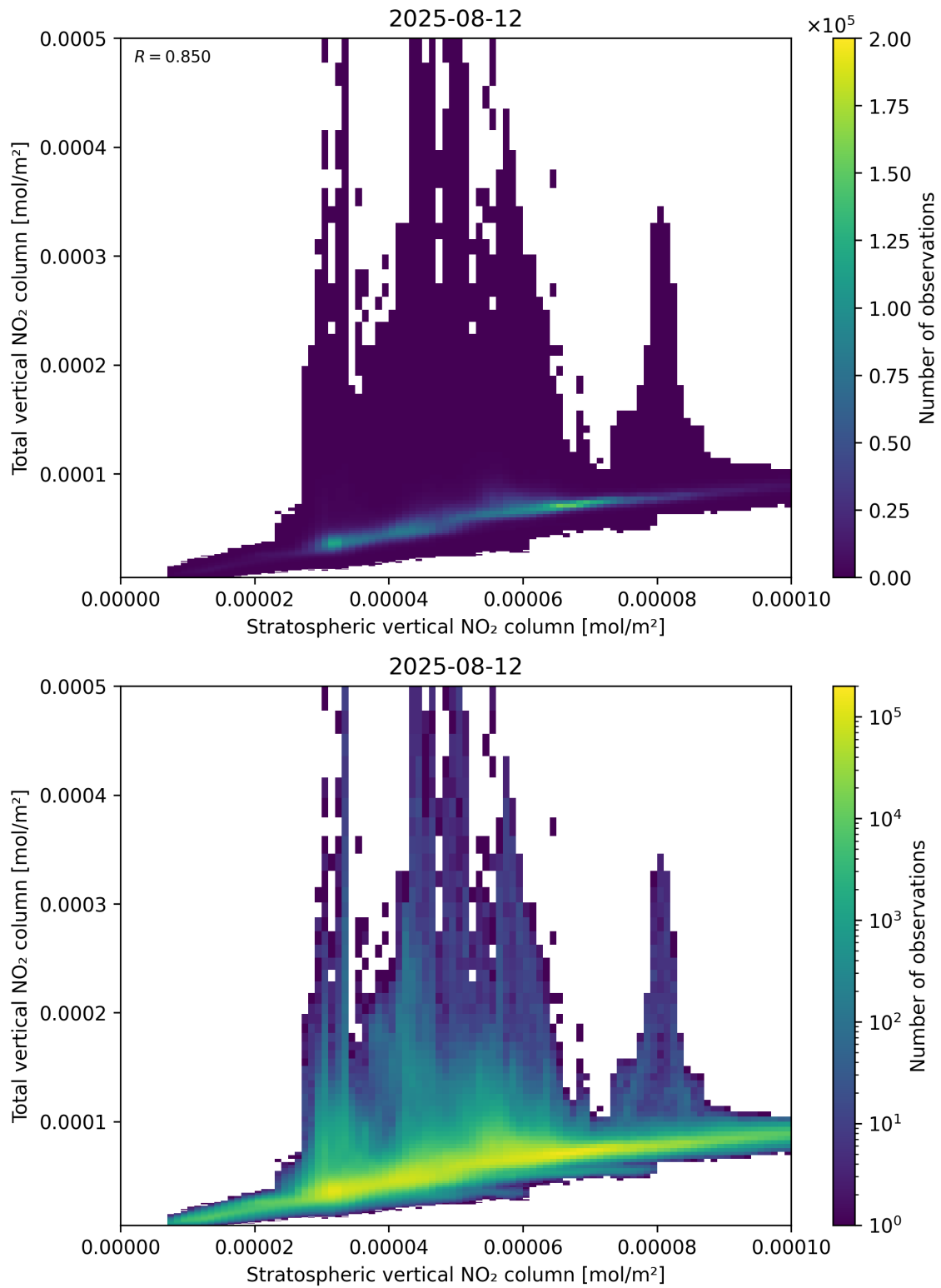
Figure 100: Scatter density plot of “Stratospheric vertical NO 2 column” against “Total vertical NO 2 column” for 2025-08-11 to 2025-08-13.
