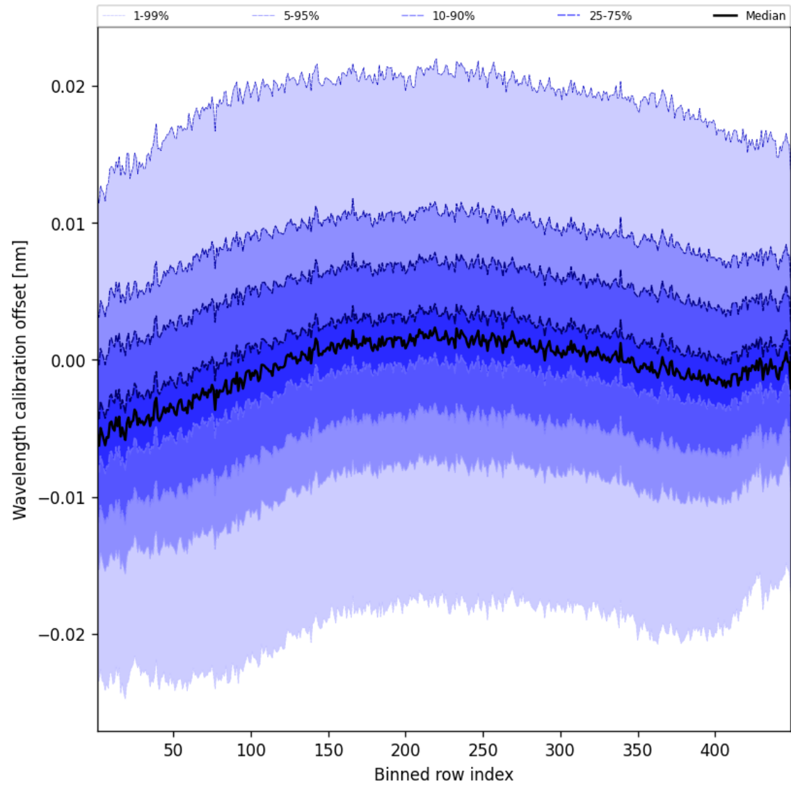
Figure 52: Along track statistics of “Wavelength calibration offset” for 2025-08-11 to 2025-08-13
