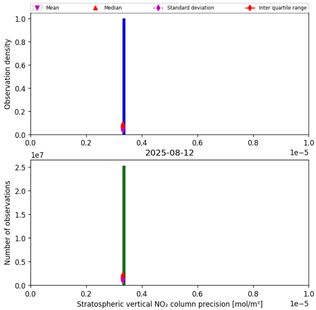
Figure 37: Histogram of “Stratospheric vertical NO 2 column precision” for 2025-08-11 to 2025-08-13
