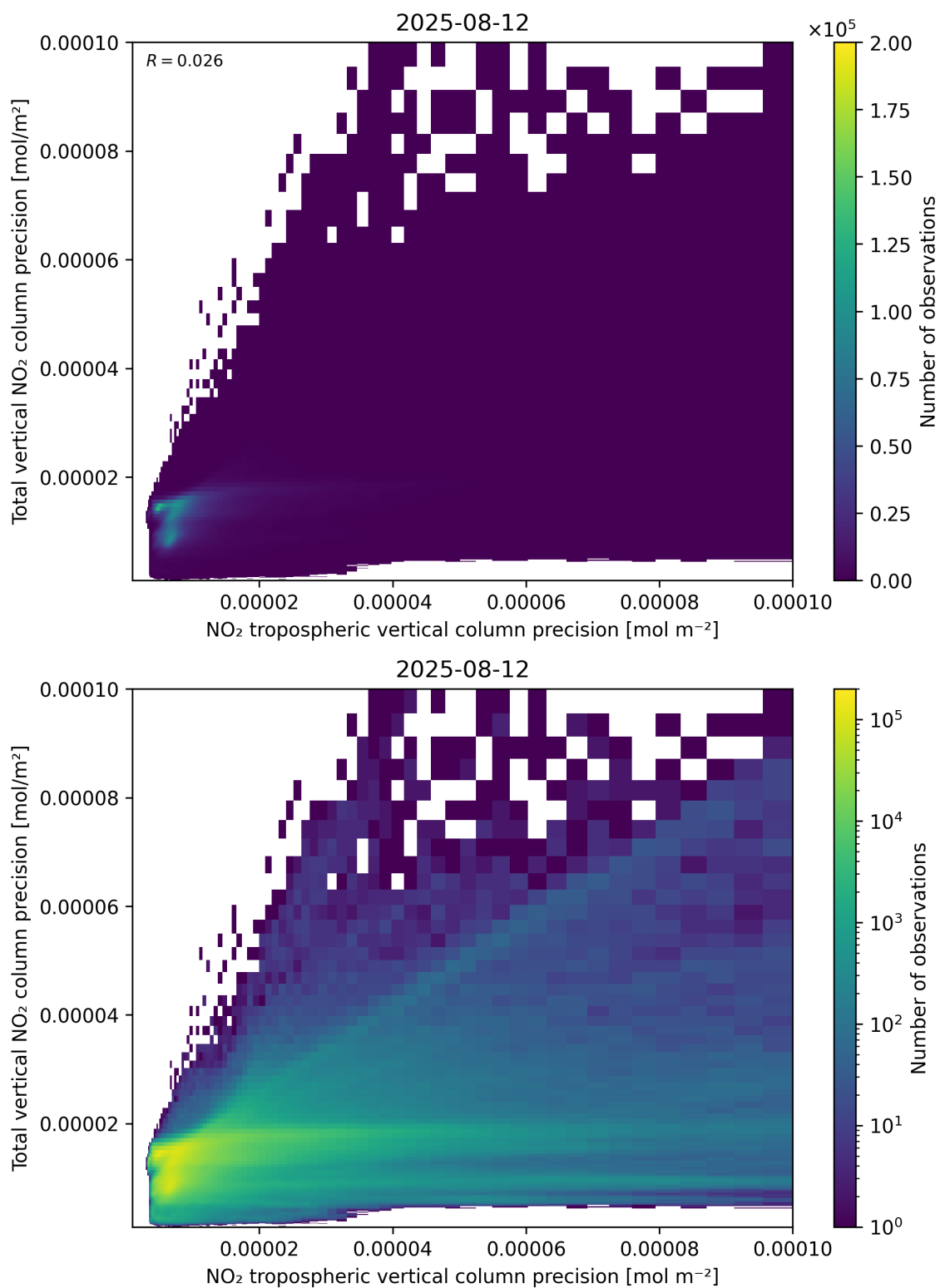
Figure 139: Scatter density plot of “NO 2 tropospheric vertical column precision” against “Total vertical NO 2 column precision” for 2025-08-11 to 2025-08-13.
