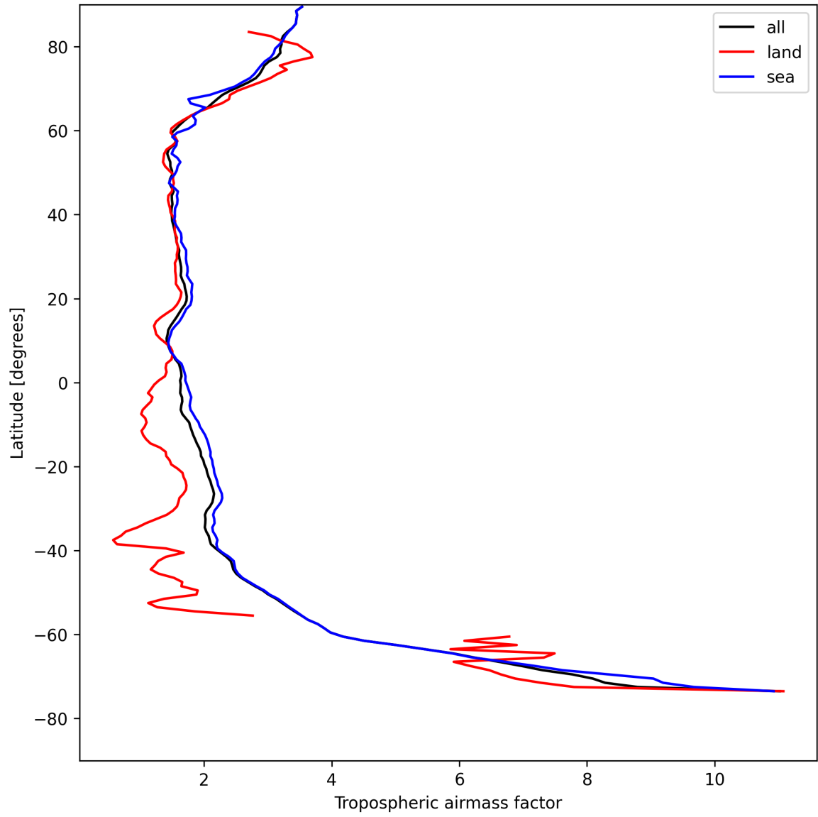
Figure 14: Zonal average of “Tropospheric air mass factor” for 2025-08-11 to 2025-08-13.
