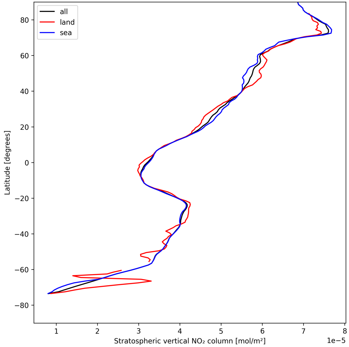
Figure 19: Zonal average of “Stratospheric vertical NO 2 column” for 2025-08-11 to 2025-08-13.
