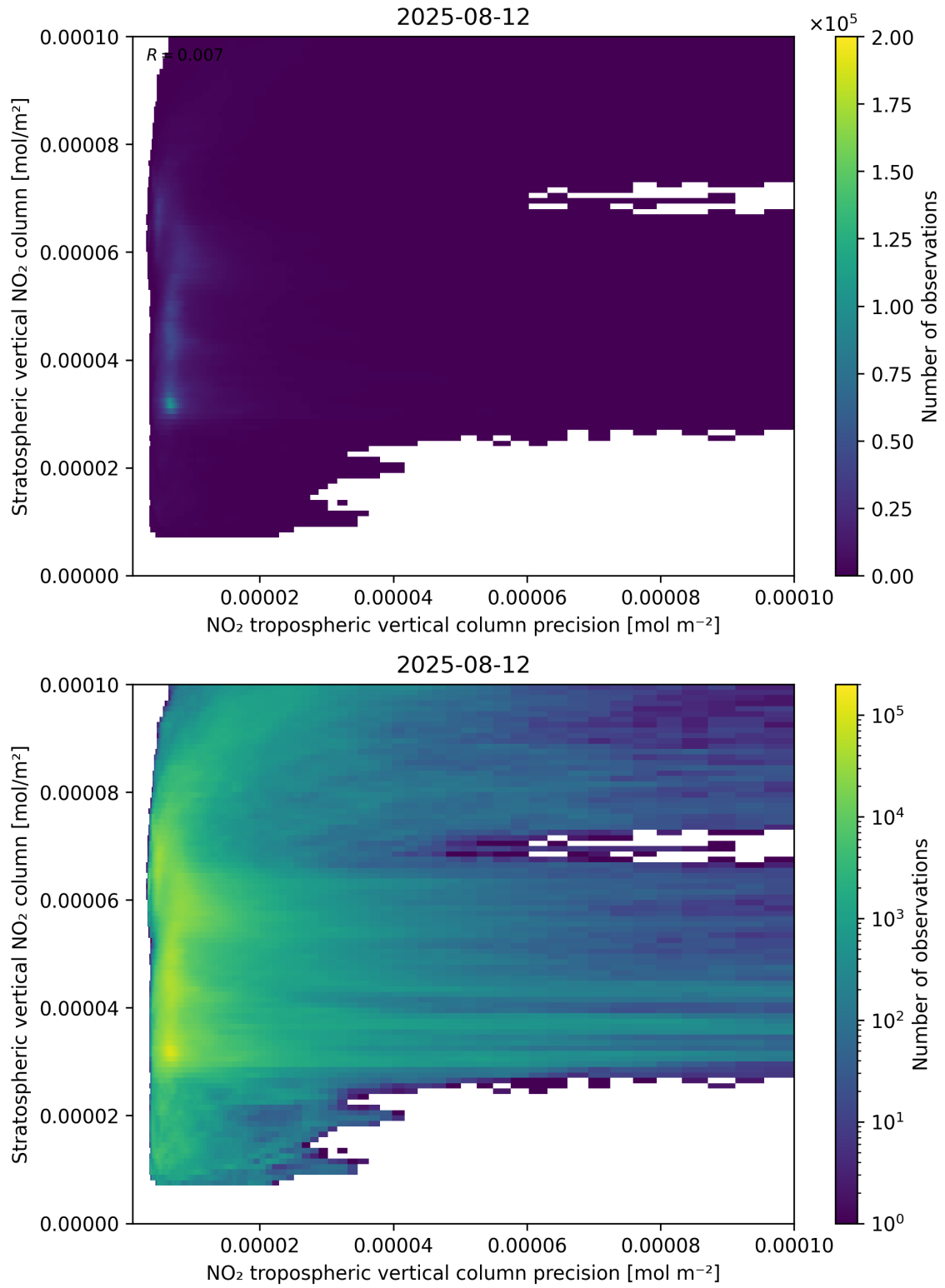
Figure 135: Scatter density plot of “NO 2 tropospheric vertical column precision” against “Stratospheric vertical NO 2 column” for 2025-08-11 to 2025-08-13.
