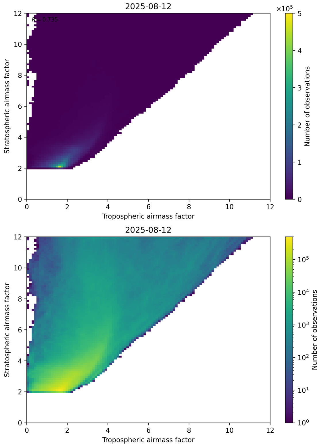
Figure 71: Scatter density plot of “Tropospheric airmass factor” against “Stratospheric airmass factor” for 2025-08-11 to 2025-08-13.
