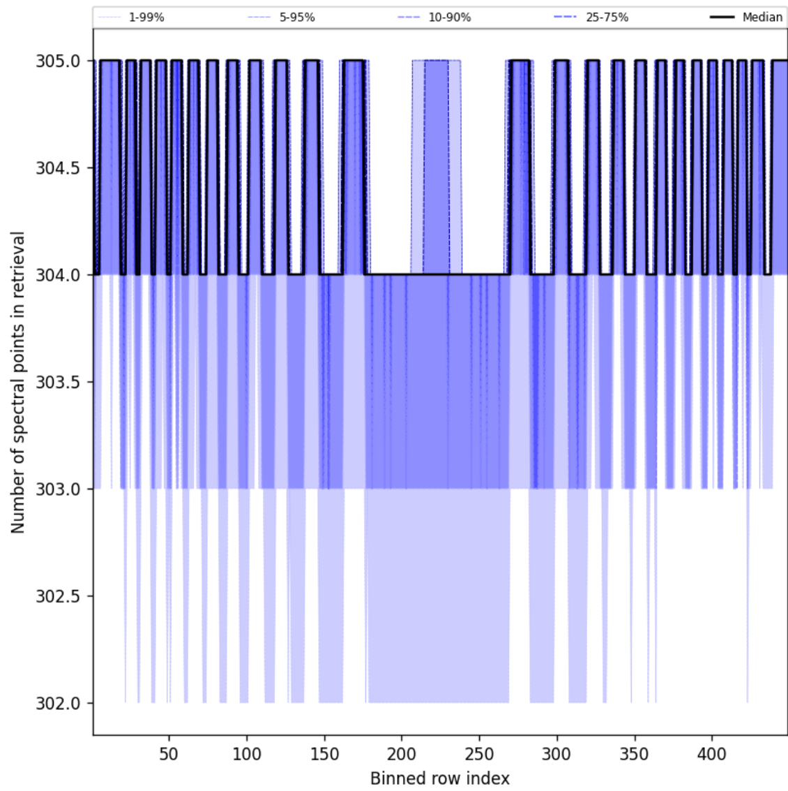
Figure 50: Along track statistics of “Number of spectral points in retrieval” for 2025-08-11 to 2025-08-13
