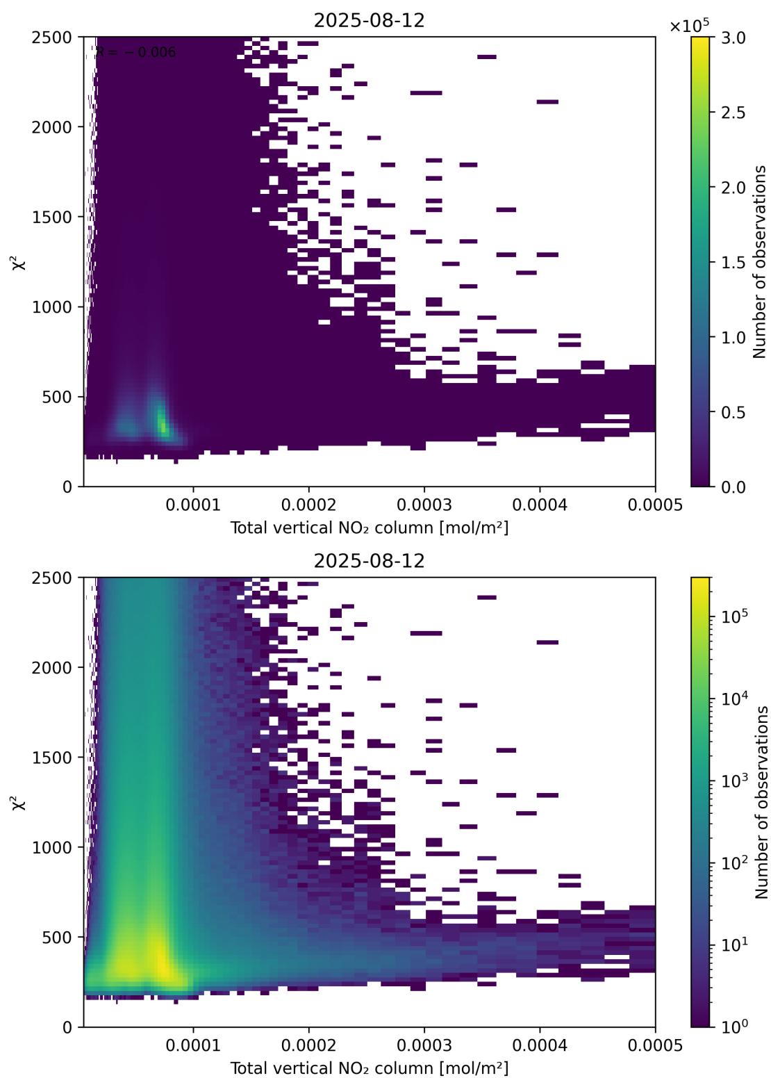
Figure 111: Scatter density plot of “Total vertical NO 2 column” against “ \chi^2 ” for 2025-08-11 to 2025-08-13.
