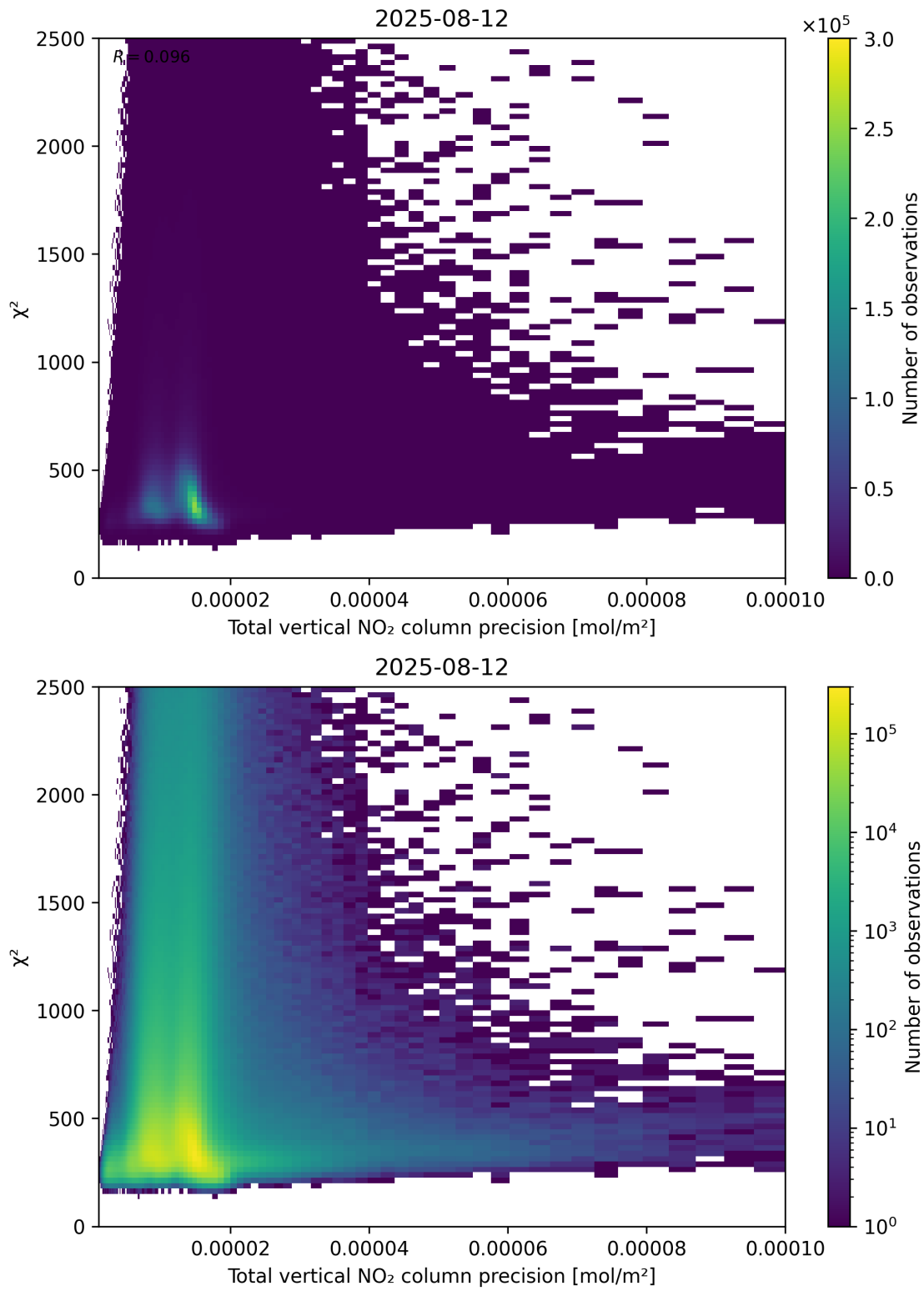
Figure 116: Scatter density plot of “Total vertical NO 2 column precision” against “ \chi^2 ” for 2025-08-11 to 2025-08-13.
