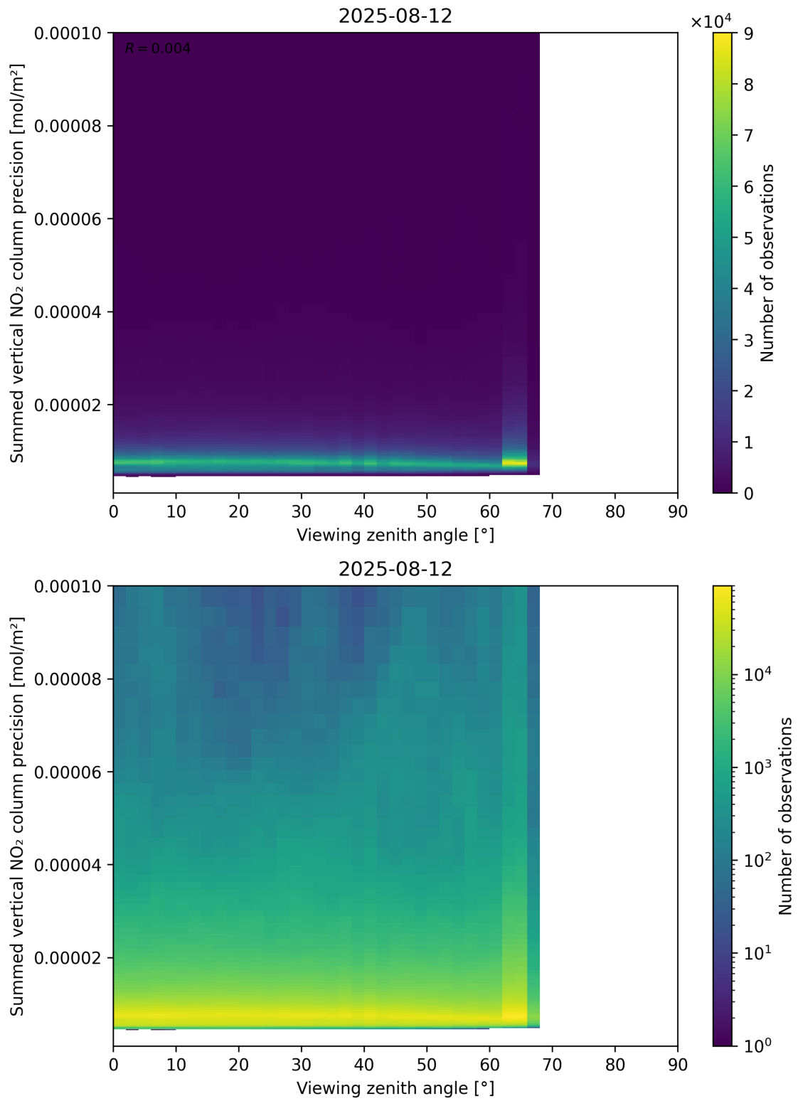
Figure 166: Scatter density plot of “Viewing zenith angle” against “Summed vertical NO 2 column precision” for 2025-08-11 to 2025-08-13.
