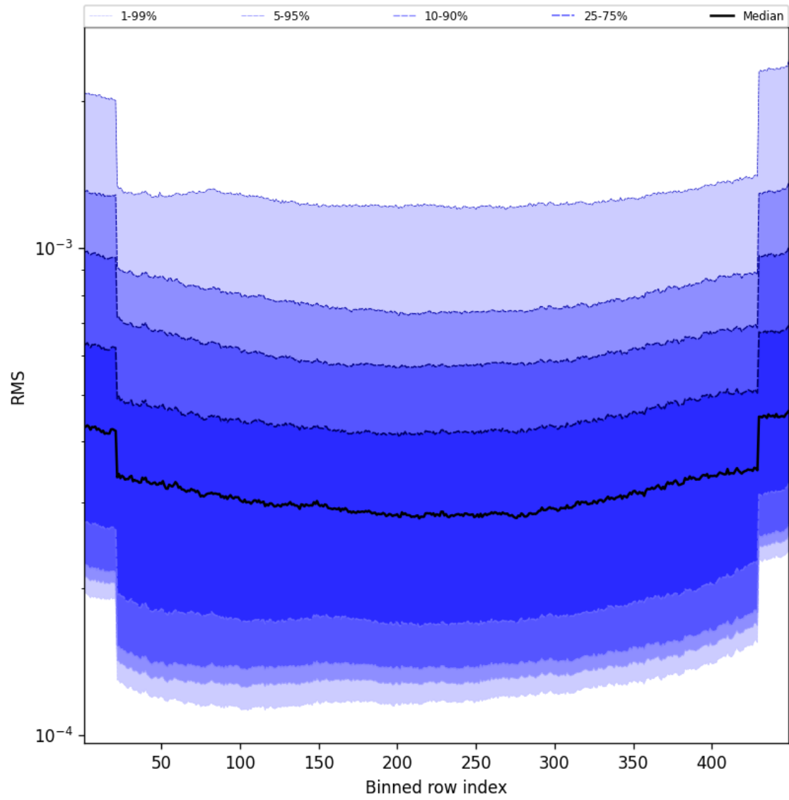
Figure 60: Along track statistics of “RMS” for 2025-08-11 to 2025-08-13
