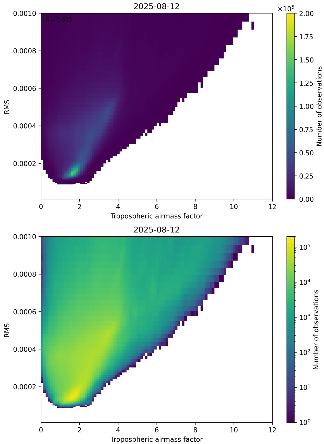
Figure 79: Scatter density plot of “Tropospheric airmass factor” against “RMS” for 2025-08-11 to 2025-08-13.
