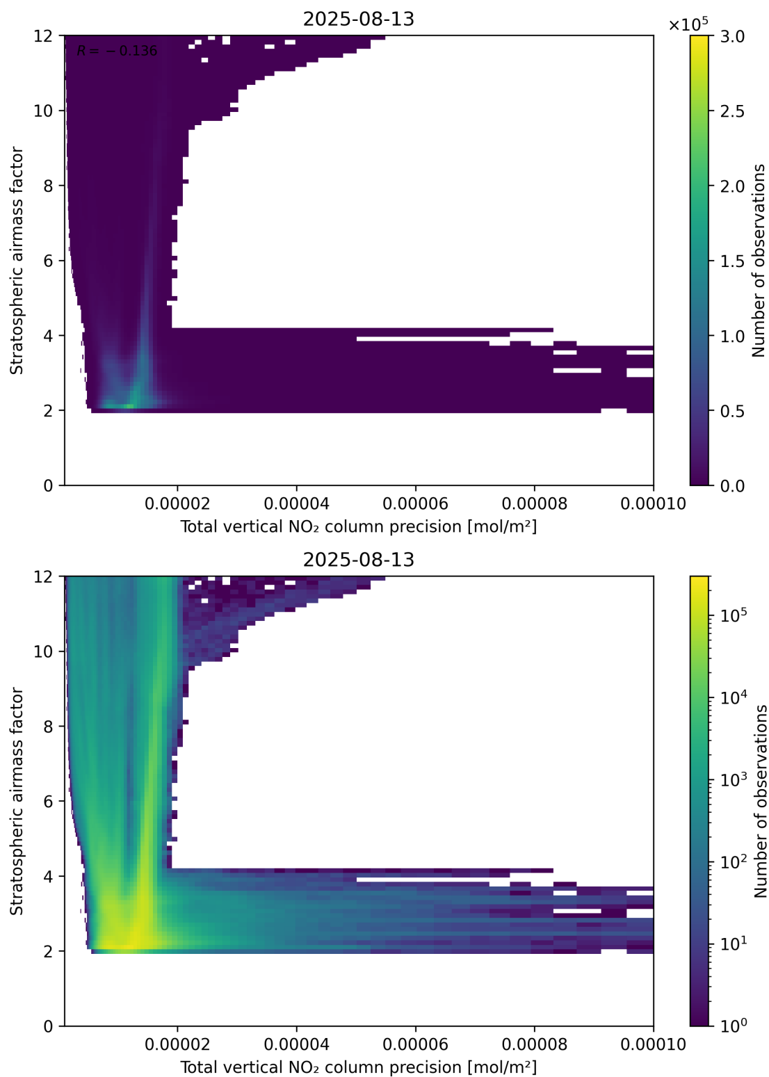
Figure 115: Scatter density plot of “Total vertical NO 2 column precision” against “Stratospheric air mass factor” for 2025-08-12 to 2025-08-14.
