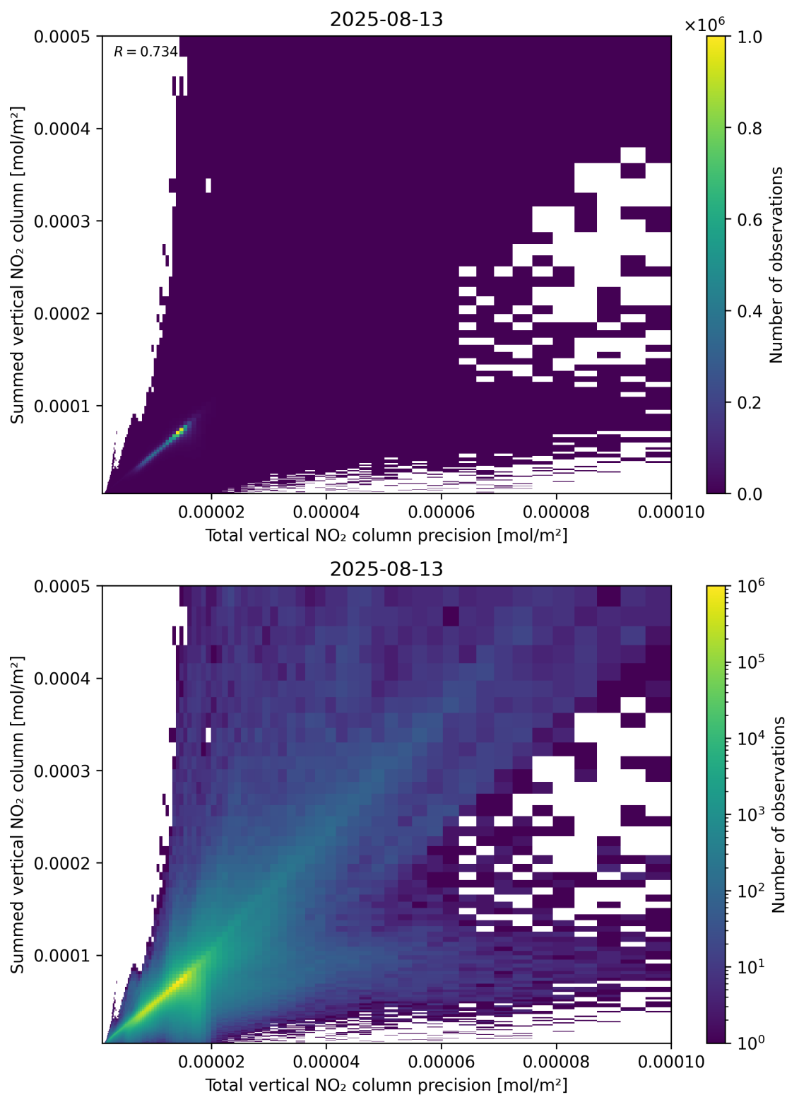
Figure 117: Scatter density plot of “Total vertical NO 2 column precision” against “Summed vertical NO 2 column” for 2025-08-12 to 2025-08-14.
