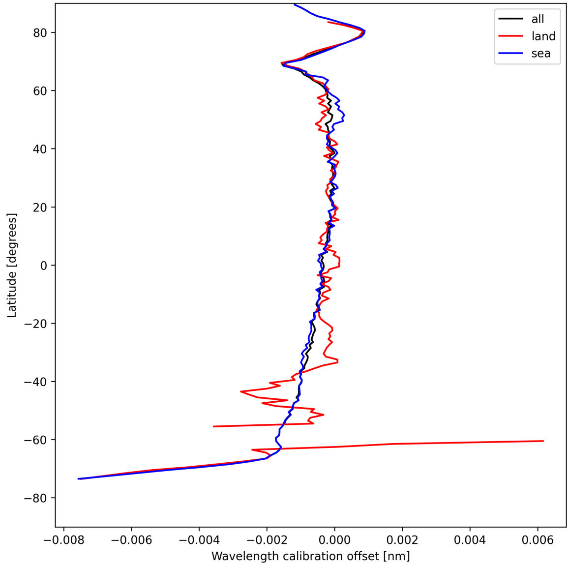
Figure 18: Zonal average of “Wavelength calibration offset” for 2025-08-12 to 2025-08-14.
