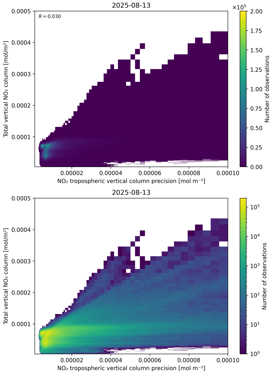
Figure 138: Scatter density plot of “NO 2 tropospheric vertical column precision” against “Total vertical NO 2 column” for 2025-08-12 to 2025-08-14.
