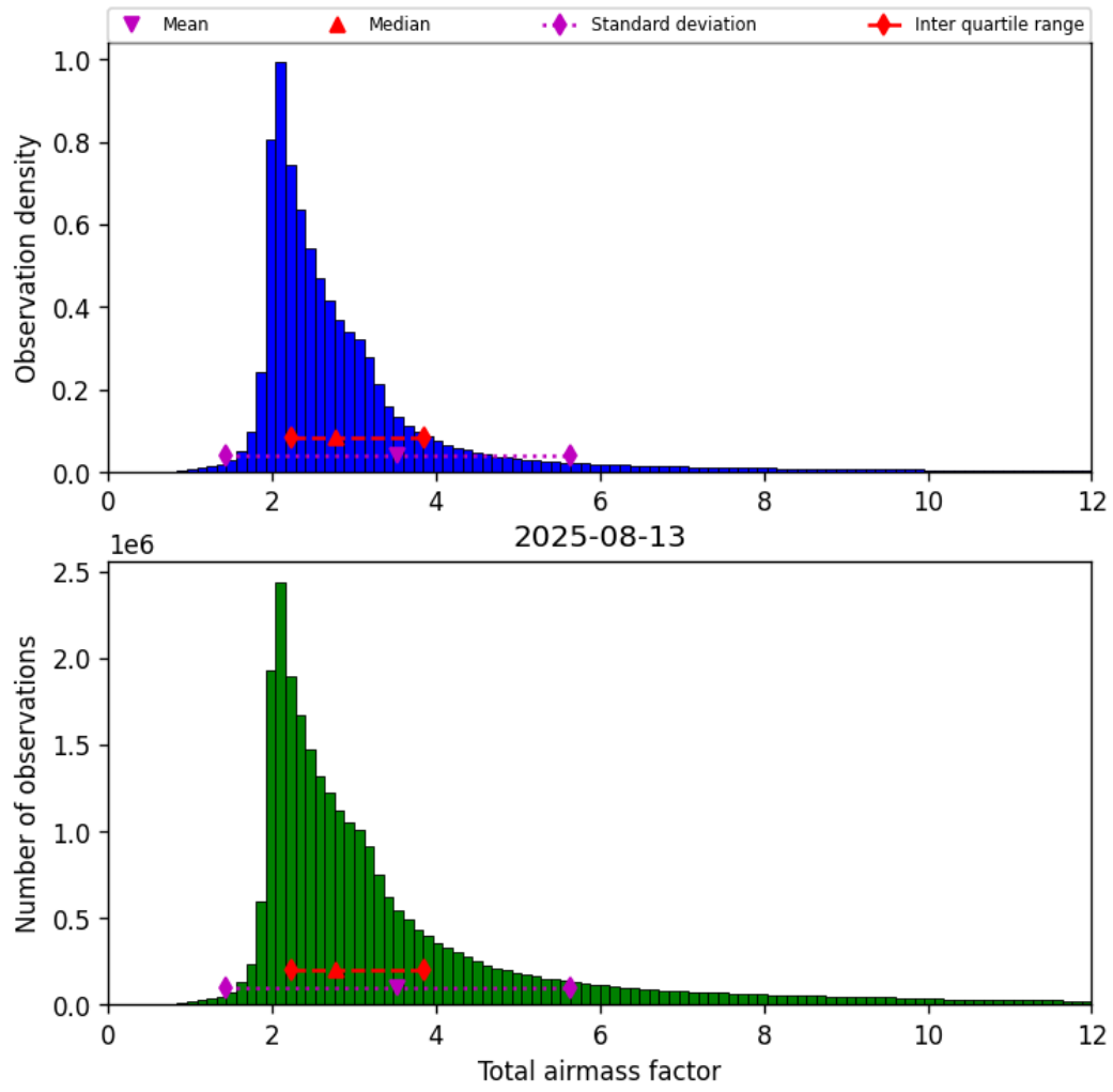
Figure 32: Histogram of “Total airmass factor” for 2025-08-12 to 2025-08-14
