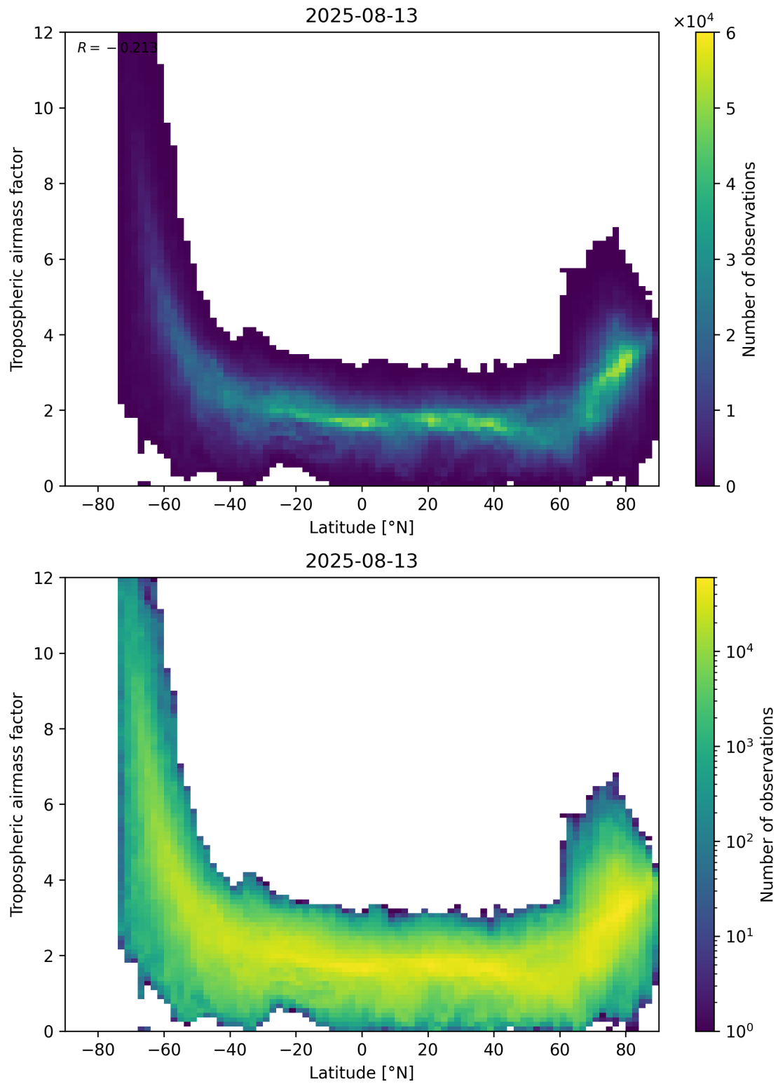
Figure 85: Scatter density plot of “Latitude” against “Tropospheric airmass factor” for 2025-08-12 to 2025-08-14.
