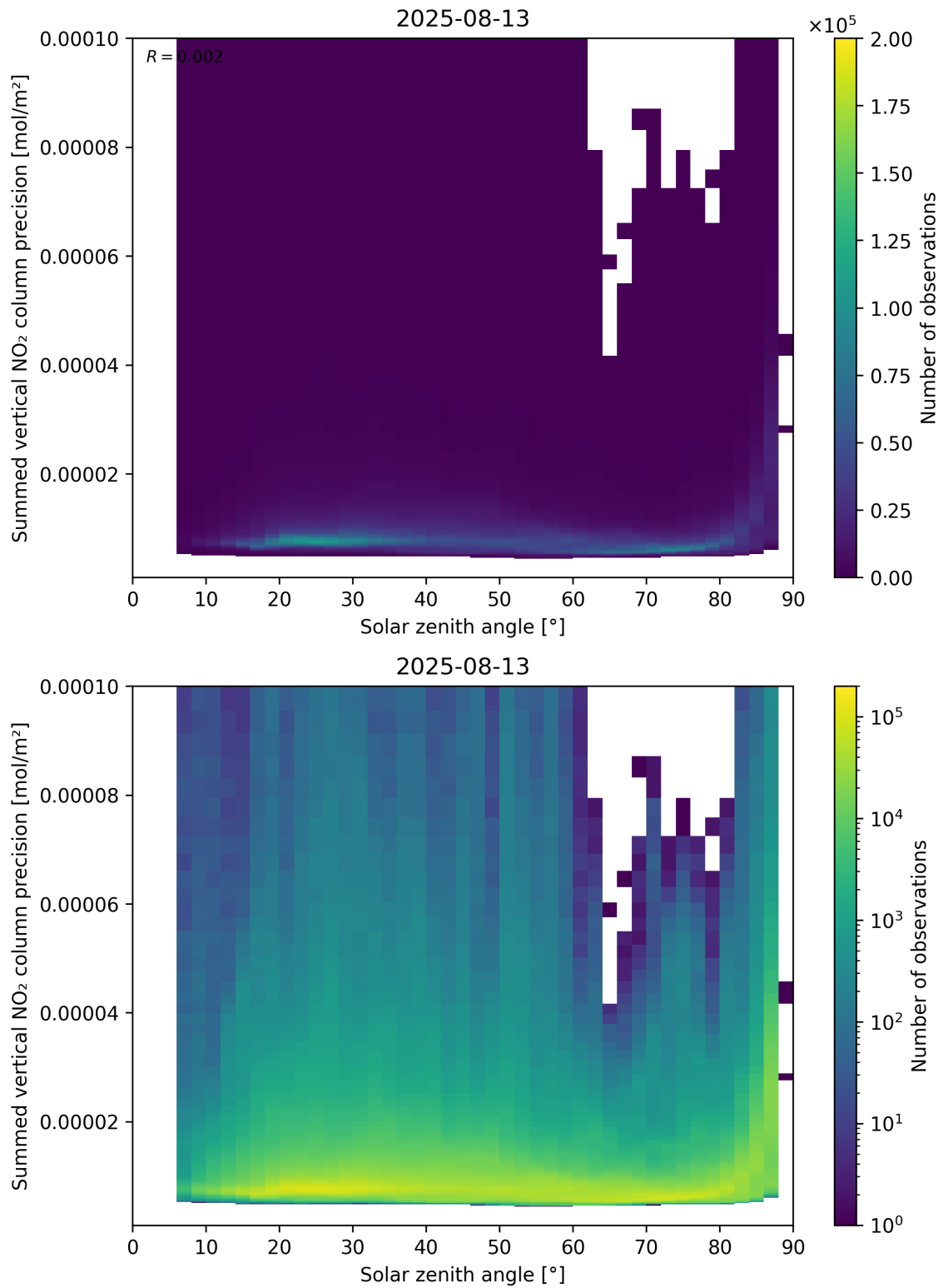
Figure 152: Scatter density plot of “Solar zenith angle” against “Summed vertical NO 2 column precision” for 2025-08-12 to 2025-08-14.
