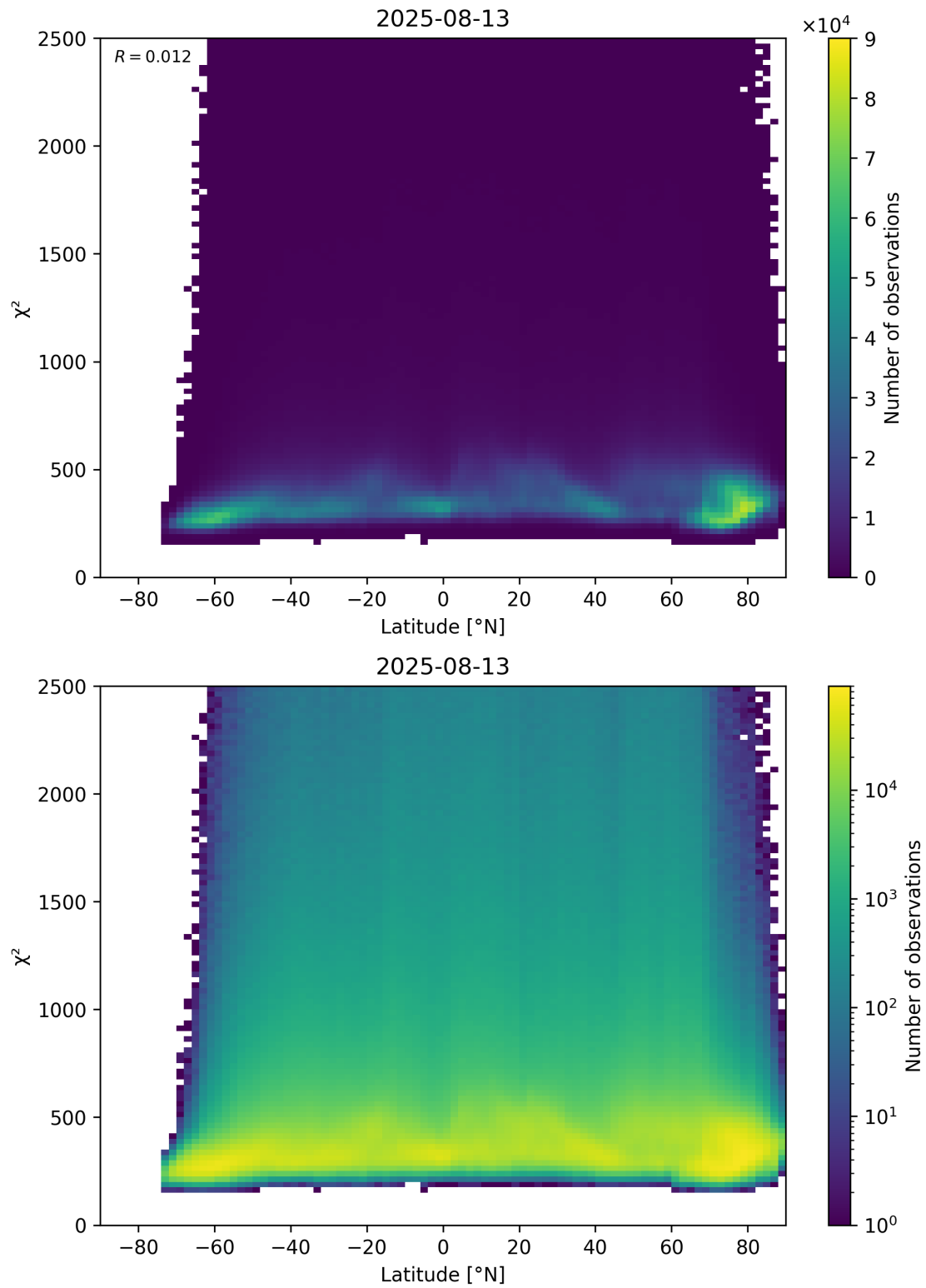
Figure 86: Scatter density plot of “Latitude” against “ \chi^2 ” for 2025-08-12 to 2025-08-14.
