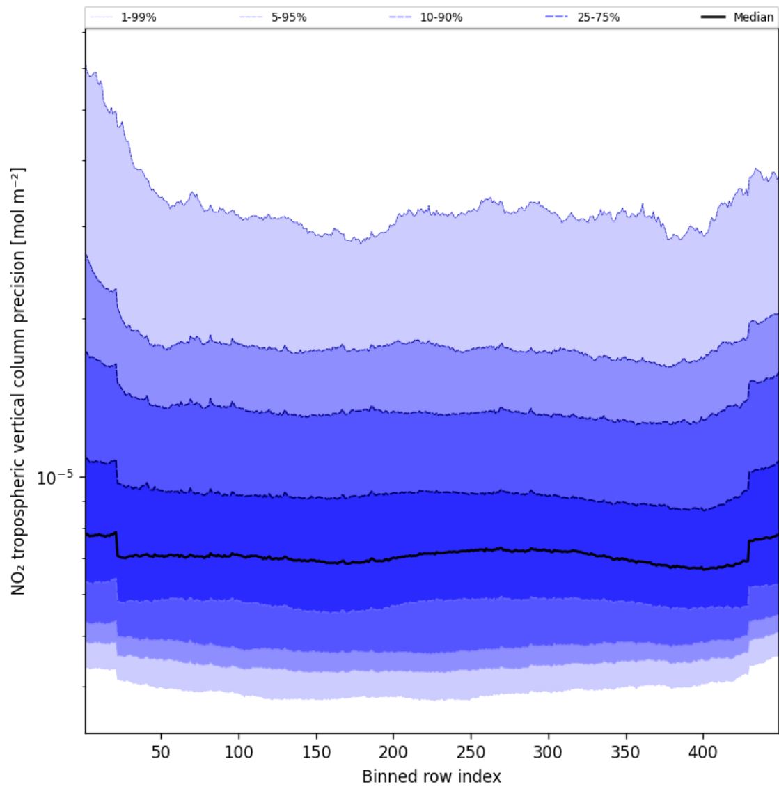
Figure 47: Along track statistics of “NO 2 tropospheric vertical column precision” for 2025-08-12 to 2025-08-14
