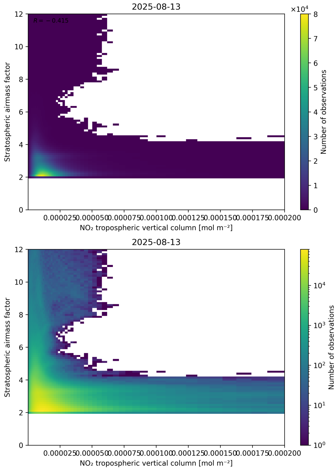
Figure 121: Scatter density plot of “NO 2 tropospheric vertical column” against “Stratospheric air mass factor” for 2025-08-12 to 2025-08-14.
