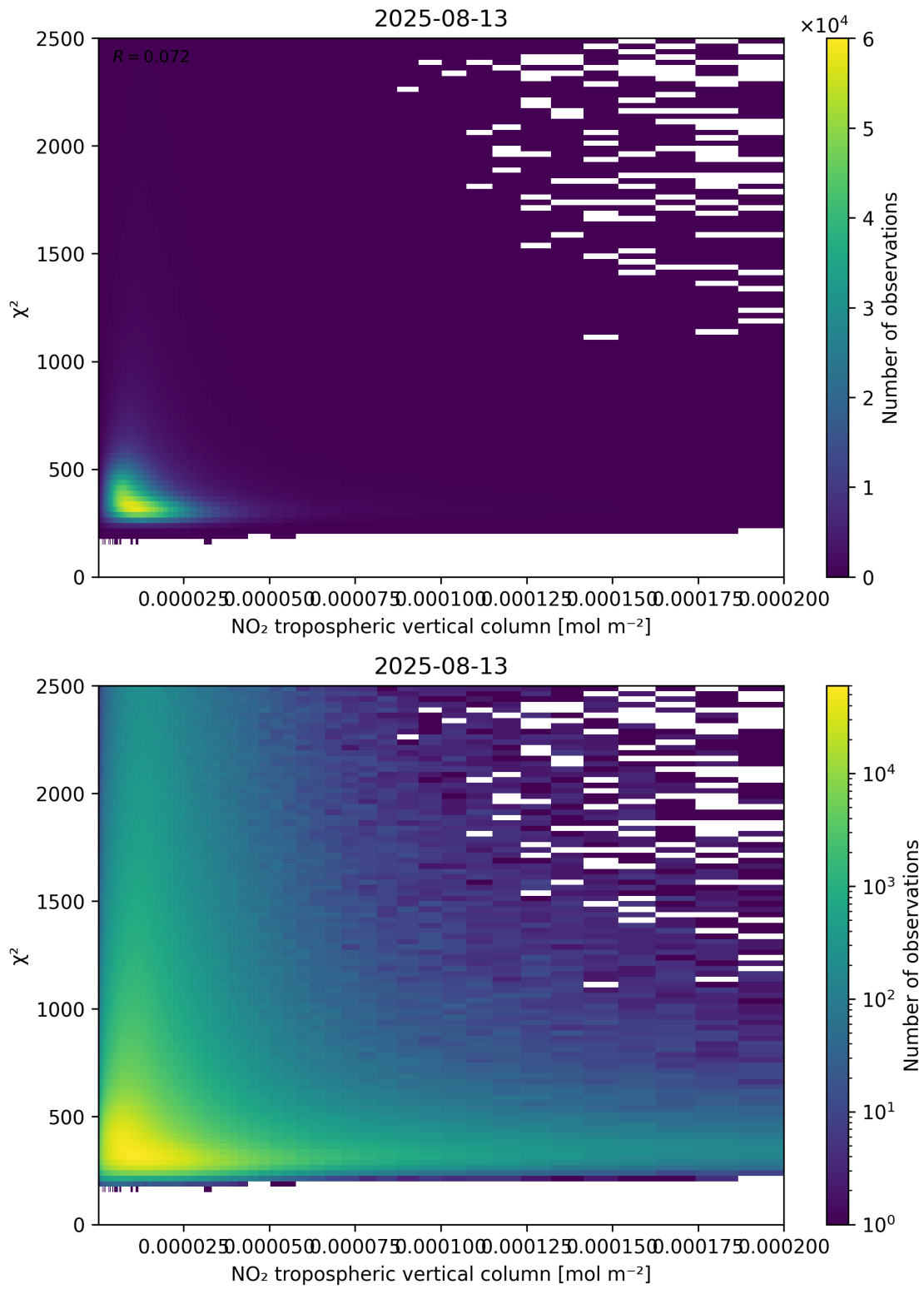
Figure 124: Scatter density plot of “NO 2 tropospheric vertical column” against “ \chi^2 ” for 2025-08-12 to 2025-08-14.
