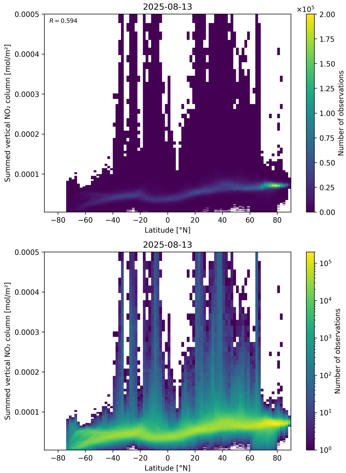
Figure 88: Scatter density plot of “Latitude” against “Summed vertical NO 2 column” for 2025-08-12 to 2025-08-14.
