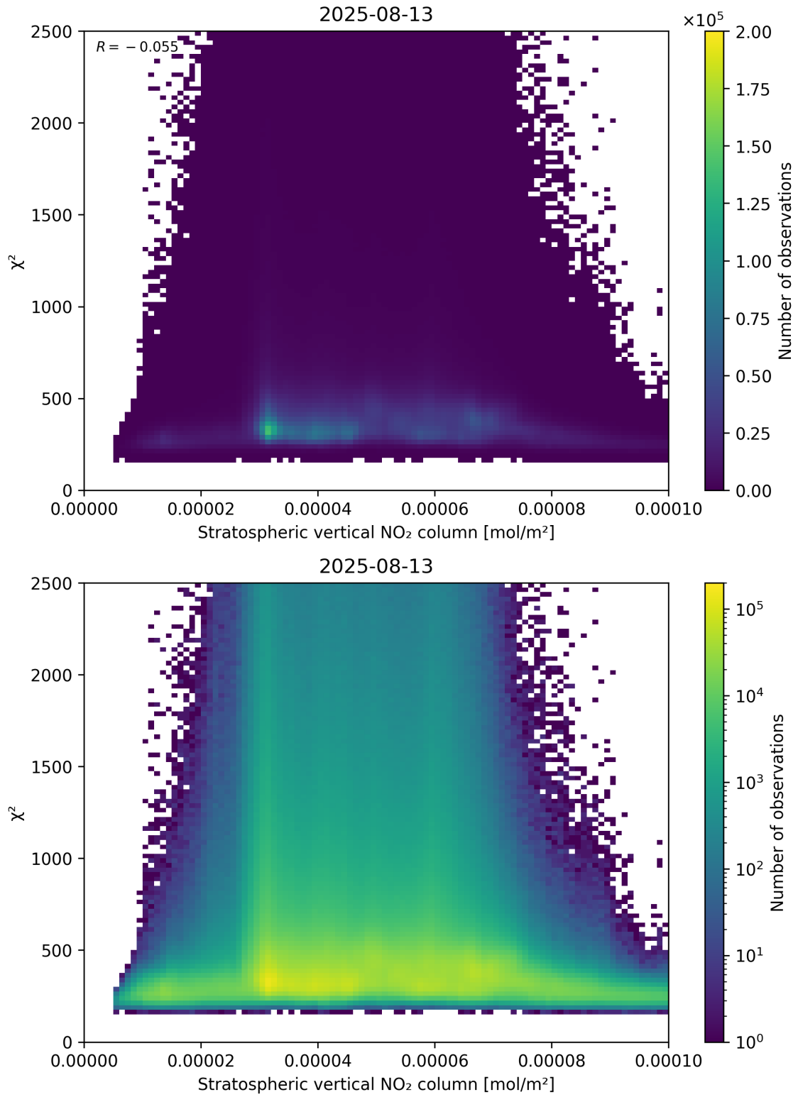
Figure 97: Scatter density plot of “Stratospheric vertical NO 2 column” against “ \chi^2 ” for 2025-08-12 to 2025-08-14.
