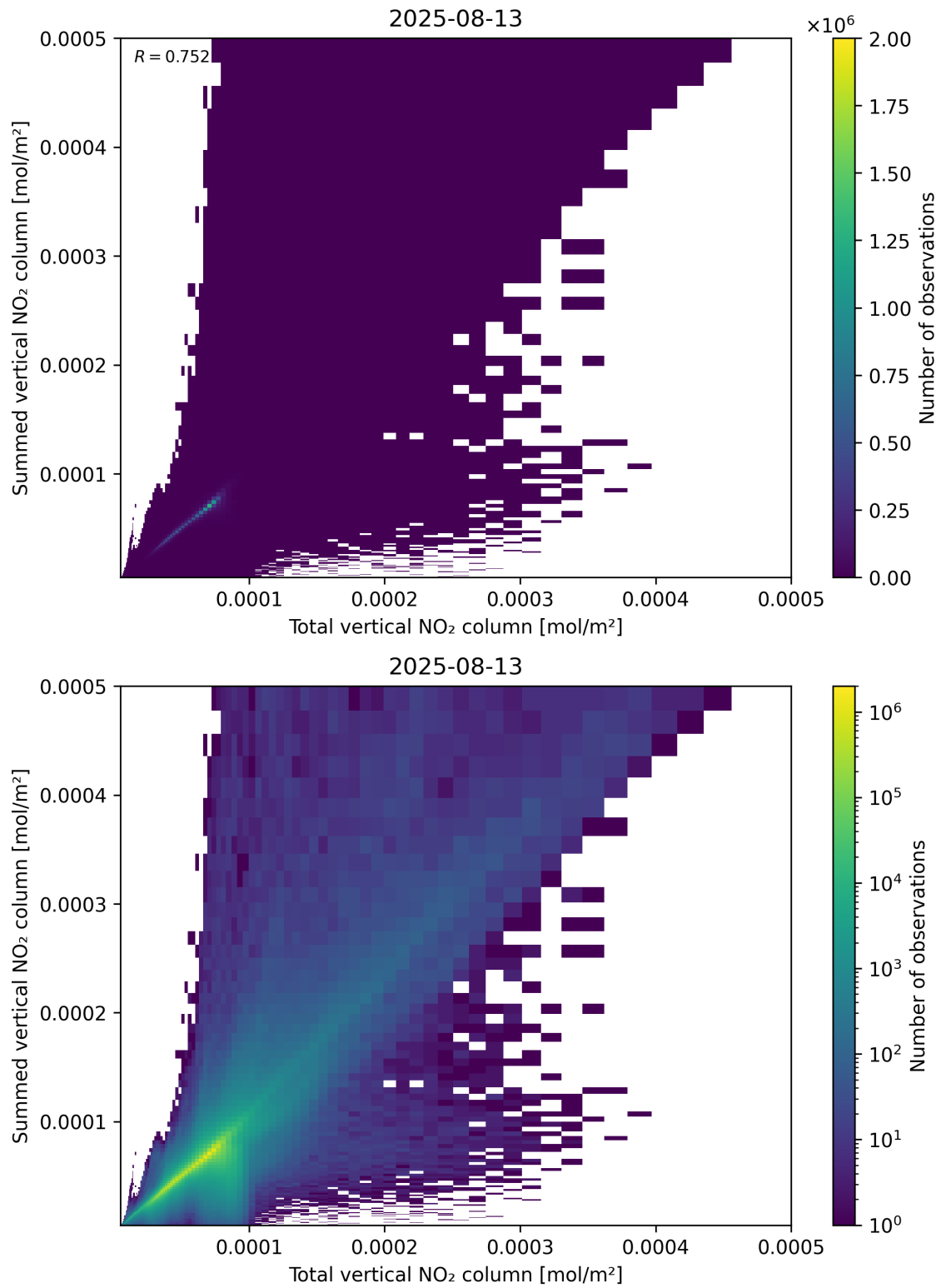
Figure 112: Scatter density plot of “Total vertical NO 2 column” against “Summed vertical NO 2 column” for 2025-08-12 to 2025-08-14.
