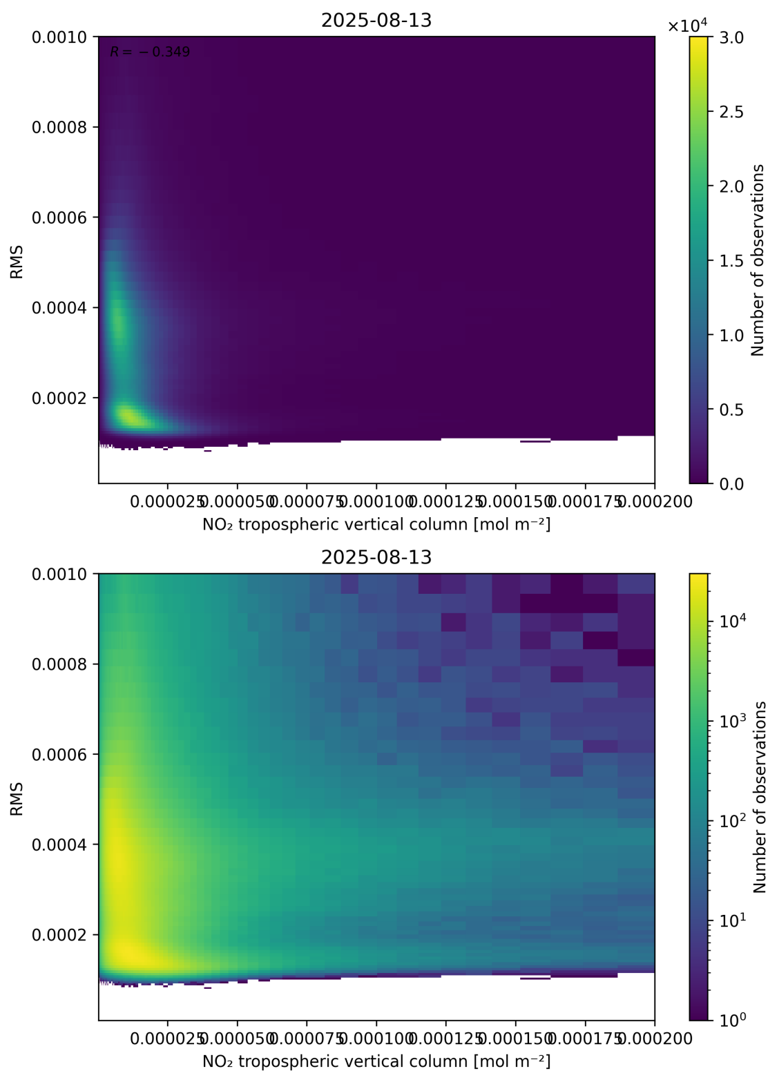
Figure 142: Scatter density plot of “NO 2 tropospheric vertical column” against “RMS” for 2025-08-12 to 2025-08-14.
