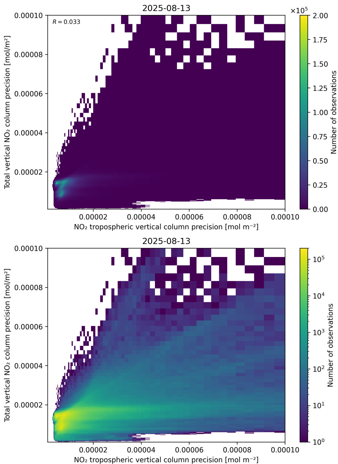
Figure 139: Scatter density plot of “NO 2 tropospheric vertical column precision” against “Total vertical NO 2 column precision” for 2025-08-12 to 2025-08-14.
