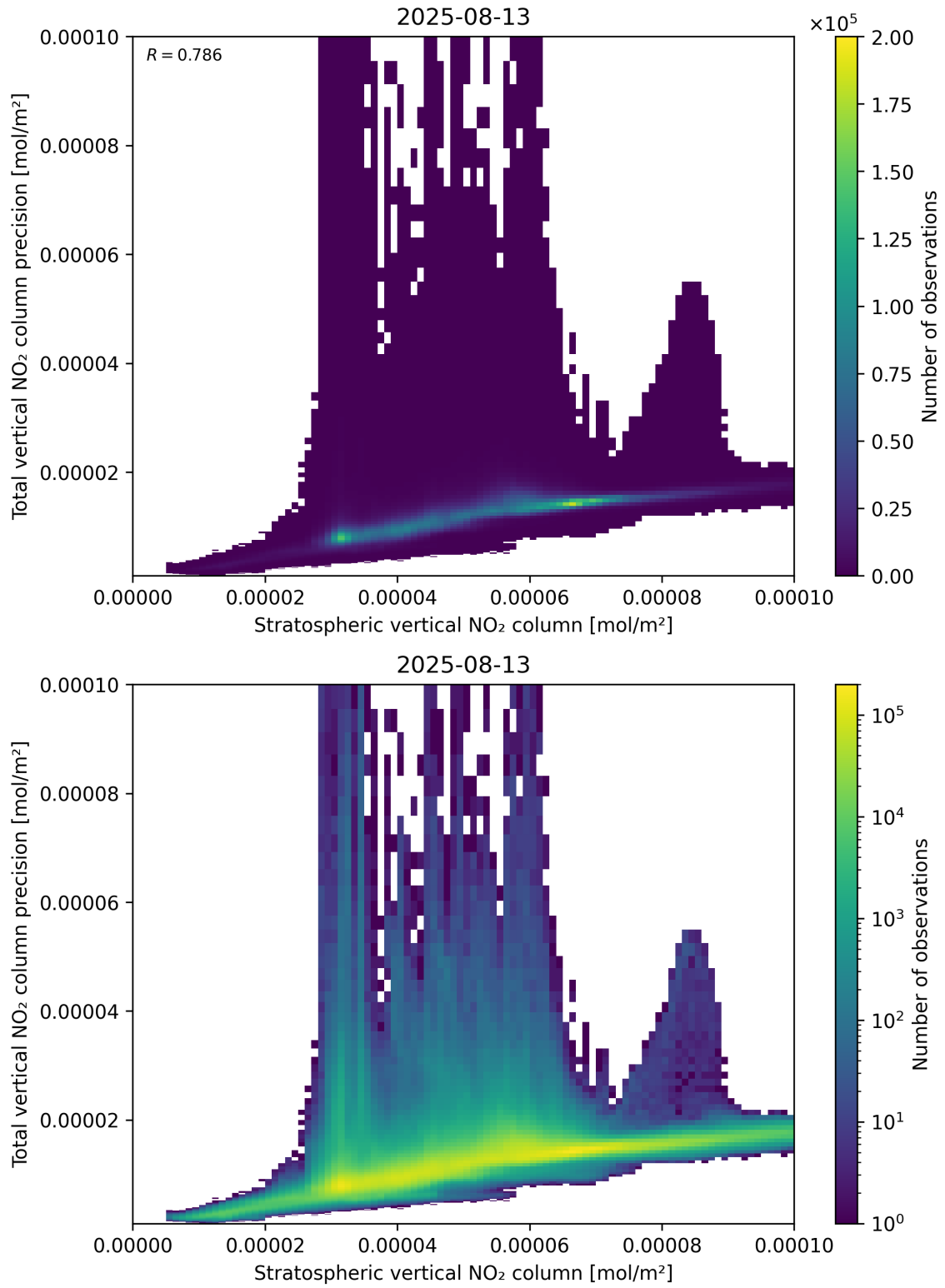
Figure 101: Scatter density plot of “Stratospheric vertical NO 2 column” against “Total vertical NO 2 column precision” for 2025-08-12 to 2025-08-14.
