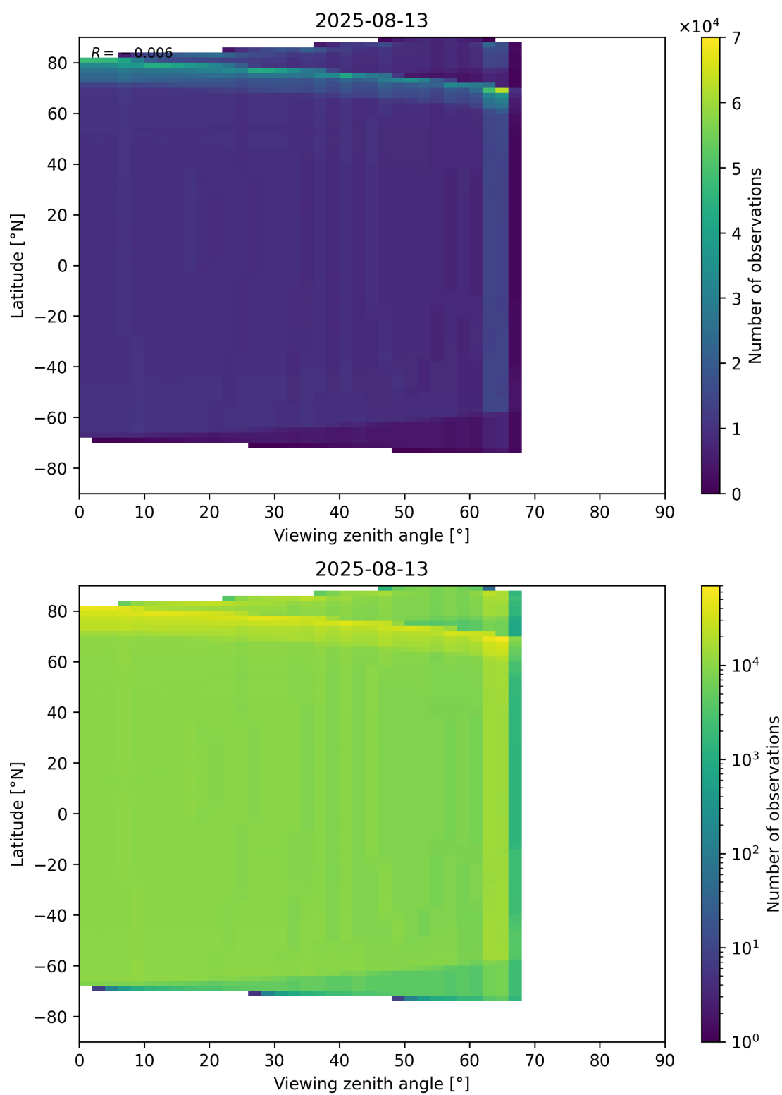
Figure 163: Scatter density plot of “Viewing zenith angle” against “Latitude” for 2025-08-12 to 2025-08-14.
