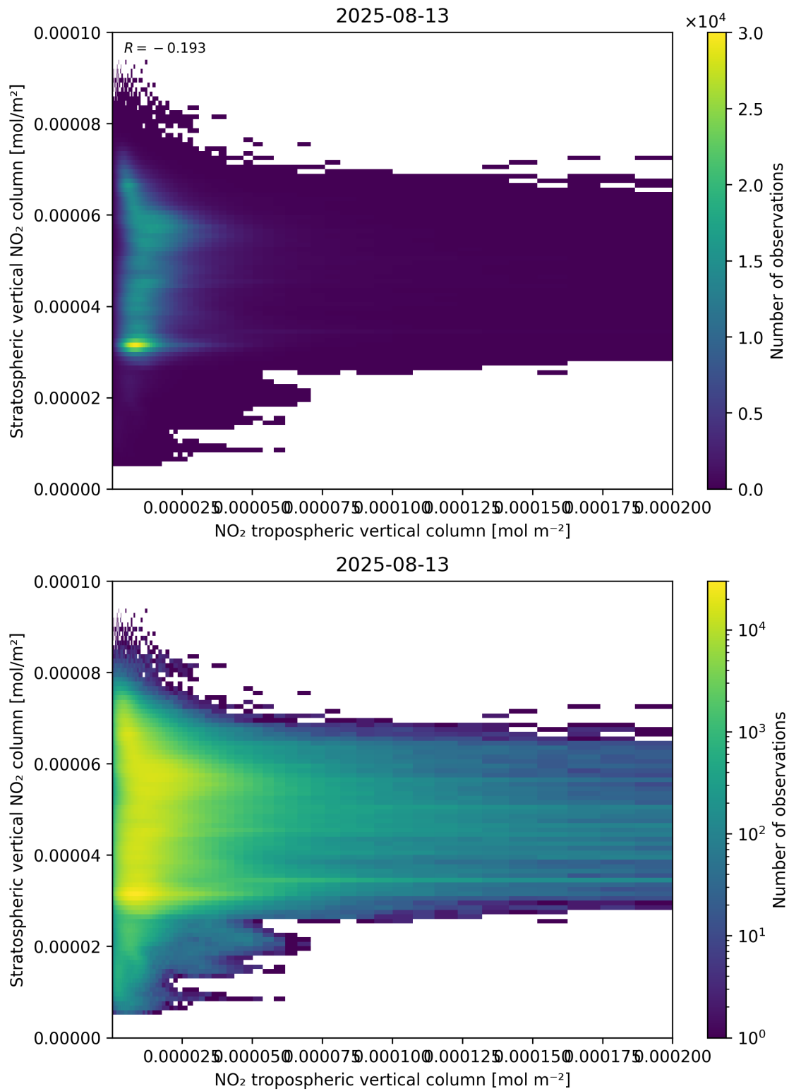
Figure 125: Scatter density plot of “NO 2 tropospheric vertical column” against “Stratospheric vertical NO 2 column” for 2025-08-12 to 2025-08-14.
