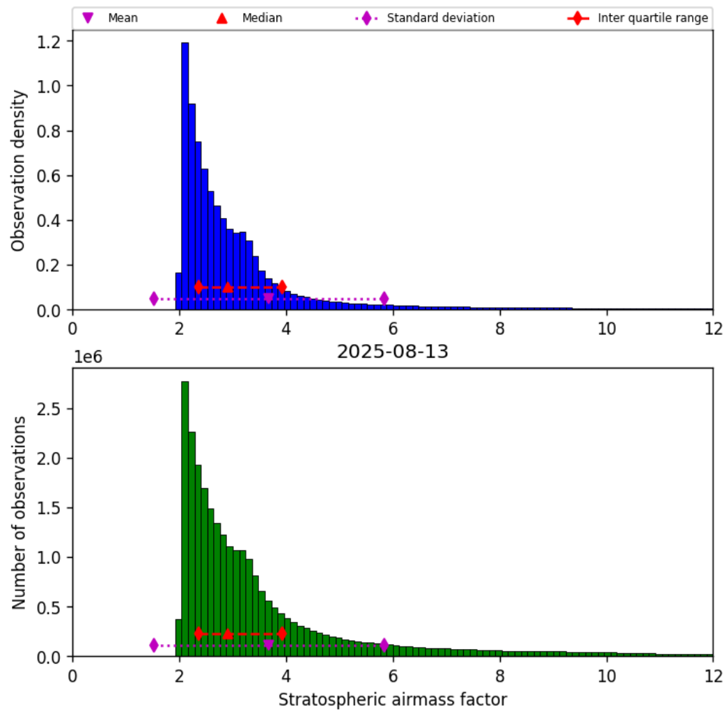
Figure 44: Histogram of “Stratospheric airmass factor” for 2025-08-12 to 2025-08-14
