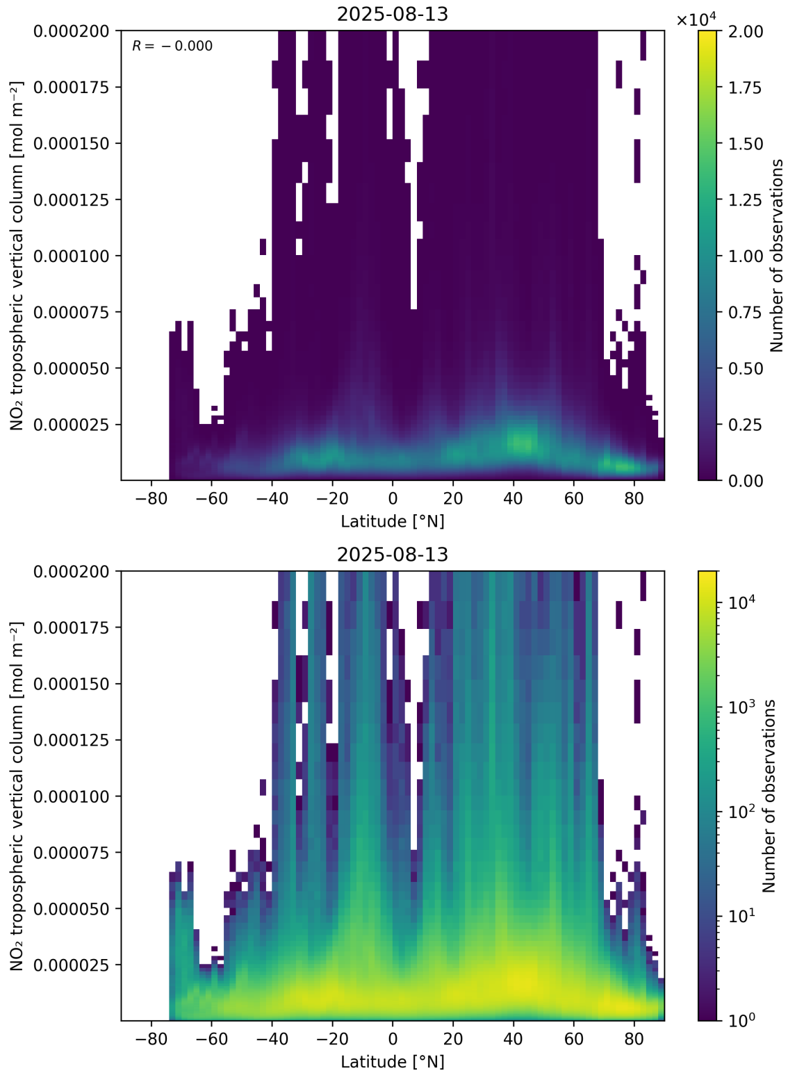
Figure 92: Scatter density plot of “Latitude” against “NO 2 tropospheric vertical column” for 2025-08-12 to 2025-08-14.
