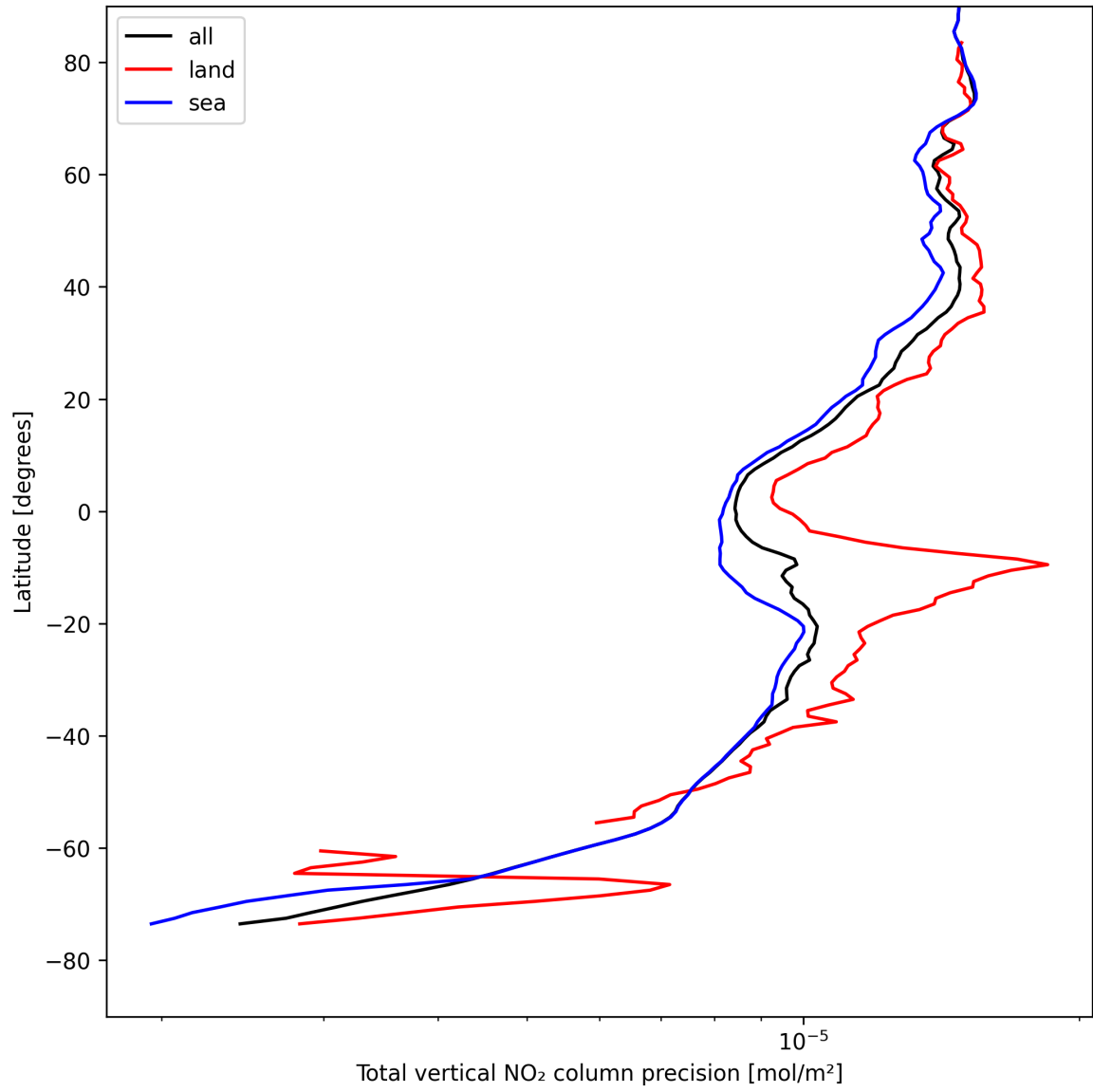
Figure 22: Zonal average of “Total vertical NO 2 column precision” for 2025-08-12 to 2025-08-14.
