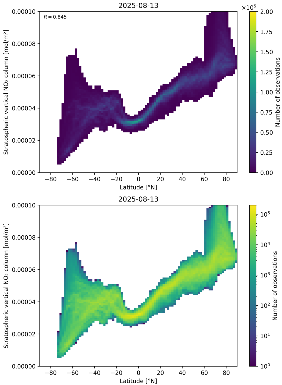
Figure 87: Scatter density plot of “Latitude” against “Stratospheric vertical NO 2 column” for 2025-08-12 to 2025-08-14.
