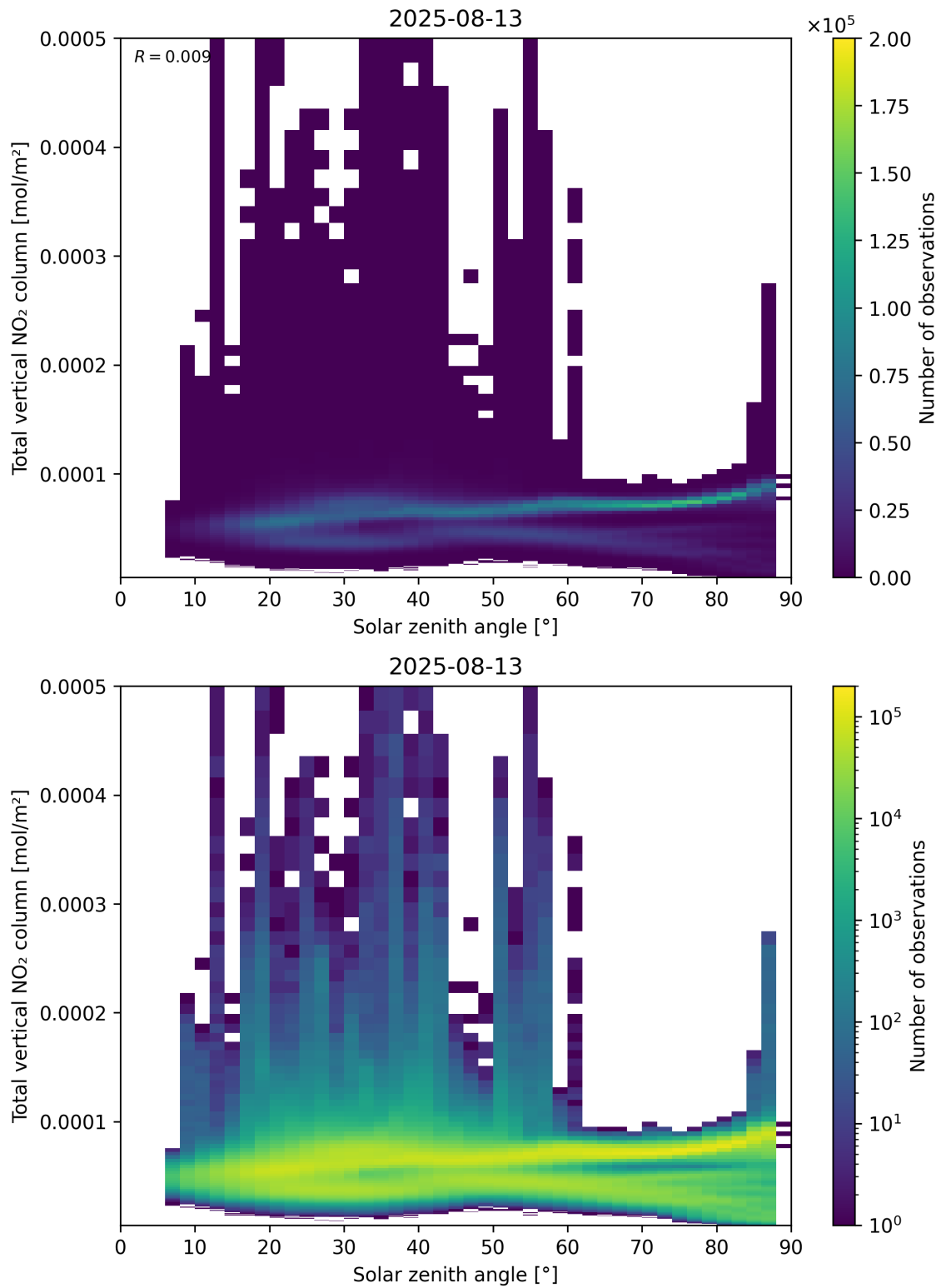
Figure 153: Scatter density plot of “Solar zenith angle” against “Total vertical NO 2 column” for 2025-08-12 to 2025-08-14.
