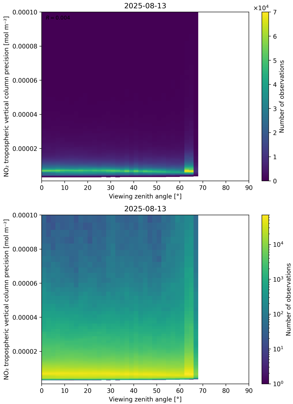
Figure 170: Scatter density plot of “Viewing zenith angle” against “NO 2 tropospheric vertical column precision” for 2025-08-12 to 2025-08-14.
