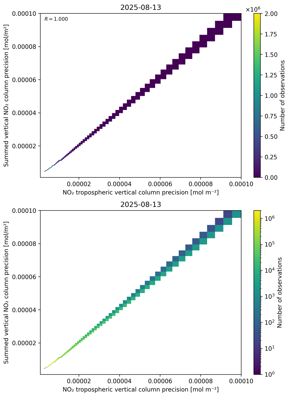
Figure 137: Scatter density plot of “NO 2 tropospheric vertical column precision” against “Summed vertical NO 2 column precision” for 2025-08-12 to 2025-08-14.
