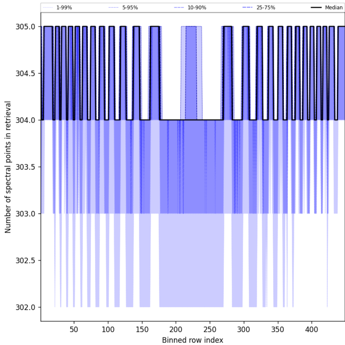
Figure 50: Along track statistics of “Number of spectral points in retrieval” for 2025-08-12 to 2025-08-14
