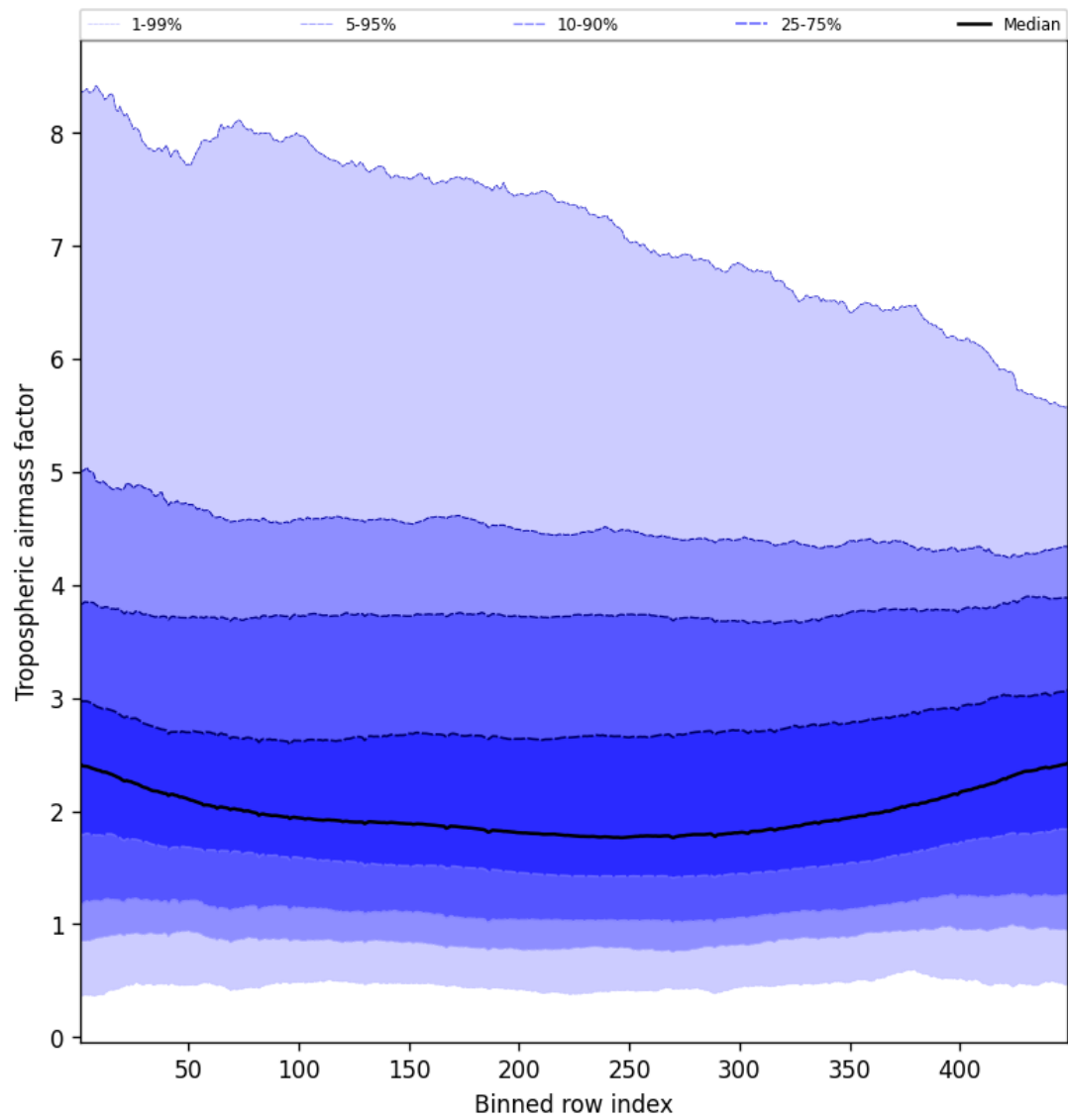
Figure 48: Along track statistics of “Tropospheric air mass factor” for 2025-08-12 to 2025-08-14
