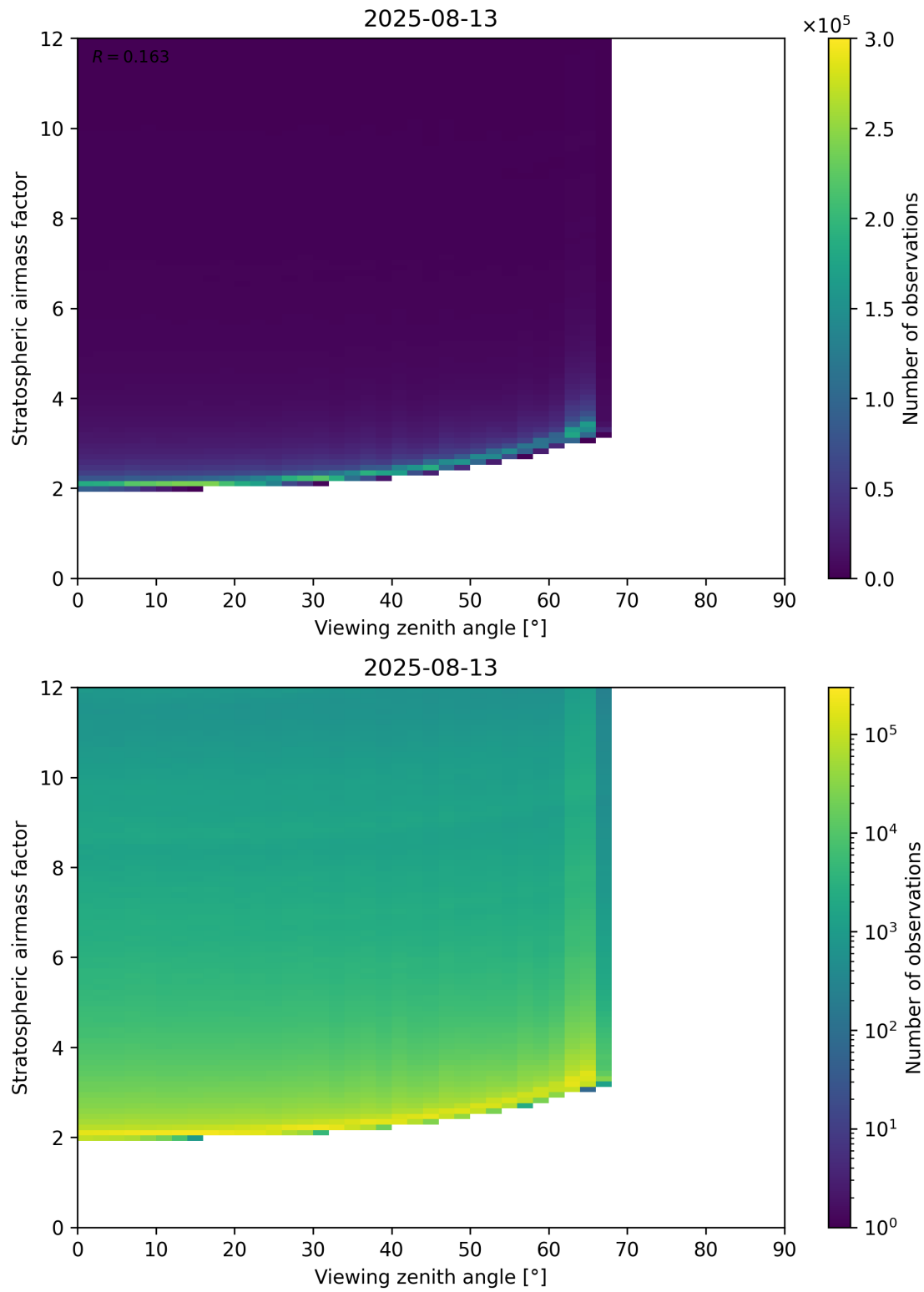
Figure 159: Scatter density plot of “Viewing zenith angle” against “Stratospheric airmass factor” for 2025-08-12 to 2025-08-14.
