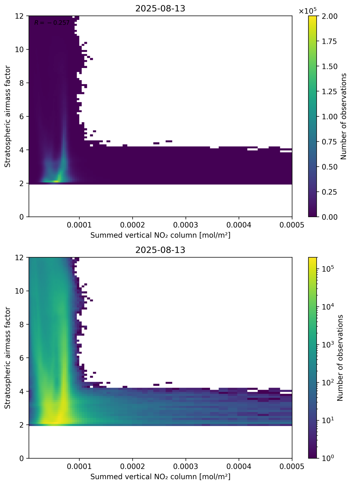
Figure 103: Scatter density plot of “Summed vertical NO 2 column” against “Stratospheric air mass factor” for 2025-08-12 to 2025-08-14.
