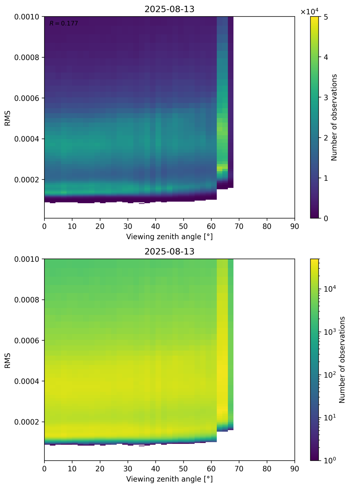
Figure 171: Scatter density plot of “Viewing zenith angle” against “RMS” for 2025-08-12 to 2025-08-14.
