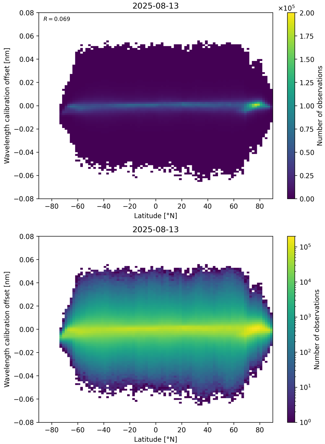
Figure 95: Scatter density plot of “Latitude” against “Wavelength calibration offset” for 2025-08-12 to 2025-08-14.
