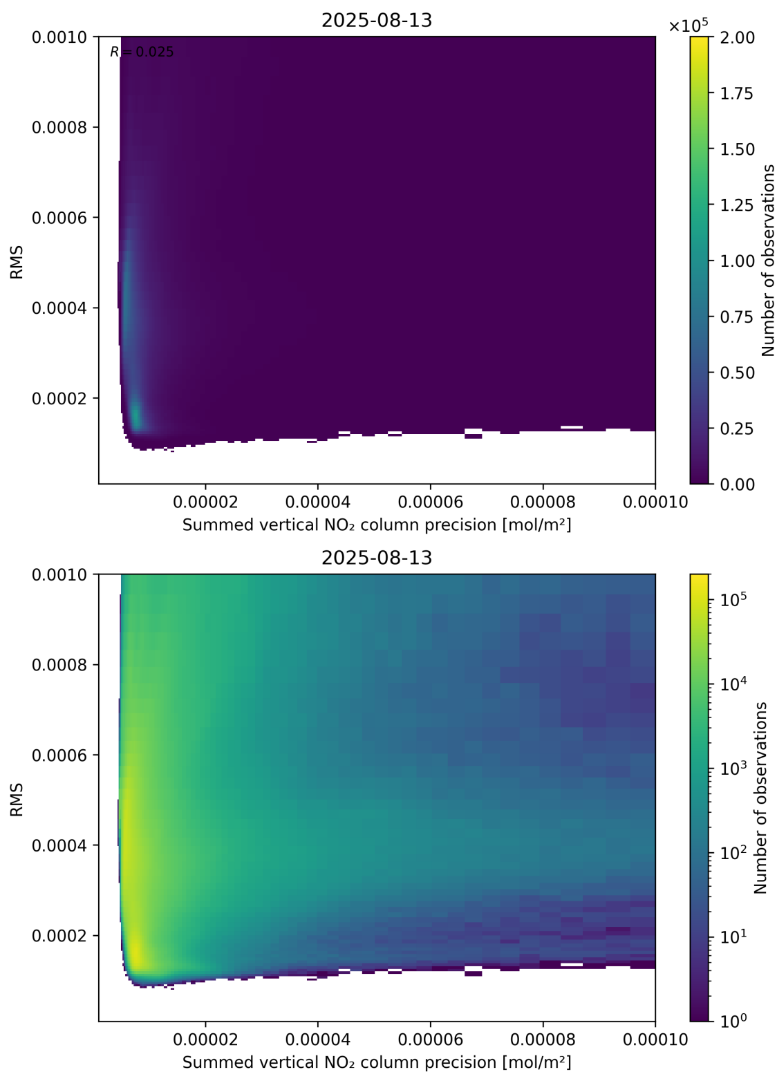
Figure 108: Scatter density plot of “Summed vertical NO 2 column precision” against “RMS” for 2025-08-12 to 2025-08-14.
