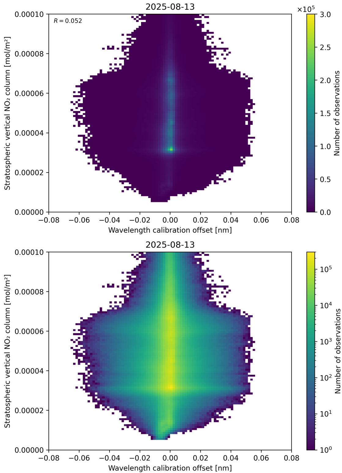
Figure 176: Scatter density plot of “Wavelength calibration offset” against “Stratospheric vertical NO 2 column” for 2025-08-12 to 2025-08-14.
