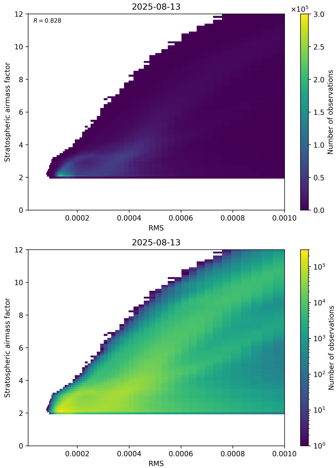
Figure 144: Scatter density plot of “RMS” against “Stratospheric airmass factor” for 2025-08-12 to 2025-08-14.
