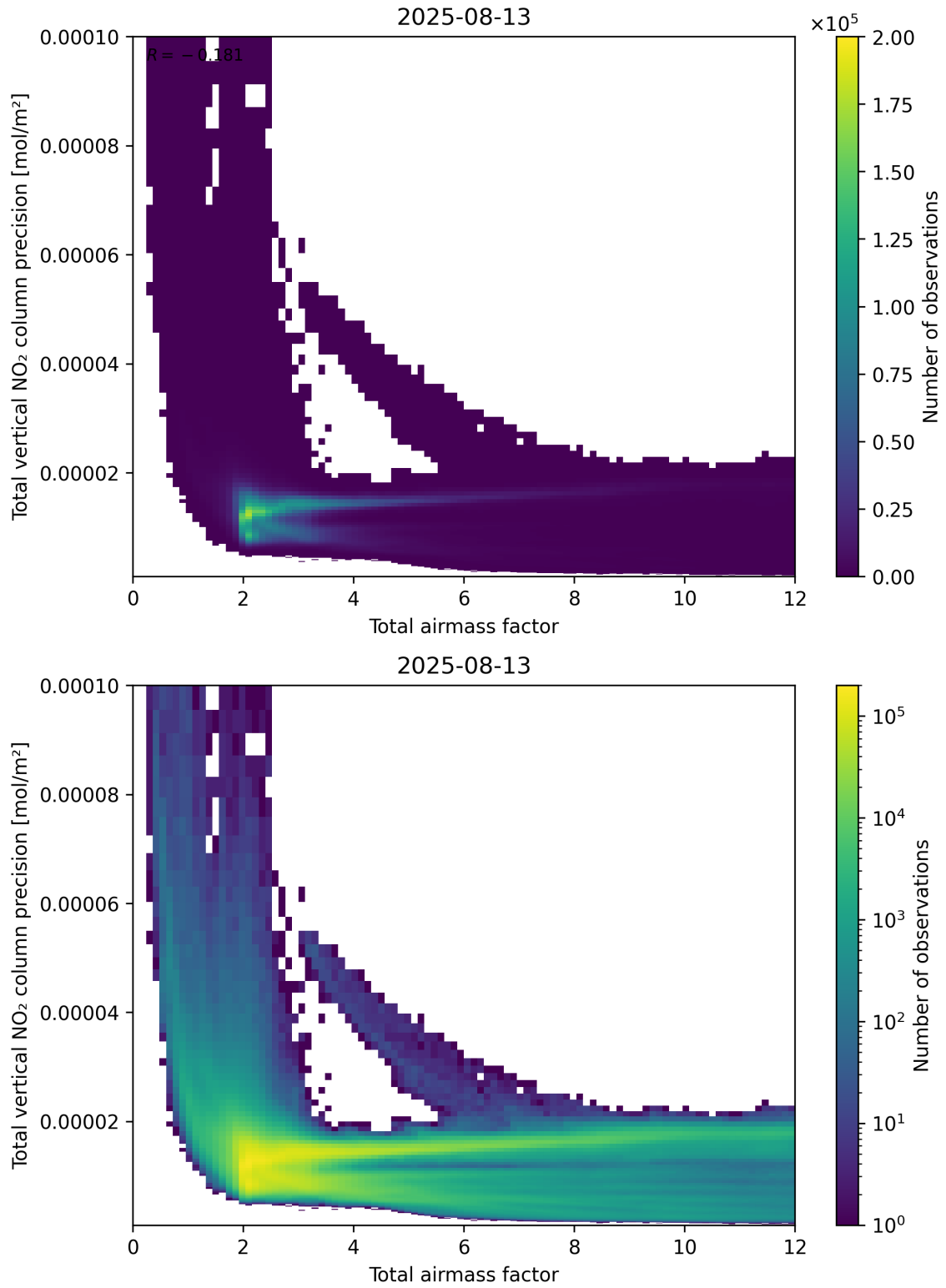
Figure 68: Scatter density plot of “Total airmass factor” against “Total vertical NO 2 column precision” for 2025-08-12 to 2025-08-14.
