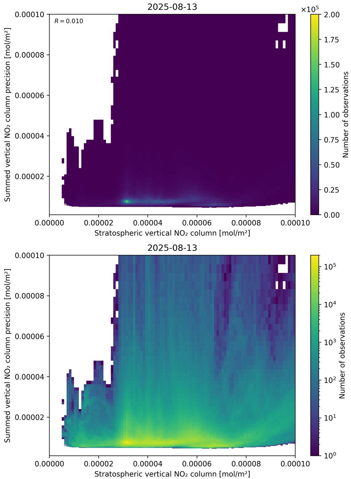
Figure 99: Scatter density plot of “Stratospheric vertical NO 2 column” against “Summed vertical NO 2 column precision” for 2025-08-12 to 2025-08-14.
