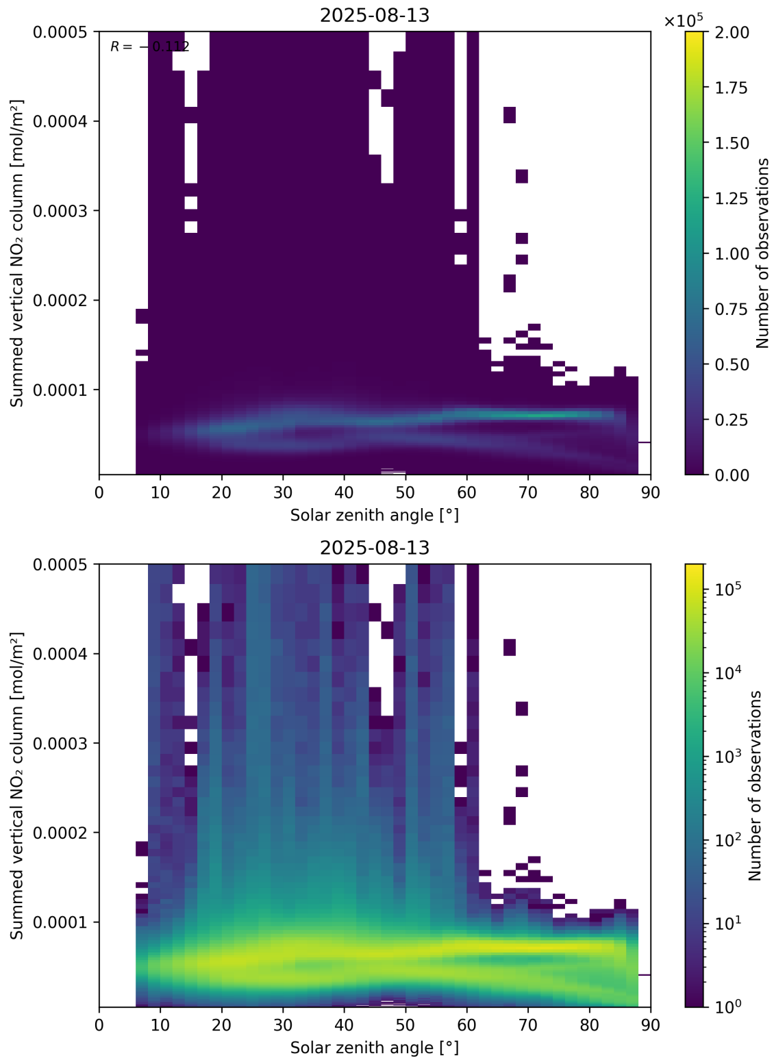
Figure 151: Scatter density plot of “Solar zenith angle” against “Summed vertical NO 2 column” for 2025-08-12 to 2025-08-14.
