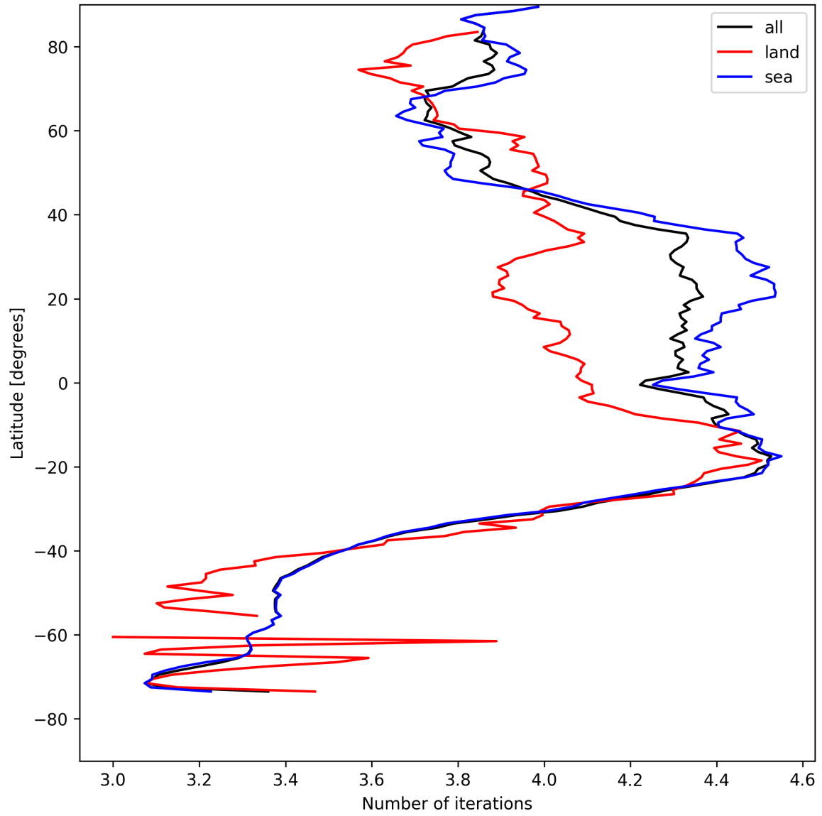
Figure 17: Zonal average of “Number of iterations” for 2025-08-12 to 2025-08-14.
