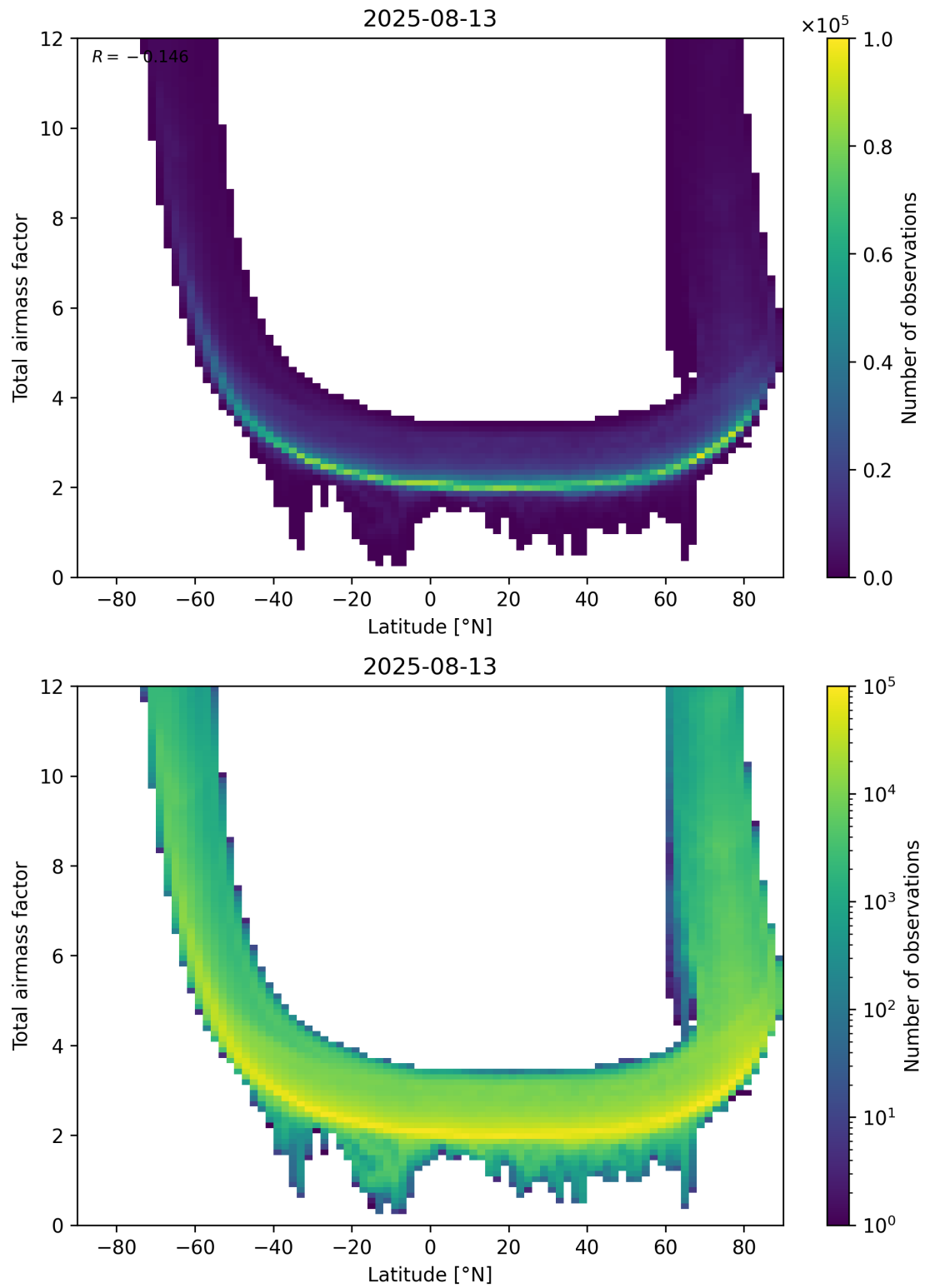
Figure 84: Scatter density plot of “Latitude” against “Total airmass factor” for 2025-08-12 to 2025-08-14.
