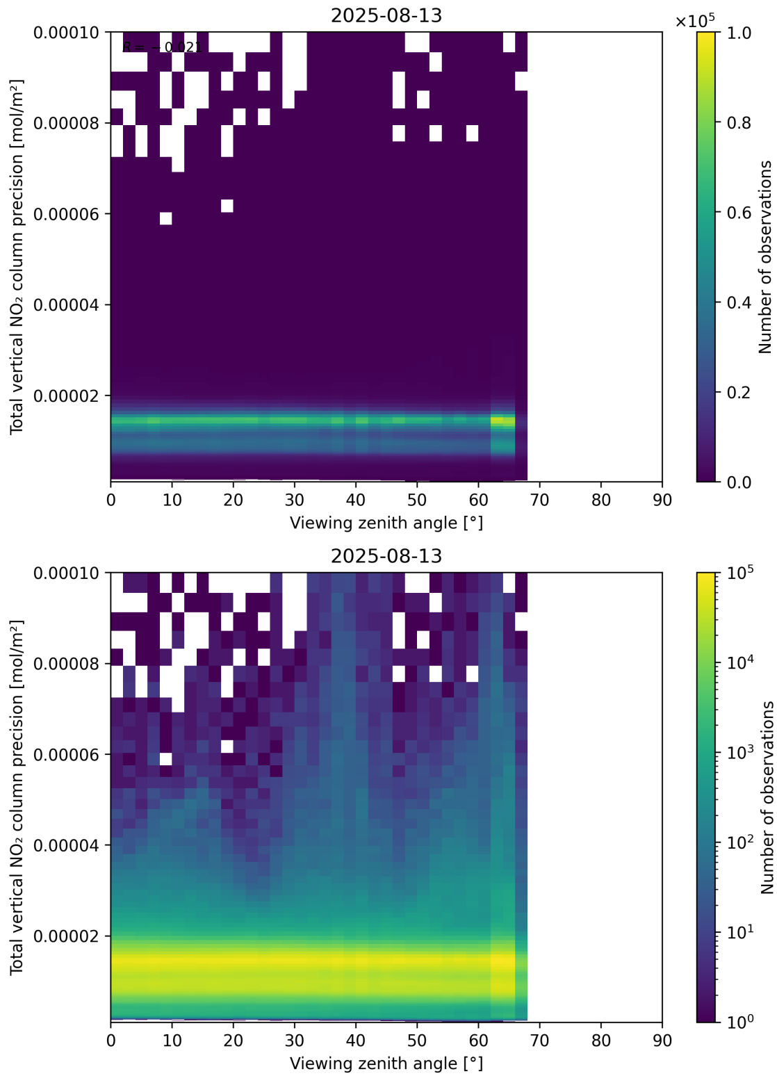
Figure 168: Scatter density plot of “Viewing zenith angle” against “Total vertical NO 2 column precision” for 2025-08-12 to 2025-08-14.
