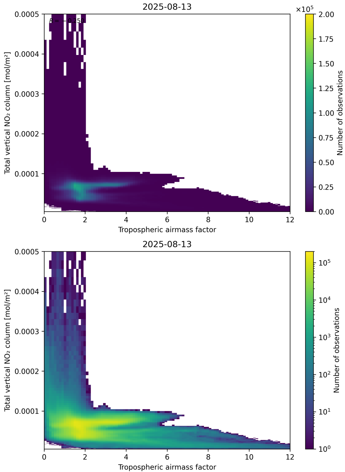
Figure 77: Scatter density plot of “Tropospheric airmass factor” against “Total vertical NO 2 column” for 2025-08-12 to 2025-08-14.
