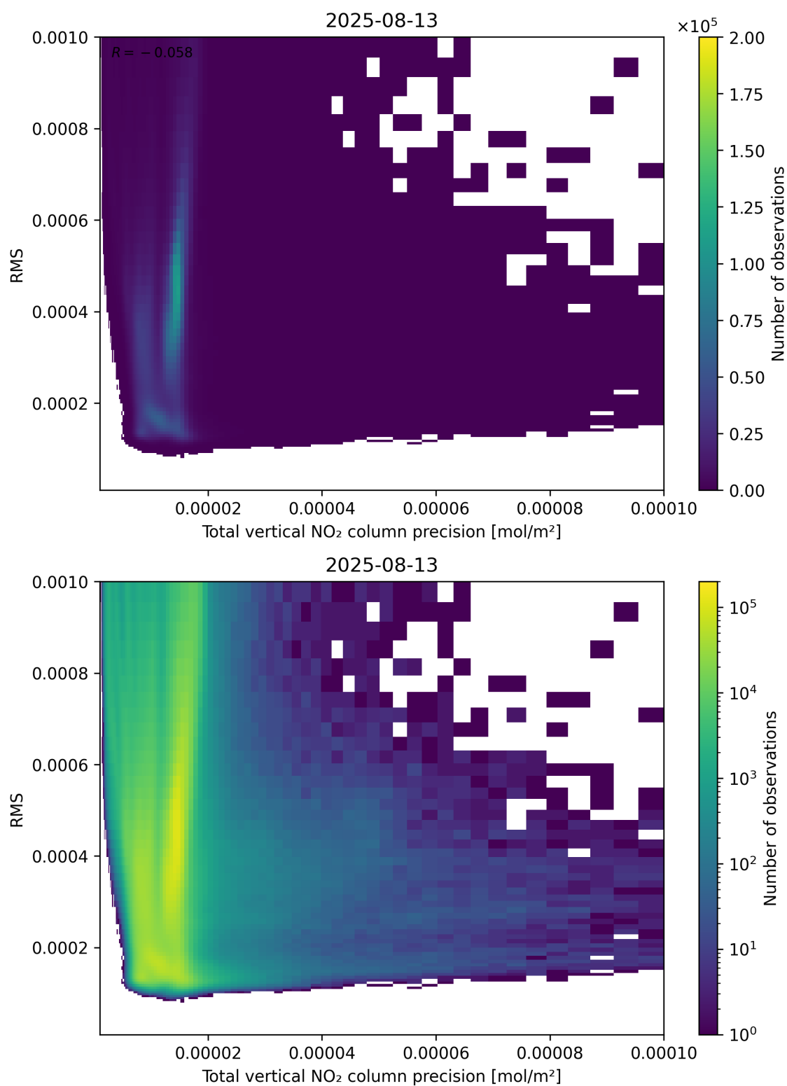
Figure 119: Scatter density plot of “Total vertical NO 2 column precision” against “RMS” for 2025-08-12 to 2025-08-14.
