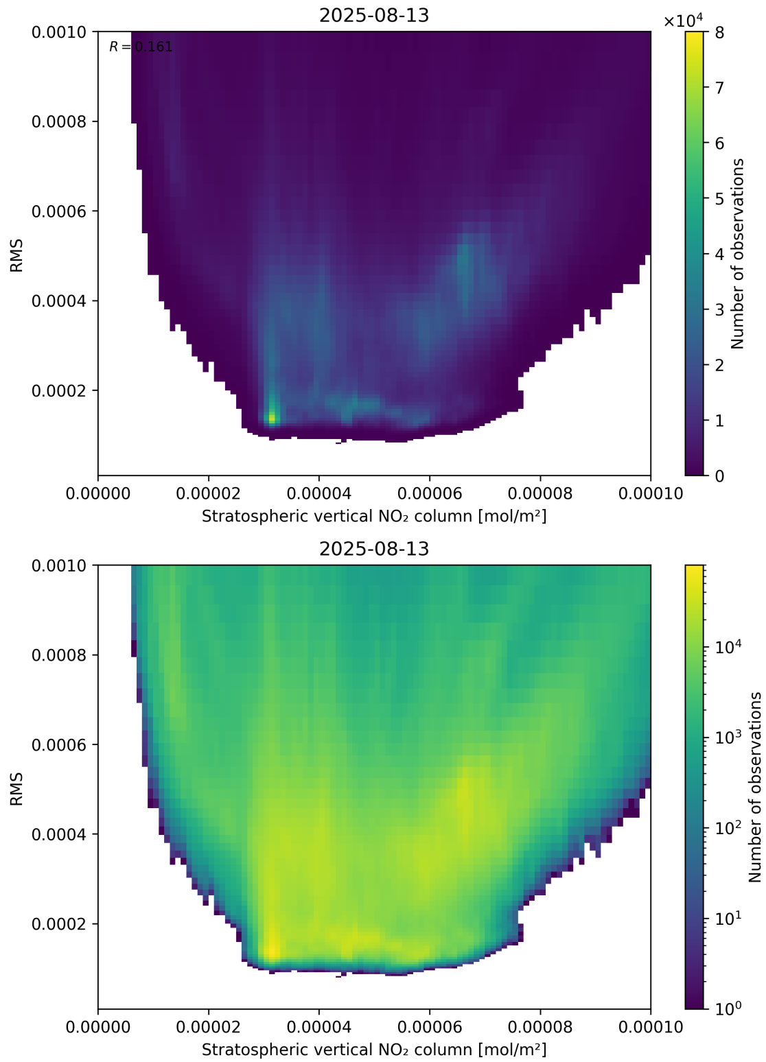
Figure 102: Scatter density plot of “Stratospheric vertical NO 2 column” against “RMS” for 2025-08-12 to 2025-08-14.
