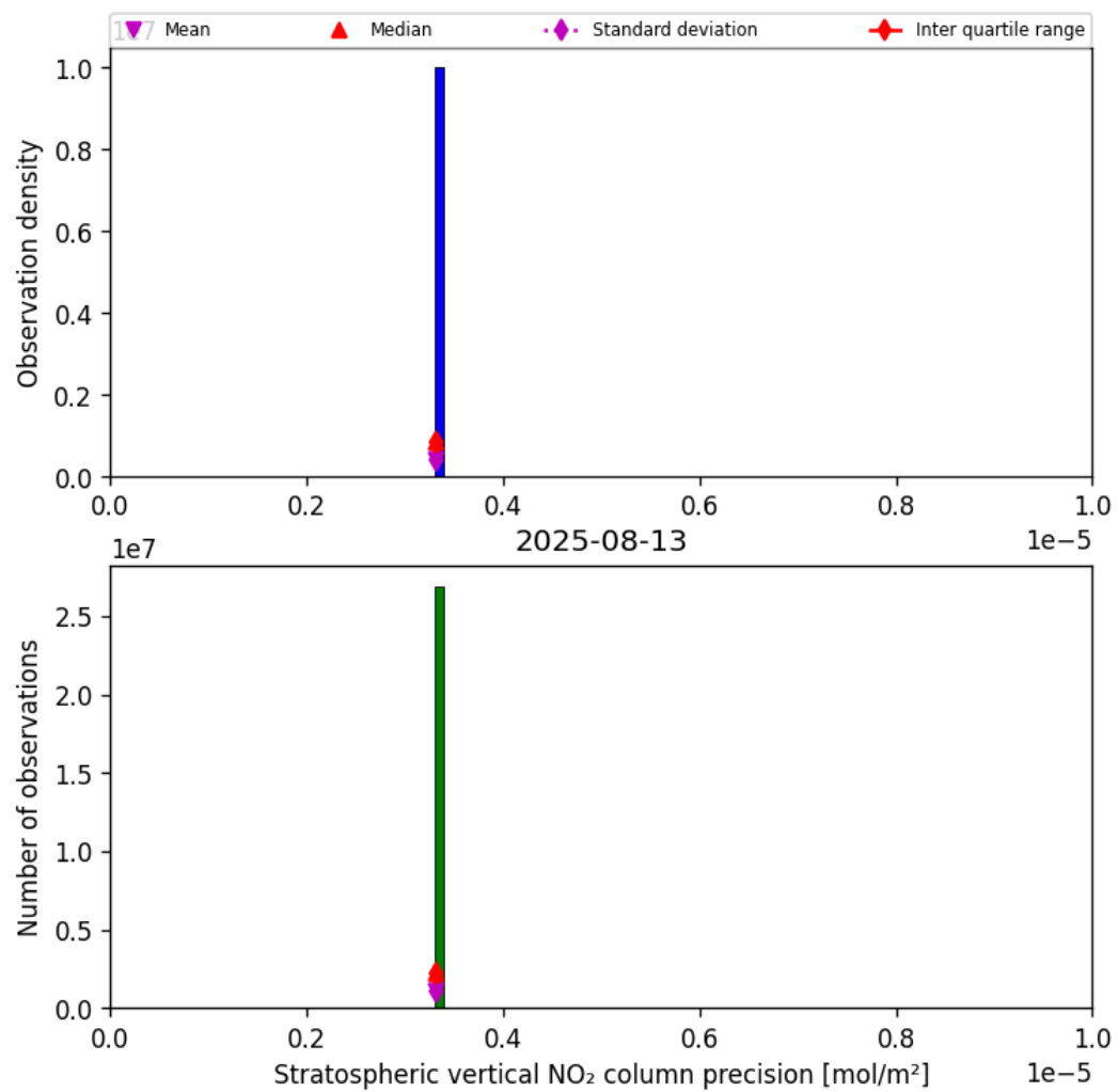
Figure 37: Histogram of “Stratospheric vertical NO 2 column precision” for 2025-08-12 to 2025-08-14
