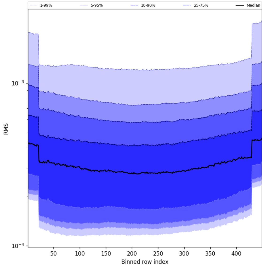
Figure 60: Along track statistics of “RMS” for 2025-08-12 to 2025-08-14
