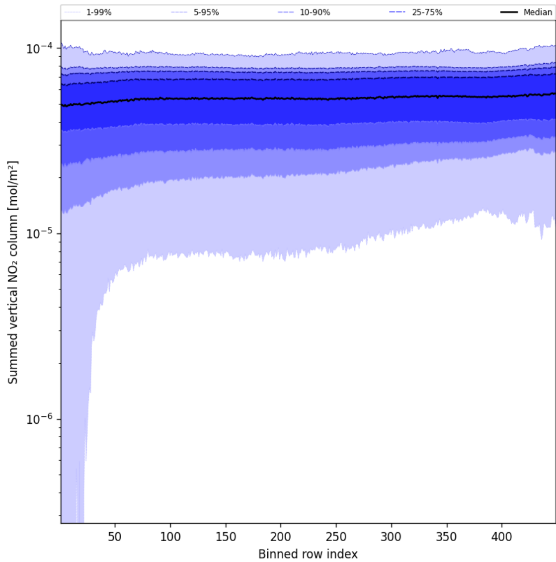
Figure 57: Along track statistics of “Summed vertical NO 2 column” for 2025-08-12 to 2025-08-14
