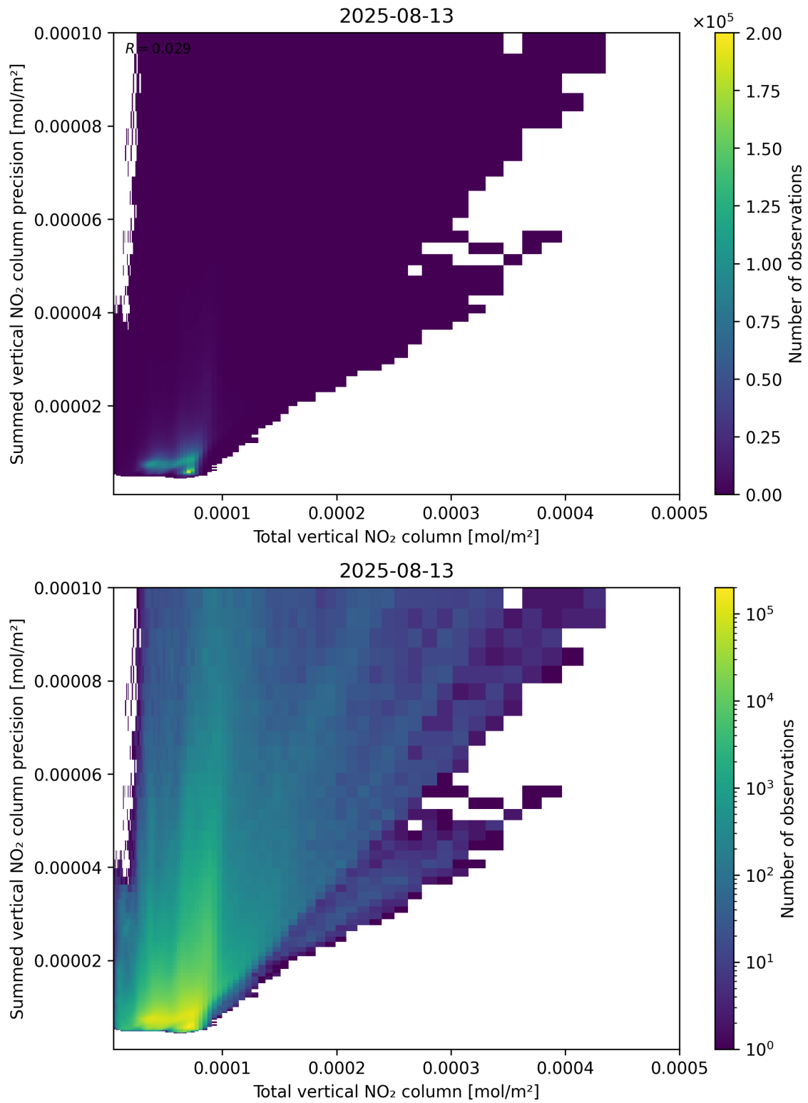
Figure 113: Scatter density plot of “Total vertical NO 2 column” against “Summed vertical NO 2 column precision” for 2025-08-12 to 2025-08-14.
