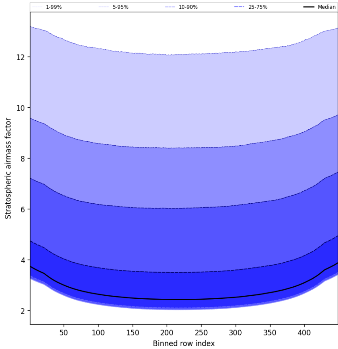
Figure 61: Along track statistics of “Stratospheric airmass factor” for 2025-08-12 to 2025-08-14
