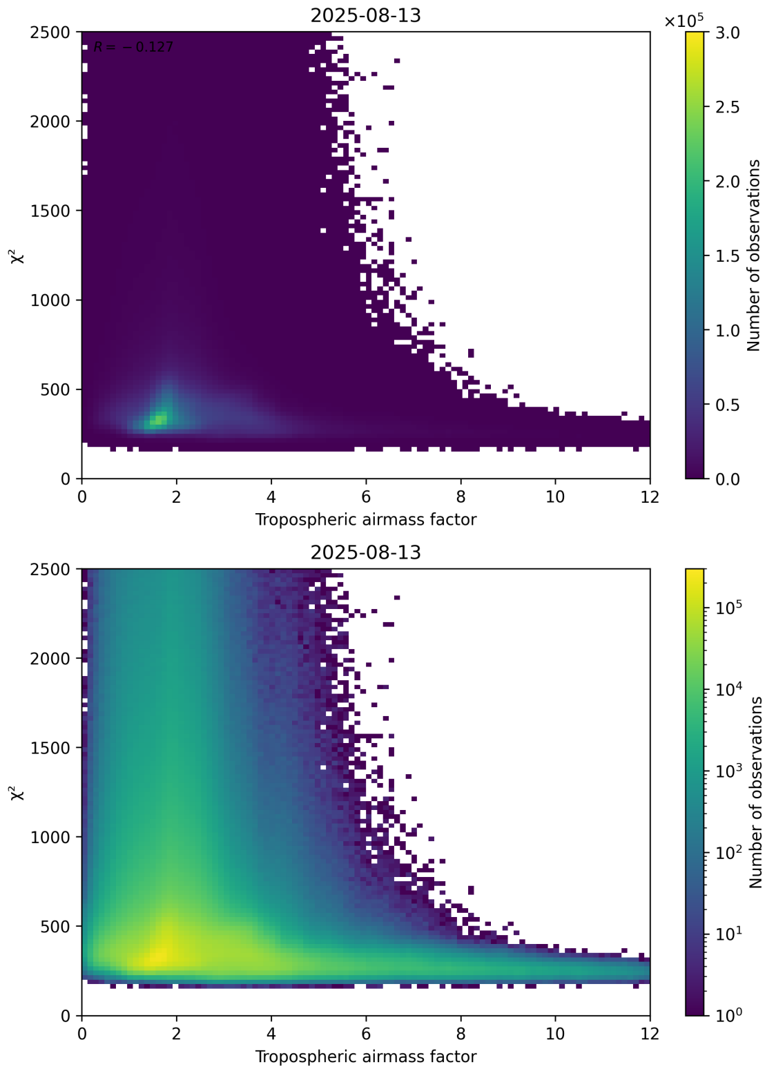
Figure 73: Scatter density plot of “Tropospheric airmass factor” against “ \chi^2 ” for 2025-08-12 to 2025-08-14.
