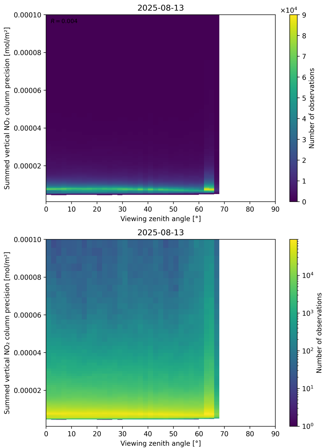
Figure 166: Scatter density plot of “Viewing zenith angle” against “Summed vertical NO 2 column precision” for 2025-08-12 to 2025-08-14.
