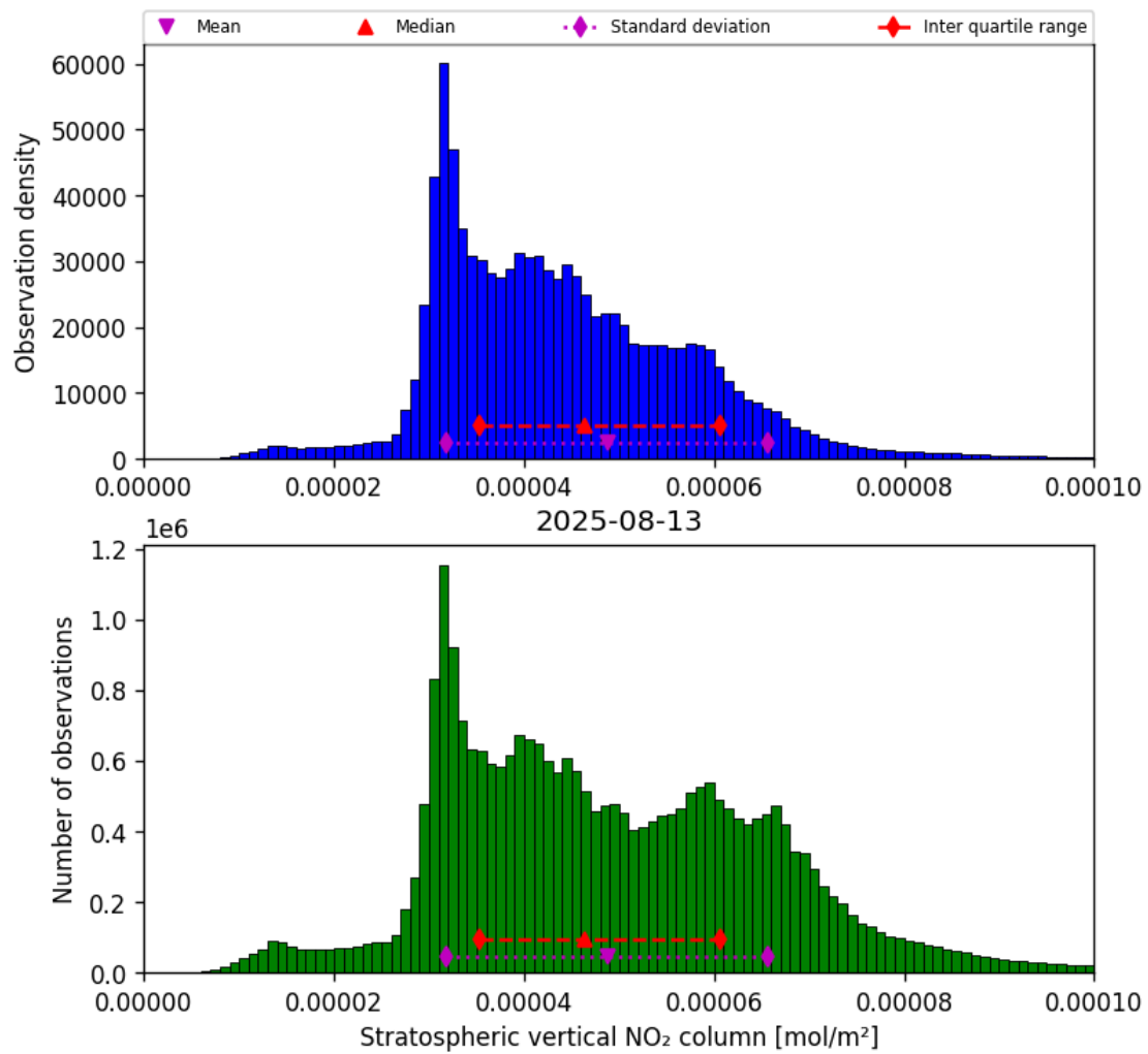
Figure 36: Histogram of “Stratospheric vertical NO 2 column” for 2025-08-12 to 2025-08-14
