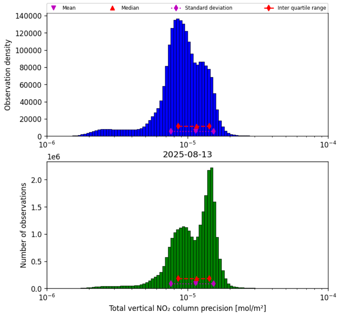
Figure 39: Histogram of “Total vertical NO 2 column precision” for 2025-08-12 to 2025-08-14
