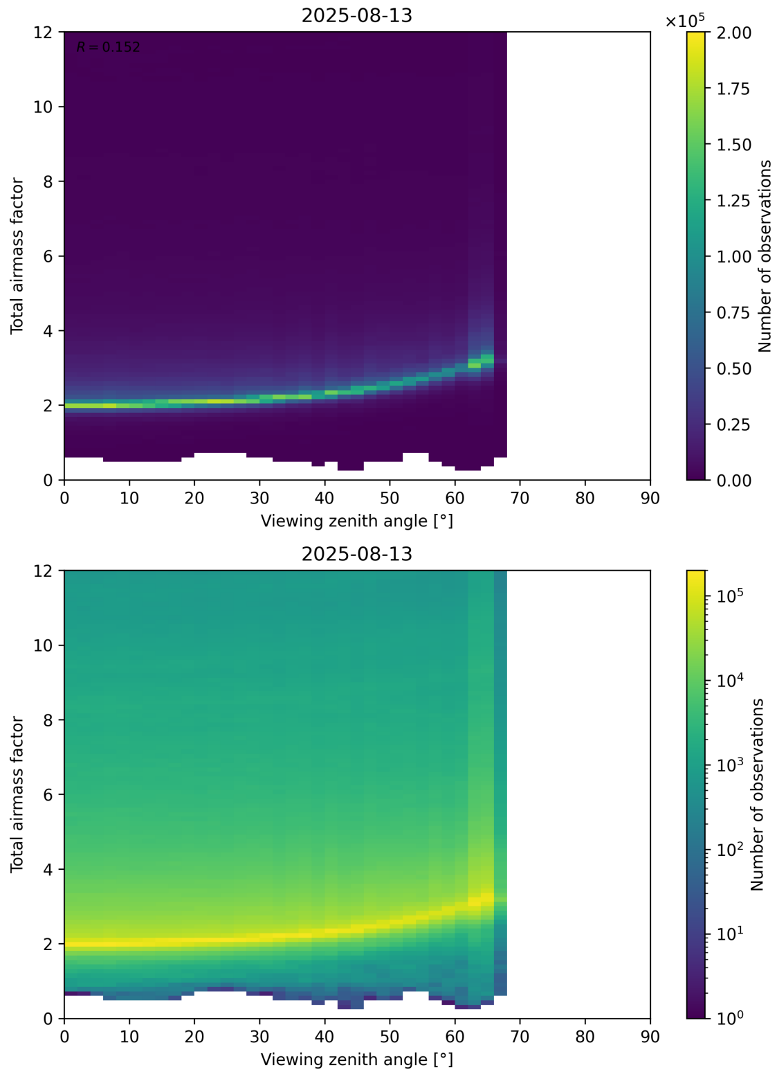
Figure 160: Scatter density plot of “Viewing zenith angle” against “Total airmass factor” for 2025-08-12 to 2025-08-14.
