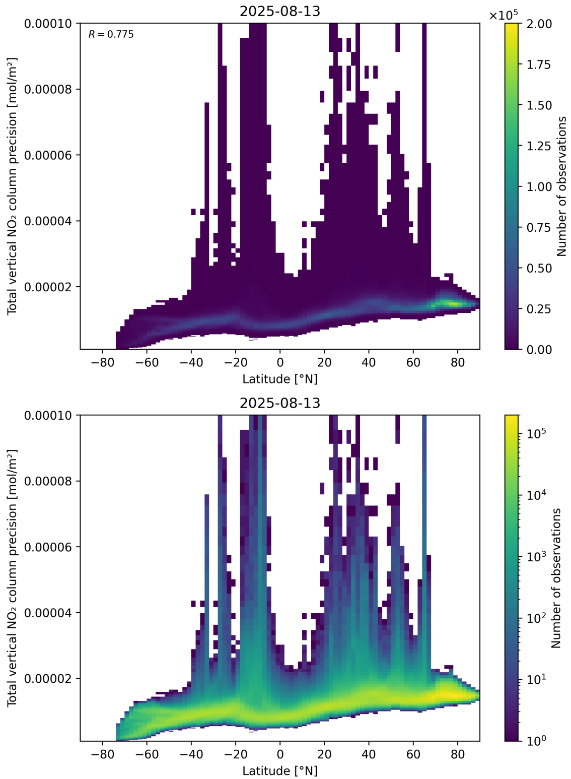
Figure 91: Scatter density plot of “Latitude” against “Total vertical NO 2 column precision” for 2025-08-12 to 2025-08-14.
