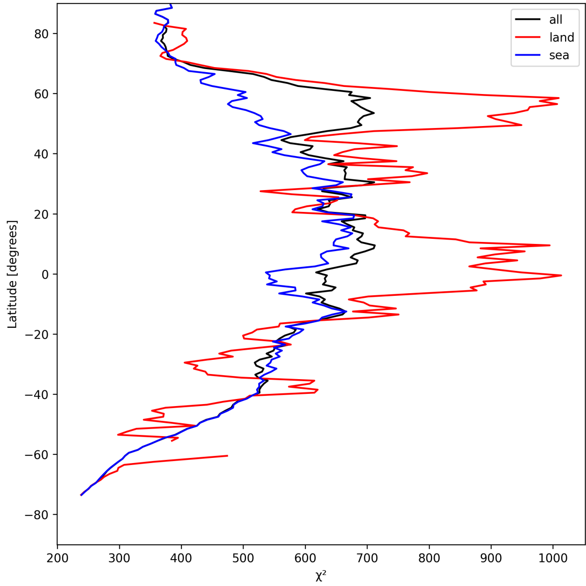
Figure 25: Zonal average of “ \chi^2 ” for 2025-08-12 to 2025-08-14.
