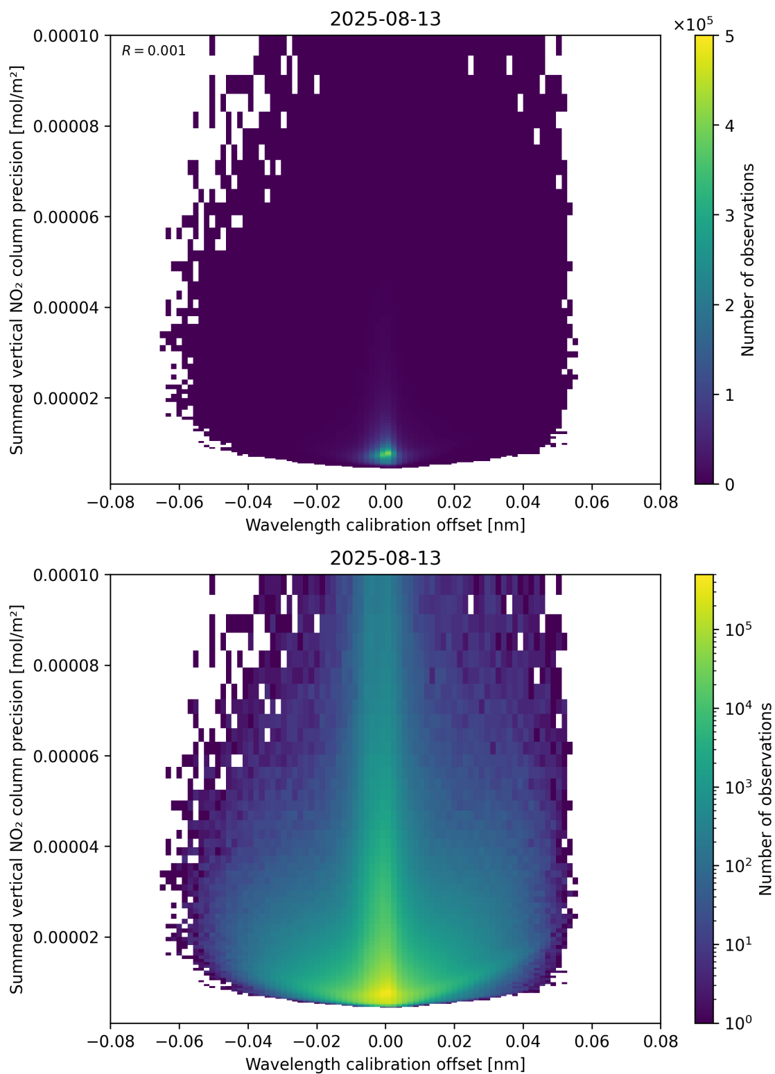
Figure 178: Scatter density plot of “Wavelength calibration offset” against “Summed vertical NO 2 column precision” for 2025-08-12 to 2025-08-14.
