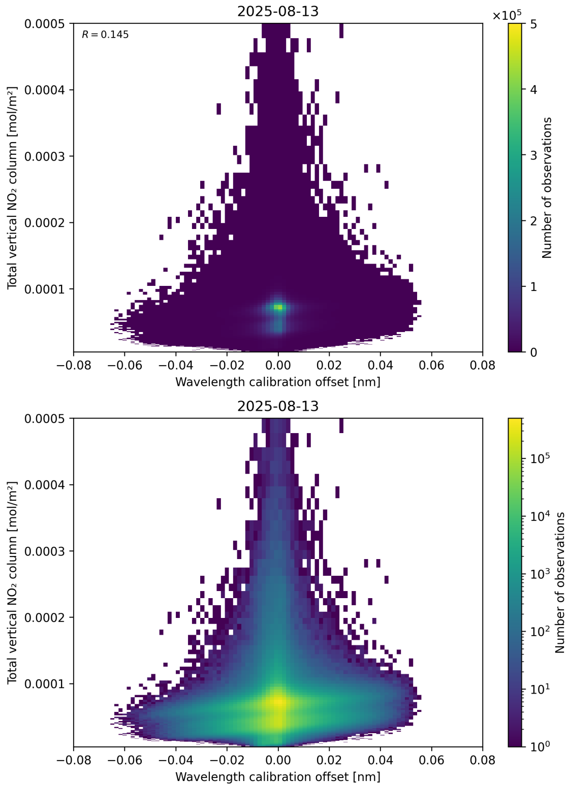
Figure 179: Scatter density plot of “Wavelength calibration offset” against “Total vertical NO 2 column” for 2025-08-12 to 2025-08-14.
