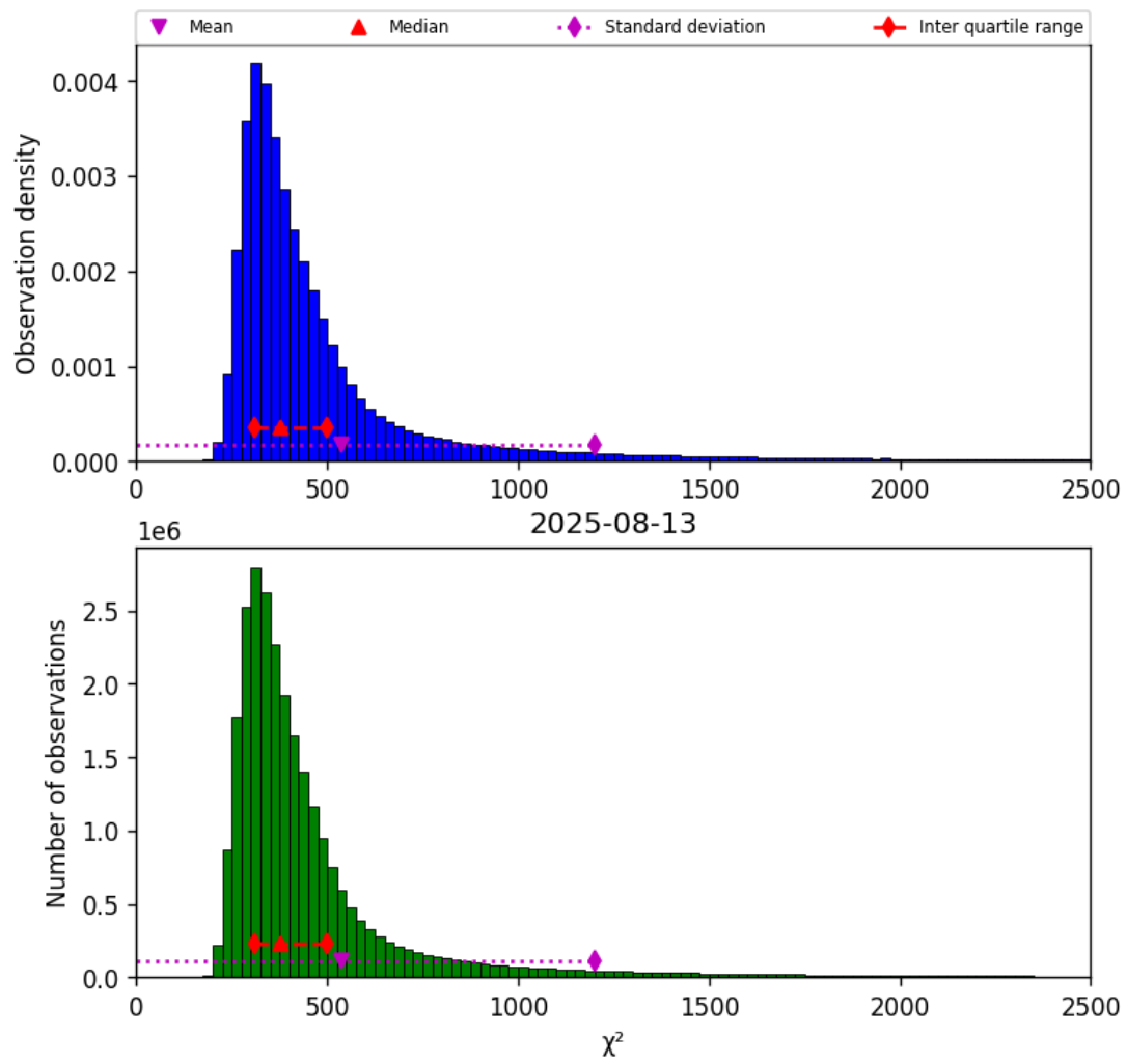
Figure 42: Histogram of “ \chi^2 ” for 2025-08-12 to 2025-08-14
