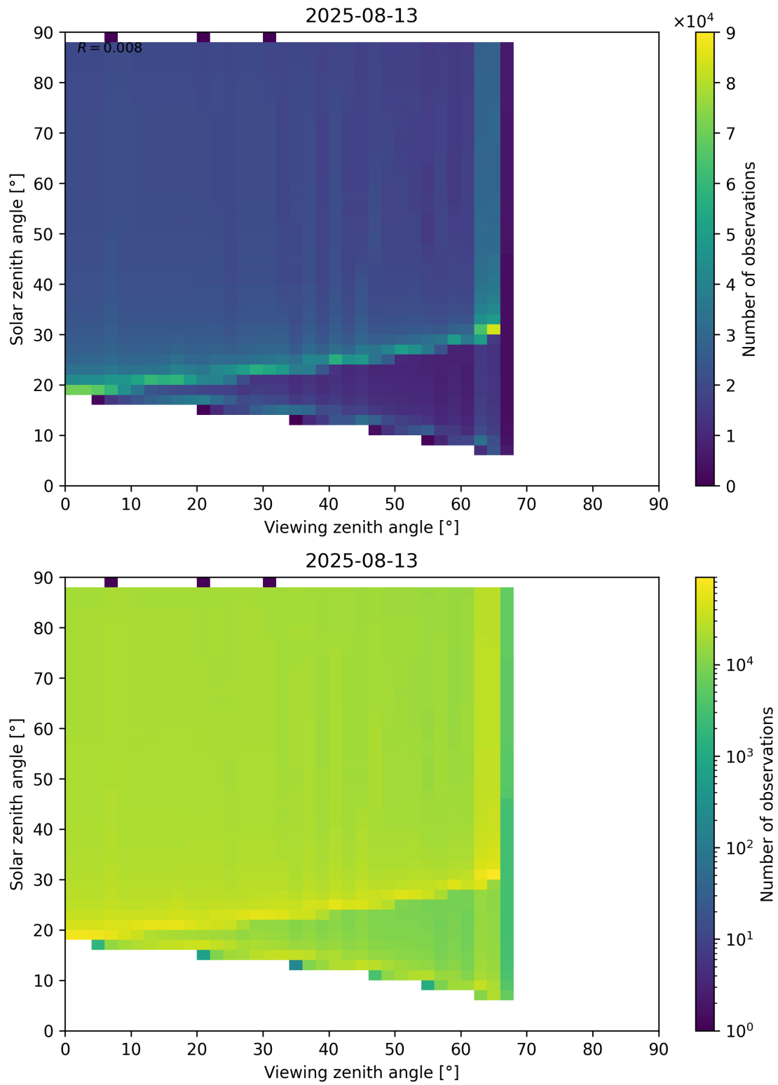
Figure 172: Scatter density plot of “Viewing zenith angle” against “Solar zenith angle” for 2025-08-12 to 2025-08-14.
