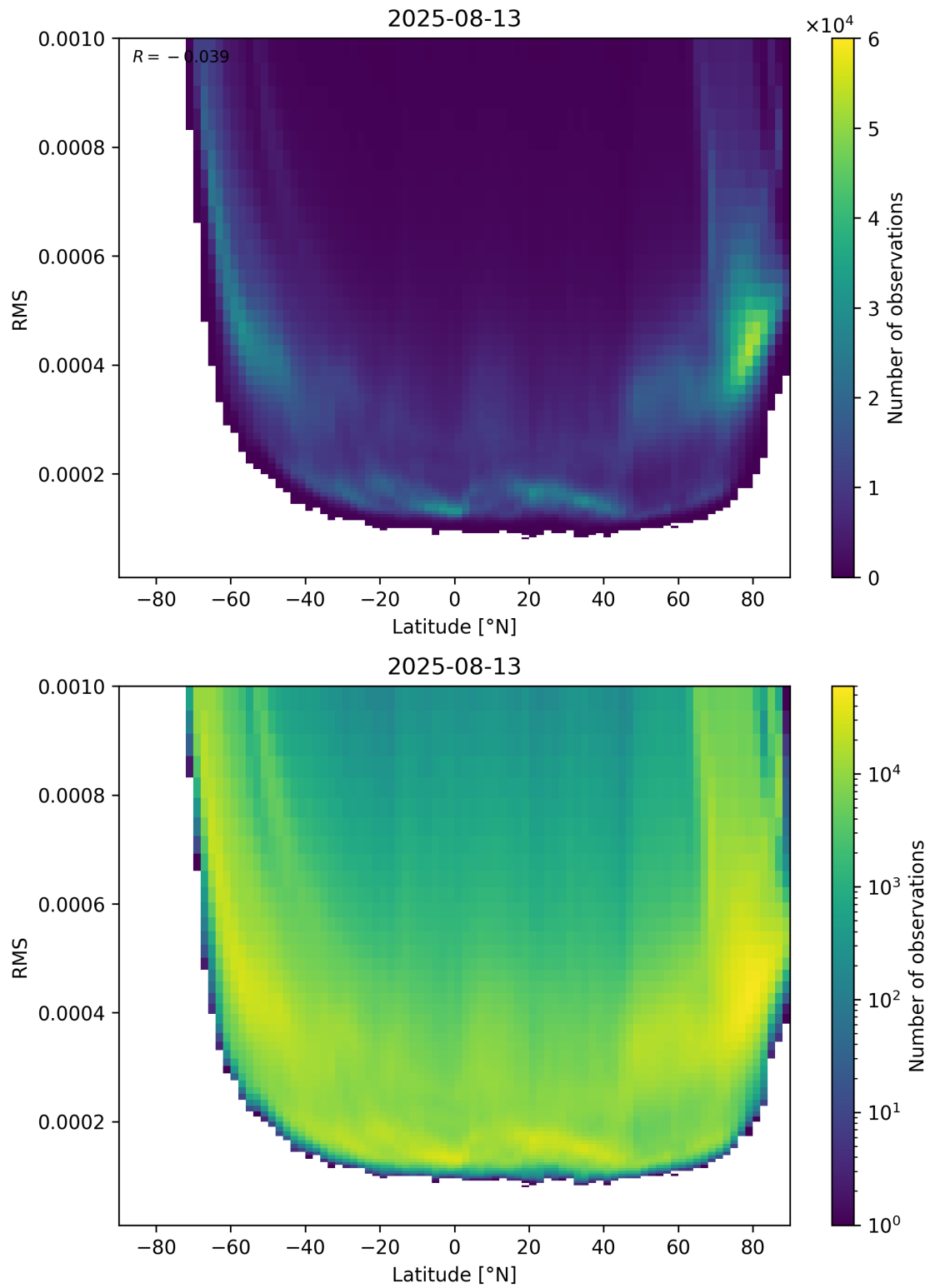
Figure 94: Scatter density plot of “Latitude” against “RMS” for 2025-08-12 to 2025-08-14.
