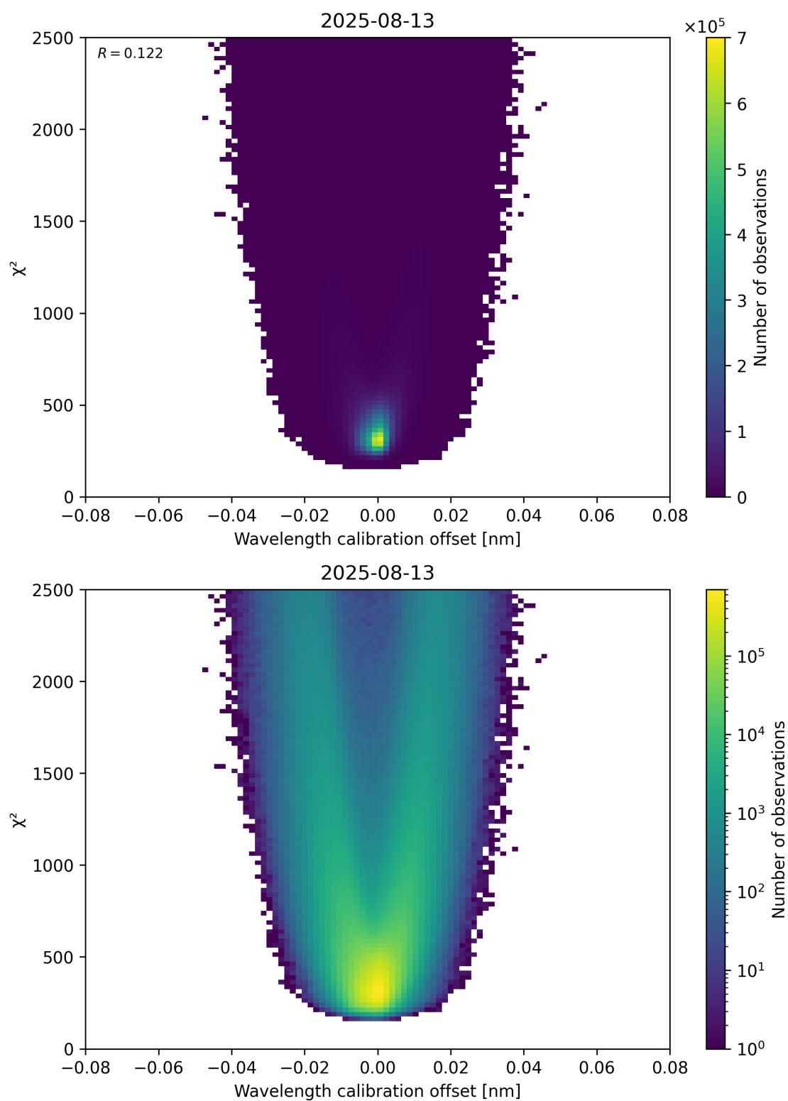
Figure 175: Scatter density plot of “Wavelength calibration offset” against “ \chi^2 ” for 2025-08-12 to 2025-08-14.
