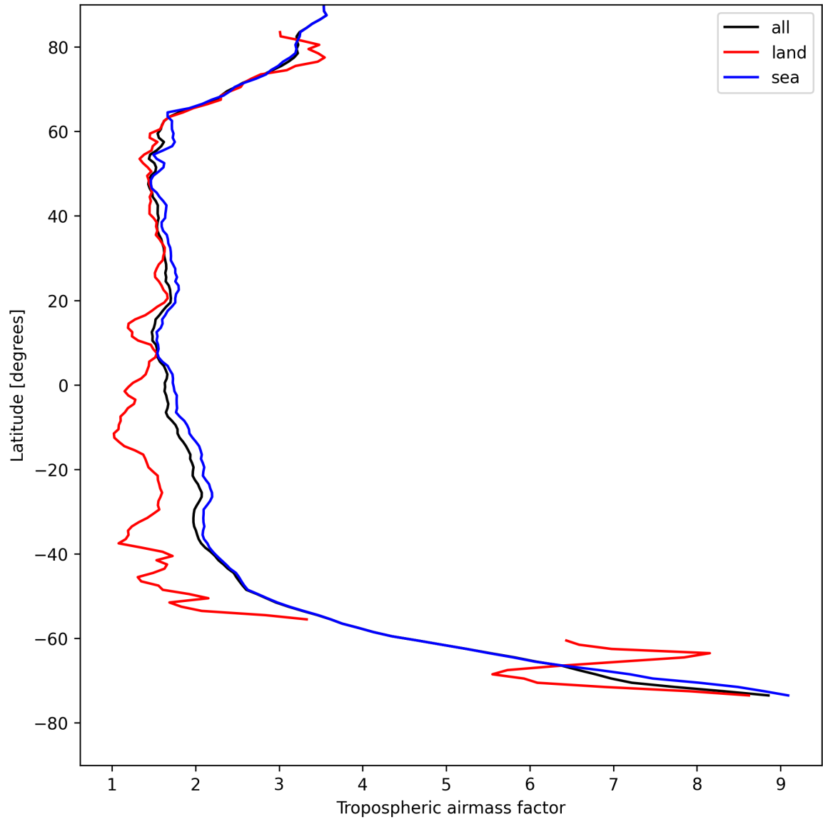
Figure 14: Zonal average of “Tropospheric airmass factor” for 2025-08-12 to 2025-08-14.
