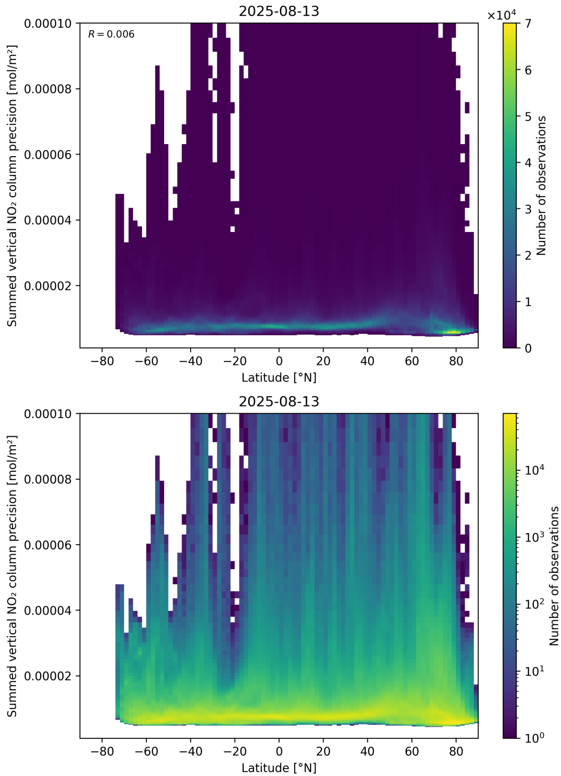
Figure 89: Scatter density plot of “Latitude” against “Summed vertical NO 2 column precision” for 2025-08-12 to 2025-08-14.
