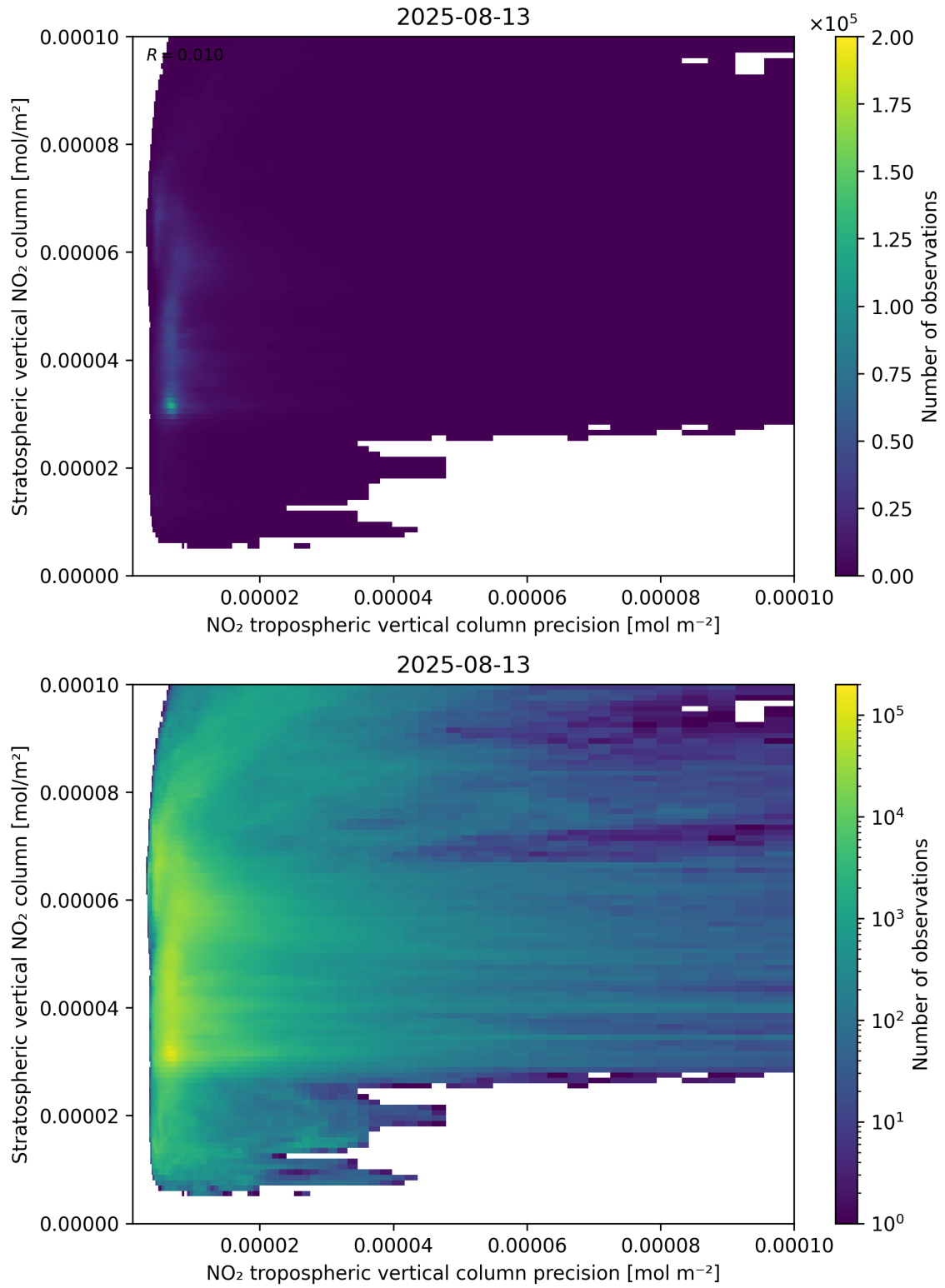
Figure 135: Scatter density plot of “NO 2 tropospheric vertical column precision” against “Stratospheric vertical NO 2 column” for 2025-08-12 to 2025-08-14.
