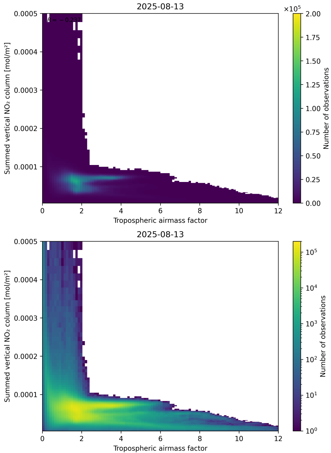
Figure 75: Scatter density plot of “Tropospheric air mass factor” against “Summed vertical NO 2 column” for 2025-08-12 to 2025-08-14.
