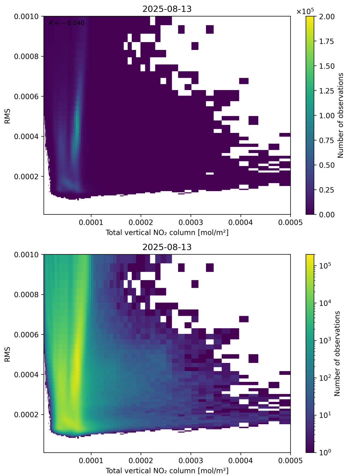
Figure 120: Scatter density plot of “Total vertical NO 2 column” against “RMS” for 2025-08-12 to 2025-08-14.
