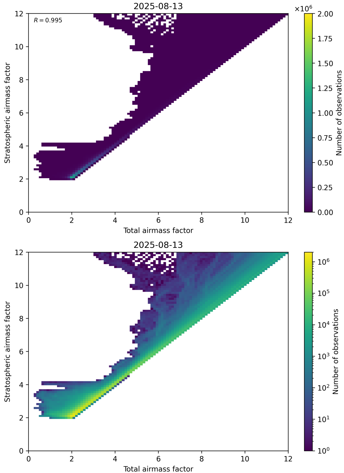
Figure 62: Scatter density plot of “Total airmass factor” against “Stratospheric airmass factor” for 2025-08-12 to 2025-08-14.
