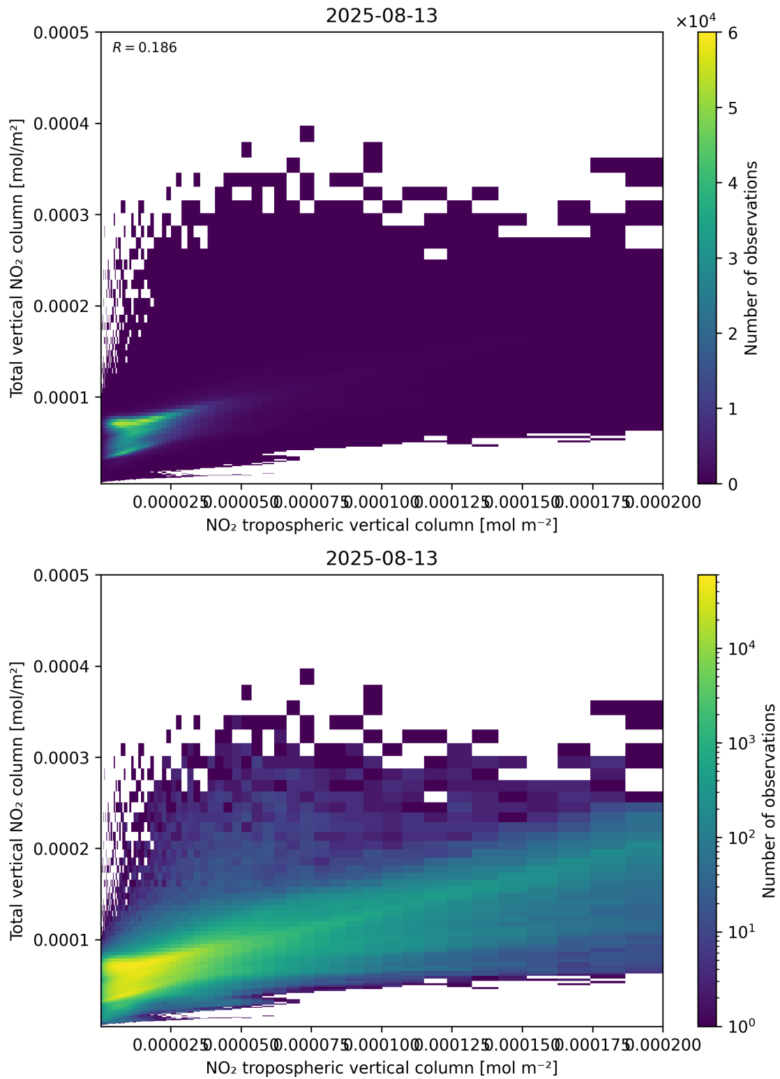
Figure 128: Scatter density plot of “NO 2 tropospheric vertical column” against “Total vertical NO 2 column” for 2025-08-12 to 2025-08-14.
