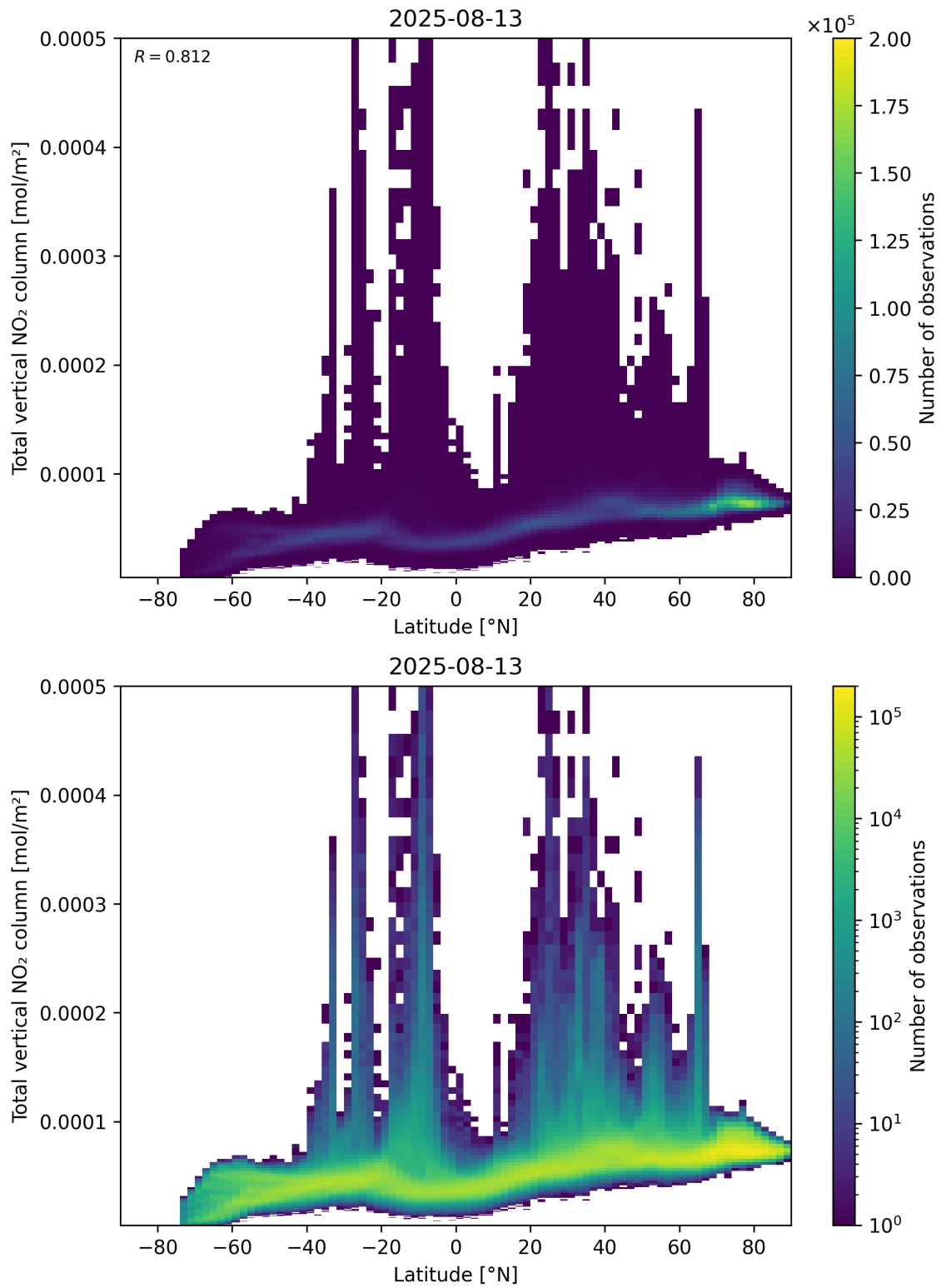
Figure 90: Scatter density plot of “Latitude” against “Total vertical NO 2 column” for 2025-08-12 to 2025-08-14.
