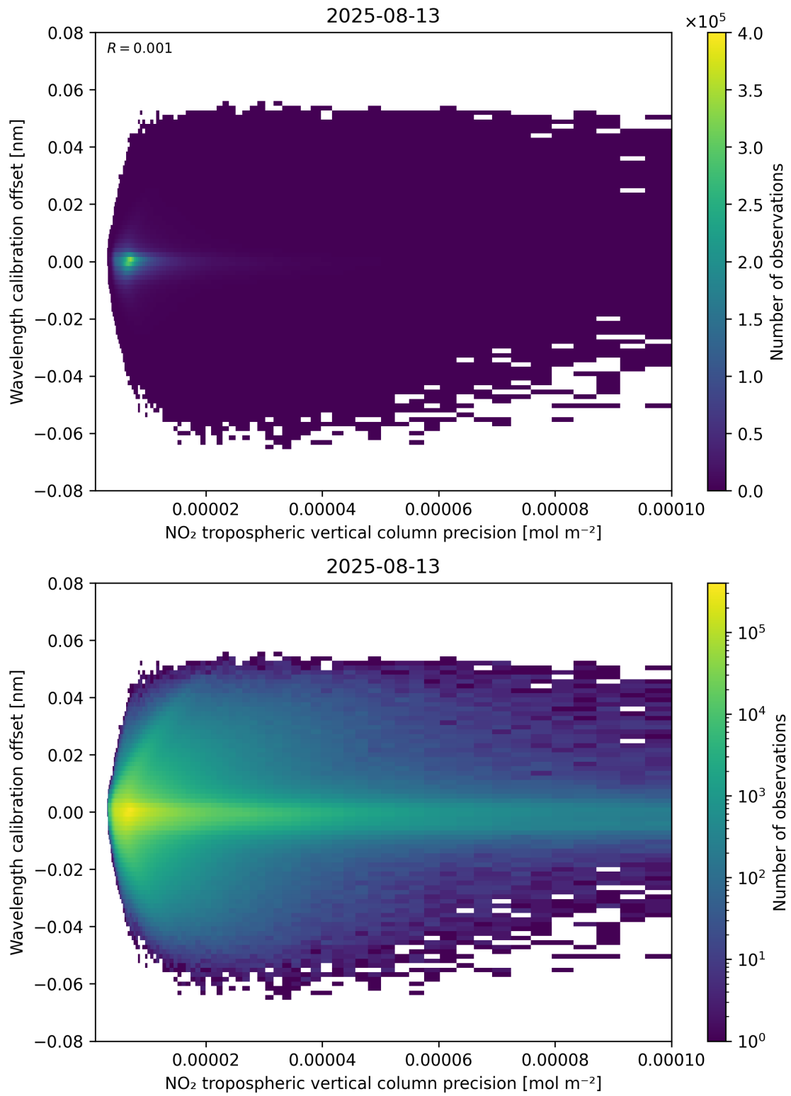
Figure 141: Scatter density plot of “NO 2 tropospheric vertical column precision” against “Wavelength calibration offset” for 2025-08-12 to 2025-08-14.
