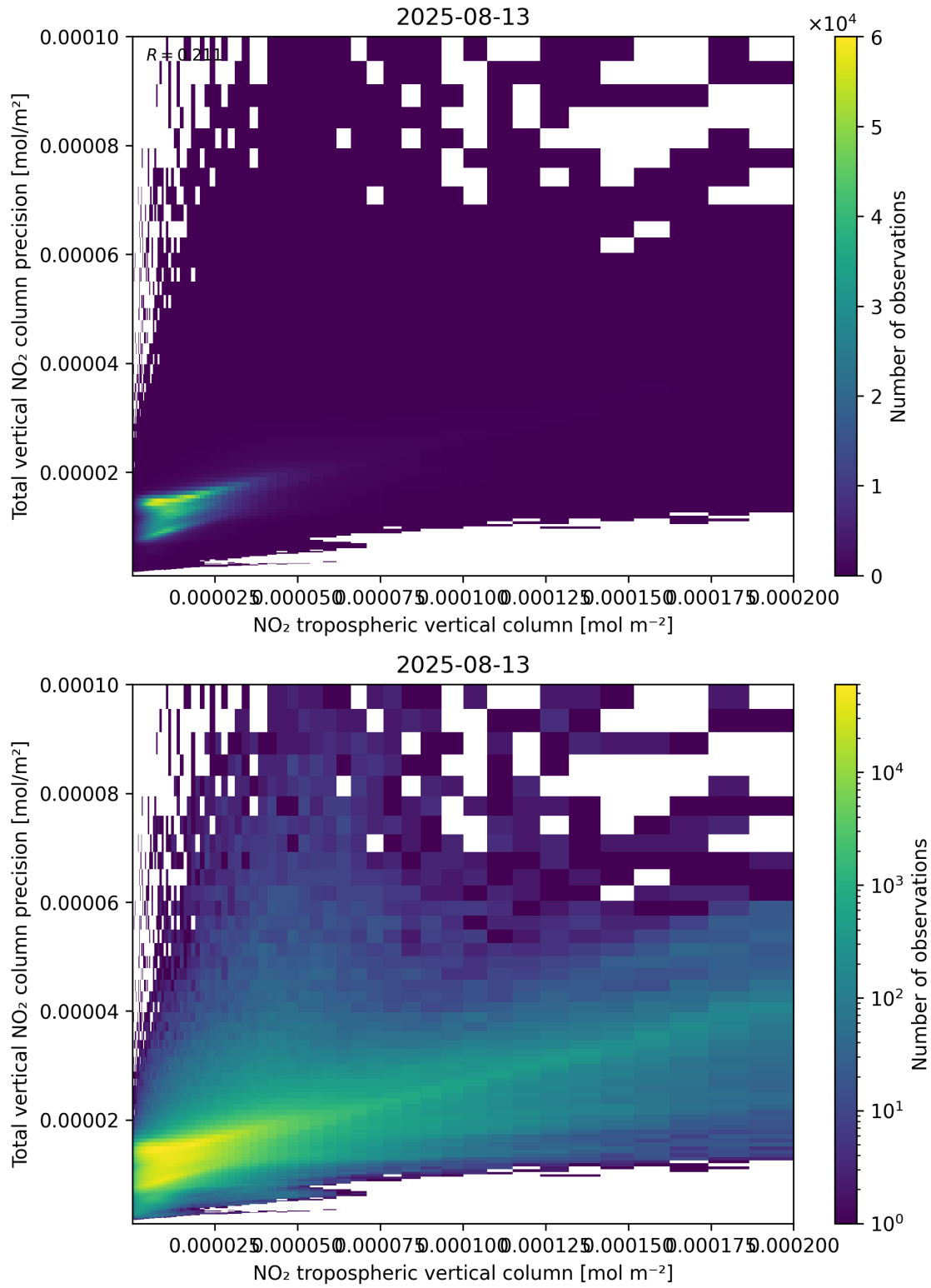
Figure 129: Scatter density plot of “NO 2 tropospheric vertical column” against “Total vertical NO 2 column precision” for 2025-08-12 to 2025-08-14.
