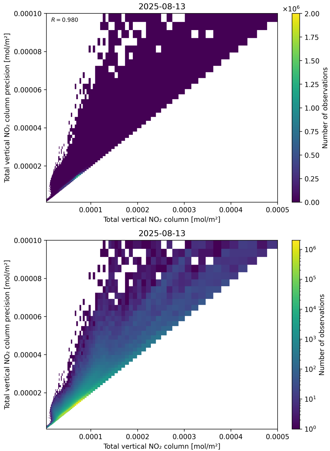
Figure 114: Scatter density plot of “Total vertical NO 2 column” against “Total vertical NO 2 column precision” for 2025-08-12 to 2025-08-14.
