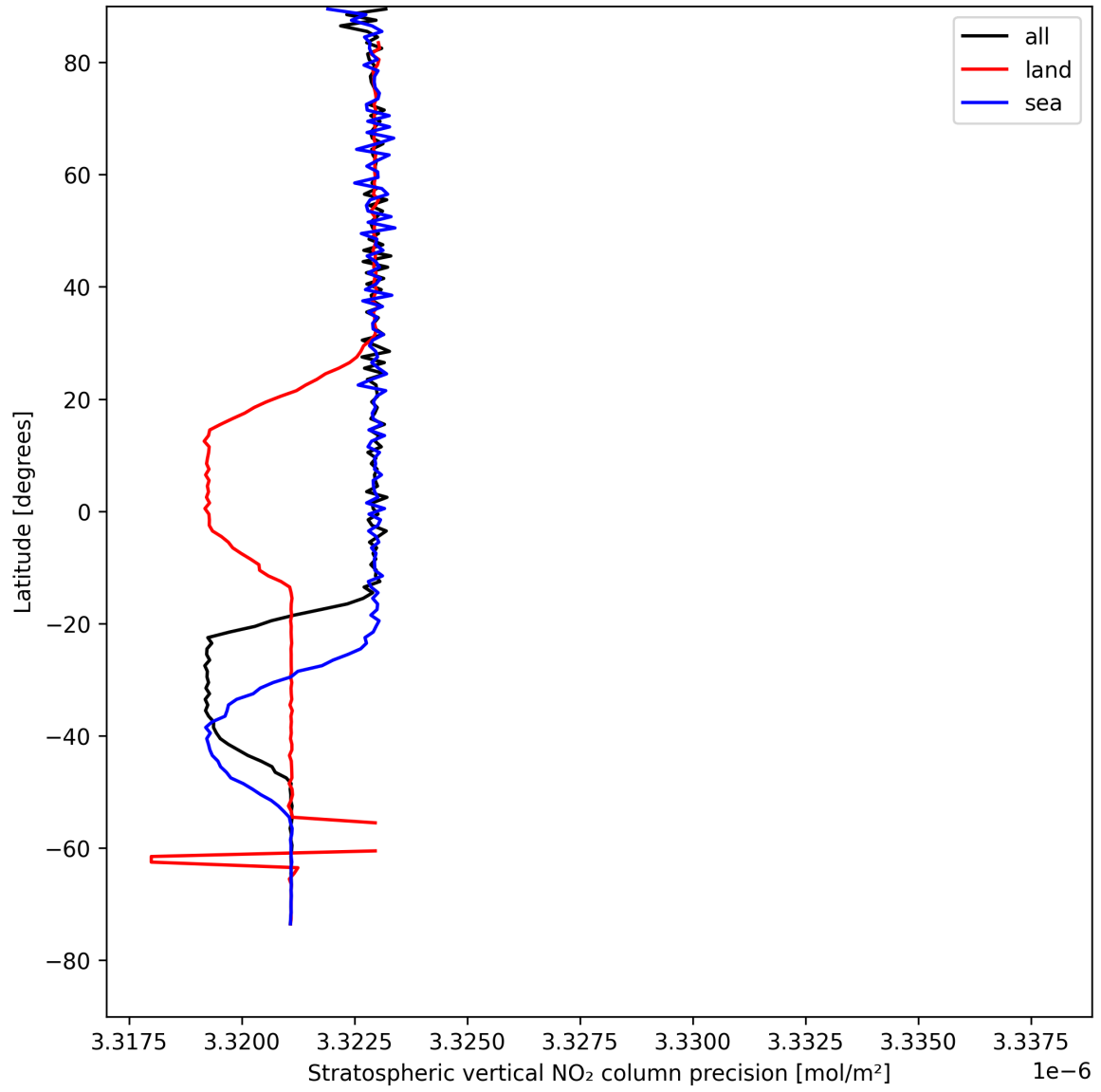
Figure 20: Zonal average of “Stratospheric vertical NO 2 column precision” for 2025-08-12 to 2025-08-14.
