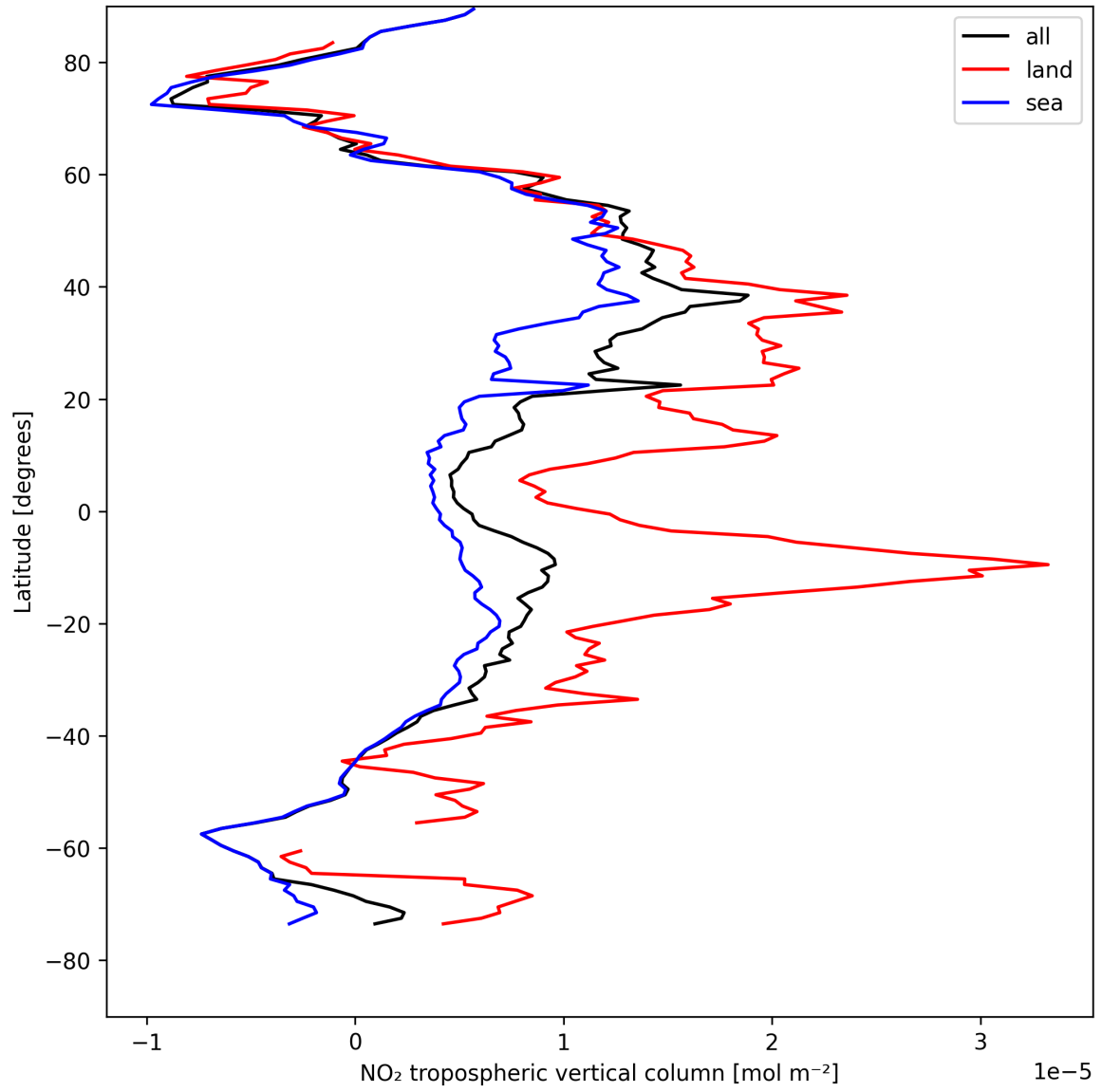
Figure 12: Zonal average of “NO 2 tropospheric vertical column” for 2025-08-12 to 2025-08-14.
