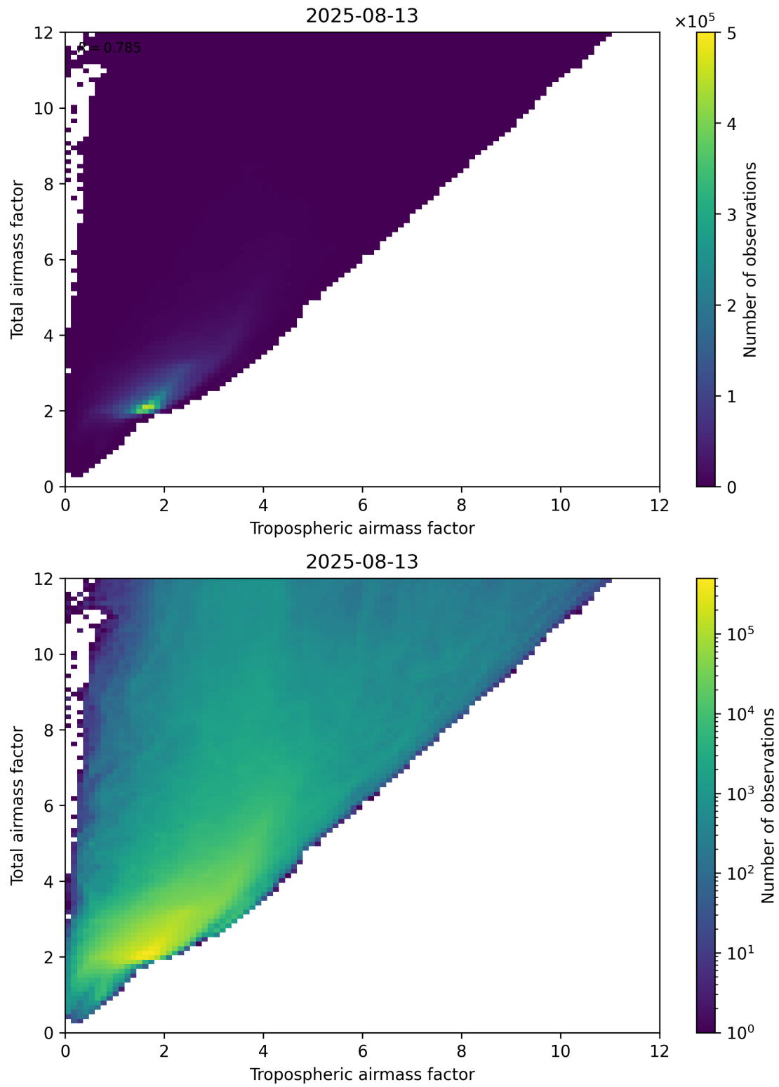
Figure 72: Scatter density plot of “Tropospheric airmass factor” against “Total airmass factor” for 2025-08-12 to 2025-08-14.
