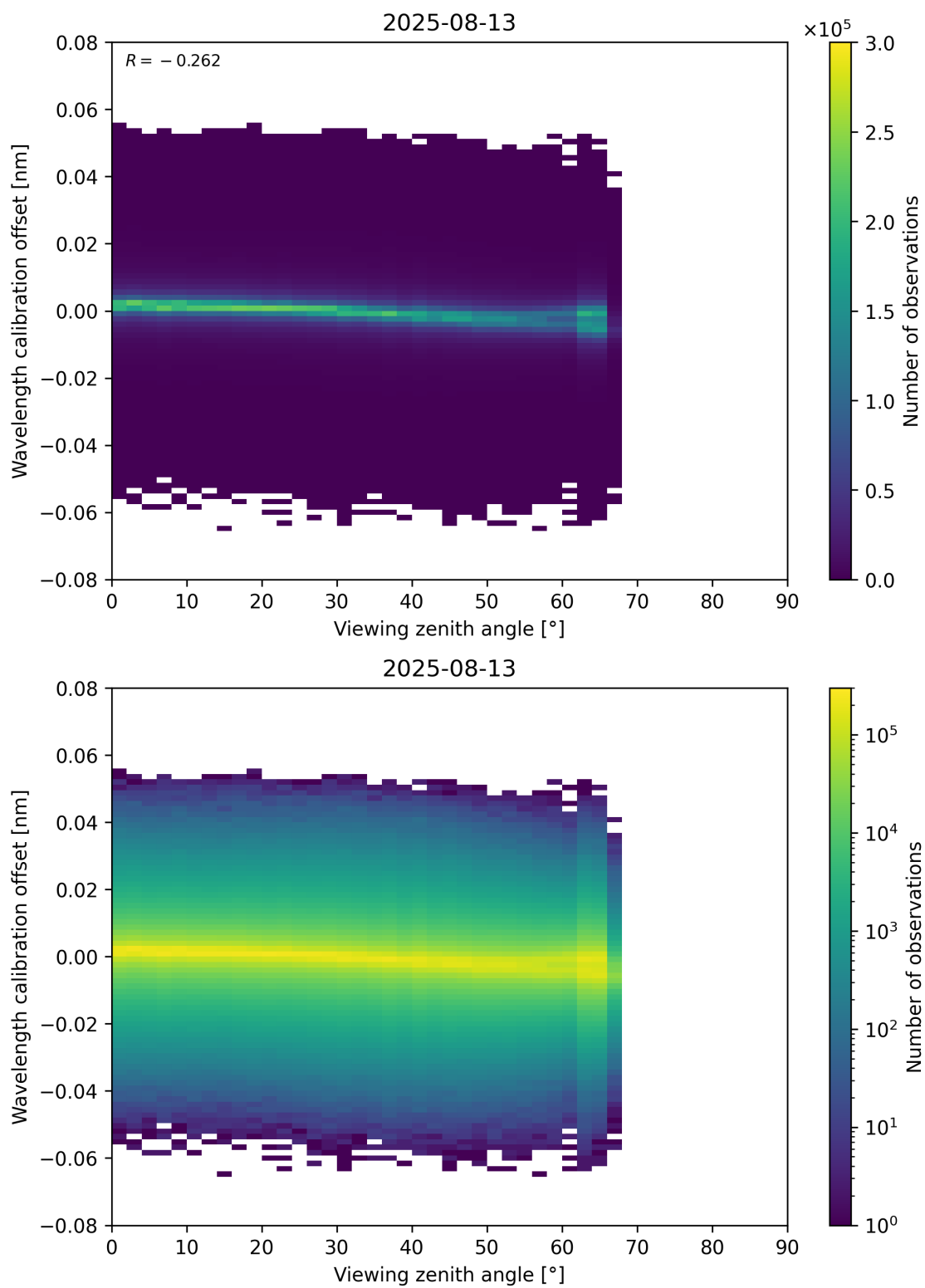
Figure 173: Scatter density plot of “Viewing zenith angle” against “Wavelength calibration offset” for 2025-08-12 to 2025-08-14.
