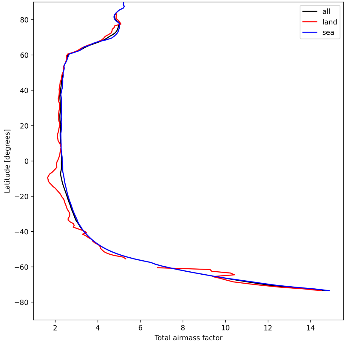
Figure 15: Zonal average of “Total airmass factor” for 2025-08-12 to 2025-08-14.
