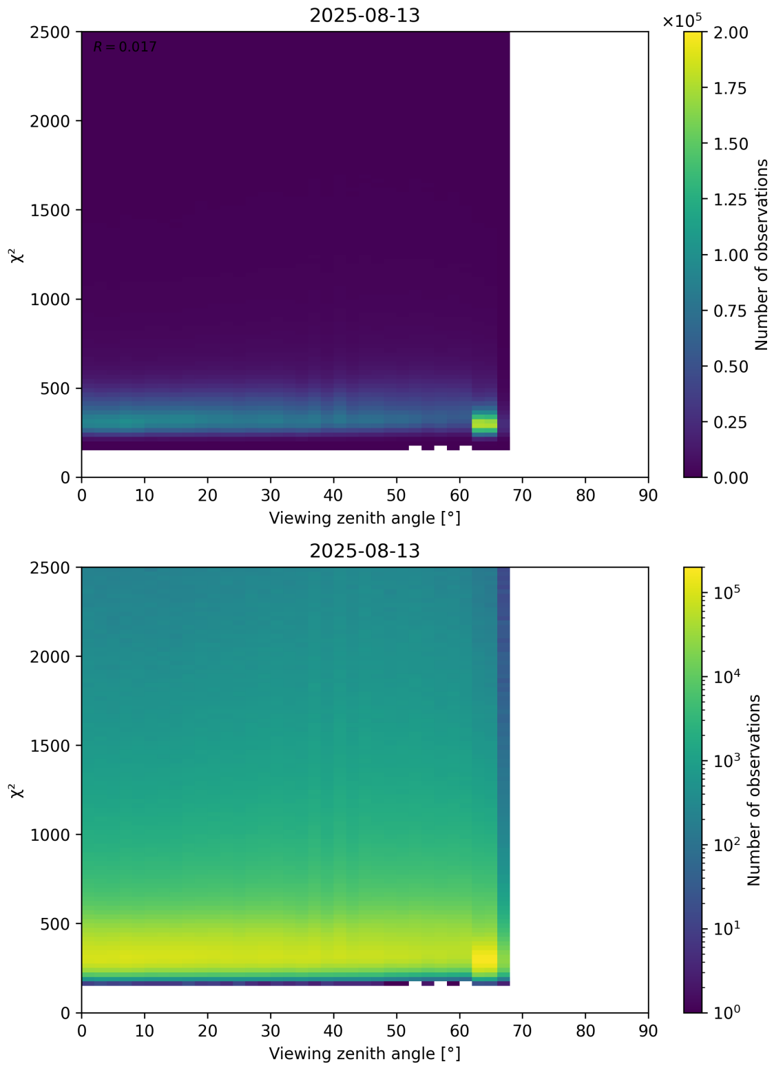
Figure 162: Scatter density plot of “Viewing zenith angle” against “ \chi^2 ” for 2025-08-12 to 2025-08-14.
