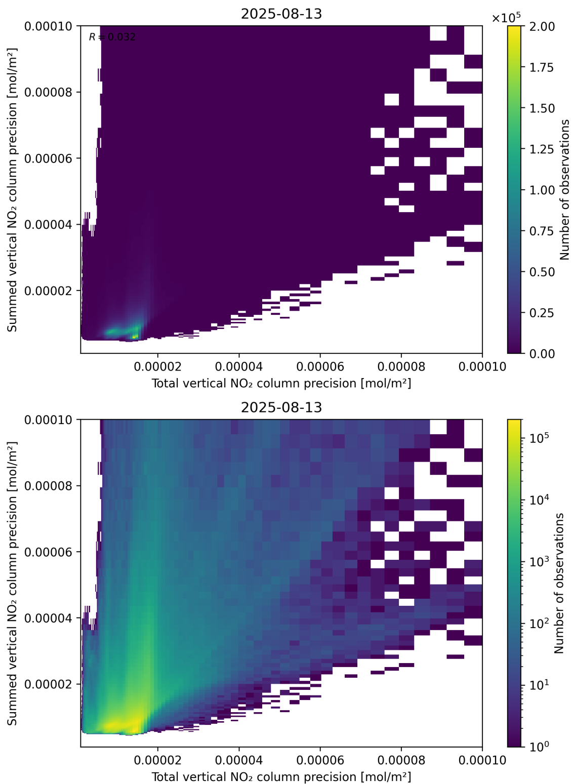
Figure 118: Scatter density plot of “Total vertical NO 2 column precision” against “Summed vertical NO 2 column precision” for 2025-08-12 to 2025-08-14.
