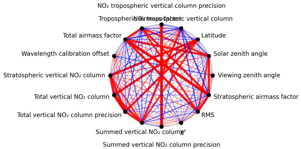
Figure 1: Map of correlation graph for 2025-08-12 to 2025-08-14.
