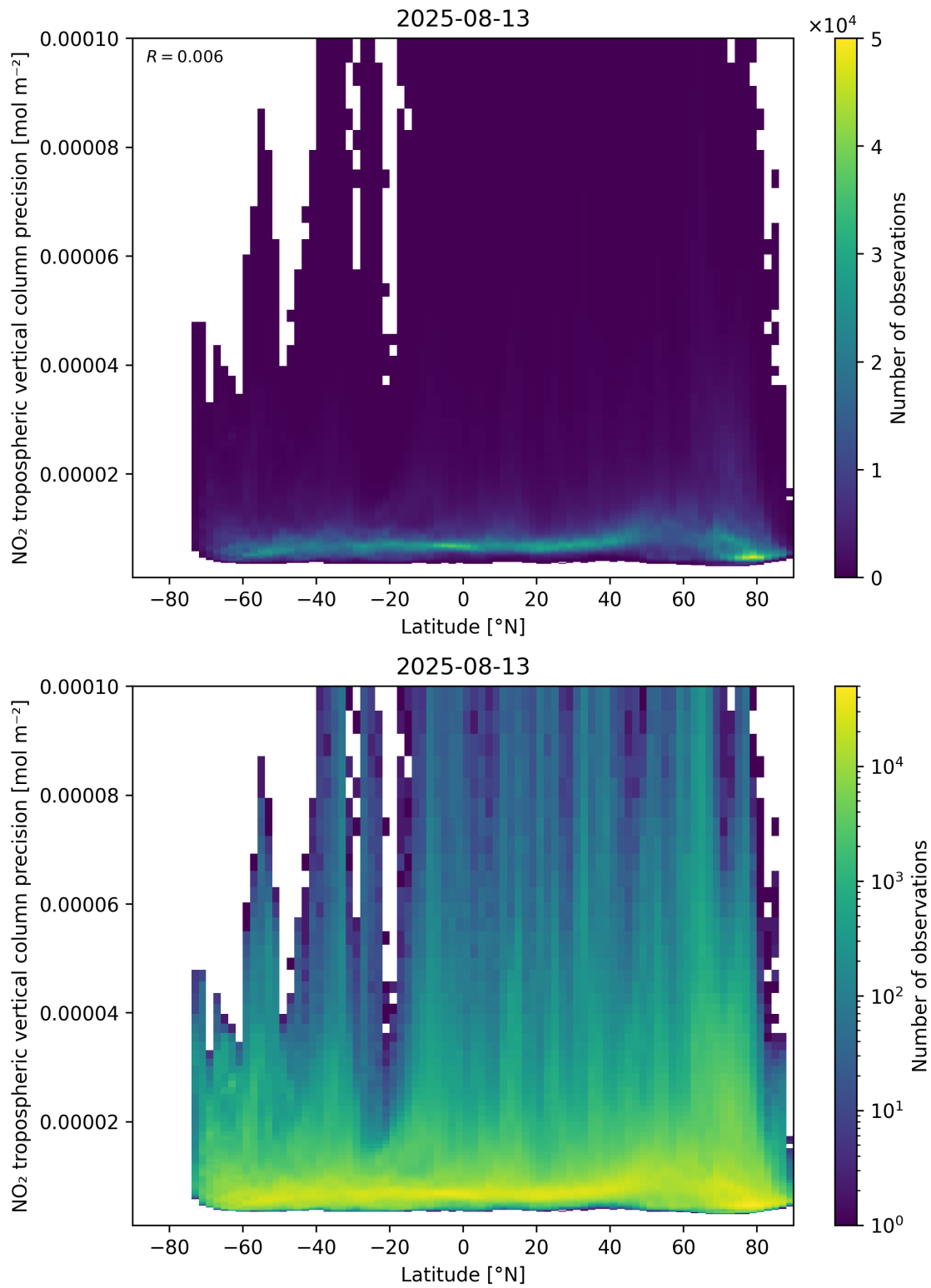
Figure 93: Scatter density plot of “Latitude” against “NO 2 tropospheric vertical column precision” for 2025-08-12 to 2025-08-14.
