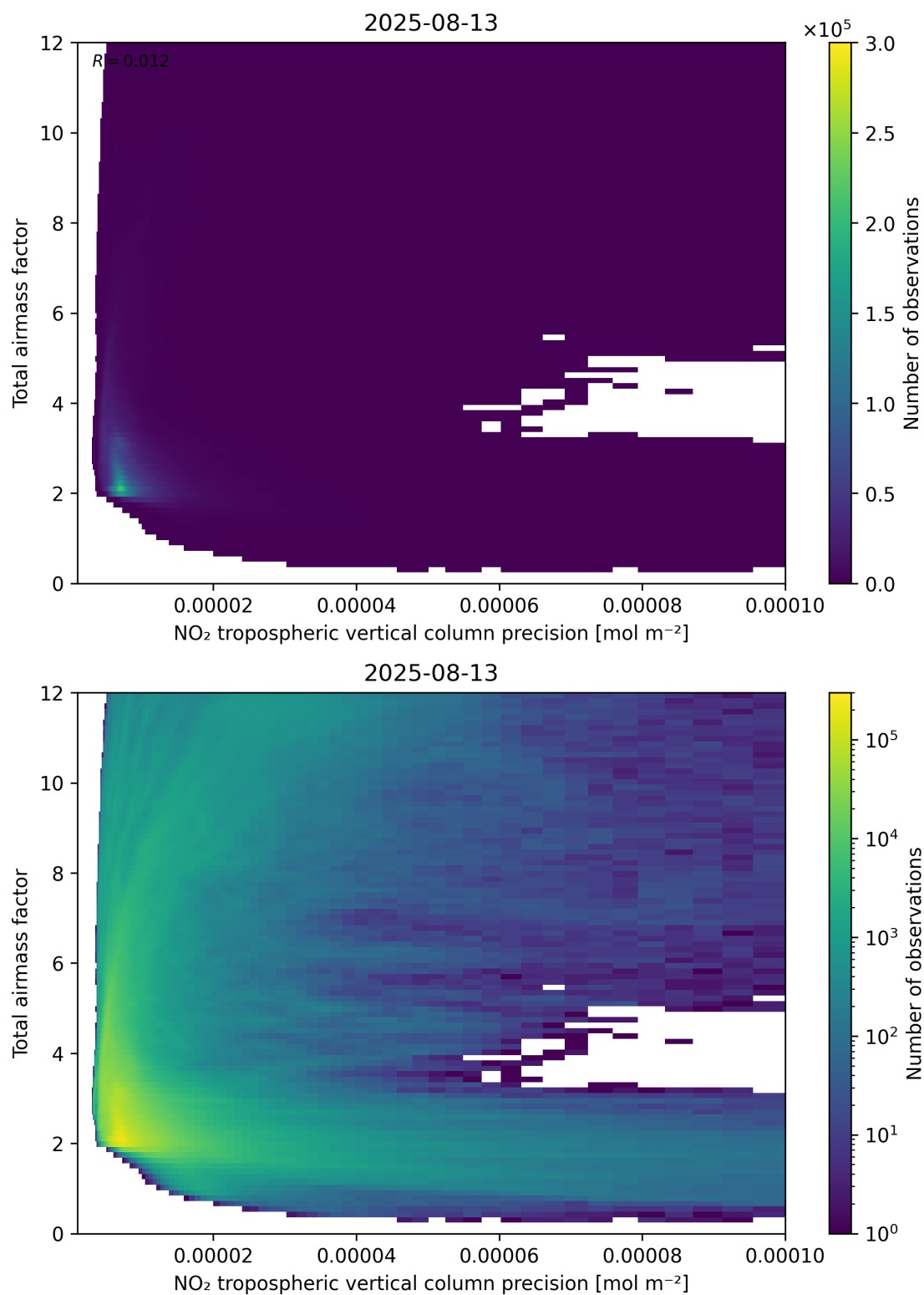
Figure 132: Scatter density plot of “NO 2 tropospheric vertical column precision” against “Total air mass factor” for 2025-08-12 to 2025-08-14.
