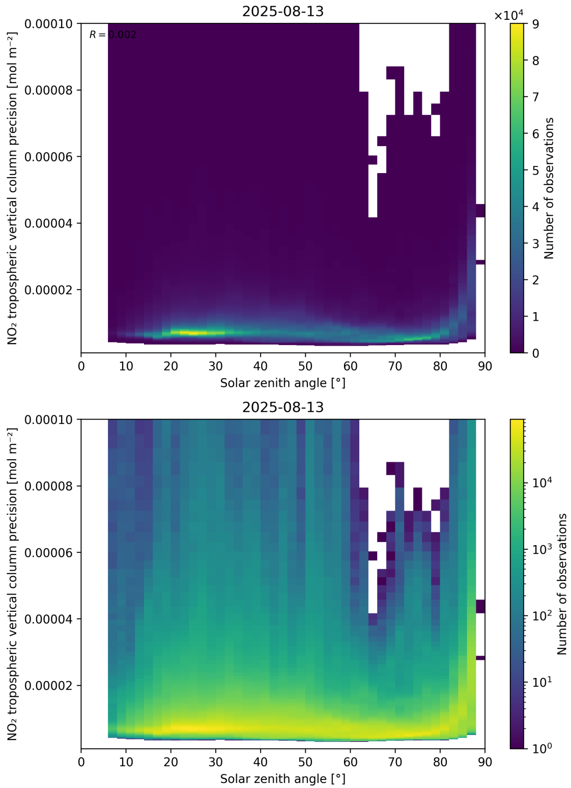
Figure 156: Scatter density plot of “Solar zenith angle” against “NO 2 tropospheric vertical column precision” for 2025-08-12 to 2025-08-14.
