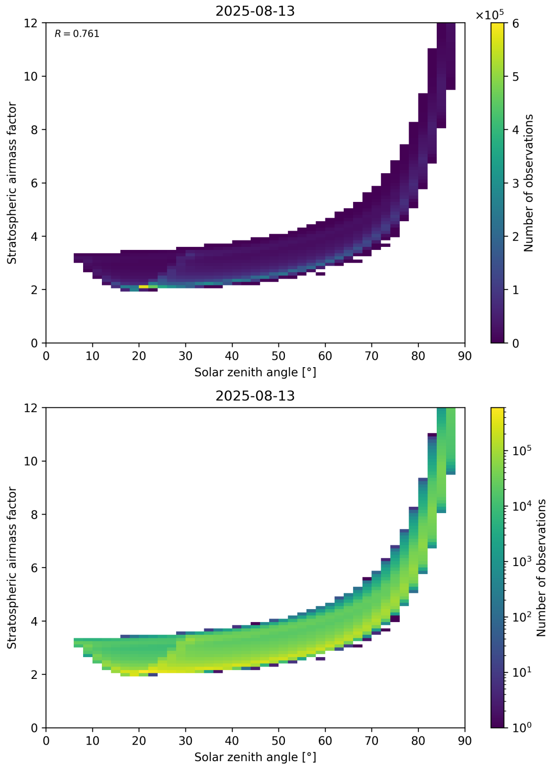
Figure 145: Scatter density plot of “Solar zenith angle” against “Stratospheric airmass factor” for 2025-08-12 to 2025-08-14.
