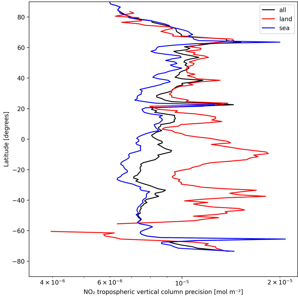
Figure 13: Zonal average of “NO 2 tropospheric vertical column precision” for 2025-08-12 to 2025-08-14.
