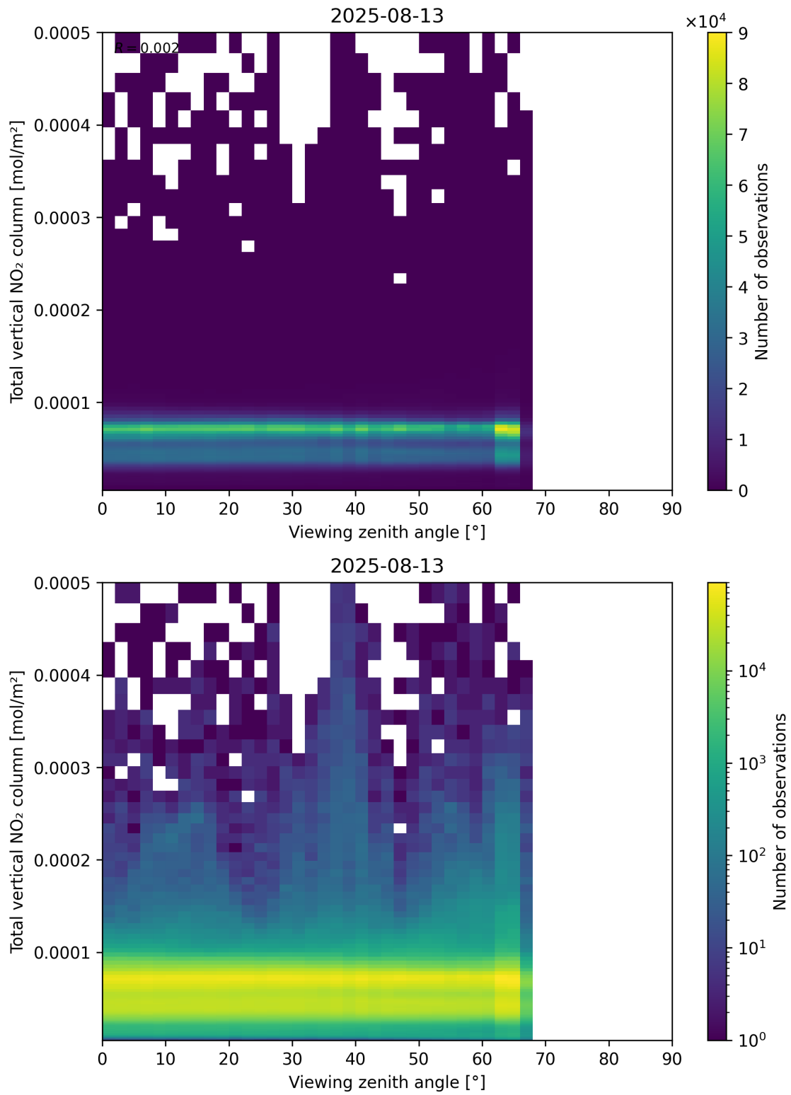
Figure 167: Scatter density plot of “Viewing zenith angle” against “Total vertical NO 2 column” for 2025-08-12 to 2025-08-14.
