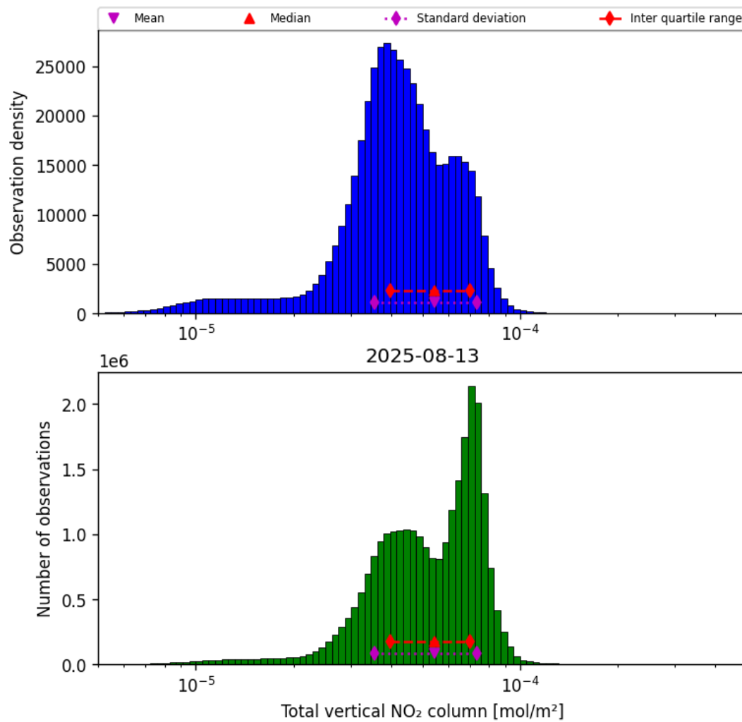
Figure 38: Histogram of “Total vertical NO 2 column” for 2025-08-12 to 2025-08-14
