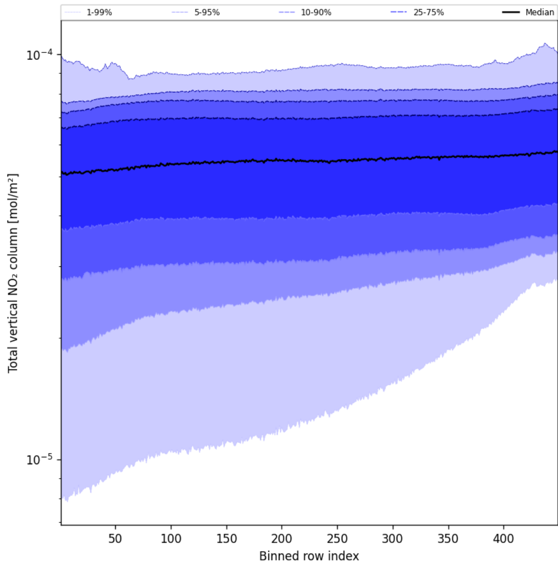
Figure 55: Along track statistics of “Total vertical NO 2 column” for 2025-08-12 to 2025-08-14
