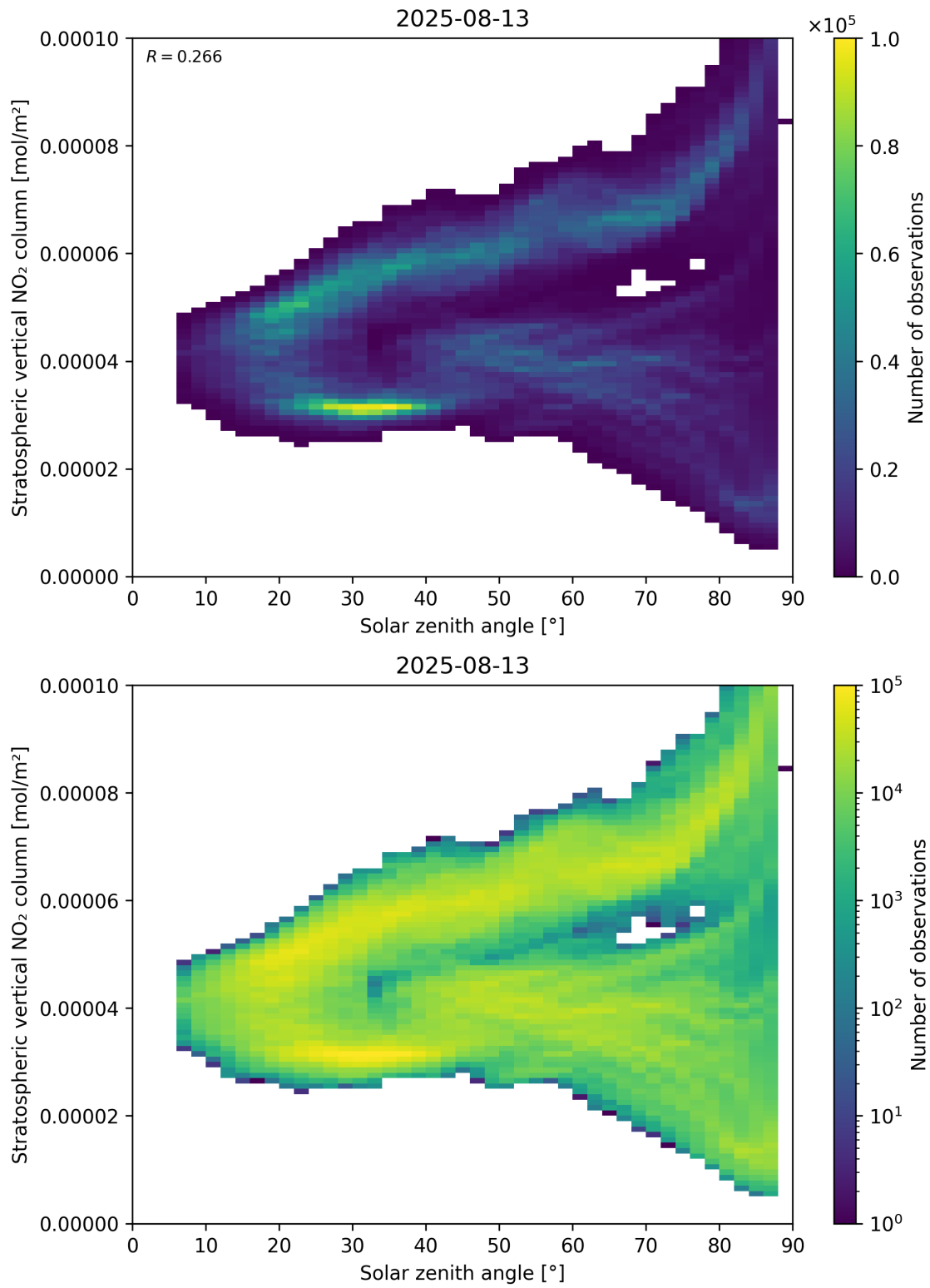
Figure 150: Scatter density plot of “Solar zenith angle” against “Stratospheric vertical NO 2 column” for 2025-08-12 to 2025-08-14.
