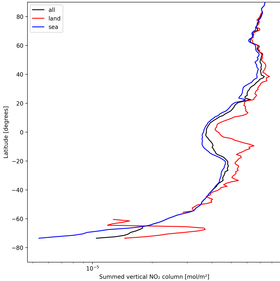
Figure 23: Zonal average of “Summed vertical NO 2 column” for 2025-08-12 to 2025-08-14.
