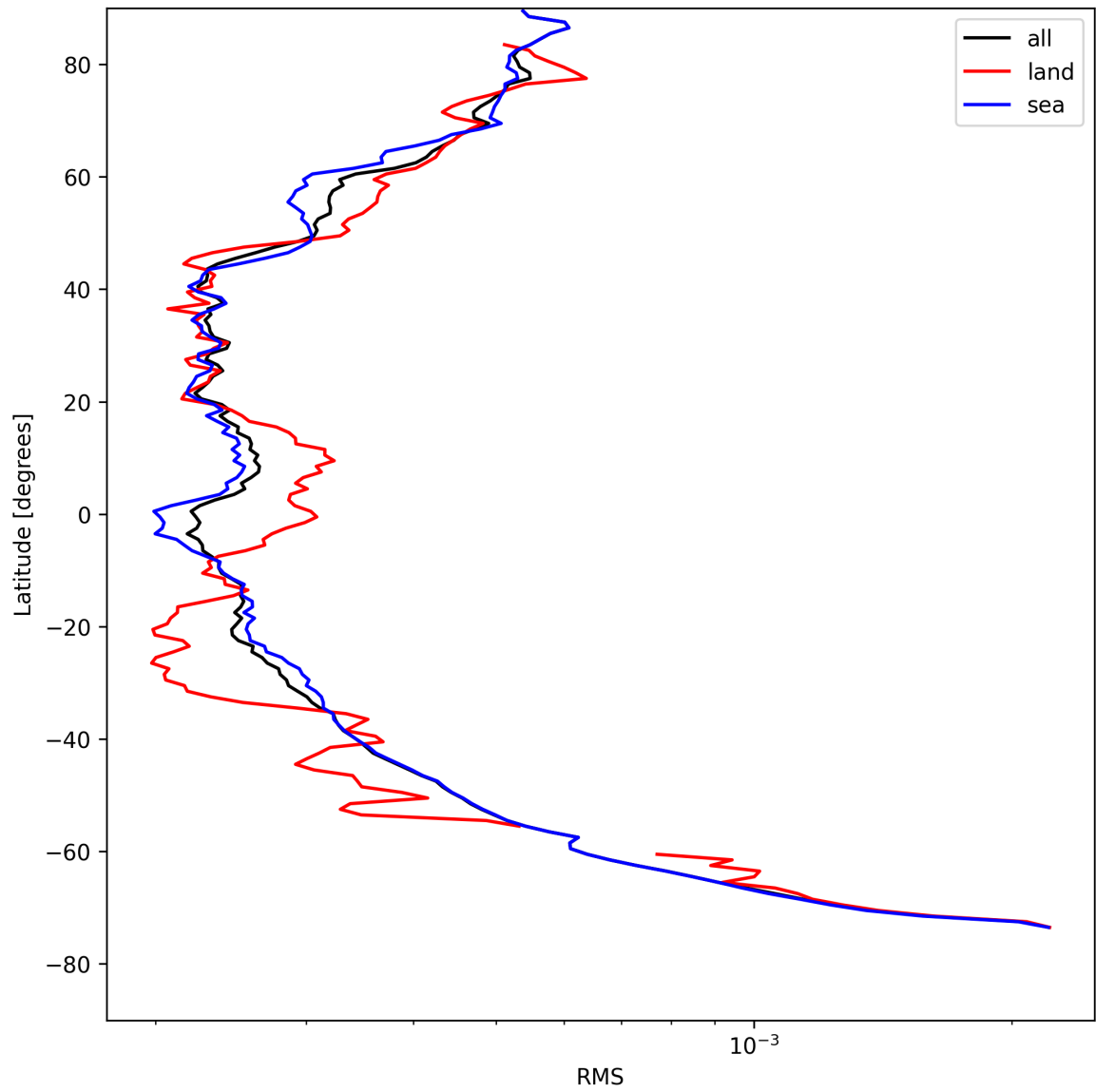
Figure 26: Zonal average of “RMS” for 2025-08-12 to 2025-08-14.
