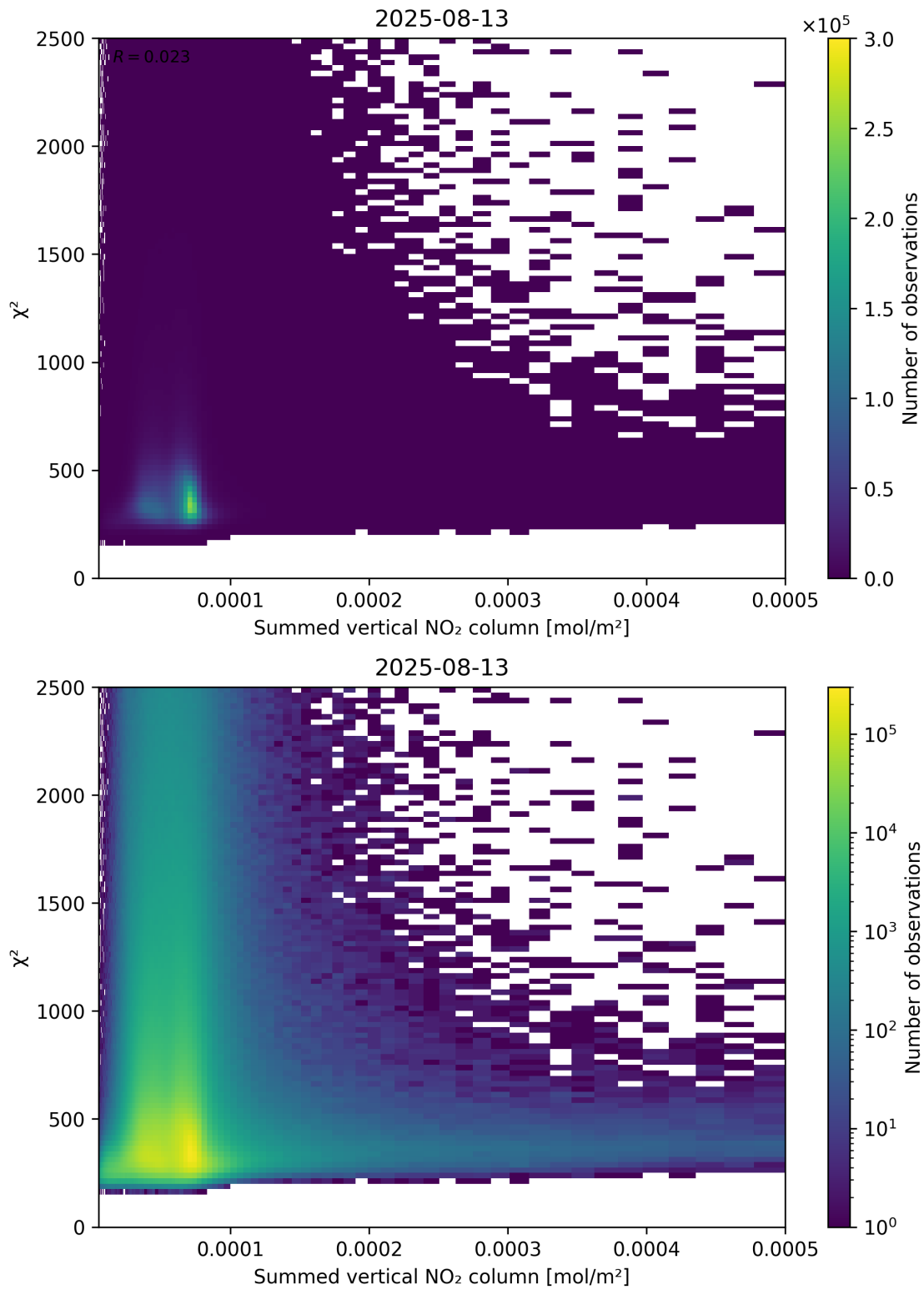
Figure 104: Scatter density plot of “Summed vertical NO 2 column” against “ \chi^2 ” for 2025-08-12 to 2025-08-14.
