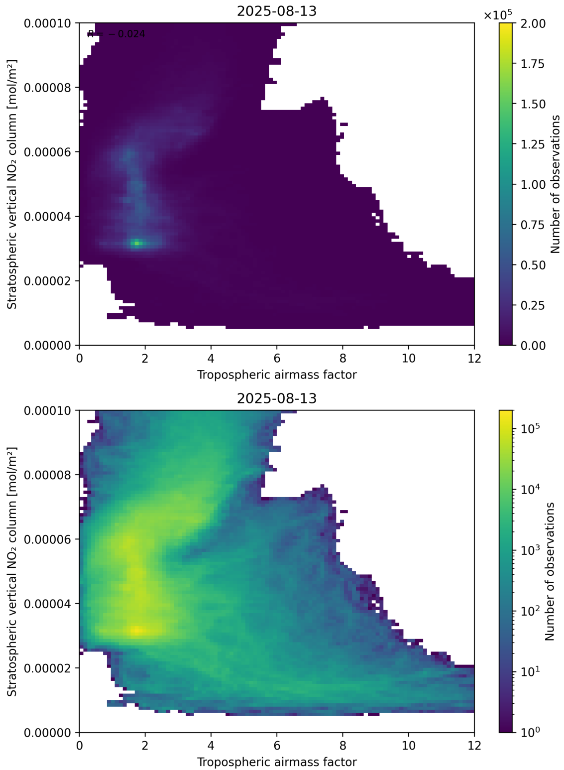
Figure 74: Scatter density plot of “Tropospheric air mass factor” against “Stratospheric vertical NO 2 column” for 2025-08-12 to 2025-08-14.
