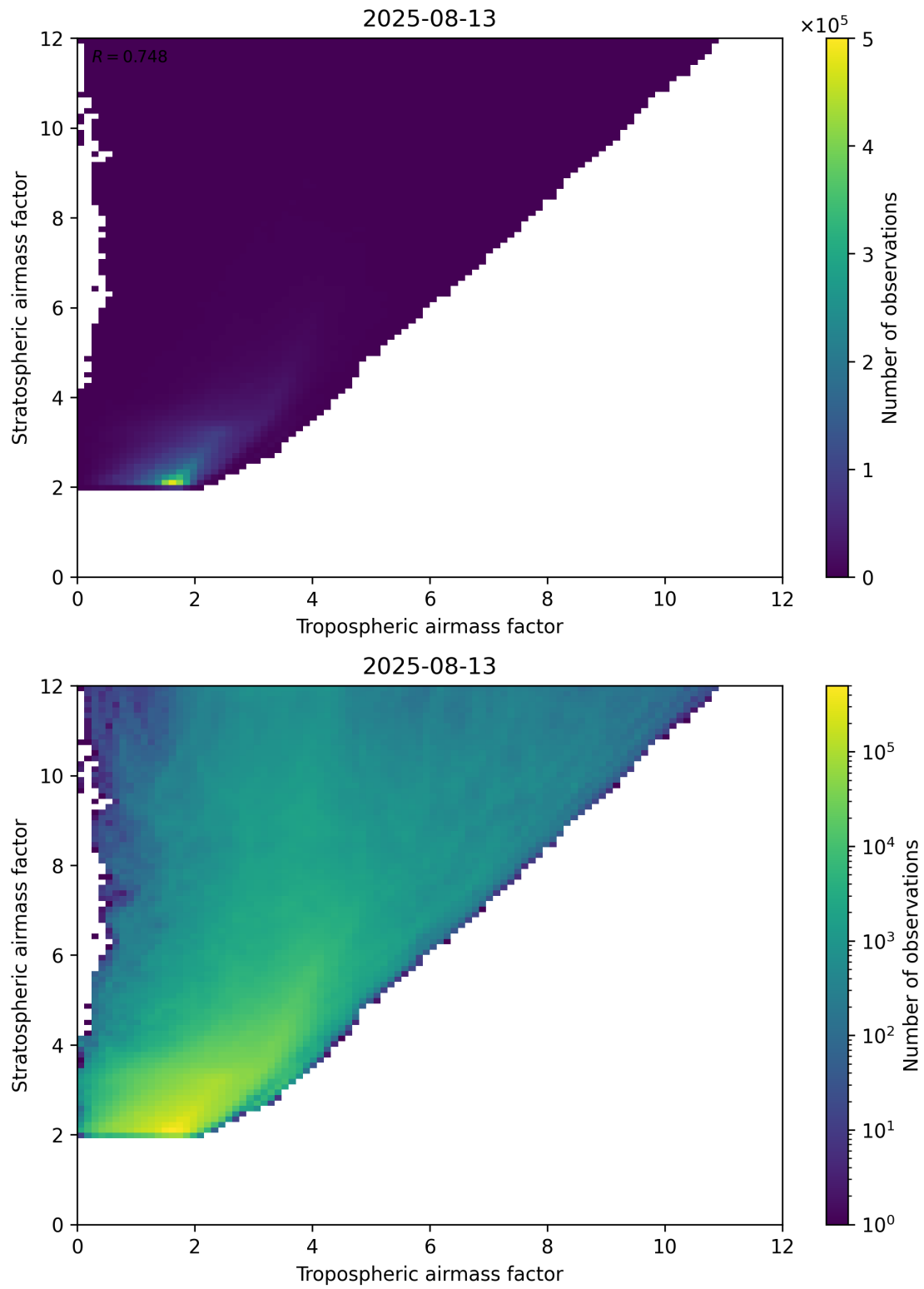
Figure 71: Scatter density plot of “Tropospheric airmass factor” against “Stratospheric airmass factor” for 2025-08-12 to 2025-08-14.
