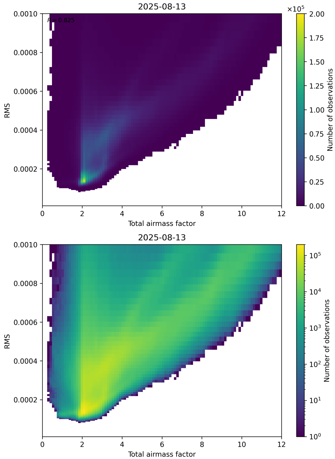
Figure 69: Scatter density plot of “Total airmass factor” against “RMS” for 2025-08-12 to 2025-08-14.
