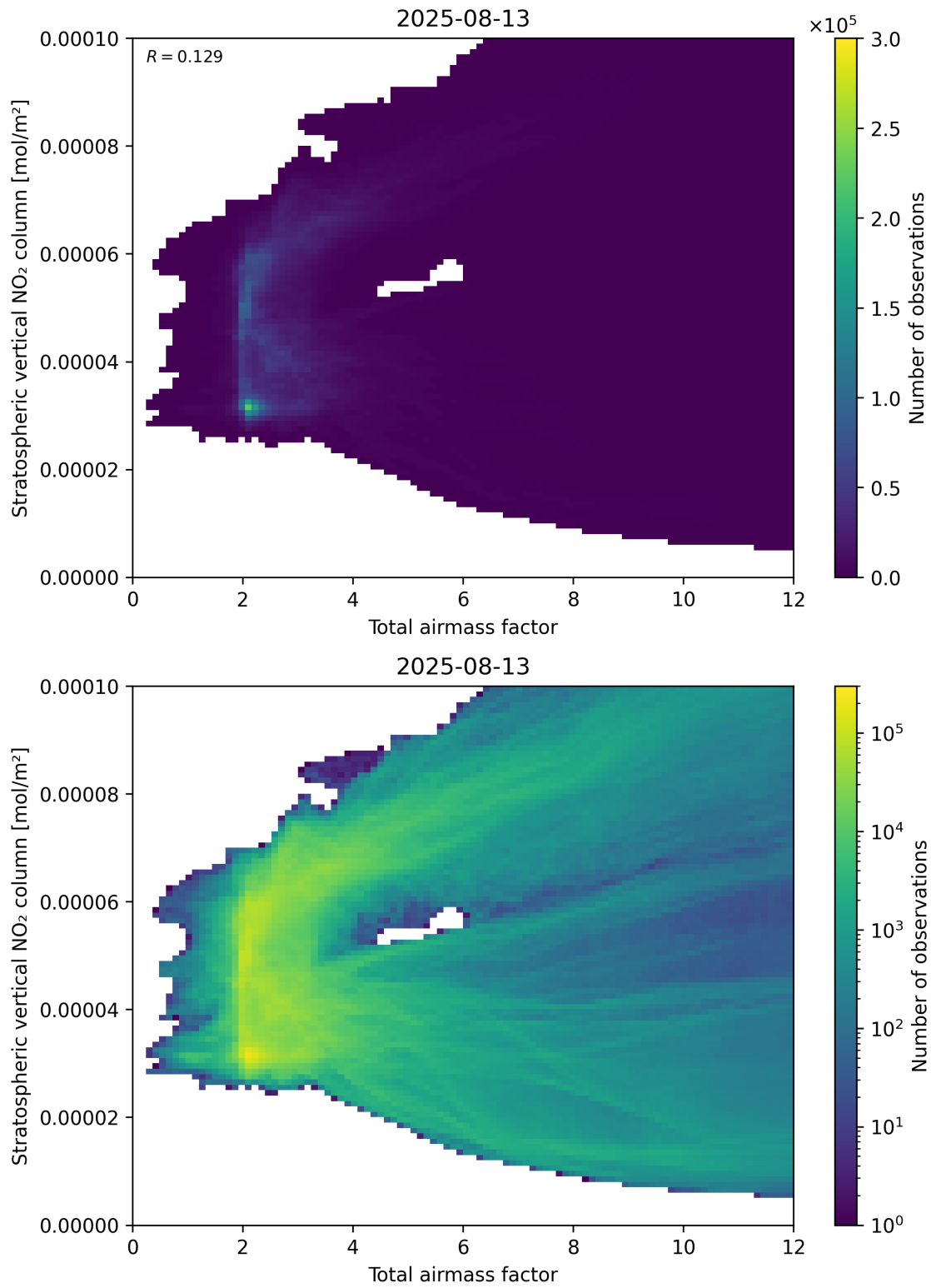
Figure 64: Scatter density plot of “Total airmass factor” against “Stratospheric vertical \text{NO}_2 column” for 2025-08-12 to 2025-08-14.
