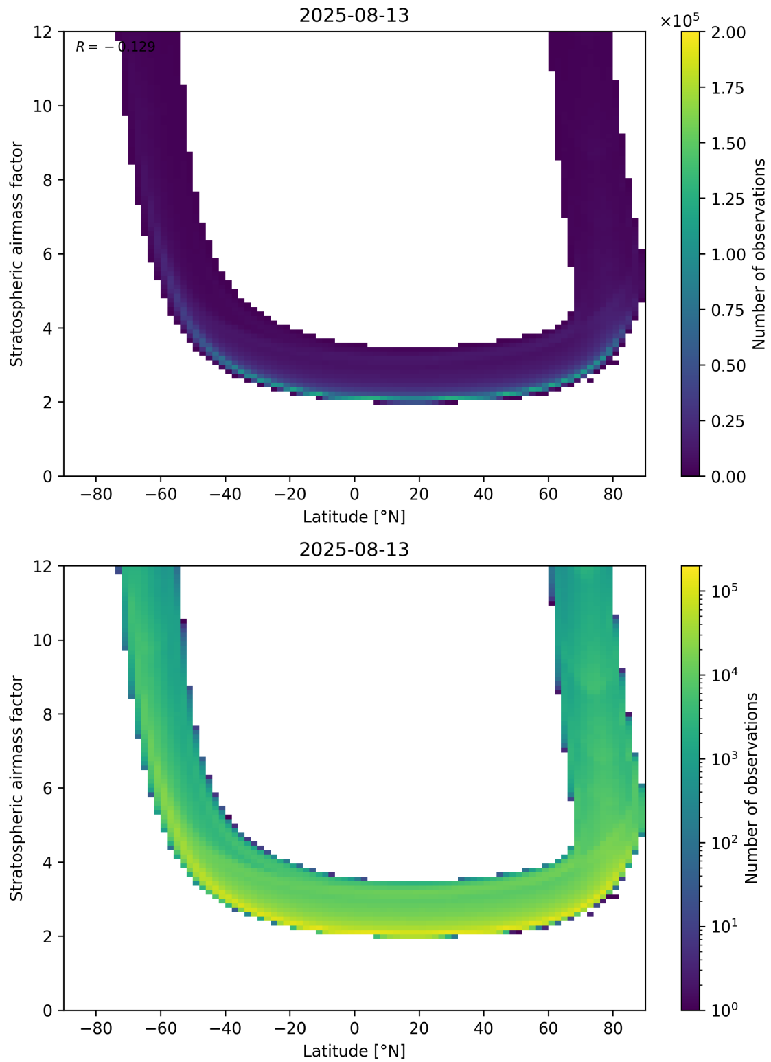
Figure 83: Scatter density plot of “Latitude” against “Stratospheric airmass factor” for 2025-08-12 to 2025-08-14.
