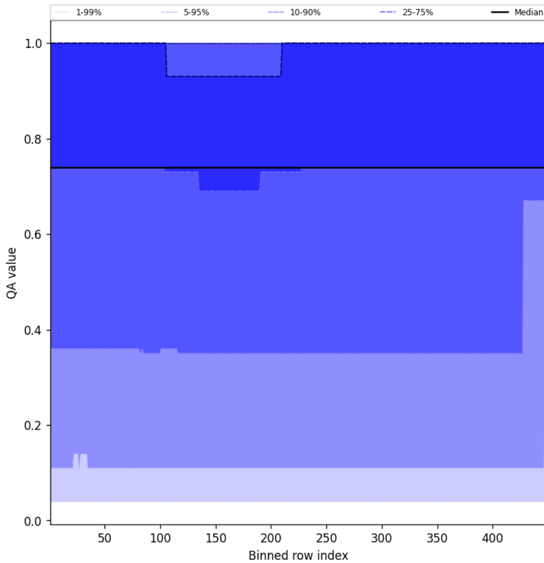
Figure 45: Along track statistics of “QA value” for 2025-08-12 to 2025-08-14
