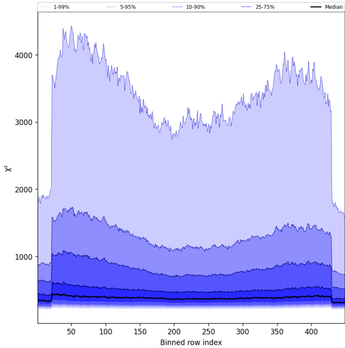
Figure 59: Along track statistics of “ \chi^2 ” for 2025-08-12 to 2025-08-14
