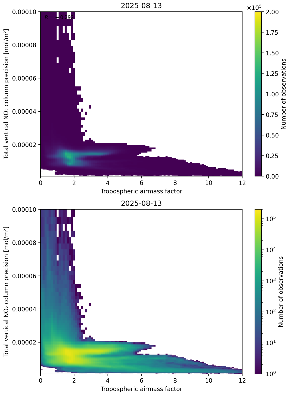
Figure 78: Scatter density plot of “Tropospheric air mass factor” against “Total vertical NO 2 column precision” for 2025-08-12 to 2025-08-14.
