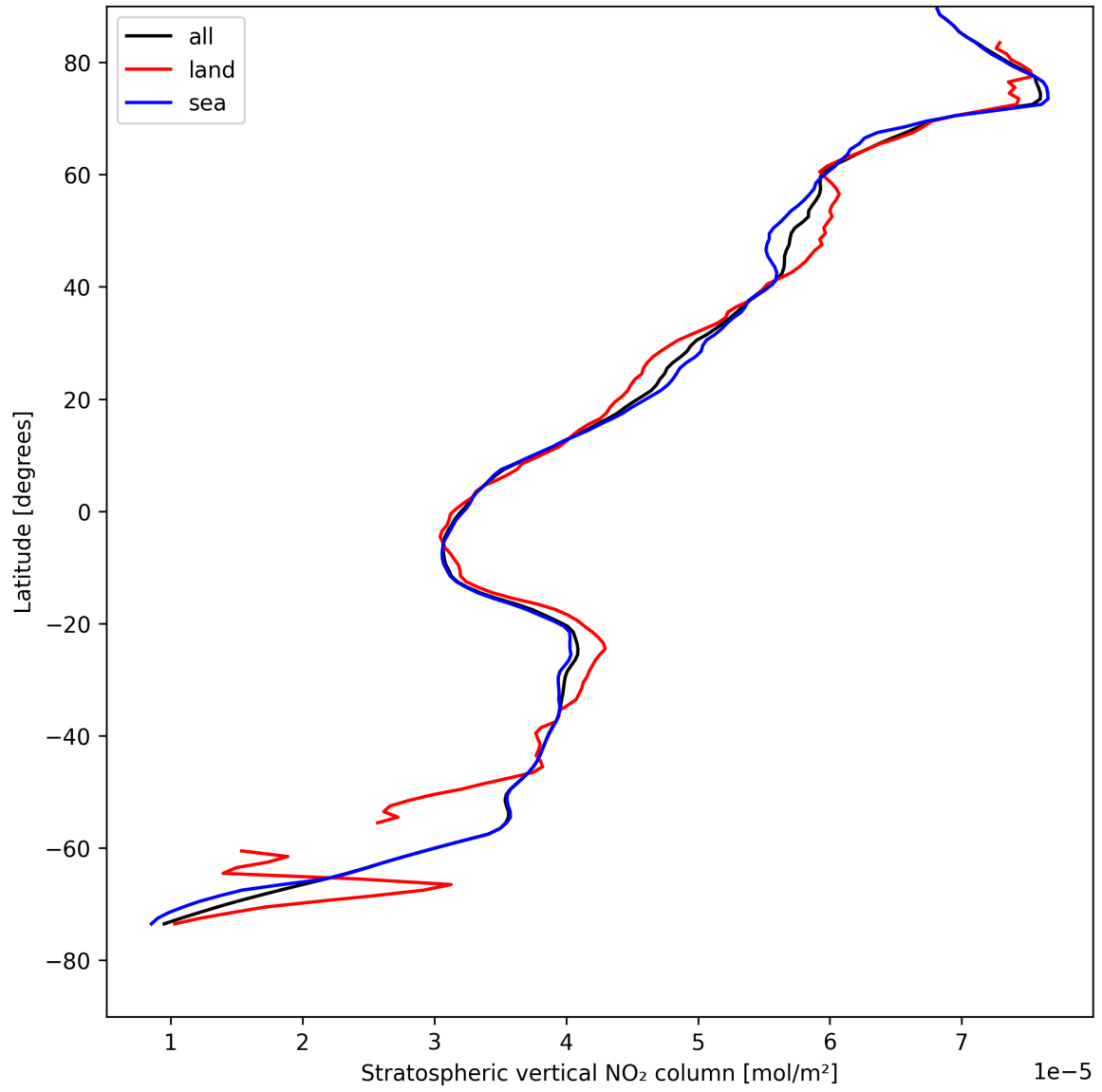
Figure 19: Zonal average of “Stratospheric vertical NO 2 column” for 2025-08-12 to 2025-08-14.
