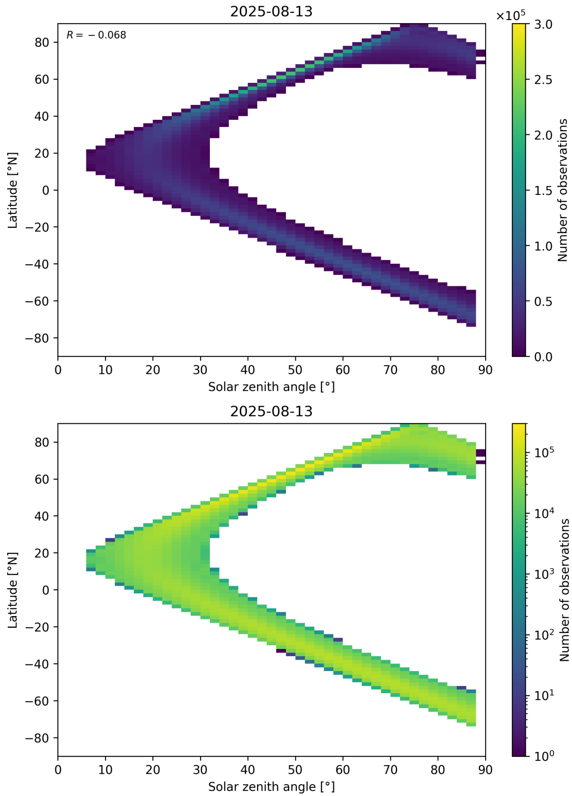
Figure 149: Scatter density plot of “Solar zenith angle” against “Latitude” for 2025-08-12 to 2025-08-14.
