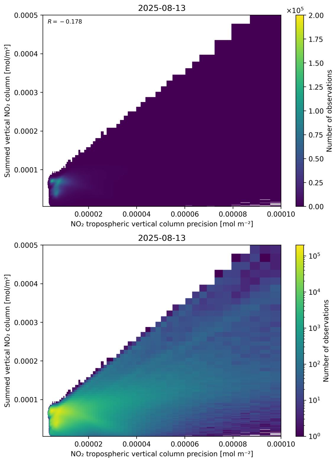
Figure 136: Scatter density plot of “NO 2 tropospheric vertical column precision” against “Summed vertical NO 2 column” for 2025-08-12 to 2025-08-14.
