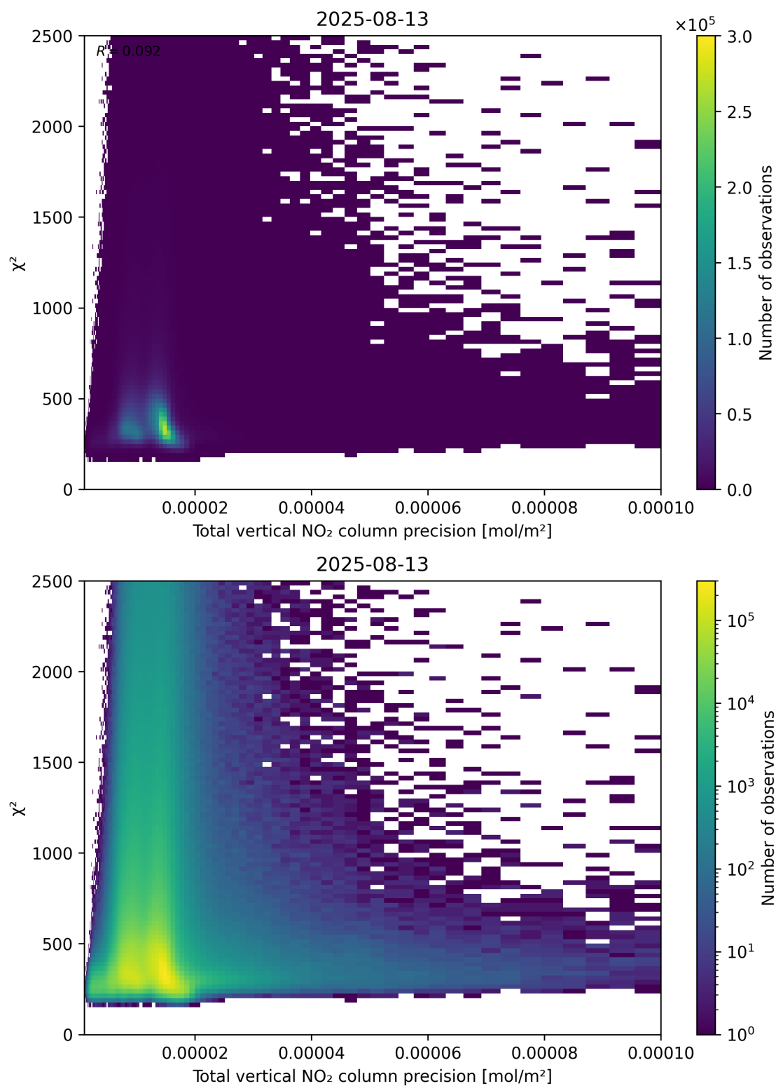
Figure 116: Scatter density plot of “Total vertical NO 2 column precision” against “ \chi^2 ” for 2025-08-12 to 2025-08-14.
