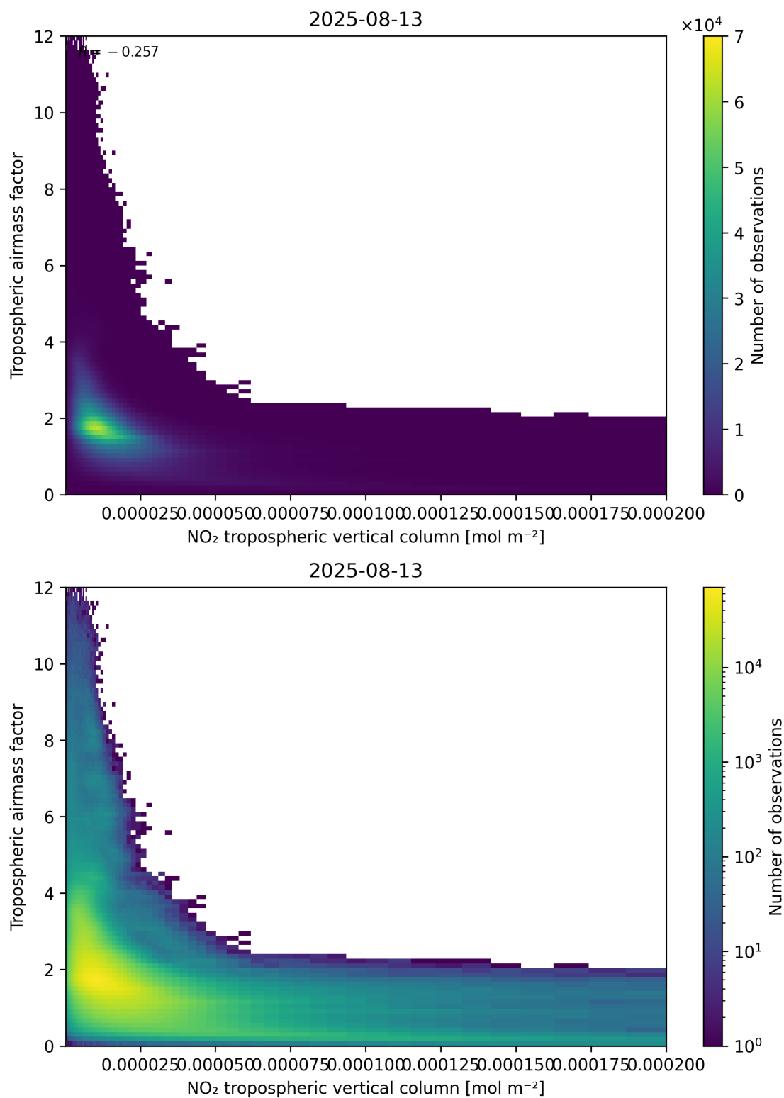
Figure 123: Scatter density plot of “NO 2 tropospheric vertical column” against “Tropospheric air mass factor” for 2025-08-12 to 2025-08-14.
