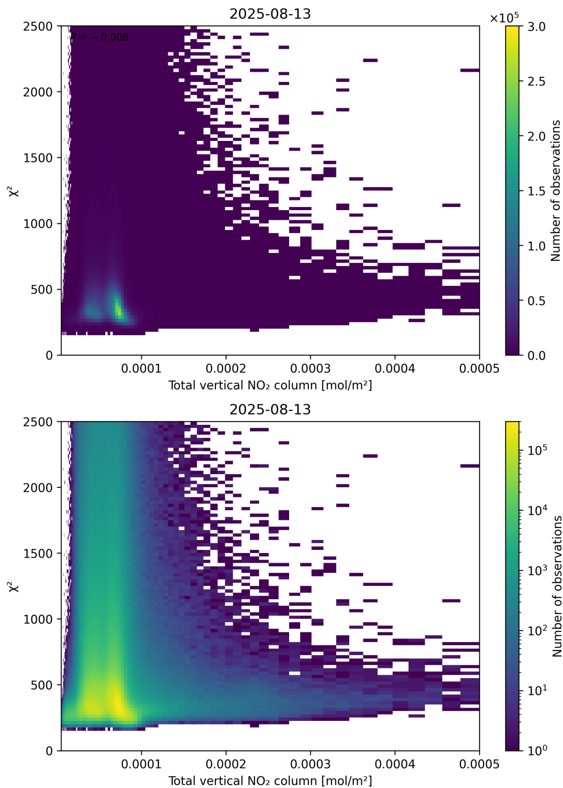
Figure 111: Scatter density plot of “Total vertical NO 2 column” against “ \chi^2 ” for 2025-08-12 to 2025-08-14.
