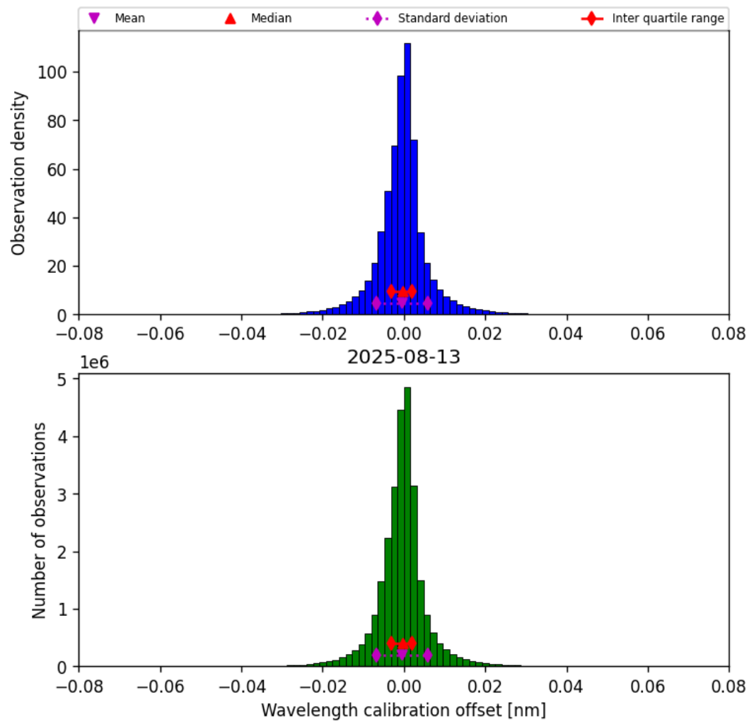
Figure 35: Histogram of “Wavelength calibration offset” for 2025-08-12 to 2025-08-14
