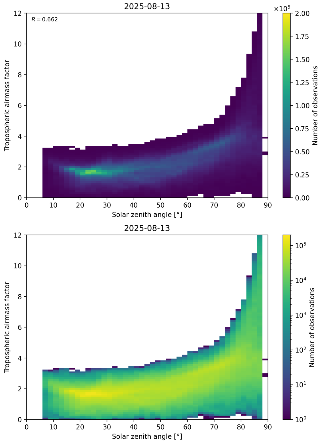
Figure 147: Scatter density plot of “Solar zenith angle” against “Tropospheric airmass factor” for 2025-08-12 to 2025-08-14.
