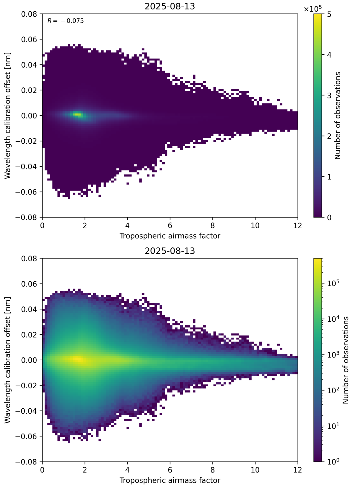
Figure 80: Scatter density plot of “Tropospheric airmass factor” against “Wavelength calibration offset” for 2025-08-12 to 2025-08-14.
