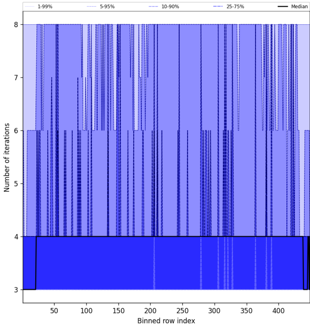
Figure 51: Along track statistics of “Number of iterations” for 2025-08-12 to 2025-08-14
