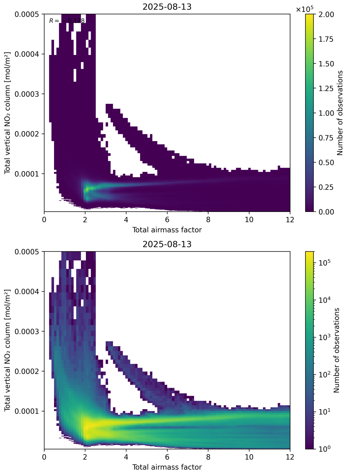
Figure 67: Scatter density plot of “Total airmass factor” against “Total vertical NO 2 column” for 2025-08-12 to 2025-08-14.
