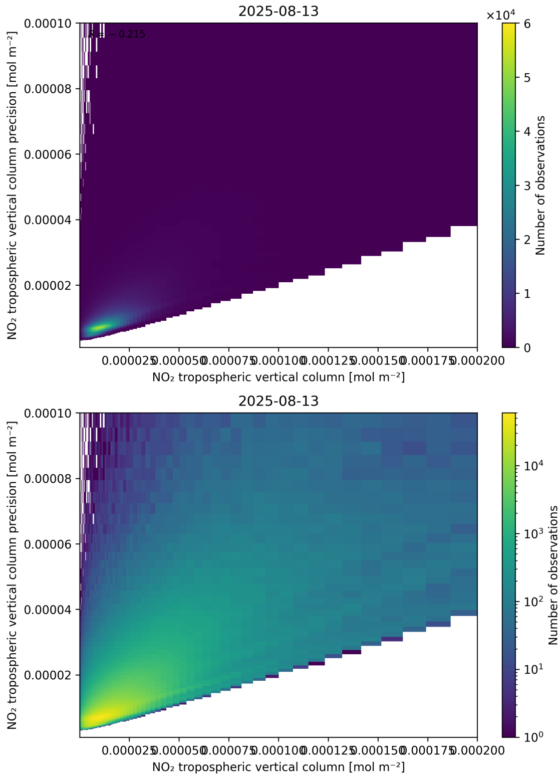
Figure 130: Scatter density plot of “NO 2 tropospheric vertical column” against “NO 2 tropospheric vertical column precision” for 2025-08-12 to 2025-08-14.
