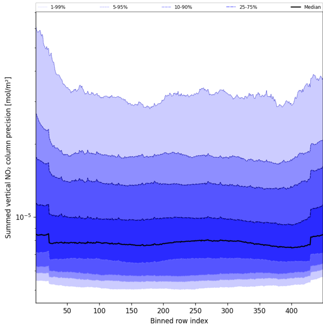
Figure 58: Along track statistics of “Summed vertical NO 2 column precision” for 2025-08-12 to 2025-08-14
