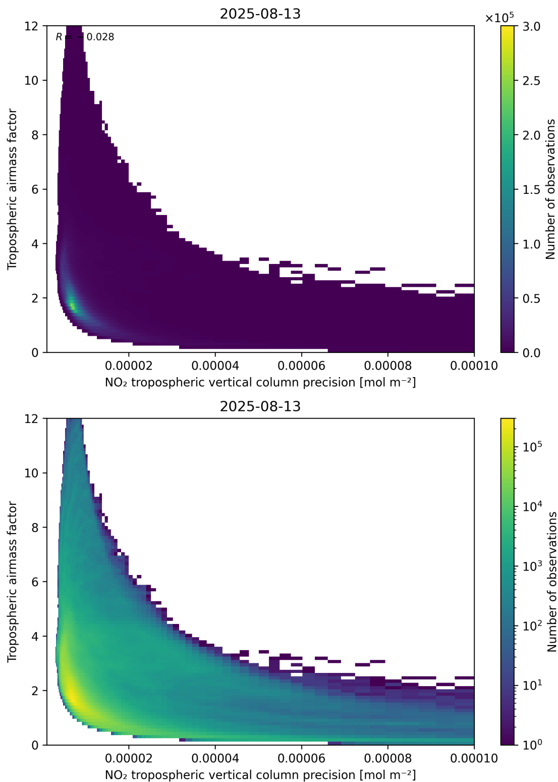
Figure 133: Scatter density plot of “NO 2 tropospheric vertical column precision” against “Tropospheric airmass factor” for 2025-08-12 to 2025-08-14.
