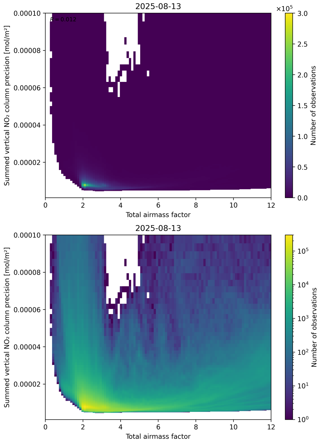
Figure 66: Scatter density plot of “Total airmass factor” against “Summed vertical NO 2 column precision” for 2025-08-12 to 2025-08-14.
