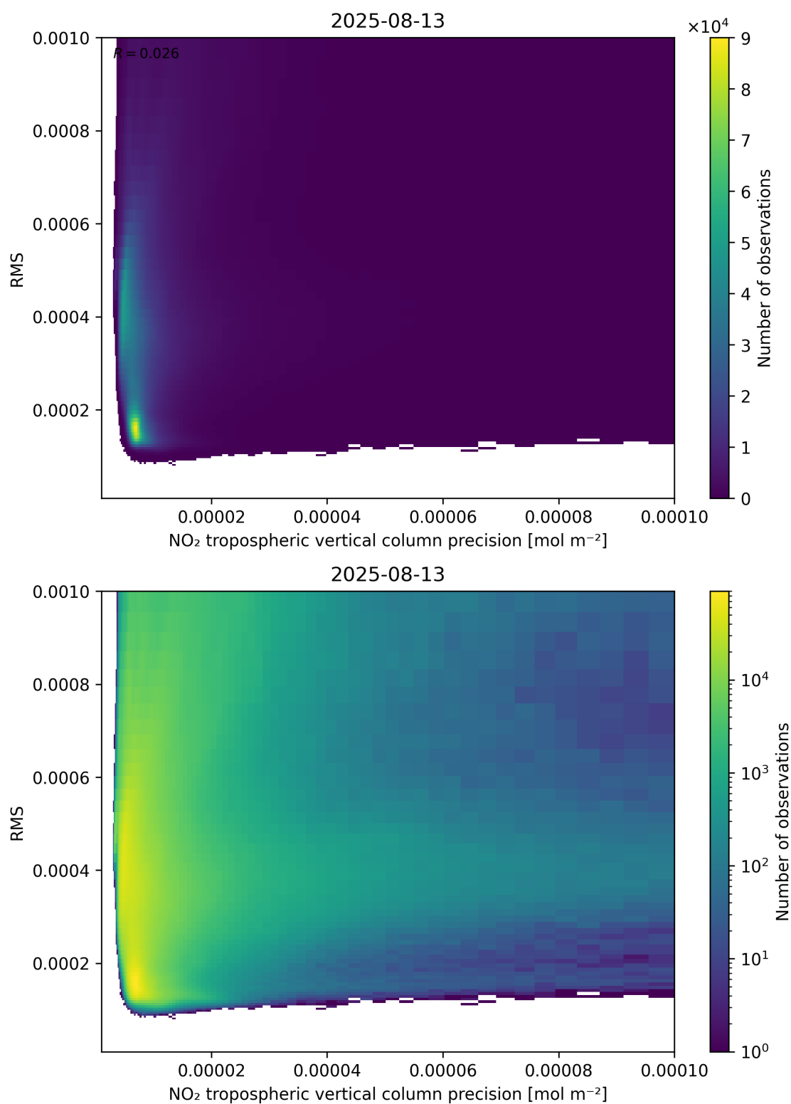
Figure 140: Scatter density plot of “NO 2 tropospheric vertical column precision” against “RMS” for 2025-08-12 to 2025-08-14.
