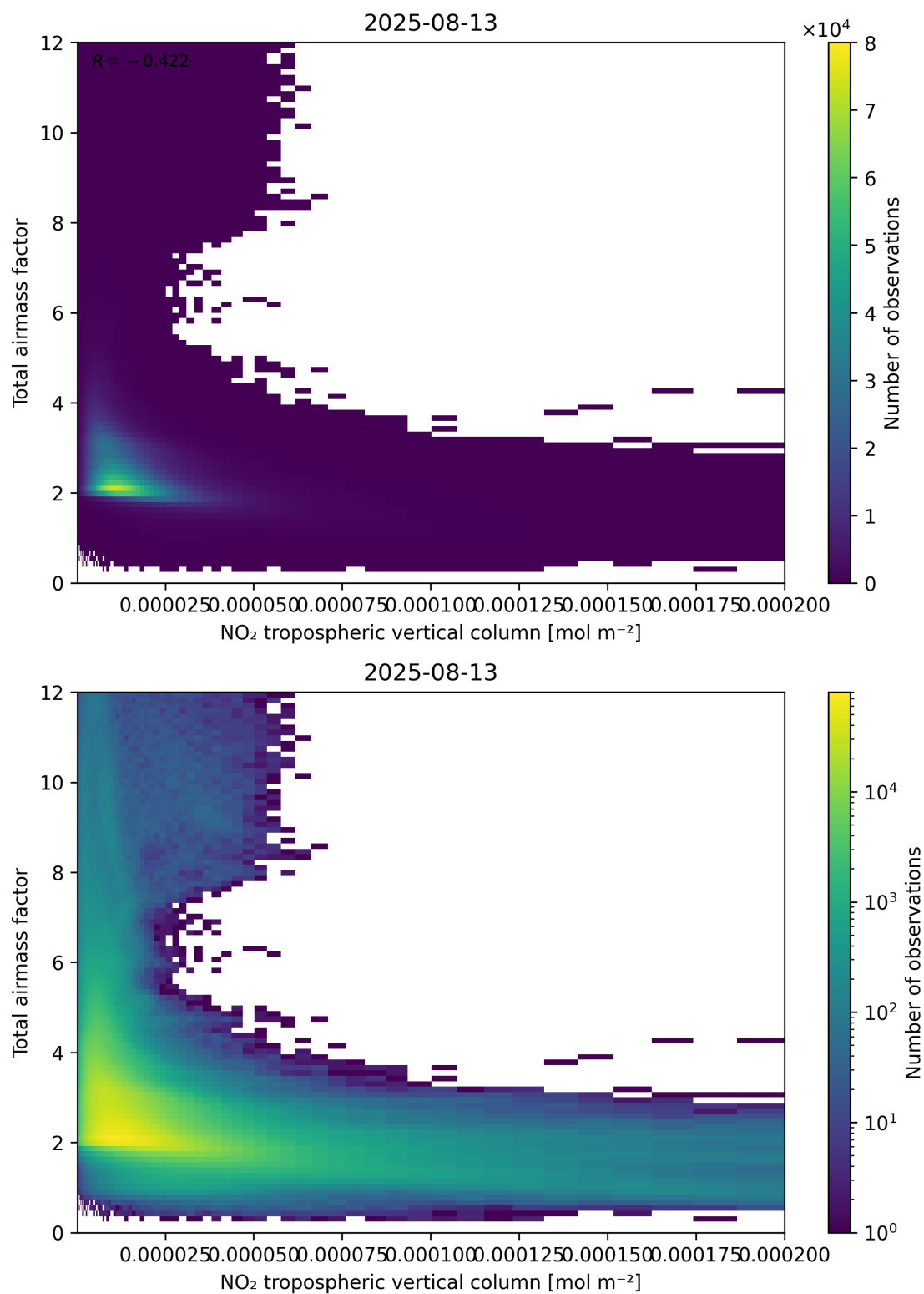
Figure 122: Scatter density plot of “NO 2 tropospheric vertical column” against “Total air mass factor” for 2025-08-12 to 2025-08-14.
