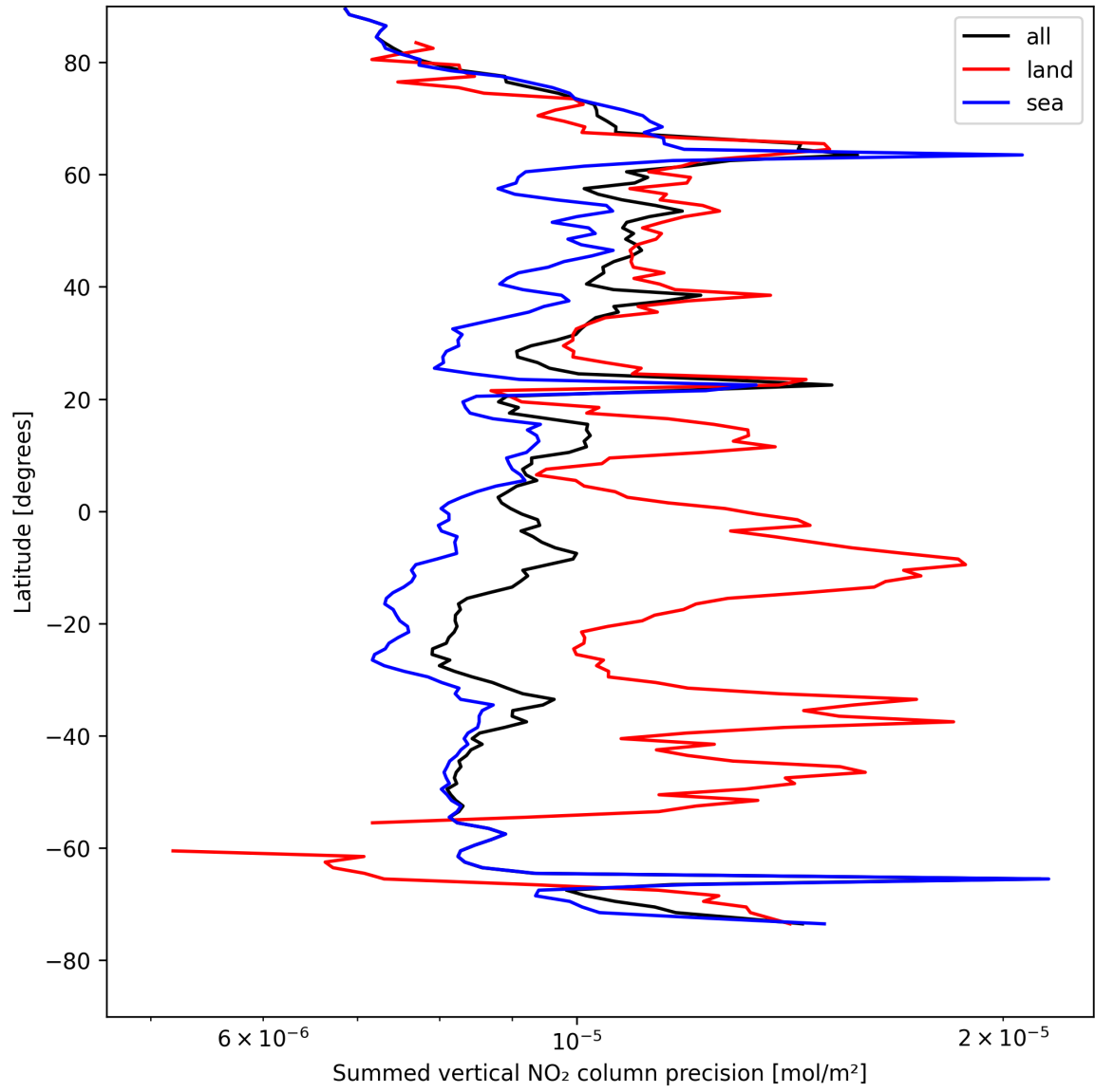
Figure 24: Zonal average of “Summed vertical NO 2 column precision” for 2025-08-12 to 2025-08-14.
