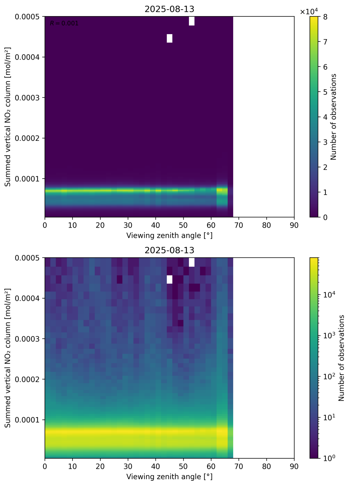
Figure 165: Scatter density plot of “Viewing zenith angle” against “Summed vertical NO 2 column” for 2025-08-12 to 2025-08-14.
