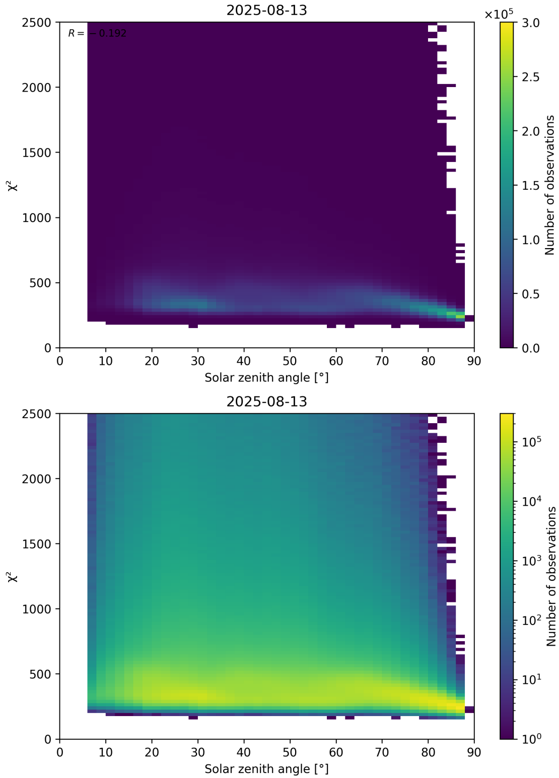
Figure 148: Scatter density plot of “Solar zenith angle” against “ \chi^2 ” for 2025-08-12 to 2025-08-14.
