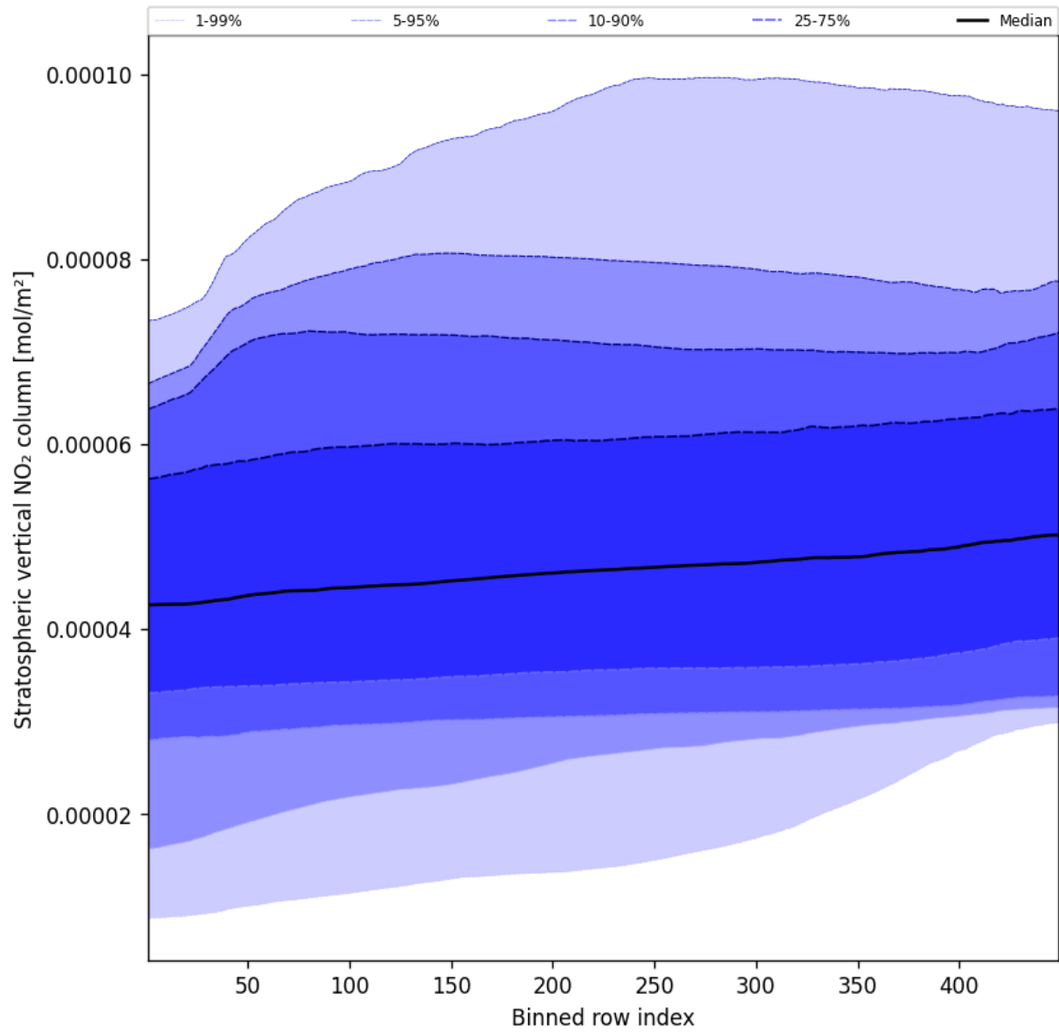
Figure 53: Along track statistics of “Stratospheric vertical NO 2 column” for 2025-08-12 to 2025-08-14
