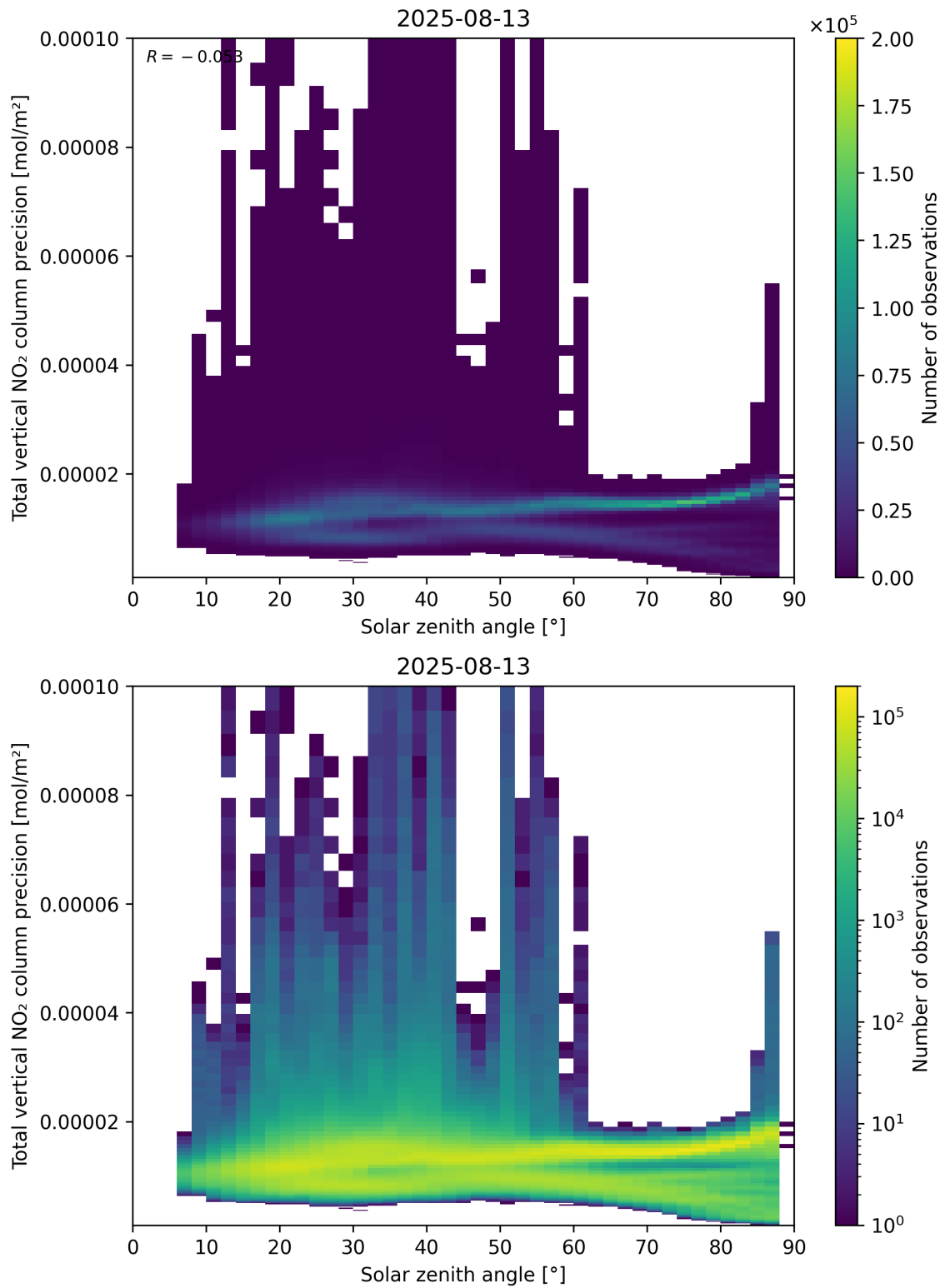
Figure 154: Scatter density plot of “Solar zenith angle” against “Total vertical NO 2 column precision” for 2025-08-12 to 2025-08-14.
