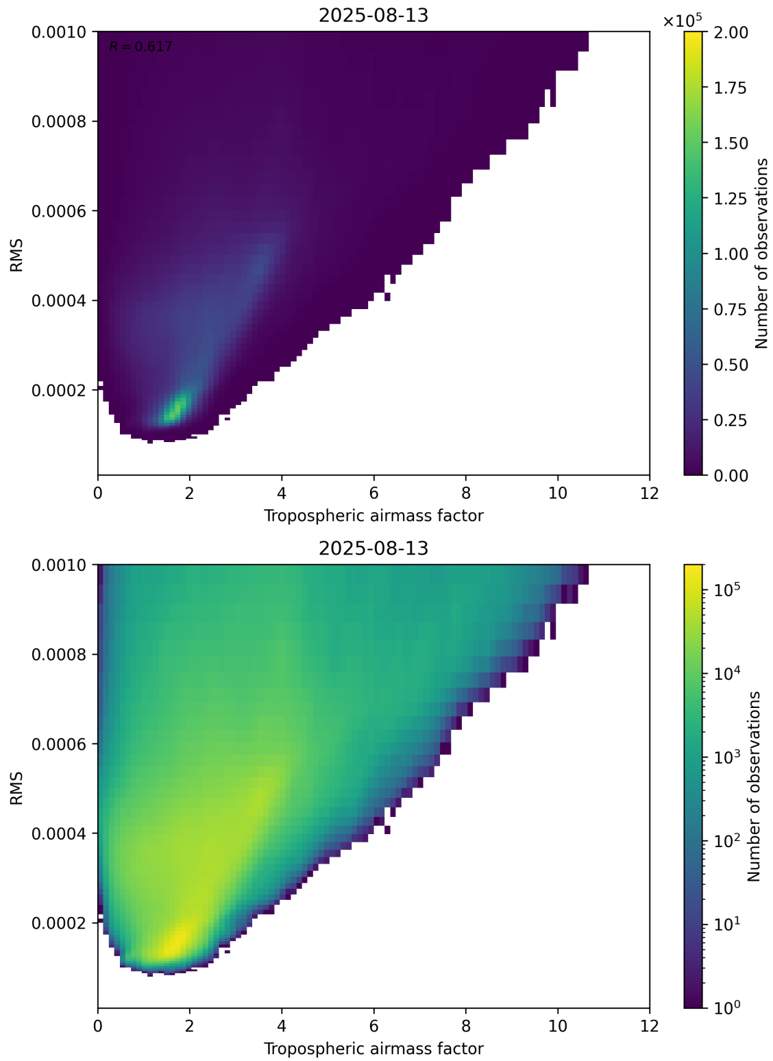
Figure 79: Scatter density plot of “Tropospheric airmass factor” against “RMS” for 2025-08-12 to 2025-08-14.
