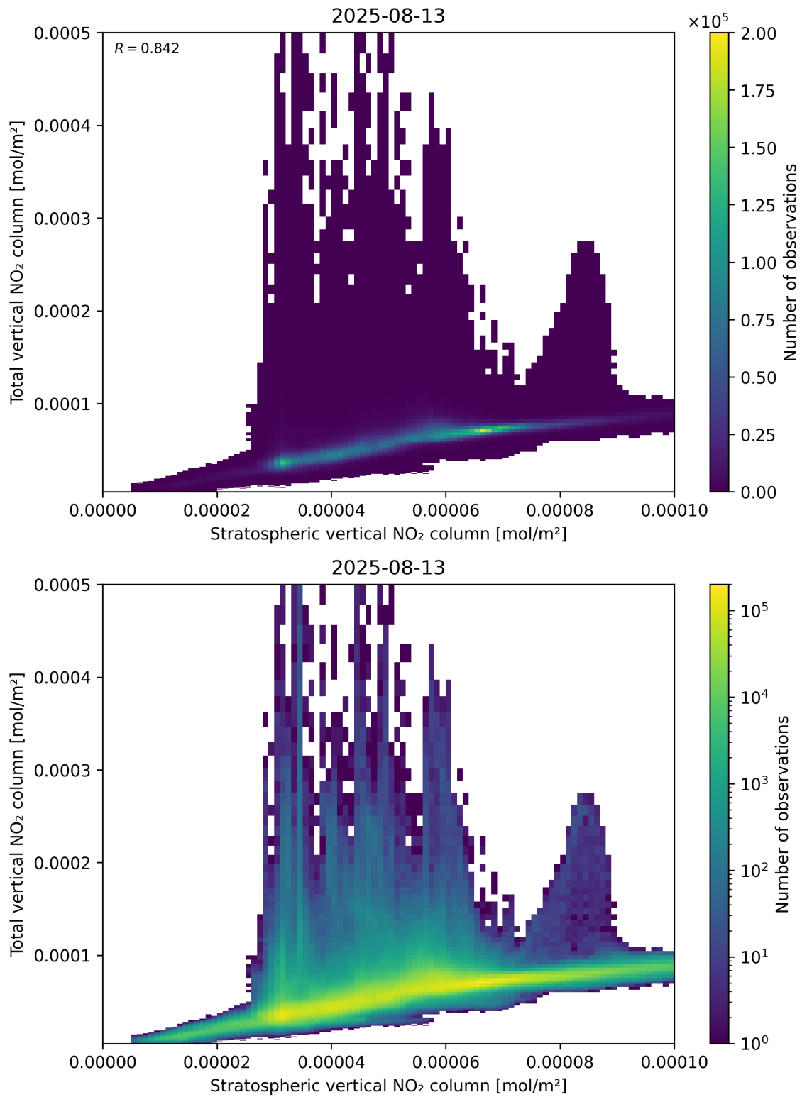
Figure 100: Scatter density plot of “Stratospheric vertical NO 2 column” against “Total vertical NO 2 column” for 2025-08-12 to 2025-08-14.
