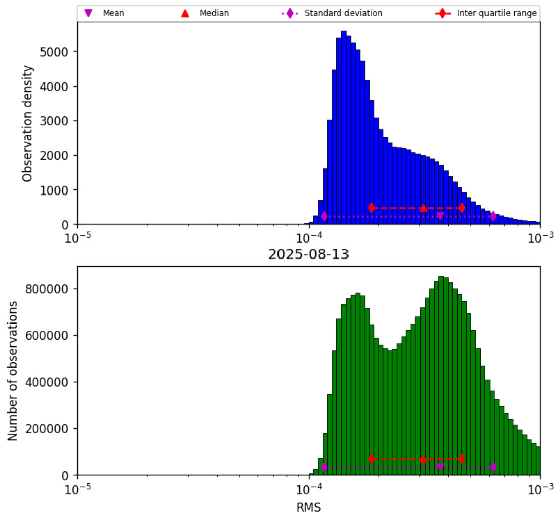
Figure 43: Histogram of “RMS” for 2025-08-12 to 2025-08-14
