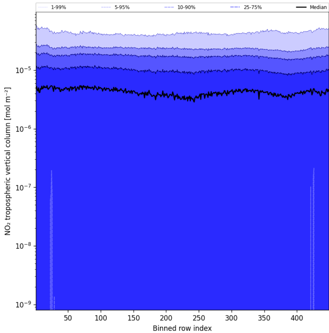
Figure 46: Along track statistics of “NO 2 tropospheric vertical column” for 2025-08-12 to 2025-08-14
