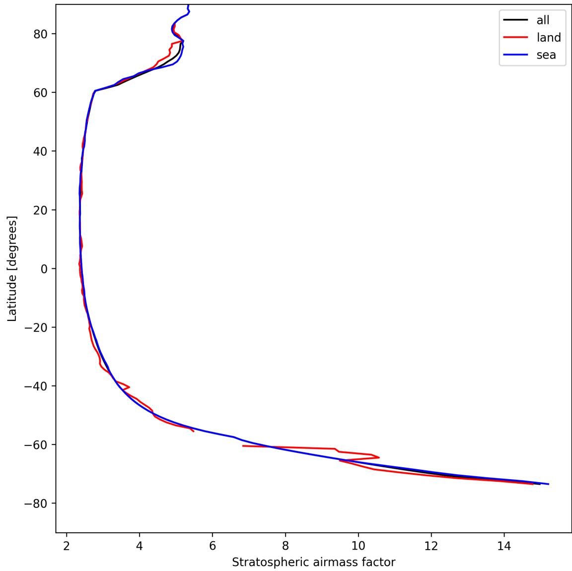
Figure 27: Zonal average of “Stratospheric airmass factor” for 2025-08-12 to 2025-08-14.
