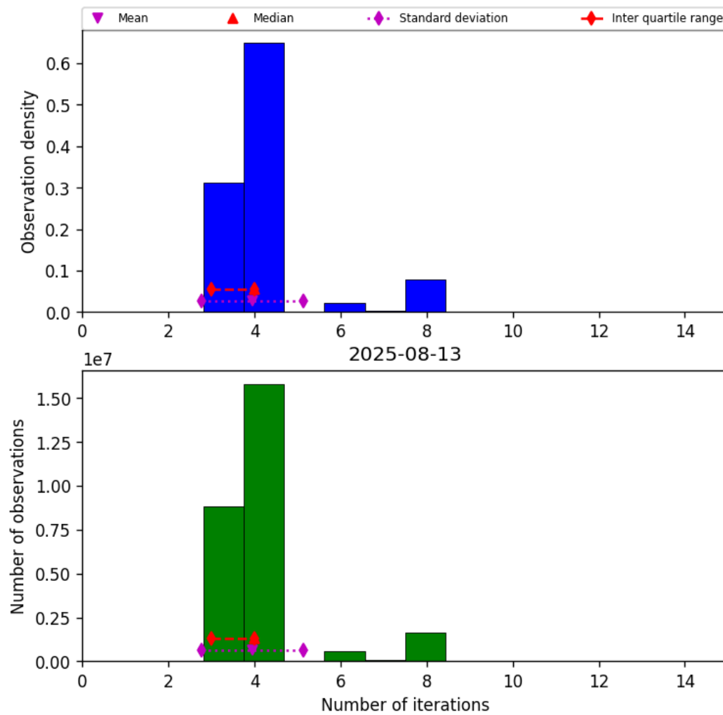
Figure 34: Histogram of “Number of iterations” for 2025-08-12 to 2025-08-14
