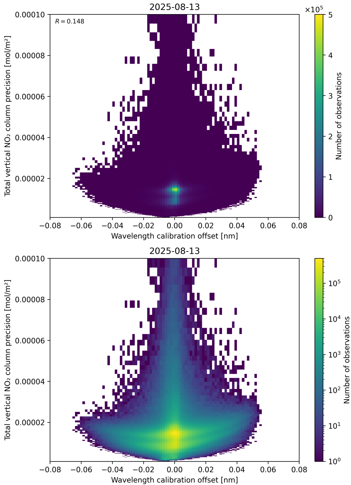
Figure 180: Scatter density plot of “Wavelength calibration offset” against “Total vertical NO 2 column precision” for 2025-08-12 to 2025-08-14.
