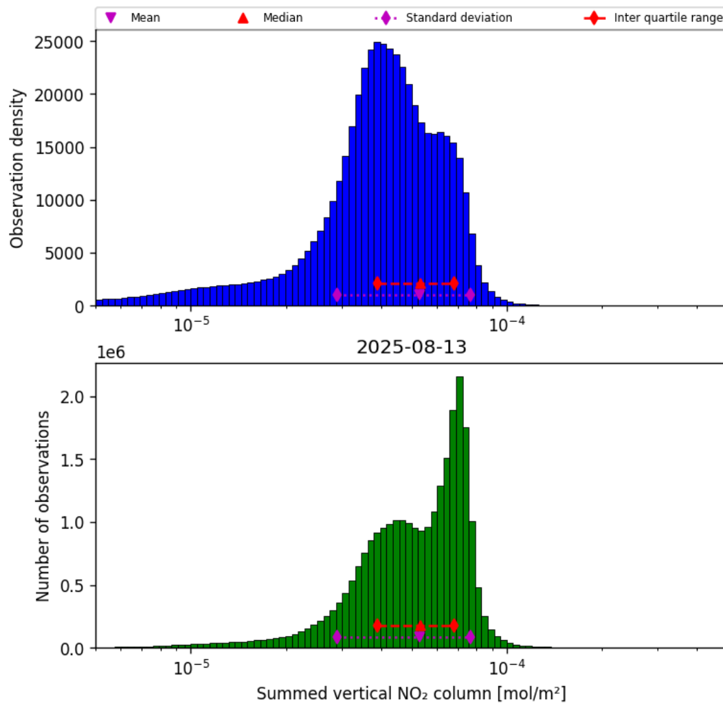
Figure 40: Histogram of “Summed vertical NO 2 column” for 2025-08-12 to 2025-08-14
