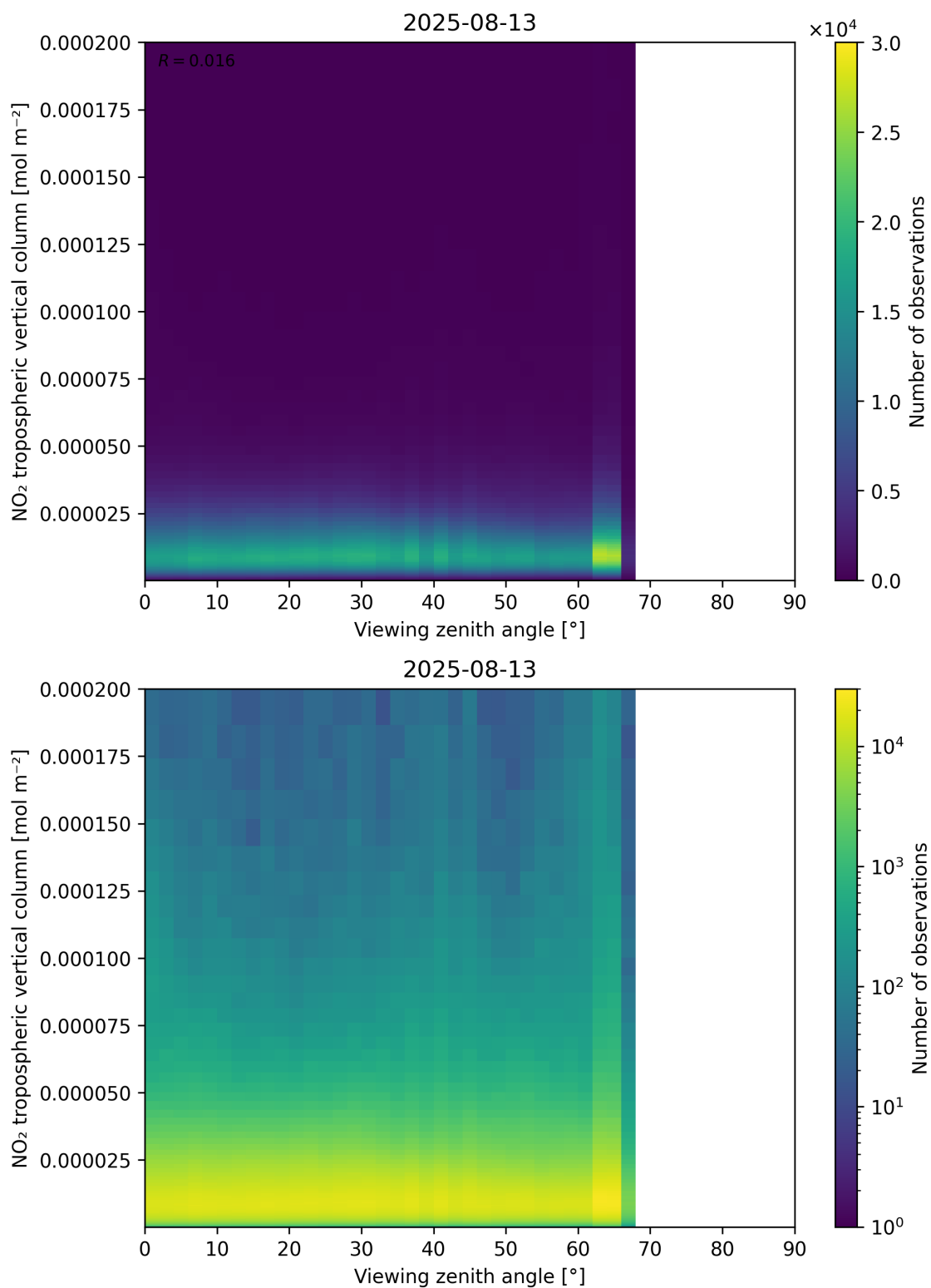
Figure 169: Scatter density plot of “Viewing zenith angle” against “NO 2 tropospheric vertical column” for 2025-08-12 to 2025-08-14.
