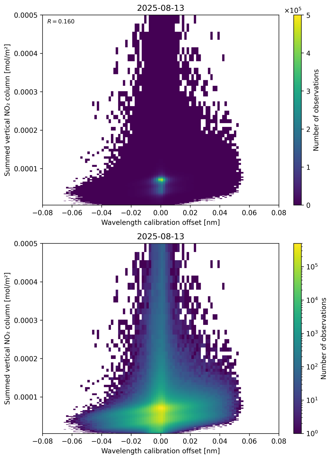
Figure 177: Scatter density plot of “Wavelength calibration offset” against “Summed vertical NO 2 column” for 2025-08-12 to 2025-08-14.
