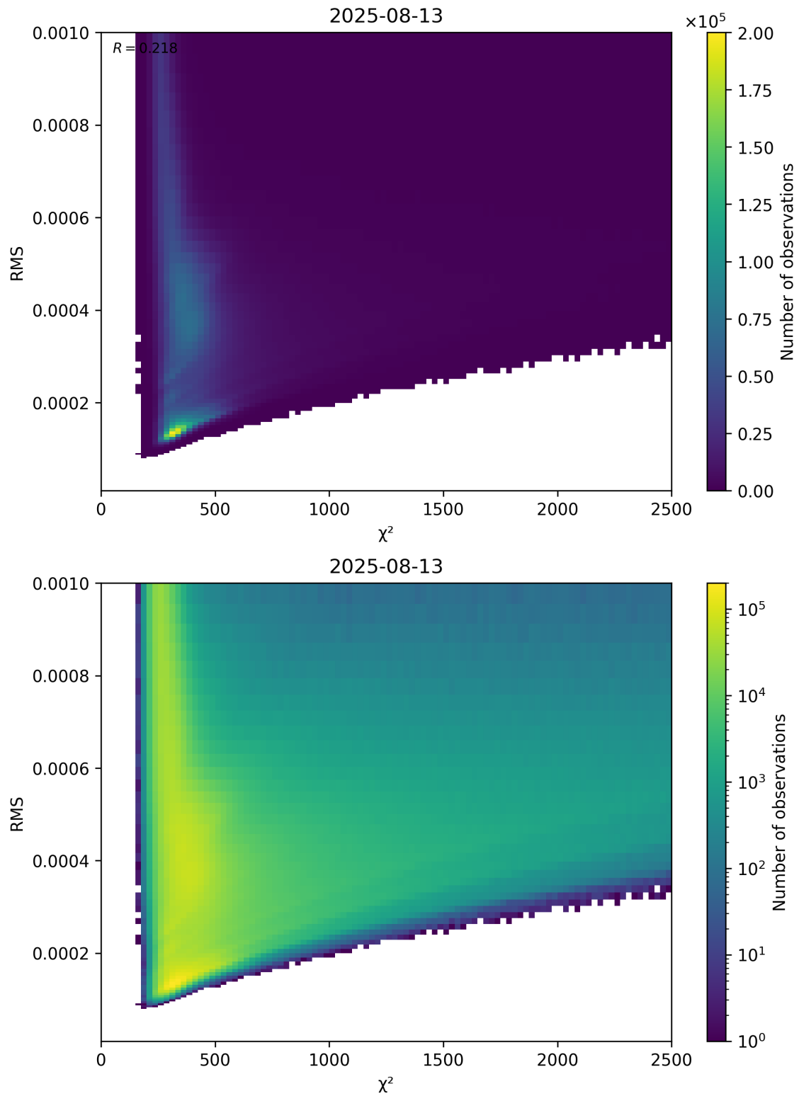
Figure 82: Scatter density plot of “ \chi^2 ” against “RMS” for 2025-08-12 to 2025-08-14.
