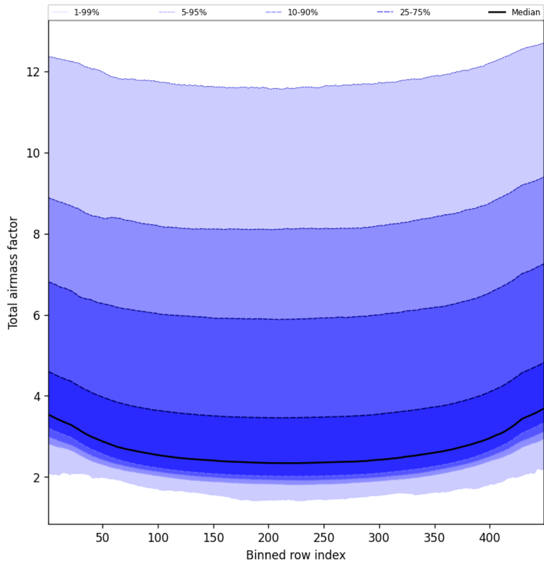
Figure 49: Along track statistics of “Total airmass factor” for 2025-08-12 to 2025-08-14
