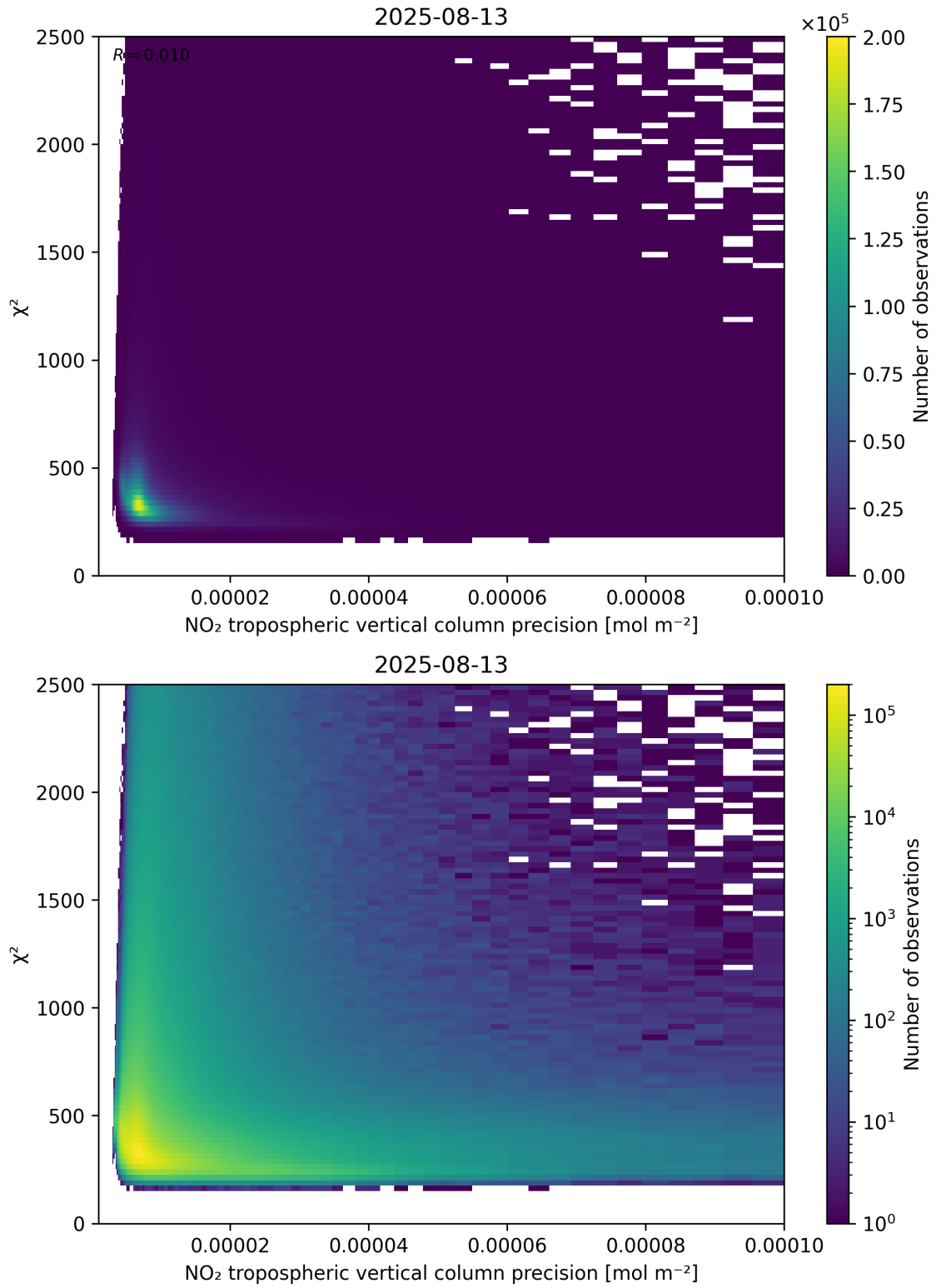
Figure 134: Scatter density plot of “NO 2 tropospheric vertical column precision” against “ \chi^2 ” for 2025-08-12 to 2025-08-14.
