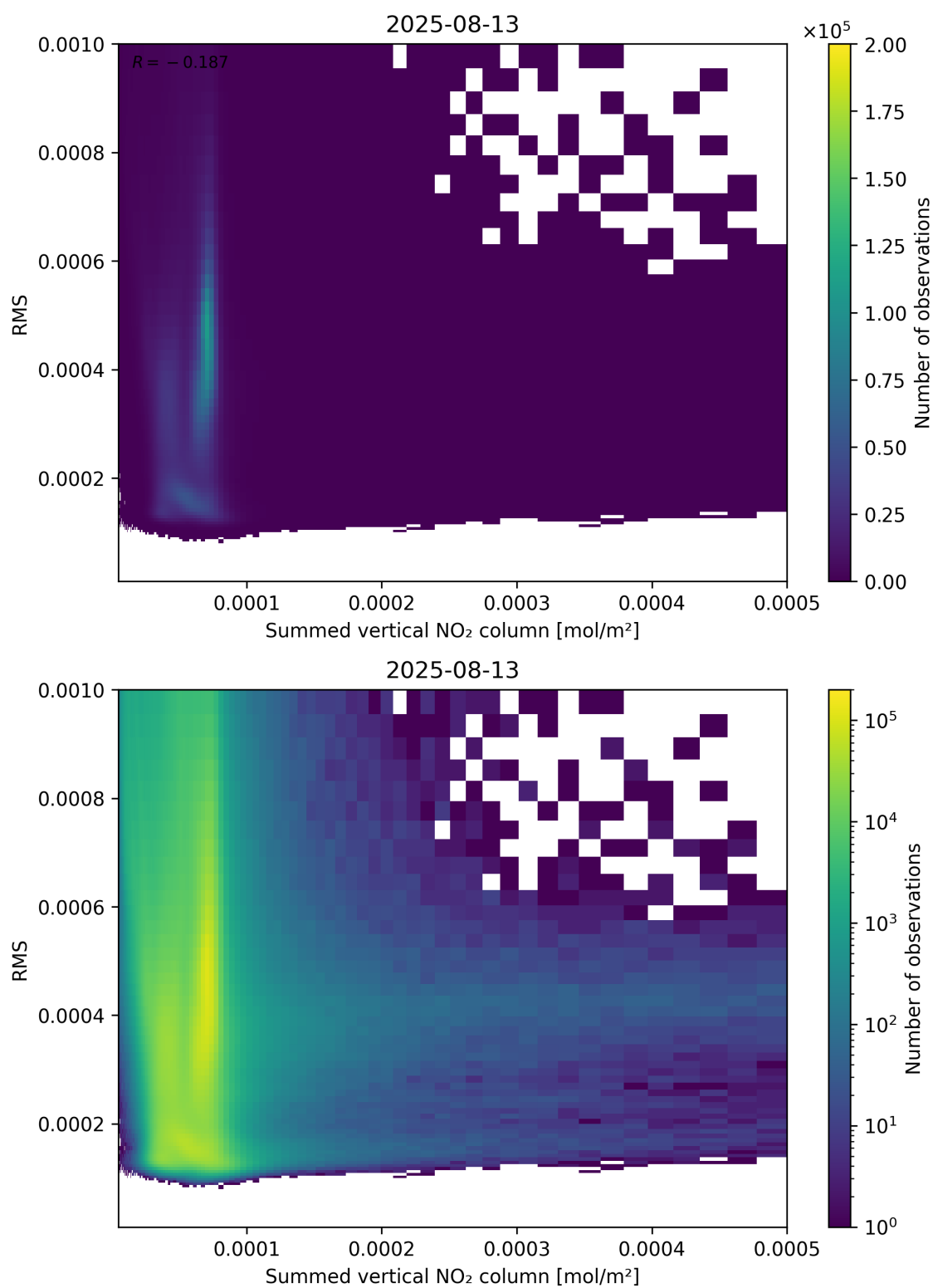
Figure 109: Scatter density plot of “Summed vertical NO 2 column” against “RMS” for 2025-08-12 to 2025-08-14.
