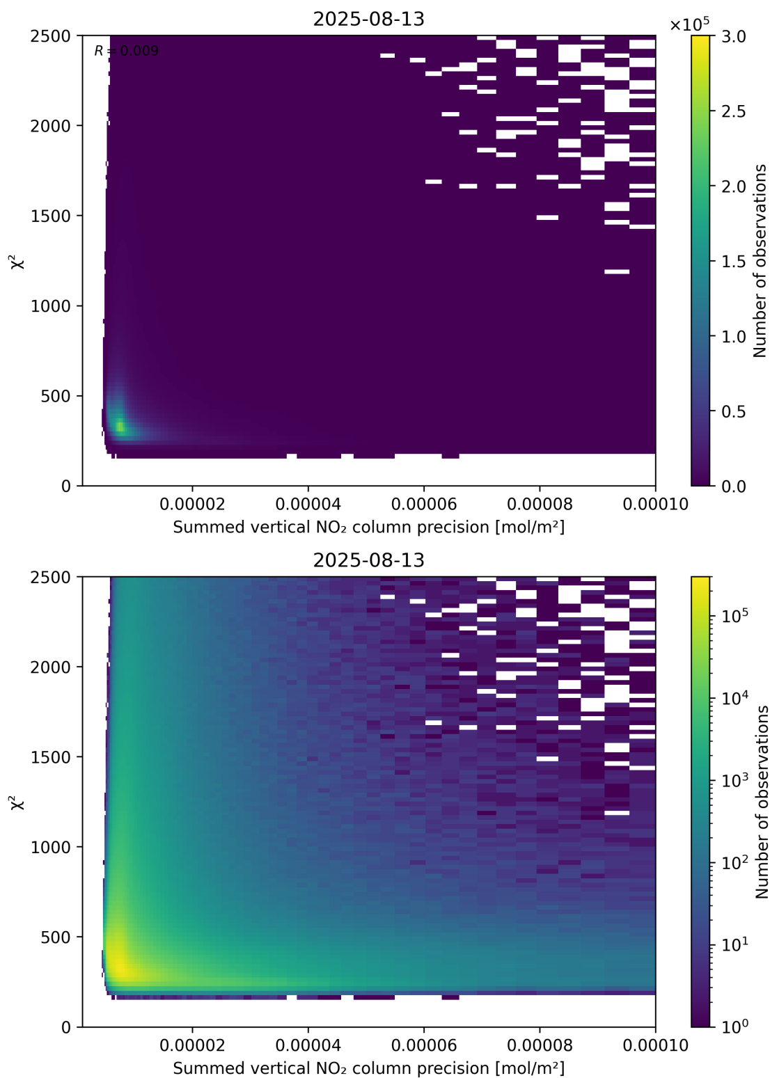
Figure 107: Scatter density plot of “Summed vertical NO 2 column precision” against “ \chi^2 ” for 2025-08-12 to 2025-08-14.
