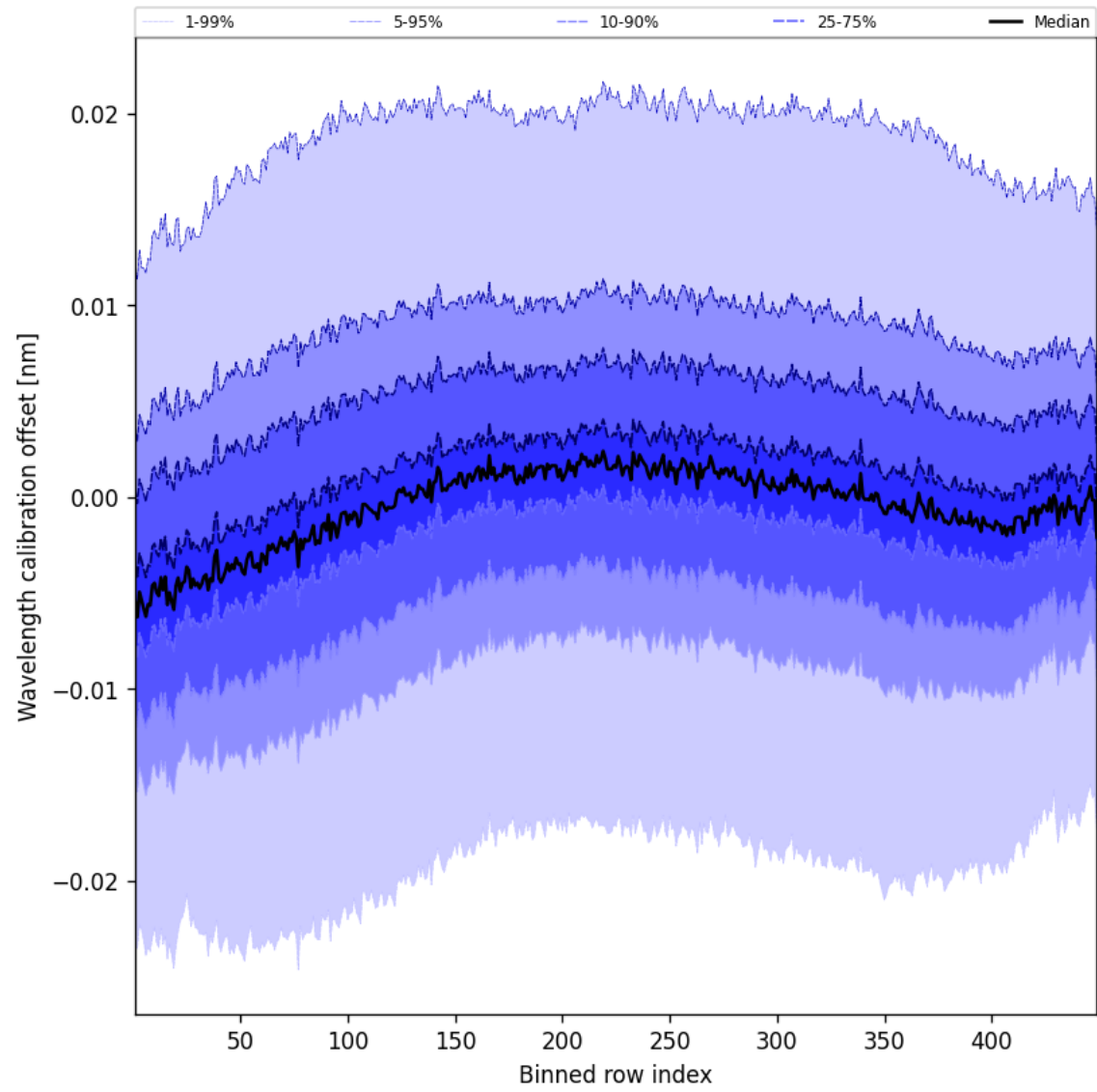
Figure 52: Along track statistics of “Wavelength calibration offset” for 2025-08-12 to 2025-08-14
