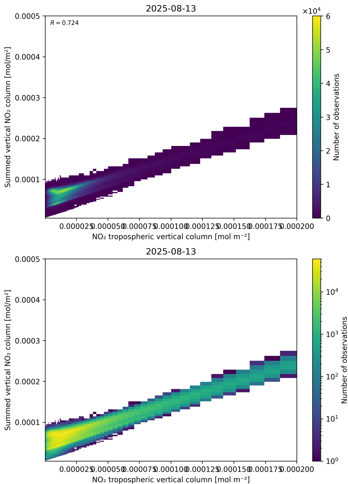
Figure 126: Scatter density plot of “NO 2 tropospheric vertical column” against “Summed vertical NO 2 column” for 2025-08-12 to 2025-08-14.
