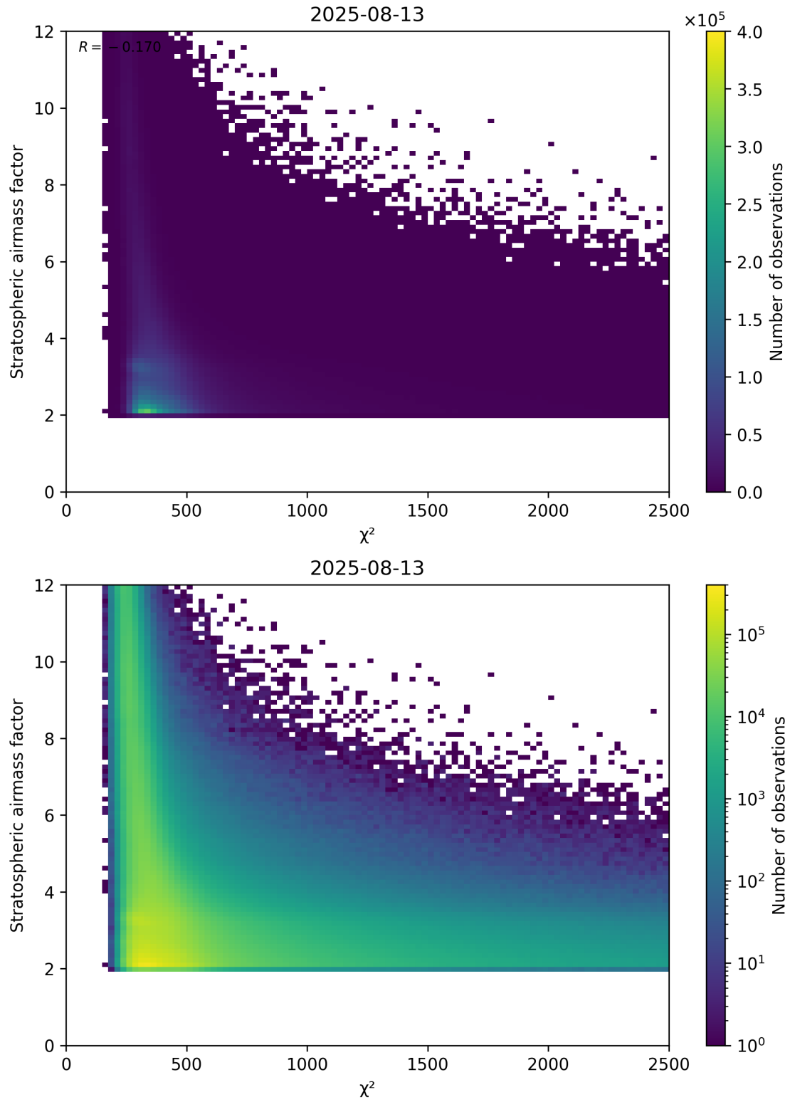
Figure 81: Scatter density plot of “ \chi^2 ” against “Stratospheric airmass factor” for 2025-08-12 to 2025-08-14.
