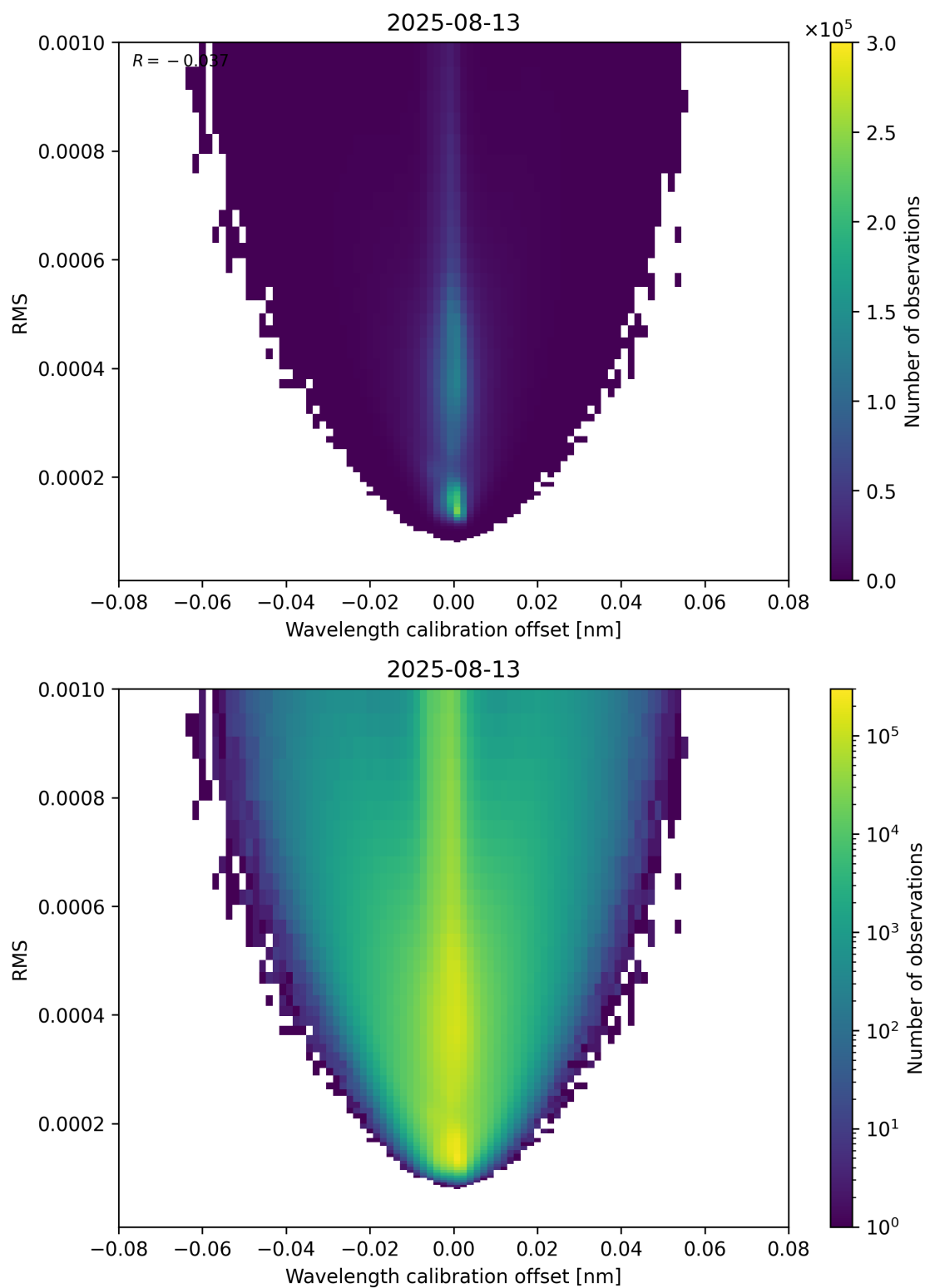
Figure 181: Scatter density plot of “Wavelength calibration offset” against “RMS” for 2025-08-12 to 2025-08-14.
