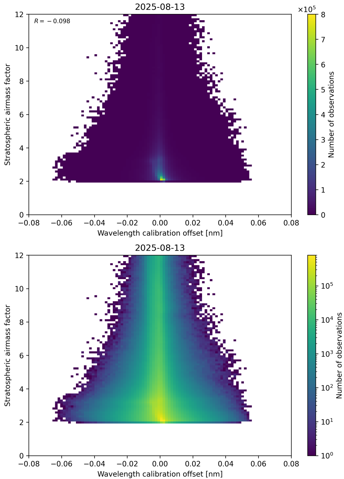
Figure 174: Scatter density plot of “Wavelength calibration offset” against “Stratospheric airmass factor” for 2025-08-12 to 2025-08-14.
