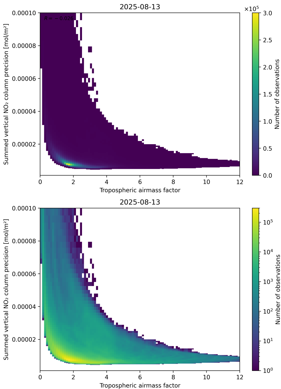
Figure 76: Scatter density plot of “Tropospheric air mass factor” against “Summed vertical NO 2 column precision” for 2025-08-12 to 2025-08-14.
