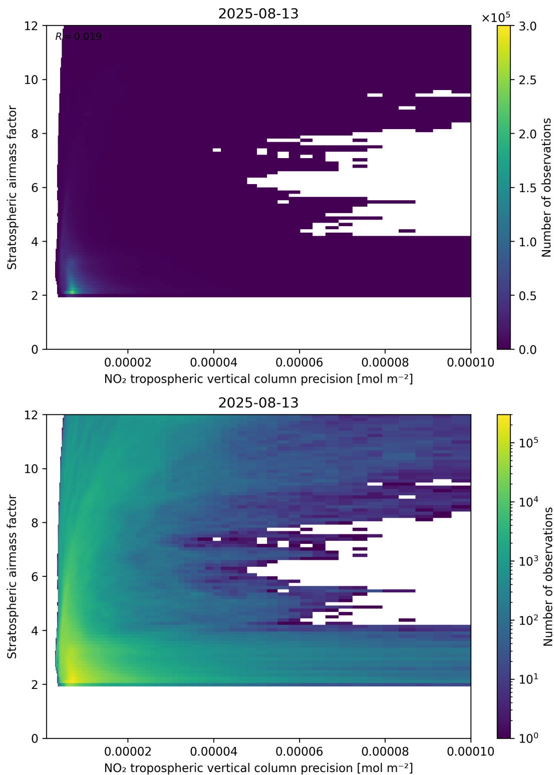
Figure 131: Scatter density plot of “NO 2 tropospheric vertical column precision” against “Stratospheric airmass factor” for 2025-08-12 to 2025-08-14.
