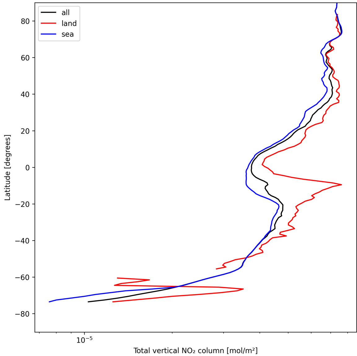
Figure 21: Zonal average of “Total vertical NO 2 column” for 2025-08-12 to 2025-08-14.
