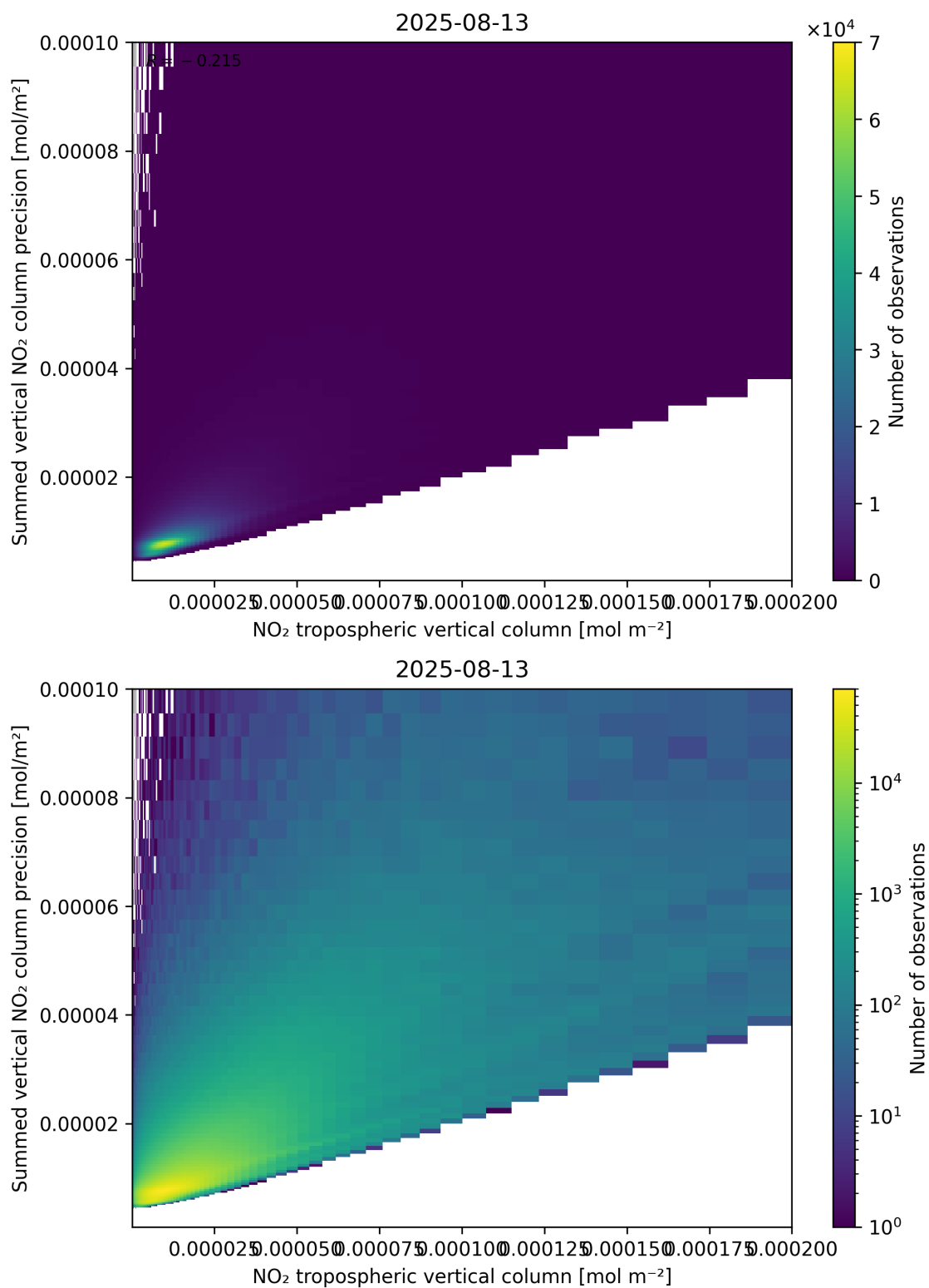
Figure 127: Scatter density plot of “NO 2 tropospheric vertical column” against “Summed vertical NO 2 column precision” for 2025-08-12 to 2025-08-14.
