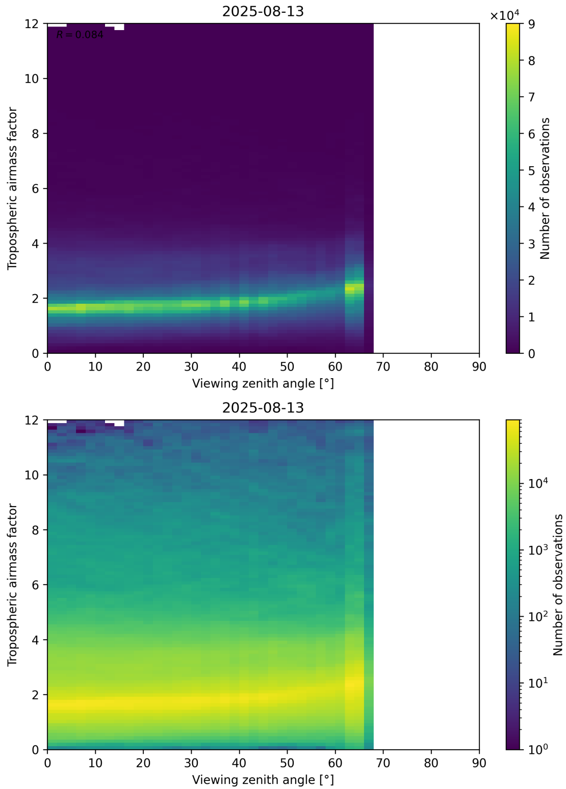
Figure 161: Scatter density plot of “Viewing zenith angle” against “Tropospheric airmass factor” for 2025-08-12 to 2025-08-14.
