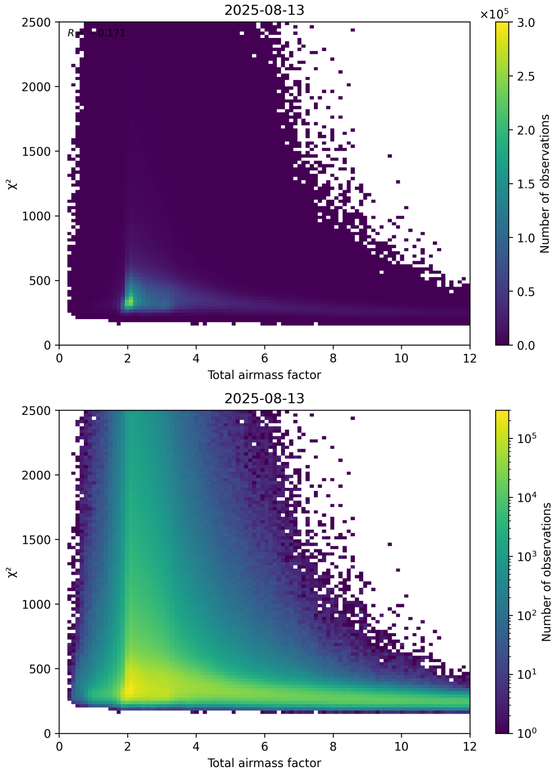
Figure 63: Scatter density plot of “Total airmass factor” against “ \chi^2 ” for 2025-08-12 to 2025-08-14.
