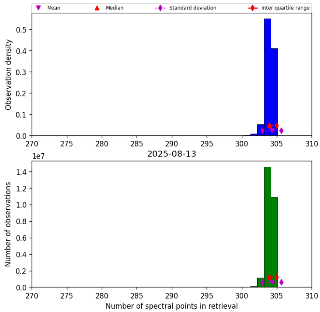
Figure 33: Histogram of “Number of spectral points in retrieval” for 2025-08-12 to 2025-08-14
