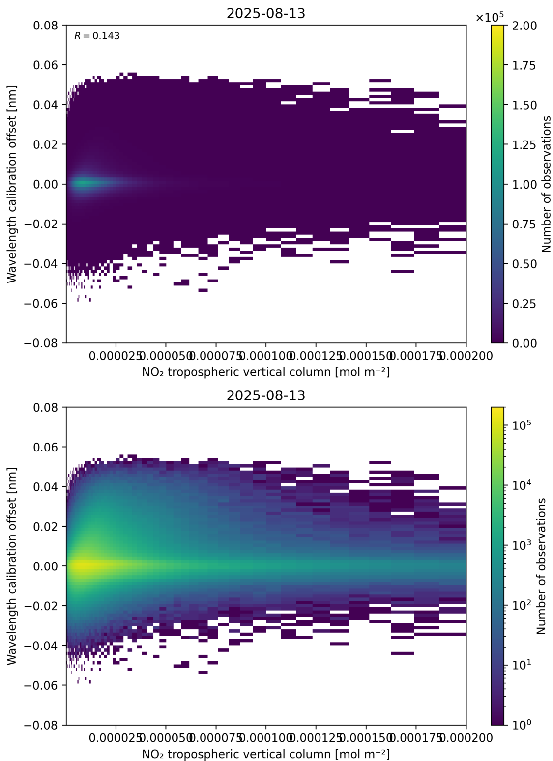
Figure 143: Scatter density plot of “NO 2 tropospheric vertical column” against “Wavelength calibration offset” for 2025-08-12 to 2025-08-14.
