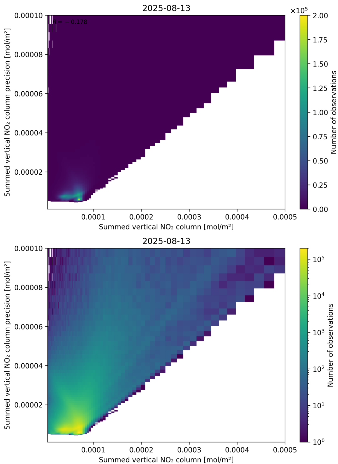
Figure 105: Scatter density plot of “Summed vertical NO 2 column” against “Summed vertical NO 2 column precision” for 2025-08-12 to 2025-08-14.
