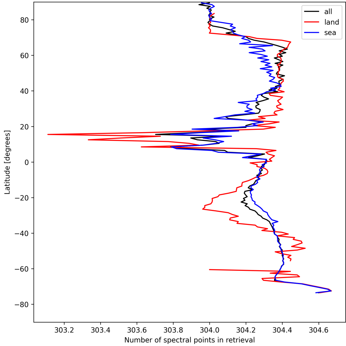
Figure 16: Zonal average of “Number of spectral points in retrieval” for 2025-08-12 to 2025-08-14.
