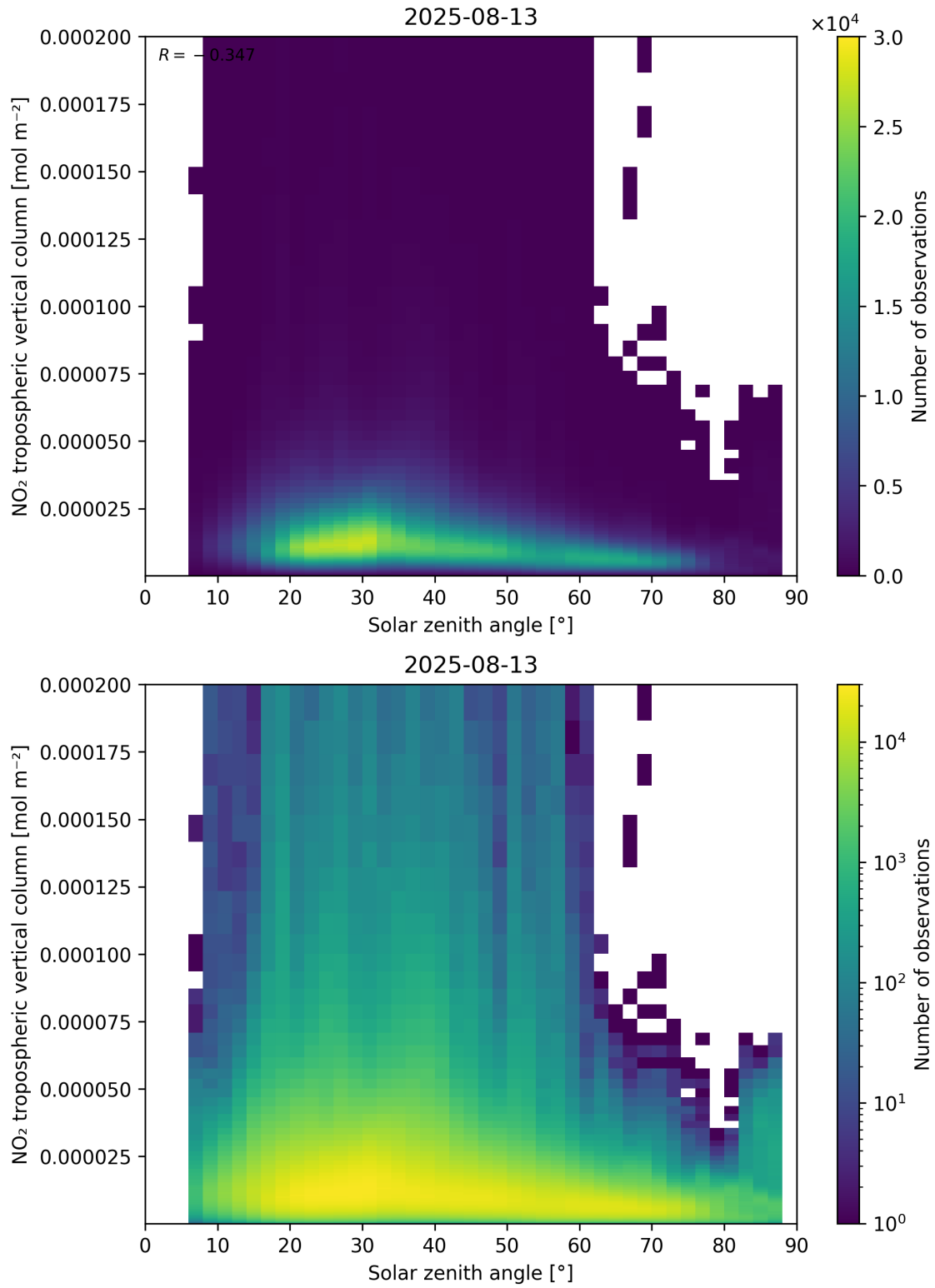
Figure 155: Scatter density plot of “Solar zenith angle” against “NO 2 tropospheric vertical column” for 2025-08-12 to 2025-08-14.
