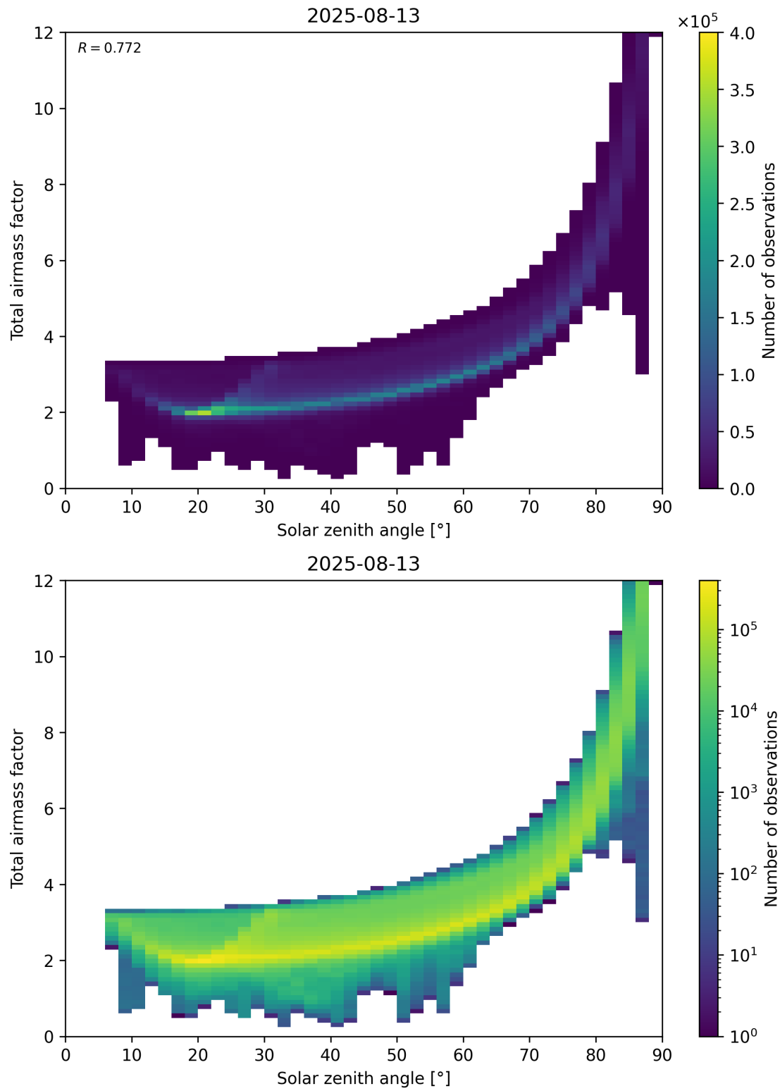
Figure 146: Scatter density plot of “Solar zenith angle” against “Total air mass factor” for 2025-08-12 to 2025-08-14.
