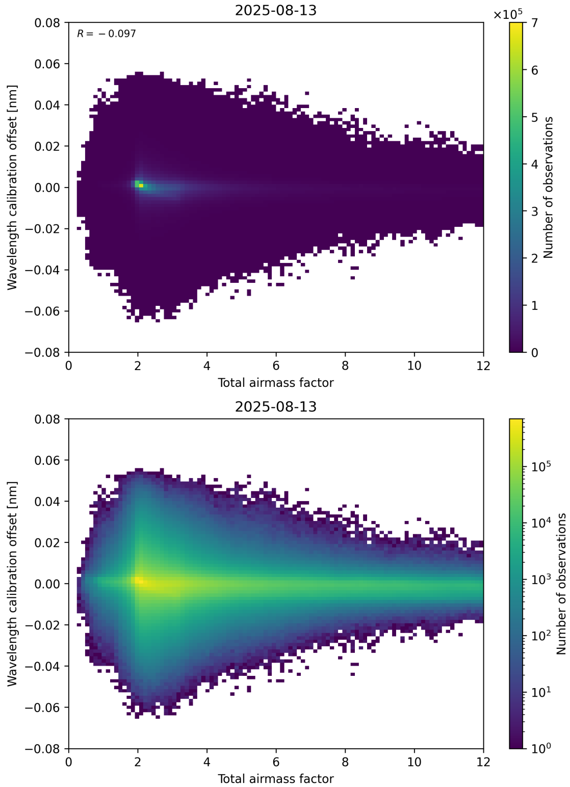
Figure 70: Scatter density plot of “Total airmass factor” against “Wavelength calibration offset” for 2025-08-12 to 2025-08-14.
