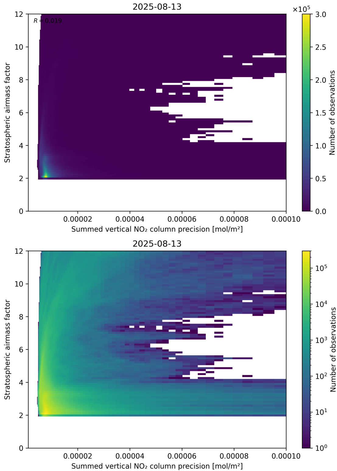
Figure 106: Scatter density plot of “Summed vertical NO 2 column precision” against “Stratospheric airmass factor” for 2025-08-12 to 2025-08-14.
