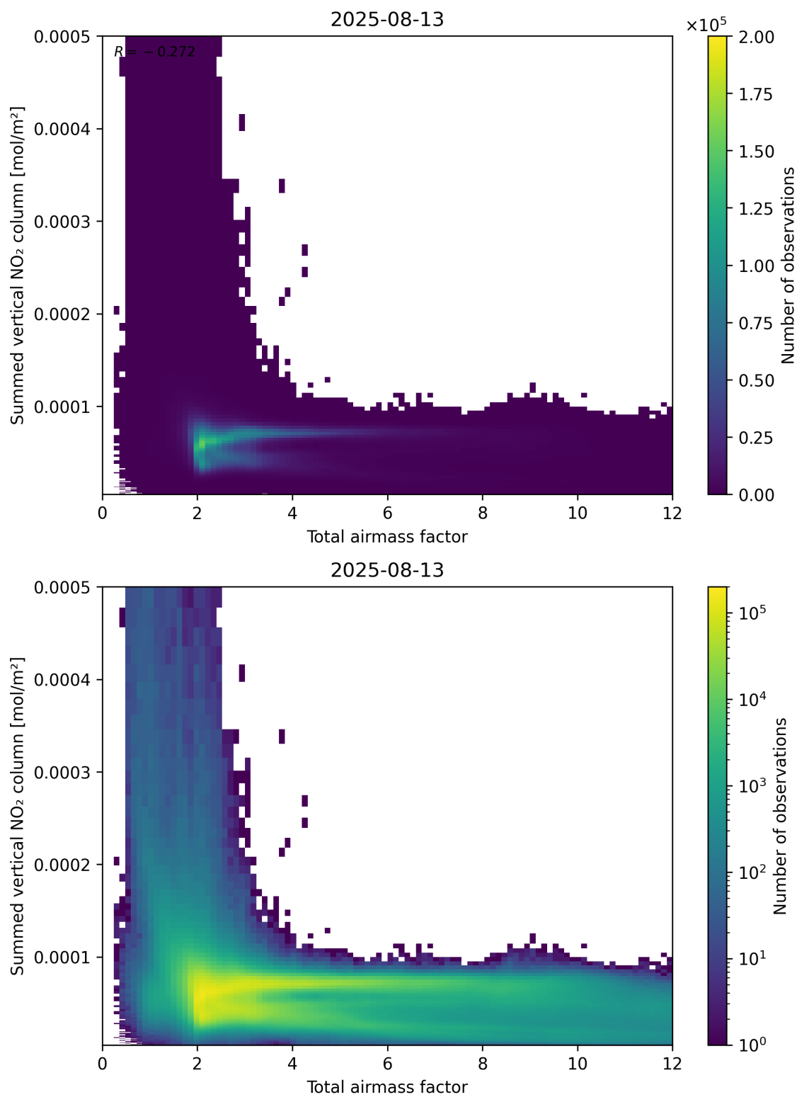
Figure 65: Scatter density plot of “Total airmass factor” against “Summed vertical NO 2 column” for 2025-08-12 to 2025-08-14.
