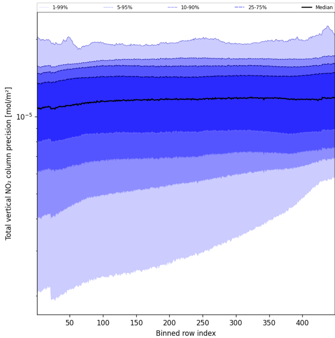
Figure 56: Along track statistics of “Total vertical NO 2 column precision” for 2025-08-12 to 2025-08-14
