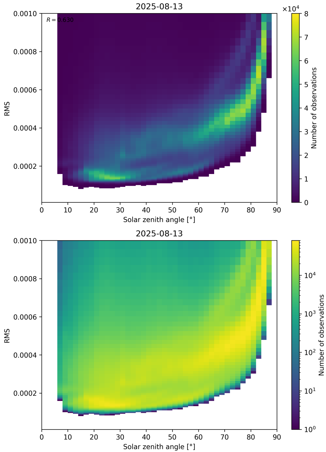
Figure 157: Scatter density plot of “Solar zenith angle” against “RMS” for 2025-08-12 to 2025-08-14.
