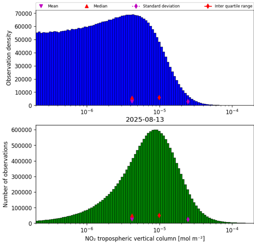
Figure 29: Histogram of “NO 2 tropospheric vertical column” for 2025-08-12 to 2025-08-14
