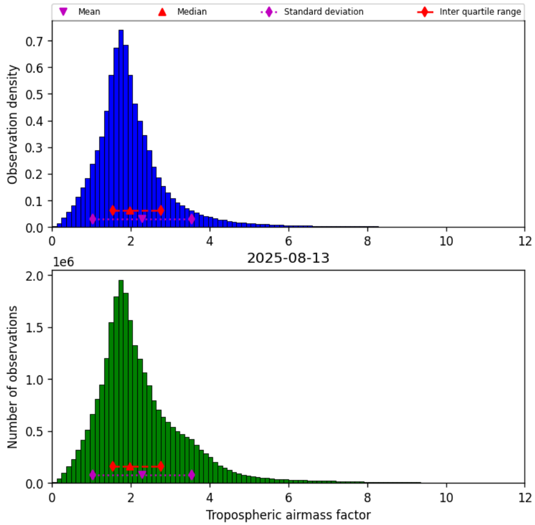
Figure 31: Histogram of “Tropospheric airmass factor” for 2025-08-12 to 2025-08-14
