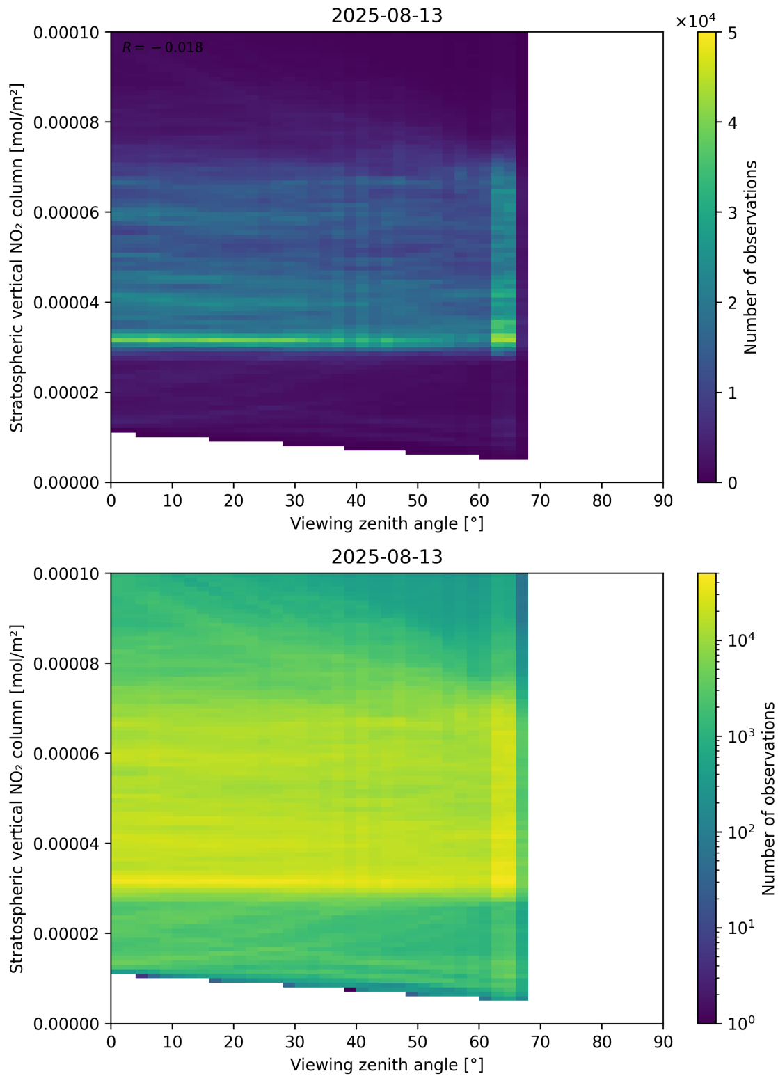
Figure 164: Scatter density plot of “Viewing zenith angle” against “Stratospheric vertical NO 2 column” for 2025-08-12 to 2025-08-14.
