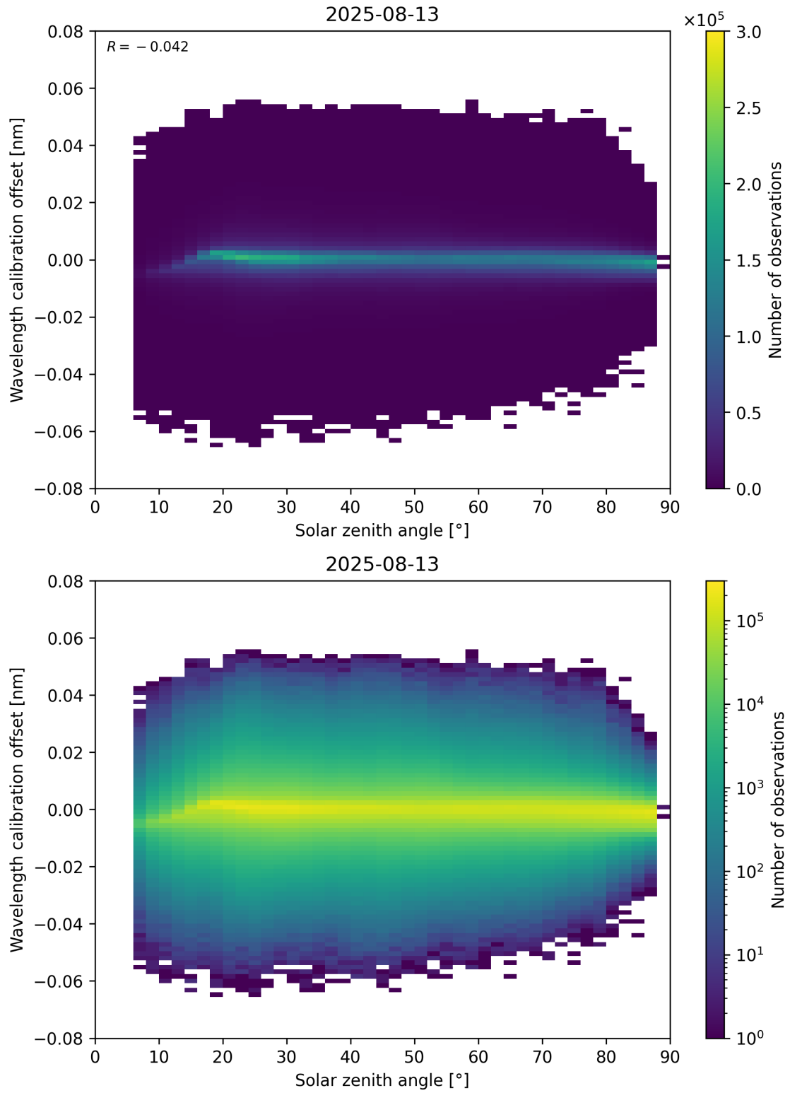
Figure 158: Scatter density plot of “Solar zenith angle” against “Wavelength calibration offset” for 2025-08-12 to 2025-08-14.
