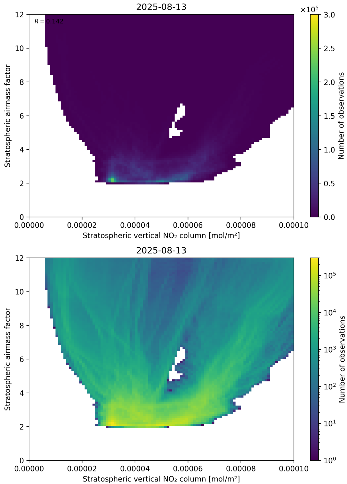
Figure 96: Scatter density plot of “Stratospheric vertical NO 2 column” against “Stratospheric airmass factor” for 2025-08-12 to 2025-08-14.
