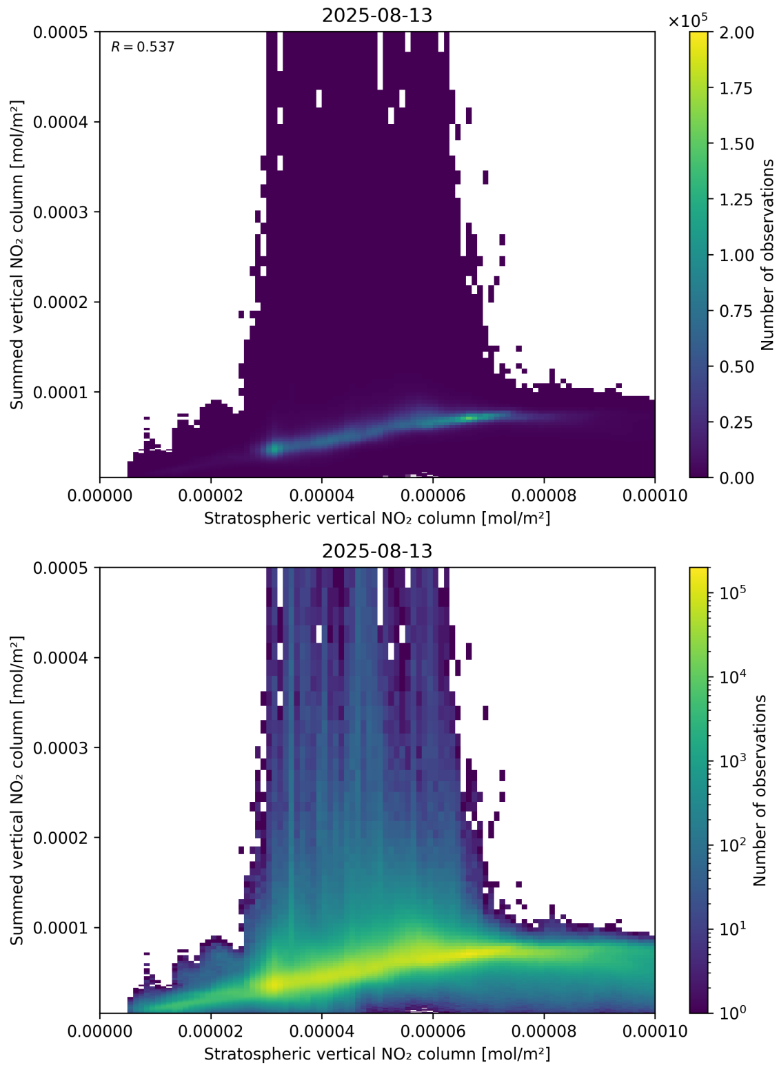
Figure 98: Scatter density plot of “Stratospheric vertical NO 2 column” against “Summed vertical NO 2 column” for 2025-08-12 to 2025-08-14.
