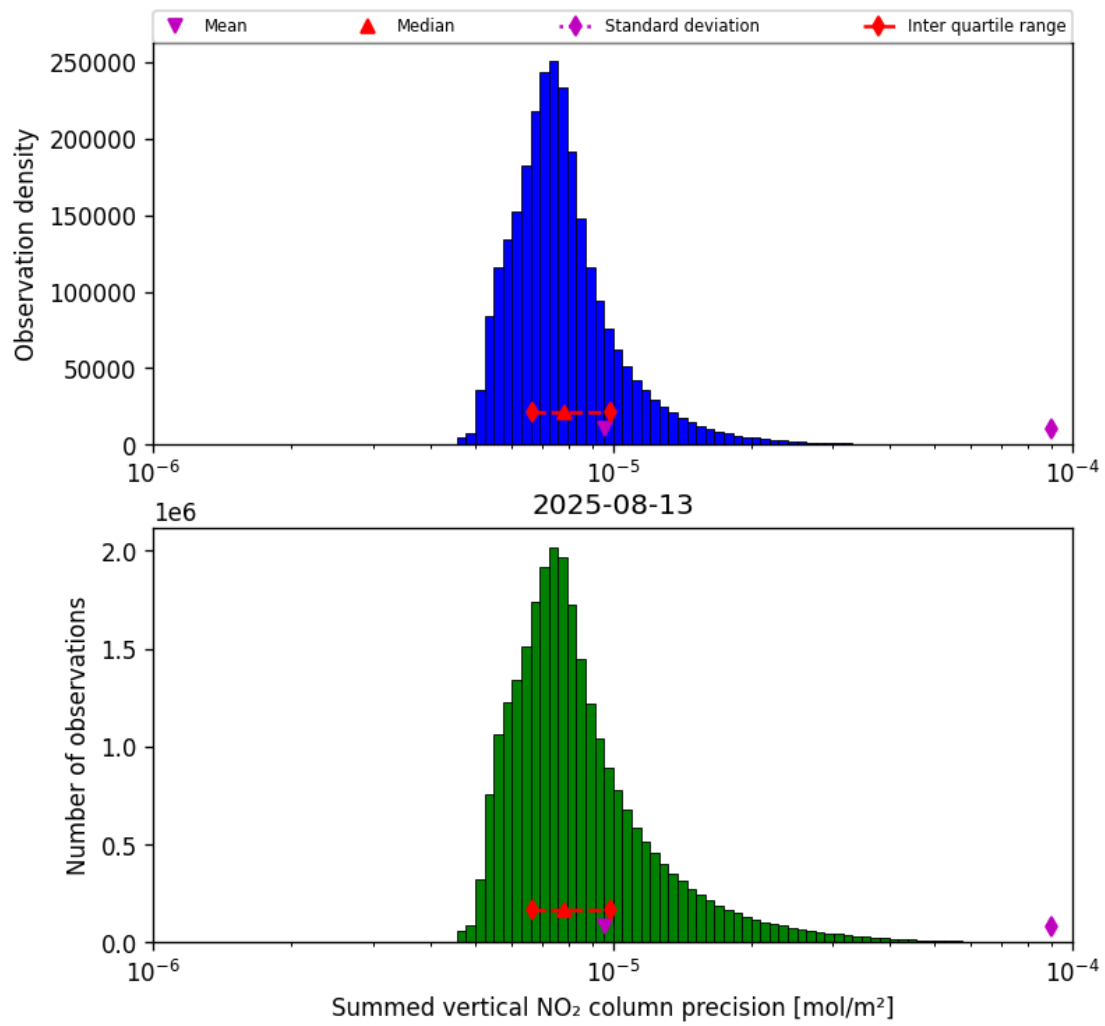
Figure 41: Histogram of "Summed vertical NO 2 column precision" for 2025-08-12 to 2025-08-14
