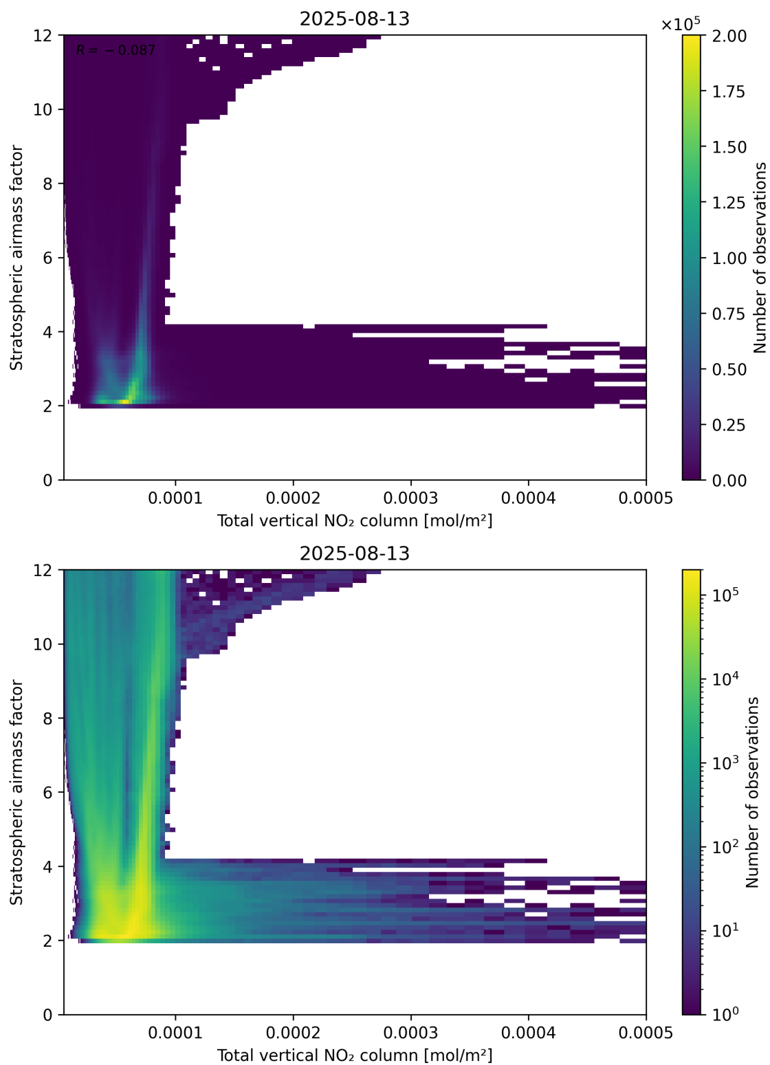
Figure 110: Scatter density plot of “Total vertical NO 2 column” against “Stratospheric air mass factor” for 2025-08-12 to 2025-08-14.
