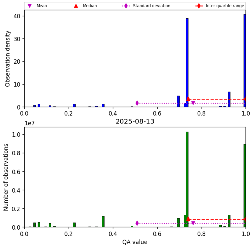
Figure 28: Histogram of “QA value” for 2025-08-12 to 2025-08-14
