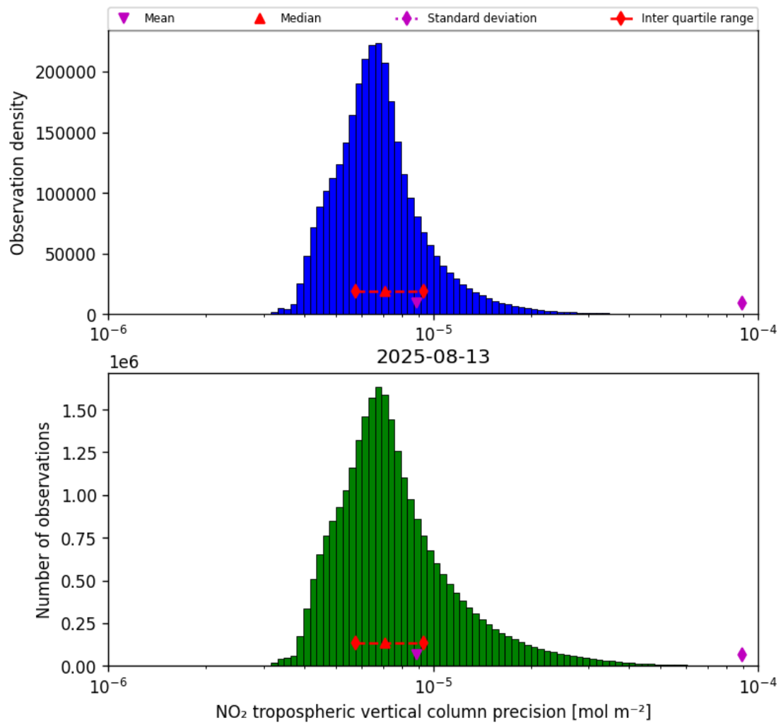
Figure 30: Histogram of “NO 2 tropospheric vertical column precision” for 2025-08-12 to 2025-08-14
