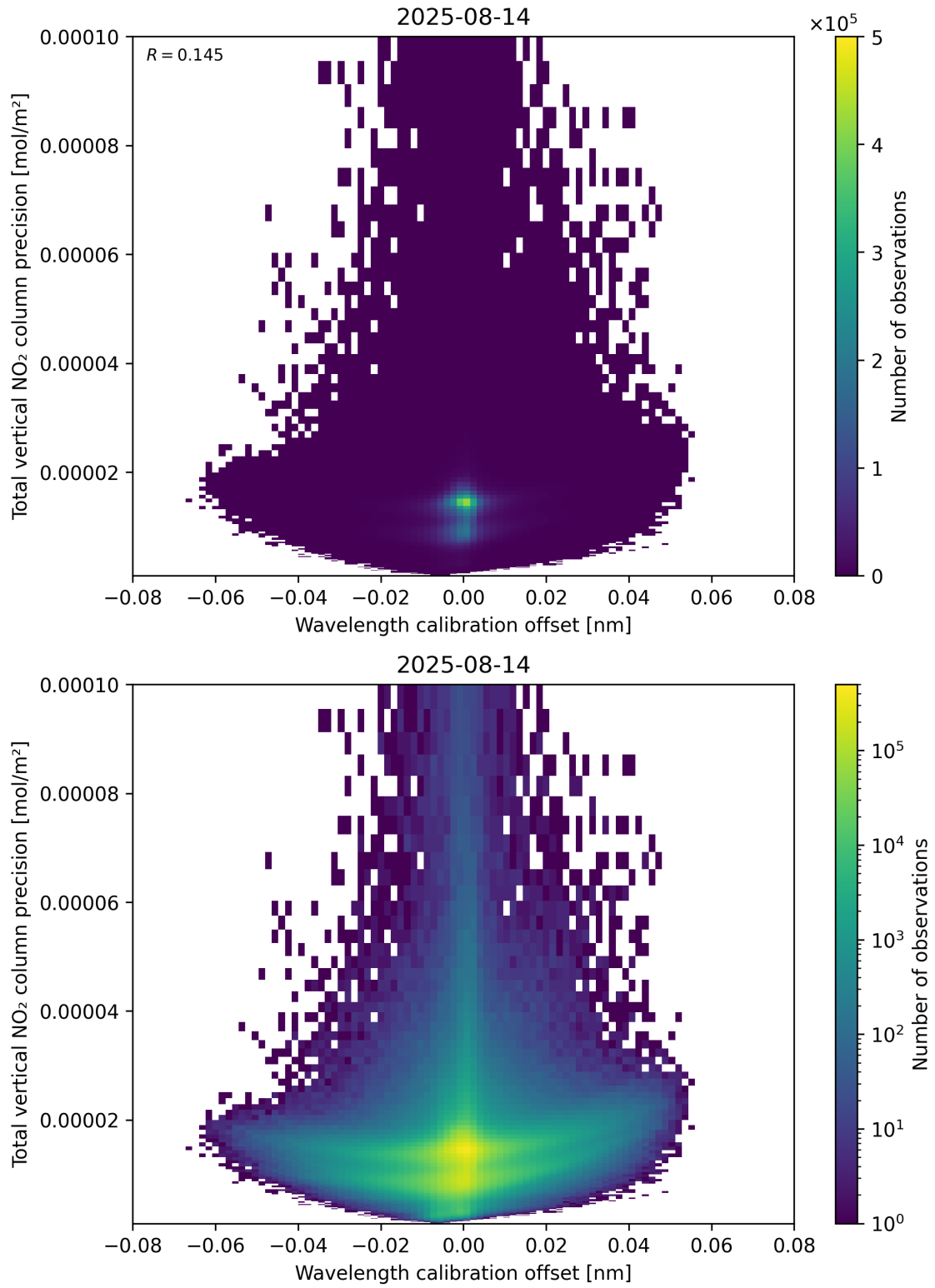
Figure 180: Scatter density plot of “Wavelength calibration offset” against “Total vertical NO 2 column precision” for 2025-08-14 to 2025-08-15.
