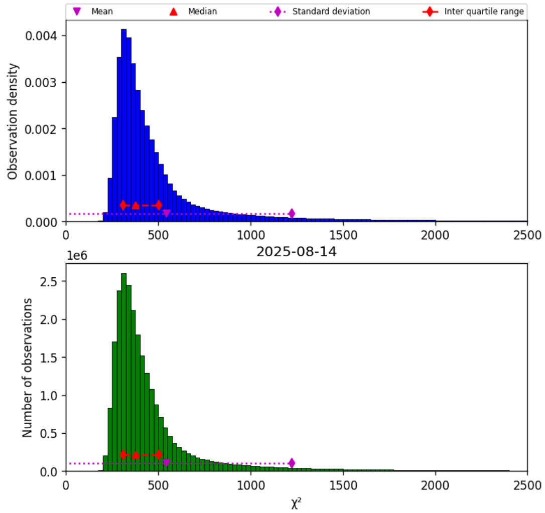
Figure 42: Histogram of “ \chi^2 ” for 2025-08-14 to 2025-08-15
