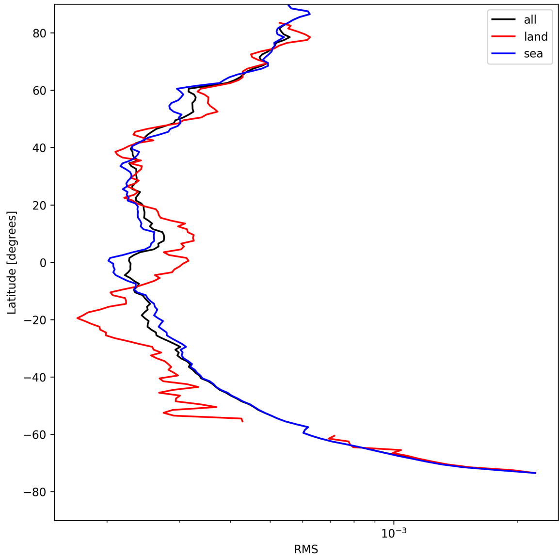
Figure 26: Zonal average of “RMS” for 2025-08-14 to 2025-08-15.
