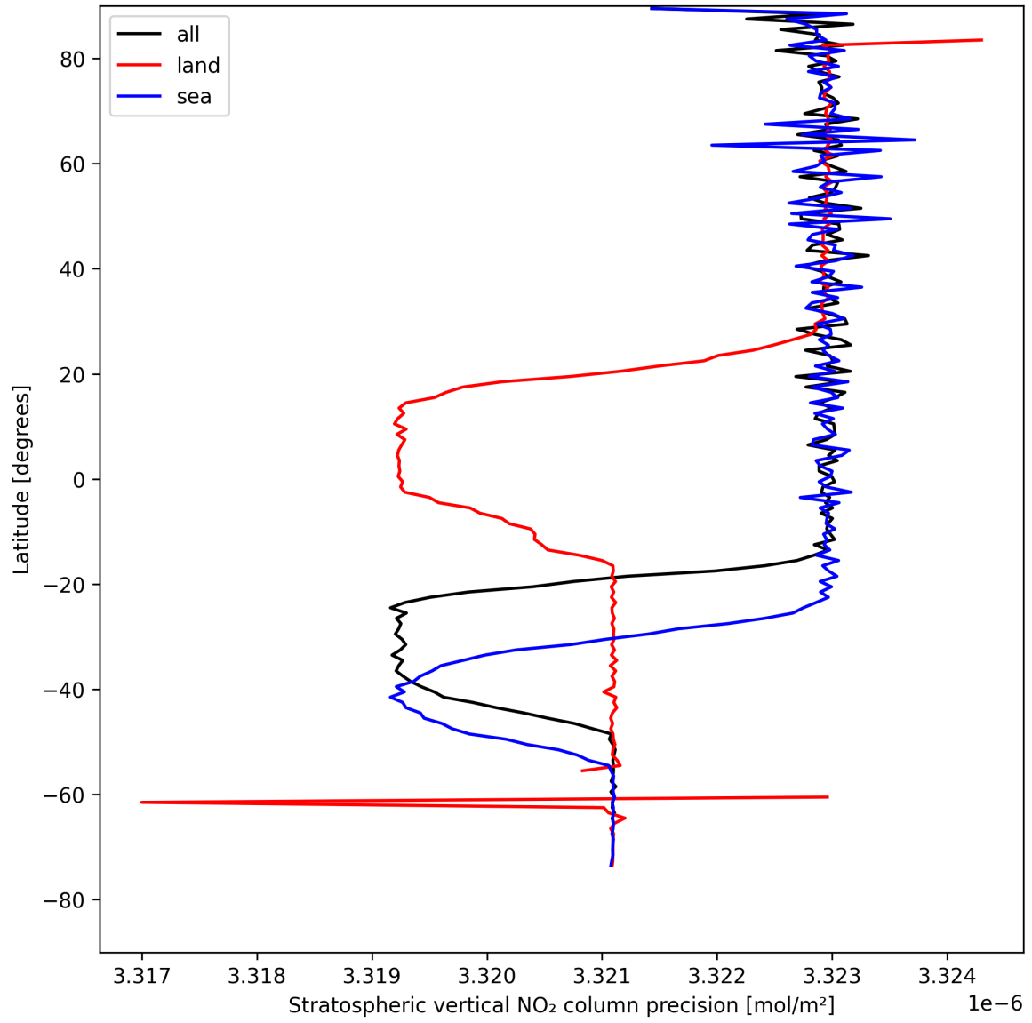
Figure 20: Zonal average of “Stratospheric vertical NO 2 column precision” for 2025-08-14 to 2025-08-15.
