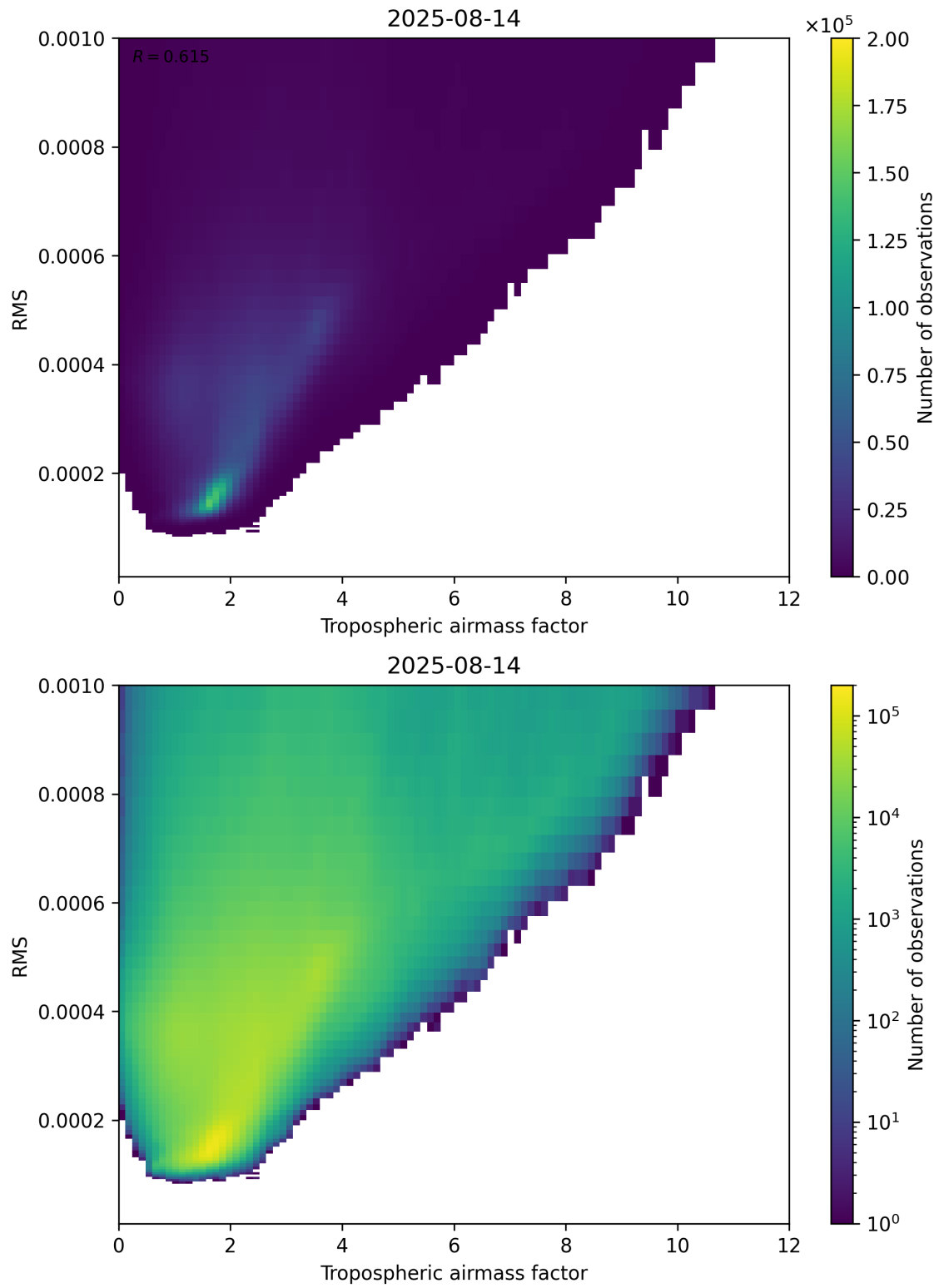
Figure 79: Scatter density plot of “Tropospheric airmass factor” against “RMS” for 2025-08-14 to 2025-08-15.
