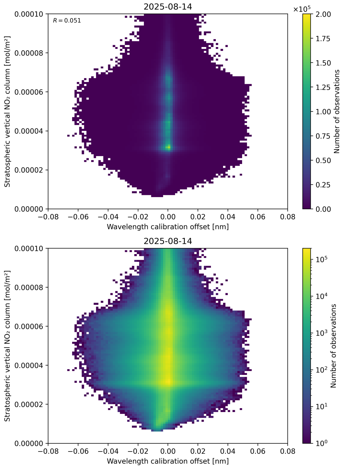
Figure 176: Scatter density plot of “Wavelength calibration offset” against “Stratospheric vertical NO 2 column” for 2025-08-14 to 2025-08-15.
