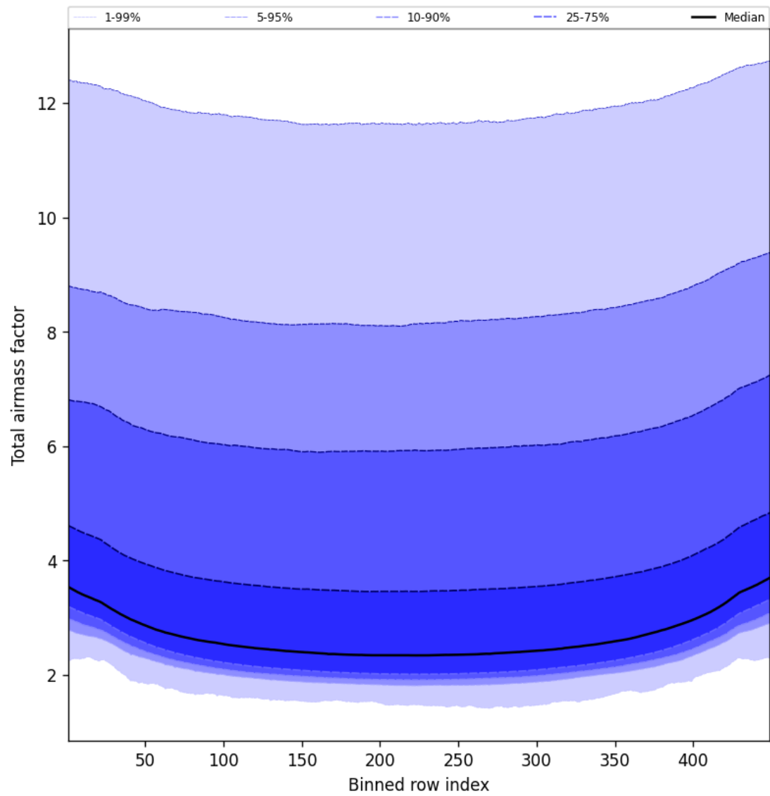
Figure 49: Along track statistics of “Total airmass factor” for 2025-08-14 to 2025-08-15
