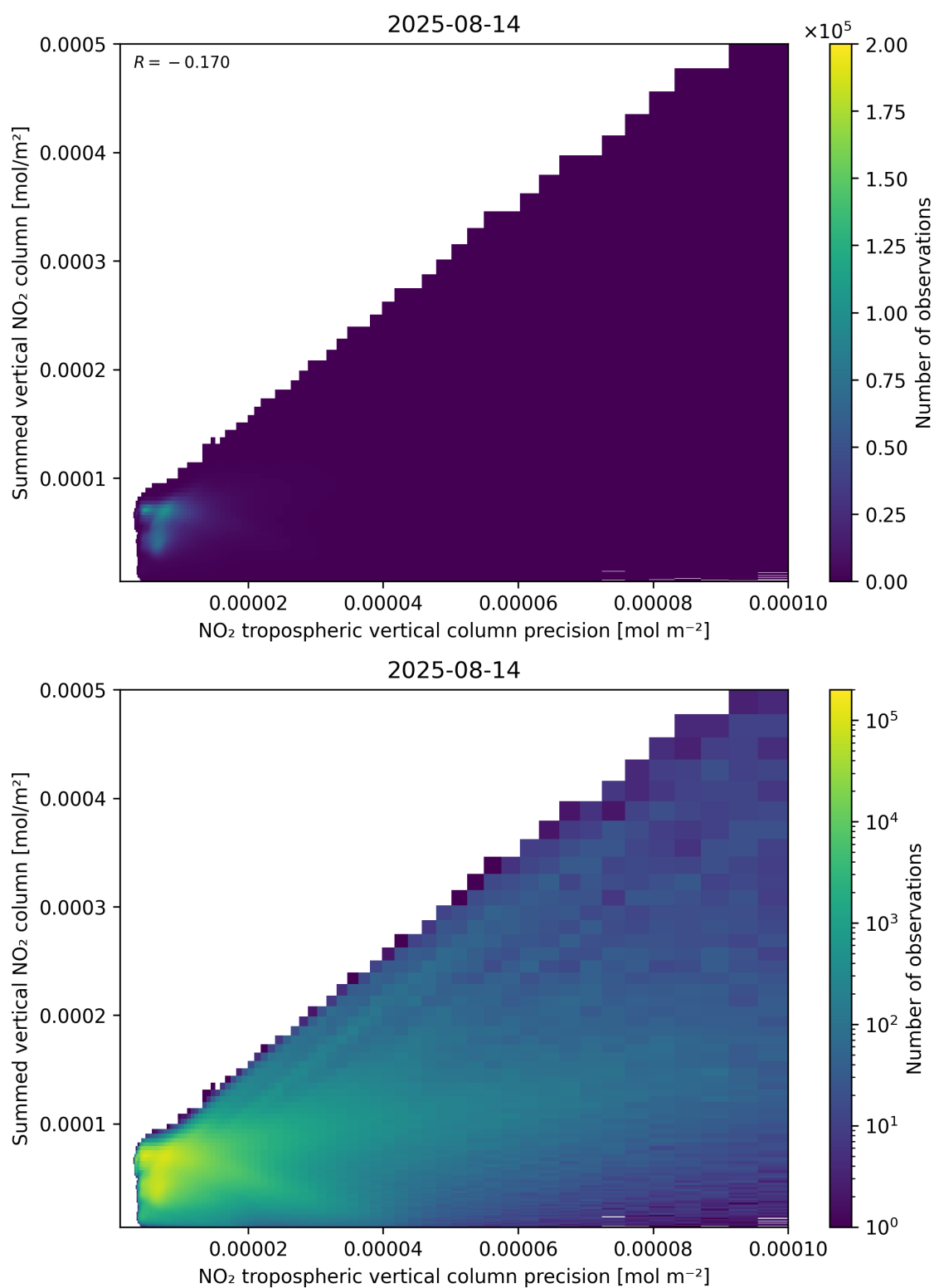
Figure 136: Scatter density plot of “NO 2 tropospheric vertical column precision” against “Summed vertical NO 2 column” for 2025-08-14 to 2025-08-15.
