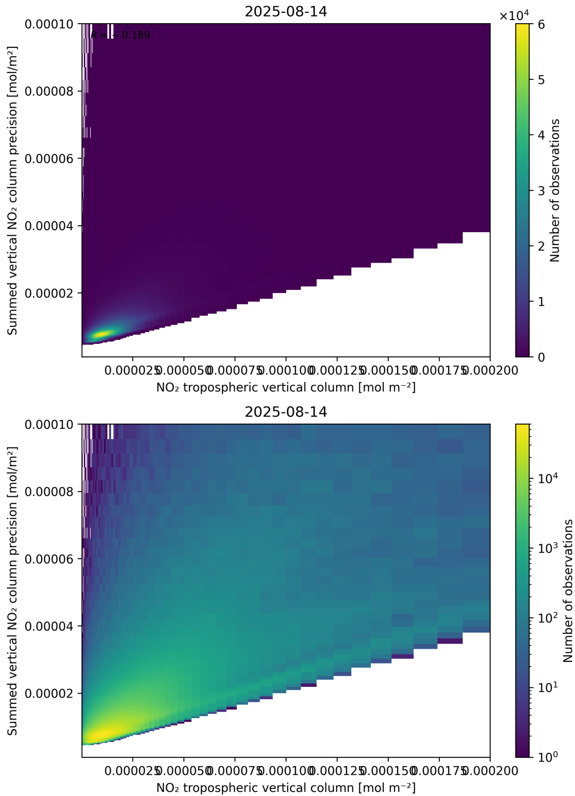
Figure 127: Scatter density plot of “NO 2 tropospheric vertical column” against “Summed vertical NO 2 column precision” for 2025-08-14 to 2025-08-15.
