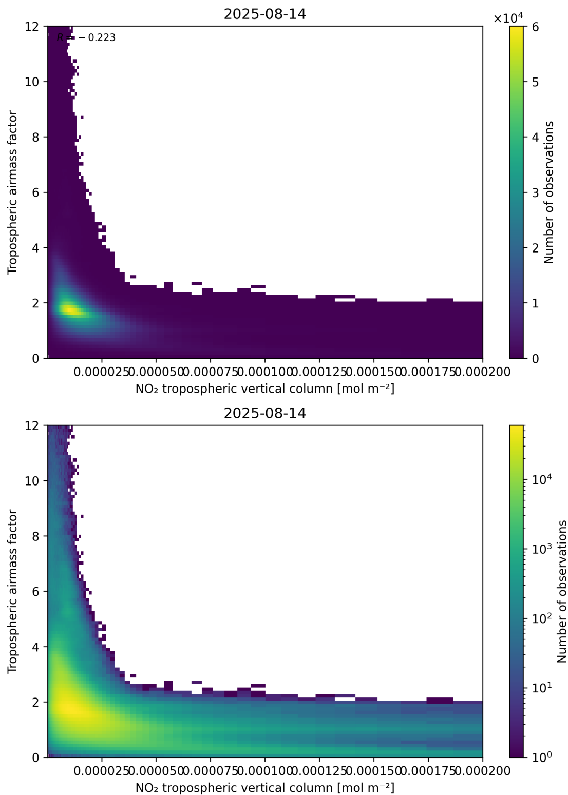
Figure 123: Scatter density plot of “NO 2 tropospheric vertical column” against “Tropospheric air mass factor” for 2025-08-14 to 2025-08-15.
