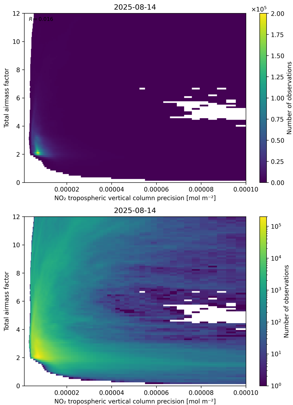
Figure 132: Scatter density plot of “NO 2 tropospheric vertical column precision” against “Total air mass factor” for 2025-08-14 to 2025-08-15.
