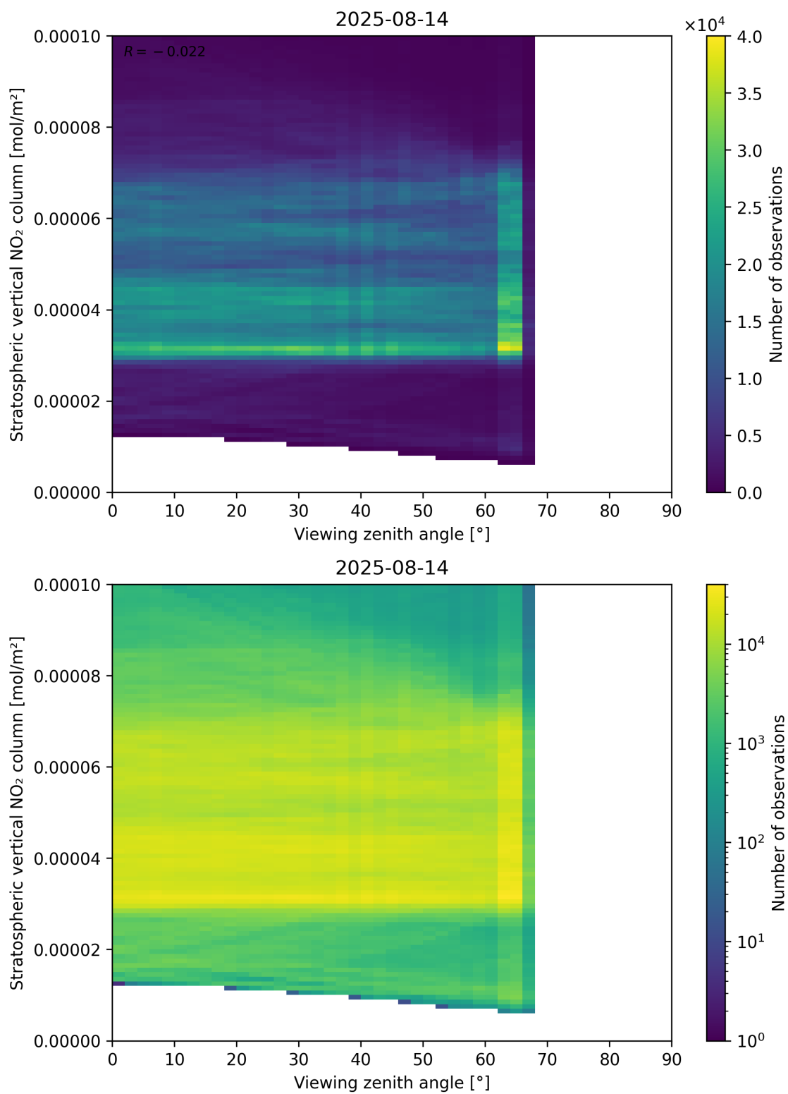
Figure 164: Scatter density plot of “Viewing zenith angle” against “Stratospheric vertical NO 2 column” for 2025-08-14 to 2025-08-15.
