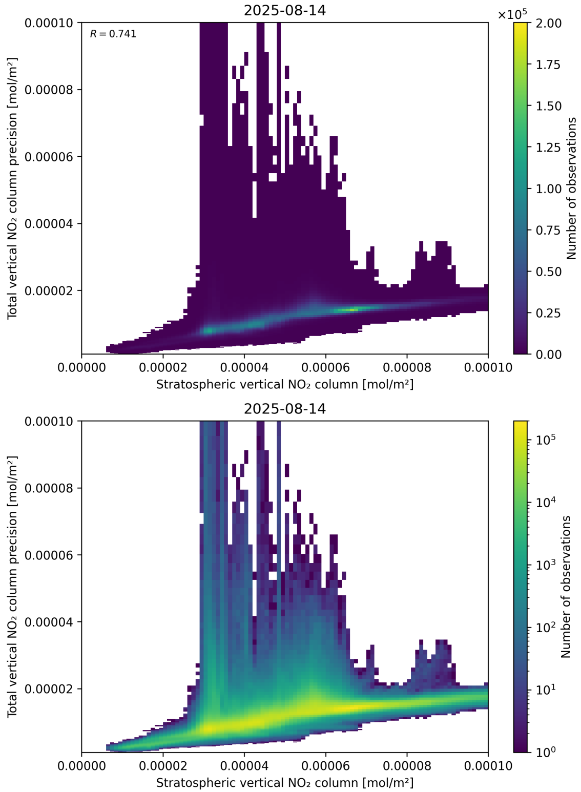
Figure 101: Scatter density plot of “Stratospheric vertical NO 2 column” against “Total vertical NO 2 column precision” for 2025-08-14 to 2025-08-15.
