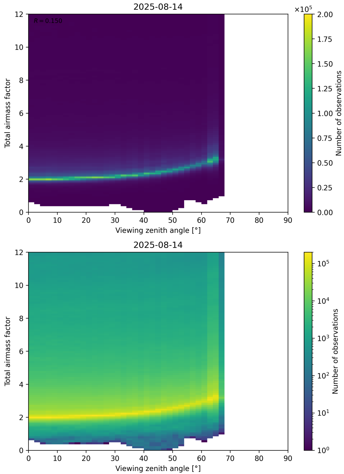
Figure 160: Scatter density plot of “Viewing zenith angle” against “Total airmass factor” for 2025-08-14 to 2025-08-15.
