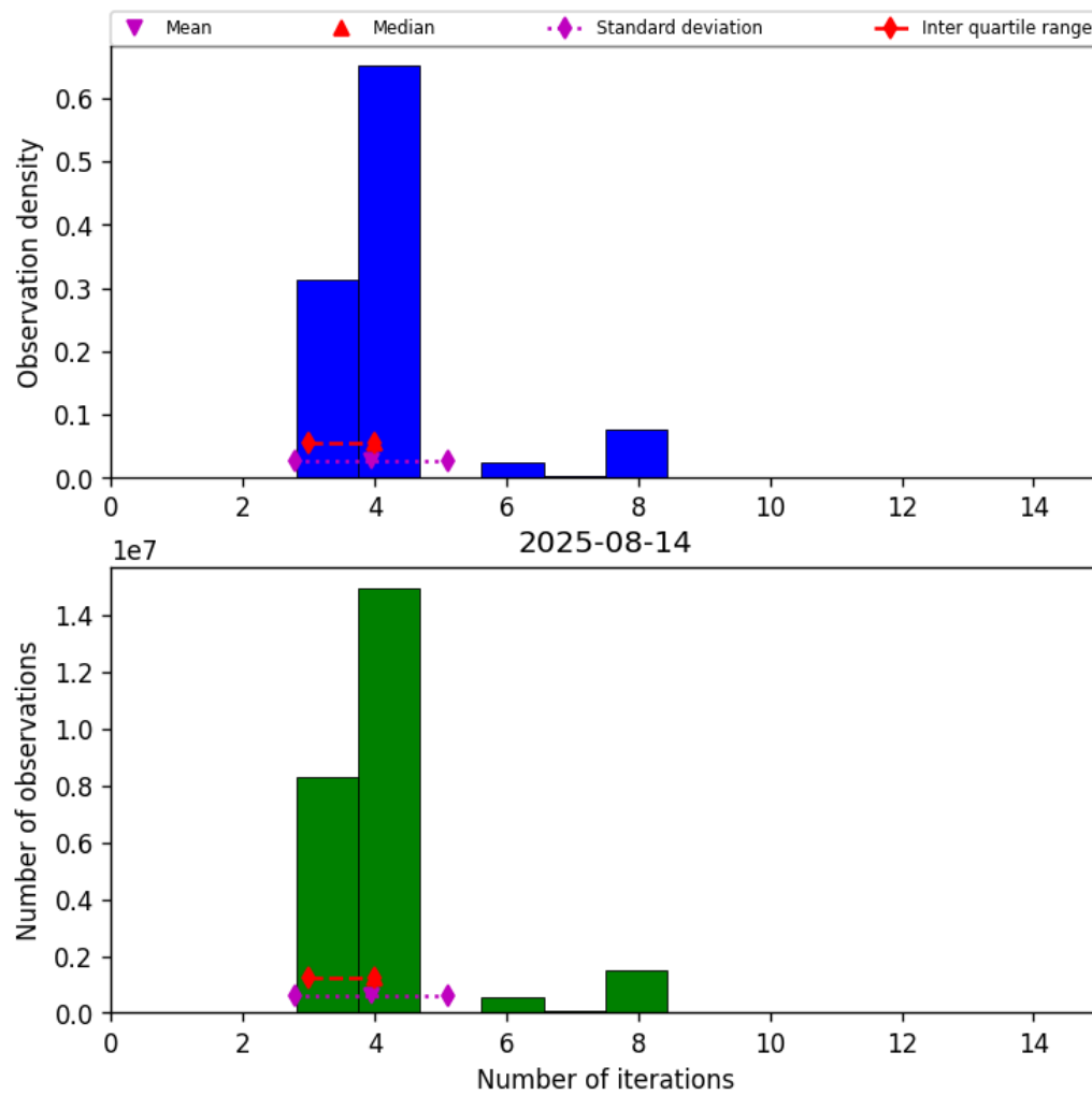
Figure 34: Histogram of “Number of iterations” for 2025-08-14 to 2025-08-15
