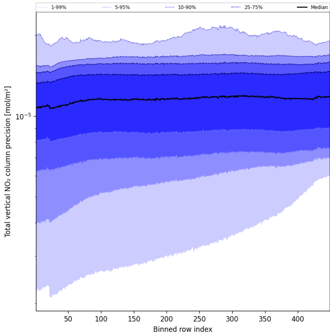
Figure 56: Along track statistics of “Total vertical NO 2 column precision” for 2025-08-14 to 2025-08-15
