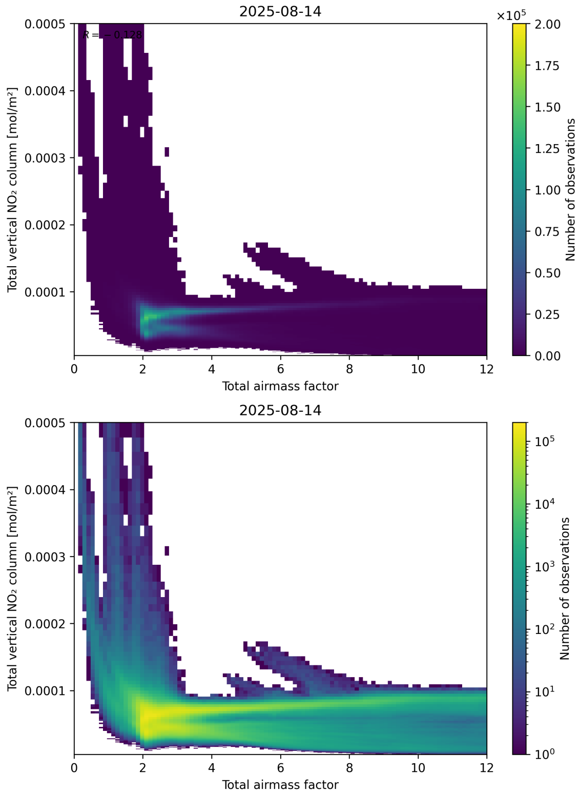
Figure 67: Scatter density plot of “Total airmass factor” against “Total vertical NO 2 column” for 2025-08-14 to 2025-08-15.
