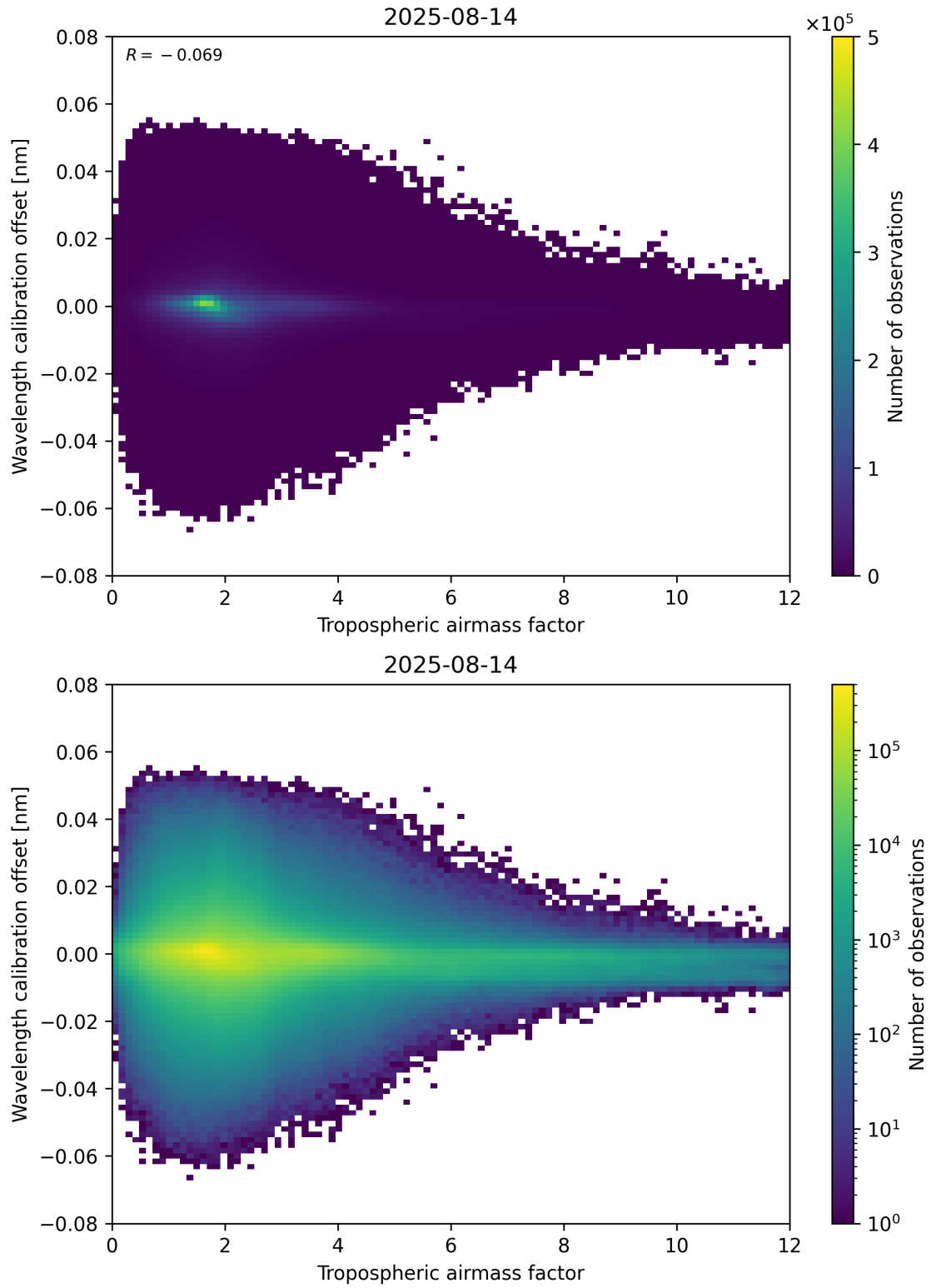
Figure 80: Scatter density plot of “Tropospheric air mass factor” against “Wavelength calibration offset” for 2025-08-14 to 2025-08-15.
