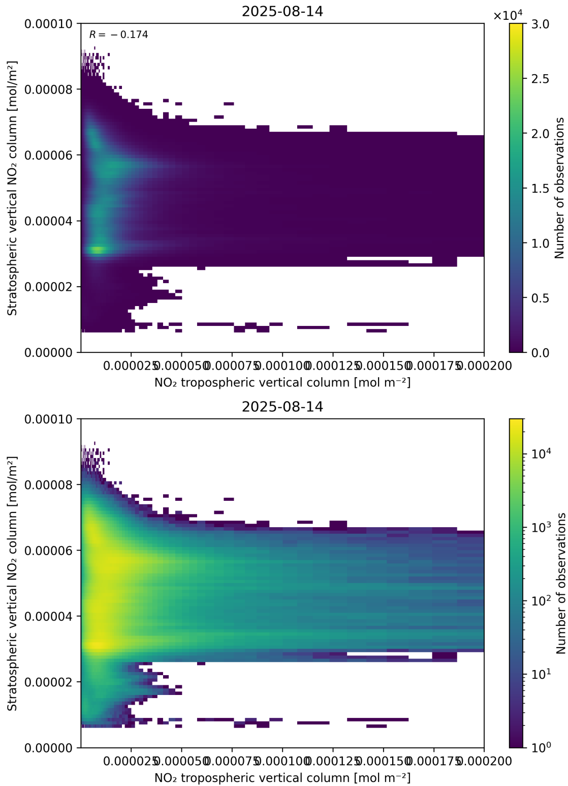
Figure 125: Scatter density plot of “NO 2 tropospheric vertical column” against “Stratospheric vertical NO 2 column” for 2025-08-14 to 2025-08-15.
