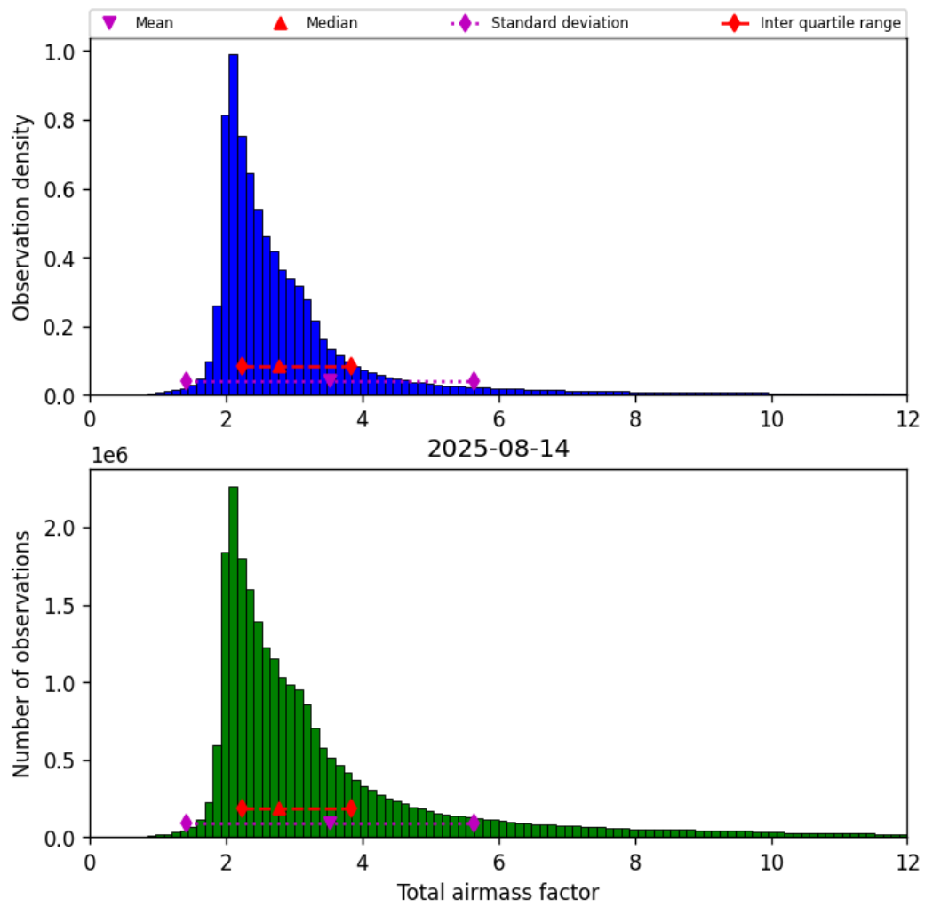
Figure 32: Histogram of “Total airmass factor” for 2025-08-14 to 2025-08-15
