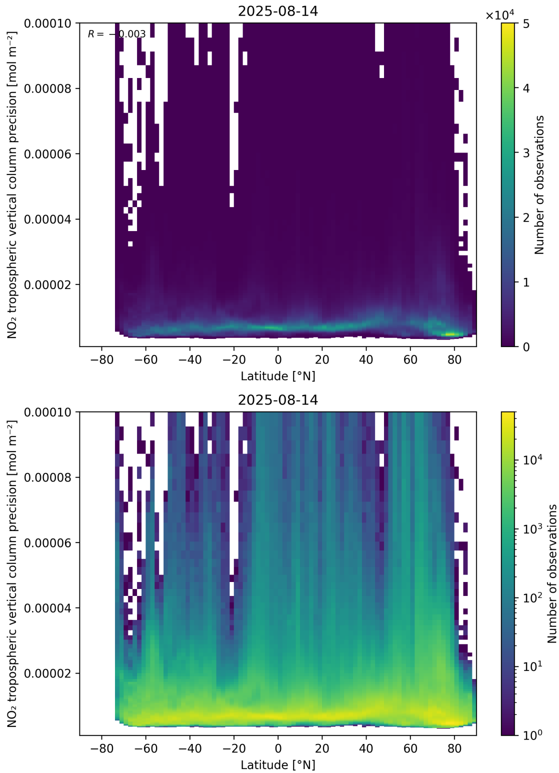
Figure 93: Scatter density plot of “Latitude” against “NO 2 tropospheric vertical column precision” for 2025-08-14 to 2025-08-15.
