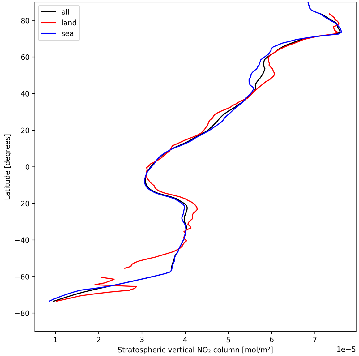
Figure 19: Zonal average of “Stratospheric vertical NO 2 column” for 2025-08-14 to 2025-08-15.
