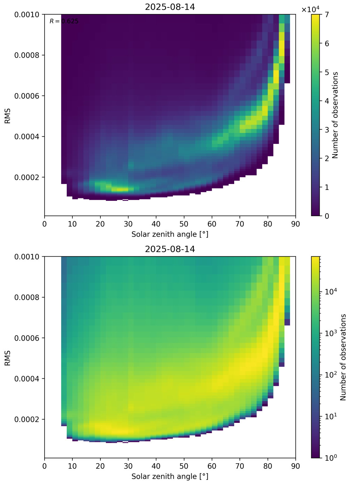
Figure 157: Scatter density plot of “Solar zenith angle” against “RMS” for 2025-08-14 to 2025-08-15.
