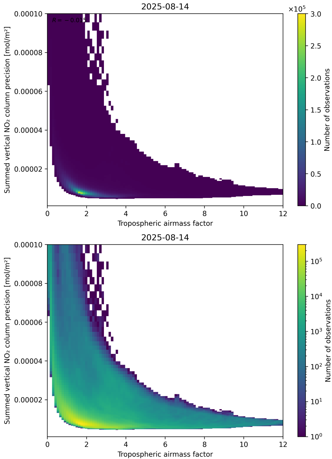
Figure 76: Scatter density plot of “Tropospheric air mass factor” against “Summed vertical NO 2 column precision” for 2025-08-14 to 2025-08-15.
