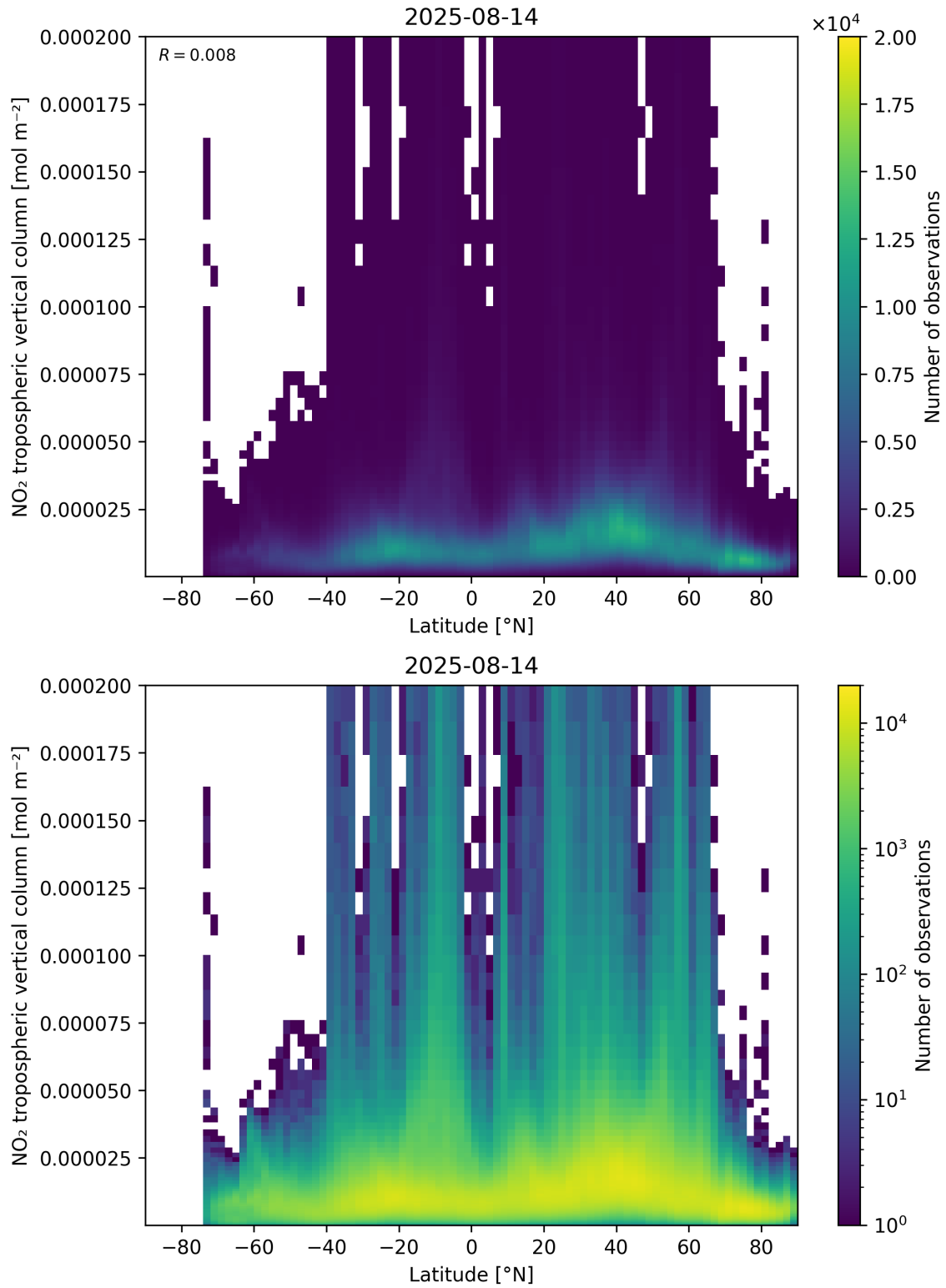
Figure 92: Scatter density plot of “Latitude” against “NO 2 tropospheric vertical column” for 2025-08-14 to 2025-08-15.
