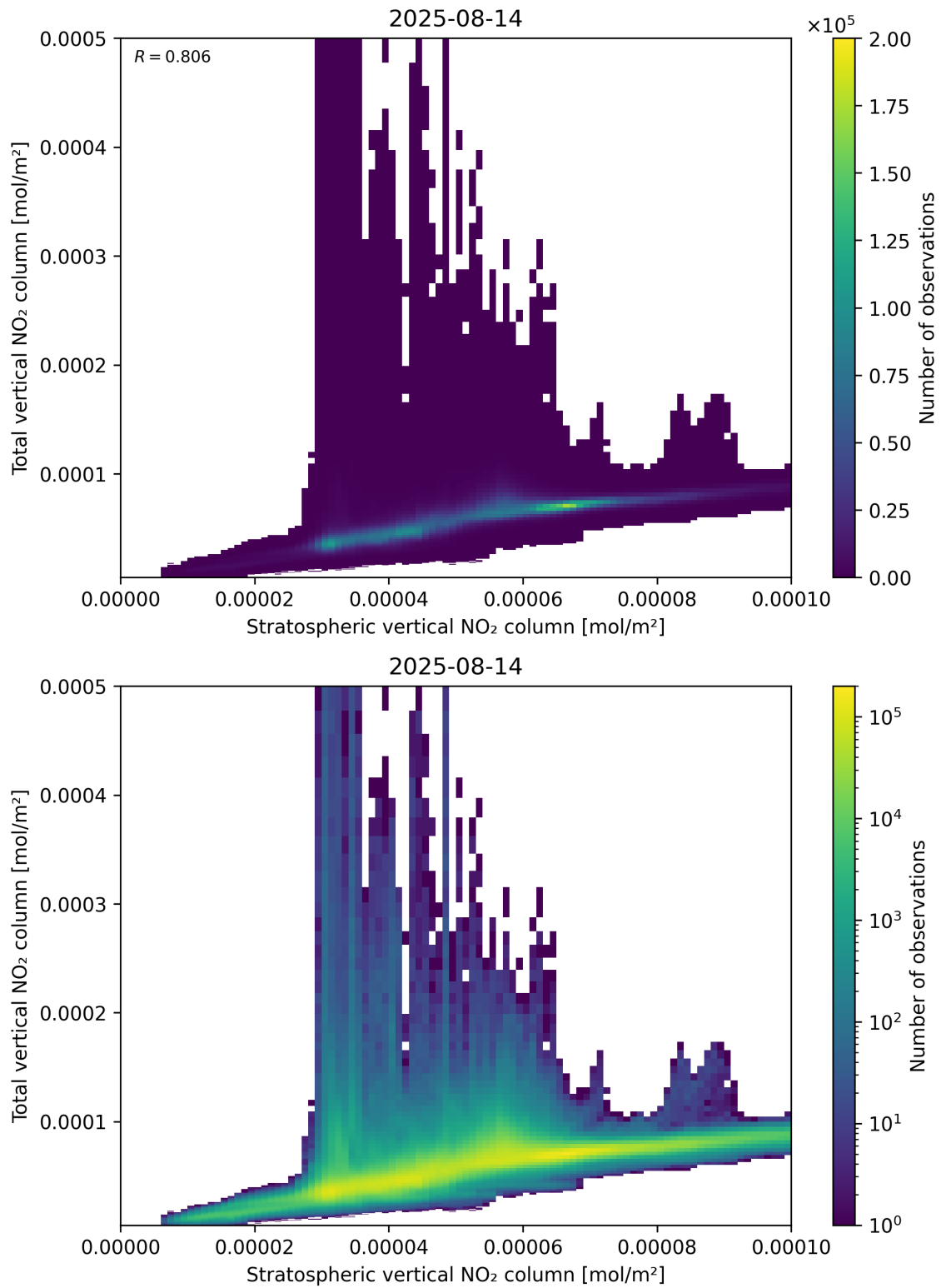
Figure 100: Scatter density plot of “Stratospheric vertical NO 2 column” against “Total vertical NO 2 column” for 2025-08-14 to 2025-08-15.
