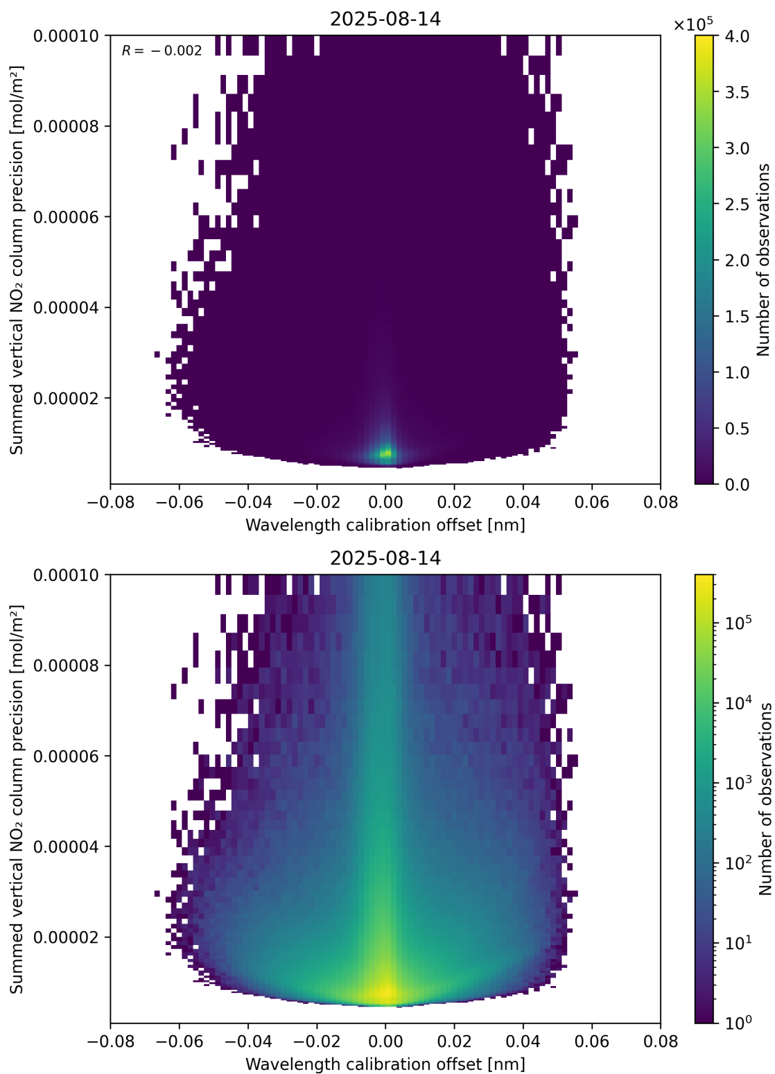
Figure 178: Scatter density plot of “Wavelength calibration offset” against “Summed vertical NO 2 column precision” for 2025-08-14 to 2025-08-15.
