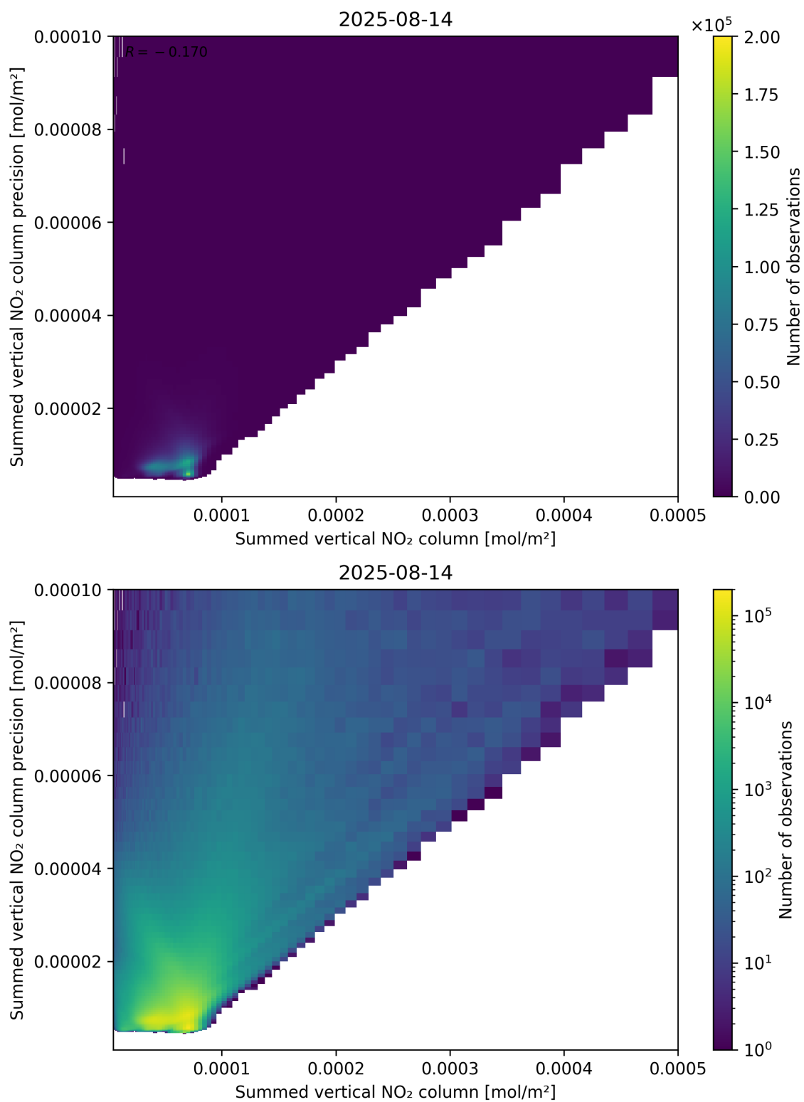
Figure 105: Scatter density plot of “Summed vertical NO 2 column” against “Summed vertical NO 2 column precision” for 2025-08-14 to 2025-08-15.
