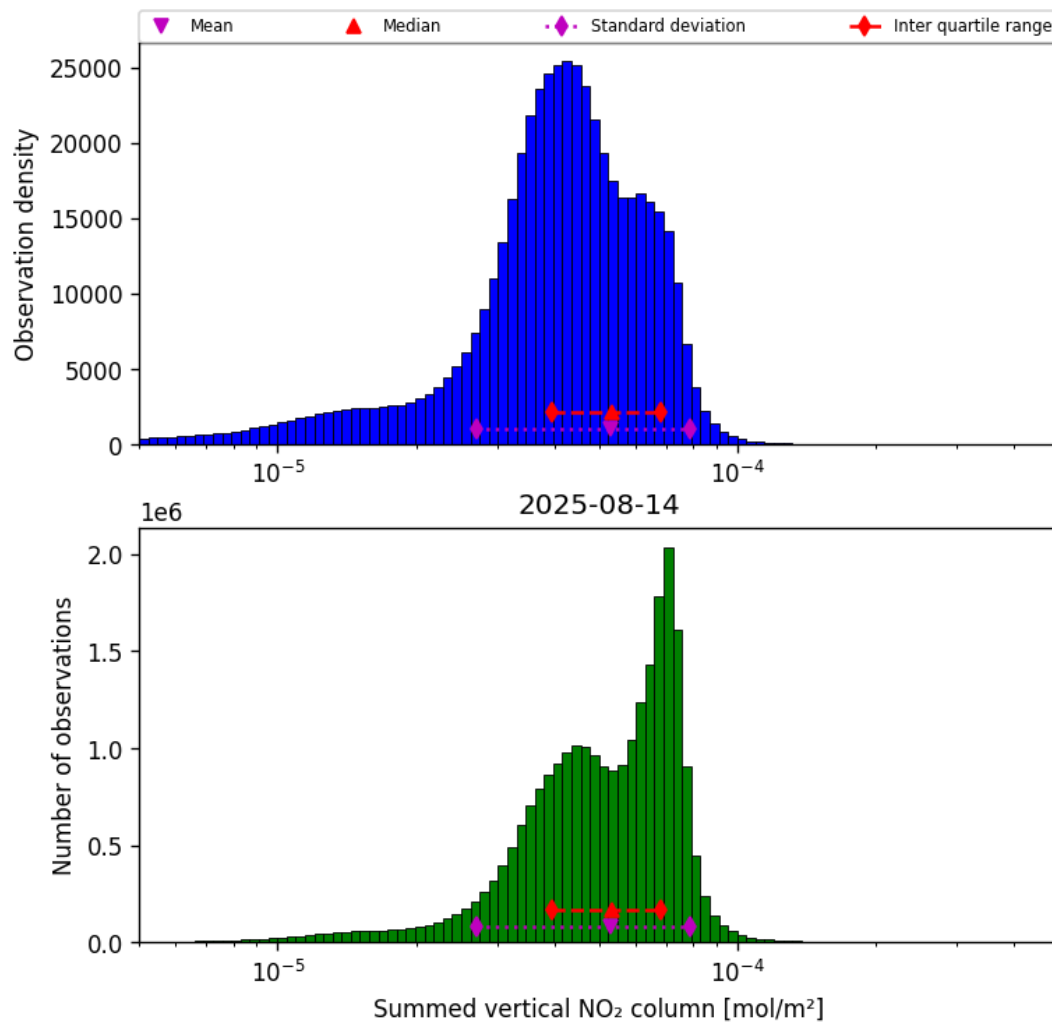
Figure 40: Histogram of “Summed vertical NO 2 column” for 2025-08-14 to 2025-08-15
