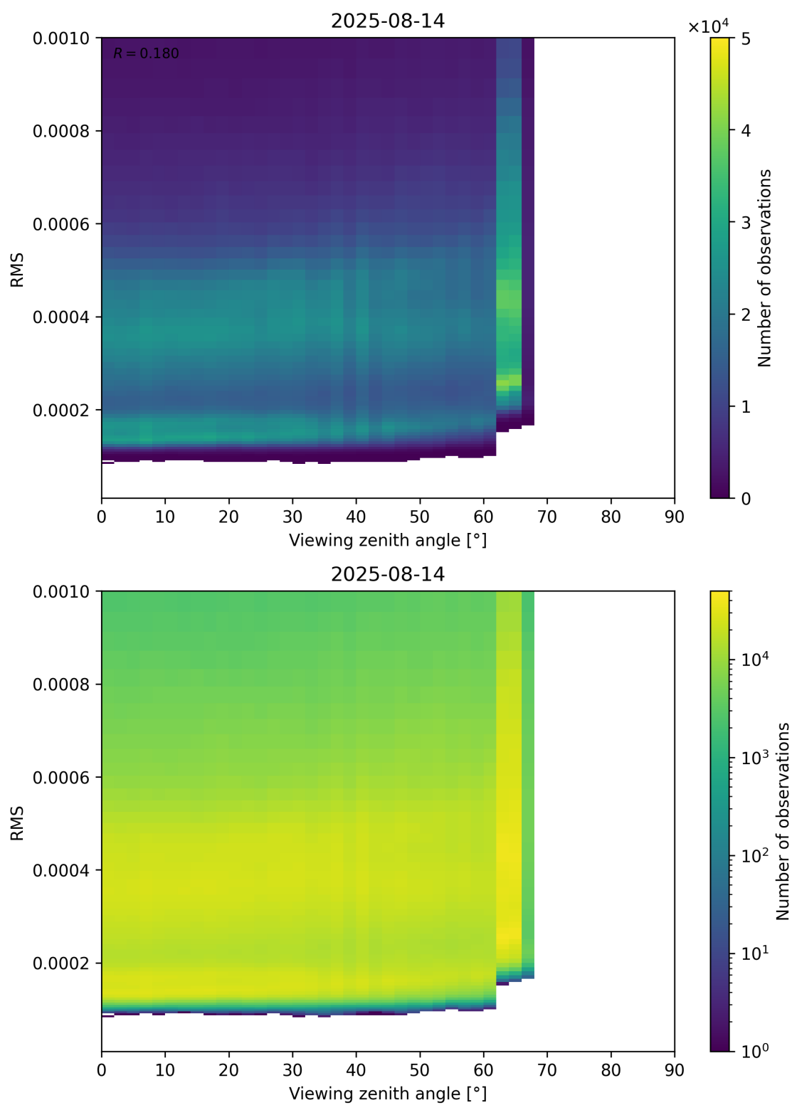
Figure 171: Scatter density plot of “Viewing zenith angle” against “RMS” for 2025-08-14 to 2025-08-15.
