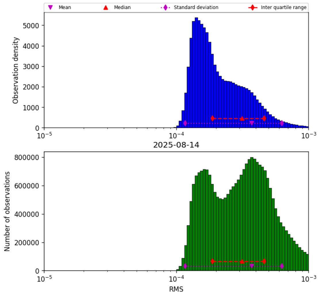
Figure 43: Histogram of “RMS” for 2025-08-14 to 2025-08-15
