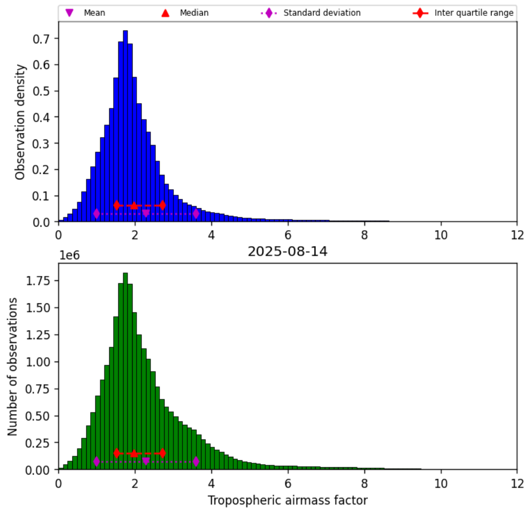
Figure 31: Histogram of “Tropospheric airmass factor” for 2025-08-14 to 2025-08-15
