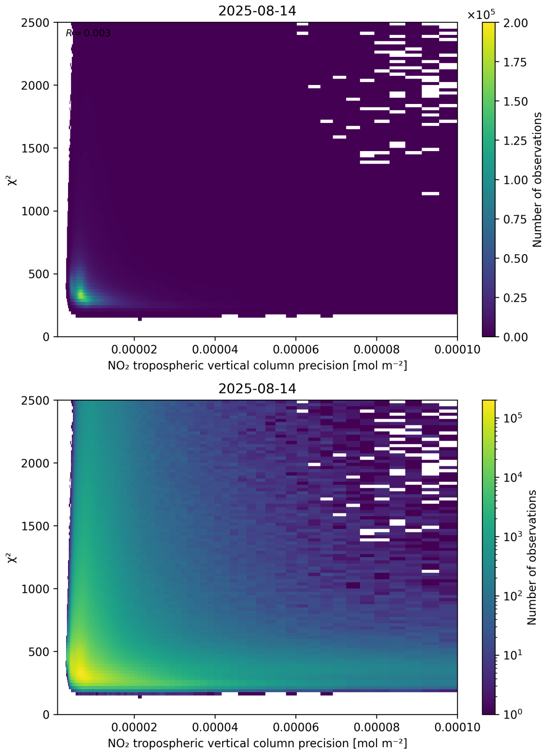
Figure 134: Scatter density plot of “NO 2 tropospheric vertical column precision” against “ \chi^2 ” for 2025-08-14 to 2025-08-15.
