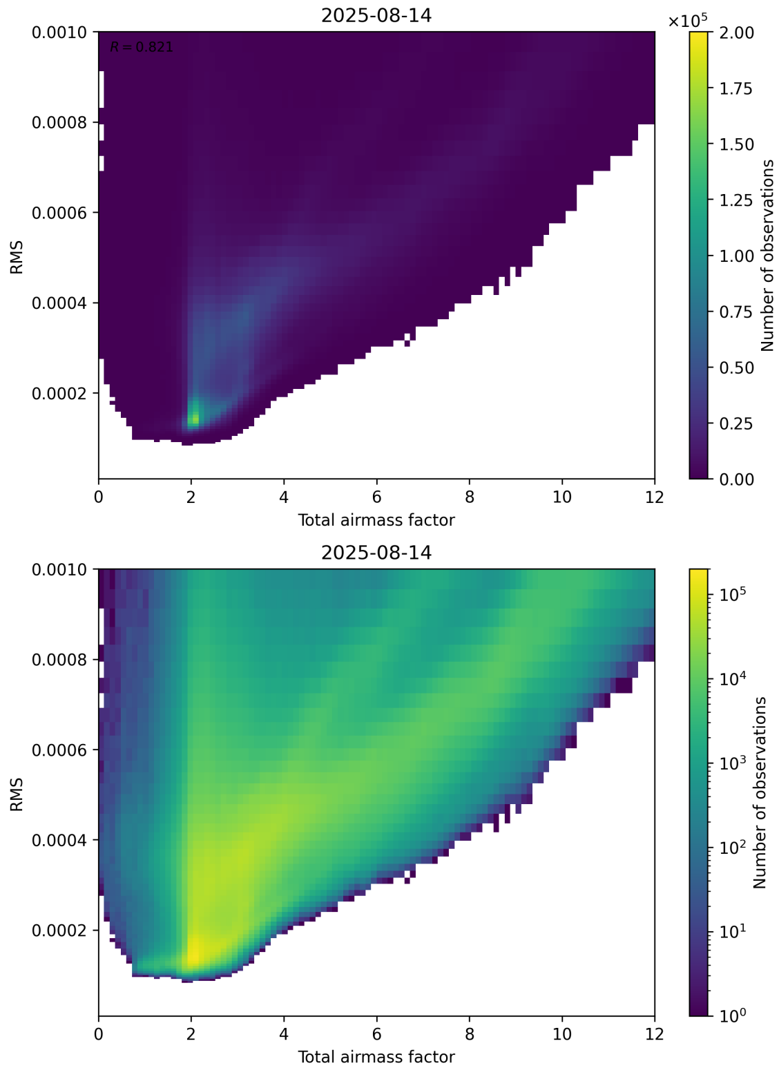
Figure 69: Scatter density plot of “Total airmass factor” against “RMS” for 2025-08-14 to 2025-08-15.
