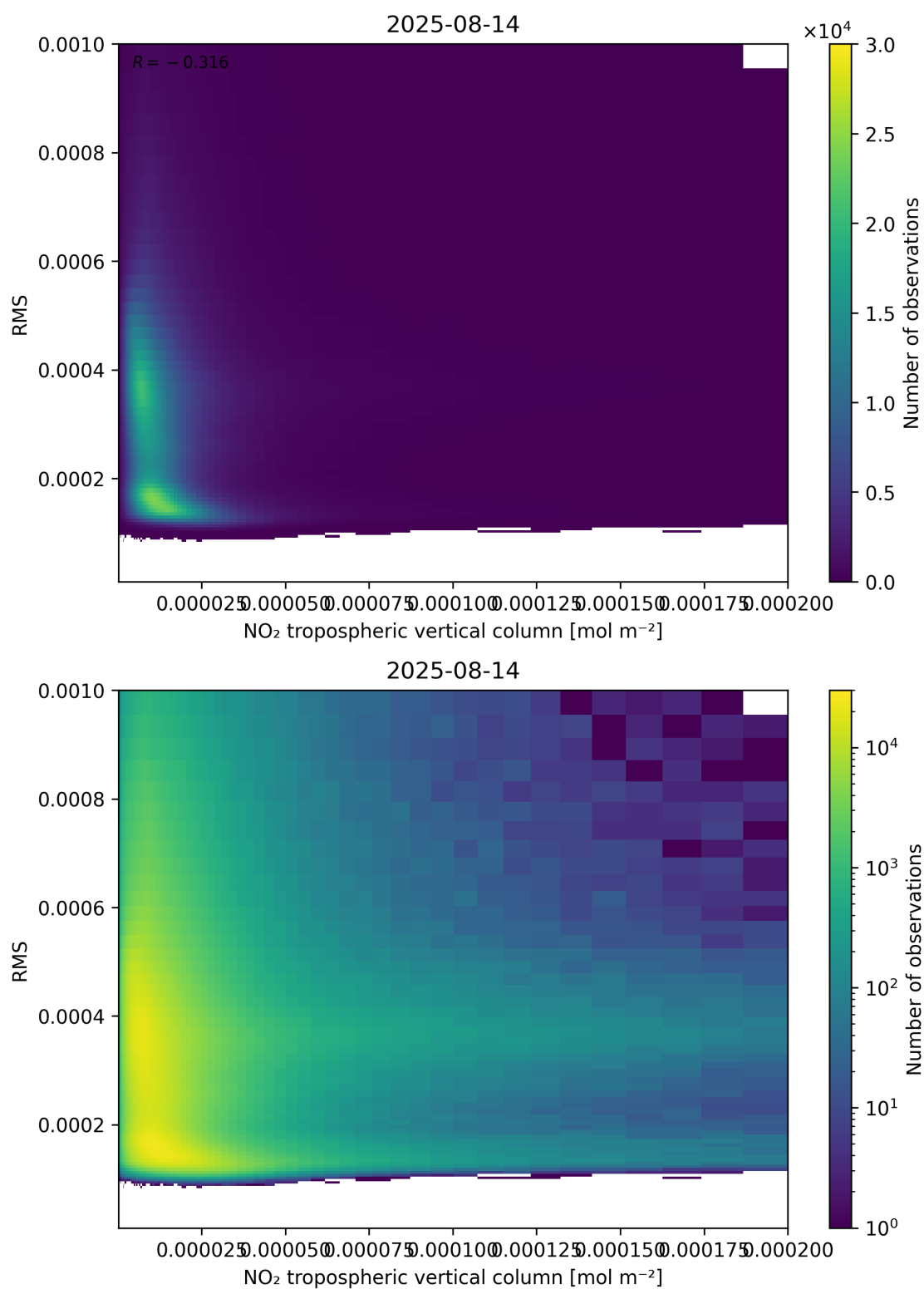
Figure 142: Scatter density plot of “NO 2 tropospheric vertical column” against “RMS” for 2025-08-14 to 2025-08-15.
