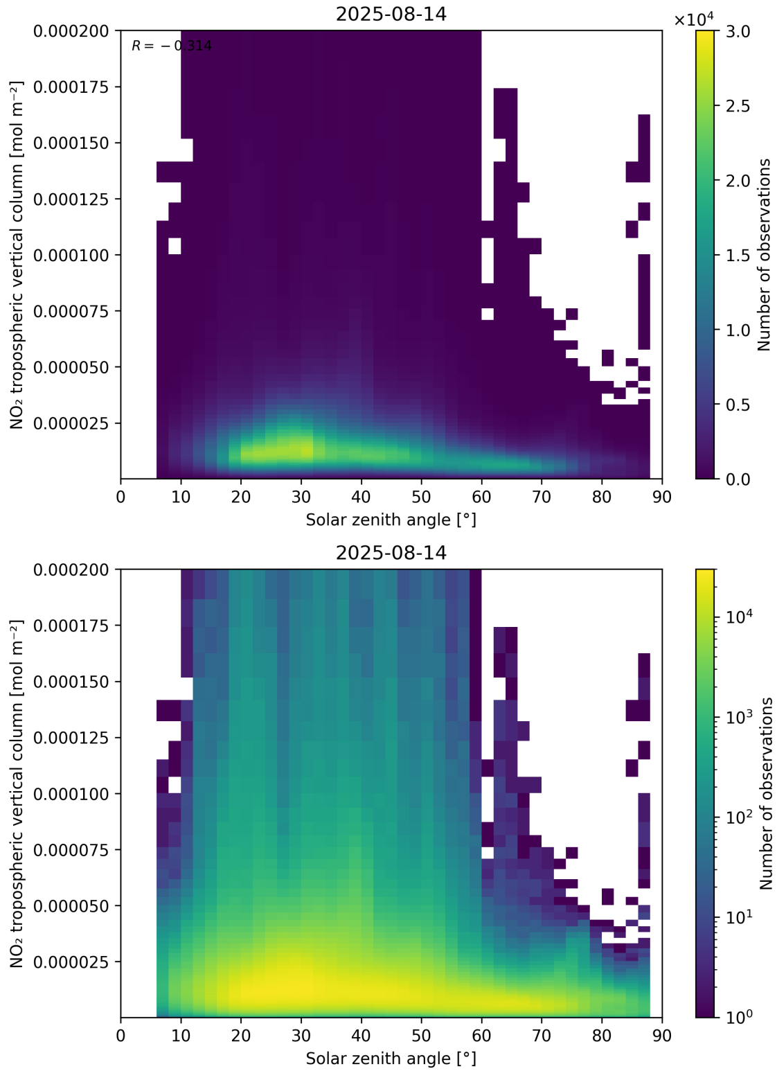
Figure 155: Scatter density plot of “Solar zenith angle” against “NO 2 tropospheric vertical column” for 2025-08-14 to 2025-08-15.
