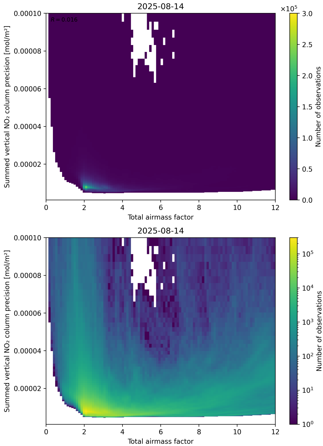
Figure 66: Scatter density plot of “Total airmass factor” against “Summed vertical NO 2 column precision” for 2025-08-14 to 2025-08-15.
