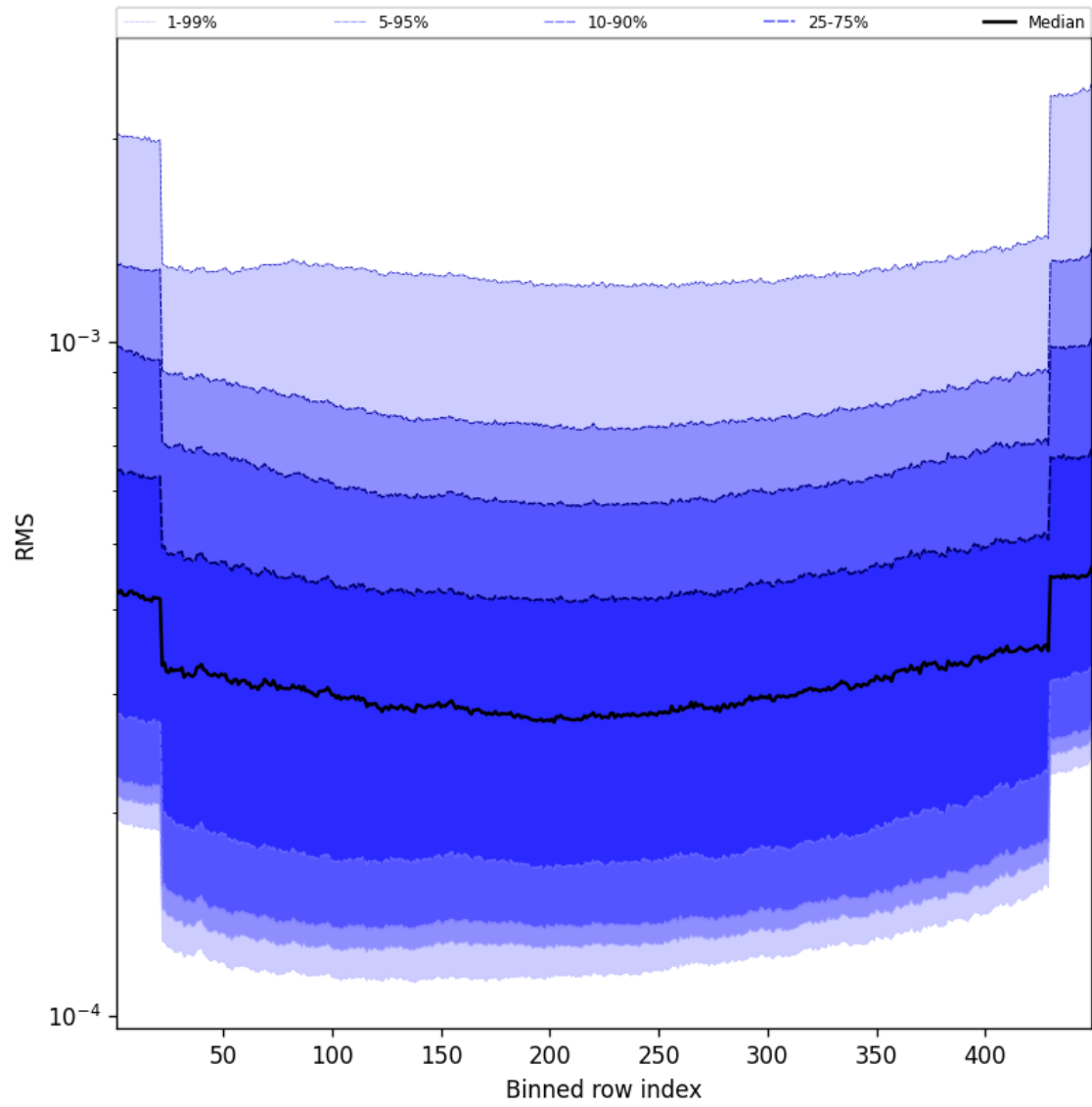
Figure 60: Along track statistics of “RMS” for 2025-08-14 to 2025-08-15
