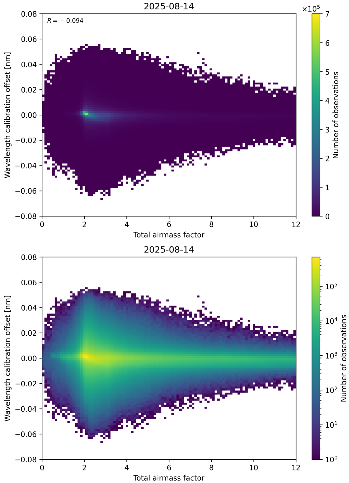
Figure 70: Scatter density plot of “Total airmass factor” against “Wavelength calibration offset” for 2025-08-14 to 2025-08-15.
