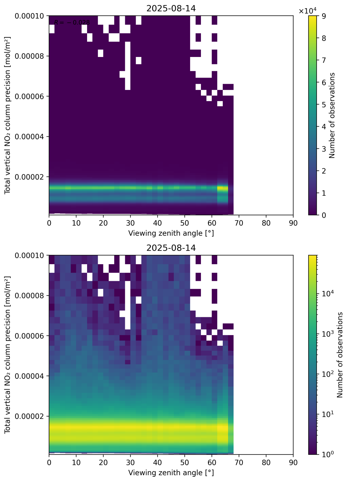
Figure 168: Scatter density plot of “Viewing zenith angle” against “Total vertical NO 2 column precision” for 2025-08-14 to 2025-08-15.
