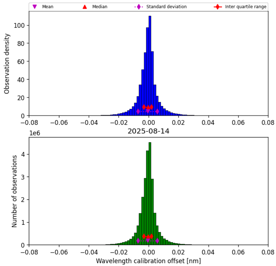
Figure 35: Histogram of “Wavelength calibration offset” for 2025-08-14 to 2025-08-15
