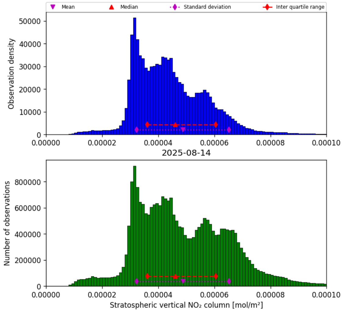
Figure 36: Histogram of “Stratospheric vertical NO 2 column” for 2025-08-14 to 2025-08-15
