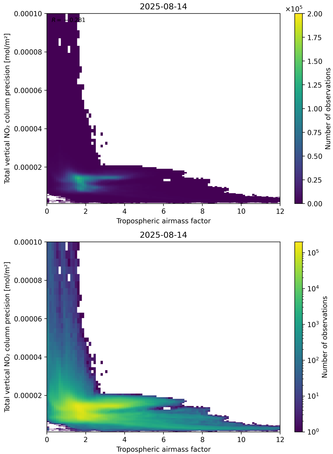
Figure 78: Scatter density plot of “Tropospheric air mass factor” against “Total vertical NO 2 column precision” for 2025-08-14 to 2025-08-15.
