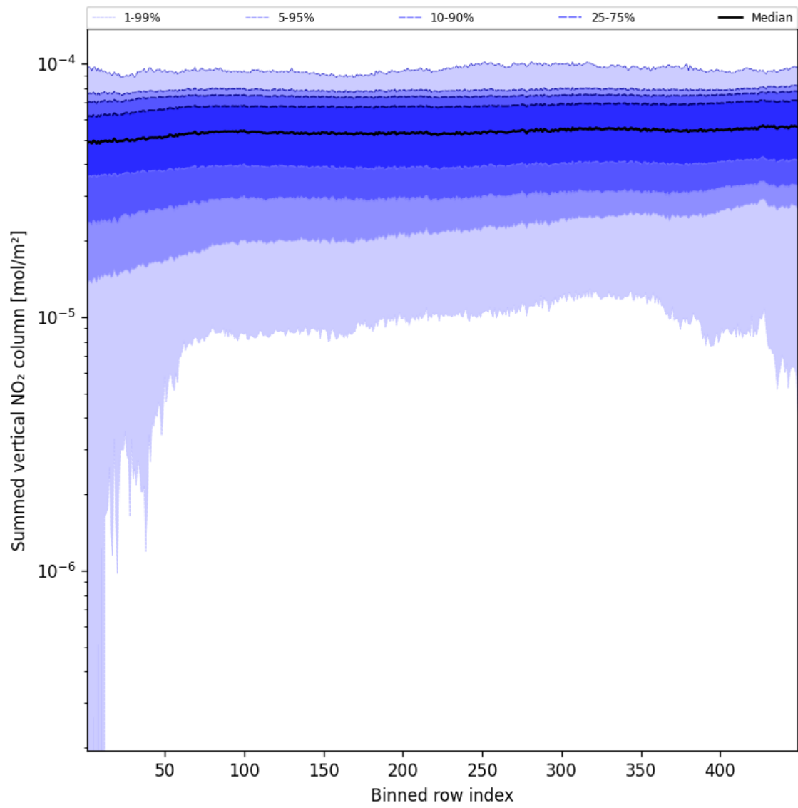
Figure 57: Along track statistics of “Summed vertical NO 2 column” for 2025-08-14 to 2025-08-15
