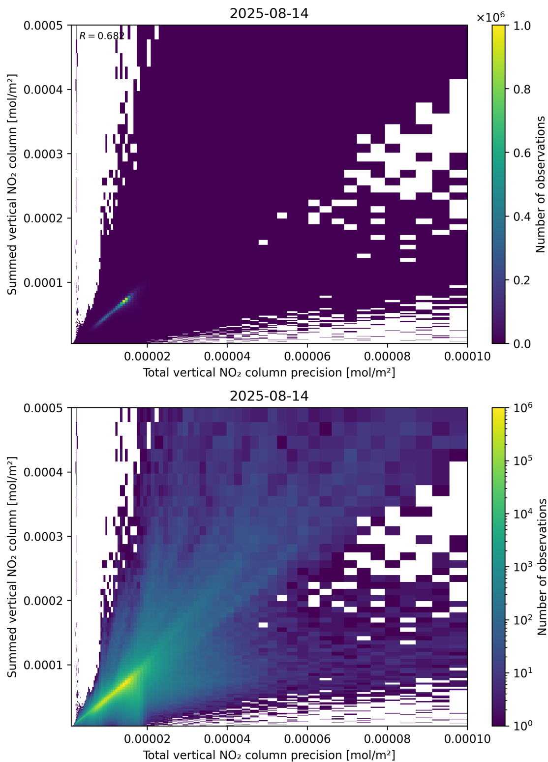
Figure 117: Scatter density plot of “Total vertical NO 2 column precision” against “Summed vertical NO 2 column” for 2025-08-14 to 2025-08-15.
