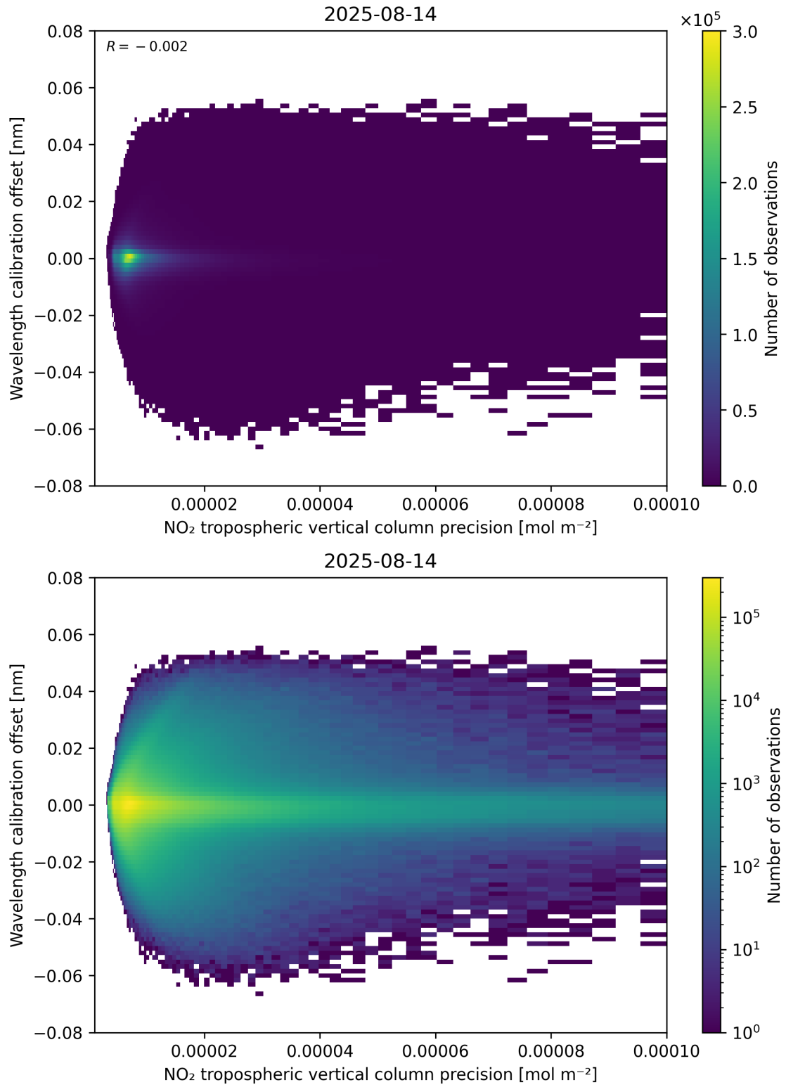
Figure 141: Scatter density plot of “NO 2 tropospheric vertical column precision” against “Wavelength calibration offset” for 2025-08-14 to 2025-08-15.
