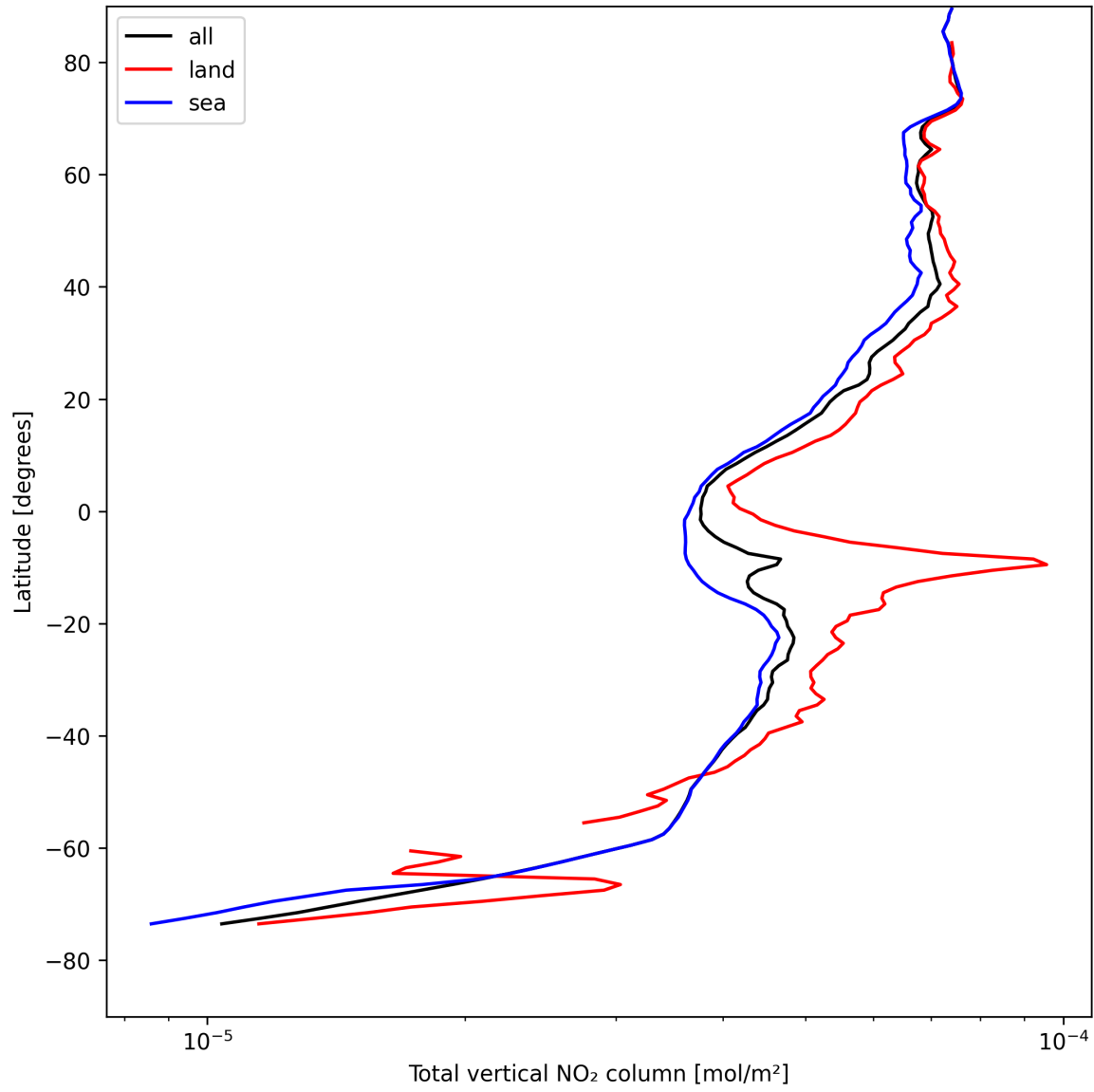
Figure 21: Zonal average of “Total vertical NO 2 column” for 2025-08-14 to 2025-08-15.
