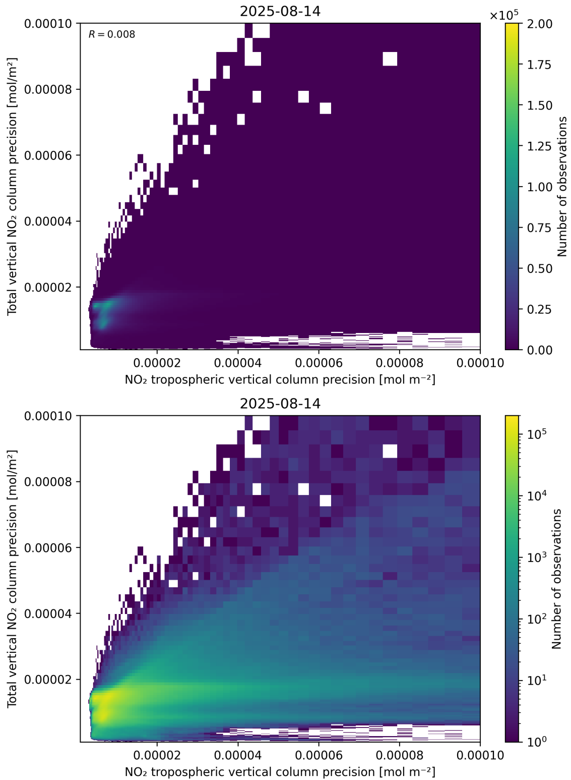
Figure 139: Scatter density plot of “NO 2 tropospheric vertical column precision” against “Total vertical NO 2 column precision” for 2025-08-14 to 2025-08-15.
