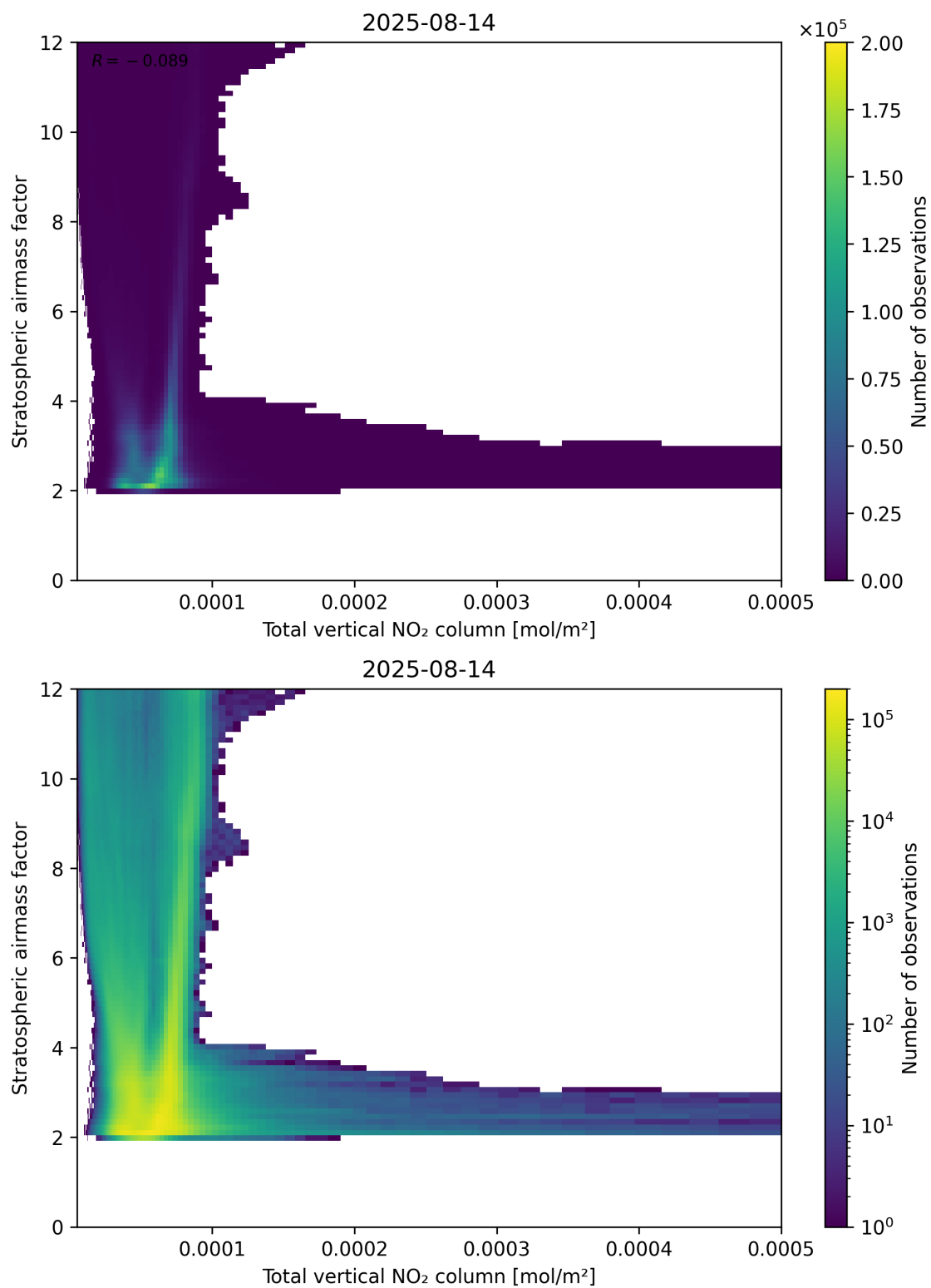
Figure 110: Scatter density plot of “Total vertical NO 2 column” against “Stratospheric airmass factor” for 2025-08-14 to 2025-08-15.
