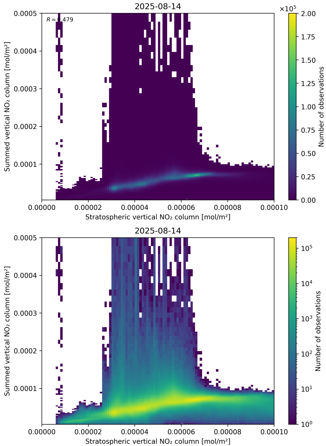
Figure 98: Scatter density plot of “Stratospheric vertical NO 2 column” against “Summed vertical NO 2 column” for 2025-08-14 to 2025-08-15.
