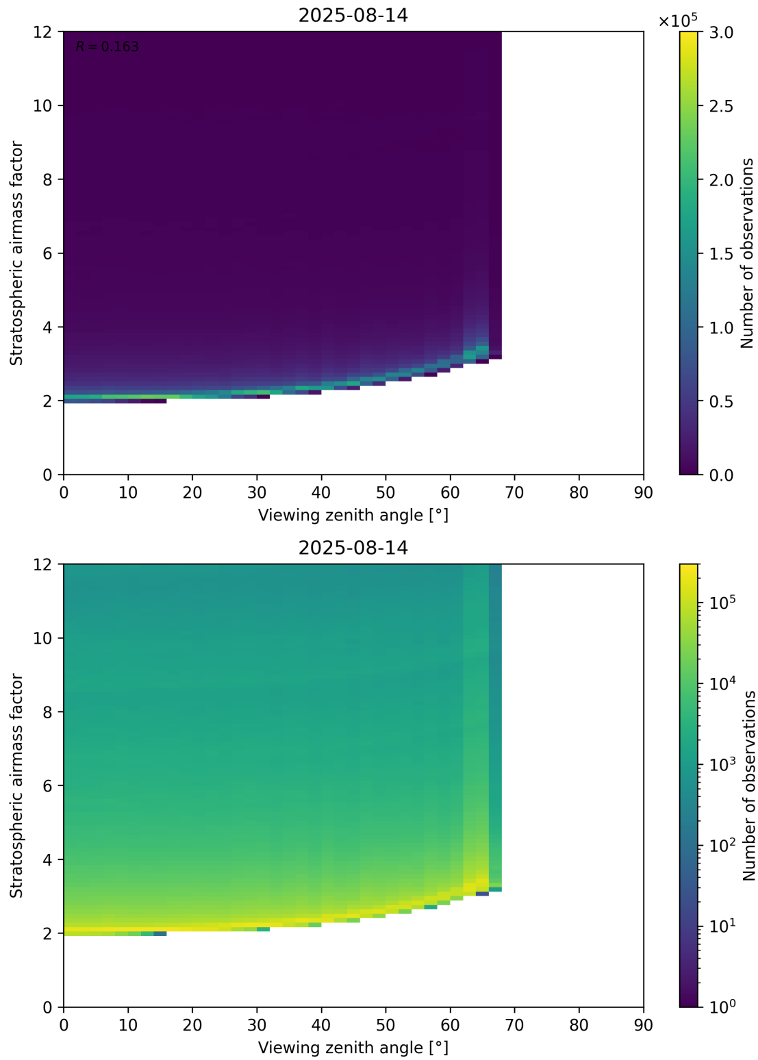
Figure 159: Scatter density plot of “Viewing zenith angle” against “Stratospheric airmass factor” for 2025-08-14 to 2025-08-15.
