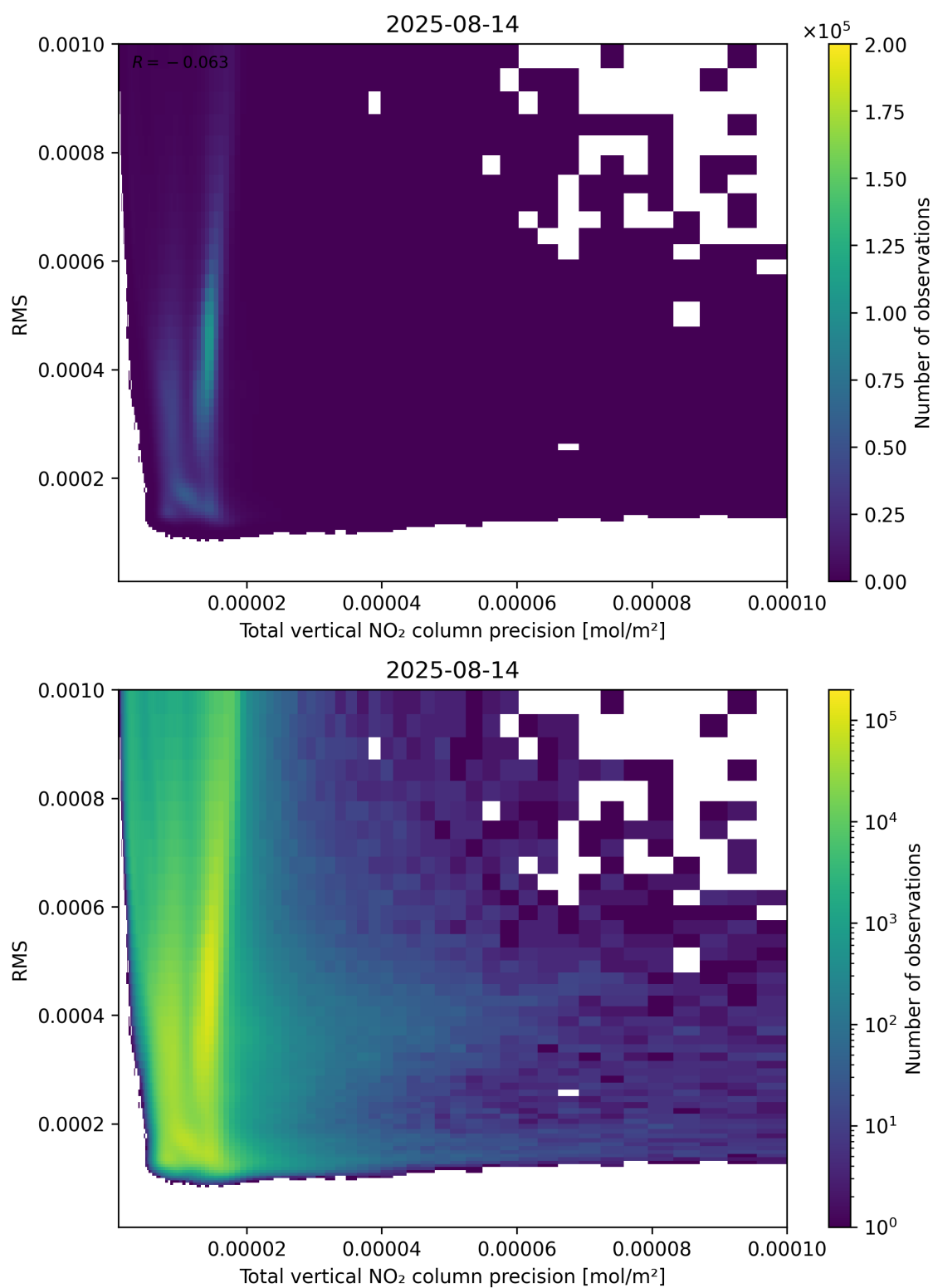
Figure 119: Scatter density plot of “Total vertical NO 2 column precision” against “RMS” for 2025-08-14 to 2025-08-15.
