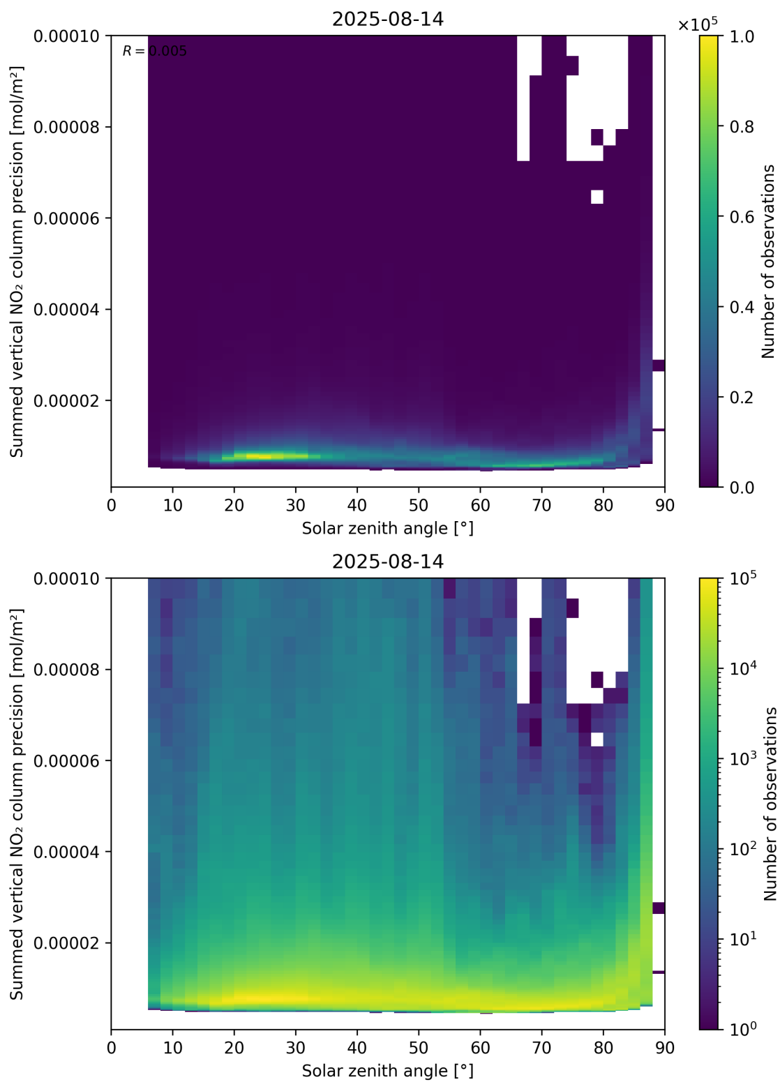
Figure 152: Scatter density plot of “Solar zenith angle” against “Summed vertical NO 2 column precision” for 2025-08-14 to 2025-08-15.
