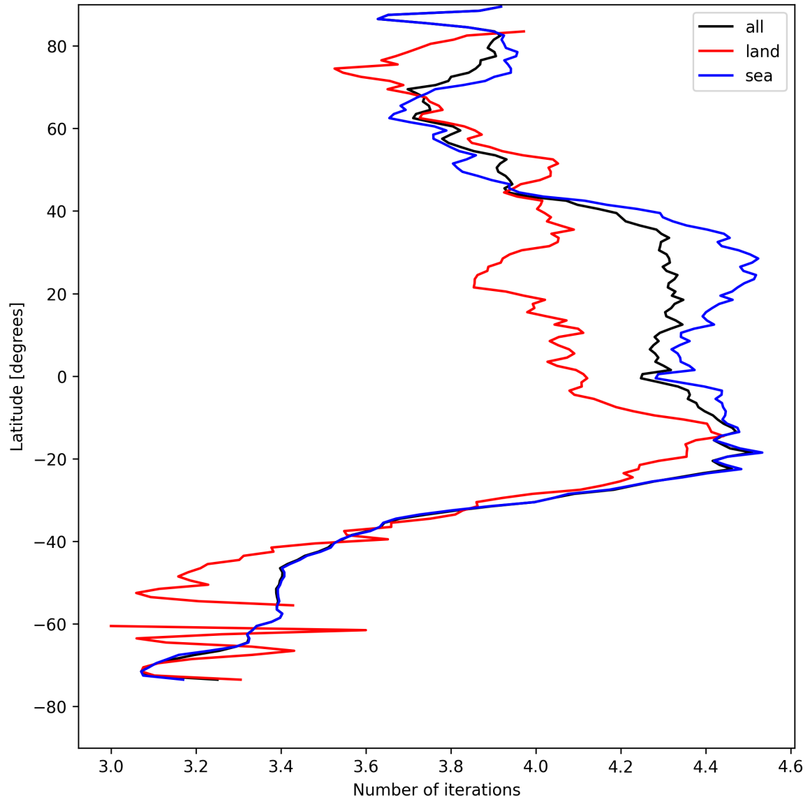
Figure 17: Zonal average of “Number of iterations” for 2025-08-14 to 2025-08-15.
