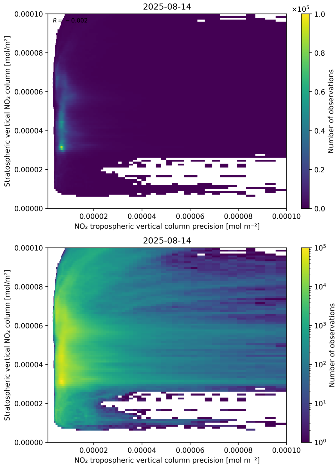
Figure 135: Scatter density plot of “NO 2 tropospheric vertical column precision” against “Stratospheric vertical NO 2 column” for 2025-08-14 to 2025-08-15.
