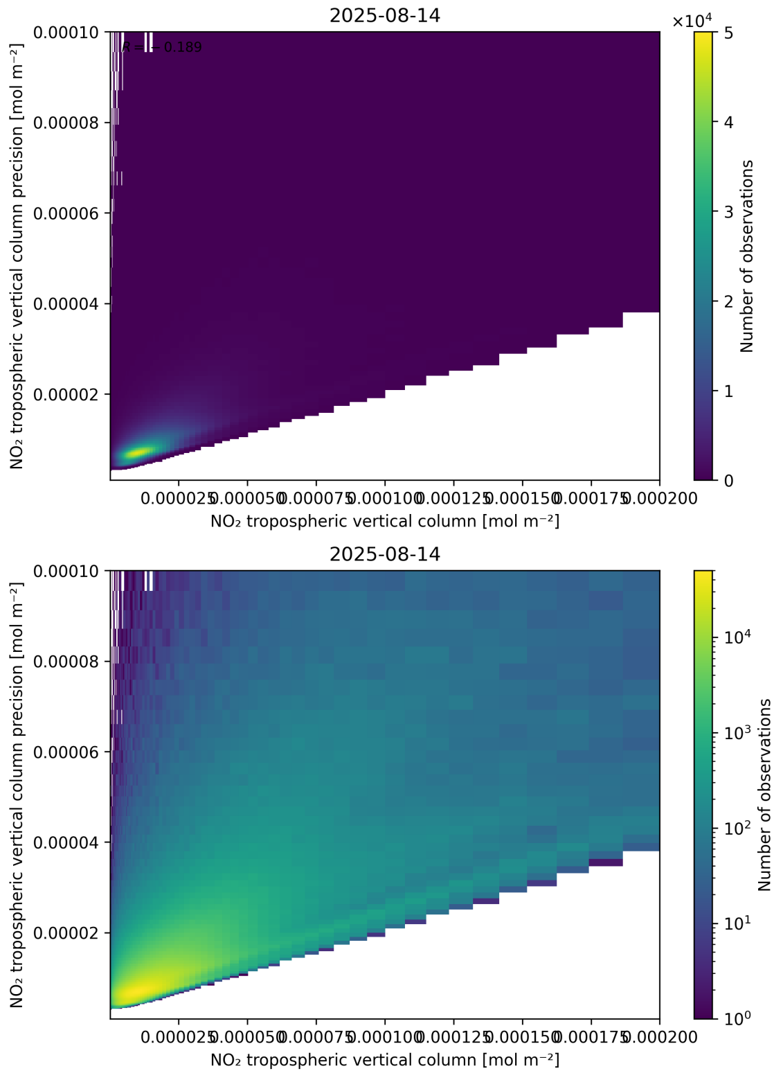
Figure 130: Scatter density plot of “NO 2 tropospheric vertical column” against “NO 2 tropospheric vertical column precision” for 2025-08-14 to 2025-08-15.
