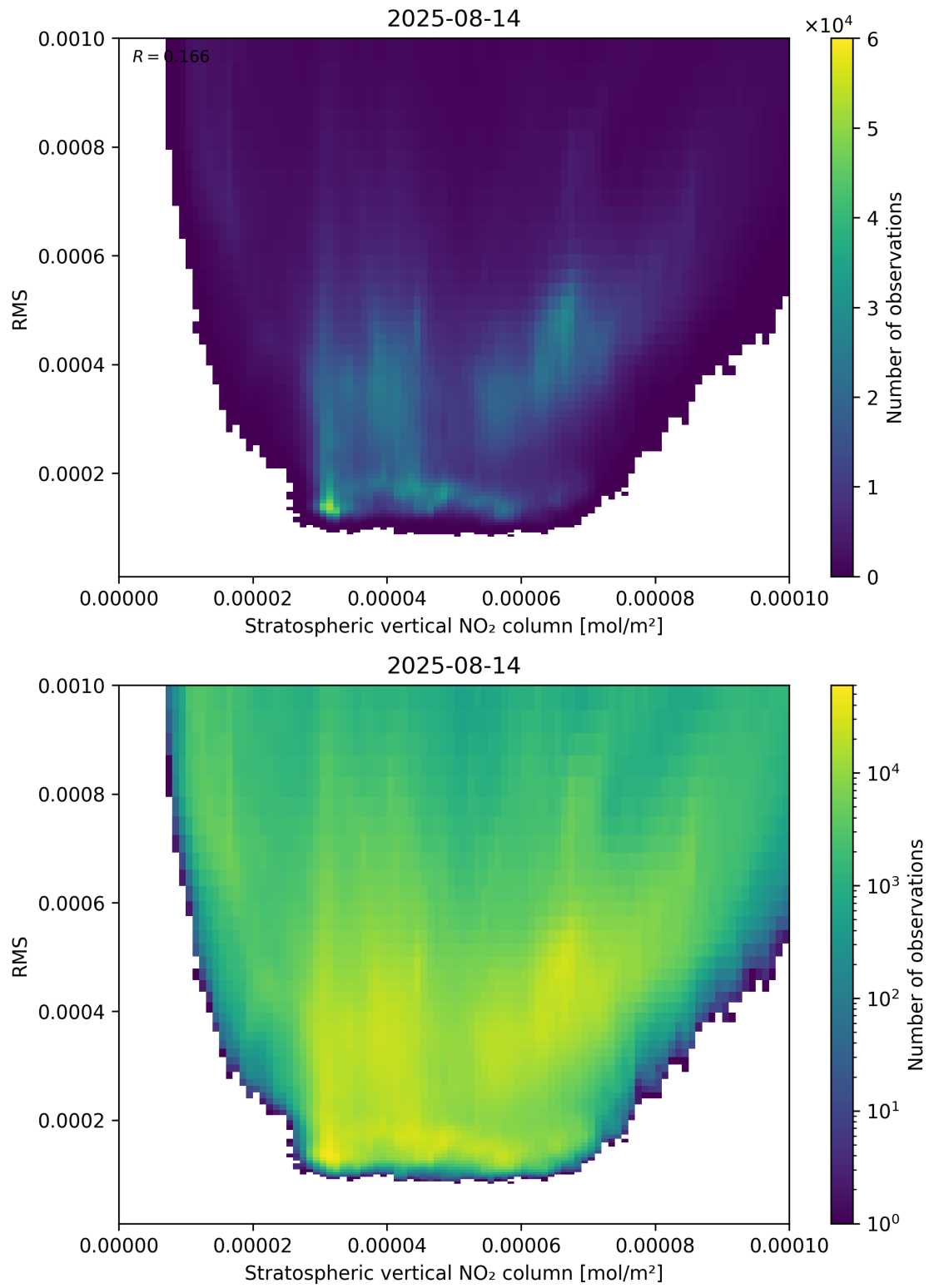
Figure 102: Scatter density plot of “Stratospheric vertical NO 2 column” against “RMS” for 2025-08-14 to 2025-08-15.
