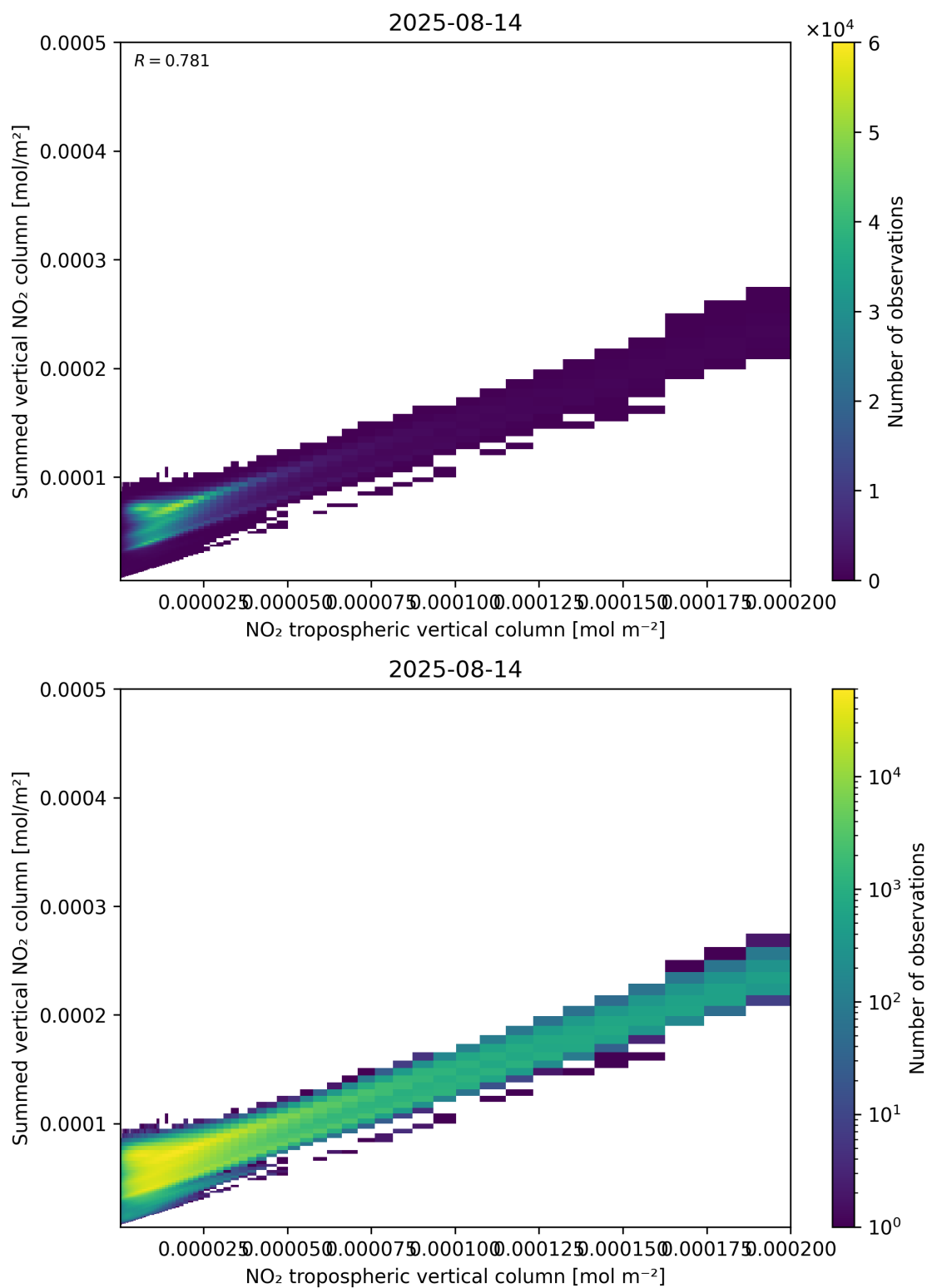
Figure 126: Scatter density plot of “NO 2 tropospheric vertical column” against “Summed vertical NO 2 column” for 2025-08-14 to 2025-08-15.
