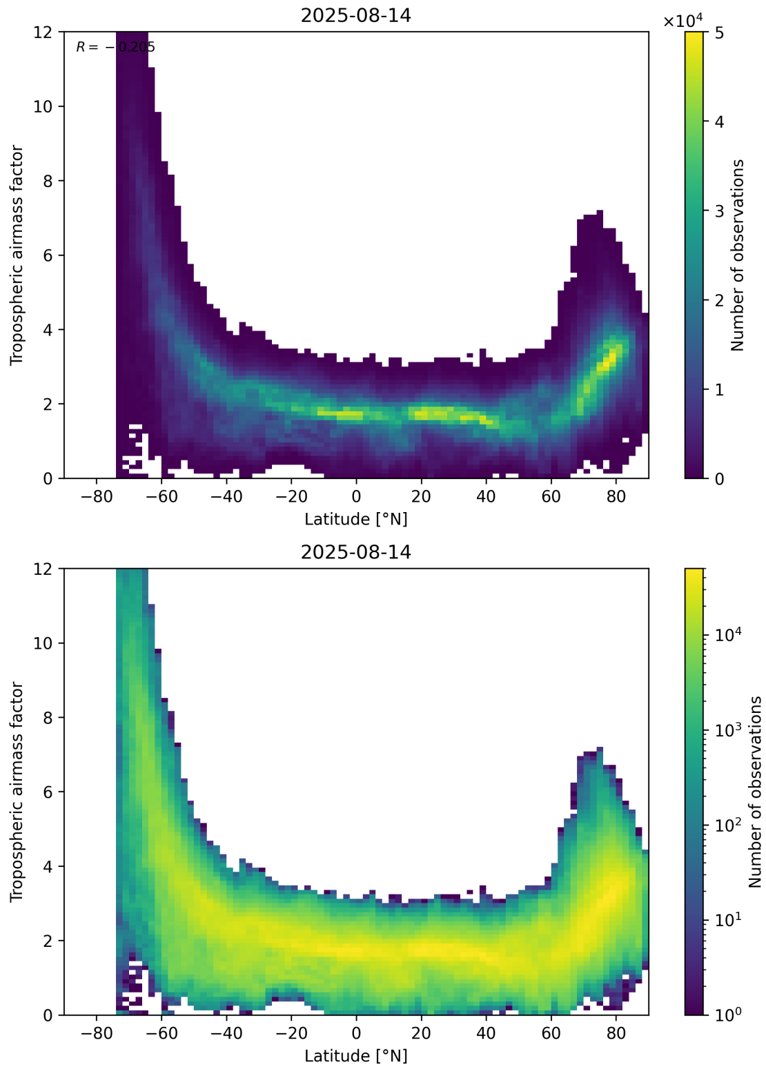
Figure 85: Scatter density plot of “Latitude” against “Tropospheric air mass factor” for 2025-08-14 to 2025-08-15.
