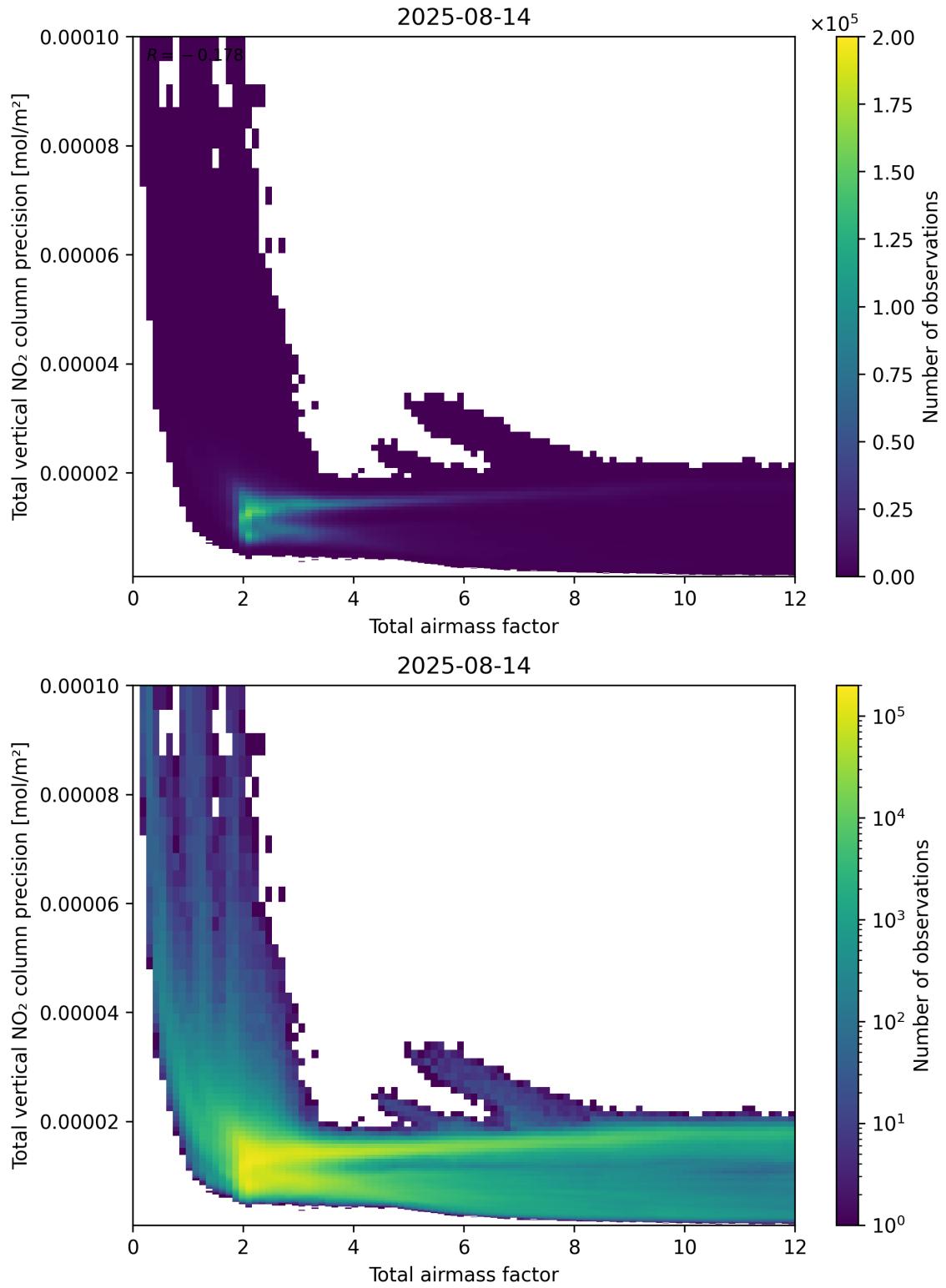
Figure 68: Scatter density plot of “Total airmass factor” against “Total vertical NO 2 column precision” for 2025-08-14 to 2025-08-15.
