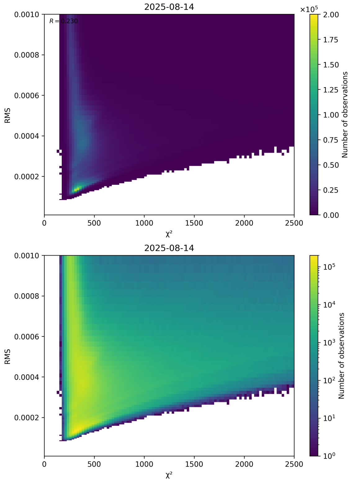
Figure 82: Scatter density plot of “ \chi^2 ” against “RMS” for 2025-08-14 to 2025-08-15.
