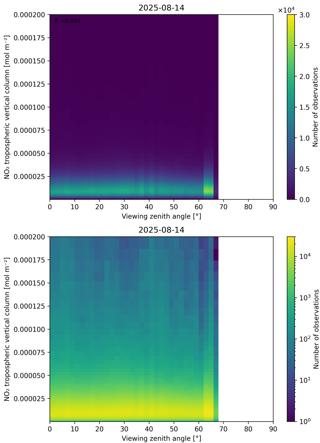
Figure 169: Scatter density plot of “Viewing zenith angle” against “NO 2 tropospheric vertical column” for 2025-08-14 to 2025-08-15.
