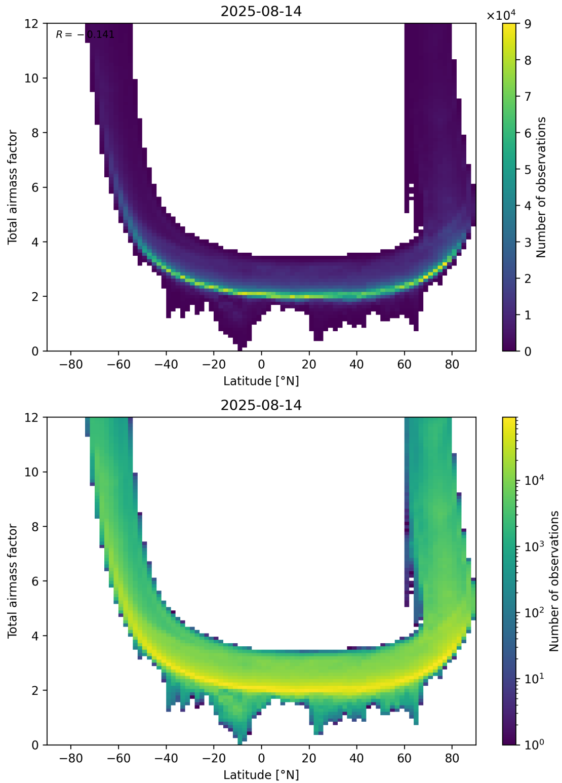
Figure 84: Scatter density plot of “Latitude” against “Total airmass factor” for 2025-08-14 to 2025-08-15.
