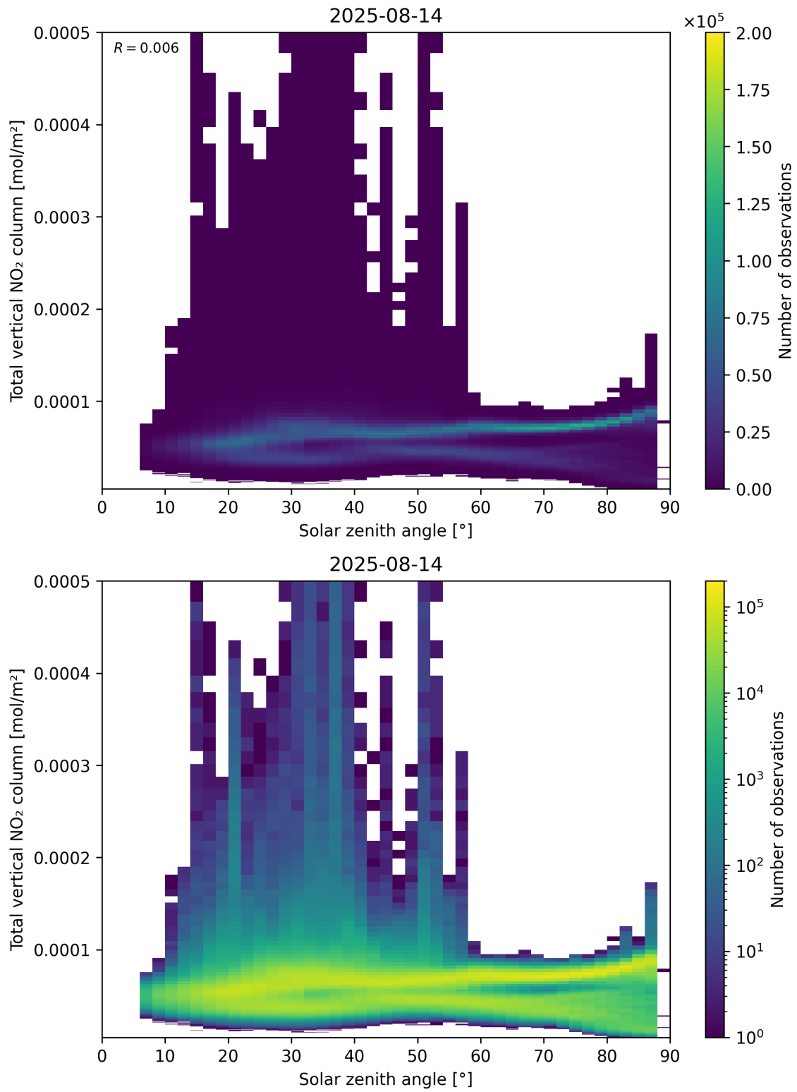
Figure 153: Scatter density plot of “Solar zenith angle” against “Total vertical NO 2 column” for 2025-08-14 to 2025-08-15.
