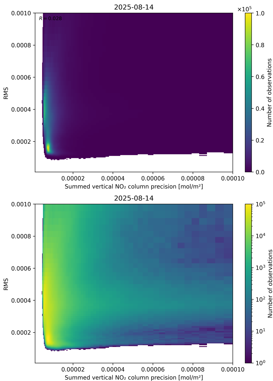
Figure 108: Scatter density plot of “Summed vertical NO 2 column precision” against “RMS” for 2025-08-14 to 2025-08-15.
