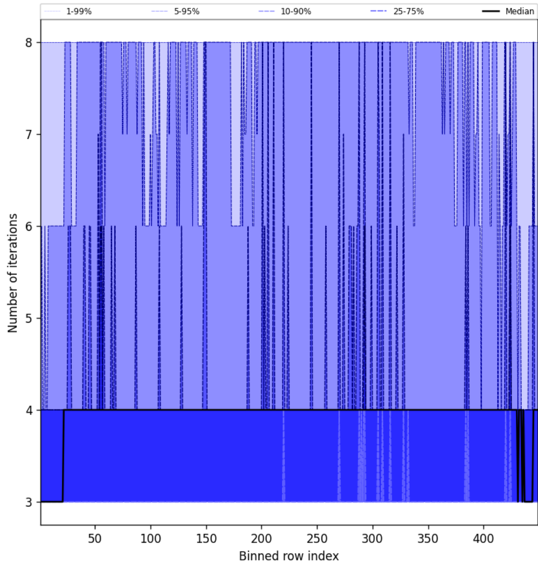
Figure 51: Along track statistics of “Number of iterations” for 2025-08-14 to 2025-08-15
