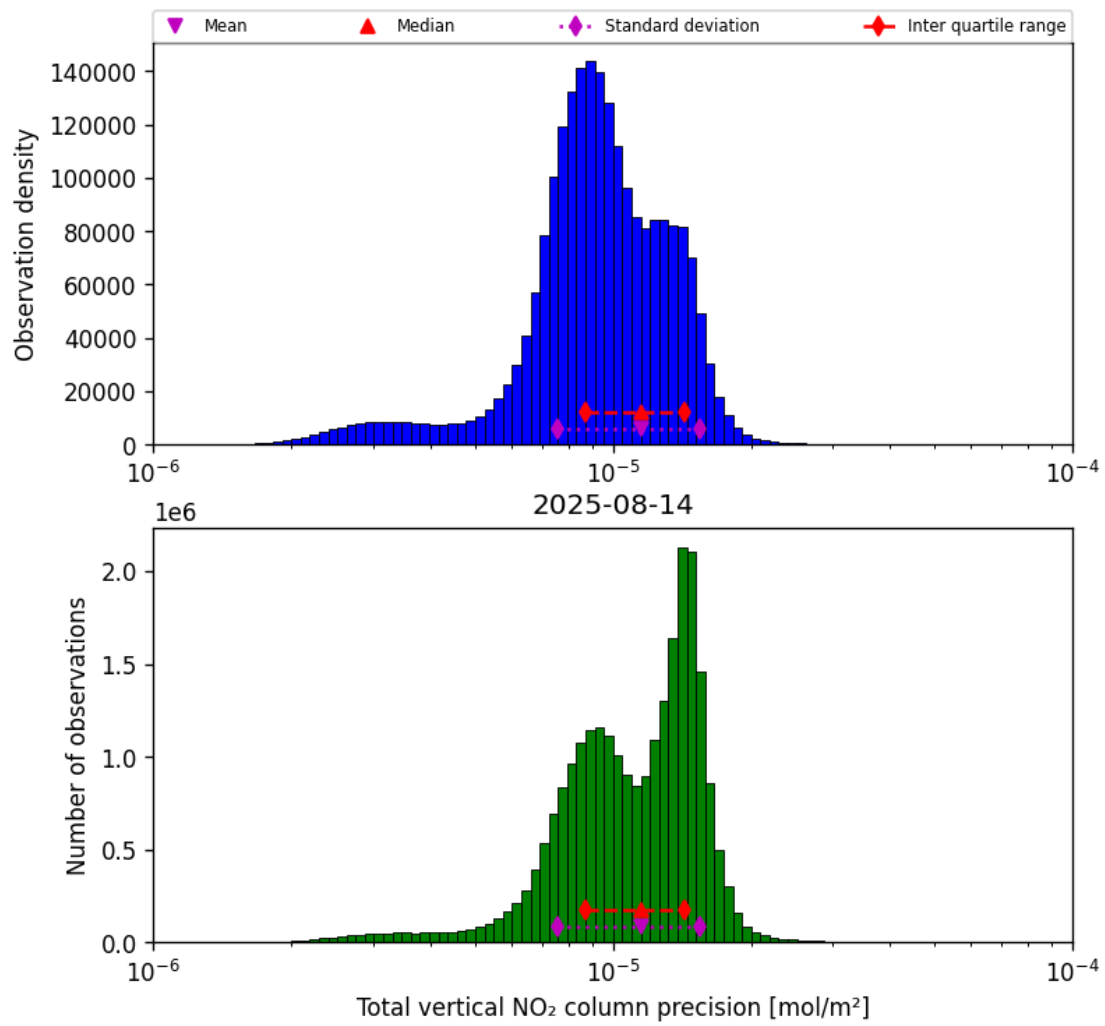
Figure 39: Histogram of “Total vertical NO 2 column precision” for 2025-08-14 to 2025-08-15
