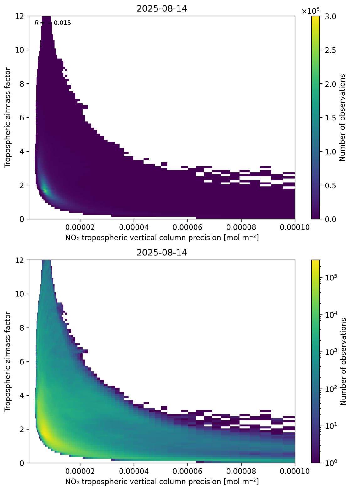
Figure 133: Scatter density plot of “NO 2 tropospheric vertical column precision” against “Tropospheric airmass factor” for 2025-08-14 to 2025-08-15.
