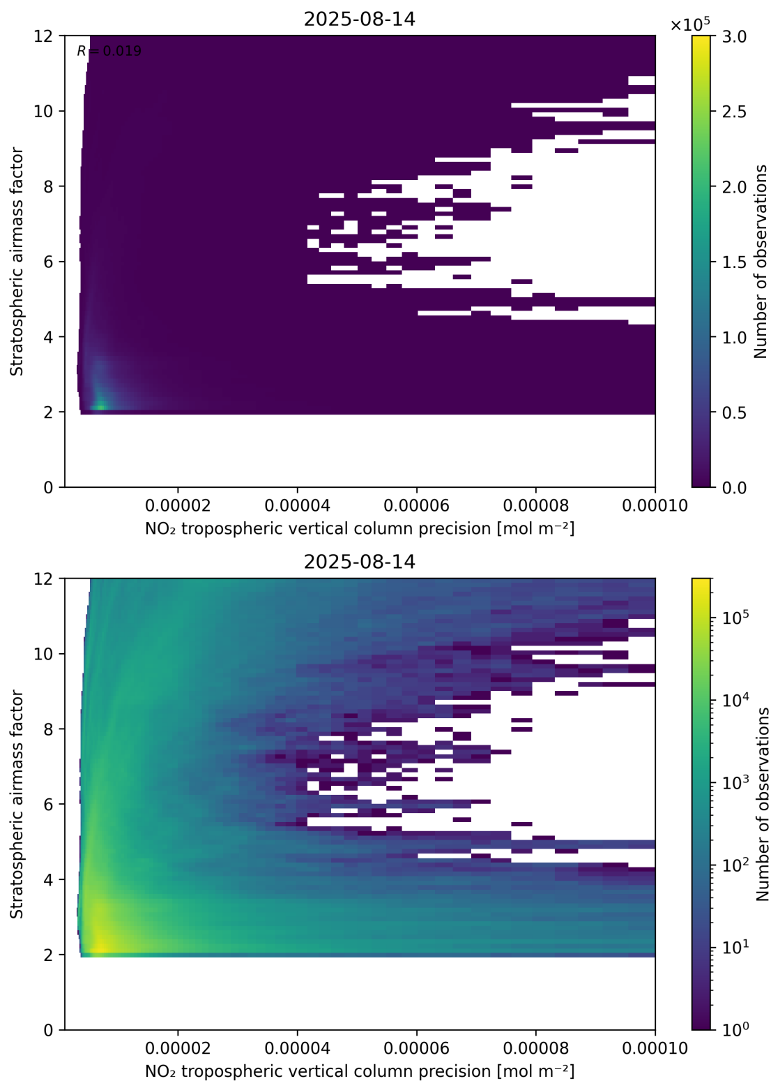
Figure 131: Scatter density plot of “NO 2 tropospheric vertical column precision” against “Stratospheric airmass factor” for 2025-08-14 to 2025-08-15.
