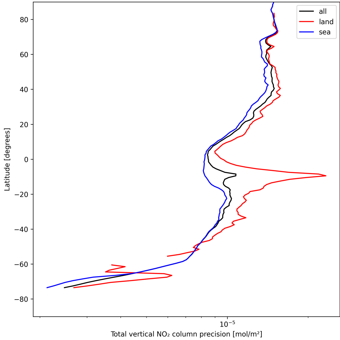
Figure 22: Zonal average of “Total vertical NO 2 column precision” for 2025-08-14 to 2025-08-15.
