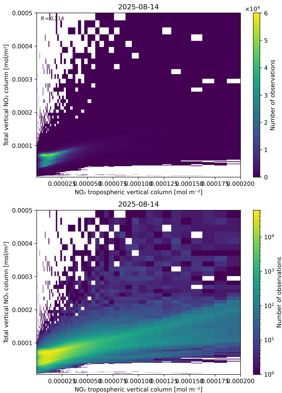
Figure 128: Scatter density plot of “NO 2 tropospheric vertical column” against “Total vertical NO 2 column” for 2025-08-14 to 2025-08-15.
