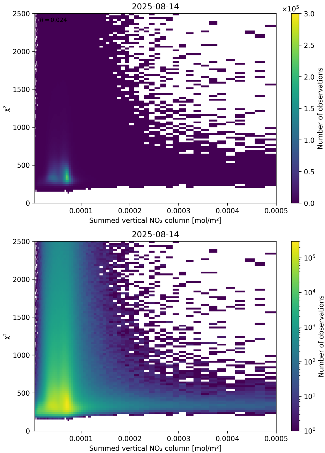
Figure 104: Scatter density plot of “Summed vertical NO 2 column” against “ \chi^2 ” for 2025-08-14 to 2025-08-15.
