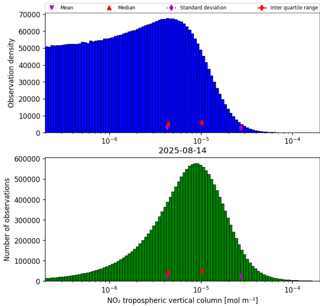
Figure 29: Histogram of “NO 2 tropospheric vertical column” for 2025-08-14 to 2025-08-15
