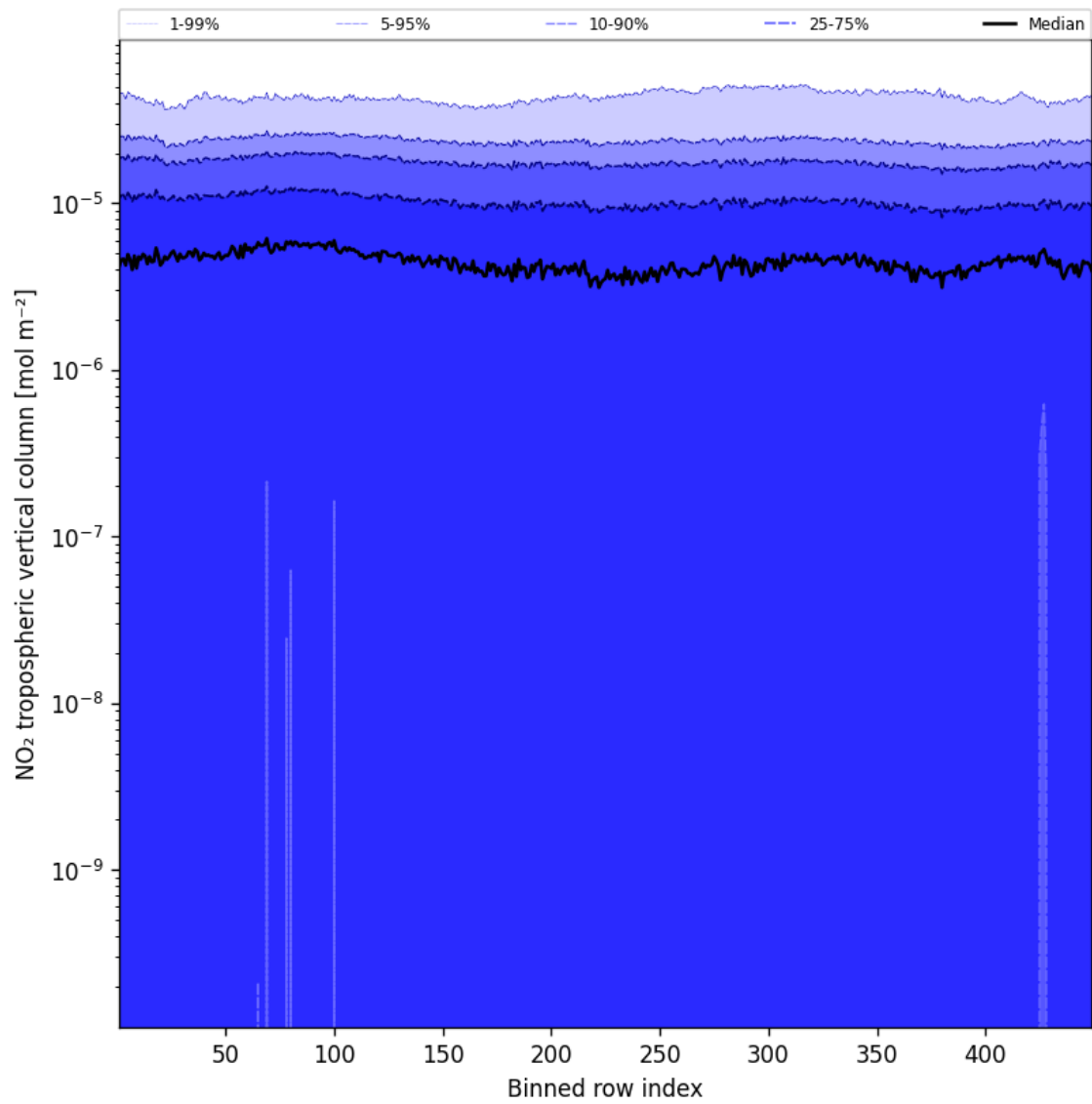
Figure 46: Along track statistics of “NO 2 tropospheric vertical column” for 2025-08-14 to 2025-08-15
