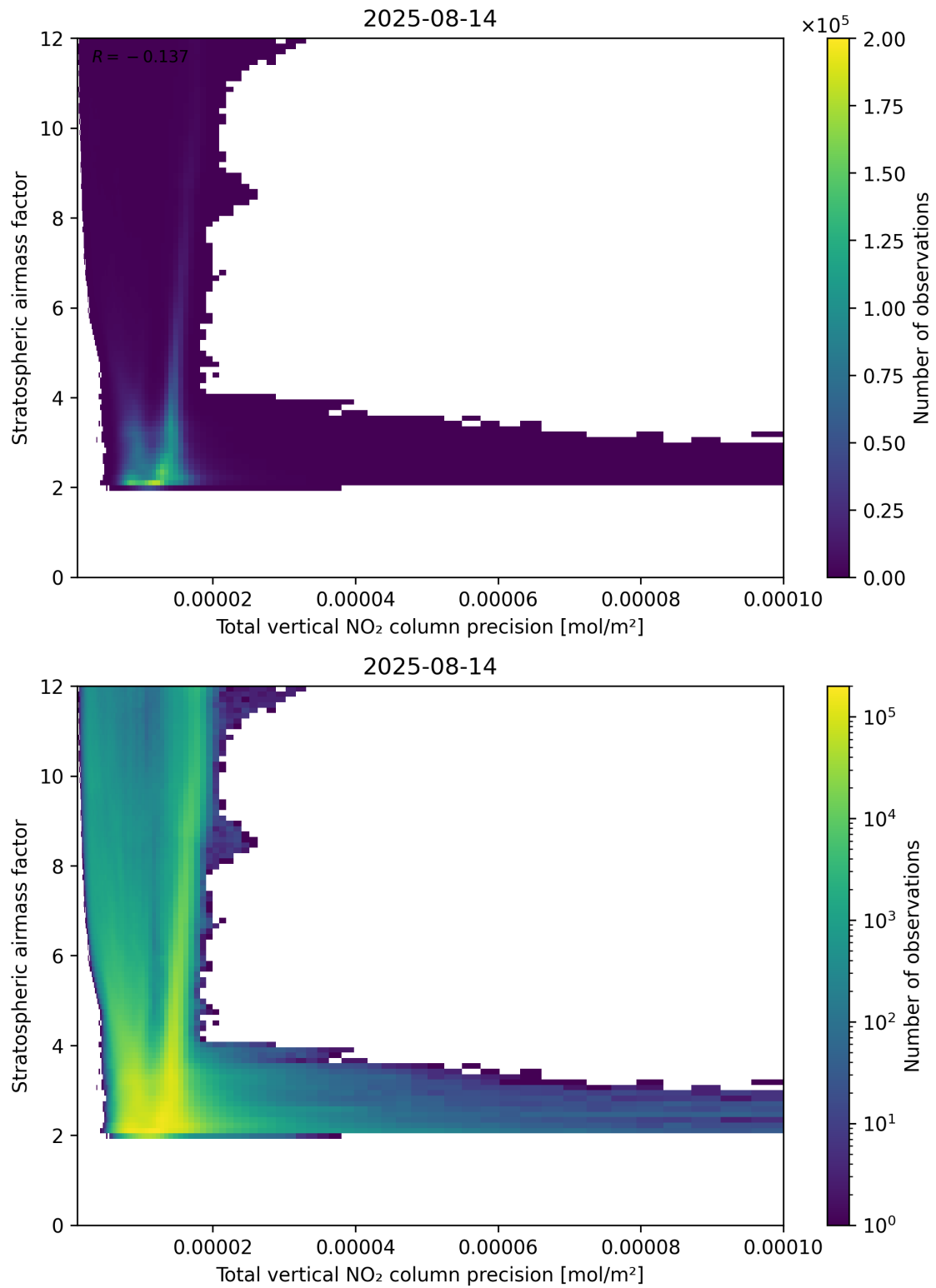
Figure 115: Scatter density plot of “Total vertical NO 2 column precision” against “Stratospheric airmass factor” for 2025-08-14 to 2025-08-15.
