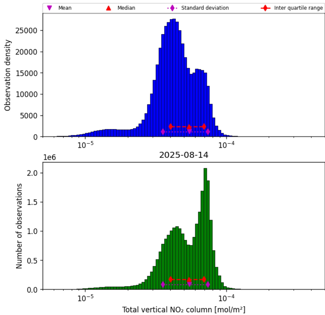
Figure 38: Histogram of “Total vertical NO 2 column” for 2025-08-14 to 2025-08-15
