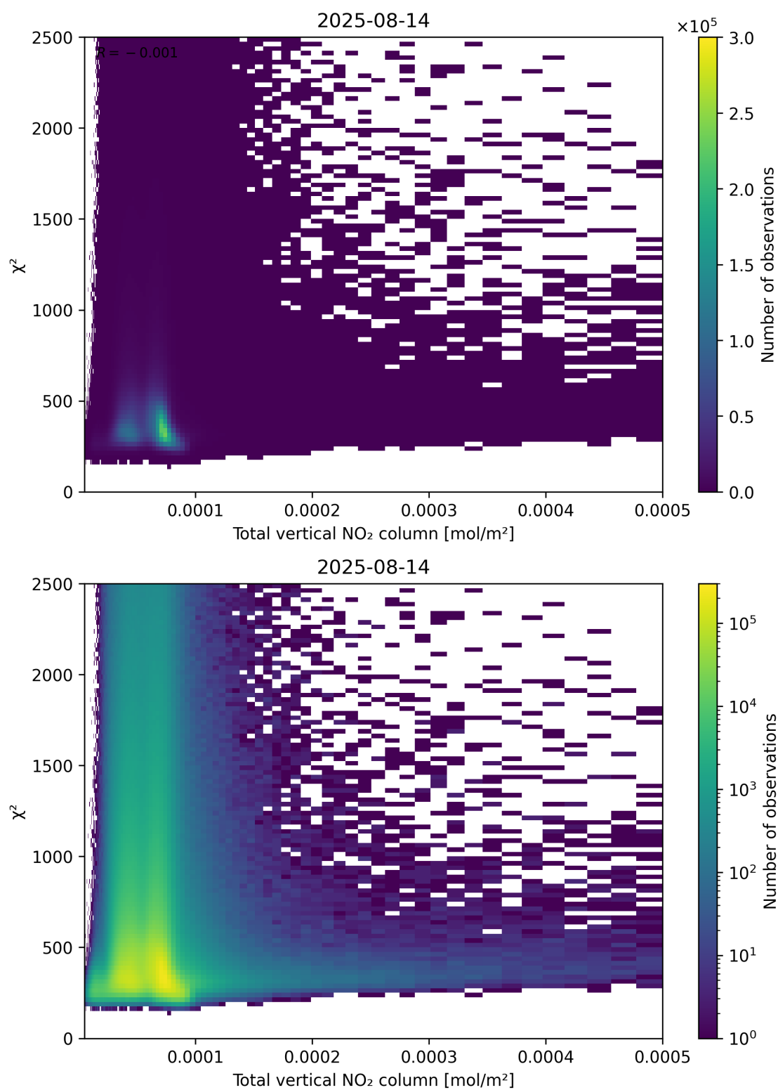
Figure 111: Scatter density plot of “Total vertical NO 2 column” against “ \chi^2 ” for 2025-08-14 to 2025-08-15.
