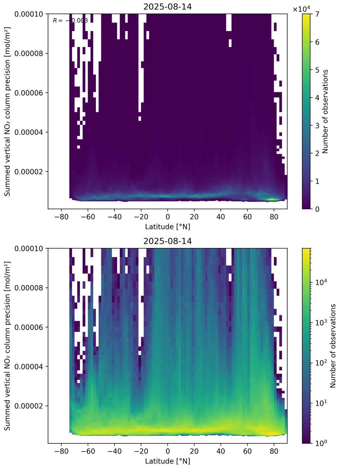
Figure 89: Scatter density plot of “Latitude” against “Summed vertical NO 2 column precision” for 2025-08-14 to 2025-08-15.
