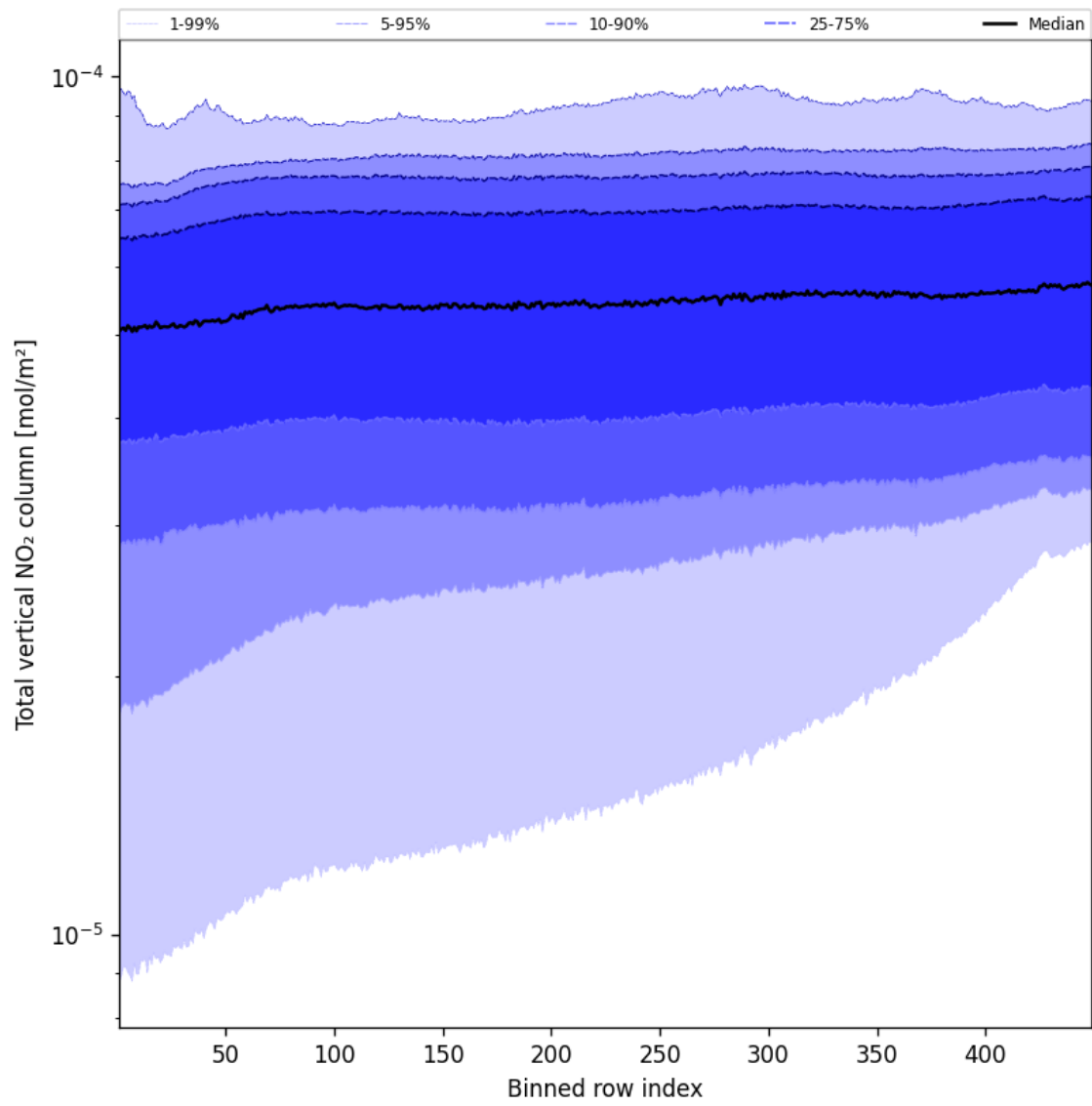
Figure 55: Along track statistics of “Total vertical NO 2 column” for 2025-08-14 to 2025-08-15
