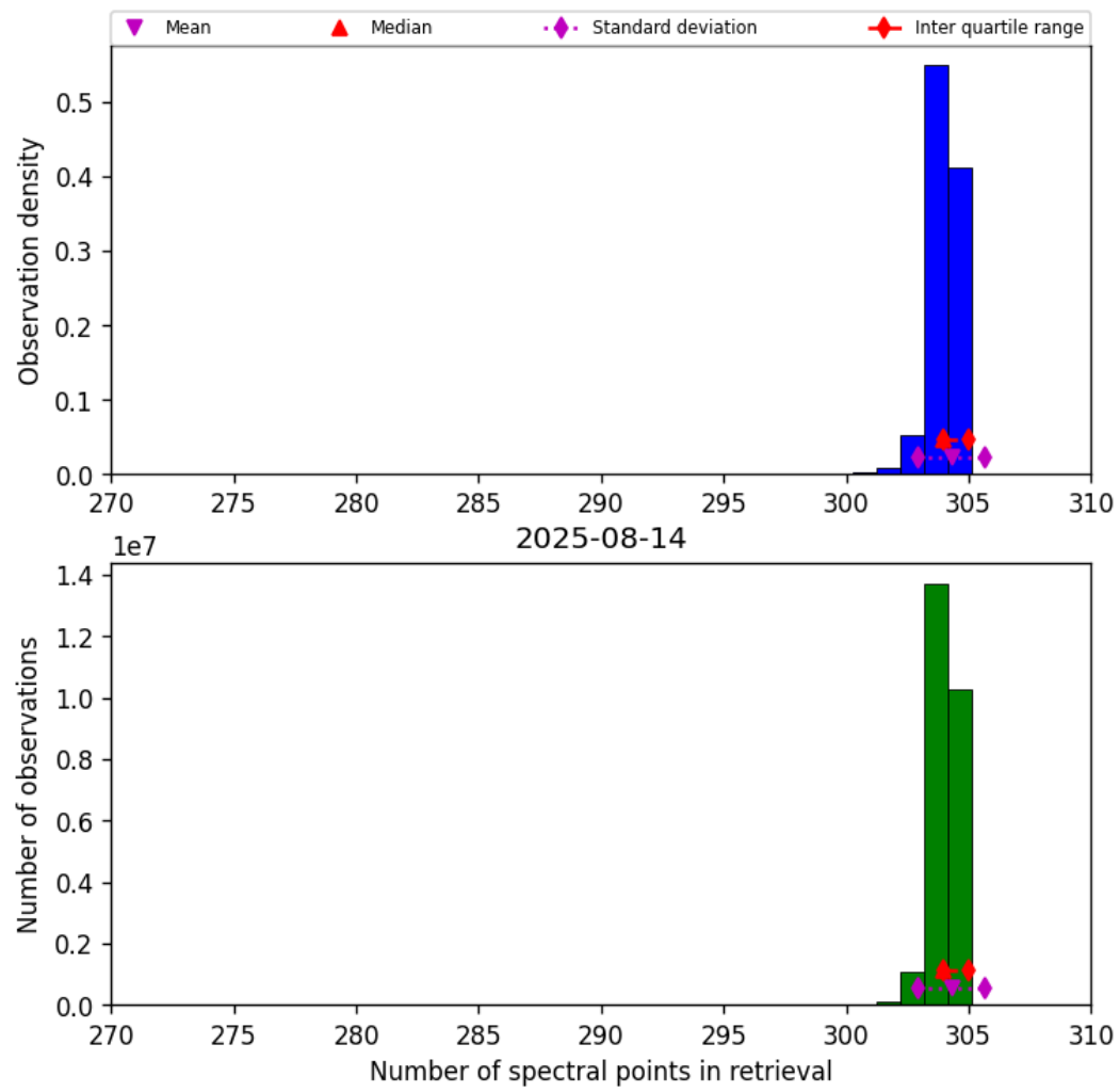
Figure 33: Histogram of “Number of spectral points in retrieval” for 2025-08-14 to 2025-08-15
