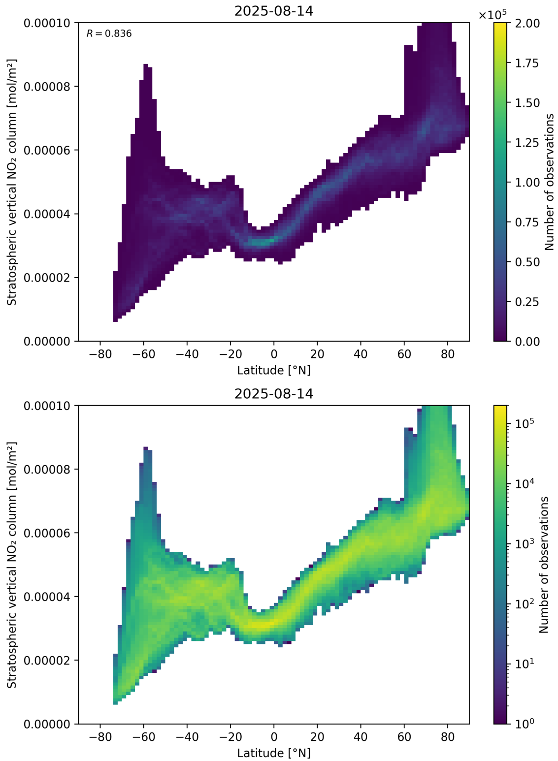
Figure 87: Scatter density plot of “Latitude” against “Stratospheric vertical NO 2 column” for 2025-08-14 to 2025-08-15.
