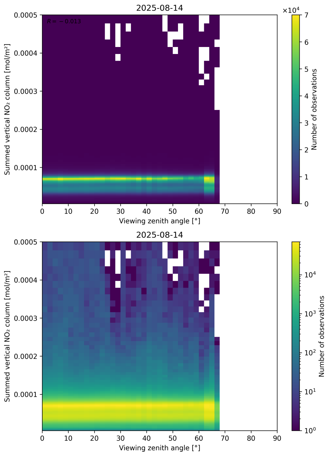
Figure 165: Scatter density plot of “Viewing zenith angle” against “Summed vertical NO 2 column” for 2025-08-14 to 2025-08-15.
