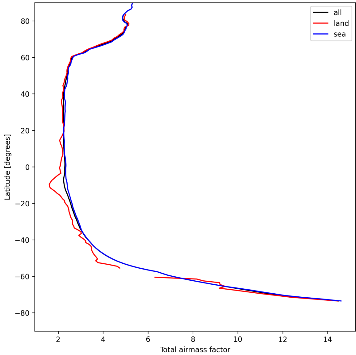
Figure 15: Zonal average of “Total airmass factor” for 2025-08-14 to 2025-08-15.
