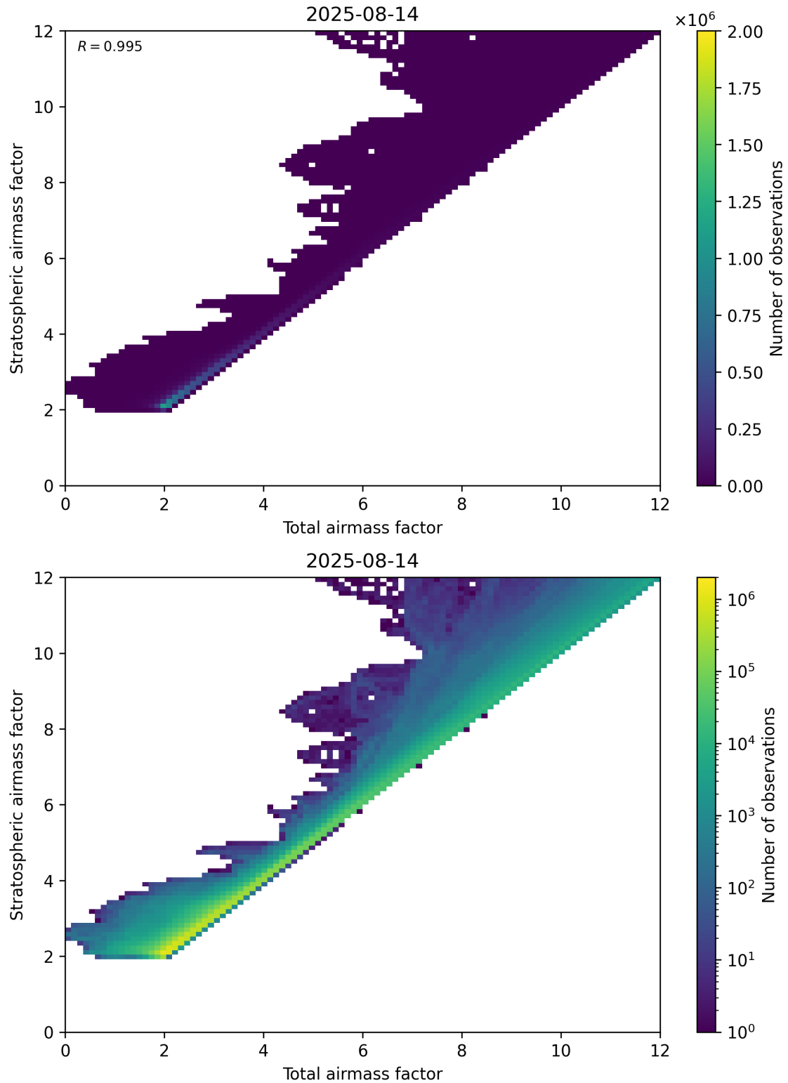
Figure 62: Scatter density plot of “Total airmass factor” against “Stratospheric airmass factor” for 2025-08-14 to 2025-08-15.
