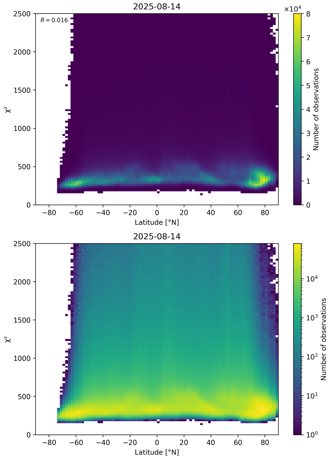
Figure 86: Scatter density plot of “Latitude” against “ \chi^2 ” for 2025-08-14 to 2025-08-15.
