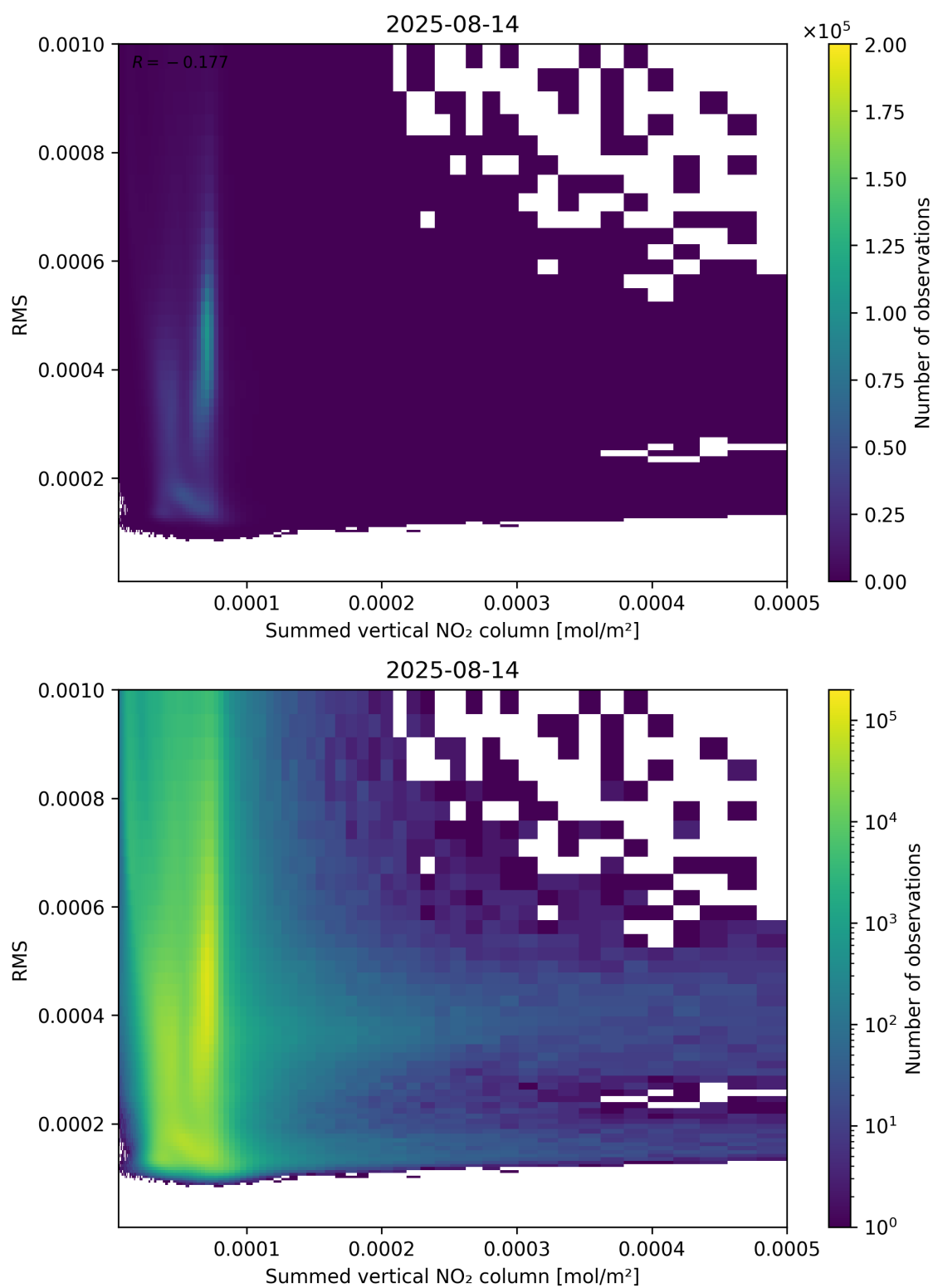
Figure 109: Scatter density plot of “Summed vertical NO 2 column” against “RMS” for 2025-08-14 to 2025-08-15.
