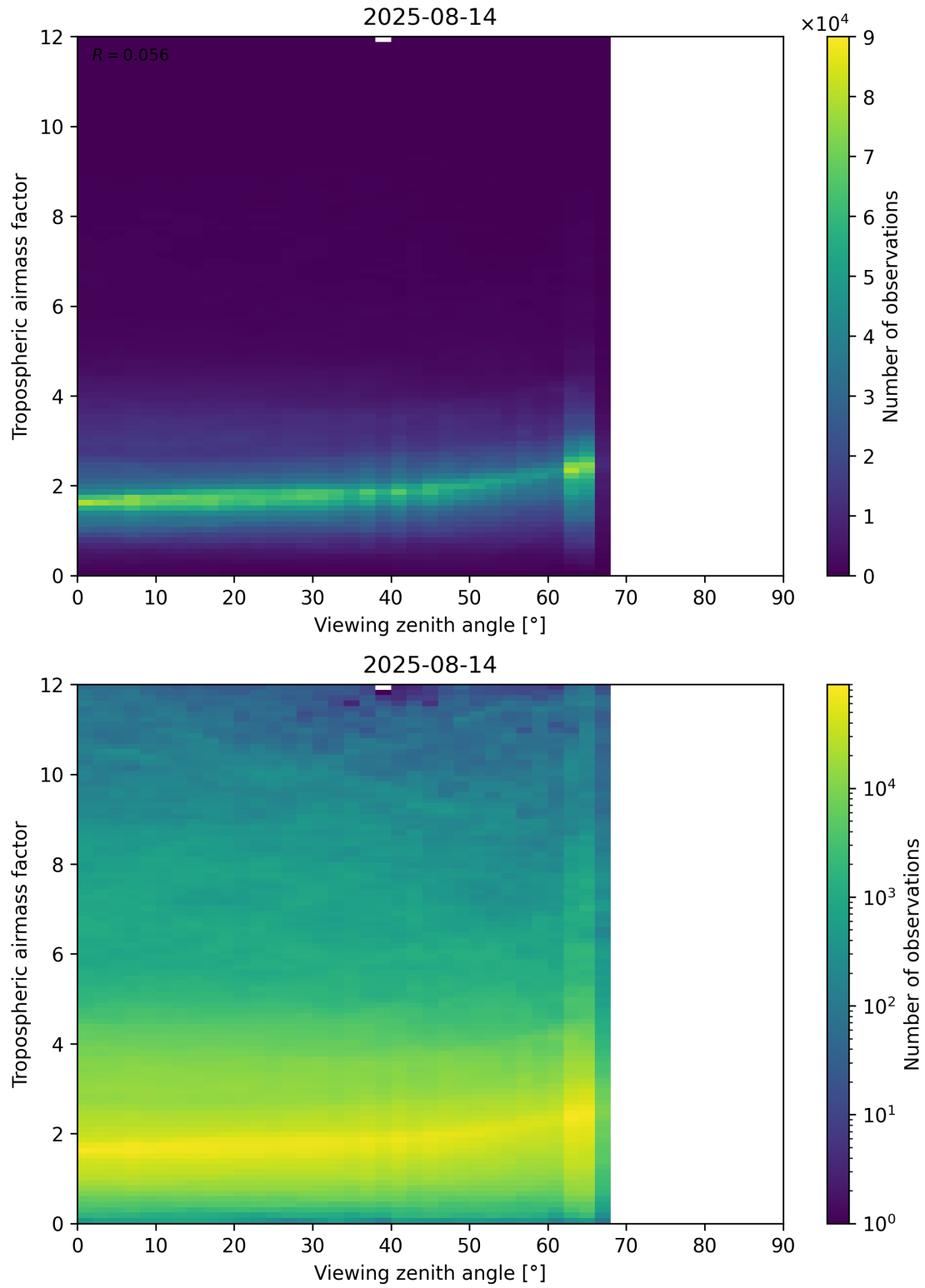
Figure 161: Scatter density plot of “Viewing zenith angle” against “Tropospheric airmass factor” for 2025-08-14 to 2025-08-15.
