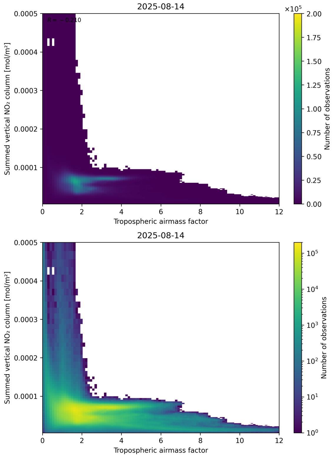
Figure 75: Scatter density plot of “Tropospheric air mass factor” against “Summed vertical NO 2 column” for 2025-08-14 to 2025-08-15.
