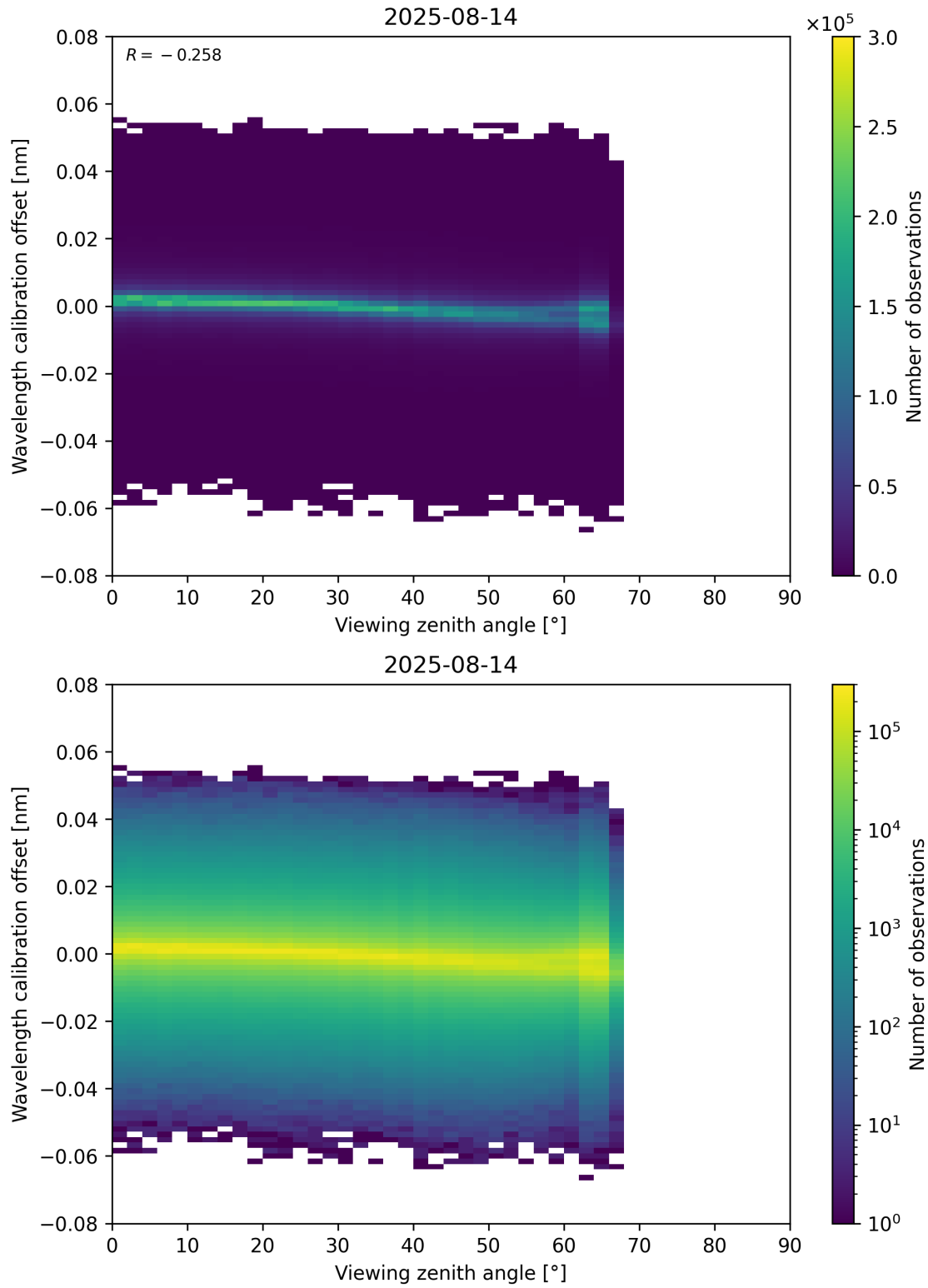
Figure 173: Scatter density plot of “Viewing zenith angle” against “Wavelength calibration offset” for 2025-08-14 to 2025-08-15.
