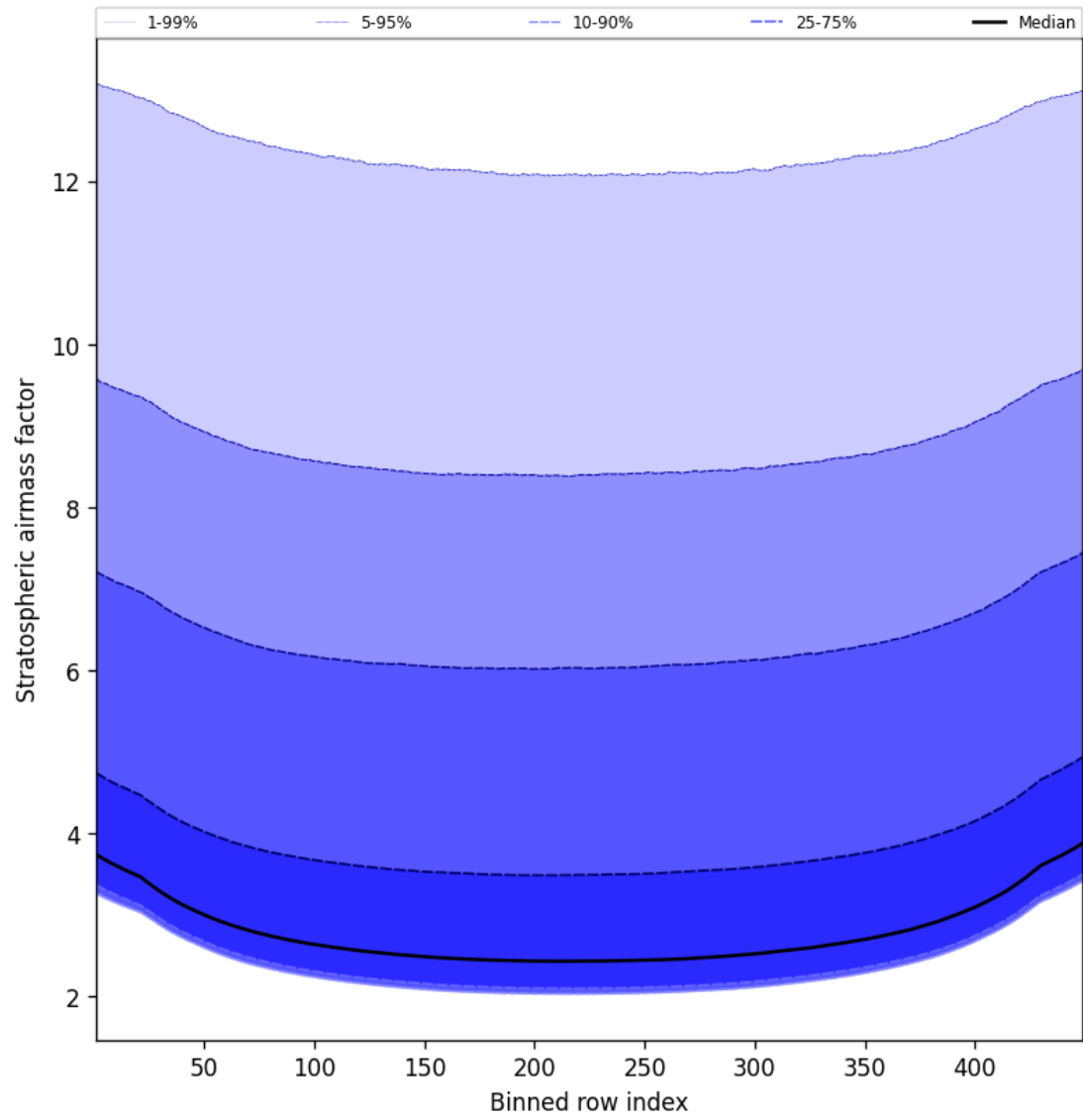
Figure 61: Along track statistics of “Stratospheric airmass factor” for 2025-08-14 to 2025-08-15
