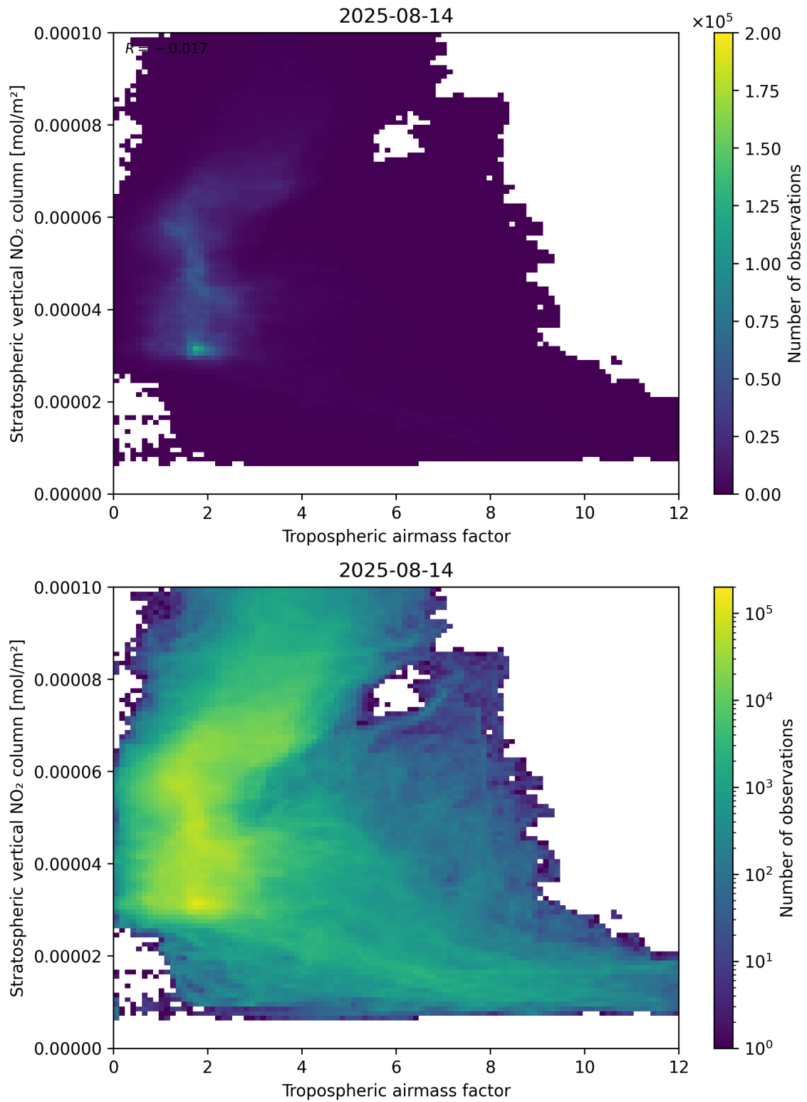
Figure 74: Scatter density plot of “Tropospheric air mass factor” against “Stratospheric vertical NO 2 column” for 2025-08-14 to 2025-08-15.
