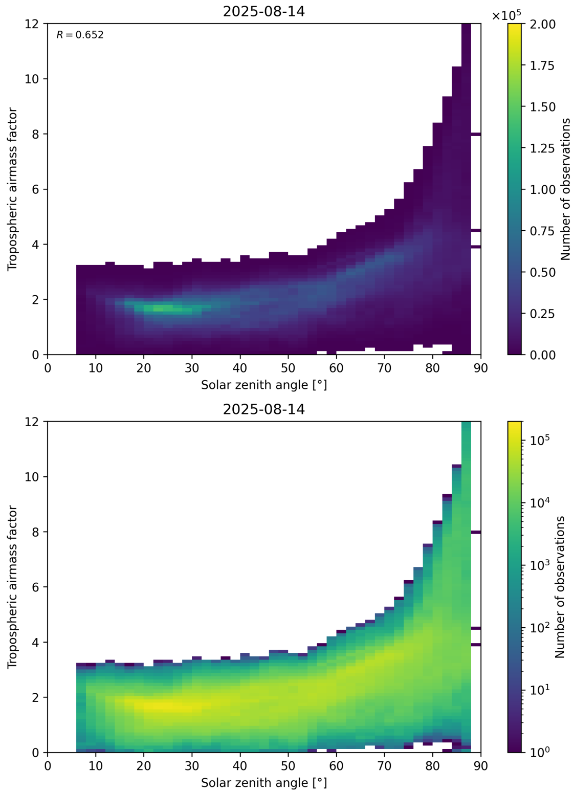
Figure 147: Scatter density plot of “Solar zenith angle” against “Tropospheric airmass factor” for 2025-08-14 to 2025-08-15.
