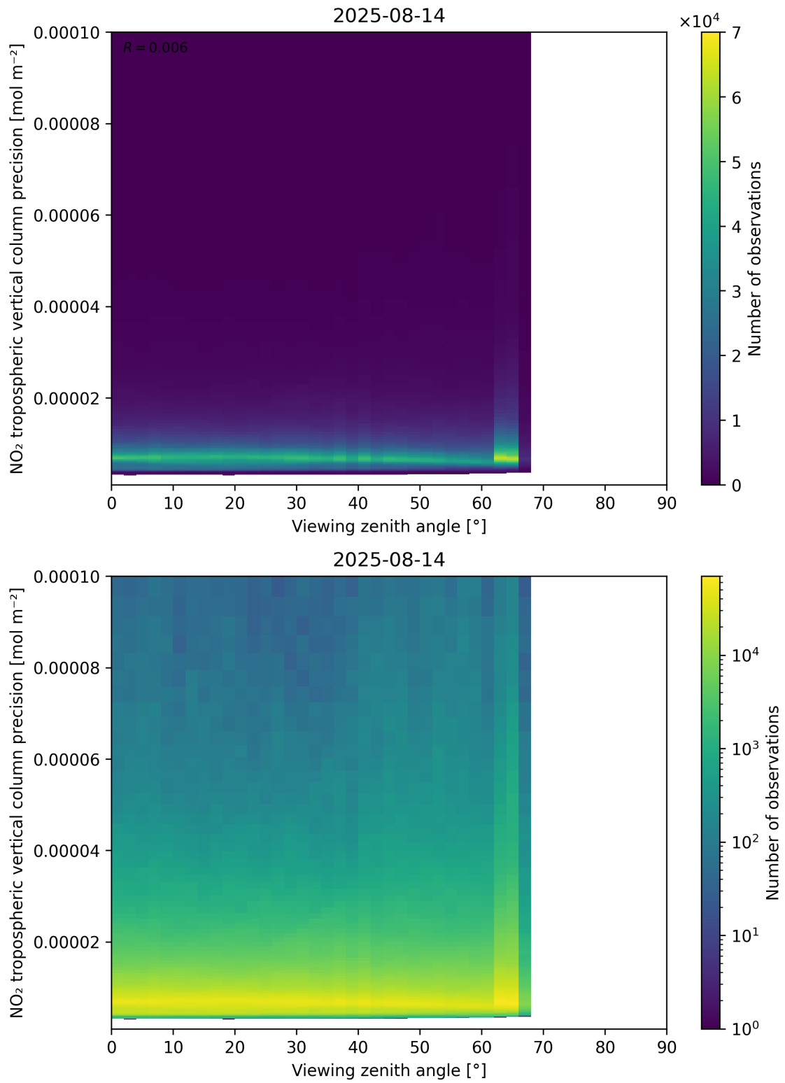
Figure 170: Scatter density plot of “Viewing zenith angle” against “NO 2 tropospheric vertical column precision” for 2025-08-14 to 2025-08-15.
