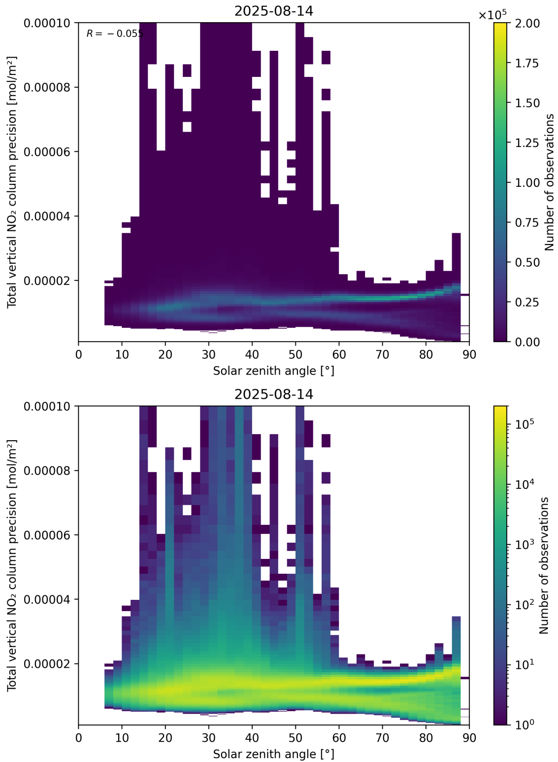
Figure 154: Scatter density plot of “Solar zenith angle” against “Total vertical NO 2 column precision” for 2025-08-14 to 2025-08-15.
