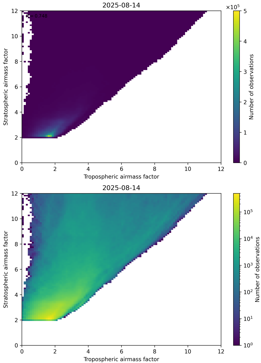
Figure 71: Scatter density plot of “Tropospheric airmass factor” against “Stratospheric airmass factor” for 2025-08-14 to 2025-08-15.
