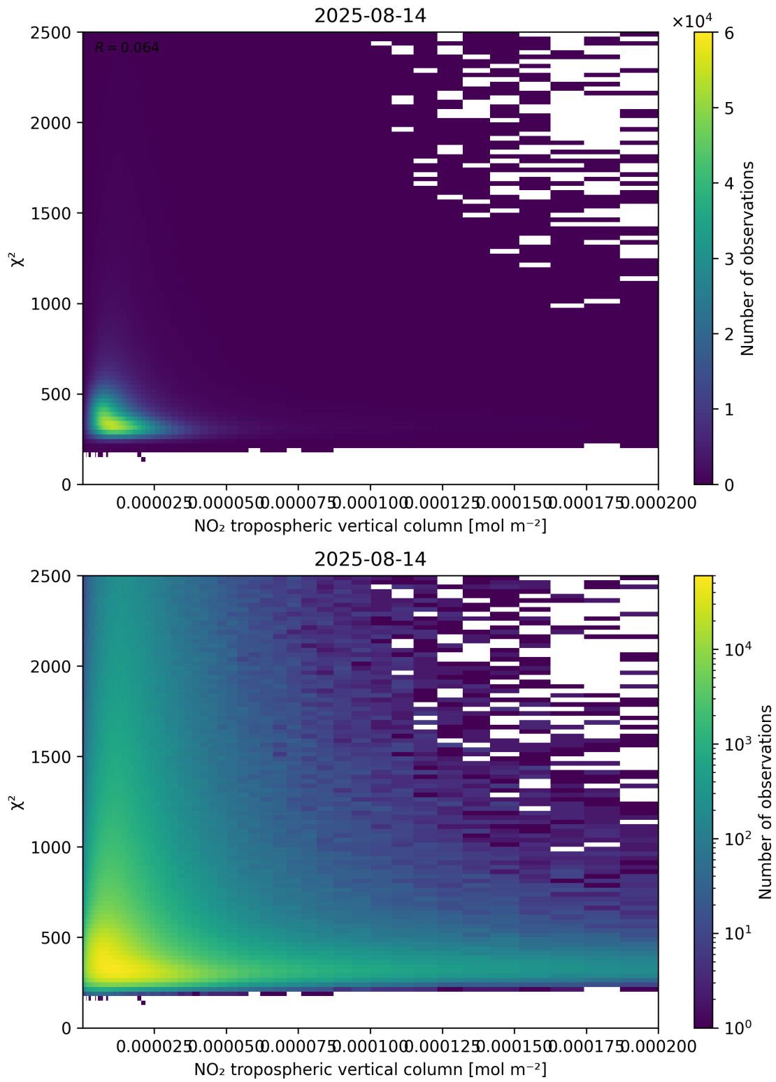
Figure 124: Scatter density plot of “NO 2 tropospheric vertical column” against “ \chi^2 ” for 2025-08-14 to 2025-08-15.
