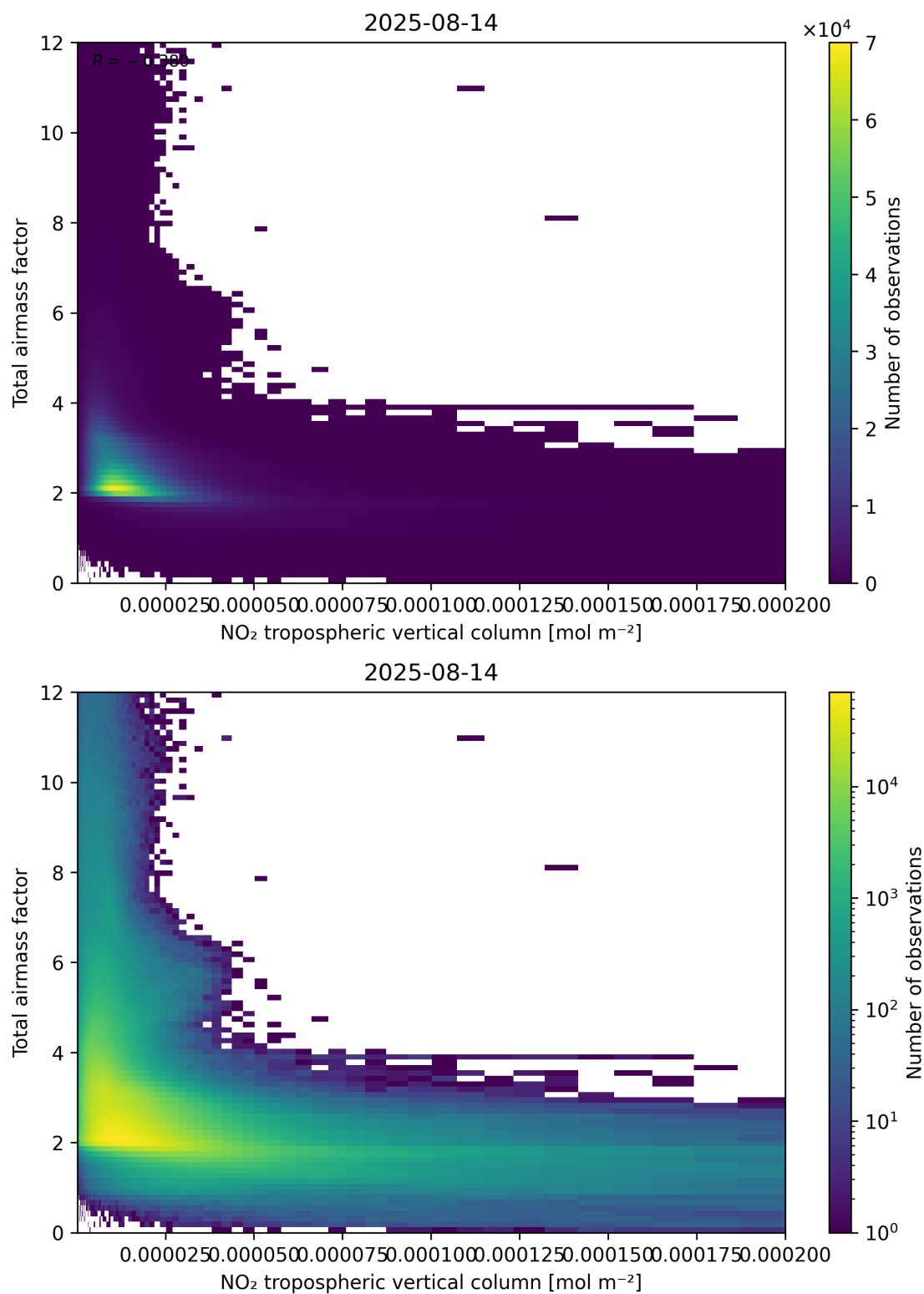
Figure 122: Scatter density plot of “NO 2 tropospheric vertical column” against “Total air mass factor” for 2025-08-14 to 2025-08-15.
