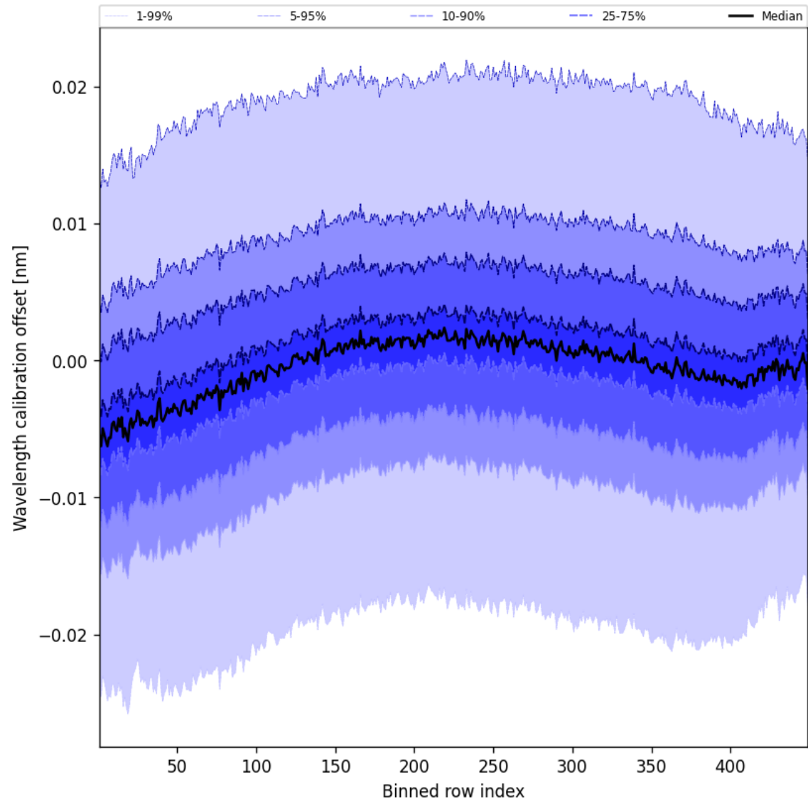
Figure 52: Along track statistics of “Wavelength calibration offset” for 2025-08-14 to 2025-08-15
