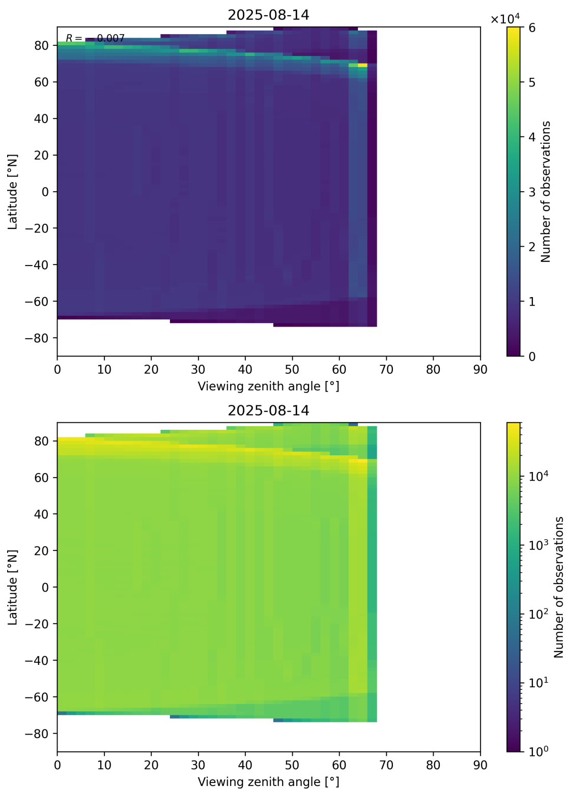
Figure 163: Scatter density plot of “Viewing zenith angle” against “Latitude” for 2025-08-14 to 2025-08-15.
