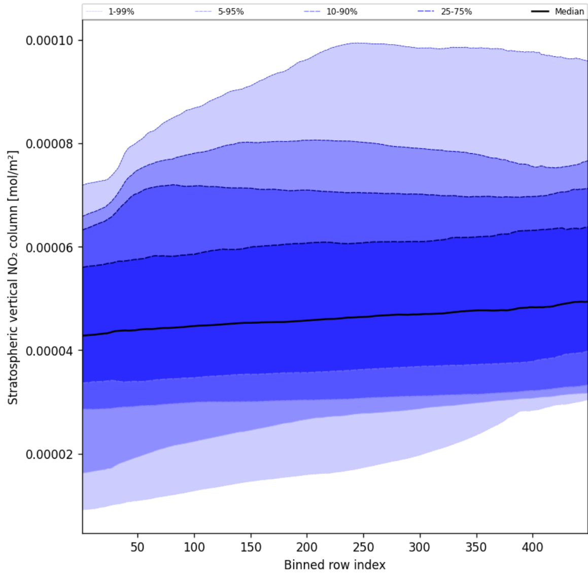
Figure 53: Along track statistics of “Stratospheric vertical NO 2 column” for 2025-08-14 to 2025-08-15
