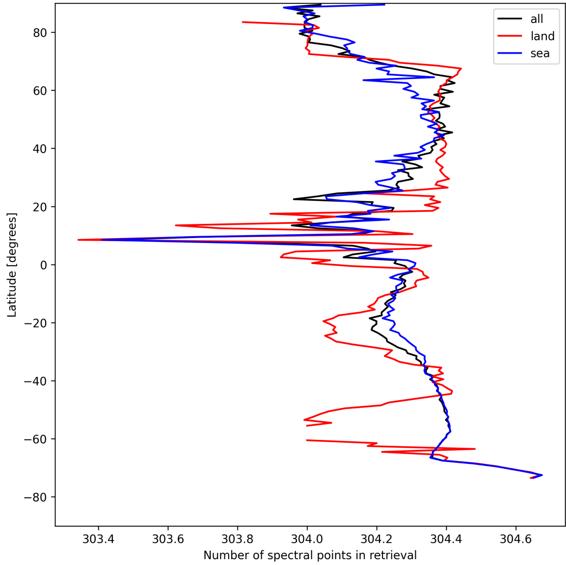
Figure 16: Zonal average of “Number of spectral points in retrieval” for 2025-08-14 to 2025-08-15.
