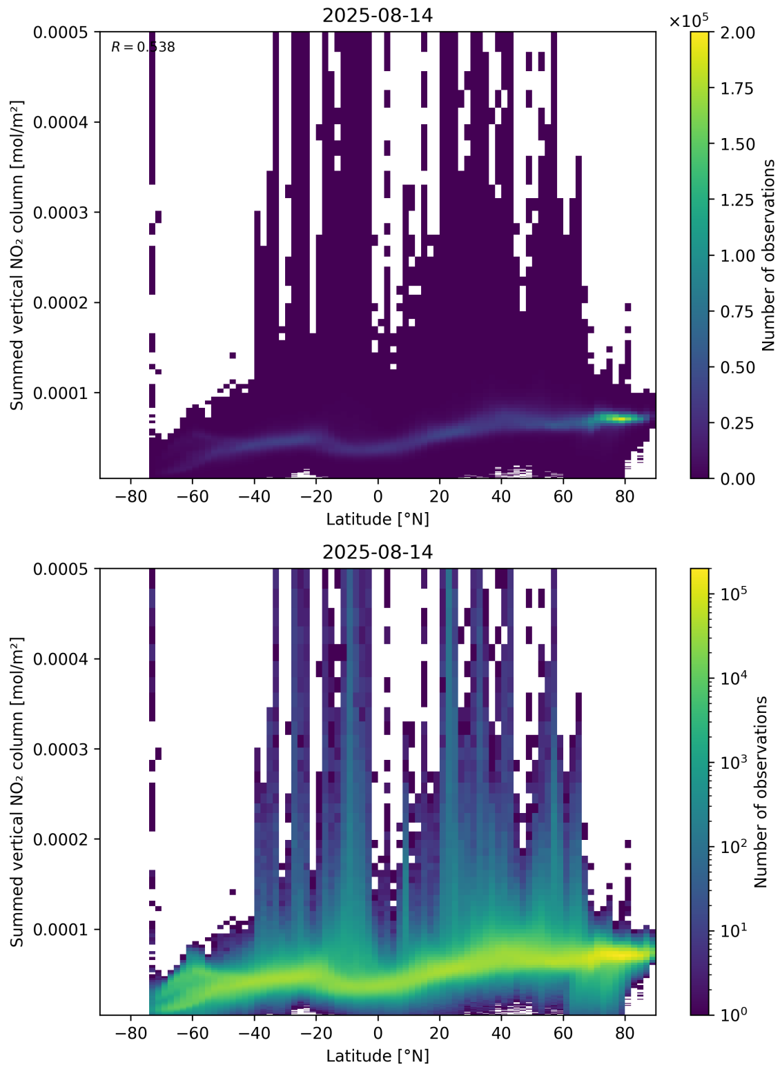
Figure 88: Scatter density plot of “Latitude” against “Summed vertical NO 2 column” for 2025-08-14 to 2025-08-15.
