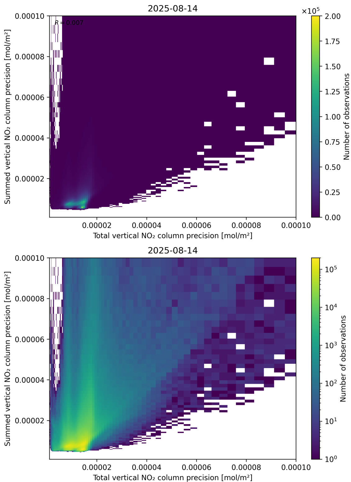
Figure 118: Scatter density plot of “Total vertical NO 2 column precision” against “Summed vertical NO 2 column precision” for 2025-08-14 to 2025-08-15.
