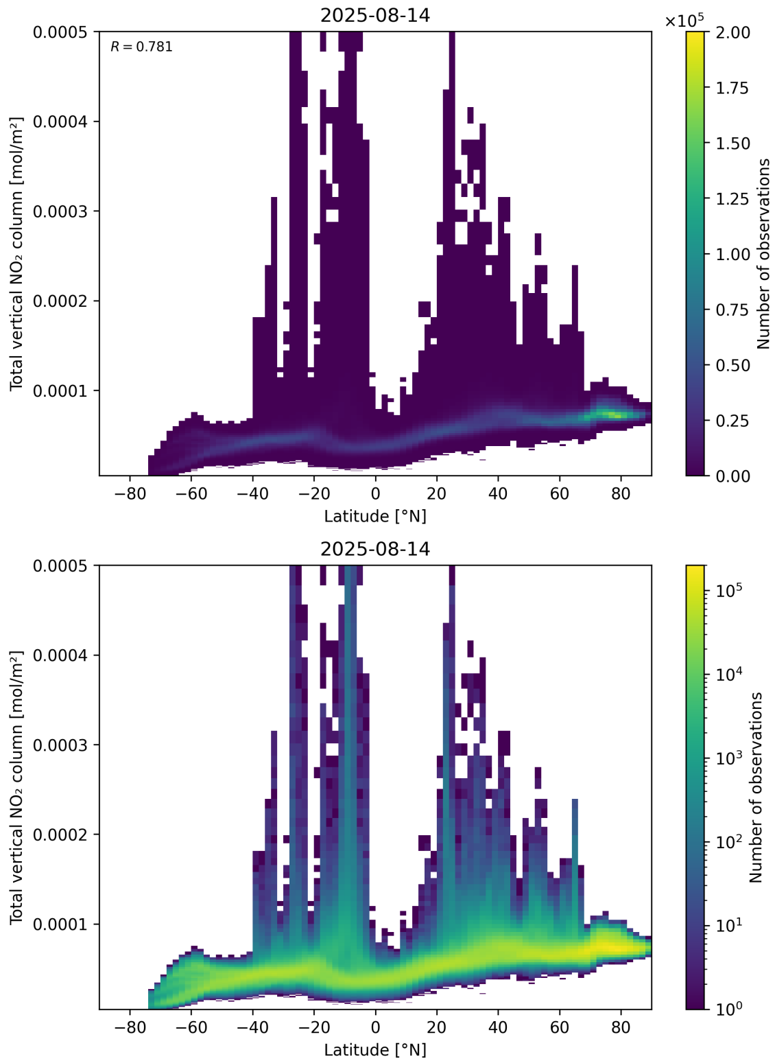
Figure 90: Scatter density plot of “Latitude” against “Total vertical NO 2 column” for 2025-08-14 to 2025-08-15.
