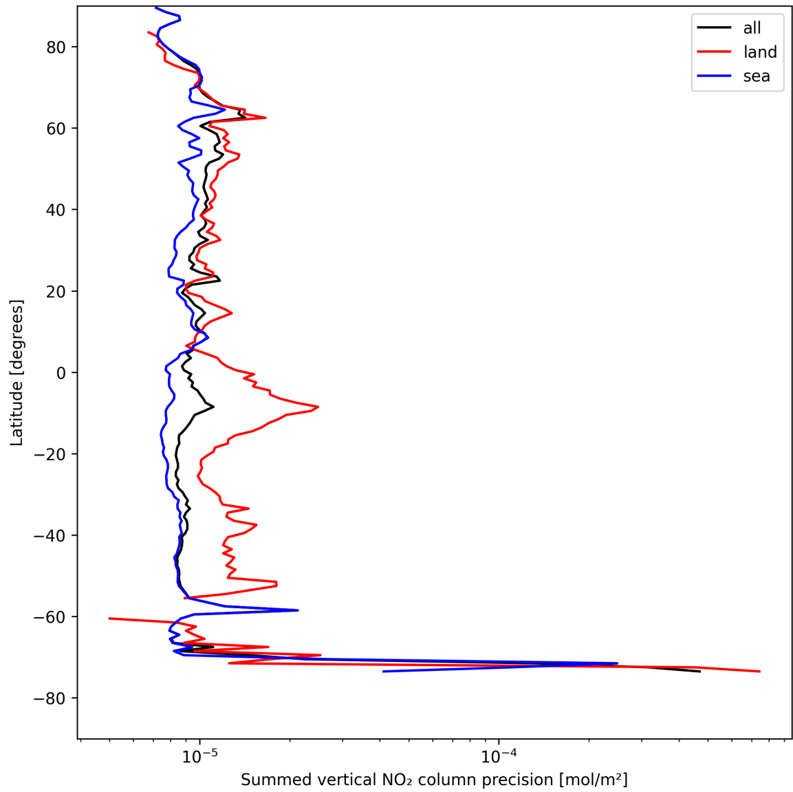
Figure 24: Zonal average of “Summed vertical NO 2 column precision” for 2025-08-14 to 2025-08-15.
