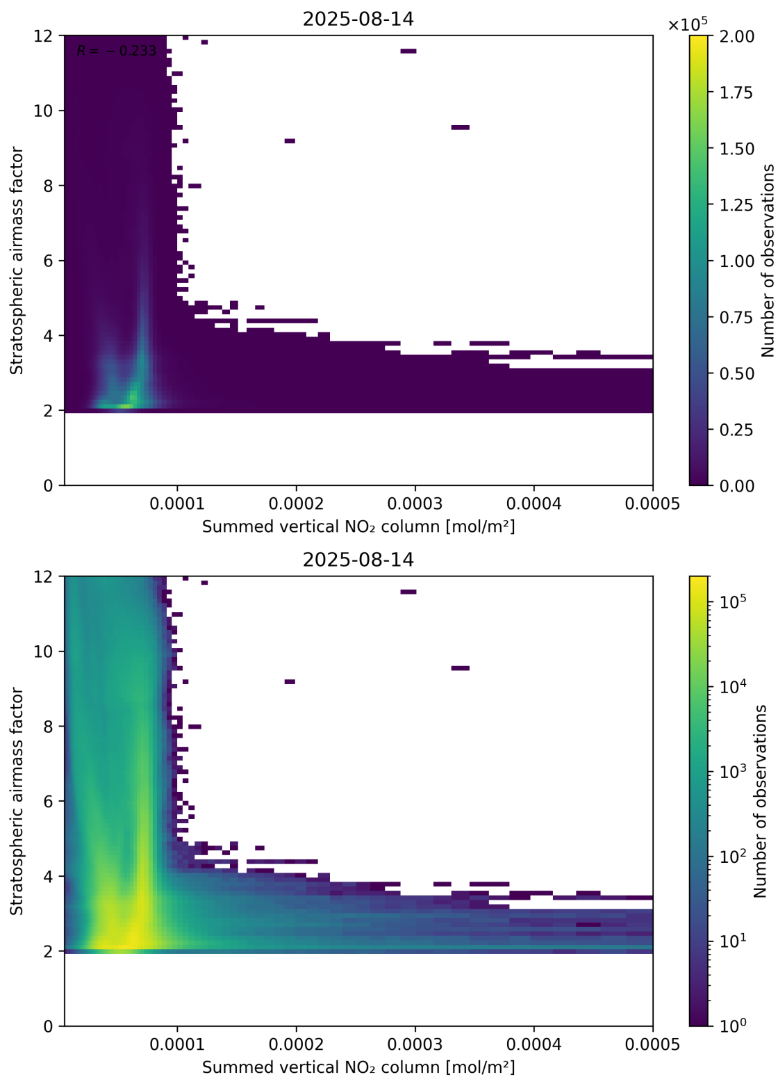
Figure 103: Scatter density plot of “Summed vertical NO 2 column” against “Stratospheric airmass factor” for 2025-08-14 to 2025-08-15.
