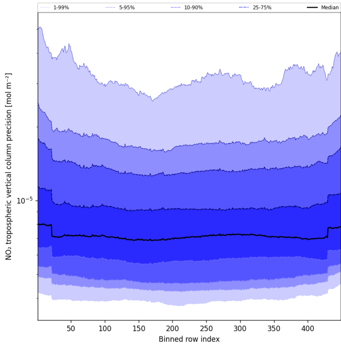
Figure 47: Along track statistics of “NO 2 tropospheric vertical column precision” for 2025-08-14 to 2025-08-15
