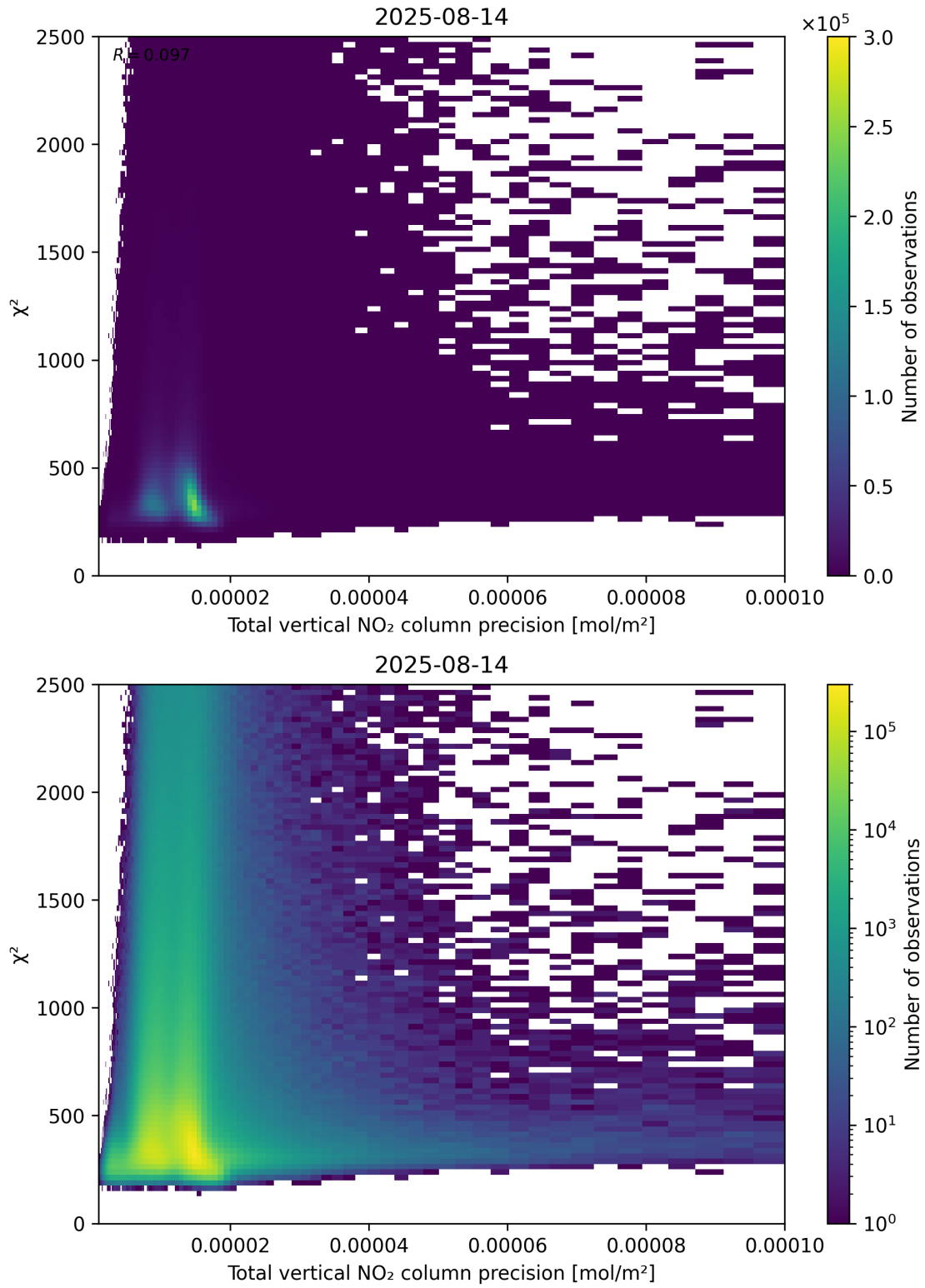
Figure 116: Scatter density plot of “Total vertical NO 2 column precision” against “ \chi^2 ” for 2025-08-14 to 2025-08-15.
