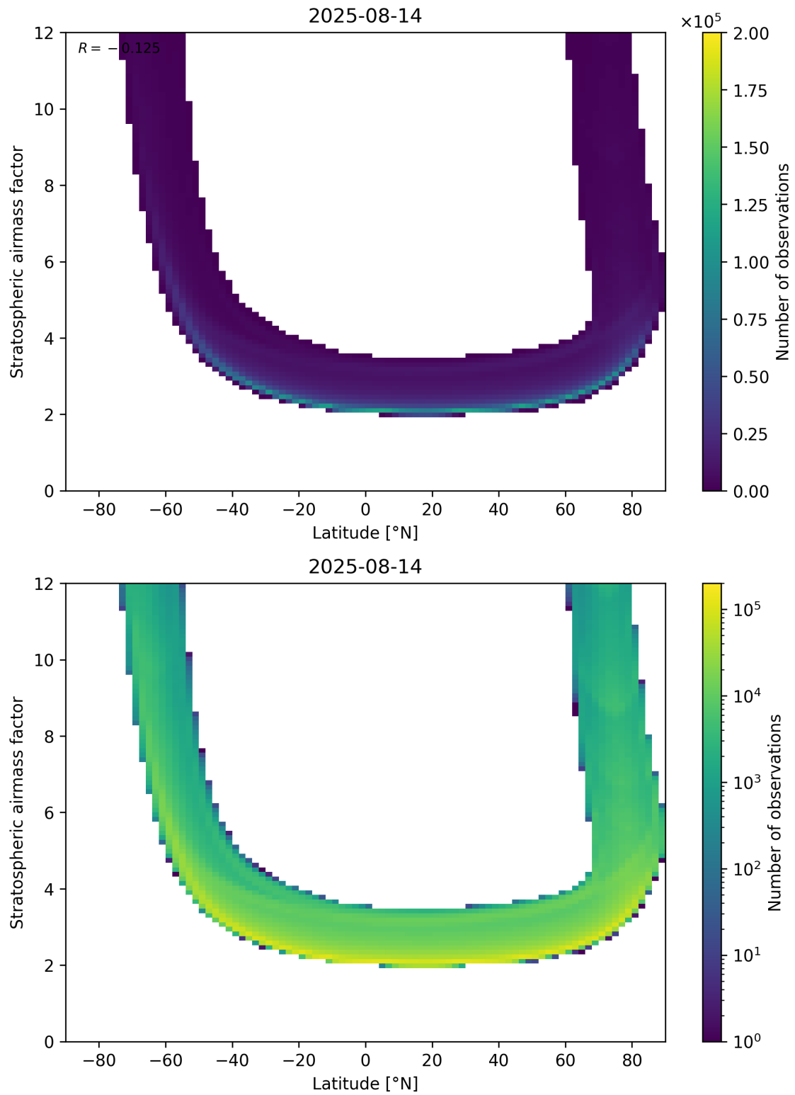
Figure 83: Scatter density plot of “Latitude” against “Stratospheric air mass factor” for 2025-08-14 to 2025-08-15.
