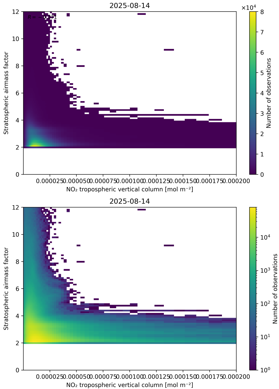
Figure 121: Scatter density plot of “NO 2 tropospheric vertical column” against “Stratospheric air mass factor” for 2025-08-14 to 2025-08-15.
