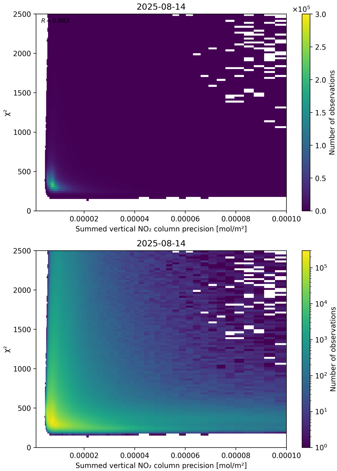
Figure 107: Scatter density plot of “Summed vertical NO 2 column precision” against “ \chi^2 ” for 2025-08-14 to 2025-08-15.
