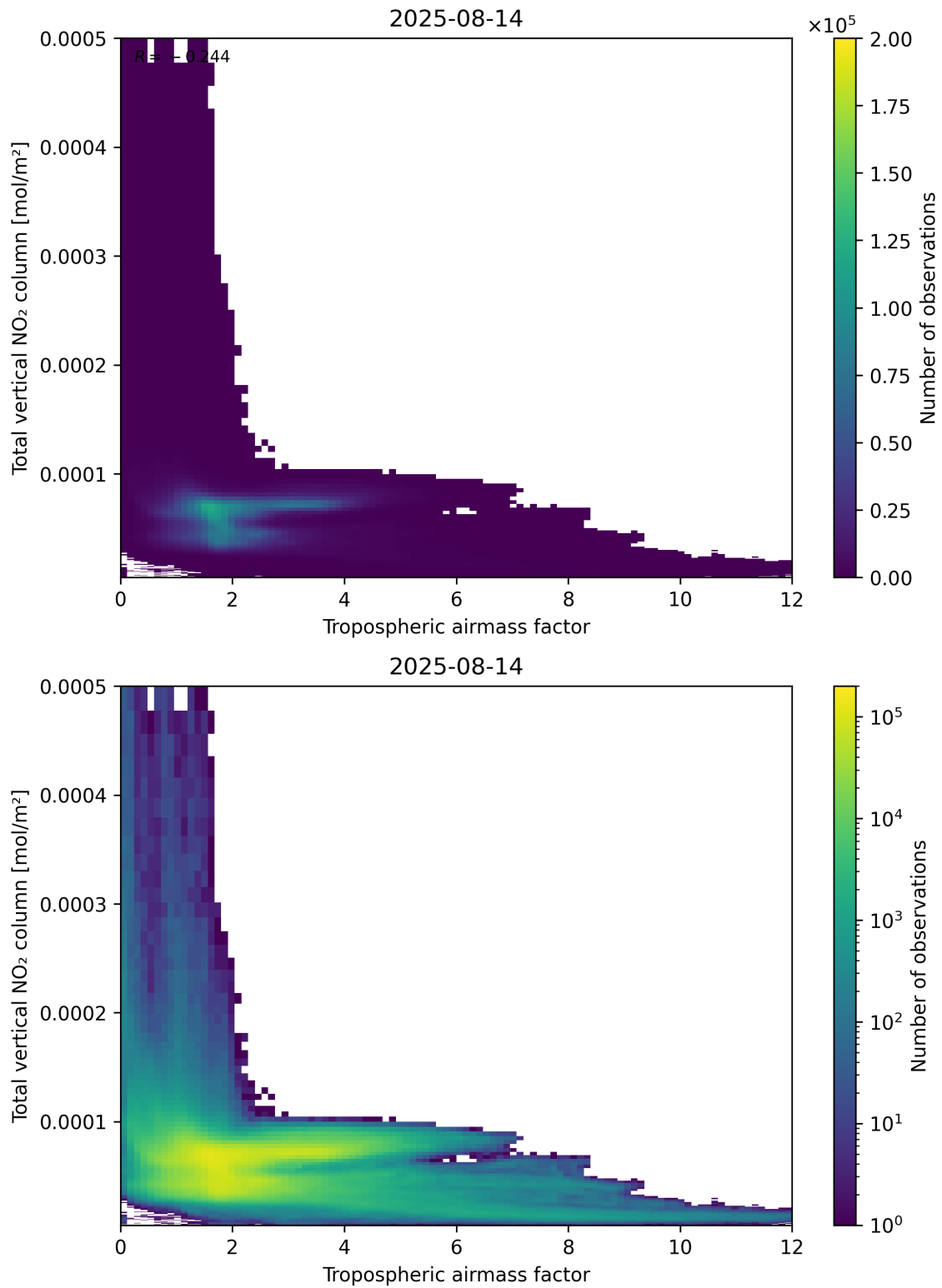
Figure 77: Scatter density plot of “Tropospheric airmass factor” against “Total vertical NO 2 column” for 2025-08-14 to 2025-08-15.
