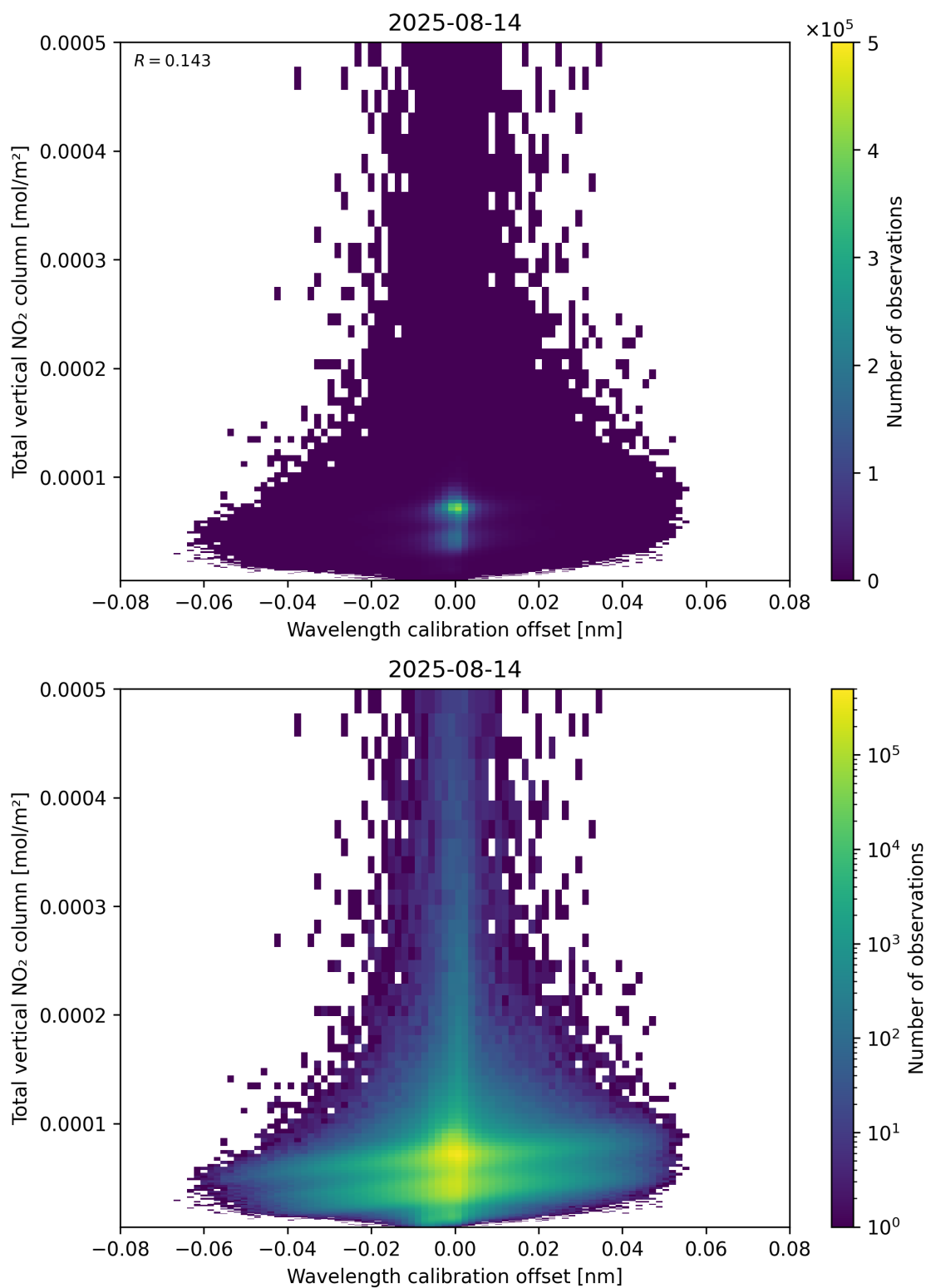
Figure 179: Scatter density plot of “Wavelength calibration offset” against “Total vertical NO 2 column” for 2025-08-14 to 2025-08-15.
