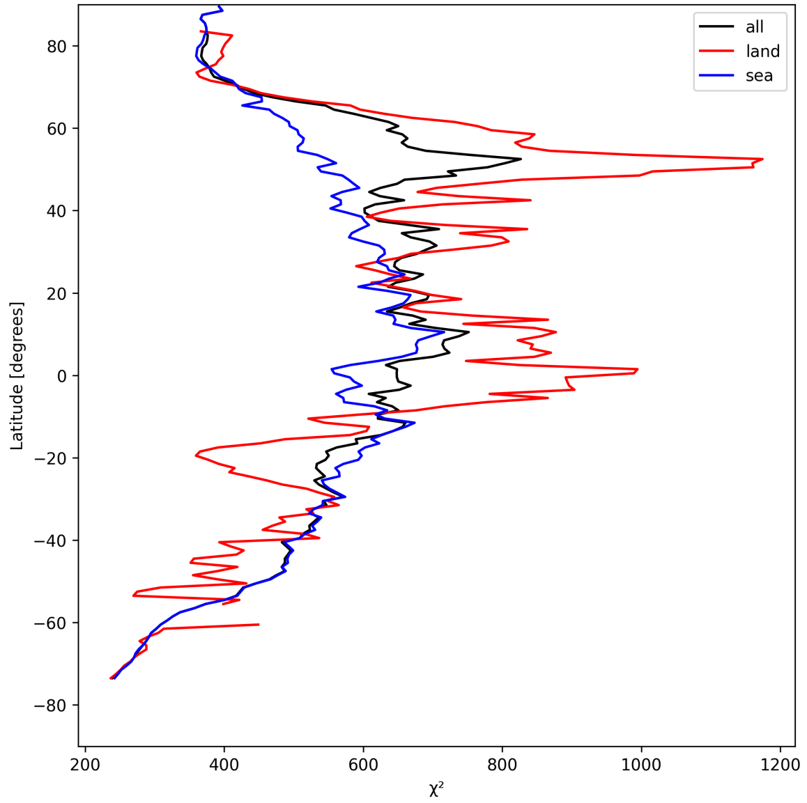
Figure 25: Zonal average of “ \chi^2 ” for 2025-08-14 to 2025-08-15.
