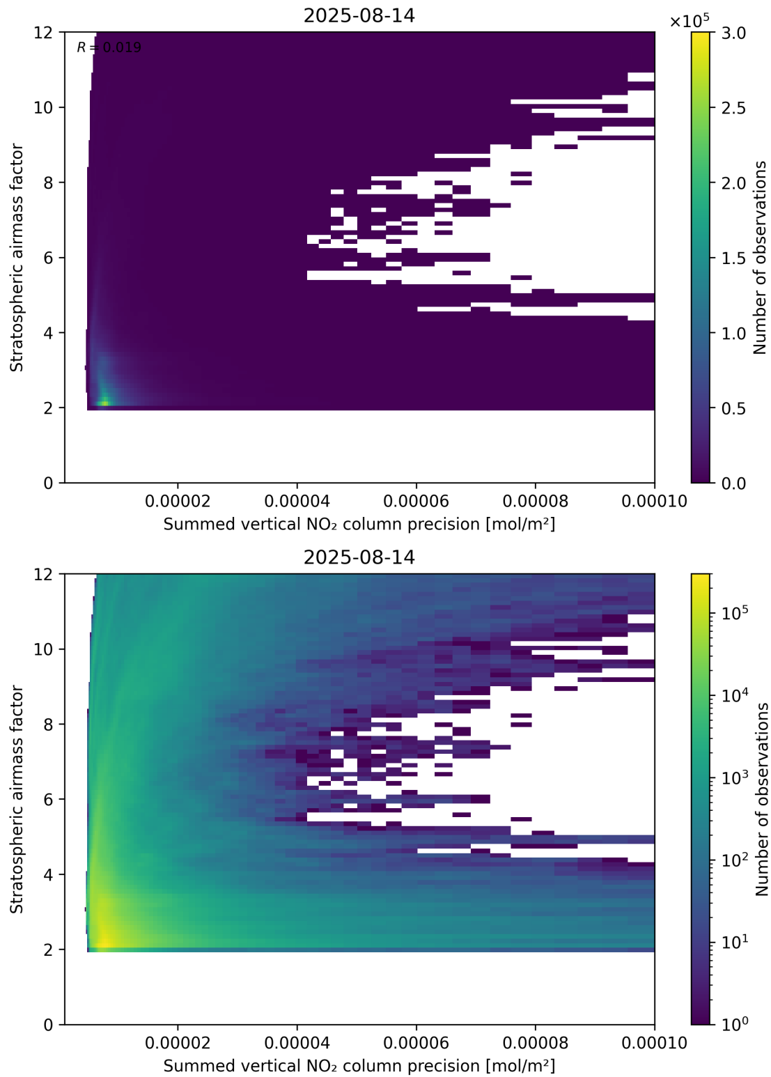
Figure 106: Scatter density plot of “Summed vertical NO 2 column precision” against “Stratospheric airmass factor” for 2025-08-14 to 2025-08-15.
