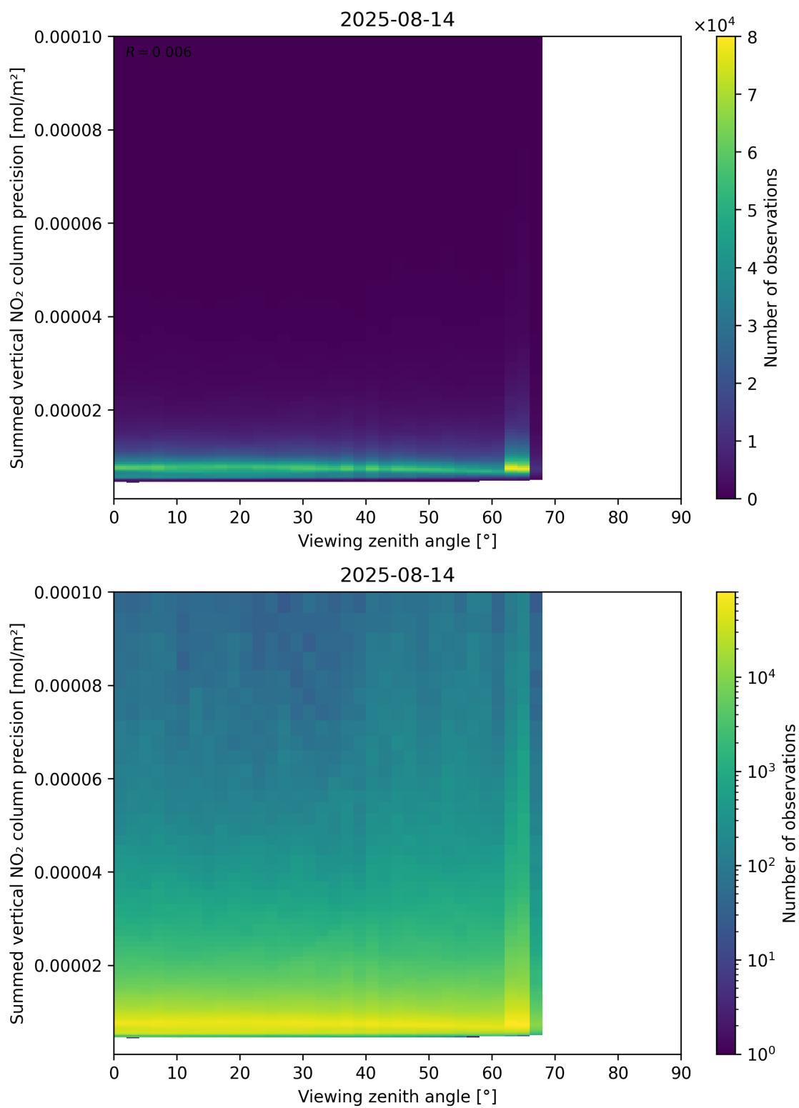
Figure 166: Scatter density plot of “Viewing zenith angle” against “Summed vertical NO 2 column precision” for 2025-08-14 to 2025-08-15.
