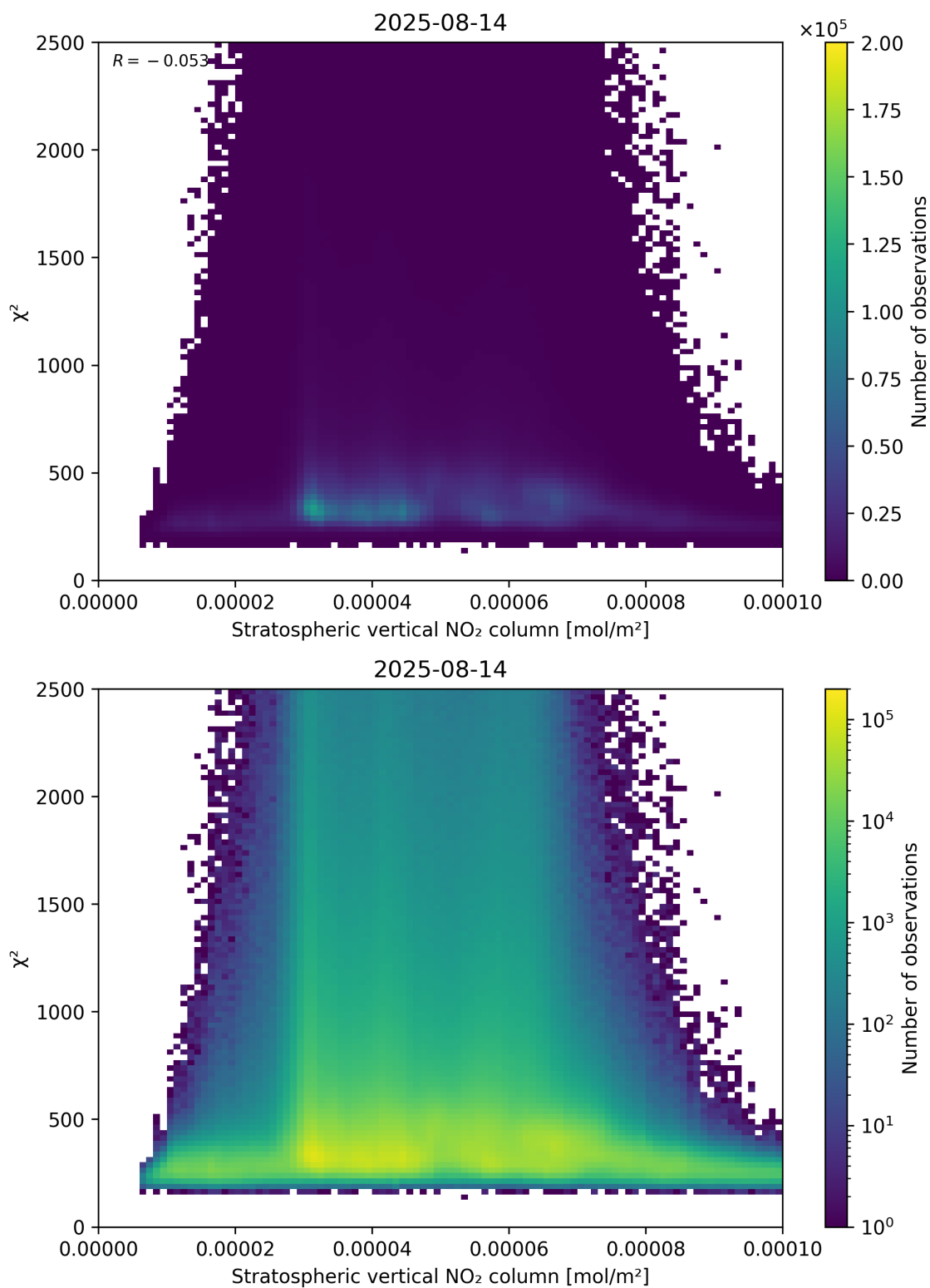
Figure 97: Scatter density plot of “Stratospheric vertical NO 2 column” against “ \chi^2 ” for 2025-08-14 to 2025-08-15.
