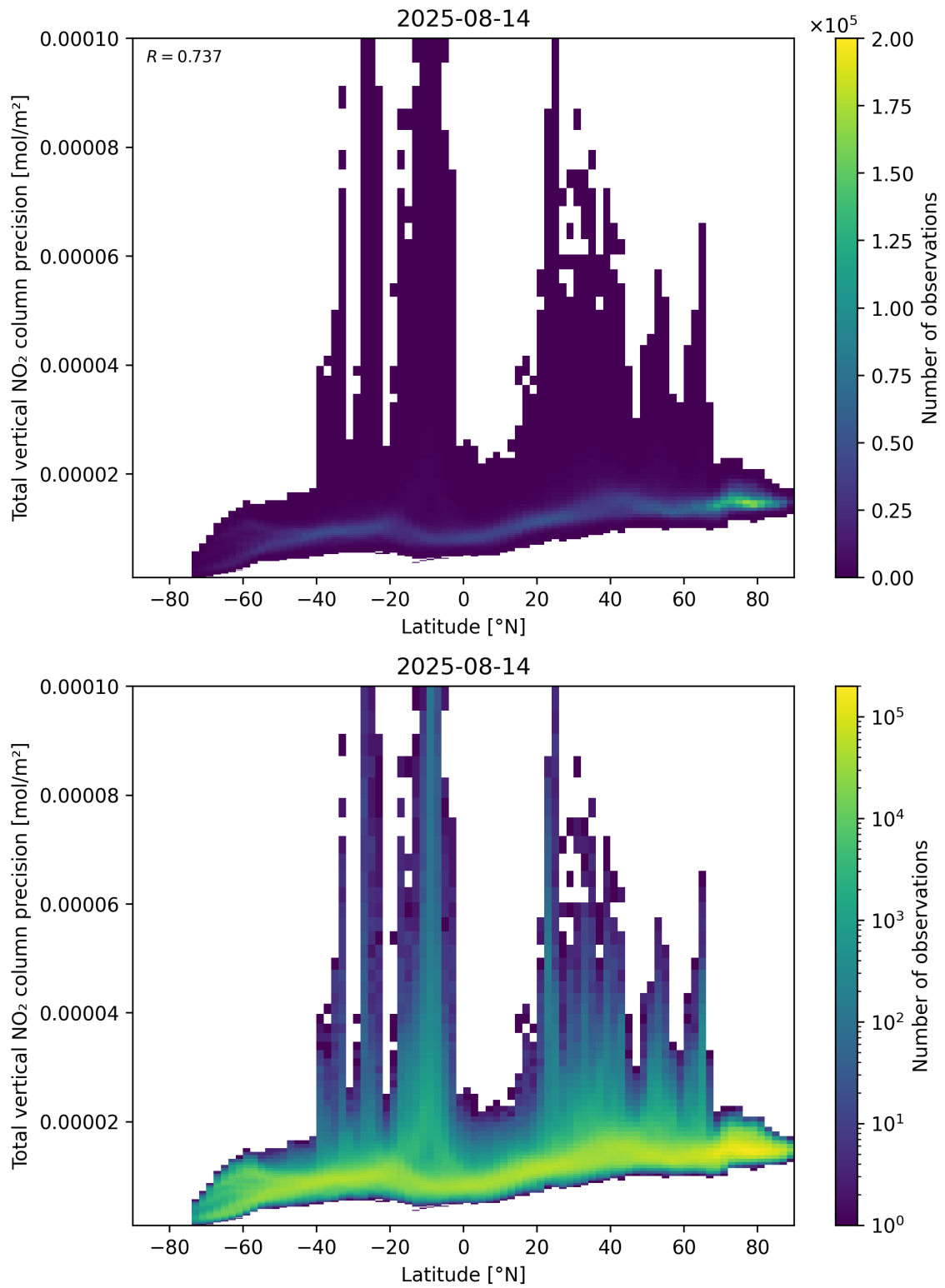
Figure 91: Scatter density plot of “Latitude” against “Total vertical NO 2 column precision” for 2025-08-14 to 2025-08-15.
