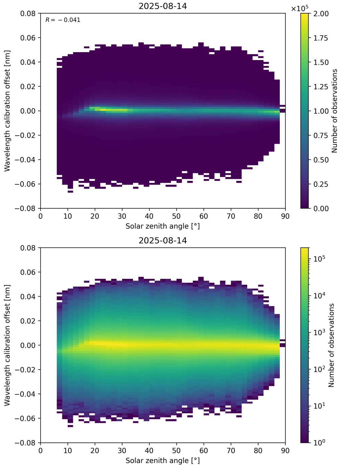
Figure 158: Scatter density plot of “Solar zenith angle” against “Wavelength calibration offset” for 2025-08-14 to 2025-08-15.
