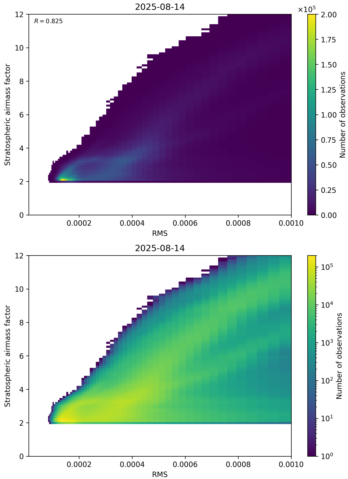
Figure 144: Scatter density plot of “RMS” against “Stratospheric airmass factor” for 2025-08-14 to 2025-08-15.
