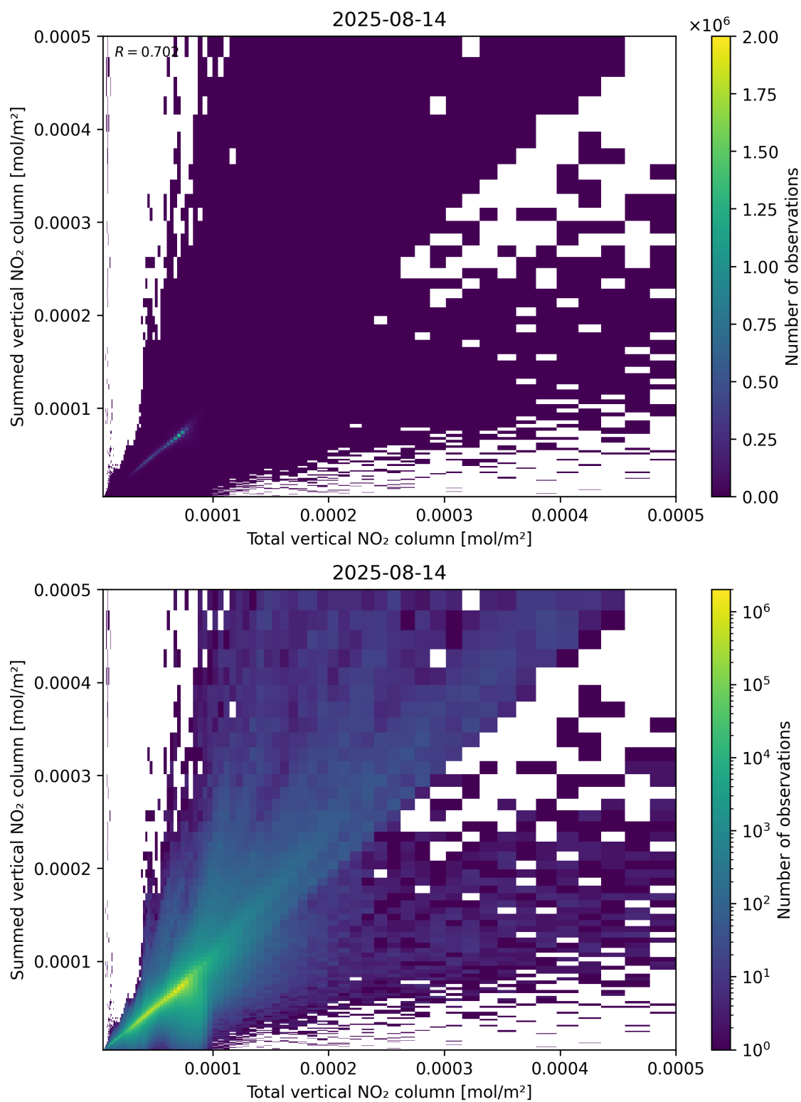
Figure 112: Scatter density plot of “Total vertical NO 2 column” against “Summed vertical NO 2 column” for 2025-08-14 to 2025-08-15.
