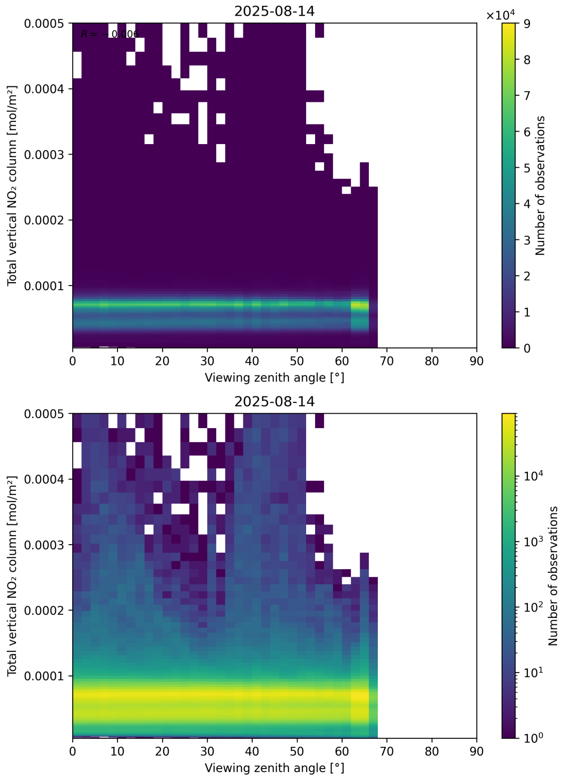
Figure 167: Scatter density plot of “Viewing zenith angle” against “Total vertical NO 2 column” for 2025-08-14 to 2025-08-15.
