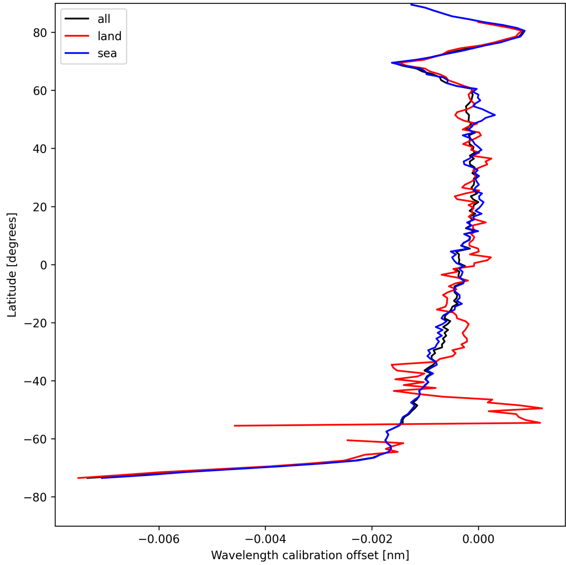
Figure 18: Zonal average of “Wavelength calibration offset” for 2025-08-14 to 2025-08-15.
