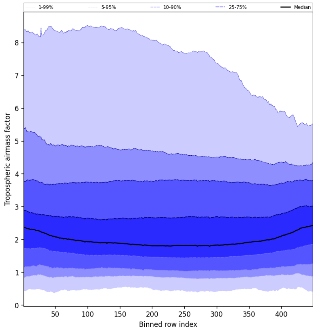
Figure 48: Along track statistics of “Tropospheric air mass factor” for 2025-08-14 to 2025-08-15
