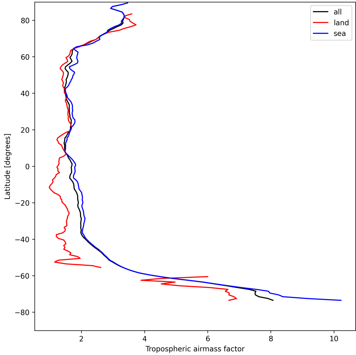
Figure 14: Zonal average of “Tropospheric air mass factor” for 2025-08-14 to 2025-08-15.
