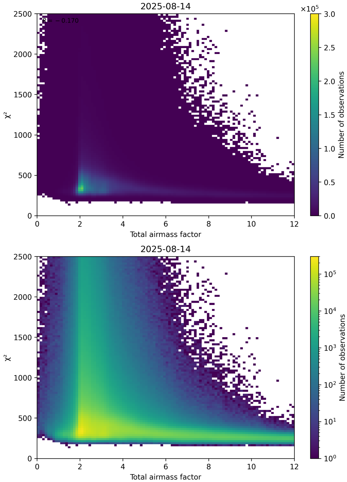
Figure 63: Scatter density plot of “Total airmass factor” against “ \chi^2 ” for 2025-08-14 to 2025-08-15.
