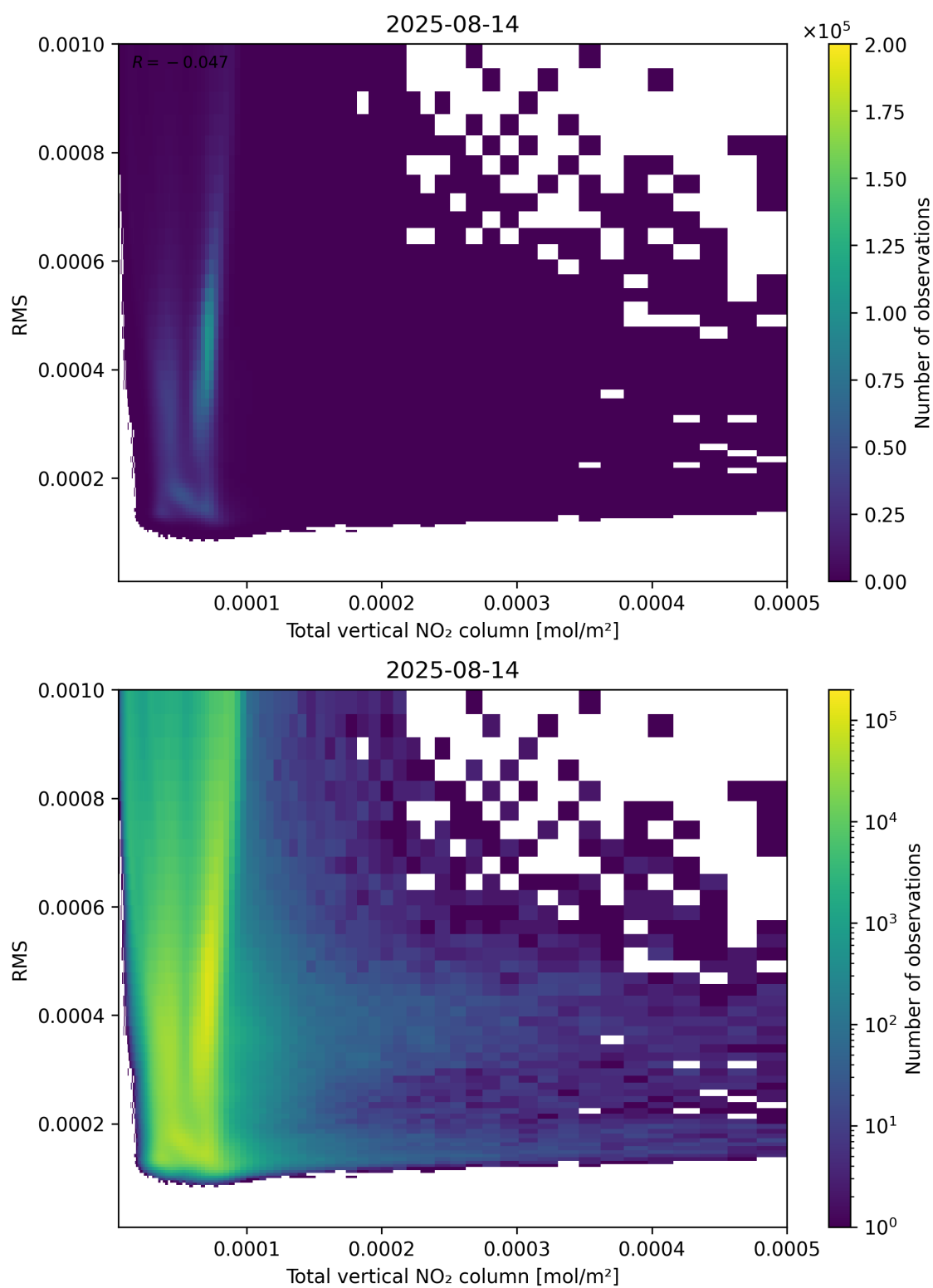
Figure 120: Scatter density plot of “Total vertical NO 2 column” against “RMS” for 2025-08-14 to 2025-08-15.
