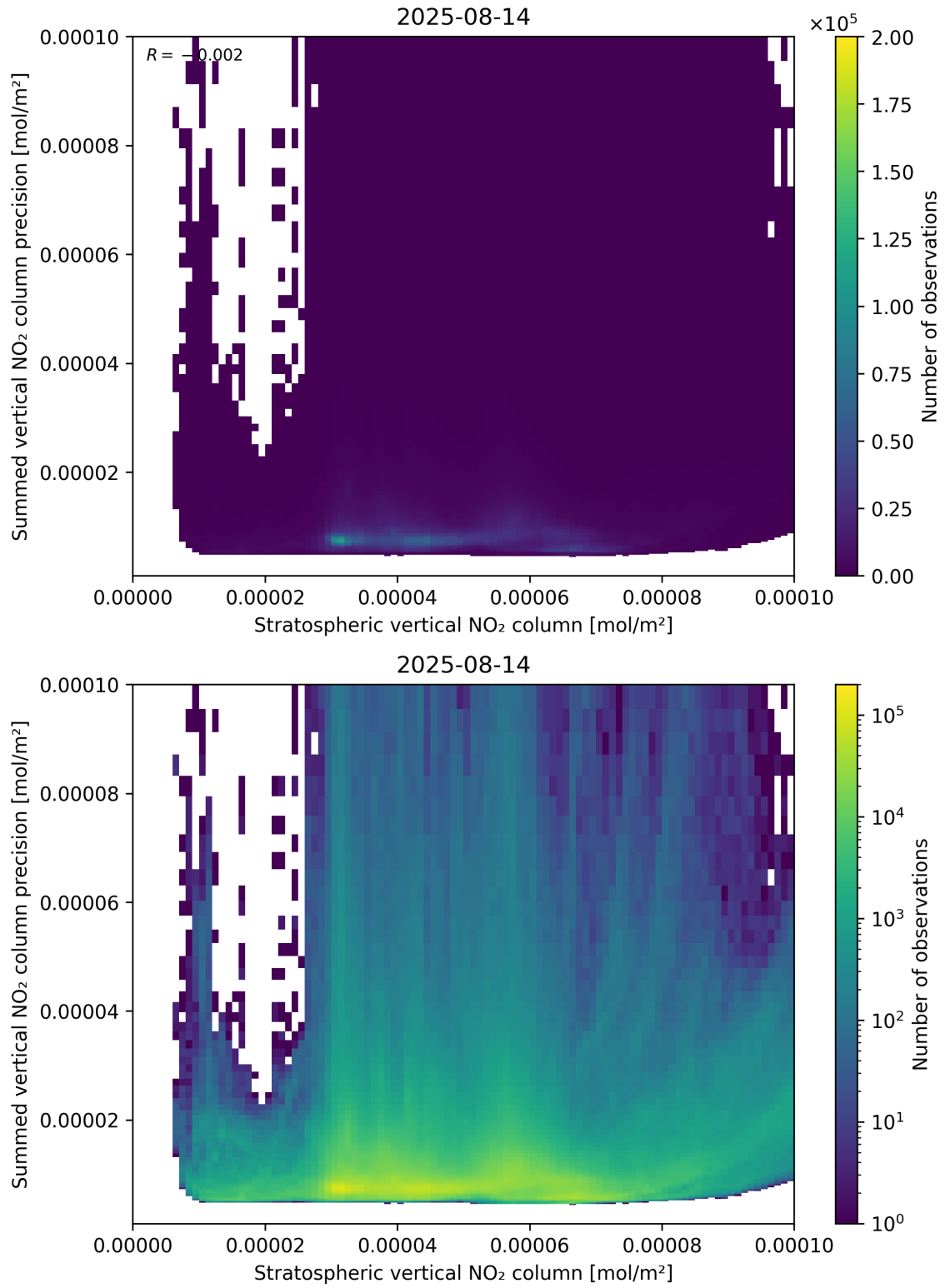
Figure 99: Scatter density plot of “Stratospheric vertical NO 2 column” against “Summed vertical NO 2 column precision” for 2025-08-14 to 2025-08-15.
