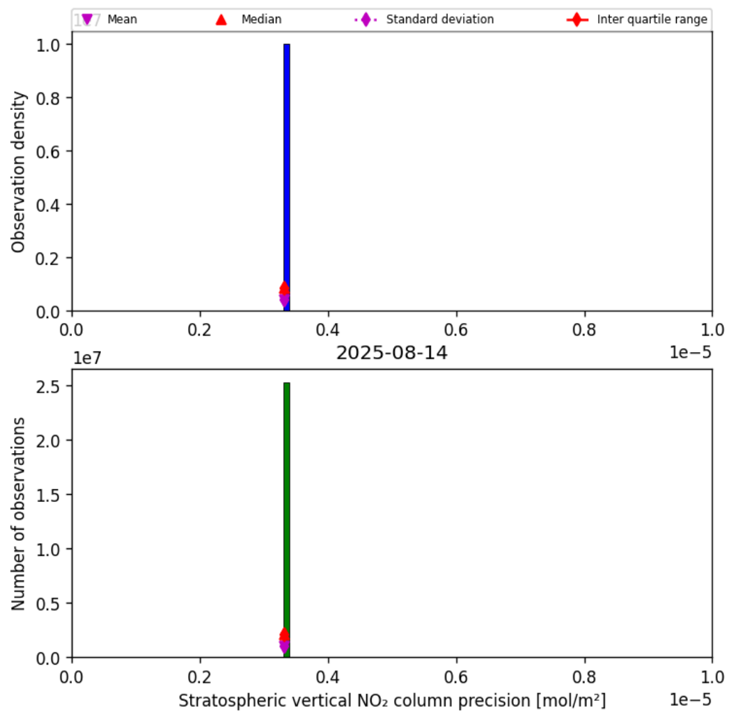
Figure 37: Histogram of “Stratospheric vertical NO 2 column precision” for 2025-08-14 to 2025-08-15
