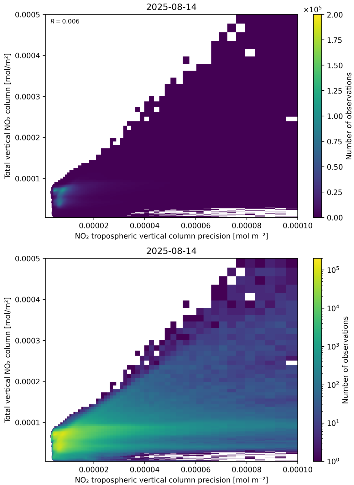
Figure 138: Scatter density plot of “NO 2 tropospheric vertical column precision” against “Total vertical NO 2 column” for 2025-08-14 to 2025-08-15.
