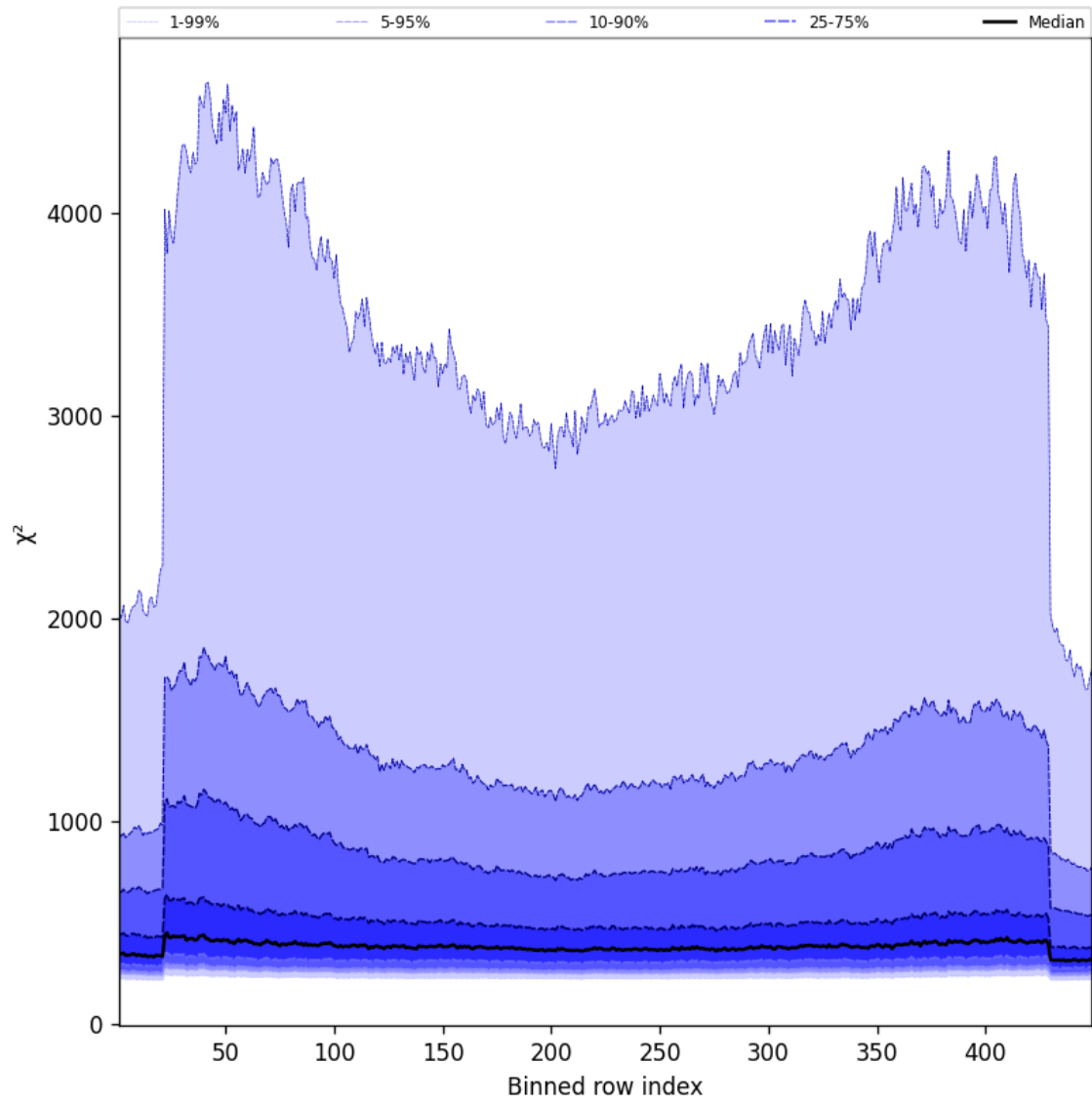
Figure 59: Along track statistics of “ \chi^2 ” for 2025-08-14 to 2025-08-15
