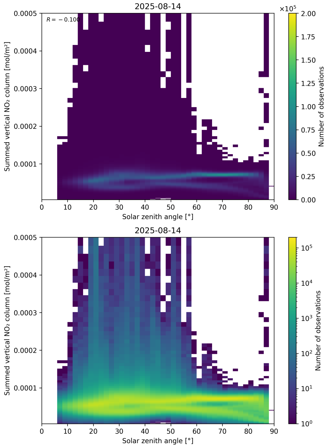
Figure 151: Scatter density plot of “Solar zenith angle” against “Summed vertical NO 2 column” for 2025-08-14 to 2025-08-15.
