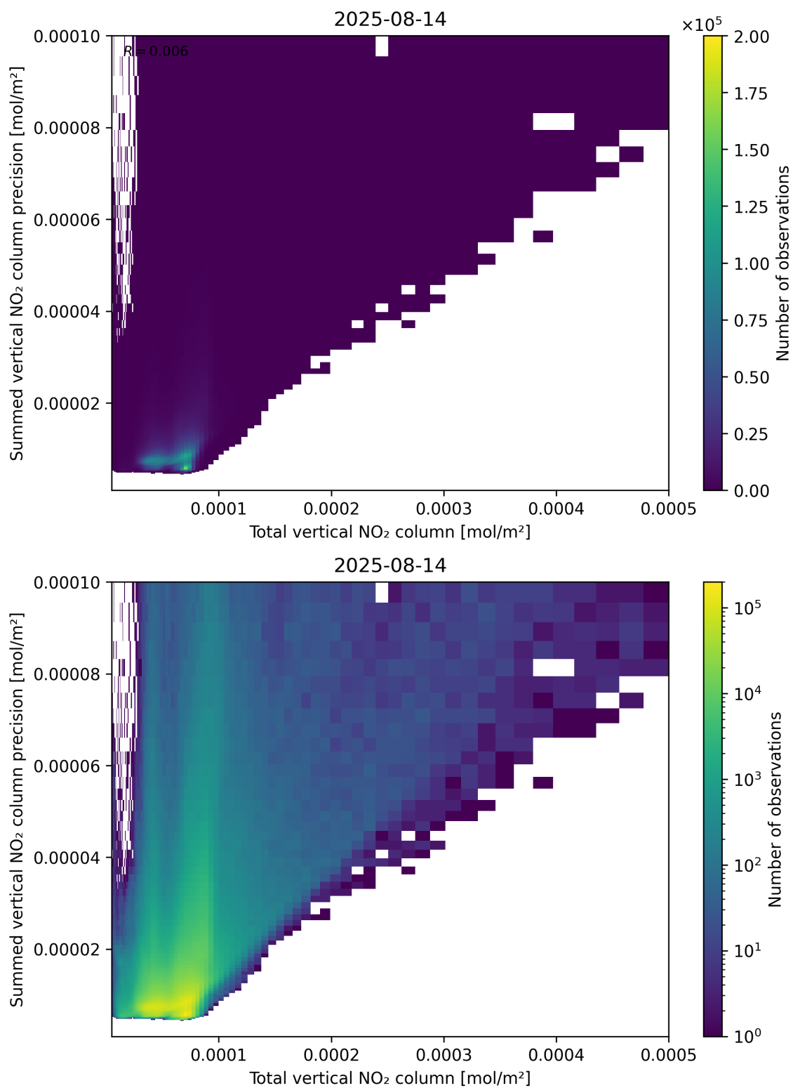
Figure 113: Scatter density plot of “Total vertical NO 2 column” against “Summed vertical NO 2 column precision” for 2025-08-14 to 2025-08-15.
