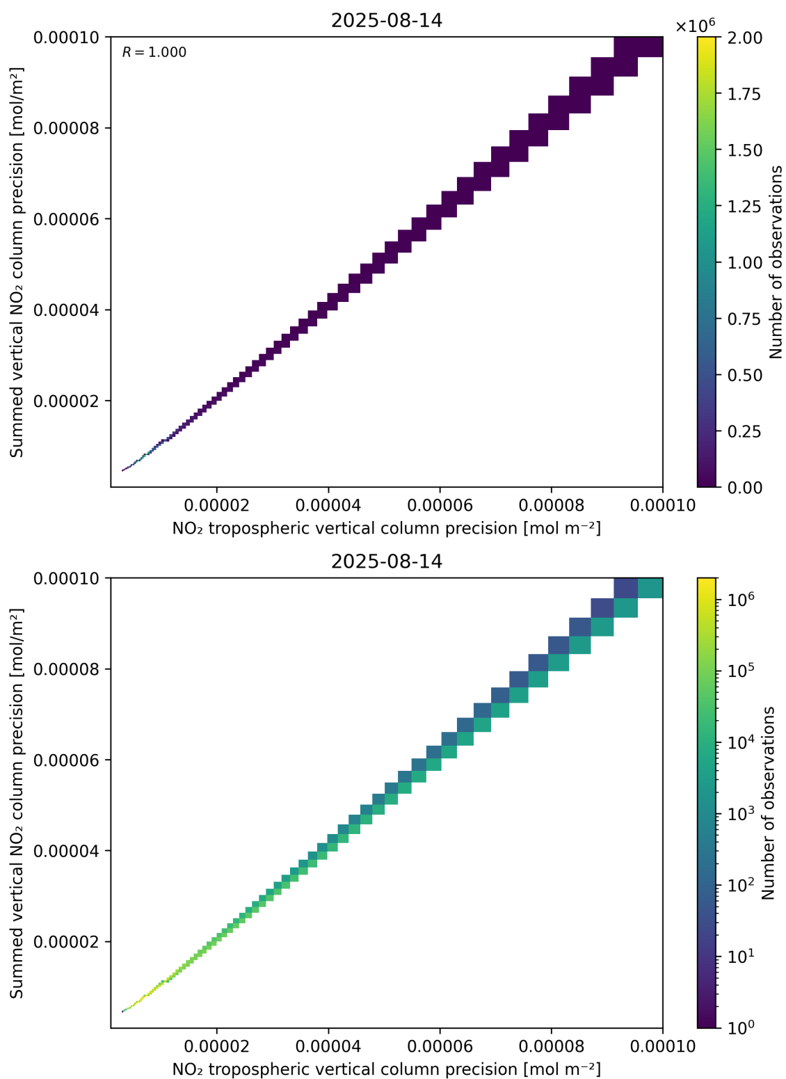
Figure 137: Scatter density plot of “NO 2 tropospheric vertical column precision” against “Summed vertical NO 2 column precision” for 2025-08-14 to 2025-08-15.
