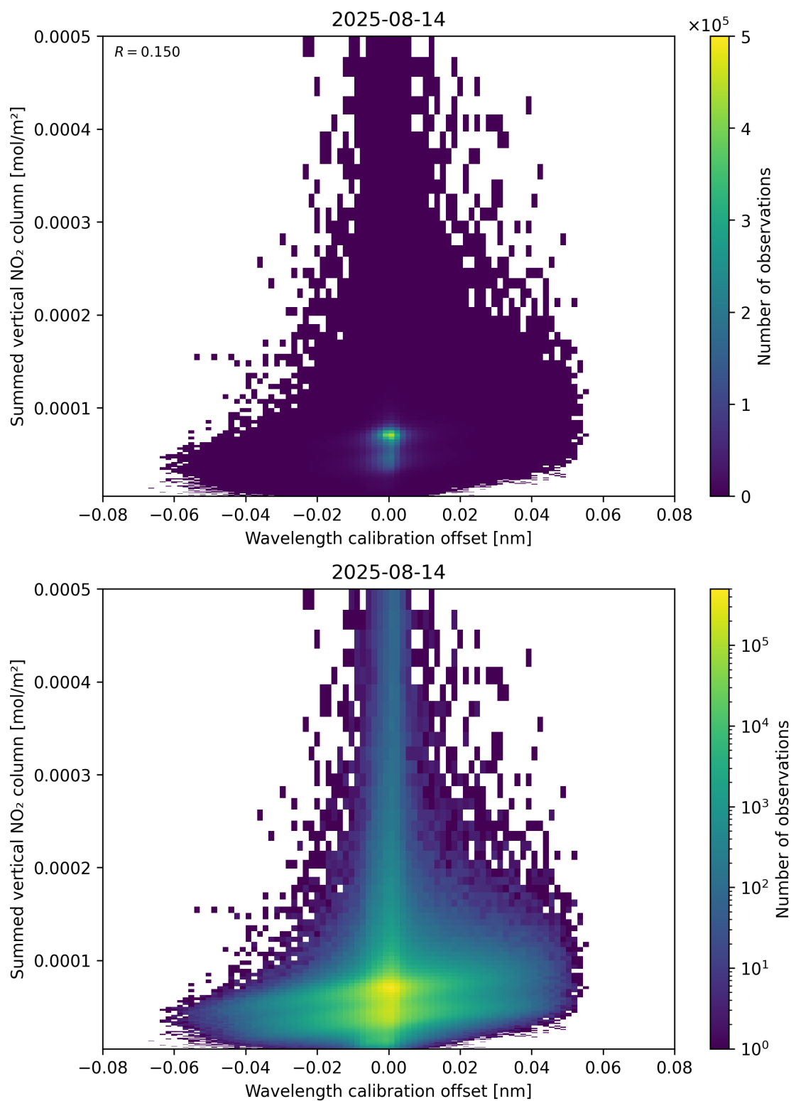
Figure 177: Scatter density plot of “Wavelength calibration offset” against “Summed vertical NO 2 column” for 2025-08-14 to 2025-08-15.
