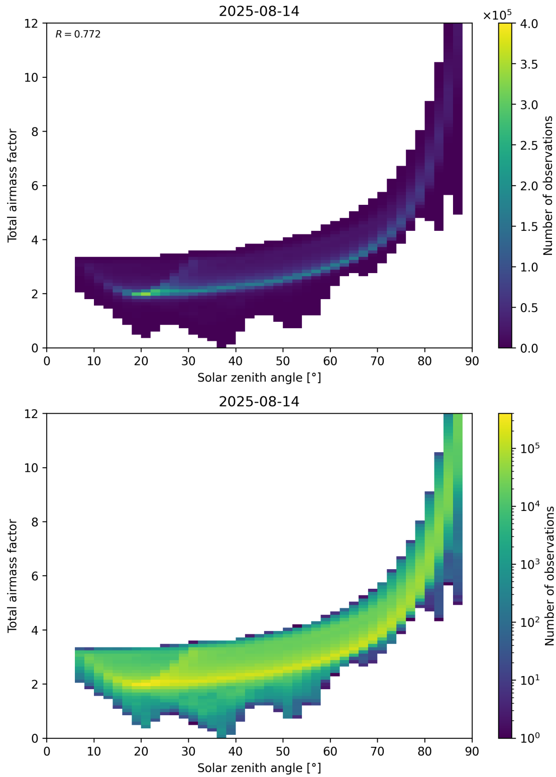
Figure 146: Scatter density plot of “Solar zenith angle” against “Total air mass factor” for 2025-08-14 to 2025-08-15.
