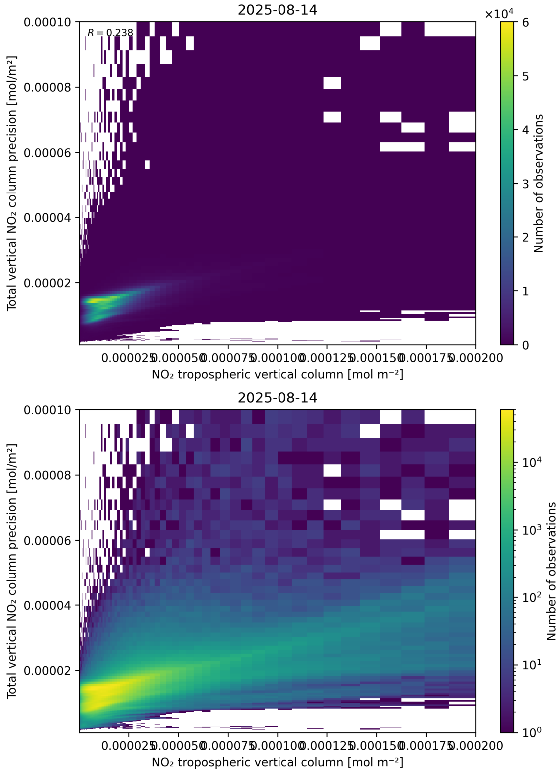
Figure 129: Scatter density plot of “NO 2 tropospheric vertical column” against “Total vertical NO 2 column precision” for 2025-08-14 to 2025-08-15.
