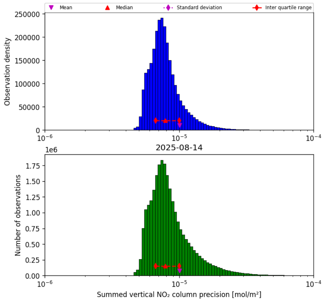
Figure 41: Histogram of “Summed vertical NO 2 column precision” for 2025-08-14 to 2025-08-15
