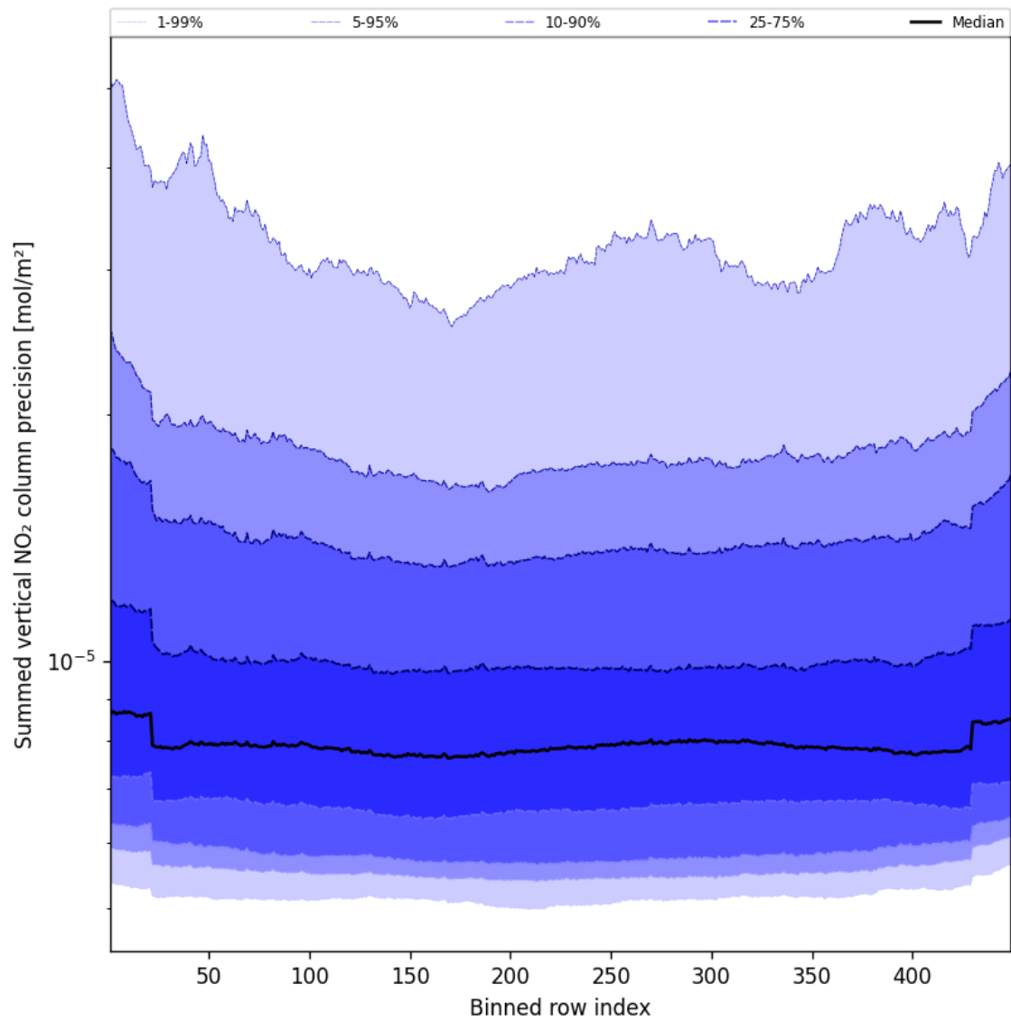
Figure 58: Along track statistics of “Summed vertical NO 2 column precision” for 2025-08-14 to 2025-08-15
