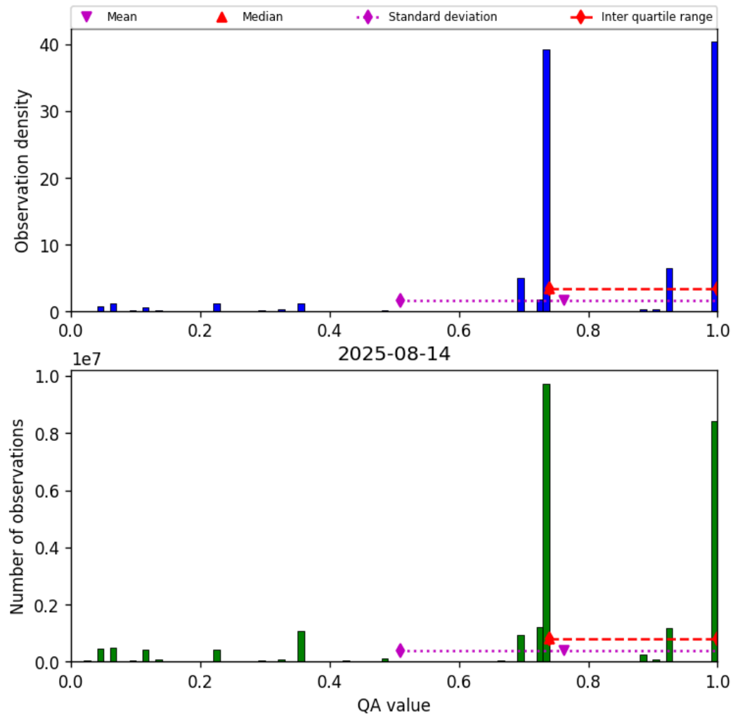
Figure 28: Histogram of “QA value” for 2025-08-14 to 2025-08-15
