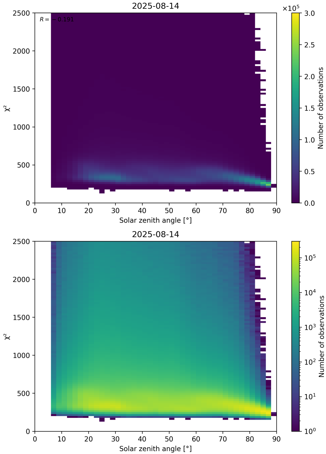
Figure 148: Scatter density plot of “Solar zenith angle” against “ \chi^2 ” for 2025-08-14 to 2025-08-15.
