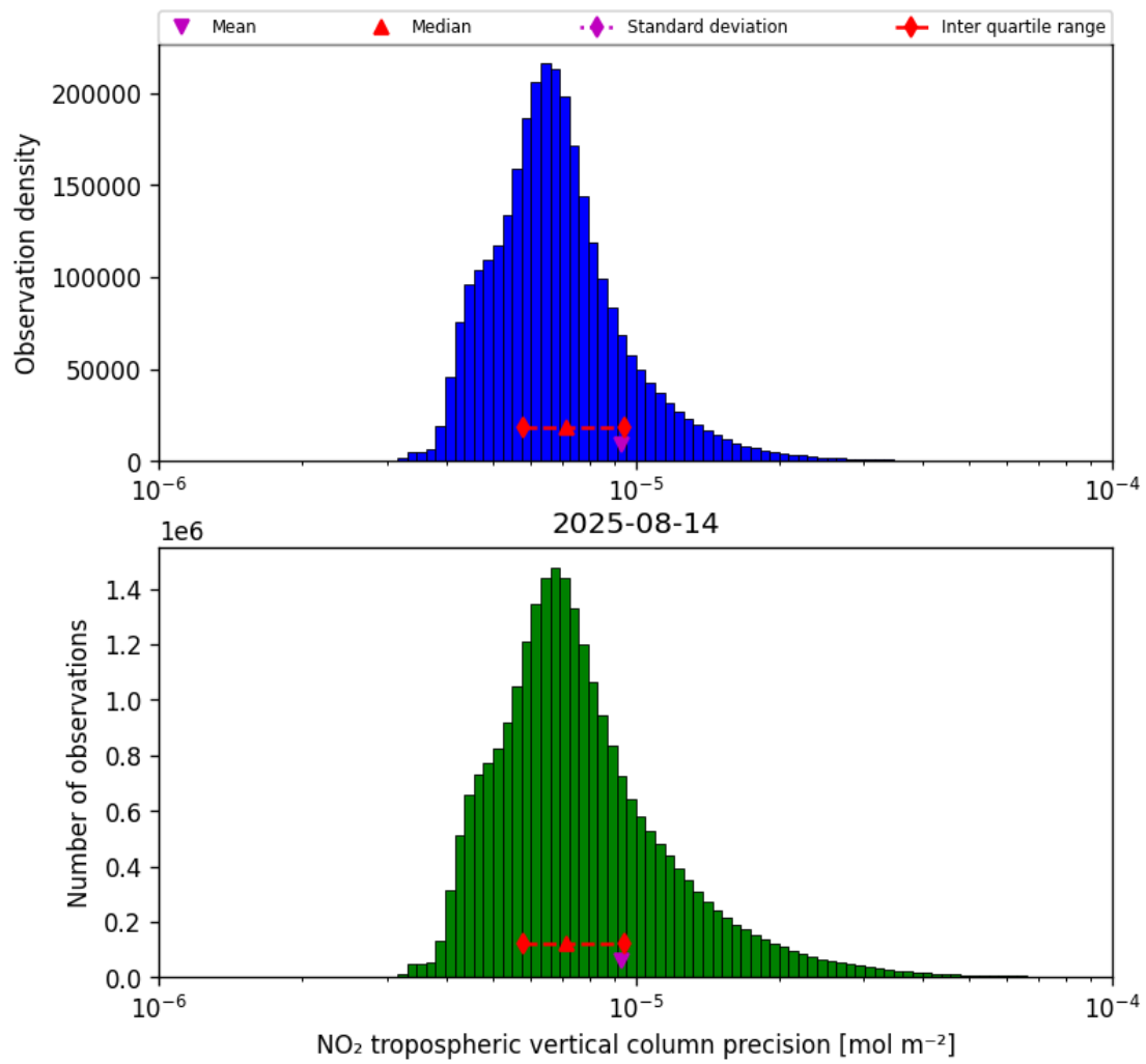
Figure 30: Histogram of “NO 2 tropospheric vertical column precision” for 2025-08-14 to 2025-08-15
