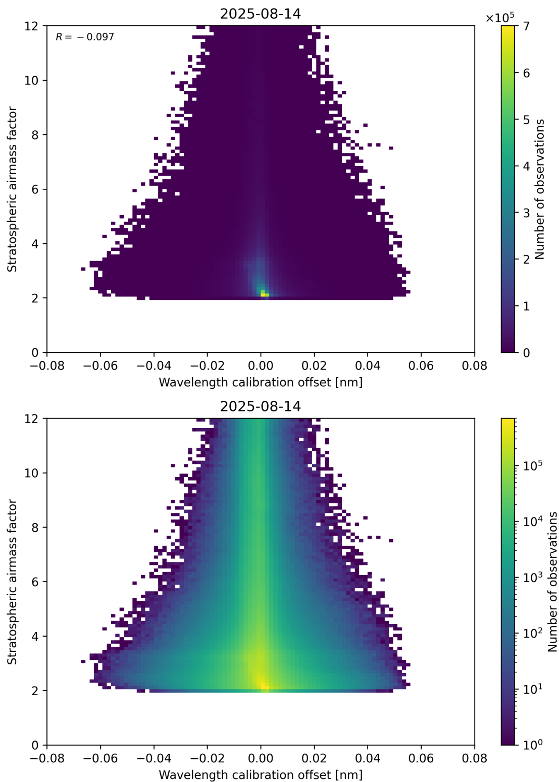
Figure 174: Scatter density plot of “Wavelength calibration offset” against “Stratospheric air mass factor” for 2025-08-14 to 2025-08-15.
