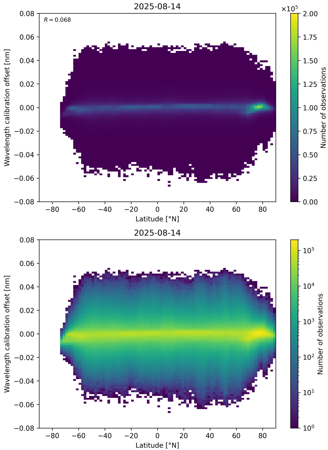
Figure 95: Scatter density plot of “Latitude” against “Wavelength calibration offset” for 2025-08-14 to 2025-08-15.
