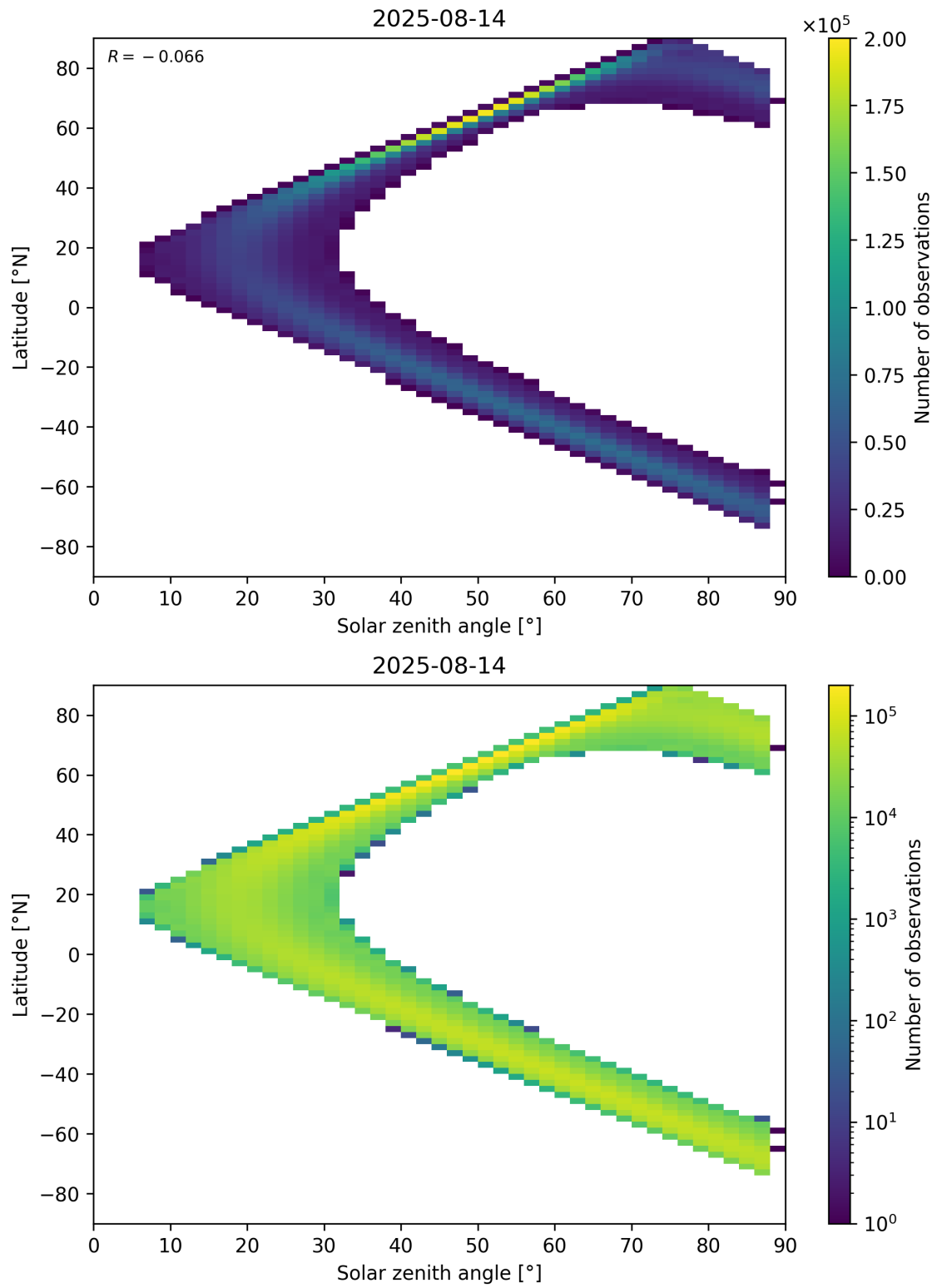
Figure 149: Scatter density plot of “Solar zenith angle” against “Latitude” for 2025-08-14 to 2025-08-15.
