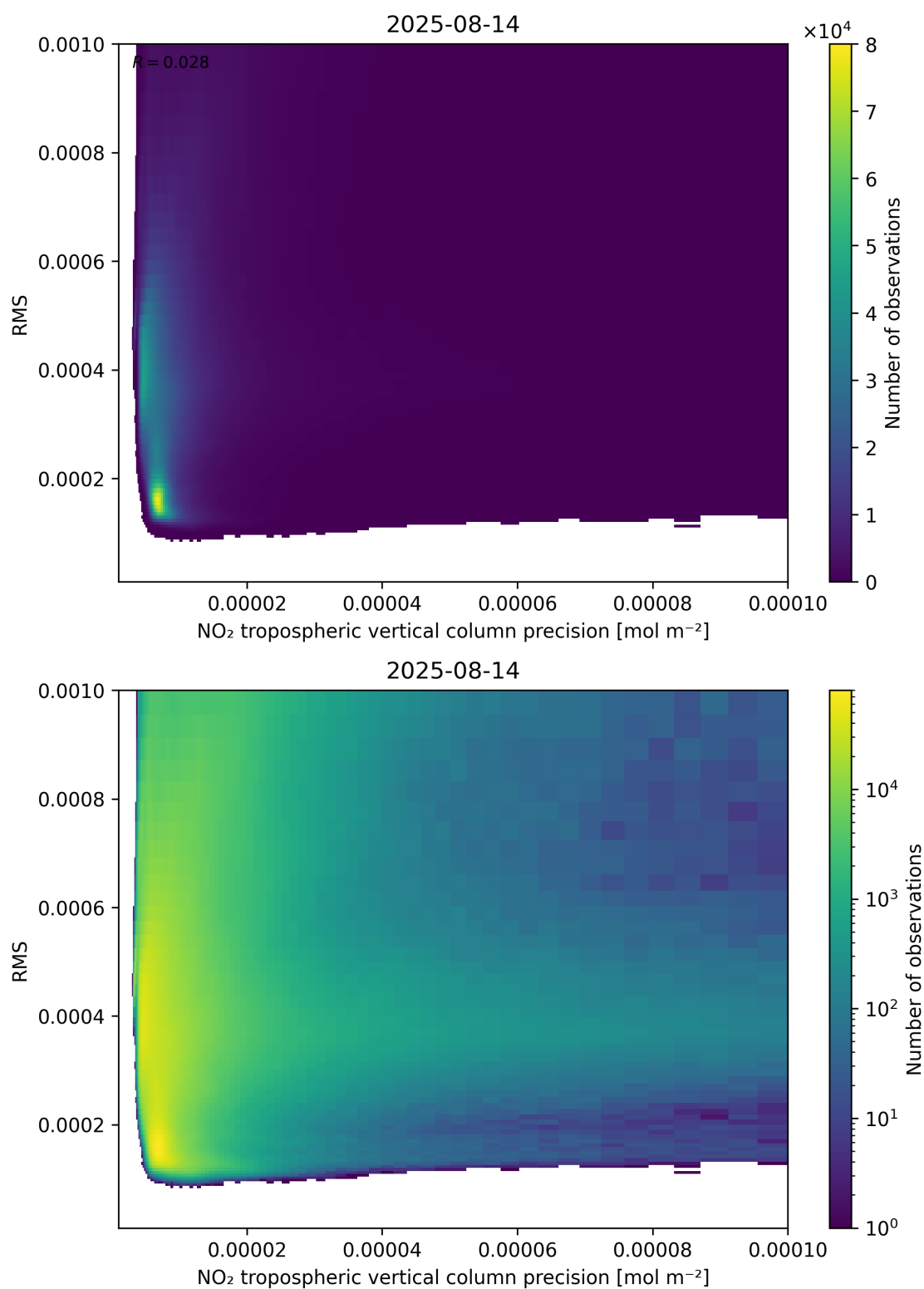
Figure 140: Scatter density plot of “NO 2 tropospheric vertical column precision” against “RMS” for 2025-08-14 to 2025-08-15.
