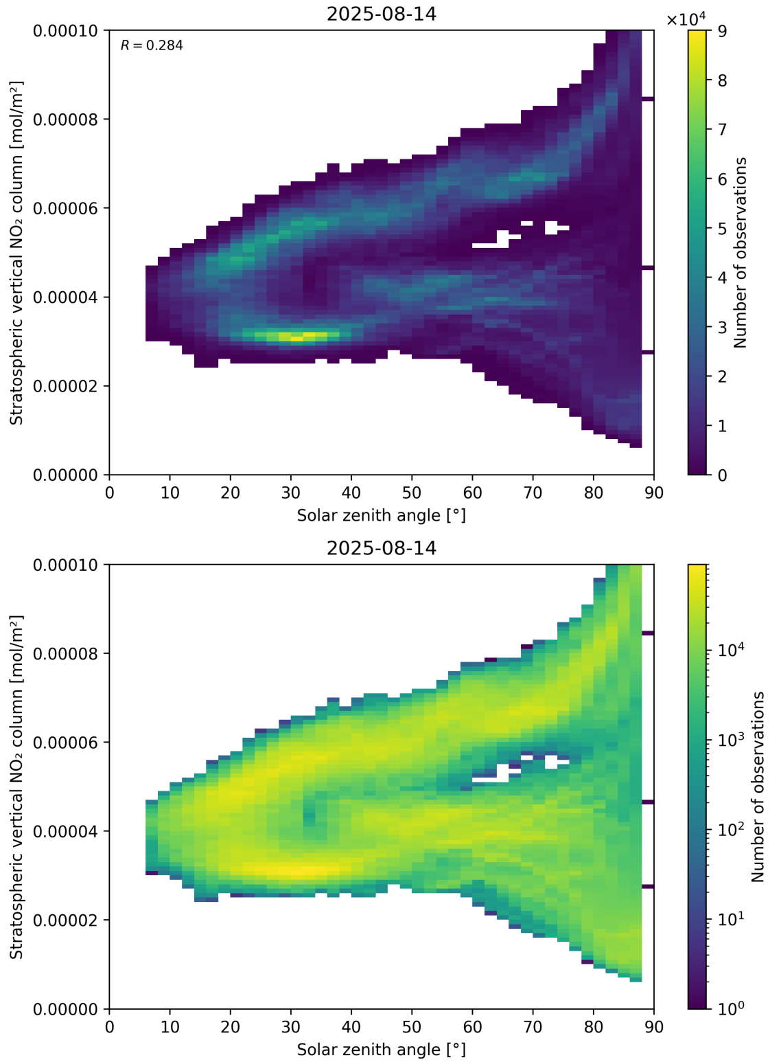
Figure 150: Scatter density plot of “Solar zenith angle” against “Stratospheric vertical NO 2 column” for 2025-08-14 to 2025-08-15.
