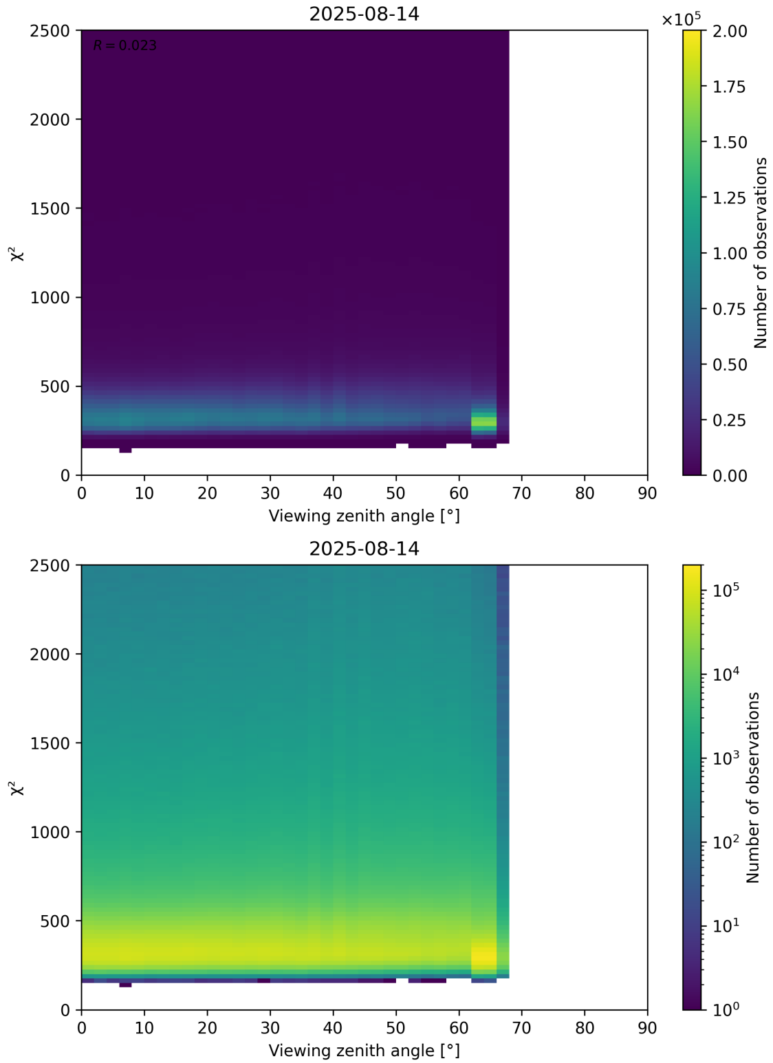
Figure 162: Scatter density plot of “Viewing zenith angle” against “ \chi^2 ” for 2025-08-14 to 2025-08-15.
