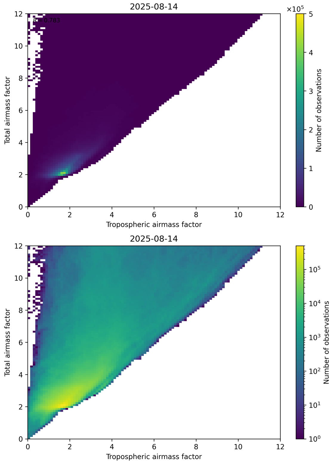
Figure 72: Scatter density plot of “Tropospheric airmass factor” against “Total airmass factor” for 2025-08-14 to 2025-08-15.
