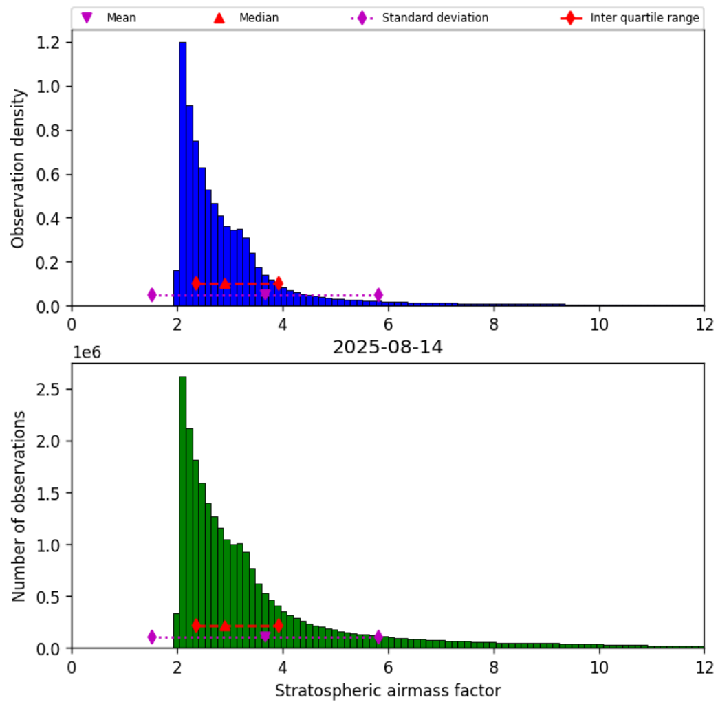
Figure 44: Histogram of “Stratospheric airmass factor” for 2025-08-14 to 2025-08-15
