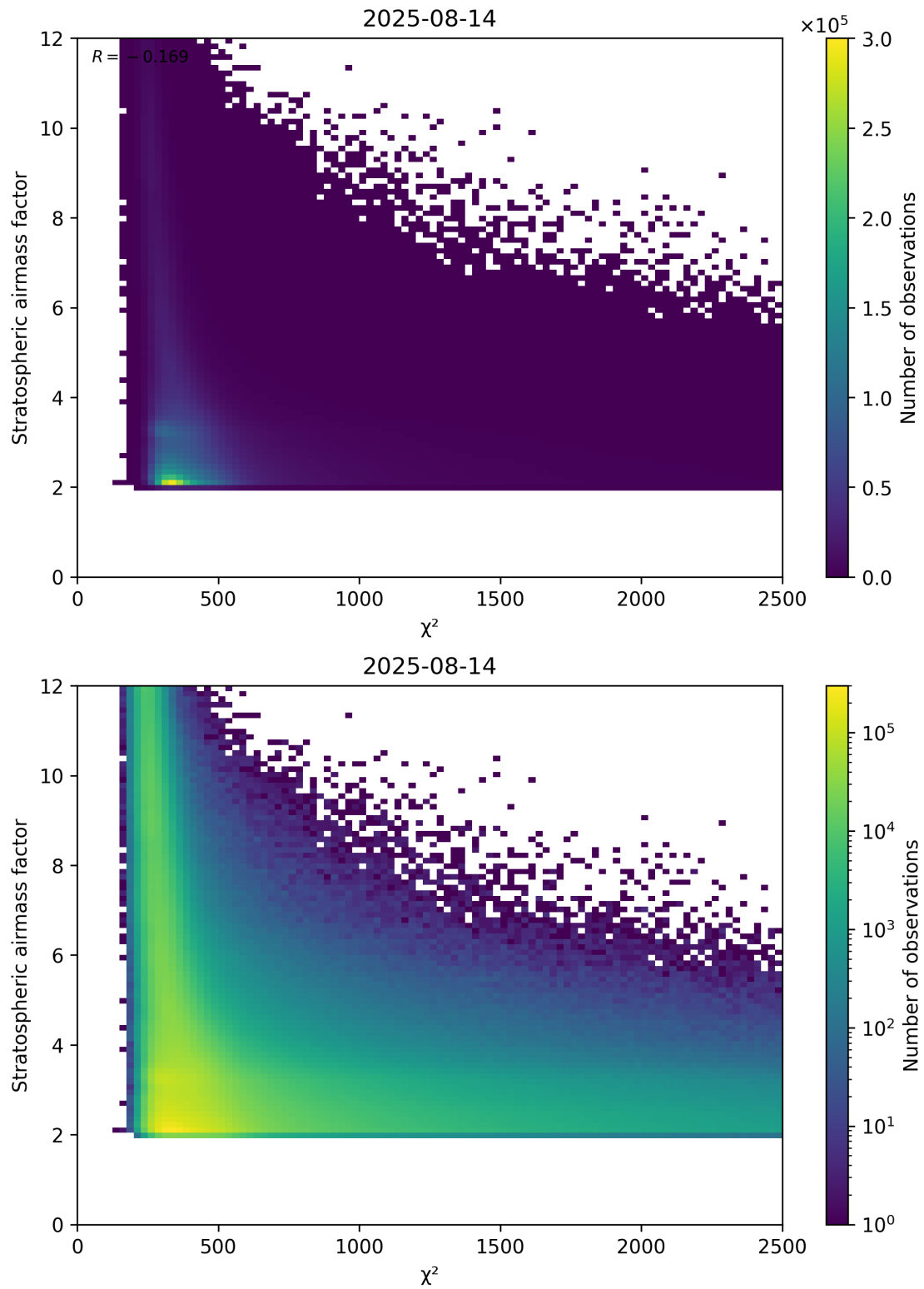
Figure 81: Scatter density plot of " \chi^2 " against "Stratospheric airmass factor" for 2025-08-14 to 2025-08-15.
