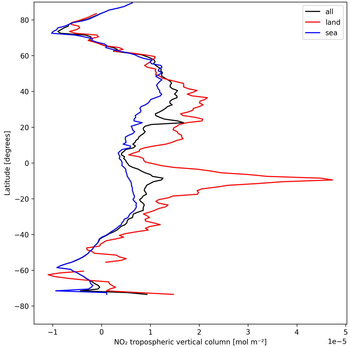
Figure 12: Zonal average of “NO 2 tropospheric vertical column” for 2025-08-14 to 2025-08-15.
