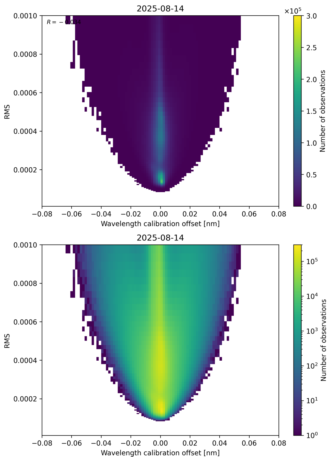
Figure 181: Scatter density plot of “Wavelength calibration offset” against “RMS” for 2025-08-14 to 2025-08-15.
