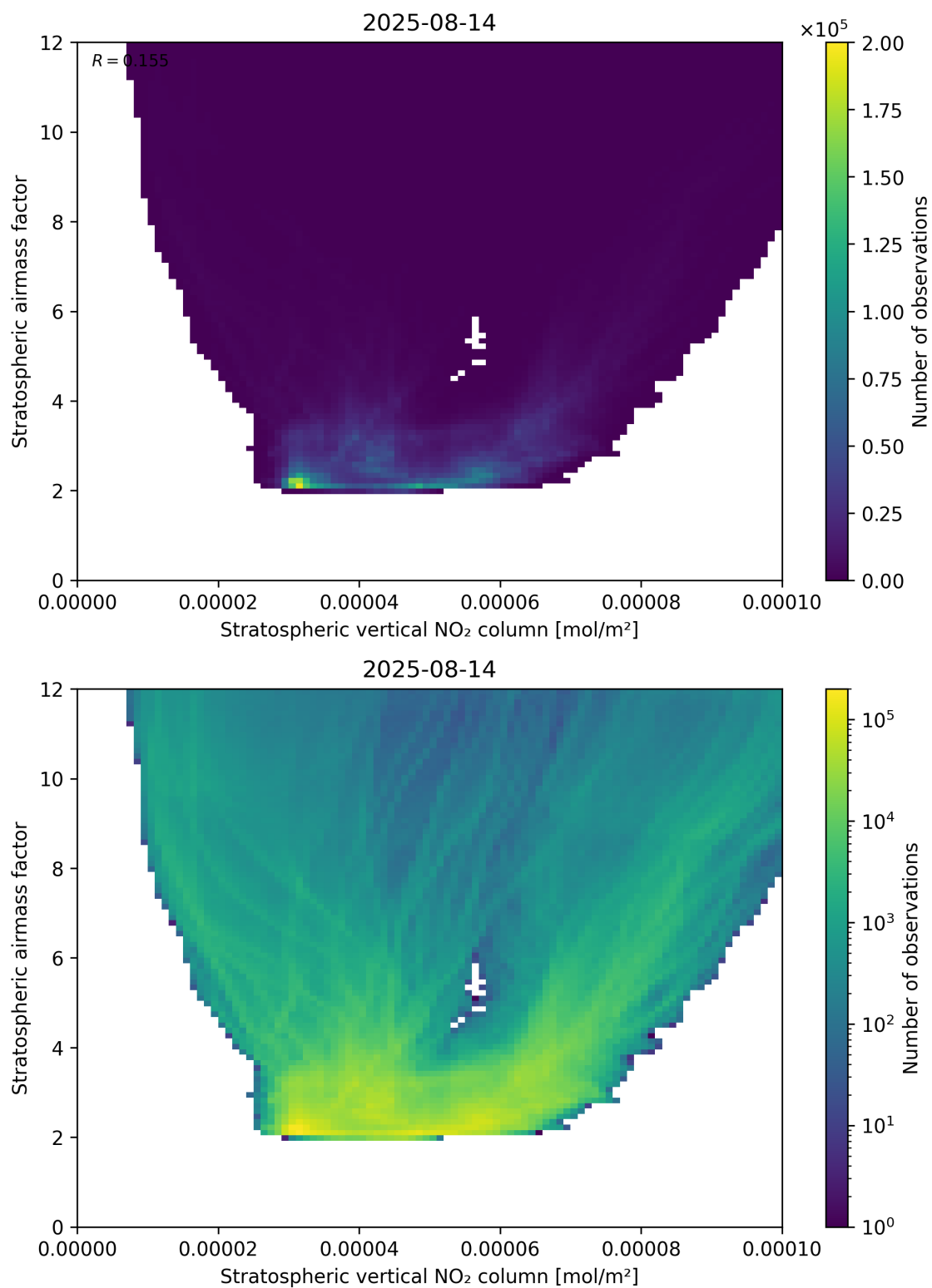
Figure 96: Scatter density plot of “Stratospheric vertical NO 2 column” against “Stratospheric airmass factor” for 2025-08-14 to 2025-08-15.
