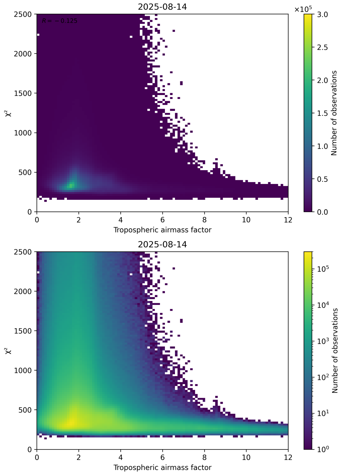
Figure 73: Scatter density plot of “Tropospheric airmass factor” against “ \chi^2 ” for 2025-08-14 to 2025-08-15.
