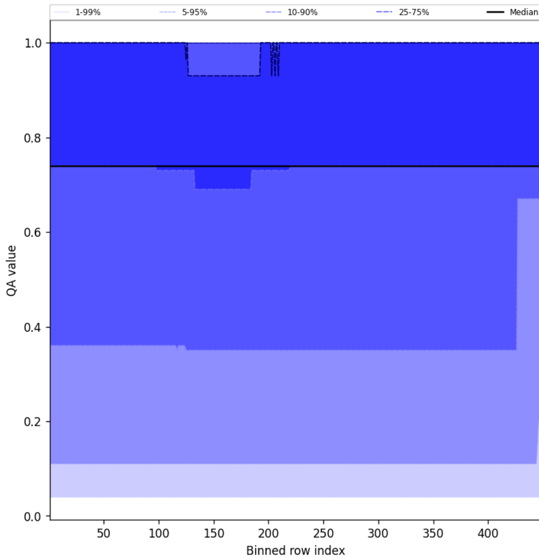
Figure 45: Along track statistics of “QA value” for 2025-08-14 to 2025-08-15
