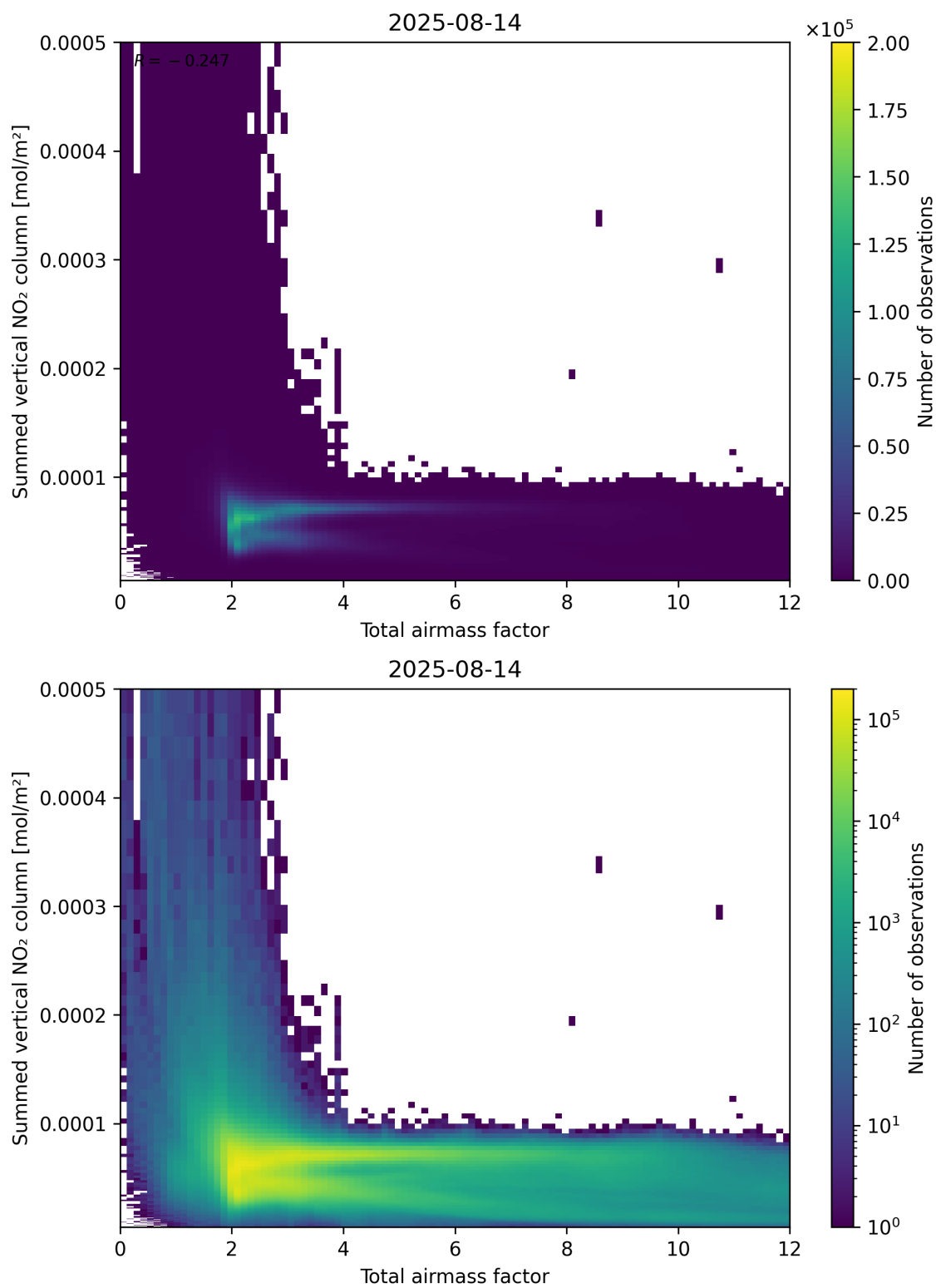
Figure 65: Scatter density plot of “Total airmass factor” against “Summed vertical NO 2 column” for 2025-08-14 to 2025-08-15.
