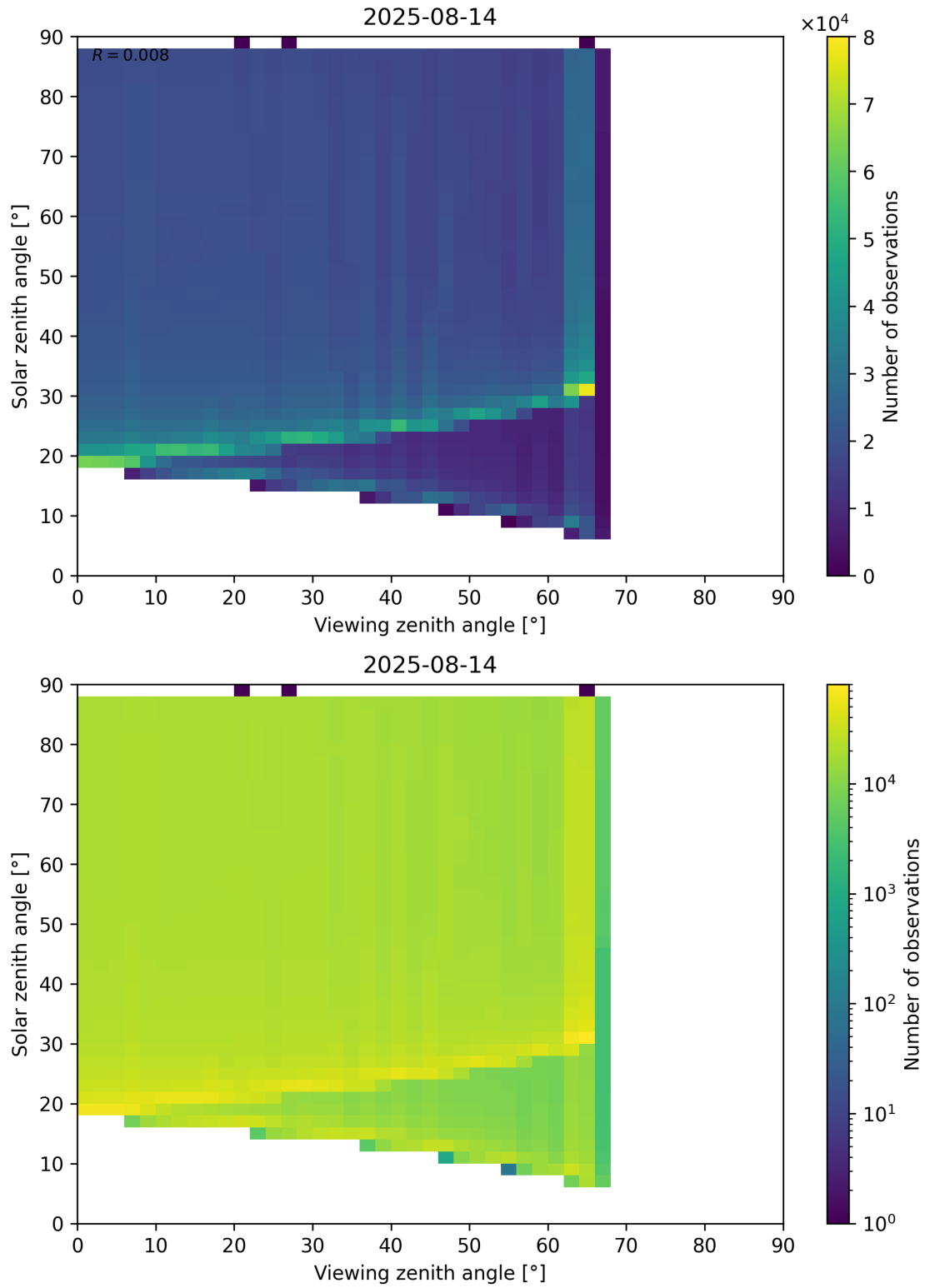
Figure 172: Scatter density plot of “Viewing zenith angle” against “Solar zenith angle” for 2025-08-14 to 2025-08-15.
