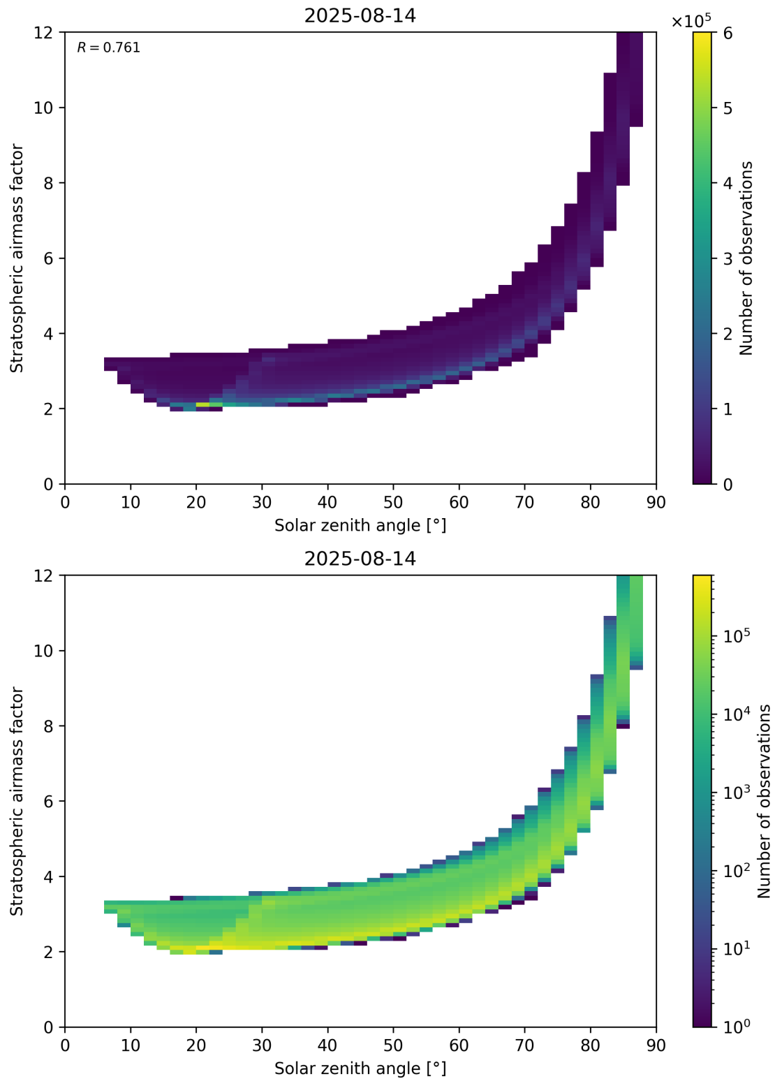
Figure 145: Scatter density plot of “Solar zenith angle” against “Stratospheric airmass factor” for 2025-08-14 to 2025-08-15.
