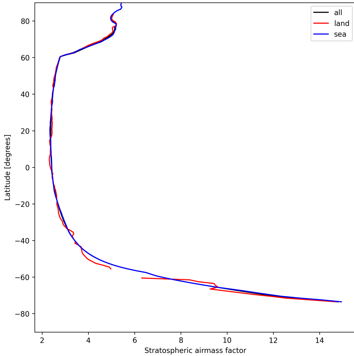
Figure 27: Zonal average of “Stratospheric airmass factor” for 2025-08-14 to 2025-08-15.
