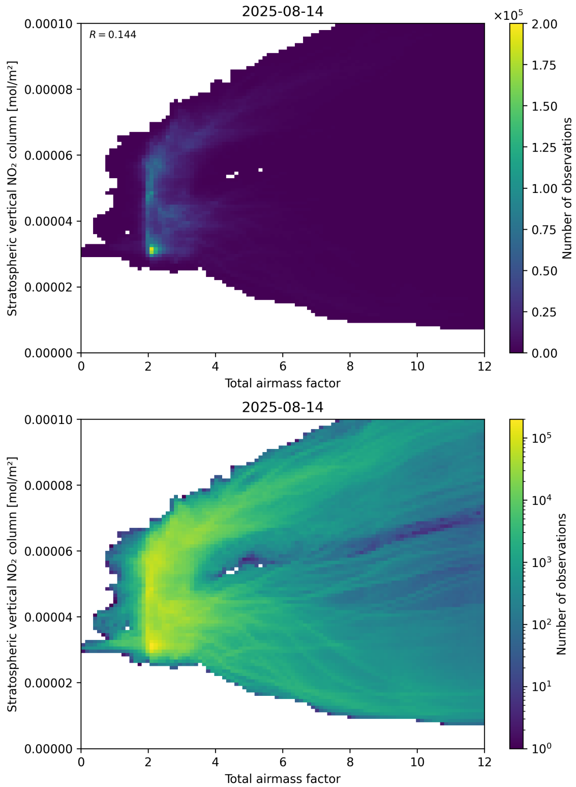
Figure 64: Scatter density plot of “Total airmass factor” against “Stratospheric vertical NO 2 column” for 2025-08-14 to 2025-08-15.
