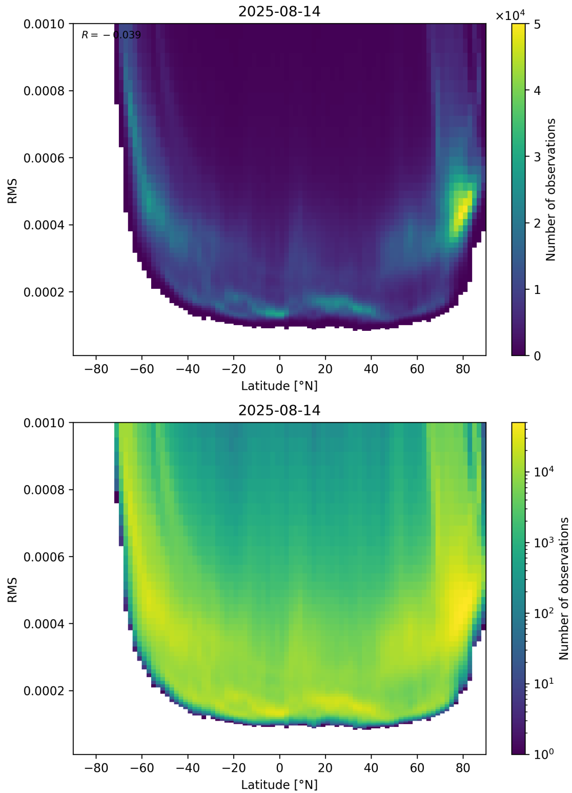
Figure 94: Scatter density plot of “Latitude” against “RMS” for 2025-08-14 to 2025-08-15.
