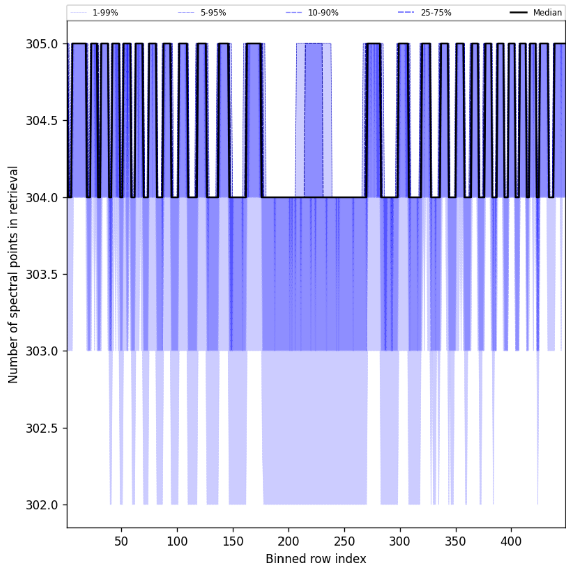
Figure 50: Along track statistics of “Number of spectral points in retrieval” for 2025-08-14 to 2025-08-15
