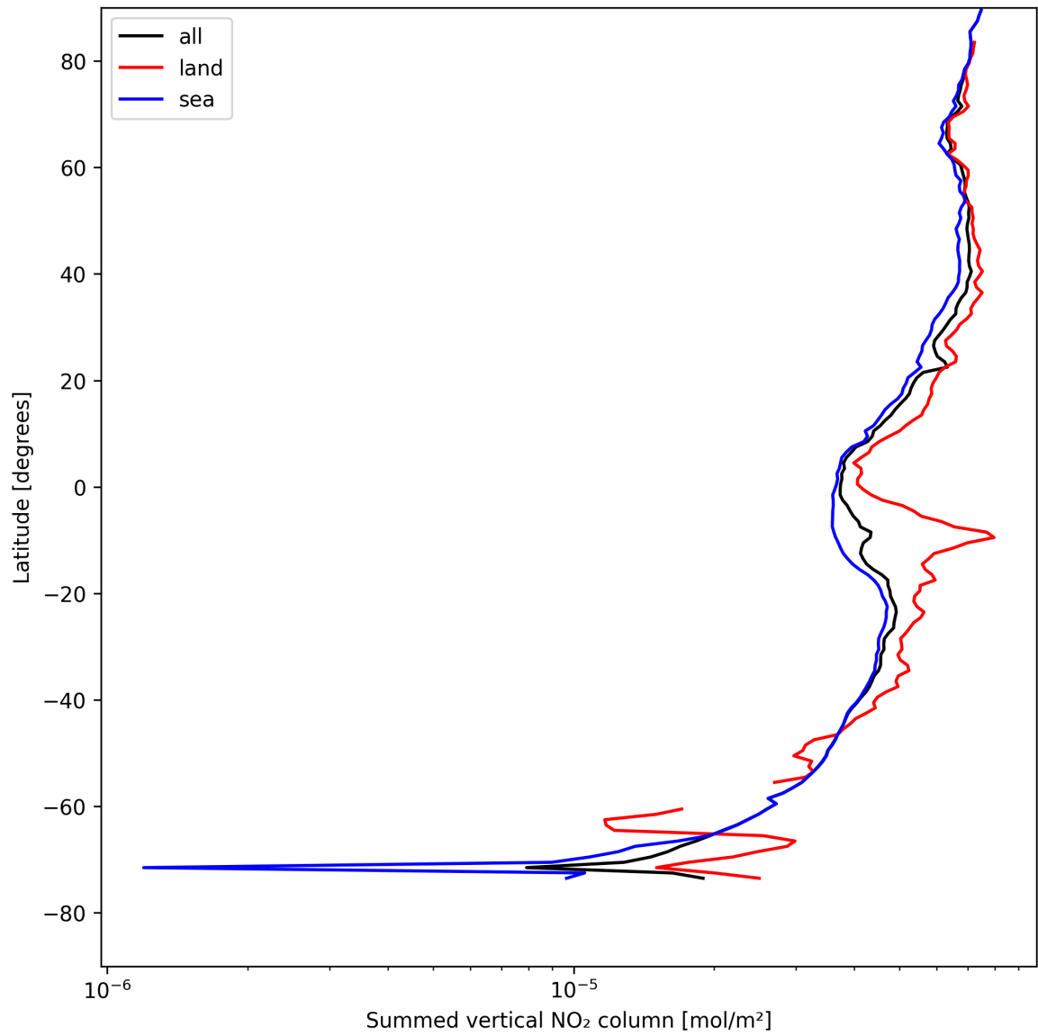
Figure 23: Zonal average of “Summed vertical NO 2 column” for 2025-08-14 to 2025-08-15.
