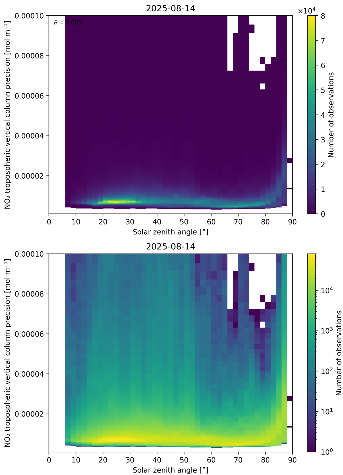
Figure 156: Scatter density plot of “Solar zenith angle” against “NO 2 tropospheric vertical column precision” for 2025-08-14 to 2025-08-15.
