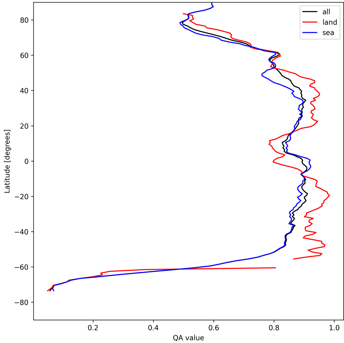
Figure 11: Zonal average of “QA value” for 2025-08-14 to 2025-08-15.
