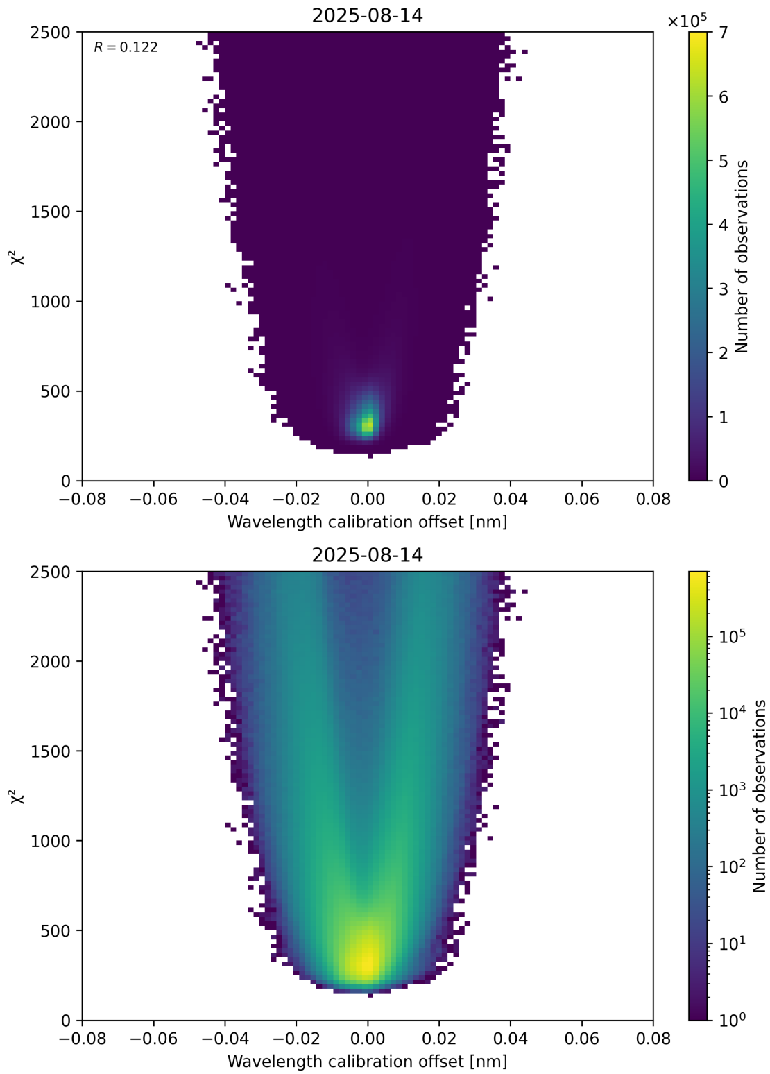
Figure 175: Scatter density plot of “Wavelength calibration offset” against “ \chi^2 ” for 2025-08-14 to 2025-08-15.
