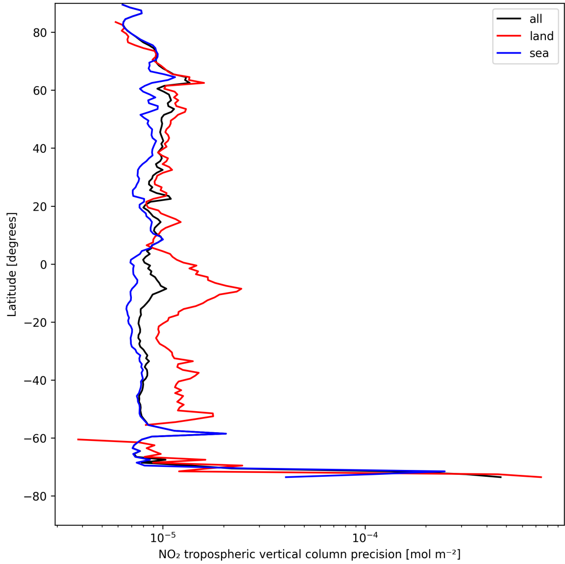
Figure 13: Zonal average of “NO 2 tropospheric vertical column precision” for 2025-08-14 to 2025-08-15.
