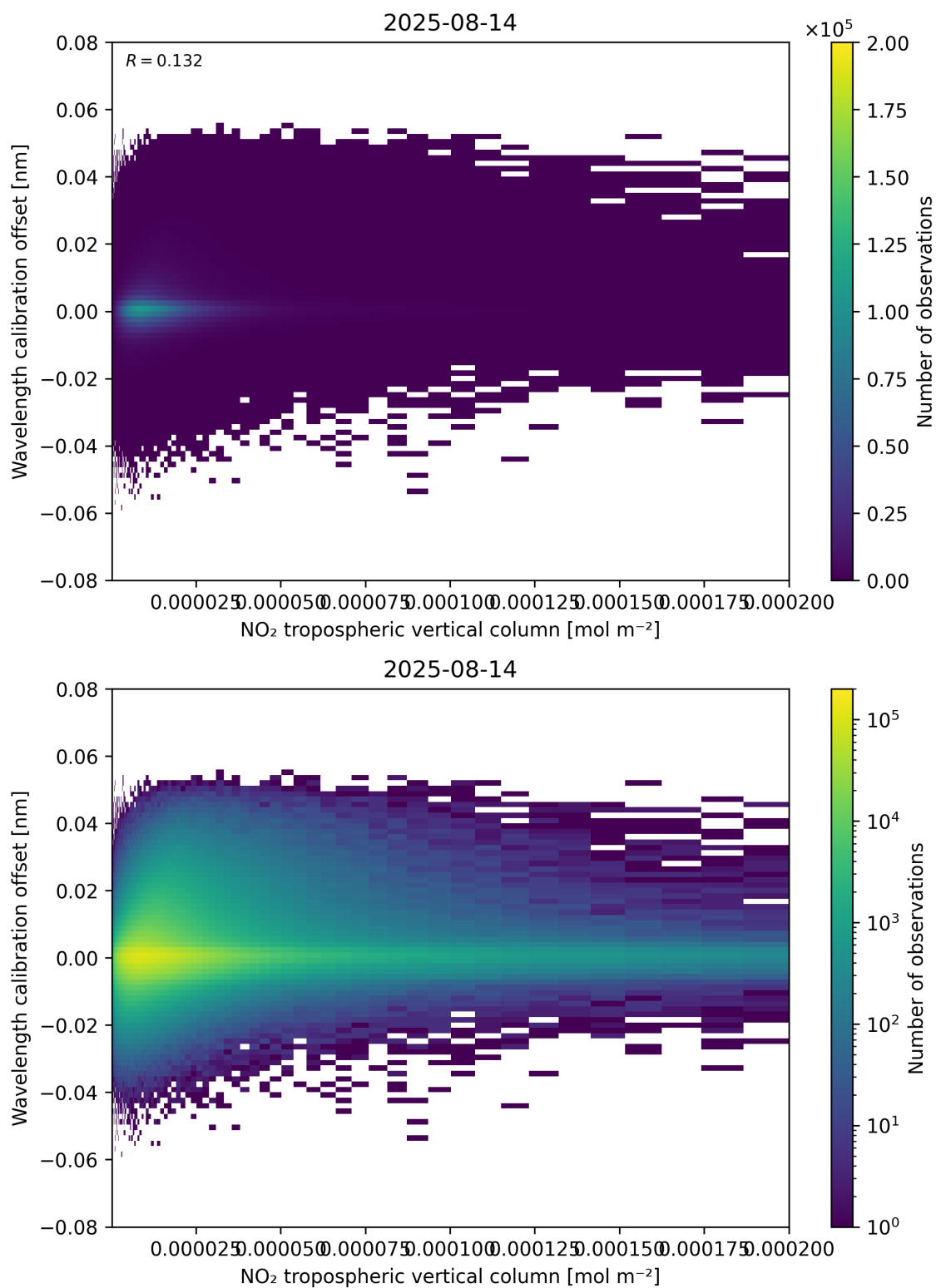
Figure 143: Scatter density plot of “NO 2 tropospheric vertical column” against “Wavelength calibration offset” for 2025-08-14 to 2025-08-15.
