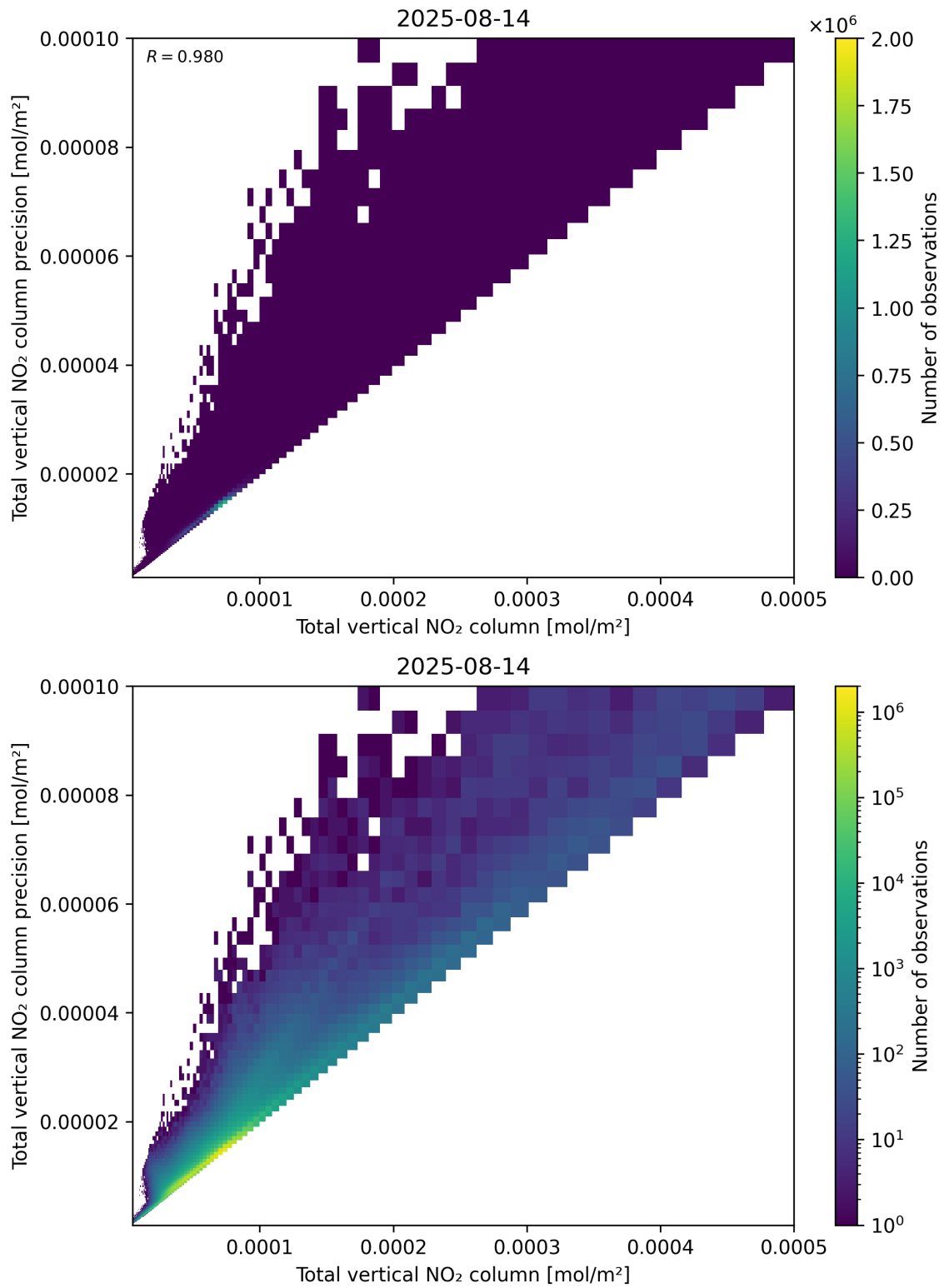
Figure 114: Scatter density plot of “Total vertical NO 2 column” against “Total vertical NO 2 column precision” for 2025-08-14 to 2025-08-15.
