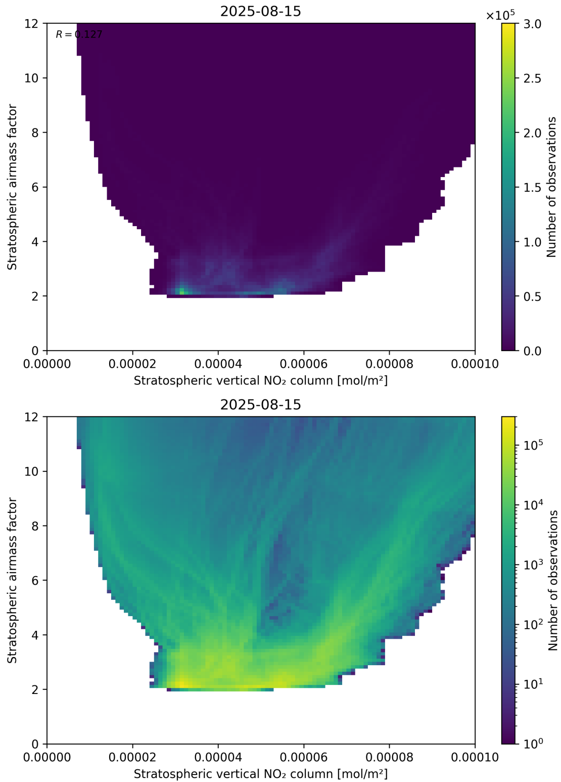
Figure 96: Scatter density plot of “Stratospheric vertical NO 2 column” against “Stratospheric airmass factor” for 2025-08-14 to 2025-08-16.
