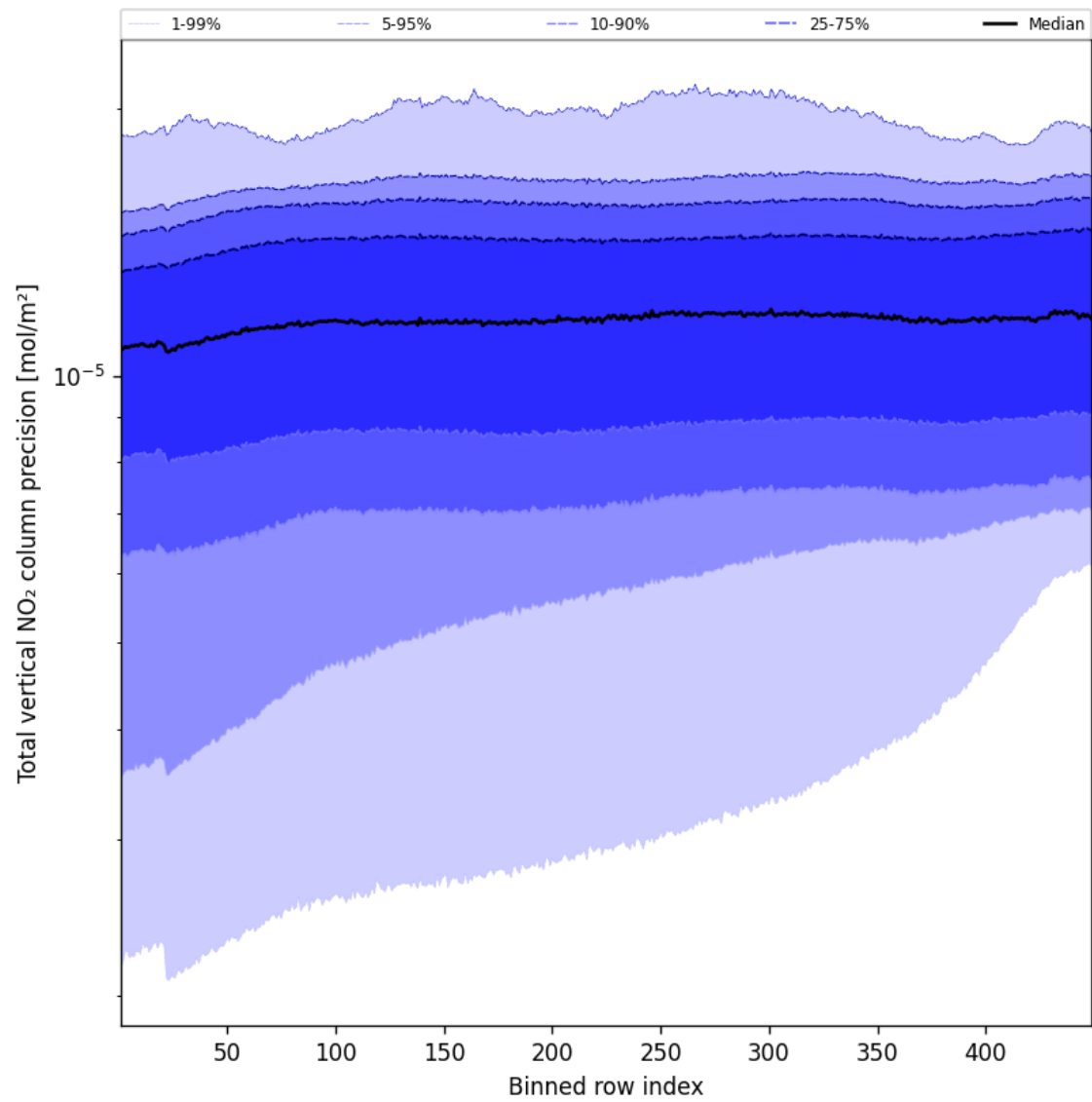
Figure 56: Along track statistics of “Total vertical NO 2 column precision” for 2025-08-14 to 2025-08-16
