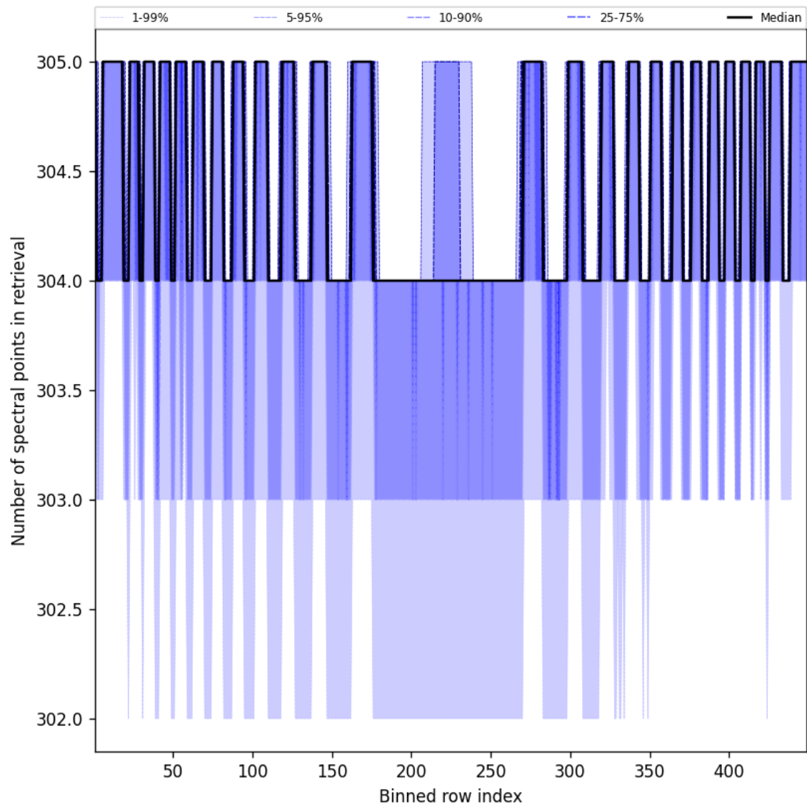
Figure 50: Along track statistics of “Number of spectral points in retrieval” for 2025-08-14 to 2025-08-16
