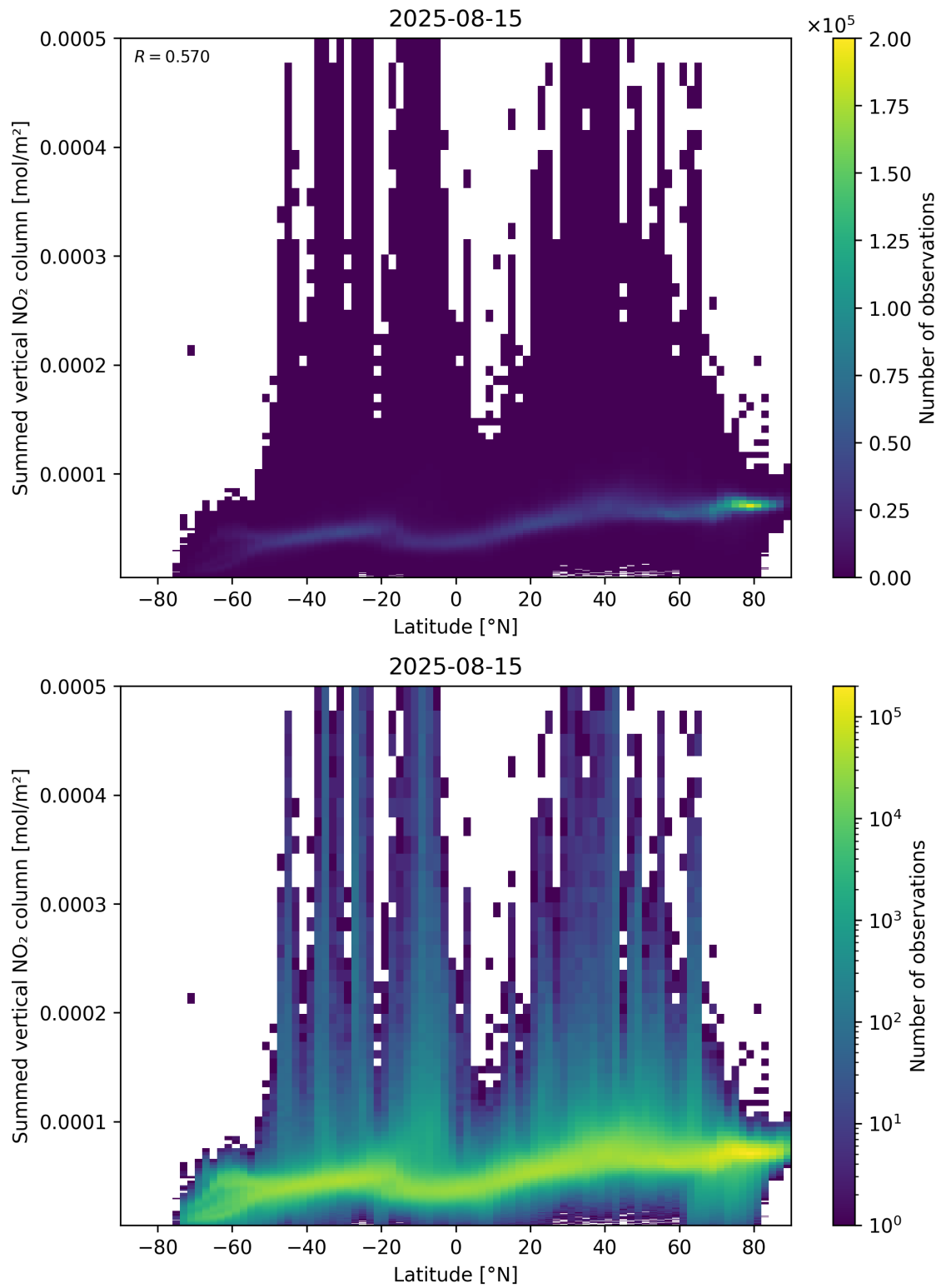
Figure 88: Scatter density plot of “Latitude” against “Summed vertical NO 2 column” for 2025-08-14 to 2025-08-16.
