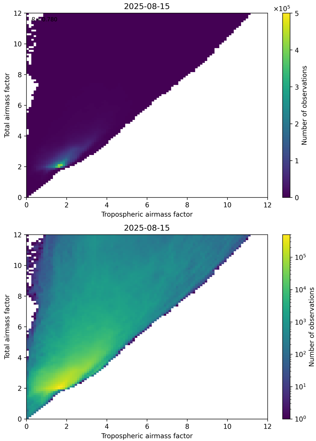
Figure 72: Scatter density plot of “Tropospheric airmass factor” against “Total airmass factor” for 2025-08-14 to 2025-08-16.
