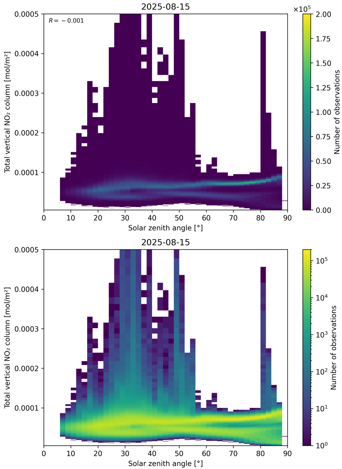
Figure 153: Scatter density plot of “Solar zenith angle” against “Total vertical NO 2 column” for 2025-08-14 to 2025-08-16.
