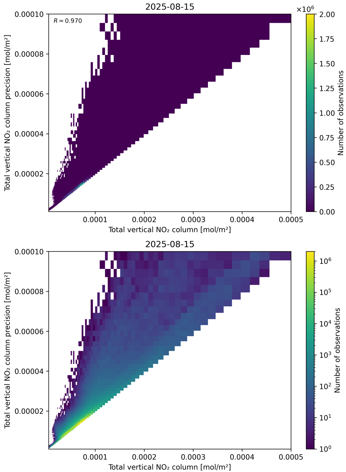
Figure 114: Scatter density plot of “Total vertical NO 2 column” against “Total vertical NO 2 column precision” for 2025-08-14 to 2025-08-16.
