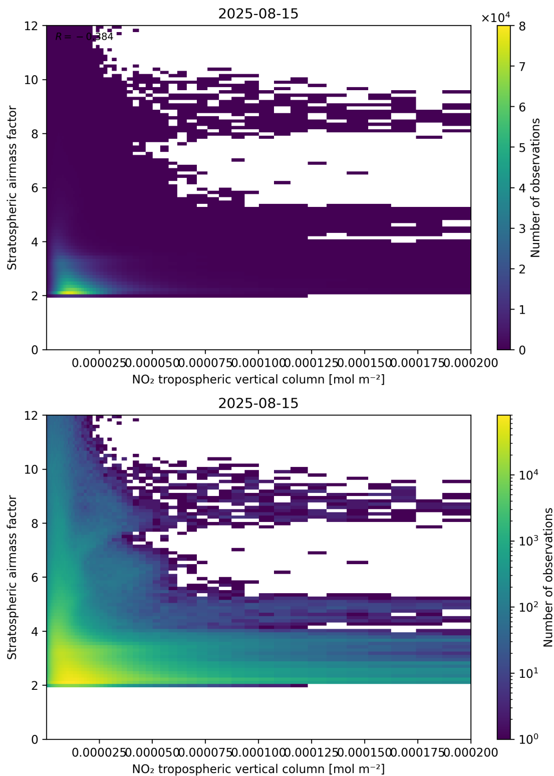
Figure 121: Scatter density plot of “NO 2 tropospheric vertical column” against “Stratospheric air mass factor” for 2025-08-14 to 2025-08-16.
