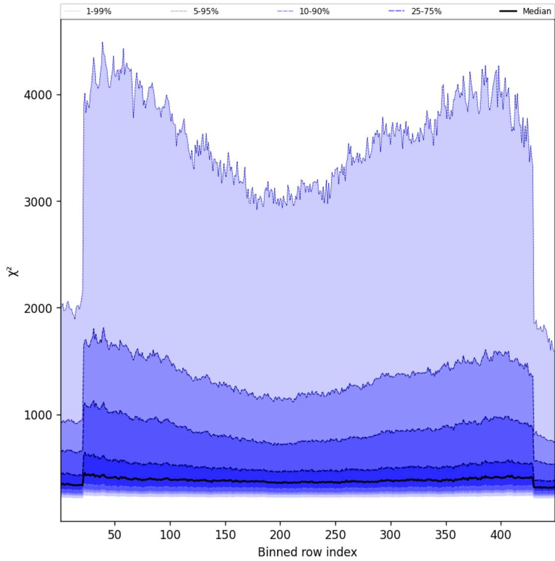
Figure 59: Along track statistics of “ \chi^2 ” for 2025-08-14 to 2025-08-16
