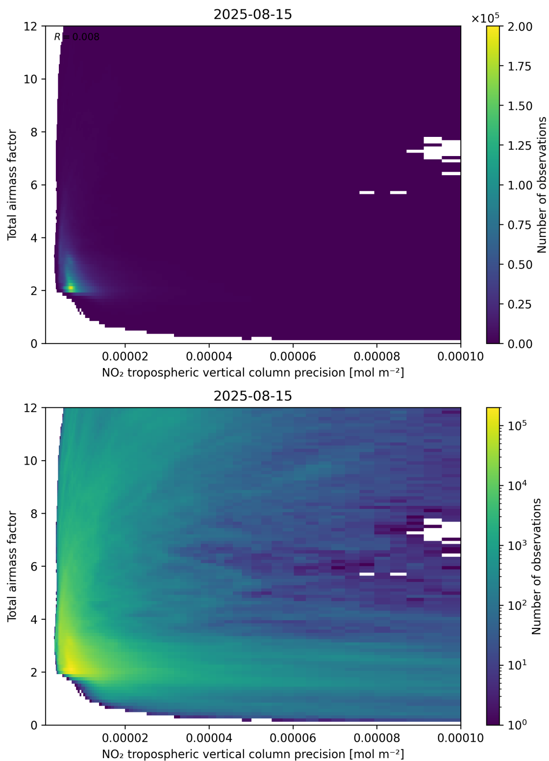
Figure 132: Scatter density plot of “NO 2 tropospheric vertical column precision” against “Total air mass factor” for 2025-08-14 to 2025-08-16.
