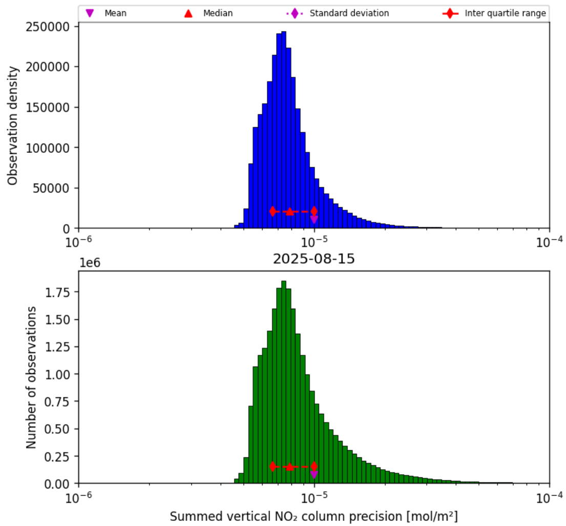
Figure 41: Histogram of "Summed vertical NO 2 column precision" for 2025-08-14 to 2025-08-16
