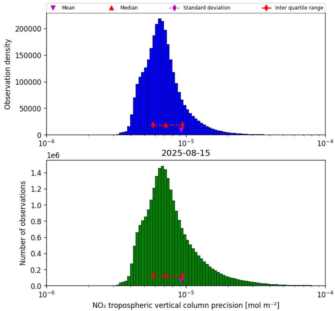
Figure 30: Histogram of “NO 2 tropospheric vertical column precision” for 2025-08-14 to 2025-08-16
