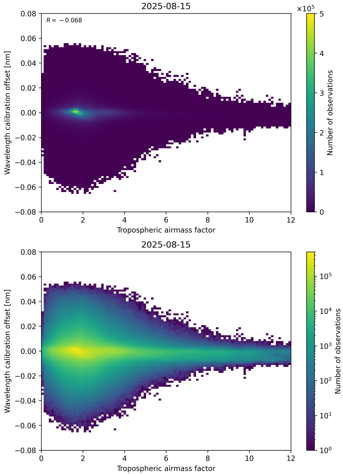
Figure 80: Scatter density plot of “Tropospheric airmass factor” against “Wavelength calibration offset” for 2025-08-14 to 2025-08-16.
