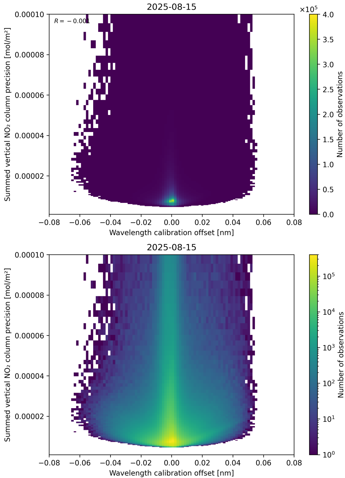
Figure 178: Scatter density plot of “Wavelength calibration offset” against “Summed vertical NO 2 column precision” for 2025-08-14 to 2025-08-16.
