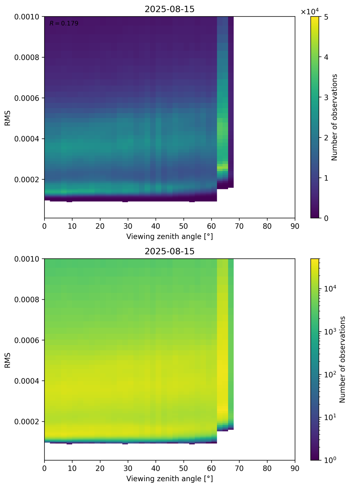
Figure 171: Scatter density plot of “Viewing zenith angle” against “RMS” for 2025-08-14 to 2025-08-16.
