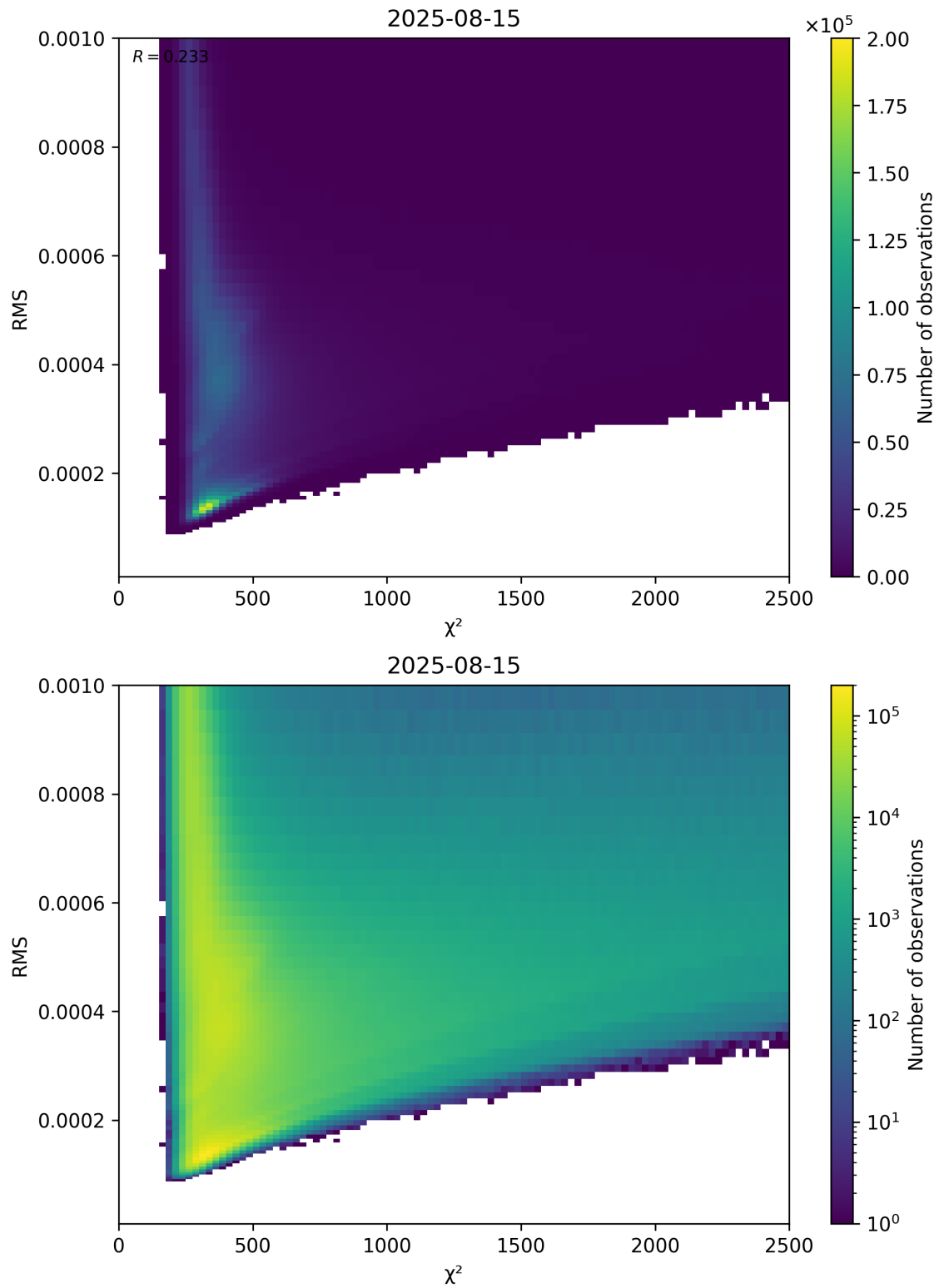
Figure 82: Scatter density plot of “ \chi^2 ” against “RMS” for 2025-08-14 to 2025-08-16.
