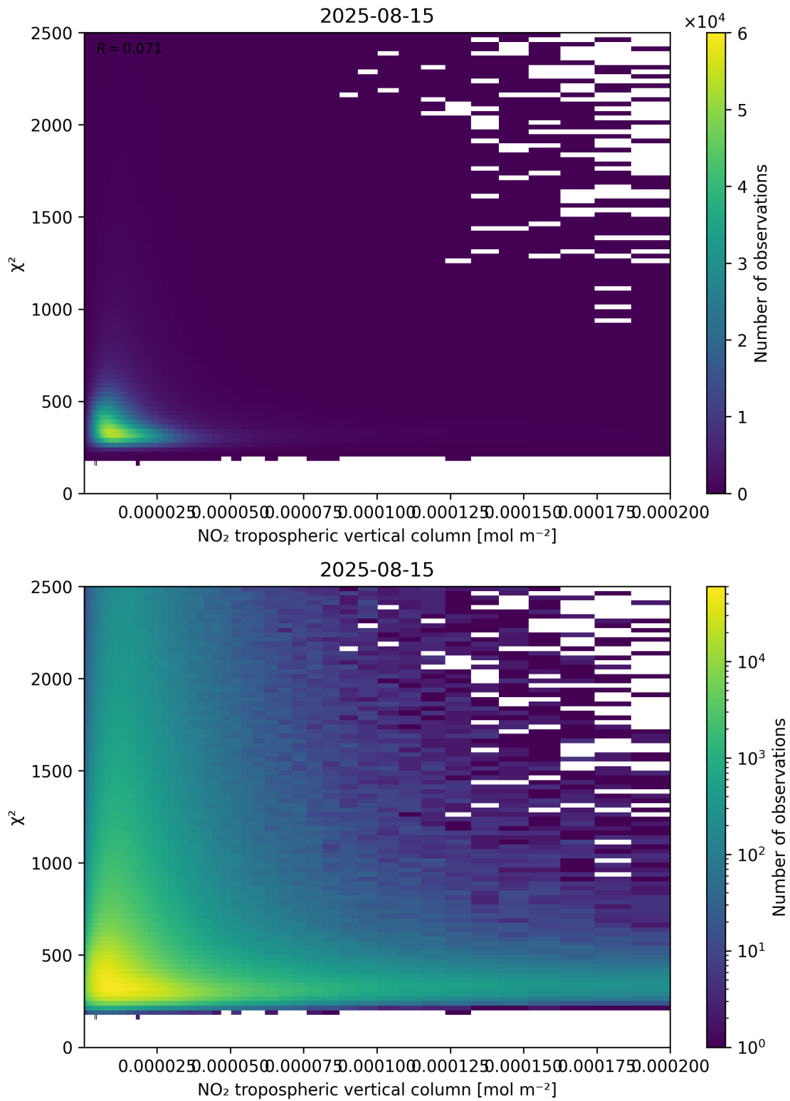
Figure 124: Scatter density plot of “NO 2 tropospheric vertical column” against “ \chi^2 ” for 2025-08-14 to 2025-08-16.
