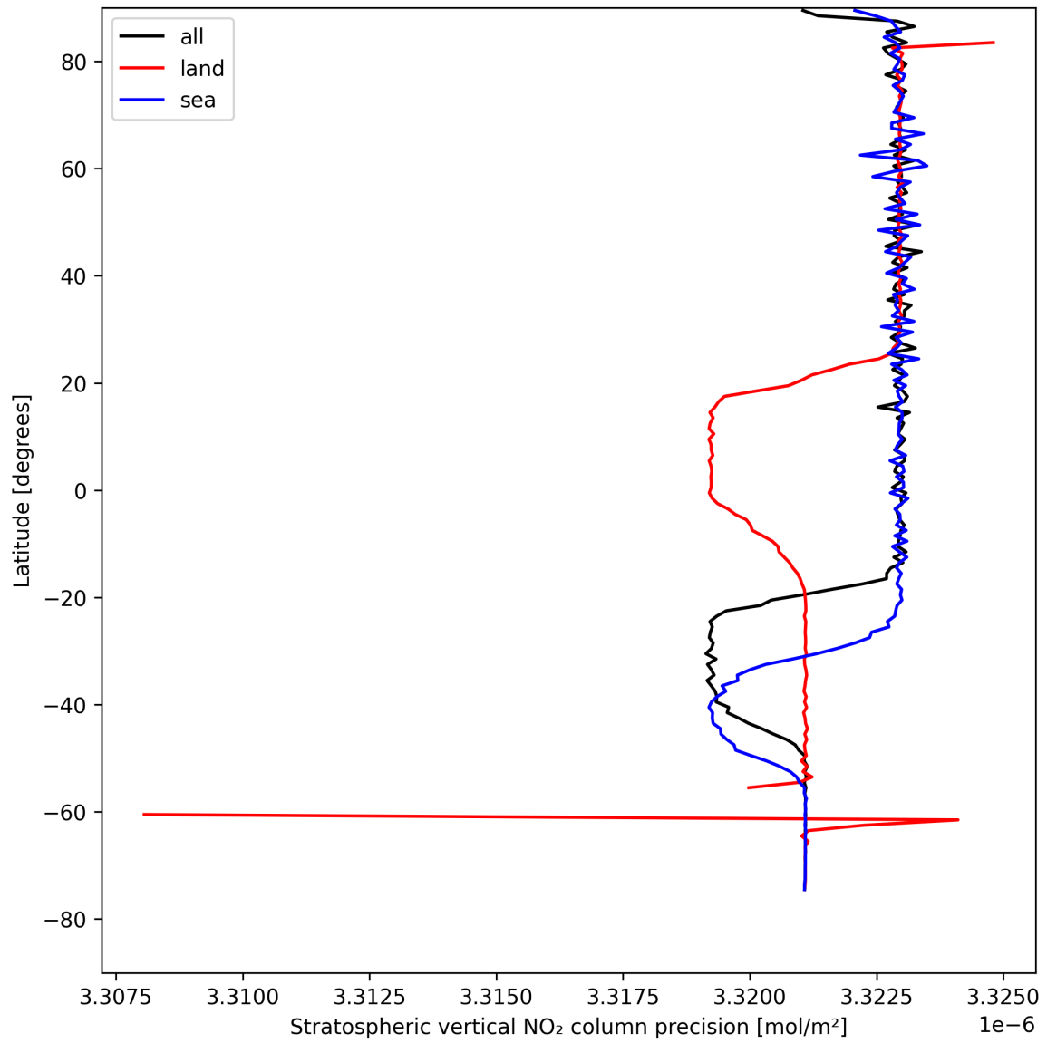
Figure 20: Zonal average of “Stratospheric vertical NO 2 column precision” for 2025-08-14 to 2025-08-16.
