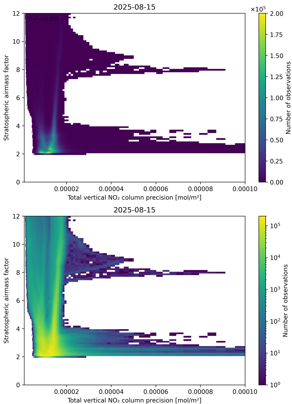
Figure 115: Scatter density plot of “Total vertical NO 2 column precision” against “Stratospheric air mass factor” for 2025-08-14 to 2025-08-16.
