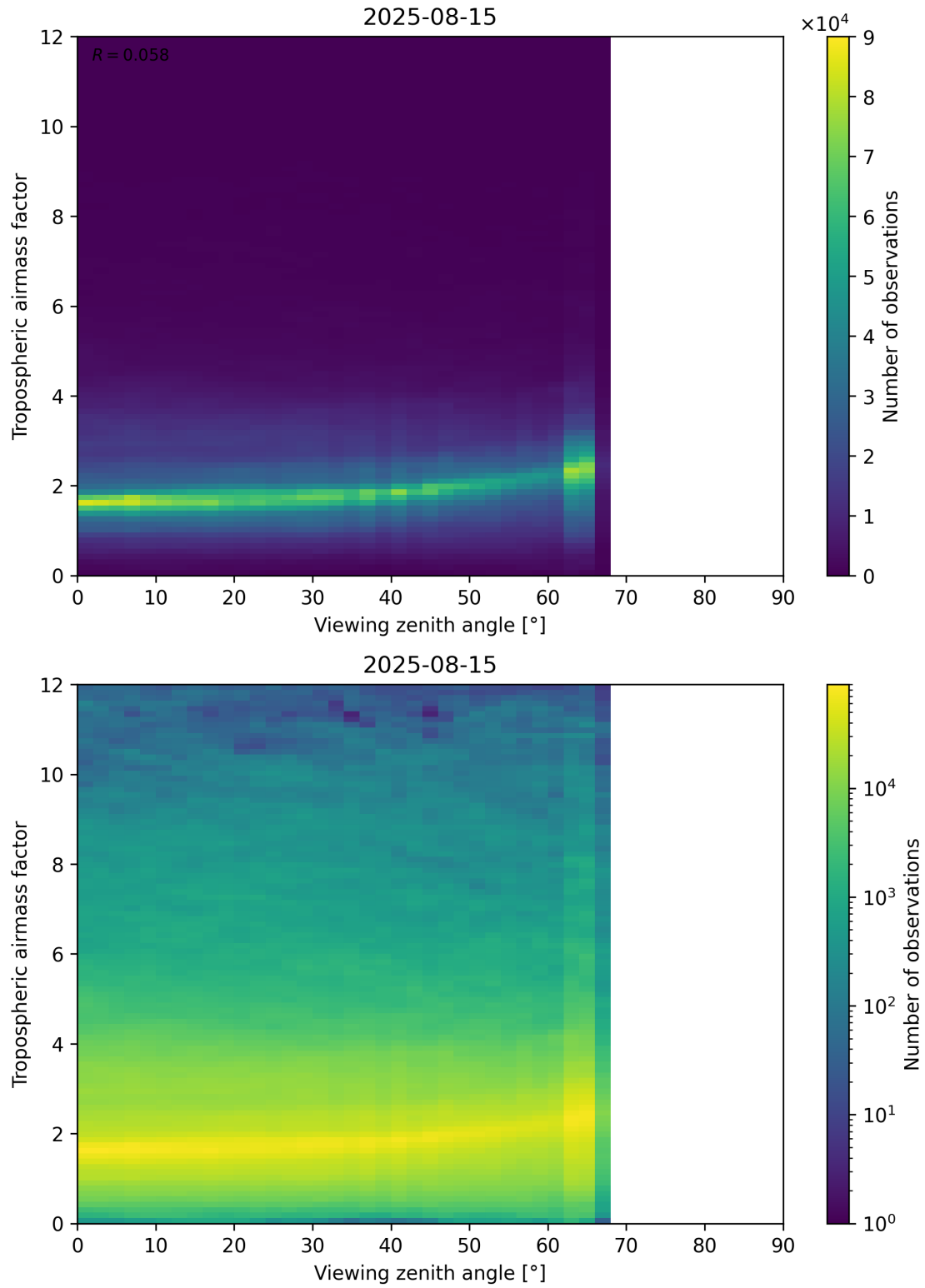
Figure 161: Scatter density plot of “Viewing zenith angle” against “Tropospheric airmass factor” for 2025-08-14 to 2025-08-16.
