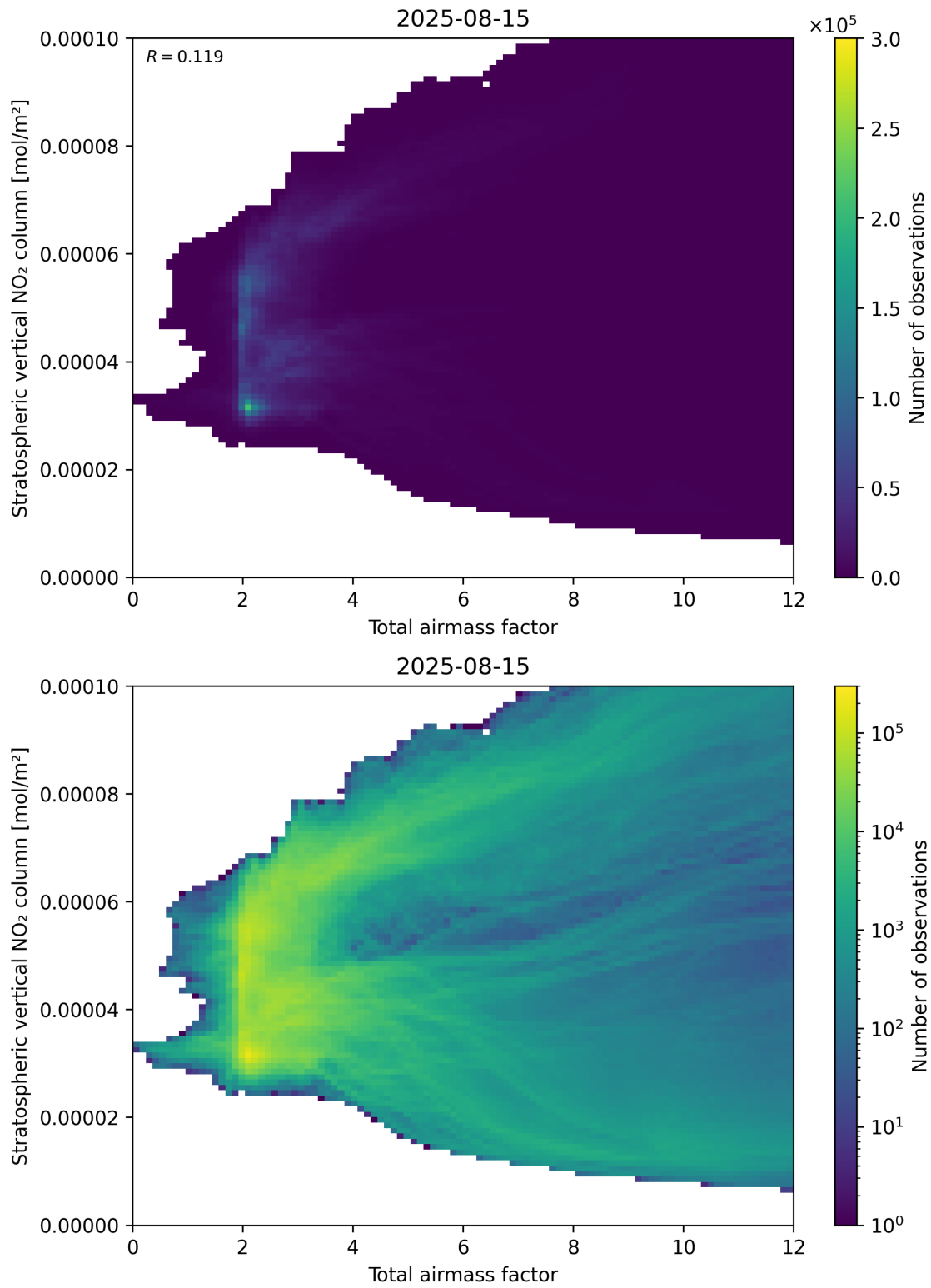
Figure 64: Scatter density plot of “Total airmass factor” against “Stratospheric vertical NO 2 column” for 2025-08-14 to 2025-08-16.
