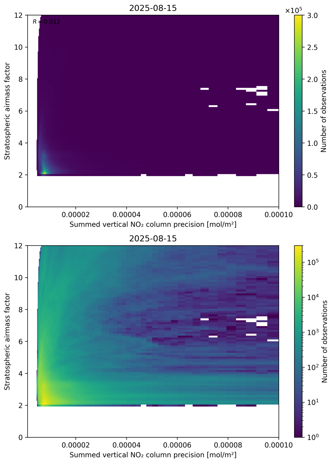
Figure 106: Scatter density plot of “Summed vertical NO 2 column precision” against “Stratospheric airmass factor” for 2025-08-14 to 2025-08-16.
