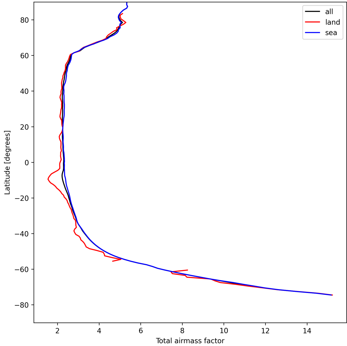
Figure 15: Zonal average of “Total airmass factor” for 2025-08-14 to 2025-08-16.
