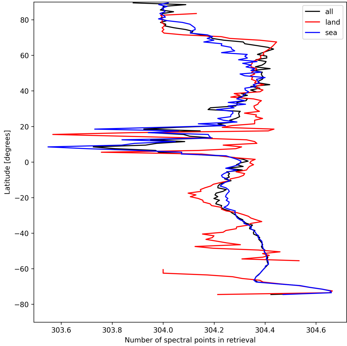
Figure 16: Zonal average of “Number of spectral points in retrieval” for 2025-08-14 to 2025-08-16.
