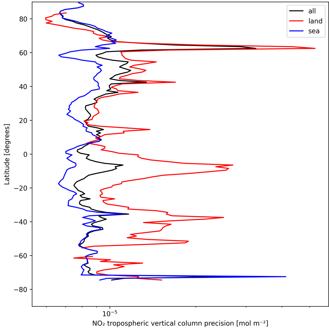
Figure 13: Zonal average of “NO 2 tropospheric vertical column precision” for 2025-08-14 to 2025-08-16.
