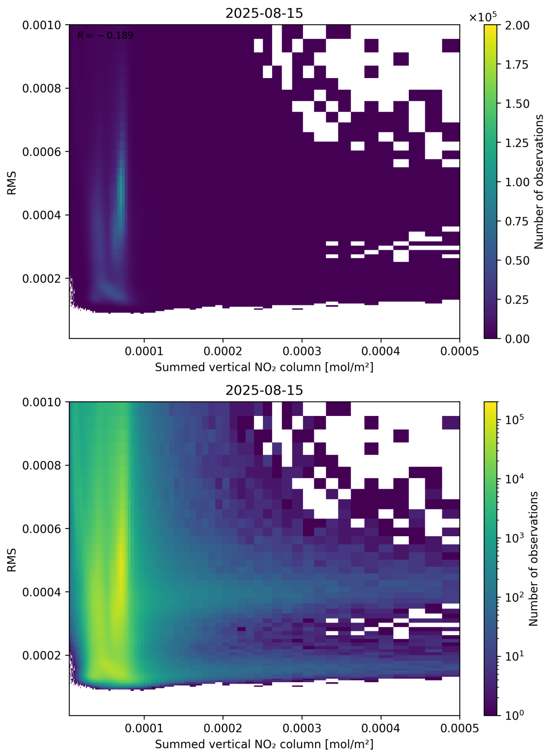
Figure 109: Scatter density plot of “Summed vertical NO 2 column” against “RMS” for 2025-08-14 to 2025-08-16.
