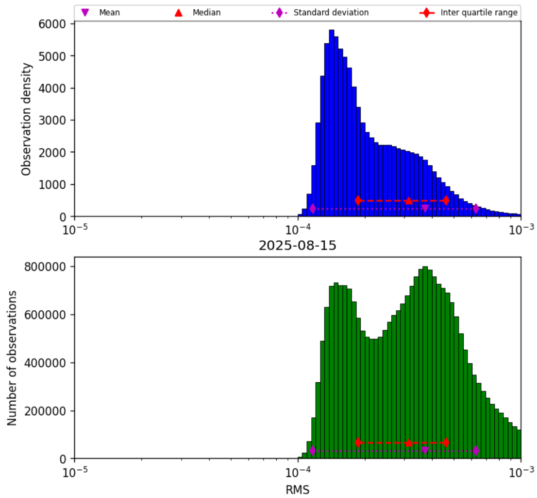
Figure 43: Histogram of “RMS” for 2025-08-14 to 2025-08-16
