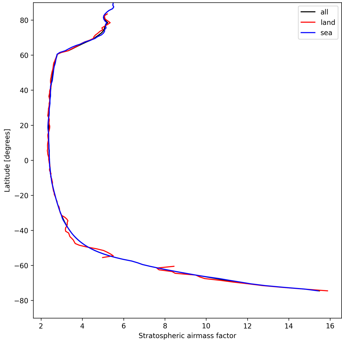
Figure 27: Zonal average of “Stratospheric airmass factor” for 2025-08-14 to 2025-08-16.
