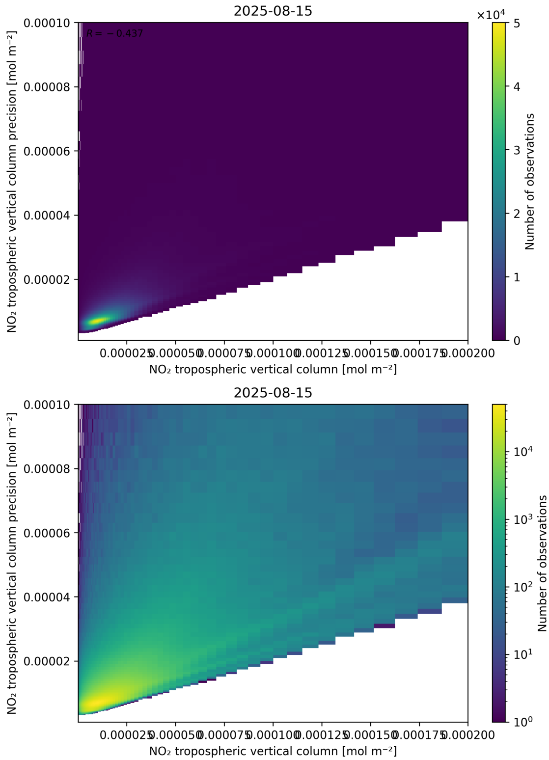
Figure 130: Scatter density plot of “NO 2 tropospheric vertical column” against “NO 2 tropospheric vertical column precision” for 2025-08-14 to 2025-08-16.
