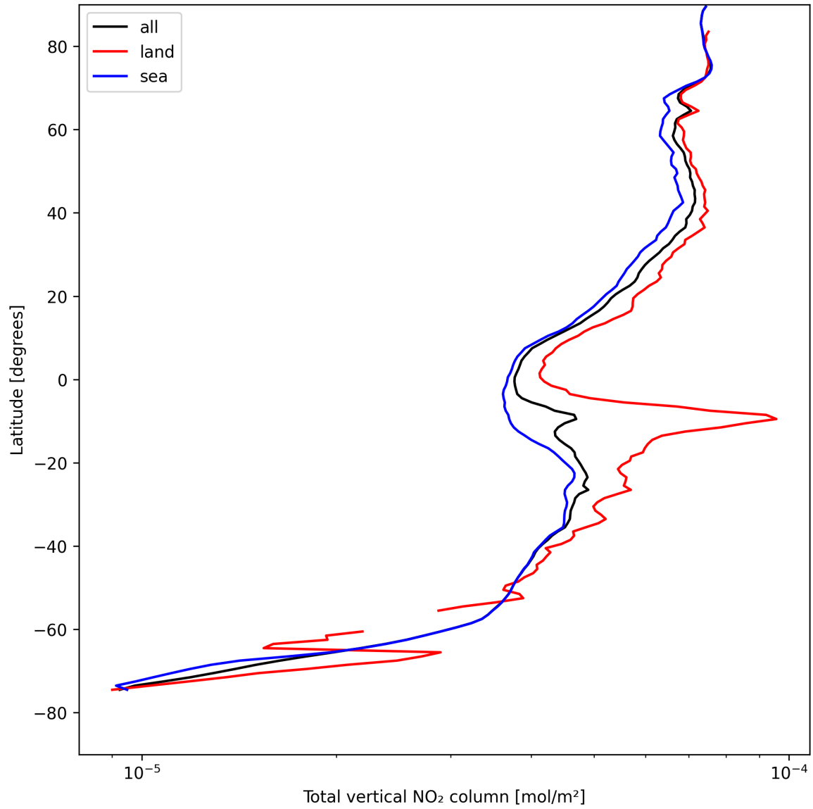
Figure 21: Zonal average of “Total vertical NO 2 column” for 2025-08-14 to 2025-08-16.
