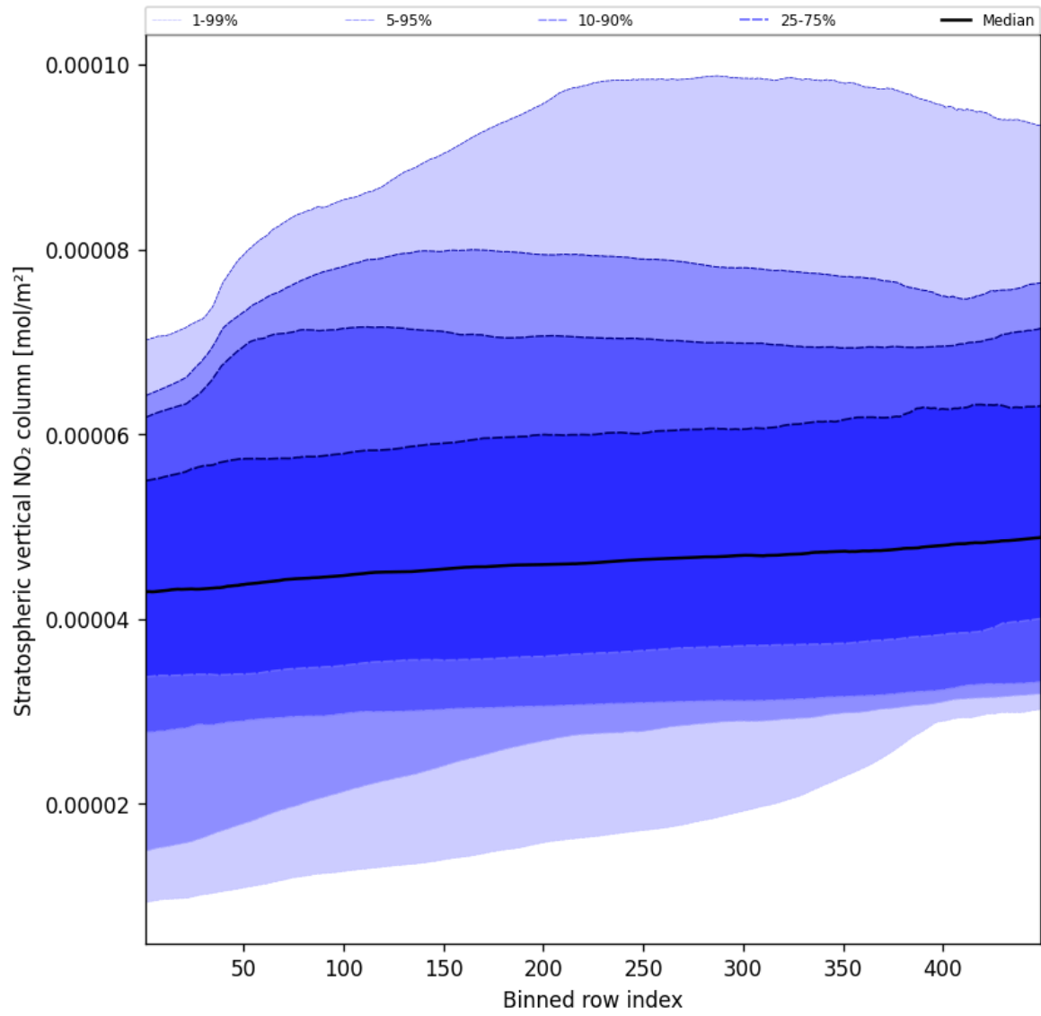
Figure 53: Along track statistics of “Stratospheric vertical NO 2 column” for 2025-08-14 to 2025-08-16
