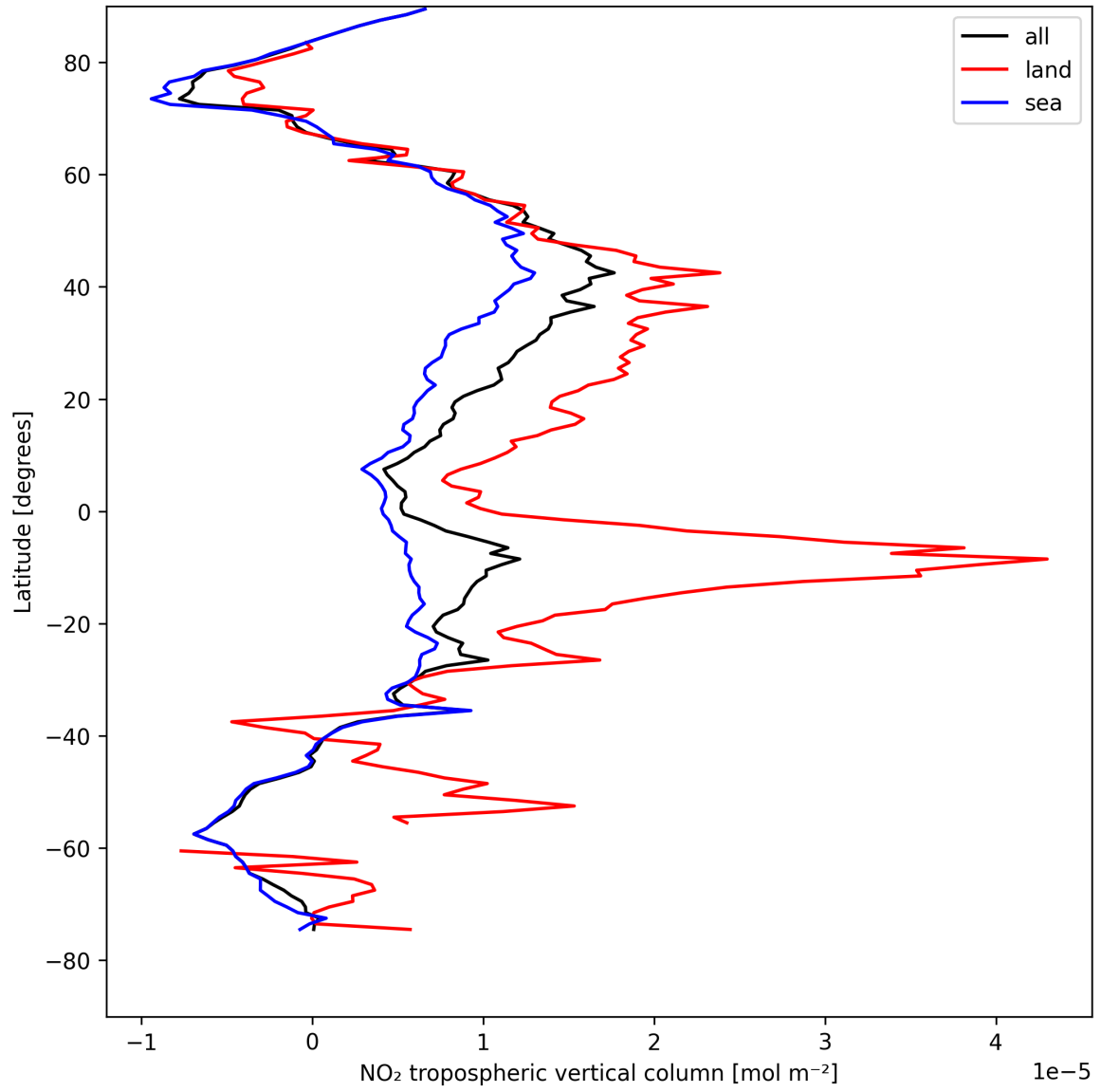
Figure 12: Zonal average of “NO 2 tropospheric vertical column” for 2025-08-14 to 2025-08-16.
