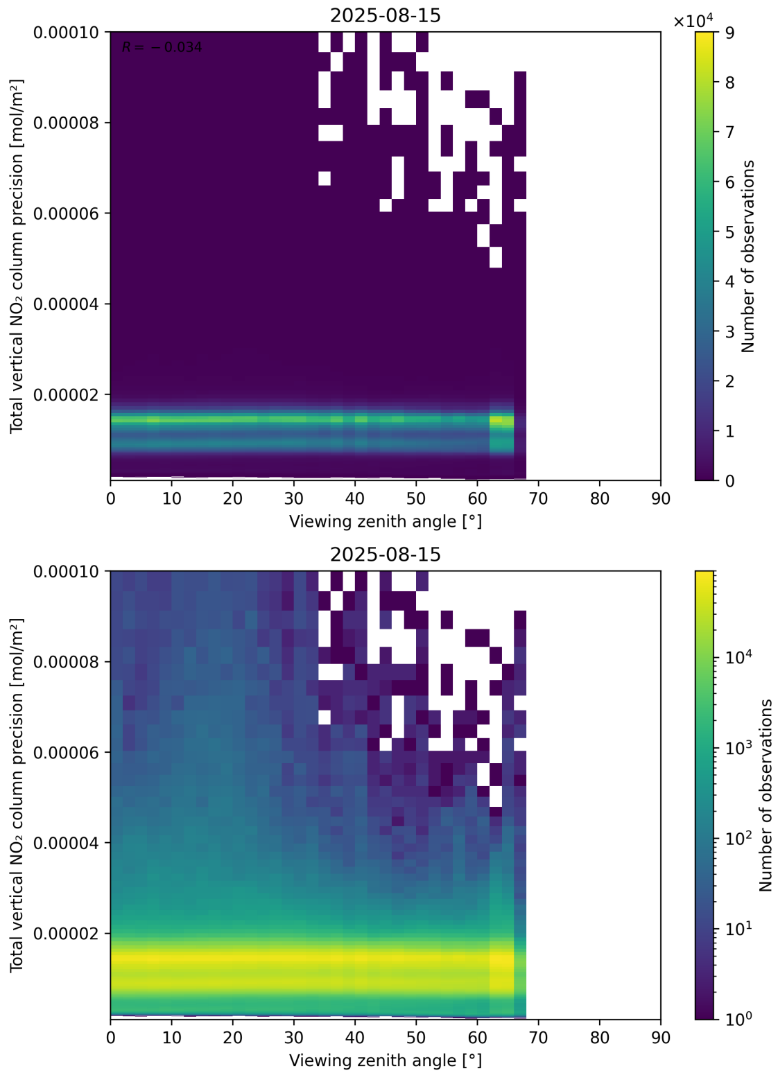
Figure 168: Scatter density plot of “Viewing zenith angle” against “Total vertical NO 2 column precision” for 2025-08-14 to 2025-08-16.
