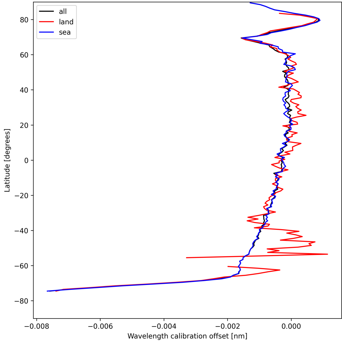
Figure 18: Zonal average of “Wavelength calibration offset” for 2025-08-14 to 2025-08-16.
