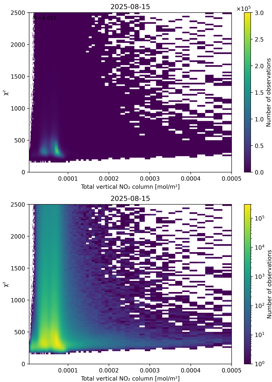
Figure 111: Scatter density plot of “Total vertical NO 2 column” against “ \chi^2 ” for 2025-08-14 to 2025-08-16.
