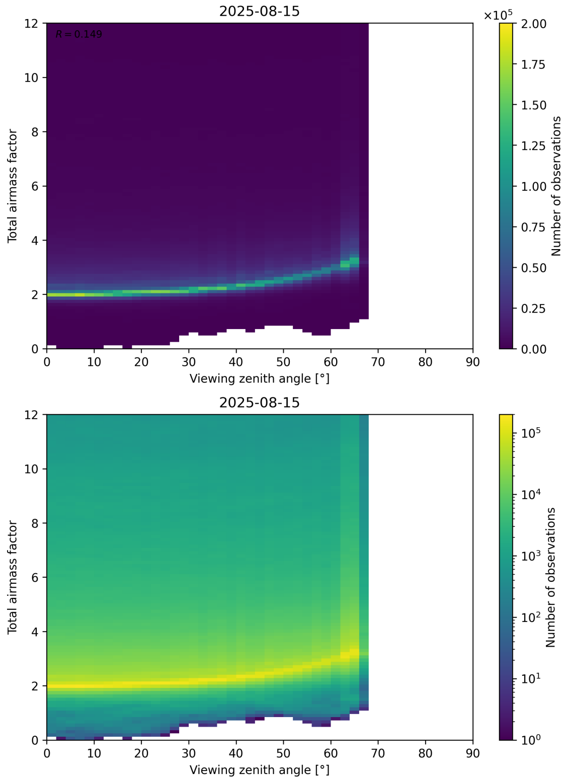
Figure 160: Scatter density plot of “Viewing zenith angle” against “Total airmass factor” for 2025-08-14 to 2025-08-16.
