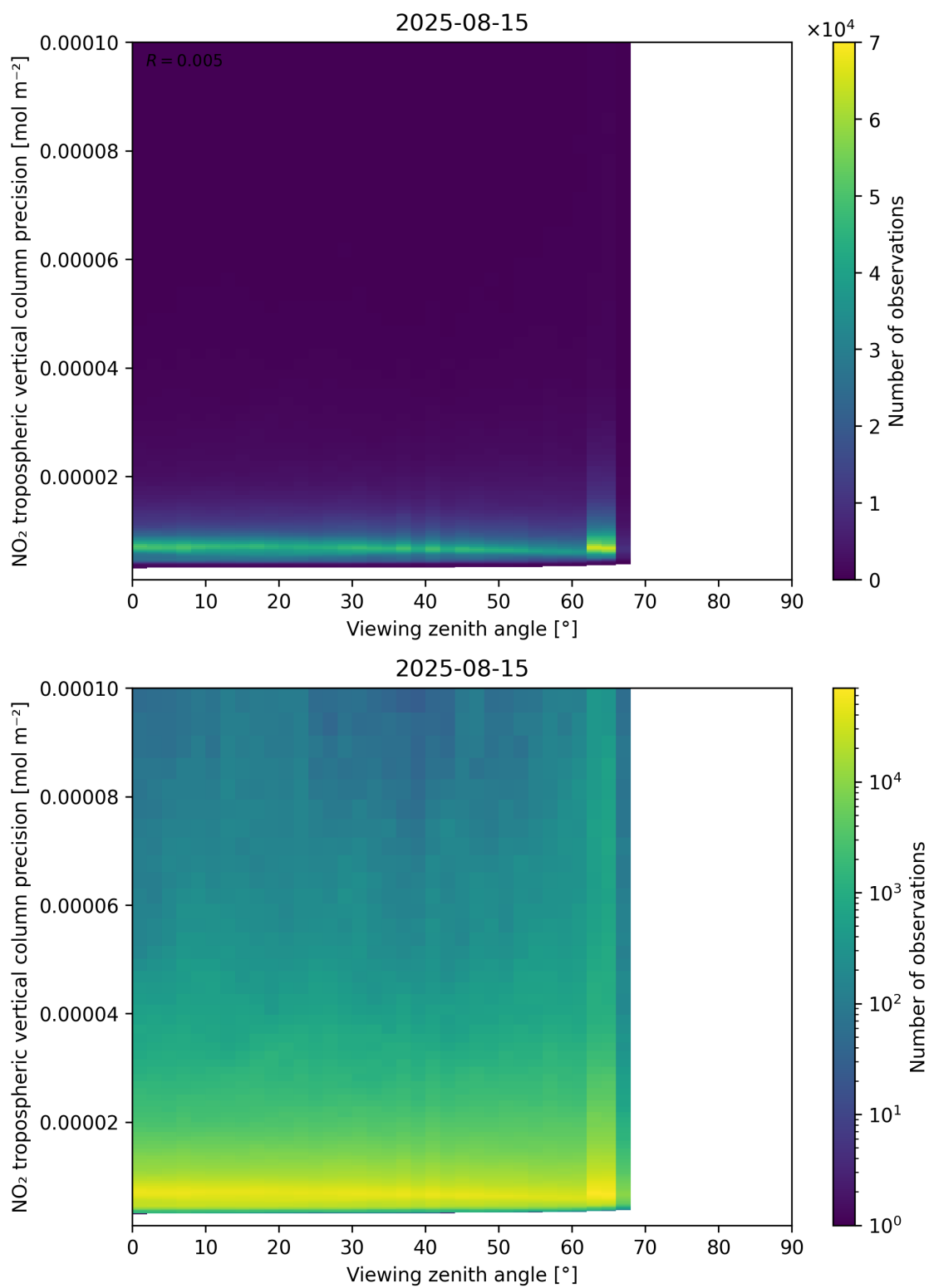
Figure 170: Scatter density plot of “Viewing zenith angle” against “NO 2 tropospheric vertical column precision” for 2025-08-14 to 2025-08-16.
