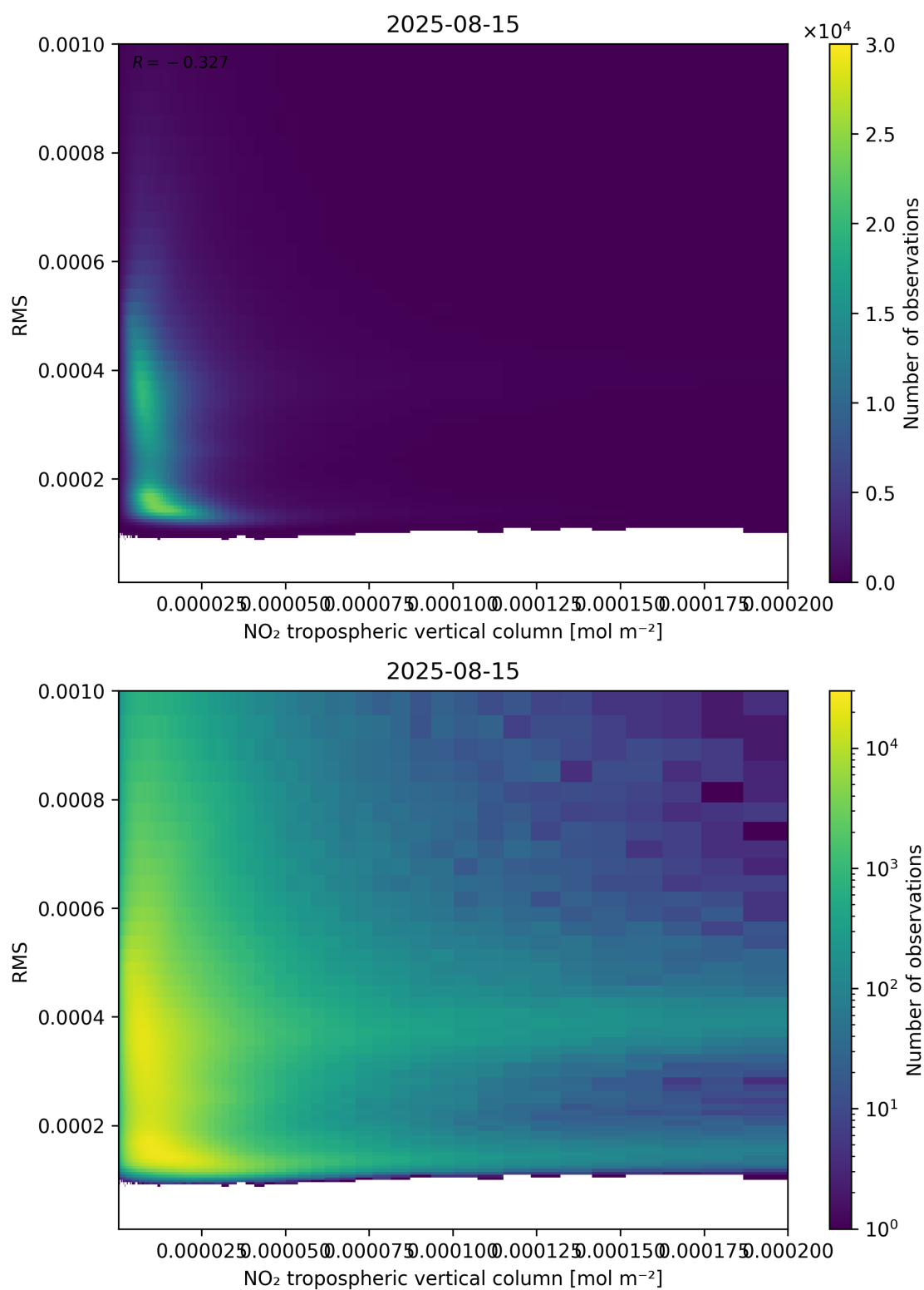
Figure 142: Scatter density plot of “NO 2 tropospheric vertical column” against “RMS” for 2025-08-14 to 2025-08-16.
