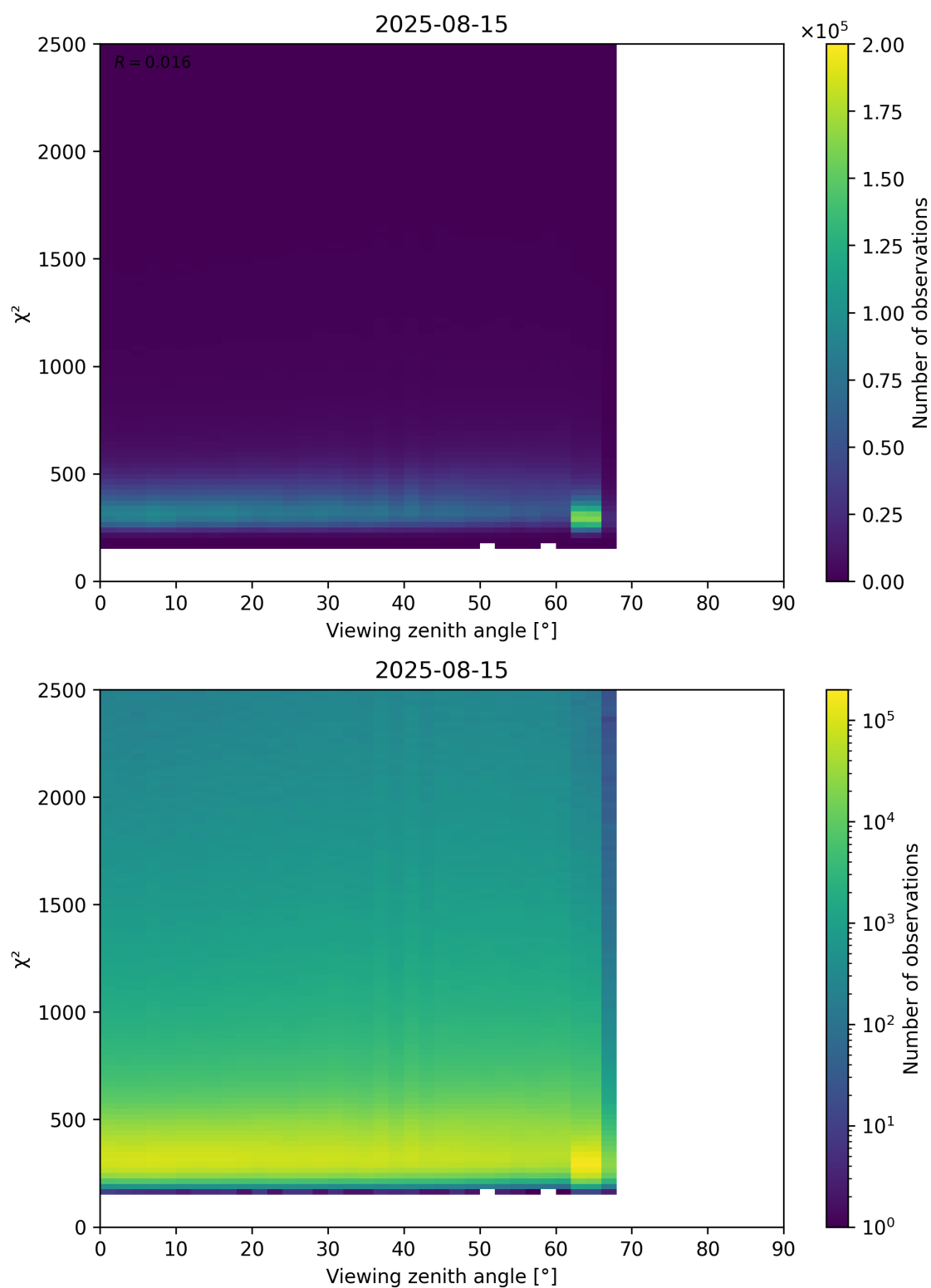
Figure 162: Scatter density plot of “Viewing zenith angle” against “ \chi^2 ” for 2025-08-14 to 2025-08-16.
