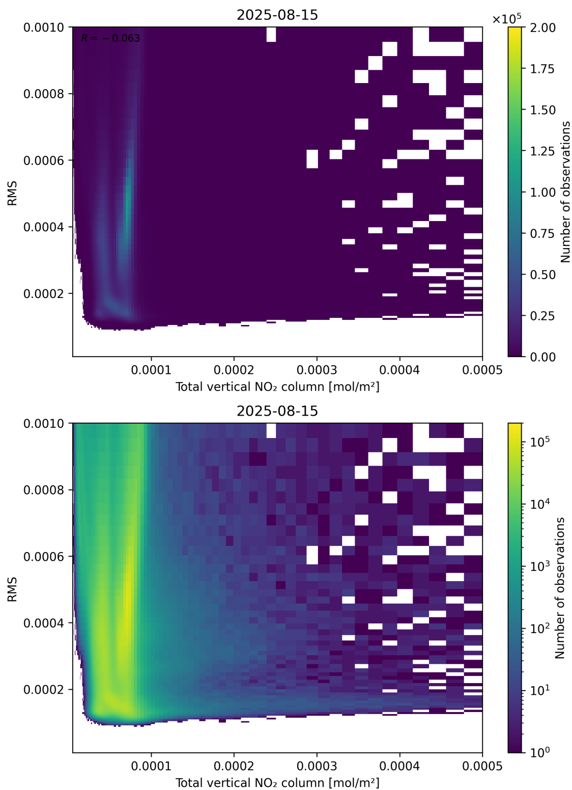
Figure 120: Scatter density plot of “Total vertical NO 2 column” against “RMS” for 2025-08-14 to 2025-08-16.
