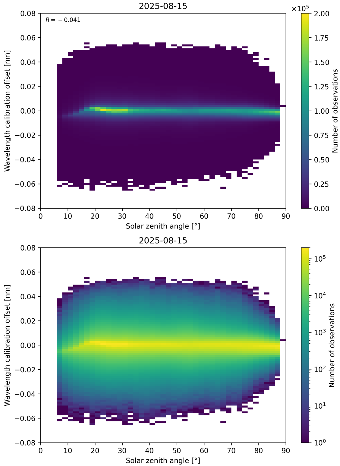
Figure 158: Scatter density plot of “Solar zenith angle” against “Wavelength calibration offset” for 2025-08-14 to 2025-08-16.
