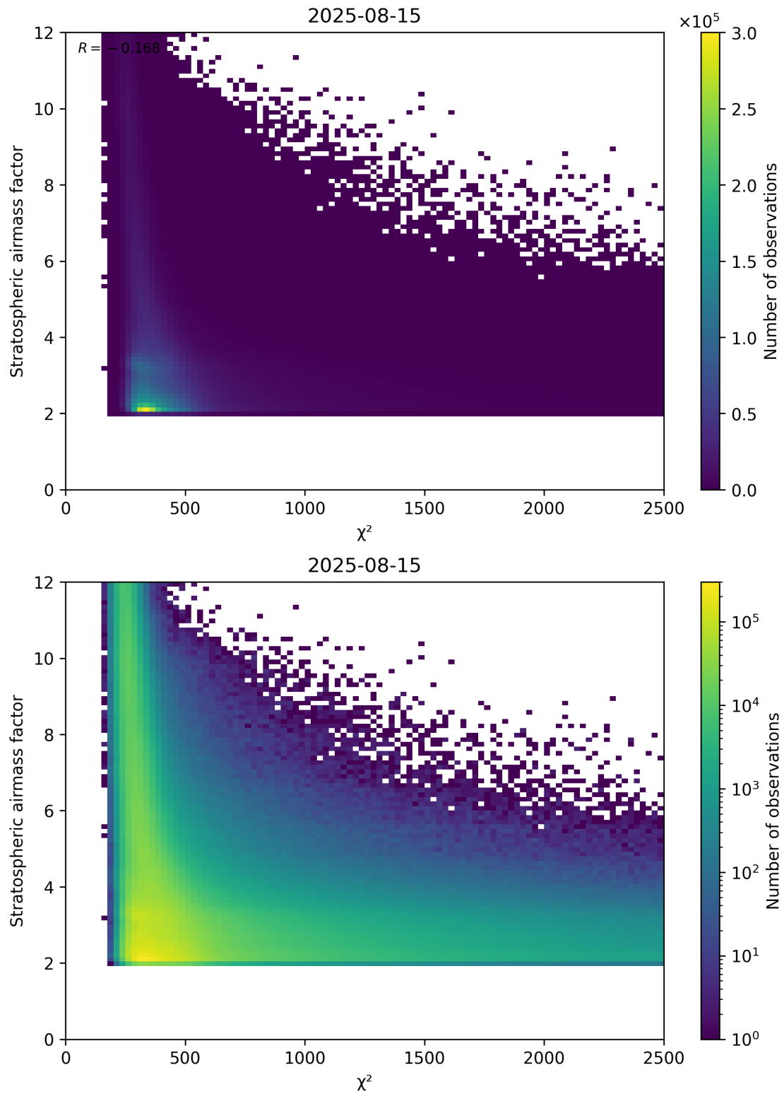
Figure 81: Scatter density plot of “ \chi^2 ” against “Stratospheric airmass factor” for 2025-08-14 to 2025-08-16.
