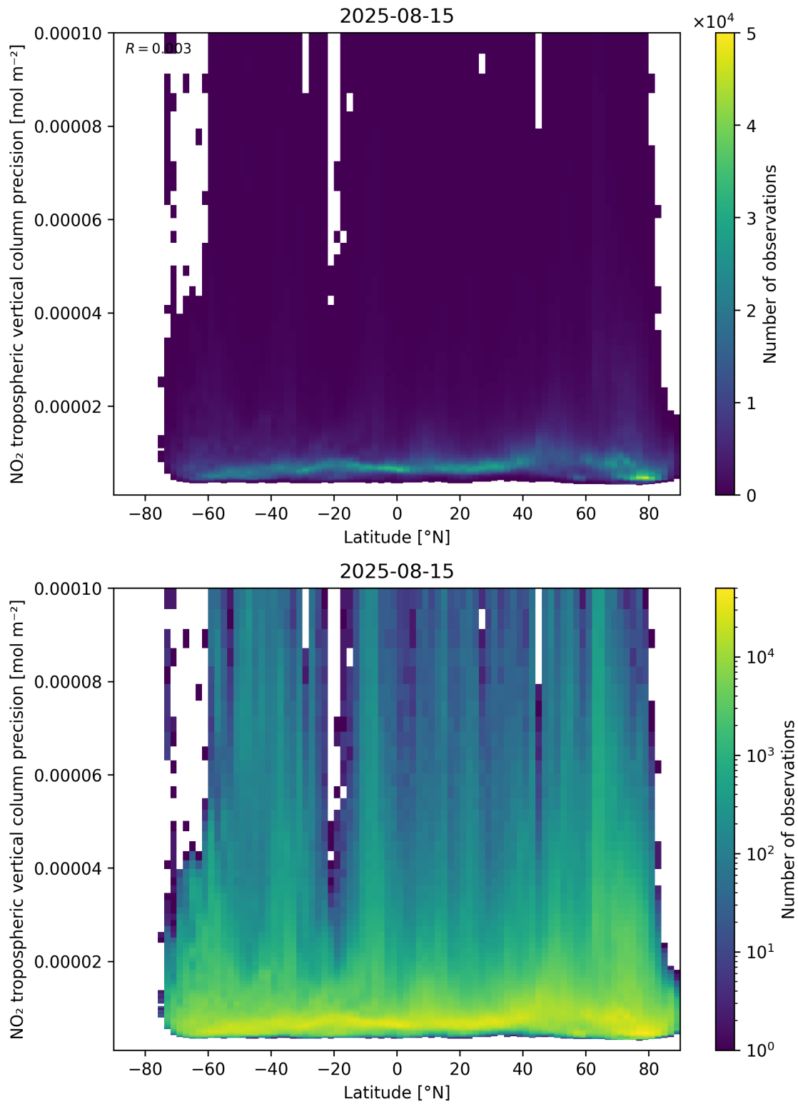
Figure 93: Scatter density plot of “Latitude” against “NO 2 tropospheric vertical column precision” for 2025-08-14 to 2025-08-16.
