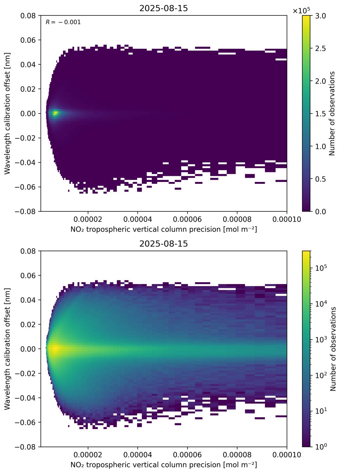
Figure 141: Scatter density plot of “NO 2 tropospheric vertical column precision” against “Wavelength calibration offset” for 2025-08-14 to 2025-08-16.
