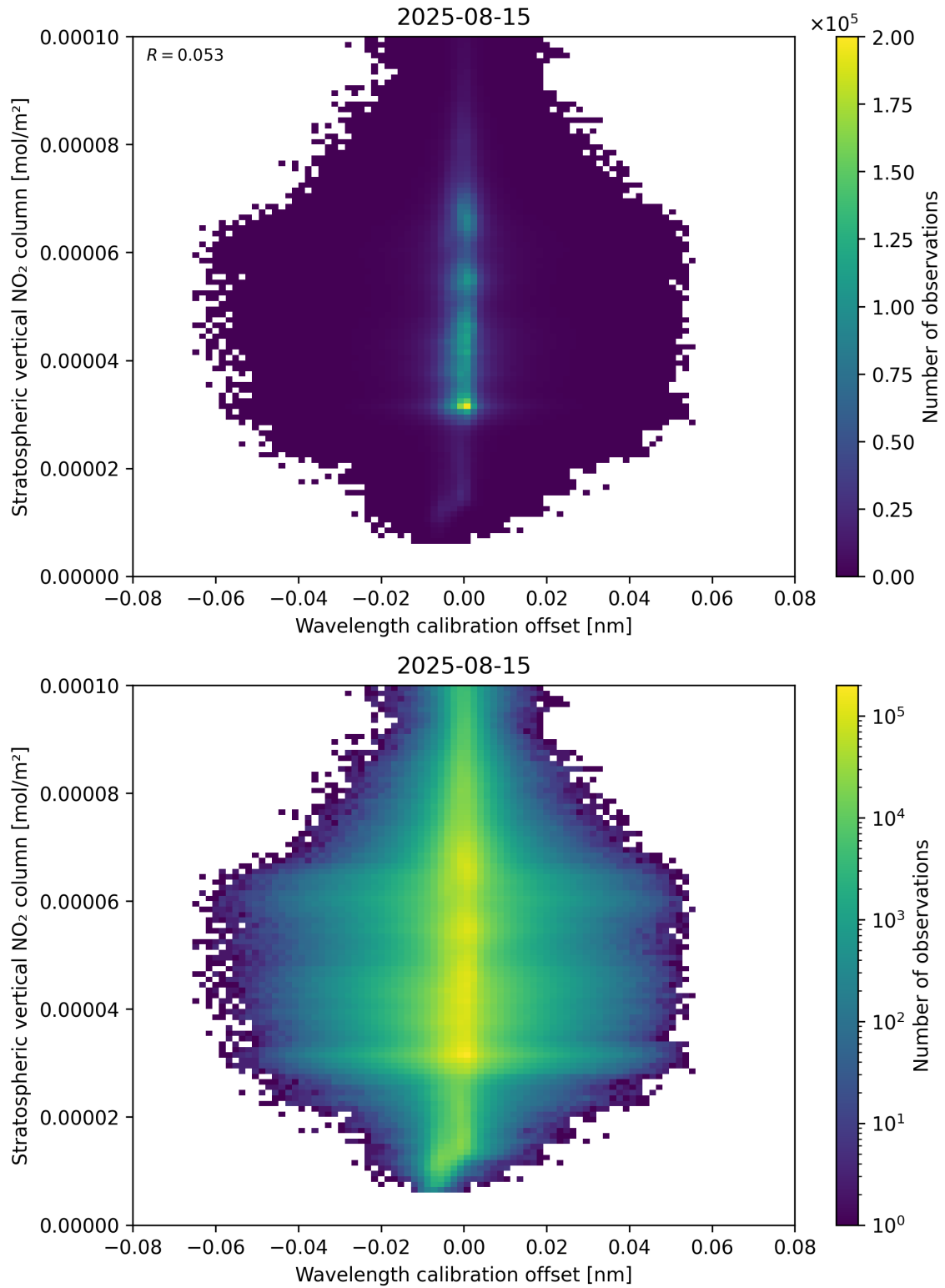
Figure 176: Scatter density plot of “Wavelength calibration offset” against “Stratospheric vertical NO 2 column” for 2025-08-14 to 2025-08-16.
