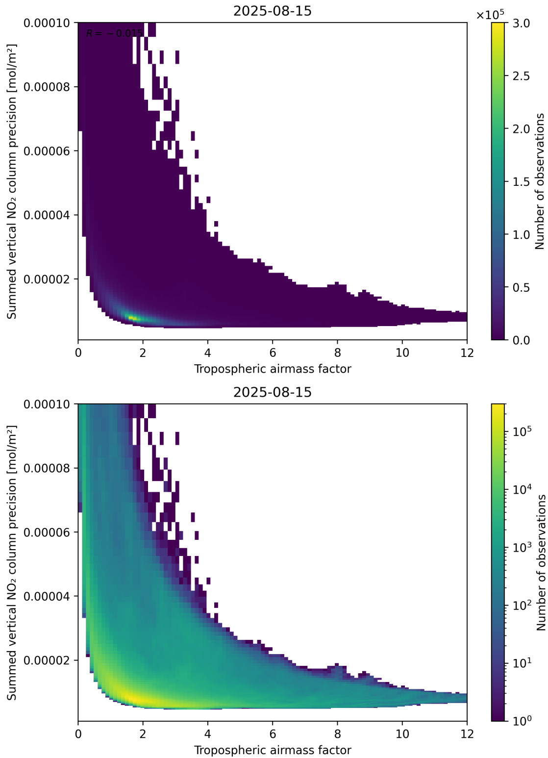
Figure 76: Scatter density plot of “Tropospheric air mass factor” against “Summed vertical NO 2 column precision” for 2025-08-14 to 2025-08-16.
