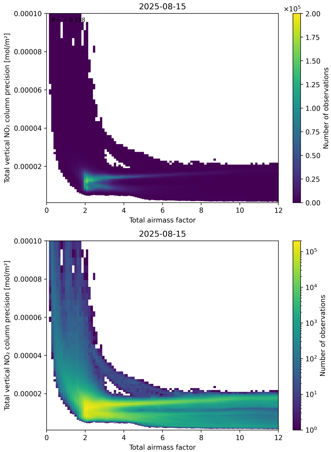
Figure 68: Scatter density plot of “Total airmass factor” against “Total vertical NO 2 column precision” for 2025-08-14 to 2025-08-16.
