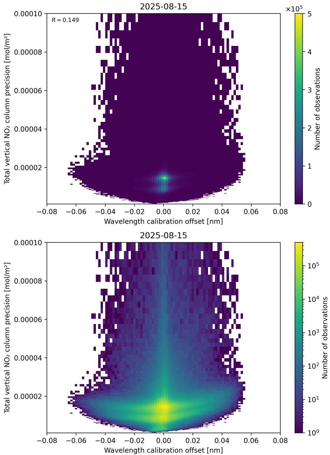
Figure 180: Scatter density plot of “Wavelength calibration offset” against “Total vertical NO 2 column precision” for 2025-08-14 to 2025-08-16.
