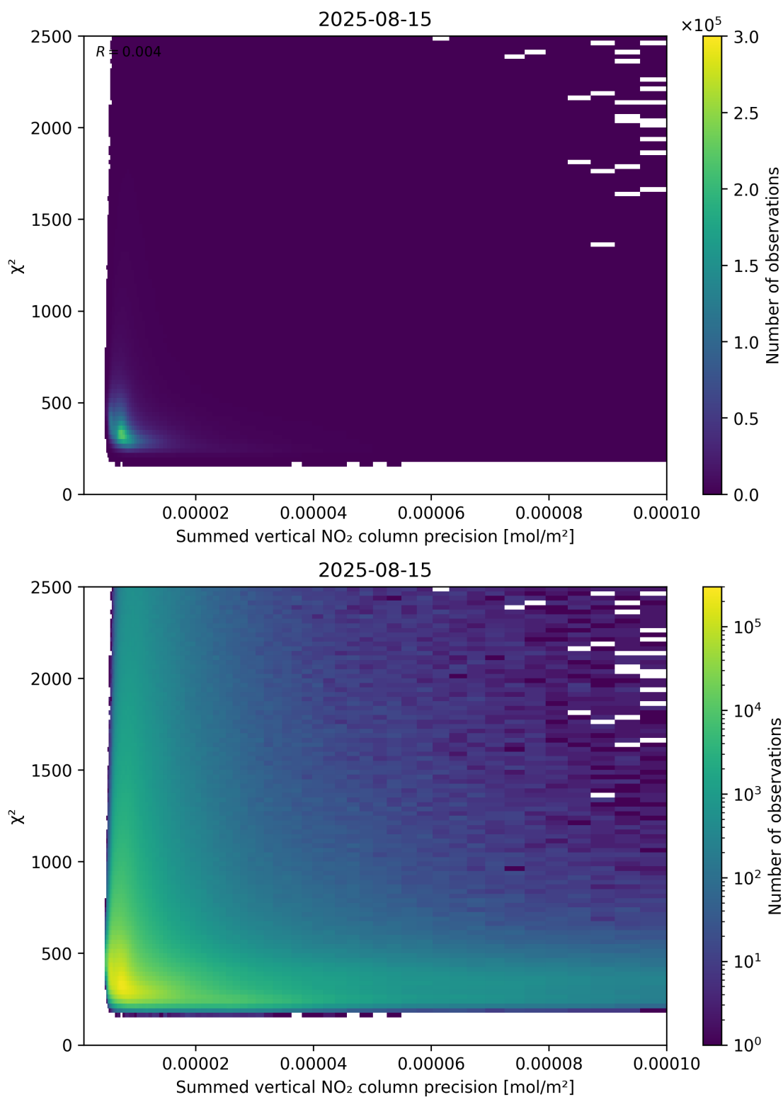
Figure 107: Scatter density plot of “Summed vertical NO 2 column precision” against “ \chi^2 ” for 2025-08-14 to 2025-08-16.
