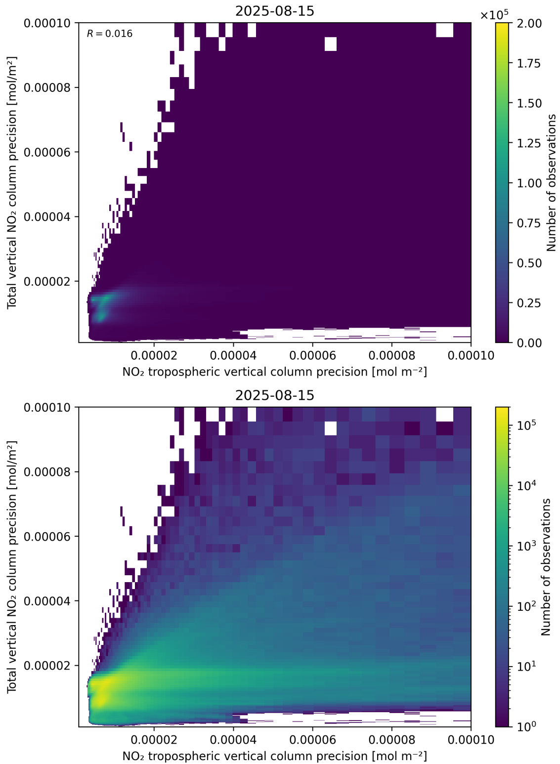
Figure 139: Scatter density plot of “NO 2 tropospheric vertical column precision” against “Total vertical NO 2 column precision” for 2025-08-14 to 2025-08-16.
