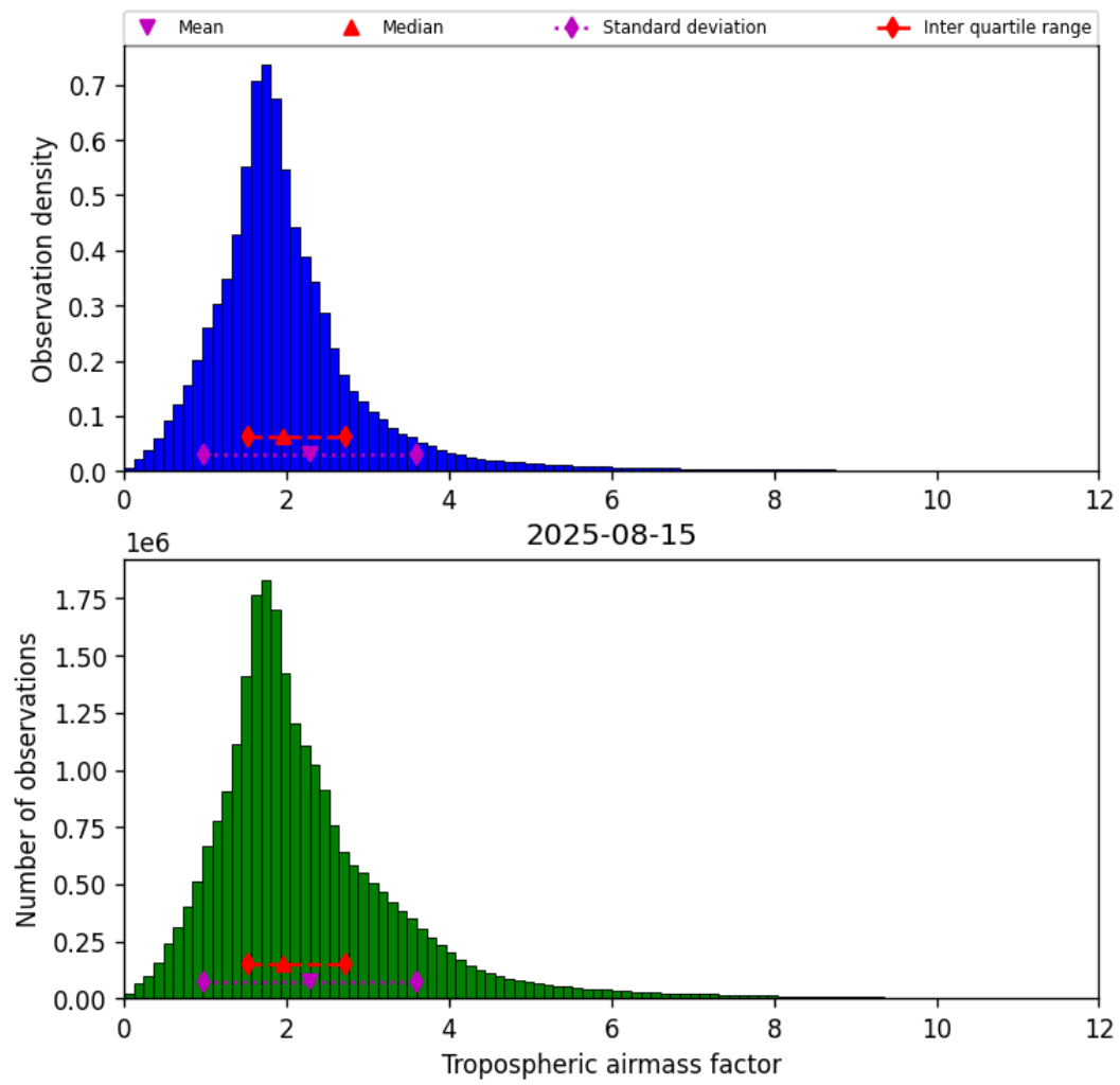
Figure 31: Histogram of “Tropospheric airmass factor” for 2025-08-14 to 2025-08-16
