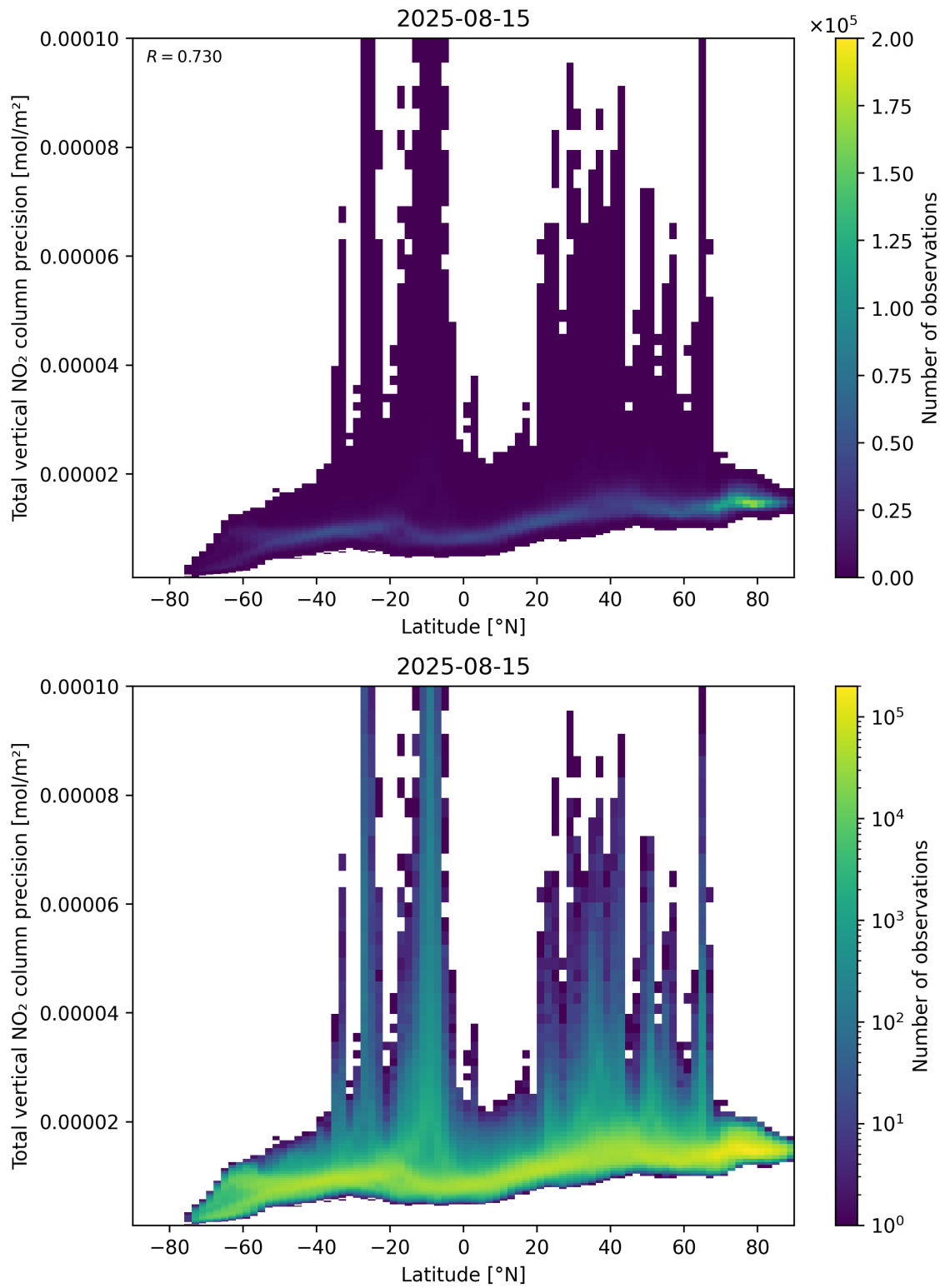
Figure 91: Scatter density plot of “Latitude” against “Total vertical NO 2 column precision” for 2025-08-14 to 2025-08-16.
