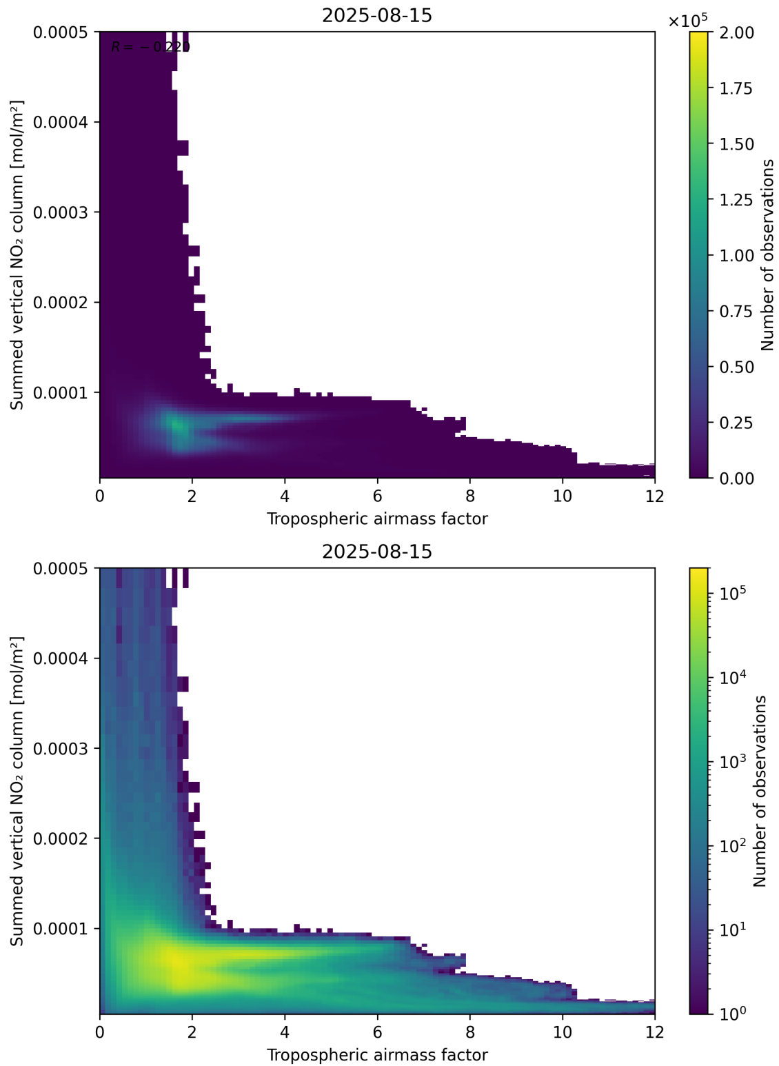
Figure 75: Scatter density plot of “Tropospheric air mass factor” against “Summed vertical NO 2 column” for 2025-08-14 to 2025-08-16.
