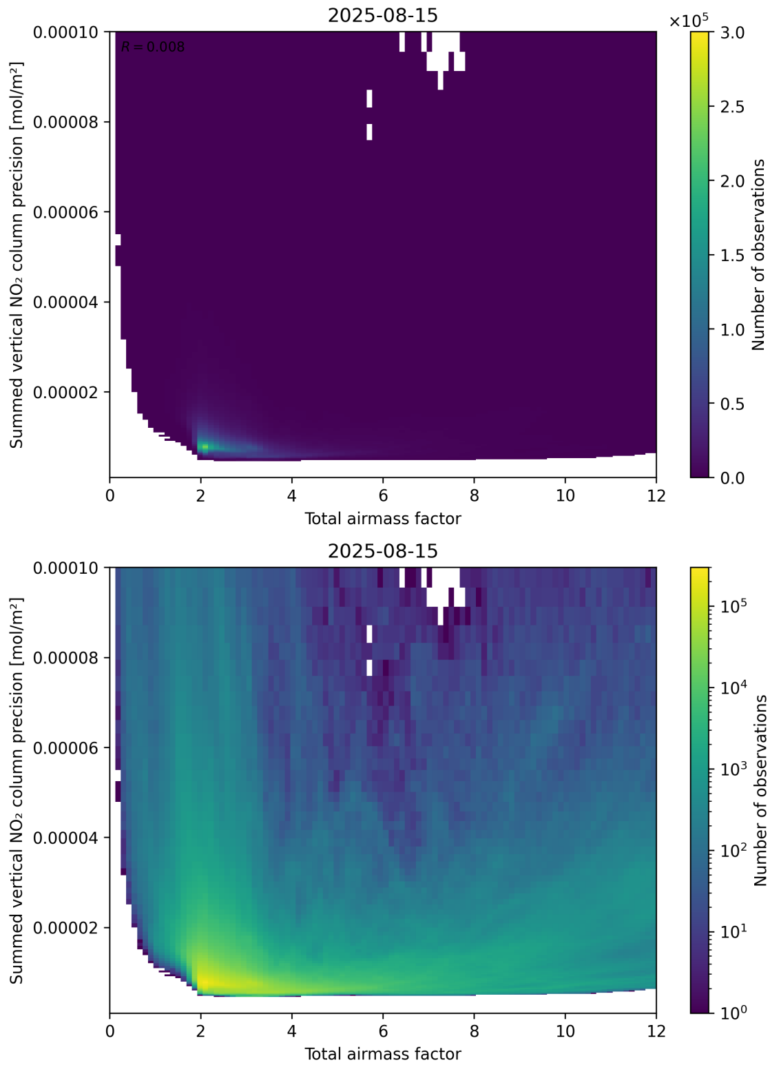
Figure 66: Scatter density plot of “Total airmass factor” against “Summed vertical NO 2 column precision” for 2025-08-14 to 2025-08-16.
