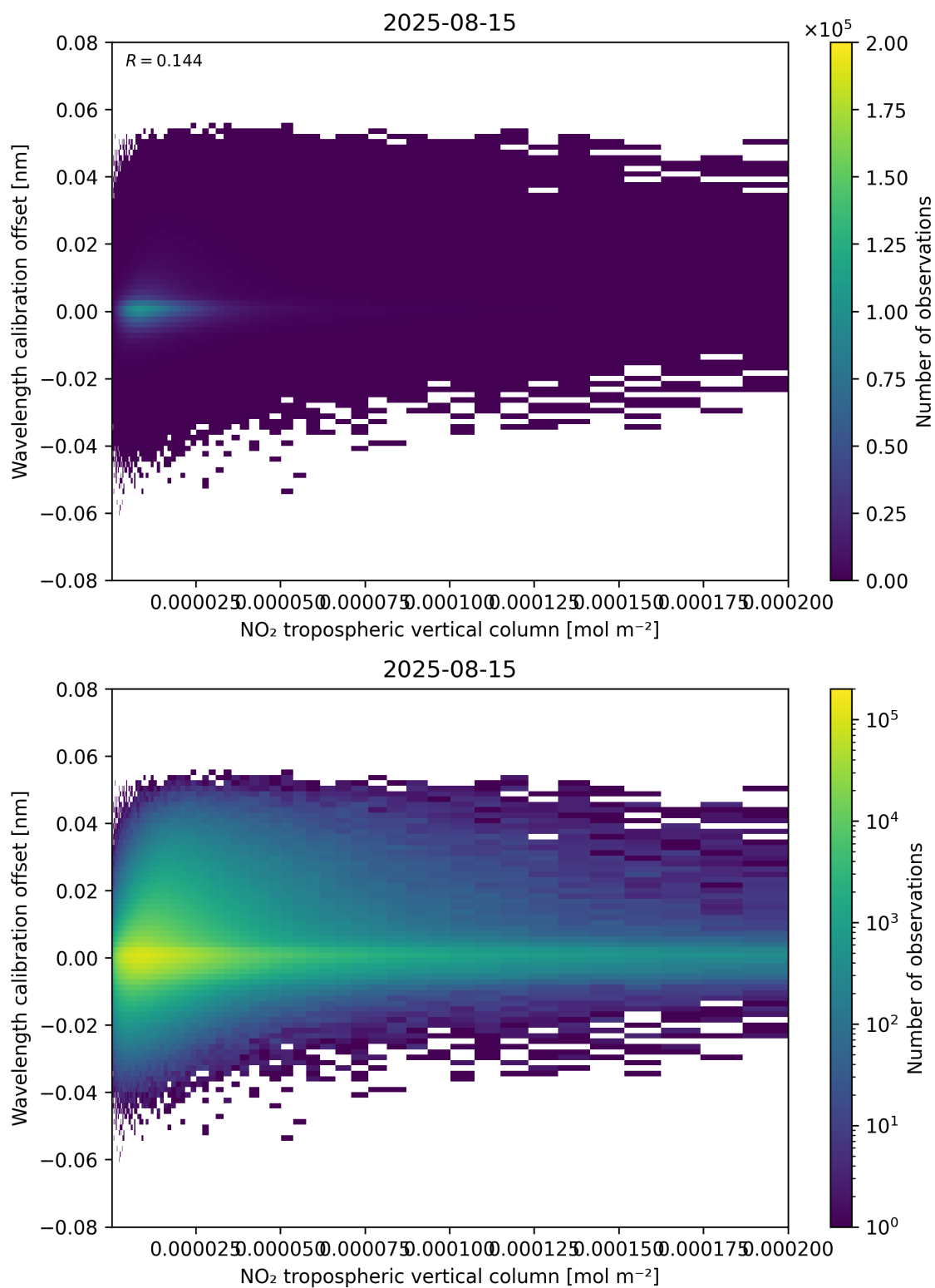
Figure 143: Scatter density plot of “NO 2 tropospheric vertical column” against “Wavelength calibration offset” for 2025-08-14 to 2025-08-16.
