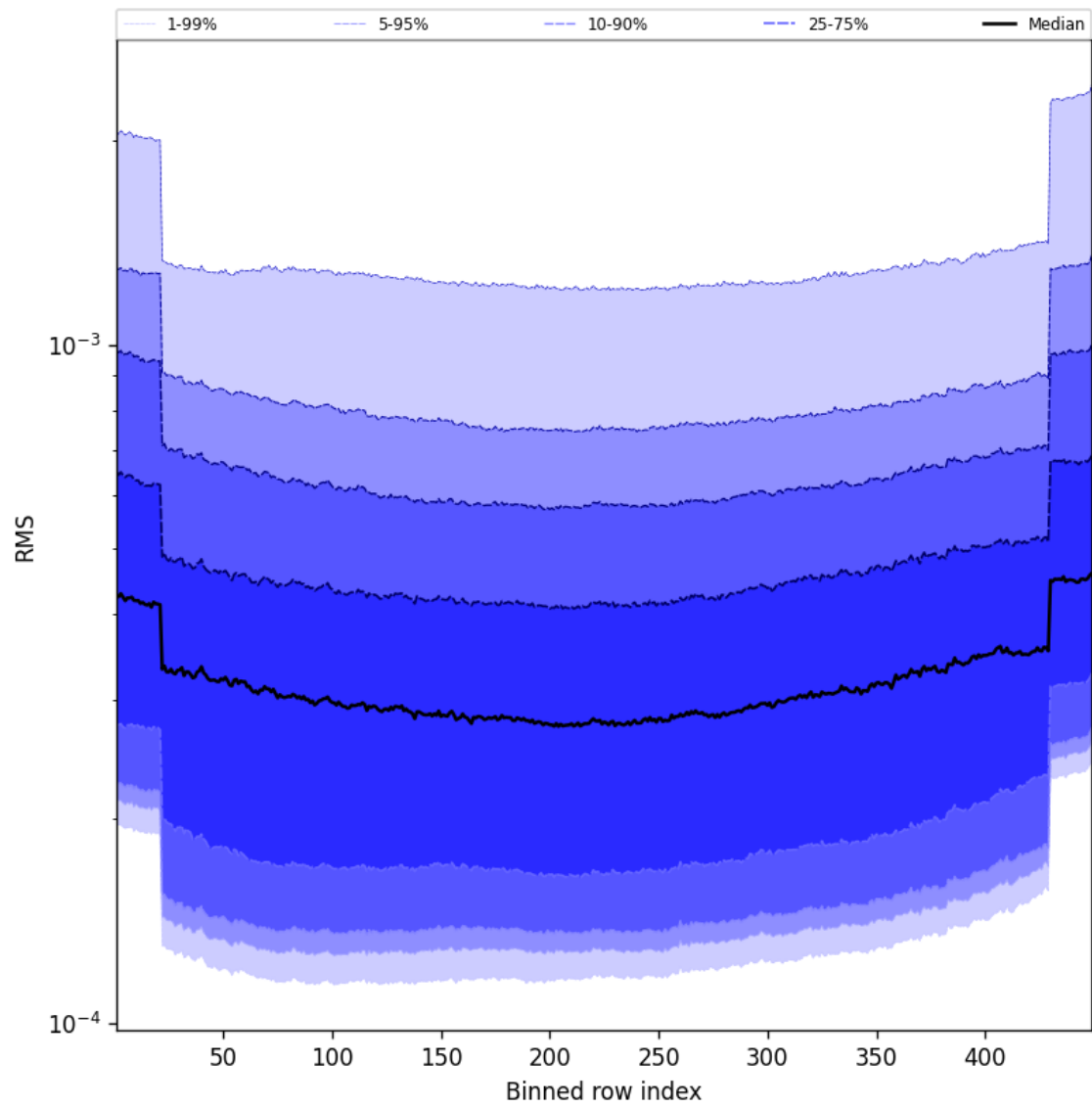
Figure 60: Along track statistics of “RMS” for 2025-08-14 to 2025-08-16
