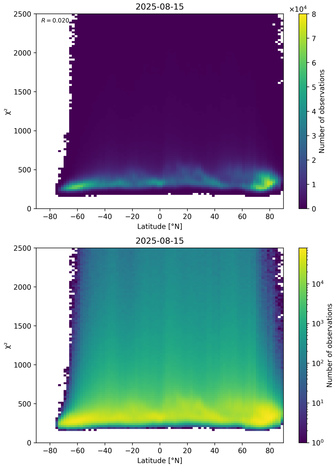
Figure 86: Scatter density plot of “Latitude” against “ \chi^2 ” for 2025-08-14 to 2025-08-16.
