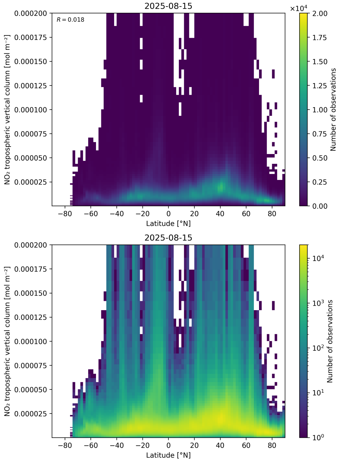
Figure 92: Scatter density plot of “Latitude” against “NO 2 tropospheric vertical column” for 2025-08-14 to 2025-08-16.
