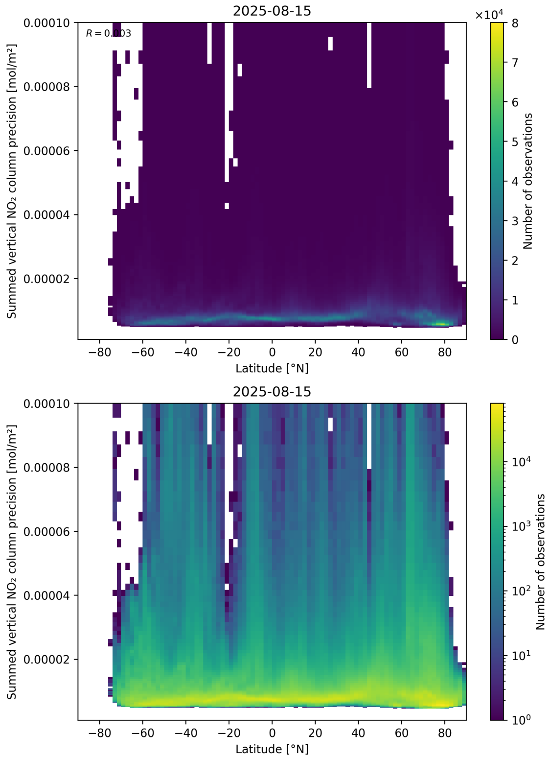
Figure 89: Scatter density plot of “Latitude” against “Summed vertical NO 2 column precision” for 2025-08-14 to 2025-08-16.
