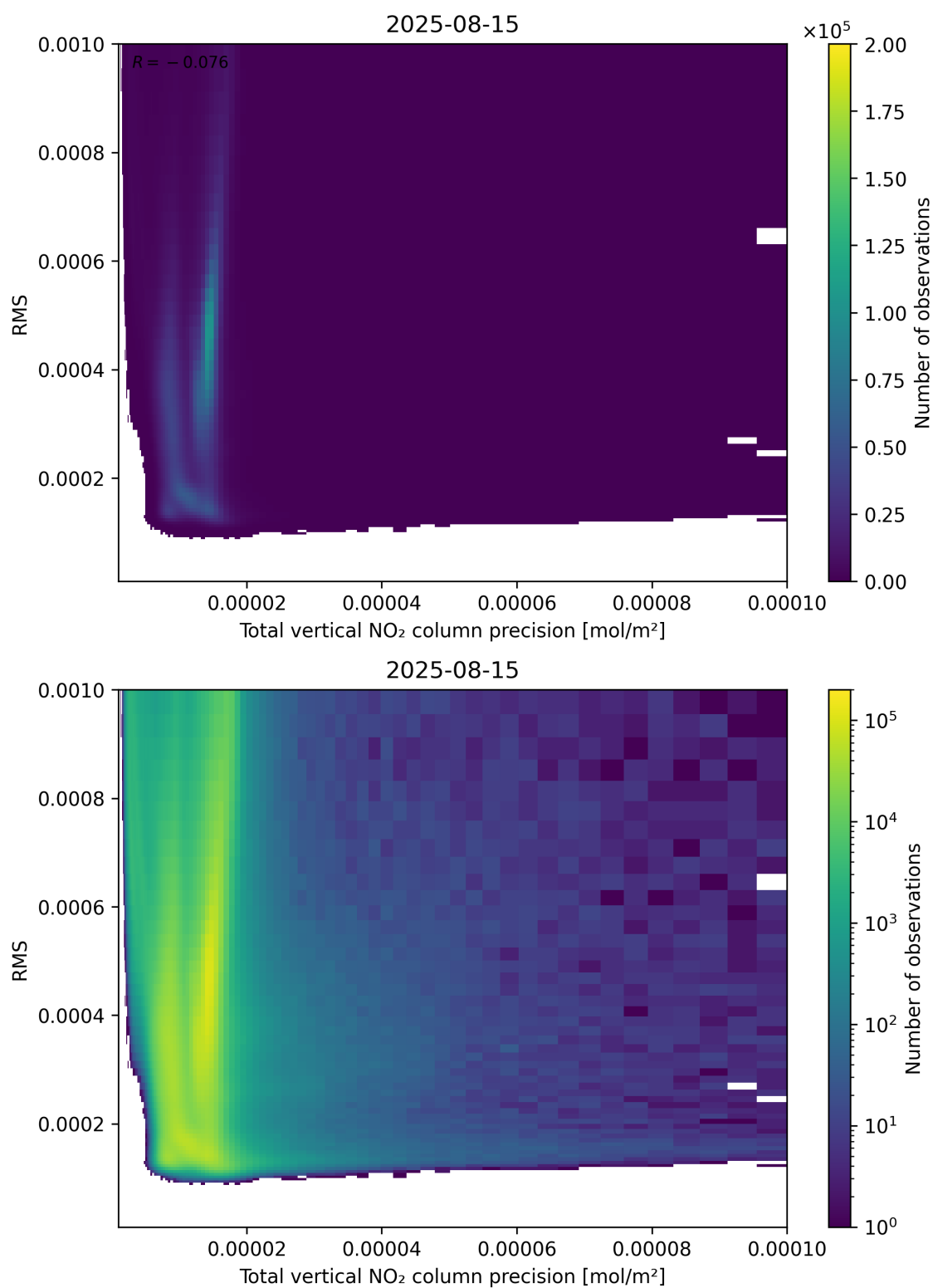
Figure 119: Scatter density plot of “Total vertical NO 2 column precision” against “RMS” for 2025-08-14 to 2025-08-16.
