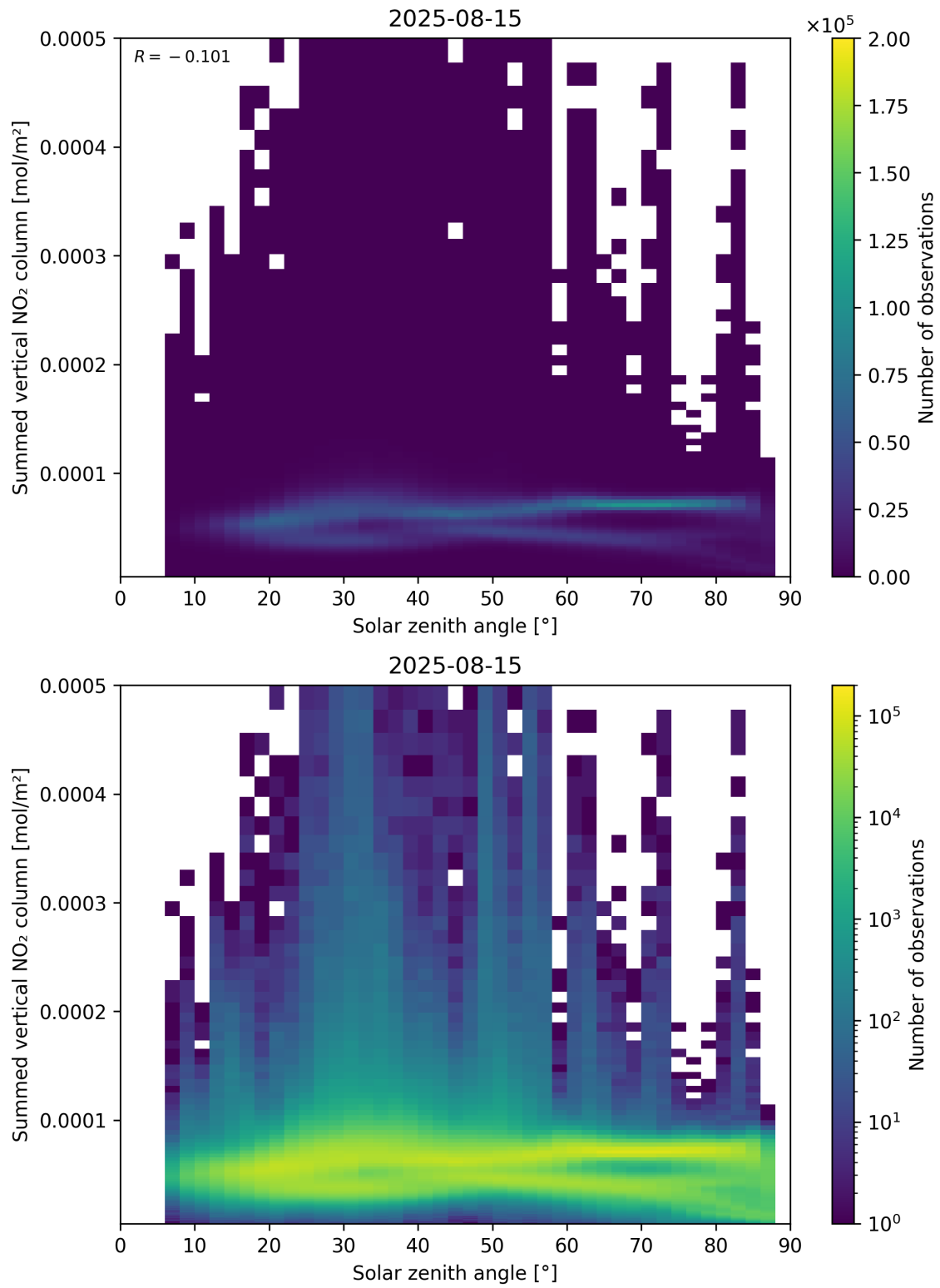
Figure 151: Scatter density plot of “Solar zenith angle” against “Summed vertical NO 2 column” for 2025-08-14 to 2025-08-16.
