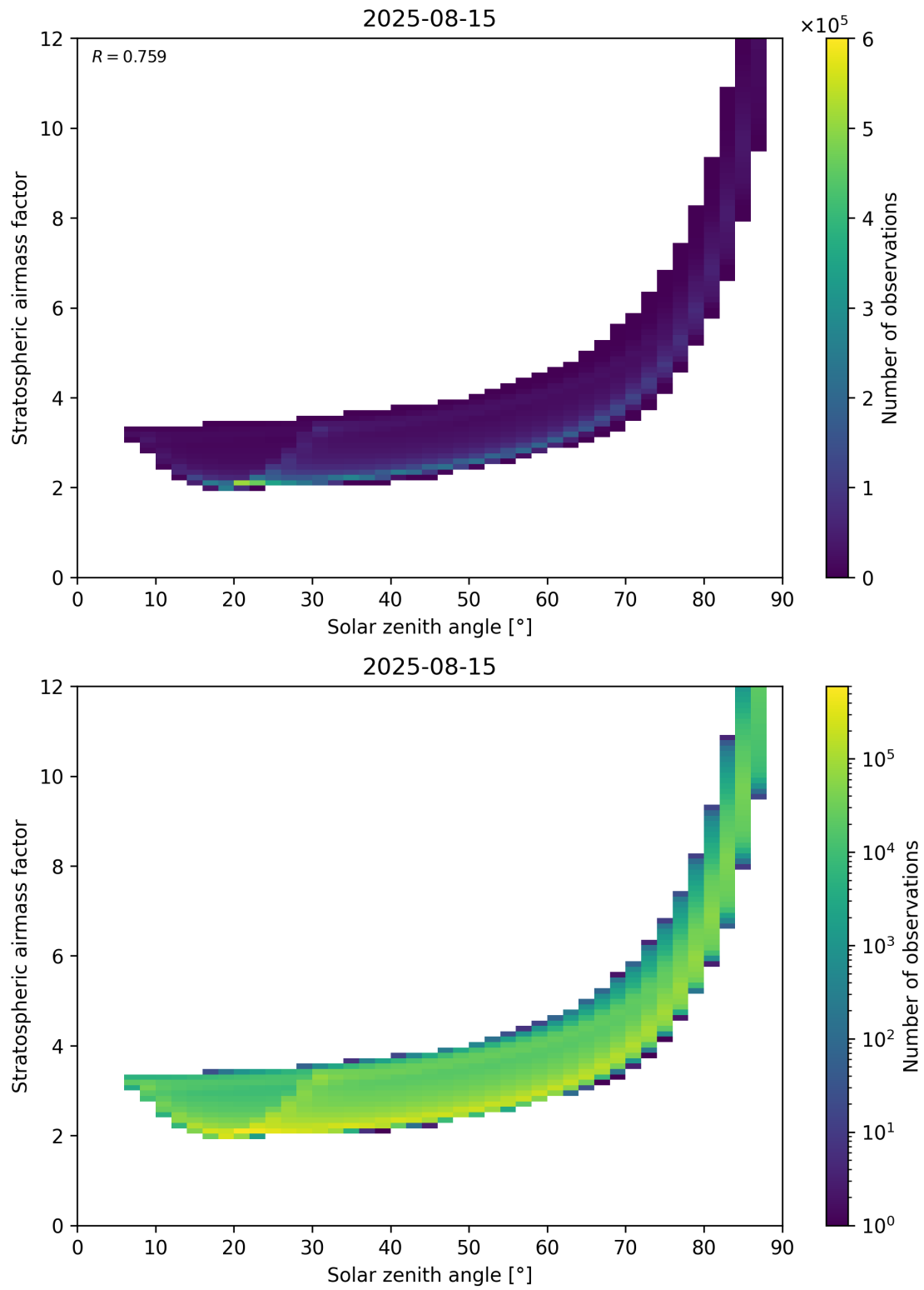
Figure 145: Scatter density plot of “Solar zenith angle” against “Stratospheric airmass factor” for 2025-08-14 to 2025-08-16.
