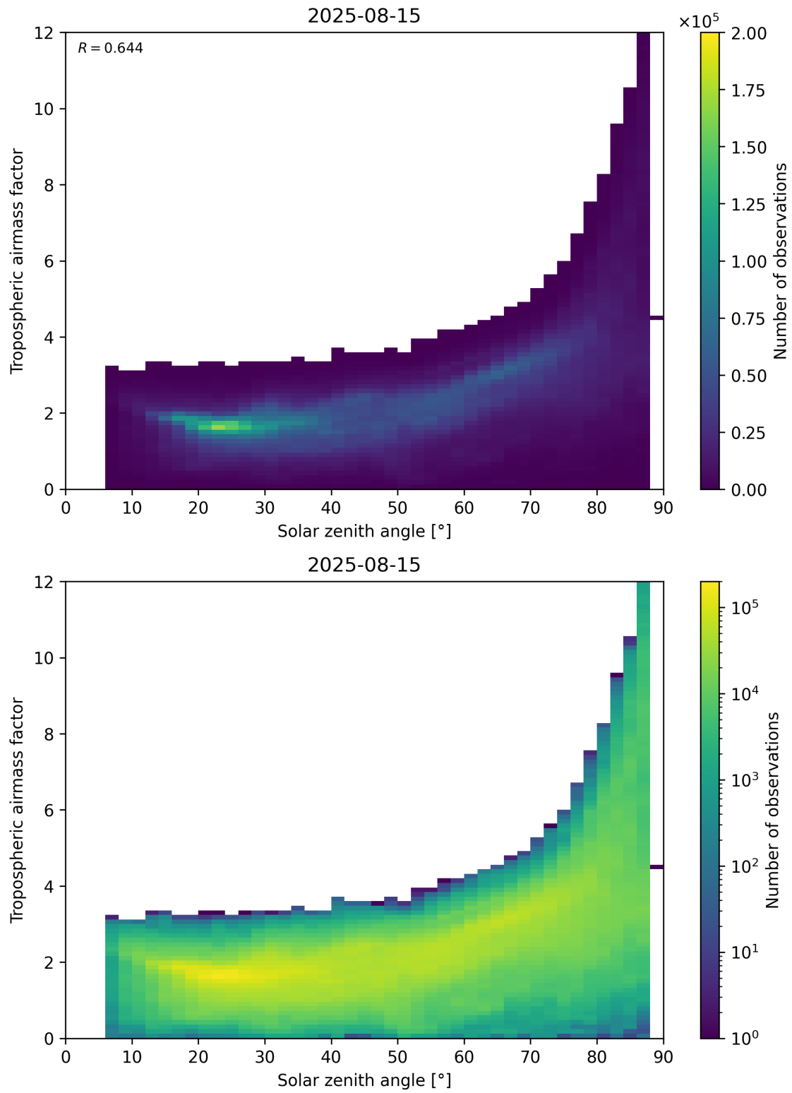
Figure 147: Scatter density plot of “Solar zenith angle” against “Tropospheric airmass factor” for 2025-08-14 to 2025-08-16.
