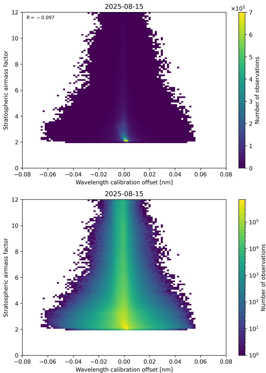
Figure 174: Scatter density plot of “Wavelength calibration offset” against “Stratospheric airmass factor” for 2025-08-14 to 2025-08-16.
