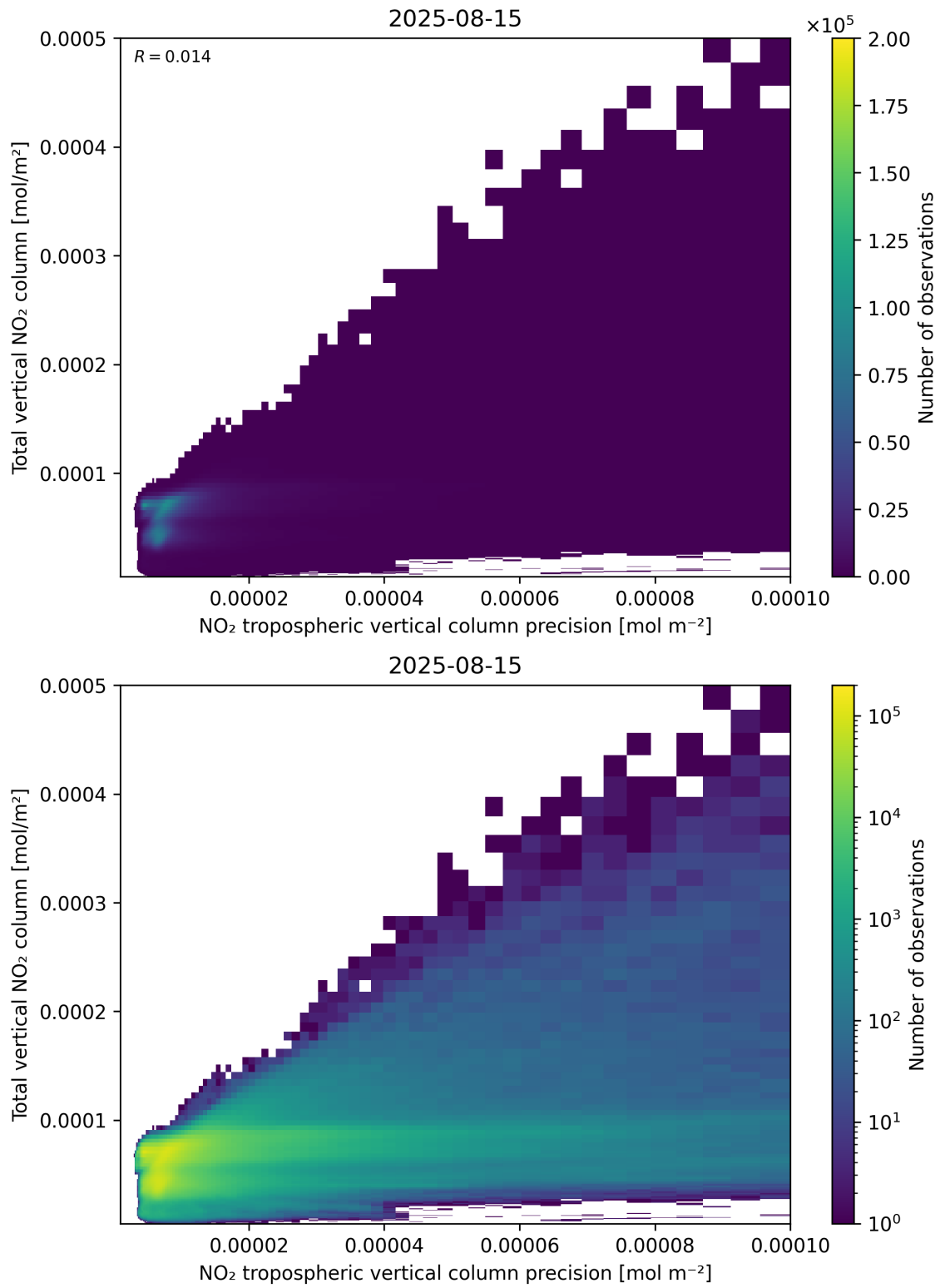
Figure 138: Scatter density plot of “NO 2 tropospheric vertical column precision” against “Total vertical NO 2 column” for 2025-08-14 to 2025-08-16.
