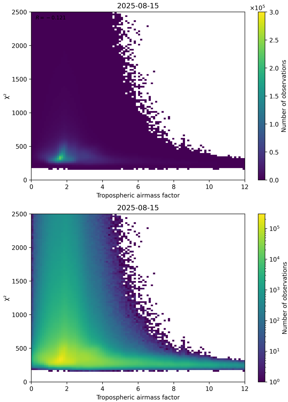
Figure 73: Scatter density plot of “Tropospheric airmass factor” against “ \chi^2 ” for 2025-08-14 to 2025-08-16.
