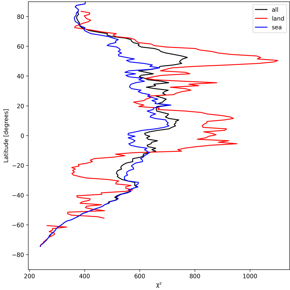
Figure 25: Zonal average of “ \chi^2 ” for 2025-08-14 to 2025-08-16.
