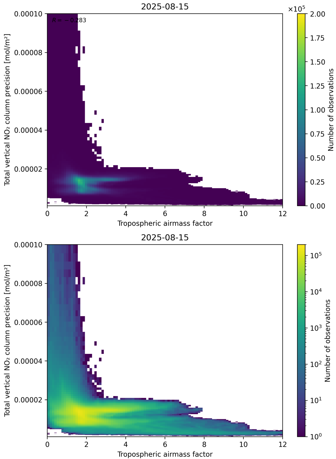
Figure 78: Scatter density plot of “Tropospheric air mass factor” against “Total vertical NO 2 column precision” for 2025-08-14 to 2025-08-16.
