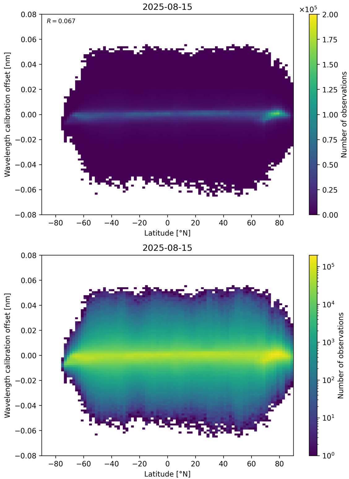
Figure 95: Scatter density plot of “Latitude” against “Wavelength calibration offset” for 2025-08-14 to 2025-08-16.
