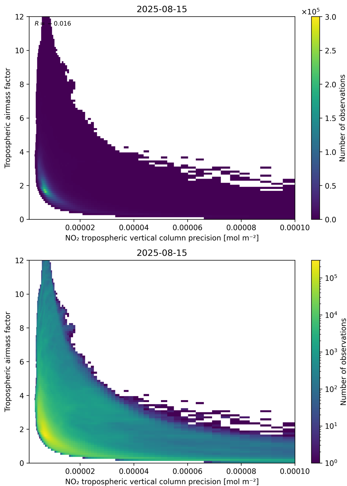
Figure 133: Scatter density plot of “NO 2 tropospheric vertical column precision” against “Tropospheric air mass factor” for 2025-08-14 to 2025-08-16.
