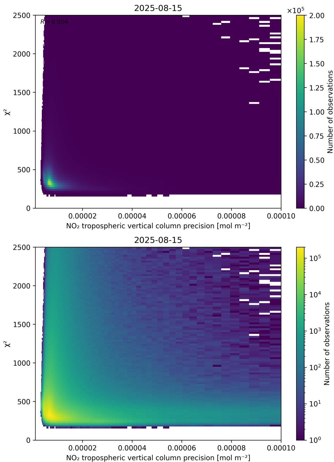
Figure 134: Scatter density plot of “NO 2 tropospheric vertical column precision” against “ \chi^2 ” for 2025-08-14 to 2025-08-16.
