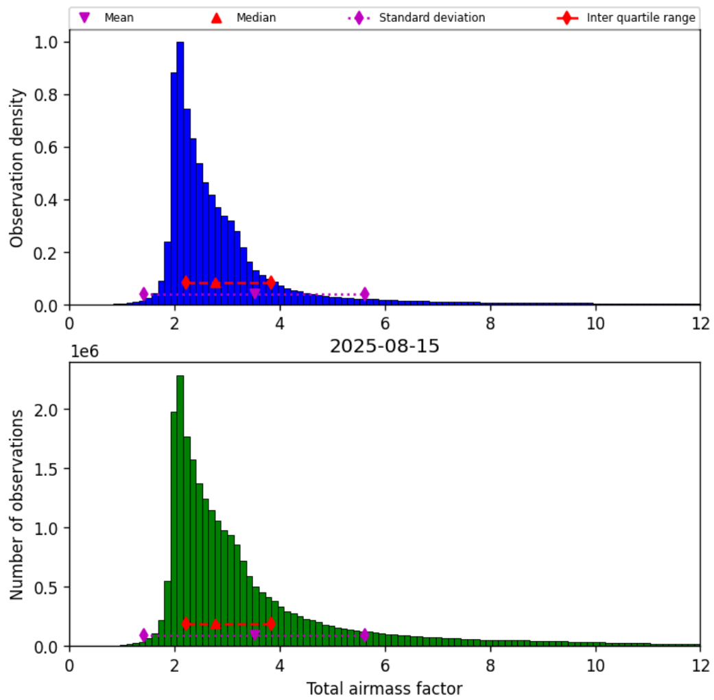
Figure 32: Histogram of “Total airmass factor” for 2025-08-14 to 2025-08-16
