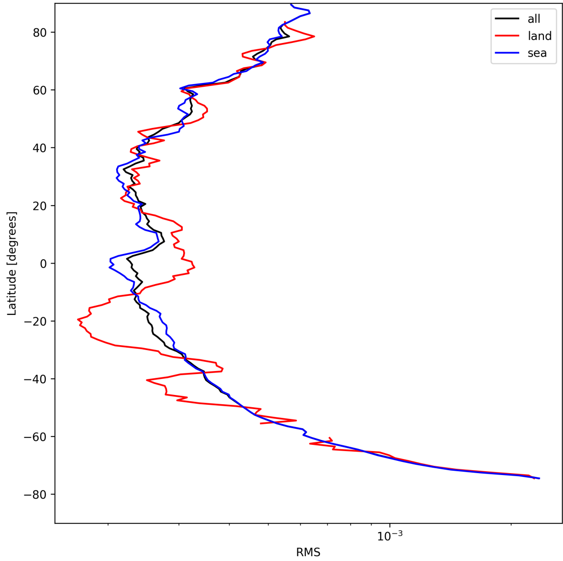
Figure 26: Zonal average of “RMS” for 2025-08-14 to 2025-08-16.
