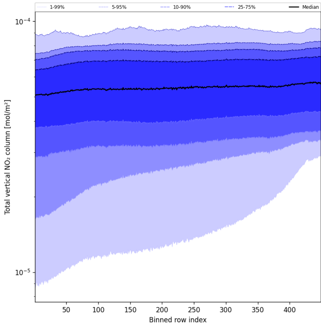
Figure 55: Along track statistics of “Total vertical NO 2 column” for 2025-08-14 to 2025-08-16
