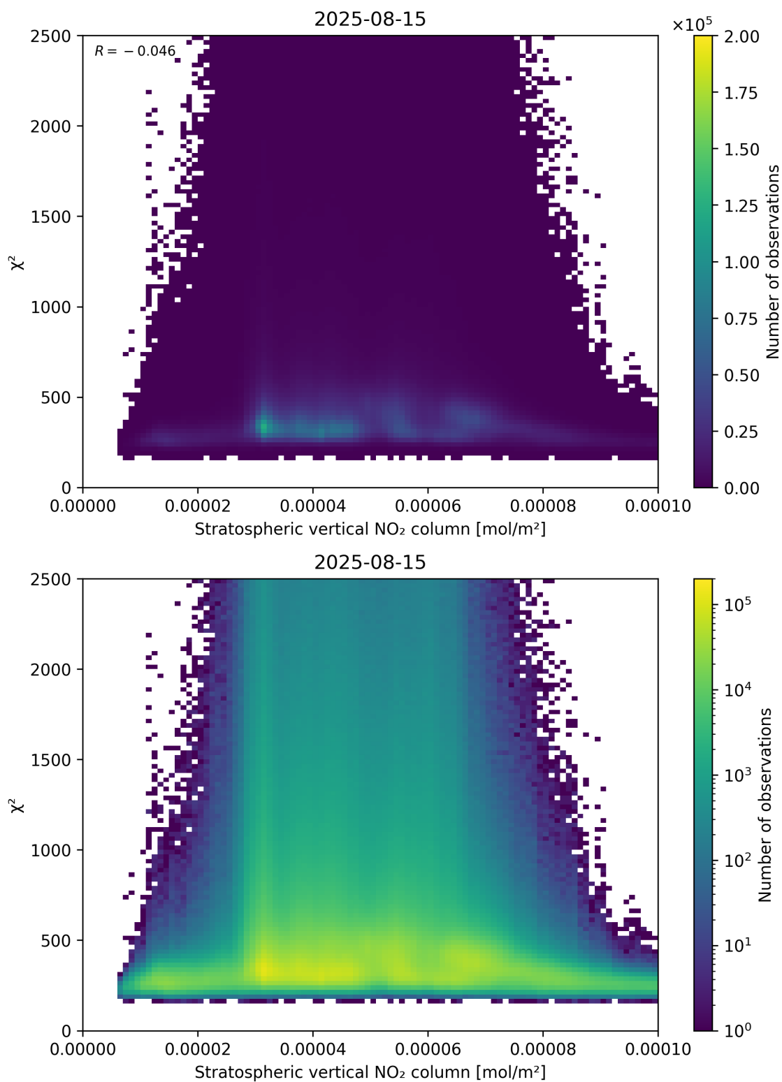
Figure 97: Scatter density plot of “Stratospheric vertical NO 2 column” against “ \chi^2 ” for 2025-08-14 to 2025-08-16.
