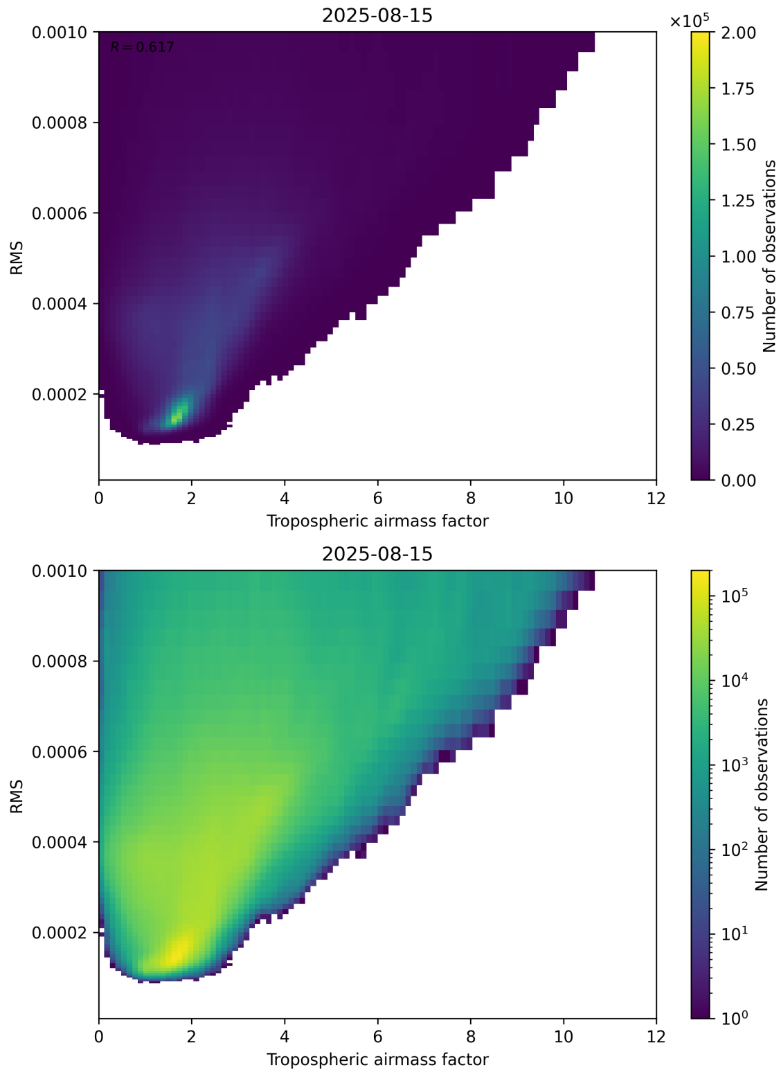
Figure 79: Scatter density plot of “Tropospheric airmass factor” against “RMS” for 2025-08-14 to 2025-08-16.
