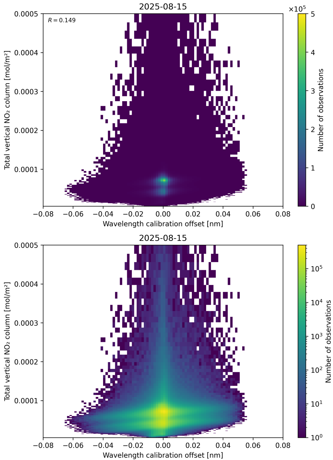
Figure 179: Scatter density plot of “Wavelength calibration offset” against “Total vertical NO 2 column” for 2025-08-14 to 2025-08-16.
