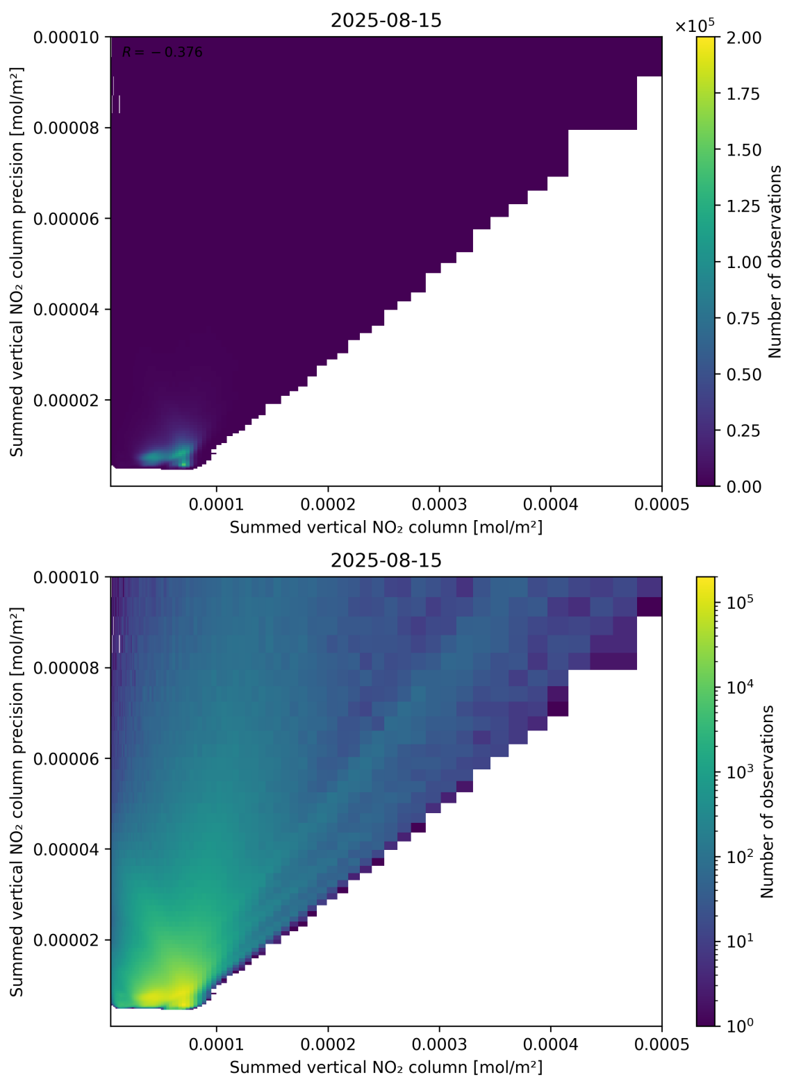
Figure 105: Scatter density plot of “Summed vertical NO 2 column” against “Summed vertical NO 2 column precision” for 2025-08-14 to 2025-08-16.
