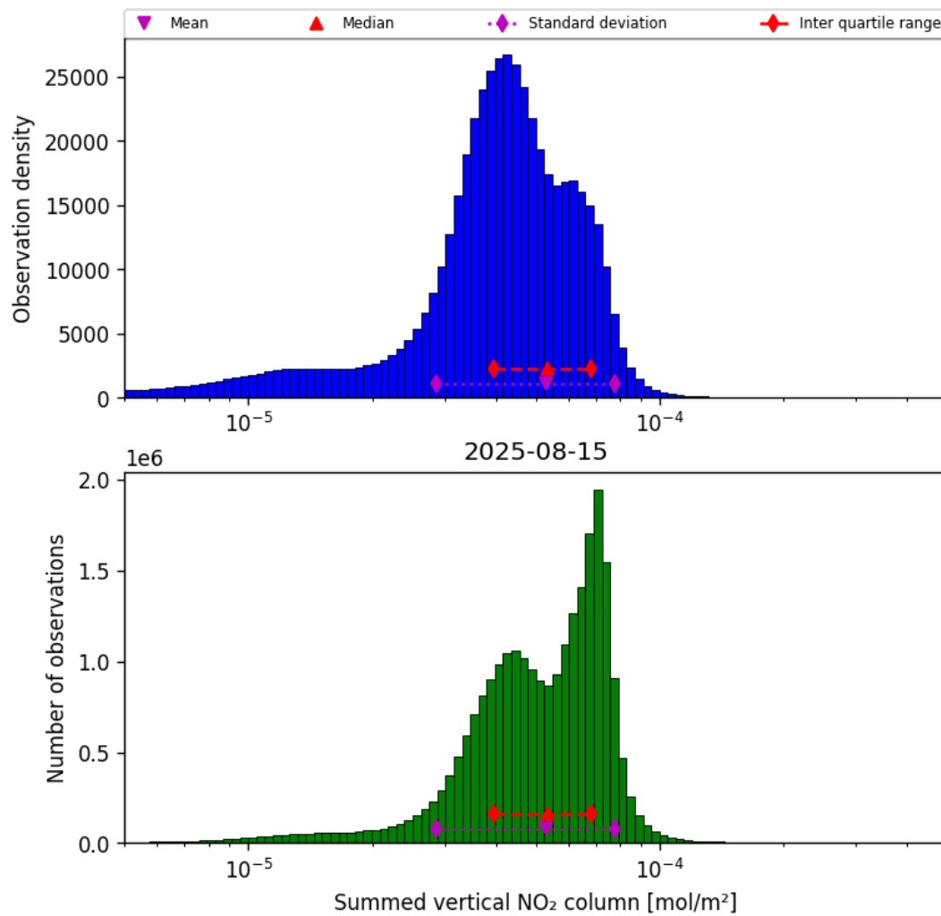
Figure 40: Histogram of “Summed vertical NO 2 column” for 2025-08-14 to 2025-08-16
