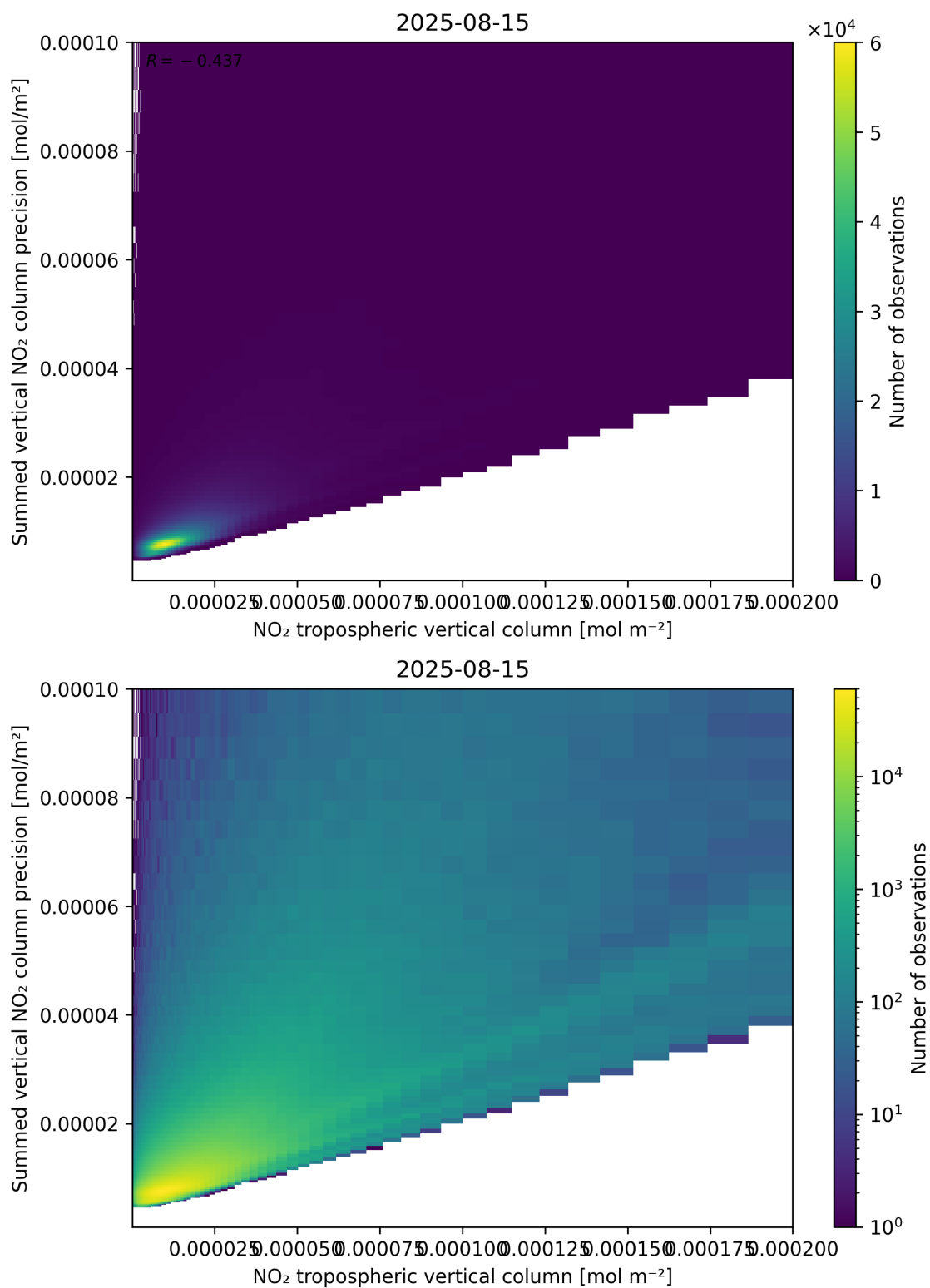
Figure 127: Scatter density plot of “NO 2 tropospheric vertical column” against “Summed vertical NO 2 column precision” for 2025-08-14 to 2025-08-16.
