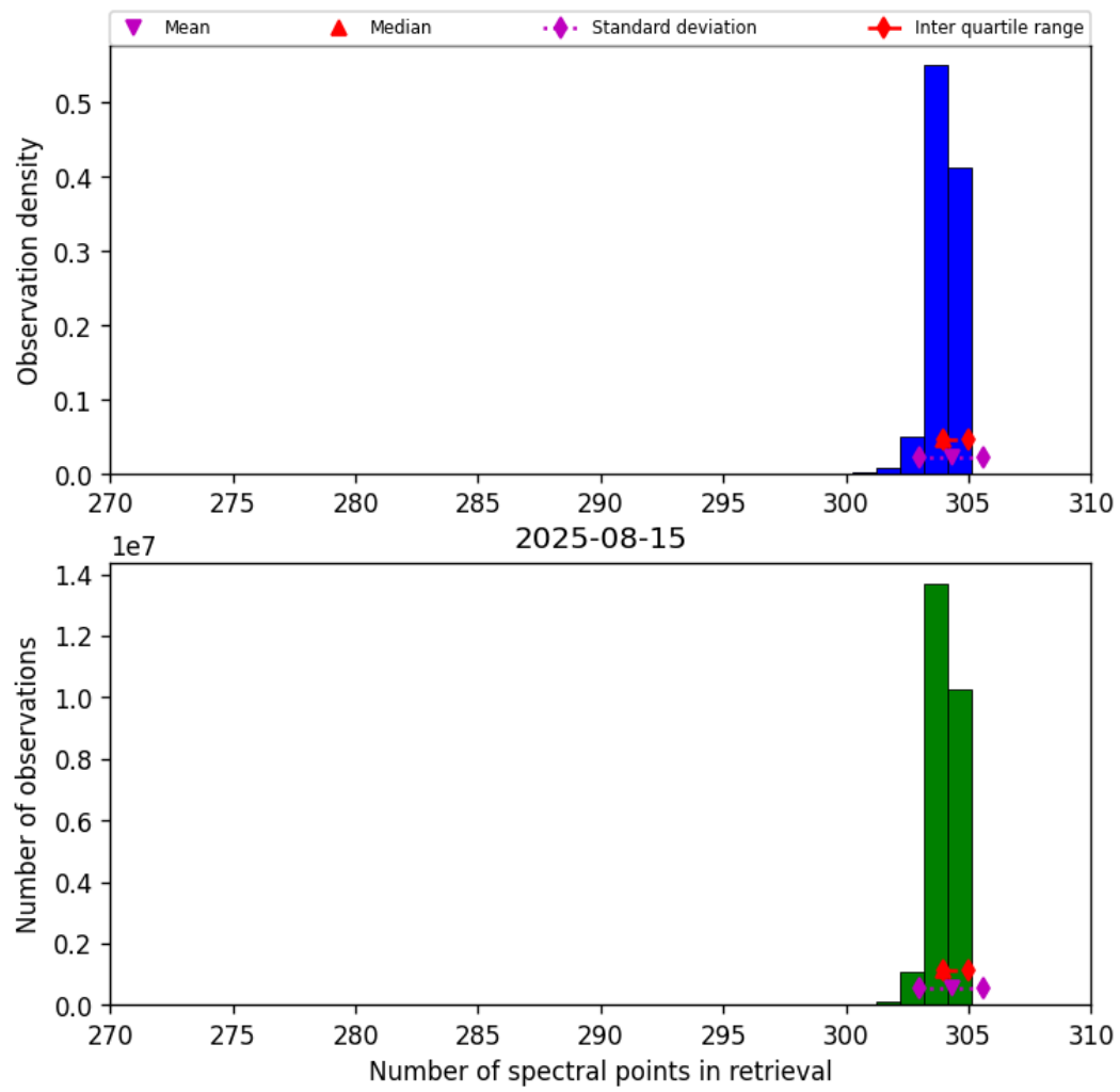
Figure 33: Histogram of “Number of spectral points in retrieval” for 2025-08-14 to 2025-08-16
