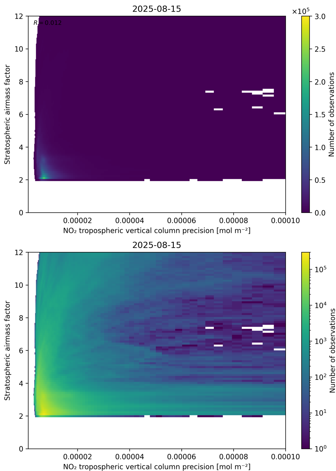
Figure 131: Scatter density plot of “NO 2 tropospheric vertical column precision” against “Stratospheric airmass factor” for 2025-08-14 to 2025-08-16.
