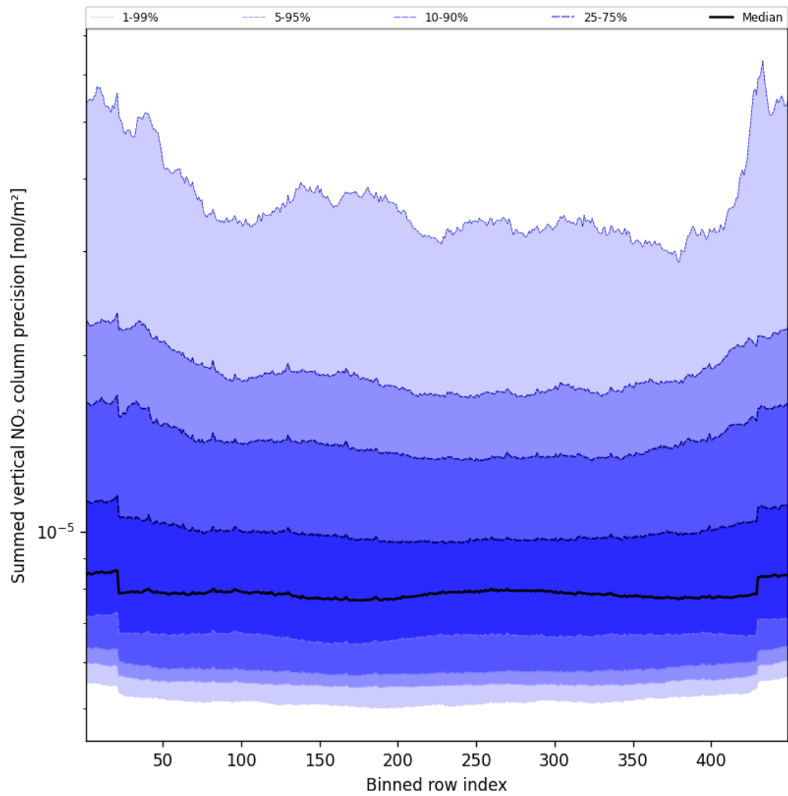
Figure 58: Along track statistics of “Summed vertical NO 2 column precision” for 2025-08-14 to 2025-08-16
