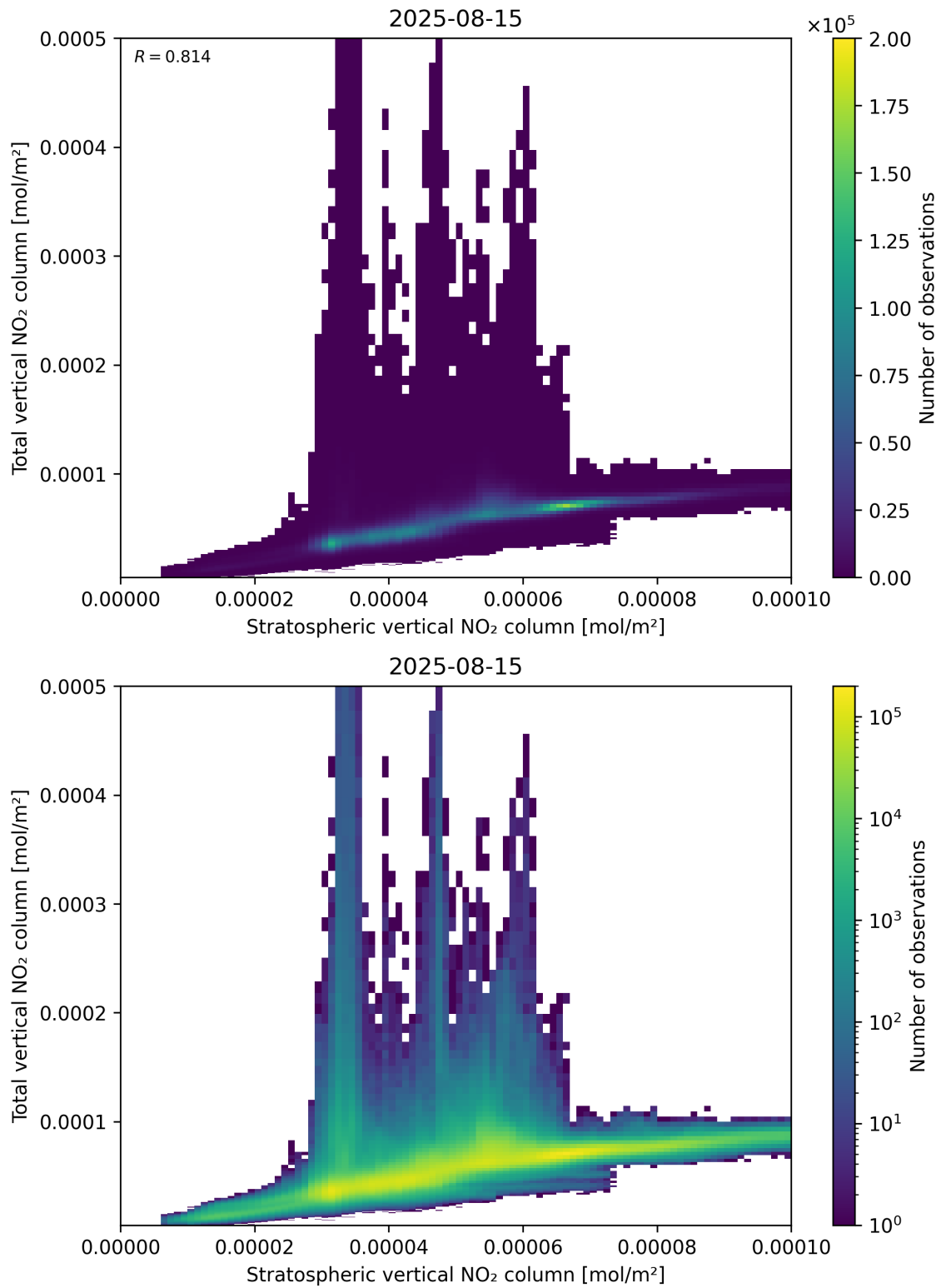
Figure 100: Scatter density plot of “Stratospheric vertical NO 2 column” against “Total vertical NO 2 column” for 2025-08-14 to 2025-08-16.
