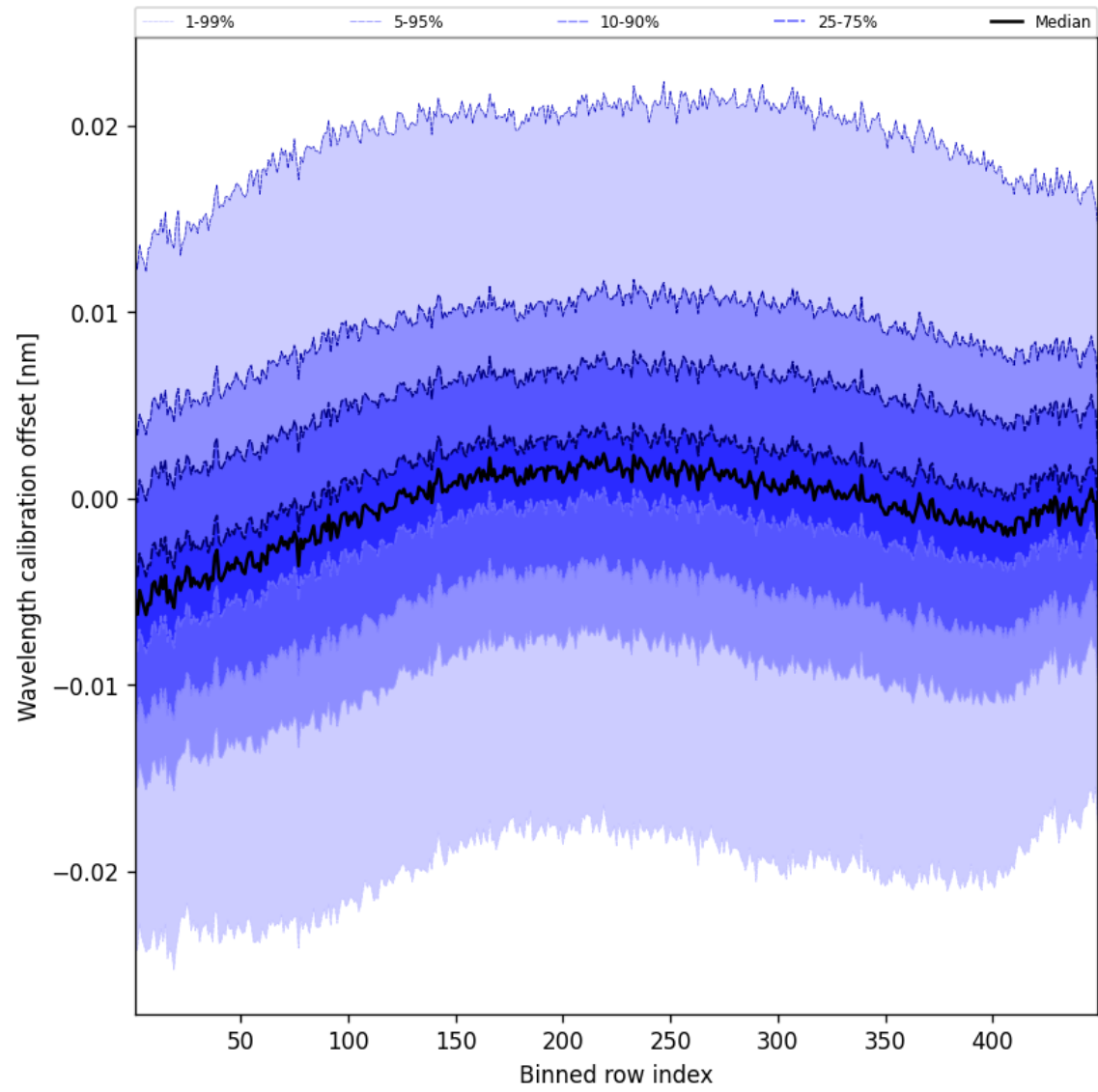
Figure 52: Along track statistics of “Wavelength calibration offset” for 2025-08-14 to 2025-08-16
