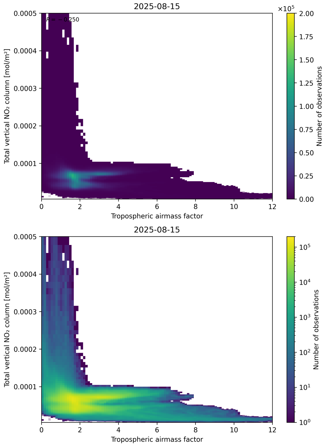
Figure 77: Scatter density plot of “Tropospheric airmass factor” against “Total vertical NO 2 column” for 2025-08-14 to 2025-08-16.
