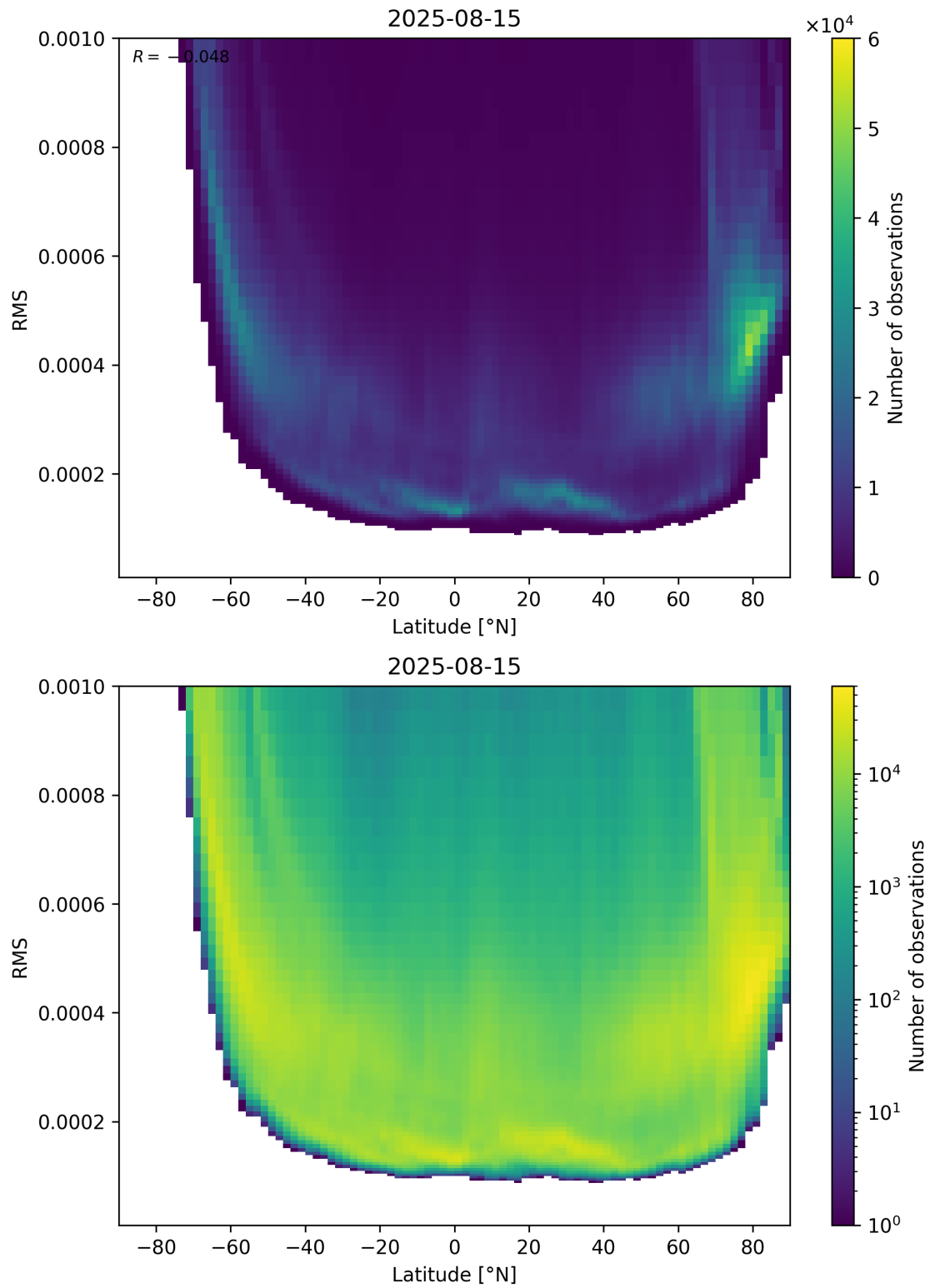
Figure 94: Scatter density plot of “Latitude” against “RMS” for 2025-08-14 to 2025-08-16.
