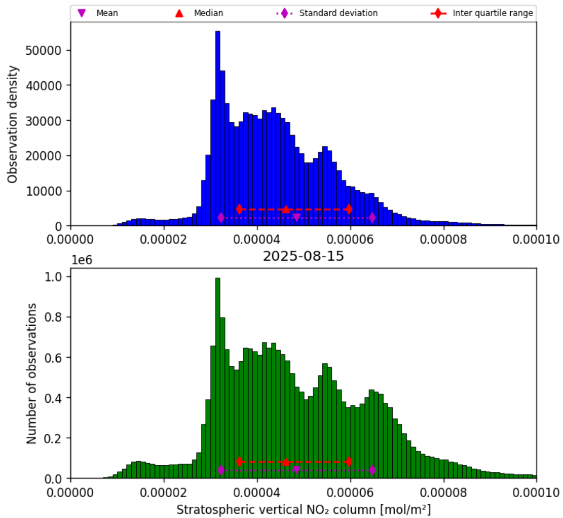
Figure 36: Histogram of “Stratospheric vertical NO 2 column” for 2025-08-14 to 2025-08-16
