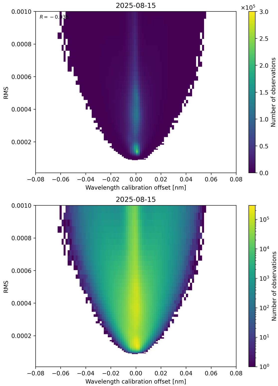
Figure 181: Scatter density plot of “Wavelength calibration offset” against “RMS” for 2025-08-14 to 2025-08-16.
