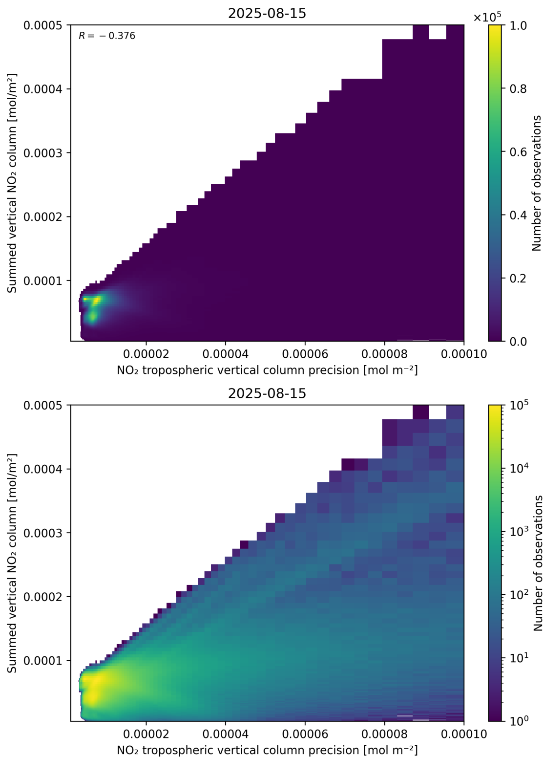
Figure 136: Scatter density plot of “NO 2 tropospheric vertical column precision” against “Summed vertical NO 2 column” for 2025-08-14 to 2025-08-16.
