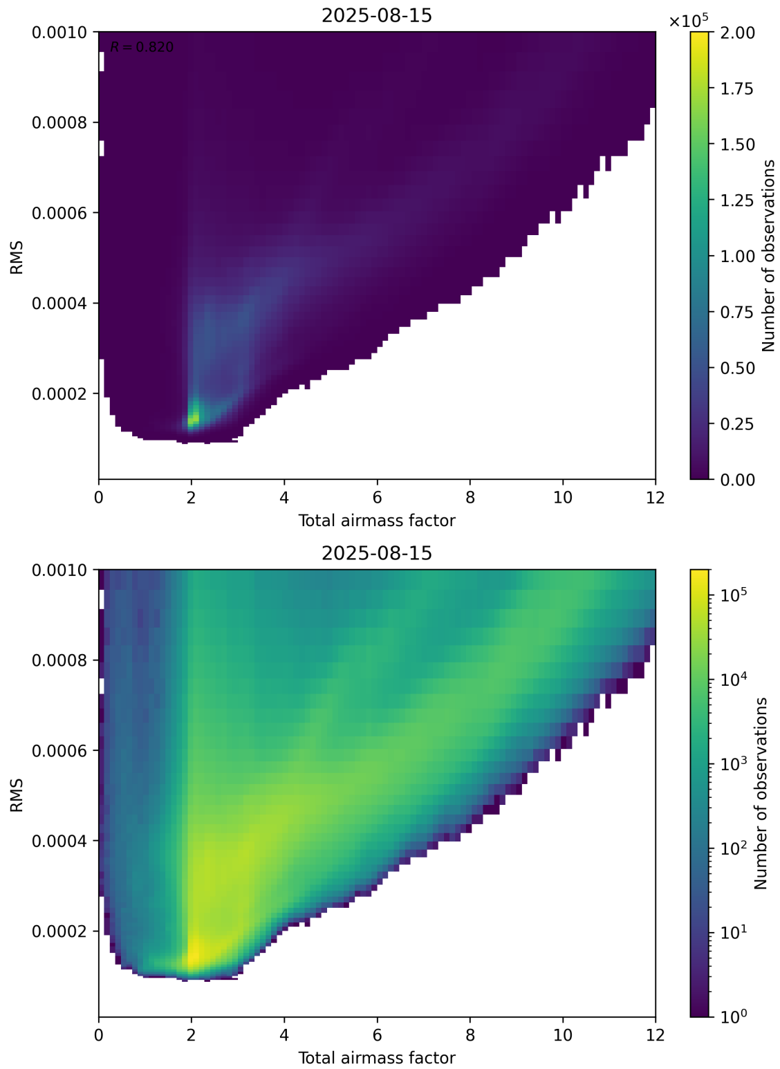
Figure 69: Scatter density plot of “Total airmass factor” against “RMS” for 2025-08-14 to 2025-08-16.
