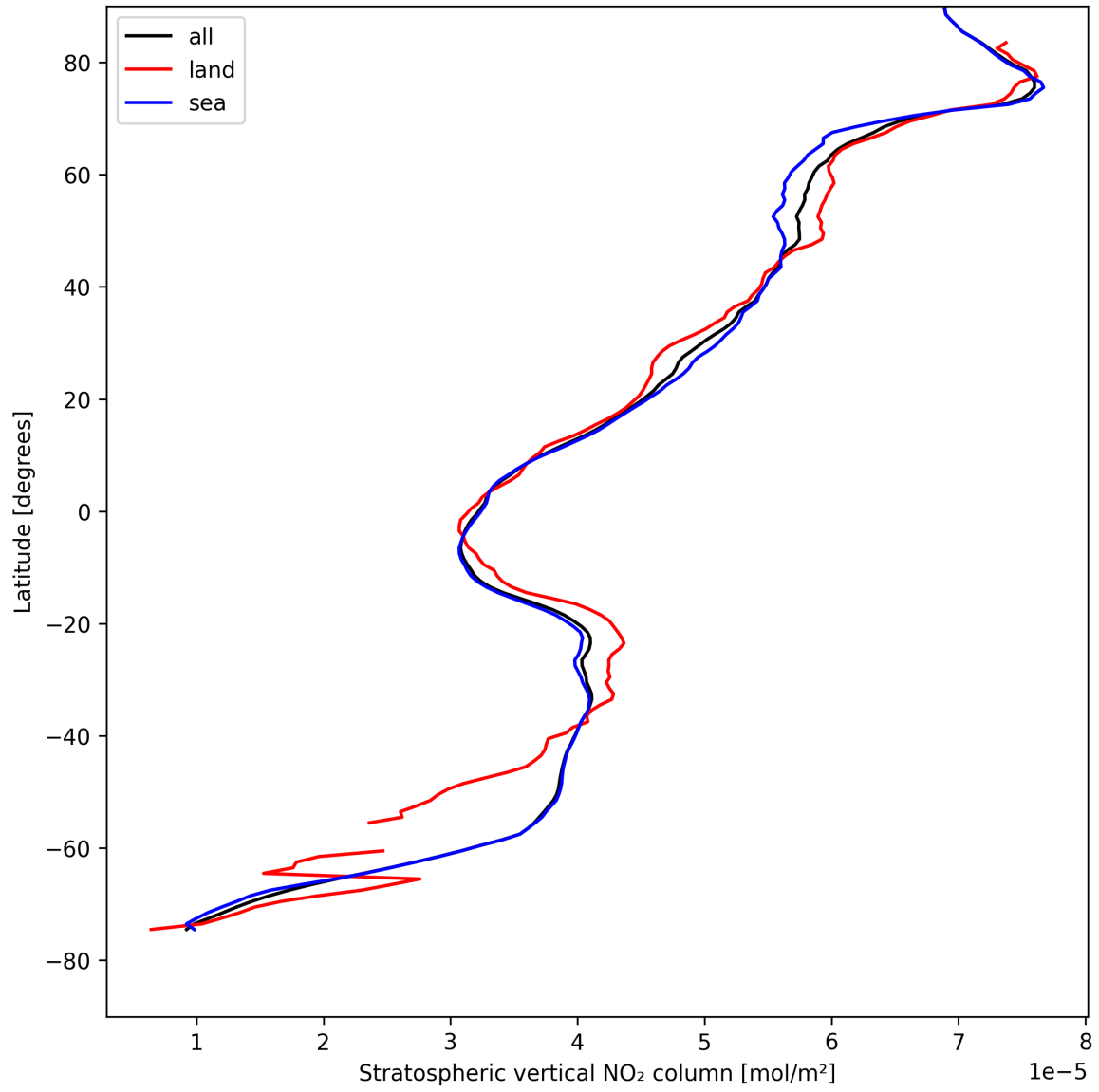
Figure 19: Zonal average of “Stratospheric vertical NO 2 column” for 2025-08-14 to 2025-08-16.
