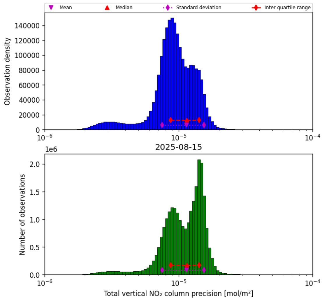
Figure 39: Histogram of “Total vertical NO 2 column precision” for 2025-08-14 to 2025-08-16
