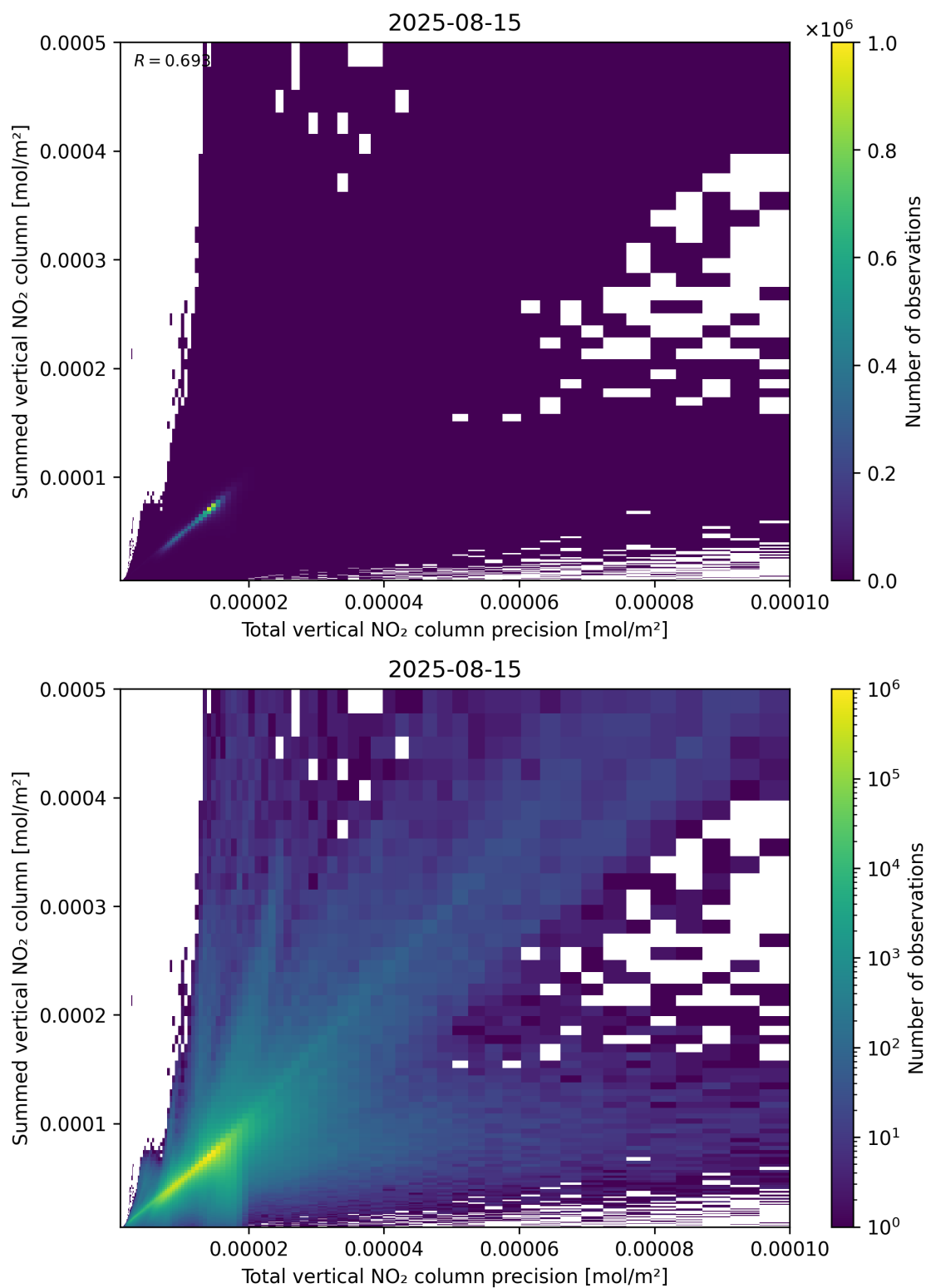
Figure 117: Scatter density plot of “Total vertical NO 2 column precision” against “Summed vertical NO 2 column” for 2025-08-14 to 2025-08-16.
