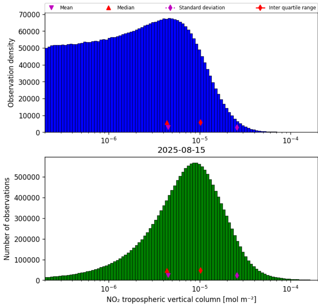
Figure 29: Histogram of “NO 2 tropospheric vertical column” for 2025-08-14 to 2025-08-16
