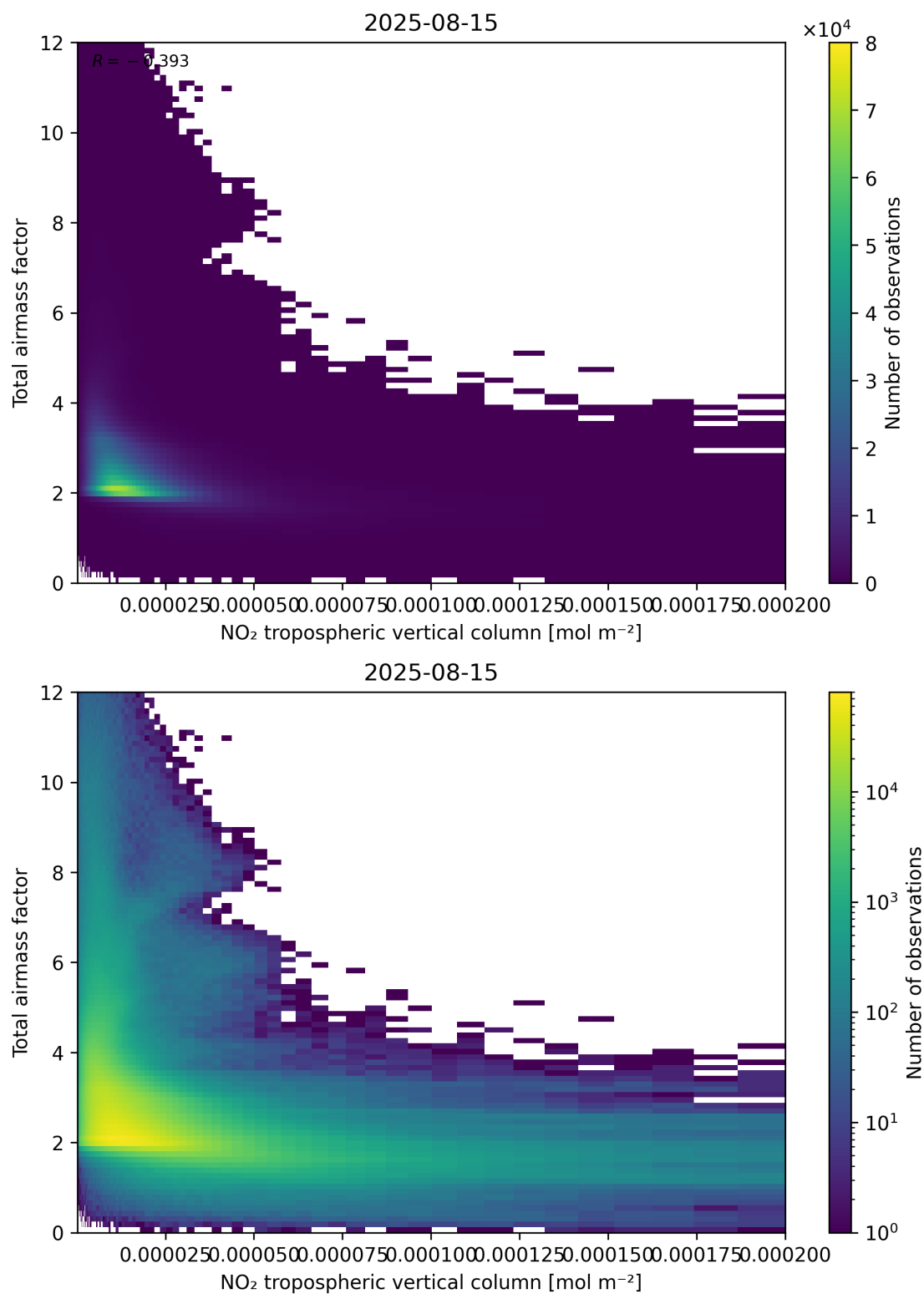
Figure 122: Scatter density plot of “NO 2 tropospheric vertical column” against “Total air mass factor” for 2025-08-14 to 2025-08-16.
