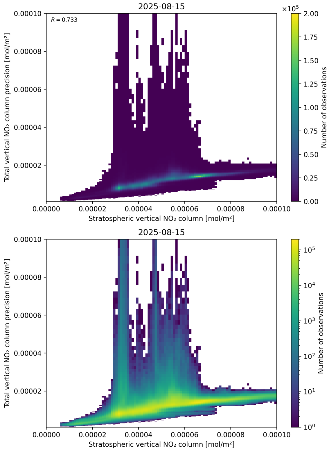
Figure 101: Scatter density plot of “Stratospheric vertical NO 2 column” against “Total vertical NO 2 column precision” for 2025-08-14 to 2025-08-16.
