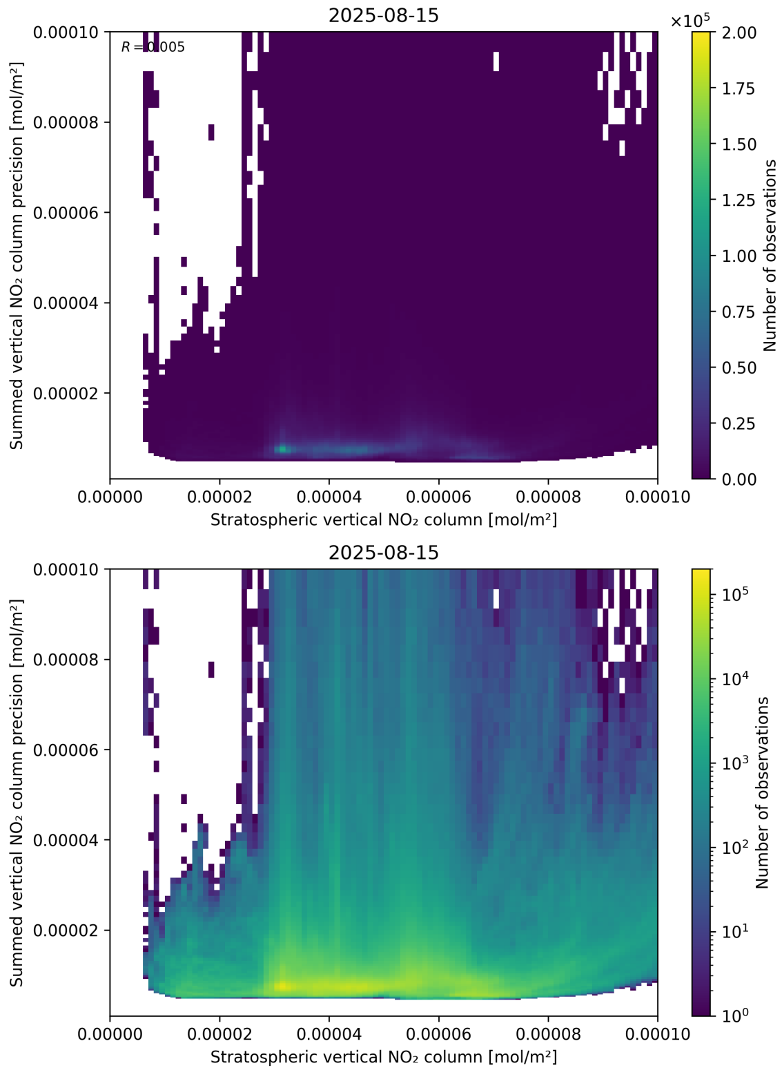
Figure 99: Scatter density plot of “Stratospheric vertical NO 2 column” against “Summed vertical NO 2 column precision” for 2025-08-14 to 2025-08-16.
