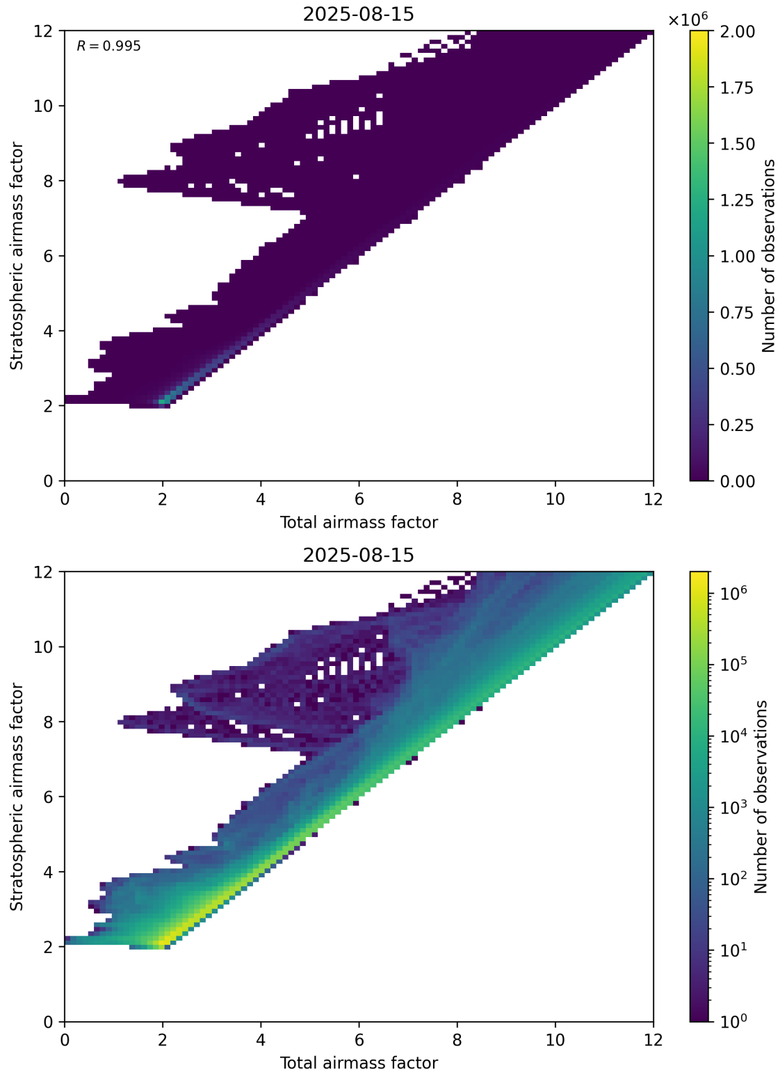
Figure 62: Scatter density plot of “Total airmass factor” against “Stratospheric airmass factor” for 2025-08-14 to 2025-08-16.
