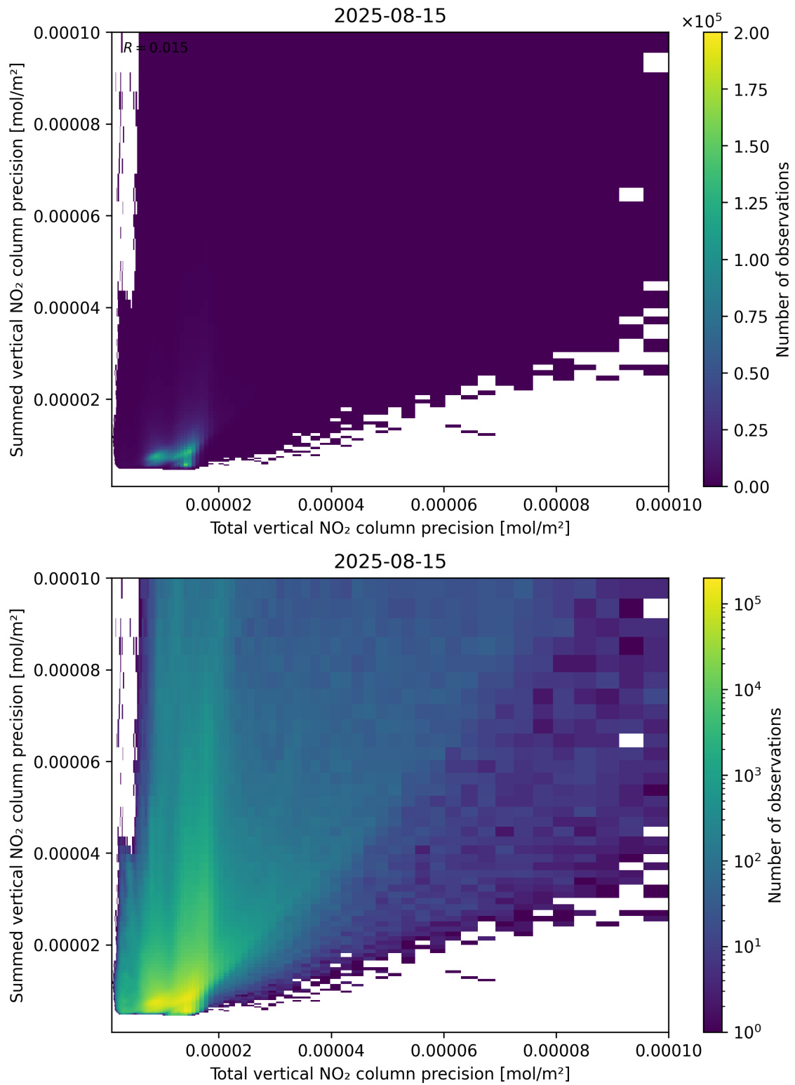
Figure 118: Scatter density plot of “Total vertical NO 2 column precision” against “Summed vertical NO 2 column precision” for 2025-08-14 to 2025-08-16.
