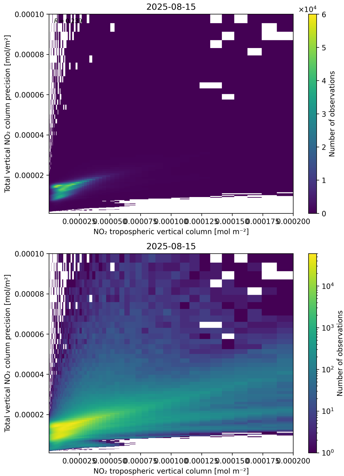
Figure 129: Scatter density plot of “NO 2 tropospheric vertical column” against “Total vertical NO 2 column precision” for 2025-08-14 to 2025-08-16.
