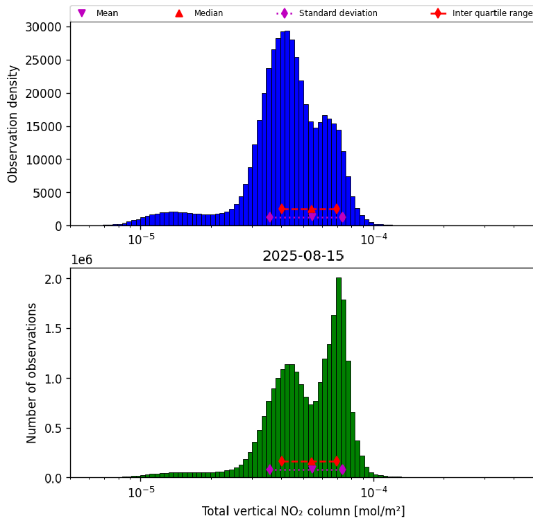
Figure 38: Histogram of “Total vertical NO 2 column” for 2025-08-14 to 2025-08-16
