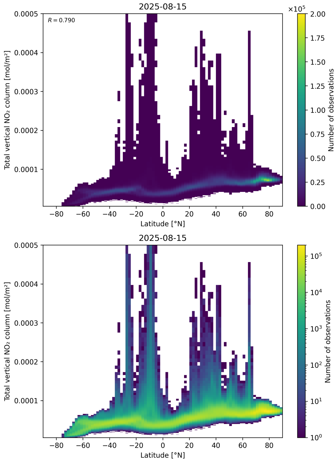
Figure 90: Scatter density plot of “Latitude” against “Total vertical NO 2 column” for 2025-08-14 to 2025-08-16.
