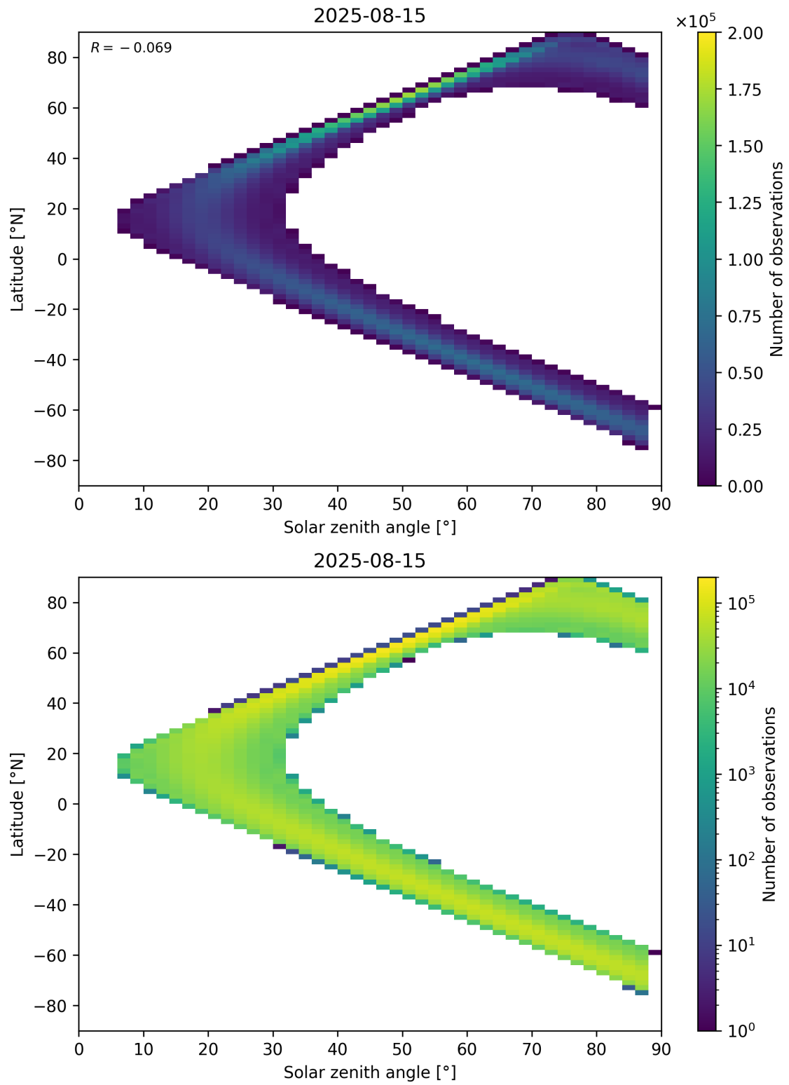
Figure 149: Scatter density plot of “Solar zenith angle” against “Latitude” for 2025-08-14 to 2025-08-16.
