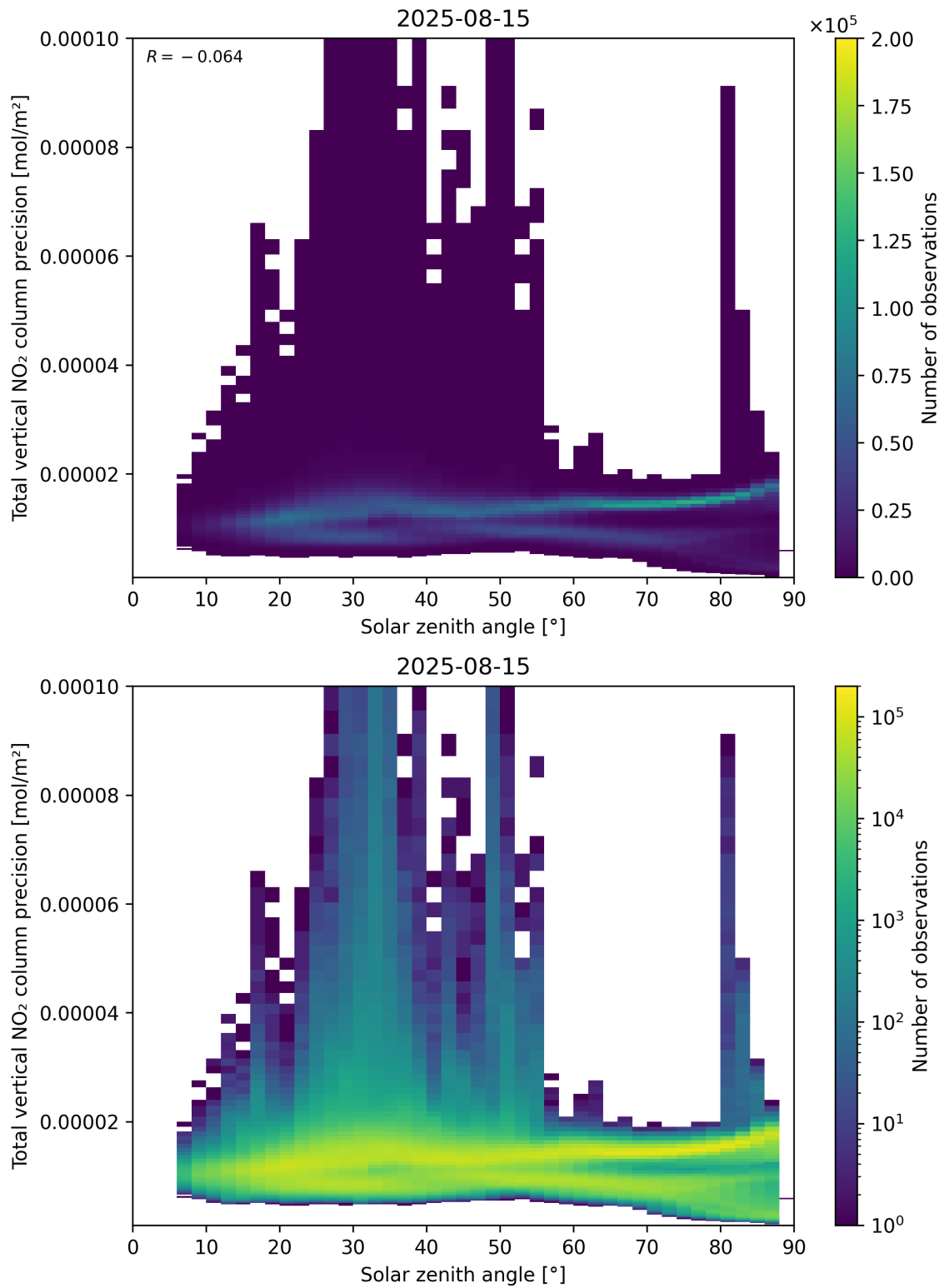
Figure 154: Scatter density plot of “Solar zenith angle” against “Total vertical NO 2 column precision” for 2025-08-14 to 2025-08-16.
