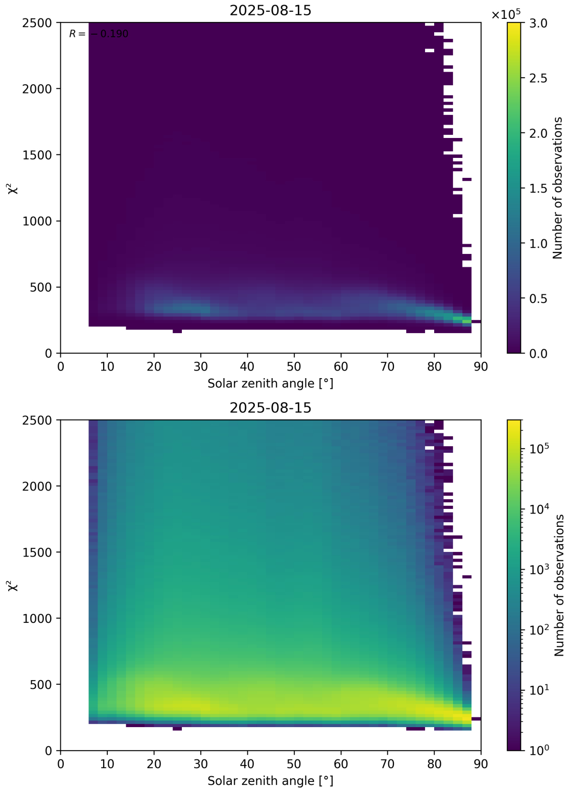
Figure 148: Scatter density plot of “Solar zenith angle” against “ \chi^2 ” for 2025-08-14 to 2025-08-16.
