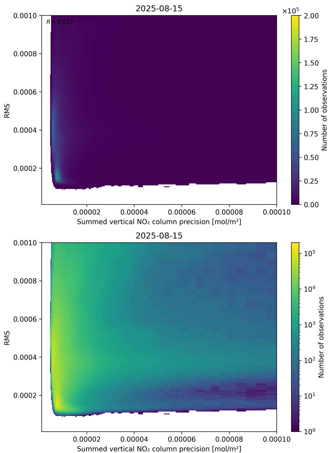
Figure 108: Scatter density plot of “Summed vertical NO 2 column precision” against “RMS” for 2025-08-14 to 2025-08-16.
