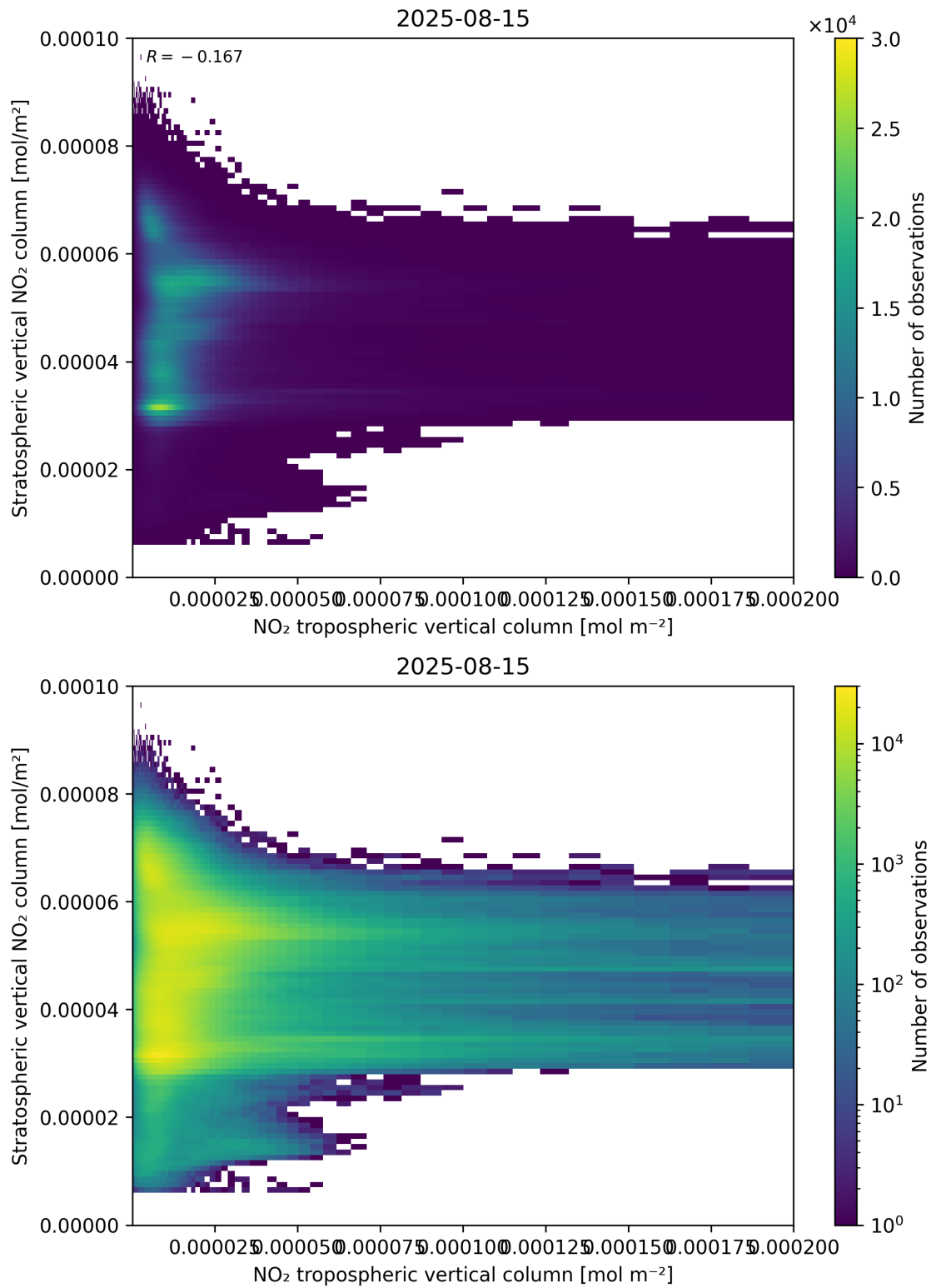
Figure 125: Scatter density plot of “NO 2 tropospheric vertical column” against “Stratospheric vertical NO 2 column” for 2025-08-14 to 2025-08-16.
