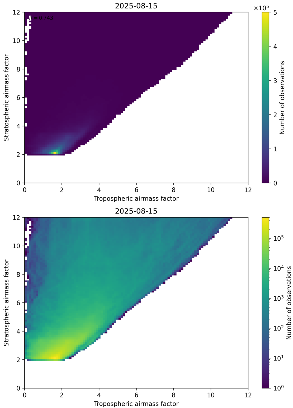
Figure 71: Scatter density plot of “Tropospheric airmass factor” against “Stratospheric airmass factor” for 2025-08-14 to 2025-08-16.
