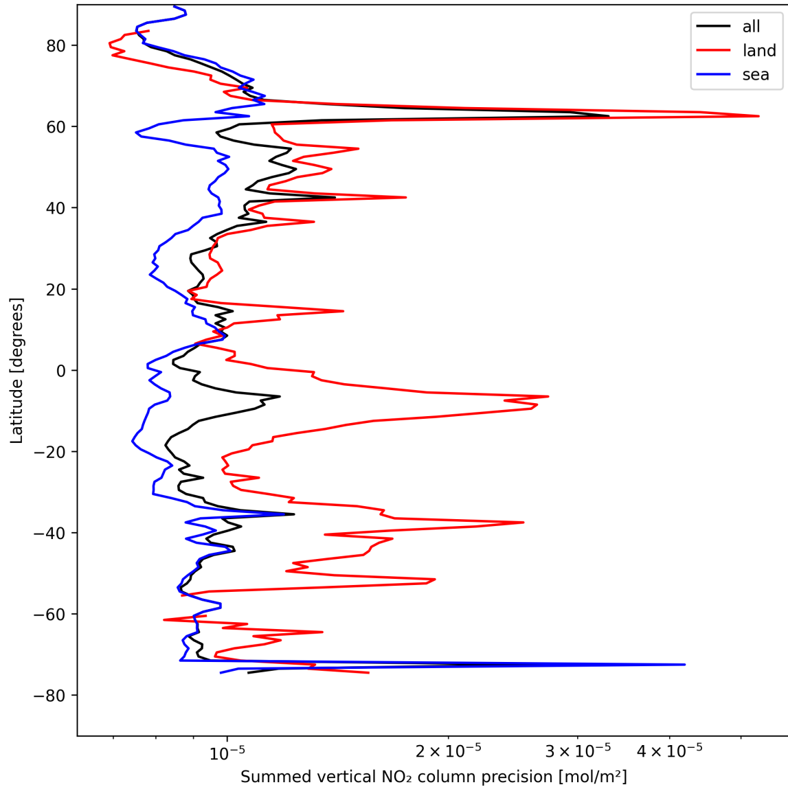
Figure 24: Zonal average of “Summed vertical NO 2 column precision” for 2025-08-14 to 2025-08-16.
