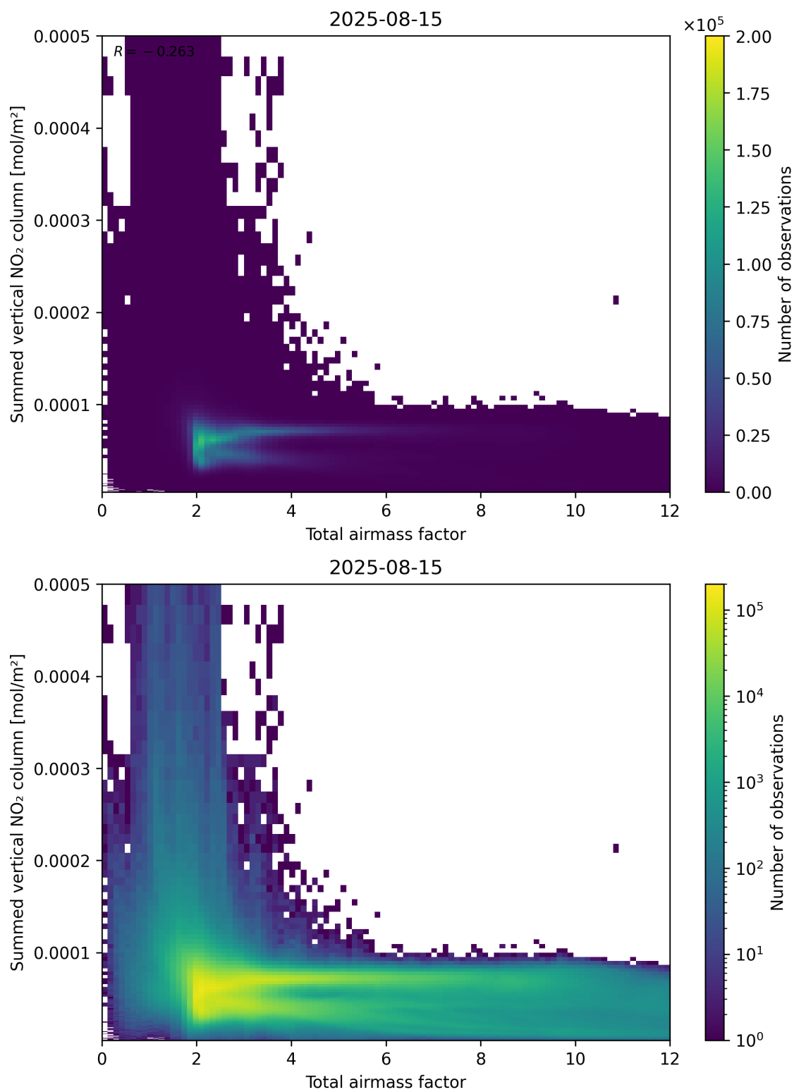
Figure 65: Scatter density plot of “Total airmass factor” against “Summed vertical NO 2 column” for 2025-08-14 to 2025-08-16.
