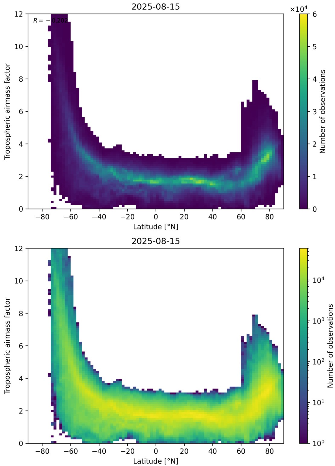
Figure 85: Scatter density plot of “Latitude” against “Tropospheric air mass factor” for 2025-08-14 to 2025-08-16.
