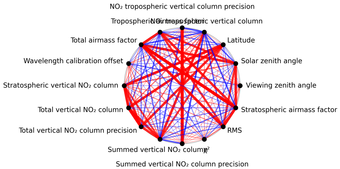
Figure 1: Map of correlation graph for 2025-08-14 to 2025-08-16.
