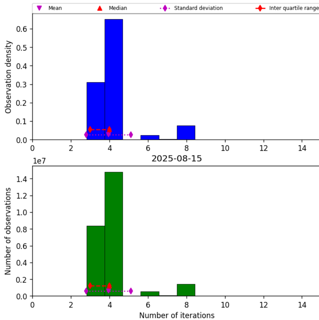
Figure 34: Histogram of “Number of iterations” for 2025-08-14 to 2025-08-16
