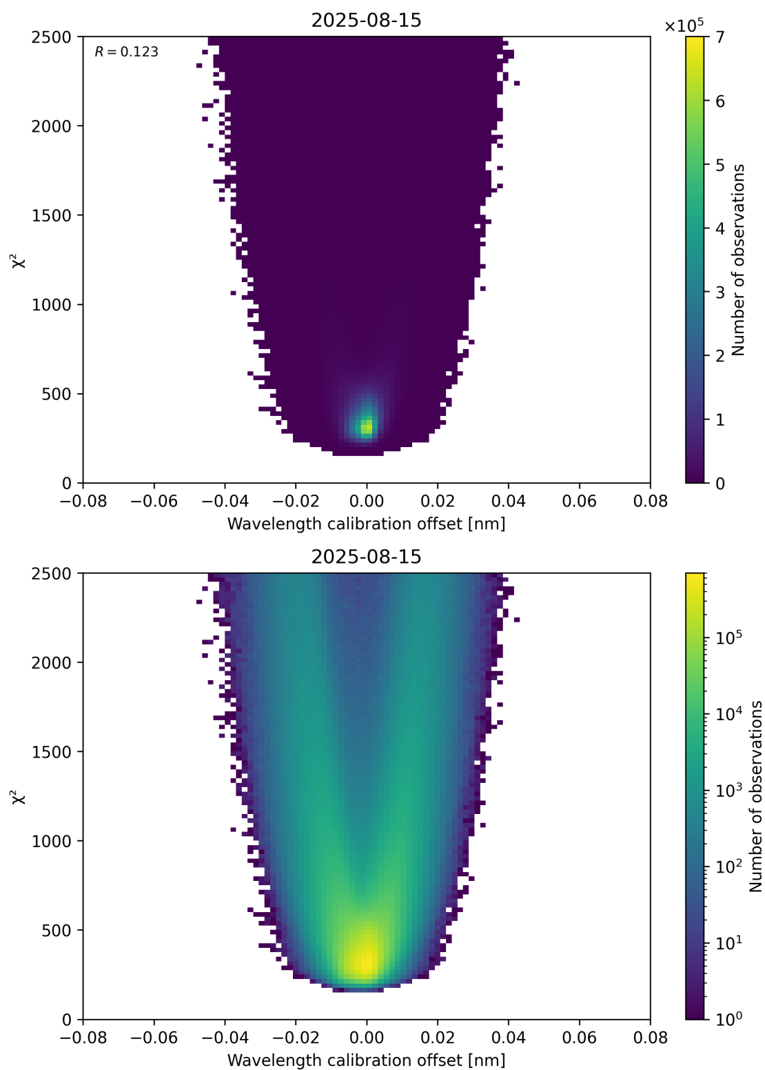
Figure 175: Scatter density plot of “Wavelength calibration offset” against “ \chi^2 ” for 2025-08-14 to 2025-08-16.
