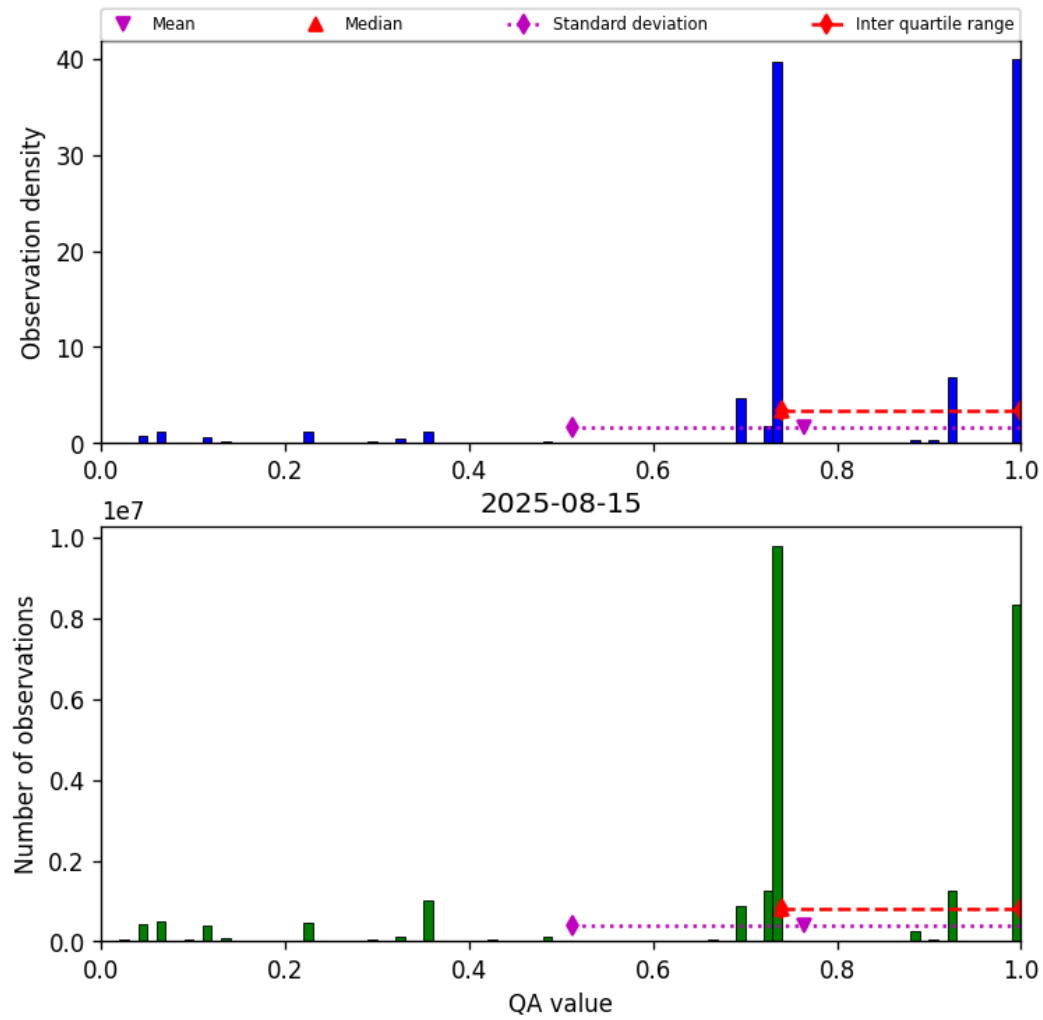
Figure 28: Histogram of “QA value” for 2025-08-14 to 2025-08-16
