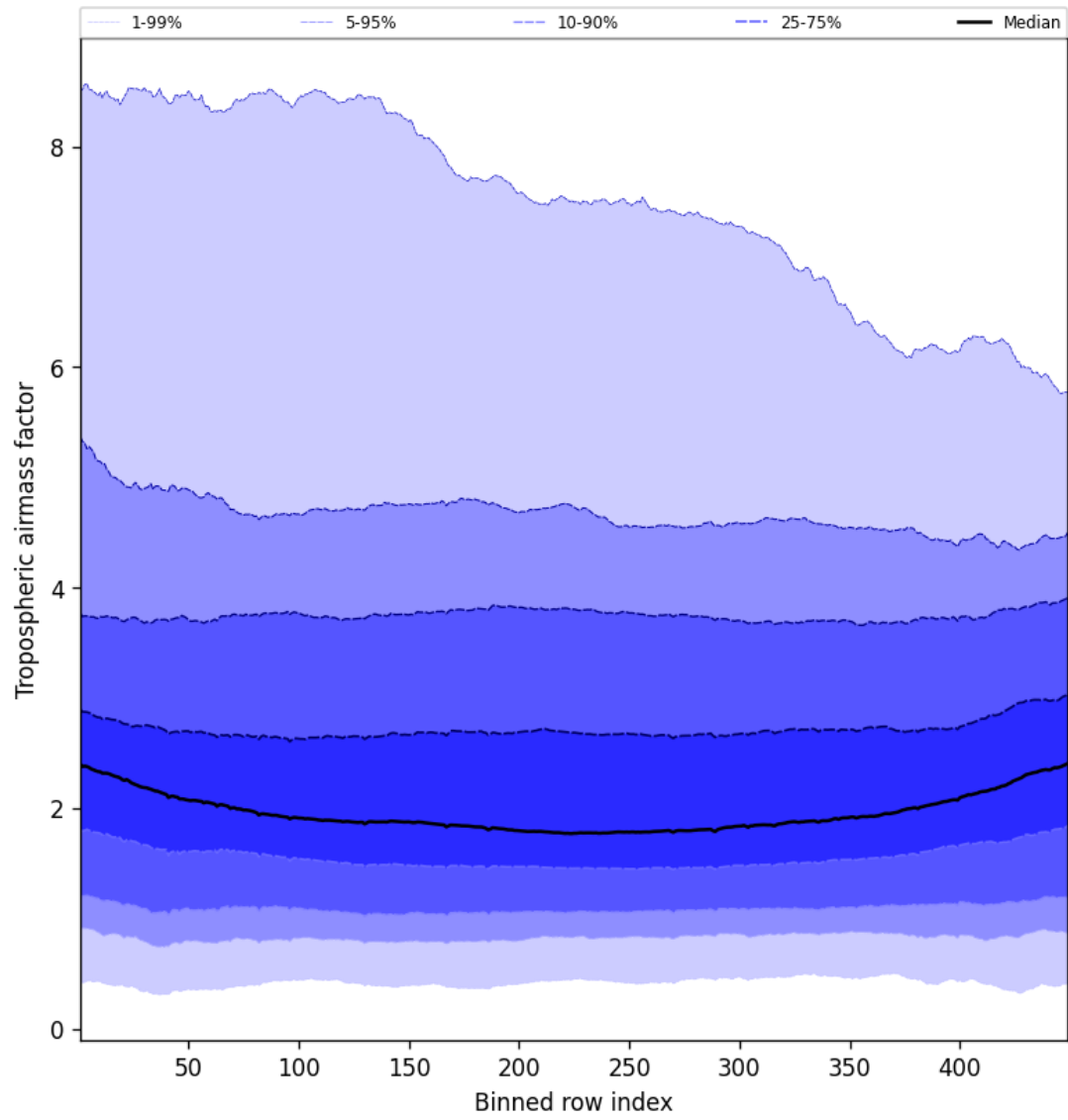
Figure 48: Along track statistics of “Tropospheric airmass factor” for 2025-08-14 to 2025-08-16
