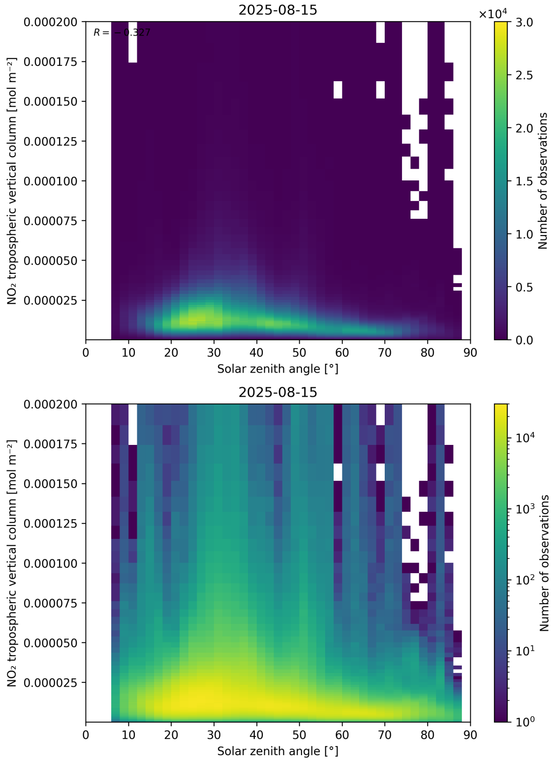
Figure 155: Scatter density plot of “Solar zenith angle” against “NO 2 tropospheric vertical column” for 2025-08-14 to 2025-08-16.
