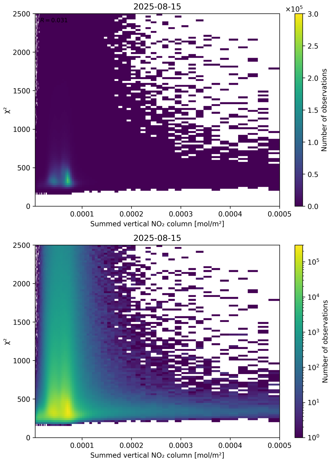
Figure 104: Scatter density plot of “Summed vertical NO 2 column” against “ \chi^2 ” for 2025-08-14 to 2025-08-16.
