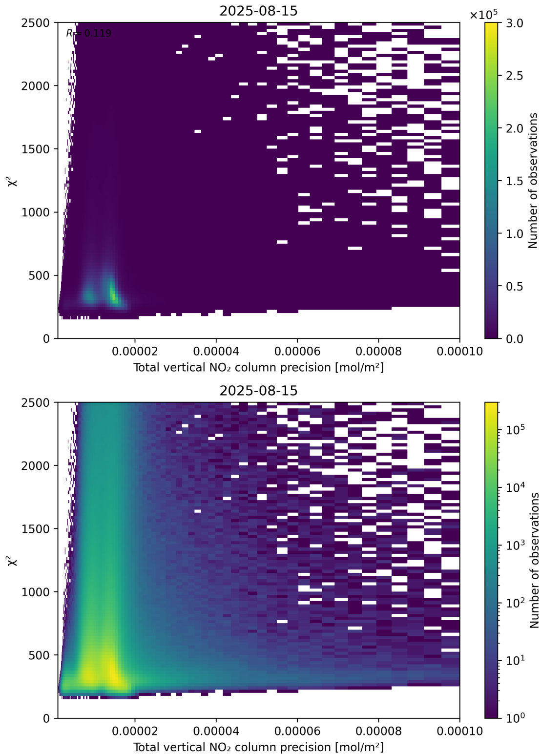
Figure 116: Scatter density plot of “Total vertical NO 2 column precision” against “ \chi^2 ” for 2025-08-14 to 2025-08-16.
