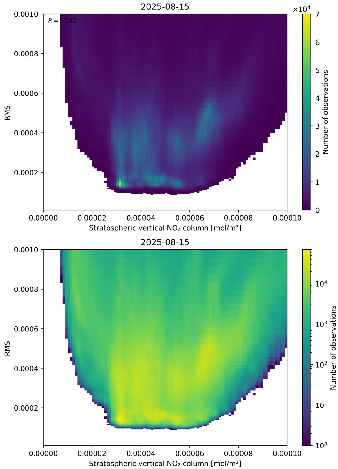
Figure 102: Scatter density plot of “Stratospheric vertical NO 2 column” against “RMS” for 2025-08-14 to 2025-08-16.
