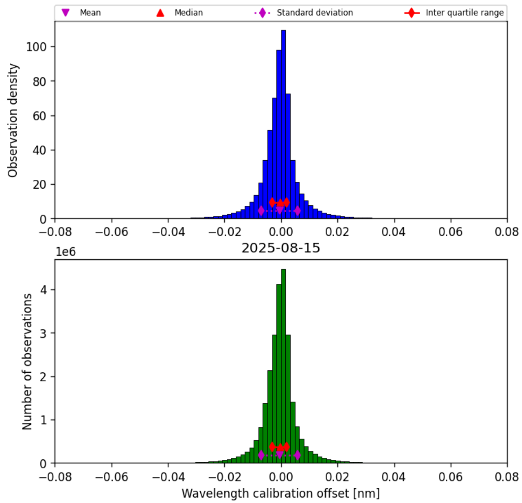
Figure 35: Histogram of “Wavelength calibration offset” for 2025-08-14 to 2025-08-16
