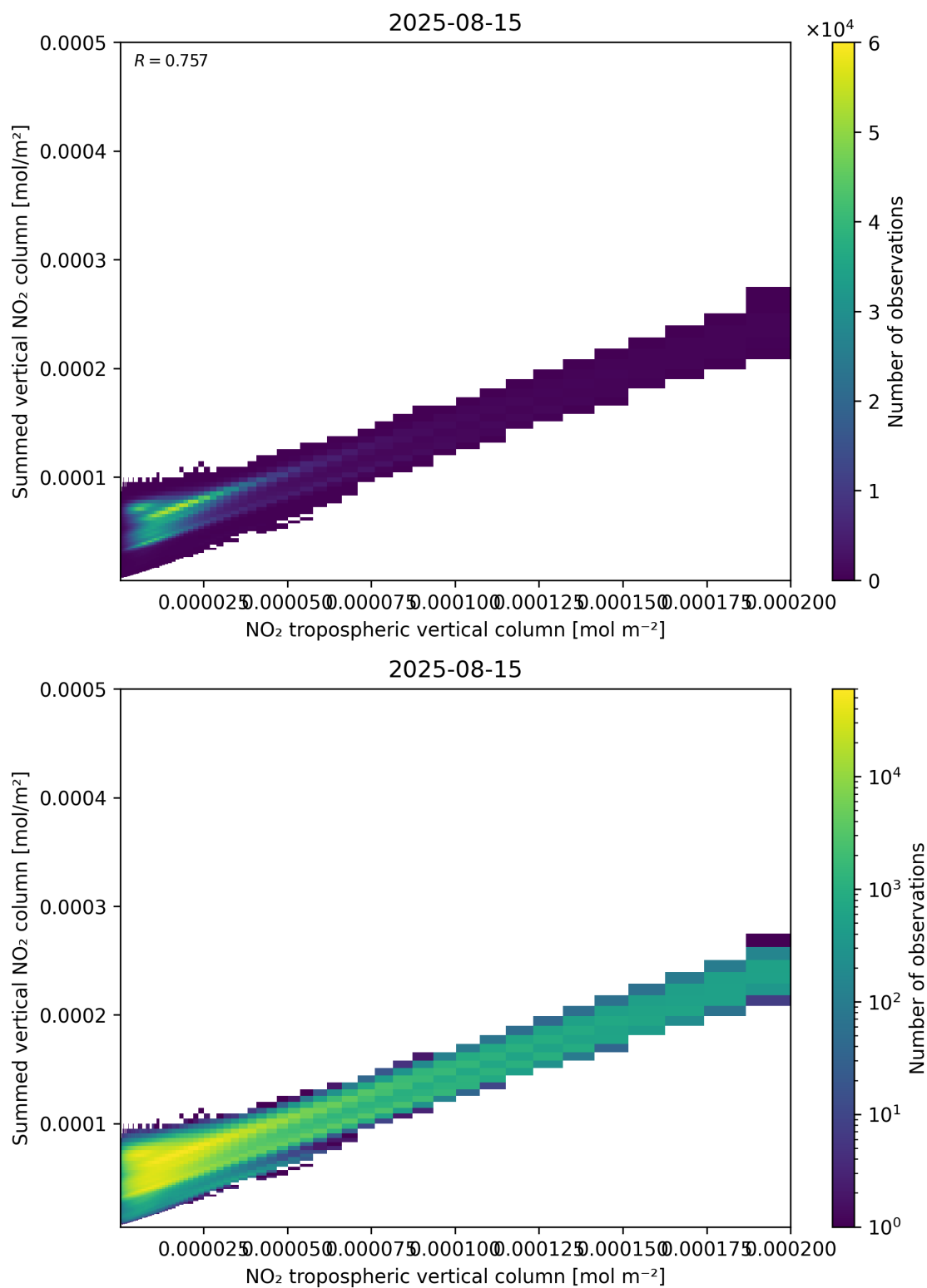
Figure 126: Scatter density plot of “NO 2 tropospheric vertical column” against “Summed vertical NO 2 column” for 2025-08-14 to 2025-08-16.
