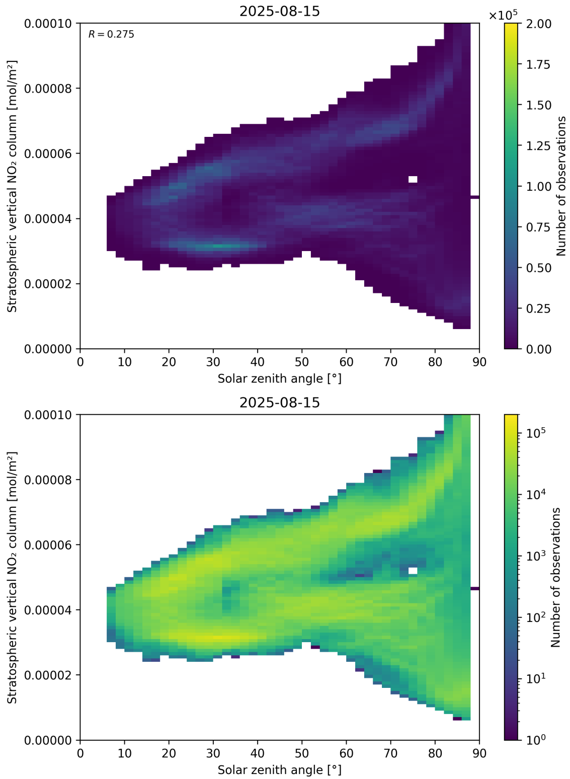
Figure 150: Scatter density plot of “Solar zenith angle” against “Stratospheric vertical NO 2 column” for 2025-08-14 to 2025-08-16.
