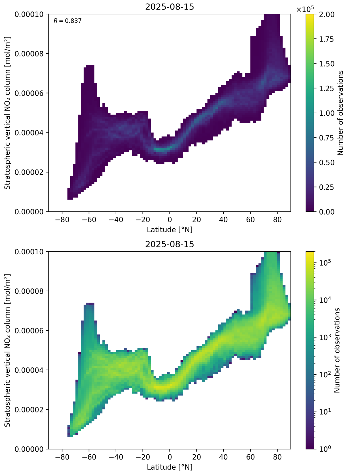
Figure 87: Scatter density plot of “Latitude” against “Stratospheric vertical NO 2 column” for 2025-08-14 to 2025-08-16.
