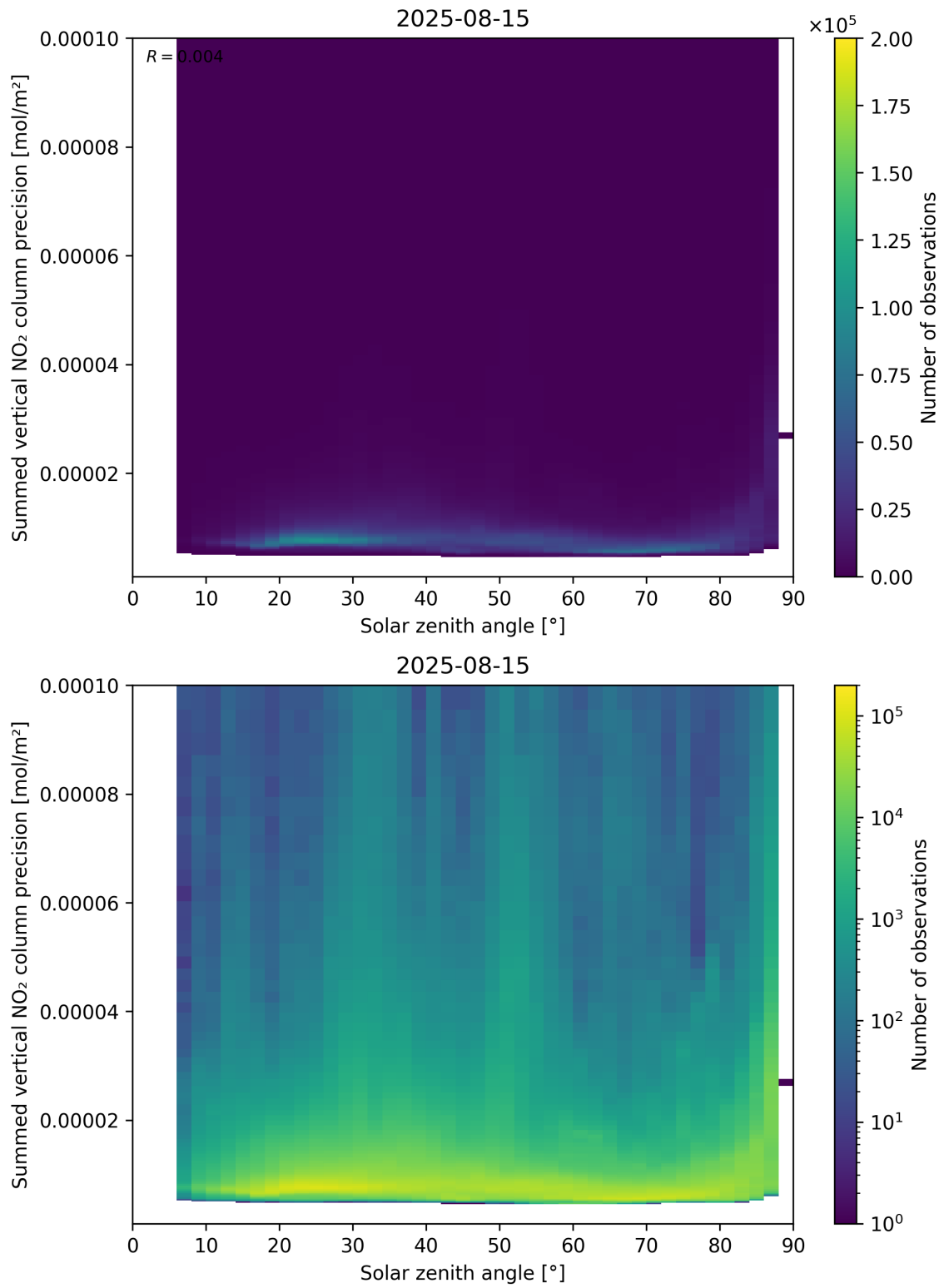
Figure 152: Scatter density plot of “Solar zenith angle” against “Summed vertical NO 2 column precision” for 2025-08-14 to 2025-08-16.
