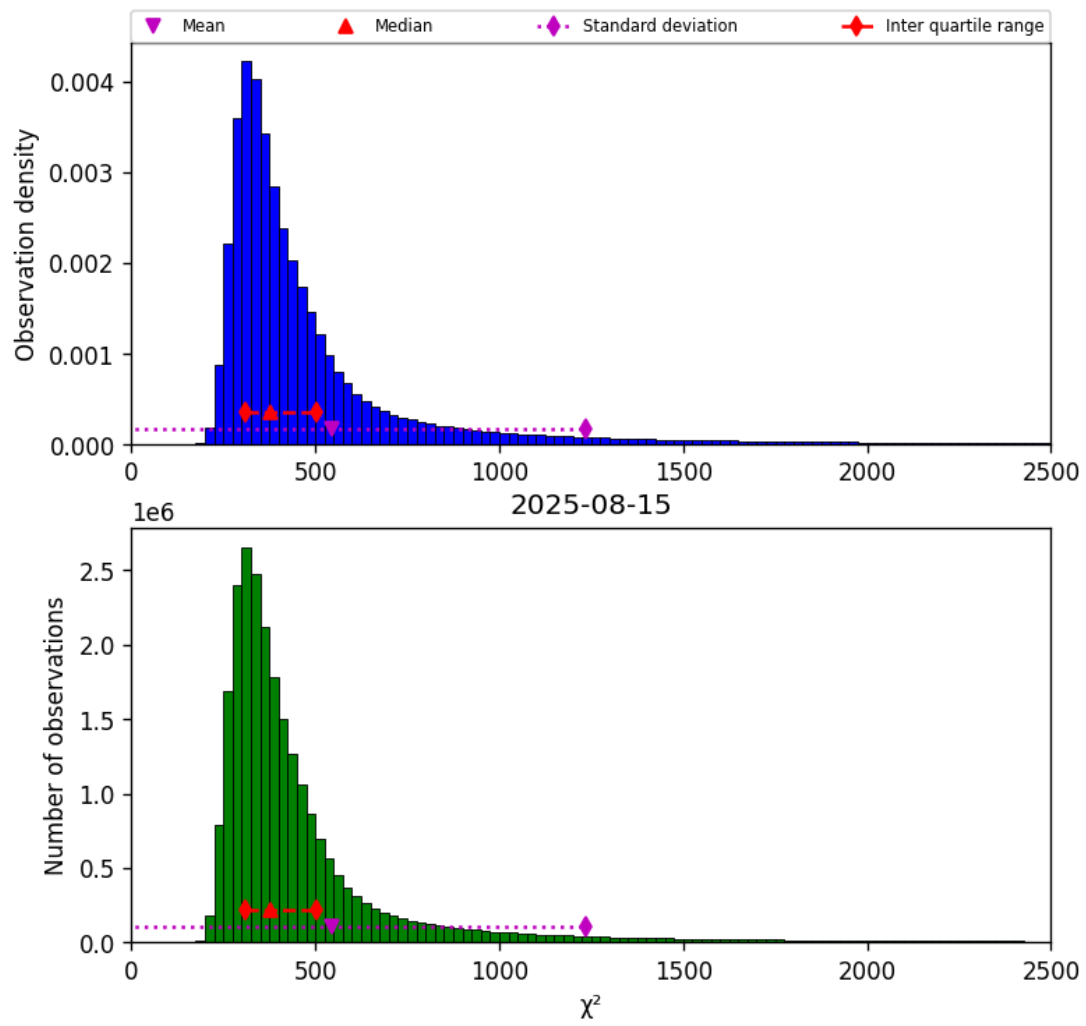
Figure 42: Histogram of " \chi^2 " for 2025-08-14 to 2025-08-16
