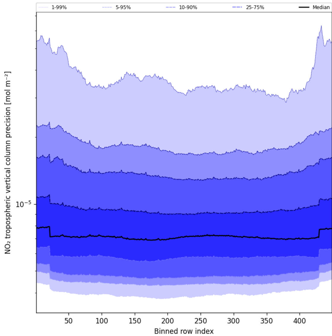
Figure 47: Along track statistics of “NO 2 tropospheric vertical column precision” for 2025-08-14 to 2025-08-16
