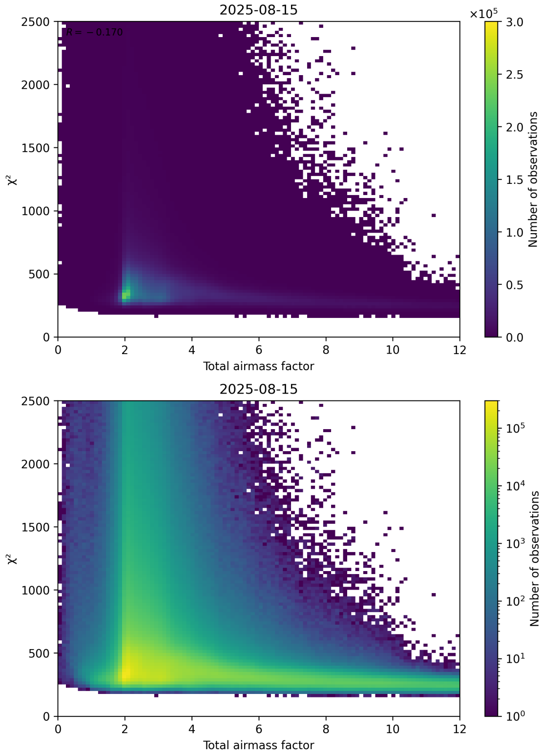
Figure 63: Scatter density plot of “Total airmass factor” against “ \chi^2 ” for 2025-08-14 to 2025-08-16.
