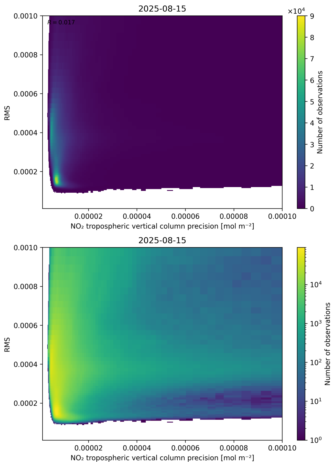
Figure 140: Scatter density plot of “NO 2 tropospheric vertical column precision” against “RMS” for 2025-08-14 to 2025-08-16.
