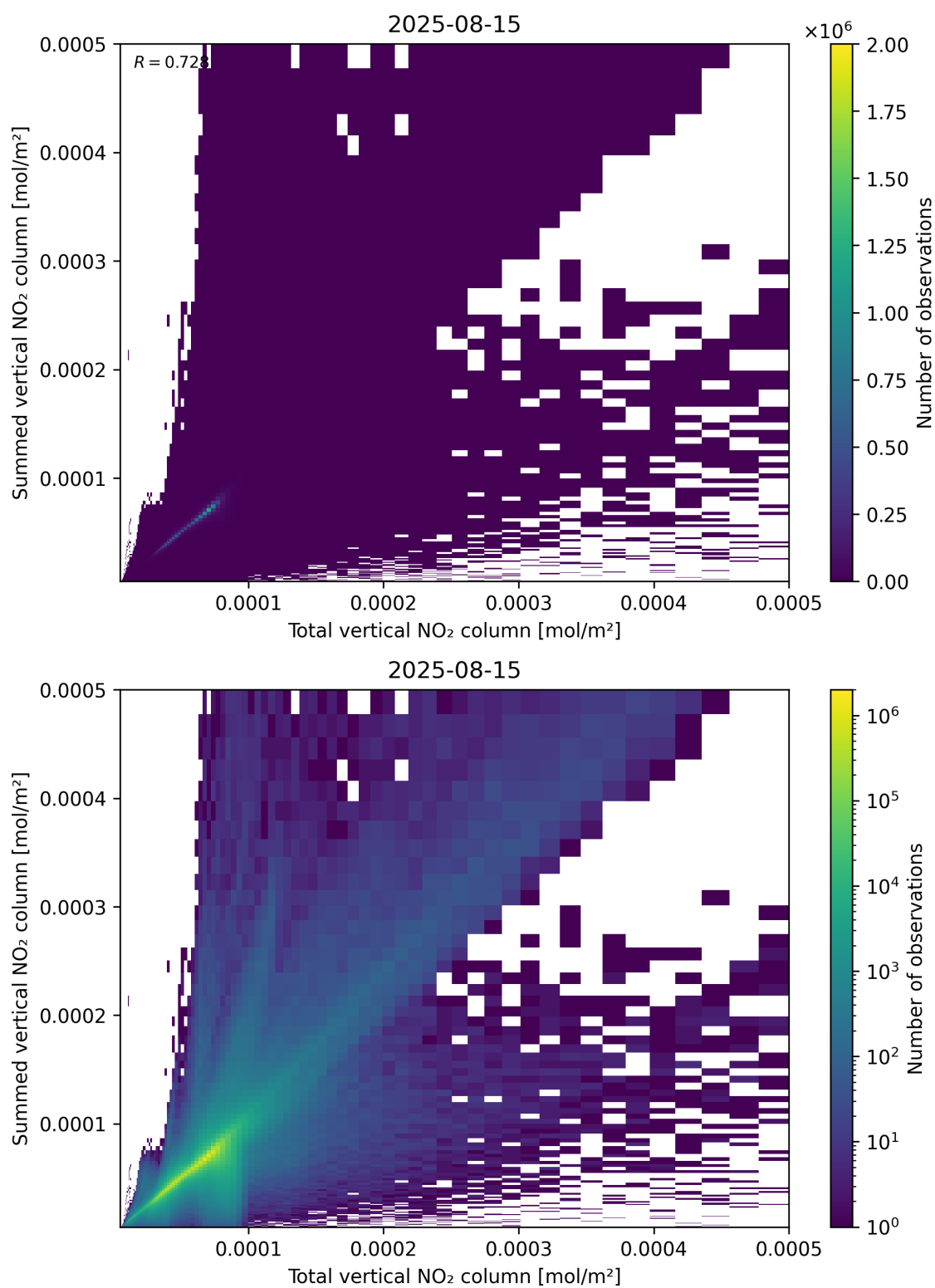
Figure 112: Scatter density plot of “Total vertical NO 2 column” against “Summed vertical NO 2 column” for 2025-08-14 to 2025-08-16.
