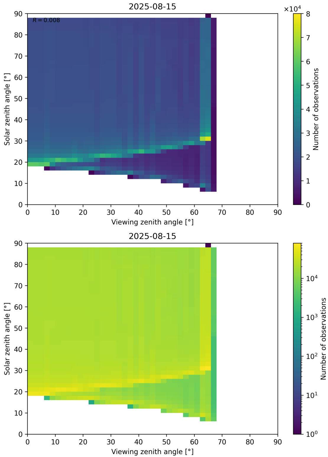
Figure 172: Scatter density plot of “Viewing zenith angle” against “Solar zenith angle” for 2025-08-14 to 2025-08-16.
