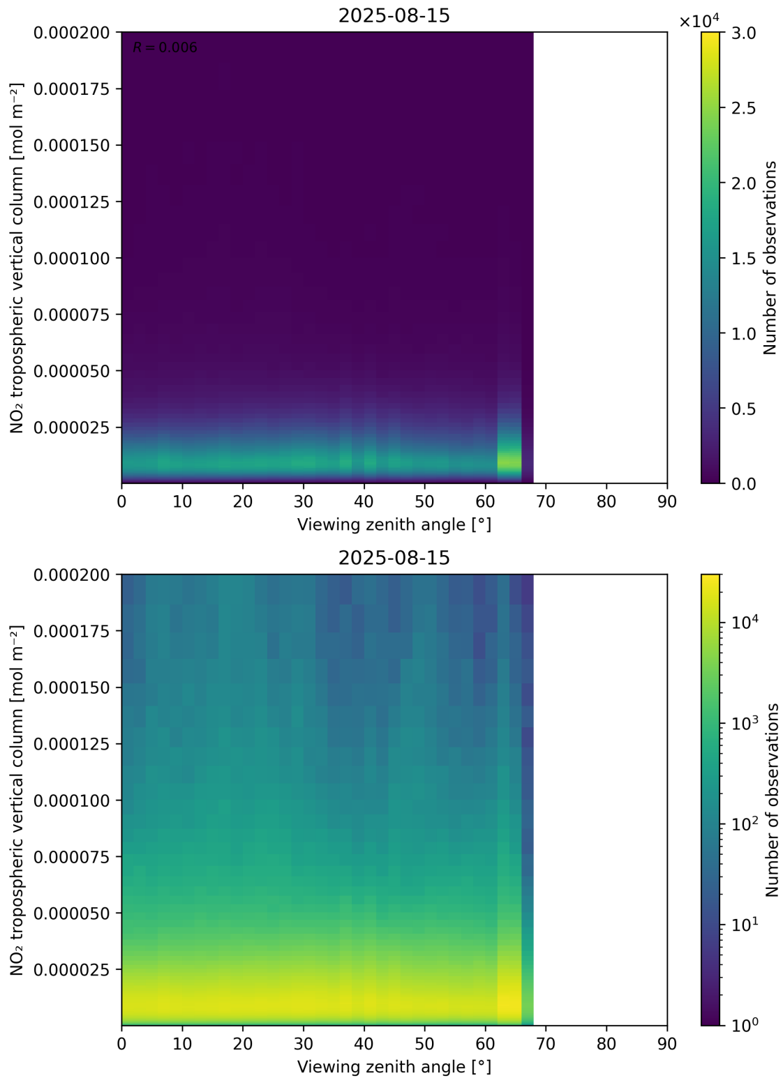
Figure 169: Scatter density plot of “Viewing zenith angle” against “NO 2 tropospheric vertical column” for 2025-08-14 to 2025-08-16.
