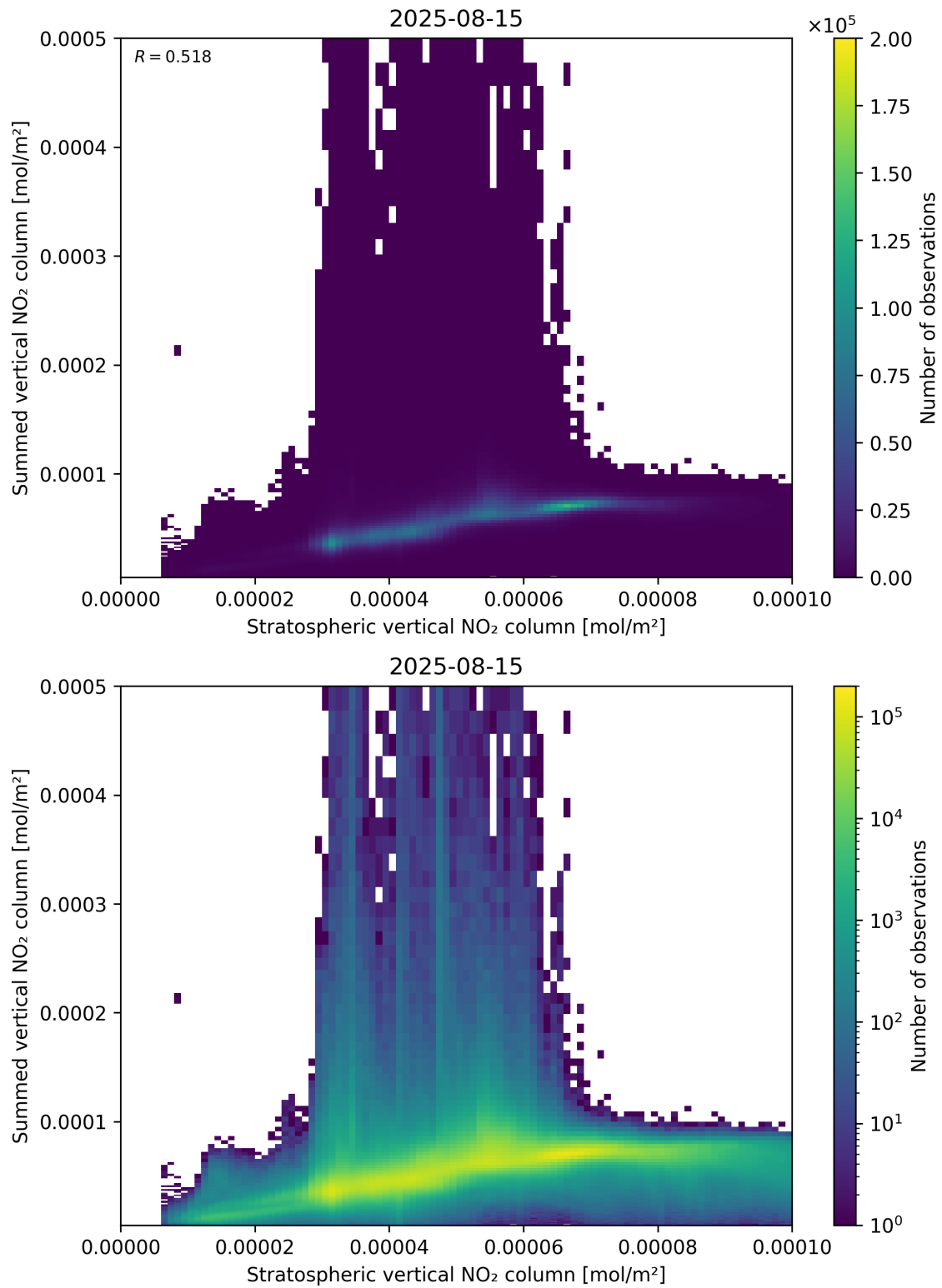
Figure 98: Scatter density plot of “Stratospheric vertical NO 2 column” against “Summed vertical NO 2 column” for 2025-08-14 to 2025-08-16.
