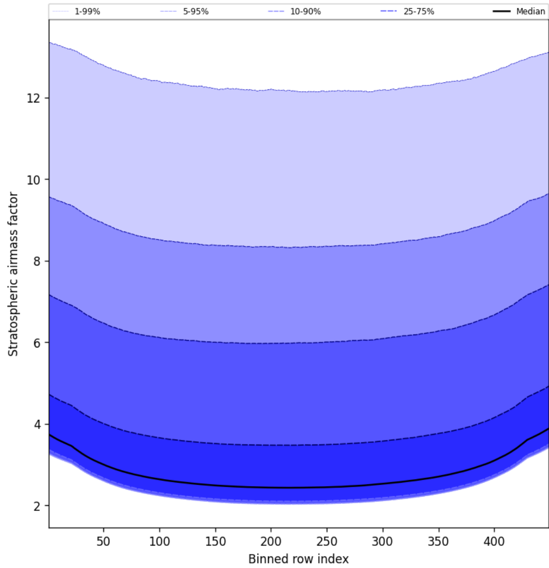
Figure 61: Along track statistics of “Stratospheric airmass factor” for 2025-08-14 to 2025-08-16
