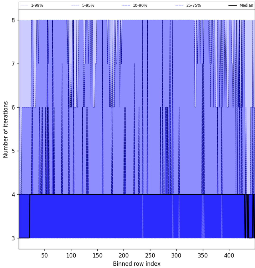
Figure 51: Along track statistics of “Number of iterations” for 2025-08-14 to 2025-08-16
