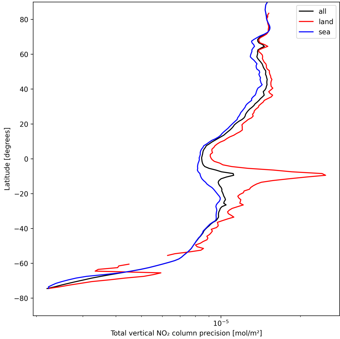
Figure 22: Zonal average of “Total vertical NO 2 column precision” for 2025-08-14 to 2025-08-16.
