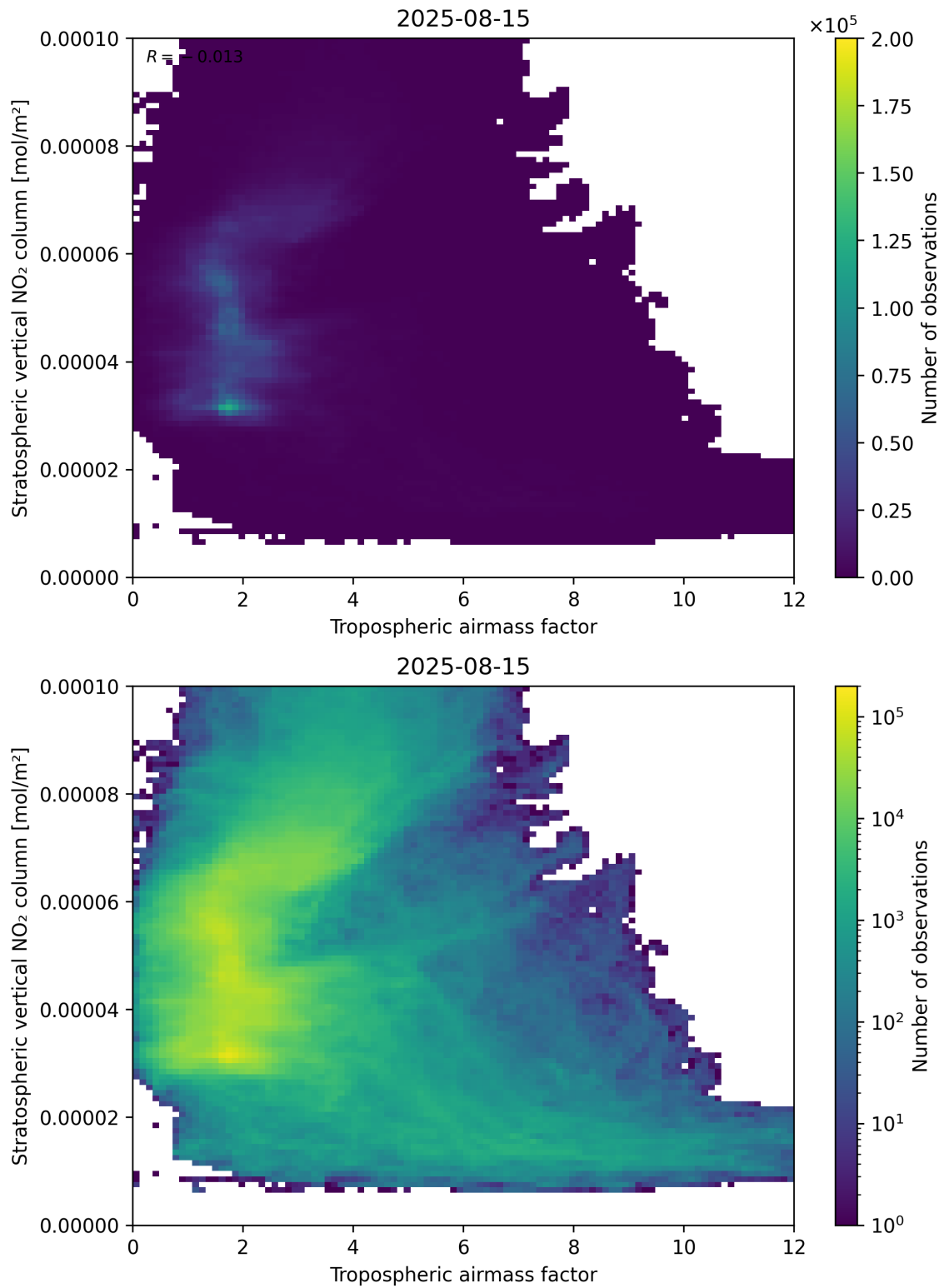
Figure 74: Scatter density plot of “Tropospheric air mass factor” against “Stratospheric vertical NO 2 column” for 2025-08-14 to 2025-08-16.
