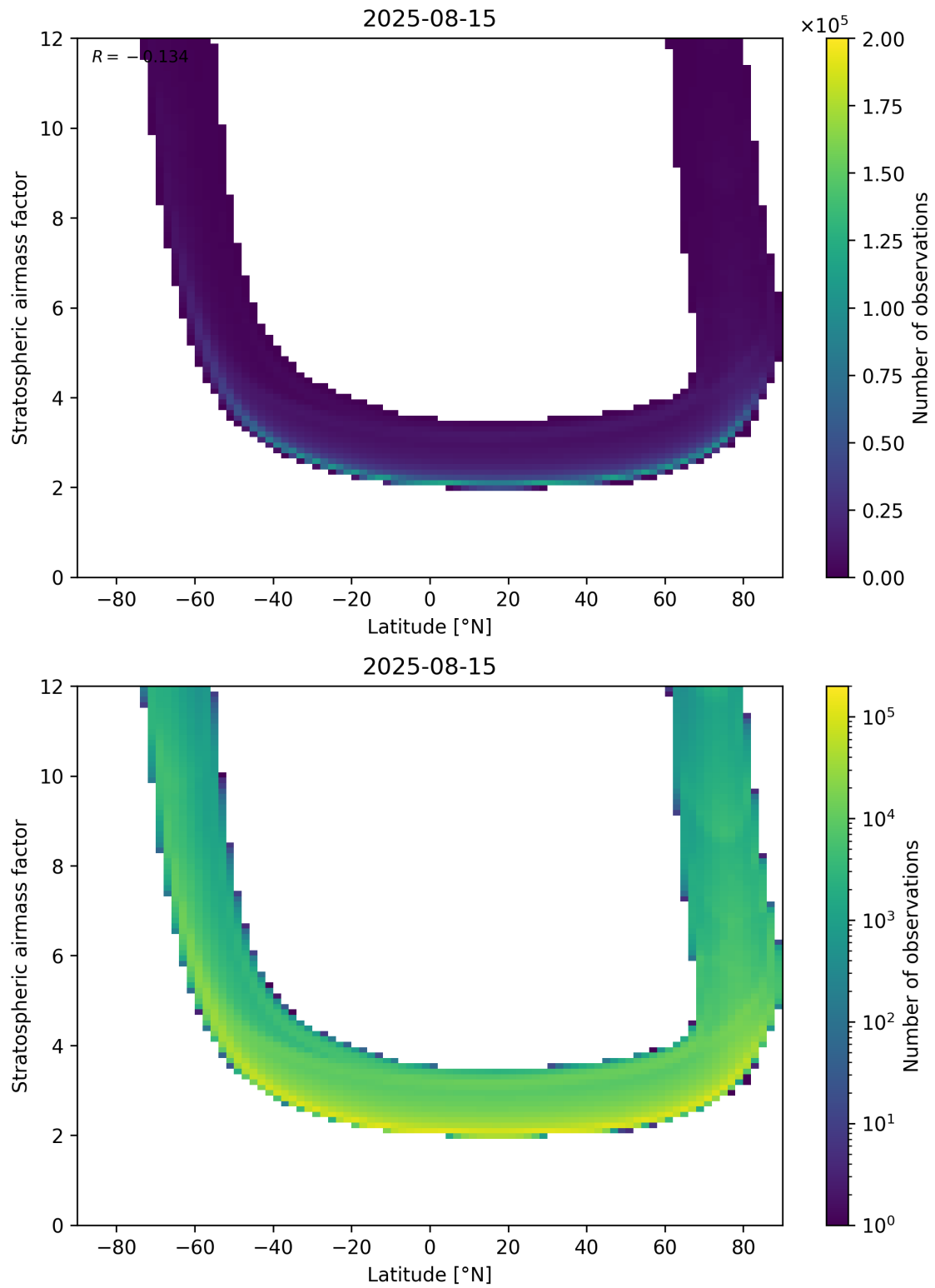
Figure 83: Scatter density plot of “Latitude” against “Stratospheric air mass factor” for 2025-08-14 to 2025-08-16.
