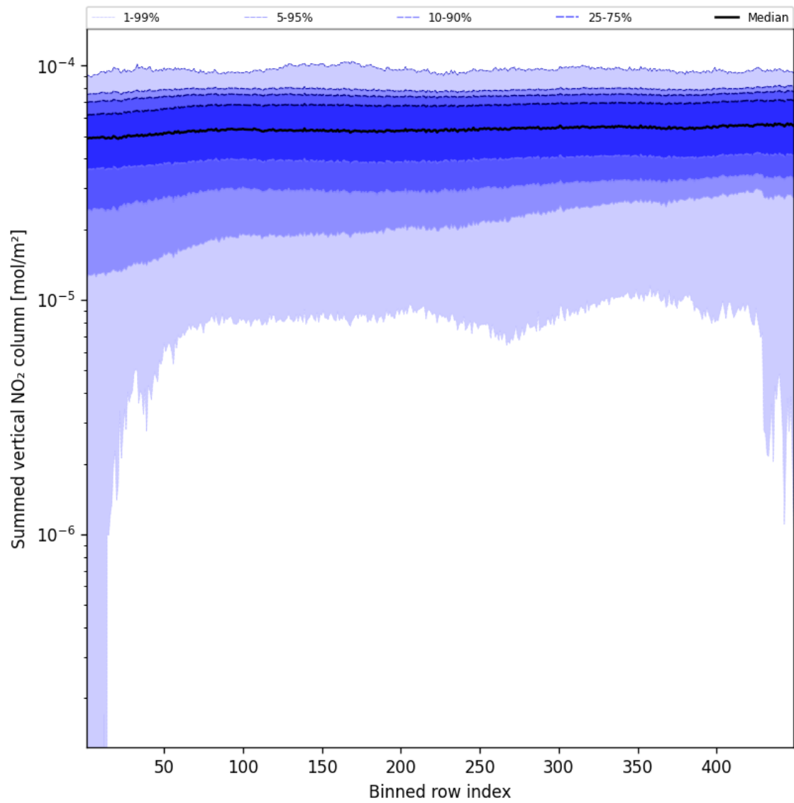
Figure 57: Along track statistics of “Summed vertical NO 2 column” for 2025-08-14 to 2025-08-16
