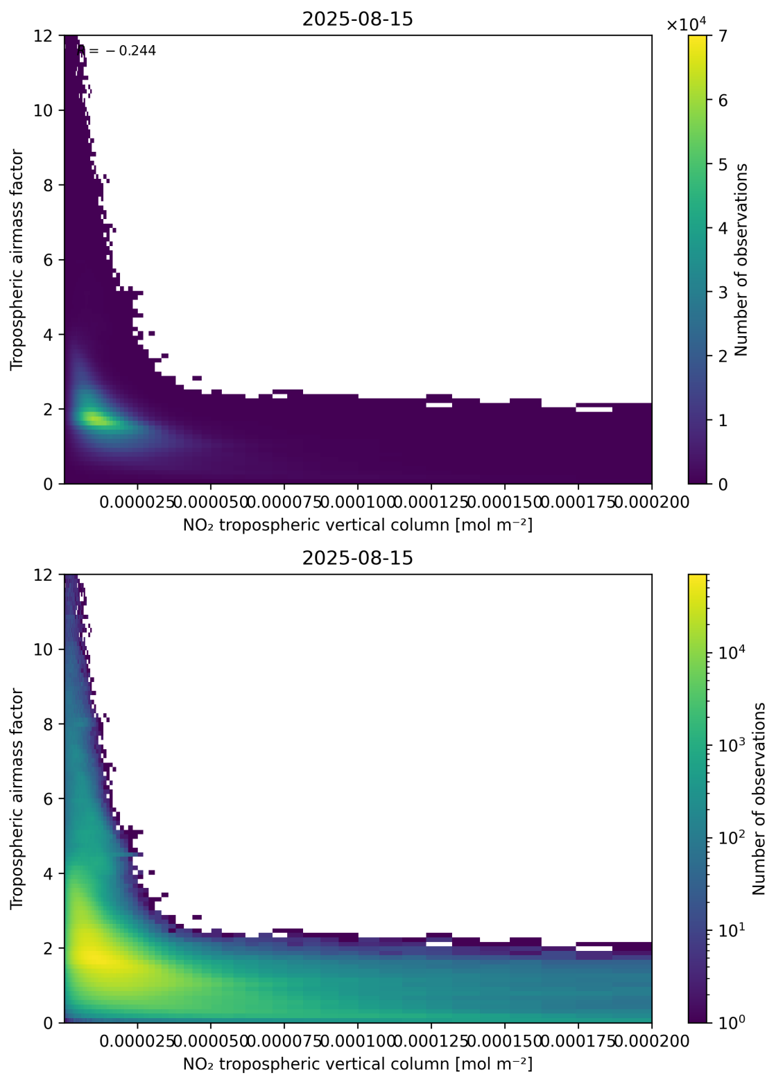
Figure 123: Scatter density plot of “NO 2 tropospheric vertical column” against “Tropospheric air mass factor” for 2025-08-14 to 2025-08-16.
