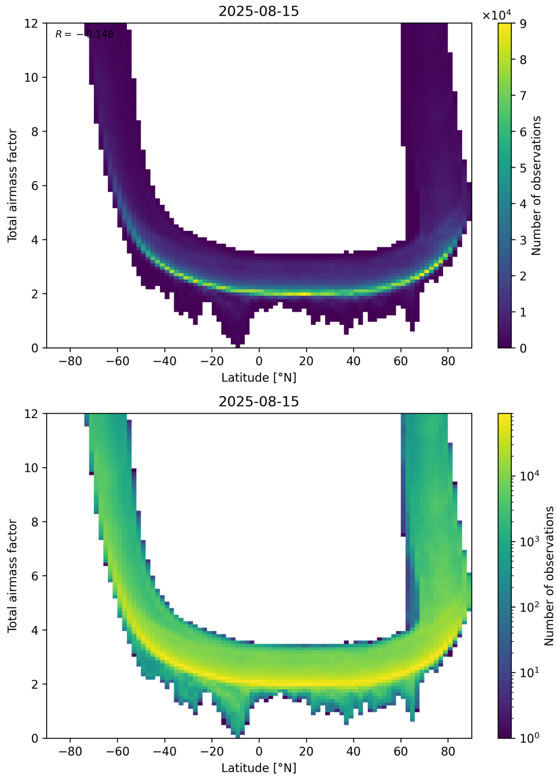
Figure 84: Scatter density plot of “Latitude” against “Total airmass factor” for 2025-08-14 to 2025-08-16.
