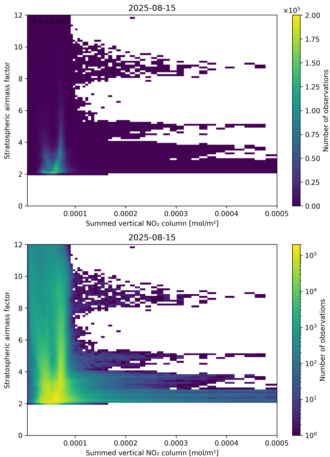
Figure 103: Scatter density plot of “Summed vertical NO 2 column” against “Stratospheric airmass factor” for 2025-08-14 to 2025-08-16.
