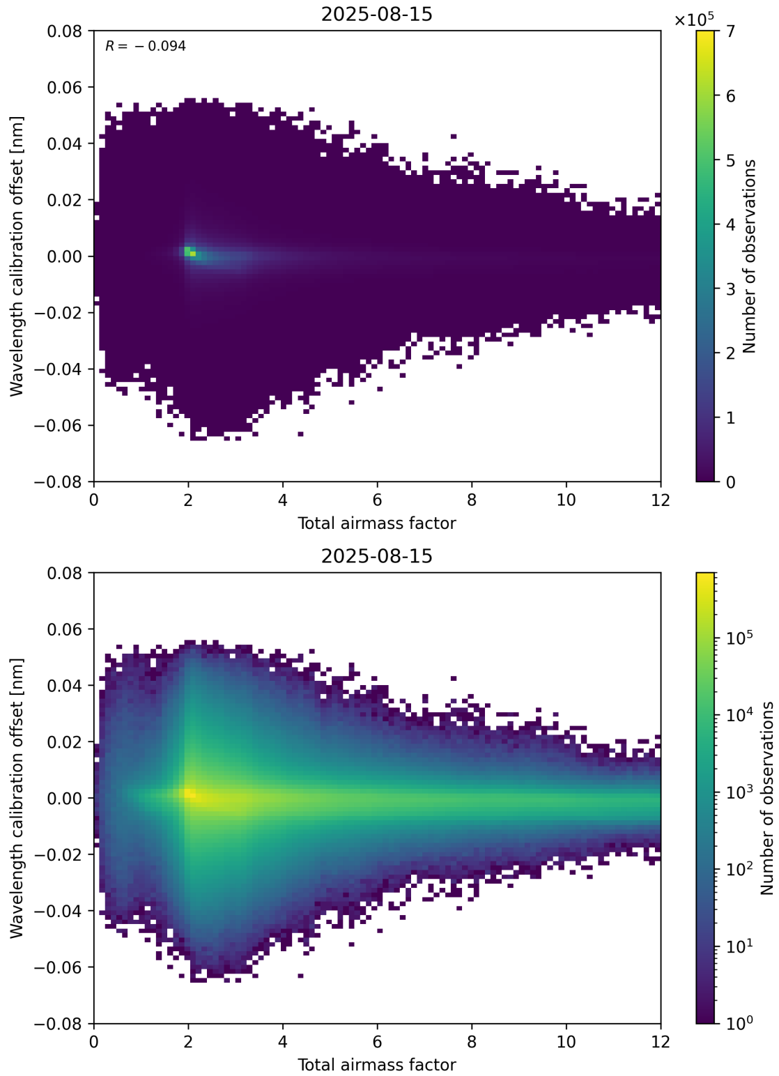
Figure 70: Scatter density plot of “Total airmass factor” against “Wavelength calibration offset” for 2025-08-14 to 2025-08-16.
