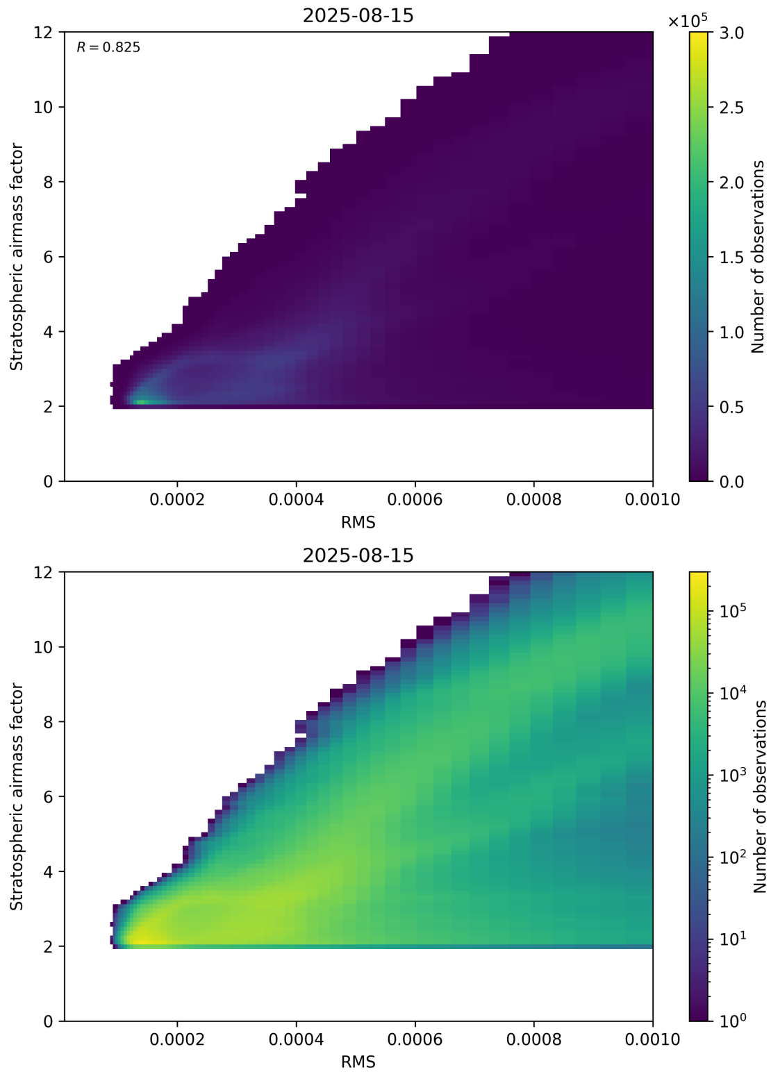
Figure 144: Scatter density plot of “RMS” against “Stratospheric airmass factor” for 2025-08-14 to 2025-08-16.
