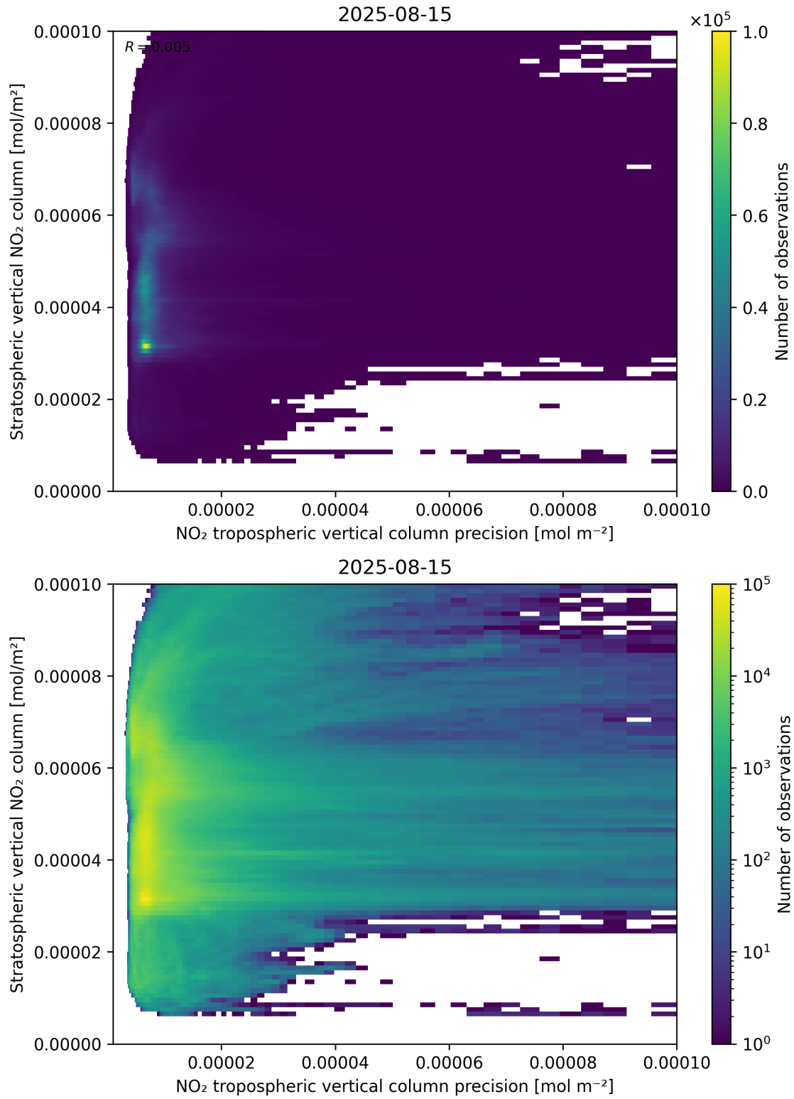
Figure 135: Scatter density plot of “NO 2 tropospheric vertical column precision” against “Stratospheric vertical NO 2 column” for 2025-08-14 to 2025-08-16.
