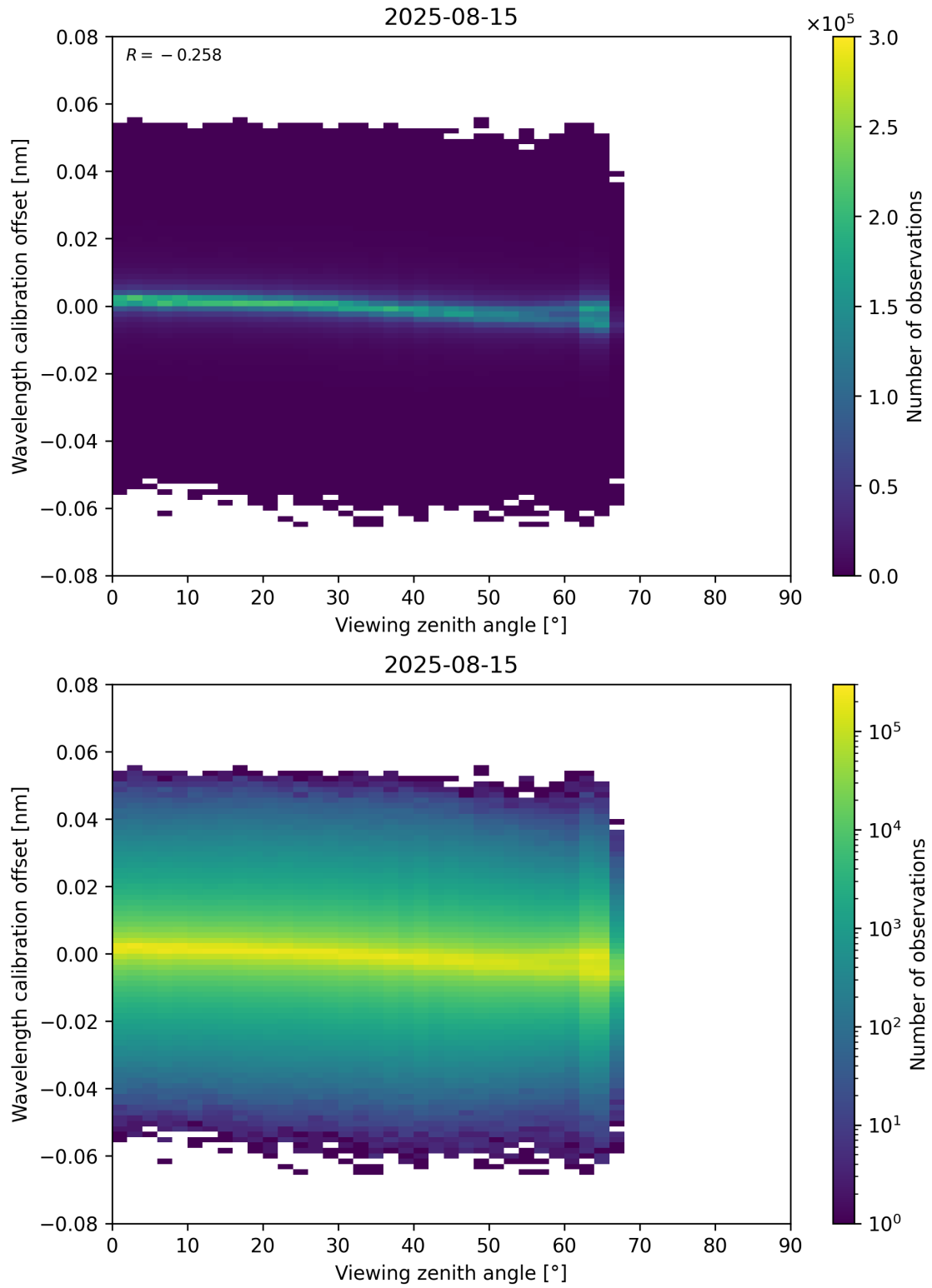
Figure 173: Scatter density plot of “Viewing zenith angle” against “Wavelength calibration offset” for 2025-08-14 to 2025-08-16.
