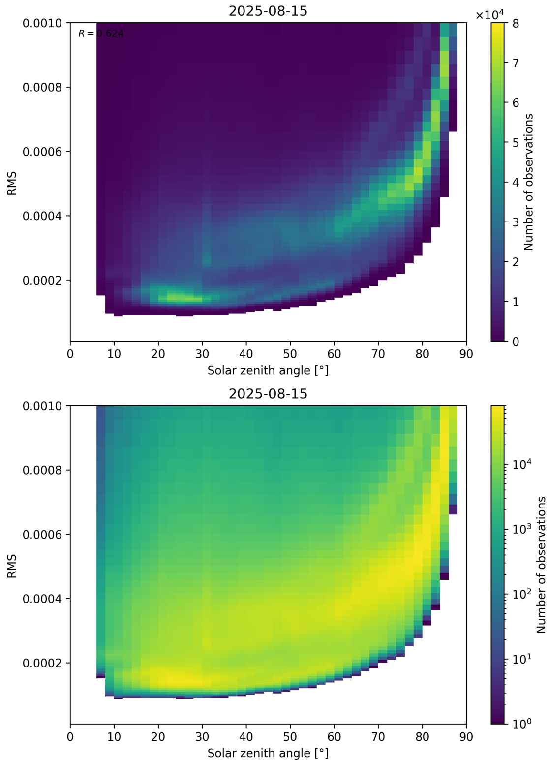
Figure 157: Scatter density plot of “Solar zenith angle” against “RMS” for 2025-08-14 to 2025-08-16.
