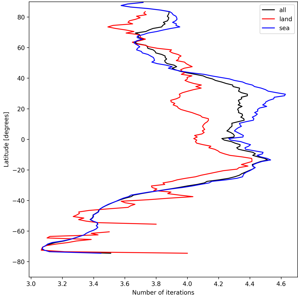
Figure 17: Zonal average of “Number of iterations” for 2025-08-14 to 2025-08-16.
