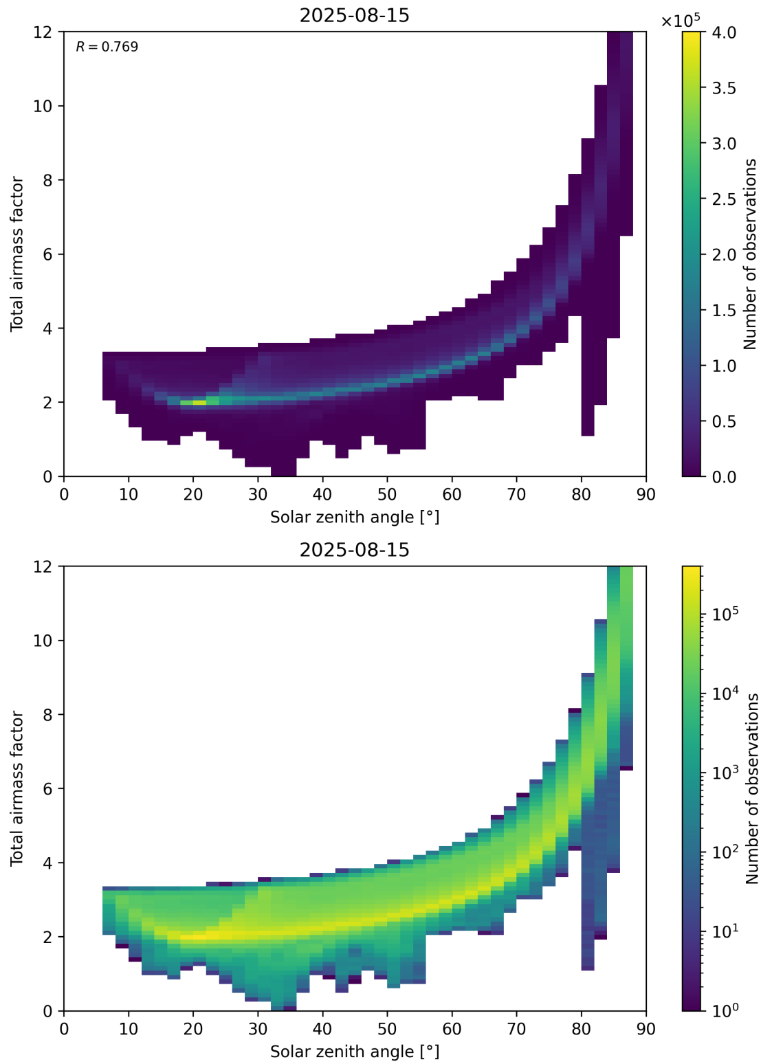
Figure 146: Scatter density plot of “Solar zenith angle” against “Total air mass factor” for 2025-08-14 to 2025-08-16.
