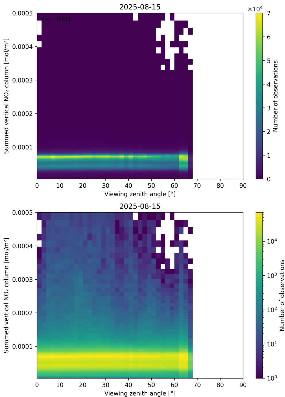
Figure 165: Scatter density plot of “Viewing zenith angle” against “Summed vertical NO 2 column” for 2025-08-14 to 2025-08-16.
