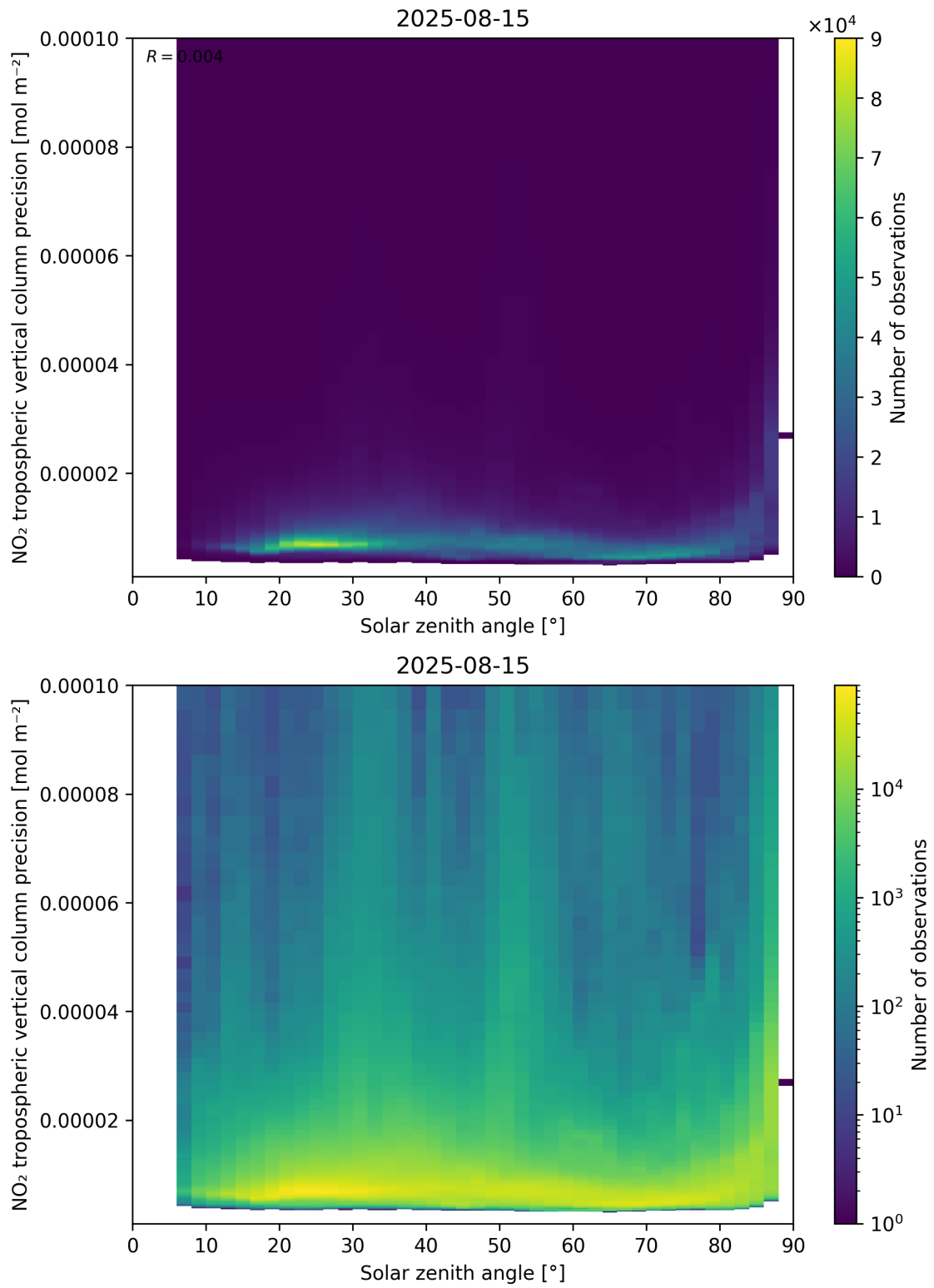
Figure 156: Scatter density plot of “Solar zenith angle” against “NO 2 tropospheric vertical column precision” for 2025-08-14 to 2025-08-16.
