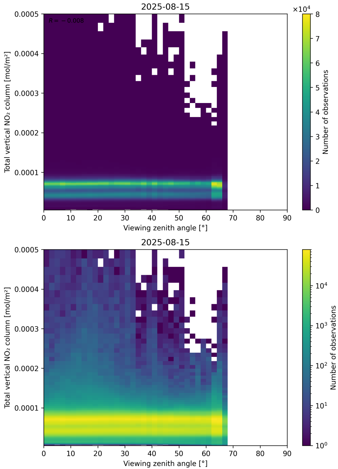
Figure 167: Scatter density plot of “Viewing zenith angle” against “Total vertical NO 2 column” for 2025-08-14 to 2025-08-16.
