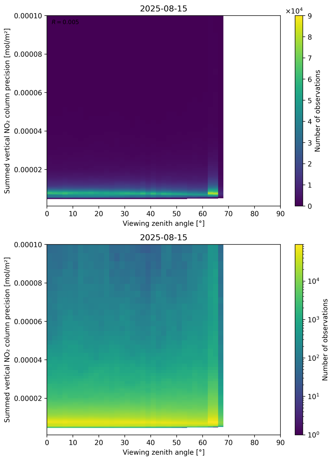
Figure 166: Scatter density plot of “Viewing zenith angle” against “Summed vertical NO 2 column precision” for 2025-08-14 to 2025-08-16.
