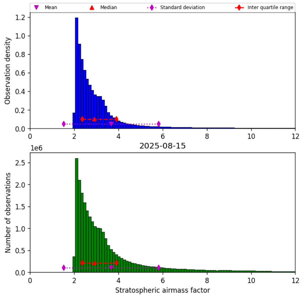
Figure 44: Histogram of “Stratospheric airmass factor” for 2025-08-14 to 2025-08-16
