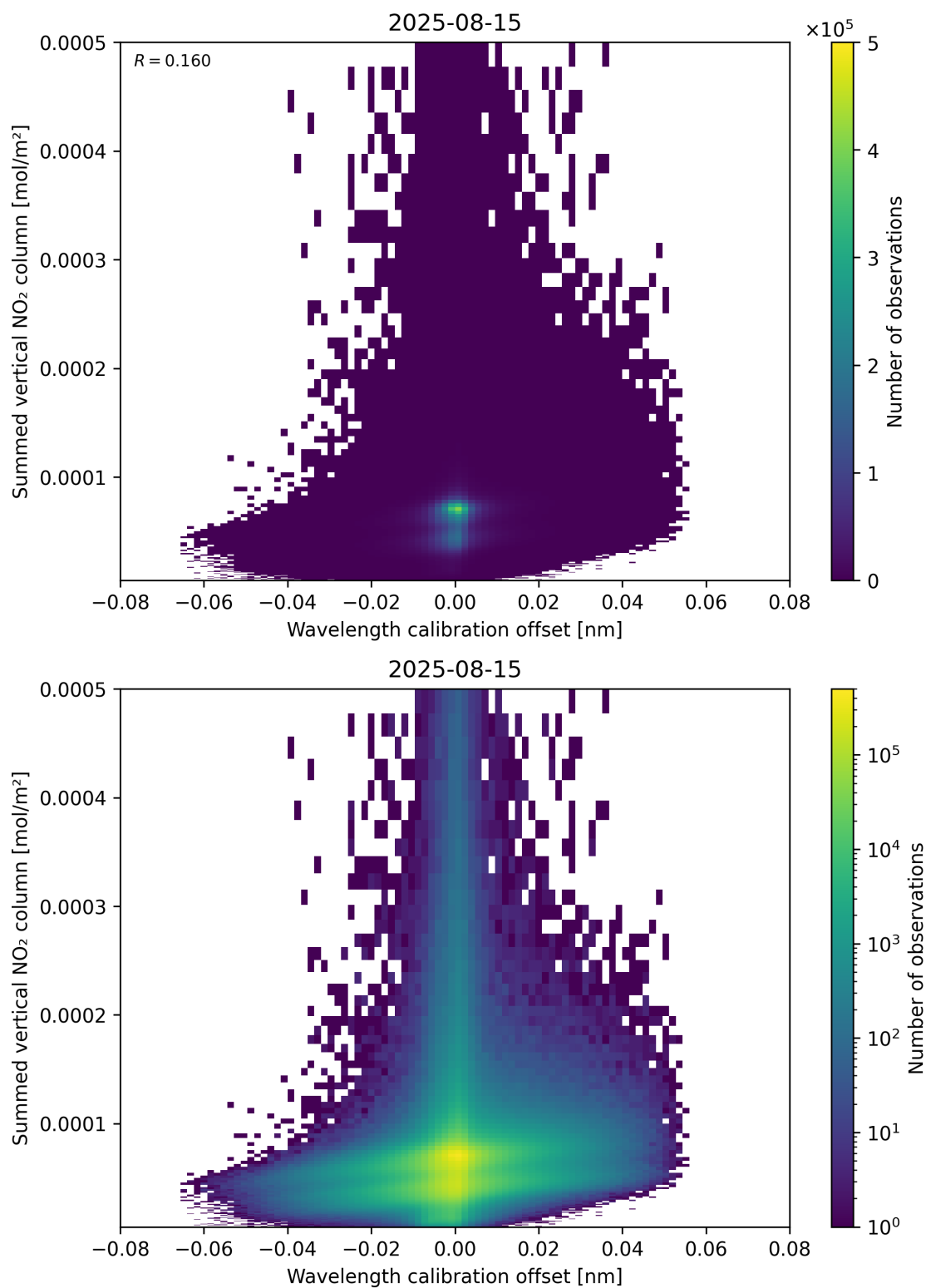
Figure 177: Scatter density plot of “Wavelength calibration offset” against “Summed vertical NO 2 column” for 2025-08-14 to 2025-08-16.
