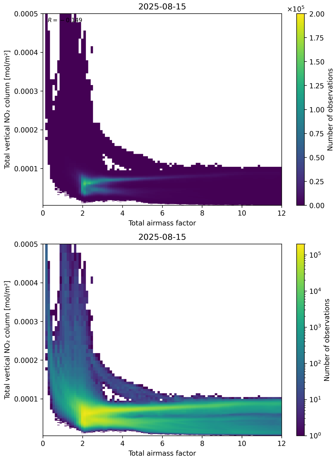
Figure 67: Scatter density plot of “Total airmass factor” against “Total vertical NO 2 column” for 2025-08-14 to 2025-08-16.
