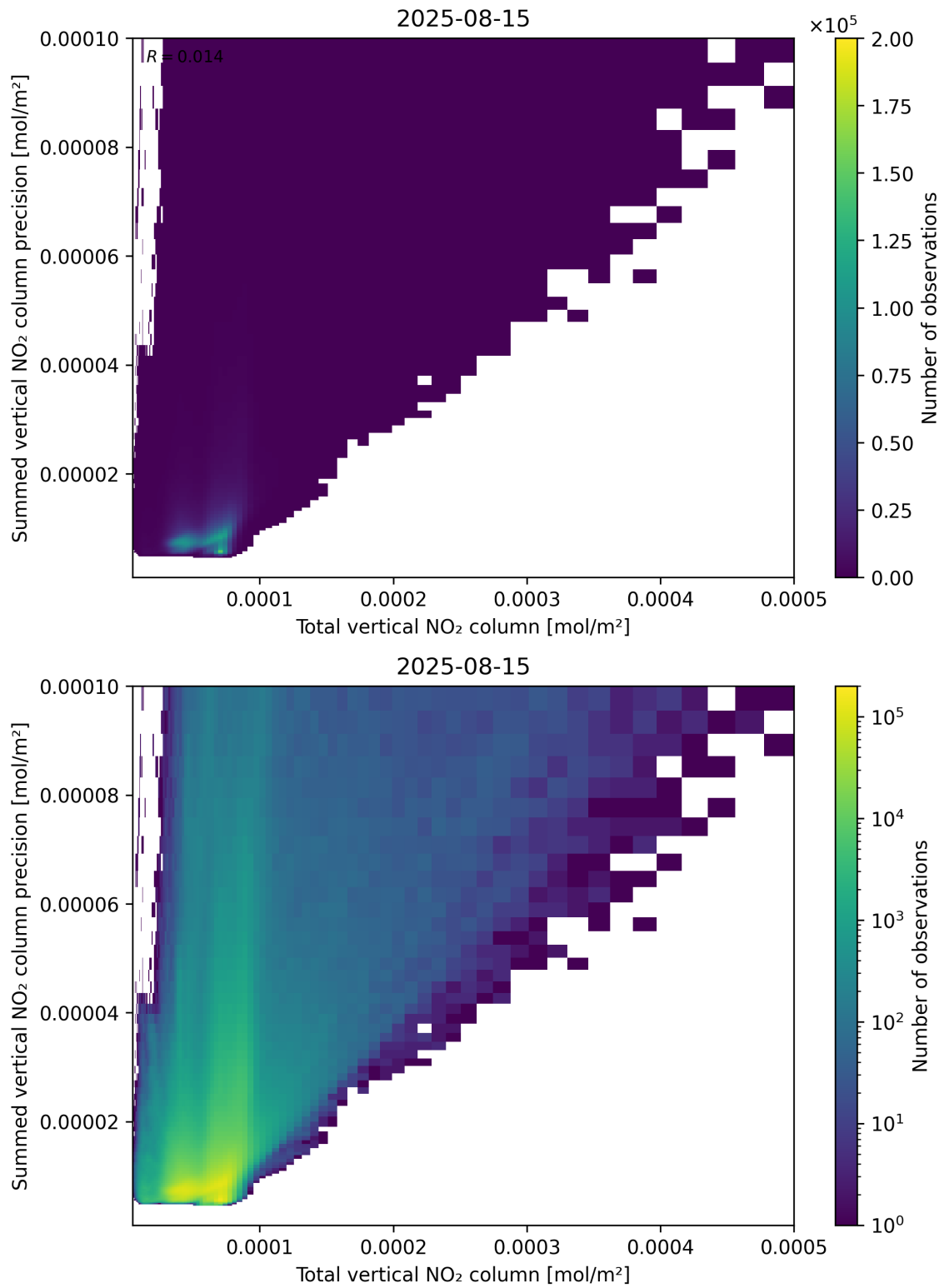
Figure 113: Scatter density plot of “Total vertical NO 2 column” against “Summed vertical NO 2 column precision” for 2025-08-14 to 2025-08-16.
