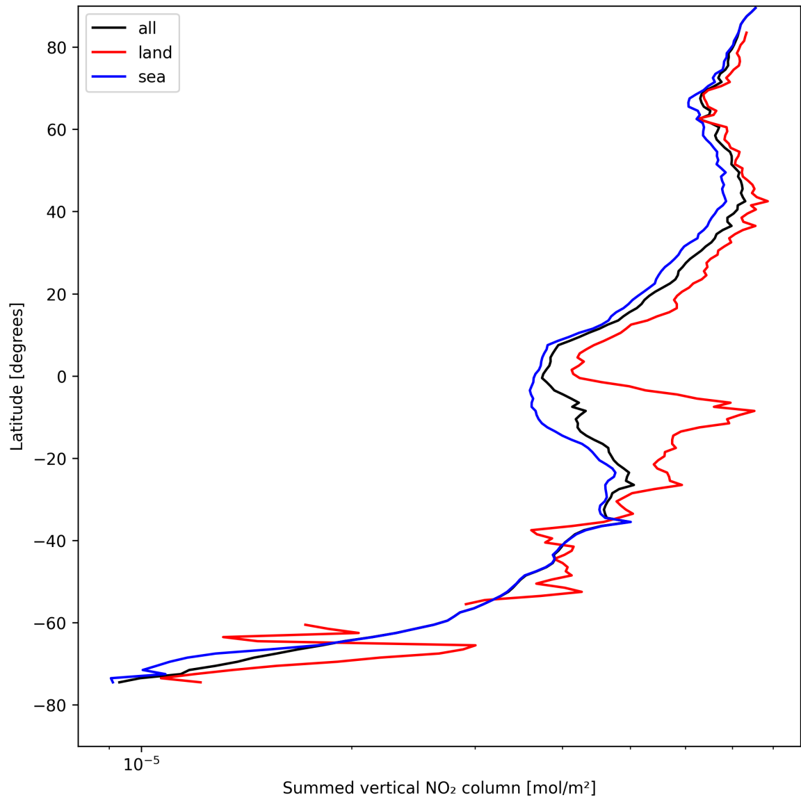
Figure 23: Zonal average of “Summed vertical NO 2 column” for 2025-08-14 to 2025-08-16.
