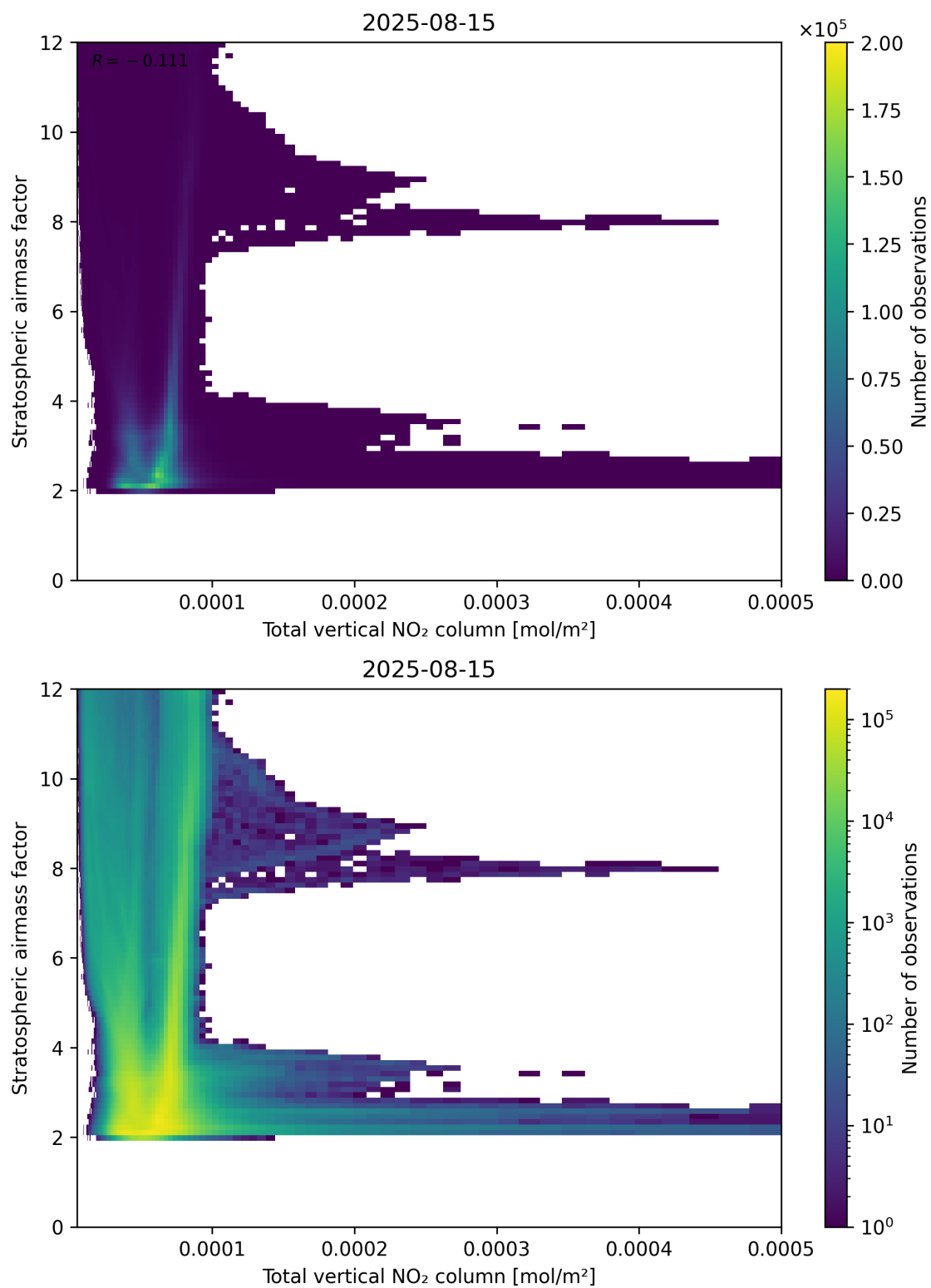
Figure 110: Scatter density plot of “Total vertical NO 2 column” against “Stratospheric airmass factor” for 2025-08-14 to 2025-08-16.
