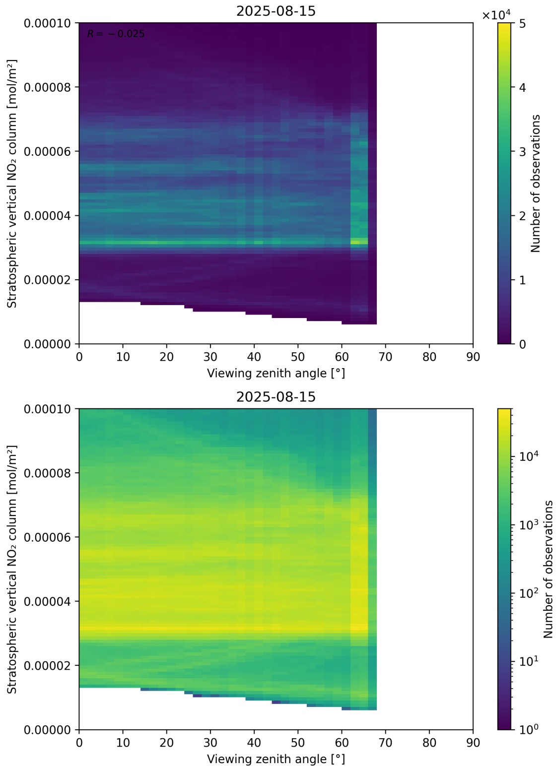
Figure 164: Scatter density plot of “Viewing zenith angle” against “Stratospheric vertical NO 2 column” for 2025-08-14 to 2025-08-16.
