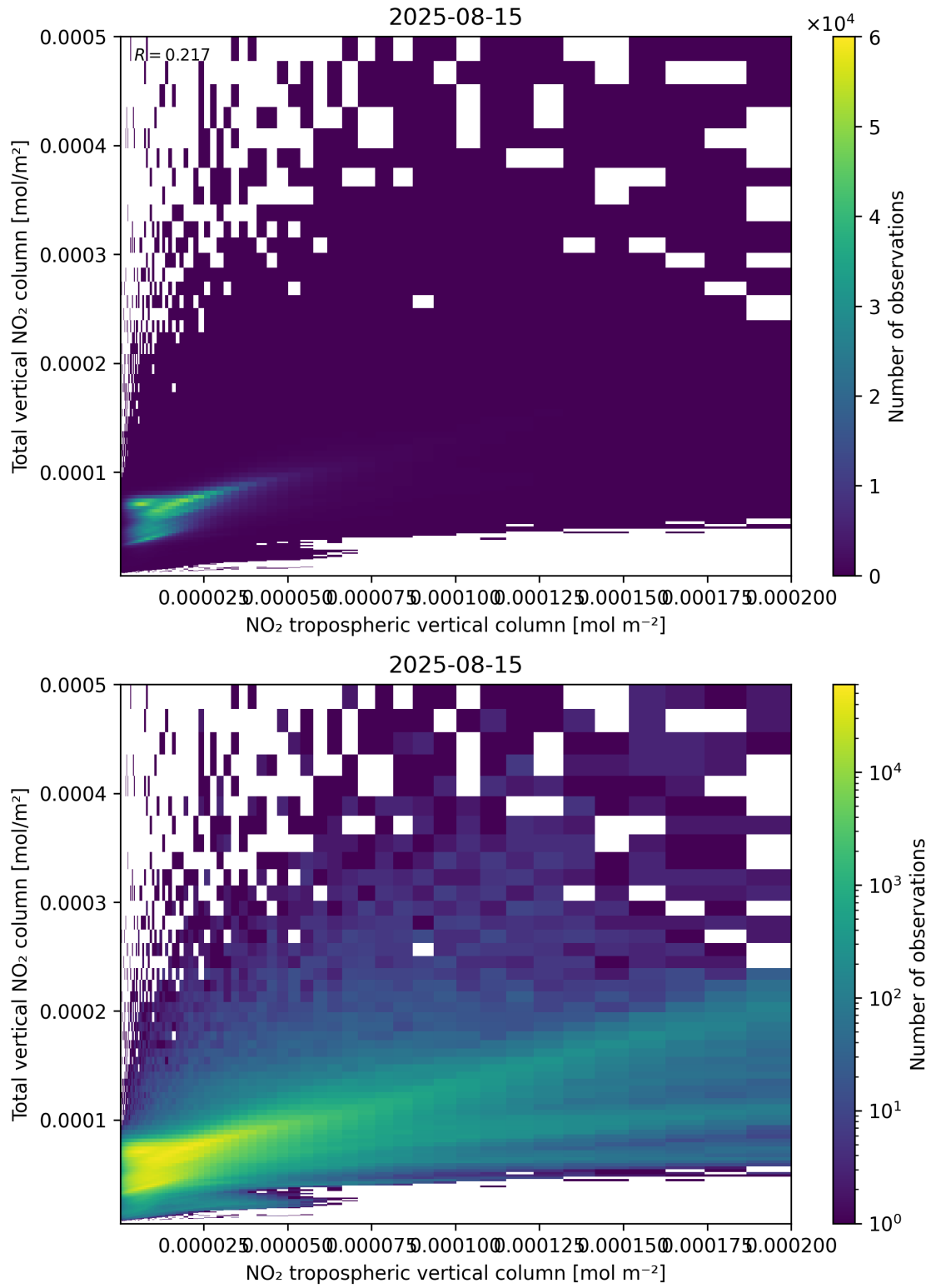
Figure 128: Scatter density plot of “NO 2 tropospheric vertical column” against “Total vertical NO 2 column” for 2025-08-14 to 2025-08-16.
