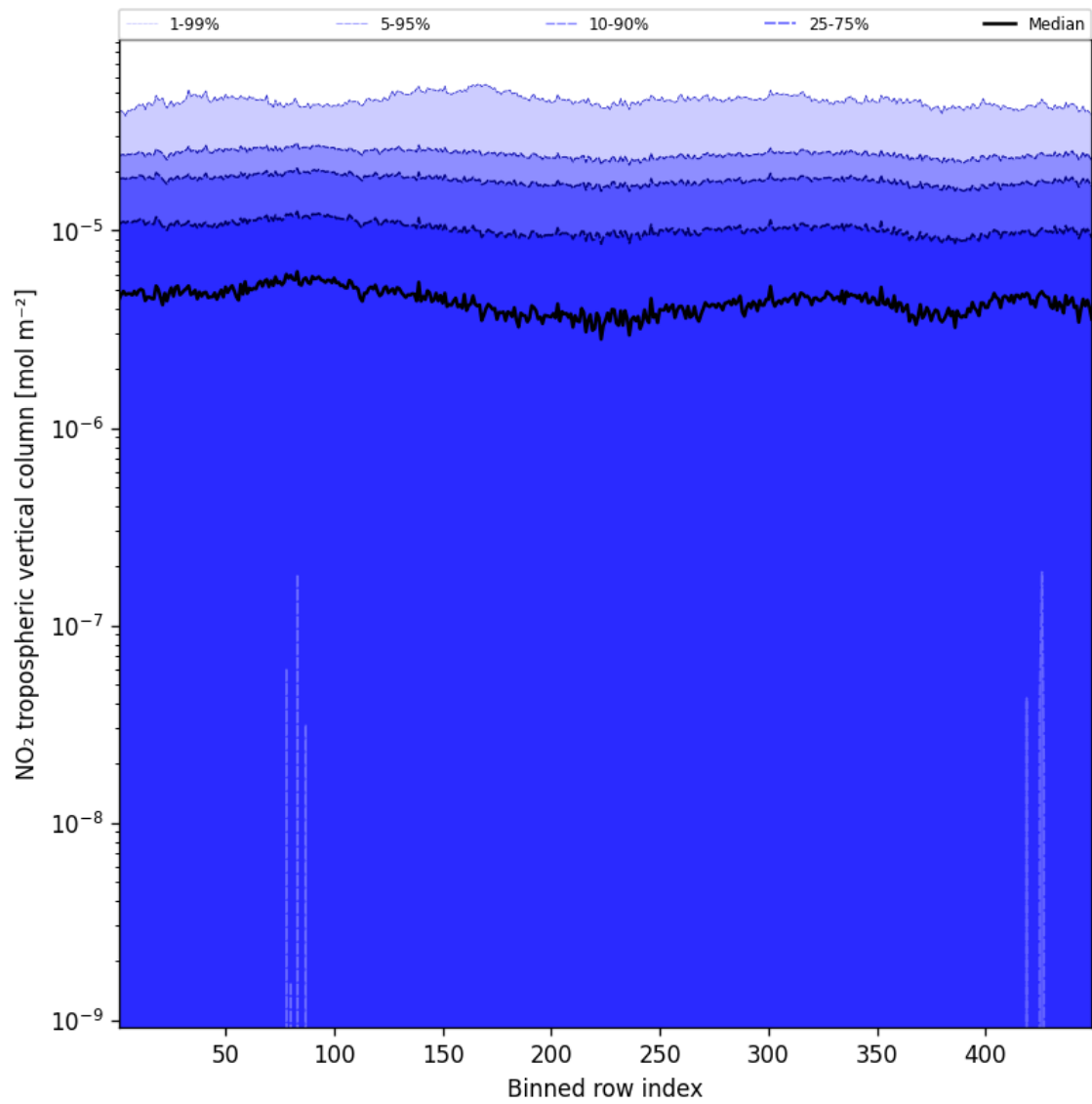
Figure 46: Along track statistics of "NO 2 tropospheric vertical column" for 2025-08-14 to 2025-08-16
