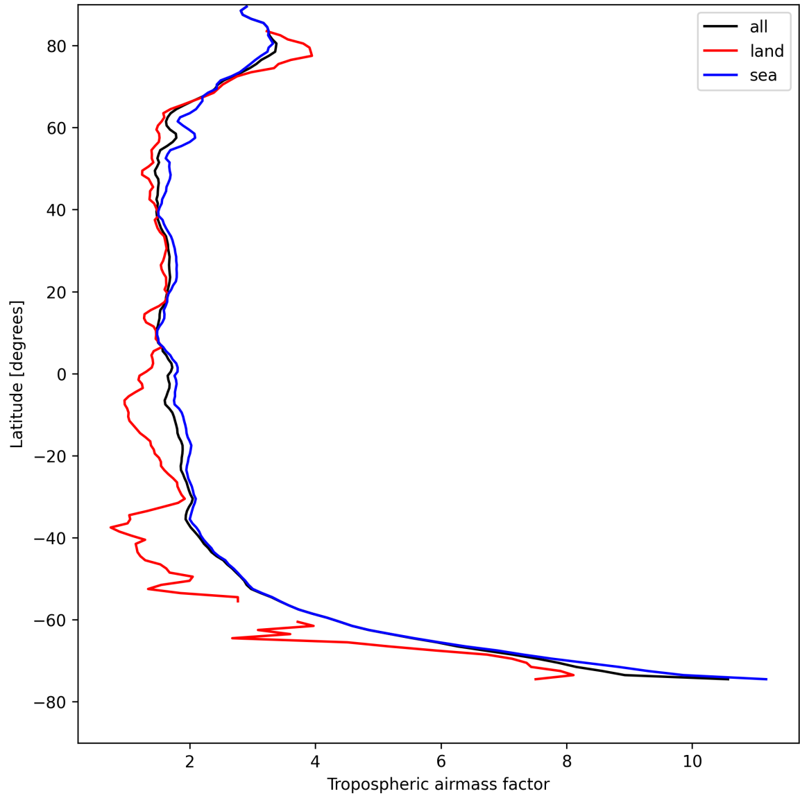
Figure 14: Zonal average of “Tropospheric airmass factor” for 2025-08-14 to 2025-08-16.
