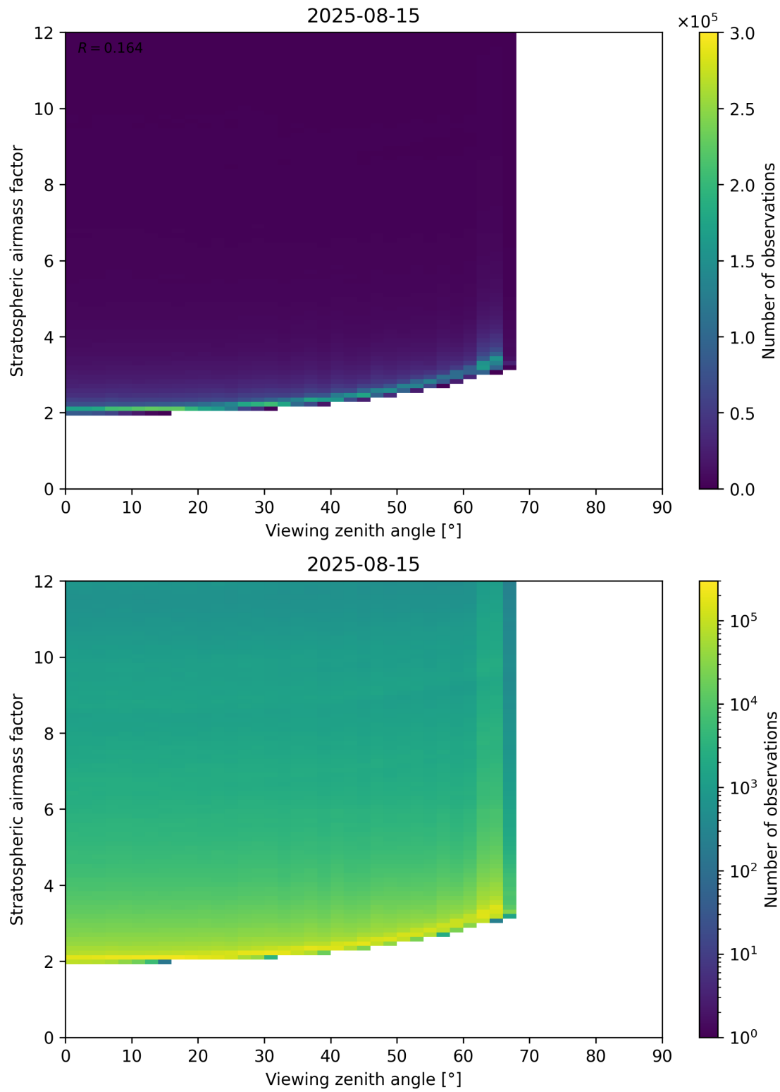
Figure 159: Scatter density plot of “Viewing zenith angle” against “Stratospheric airmass factor” for 2025-08-14 to 2025-08-16.
