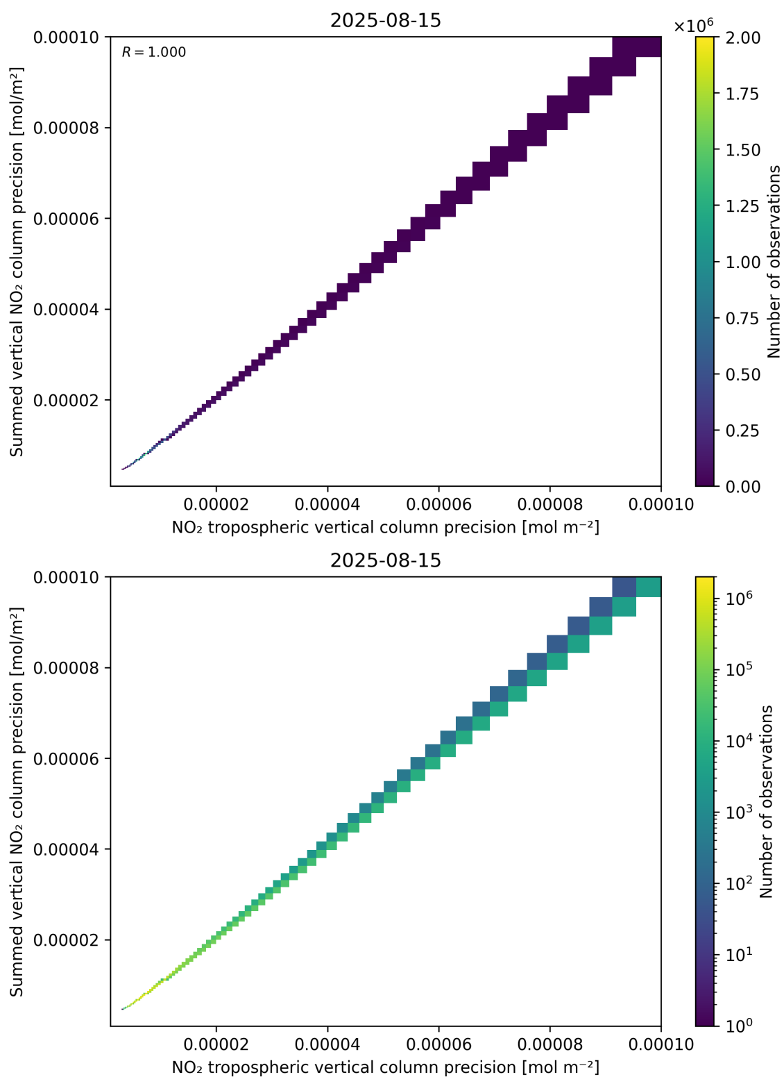
Figure 137: Scatter density plot of “NO 2 tropospheric vertical column precision” against “Summed vertical NO 2 column precision” for 2025-08-14 to 2025-08-16.
