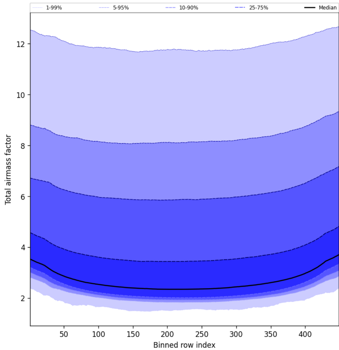
Figure 49: Along track statistics of “Total airmass factor” for 2025-08-14 to 2025-08-16
