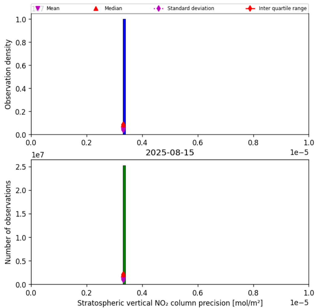
Figure 37: Histogram of “Stratospheric vertical NO 2 column precision” for 2025-08-14 to 2025-08-16
