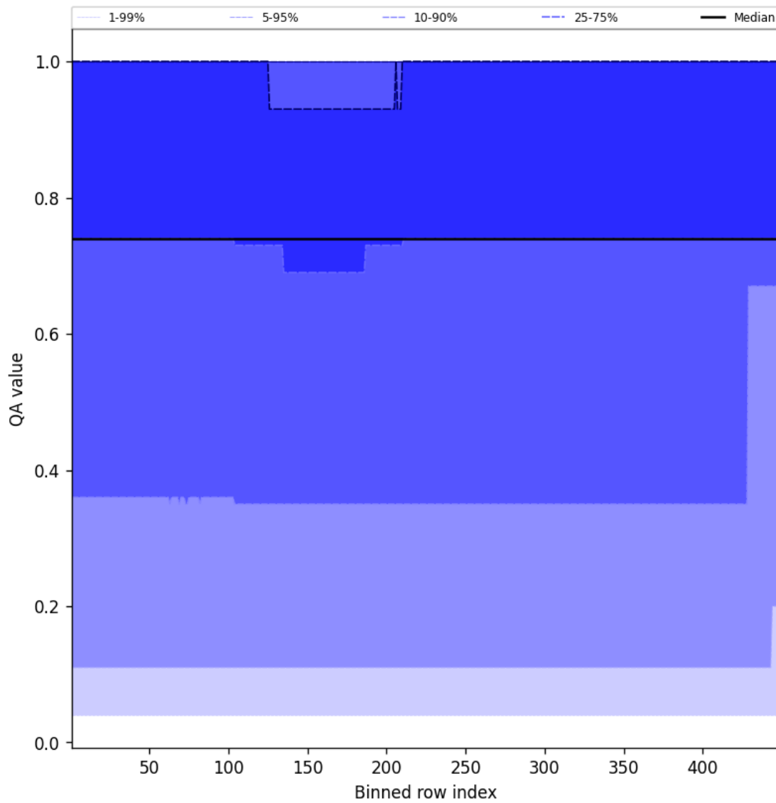
Figure 45: Along track statistics of “QA value” for 2025-08-14 to 2025-08-16
