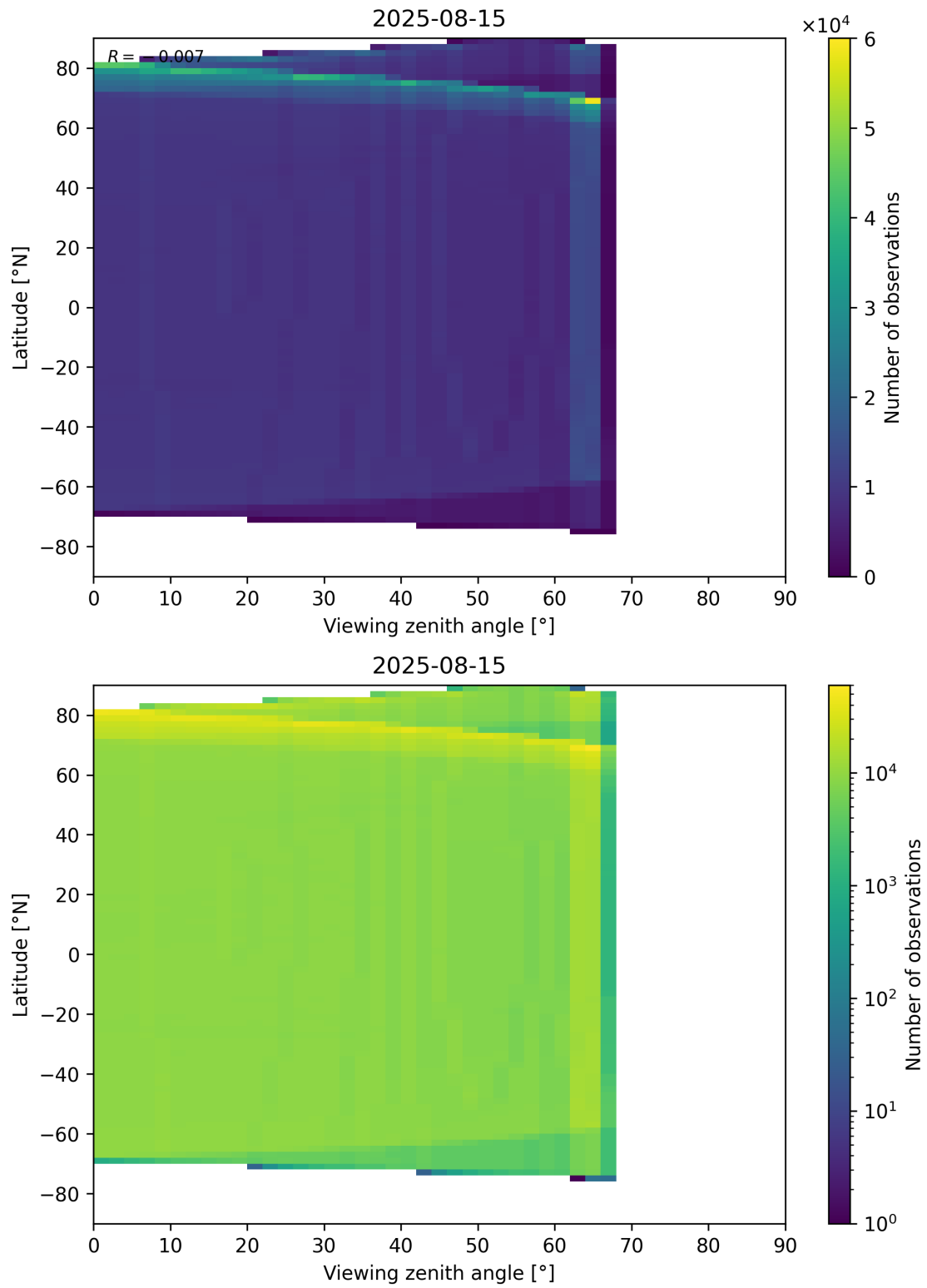
Figure 163: Scatter density plot of “Viewing zenith angle” against “Latitude” for 2025-08-14 to 2025-08-16.
