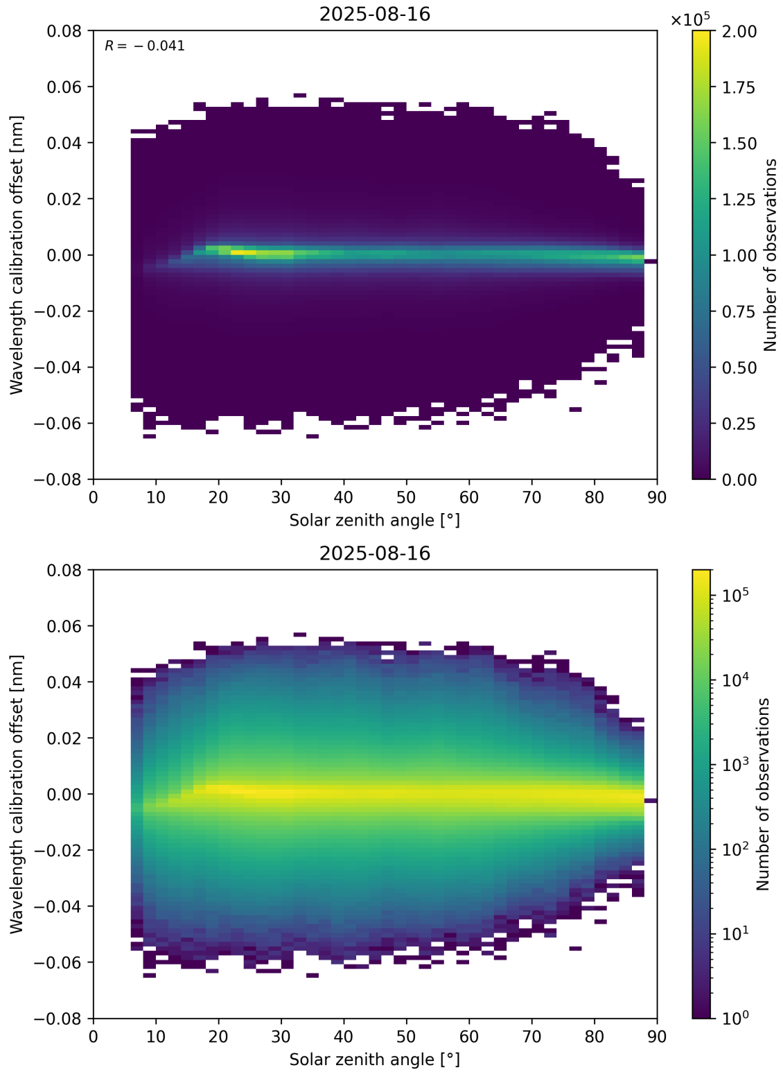
Figure 158: Scatter density plot of “Solar zenith angle” against “Wavelength calibration offset” for 2025-08-15 to 2025-08-17.
