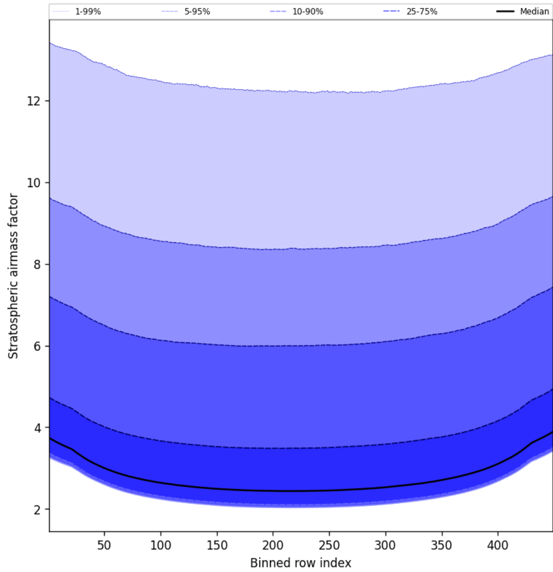
Figure 61: Along track statistics of “Stratospheric airmass factor” for 2025-08-15 to 2025-08-17
