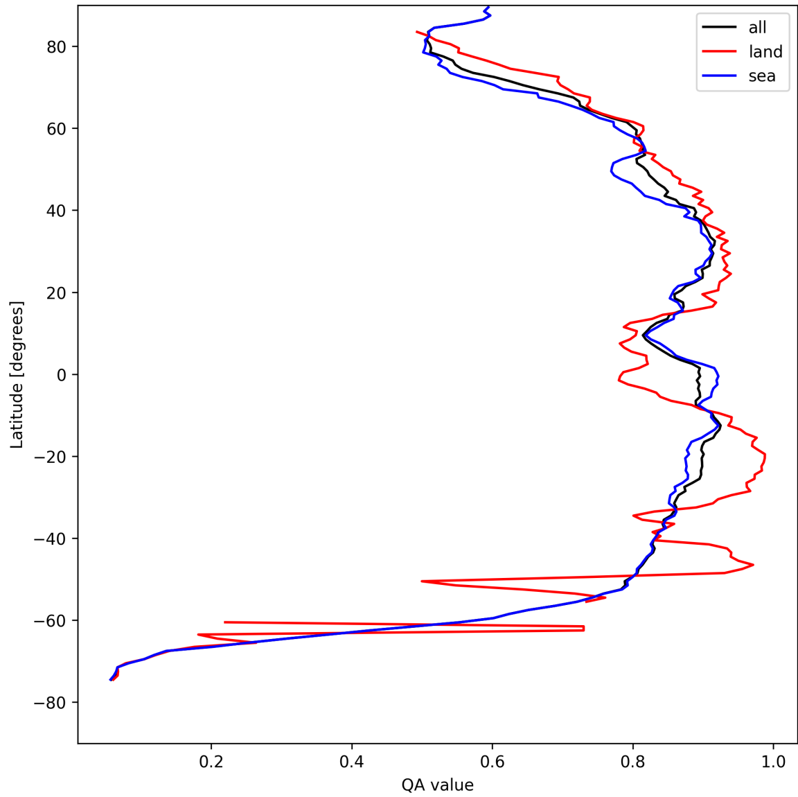
Figure 11: Zonal average of “QA value” for 2025-08-15 to 2025-08-17.
