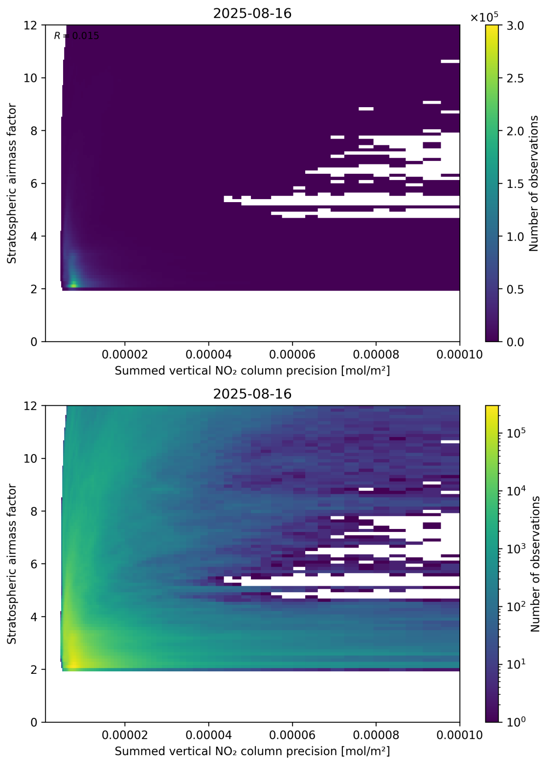
Figure 106: Scatter density plot of “Summed vertical NO 2 column precision” against “Stratospheric airmass factor” for 2025-08-15 to 2025-08-17.
