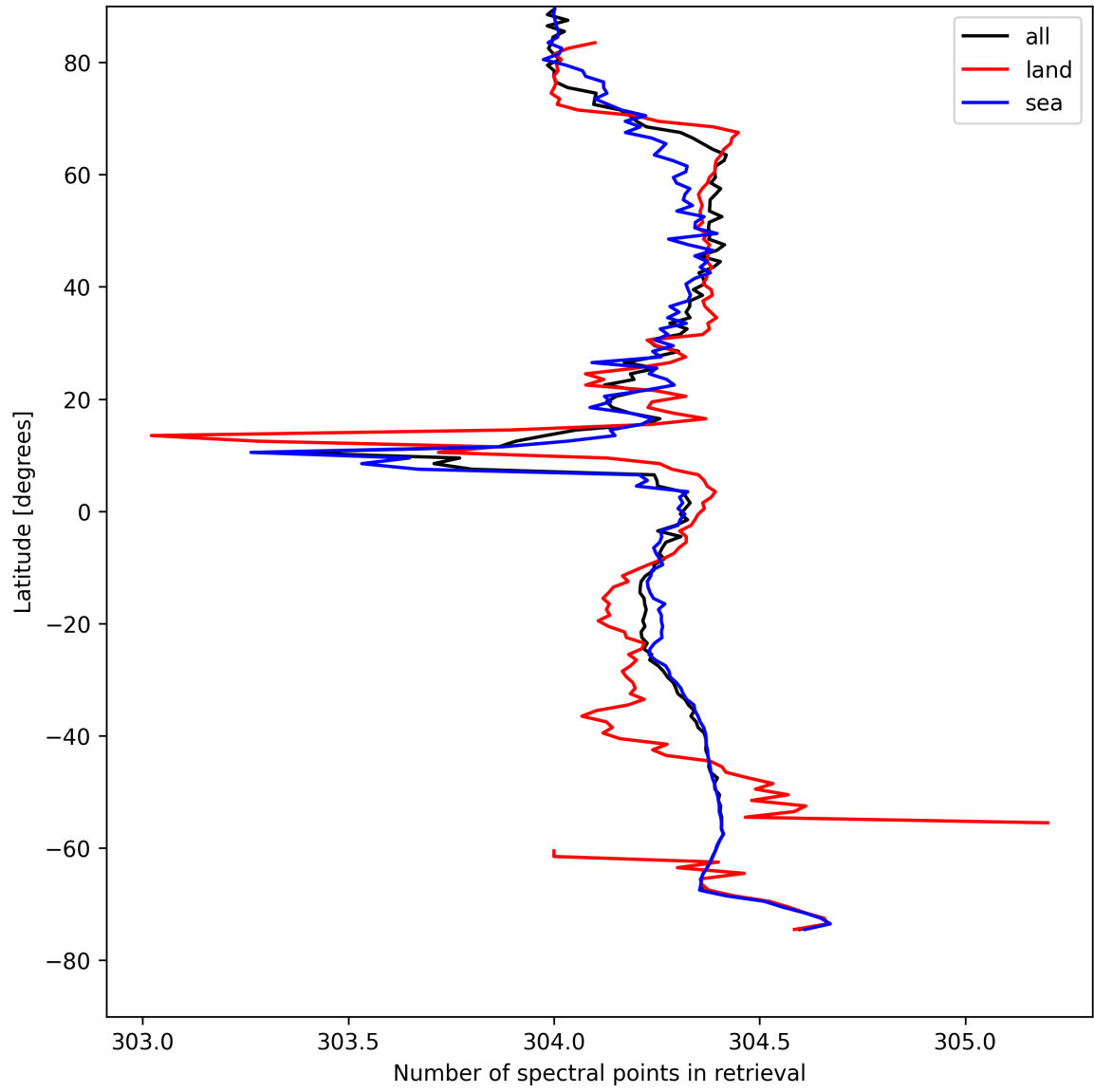
Figure 16: Zonal average of “Number of spectral points in retrieval” for 2025-08-15 to 2025-08-17.
