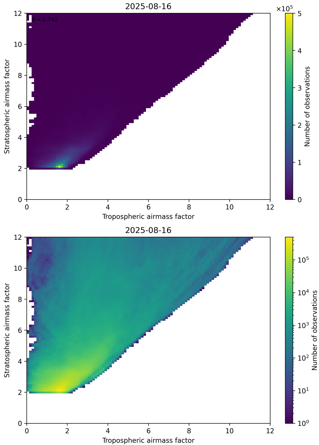
Figure 71: Scatter density plot of “Tropospheric airmass factor” against “Stratospheric airmass factor” for 2025-08-15 to 2025-08-17.
