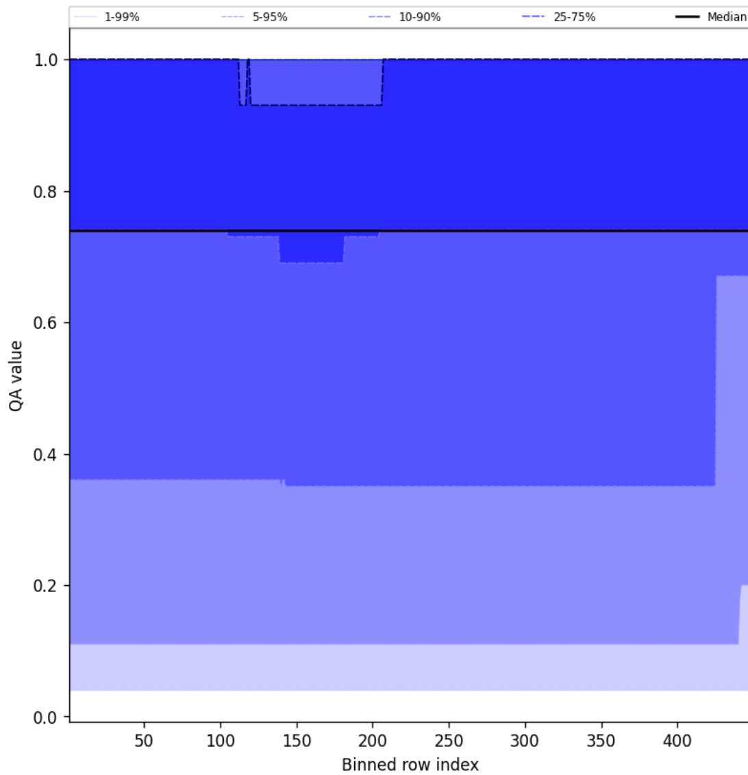
Figure 45: Along track statistics of “QA value” for 2025-08-15 to 2025-08-17
