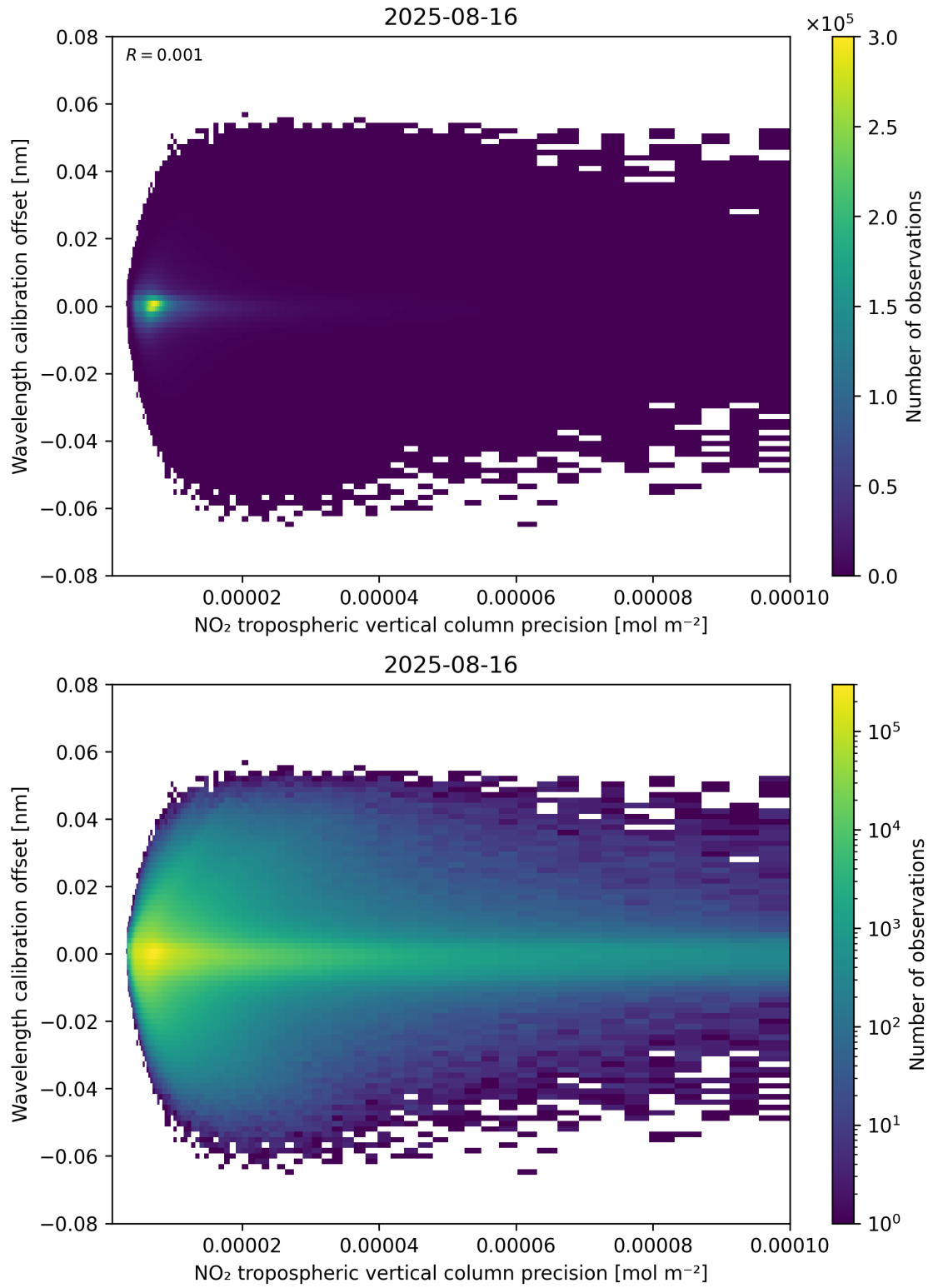
Figure 141: Scatter density plot of “NO 2 tropospheric vertical column precision” against “Wavelength calibration offset” for 2025-08-15 to 2025-08-17.
