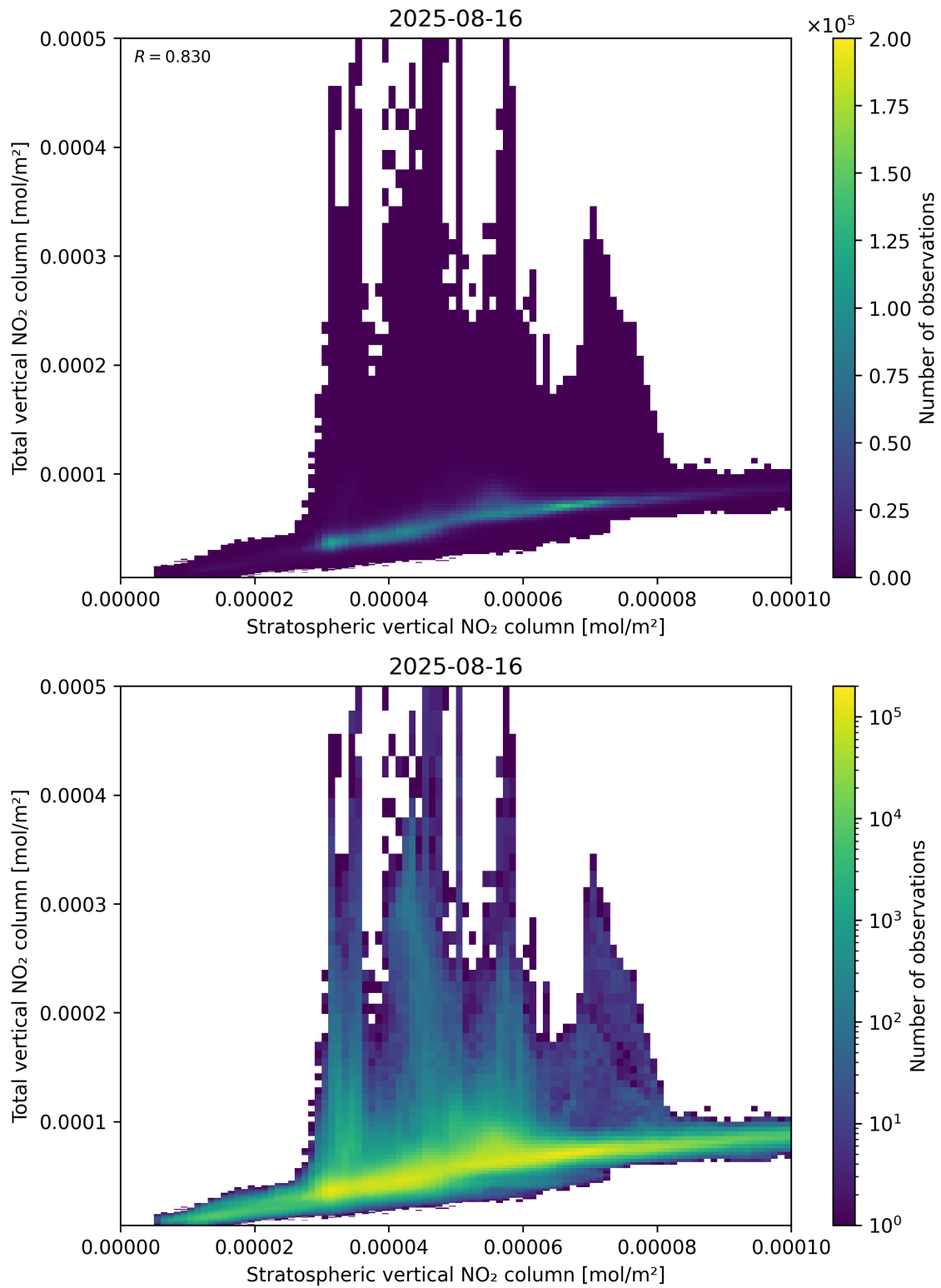
Figure 100: Scatter density plot of “Stratospheric vertical NO 2 column” against “Total vertical NO 2 column” for 2025-08-15 to 2025-08-17.
