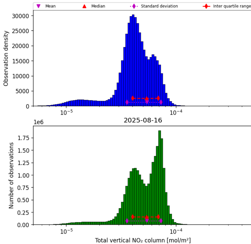
Figure 38: Histogram of “Total vertical NO 2 column” for 2025-08-15 to 2025-08-17
