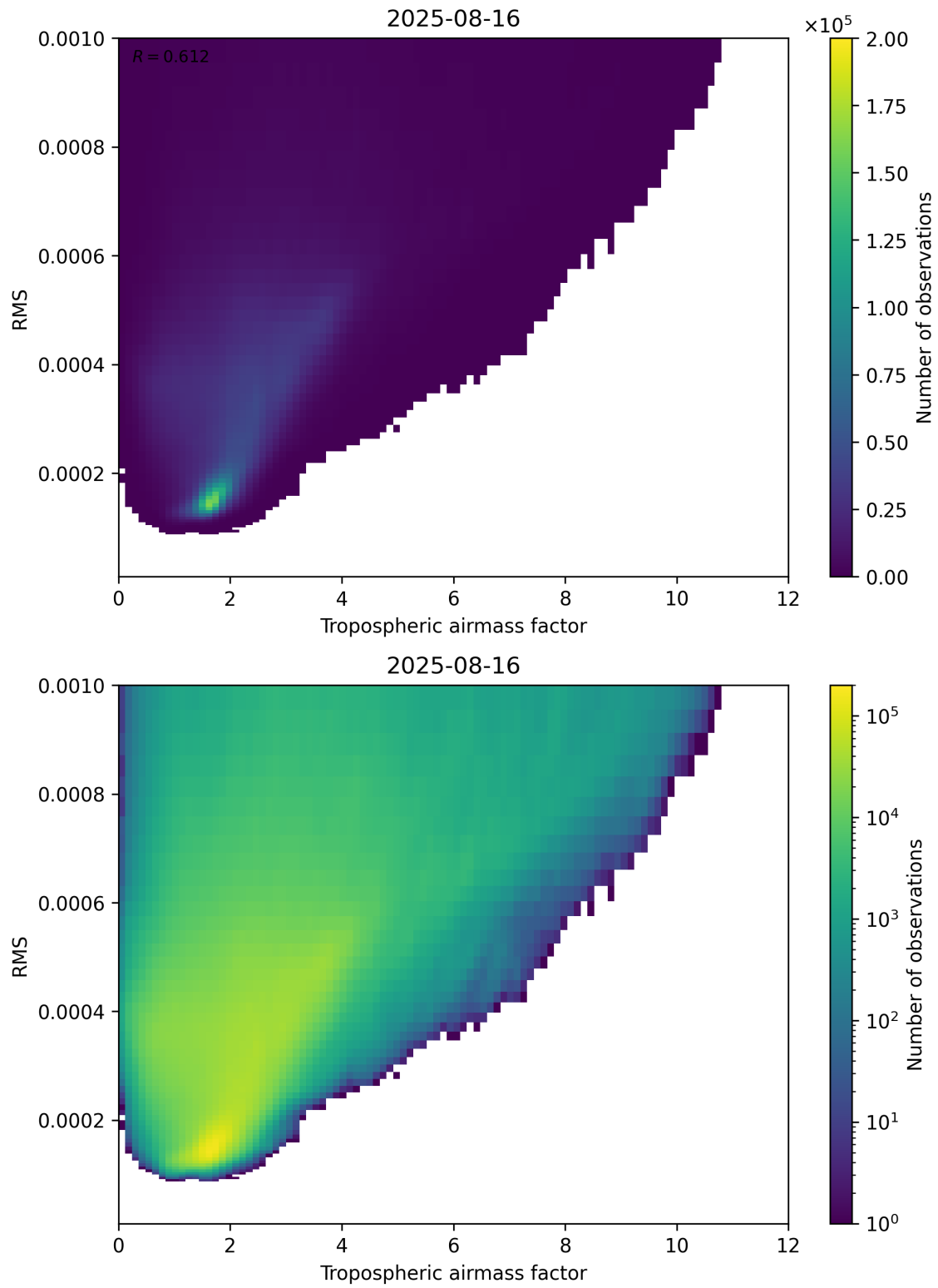
Figure 79: Scatter density plot of “Tropospheric airmass factor” against “RMS” for 2025-08-15 to 2025-08-17.
