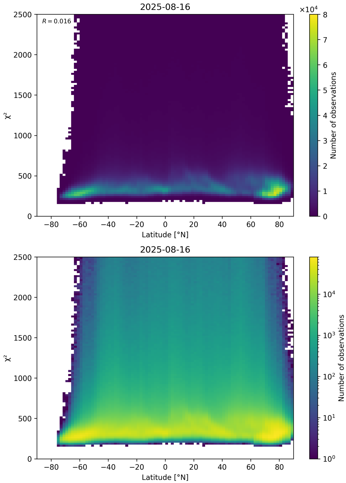
Figure 86: Scatter density plot of “Latitude” against “ \chi^2 ” for 2025-08-15 to 2025-08-17.
