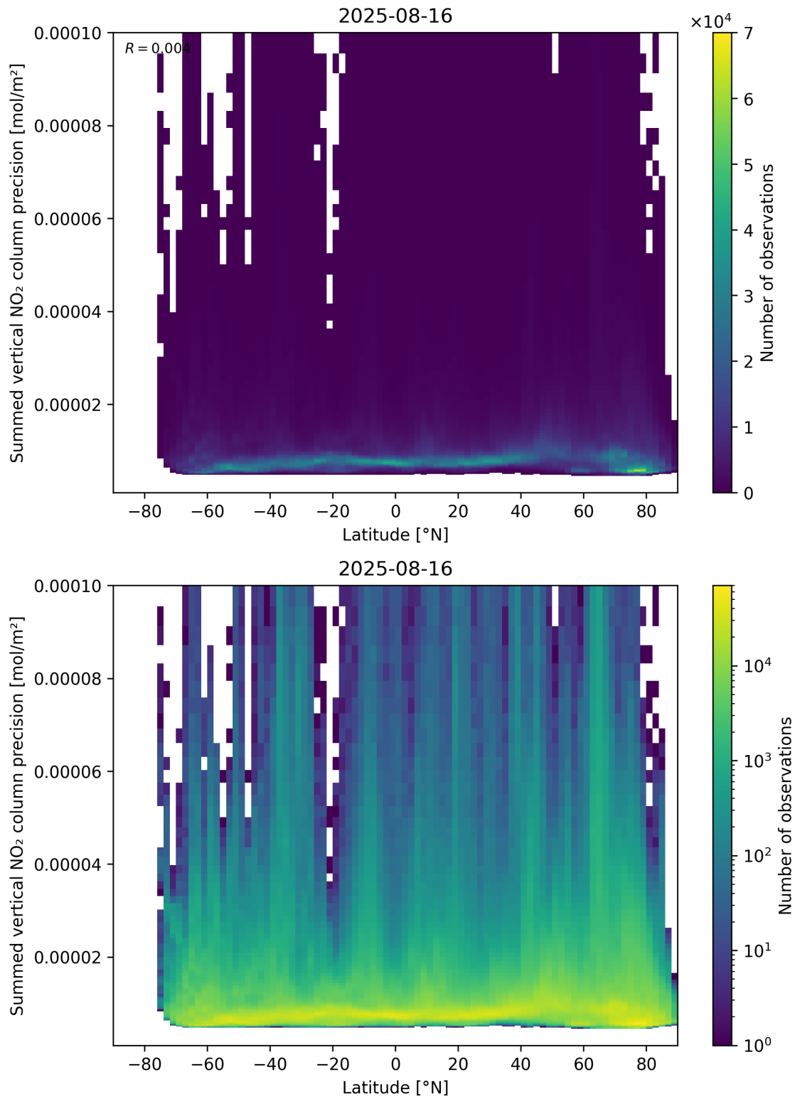
Figure 89: Scatter density plot of “Latitude” against “Summed vertical NO 2 column precision” for 2025-08-15 to 2025-08-17.
