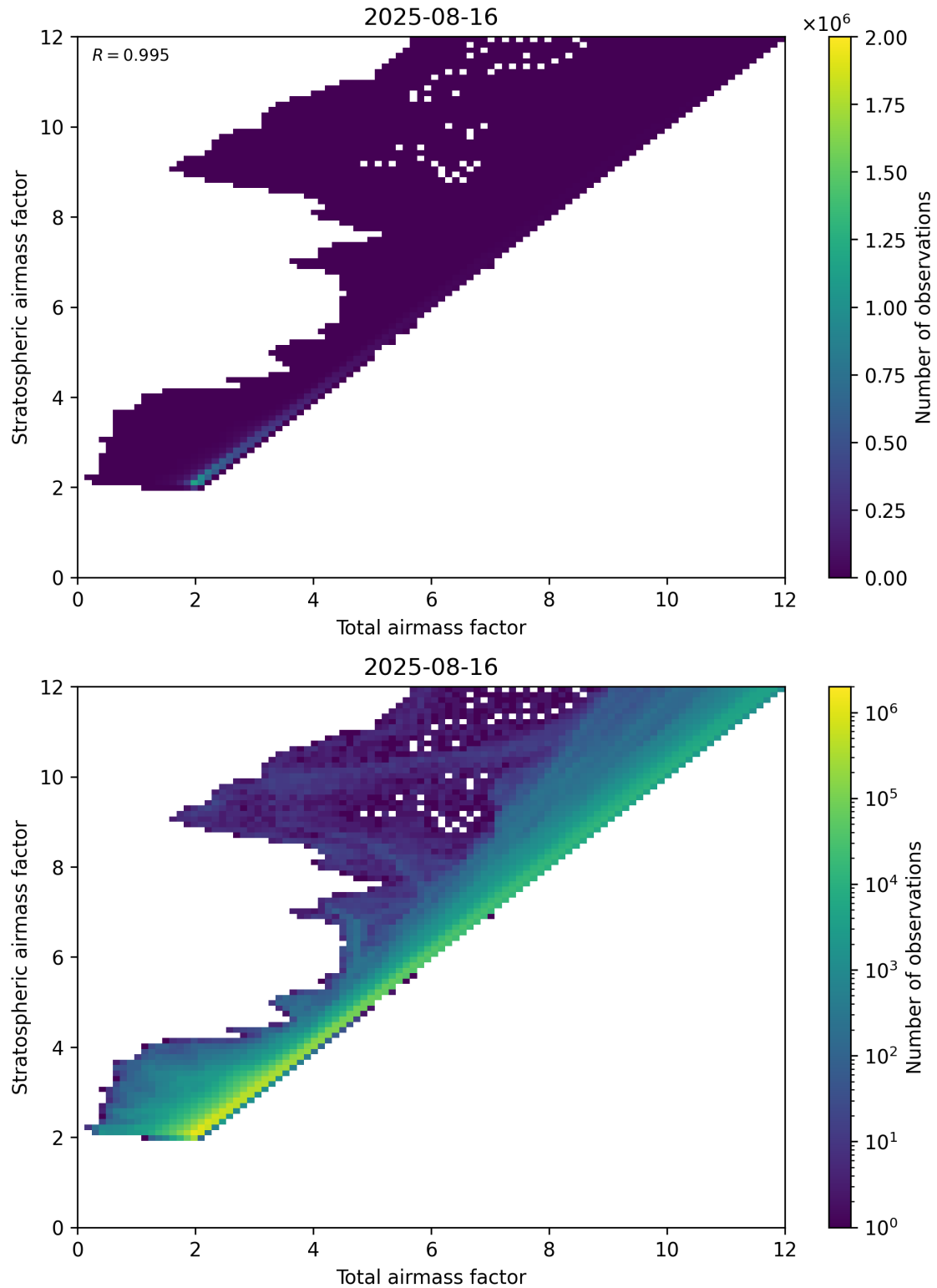
Figure 62: Scatter density plot of “Total airmass factor” against “Stratospheric airmass factor” for 2025-08-15 to 2025-08-17.
