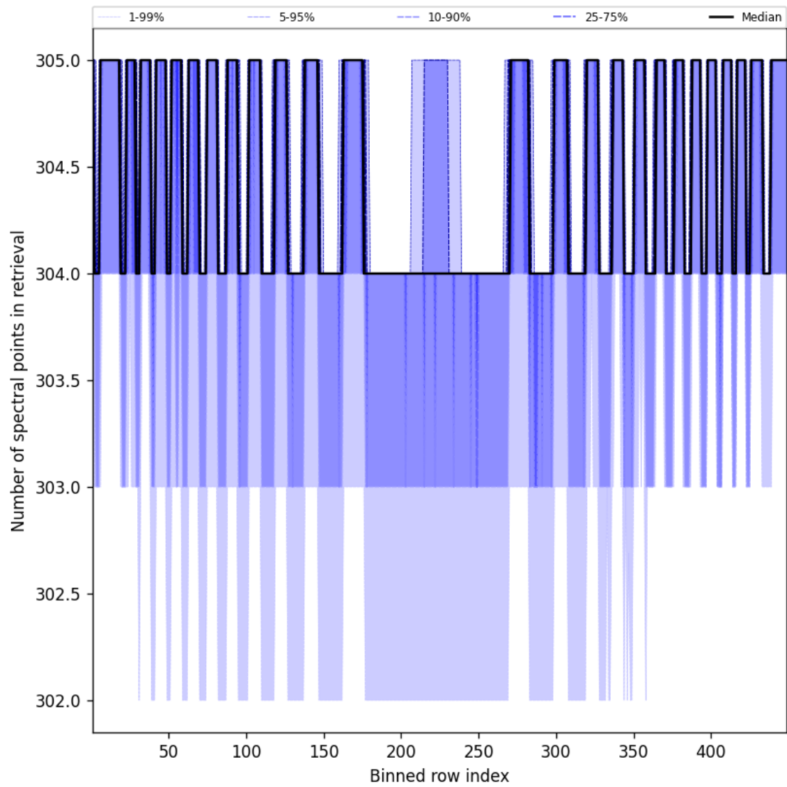
Figure 50: Along track statistics of “Number of spectral points in retrieval” for 2025-08-15 to 2025-08-17
