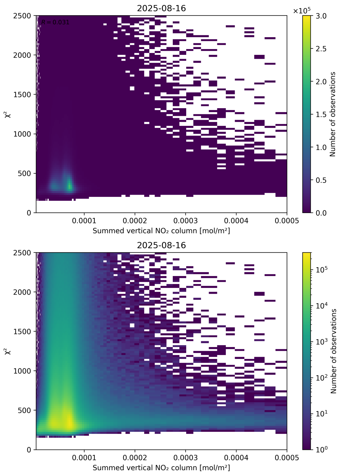
Figure 104: Scatter density plot of “Summed vertical NO 2 column” against “ \chi^2 ” for 2025-08-15 to 2025-08-17.
