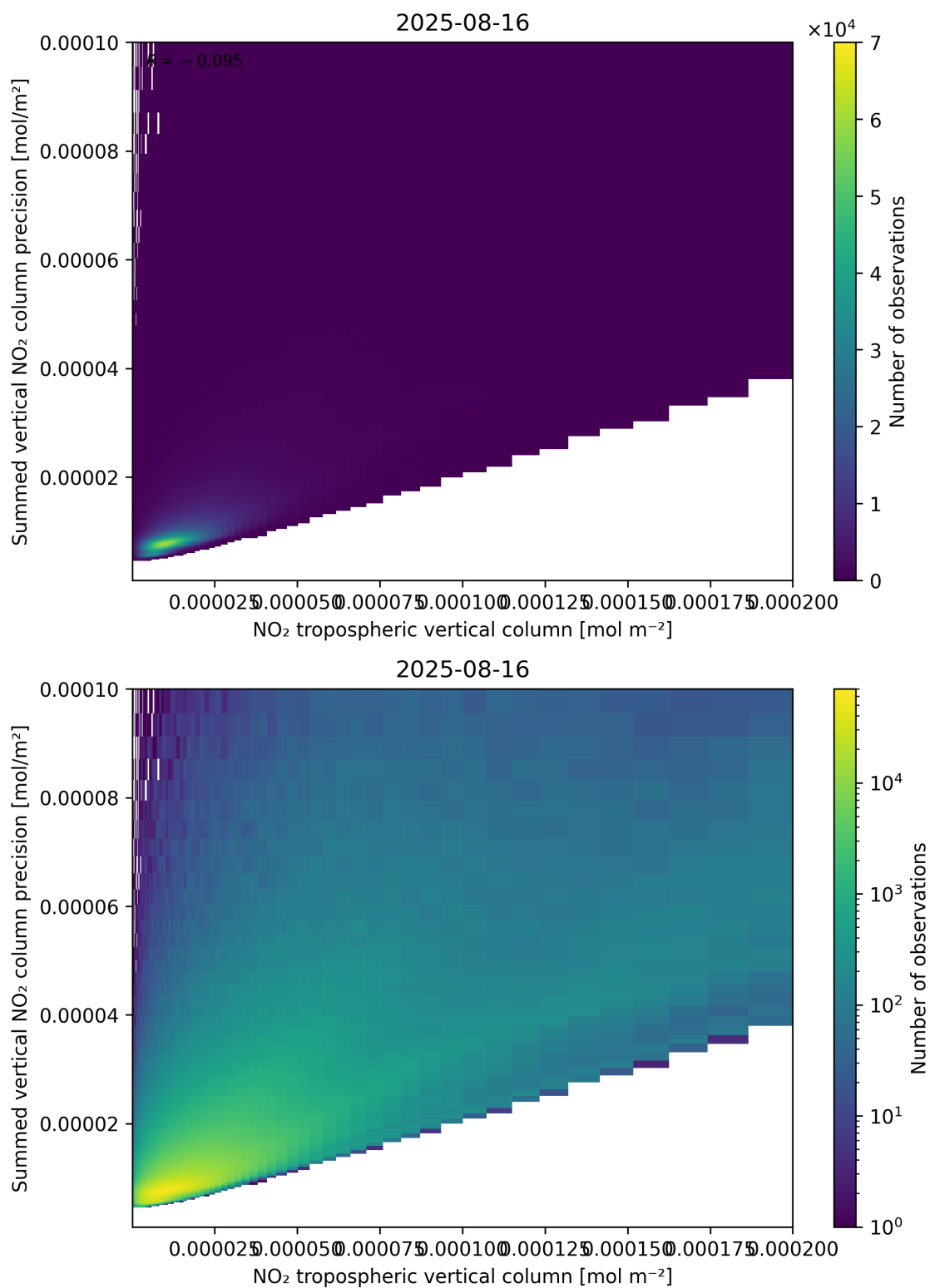
Figure 127: Scatter density plot of “NO 2 tropospheric vertical column” against “Summed vertical NO 2 column precision” for 2025-08-15 to 2025-08-17.
