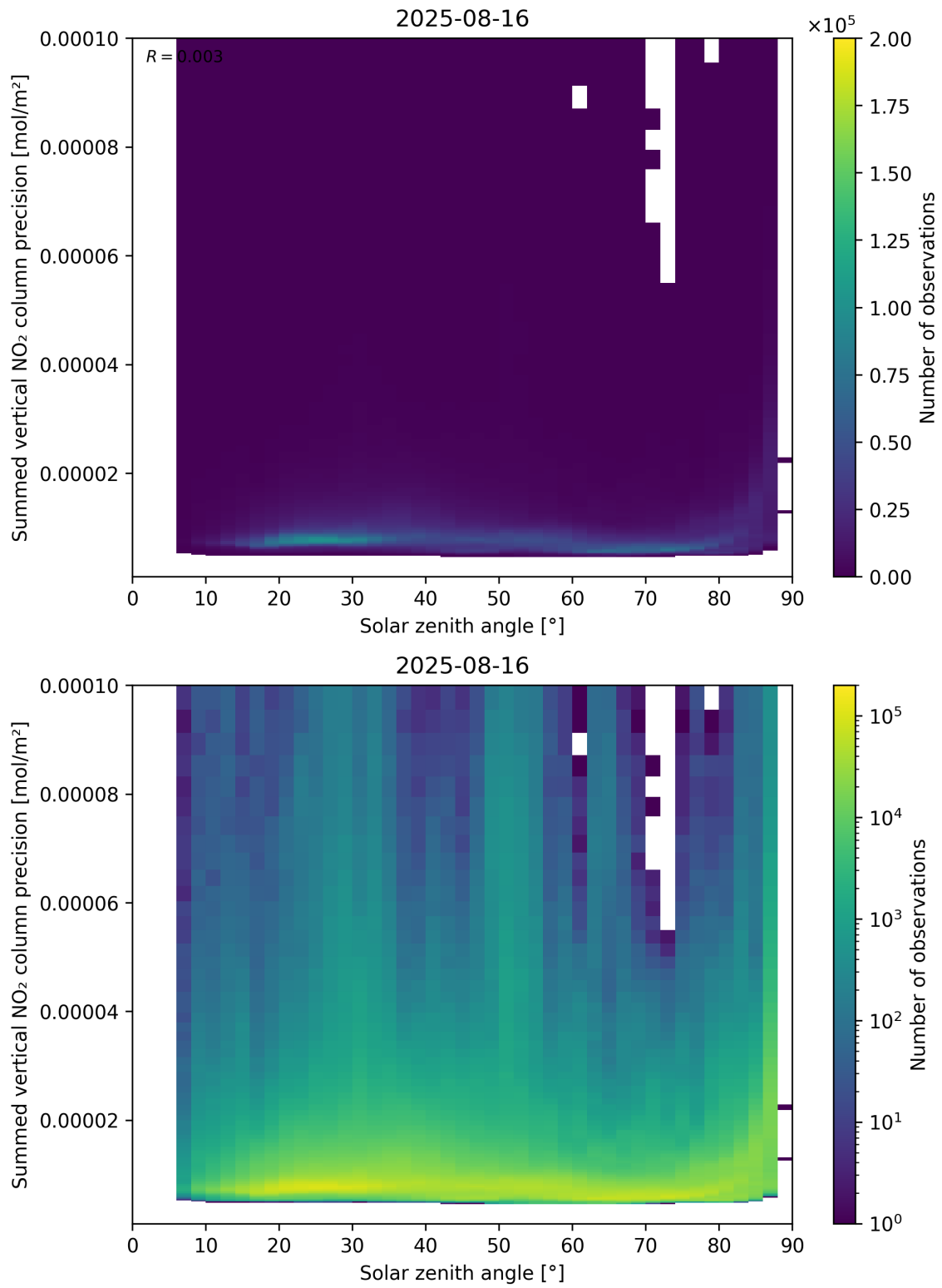
Figure 152: Scatter density plot of “Solar zenith angle” against “Summed vertical NO 2 column precision” for 2025-08-15 to 2025-08-17.
