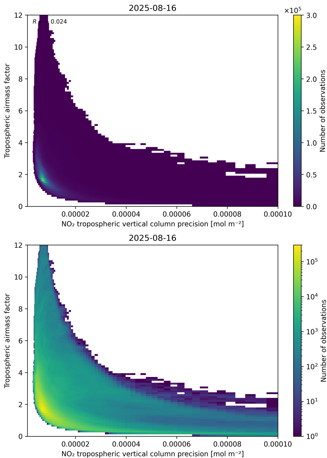
Figure 133: Scatter density plot of “NO 2 tropospheric vertical column precision” against “Tropospheric airmass factor” for 2025-08-15 to 2025-08-17.
