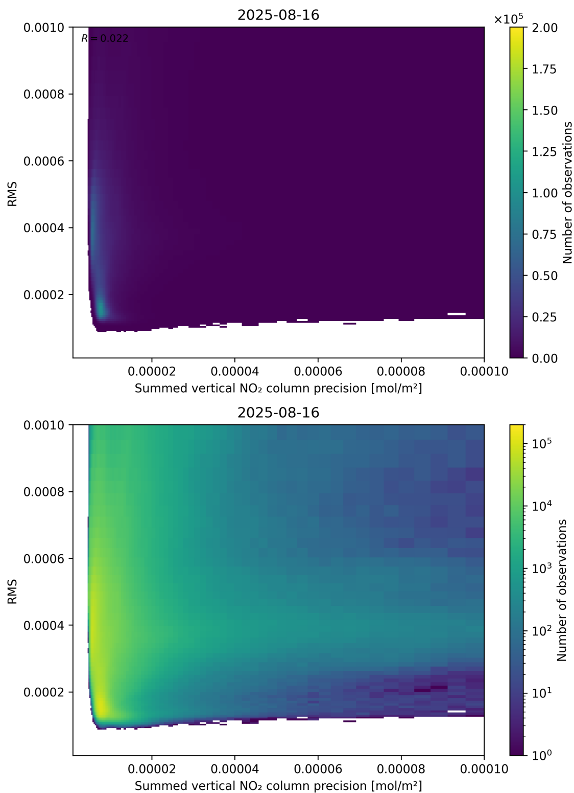
Figure 108: Scatter density plot of “Summed vertical NO 2 column precision” against “RMS” for 2025-08-15 to 2025-08-17.
