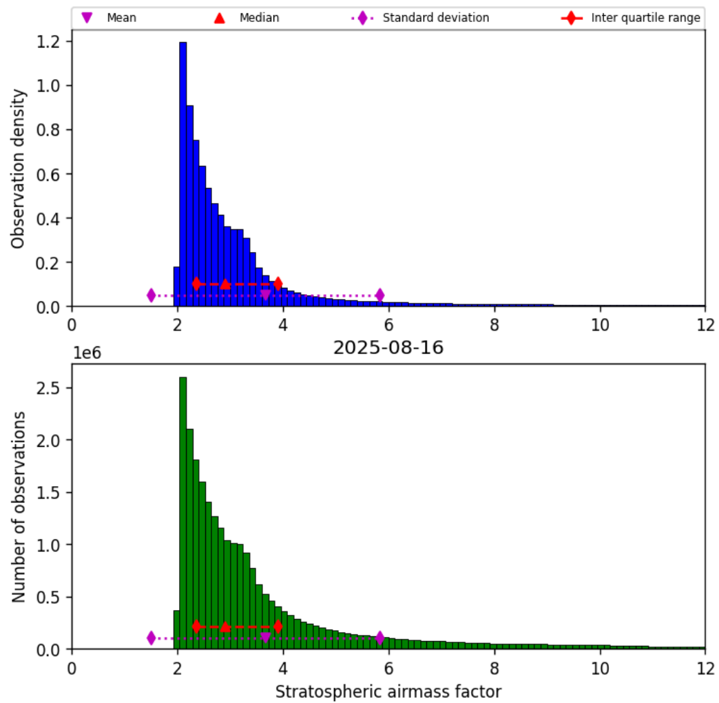
Figure 44: Histogram of “Stratospheric airmass factor” for 2025-08-15 to 2025-08-17
