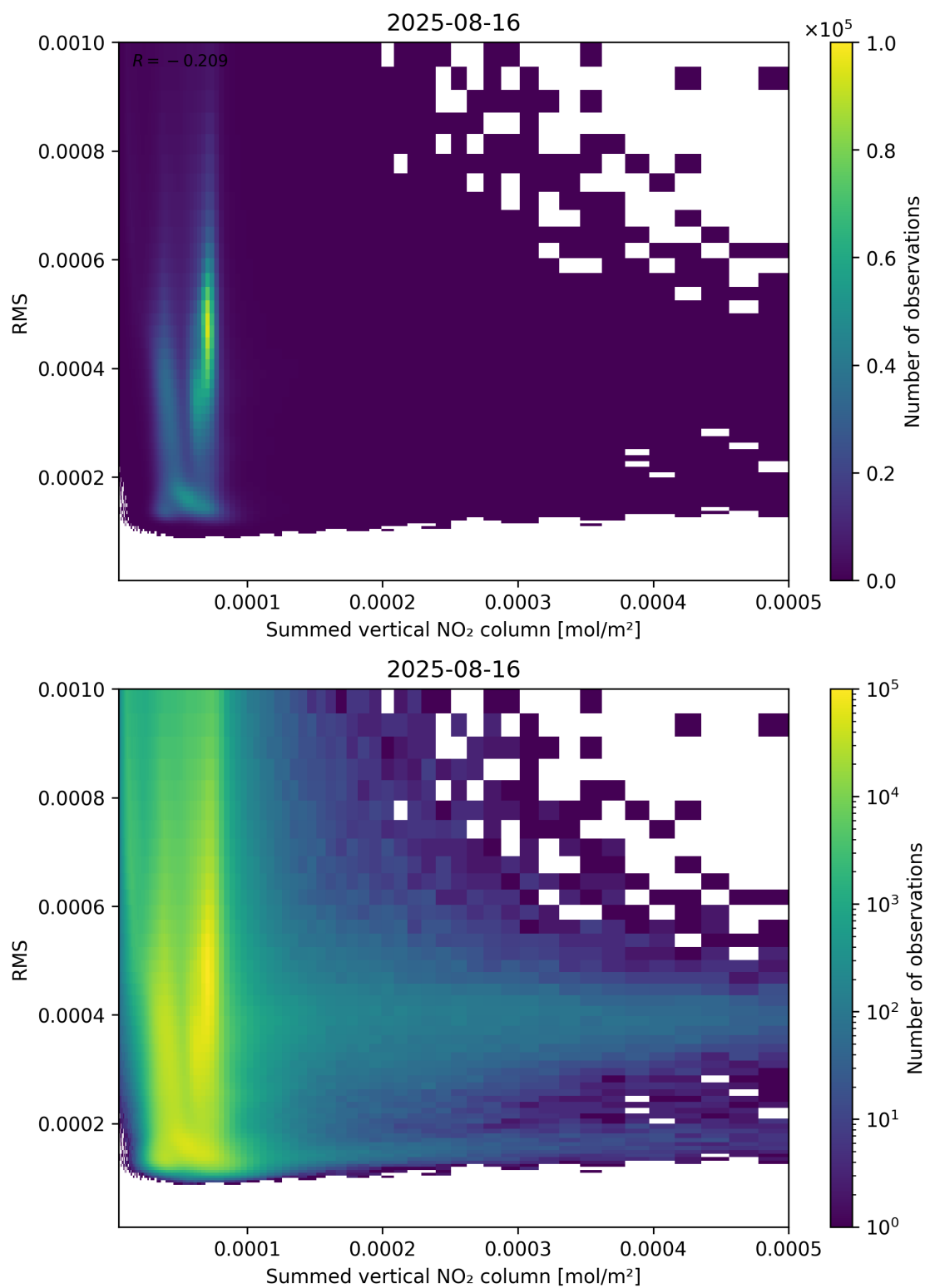
Figure 109: Scatter density plot of “Summed vertical NO 2 column” against “RMS” for 2025-08-15 to 2025-08-17.
