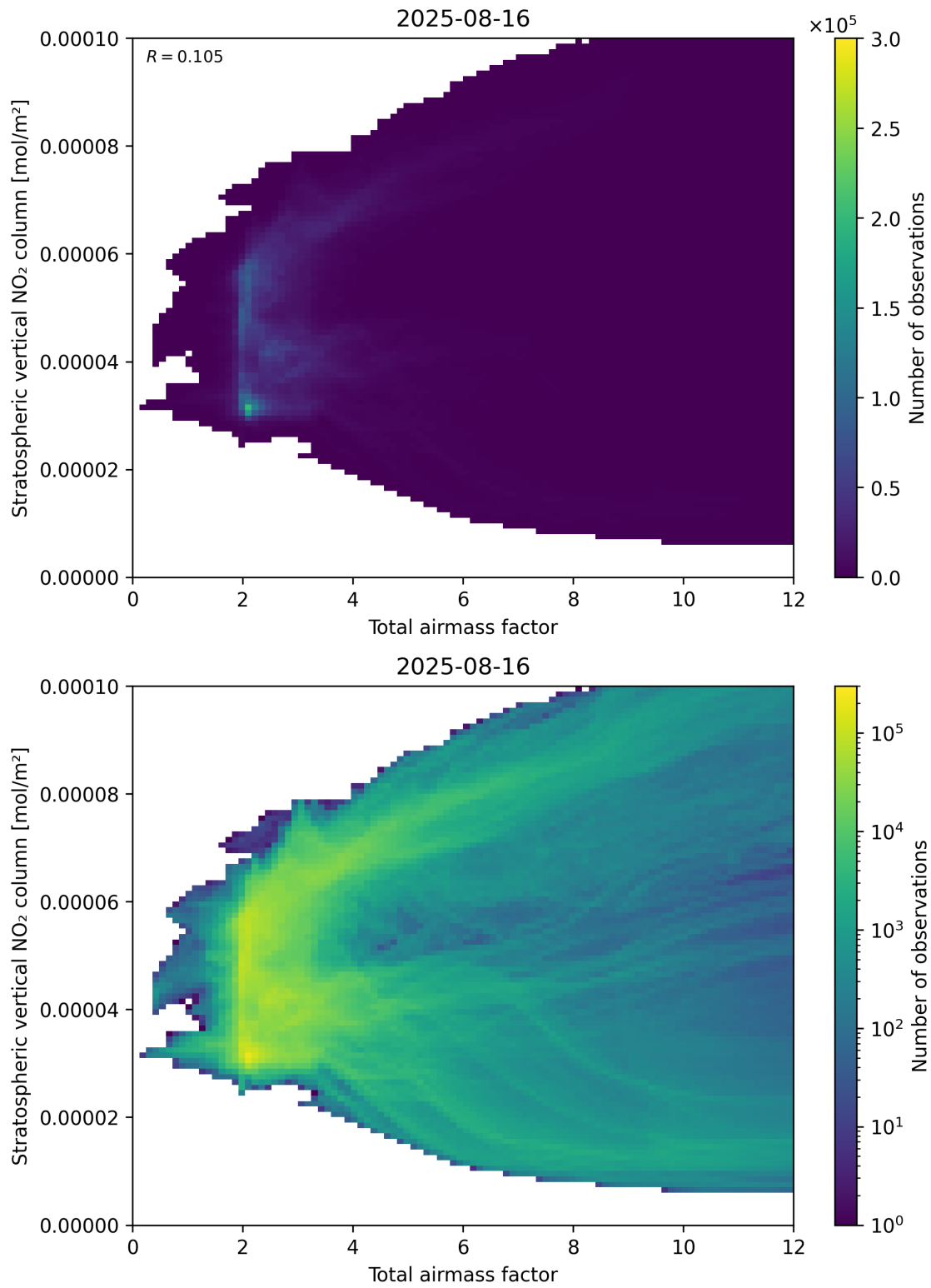
Figure 64: Scatter density plot of “Total airmass factor” against “Stratospheric vertical NO 2 column” for 2025-08-15 to 2025-08-17.
