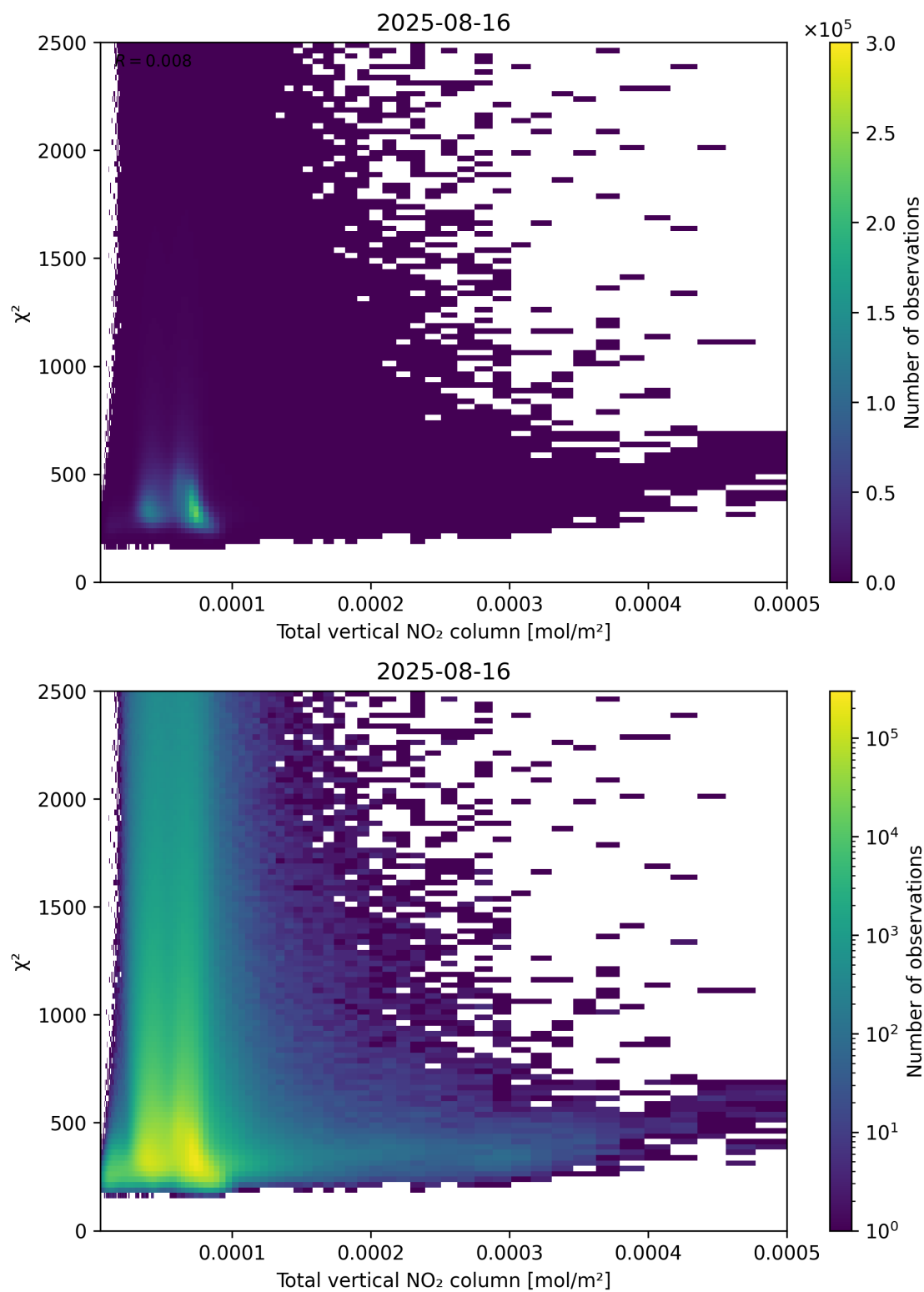
Figure 111: Scatter density plot of “Total vertical NO 2 column” against “ \chi^2 ” for 2025-08-15 to 2025-08-17.
