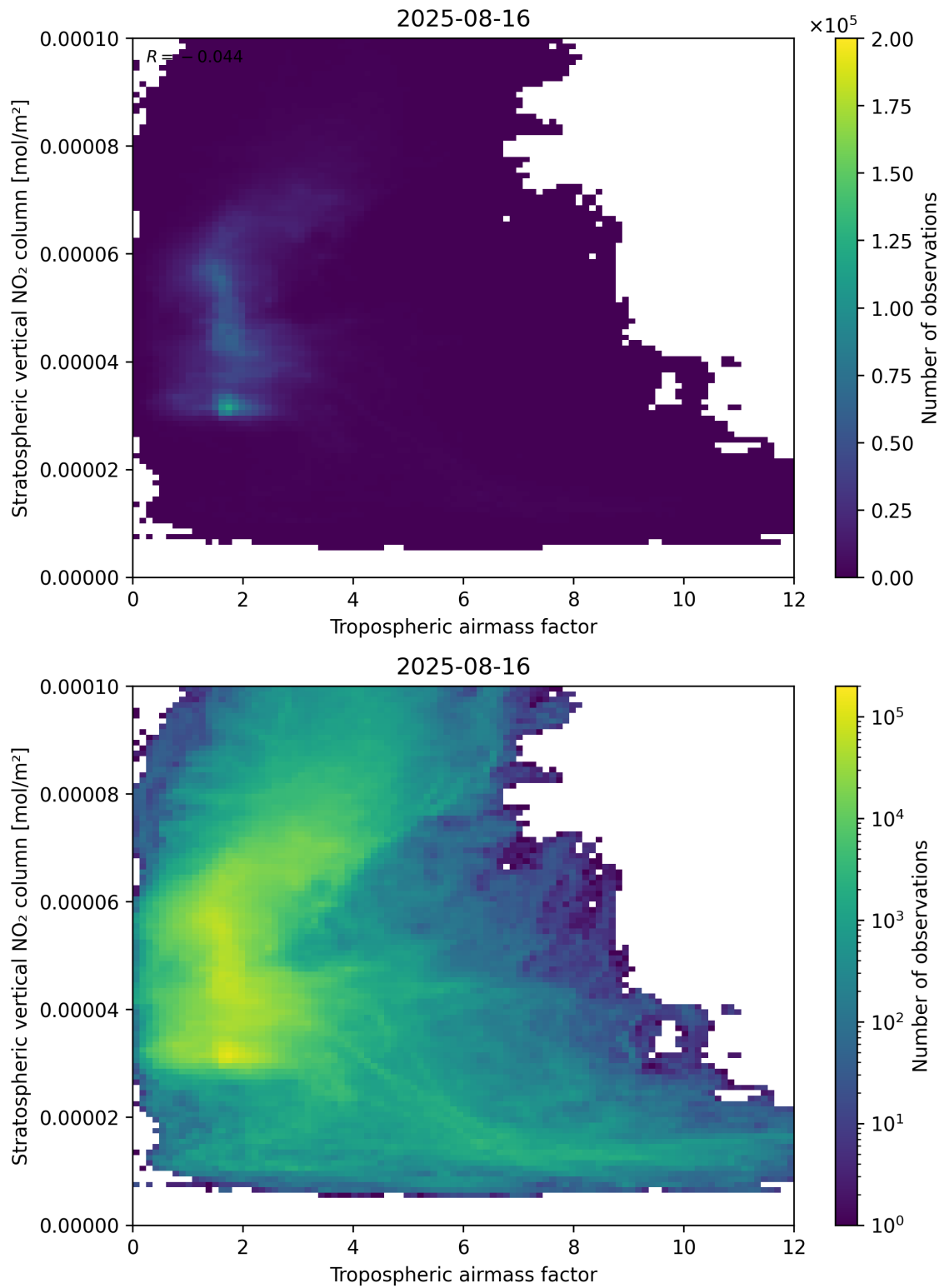
Figure 74: Scatter density plot of “Tropospheric air mass factor” against “Stratospheric vertical NO 2 column” for 2025-08-15 to 2025-08-17.
