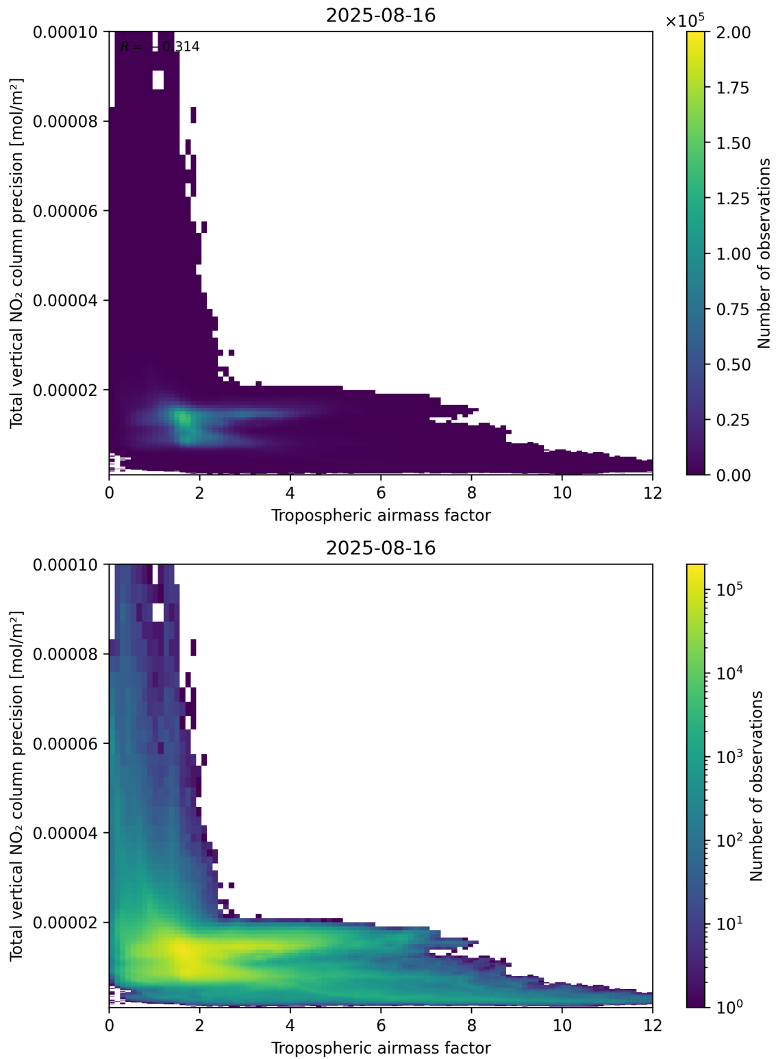
Figure 78: Scatter density plot of “Tropospheric airmass factor” against “Total vertical NO 2 column precision” for 2025-08-15 to 2025-08-17.
