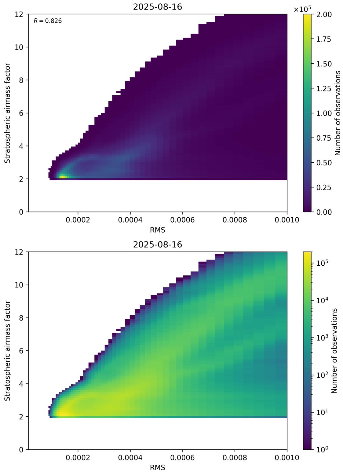
Figure 144: Scatter density plot of “RMS” against “Stratospheric airmass factor” for 2025-08-15 to 2025-08-17.
