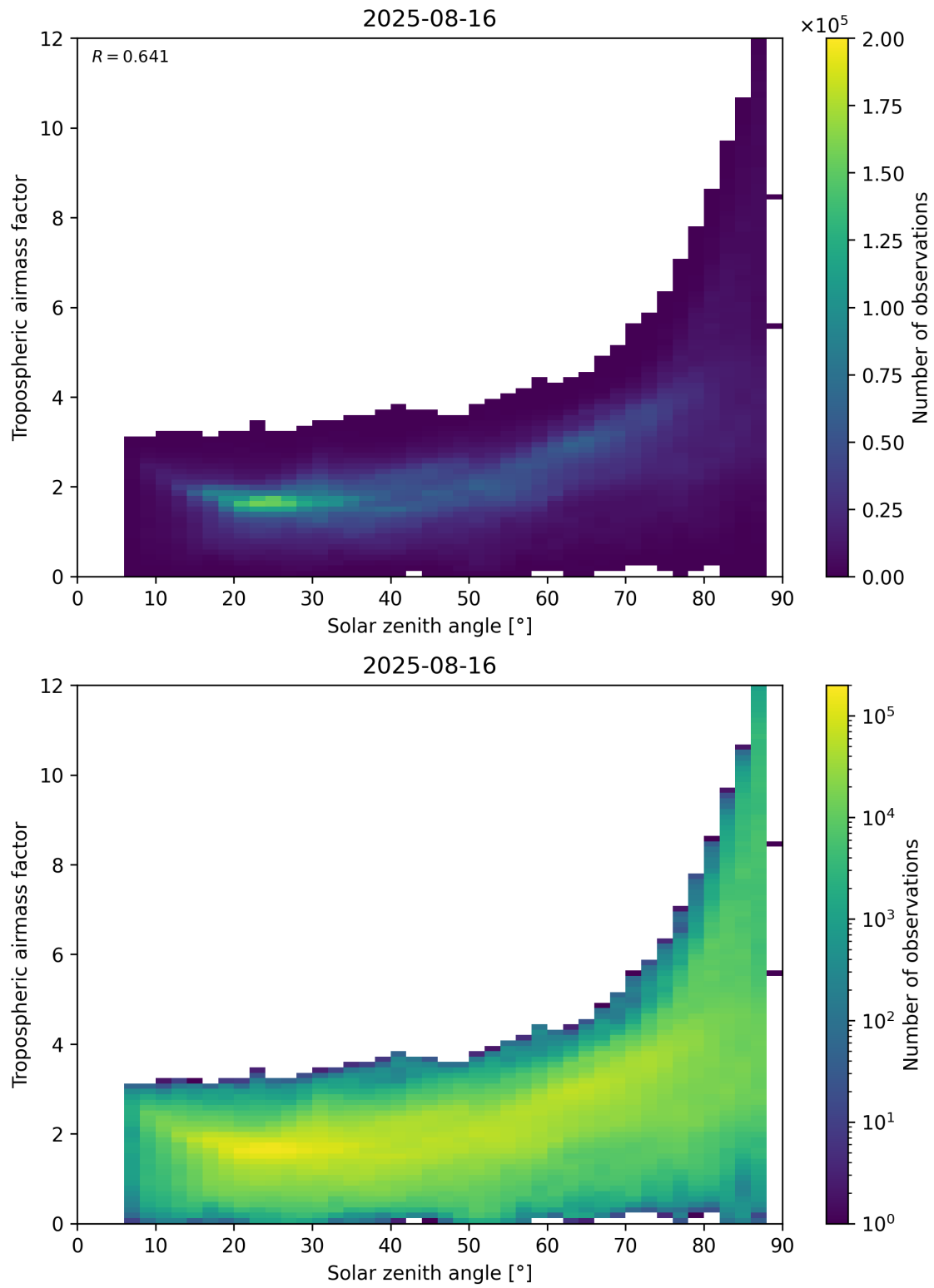
Figure 147: Scatter density plot of “Solar zenith angle” against “Tropospheric airmass factor” for 2025-08-15 to 2025-08-17.
