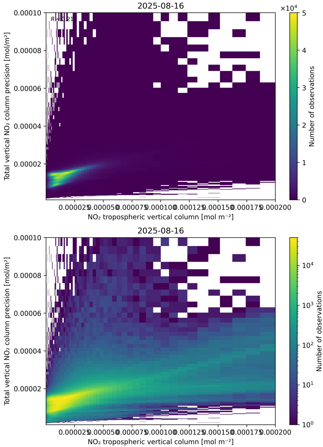
Figure 129: Scatter density plot of “NO 2 tropospheric vertical column” against “Total vertical NO 2 column precision” for 2025-08-15 to 2025-08-17.
