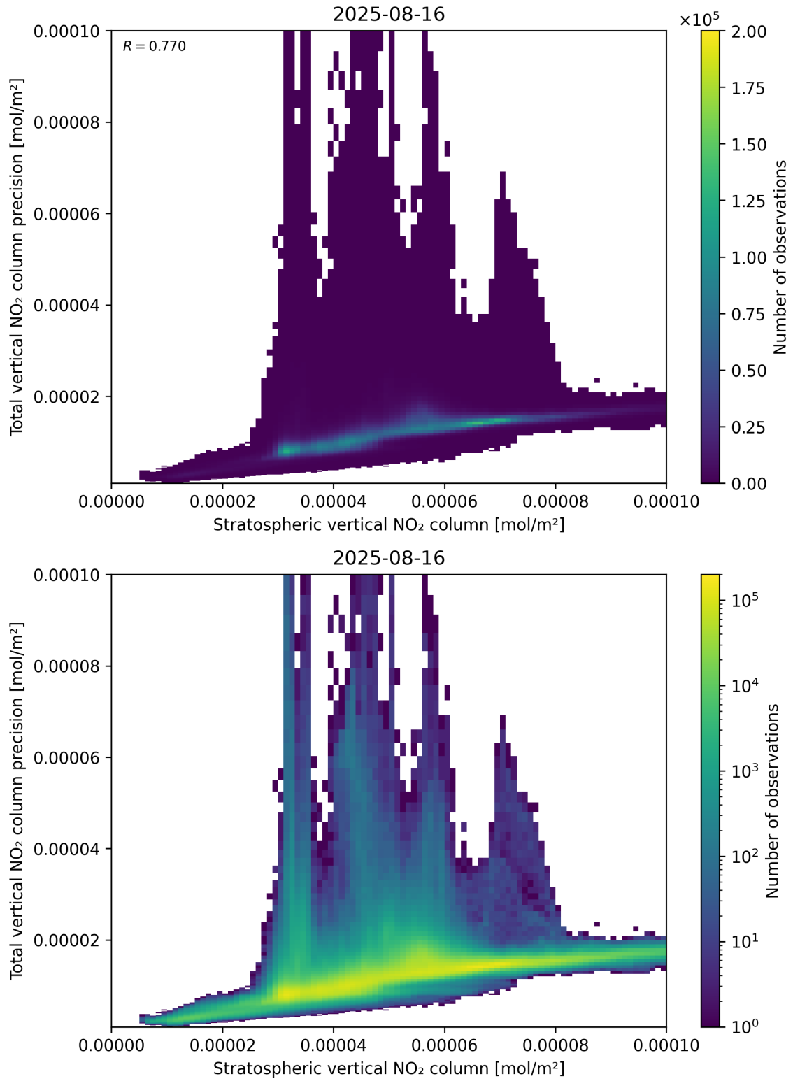
Figure 101: Scatter density plot of “Stratospheric vertical NO 2 column” against “Total vertical NO 2 column precision” for 2025-08-15 to 2025-08-17.
