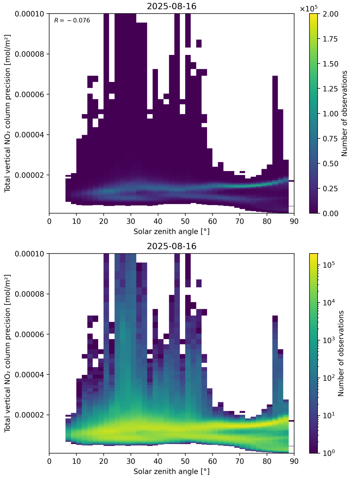
Figure 154: Scatter density plot of “Solar zenith angle” against “Total vertical NO 2 column precision” for 2025-08-15 to 2025-08-17.
