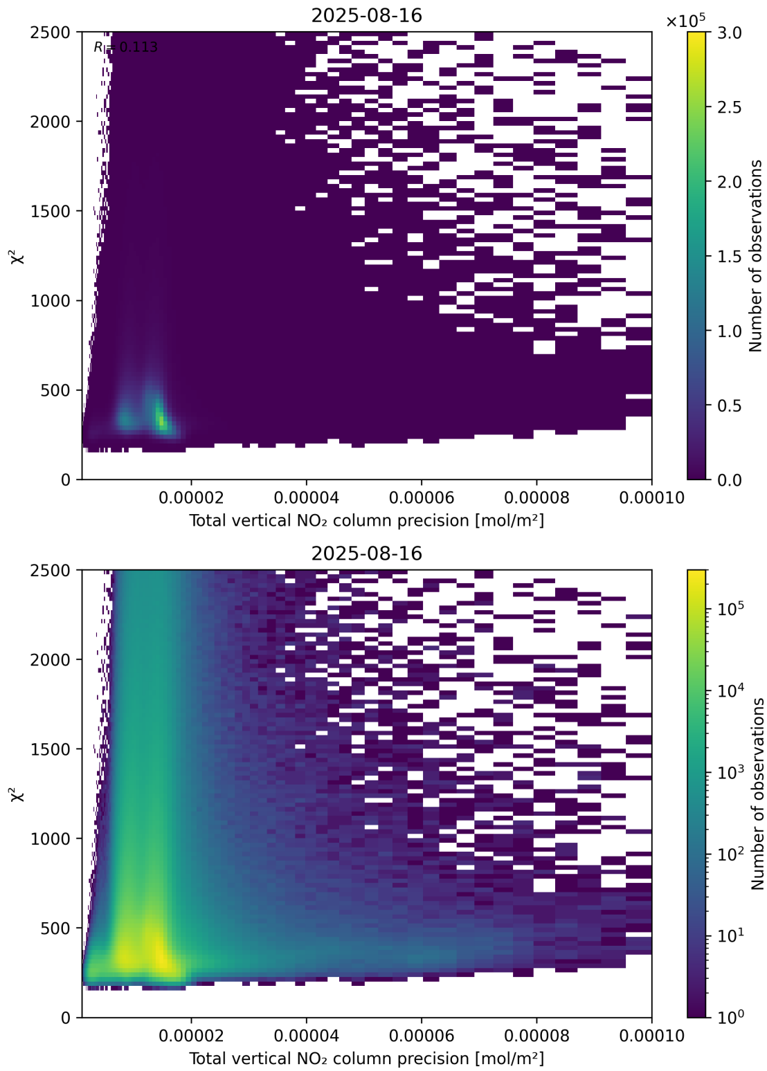
Figure 116: Scatter density plot of “Total vertical NO 2 column precision” against “ \chi^2 ” for 2025-08-15 to 2025-08-17.
