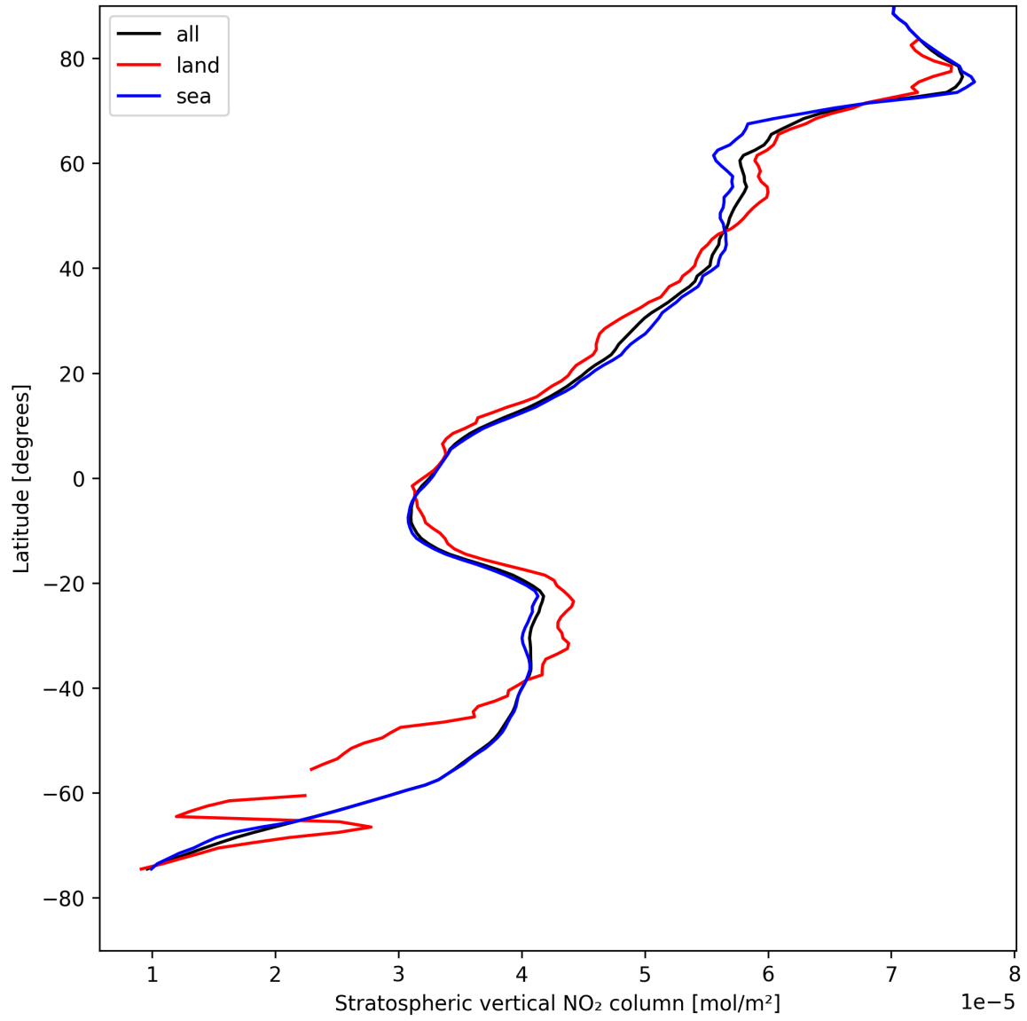
Figure 19: Zonal average of “Stratospheric vertical NO 2 column” for 2025-08-15 to 2025-08-17.
