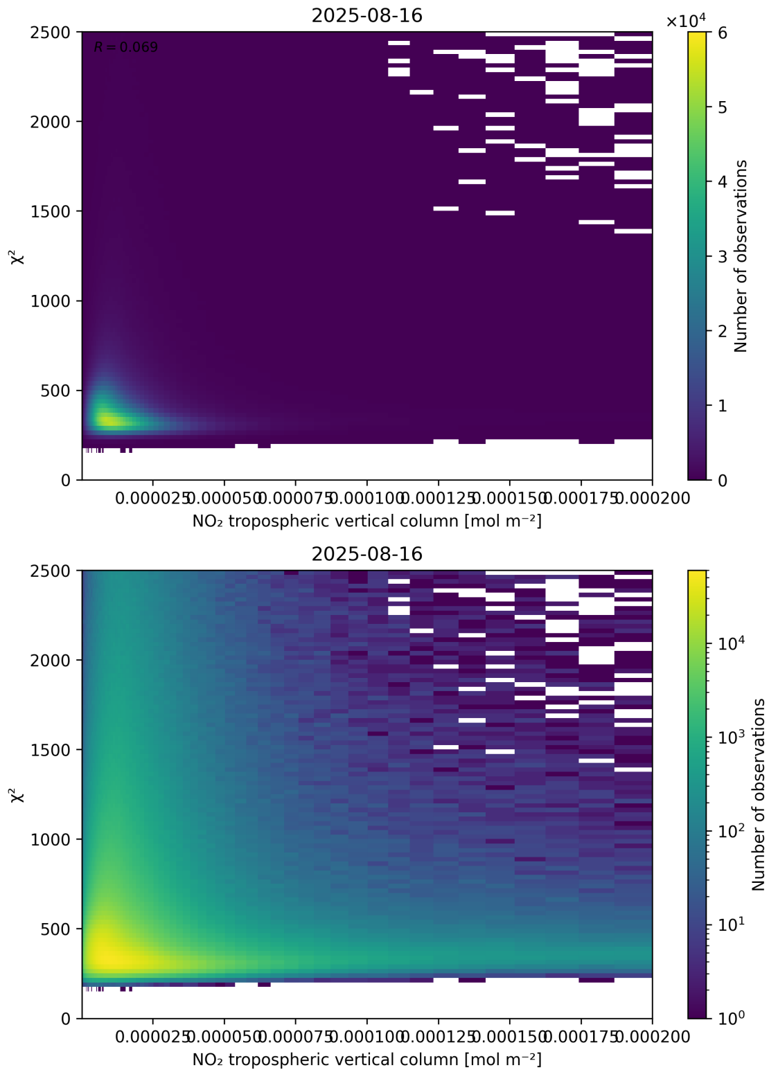
Figure 124: Scatter density plot of “NO 2 tropospheric vertical column” against “ \chi^2 ” for 2025-08-15 to 2025-08-17.
