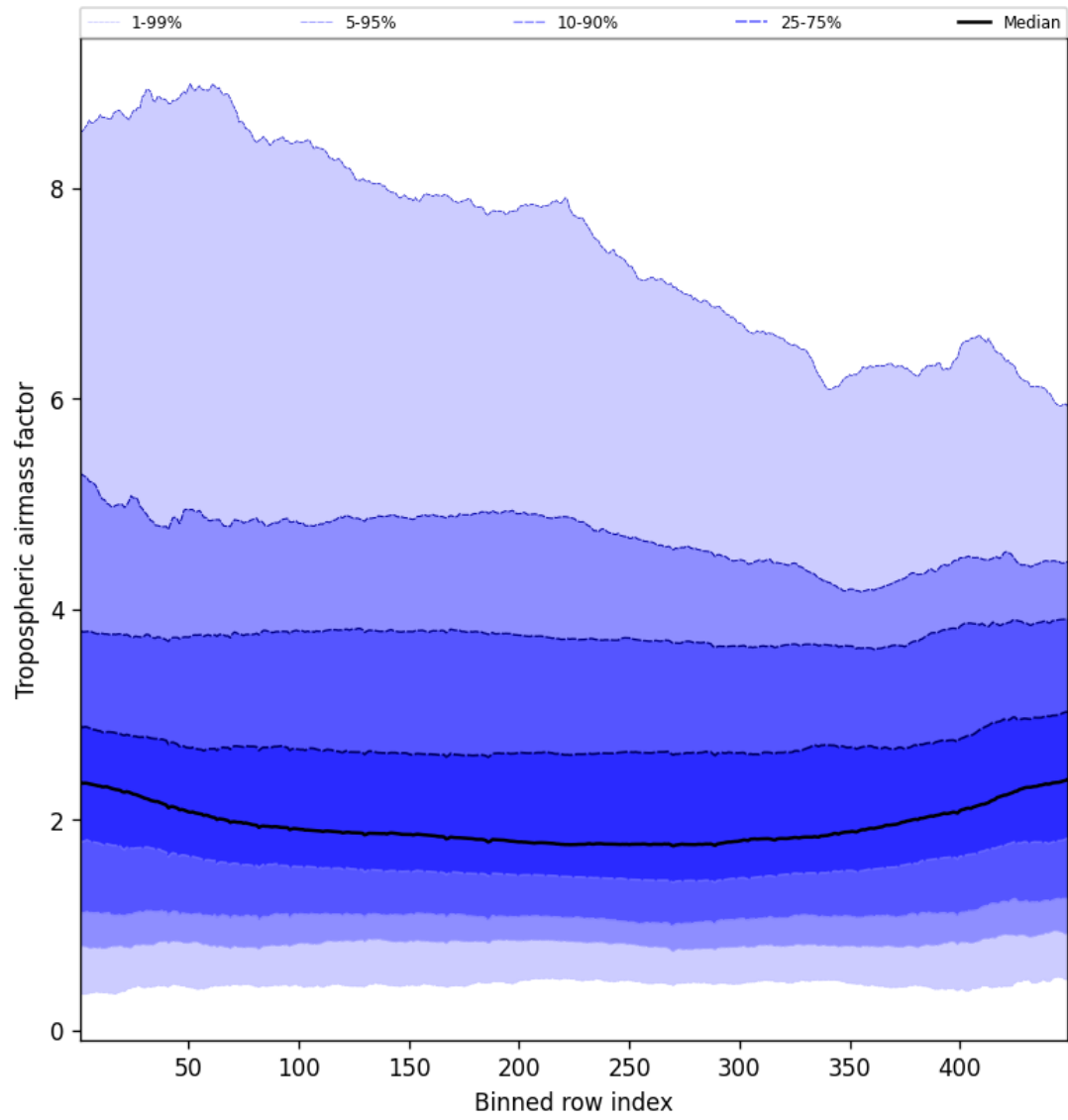
Figure 48: Along track statistics of “Tropospheric airmass factor” for 2025-08-15 to 2025-08-17
