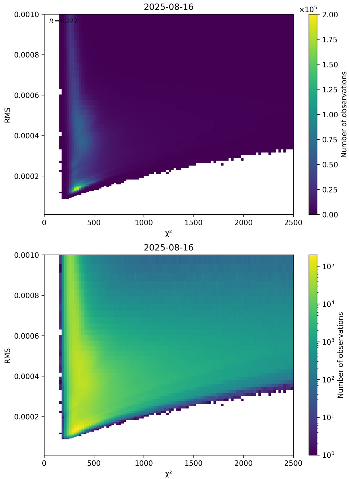
Figure 82: Scatter density plot of “ \chi^2 ” against “RMS” for 2025-08-15 to 2025-08-17.
