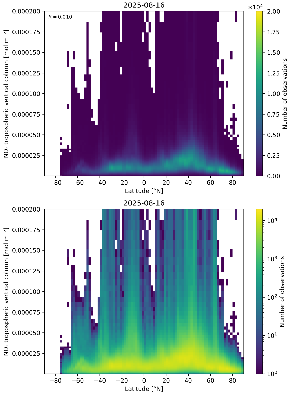
Figure 92: Scatter density plot of “Latitude” against “NO 2 tropospheric vertical column” for 2025-08-15 to 2025-08-17.
