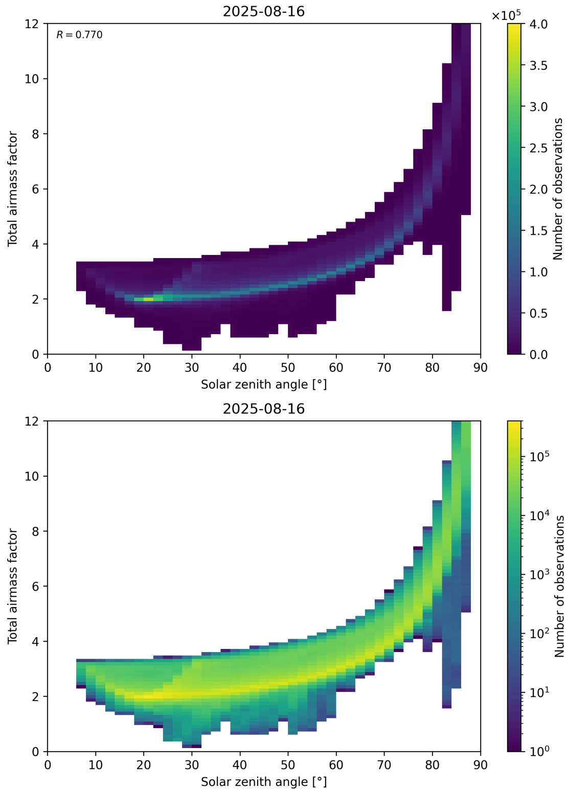
Figure 146: Scatter density plot of “Solar zenith angle” against “Total air mass factor” for 2025-08-15 to 2025-08-17.
