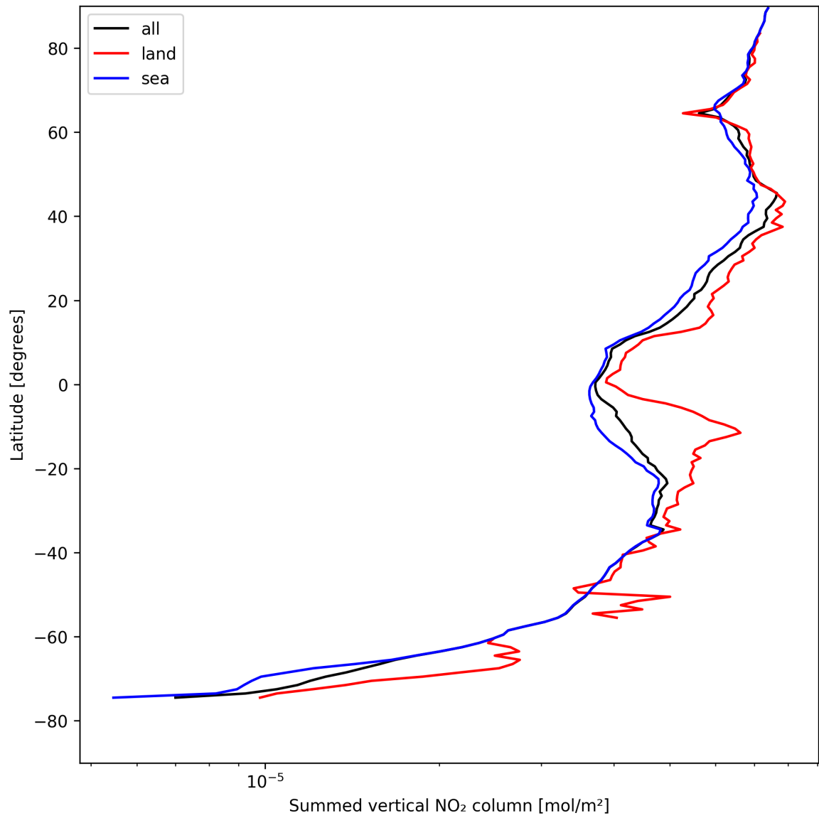
Figure 23: Zonal average of “Summed vertical NO 2 column” for 2025-08-15 to 2025-08-17.
