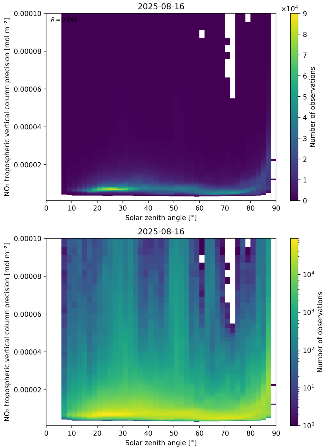
Figure 156: Scatter density plot of “Solar zenith angle” against “NO 2 tropospheric vertical column precision” for 2025-08-15 to 2025-08-17.
