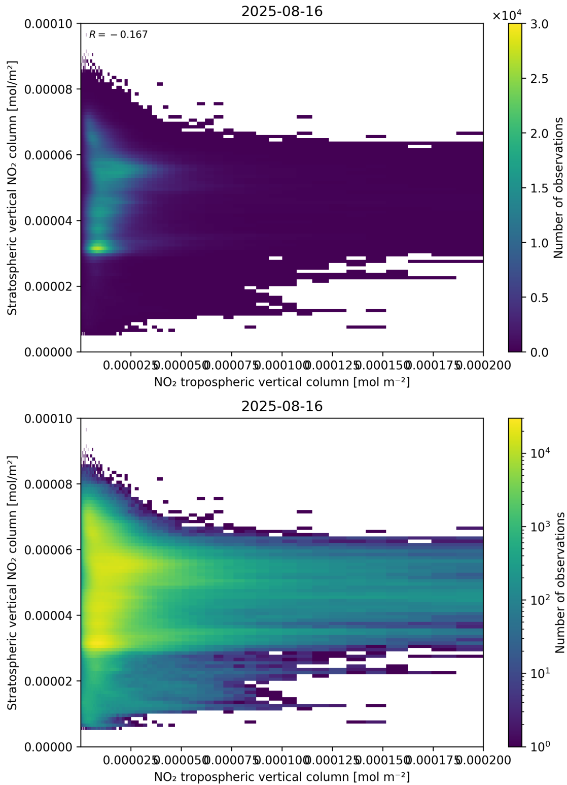
Figure 125: Scatter density plot of “NO 2 tropospheric vertical column” against “Stratospheric vertical NO 2 column” for 2025-08-15 to 2025-08-17.
