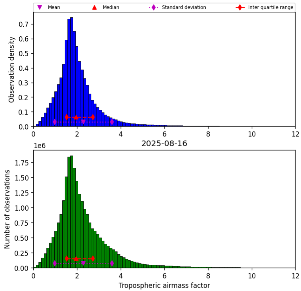
Figure 31: Histogram of “Tropospheric airmass factor” for 2025-08-15 to 2025-08-17
