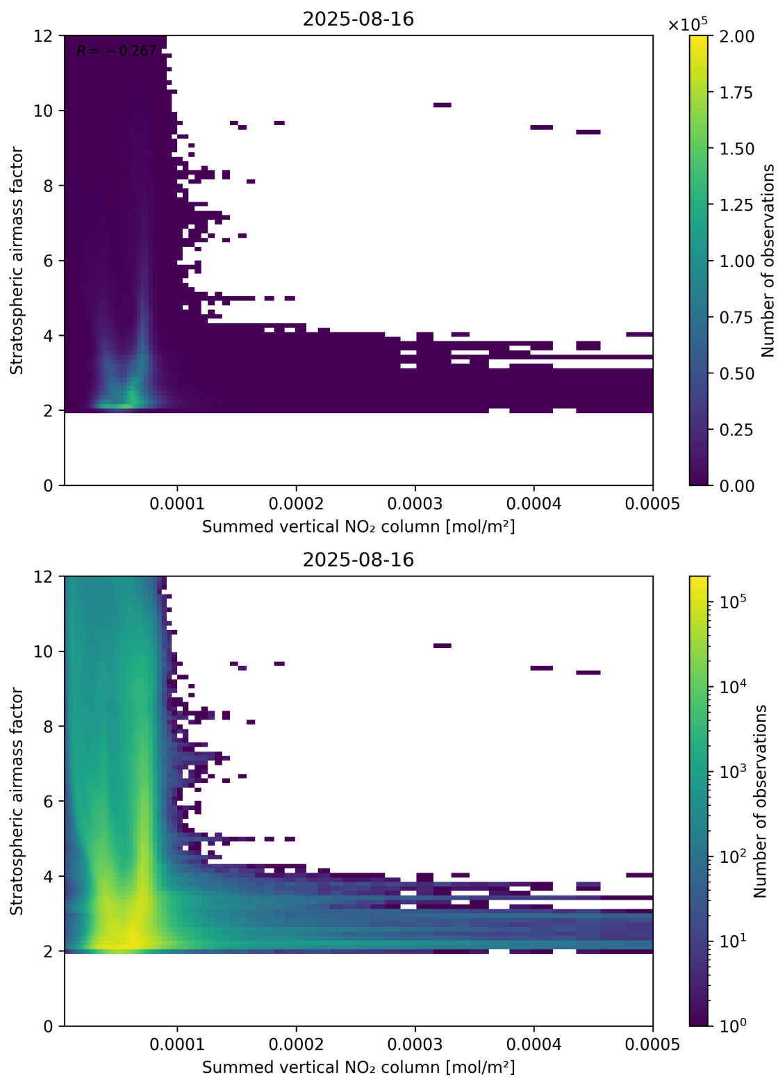
Figure 103: Scatter density plot of “Summed vertical NO 2 column” against “Stratospheric airmass factor” for 2025-08-15 to 2025-08-17.
