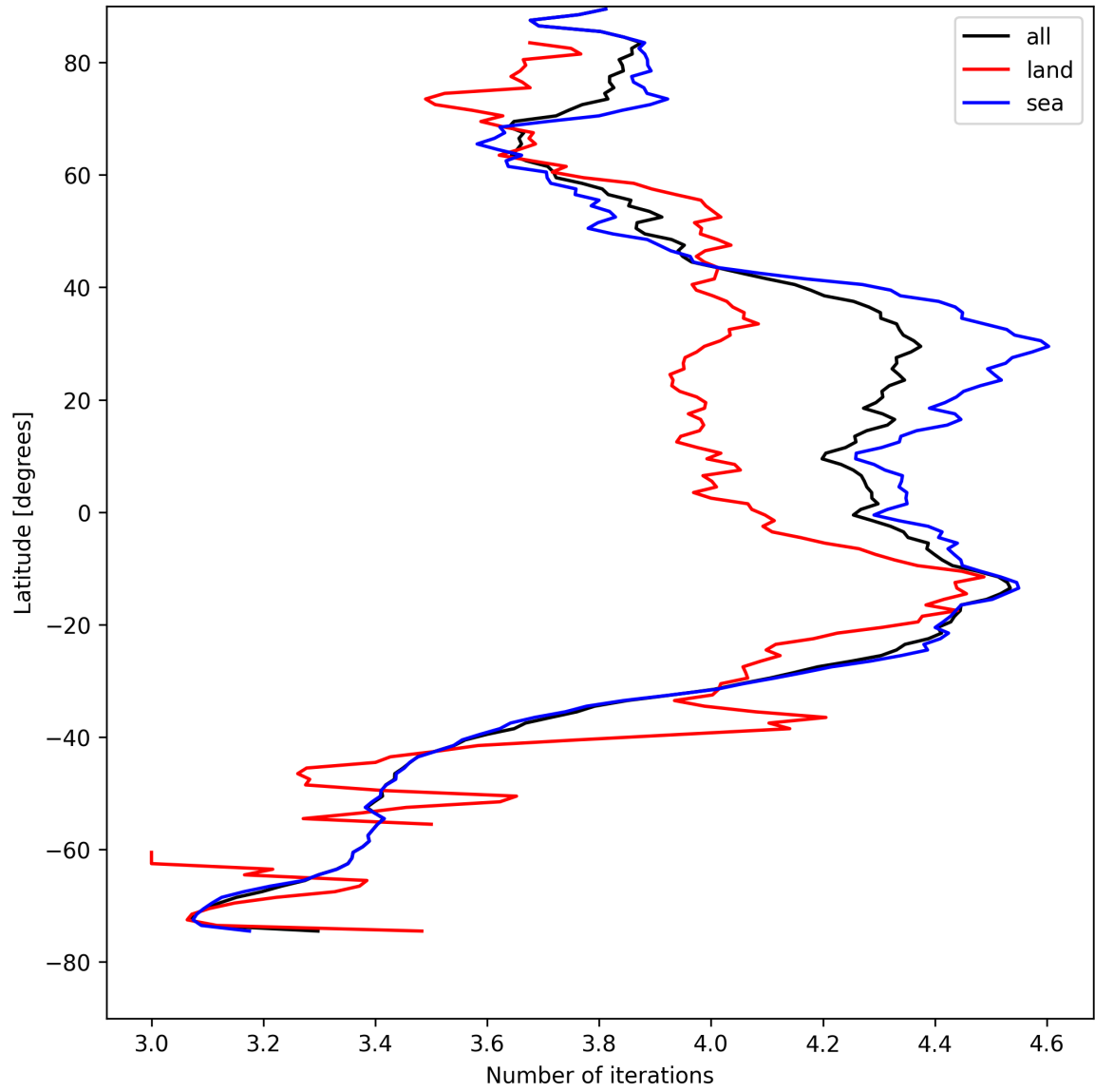
Figure 17: Zonal average of “Number of iterations” for 2025-08-15 to 2025-08-17.
