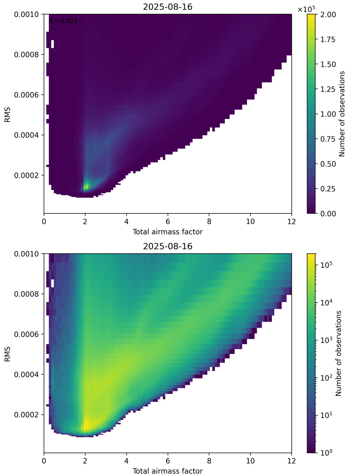
Figure 69: Scatter density plot of “Total airmass factor” against “RMS” for 2025-08-15 to 2025-08-17.
