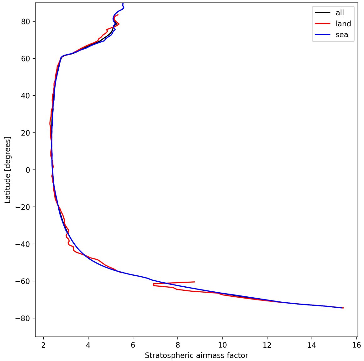
Figure 27: Zonal average of “Stratospheric airmass factor” for 2025-08-15 to 2025-08-17.
