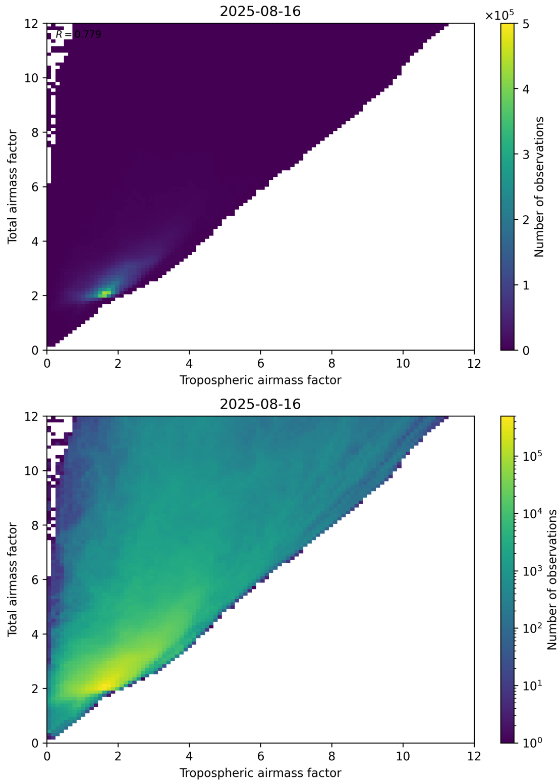
Figure 72: Scatter density plot of “Tropospheric airmass factor” against “Total airmass factor” for 2025-08-15 to 2025-08-17.
