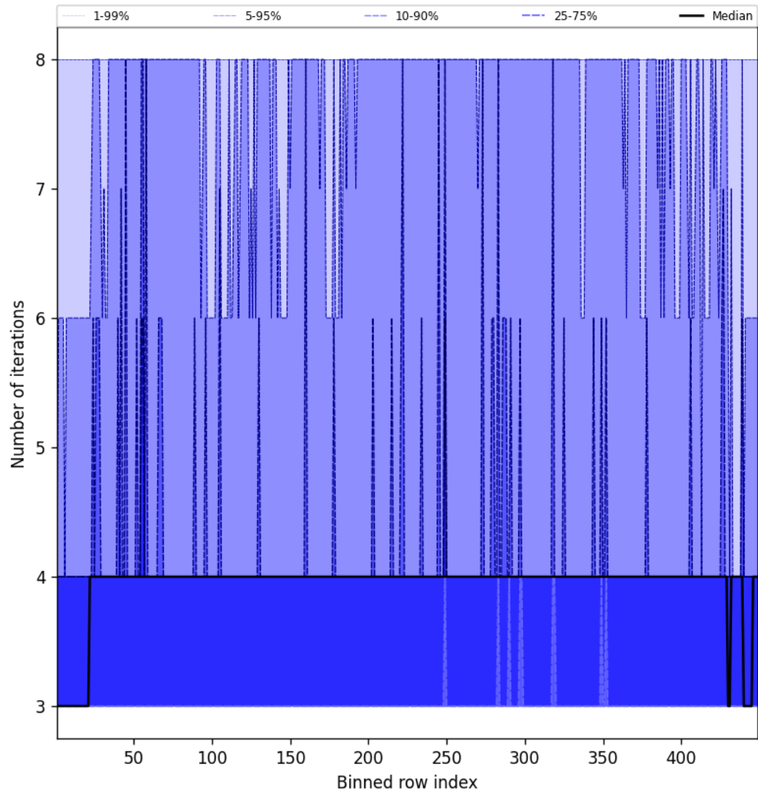
Figure 51: Along track statistics of “Number of iterations” for 2025-08-15 to 2025-08-17
