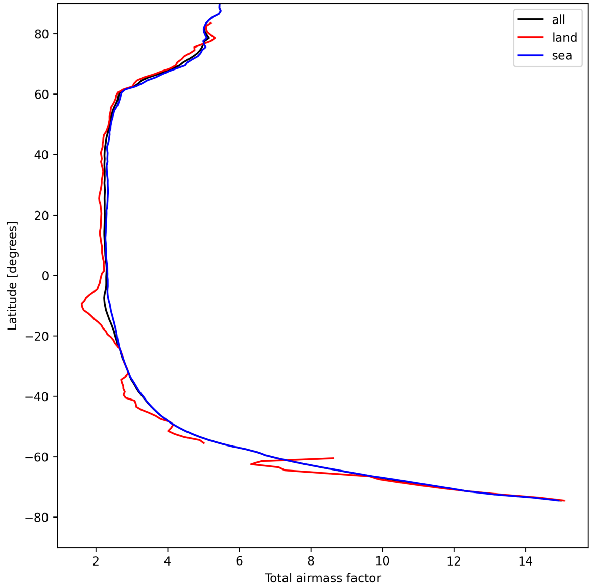
Figure 15: Zonal average of “Total airmass factor” for 2025-08-15 to 2025-08-17.
