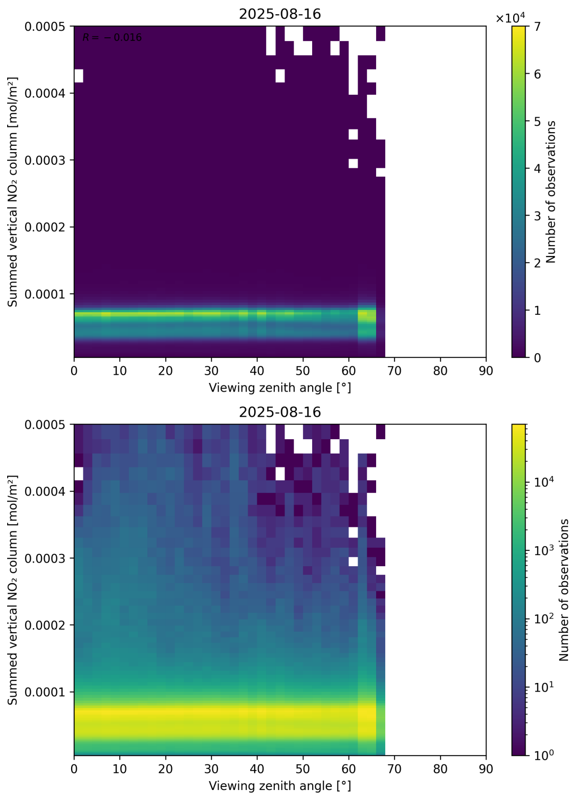
Figure 165: Scatter density plot of “Viewing zenith angle” against “Summed vertical NO 2 column” for 2025-08-15 to 2025-08-17.
