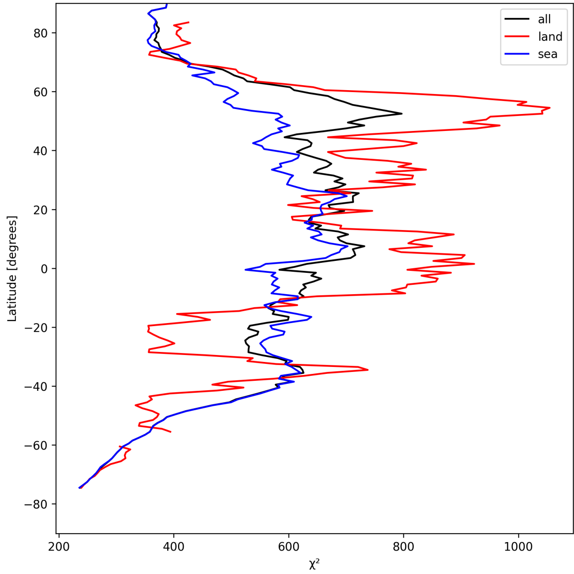
Figure 25: Zonal average of “ \chi^2 ” for 2025-08-15 to 2025-08-17.
