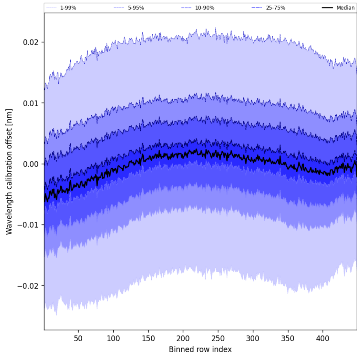
Figure 52: Along track statistics of “Wavelength calibration offset” for 2025-08-15 to 2025-08-17
