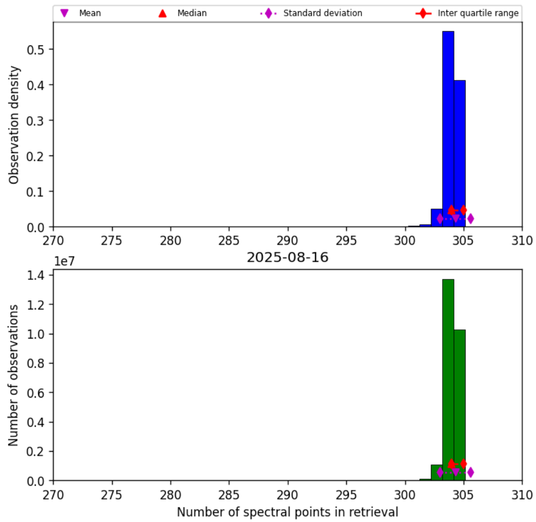
Figure 33: Histogram of “Number of spectral points in retrieval” for 2025-08-15 to 2025-08-17
