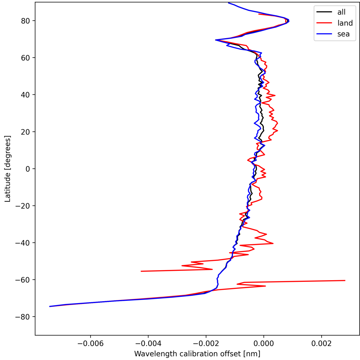
Figure 18: Zonal average of “Wavelength calibration offset” for 2025-08-15 to 2025-08-17.
