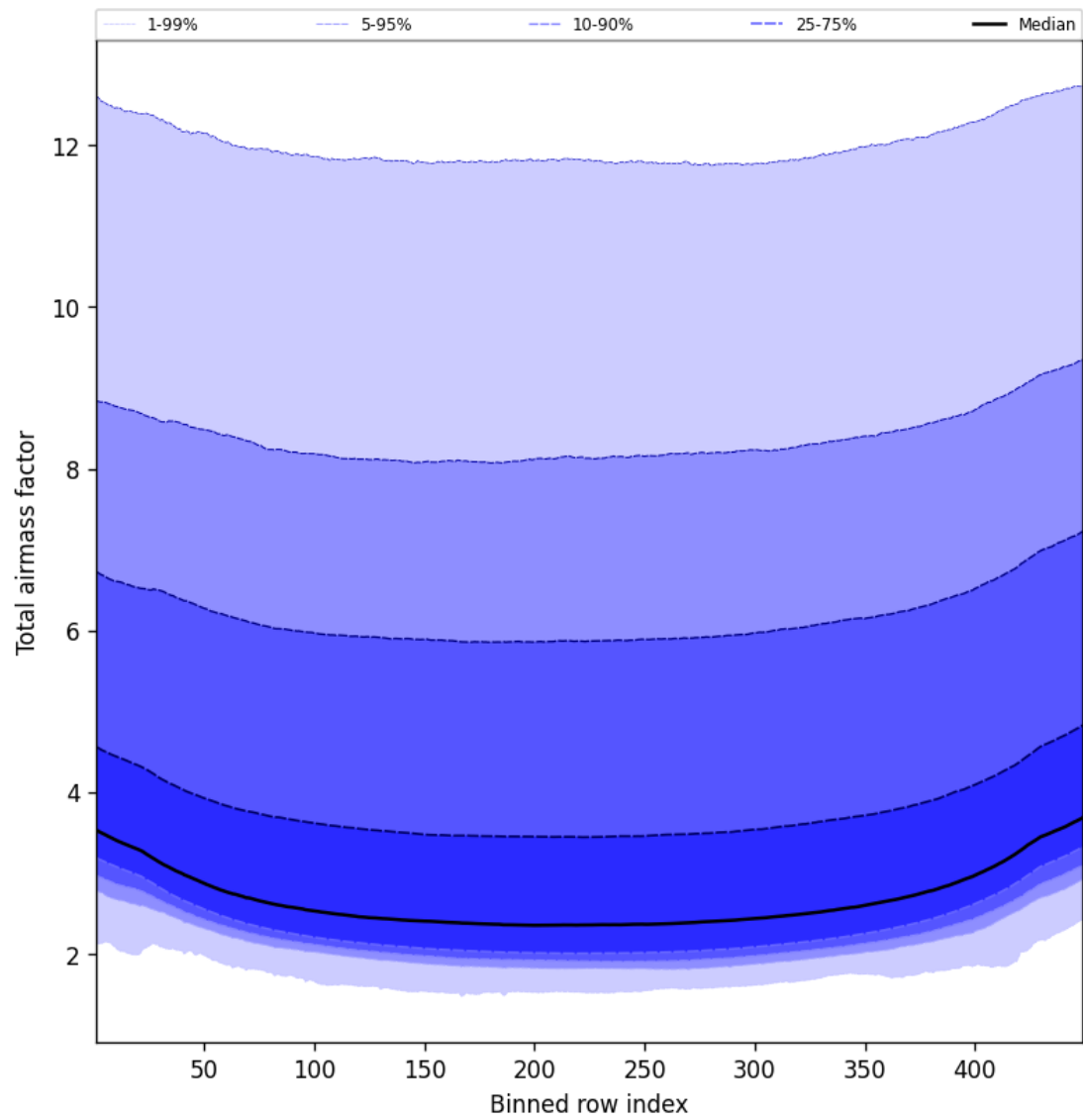
Figure 49: Along track statistics of “Total airmass factor” for 2025-08-15 to 2025-08-17
