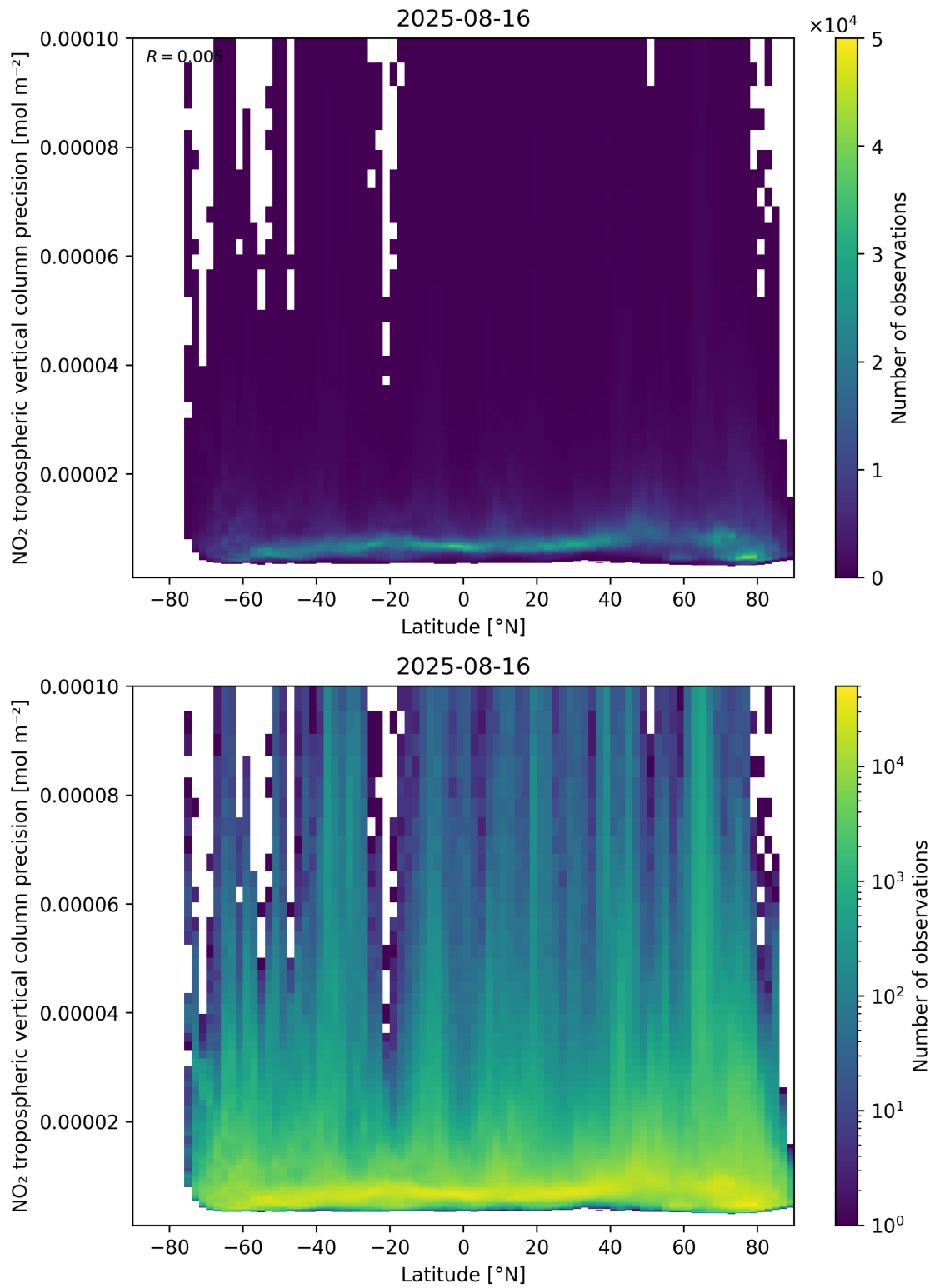
Figure 93: Scatter density plot of “Latitude” against “NO 2 tropospheric vertical column precision” for 2025-08-15 to 2025-08-17.
