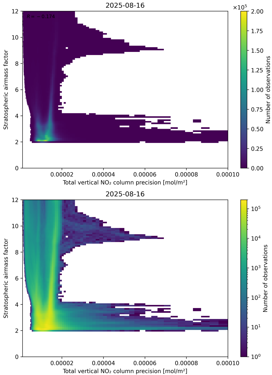
Figure 115: Scatter density plot of “Total vertical NO 2 column precision” against “Stratospheric air mass factor” for 2025-08-15 to 2025-08-17.
