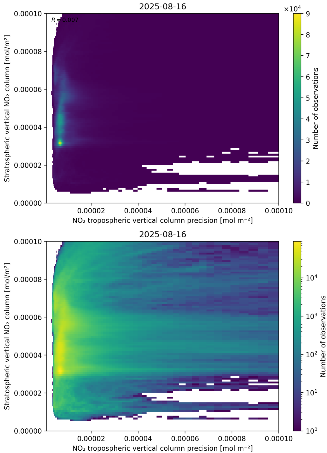
Figure 135: Scatter density plot of “NO 2 tropospheric vertical column precision” against “Stratospheric vertical NO 2 column” for 2025-08-15 to 2025-08-17.
