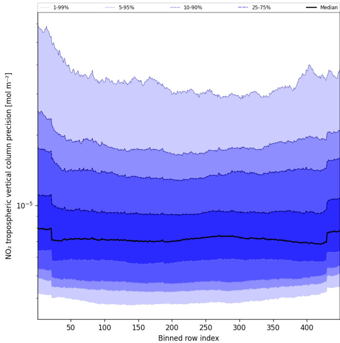
Figure 47: Along track statistics of “NO 2 tropospheric vertical column precision” for 2025-08-15 to 2025-08-17
