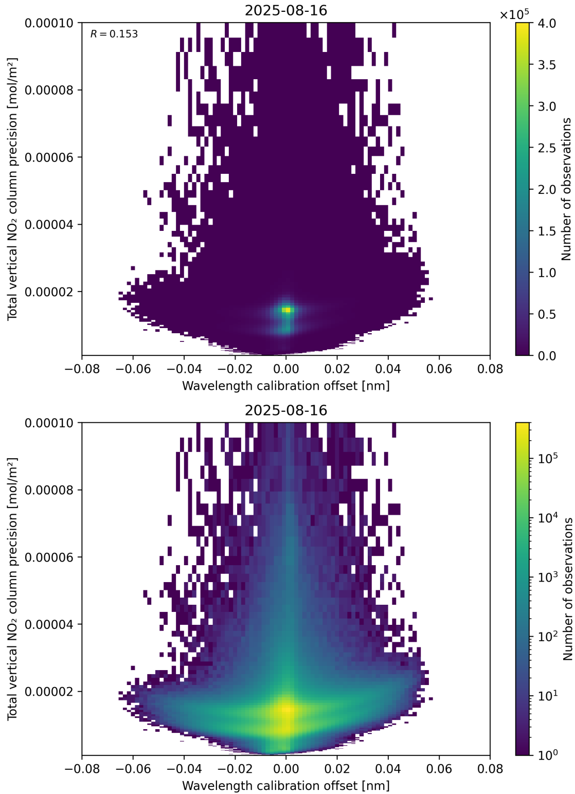
Figure 180: Scatter density plot of “Wavelength calibration offset” against “Total vertical NO 2 column precision” for 2025-08-15 to 2025-08-17.
