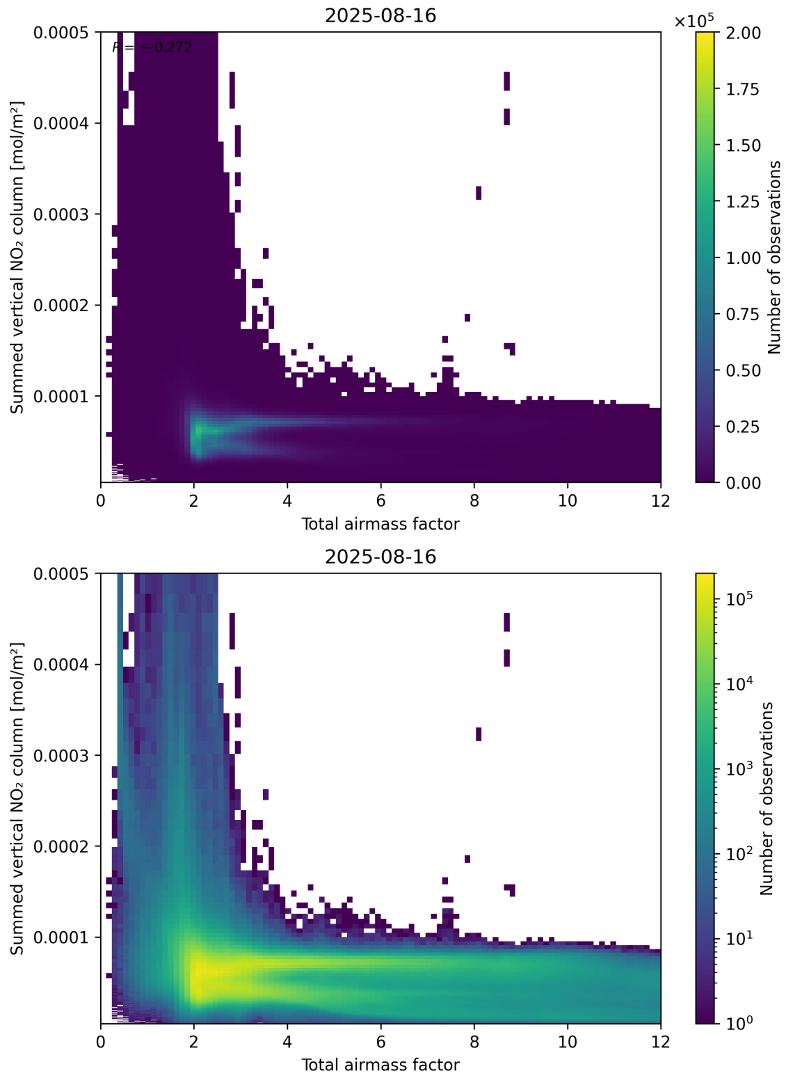
Figure 65: Scatter density plot of “Total airmass factor” against “Summed vertical NO 2 column” for 2025-08-15 to 2025-08-17.
