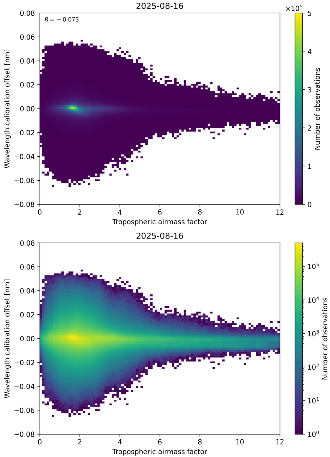
Figure 80: Scatter density plot of “Tropospheric airmass factor” against “Wavelength calibration offset” for 2025-08-15 to 2025-08-17.
