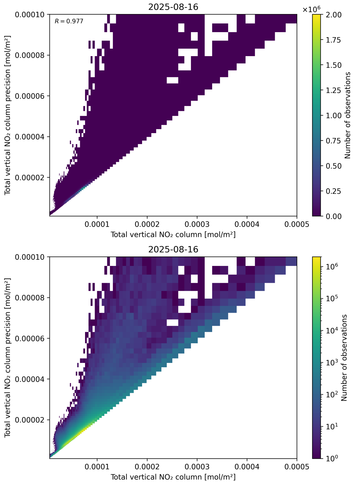
Figure 114: Scatter density plot of “Total vertical NO 2 column” against “Total vertical NO 2 column precision” for 2025-08-15 to 2025-08-17.
