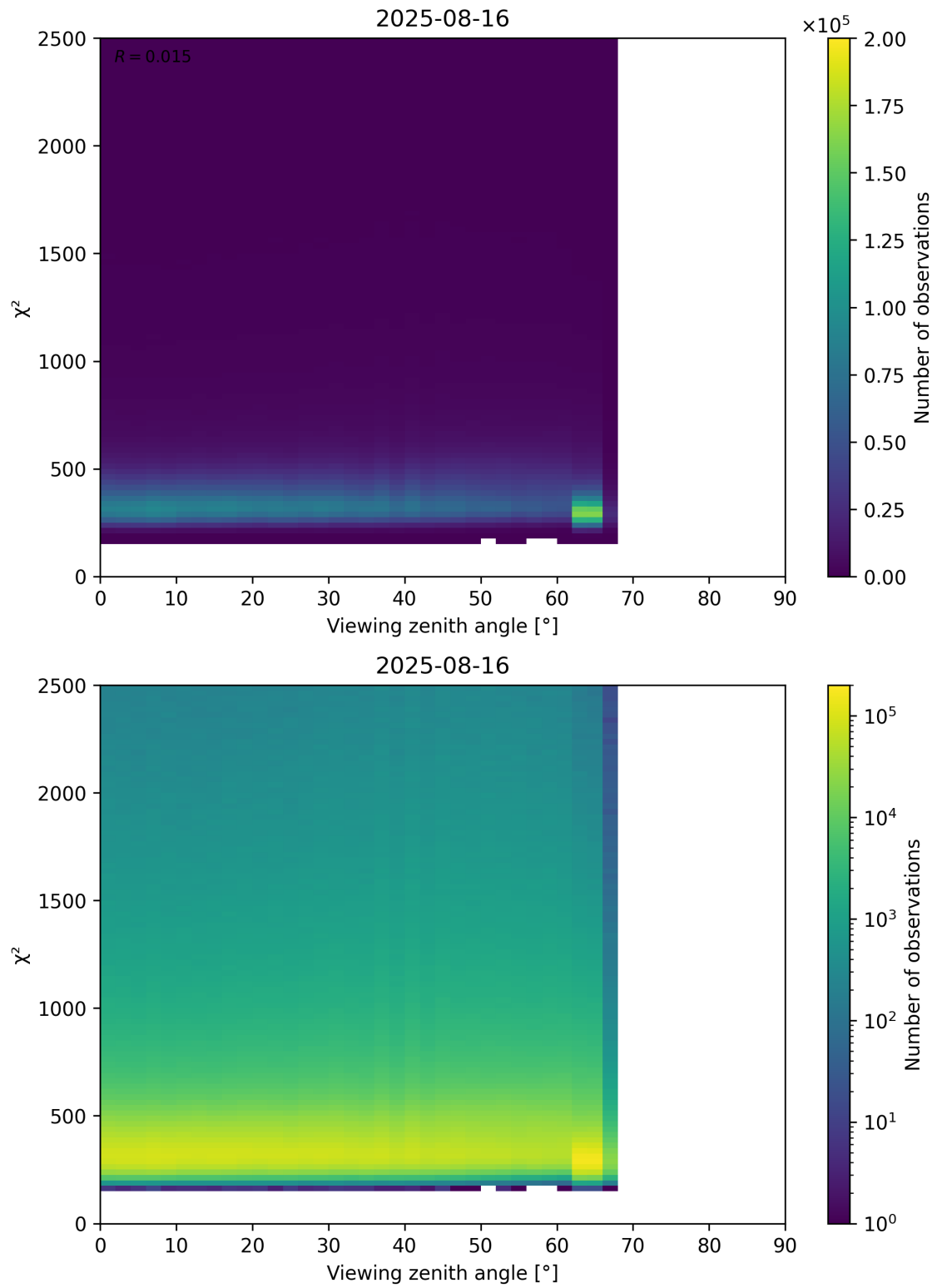
Figure 162: Scatter density plot of “Viewing zenith angle” against “ \chi^2 ” for 2025-08-15 to 2025-08-17.
