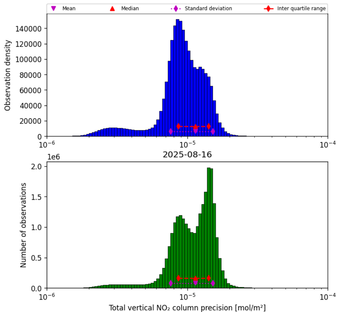
Figure 39: Histogram of “Total vertical NO 2 column precision” for 2025-08-15 to 2025-08-17
