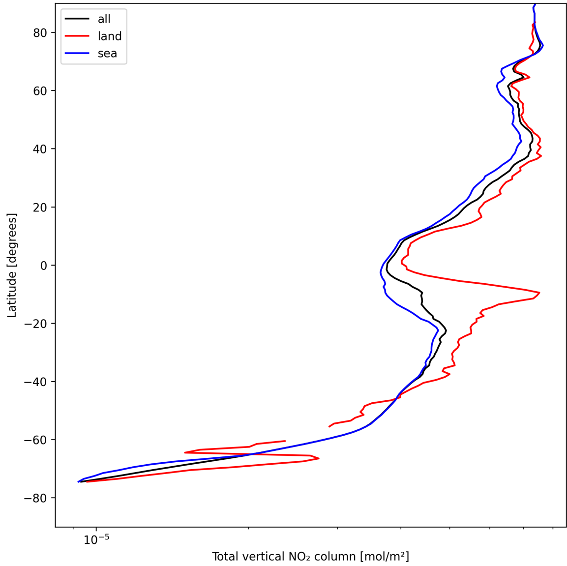
Figure 21: Zonal average of “Total vertical NO 2 column” for 2025-08-15 to 2025-08-17.
