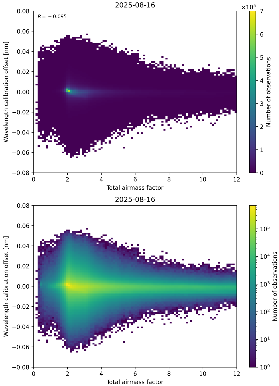
Figure 70: Scatter density plot of “Total airmass factor” against “Wavelength calibration offset” for 2025-08-15 to 2025-08-17.
