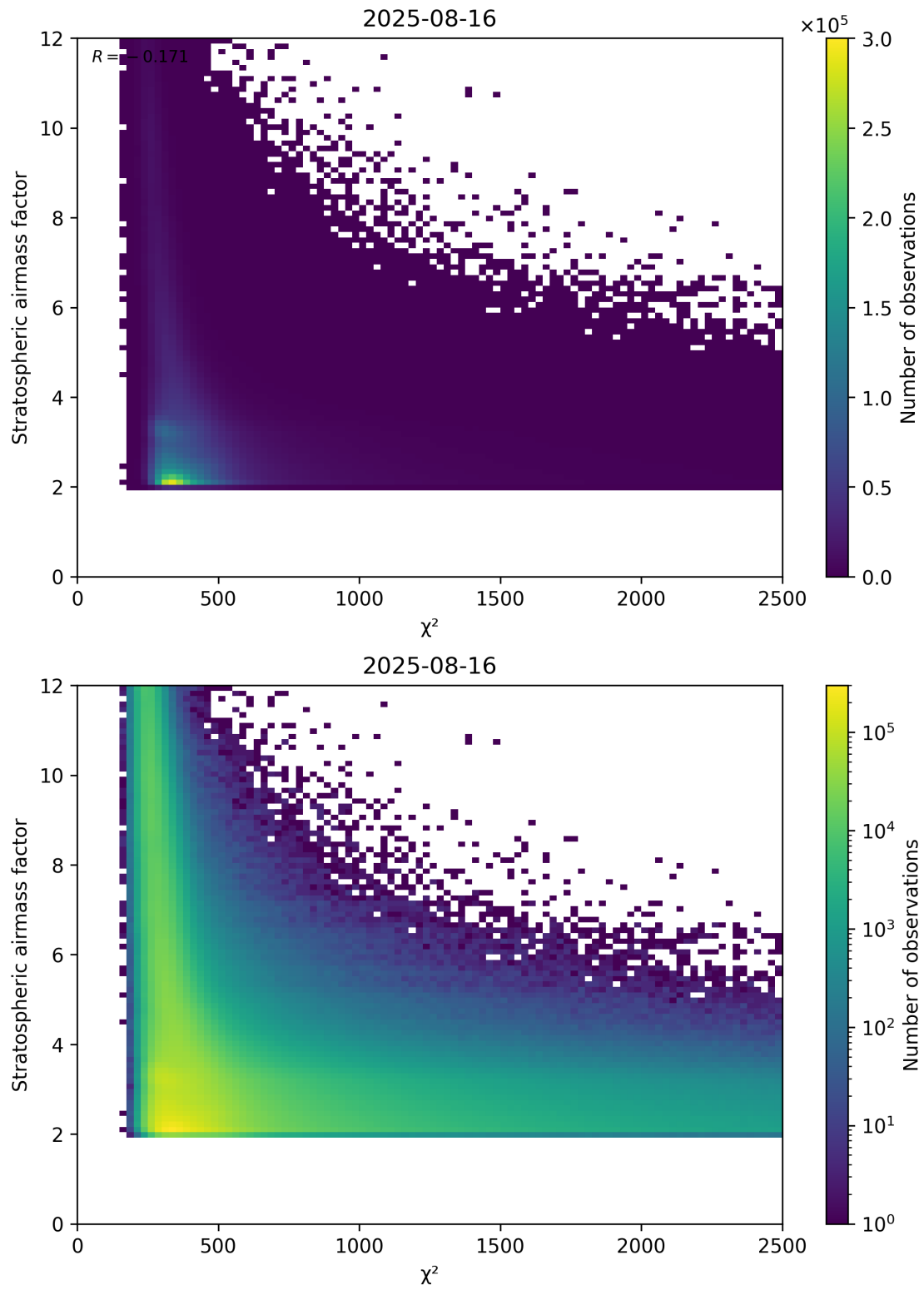
Figure 81: Scatter density plot of “ \chi^2 ” against “Stratospheric airmass factor” for 2025-08-15 to 2025-08-17.
