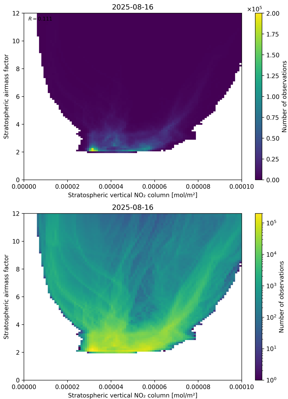
Figure 96: Scatter density plot of “Stratospheric vertical NO 2 column” against “Stratospheric airmass factor” for 2025-08-15 to 2025-08-17.
