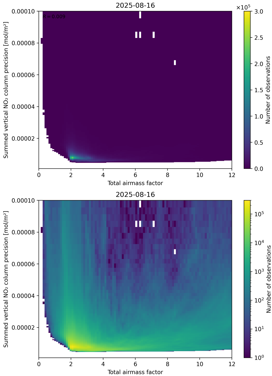
Figure 66: Scatter density plot of “Total airmass factor” against “Summed vertical NO 2 column precision” for 2025-08-15 to 2025-08-17.
