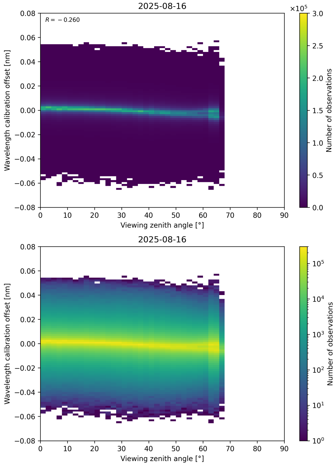
Figure 173: Scatter density plot of “Viewing zenith angle” against “Wavelength calibration offset” for 2025-08-15 to 2025-08-17.
