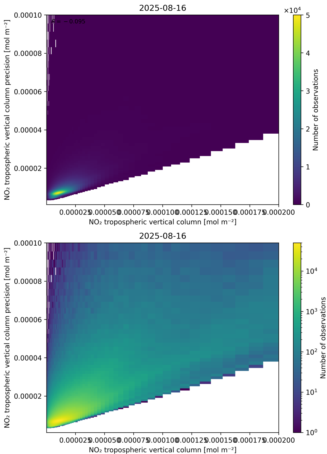
Figure 130: Scatter density plot of “NO 2 tropospheric vertical column” against “NO 2 tropospheric vertical column precision” for 2025-08-15 to 2025-08-17.
