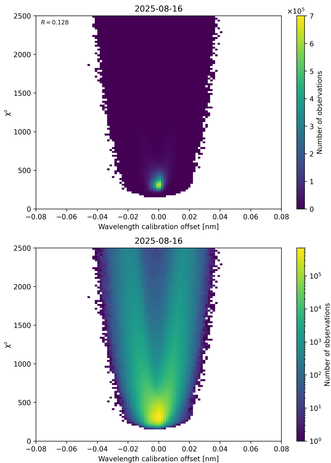
Figure 175: Scatter density plot of “Wavelength calibration offset” against “ \chi^2 ” for 2025-08-15 to 2025-08-17.
