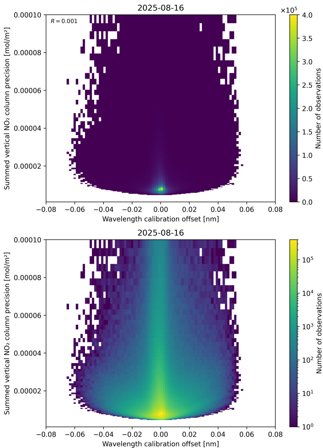
Figure 178: Scatter density plot of “Wavelength calibration offset” against “Summed vertical NO 2 column precision” for 2025-08-15 to 2025-08-17.
