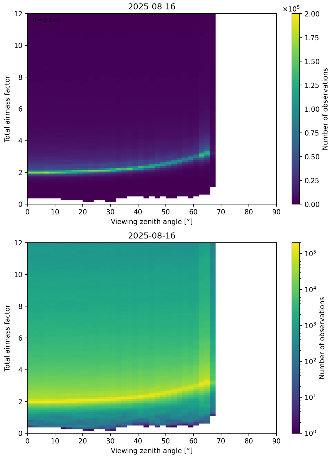
Figure 160: Scatter density plot of “Viewing zenith angle” against “Total airmass factor” for 2025-08-15 to 2025-08-17.
