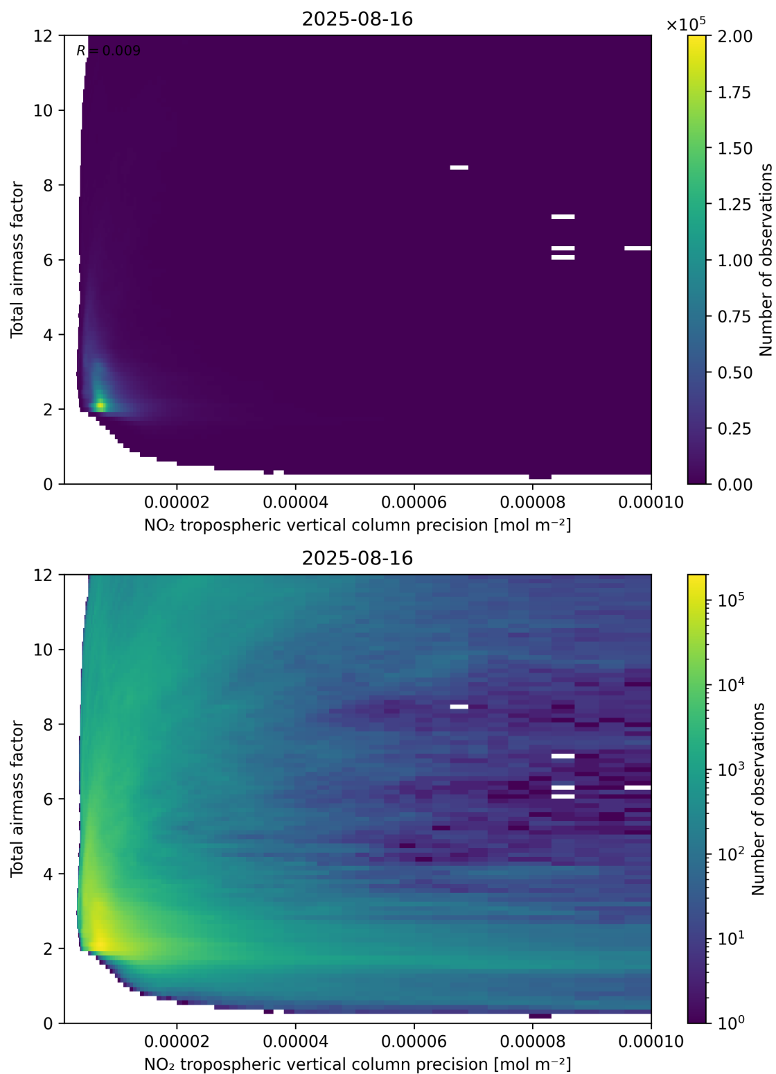
Figure 132: Scatter density plot of “NO 2 tropospheric vertical column precision” against “Total air mass factor” for 2025-08-15 to 2025-08-17.
