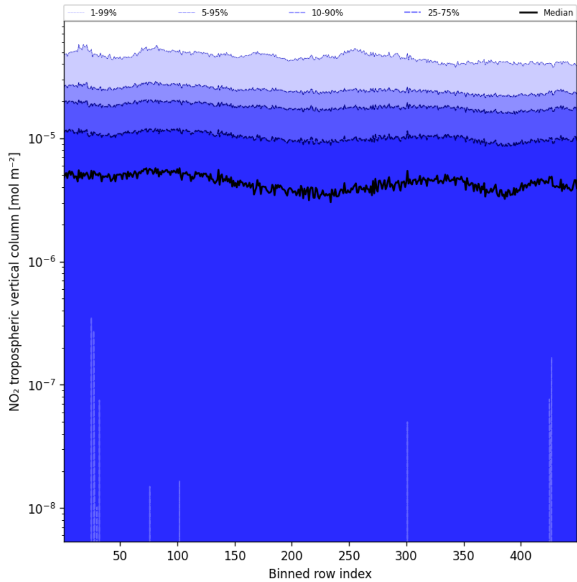
Figure 46: Along track statistics of “NO 2 tropospheric vertical column” for 2025-08-15 to 2025-08-17
