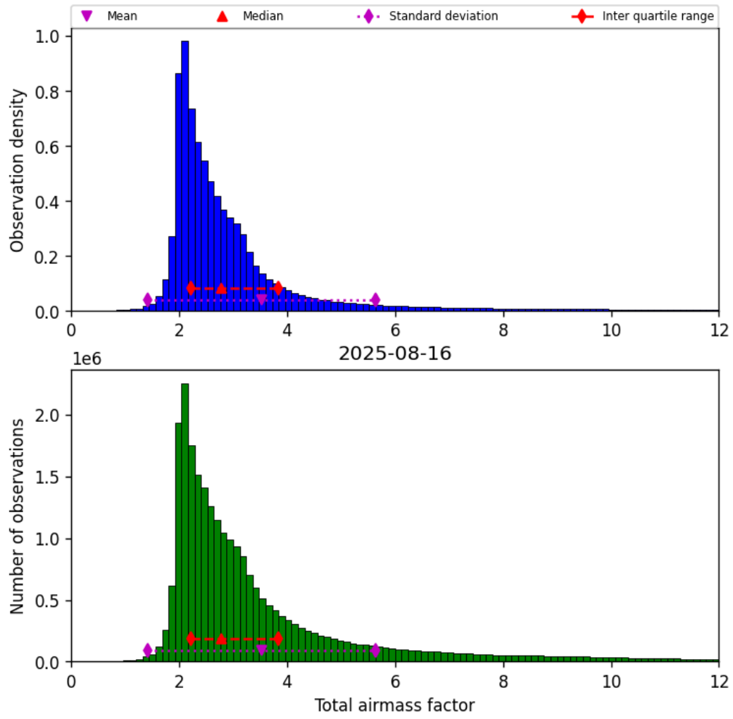
Figure 32: Histogram of “Total airmass factor” for 2025-08-15 to 2025-08-17
