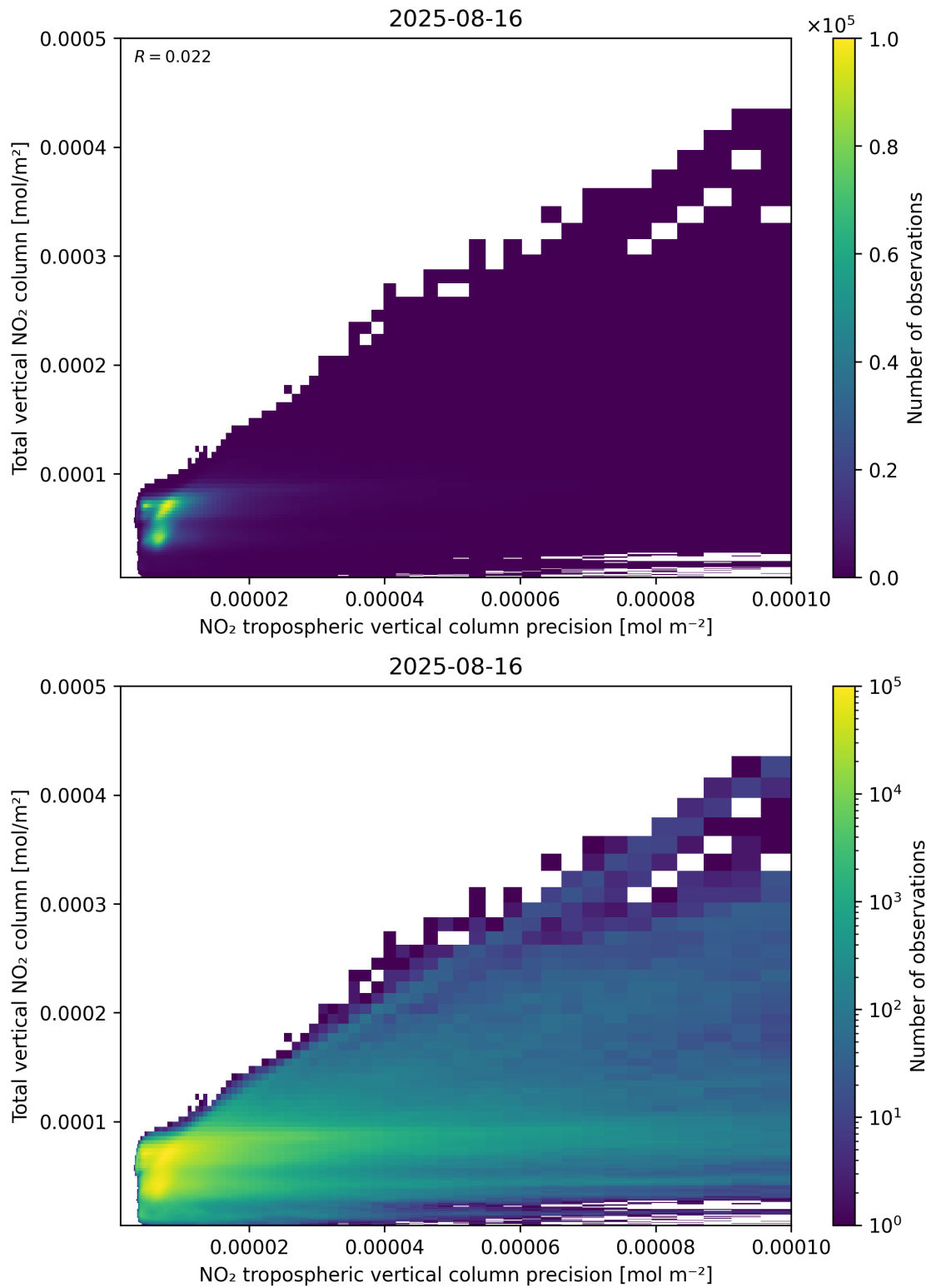
Figure 138: Scatter density plot of “NO 2 tropospheric vertical column precision” against “Total vertical NO 2 column” for 2025-08-15 to 2025-08-17.
