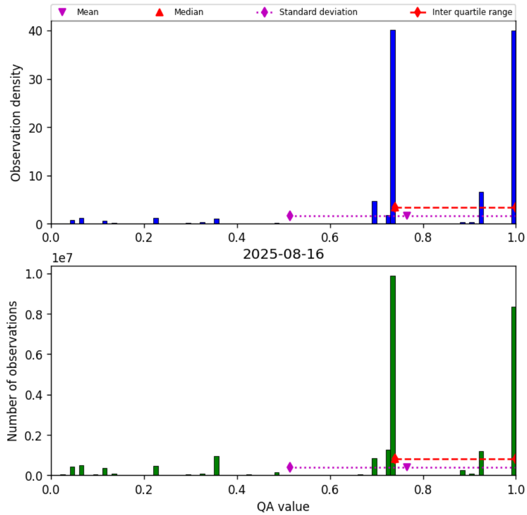
Figure 28: Histogram of “QA value” for 2025-08-15 to 2025-08-17
