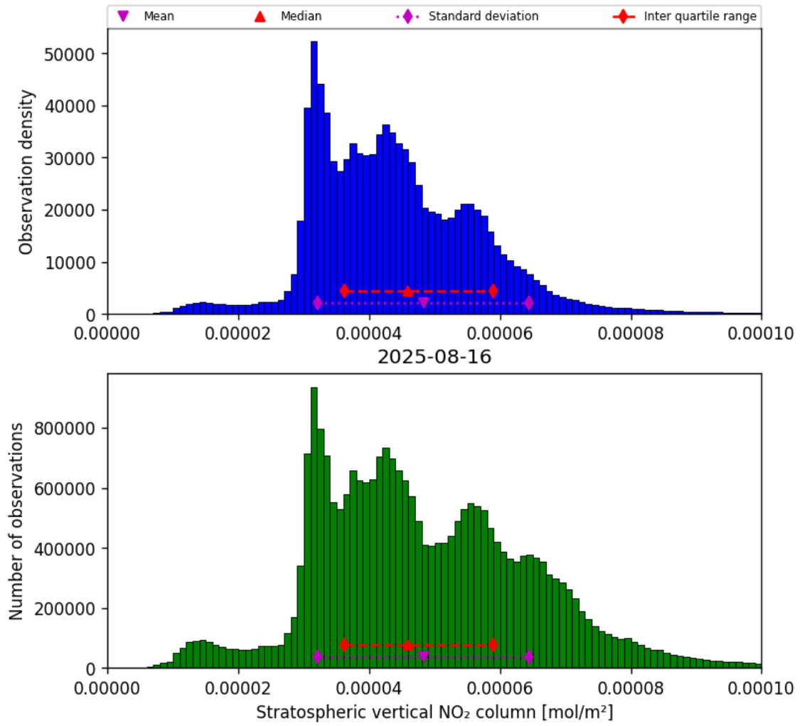
Figure 36: Histogram of “Stratospheric vertical NO 2 column” for 2025-08-15 to 2025-08-17
