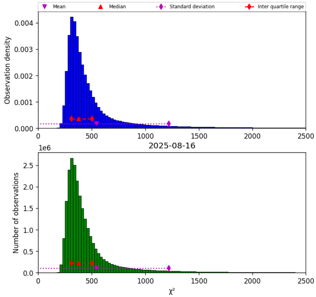
Figure 42: Histogram of “ \chi^2 ” for 2025-08-15 to 2025-08-17
