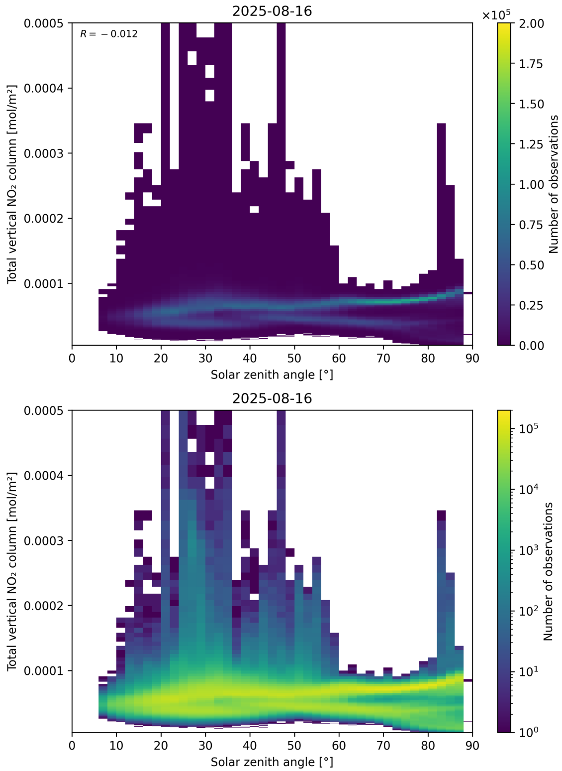
Figure 153: Scatter density plot of “Solar zenith angle” against “Total vertical NO 2 column” for 2025-08-15 to 2025-08-17.
