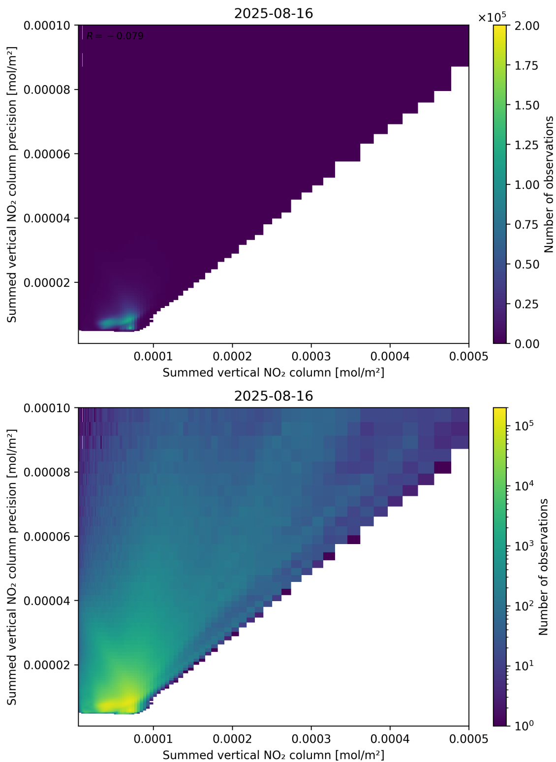
Figure 105: Scatter density plot of “Summed vertical NO 2 column” against “Summed vertical NO 2 column precision” for 2025-08-15 to 2025-08-17.
