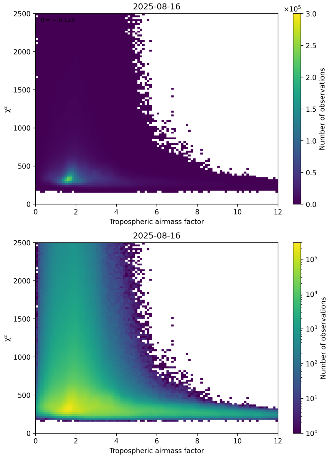
Figure 73: Scatter density plot of “Tropospheric airmass factor” against “ \chi^2 ” for 2025-08-15 to 2025-08-17.
