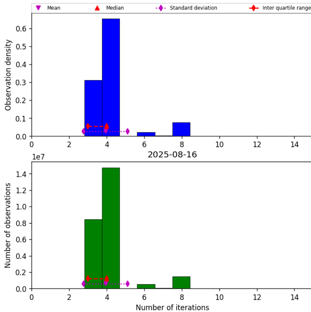
Figure 34: Histogram of “Number of iterations” for 2025-08-15 to 2025-08-17
