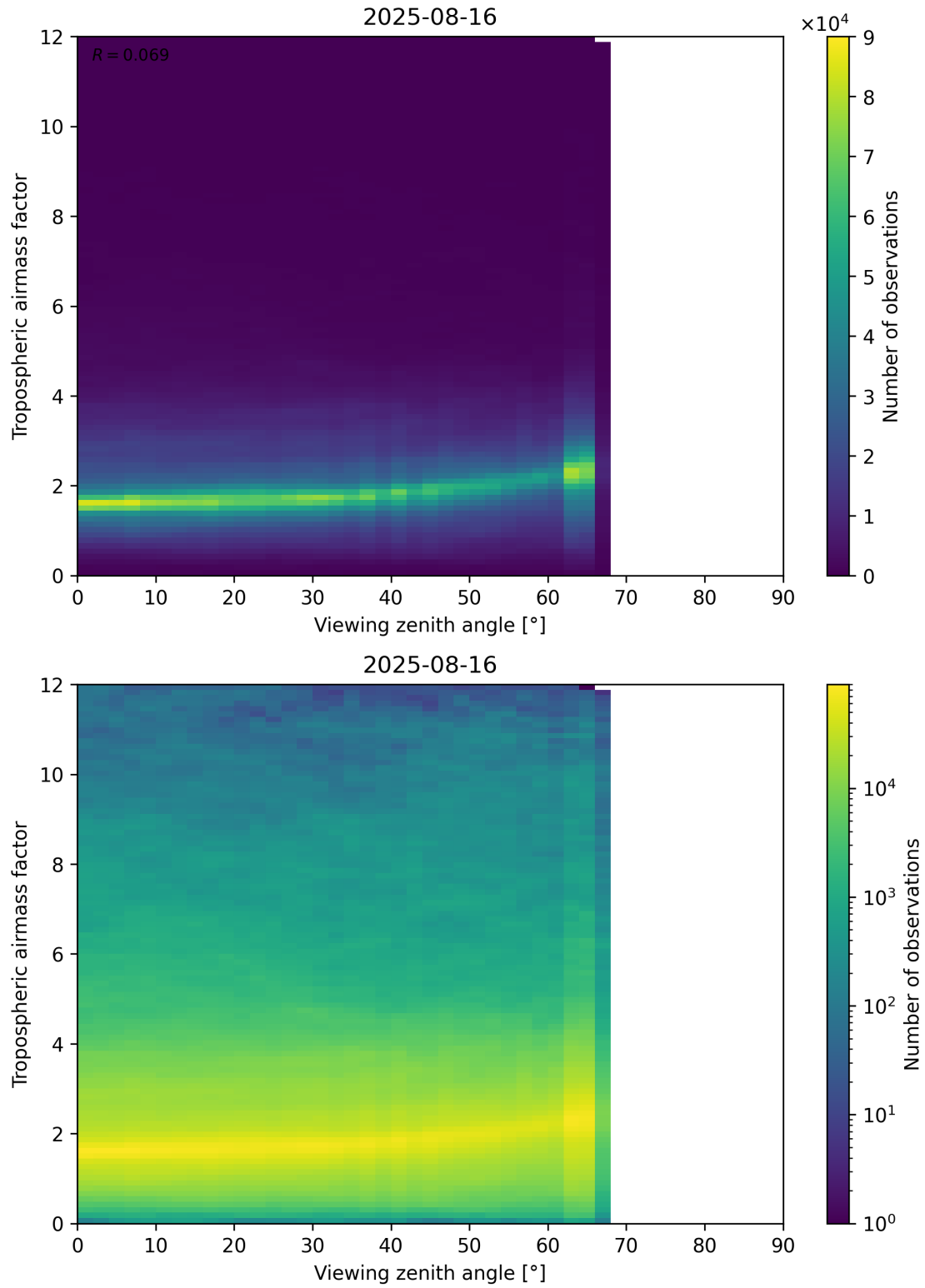
Figure 161: Scatter density plot of “Viewing zenith angle” against “Tropospheric airmass factor” for 2025-08-15 to 2025-08-17.
