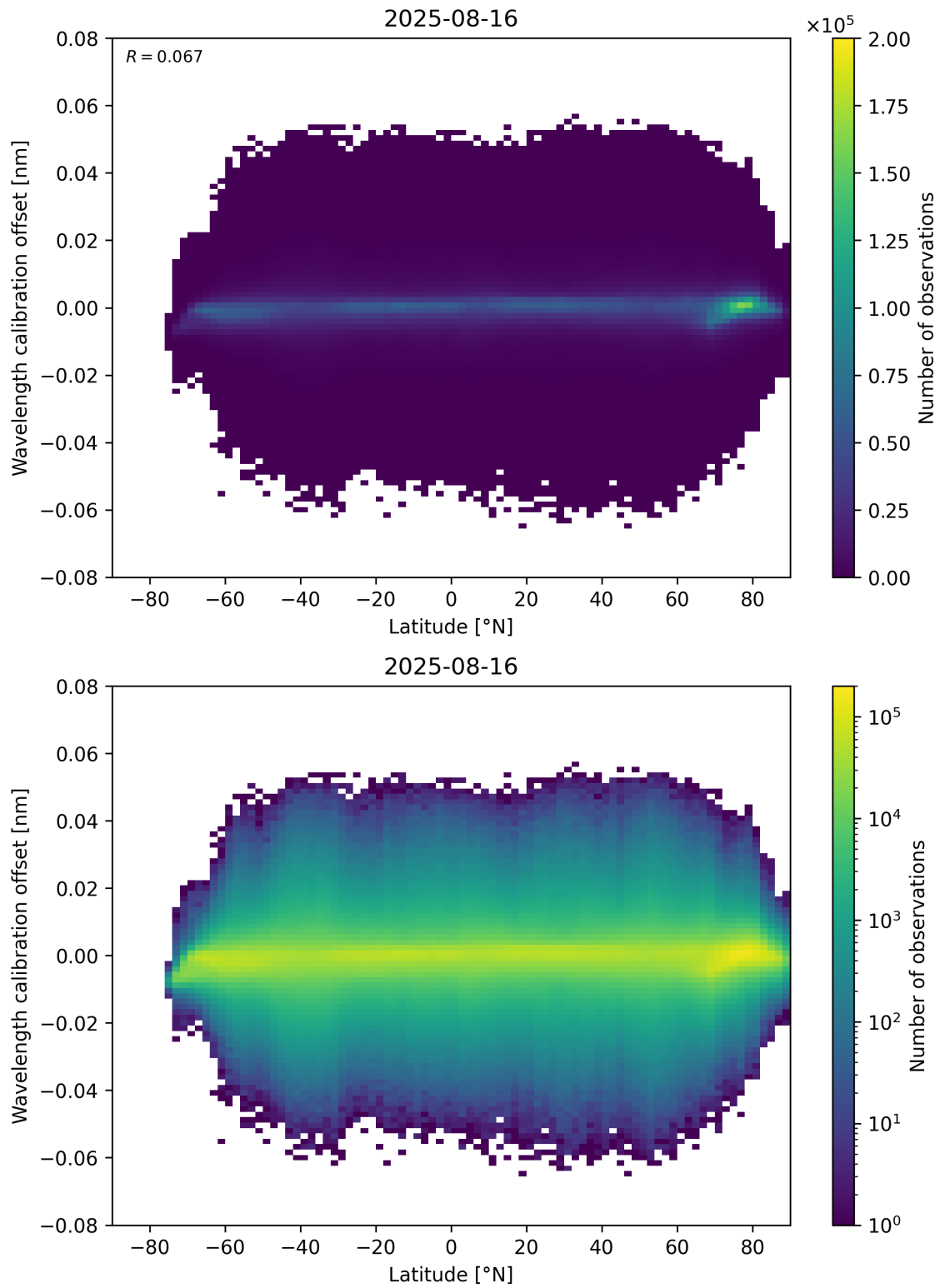
Figure 95: Scatter density plot of “Latitude” against “Wavelength calibration offset” for 2025-08-15 to 2025-08-17.
