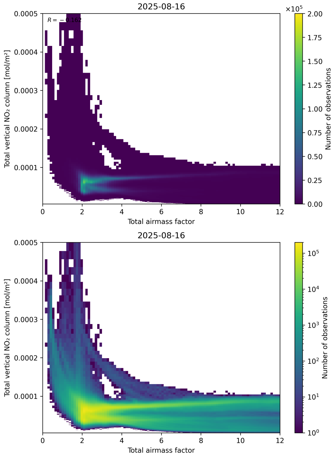
Figure 67: Scatter density plot of “Total airmass factor” against “Total vertical NO 2 column” for 2025-08-15 to 2025-08-17.
