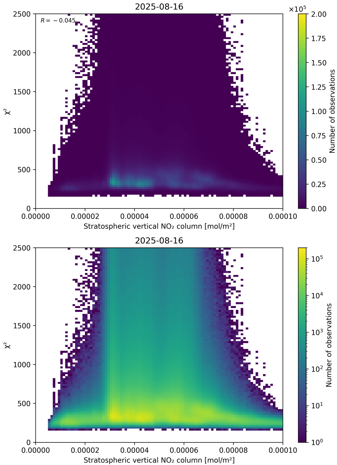
Figure 97: Scatter density plot of “Stratospheric vertical NO 2 column” against “ \chi^2 ” for 2025-08-15 to 2025-08-17.
