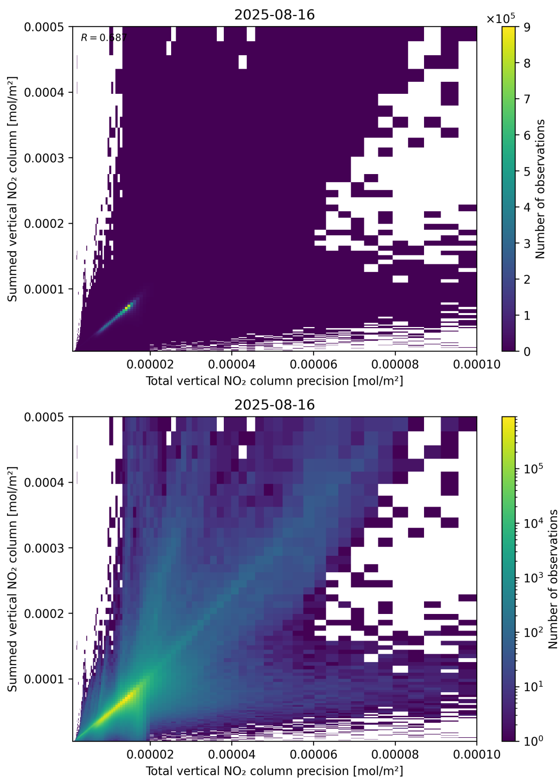
Figure 117: Scatter density plot of “Total vertical NO 2 column precision” against “Summed vertical NO 2 column” for 2025-08-15 to 2025-08-17.
