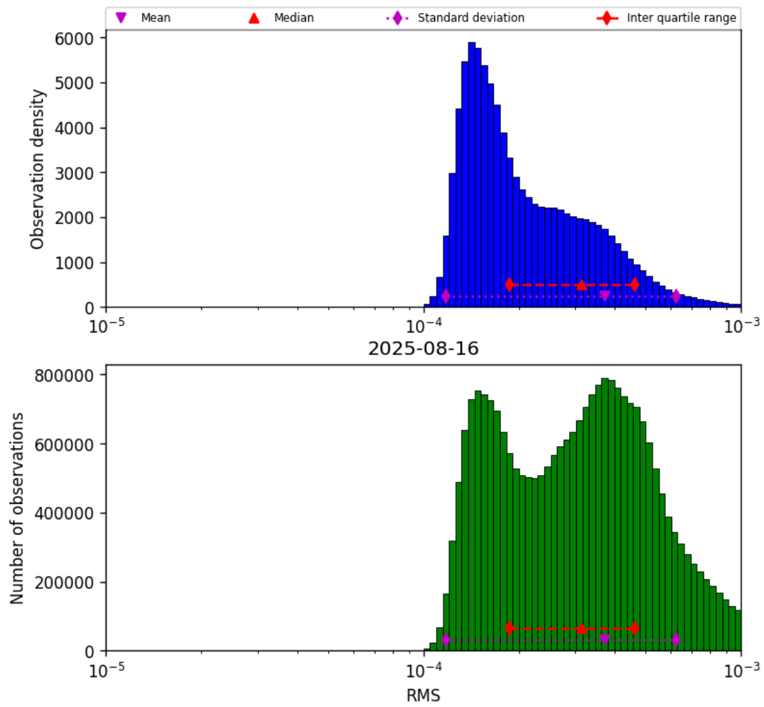
Figure 43: Histogram of “RMS” for 2025-08-15 to 2025-08-17
