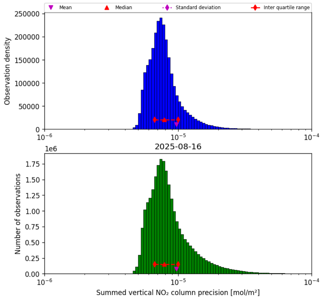
Figure 41: Histogram of "Summed vertical NO 2 column precision" for 2025-08-15 to 2025-08-17
