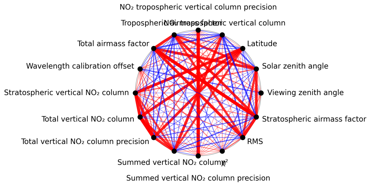
Figure 1: Map of correlation graph for 2025-08-15 to 2025-08-17.
