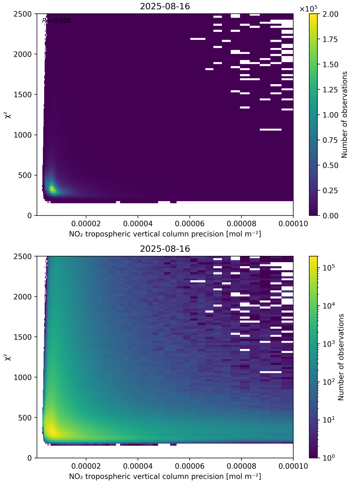
Figure 134: Scatter density plot of “NO 2 tropospheric vertical column precision” against “ \chi^2 ” for 2025-08-15 to 2025-08-17.
