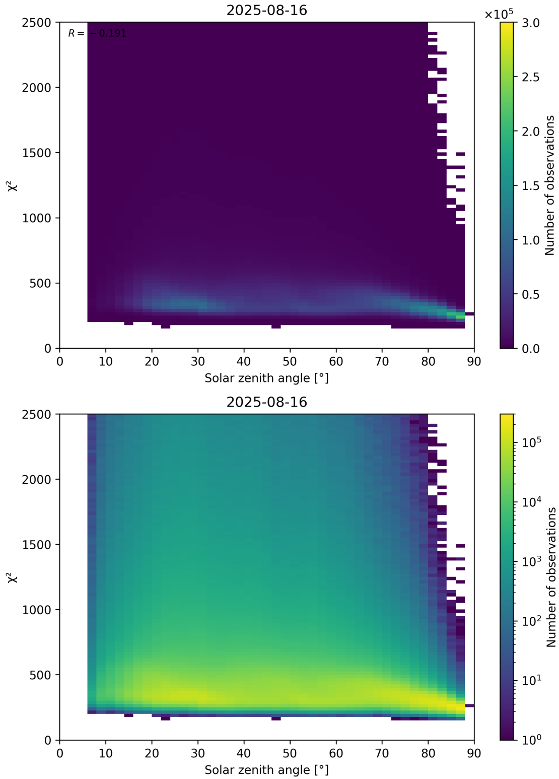
Figure 148: Scatter density plot of “Solar zenith angle” against “ \chi^2 ” for 2025-08-15 to 2025-08-17.
