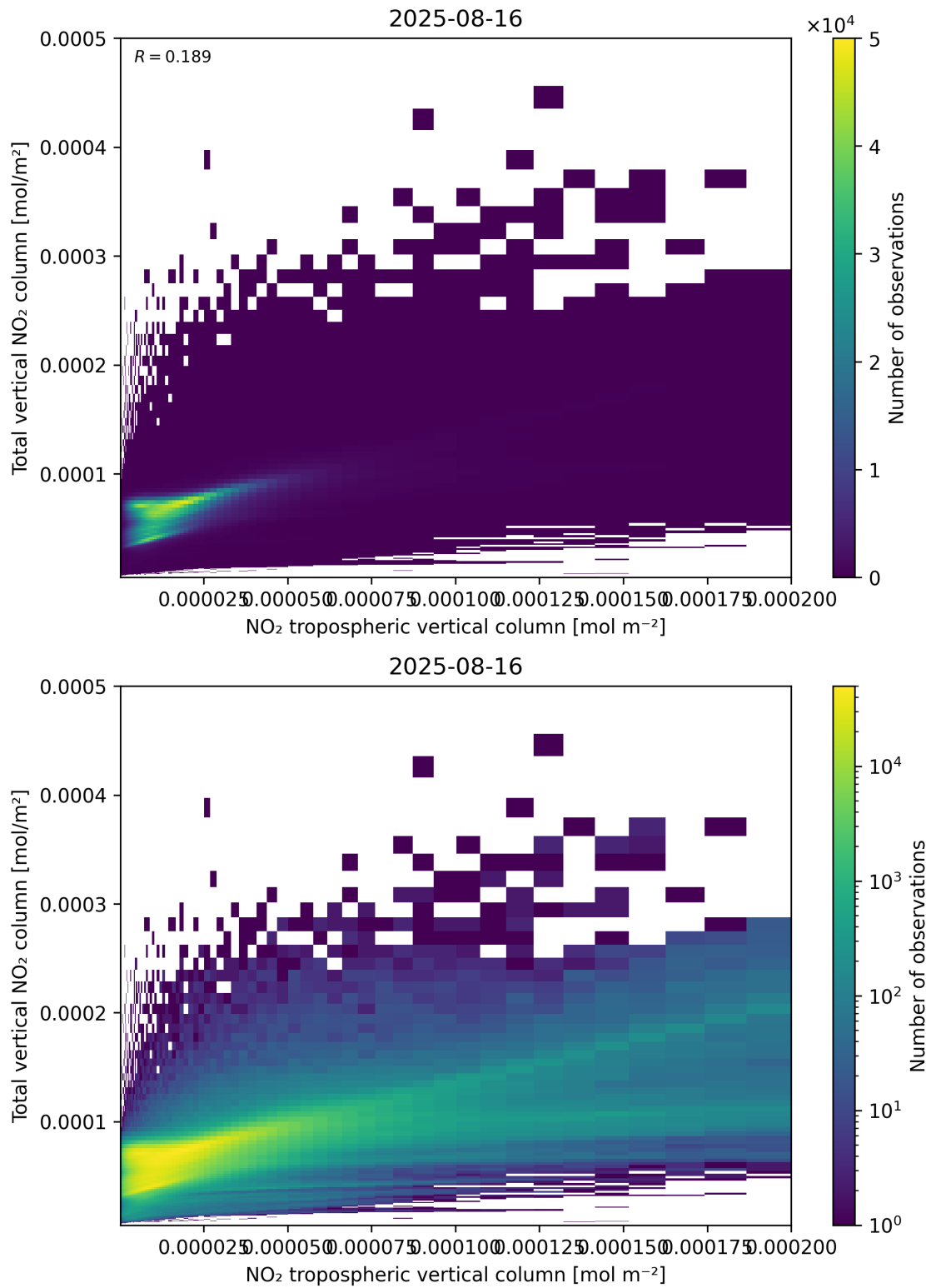
Figure 128: Scatter density plot of “NO 2 tropospheric vertical column” against “Total vertical NO 2 column” for 2025-08-15 to 2025-08-17.
