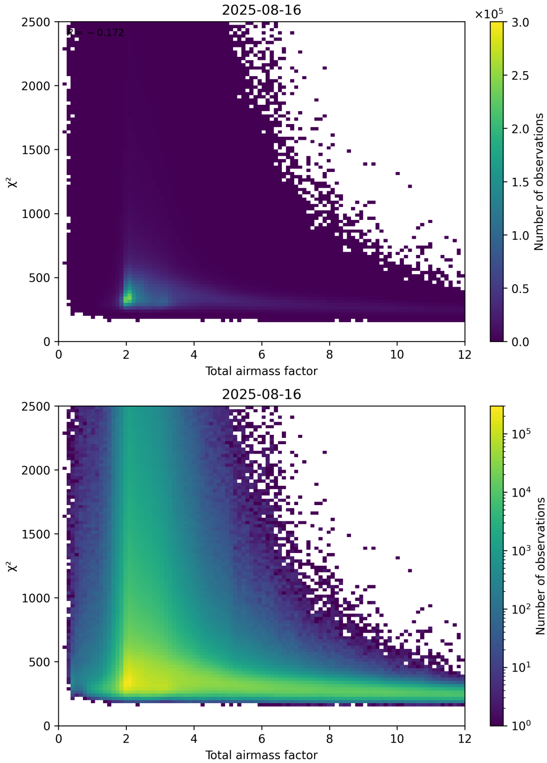
Figure 63: Scatter density plot of “Total airmass factor” against “ \chi^2 ” for 2025-08-15 to 2025-08-17.
