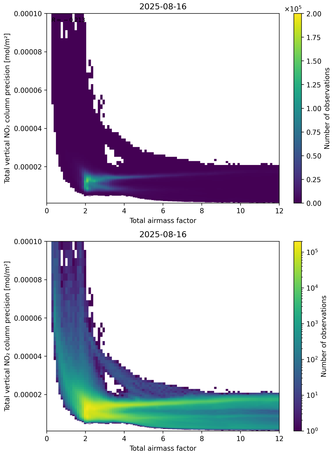
Figure 68: Scatter density plot of “Total airmass factor” against “Total vertical NO 2 column precision” for 2025-08-15 to 2025-08-17.
