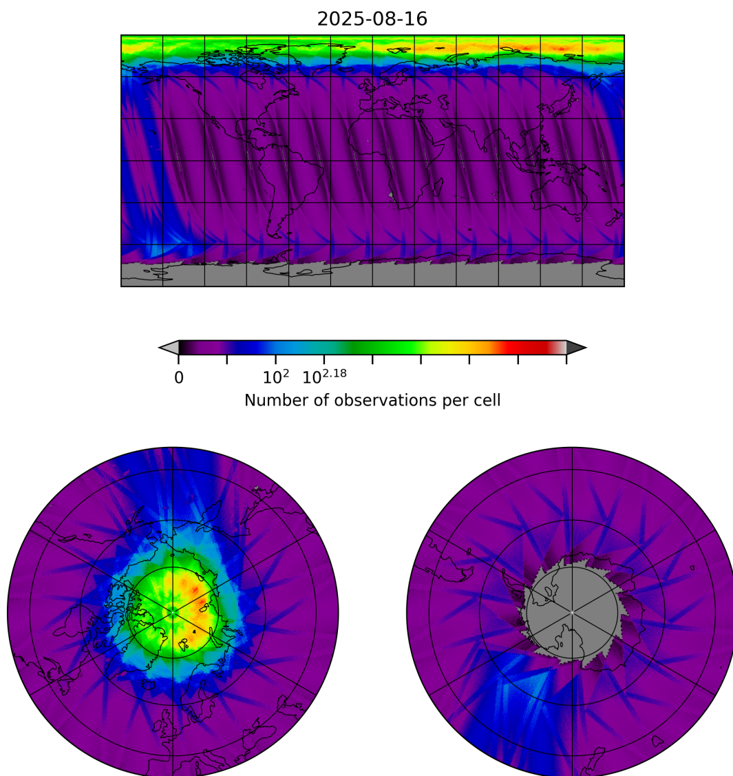
Figure 10: Map of the number of observations for 2025-08-15 to 2025-08-17
