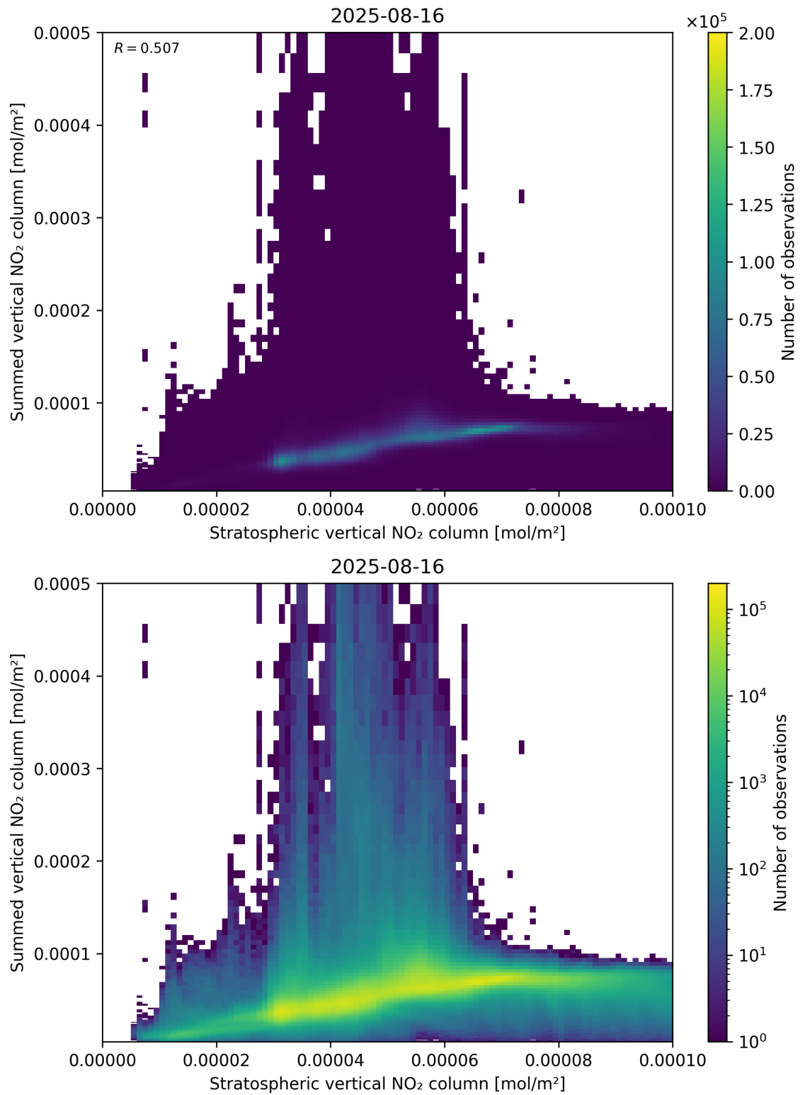
Figure 98: Scatter density plot of “Stratospheric vertical NO 2 column” against “Summed vertical NO 2 column” for 2025-08-15 to 2025-08-17.
