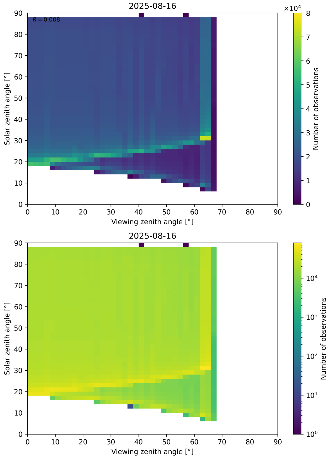
Figure 172: Scatter density plot of “Viewing zenith angle” against “Solar zenith angle” for 2025-08-15 to 2025-08-17.
