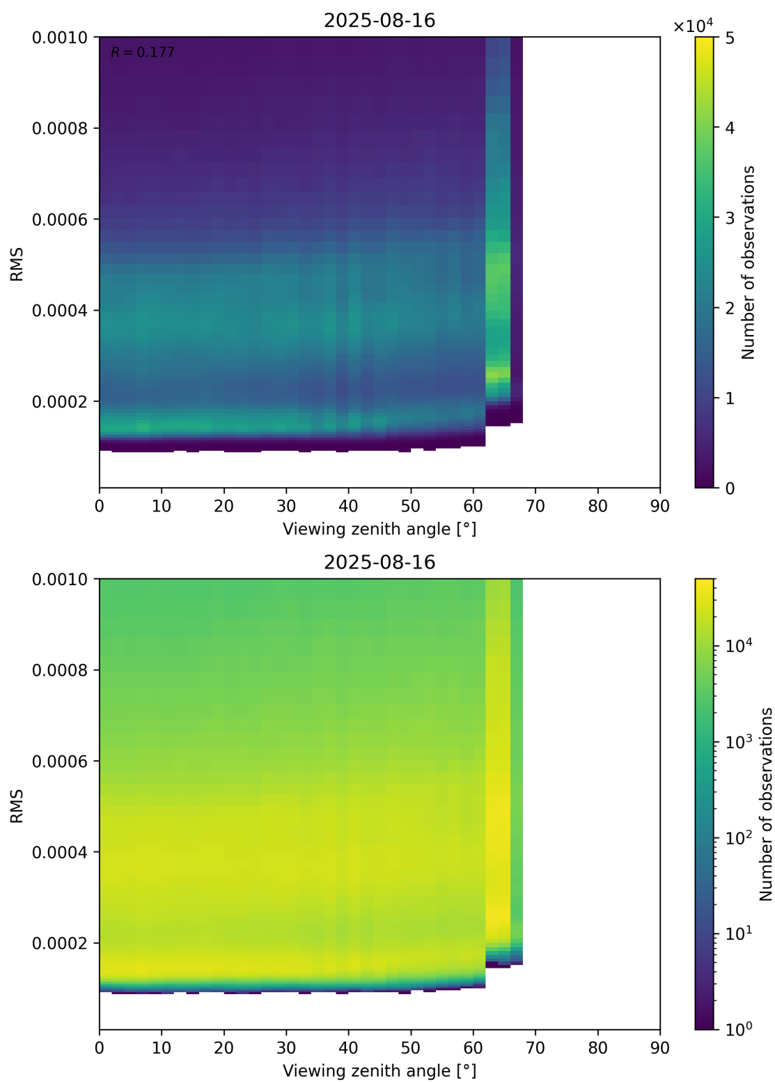
Figure 171: Scatter density plot of “Viewing zenith angle” against “RMS” for 2025-08-15 to 2025-08-17.
