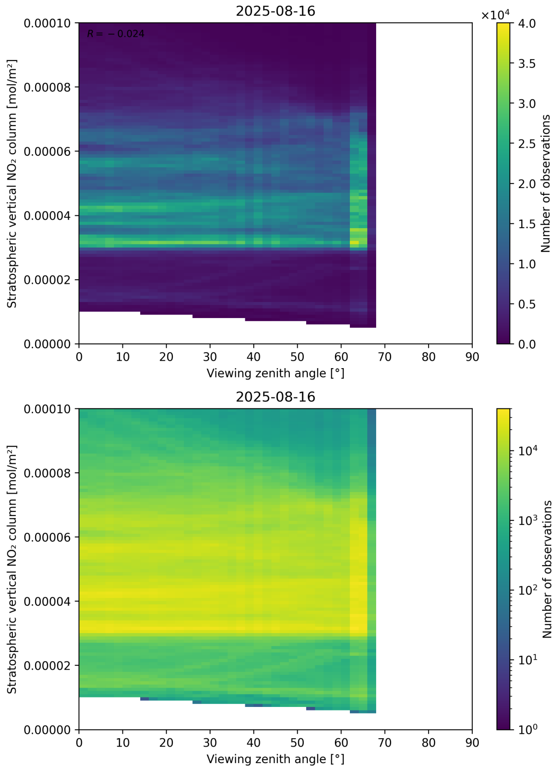
Figure 164: Scatter density plot of “Viewing zenith angle” against “Stratospheric vertical NO 2 column” for 2025-08-15 to 2025-08-17.
