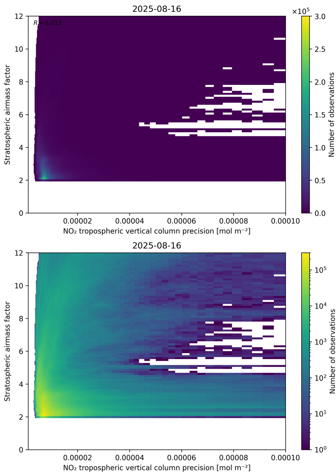
Figure 131: Scatter density plot of “NO 2 tropospheric vertical column precision” against “Stratospheric airmass factor” for 2025-08-15 to 2025-08-17.
