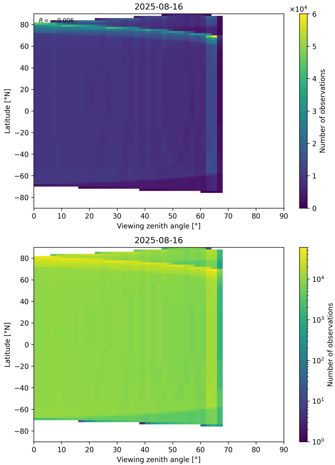
Figure 163: Scatter density plot of “Viewing zenith angle” against “Latitude” for 2025-08-15 to 2025-08-17.
