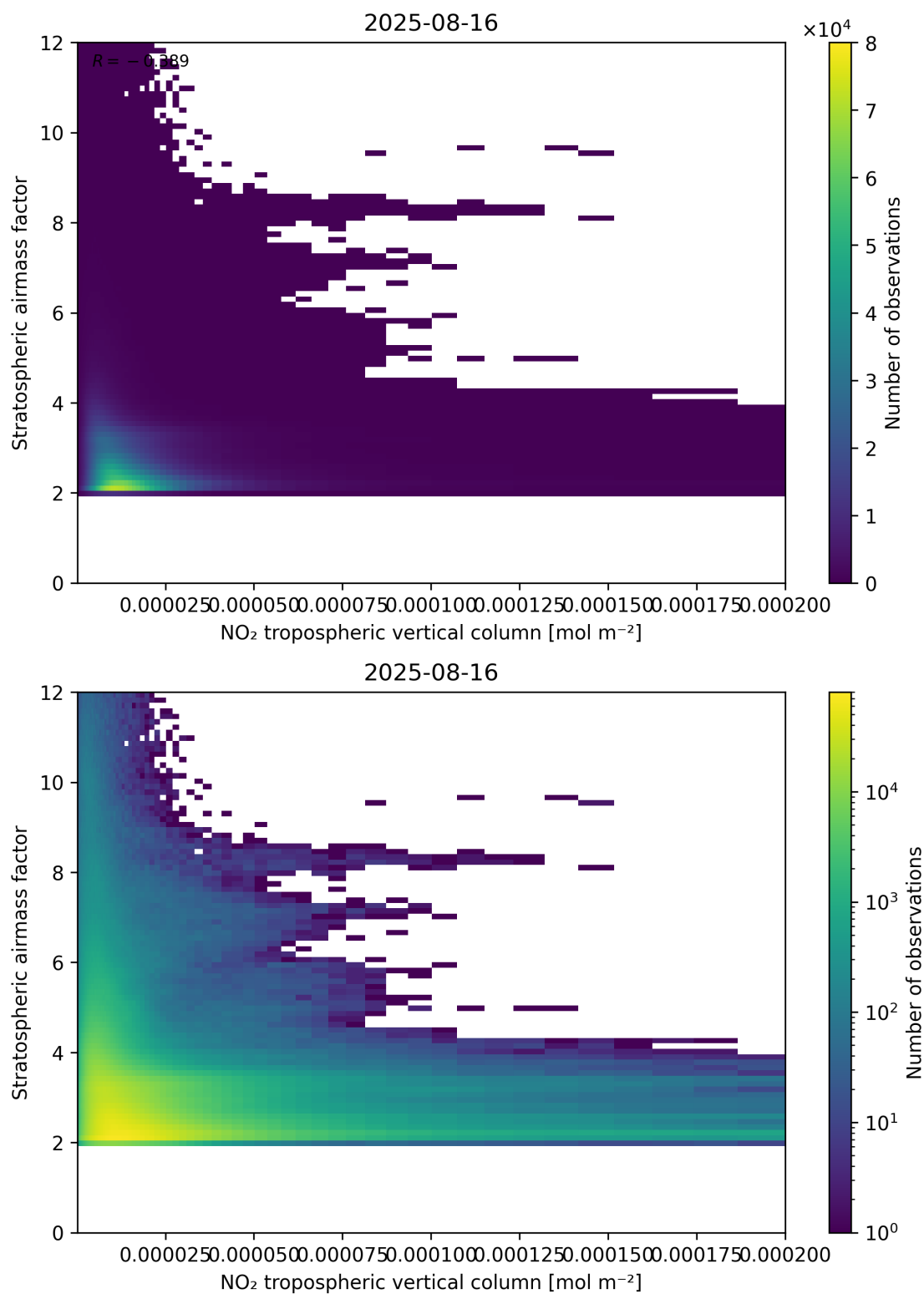
Figure 121: Scatter density plot of “NO 2 tropospheric vertical column” against “Stratospheric air mass factor” for 2025-08-15 to 2025-08-17.
