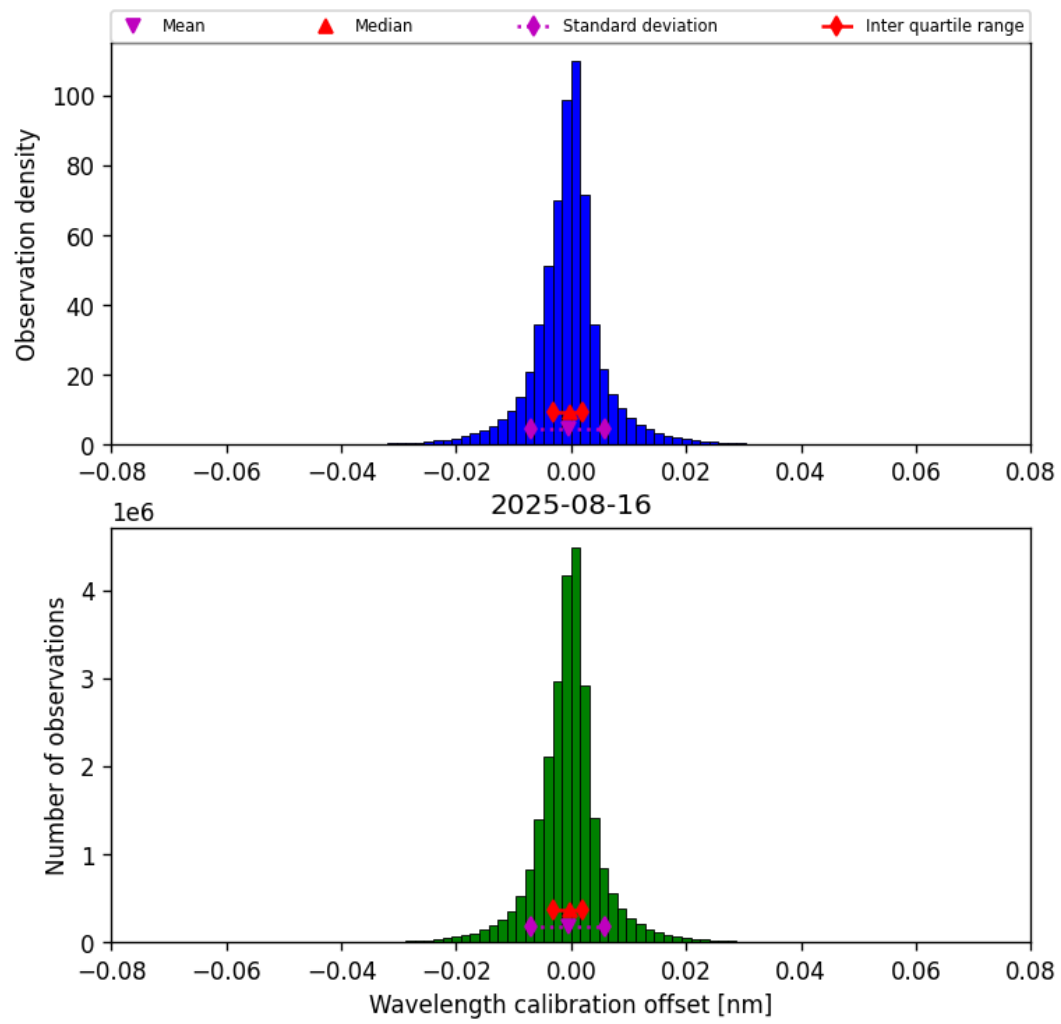
Figure 35: Histogram of “Wavelength calibration offset” for 2025-08-15 to 2025-08-17
