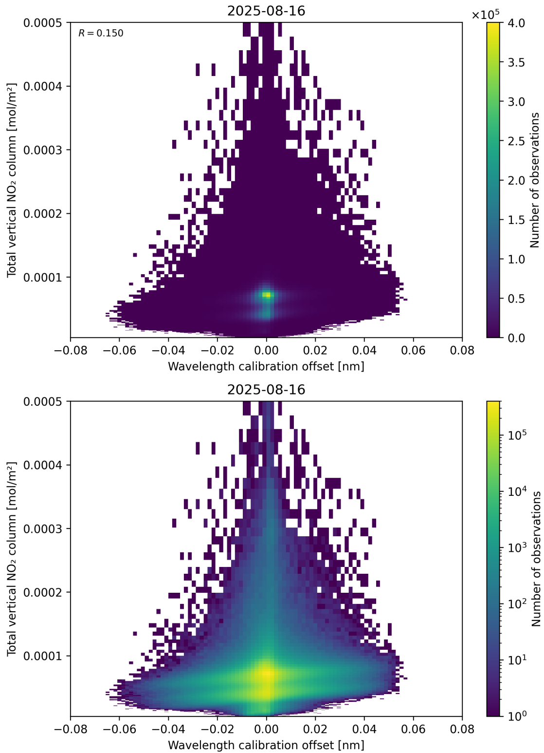
Figure 179: Scatter density plot of “Wavelength calibration offset” against “Total vertical NO 2 column” for 2025-08-15 to 2025-08-17.
