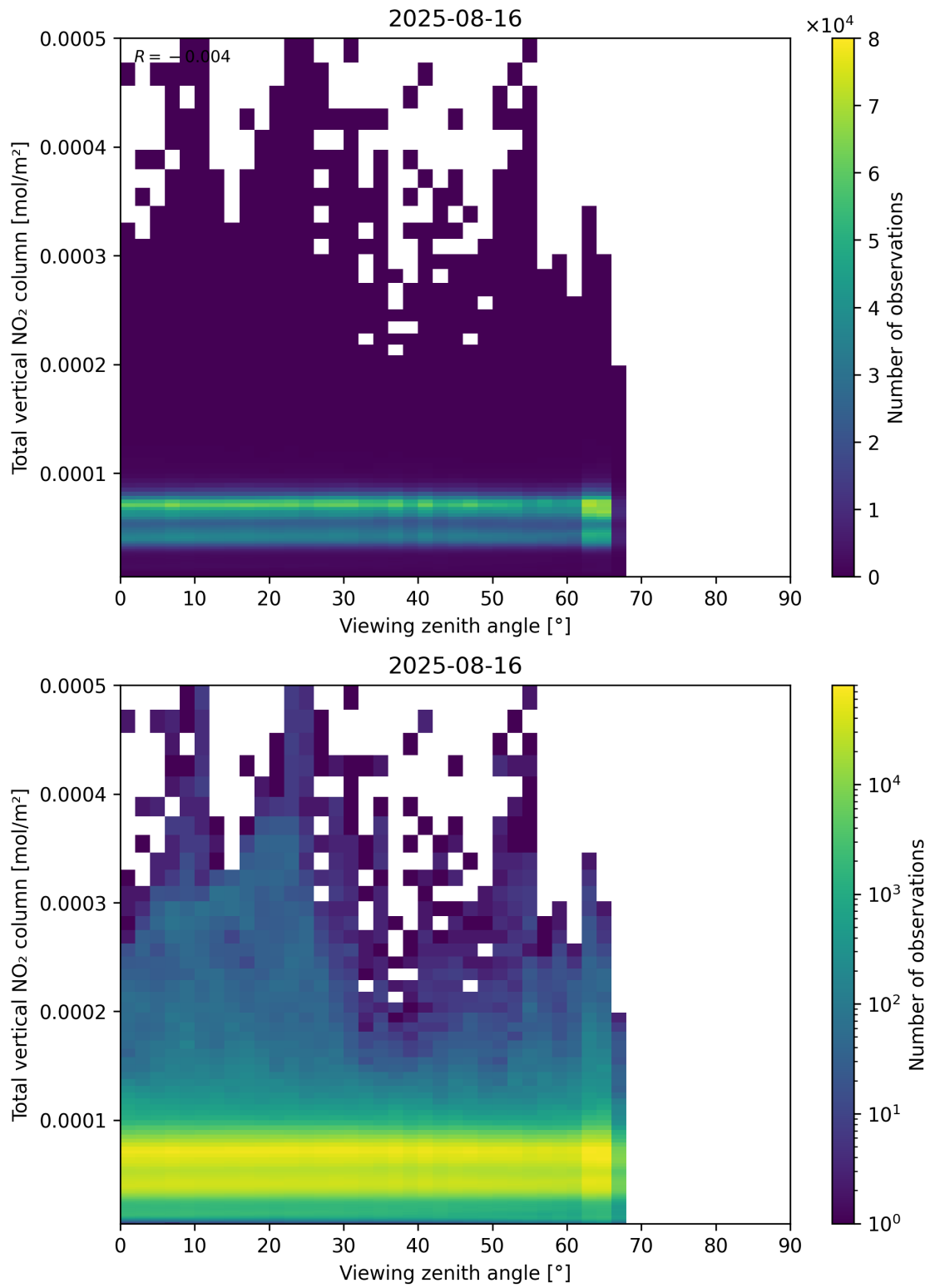
Figure 167: Scatter density plot of “Viewing zenith angle” against “Total vertical NO 2 column” for 2025-08-15 to 2025-08-17.
