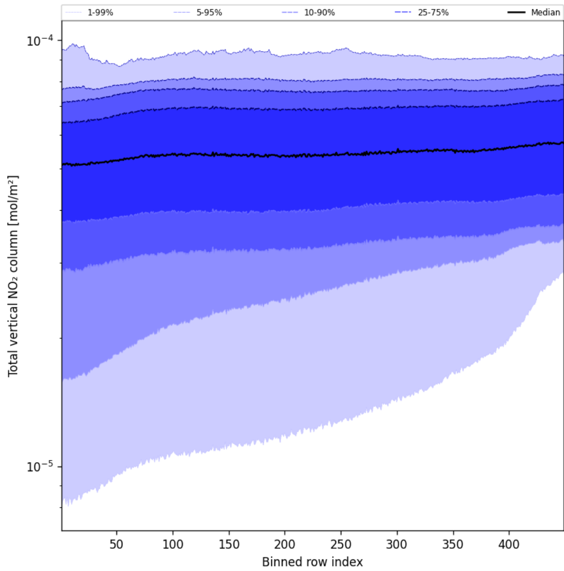
Figure 55: Along track statistics of "Total vertical NO 2 column" for 2025-08-15 to 2025-08-17
