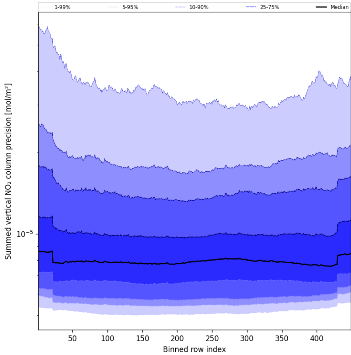
Figure 58: Along track statistics of “Summed vertical NO 2 column precision” for 2025-08-15 to 2025-08-17
