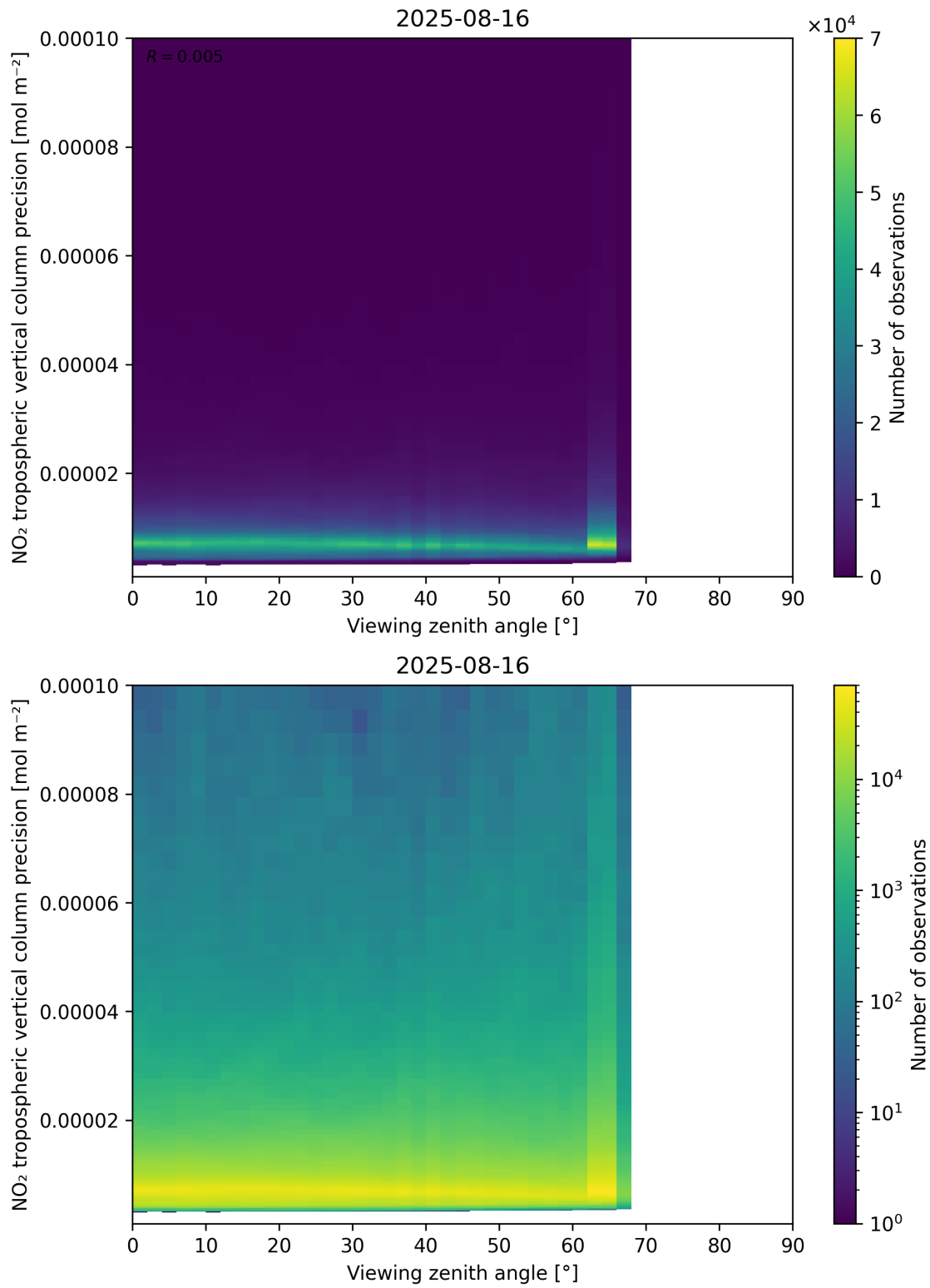
Figure 170: Scatter density plot of “Viewing zenith angle” against “NO 2 tropospheric vertical column precision” for 2025-08-15 to 2025-08-17.
