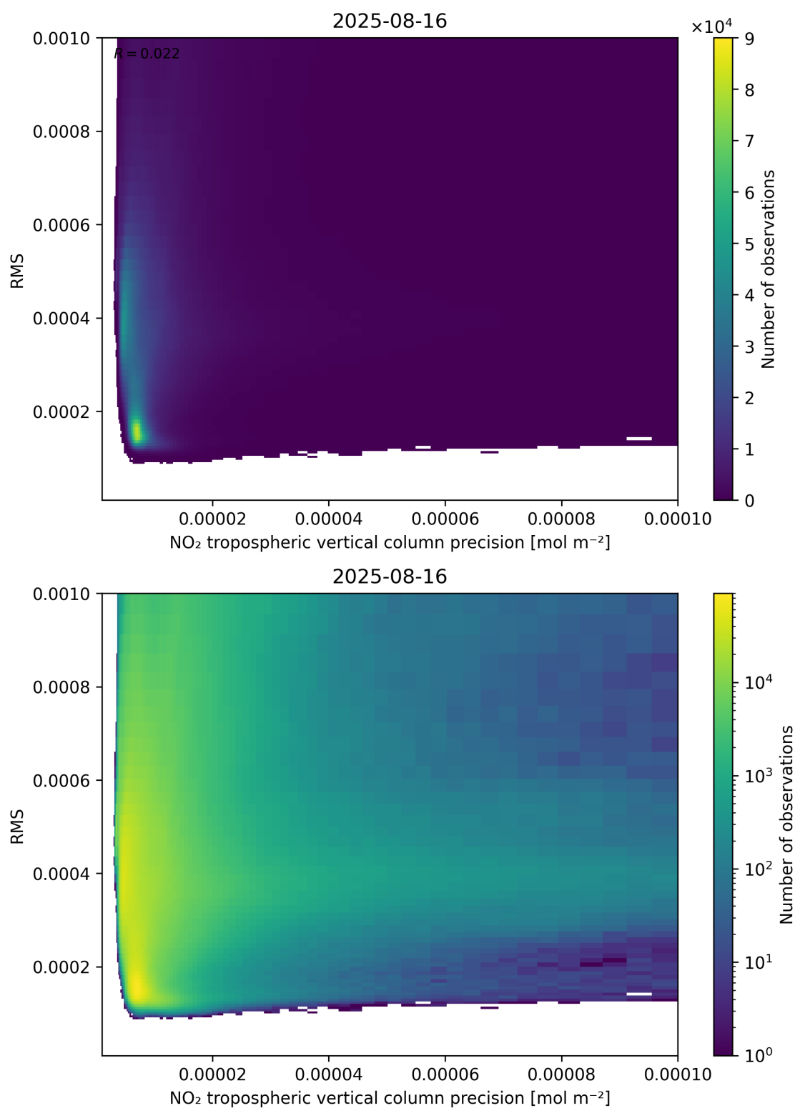
Figure 140: Scatter density plot of “NO 2 tropospheric vertical column precision” against “RMS” for 2025-08-15 to 2025-08-17.
