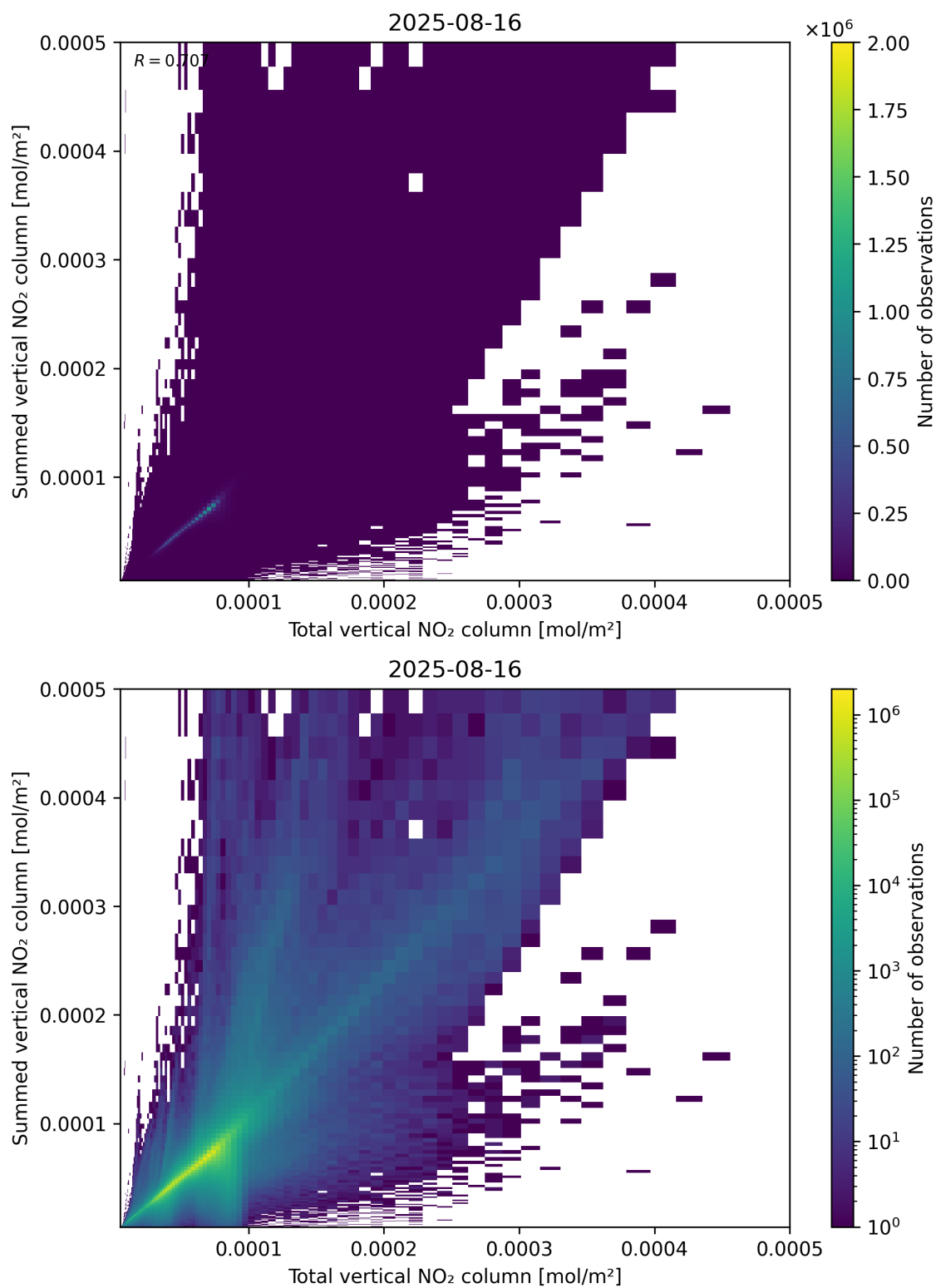
Figure 112: Scatter density plot of “Total vertical NO 2 column” against “Summed vertical NO 2 column” for 2025-08-15 to 2025-08-17.
