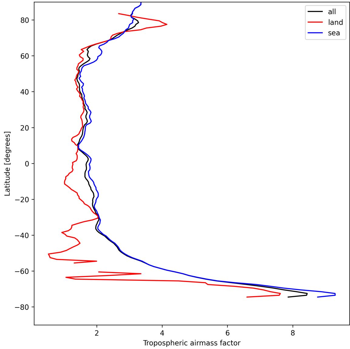
Figure 14: Zonal average of “Tropospheric airmass factor” for 2025-08-15 to 2025-08-17.
