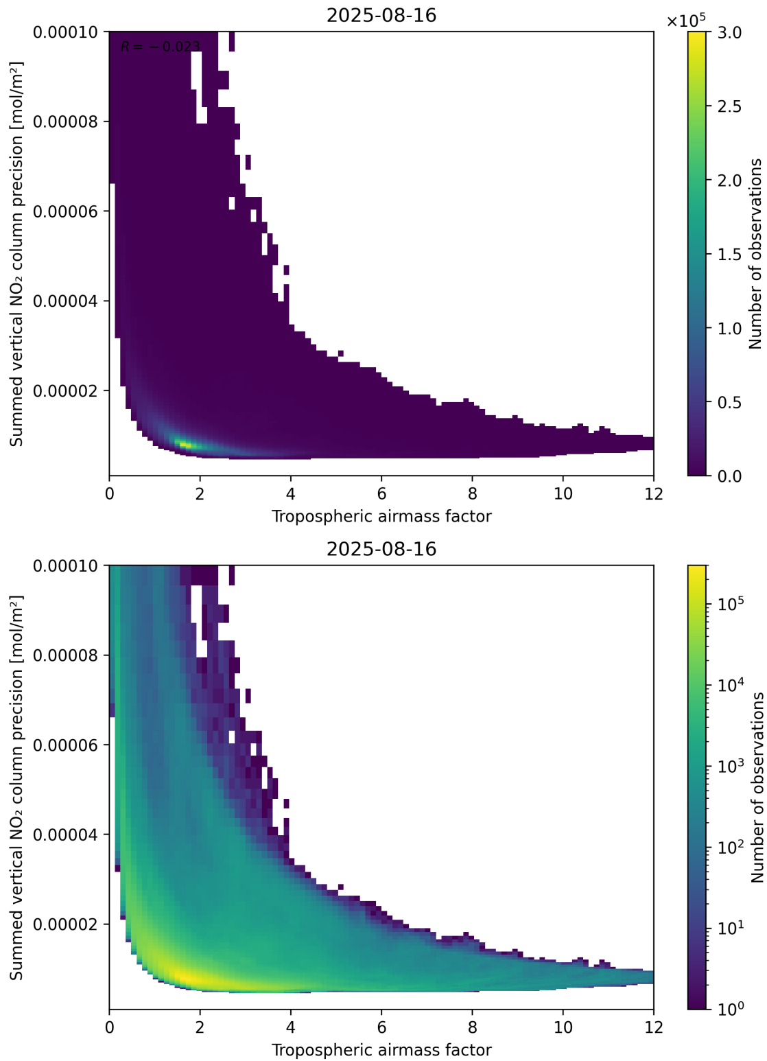
Figure 76: Scatter density plot of “Tropospheric air mass factor” against “Summed vertical NO 2 column precision” for 2025-08-15 to 2025-08-17.
