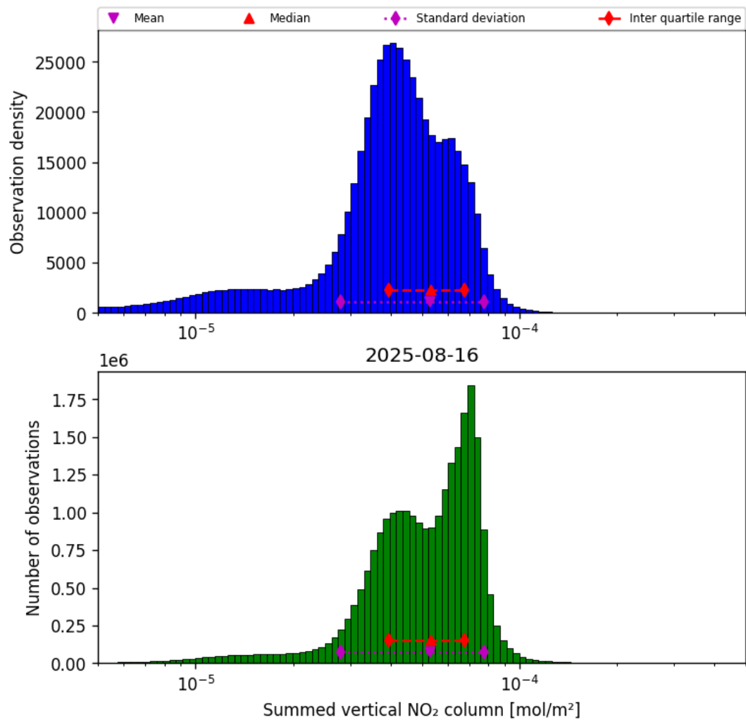
Figure 40: Histogram of “Summed vertical NO 2 column” for 2025-08-15 to 2025-08-17
