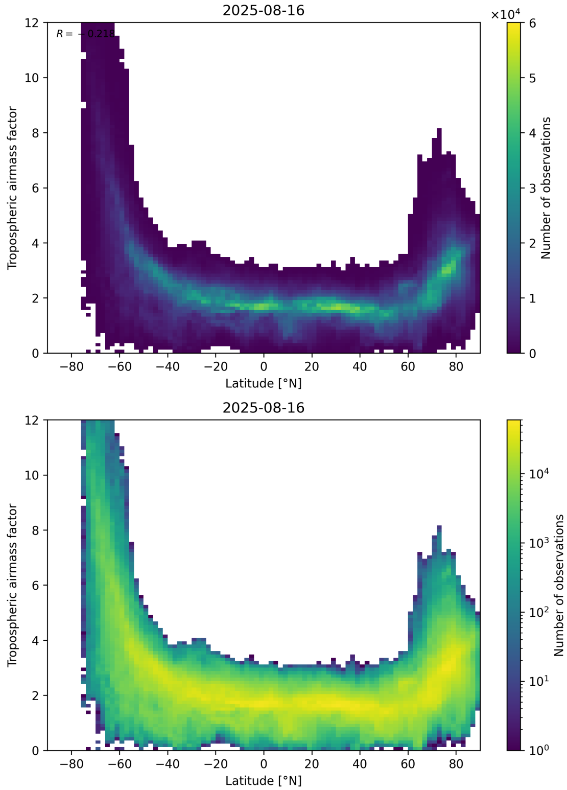
Figure 85: Scatter density plot of “Latitude” against “Tropospheric air mass factor” for 2025-08-15 to 2025-08-17.
