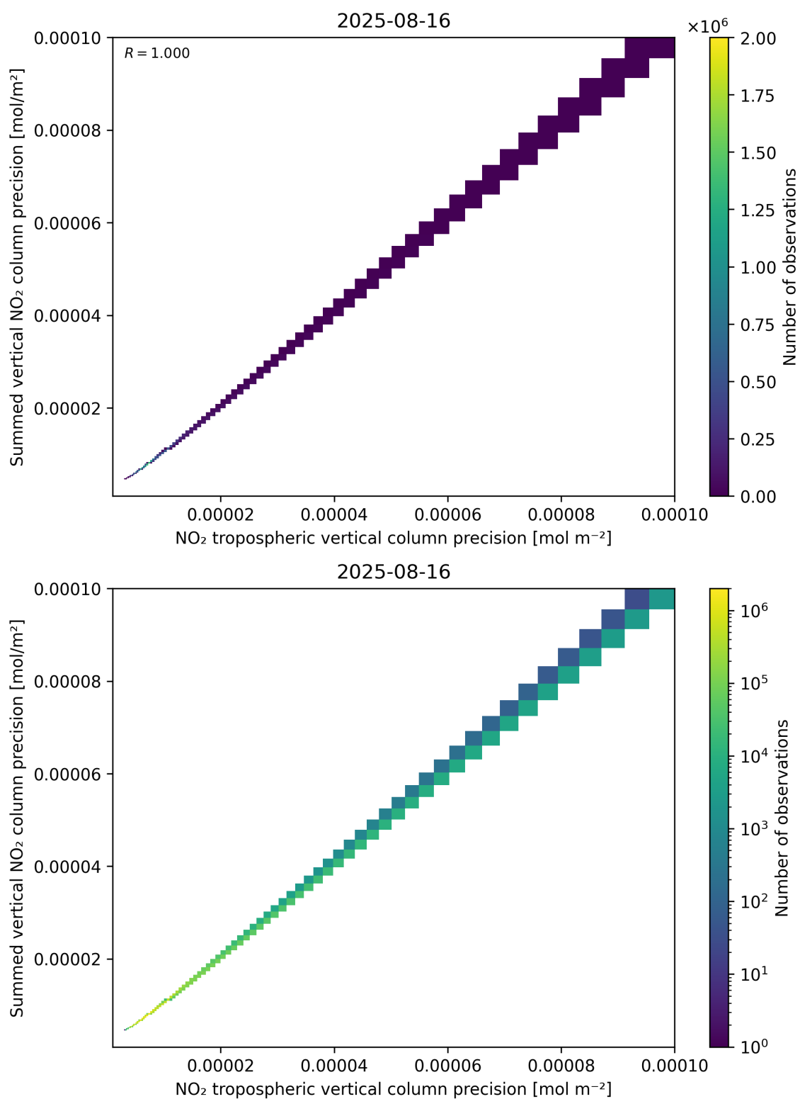
Figure 137: Scatter density plot of “NO 2 tropospheric vertical column precision” against “Summed vertical NO 2 column precision” for 2025-08-15 to 2025-08-17.
