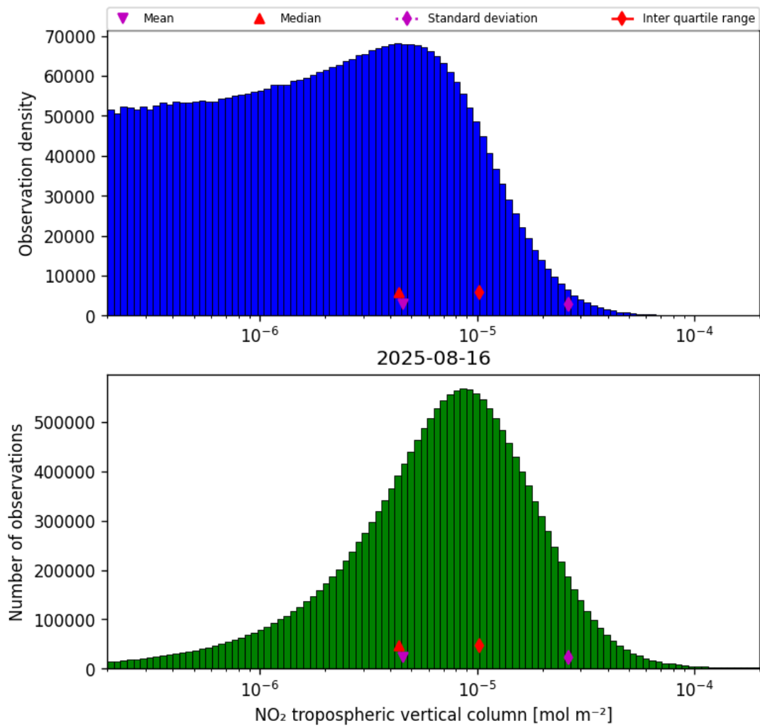
Figure 29: Histogram of “NO 2 tropospheric vertical column” for 2025-08-15 to 2025-08-17
