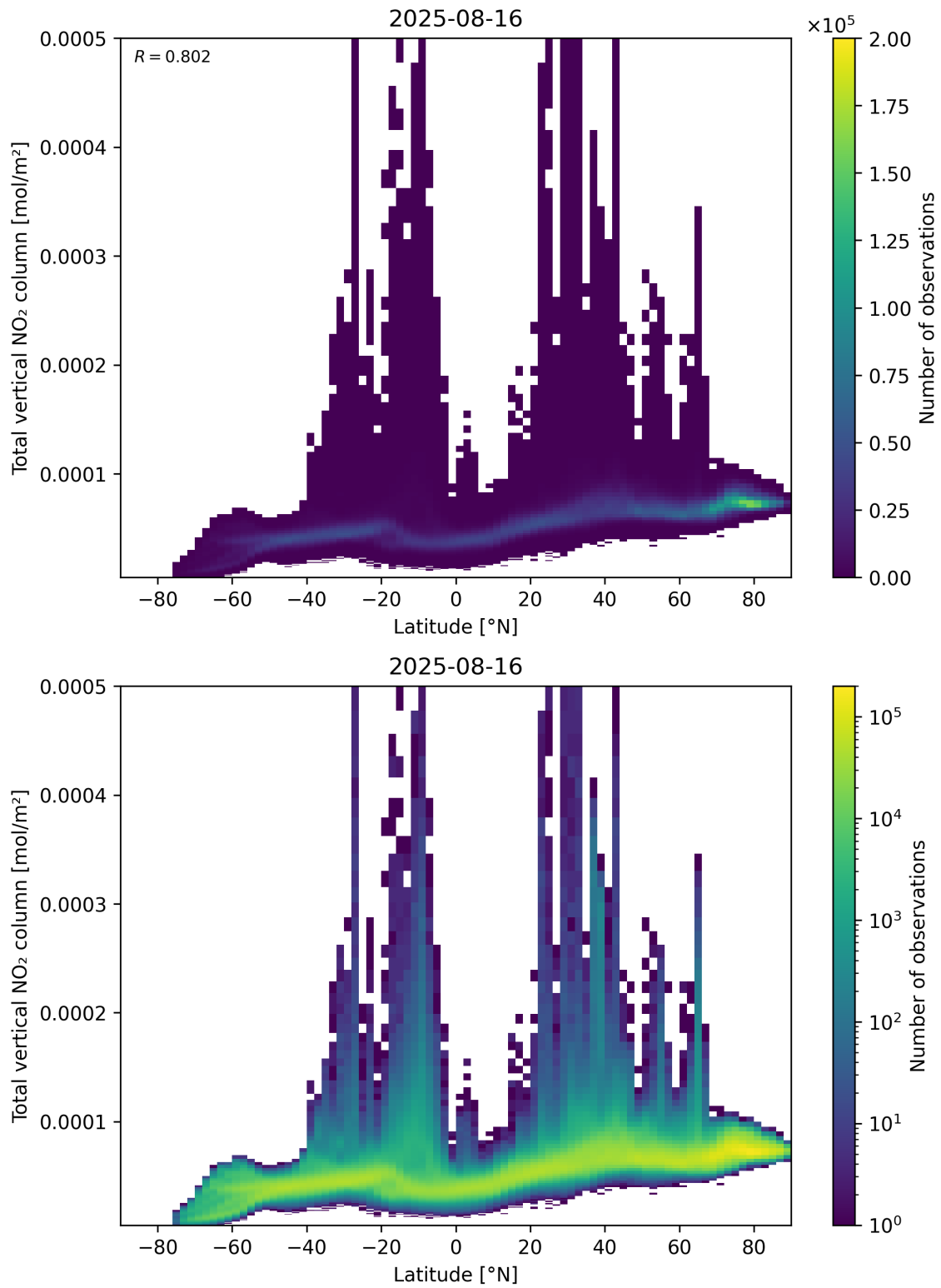
Figure 90: Scatter density plot of “Latitude” against “Total vertical NO 2 column” for 2025-08-15 to 2025-08-17.
