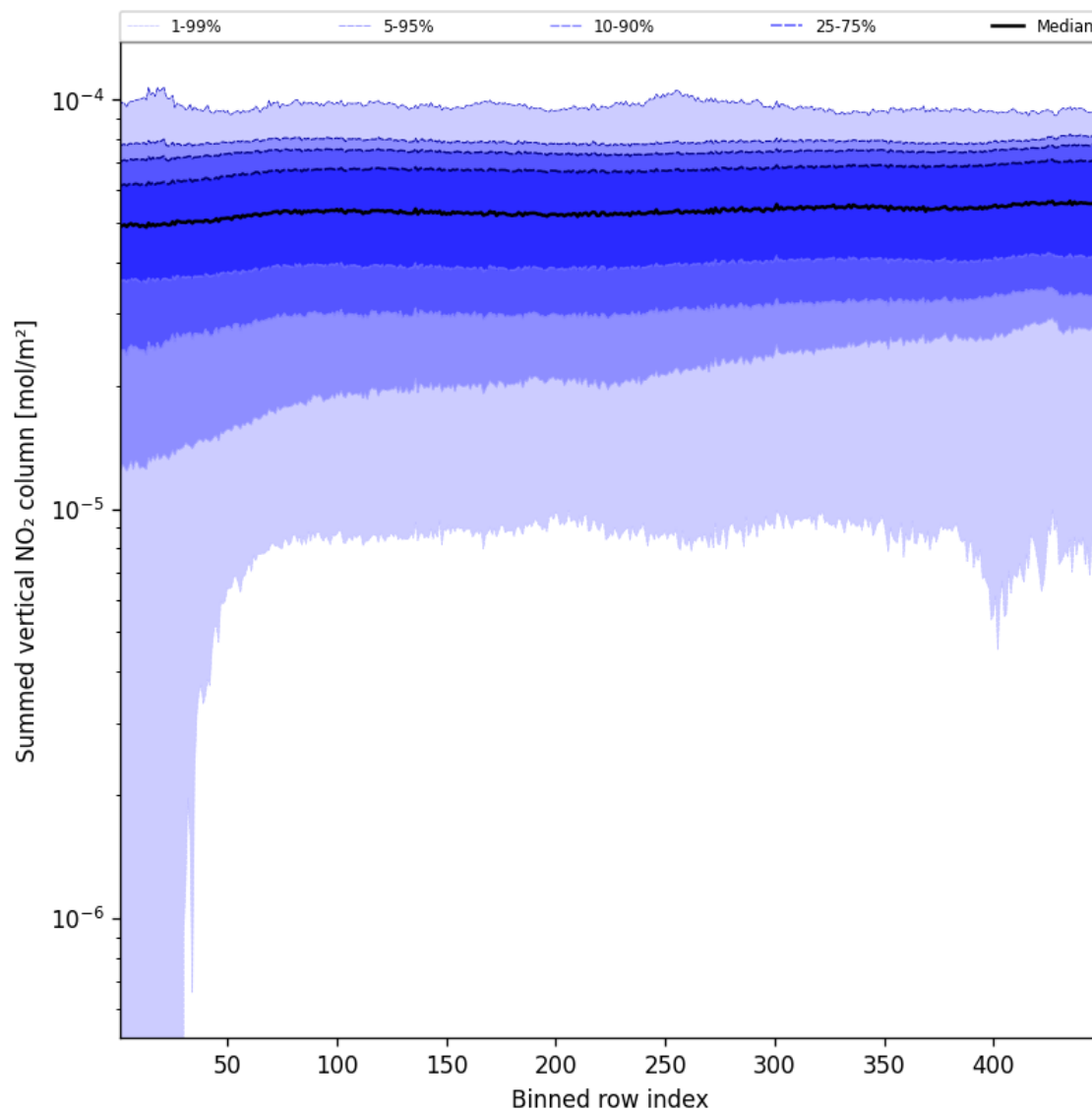
Figure 57: Along track statistics of “Summed vertical NO 2 column” for 2025-08-15 to 2025-08-17
