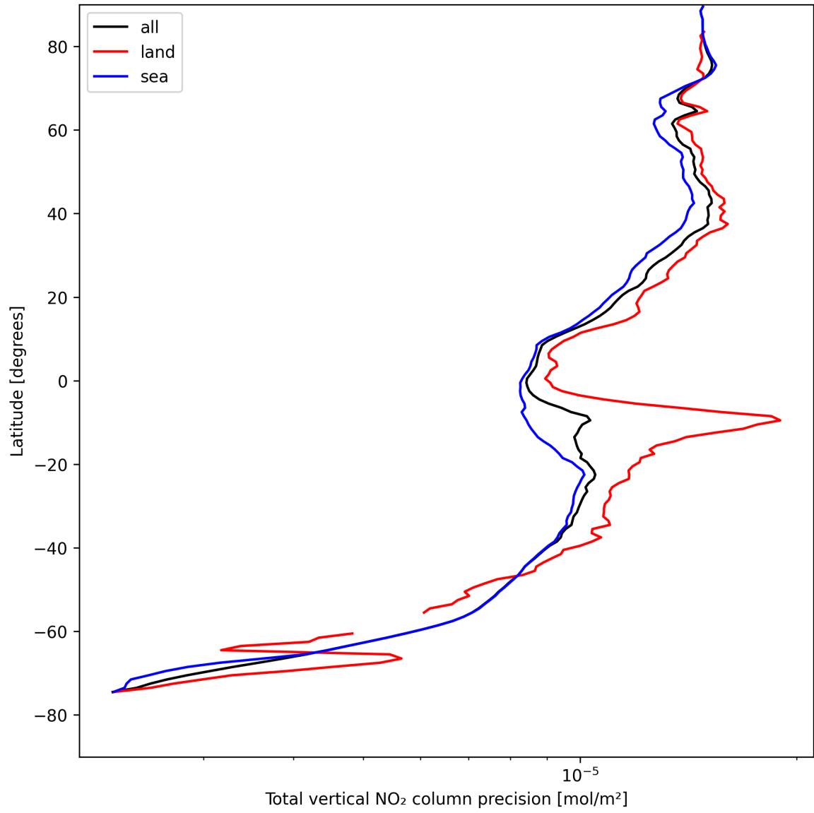
Figure 22: Zonal average of “Total vertical NO 2 column precision” for 2025-08-15 to 2025-08-17.
