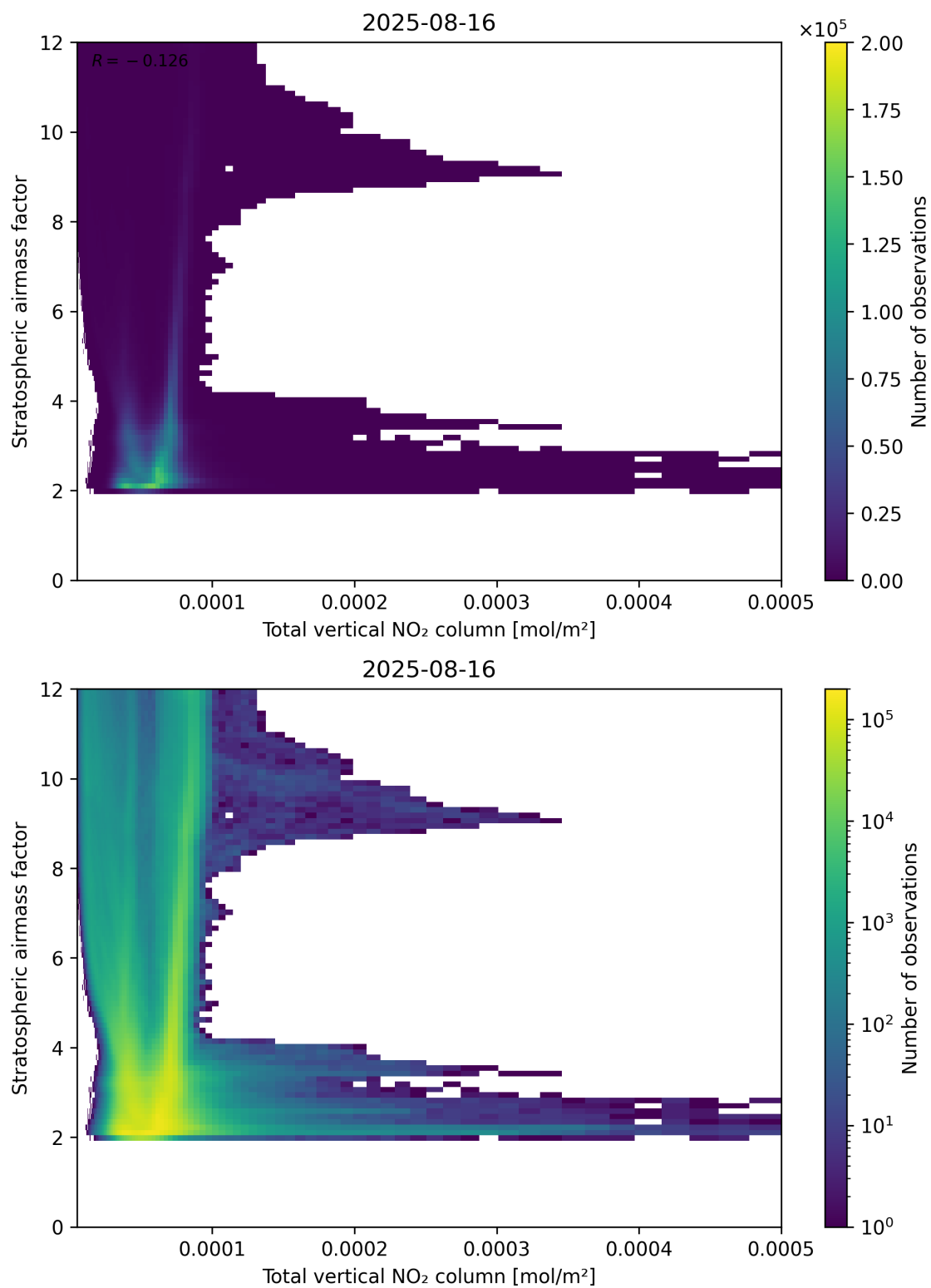
Figure 110: Scatter density plot of “Total vertical NO 2 column” against “Stratospheric airmass factor” for 2025-08-15 to 2025-08-17.
