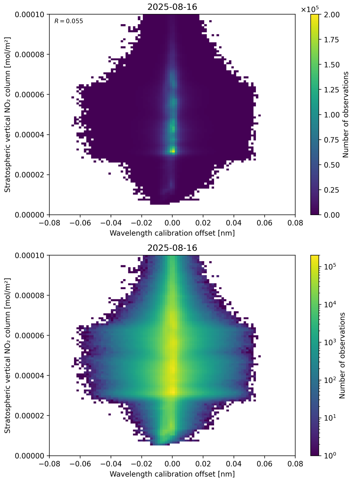
Figure 176: Scatter density plot of “Wavelength calibration offset” against “Stratospheric vertical NO 2 column” for 2025-08-15 to 2025-08-17.
