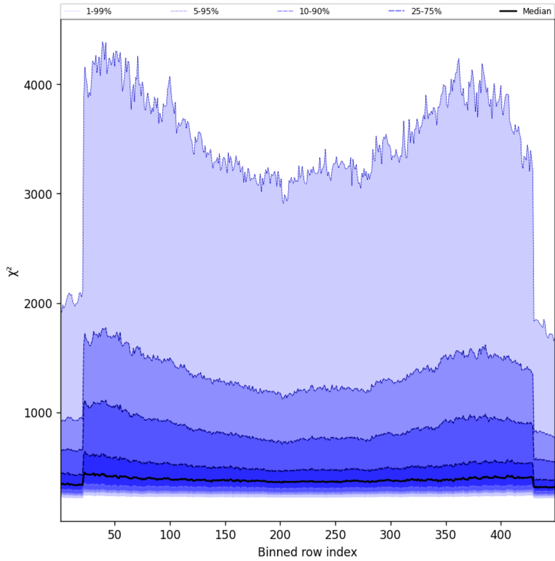
Figure 59: Along track statistics of “ \chi^2 ” for 2025-08-15 to 2025-08-17
