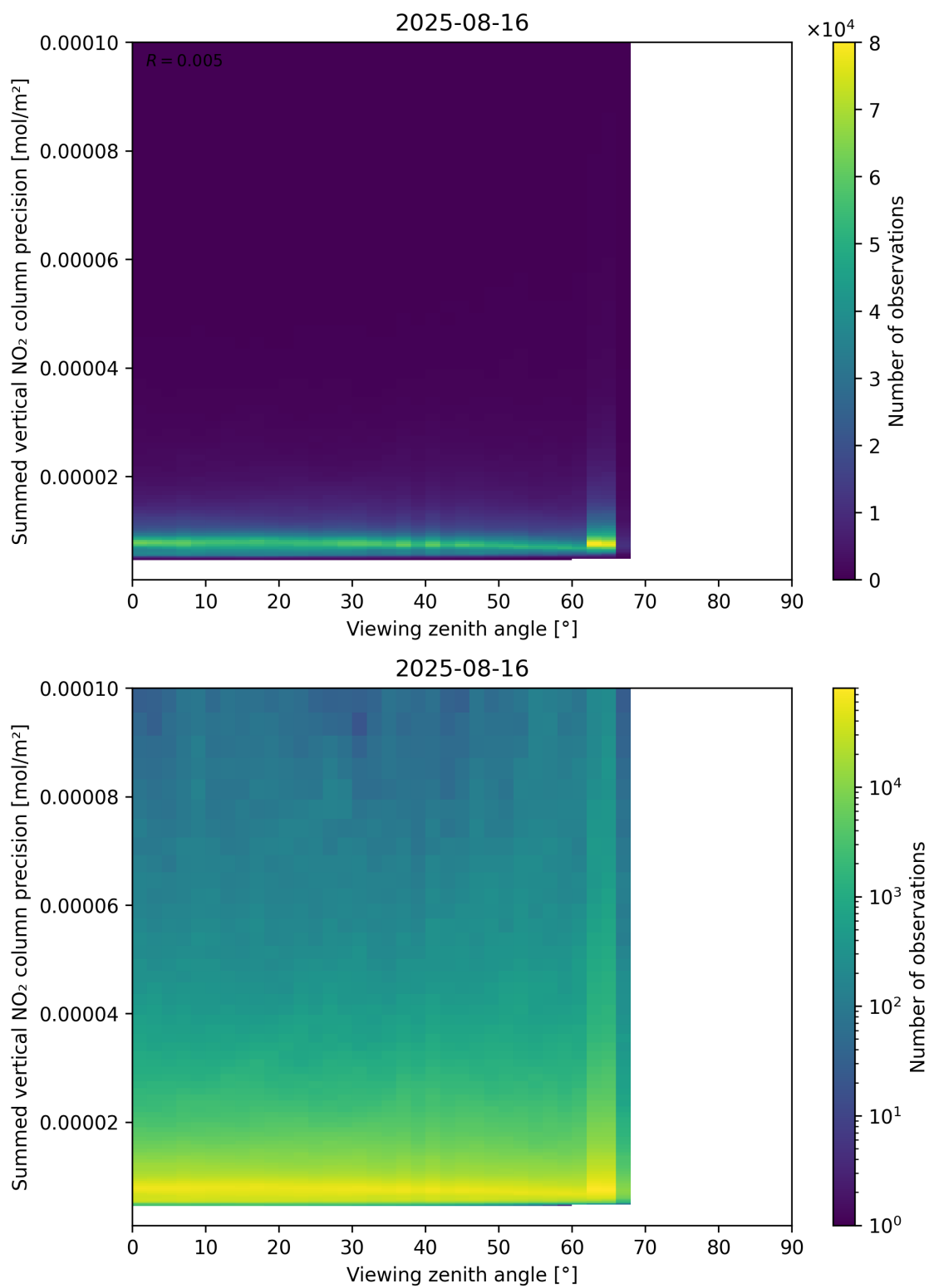
Figure 166: Scatter density plot of “Viewing zenith angle” against “Summed vertical NO 2 column precision” for 2025-08-15 to 2025-08-17.
