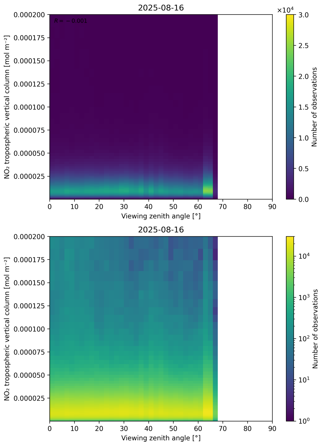
Figure 169: Scatter density plot of “Viewing zenith angle” against “NO 2 tropospheric vertical column” for 2025-08-15 to 2025-08-17.
