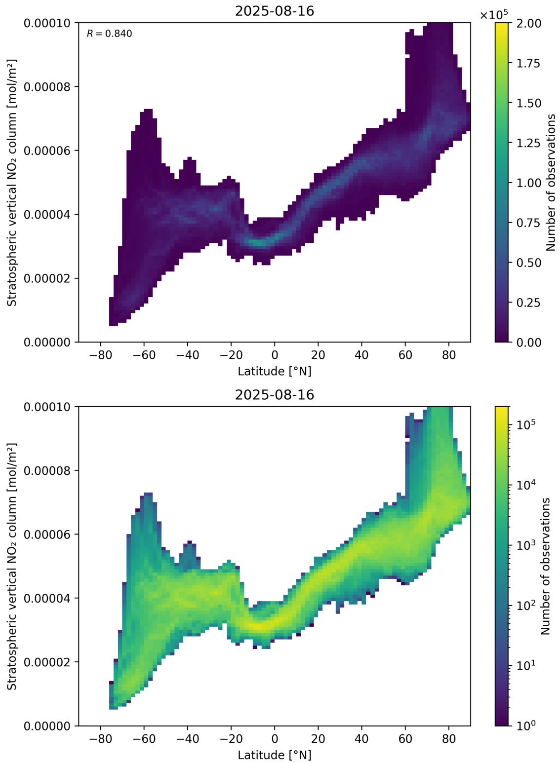
Figure 87: Scatter density plot of “Latitude” against “Stratospheric vertical NO 2 column” for 2025-08-15 to 2025-08-17.
