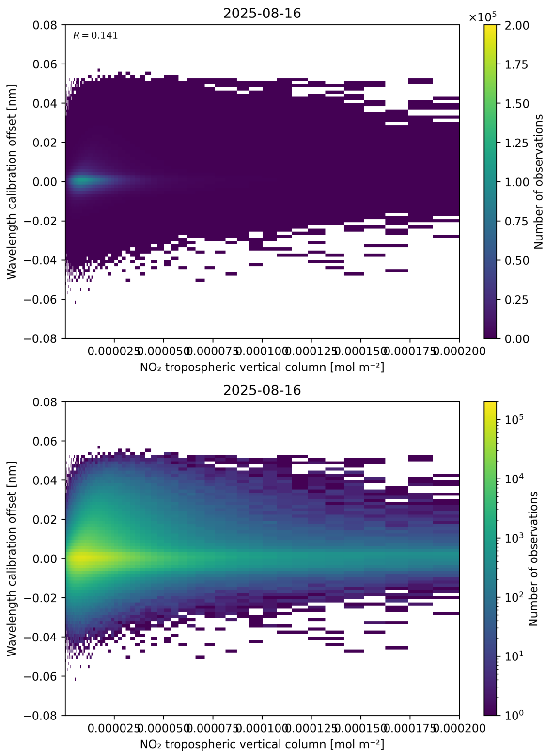
Figure 143: Scatter density plot of “NO 2 tropospheric vertical column” against “Wavelength calibration offset” for 2025-08-15 to 2025-08-17.
