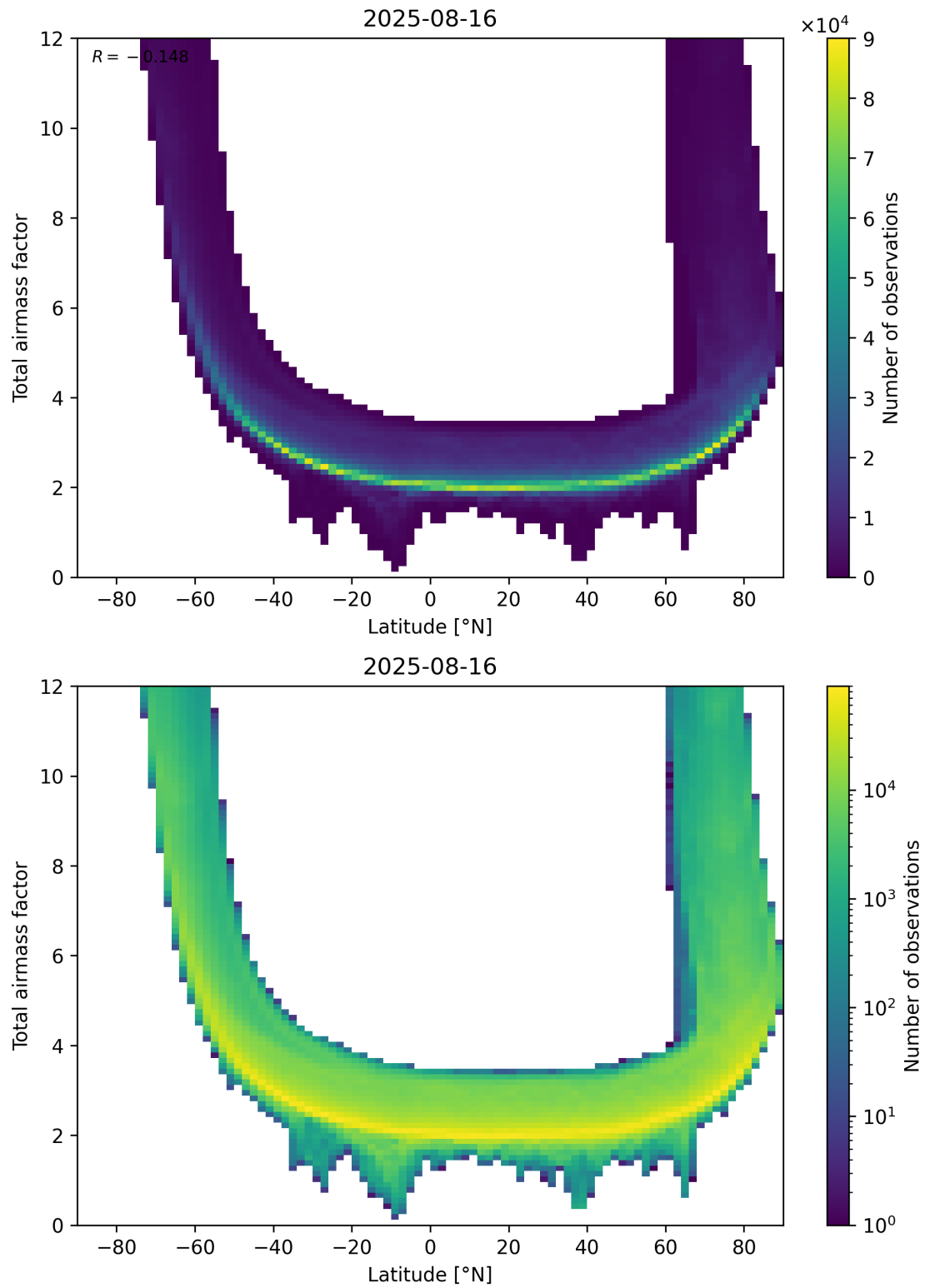
Figure 84: Scatter density plot of “Latitude” against “Total airmass factor” for 2025-08-15 to 2025-08-17.
