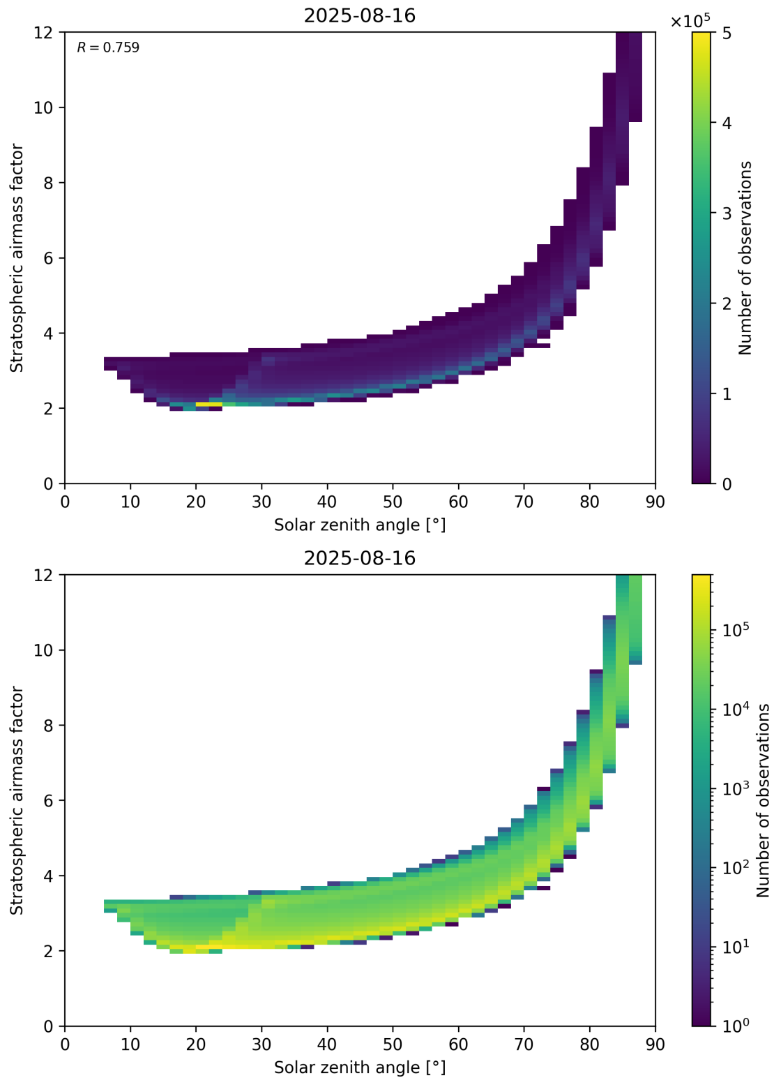
Figure 145: Scatter density plot of “Solar zenith angle” against “Stratospheric airmass factor” for 2025-08-15 to 2025-08-17.
