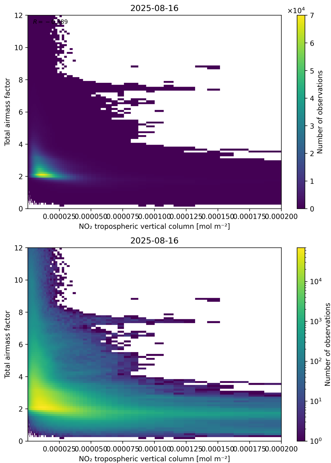
Figure 122: Scatter density plot of “NO 2 tropospheric vertical column” against “Total airmass factor” for 2025-08-15 to 2025-08-17.
