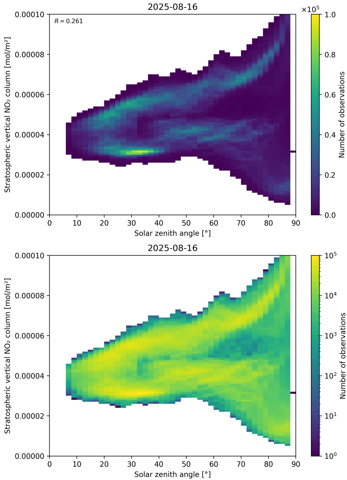
Figure 150: Scatter density plot of “Solar zenith angle” against “Stratospheric vertical NO 2 column” for 2025-08-15 to 2025-08-17.
