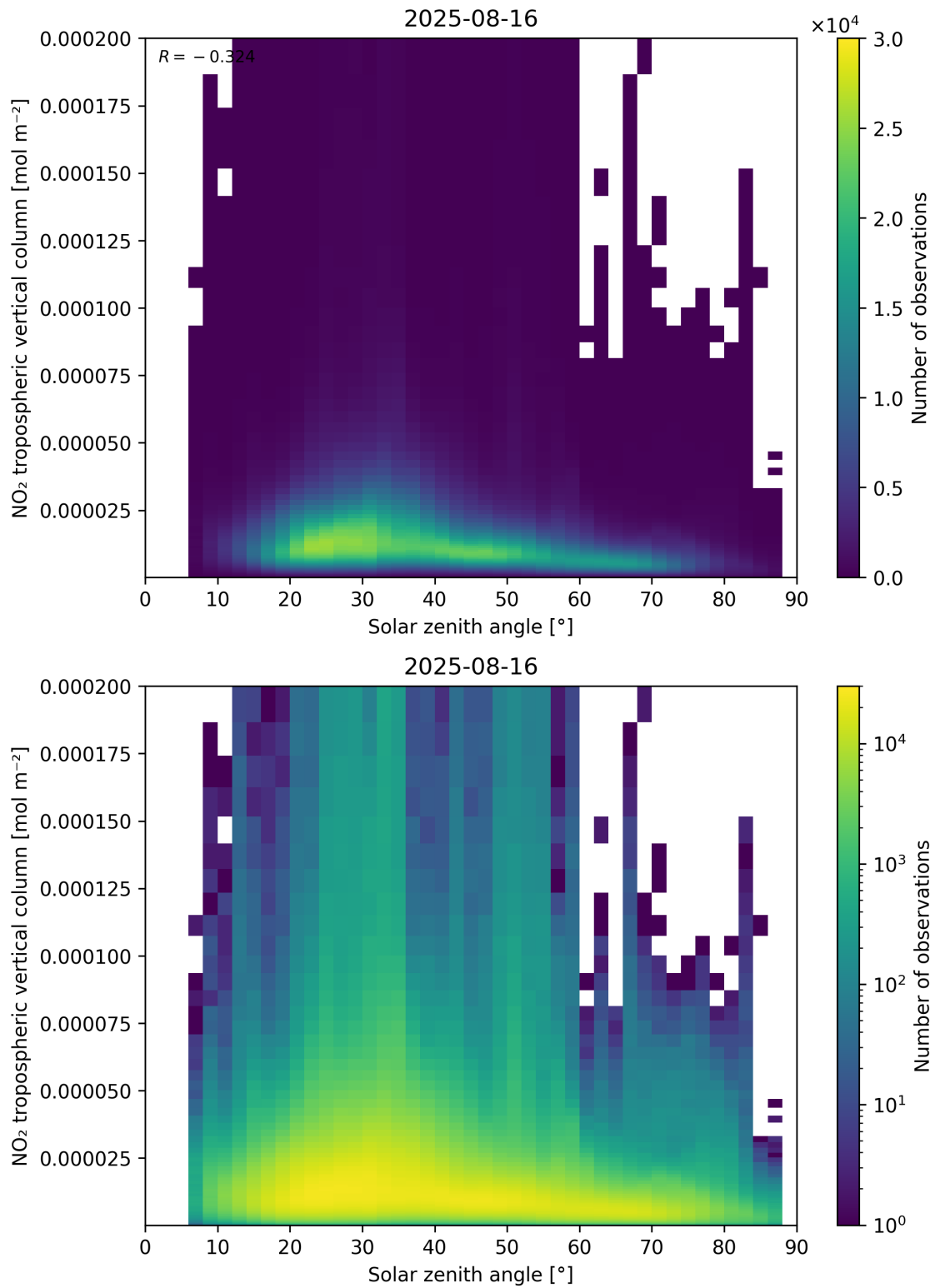
Figure 155: Scatter density plot of “Solar zenith angle” against “NO 2 tropospheric vertical column” for 2025-08-15 to 2025-08-17.
