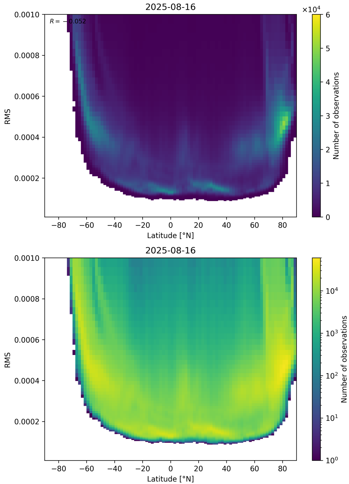
Figure 94: Scatter density plot of “Latitude” against “RMS” for 2025-08-15 to 2025-08-17.
