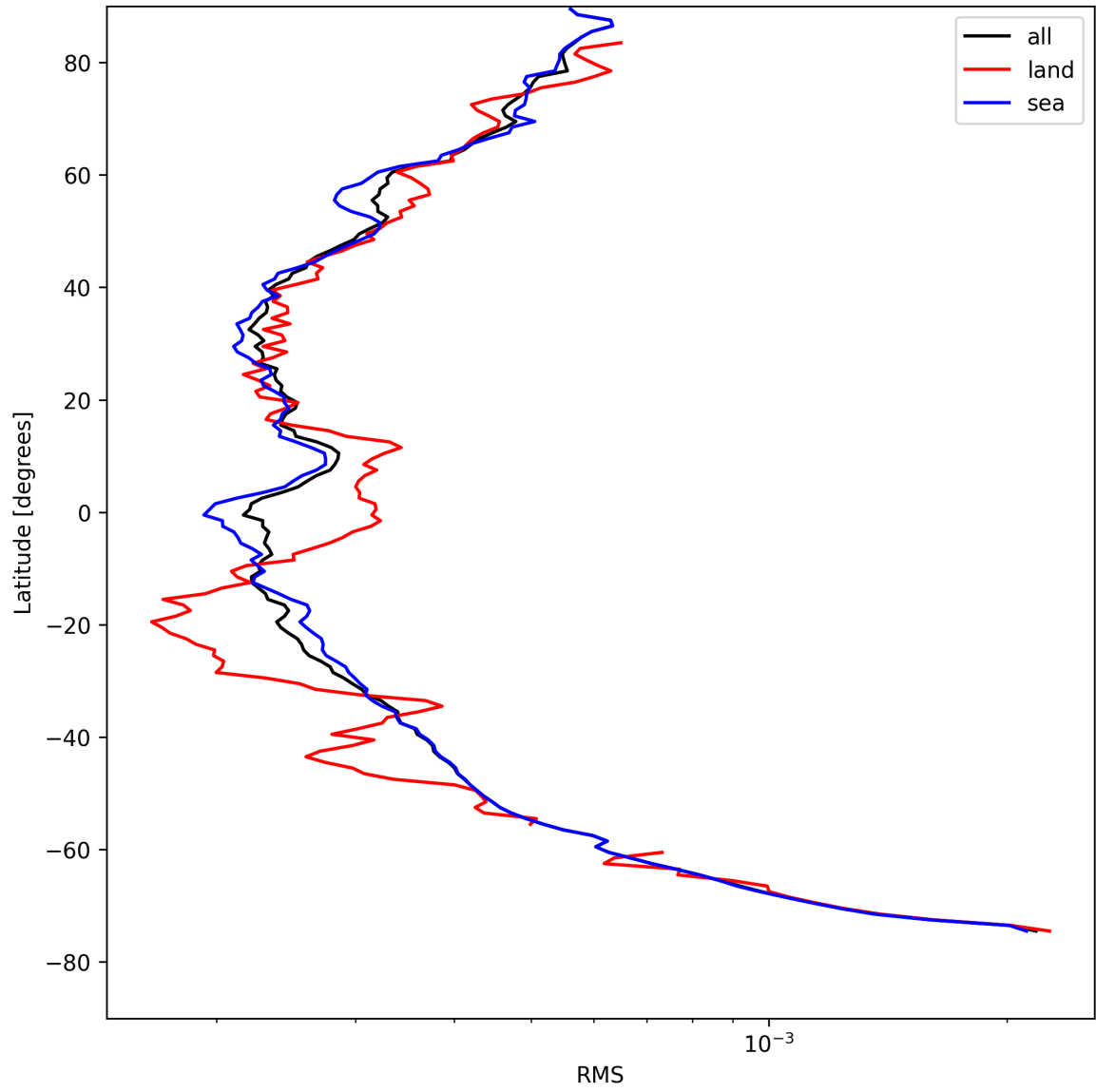
Figure 26: Zonal average of “RMS” for 2025-08-15 to 2025-08-17.
