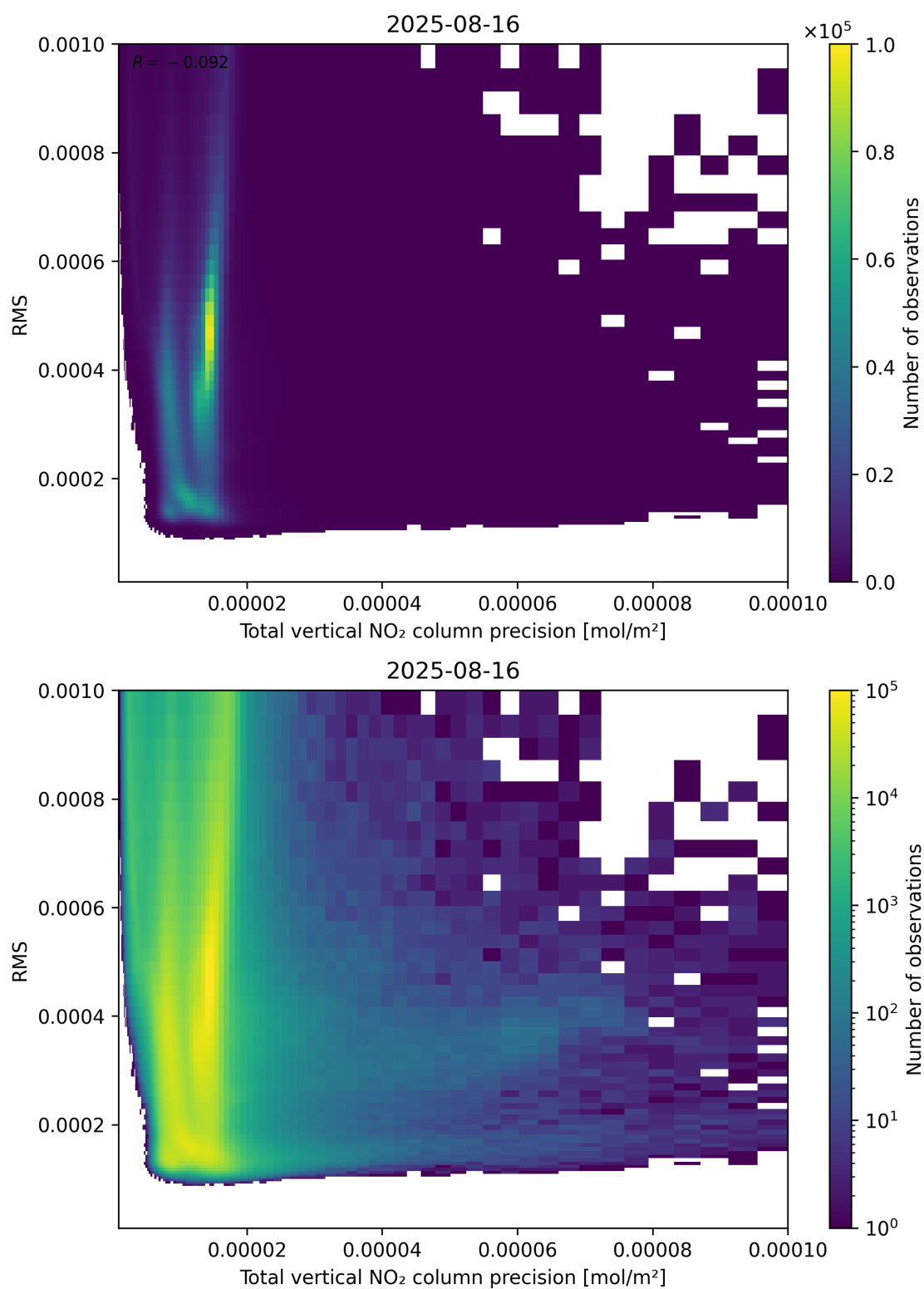
Figure 119: Scatter density plot of “Total vertical NO 2 column precision” against “RMS” for 2025-08-15 to 2025-08-17.
