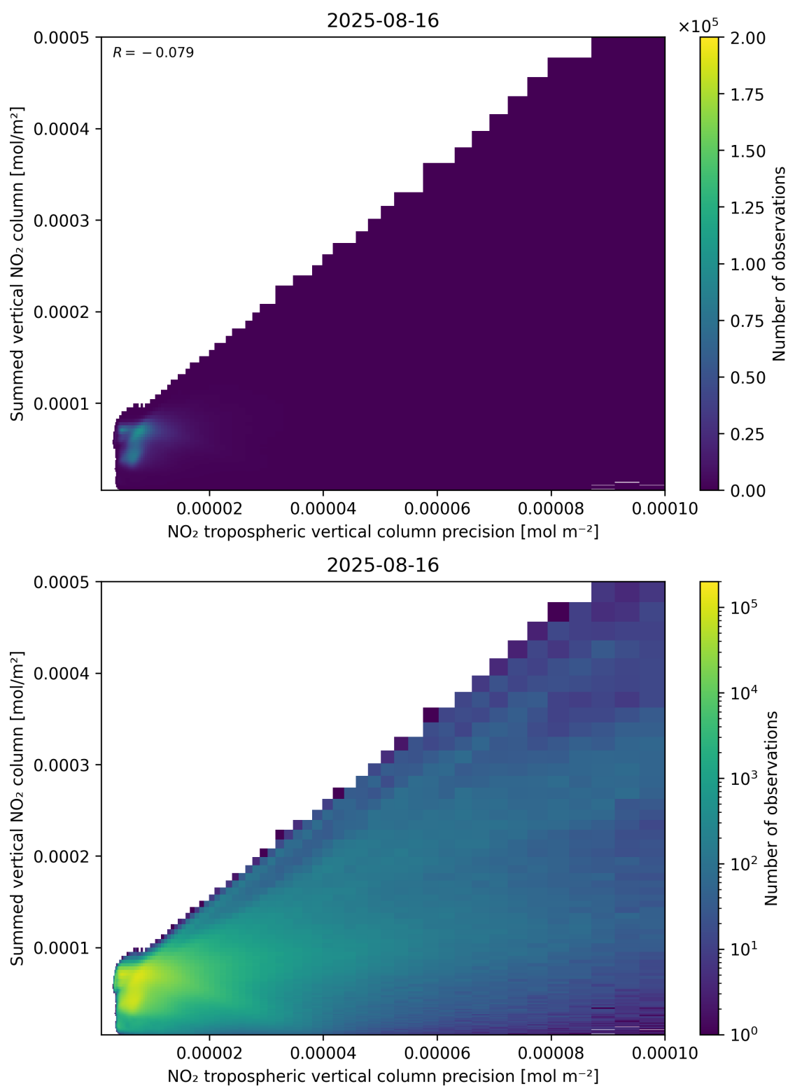
Figure 136: Scatter density plot of “NO 2 tropospheric vertical column precision” against “Summed vertical NO 2 column” for 2025-08-15 to 2025-08-17.
