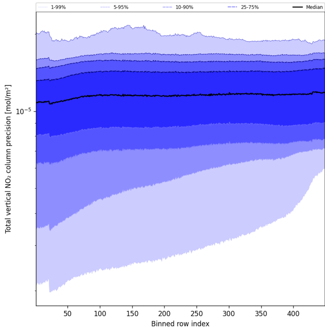
Figure 56: Along track statistics of “Total vertical NO 2 column precision” for 2025-08-15 to 2025-08-17
