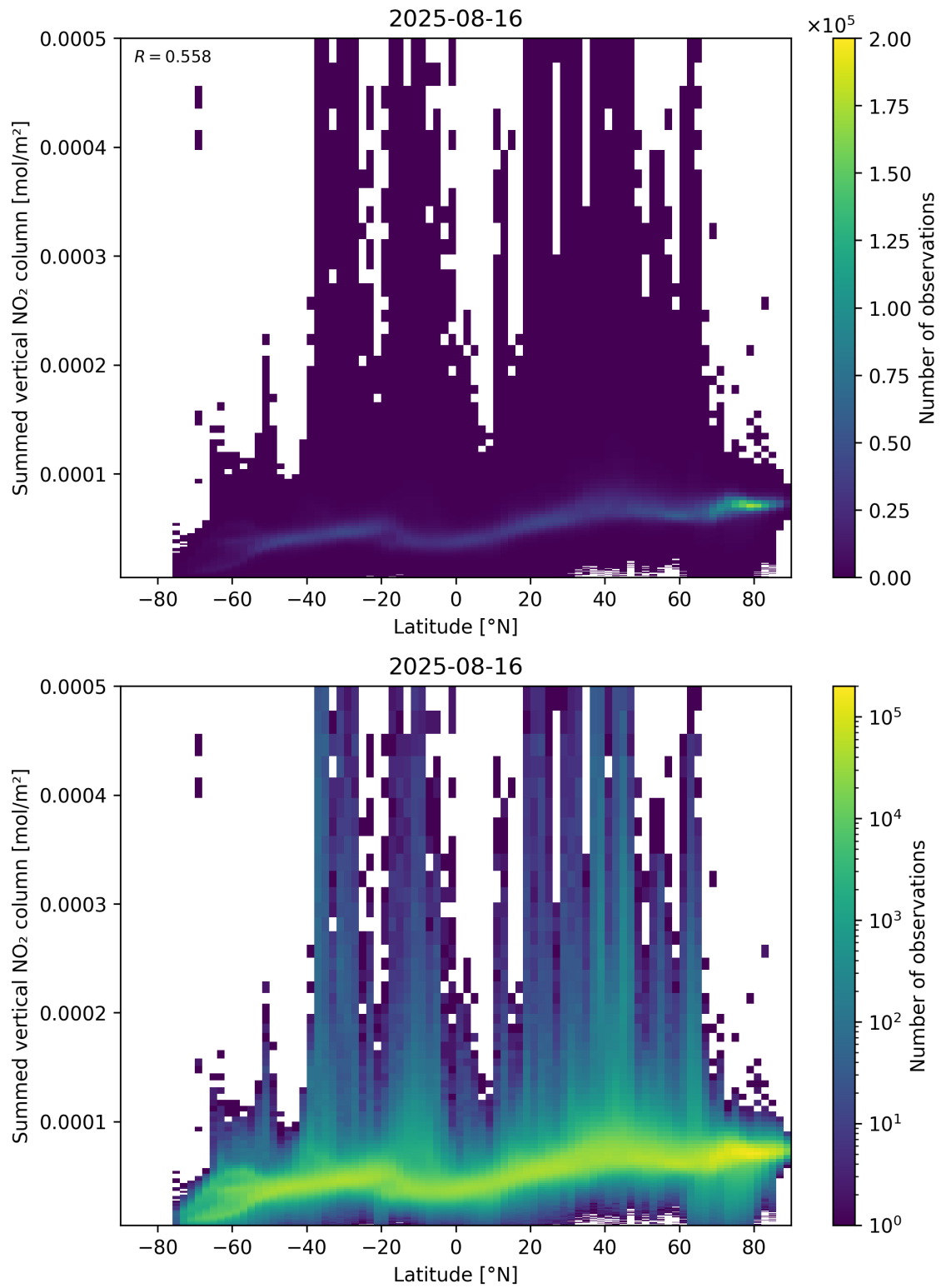
Figure 88: Scatter density plot of “Latitude” against “Summed vertical NO 2 column” for 2025-08-15 to 2025-08-17.
