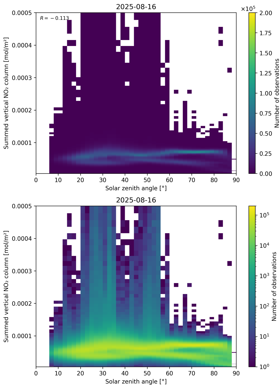
Figure 151: Scatter density plot of “Solar zenith angle” against “Summed vertical NO 2 column” for 2025-08-15 to 2025-08-17.
