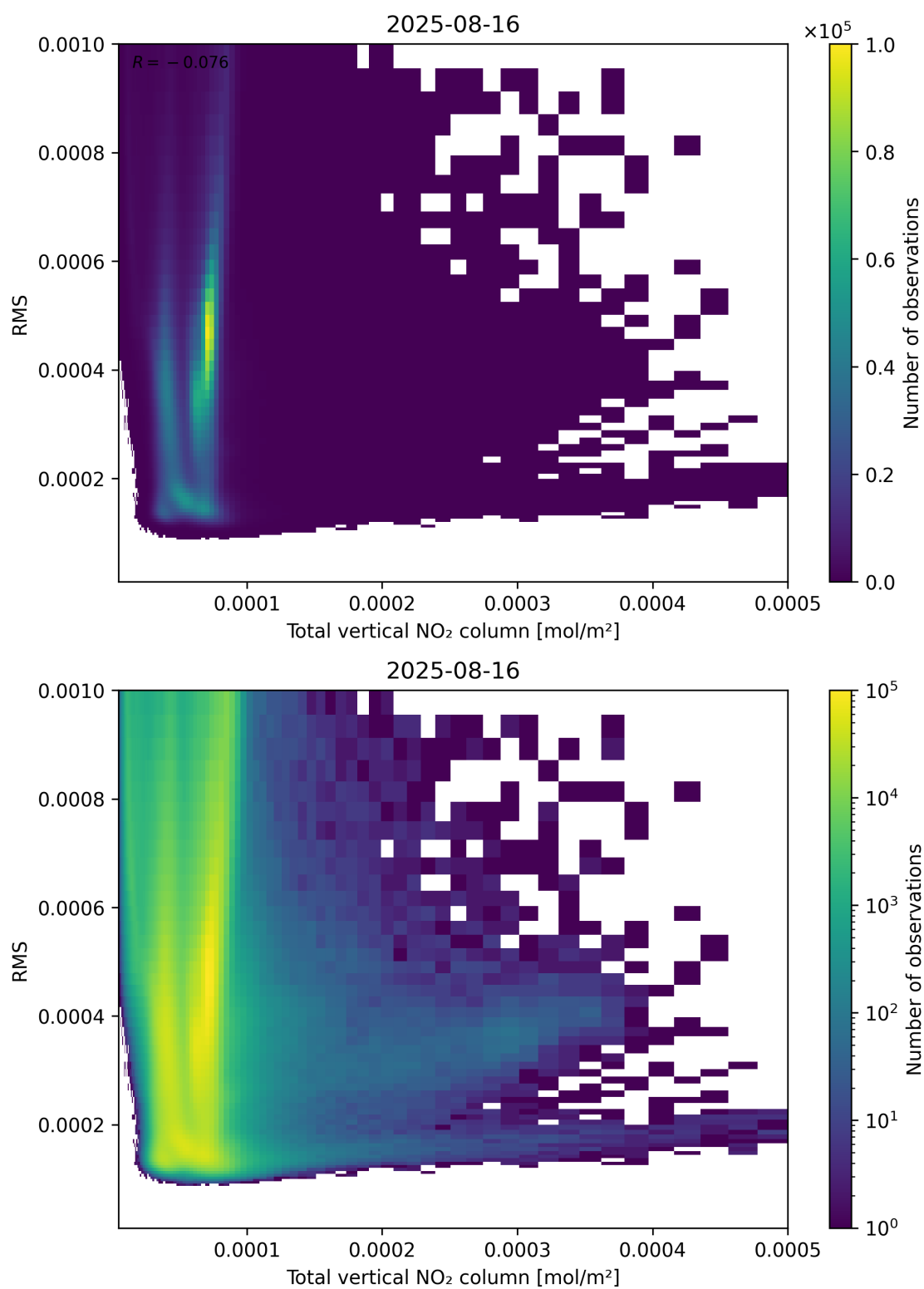
Figure 120: Scatter density plot of “Total vertical NO 2 column” against “RMS” for 2025-08-15 to 2025-08-17.
