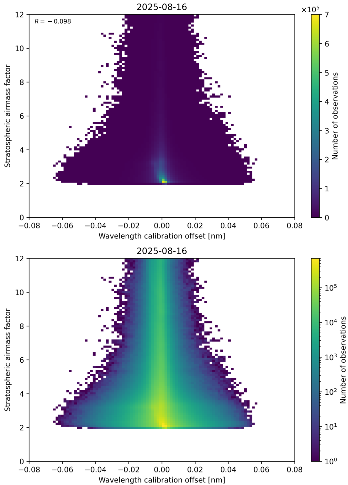
Figure 174: Scatter density plot of “Wavelength calibration offset” against “Stratospheric airmass factor” for 2025-08-15 to 2025-08-17.
