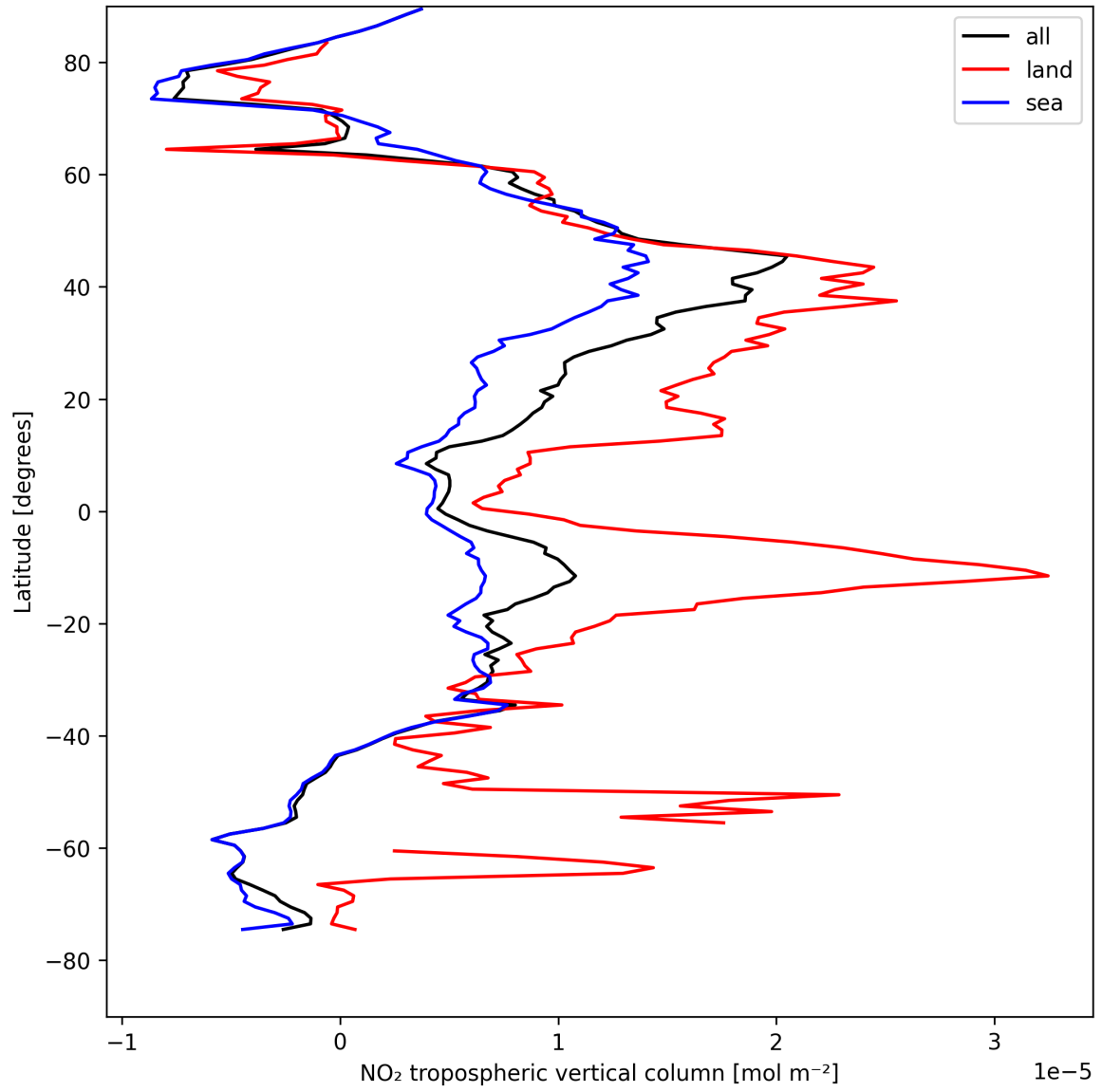
Figure 12: Zonal average of “NO 2 tropospheric vertical column” for 2025-08-15 to 2025-08-17.
