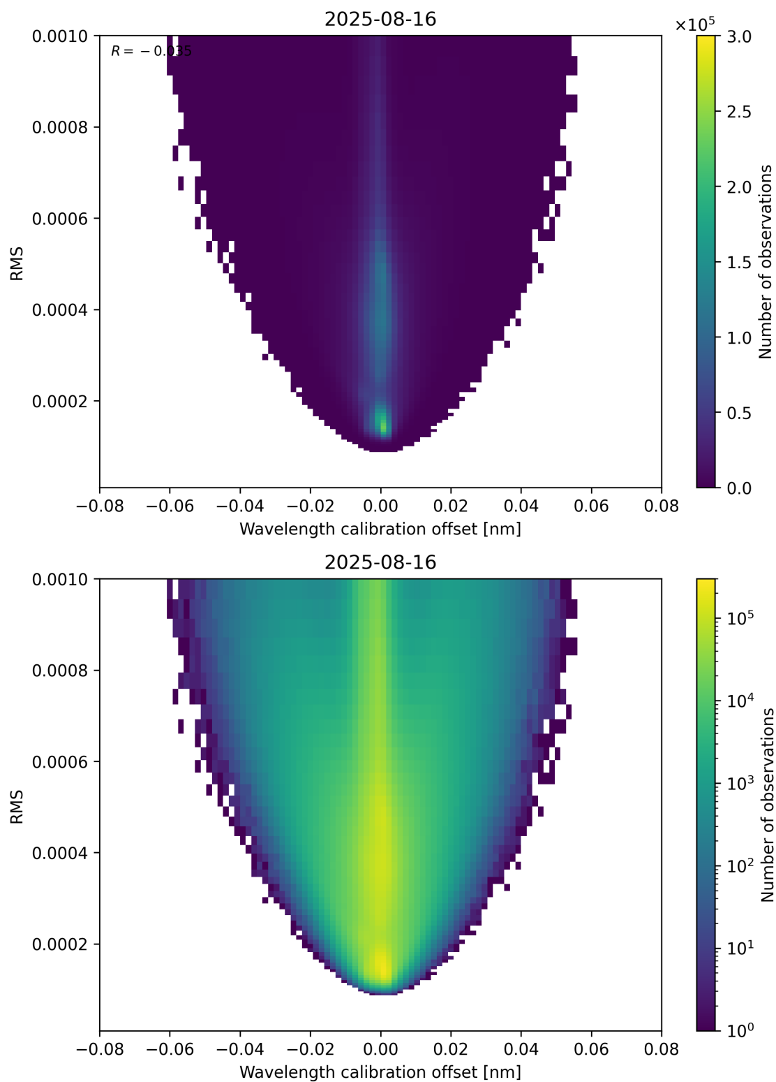
Figure 181: Scatter density plot of “Wavelength calibration offset” against “RMS” for 2025-08-15 to 2025-08-17.
