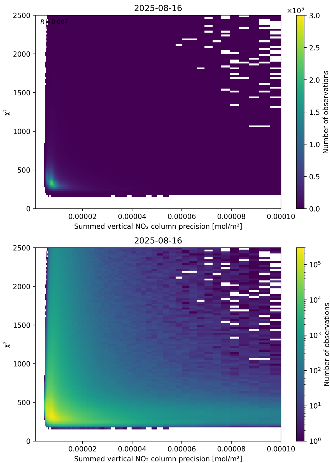
Figure 107: Scatter density plot of “Summed vertical NO 2 column precision” against “ \chi^2 ” for 2025-08-15 to 2025-08-17.
