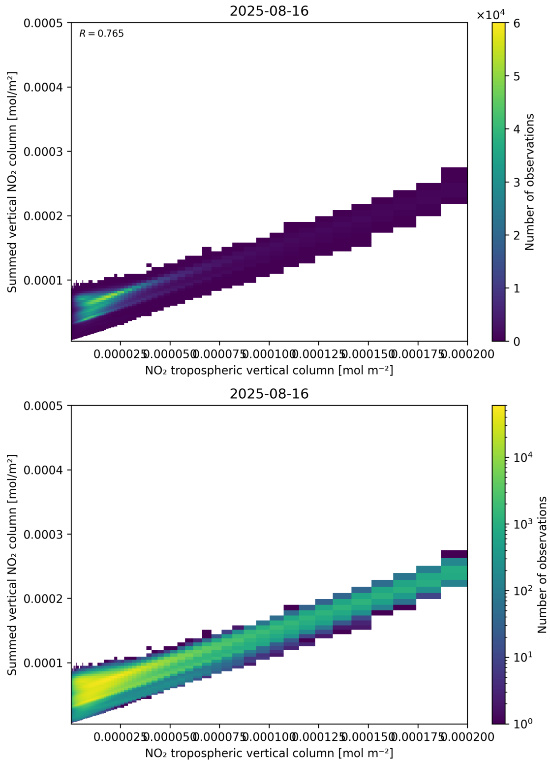
Figure 126: Scatter density plot of “NO 2 tropospheric vertical column” against “Summed vertical NO 2 column” for 2025-08-15 to 2025-08-17.
