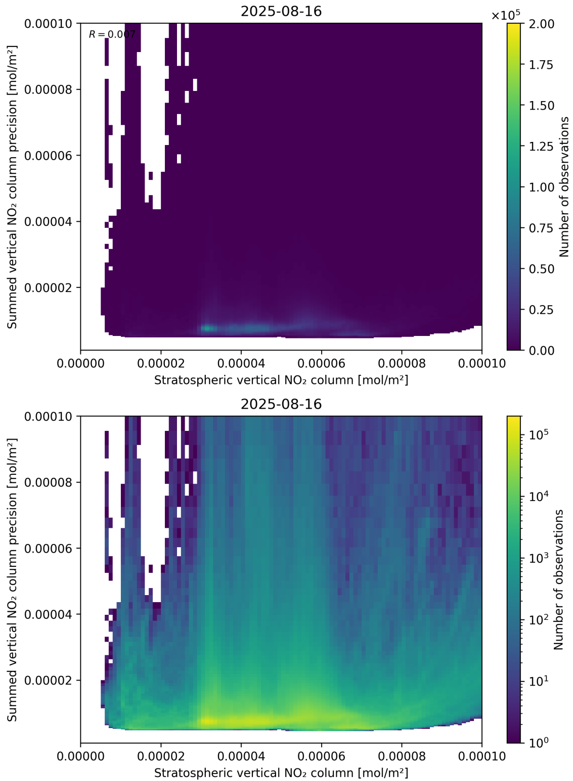
Figure 99: Scatter density plot of “Stratospheric vertical NO 2 column” against “Summed vertical NO 2 column precision” for 2025-08-15 to 2025-08-17.
