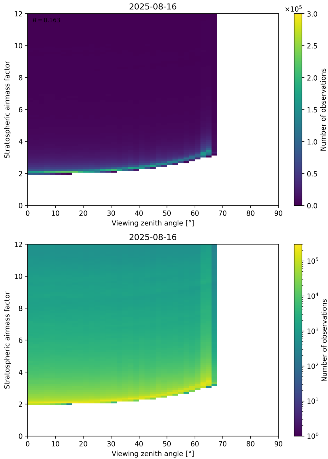
Figure 159: Scatter density plot of “Viewing zenith angle” against “Stratospheric airmass factor” for 2025-08-15 to 2025-08-17.
