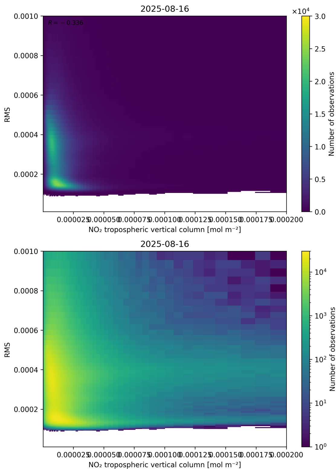
Figure 142: Scatter density plot of “NO 2 tropospheric vertical column” against “RMS” for 2025-08-15 to 2025-08-17.
