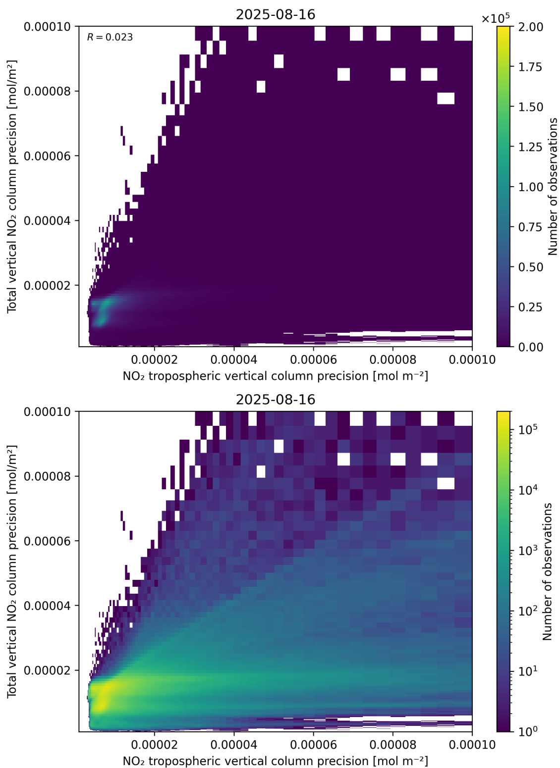
Figure 139: Scatter density plot of “NO 2 tropospheric vertical column precision” against “Total vertical NO 2 column precision” for 2025-08-15 to 2025-08-17.
