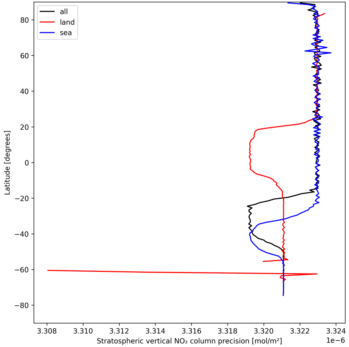
Figure 20: Zonal average of “Stratospheric vertical NO 2 column precision” for 2025-08-15 to 2025-08-17.
