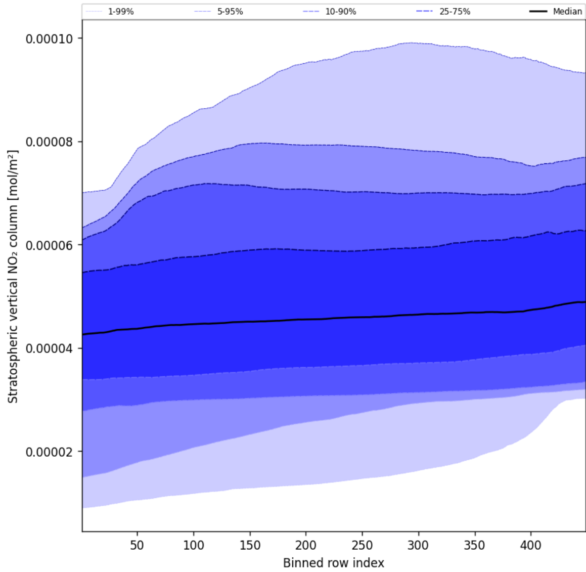
Figure 53: Along track statistics of “Stratospheric vertical NO 2 column” for 2025-08-15 to 2025-08-17
