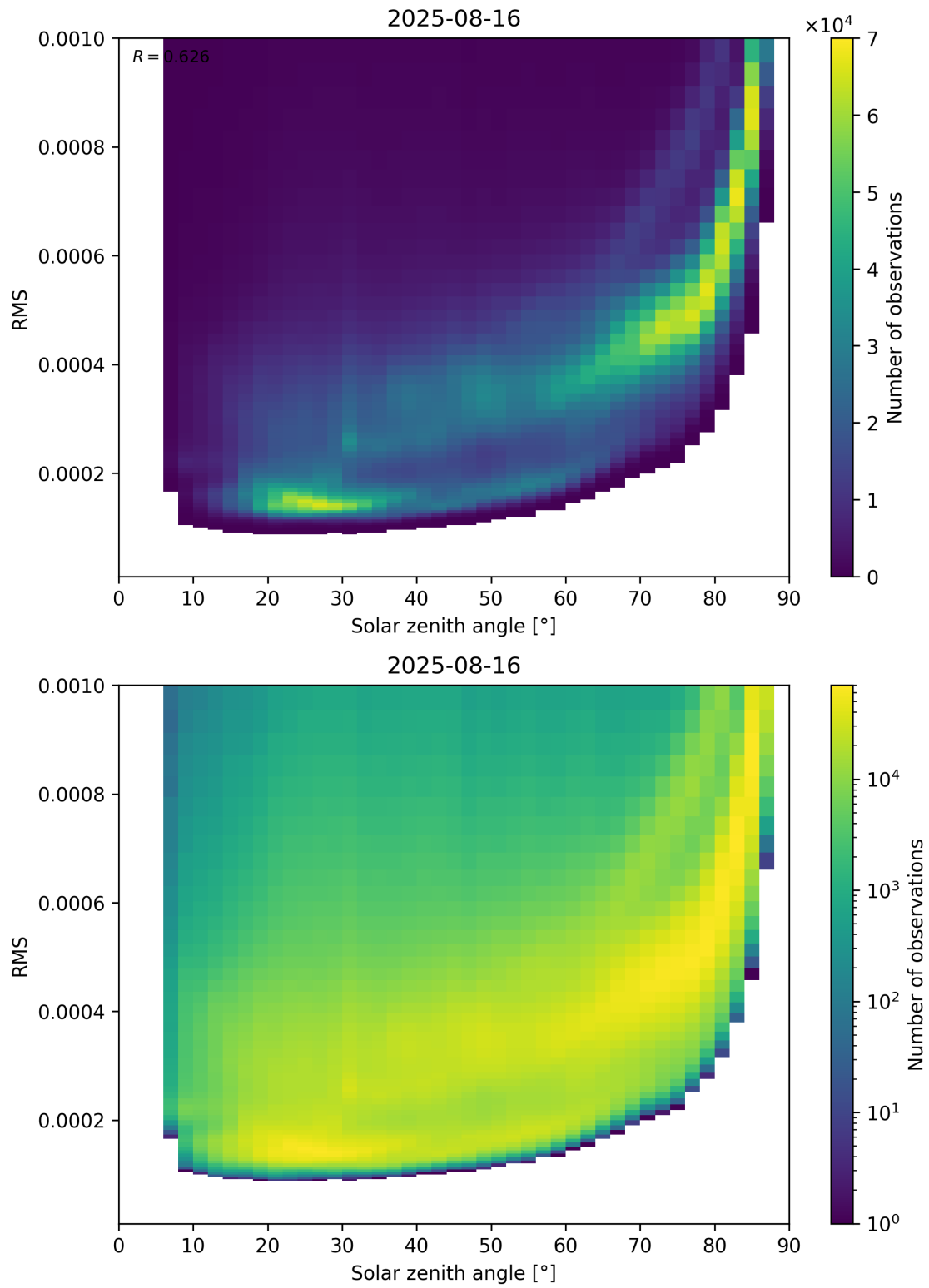
Figure 157: Scatter density plot of “Solar zenith angle” against “RMS” for 2025-08-15 to 2025-08-17.
