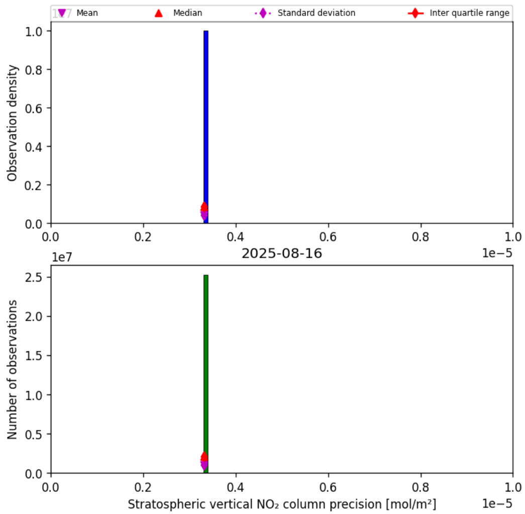
Figure 37: Histogram of “Stratospheric vertical NO 2 column precision” for 2025-08-15 to 2025-08-17
