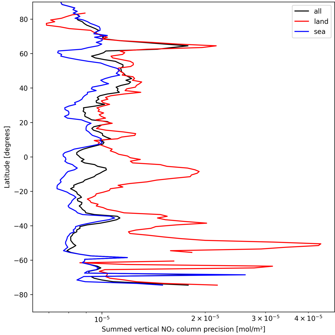
Figure 24: Zonal average of "Summed vertical NO 2 column precision" for 2025-08-15 to 2025-08-17.
