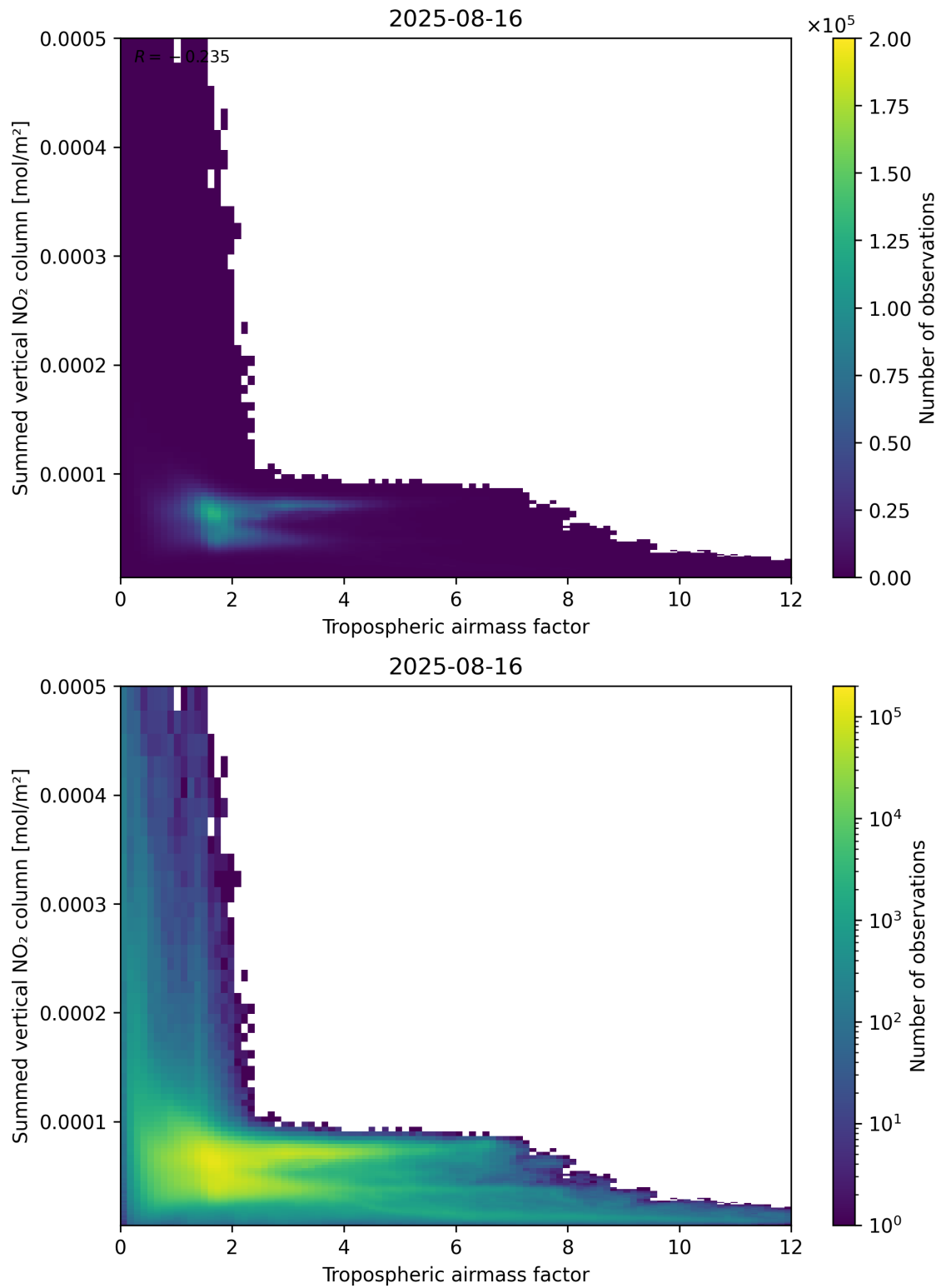
Figure 75: Scatter density plot of “Tropospheric airmass factor” against “Summed vertical NO 2 column” for 2025-08-15 to 2025-08-17.
