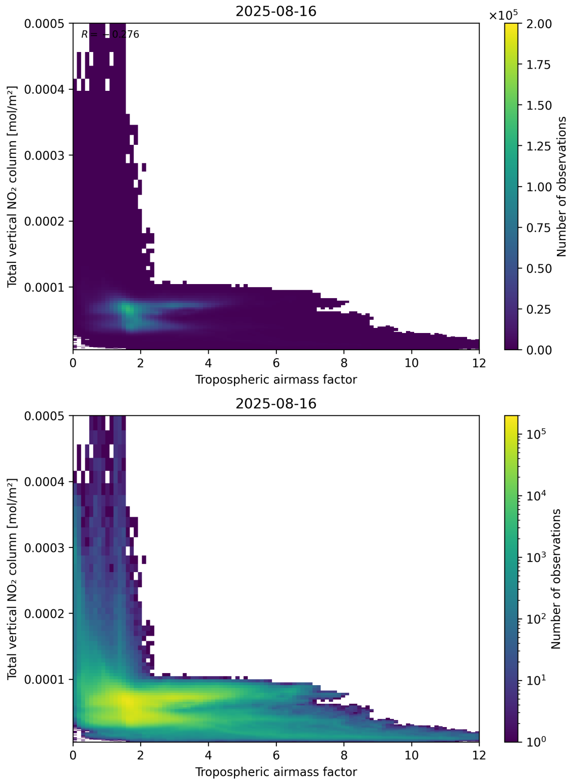
Figure 77: Scatter density plot of “Tropospheric airmass factor” against “Total vertical NO 2 column” for 2025-08-15 to 2025-08-17.
