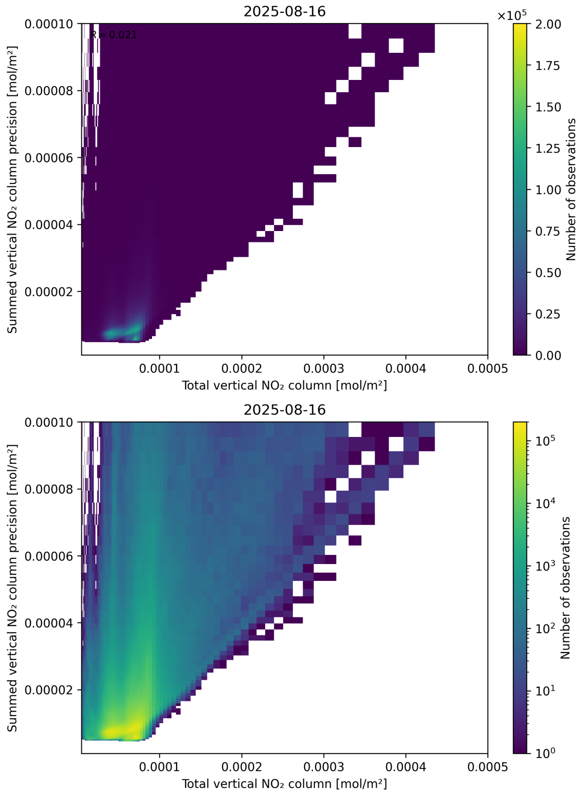
Figure 113: Scatter density plot of “Total vertical NO 2 column” against “Summed vertical NO 2 column precision” for 2025-08-15 to 2025-08-17.
