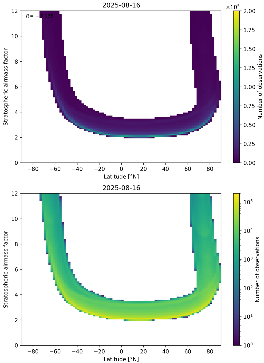
Figure 83: Scatter density plot of “Latitude” against “Stratospheric air mass factor” for 2025-08-15 to 2025-08-17.
