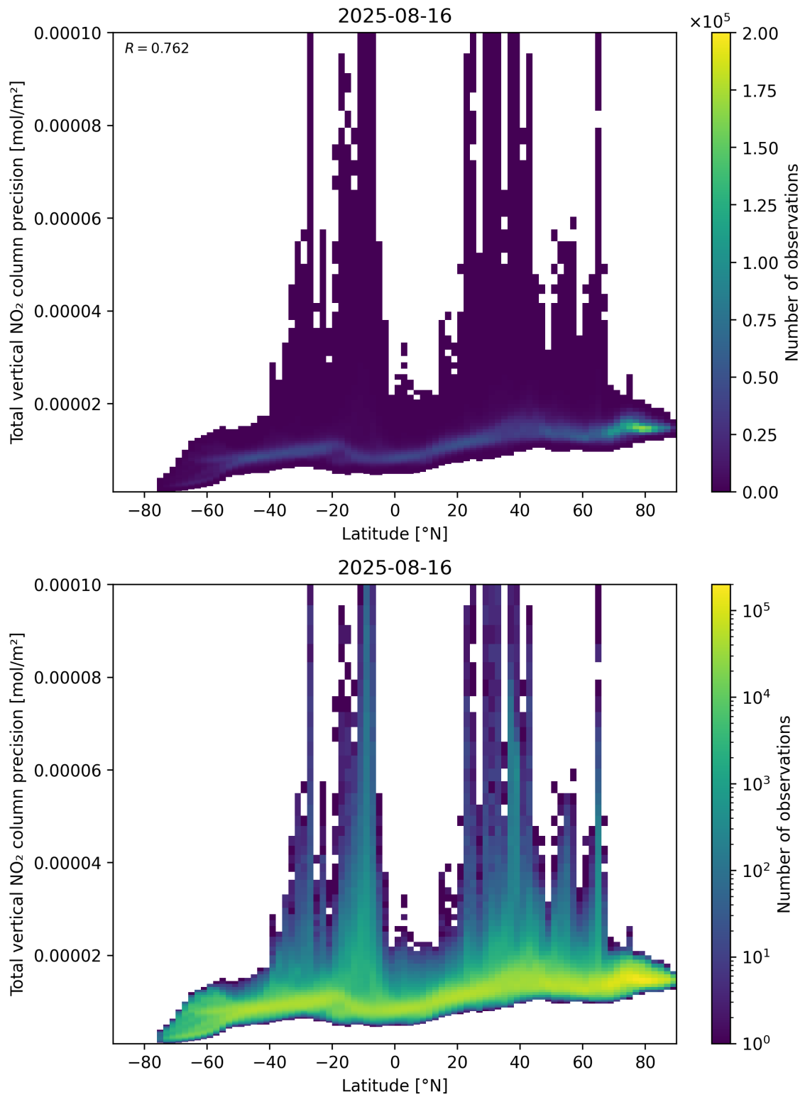
Figure 91: Scatter density plot of “Latitude” against “Total vertical NO 2 column precision” for 2025-08-15 to 2025-08-17.
