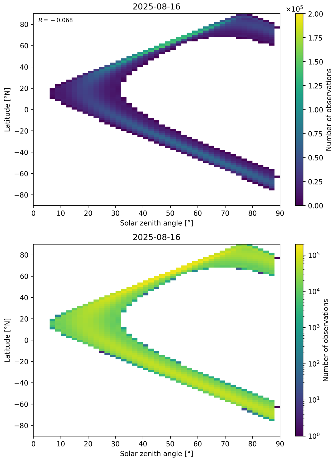
Figure 149: Scatter density plot of “Solar zenith angle” against “Latitude” for 2025-08-15 to 2025-08-17.
