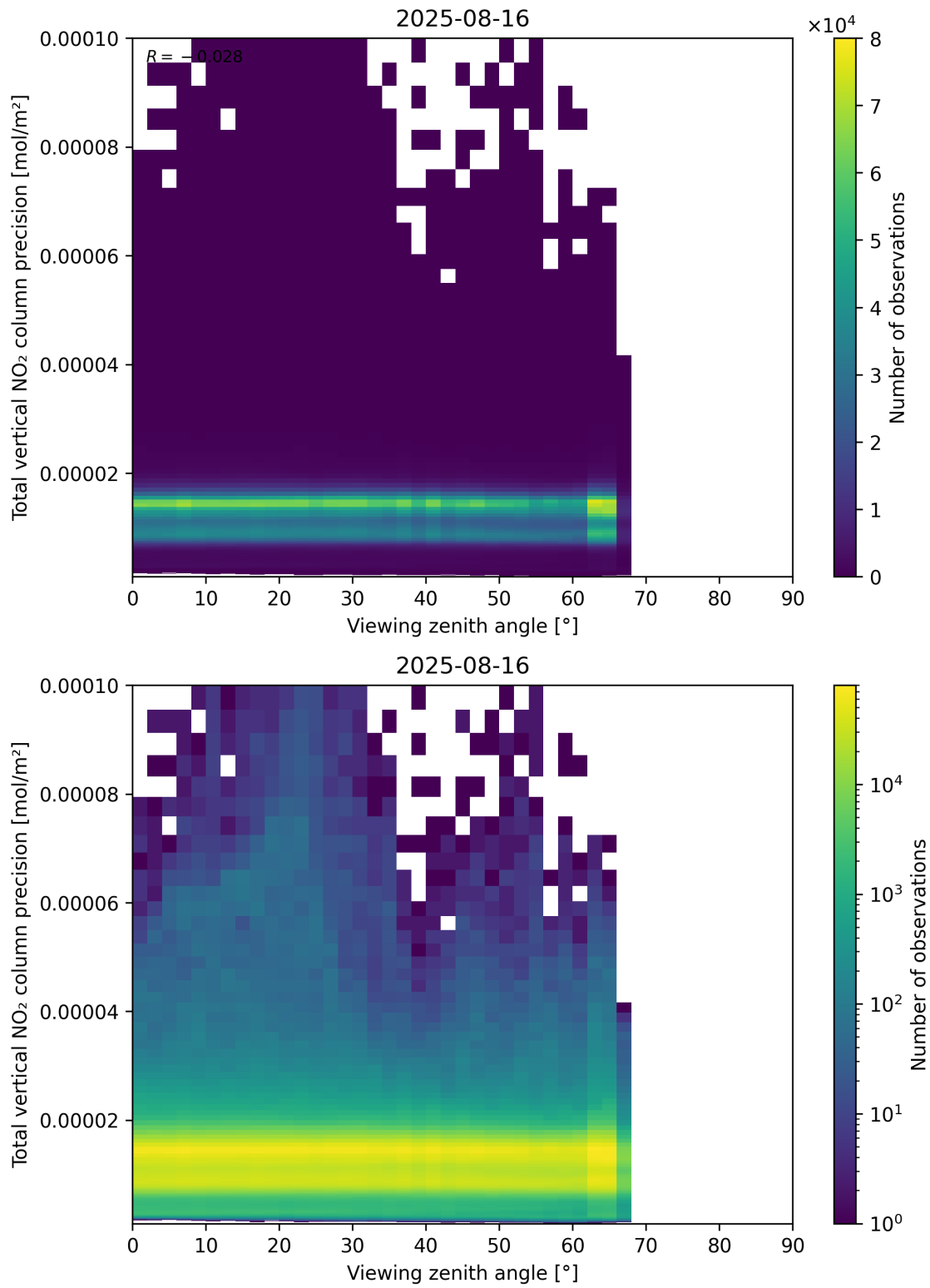
Figure 168: Scatter density plot of “Viewing zenith angle” against “Total vertical NO 2 column precision” for 2025-08-15 to 2025-08-17.
