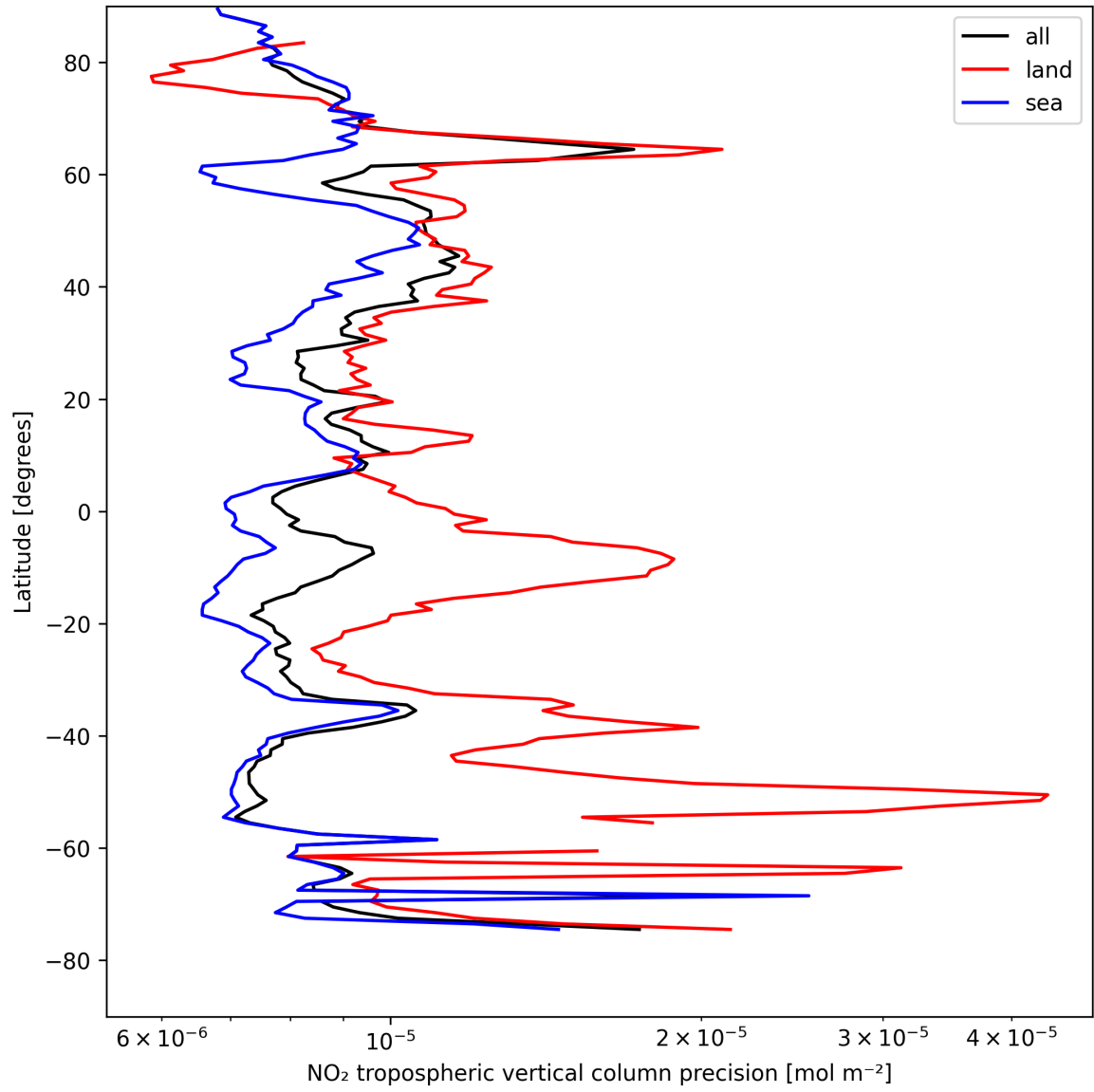
Figure 13: Zonal average of “NO 2 tropospheric vertical column precision” for 2025-08-15 to 2025-08-17.
