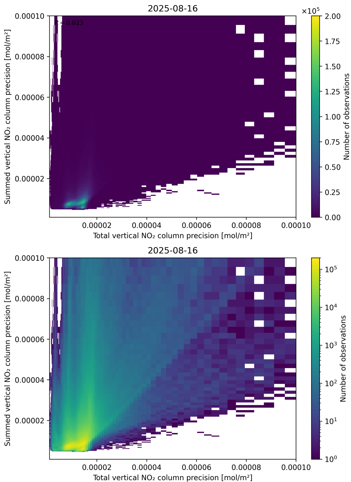
Figure 118: Scatter density plot of “Total vertical NO 2 column precision” against “Summed vertical NO 2 column precision” for 2025-08-15 to 2025-08-17.
