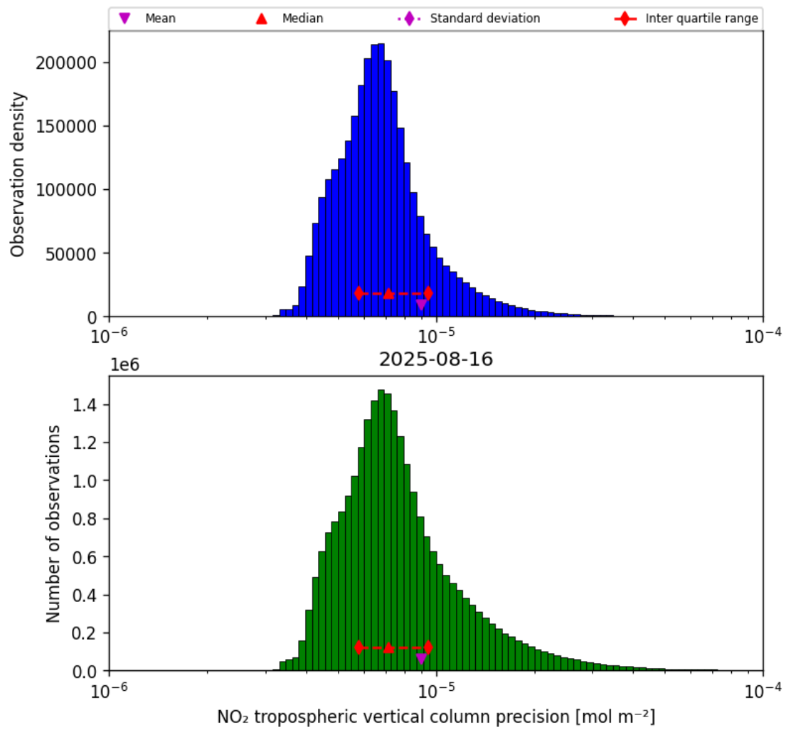
Figure 30: Histogram of "NO 2 tropospheric vertical column precision" for 2025-08-15 to 2025-08-17
