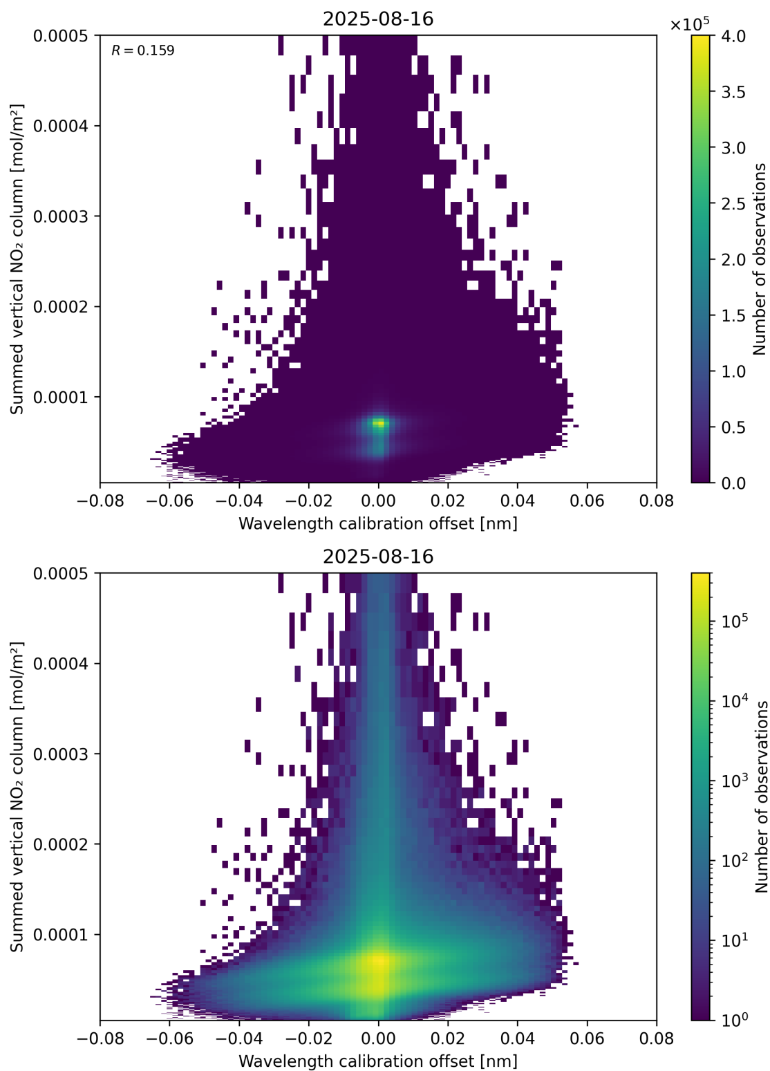
Figure 177: Scatter density plot of “Wavelength calibration offset” against “Summed vertical NO 2 column” for 2025-08-15 to 2025-08-17.
