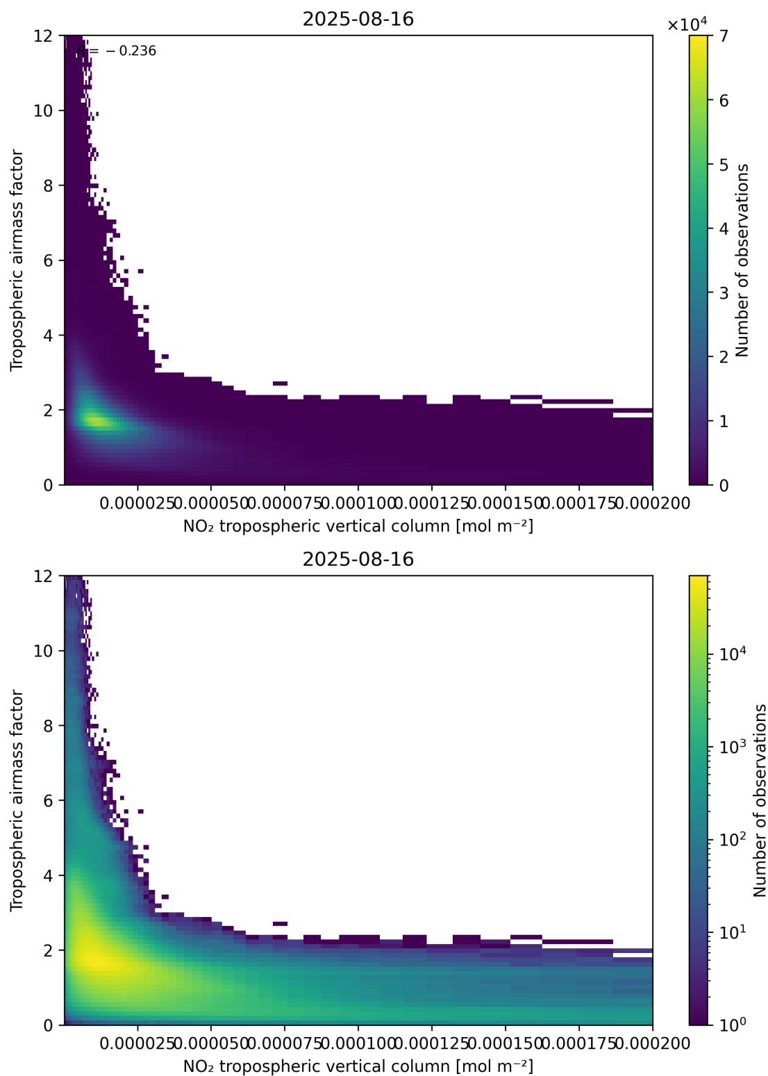
Figure 123: Scatter density plot of “NO 2 tropospheric vertical column” against “Tropospheric air mass factor” for 2025-08-15 to 2025-08-17.
