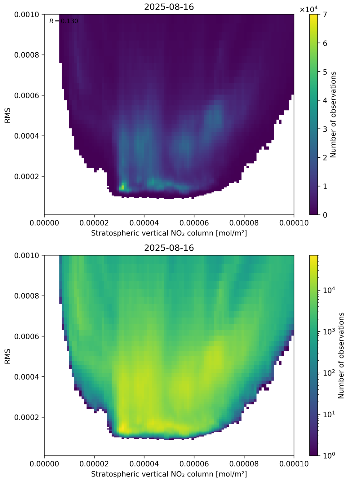
Figure 102: Scatter density plot of “Stratospheric vertical NO 2 column” against “RMS” for 2025-08-15 to 2025-08-17.
