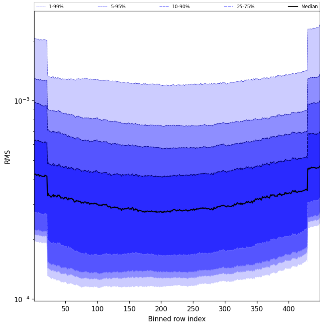
Figure 60: Along track statistics of “RMS” for 2025-08-15 to 2025-08-17
