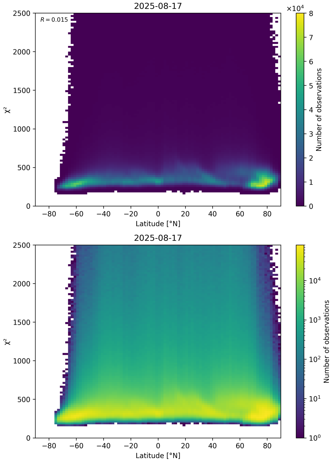
Figure 86: Scatter density plot of “Latitude” against “ \chi^2 ” for 2025-08-16 to 2025-08-18.
