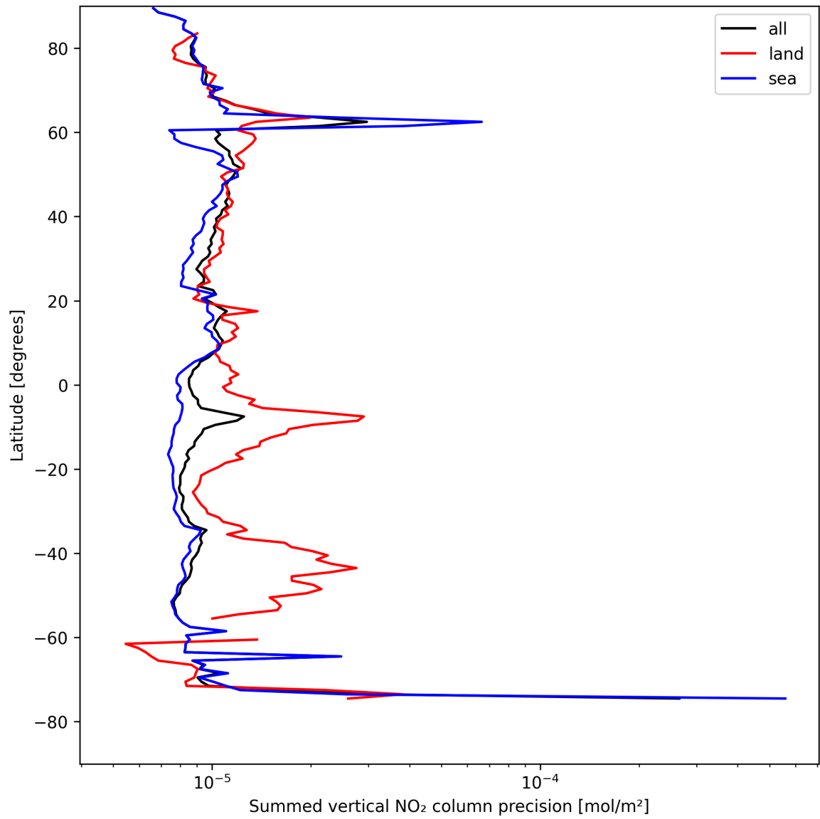
Figure 24: Zonal average of “Summed vertical NO 2 column precision” for 2025-08-16 to 2025-08-18.
