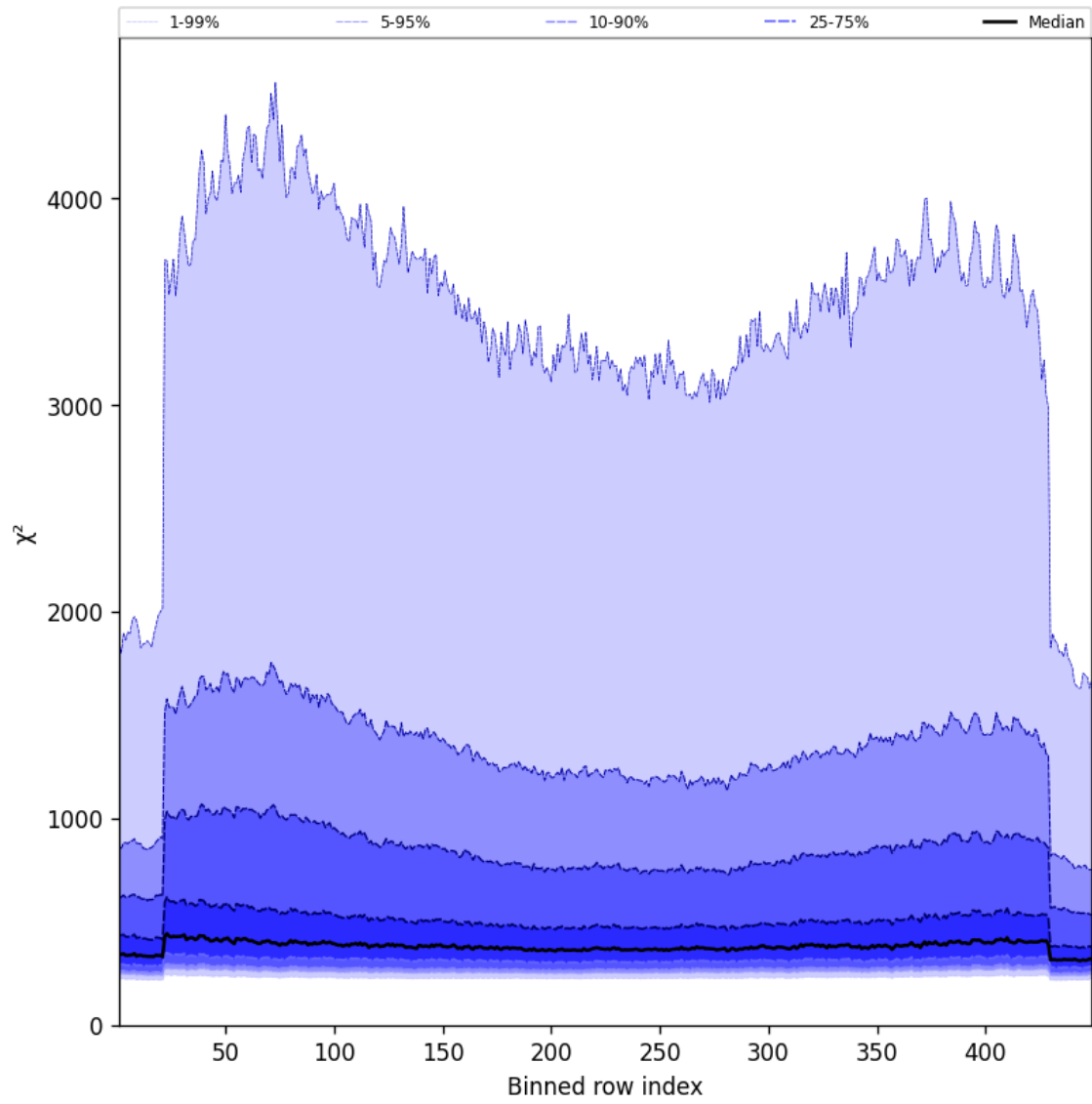
Figure 59: Along track statistics of “ \chi^2 ” for 2025-08-16 to 2025-08-18
