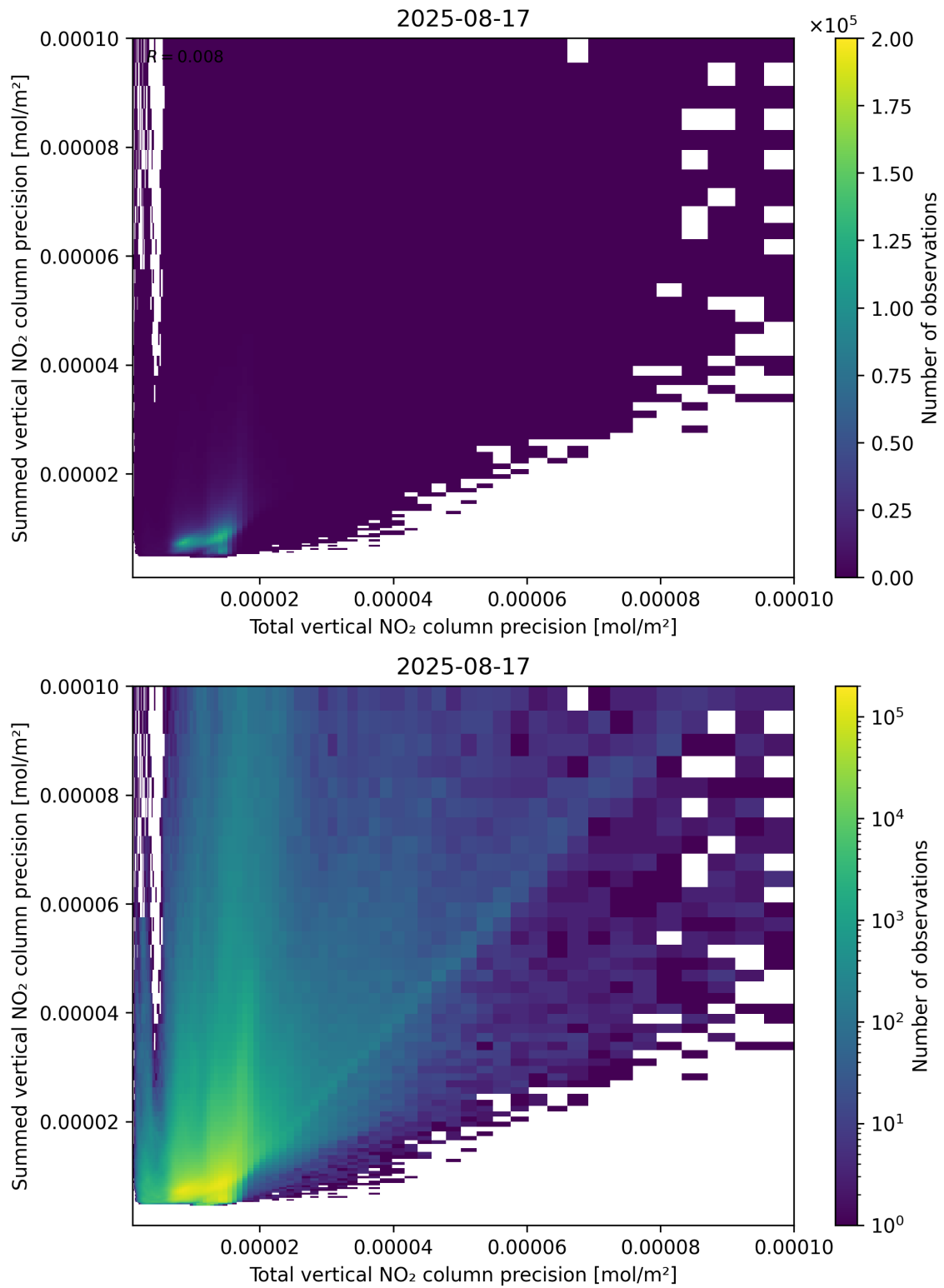
Figure 118: Scatter density plot of “Total vertical NO 2 column precision” against “Summed vertical NO 2 column precision” for 2025-08-16 to 2025-08-18.
