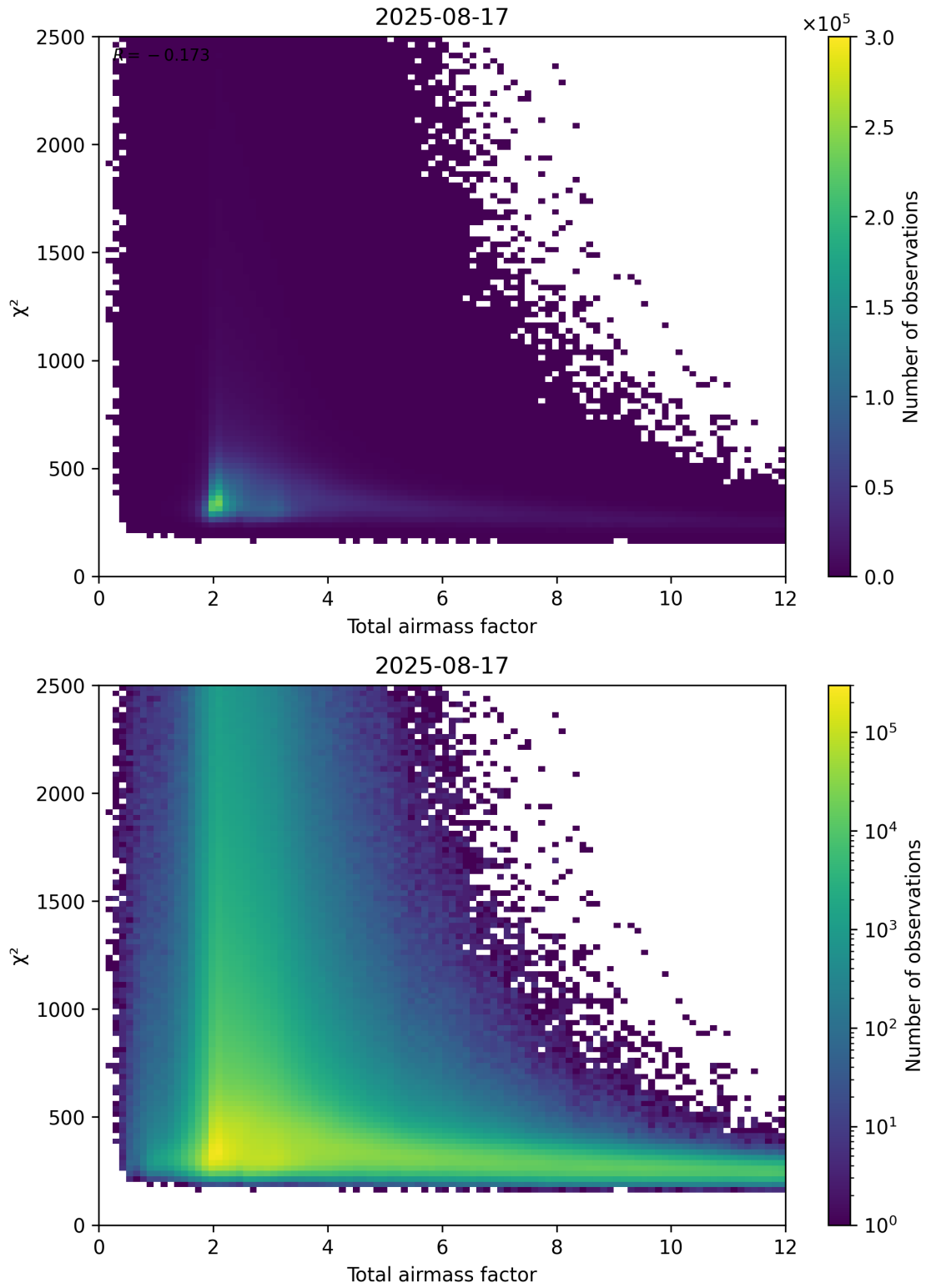
Figure 63: Scatter density plot of “Total airmass factor” against “ \chi^2 ” for 2025-08-16 to 2025-08-18.
