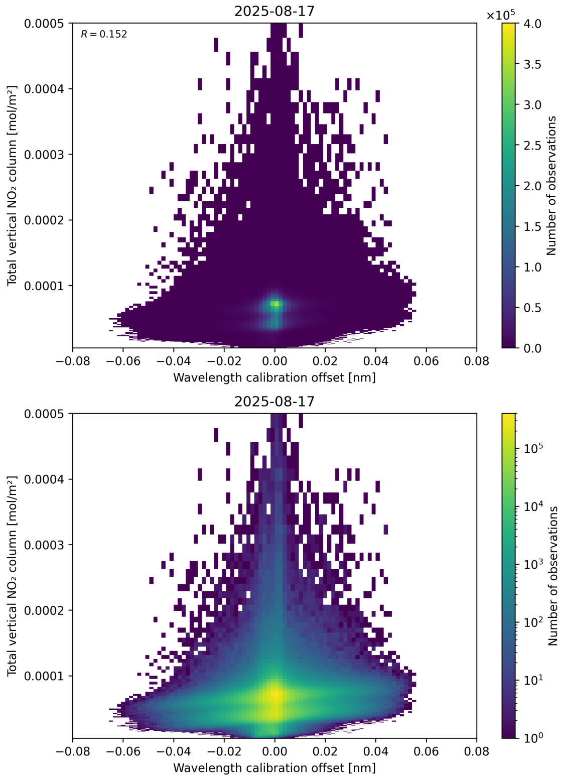
Figure 179: Scatter density plot of “Wavelength calibration offset” against “Total vertical NO 2 column” for 2025-08-16 to 2025-08-18.
