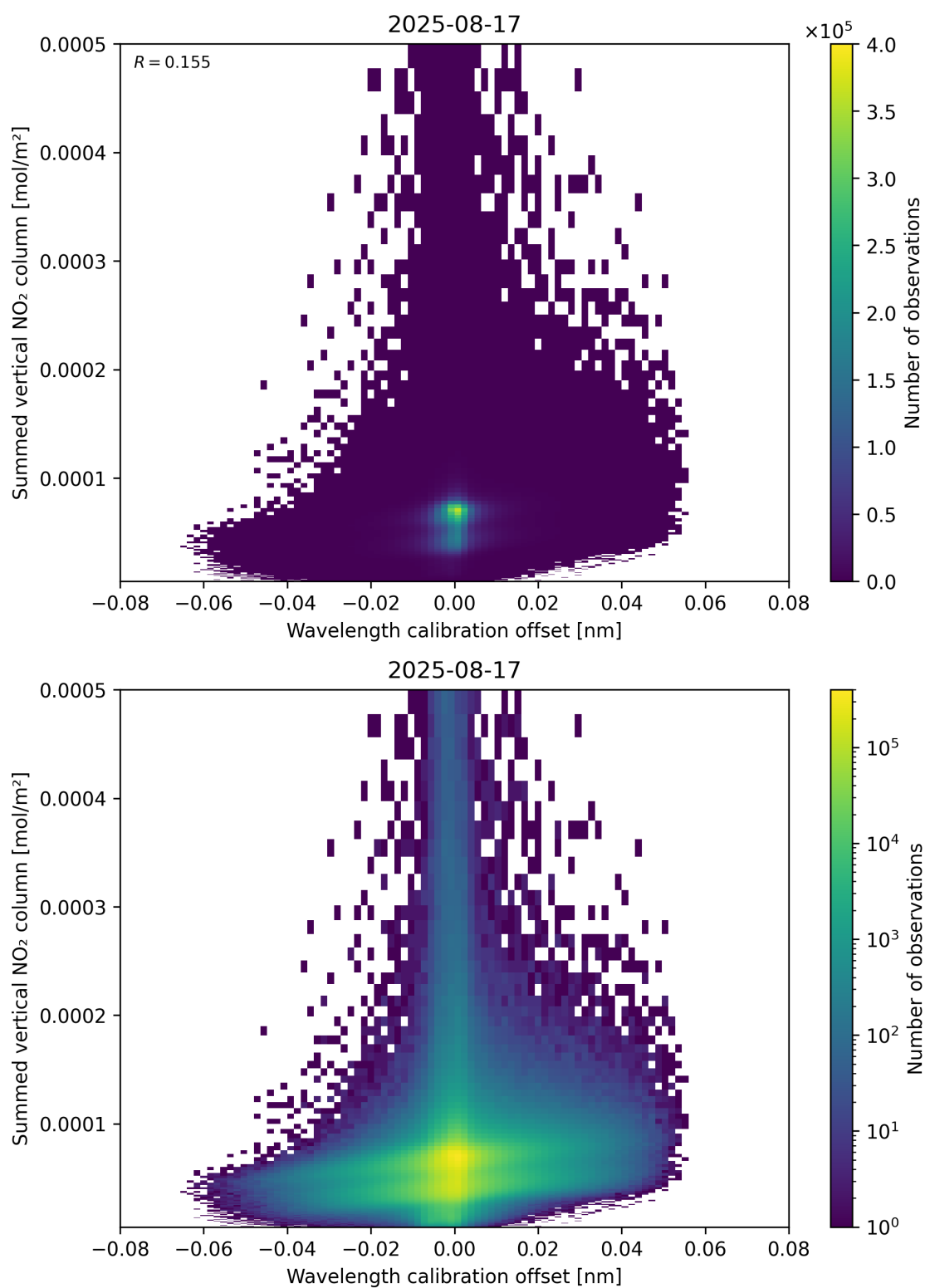
Figure 177: Scatter density plot of “Wavelength calibration offset” against “Summed vertical NO 2 column” for 2025-08-16 to 2025-08-18.
