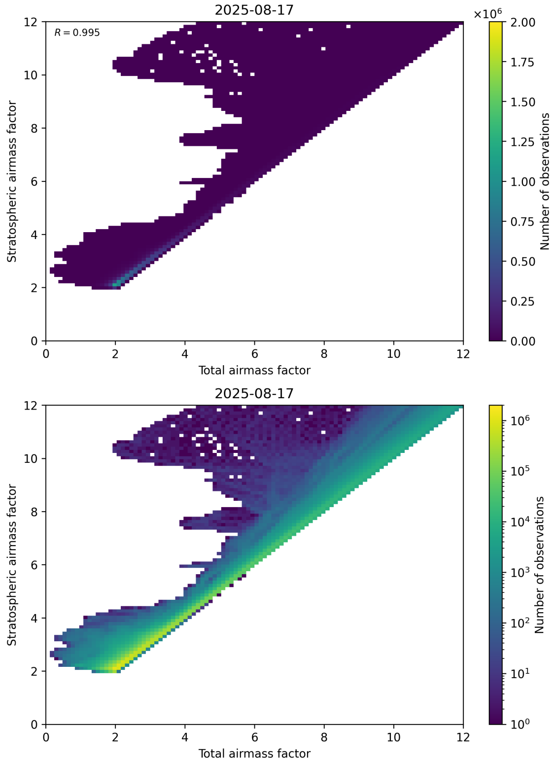
Figure 62: Scatter density plot of “Total airmass factor” against “Stratospheric airmass factor” for 2025-08-16 to 2025-08-18.
