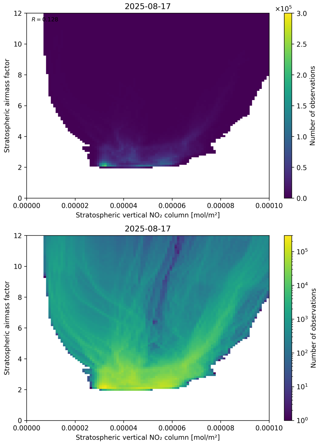
Figure 96: Scatter density plot of “Stratospheric vertical NO 2 column” against “Stratospheric airmass factor” for 2025-08-16 to 2025-08-18.
