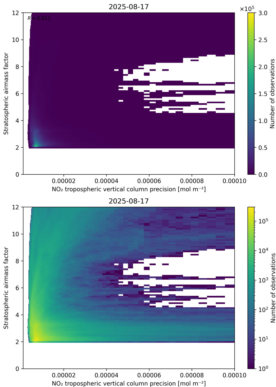
Figure 131: Scatter density plot of “NO 2 tropospheric vertical column precision” against “Stratospheric airmass factor” for 2025-08-16 to 2025-08-18.
