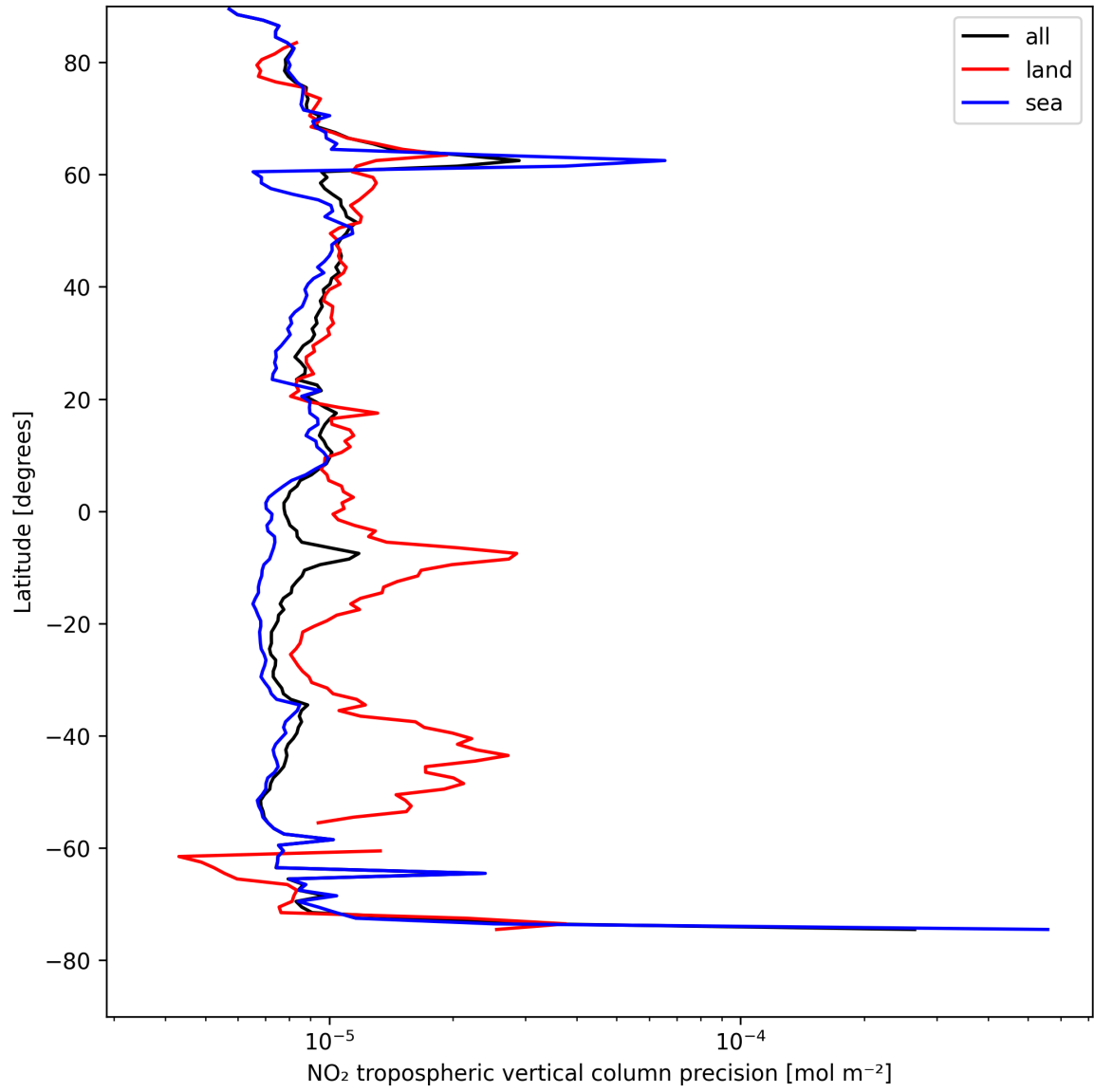
Figure 13: Zonal average of “NO 2 tropospheric vertical column precision” for 2025-08-16 to 2025-08-18.
