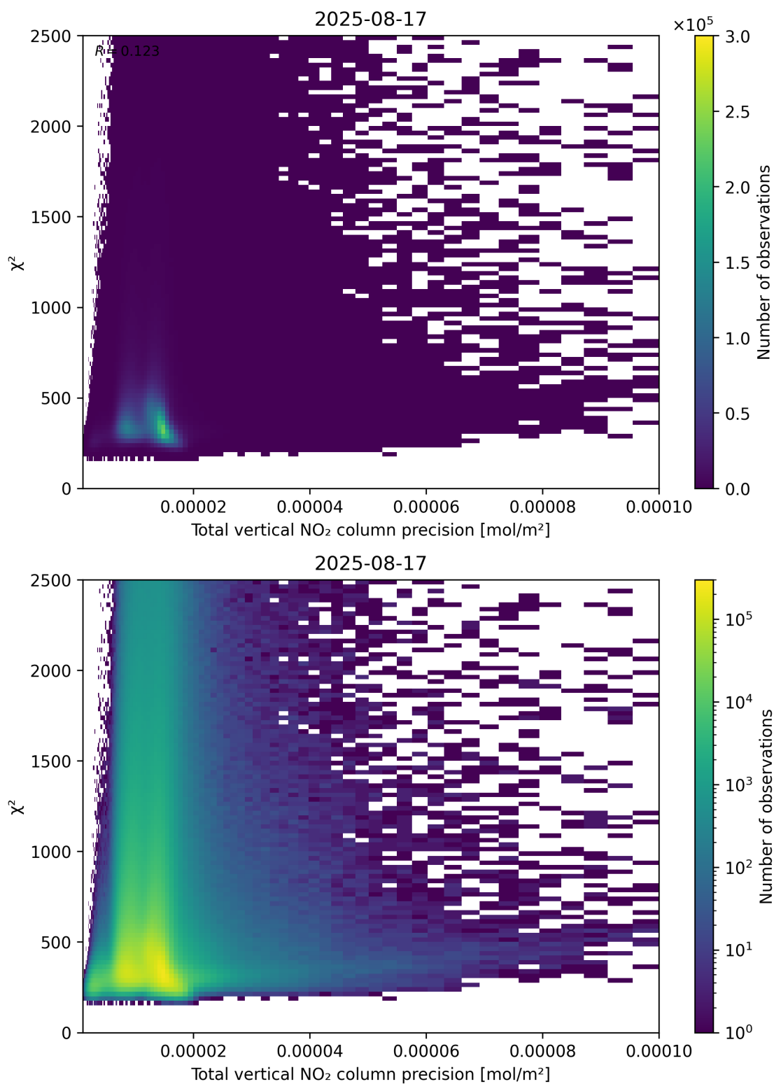
Figure 116: Scatter density plot of “Total vertical NO 2 column precision” against “ \chi^2 ” for 2025-08-16 to 2025-08-18.
