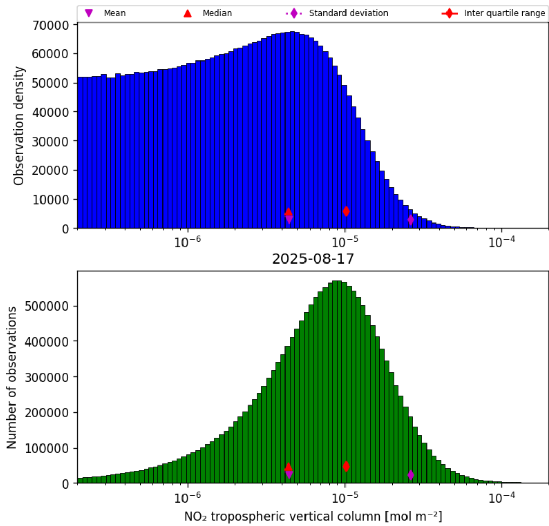
Figure 29: Histogram of “NO 2 tropospheric vertical column” for 2025-08-16 to 2025-08-18
