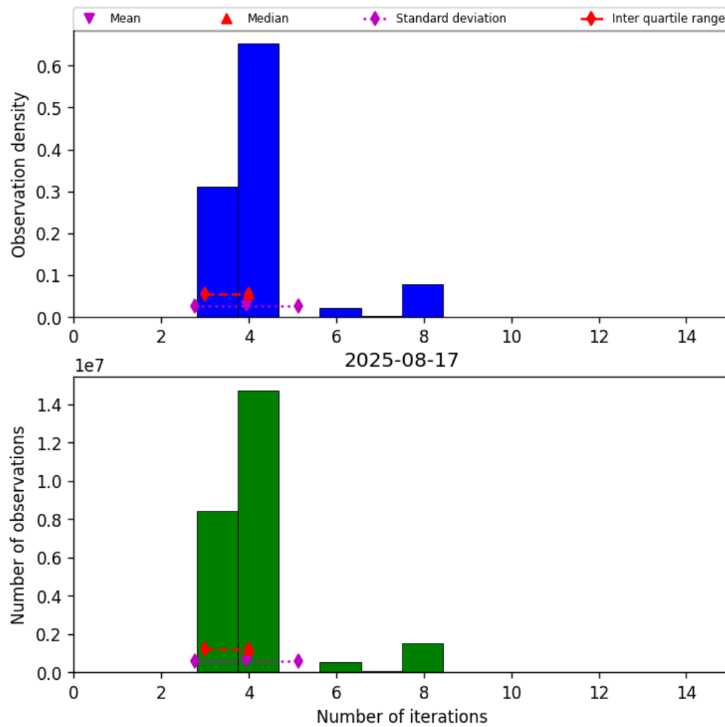
Figure 34: Histogram of “Number of iterations” for 2025-08-16 to 2025-08-18
