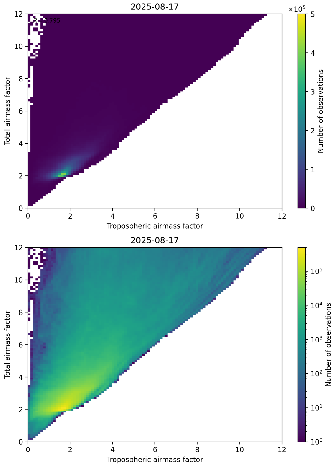
Figure 72: Scatter density plot of “Tropospheric airmass factor” against “Total airmass factor” for 2025-08-16 to 2025-08-18.
