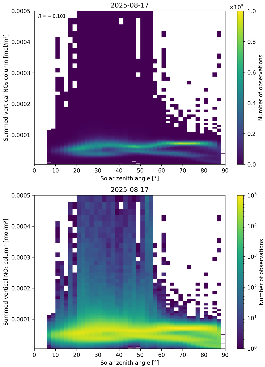
Figure 151: Scatter density plot of “Solar zenith angle” against “Summed vertical NO 2 column” for 2025-08-16 to 2025-08-18.
