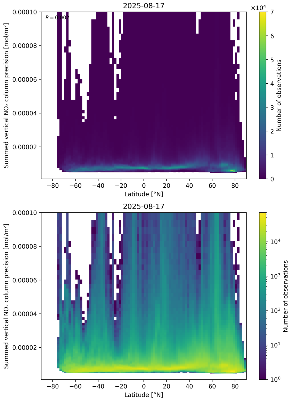
Figure 89: Scatter density plot of “Latitude” against “Summed vertical NO 2 column precision” for 2025-08-16 to 2025-08-18.
