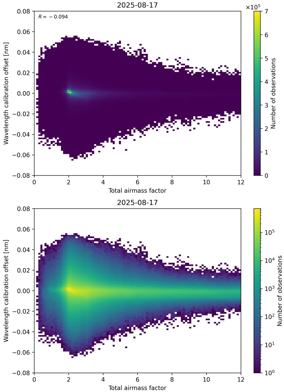
Figure 70: Scatter density plot of “Total airmass factor” against “Wavelength calibration offset” for 2025-08-16 to 2025-08-18.
