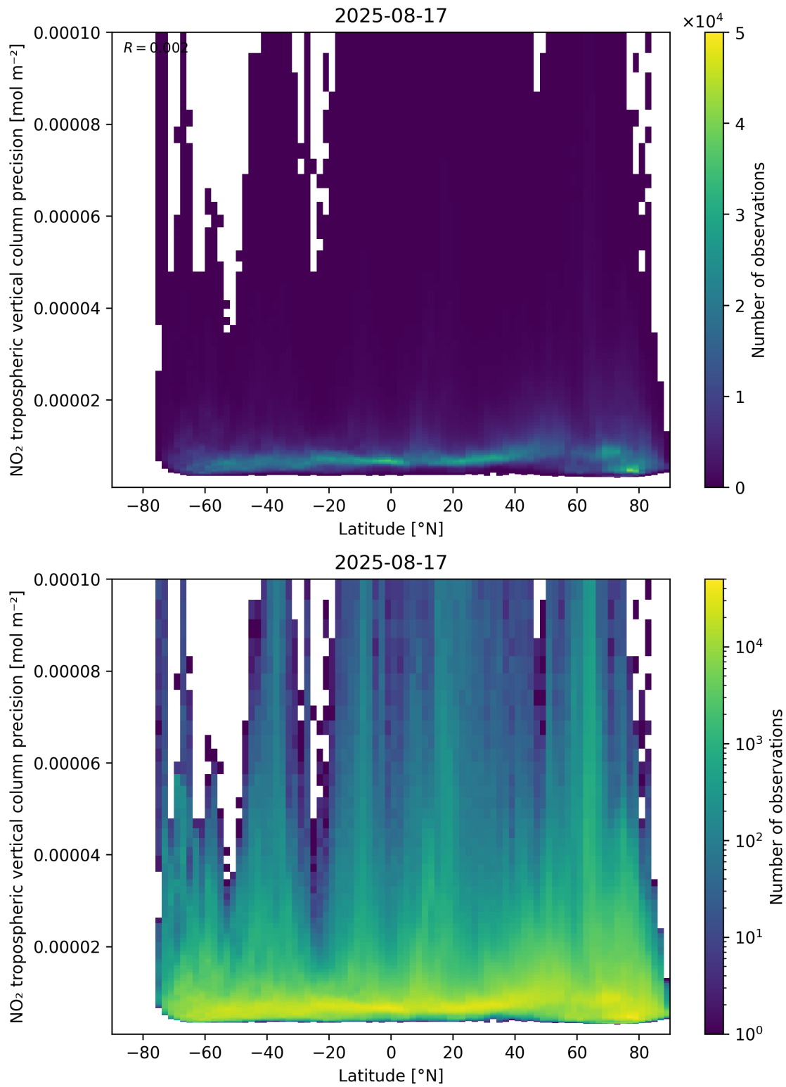
Figure 93: Scatter density plot of “Latitude” against “NO 2 tropospheric vertical column precision” for 2025-08-16 to 2025-08-18.
