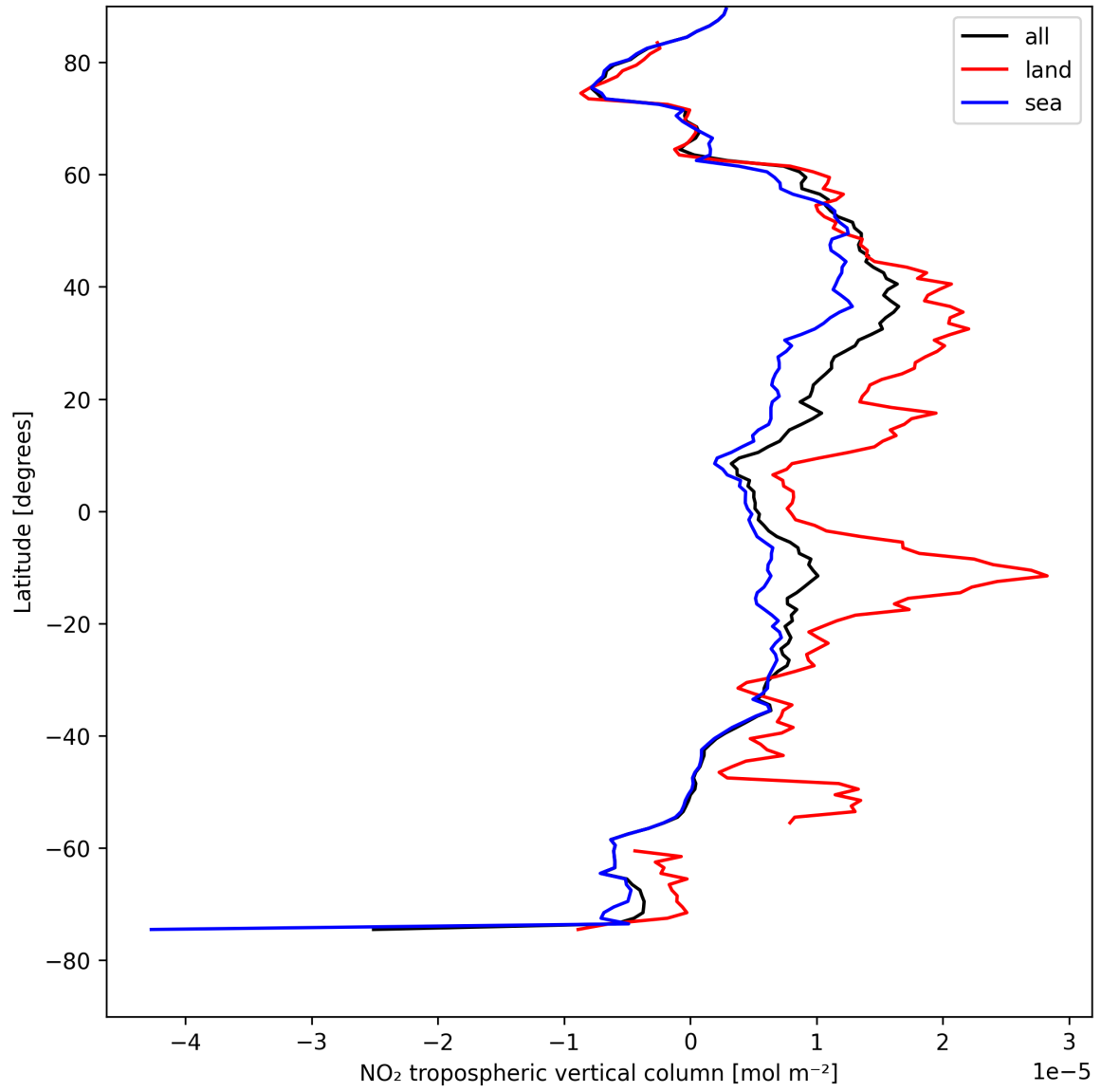
Figure 12: Zonal average of “NO 2 tropospheric vertical column” for 2025-08-16 to 2025-08-18.
