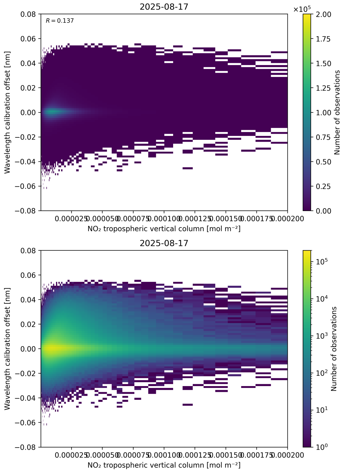
Figure 143: Scatter density plot of “NO 2 tropospheric vertical column” against “Wavelength calibration offset” for 2025-08-16 to 2025-08-18.
