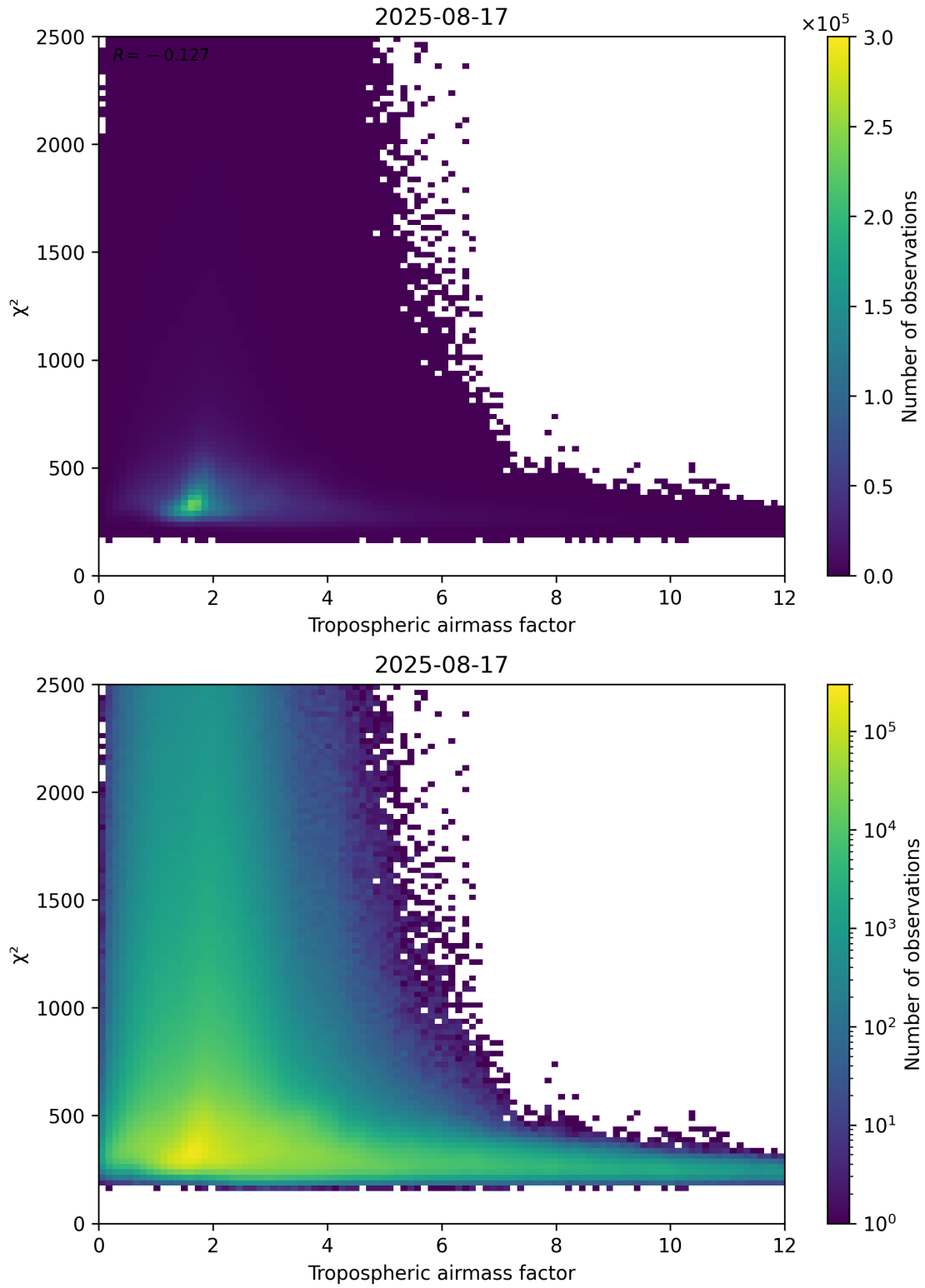
Figure 73: Scatter density plot of “Tropospheric airmass factor” against “ \chi^2 ” for 2025-08-16 to 2025-08-18.
