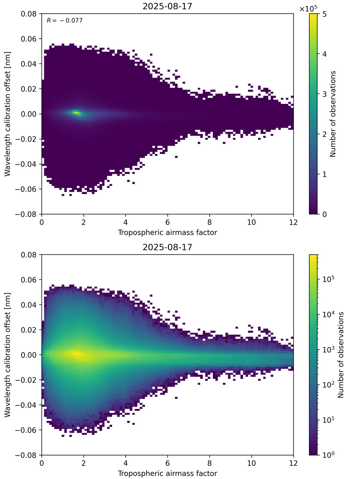
Figure 80: Scatter density plot of “Tropospheric airmass factor” against “Wavelength calibration offset” for 2025-08-16 to 2025-08-18.
