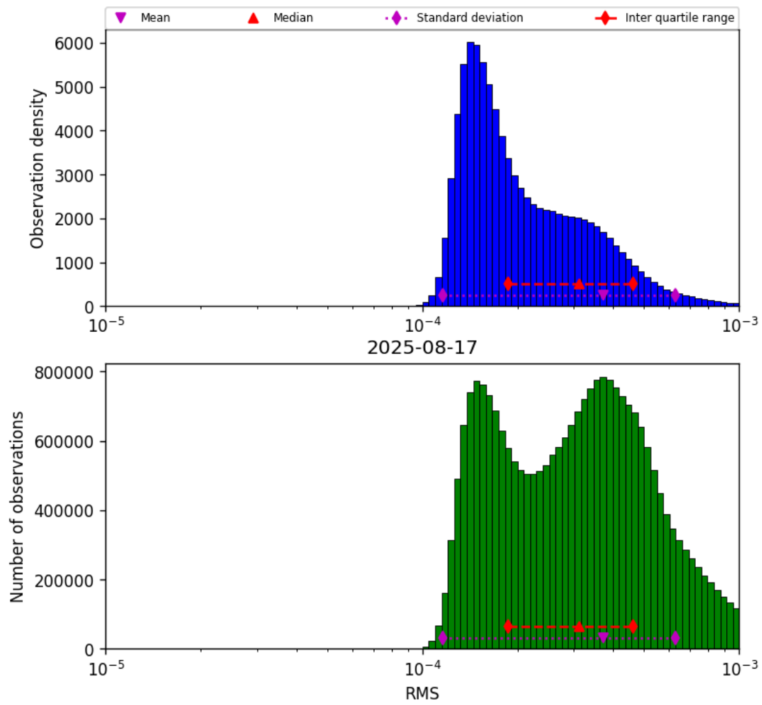
Figure 43: Histogram of “RMS” for 2025-08-16 to 2025-08-18
