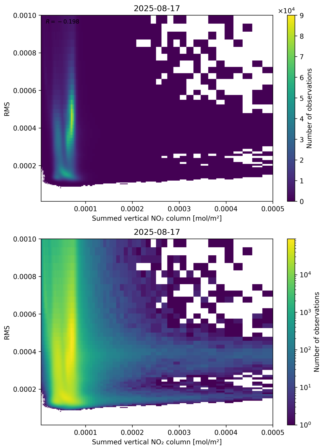
Figure 109: Scatter density plot of “Summed vertical NO 2 column” against “RMS” for 2025-08-16 to 2025-08-18.
