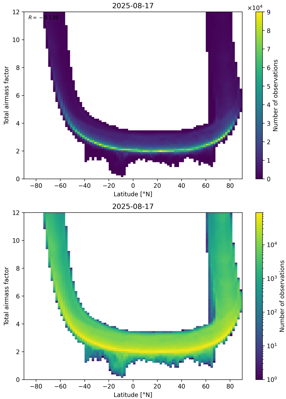
Figure 84: Scatter density plot of “Latitude” against “Total airmass factor” for 2025-08-16 to 2025-08-18.
