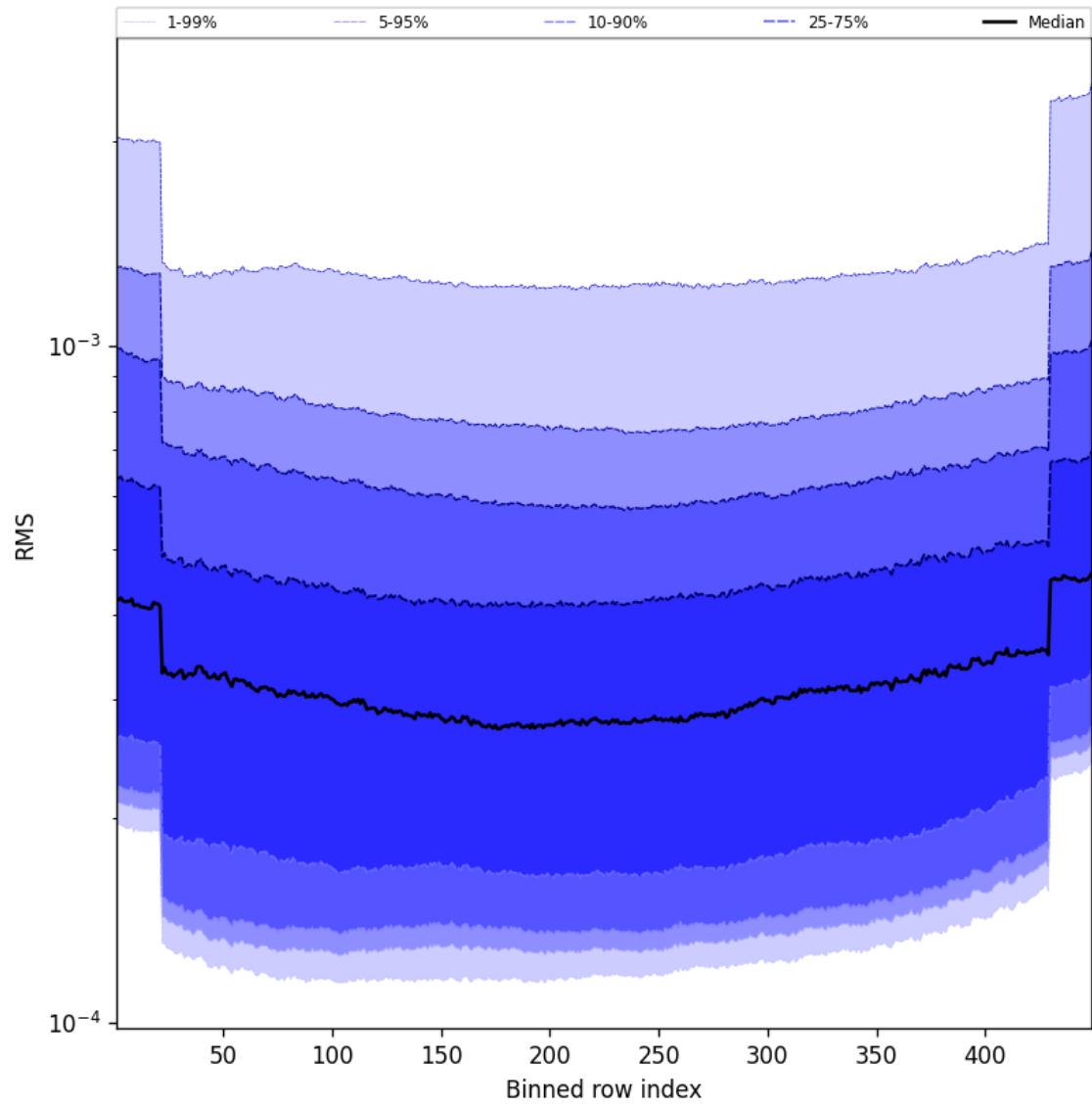
Figure 60: Along track statistics of “RMS” for 2025-08-16 to 2025-08-18
