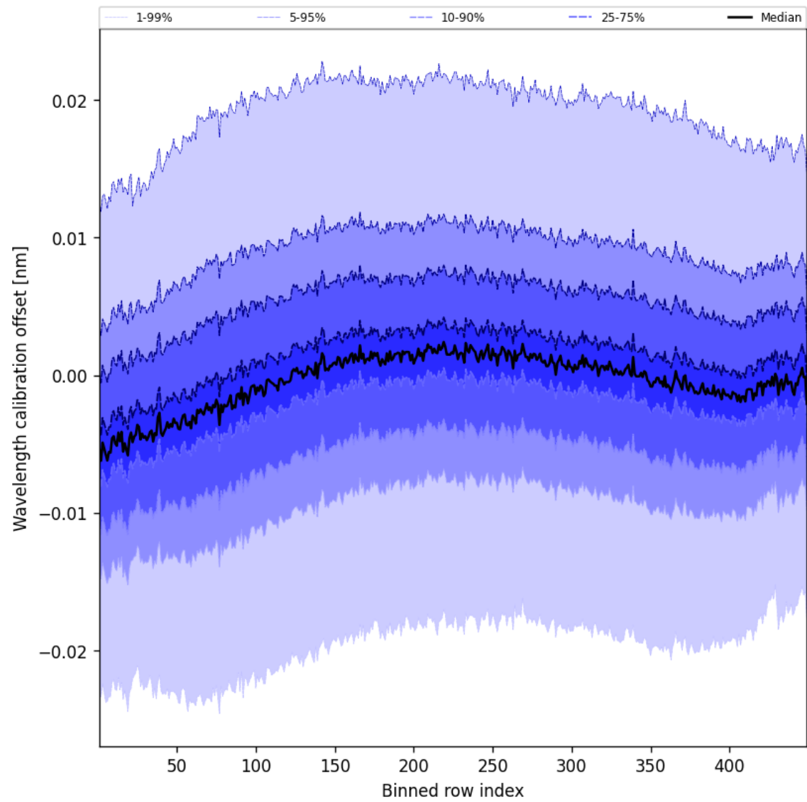
Figure 52: Along track statistics of “Wavelength calibration offset” for 2025-08-16 to 2025-08-18
