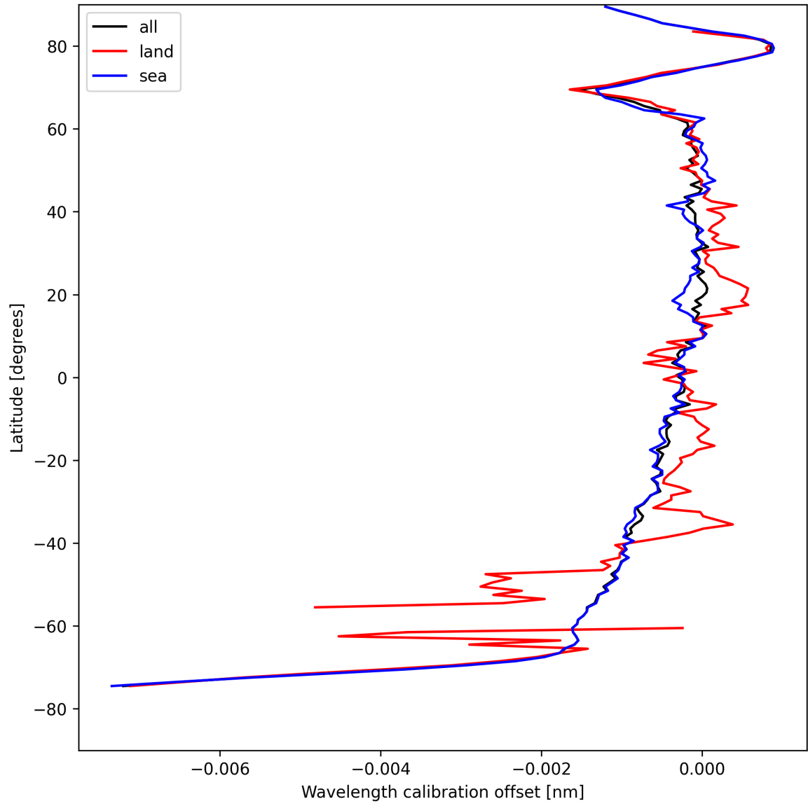
Figure 18: Zonal average of “Wavelength calibration offset” for 2025-08-16 to 2025-08-18.
