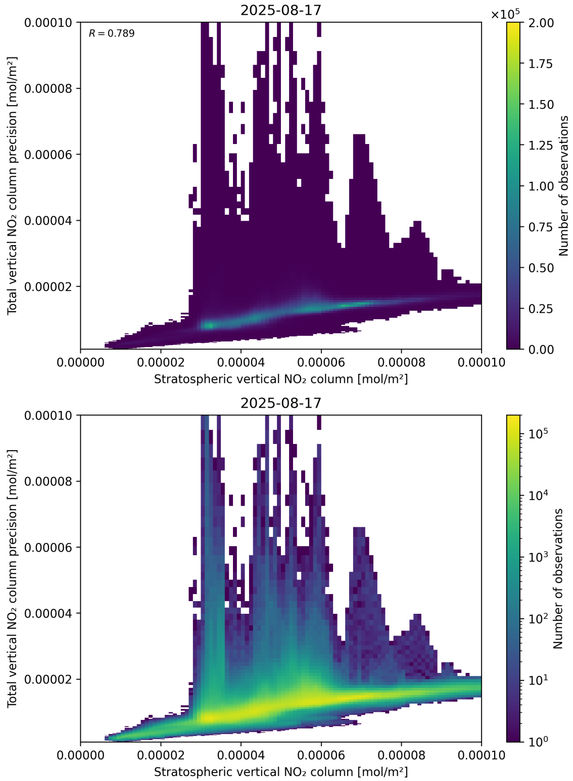
Figure 101: Scatter density plot of “Stratospheric vertical NO 2 column” against “Total vertical NO 2 column precision” for 2025-08-16 to 2025-08-18.
