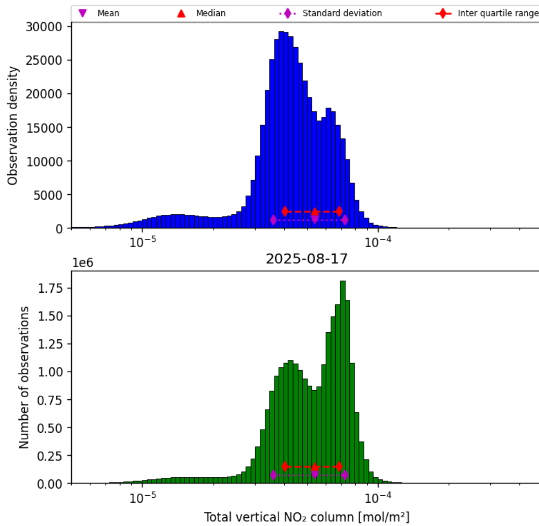
Figure 38: Histogram of “Total vertical NO 2 column” for 2025-08-16 to 2025-08-18
