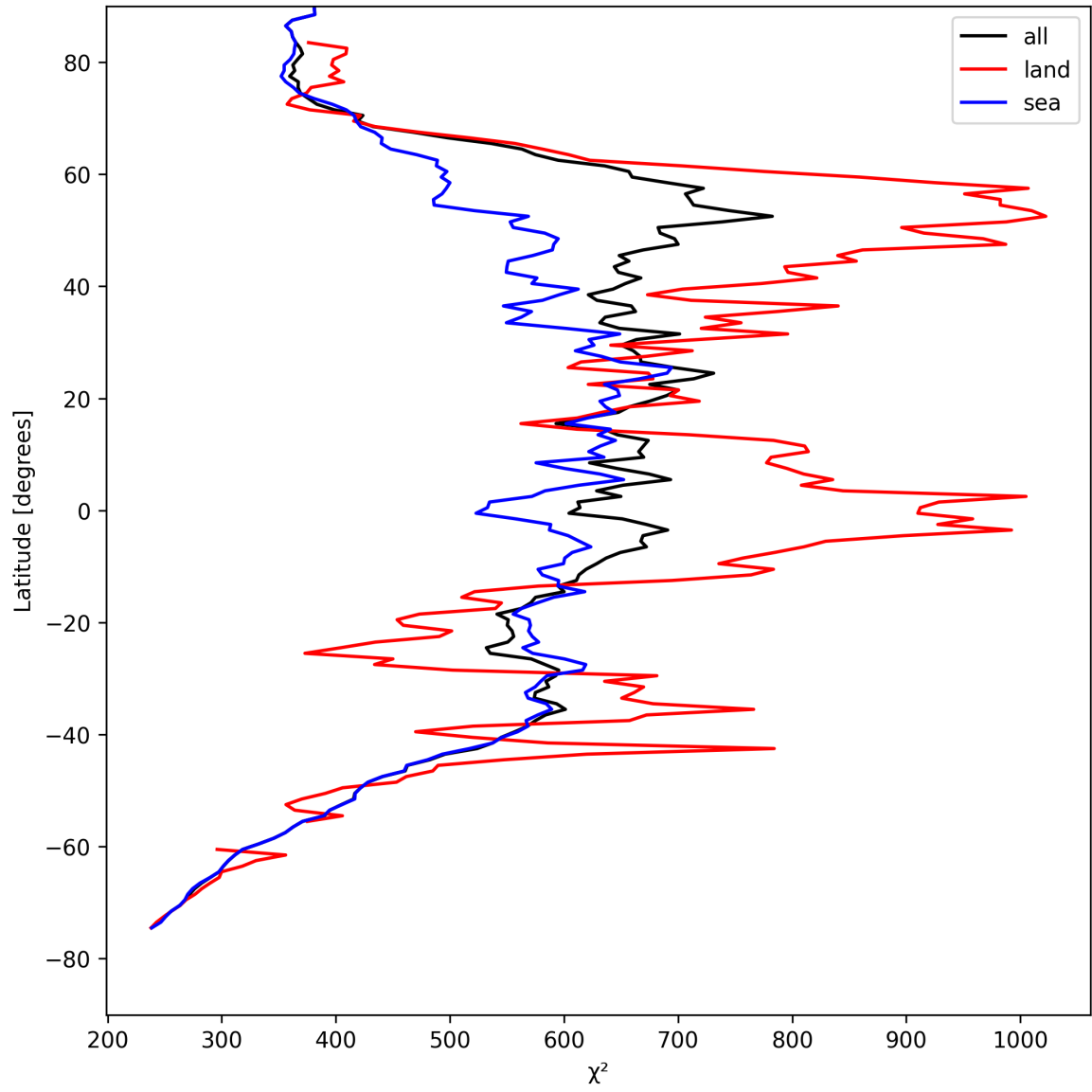
Figure 25: Zonal average of “ \chi^2 ” for 2025-08-16 to 2025-08-18.
