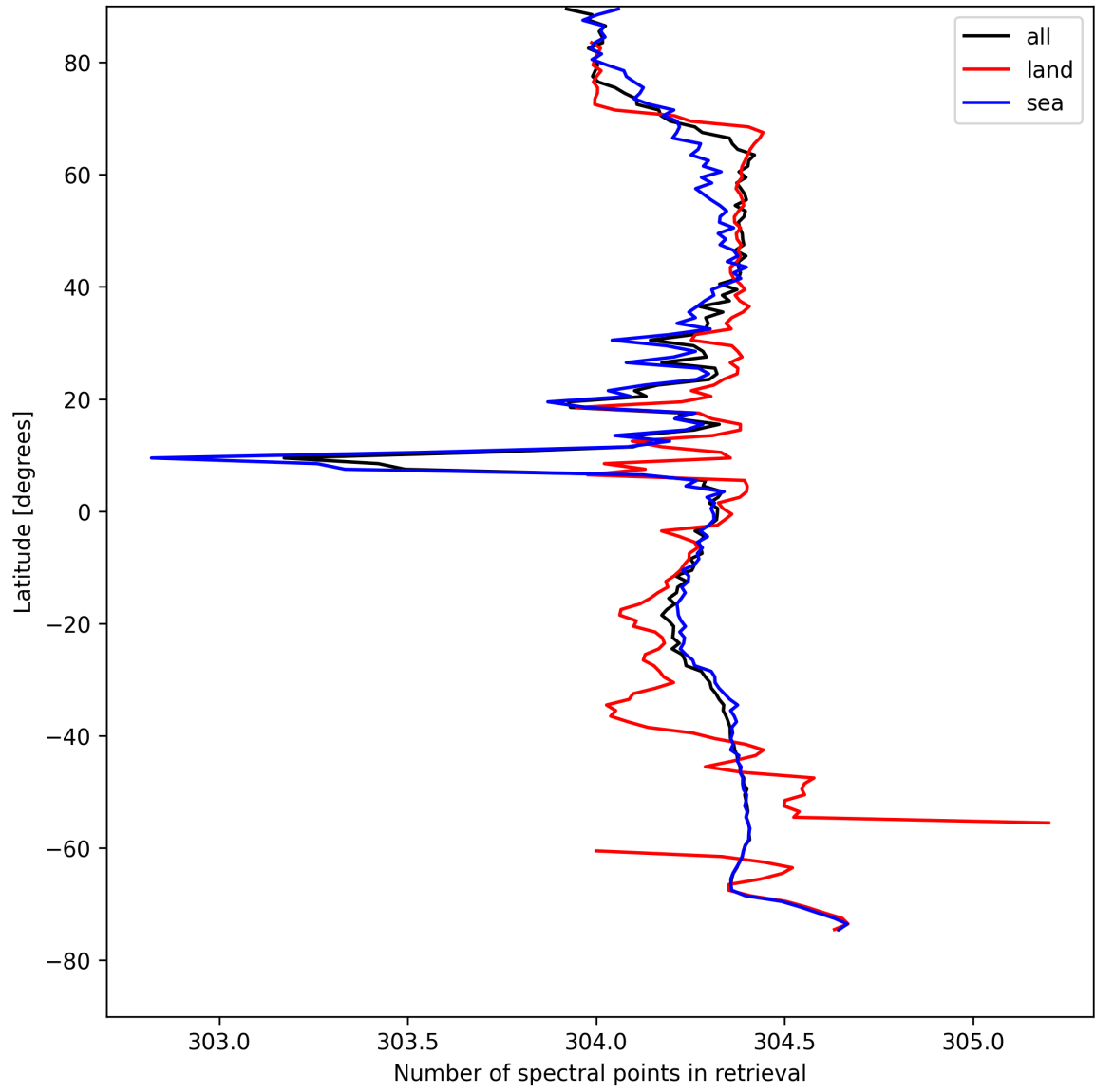
Figure 16: Zonal average of “Number of spectral points in retrieval” for 2025-08-16 to 2025-08-18.
