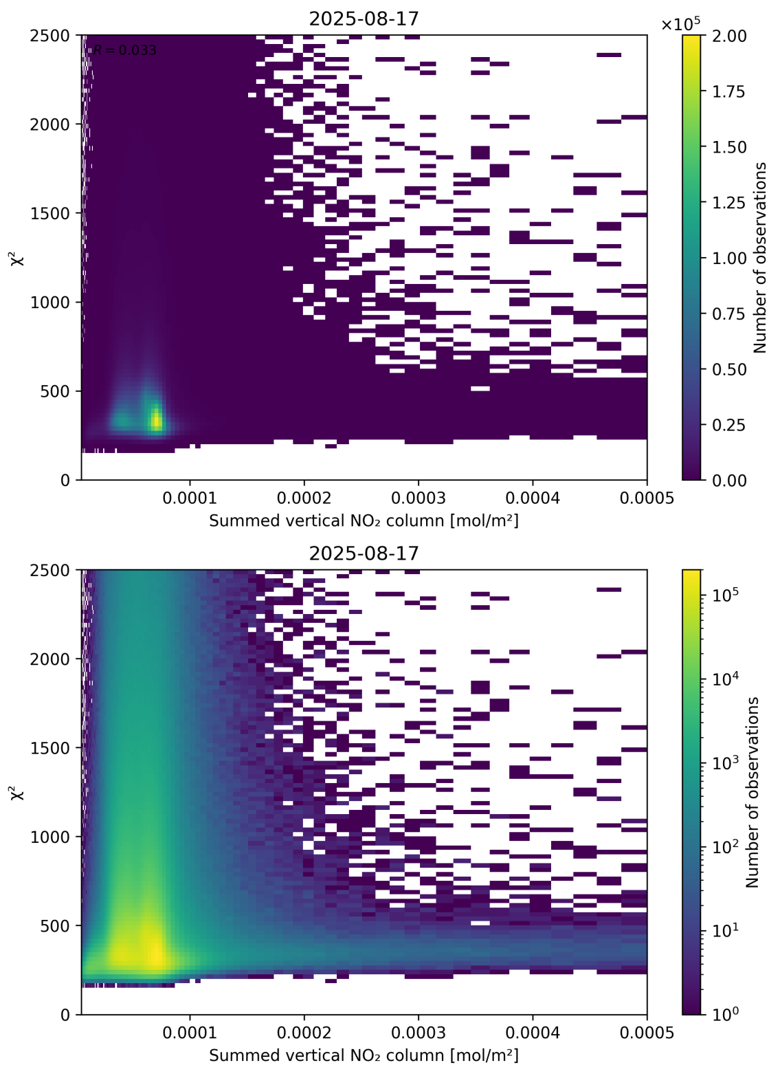
Figure 104: Scatter density plot of “Summed vertical NO 2 column” against “ \chi^2 ” for 2025-08-16 to 2025-08-18.
