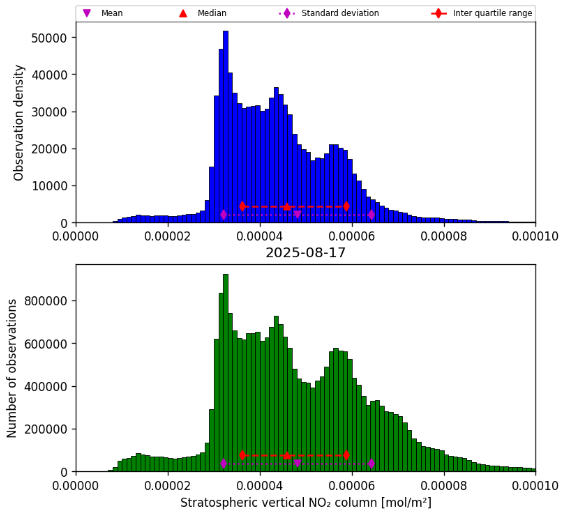
Figure 36: Histogram of “Stratospheric vertical NO 2 column” for 2025-08-16 to 2025-08-18
