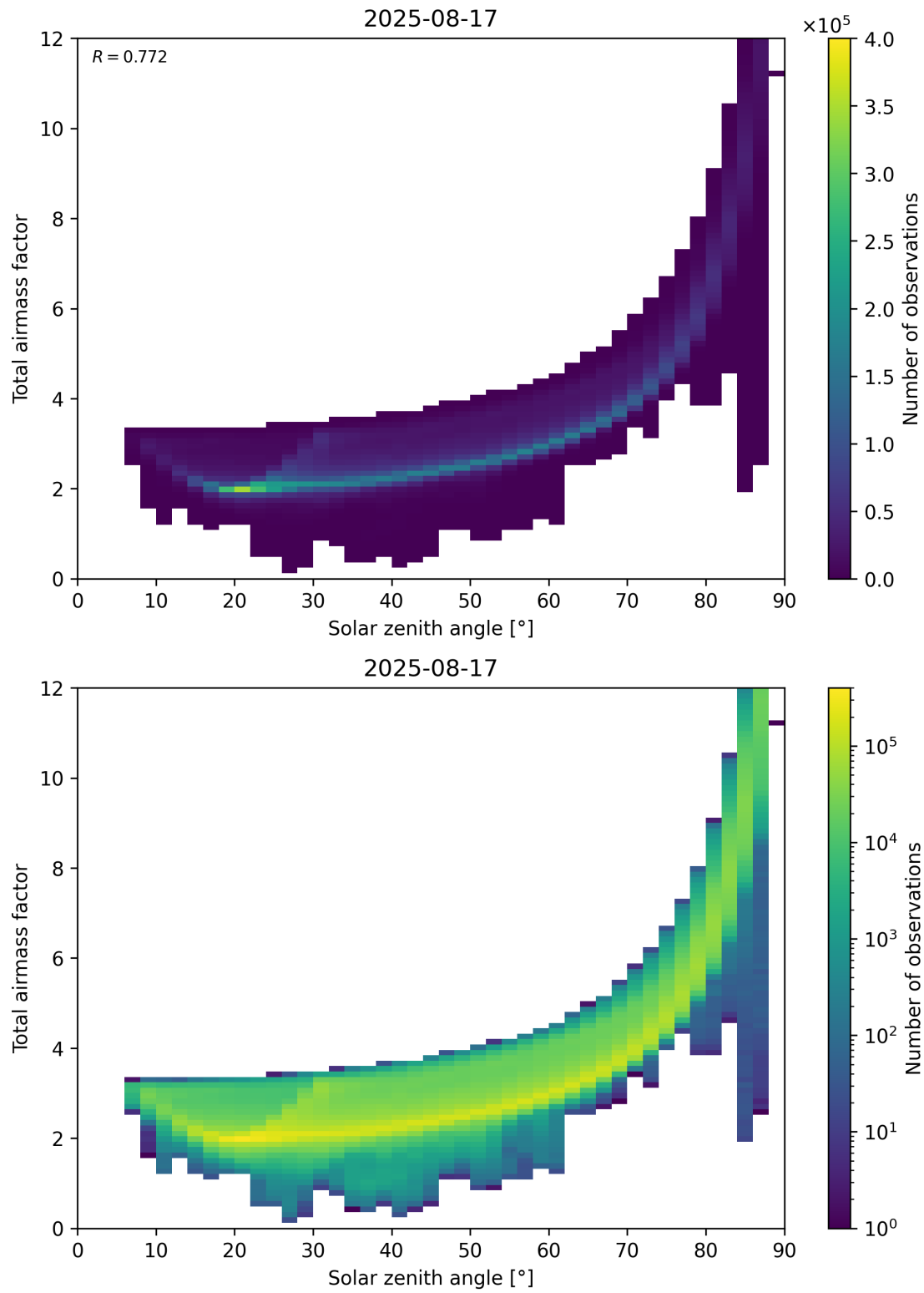
Figure 146: Scatter density plot of “Solar zenith angle” against “Total air mass factor” for 2025-08-16 to 2025-08-18.
