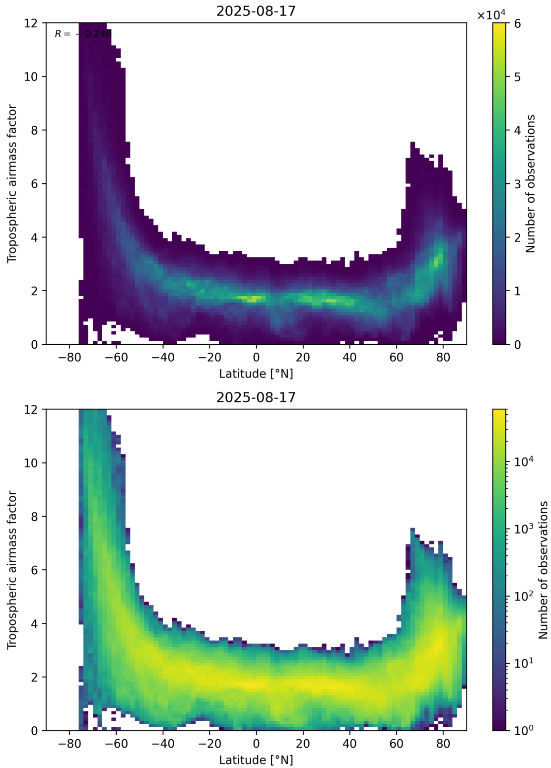
Figure 85: Scatter density plot of “Latitude” against “Tropospheric air mass factor” for 2025-08-16 to 2025-08-18.
