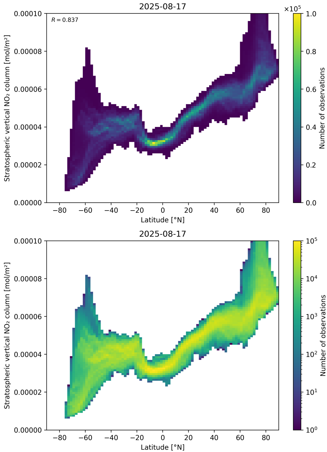
Figure 87: Scatter density plot of “Latitude” against “Stratospheric vertical \text{NO}_2 column” for 2025-08-16 to 2025-08-18.
