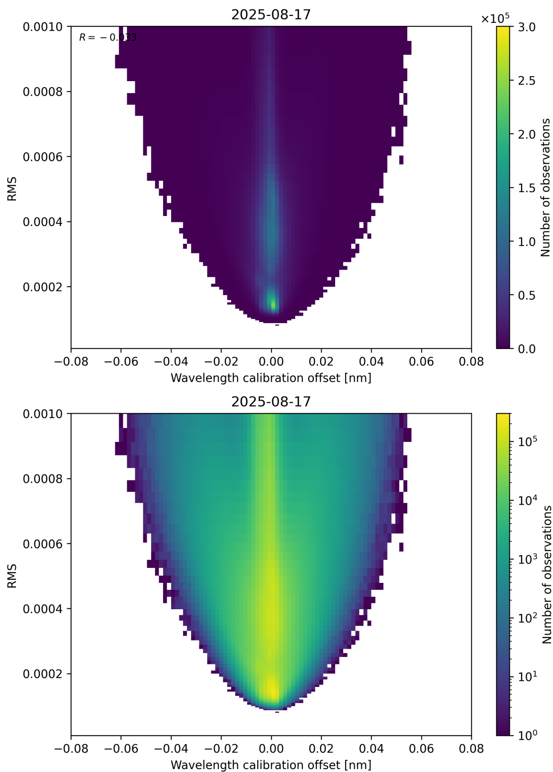
Figure 181: Scatter density plot of “Wavelength calibration offset” against “RMS” for 2025-08-16 to 2025-08-18.
