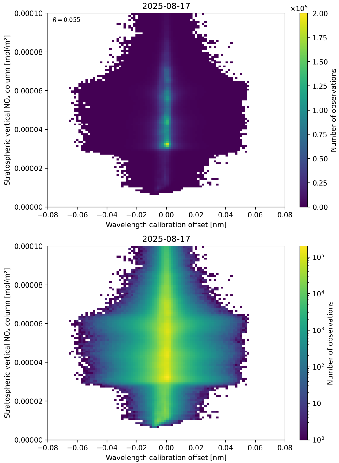
Figure 176: Scatter density plot of “Wavelength calibration offset” against “Stratospheric vertical NO 2 column” for 2025-08-16 to 2025-08-18.
