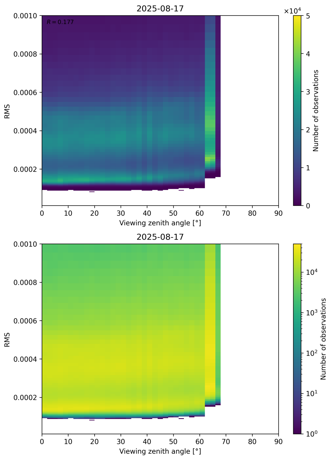
Figure 171: Scatter density plot of “Viewing zenith angle” against “RMS” for 2025-08-16 to 2025-08-18.
