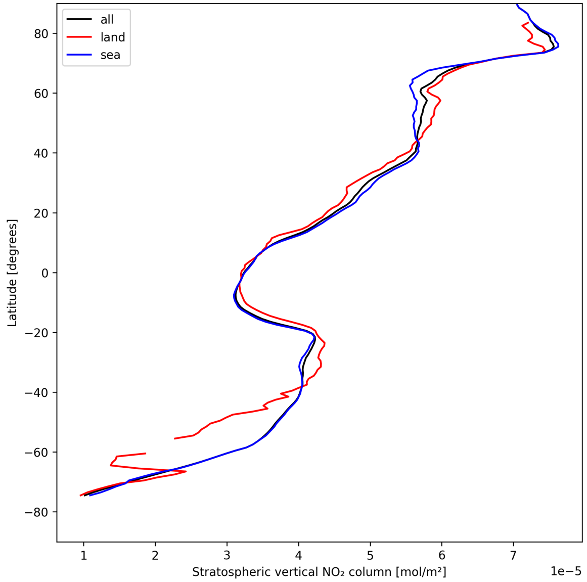
Figure 19: Zonal average of “Stratospheric vertical NO 2 column” for 2025-08-16 to 2025-08-18.
