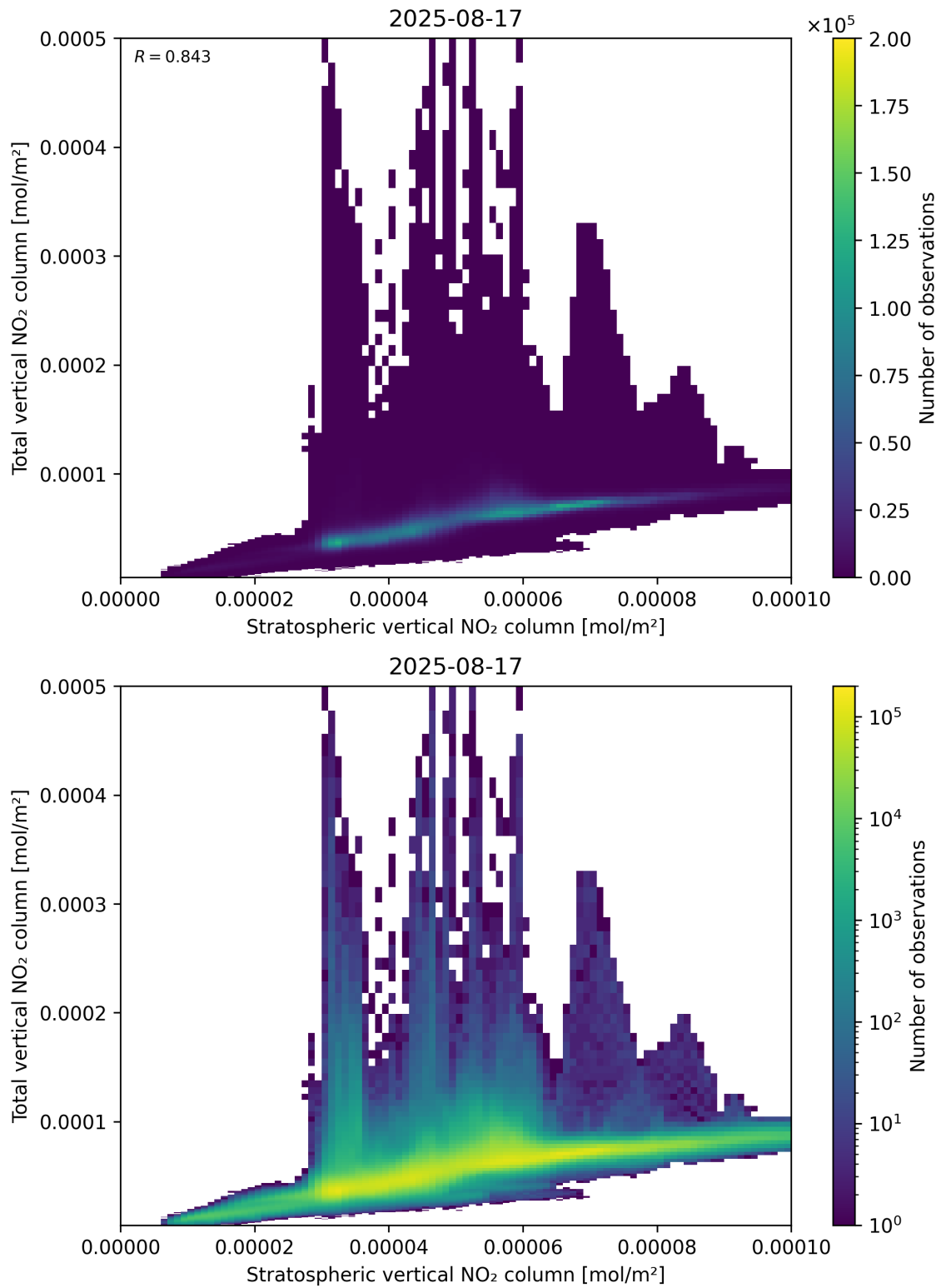
Figure 100: Scatter density plot of “Stratospheric vertical NO 2 column” against “Total vertical NO 2 column” for 2025-08-16 to 2025-08-18.
