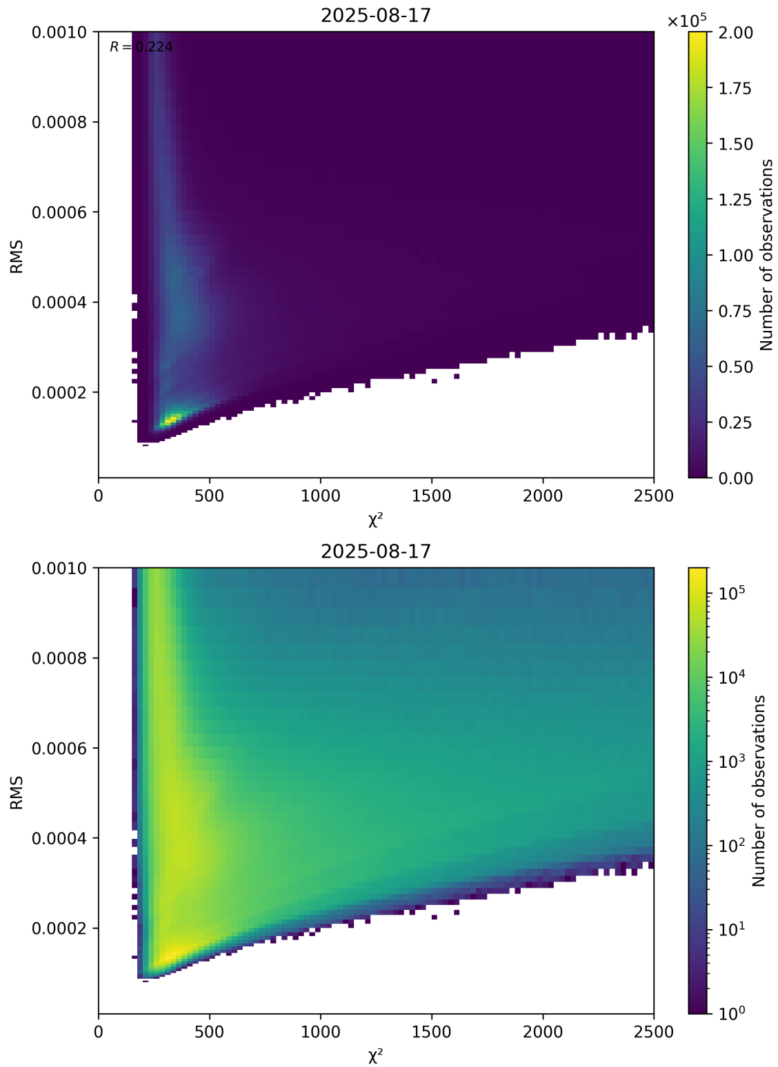
Figure 82: Scatter density plot of “ \chi^2 ” against “RMS” for 2025-08-16 to 2025-08-18.
