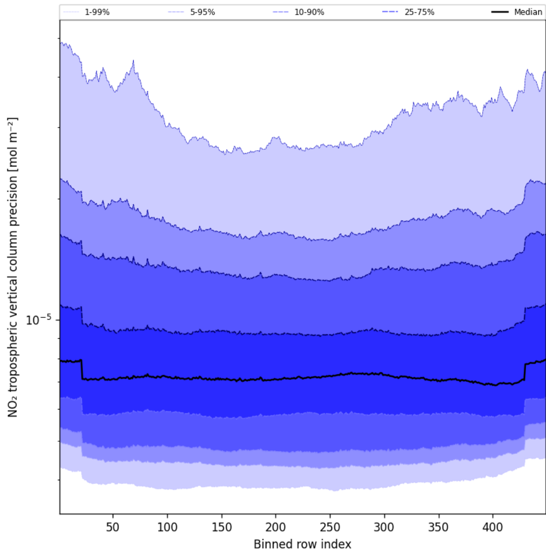
Figure 47: Along track statistics of “NO 2 tropospheric vertical column precision” for 2025-08-16 to 2025-08-18
