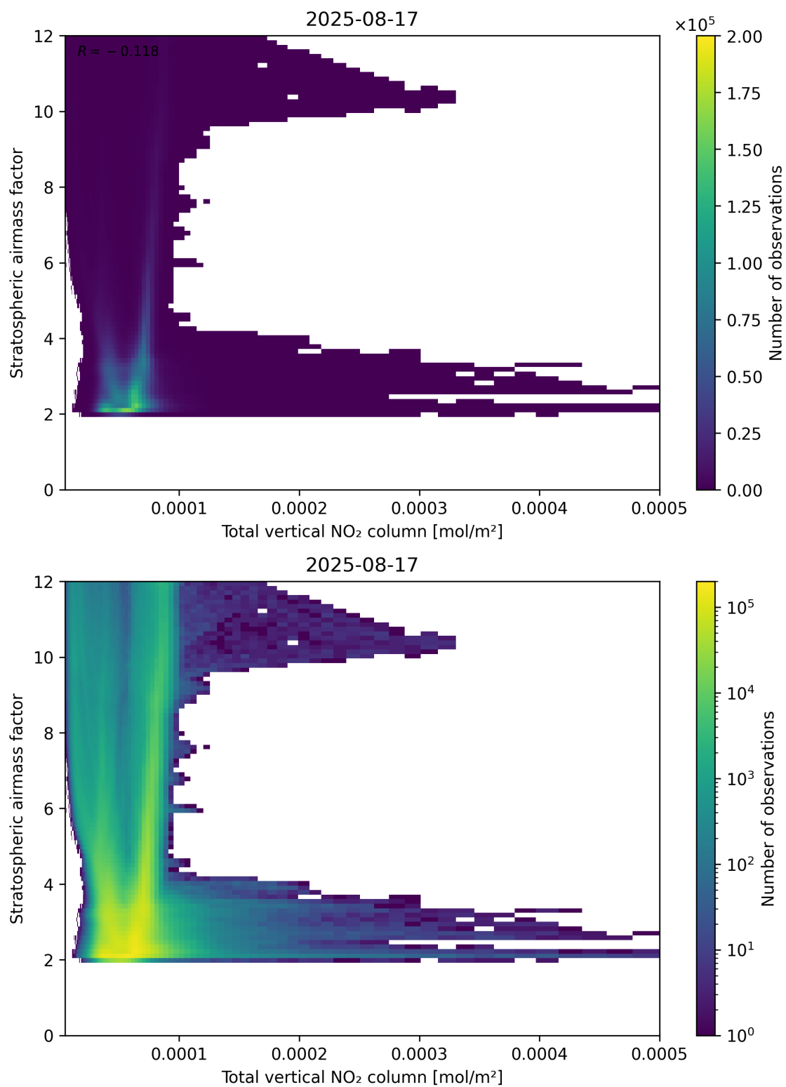
Figure 110: Scatter density plot of “Total vertical NO 2 column” against “Stratospheric airmass factor” for 2025-08-16 to 2025-08-18.
