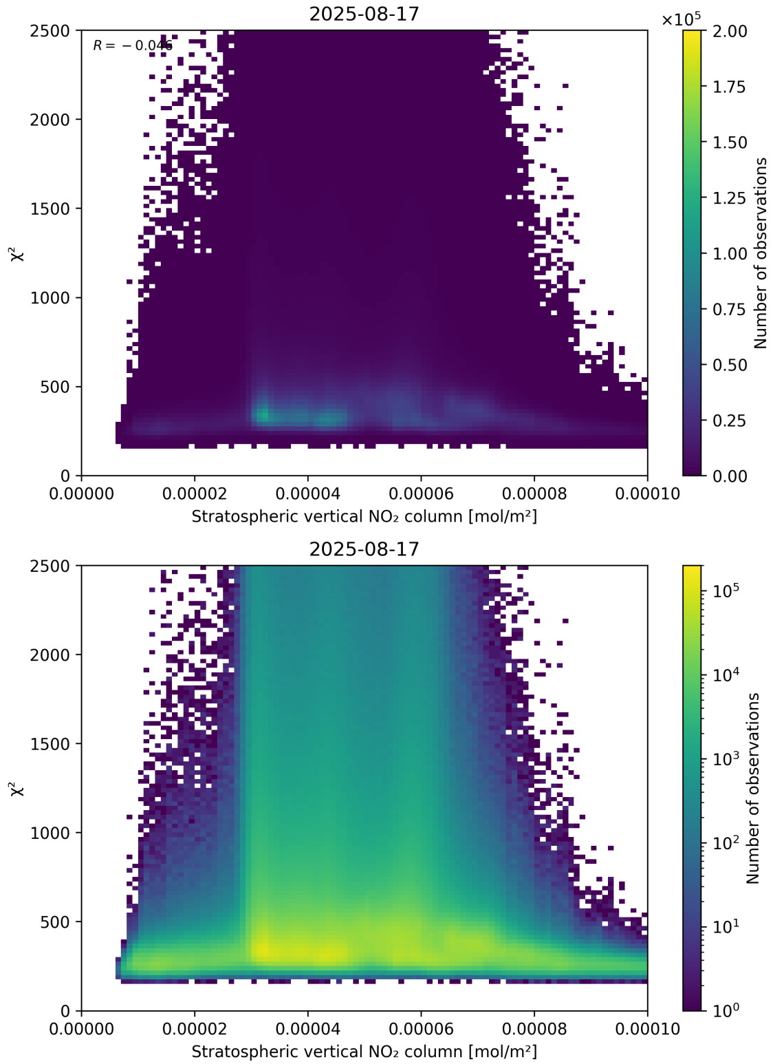
Figure 97: Scatter density plot of “Stratospheric vertical NO 2 column” against “ \chi^2 ” for 2025-08-16 to 2025-08-18.
