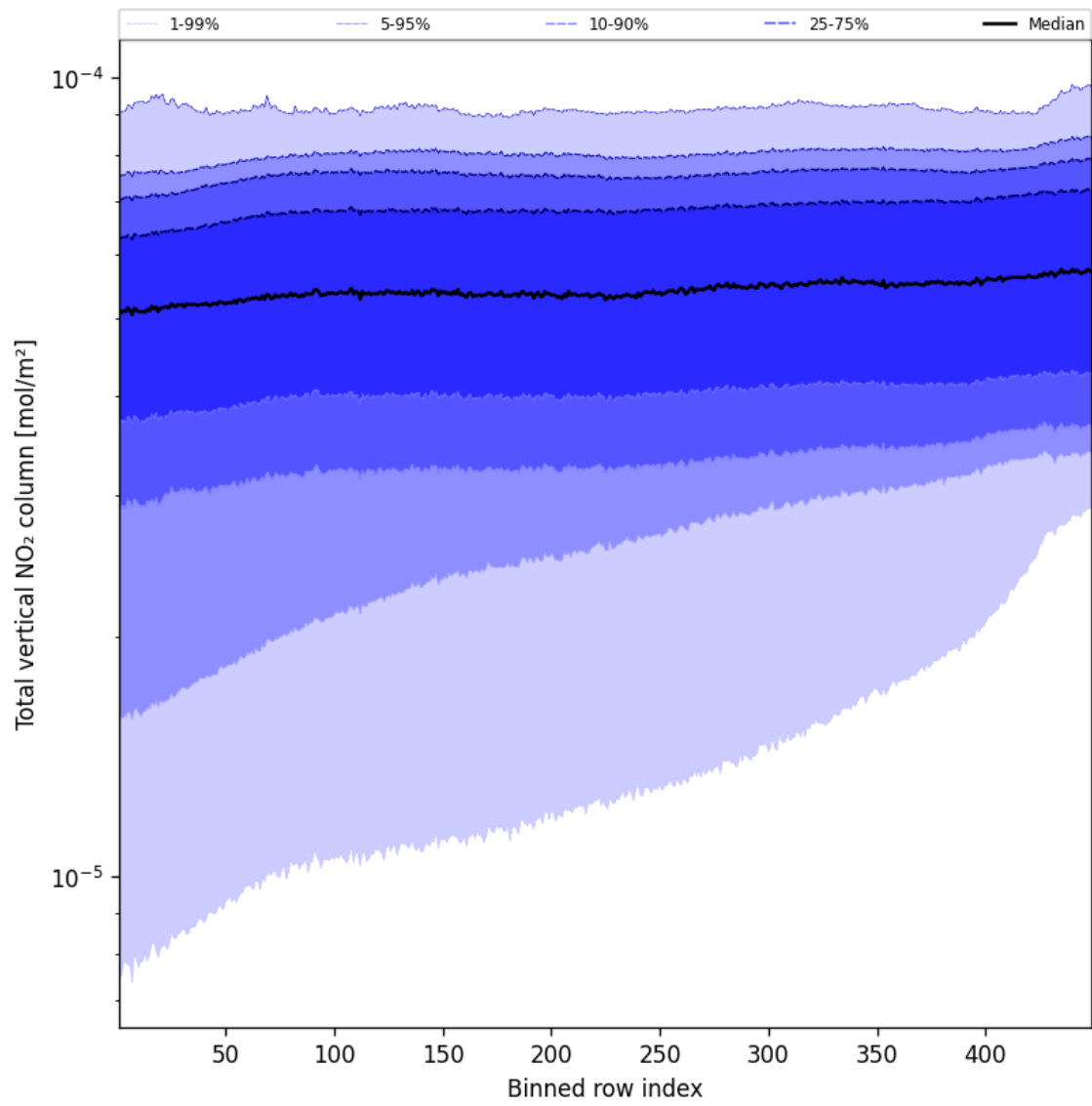
Figure 55: Along track statistics of “Total vertical NO 2 column” for 2025-08-16 to 2025-08-18
