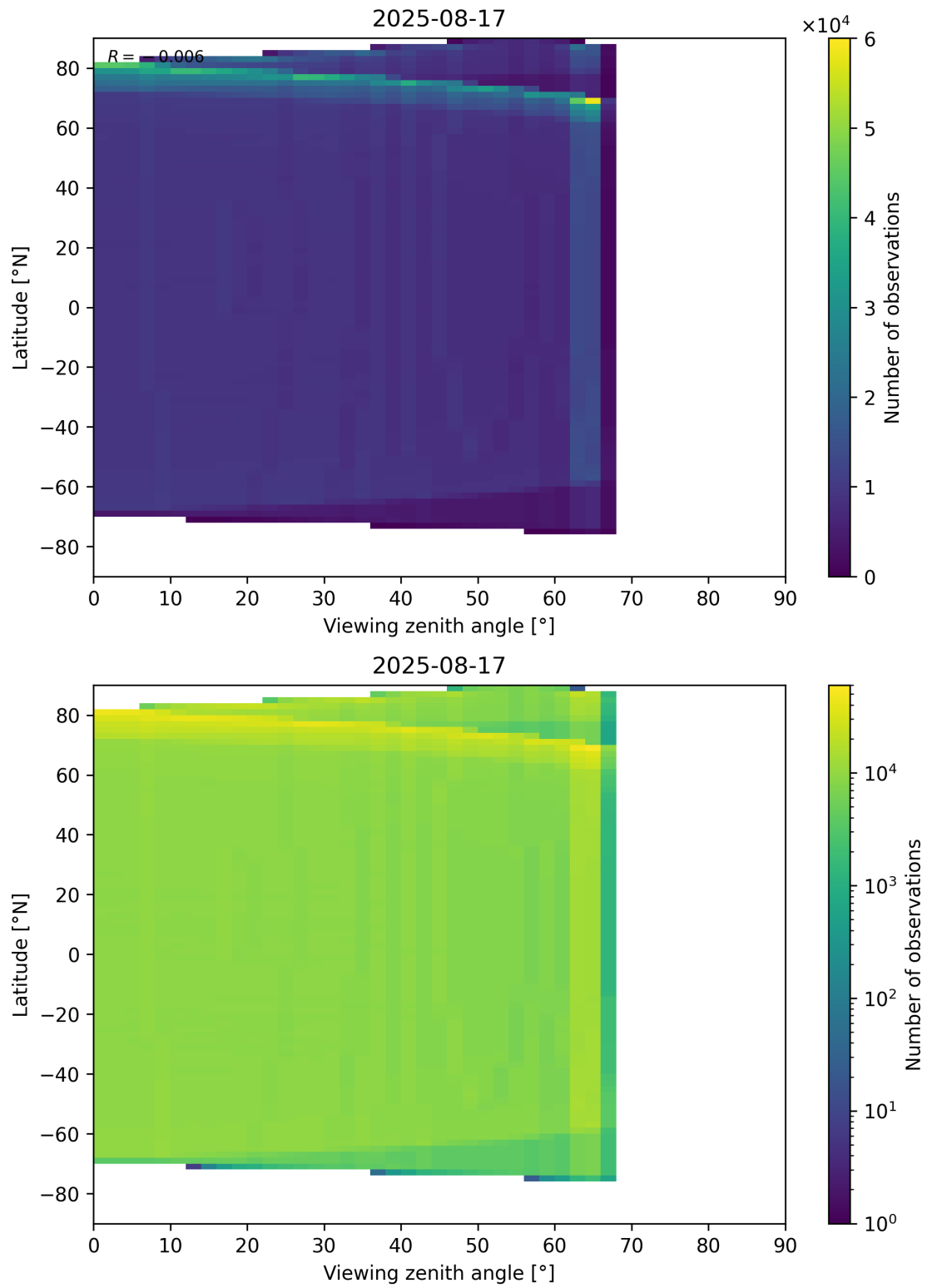
Figure 163: Scatter density plot of “Viewing zenith angle” against “Latitude” for 2025-08-16 to 2025-08-18.
