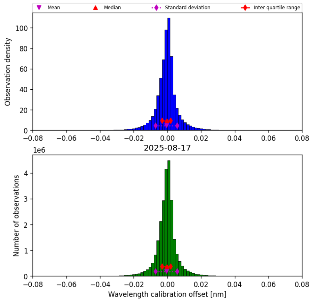
Figure 35: Histogram of “Wavelength calibration offset” for 2025-08-16 to 2025-08-18
