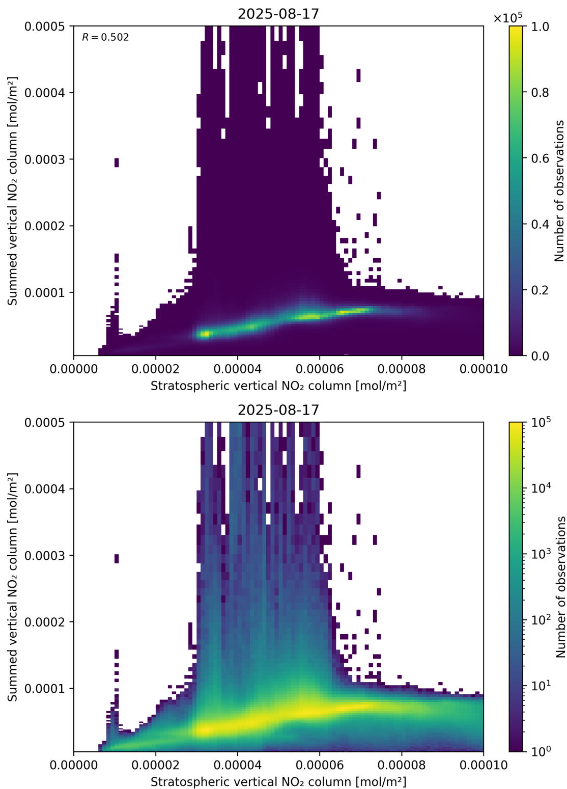
Figure 98: Scatter density plot of “Stratospheric vertical NO 2 column” against “Summed vertical NO 2 column” for 2025-08-16 to 2025-08-18.
