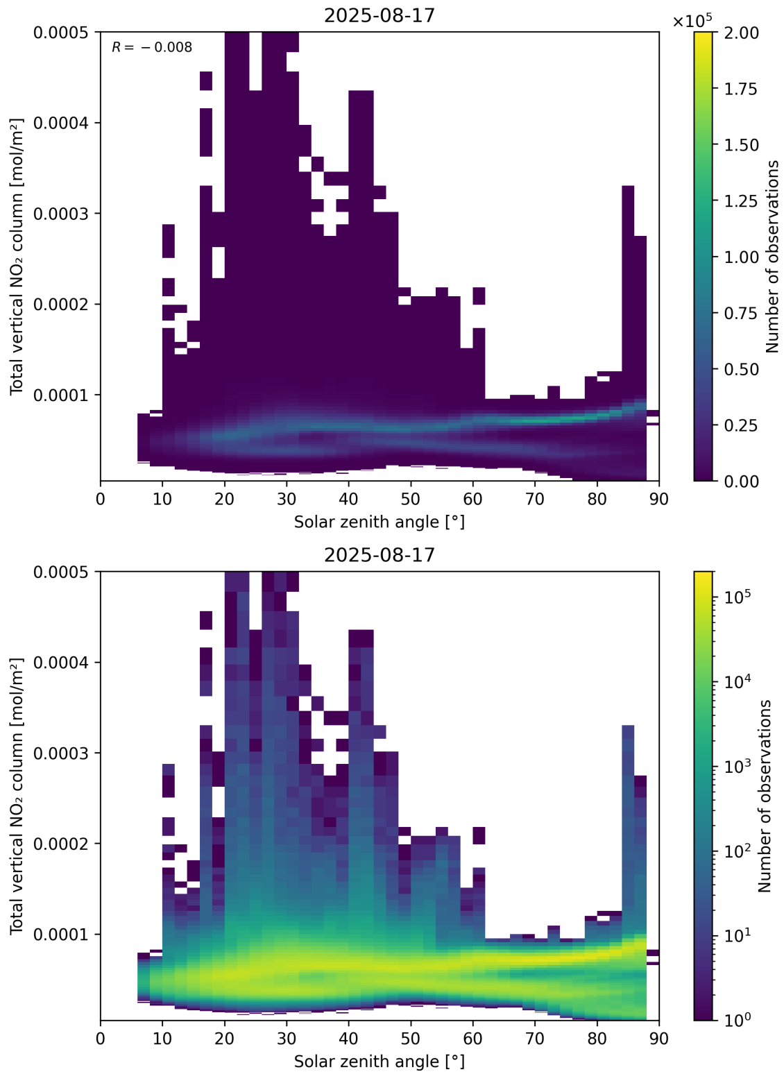
Figure 153: Scatter density plot of “Solar zenith angle” against “Total vertical NO 2 column” for 2025-08-16 to 2025-08-18.
