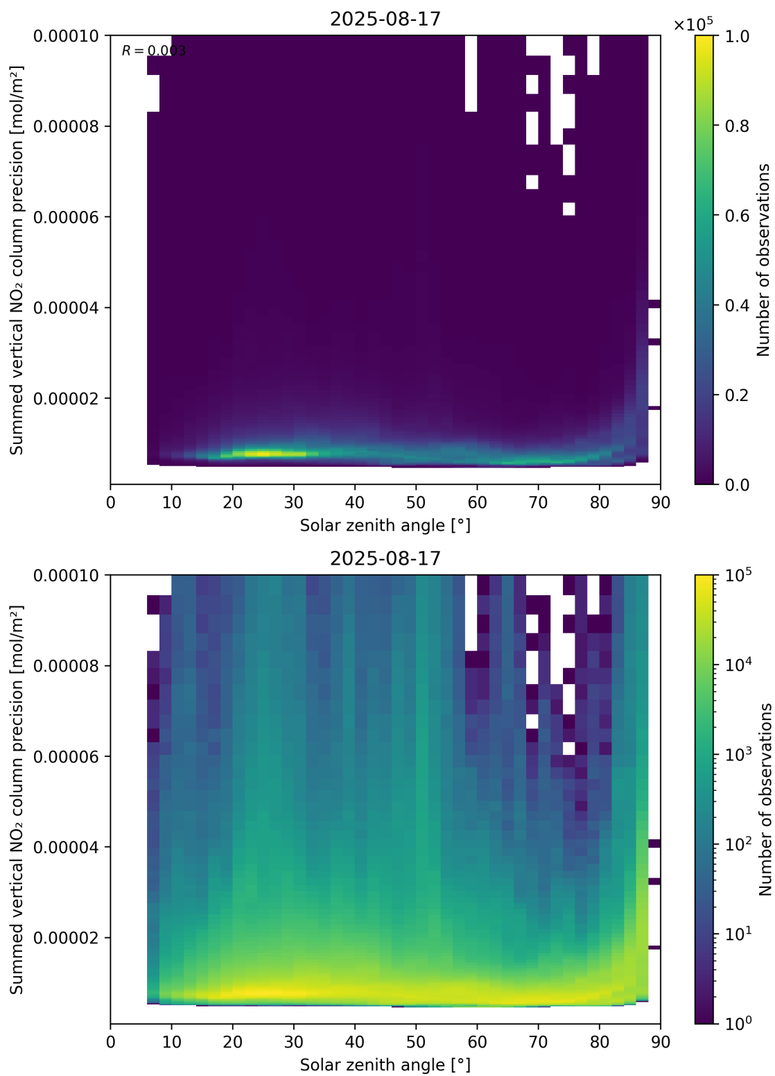
Figure 152: Scatter density plot of “Solar zenith angle” against “Summed vertical NO 2 column precision” for 2025-08-16 to 2025-08-18.
