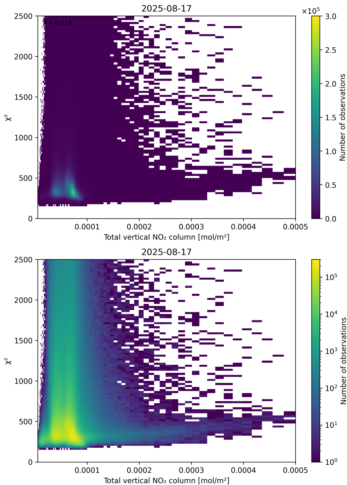
Figure 111: Scatter density plot of “Total vertical NO 2 column” against “ \chi^2 ” for 2025-08-16 to 2025-08-18.
