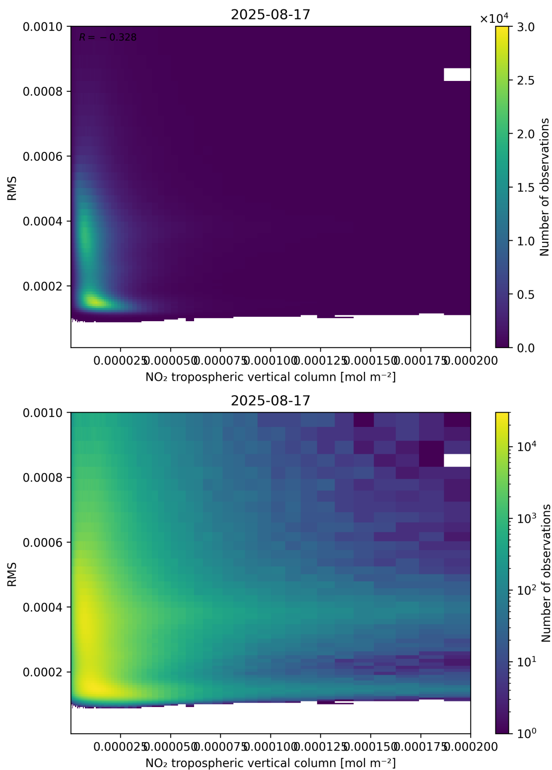
Figure 142: Scatter density plot of “NO 2 tropospheric vertical column” against “RMS” for 2025-08-16 to 2025-08-18.
