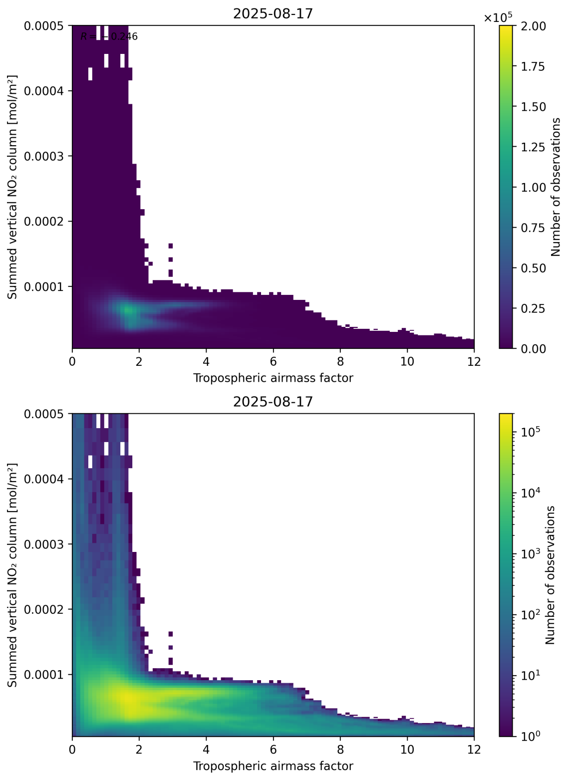
Figure 75: Scatter density plot of “Tropospheric air mass factor” against “Summed vertical NO 2 column” for 2025-08-16 to 2025-08-18.
