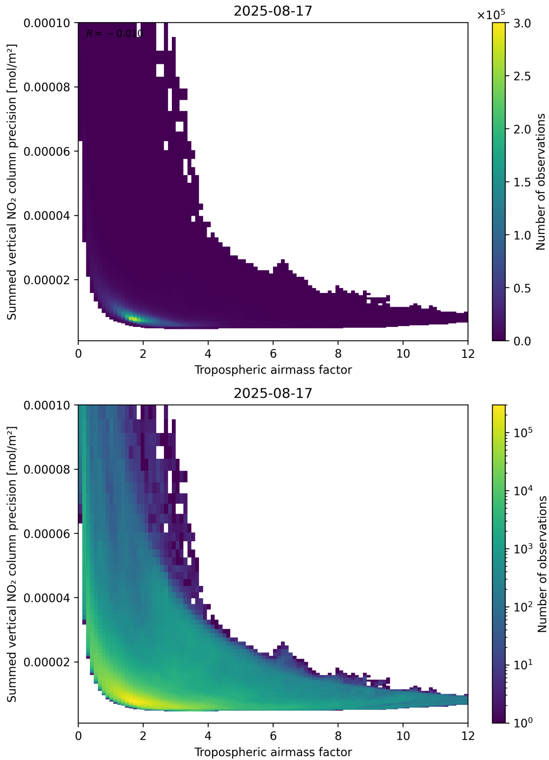
Figure 76: Scatter density plot of “Tropospheric air mass factor” against “Summed vertical NO 2 column precision” for 2025-08-16 to 2025-08-18.
