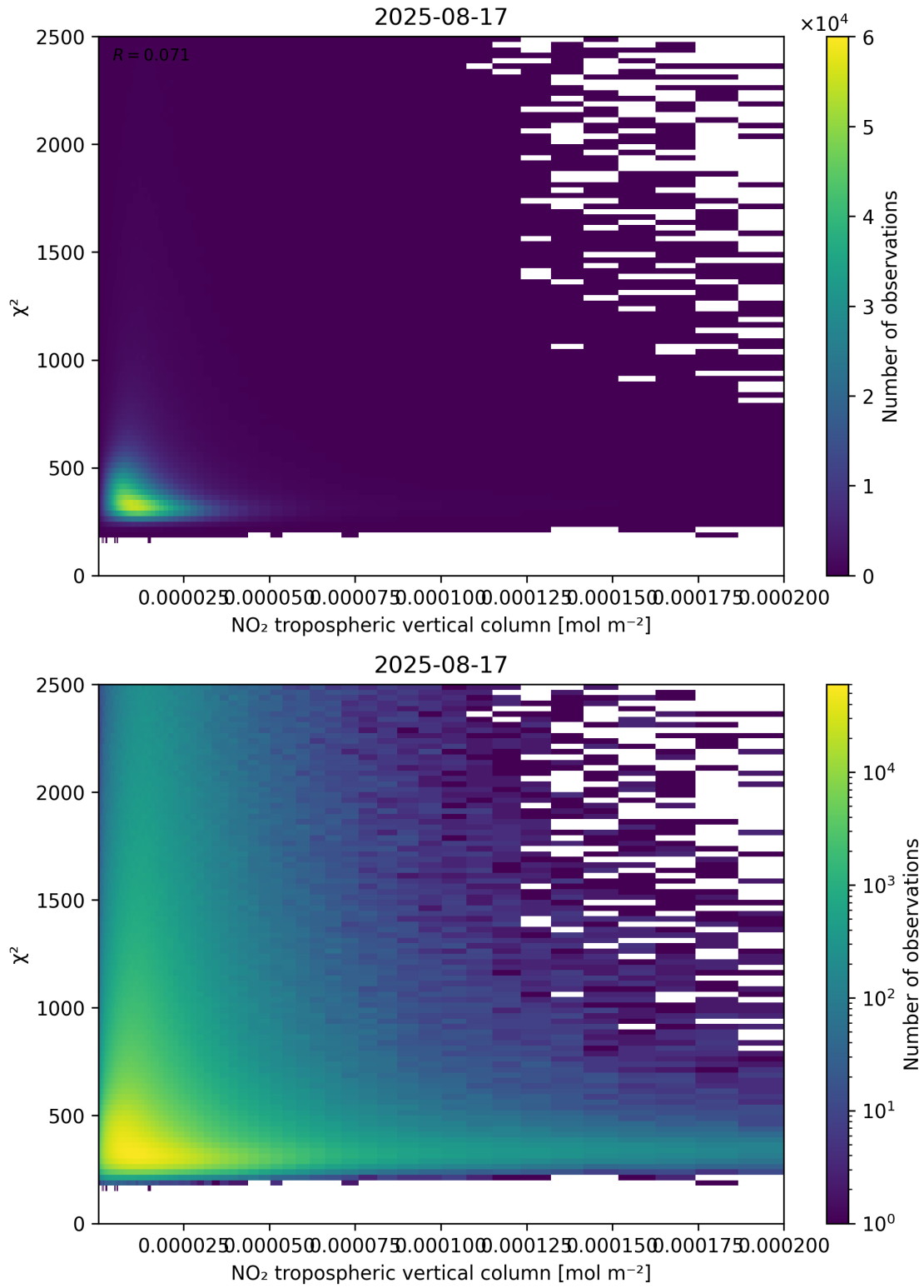
Figure 124: Scatter density plot of “NO 2 tropospheric vertical column” against “ \chi^2 ” for 2025-08-16 to 2025-08-18.
