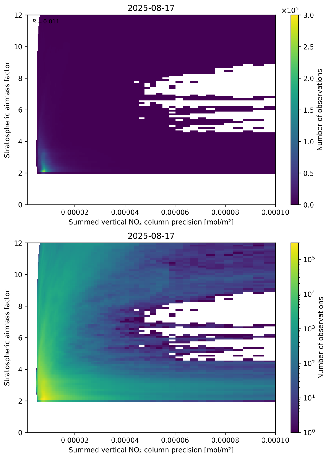
Figure 106: Scatter density plot of “Summed vertical NO 2 column precision” against “Stratospheric airmass factor” for 2025-08-16 to 2025-08-18.
