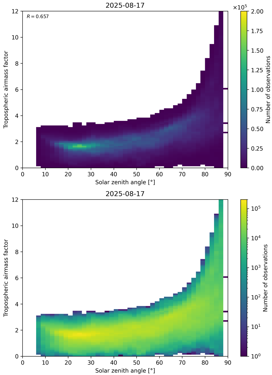
Figure 147: Scatter density plot of “Solar zenith angle” against “Tropospheric airmass factor” for 2025-08-16 to 2025-08-18.
