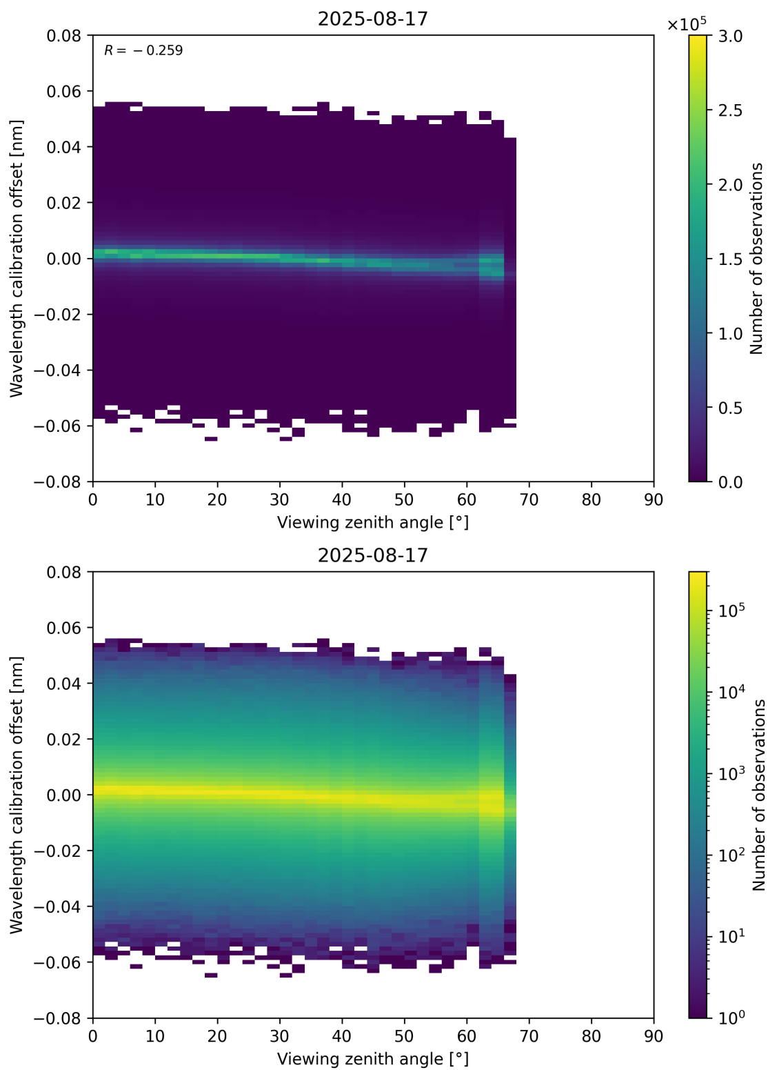
Figure 173: Scatter density plot of “Viewing zenith angle” against “Wavelength calibration offset” for 2025-08-16 to 2025-08-18.
