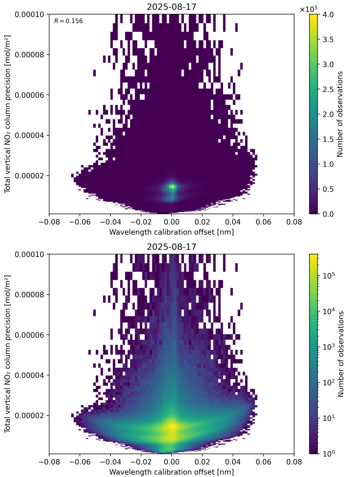
Figure 180: Scatter density plot of “Wavelength calibration offset” against “Total vertical NO 2 column precision” for 2025-08-16 to 2025-08-18.
