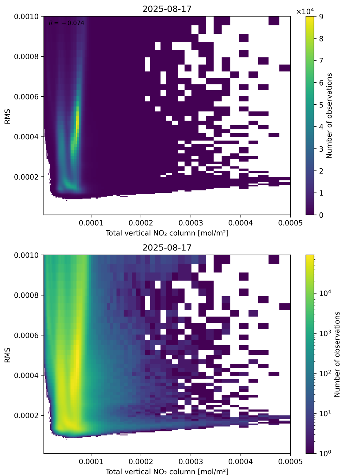
Figure 120: Scatter density plot of “Total vertical NO 2 column” against “RMS” for 2025-08-16 to 2025-08-18.
