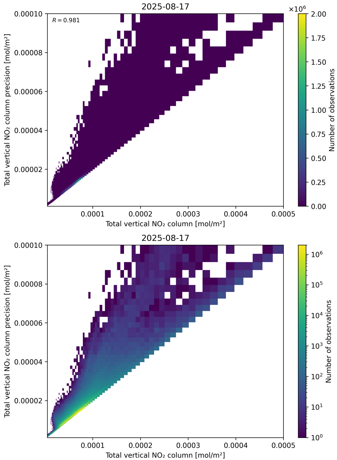
Figure 114: Scatter density plot of “Total vertical NO 2 column” against “Total vertical NO 2 column precision” for 2025-08-16 to 2025-08-18.
