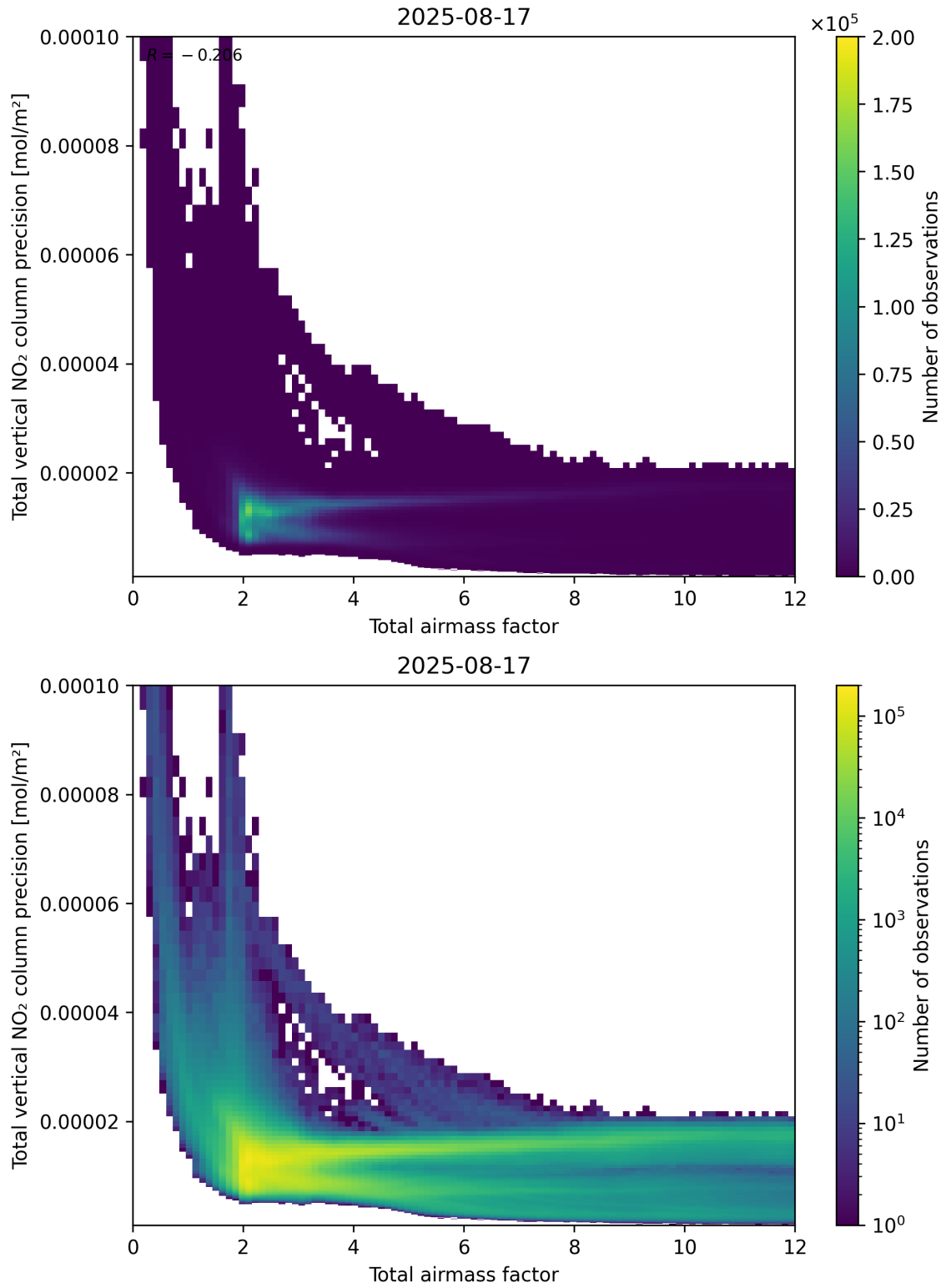
Figure 68: Scatter density plot of “Total airmass factor” against “Total vertical NO 2 column precision” for 2025-08-16 to 2025-08-18.
