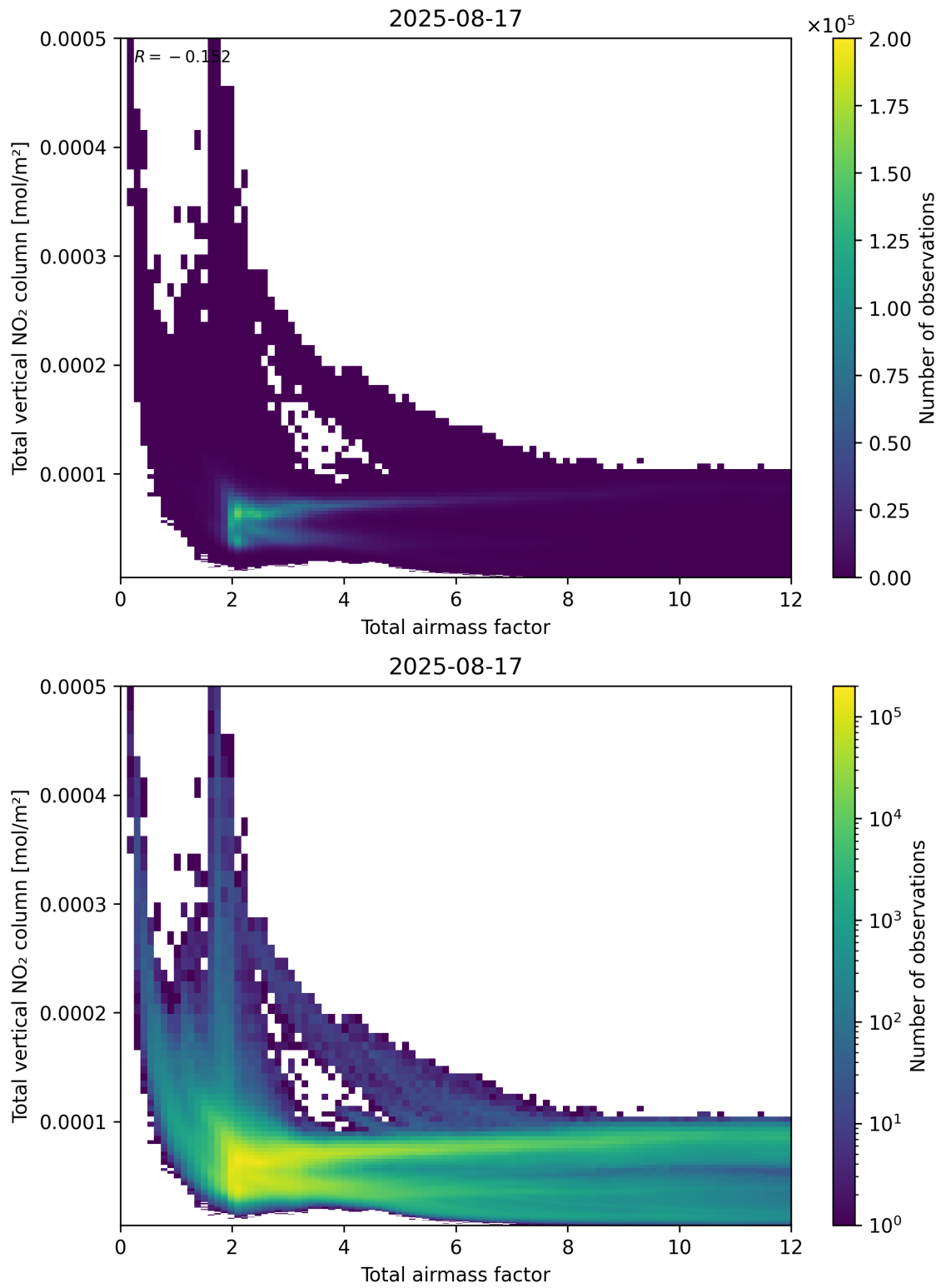
Figure 67: Scatter density plot of “Total airmass factor” against “Total vertical NO 2 column” for 2025-08-16 to 2025-08-18.
