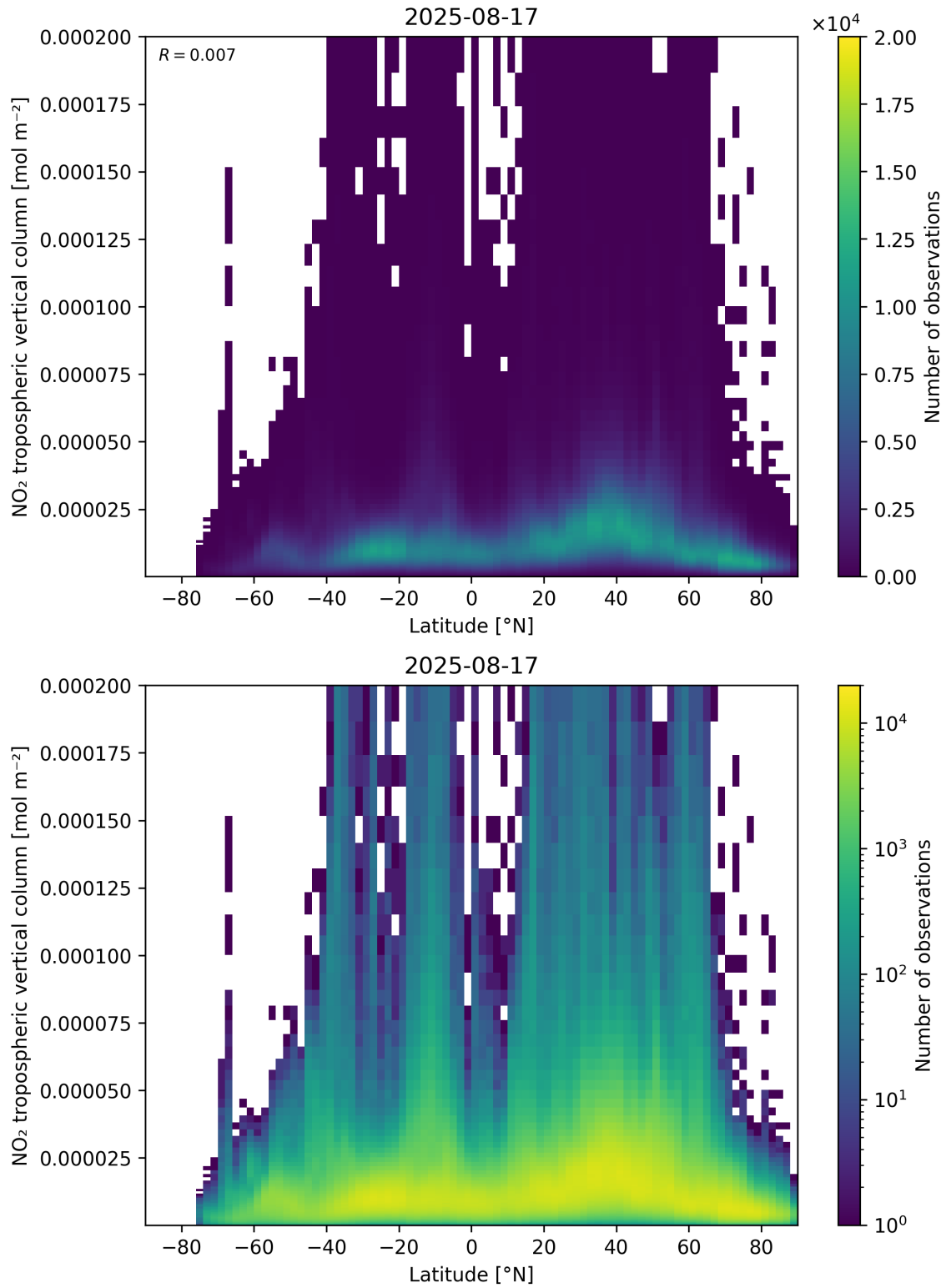
Figure 92: Scatter density plot of “Latitude” against “NO 2 tropospheric vertical column” for 2025-08-16 to 2025-08-18.
