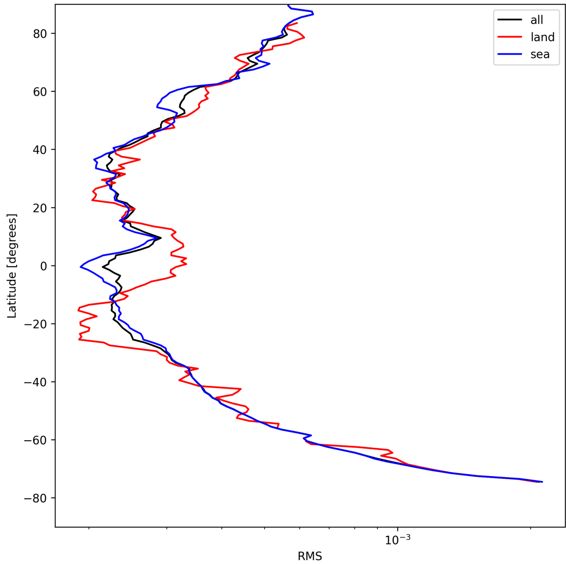
Figure 26: Zonal average of “RMS” for 2025-08-16 to 2025-08-18.
