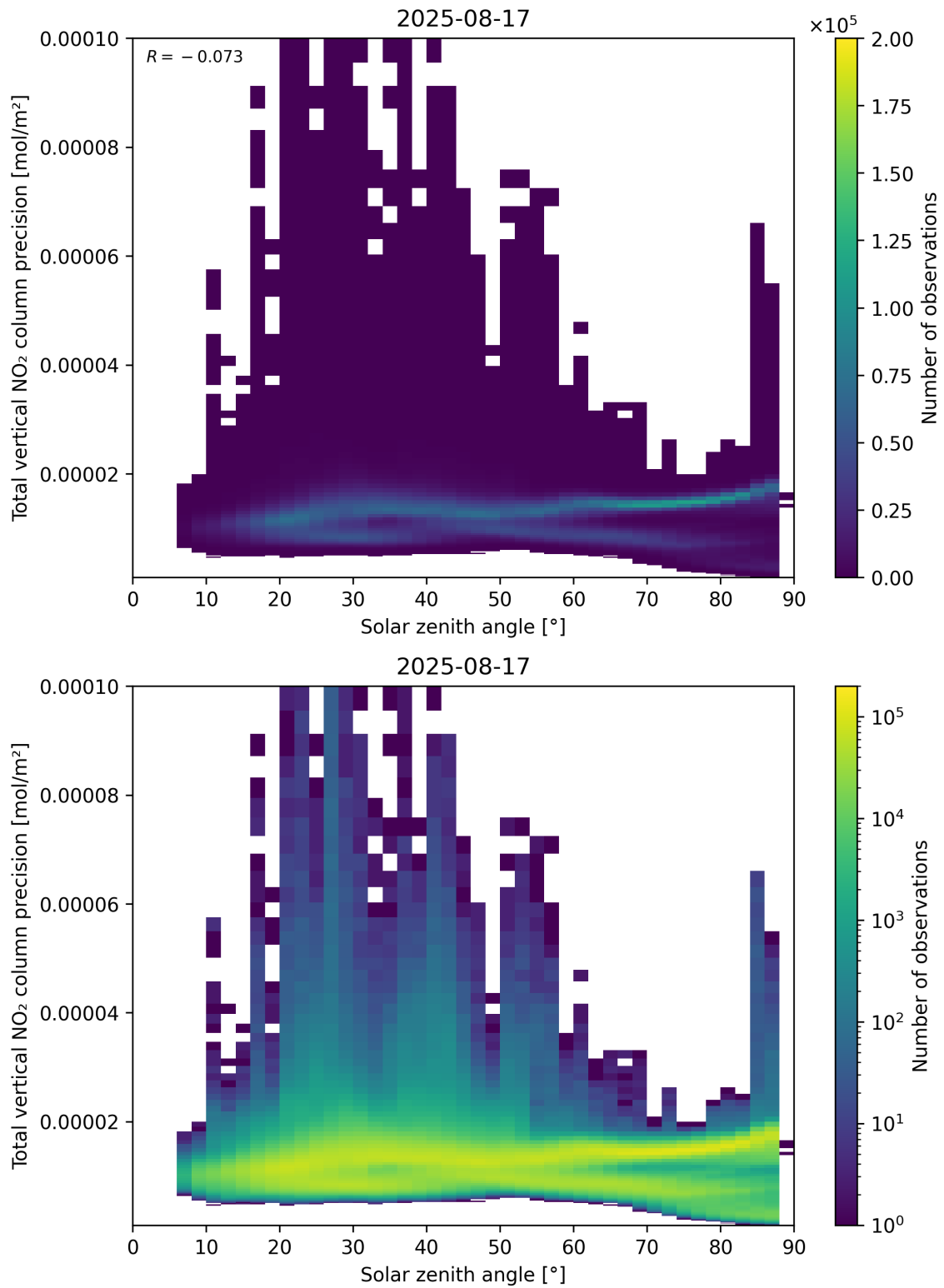
Figure 154: Scatter density plot of “Solar zenith angle” against “Total vertical NO 2 column precision” for 2025-08-16 to 2025-08-18.
