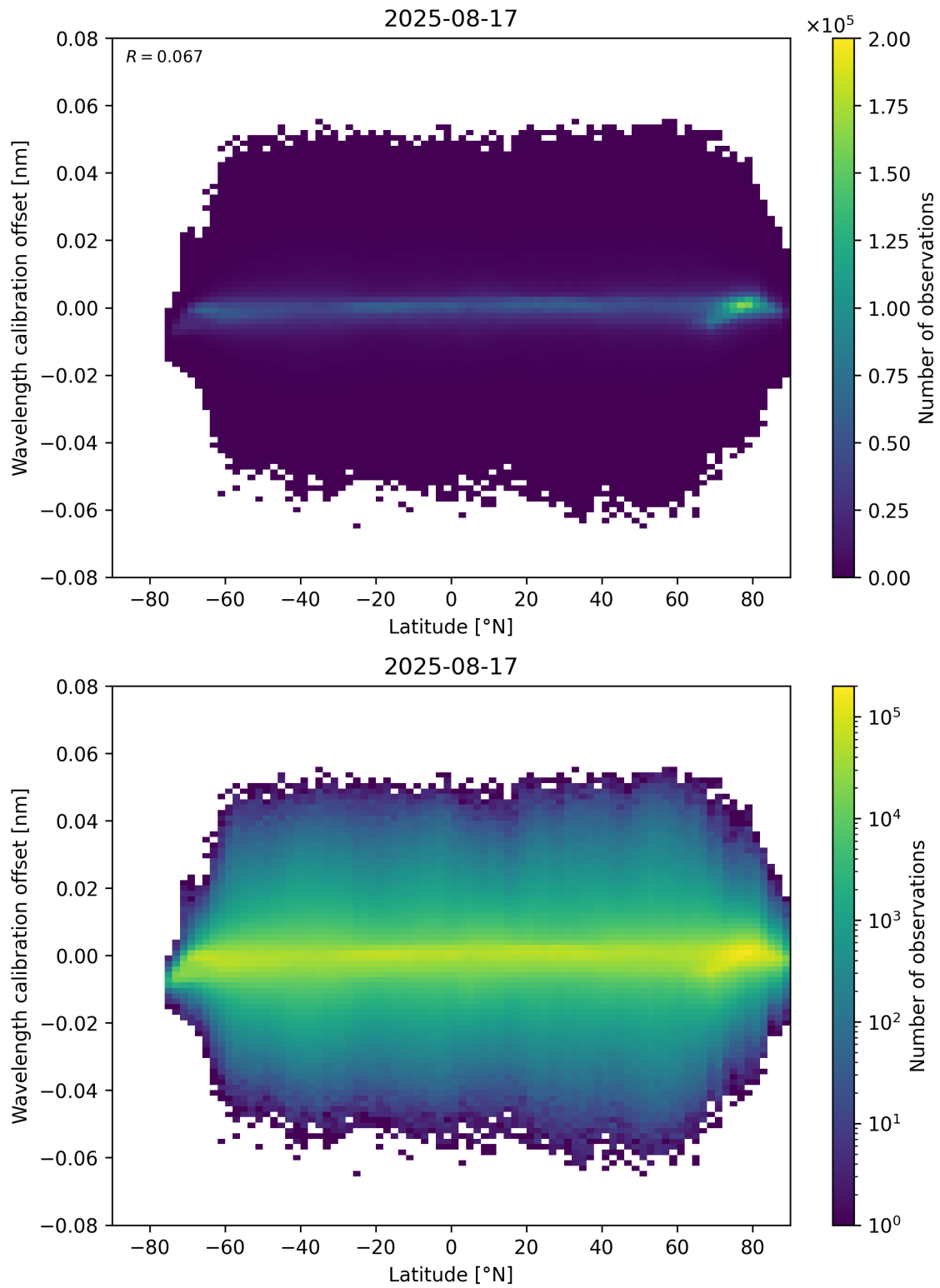
Figure 95: Scatter density plot of “Latitude” against “Wavelength calibration offset” for 2025-08-16 to 2025-08-18.
