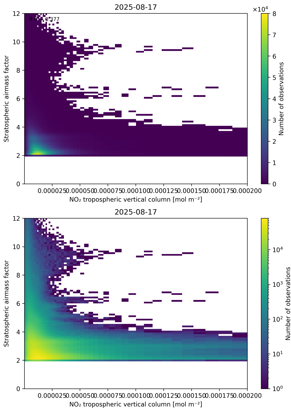
Figure 121: Scatter density plot of “NO 2 tropospheric vertical column” against “Stratospheric air mass factor” for 2025-08-16 to 2025-08-18.
