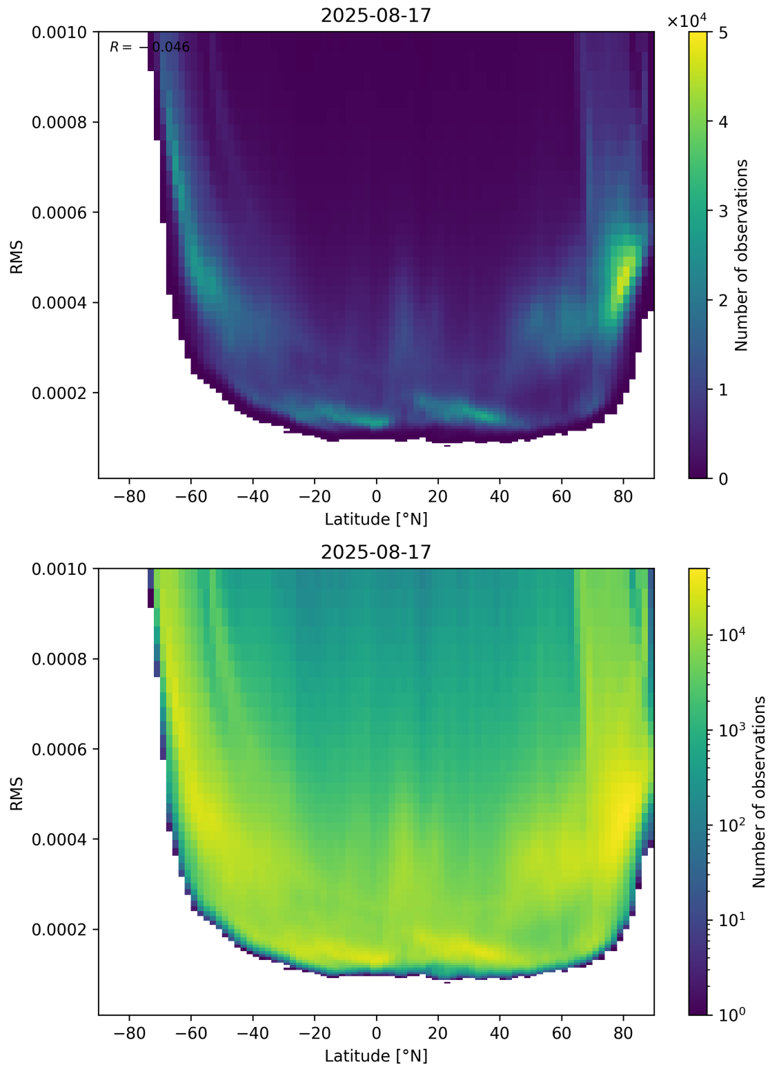
Figure 94: Scatter density plot of “Latitude” against “RMS” for 2025-08-16 to 2025-08-18.
