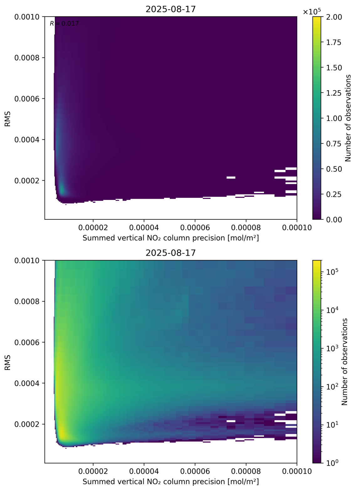
Figure 108: Scatter density plot of “Summed vertical NO 2 column precision” against “RMS” for 2025-08-16 to 2025-08-18.
