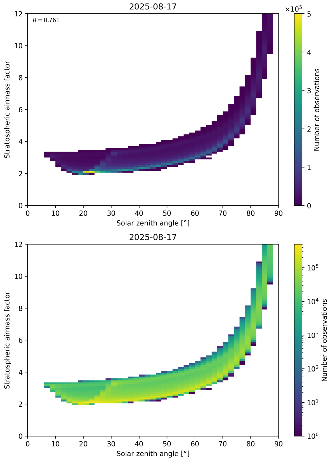
Figure 145: Scatter density plot of “Solar zenith angle” against “Stratospheric airmass factor” for 2025-08-16 to 2025-08-18.
