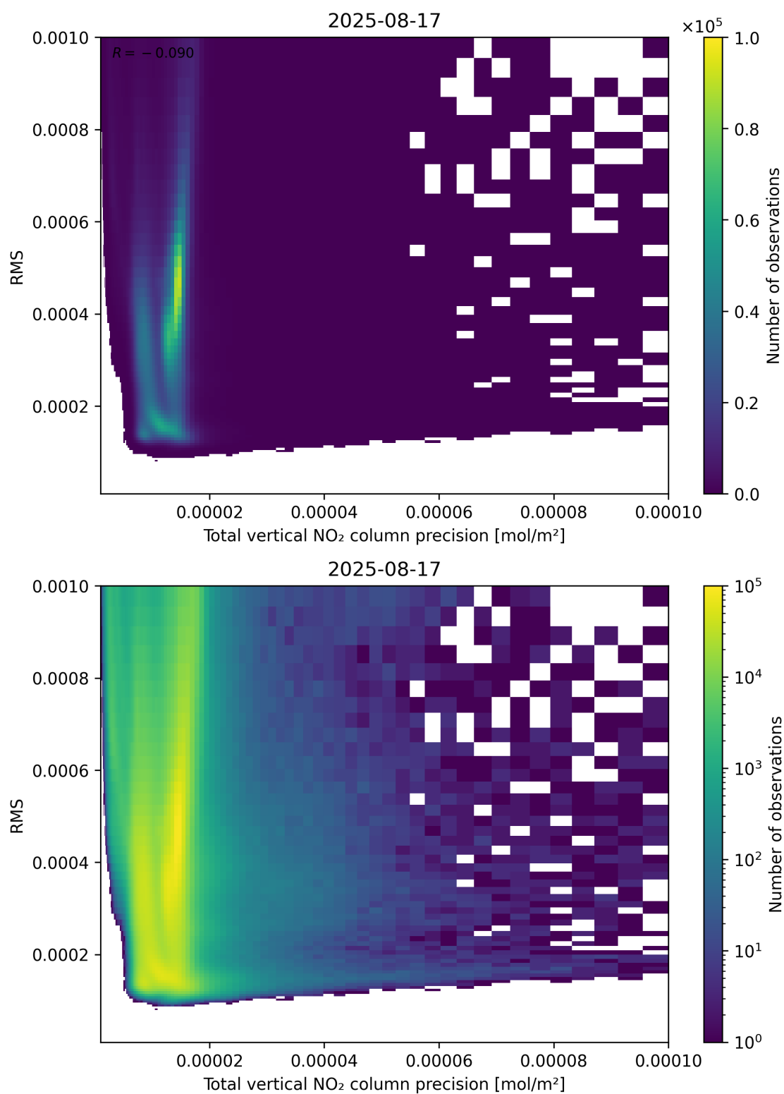
Figure 119: Scatter density plot of “Total vertical NO 2 column precision” against “RMS” for 2025-08-16 to 2025-08-18.
