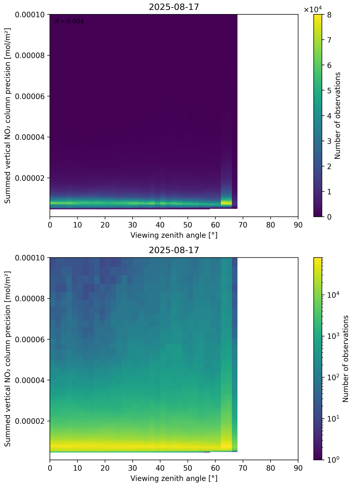
Figure 166: Scatter density plot of “Viewing zenith angle” against “Summed vertical NO 2 column precision” for 2025-08-16 to 2025-08-18.
