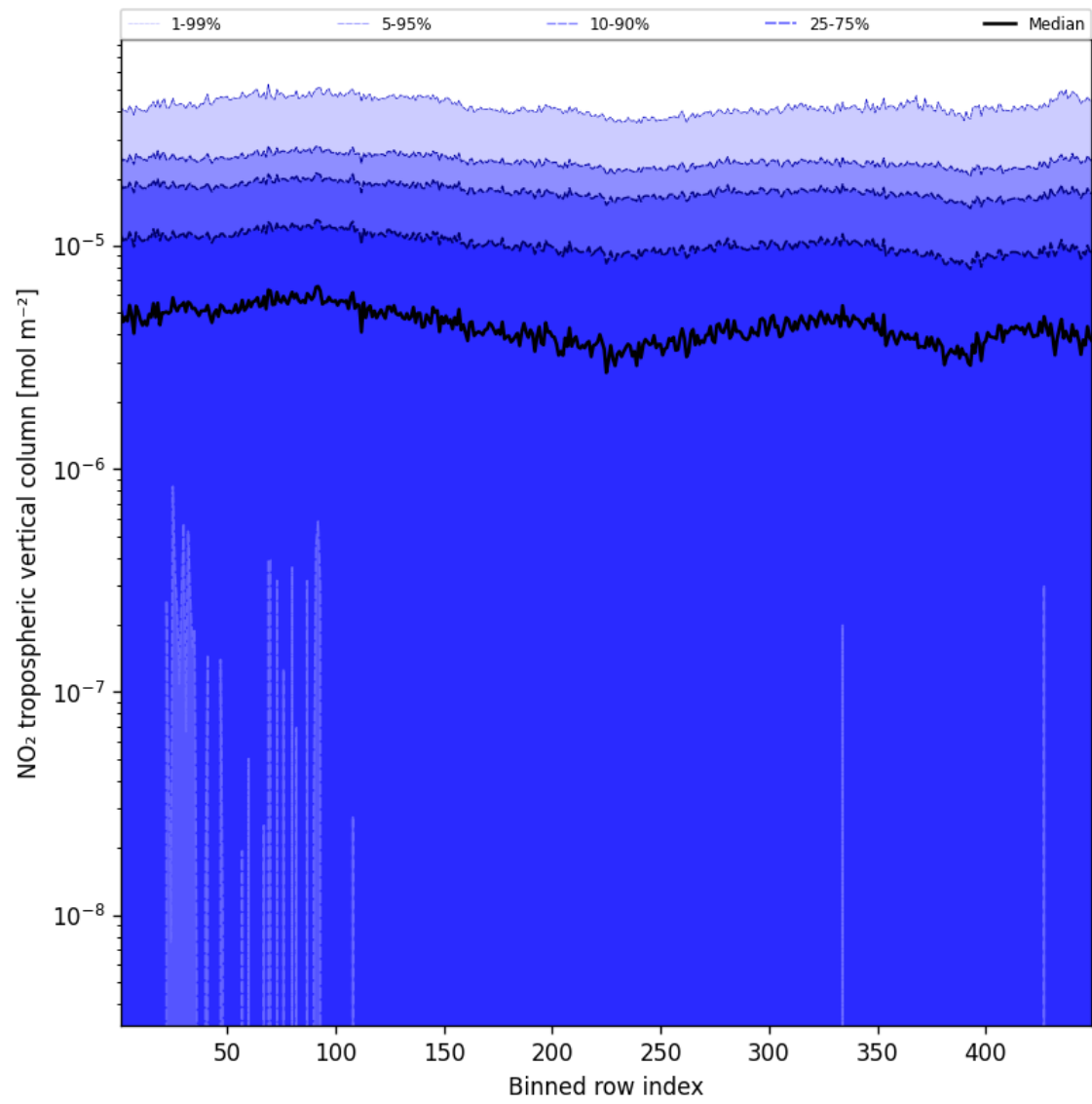
Figure 46: Along track statistics of “NO 2 tropospheric vertical column” for 2025-08-16 to 2025-08-18
