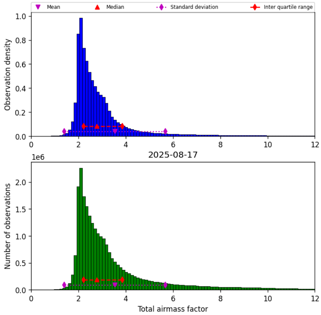
Figure 32: Histogram of “Total airmass factor” for 2025-08-16 to 2025-08-18
