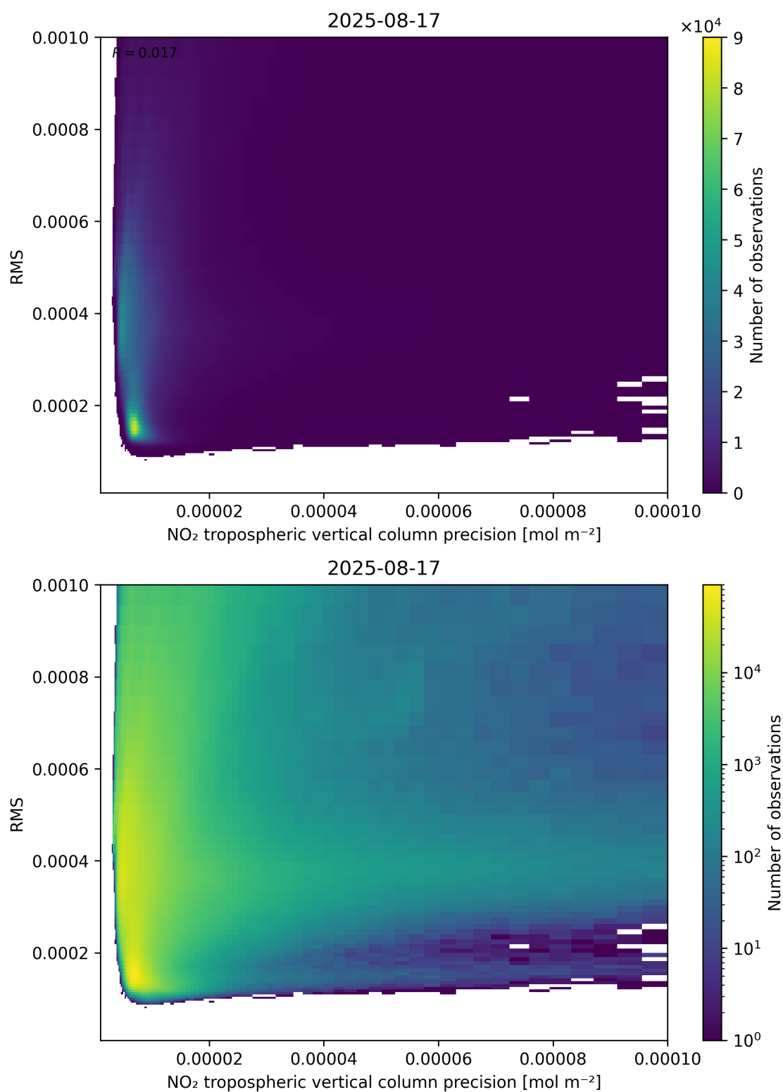
Figure 140: Scatter density plot of “NO 2 tropospheric vertical column precision” against “RMS” for 2025-08-16 to 2025-08-18.
