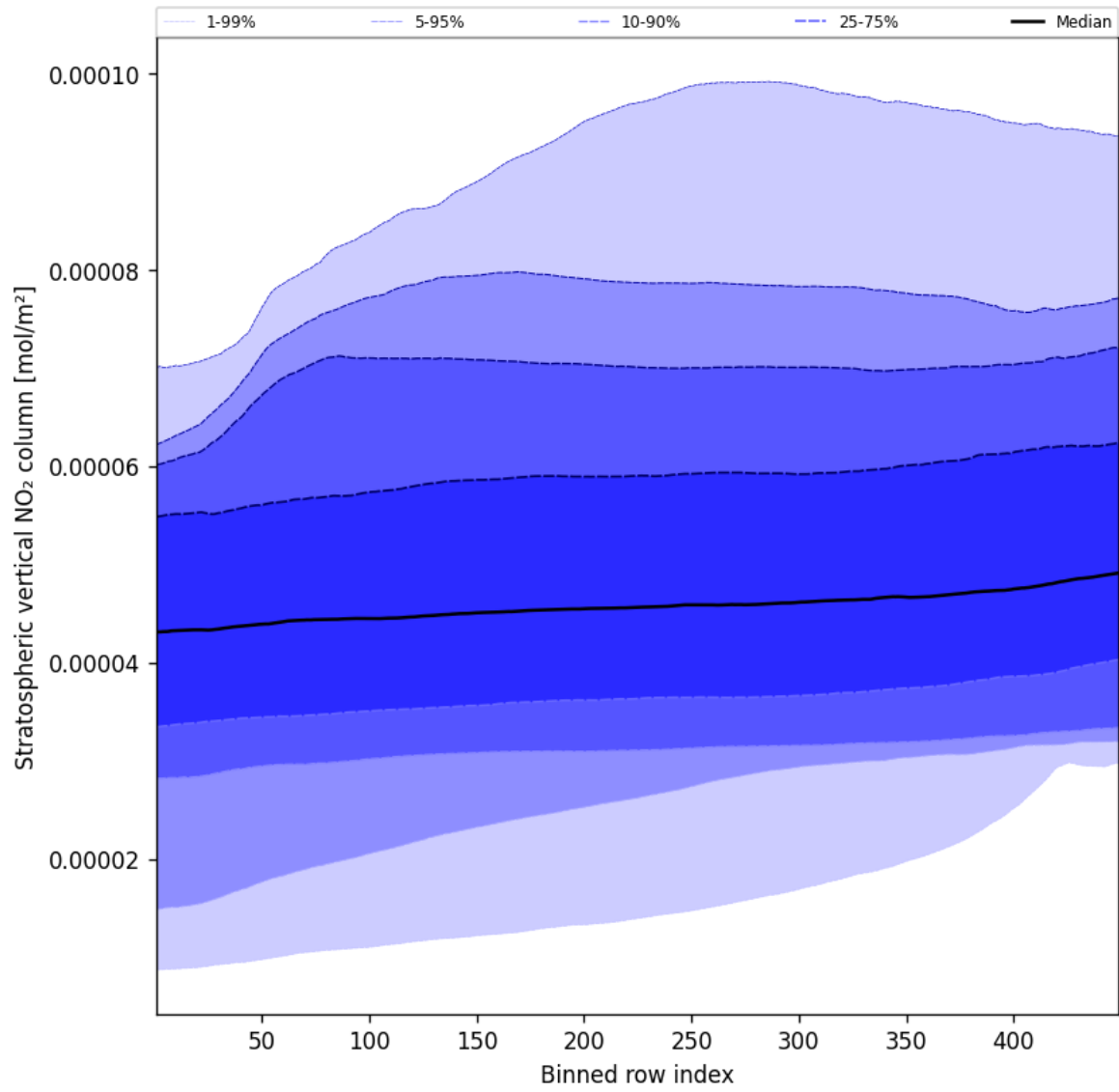
Figure 53: Along track statistics of “Stratospheric vertical NO 2 column” for 2025-08-16 to 2025-08-18
