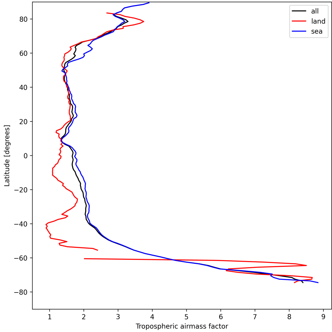
Figure 14: Zonal average of “Tropospheric airmass factor” for 2025-08-16 to 2025-08-18.
