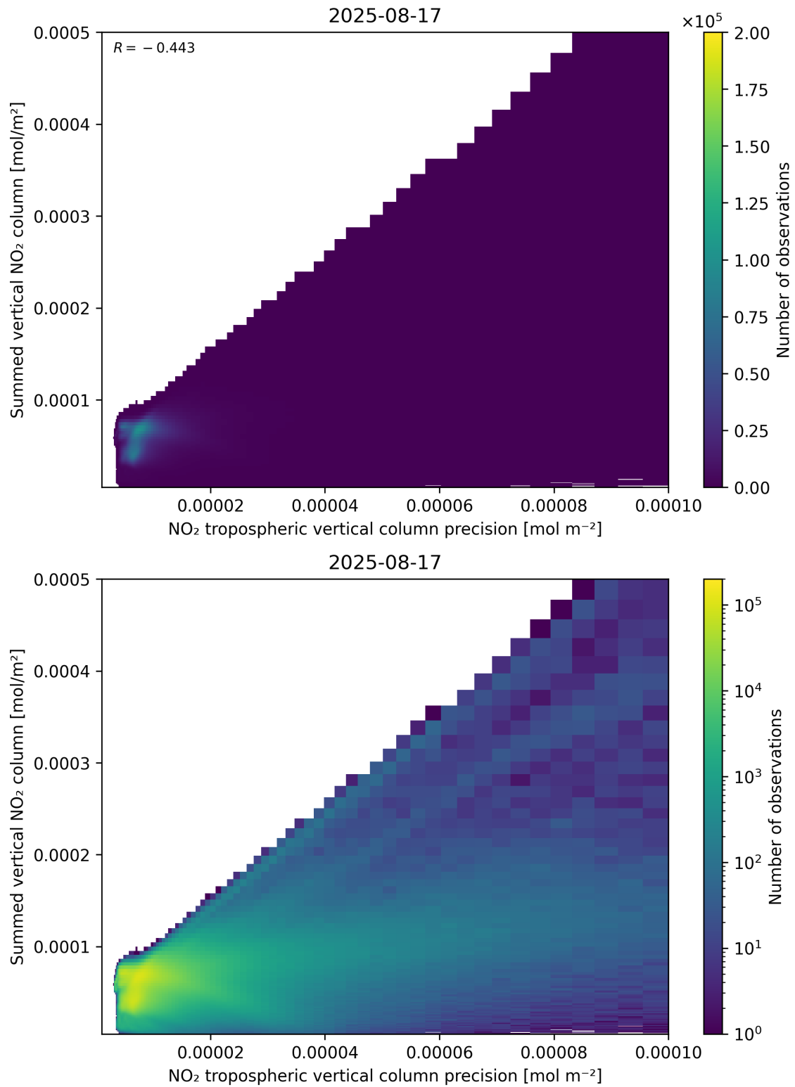
Figure 136: Scatter density plot of “NO 2 tropospheric vertical column precision” against “Summed vertical NO 2 column” for 2025-08-16 to 2025-08-18.
