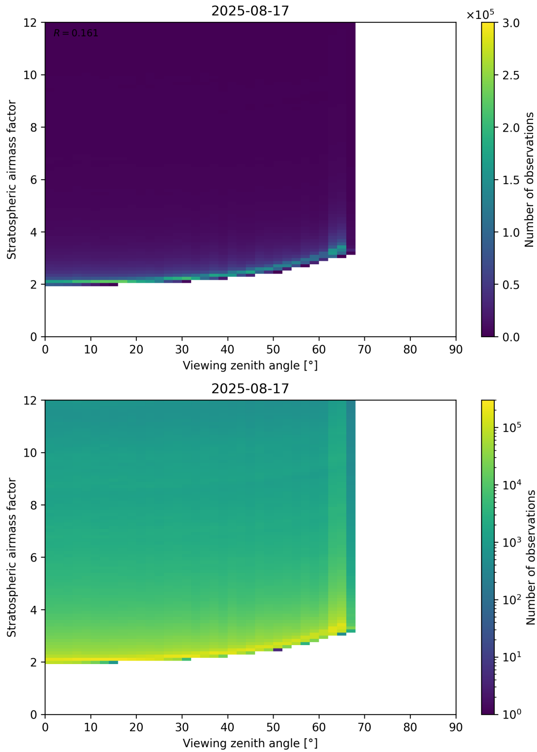
Figure 159: Scatter density plot of “Viewing zenith angle” against “Stratospheric airmass factor” for 2025-08-16 to 2025-08-18.
