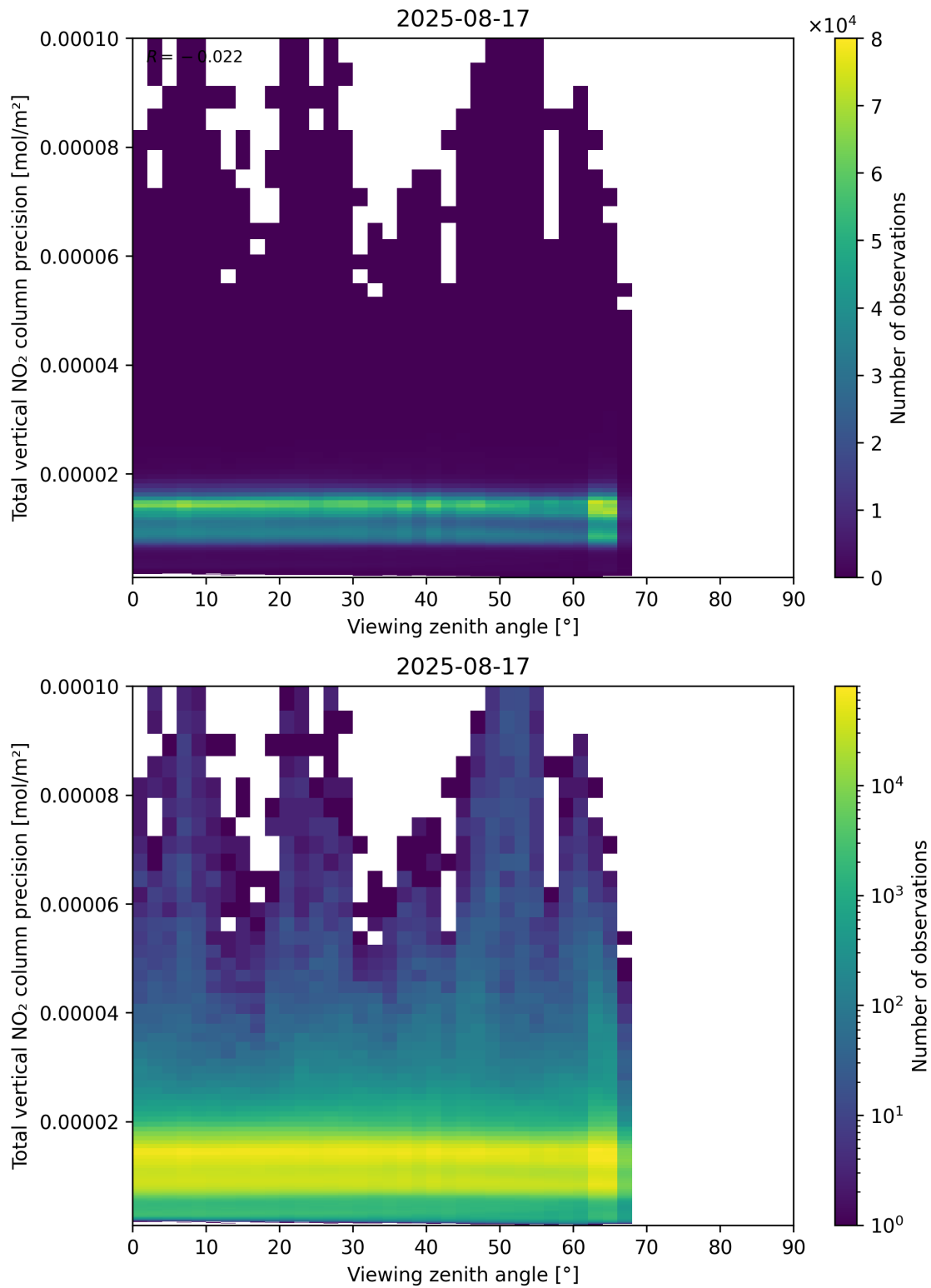
Figure 168: Scatter density plot of “Viewing zenith angle” against “Total vertical NO 2 column precision” for 2025-08-16 to 2025-08-18.
