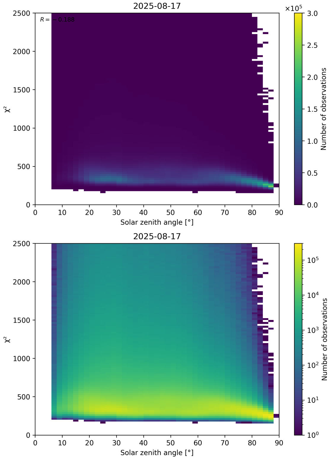
Figure 148: Scatter density plot of “Solar zenith angle” against “ \chi^2 ” for 2025-08-16 to 2025-08-18.
