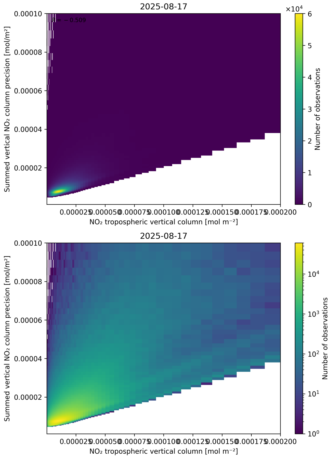
Figure 127: Scatter density plot of “NO 2 tropospheric vertical column” against “Summed vertical NO 2 column precision” for 2025-08-16 to 2025-08-18.
