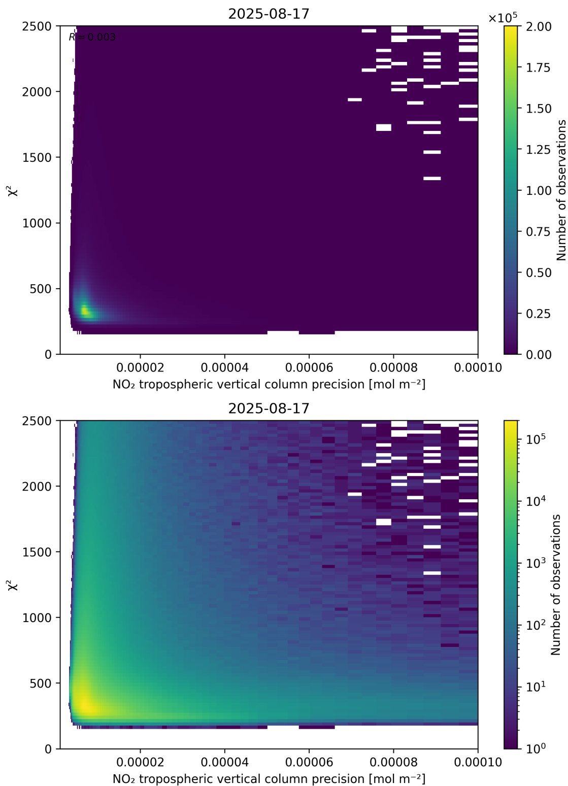
Figure 134: Scatter density plot of “NO 2 tropospheric vertical column precision” against “ \chi^2 ” for 2025-08-16 to 2025-08-18.
