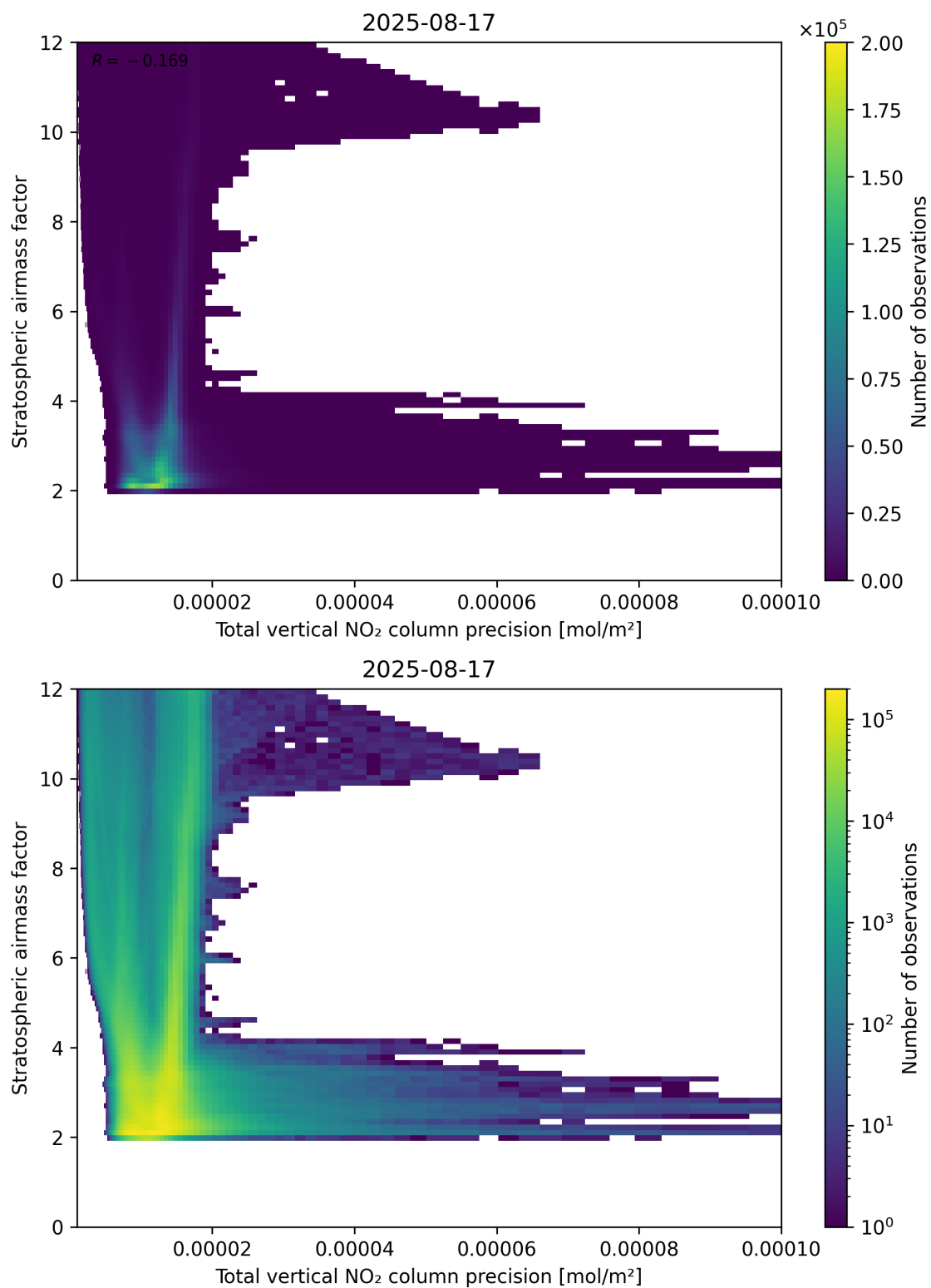
Figure 115: Scatter density plot of “Total vertical NO 2 column precision” against “Stratospheric air mass factor” for 2025-08-16 to 2025-08-18.
