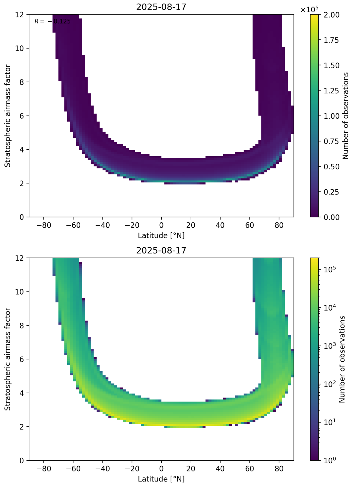
Figure 83: Scatter density plot of “Latitude” against “Stratospheric air mass factor” for 2025-08-16 to 2025-08-18.
