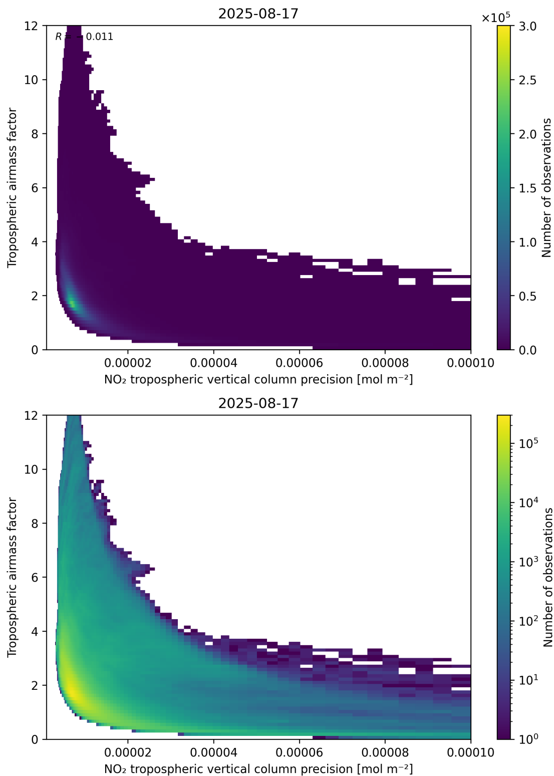
Figure 133: Scatter density plot of “NO 2 tropospheric vertical column precision” against “Tropospheric airmass factor” for 2025-08-16 to 2025-08-18.
