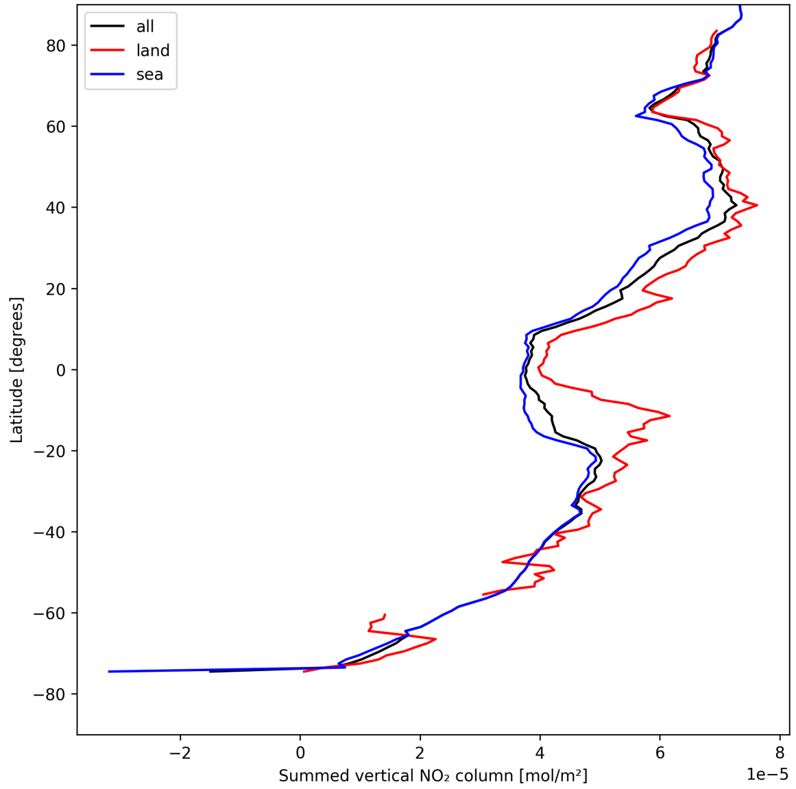
Figure 23: Zonal average of “Summed vertical NO 2 column” for 2025-08-16 to 2025-08-18.
