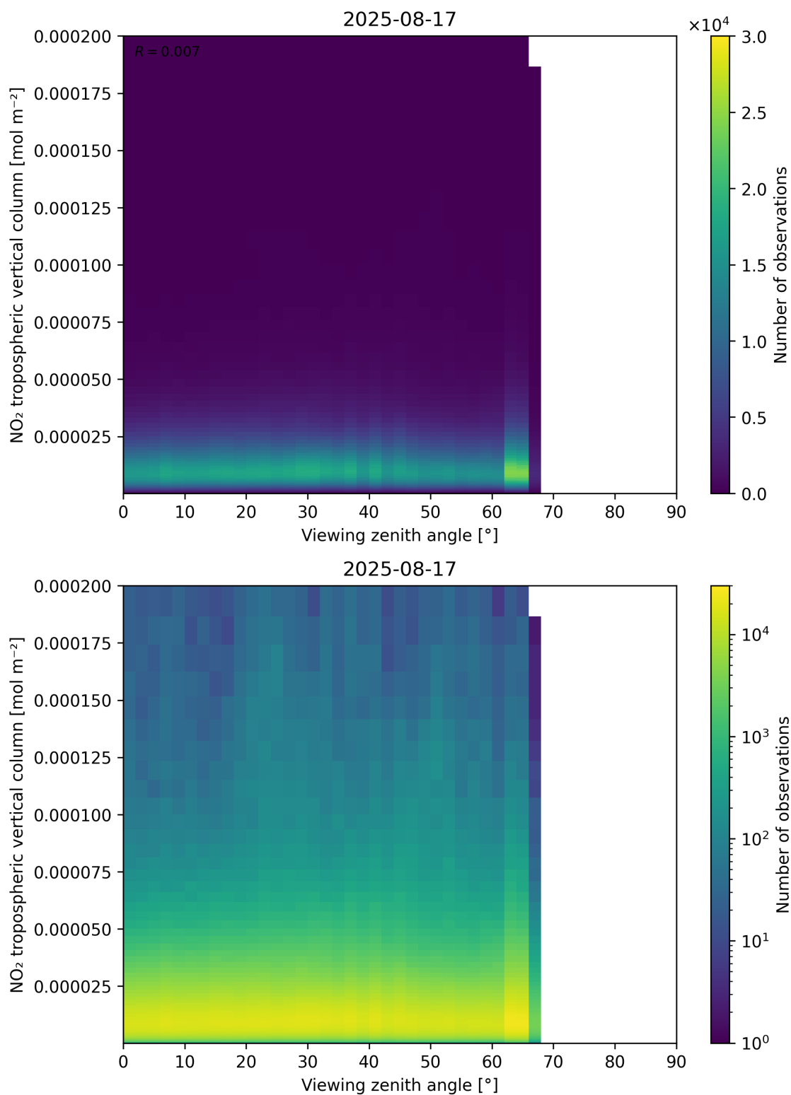
Figure 169: Scatter density plot of “Viewing zenith angle” against “NO 2 tropospheric vertical column” for 2025-08-16 to 2025-08-18.
