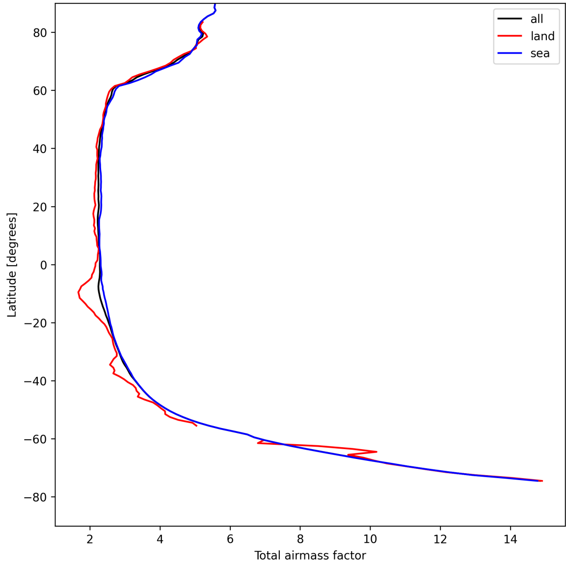
Figure 15: Zonal average of “Total airmass factor” for 2025-08-16 to 2025-08-18.
