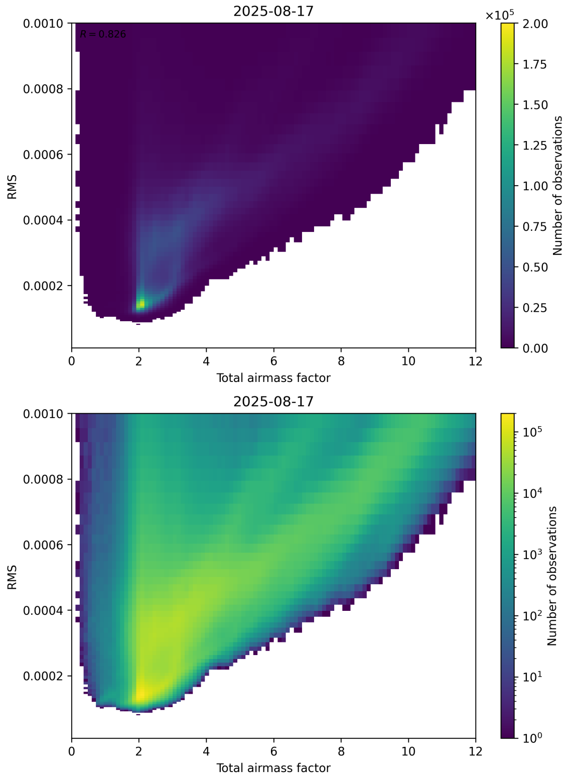
Figure 69: Scatter density plot of “Total airmass factor” against “RMS” for 2025-08-16 to 2025-08-18.
