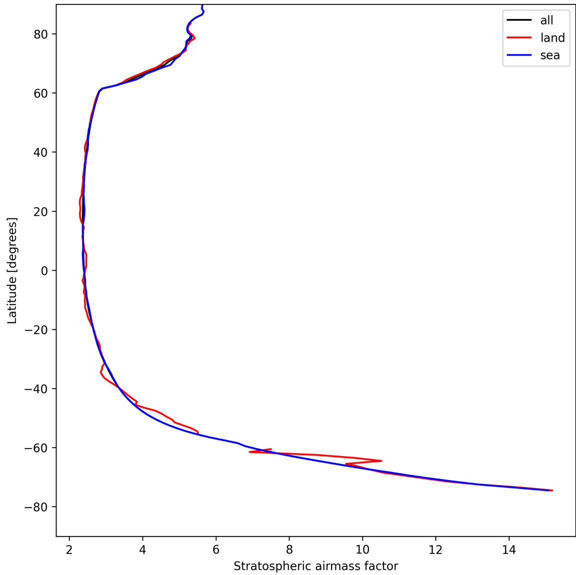
Figure 27: Zonal average of “Stratospheric airmass factor” for 2025-08-16 to 2025-08-18.
