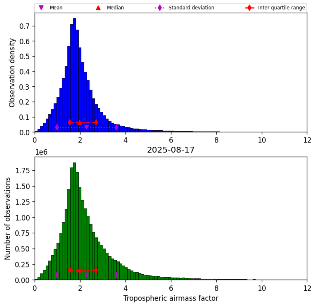
Figure 31: Histogram of “Tropospheric airmass factor” for 2025-08-16 to 2025-08-18
