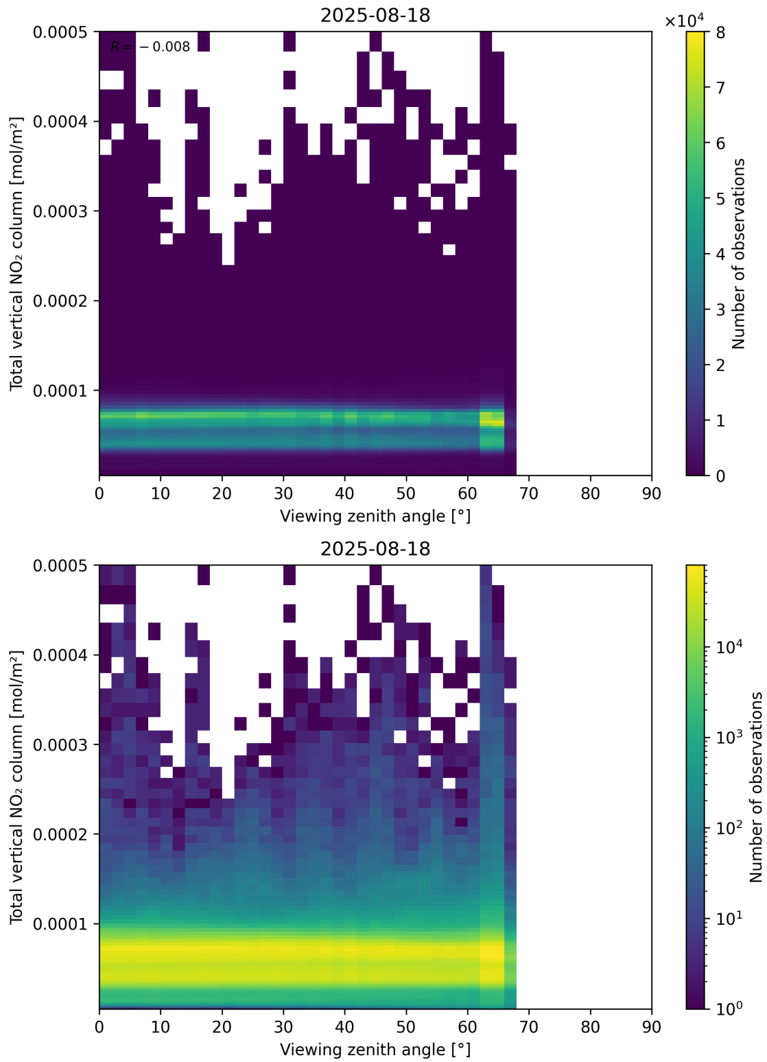
Figure 167: Scatter density plot of “Viewing zenith angle” against “Total vertical NO 2 column” for 2025-08-17 to 2025-08-19.
