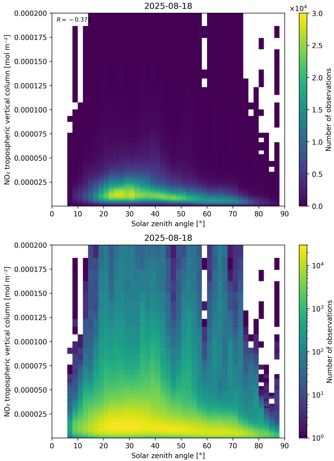
Figure 155: Scatter density plot of “Solar zenith angle” against “NO 2 tropospheric vertical column” for 2025-08-17 to 2025-08-19.
