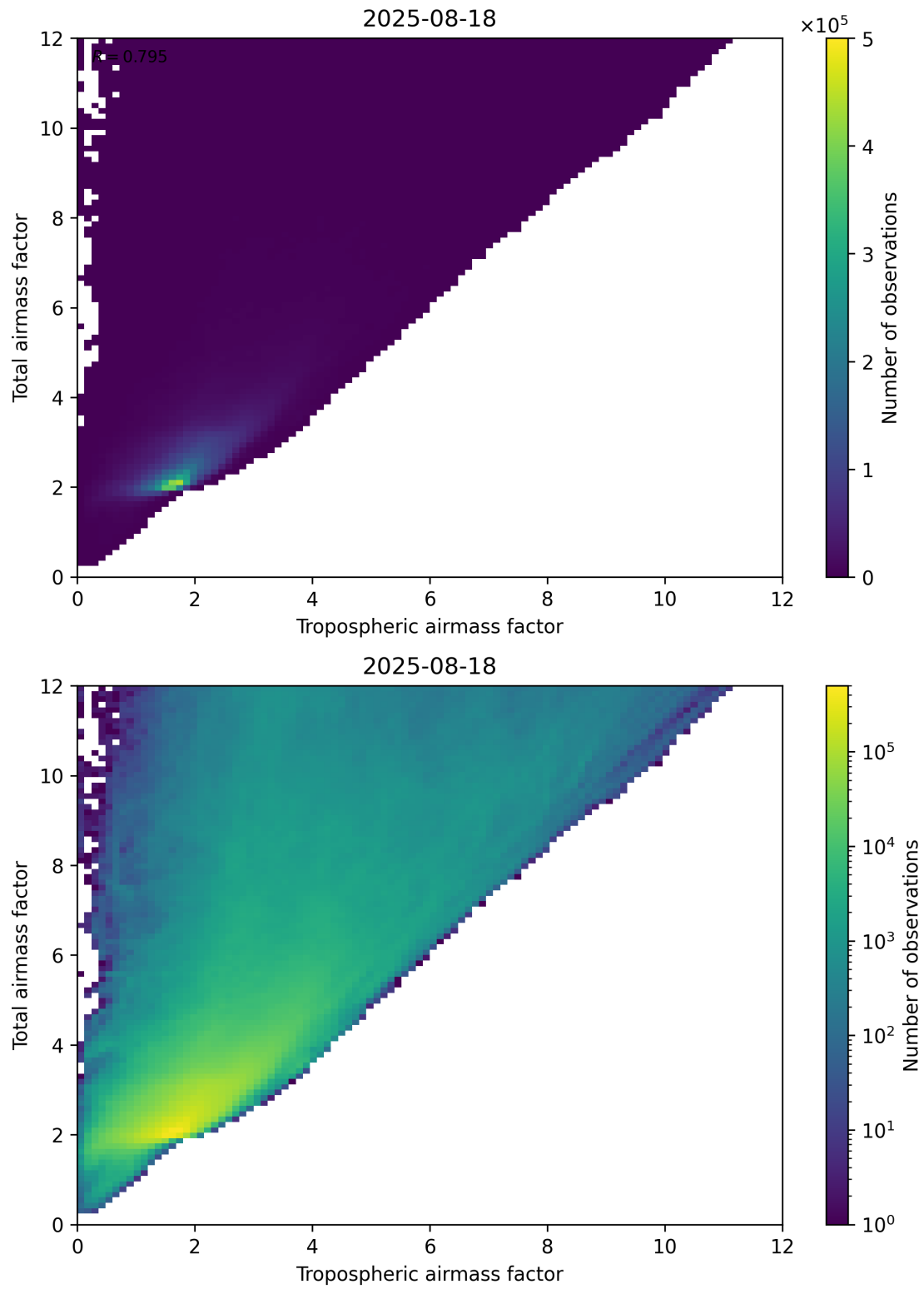
Figure 72: Scatter density plot of “Tropospheric airmass factor” against “Total airmass factor” for 2025-08-17 to 2025-08-19.
