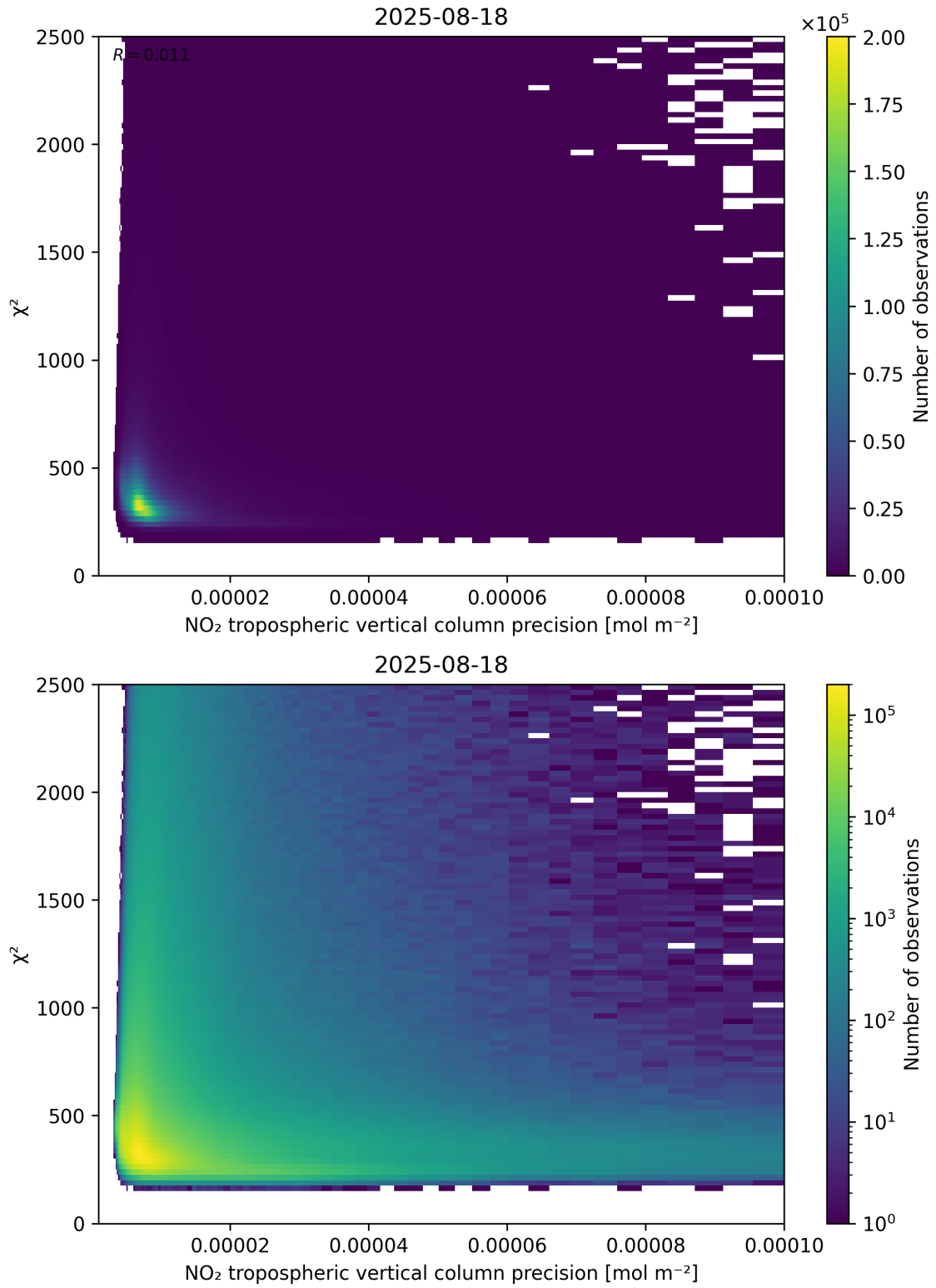
Figure 134: Scatter density plot of “NO 2 tropospheric vertical column precision” against “ \chi^2 ” for 2025-08-17 to 2025-08-19.
