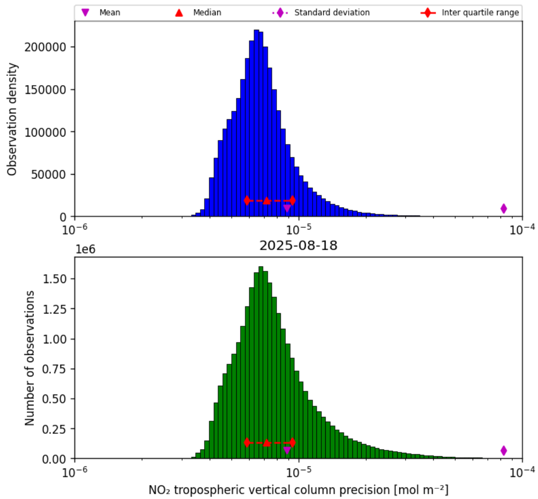
Figure 30: Histogram of “NO 2 tropospheric vertical column precision” for 2025-08-17 to 2025-08-19
