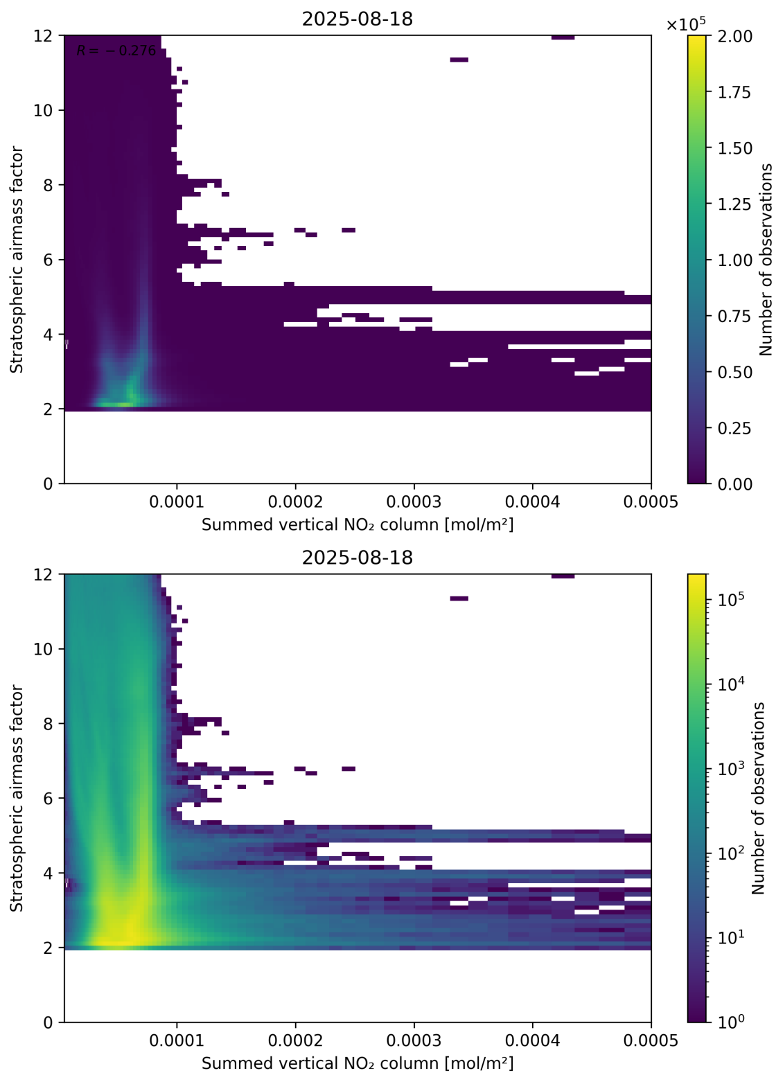
Figure 103: Scatter density plot of “Summed vertical NO 2 column” against “Stratospheric air mass factor” for 2025-08-17 to 2025-08-19.
