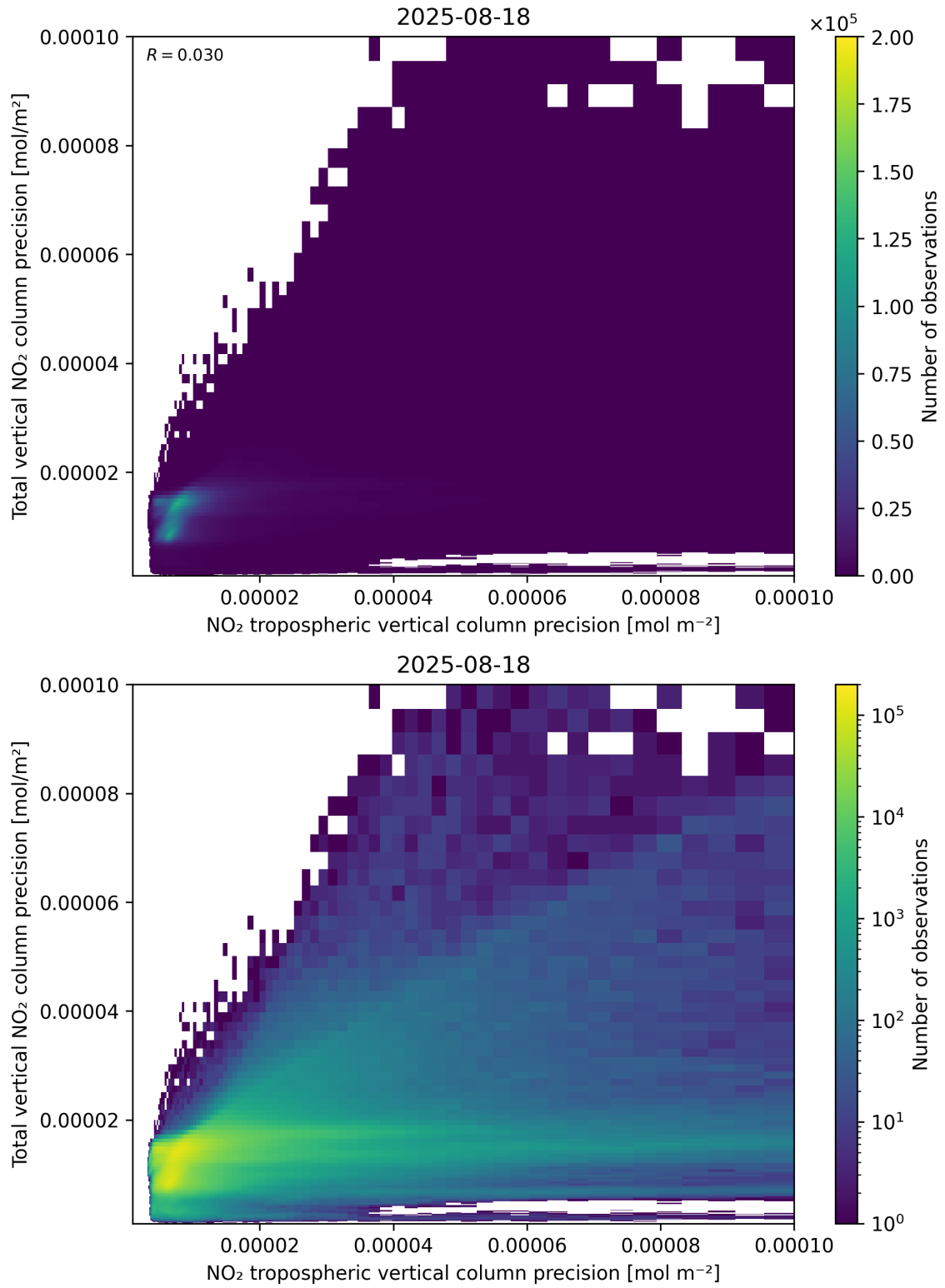
Figure 139: Scatter density plot of “NO 2 tropospheric vertical column precision” against “Total vertical NO 2 column precision” for 2025-08-17 to 2025-08-19.
