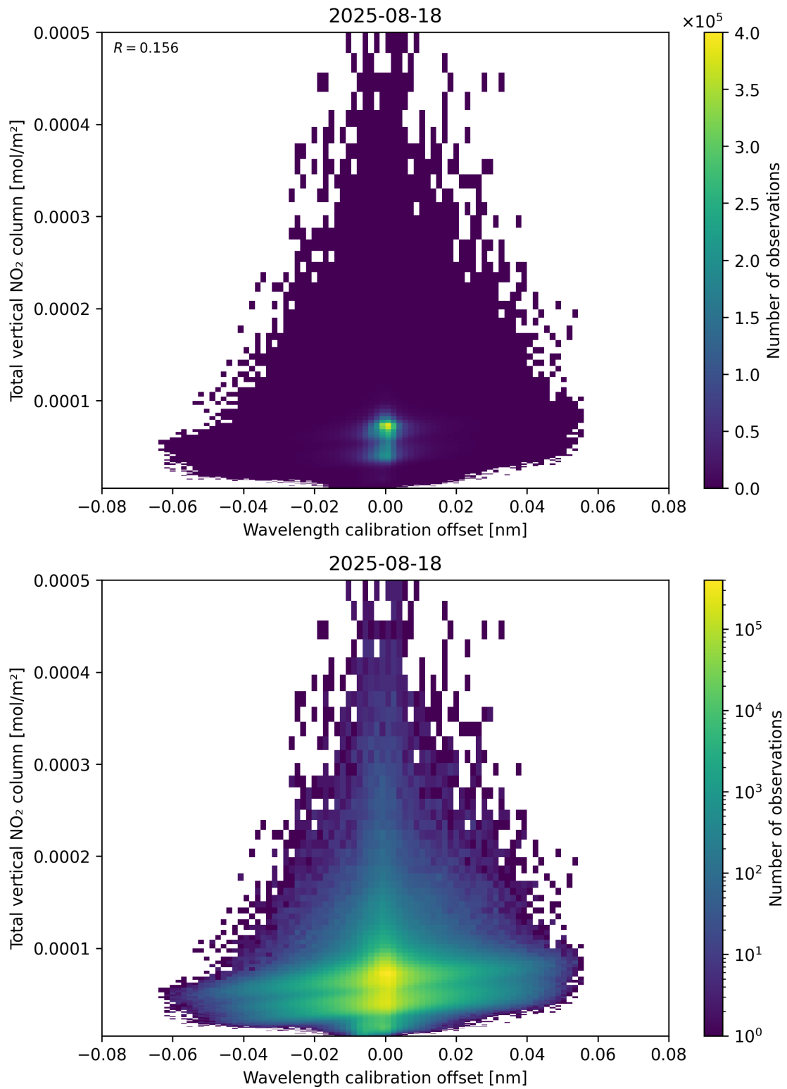
Figure 179: Scatter density plot of “Wavelength calibration offset” against “Total vertical NO 2 column” for 2025-08-17 to 2025-08-19.
