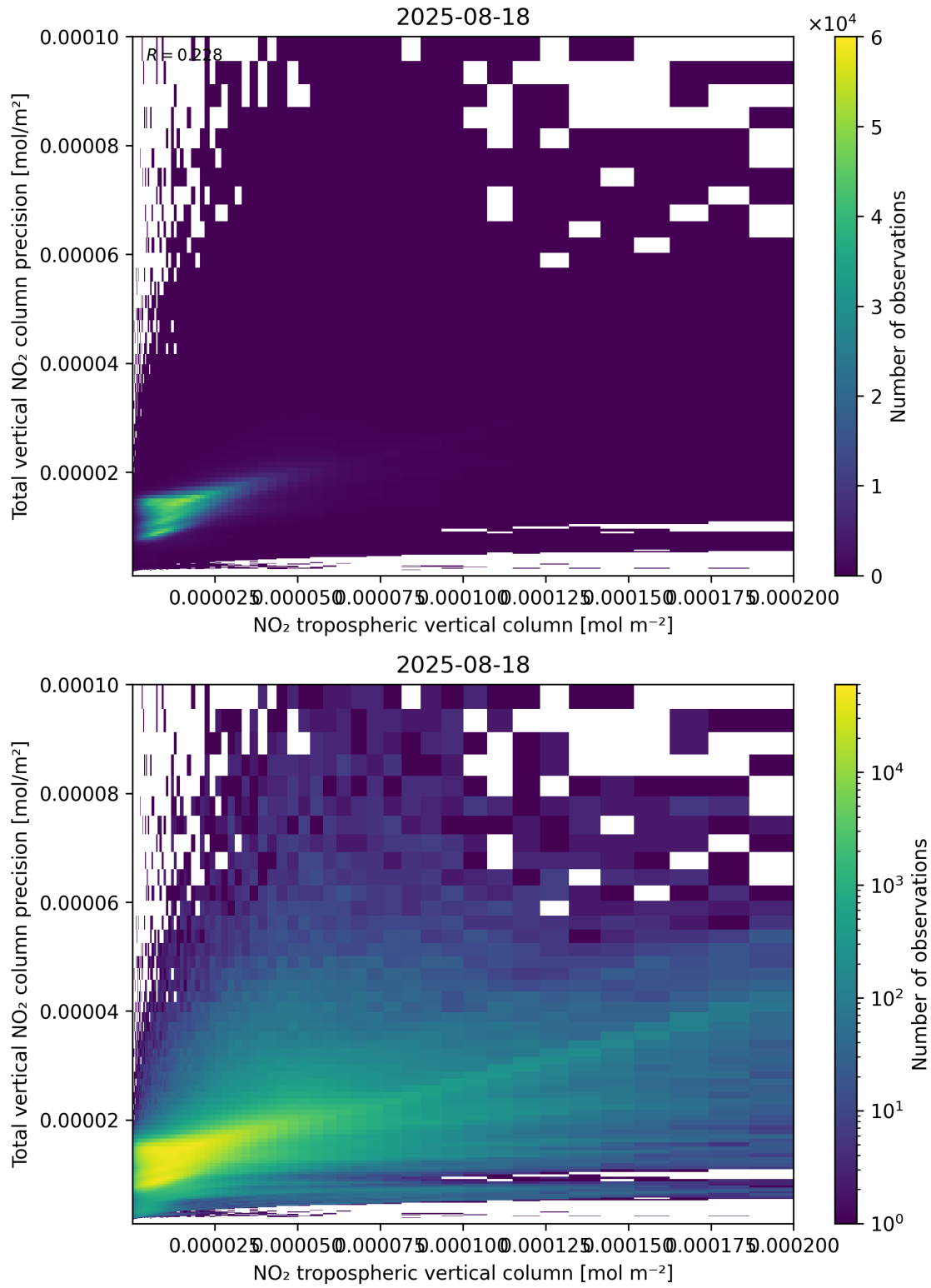
Figure 129: Scatter density plot of “NO 2 tropospheric vertical column” against “Total vertical NO 2 column precision” for 2025-08-17 to 2025-08-19.
