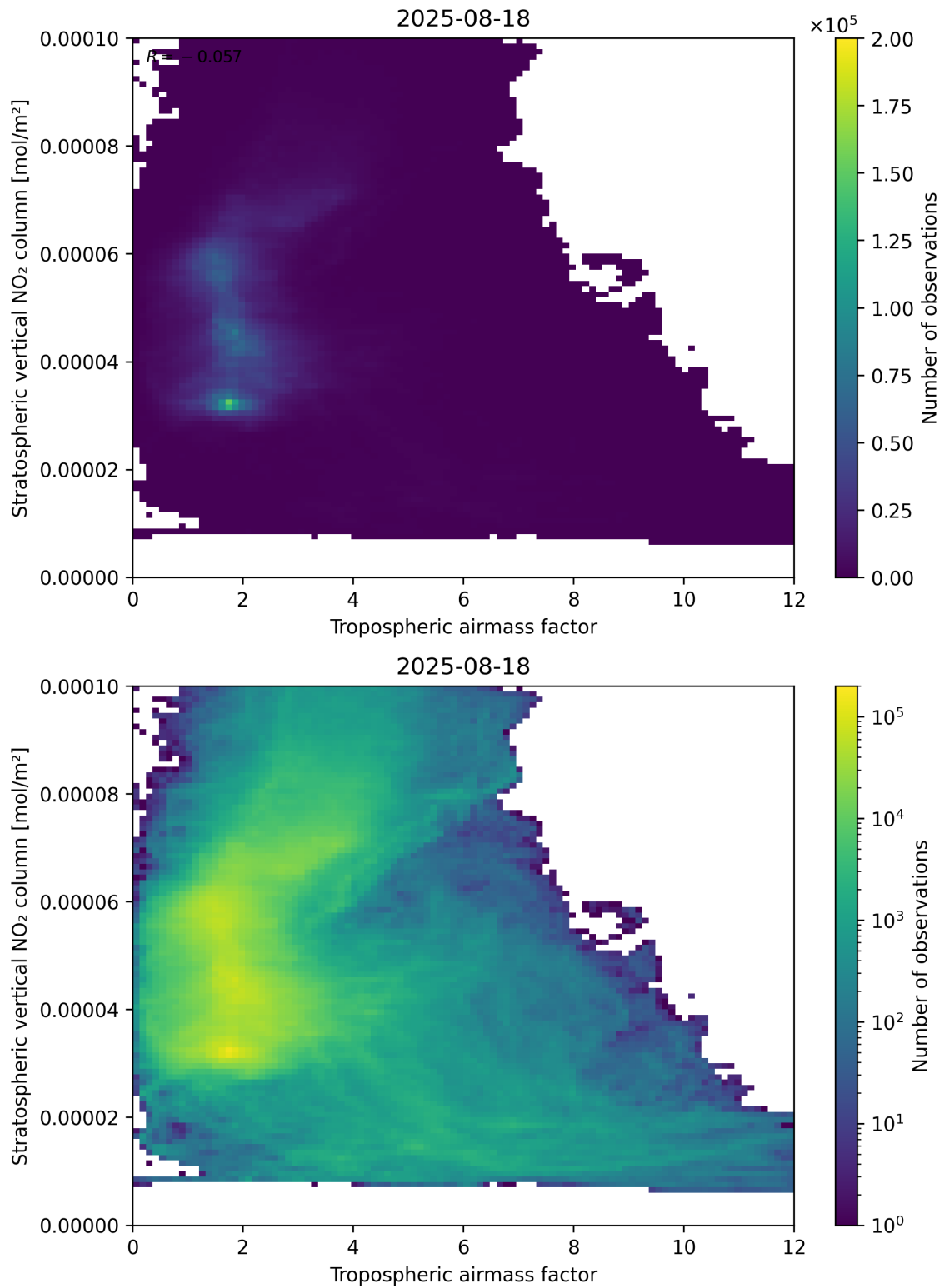
Figure 74: Scatter density plot of “Tropospheric air mass factor” against “Stratospheric vertical NO 2 column” for 2025-08-17 to 2025-08-19.
