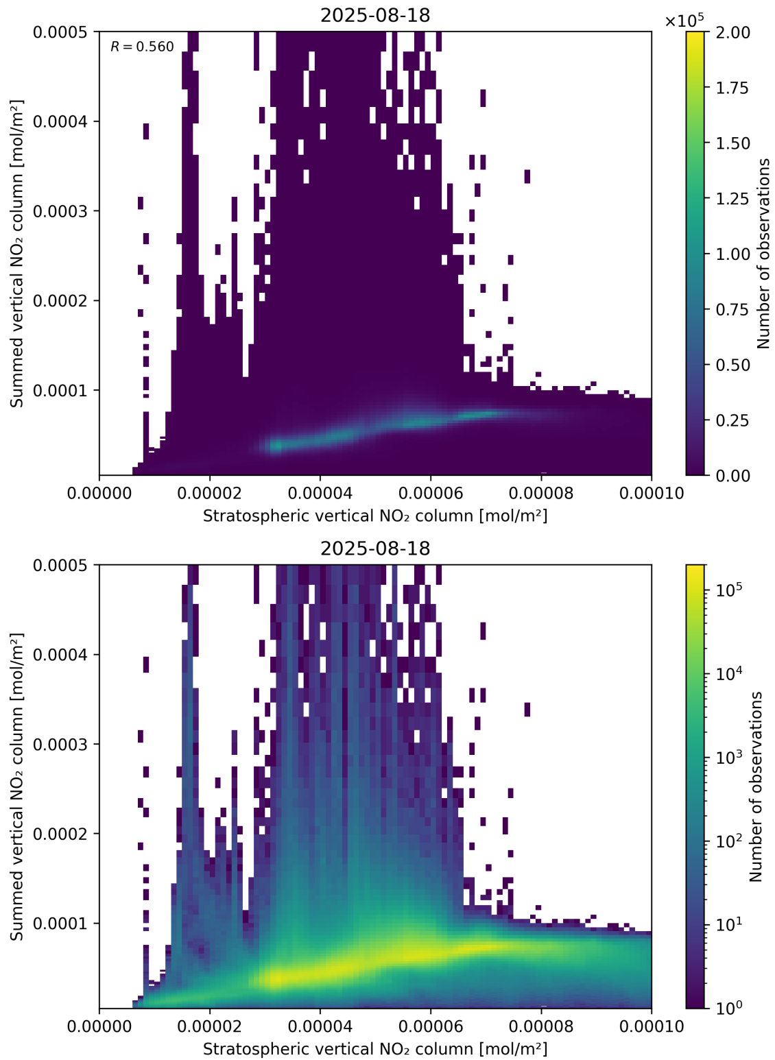
Figure 98: Scatter density plot of “Stratospheric vertical NO 2 column” against “Summed vertical NO 2 column” for 2025-08-17 to 2025-08-19.
