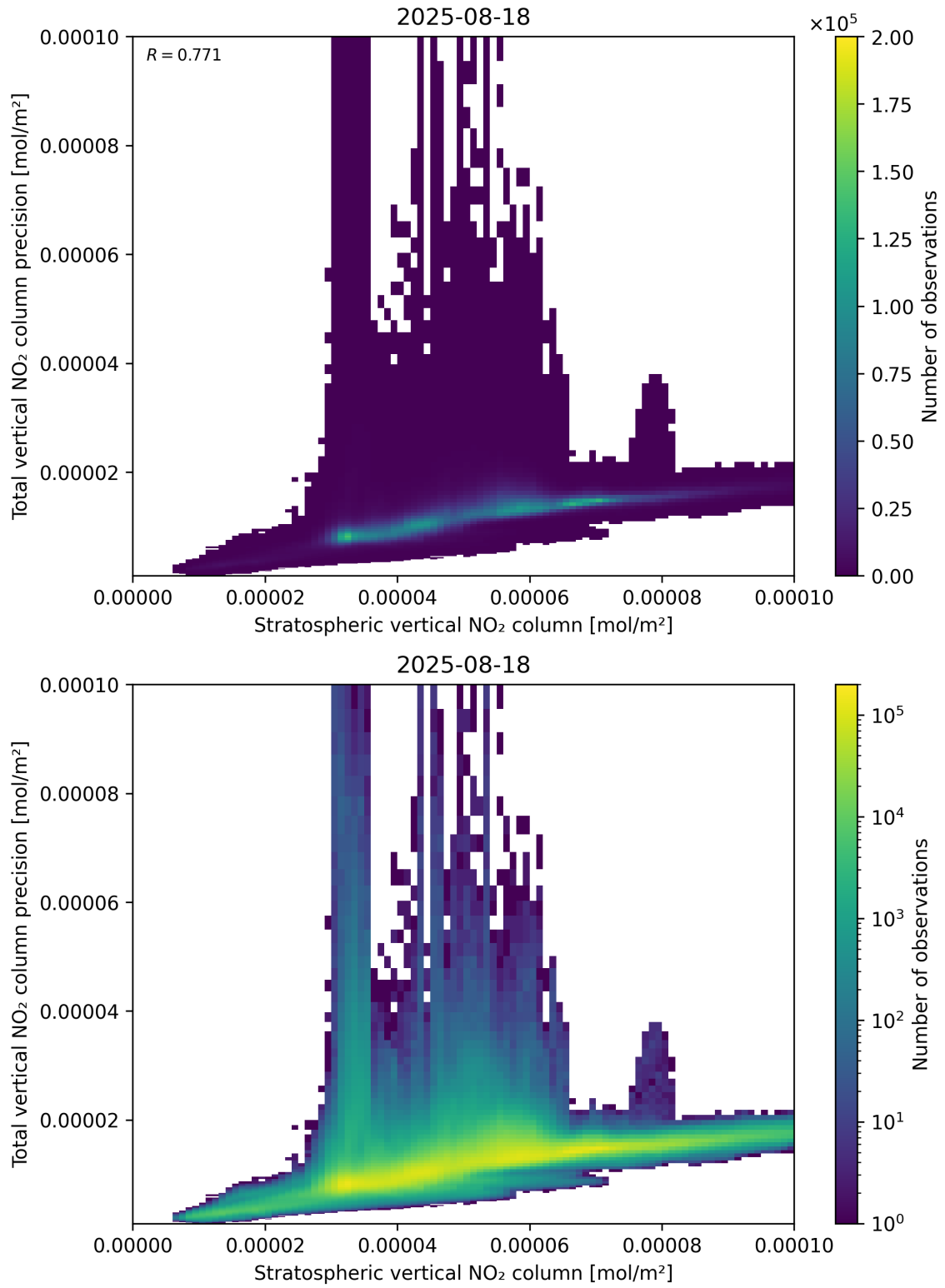
Figure 101: Scatter density plot of “Stratospheric vertical NO 2 column” against “Total vertical NO 2 column precision” for 2025-08-17 to 2025-08-19.
