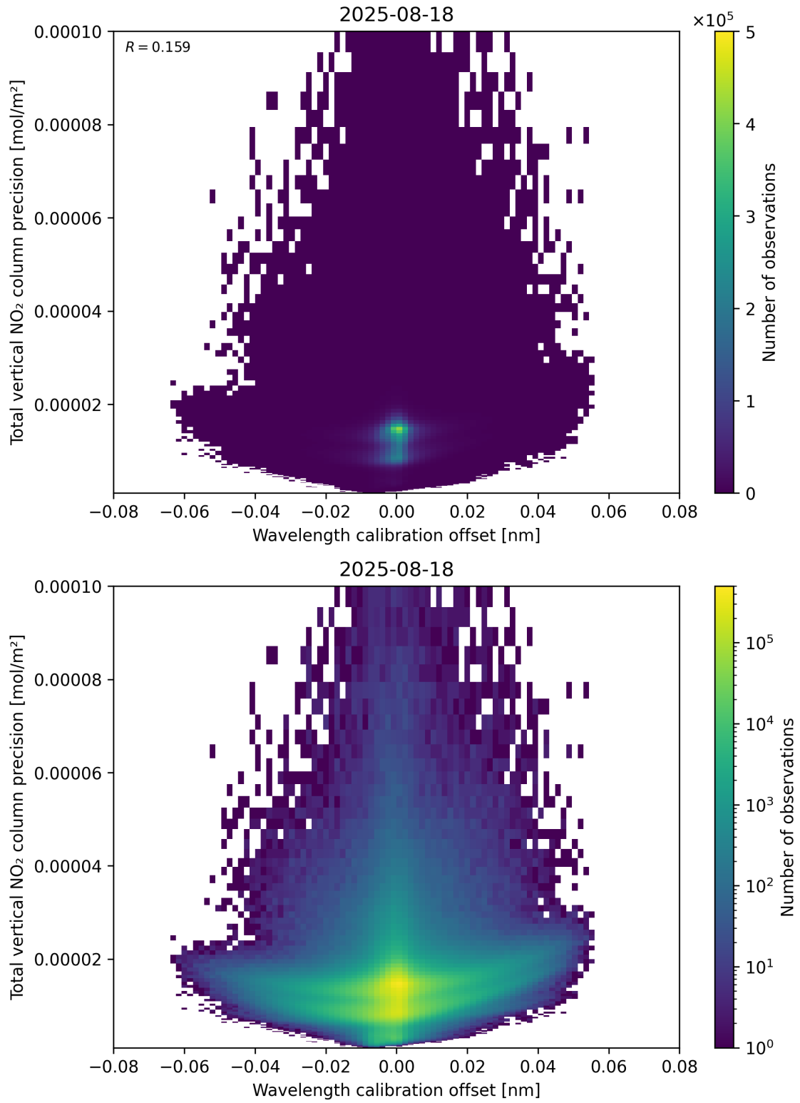
Figure 180: Scatter density plot of “Wavelength calibration offset” against “Total vertical NO 2 column precision” for 2025-08-17 to 2025-08-19.
