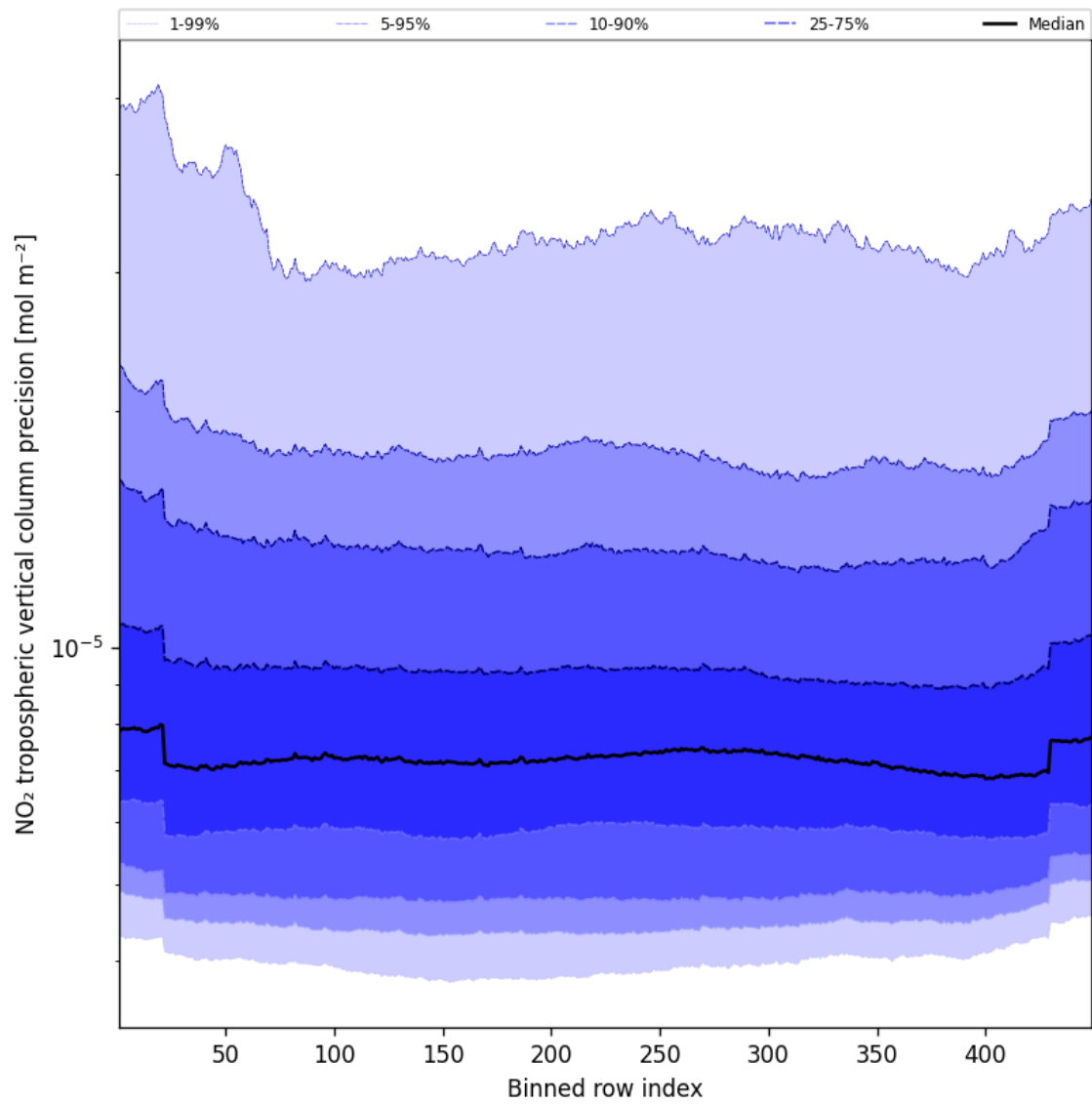
Figure 47: Along track statistics of “NO 2 tropospheric vertical column precision” for 2025-08-17 to 2025-08-19
