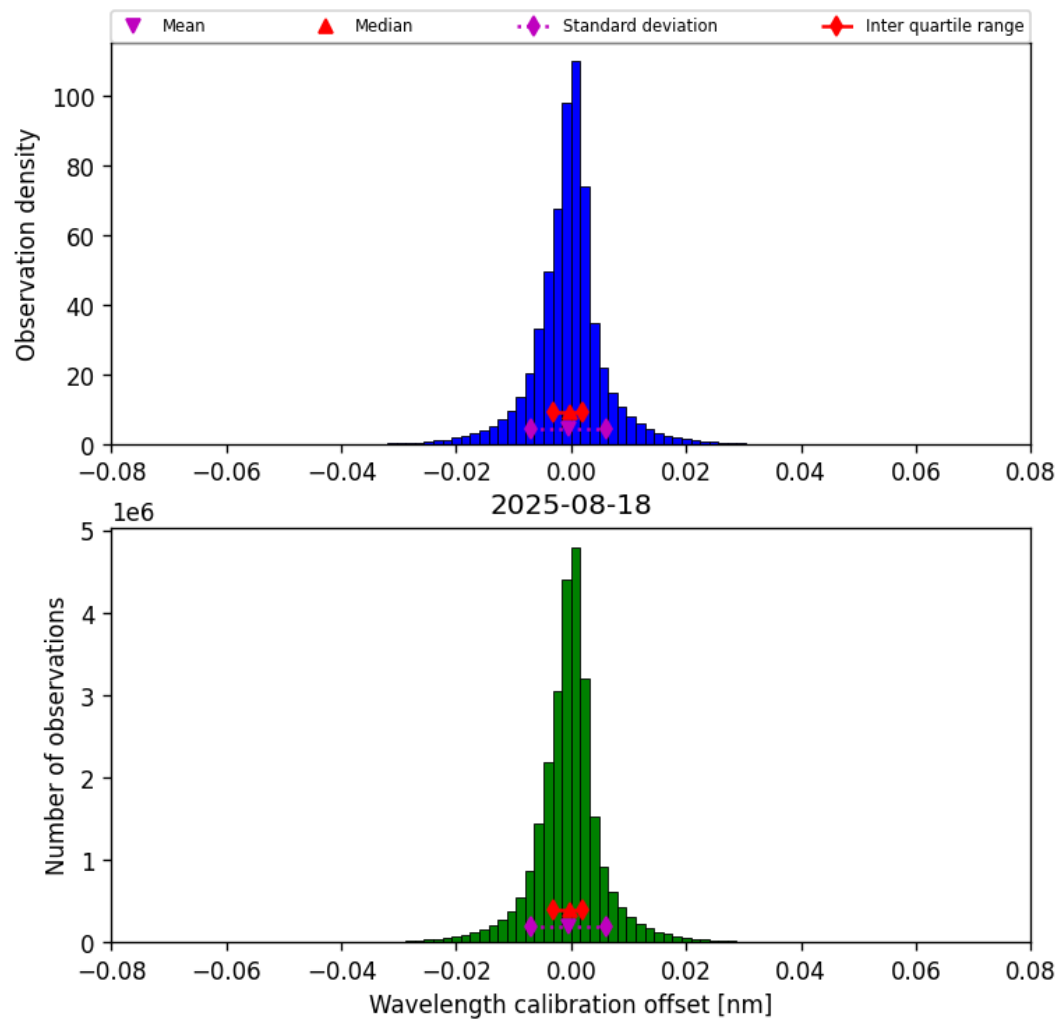
Figure 35: Histogram of “Wavelength calibration offset” for 2025-08-17 to 2025-08-19
