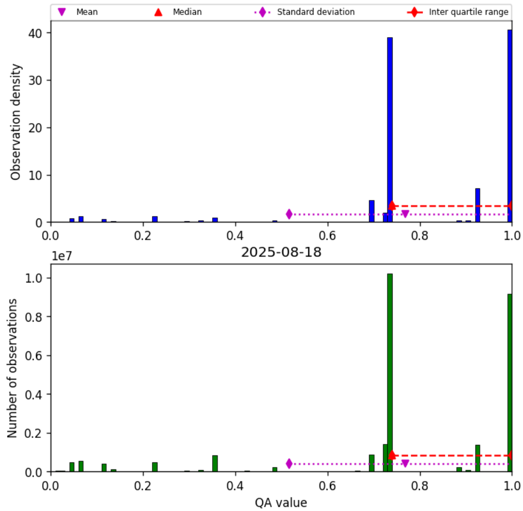
Figure 28: Histogram of “QA value” for 2025-08-17 to 2025-08-19
