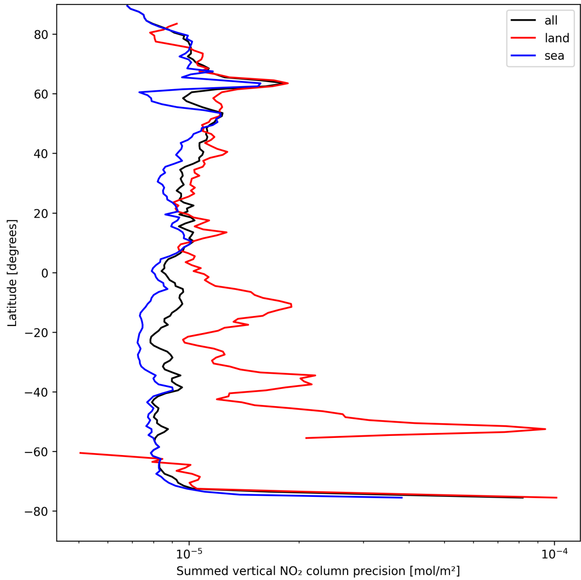
Figure 24: Zonal average of “Summed vertical NO 2 column precision” for 2025-08-17 to 2025-08-19.
