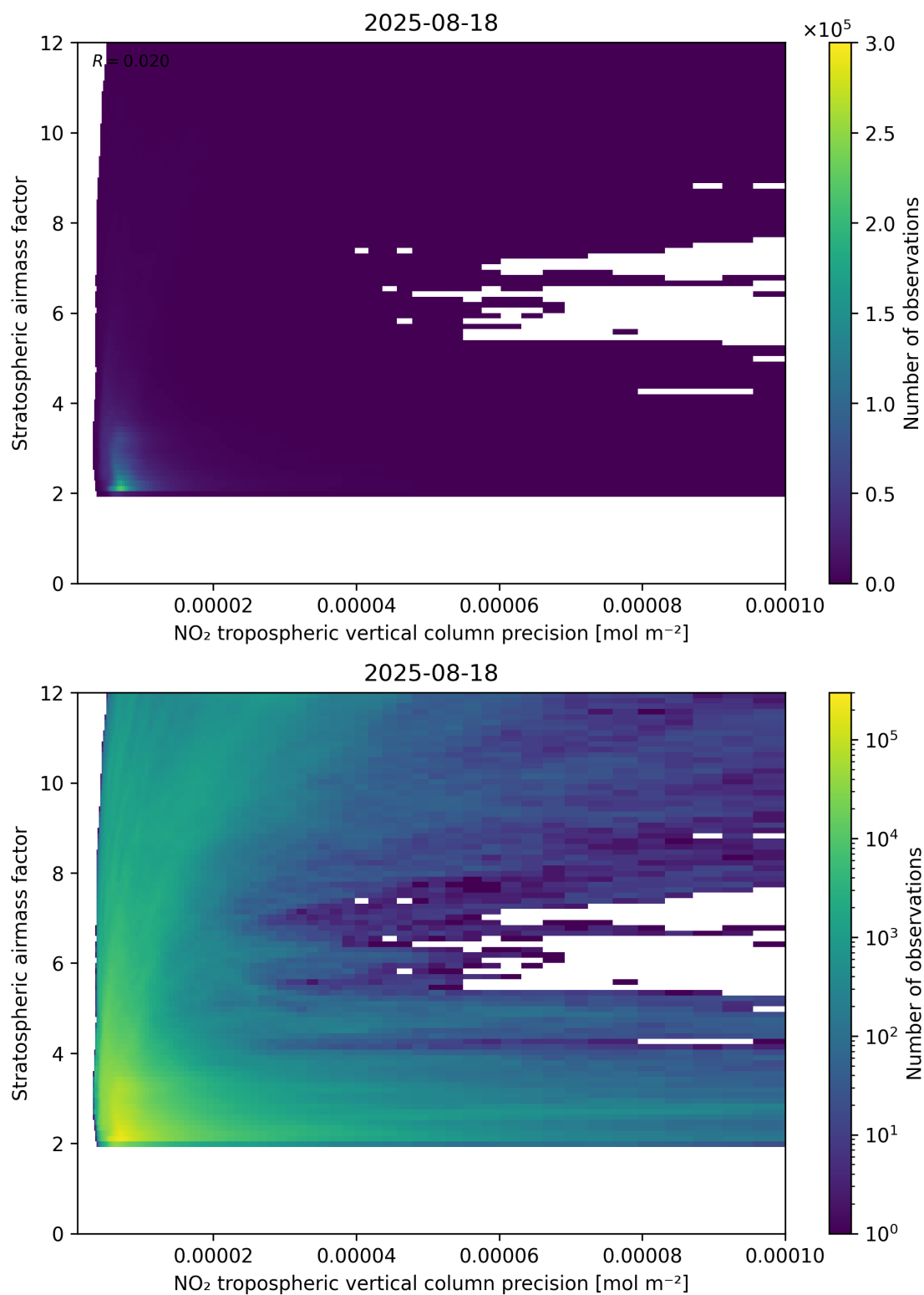
Figure 131: Scatter density plot of “NO 2 tropospheric vertical column precision” against “Stratospheric airmass factor” for 2025-08-17 to 2025-08-19.
