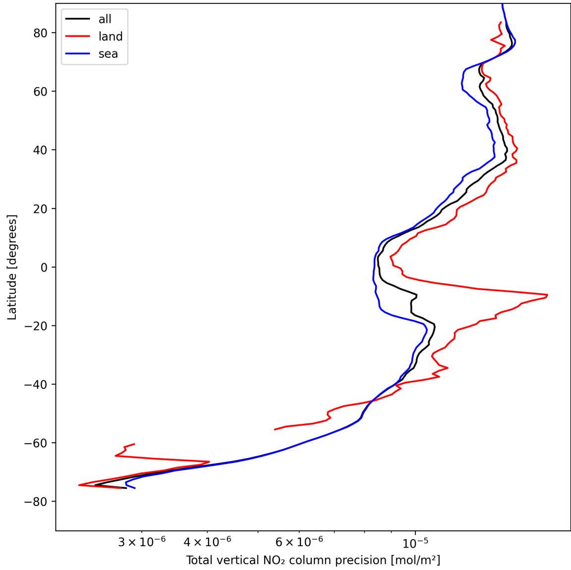
Figure 22: Zonal average of “Total vertical NO 2 column precision” for 2025-08-17 to 2025-08-19.
