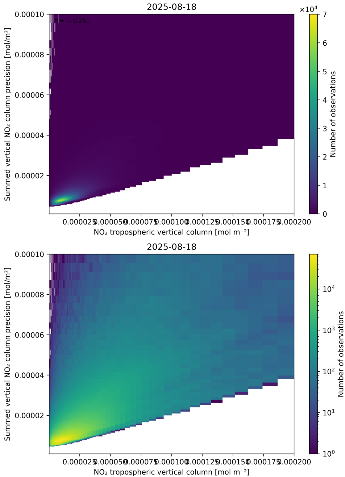
Figure 127: Scatter density plot of “NO 2 tropospheric vertical column” against “Summed vertical NO 2 column precision” for 2025-08-17 to 2025-08-19.
