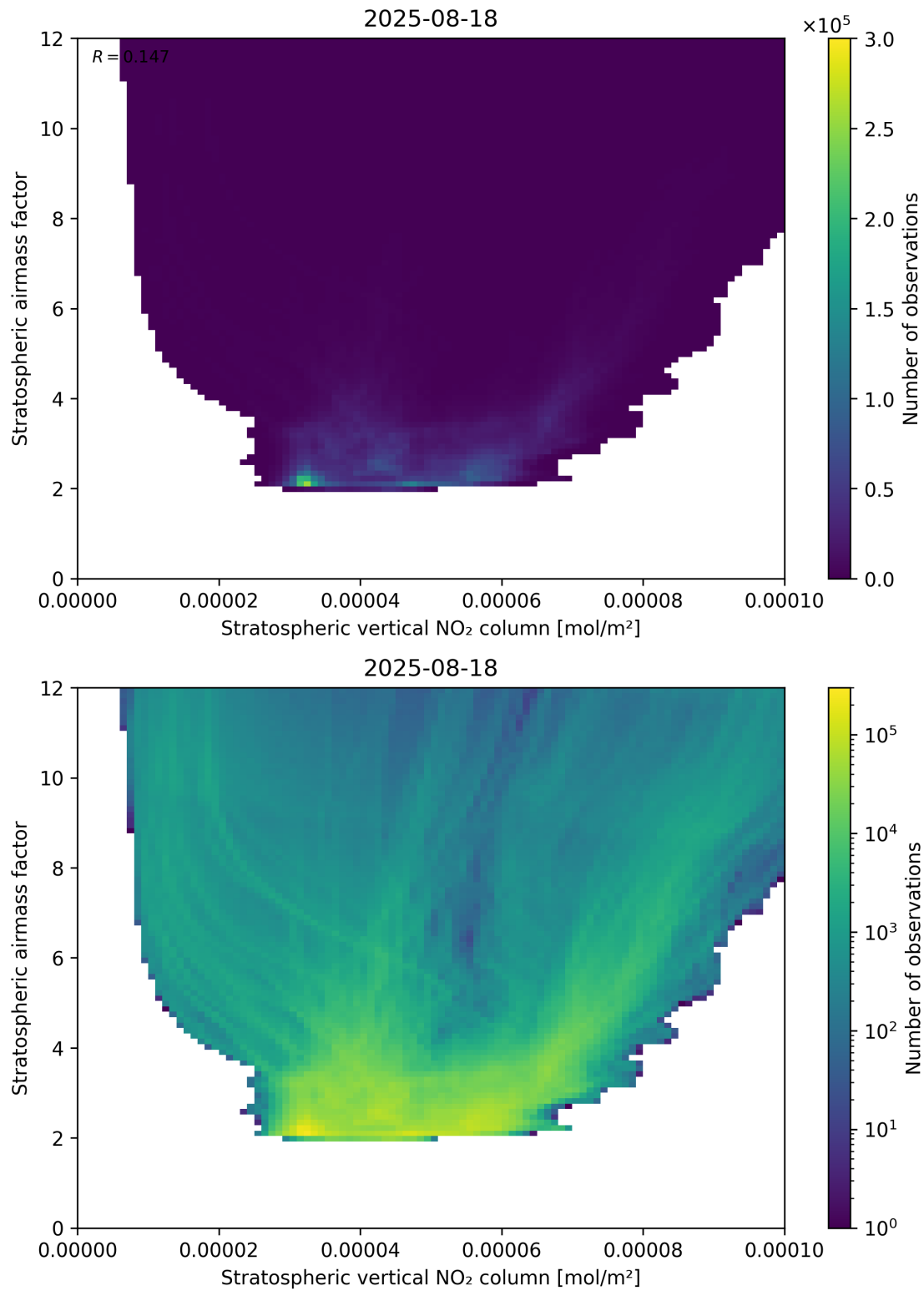
Figure 96: Scatter density plot of “Stratospheric vertical NO 2 column” against “Stratospheric airmass factor” for 2025-08-17 to 2025-08-19.
