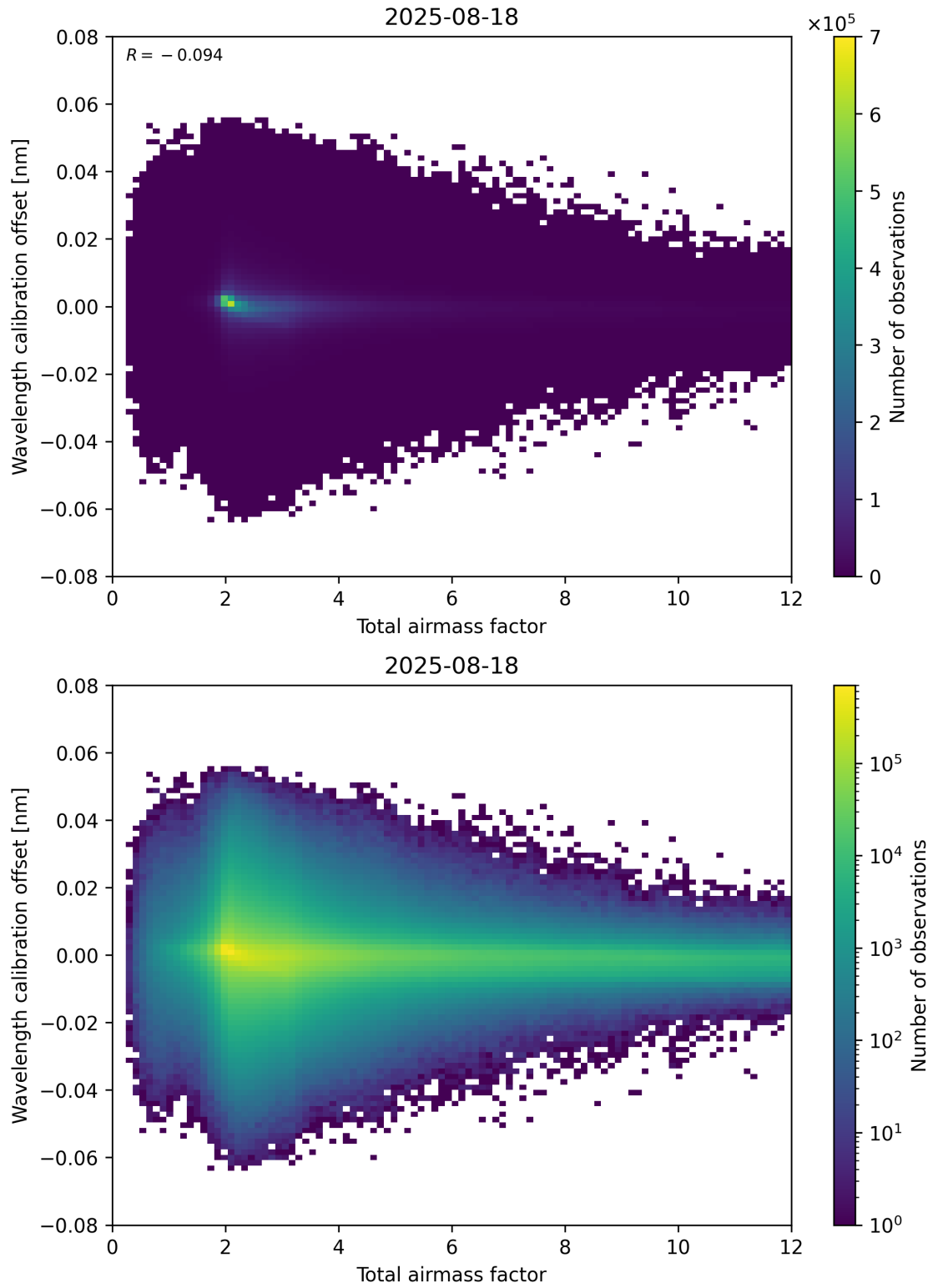
Figure 70: Scatter density plot of “Total airmass factor” against “Wavelength calibration offset” for 2025-08-17 to 2025-08-19.
