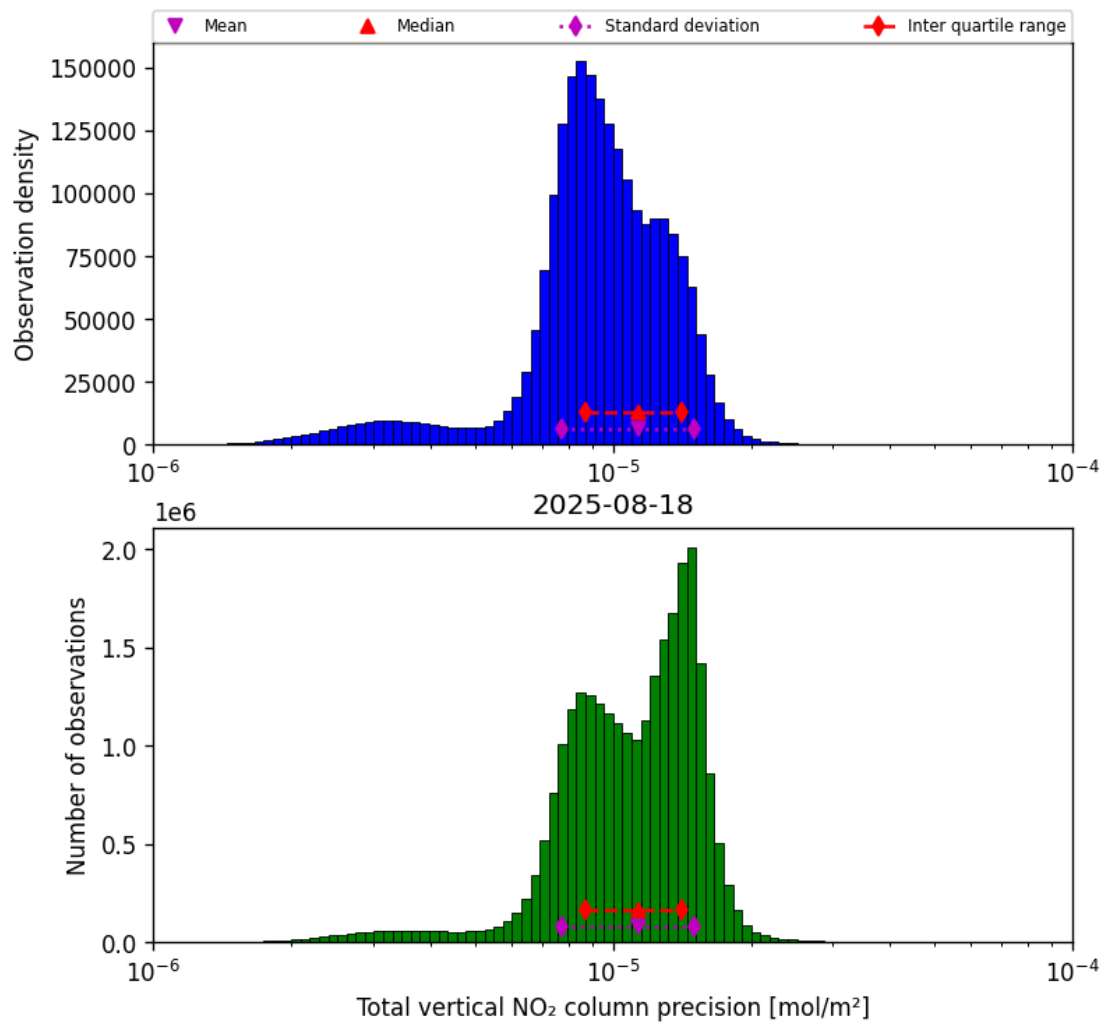
Figure 39: Histogram of “Total vertical NO 2 column precision” for 2025-08-17 to 2025-08-19
