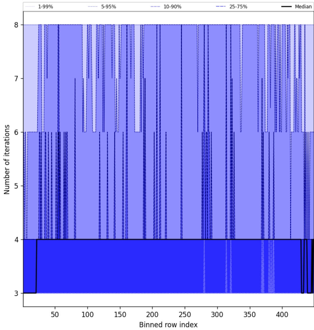
Figure 51: Along track statistics of "Number of iterations" for 2025-08-17 to 2025-08-19
