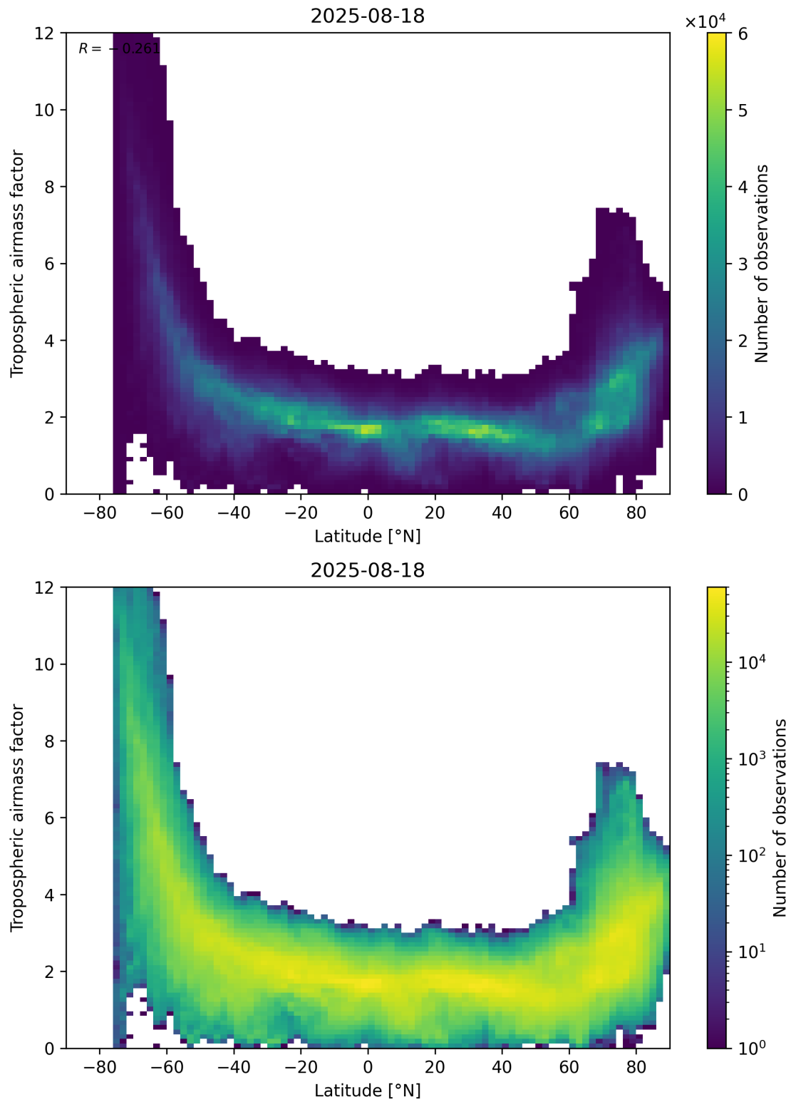
Figure 85: Scatter density plot of “Latitude” against “Tropospheric air mass factor” for 2025-08-17 to 2025-08-19.
