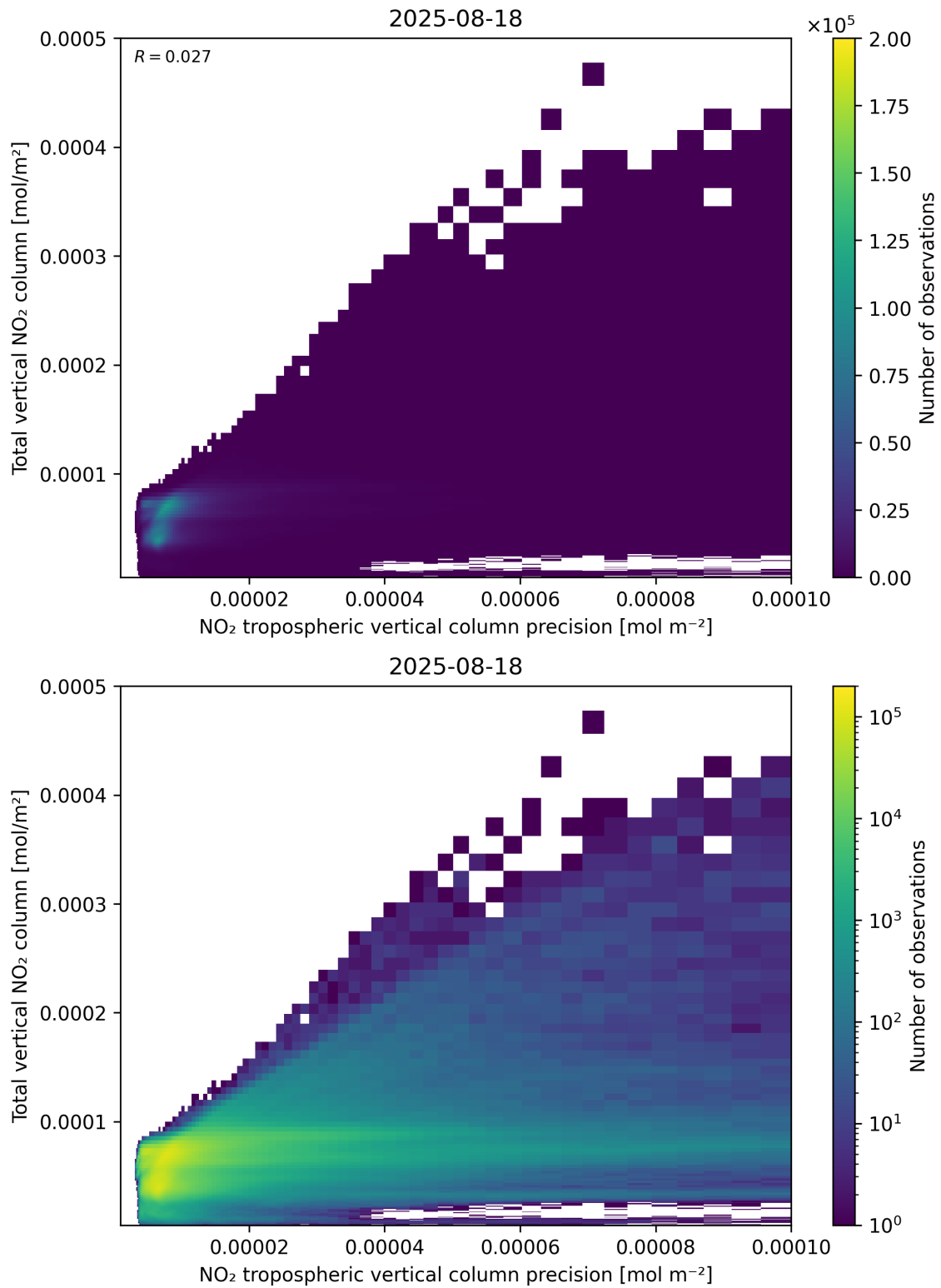
Figure 138: Scatter density plot of “NO 2 tropospheric vertical column precision” against “Total vertical NO 2 column” for 2025-08-17 to 2025-08-19.
