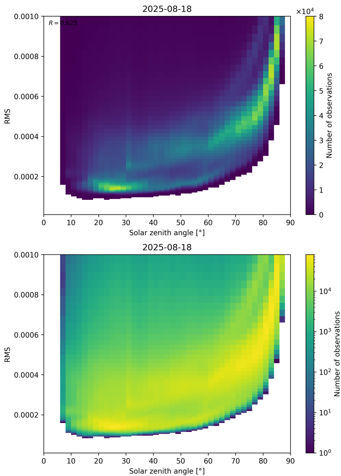
Figure 157: Scatter density plot of “Solar zenith angle” against “RMS” for 2025-08-17 to 2025-08-19.
