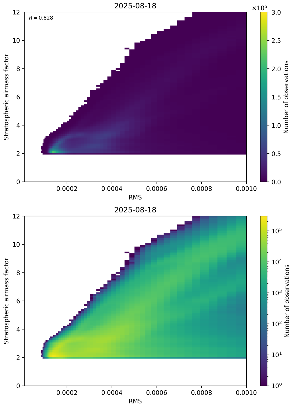
Figure 144: Scatter density plot of “RMS” against “Stratospheric airmass factor” for 2025-08-17 to 2025-08-19.
