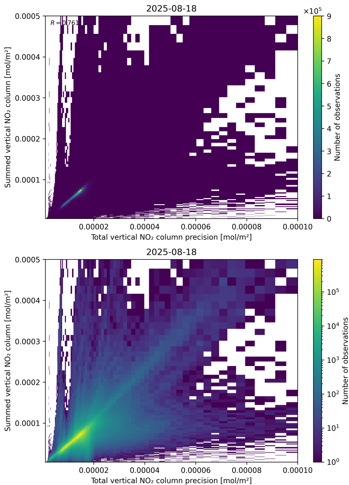
Figure 117: Scatter density plot of “Total vertical NO 2 column precision” against “Summed vertical NO 2 column” for 2025-08-17 to 2025-08-19.
