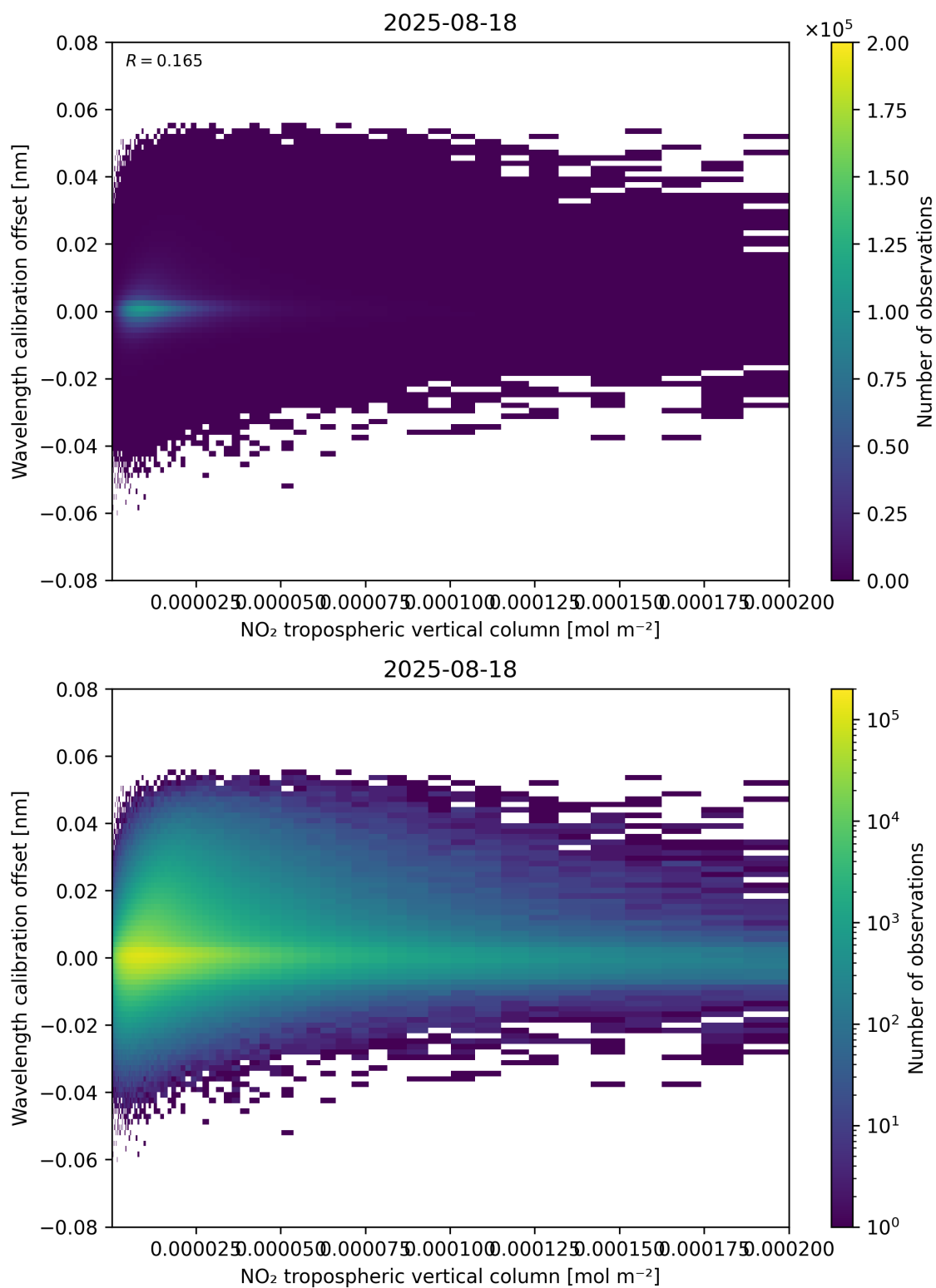
Figure 143: Scatter density plot of “NO 2 tropospheric vertical column” against “Wavelength calibration offset” for 2025-08-17 to 2025-08-19.
