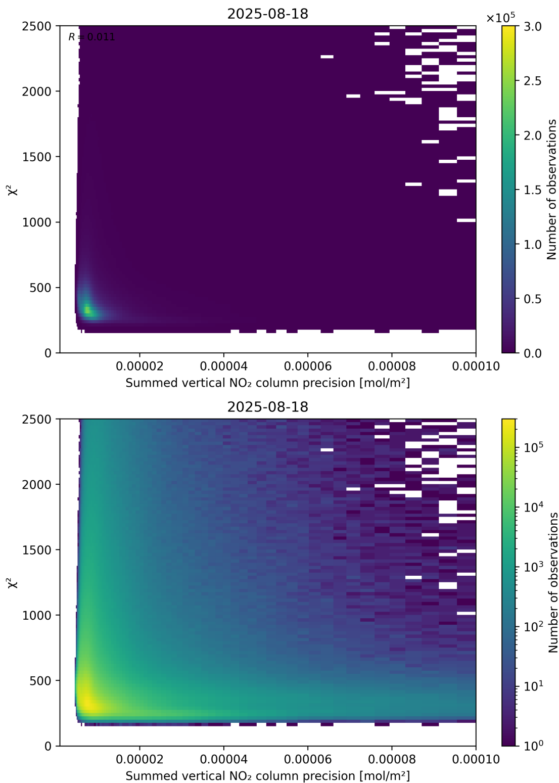
Figure 107: Scatter density plot of “Summed vertical NO 2 column precision” against “ \chi^2 ” for 2025-08-17 to 2025-08-19.
