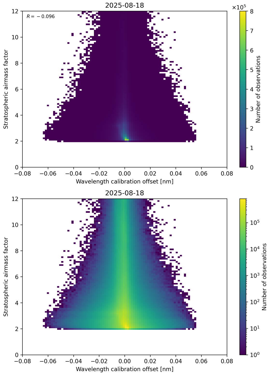
Figure 174: Scatter density plot of “Wavelength calibration offset” against “Stratospheric airmass factor” for 2025-08-17 to 2025-08-19.
