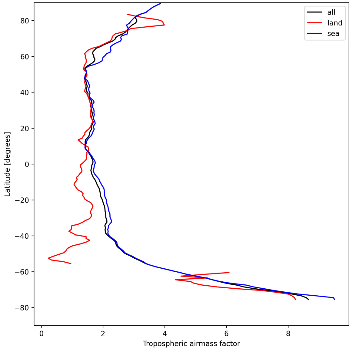
Figure 14: Zonal average of “Tropospheric airmass factor” for 2025-08-17 to 2025-08-19.
