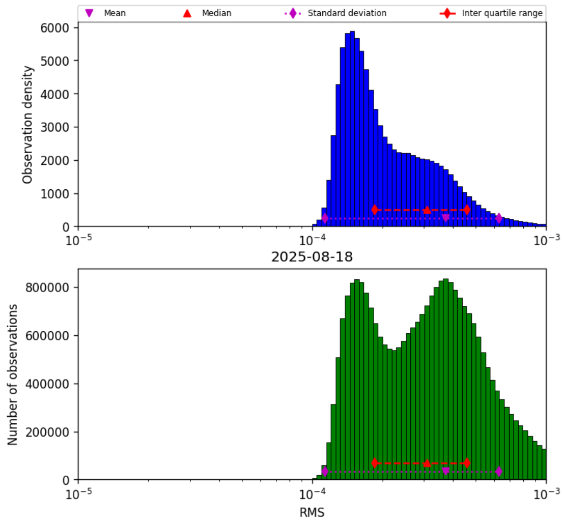
Figure 43: Histogram of “RMS” for 2025-08-17 to 2025-08-19
