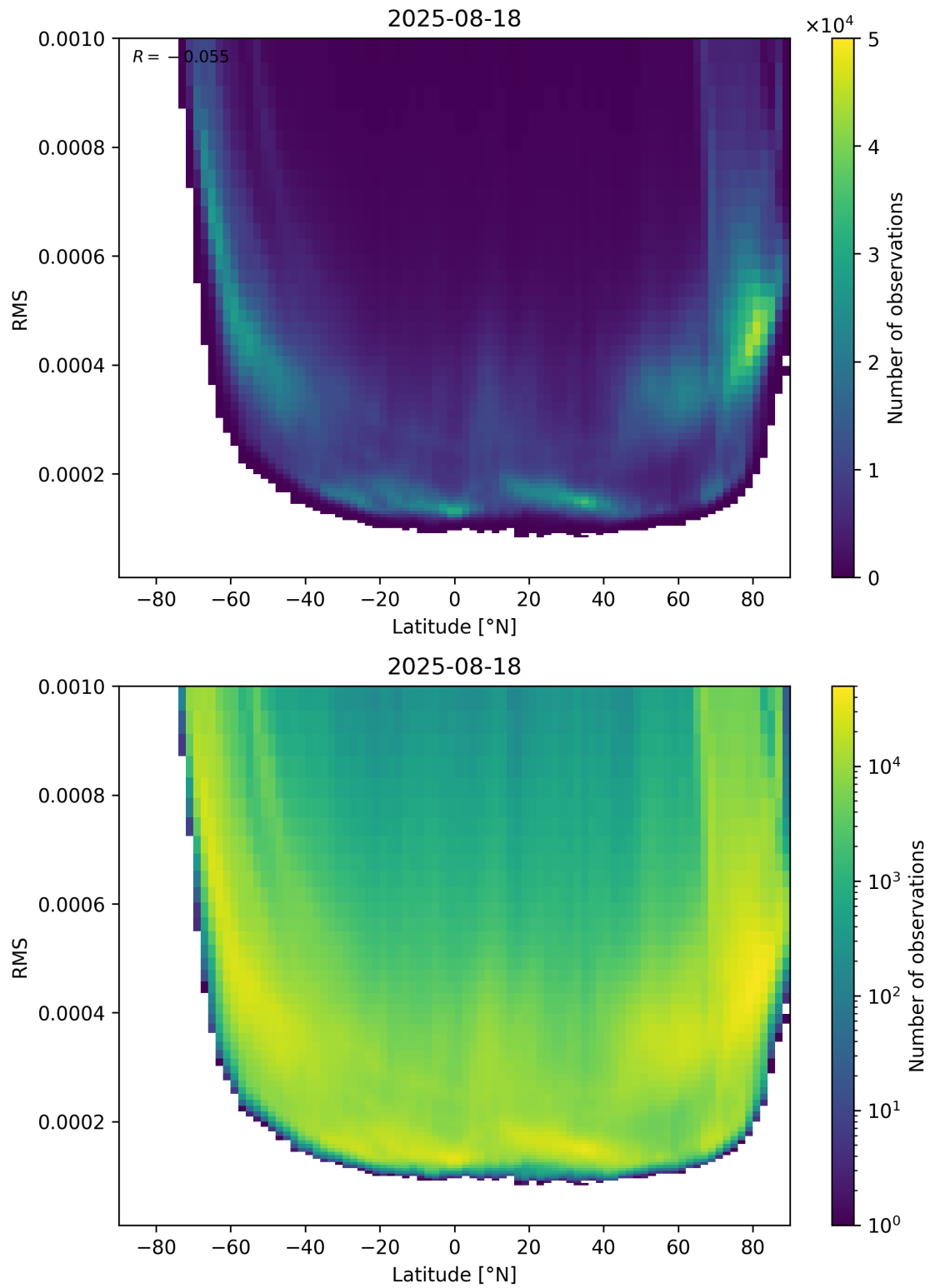
Figure 94: Scatter density plot of “Latitude” against “RMS” for 2025-08-17 to 2025-08-19.
