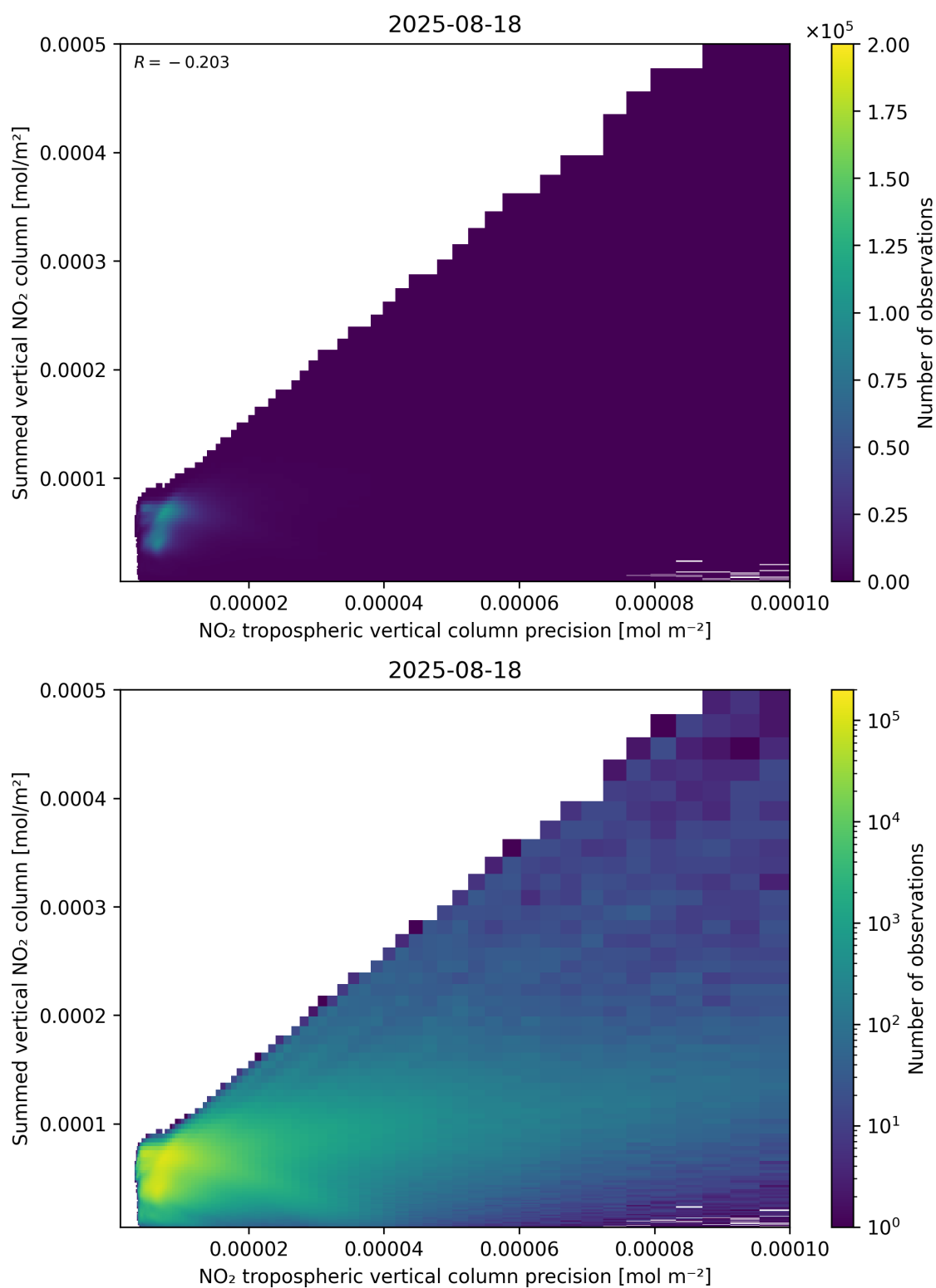
Figure 136: Scatter density plot of “NO 2 tropospheric vertical column precision” against “Summed vertical NO 2 column” for 2025-08-17 to 2025-08-19.
