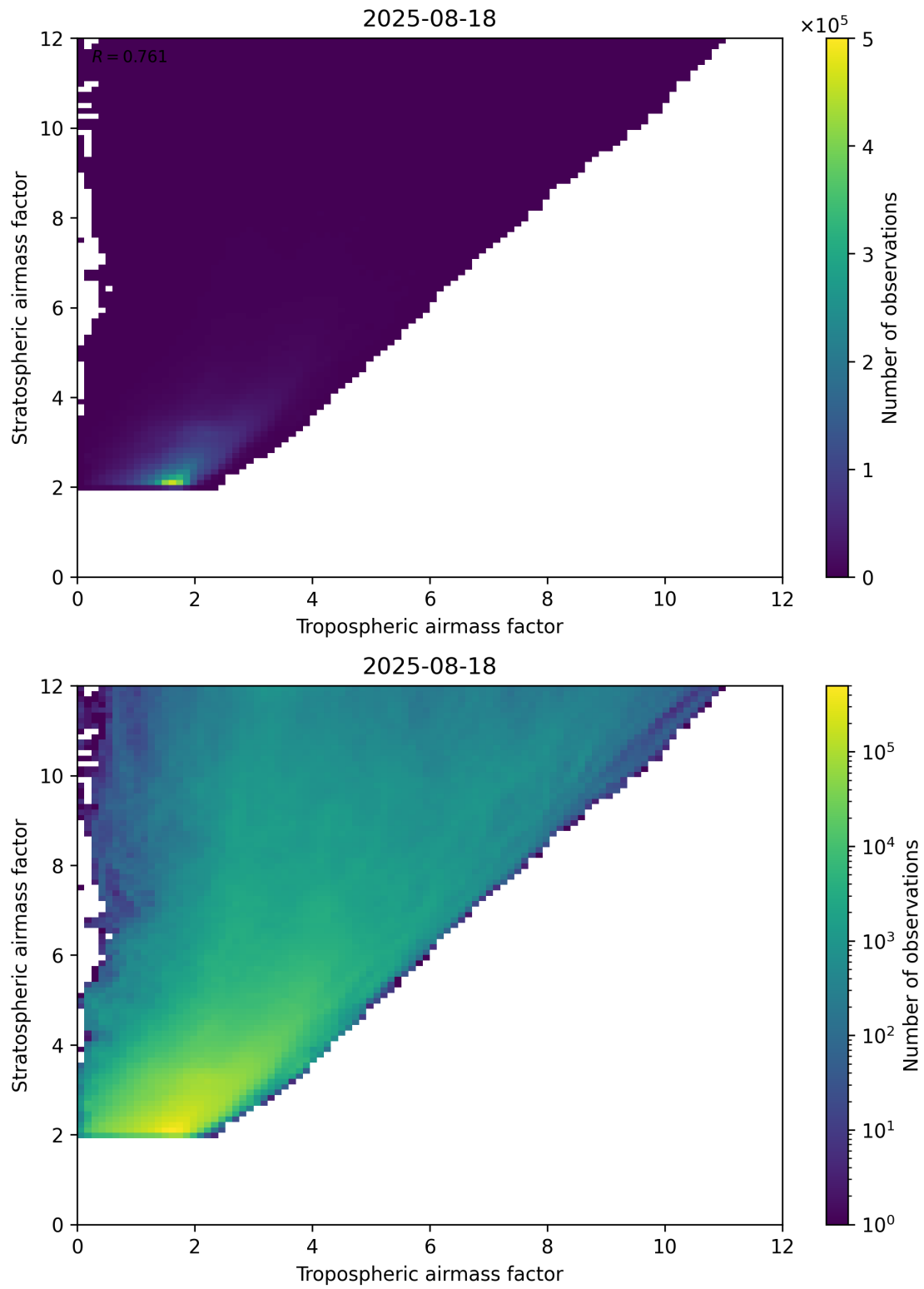
Figure 71: Scatter density plot of “Tropospheric airmass factor” against “Stratospheric airmass factor” for 2025-08-17 to 2025-08-19.
