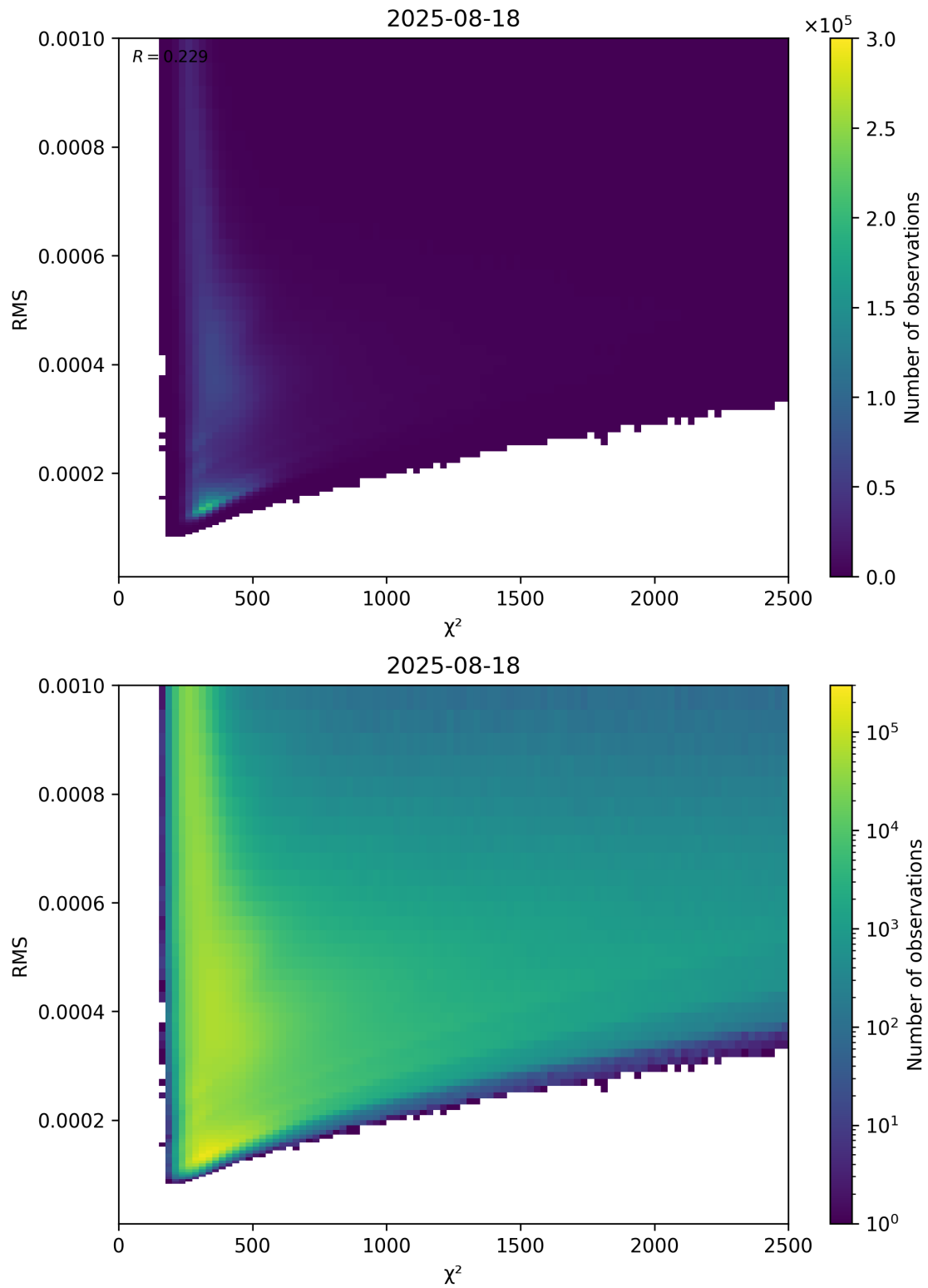
Figure 82: Scatter density plot of “ \chi^2 ” against “RMS” for 2025-08-17 to 2025-08-19.
