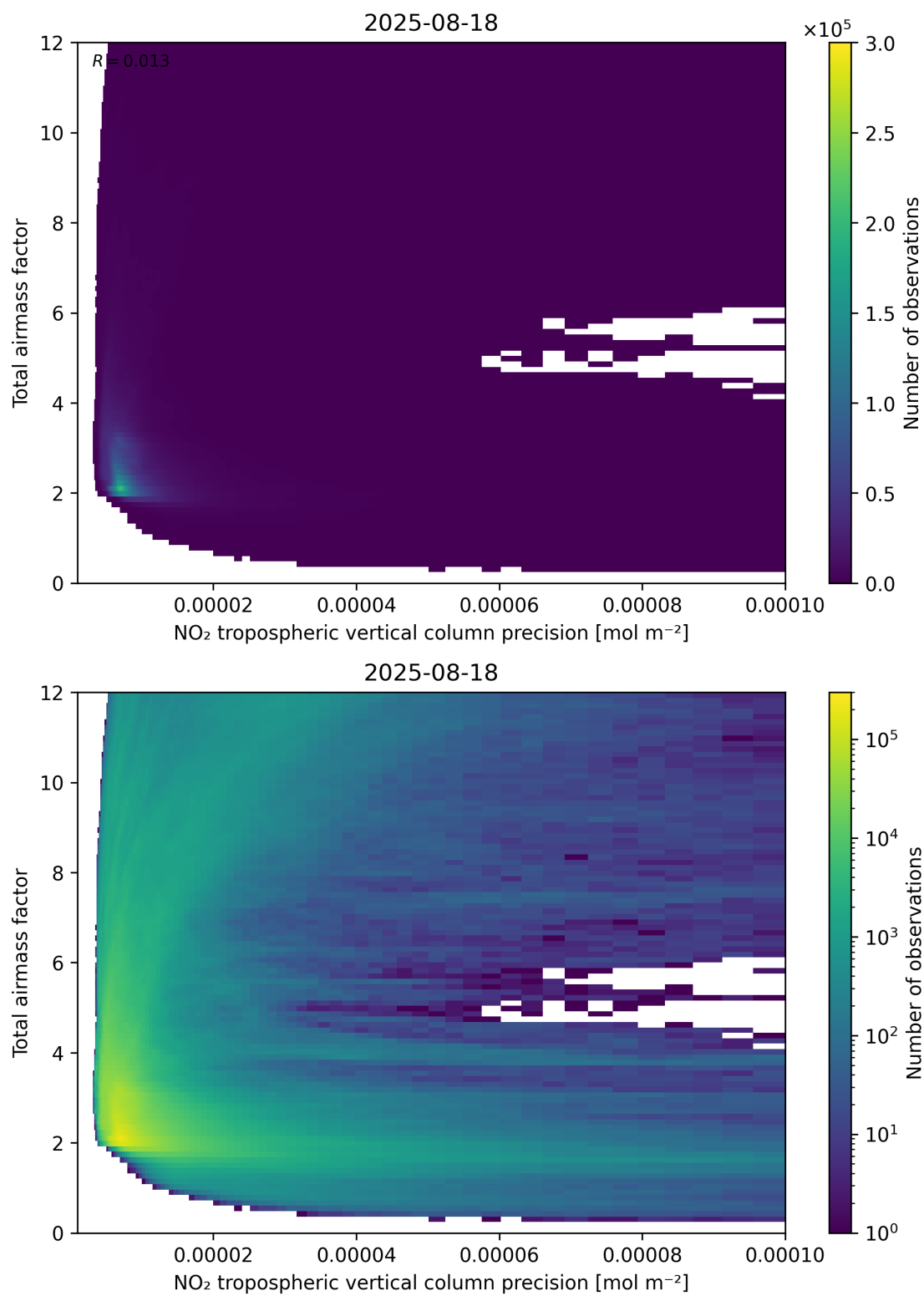
Figure 132: Scatter density plot of “NO 2 tropospheric vertical column precision” against “Total air mass factor” for 2025-08-17 to 2025-08-19.
