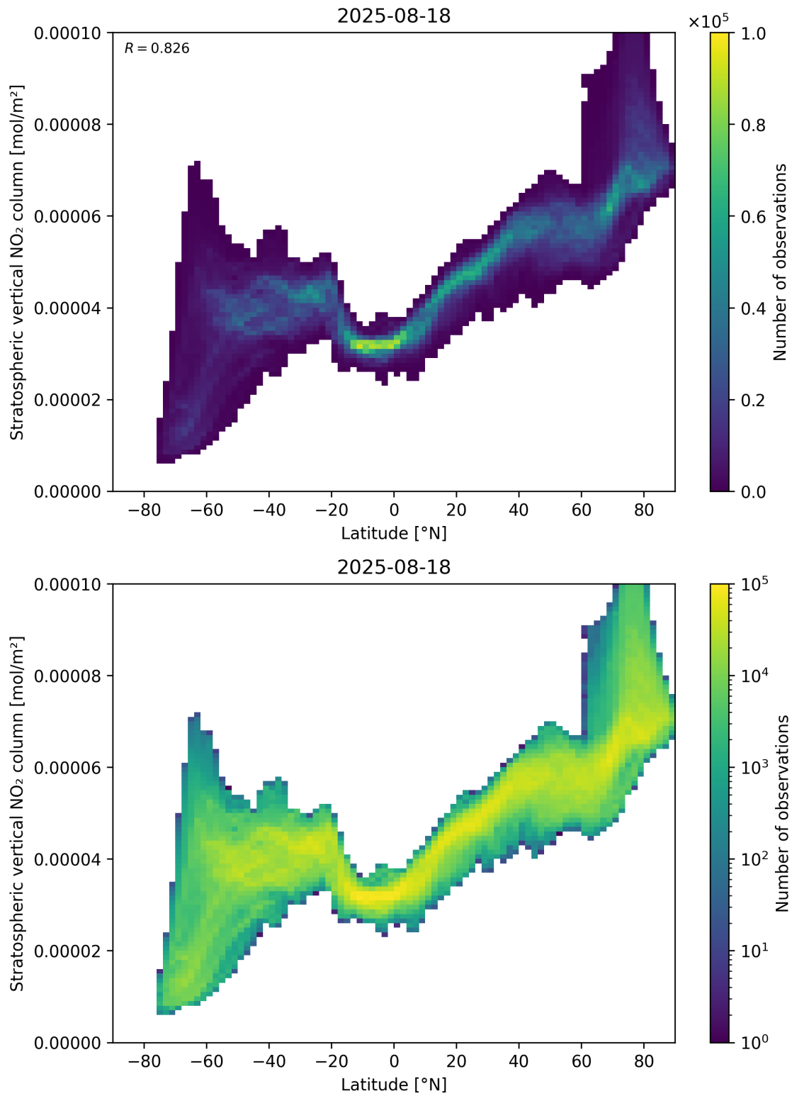
Figure 87: Scatter density plot of “Latitude” against “Stratospheric vertical NO 2 column” for 2025-08-17 to 2025-08-19.
