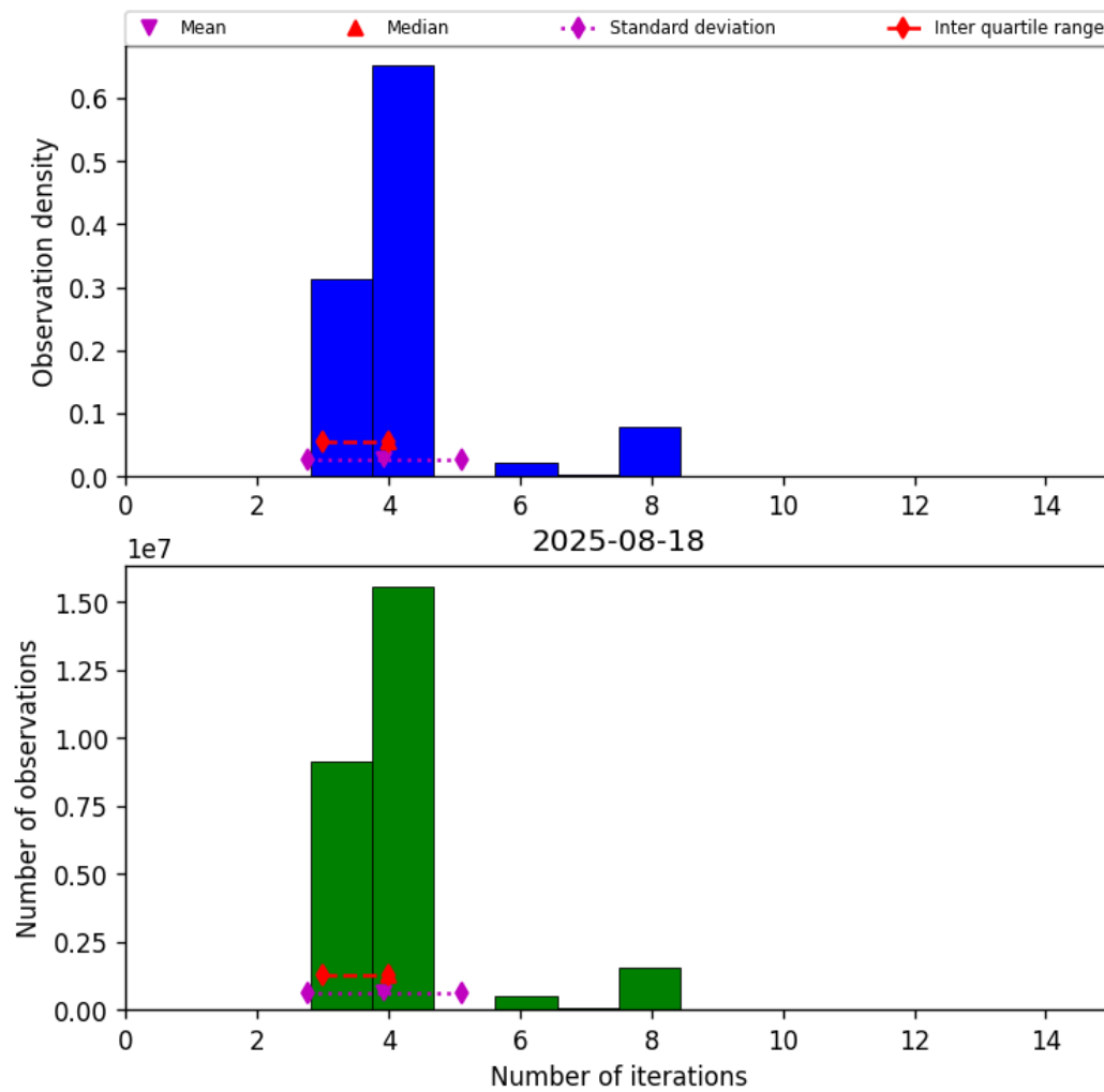
Figure 34: Histogram of “Number of iterations” for 2025-08-17 to 2025-08-19
