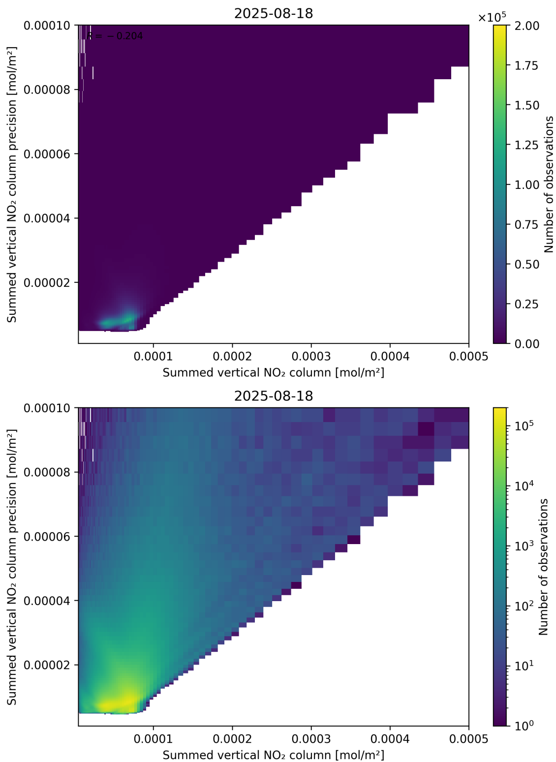
Figure 105: Scatter density plot of “Summed vertical NO 2 column” against “Summed vertical NO 2 column precision” for 2025-08-17 to 2025-08-19.
