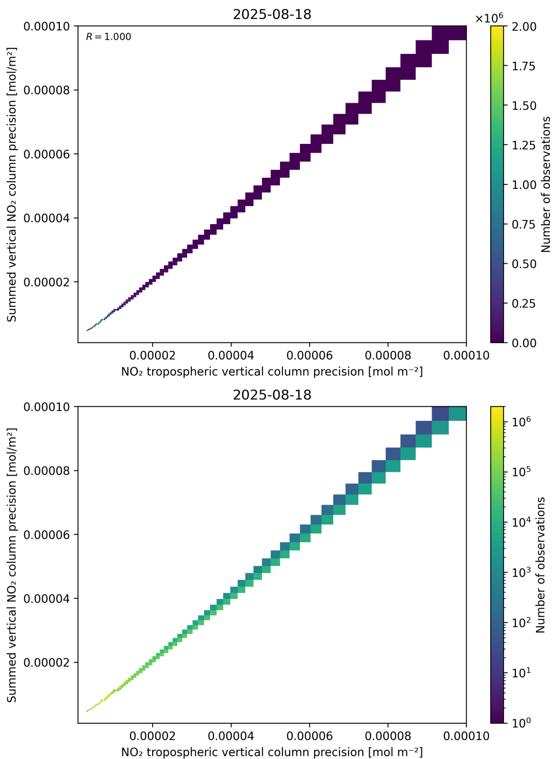
Figure 137: Scatter density plot of “NO 2 tropospheric vertical column precision” against “Summed vertical NO 2 column precision” for 2025-08-17 to 2025-08-19.
