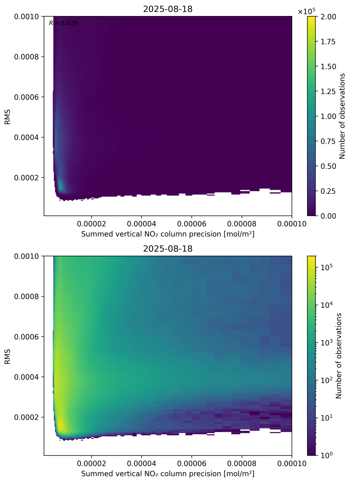
Figure 108: Scatter density plot of “Summed vertical NO 2 column precision” against “RMS” for 2025-08-17 to 2025-08-19.
