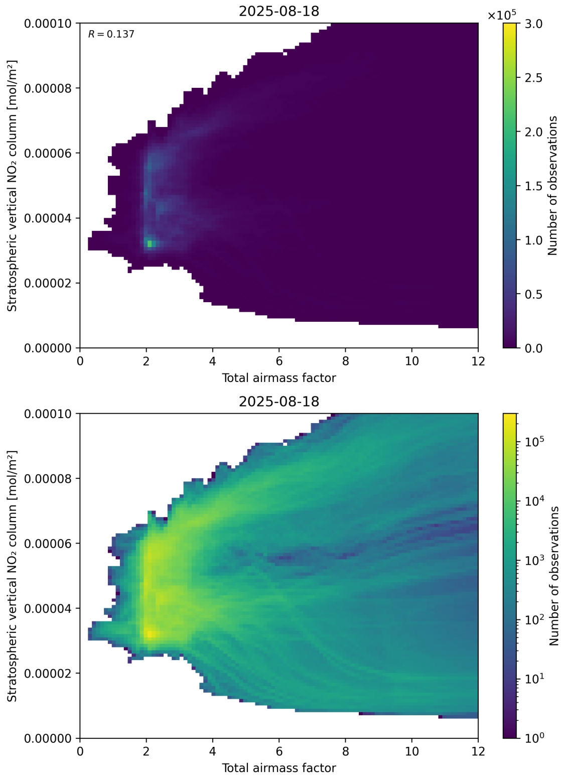
Figure 64: Scatter density plot of “Total airmass factor” against “Stratospheric vertical \text{NO}_2 column” for 2025-08-17 to 2025-08-19.
