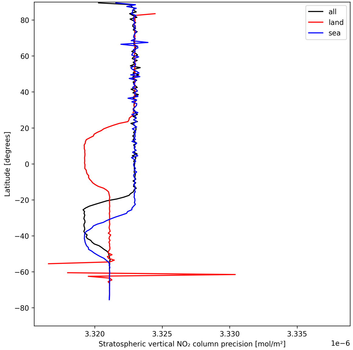
Figure 20: Zonal average of “Stratospheric vertical NO 2 column precision” for 2025-08-17 to 2025-08-19.
