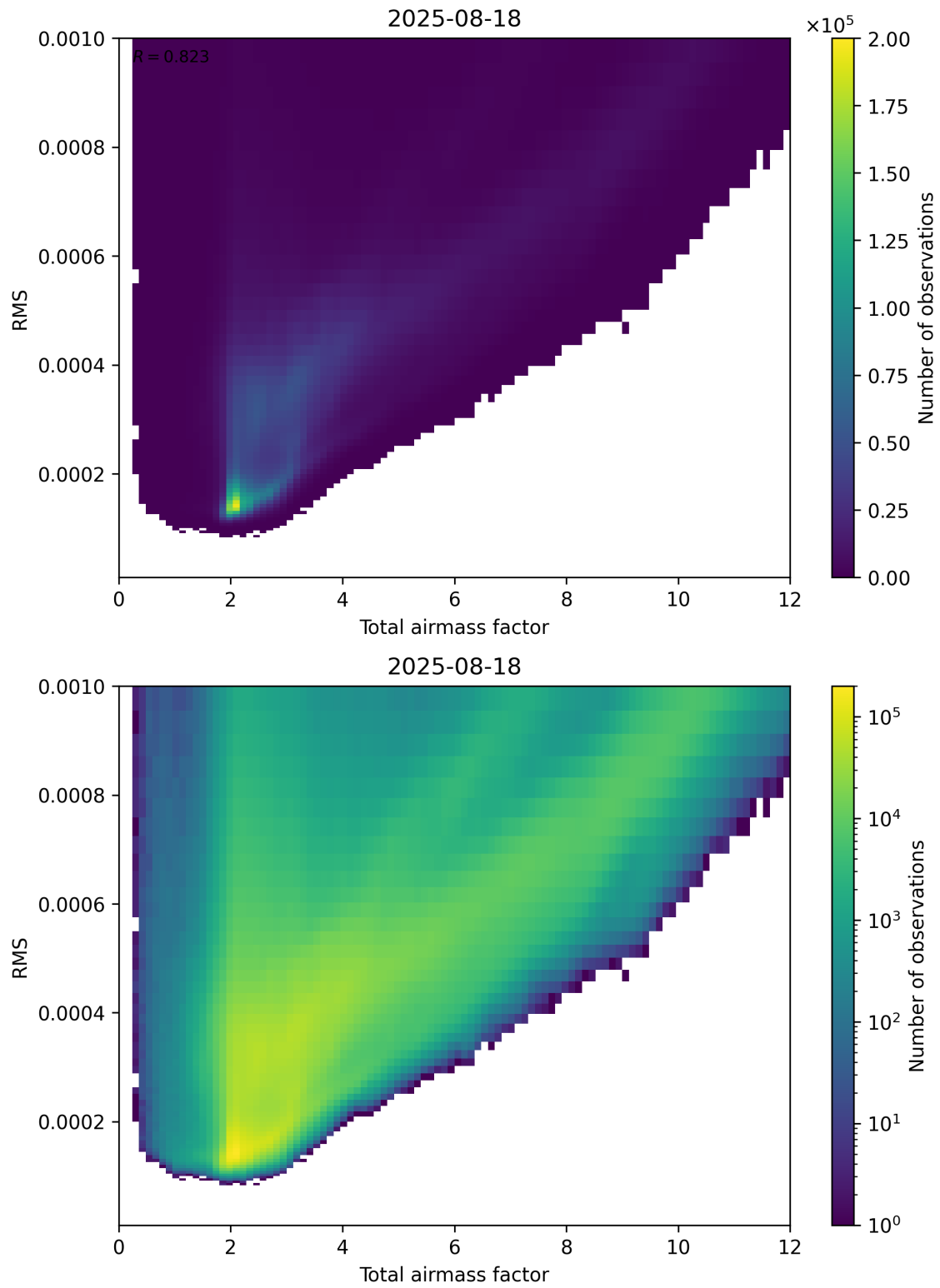
Figure 69: Scatter density plot of “Total airmass factor” against “RMS” for 2025-08-17 to 2025-08-19.
