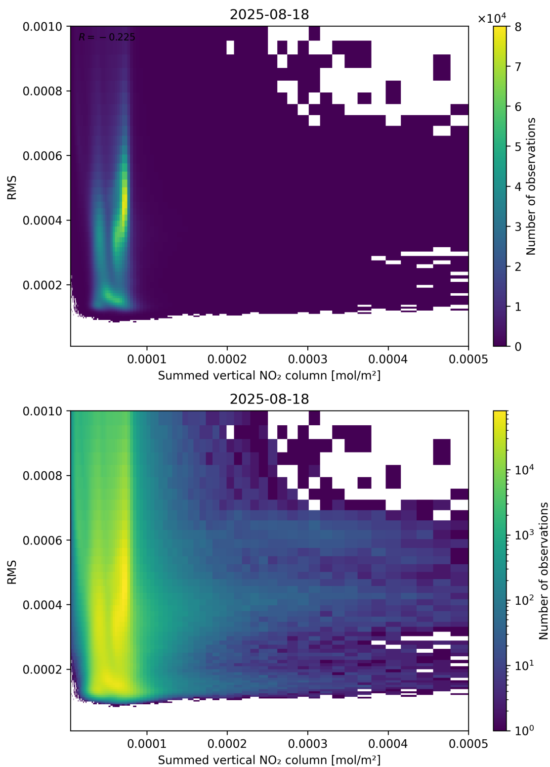
Figure 109: Scatter density plot of “Summed vertical NO 2 column” against “RMS” for 2025-08-17 to 2025-08-19.
