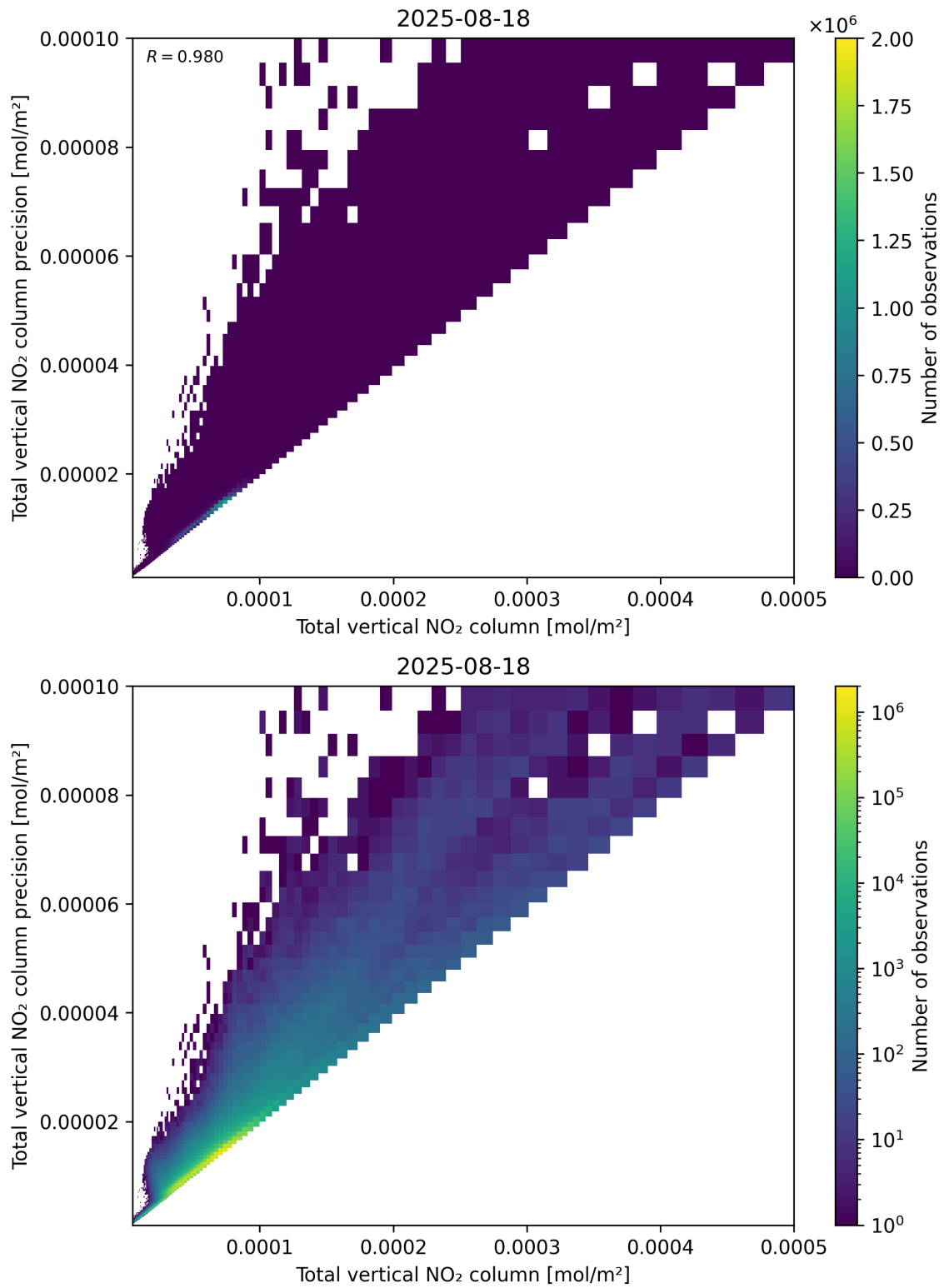
Figure 114: Scatter density plot of “Total vertical NO 2 column” against “Total vertical NO 2 column precision” for 2025-08-17 to 2025-08-19.
