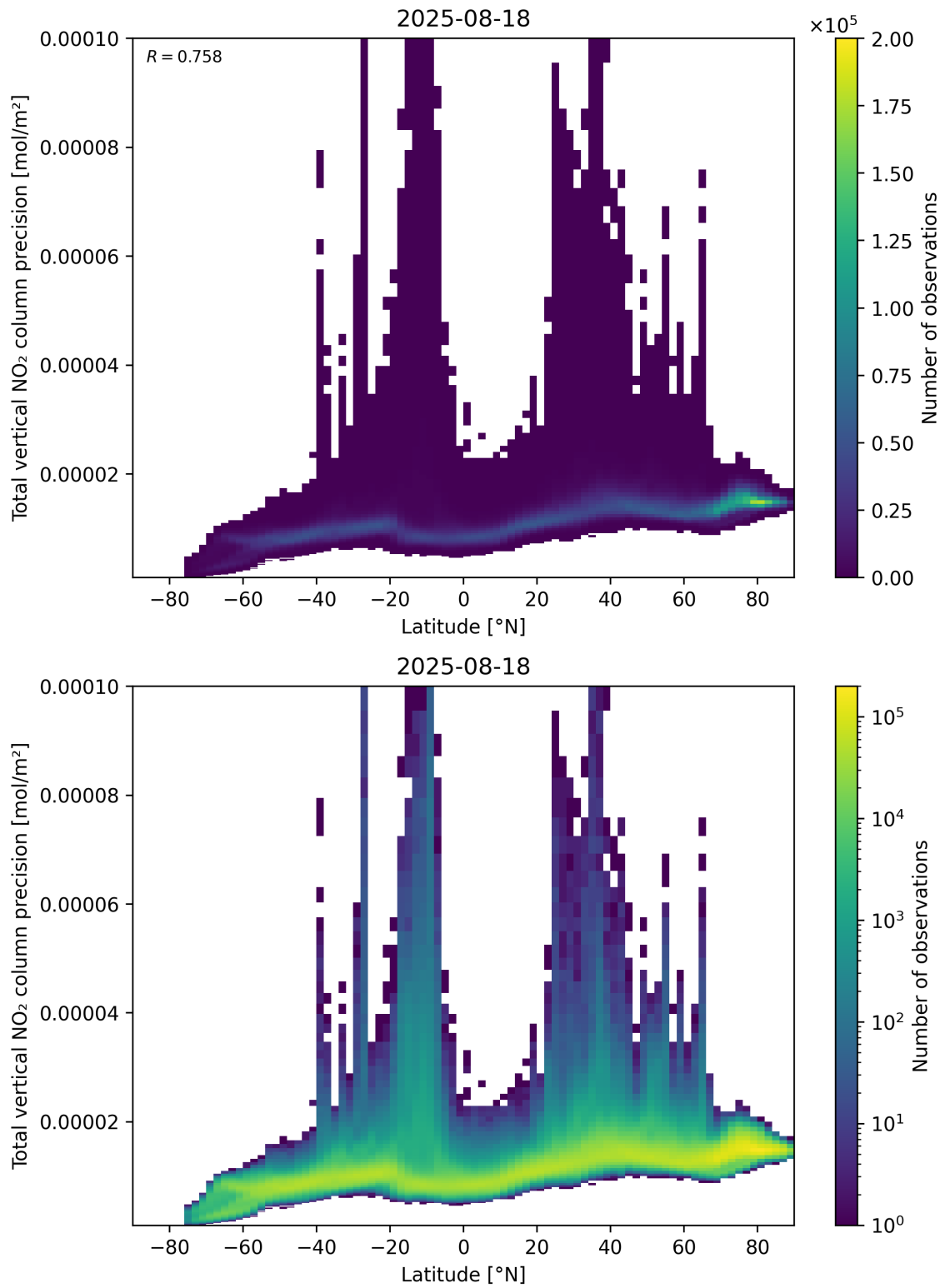
Figure 91: Scatter density plot of “Latitude” against “Total vertical NO 2 column precision” for 2025-08-17 to 2025-08-19.
