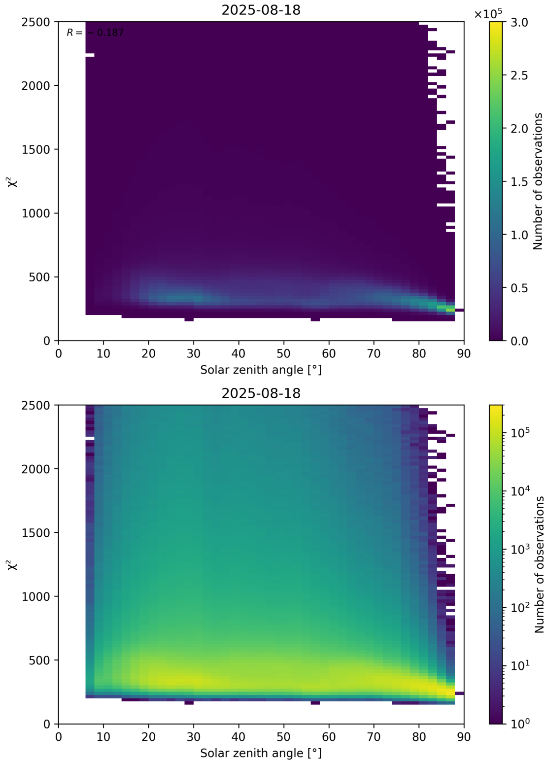
Figure 148: Scatter density plot of “Solar zenith angle” against “ \chi^2 ” for 2025-08-17 to 2025-08-19.
