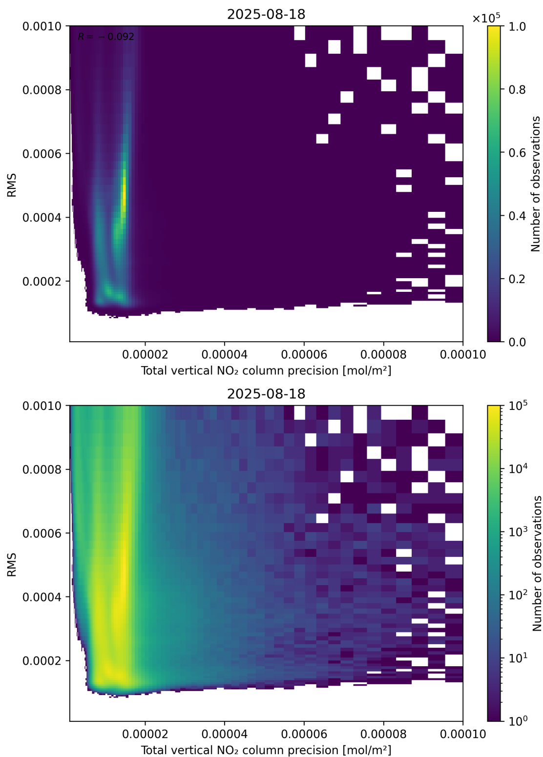
Figure 119: Scatter density plot of “Total vertical NO 2 column precision” against “RMS” for 2025-08-17 to 2025-08-19.
