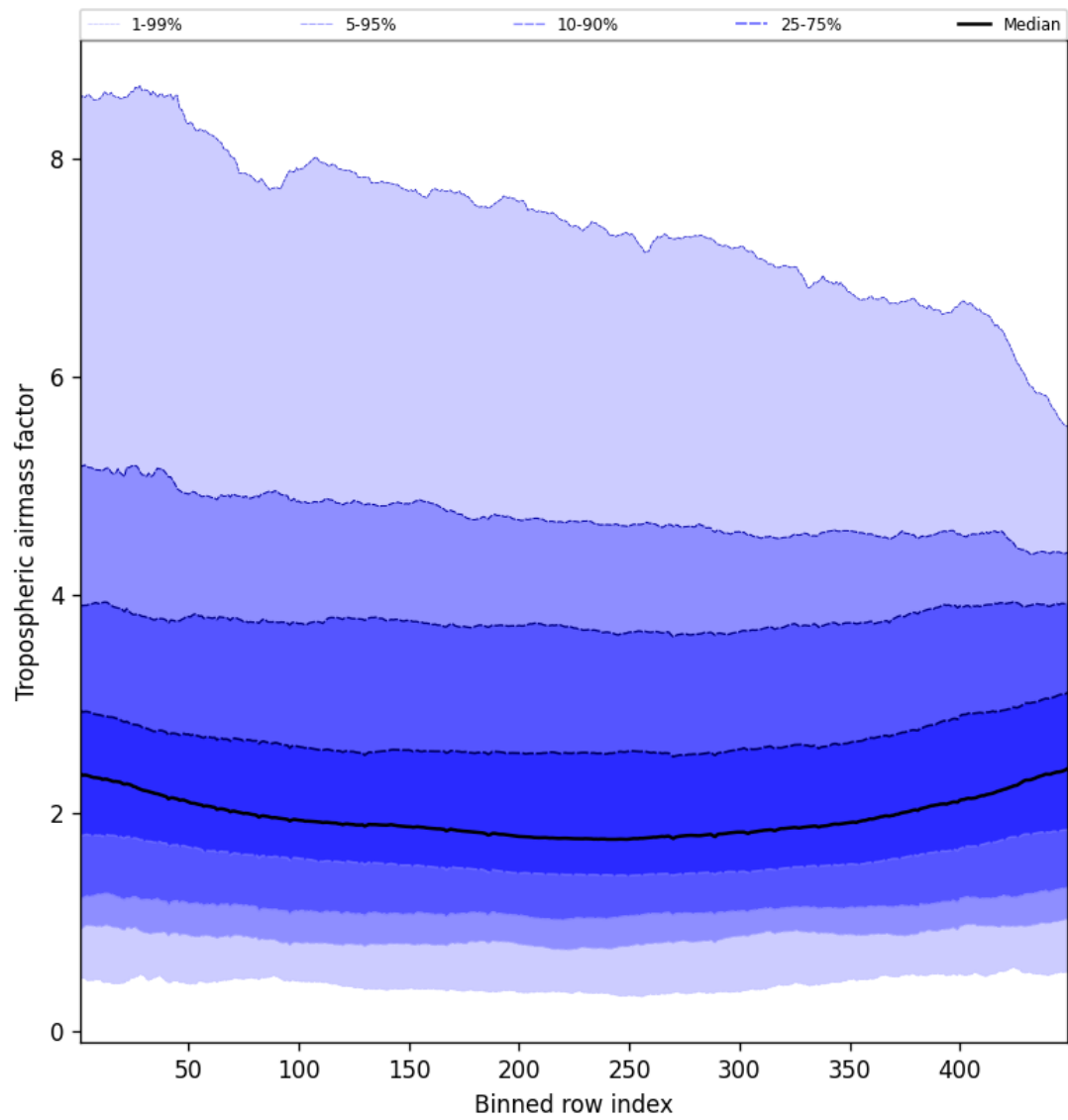
Figure 48: Along track statistics of “Tropospheric air mass factor” for 2025-08-17 to 2025-08-19
