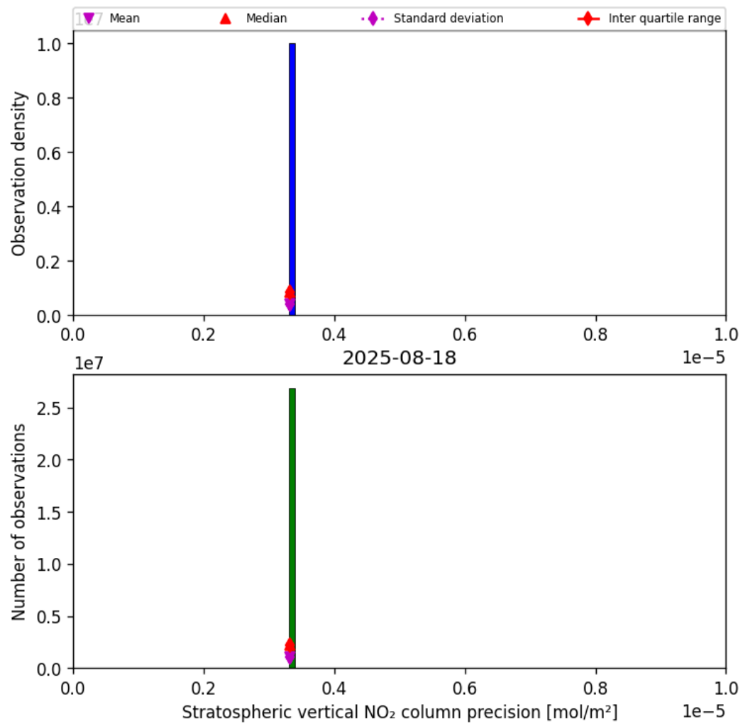
Figure 37: Histogram of “Stratospheric vertical NO 2 column precision” for 2025-08-17 to 2025-08-19
