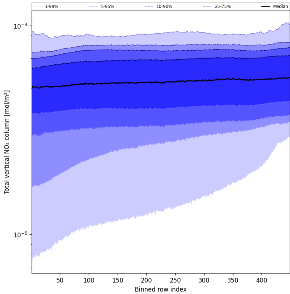
Figure 55: Along track statistics of “Total vertical NO 2 column” for 2025-08-17 to 2025-08-19
