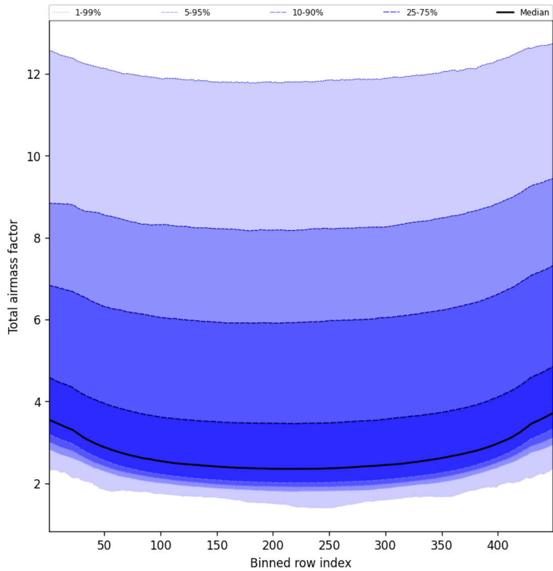
Figure 49: Along track statistics of “Total airmass factor” for 2025-08-17 to 2025-08-19
