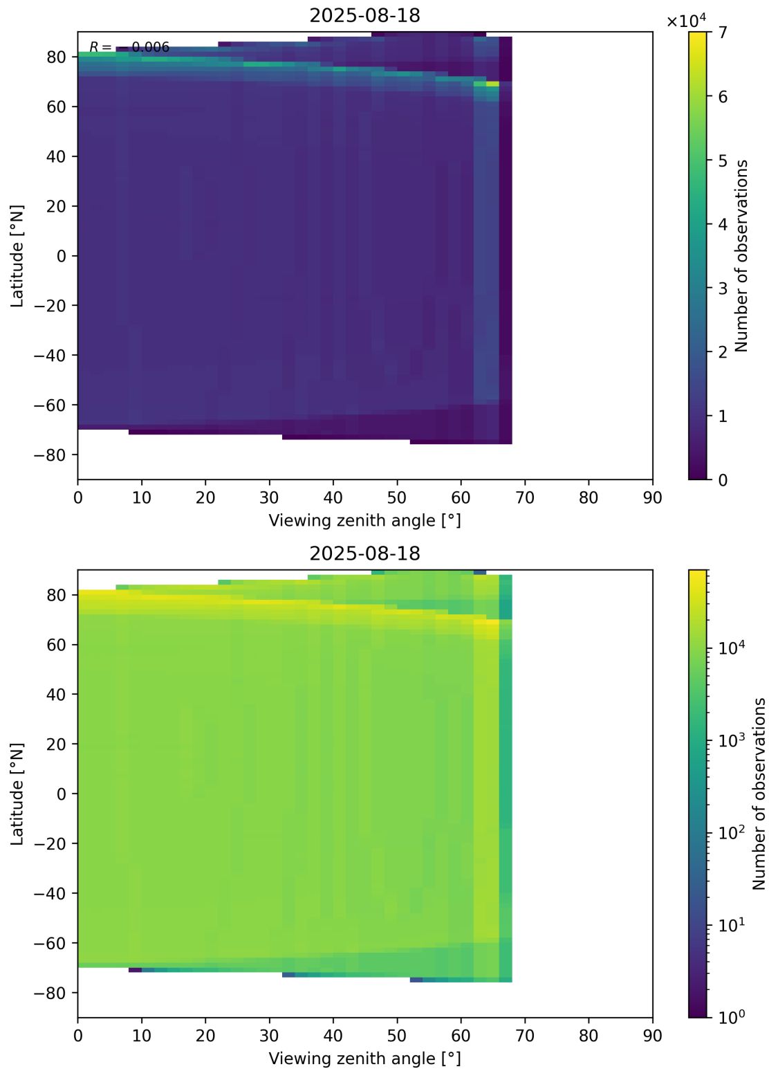
Figure 163: Scatter density plot of “Viewing zenith angle” against “Latitude” for 2025-08-17 to 2025-08-19.
