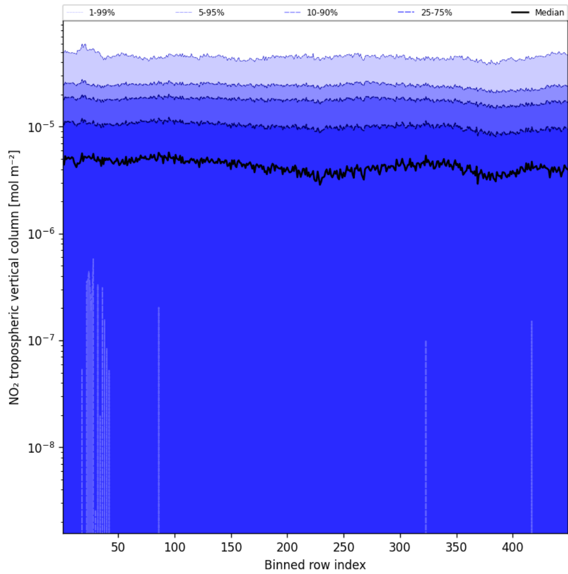
Figure 46: Along track statistics of “NO 2 tropospheric vertical column” for 2025-08-17 to 2025-08-19
