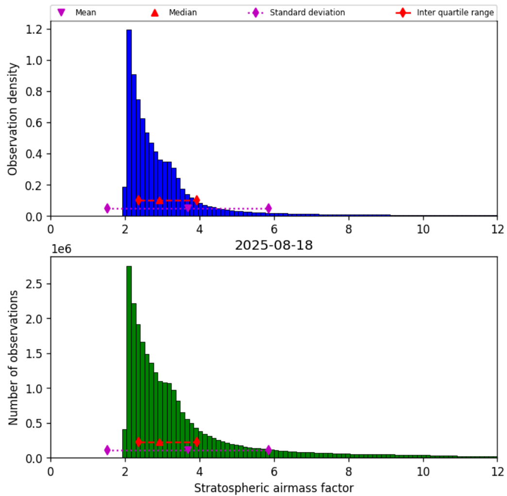
Figure 44: Histogram of “Stratospheric airmass factor” for 2025-08-17 to 2025-08-19
