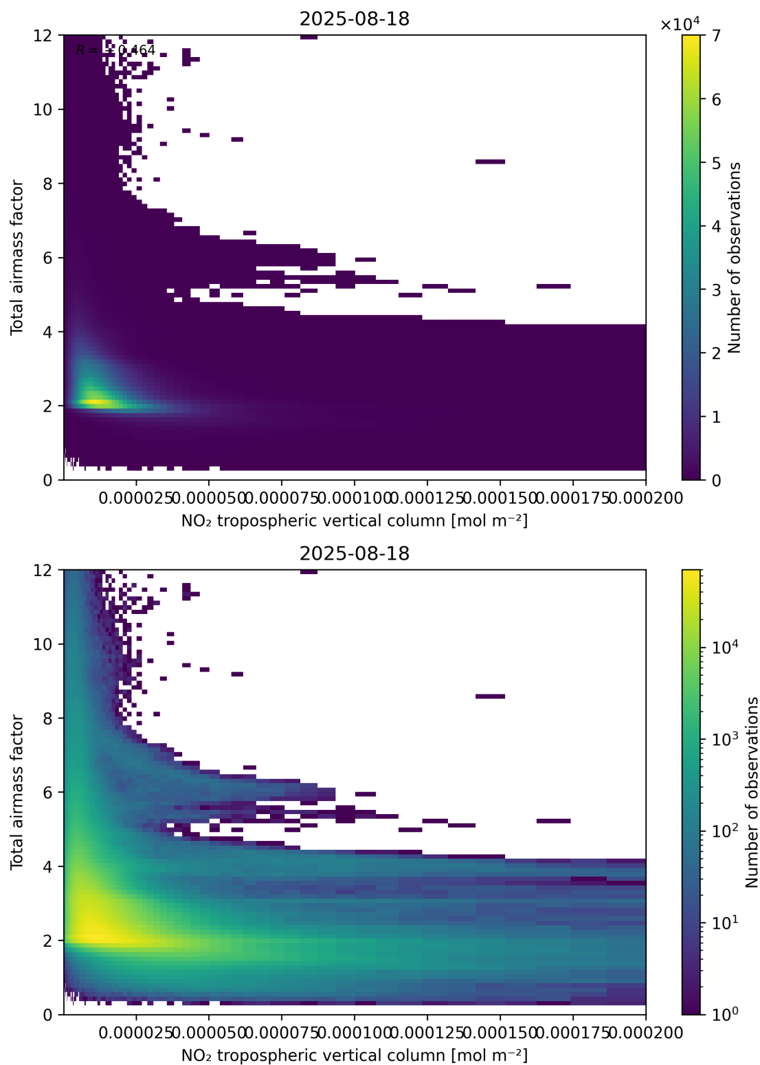
Figure 122: Scatter density plot of “NO 2 tropospheric vertical column” against “Total air mass factor” for 2025-08-17 to 2025-08-19.
