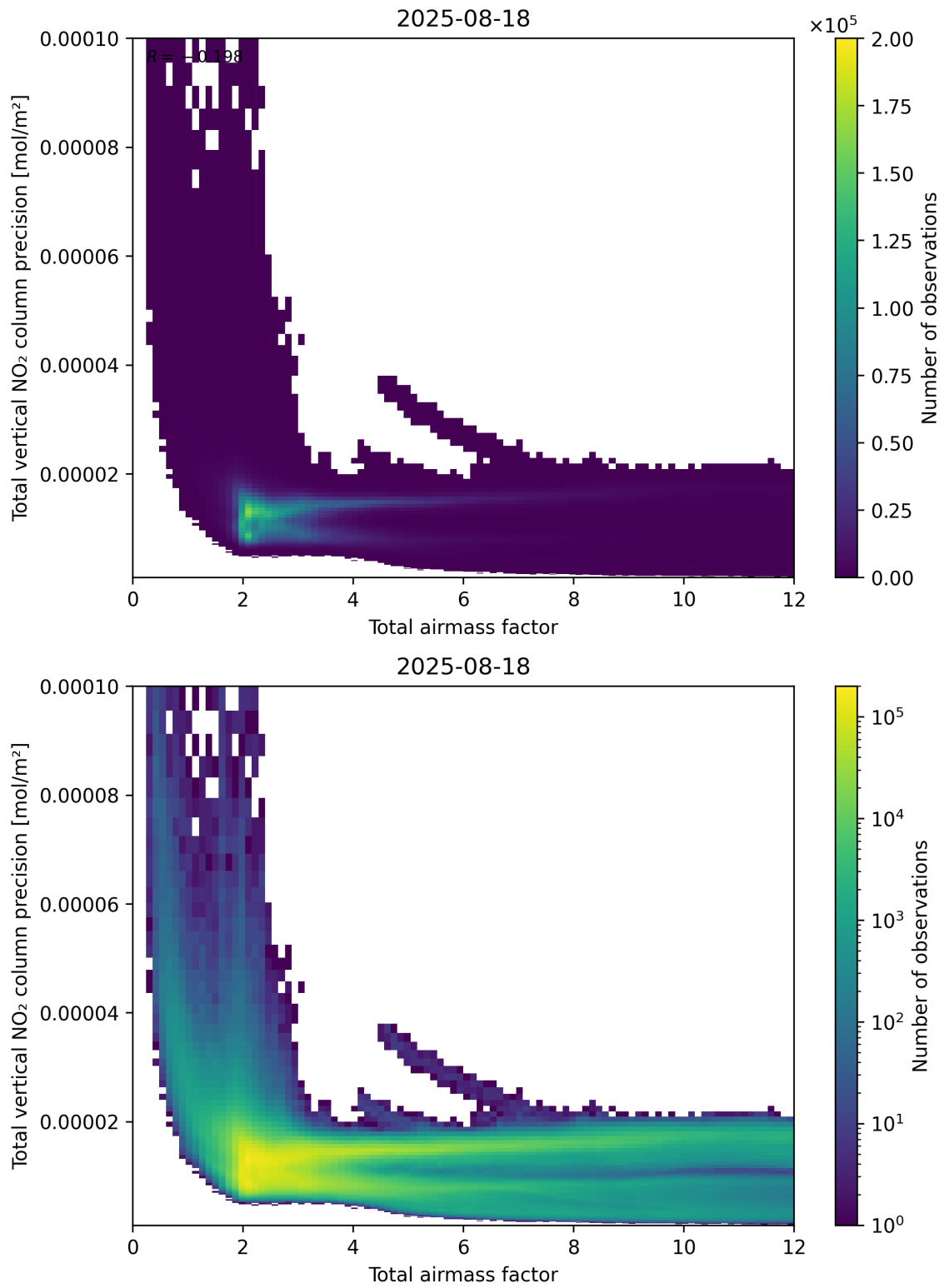
Figure 68: Scatter density plot of “Total airmass factor” against “Total vertical NO 2 column precision” for 2025-08-17 to 2025-08-19.
