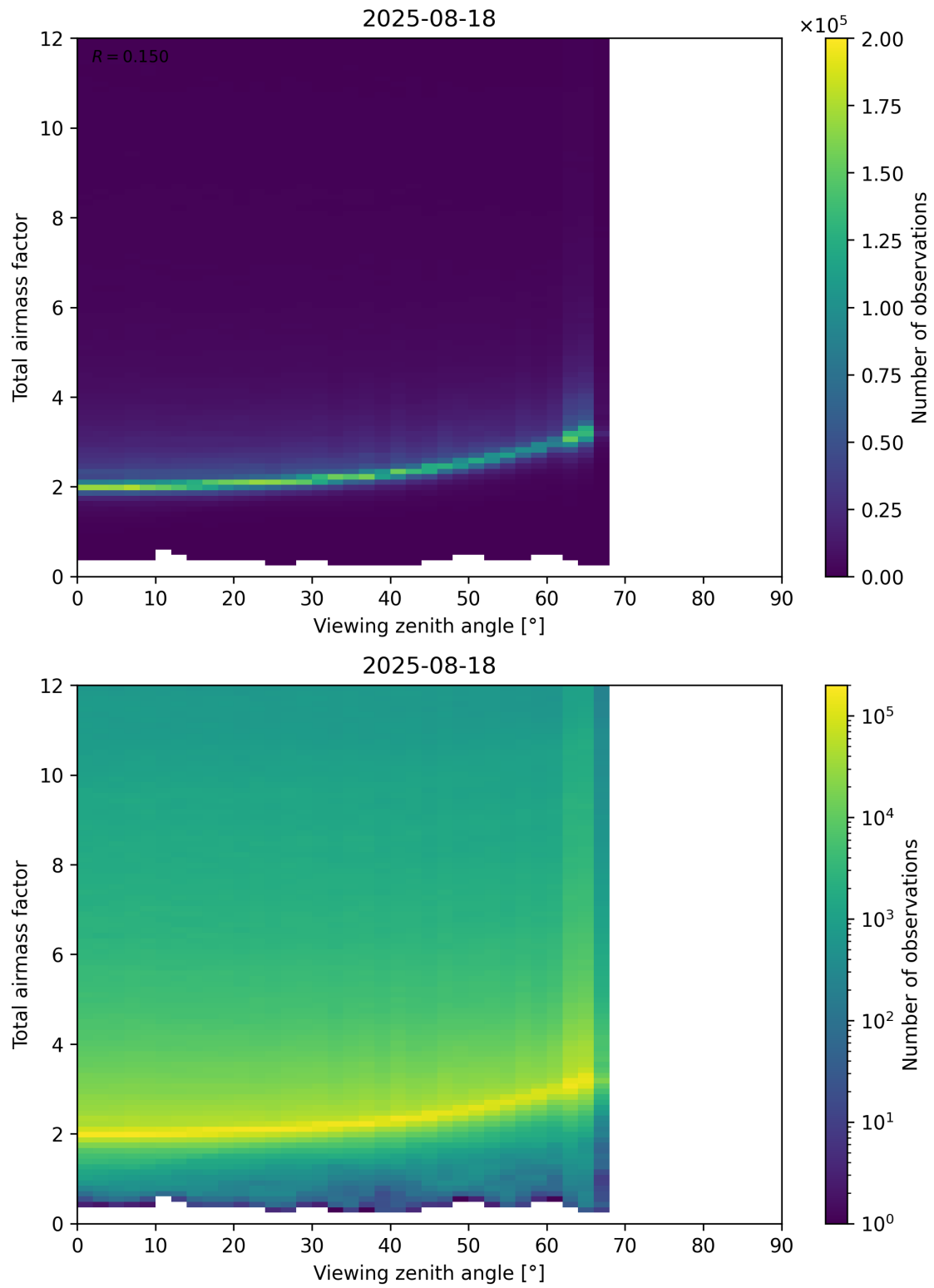
Figure 160: Scatter density plot of “Viewing zenith angle” against “Total airmass factor” for 2025-08-17 to 2025-08-19.
