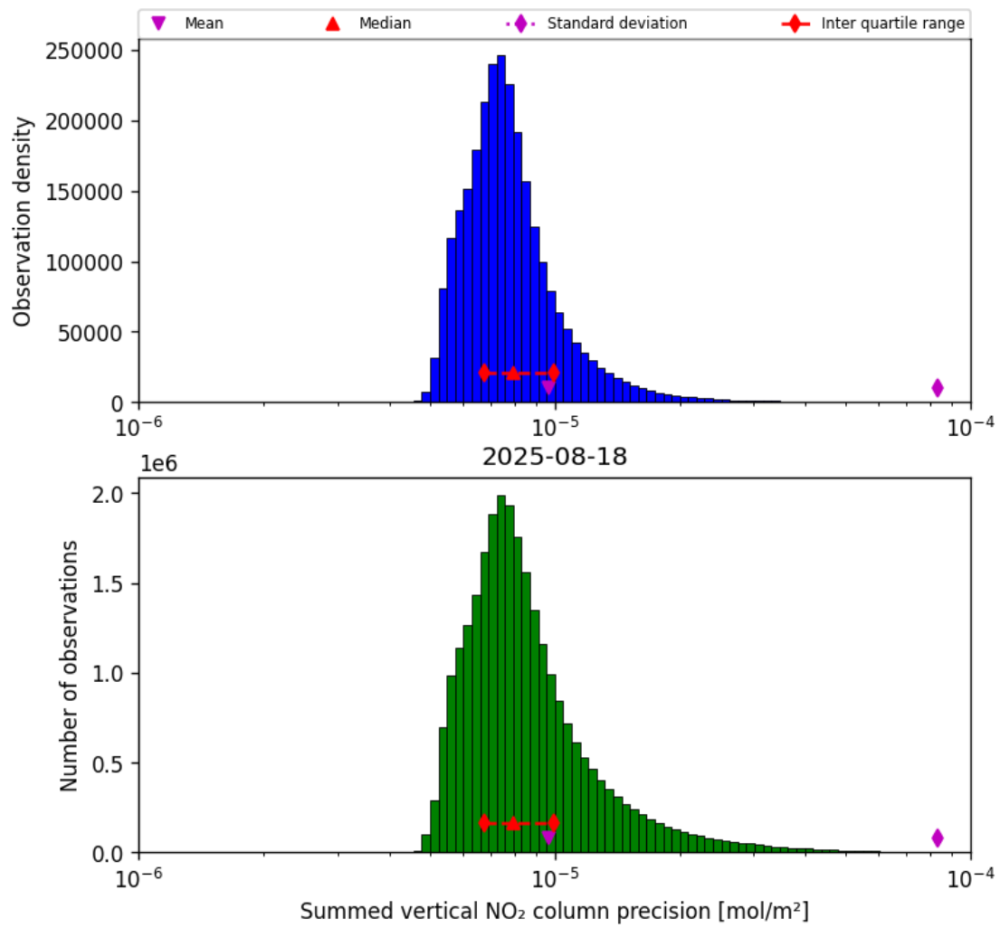
Figure 41: Histogram of "Summed vertical NO 2 column precision" for 2025-08-17 to 2025-08-19
