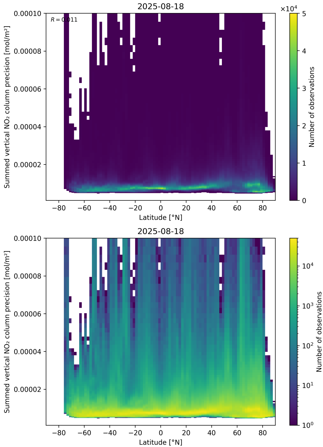
Figure 89: Scatter density plot of “Latitude” against “Summed vertical NO 2 column precision” for 2025-08-17 to 2025-08-19.
