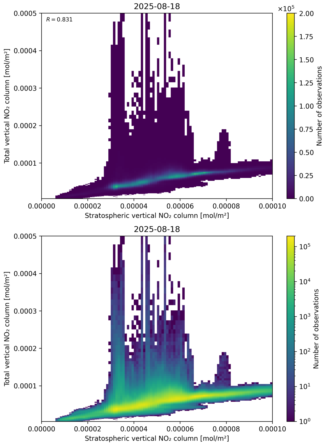
Figure 100: Scatter density plot of “Stratospheric vertical NO 2 column” against “Total vertical NO 2 column” for 2025-08-17 to 2025-08-19.
