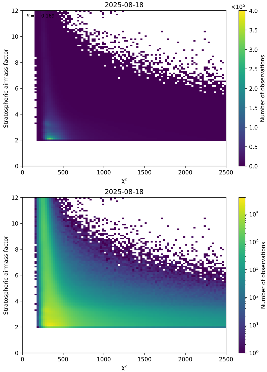
Figure 81: Scatter density plot of “ \chi^2 ” against “Stratospheric air mass factor” for 2025-08-17 to 2025-08-19.
