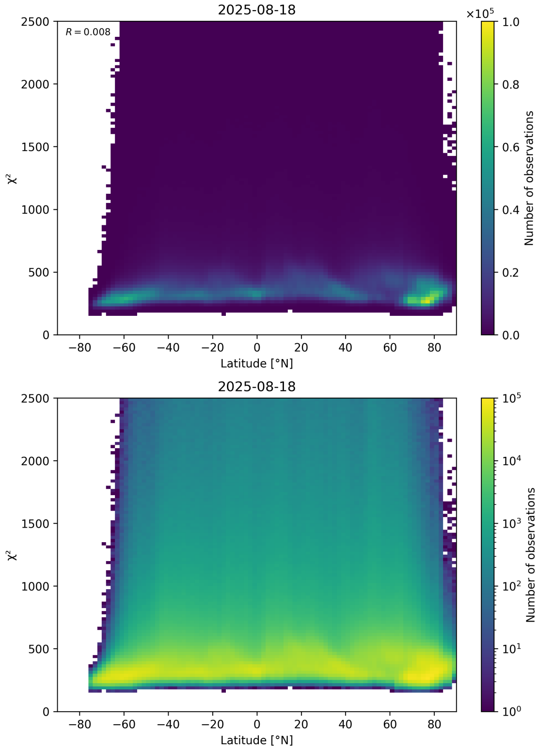
Figure 86: Scatter density plot of “Latitude” against “ \chi^2 ” for 2025-08-17 to 2025-08-19.
