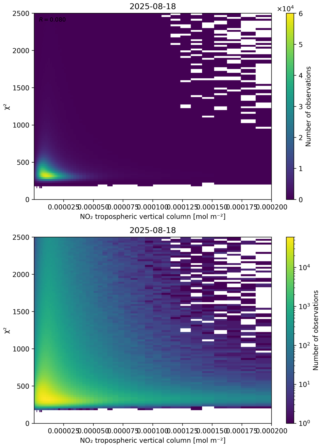
Figure 124: Scatter density plot of “NO 2 tropospheric vertical column” against “ \chi^2 ” for 2025-08-17 to 2025-08-19.
