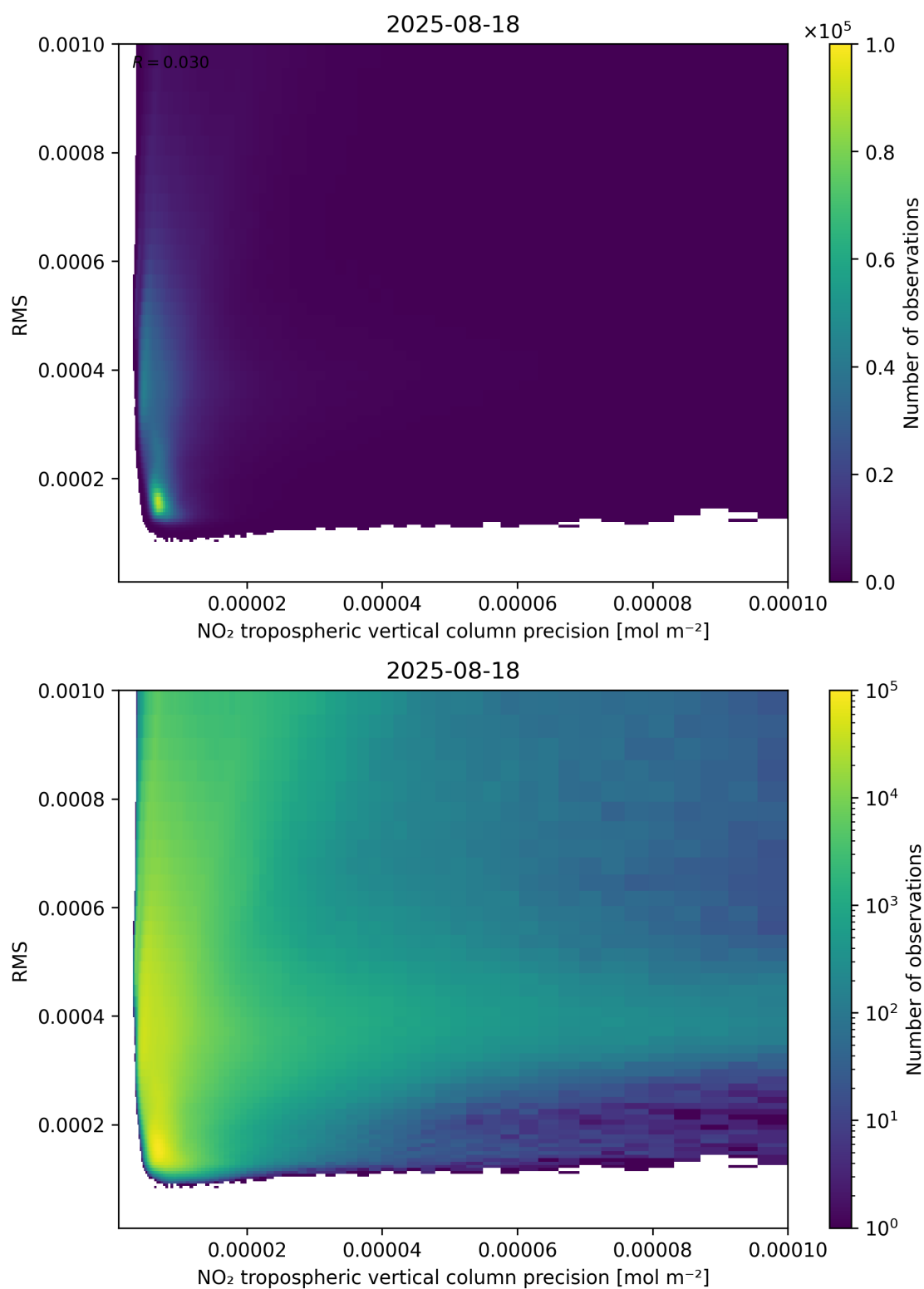
Figure 140: Scatter density plot of “NO 2 tropospheric vertical column precision” against “RMS” for 2025-08-17 to 2025-08-19.
