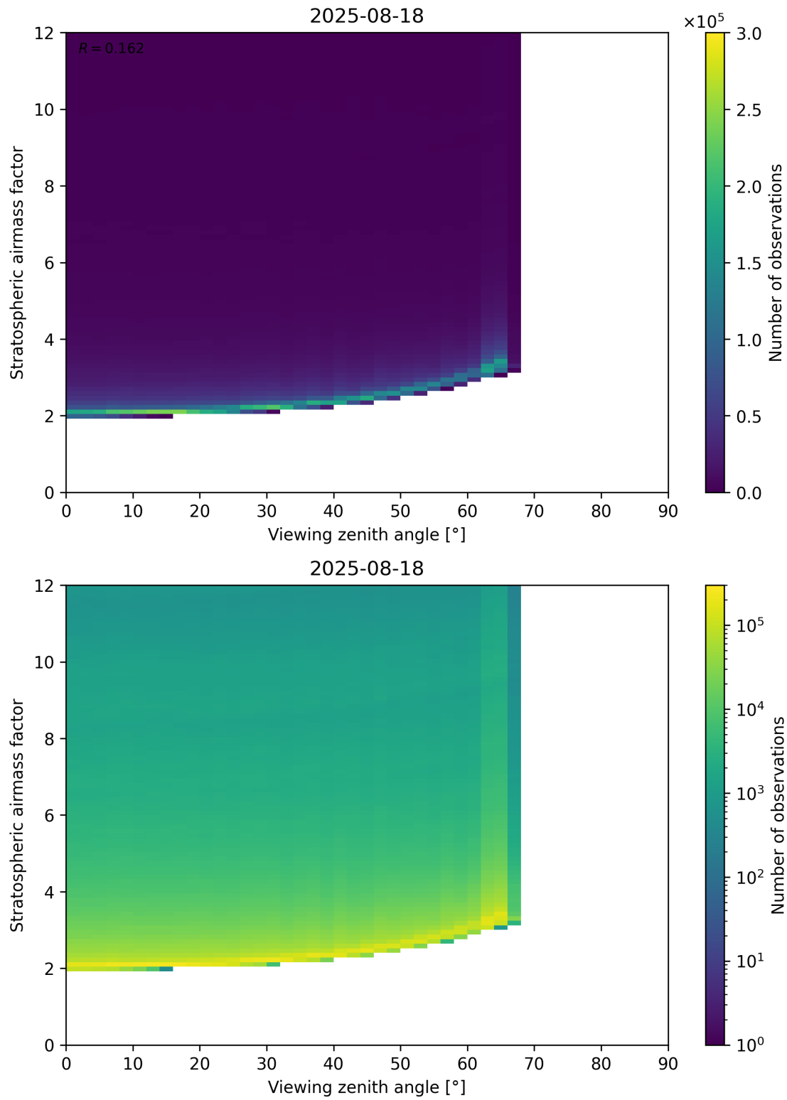
Figure 159: Scatter density plot of “Viewing zenith angle” against “Stratospheric airmass factor” for 2025-08-17 to 2025-08-19.
