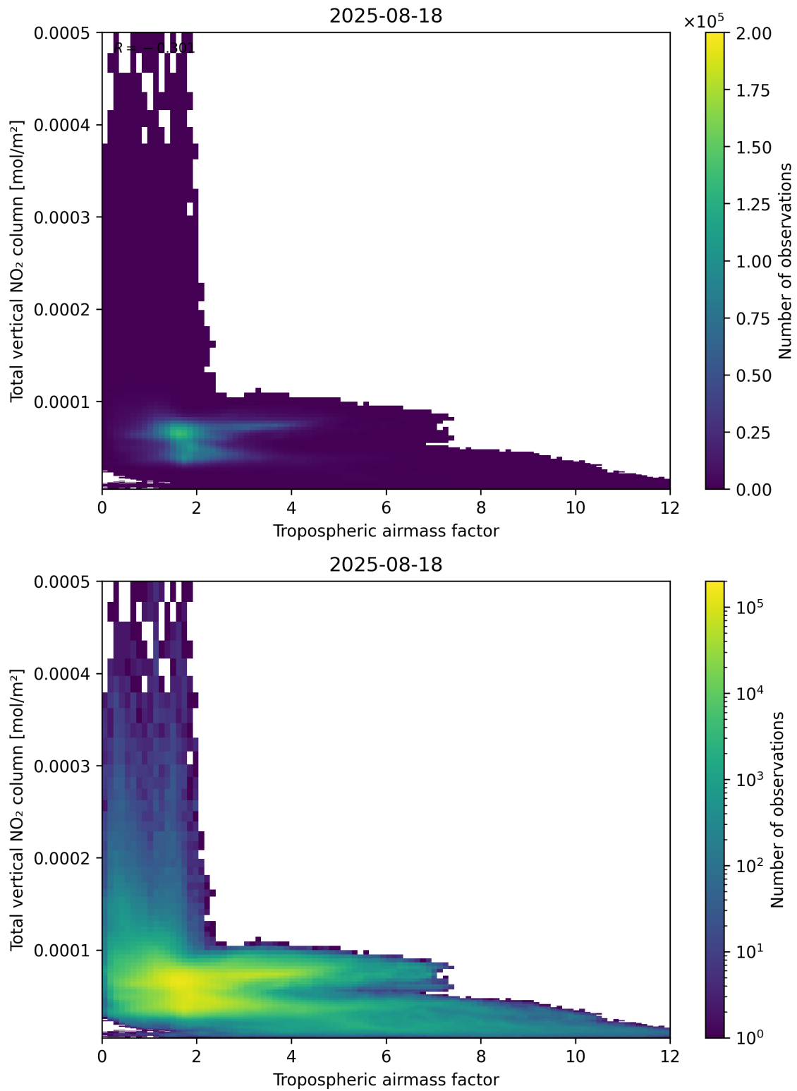
Figure 77: Scatter density plot of “Tropospheric airmass factor” against “Total vertical NO 2 column” for 2025-08-17 to 2025-08-19.
