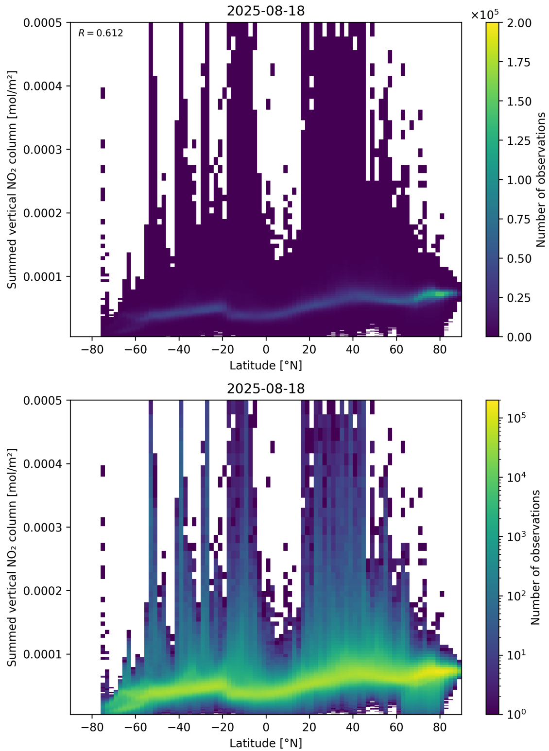
Figure 88: Scatter density plot of “Latitude” against “Summed vertical NO 2 column” for 2025-08-17 to 2025-08-19.
