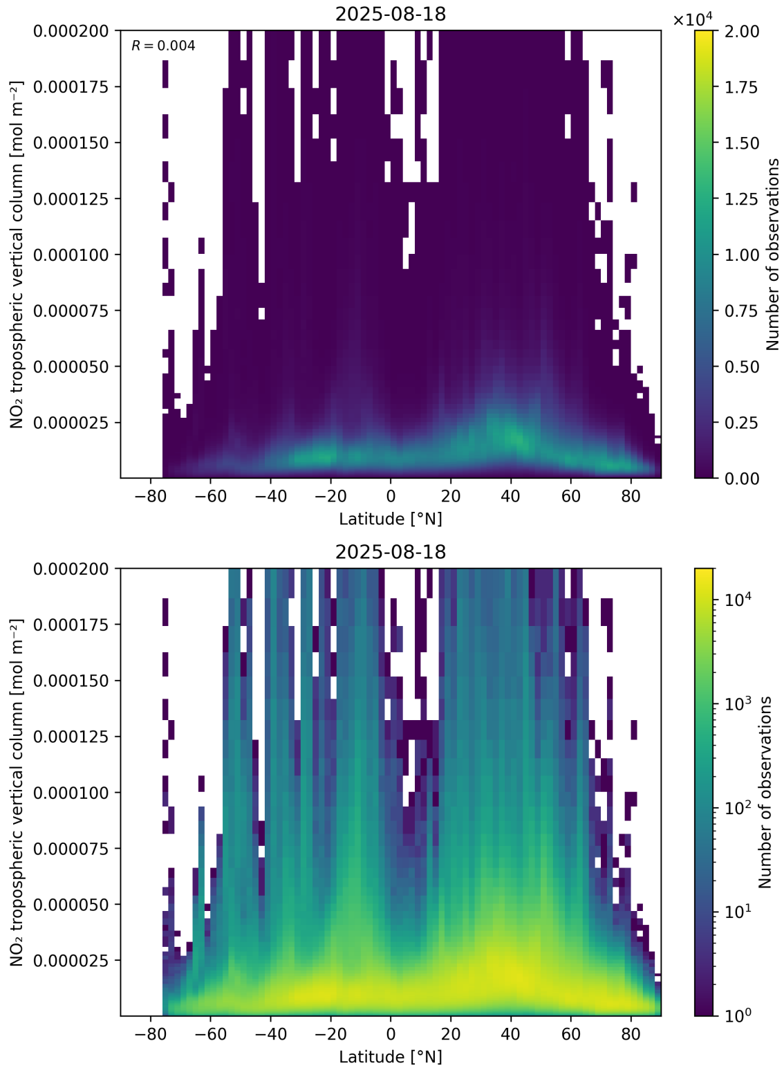
Figure 92: Scatter density plot of “Latitude” against “NO 2 tropospheric vertical column” for 2025-08-17 to 2025-08-19.
