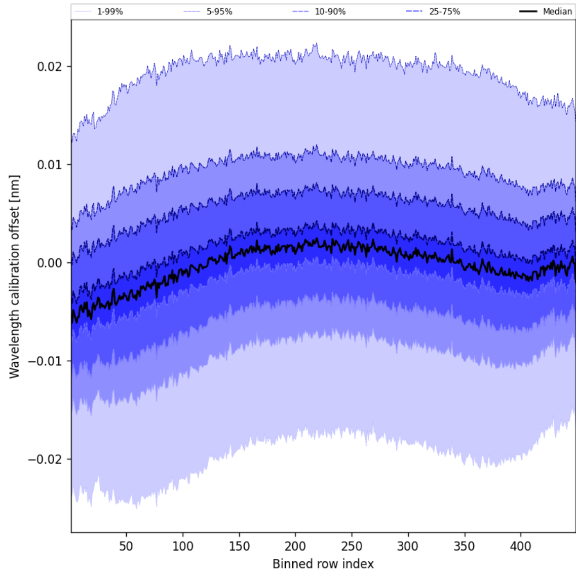
Figure 52: Along track statistics of “Wavelength calibration offset” for 2025-08-17 to 2025-08-19
