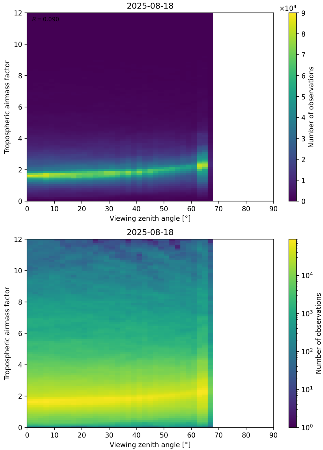
Figure 161: Scatter density plot of “Viewing zenith angle” against “Tropospheric airmass factor” for 2025-08-17 to 2025-08-19.
