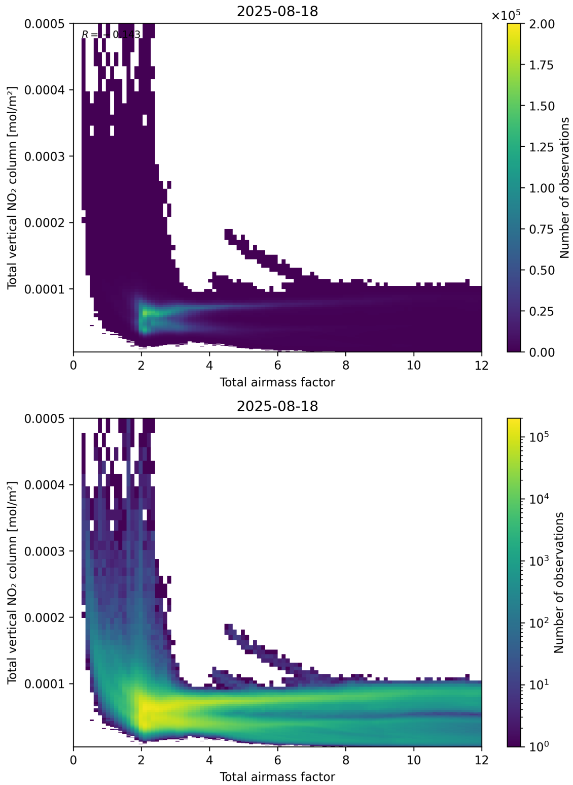
Figure 67: Scatter density plot of “Total airmass factor” against “Total vertical NO 2 column” for 2025-08-17 to 2025-08-19.
