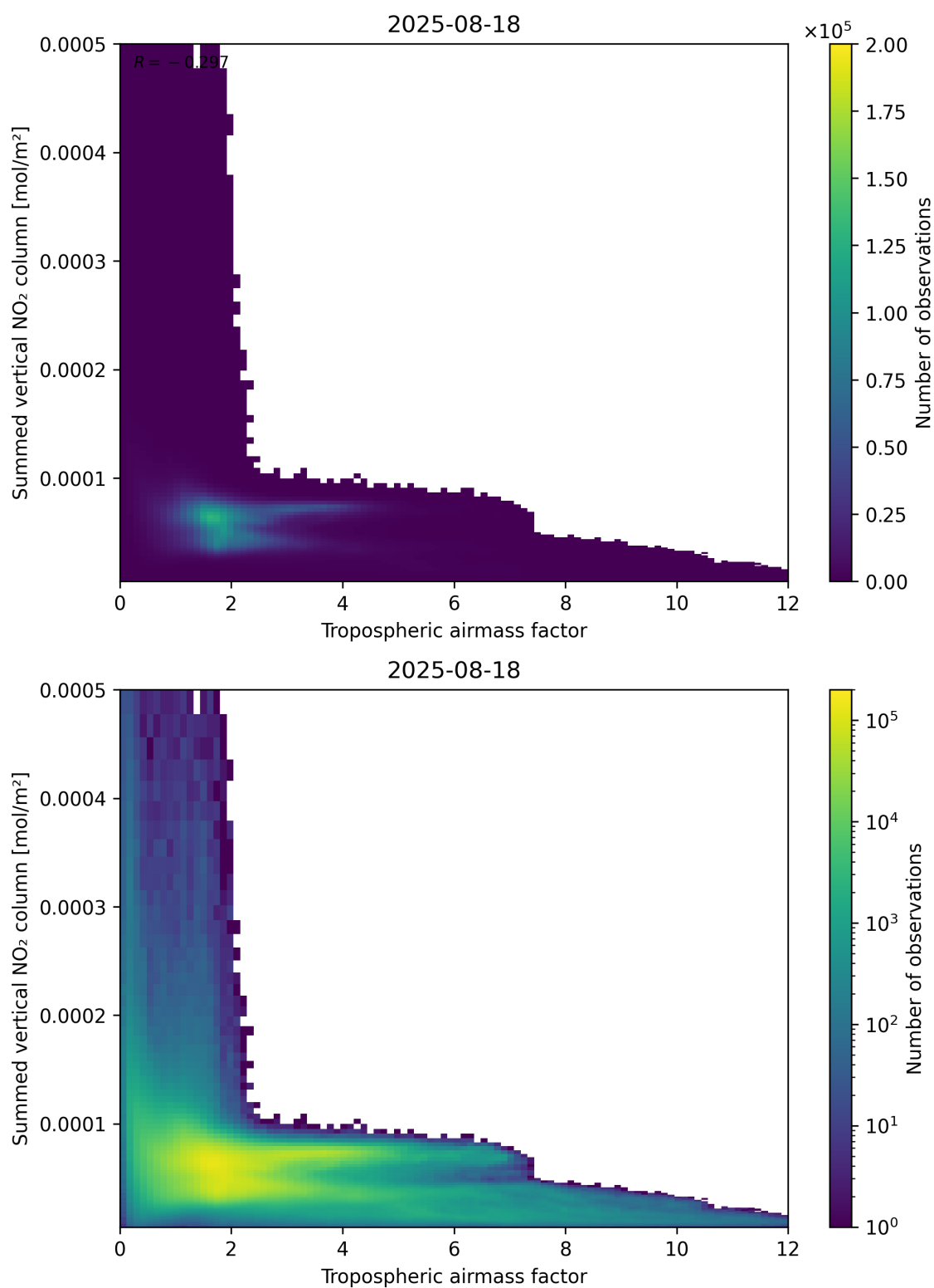
Figure 75: Scatter density plot of “Tropospheric airmass factor” against “Summed vertical NO 2 column” for 2025-08-17 to 2025-08-19.
