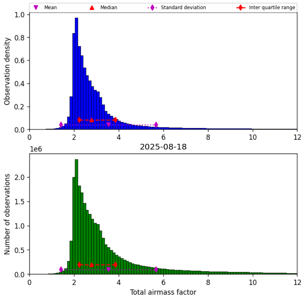
Figure 32: Histogram of “Total airmass factor” for 2025-08-17 to 2025-08-19
