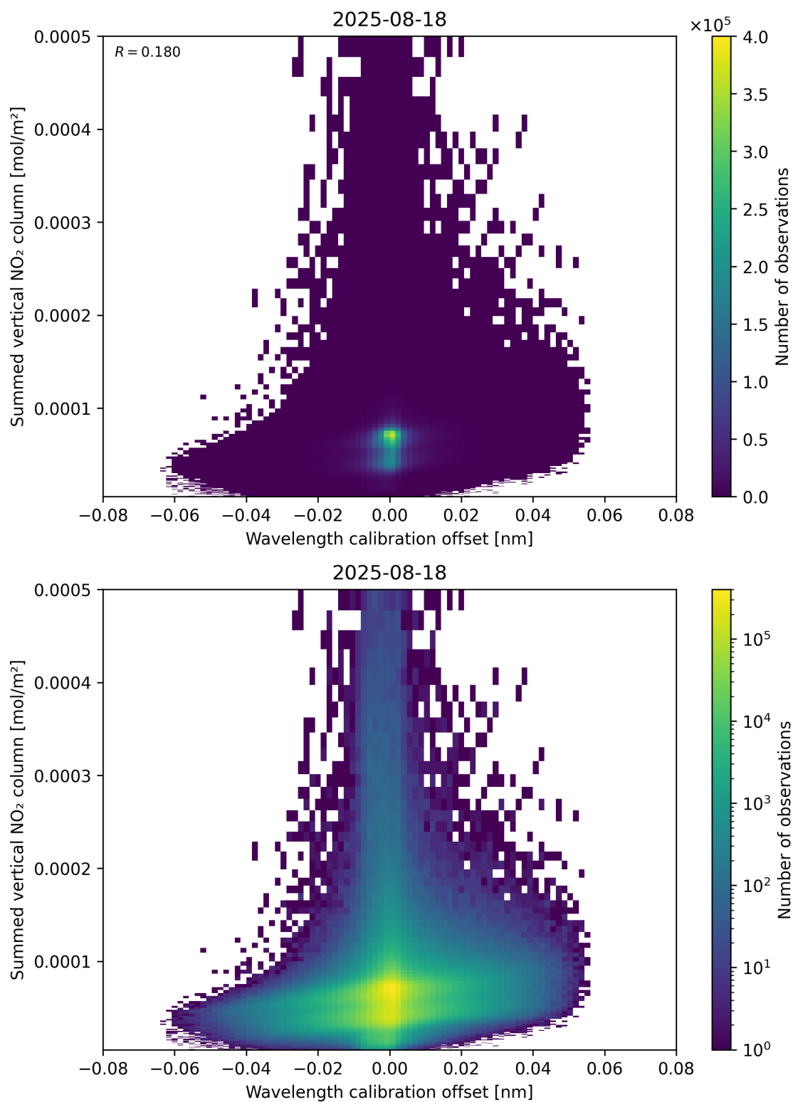
Figure 177: Scatter density plot of “Wavelength calibration offset” against “Summed vertical NO 2 column” for 2025-08-17 to 2025-08-19.
