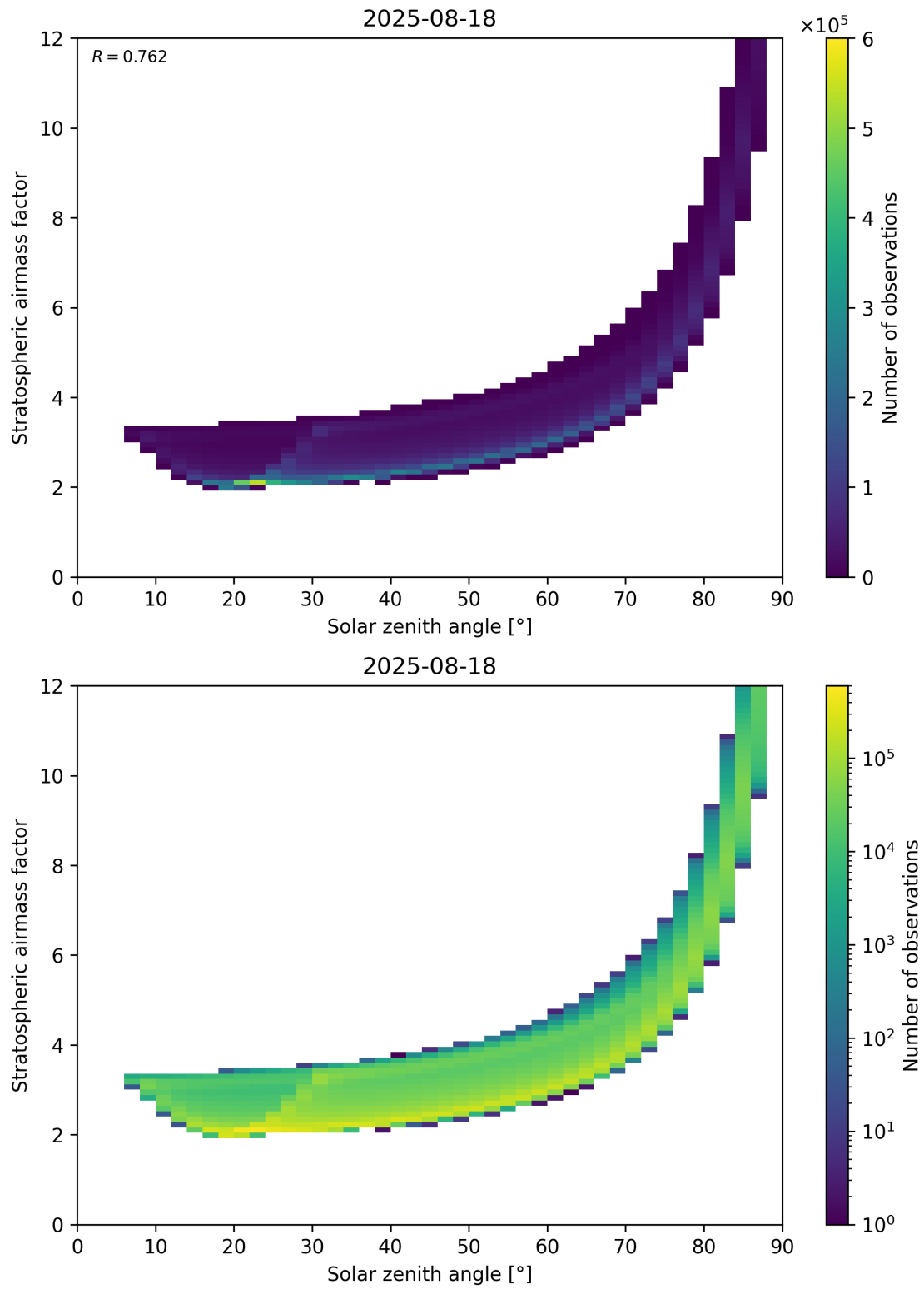
Figure 145: Scatter density plot of “Solar zenith angle” against “Stratospheric airmass factor” for 2025-08-17 to 2025-08-19.
