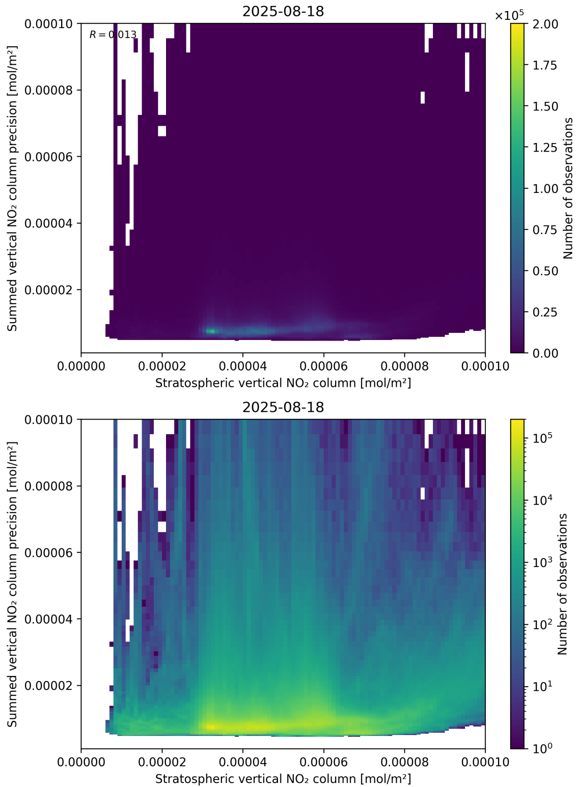
Figure 99: Scatter density plot of “Stratospheric vertical NO 2 column” against “Summed vertical NO 2 column precision” for 2025-08-17 to 2025-08-19.
