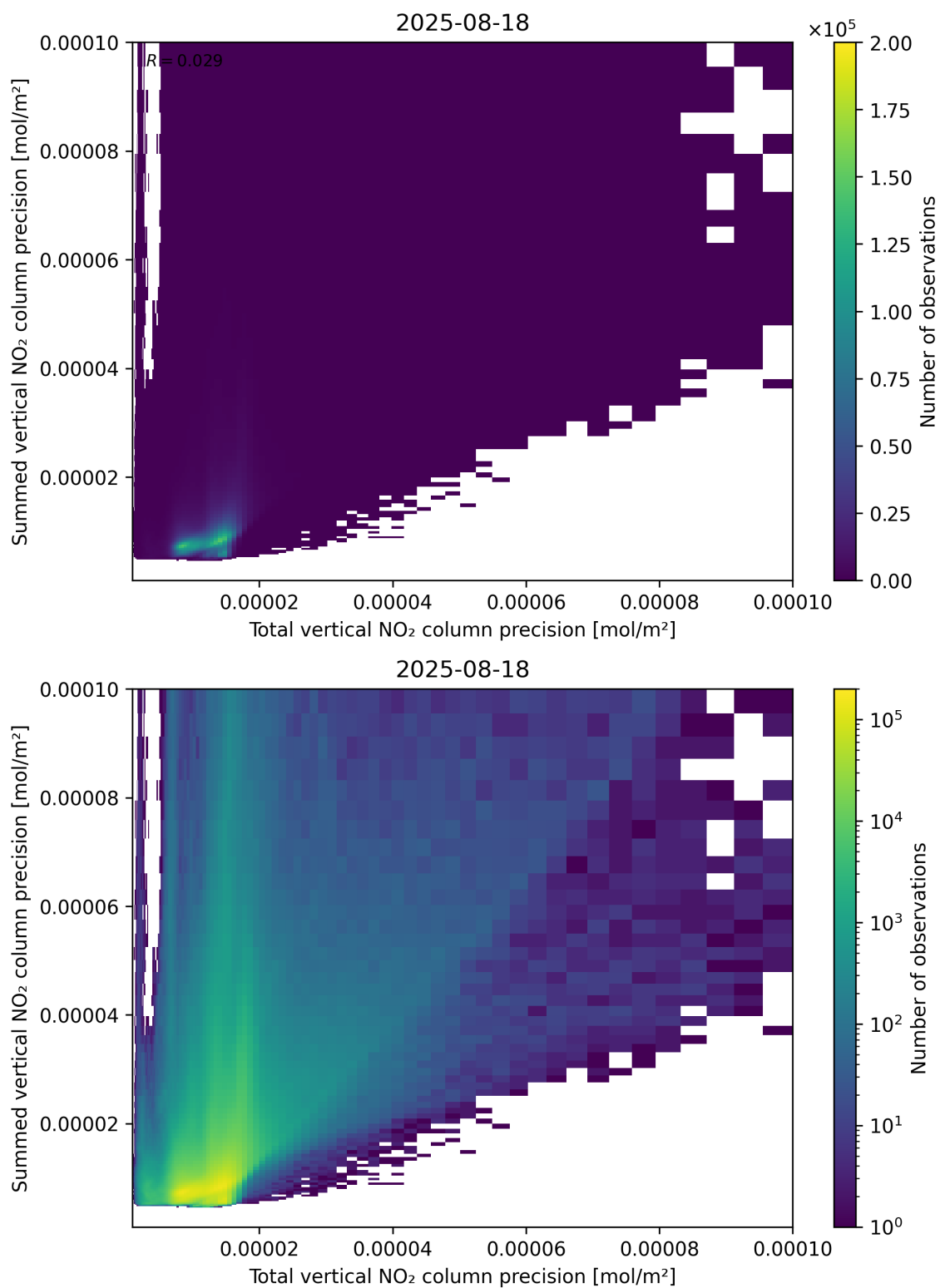
Figure 118: Scatter density plot of “Total vertical NO 2 column precision” against “Summed vertical NO 2 column precision” for 2025-08-17 to 2025-08-19.
