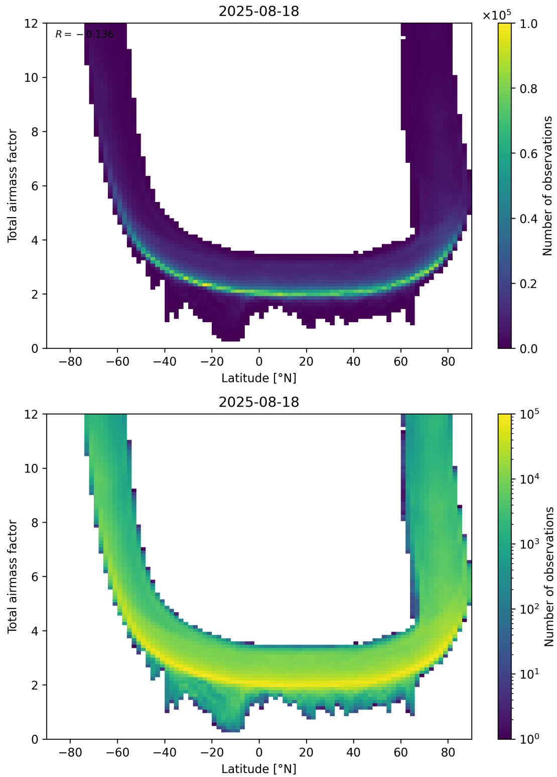
Figure 84: Scatter density plot of “Latitude” against “Total airmass factor” for 2025-08-17 to 2025-08-19.
