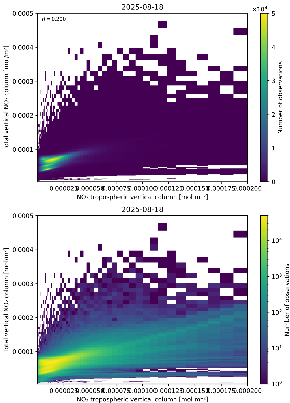
Figure 128: Scatter density plot of “NO 2 tropospheric vertical column” against “Total vertical NO 2 column” for 2025-08-17 to 2025-08-19.
