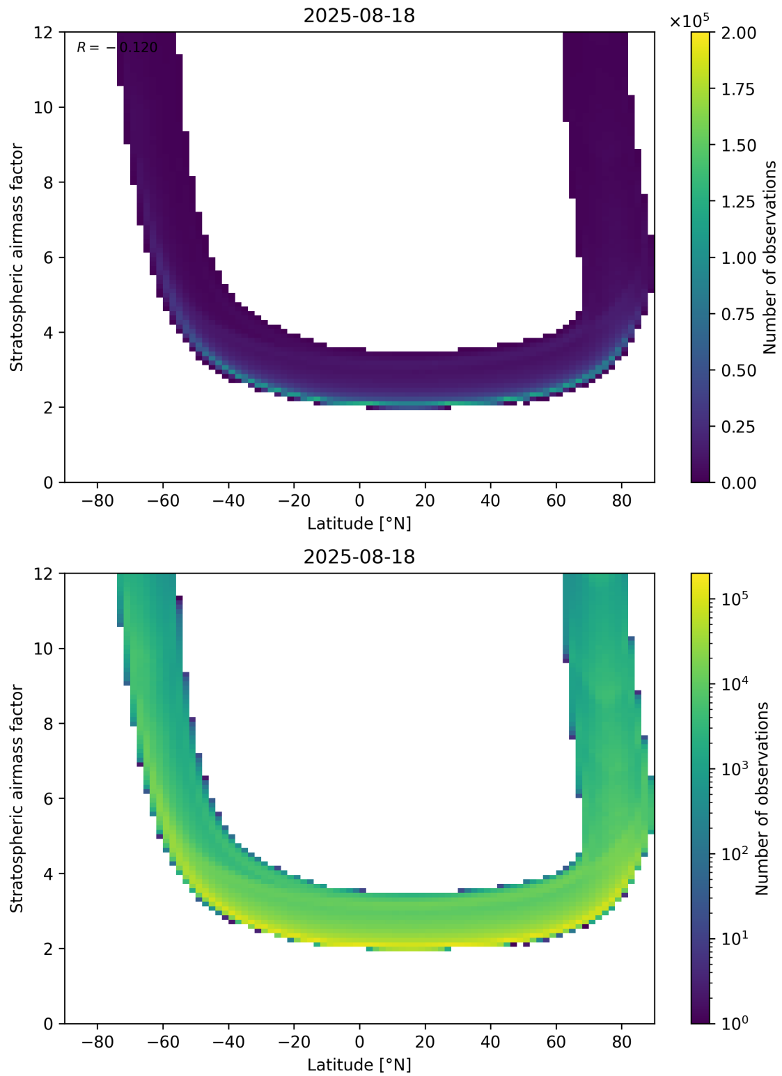
Figure 83: Scatter density plot of “Latitude” against “Stratospheric air mass factor” for 2025-08-17 to 2025-08-19.
