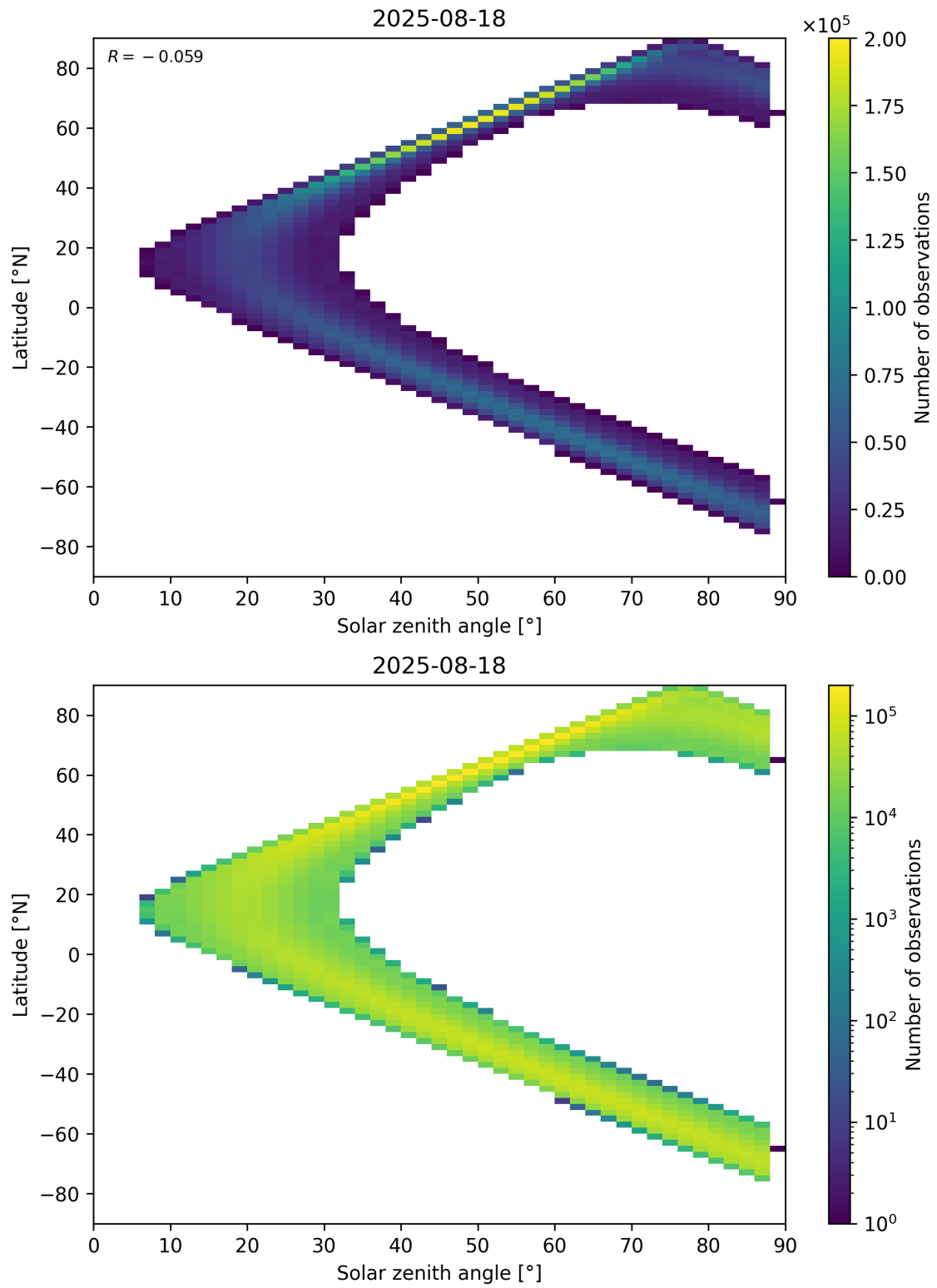
Figure 149: Scatter density plot of “Solar zenith angle” against “Latitude” for 2025-08-17 to 2025-08-19.
