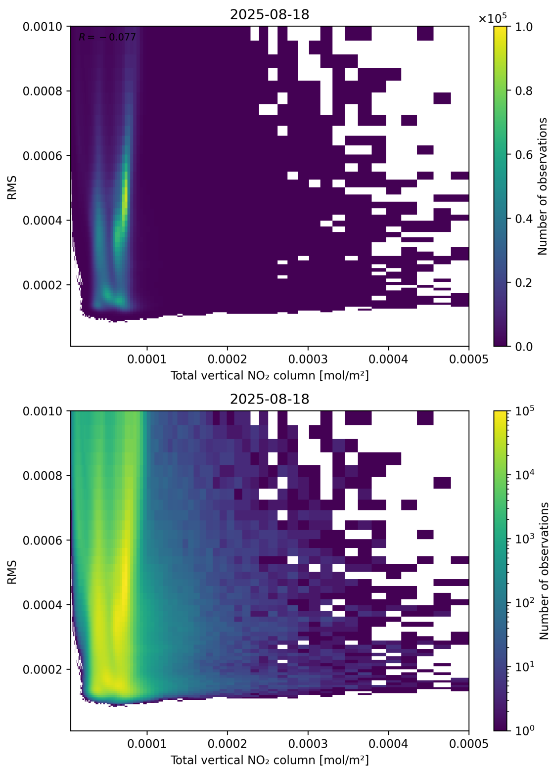
Figure 120: Scatter density plot of “Total vertical NO 2 column” against “RMS” for 2025-08-17 to 2025-08-19.
