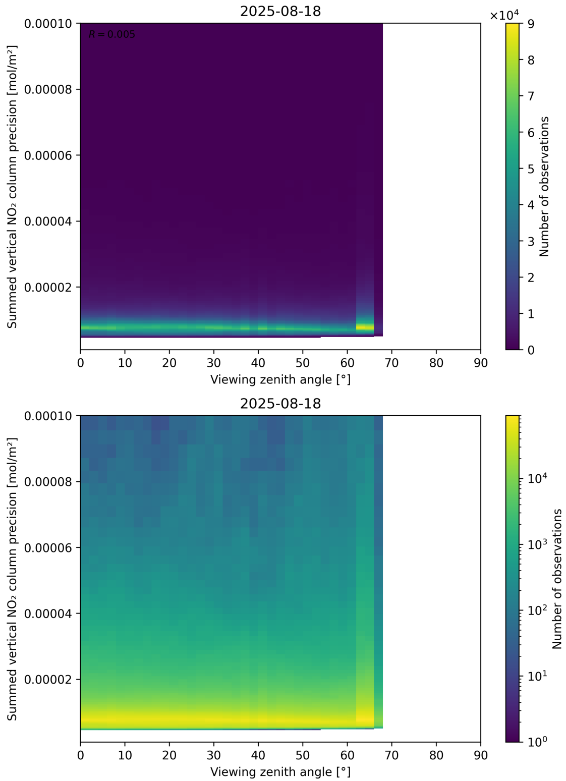
Figure 166: Scatter density plot of “Viewing zenith angle” against “Summed vertical NO 2 column precision” for 2025-08-17 to 2025-08-19.
