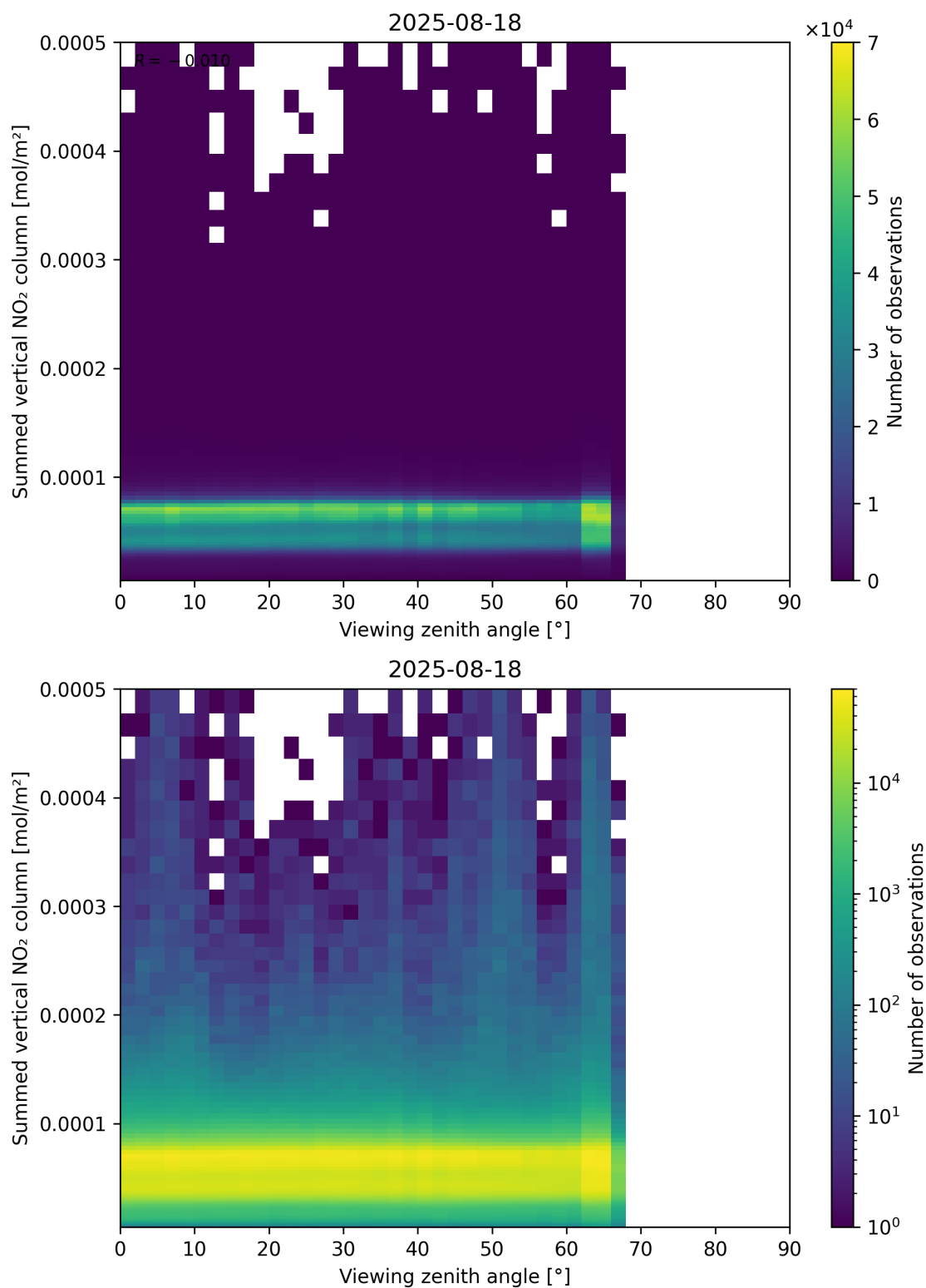
Figure 165: Scatter density plot of “Viewing zenith angle” against “Summed vertical NO 2 column” for 2025-08-17 to 2025-08-19.
