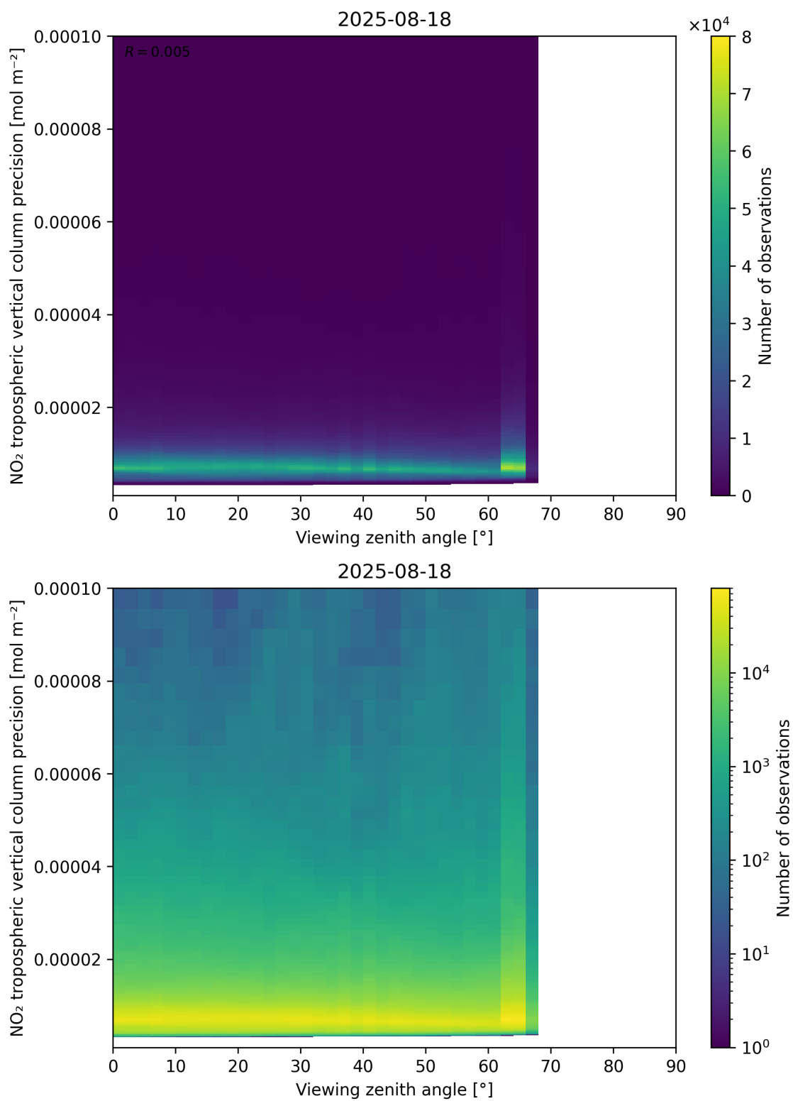
Figure 170: Scatter density plot of “Viewing zenith angle” against “NO 2 tropospheric vertical column precision” for 2025-08-17 to 2025-08-19.
