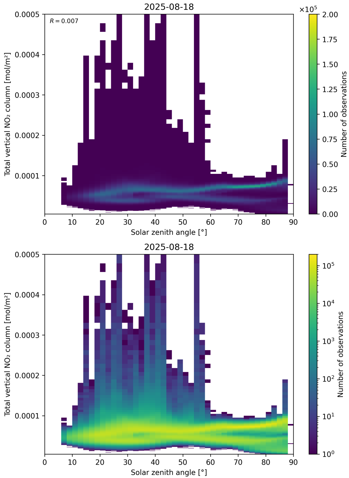
Figure 153: Scatter density plot of “Solar zenith angle” against “Total vertical NO 2 column” for 2025-08-17 to 2025-08-19.
