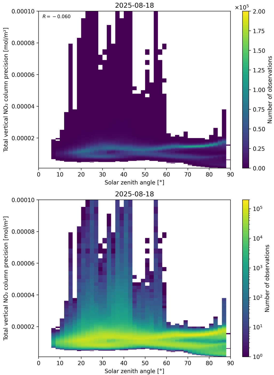
Figure 154: Scatter density plot of “Solar zenith angle” against “Total vertical NO 2 column precision” for 2025-08-17 to 2025-08-19.
