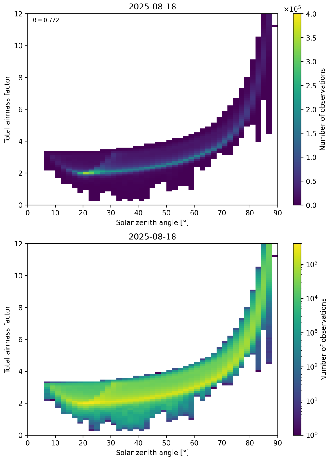
Figure 146: Scatter density plot of “Solar zenith angle” against “Total air mass factor” for 2025-08-17 to 2025-08-19.
