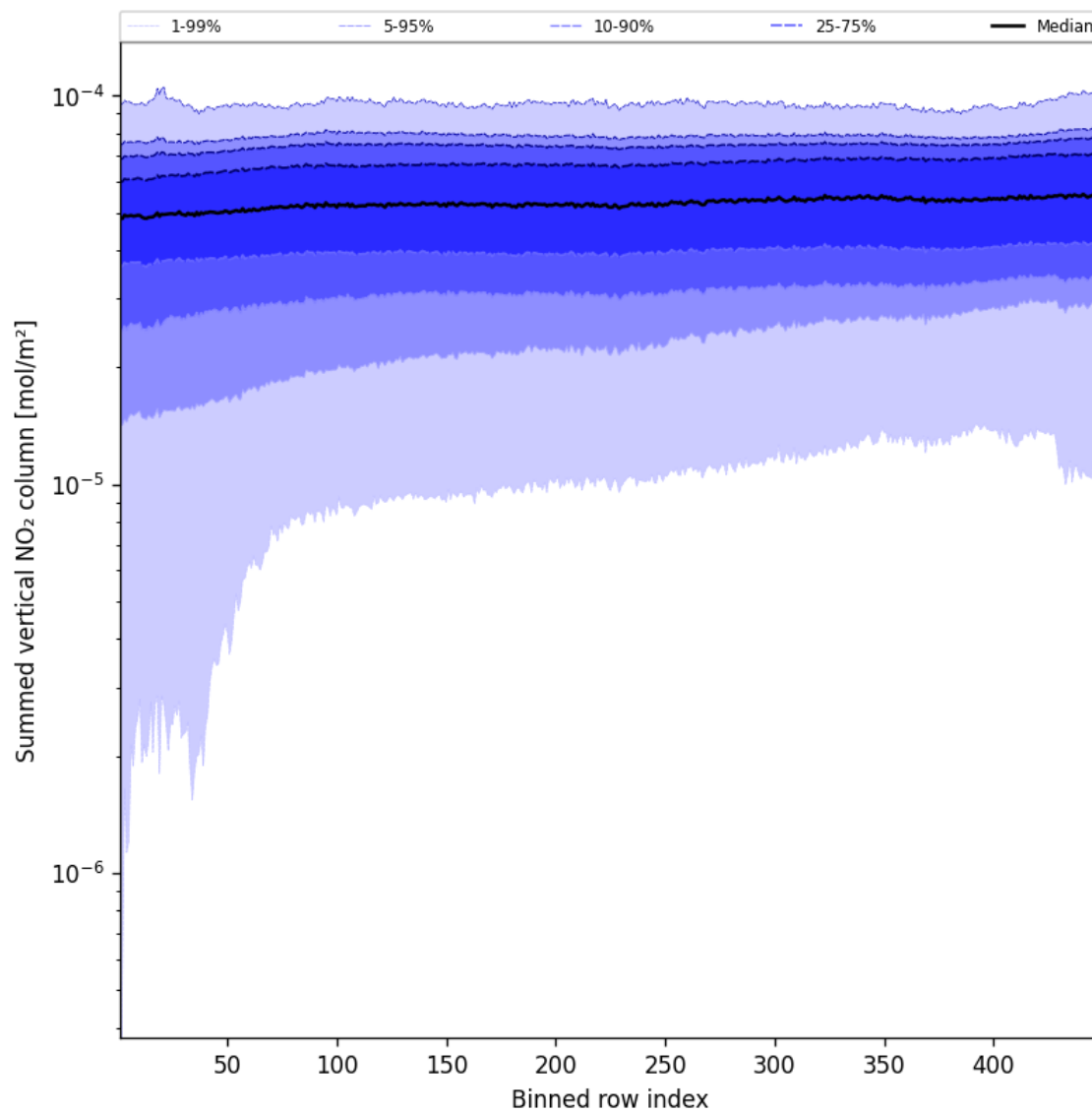
Figure 57: Along track statistics of “Summed vertical NO 2 column” for 2025-08-17 to 2025-08-19
