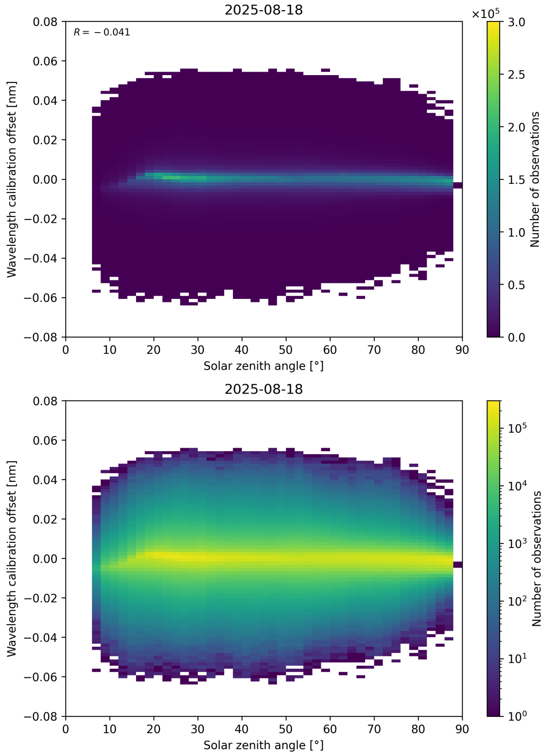
Figure 158: Scatter density plot of “Solar zenith angle” against “Wavelength calibration offset” for 2025-08-17 to 2025-08-19.
