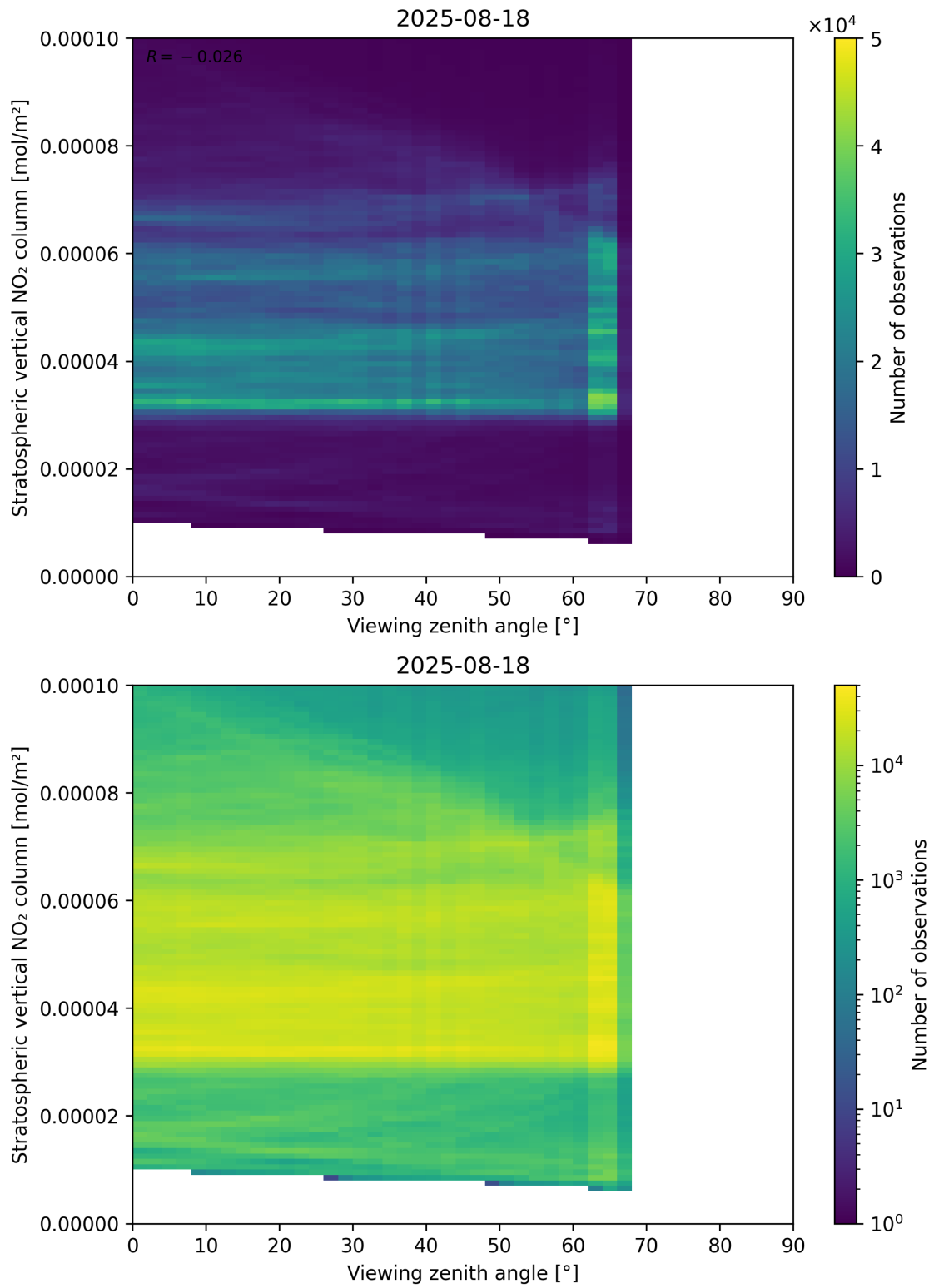
Figure 164: Scatter density plot of “Viewing zenith angle” against “Stratospheric vertical NO 2 column” for 2025-08-17 to 2025-08-19.
