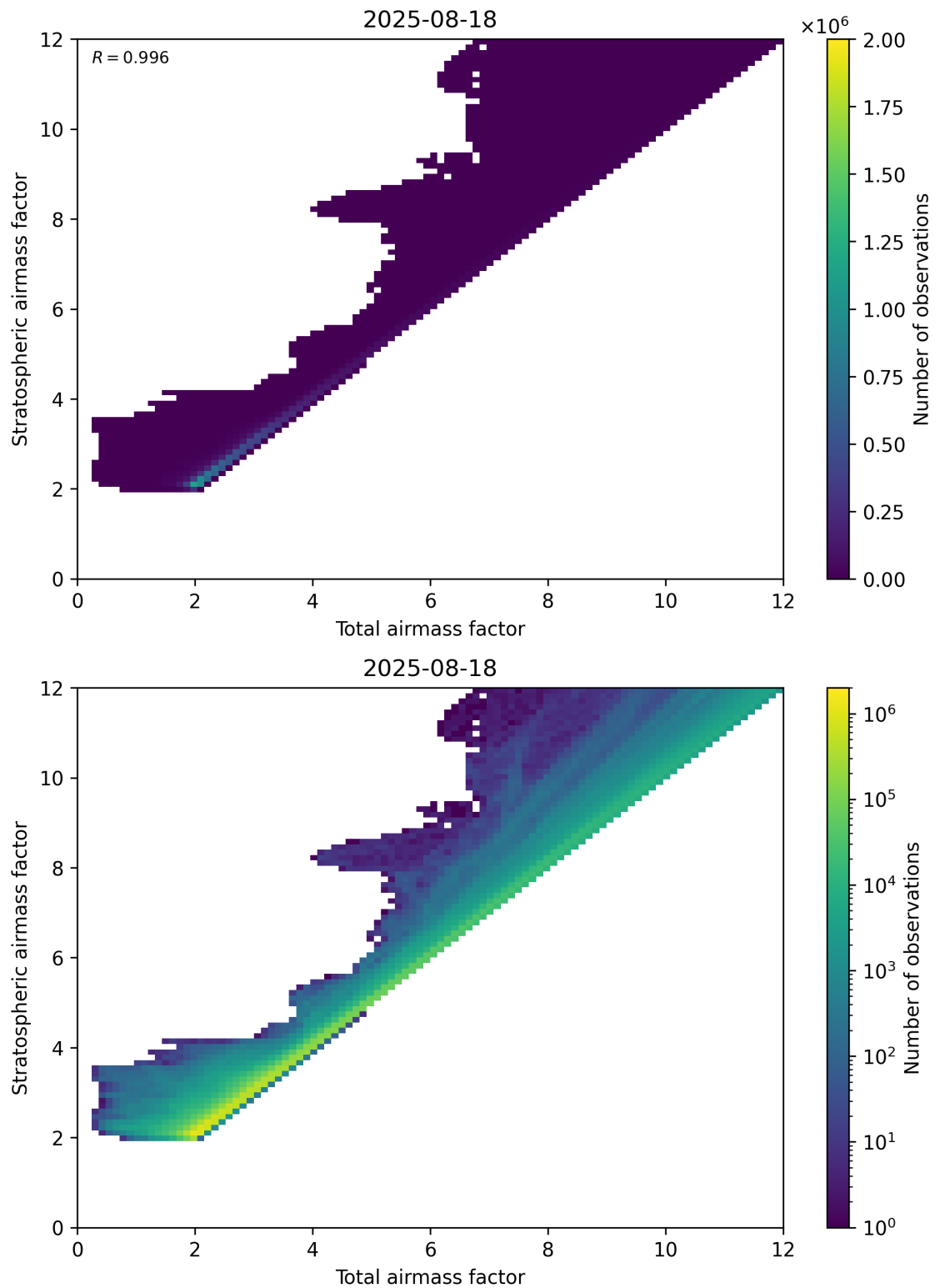
Figure 62: Scatter density plot of “Total air mass factor” against “Stratospheric air mass factor” for 2025-08-17 to 2025-08-19.
