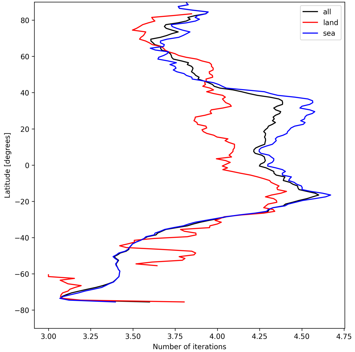
Figure 17: Zonal average of “Number of iterations” for 2025-08-17 to 2025-08-19.
