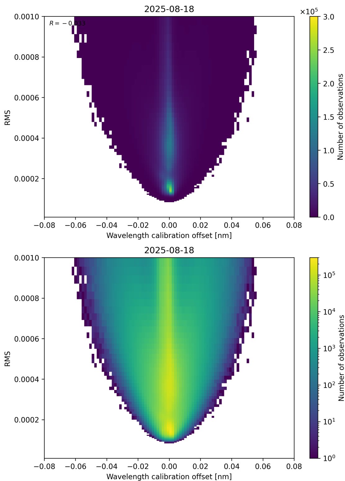
Figure 181: Scatter density plot of “Wavelength calibration offset” against “RMS” for 2025-08-17 to 2025-08-19.
