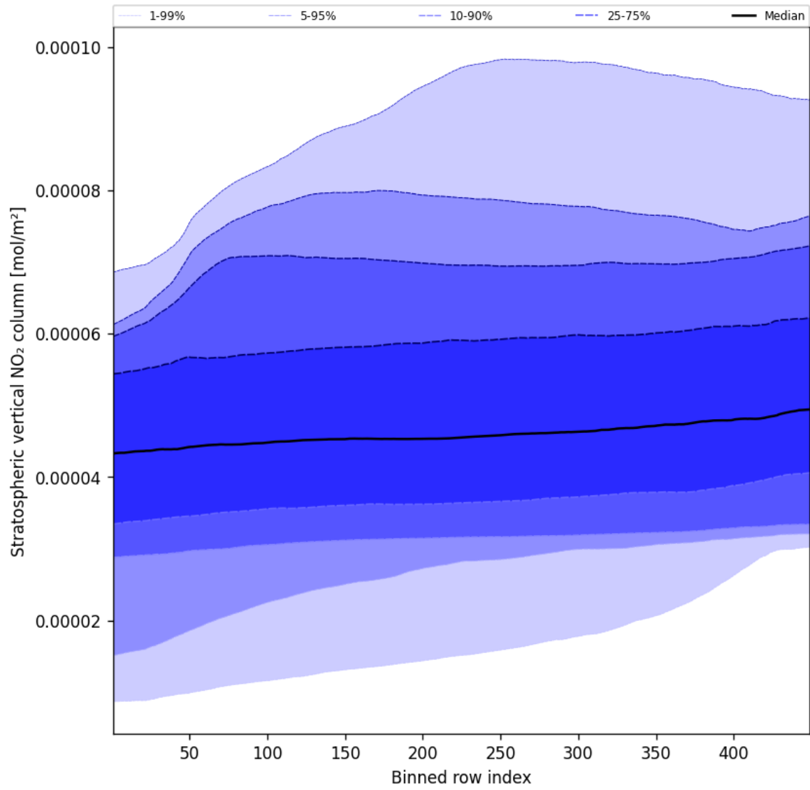
Figure 53: Along track statistics of “Stratospheric vertical NO 2 column” for 2025-08-17 to 2025-08-19
