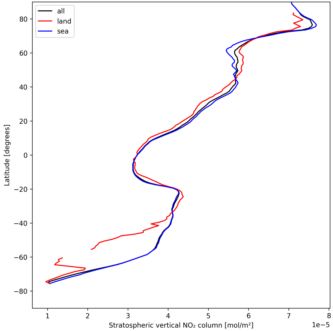
Figure 19: Zonal average of “Stratospheric vertical NO 2 column” for 2025-08-17 to 2025-08-19.
