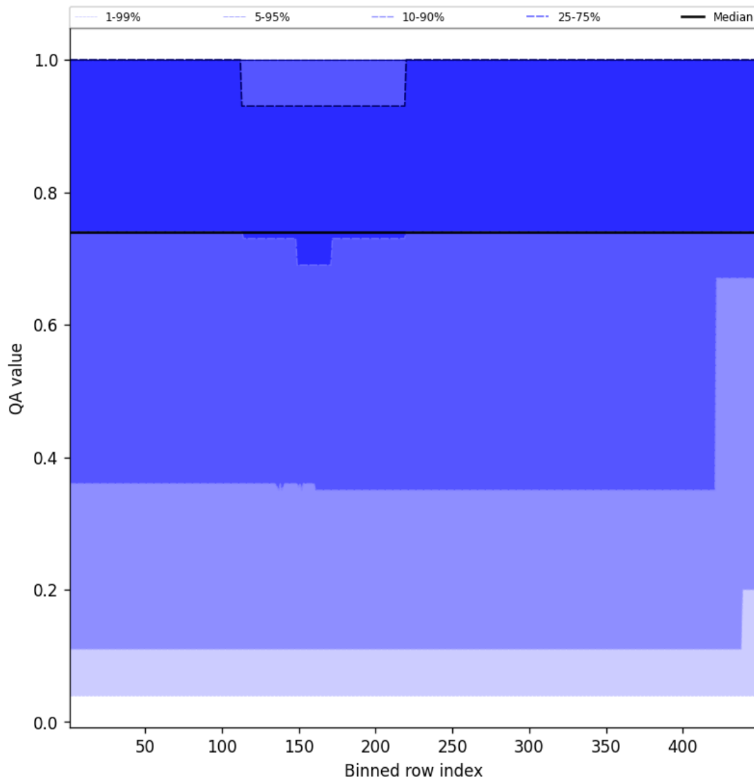
Figure 45: Along track statistics of “QA value” for 2025-08-17 to 2025-08-19
