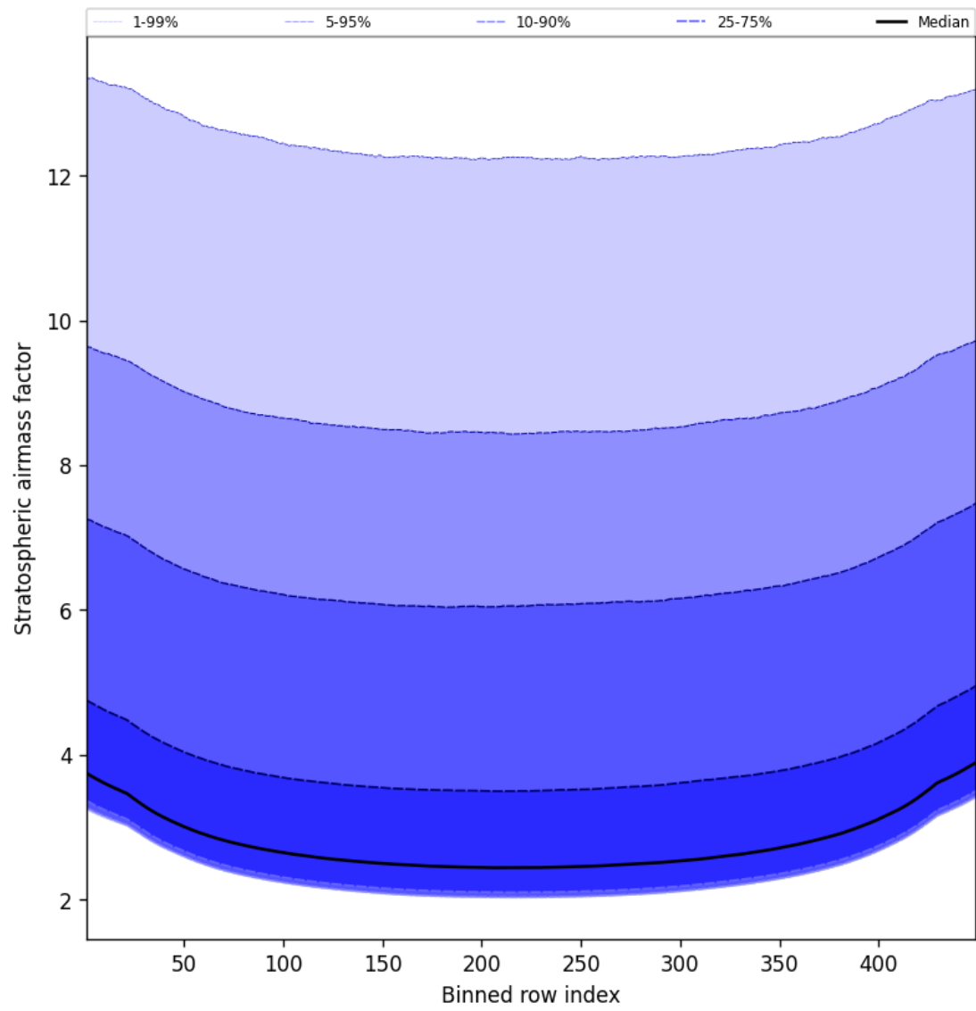
Figure 61: Along track statistics of “Stratospheric airmass factor” for 2025-08-17 to 2025-08-19
