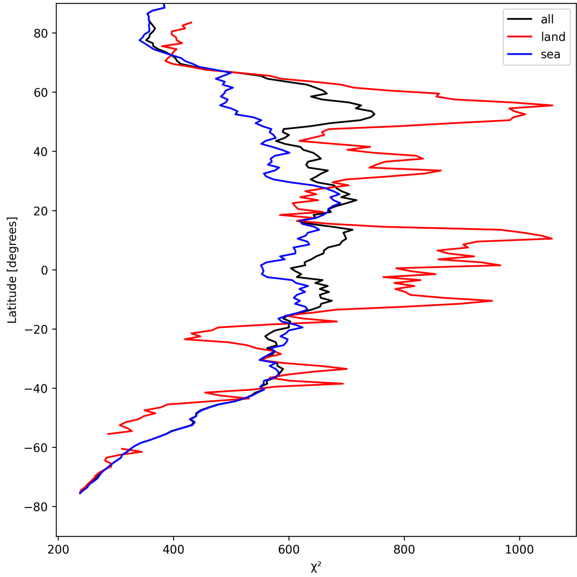
Figure 25: Zonal average of “ \chi^2 ” for 2025-08-17 to 2025-08-19.
