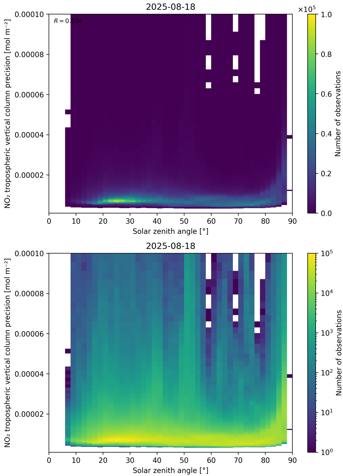
Figure 156: Scatter density plot of “Solar zenith angle” against “NO 2 tropospheric vertical column precision” for 2025-08-17 to 2025-08-19.
