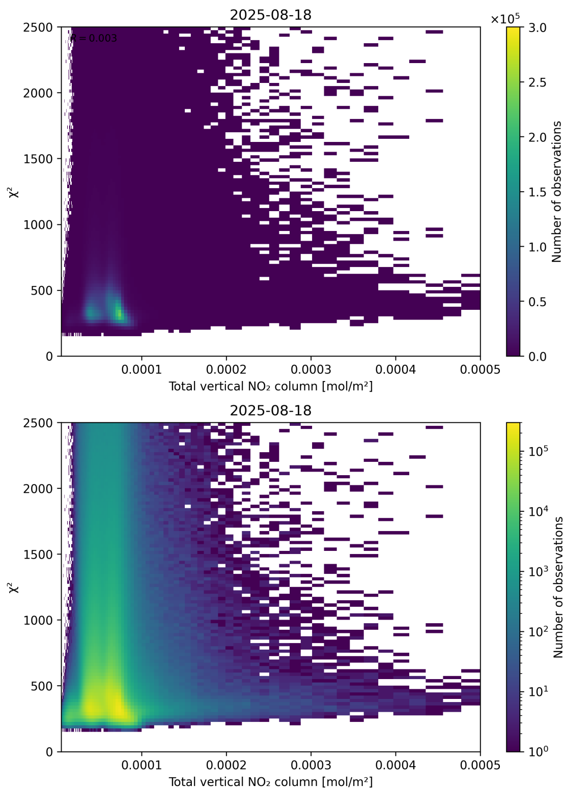
Figure 111: Scatter density plot of “Total vertical NO 2 column” against “ \chi^2 ” for 2025-08-17 to 2025-08-19.
