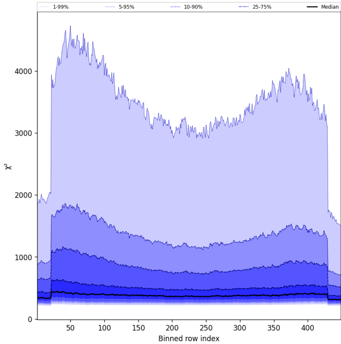
Figure 59: Along track statistics of “ \chi^2 ” for 2025-08-17 to 2025-08-19
