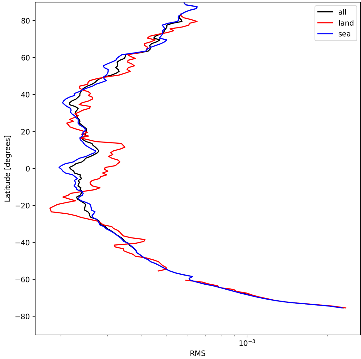
Figure 26: Zonal average of “RMS” for 2025-08-17 to 2025-08-19.
