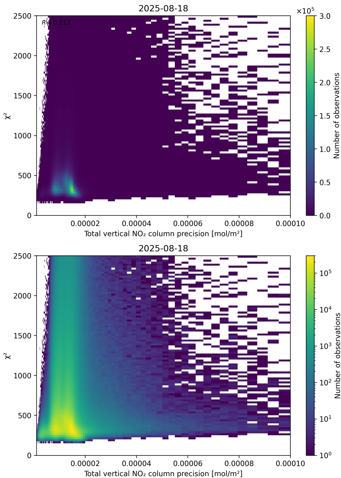
Figure 116: Scatter density plot of “Total vertical NO 2 column precision” against “ \chi^2 ” for 2025-08-17 to 2025-08-19.
