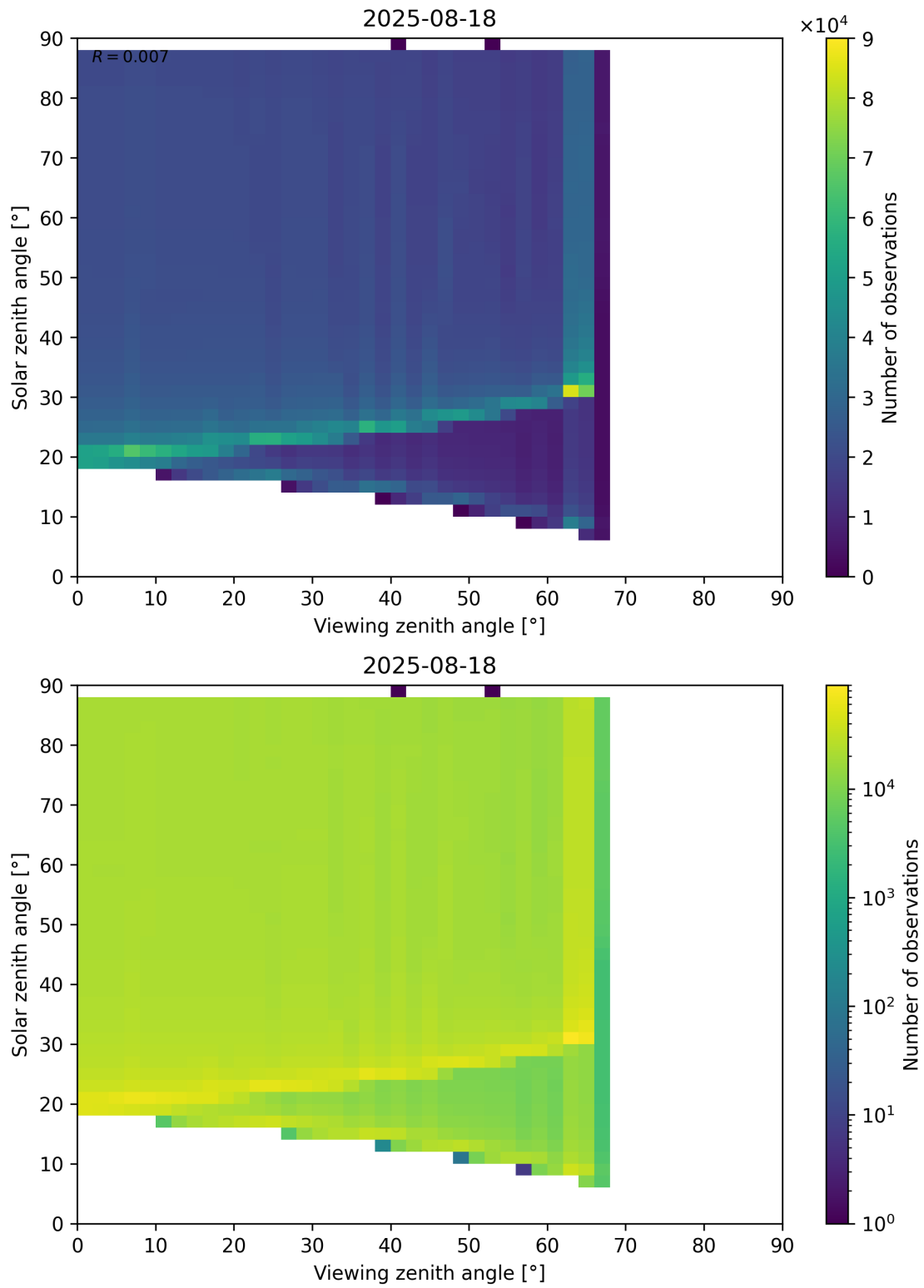
Figure 172: Scatter density plot of “Viewing zenith angle” against “Solar zenith angle” for 2025-08-17 to 2025-08-19.
