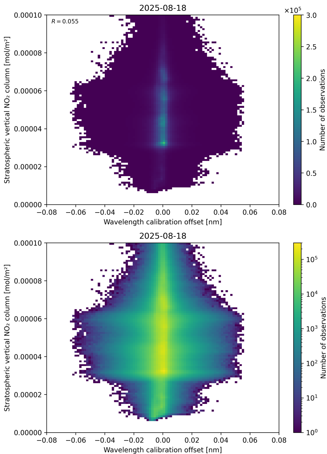
Figure 176: Scatter density plot of “Wavelength calibration offset” against “Stratospheric vertical NO 2 column” for 2025-08-17 to 2025-08-19.
