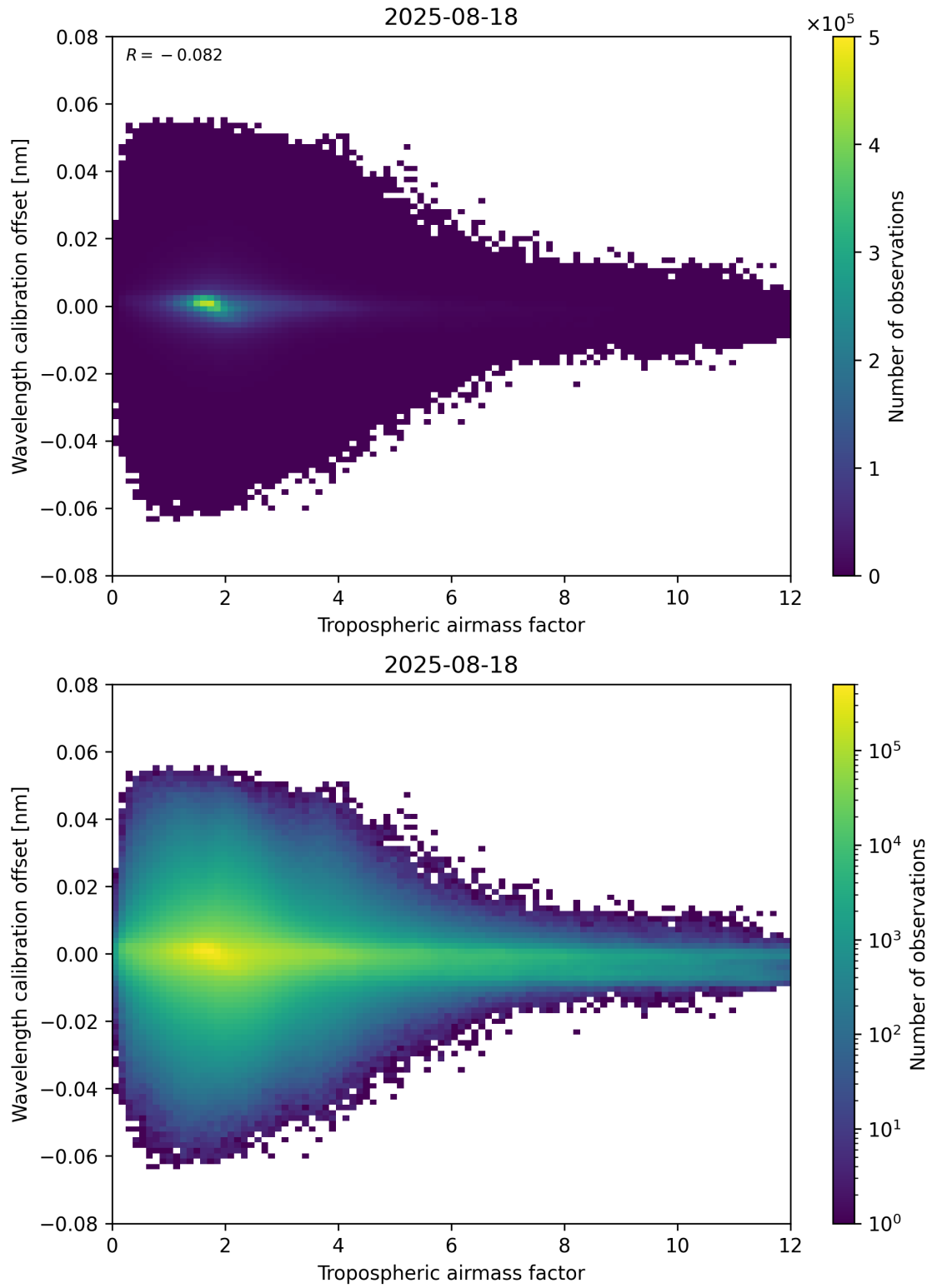
Figure 80: Scatter density plot of “Tropospheric airmass factor” against “Wavelength calibration offset” for 2025-08-17 to 2025-08-19.
