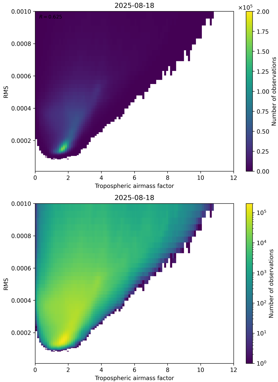
Figure 79: Scatter density plot of “Tropospheric airmass factor” against “RMS” for 2025-08-17 to 2025-08-19.
