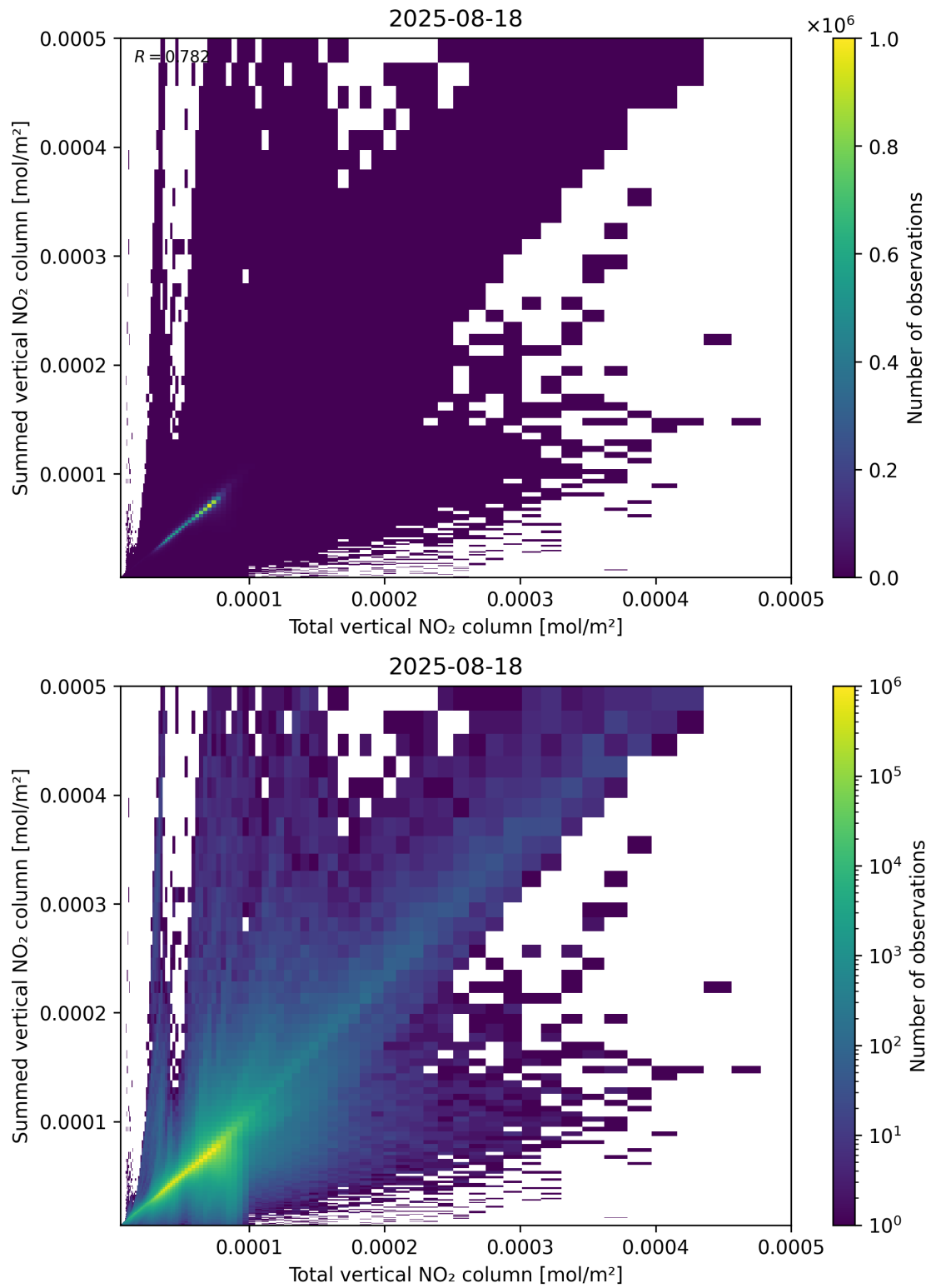
Figure 112: Scatter density plot of “Total vertical NO 2 column” against “Summed vertical NO 2 column” for 2025-08-17 to 2025-08-19.
