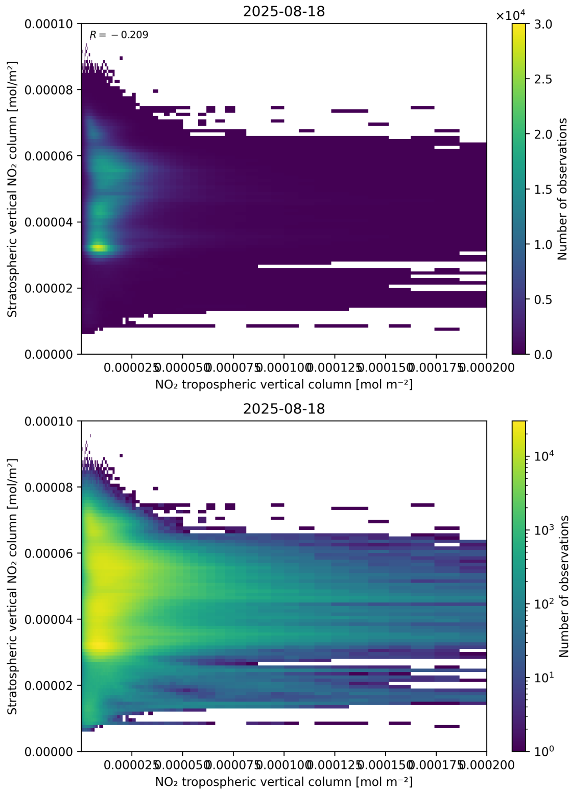
Figure 125: Scatter density plot of “NO 2 tropospheric vertical column” against “Stratospheric vertical NO 2 column” for 2025-08-17 to 2025-08-19.
