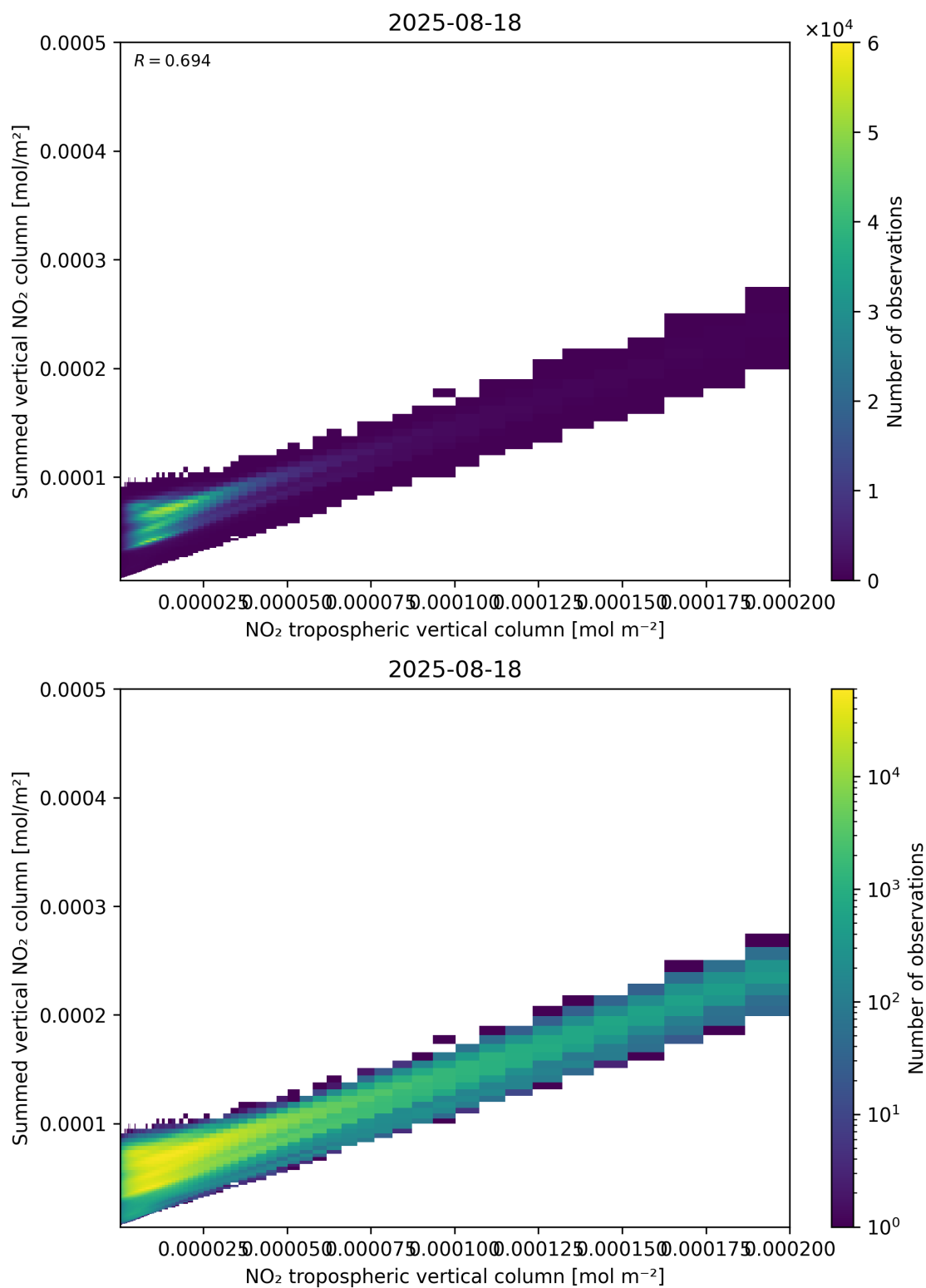
Figure 126: Scatter density plot of “NO 2 tropospheric vertical column” against “Summed vertical NO 2 column” for 2025-08-17 to 2025-08-19.
