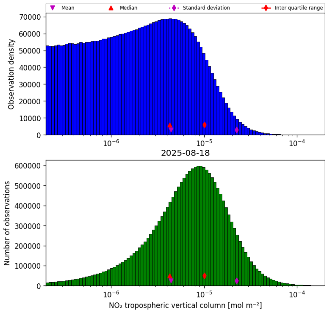
Figure 29: Histogram of “NO 2 tropospheric vertical column” for 2025-08-17 to 2025-08-19
