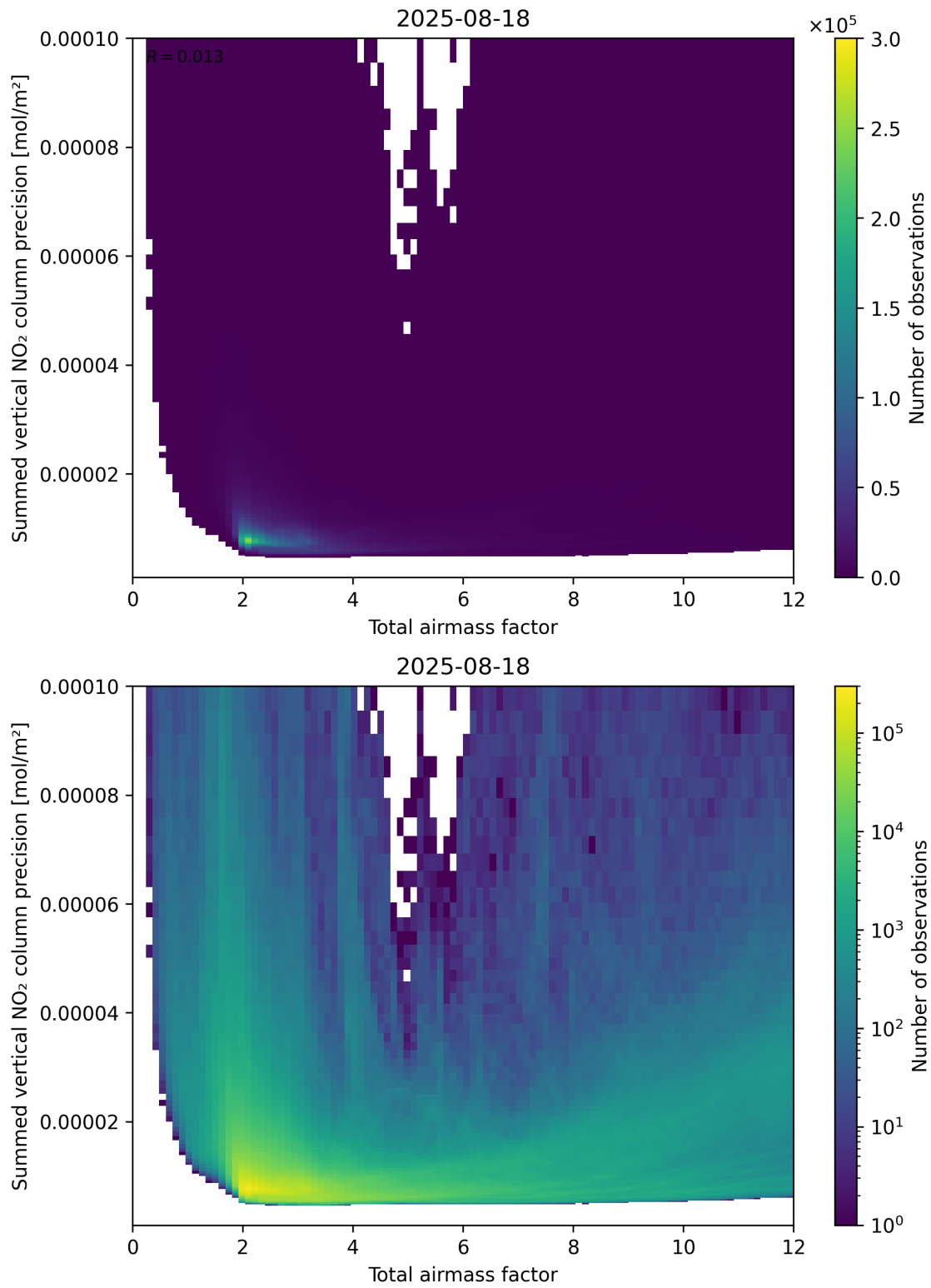
Figure 66: Scatter density plot of “Total airmass factor” against “Summed vertical NO 2 column precision” for 2025-08-17 to 2025-08-19.
