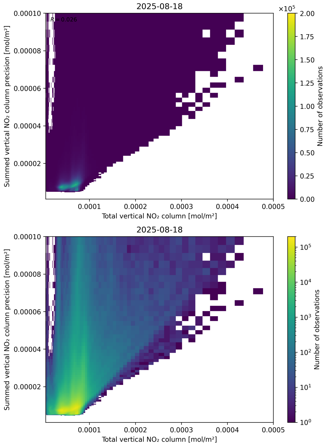
Figure 113: Scatter density plot of “Total vertical NO 2 column” against “Summed vertical NO 2 column precision” for 2025-08-17 to 2025-08-19.
