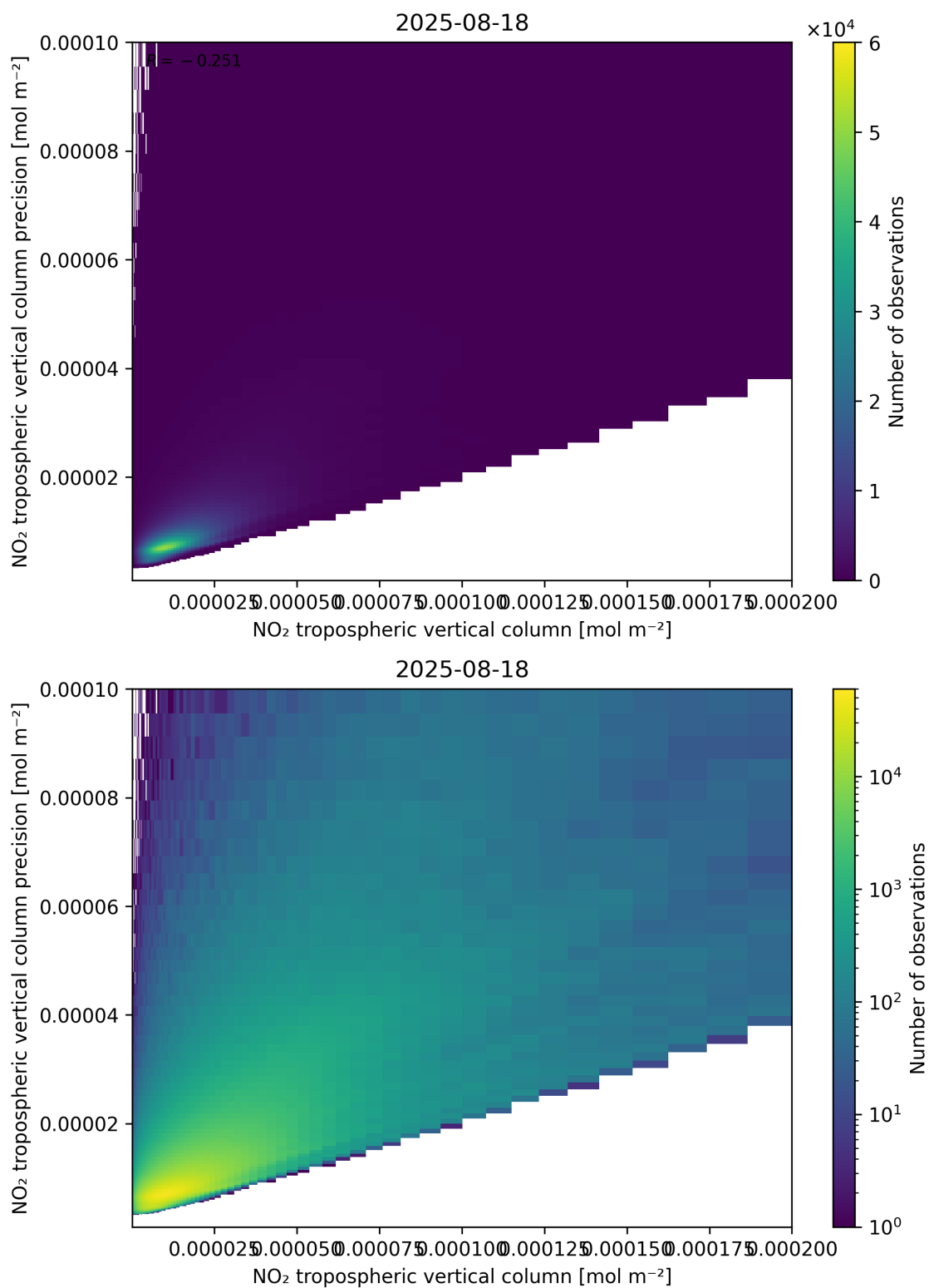
Figure 130: Scatter density plot of “NO 2 tropospheric vertical column” against “NO 2 tropospheric vertical column precision” for 2025-08-17 to 2025-08-19.
