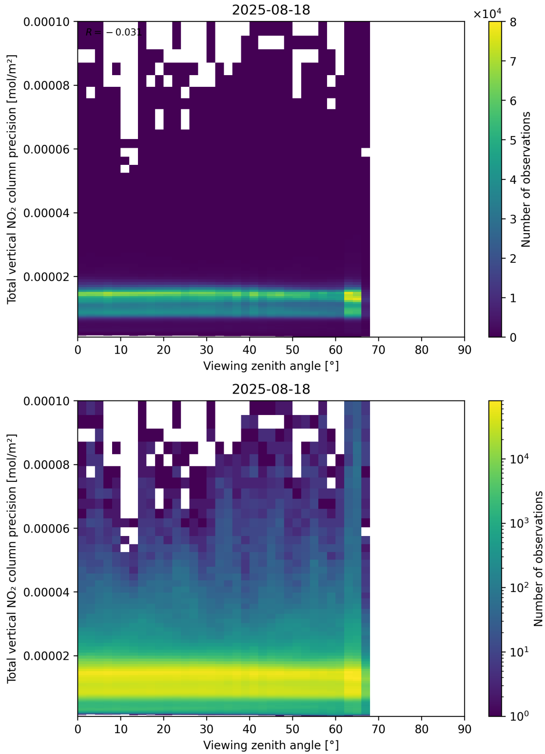
Figure 168: Scatter density plot of “Viewing zenith angle” against “Total vertical NO 2 column precision” for 2025-08-17 to 2025-08-19.
