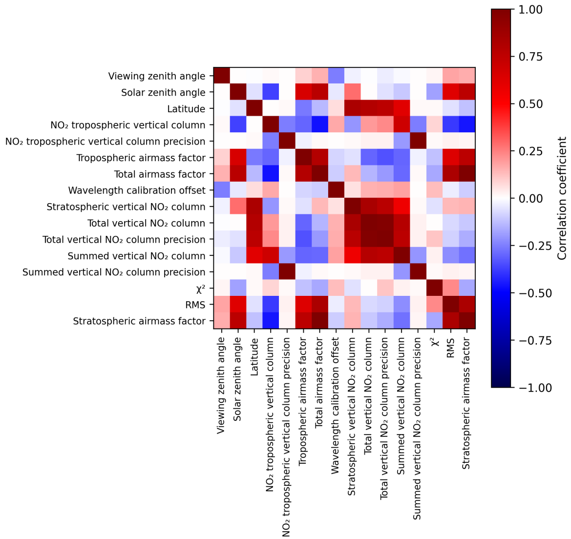
Figure 2: Map of correlation matrix for 2025-08-17 to 2025-08-19.
