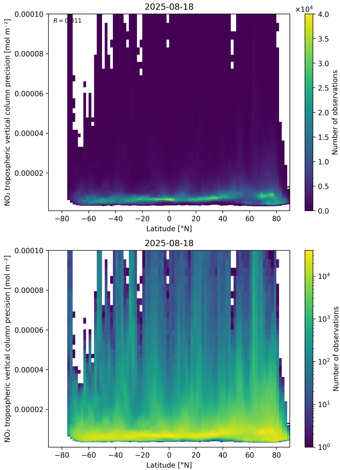
Figure 93: Scatter density plot of “Latitude” against “NO 2 tropospheric vertical column precision” for 2025-08-17 to 2025-08-19.
