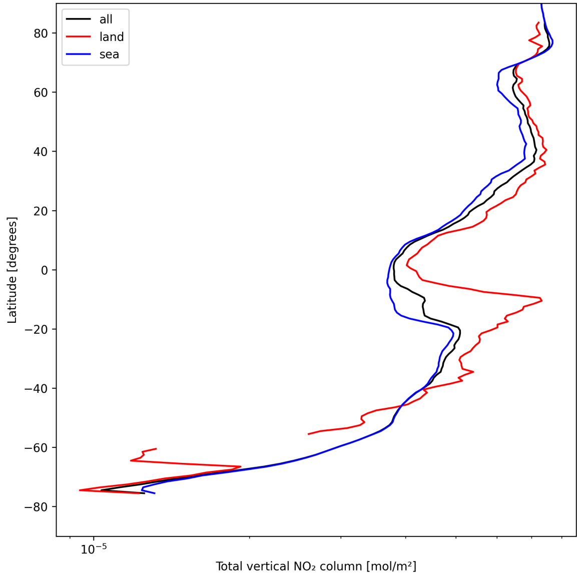
Figure 21: Zonal average of “Total vertical NO 2 column” for 2025-08-17 to 2025-08-19.
