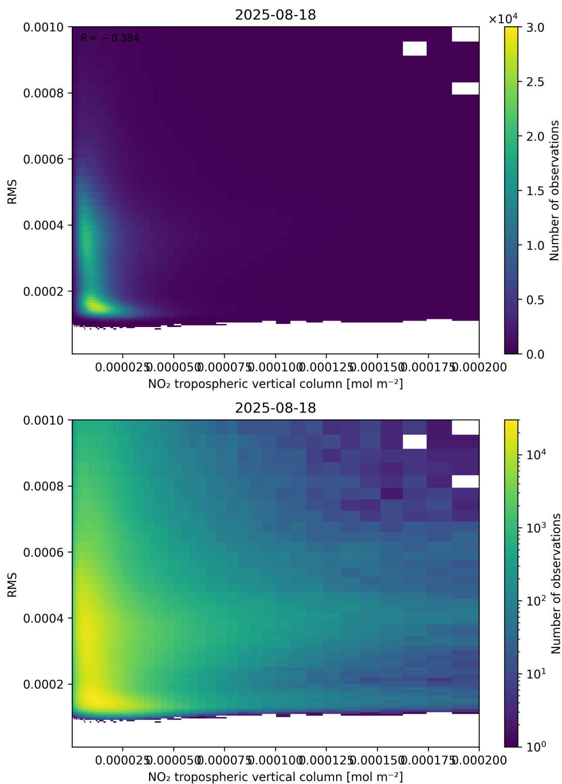
Figure 142: Scatter density plot of “NO 2 tropospheric vertical column” against “RMS” for 2025-08-17 to 2025-08-19.
