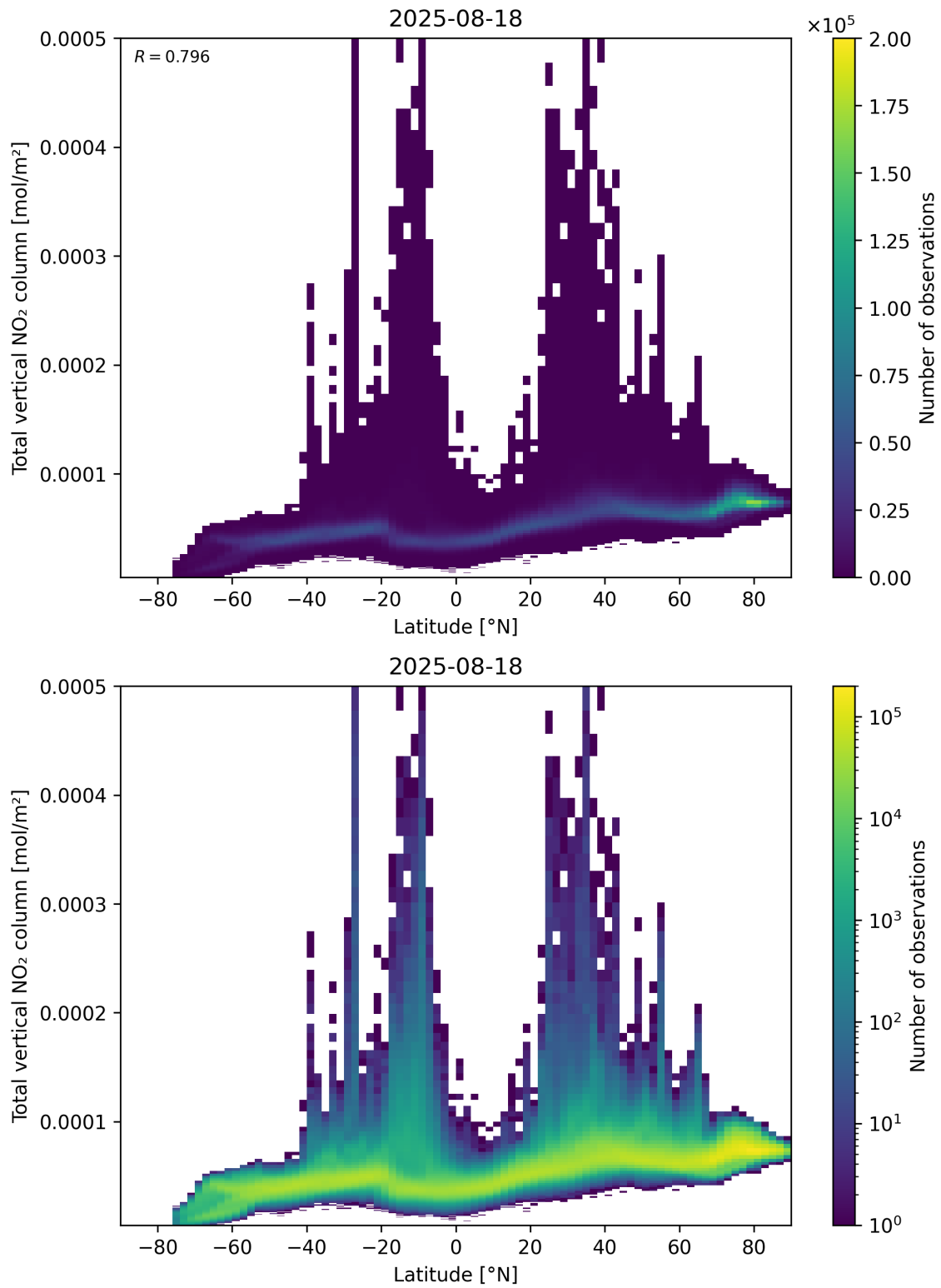
Figure 90: Scatter density plot of “Latitude” against “Total vertical NO 2 column” for 2025-08-17 to 2025-08-19.
