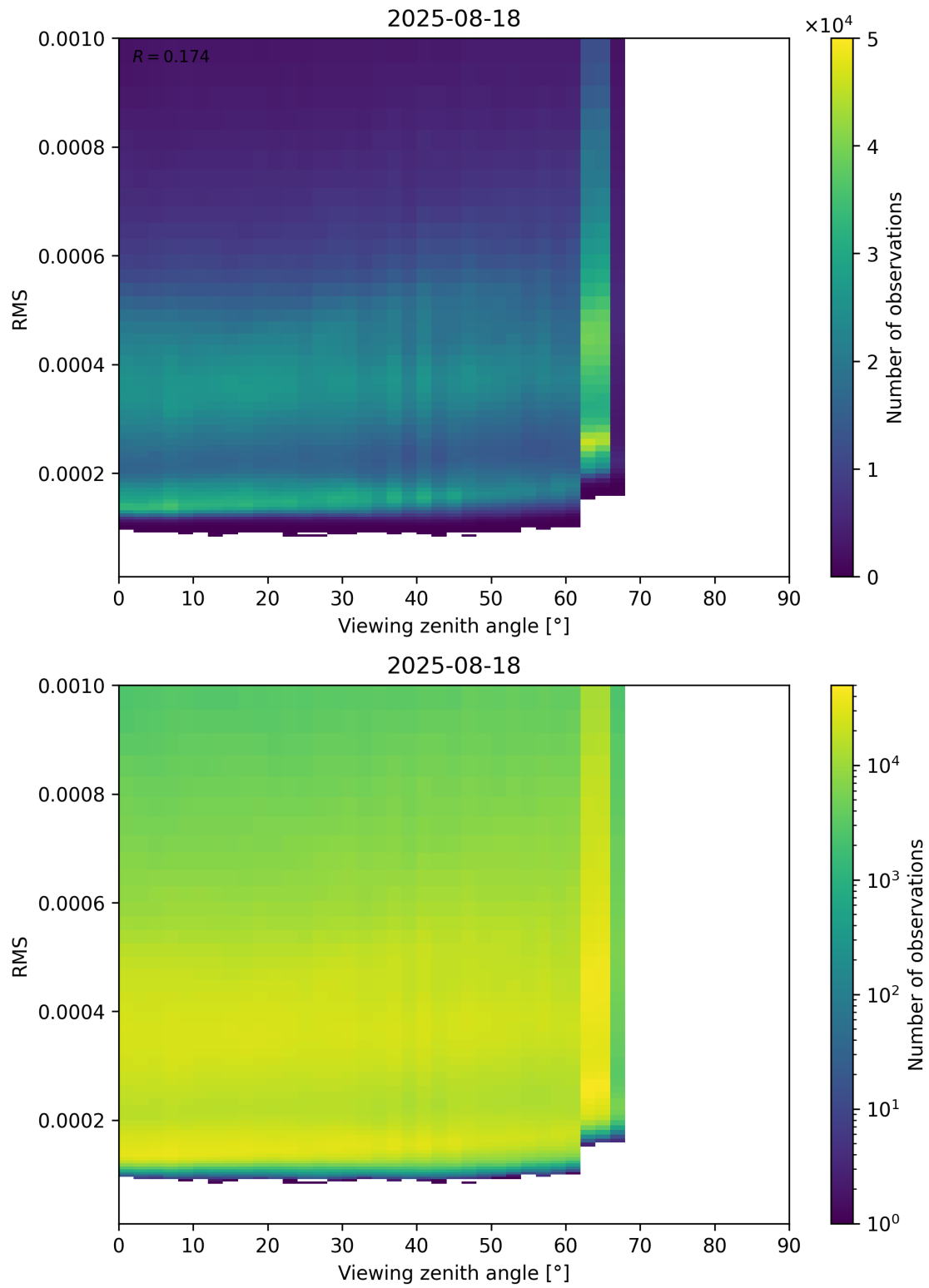
Figure 171: Scatter density plot of “Viewing zenith angle” against “RMS” for 2025-08-17 to 2025-08-19.
