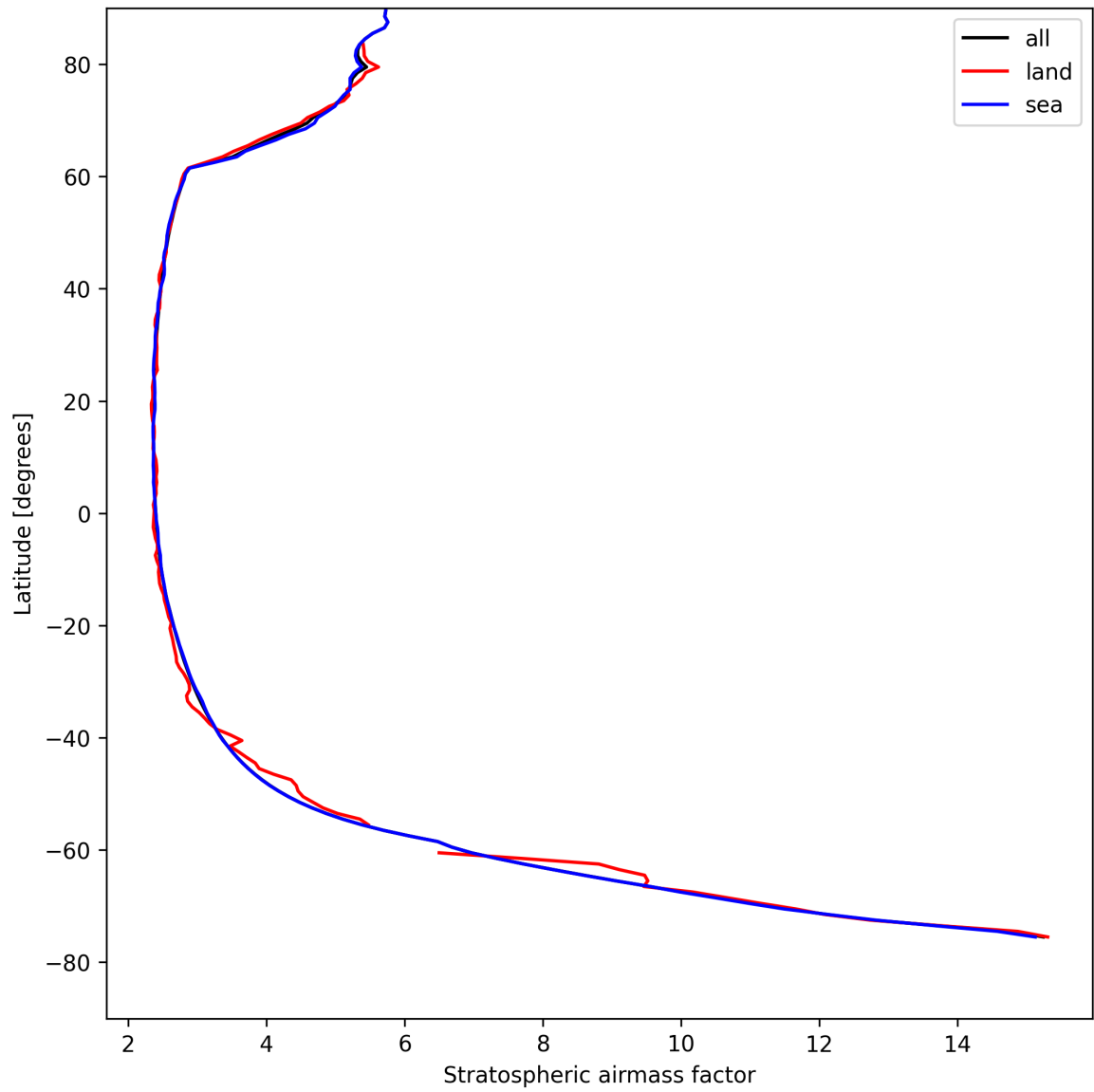
Figure 27: Zonal average of “Stratospheric airmass factor” for 2025-08-17 to 2025-08-19.
