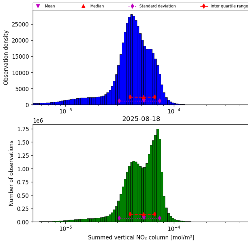
Figure 40: Histogram of “Summed vertical NO 2 column” for 2025-08-17 to 2025-08-19
