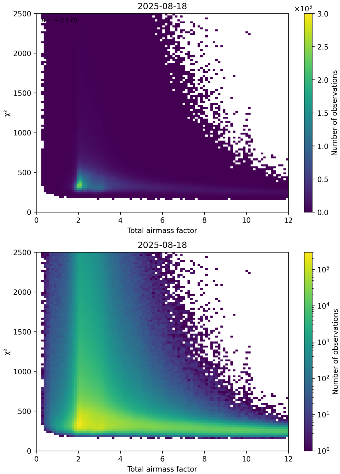
Figure 63: Scatter density plot of “Total airmass factor” against “ \chi^2 ” for 2025-08-17 to 2025-08-19.
