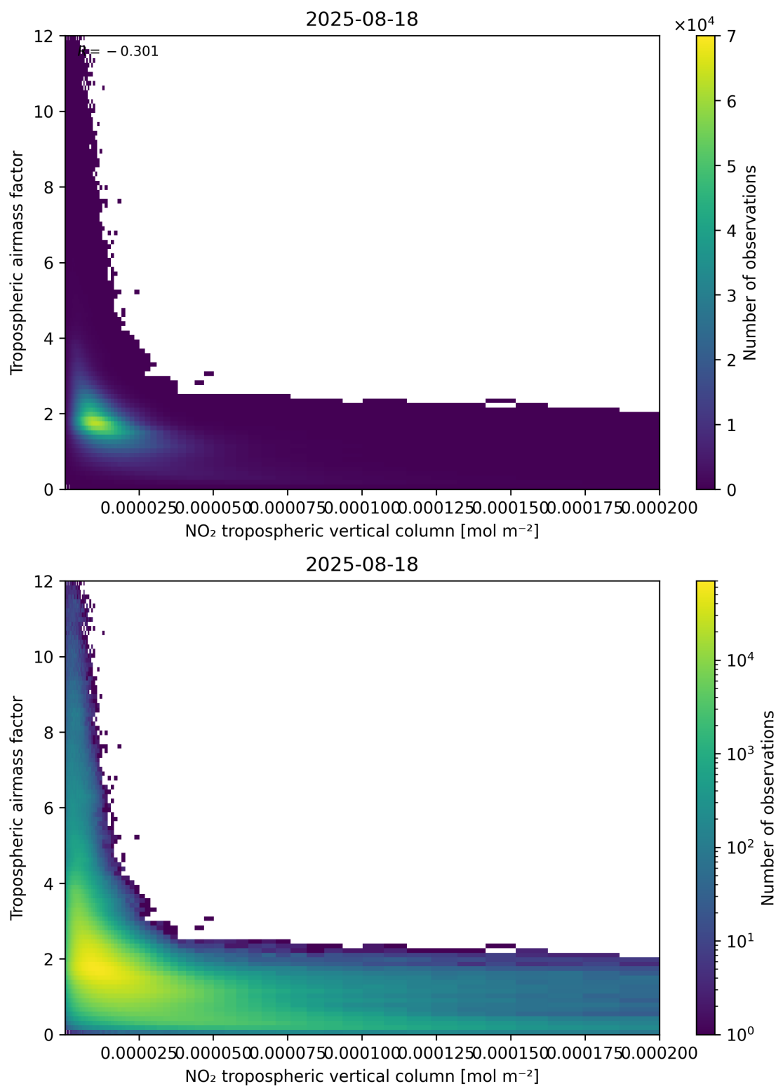
Figure 123: Scatter density plot of “NO 2 tropospheric vertical column” against “Tropospheric air mass factor” for 2025-08-17 to 2025-08-19.
