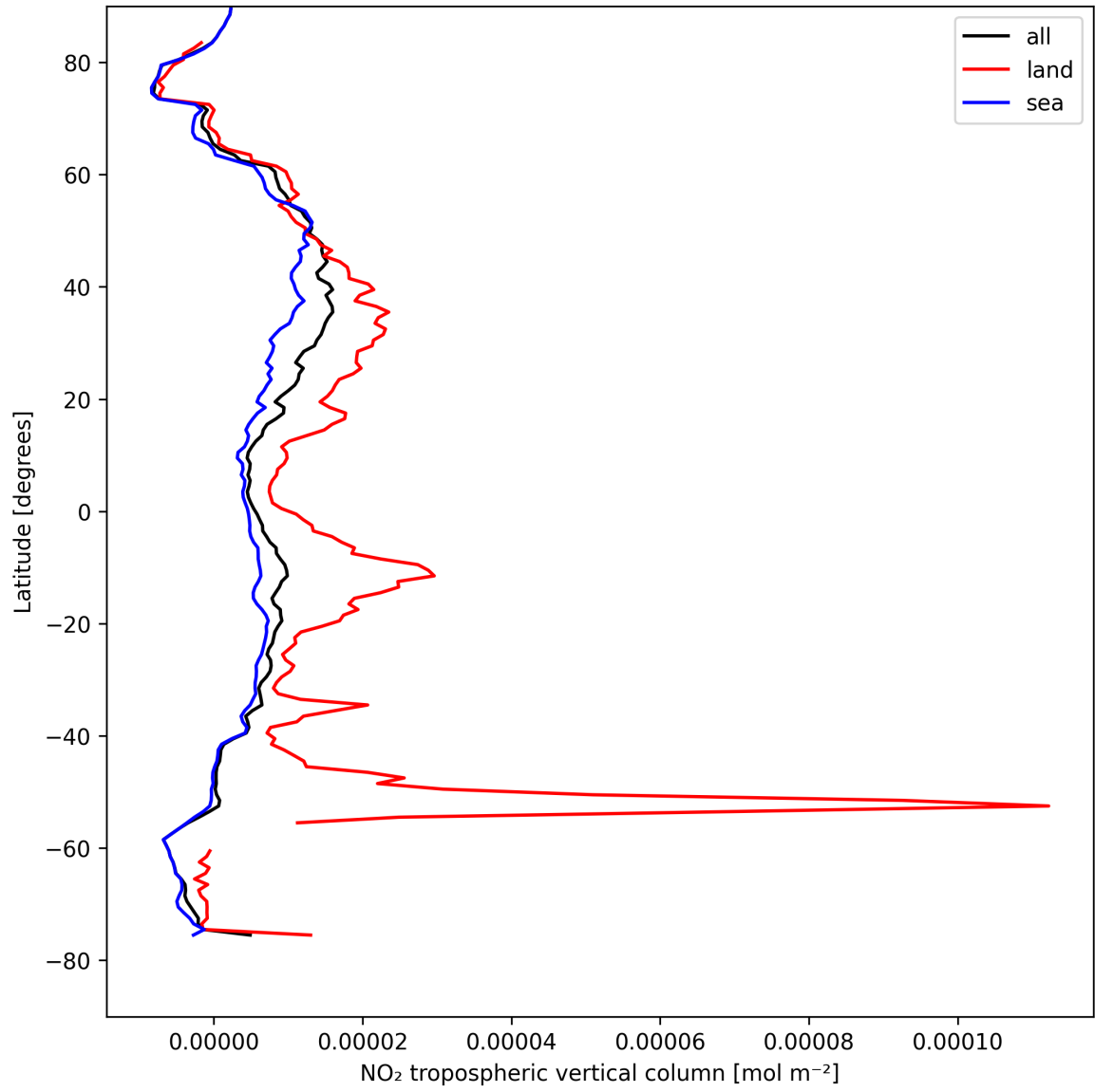
Figure 12: Zonal average of “NO 2 tropospheric vertical column” for 2025-08-17 to 2025-08-19.
