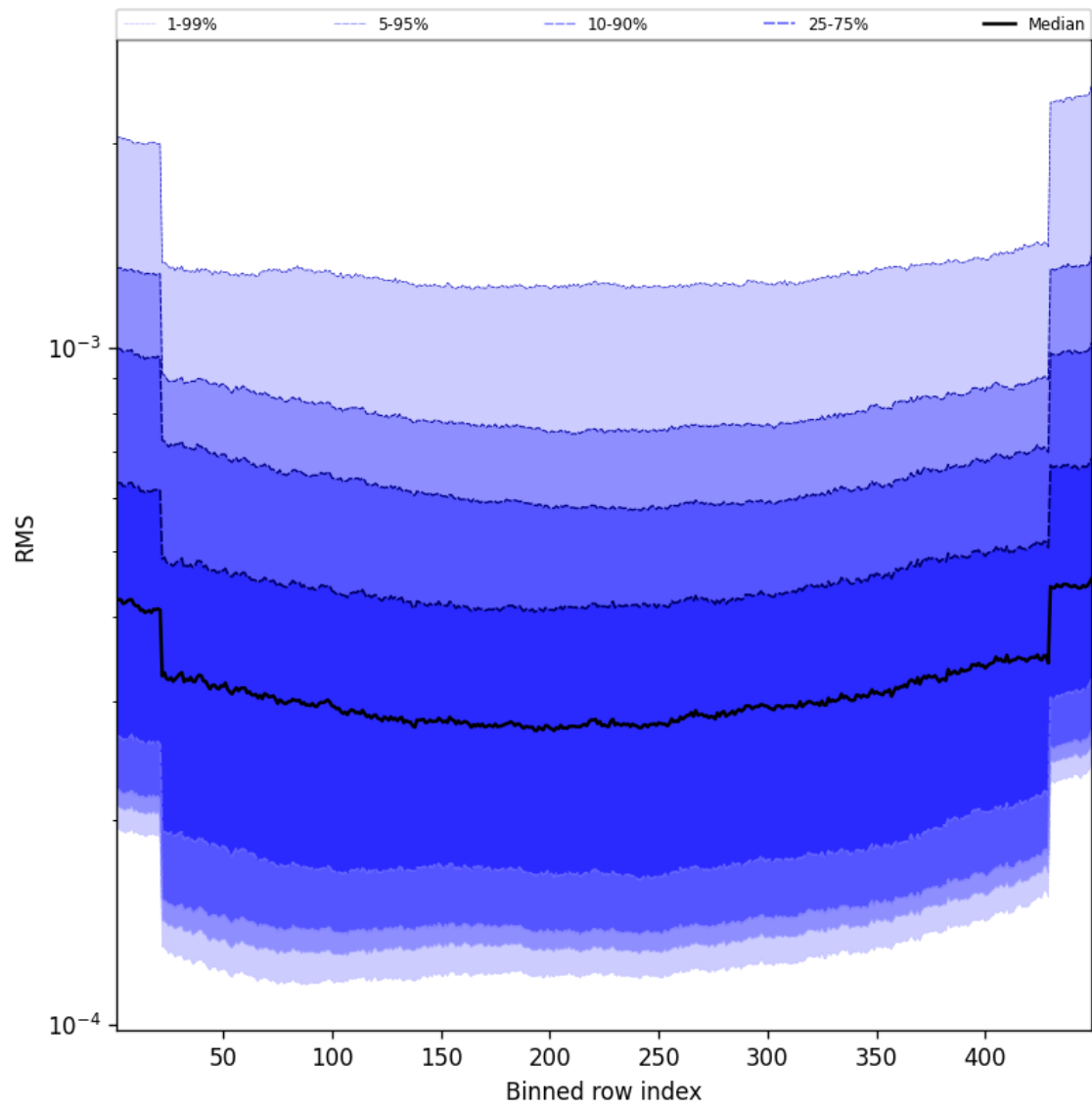
Figure 60: Along track statistics of “RMS” for 2025-08-17 to 2025-08-19
