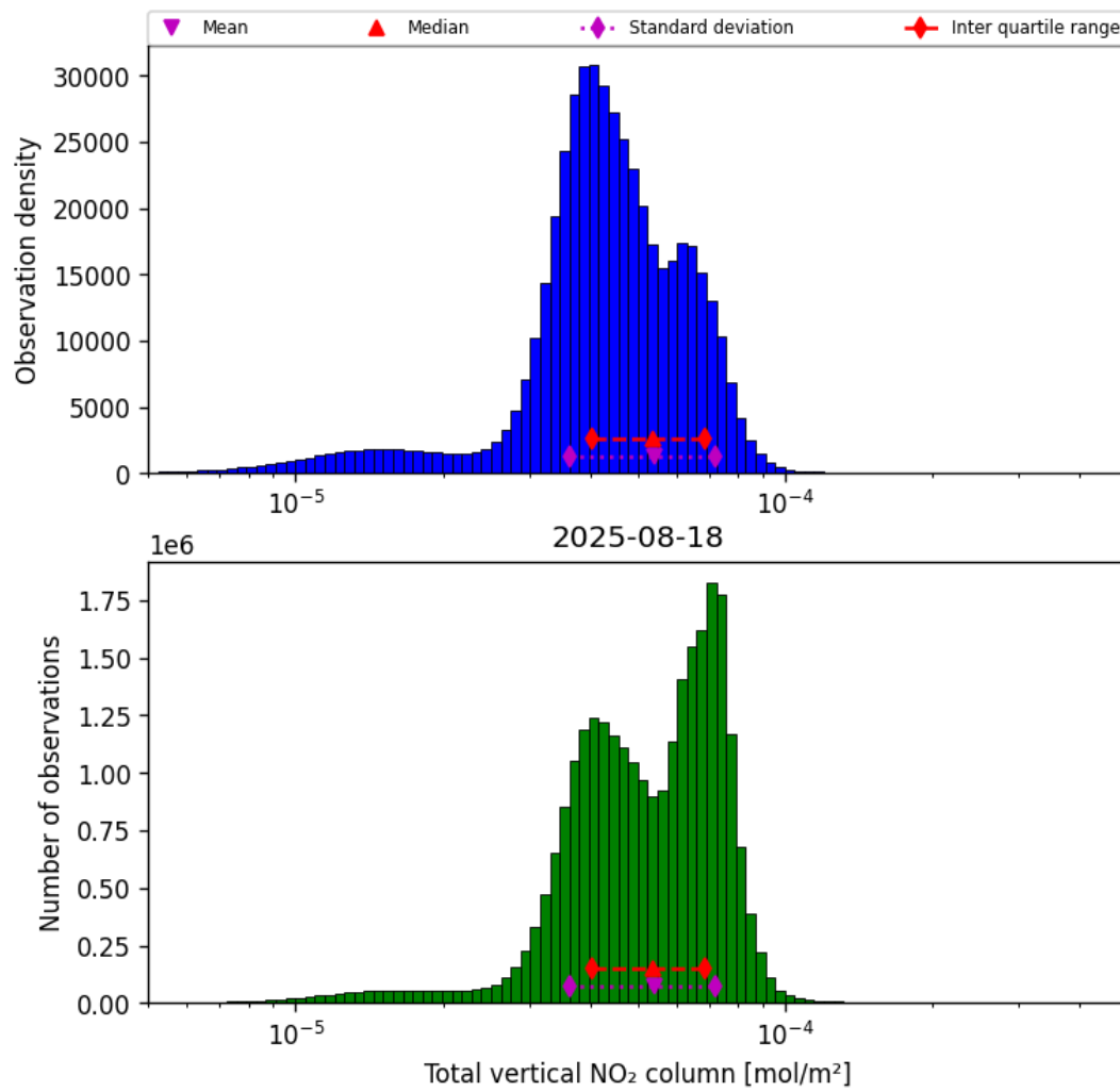
Figure 38: Histogram of “Total vertical NO 2 column” for 2025-08-17 to 2025-08-19
