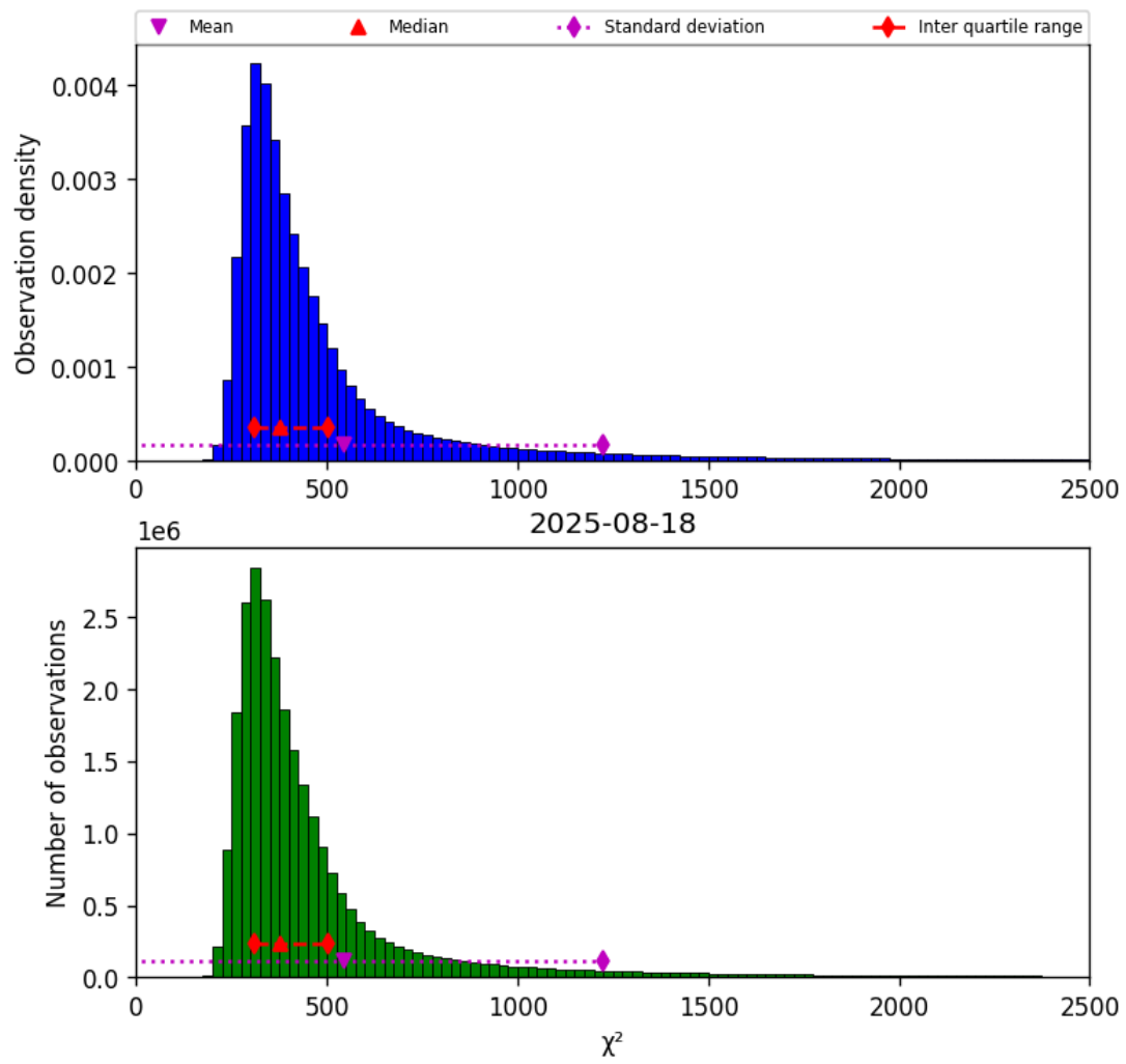
Figure 42: Histogram of “ \chi^2 ” for 2025-08-17 to 2025-08-19
