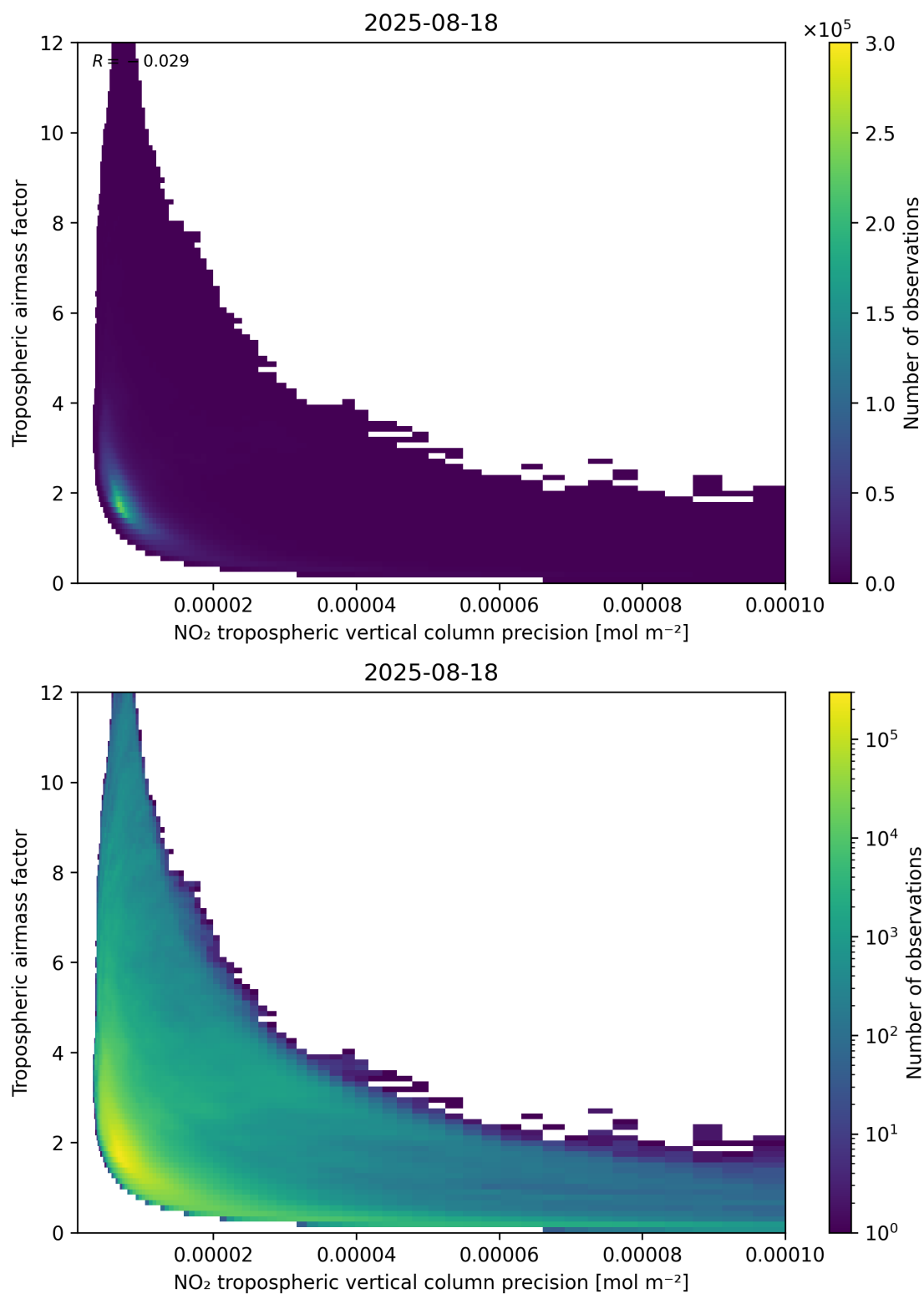
Figure 133: Scatter density plot of “NO 2 tropospheric vertical column precision” against “Tropospheric air mass factor” for 2025-08-17 to 2025-08-19.
