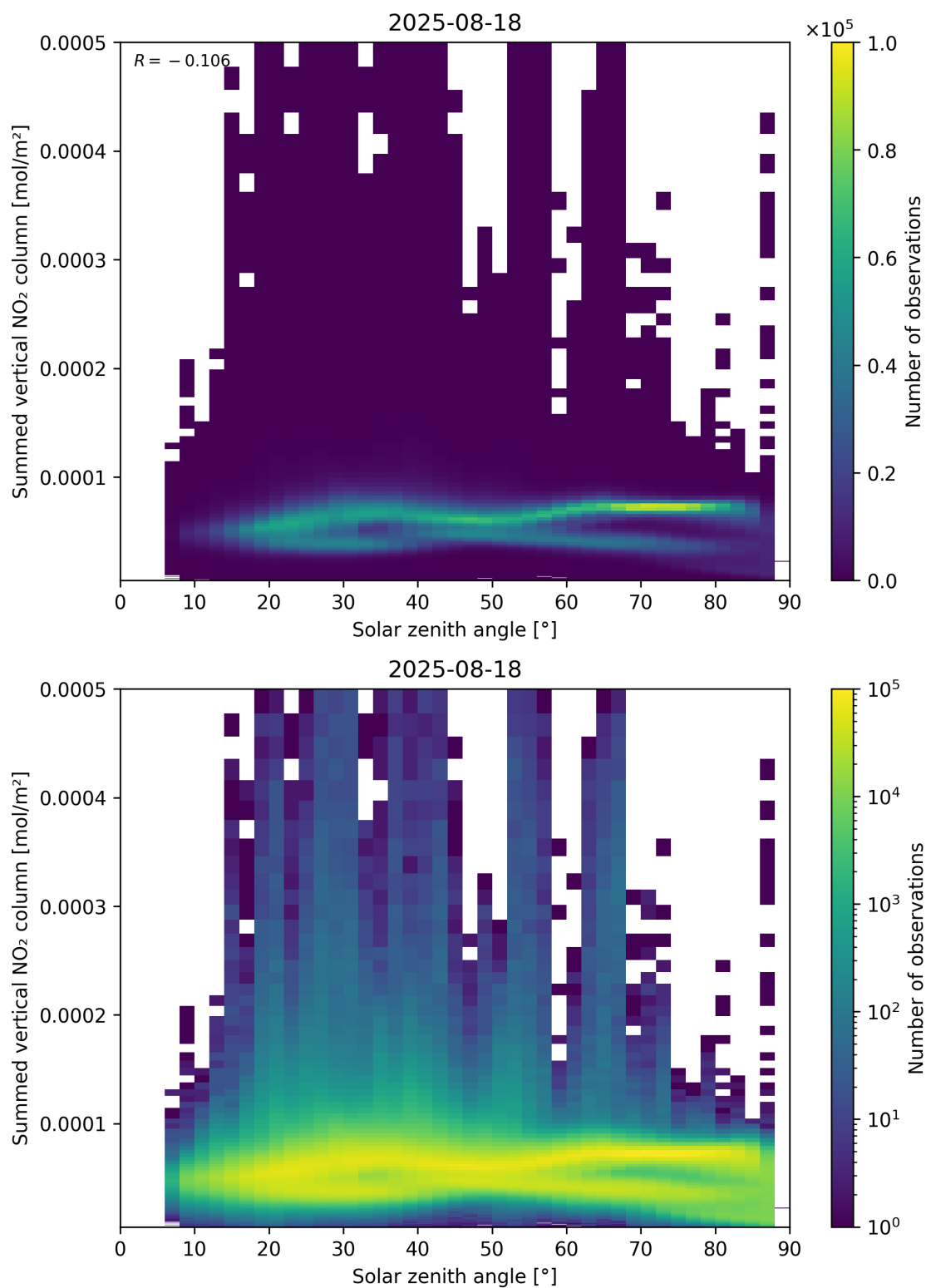
Figure 151: Scatter density plot of “Solar zenith angle” against “Summed vertical NO 2 column” for 2025-08-17 to 2025-08-19.
