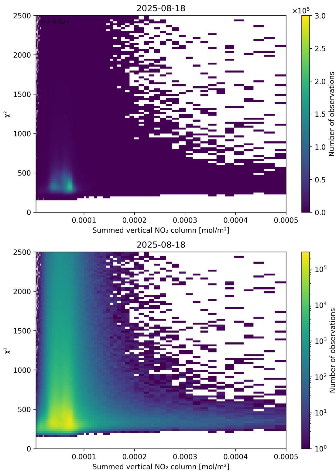
Figure 104: Scatter density plot of “Summed vertical NO 2 column” against “ \chi^2 ” for 2025-08-17 to 2025-08-19.
