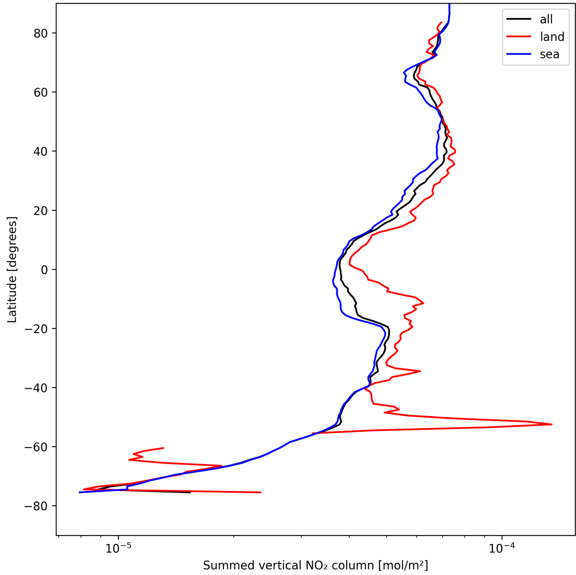
Figure 23: Zonal average of “Summed vertical NO 2 column” for 2025-08-17 to 2025-08-19.
