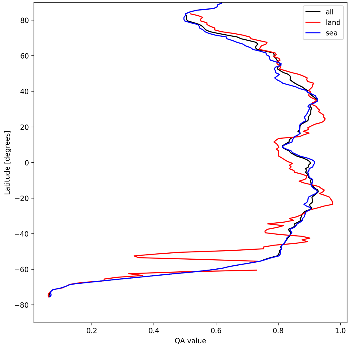
Figure 11: Zonal average of “QA value” for 2025-08-17 to 2025-08-19.
