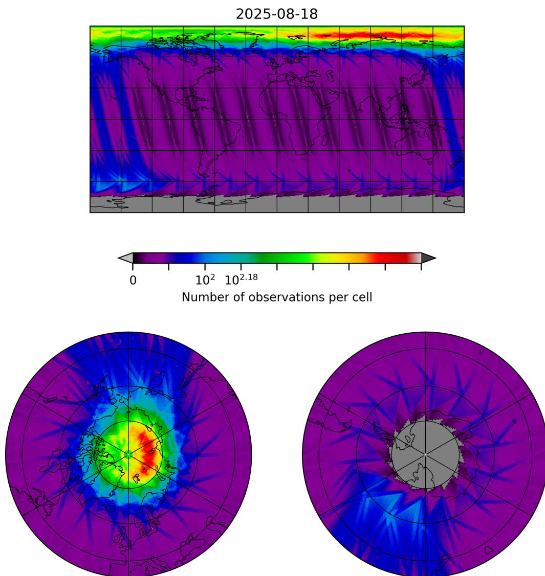
Figure 10: Map of the number of observations for 2025-08-17 to 2025-08-19
