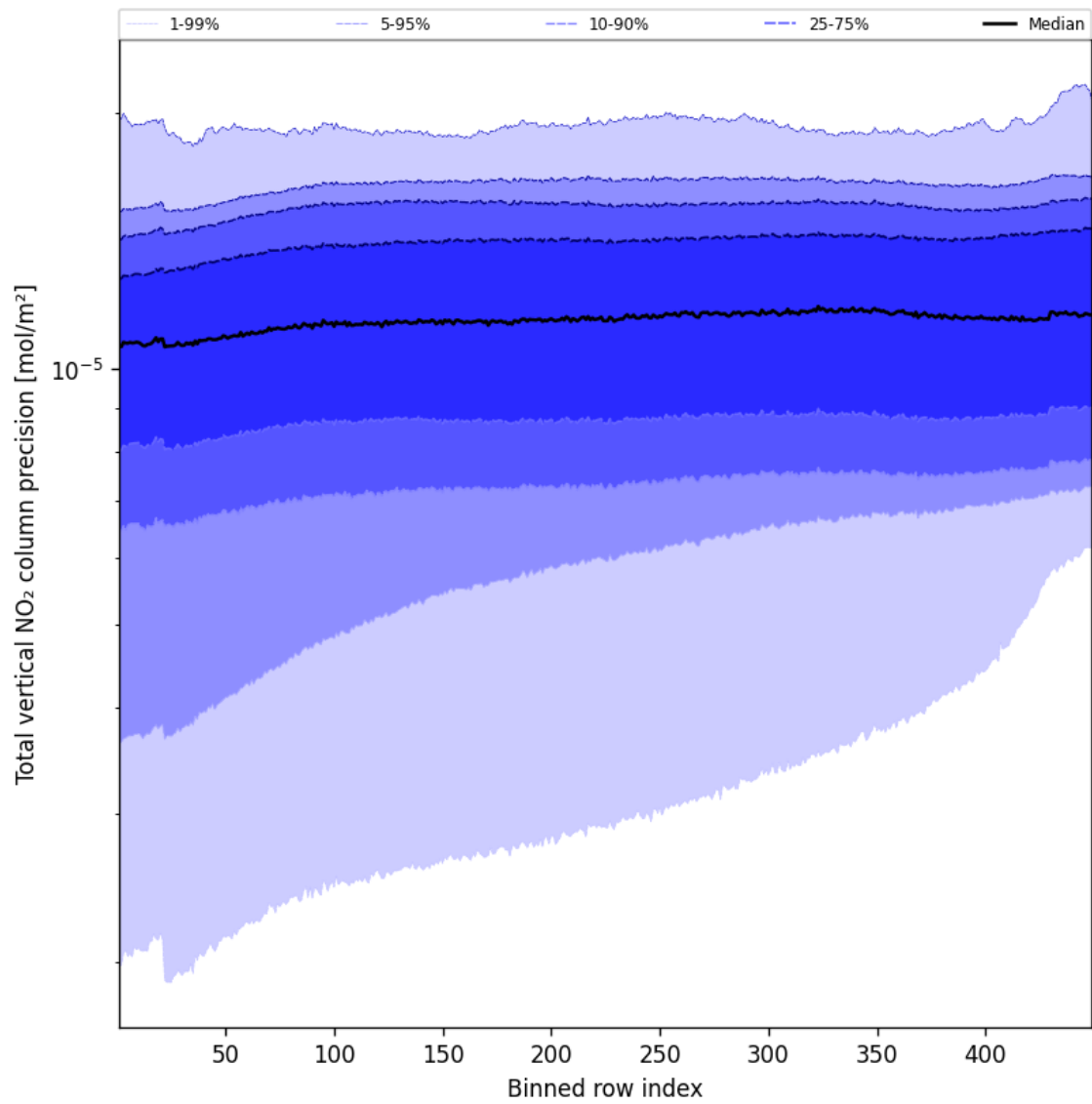
Figure 56: Along track statistics of “Total vertical NO 2 column precision” for 2025-08-17 to 2025-08-19
