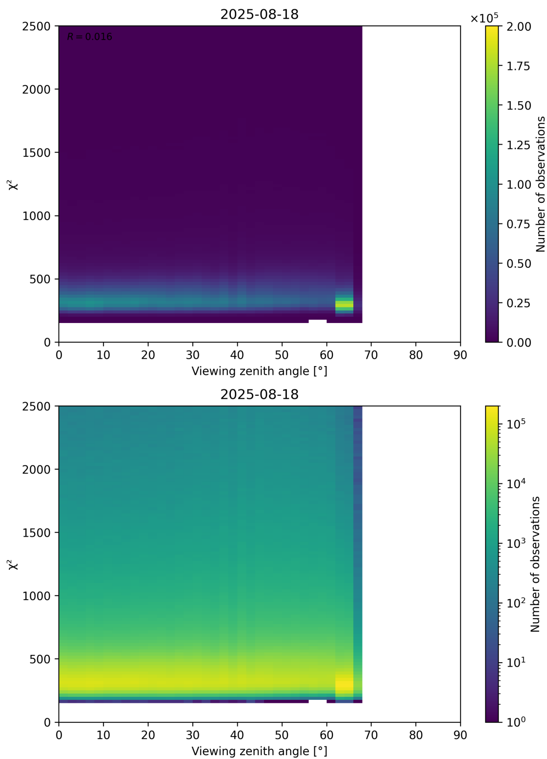
Figure 162: Scatter density plot of “Viewing zenith angle” against “ \chi^2 ” for 2025-08-17 to 2025-08-19.
