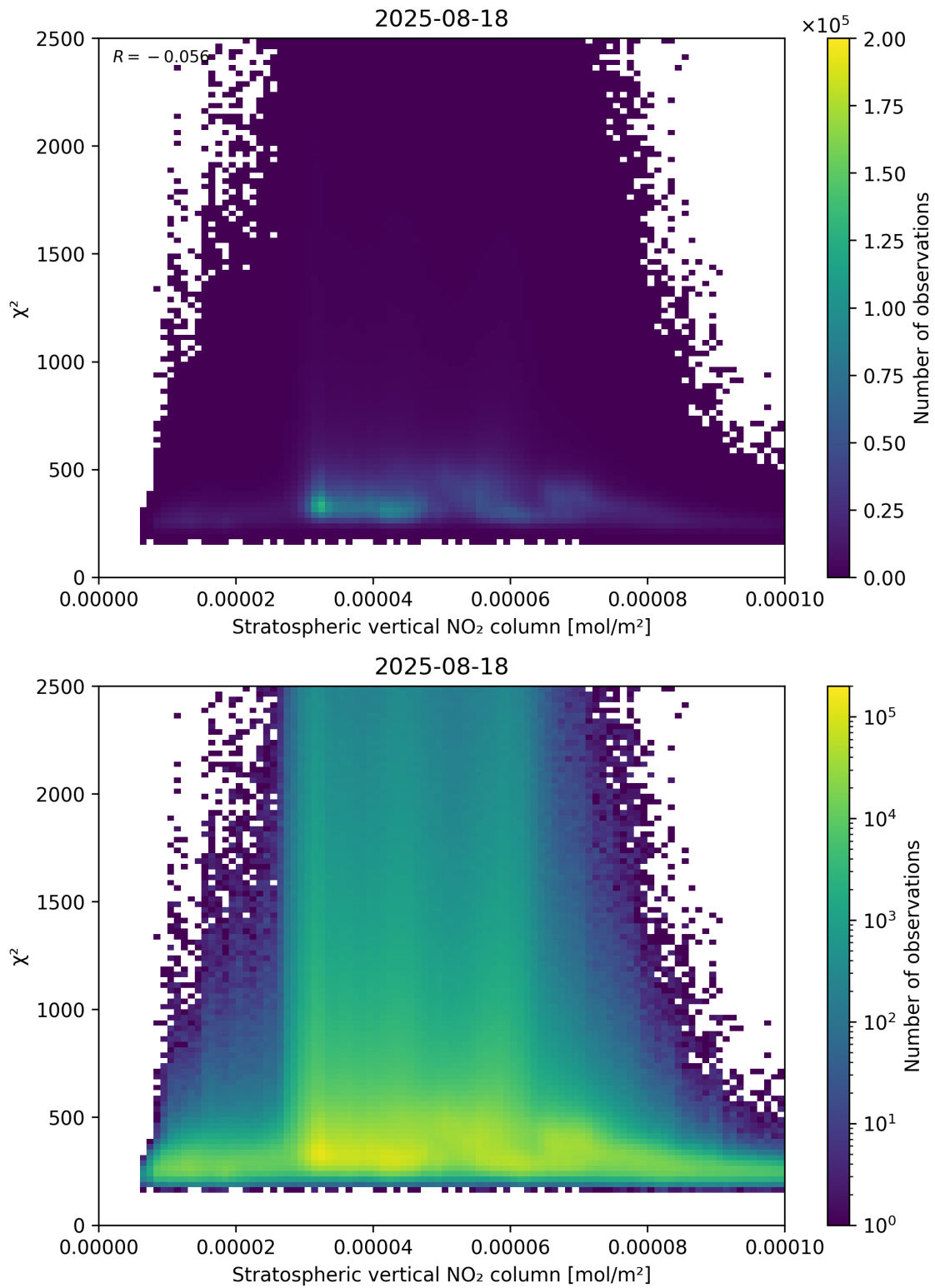
Figure 97: Scatter density plot of “Stratospheric vertical NO 2 column” against “ \chi^2 ” for 2025-08-17 to 2025-08-19.
