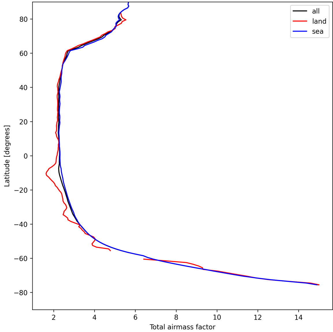
Figure 15: Zonal average of “Total airmass factor” for 2025-08-17 to 2025-08-19.
