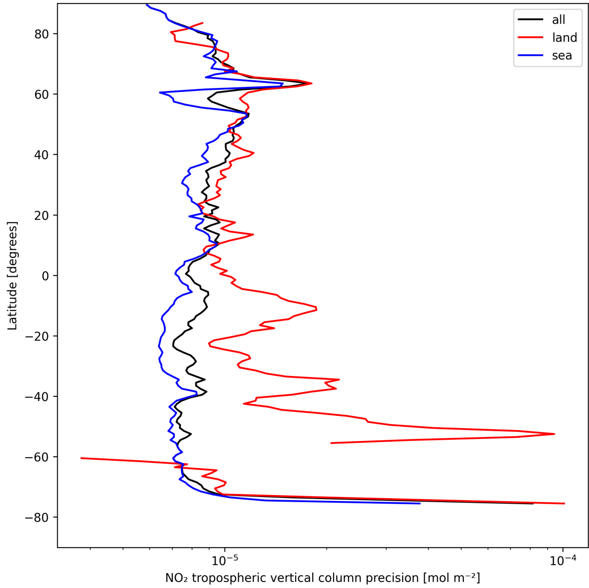
Figure 13: Zonal average of “NO 2 tropospheric vertical column precision” for 2025-08-17 to 2025-08-19.
