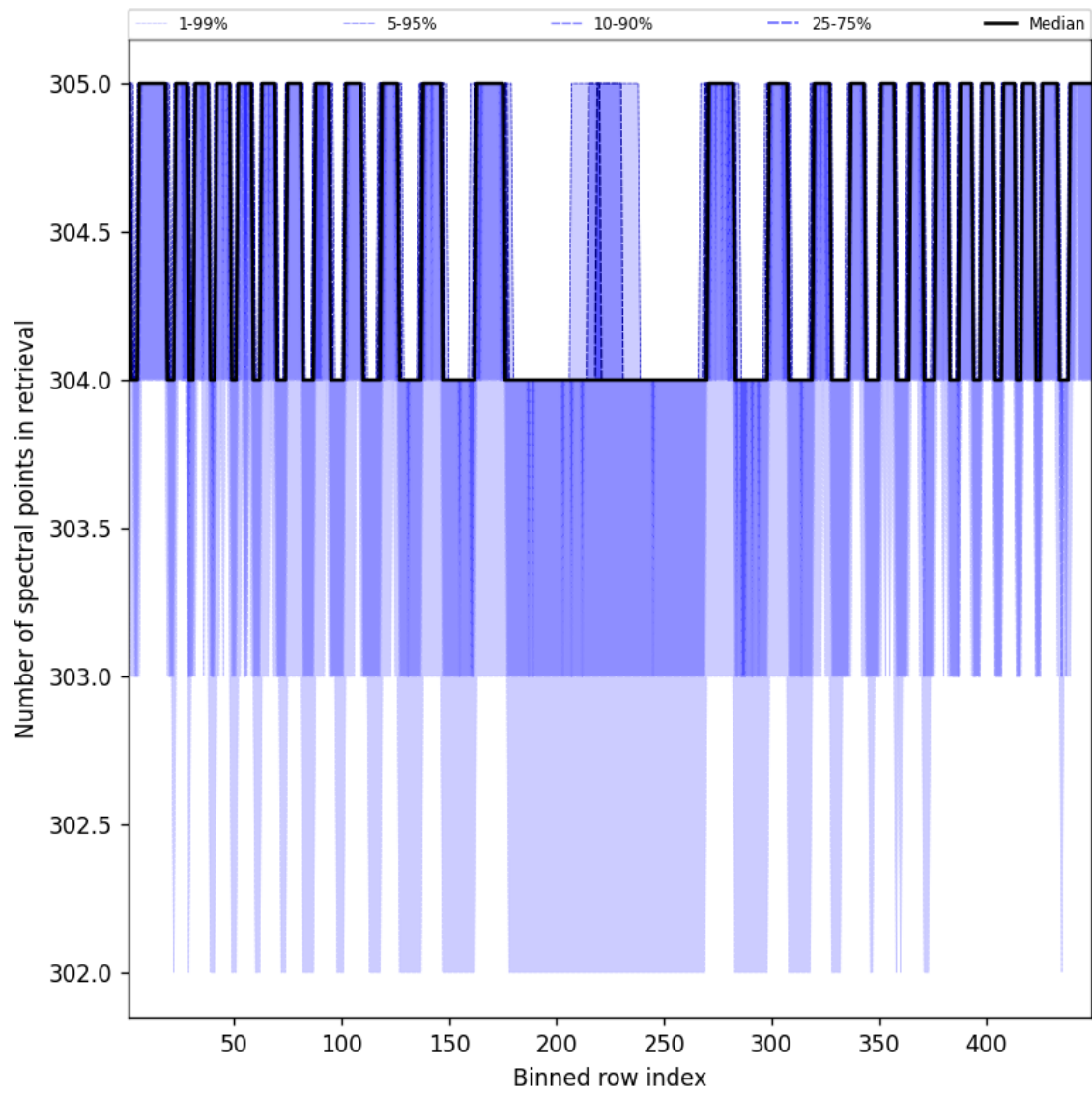
Figure 50: Along track statistics of “Number of spectral points in retrieval” for 2025-08-17 to 2025-08-19
