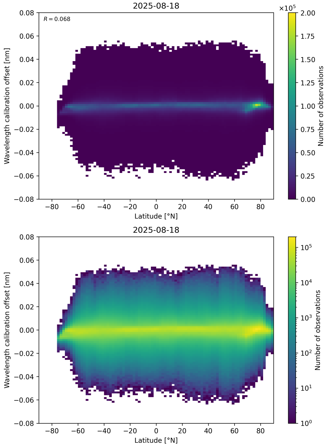
Figure 95: Scatter density plot of “Latitude” against “Wavelength calibration offset” for 2025-08-17 to 2025-08-19.
