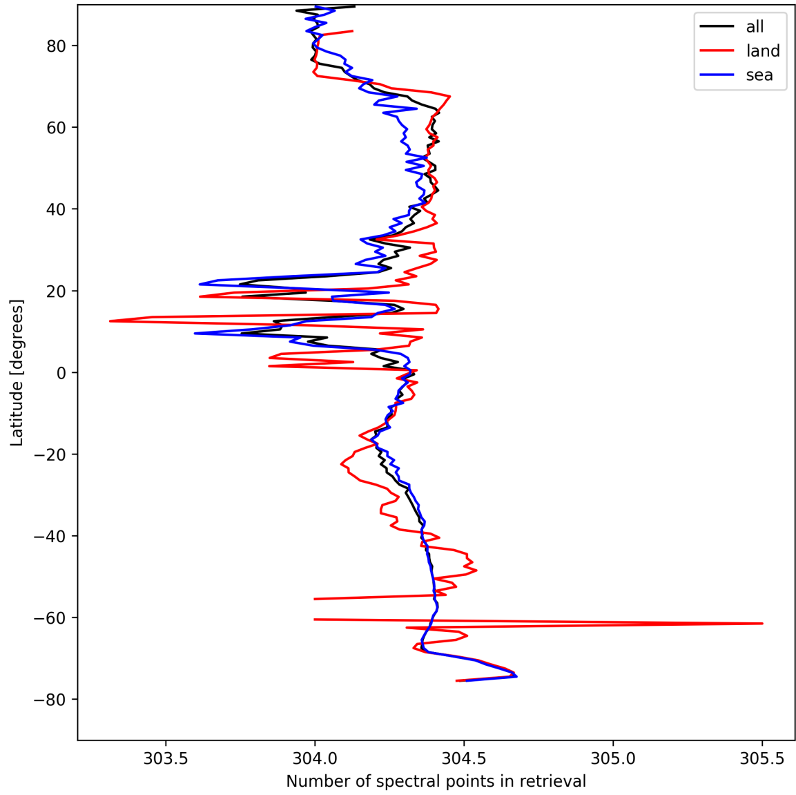
Figure 16: Zonal average of “Number of spectral points in retrieval” for 2025-08-17 to 2025-08-19.
