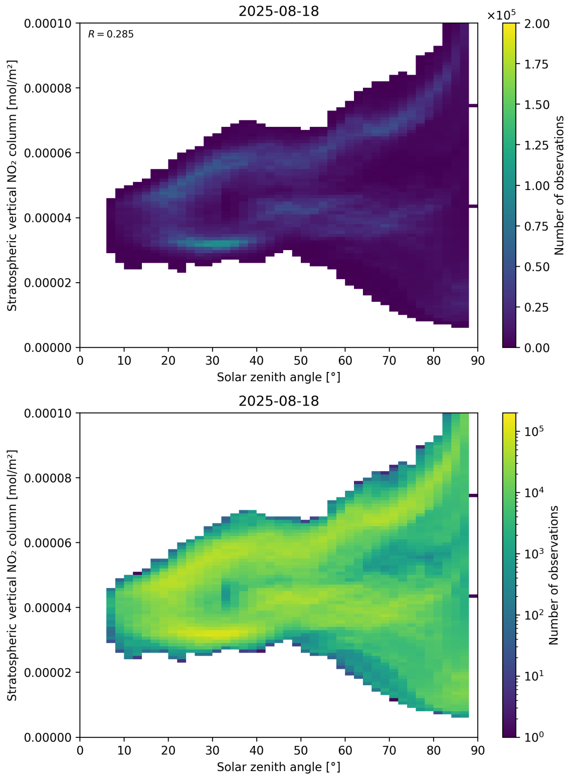
Figure 150: Scatter density plot of “Solar zenith angle” against “Stratospheric vertical NO 2 column” for 2025-08-17 to 2025-08-19.
