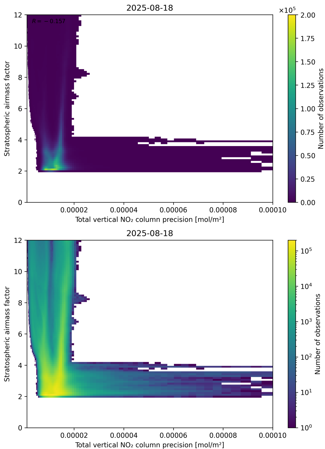
Figure 115: Scatter density plot of “Total vertical NO 2 column precision” against “Stratospheric air mass factor” for 2025-08-17 to 2025-08-19.
