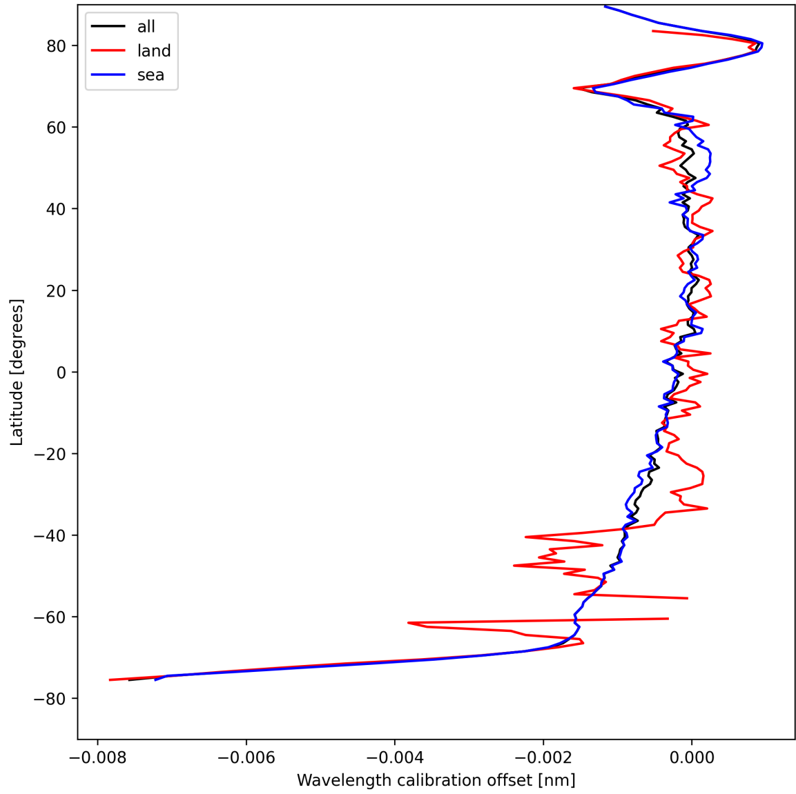
Figure 18: Zonal average of “Wavelength calibration offset” for 2025-08-17 to 2025-08-19.
