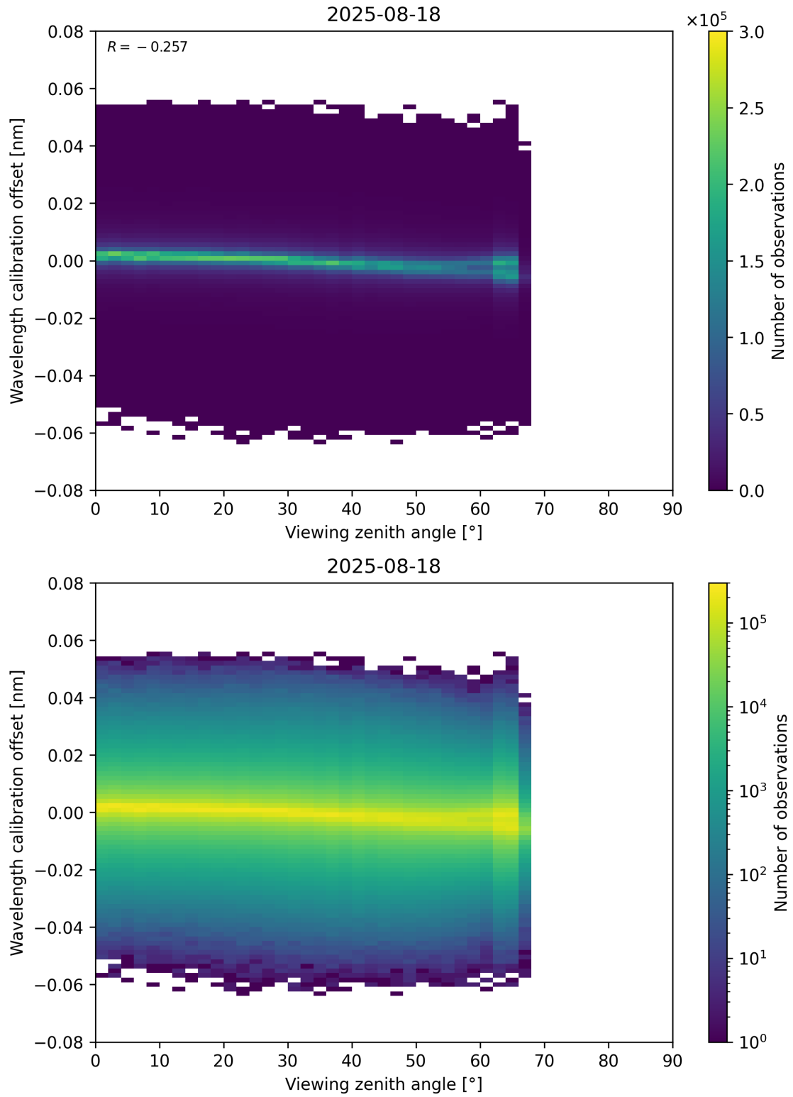
Figure 173: Scatter density plot of “Viewing zenith angle” against “Wavelength calibration offset” for 2025-08-17 to 2025-08-19.
