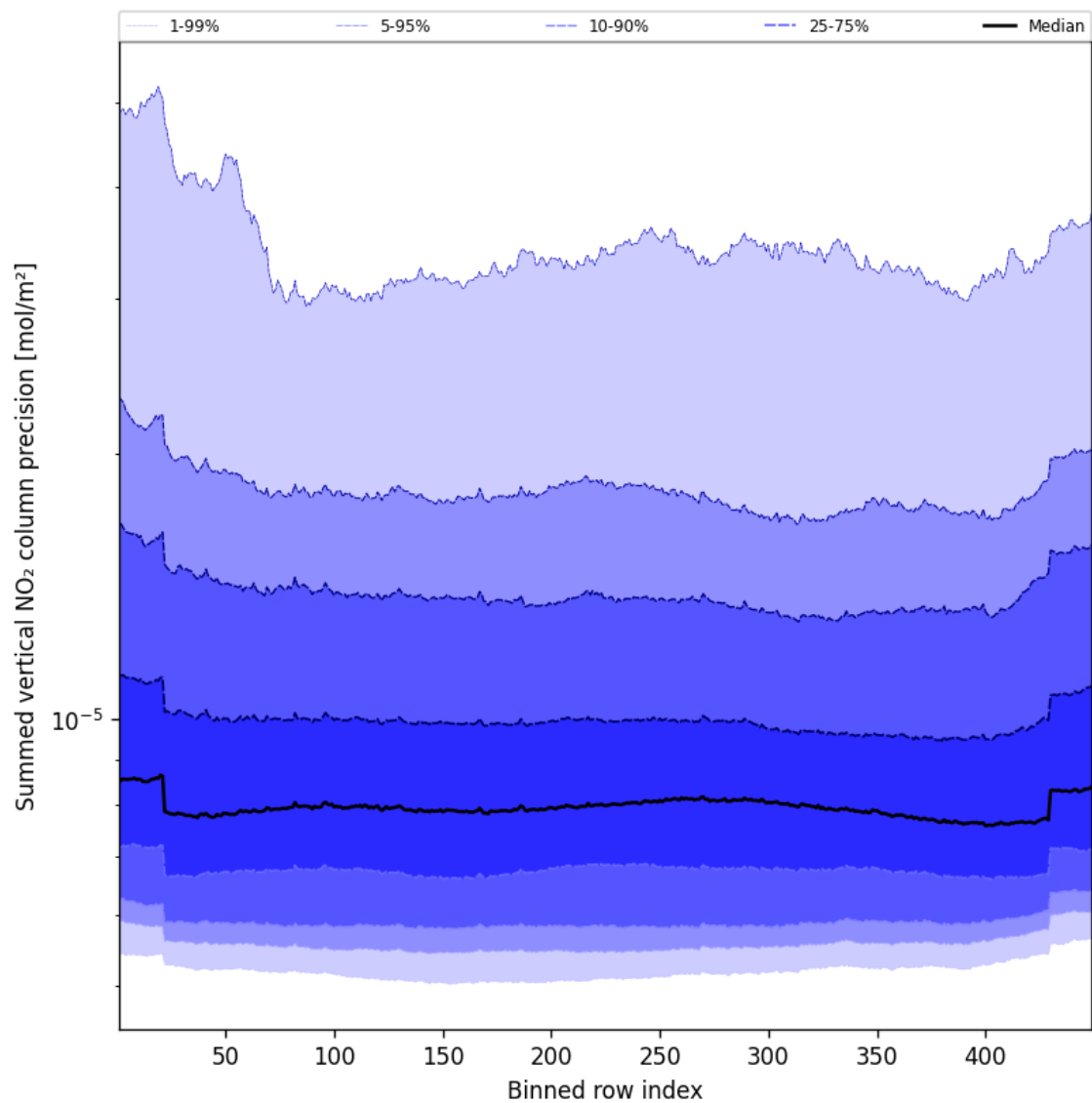
Figure 58: Along track statistics of “Summed vertical NO 2 column precision” for 2025-08-17 to 2025-08-19
