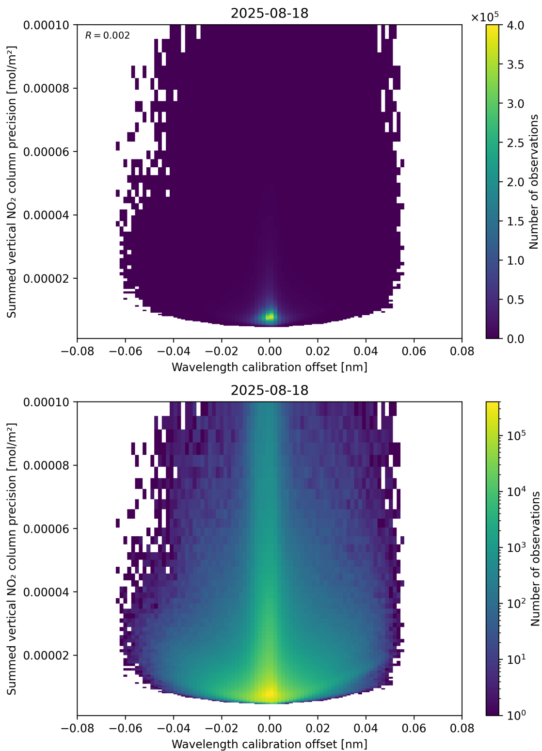
Figure 178: Scatter density plot of “Wavelength calibration offset” against “Summed vertical NO 2 column precision” for 2025-08-17 to 2025-08-19.
