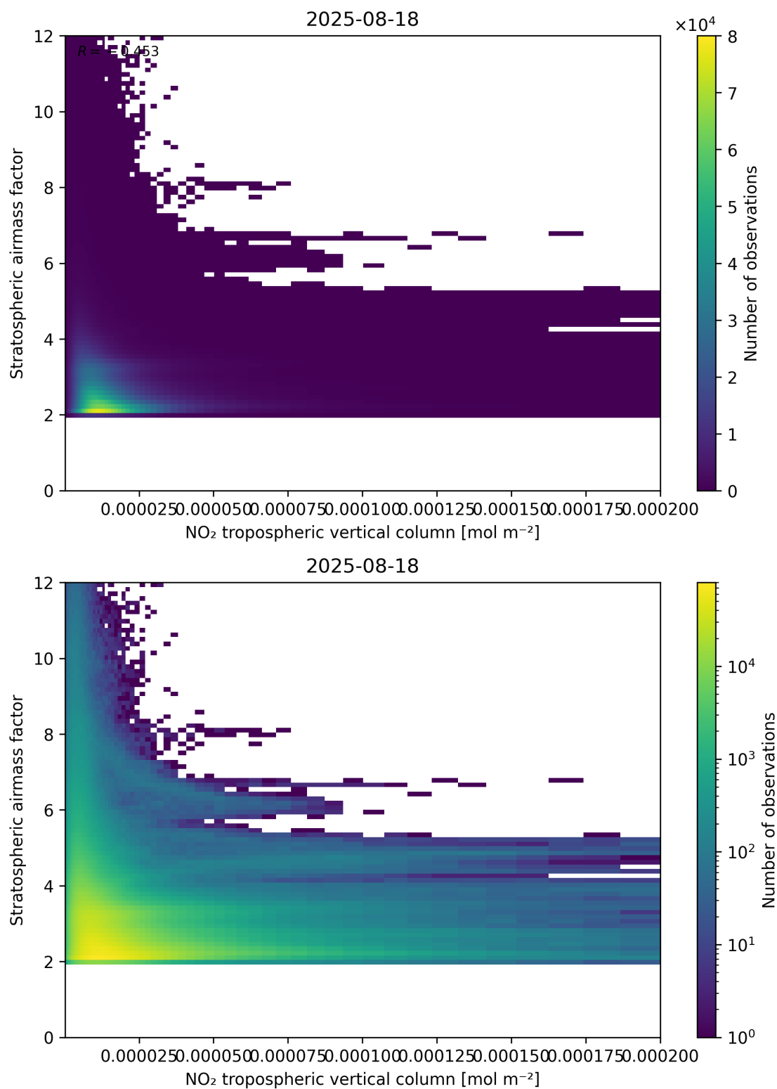
Figure 121: Scatter density plot of “NO 2 tropospheric vertical column” against “Stratospheric air mass factor” for 2025-08-17 to 2025-08-19.
