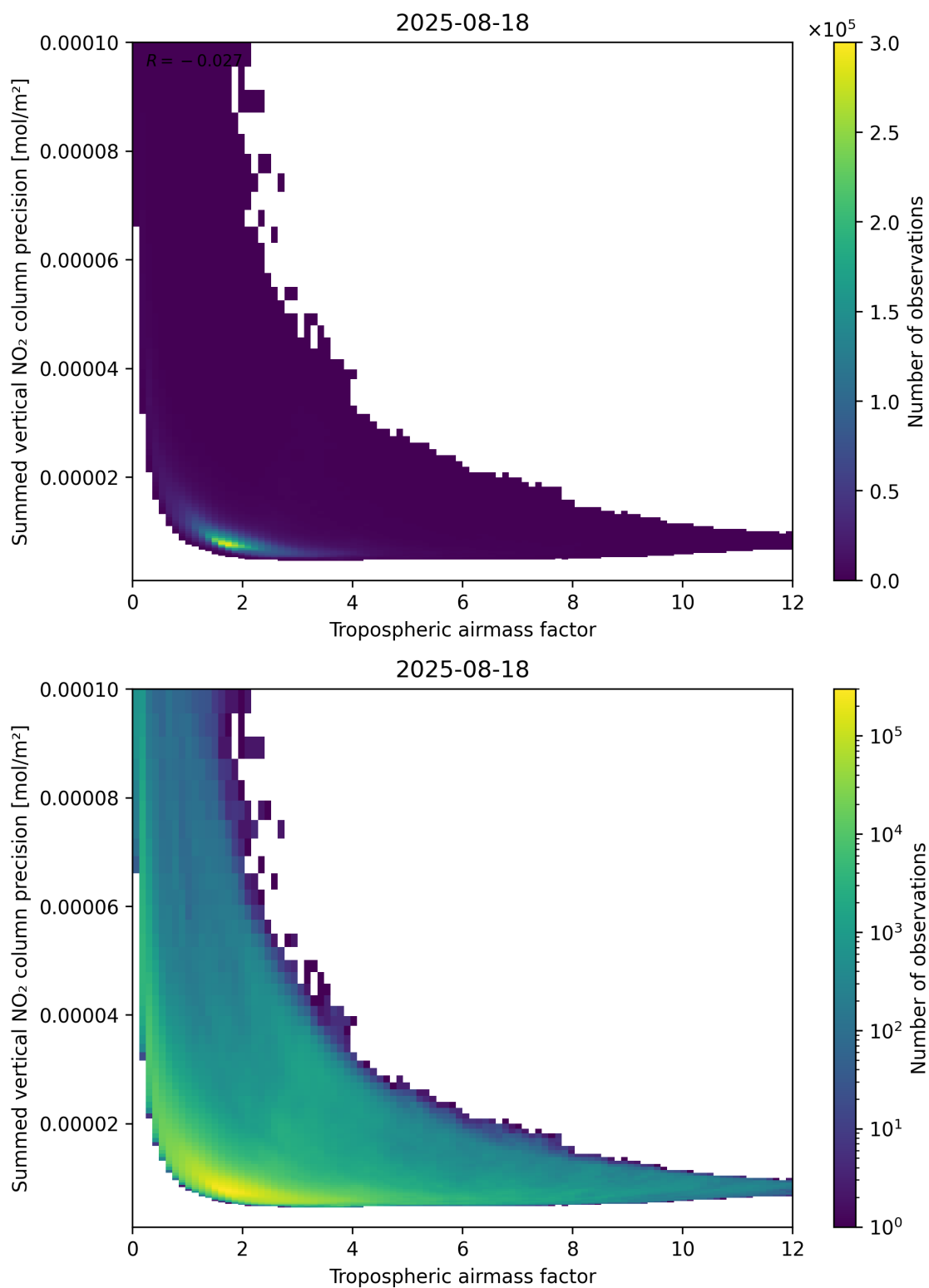
Figure 76: Scatter density plot of “Tropospheric airmass factor” against “Summed vertical NO 2 column precision” for 2025-08-17 to 2025-08-19.
