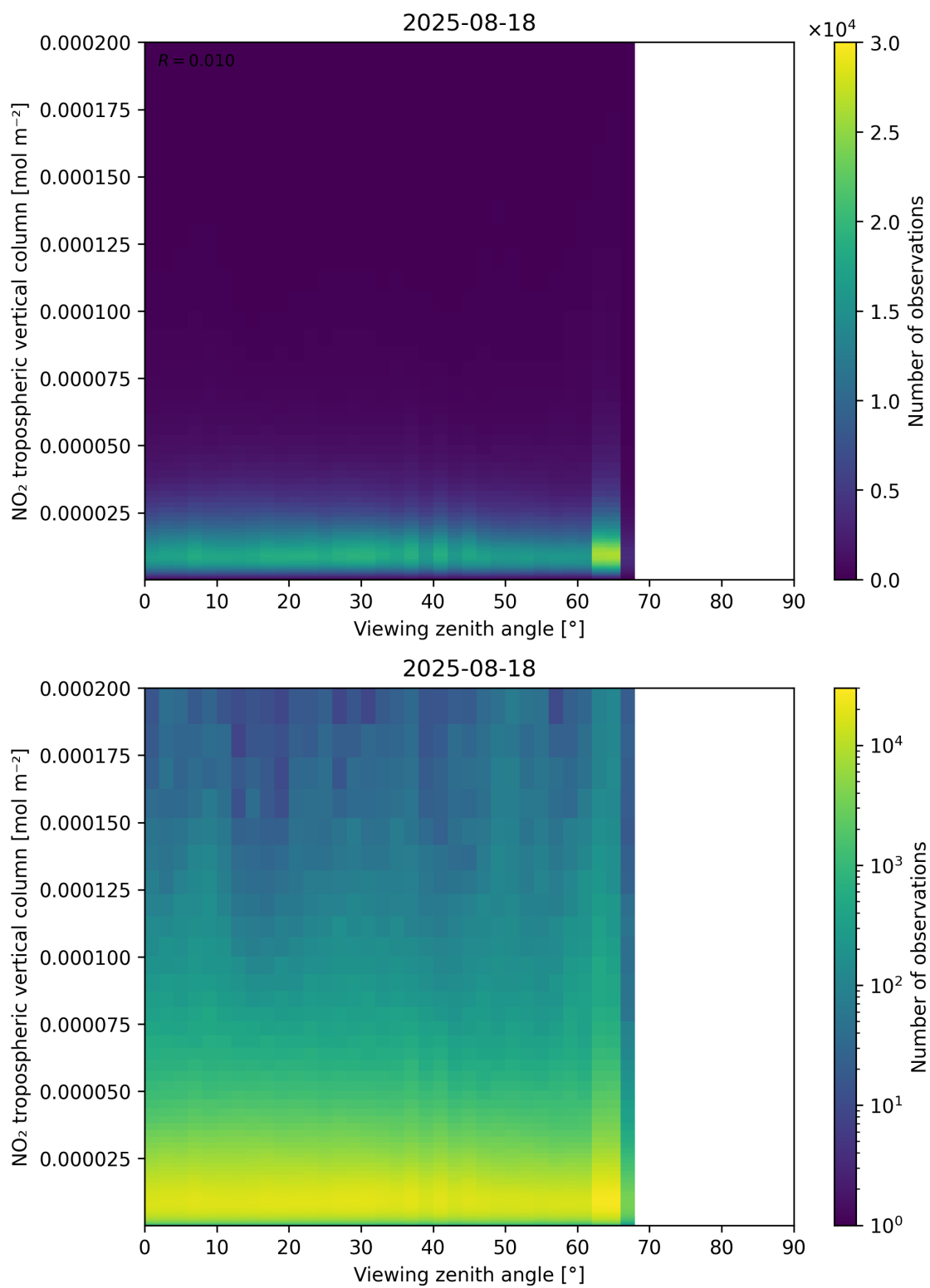
Figure 169: Scatter density plot of “Viewing zenith angle” against “NO 2 tropospheric vertical column” for 2025-08-17 to 2025-08-19.
