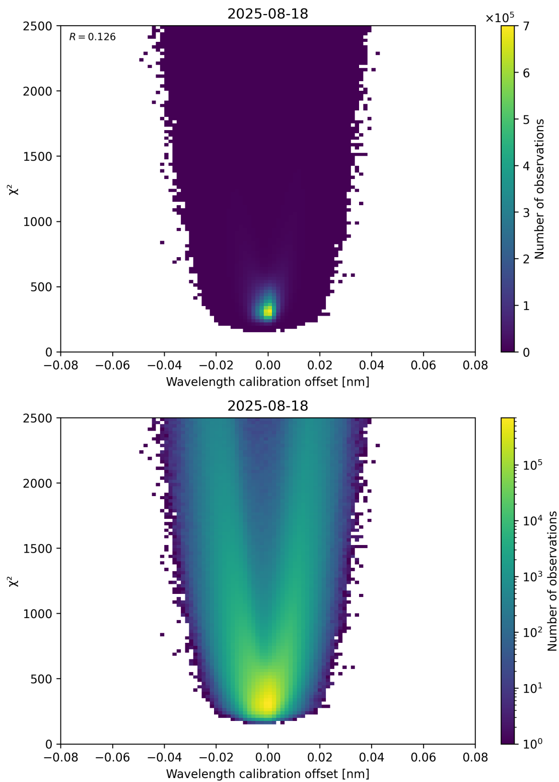
Figure 175: Scatter density plot of “Wavelength calibration offset” against “ \chi^2 ” for 2025-08-17 to 2025-08-19.
