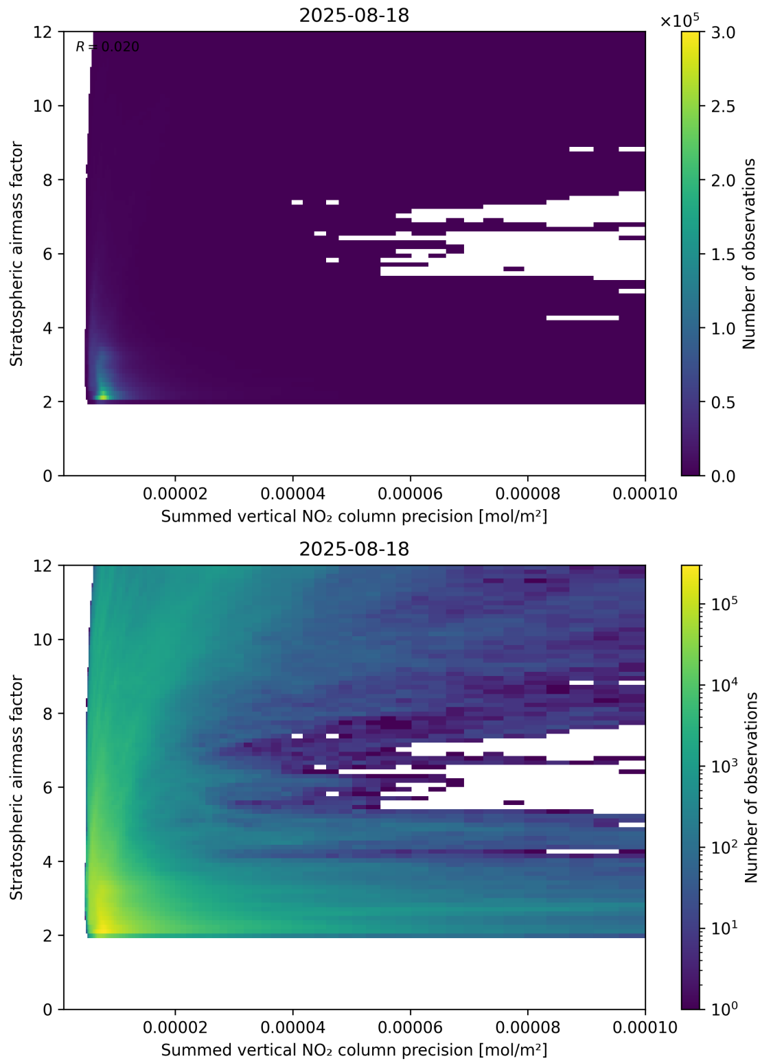
Figure 106: Scatter density plot of “Summed vertical NO 2 column precision” against “Stratospheric airmass factor” for 2025-08-17 to 2025-08-19.
