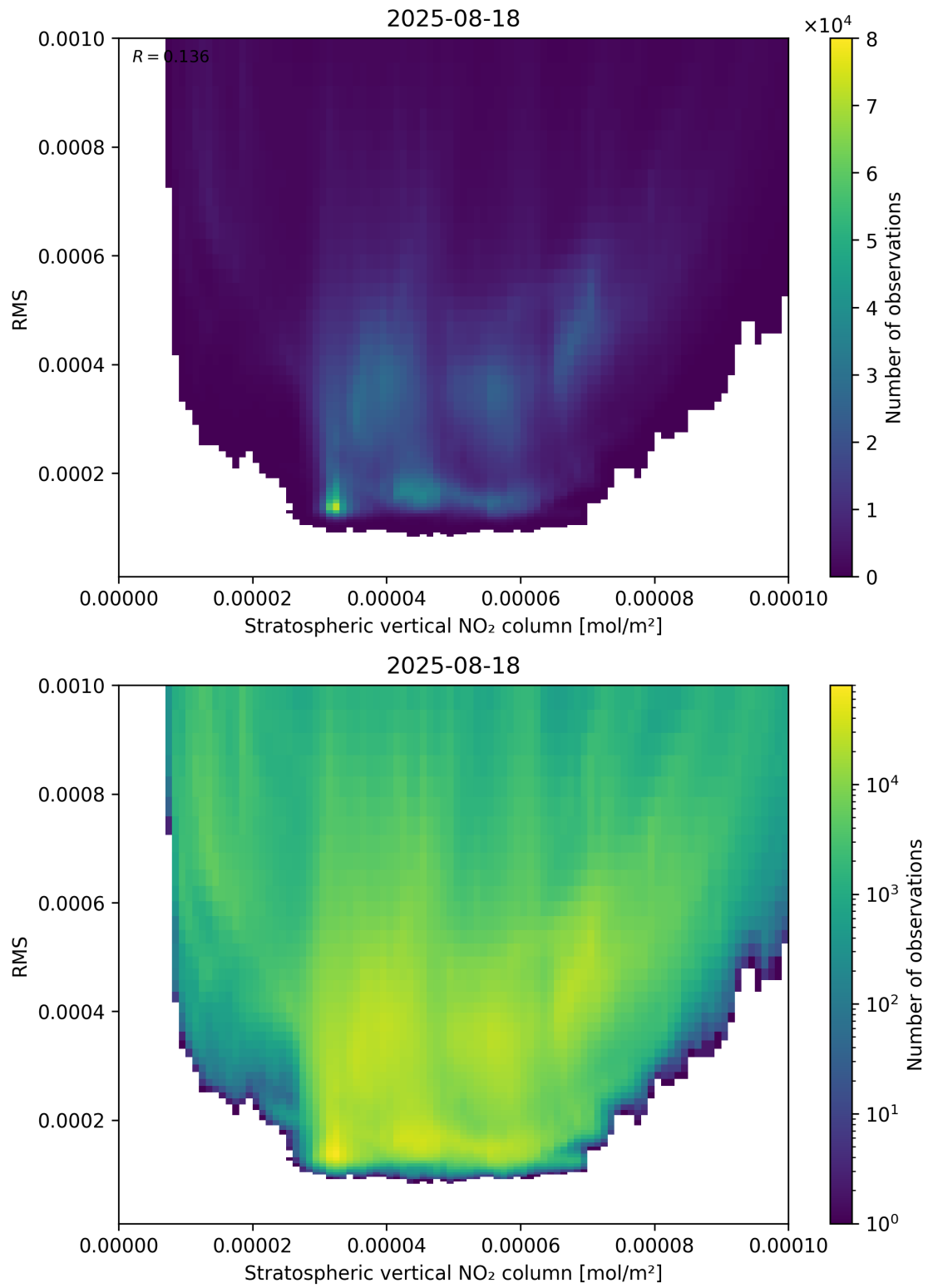
Figure 102: Scatter density plot of “Stratospheric vertical NO 2 column” against “RMS” for 2025-08-17 to 2025-08-19.
