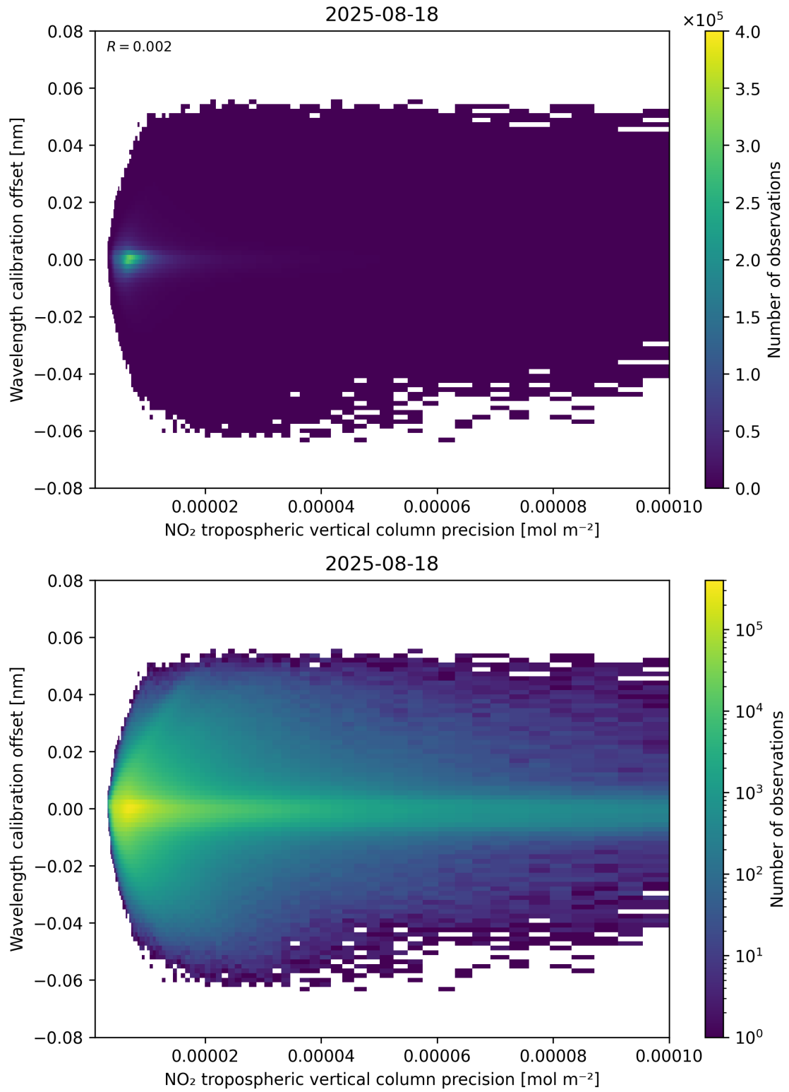
Figure 141: Scatter density plot of “NO 2 tropospheric vertical column precision” against “Wavelength calibration offset” for 2025-08-17 to 2025-08-19.
