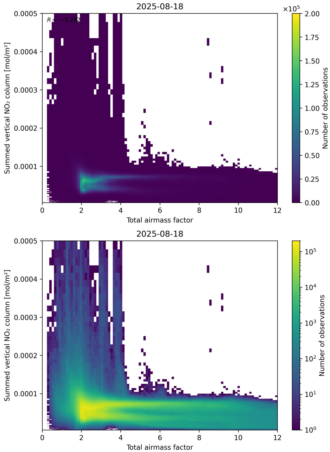
Figure 65: Scatter density plot of “Total airmass factor” against “Summed vertical NO 2 column” for 2025-08-17 to 2025-08-19.
