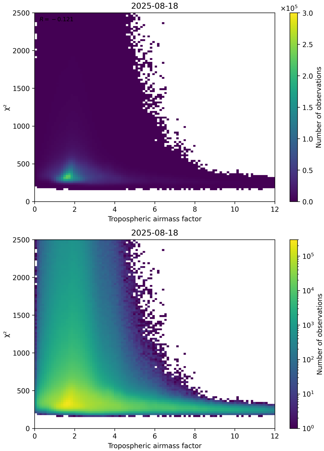
Figure 73: Scatter density plot of “Tropospheric airmass factor” against “ \chi^2 ” for 2025-08-17 to 2025-08-19.
