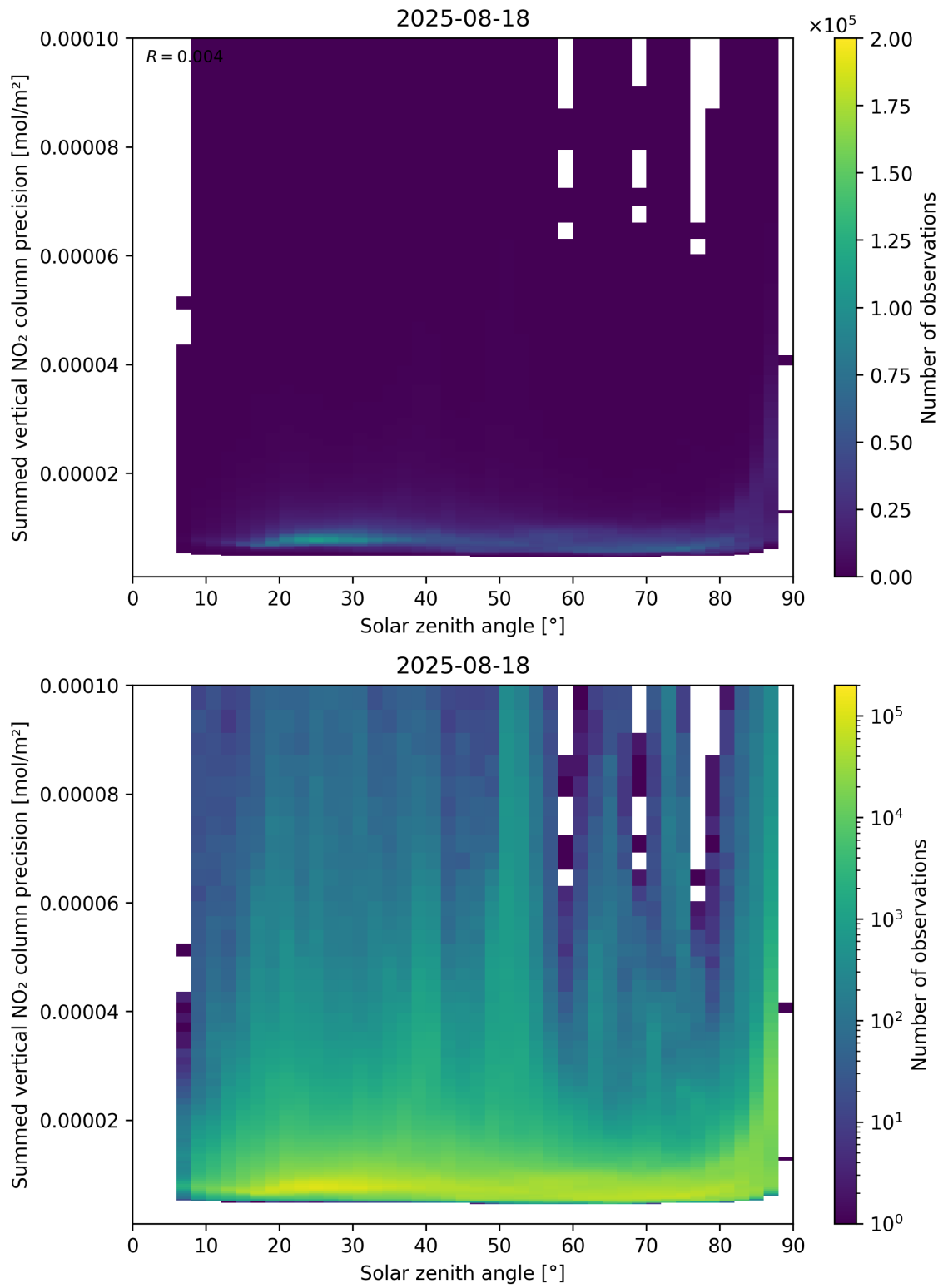
Figure 152: Scatter density plot of “Solar zenith angle” against “Summed vertical NO 2 column precision” for 2025-08-17 to 2025-08-19.
