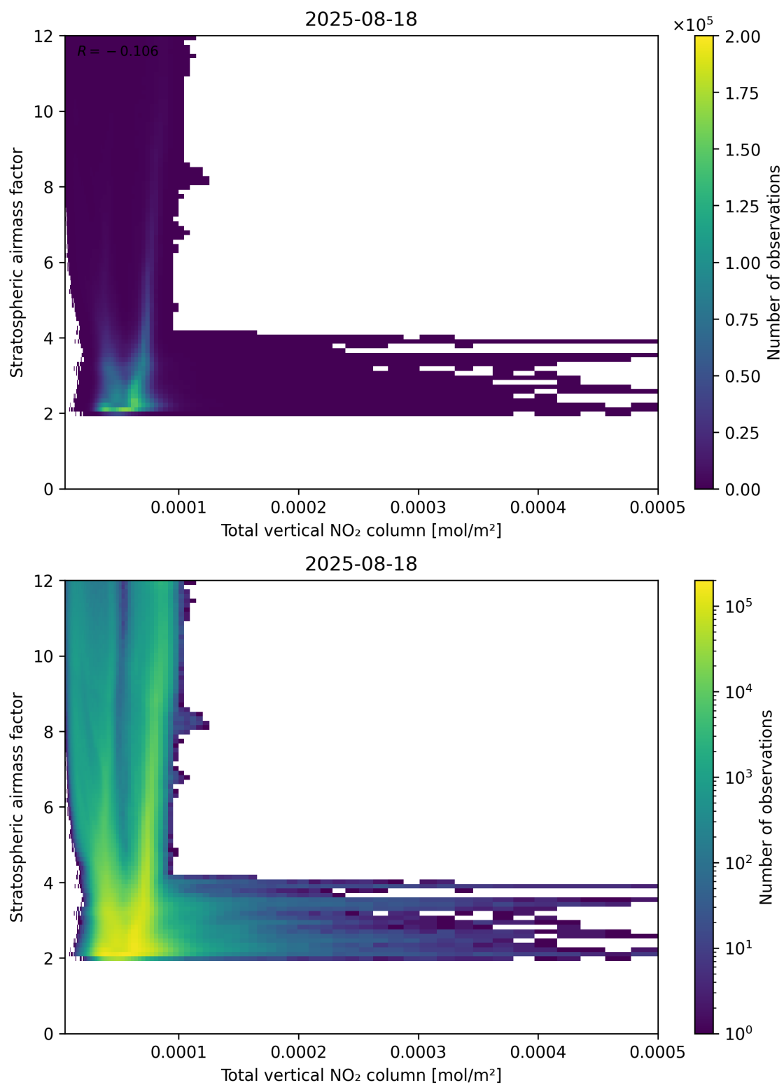
Figure 110: Scatter density plot of “Total vertical NO 2 column” against “Stratospheric airmass factor” for 2025-08-17 to 2025-08-19.
