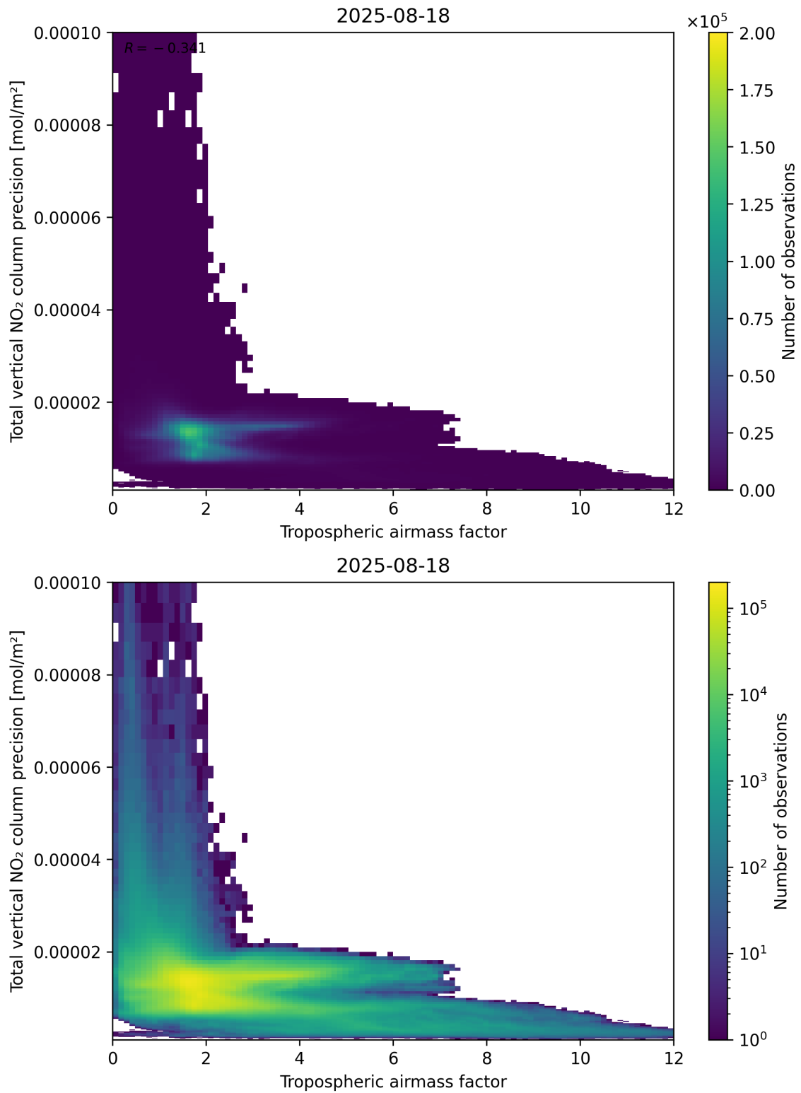
Figure 78: Scatter density plot of “Tropospheric airmass factor” against “Total vertical NO 2 column precision” for 2025-08-17 to 2025-08-19.
