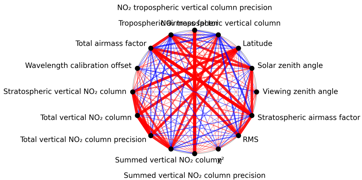
Figure 1: Map of correlation graph for 2025-08-17 to 2025-08-19.
