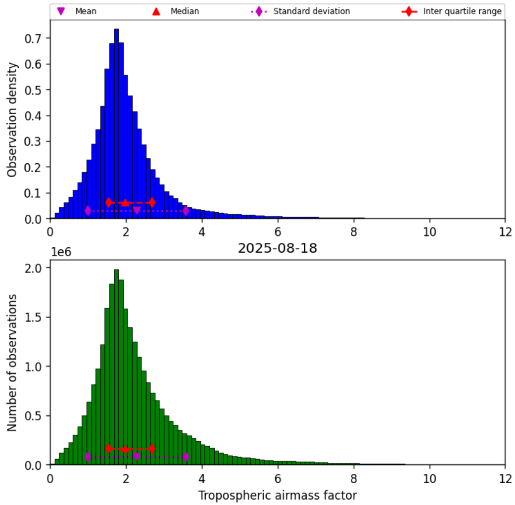
Figure 31: Histogram of “Tropospheric airmass factor” for 2025-08-17 to 2025-08-19
