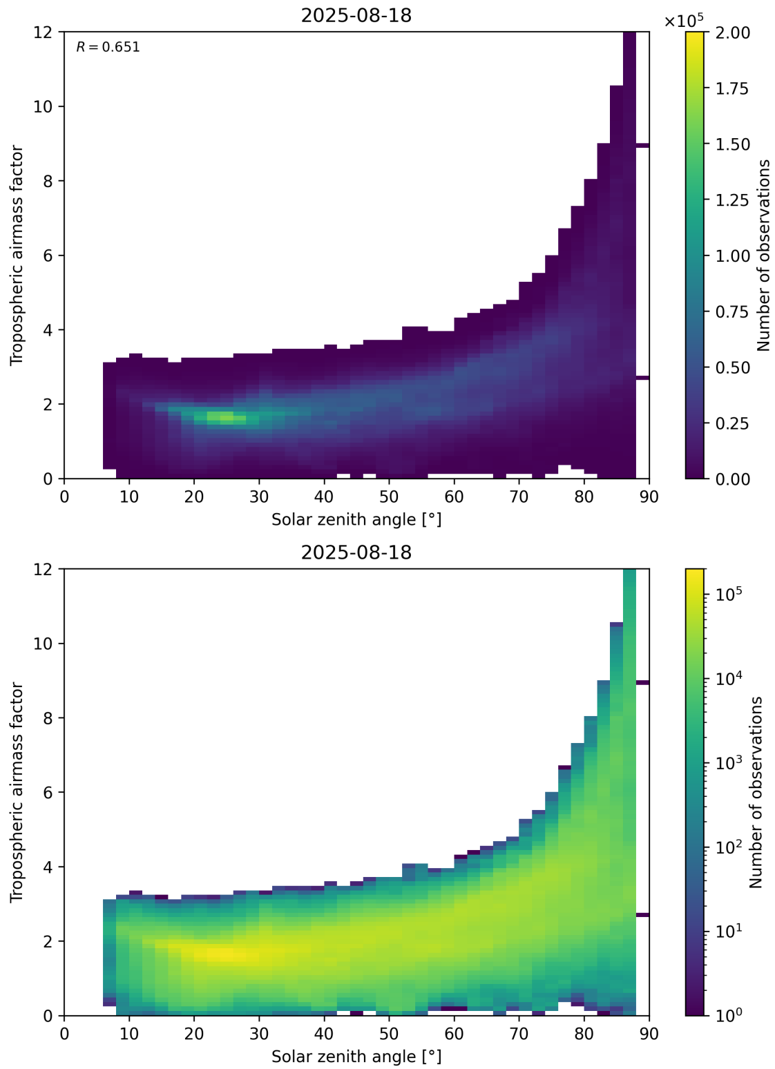
Figure 147: Scatter density plot of “Solar zenith angle” against “Tropospheric airmass factor” for 2025-08-17 to 2025-08-19.
