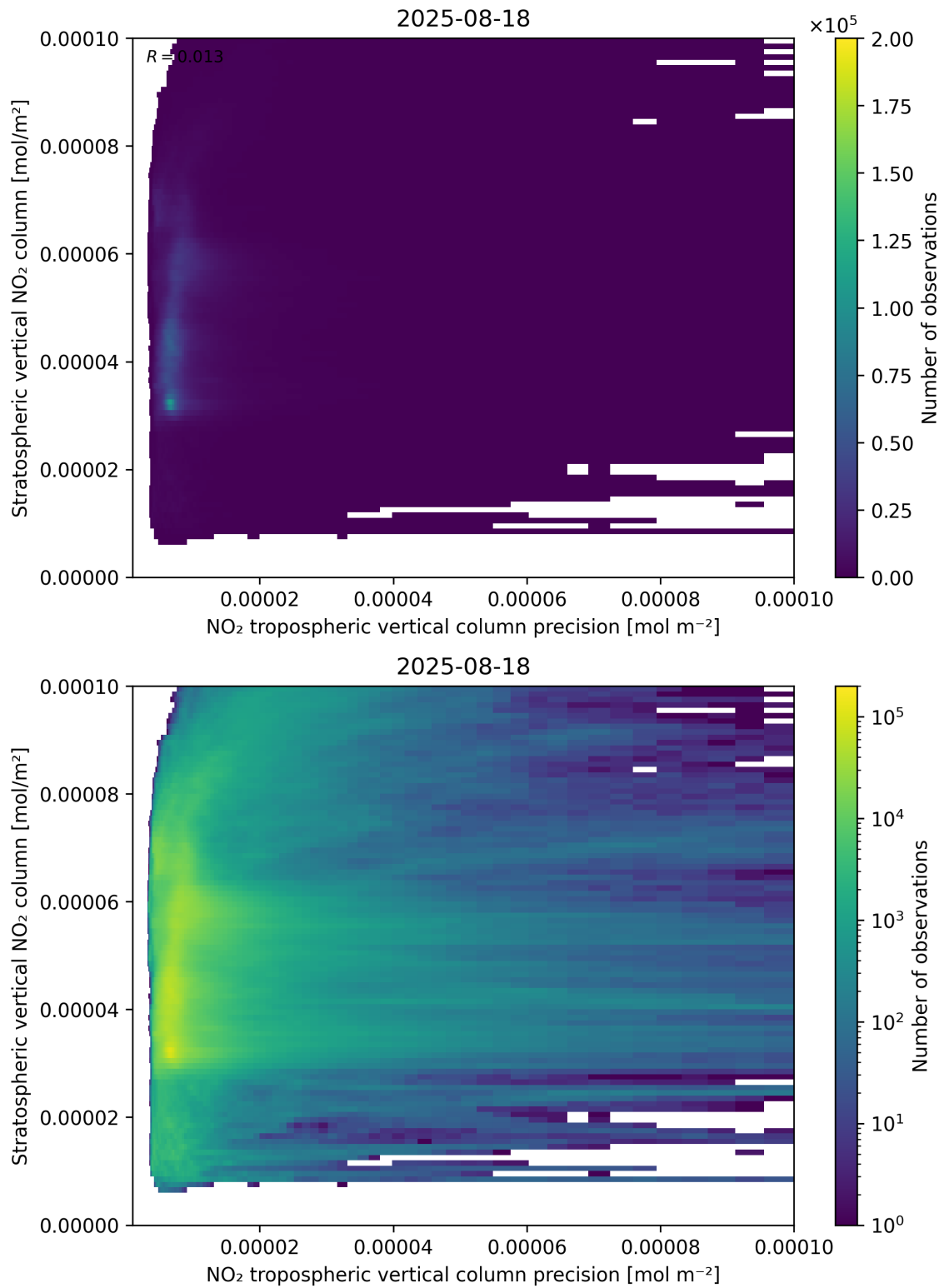
Figure 135: Scatter density plot of “NO 2 tropospheric vertical column precision” against “Stratospheric vertical NO 2 column” for 2025-08-17 to 2025-08-19.
