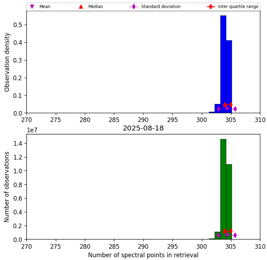
Figure 33: Histogram of “Number of spectral points in retrieval” for 2025-08-17 to 2025-08-19
