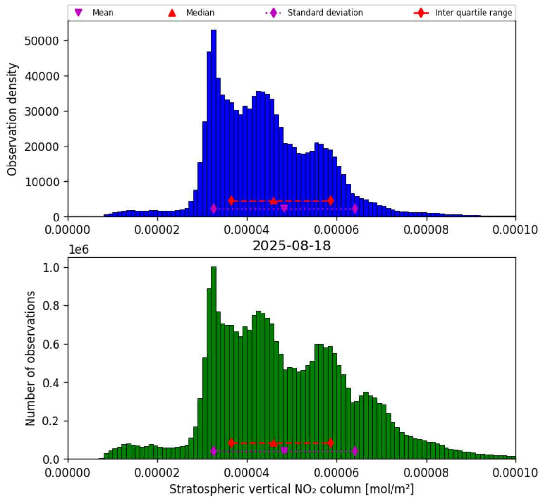
Figure 36: Histogram of “Stratospheric vertical NO 2 column” for 2025-08-17 to 2025-08-19
