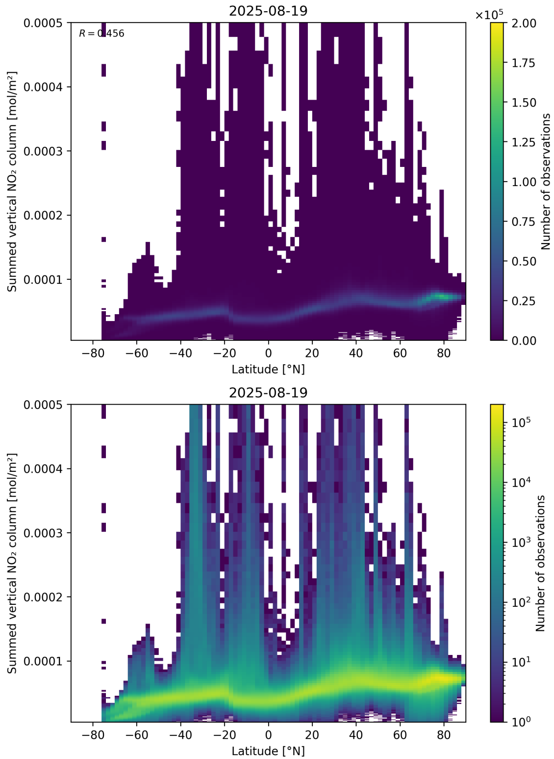
Figure 88: Scatter density plot of “Latitude” against “Summed vertical NO 2 column” for 2025-08-19 to 2025-08-20.
