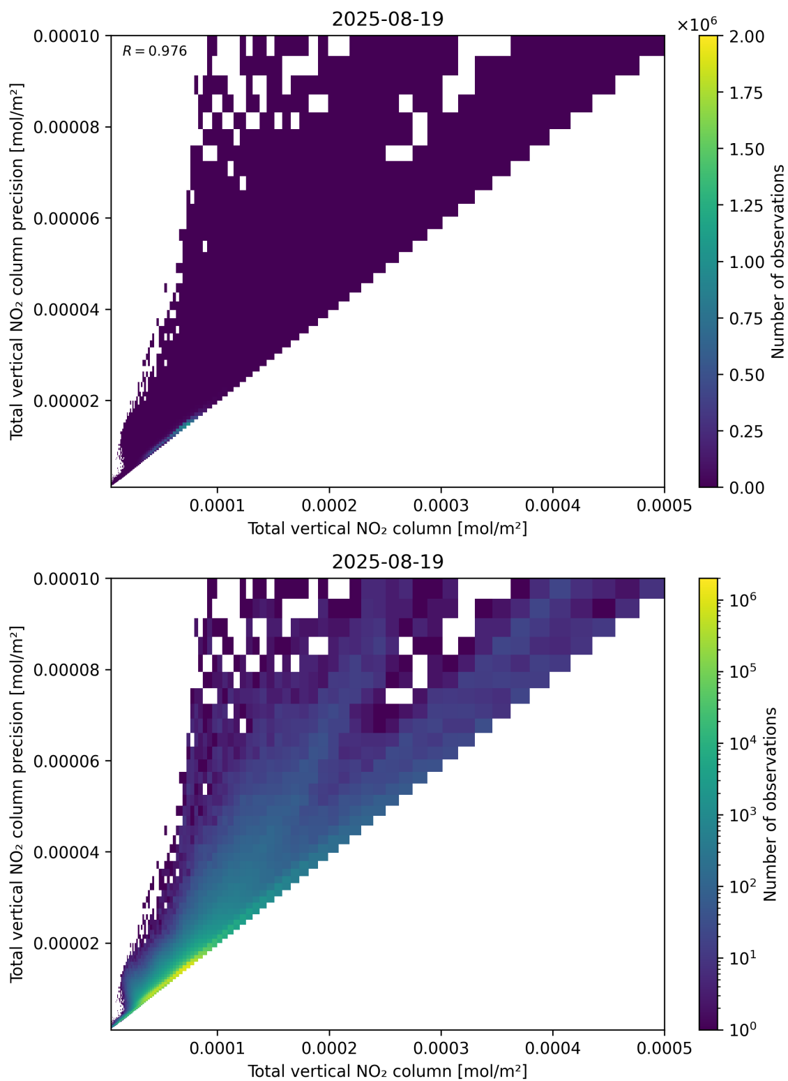
Figure 114: Scatter density plot of “Total vertical NO 2 column” against “Total vertical NO 2 column precision” for 2025-08-19 to 2025-08-20.
