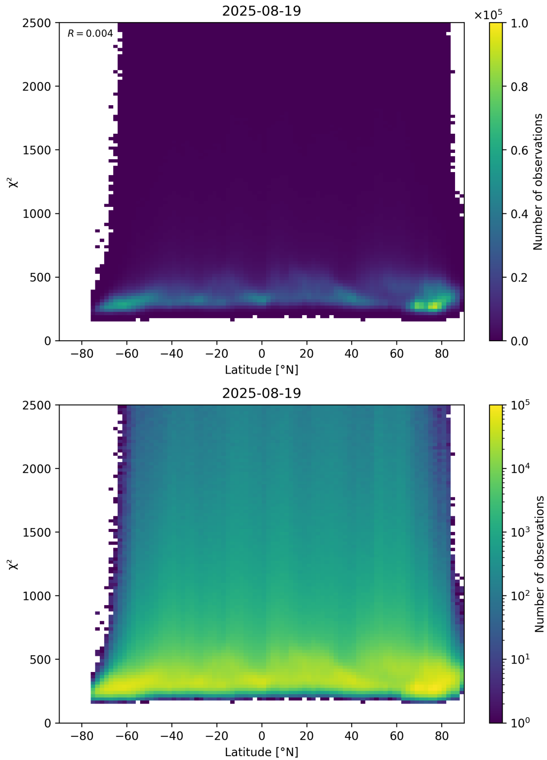
Figure 86: Scatter density plot of “Latitude” against “ \chi^2 ” for 2025-08-19 to 2025-08-20.
