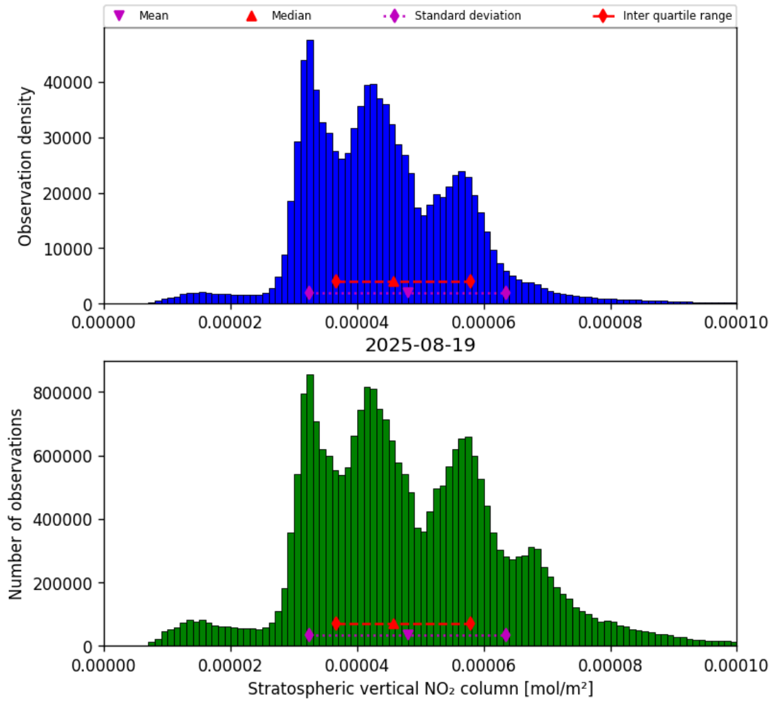
Figure 36: Histogram of “Stratospheric vertical NO 2 column” for 2025-08-19 to 2025-08-20
