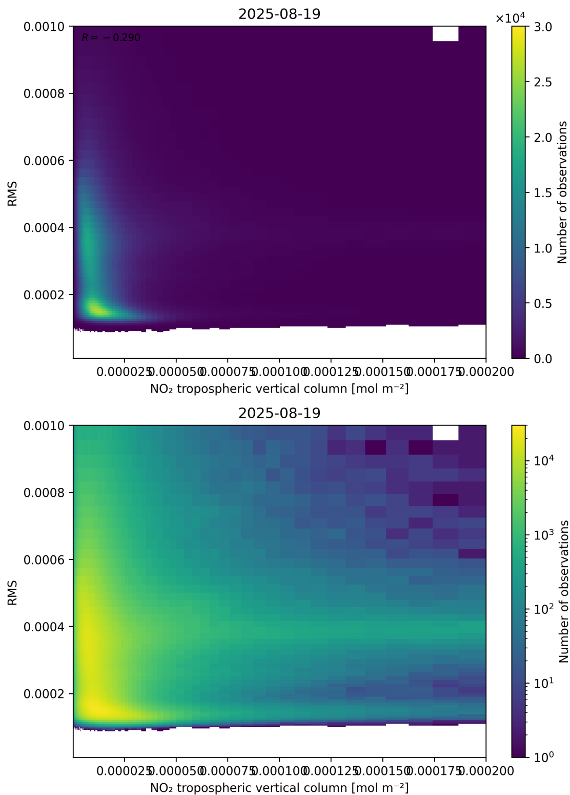
Figure 142: Scatter density plot of “NO 2 tropospheric vertical column” against “RMS” for 2025-08-19 to 2025-08-20.
