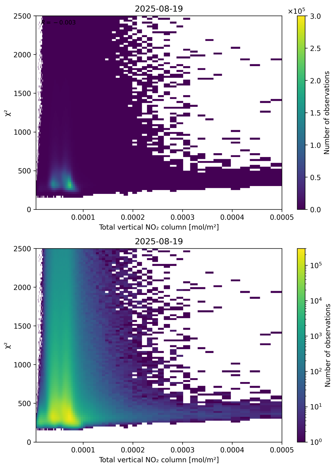
Figure 111: Scatter density plot of “Total vertical NO 2 column” against “ \chi^2 ” for 2025-08-19 to 2025-08-20.
