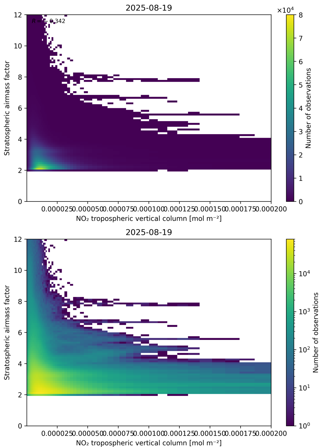
Figure 121: Scatter density plot of “NO 2 tropospheric vertical column” against “Stratospheric air mass factor” for 2025-08-19 to 2025-08-20.
