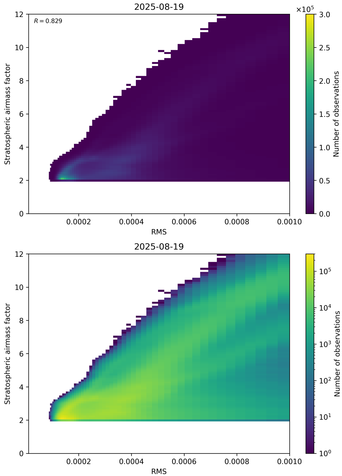
Figure 144: Scatter density plot of “RMS” against “Stratospheric airmass factor” for 2025-08-19 to 2025-08-20.
