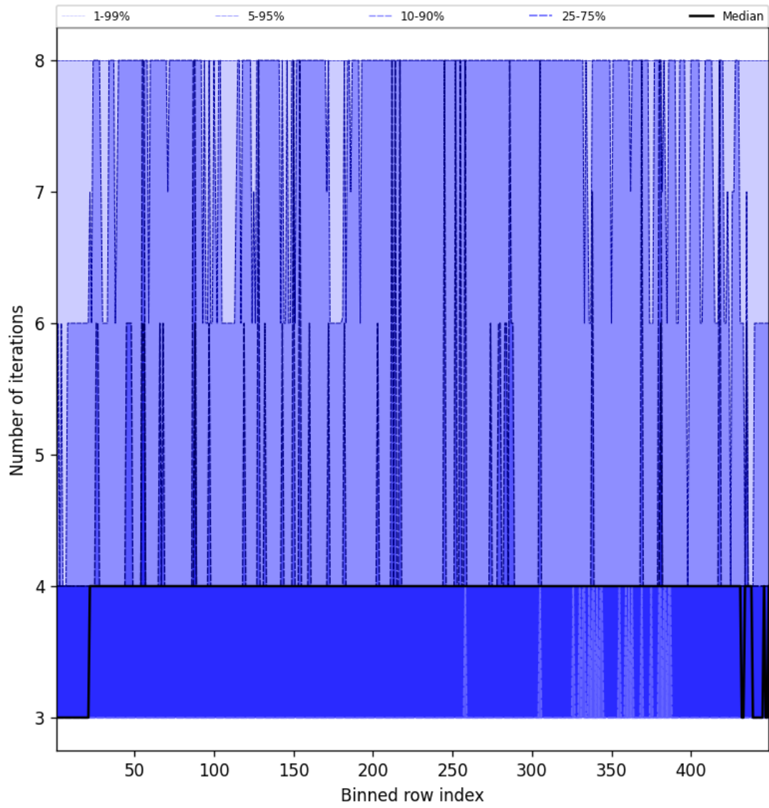
Figure 51: Along track statistics of “Number of iterations” for 2025-08-19 to 2025-08-20
