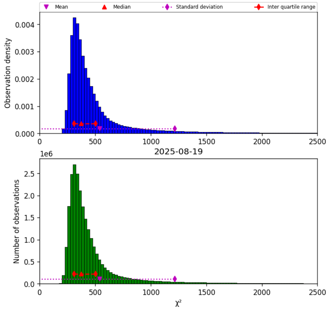
Figure 42: Histogram of “ \chi^2 ” for 2025-08-19 to 2025-08-20
