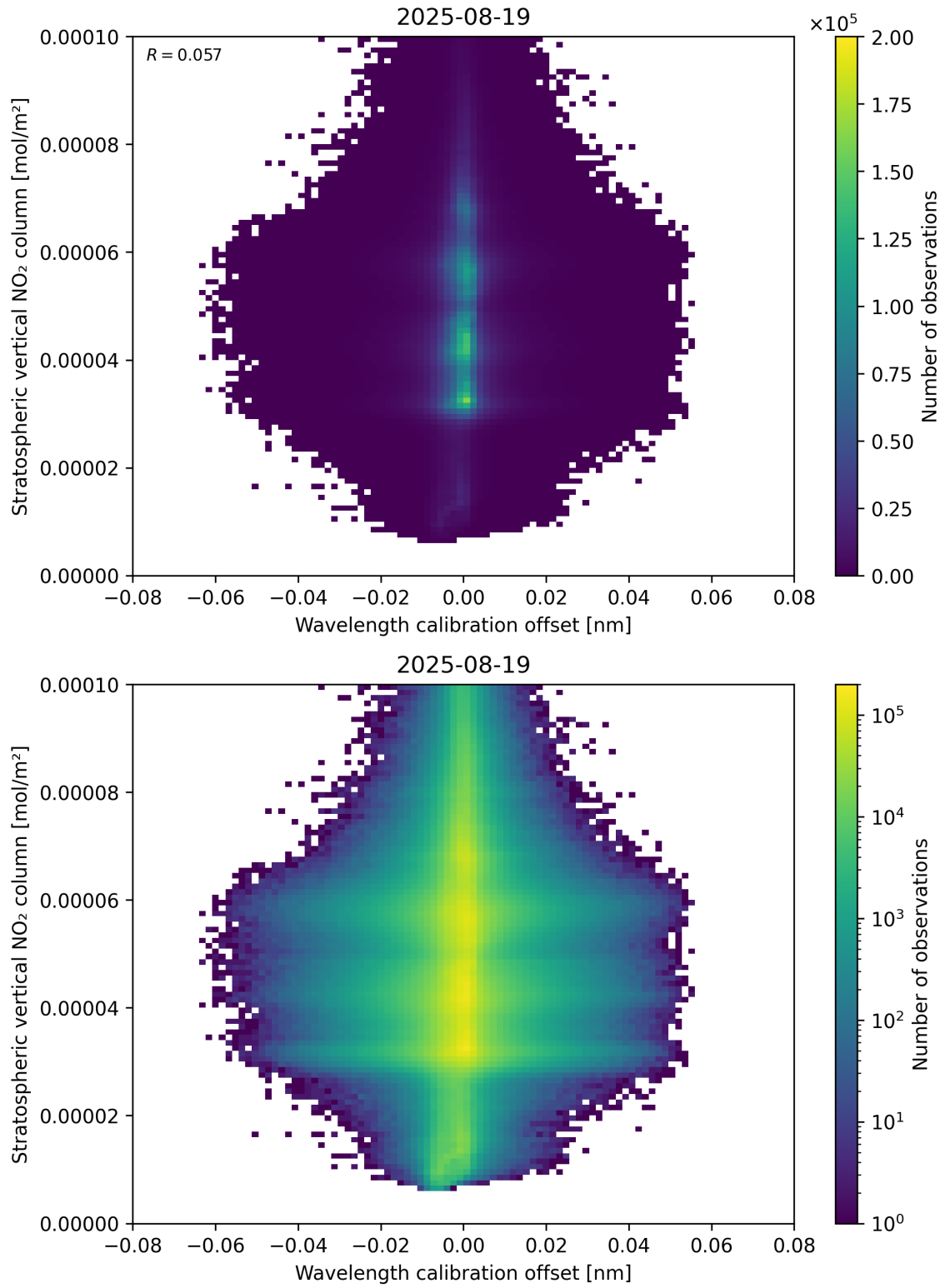
Figure 176: Scatter density plot of “Wavelength calibration offset” against “Stratospheric vertical NO 2 column” for 2025-08-19 to 2025-08-20.
