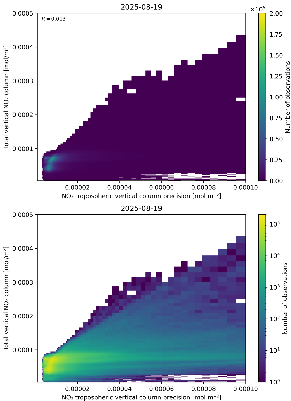
Figure 138: Scatter density plot of “NO 2 tropospheric vertical column precision” against “Total vertical NO 2 column” for 2025-08-19 to 2025-08-20.
