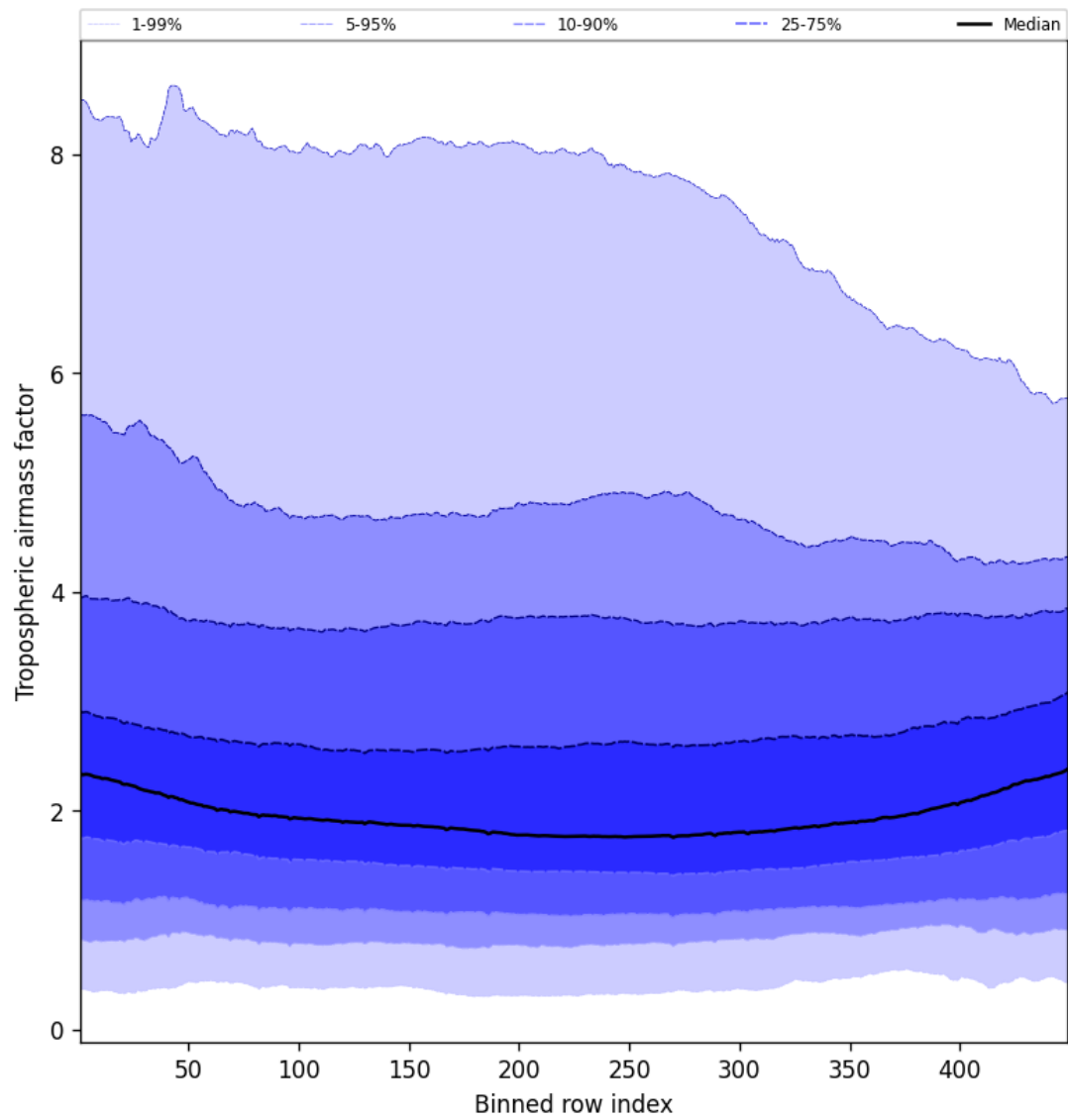
Figure 48: Along track statistics of “Tropospheric air mass factor” for 2025-08-19 to 2025-08-20
