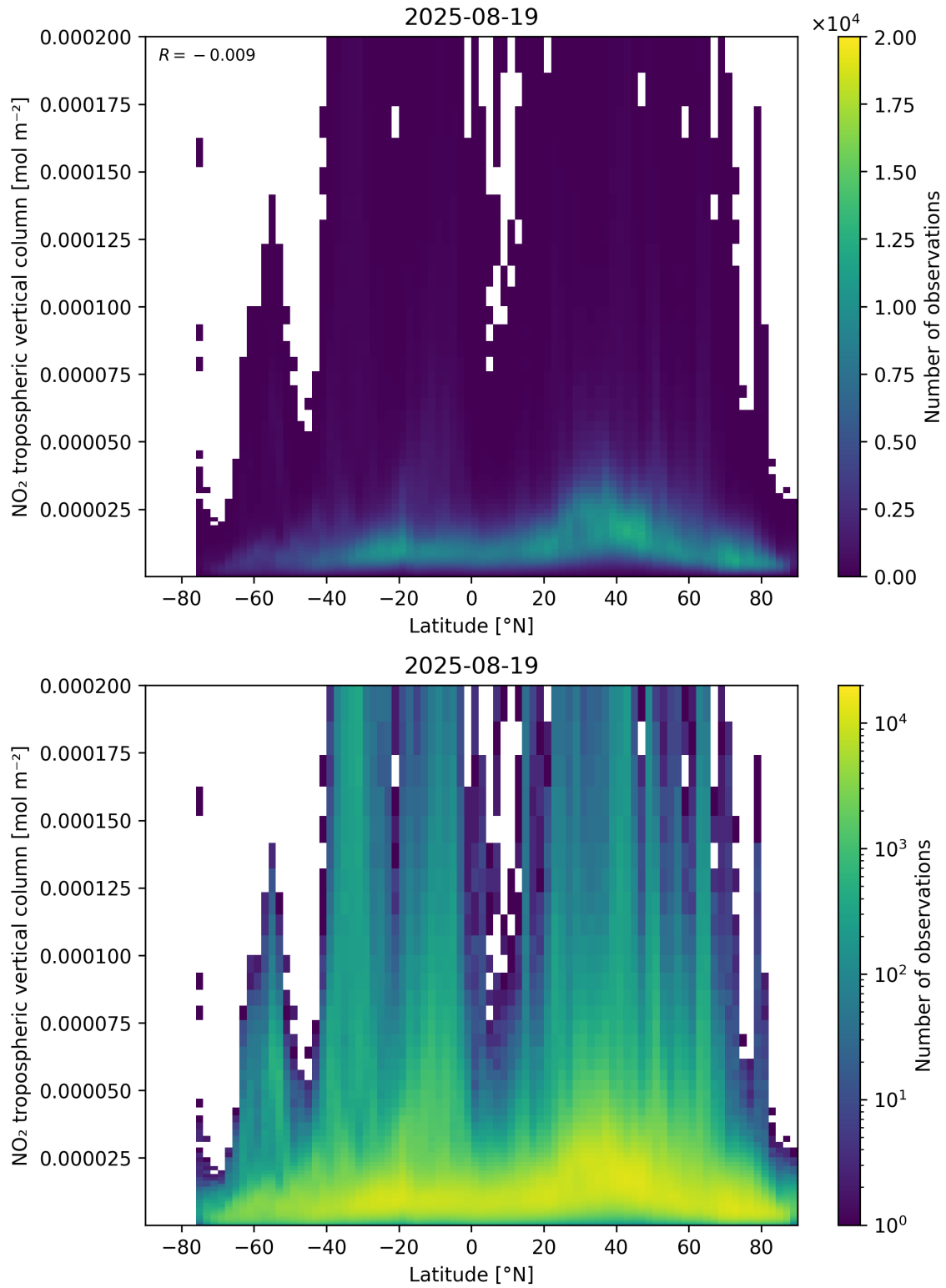
Figure 92: Scatter density plot of “Latitude” against “NO 2 tropospheric vertical column” for 2025-08-19 to 2025-08-20.
