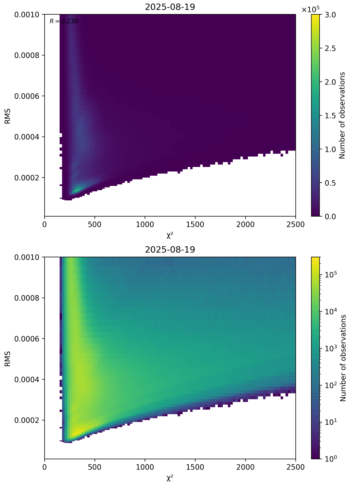
Figure 82: Scatter density plot of “ \chi^2 ” against “RMS” for 2025-08-19 to 2025-08-20.
