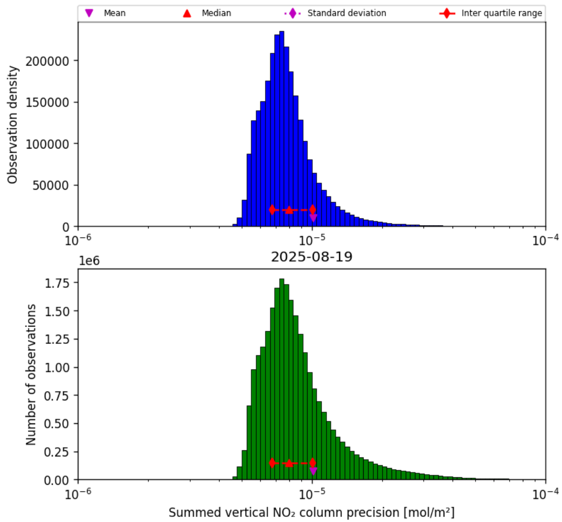
Figure 41: Histogram of “Summed vertical NO 2 column precision” for 2025-08-19 to 2025-08-20
