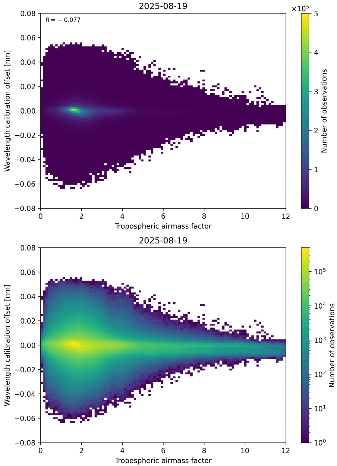
Figure 80: Scatter density plot of “Tropospheric airmass factor” against “Wavelength calibration offset” for 2025-08-19 to 2025-08-20.
