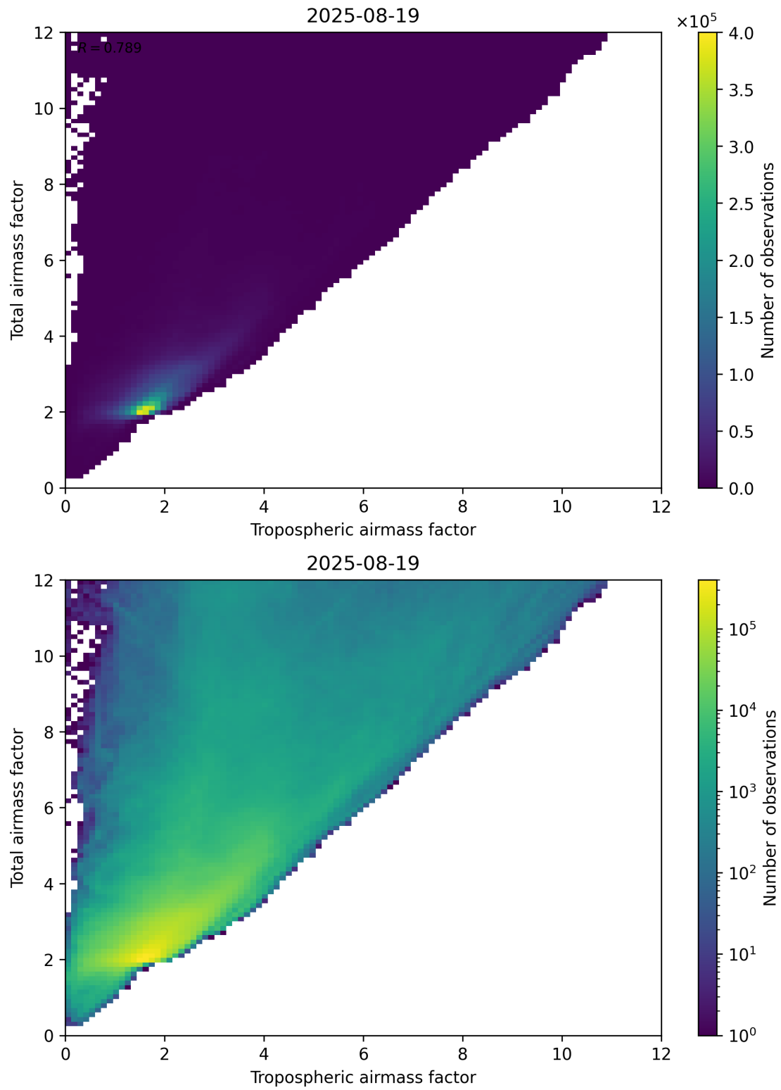
Figure 72: Scatter density plot of “Tropospheric airmass factor” against “Total airmass factor” for 2025-08-19 to 2025-08-20.
