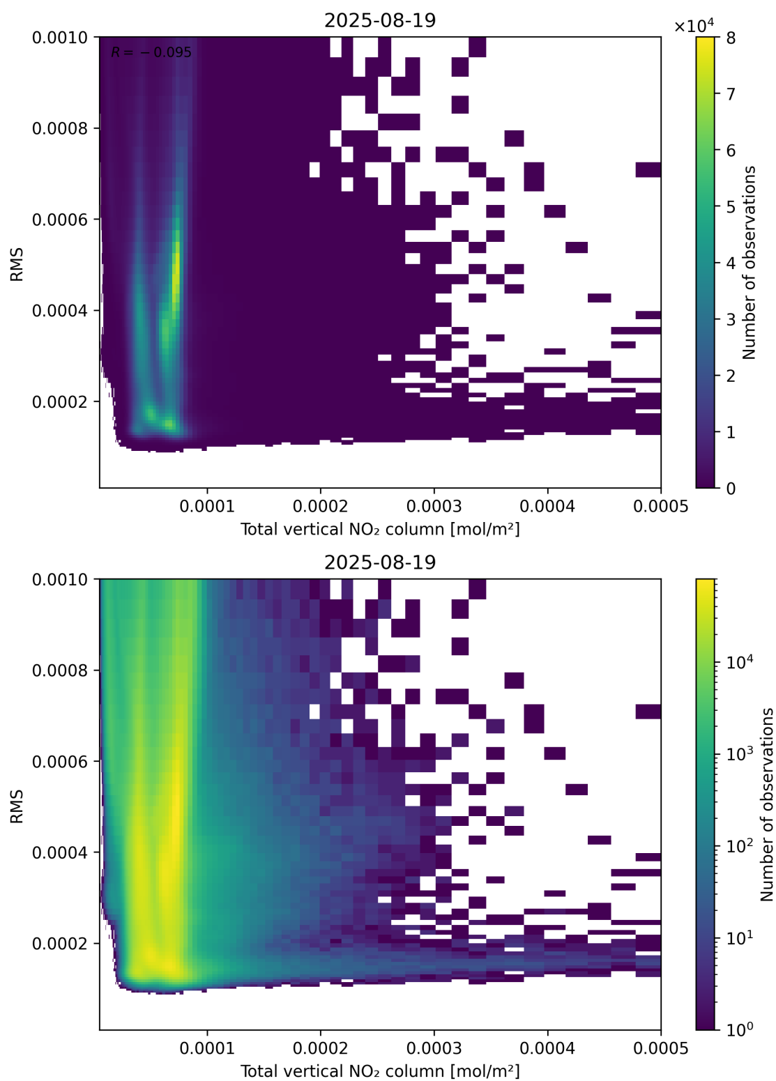
Figure 120: Scatter density plot of “Total vertical NO 2 column” against “RMS” for 2025-08-19 to 2025-08-20.
