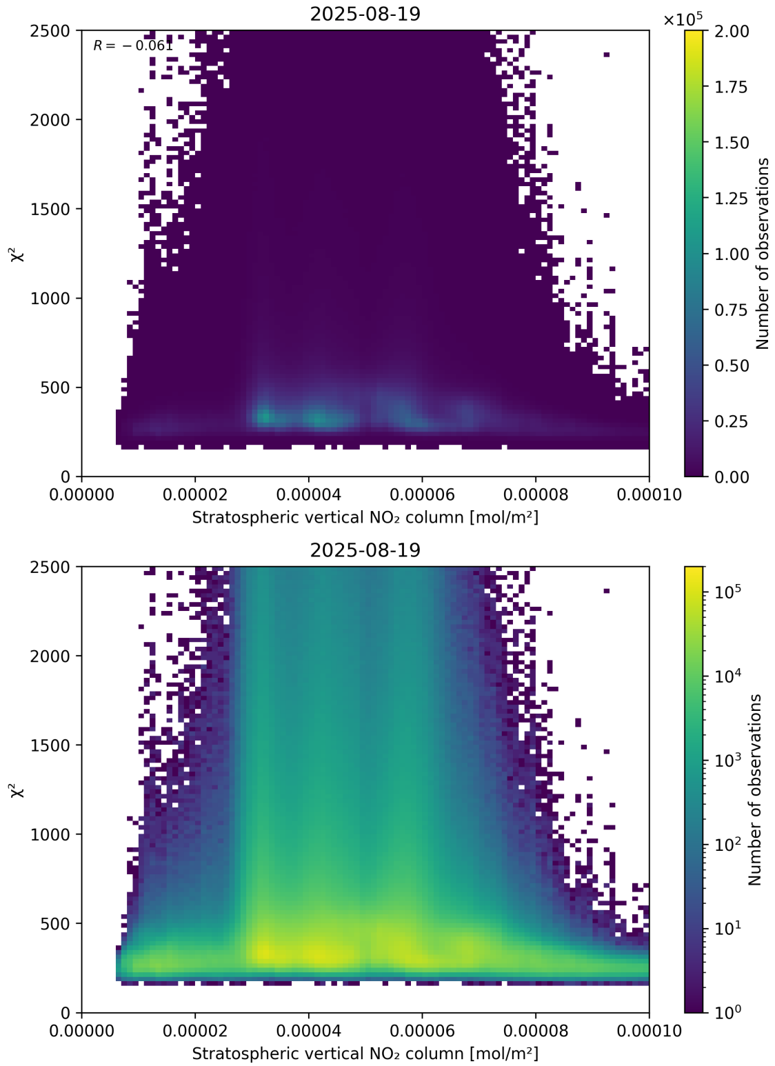
Figure 97: Scatter density plot of “Stratospheric vertical NO 2 column” against “ \chi^2 ” for 2025-08-19 to 2025-08-20.
