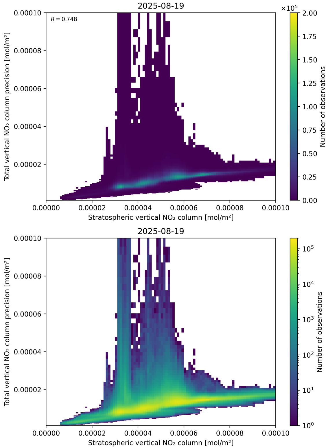
Figure 101: Scatter density plot of “Stratospheric vertical NO 2 column” against “Total vertical NO 2 column precision” for 2025-08-19 to 2025-08-20.
