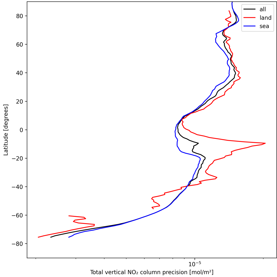
Figure 22: Zonal average of “Total vertical NO 2 column precision” for 2025-08-19 to 2025-08-20.
