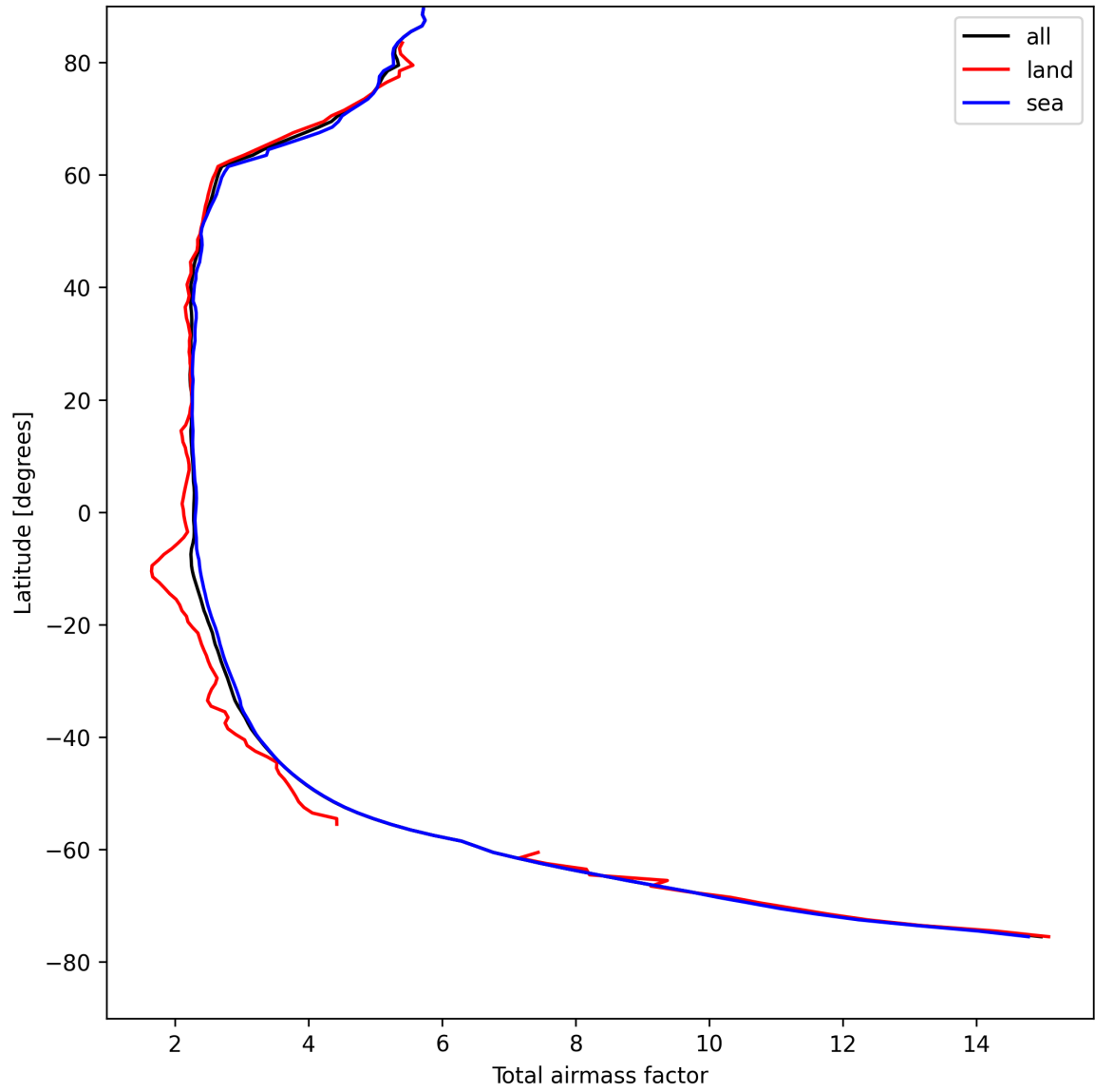
Figure 15: Zonal average of “Total airmass factor” for 2025-08-19 to 2025-08-20.
