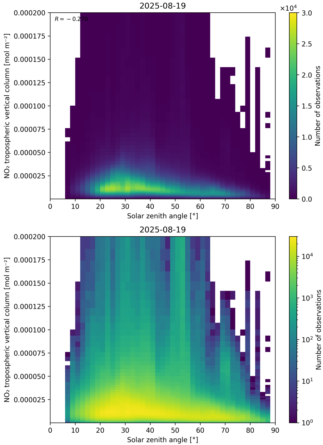
Figure 155: Scatter density plot of “Solar zenith angle” against “NO 2 tropospheric vertical column” for 2025-08-19 to 2025-08-20.
