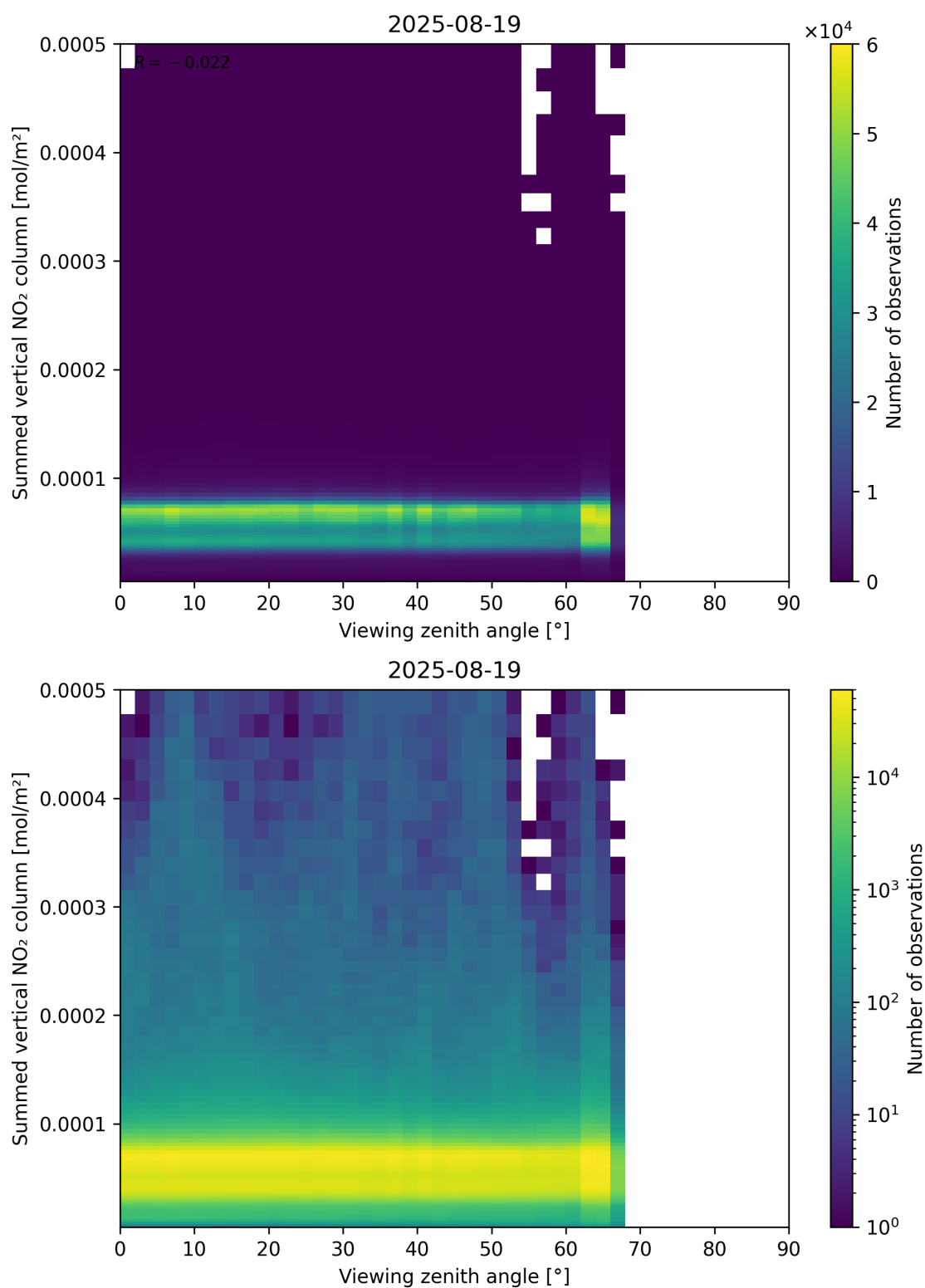
Figure 165: Scatter density plot of “Viewing zenith angle” against “Summed vertical NO 2 column” for 2025-08-19 to 2025-08-20.
