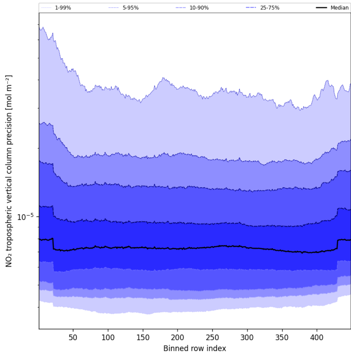
Figure 47: Along track statistics of “NO 2 tropospheric vertical column precision” for 2025-08-19 to 2025-08-20
