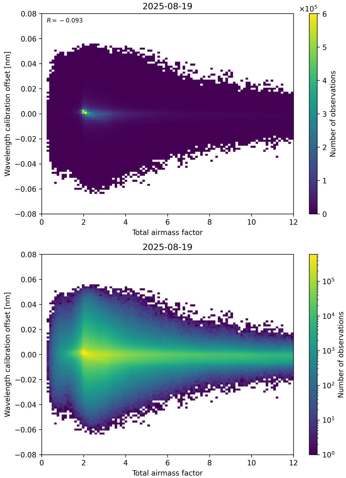
Figure 70: Scatter density plot of “Total airmass factor” against “Wavelength calibration offset” for 2025-08-19 to 2025-08-20.
