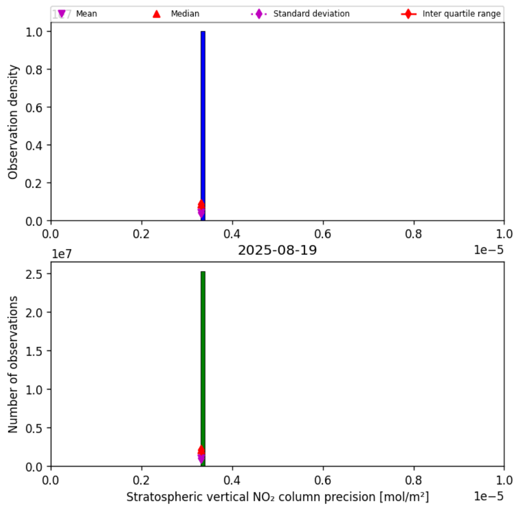
Figure 37: Histogram of “Stratospheric vertical NO 2 column precision” for 2025-08-19 to 2025-08-20
