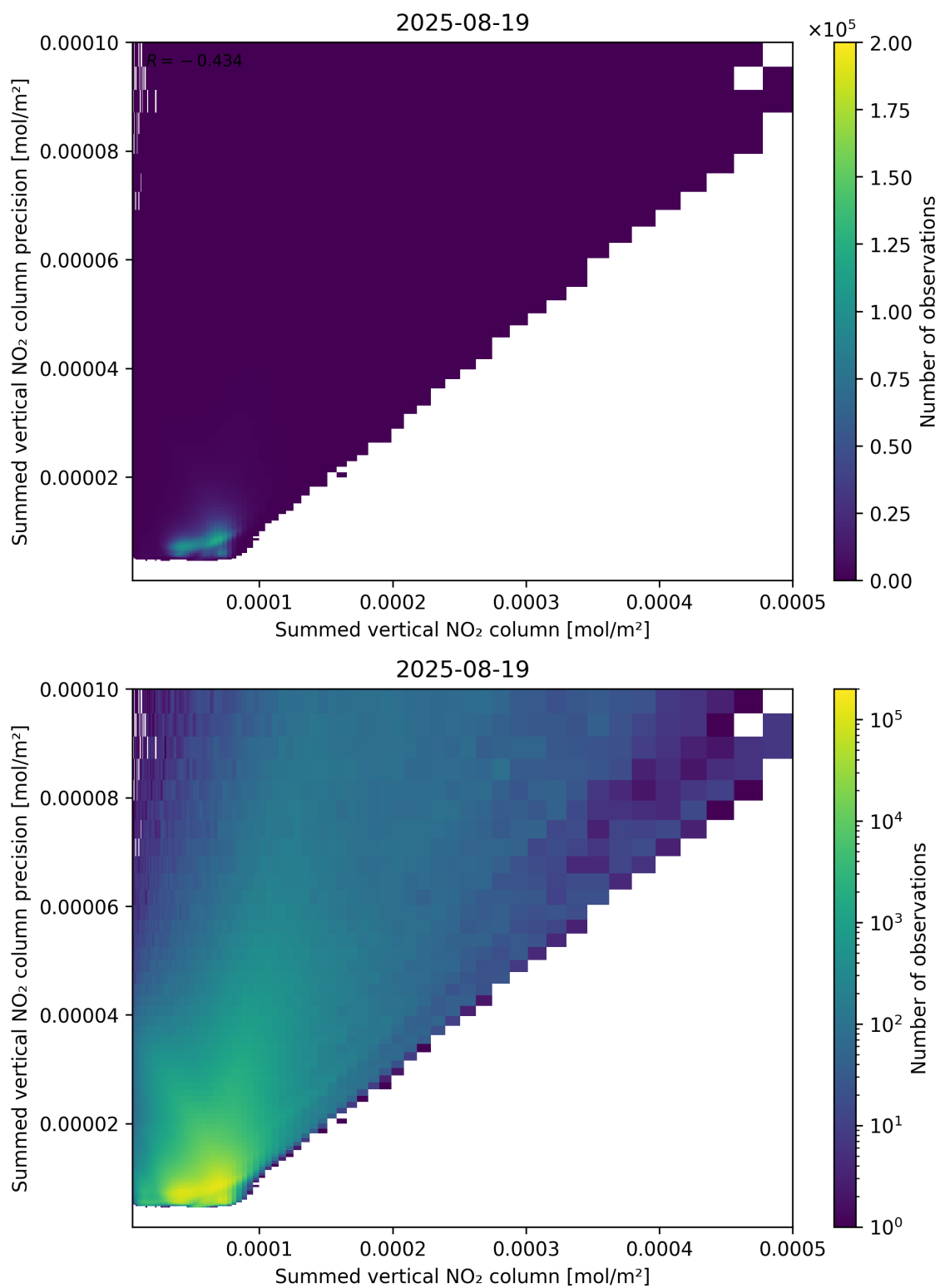
Figure 105: Scatter density plot of “Summed vertical NO 2 column” against “Summed vertical NO 2 column precision” for 2025-08-19 to 2025-08-20.
