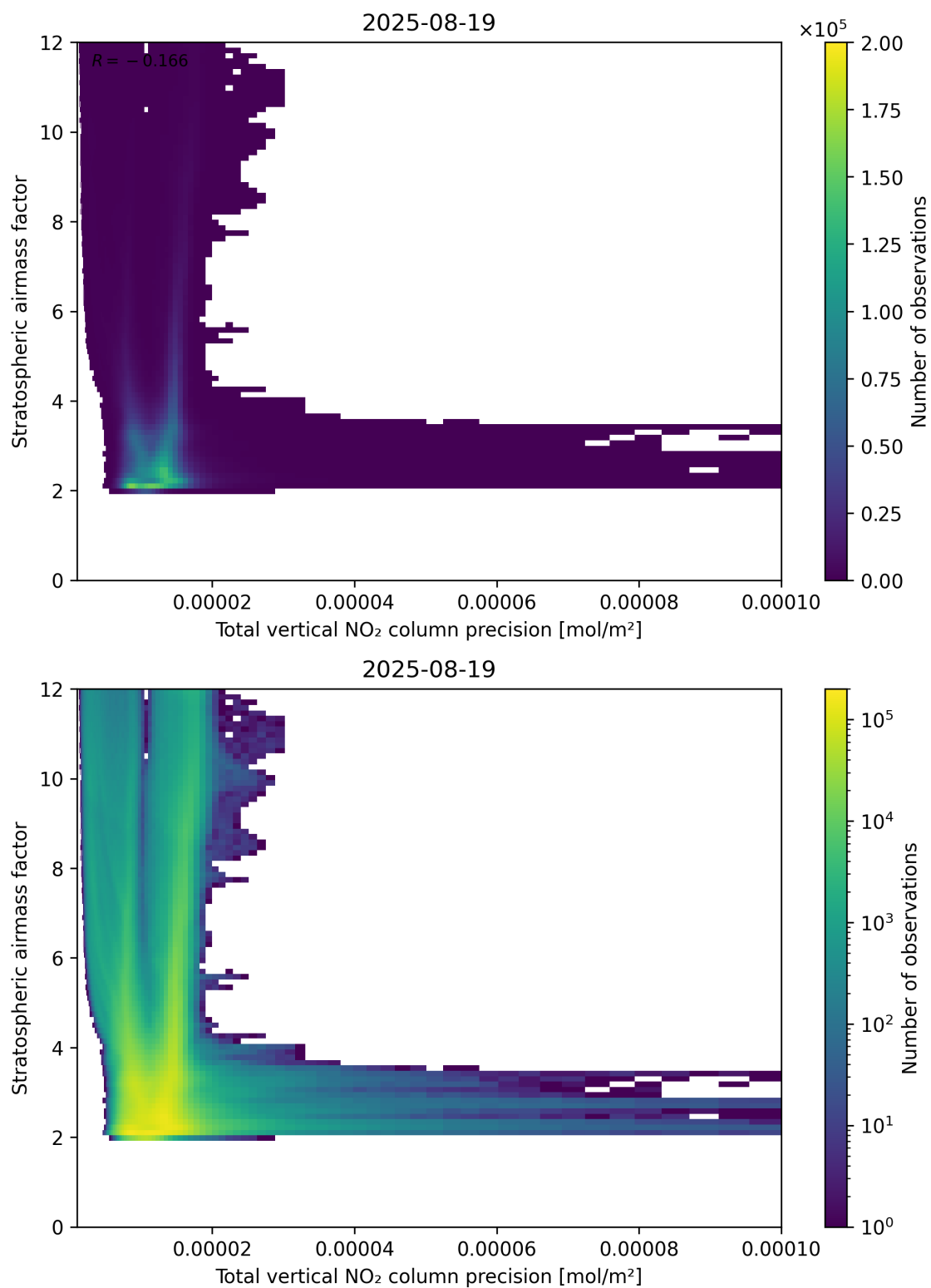
Figure 115: Scatter density plot of “Total vertical NO 2 column precision” against “Stratospheric airmass factor” for 2025-08-19 to 2025-08-20.
