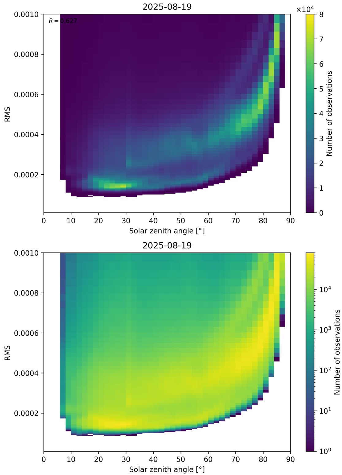
Figure 157: Scatter density plot of “Solar zenith angle” against “RMS” for 2025-08-19 to 2025-08-20.
