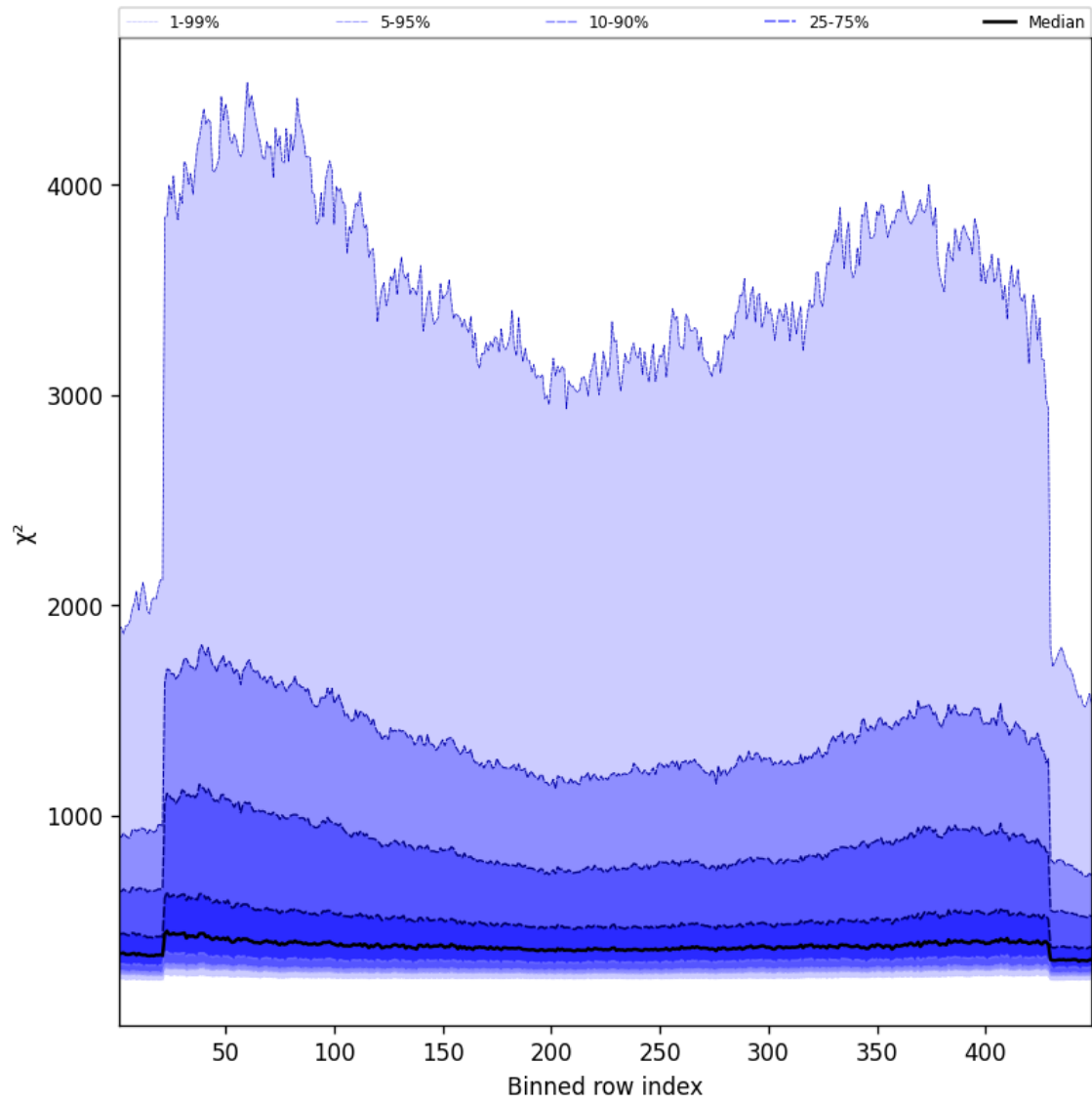
Figure 59: Along track statistics of “ \chi^2 ” for 2025-08-19 to 2025-08-20
