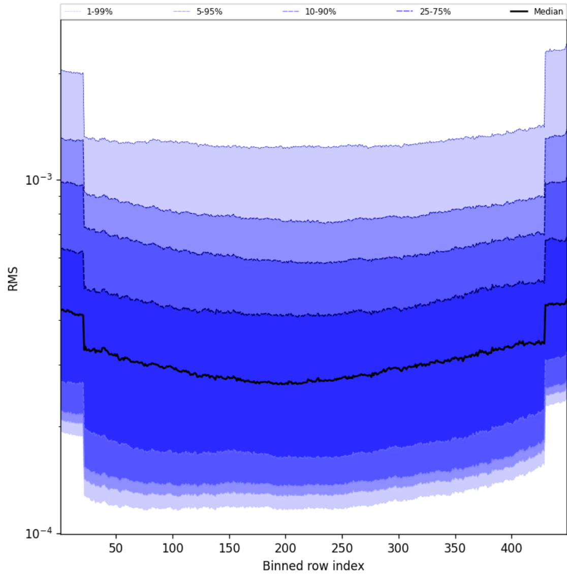
Figure 60: Along track statistics of “RMS” for 2025-08-19 to 2025-08-20
