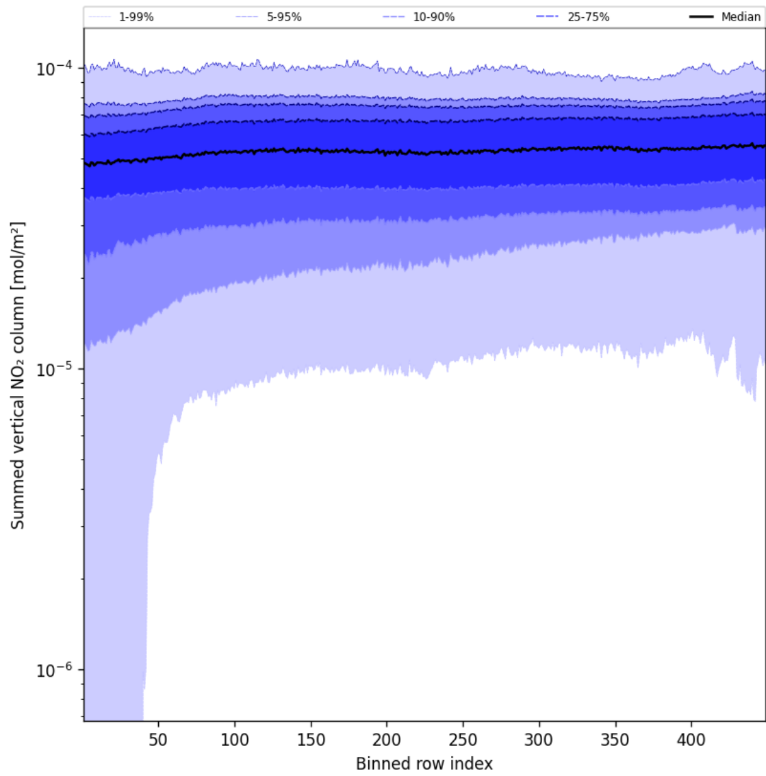
Figure 57: Along track statistics of “Summed vertical NO 2 column” for 2025-08-19 to 2025-08-20
