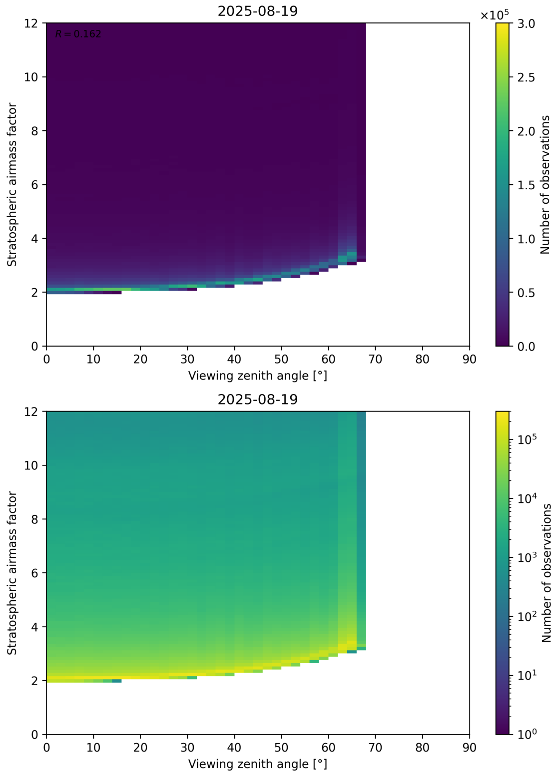
Figure 159: Scatter density plot of “Viewing zenith angle” against “Stratospheric airmass factor” for 2025-08-19 to 2025-08-20.
