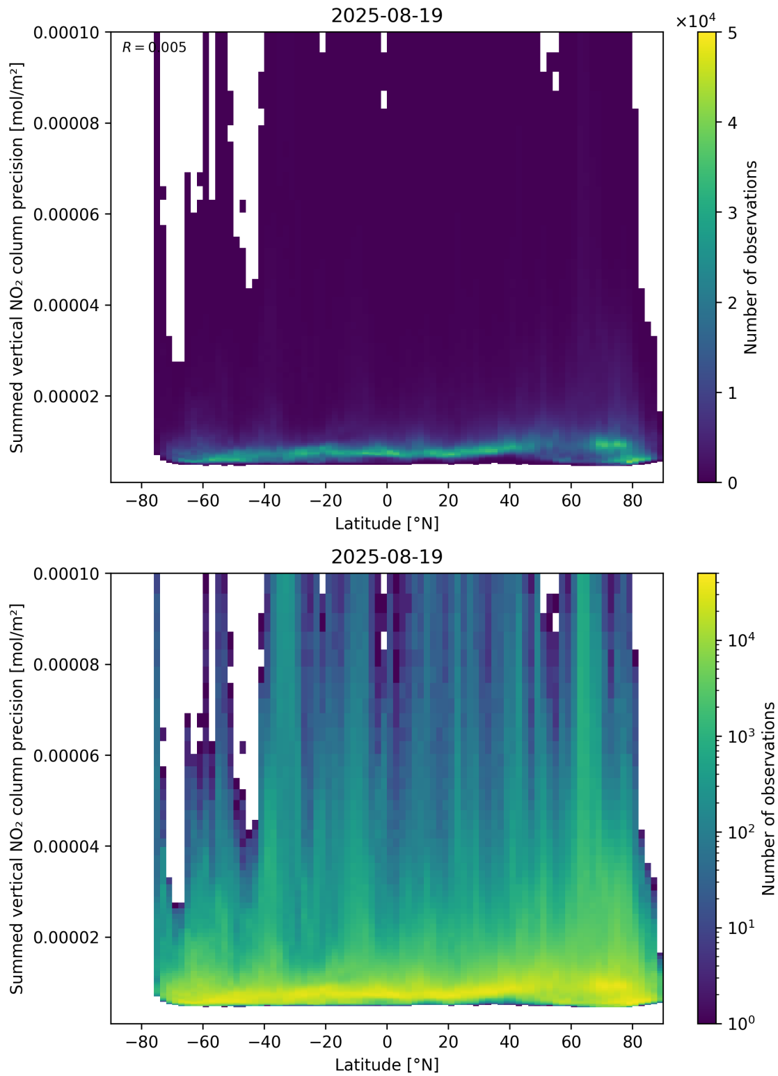
Figure 89: Scatter density plot of “Latitude” against “Summed vertical NO 2 column precision” for 2025-08-19 to 2025-08-20.
