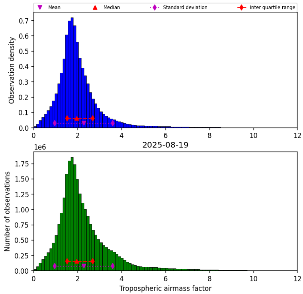
Figure 31: Histogram of “Tropospheric airmass factor” for 2025-08-19 to 2025-08-20
