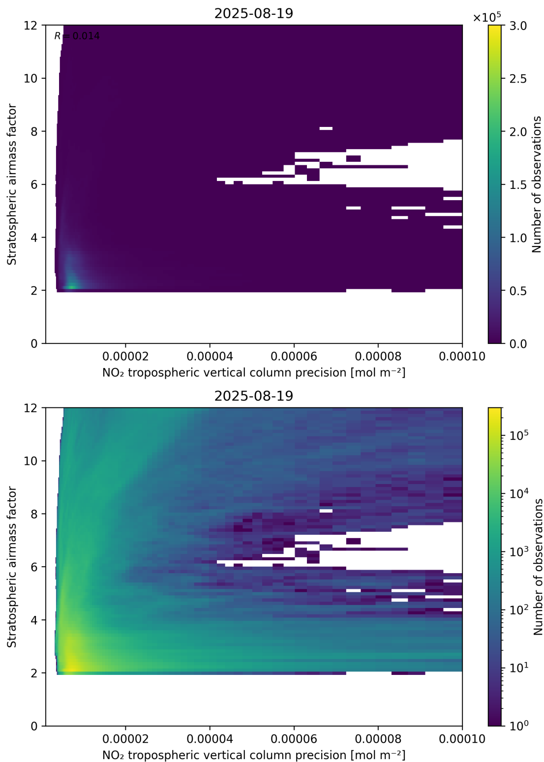
Figure 131: Scatter density plot of “NO 2 tropospheric vertical column precision” against “Stratospheric airmass factor” for 2025-08-19 to 2025-08-20.
