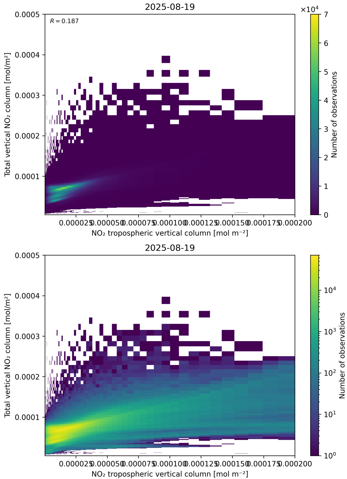
Figure 128: Scatter density plot of “NO 2 tropospheric vertical column” against “Total vertical NO 2 column” for 2025-08-19 to 2025-08-20.
