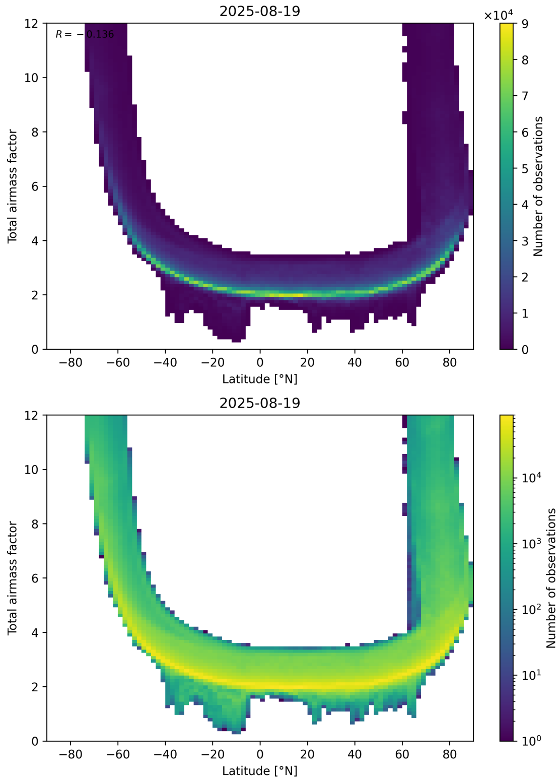
Figure 84: Scatter density plot of “Latitude” against “Total airmass factor” for 2025-08-19 to 2025-08-20.
