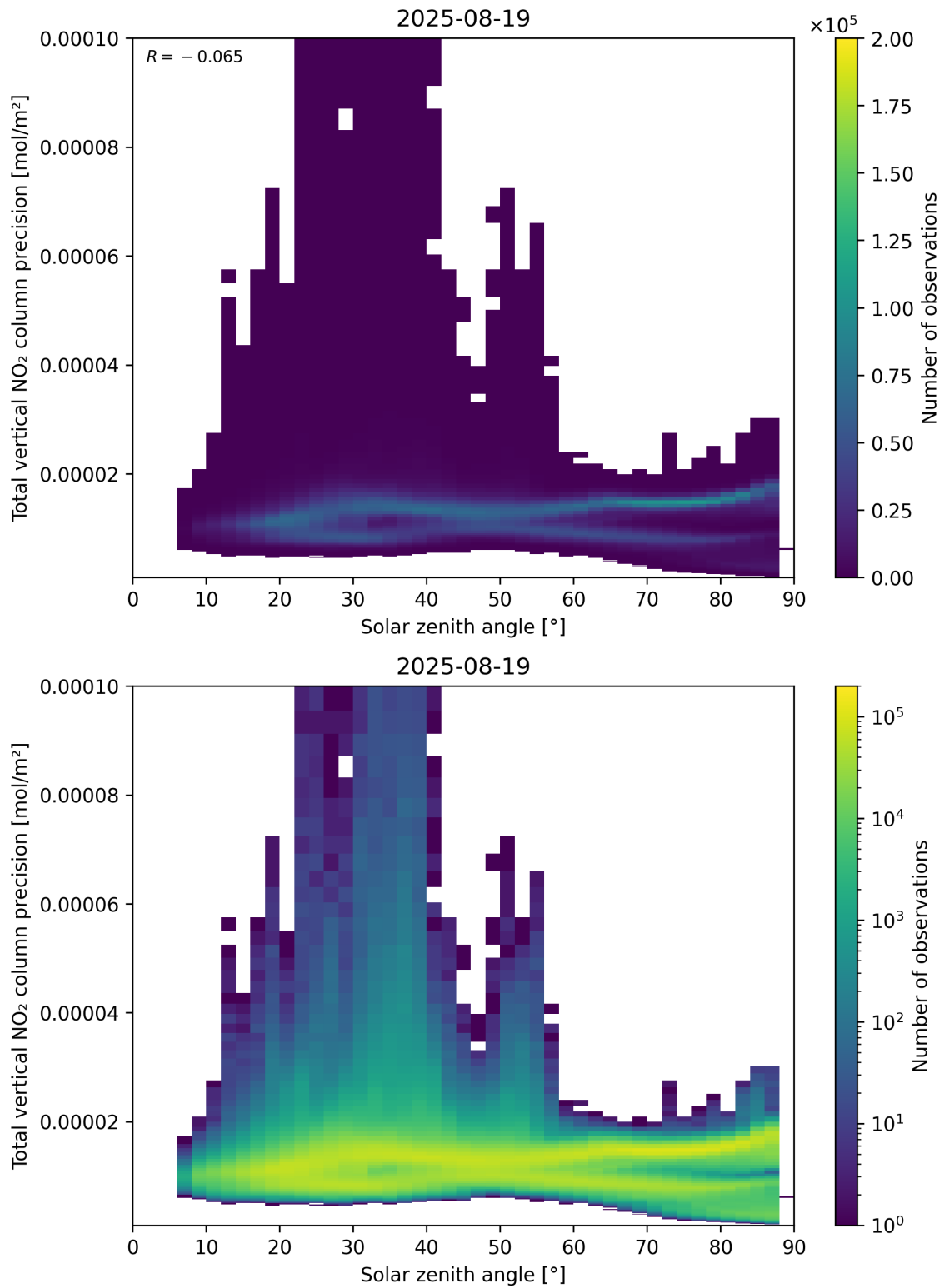
Figure 154: Scatter density plot of “Solar zenith angle” against “Total vertical NO 2 column precision” for 2025-08-19 to 2025-08-20.
