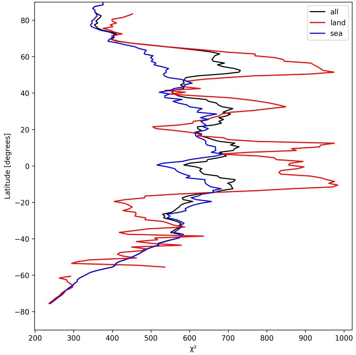
Figure 25: Zonal average of “ \chi^2 ” for 2025-08-19 to 2025-08-20.
