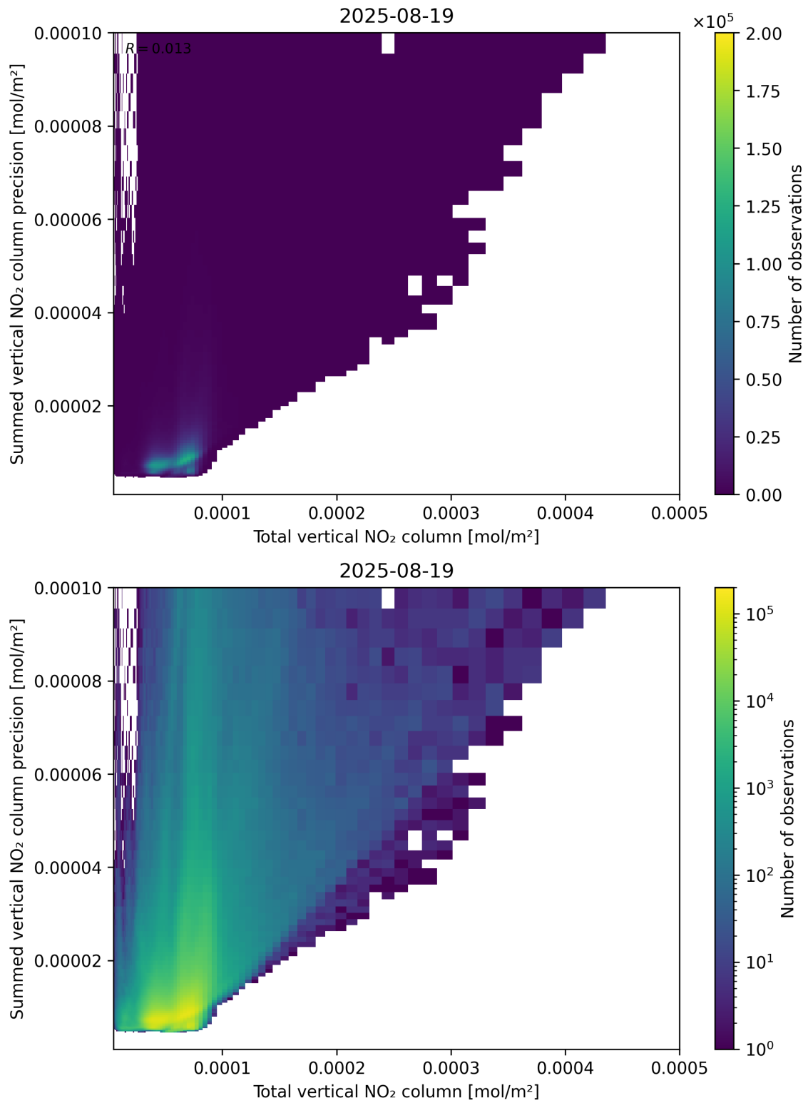
Figure 113: Scatter density plot of “Total vertical NO 2 column” against “Summed vertical NO 2 column precision” for 2025-08-19 to 2025-08-20.
