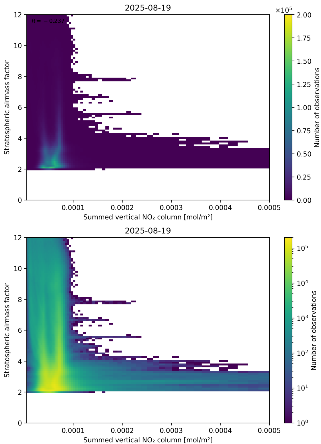
Figure 103: Scatter density plot of “Summed vertical NO 2 column” against “Stratospheric air mass factor” for 2025-08-19 to 2025-08-20.
