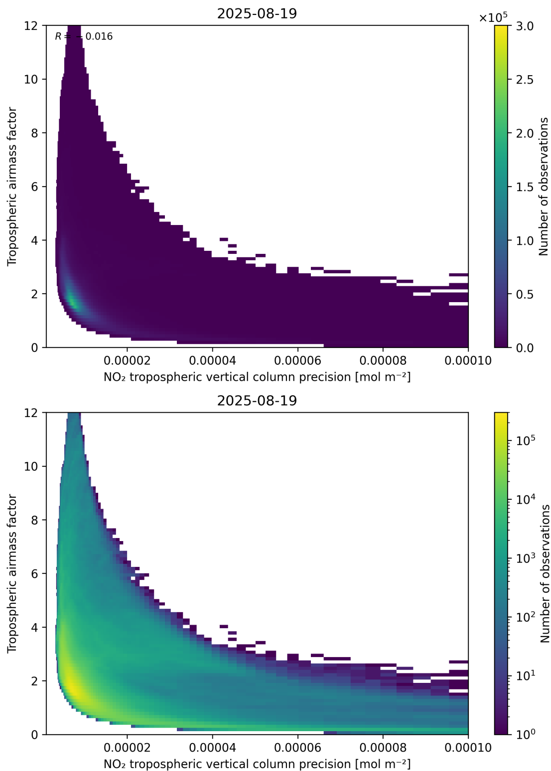
Figure 133: Scatter density plot of “NO 2 tropospheric vertical column precision” against “Tropospheric air mass factor” for 2025-08-19 to 2025-08-20.
