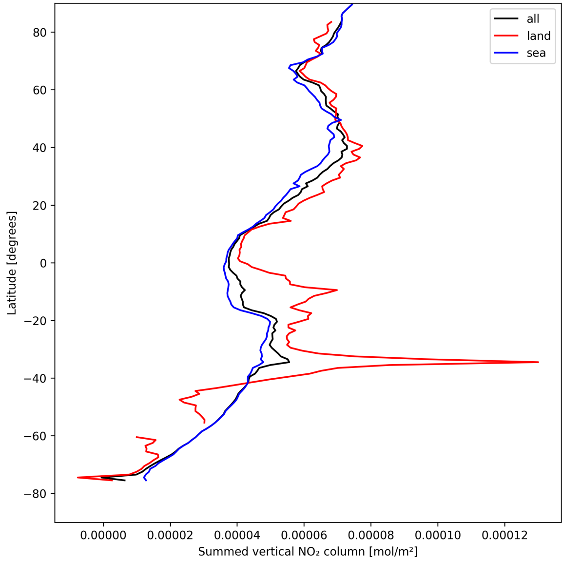
Figure 23: Zonal average of “Summed vertical NO 2 column” for 2025-08-19 to 2025-08-20.
