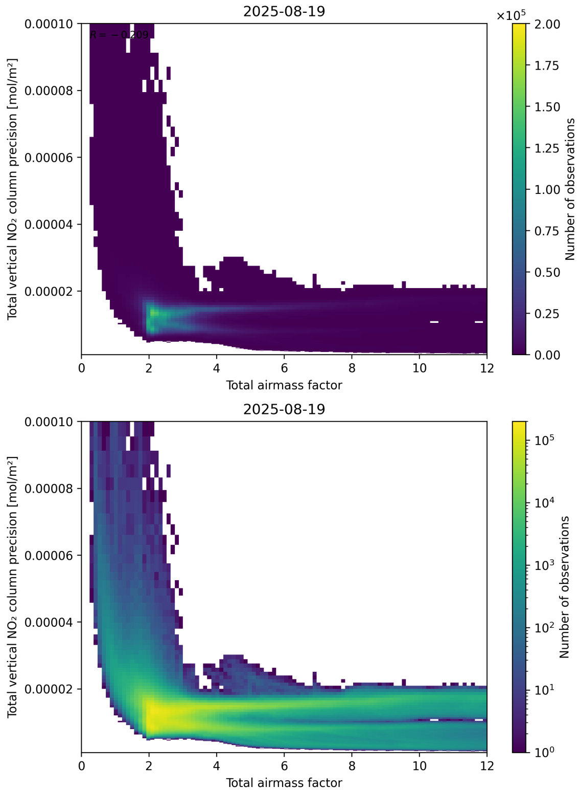
Figure 68: Scatter density plot of “Total airmass factor” against “Total vertical NO 2 column precision” for 2025-08-19 to 2025-08-20.
