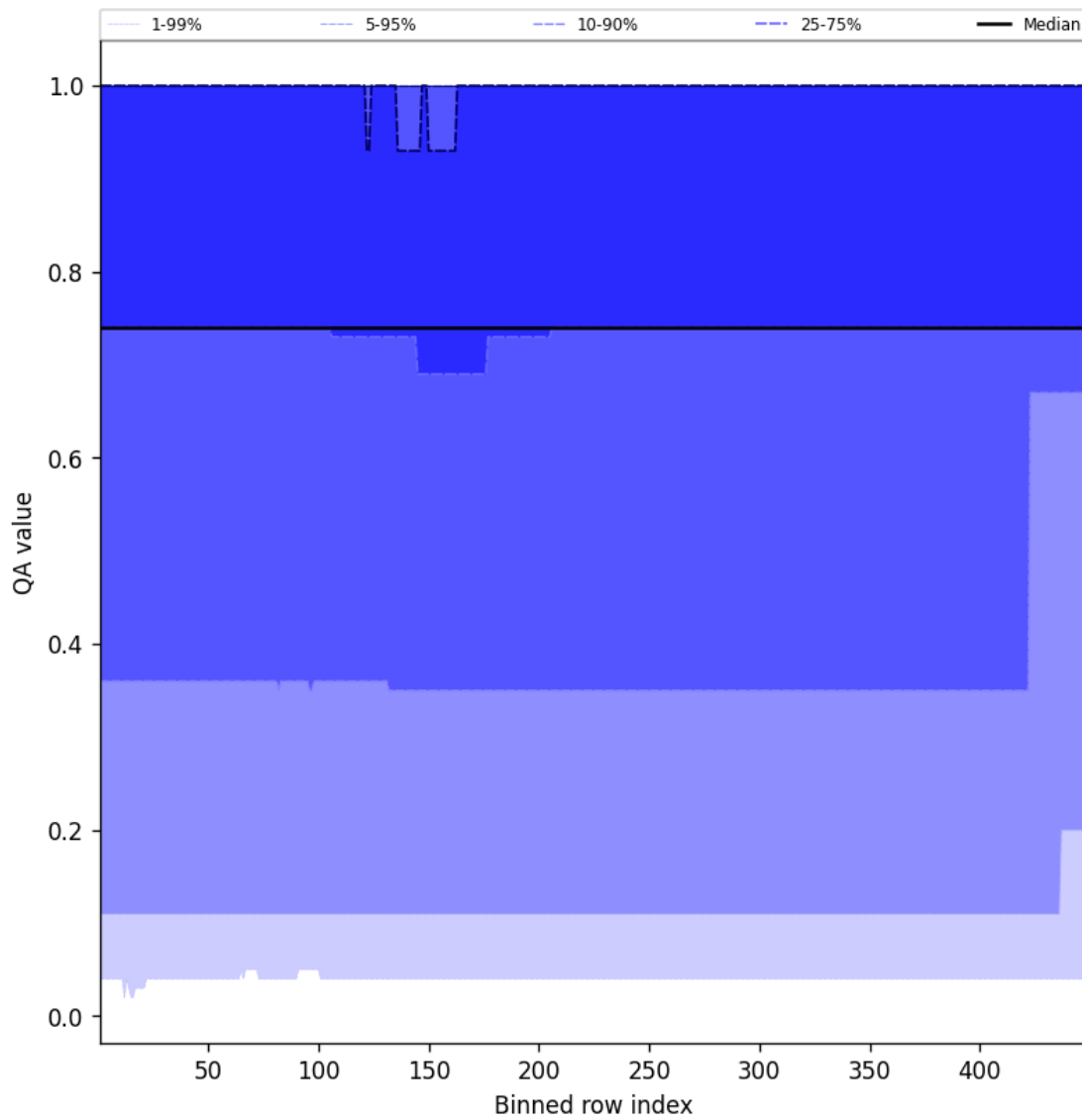
Figure 45: Along track statistics of “QA value” for 2025-08-19 to 2025-08-20
