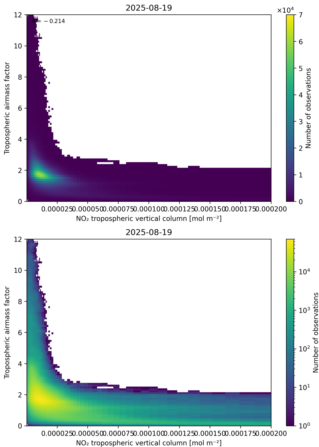
Figure 123: Scatter density plot of “NO 2 tropospheric vertical column” against “Tropospheric air mass factor” for 2025-08-19 to 2025-08-20.
