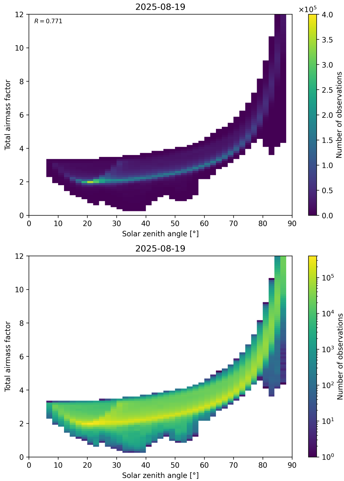
Figure 146: Scatter density plot of “Solar zenith angle” against “Total airmass factor” for 2025-08-19 to 2025-08-20.
