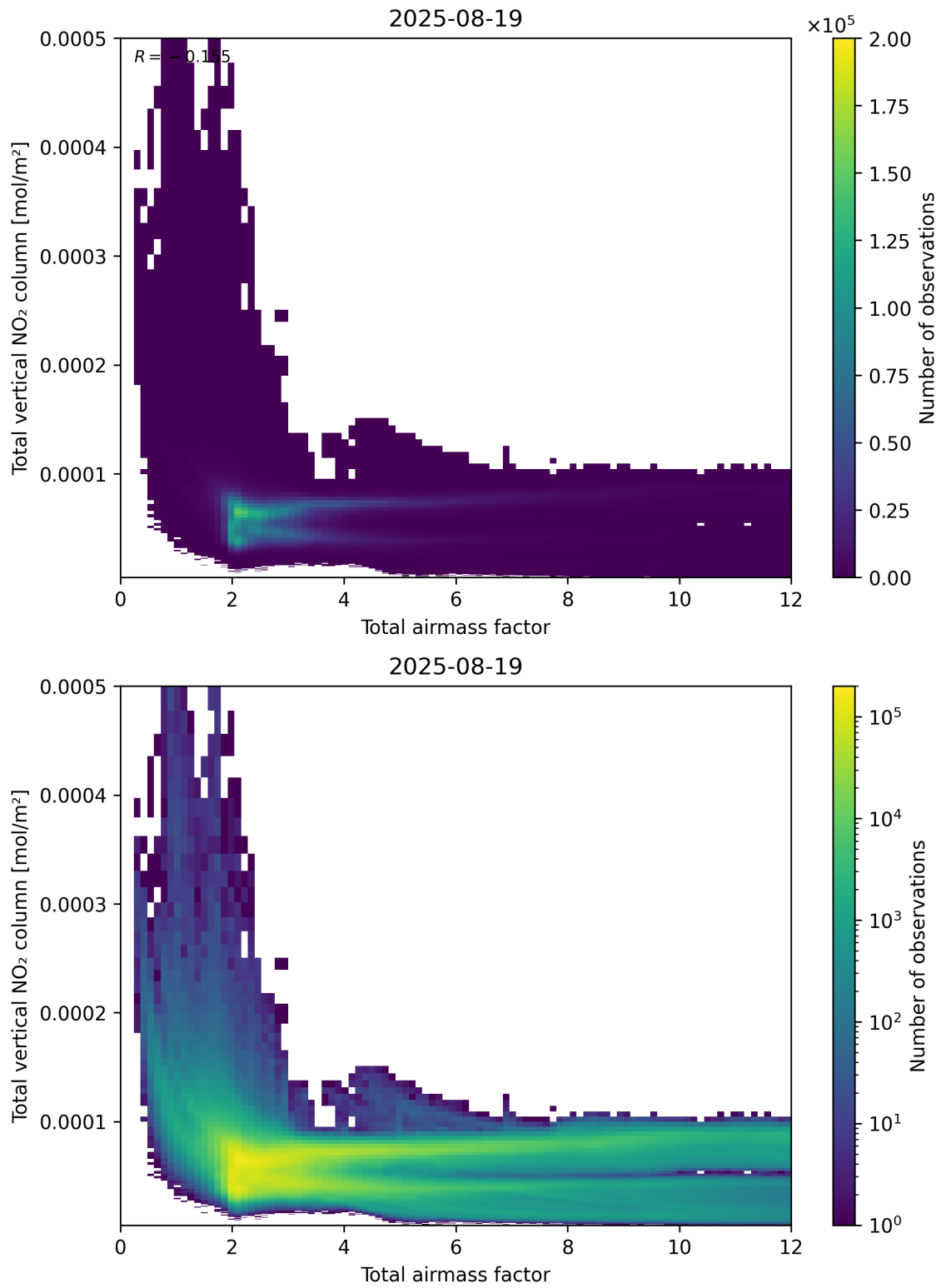
Figure 67: Scatter density plot of “Total airmass factor” against “Total vertical NO 2 column” for 2025-08-19 to 2025-08-20.
