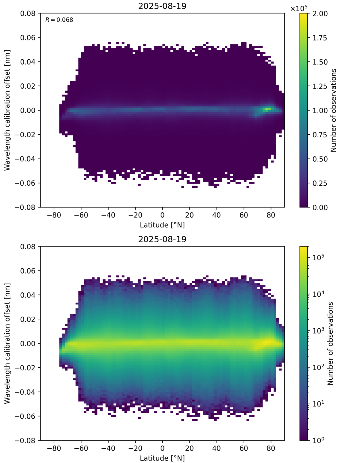
Figure 95: Scatter density plot of “Latitude” against “Wavelength calibration offset” for 2025-08-19 to 2025-08-20.
