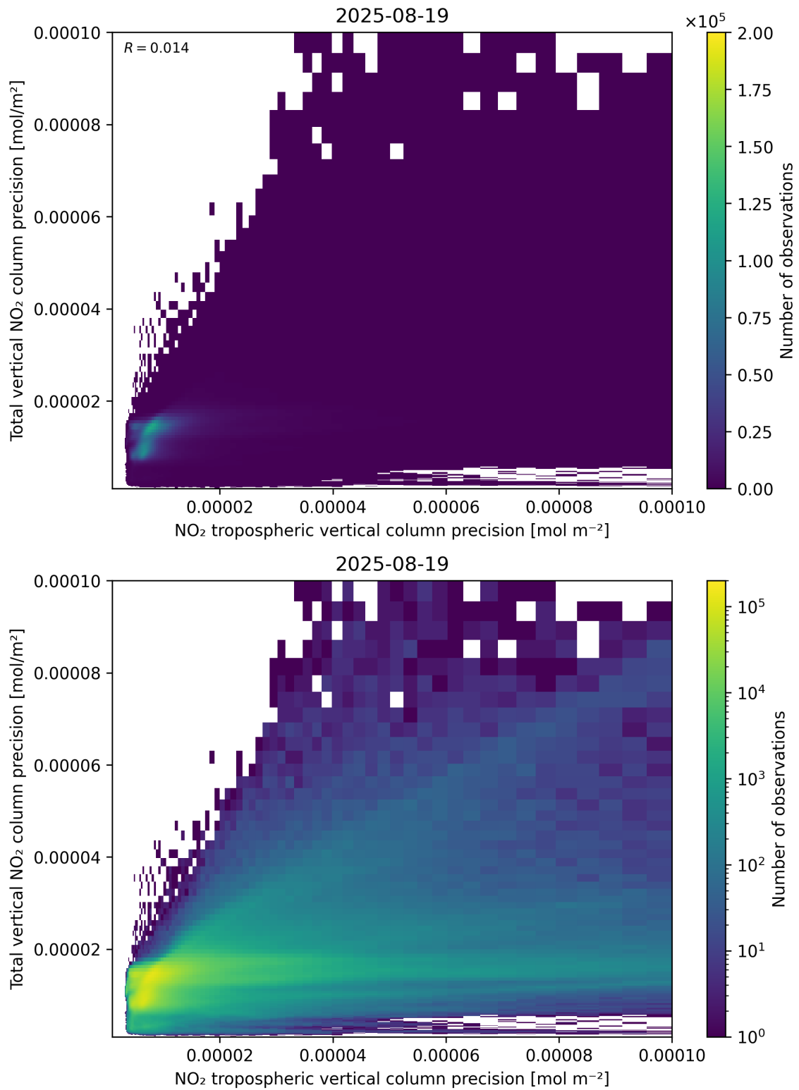
Figure 139: Scatter density plot of “NO 2 tropospheric vertical column precision” against “Total vertical NO 2 column precision” for 2025-08-19 to 2025-08-20.
