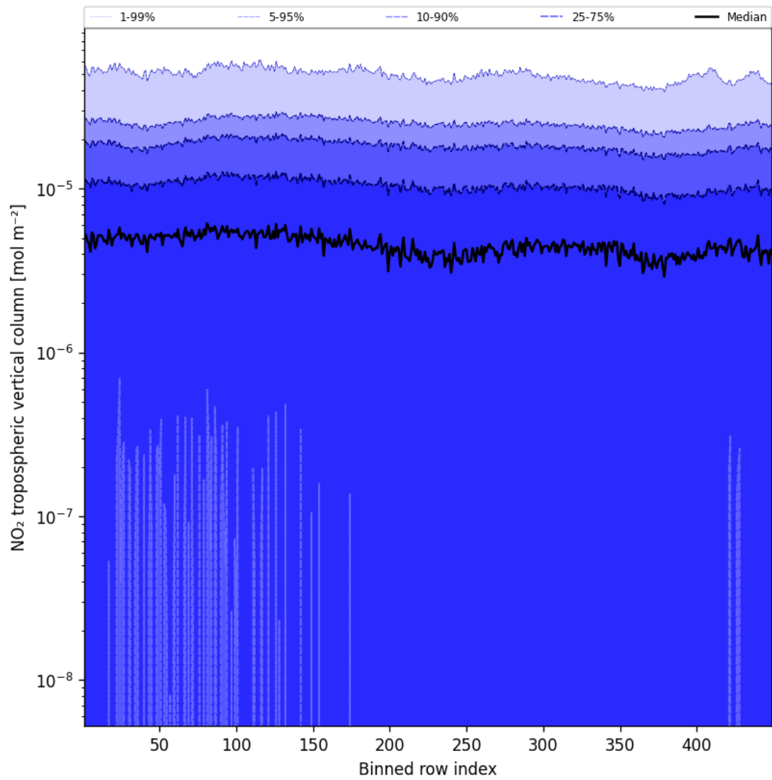
Figure 46: Along track statistics of “NO 2 tropospheric vertical column” for 2025-08-19 to 2025-08-20
