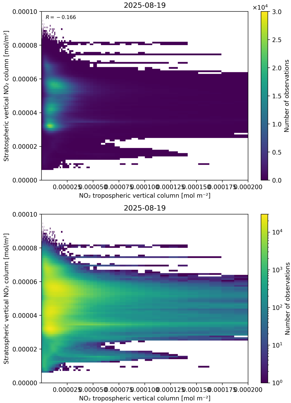
Figure 125: Scatter density plot of “NO 2 tropospheric vertical column” against “Stratospheric vertical NO 2 column” for 2025-08-19 to 2025-08-20.
