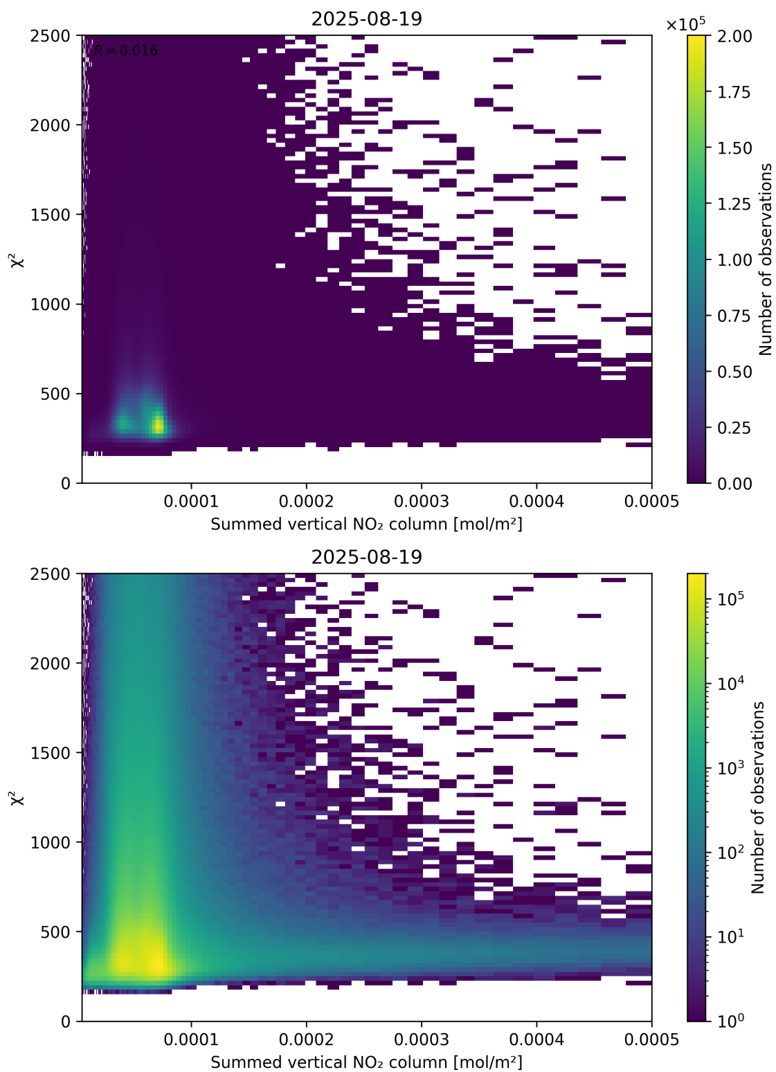
Figure 104: Scatter density plot of “Summed vertical NO 2 column” against “ \chi^2 ” for 2025-08-19 to 2025-08-20.
