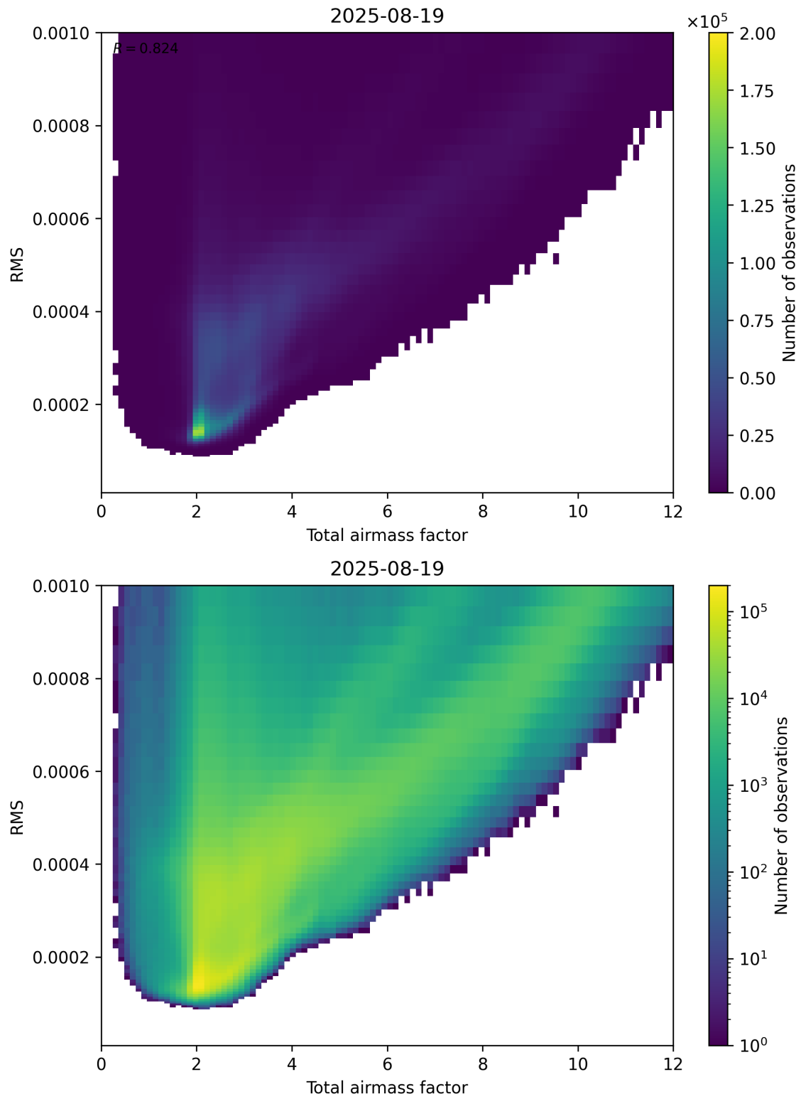
Figure 69: Scatter density plot of “Total airmass factor” against “RMS” for 2025-08-19 to 2025-08-20.
