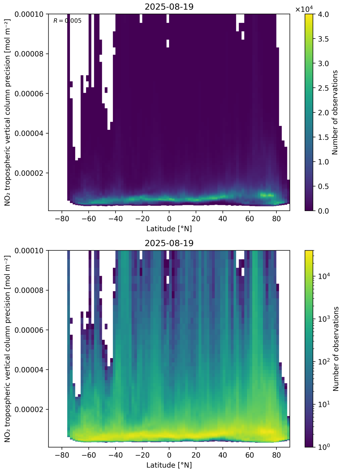
Figure 93: Scatter density plot of “Latitude” against “NO 2 tropospheric vertical column precision” for 2025-08-19 to 2025-08-20.
