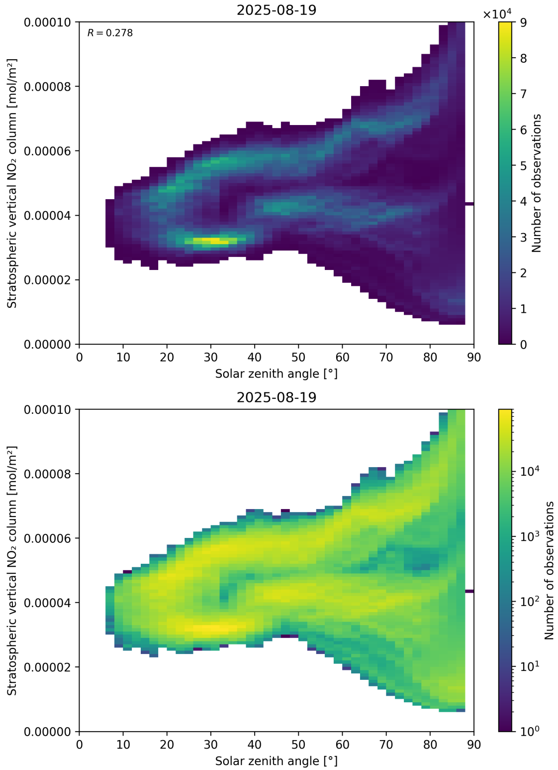
Figure 150: Scatter density plot of “Solar zenith angle” against “Stratospheric vertical NO 2 column” for 2025-08-19 to 2025-08-20.
