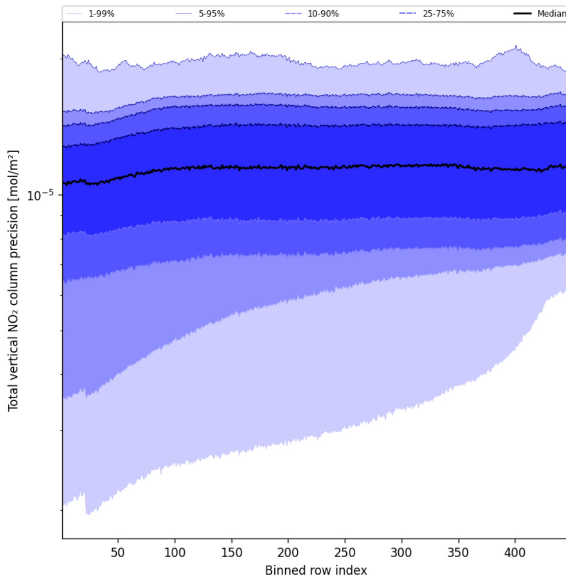
Figure 56: Along track statistics of “Total vertical NO 2 column precision” for 2025-08-19 to 2025-08-20
