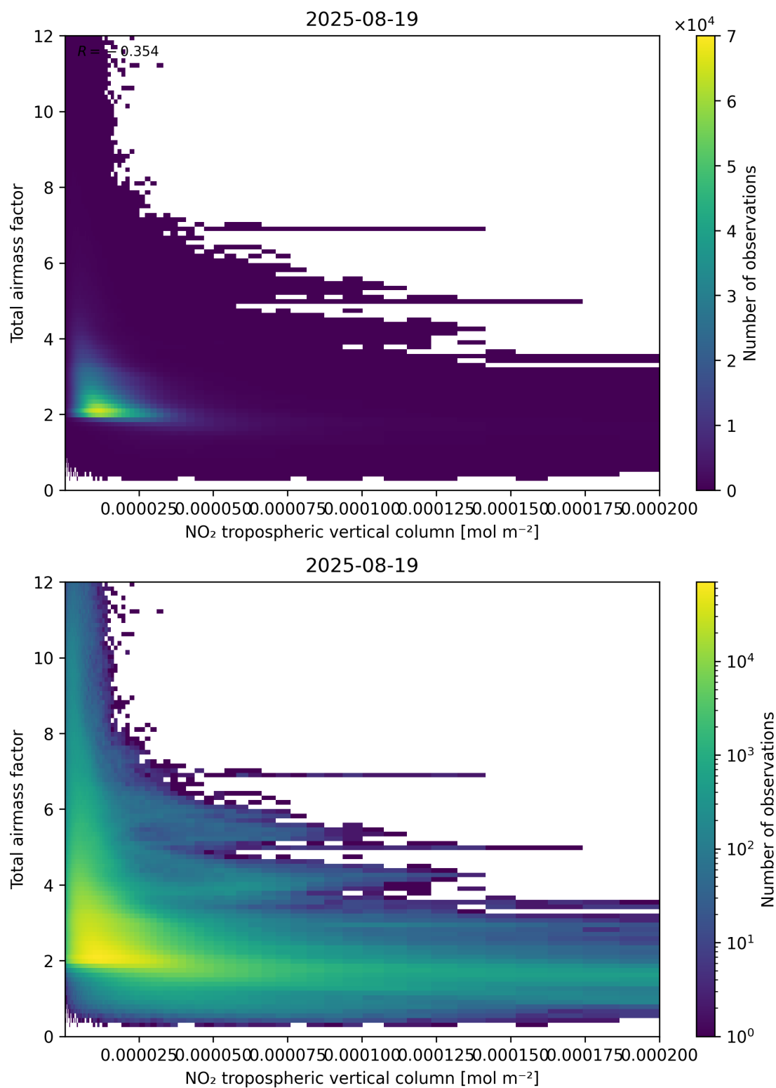
Figure 122: Scatter density plot of “NO 2 tropospheric vertical column” against “Total air mass factor” for 2025-08-19 to 2025-08-20.
