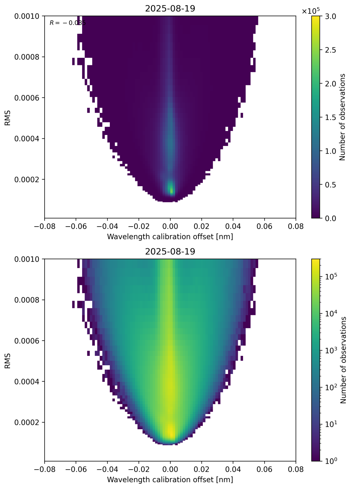
Figure 181: Scatter density plot of “Wavelength calibration offset” against “RMS” for 2025-08-19 to 2025-08-20.
