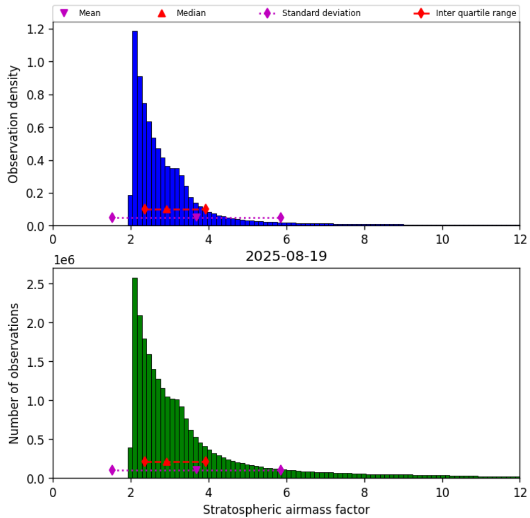
Figure 44: Histogram of “Stratospheric airmass factor” for 2025-08-19 to 2025-08-20
