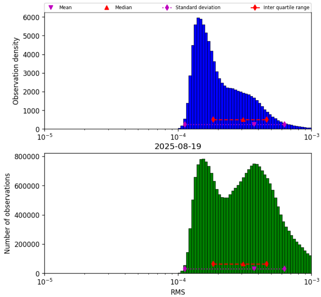
Figure 43: Histogram of “RMS” for 2025-08-19 to 2025-08-20
