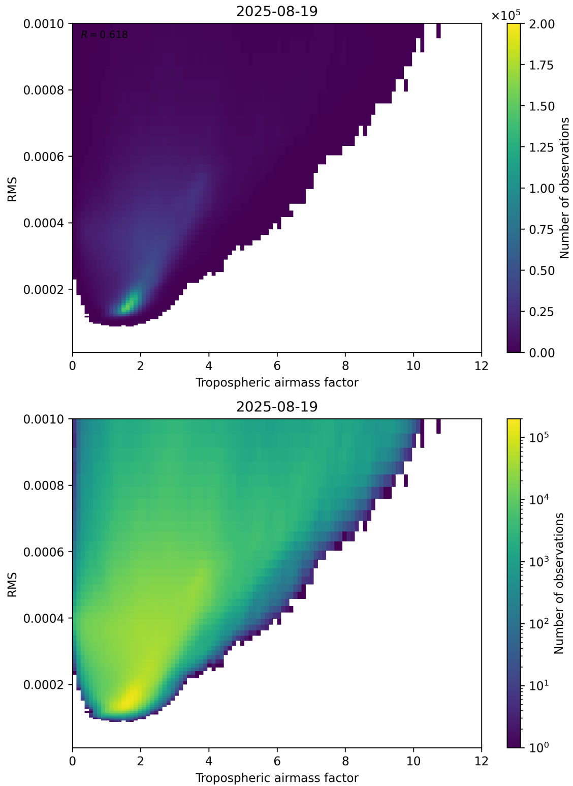
Figure 79: Scatter density plot of “Tropospheric airmass factor” against “RMS” for 2025-08-19 to 2025-08-20.
