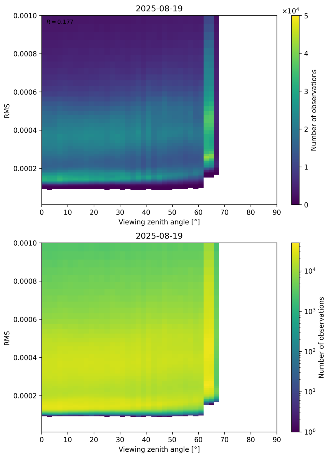
Figure 171: Scatter density plot of “Viewing zenith angle” against “RMS” for 2025-08-19 to 2025-08-20.
