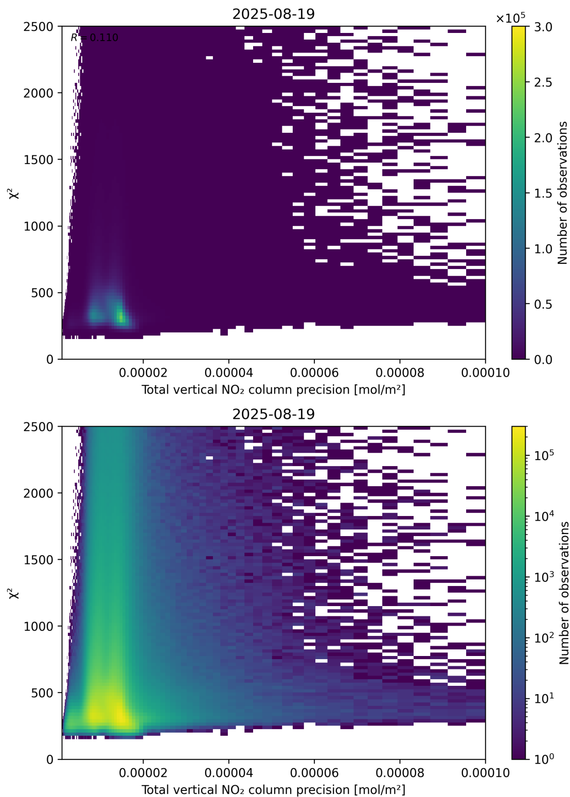
Figure 116: Scatter density plot of “Total vertical NO 2 column precision” against “ \chi^2 ” for 2025-08-19 to 2025-08-20.
