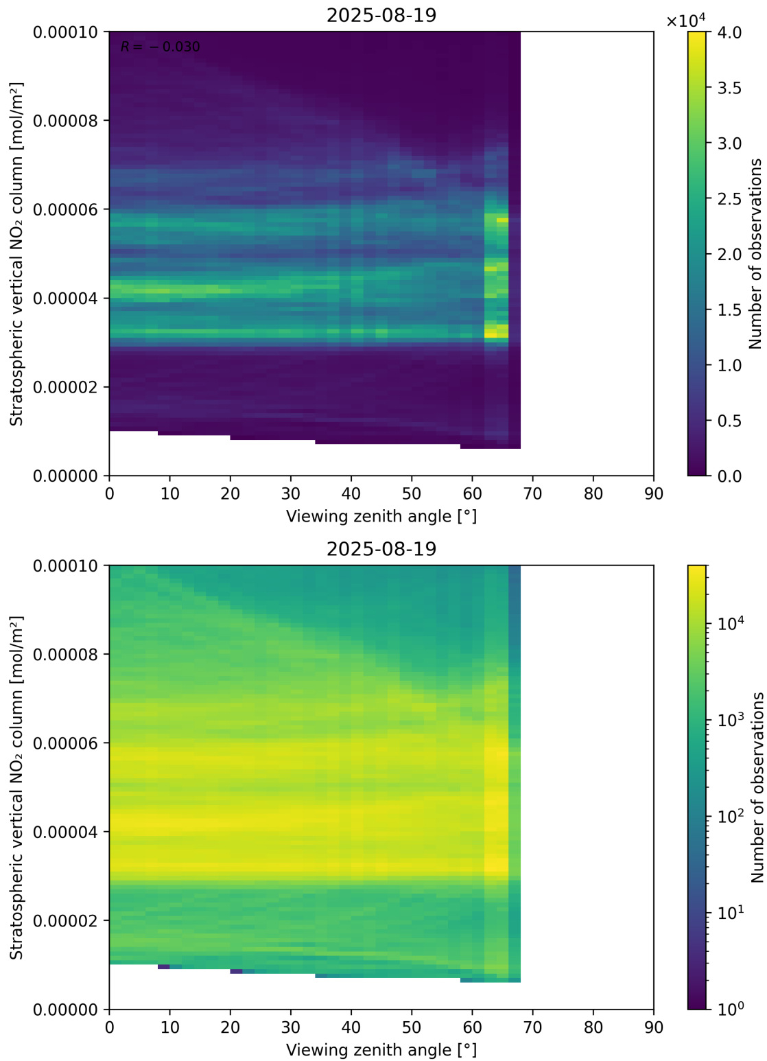
Figure 164: Scatter density plot of “Viewing zenith angle” against “Stratospheric vertical NO 2 column” for 2025-08-19 to 2025-08-20.
