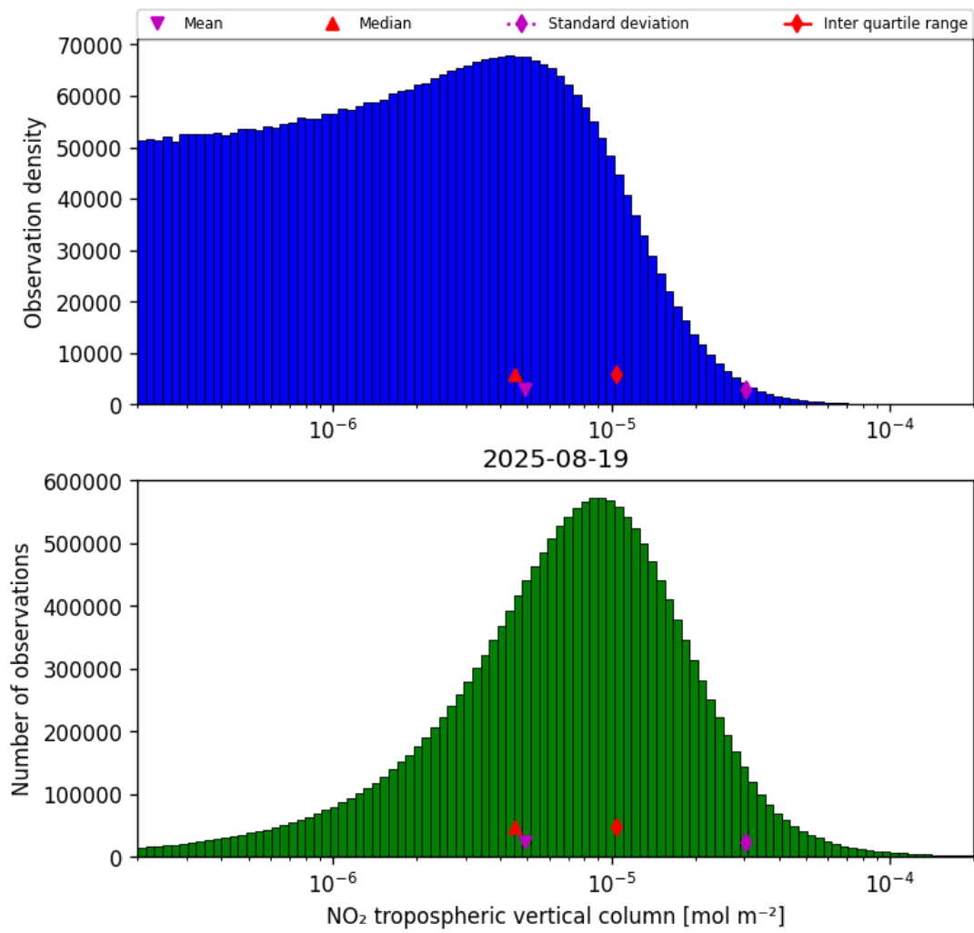
Figure 29: Histogram of “NO 2 tropospheric vertical column” for 2025-08-19 to 2025-08-20
