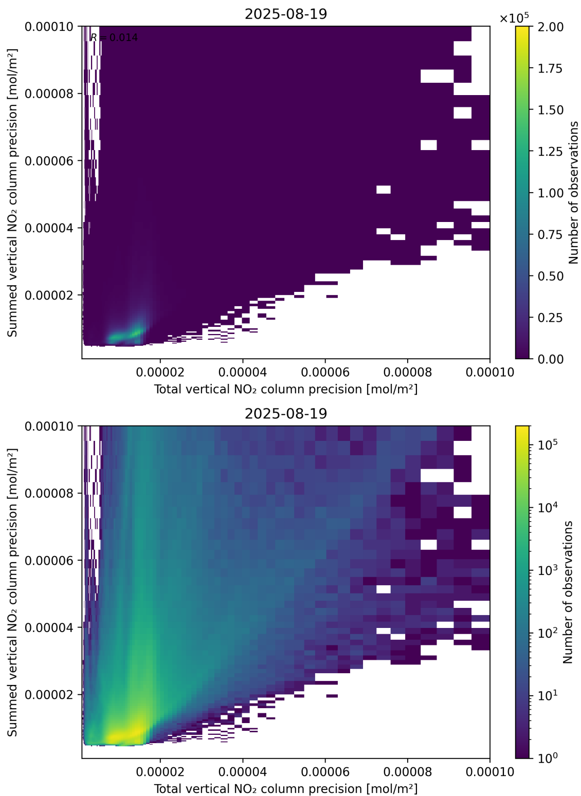
Figure 118: Scatter density plot of “Total vertical NO 2 column precision” against “Summed vertical NO 2 column precision” for 2025-08-19 to 2025-08-20.
