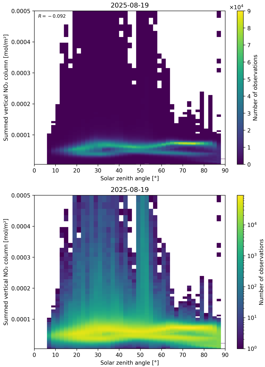
Figure 151: Scatter density plot of “Solar zenith angle” against “Summed vertical NO 2 column” for 2025-08-19 to 2025-08-20.
