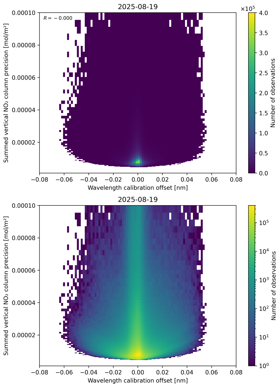
Figure 178: Scatter density plot of “Wavelength calibration offset” against “Summed vertical NO 2 column precision” for 2025-08-19 to 2025-08-20.
