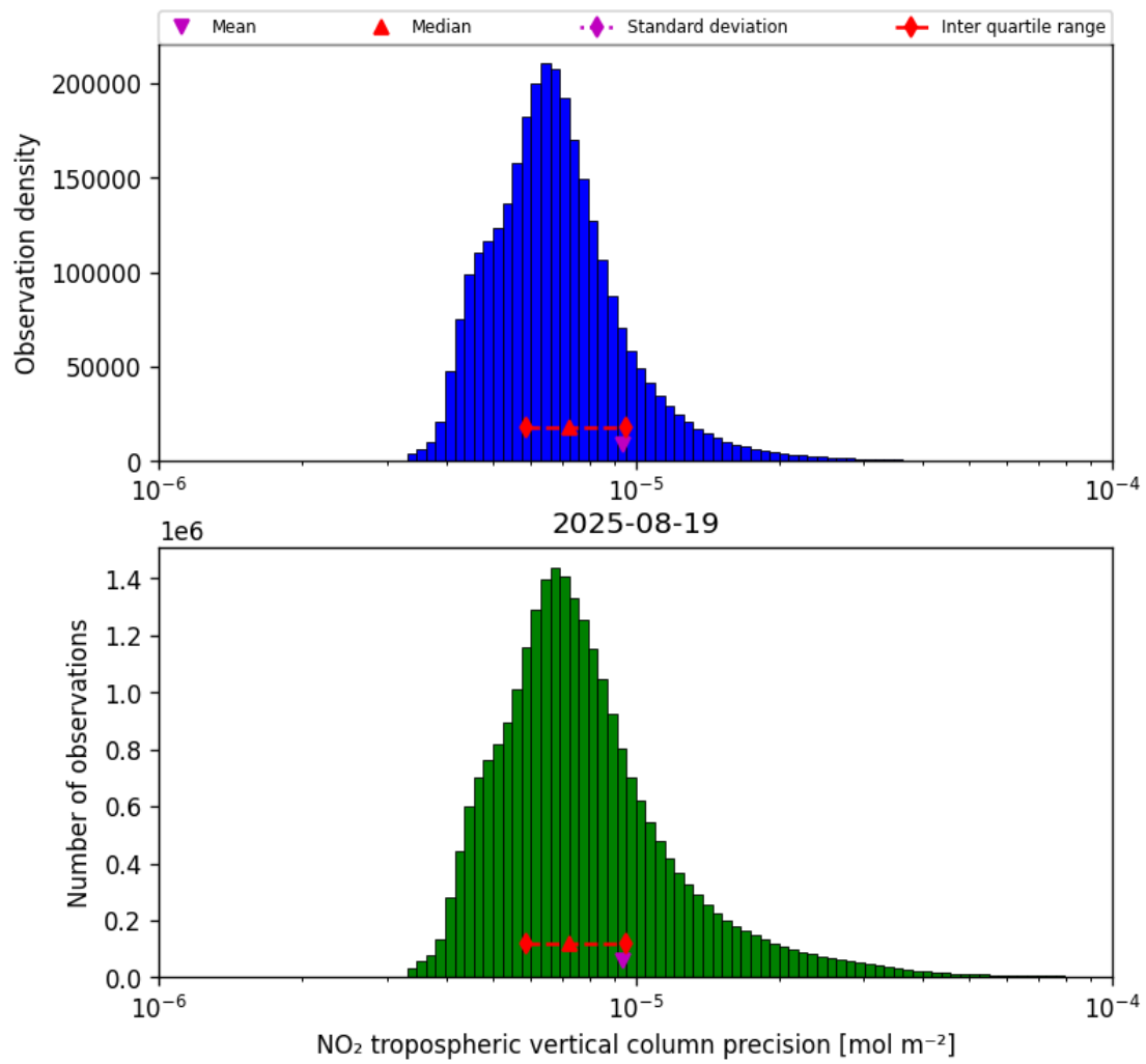
Figure 30: Histogram of “NO 2 tropospheric vertical column precision” for 2025-08-19 to 2025-08-20
