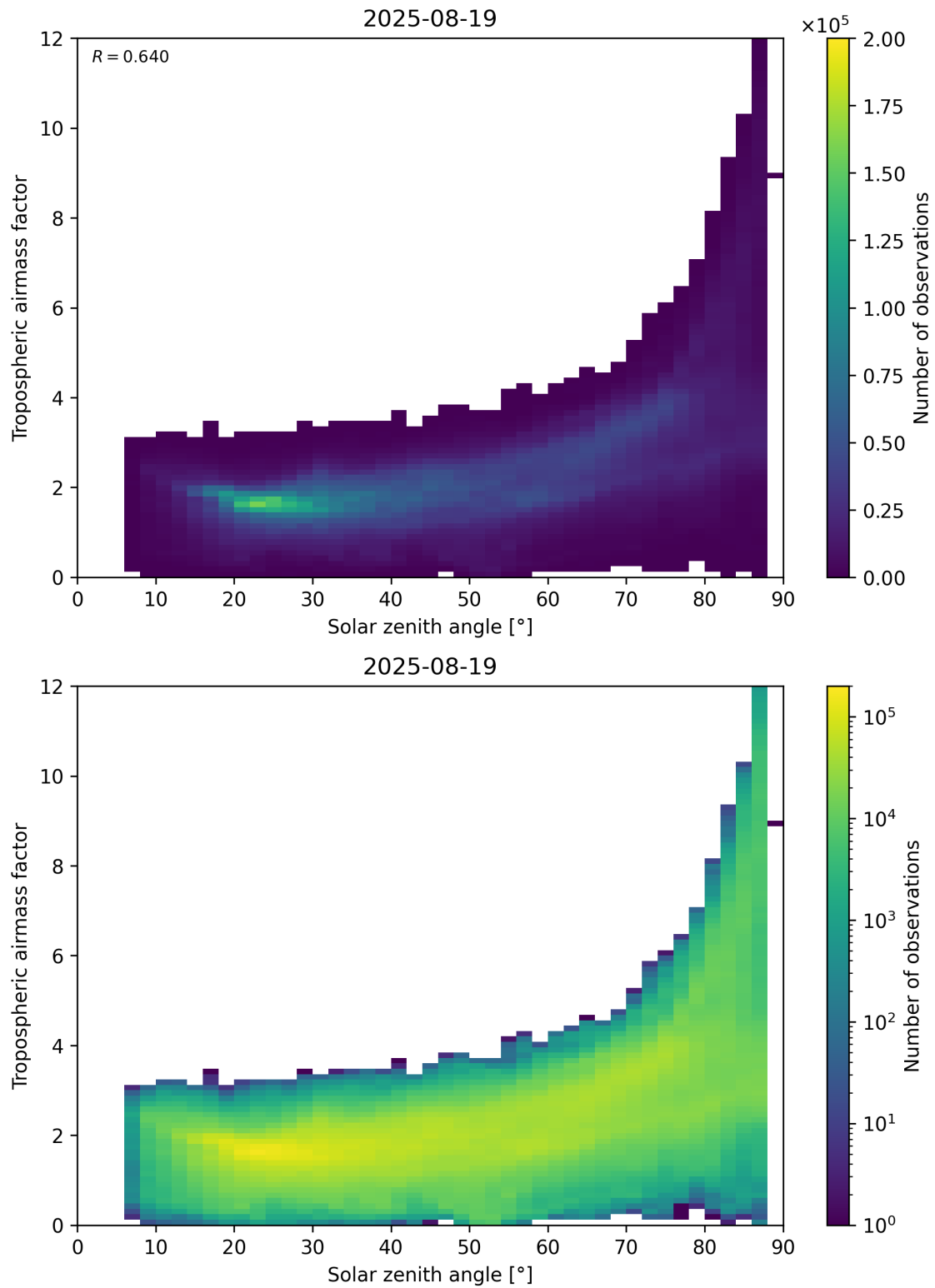
Figure 147: Scatter density plot of “Solar zenith angle” against “Tropospheric airmass factor” for 2025-08-19 to 2025-08-20.
