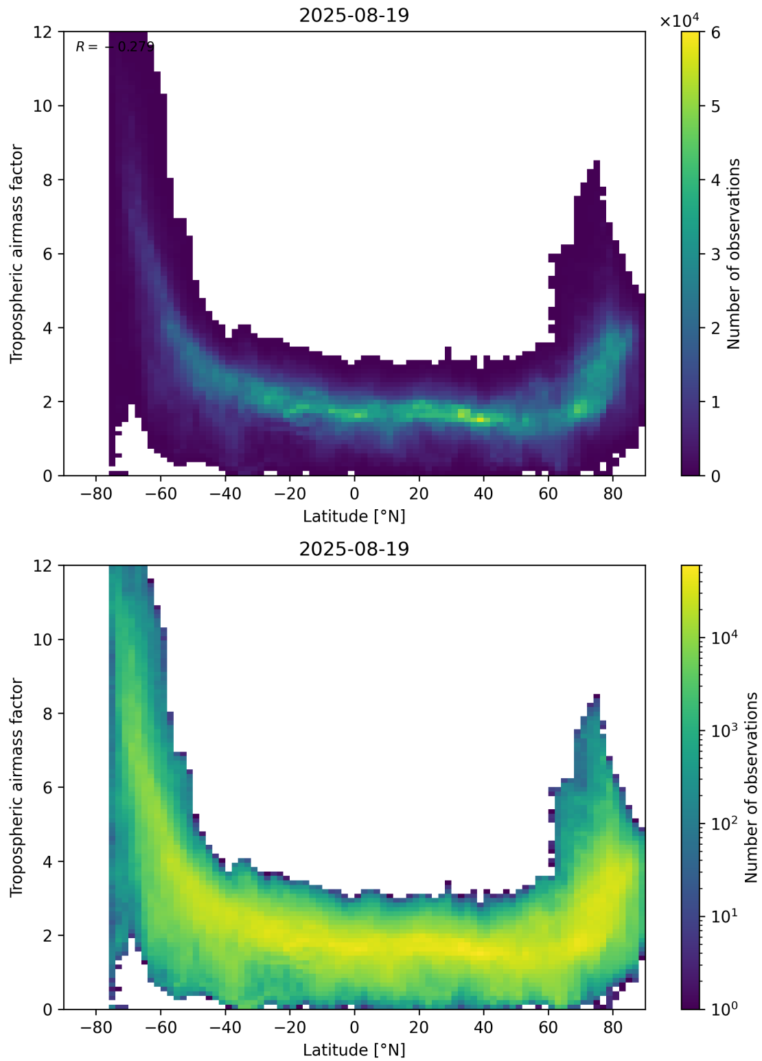
Figure 85: Scatter density plot of “Latitude” against “Tropospheric airmass factor” for 2025-08-19 to 2025-08-20.
