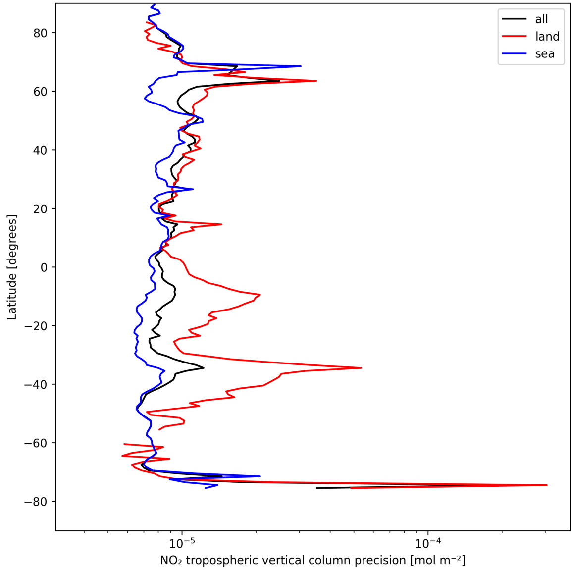
Figure 13: Zonal average of "NO 2 tropospheric vertical column precision" for 2025-08-19 to 2025-08-20.
