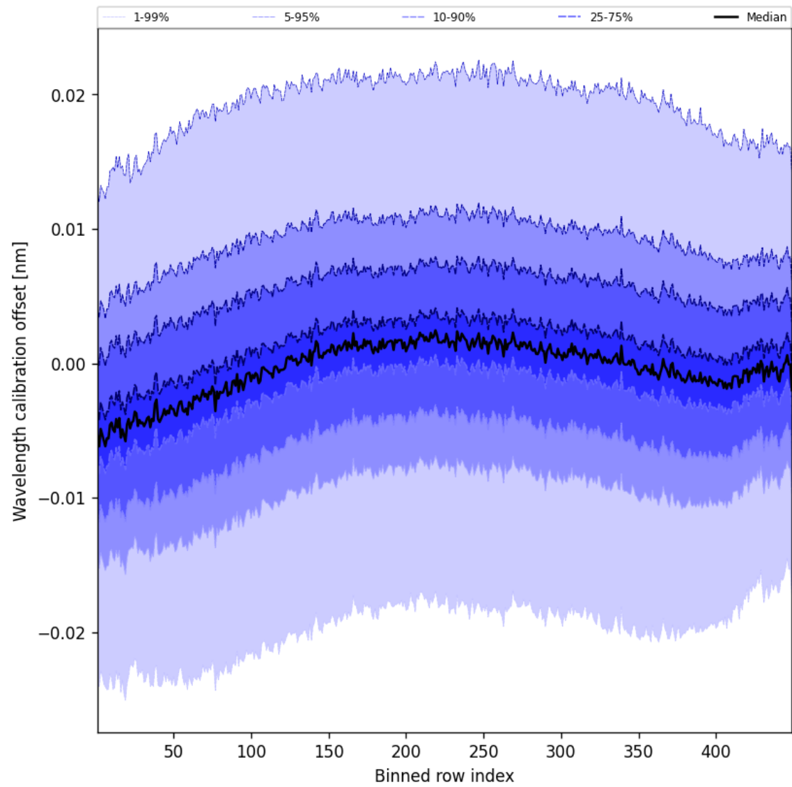
Figure 52: Along track statistics of “Wavelength calibration offset” for 2025-08-19 to 2025-08-20
