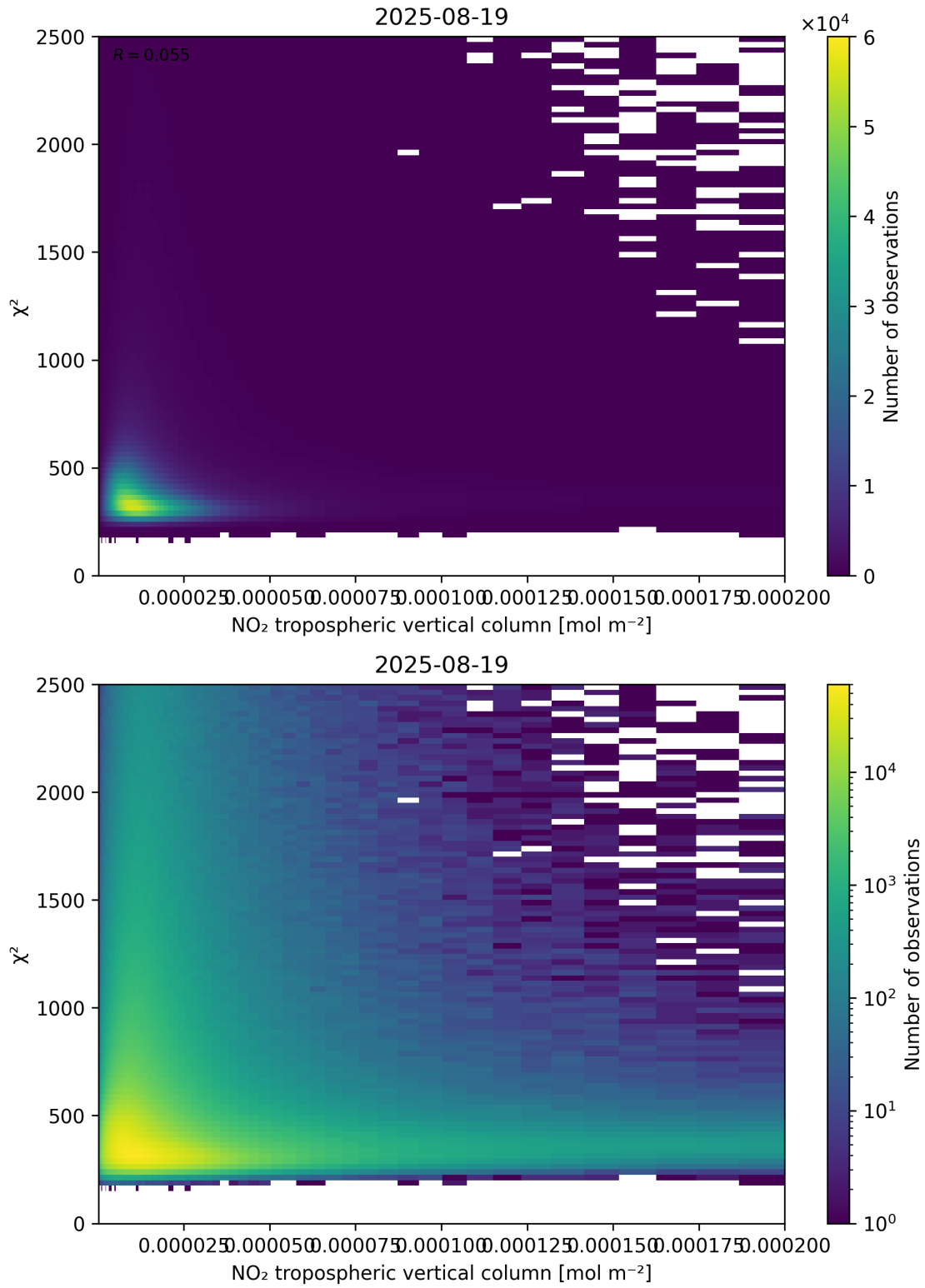
Figure 124: Scatter density plot of “NO 2 tropospheric vertical column” against “ \chi^2 ” for 2025-08-19 to 2025-08-20.
