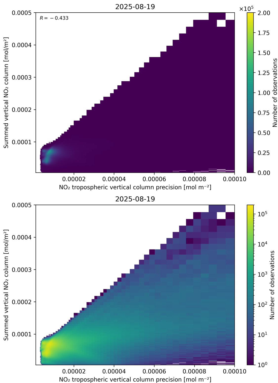
Figure 136: Scatter density plot of “NO 2 tropospheric vertical column precision” against “Summed vertical NO 2 column” for 2025-08-19 to 2025-08-20.
