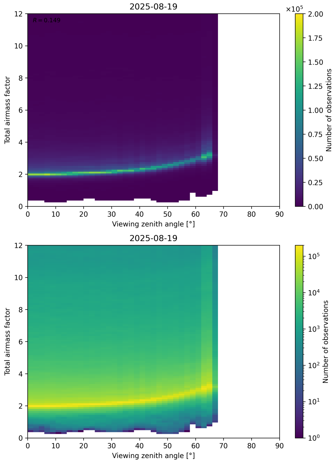
Figure 160: Scatter density plot of “Viewing zenith angle” against “Total airmass factor” for 2025-08-19 to 2025-08-20.
