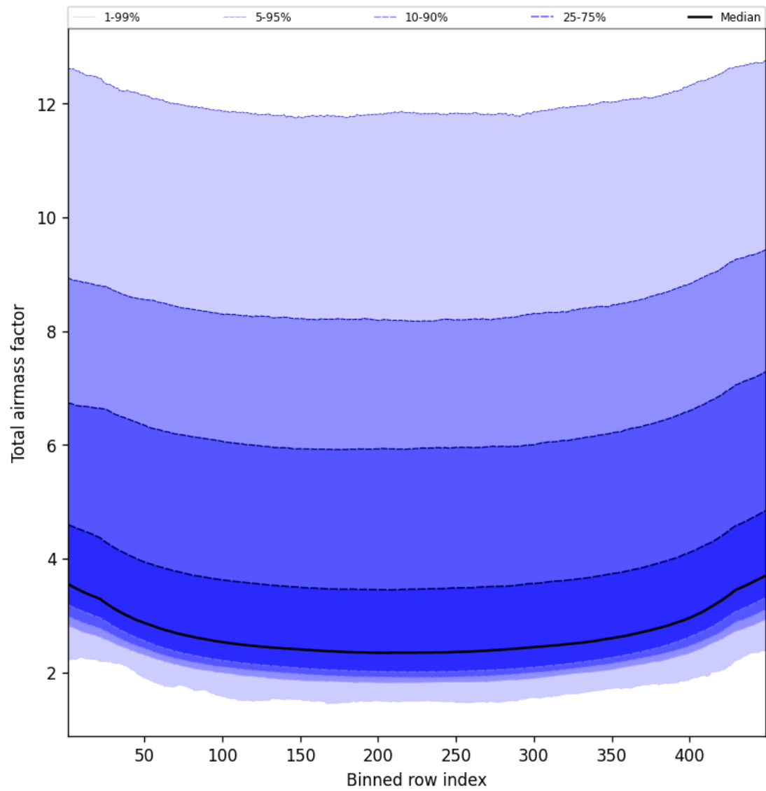
Figure 49: Along track statistics of “Total airmass factor” for 2025-08-19 to 2025-08-20
