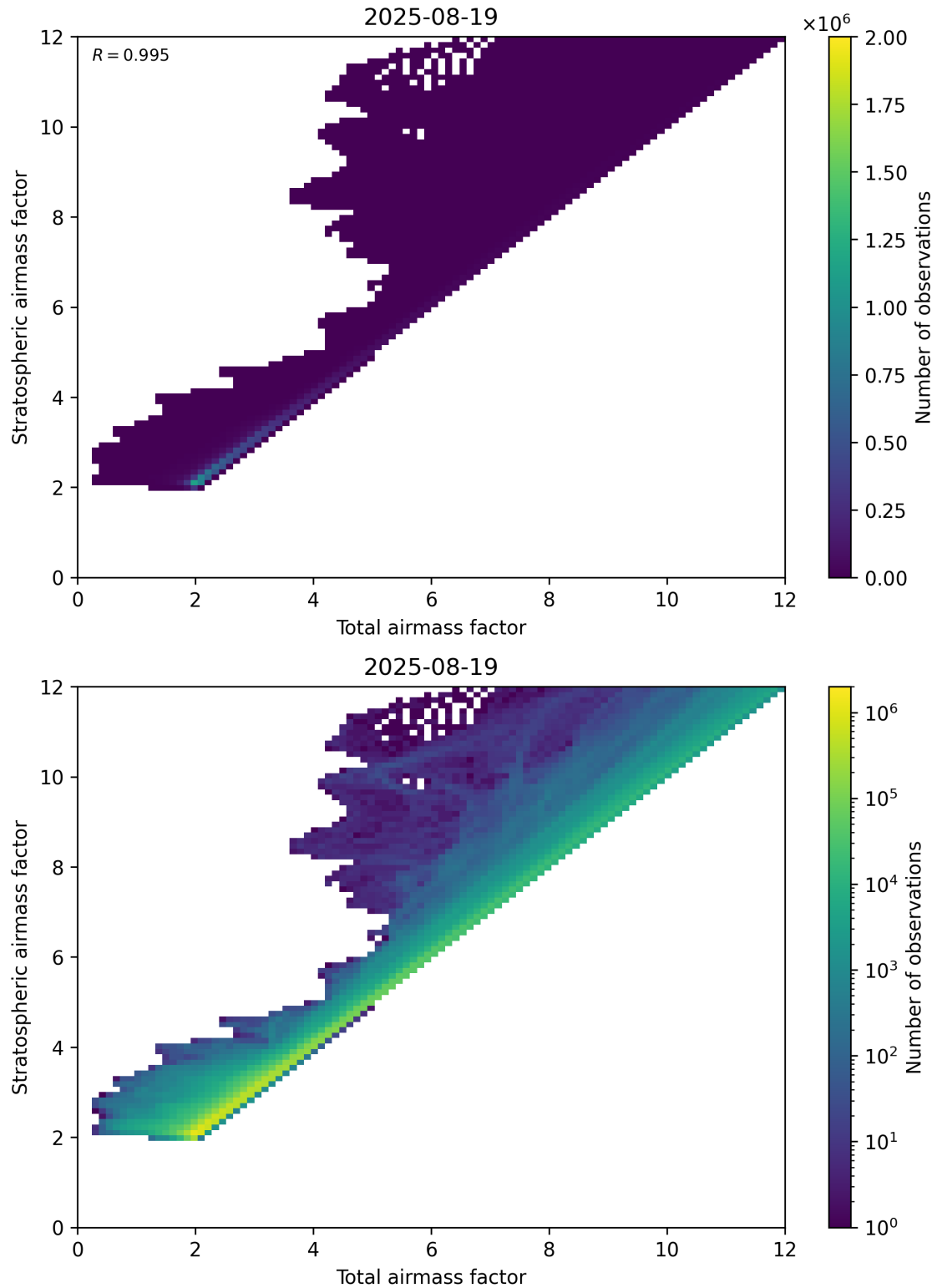
Figure 62: Scatter density plot of “Total airmass factor” against “Stratospheric airmass factor” for 2025-08-19 to 2025-08-20.
