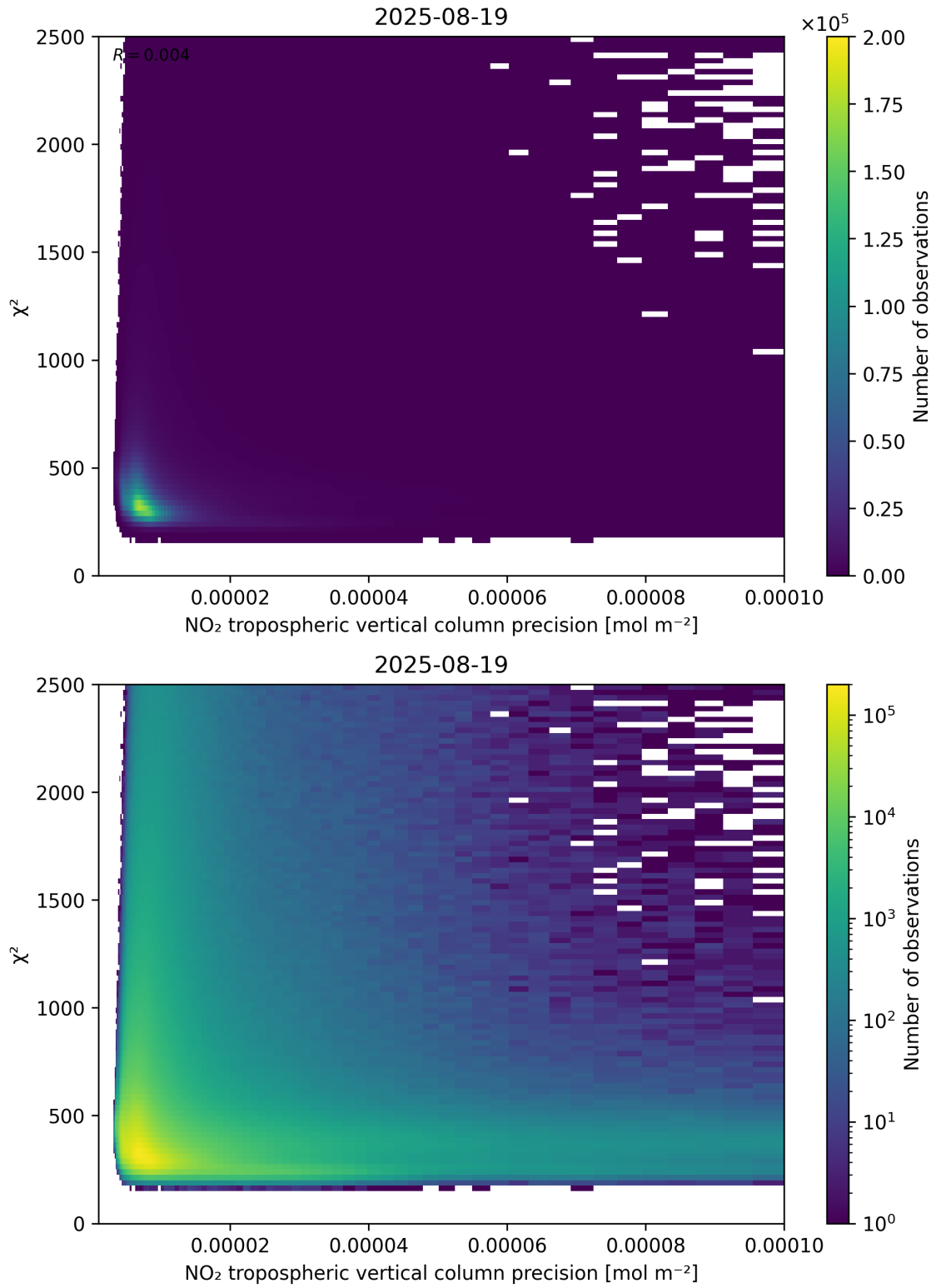
Figure 134: Scatter density plot of “NO 2 tropospheric vertical column precision” against “ \chi^2 ” for 2025-08-19 to 2025-08-20.
