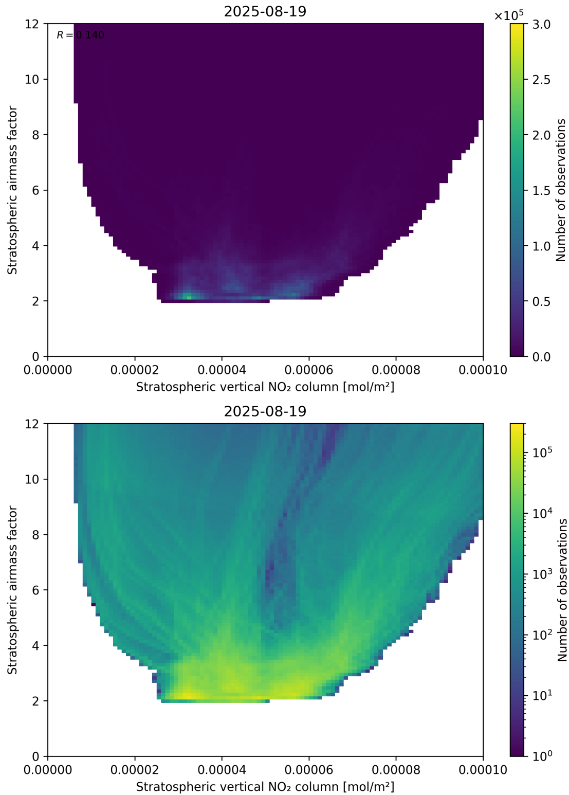
Figure 96: Scatter density plot of “Stratospheric vertical NO 2 column” against “Stratospheric airmass factor” for 2025-08-19 to 2025-08-20.
