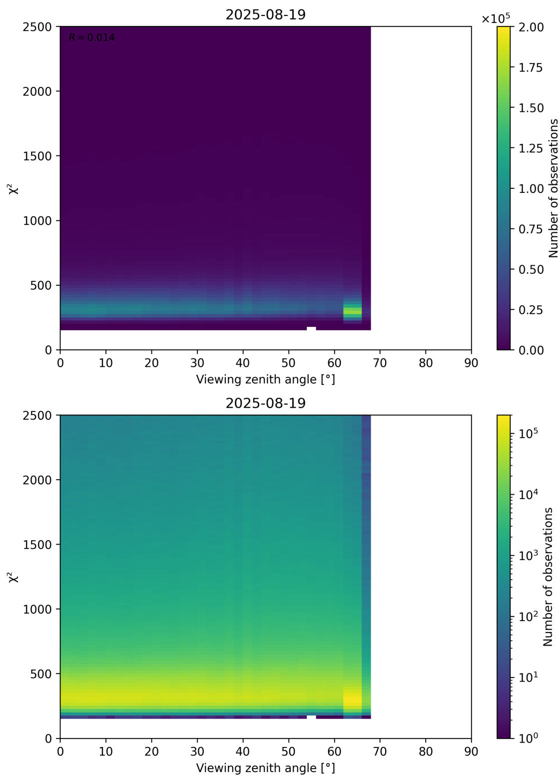
Figure 162: Scatter density plot of “Viewing zenith angle” against “ \chi^2 ” for 2025-08-19 to 2025-08-20.
