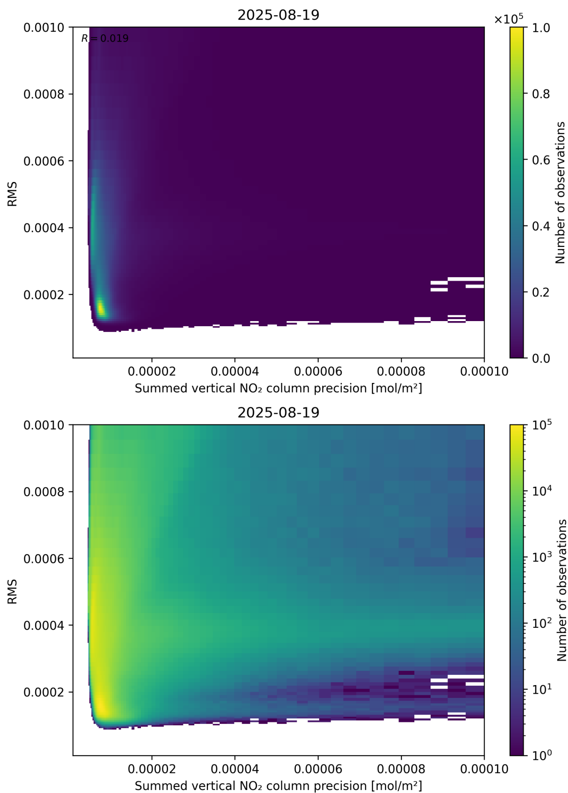
Figure 108: Scatter density plot of “Summed vertical NO 2 column precision” against “RMS” for 2025-08-19 to 2025-08-20.
