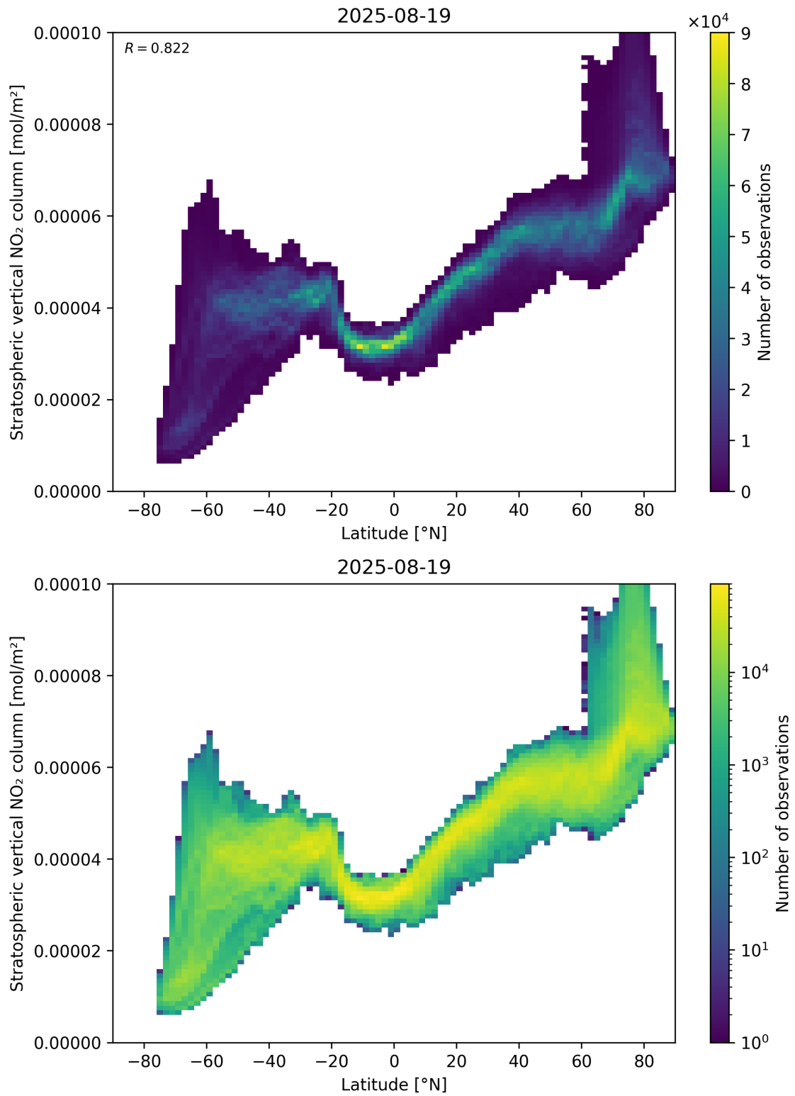
Figure 87: Scatter density plot of “Latitude” against “Stratospheric vertical \text{NO}_2 column” for 2025-08-19 to 2025-08-20.
