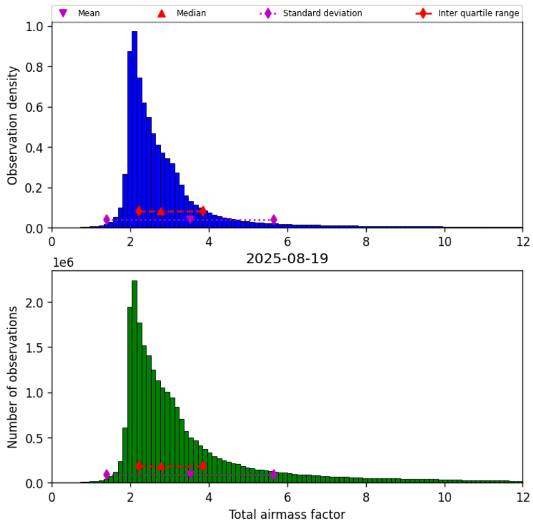
Figure 32: Histogram of “Total airmass factor” for 2025-08-19 to 2025-08-20
