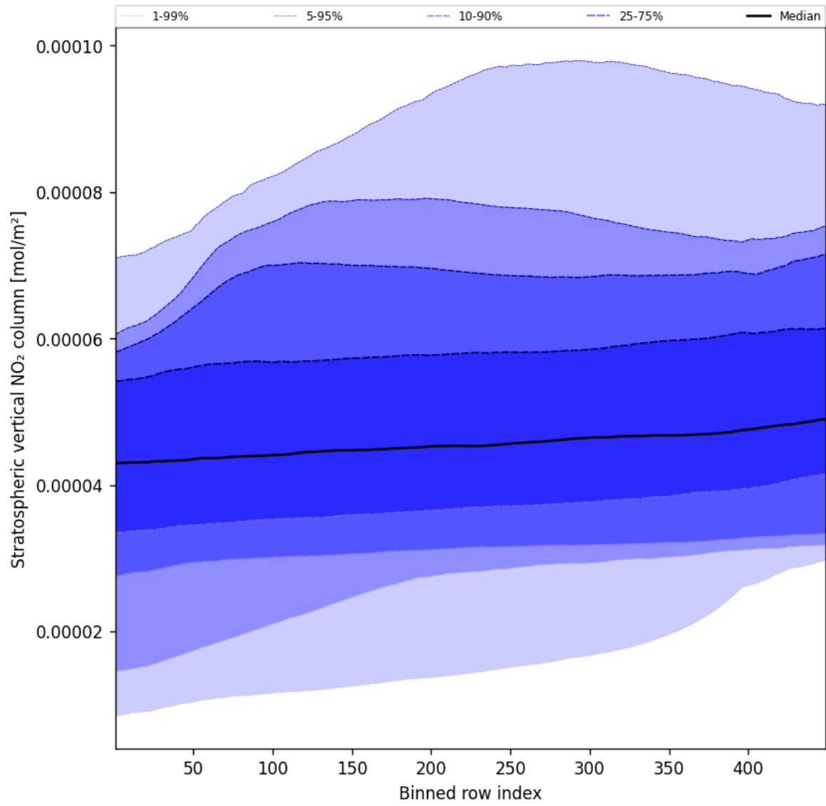
Figure 53: Along track statistics of “Stratospheric vertical NO 2 column” for 2025-08-19 to 2025-08-20
