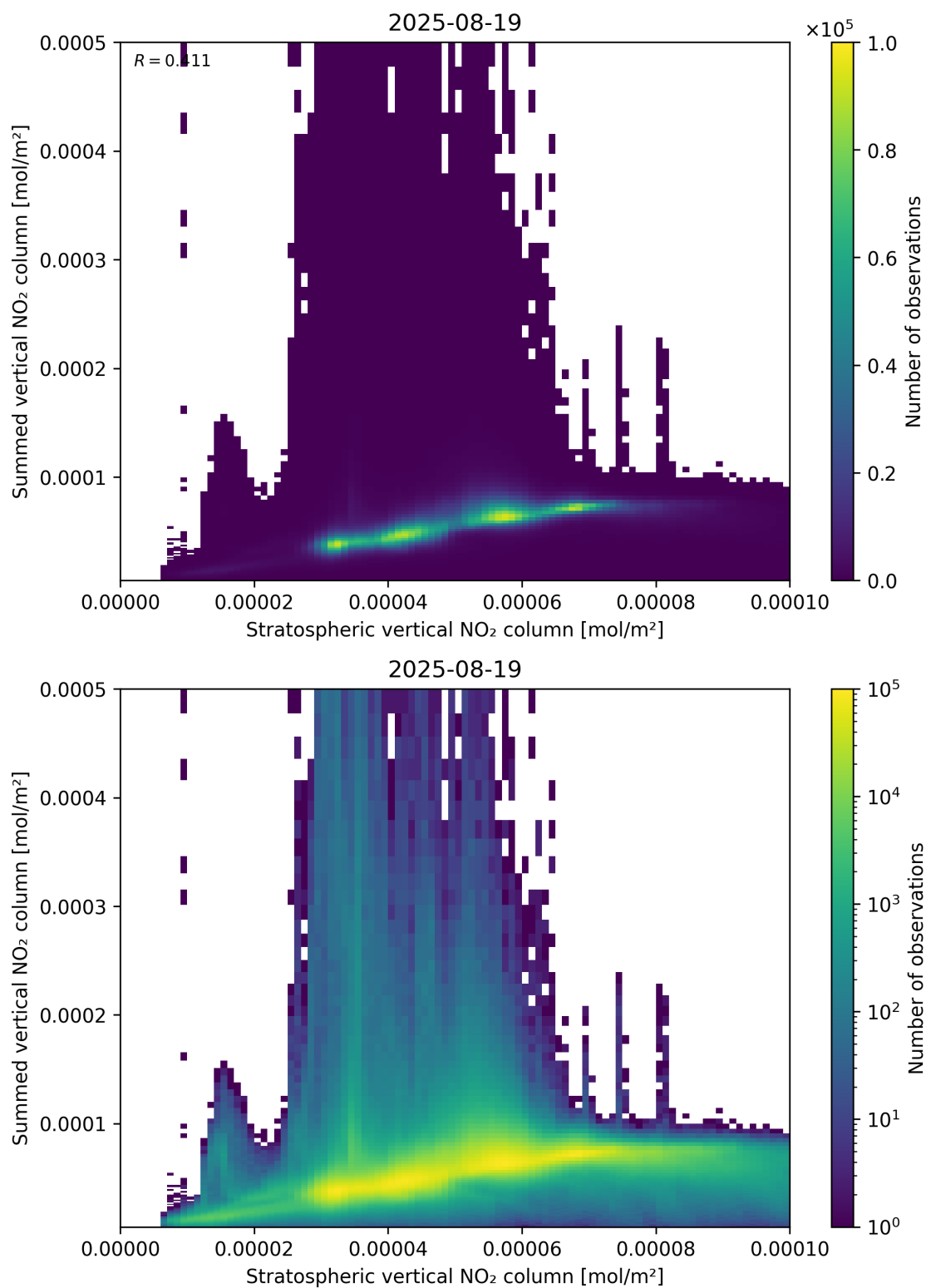
Figure 98: Scatter density plot of “Stratospheric vertical NO 2 column” against “Summed vertical NO 2 column” for 2025-08-19 to 2025-08-20.
