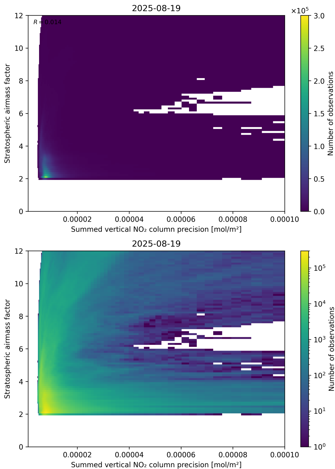
Figure 106: Scatter density plot of “Summed vertical NO 2 column precision” against “Stratospheric airmass factor” for 2025-08-19 to 2025-08-20.
