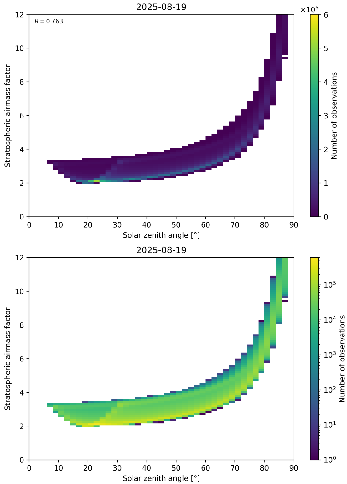
Figure 145: Scatter density plot of “Solar zenith angle” against “Stratospheric airmass factor” for 2025-08-19 to 2025-08-20.
