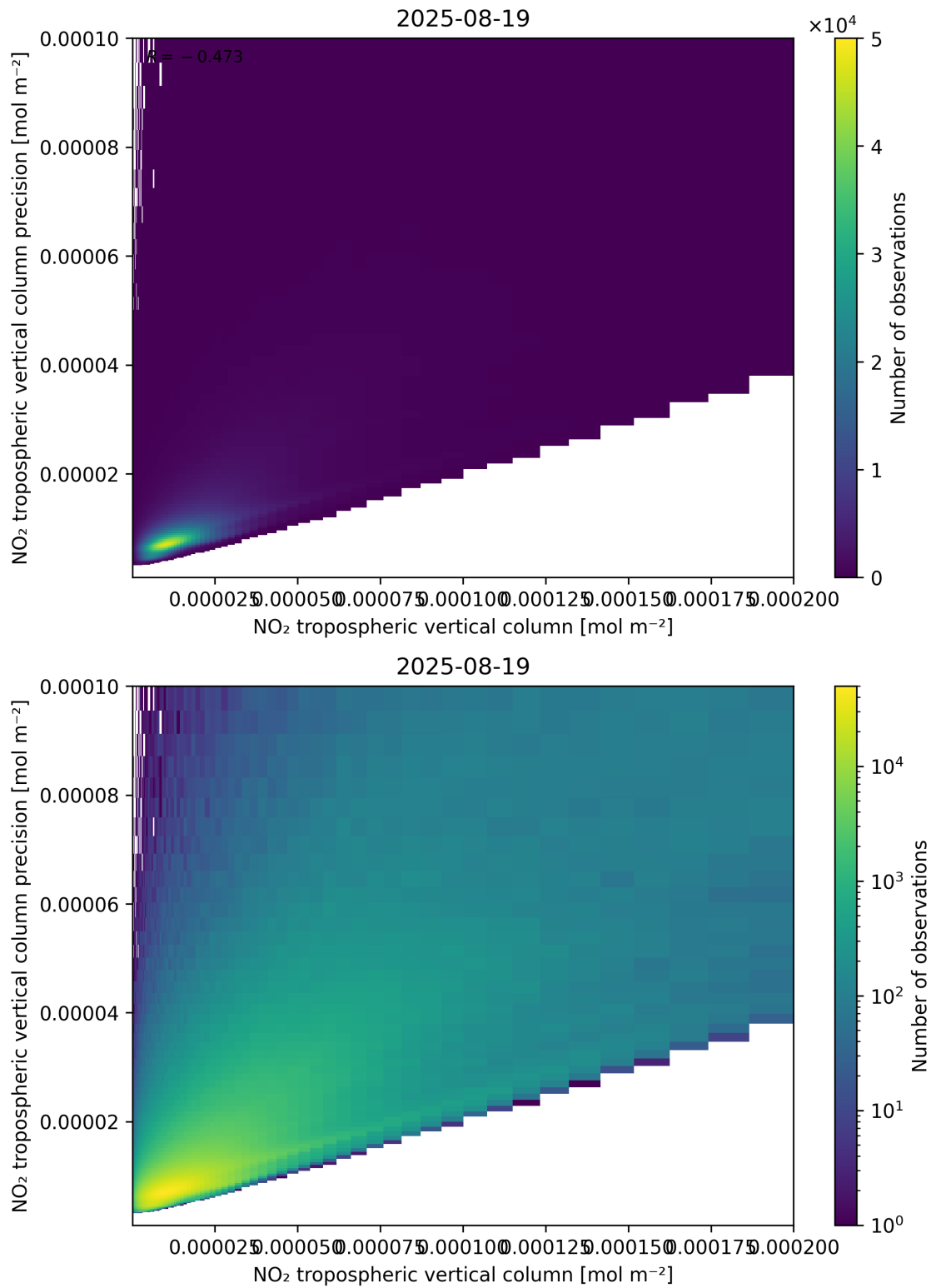
Figure 130: Scatter density plot of “NO 2 tropospheric vertical column” against “NO 2 tropospheric vertical column precision” for 2025-08-19 to 2025-08-20.
