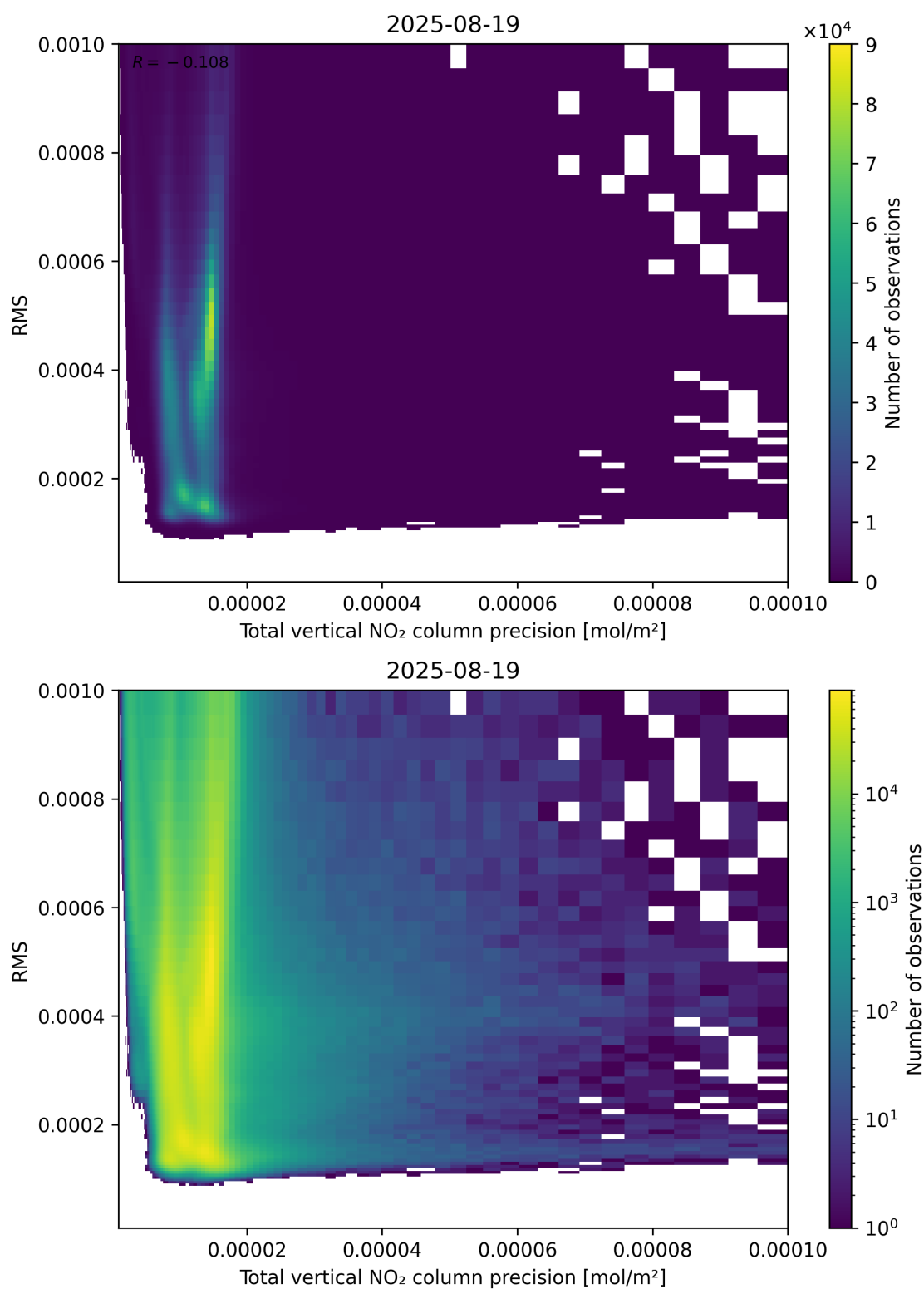
Figure 119: Scatter density plot of “Total vertical NO 2 column precision” against “RMS” for 2025-08-19 to 2025-08-20.
