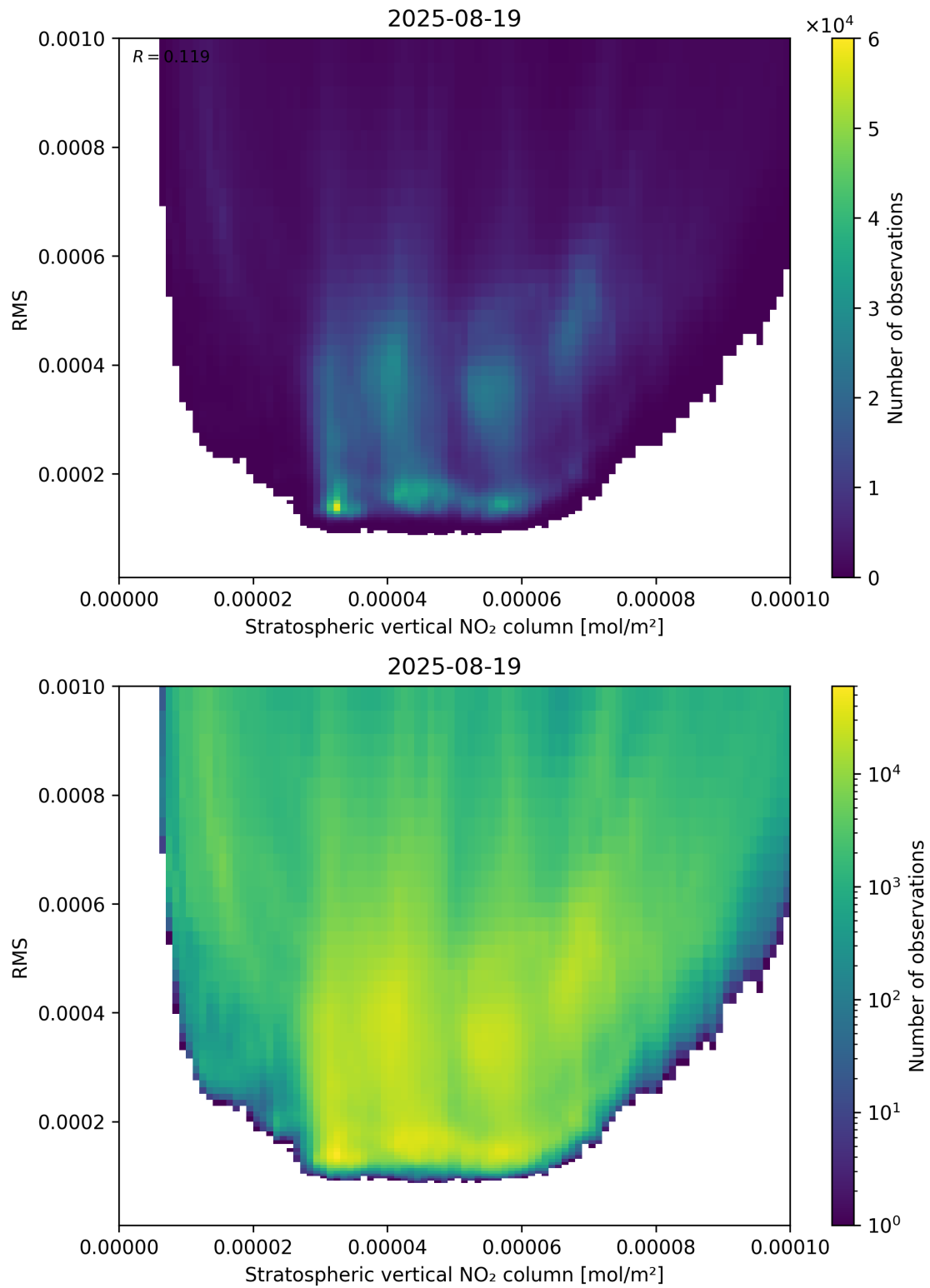
Figure 102: Scatter density plot of “Stratospheric vertical NO 2 column” against “RMS” for 2025-08-19 to 2025-08-20.
