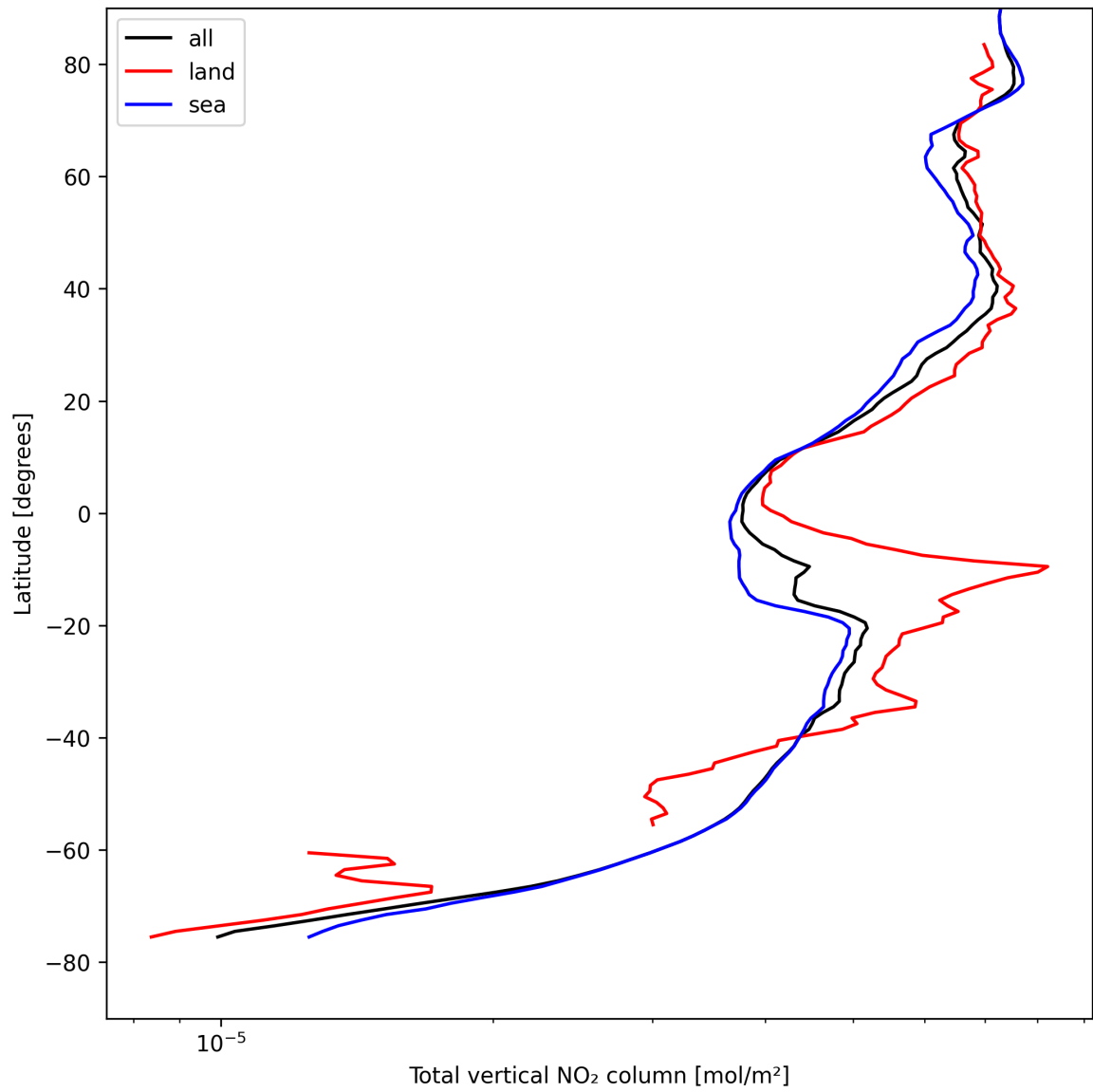
Figure 21: Zonal average of “Total vertical NO 2 column” for 2025-08-19 to 2025-08-20.
