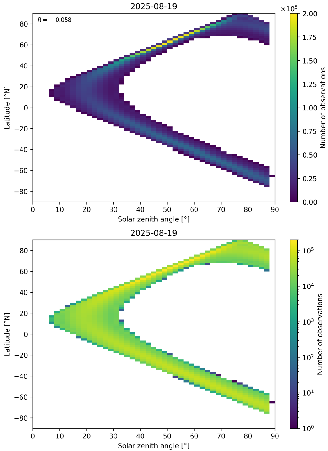
Figure 149: Scatter density plot of “Solar zenith angle” against “Latitude” for 2025-08-19 to 2025-08-20.
