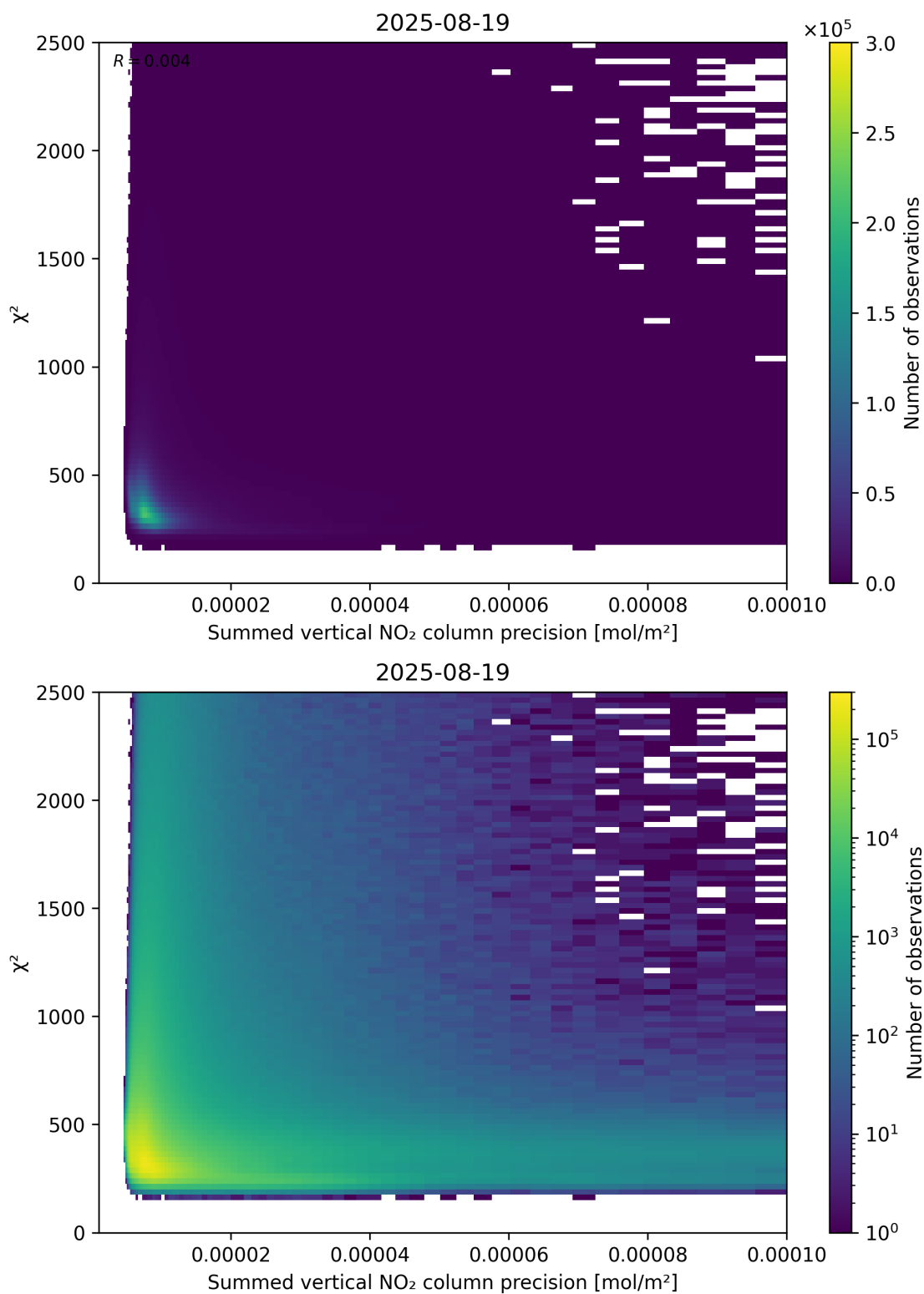
Figure 107: Scatter density plot of “Summed vertical NO 2 column precision” against “ \chi^2 ” for 2025-08-19 to 2025-08-20.
