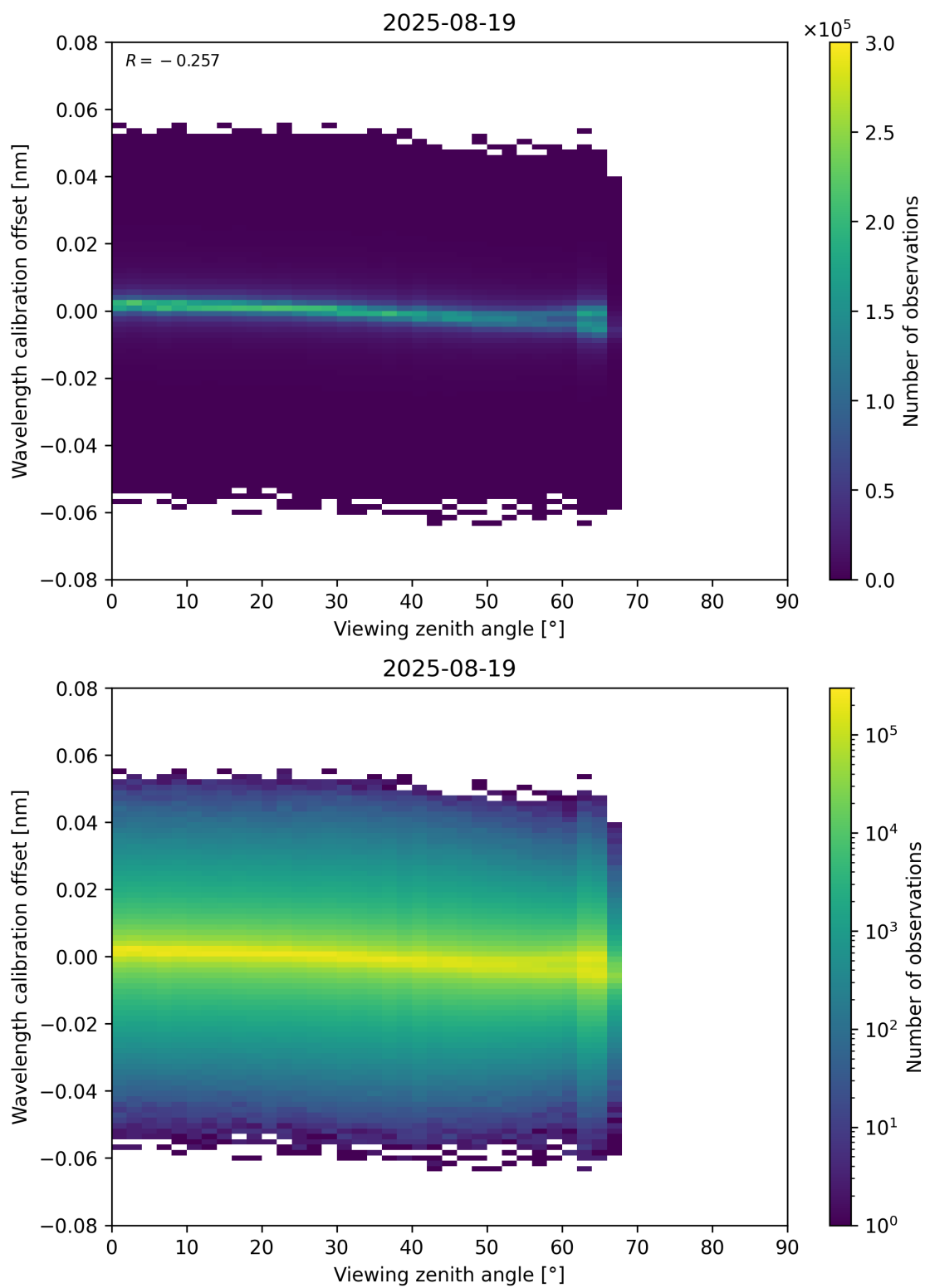
Figure 173: Scatter density plot of “Viewing zenith angle” against “Wavelength calibration offset” for 2025-08-19 to 2025-08-20.
