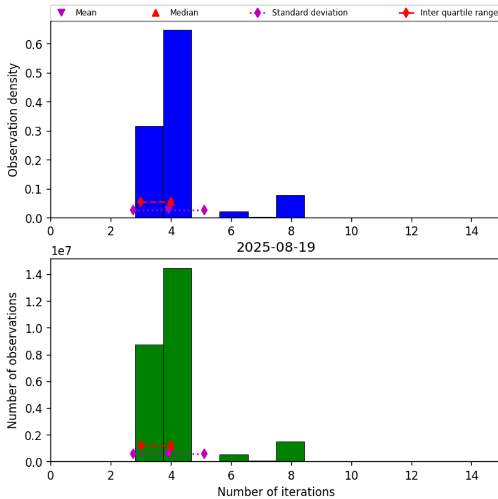
Figure 34: Histogram of “Number of iterations” for 2025-08-19 to 2025-08-20
