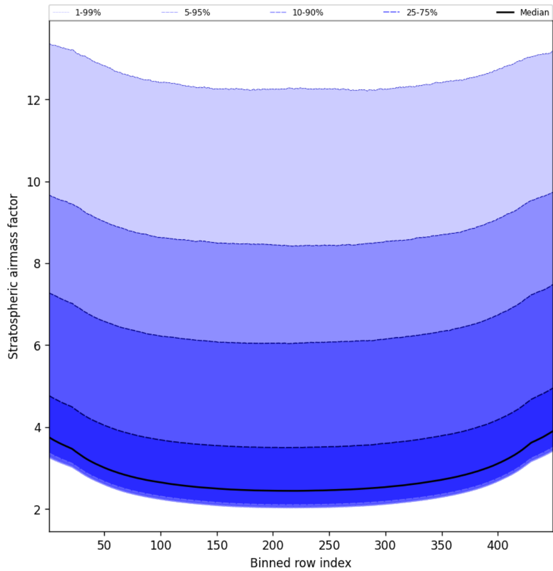
Figure 61: Along track statistics of “Stratospheric airmass factor” for 2025-08-19 to 2025-08-20
