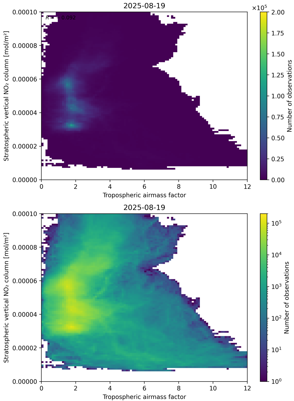
Figure 74: Scatter density plot of “Tropospheric air mass factor” against “Stratospheric vertical NO 2 column” for 2025-08-19 to 2025-08-20.
