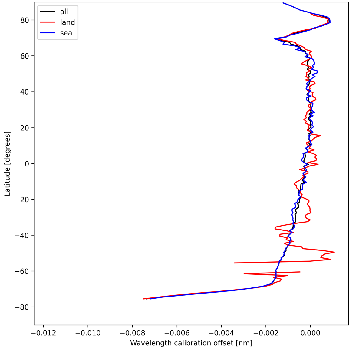
Figure 18: Zonal average of “Wavelength calibration offset” for 2025-08-19 to 2025-08-20.
