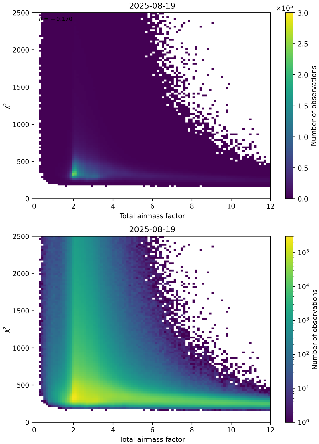
Figure 63: Scatter density plot of “Total airmass factor” against “ \chi^2 ” for 2025-08-19 to 2025-08-20.
