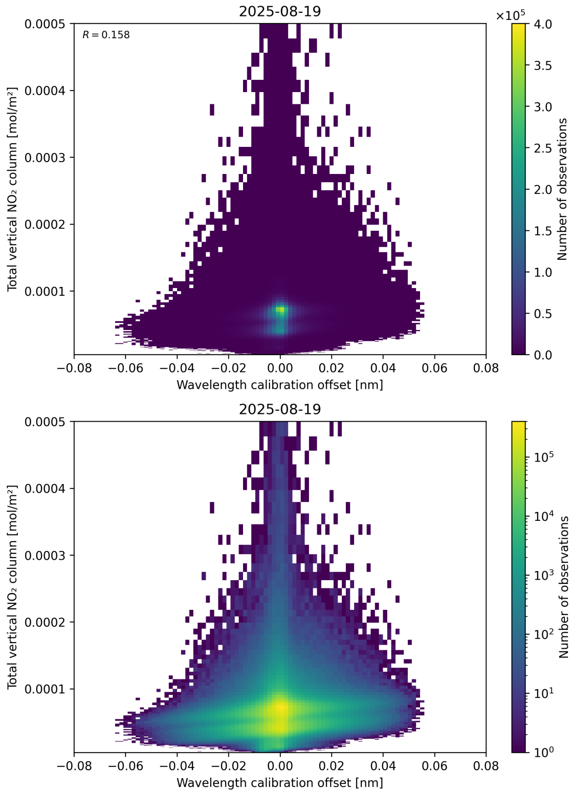
Figure 179: Scatter density plot of “Wavelength calibration offset” against “Total vertical NO 2 column” for 2025-08-19 to 2025-08-20.
