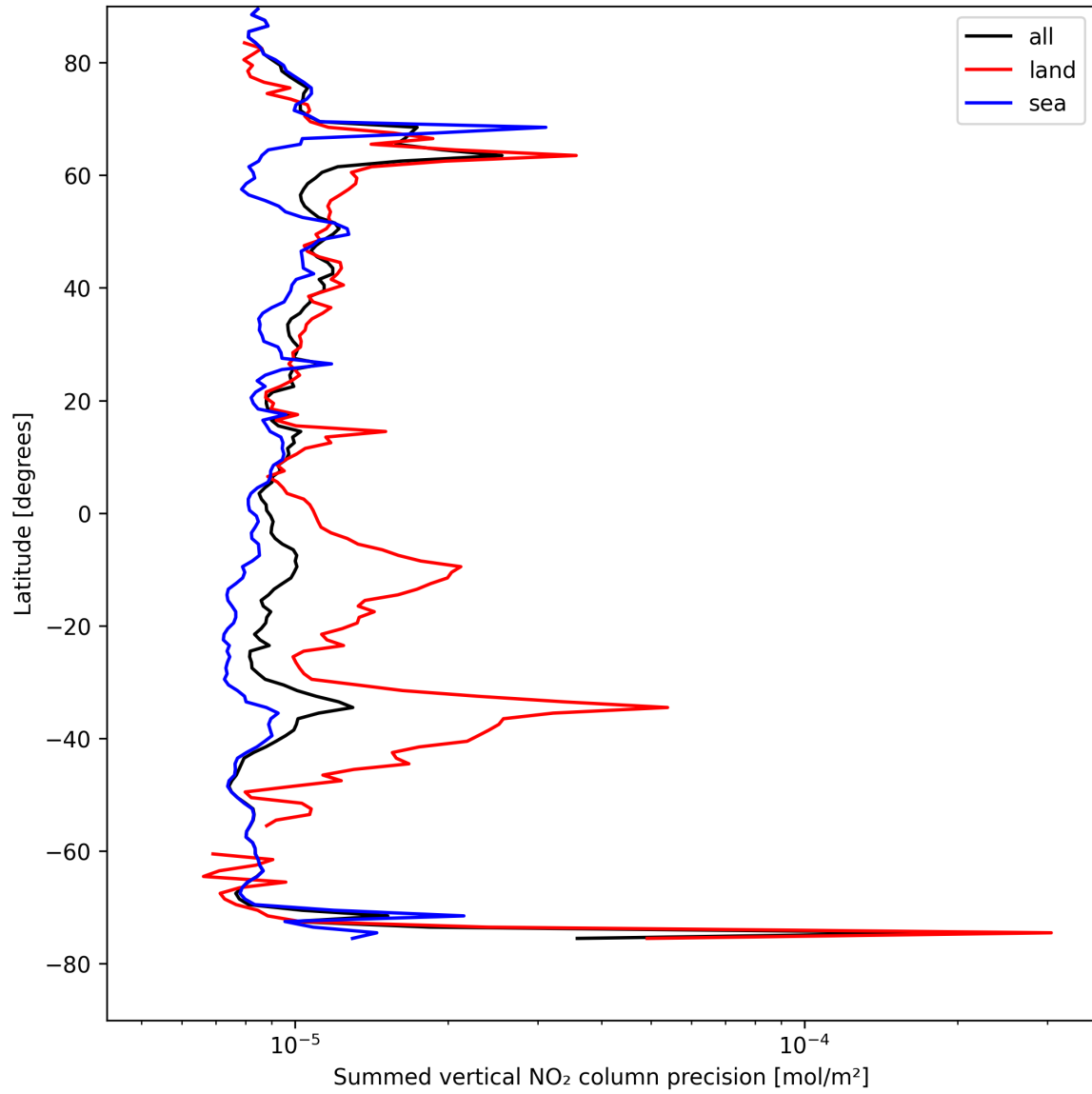
Figure 24: Zonal average of “Summed vertical NO 2 column precision” for 2025-08-19 to 2025-08-20.
