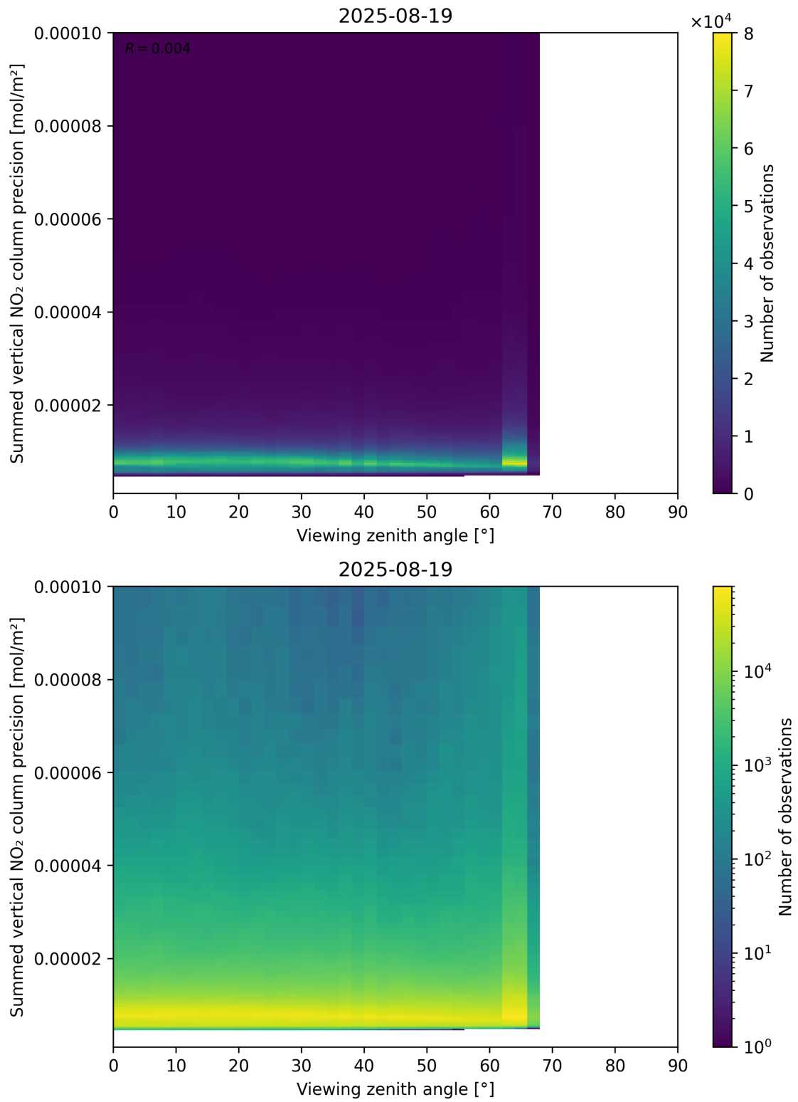
Figure 166: Scatter density plot of “Viewing zenith angle” against “Summed vertical NO 2 column precision” for 2025-08-19 to 2025-08-20.
