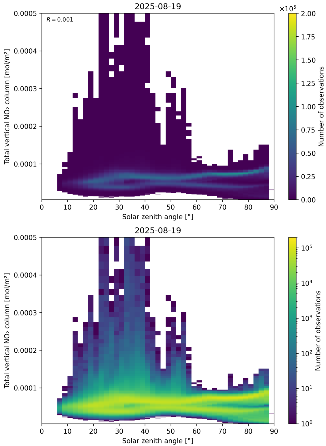
Figure 153: Scatter density plot of “Solar zenith angle” against “Total vertical NO 2 column” for 2025-08-19 to 2025-08-20.
