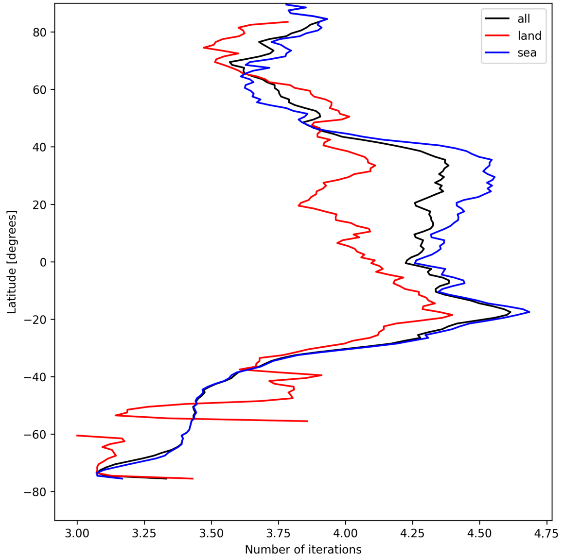
Figure 17: Zonal average of “Number of iterations” for 2025-08-19 to 2025-08-20.
