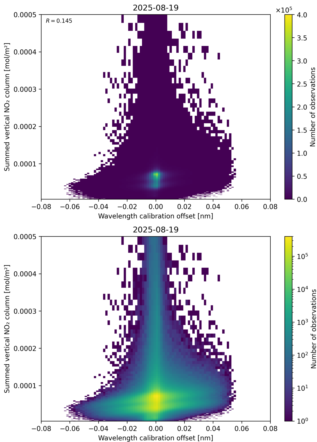
Figure 177: Scatter density plot of “Wavelength calibration offset” against “Summed vertical NO 2 column” for 2025-08-19 to 2025-08-20.
