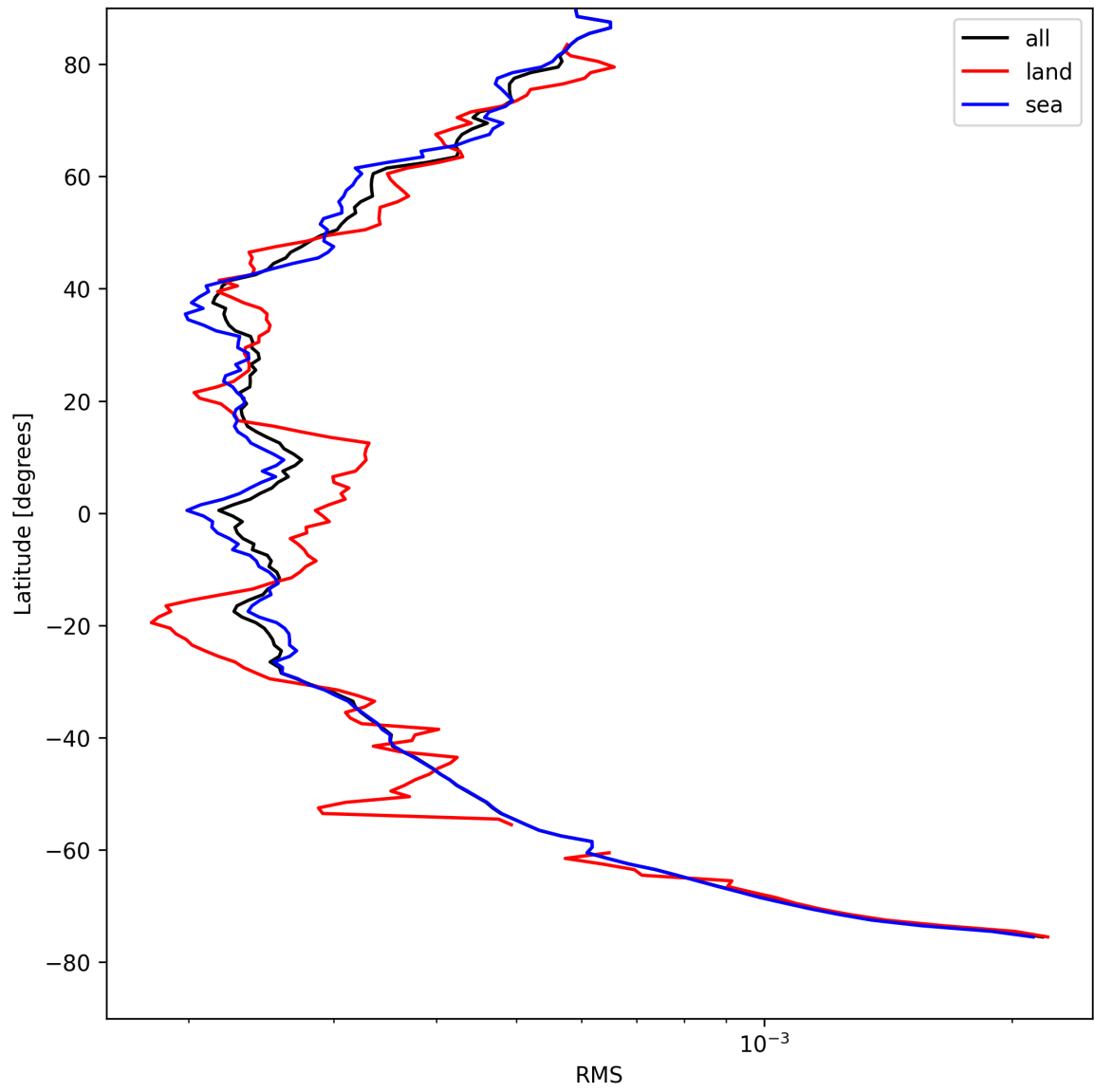
Figure 26: Zonal average of “RMS” for 2025-08-19 to 2025-08-20.
