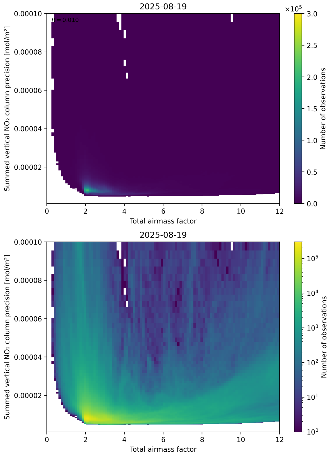
Figure 66: Scatter density plot of “Total airmass factor” against “Summed vertical NO 2 column precision” for 2025-08-19 to 2025-08-20.
