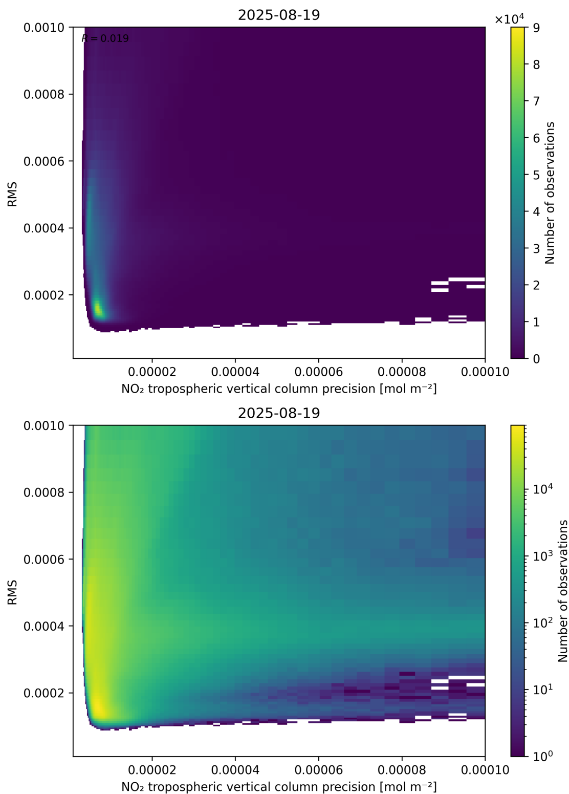
Figure 140: Scatter density plot of “NO 2 tropospheric vertical column precision” against “RMS” for 2025-08-19 to 2025-08-20.
