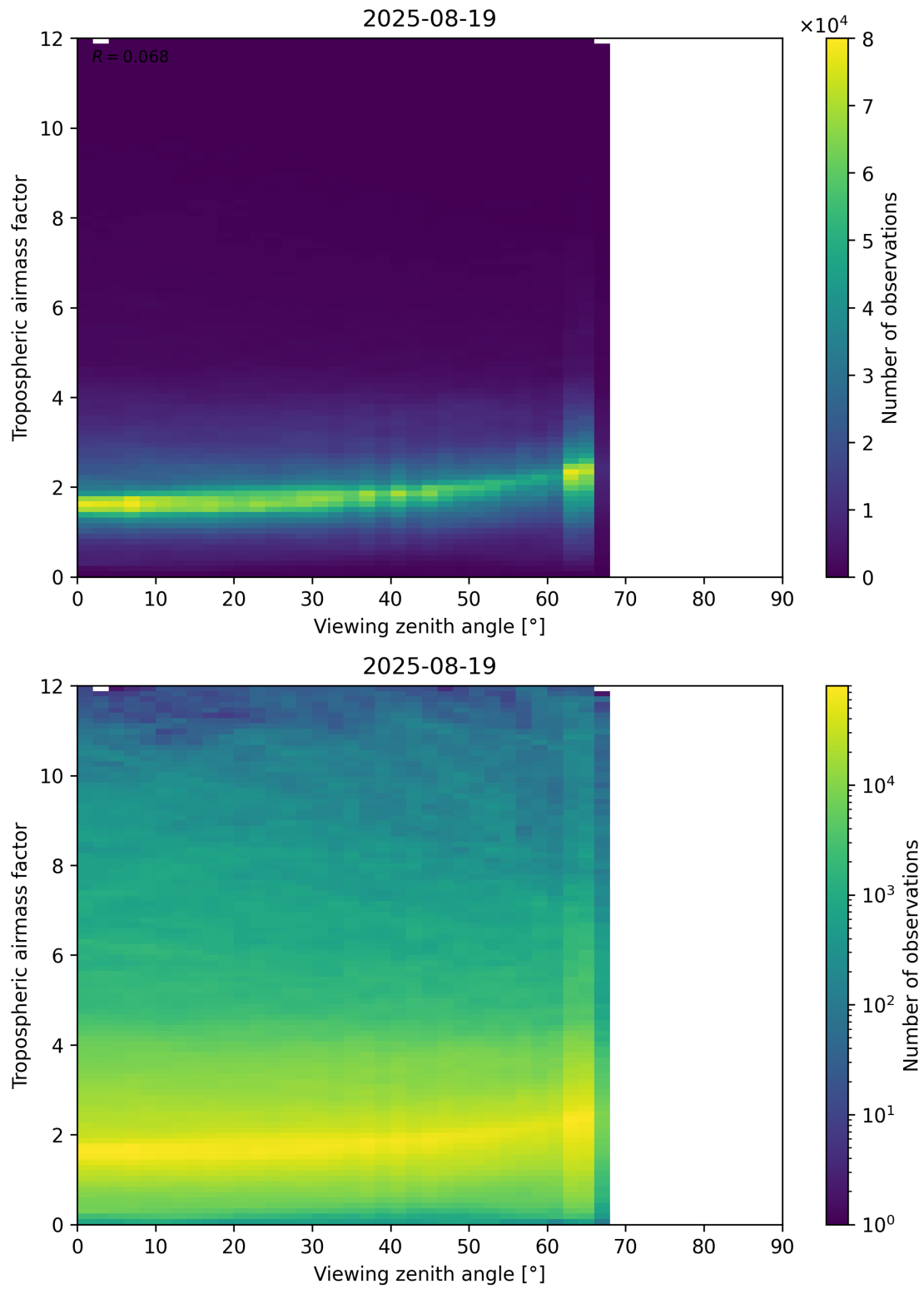
Figure 161: Scatter density plot of “Viewing zenith angle” against “Tropospheric airmass factor” for 2025-08-19 to 2025-08-20.
