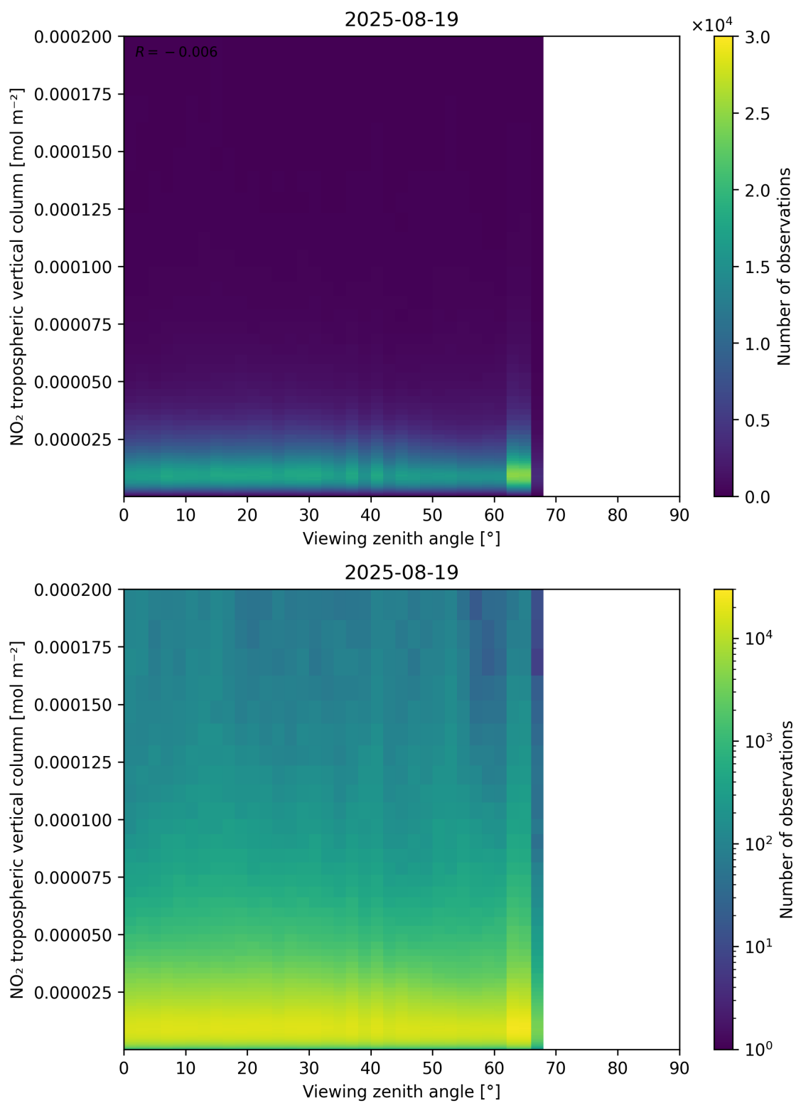
Figure 169: Scatter density plot of “Viewing zenith angle” against “NO 2 tropospheric vertical column” for 2025-08-19 to 2025-08-20.
