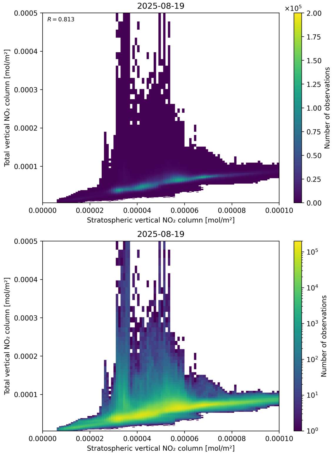
Figure 100: Scatter density plot of “Stratospheric vertical NO 2 column” against “Total vertical NO 2 column” for 2025-08-19 to 2025-08-20.
