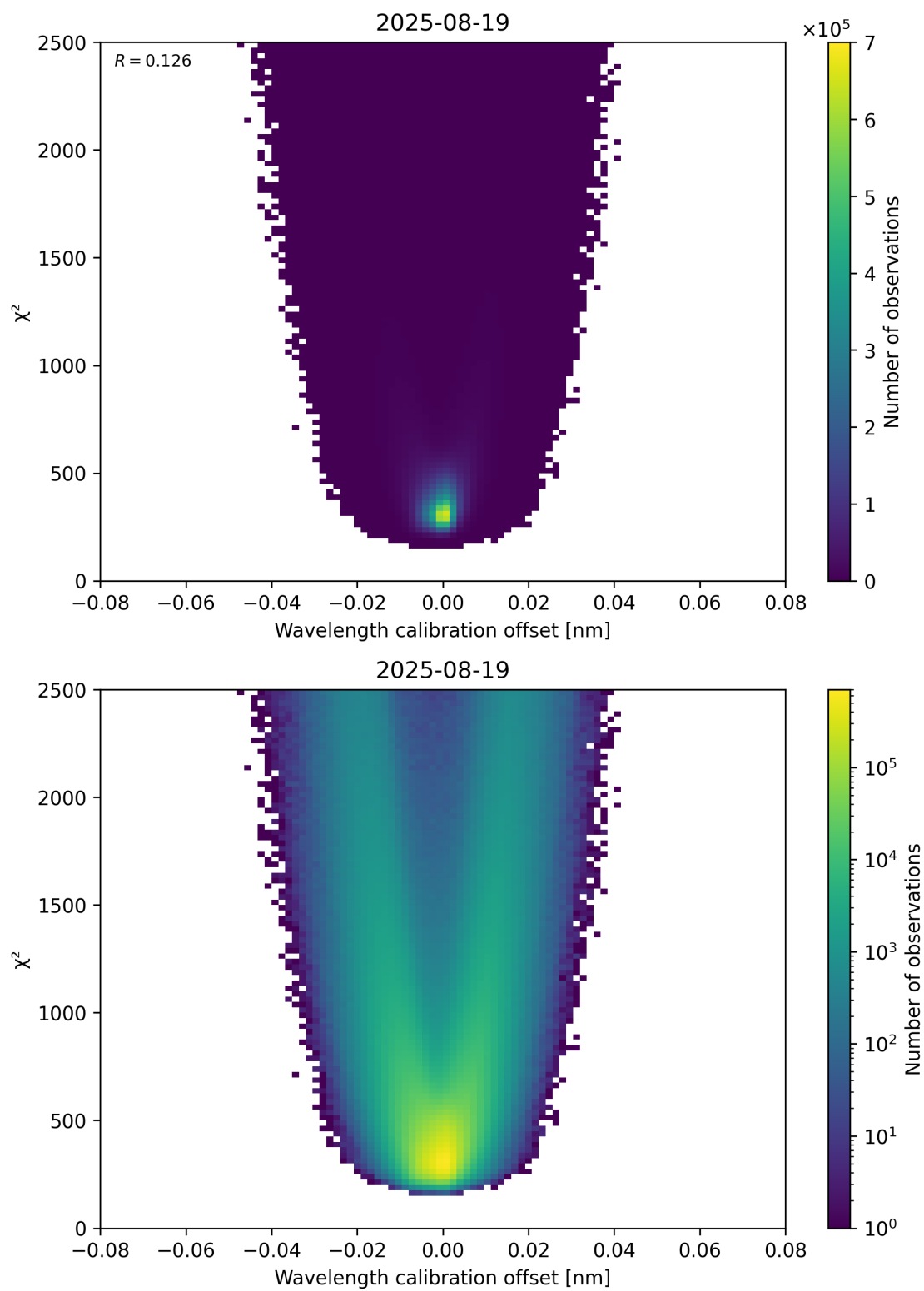
Figure 175: Scatter density plot of “Wavelength calibration offset” against “ \chi^2 ” for 2025-08-19 to 2025-08-20.
