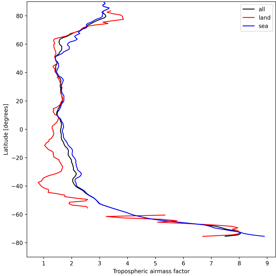
Figure 14: Zonal average of “Tropospheric air mass factor” for 2025-08-19 to 2025-08-20.
