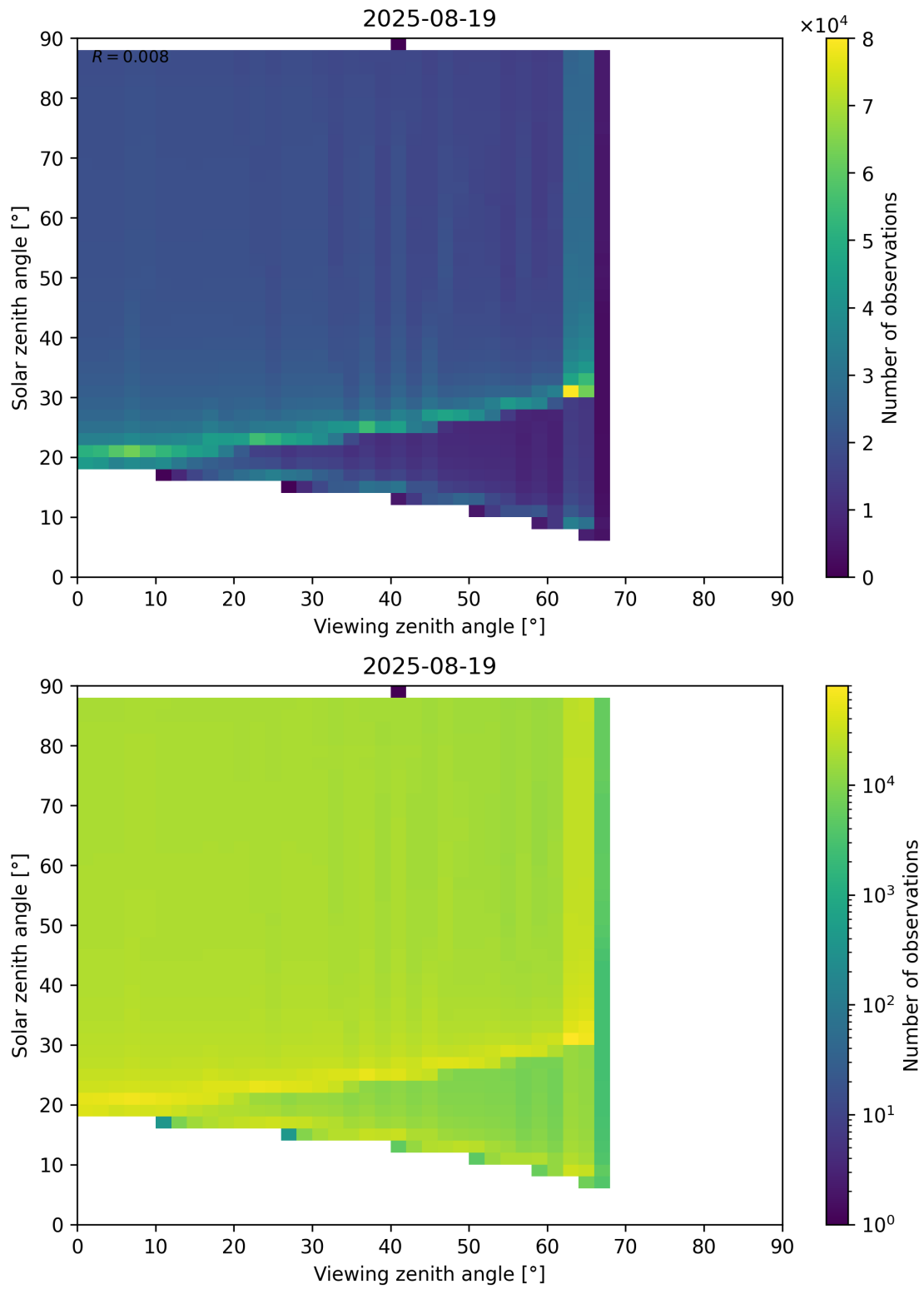
Figure 172: Scatter density plot of “Viewing zenith angle” against “Solar zenith angle” for 2025-08-19 to 2025-08-20.
