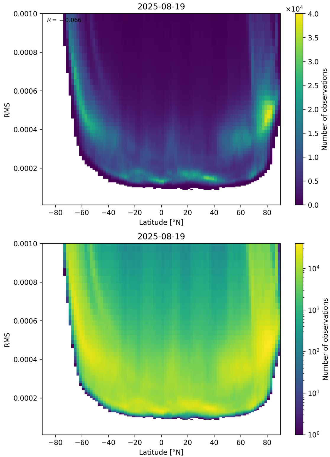
Figure 94: Scatter density plot of “Latitude” against “RMS” for 2025-08-19 to 2025-08-20.
