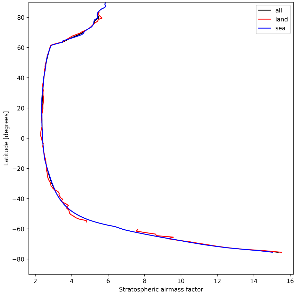
Figure 27: Zonal average of “Stratospheric airmass factor” for 2025-08-19 to 2025-08-20.
