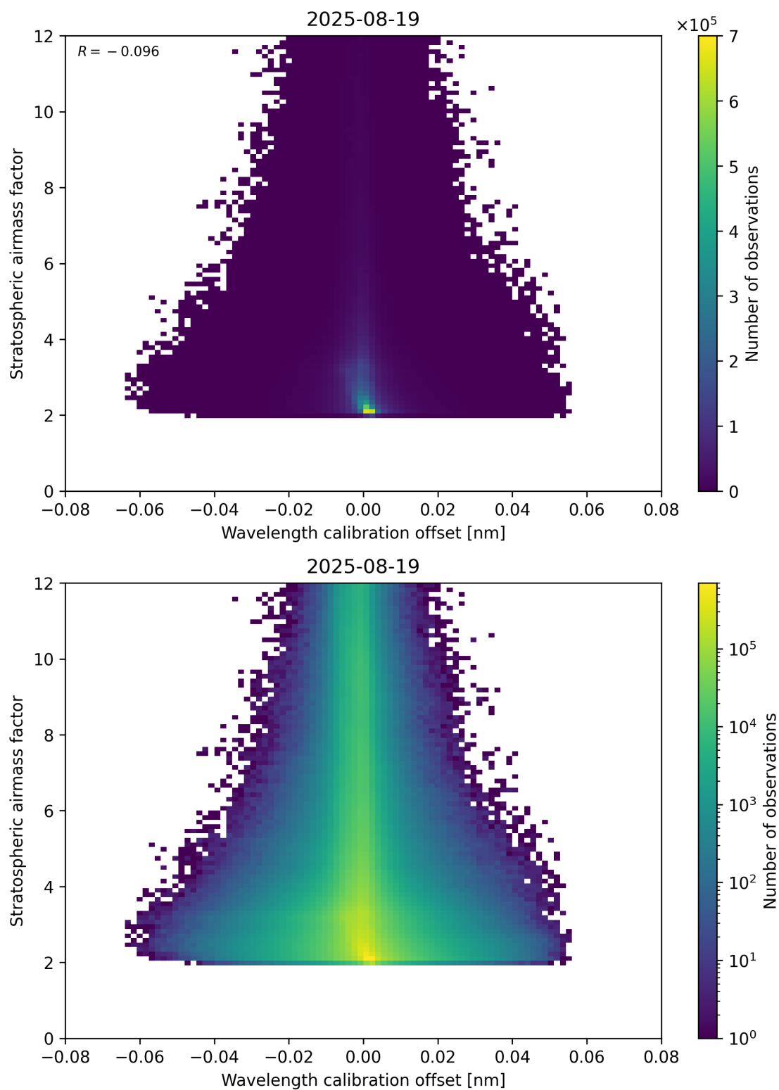
Figure 174: Scatter density plot of “Wavelength calibration offset” against “Stratospheric air mass factor” for 2025-08-19 to 2025-08-20.
