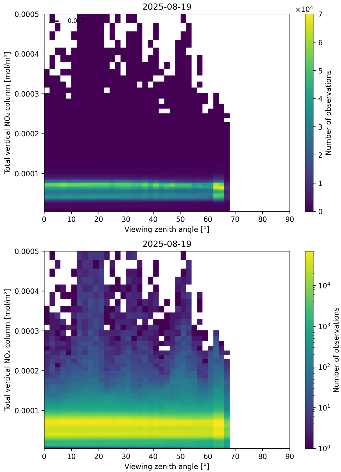
Figure 167: Scatter density plot of “Viewing zenith angle” against “Total vertical NO 2 column” for 2025-08-19 to 2025-08-20.
