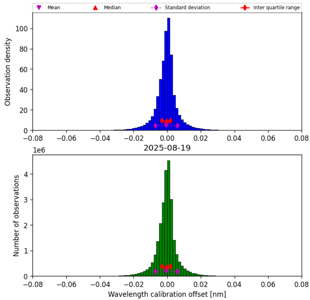
Figure 35: Histogram of “Wavelength calibration offset” for 2025-08-19 to 2025-08-20
