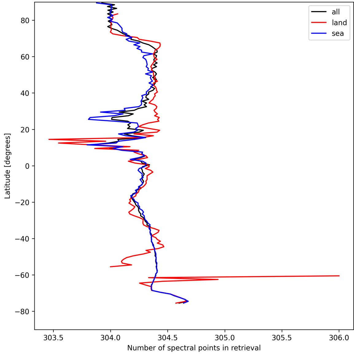
Figure 16: Zonal average of “Number of spectral points in retrieval” for 2025-08-19 to 2025-08-20.
