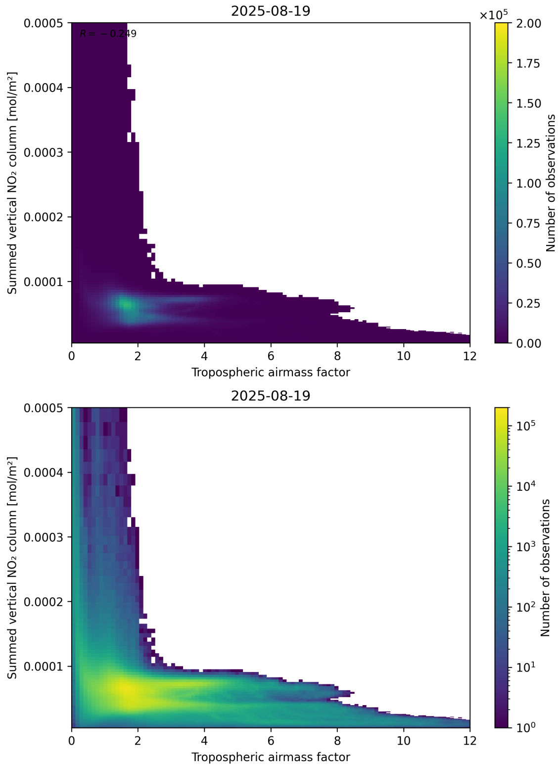
Figure 75: Scatter density plot of “Tropospheric air mass factor” against “Summed vertical NO 2 column” for 2025-08-19 to 2025-08-20.
