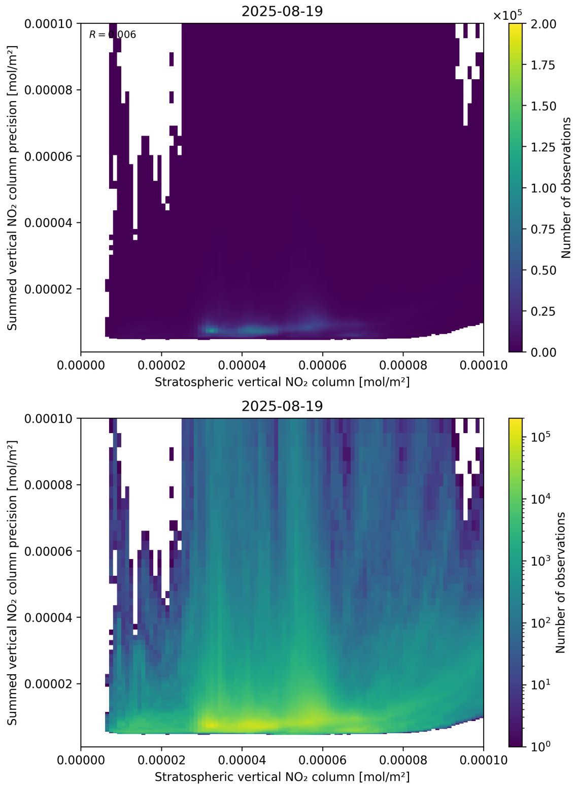
Figure 99: Scatter density plot of “Stratospheric vertical NO 2 column” against “Summed vertical NO 2 column precision” for 2025-08-19 to 2025-08-20.
