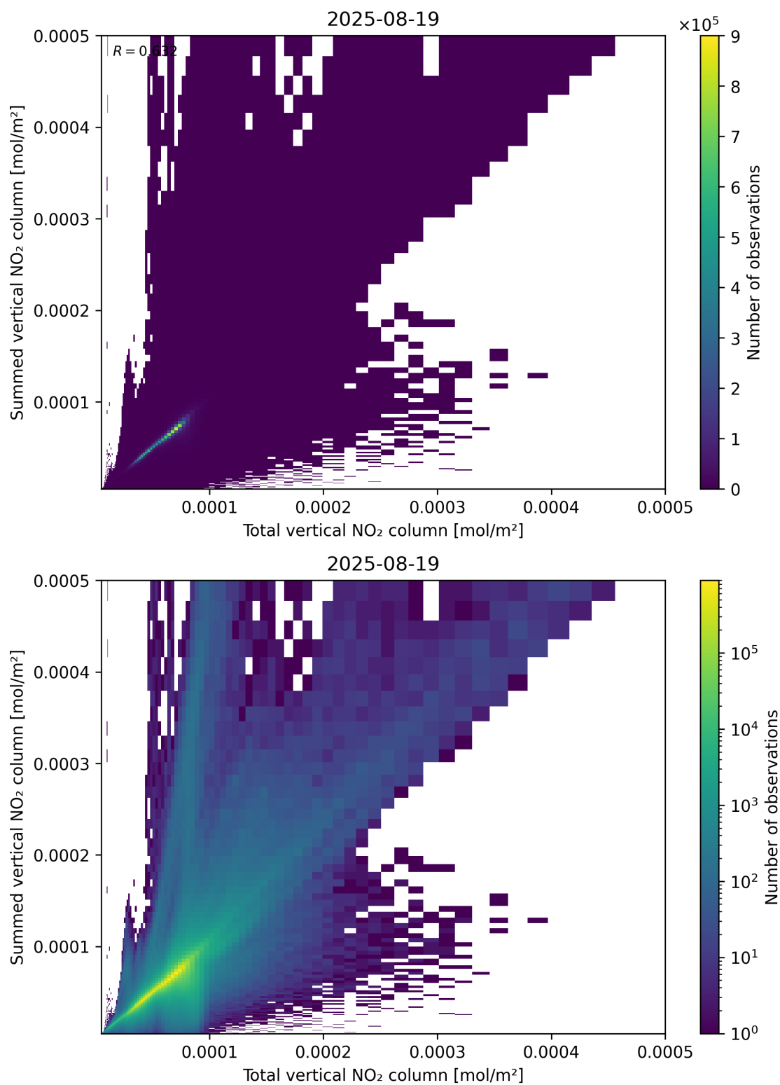
Figure 112: Scatter density plot of “Total vertical NO 2 column” against “Summed vertical NO 2 column” for 2025-08-19 to 2025-08-20.
