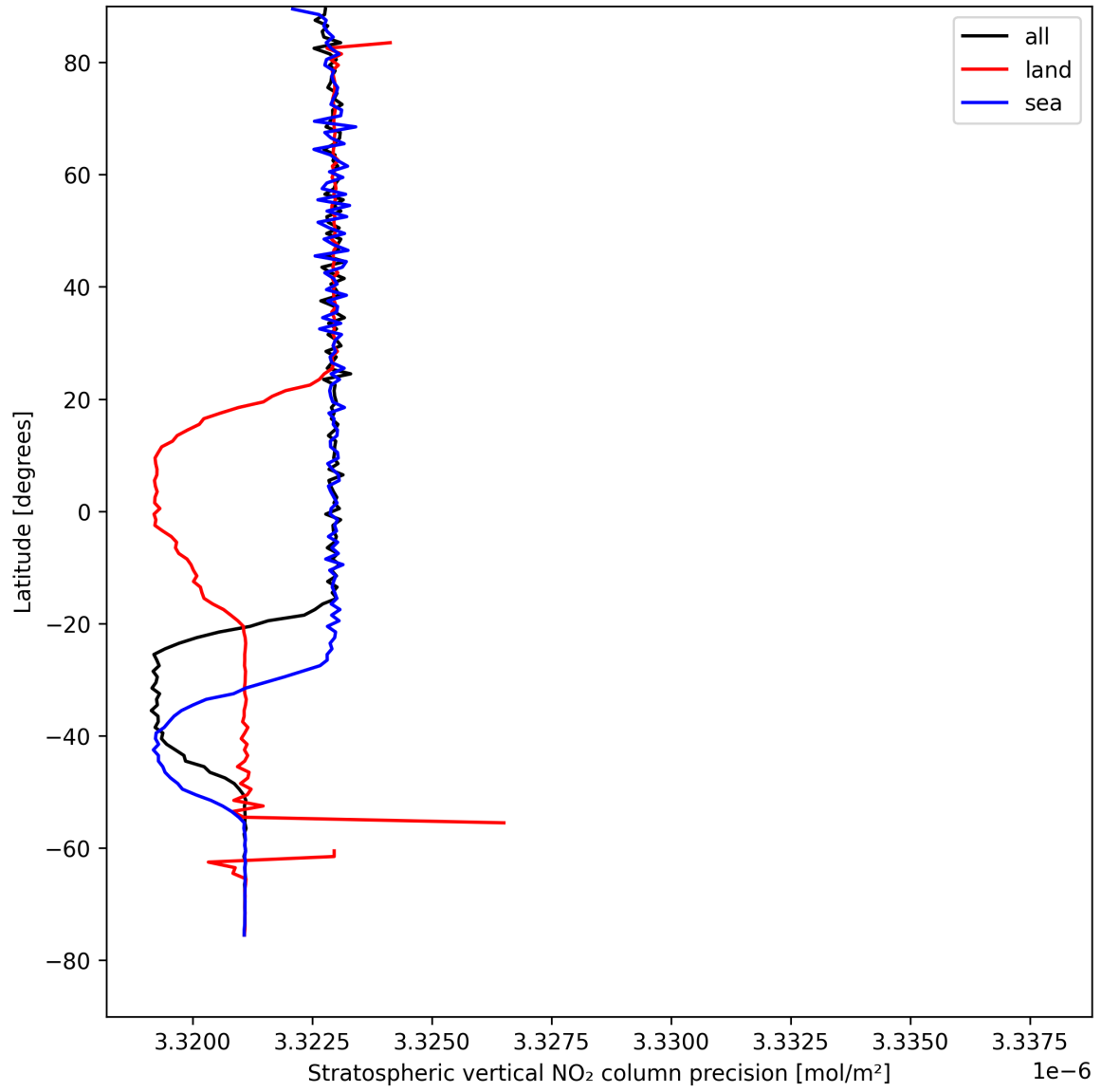
Figure 20: Zonal average of “Stratospheric vertical NO 2 column precision” for 2025-08-19 to 2025-08-20.
