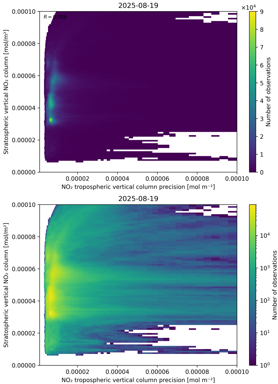
Figure 135: Scatter density plot of “NO 2 tropospheric vertical column precision” against “Stratospheric vertical NO 2 column” for 2025-08-19 to 2025-08-20.
