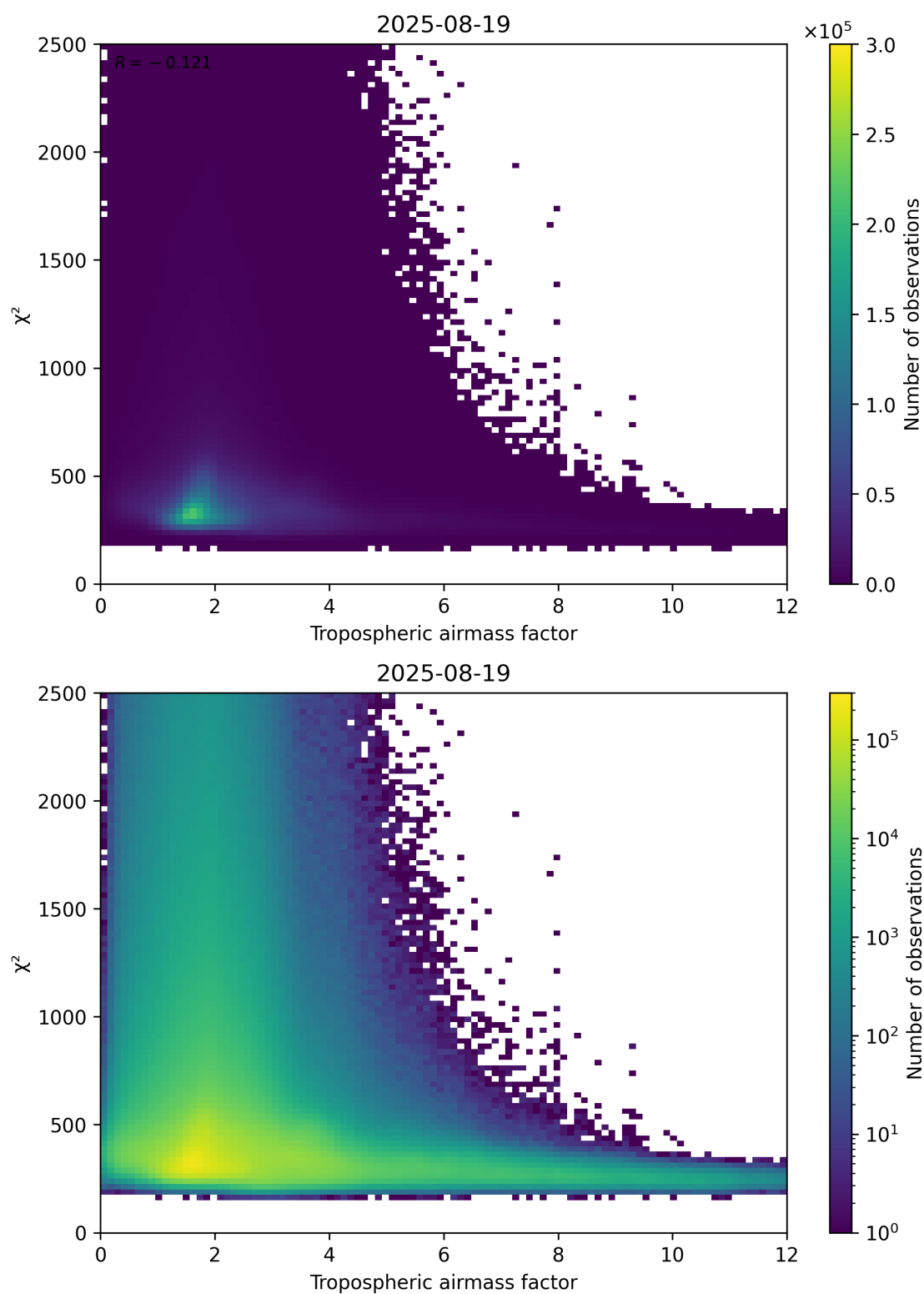
Figure 73: Scatter density plot of “Tropospheric airmass factor” against “ \chi^2 ” for 2025-08-19 to 2025-08-20.
