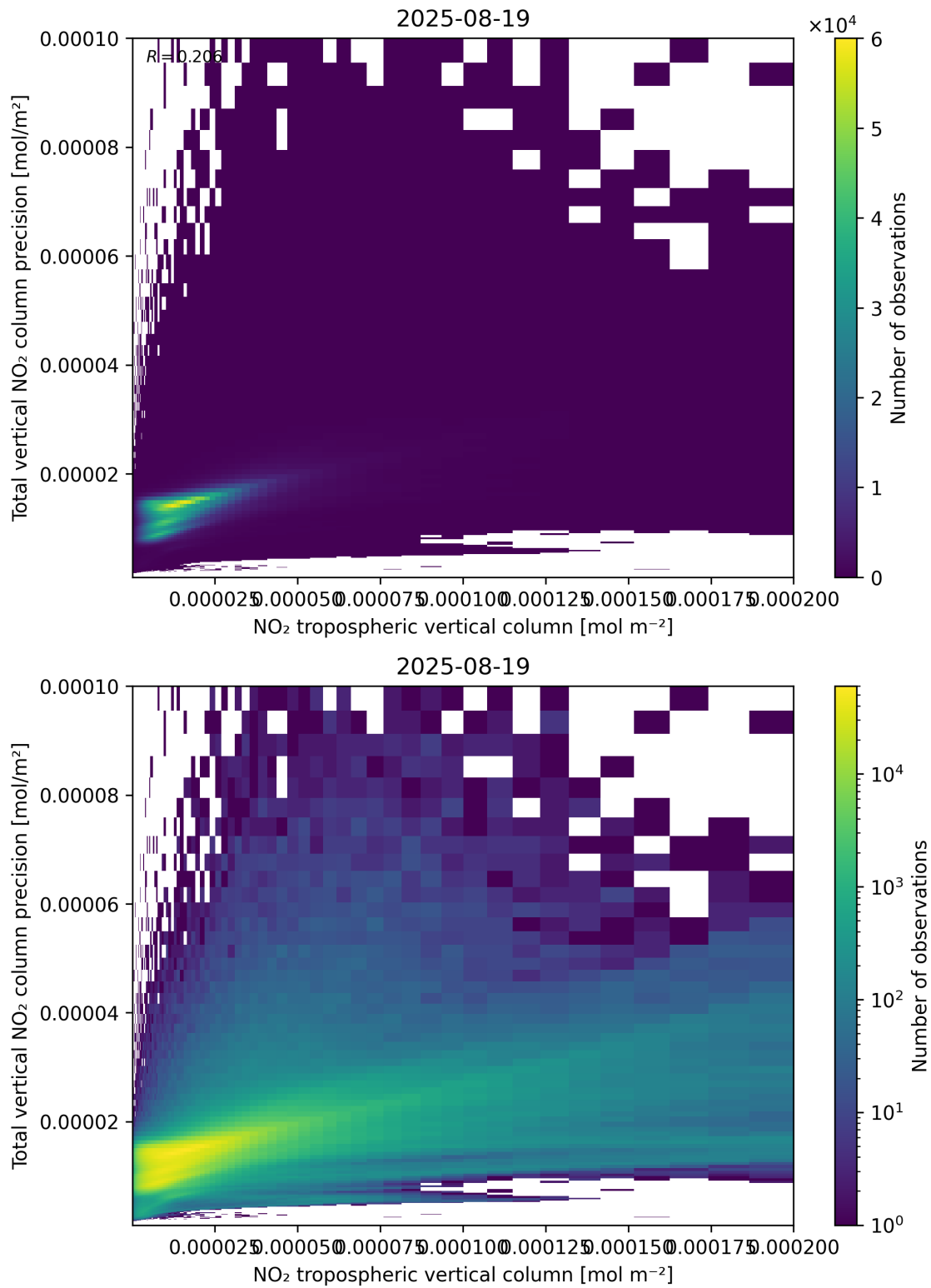
Figure 129: Scatter density plot of “NO 2 tropospheric vertical column” against “Total vertical NO 2 column precision” for 2025-08-19 to 2025-08-20.
