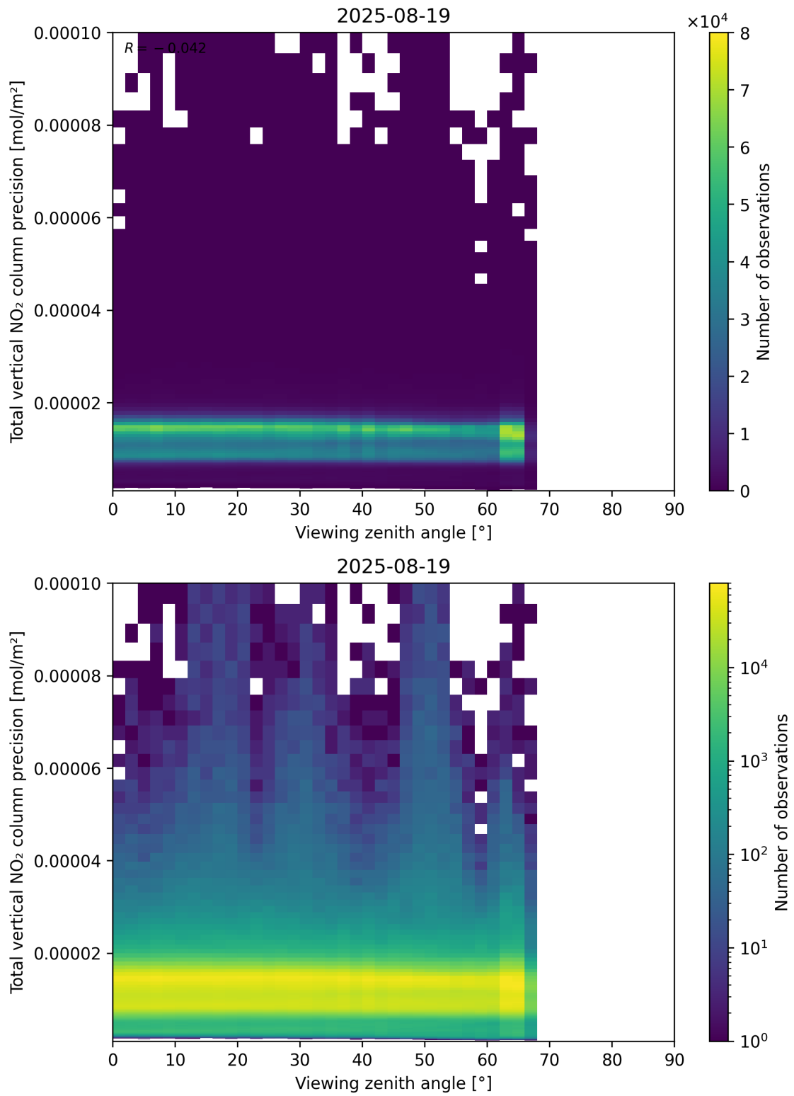
Figure 168: Scatter density plot of “Viewing zenith angle” against “Total vertical NO 2 column precision” for 2025-08-19 to 2025-08-20.
