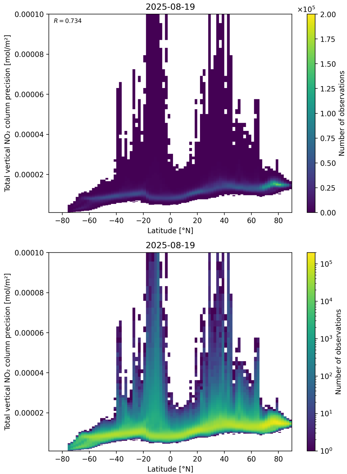
Figure 91: Scatter density plot of “Latitude” against “Total vertical NO 2 column precision” for 2025-08-19 to 2025-08-20.
