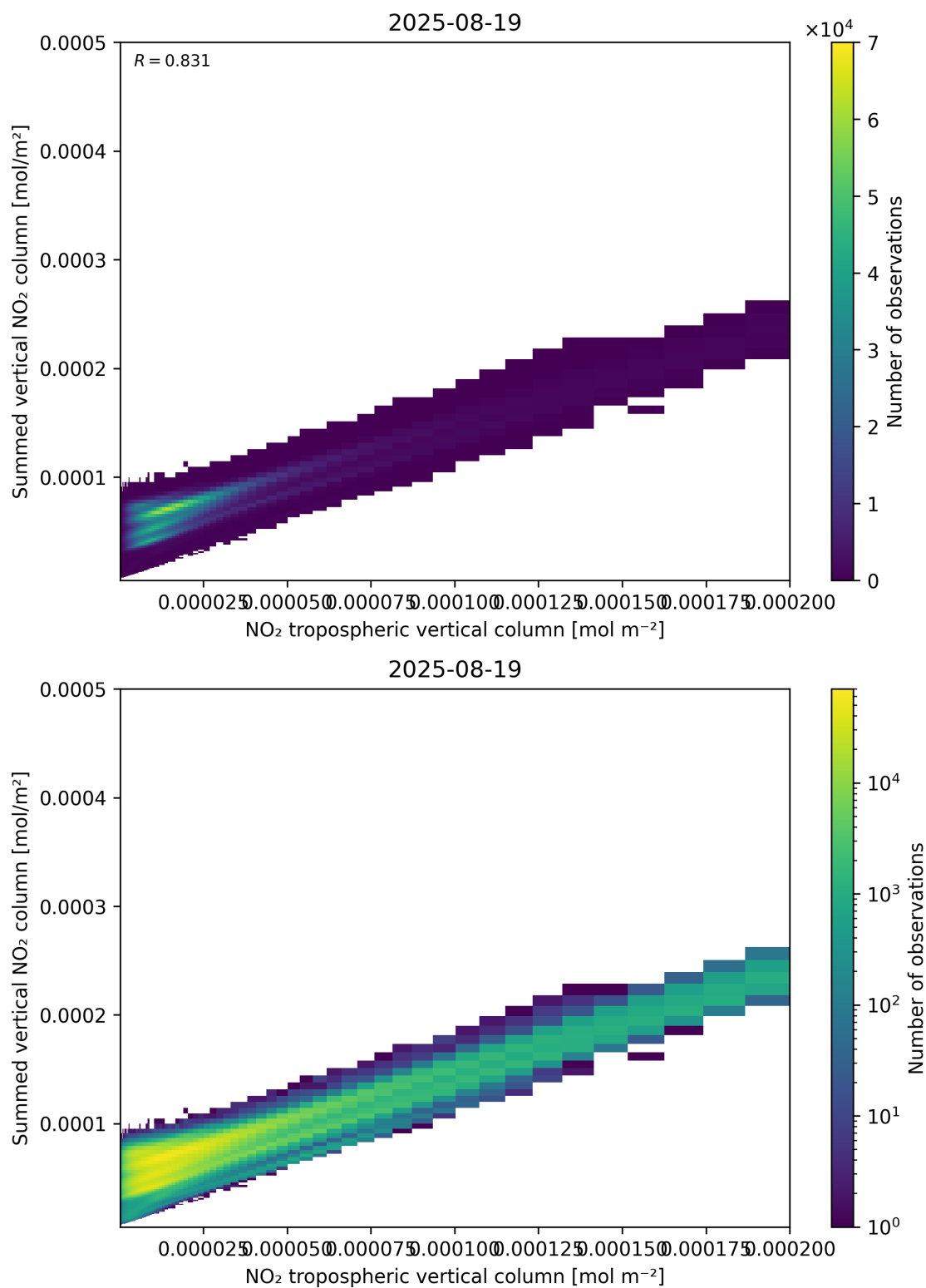
Figure 126: Scatter density plot of “NO 2 tropospheric vertical column” against “Summed vertical NO 2 column” for 2025-08-19 to 2025-08-20.
