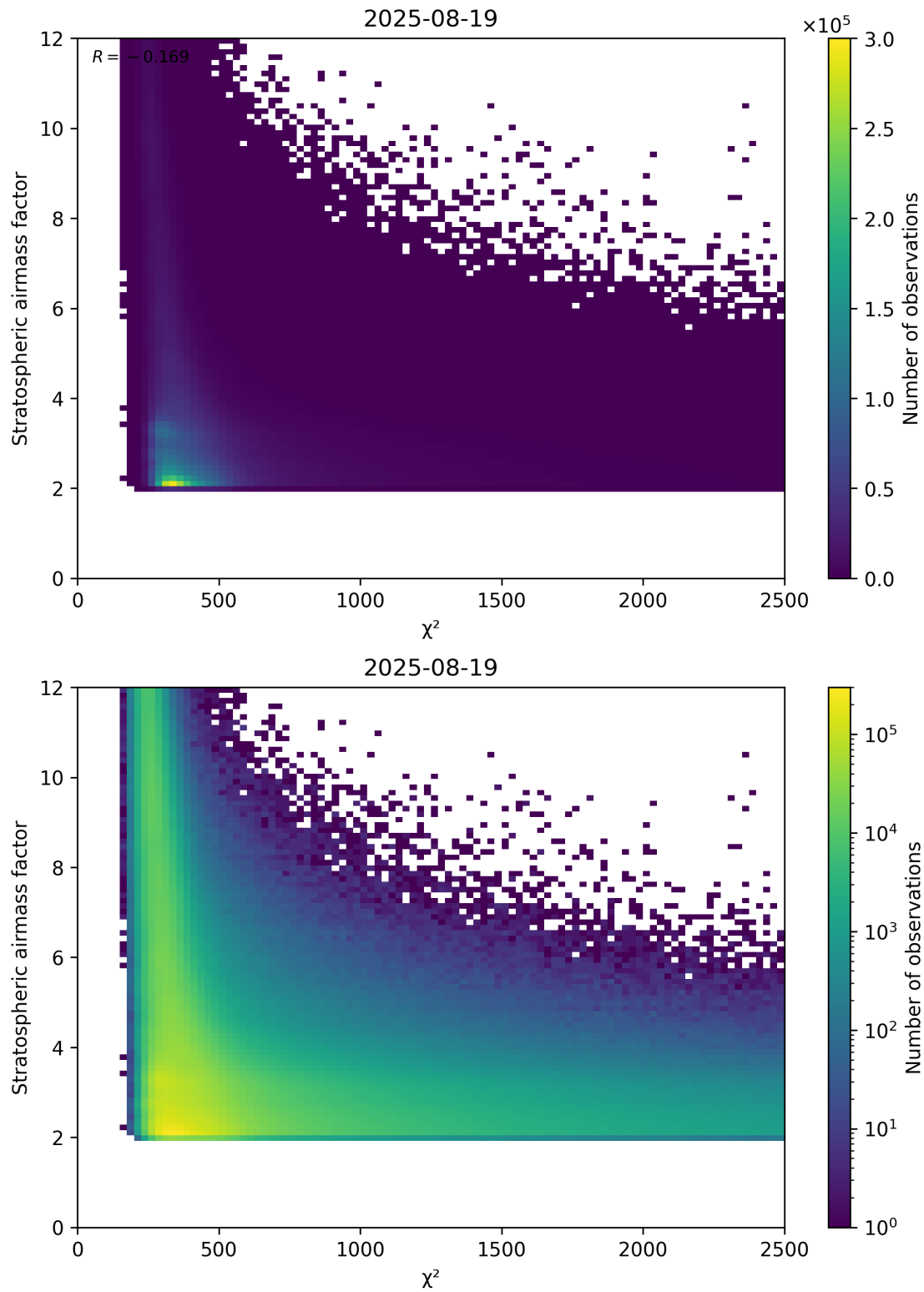
Figure 81: Scatter density plot of “ \chi^2 ” against “Stratospheric airmass factor” for 2025-08-19 to 2025-08-20.
