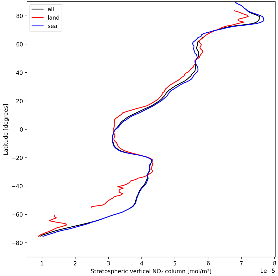
Figure 19: Zonal average of “Stratospheric vertical NO 2 column” for 2025-08-19 to 2025-08-20.
