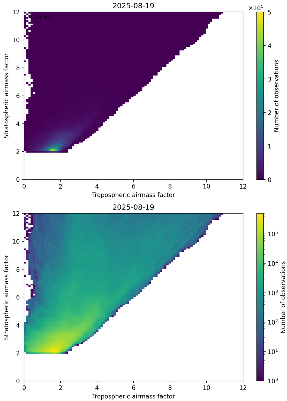
Figure 71: Scatter density plot of “Tropospheric airmass factor” against “Stratospheric airmass factor” for 2025-08-19 to 2025-08-20.
