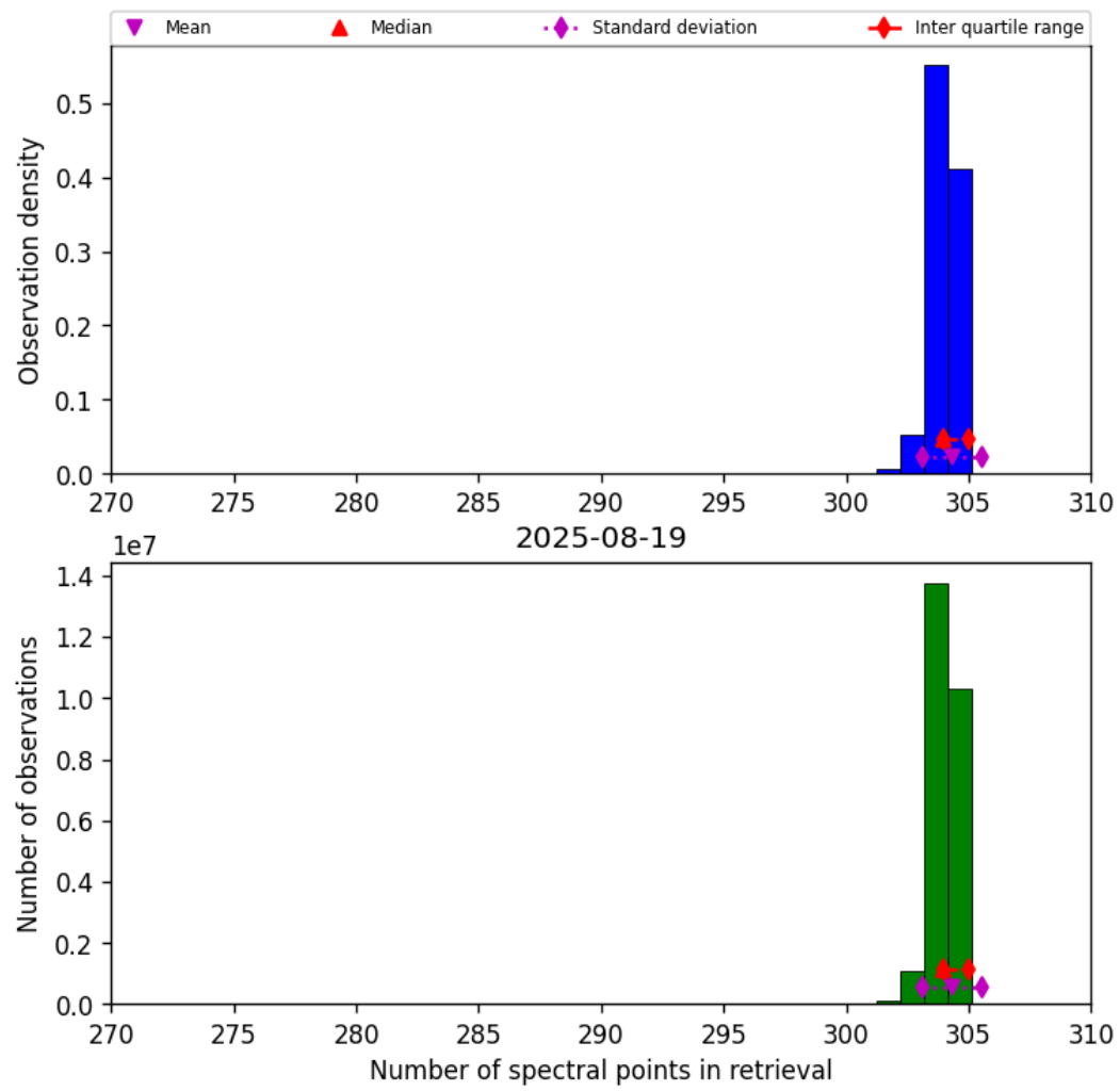
Figure 33: Histogram of “Number of spectral points in retrieval” for 2025-08-19 to 2025-08-20
