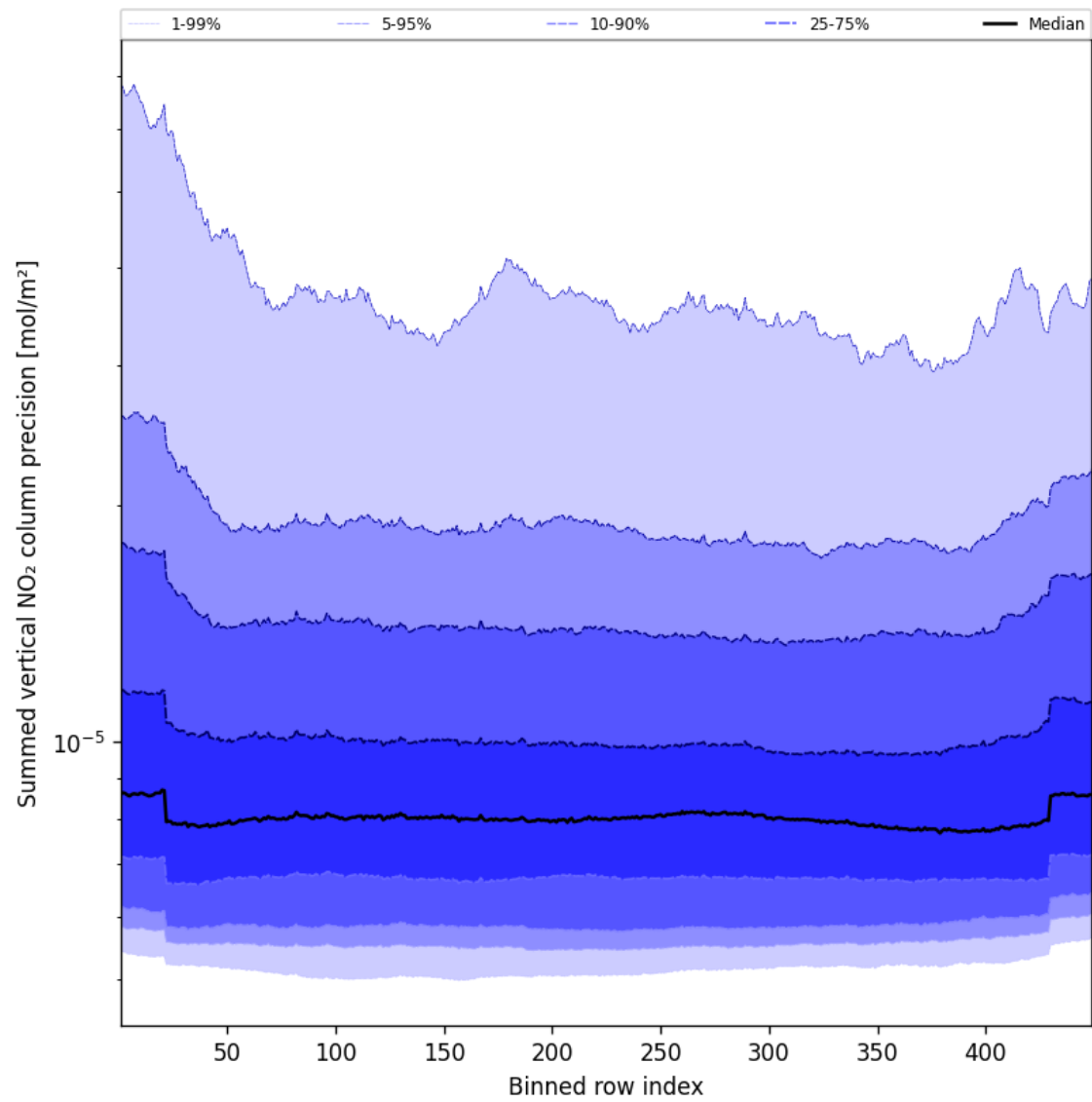
Figure 58: Along track statistics of “Summed vertical NO 2 column precision” for 2025-08-19 to 2025-08-20
