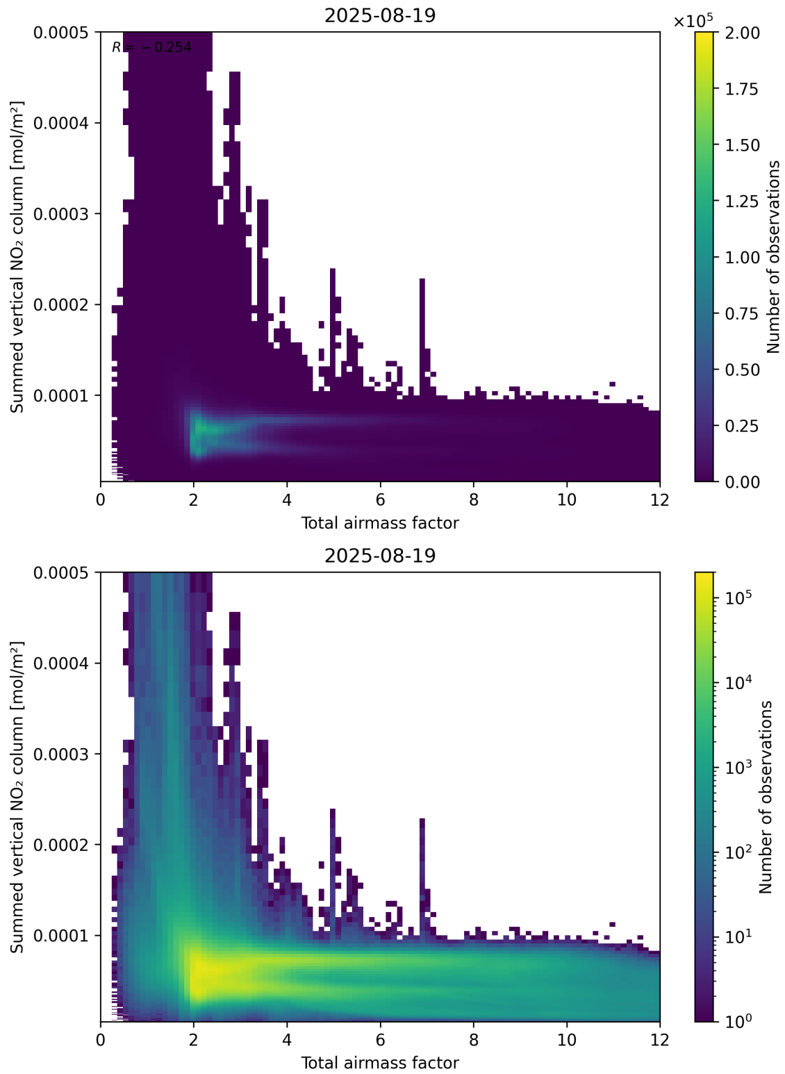
Figure 65: Scatter density plot of “Total airmass factor” against “Summed vertical NO 2 column” for 2025-08-19 to 2025-08-20.
