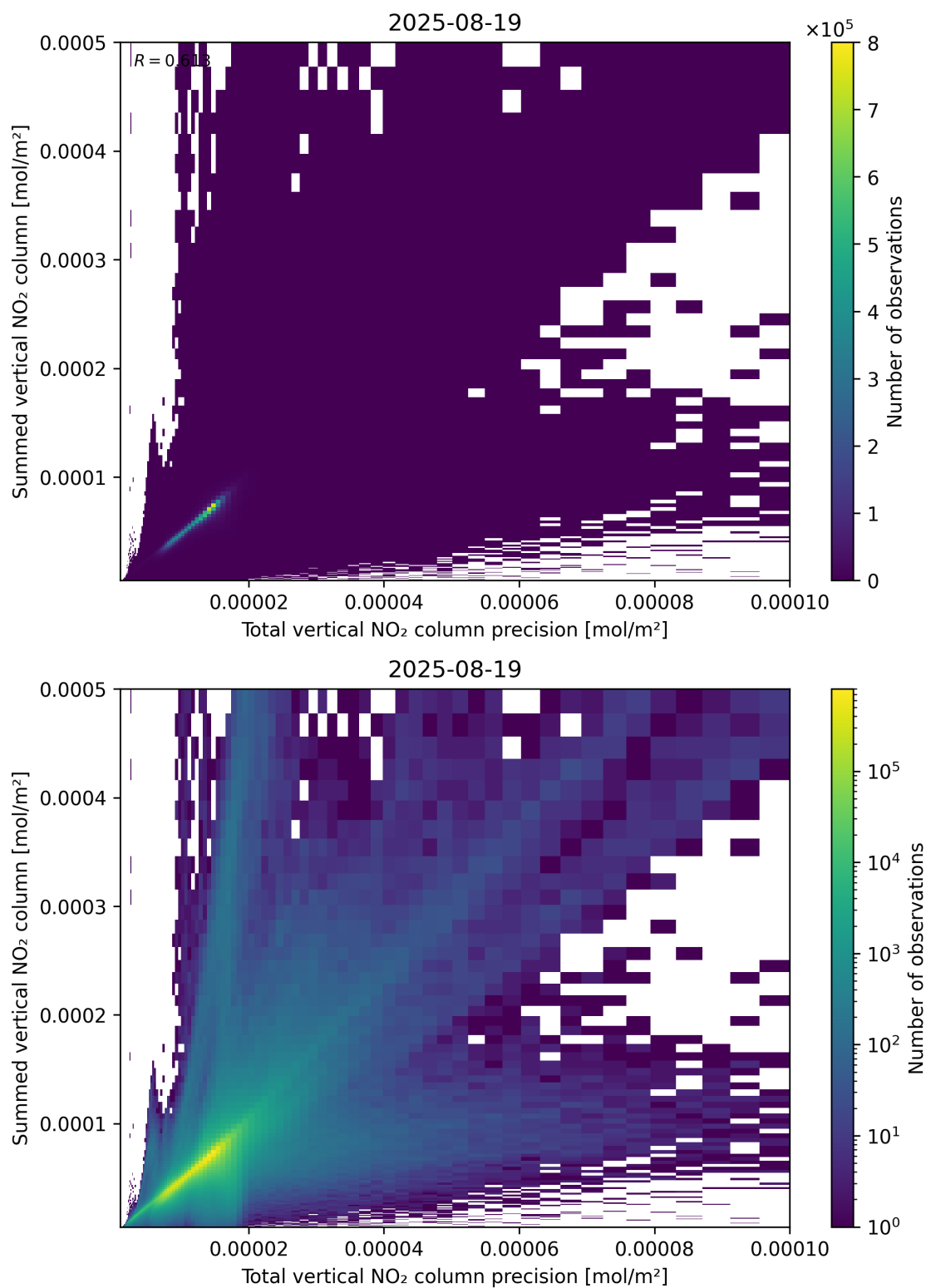
Figure 117: Scatter density plot of “Total vertical NO 2 column precision” against “Summed vertical NO 2 column” for 2025-08-19 to 2025-08-20.
