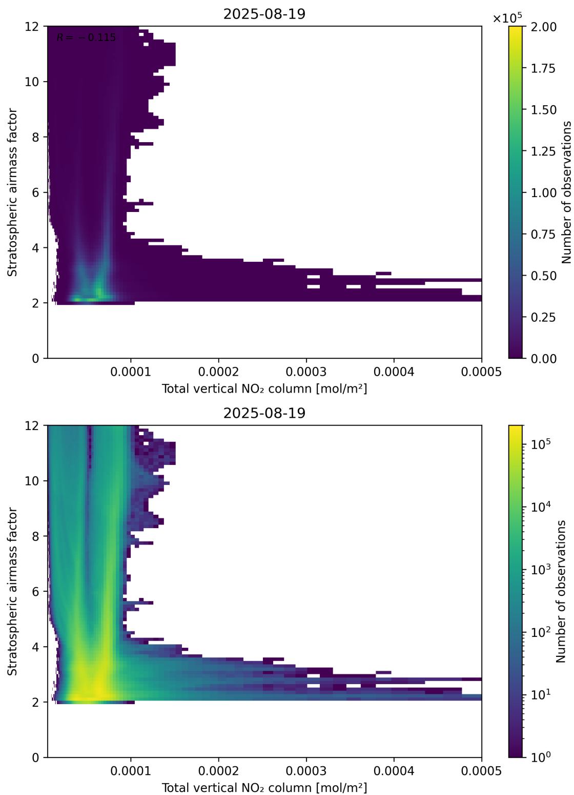
Figure 110: Scatter density plot of “Total vertical NO 2 column” against “Stratospheric airmass factor” for 2025-08-19 to 2025-08-20.
