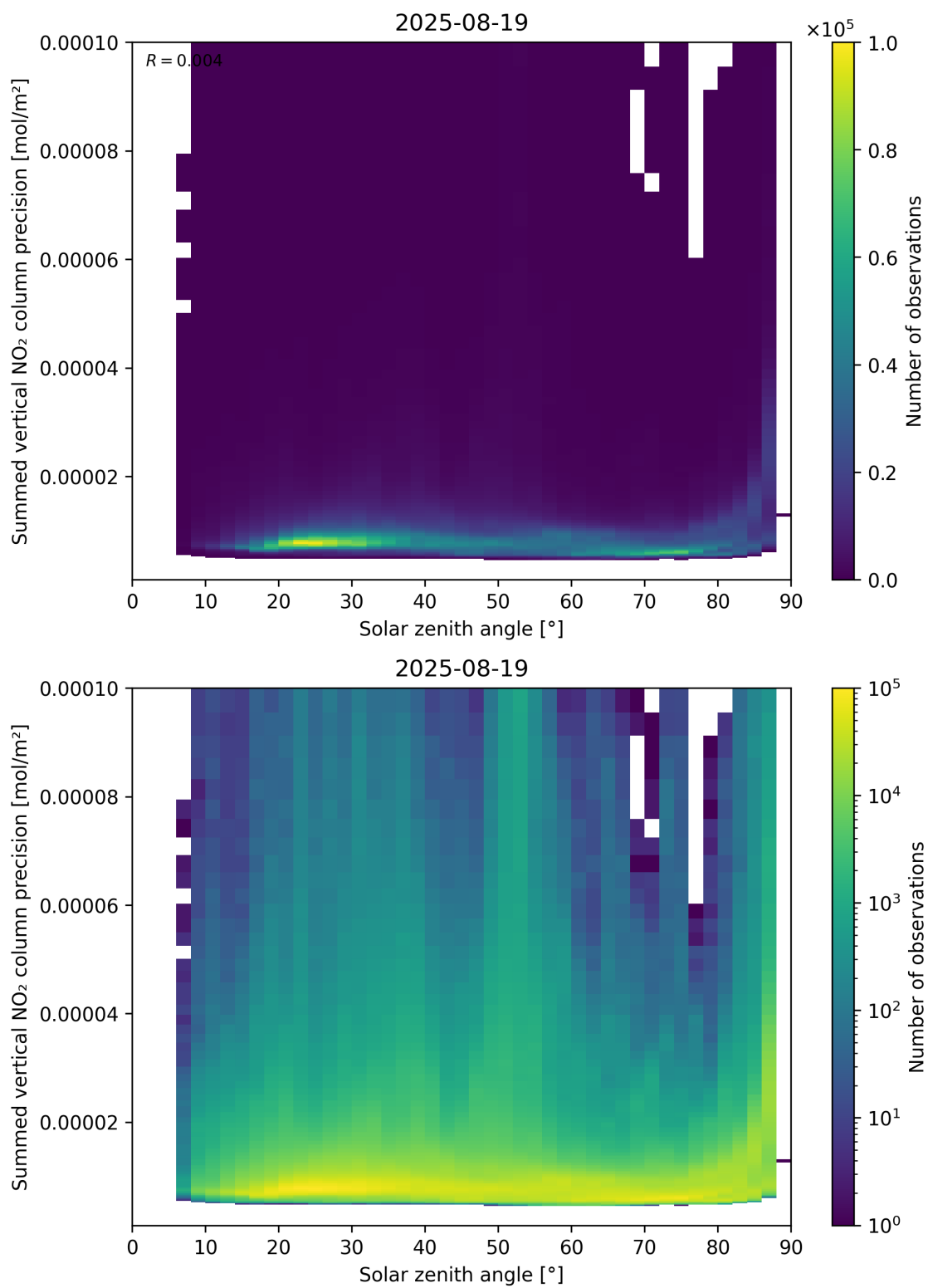
Figure 152: Scatter density plot of “Solar zenith angle” against “Summed vertical NO 2 column precision” for 2025-08-19 to 2025-08-20.
