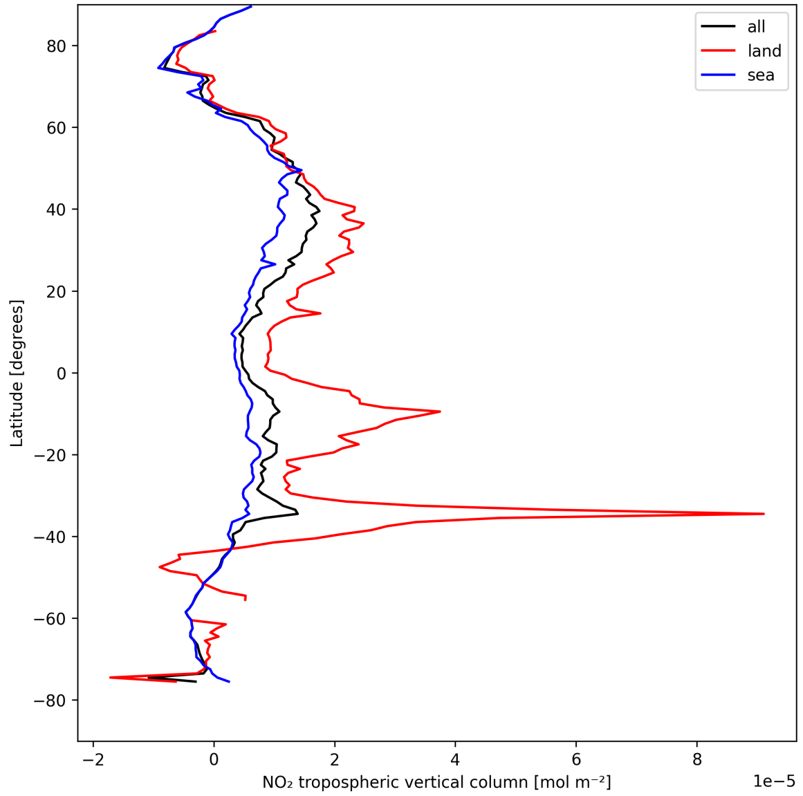
Figure 12: Zonal average of “NO 2 tropospheric vertical column” for 2025-08-19 to 2025-08-20.
