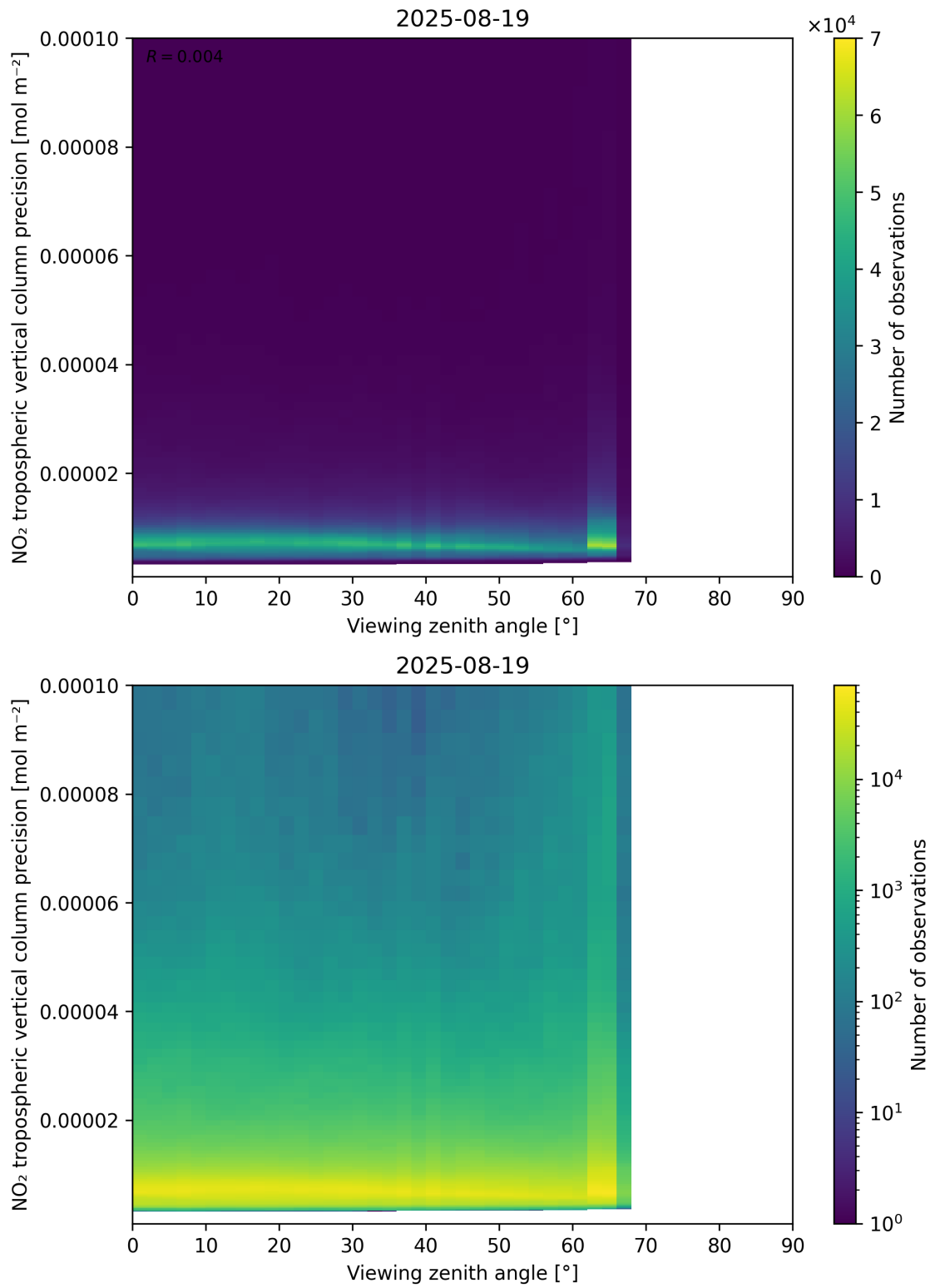
Figure 170: Scatter density plot of “Viewing zenith angle” against “NO 2 tropospheric vertical column precision” for 2025-08-19 to 2025-08-20.
