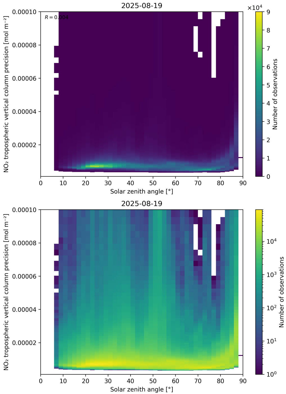
Figure 156: Scatter density plot of “Solar zenith angle” against “NO 2 tropospheric vertical column precision” for 2025-08-19 to 2025-08-20.
