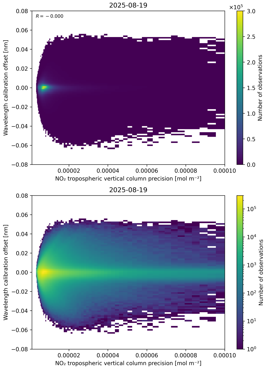
Figure 141: Scatter density plot of “NO 2 tropospheric vertical column precision” against “Wavelength calibration offset” for 2025-08-19 to 2025-08-20.
