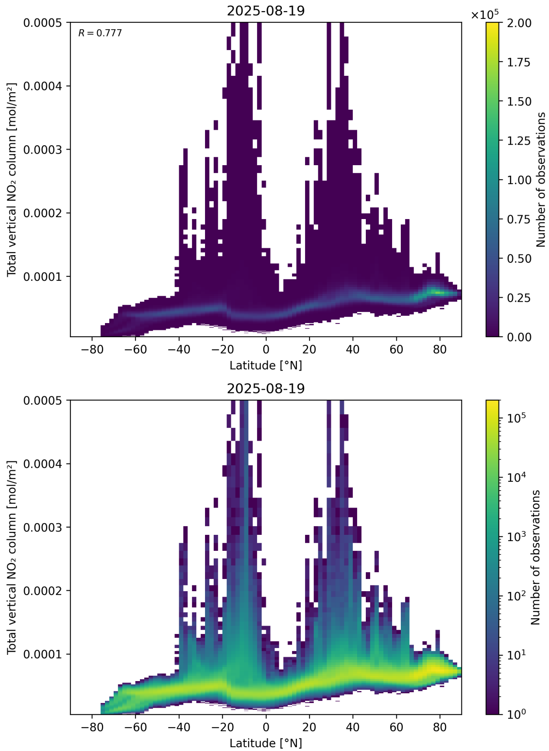
Figure 90: Scatter density plot of “Latitude” against “Total vertical NO 2 column” for 2025-08-19 to 2025-08-20.
