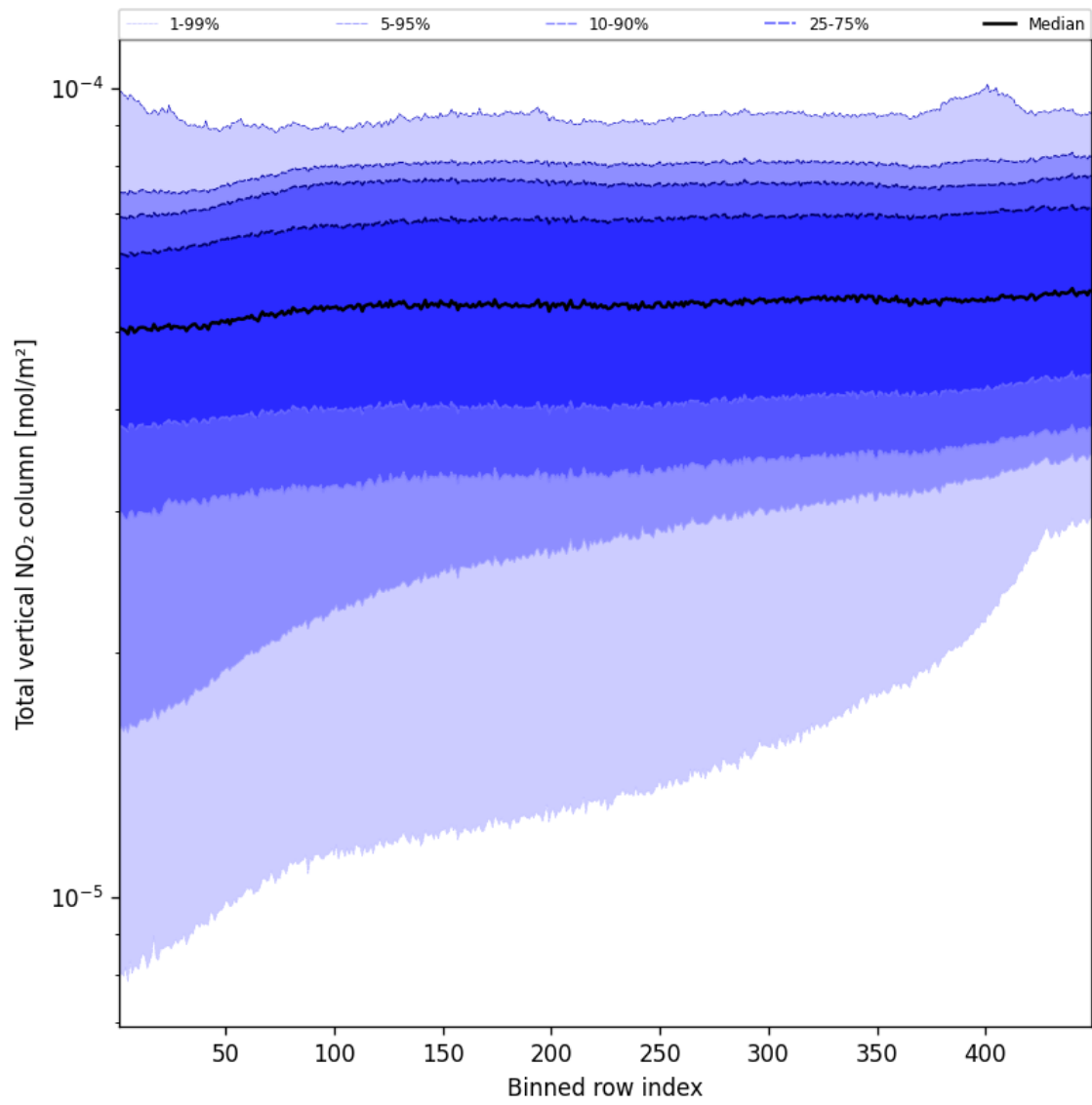
Figure 55: Along track statistics of “Total vertical NO 2 column” for 2025-08-19 to 2025-08-20
