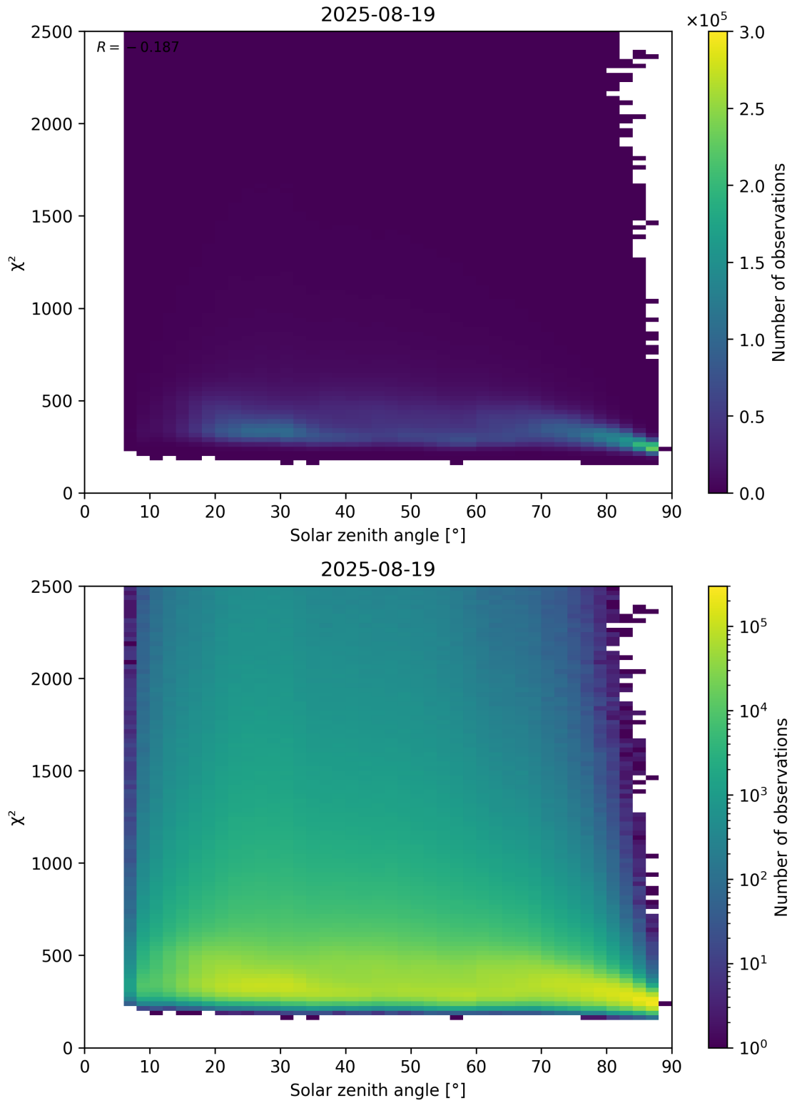
Figure 148: Scatter density plot of “Solar zenith angle” against “ \chi^2 ” for 2025-08-19 to 2025-08-20.
