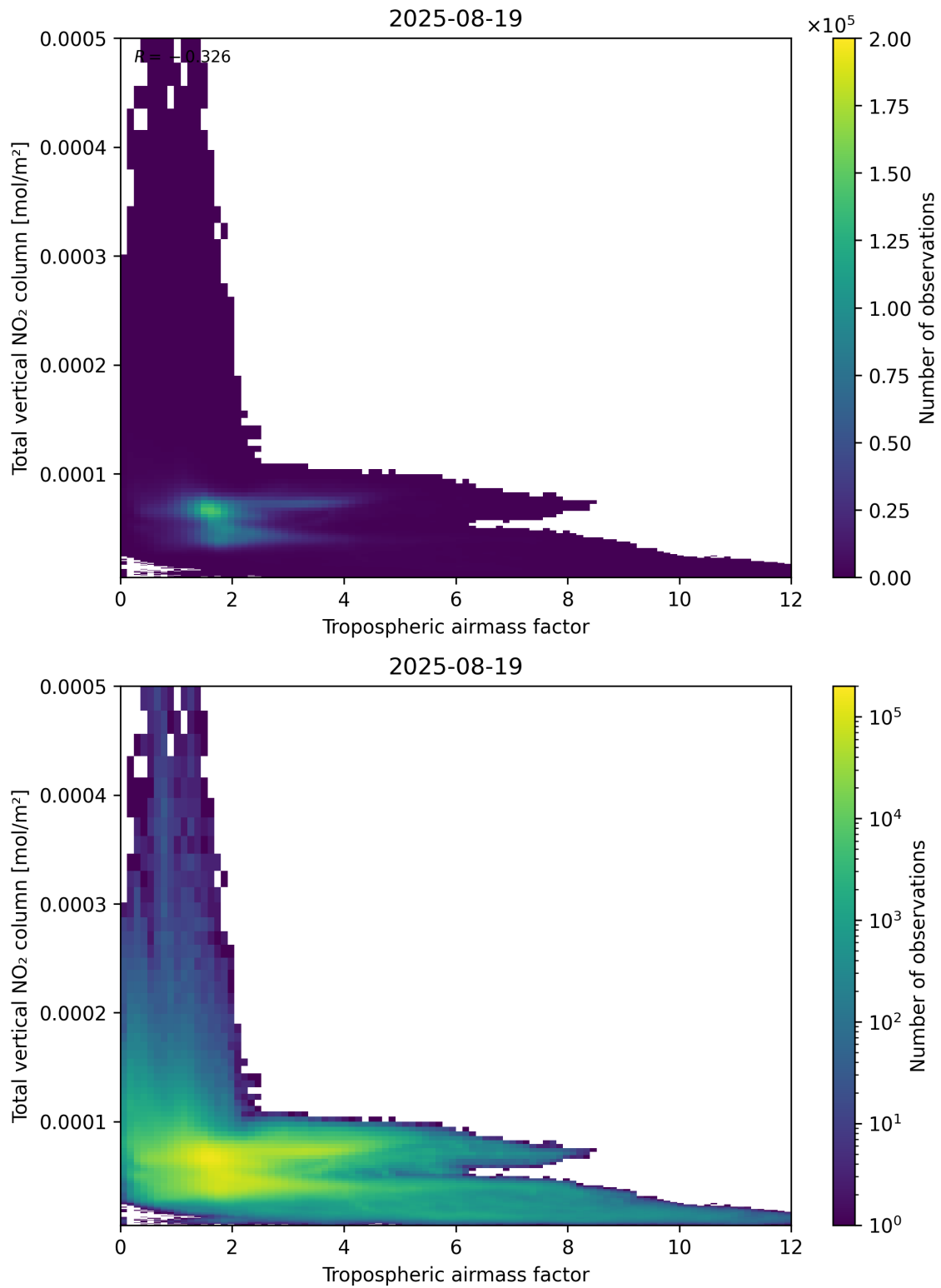
Figure 77: Scatter density plot of “Tropospheric airmass factor” against “Total vertical NO 2 column” for 2025-08-19 to 2025-08-20.
