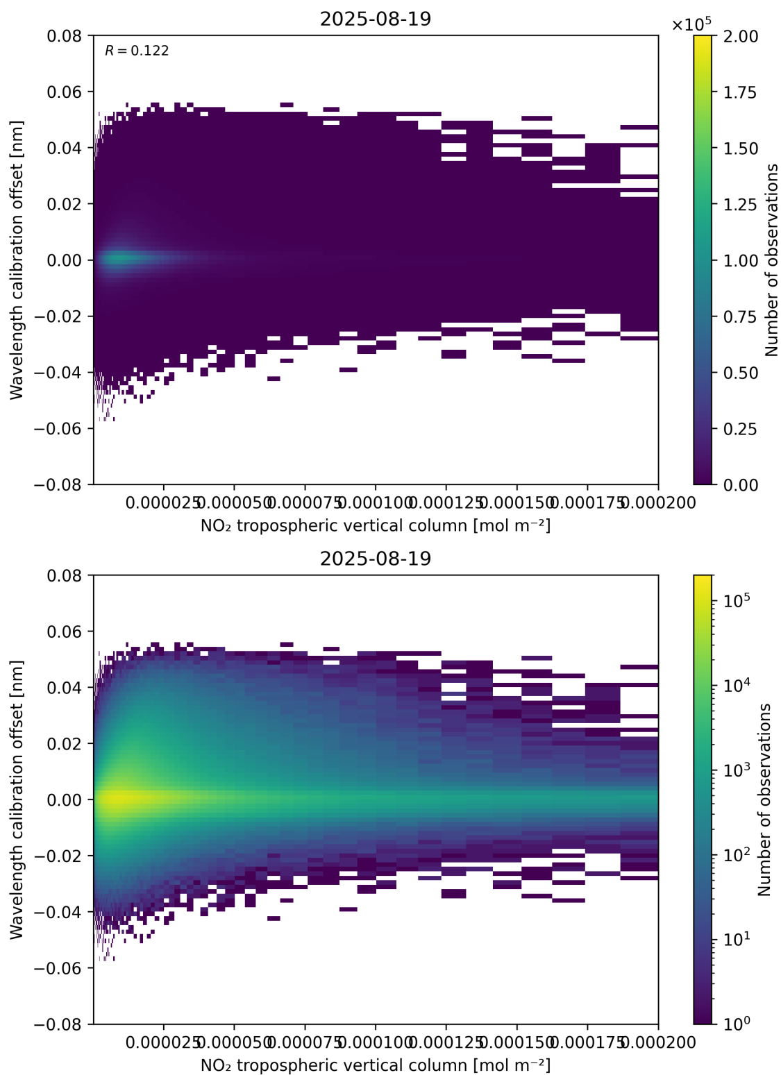
Figure 143: Scatter density plot of “NO 2 tropospheric vertical column” against “Wavelength calibration offset” for 2025-08-19 to 2025-08-20.
