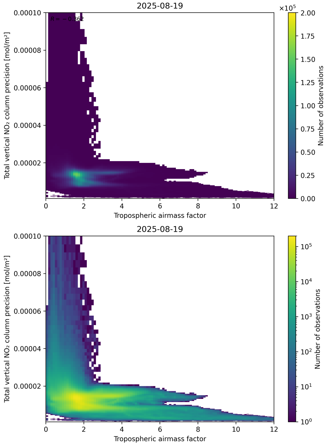
Figure 78: Scatter density plot of “Tropospheric air mass factor” against “Total vertical NO 2 column precision” for 2025-08-19 to 2025-08-20.
