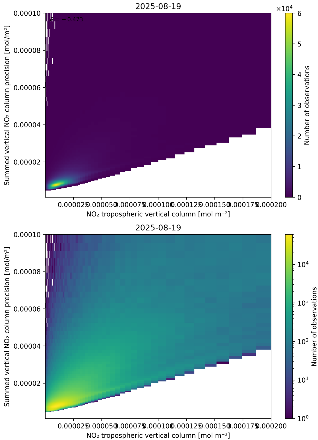
Figure 127: Scatter density plot of “NO 2 tropospheric vertical column” against “Summed vertical NO 2 column precision” for 2025-08-19 to 2025-08-20.
