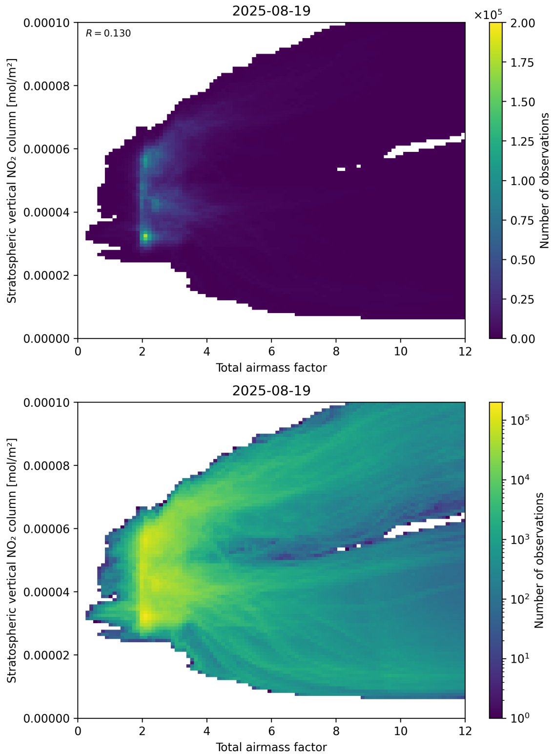
Figure 64: Scatter density plot of “Total airmass factor” against “Stratospheric vertical NO 2 column” for 2025-08-19 to 2025-08-20.
