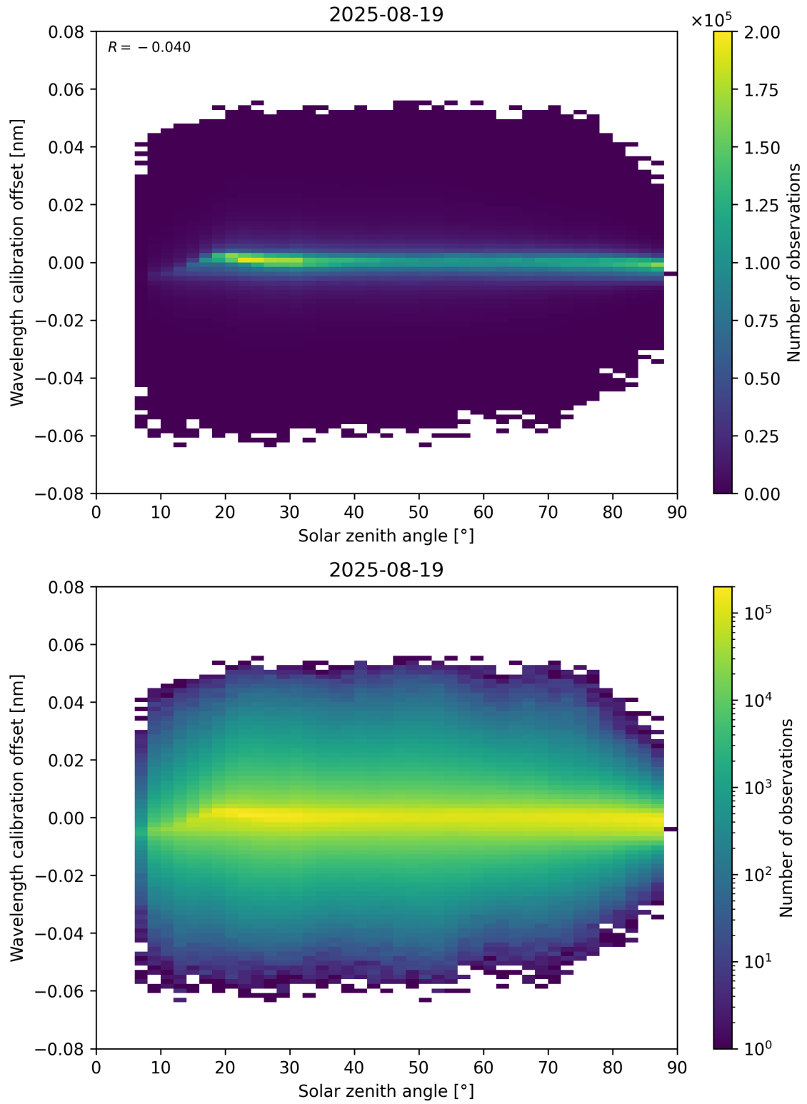
Figure 158: Scatter density plot of “Solar zenith angle” against “Wavelength calibration offset” for 2025-08-19 to 2025-08-20.
