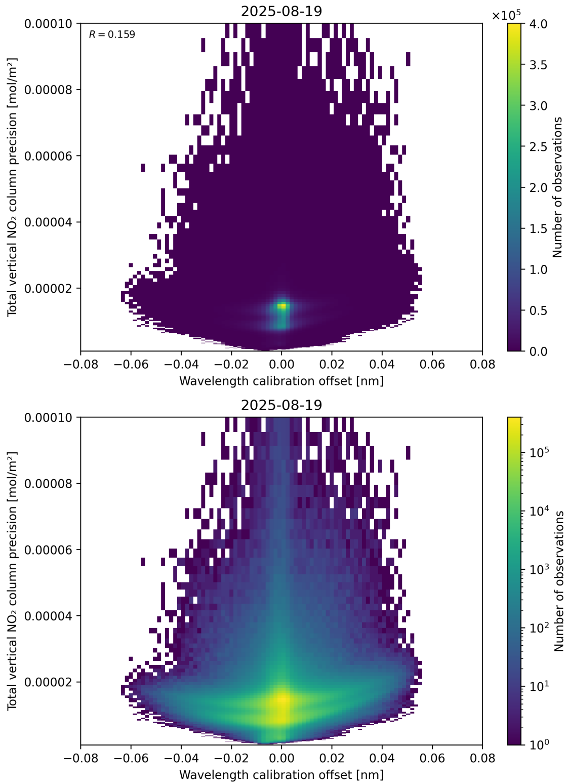
Figure 180: Scatter density plot of “Wavelength calibration offset” against “Total vertical NO 2 column precision” for 2025-08-19 to 2025-08-20.
