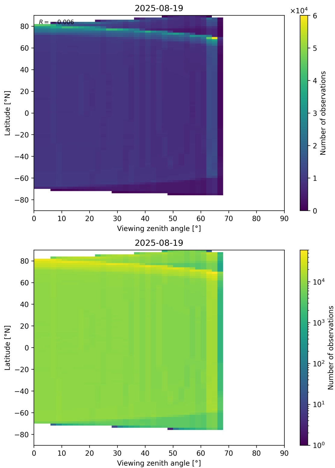
Figure 163: Scatter density plot of “Viewing zenith angle” against “Latitude” for 2025-08-19 to 2025-08-20.
