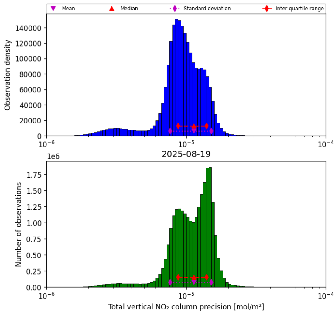
Figure 39: Histogram of “Total vertical NO 2 column precision” for 2025-08-19 to 2025-08-20
