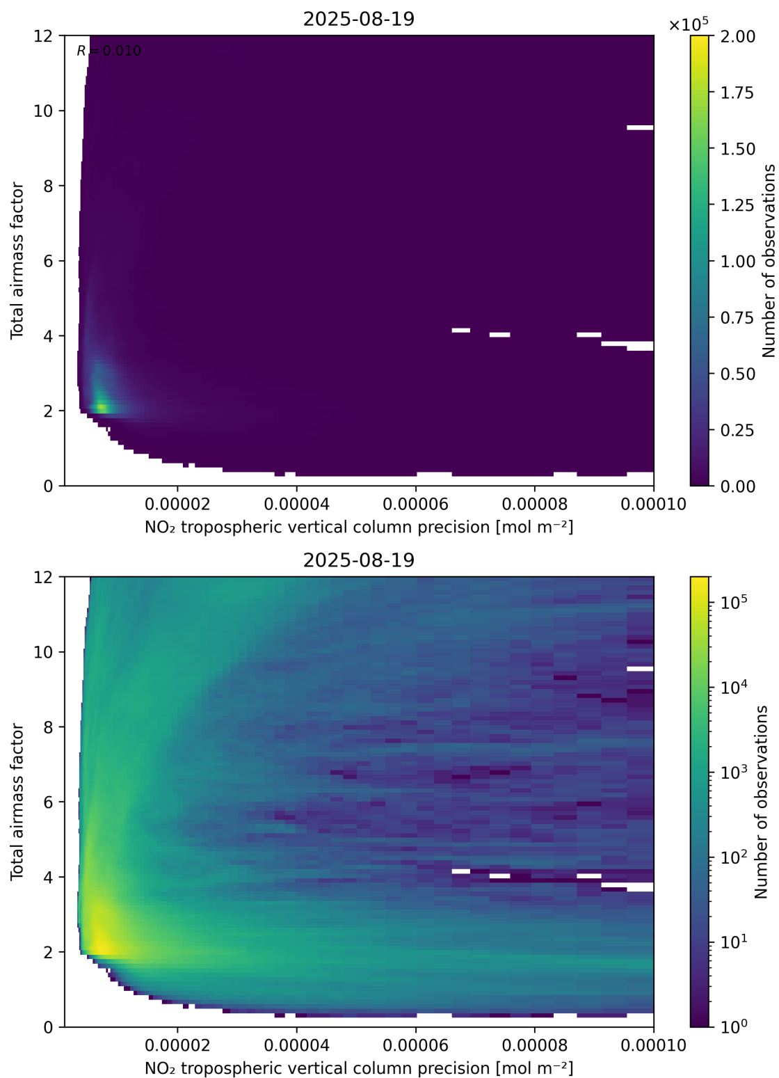
Figure 132: Scatter density plot of “NO 2 tropospheric vertical column precision” against “Total airmass factor” for 2025-08-19 to 2025-08-20.
