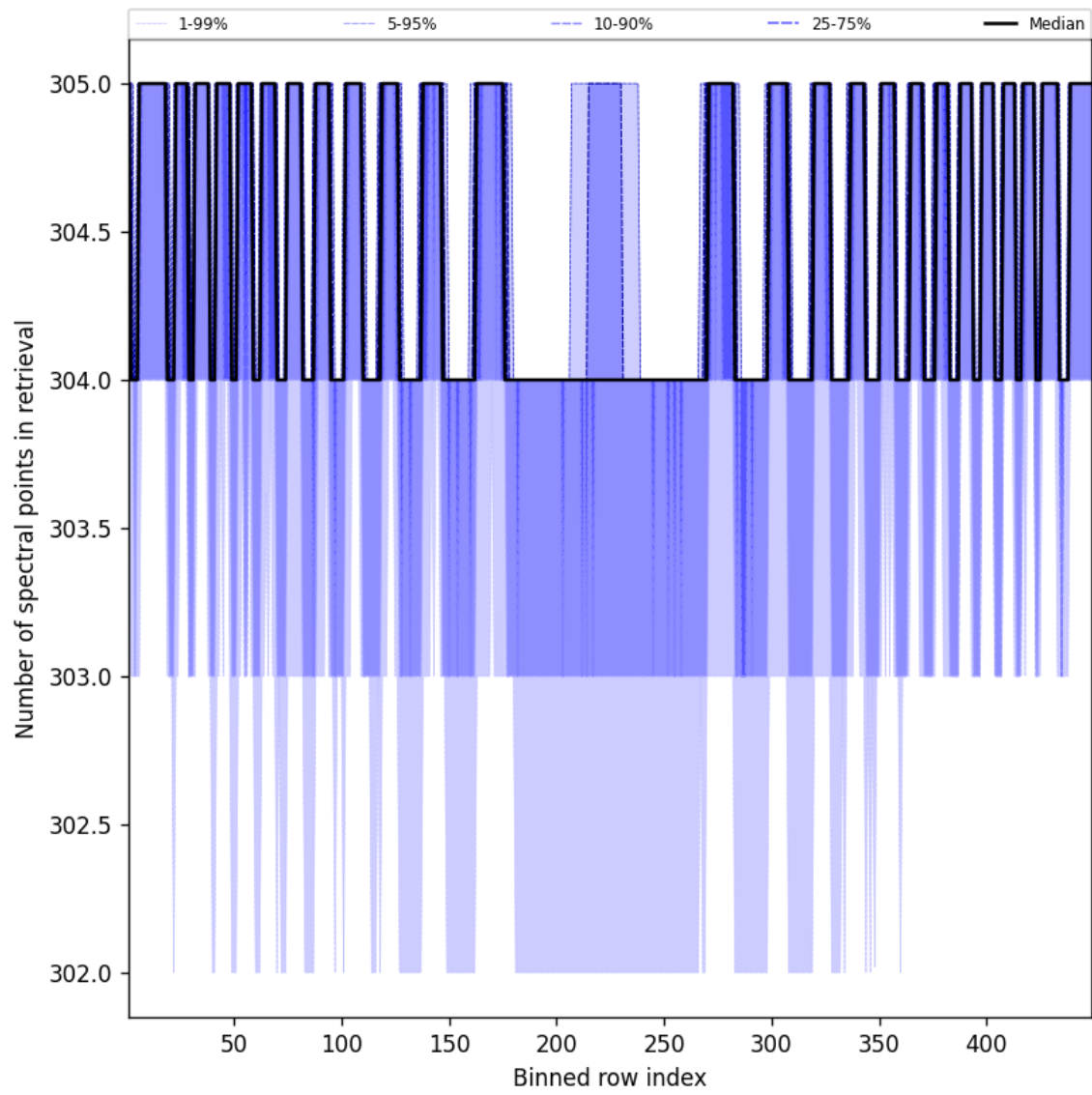
Figure 50: Along track statistics of “Number of spectral points in retrieval” for 2025-08-19 to 2025-08-20
