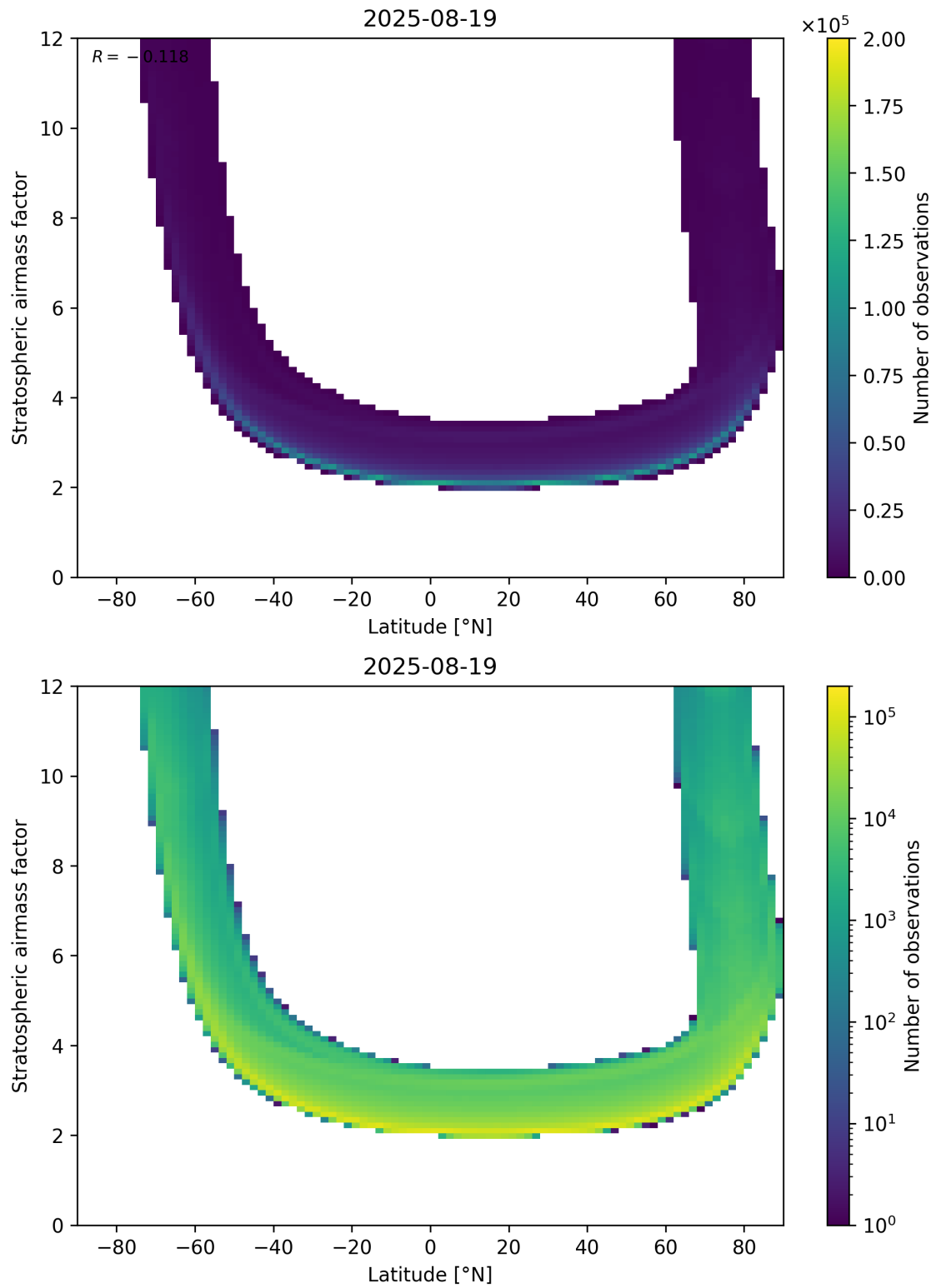
Figure 83: Scatter density plot of “Latitude” against “Stratospheric air mass factor” for 2025-08-19 to 2025-08-20.
