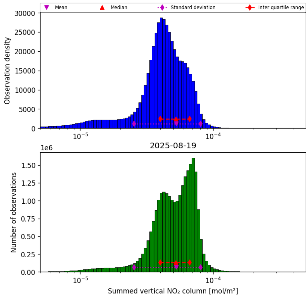
Figure 40: Histogram of “Summed vertical NO 2 column” for 2025-08-19 to 2025-08-20
