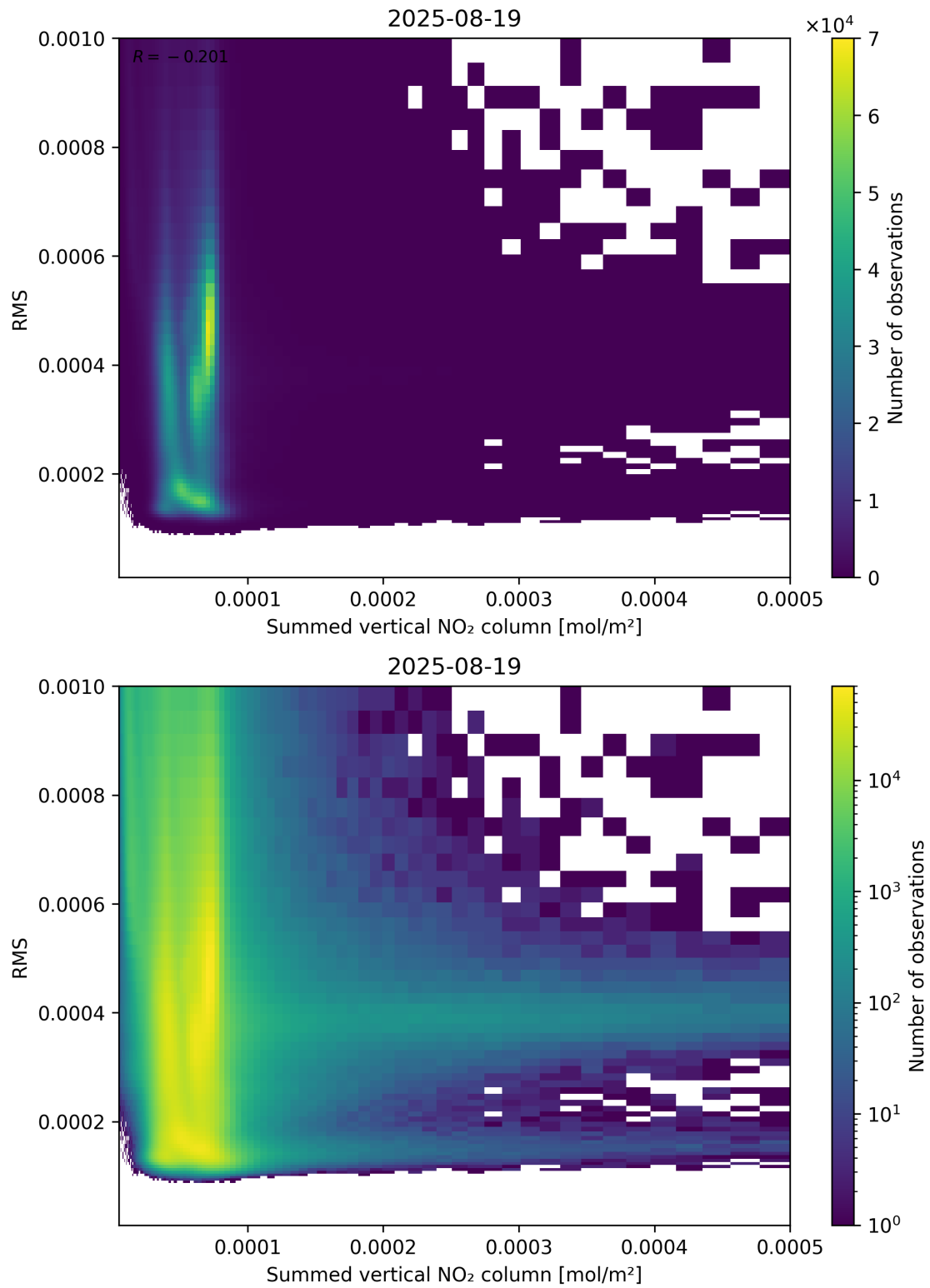
Figure 109: Scatter density plot of “Summed vertical NO 2 column” against “RMS” for 2025-08-19 to 2025-08-20.
