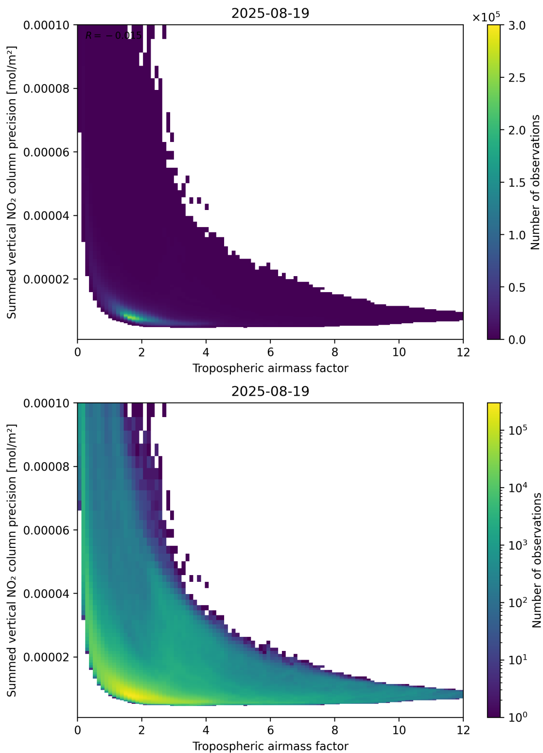
Figure 76: Scatter density plot of “Tropospheric air mass factor” against “Summed vertical NO 2 column precision” for 2025-08-19 to 2025-08-20.
