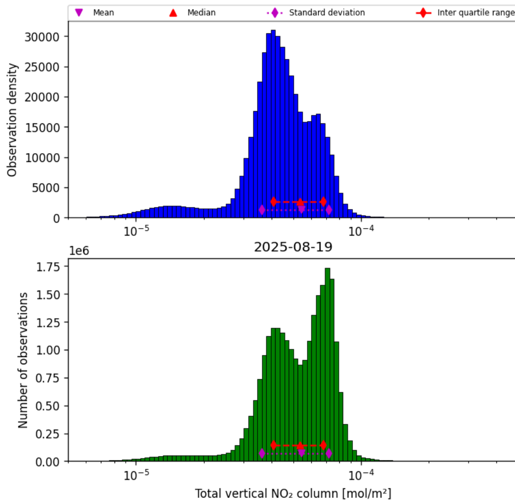
Figure 38: Histogram of “Total vertical NO 2 column” for 2025-08-19 to 2025-08-20
