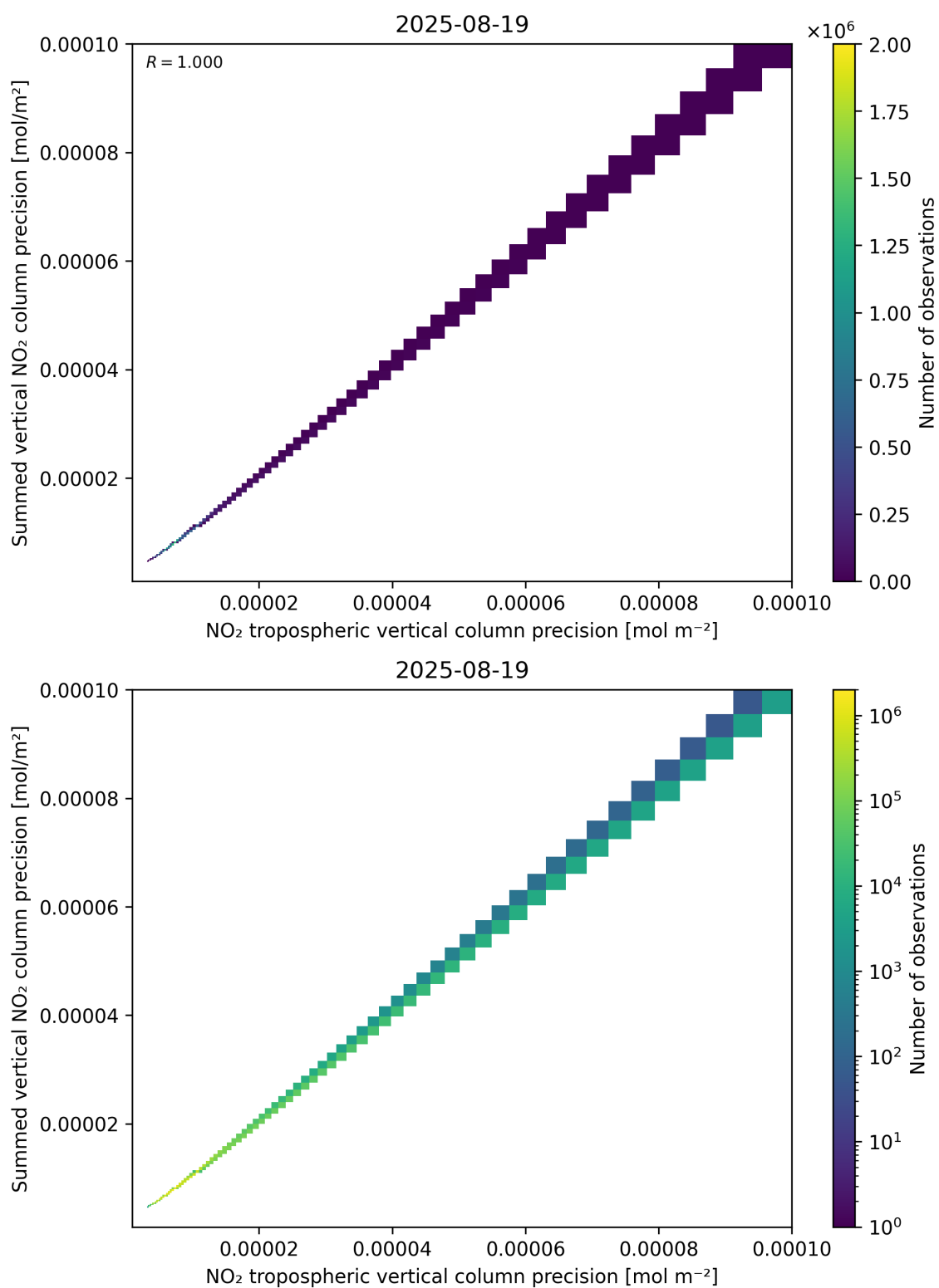
Figure 137: Scatter density plot of “NO 2 tropospheric vertical column precision” against “Summed vertical NO 2 column precision” for 2025-08-19 to 2025-08-20.
