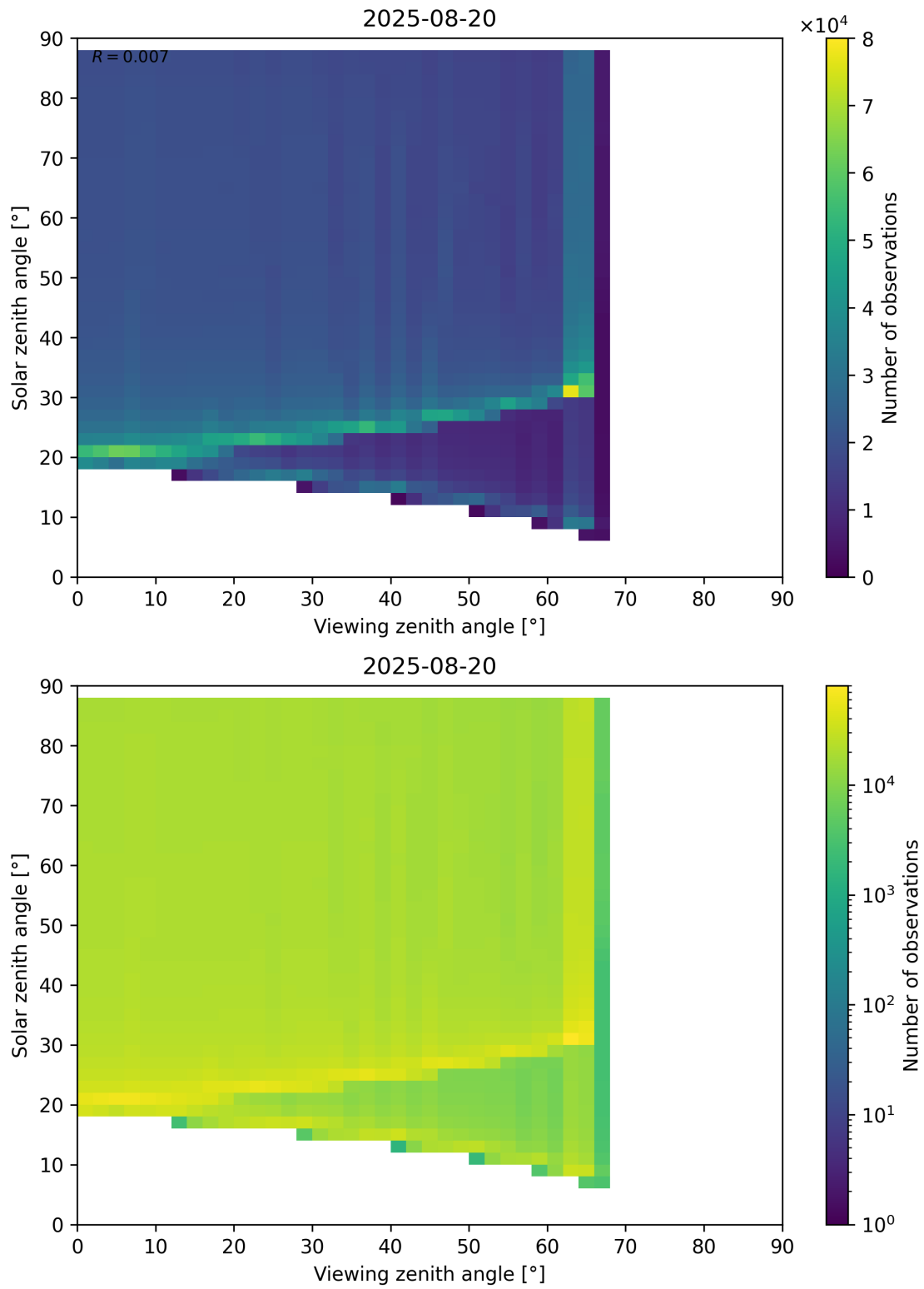
Figure 172: Scatter density plot of “Viewing zenith angle” against “Solar zenith angle” for 2025-08-19 to 2025-08-21.
