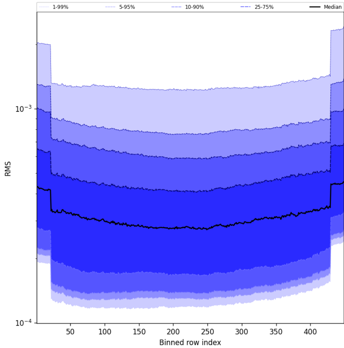
Figure 60: Along track statistics of “RMS” for 2025-08-19 to 2025-08-21
