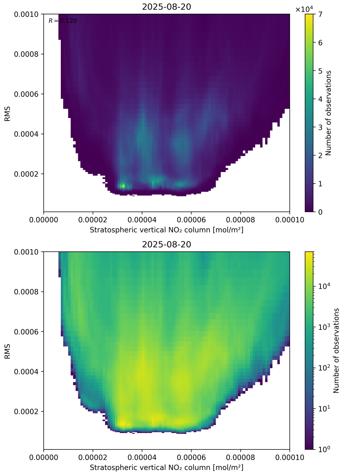
Figure 102: Scatter density plot of “Stratospheric vertical NO 2 column” against “RMS” for 2025-08-19 to 2025-08-21.
