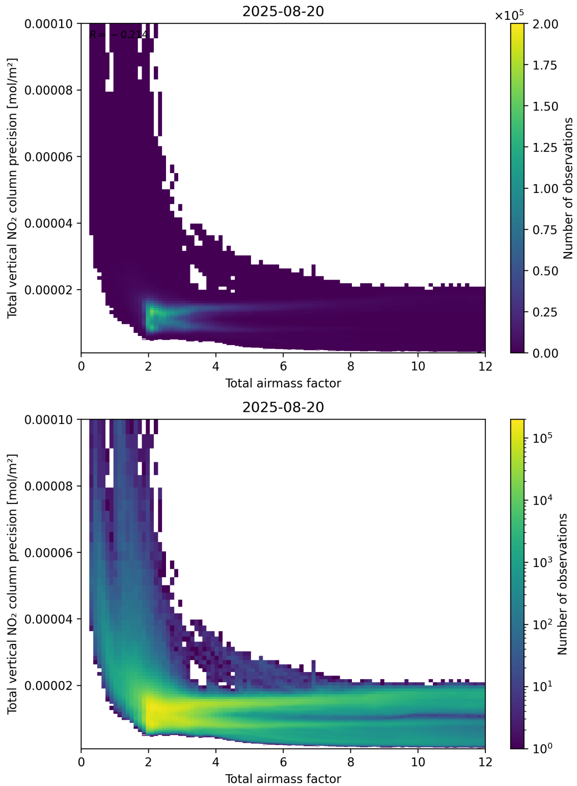
Figure 68: Scatter density plot of “Total airmass factor” against “Total vertical NO 2 column precision” for 2025-08-19 to 2025-08-21.
