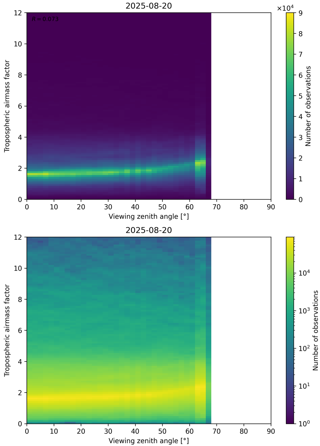
Figure 161: Scatter density plot of “Viewing zenith angle” against “Tropospheric air mass factor” for 2025-08-19 to 2025-08-21.
