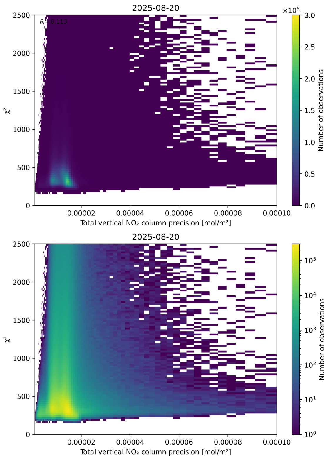
Figure 116: Scatter density plot of “Total vertical NO 2 column precision” against “ \chi^2 ” for 2025-08-19 to 2025-08-21.
