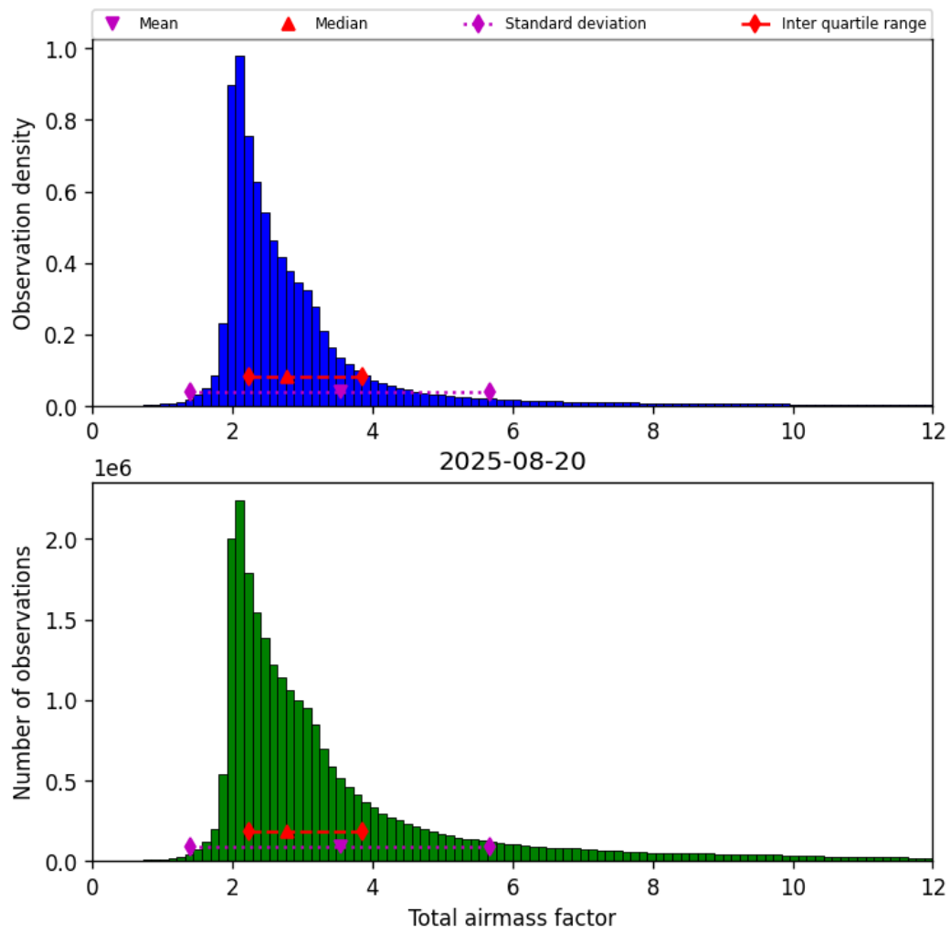
Figure 32: Histogram of “Total airmass factor” for 2025-08-19 to 2025-08-21
