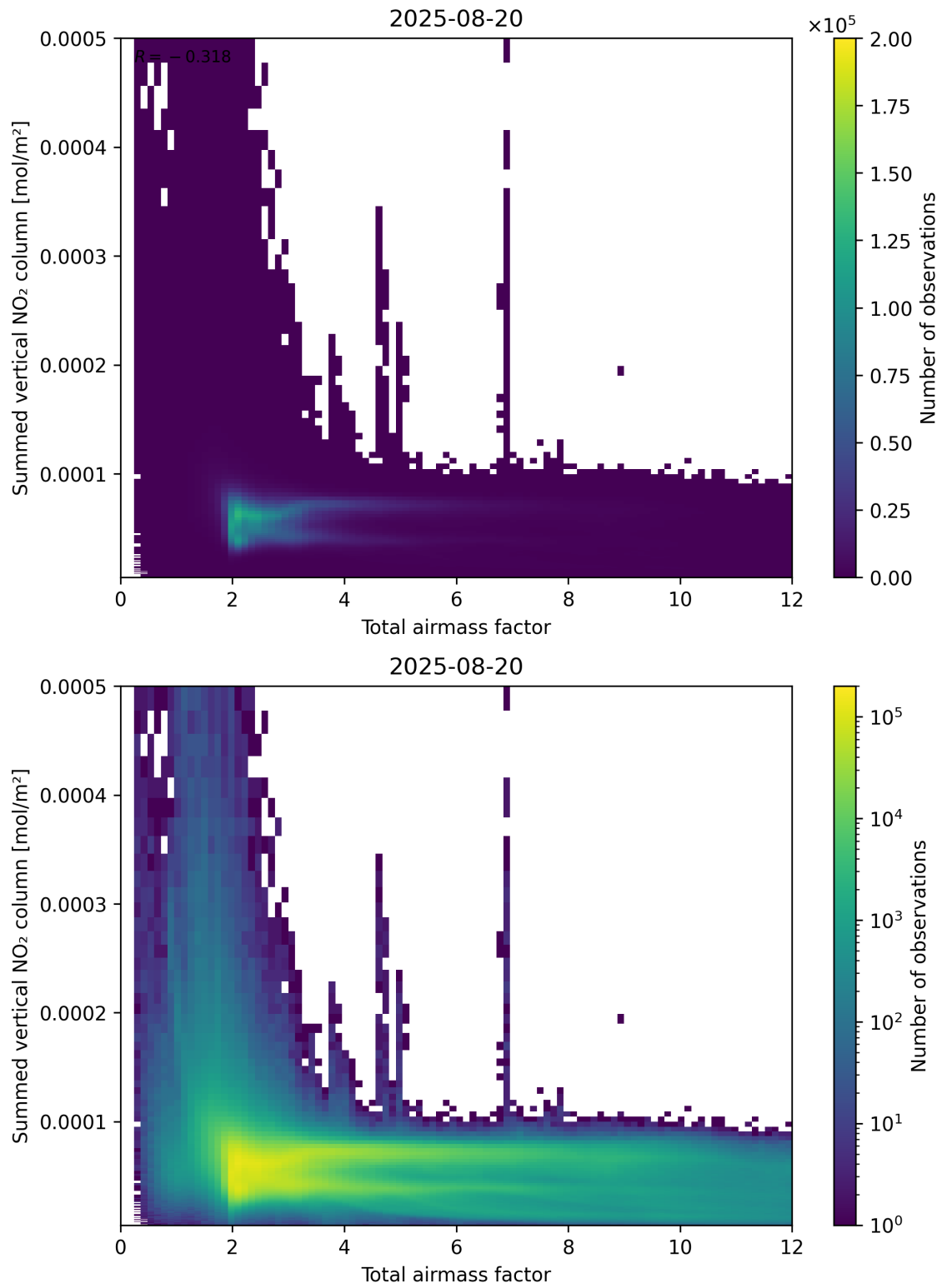
Figure 65: Scatter density plot of “Total airmass factor” against “Summed vertical NO 2 column” for 2025-08-19 to 2025-08-21.
