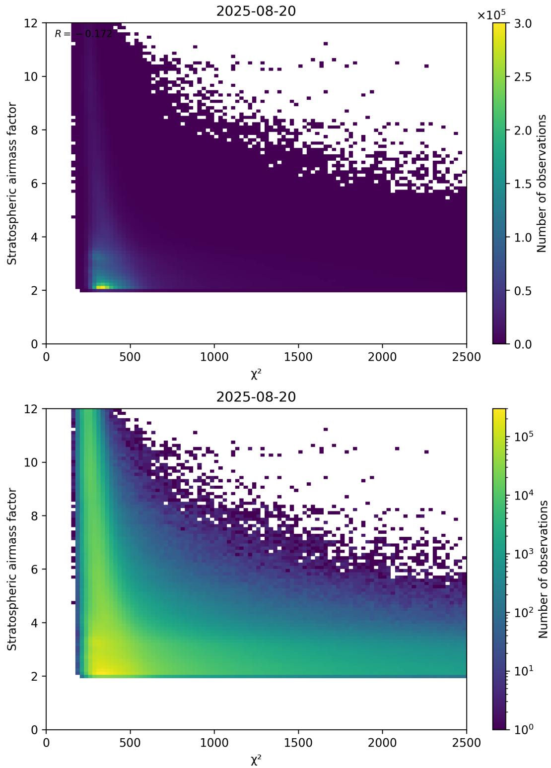
Figure 81: Scatter density plot of “ \chi^2 ” against “Stratospheric airmass factor” for 2025-08-19 to 2025-08-21.
