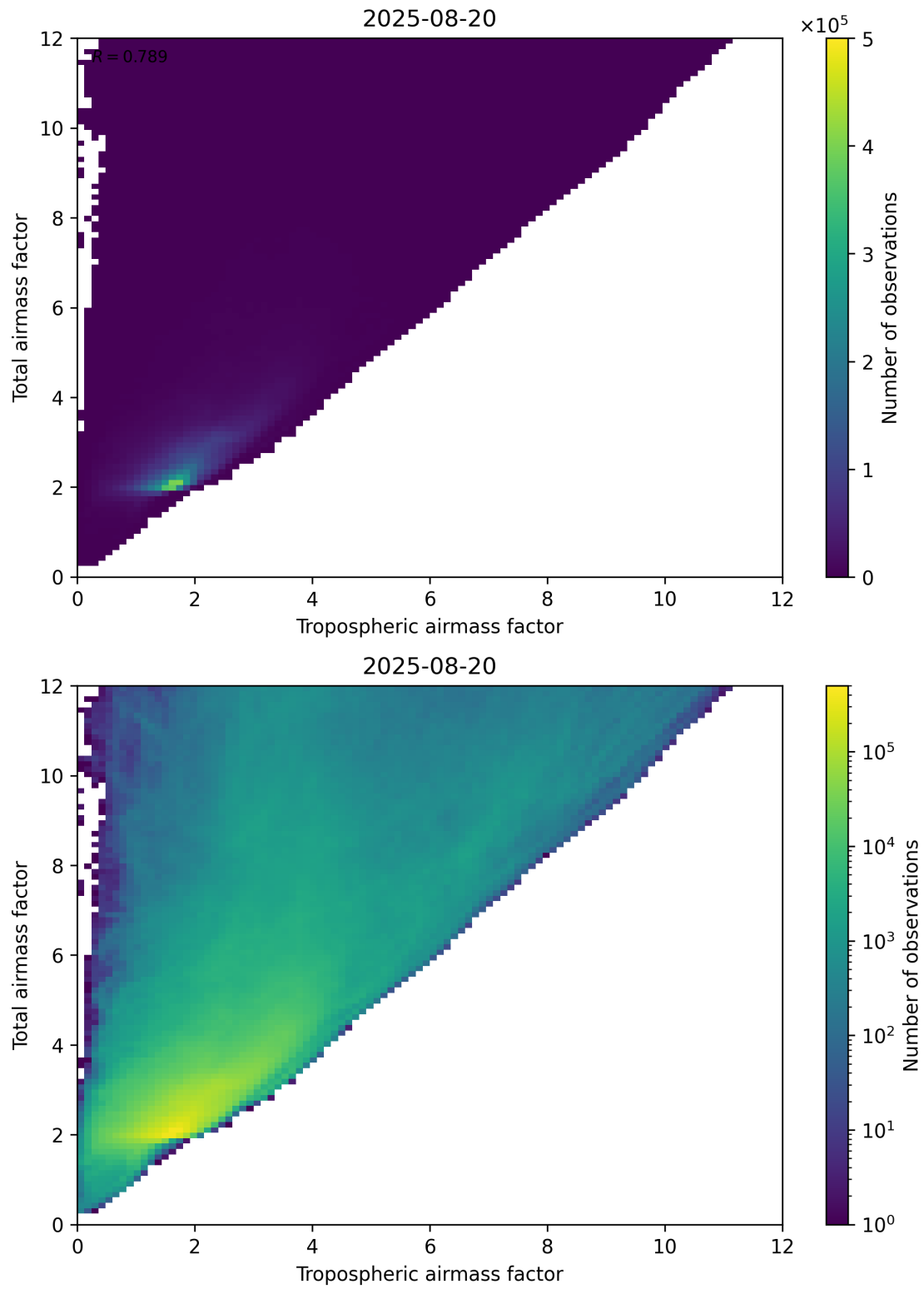
Figure 72: Scatter density plot of “Tropospheric airmass factor” against “Total airmass factor” for 2025-08-19 to 2025-08-21.
