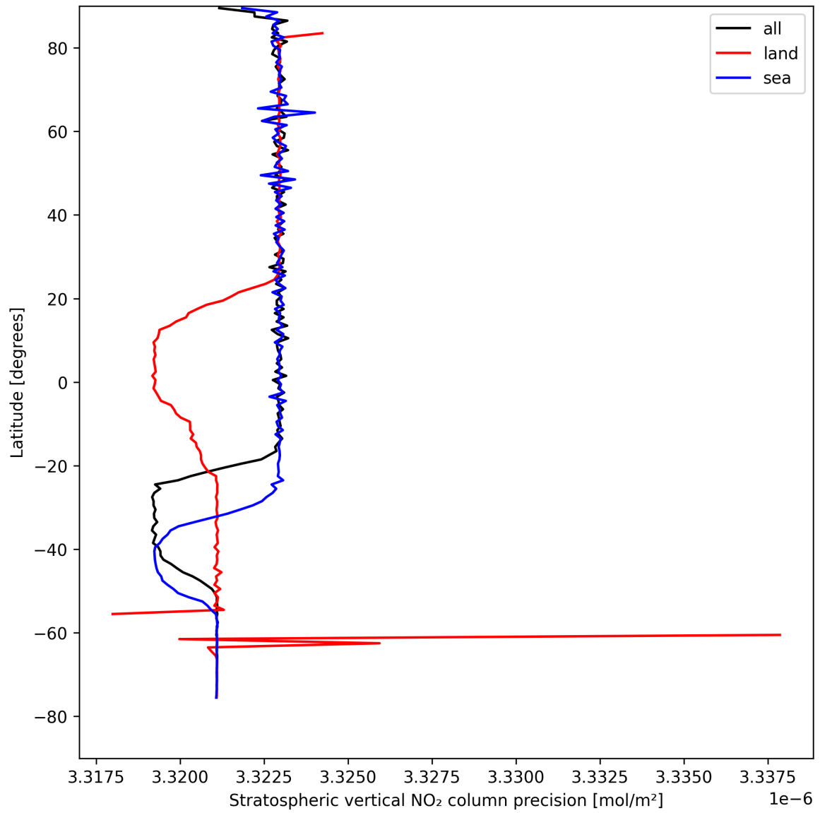
Figure 20: Zonal average of “Stratospheric vertical NO 2 column precision” for 2025-08-19 to 2025-08-21.
