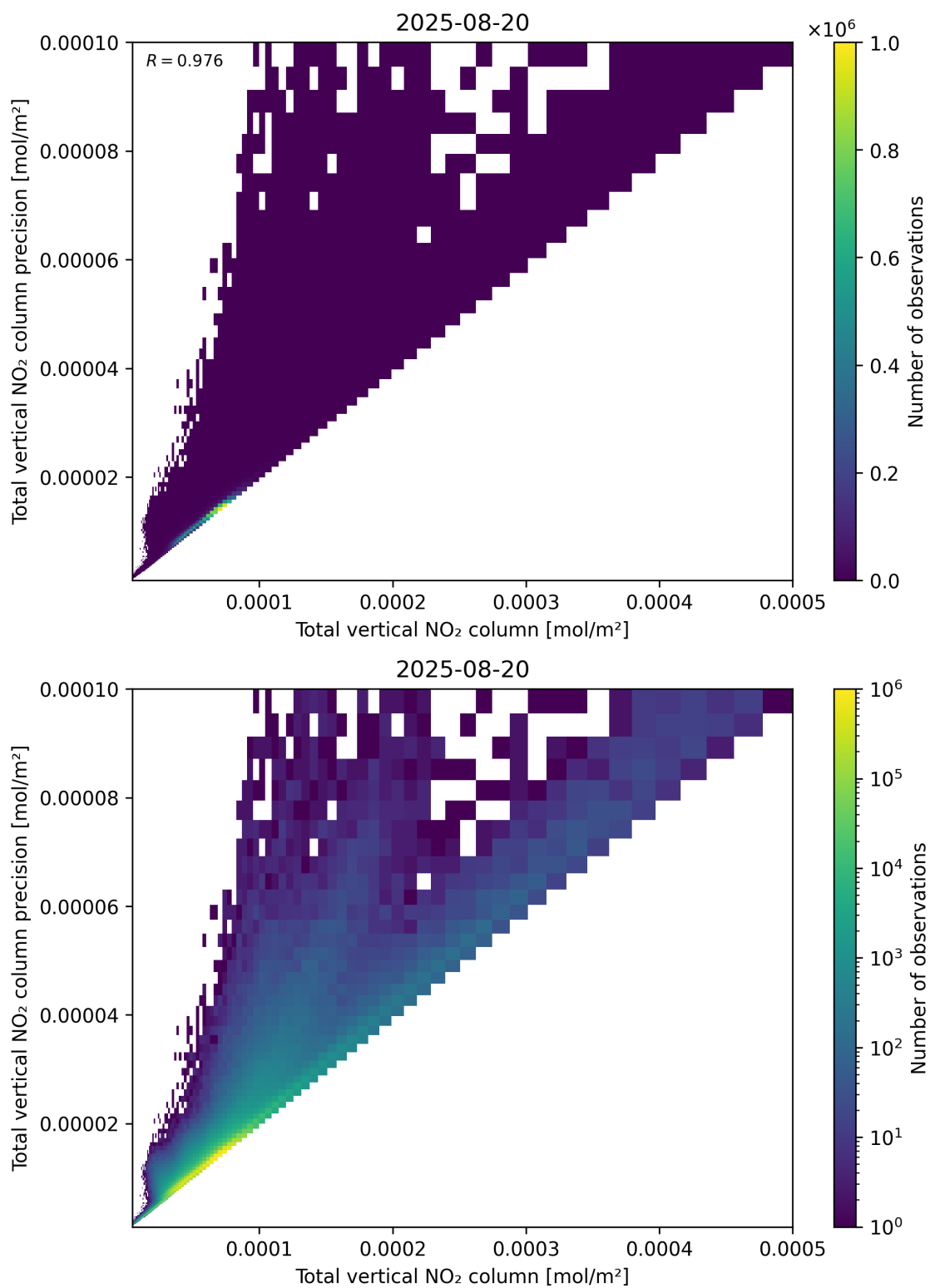
Figure 114: Scatter density plot of “Total vertical NO 2 column” against “Total vertical NO 2 column precision” for 2025-08-19 to 2025-08-21.
