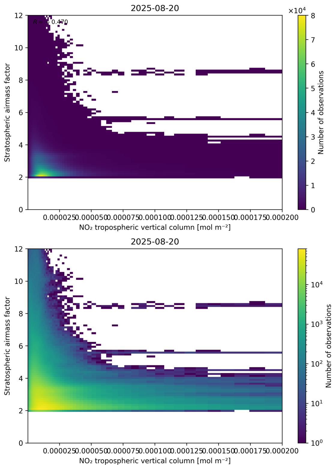
Figure 121: Scatter density plot of “NO 2 tropospheric vertical column” against “Stratospheric air mass factor” for 2025-08-19 to 2025-08-21.
