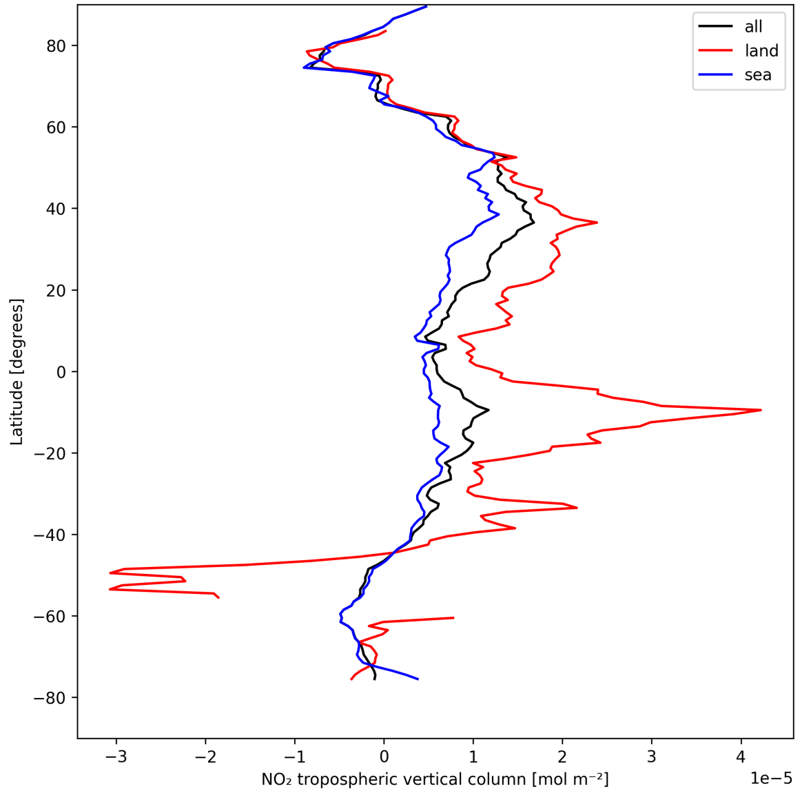
Figure 12: Zonal average of “NO 2 tropospheric vertical column” for 2025-08-19 to 2025-08-21.
