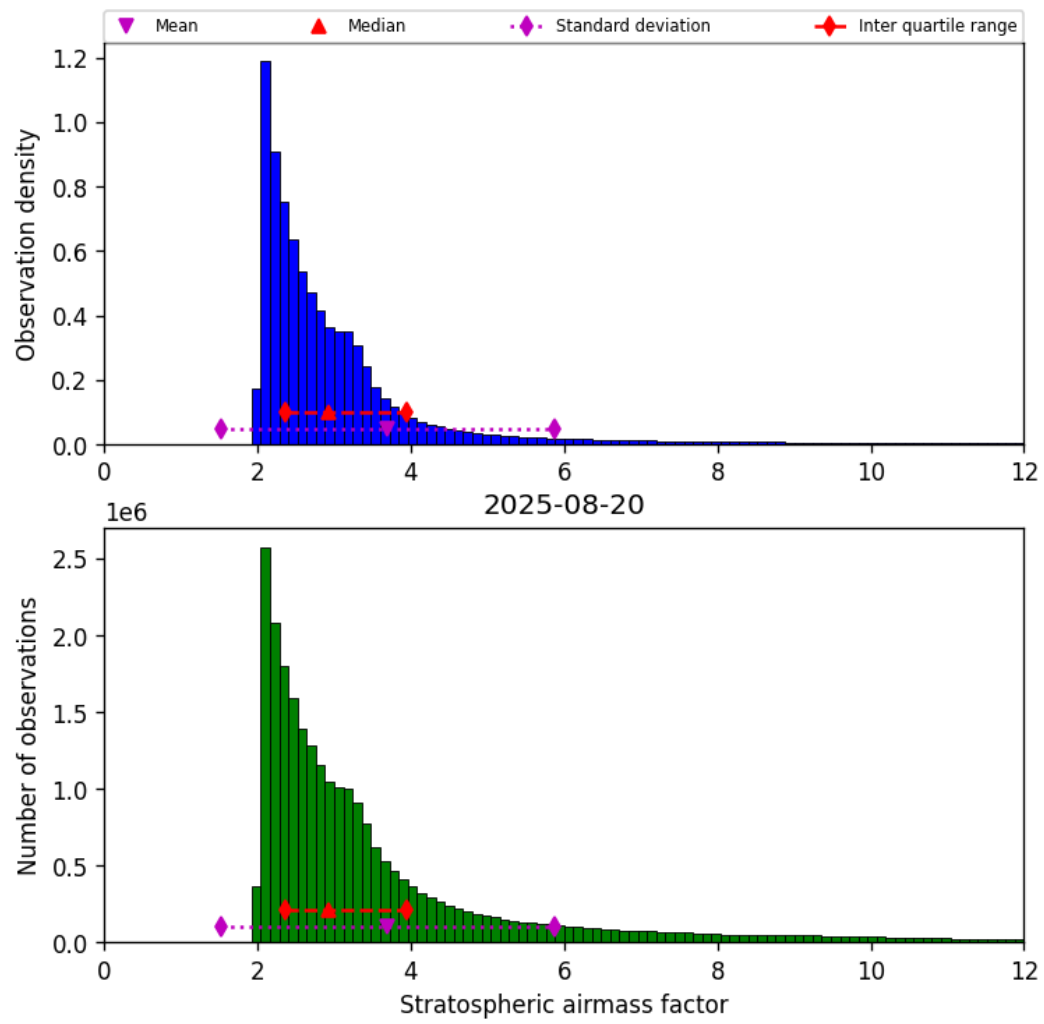
Figure 44: Histogram of “Stratospheric airmass factor” for 2025-08-19 to 2025-08-21
