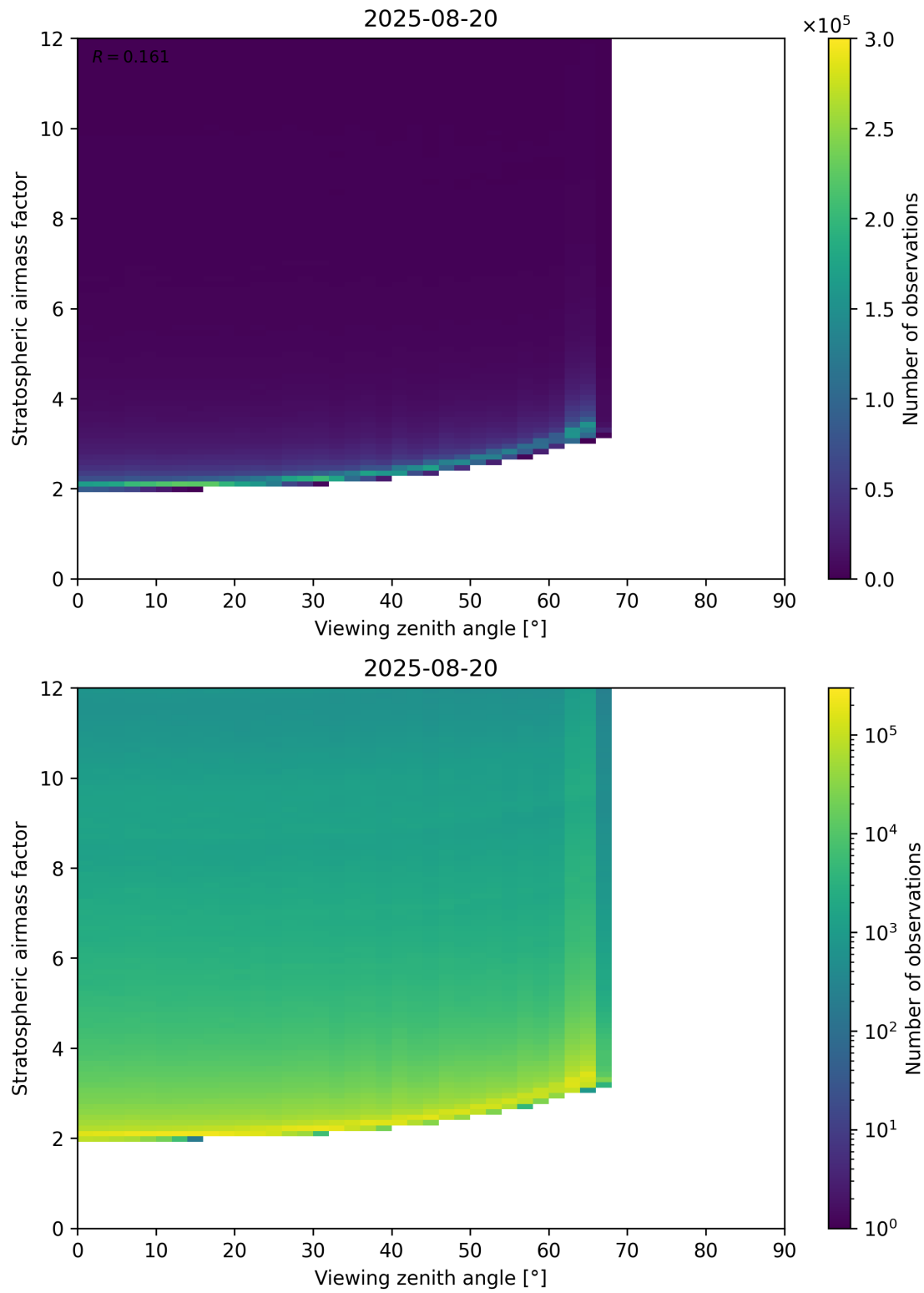
Figure 159: Scatter density plot of “Viewing zenith angle” against “Stratospheric airmass factor” for 2025-08-19 to 2025-08-21.
