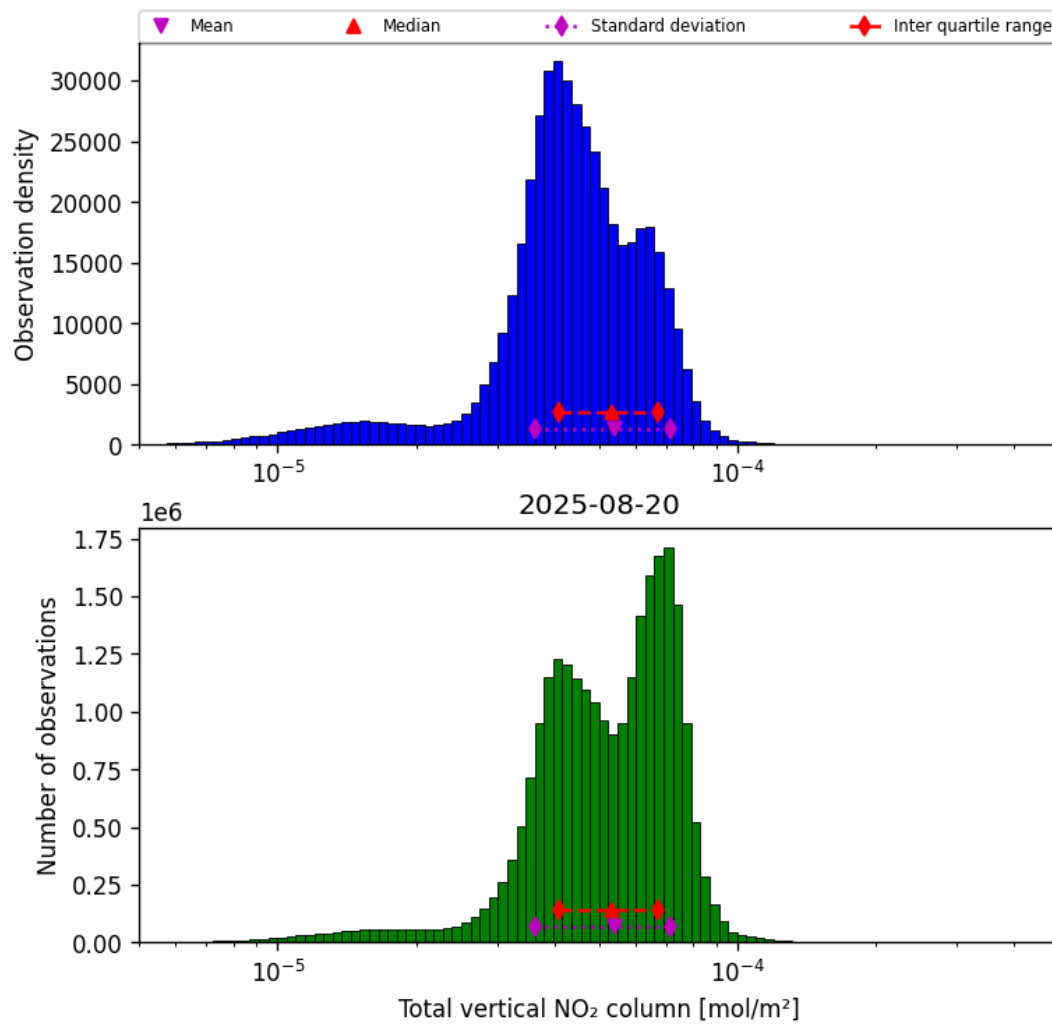
Figure 38: Histogram of “Total vertical NO 2 column” for 2025-08-19 to 2025-08-21
