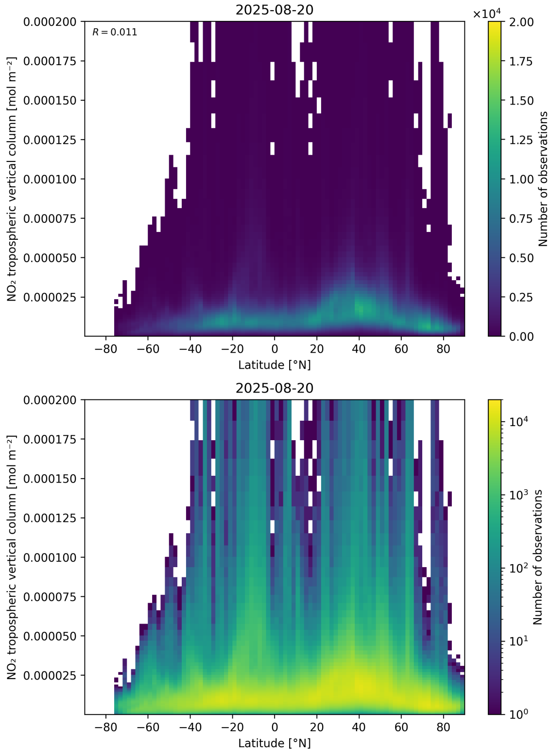
Figure 92: Scatter density plot of “Latitude” against “NO 2 tropospheric vertical column” for 2025-08-19 to 2025-08-21.
