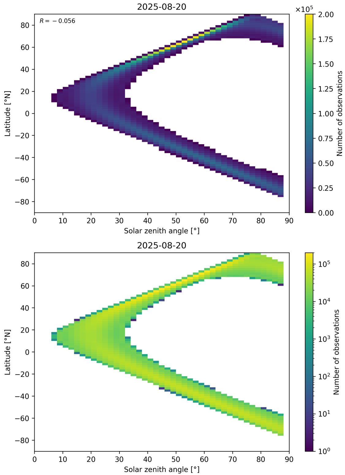
Figure 149: Scatter density plot of “Solar zenith angle” against “Latitude” for 2025-08-19 to 2025-08-21.
