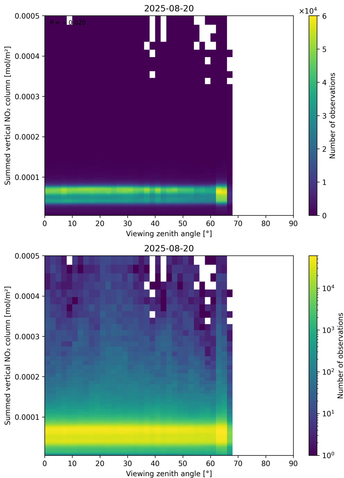
Figure 165: Scatter density plot of “Viewing zenith angle” against “Summed vertical NO 2 column” for 2025-08-19 to 2025-08-21.
