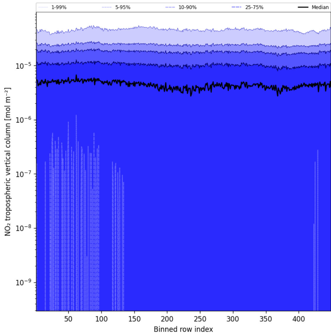
Figure 46: Along track statistics of “NO 2 tropospheric vertical column” for 2025-08-19 to 2025-08-21
