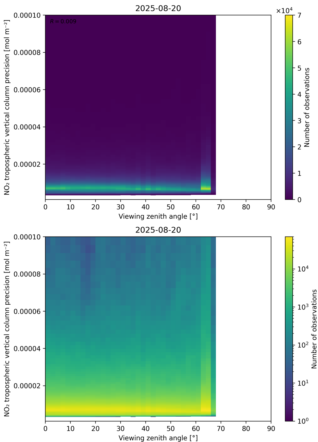
Figure 170: Scatter density plot of “Viewing zenith angle” against “NO 2 tropospheric vertical column precision” for 2025-08-19 to 2025-08-21.
