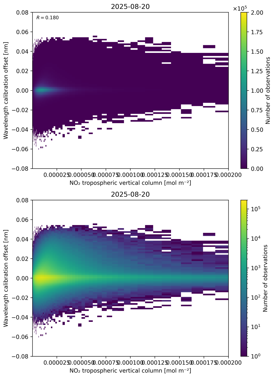
Figure 143: Scatter density plot of “NO 2 tropospheric vertical column” against “Wavelength calibration offset” for 2025-08-19 to 2025-08-21.
