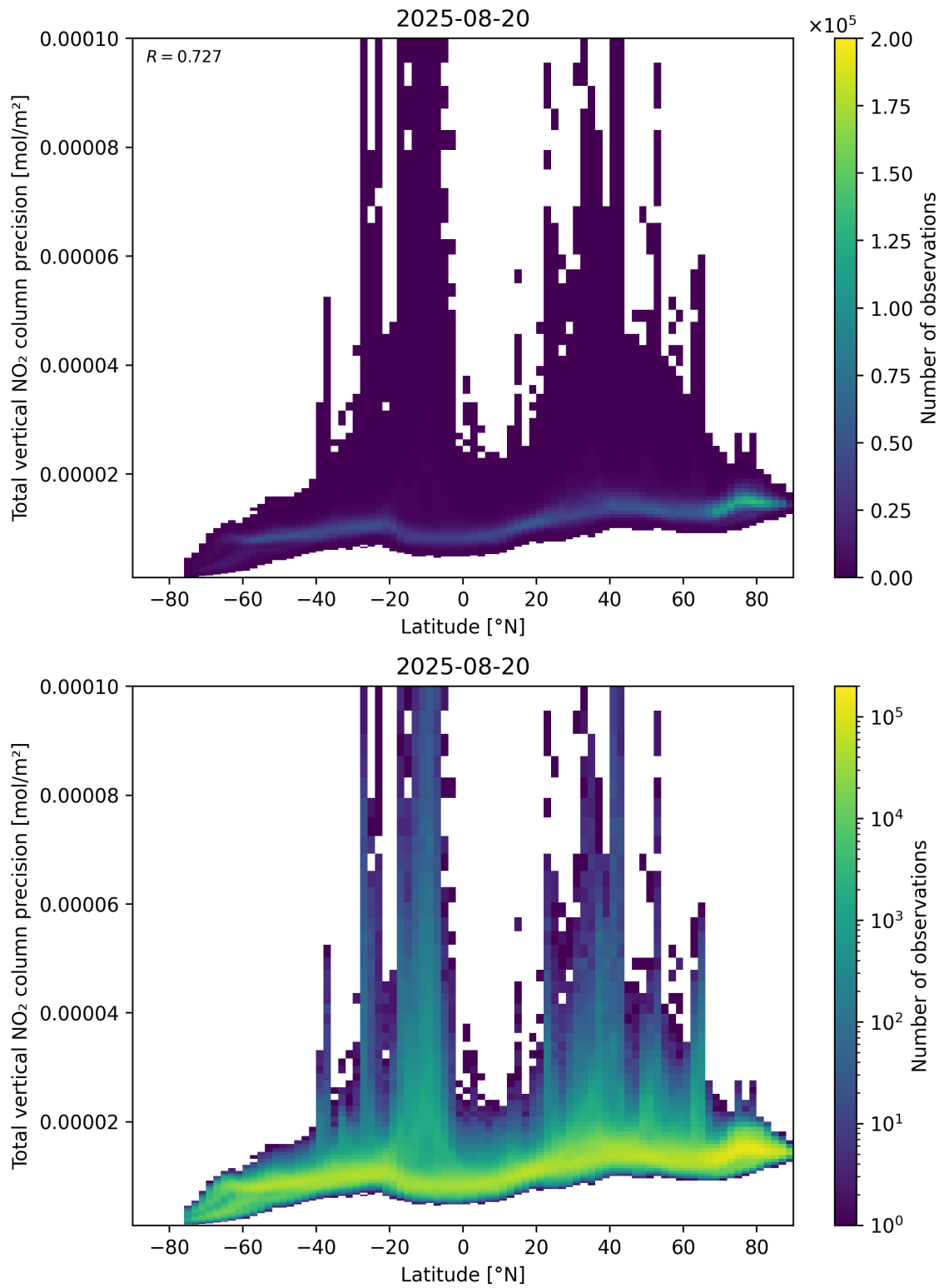
Figure 91: Scatter density plot of “Latitude” against “Total vertical NO 2 column precision” for 2025-08-19 to 2025-08-21.
