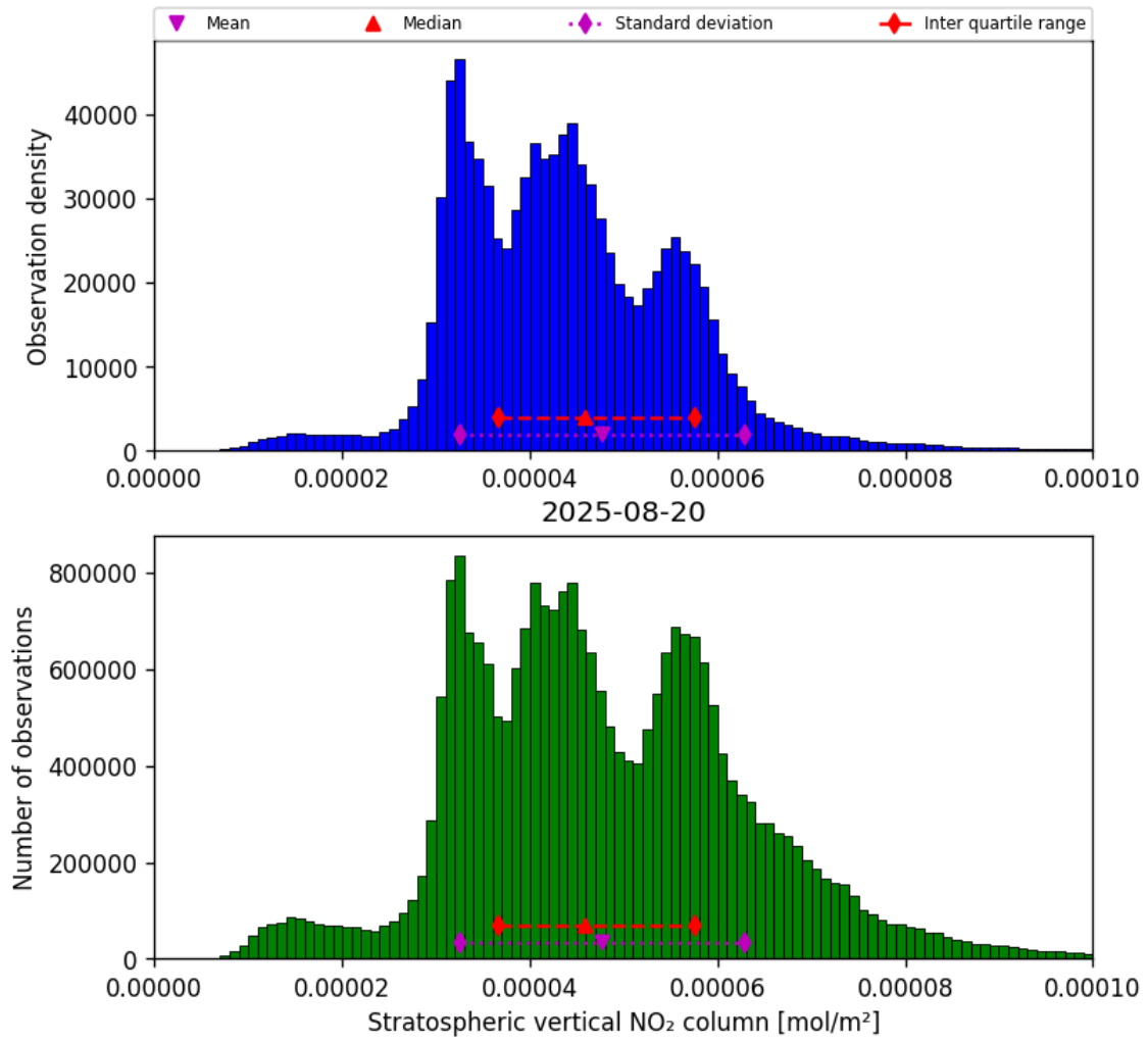
Figure 36: Histogram of “Stratospheric vertical NO 2 column” for 2025-08-19 to 2025-08-21
