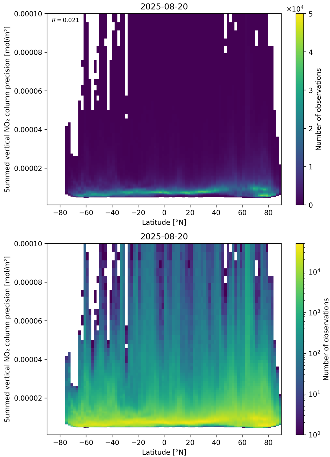
Figure 89: Scatter density plot of “Latitude” against “Summed vertical NO 2 column precision” for 2025-08-19 to 2025-08-21.
