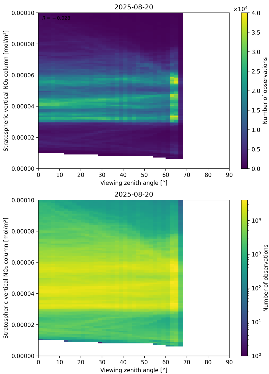
Figure 164: Scatter density plot of “Viewing zenith angle” against “Stratospheric vertical NO 2 column” for 2025-08-19 to 2025-08-21.
