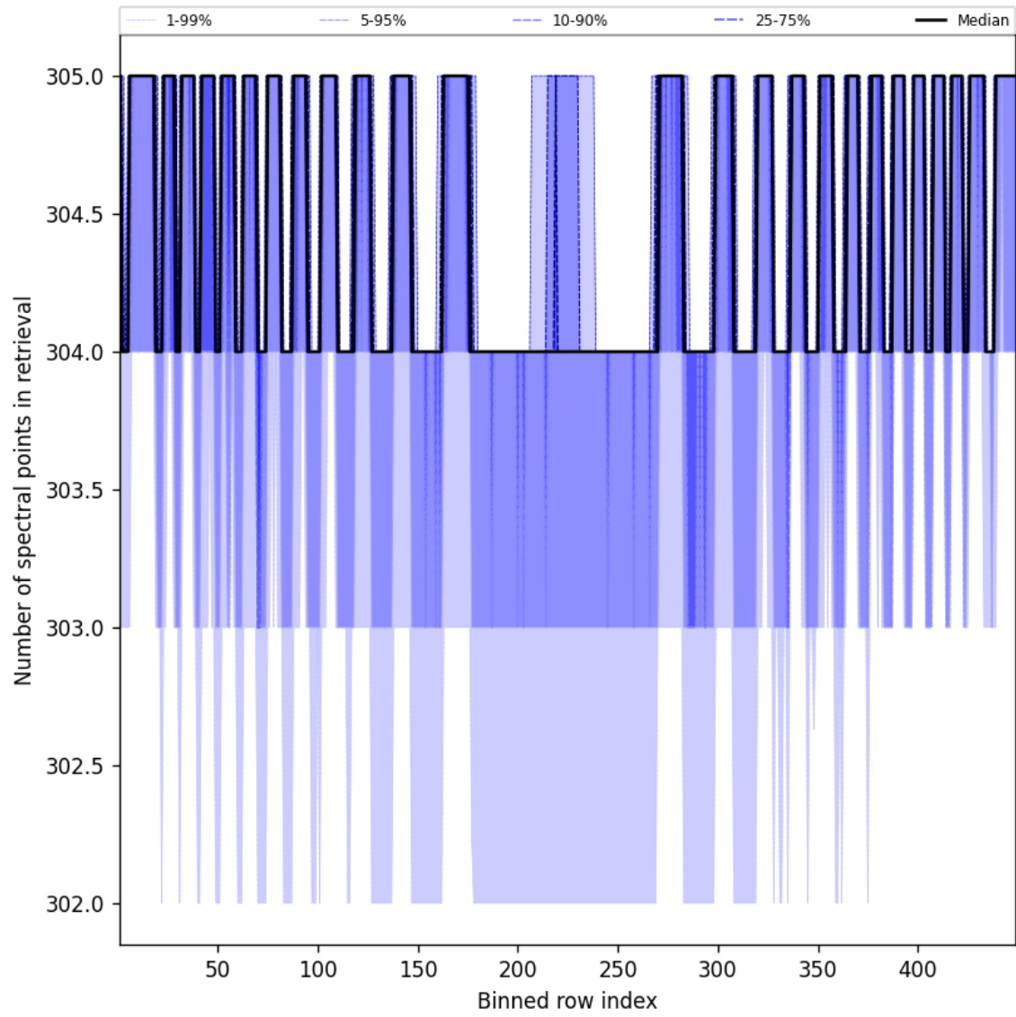
Figure 50: Along track statistics of “Number of spectral points in retrieval” for 2025-08-19 to 2025-08-21
