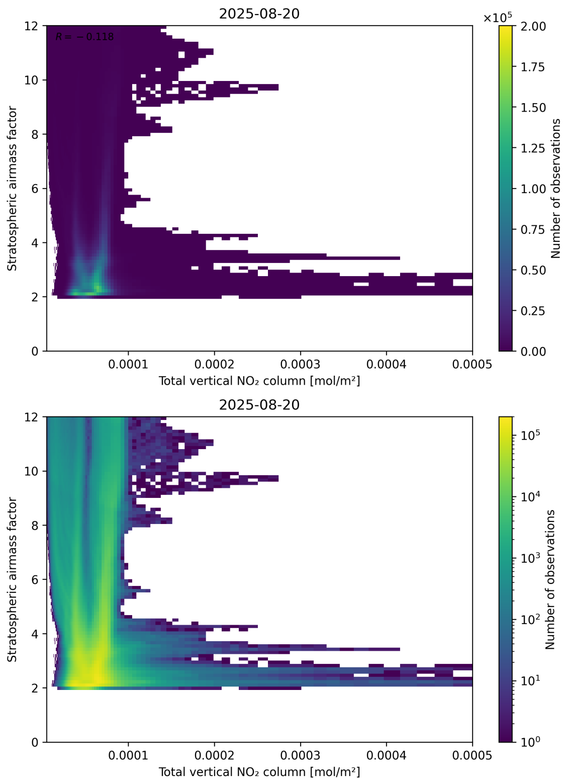
Figure 110: Scatter density plot of “Total vertical NO 2 column” against “Stratospheric airmass factor” for 2025-08-19 to 2025-08-21.
