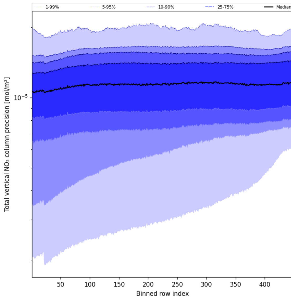
Figure 56: Along track statistics of “Total vertical NO 2 column precision” for 2025-08-19 to 2025-08-21
