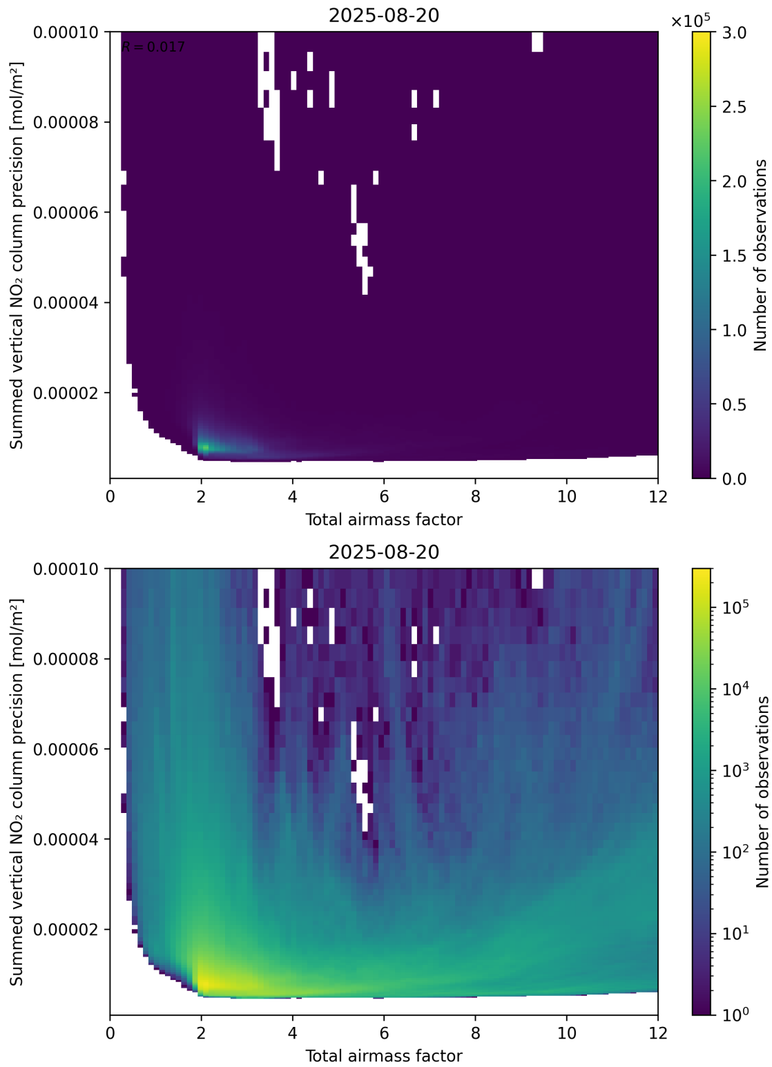
Figure 66: Scatter density plot of “Total airmass factor” against “Summed vertical NO 2 column precision” for 2025-08-19 to 2025-08-21.
