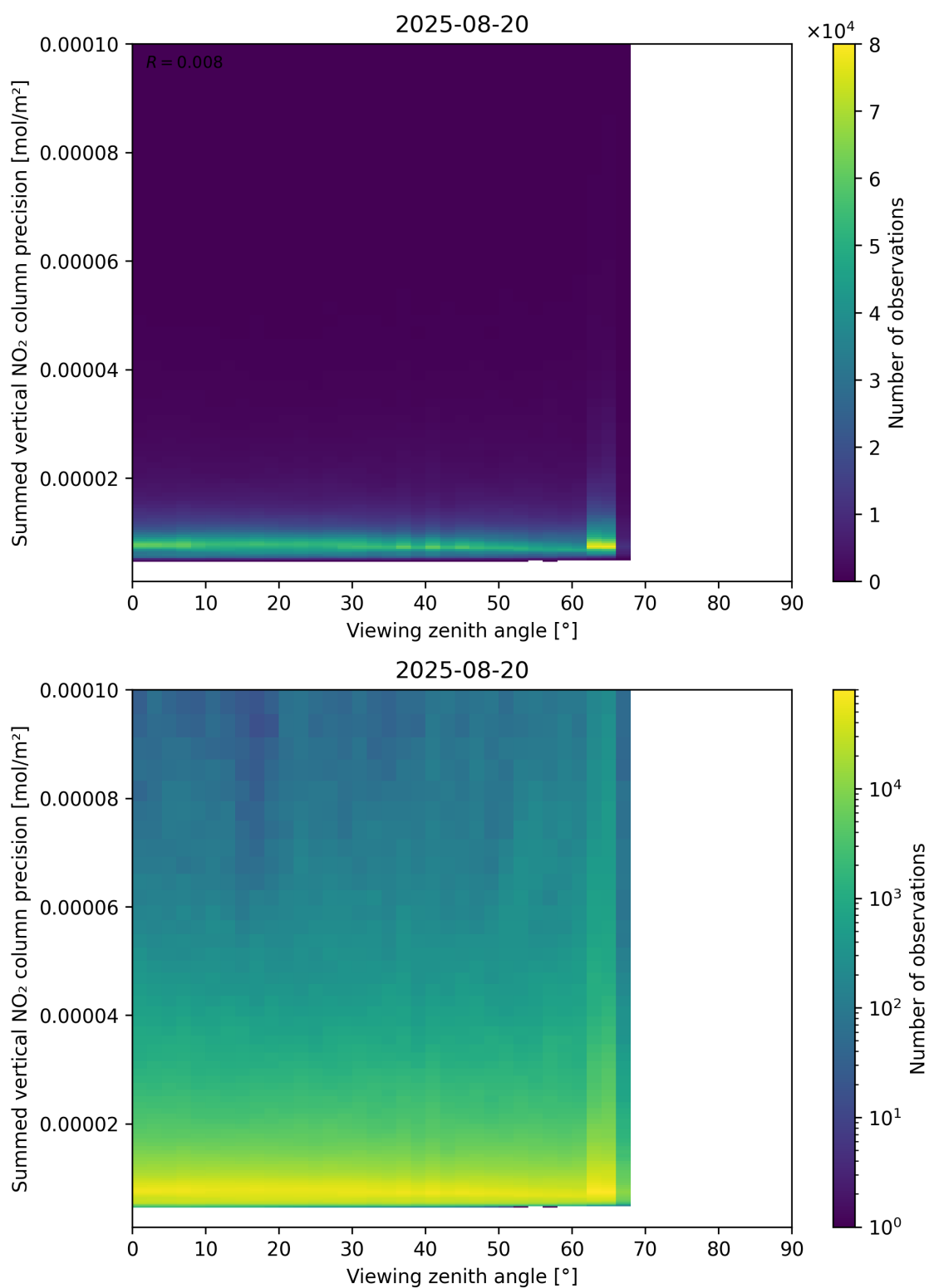
Figure 166: Scatter density plot of “Viewing zenith angle” against “Summed vertical NO 2 column precision” for 2025-08-19 to 2025-08-21.
