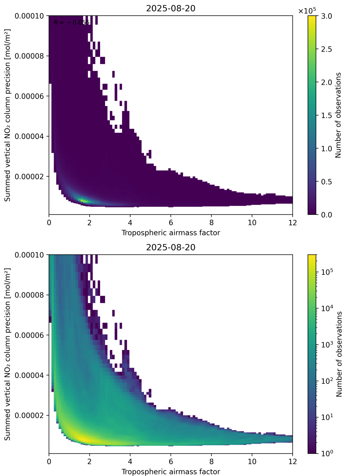
Figure 76: Scatter density plot of “Tropospheric airmass factor” against “Summed vertical NO 2 column precision” for 2025-08-19 to 2025-08-21.
