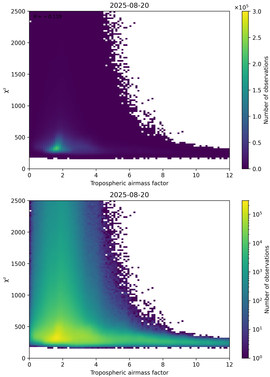
Figure 73: Scatter density plot of “Tropospheric airmass factor” against “ \chi^2 ” for 2025-08-19 to 2025-08-21.
