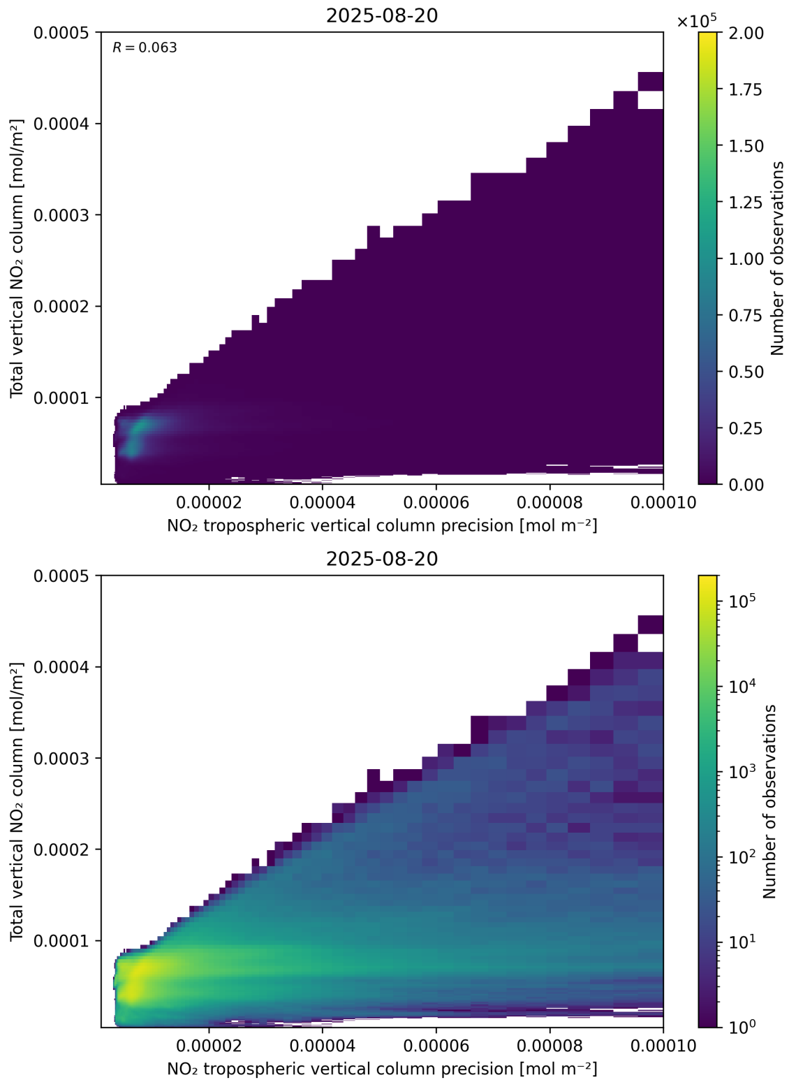
Figure 138: Scatter density plot of “NO 2 tropospheric vertical column precision” against “Total vertical NO 2 column” for 2025-08-19 to 2025-08-21.
