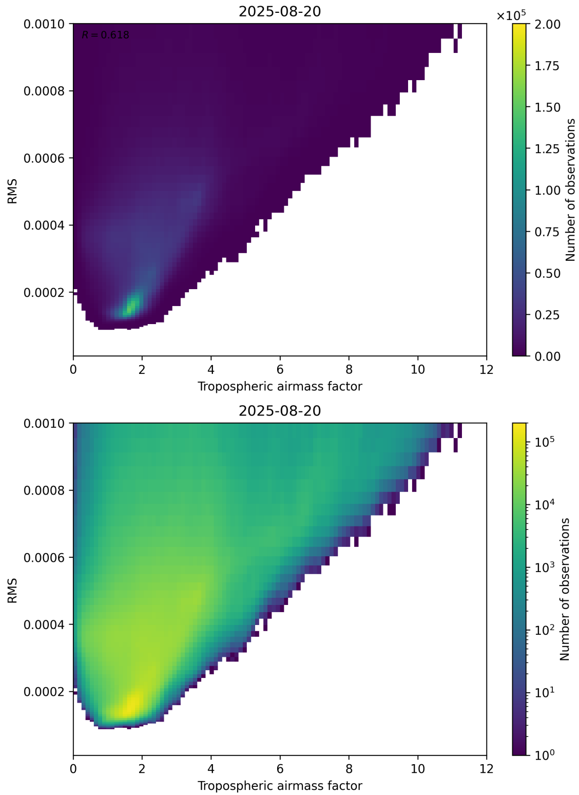
Figure 79: Scatter density plot of “Tropospheric airmass factor” against “RMS” for 2025-08-19 to 2025-08-21.
