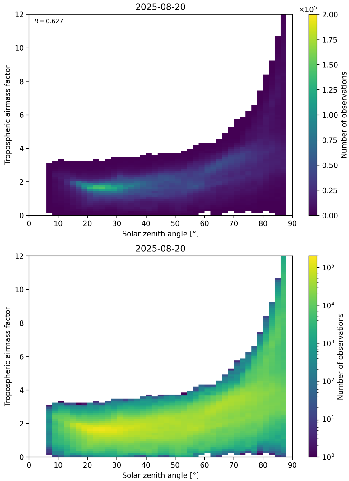
Figure 147: Scatter density plot of “Solar zenith angle” against “Tropospheric airmass factor” for 2025-08-19 to 2025-08-21.
