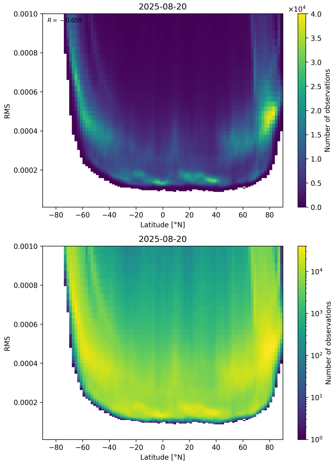
Figure 94: Scatter density plot of “Latitude” against “RMS” for 2025-08-19 to 2025-08-21.
