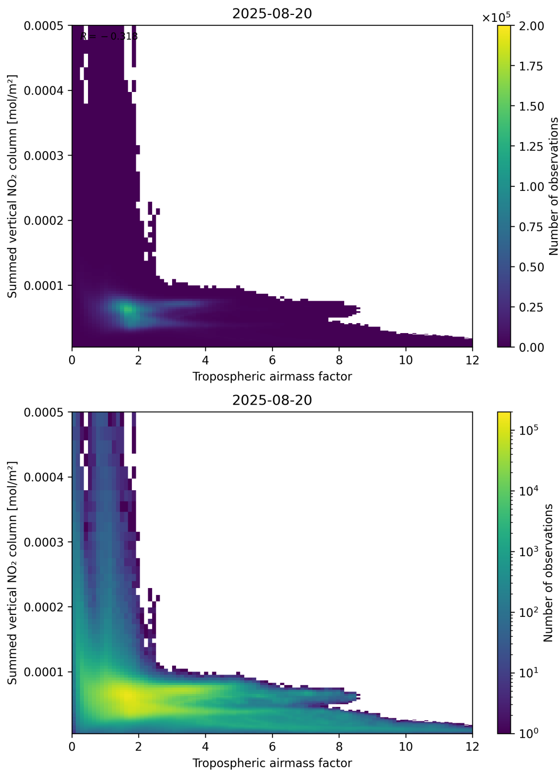
Figure 75: Scatter density plot of “Tropospheric airmass factor” against “Summed vertical NO 2 column” for 2025-08-19 to 2025-08-21.
