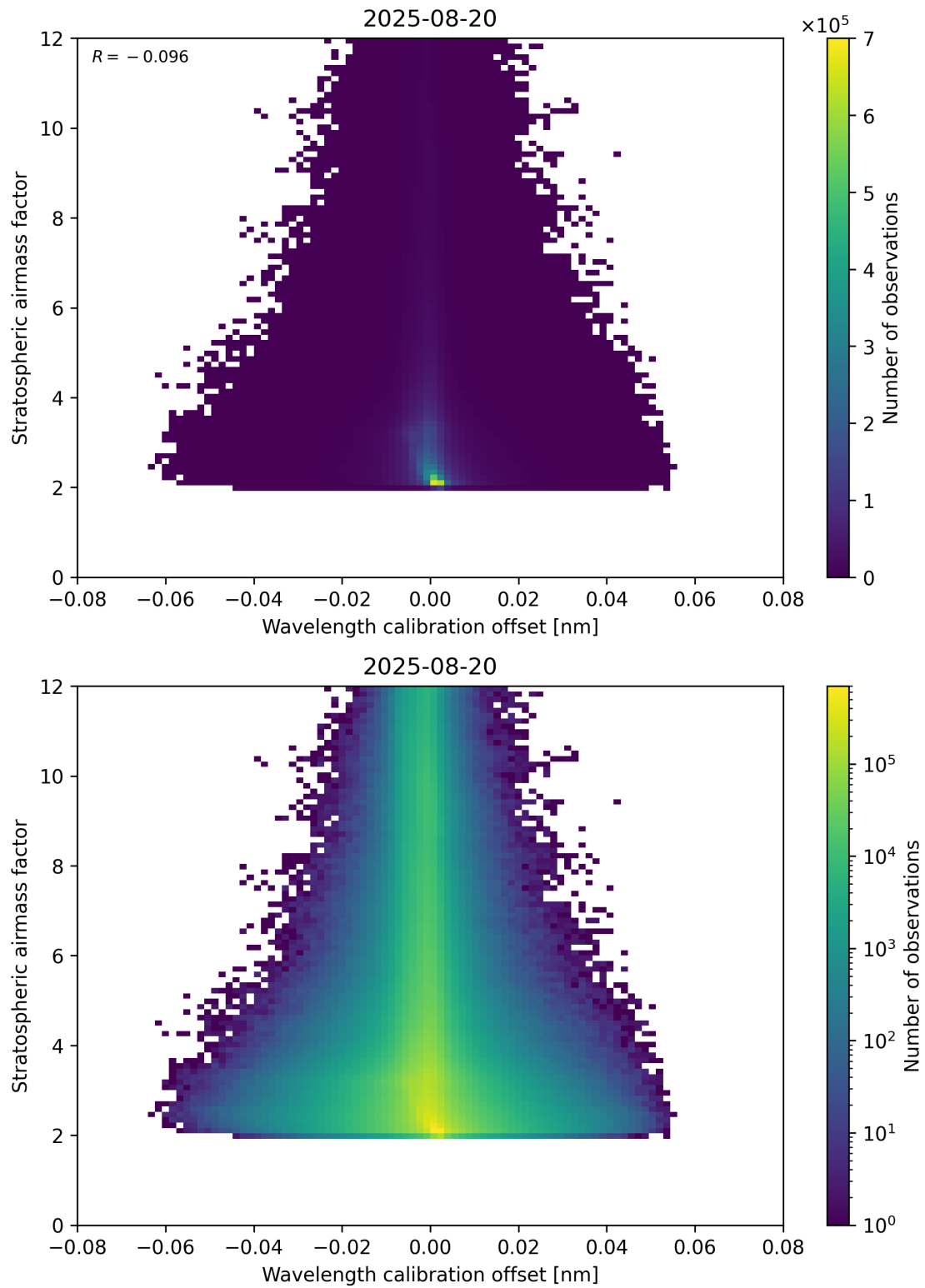
Figure 174: Scatter density plot of “Wavelength calibration offset” against “Stratospheric airmass factor” for 2025-08-19 to 2025-08-21.
