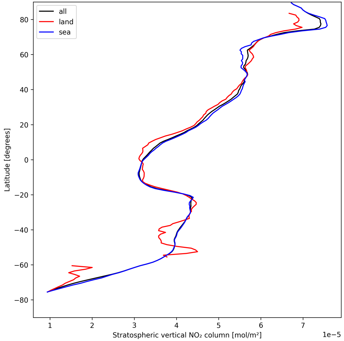
Figure 19: Zonal average of “Stratospheric vertical NO 2 column” for 2025-08-19 to 2025-08-21.
