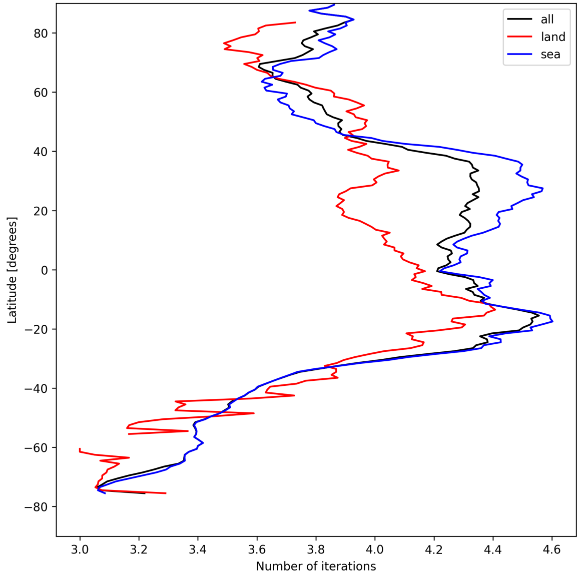
Figure 17: Zonal average of “Number of iterations” for 2025-08-19 to 2025-08-21.
