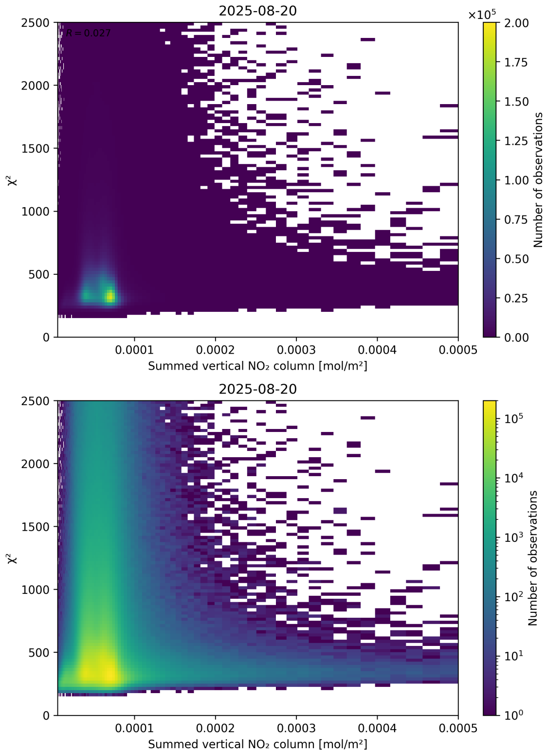
Figure 104: Scatter density plot of “Summed vertical NO 2 column” against “ \chi^2 ” for 2025-08-19 to 2025-08-21.
