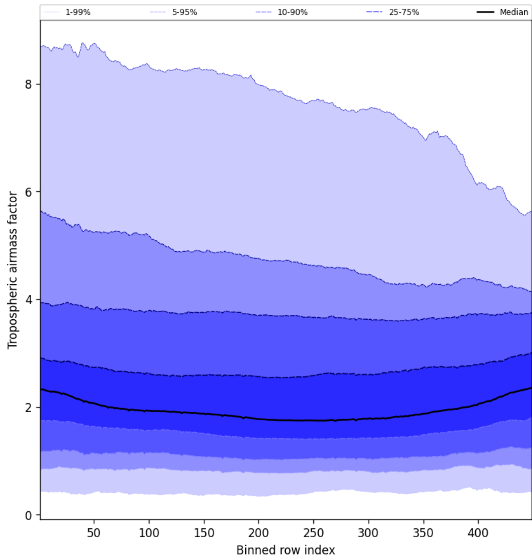
Figure 48: Along track statistics of “Tropospheric air mass factor” for 2025-08-19 to 2025-08-21
