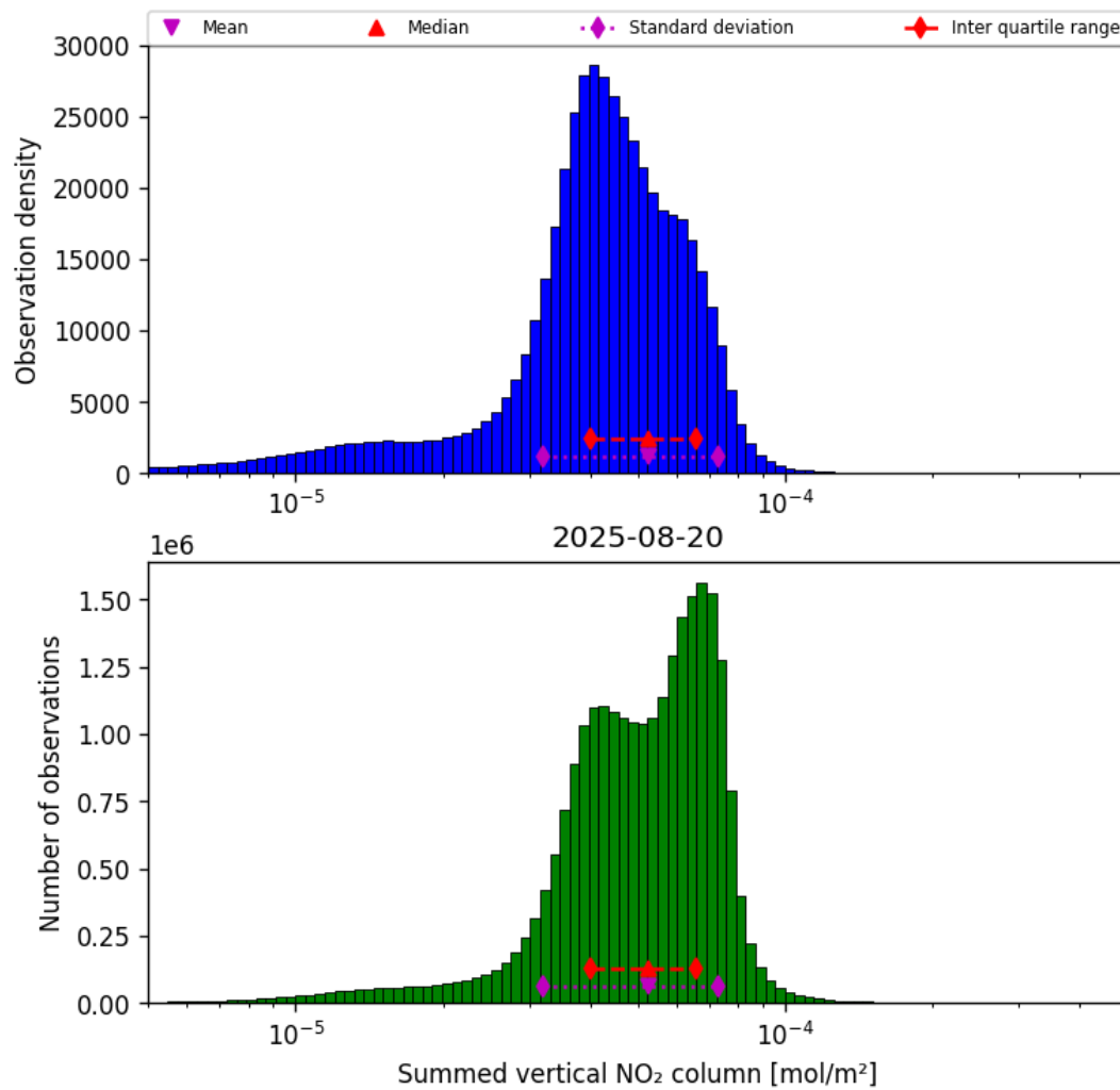
Figure 40: Histogram of “Summed vertical NO 2 column” for 2025-08-19 to 2025-08-21
