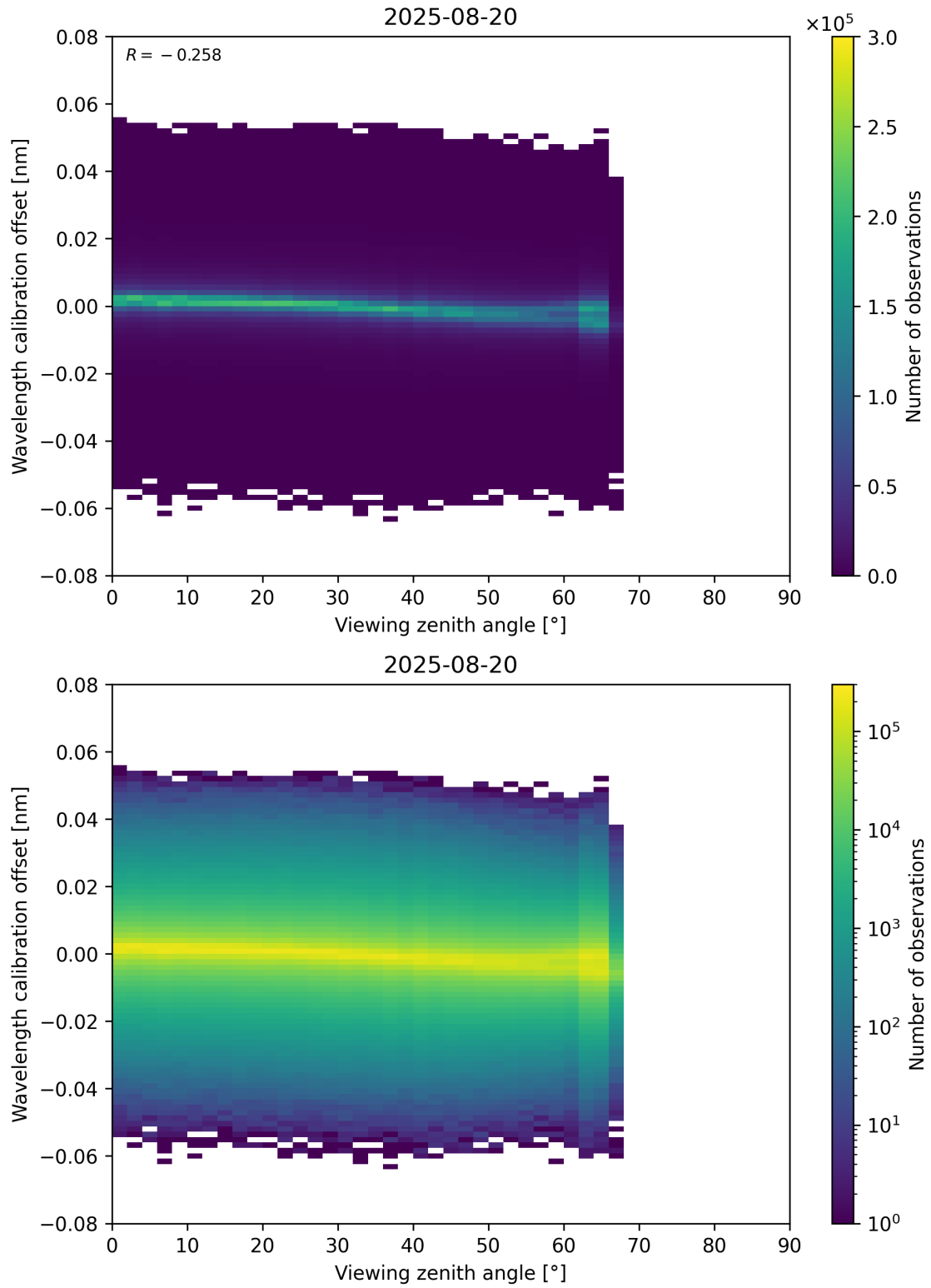
Figure 173: Scatter density plot of “Viewing zenith angle” against “Wavelength calibration offset” for 2025-08-19 to 2025-08-21.
