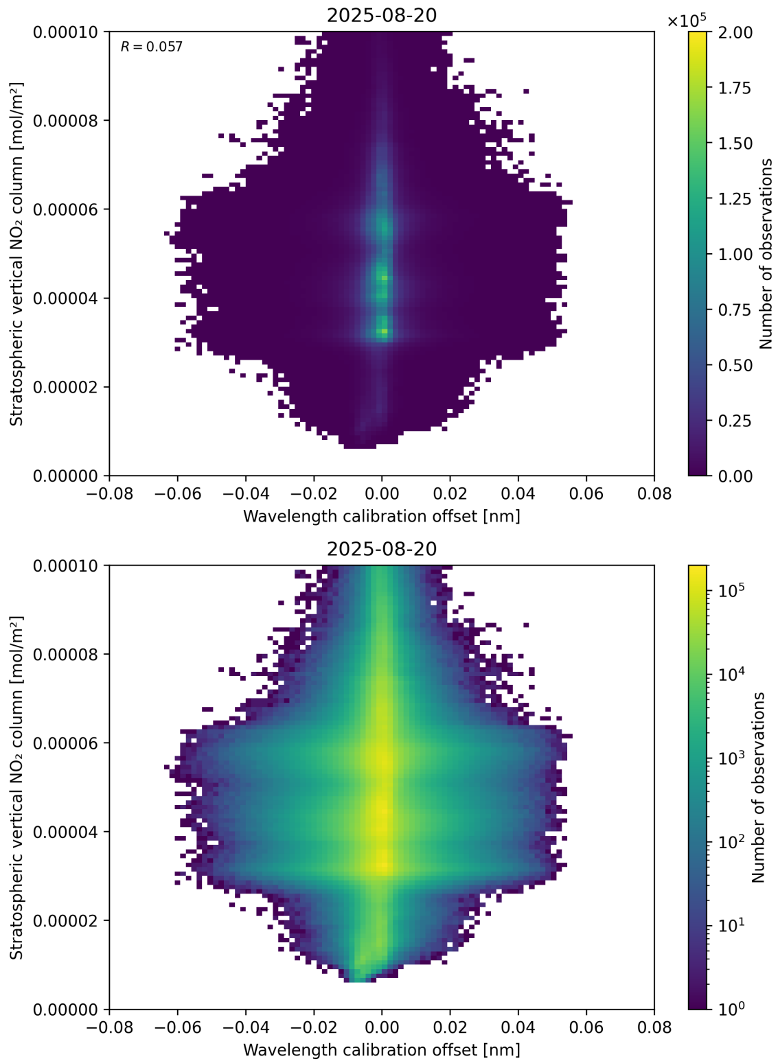
Figure 176: Scatter density plot of “Wavelength calibration offset” against “Stratospheric vertical NO 2 column” for 2025-08-19 to 2025-08-21.
