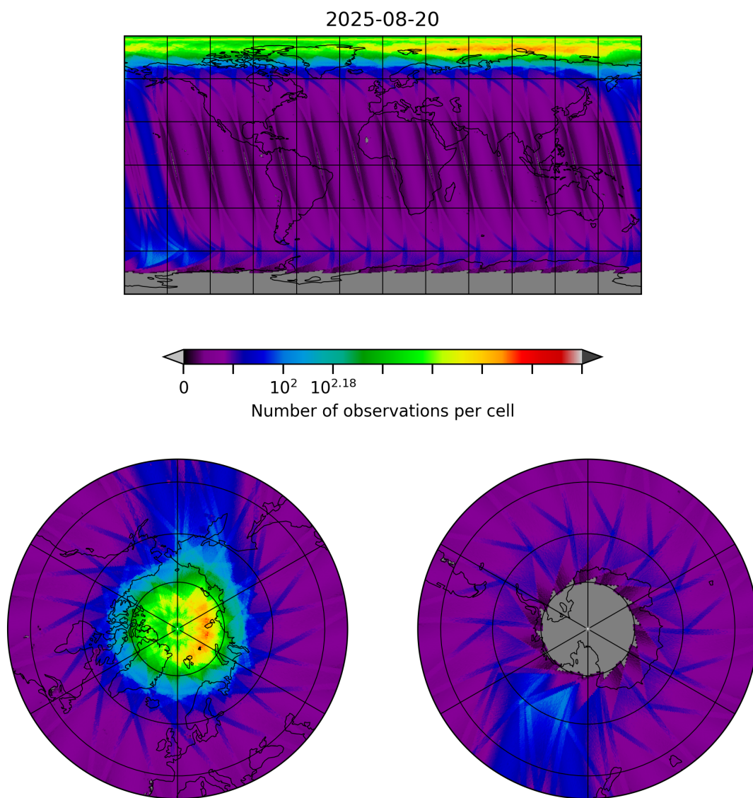
Figure 10: Map of the number of observations for 2025-08-19 to 2025-08-21
