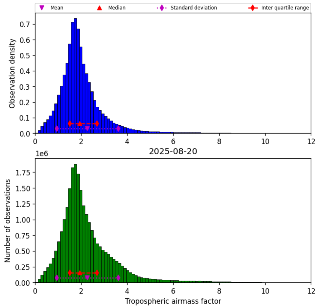
Figure 31: Histogram of “Tropospheric airmass factor” for 2025-08-19 to 2025-08-21
