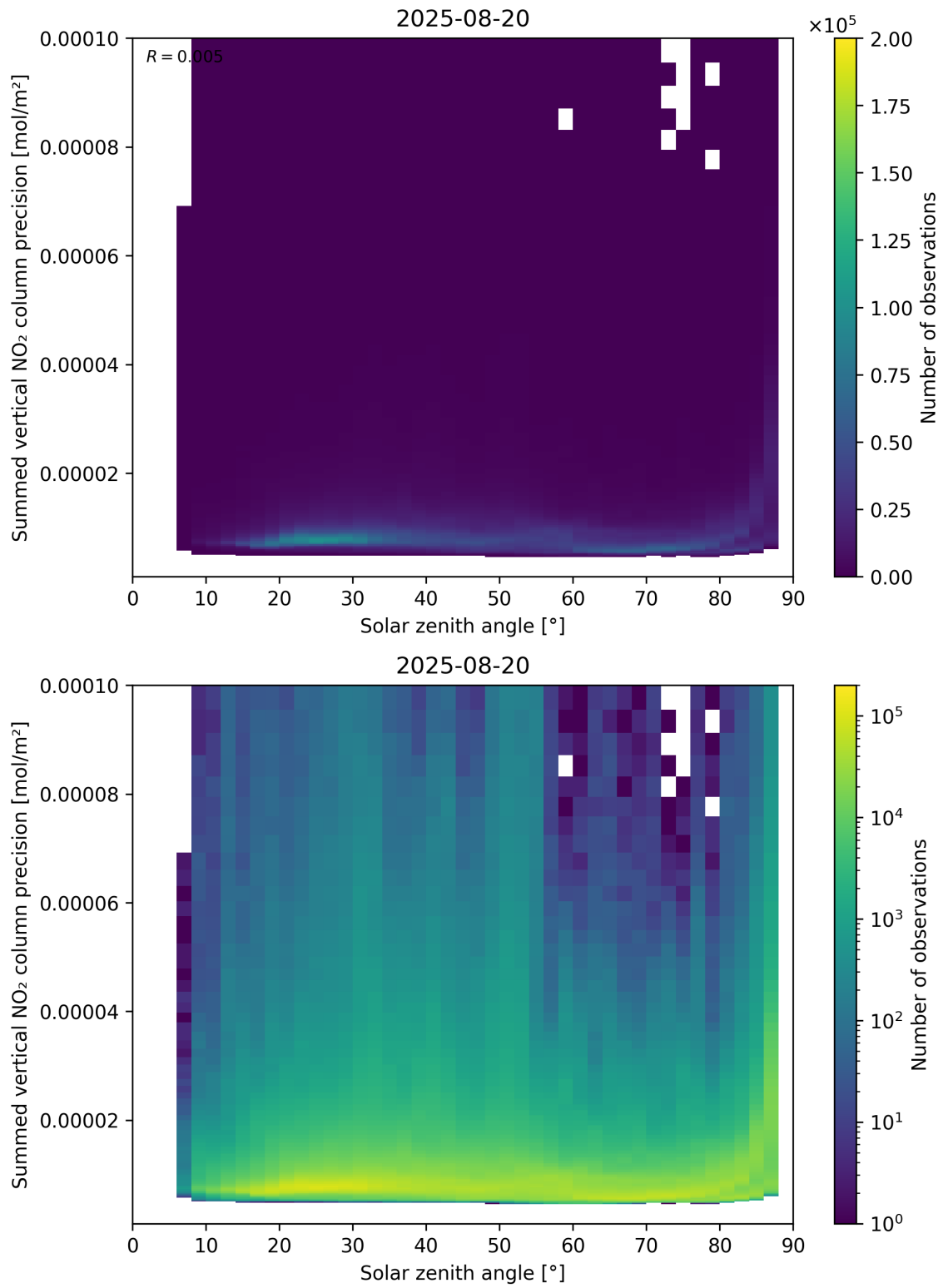
Figure 152: Scatter density plot of “Solar zenith angle” against “Summed vertical NO 2 column precision” for 2025-08-19 to 2025-08-21.
