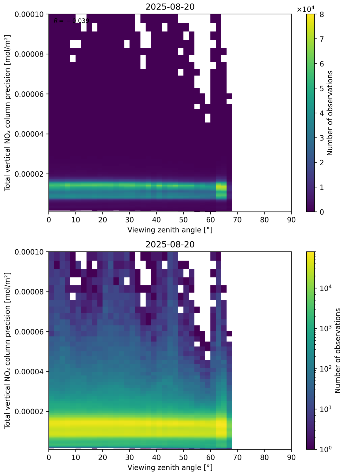
Figure 168: Scatter density plot of “Viewing zenith angle” against “Total vertical NO 2 column precision” for 2025-08-19 to 2025-08-21.
