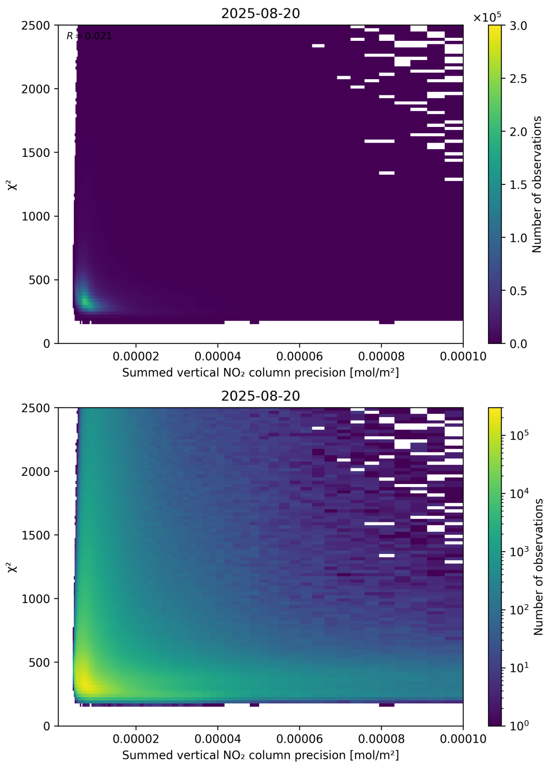
Figure 107: Scatter density plot of “Summed vertical NO 2 column precision” against “ \chi^2 ” for 2025-08-19 to 2025-08-21.
