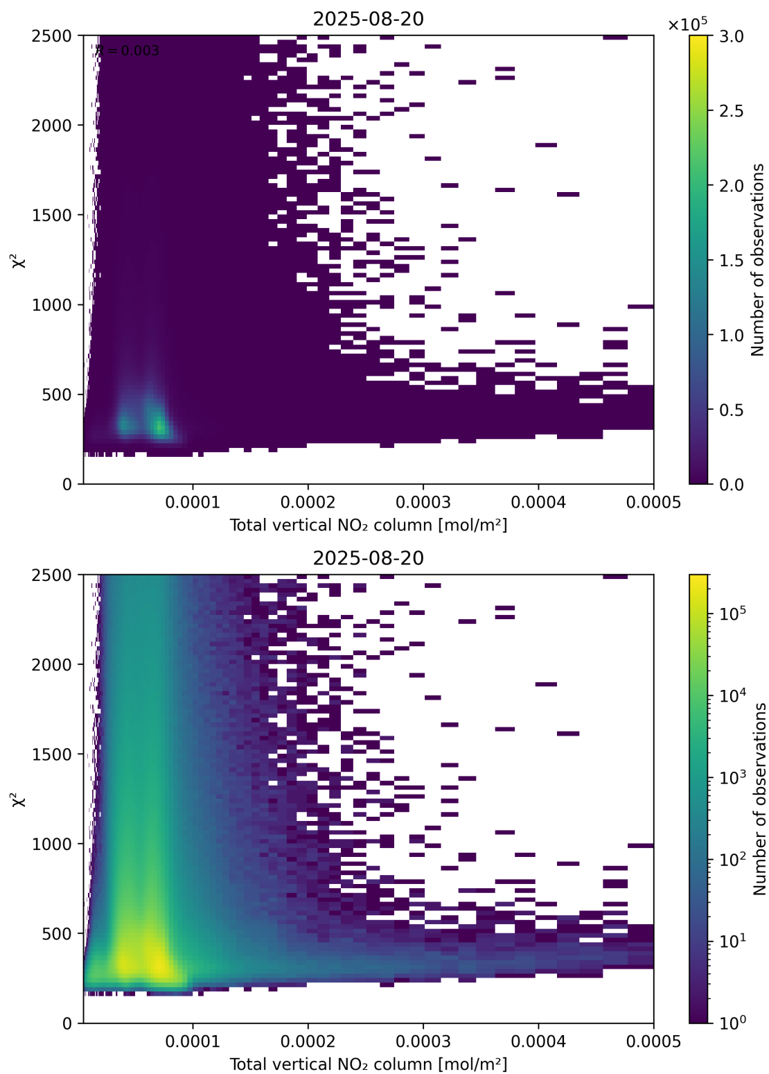
Figure 111: Scatter density plot of “Total vertical NO 2 column” against “ \chi^2 ” for 2025-08-19 to 2025-08-21.
