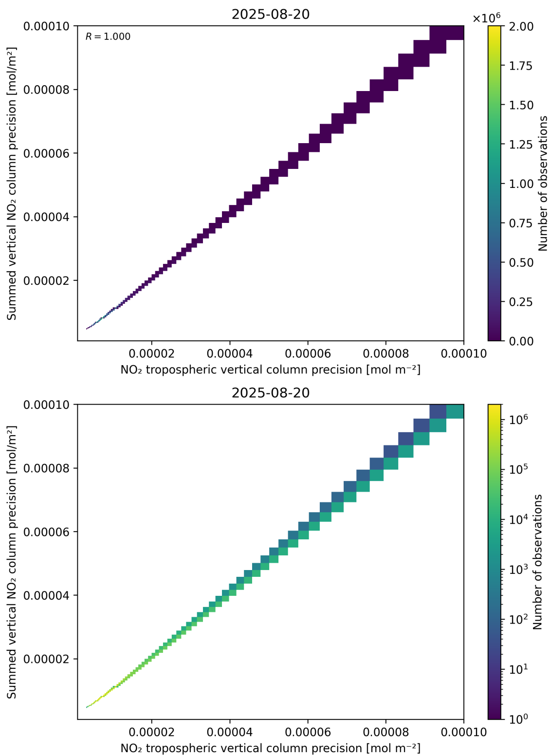
Figure 137: Scatter density plot of “NO 2 tropospheric vertical column precision” against “Summed vertical NO 2 column precision” for 2025-08-19 to 2025-08-21.
