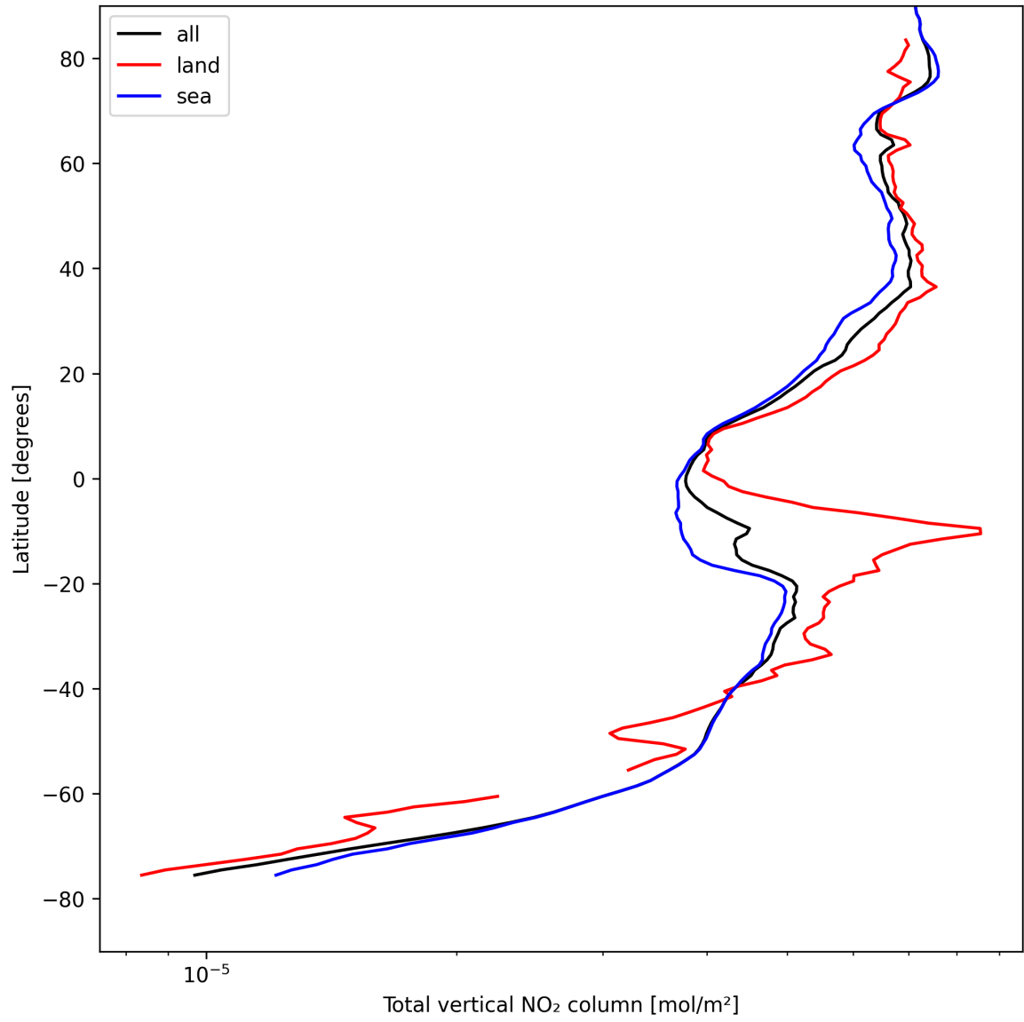
Figure 21: Zonal average of “Total vertical NO 2 column” for 2025-08-19 to 2025-08-21.
