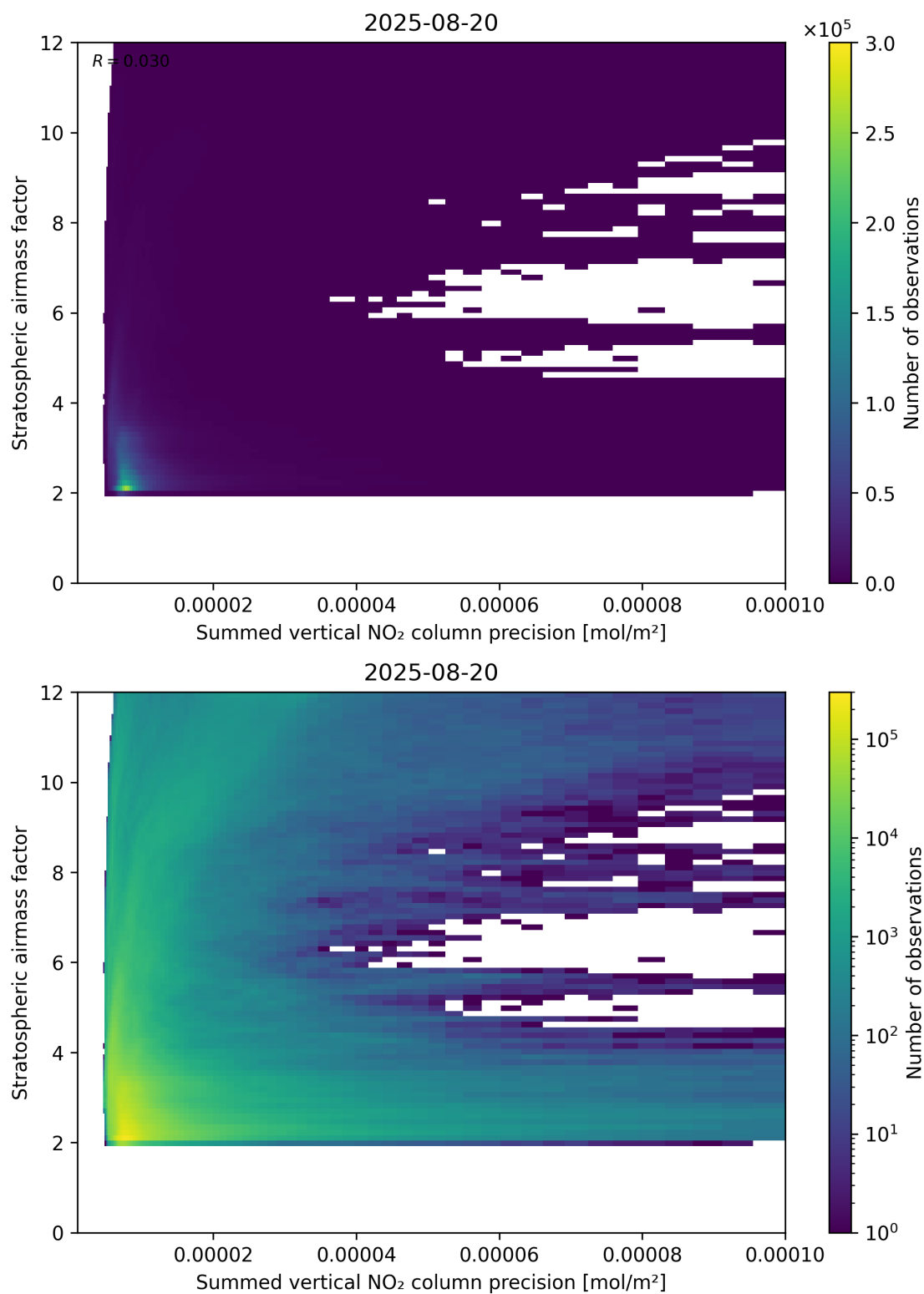
Figure 106: Scatter density plot of “Summed vertical NO 2 column precision” against “Stratospheric airmass factor” for 2025-08-19 to 2025-08-21.
