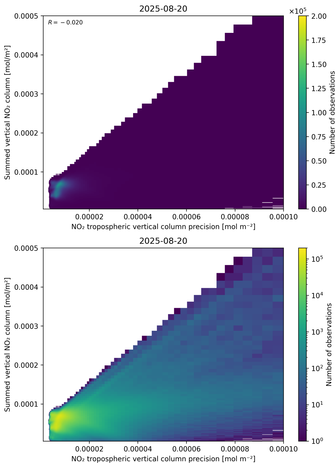
Figure 136: Scatter density plot of “NO 2 tropospheric vertical column precision” against “Summed vertical NO 2 column” for 2025-08-19 to 2025-08-21.
