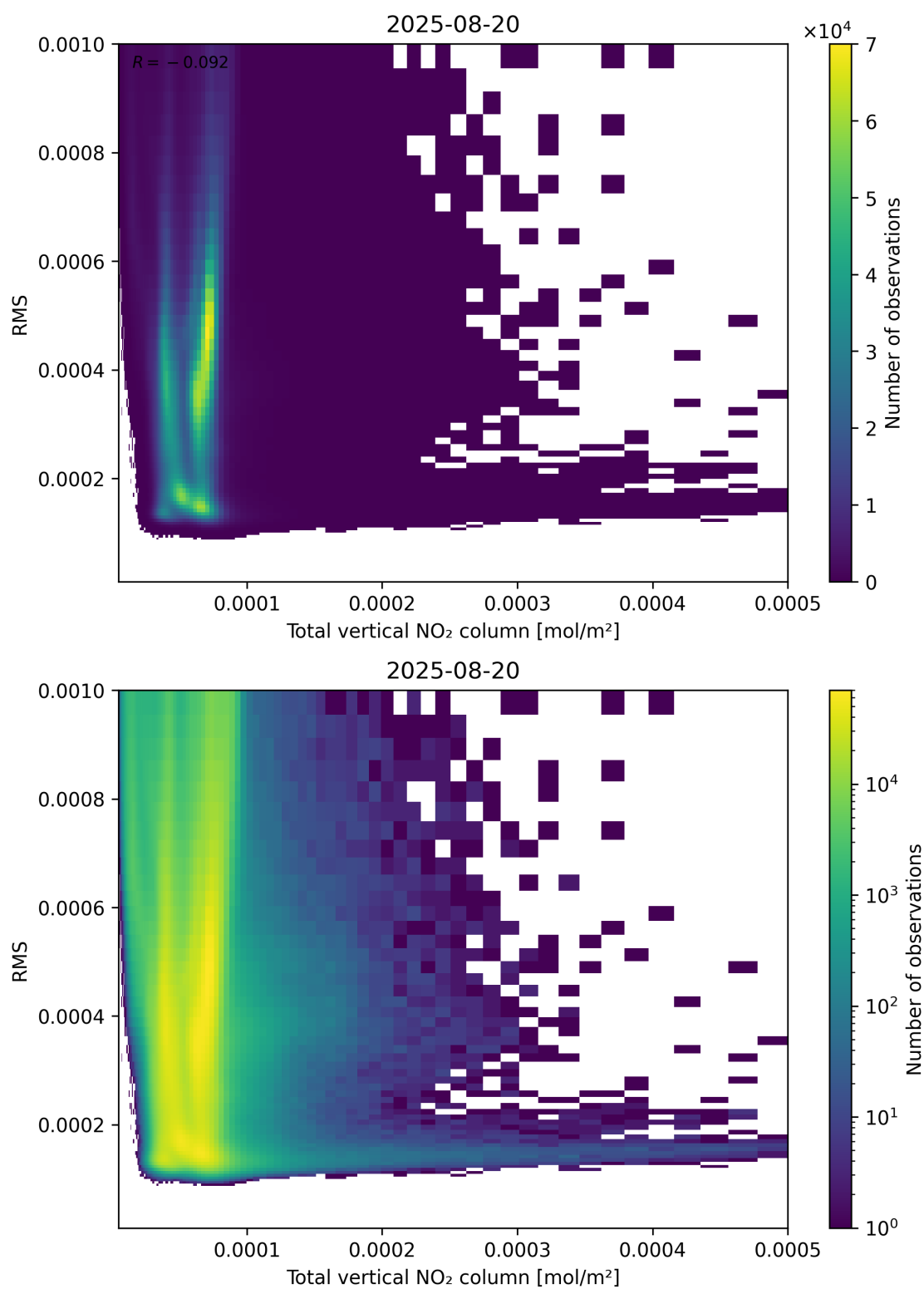
Figure 120: Scatter density plot of “Total vertical NO 2 column” against “RMS” for 2025-08-19 to 2025-08-21.
