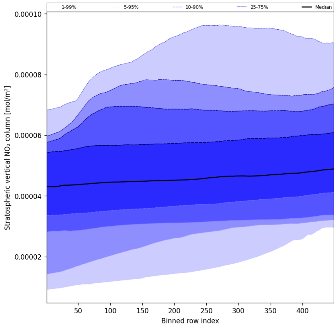
Figure 53: Along track statistics of “Stratospheric vertical NO 2 column” for 2025-08-19 to 2025-08-21
