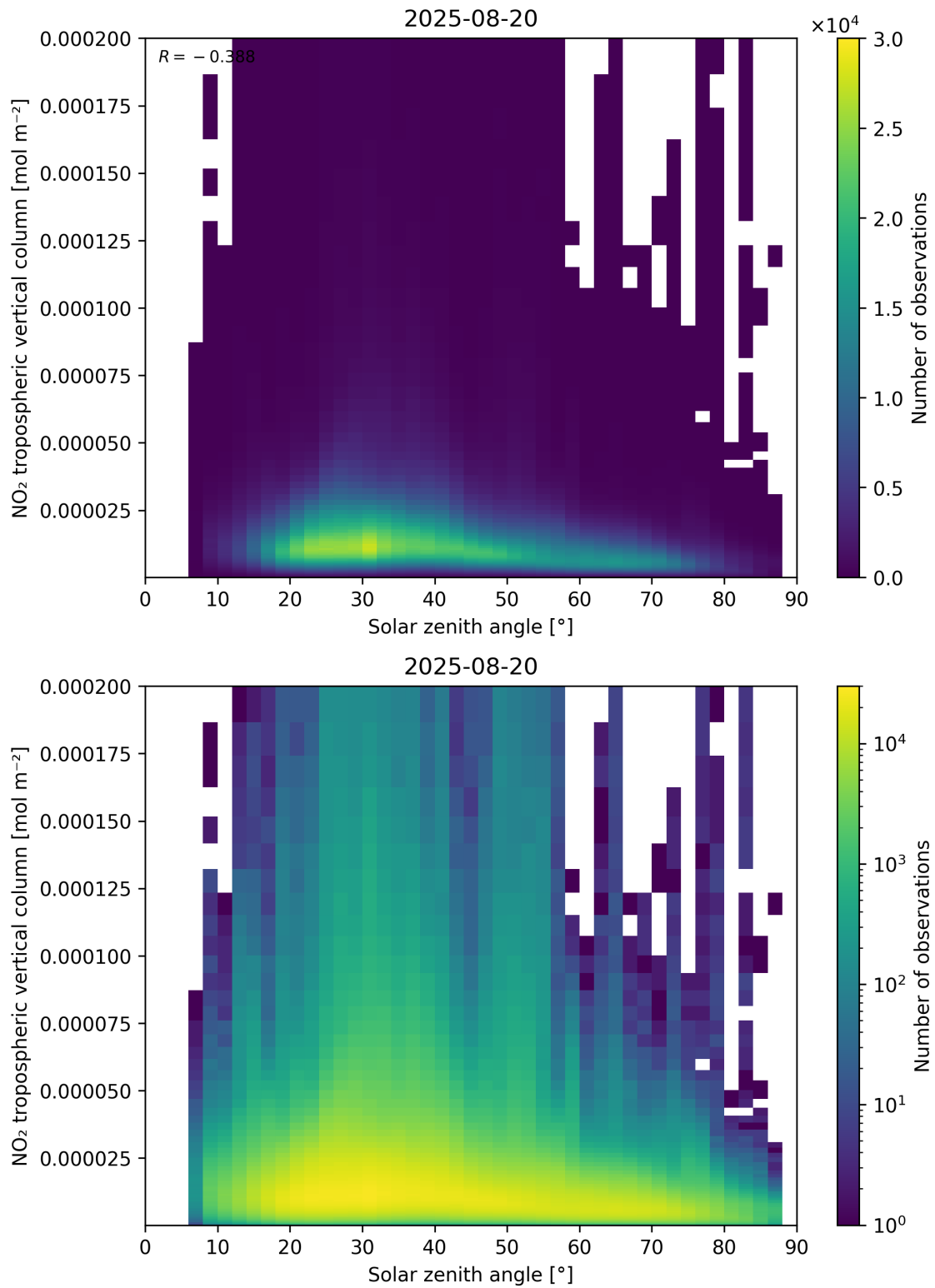
Figure 155: Scatter density plot of “Solar zenith angle” against “NO 2 tropospheric vertical column” for 2025-08-19 to 2025-08-21.
