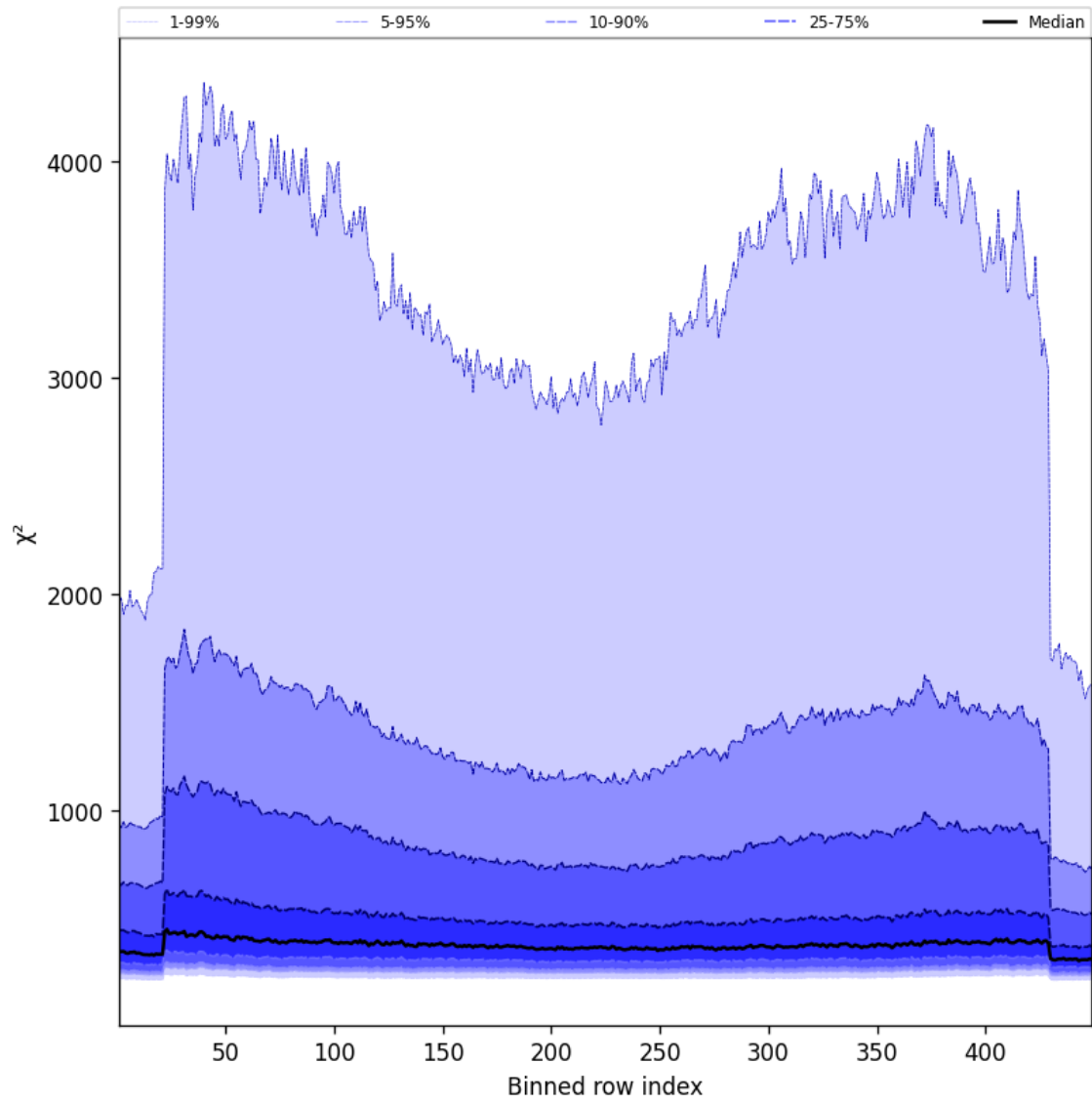
Figure 59: Along track statistics of “ \chi^2 ” for 2025-08-19 to 2025-08-21
