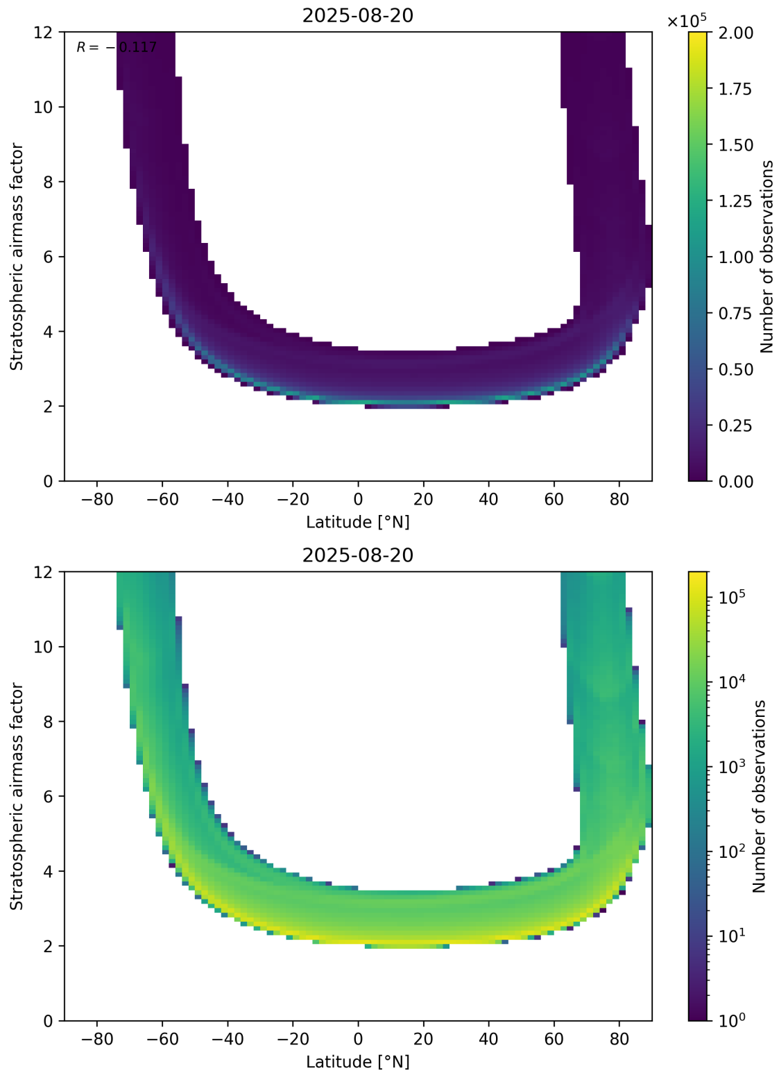
Figure 83: Scatter density plot of “Latitude” against “Stratospheric air mass factor” for 2025-08-19 to 2025-08-21.
