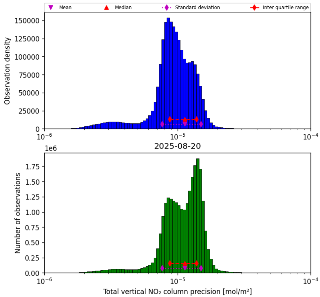
Figure 39: Histogram of “Total vertical NO 2 column precision” for 2025-08-19 to 2025-08-21
