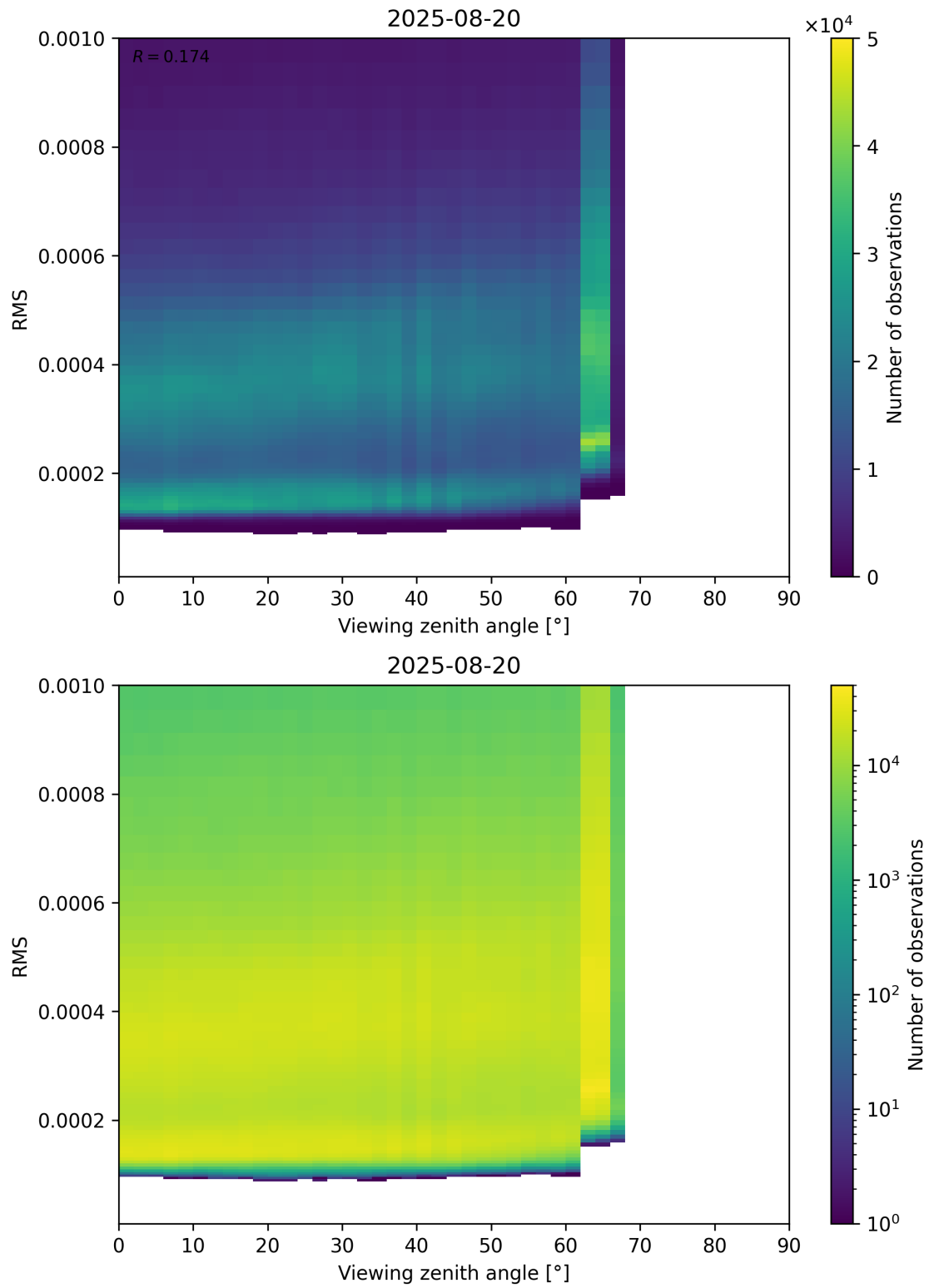
Figure 171: Scatter density plot of “Viewing zenith angle” against “RMS” for 2025-08-19 to 2025-08-21.
