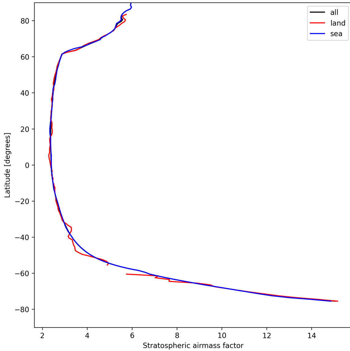
Figure 27: Zonal average of “Stratospheric airmass factor” for 2025-08-19 to 2025-08-21.
