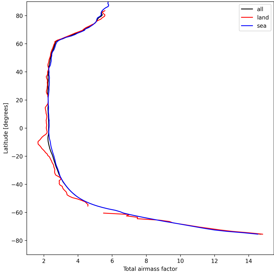
Figure 15: Zonal average of “Total airmass factor” for 2025-08-19 to 2025-08-21.
