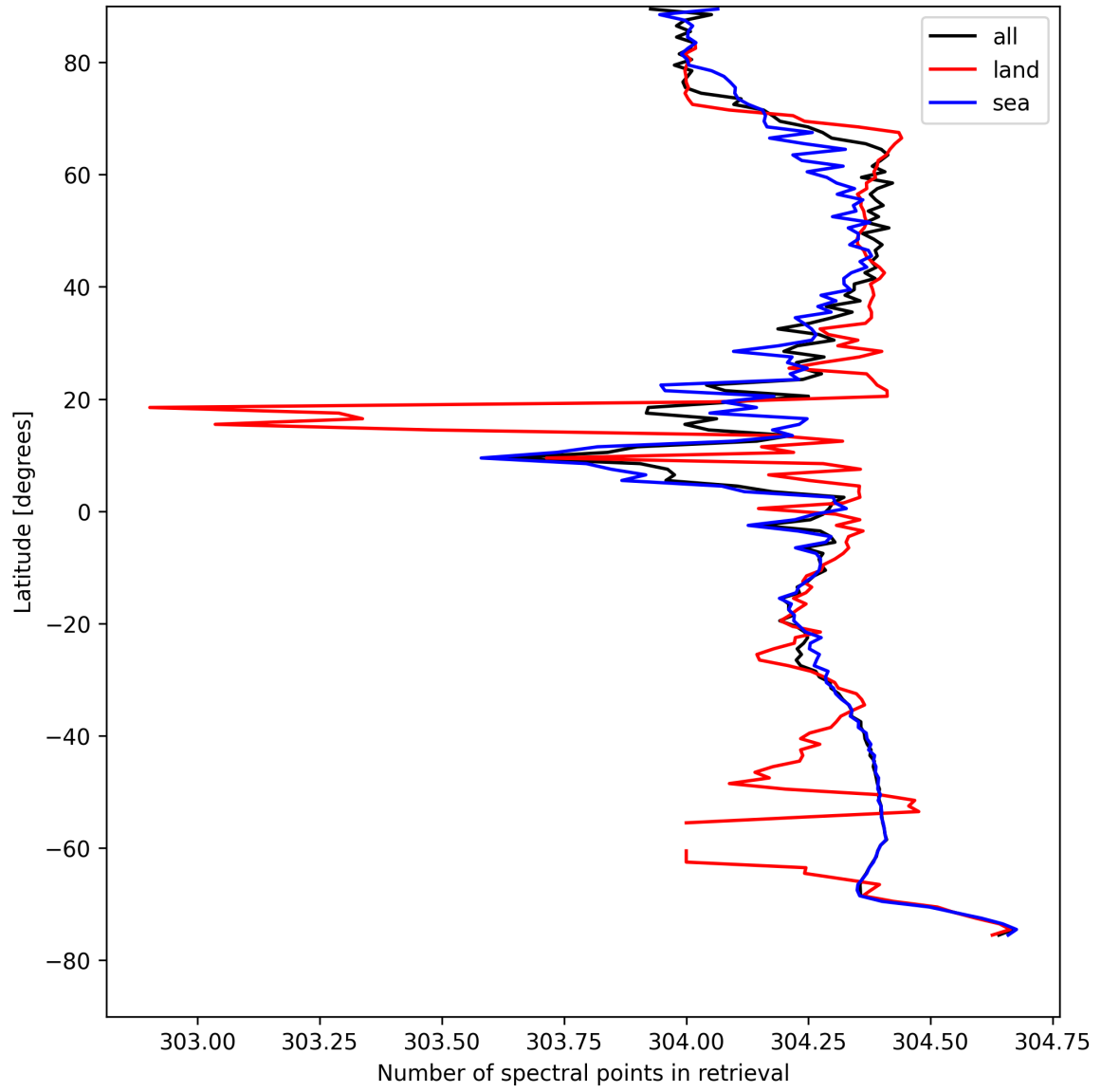
Figure 16: Zonal average of “Number of spectral points in retrieval” for 2025-08-19 to 2025-08-21.
