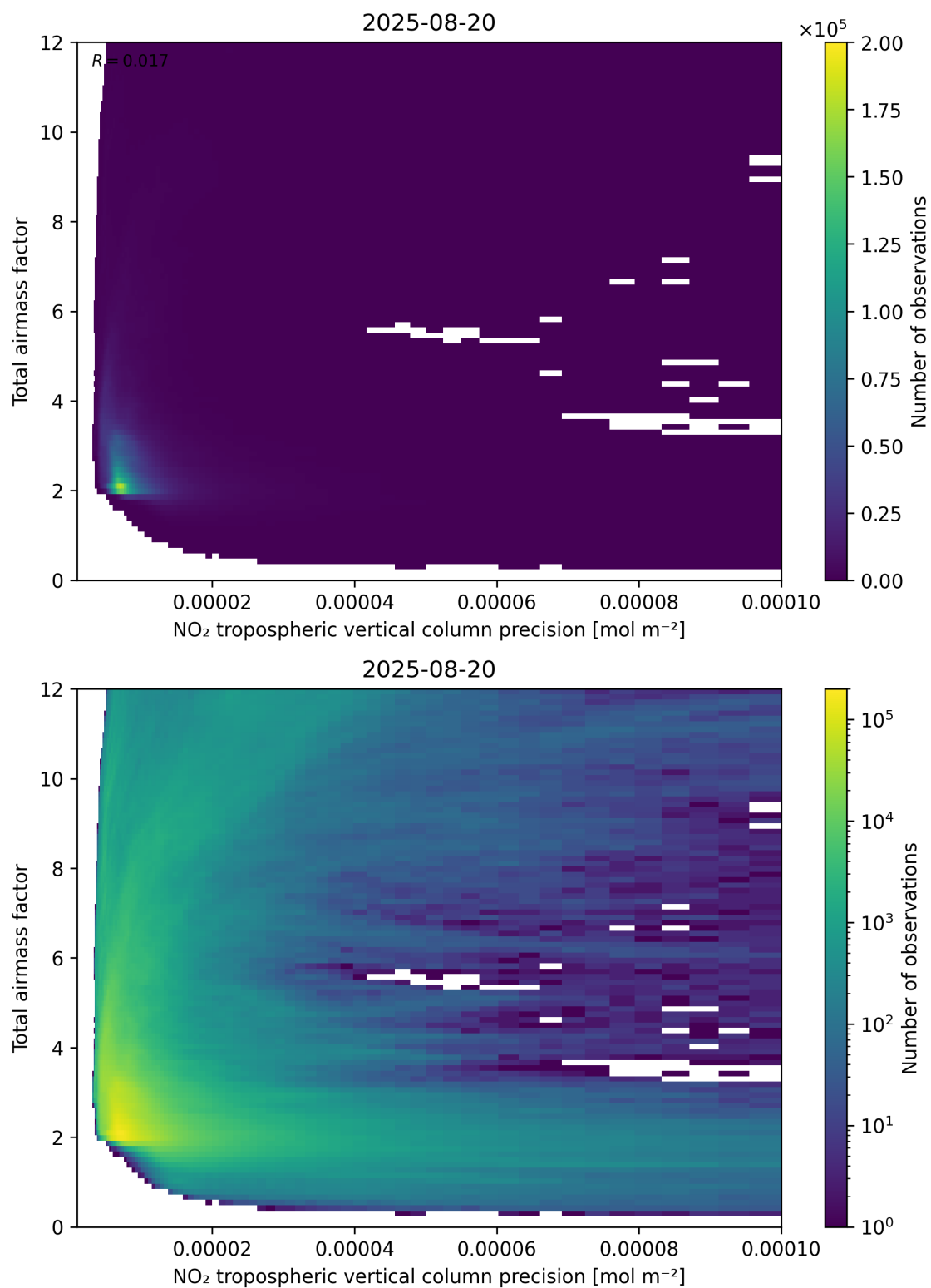
Figure 132: Scatter density plot of “NO 2 tropospheric vertical column precision” against “Total air mass factor” for 2025-08-19 to 2025-08-21.
