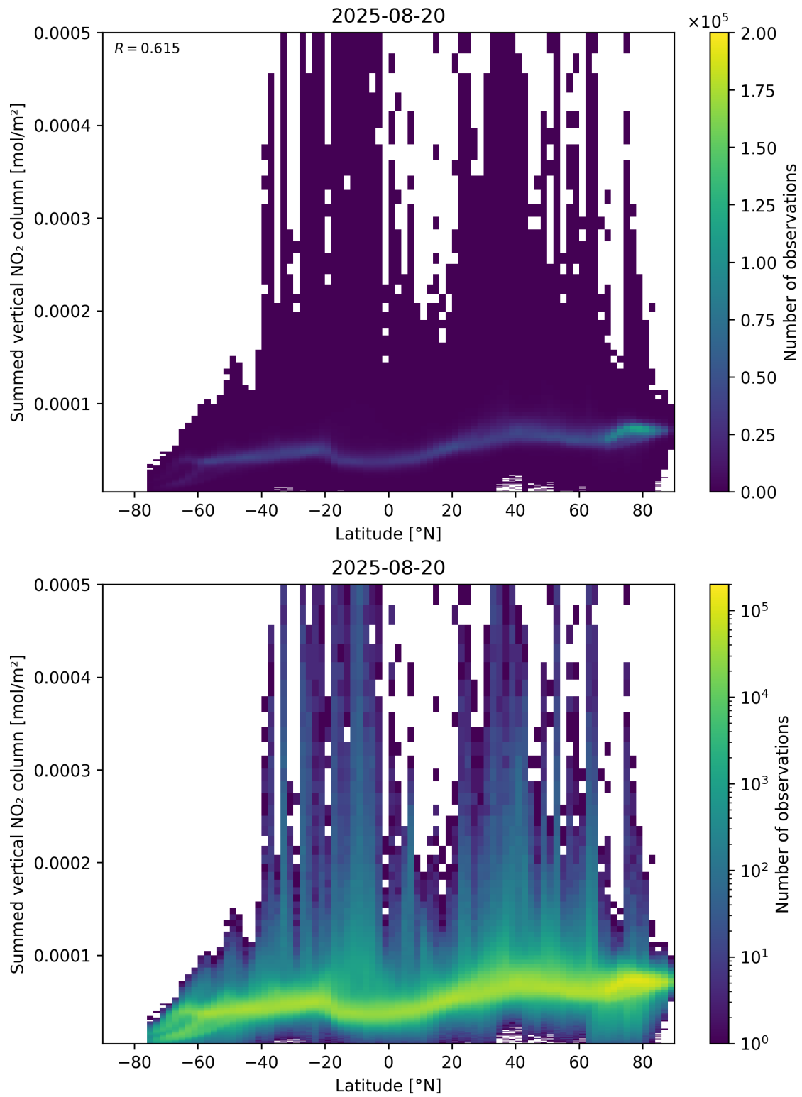
Figure 88: Scatter density plot of “Latitude” against “Summed vertical NO 2 column” for 2025-08-19 to 2025-08-21.
