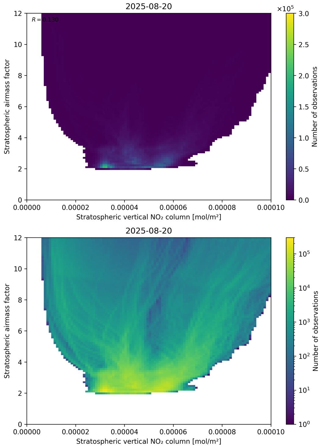
Figure 96: Scatter density plot of “Stratospheric vertical NO 2 column” against “Stratospheric airmass factor” for 2025-08-19 to 2025-08-21.
