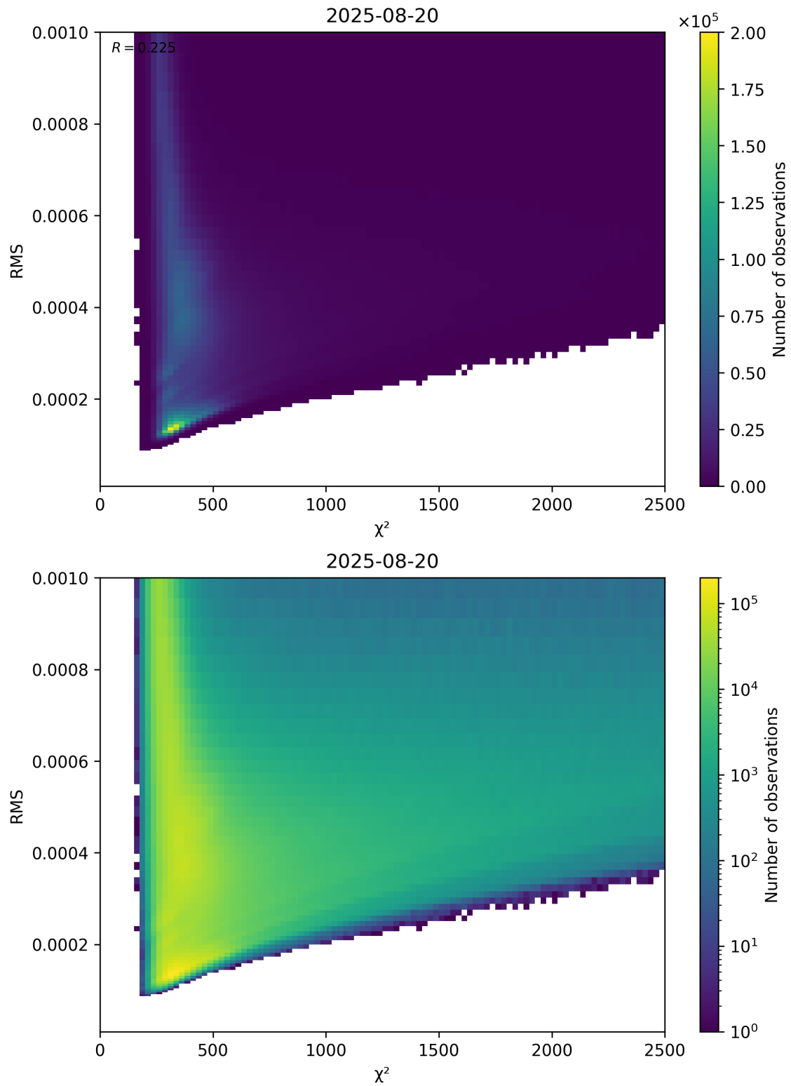
Figure 82: Scatter density plot of “ \chi^2 ” against “RMS” for 2025-08-19 to 2025-08-21.
