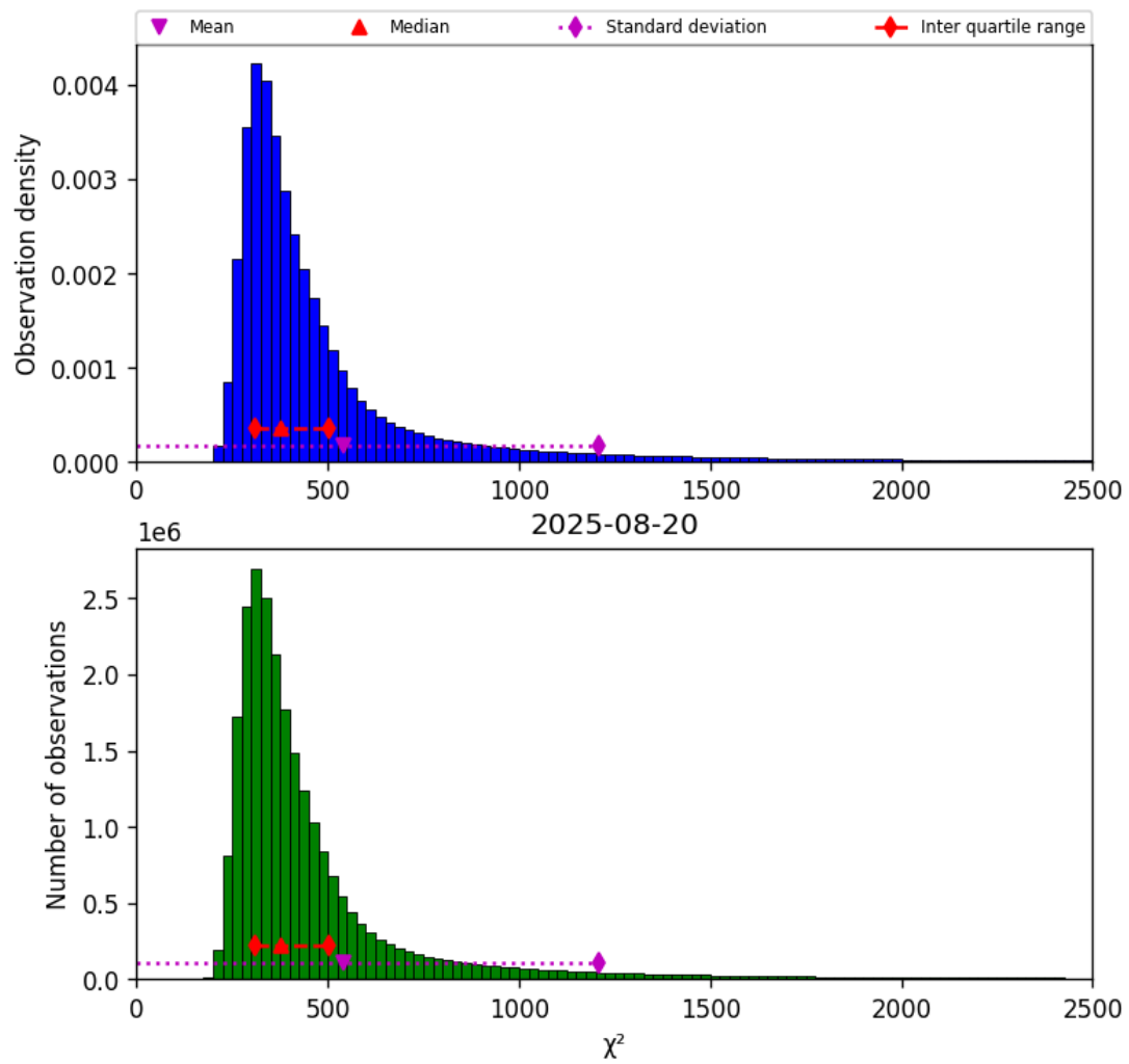
Figure 42: Histogram of “ \chi^2 ” for 2025-08-19 to 2025-08-21
