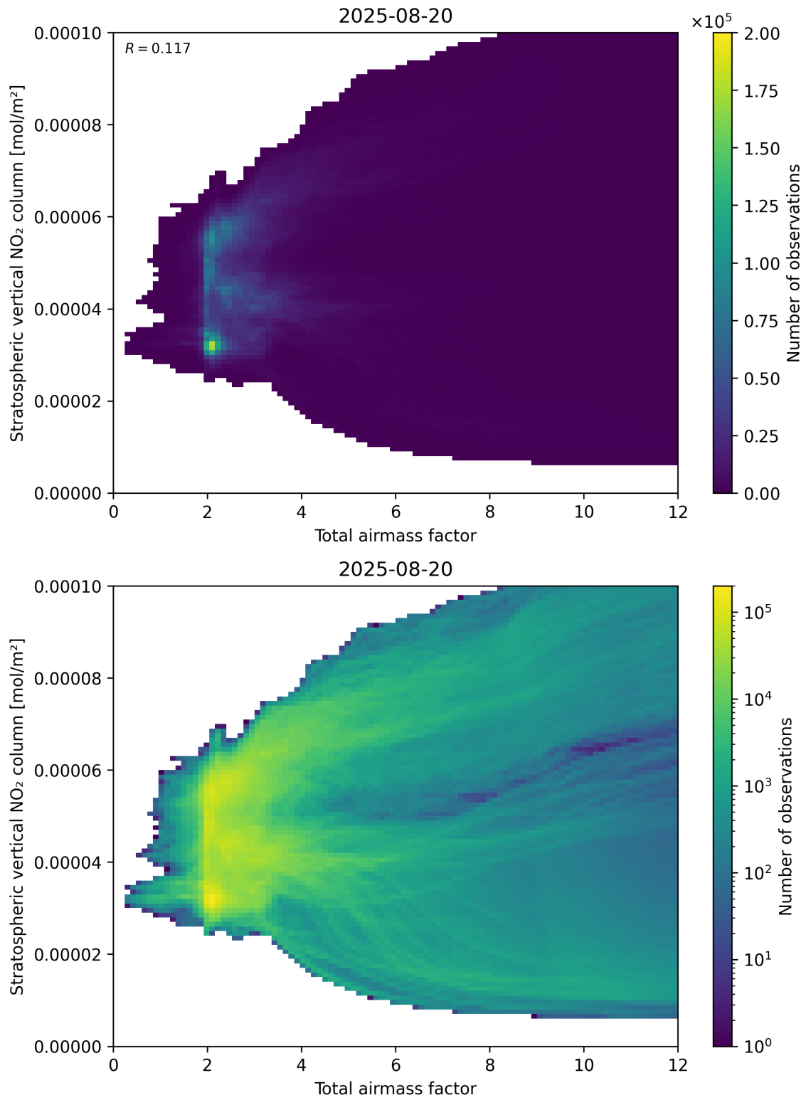
Figure 64: Scatter density plot of “Total airmass factor” against “Stratospheric vertical NO 2 column” for 2025-08-19 to 2025-08-21.
