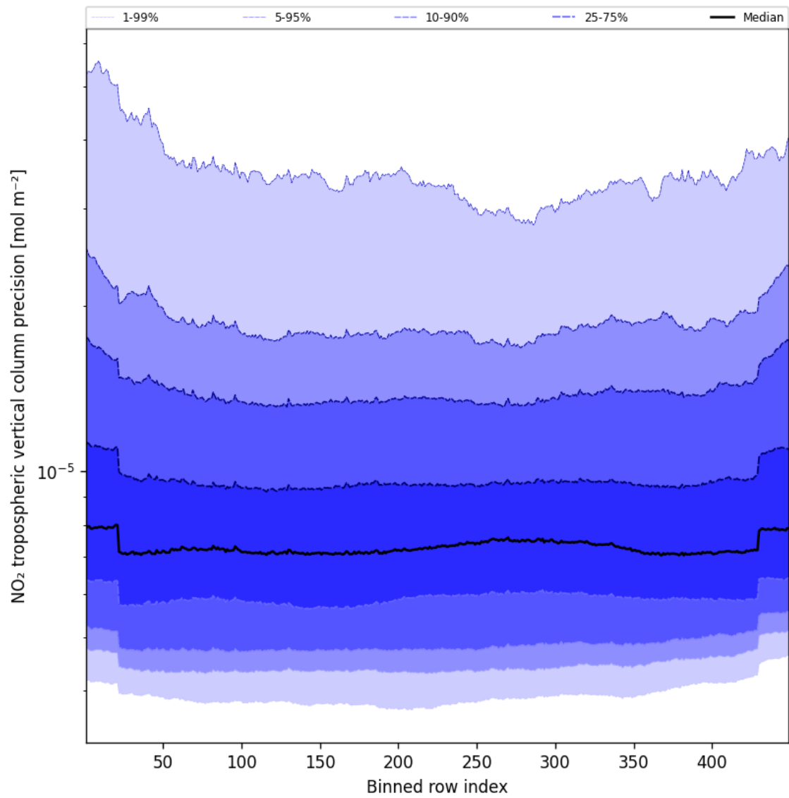
Figure 47: Along track statistics of “NO 2 tropospheric vertical column precision” for 2025-08-19 to 2025-08-21
