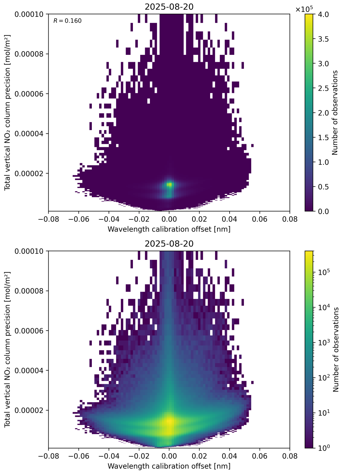
Figure 180: Scatter density plot of “Wavelength calibration offset” against “Total vertical NO 2 column precision” for 2025-08-19 to 2025-08-21.
