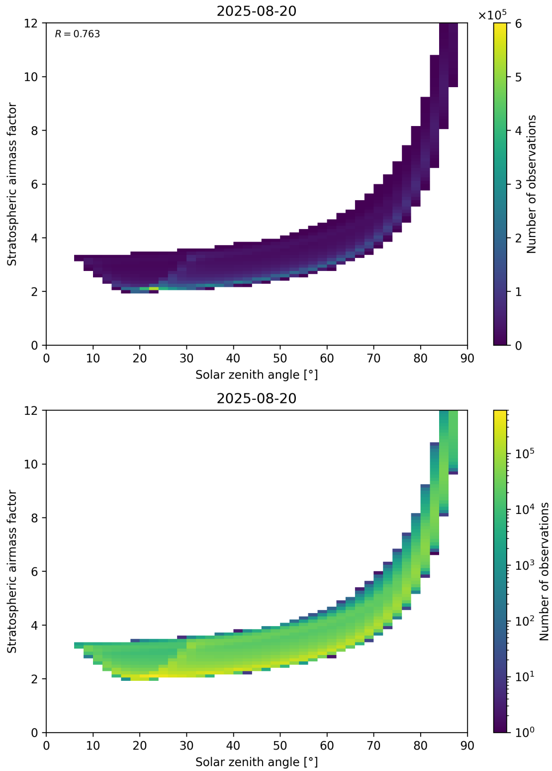
Figure 145: Scatter density plot of “Solar zenith angle” against “Stratospheric airmass factor” for 2025-08-19 to 2025-08-21.
