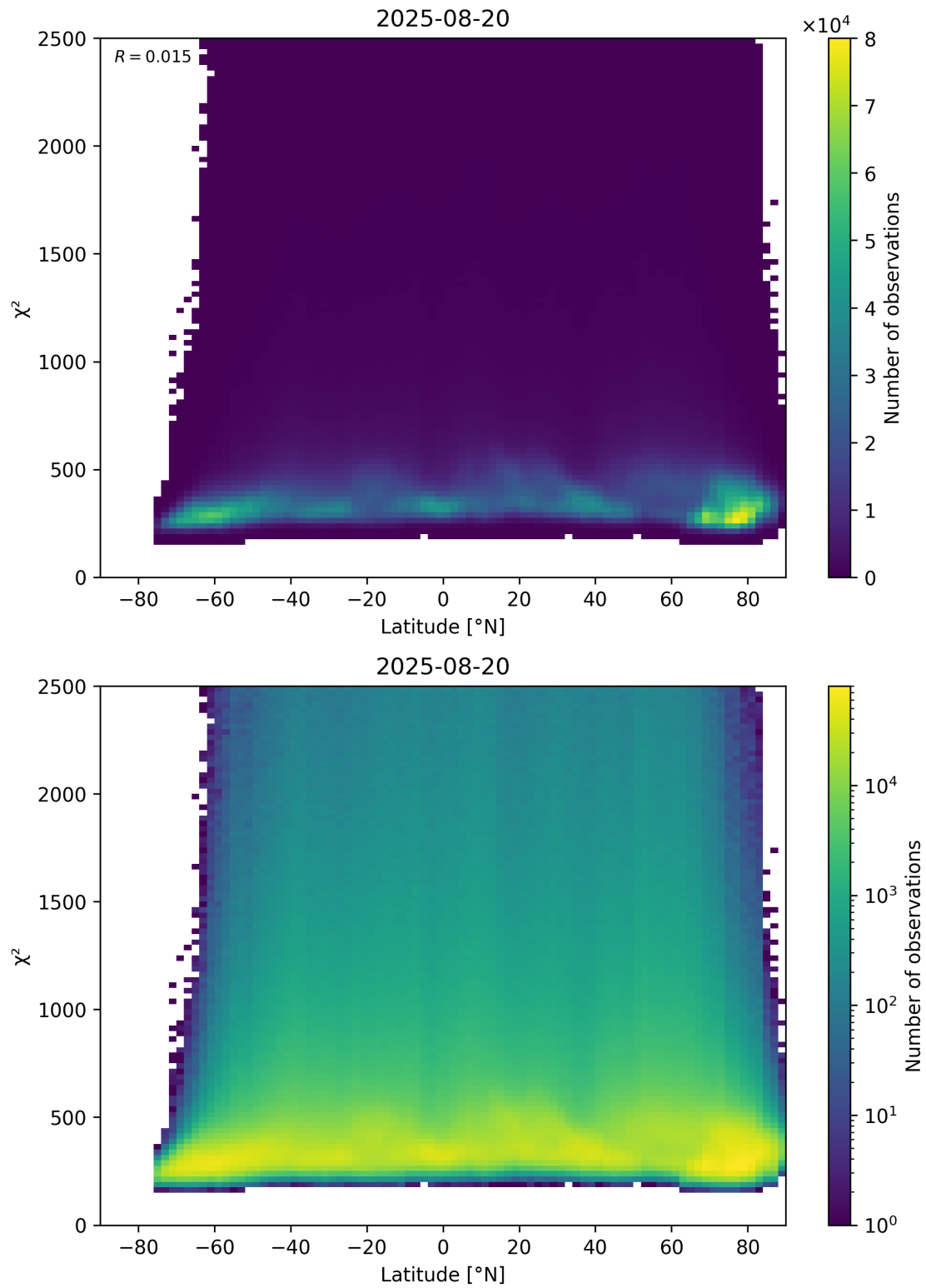
Figure 86: Scatter density plot of “Latitude” against “ \chi^2 ” for 2025-08-19 to 2025-08-21.
