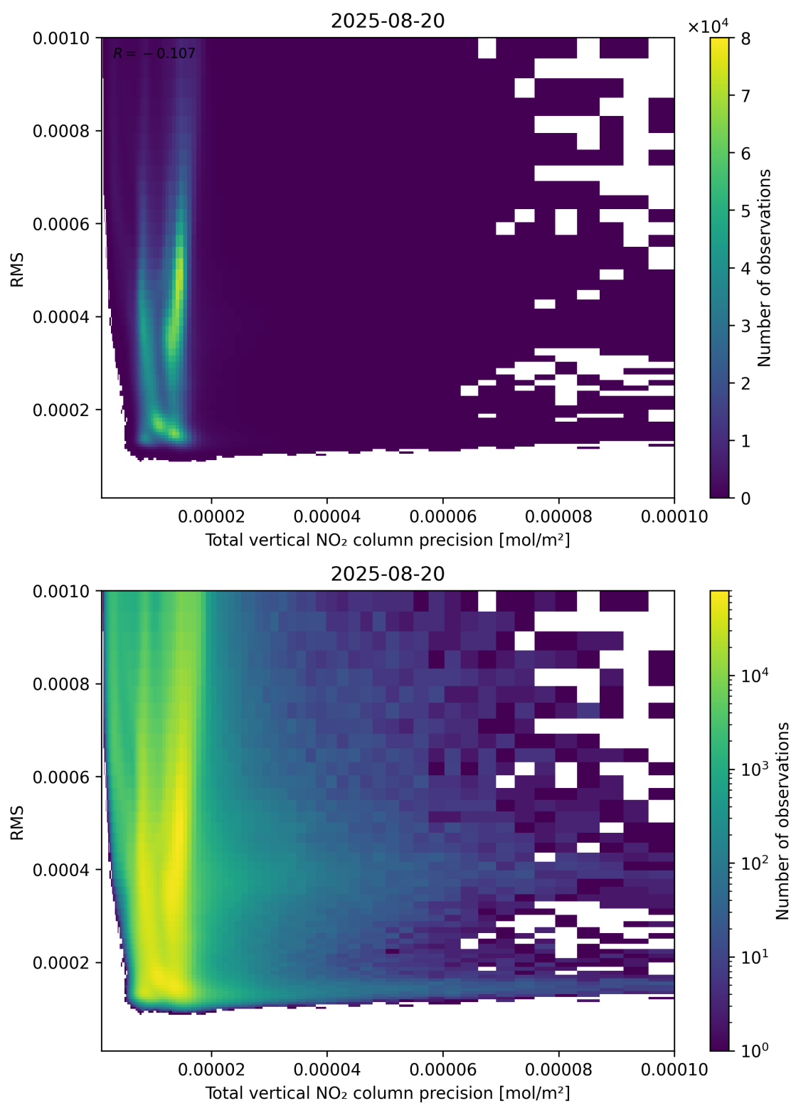
Figure 119: Scatter density plot of “Total vertical NO 2 column precision” against “RMS” for 2025-08-19 to 2025-08-21.
