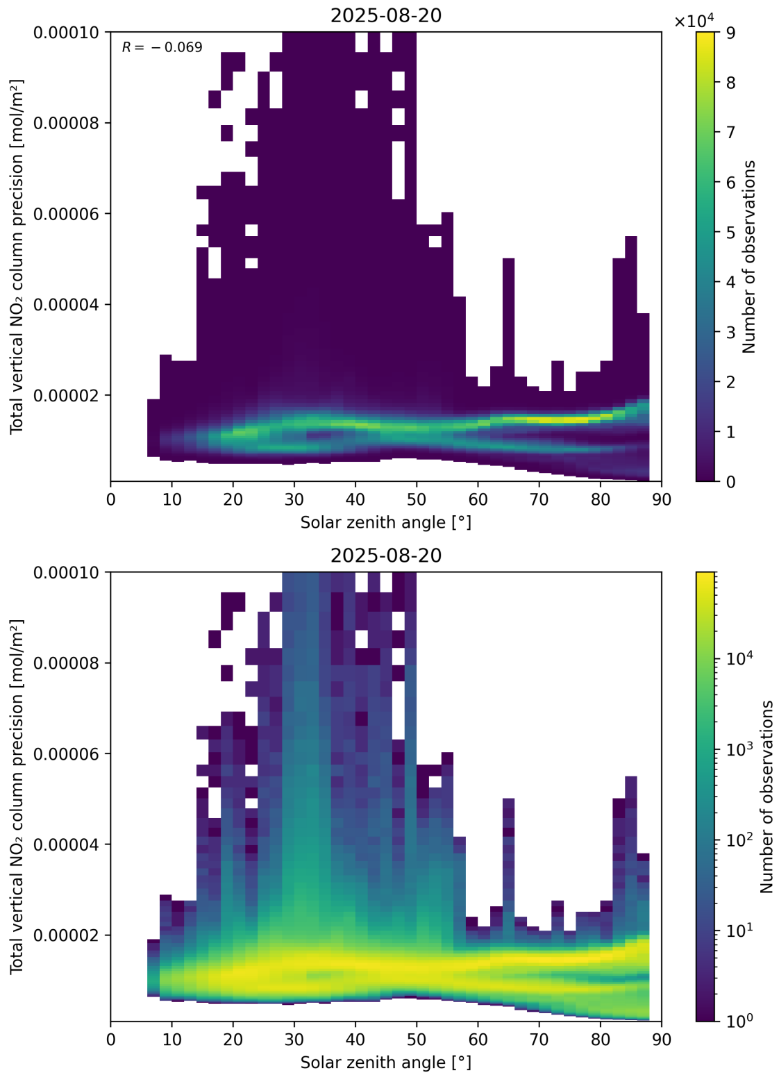
Figure 154: Scatter density plot of “Solar zenith angle” against “Total vertical NO 2 column precision” for 2025-08-19 to 2025-08-21.
