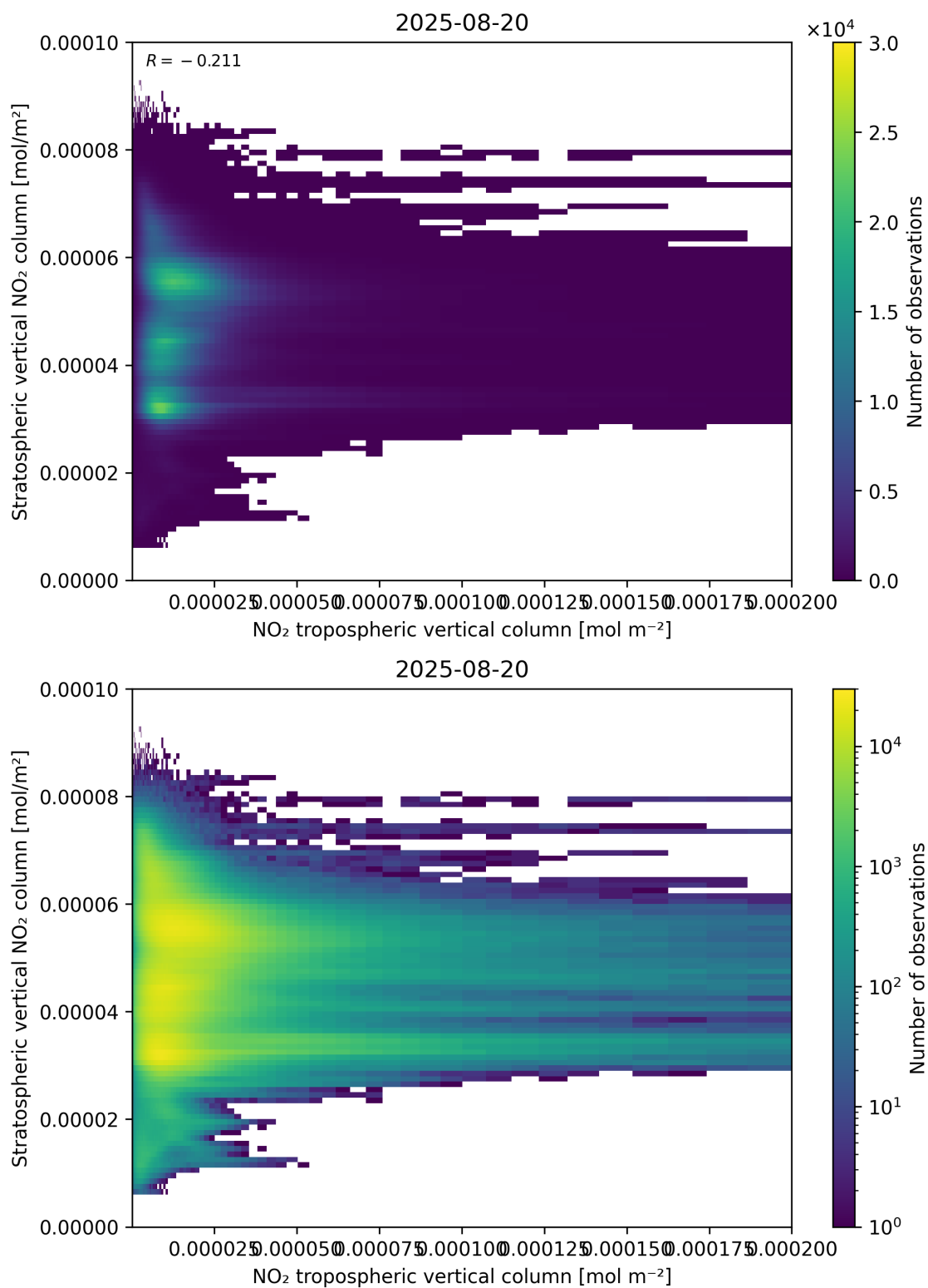
Figure 125: Scatter density plot of “NO 2 tropospheric vertical column” against “Stratospheric vertical NO 2 column” for 2025-08-19 to 2025-08-21.
