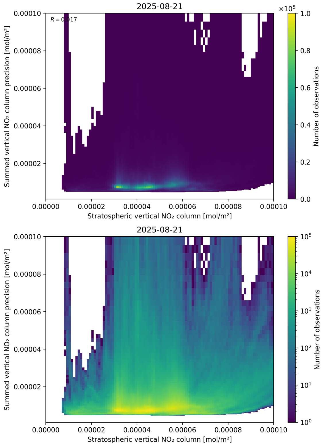
Figure 99: Scatter density plot of “Stratospheric vertical NO 2 column” against “Summed vertical NO 2 column precision” for 2025-08-20 to 2025-08-22.
