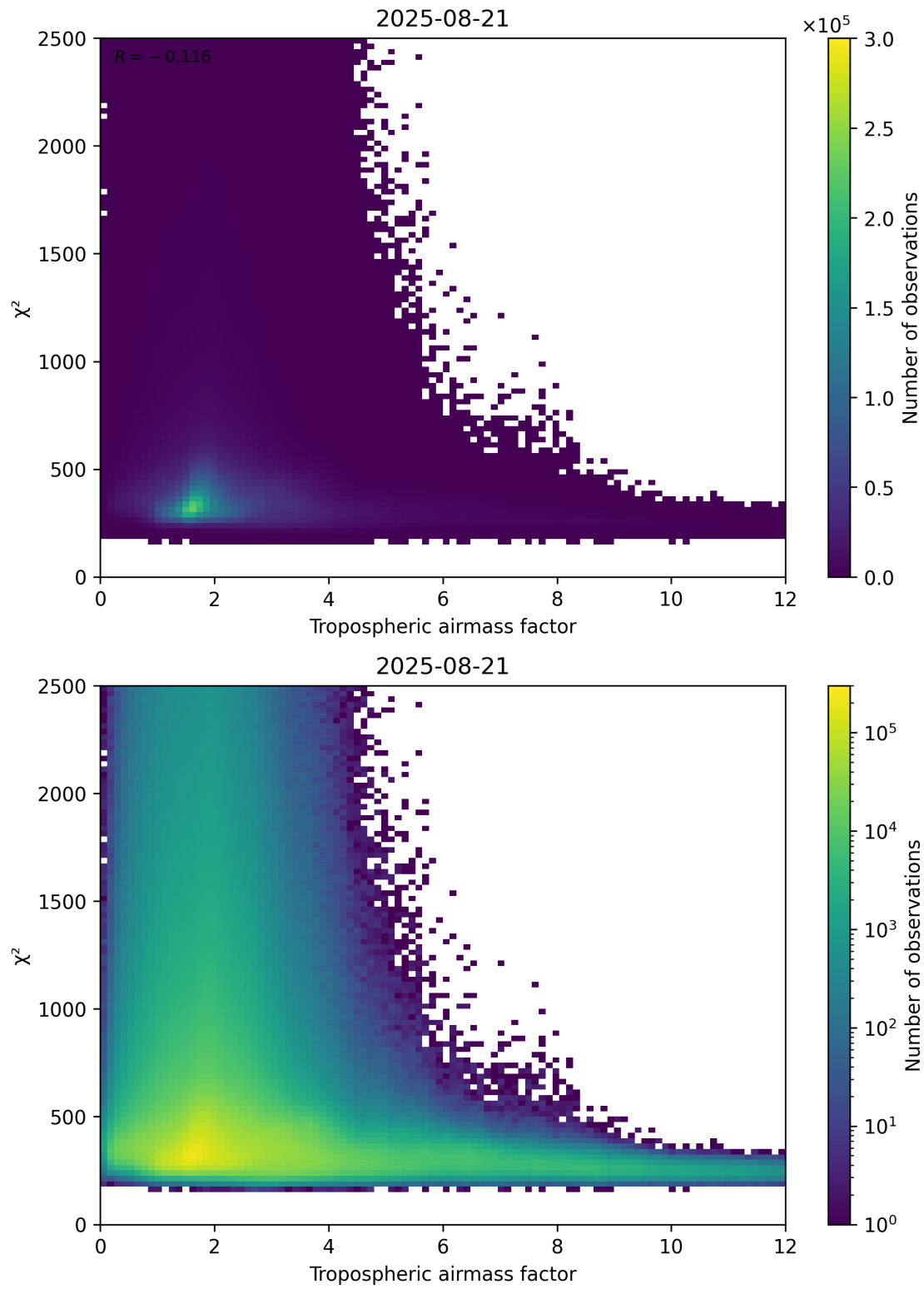
Figure 73: Scatter density plot of “Tropospheric airmass factor” against “ \chi^2 ” for 2025-08-20 to 2025-08-22.
