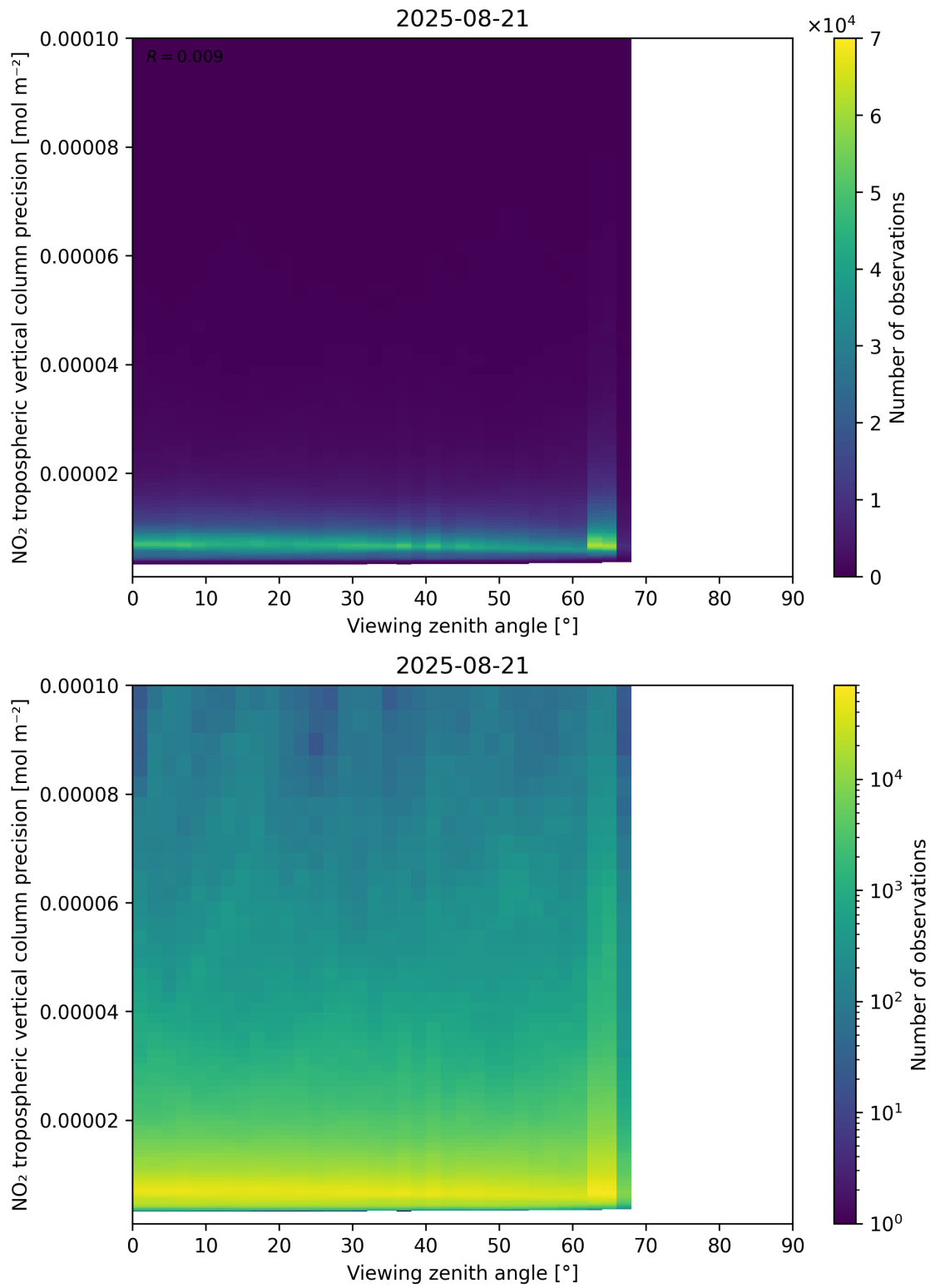
Figure 170: Scatter density plot of “Viewing zenith angle” against “NO 2 tropospheric vertical column precision” for 2025-08-20 to 2025-08-22.
