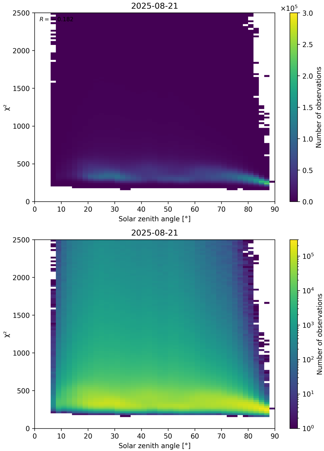
Figure 148: Scatter density plot of “Solar zenith angle” against “ \chi^2 ” for 2025-08-20 to 2025-08-22.
