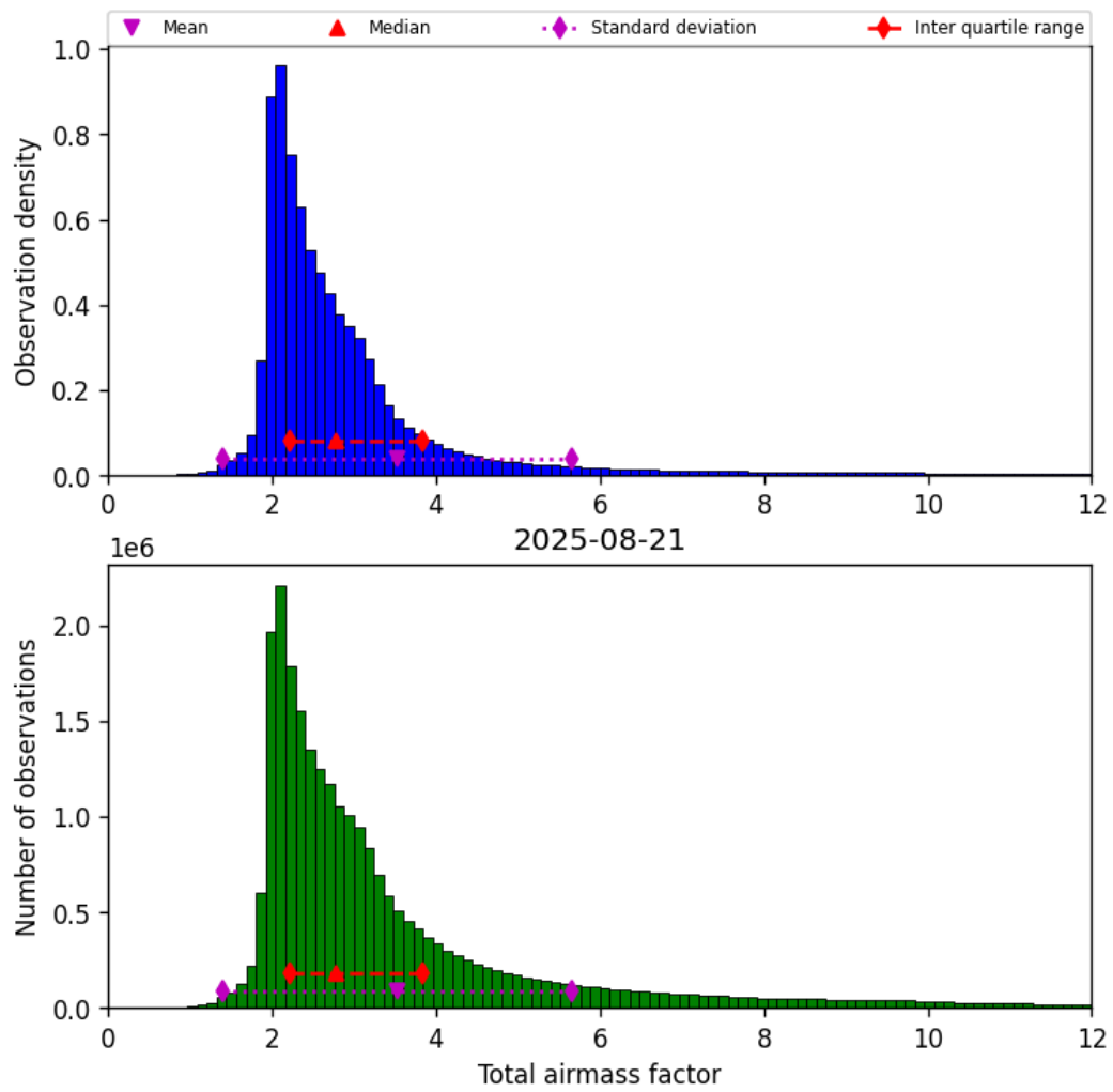
Figure 32: Histogram of “Total airmass factor” for 2025-08-20 to 2025-08-22
