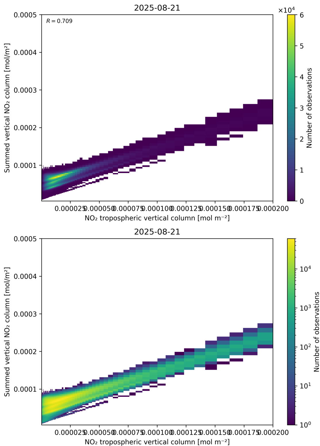
Figure 126: Scatter density plot of “NO 2 tropospheric vertical column” against “Summed vertical NO 2 column” for 2025-08-20 to 2025-08-22.
