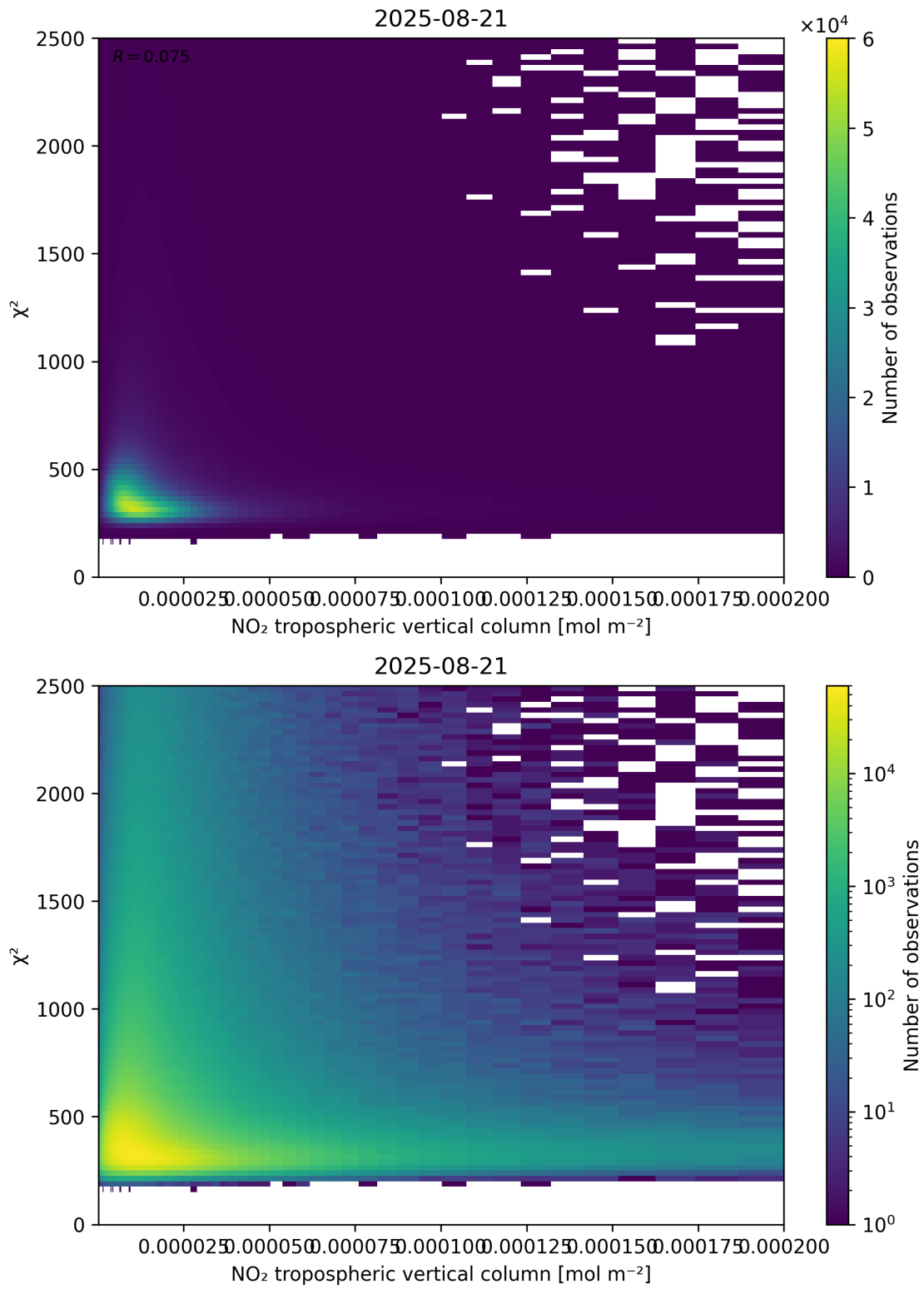
Figure 124: Scatter density plot of “NO 2 tropospheric vertical column” against “ \chi^2 ” for 2025-08-20 to 2025-08-22.
