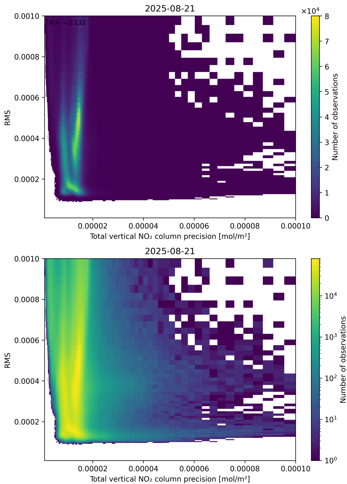
Figure 119: Scatter density plot of “Total vertical NO 2 column precision” against “RMS” for 2025-08-20 to 2025-08-22.
