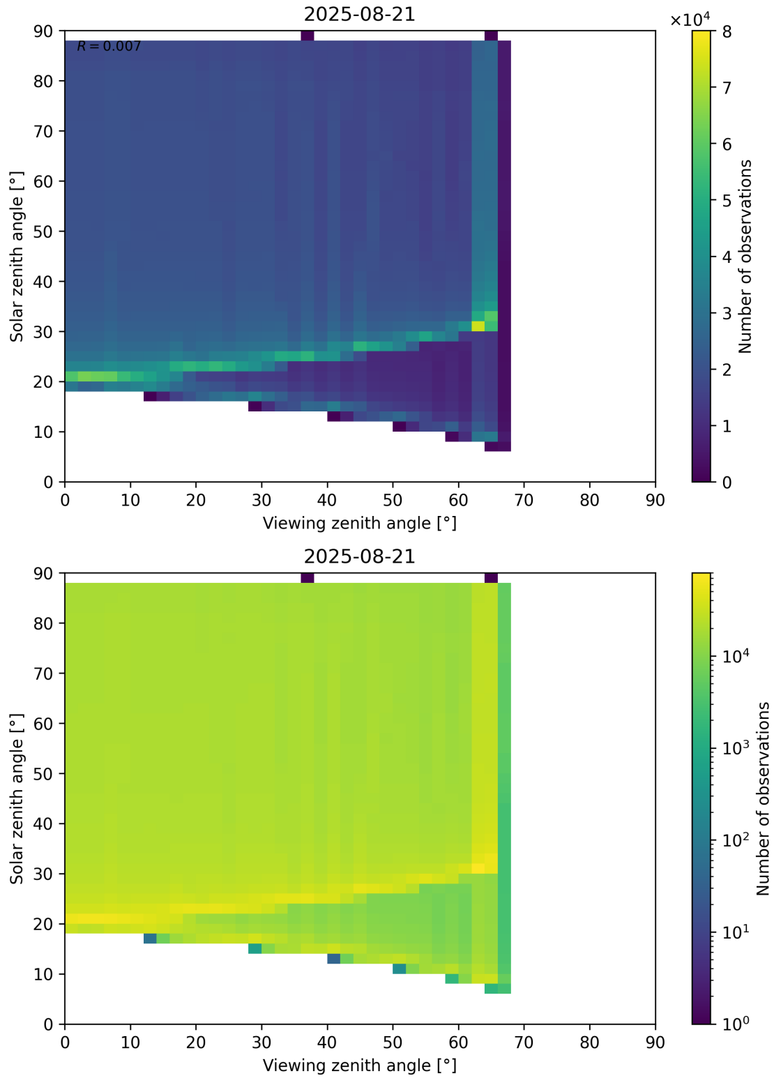
Figure 172: Scatter density plot of “Viewing zenith angle” against “Solar zenith angle” for 2025-08-20 to 2025-08-22.
