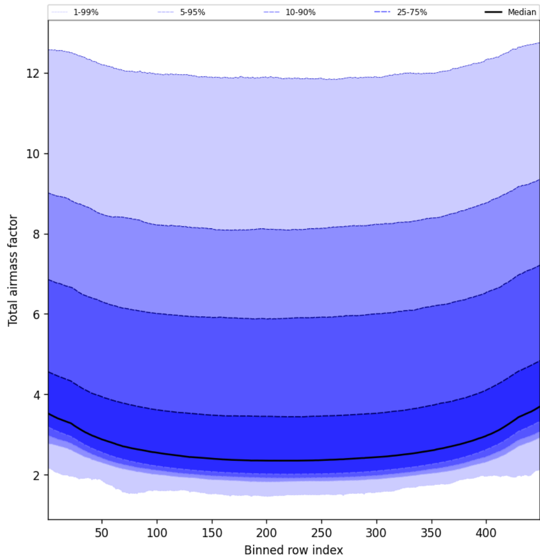
Figure 49: Along track statistics of “Total airmass factor” for 2025-08-20 to 2025-08-22
