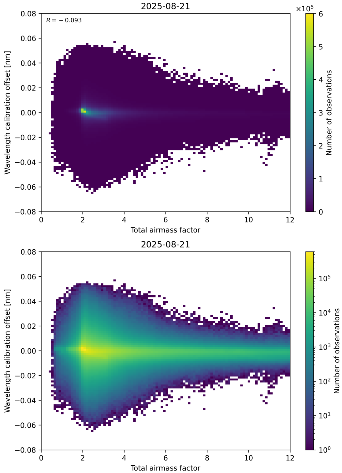
Figure 70: Scatter density plot of “Total airmass factor” against “Wavelength calibration offset” for 2025-08-20 to 2025-08-22.
