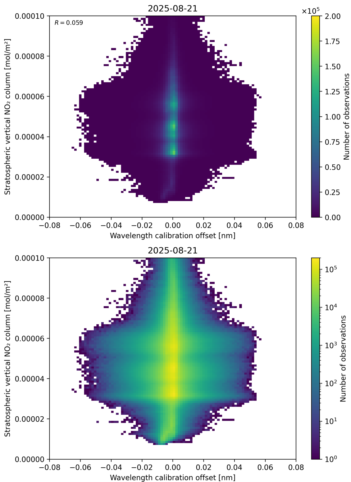
Figure 176: Scatter density plot of “Wavelength calibration offset” against “Stratospheric vertical NO 2 column” for 2025-08-20 to 2025-08-22.
