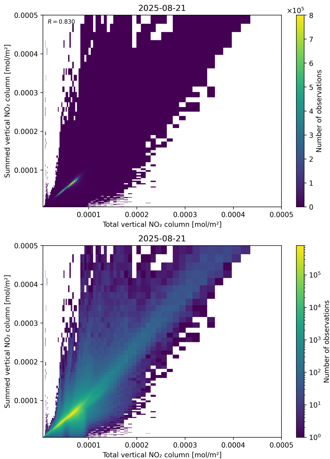
Figure 112: Scatter density plot of “Total vertical NO 2 column” against “Summed vertical NO 2 column” for 2025-08-20 to 2025-08-22.
