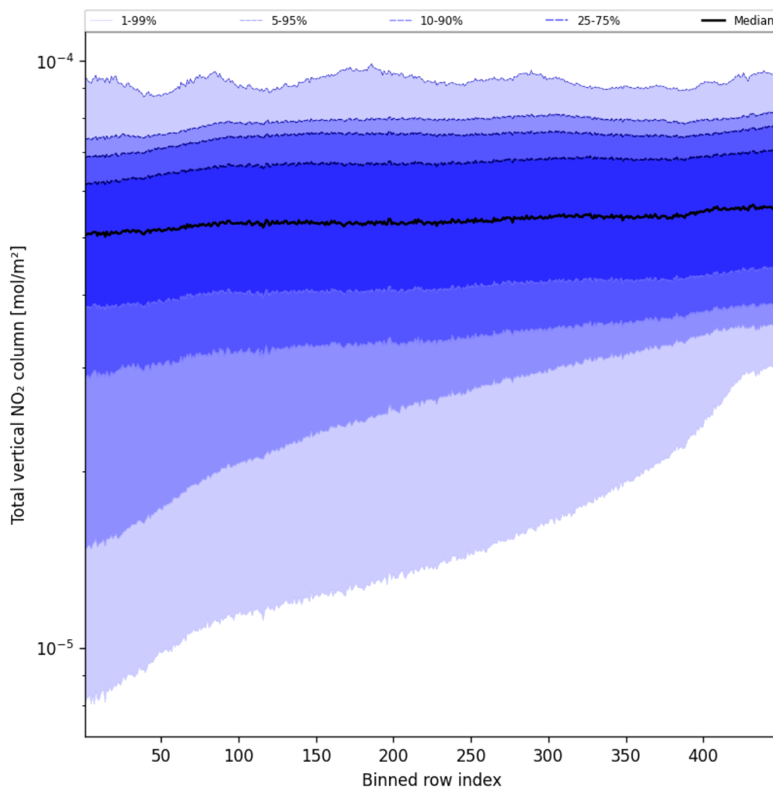
Figure 55: Along track statistics of “Total vertical NO 2 column” for 2025-08-20 to 2025-08-22
