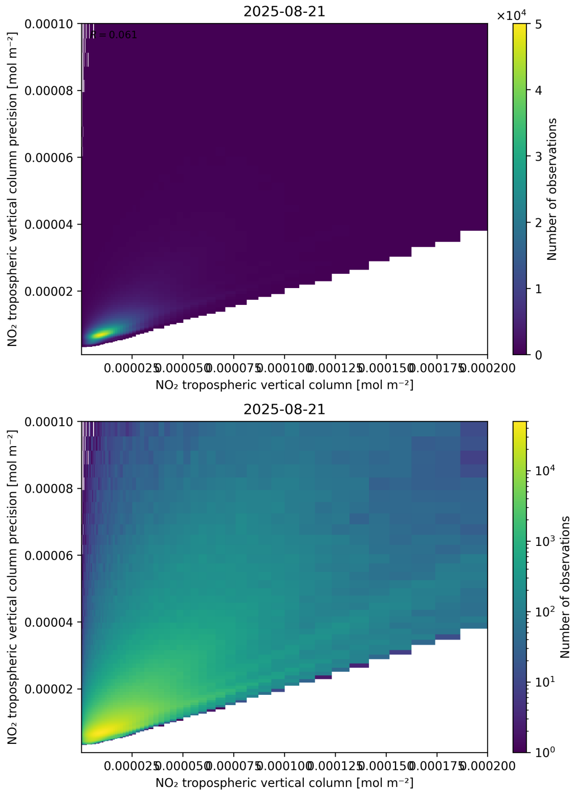
Figure 130: Scatter density plot of “NO 2 tropospheric vertical column” against “NO 2 tropospheric vertical column precision” for 2025-08-20 to 2025-08-22.
