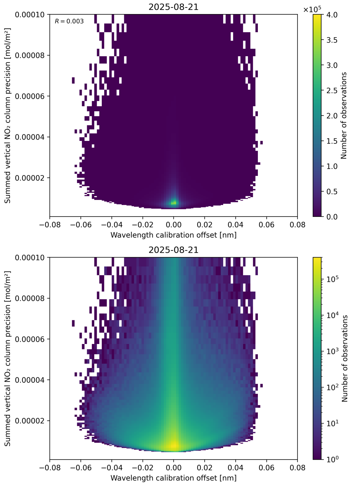
Figure 178: Scatter density plot of “Wavelength calibration offset” against “Summed vertical NO 2 column precision” for 2025-08-20 to 2025-08-22.
