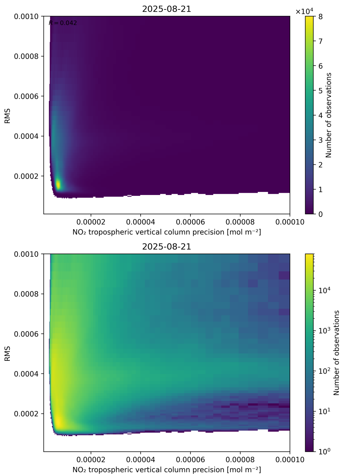
Figure 140: Scatter density plot of “NO 2 tropospheric vertical column precision” against “RMS” for 2025-08-20 to 2025-08-22.
