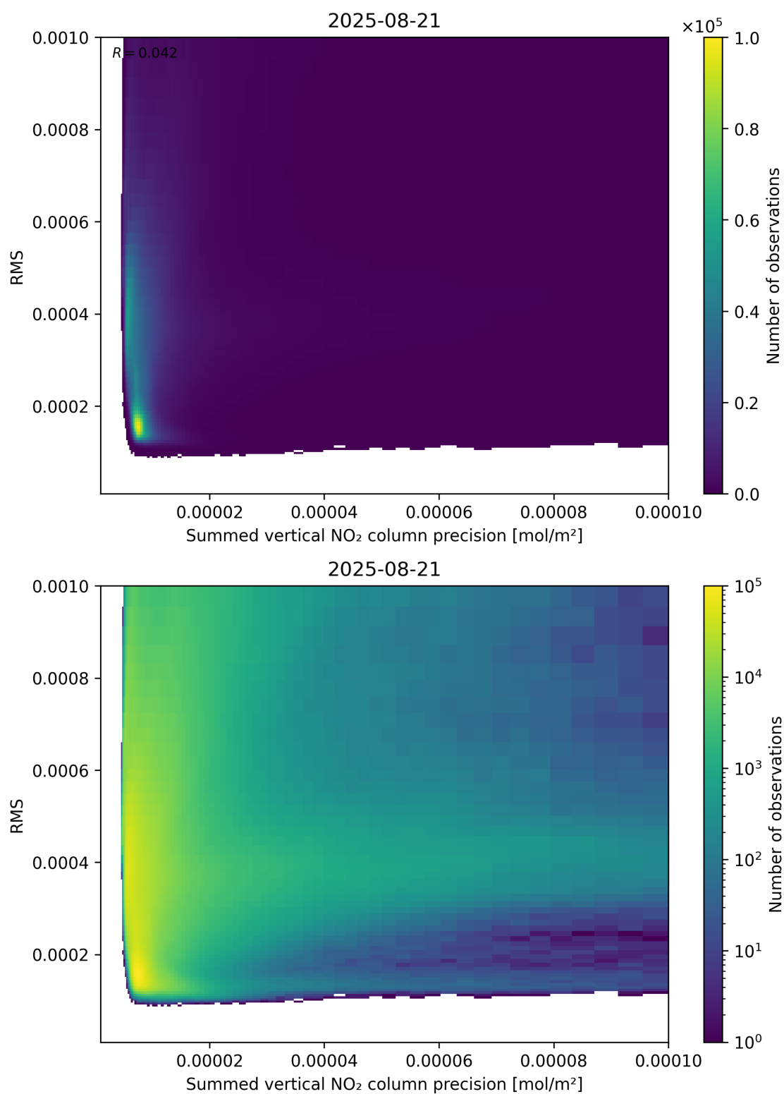
Figure 108: Scatter density plot of “Summed vertical NO 2 column precision” against “RMS” for 2025-08-20 to 2025-08-22.
