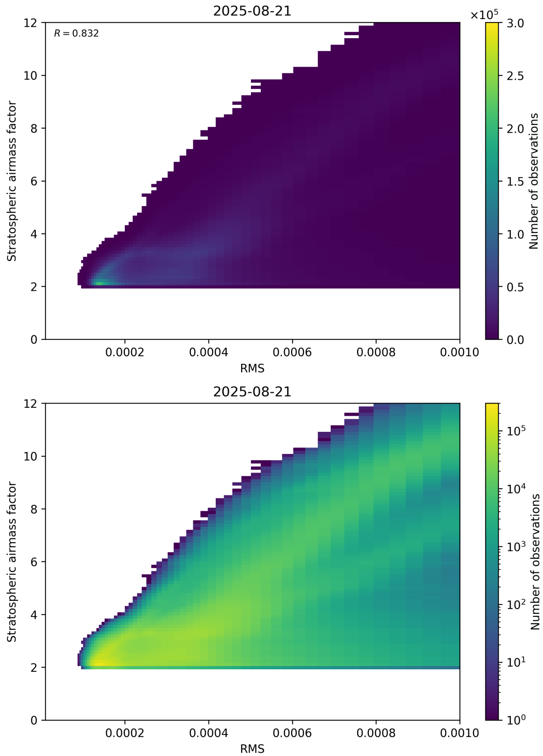
Figure 144: Scatter density plot of “RMS” against “Stratospheric airmass factor” for 2025-08-20 to 2025-08-22.
