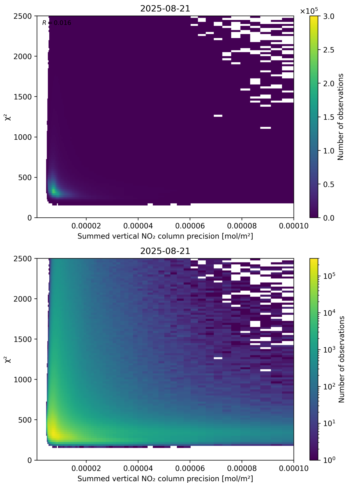
Figure 107: Scatter density plot of “Summed vertical NO 2 column precision” against “ \chi^2 ” for 2025-08-20 to 2025-08-22.
