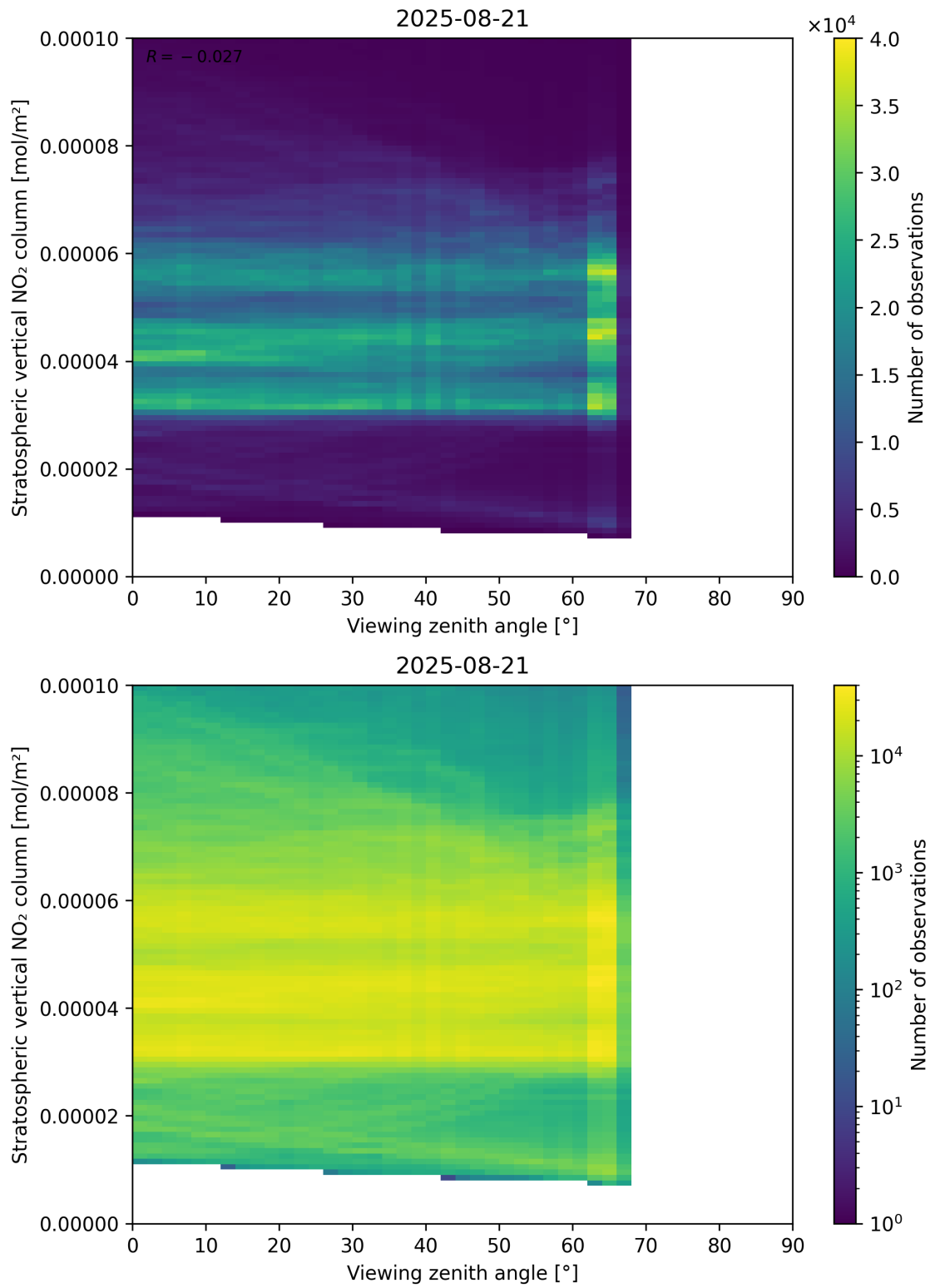
Figure 164: Scatter density plot of “Viewing zenith angle” against “Stratospheric vertical NO 2 column” for 2025-08-20 to 2025-08-22.
