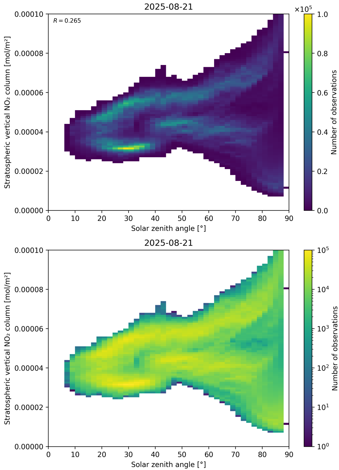
Figure 150: Scatter density plot of “Solar zenith angle” against “Stratospheric vertical NO 2 column” for 2025-08-20 to 2025-08-22.
