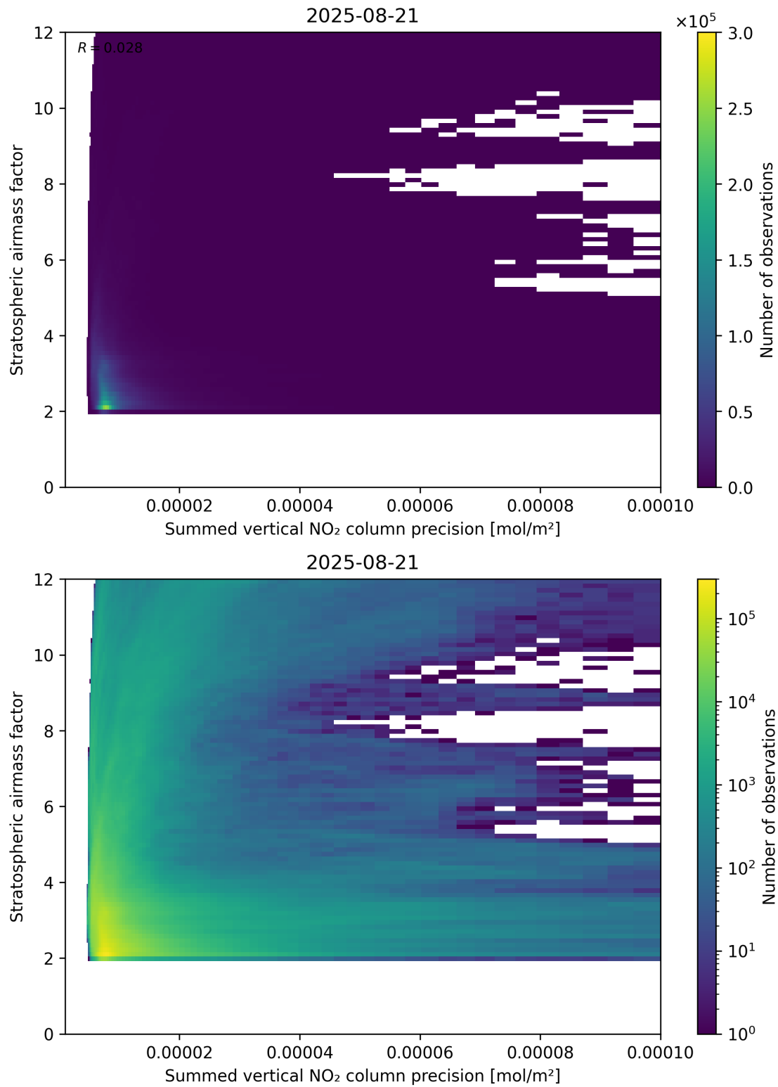
Figure 106: Scatter density plot of “Summed vertical NO 2 column precision” against “Stratospheric airmass factor” for 2025-08-20 to 2025-08-22.
