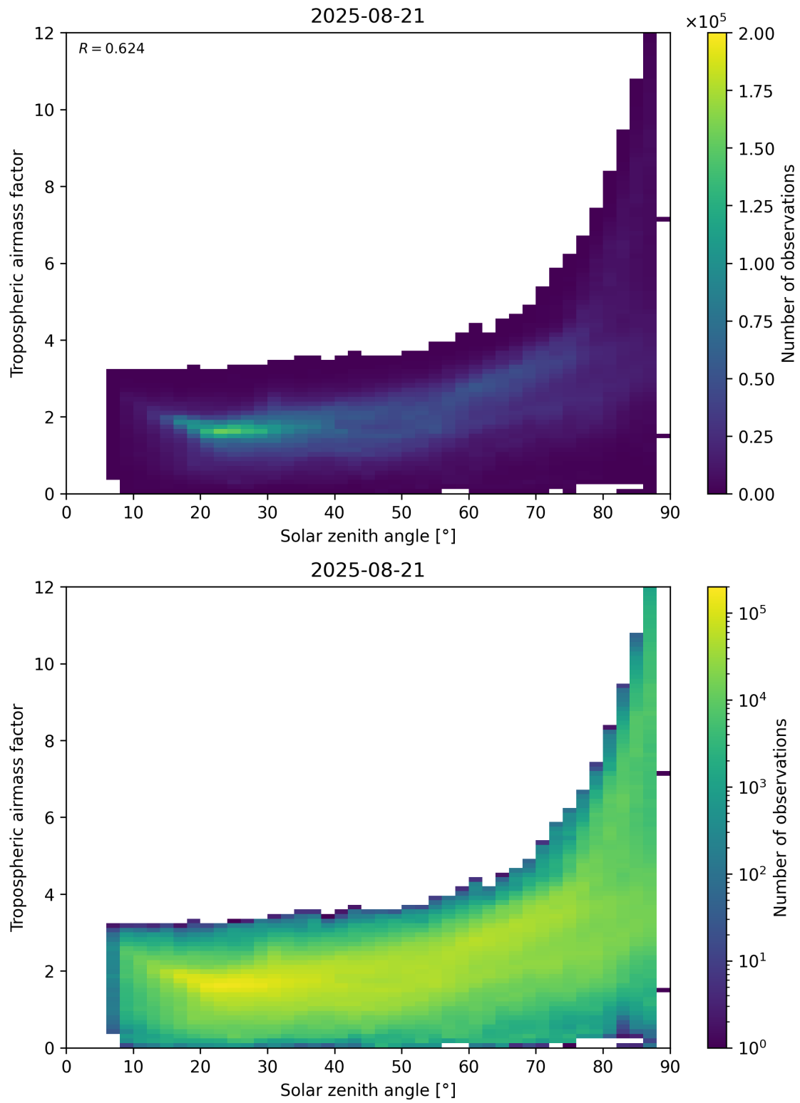
Figure 147: Scatter density plot of “Solar zenith angle” against “Tropospheric airmass factor” for 2025-08-20 to 2025-08-22.
