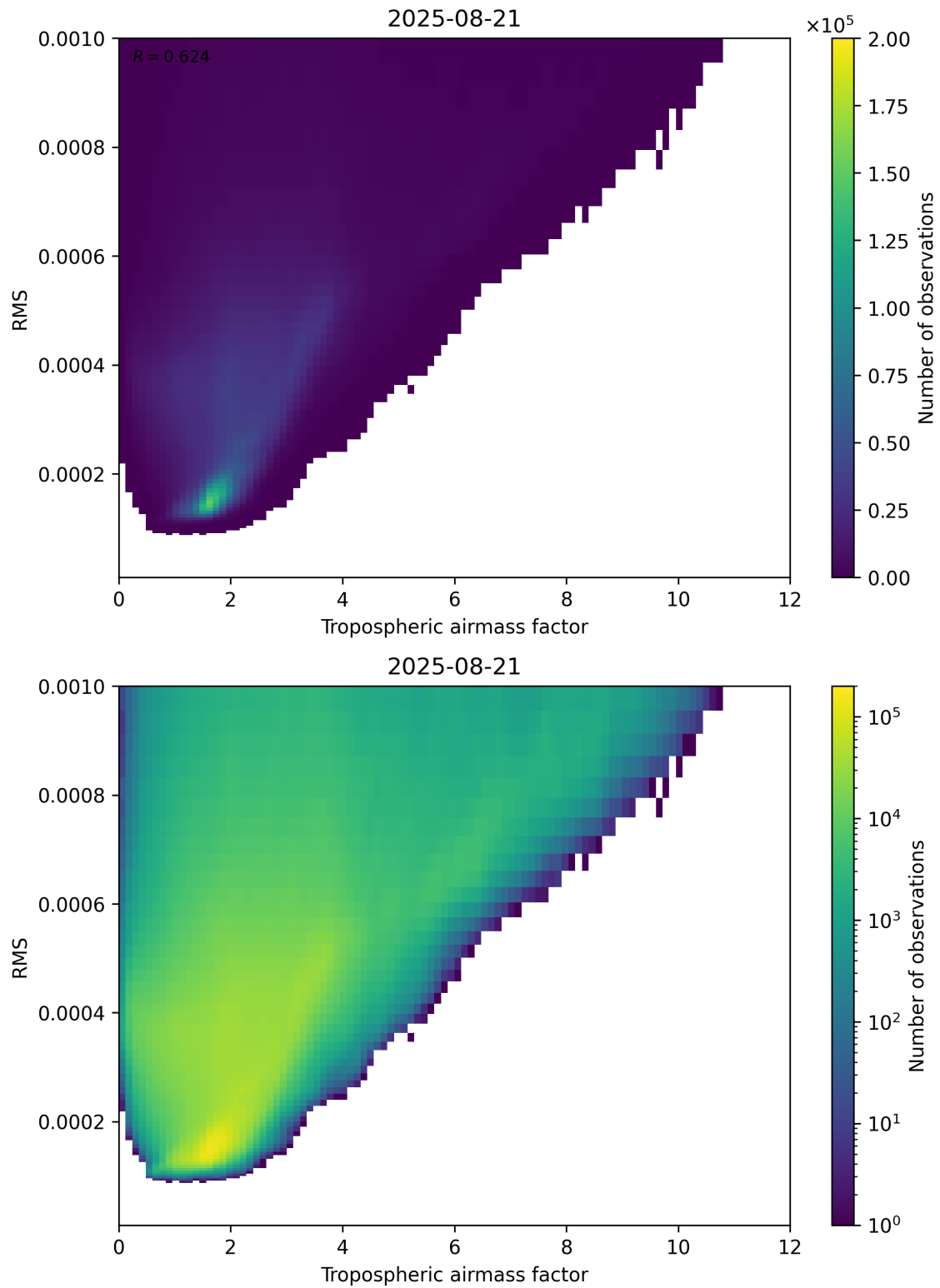
Figure 79: Scatter density plot of “Tropospheric airmass factor” against “RMS” for 2025-08-20 to 2025-08-22.
