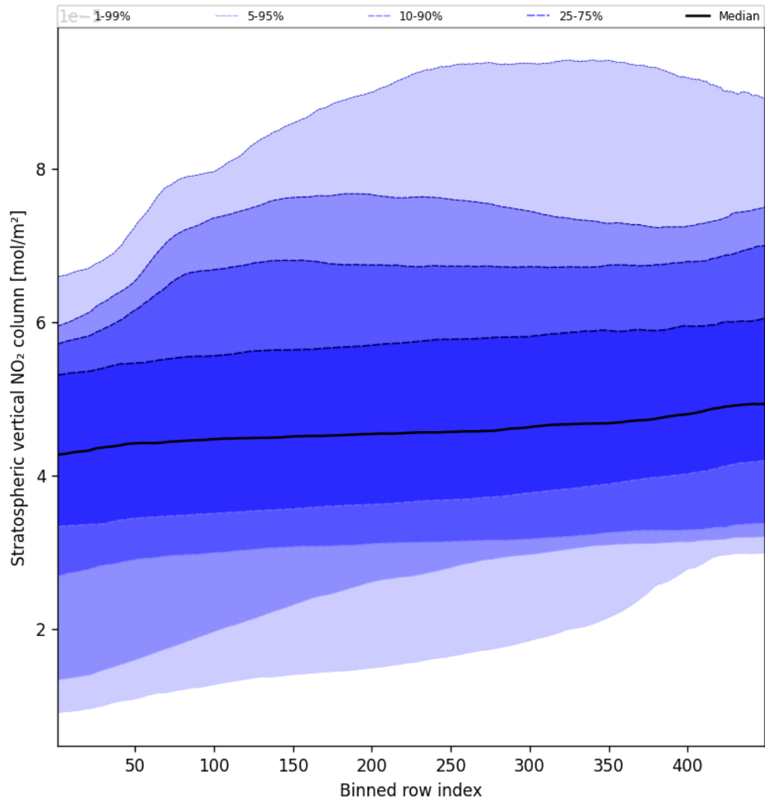
Figure 53: Along track statistics of “Stratospheric vertical NO 2 column” for 2025-08-20 to 2025-08-22
