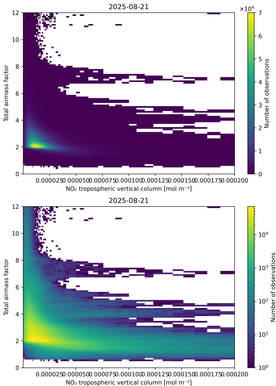
Figure 122: Scatter density plot of “NO 2 tropospheric vertical column” against “Total air mass factor” for 2025-08-20 to 2025-08-22.
