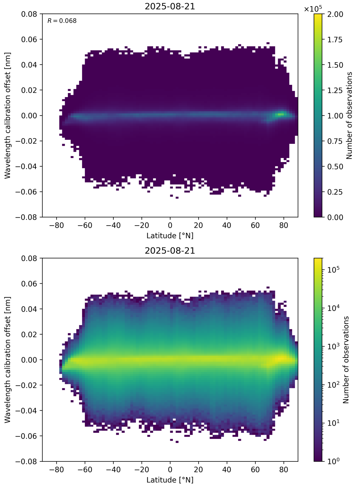
Figure 95: Scatter density plot of “Latitude” against “Wavelength calibration offset” for 2025-08-20 to 2025-08-22.
