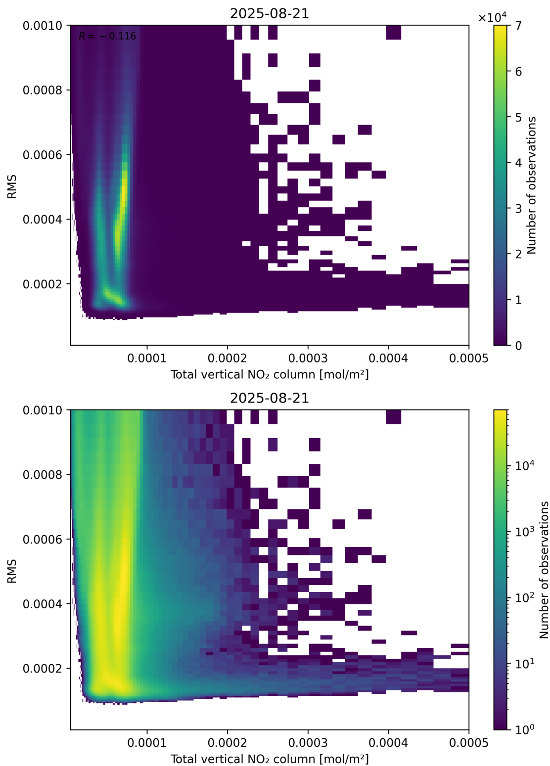
Figure 120: Scatter density plot of “Total vertical NO 2 column” against “RMS” for 2025-08-20 to 2025-08-22.
