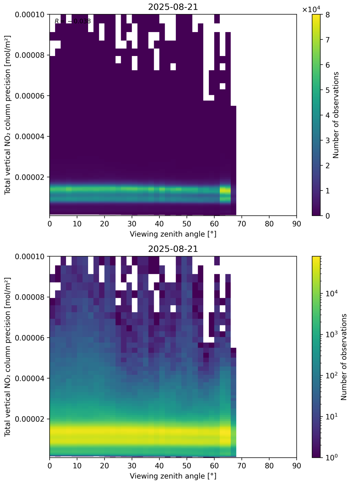
Figure 168: Scatter density plot of “Viewing zenith angle” against “Total vertical NO 2 column precision” for 2025-08-20 to 2025-08-22.
