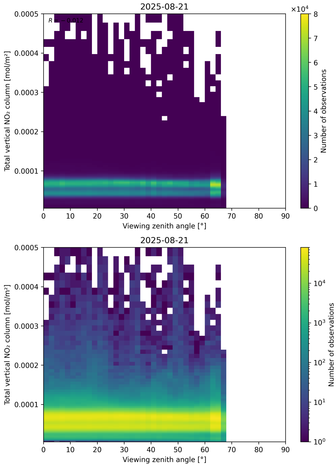
Figure 167: Scatter density plot of “Viewing zenith angle” against “Total vertical NO 2 column” for 2025-08-20 to 2025-08-22.
