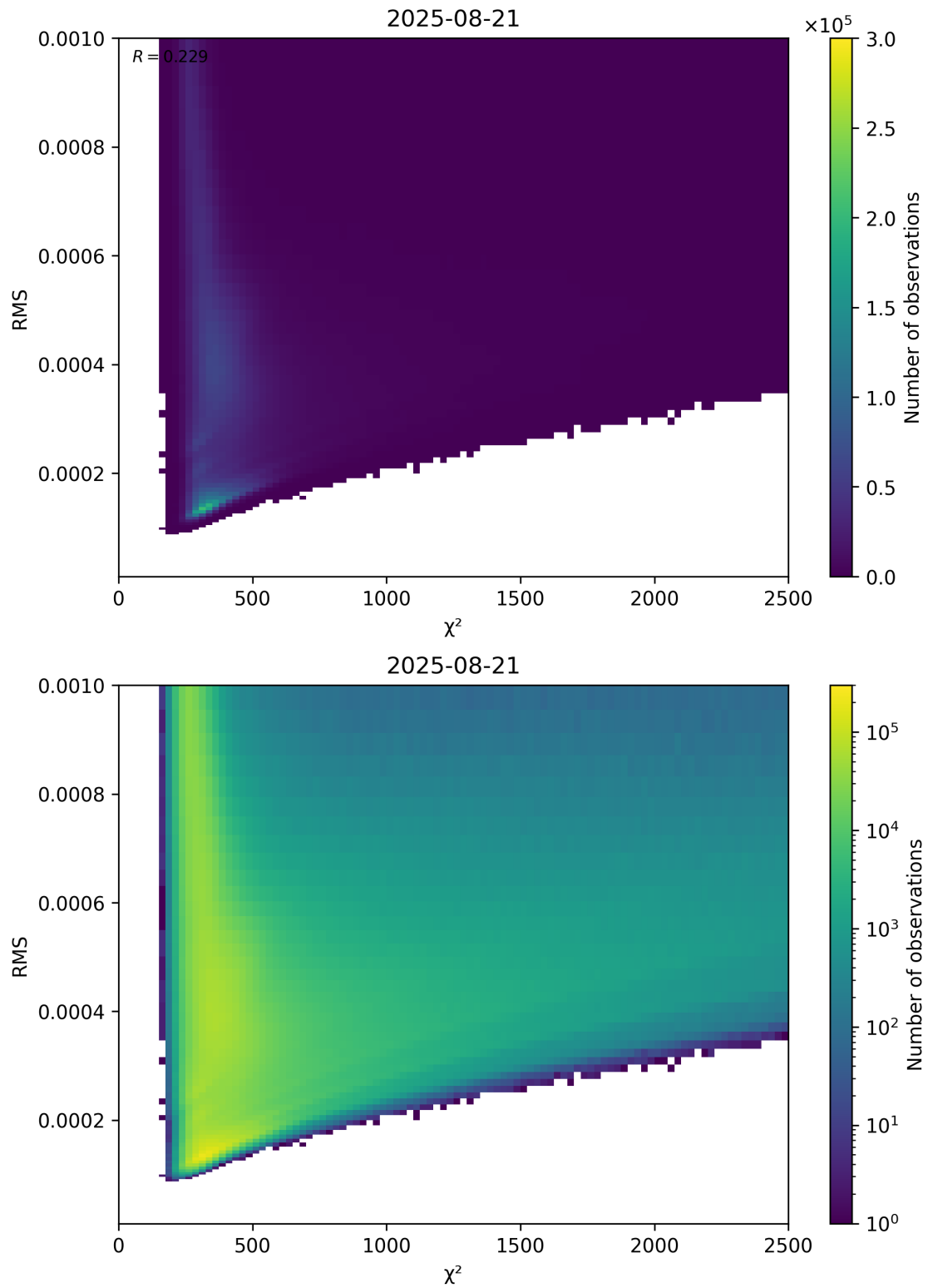
Figure 82: Scatter density plot of “ \chi^2 ” against “RMS” for 2025-08-20 to 2025-08-22.
