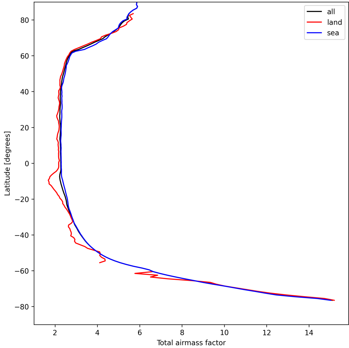
Figure 15: Zonal average of “Total airmass factor” for 2025-08-20 to 2025-08-22.
