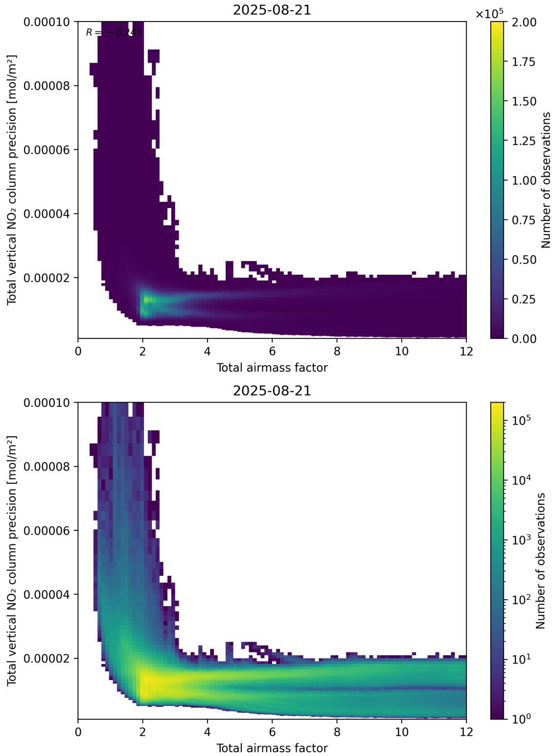
Figure 68: Scatter density plot of “Total airmass factor” against “Total vertical NO 2 column precision” for 2025-08-20 to 2025-08-22.
