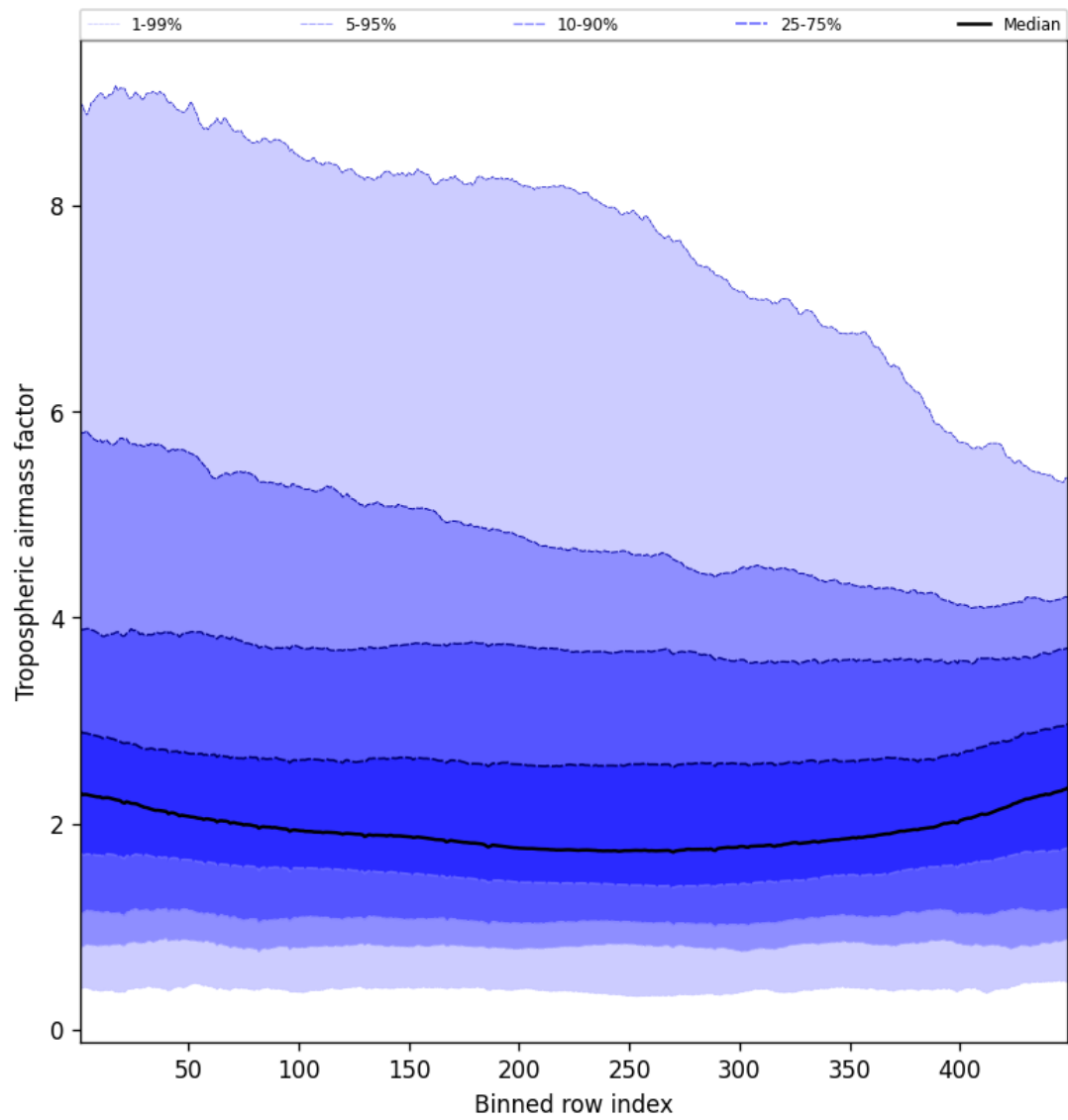
Figure 48: Along track statistics of “Tropospheric air mass factor” for 2025-08-20 to 2025-08-22
