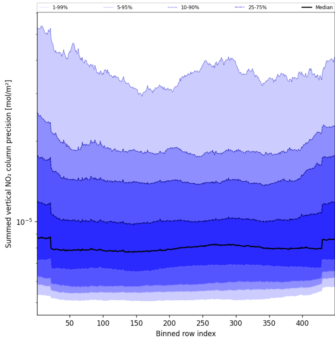
Figure 58: Along track statistics of “Summed vertical NO 2 column precision” for 2025-08-20 to 2025-08-22
