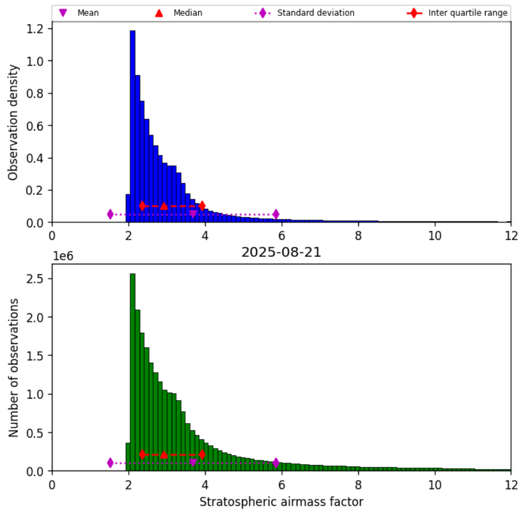
Figure 44: Histogram of “Stratospheric airmass factor” for 2025-08-20 to 2025-08-22
