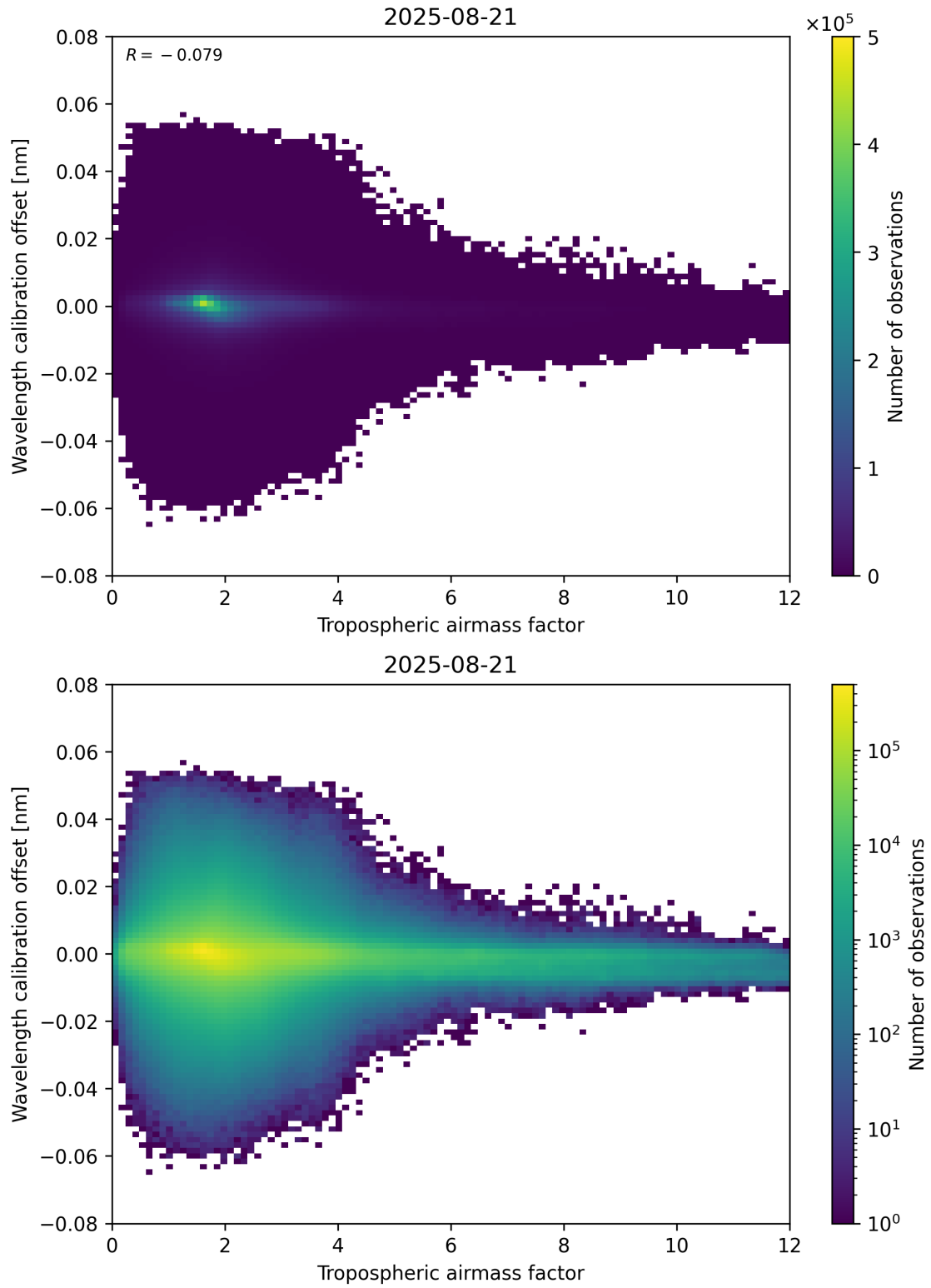
Figure 80: Scatter density plot of “Tropospheric airmass factor” against “Wavelength calibration offset” for 2025-08-20 to 2025-08-22.
