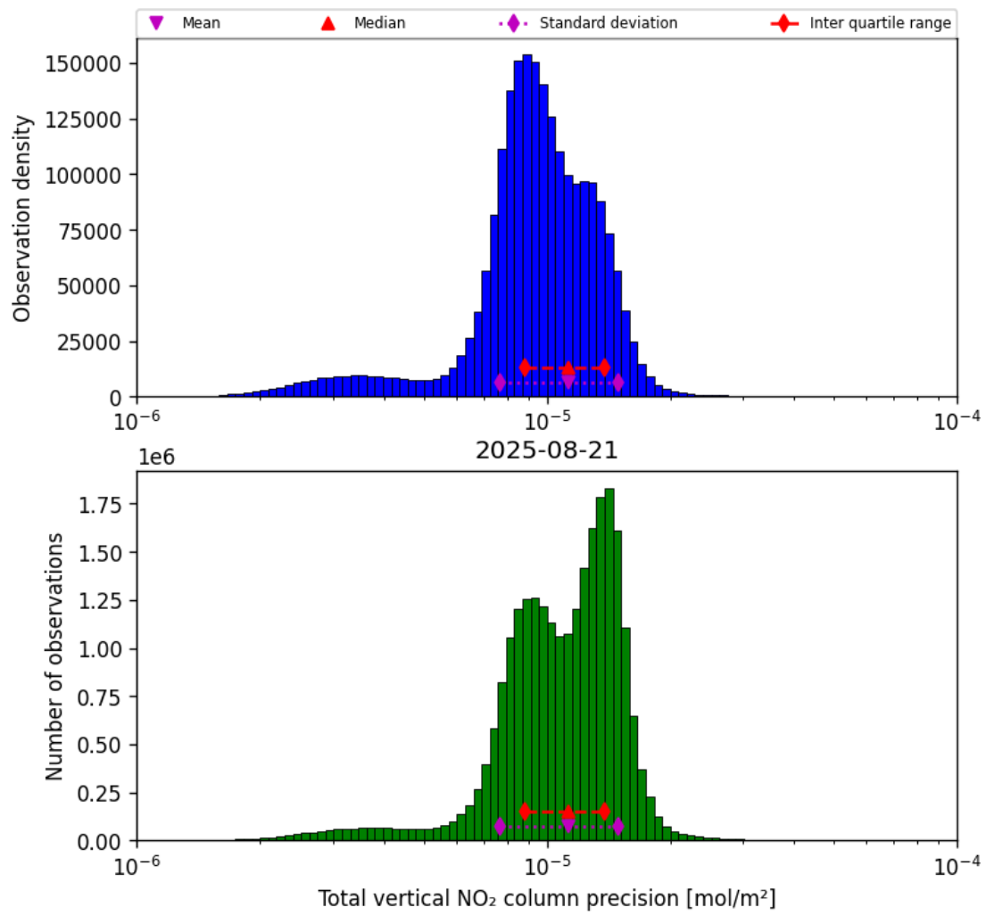
Figure 39: Histogram of “Total vertical NO 2 column precision” for 2025-08-20 to 2025-08-22
