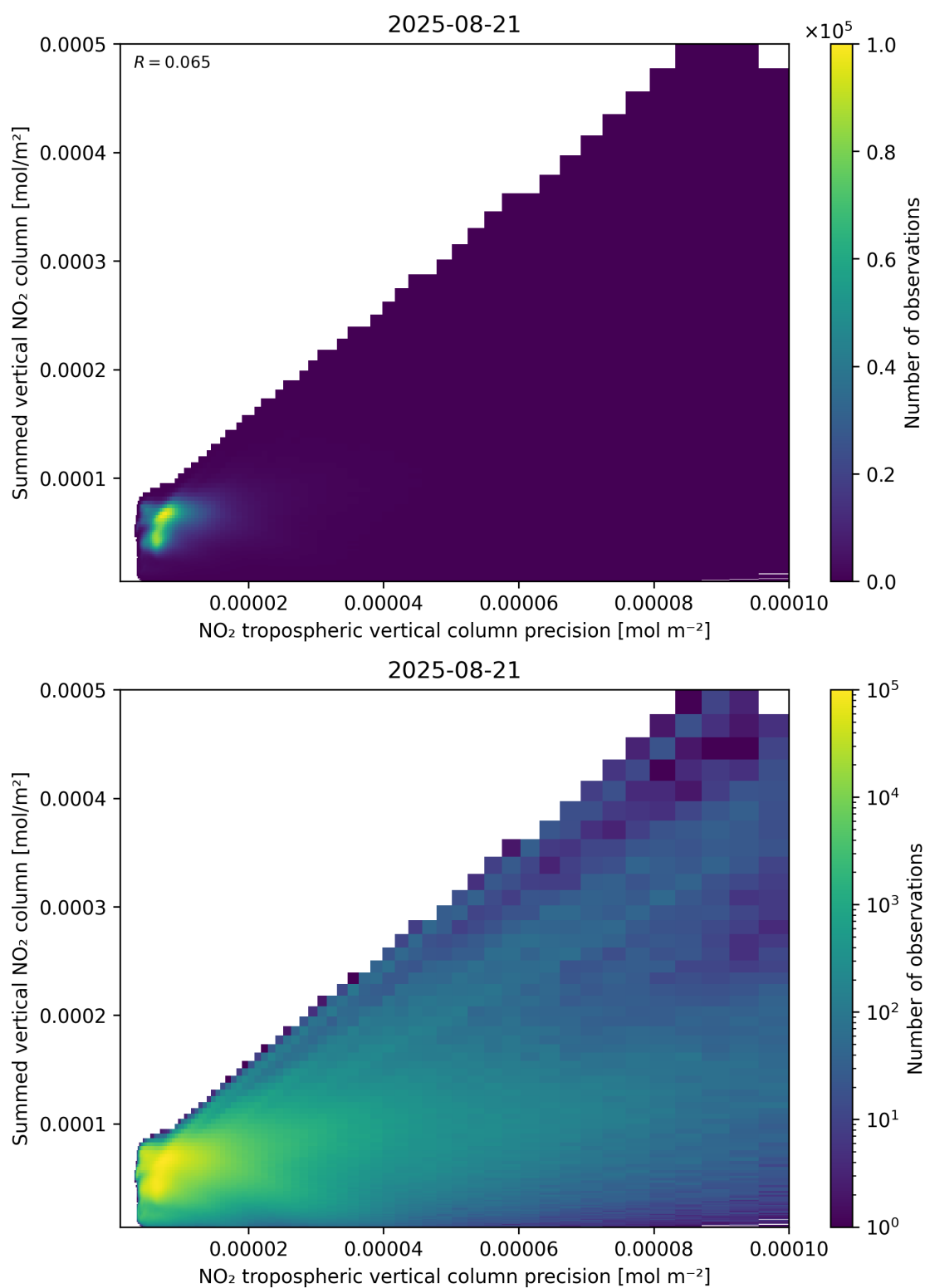
Figure 136: Scatter density plot of “NO 2 tropospheric vertical column precision” against “Summed vertical NO 2 column” for 2025-08-20 to 2025-08-22.
