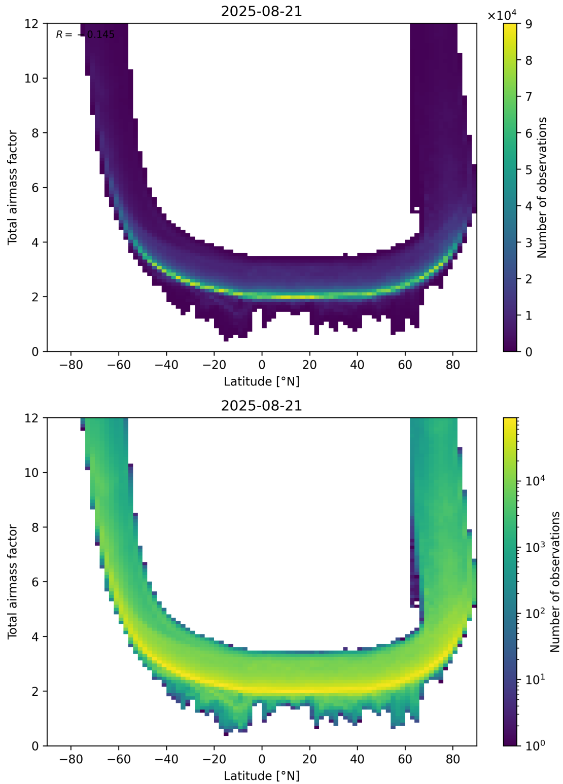
Figure 84: Scatter density plot of “Latitude” against “Total airmass factor” for 2025-08-20 to 2025-08-22.
