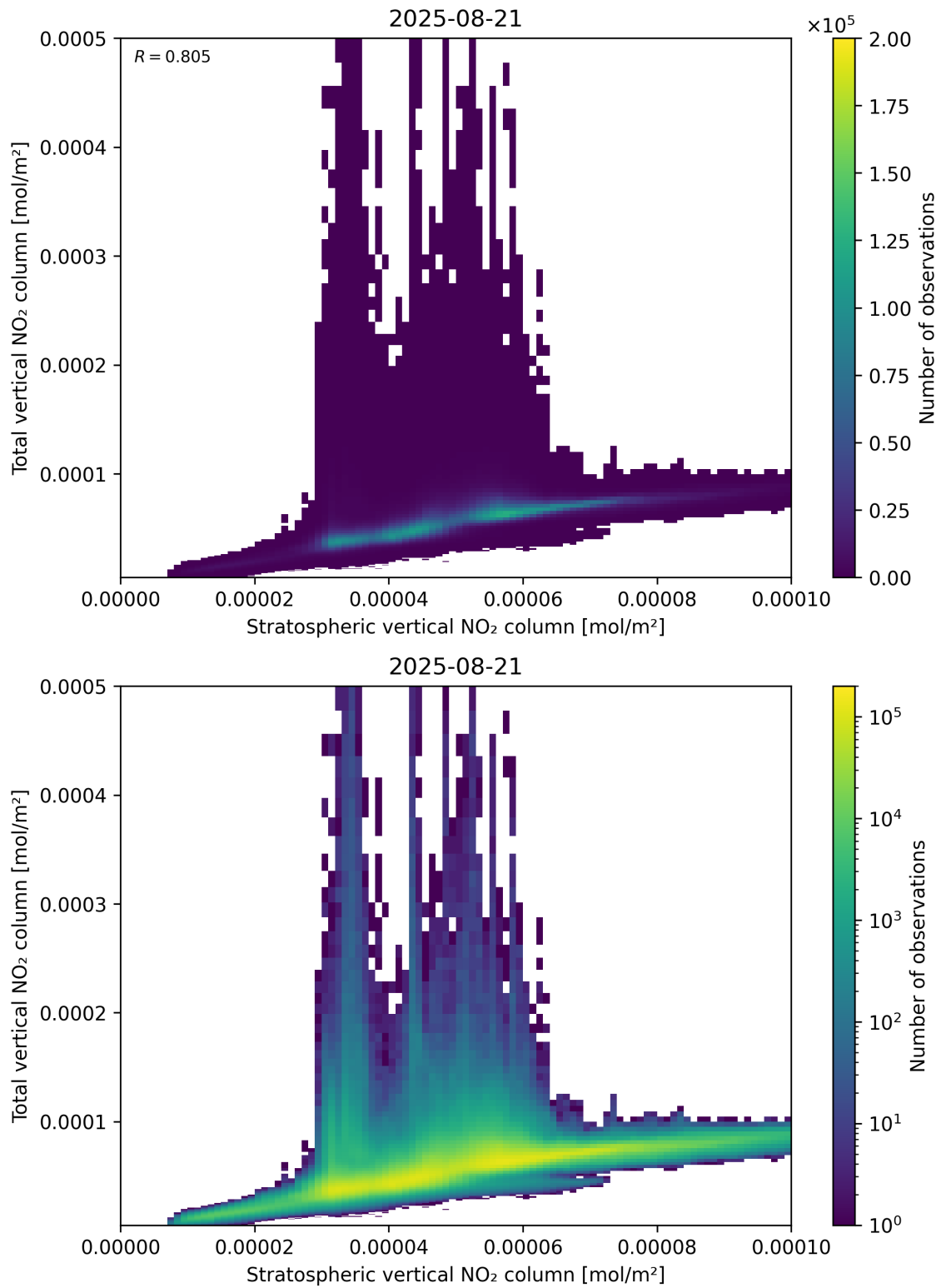
Figure 100: Scatter density plot of “Stratospheric vertical NO 2 column” against “Total vertical NO 2 column” for 2025-08-20 to 2025-08-22.
