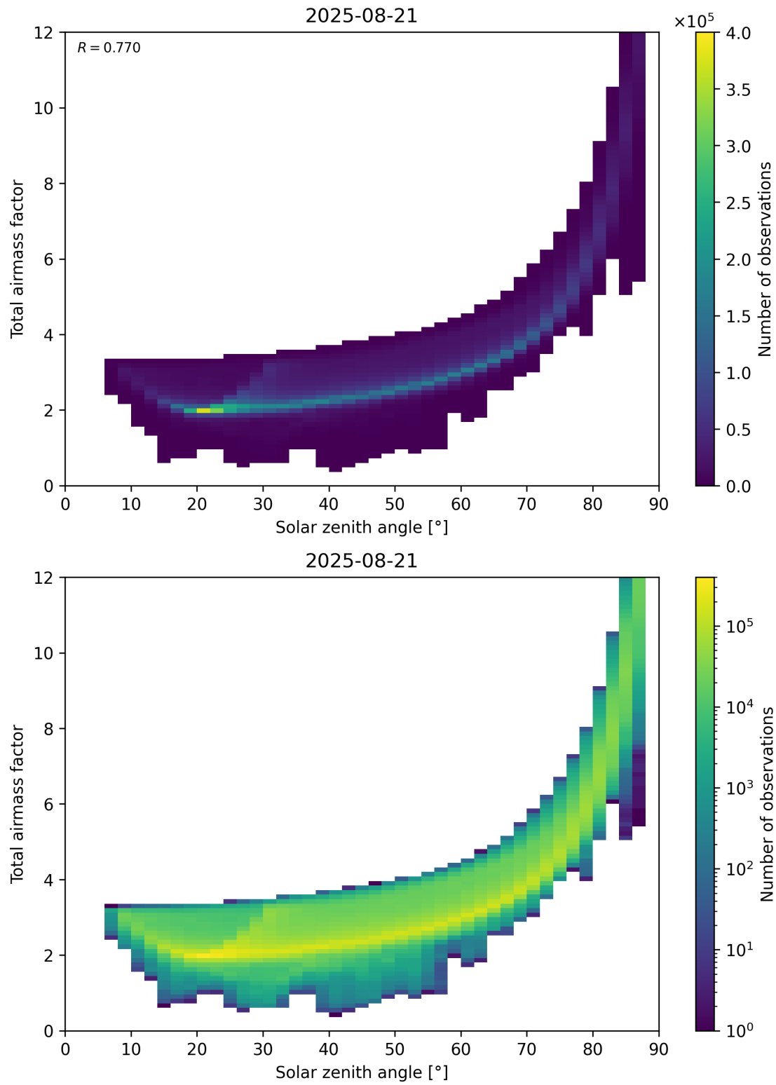
Figure 146: Scatter density plot of “Solar zenith angle” against “Total airmass factor” for 2025-08-20 to 2025-08-22.
