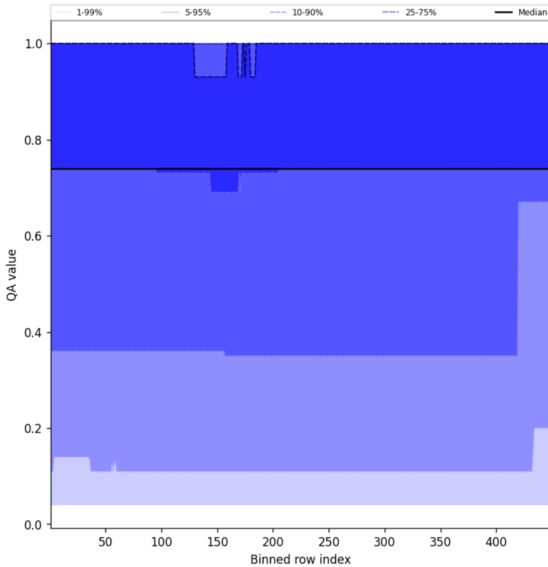
Figure 45: Along track statistics of “QA value” for 2025-08-20 to 2025-08-22
