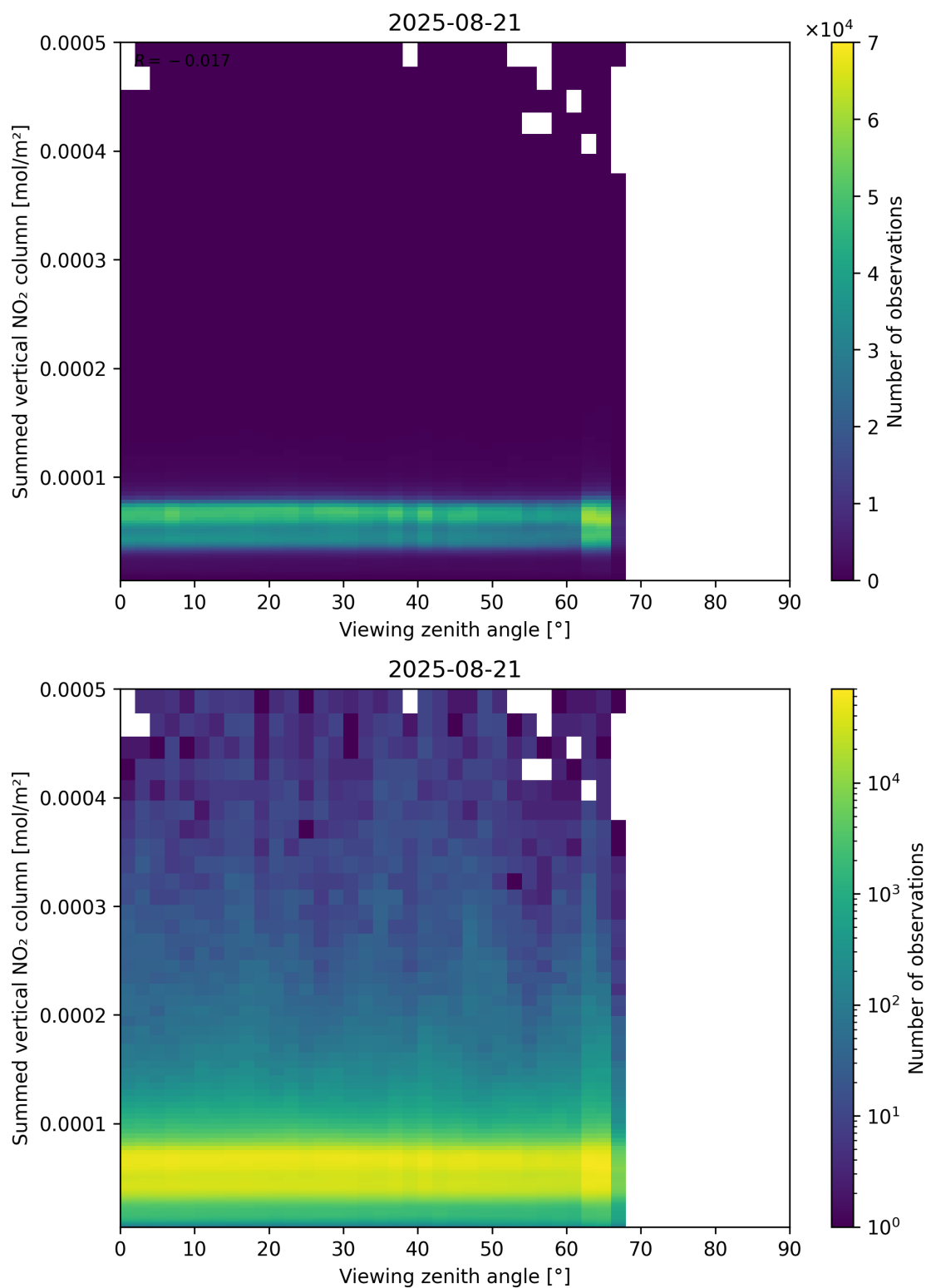
Figure 165: Scatter density plot of “Viewing zenith angle” against “Summed vertical NO 2 column” for 2025-08-20 to 2025-08-22.
