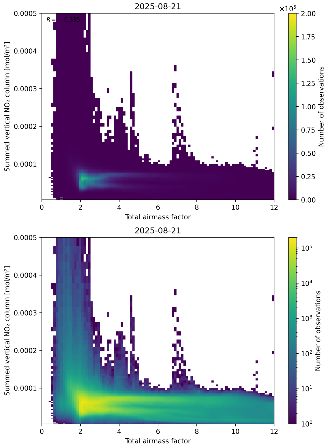
Figure 65: Scatter density plot of “Total airmass factor” against “Summed vertical NO 2 column” for 2025-08-20 to 2025-08-22.
