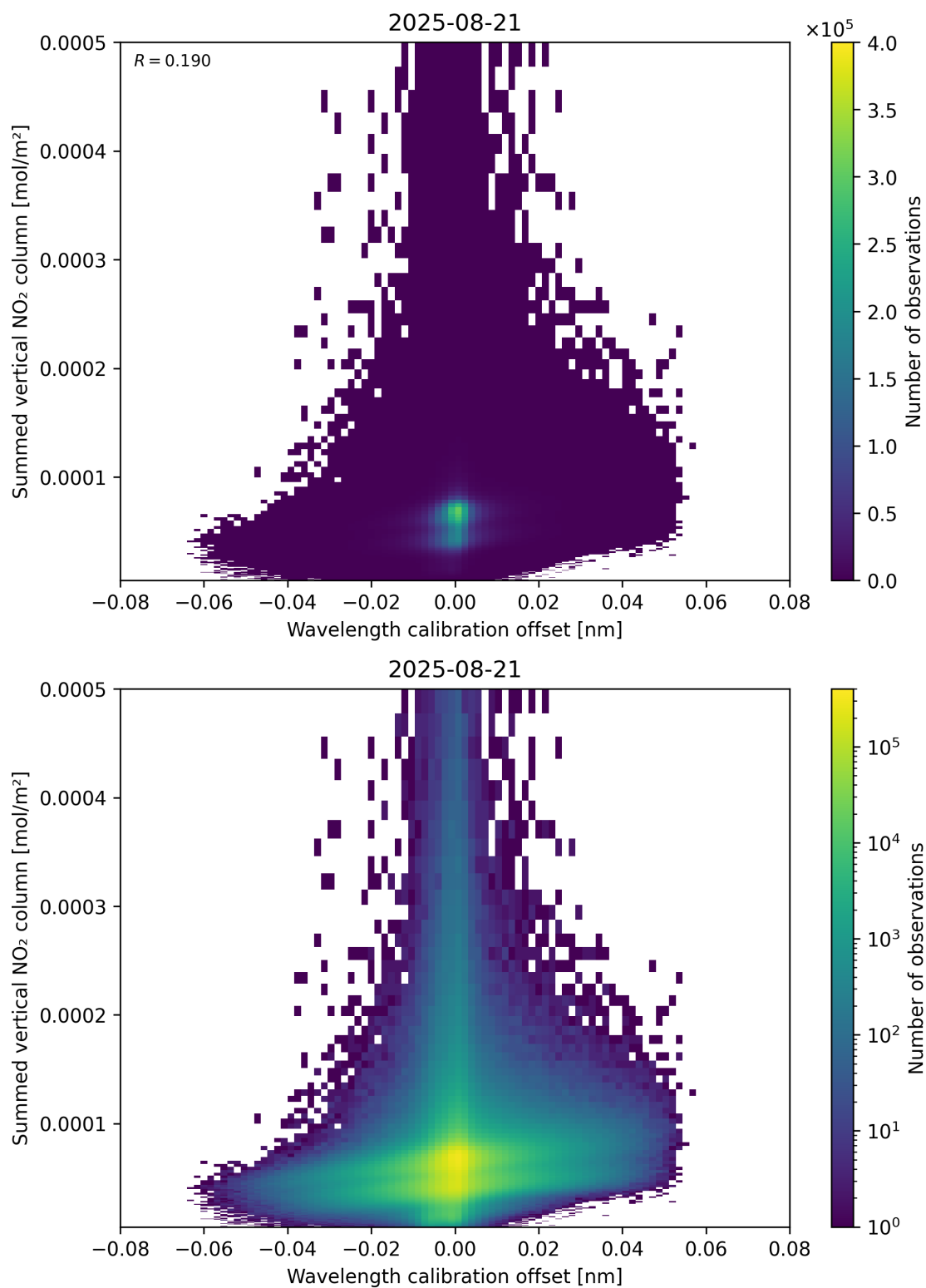
Figure 177: Scatter density plot of “Wavelength calibration offset” against “Summed vertical NO 2 column” for 2025-08-20 to 2025-08-22.
