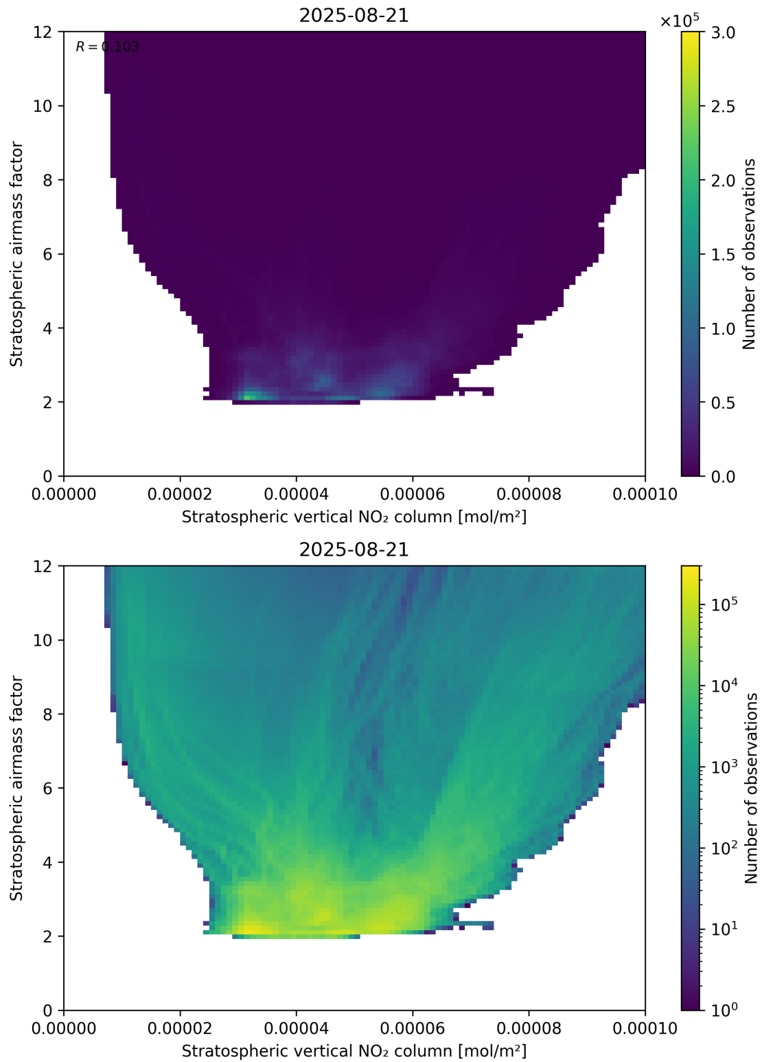
Figure 96: Scatter density plot of “Stratospheric vertical NO 2 column” against “Stratospheric airmass factor” for 2025-08-20 to 2025-08-22.
