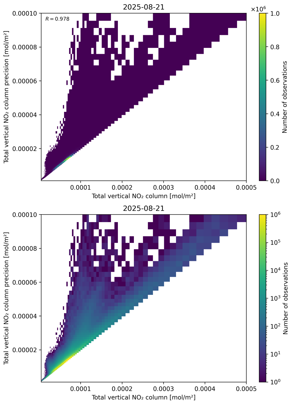
Figure 114: Scatter density plot of “Total vertical NO 2 column” against “Total vertical NO 2 column precision” for 2025-08-20 to 2025-08-22.
