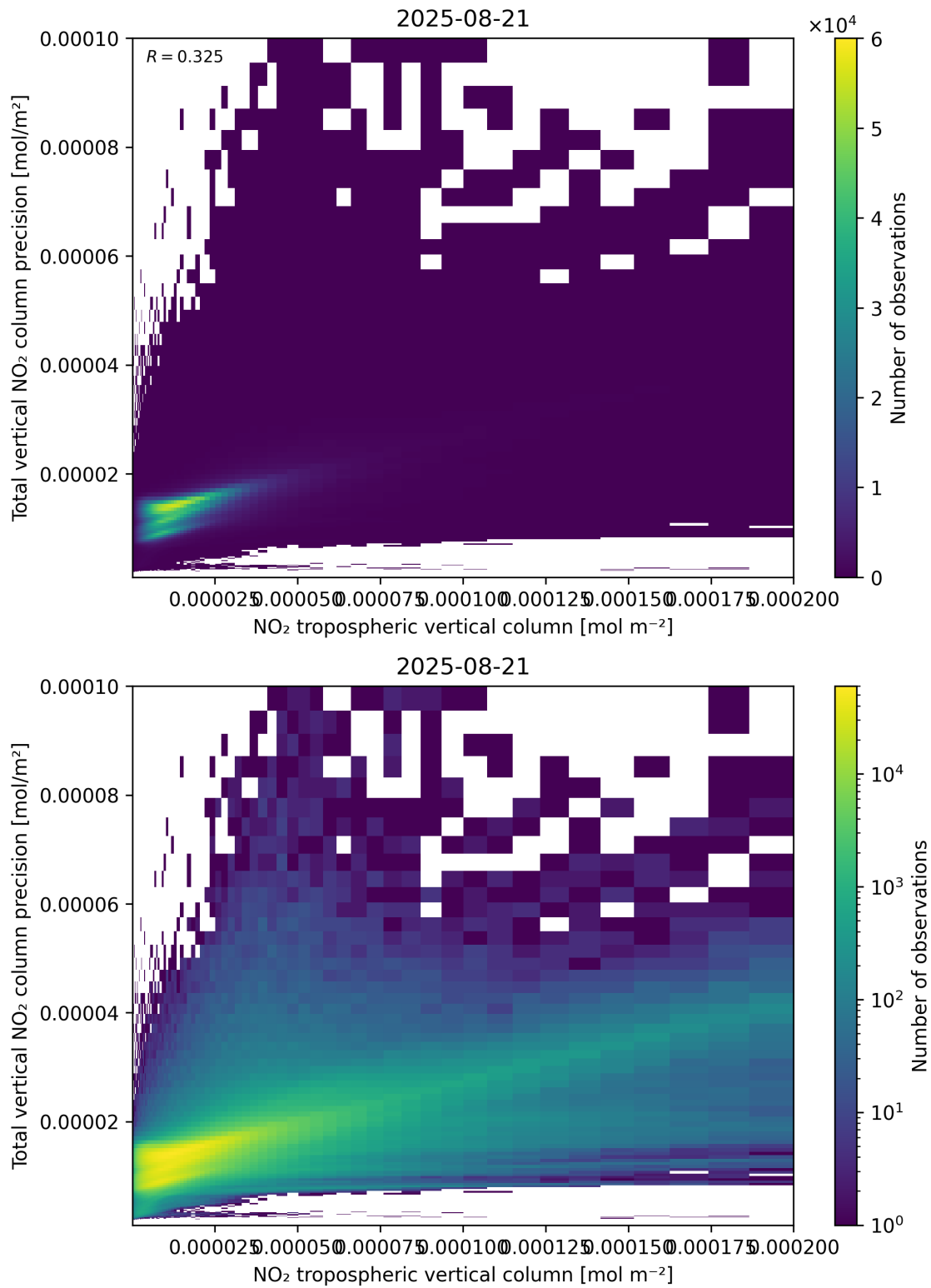
Figure 129: Scatter density plot of “NO 2 tropospheric vertical column” against “Total vertical NO 2 column precision” for 2025-08-20 to 2025-08-22.
