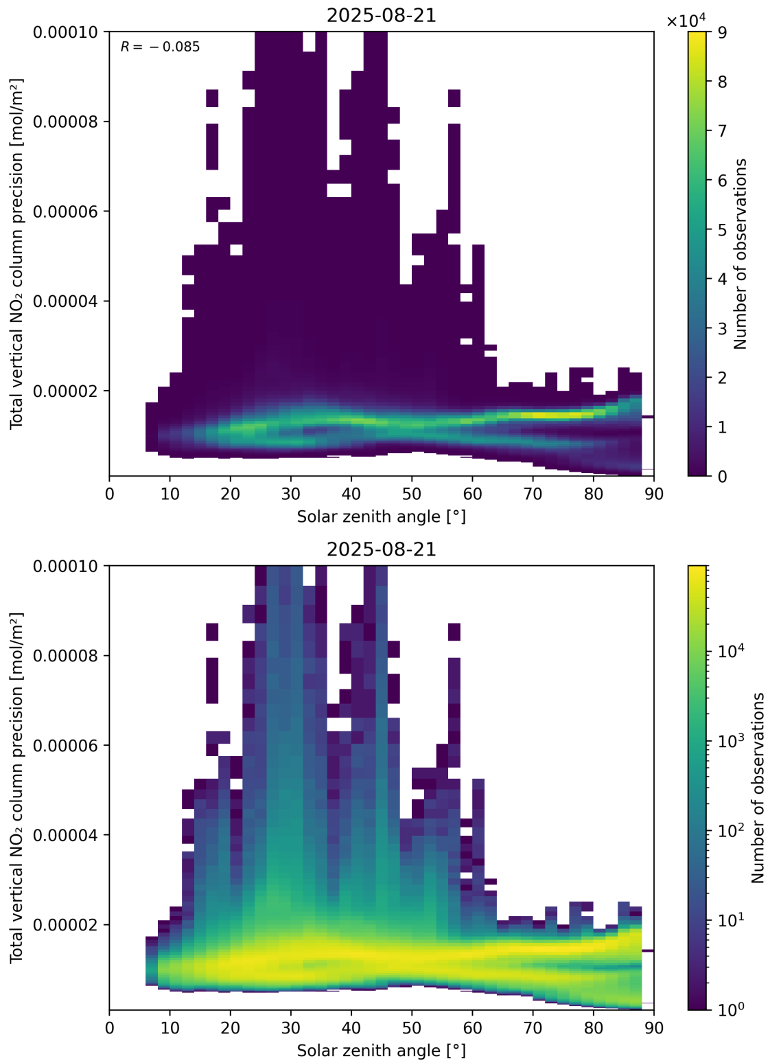
Figure 154: Scatter density plot of “Solar zenith angle” against “Total vertical NO 2 column precision” for 2025-08-20 to 2025-08-22.
