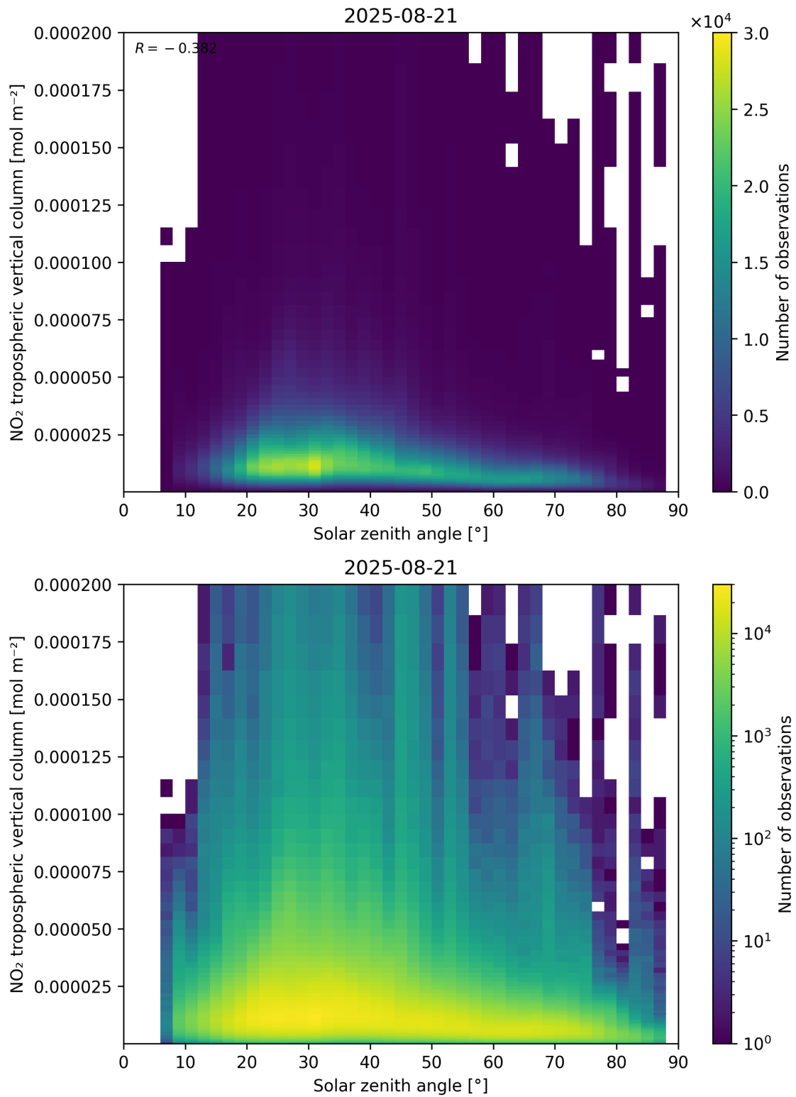
Figure 155: Scatter density plot of “Solar zenith angle” against “NO 2 tropospheric vertical column” for 2025-08-20 to 2025-08-22.
