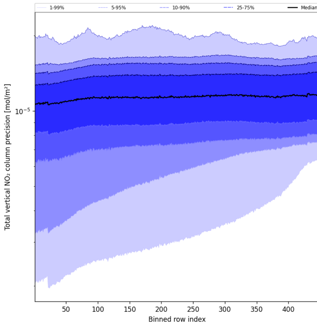
Figure 56: Along track statistics of “Total vertical NO 2 column precision” for 2025-08-20 to 2025-08-22
