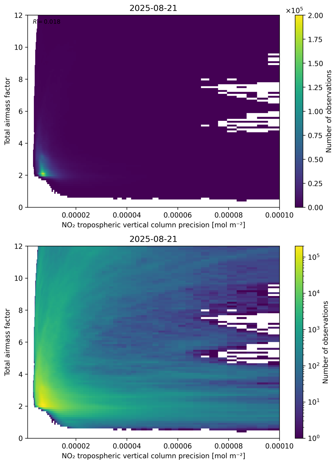
Figure 132: Scatter density plot of “NO 2 tropospheric vertical column precision” against “Total air mass factor” for 2025-08-20 to 2025-08-22.
