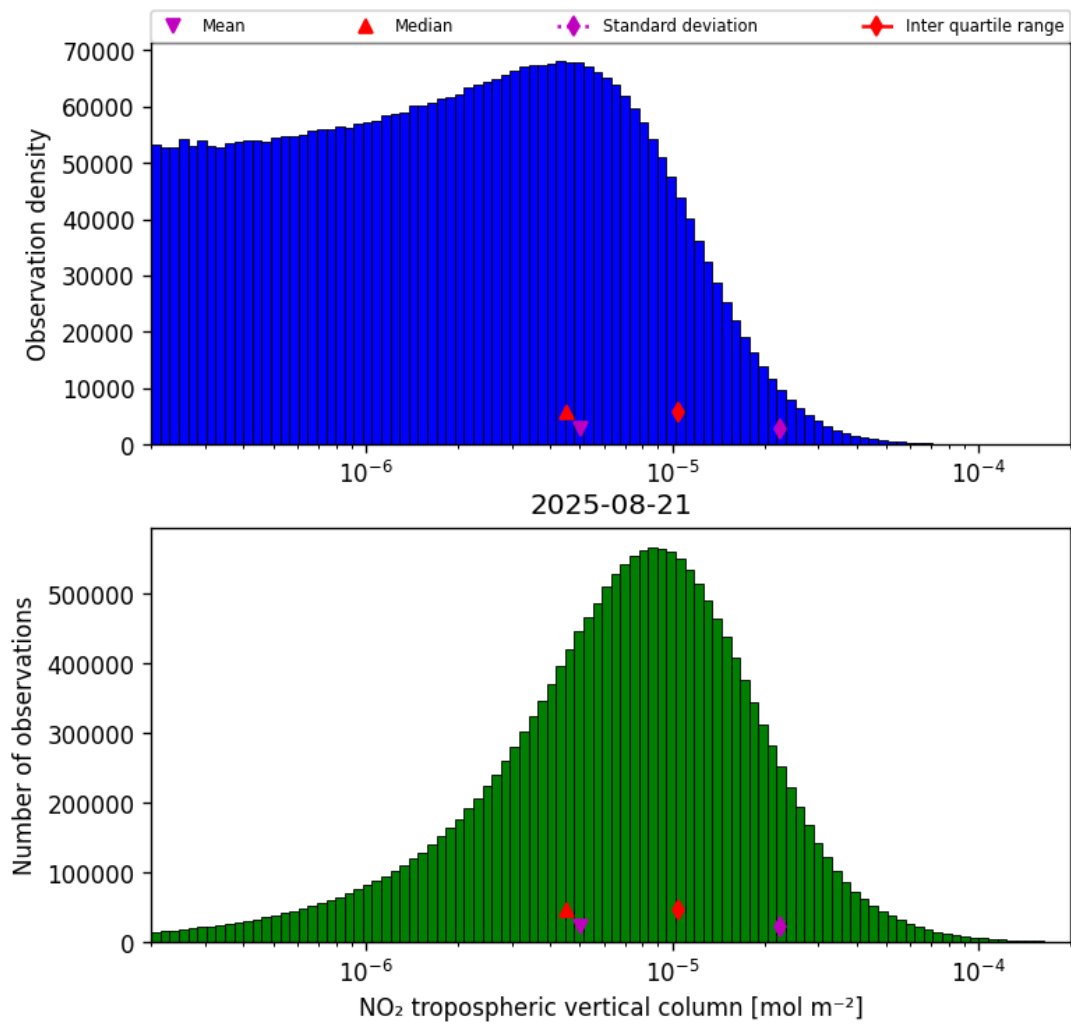
Figure 29: Histogram of “NO 2 tropospheric vertical column” for 2025-08-20 to 2025-08-22
