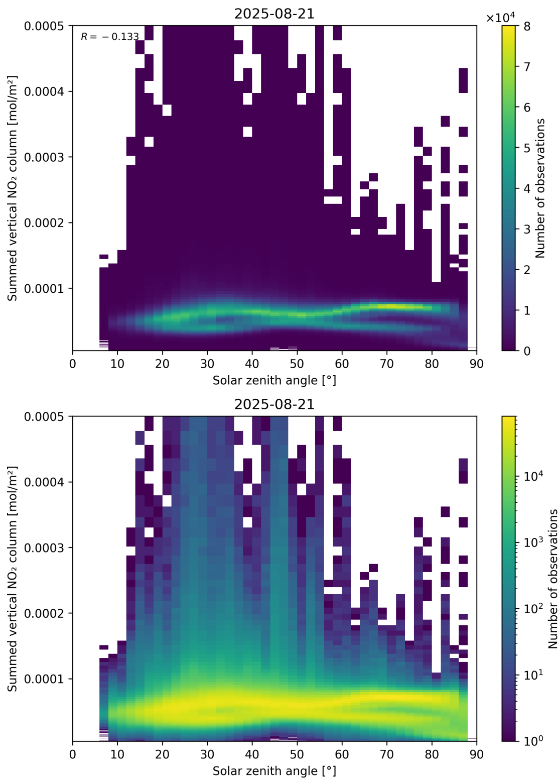
Figure 151: Scatter density plot of “Solar zenith angle” against “Summed vertical NO 2 column” for 2025-08-20 to 2025-08-22.
