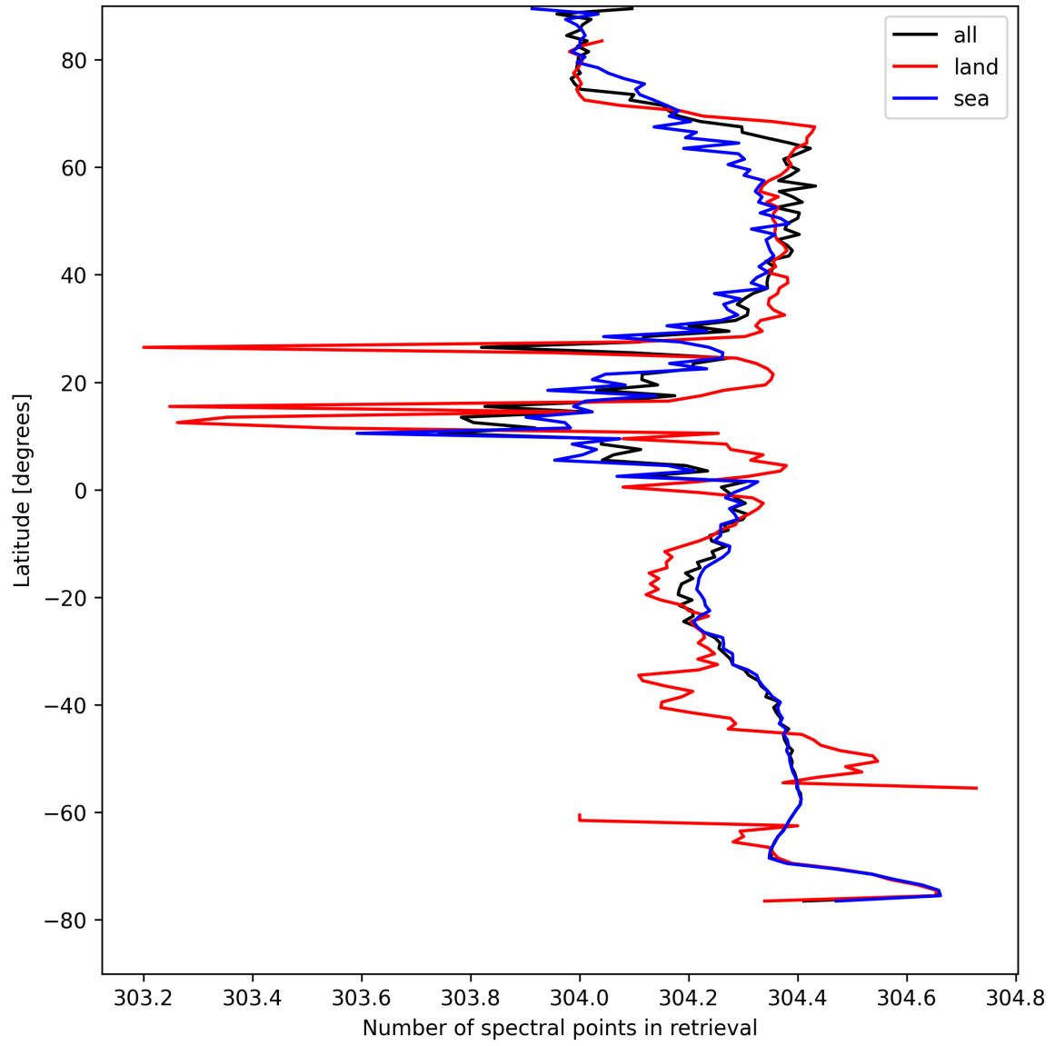
Figure 16: Zonal average of “Number of spectral points in retrieval” for 2025-08-20 to 2025-08-22.
