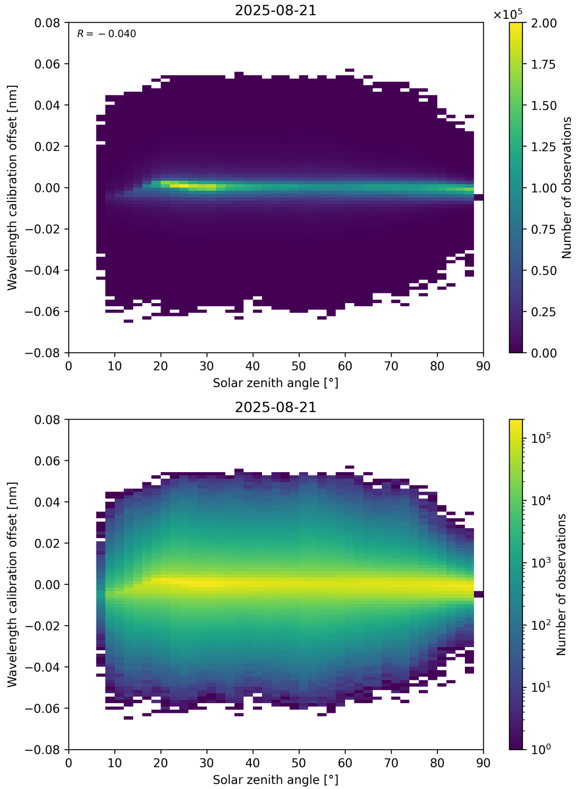
Figure 158: Scatter density plot of “Solar zenith angle” against “Wavelength calibration offset” for 2025-08-20 to 2025-08-22.
