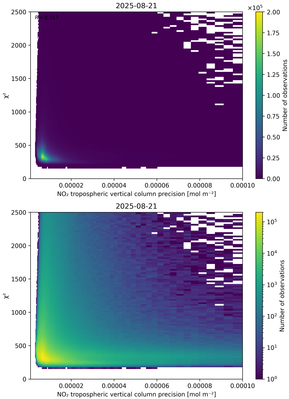
Figure 134: Scatter density plot of “NO 2 tropospheric vertical column precision” against “ \chi^2 ” for 2025-08-20 to 2025-08-22.
