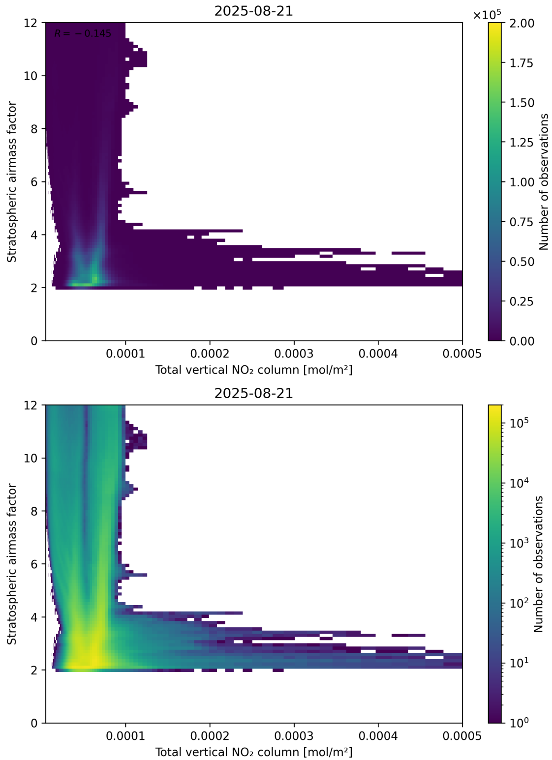
Figure 110: Scatter density plot of “Total vertical NO 2 column” against “Stratospheric airmass factor” for 2025-08-20 to 2025-08-22.
