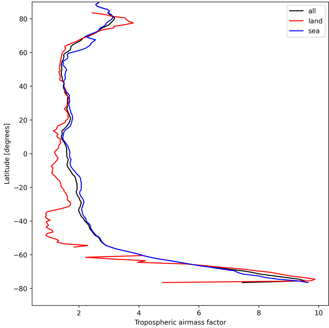
Figure 14: Zonal average of “Tropospheric airmass factor” for 2025-08-20 to 2025-08-22.
