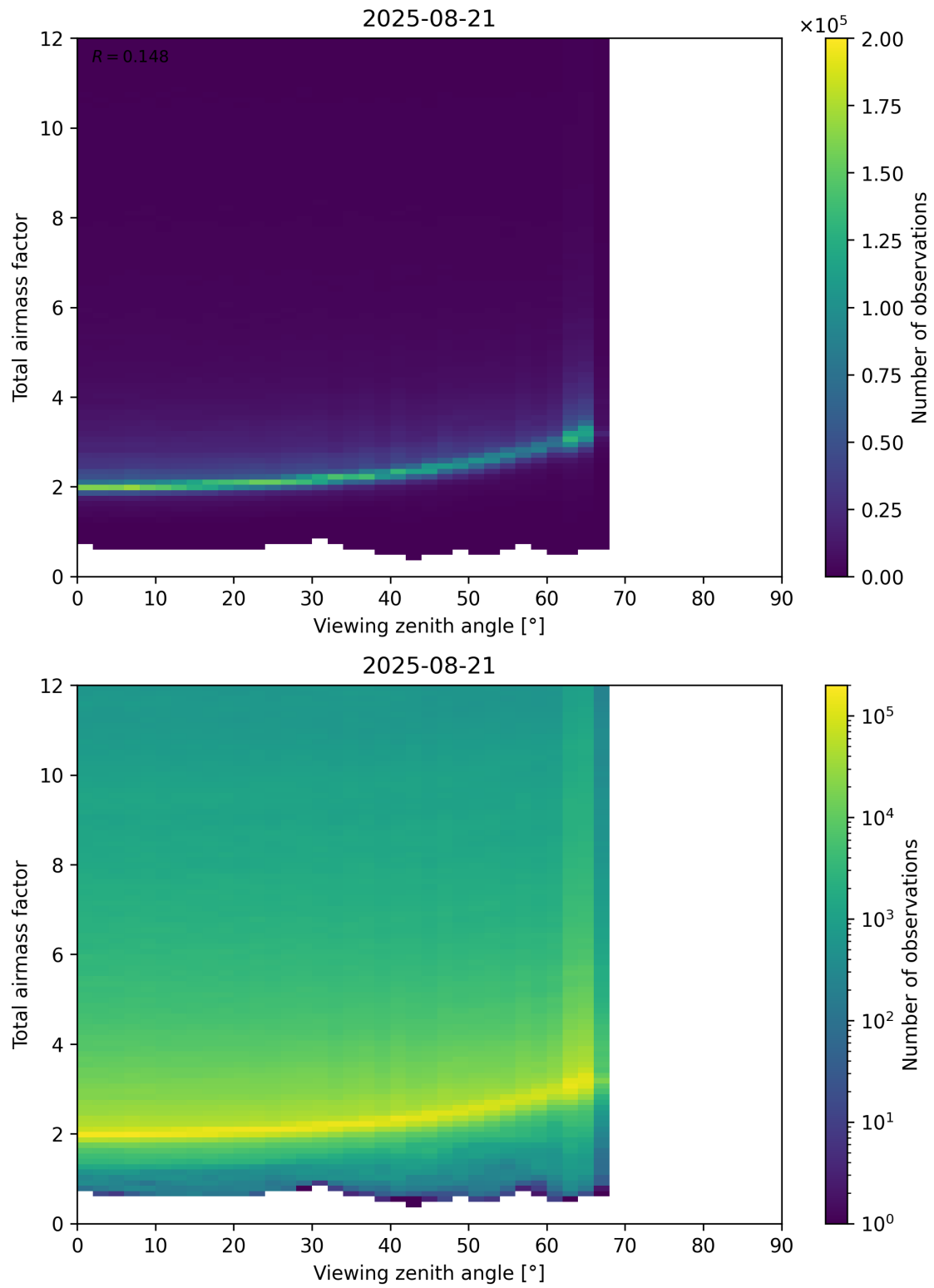
Figure 160: Scatter density plot of “Viewing zenith angle” against “Total airmass factor” for 2025-08-20 to 2025-08-22.
