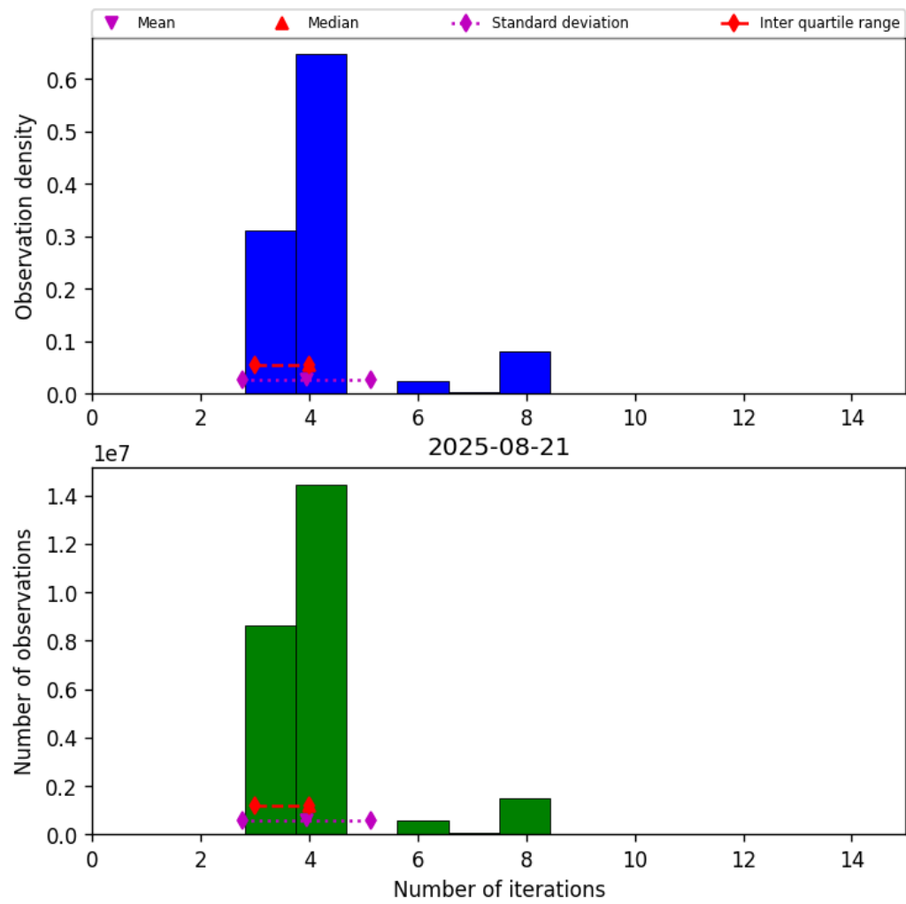
Figure 34: Histogram of "Number of iterations" for 2025-08-20 to 2025-08-22
