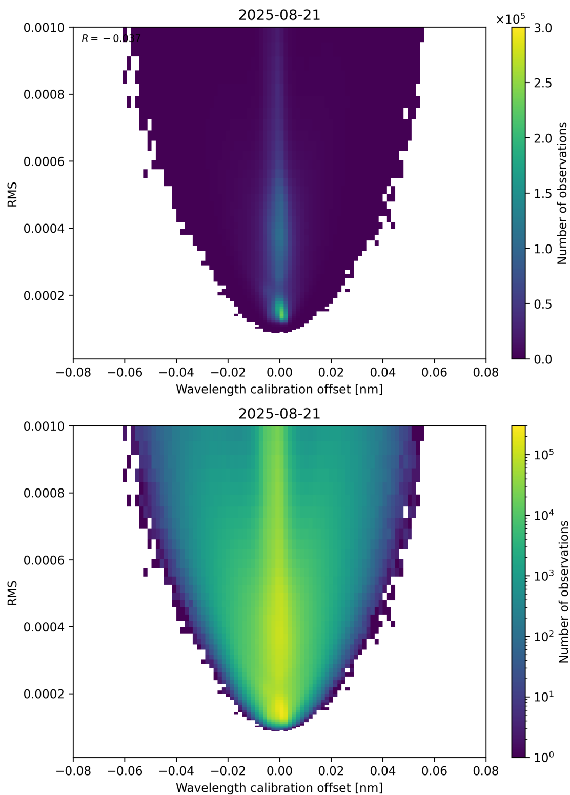
Figure 181: Scatter density plot of “Wavelength calibration offset” against “RMS” for 2025-08-20 to 2025-08-22.
