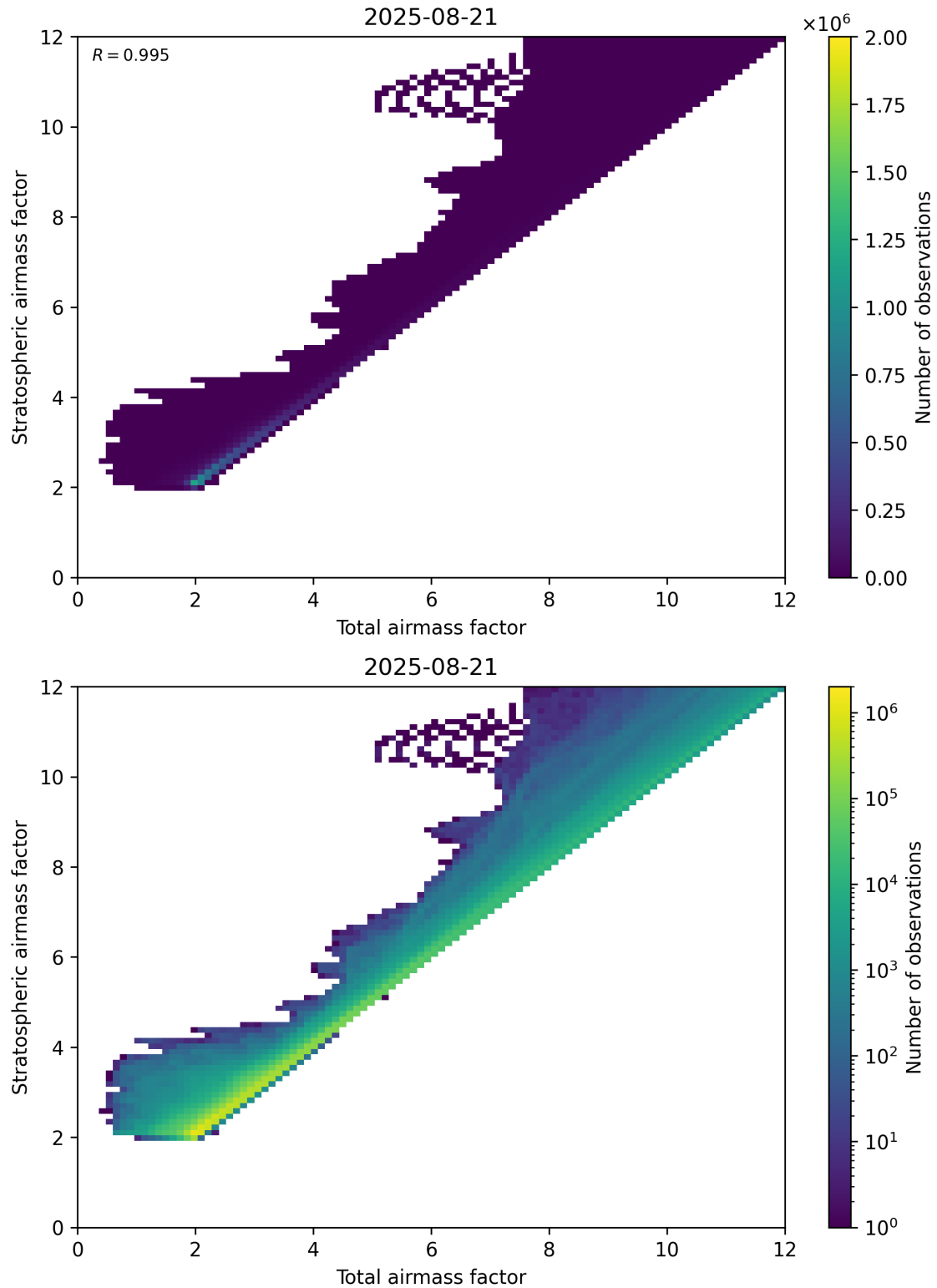
Figure 62: Scatter density plot of “Total airmass factor” against “Stratospheric airmass factor” for 2025-08-20 to 2025-08-22.
