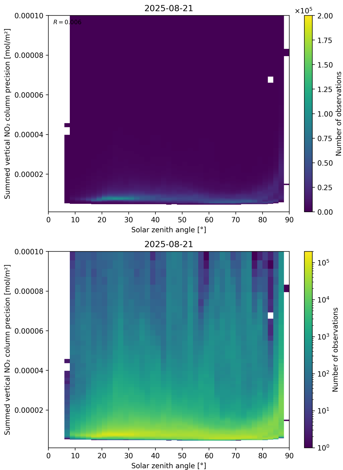
Figure 152: Scatter density plot of “Solar zenith angle” against “Summed vertical NO 2 column precision” for 2025-08-20 to 2025-08-22.
