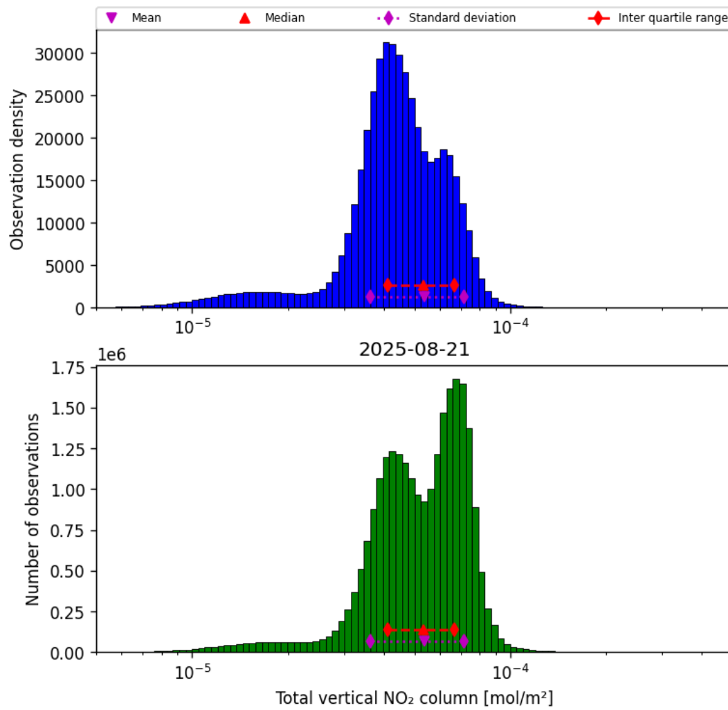
Figure 38: Histogram of “Total vertical NO 2 column” for 2025-08-20 to 2025-08-22
