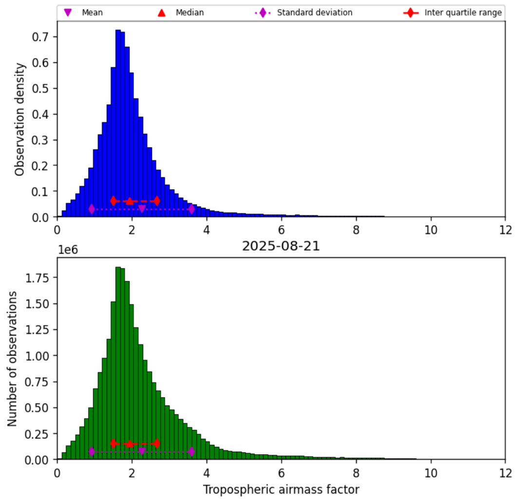
Figure 31: Histogram of “Tropospheric airmass factor” for 2025-08-20 to 2025-08-22
