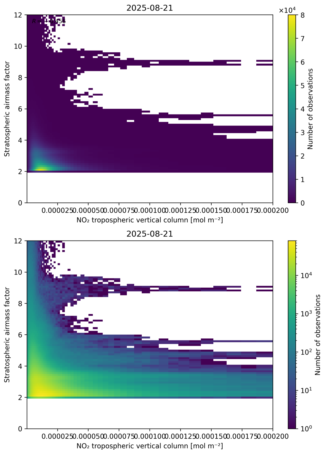
Figure 121: Scatter density plot of “NO 2 tropospheric vertical column” against “Stratospheric air mass factor” for 2025-08-20 to 2025-08-22.
