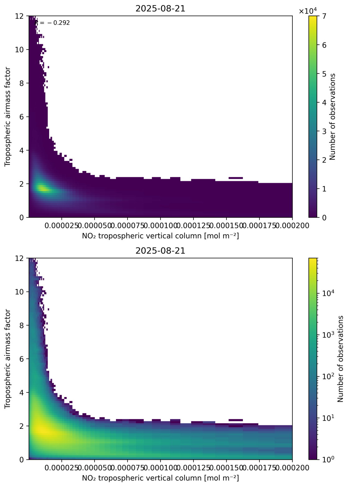
Figure 123: Scatter density plot of “NO 2 tropospheric vertical column” against “Tropospheric air mass factor” for 2025-08-20 to 2025-08-22.
