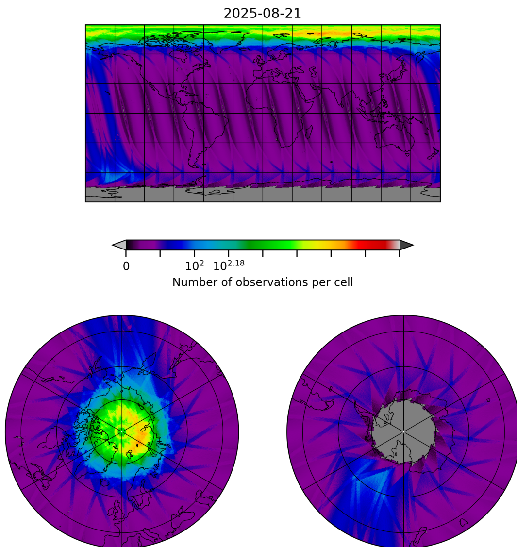
Figure 10: Map of the number of observations for 2025-08-20 to 2025-08-22
