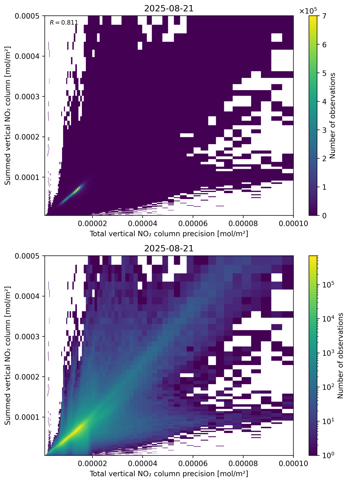
Figure 117: Scatter density plot of “Total vertical NO 2 column precision” against “Summed vertical NO 2 column” for 2025-08-20 to 2025-08-22.
