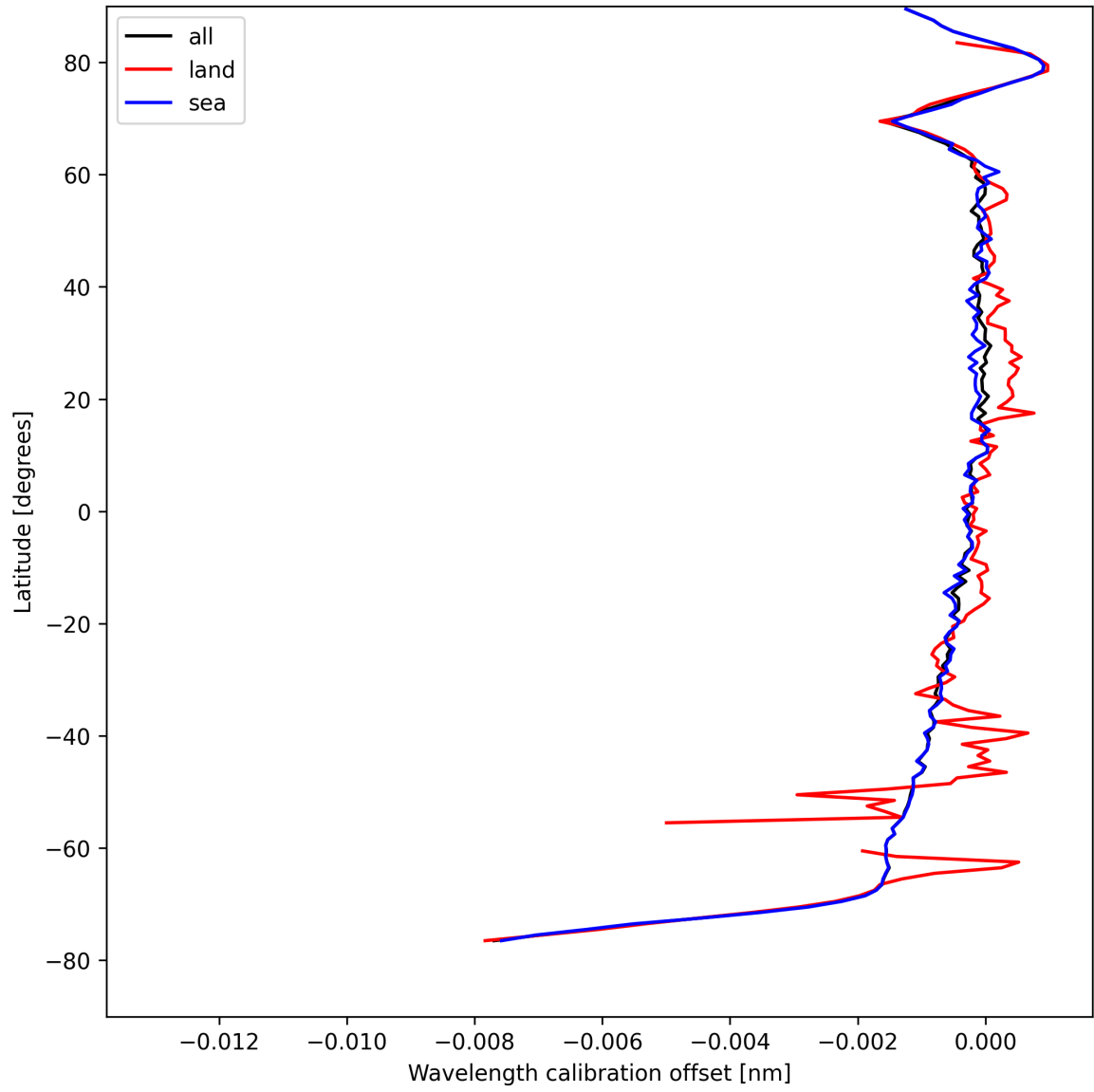
Figure 18: Zonal average of “Wavelength calibration offset” for 2025-08-20 to 2025-08-22.
