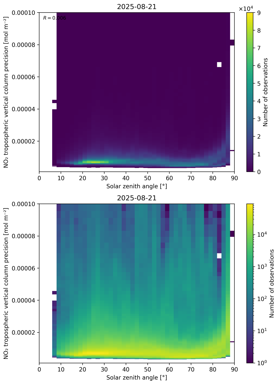
Figure 156: Scatter density plot of “Solar zenith angle” against “NO 2 tropospheric vertical column precision” for 2025-08-20 to 2025-08-22.
