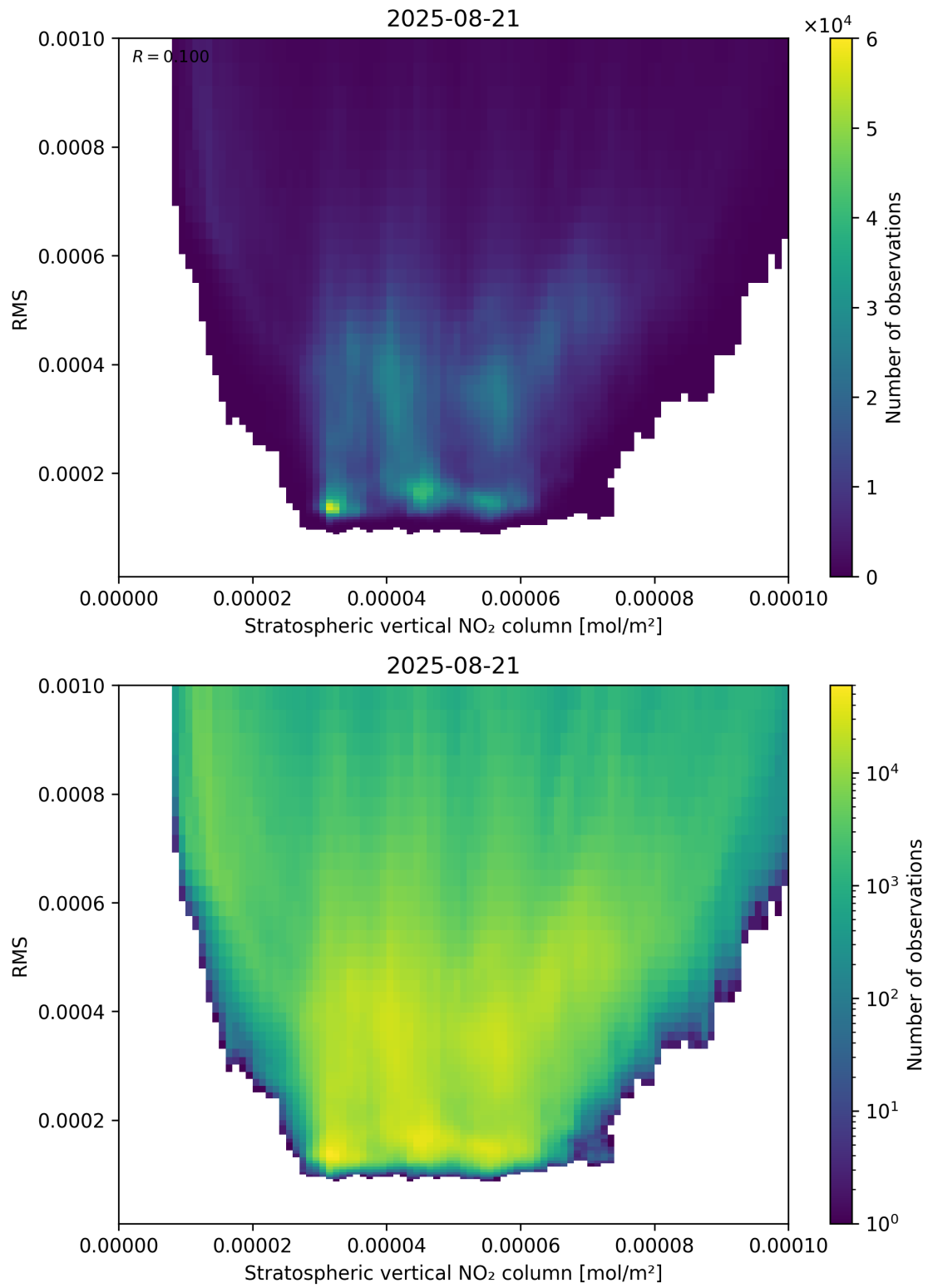
Figure 102: Scatter density plot of “Stratospheric vertical NO 2 column” against “RMS” for 2025-08-20 to 2025-08-22.
