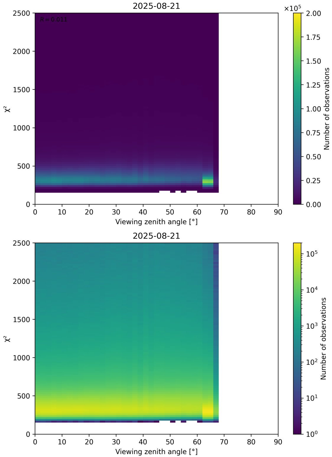
Figure 162: Scatter density plot of “Viewing zenith angle” against “ \chi^2 ” for 2025-08-20 to 2025-08-22.
