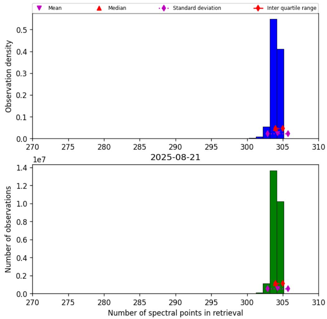
Figure 33: Histogram of “Number of spectral points in retrieval” for 2025-08-20 to 2025-08-22
