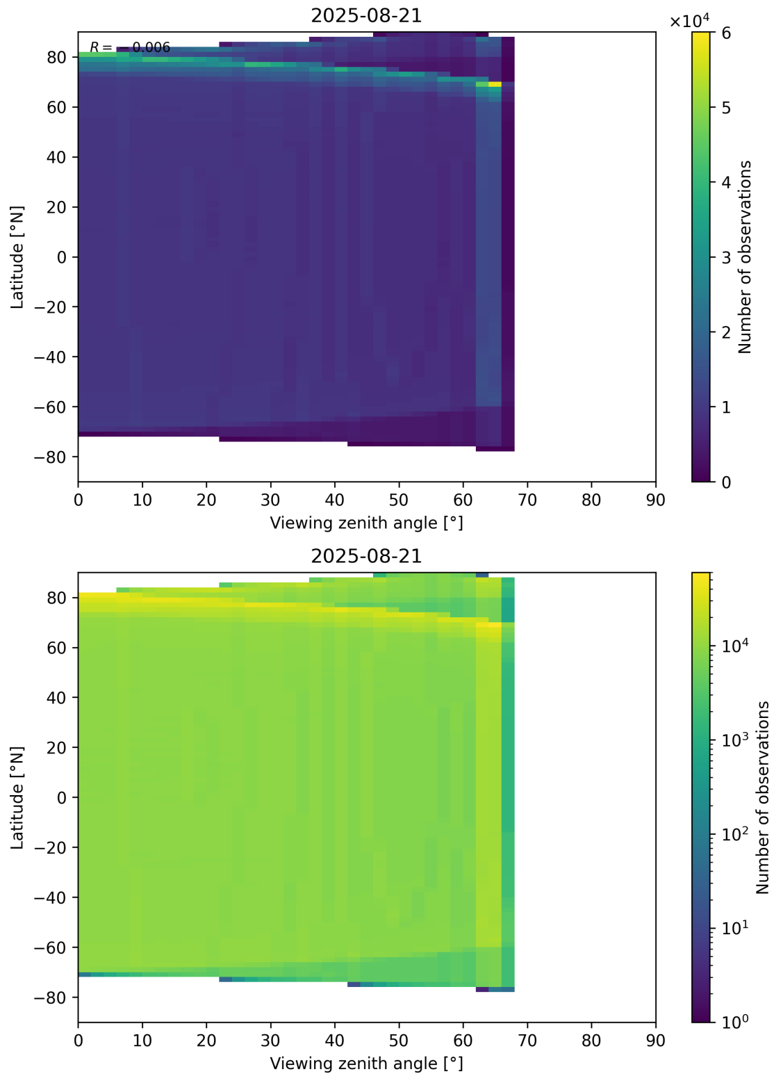
Figure 163: Scatter density plot of “Viewing zenith angle” against “Latitude” for 2025-08-20 to 2025-08-22.
