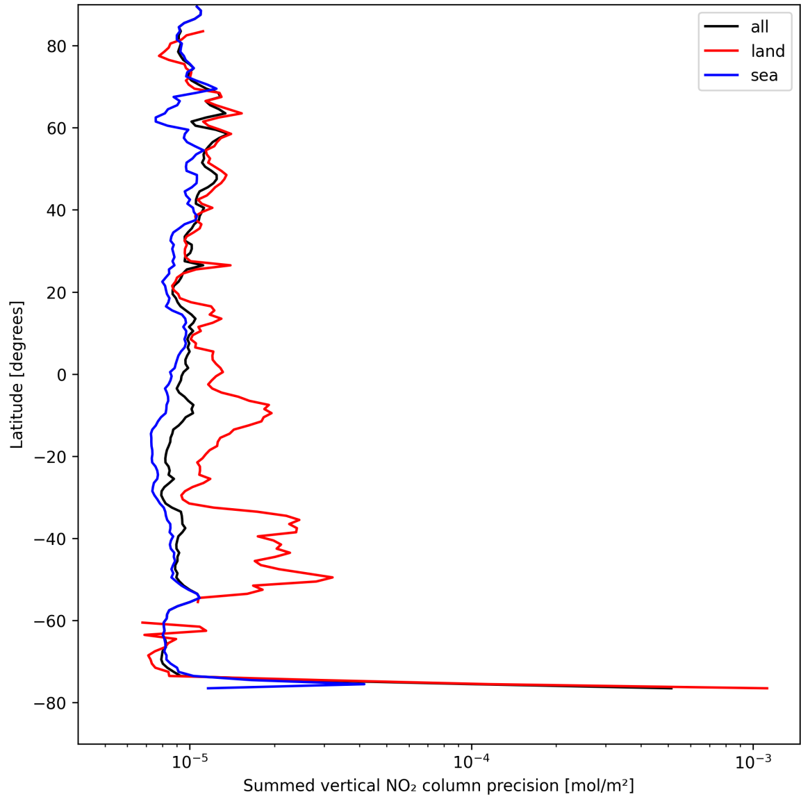
Figure 24: Zonal average of “Summed vertical NO 2 column precision” for 2025-08-20 to 2025-08-22.
