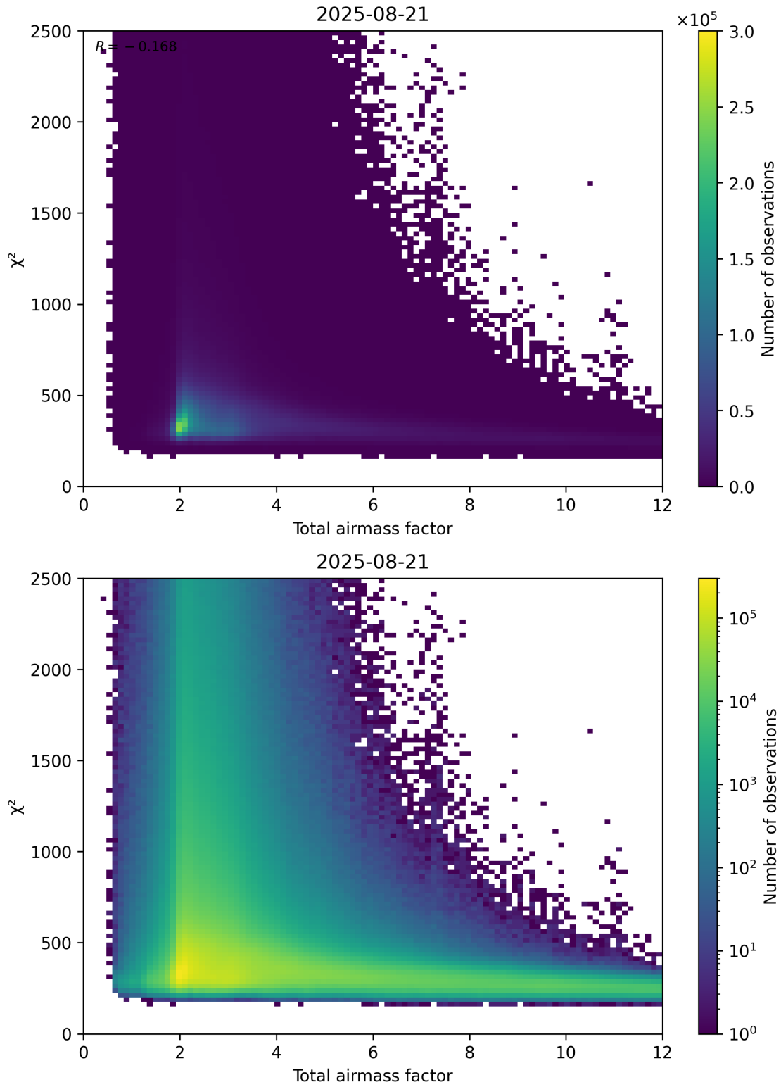
Figure 63: Scatter density plot of “Total airmass factor” against “ \chi^2 ” for 2025-08-20 to 2025-08-22.
