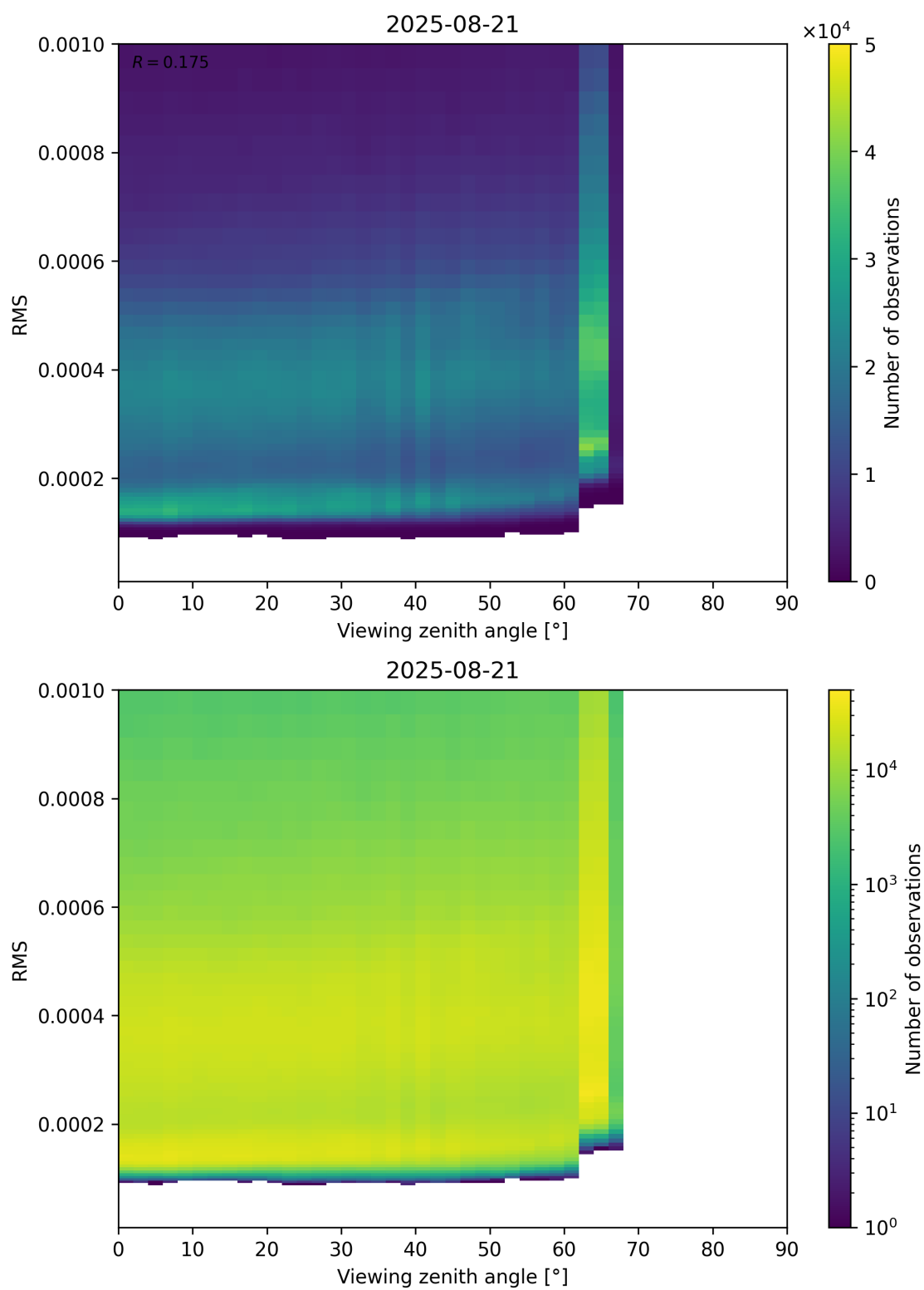
Figure 171: Scatter density plot of “Viewing zenith angle” against “RMS” for 2025-08-20 to 2025-08-22.
