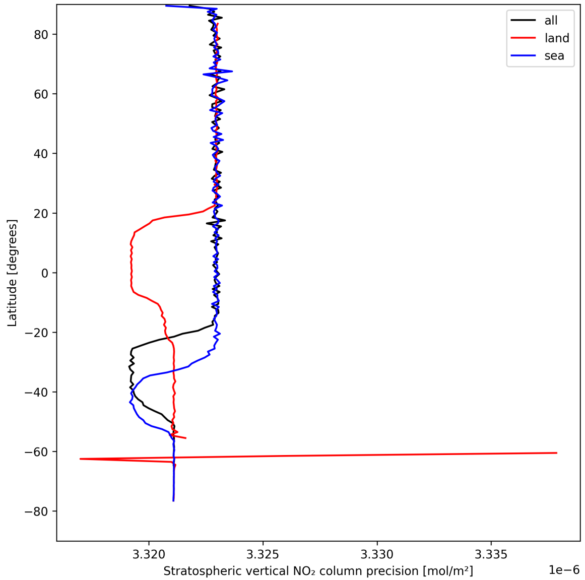
Figure 20: Zonal average of “Stratospheric vertical NO 2 column precision” for 2025-08-20 to 2025-08-22.
