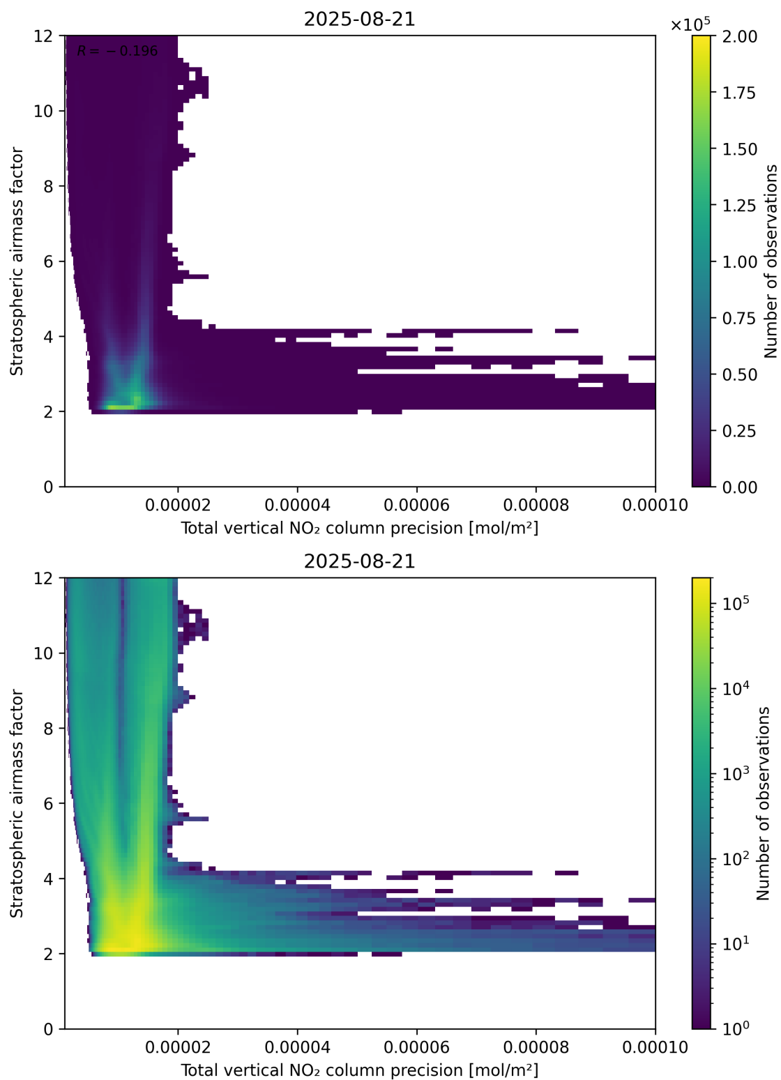
Figure 115: Scatter density plot of “Total vertical NO 2 column precision” against “Stratospheric air mass factor” for 2025-08-20 to 2025-08-22.
