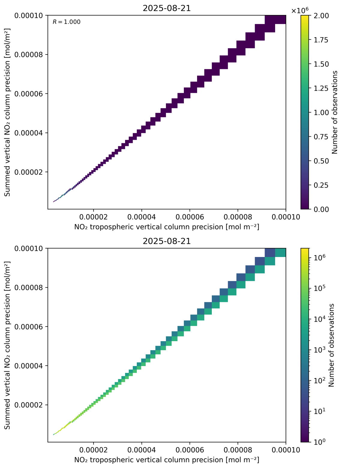
Figure 137: Scatter density plot of “NO 2 tropospheric vertical column precision” against “Summed vertical NO 2 column precision” for 2025-08-20 to 2025-08-22.
