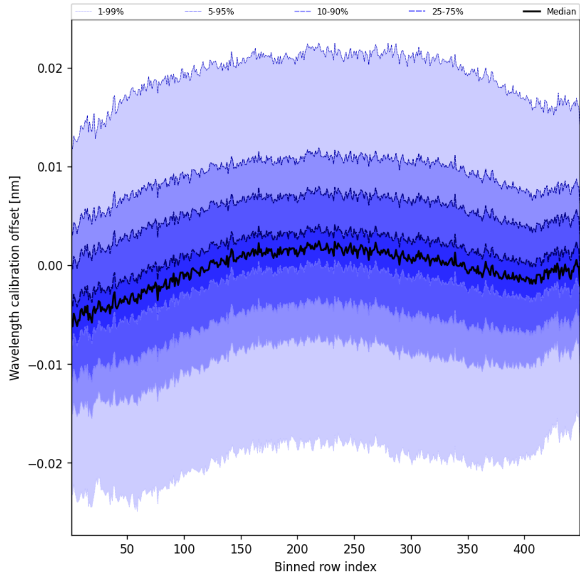
Figure 52: Along track statistics of “Wavelength calibration offset” for 2025-08-20 to 2025-08-22
