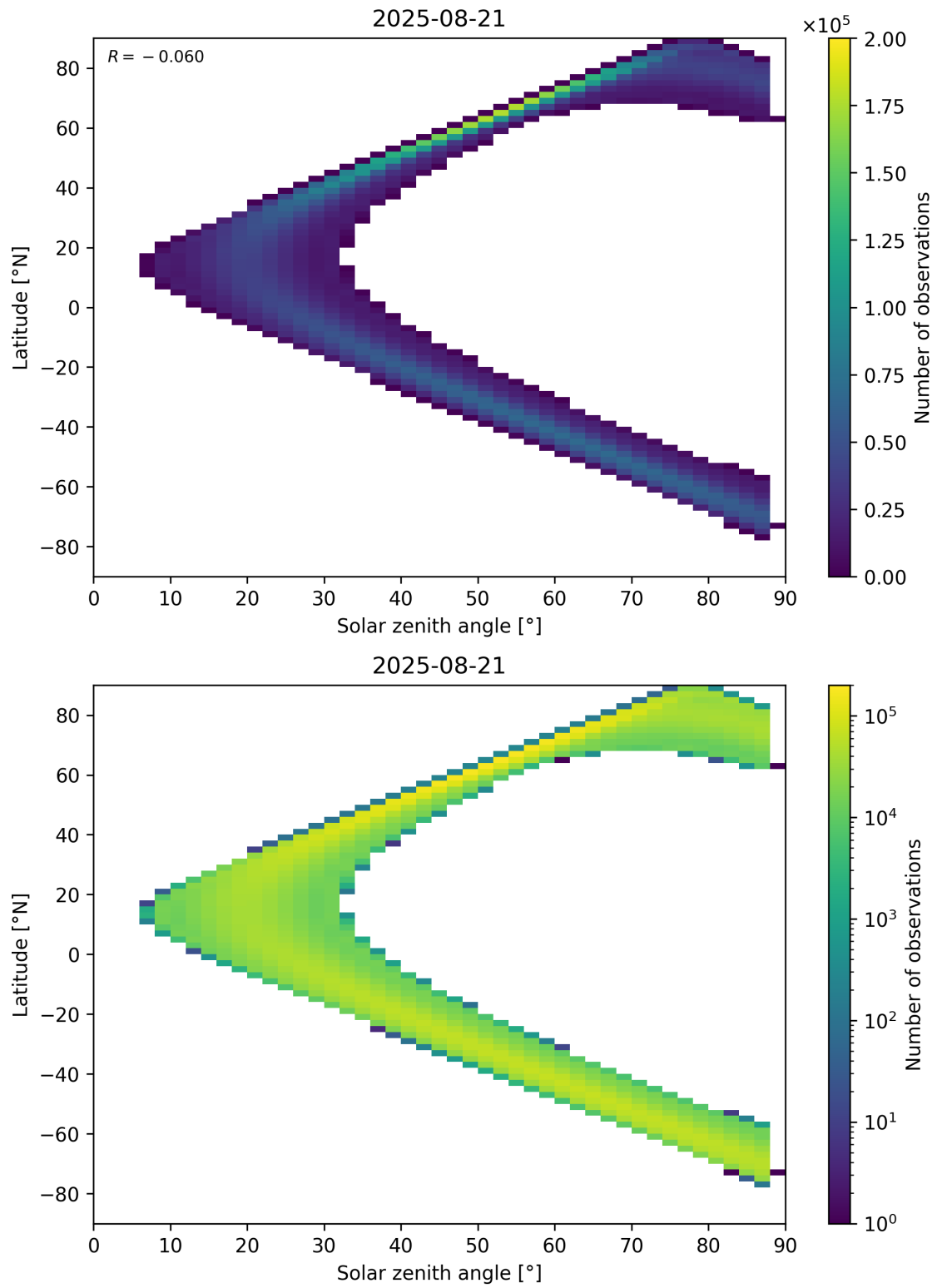
Figure 149: Scatter density plot of “Solar zenith angle” against “Latitude” for 2025-08-20 to 2025-08-22.
