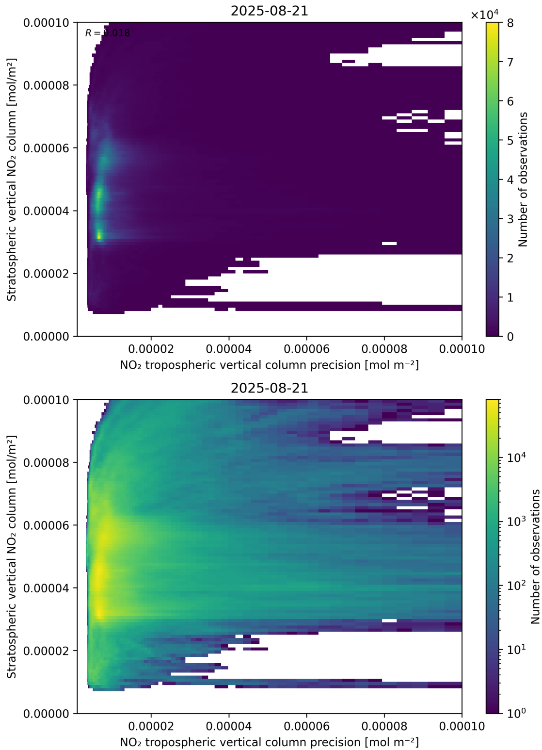
Figure 135: Scatter density plot of “NO 2 tropospheric vertical column precision” against “Stratospheric vertical NO 2 column” for 2025-08-20 to 2025-08-22.
