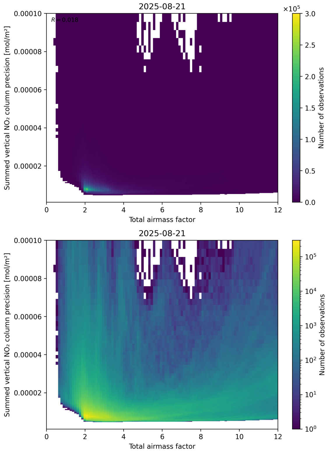
Figure 66: Scatter density plot of “Total airmass factor” against “Summed vertical NO 2 column precision” for 2025-08-20 to 2025-08-22.
