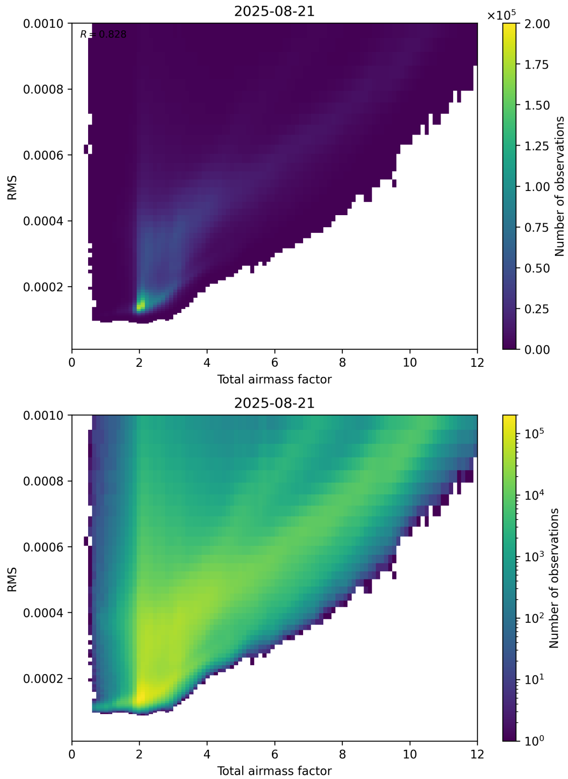
Figure 69: Scatter density plot of “Total airmass factor” against “RMS” for 2025-08-20 to 2025-08-22.
