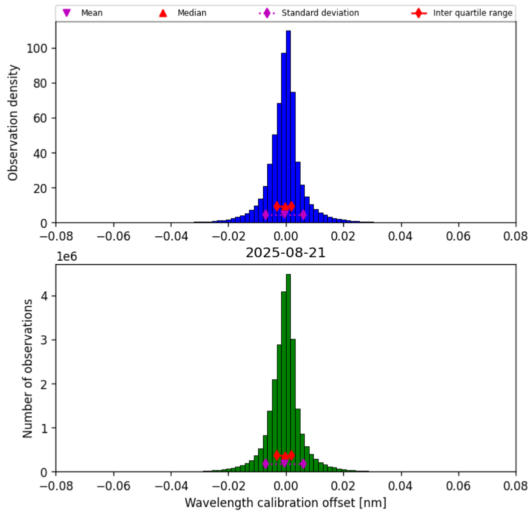
Figure 35: Histogram of “Wavelength calibration offset” for 2025-08-20 to 2025-08-22
