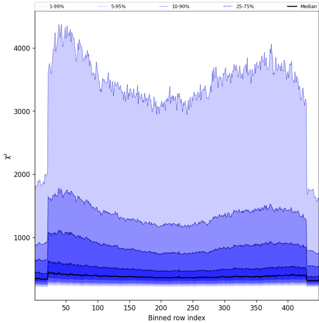
Figure 59: Along track statistics of “ \chi^2 ” for 2025-08-20 to 2025-08-22
