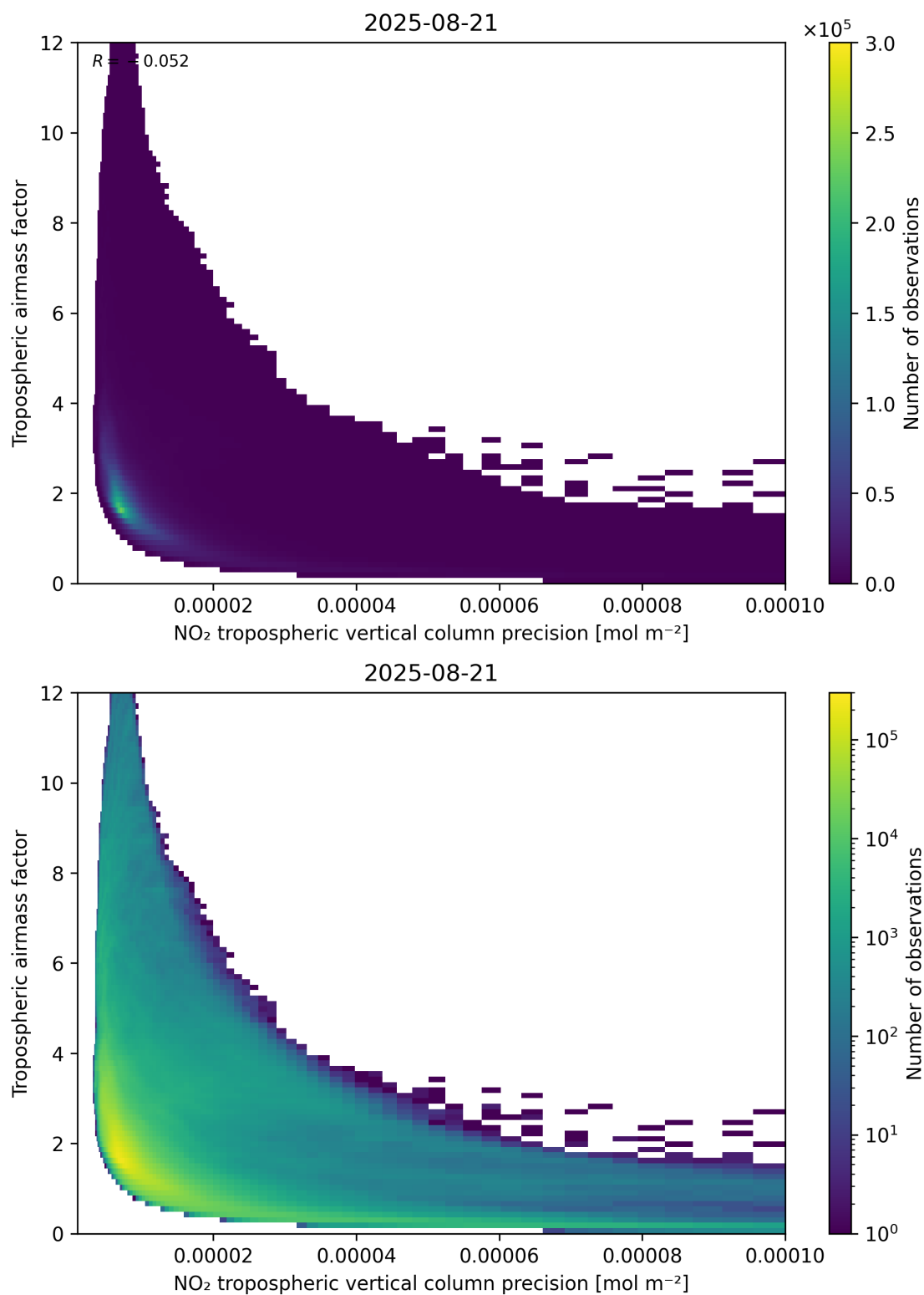
Figure 133: Scatter density plot of “NO 2 tropospheric vertical column precision” against “Tropospheric air mass factor” for 2025-08-20 to 2025-08-22.
