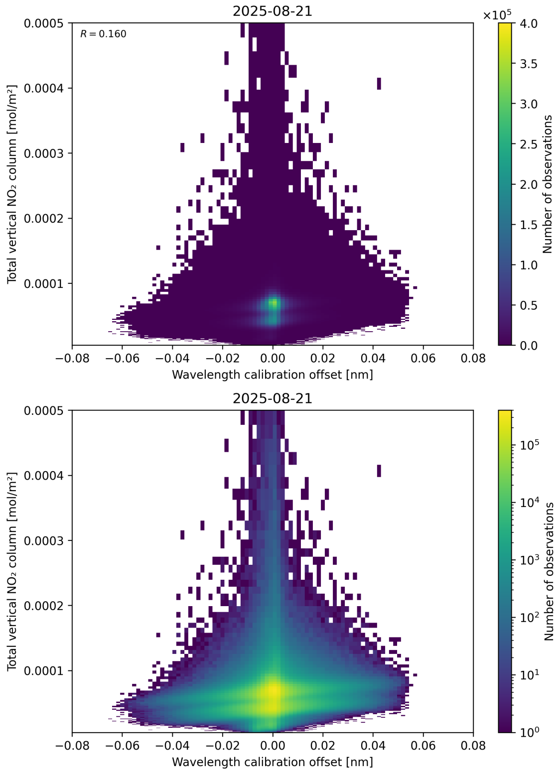
Figure 179: Scatter density plot of “Wavelength calibration offset” against “Total vertical NO 2 column” for 2025-08-20 to 2025-08-22.
