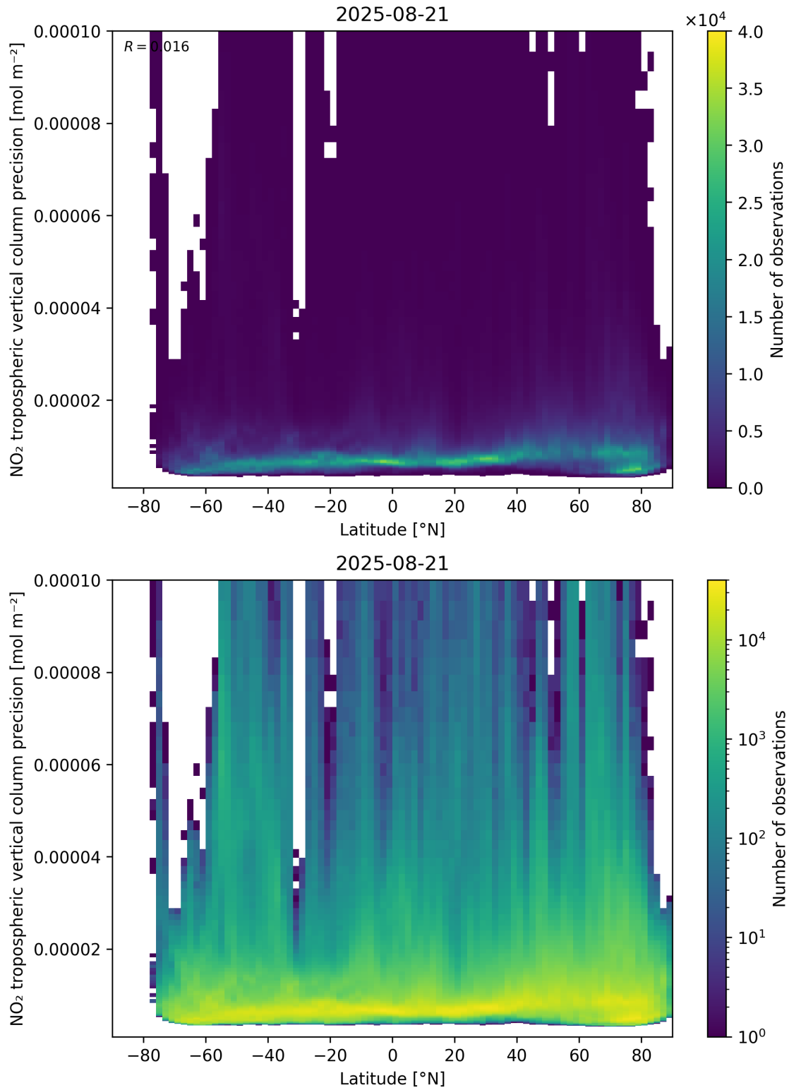
Figure 93: Scatter density plot of “Latitude” against “NO 2 tropospheric vertical column precision” for 2025-08-20 to 2025-08-22.
