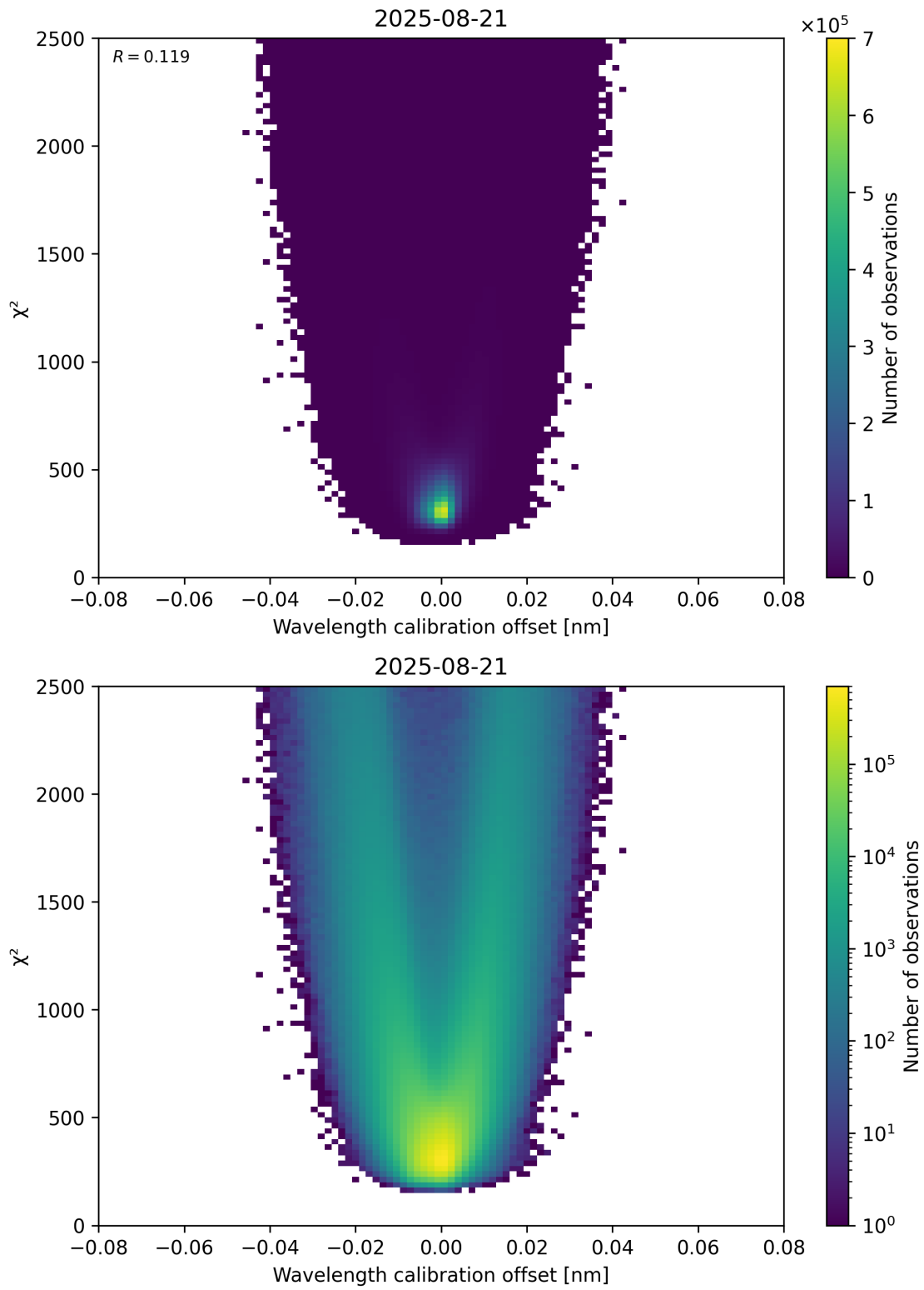
Figure 175: Scatter density plot of “Wavelength calibration offset” against “ \chi^2 ” for 2025-08-20 to 2025-08-22.
