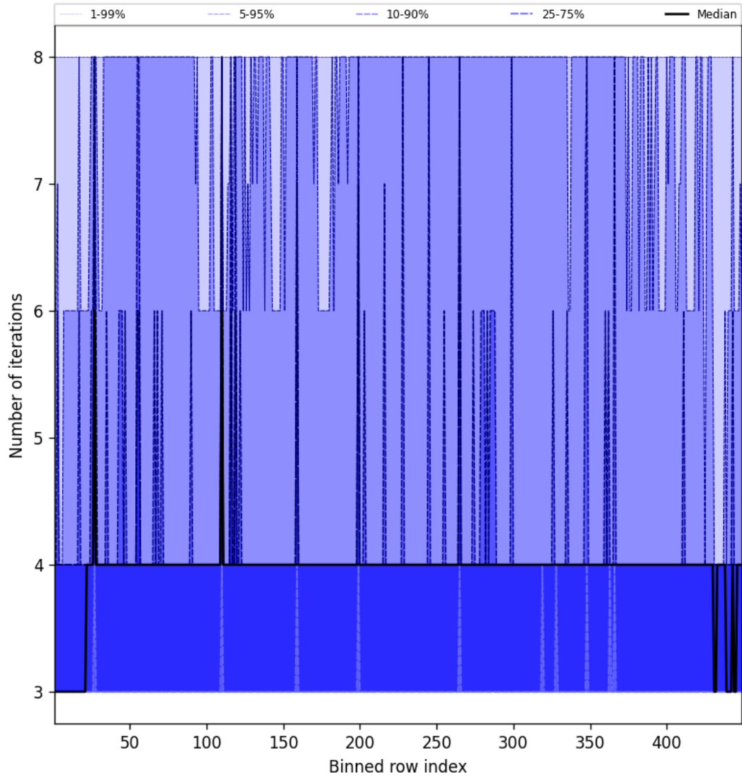
Figure 51: Along track statistics of “Number of iterations” for 2025-08-20 to 2025-08-22
