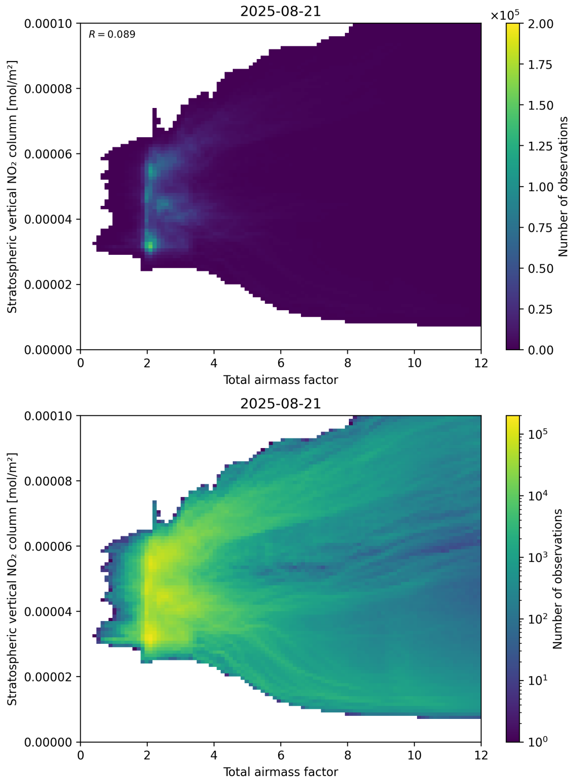
Figure 64: Scatter density plot of “Total airmass factor” against “Stratospheric vertical NO 2 column” for 2025-08-20 to 2025-08-22.
