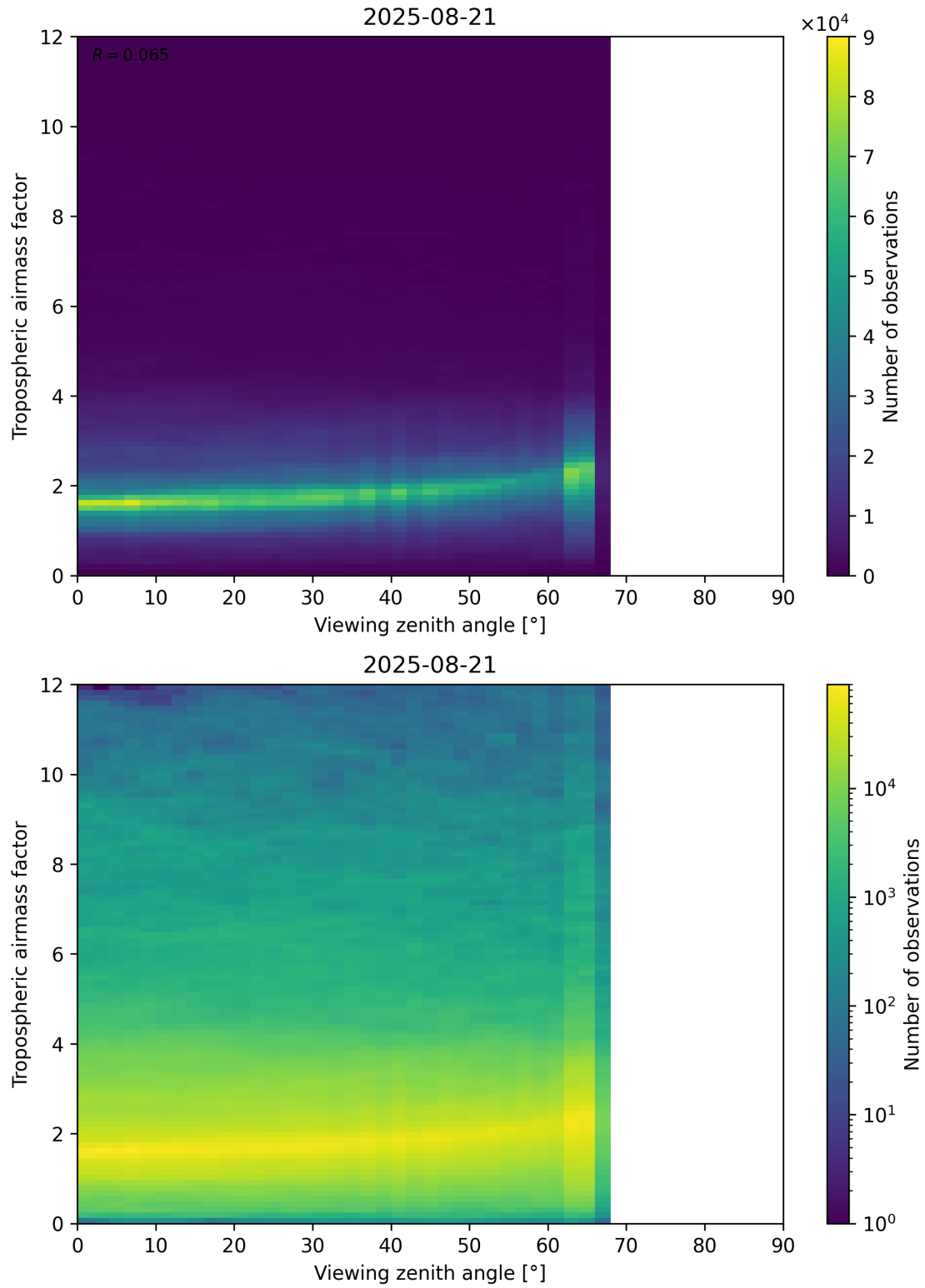
Figure 161: Scatter density plot of “Viewing zenith angle” against “Tropospheric airmass factor” for 2025-08-20 to 2025-08-22.
