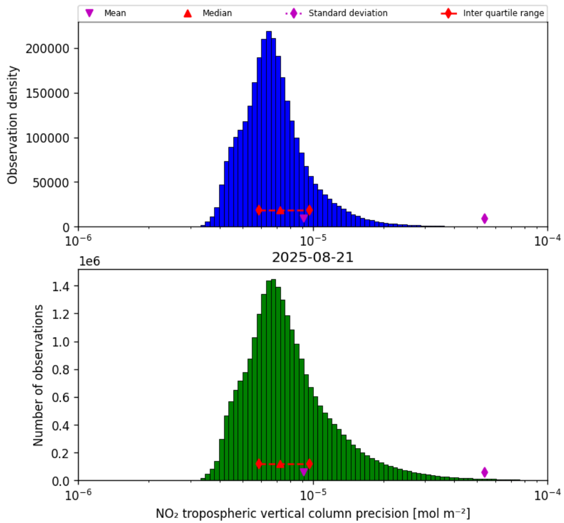
Figure 30: Histogram of “NO 2 tropospheric vertical column precision” for 2025-08-20 to 2025-08-22
