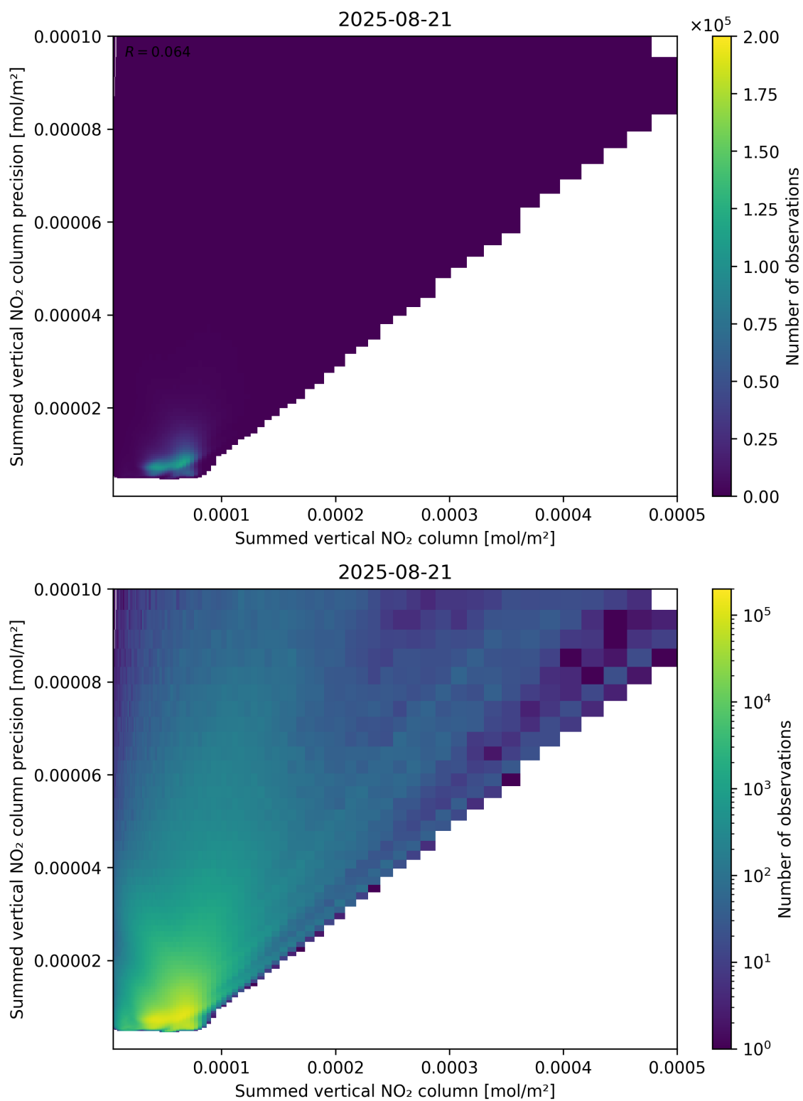
Figure 105: Scatter density plot of “Summed vertical NO 2 column” against “Summed vertical NO 2 column precision” for 2025-08-20 to 2025-08-22.
