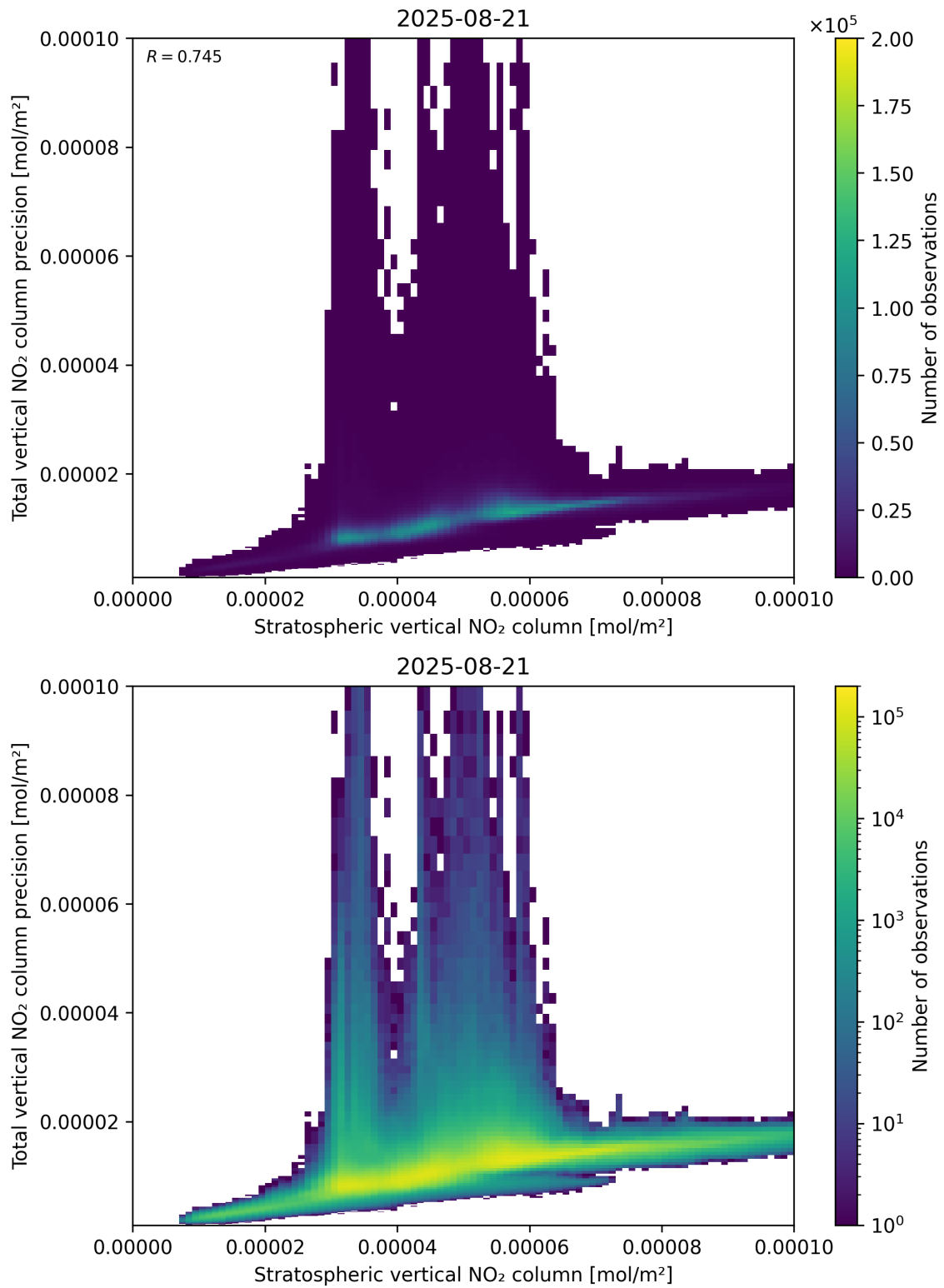
Figure 101: Scatter density plot of “Stratospheric vertical NO 2 column” against “Total vertical NO 2 column precision” for 2025-08-20 to 2025-08-22.
