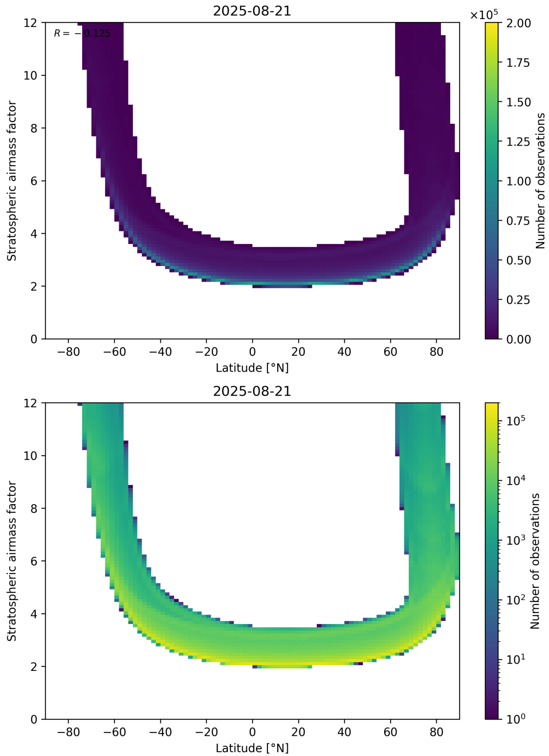
Figure 83: Scatter density plot of “Latitude” against “Stratospheric airmass factor” for 2025-08-20 to 2025-08-22.
