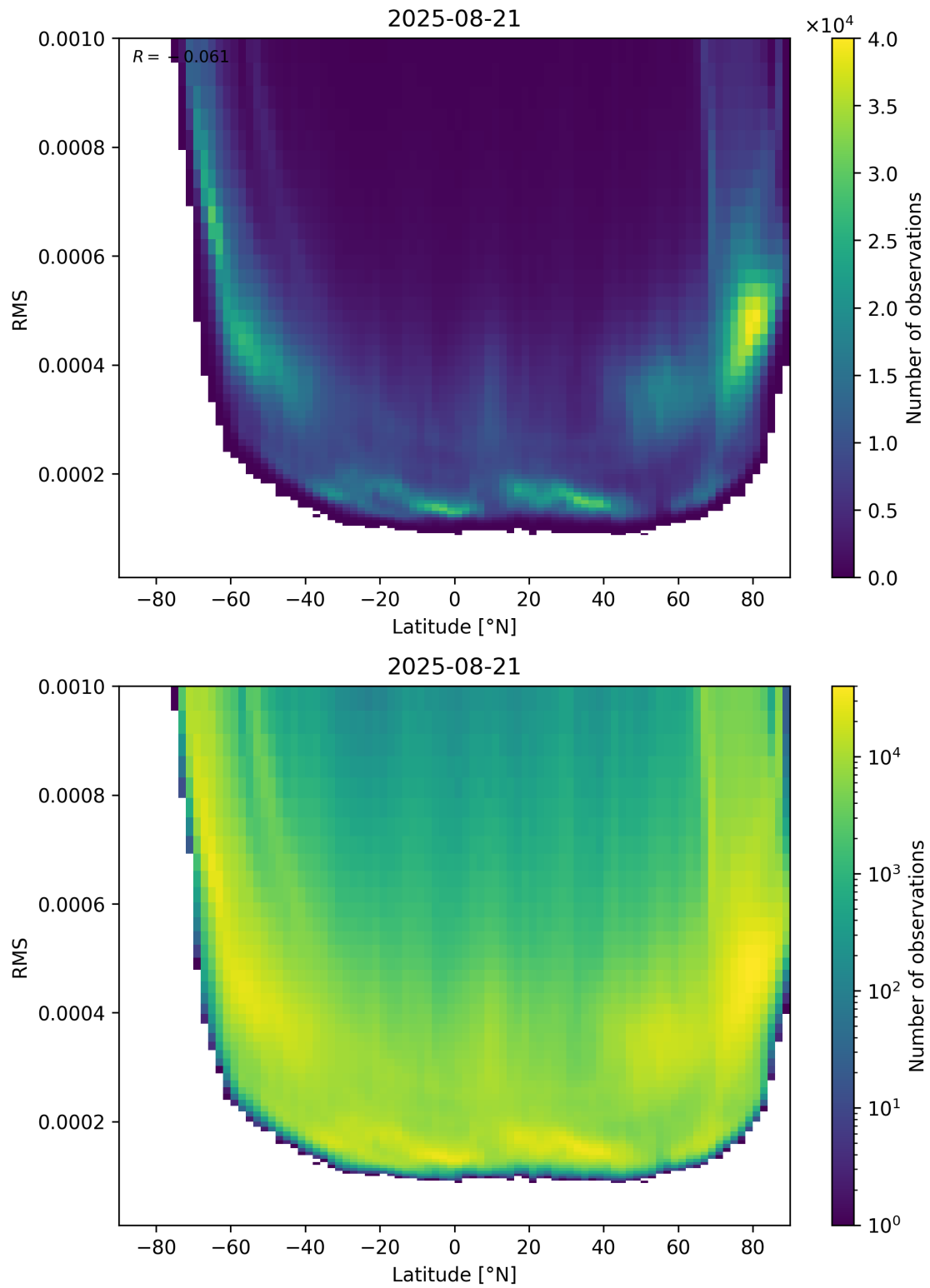
Figure 94: Scatter density plot of “Latitude” against “RMS” for 2025-08-20 to 2025-08-22.
