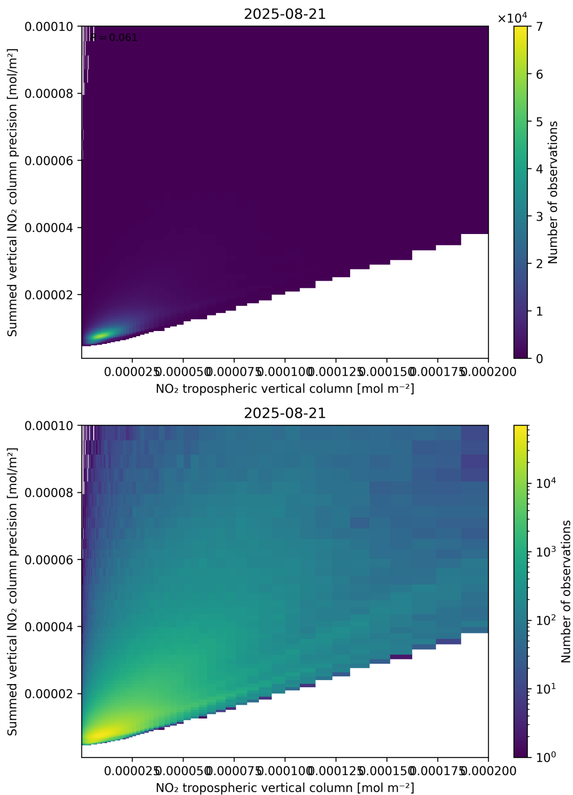
Figure 127: Scatter density plot of “NO 2 tropospheric vertical column” against “Summed vertical NO 2 column precision” for 2025-08-20 to 2025-08-22.
