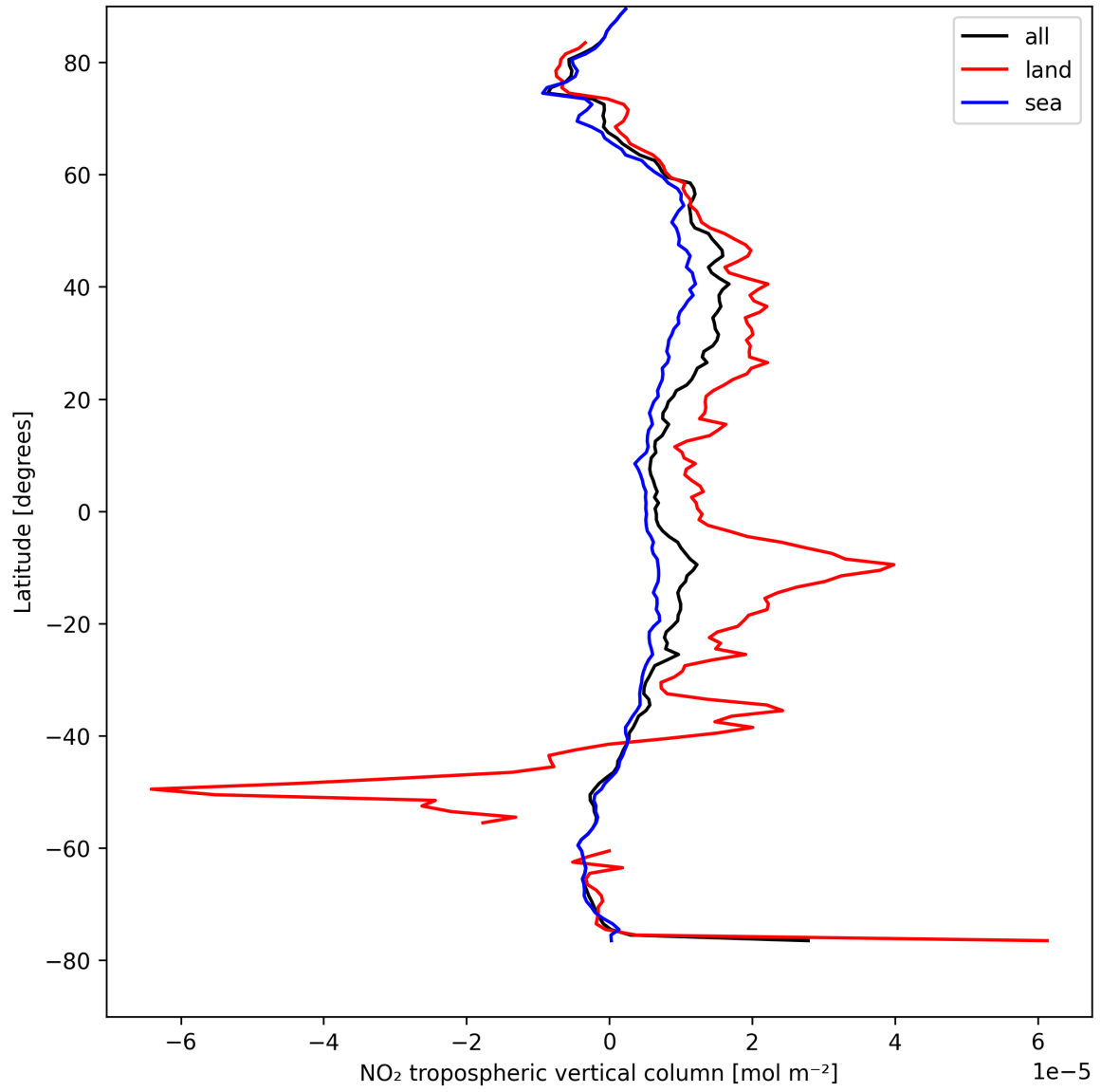
Figure 12: Zonal average of “NO 2 tropospheric vertical column” for 2025-08-20 to 2025-08-22.
