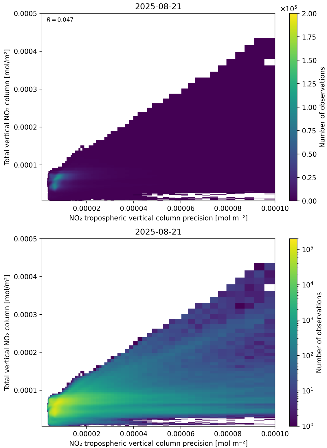
Figure 138: Scatter density plot of “NO 2 tropospheric vertical column precision” against “Total vertical NO 2 column” for 2025-08-20 to 2025-08-22.
