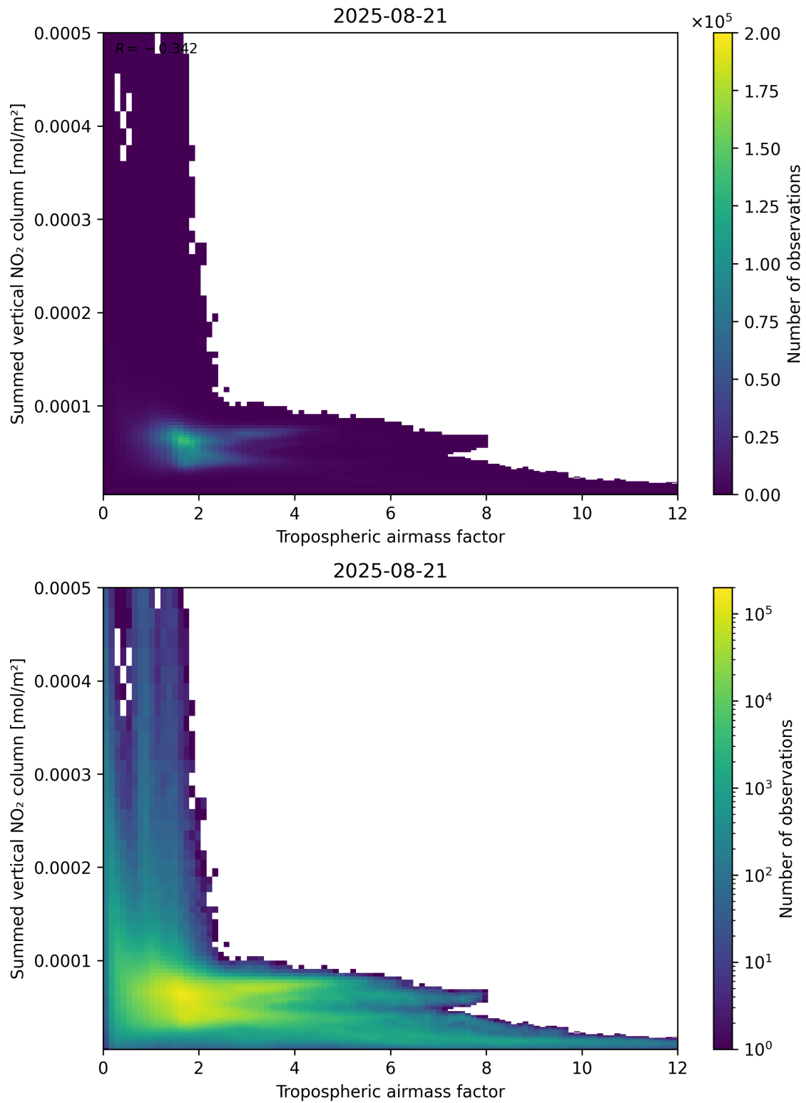
Figure 75: Scatter density plot of “Tropospheric air mass factor” against “Summed vertical NO 2 column” for 2025-08-20 to 2025-08-22.
