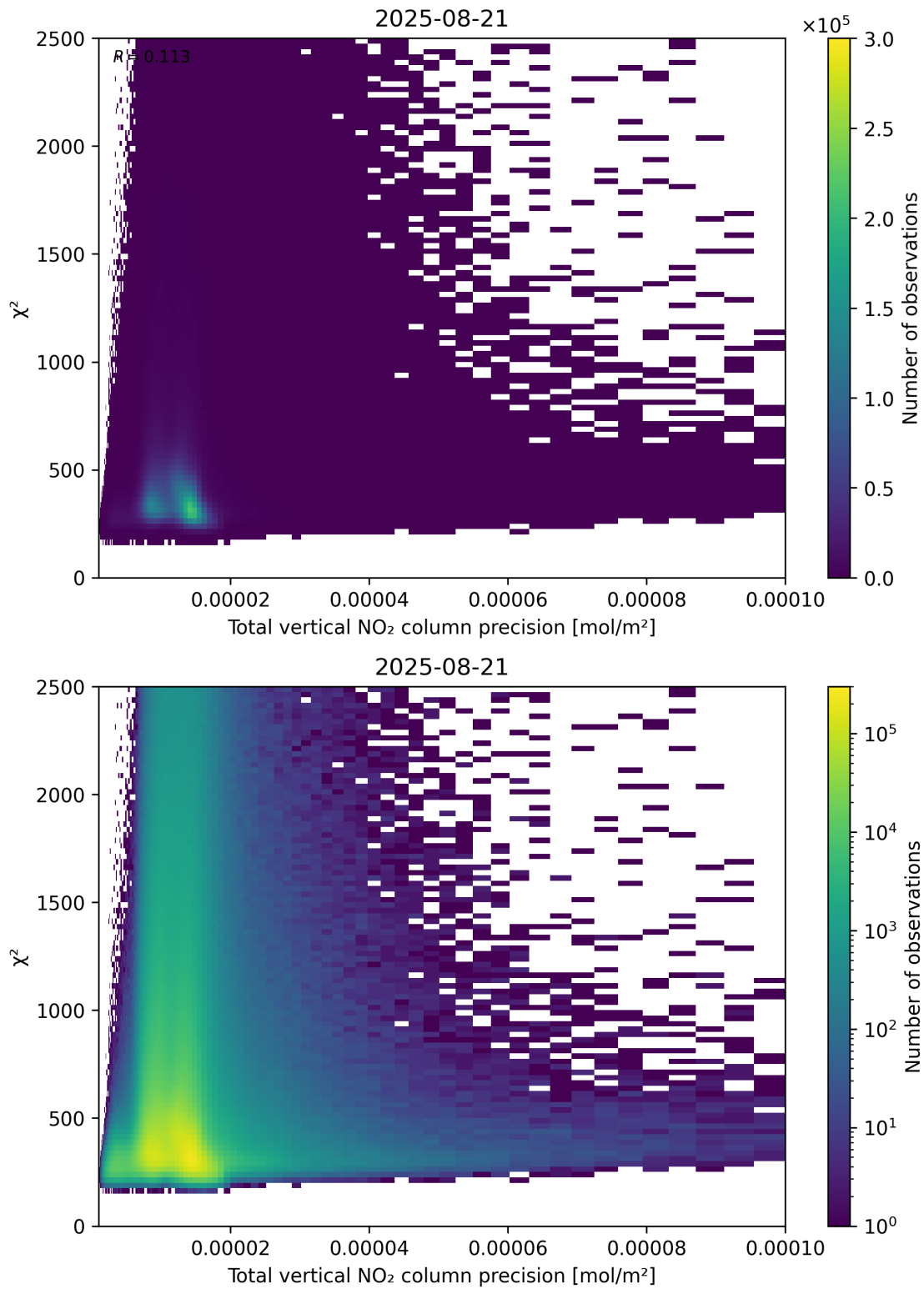
Figure 116: Scatter density plot of “Total vertical NO 2 column precision” against “ \chi^2 ” for 2025-08-20 to 2025-08-22.
