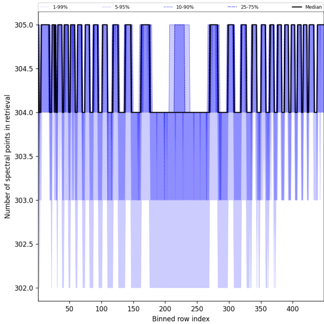
Figure 50: Along track statistics of “Number of spectral points in retrieval” for 2025-08-20 to 2025-08-22
