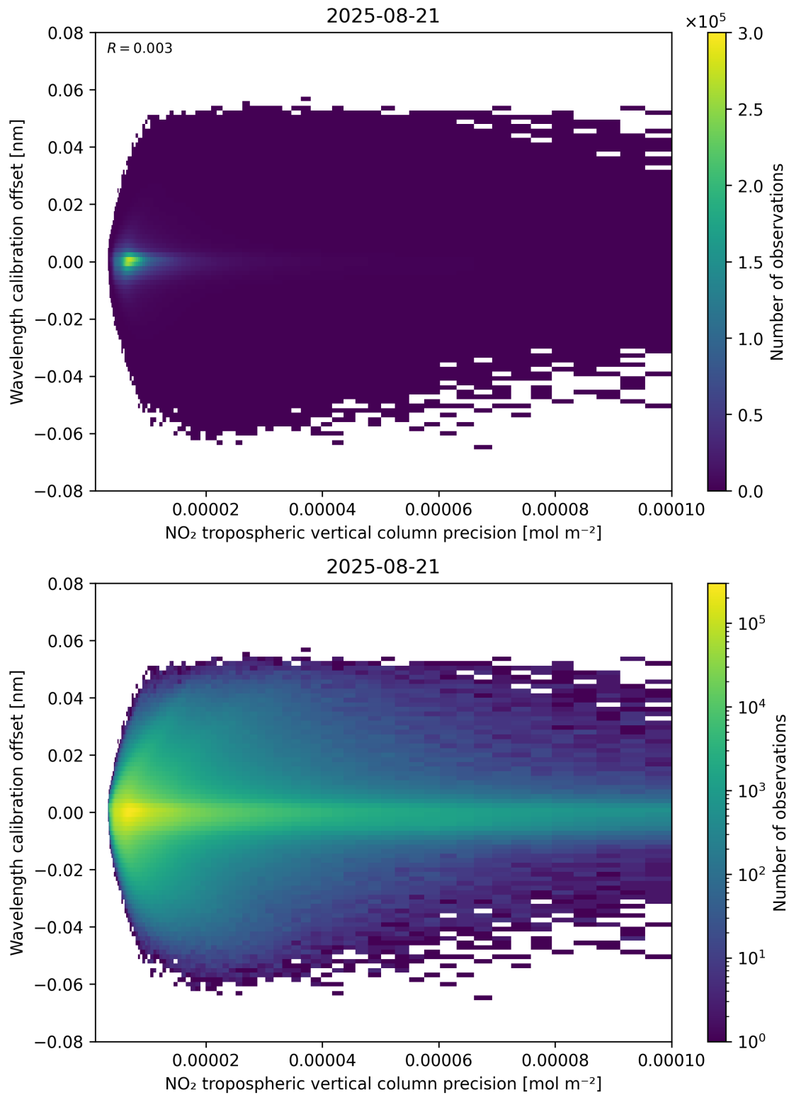
Figure 141: Scatter density plot of “NO 2 tropospheric vertical column precision” against “Wavelength calibration offset” for 2025-08-20 to 2025-08-22.
