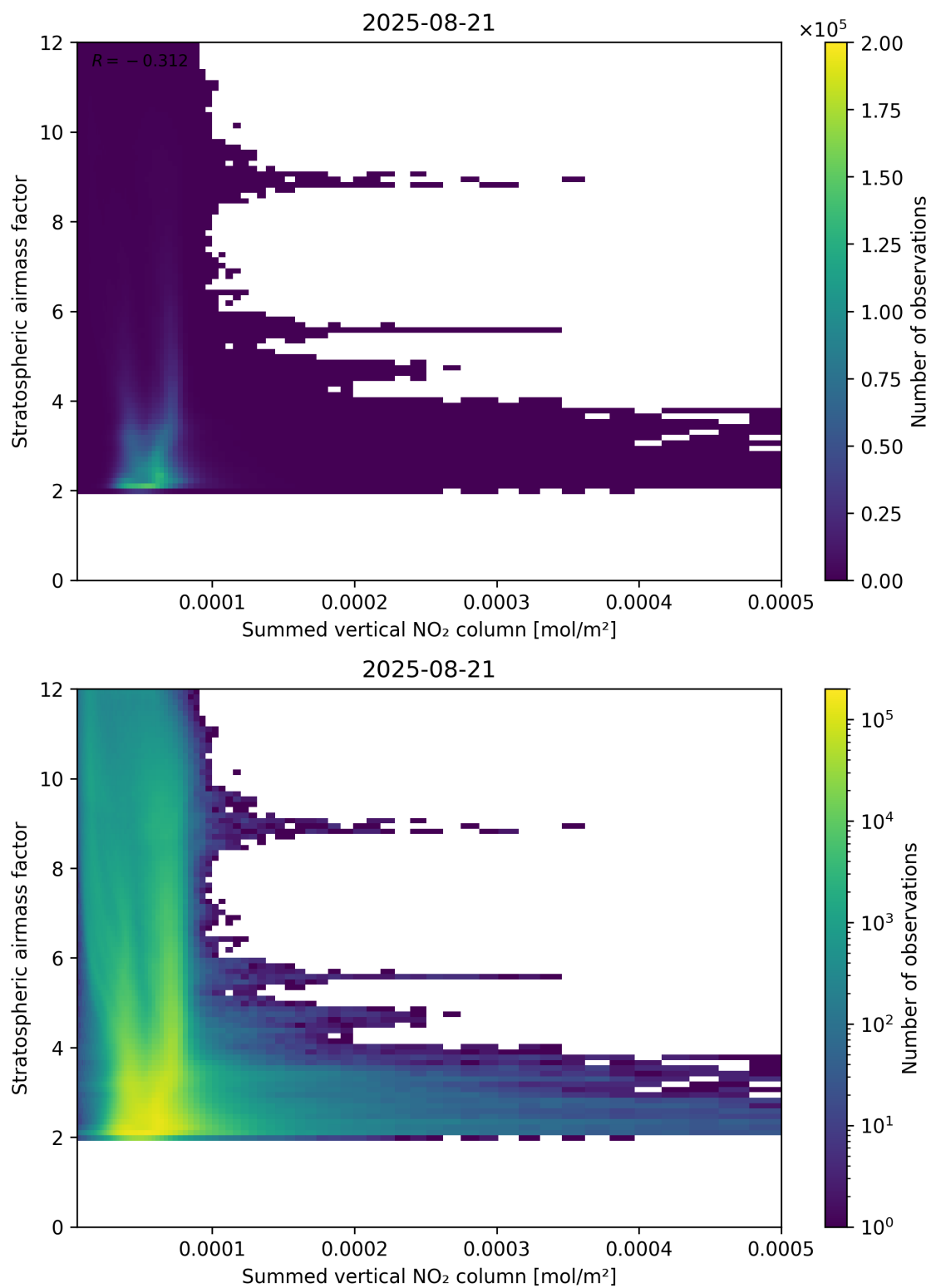
Figure 103: Scatter density plot of “Summed vertical NO 2 column” against “Stratospheric airmass factor” for 2025-08-20 to 2025-08-22.
