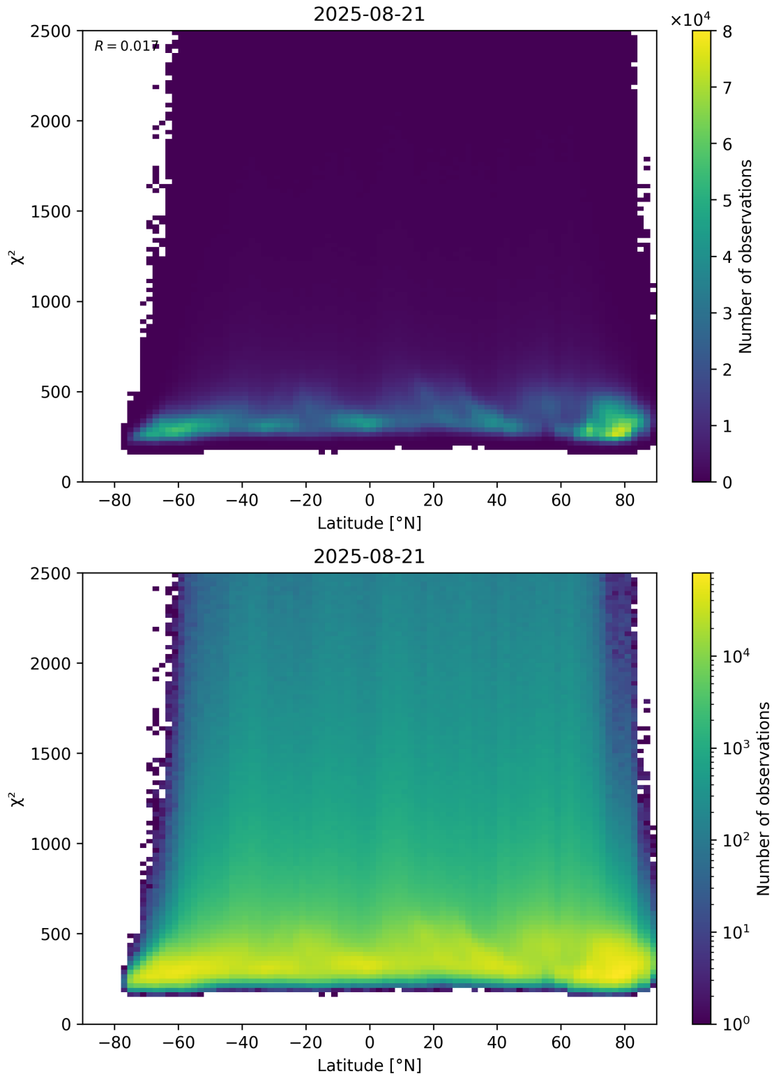
Figure 86: Scatter density plot of “Latitude” against “ \chi^2 ” for 2025-08-20 to 2025-08-22.
