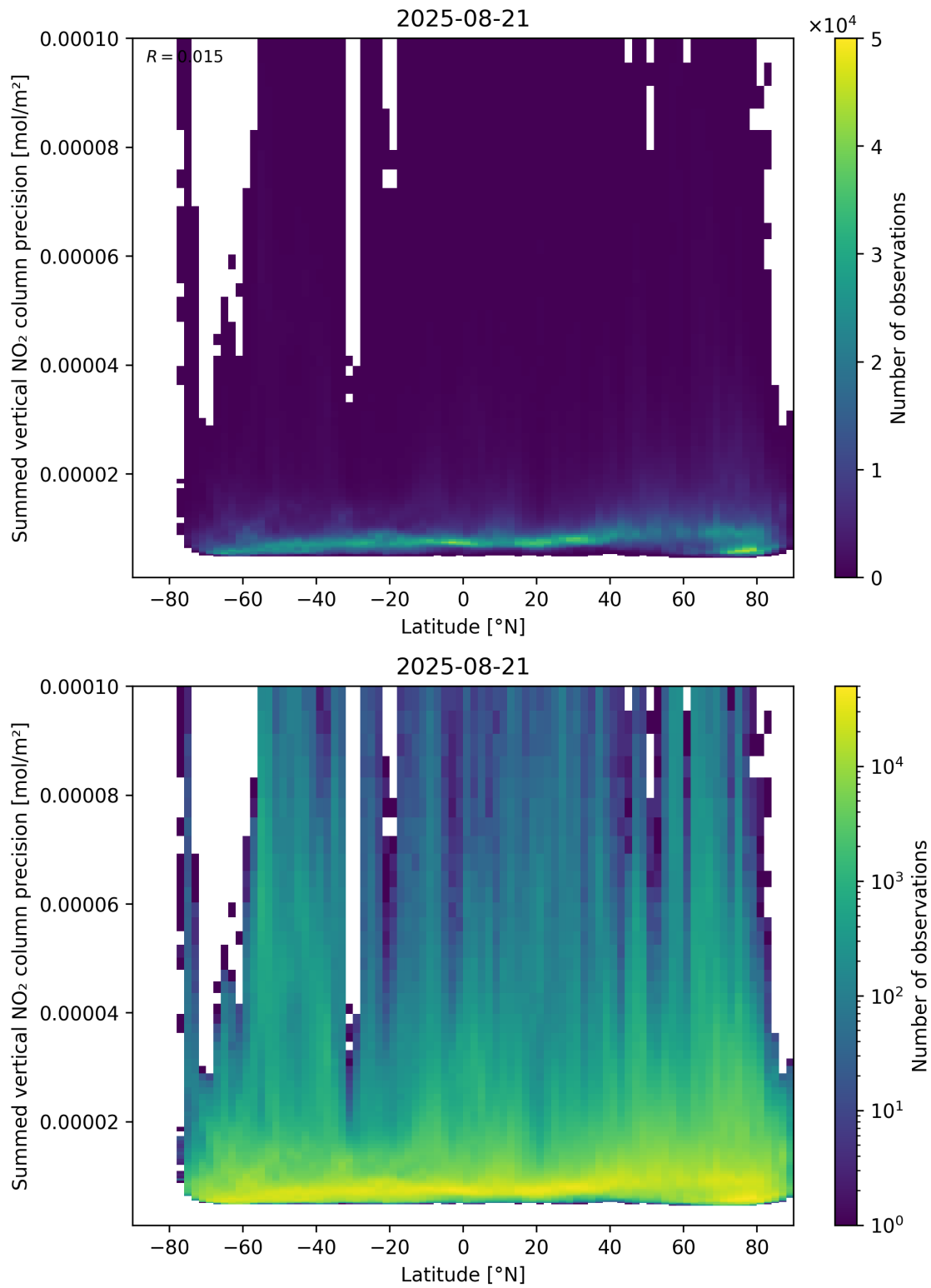
Figure 89: Scatter density plot of “Latitude” against “Summed vertical NO 2 column precision” for 2025-08-20 to 2025-08-22.
