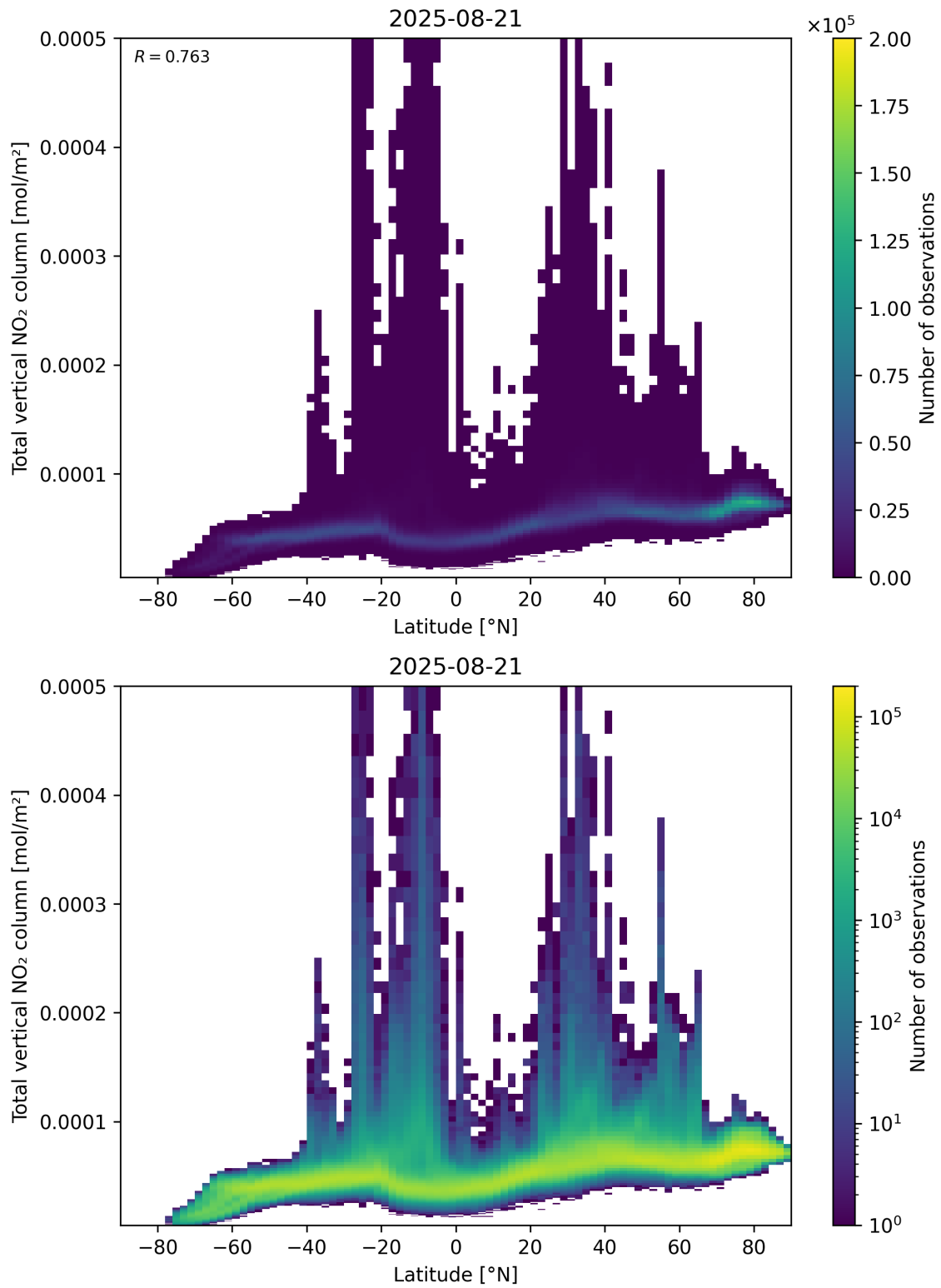
Figure 90: Scatter density plot of “Latitude” against “Total vertical NO 2 column” for 2025-08-20 to 2025-08-22.
