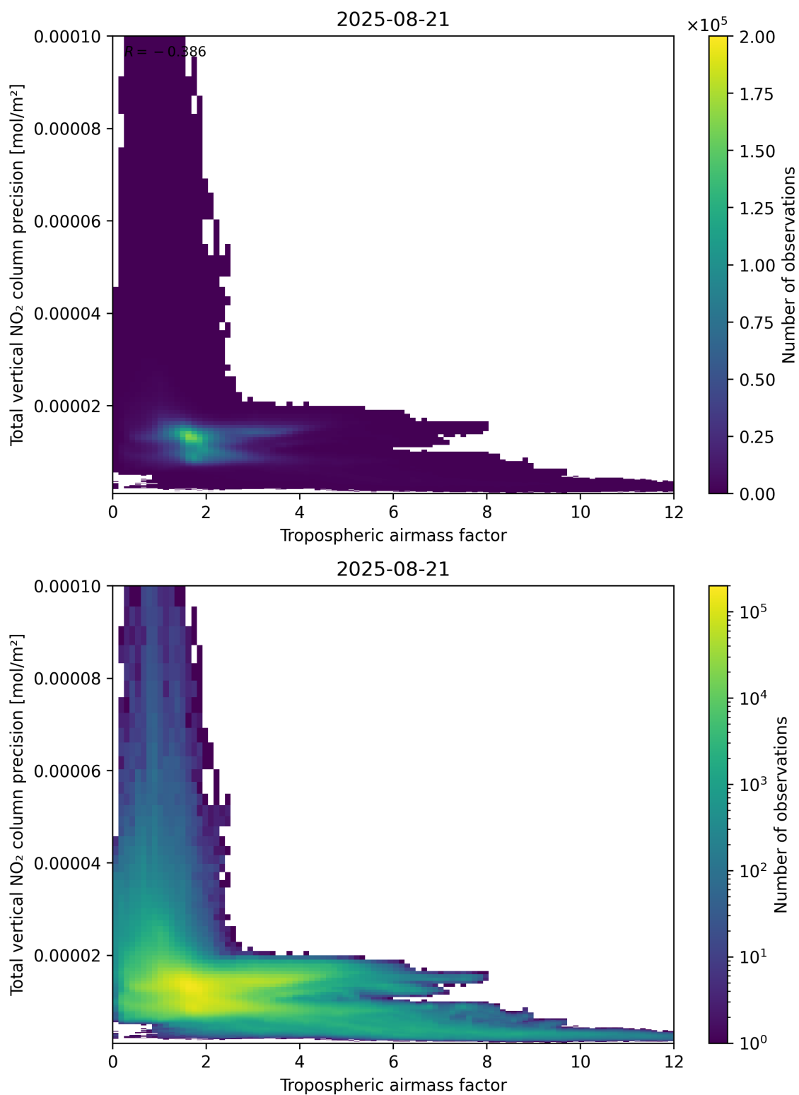
Figure 78: Scatter density plot of “Tropospheric air mass factor” against “Total vertical NO 2 column precision” for 2025-08-20 to 2025-08-22.
