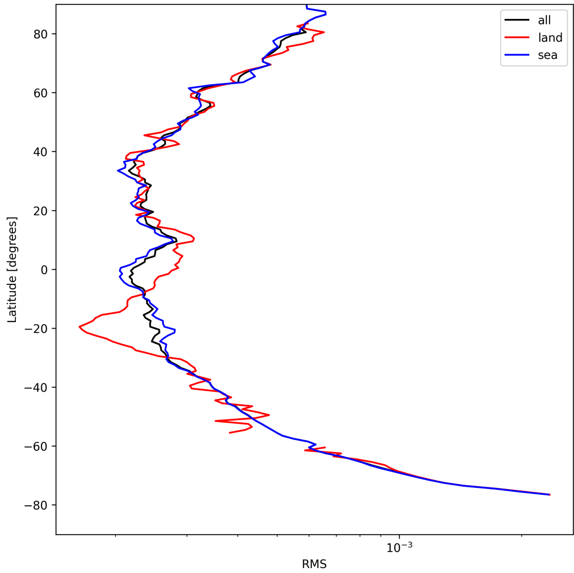
Figure 26: Zonal average of “RMS” for 2025-08-20 to 2025-08-22.
