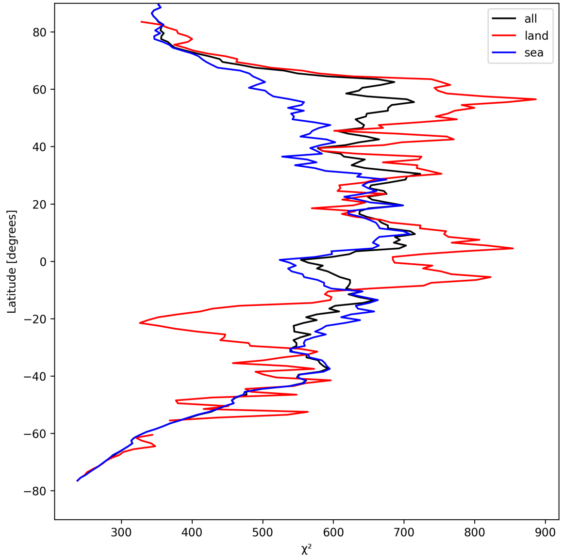
Figure 25: Zonal average of “ \chi^2 ” for 2025-08-20 to 2025-08-22.
