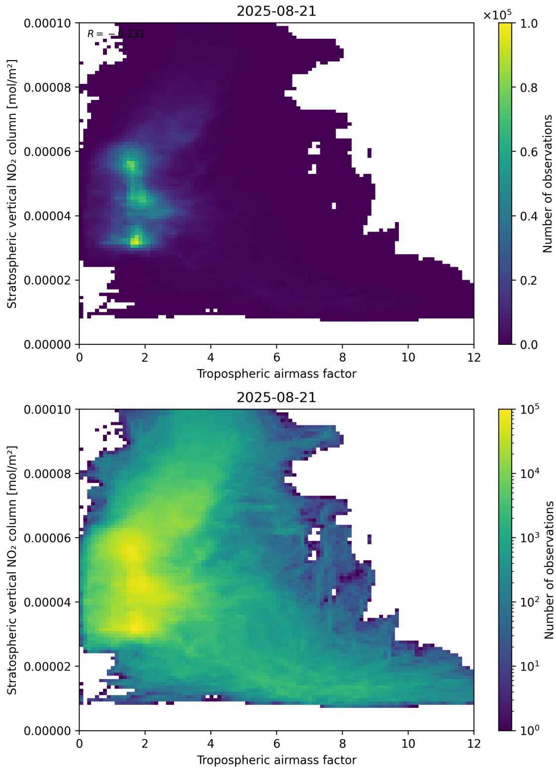
Figure 74: Scatter density plot of “Tropospheric air mass factor” against “Stratospheric vertical NO 2 column” for 2025-08-20 to 2025-08-22.
