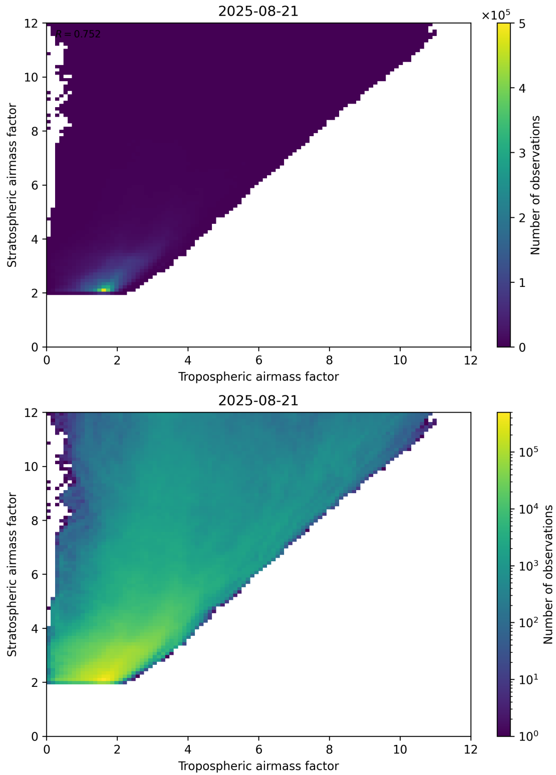
Figure 71: Scatter density plot of “Tropospheric airmass factor” against “Stratospheric airmass factor” for 2025-08-20 to 2025-08-22.
