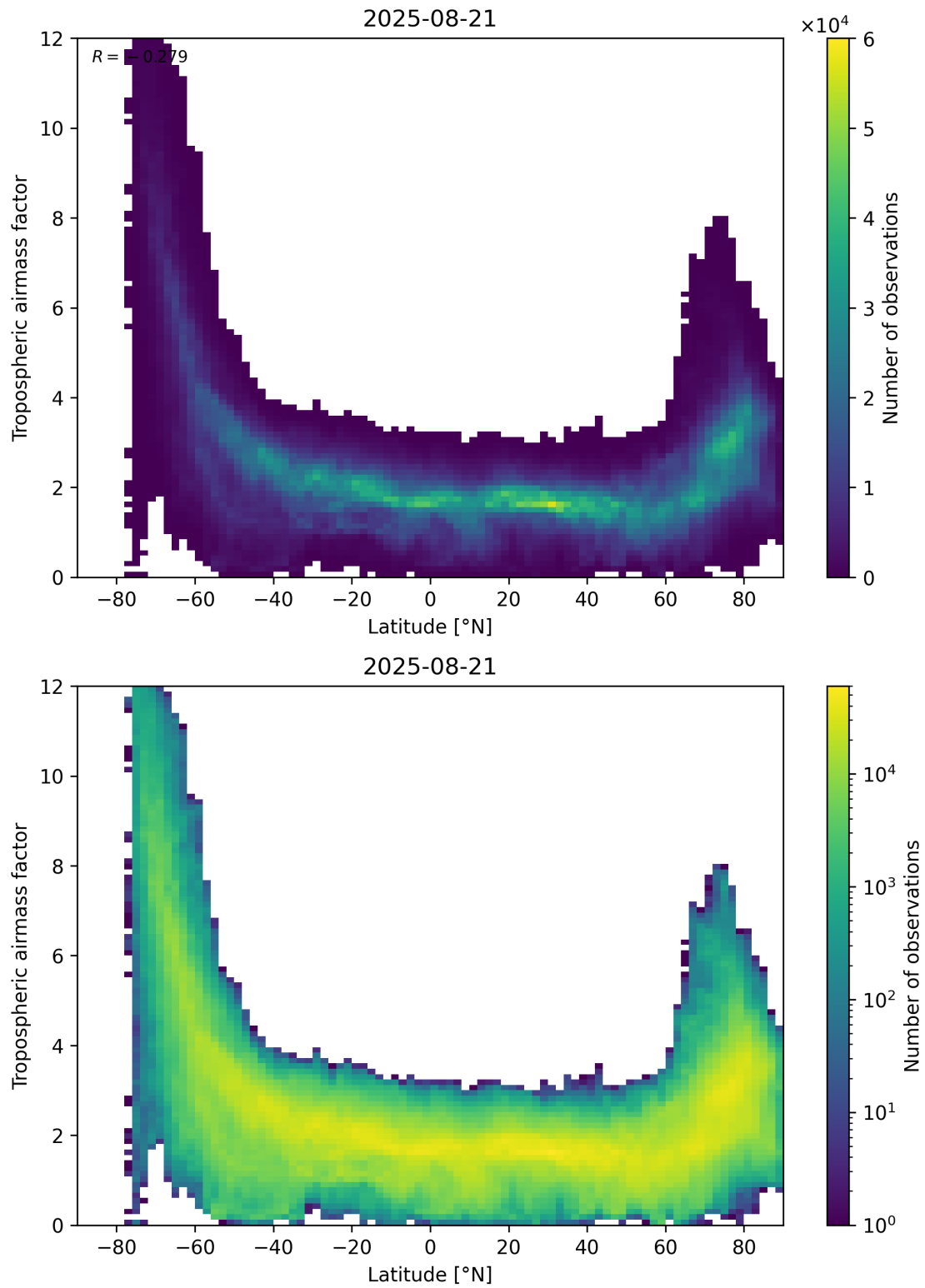
Figure 85: Scatter density plot of “Latitude” against “Tropospheric air mass factor” for 2025-08-20 to 2025-08-22.
