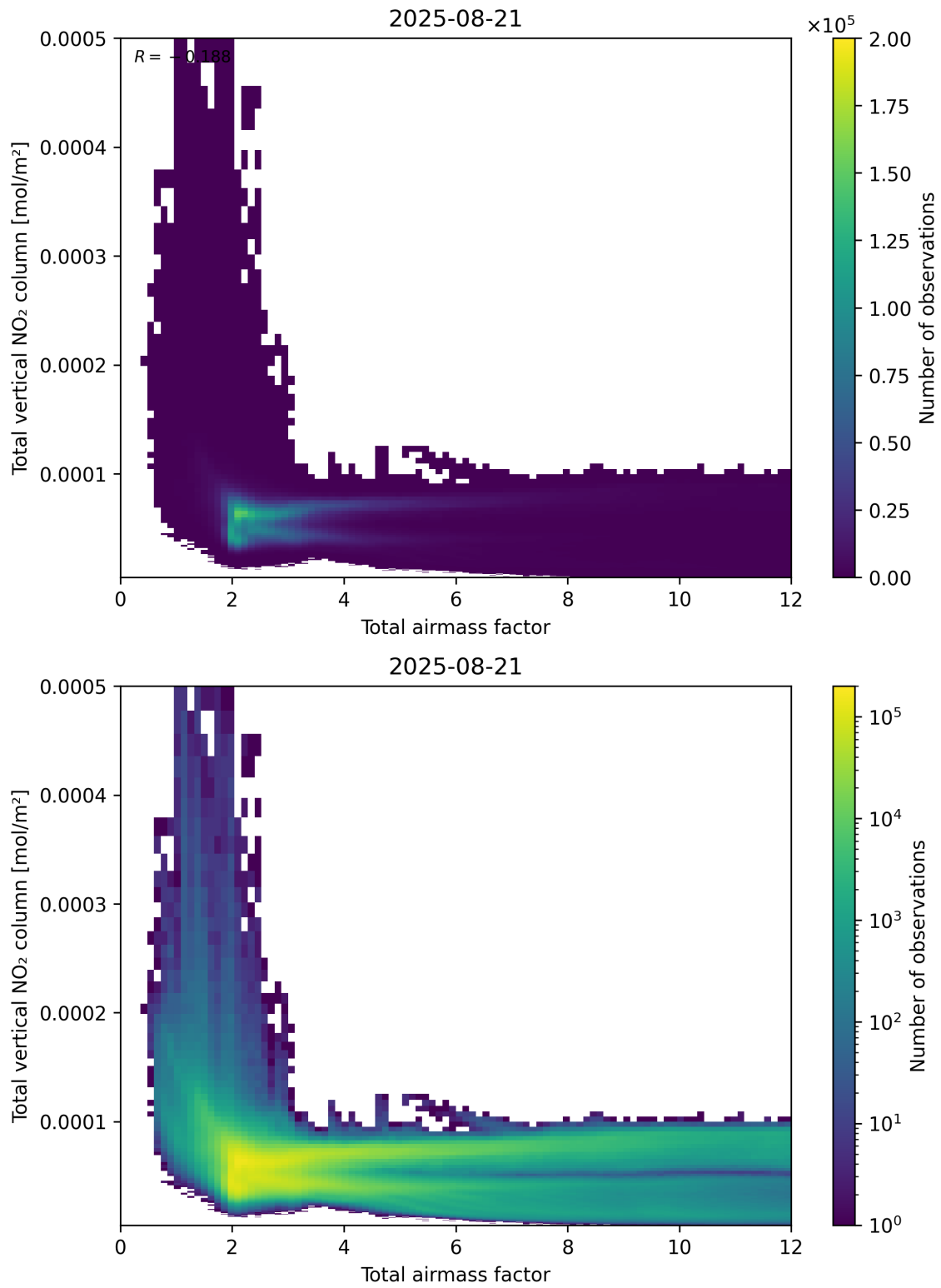
Figure 67: Scatter density plot of “Total airmass factor” against “Total vertical NO 2 column” for 2025-08-20 to 2025-08-22.
