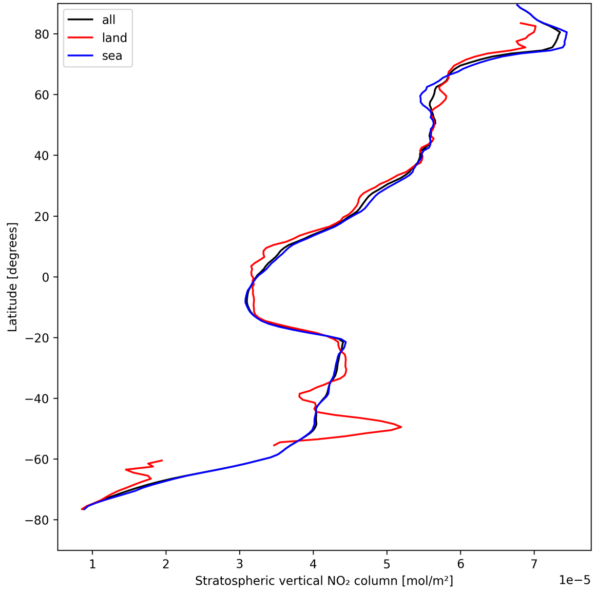
Figure 19: Zonal average of “Stratospheric vertical NO 2 column” for 2025-08-20 to 2025-08-22.
