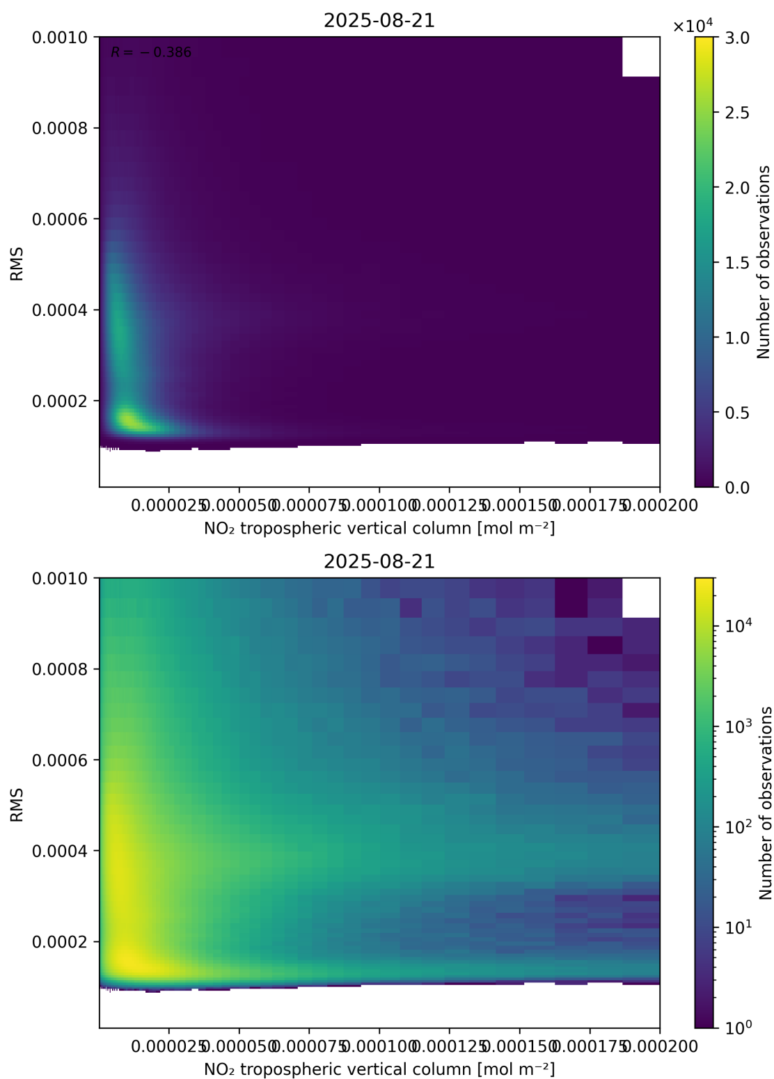
Figure 142: Scatter density plot of “NO 2 tropospheric vertical column” against “RMS” for 2025-08-20 to 2025-08-22.
