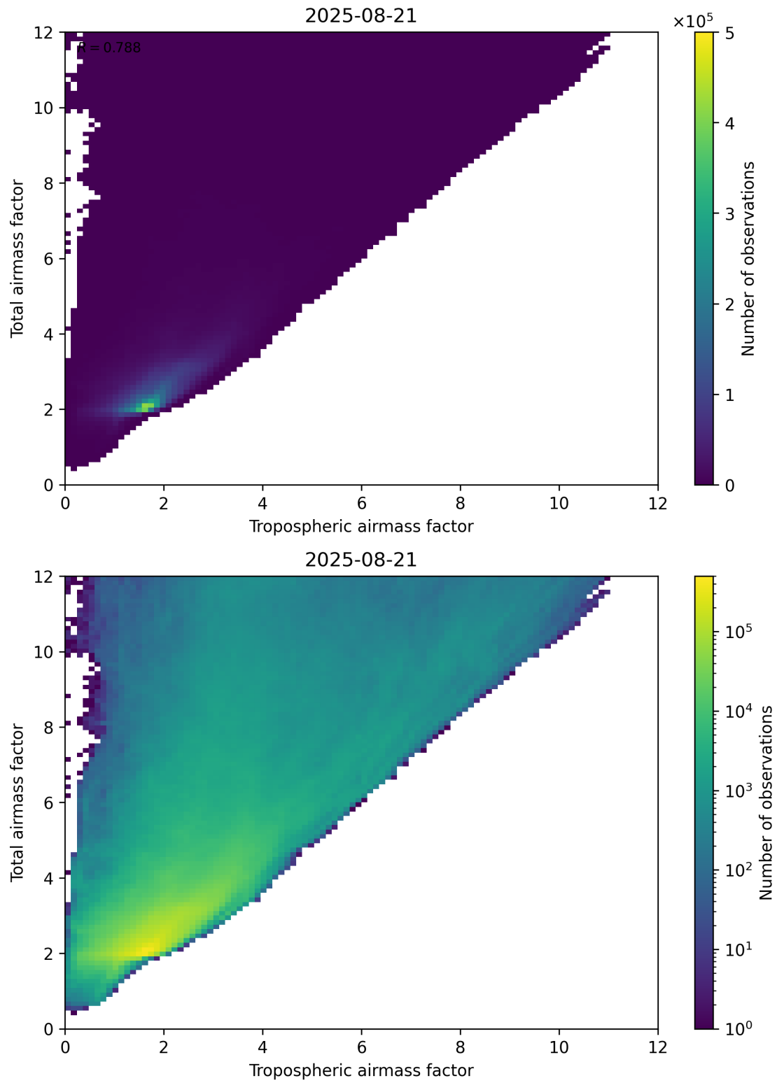
Figure 72: Scatter density plot of “Tropospheric airmass factor” against “Total airmass factor” for 2025-08-20 to 2025-08-22.
