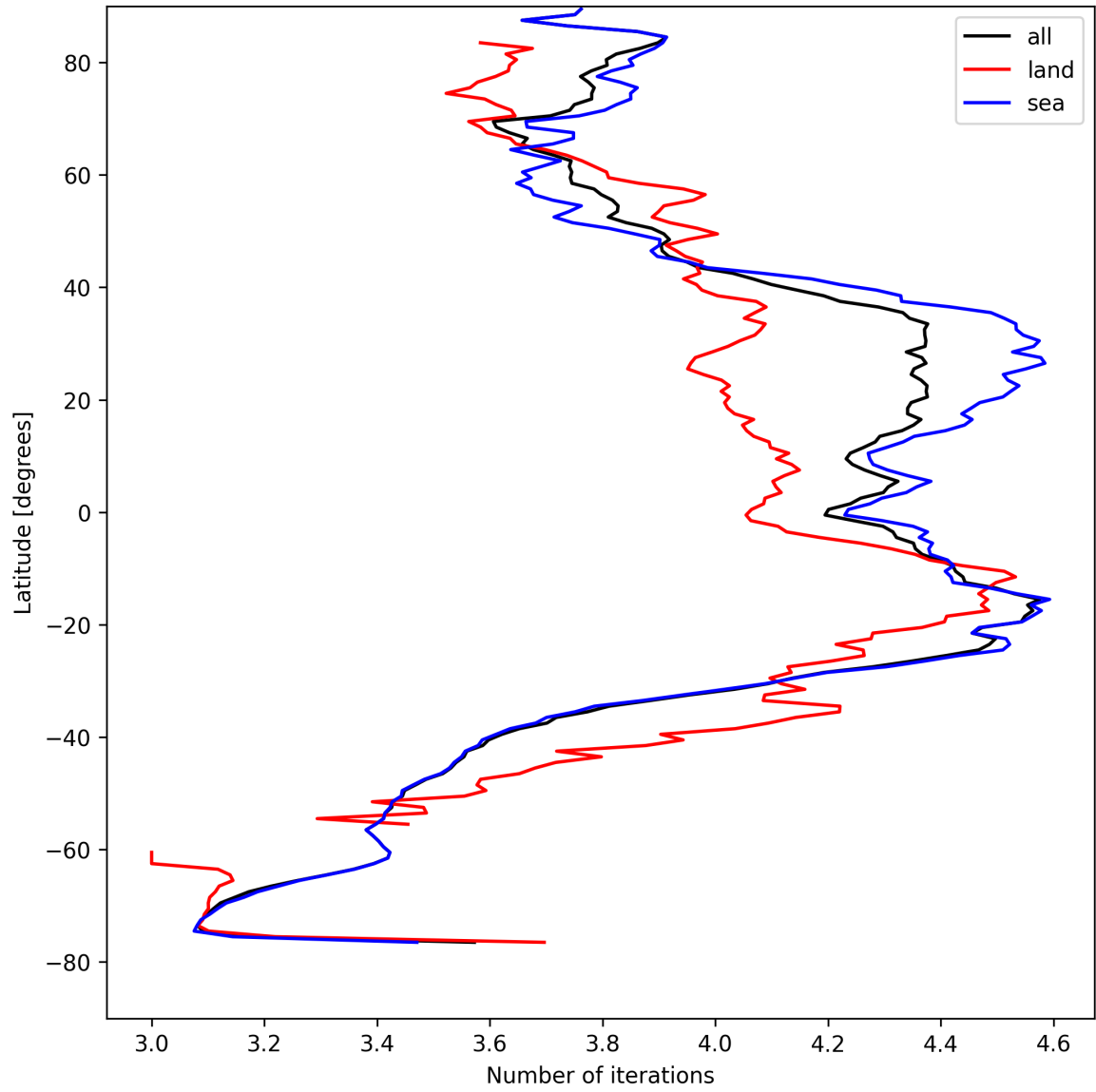
Figure 17: Zonal average of “Number of iterations” for 2025-08-20 to 2025-08-22.
