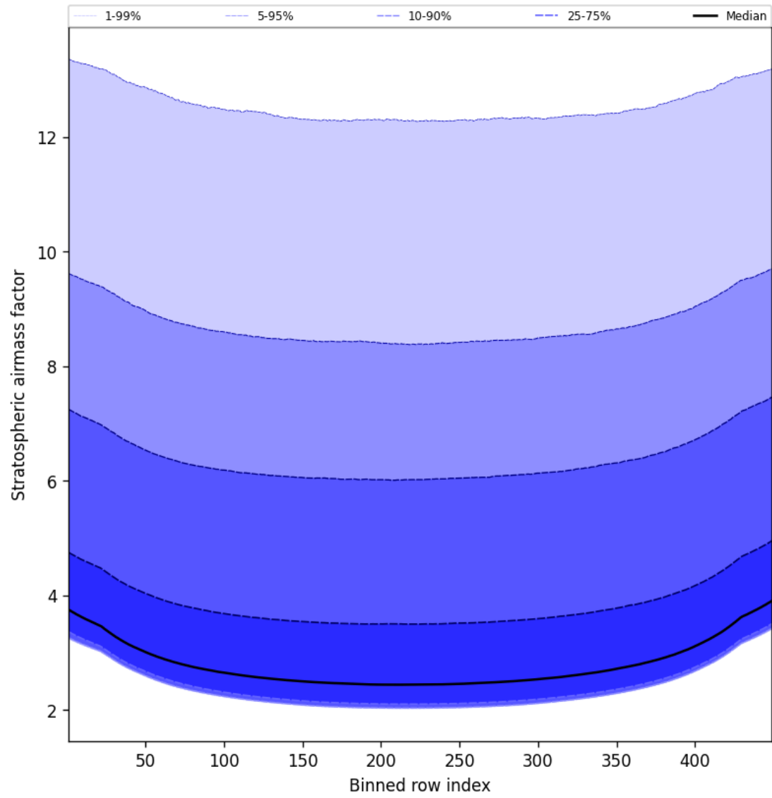
Figure 61: Along track statistics of “Stratospheric airmass factor” for 2025-08-20 to 2025-08-22
