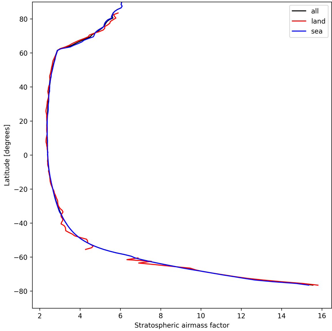
Figure 27: Zonal average of “Stratospheric airmass factor” for 2025-08-20 to 2025-08-22.
