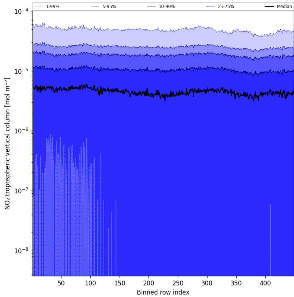
Figure 46: Along track statistics of “NO 2 tropospheric vertical column” for 2025-08-20 to 2025-08-22
