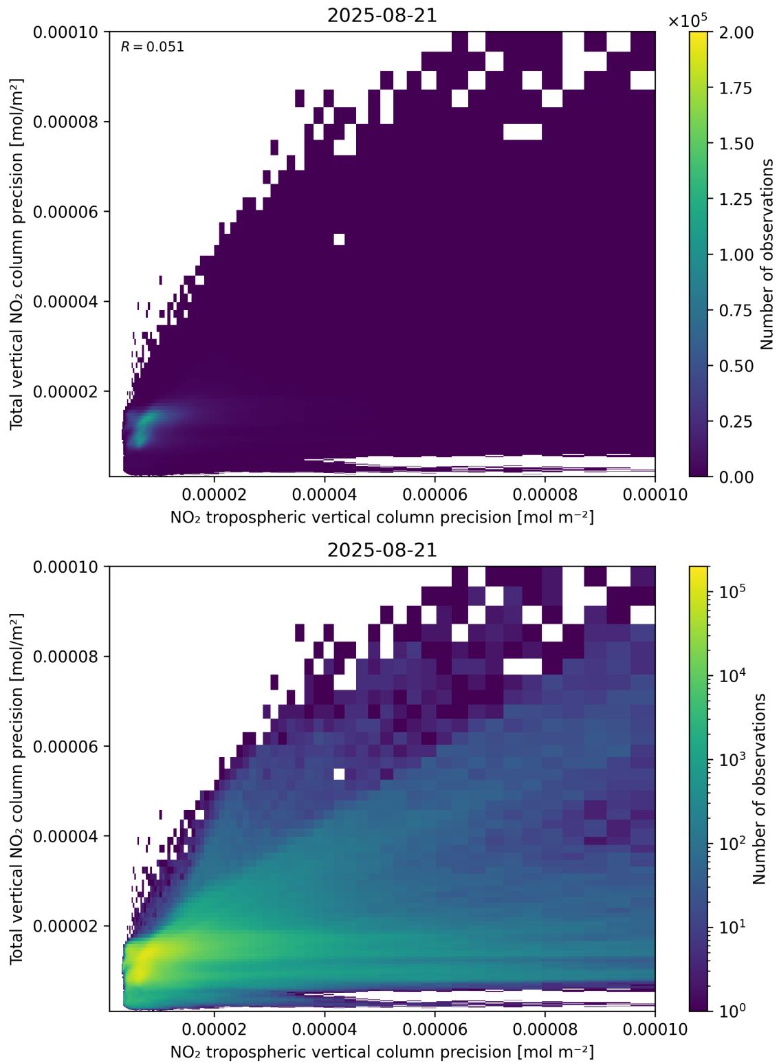
Figure 139: Scatter density plot of “NO 2 tropospheric vertical column precision” against “Total vertical NO 2 column precision” for 2025-08-20 to 2025-08-22.
