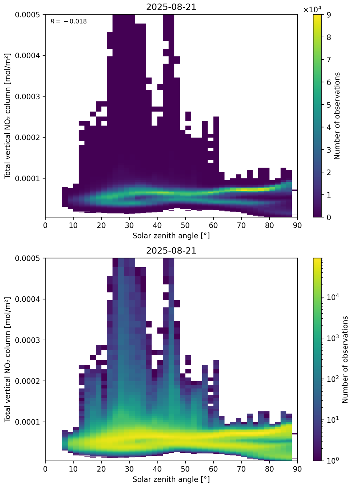
Figure 153: Scatter density plot of “Solar zenith angle” against “Total vertical NO 2 column” for 2025-08-20 to 2025-08-22.
