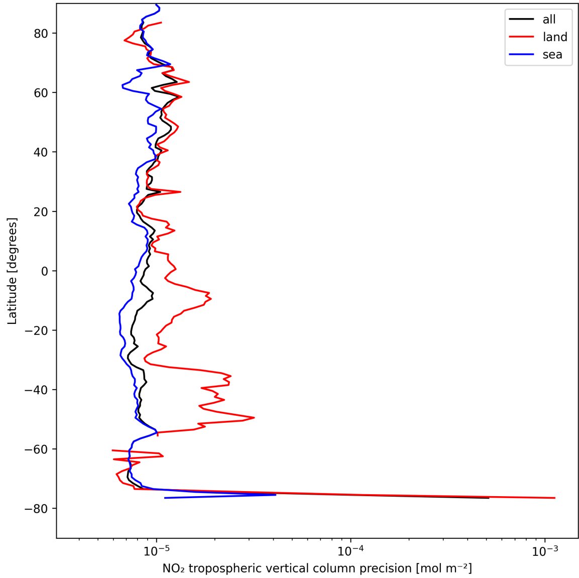
Figure 13: Zonal average of “NO 2 tropospheric vertical column precision” for 2025-08-20 to 2025-08-22.
