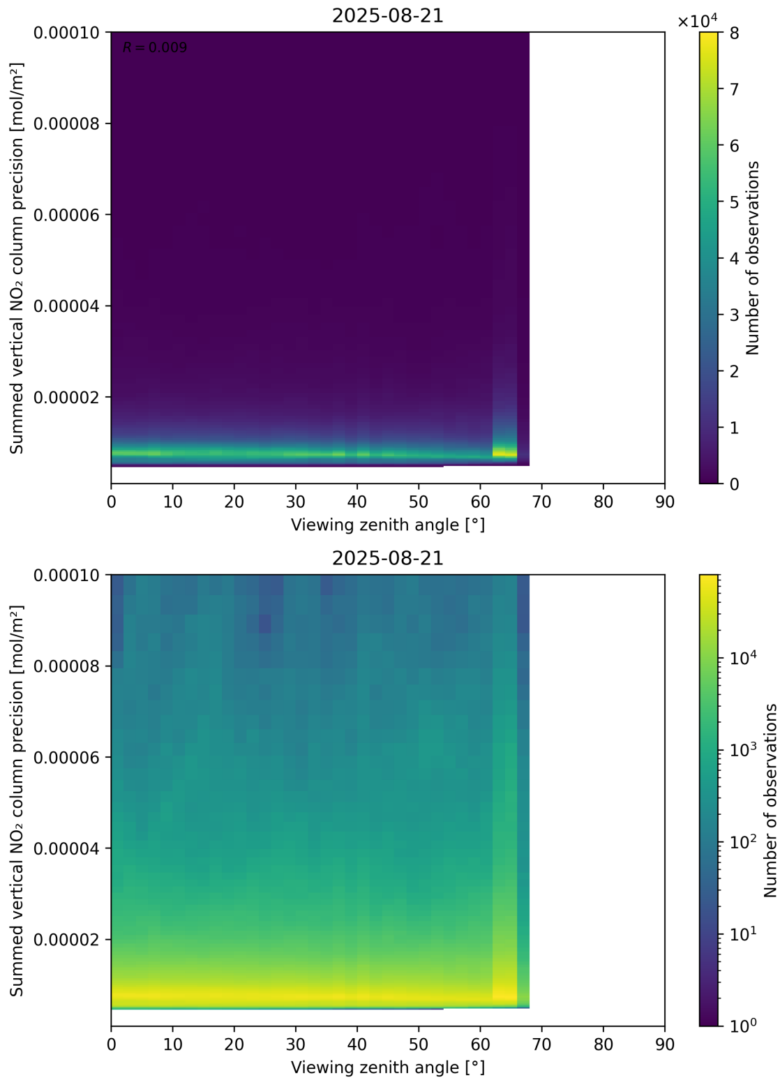
Figure 166: Scatter density plot of “Viewing zenith angle” against “Summed vertical NO 2 column precision” for 2025-08-20 to 2025-08-22.
