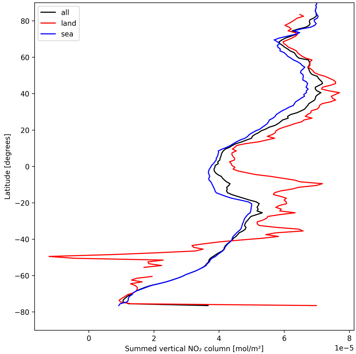
Figure 23: Zonal average of “Summed vertical NO 2 column” for 2025-08-20 to 2025-08-22.
