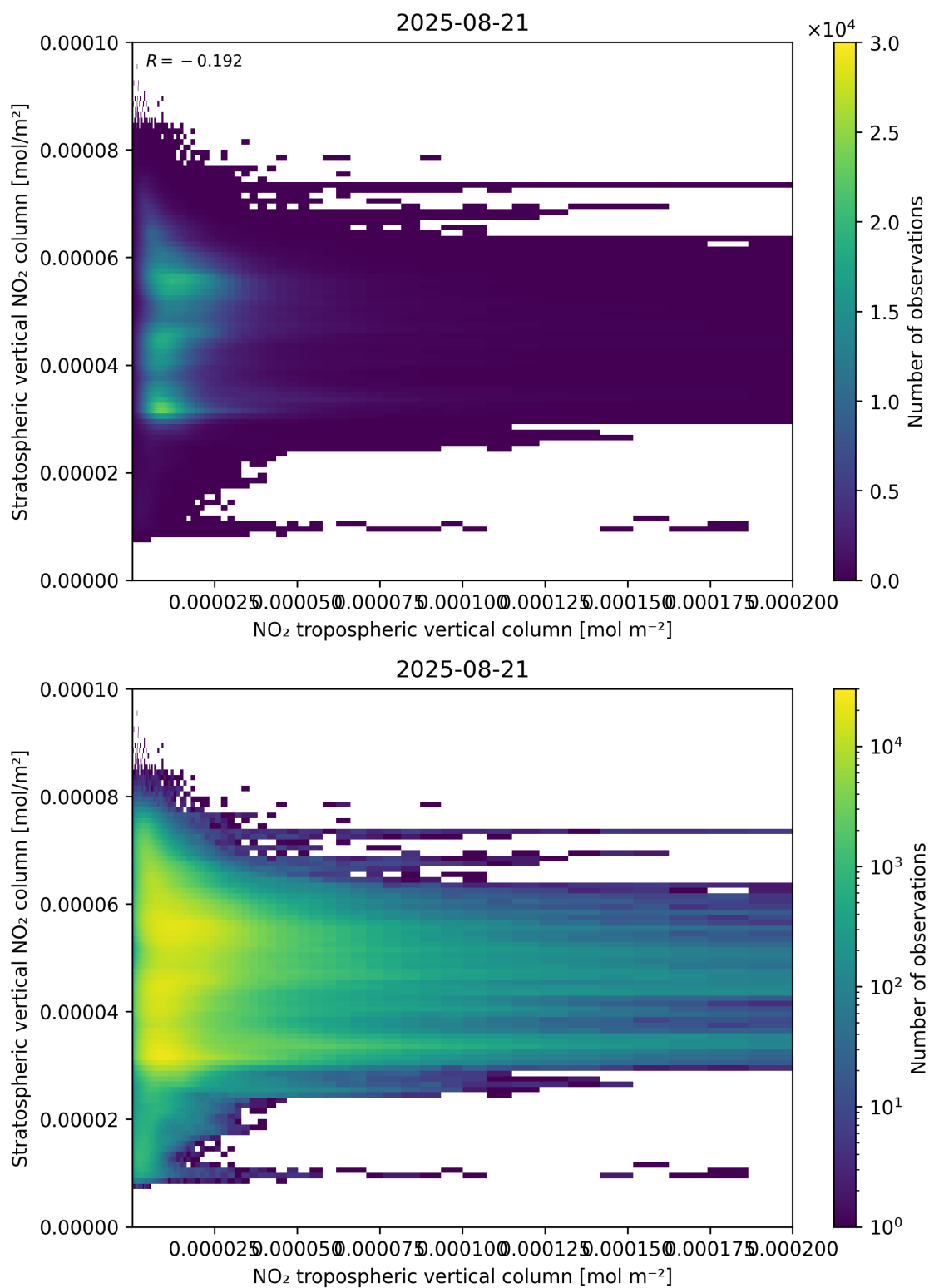
Figure 125: Scatter density plot of “NO 2 tropospheric vertical column” against “Stratospheric vertical NO 2 column” for 2025-08-20 to 2025-08-22.
