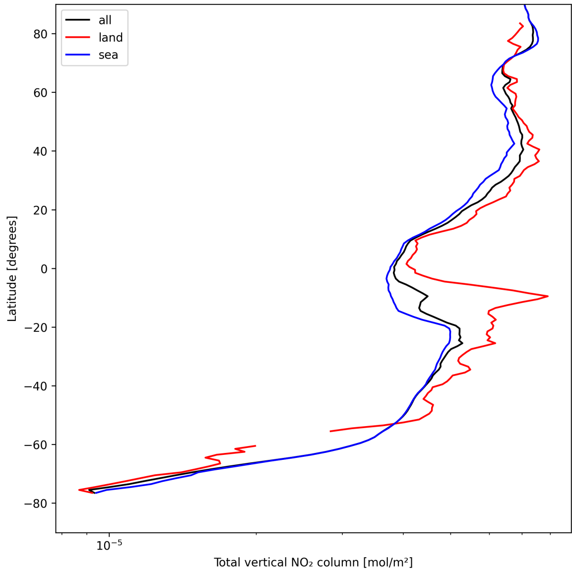
Figure 21: Zonal average of “Total vertical NO 2 column” for 2025-08-20 to 2025-08-22.
