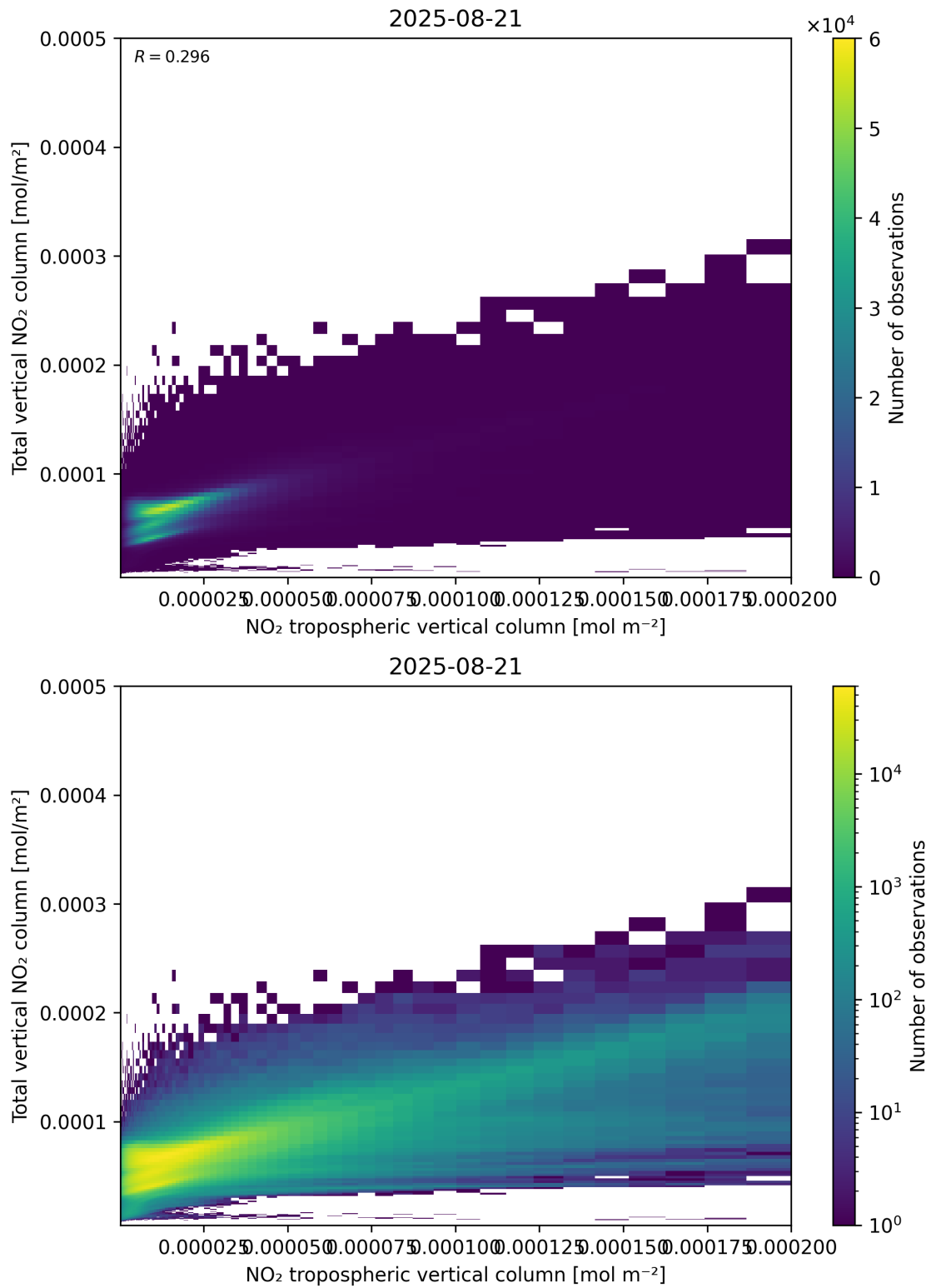
Figure 128: Scatter density plot of “NO 2 tropospheric vertical column” against “Total vertical NO 2 column” for 2025-08-20 to 2025-08-22.
