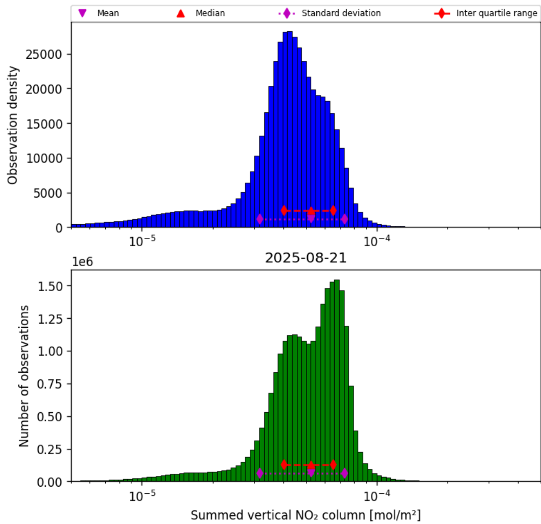
Figure 40: Histogram of “Summed vertical NO 2 column” for 2025-08-20 to 2025-08-22
