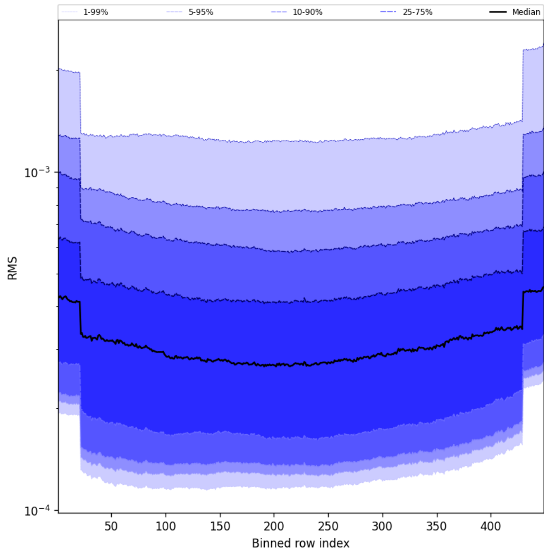
Figure 60: Along track statistics of “RMS” for 2025-08-20 to 2025-08-22
