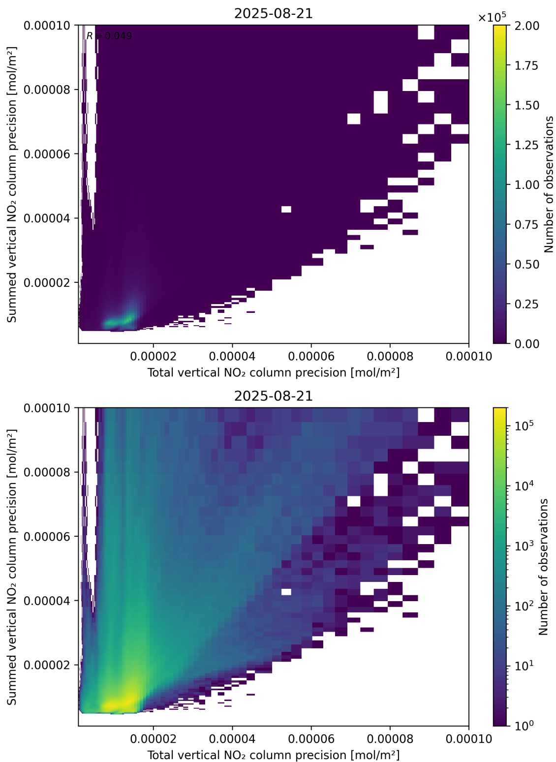
Figure 118: Scatter density plot of “Total vertical NO 2 column precision” against “Summed vertical NO 2 column precision” for 2025-08-20 to 2025-08-22.
