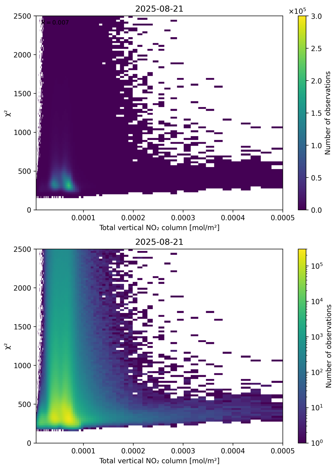
Figure 111: Scatter density plot of “Total vertical NO 2 column” against “ \chi^2 ” for 2025-08-20 to 2025-08-22.
