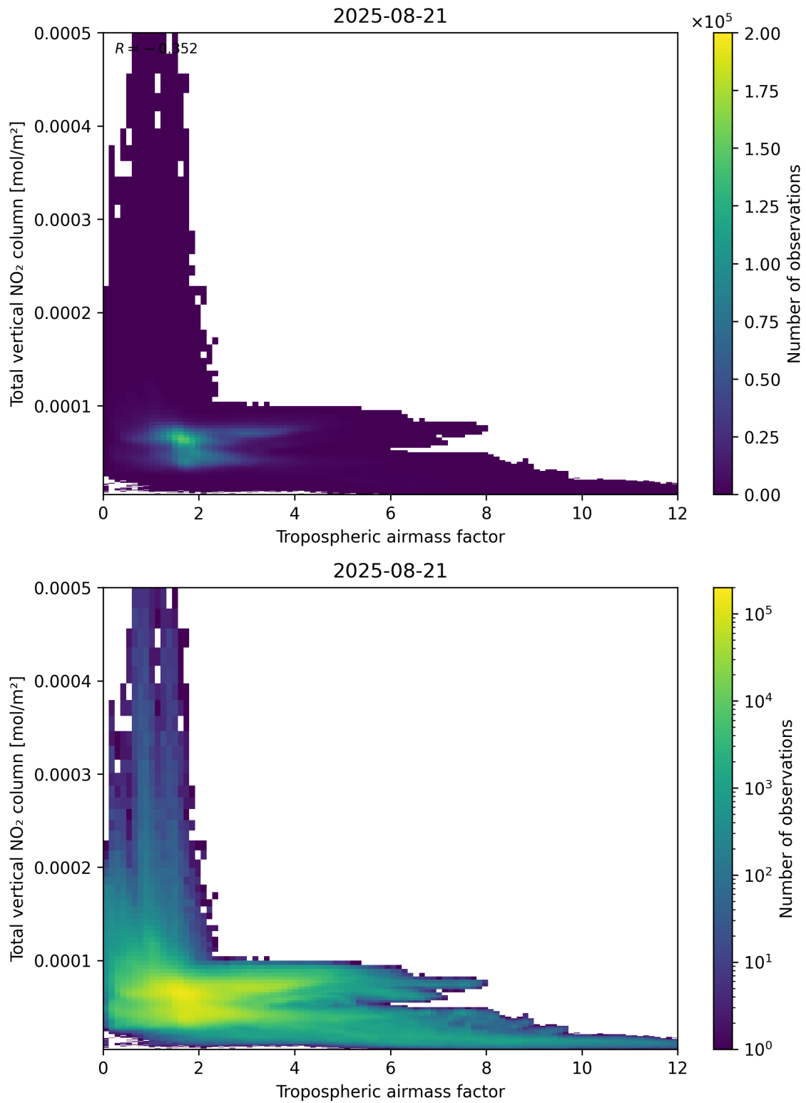
Figure 77: Scatter density plot of “Tropospheric airmass factor” against “Total vertical NO 2 column” for 2025-08-20 to 2025-08-22.
