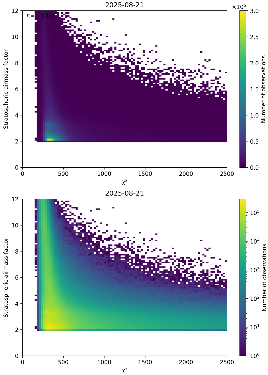
Figure 81: Scatter density plot of “ \chi^2 ” against “Stratospheric airmass factor” for 2025-08-20 to 2025-08-22.
