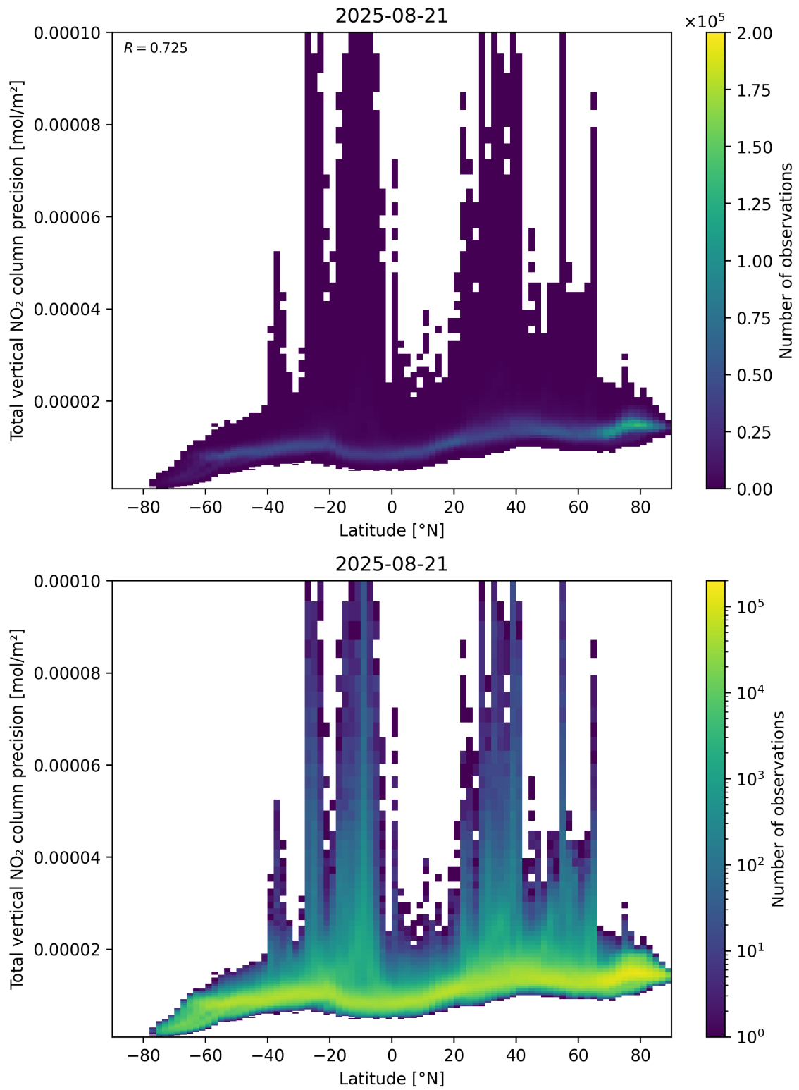
Figure 91: Scatter density plot of “Latitude” against “Total vertical NO 2 column precision” for 2025-08-20 to 2025-08-22.
