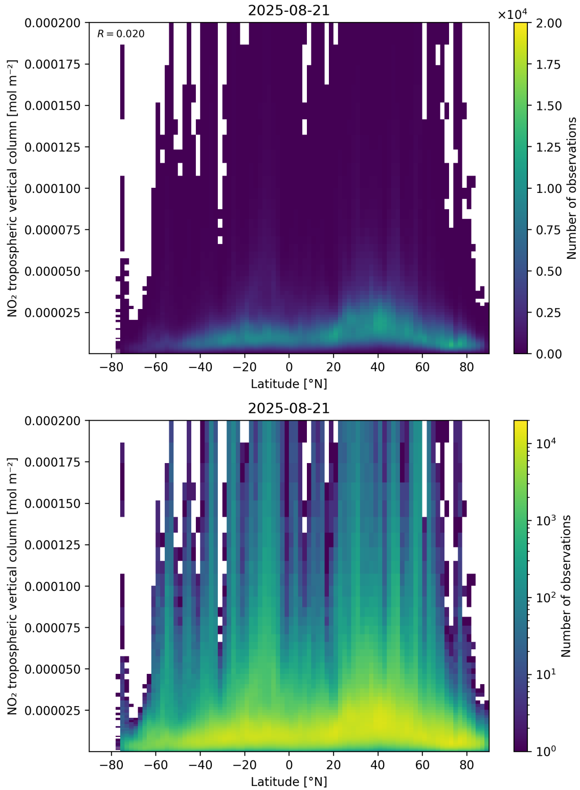
Figure 92: Scatter density plot of “Latitude” against “NO 2 tropospheric vertical column” for 2025-08-20 to 2025-08-22.
