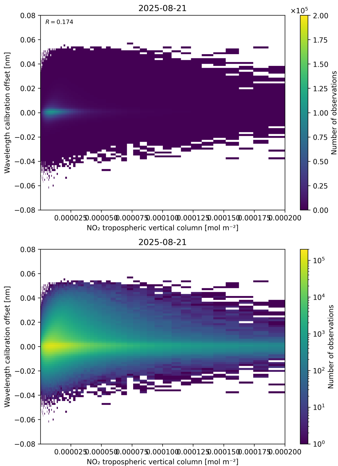
Figure 143: Scatter density plot of “NO 2 tropospheric vertical column” against “Wavelength calibration offset” for 2025-08-20 to 2025-08-22.
