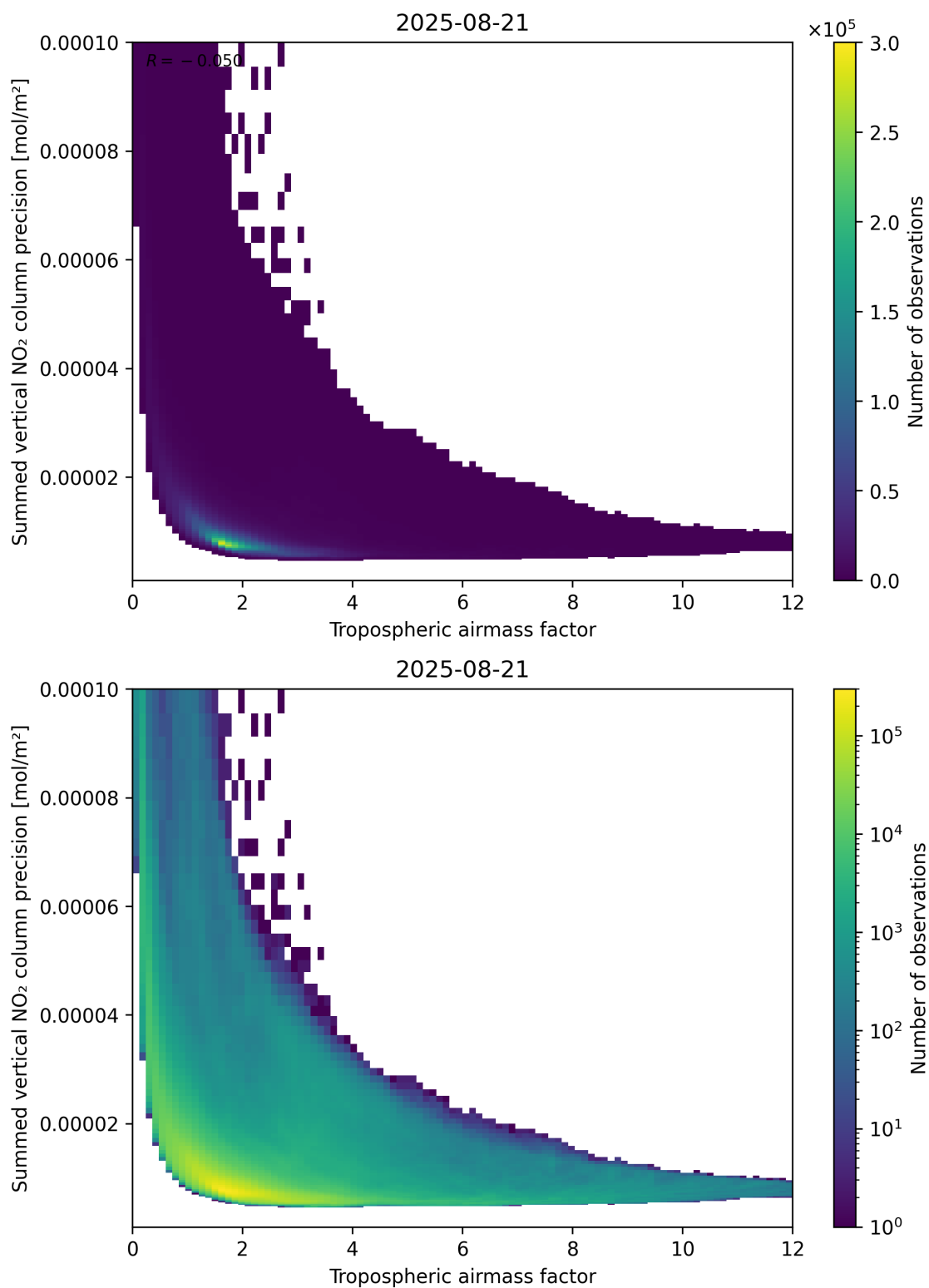
Figure 76: Scatter density plot of “Tropospheric airmass factor” against “Summed vertical NO 2 column precision” for 2025-08-20 to 2025-08-22.
