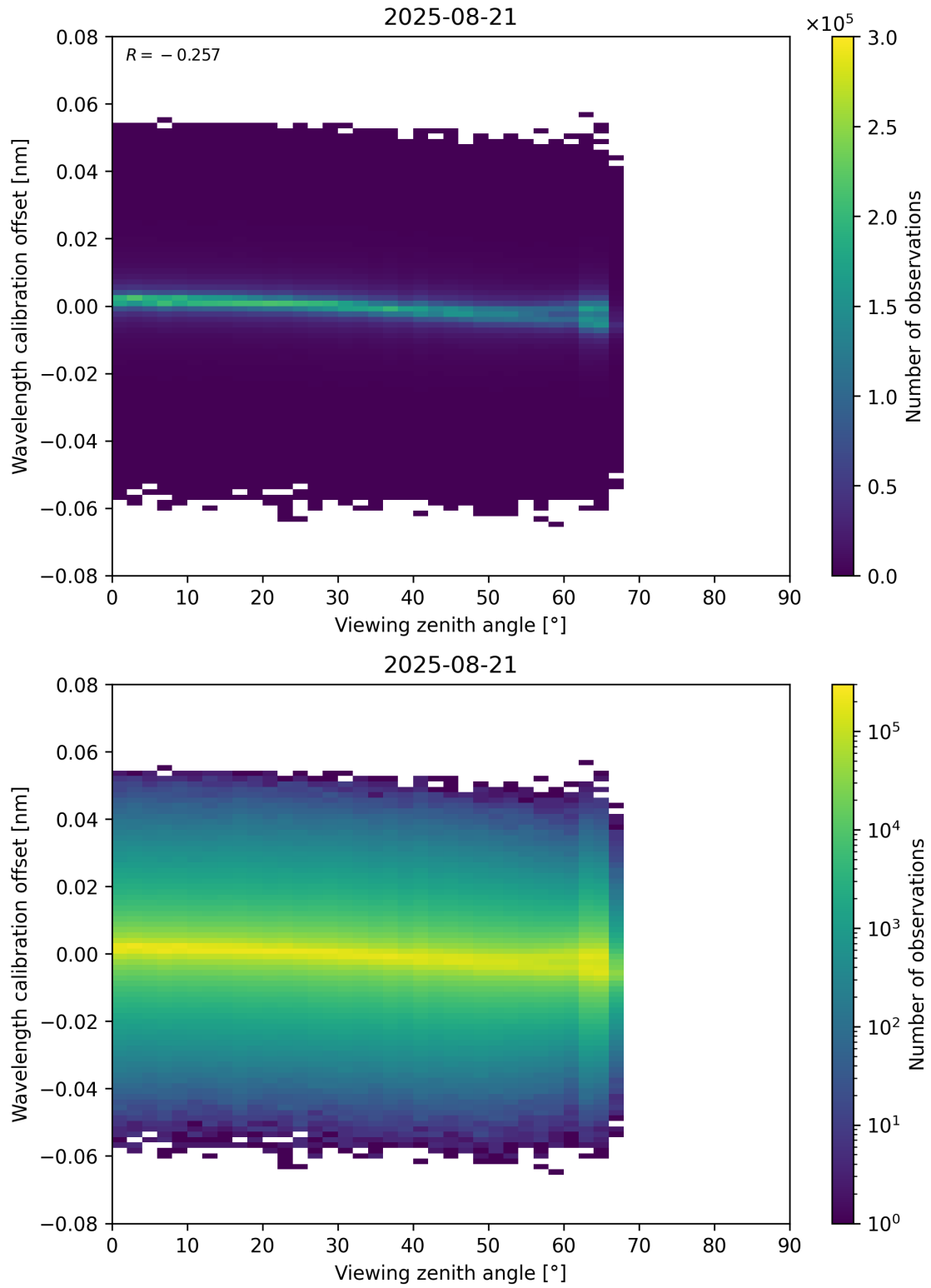
Figure 173: Scatter density plot of “Viewing zenith angle” against “Wavelength calibration offset” for 2025-08-20 to 2025-08-22.
