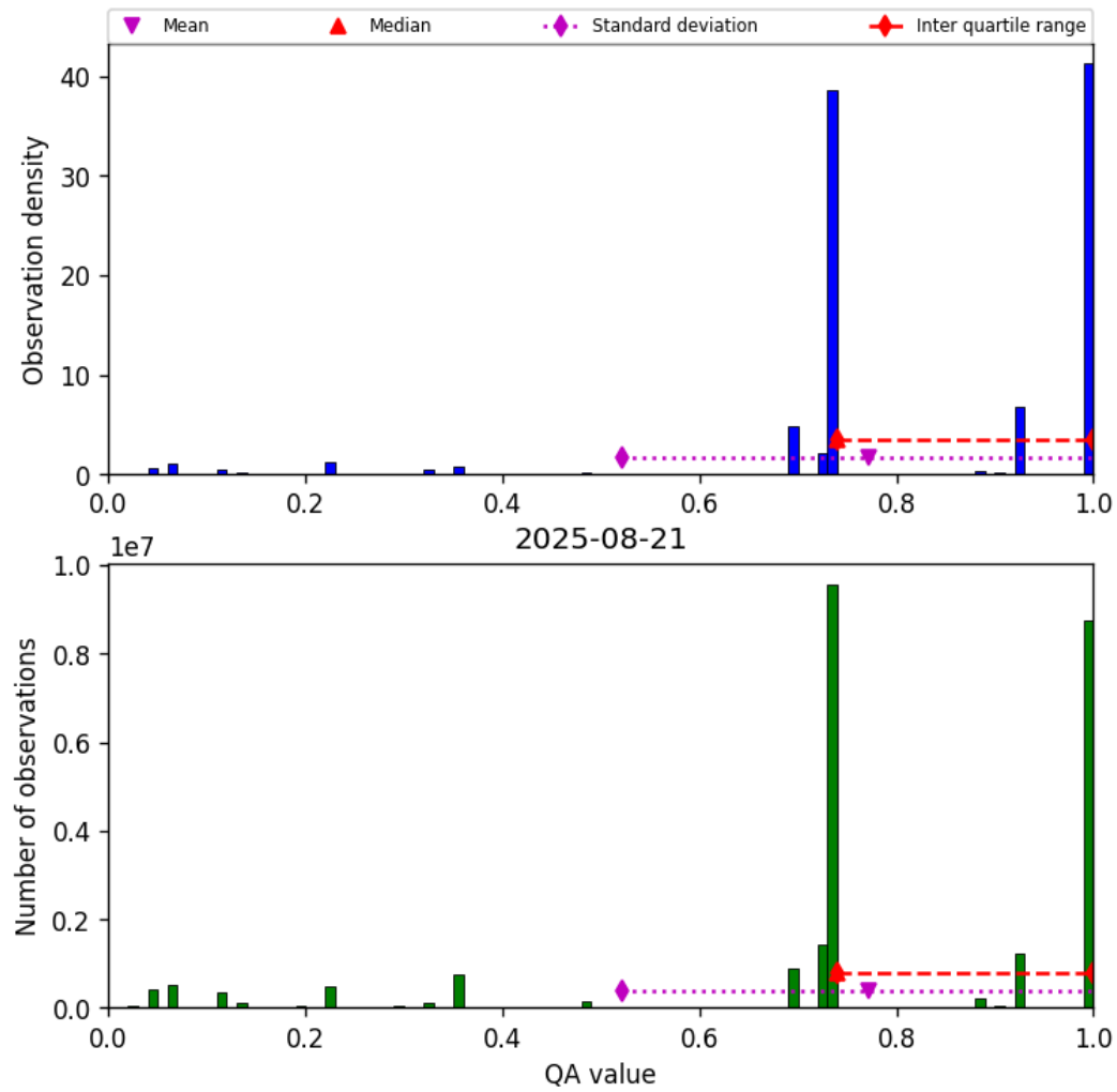
Figure 28: Histogram of “QA value” for 2025-08-20 to 2025-08-22
