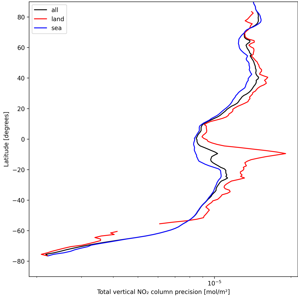
Figure 22: Zonal average of “Total vertical NO 2 column precision” for 2025-08-20 to 2025-08-22.
