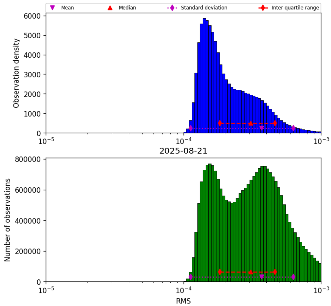
Figure 43: Histogram of “RMS” for 2025-08-20 to 2025-08-22
