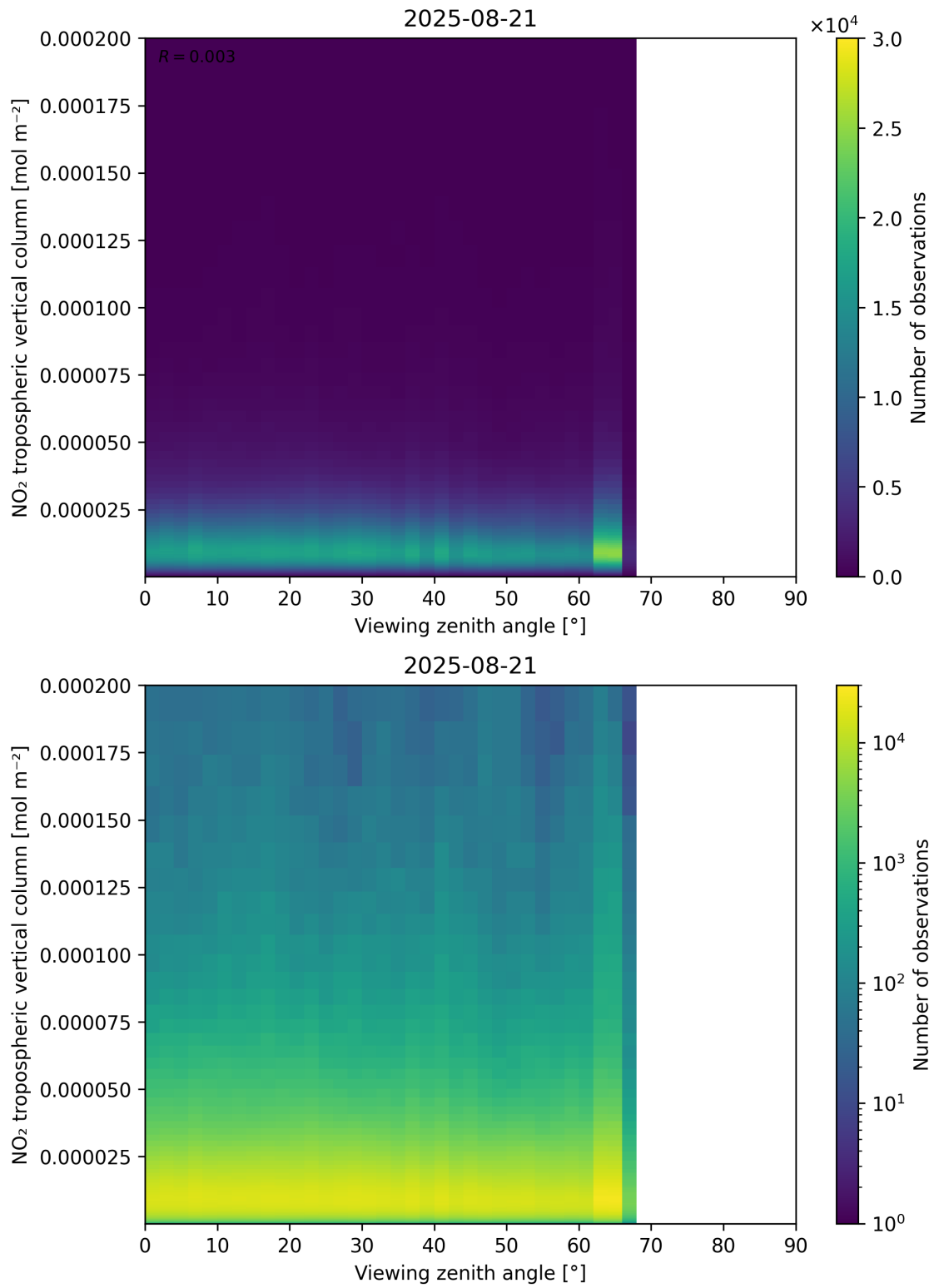
Figure 169: Scatter density plot of “Viewing zenith angle” against “NO 2 tropospheric vertical column” for 2025-08-20 to 2025-08-22.
