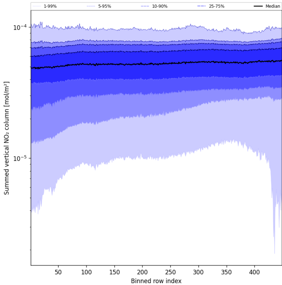
Figure 57: Along track statistics of “Summed vertical NO 2 column” for 2025-08-20 to 2025-08-22
