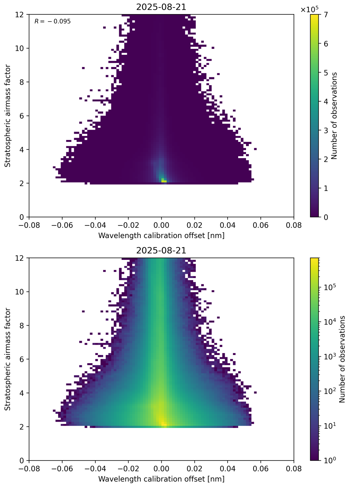
Figure 174: Scatter density plot of “Wavelength calibration offset” against “Stratospheric airmass factor” for 2025-08-20 to 2025-08-22.
