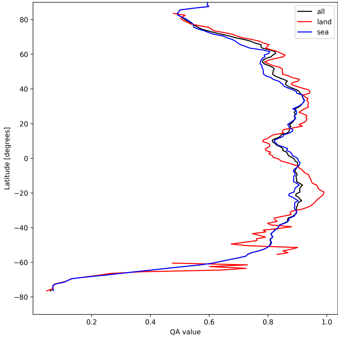
Figure 11: Zonal average of “QA value” for 2025-08-20 to 2025-08-22.
