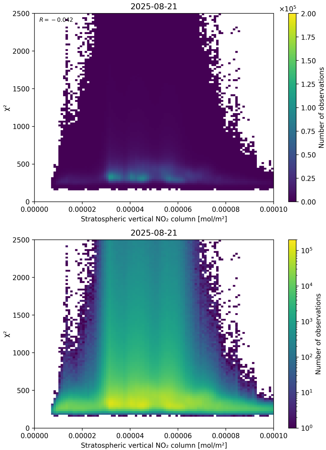
Figure 97: Scatter density plot of “Stratospheric vertical NO 2 column” against “ \chi^2 ” for 2025-08-20 to 2025-08-22.
