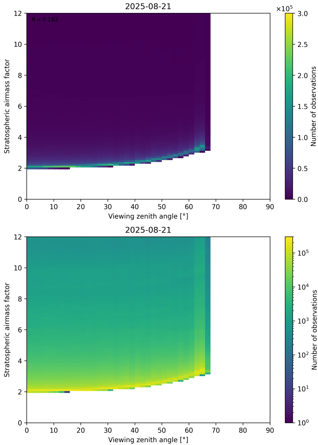
Figure 159: Scatter density plot of “Viewing zenith angle” against “Stratospheric airmass factor” for 2025-08-20 to 2025-08-22.
