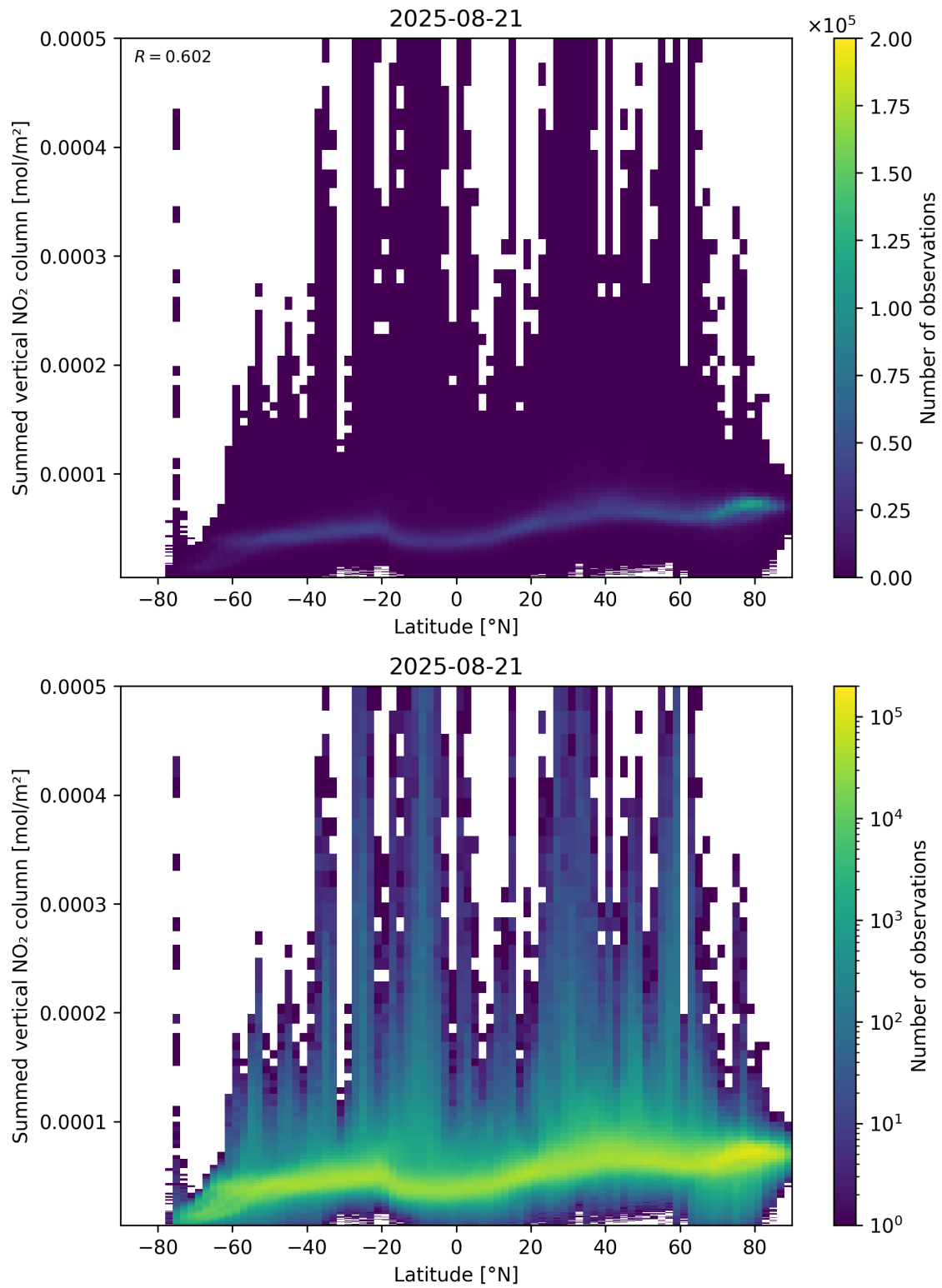
Figure 88: Scatter density plot of “Latitude” against “Summed vertical NO 2 column” for 2025-08-20 to 2025-08-22.
