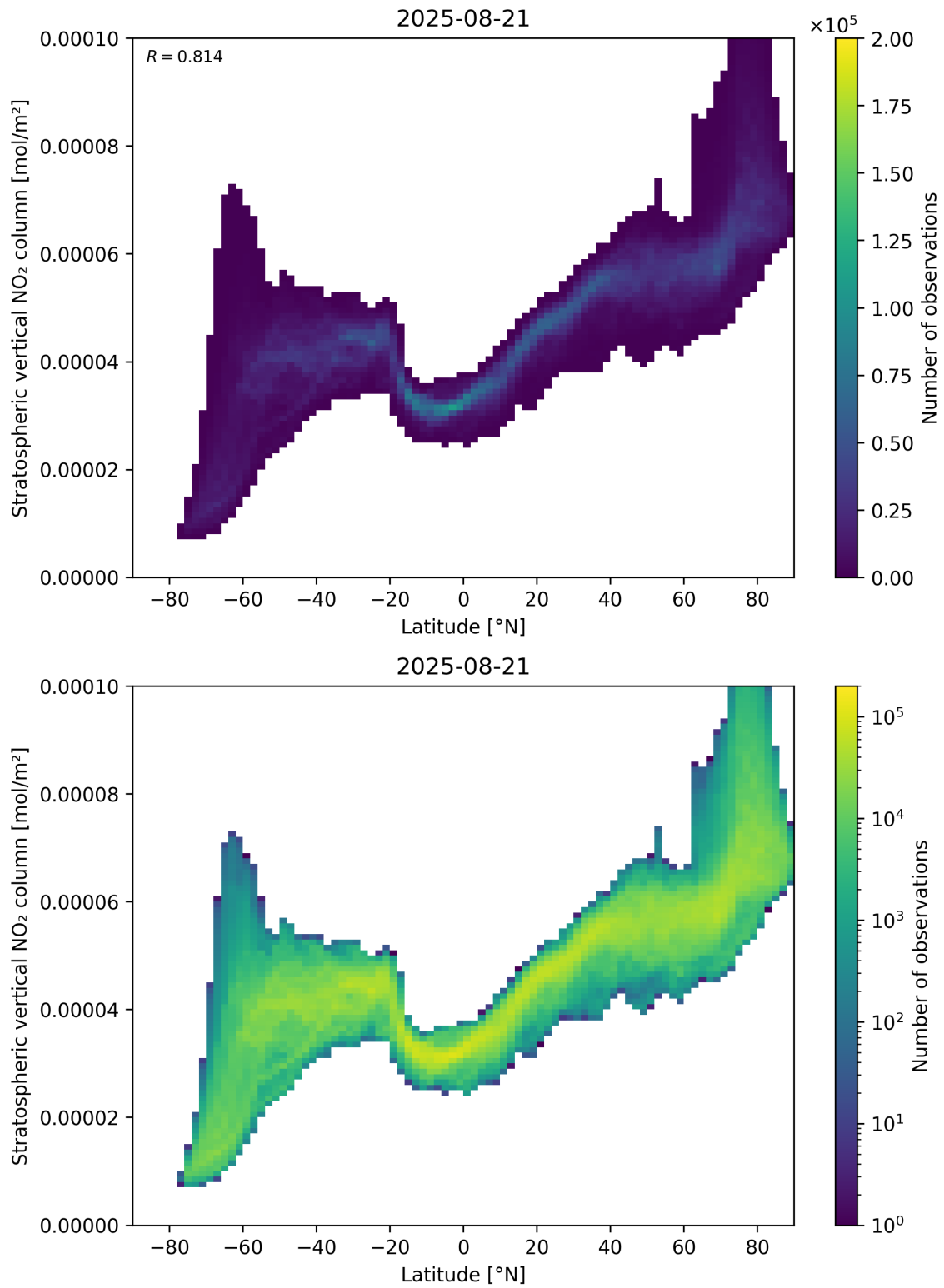
Figure 87: Scatter density plot of “Latitude” against “Stratospheric vertical NO 2 column” for 2025-08-20 to 2025-08-22.
