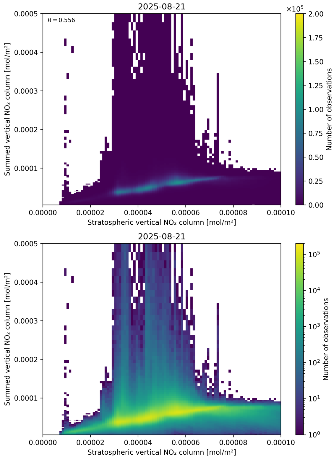
Figure 98: Scatter density plot of “Stratospheric vertical NO 2 column” against “Summed vertical NO 2 column” for 2025-08-20 to 2025-08-22.
