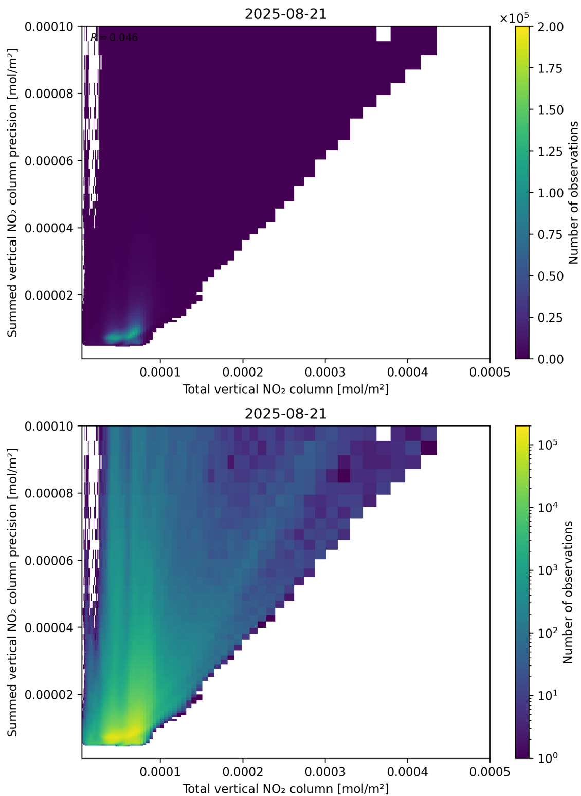
Figure 113: Scatter density plot of “Total vertical NO 2 column” against “Summed vertical NO 2 column precision” for 2025-08-20 to 2025-08-22.
