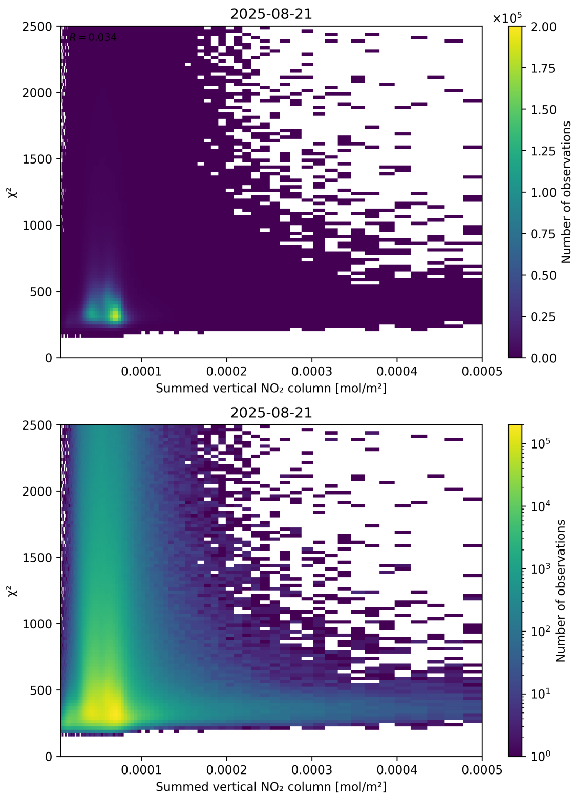
Figure 104: Scatter density plot of “Summed vertical NO 2 column” against “ \chi^2 ” for 2025-08-20 to 2025-08-22.
