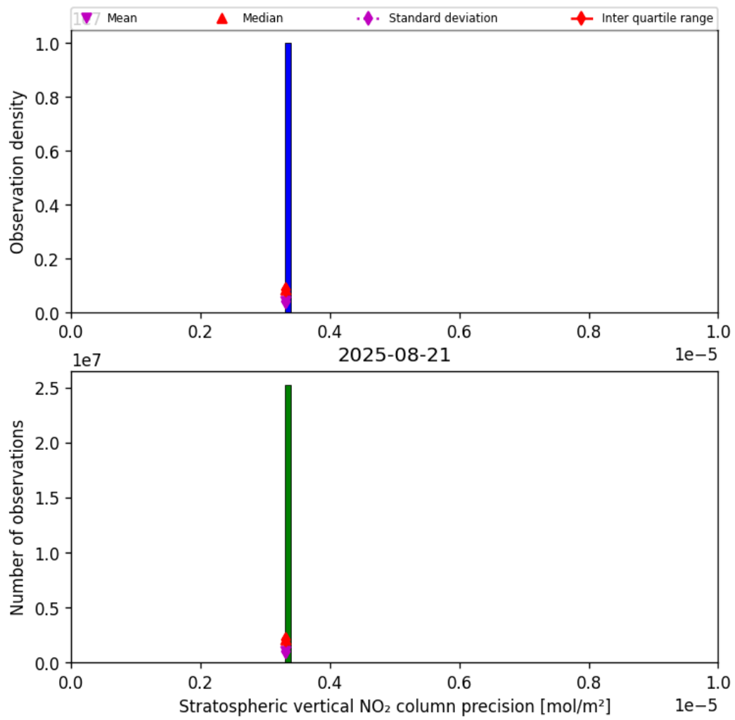
Figure 37: Histogram of “Stratospheric vertical NO 2 column precision” for 2025-08-20 to 2025-08-22
