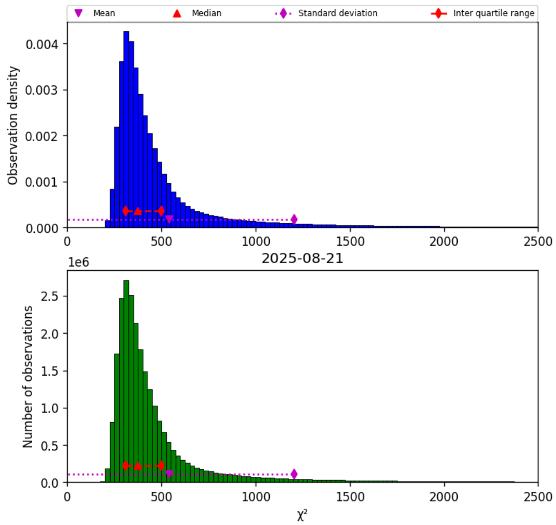
Figure 42: Histogram of “ \chi^2 ” for 2025-08-20 to 2025-08-22
