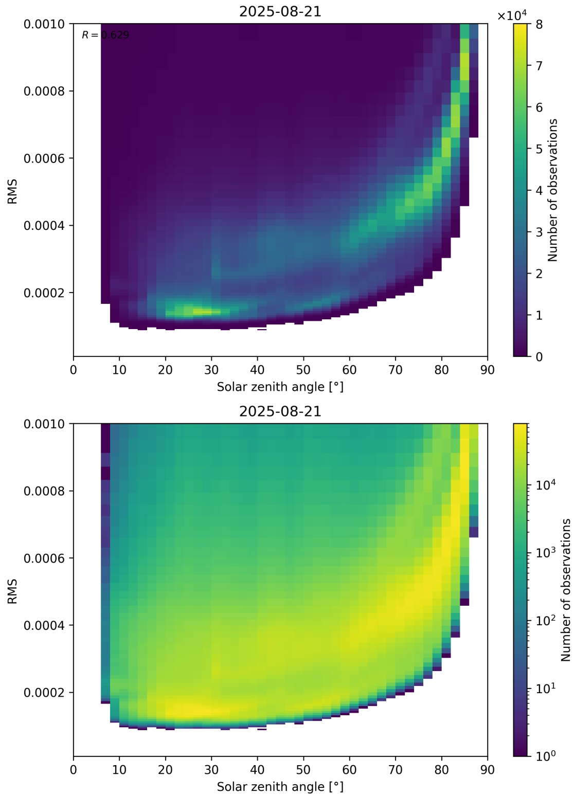
Figure 157: Scatter density plot of “Solar zenith angle” against “RMS” for 2025-08-20 to 2025-08-22.
