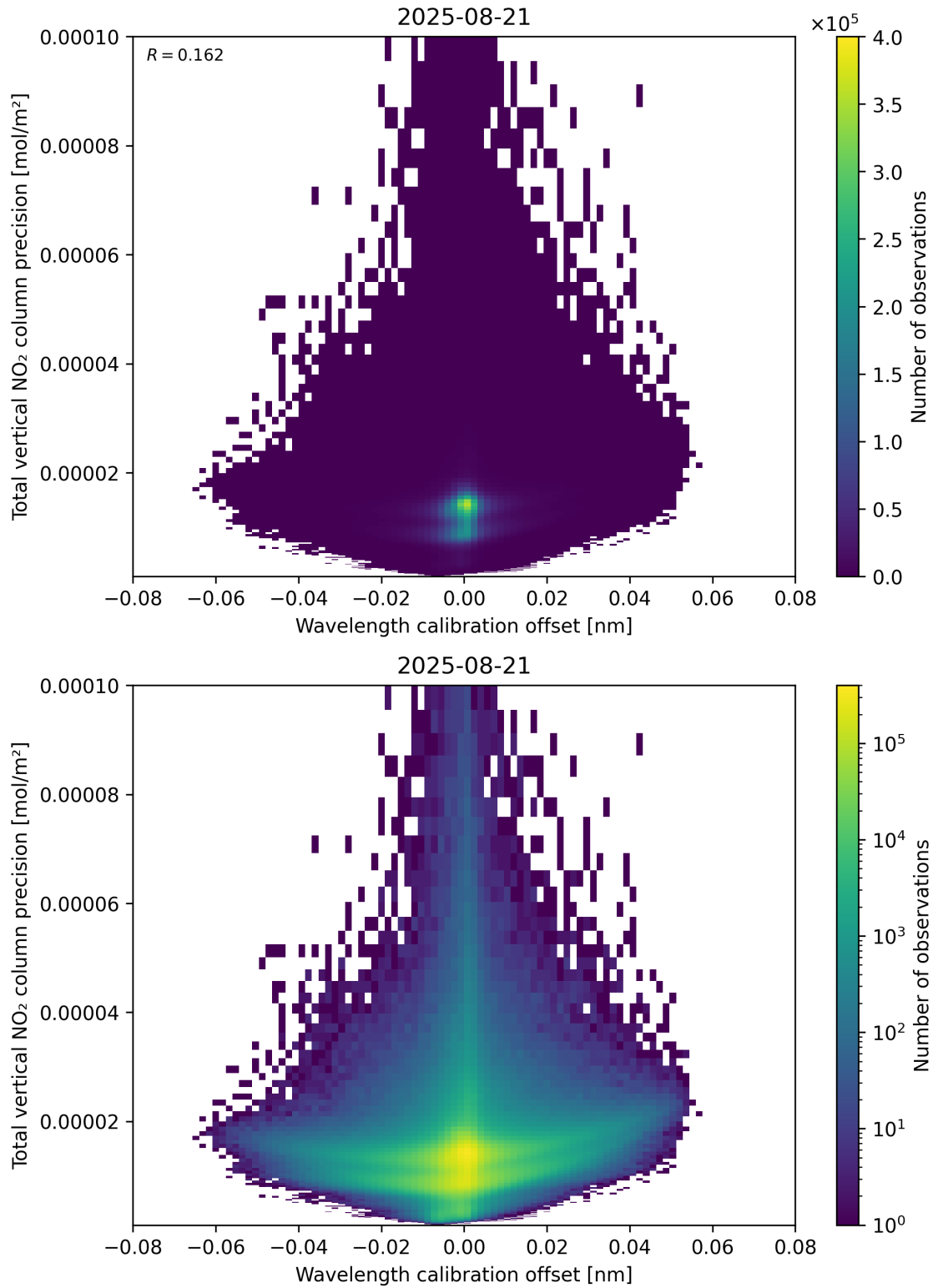
Figure 180: Scatter density plot of “Wavelength calibration offset” against “Total vertical NO 2 column precision” for 2025-08-20 to 2025-08-22.
