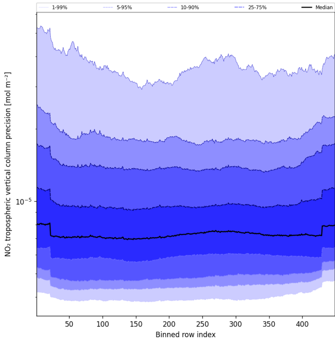
Figure 47: Along track statistics of “NO 2 tropospheric vertical column precision” for 2025-08-20 to 2025-08-22
