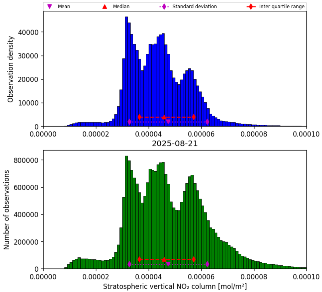
Figure 36: Histogram of “Stratospheric vertical NO 2 column” for 2025-08-20 to 2025-08-22
