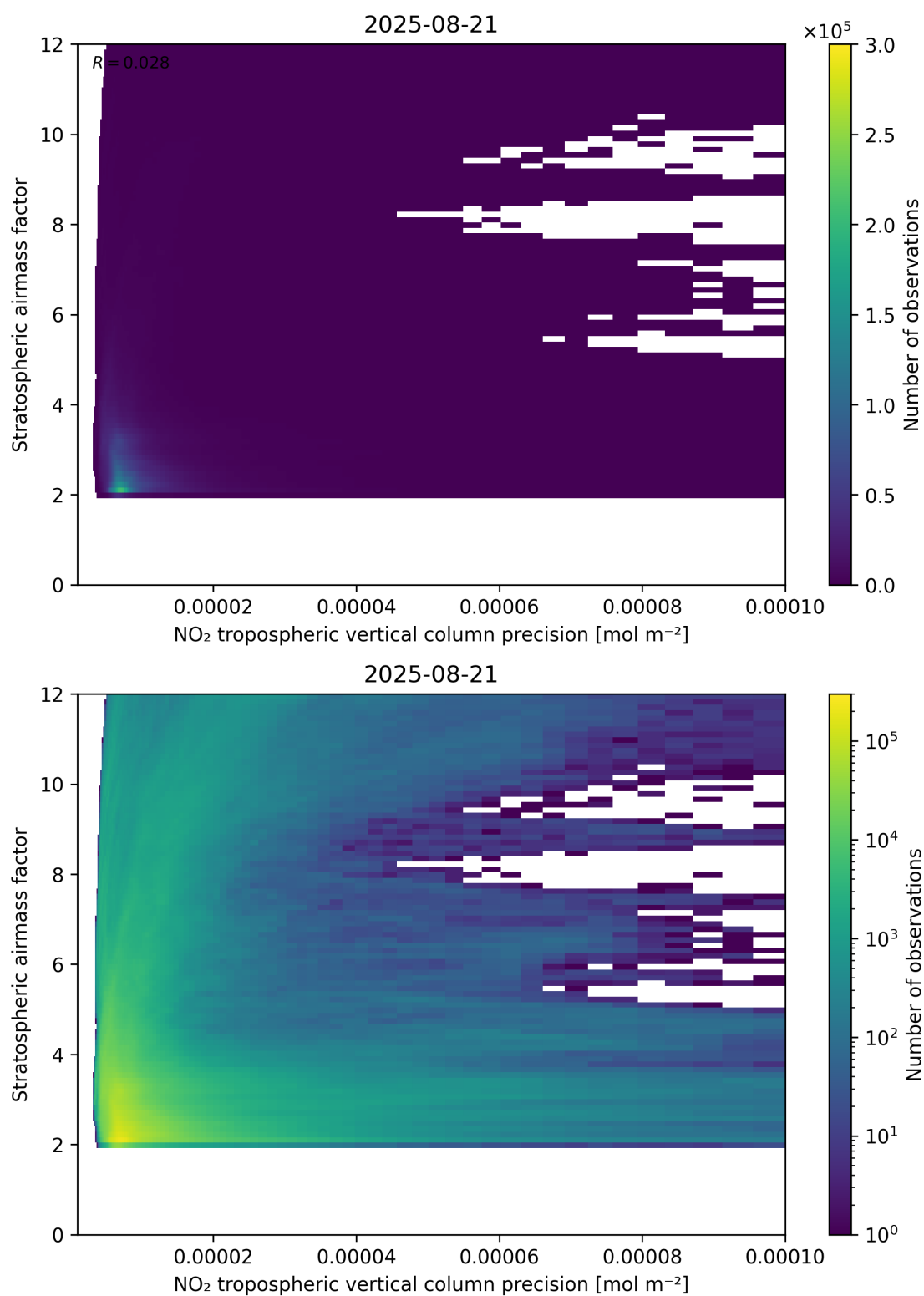
Figure 131: Scatter density plot of “NO 2 tropospheric vertical column precision” against “Stratospheric airmass factor” for 2025-08-20 to 2025-08-22.
