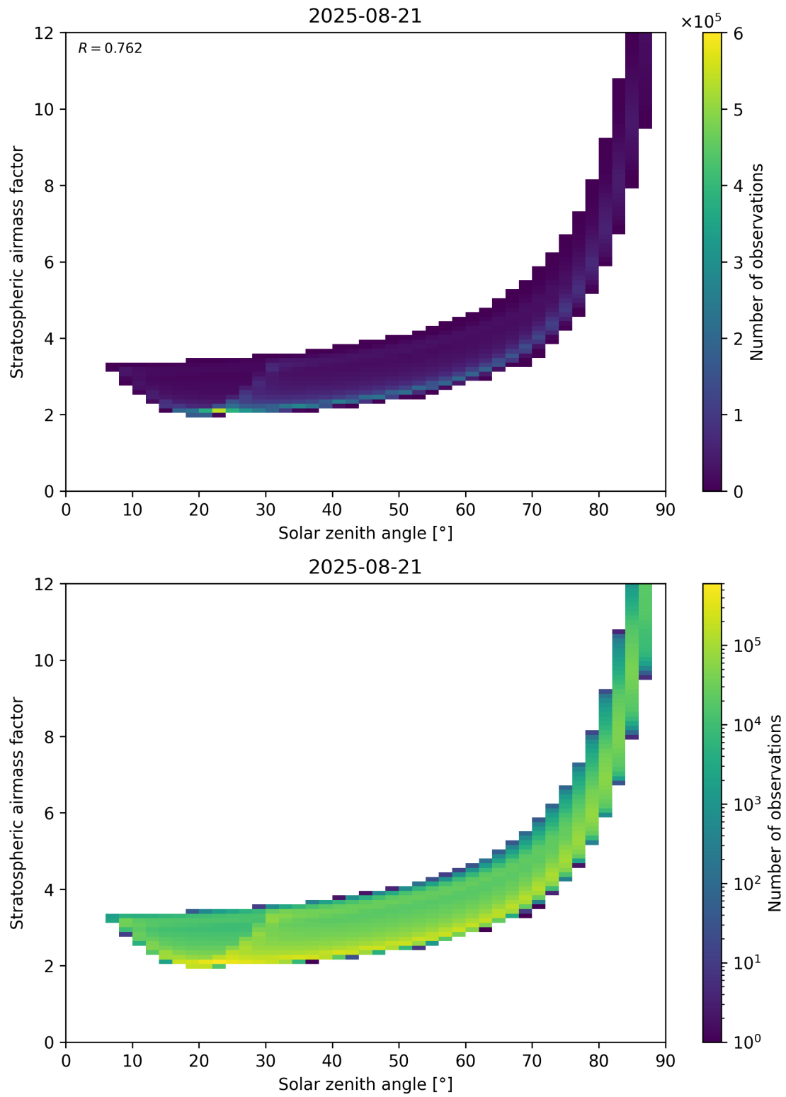
Figure 145: Scatter density plot of “Solar zenith angle” against “Stratospheric airmass factor” for 2025-08-20 to 2025-08-22.
