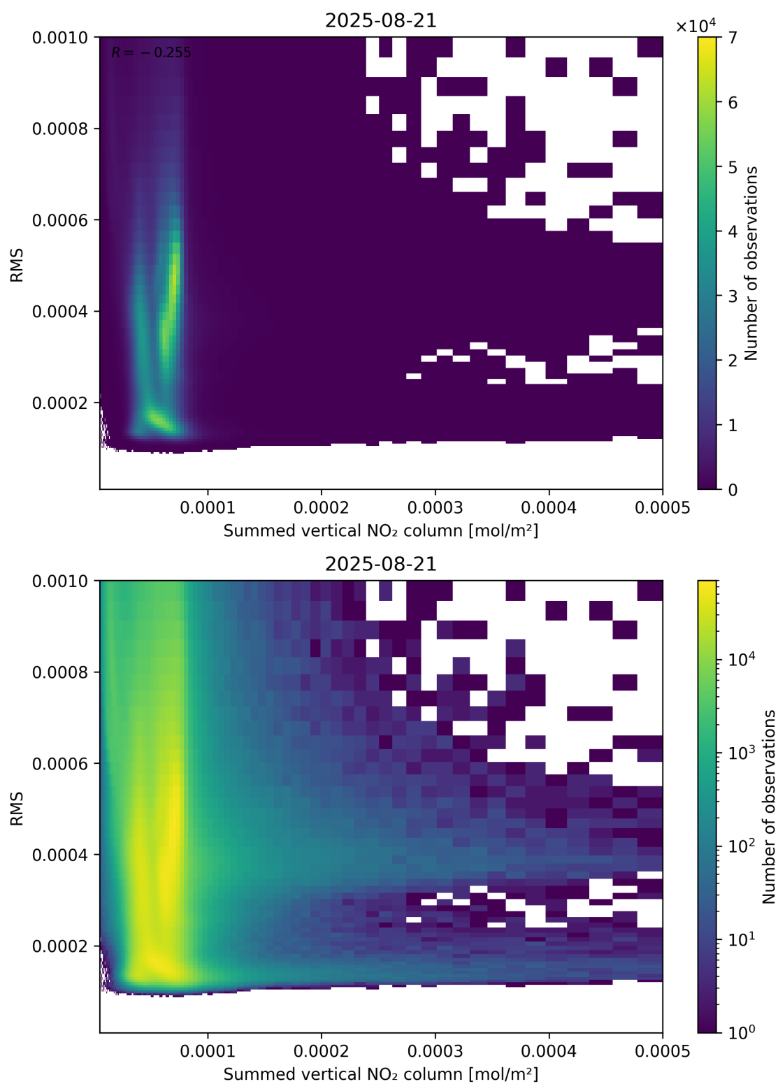
Figure 109: Scatter density plot of “Summed vertical NO 2 column” against “RMS” for 2025-08-20 to 2025-08-22.
