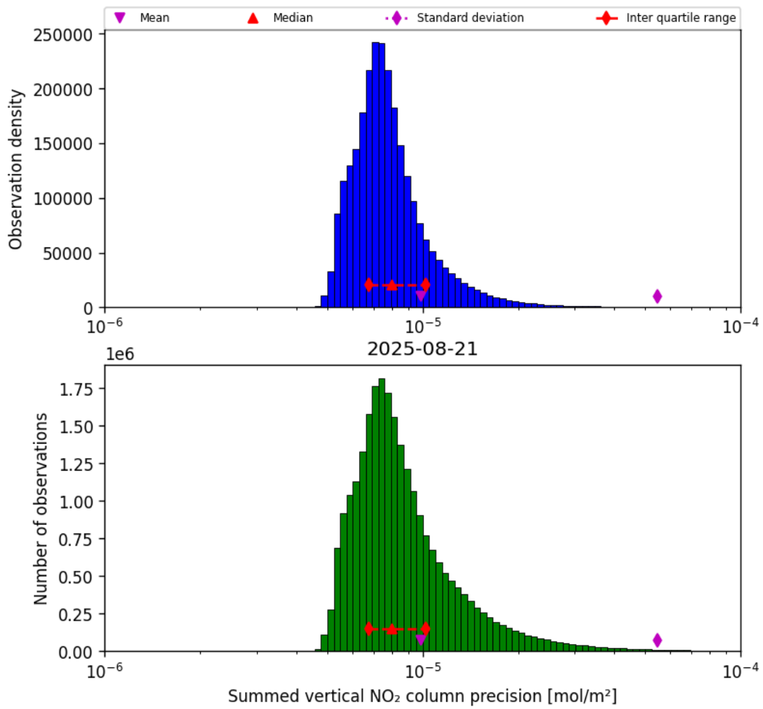
Figure 41: Histogram of "Summed vertical NO 2 column precision" for 2025-08-20 to 2025-08-22
