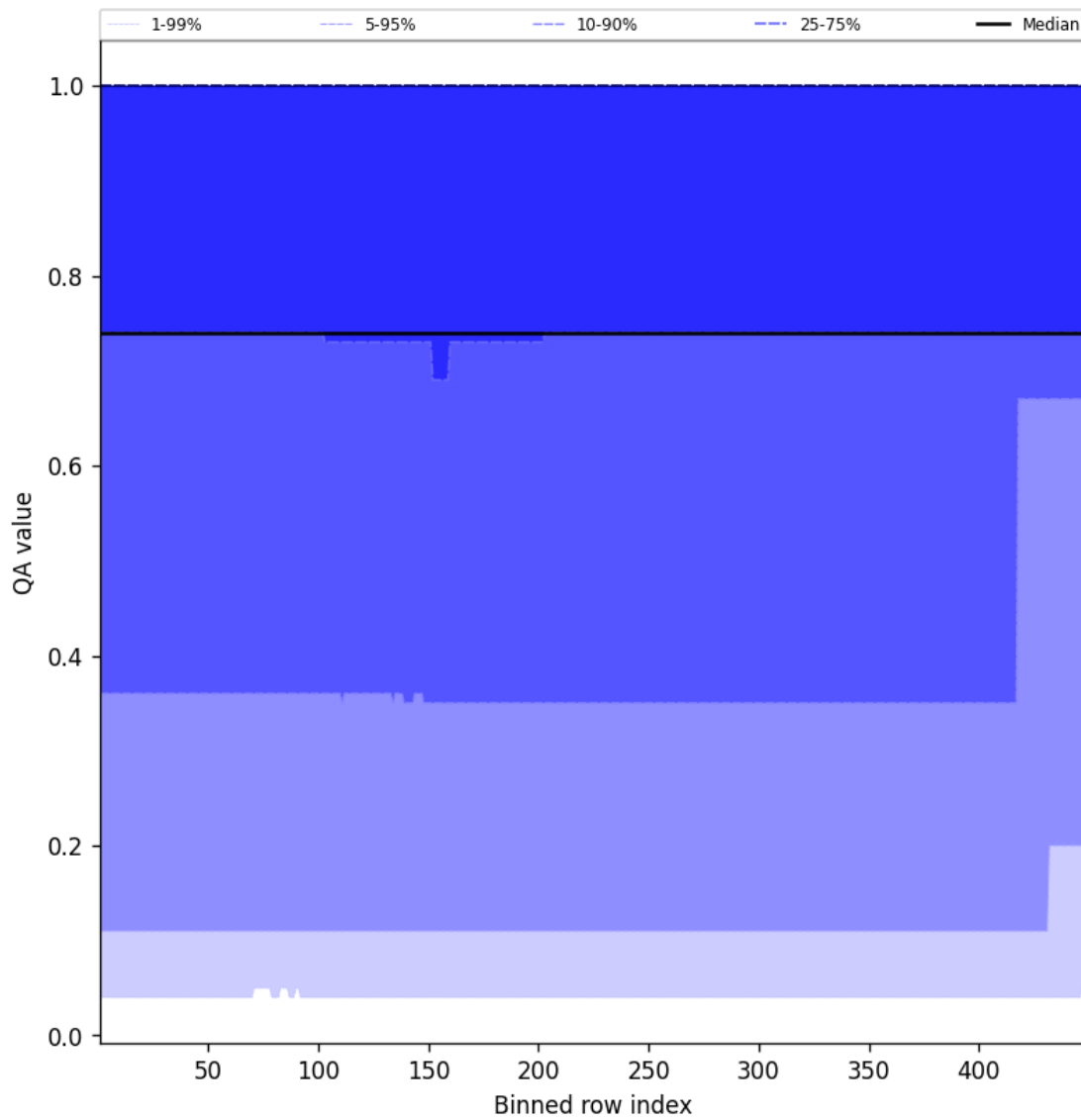
Figure 45: Along track statistics of “QA value” for 2025-08-21 to 2025-08-23
