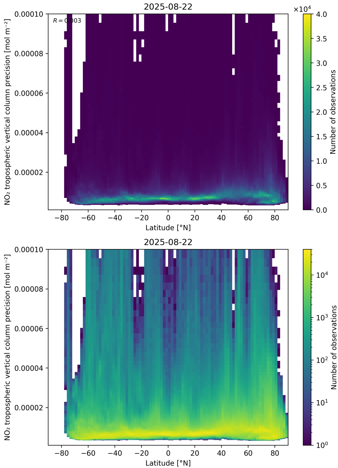
Figure 93: Scatter density plot of “Latitude” against “NO 2 tropospheric vertical column precision” for 2025-08-21 to 2025-08-23.
