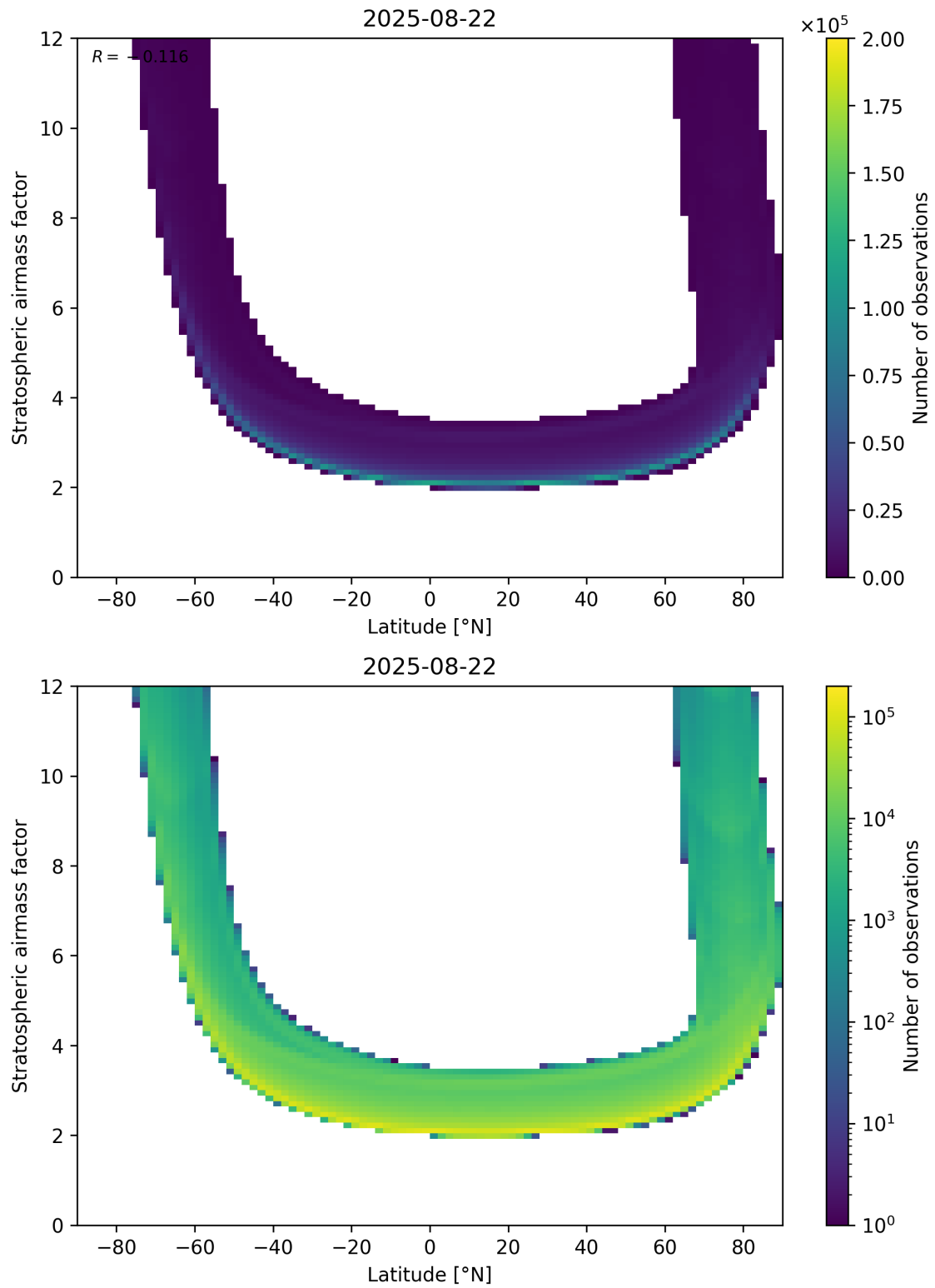
Figure 83: Scatter density plot of “Latitude” against “Stratospheric air mass factor” for 2025-08-21 to 2025-08-23.
