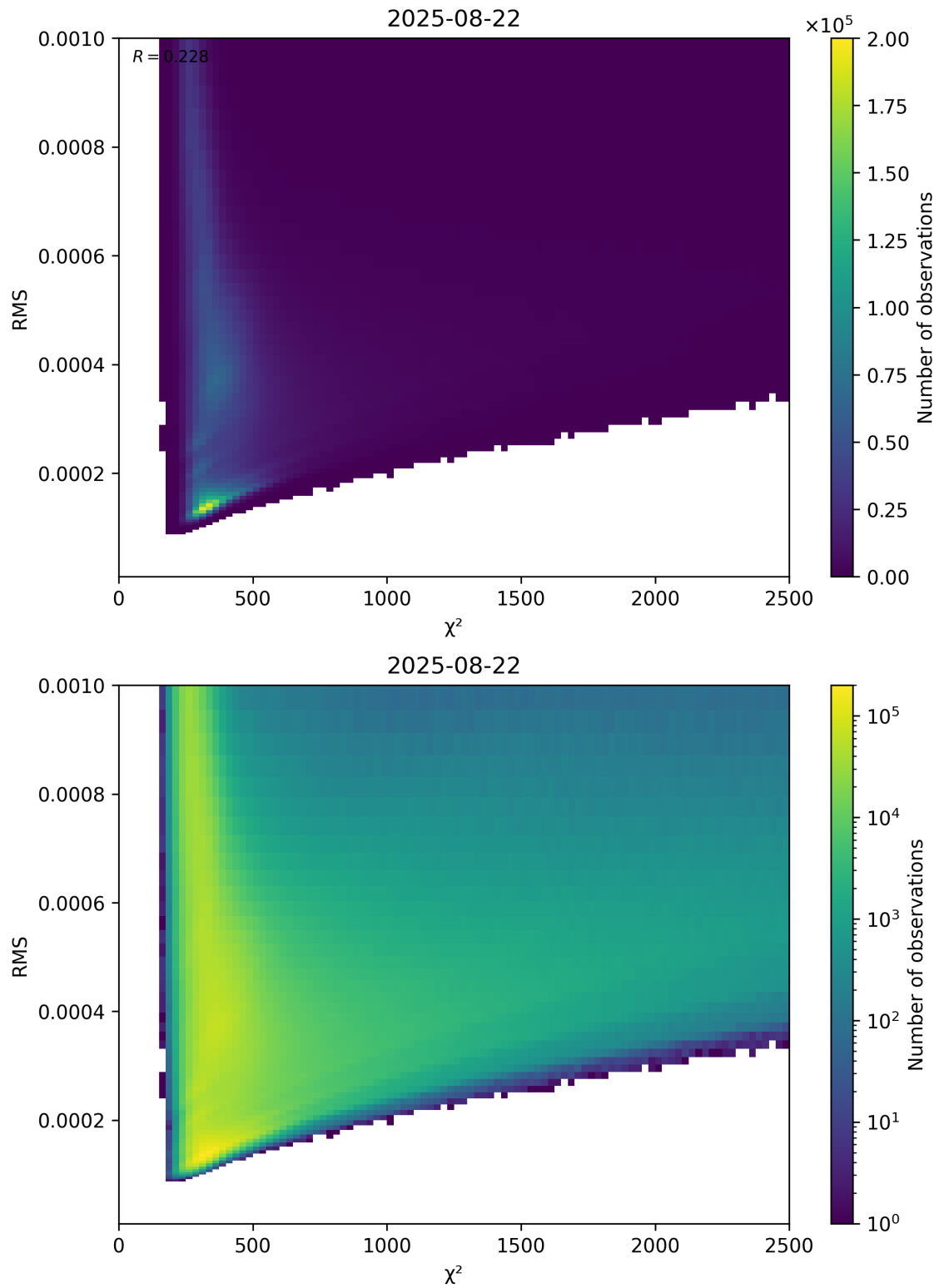
Figure 82: Scatter density plot of “ \chi^2 ” against “RMS” for 2025-08-21 to 2025-08-23.
