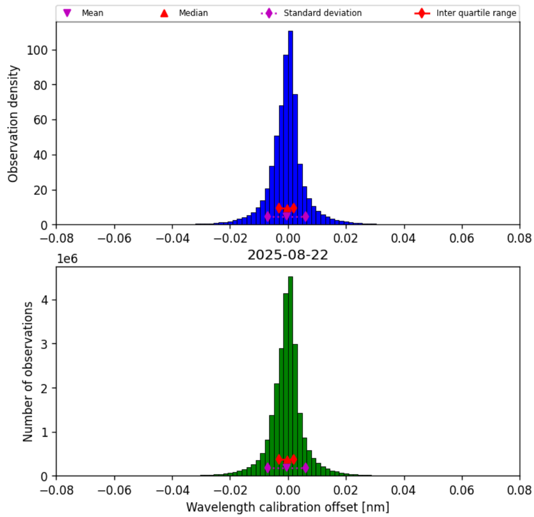
Figure 35: Histogram of “Wavelength calibration offset” for 2025-08-21 to 2025-08-23
