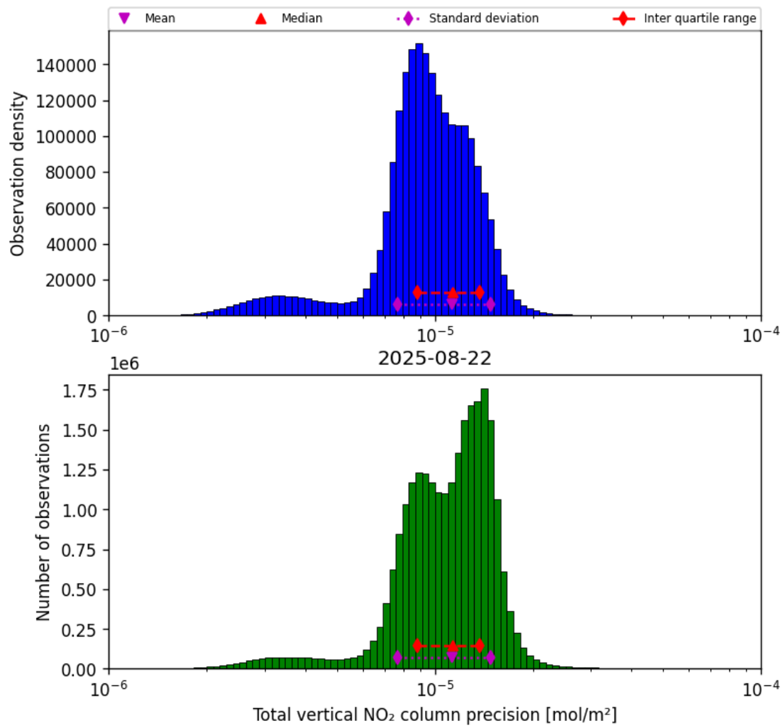
Figure 39: Histogram of “Total vertical NO 2 column precision” for 2025-08-21 to 2025-08-23
