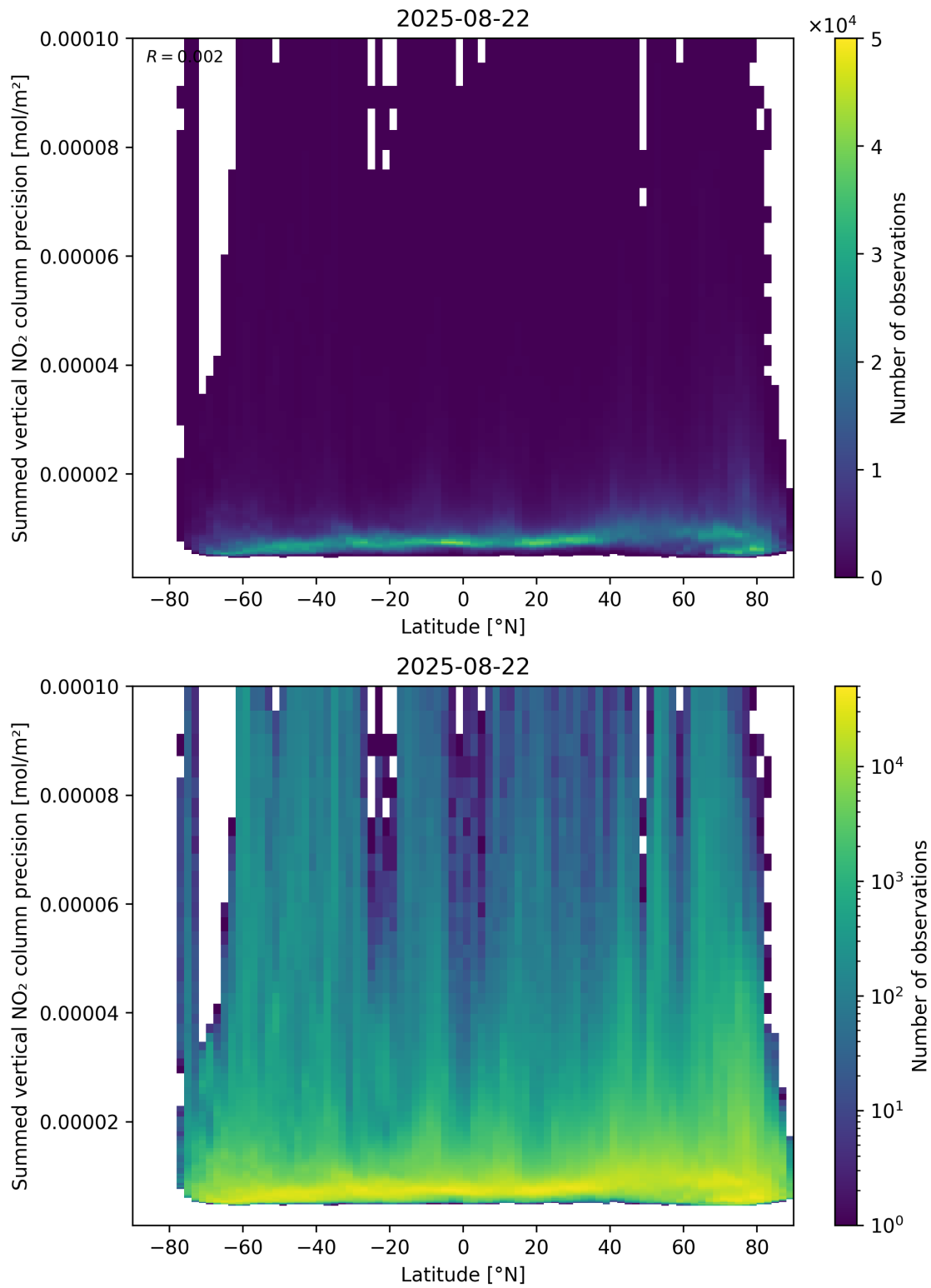
Figure 89: Scatter density plot of “Latitude” against “Summed vertical NO 2 column precision” for 2025-08-21 to 2025-08-23.
