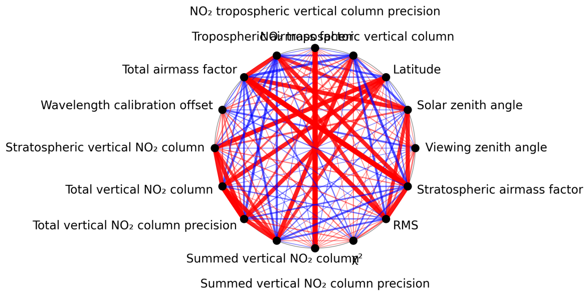
Figure 1: Map of correlation graph for 2025-08-21 to 2025-08-23.
