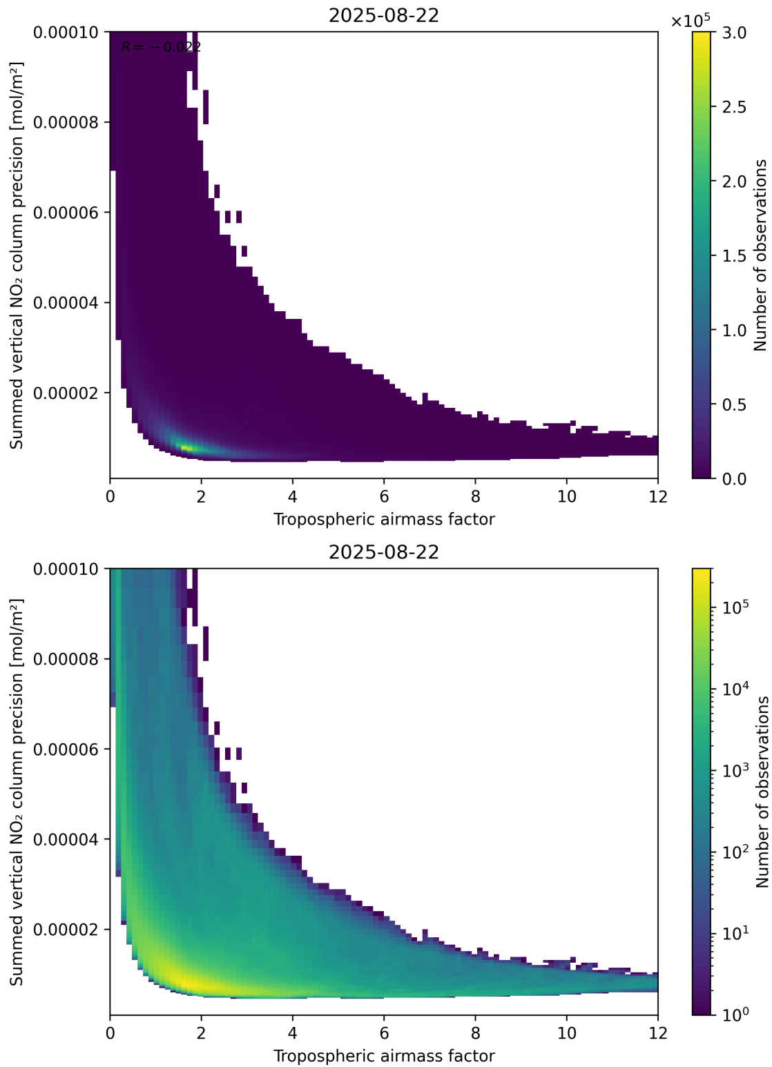
Figure 76: Scatter density plot of “Tropospheric air mass factor” against “Summed vertical NO 2 column precision” for 2025-08-21 to 2025-08-23.
