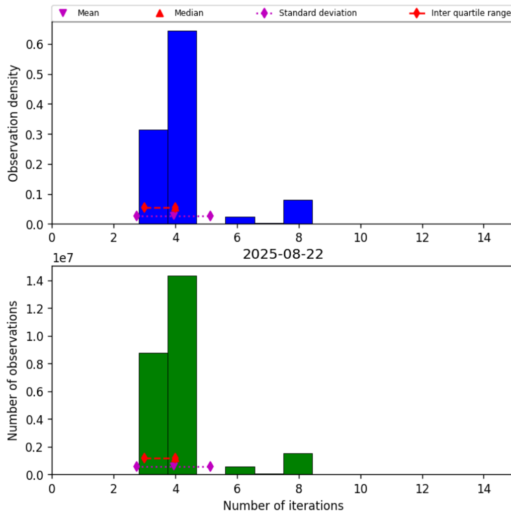
Figure 34: Histogram of “Number of iterations” for 2025-08-21 to 2025-08-23
