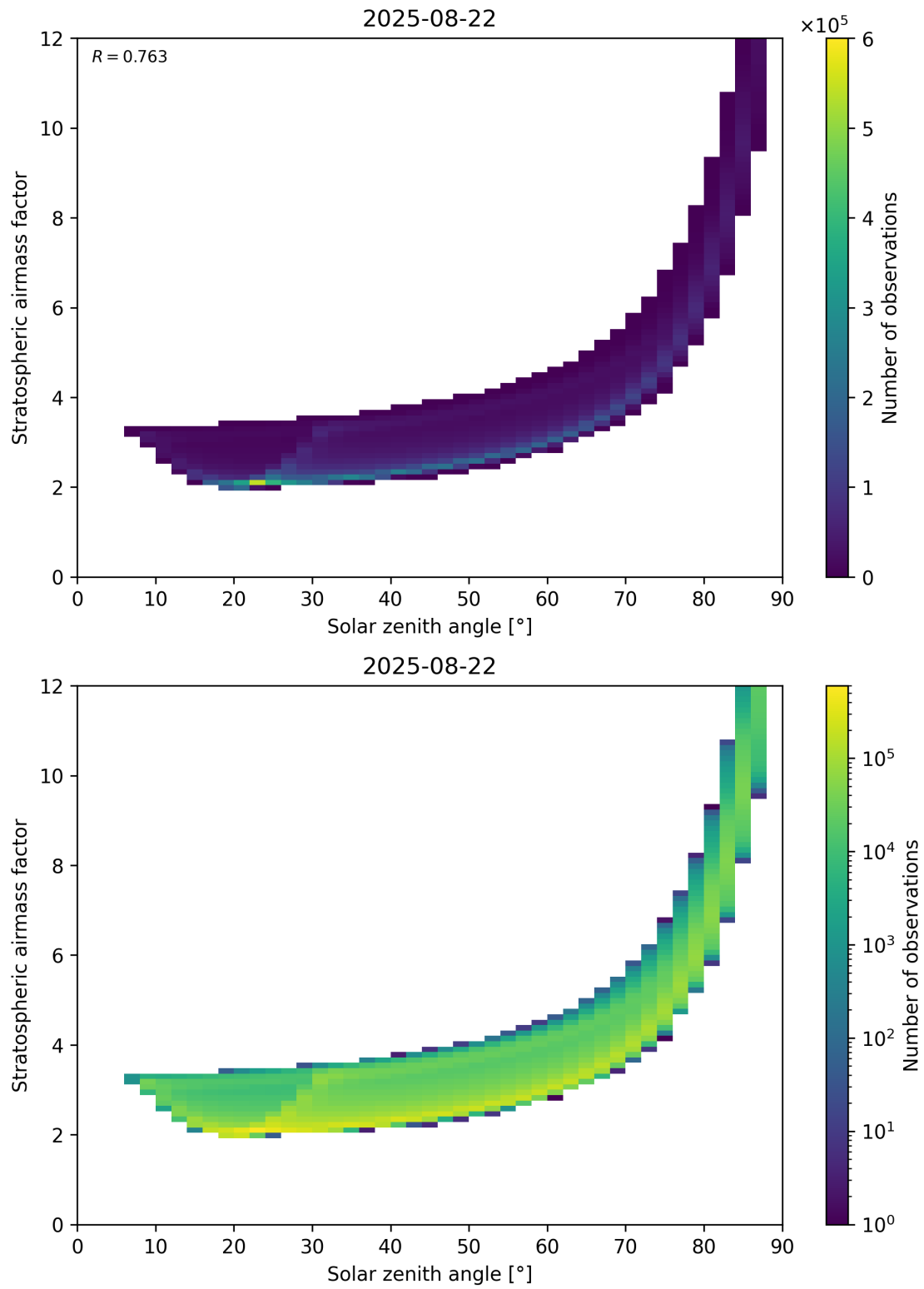
Figure 145: Scatter density plot of “Solar zenith angle” against “Stratospheric airmass factor” for 2025-08-21 to 2025-08-23.
