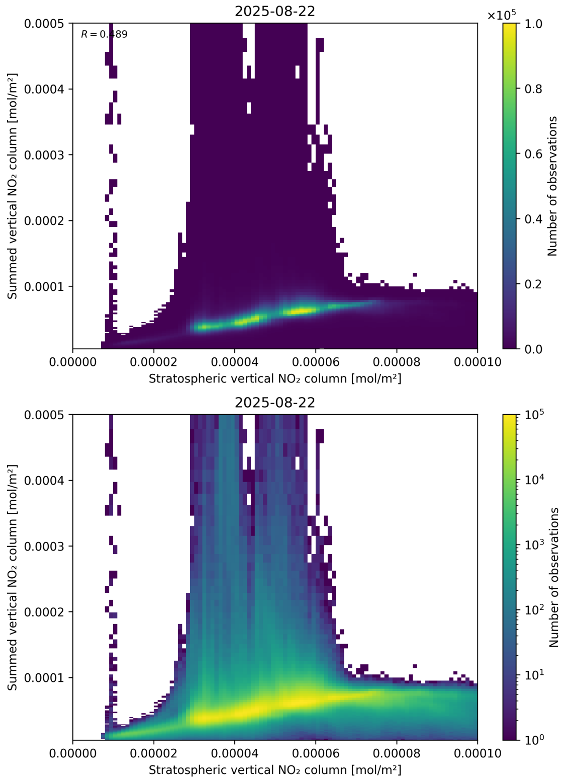
Figure 98: Scatter density plot of “Stratospheric vertical NO 2 column” against “Summed vertical NO 2 column” for 2025-08-21 to 2025-08-23.
