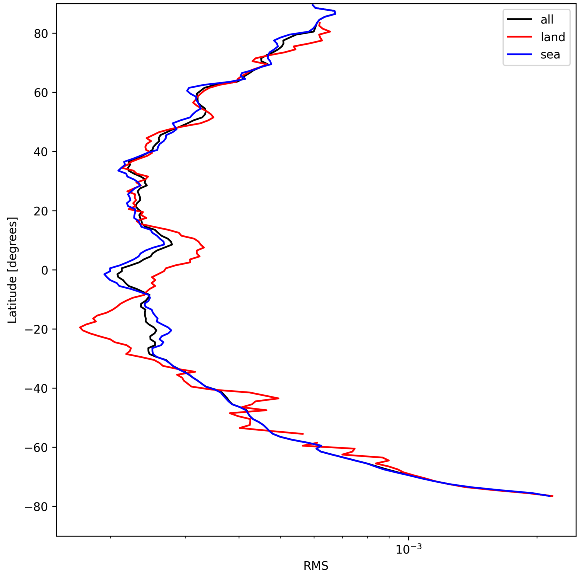
Figure 26: Zonal average of “RMS” for 2025-08-21 to 2025-08-23.
