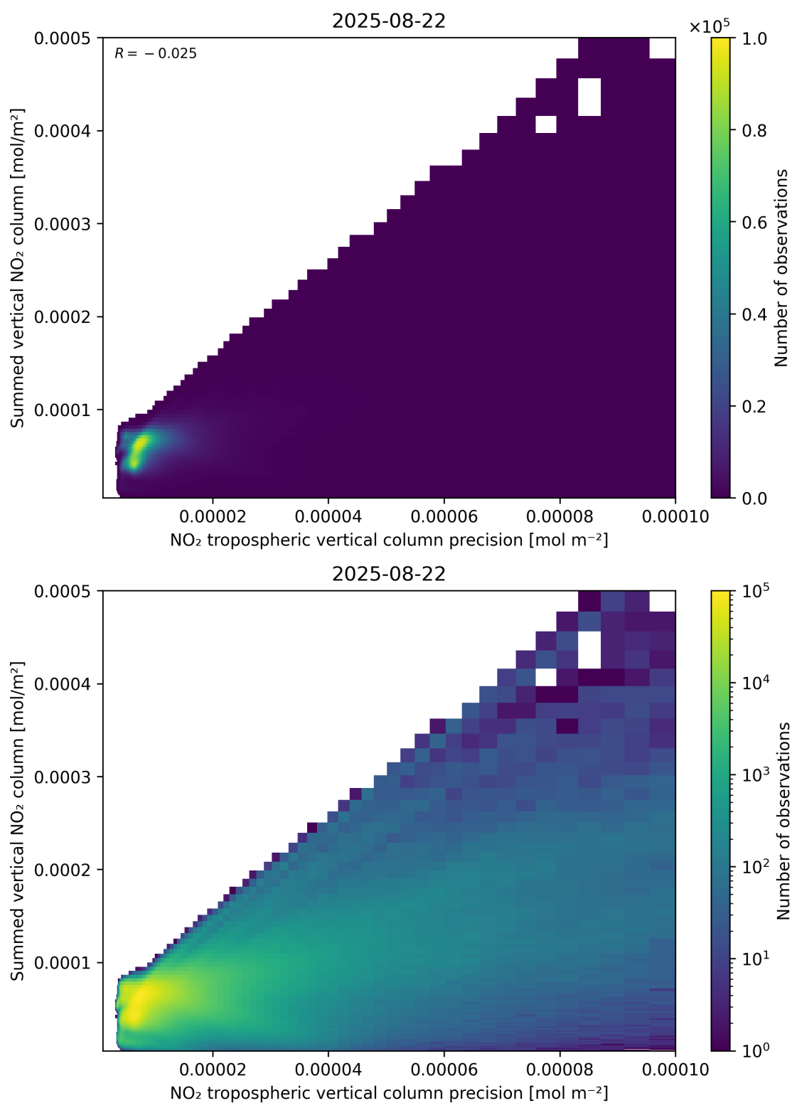
Figure 136: Scatter density plot of “NO 2 tropospheric vertical column precision” against “Summed vertical NO 2 column” for 2025-08-21 to 2025-08-23.
