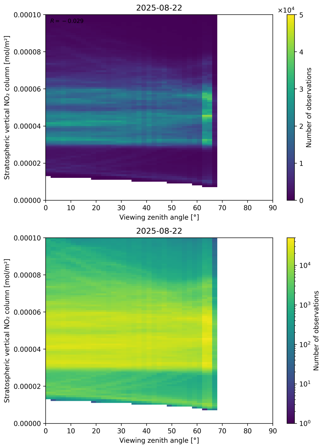
Figure 164: Scatter density plot of “Viewing zenith angle” against “Stratospheric vertical NO 2 column” for 2025-08-21 to 2025-08-23.
