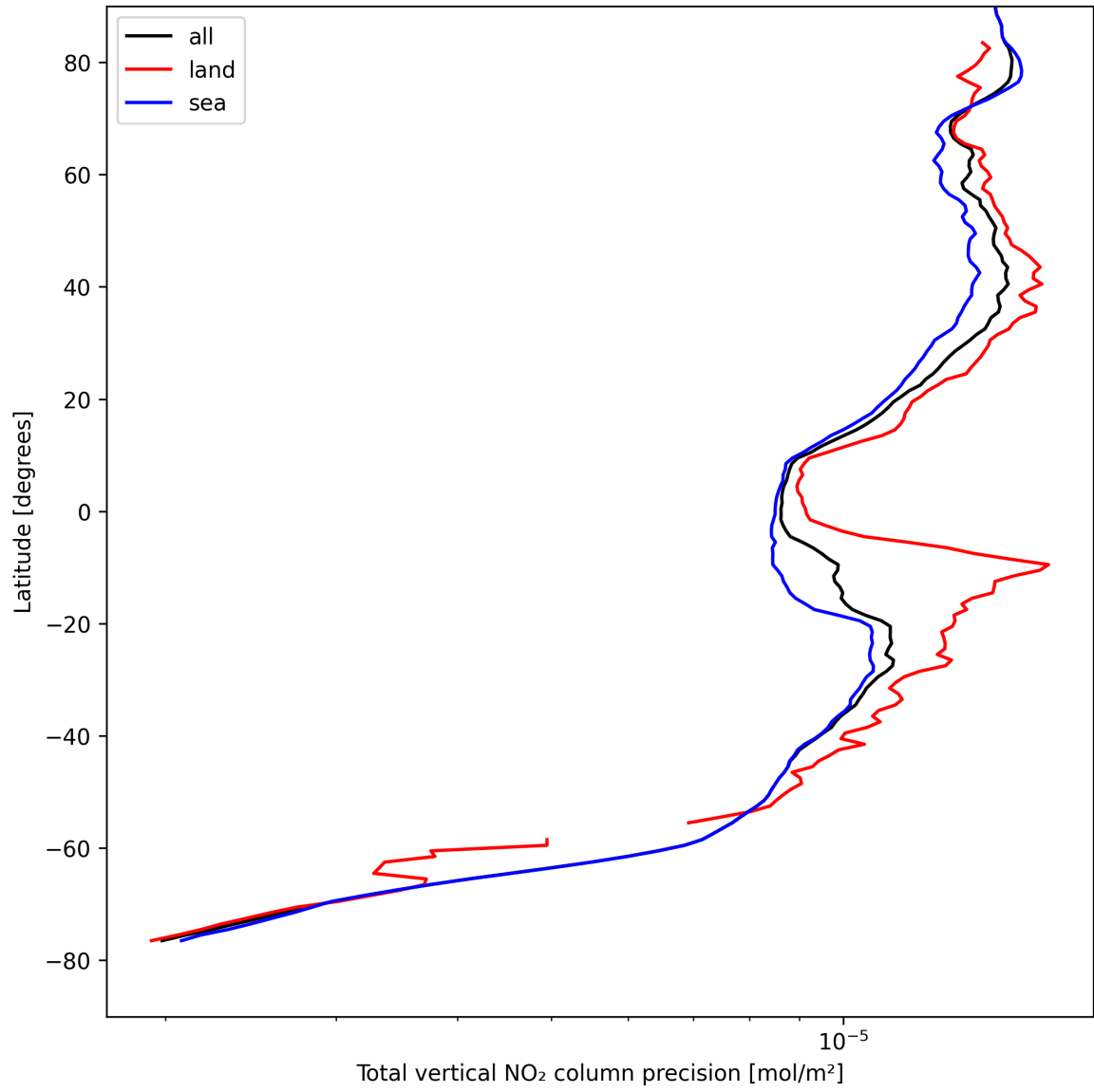
Figure 22: Zonal average of “Total vertical NO 2 column precision” for 2025-08-21 to 2025-08-23.
