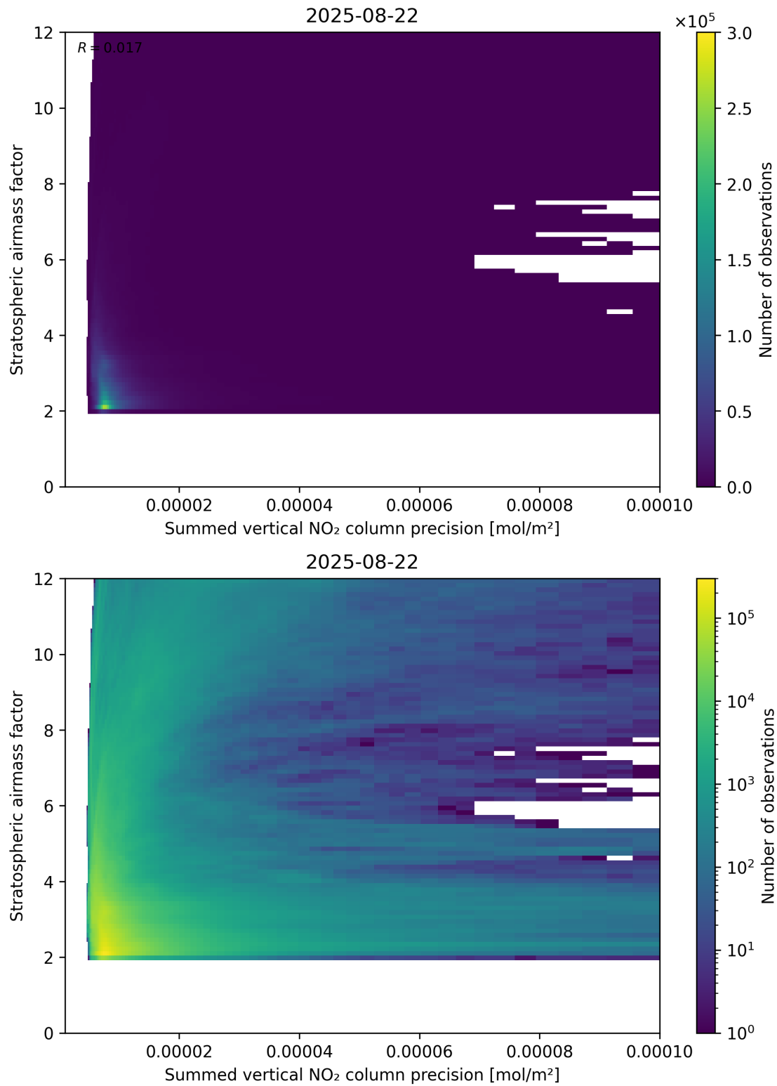
Figure 106: Scatter density plot of “Summed vertical NO 2 column precision” against “Stratospheric airmass factor” for 2025-08-21 to 2025-08-23.
