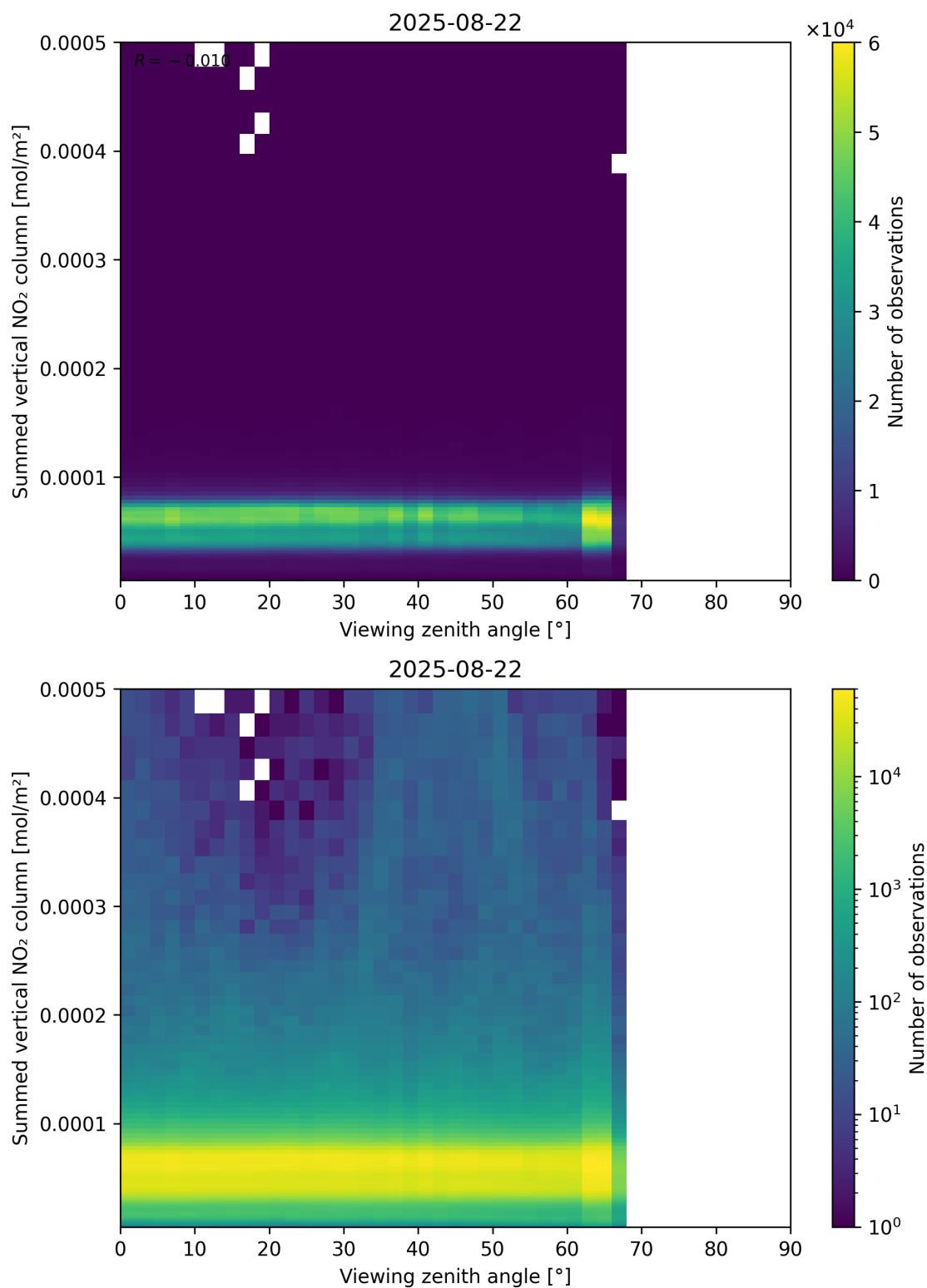
Figure 165: Scatter density plot of “Viewing zenith angle” against “Summed vertical NO 2 column” for 2025-08-21 to 2025-08-23.
