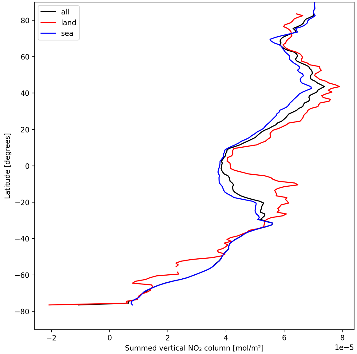
Figure 23: Zonal average of “Summed vertical NO 2 column” for 2025-08-21 to 2025-08-23.
