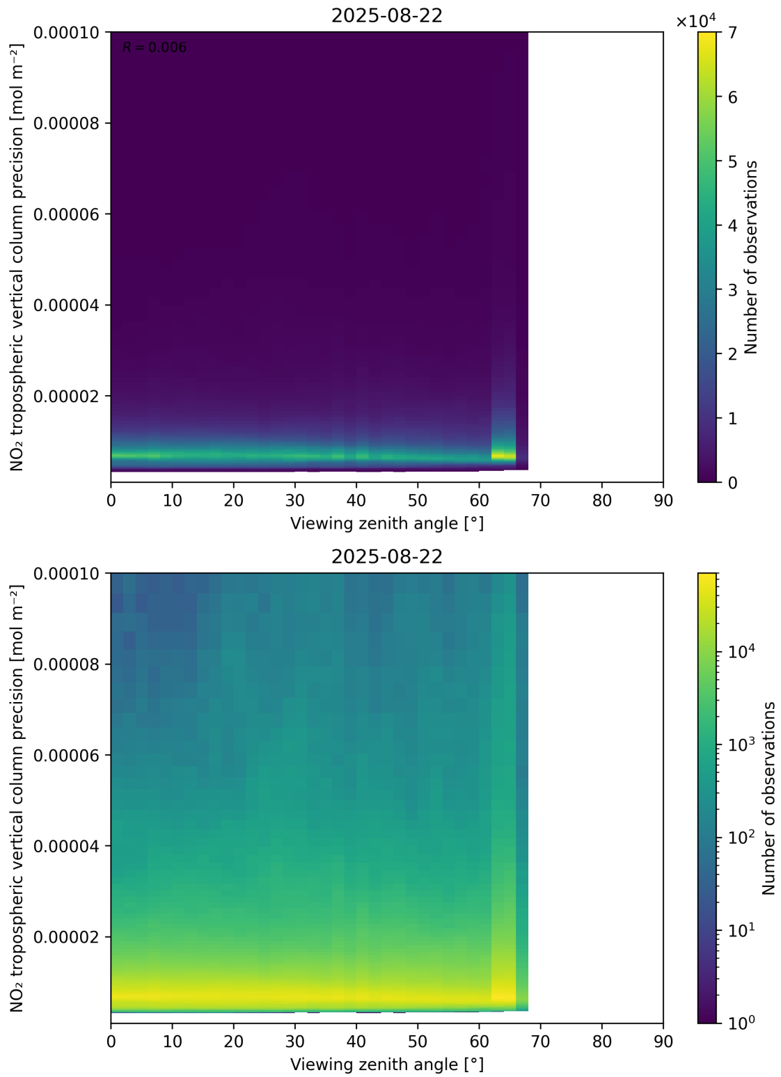
Figure 170: Scatter density plot of “Viewing zenith angle” against “NO 2 tropospheric vertical column precision” for 2025-08-21 to 2025-08-23.
