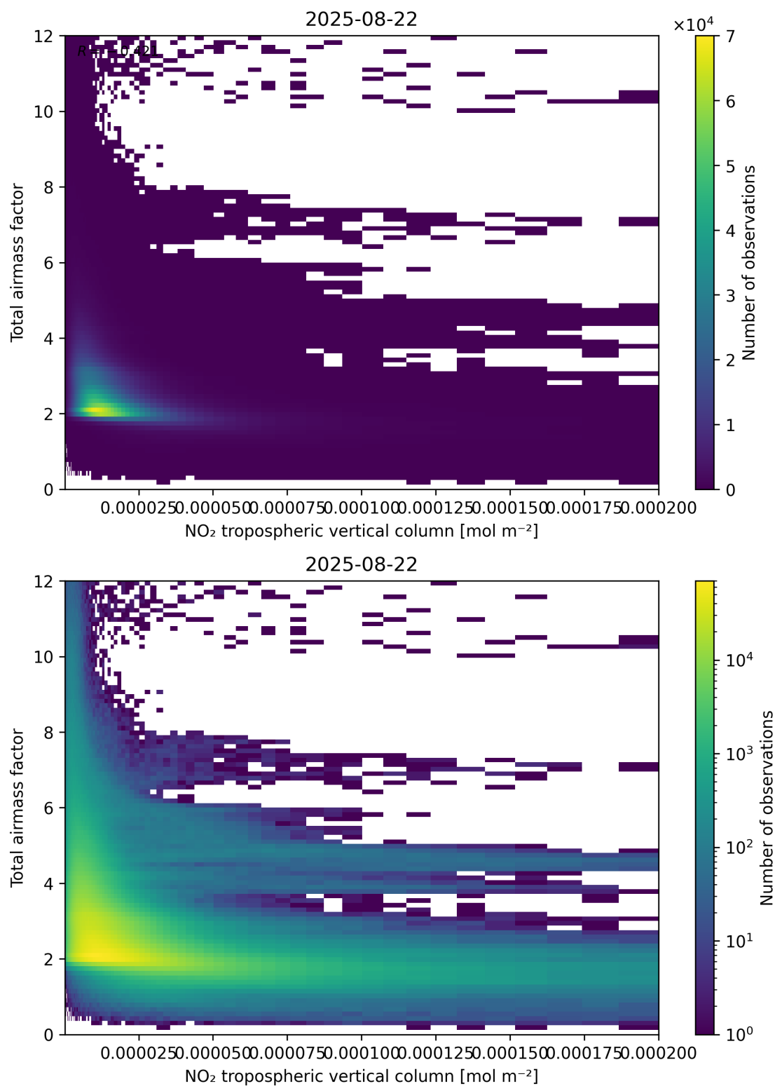
Figure 122: Scatter density plot of “NO 2 tropospheric vertical column” against “Total airmass factor” for 2025-08-21 to 2025-08-23.
