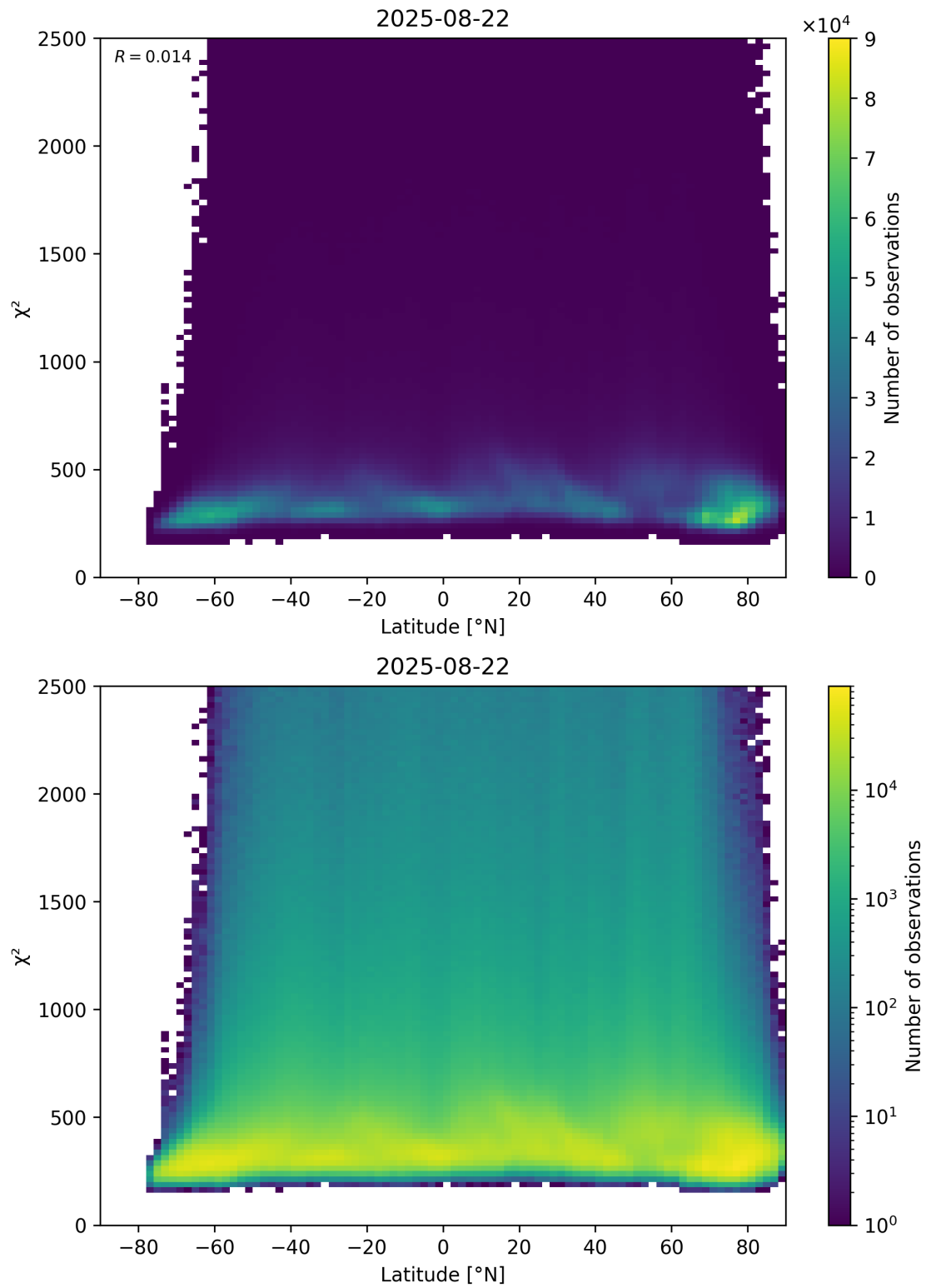
Figure 86: Scatter density plot of “Latitude” against “ \chi^2 ” for 2025-08-21 to 2025-08-23.
