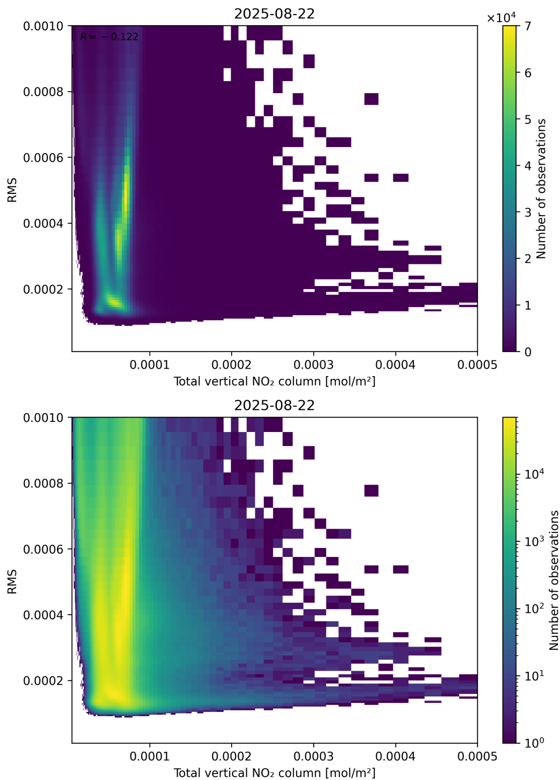
Figure 120: Scatter density plot of “Total vertical NO 2 column” against “RMS” for 2025-08-21 to 2025-08-23.
