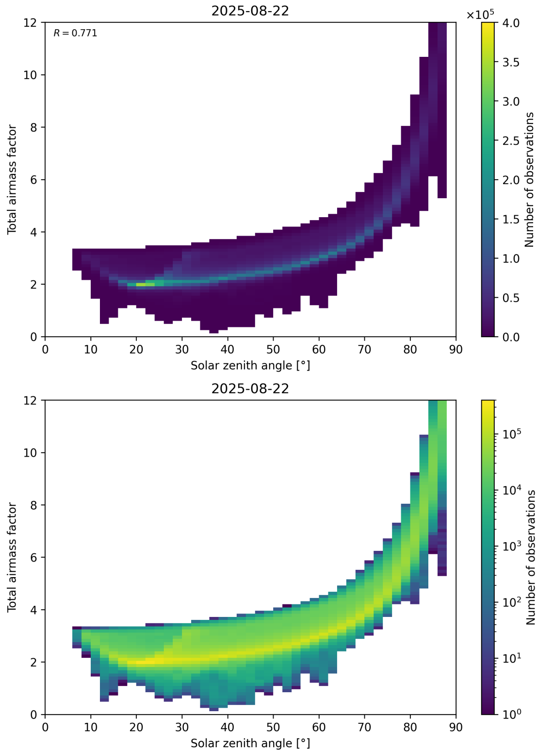
Figure 146: Scatter density plot of “Solar zenith angle” against “Total air mass factor” for 2025-08-21 to 2025-08-23.
