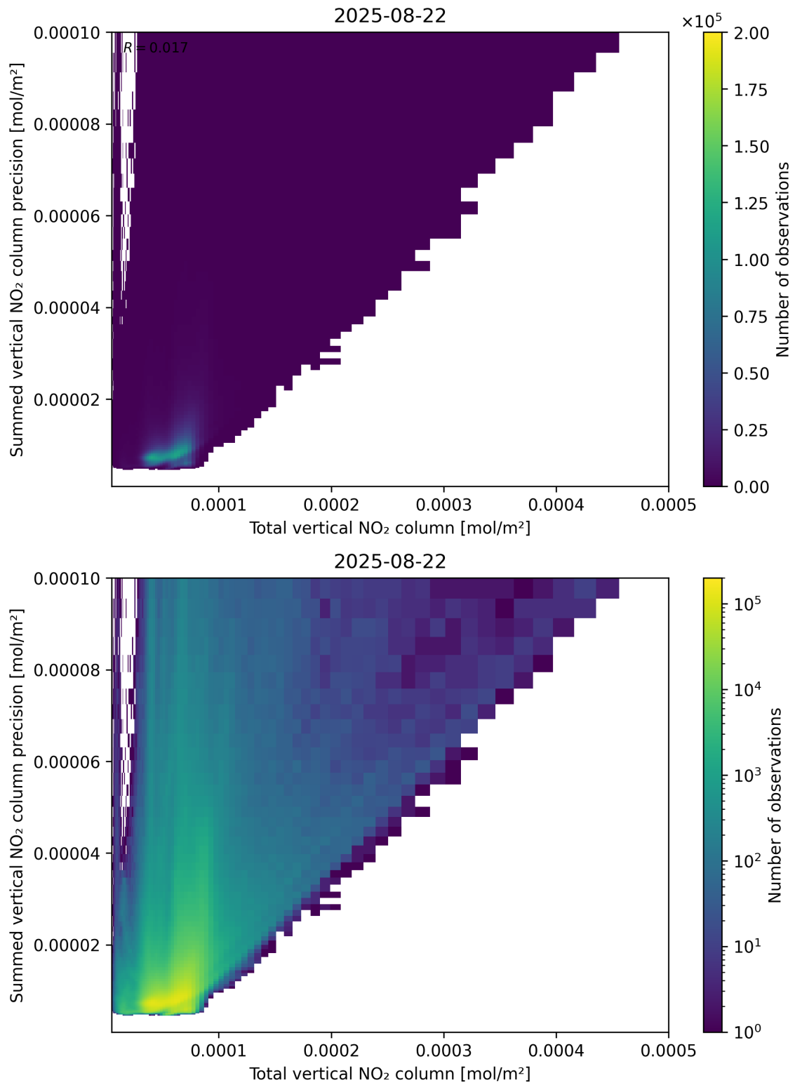
Figure 113: Scatter density plot of “Total vertical NO 2 column” against “Summed vertical NO 2 column precision” for 2025-08-21 to 2025-08-23.
