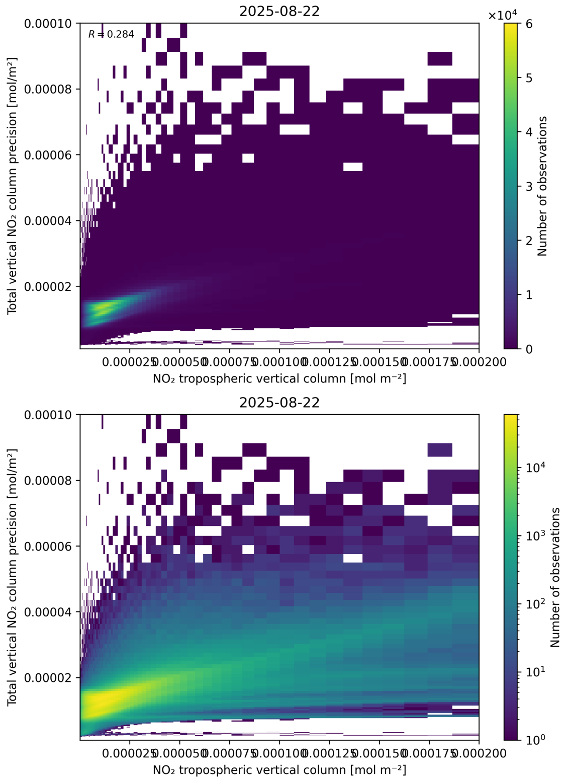
Figure 129: Scatter density plot of “NO 2 tropospheric vertical column” against “Total vertical NO 2 column precision” for 2025-08-21 to 2025-08-23.
