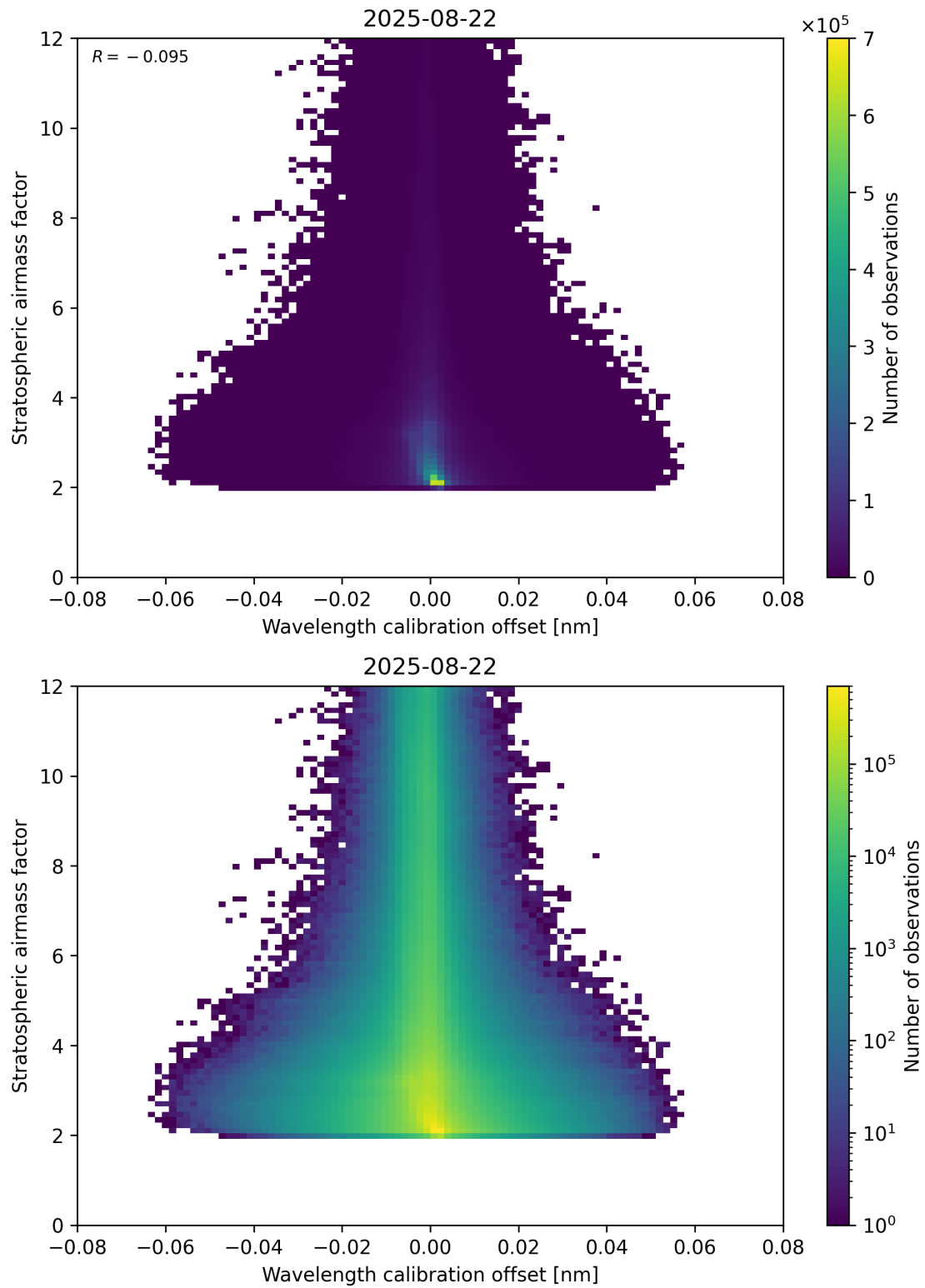
Figure 174: Scatter density plot of “Wavelength calibration offset” against “Stratospheric airmass factor” for 2025-08-21 to 2025-08-23.
