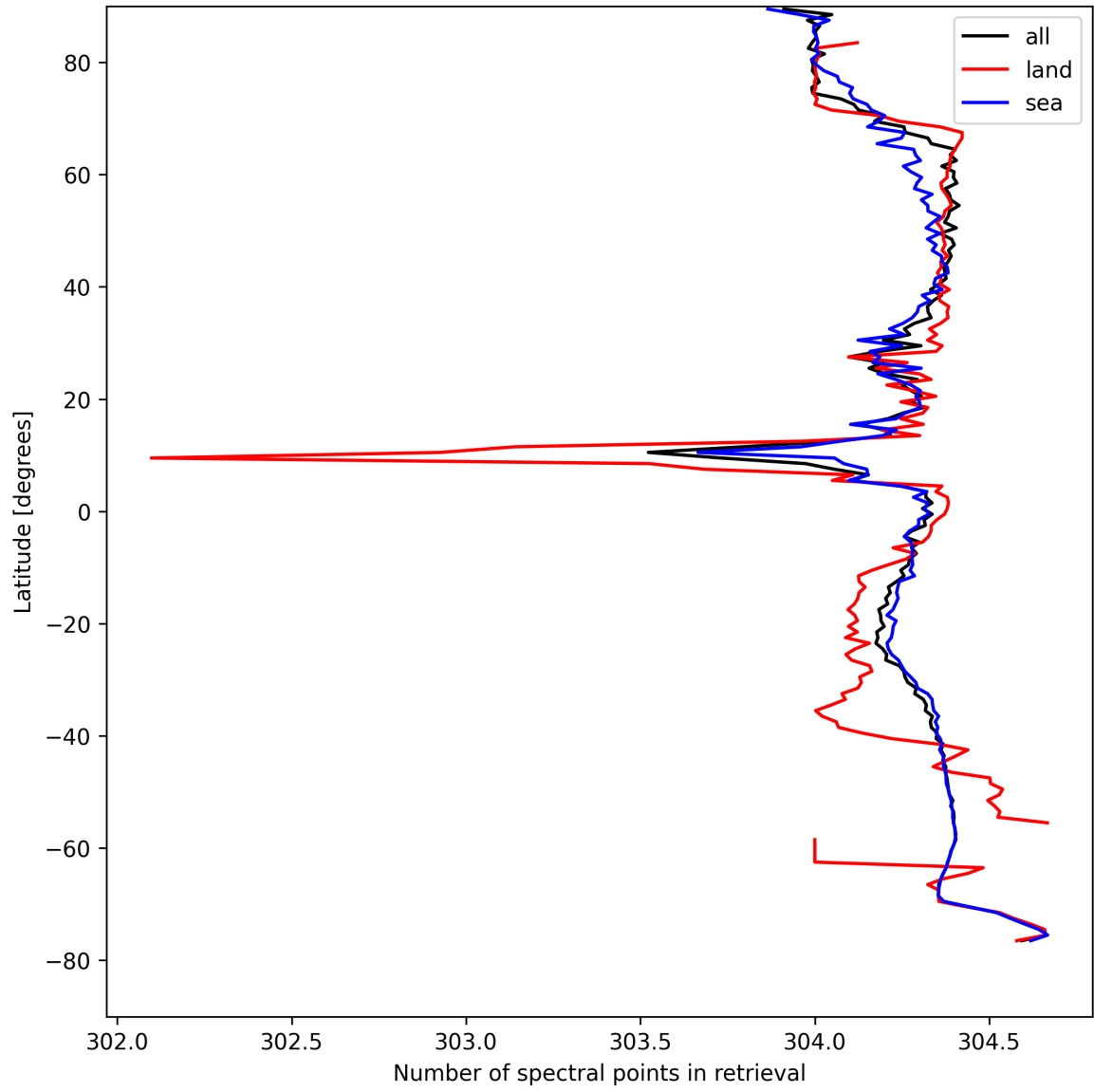
Figure 16: Zonal average of “Number of spectral points in retrieval” for 2025-08-21 to 2025-08-23.
