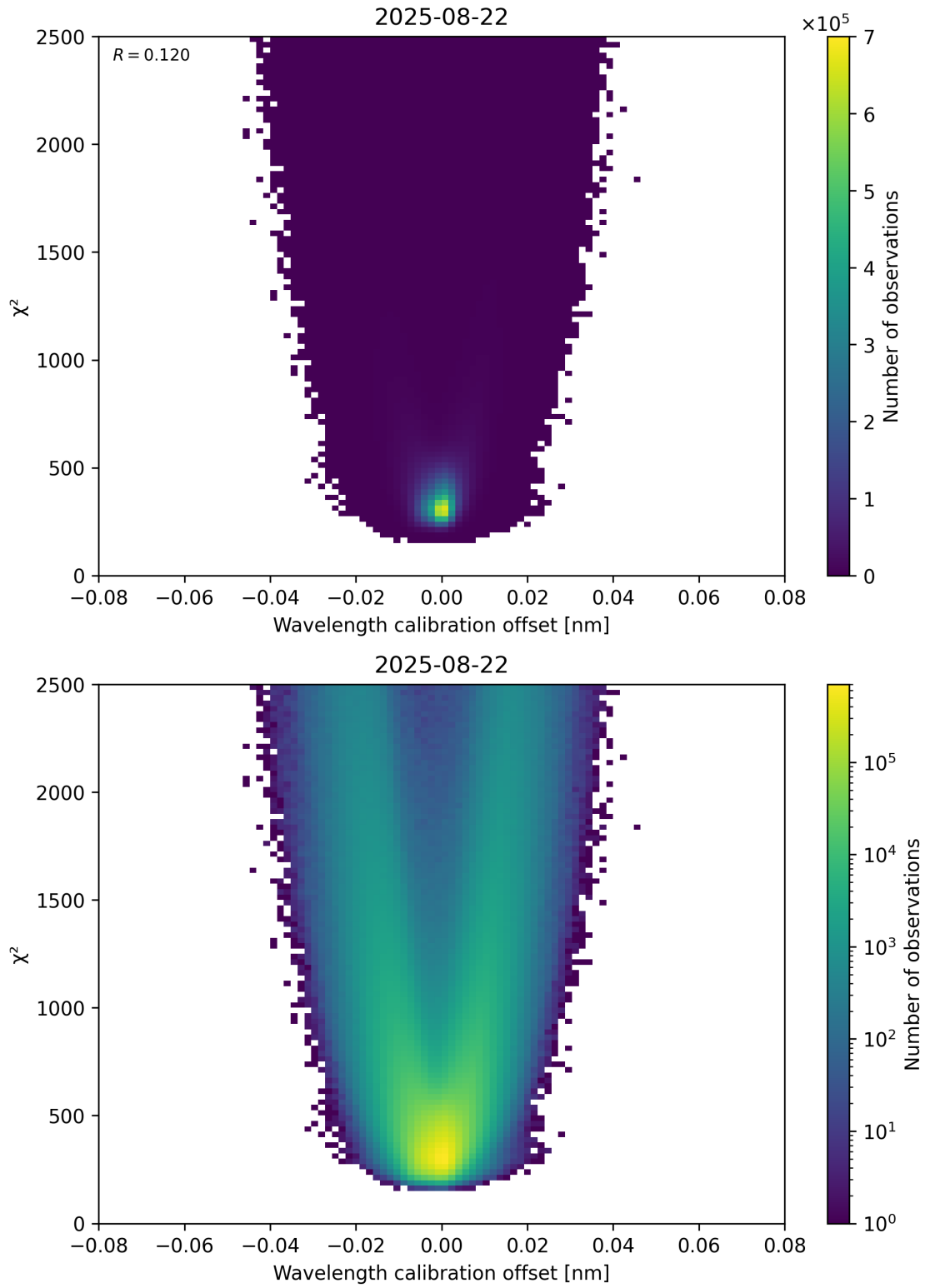
Figure 175: Scatter density plot of “Wavelength calibration offset” against “ \chi^2 ” for 2025-08-21 to 2025-08-23.
