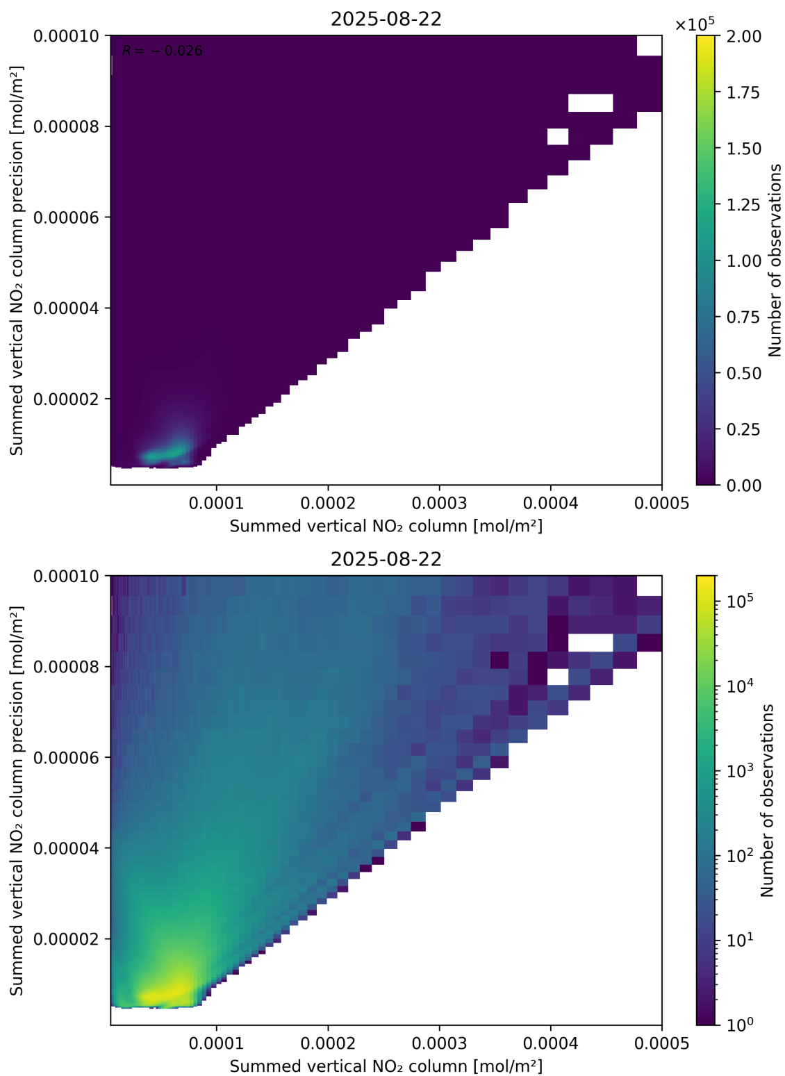
Figure 105: Scatter density plot of “Summed vertical NO 2 column” against “Summed vertical NO 2 column precision” for 2025-08-21 to 2025-08-23.
