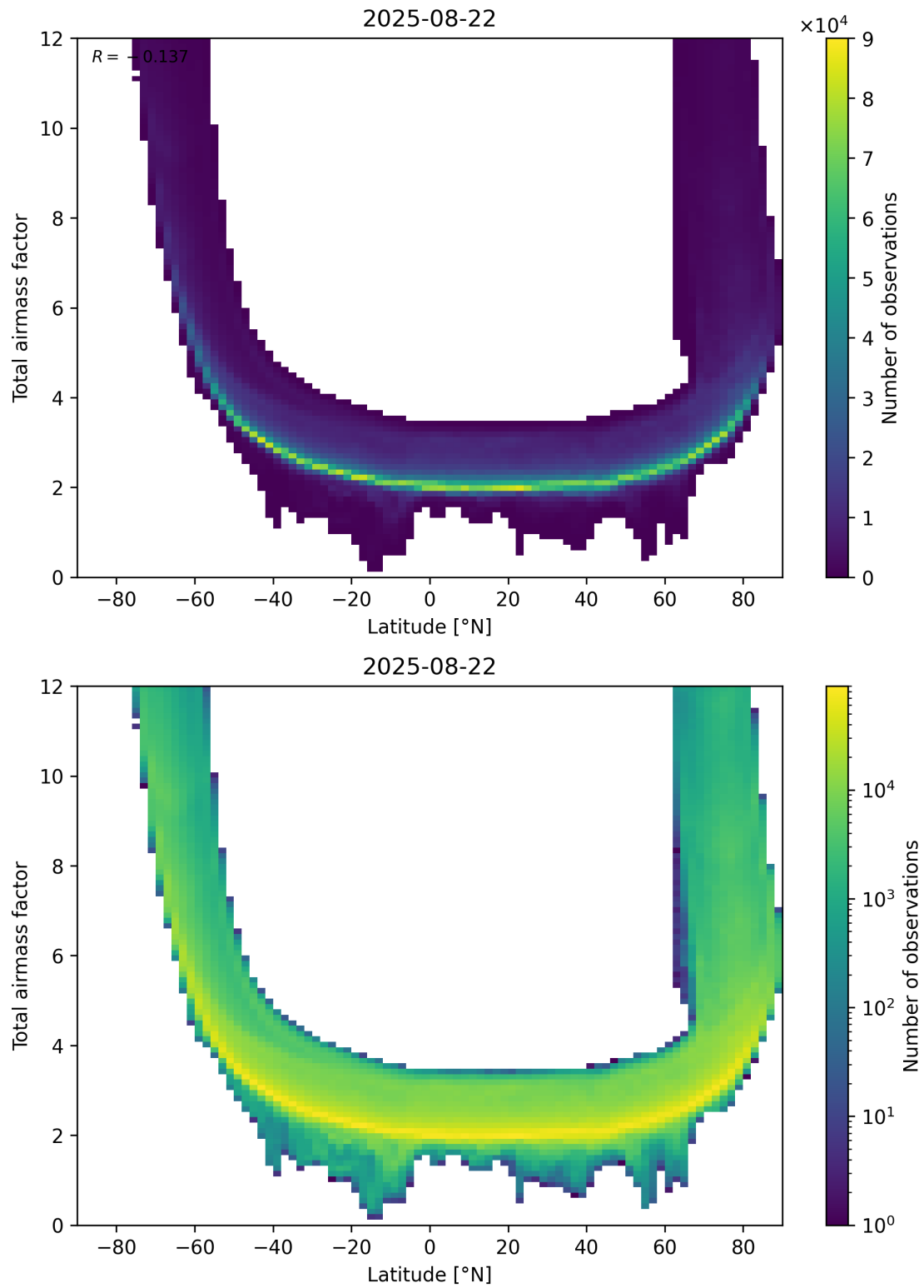
Figure 84: Scatter density plot of “Latitude” against “Total airmass factor” for 2025-08-21 to 2025-08-23.
