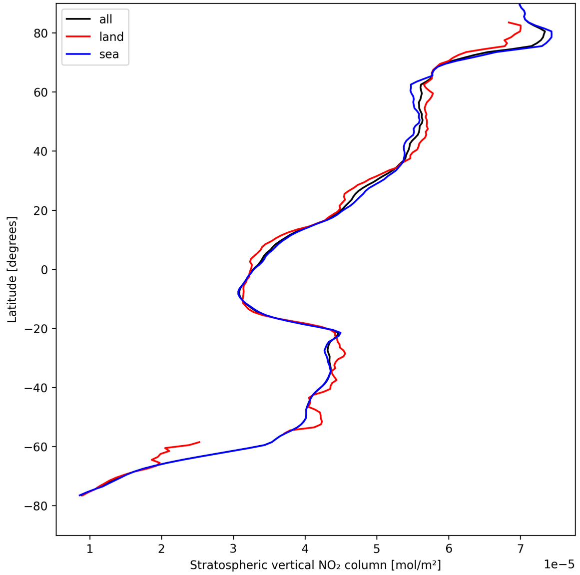
Figure 19: Zonal average of “Stratospheric vertical NO 2 column” for 2025-08-21 to 2025-08-23.
