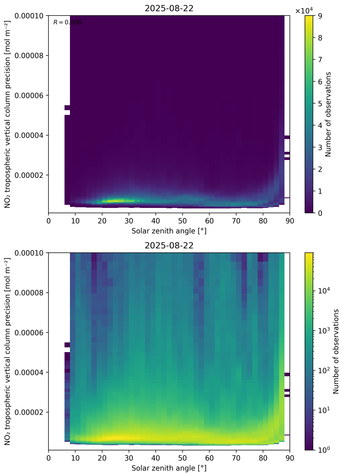
Figure 156: Scatter density plot of “Solar zenith angle” against “NO 2 tropospheric vertical column precision” for 2025-08-21 to 2025-08-23.
