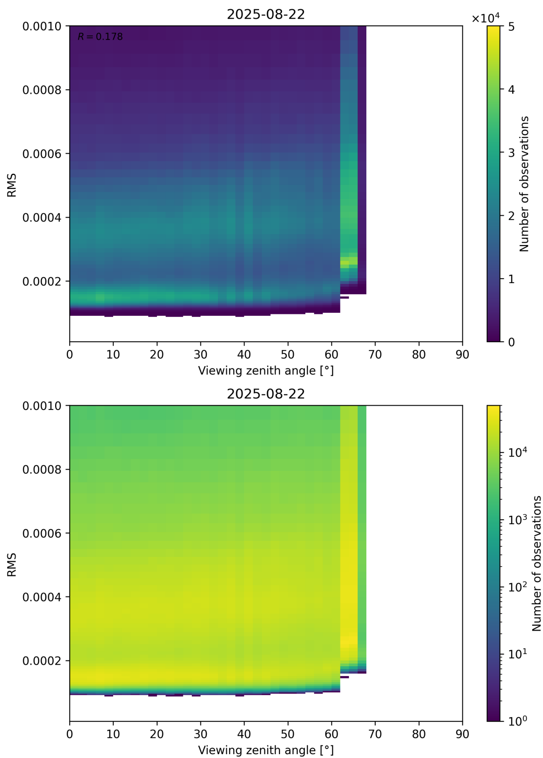
Figure 171: Scatter density plot of “Viewing zenith angle” against “RMS” for 2025-08-21 to 2025-08-23.
