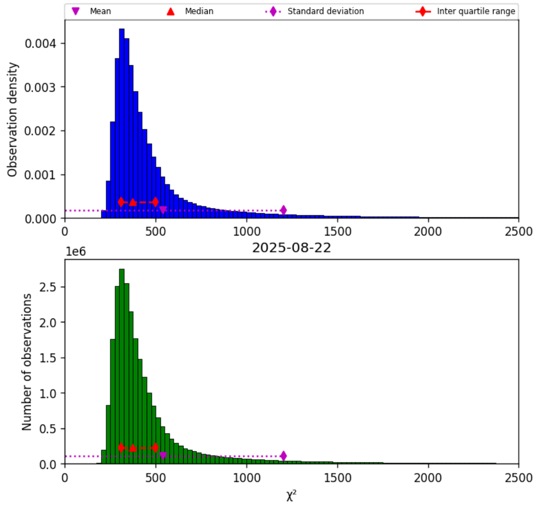
Figure 42: Histogram of " \chi^2 " for 2025-08-21 to 2025-08-23
