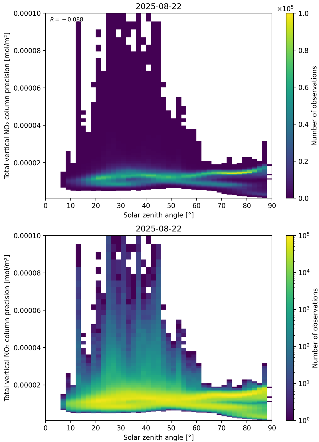
Figure 154: Scatter density plot of “Solar zenith angle” against “Total vertical NO 2 column precision” for 2025-08-21 to 2025-08-23.
