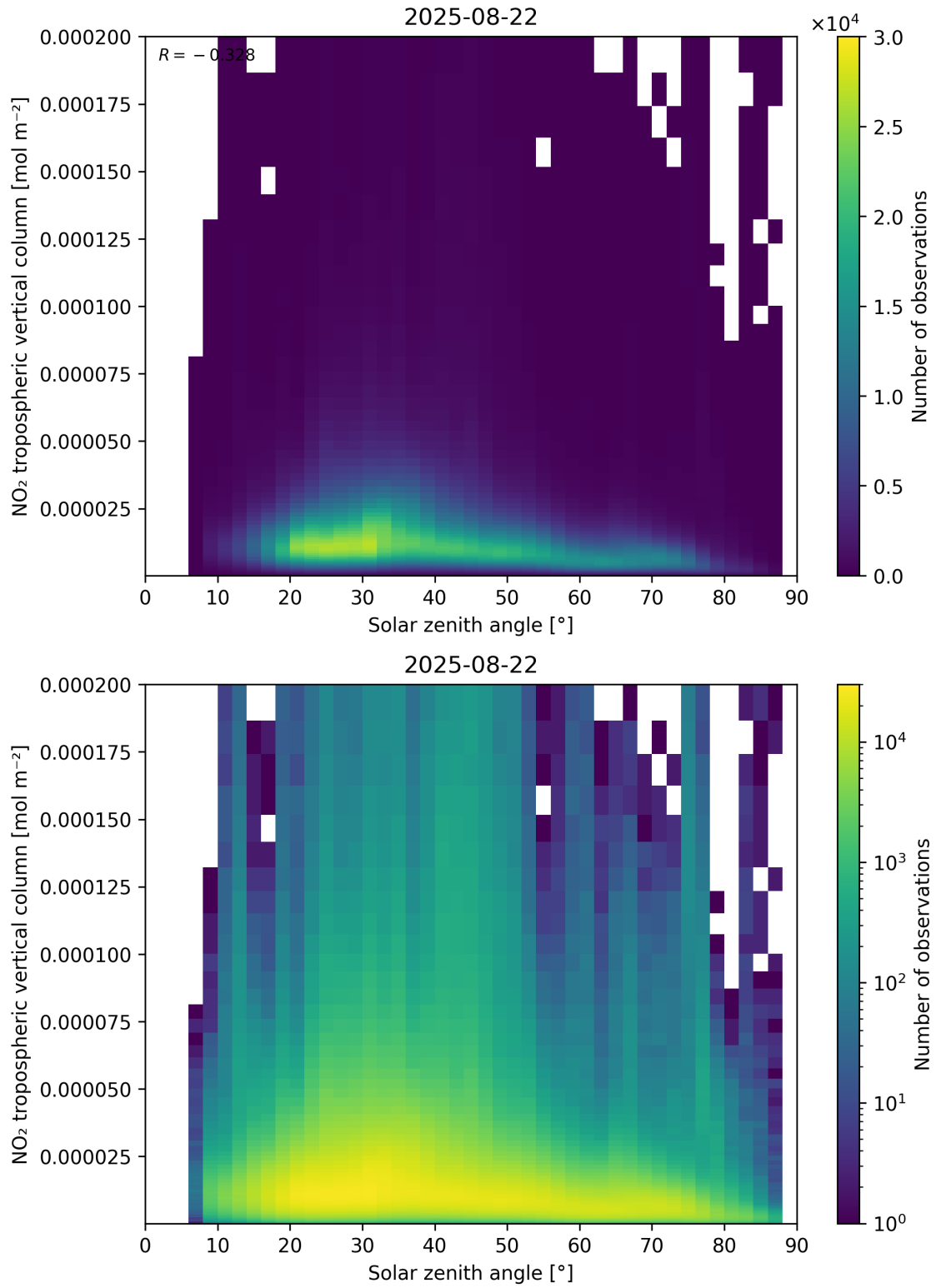
Figure 155: Scatter density plot of “Solar zenith angle” against “NO 2 tropospheric vertical column” for 2025-08-21 to 2025-08-23.
