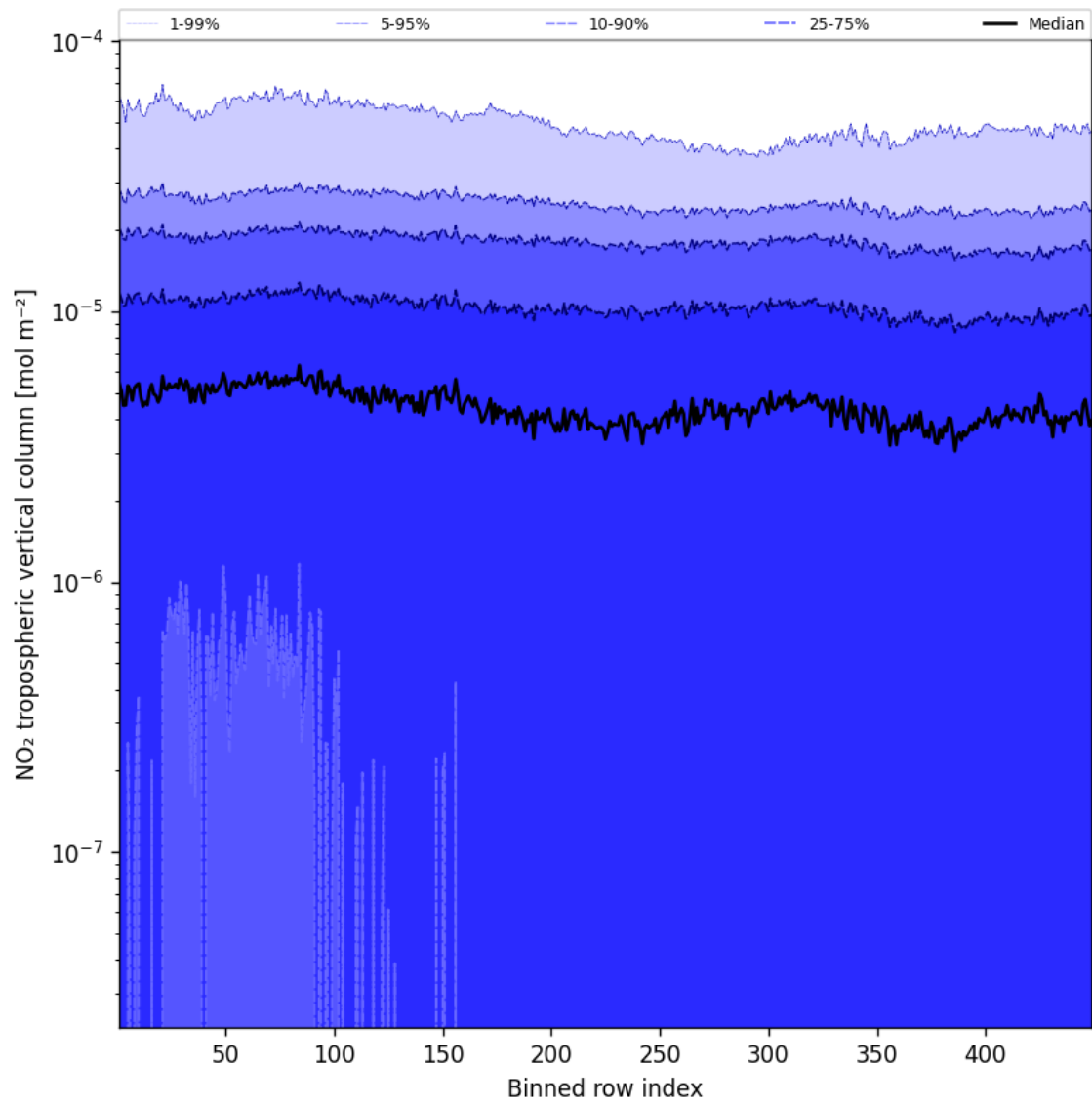
Figure 46: Along track statistics of “NO 2 tropospheric vertical column” for 2025-08-21 to 2025-08-23
