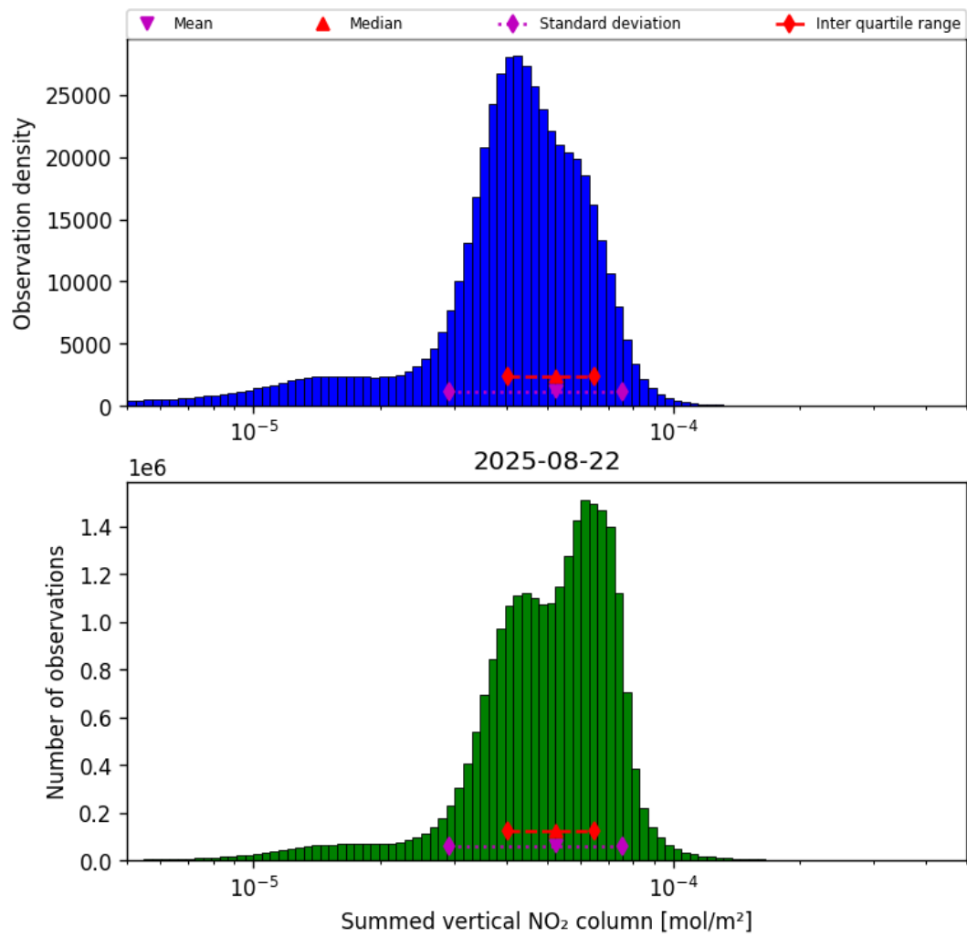
Figure 40: Histogram of “Summed vertical NO 2 column” for 2025-08-21 to 2025-08-23
