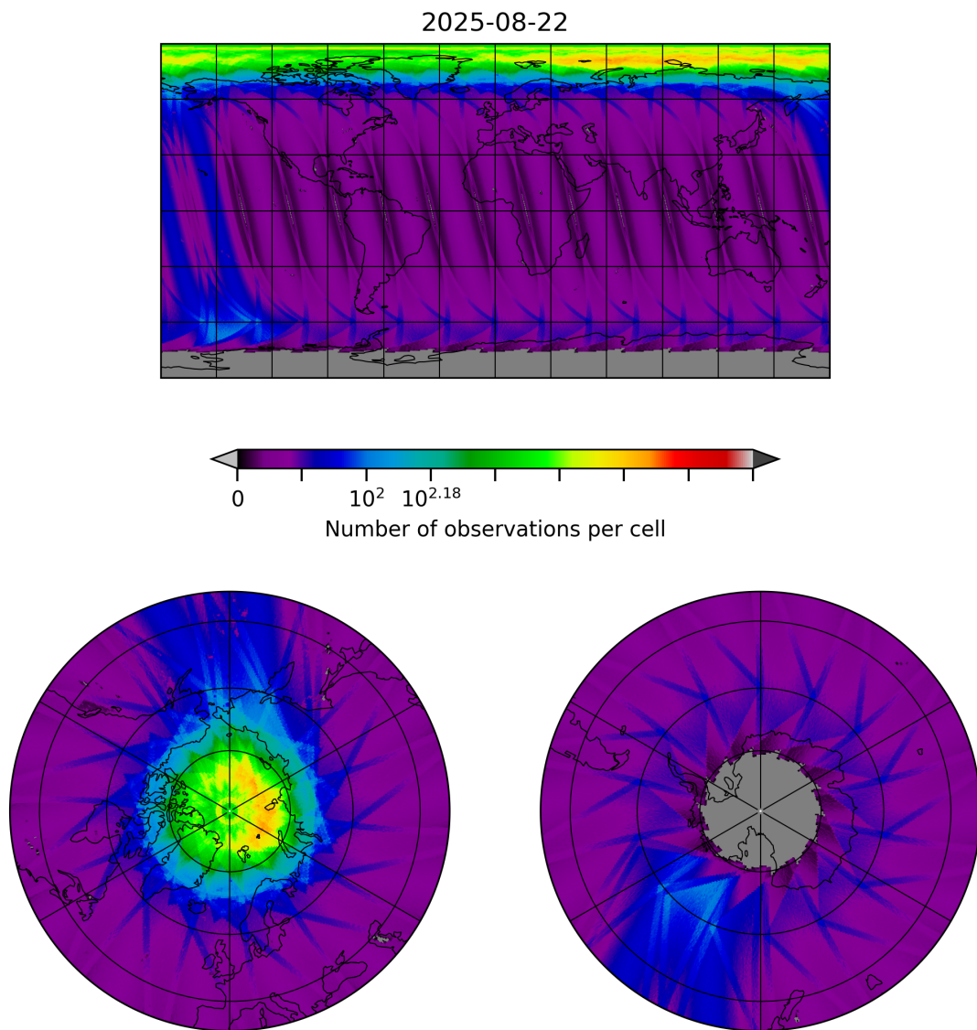
Figure 10: Map of the number of observations for 2025-08-21 to 2025-08-23
