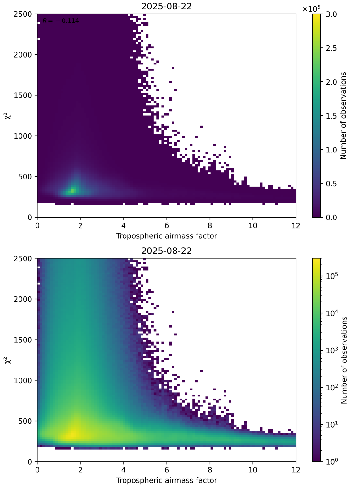
Figure 73: Scatter density plot of “Tropospheric airmass factor” against “ \chi^2 ” for 2025-08-21 to 2025-08-23.
