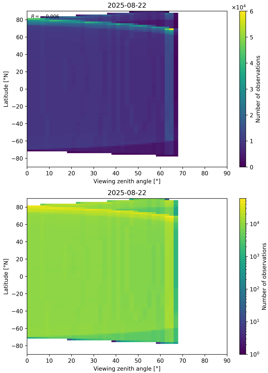
Figure 163: Scatter density plot of “Viewing zenith angle” against “Latitude” for 2025-08-21 to 2025-08-23.
