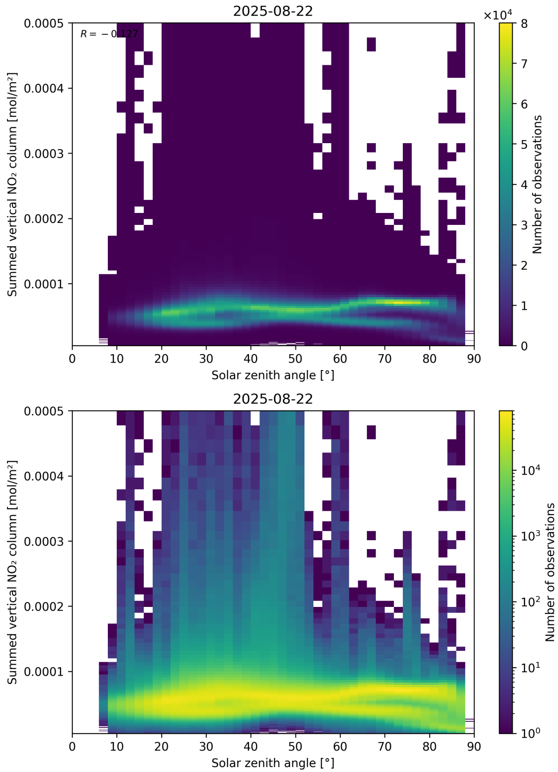
Figure 151: Scatter density plot of “Solar zenith angle” against “Summed vertical NO 2 column” for 2025-08-21 to 2025-08-23.
