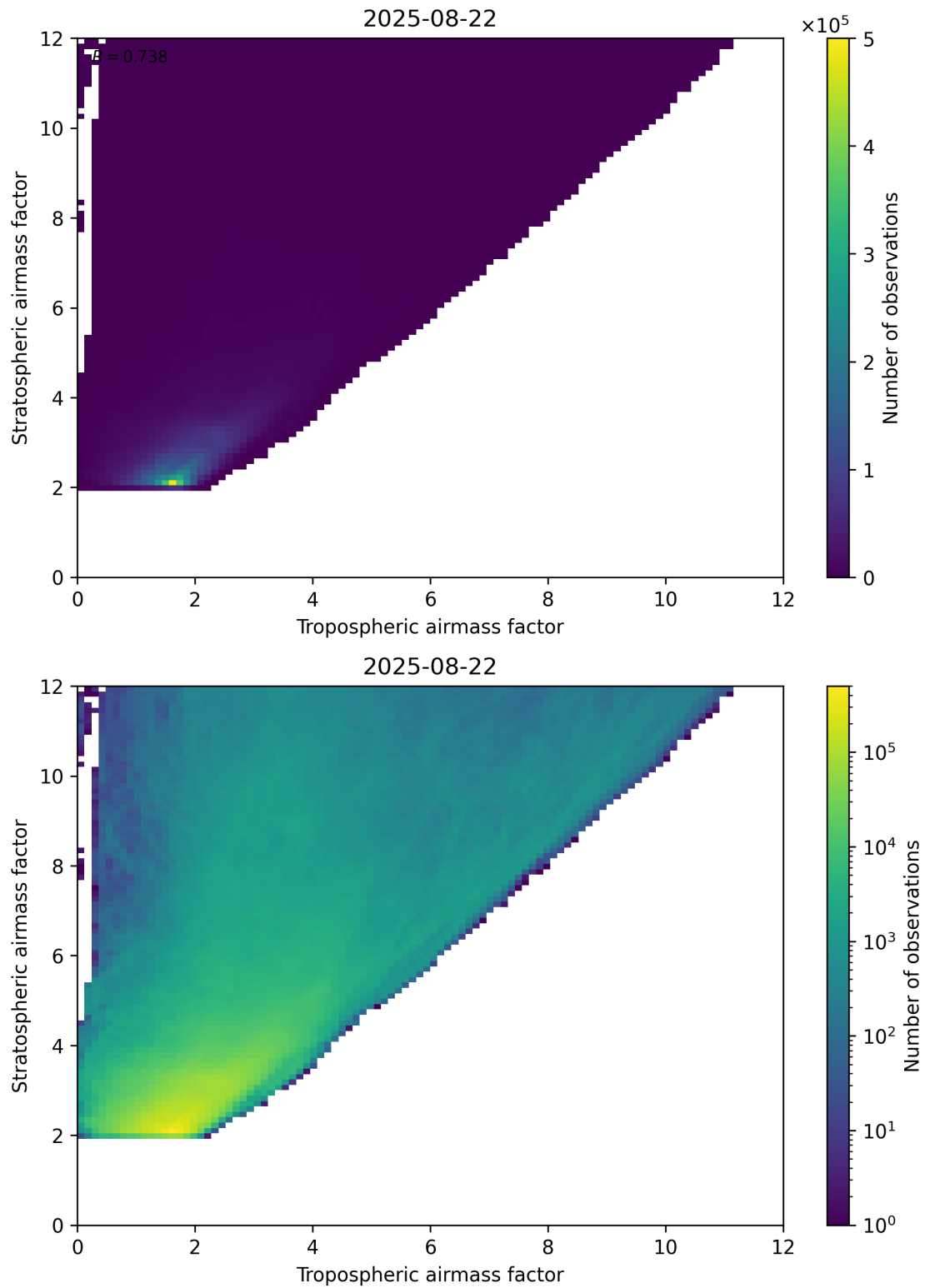
Figure 71: Scatter density plot of “Tropospheric airmass factor” against “Stratospheric airmass factor” for 2025-08-21 to 2025-08-23.
