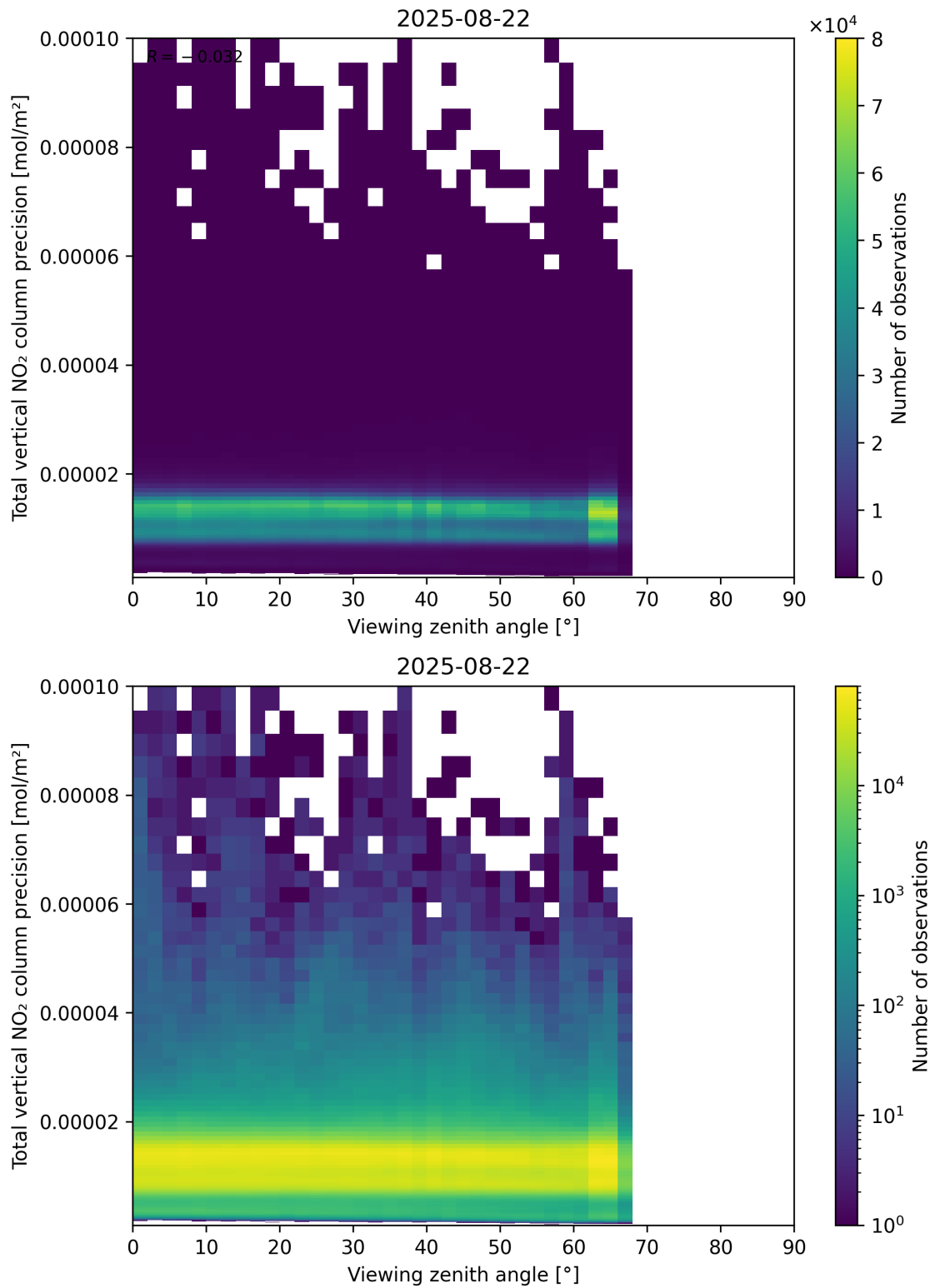
Figure 168: Scatter density plot of “Viewing zenith angle” against “Total vertical NO 2 column precision” for 2025-08-21 to 2025-08-23.
