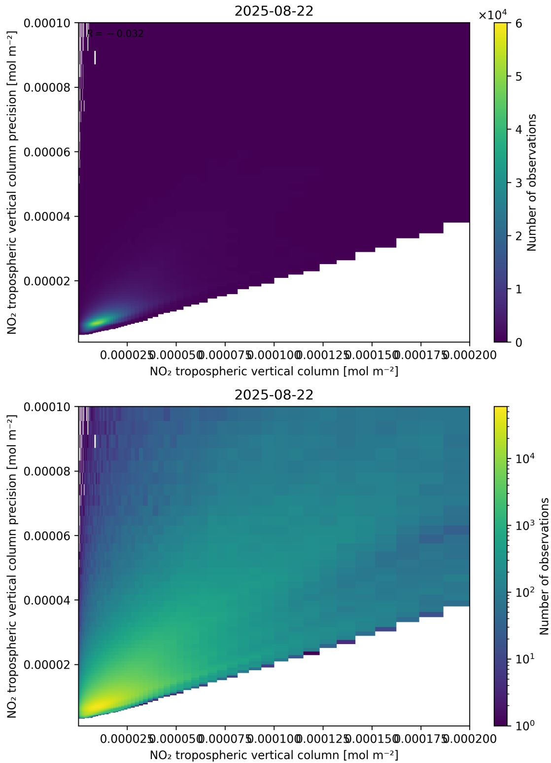
Figure 130: Scatter density plot of “NO 2 tropospheric vertical column” against “NO 2 tropospheric vertical column precision” for 2025-08-21 to 2025-08-23.
