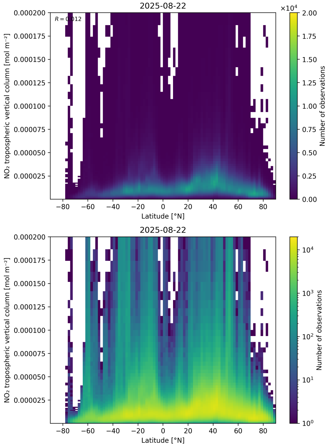
Figure 92: Scatter density plot of “Latitude” against “NO 2 tropospheric vertical column” for 2025-08-21 to 2025-08-23.
