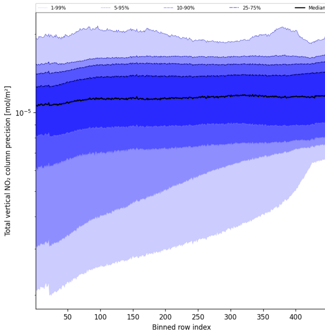
Figure 56: Along track statistics of “Total vertical NO 2 column precision” for 2025-08-21 to 2025-08-23
