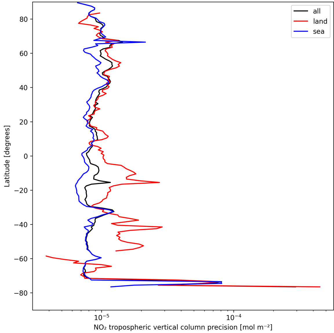
Figure 13: Zonal average of “NO 2 tropospheric vertical column precision” for 2025-08-21 to 2025-08-23.
