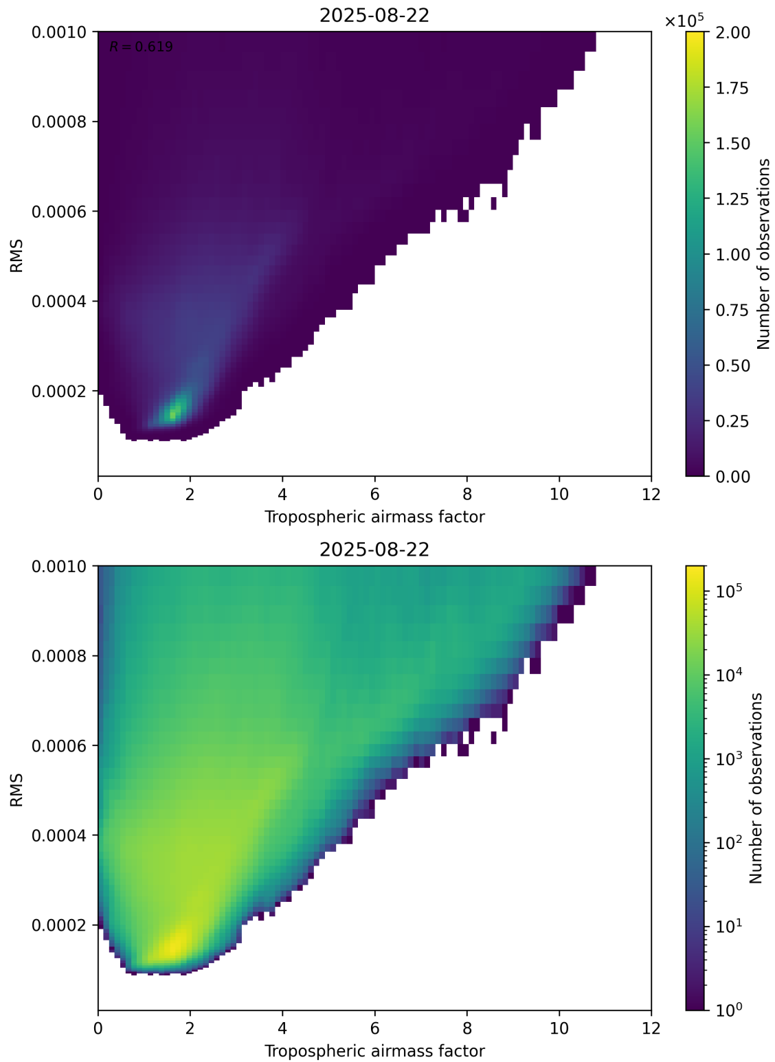
Figure 79: Scatter density plot of “Tropospheric airmass factor” against “RMS” for 2025-08-21 to 2025-08-23.
