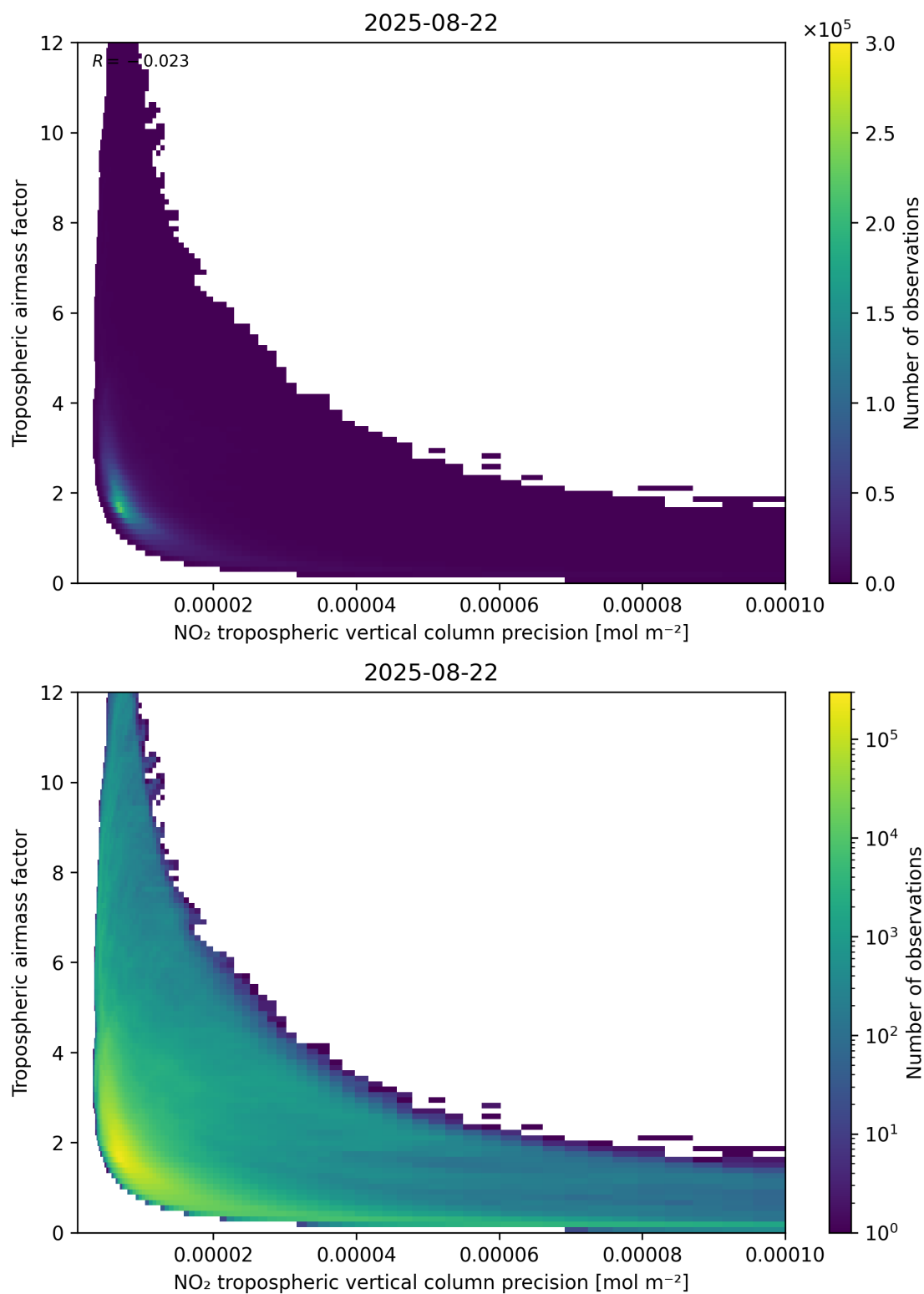
Figure 133: Scatter density plot of “NO 2 tropospheric vertical column precision” against “Tropospheric airmass factor” for 2025-08-21 to 2025-08-23.
