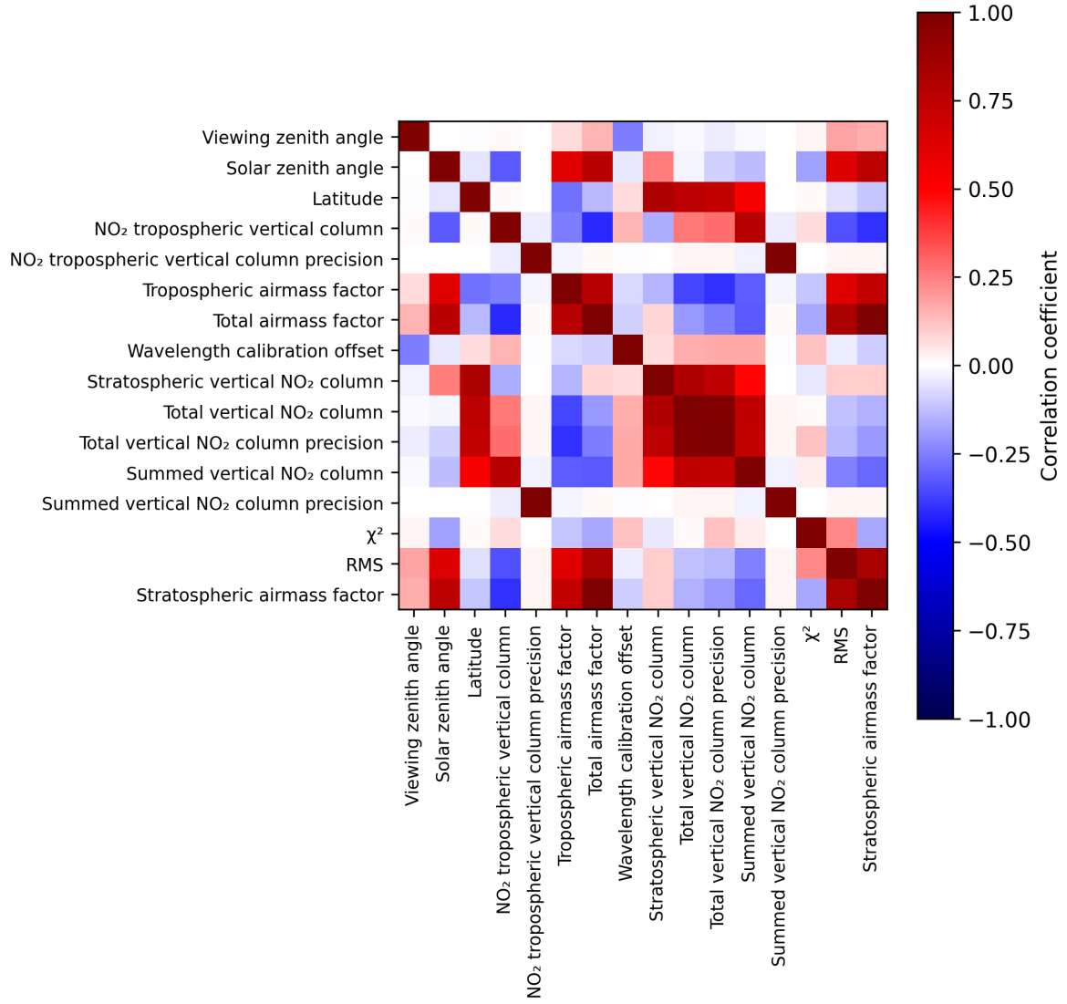
Figure 2: Map of correlation matrix for 2025-08-21 to 2025-08-23.
