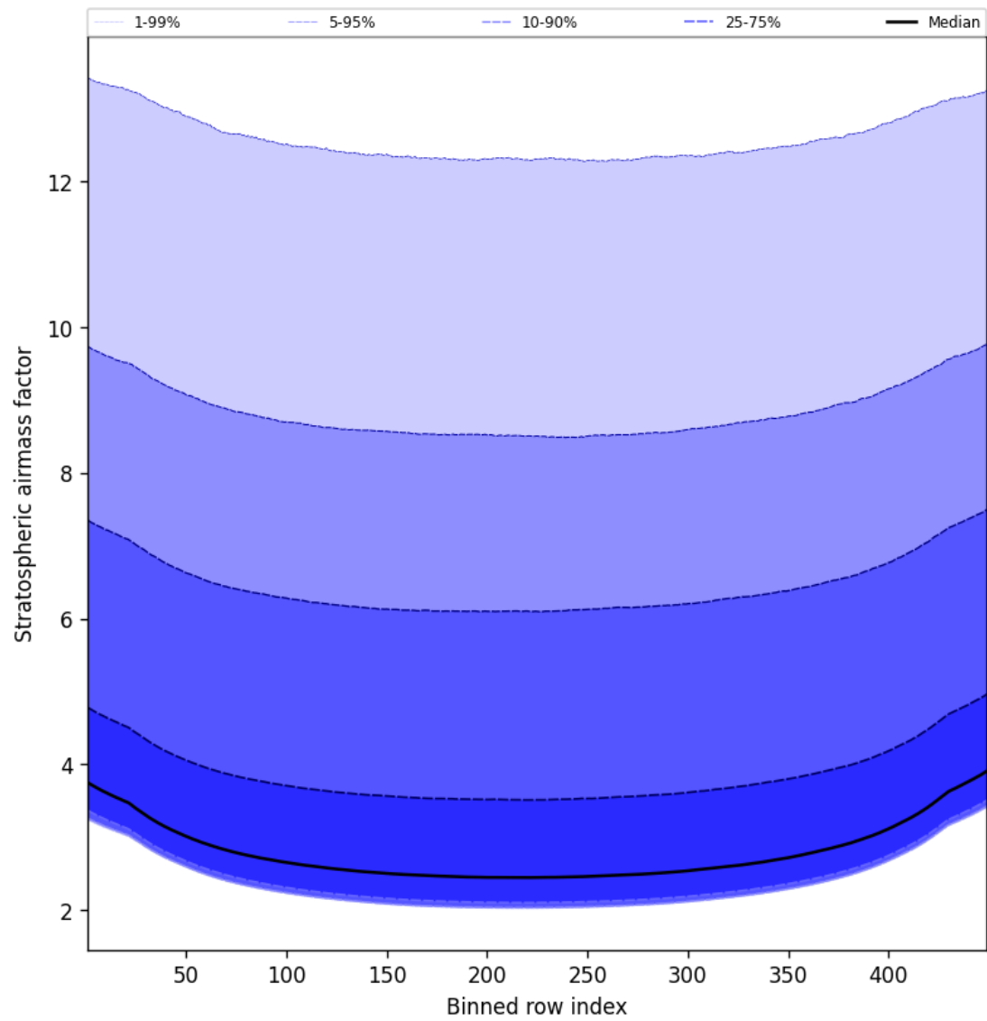
Figure 61: Along track statistics of “Stratospheric airmass factor” for 2025-08-21 to 2025-08-23
