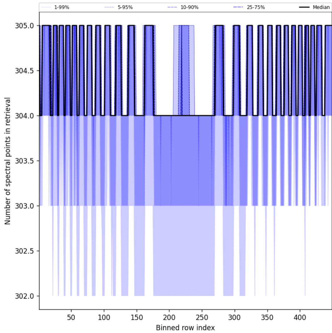
Figure 50: Along track statistics of “Number of spectral points in retrieval” for 2025-08-21 to 2025-08-23
