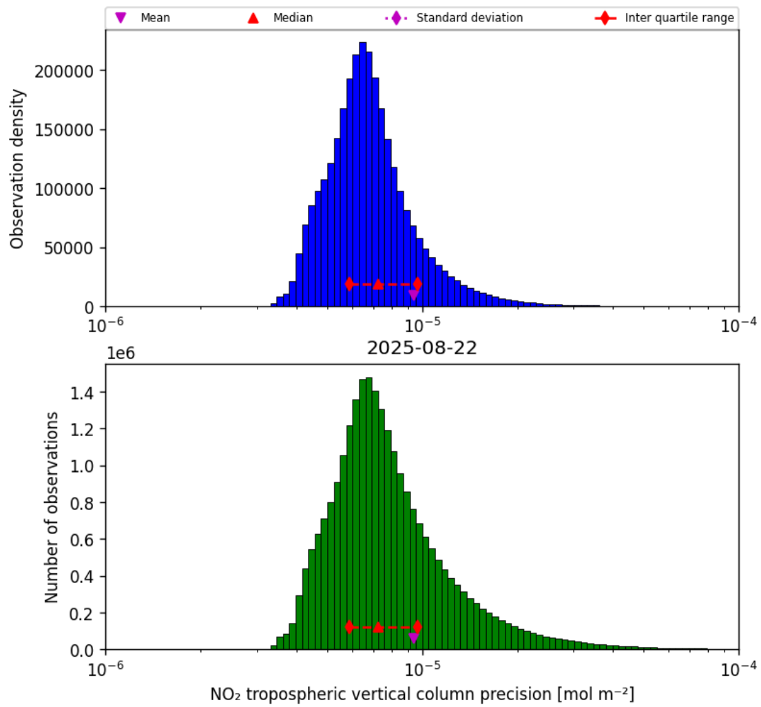
Figure 30: Histogram of "NO 2 tropospheric vertical column precision" for 2025-08-21 to 2025-08-23
