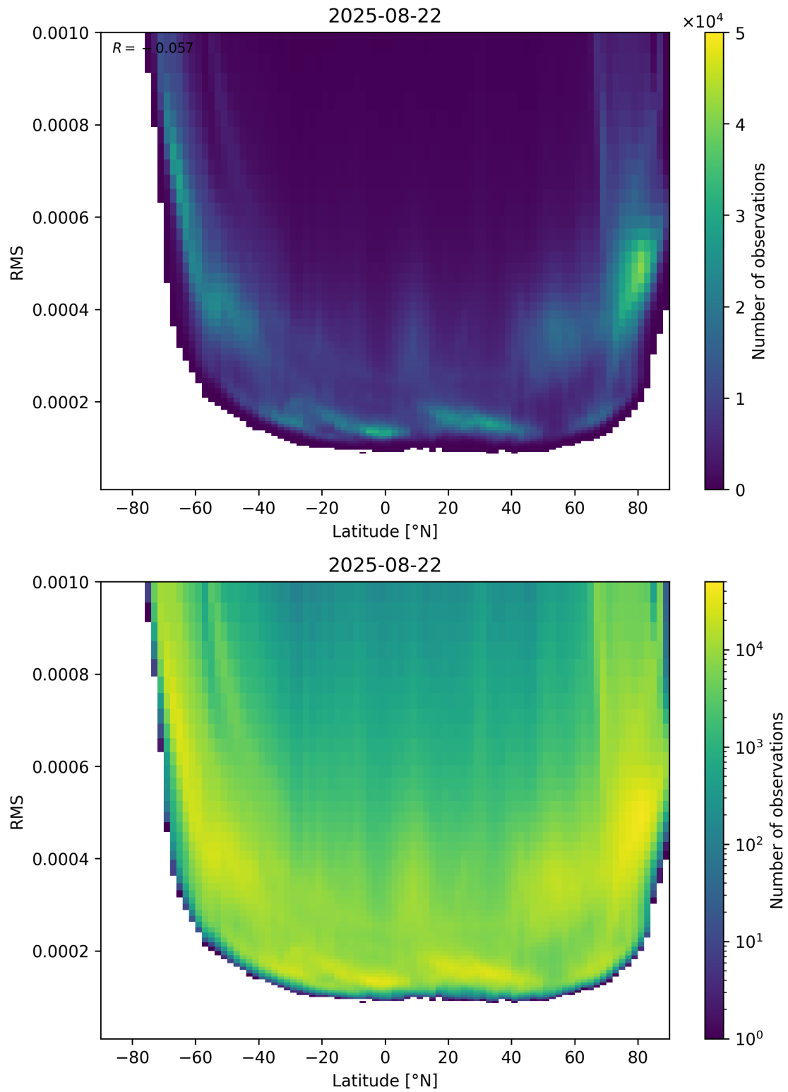
Figure 94: Scatter density plot of “Latitude” against “RMS” for 2025-08-21 to 2025-08-23.
