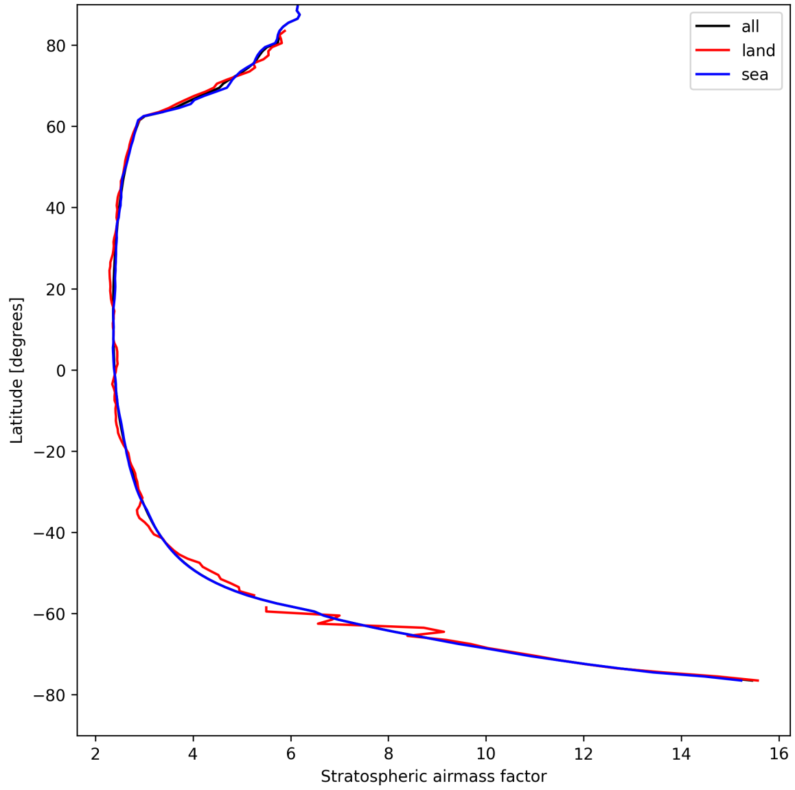
Figure 27: Zonal average of “Stratospheric airmass factor” for 2025-08-21 to 2025-08-23.
