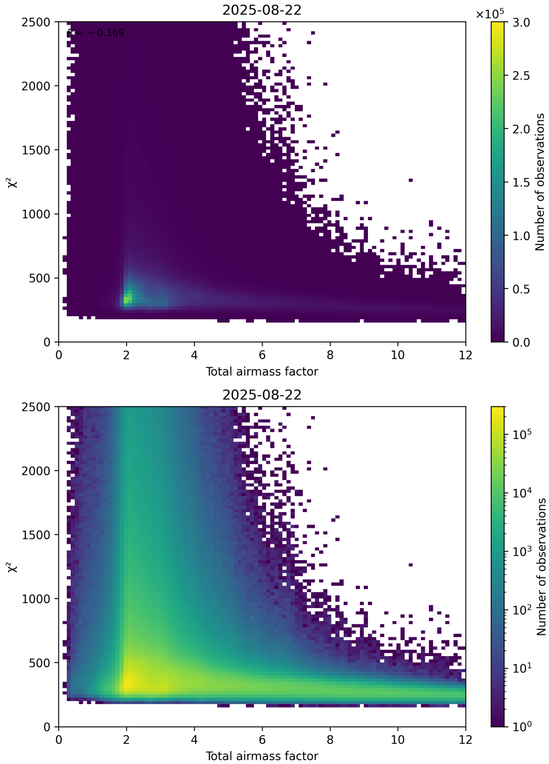
Figure 63: Scatter density plot of “Total airmass factor” against “ \chi^2 ” for 2025-08-21 to 2025-08-23.
