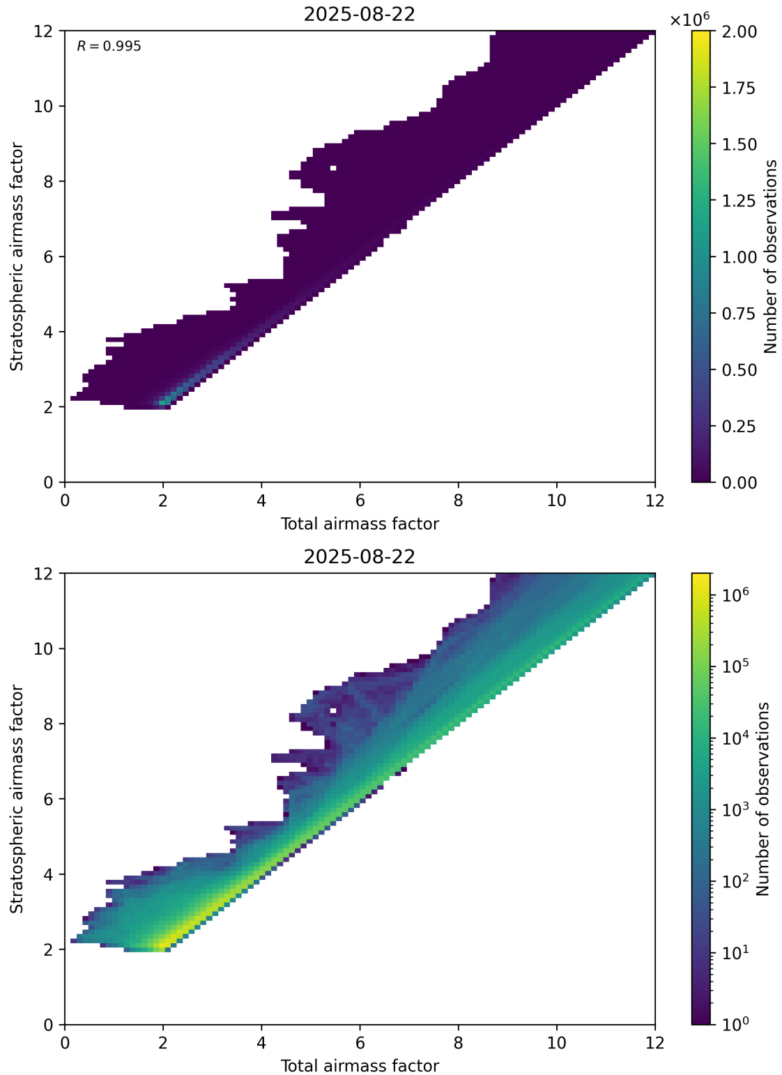
Figure 62: Scatter density plot of “Total air mass factor” against “Stratospheric air mass factor” for 2025-08-21 to 2025-08-23.
