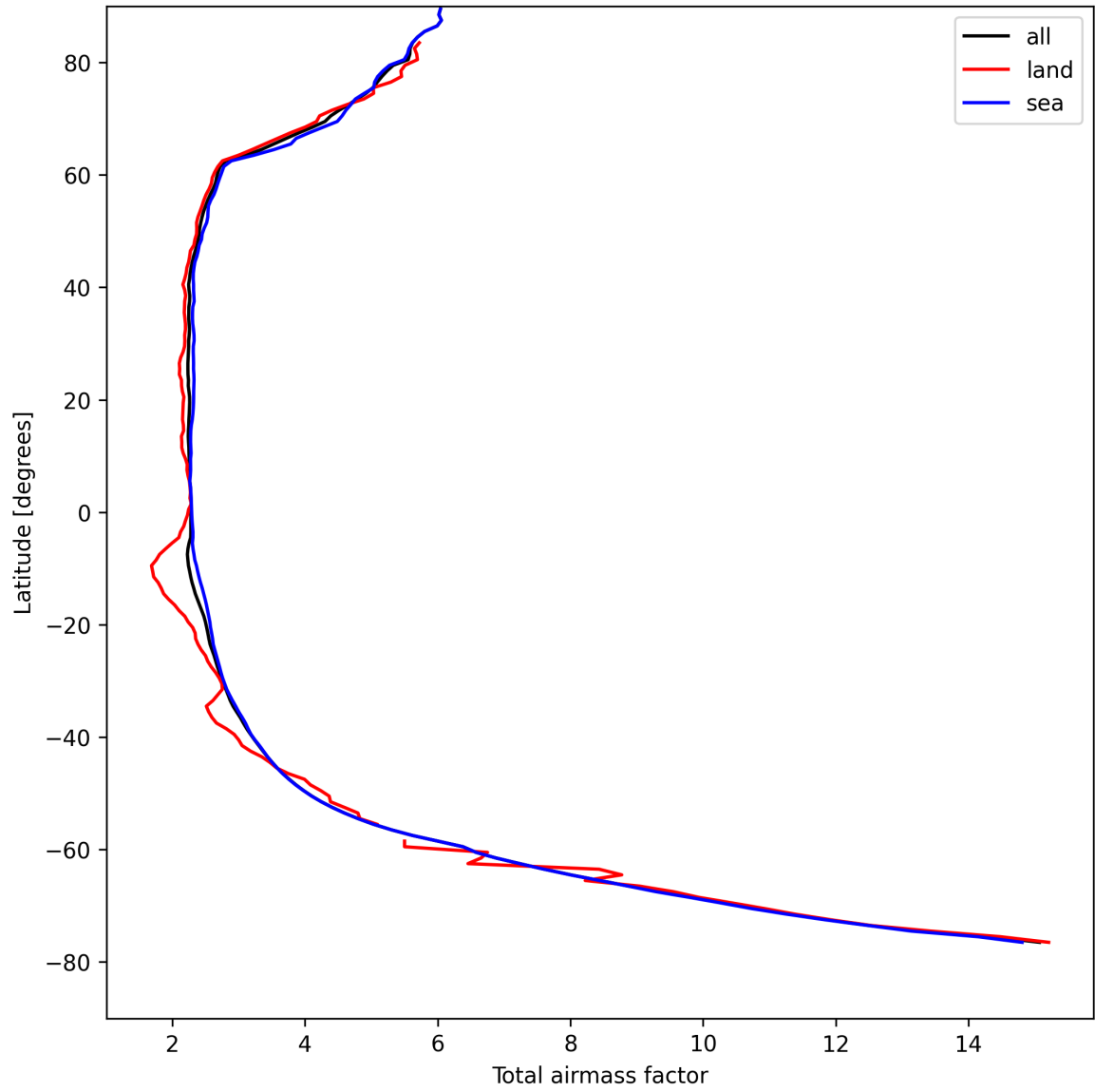
Figure 15: Zonal average of “Total airmass factor” for 2025-08-21 to 2025-08-23.
