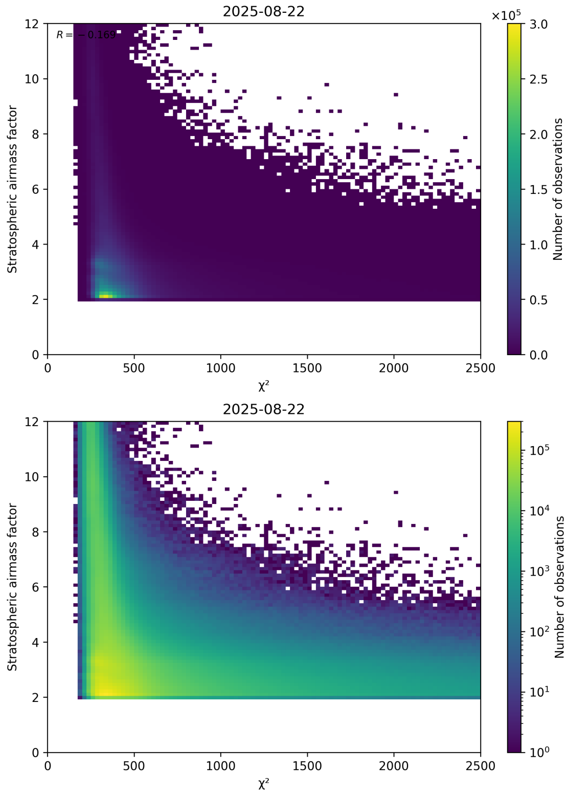
Figure 81: Scatter density plot of “ \chi^2 ” against “Stratospheric airmass factor” for 2025-08-21 to 2025-08-23.
