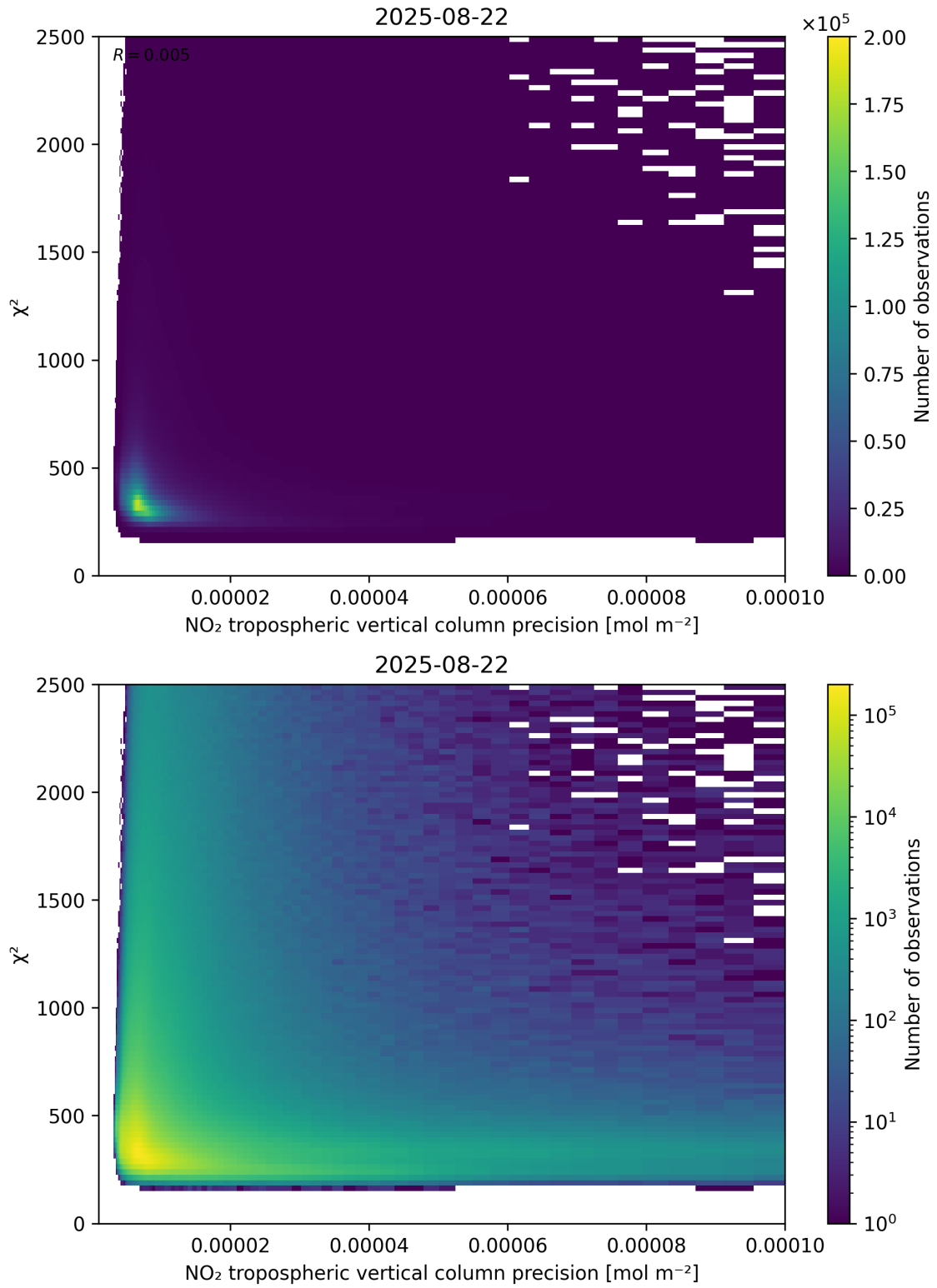
Figure 134: Scatter density plot of “NO 2 tropospheric vertical column precision” against “ \chi^2 ” for 2025-08-21 to 2025-08-23.
