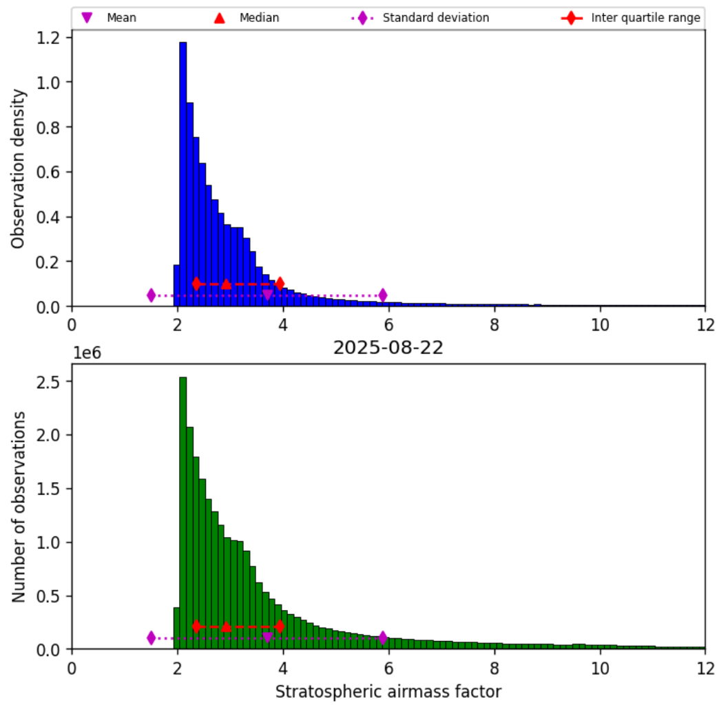
Figure 44: Histogram of “Stratospheric airmass factor” for 2025-08-21 to 2025-08-23
