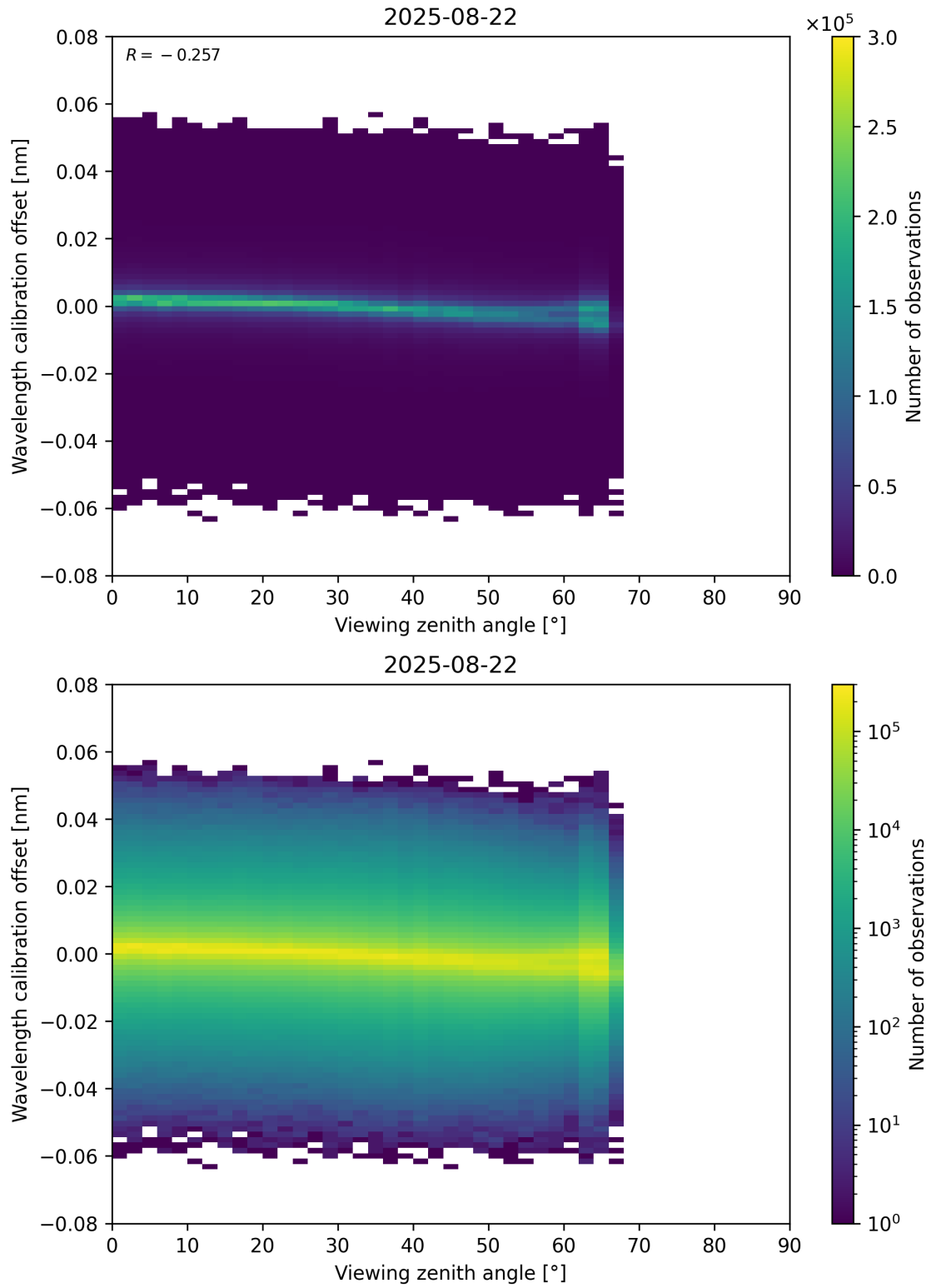
Figure 173: Scatter density plot of “Viewing zenith angle” against “Wavelength calibration offset” for 2025-08-21 to 2025-08-23.
