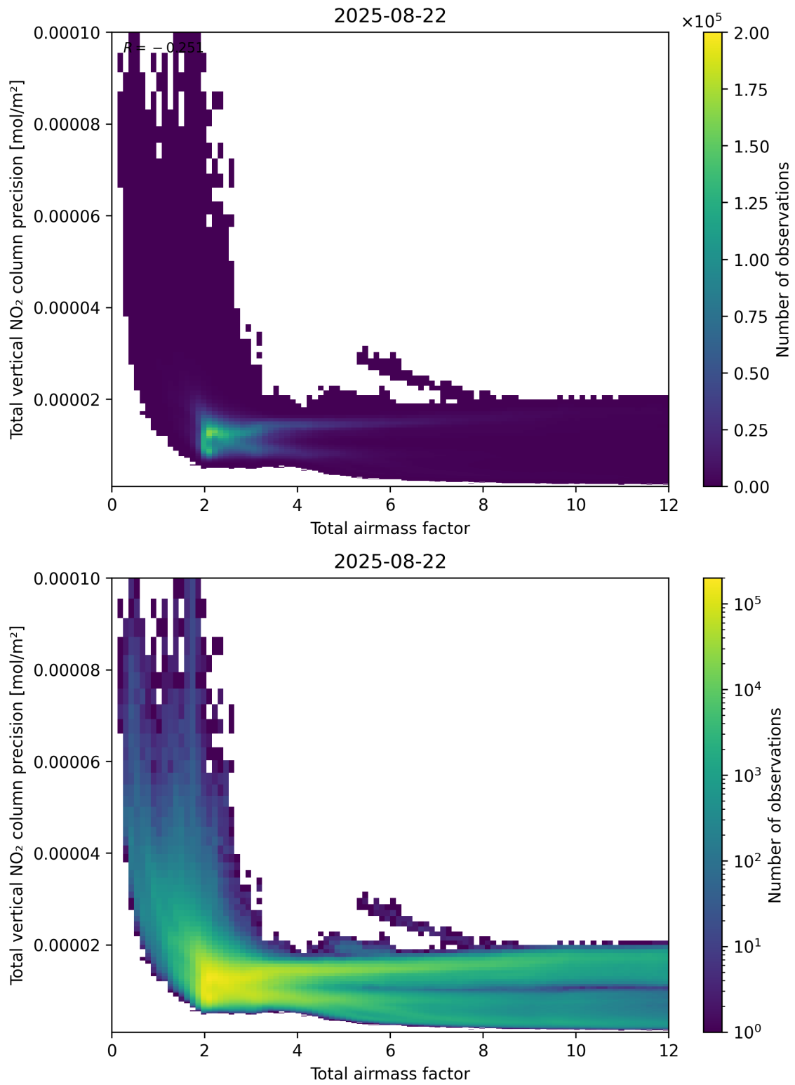
Figure 68: Scatter density plot of “Total airmass factor” against “Total vertical NO 2 column precision” for 2025-08-21 to 2025-08-23.
