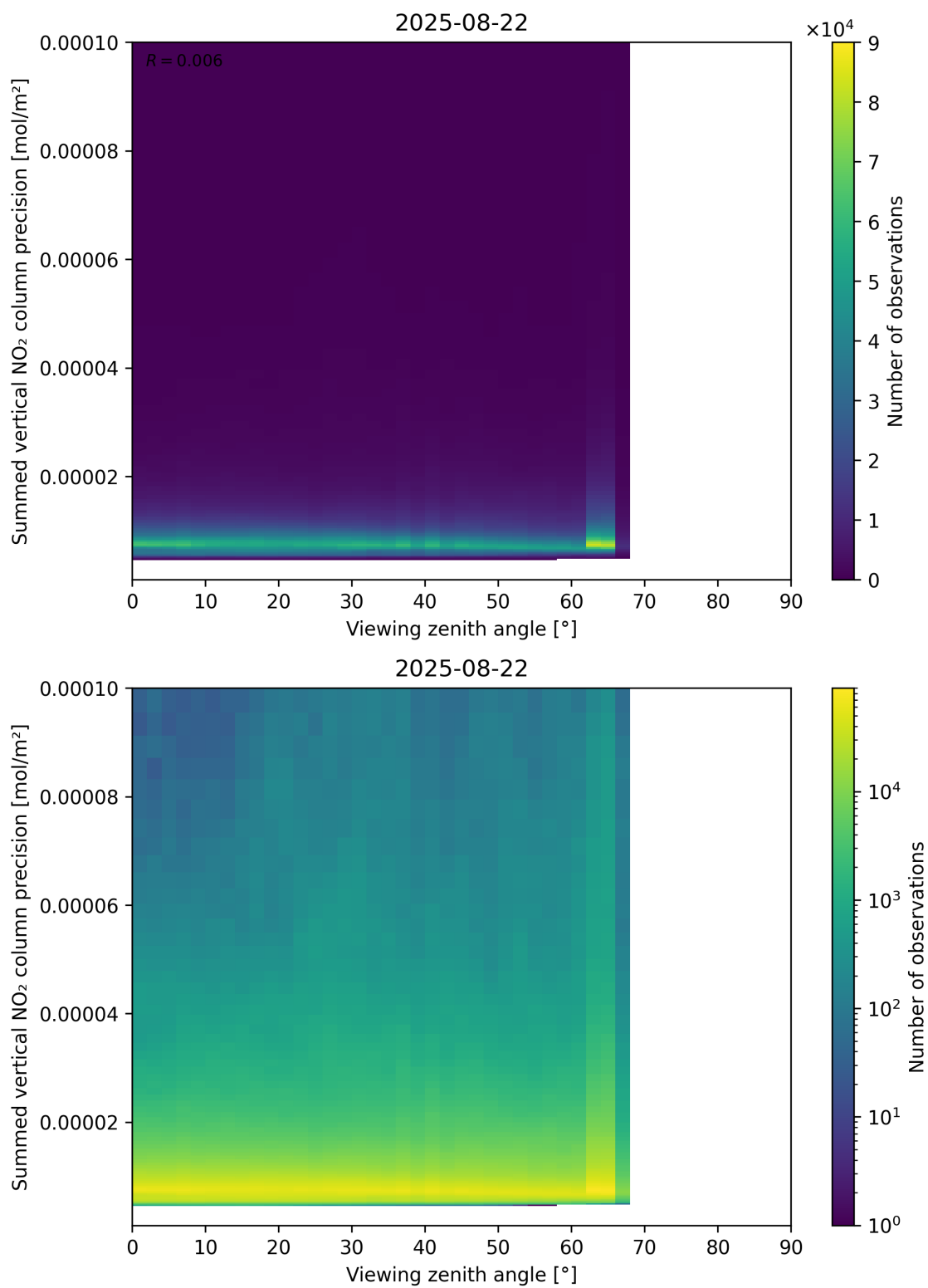
Figure 166: Scatter density plot of “Viewing zenith angle” against “Summed vertical NO 2 column precision” for 2025-08-21 to 2025-08-23.
