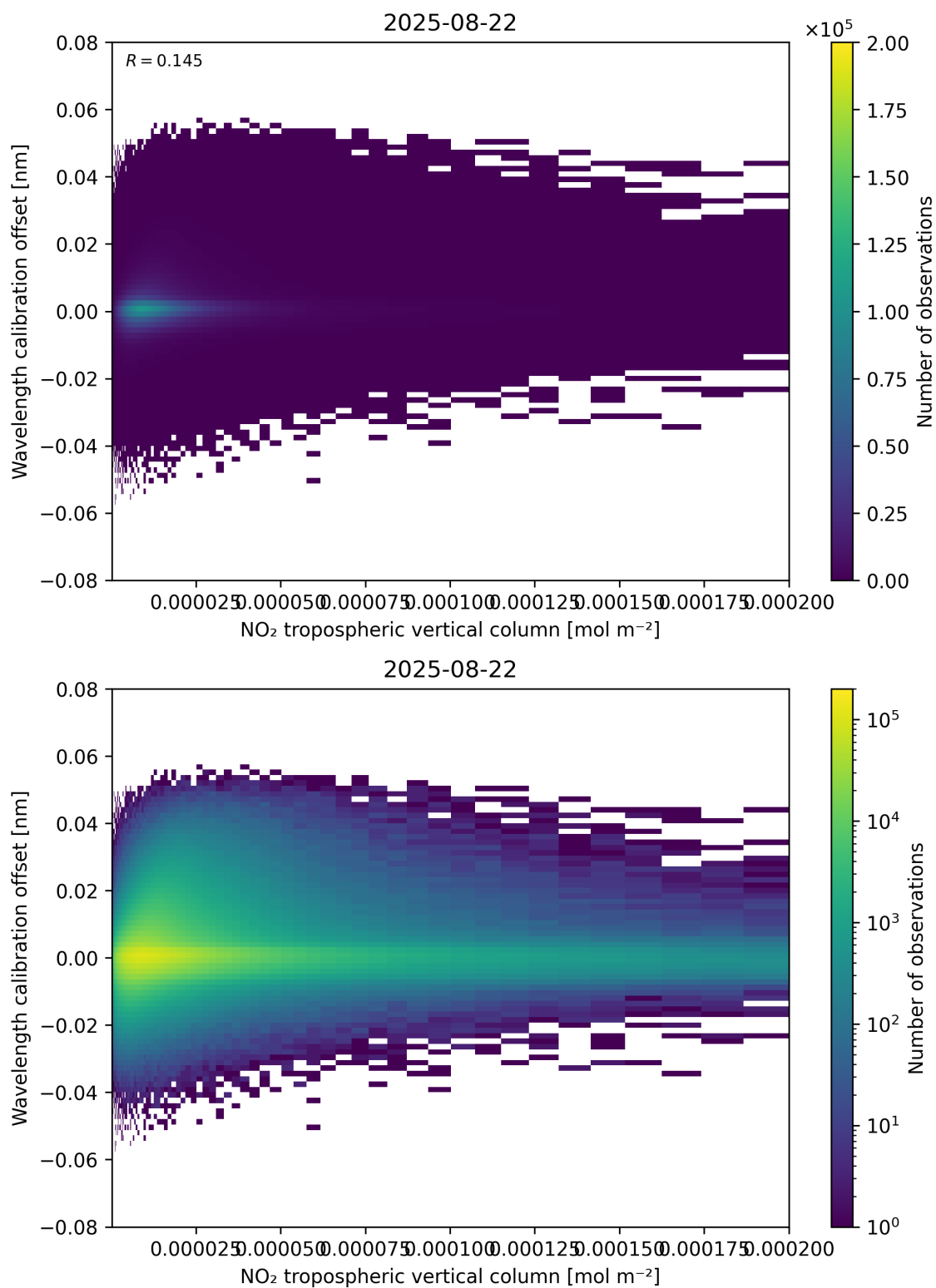
Figure 143: Scatter density plot of “NO 2 tropospheric vertical column” against “Wavelength calibration offset” for 2025-08-21 to 2025-08-23.
