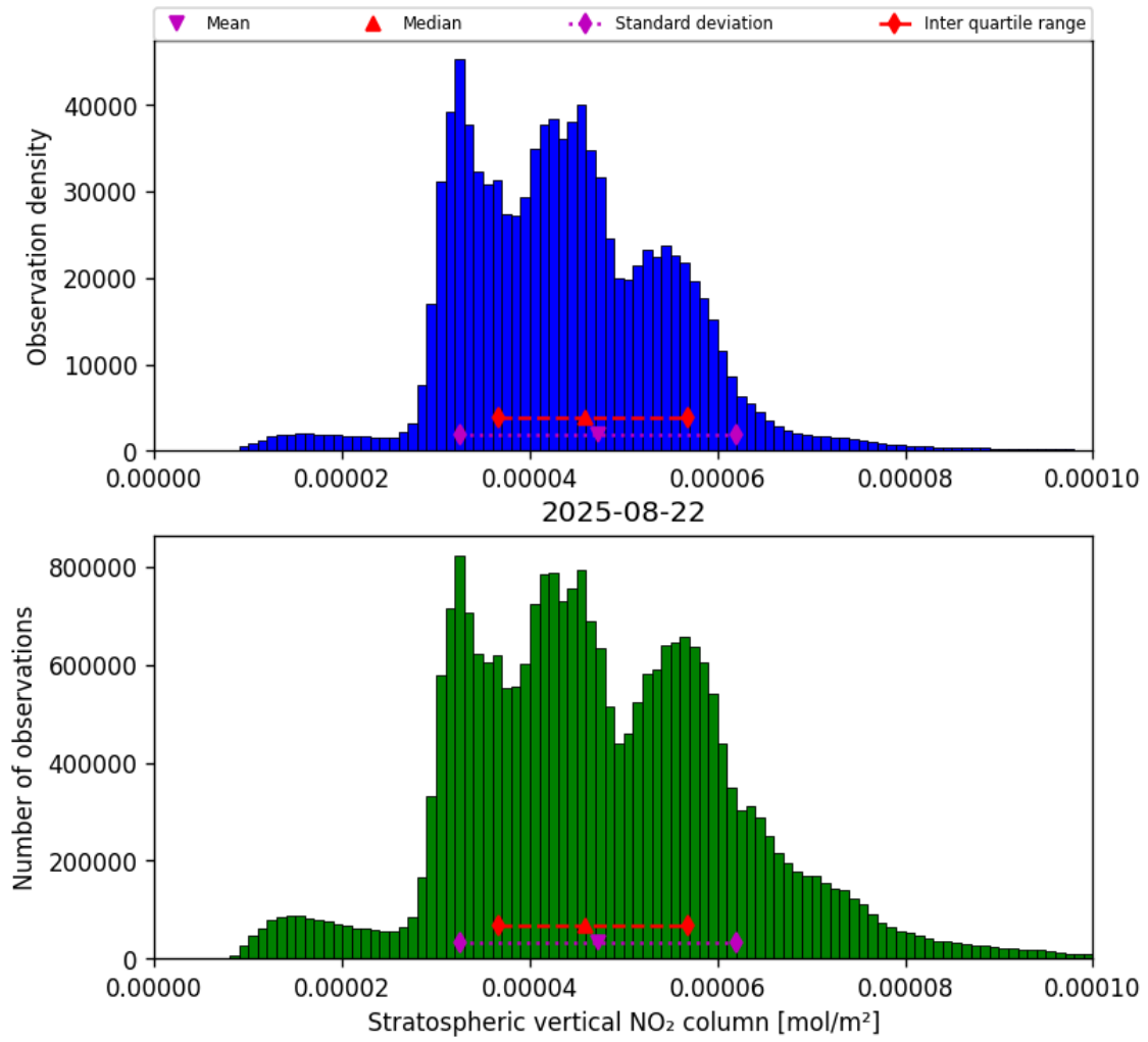
Figure 36: Histogram of “Stratospheric vertical NO 2 column” for 2025-08-21 to 2025-08-23
