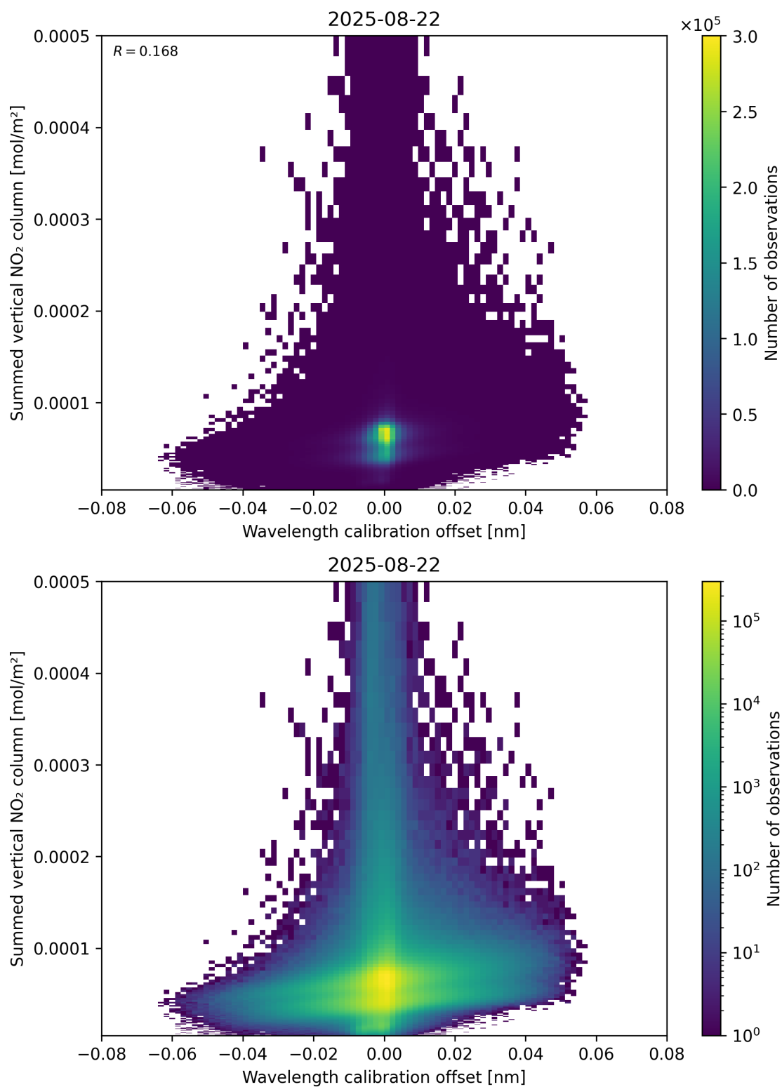
Figure 177: Scatter density plot of “Wavelength calibration offset” against “Summed vertical NO 2 column” for 2025-08-21 to 2025-08-23.
