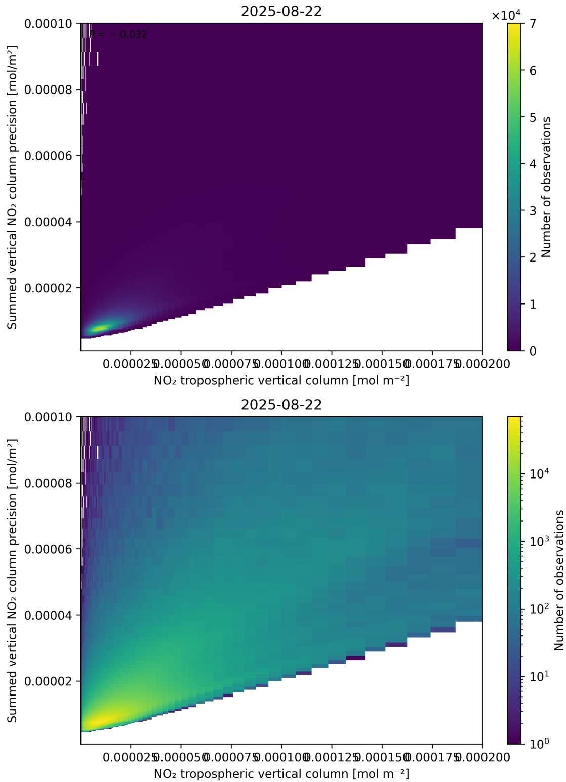
Figure 127: Scatter density plot of “NO 2 tropospheric vertical column” against “Summed vertical NO 2 column precision” for 2025-08-21 to 2025-08-23.
