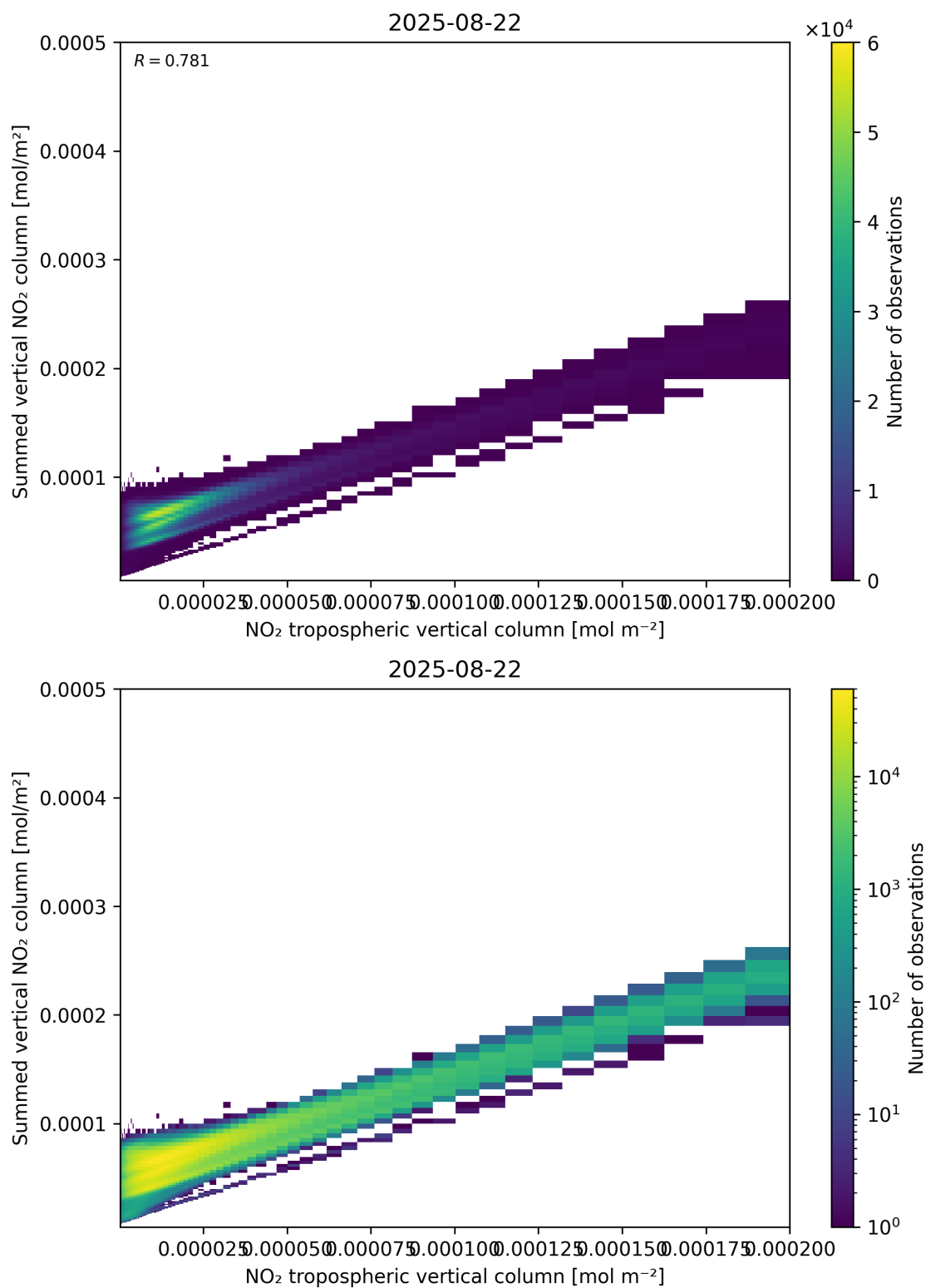
Figure 126: Scatter density plot of “NO 2 tropospheric vertical column” against “Summed vertical NO 2 column” for 2025-08-21 to 2025-08-23.
