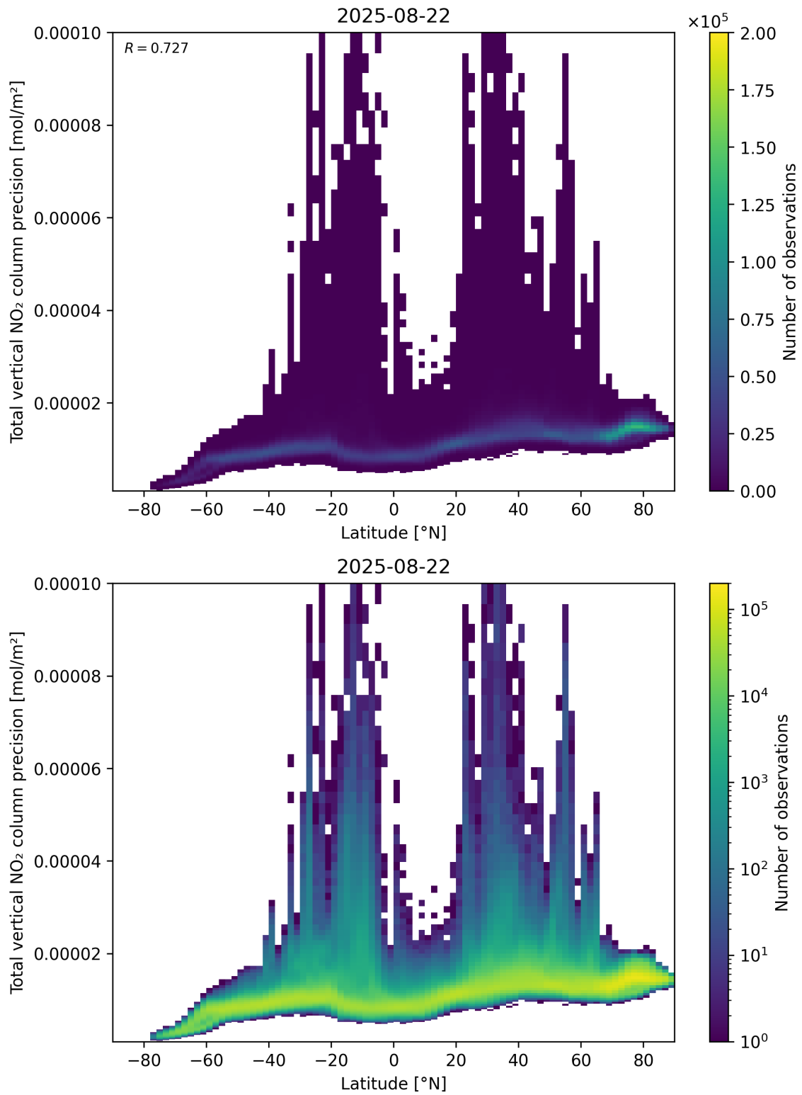
Figure 91: Scatter density plot of “Latitude” against “Total vertical NO 2 column precision” for 2025-08-21 to 2025-08-23.
