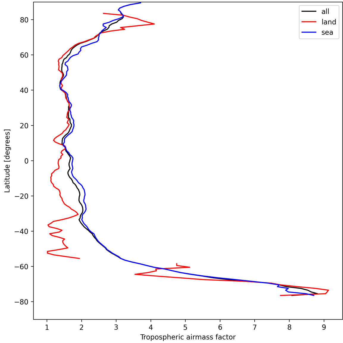
Figure 14: Zonal average of “Tropospheric airmass factor” for 2025-08-21 to 2025-08-23.
