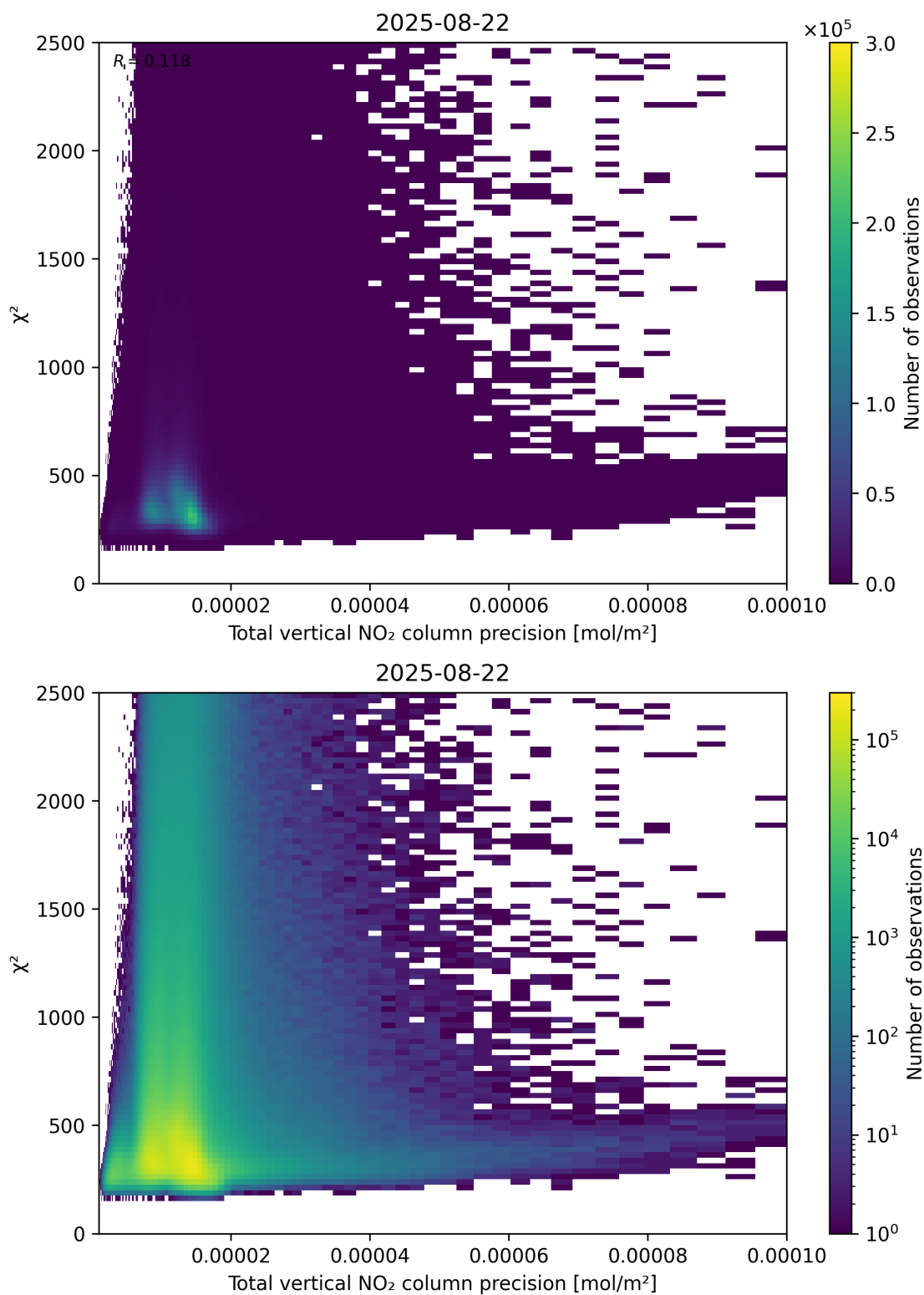
Figure 116: Scatter density plot of “Total vertical NO 2 column precision” against “ \chi^2 ” for 2025-08-21 to 2025-08-23.
