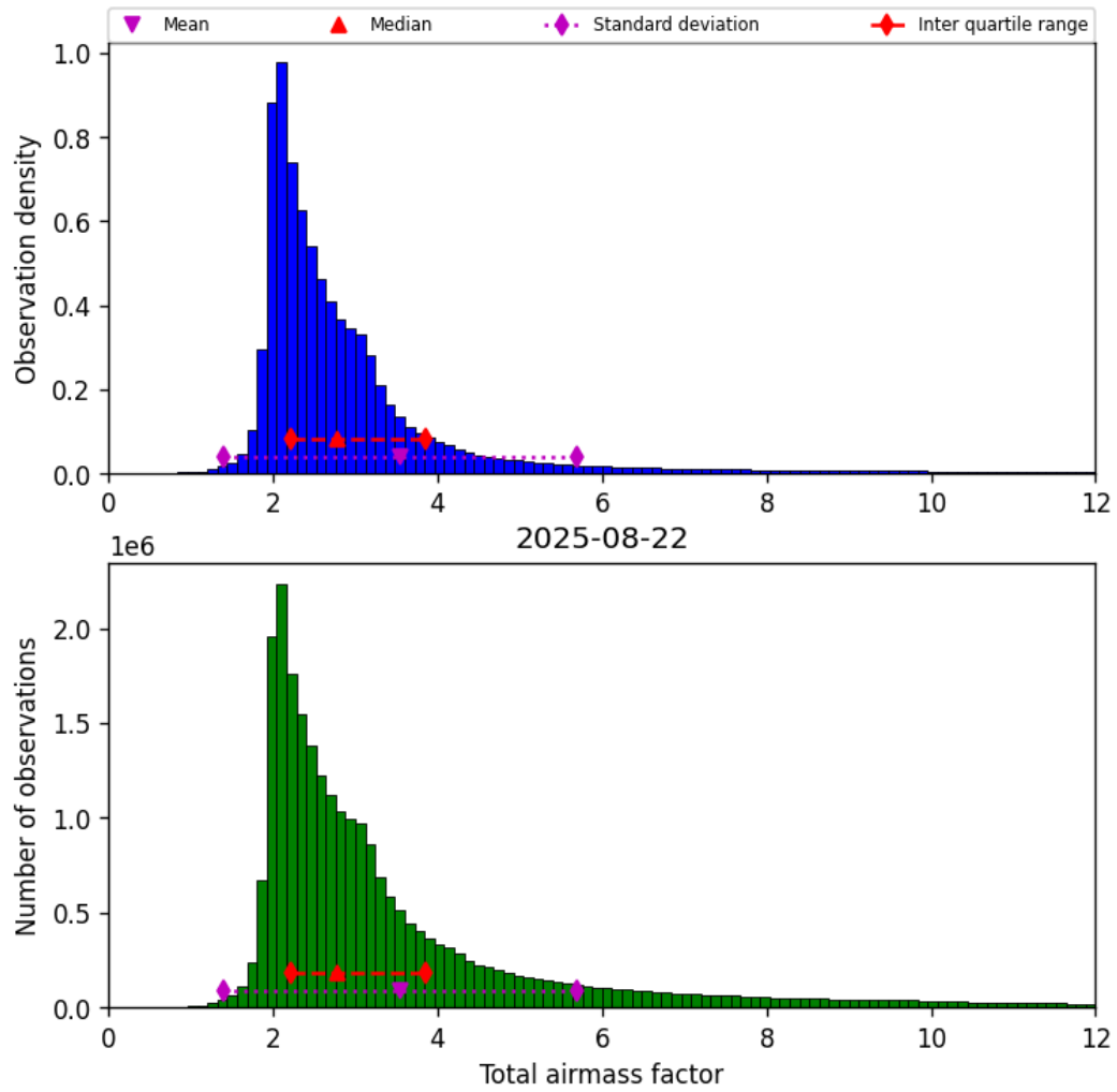
Figure 32: Histogram of “Total airmass factor” for 2025-08-21 to 2025-08-23
