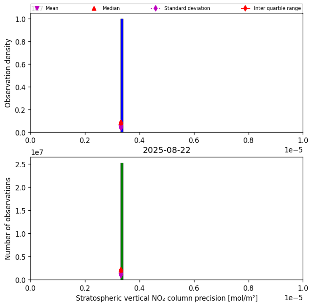
Figure 37: Histogram of “Stratospheric vertical NO 2 column precision” for 2025-08-21 to 2025-08-23
