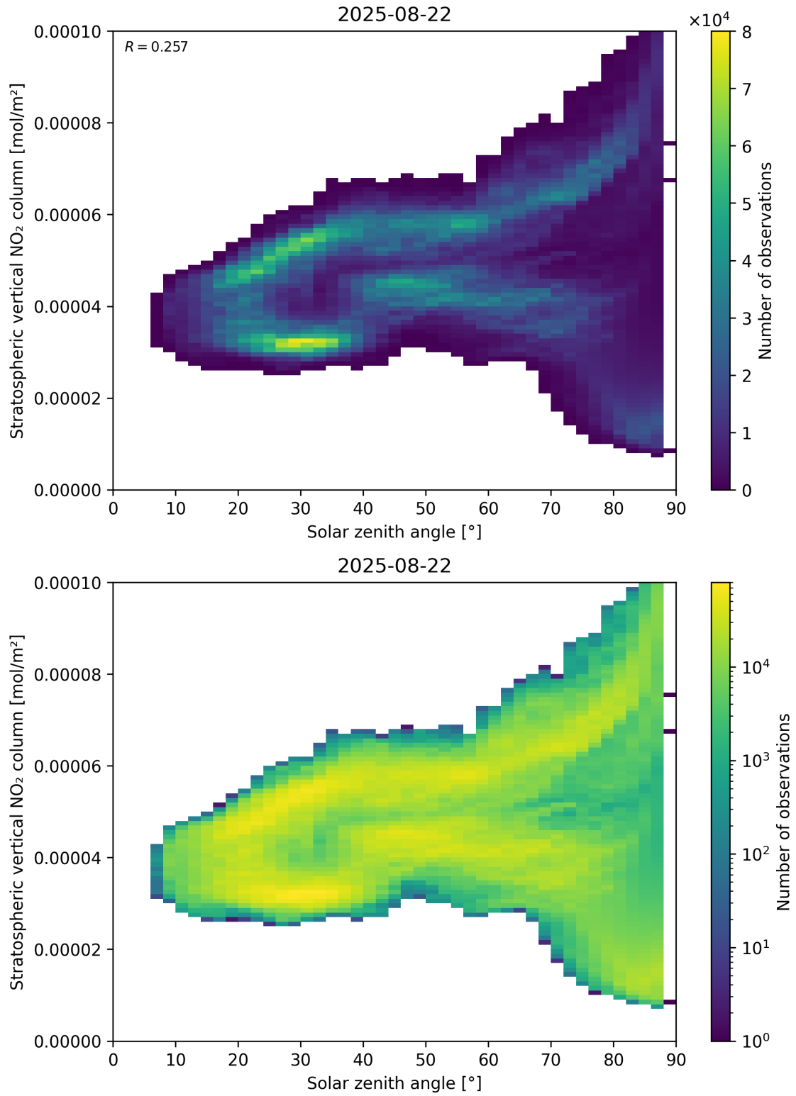
Figure 150: Scatter density plot of “Solar zenith angle” against “Stratospheric vertical NO 2 column” for 2025-08-21 to 2025-08-23.
