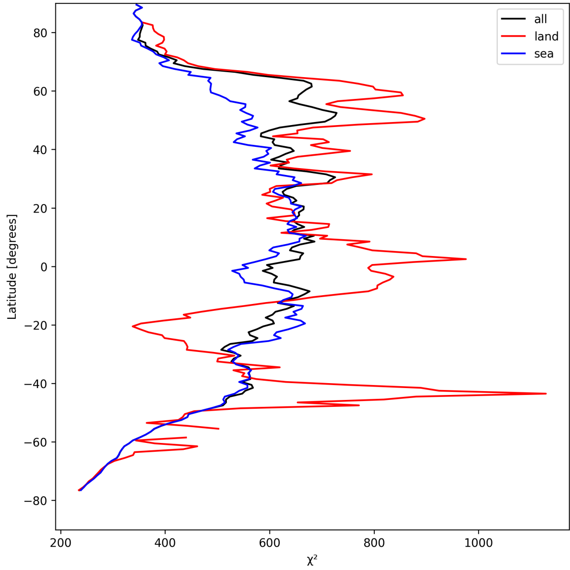
Figure 25: Zonal average of “ \chi^2 ” for 2025-08-21 to 2025-08-23.
