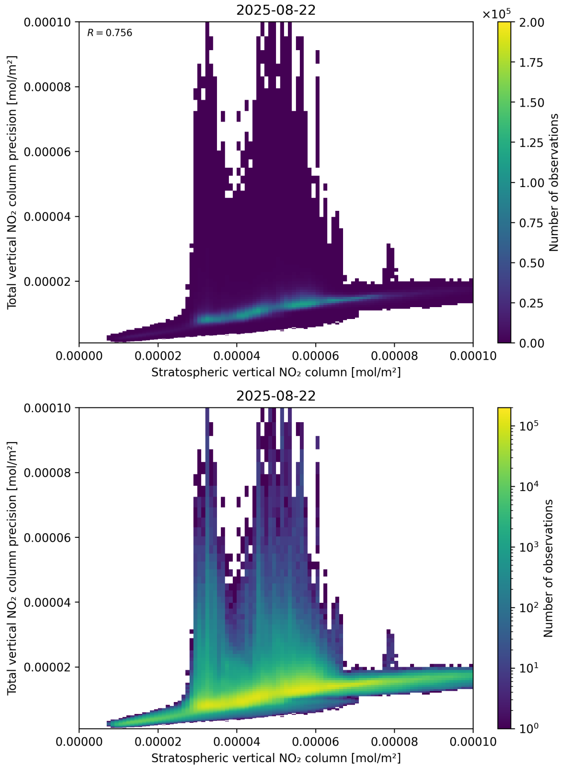
Figure 101: Scatter density plot of “Stratospheric vertical NO 2 column” against “Total vertical NO 2 column precision” for 2025-08-21 to 2025-08-23.
