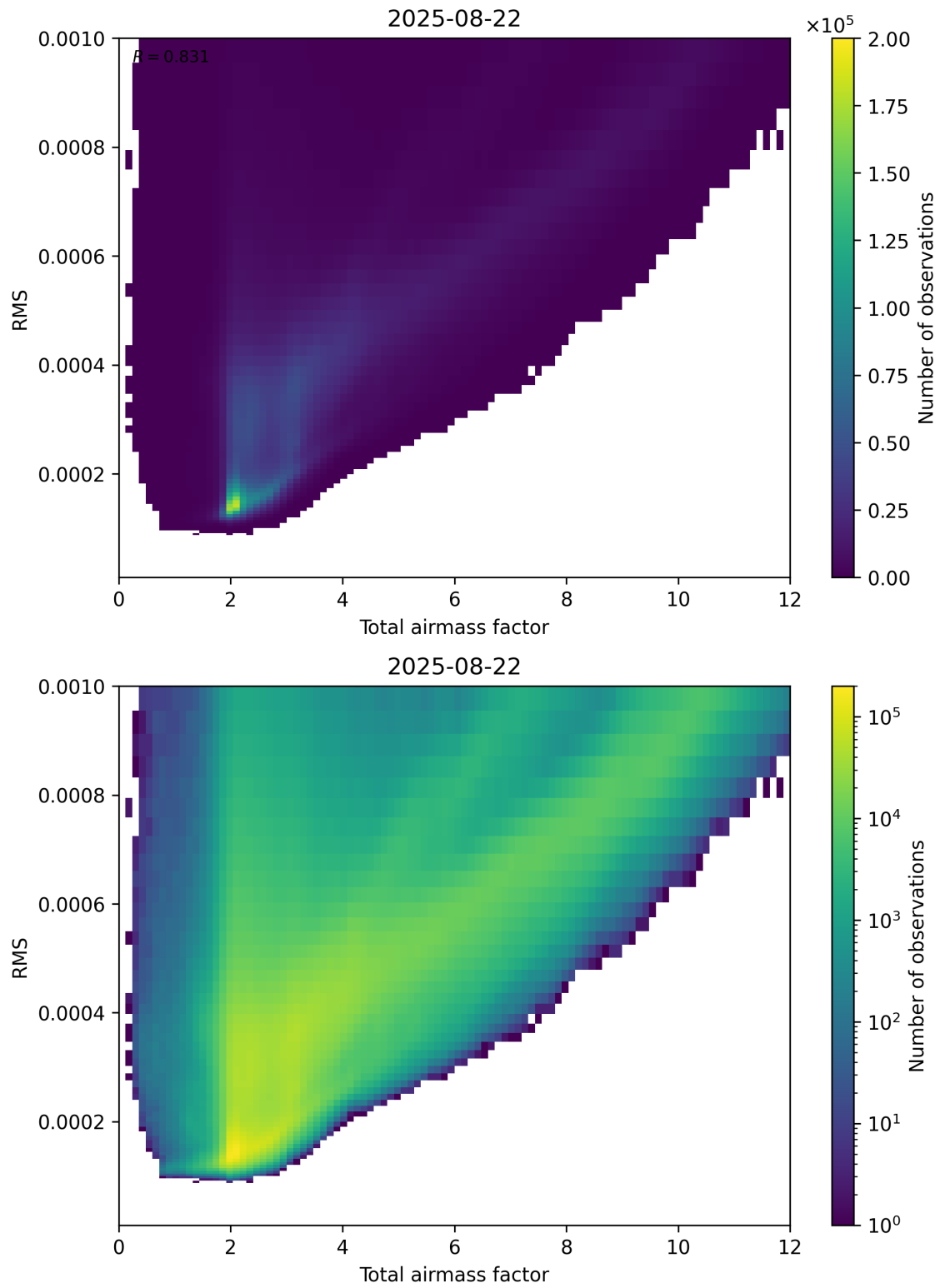
Figure 69: Scatter density plot of “Total airmass factor” against “RMS” for 2025-08-21 to 2025-08-23.
