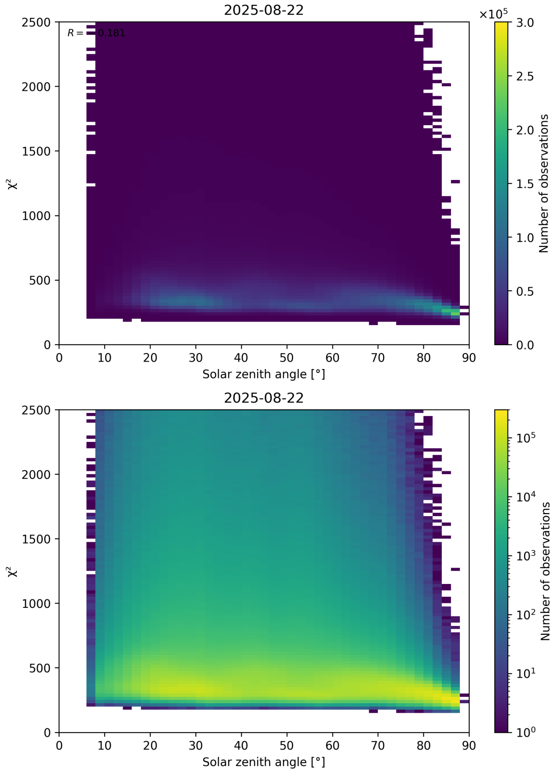
Figure 148: Scatter density plot of “Solar zenith angle” against “ \chi^2 ” for 2025-08-21 to 2025-08-23.
