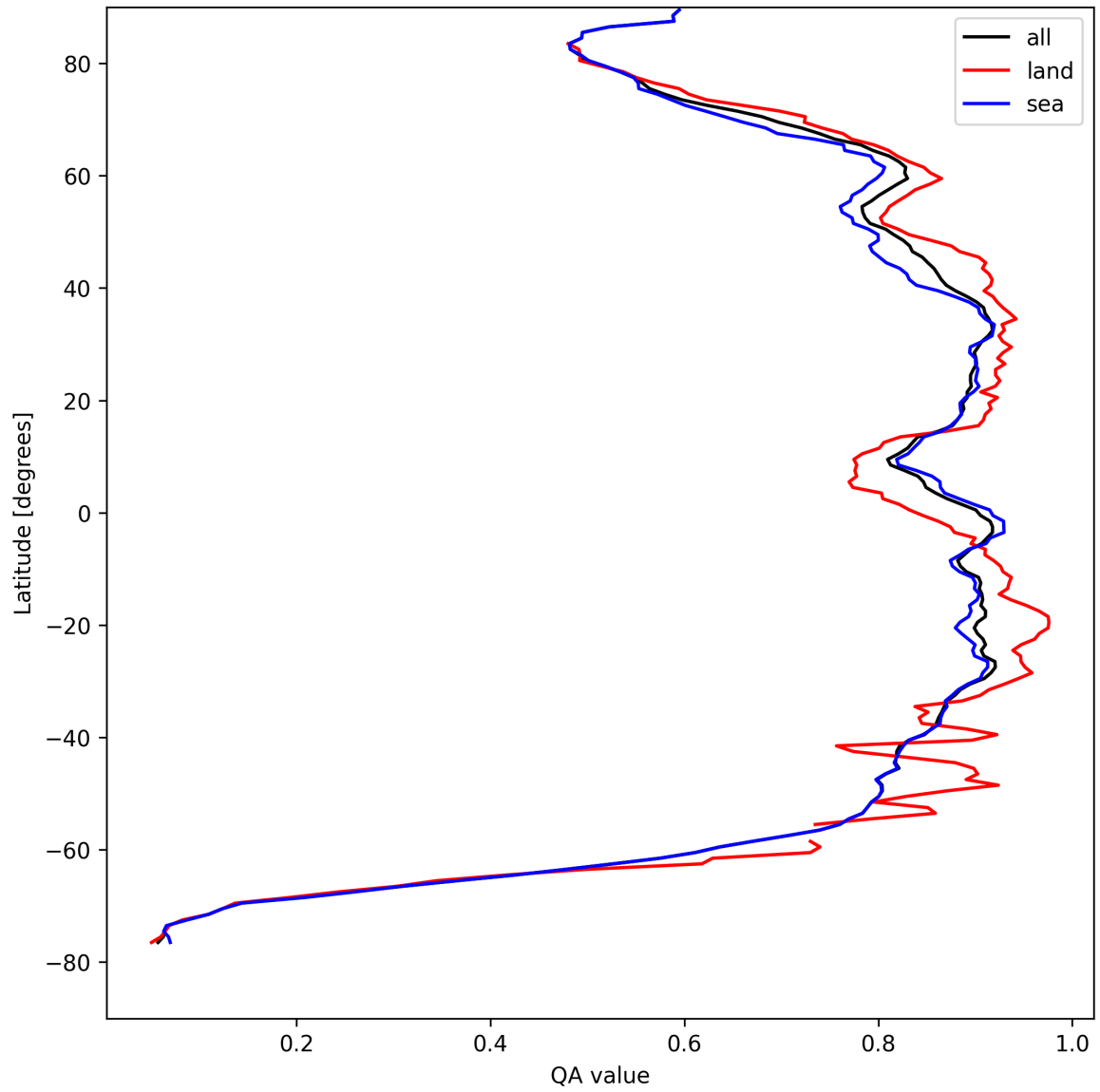
Figure 11: Zonal average of “QA value” for 2025-08-21 to 2025-08-23.
