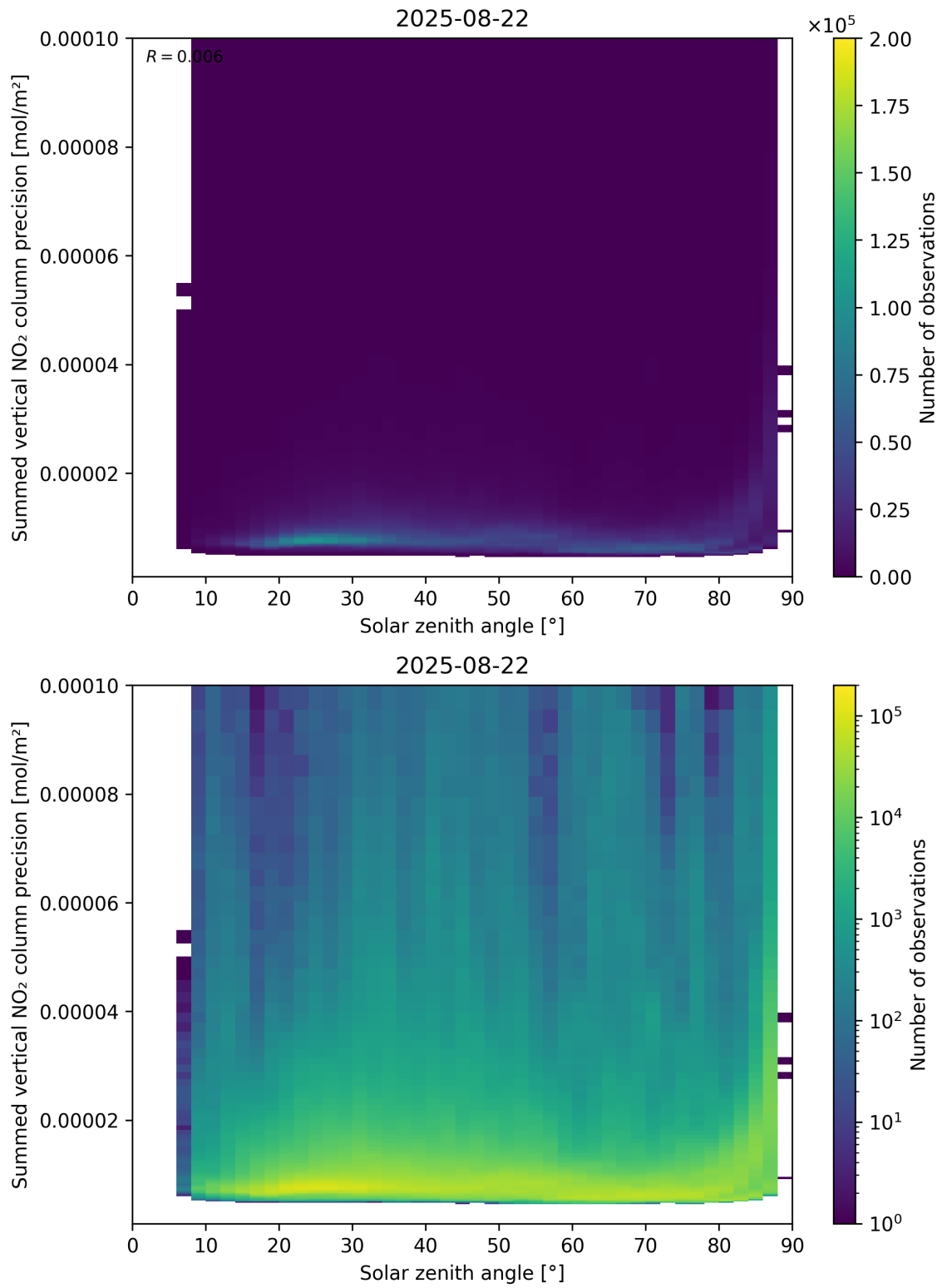
Figure 152: Scatter density plot of “Solar zenith angle” against “Summed vertical NO 2 column precision” for 2025-08-21 to 2025-08-23.
