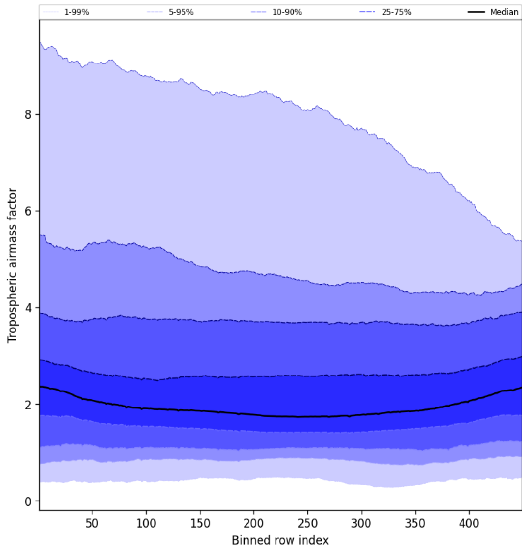
Figure 48: Along track statistics of “Tropospheric airmass factor” for 2025-08-21 to 2025-08-23
