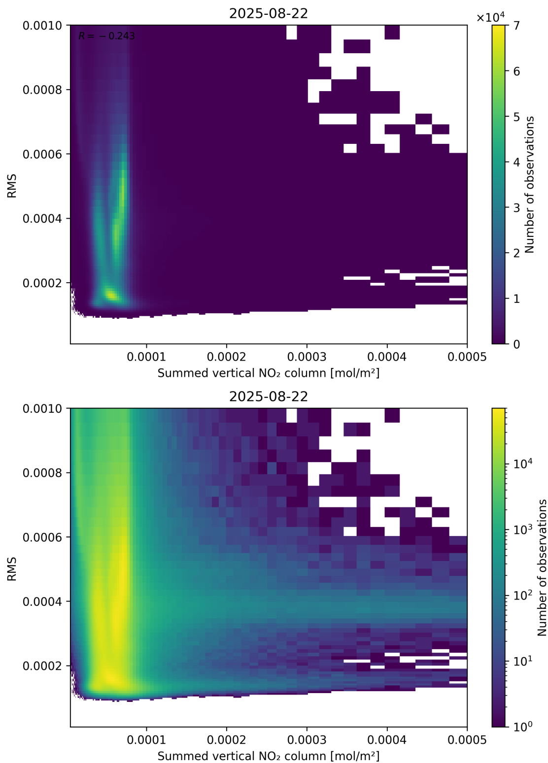
Figure 109: Scatter density plot of “Summed vertical NO 2 column” against “RMS” for 2025-08-21 to 2025-08-23.
