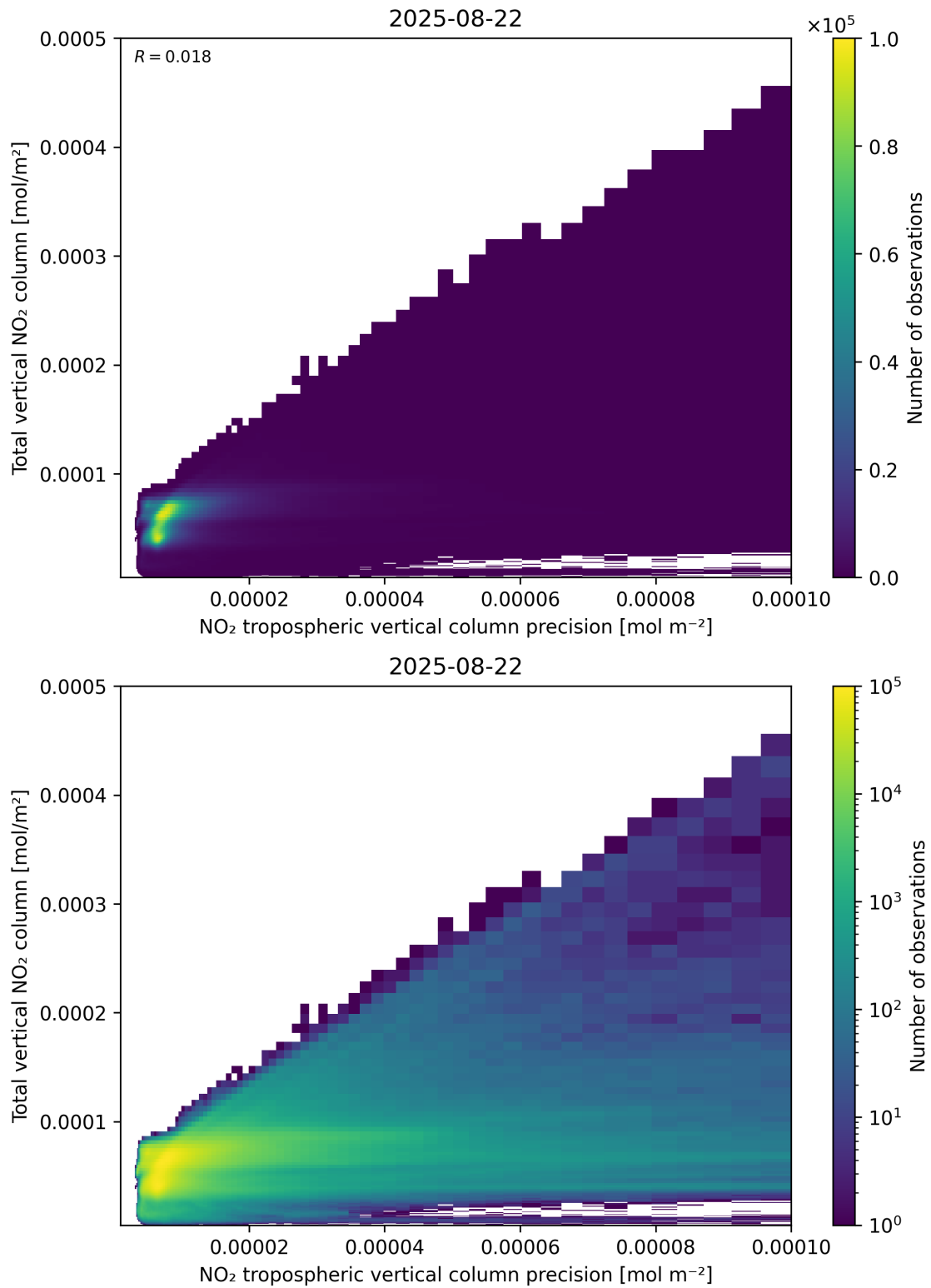
Figure 138: Scatter density plot of “NO 2 tropospheric vertical column precision” against “Total vertical NO 2 column” for 2025-08-21 to 2025-08-23.
