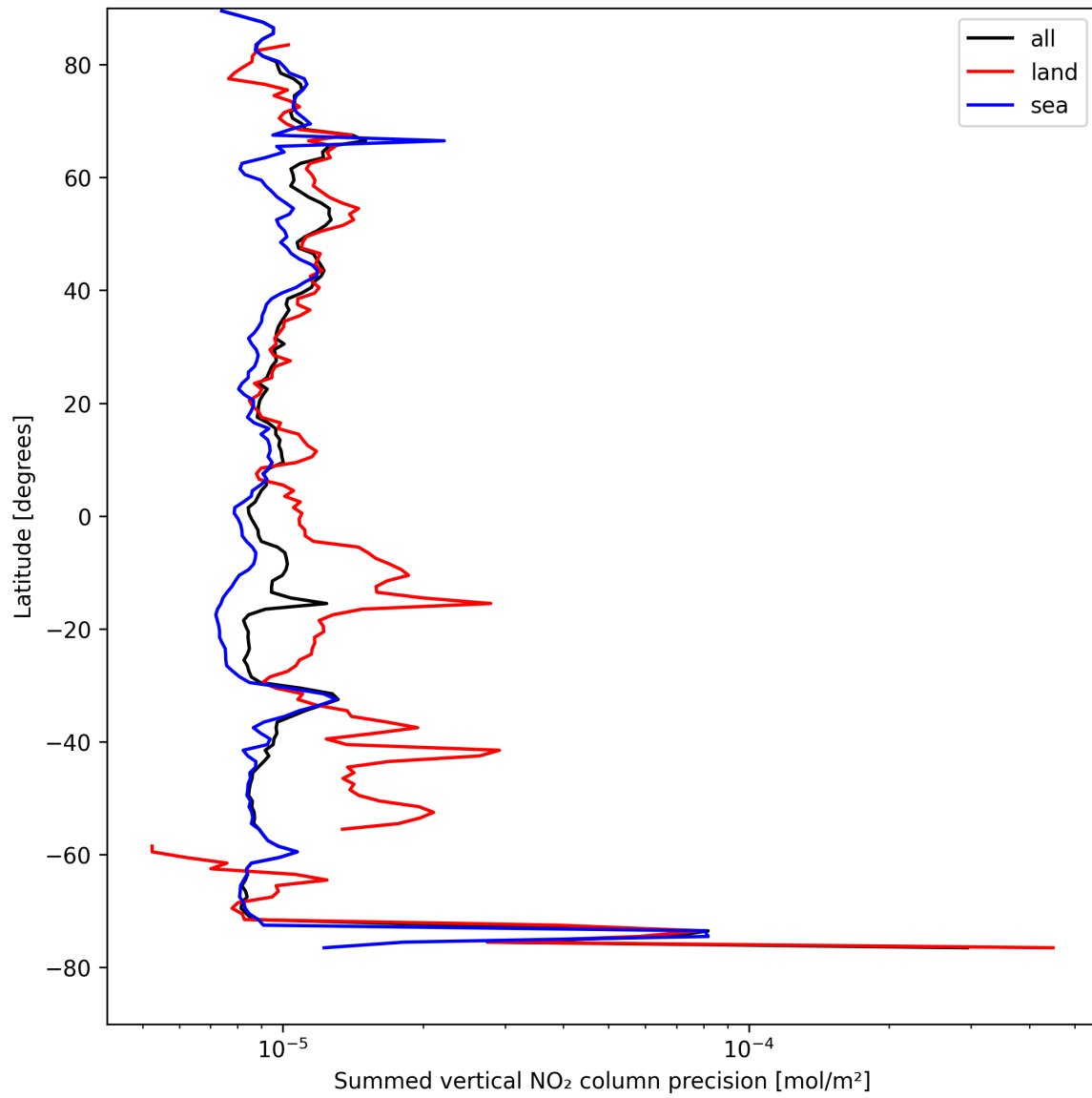
Figure 24: Zonal average of “Summed vertical NO 2 column precision” for 2025-08-21 to 2025-08-23.
