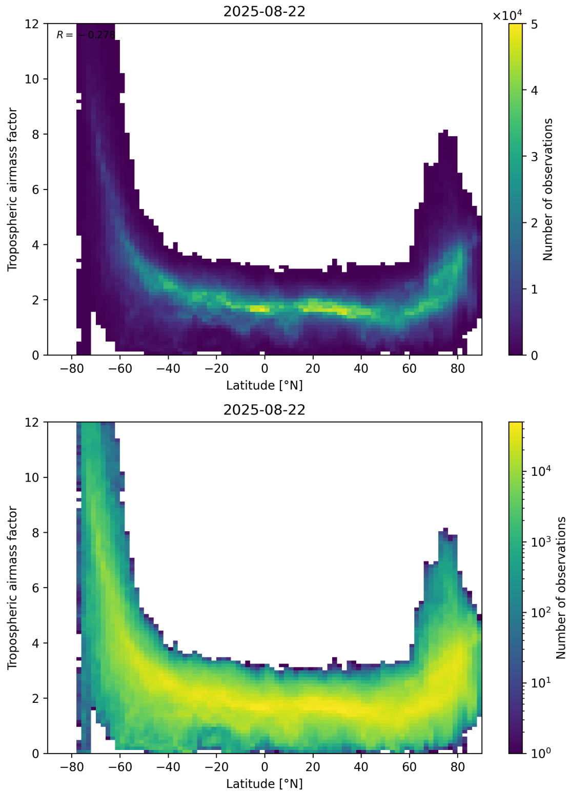
Figure 85: Scatter density plot of “Latitude” against “Tropospheric airmass factor” for 2025-08-21 to 2025-08-23.
