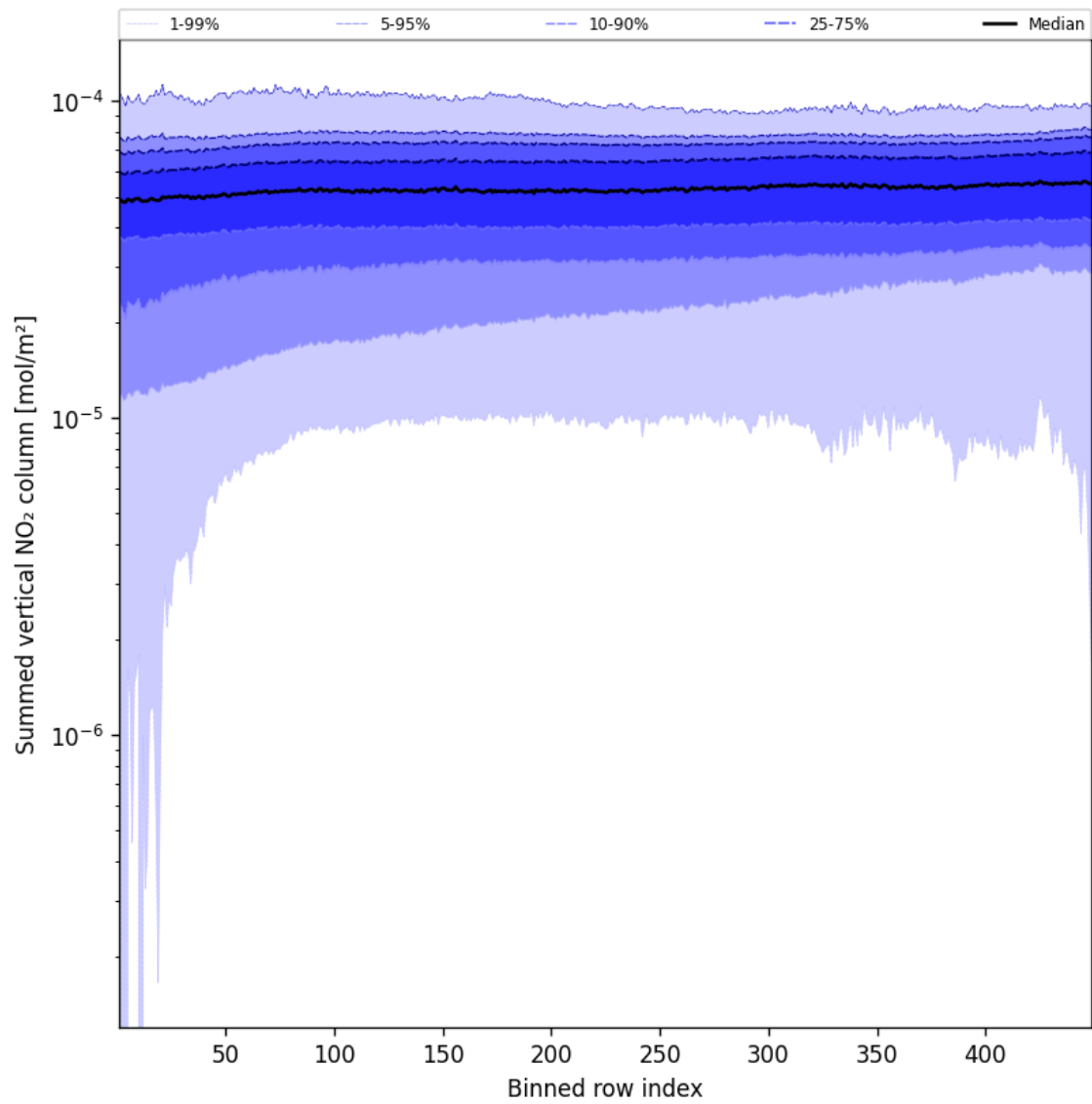
Figure 57: Along track statistics of “Summed vertical NO 2 column” for 2025-08-21 to 2025-08-23
