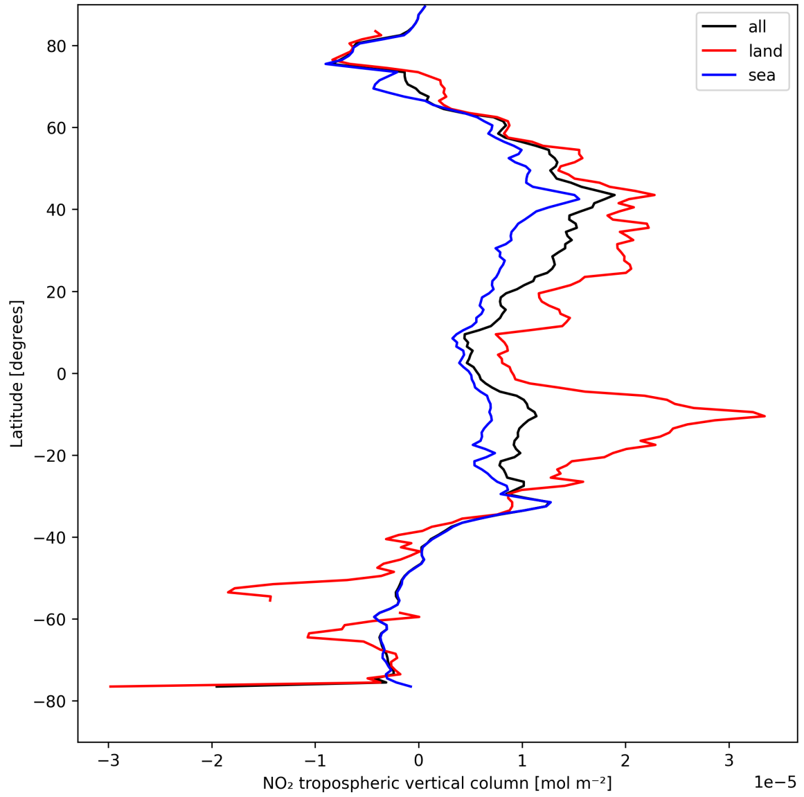
Figure 12: Zonal average of “NO 2 tropospheric vertical column” for 2025-08-21 to 2025-08-23.
