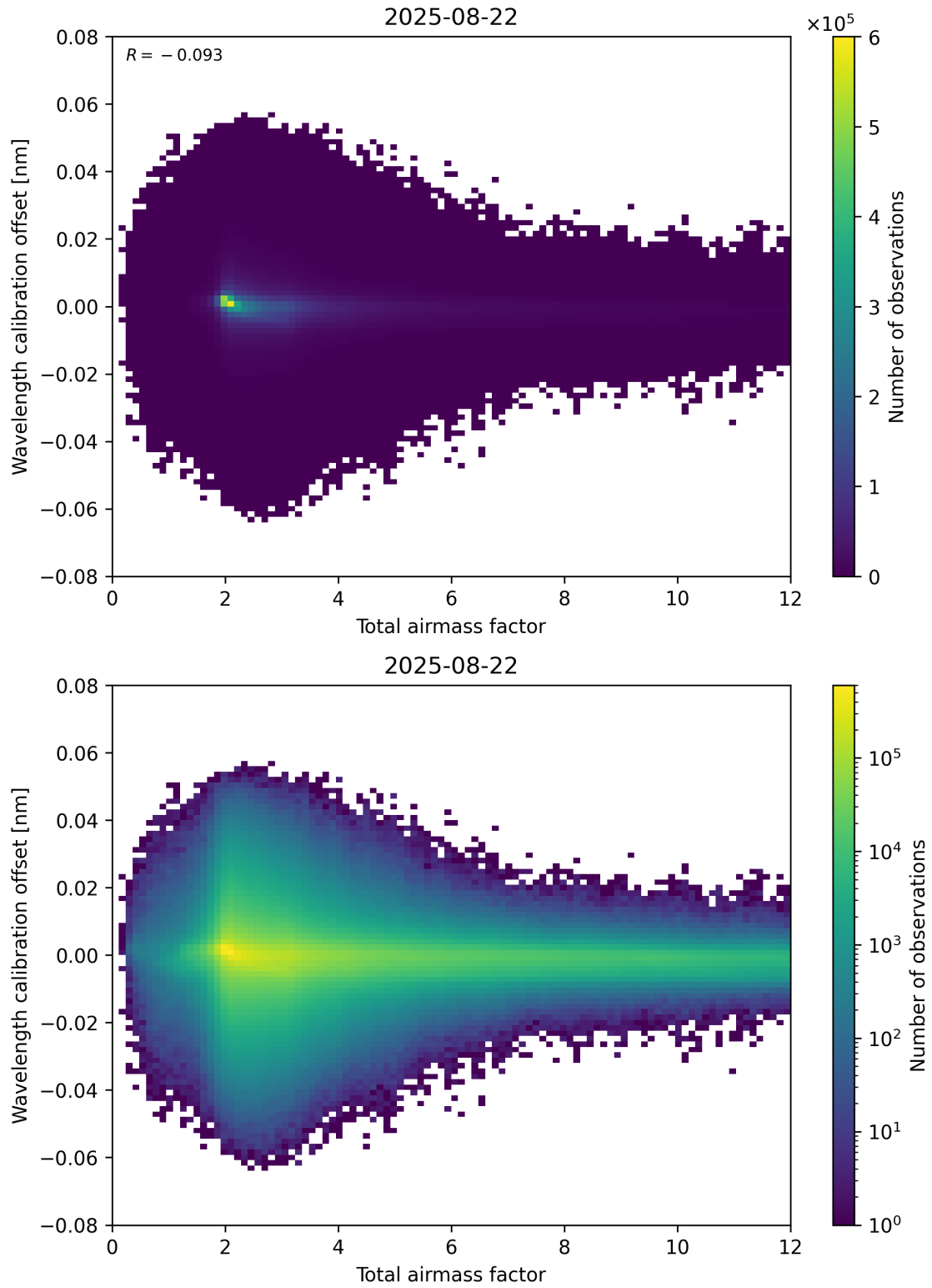
Figure 70: Scatter density plot of “Total airmass factor” against “Wavelength calibration offset” for 2025-08-21 to 2025-08-23.
