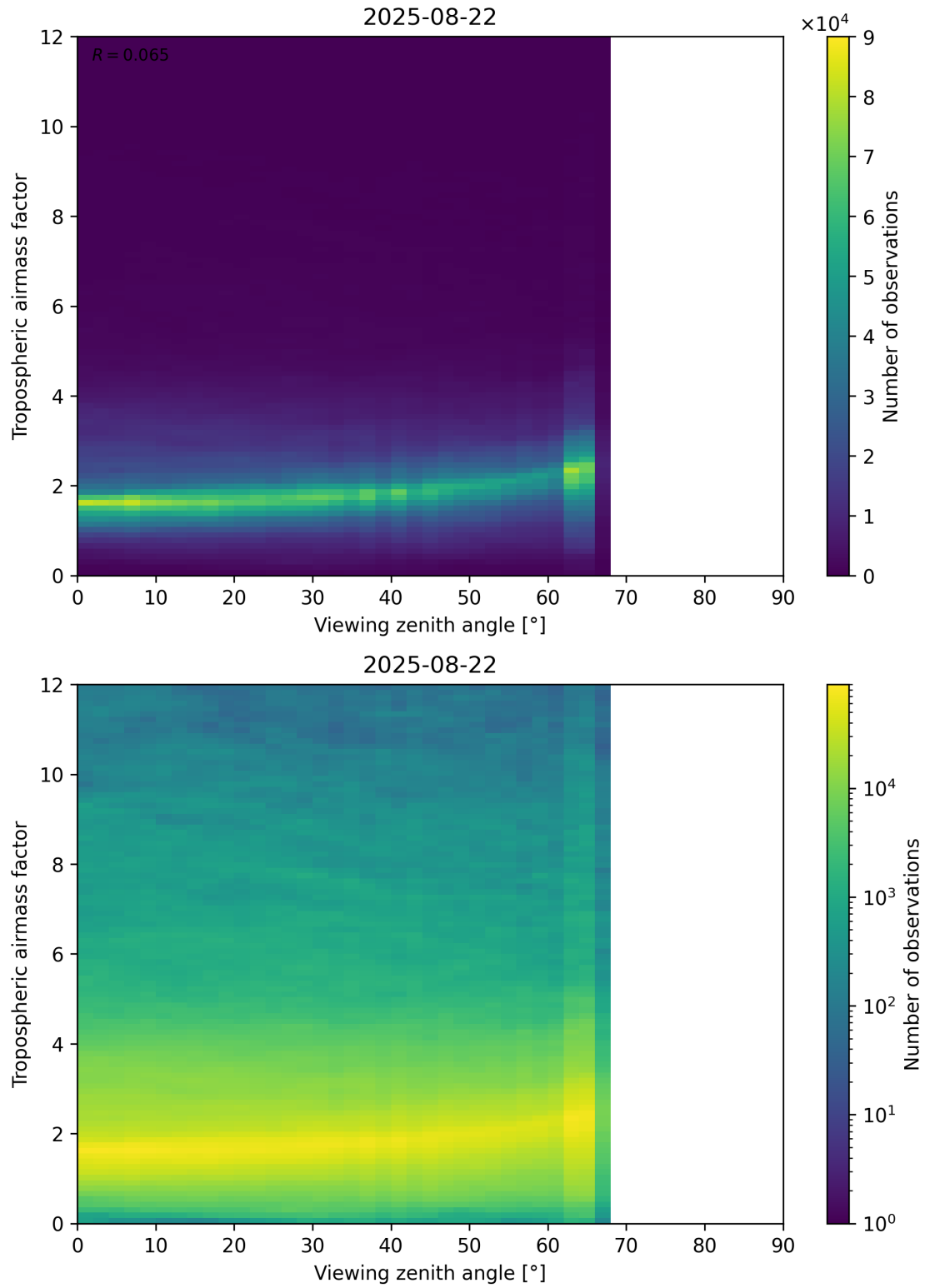
Figure 161: Scatter density plot of “Viewing zenith angle” against “Tropospheric airmass factor” for 2025-08-21 to 2025-08-23.
