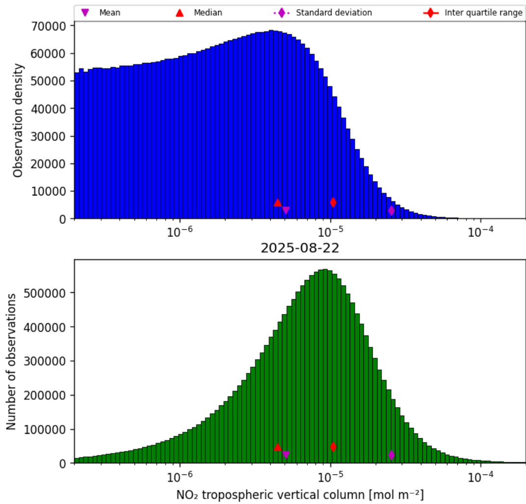
Figure 29: Histogram of “NO 2 tropospheric vertical column” for 2025-08-21 to 2025-08-23
