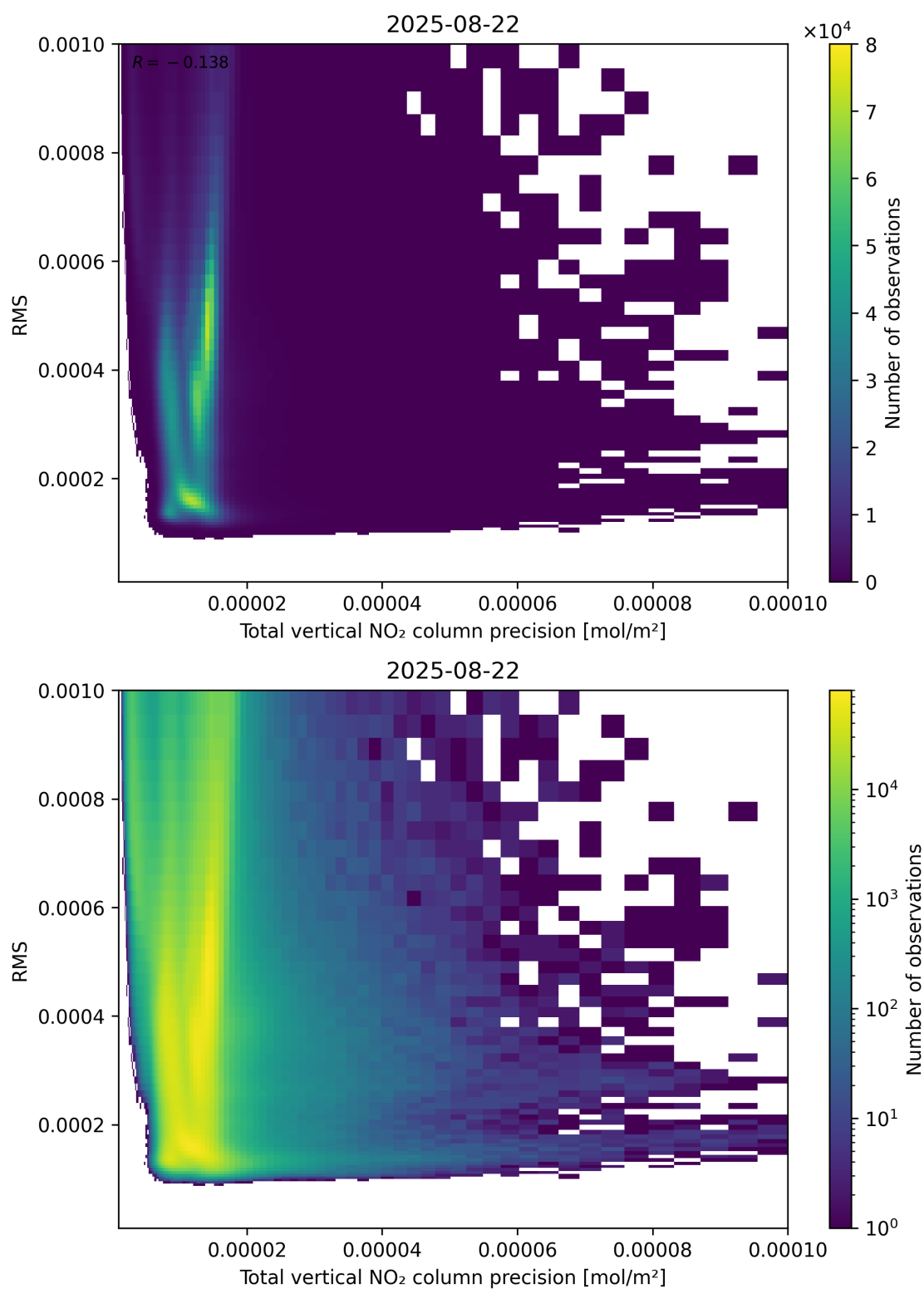
Figure 119: Scatter density plot of “Total vertical NO 2 column precision” against “RMS” for 2025-08-21 to 2025-08-23.
