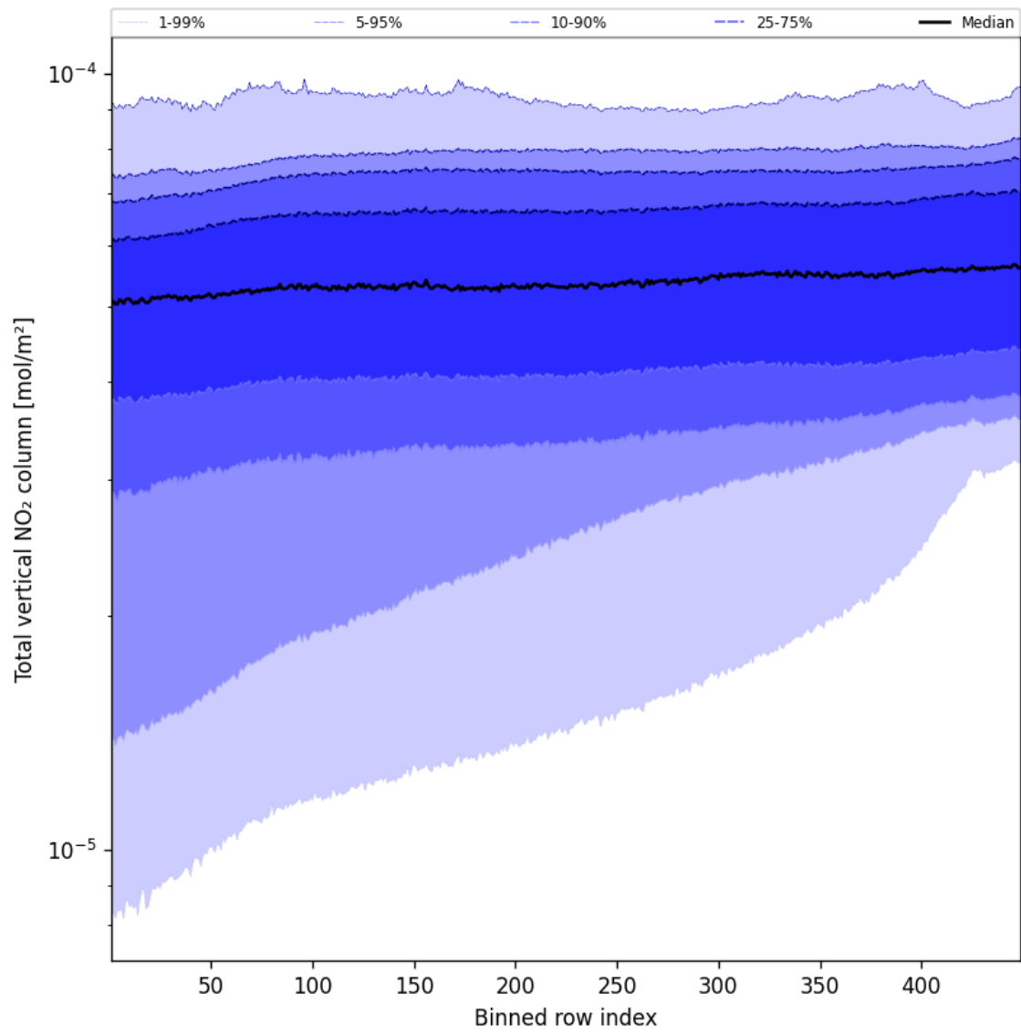
Figure 55: Along track statistics of “Total vertical NO 2 column” for 2025-08-21 to 2025-08-23
