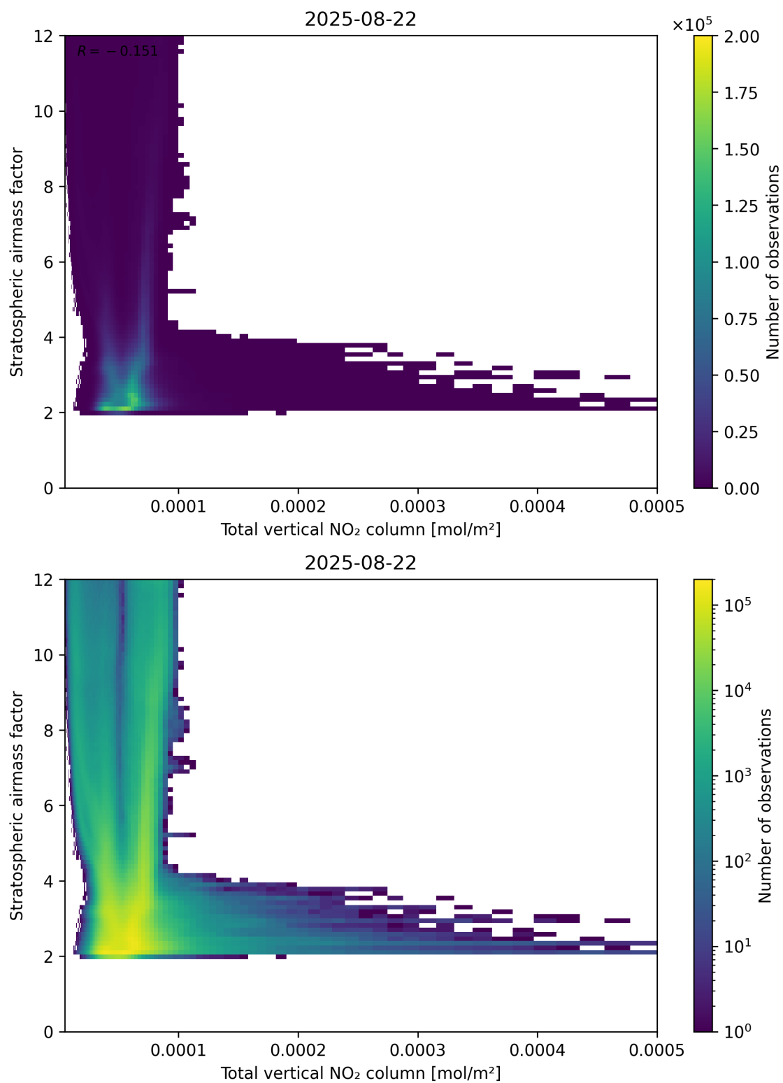
Figure 110: Scatter density plot of “Total vertical NO 2 column” against “Stratospheric airmass factor” for 2025-08-21 to 2025-08-23.
