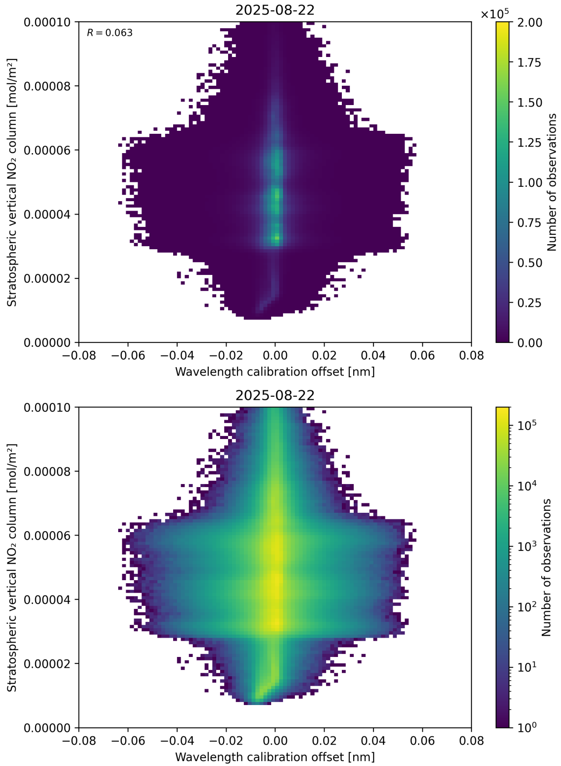
Figure 176: Scatter density plot of “Wavelength calibration offset” against “Stratospheric vertical NO 2 column” for 2025-08-21 to 2025-08-23.
