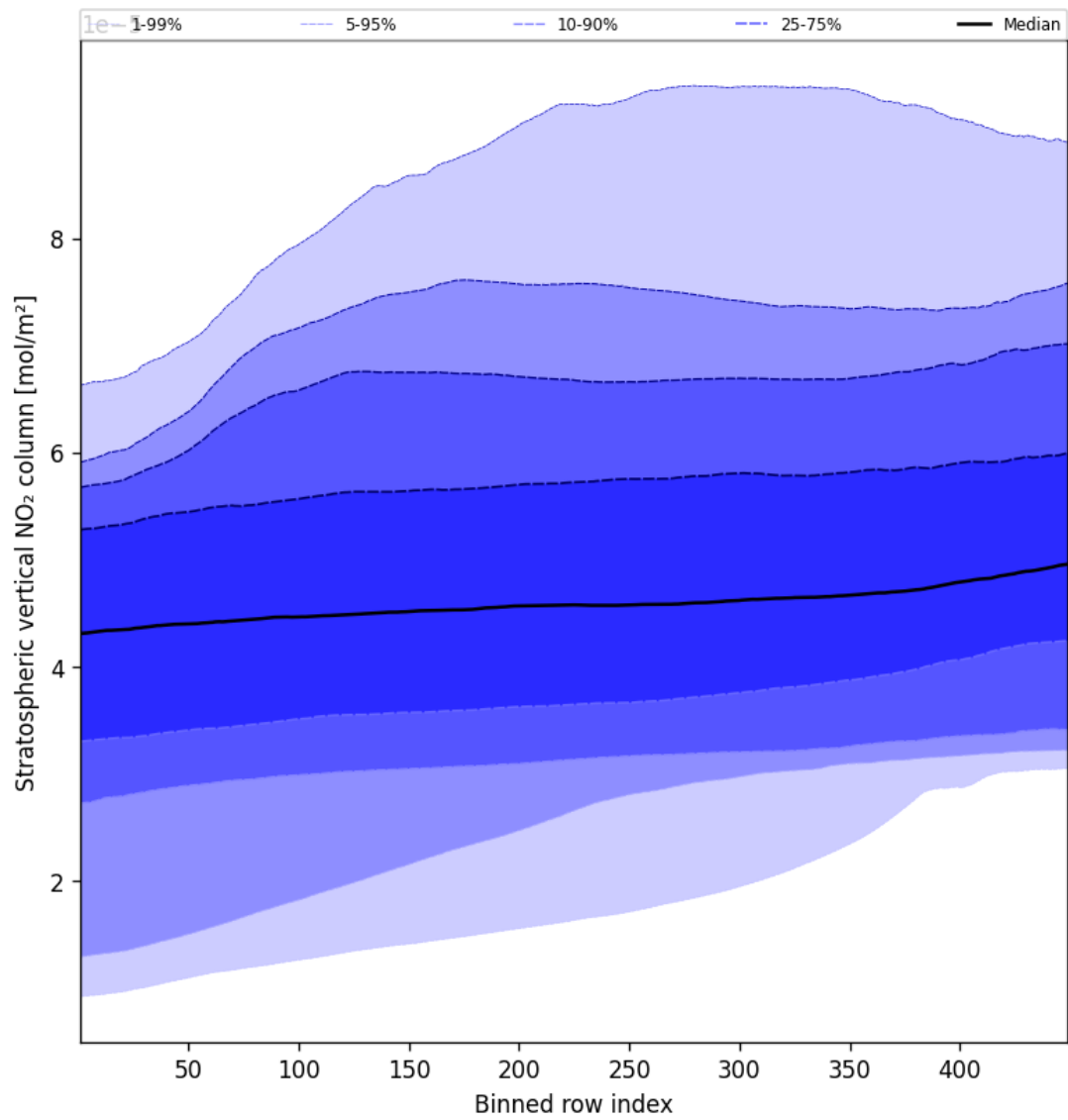
Figure 53: Along track statistics of “Stratospheric vertical NO 2 column” for 2025-08-21 to 2025-08-23
