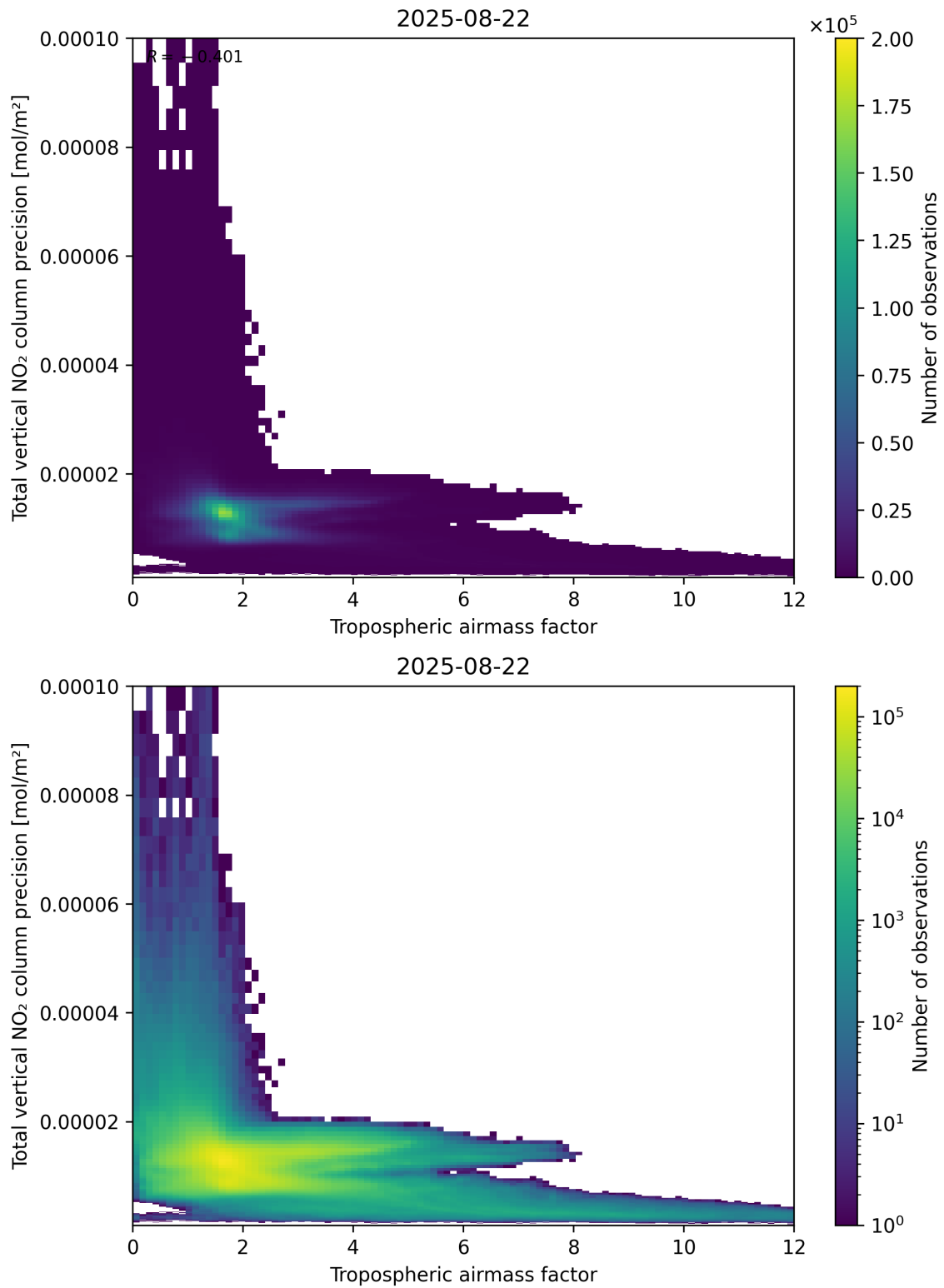
Figure 78: Scatter density plot of “Tropospheric air mass factor” against “Total vertical NO 2 column precision” for 2025-08-21 to 2025-08-23.
