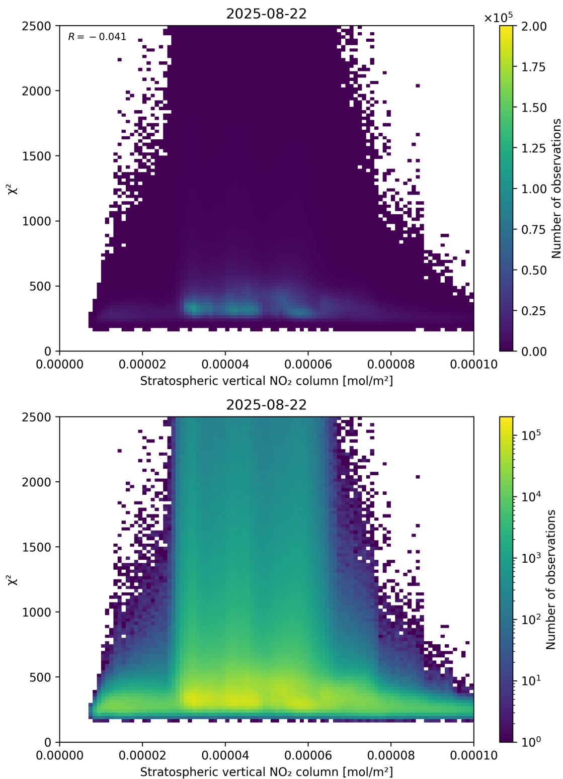
Figure 97: Scatter density plot of “Stratospheric vertical NO 2 column” against “ \chi^2 ” for 2025-08-21 to 2025-08-23.
