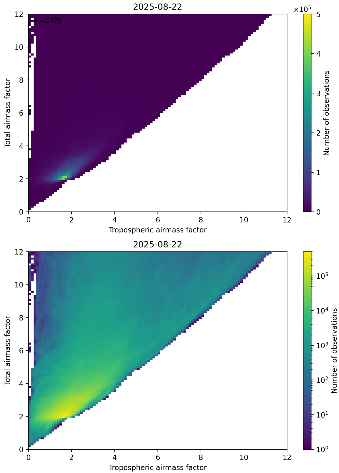
Figure 72: Scatter density plot of “Tropospheric airmass factor” against “Total airmass factor” for 2025-08-21 to 2025-08-23.
