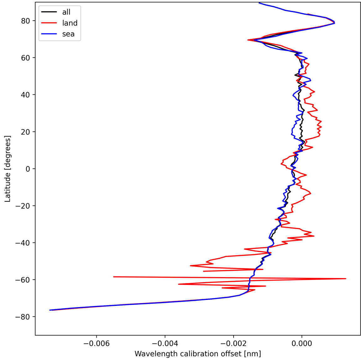
Figure 18: Zonal average of “Wavelength calibration offset” for 2025-08-21 to 2025-08-23.
