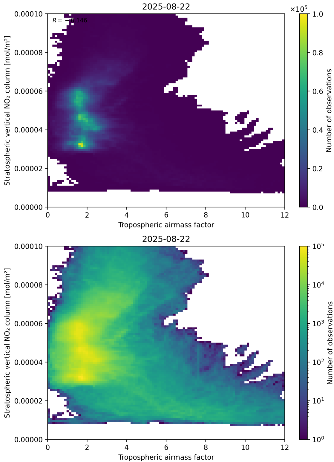
Figure 74: Scatter density plot of “Tropospheric air mass factor” against “Stratospheric vertical NO 2 column” for 2025-08-21 to 2025-08-23.
