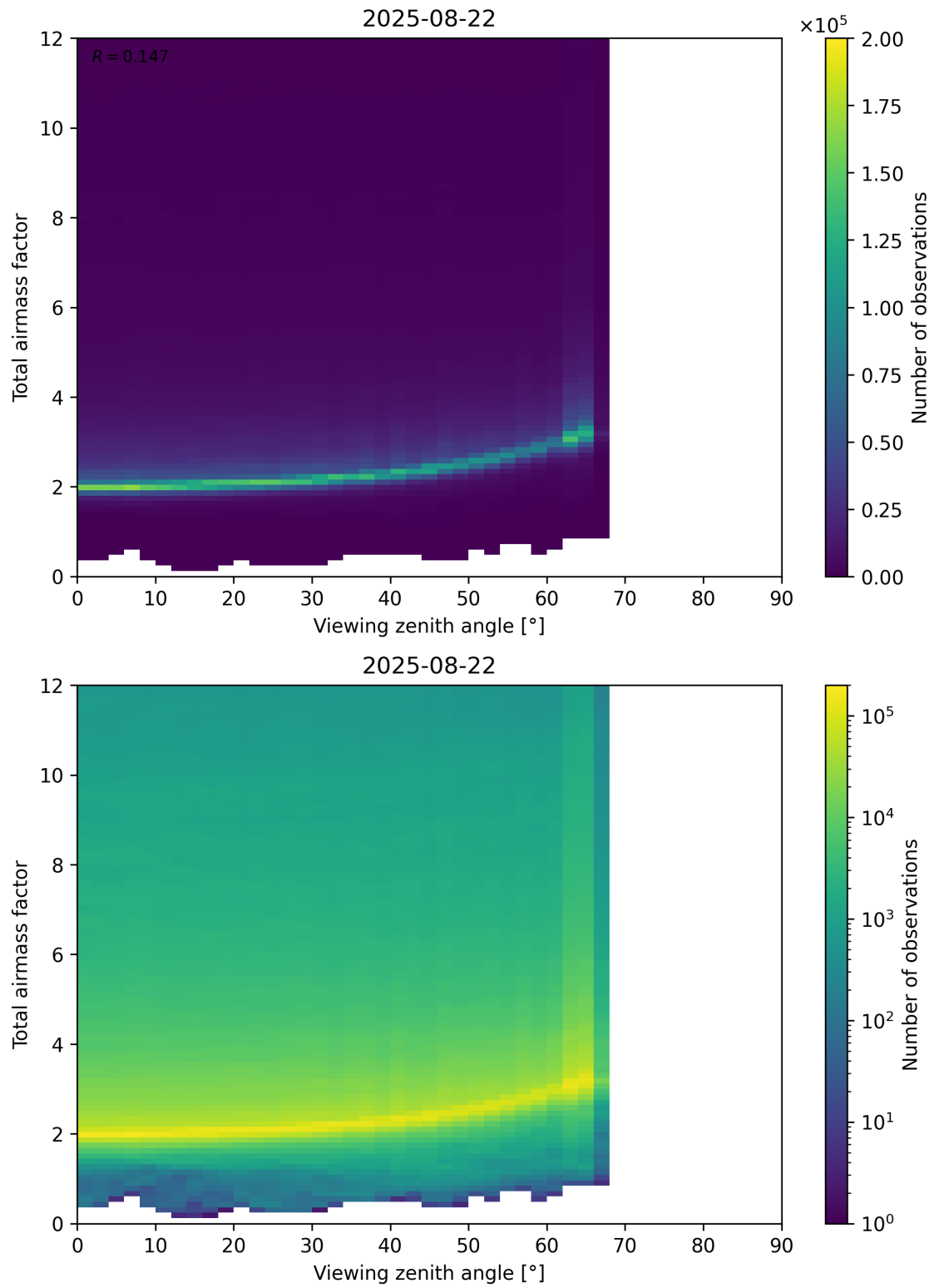
Figure 160: Scatter density plot of “Viewing zenith angle” against “Total airmass factor” for 2025-08-21 to 2025-08-23.
