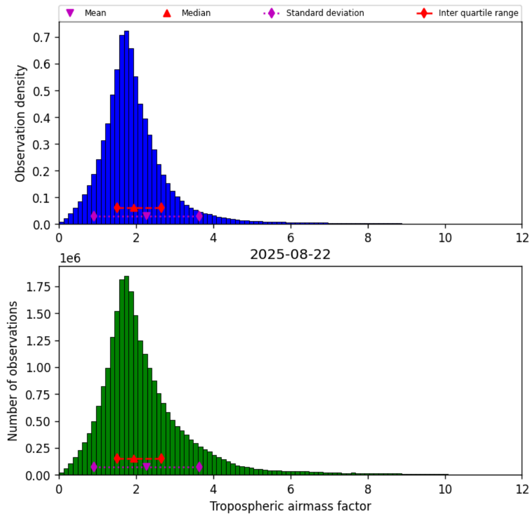
Figure 31: Histogram of “Tropospheric airmass factor” for 2025-08-21 to 2025-08-23
