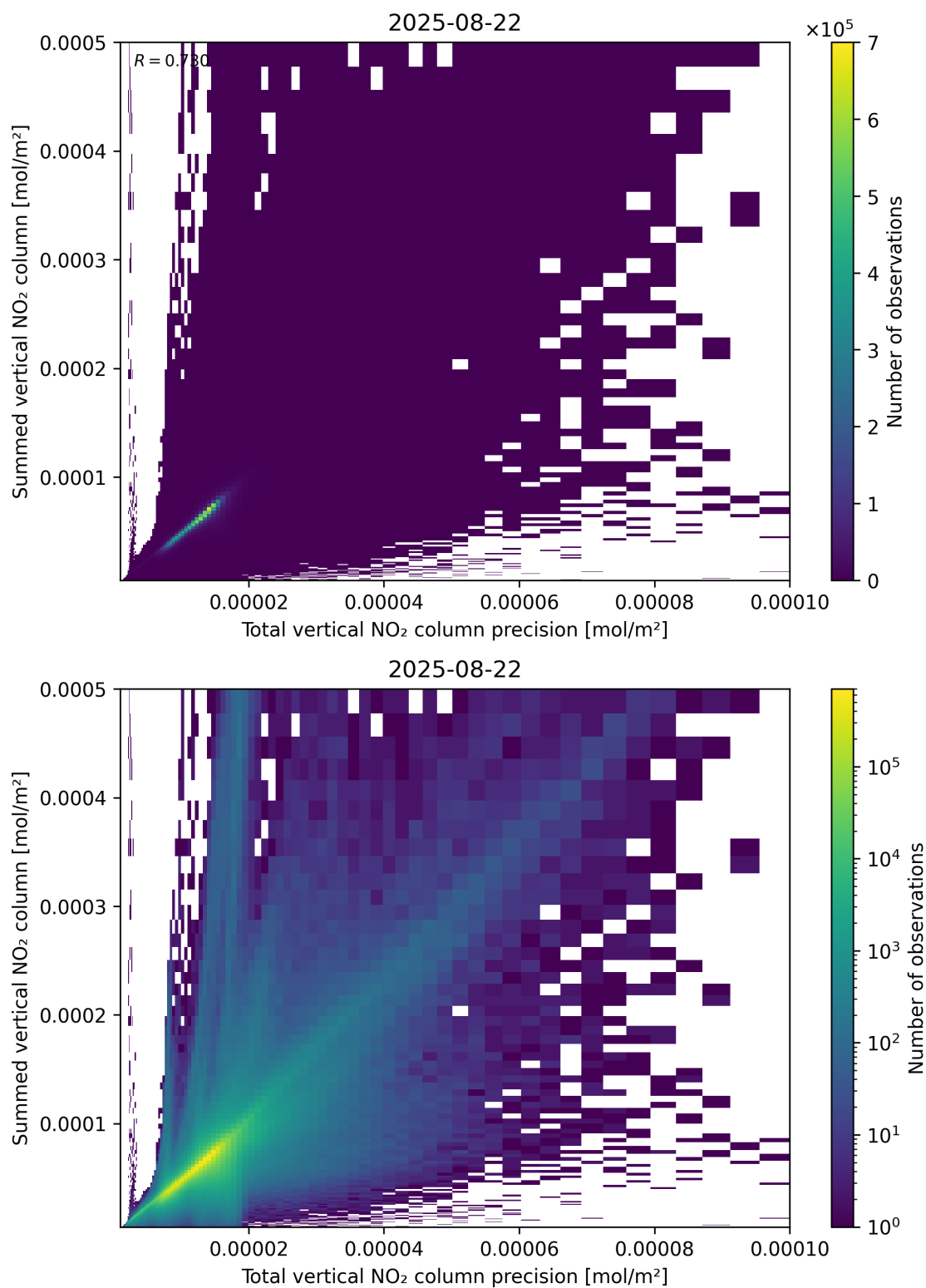
Figure 117: Scatter density plot of “Total vertical NO 2 column precision” against “Summed vertical NO 2 column” for 2025-08-21 to 2025-08-23.
