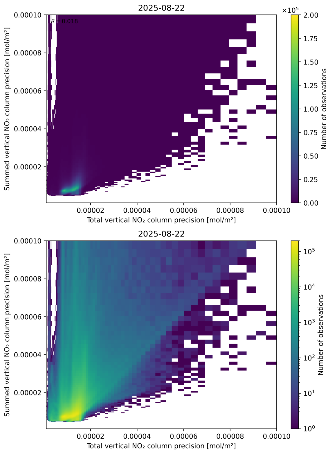
Figure 118: Scatter density plot of “Total vertical NO 2 column precision” against “Summed vertical NO 2 column precision” for 2025-08-21 to 2025-08-23.
