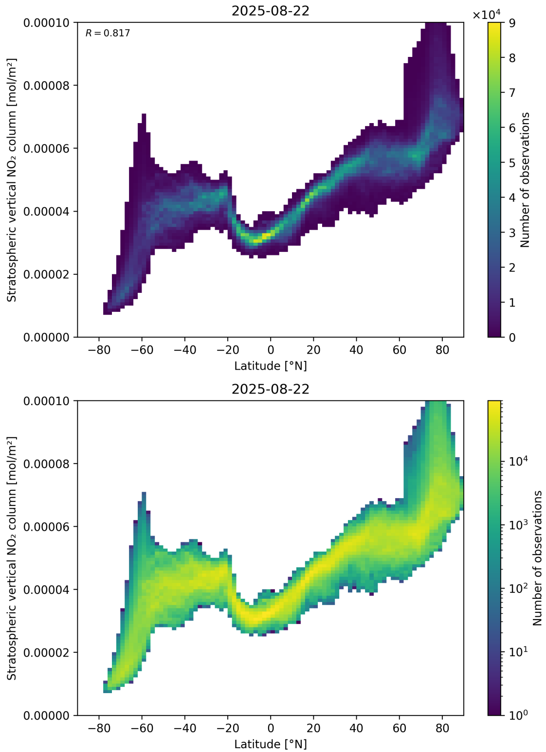
Figure 87: Scatter density plot of “Latitude” against “Stratospheric vertical NO 2 column” for 2025-08-21 to 2025-08-23.
