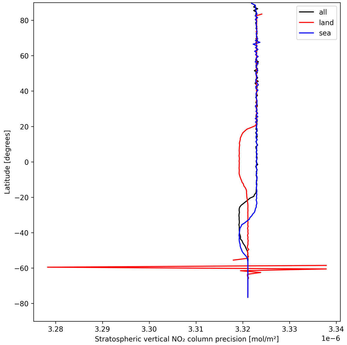
Figure 20: Zonal average of “Stratospheric vertical NO 2 column precision” for 2025-08-21 to 2025-08-23.
