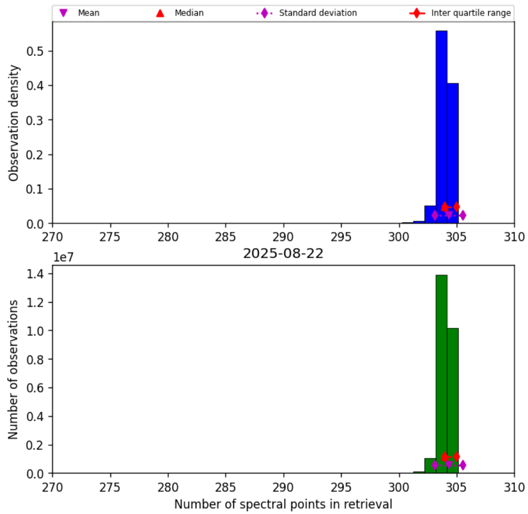
Figure 33: Histogram of “Number of spectral points in retrieval” for 2025-08-21 to 2025-08-23
