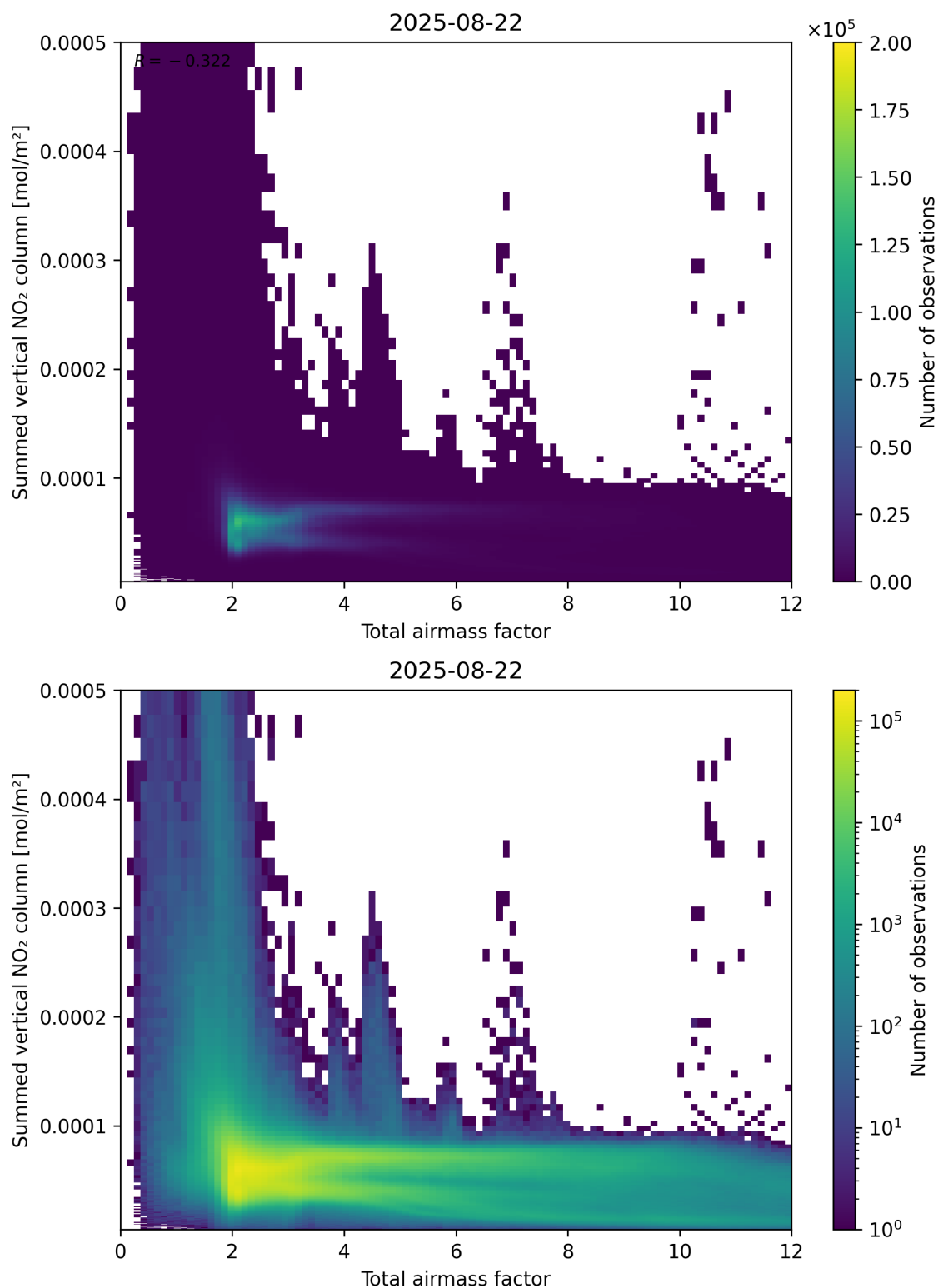
Figure 65: Scatter density plot of “Total airmass factor” against “Summed vertical NO 2 column” for 2025-08-21 to 2025-08-23.
