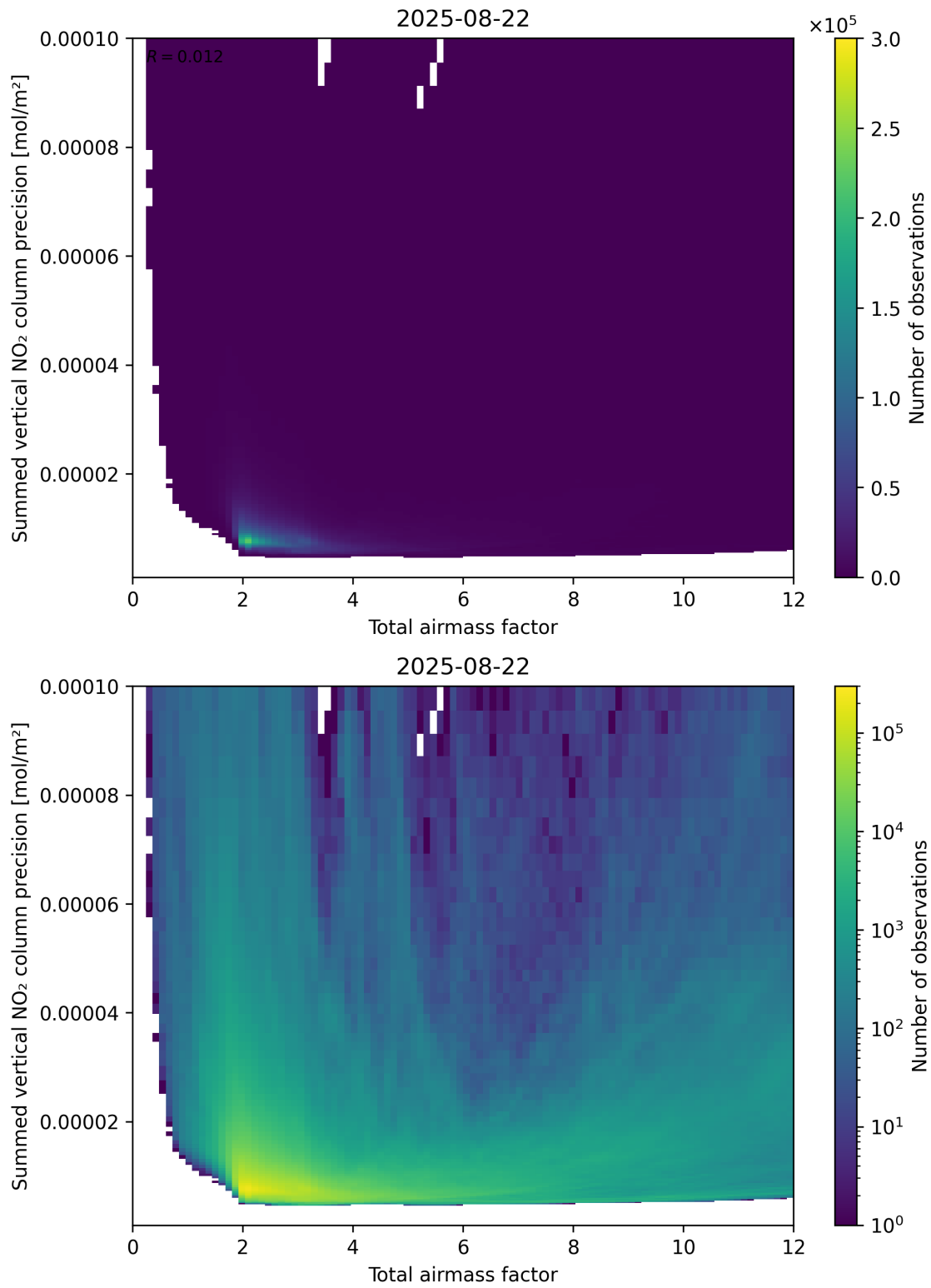
Figure 66: Scatter density plot of “Total airmass factor” against “Summed vertical NO 2 column precision” for 2025-08-21 to 2025-08-23.
