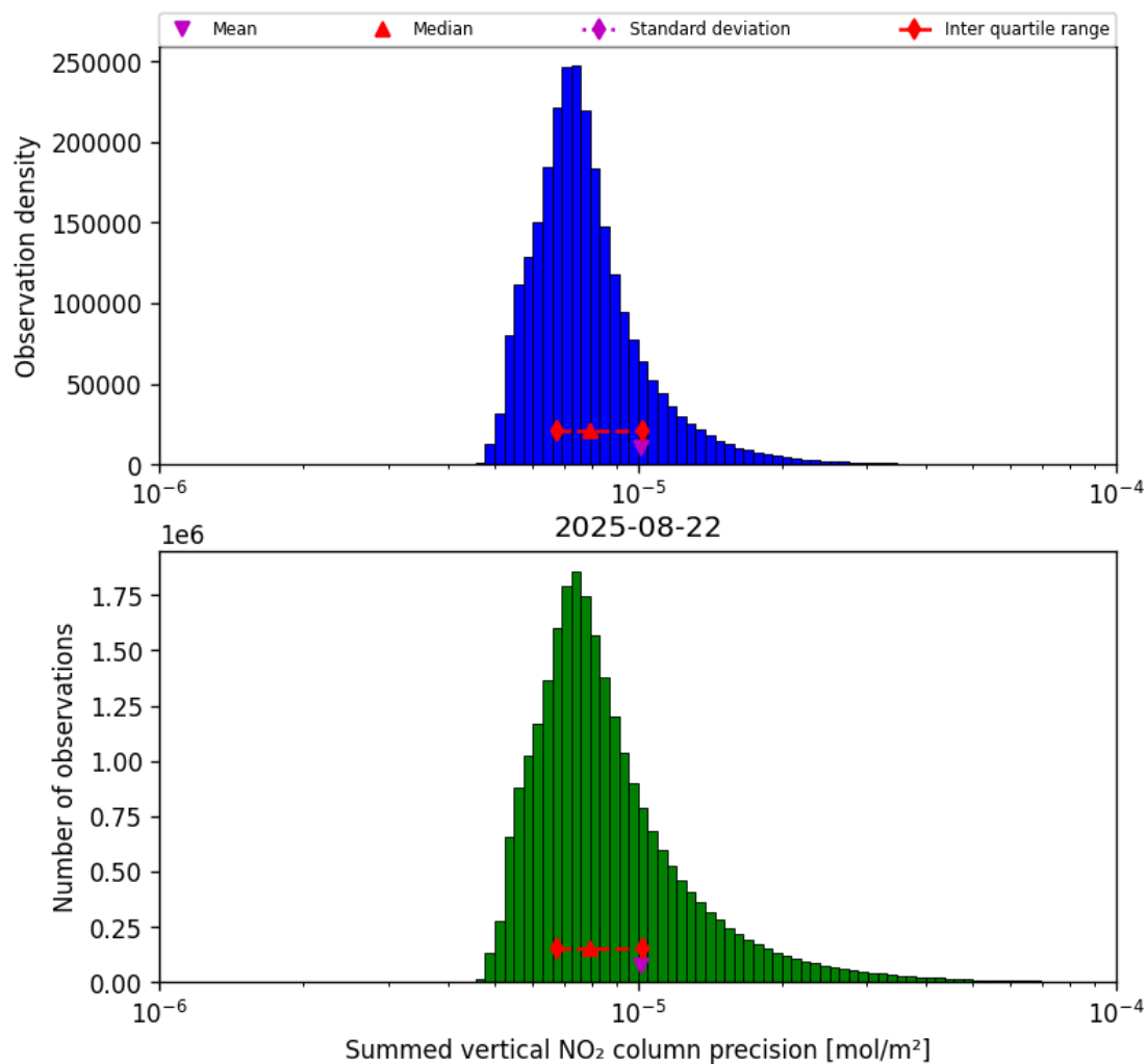
Figure 41: Histogram of “Summed vertical NO 2 column precision” for 2025-08-21 to 2025-08-23
