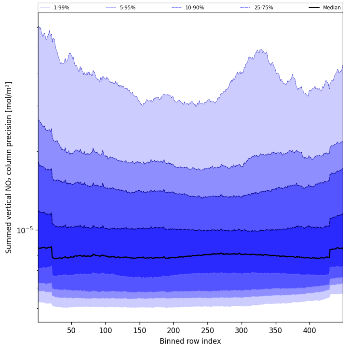
Figure 58: Along track statistics of “Summed vertical NO 2 column precision” for 2025-08-21 to 2025-08-23
