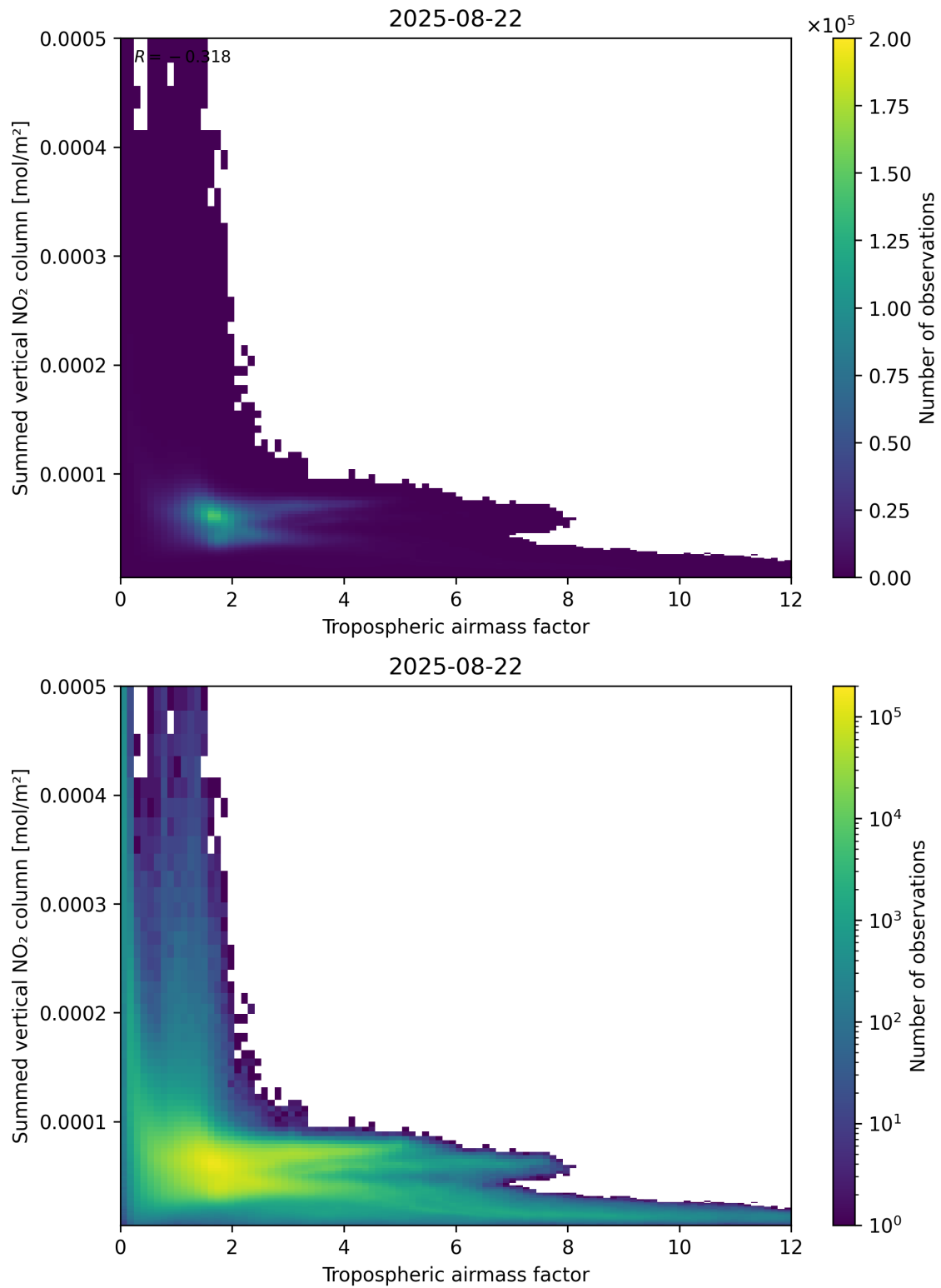
Figure 75: Scatter density plot of “Tropospheric air mass factor” against “Summed vertical NO 2 column” for 2025-08-21 to 2025-08-23.
