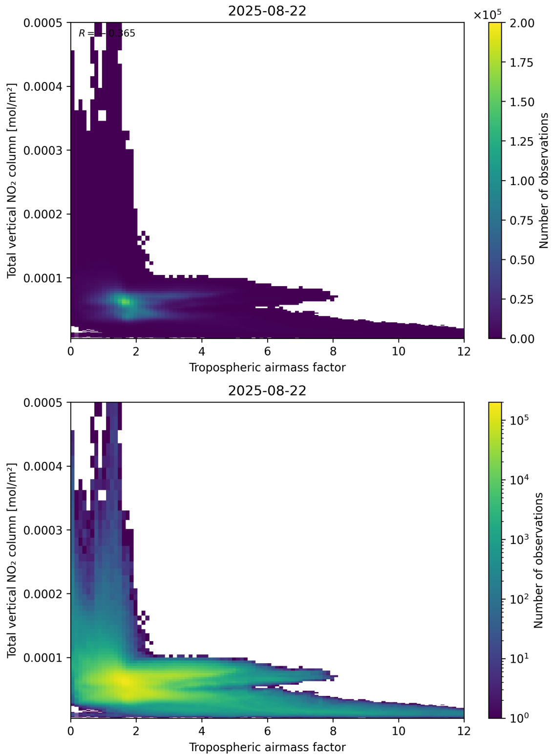
Figure 77: Scatter density plot of “Tropospheric airmass factor” against “Total vertical NO 2 column” for 2025-08-21 to 2025-08-23.
