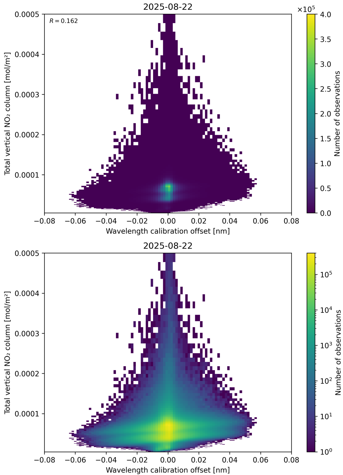
Figure 179: Scatter density plot of “Wavelength calibration offset” against “Total vertical NO 2 column” for 2025-08-21 to 2025-08-23.
