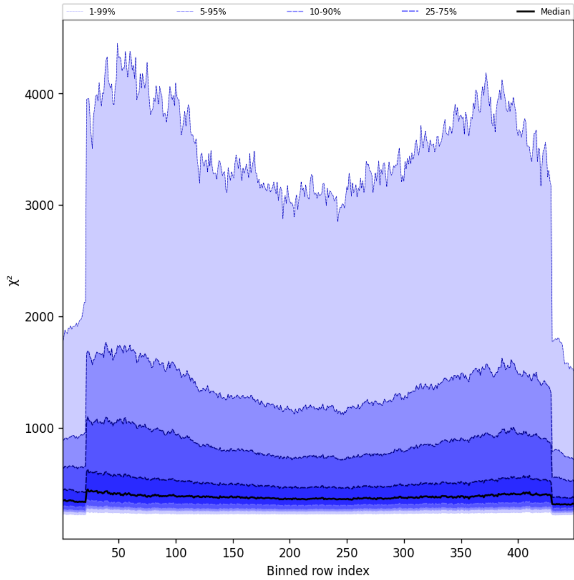
Figure 59: Along track statistics of “ \chi^2 ” for 2025-08-21 to 2025-08-23
