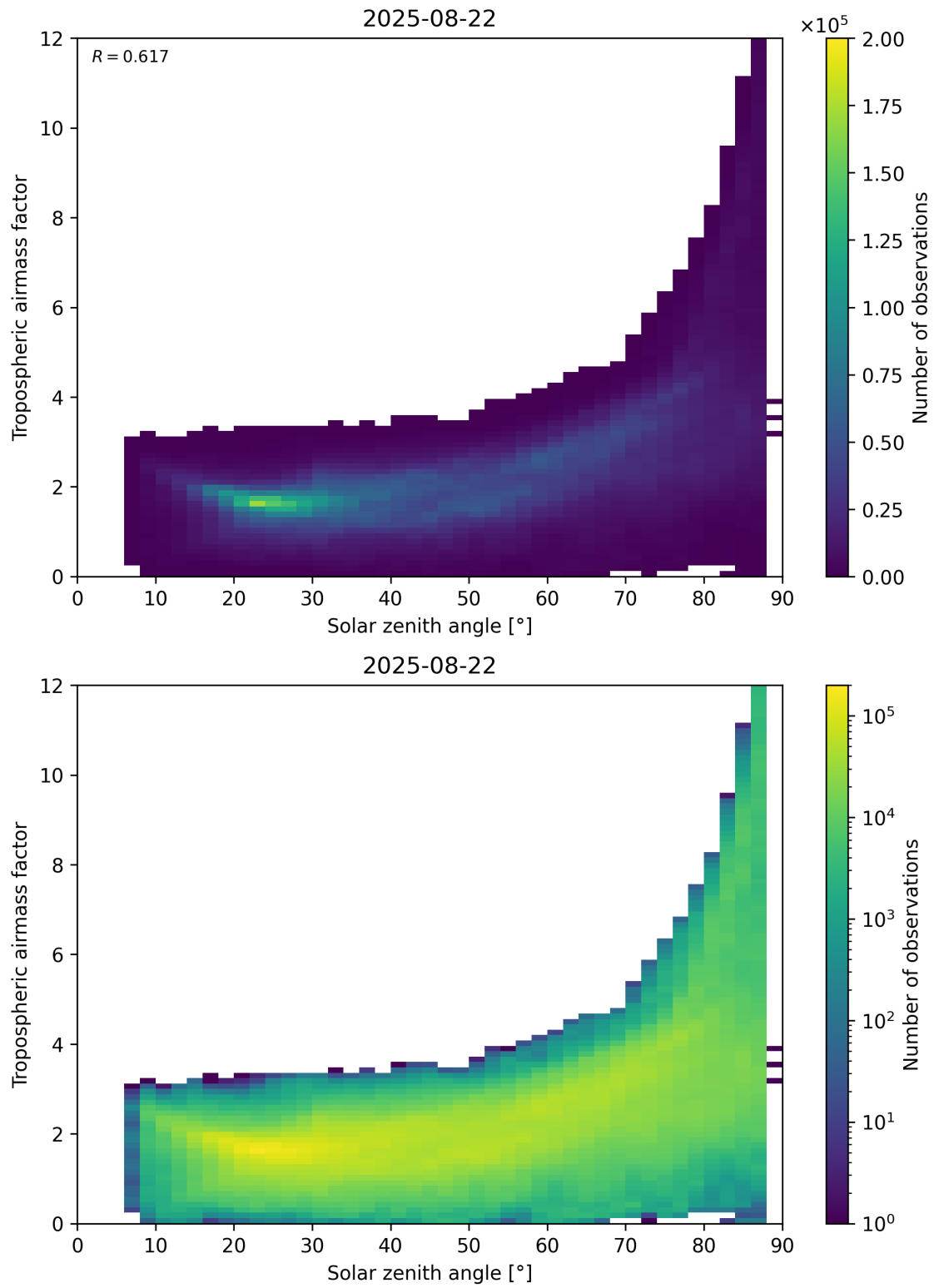
Figure 147: Scatter density plot of “Solar zenith angle” against “Tropospheric airmass factor” for 2025-08-21 to 2025-08-23.
