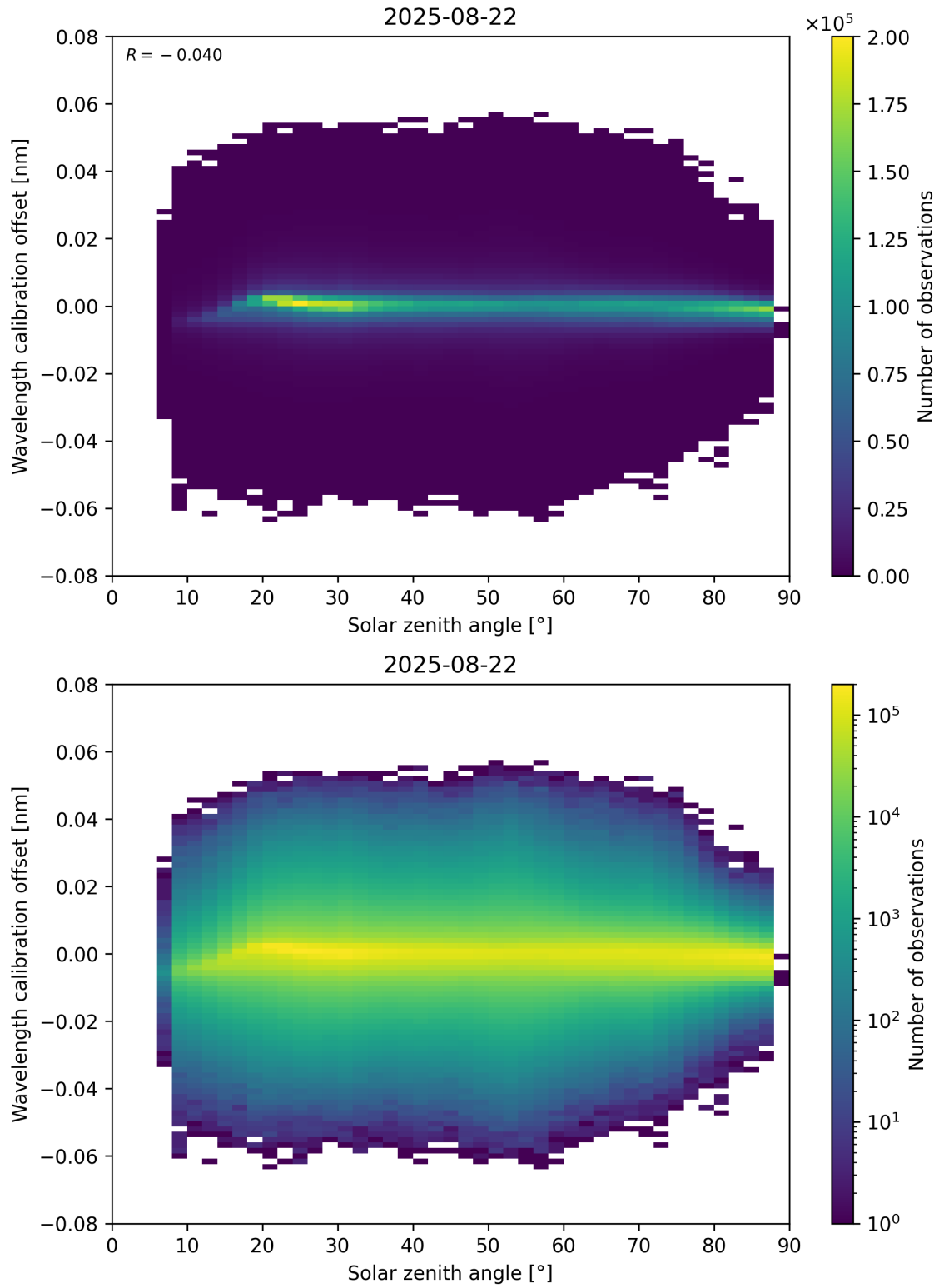
Figure 158: Scatter density plot of “Solar zenith angle” against “Wavelength calibration offset” for 2025-08-21 to 2025-08-23.
