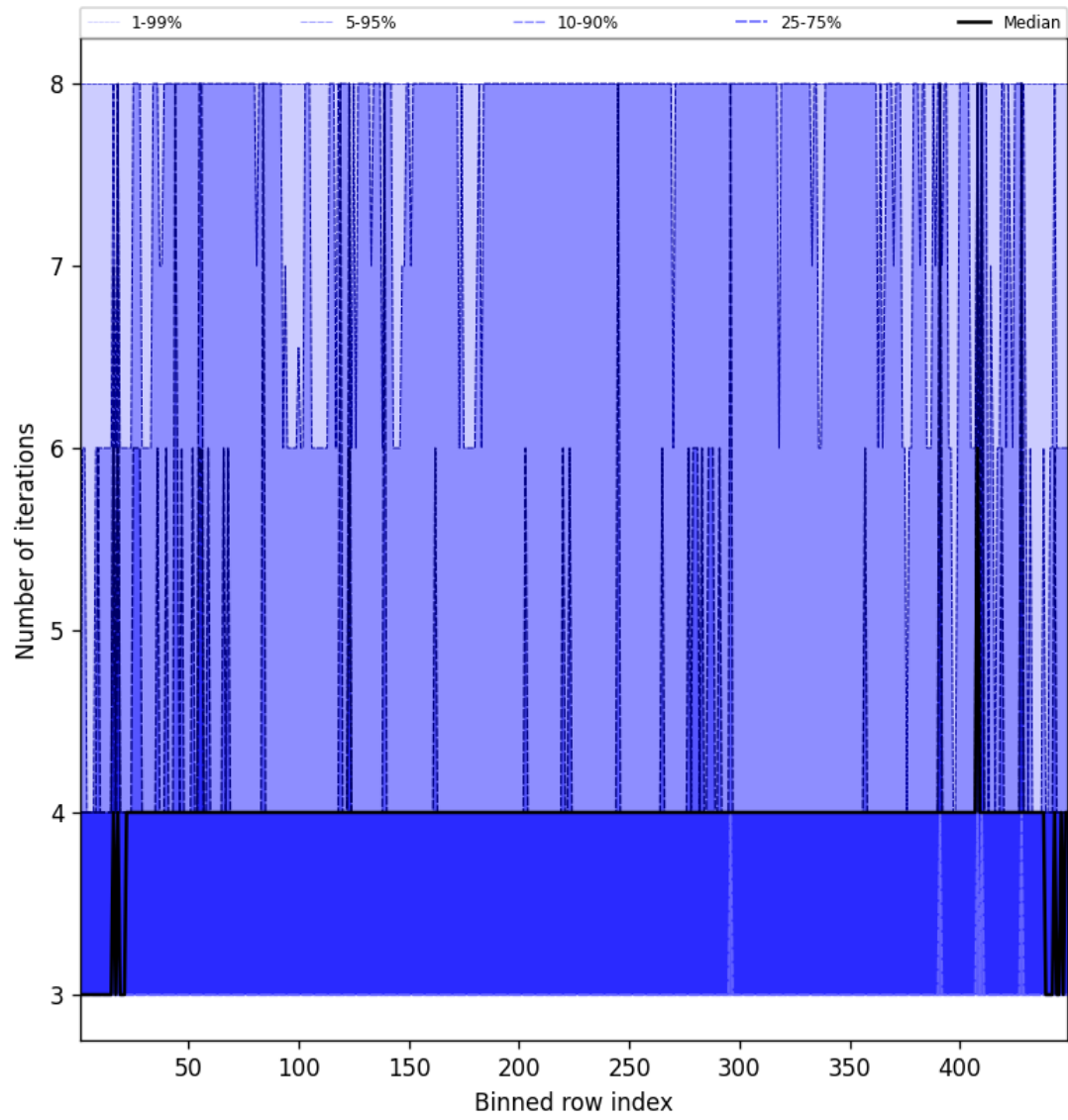
Figure 51: Along track statistics of “Number of iterations” for 2025-08-21 to 2025-08-23
