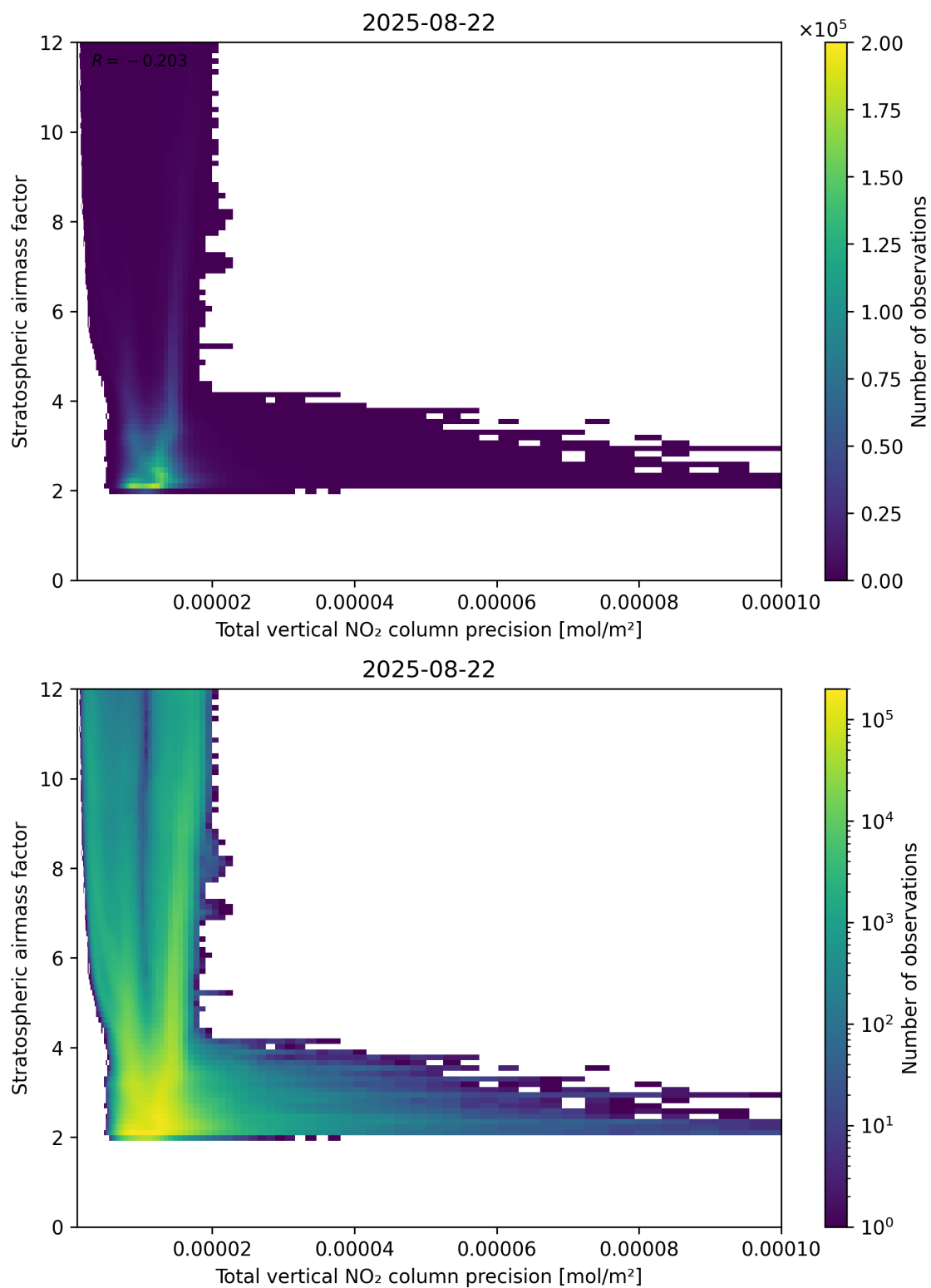
Figure 115: Scatter density plot of “Total vertical NO 2 column precision” against “Stratospheric air mass factor” for 2025-08-21 to 2025-08-23.
