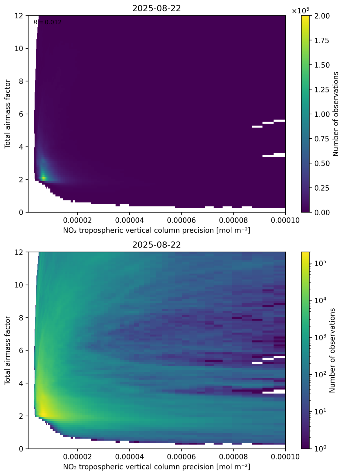
Figure 132: Scatter density plot of “NO 2 tropospheric vertical column precision” against “Total air mass factor” for 2025-08-21 to 2025-08-23.
