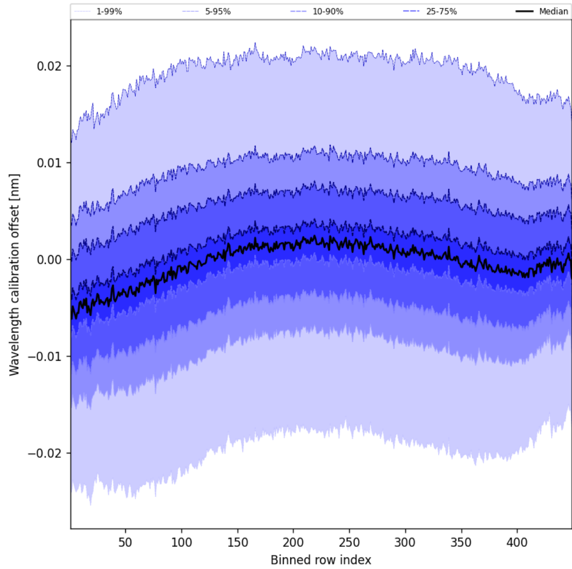
Figure 52: Along track statistics of “Wavelength calibration offset” for 2025-08-21 to 2025-08-23
