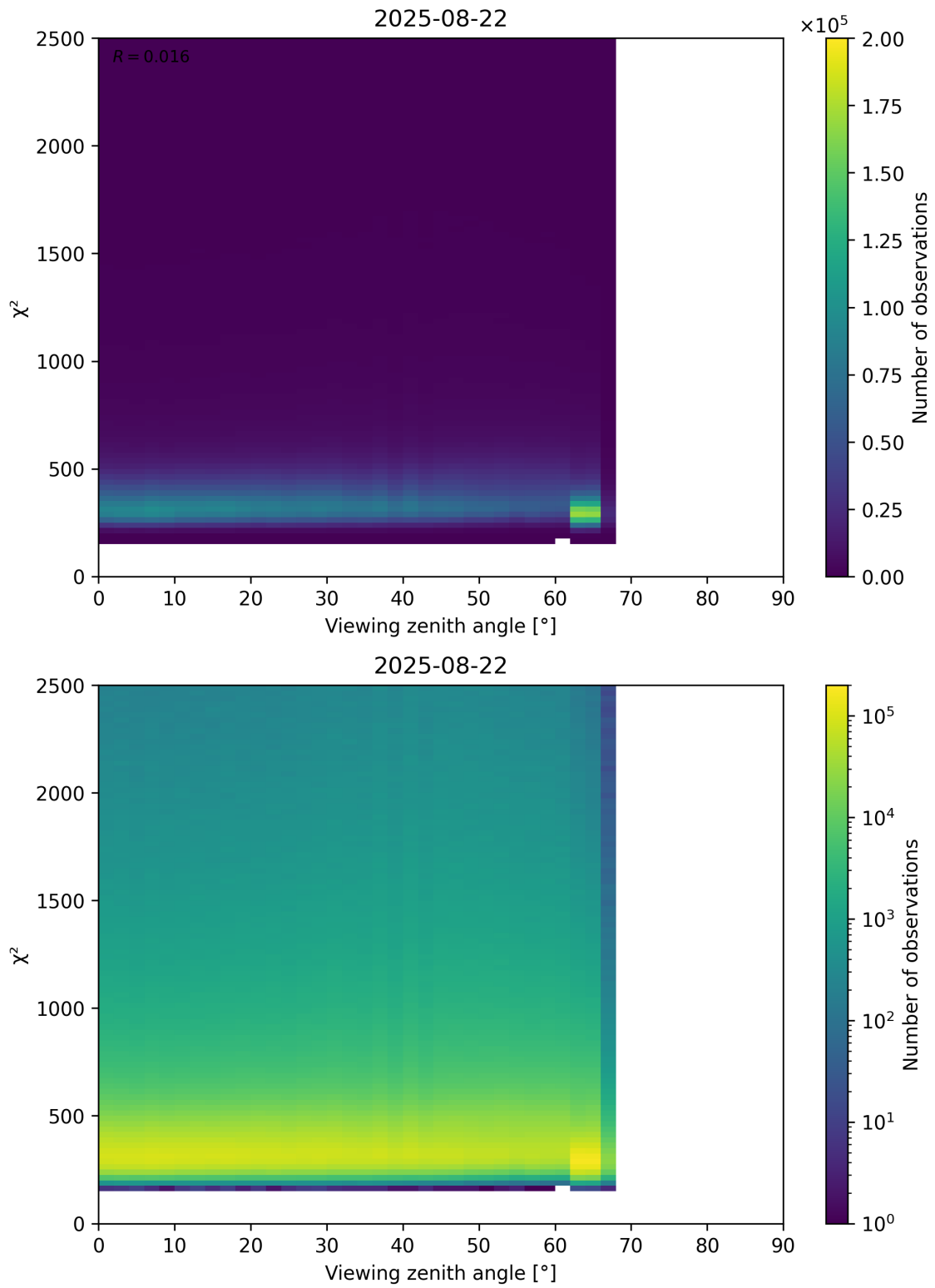
Figure 162: Scatter density plot of “Viewing zenith angle” against “ \chi^2 ” for 2025-08-21 to 2025-08-23.
