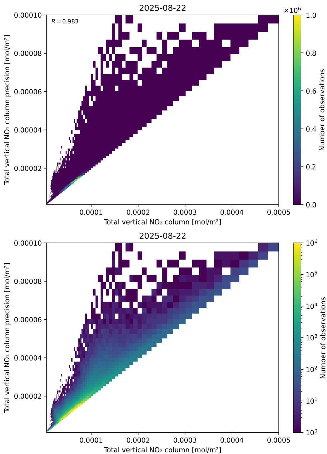
Figure 114: Scatter density plot of “Total vertical NO 2 column” against “Total vertical NO 2 column precision” for 2025-08-21 to 2025-08-23.
