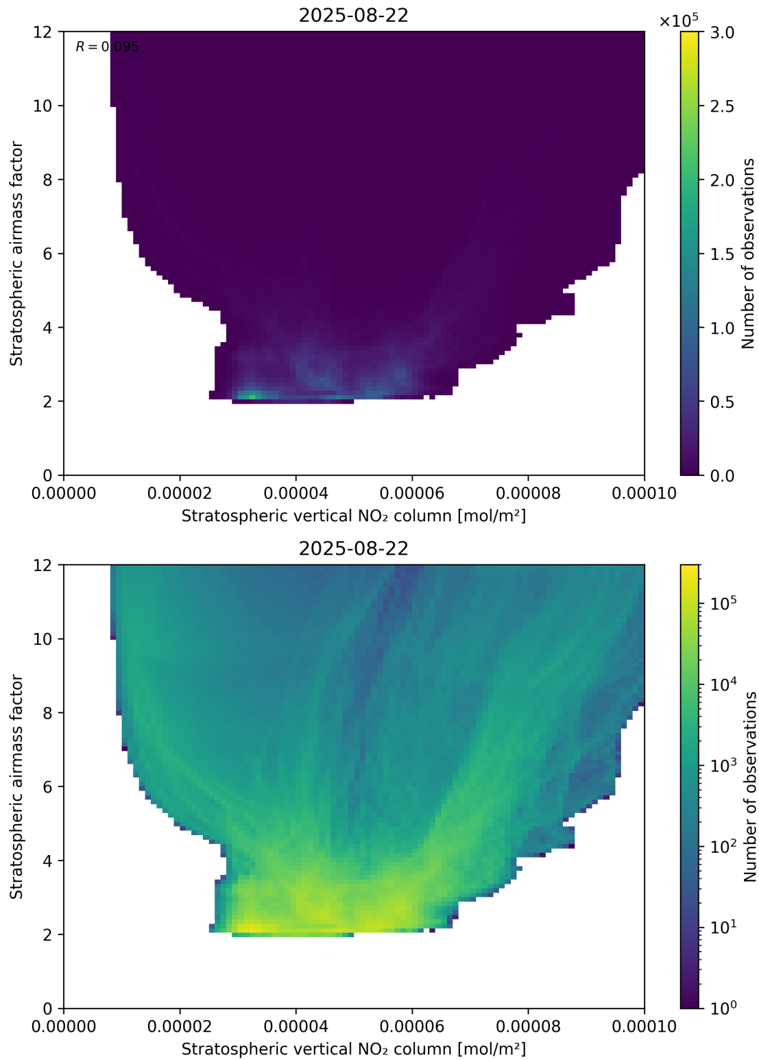
Figure 96: Scatter density plot of “Stratospheric vertical NO 2 column” against “Stratospheric airmass factor” for 2025-08-21 to 2025-08-23.
