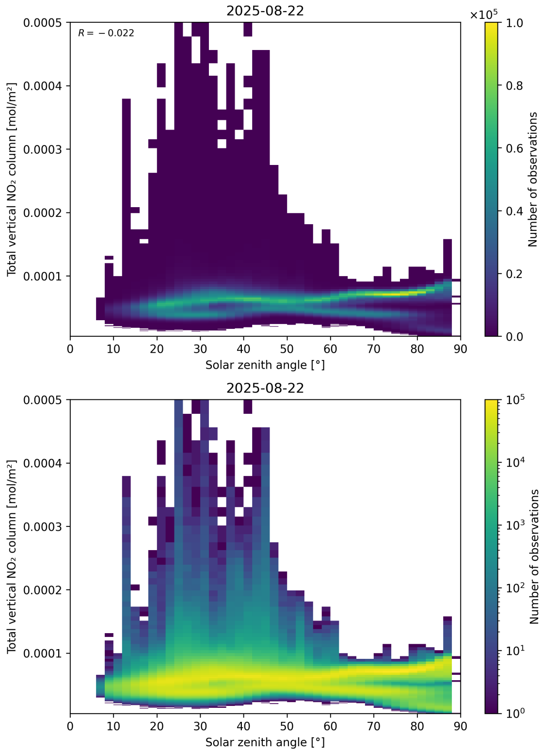
Figure 153: Scatter density plot of “Solar zenith angle” against “Total vertical NO 2 column” for 2025-08-21 to 2025-08-23.
