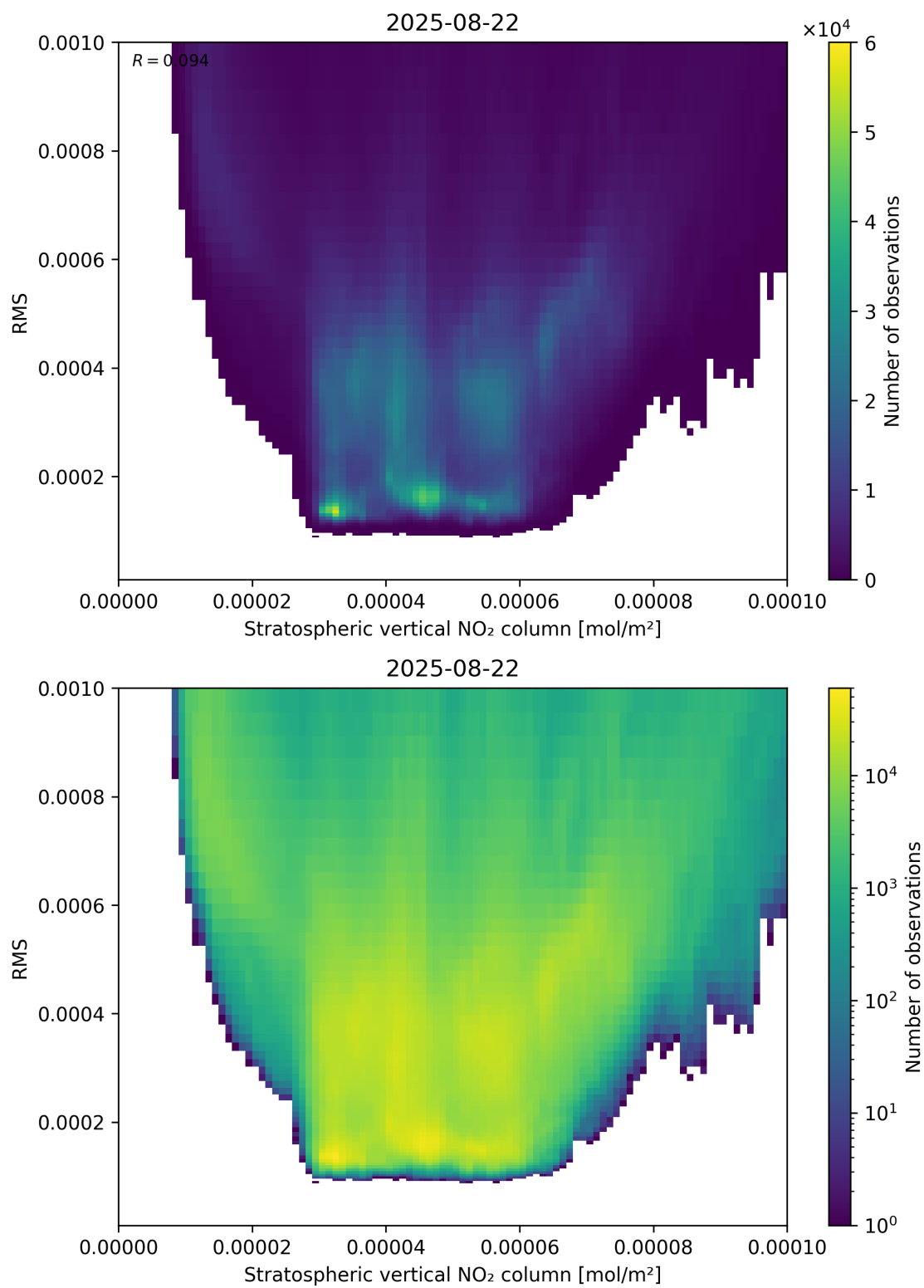
Figure 102: Scatter density plot of “Stratospheric vertical NO 2 column” against “RMS” for 2025-08-21 to 2025-08-23.
