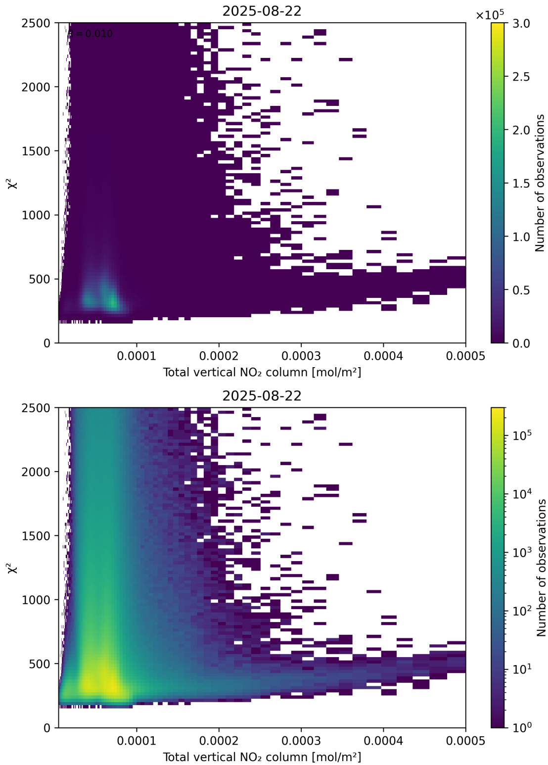
Figure 111: Scatter density plot of “Total vertical NO 2 column” against “ \chi^2 ” for 2025-08-21 to 2025-08-23.
