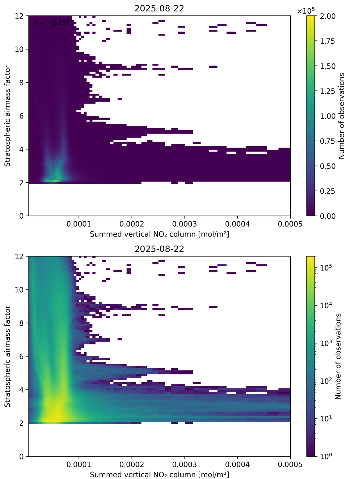
Figure 103: Scatter density plot of “Summed vertical NO 2 column” against “Stratospheric airmass factor” for 2025-08-21 to 2025-08-23.
