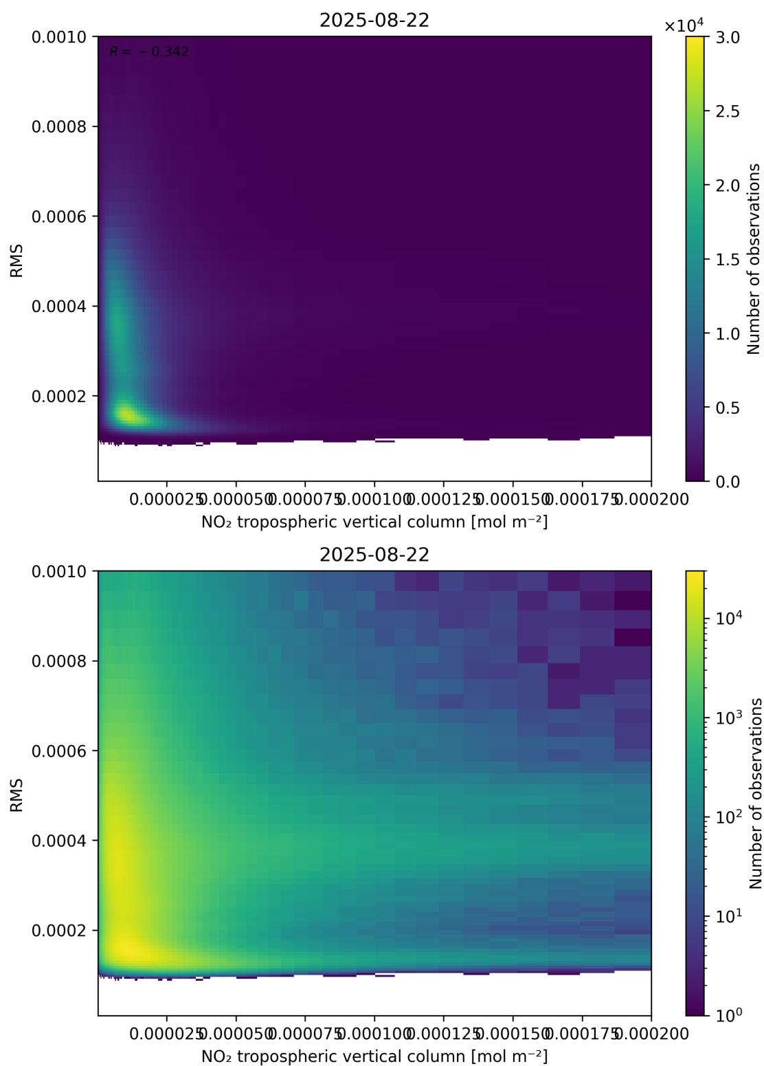
Figure 142: Scatter density plot of “NO 2 tropospheric vertical column” against “RMS” for 2025-08-21 to 2025-08-23.
