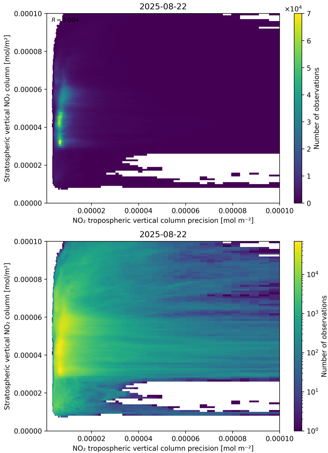
Figure 135: Scatter density plot of “NO 2 tropospheric vertical column precision” against “Stratospheric vertical NO 2 column” for 2025-08-21 to 2025-08-23.
