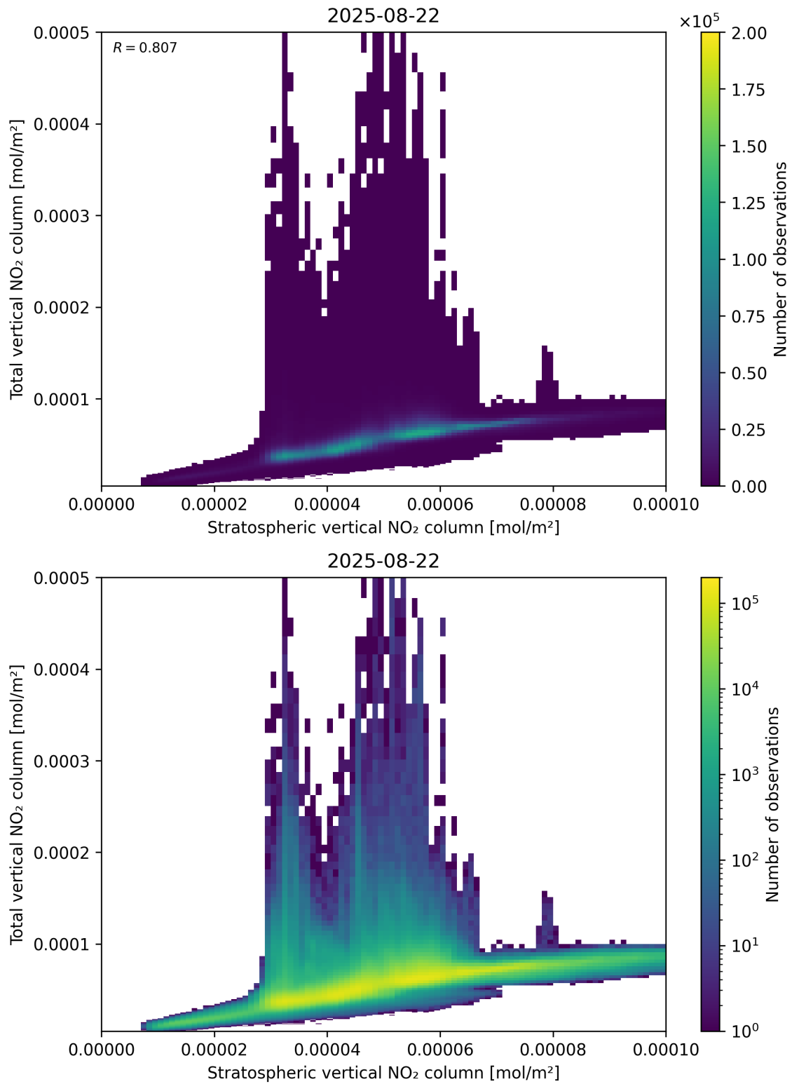
Figure 100: Scatter density plot of “Stratospheric vertical NO 2 column” against “Total vertical NO 2 column” for 2025-08-21 to 2025-08-23.
