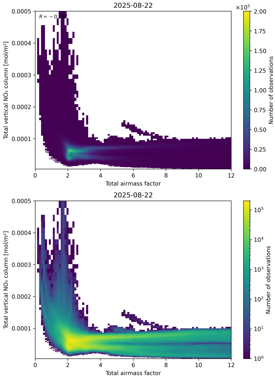
Figure 67: Scatter density plot of “Total airmass factor” against “Total vertical NO 2 column” for 2025-08-21 to 2025-08-23.
