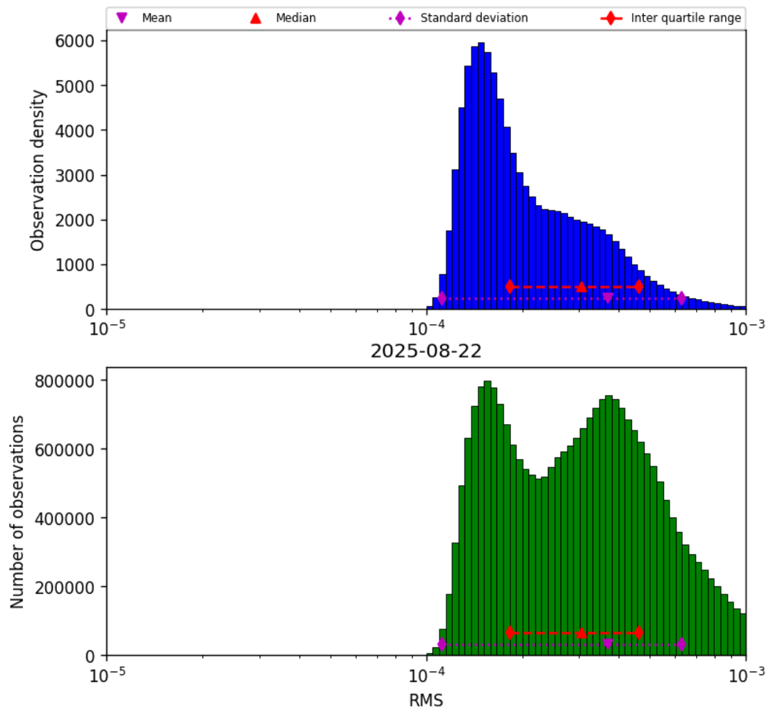
Figure 43: Histogram of “RMS” for 2025-08-21 to 2025-08-23
