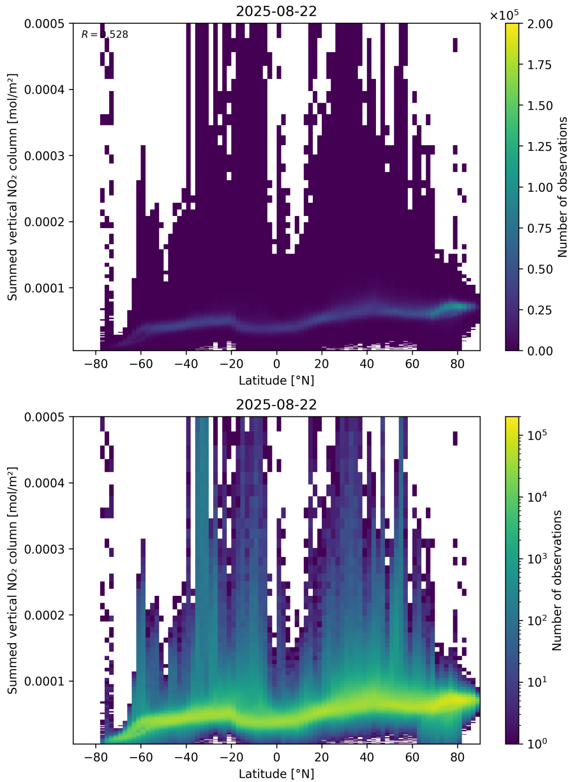
Figure 88: Scatter density plot of “Latitude” against “Summed vertical NO 2 column” for 2025-08-21 to 2025-08-23.
