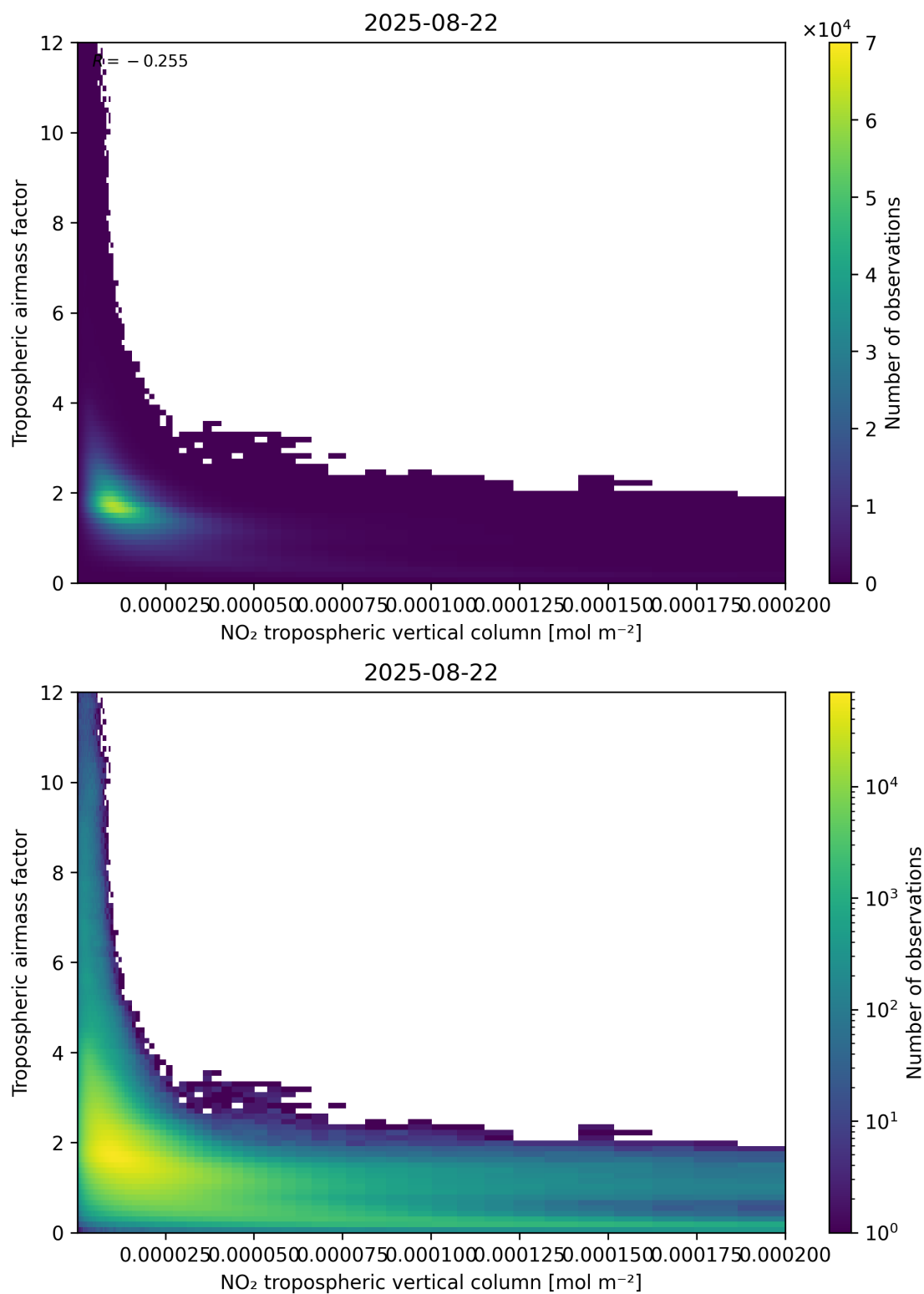
Figure 123: Scatter density plot of “NO 2 tropospheric vertical column” against “Tropospheric air mass factor” for 2025-08-21 to 2025-08-23.
