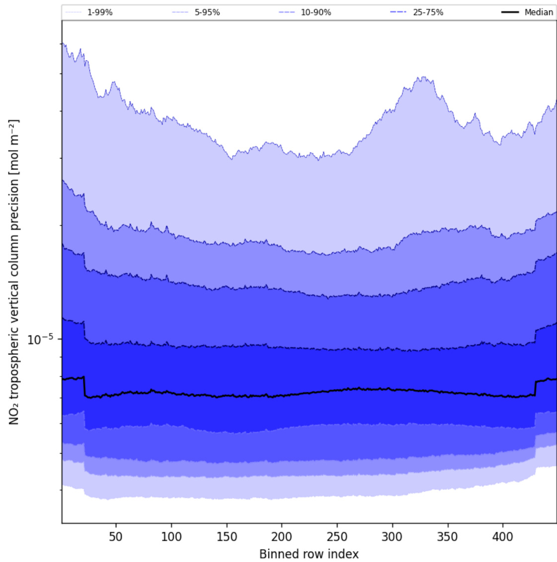
Figure 47: Along track statistics of “NO 2 tropospheric vertical column precision” for 2025-08-21 to 2025-08-23
