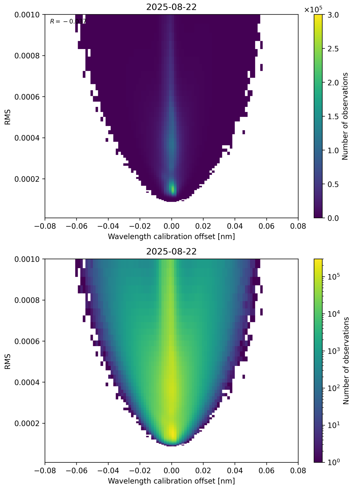
Figure 181: Scatter density plot of “Wavelength calibration offset” against “RMS” for 2025-08-21 to 2025-08-23.
