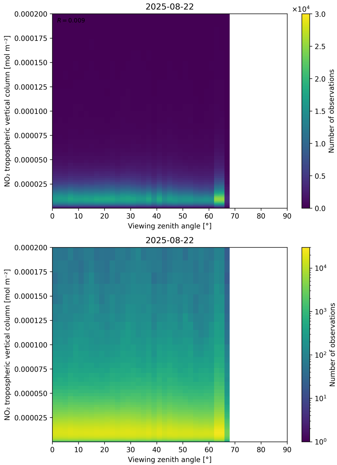
Figure 169: Scatter density plot of “Viewing zenith angle” against “NO 2 tropospheric vertical column” for 2025-08-21 to 2025-08-23.
