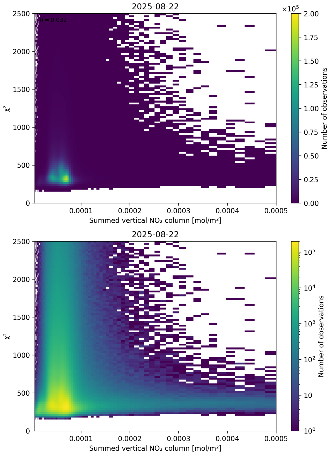
Figure 104: Scatter density plot of “Summed vertical NO 2 column” against “ \chi^2 ” for 2025-08-21 to 2025-08-23.
