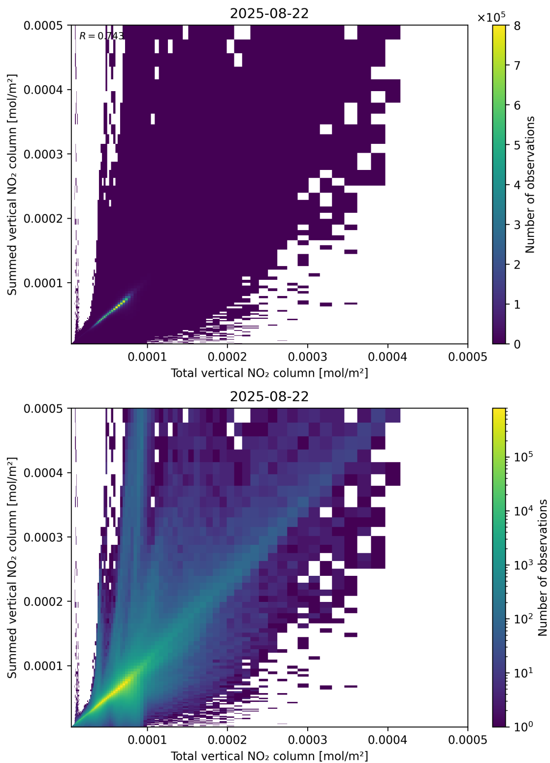
Figure 112: Scatter density plot of “Total vertical NO 2 column” against “Summed vertical NO 2 column” for 2025-08-21 to 2025-08-23.
