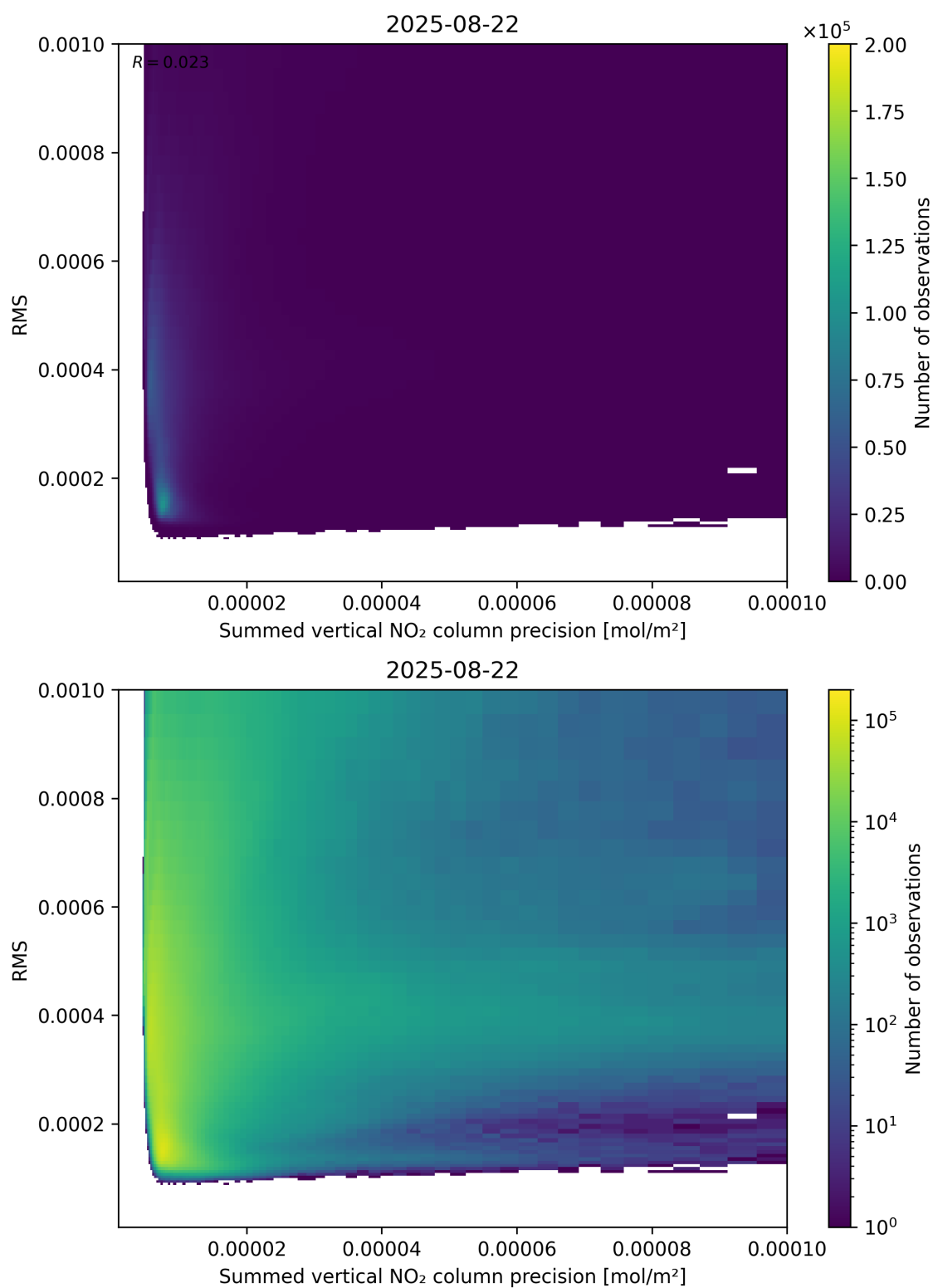
Figure 108: Scatter density plot of “Summed vertical NO 2 column precision” against “RMS” for 2025-08-21 to 2025-08-23.
