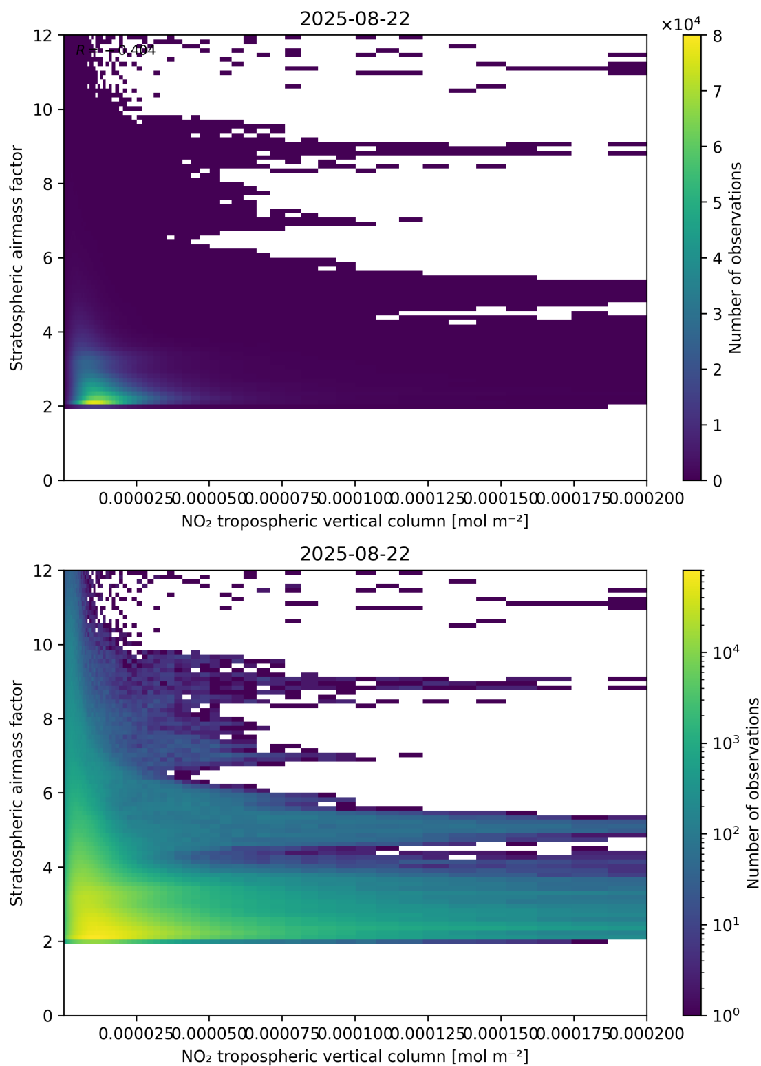
Figure 121: Scatter density plot of “NO 2 tropospheric vertical column” against “Stratospheric airmass factor” for 2025-08-21 to 2025-08-23.
