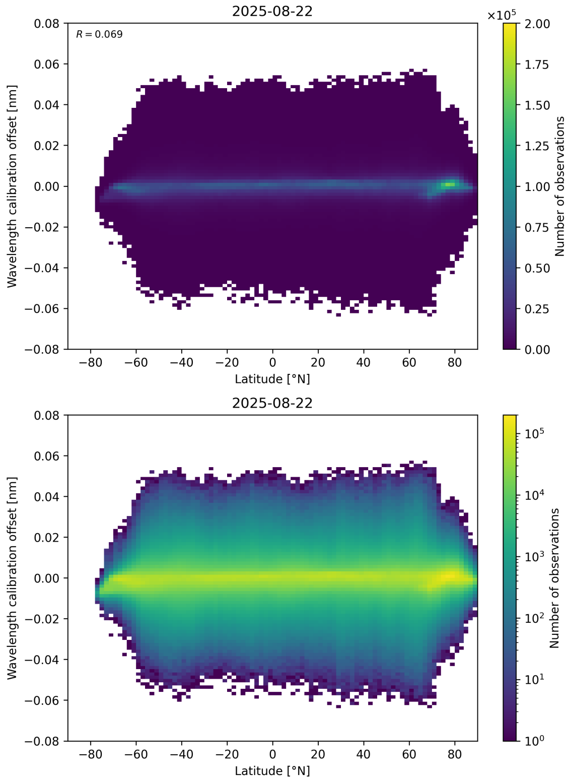
Figure 95: Scatter density plot of “Latitude” against “Wavelength calibration offset” for 2025-08-21 to 2025-08-23.
