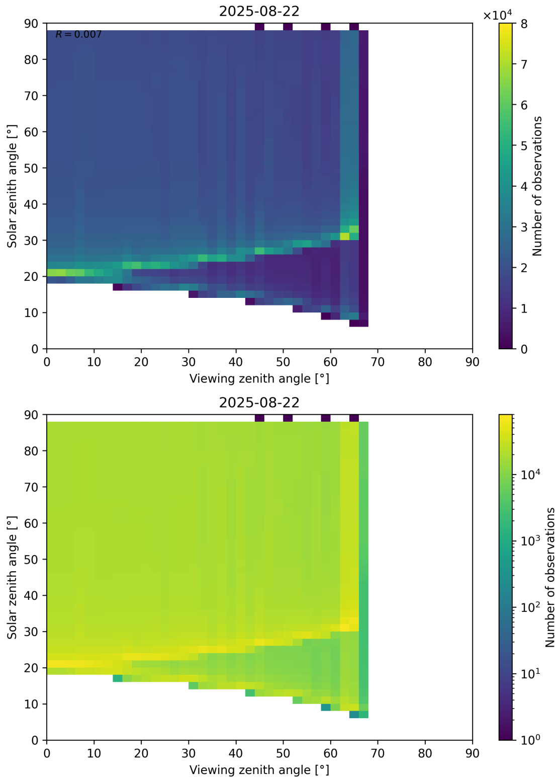
Figure 172: Scatter density plot of “Viewing zenith angle” against “Solar zenith angle” for 2025-08-21 to 2025-08-23.
