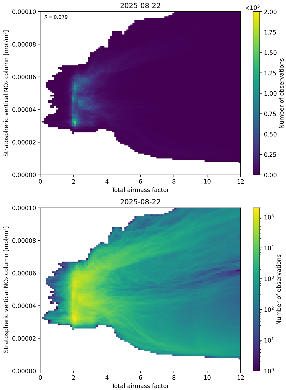
Figure 64: Scatter density plot of “Total airmass factor” against “Stratospheric vertical NO 2 column” for 2025-08-21 to 2025-08-23.
