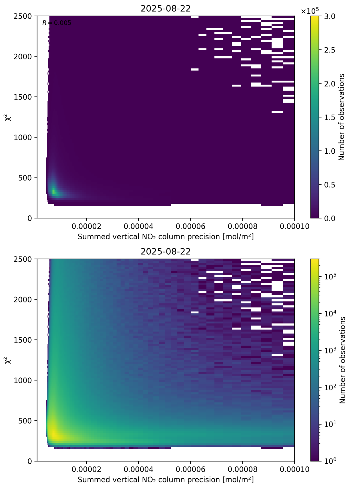
Figure 107: Scatter density plot of “Summed vertical NO 2 column precision” against “ \chi^2 ” for 2025-08-21 to 2025-08-23.
