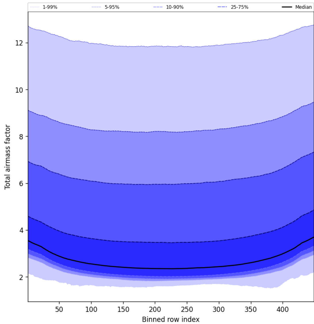
Figure 49: Along track statistics of “Total airmass factor” for 2025-08-21 to 2025-08-23
