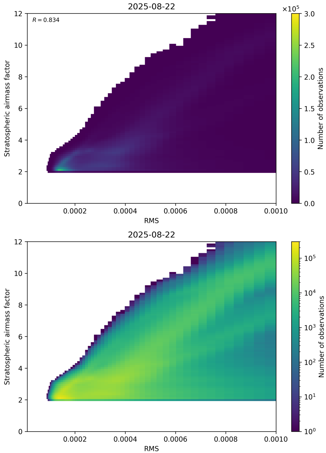
Figure 144: Scatter density plot of “RMS” against “Stratospheric airmass factor” for 2025-08-21 to 2025-08-23.
