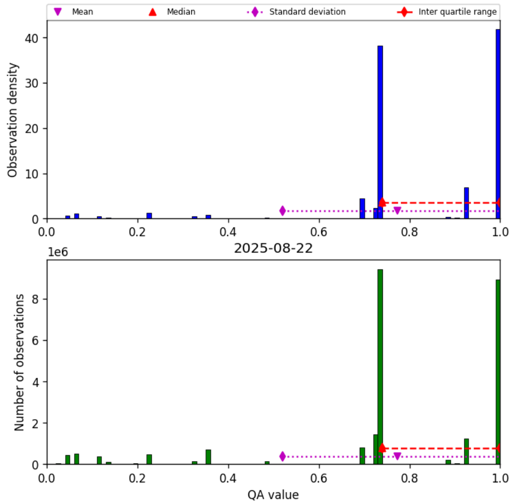
Figure 28: Histogram of “QA value” for 2025-08-21 to 2025-08-23
