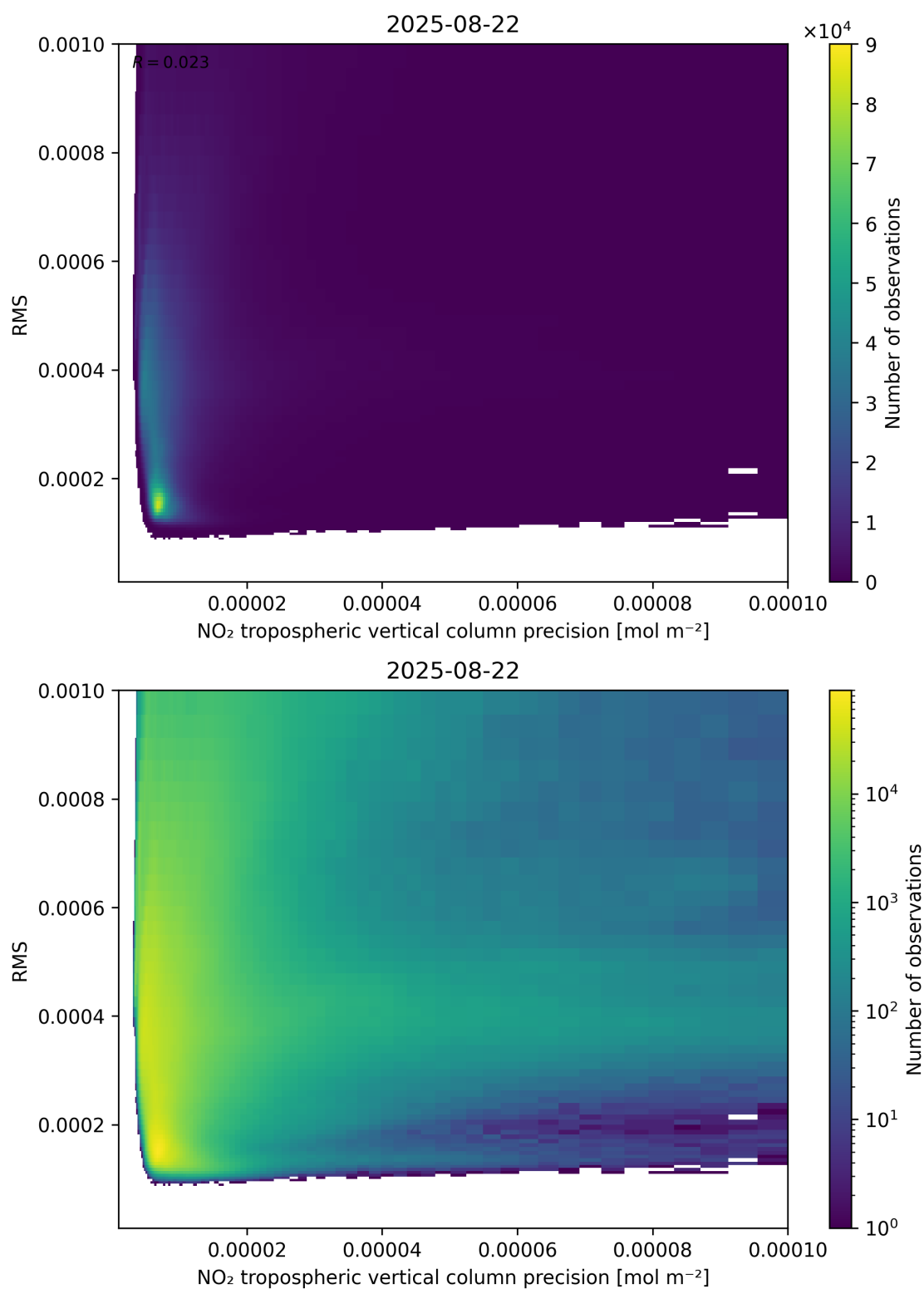
Figure 140: Scatter density plot of “NO 2 tropospheric vertical column precision” against “RMS” for 2025-08-21 to 2025-08-23.
