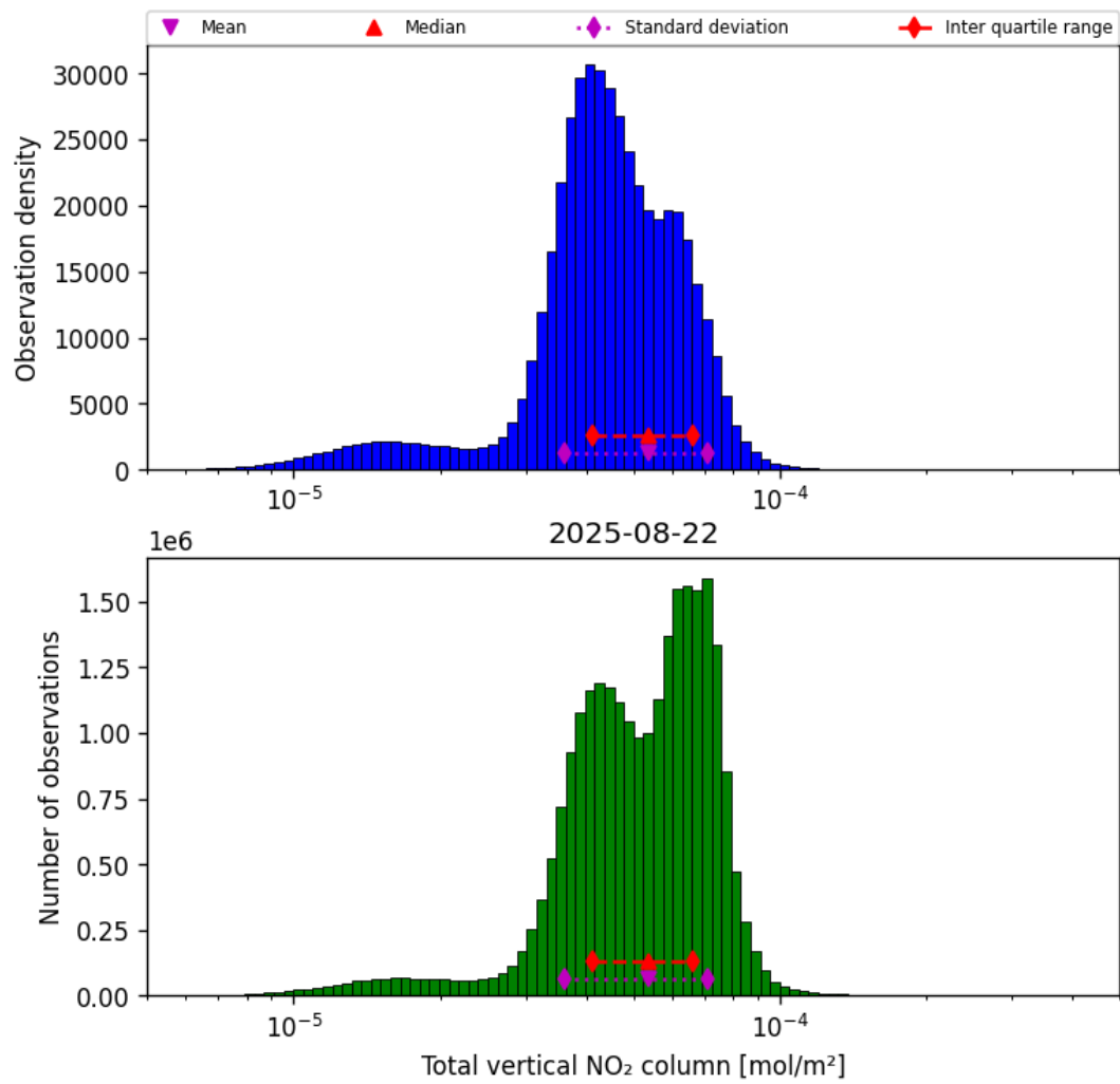
Figure 38: Histogram of “Total vertical NO 2 column” for 2025-08-21 to 2025-08-23
