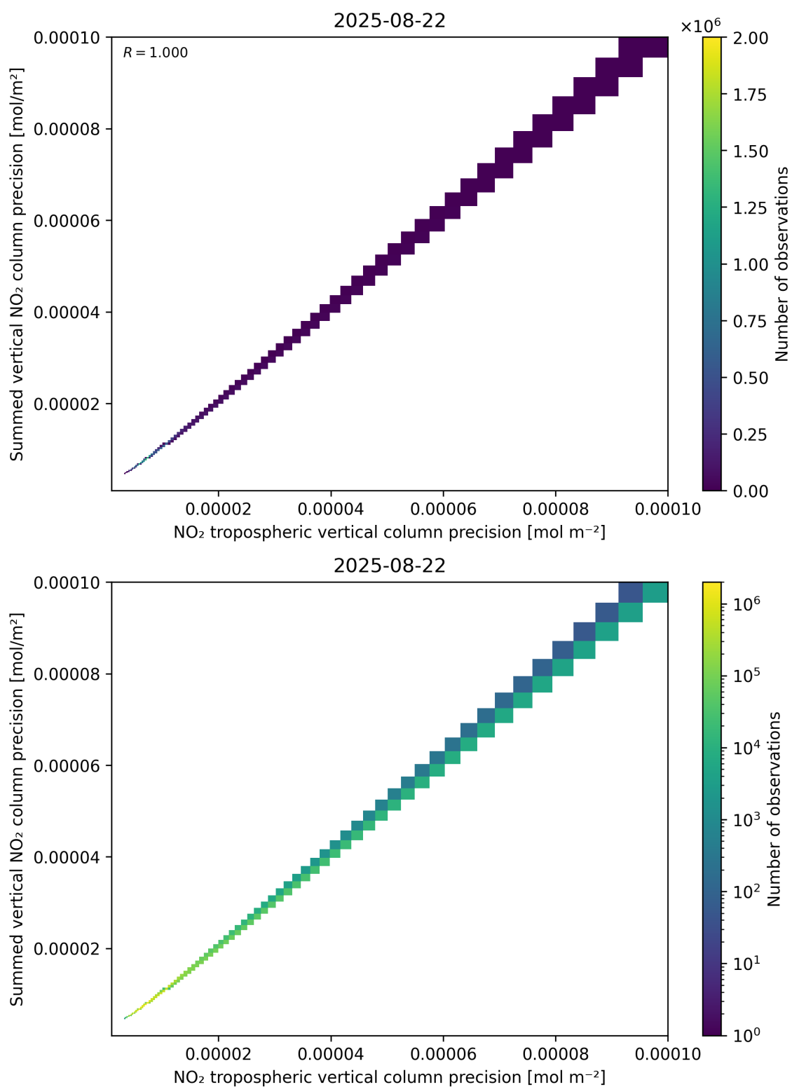
Figure 137: Scatter density plot of “NO 2 tropospheric vertical column precision” against “Summed vertical NO 2 column precision” for 2025-08-21 to 2025-08-23.
