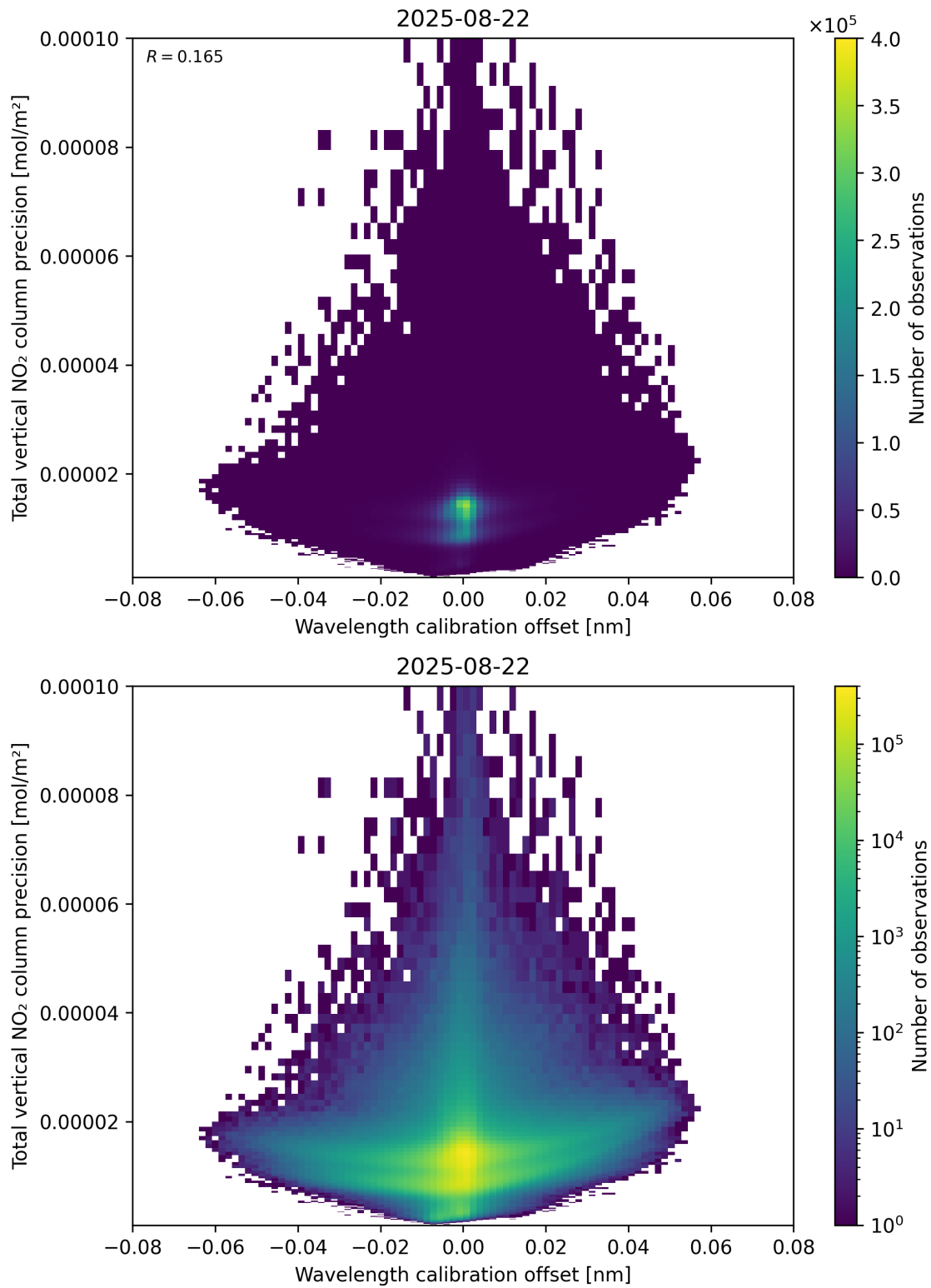
Figure 180: Scatter density plot of “Wavelength calibration offset” against “Total vertical NO 2 column precision” for 2025-08-21 to 2025-08-23.
