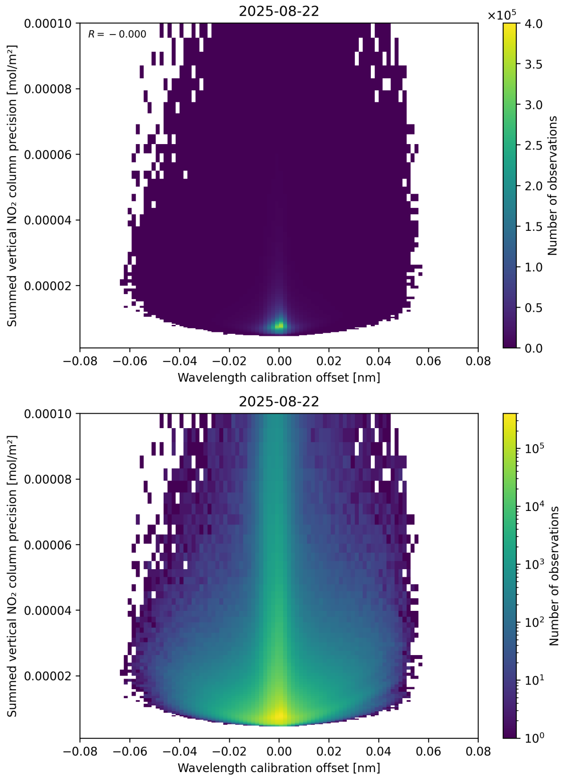
Figure 178: Scatter density plot of “Wavelength calibration offset” against “Summed vertical NO 2 column precision” for 2025-08-21 to 2025-08-23.
