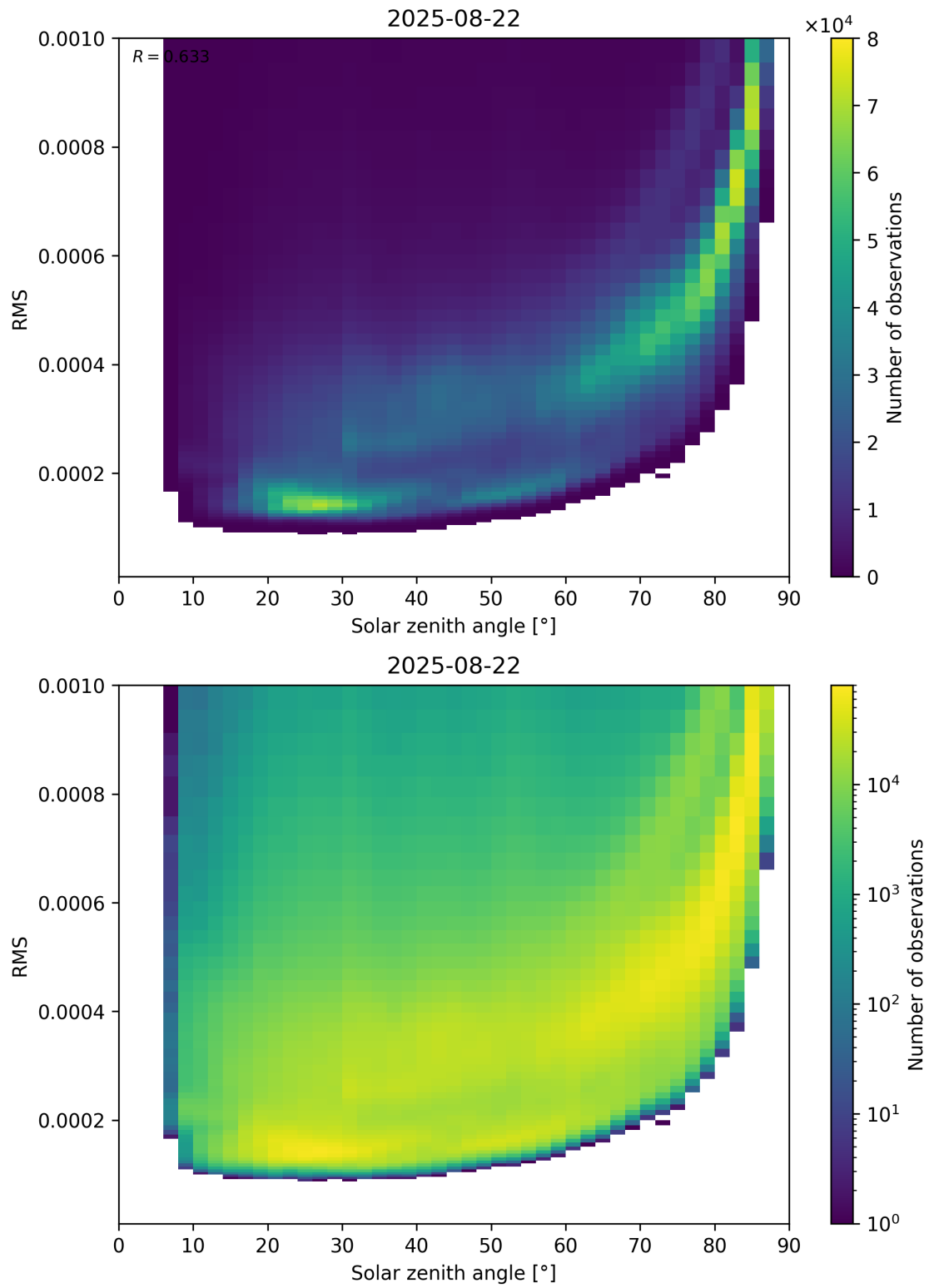
Figure 157: Scatter density plot of “Solar zenith angle” against “RMS” for 2025-08-21 to 2025-08-23.
