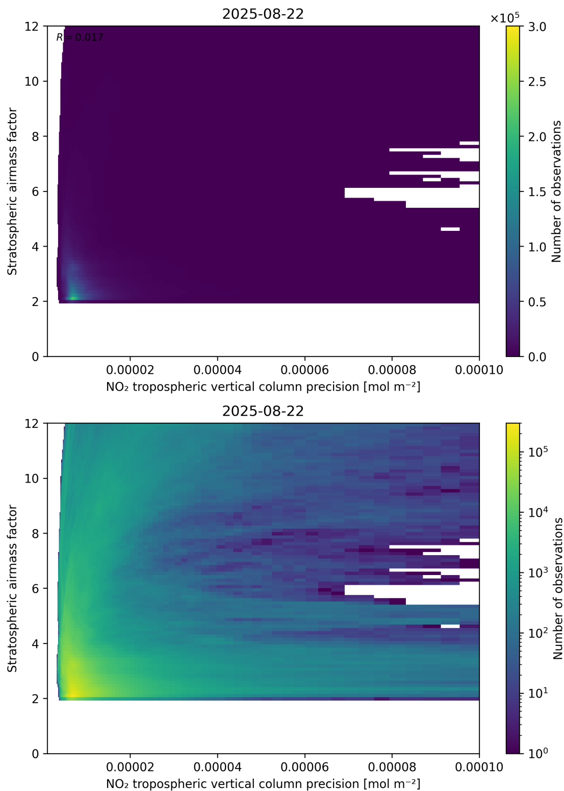
Figure 131: Scatter density plot of “NO 2 tropospheric vertical column precision” against “Stratospheric airmass factor” for 2025-08-21 to 2025-08-23.
