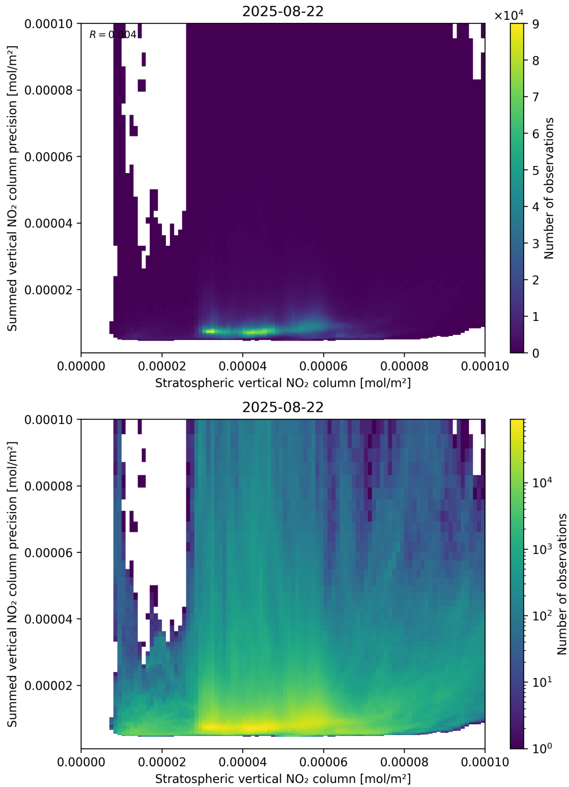
Figure 99: Scatter density plot of “Stratospheric vertical NO 2 column” against “Summed vertical NO 2 column precision” for 2025-08-21 to 2025-08-23.
