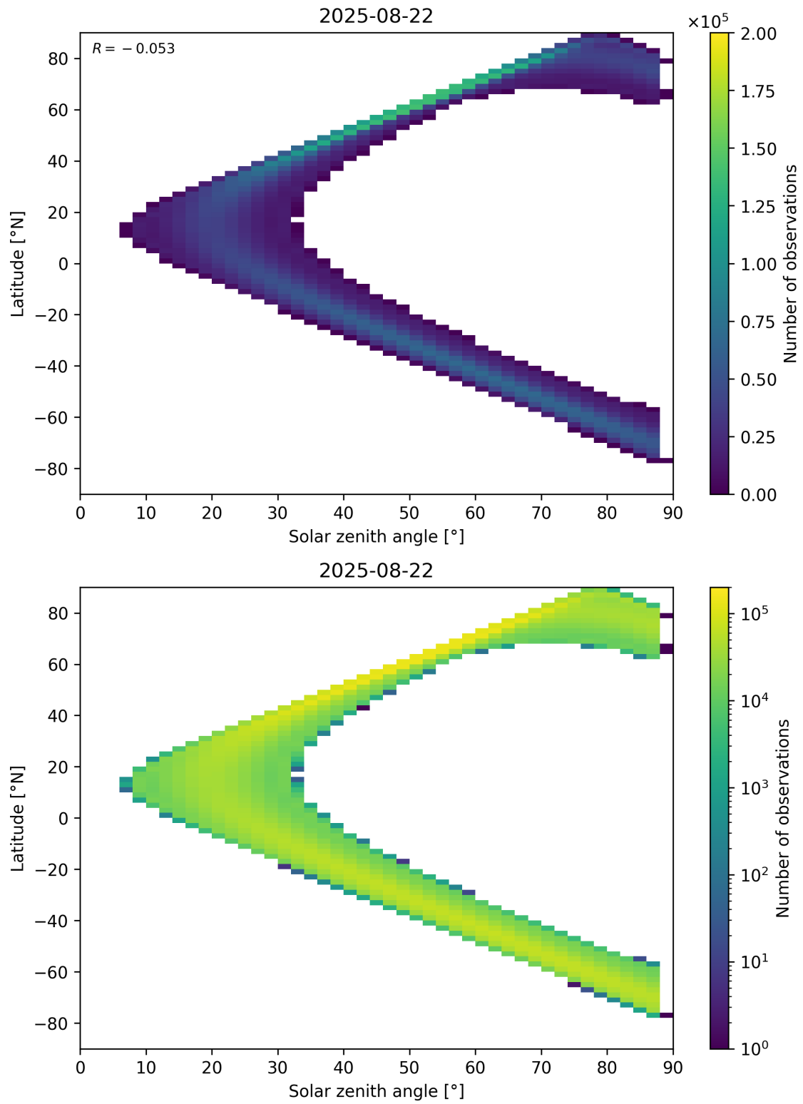
Figure 149: Scatter density plot of “Solar zenith angle” against “Latitude” for 2025-08-21 to 2025-08-23.
