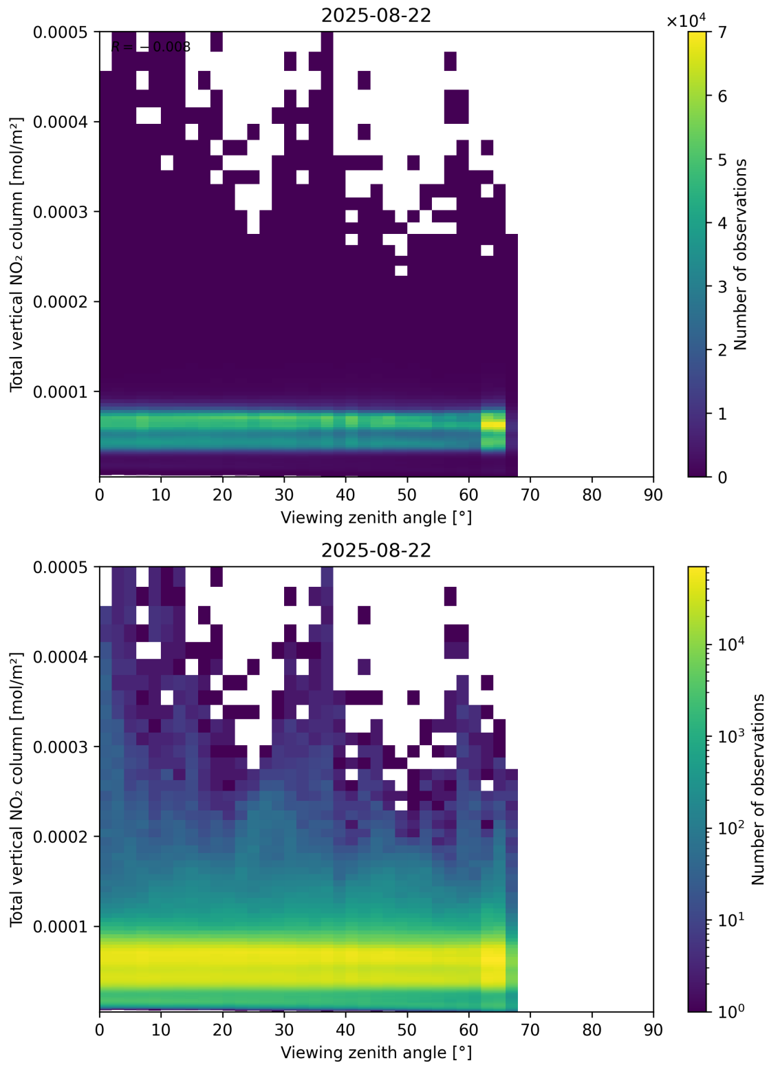
Figure 167: Scatter density plot of “Viewing zenith angle” against “Total vertical NO 2 column” for 2025-08-21 to 2025-08-23.
