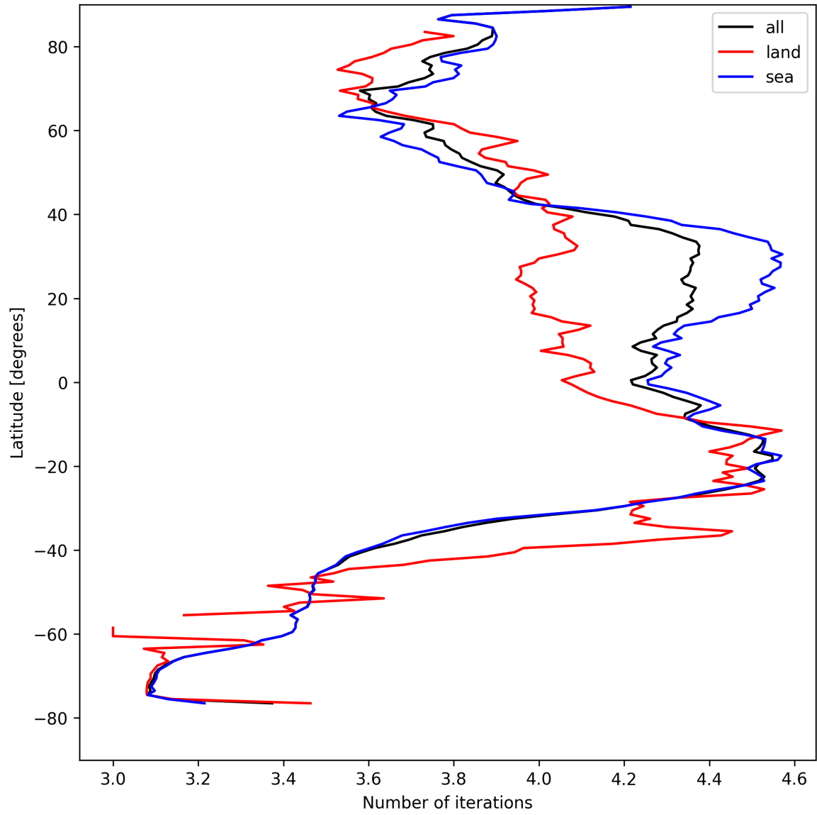
Figure 17: Zonal average of “Number of iterations” for 2025-08-21 to 2025-08-23.
