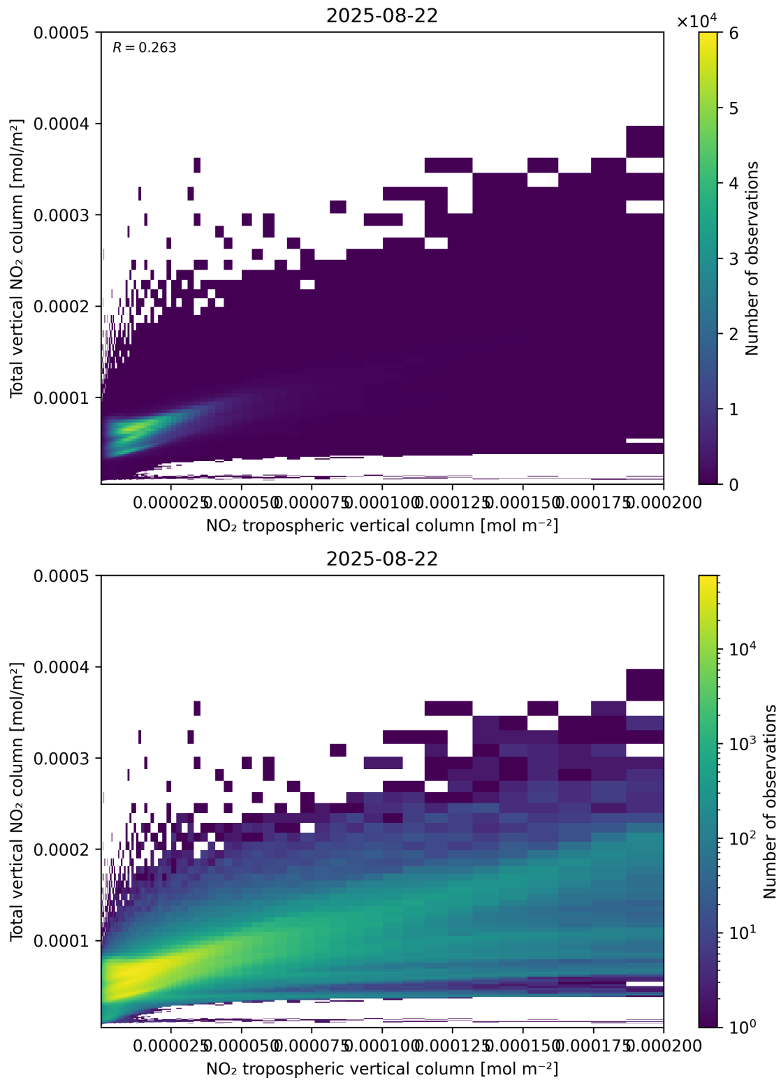
Figure 128: Scatter density plot of “NO 2 tropospheric vertical column” against “Total vertical NO 2 column” for 2025-08-21 to 2025-08-23.
