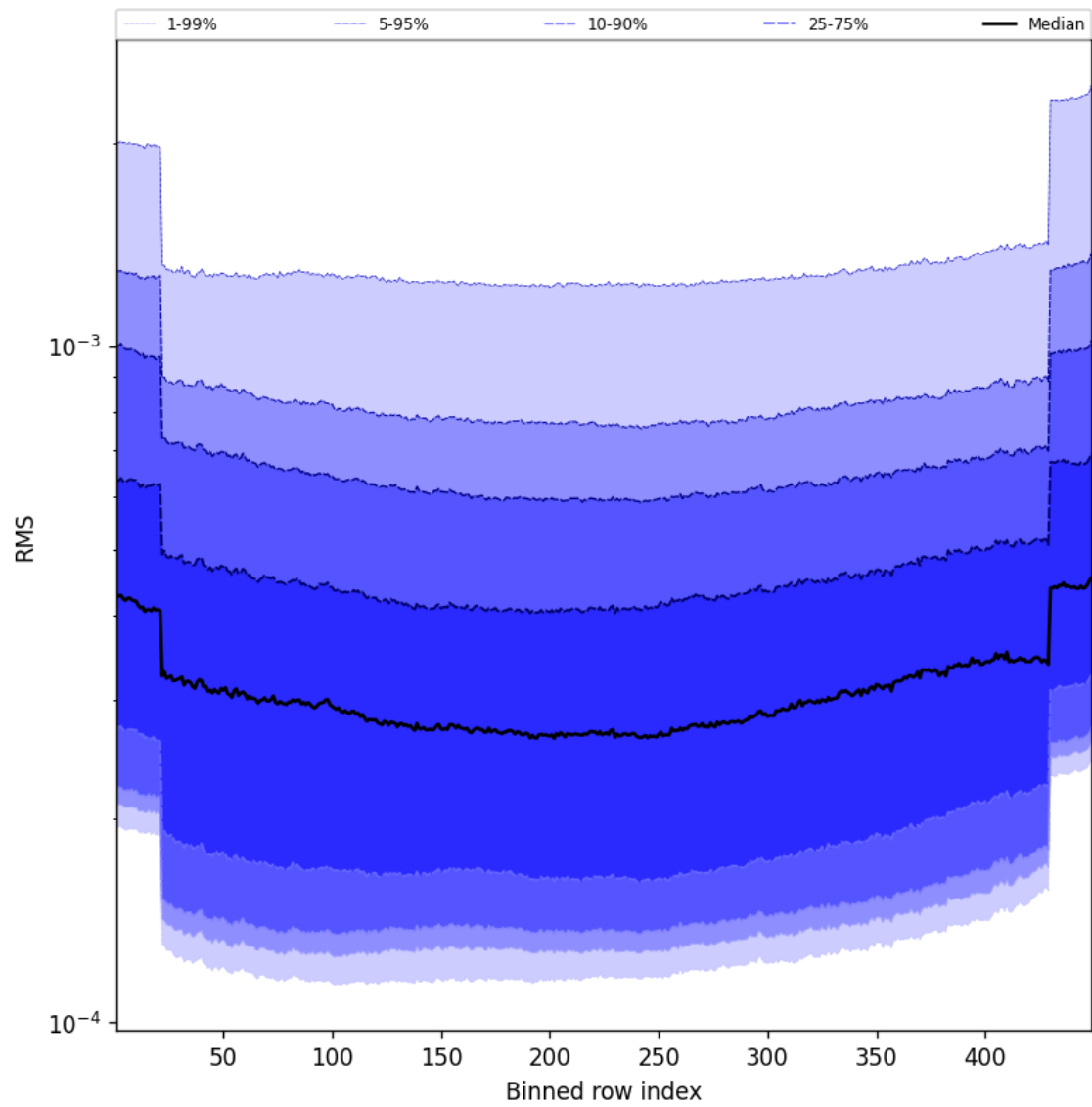
Figure 60: Along track statistics of “RMS” for 2025-08-21 to 2025-08-23
