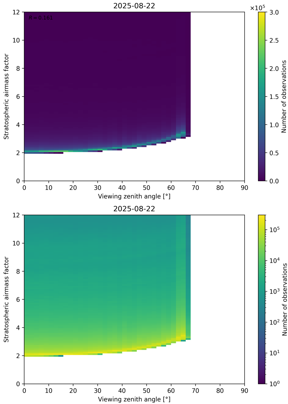
Figure 159: Scatter density plot of “Viewing zenith angle” against “Stratospheric airmass factor” for 2025-08-21 to 2025-08-23.
