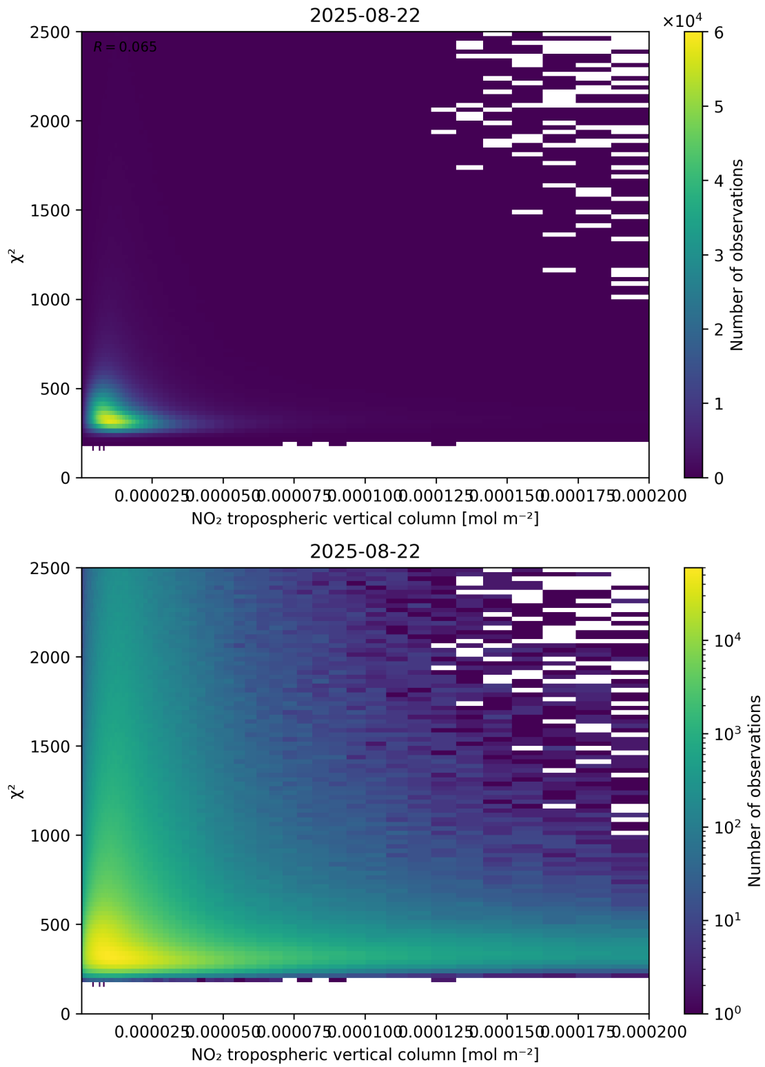
Figure 124: Scatter density plot of “NO 2 tropospheric vertical column” against “ \chi^2 ” for 2025-08-21 to 2025-08-23.
