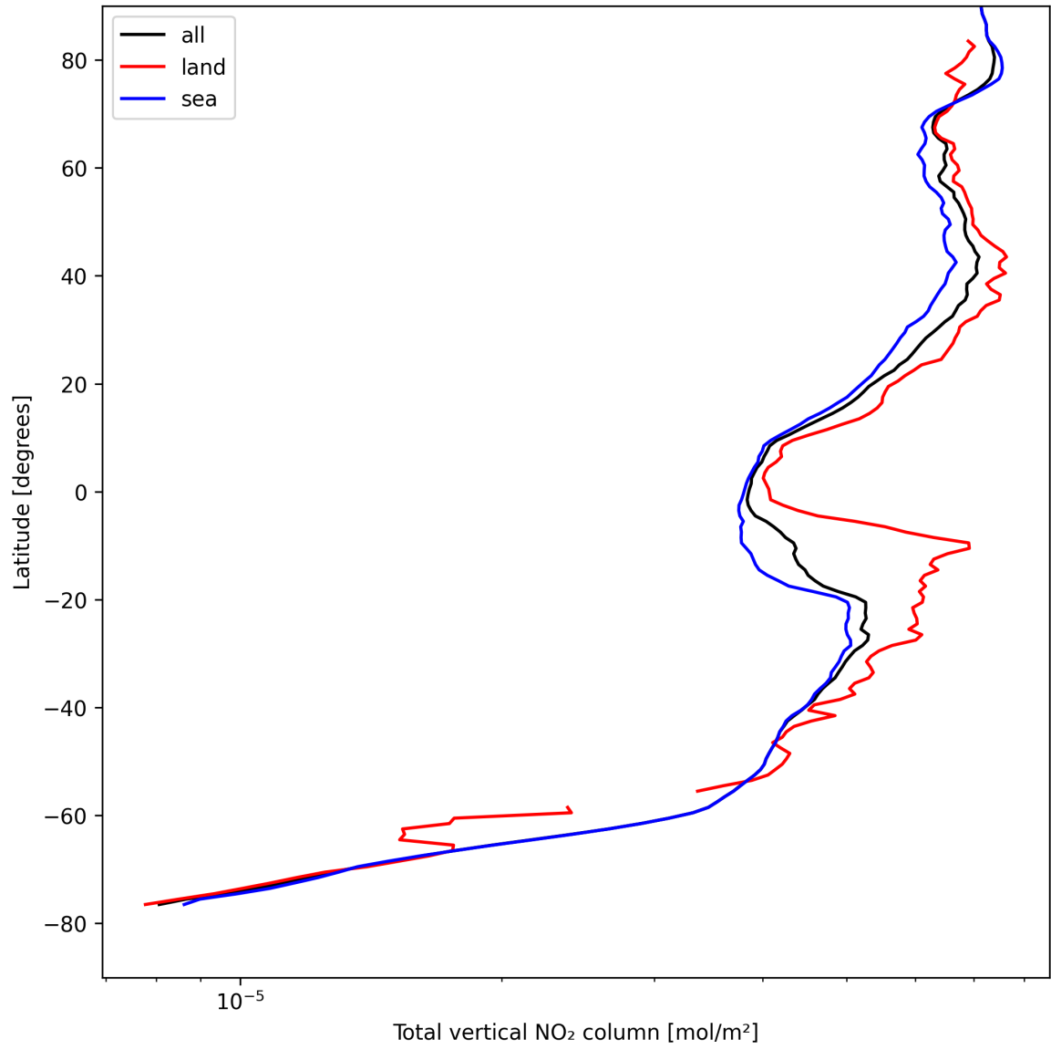
Figure 21: Zonal average of “Total vertical NO 2 column” for 2025-08-21 to 2025-08-23.
