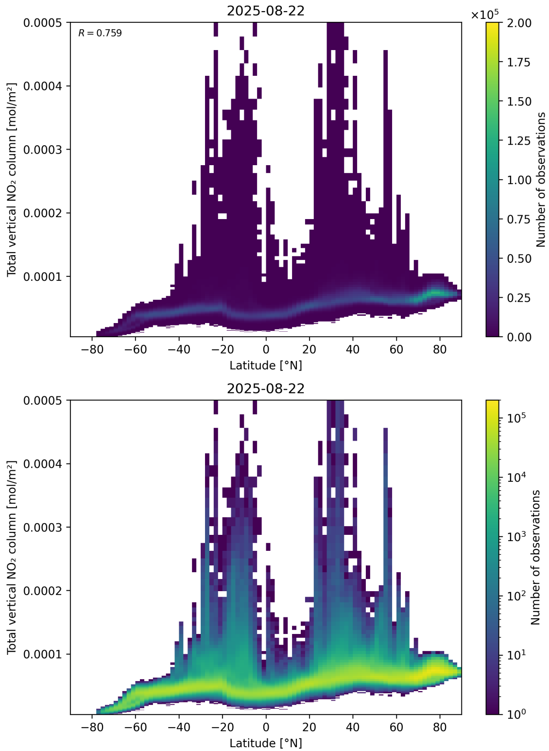
Figure 90: Scatter density plot of “Latitude” against “Total vertical NO 2 column” for 2025-08-21 to 2025-08-23.
