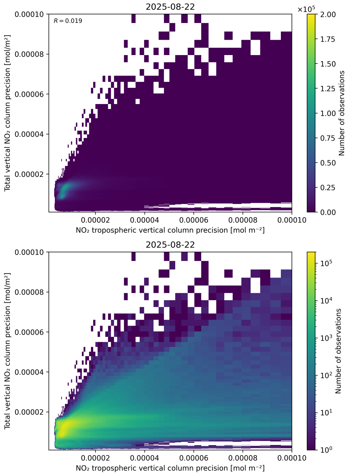
Figure 139: Scatter density plot of “NO 2 tropospheric vertical column precision” against “Total vertical NO 2 column precision” for 2025-08-21 to 2025-08-23.
