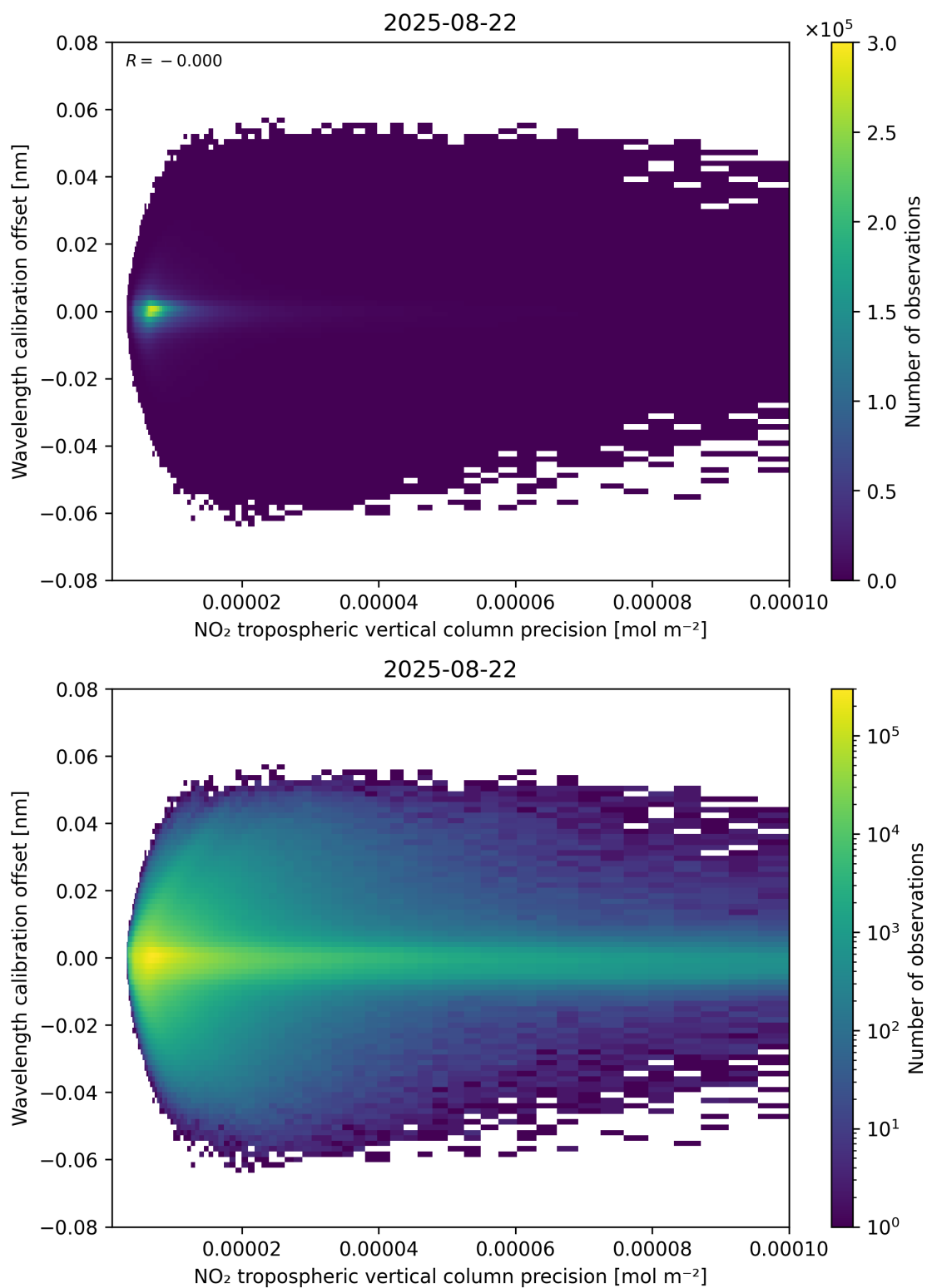
Figure 141: Scatter density plot of “NO 2 tropospheric vertical column precision” against “Wavelength calibration offset” for 2025-08-21 to 2025-08-23.
