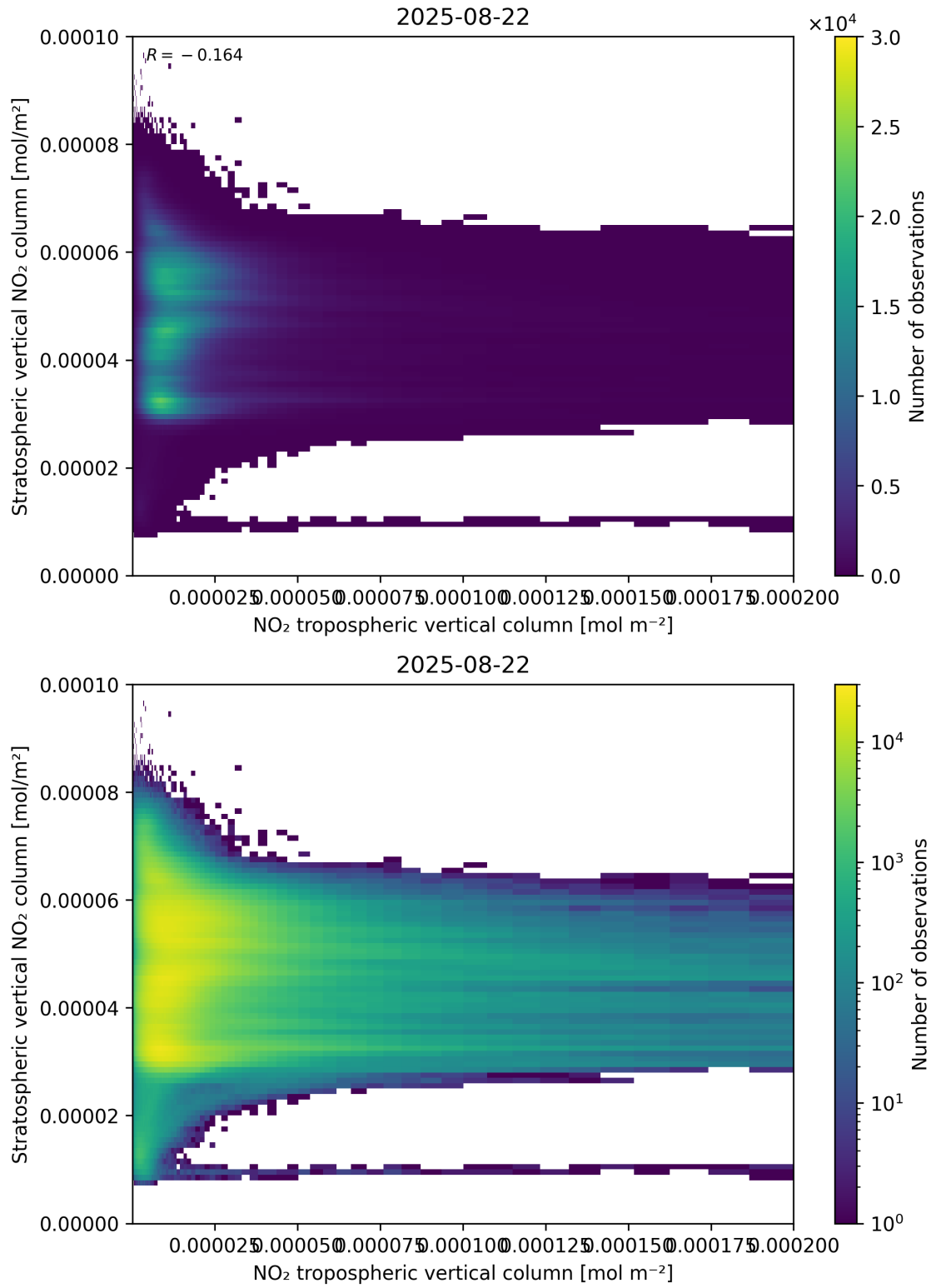
Figure 125: Scatter density plot of “NO 2 tropospheric vertical column” against “Stratospheric vertical NO 2 column” for 2025-08-21 to 2025-08-23.
