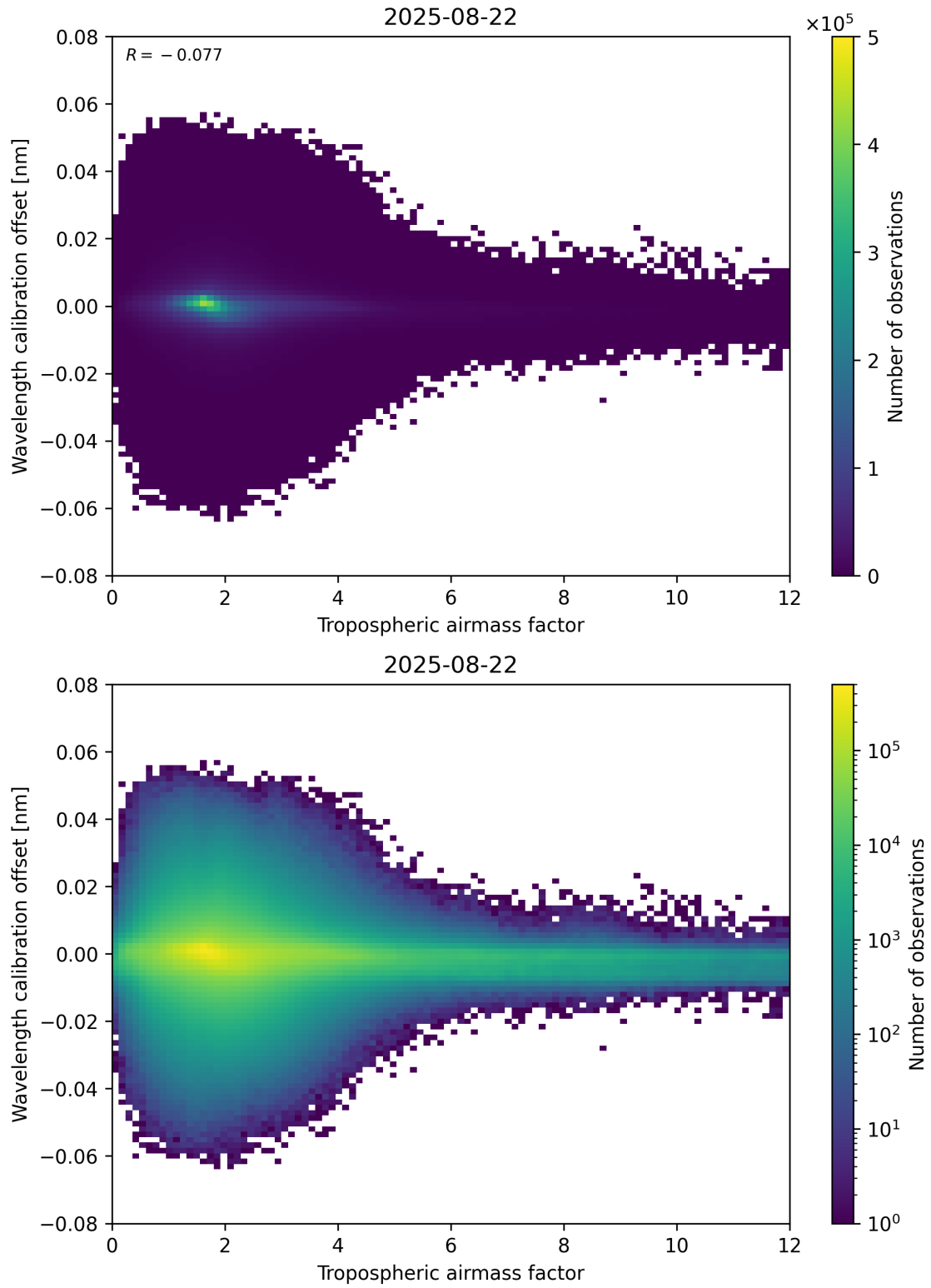
Figure 80: Scatter density plot of “Tropospheric airmass factor” against “Wavelength calibration offset” for 2025-08-21 to 2025-08-23.
