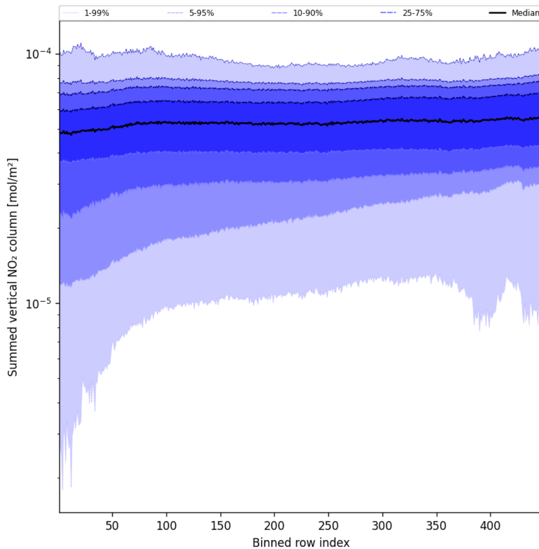
Figure 57: Along track statistics of “Summed vertical NO 2 column” for 2025-08-22 to 2025-08-24
