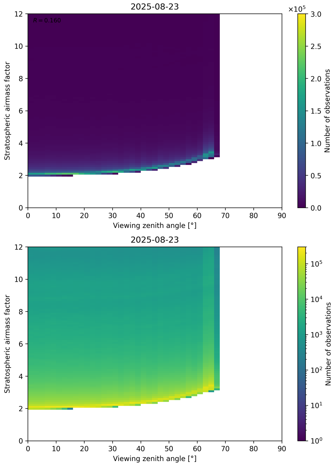
Figure 159: Scatter density plot of “Viewing zenith angle” against “Stratospheric airmass factor” for 2025-08-22 to 2025-08-24.
