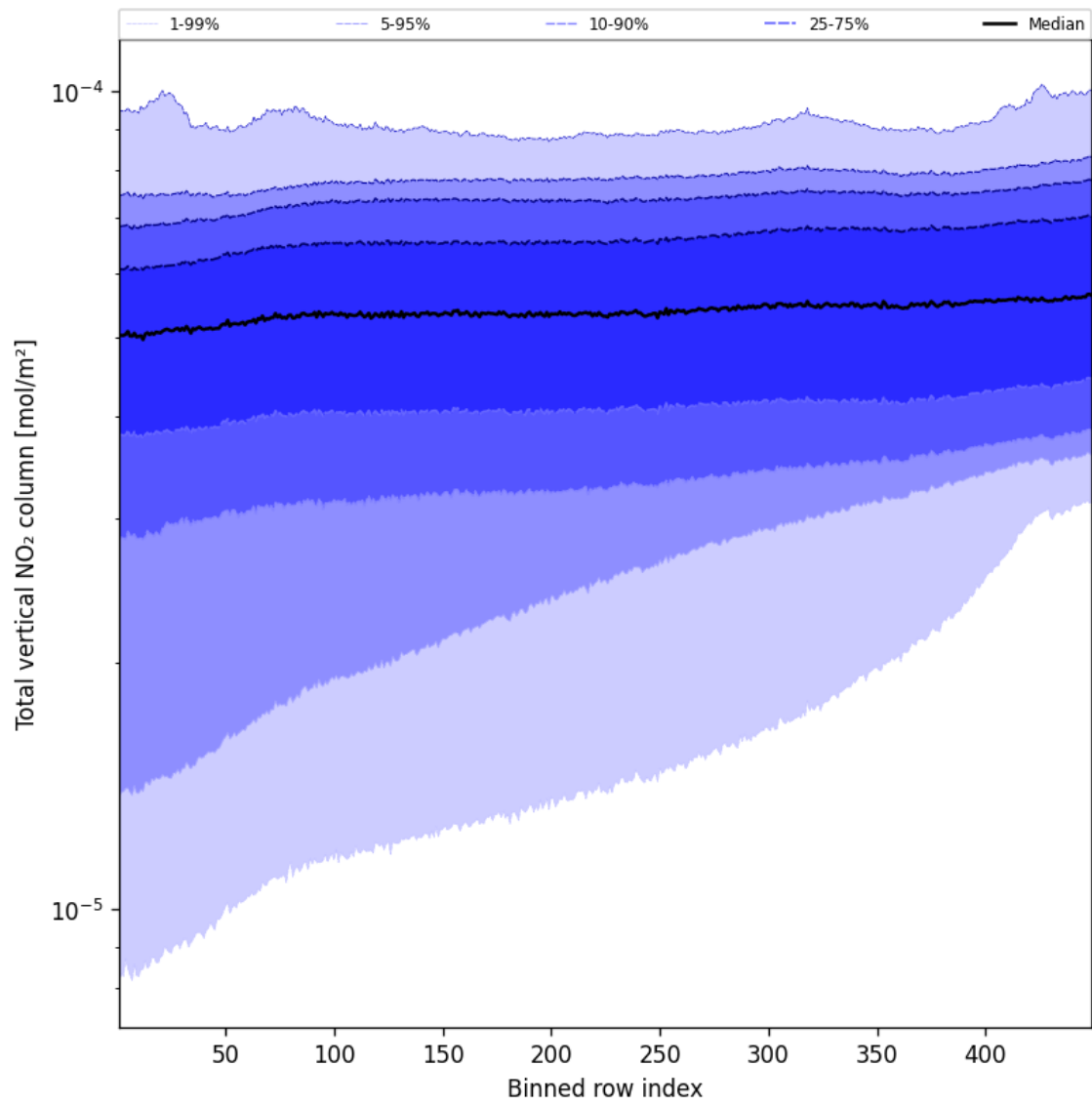
Figure 55: Along track statistics of “Total vertical NO 2 column” for 2025-08-22 to 2025-08-24
