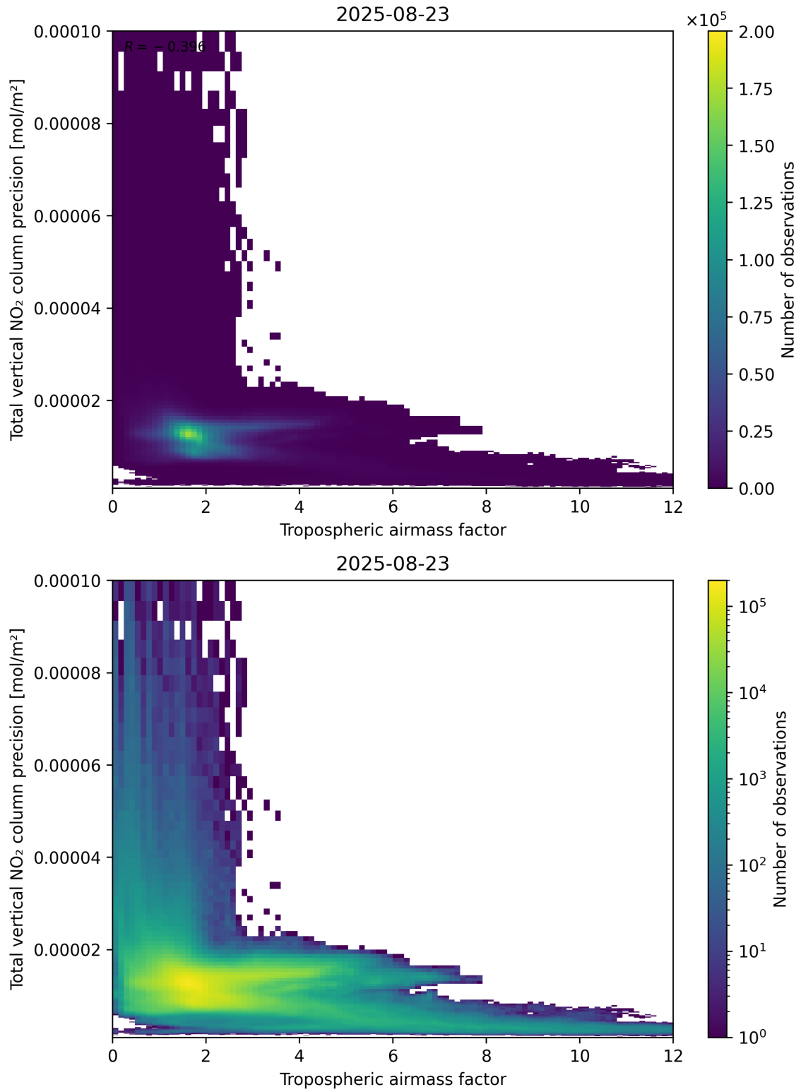
Figure 78: Scatter density plot of “Tropospheric air mass factor” against “Total vertical NO 2 column precision” for 2025-08-22 to 2025-08-24.
