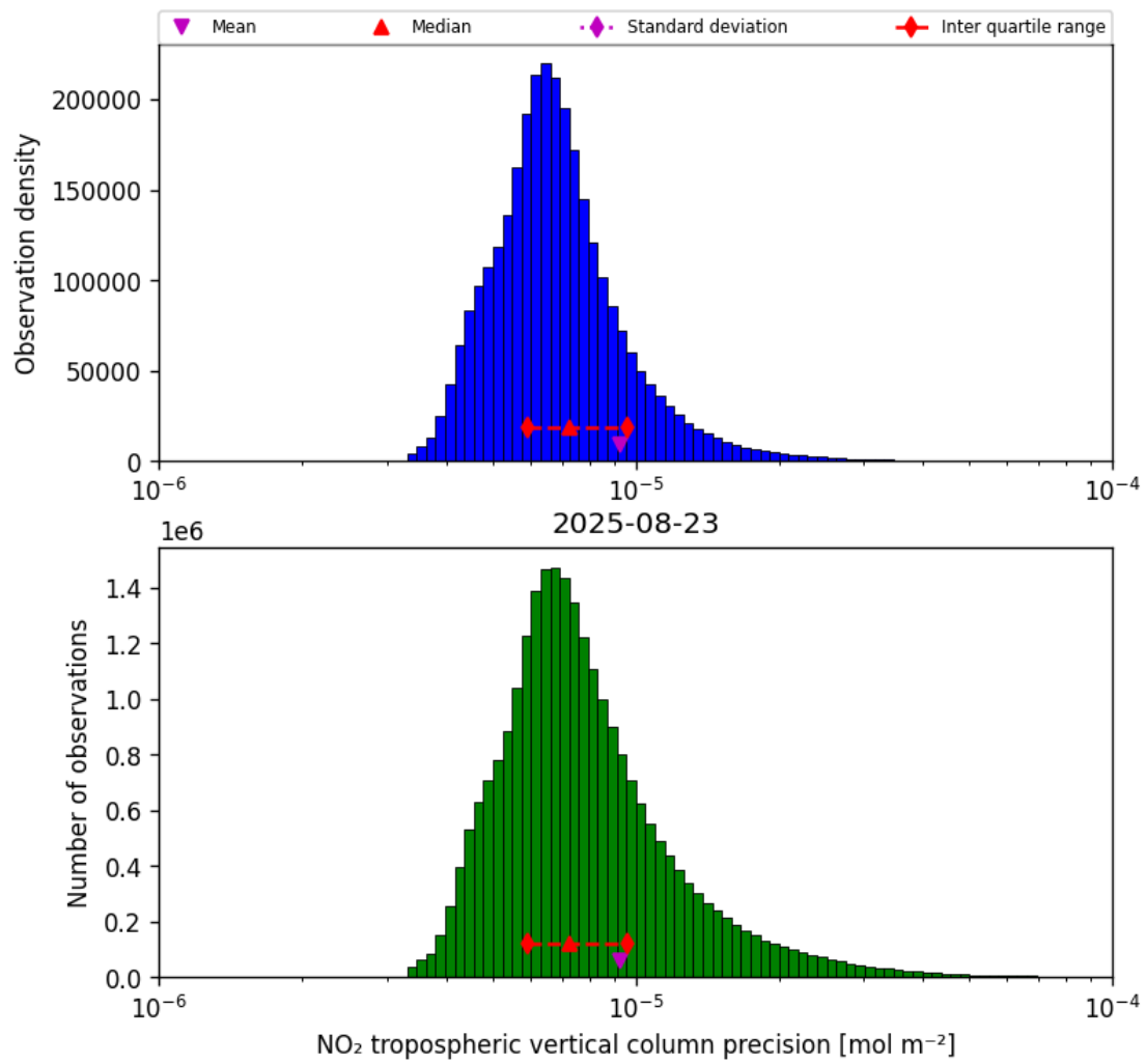
Figure 30: Histogram of “NO 2 tropospheric vertical column precision” for 2025-08-22 to 2025-08-24
