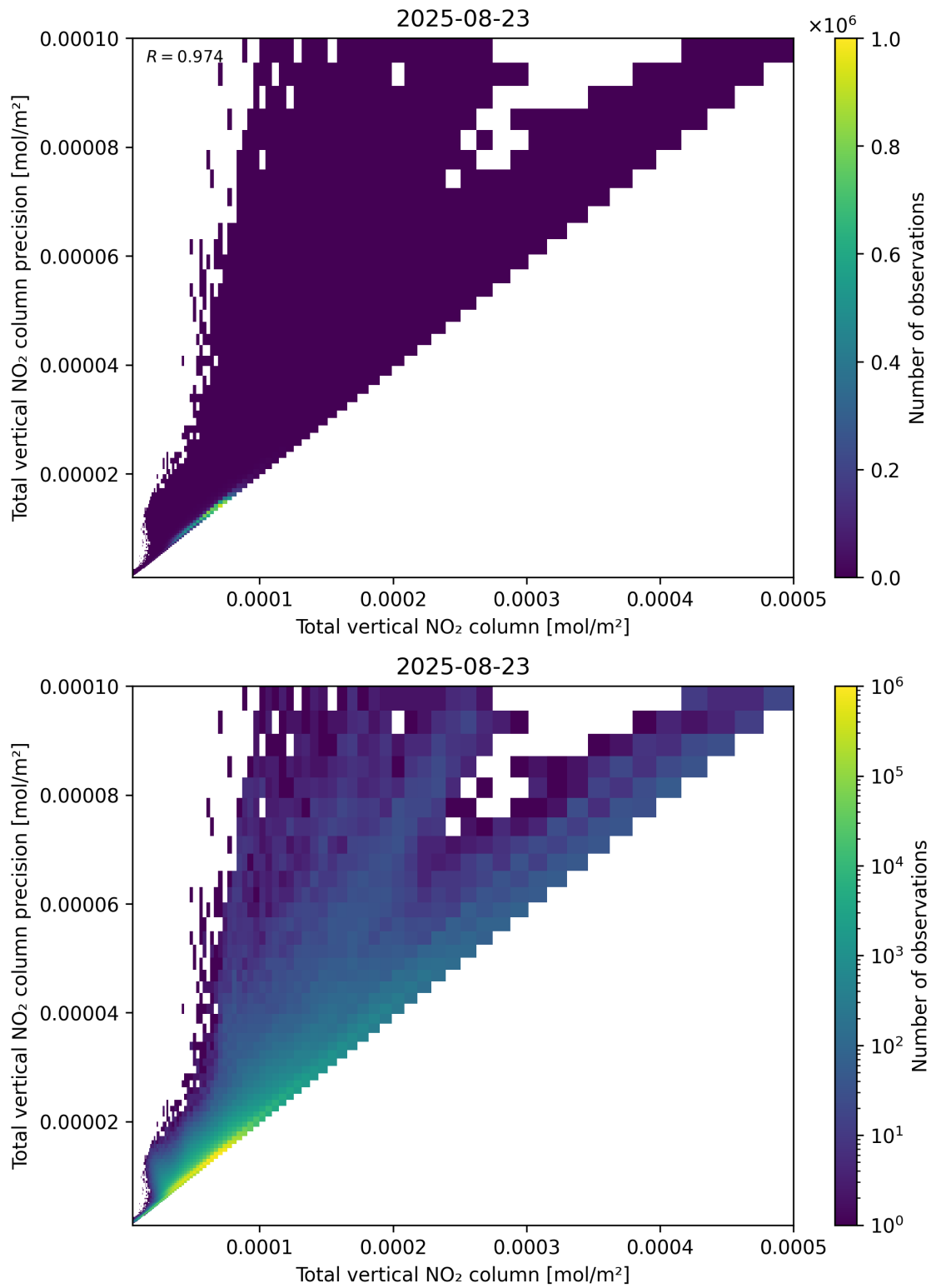
Figure 114: Scatter density plot of “Total vertical NO 2 column” against “Total vertical NO 2 column precision” for 2025-08-22 to 2025-08-24.
