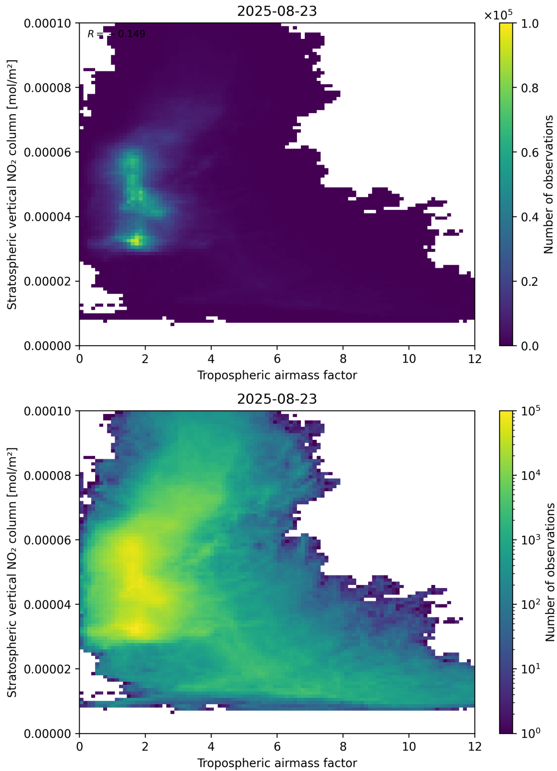
Figure 74: Scatter density plot of “Tropospheric air mass factor” against “Stratospheric vertical NO 2 column” for 2025-08-22 to 2025-08-24.
