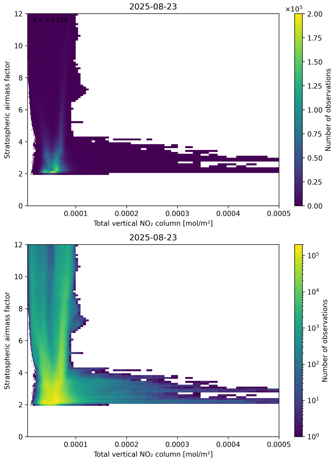
Figure 110: Scatter density plot of “Total vertical NO 2 column” against “Stratospheric airmass factor” for 2025-08-22 to 2025-08-24.
