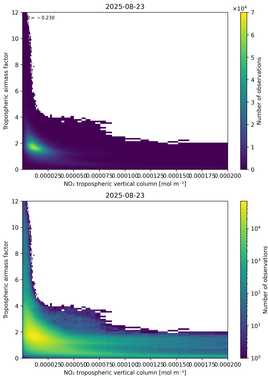
Figure 123: Scatter density plot of “NO 2 tropospheric vertical column” against “Tropospheric air mass factor” for 2025-08-22 to 2025-08-24.
