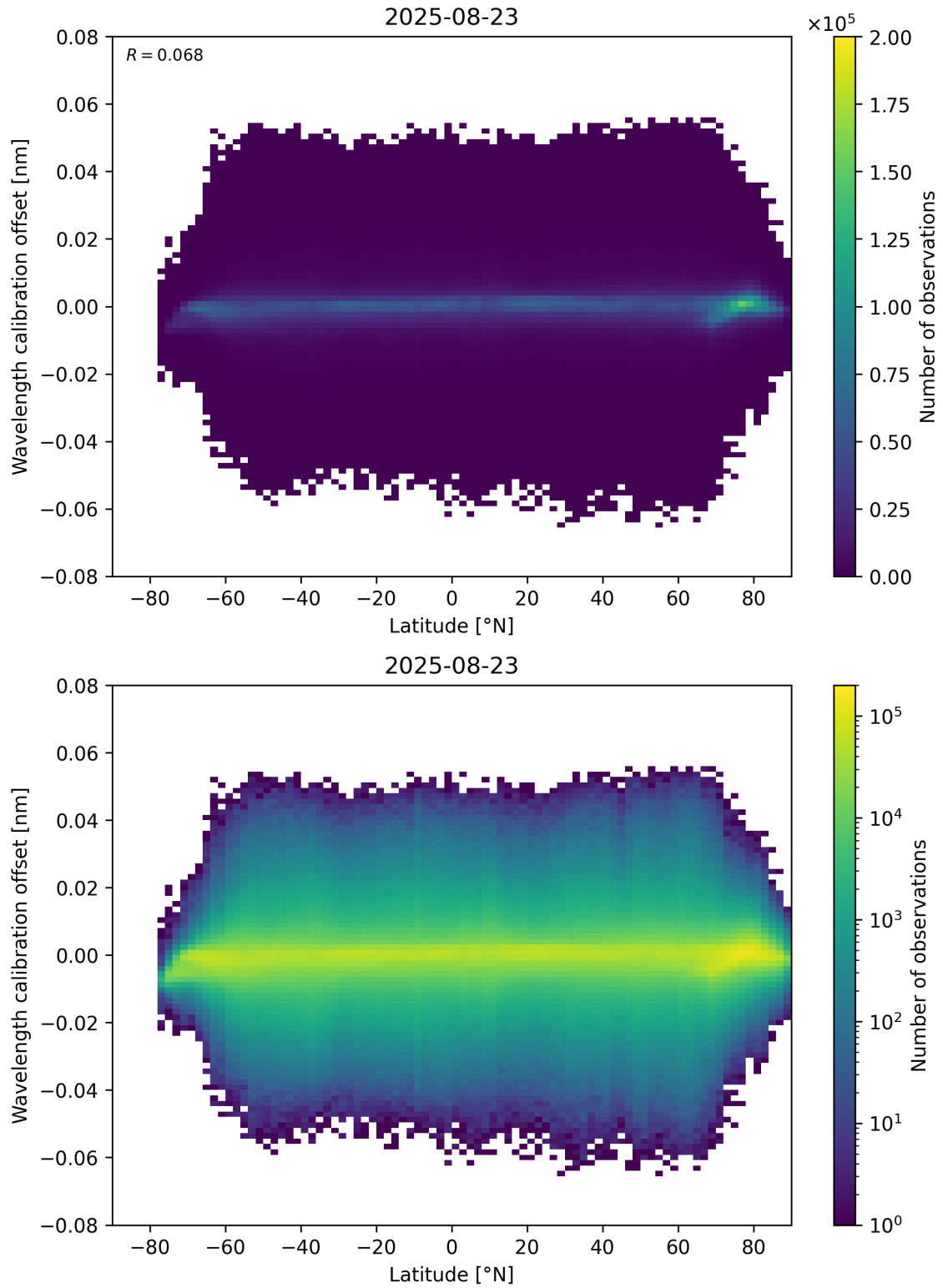
Figure 95: Scatter density plot of “Latitude” against “Wavelength calibration offset” for 2025-08-22 to 2025-08-24.
