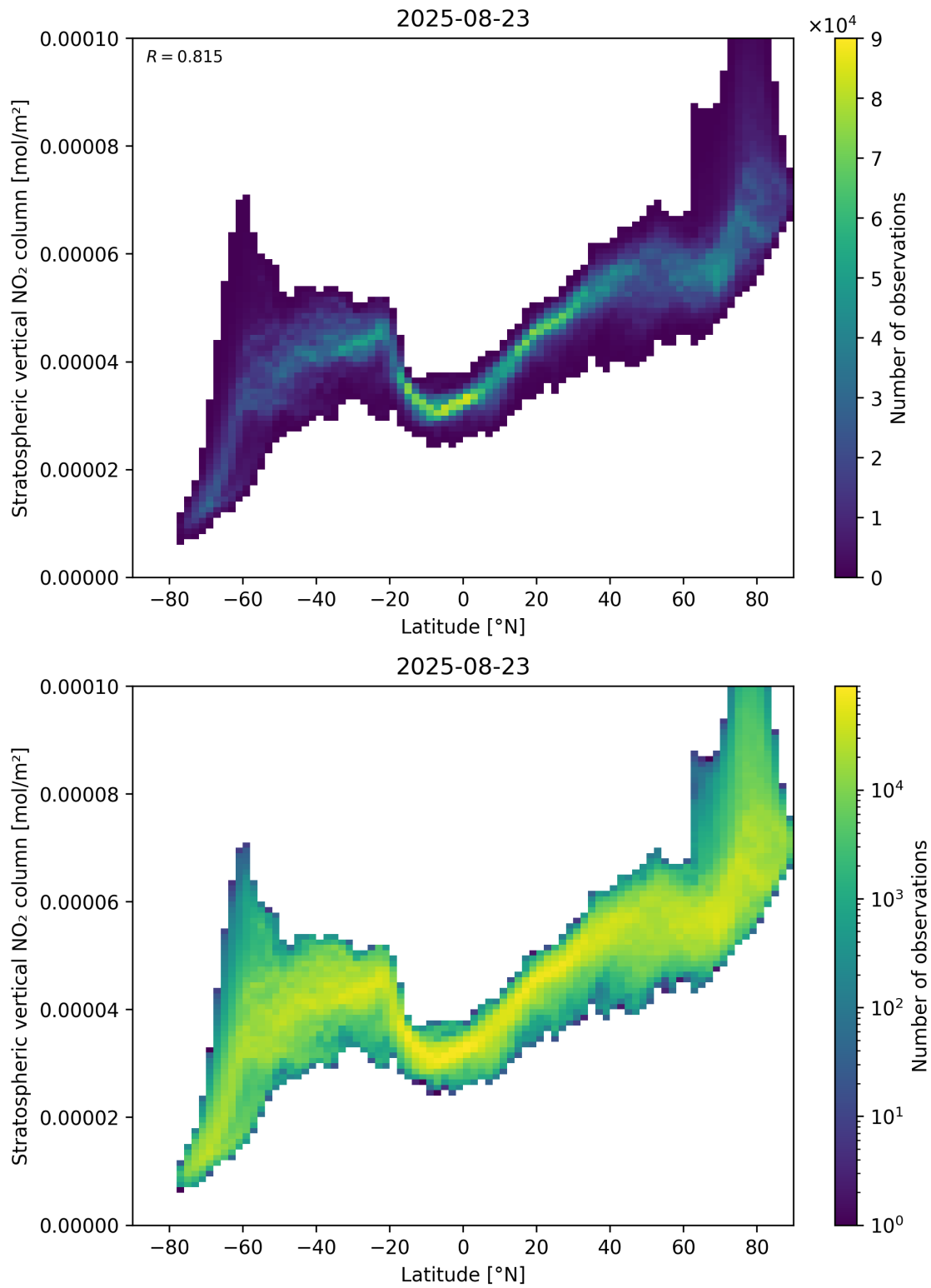
Figure 87: Scatter density plot of “Latitude” against “Stratospheric vertical \text{NO}_2 column” for 2025-08-22 to 2025-08-24.
