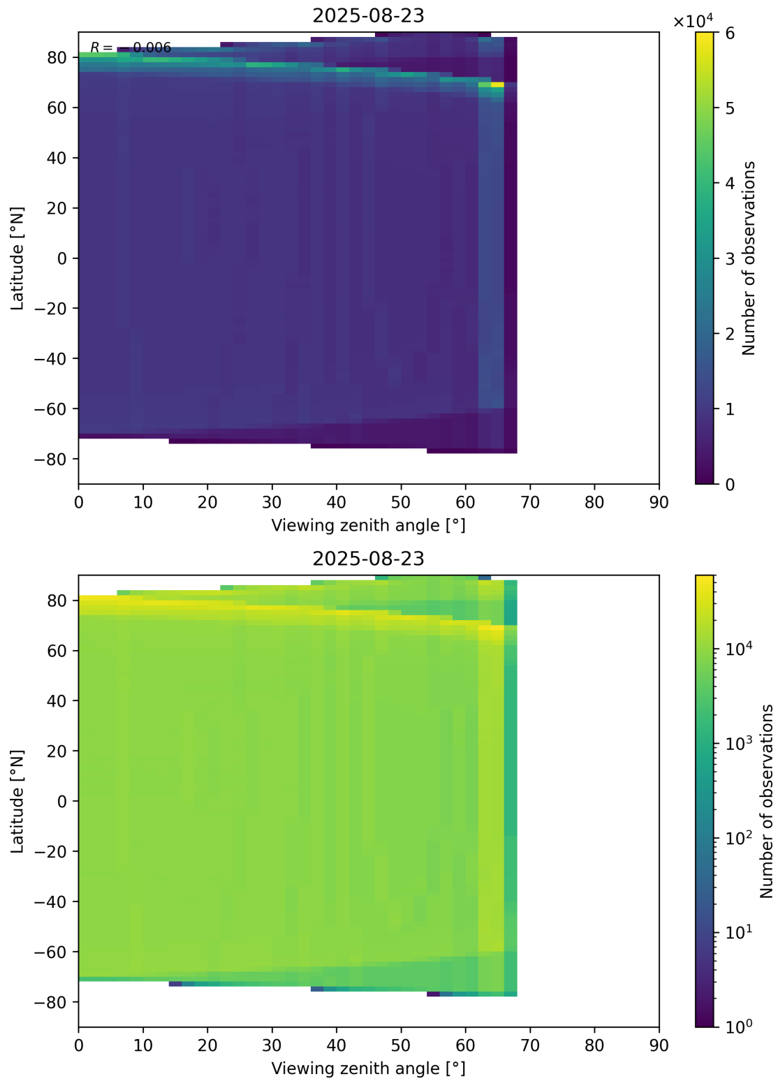
Figure 163: Scatter density plot of “Viewing zenith angle” against “Latitude” for 2025-08-22 to 2025-08-24.
