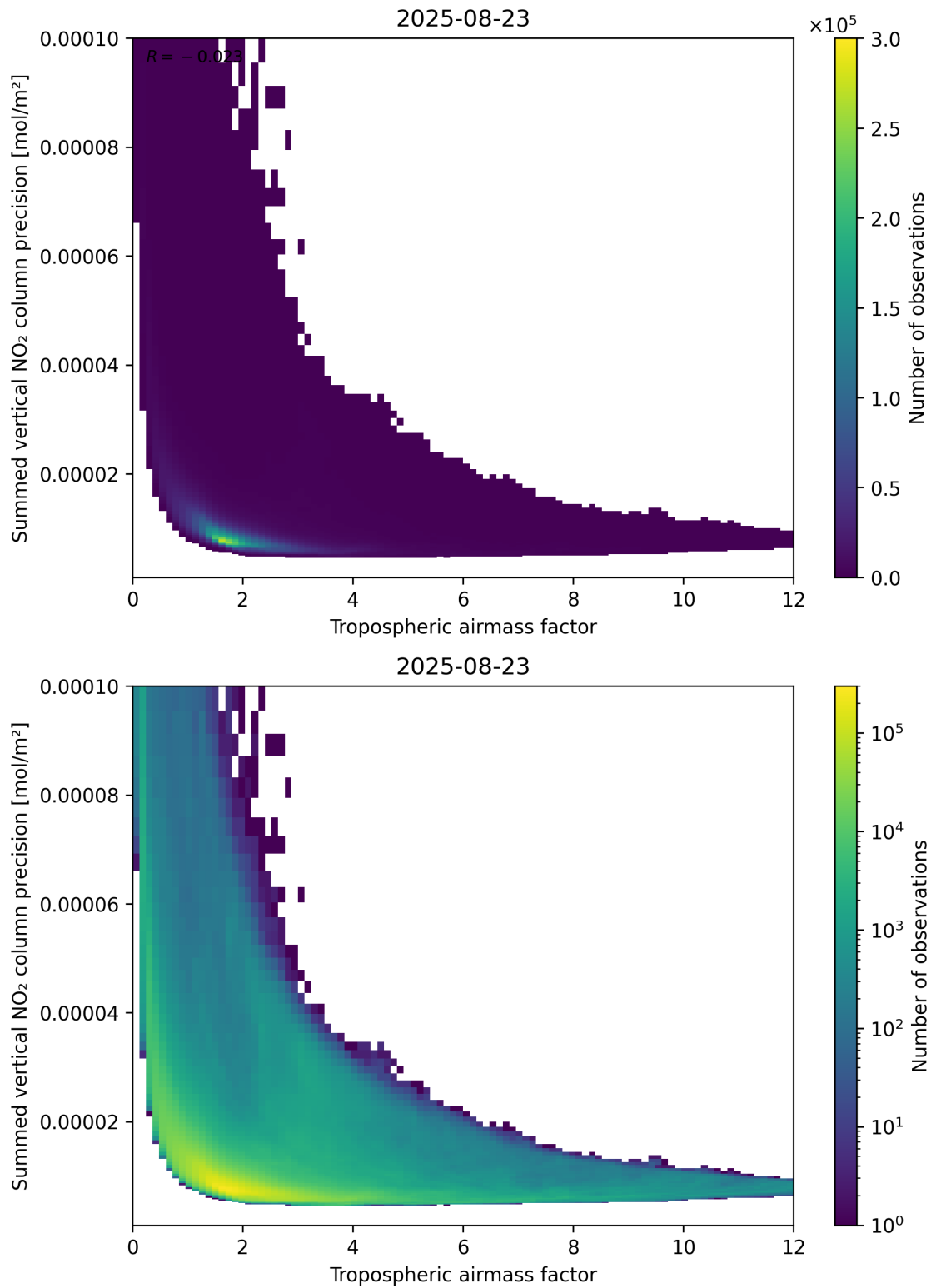
Figure 76: Scatter density plot of “Tropospheric air mass factor” against “Summed vertical NO 2 column precision” for 2025-08-22 to 2025-08-24.
