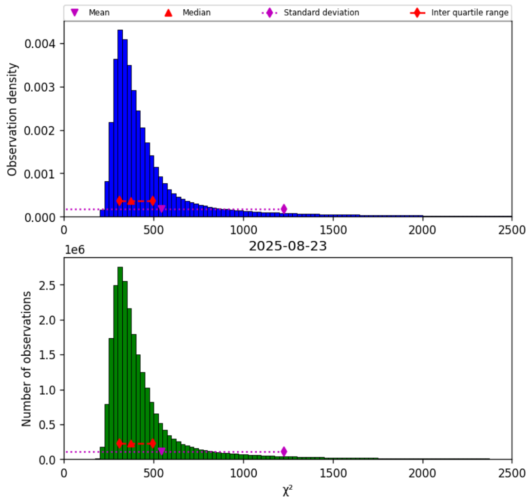
Figure 42: Histogram of “ \chi^2 ” for 2025-08-22 to 2025-08-24
