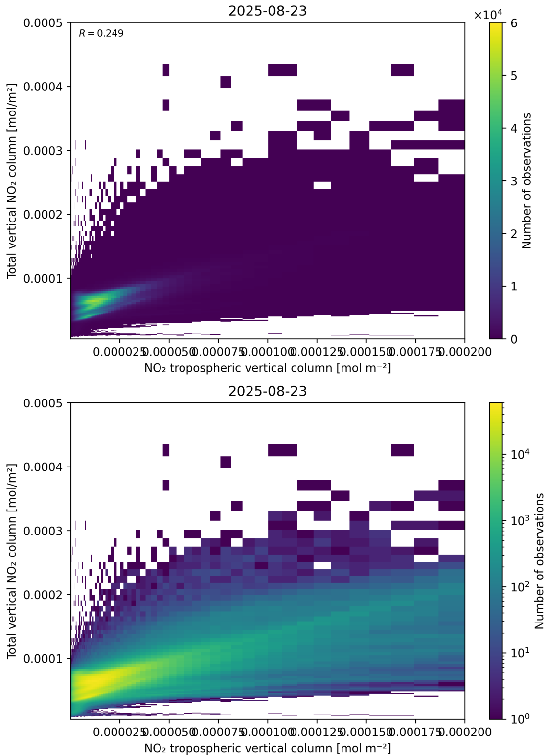
Figure 128: Scatter density plot of “NO 2 tropospheric vertical column” against “Total vertical NO 2 column” for 2025-08-22 to 2025-08-24.
