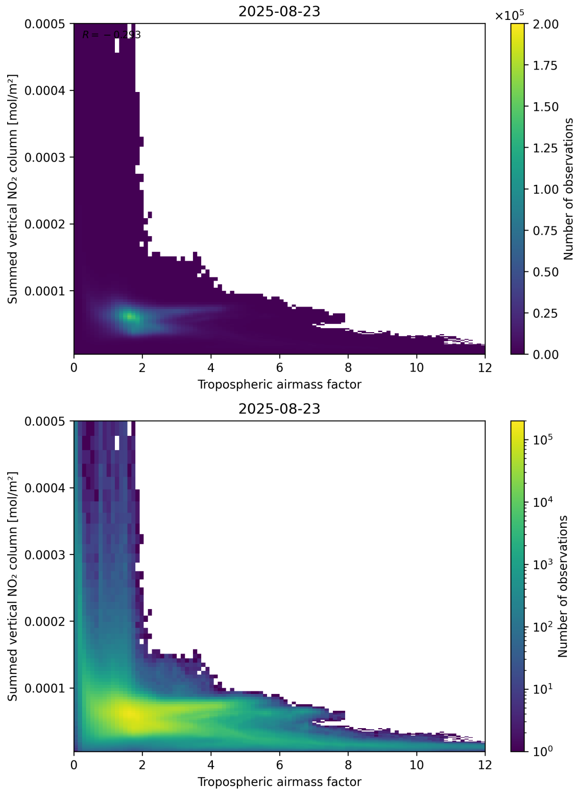
Figure 75: Scatter density plot of “Tropospheric air mass factor” against “Summed vertical NO 2 column” for 2025-08-22 to 2025-08-24.
