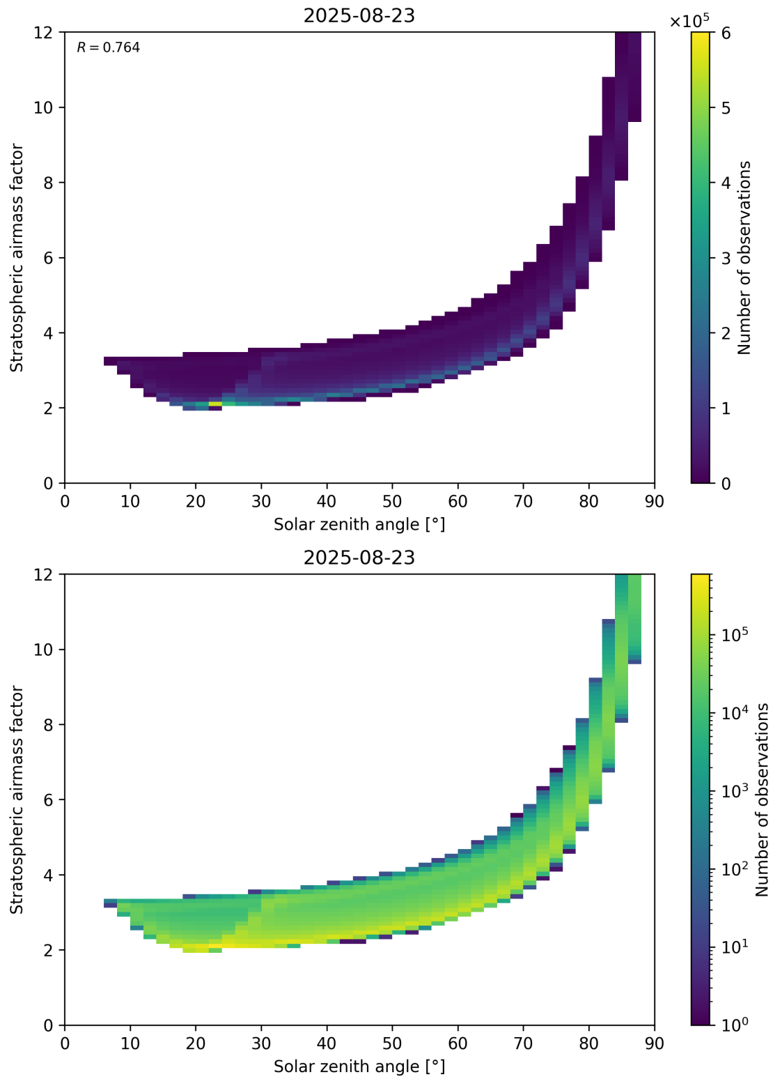
Figure 145: Scatter density plot of “Solar zenith angle” against “Stratospheric airmass factor” for 2025-08-22 to 2025-08-24.
