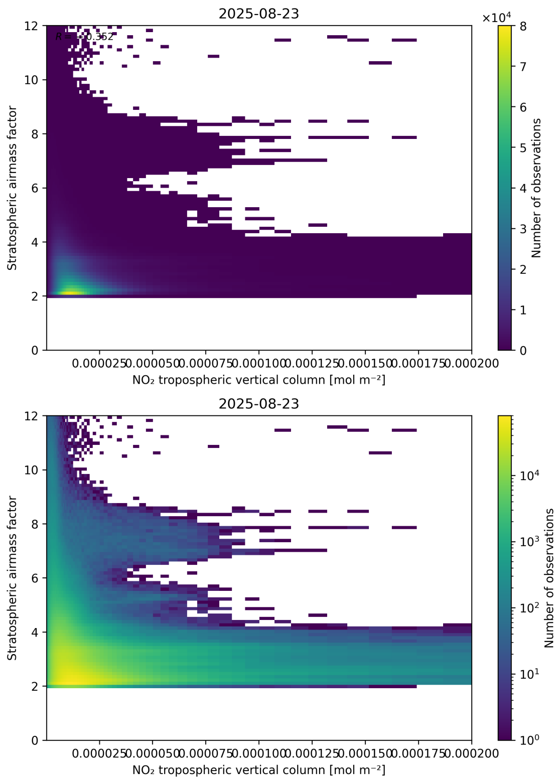
Figure 121: Scatter density plot of “NO 2 tropospheric vertical column” against “Stratospheric air mass factor” for 2025-08-22 to 2025-08-24.
