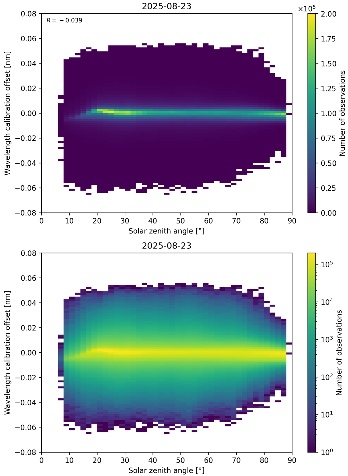
Figure 158: Scatter density plot of “Solar zenith angle” against “Wavelength calibration offset” for 2025-08-22 to 2025-08-24.
