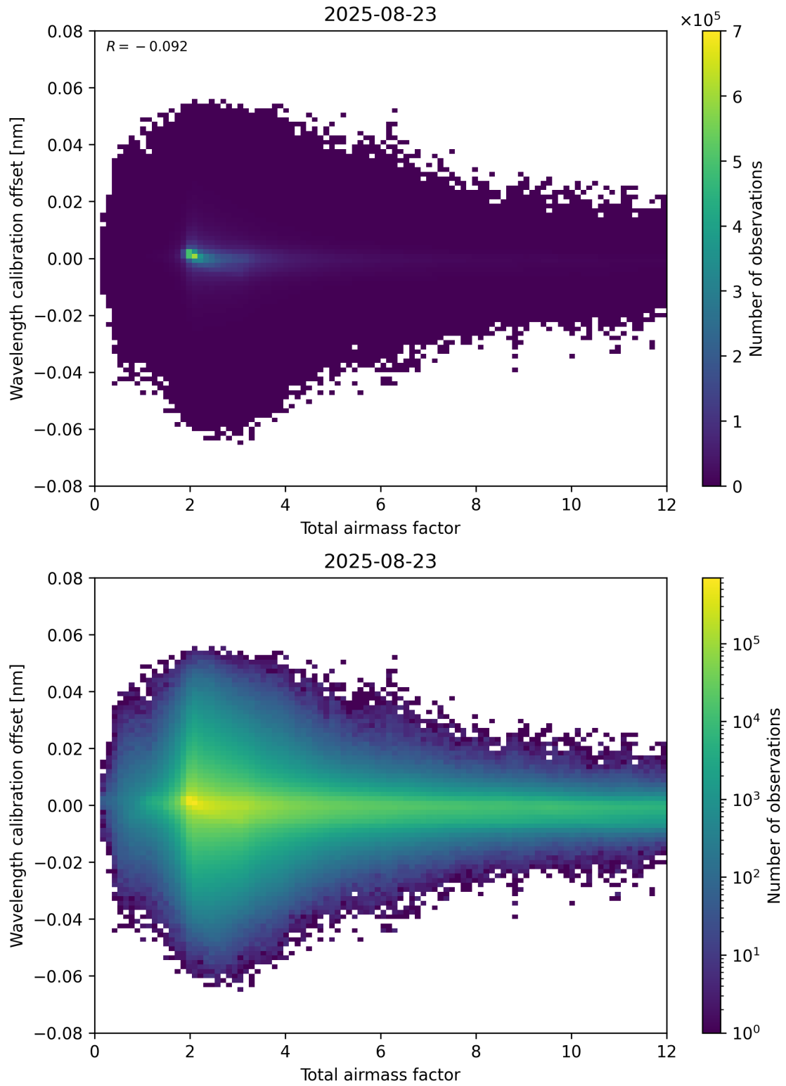
Figure 70: Scatter density plot of “Total airmass factor” against “Wavelength calibration offset” for 2025-08-22 to 2025-08-24.
