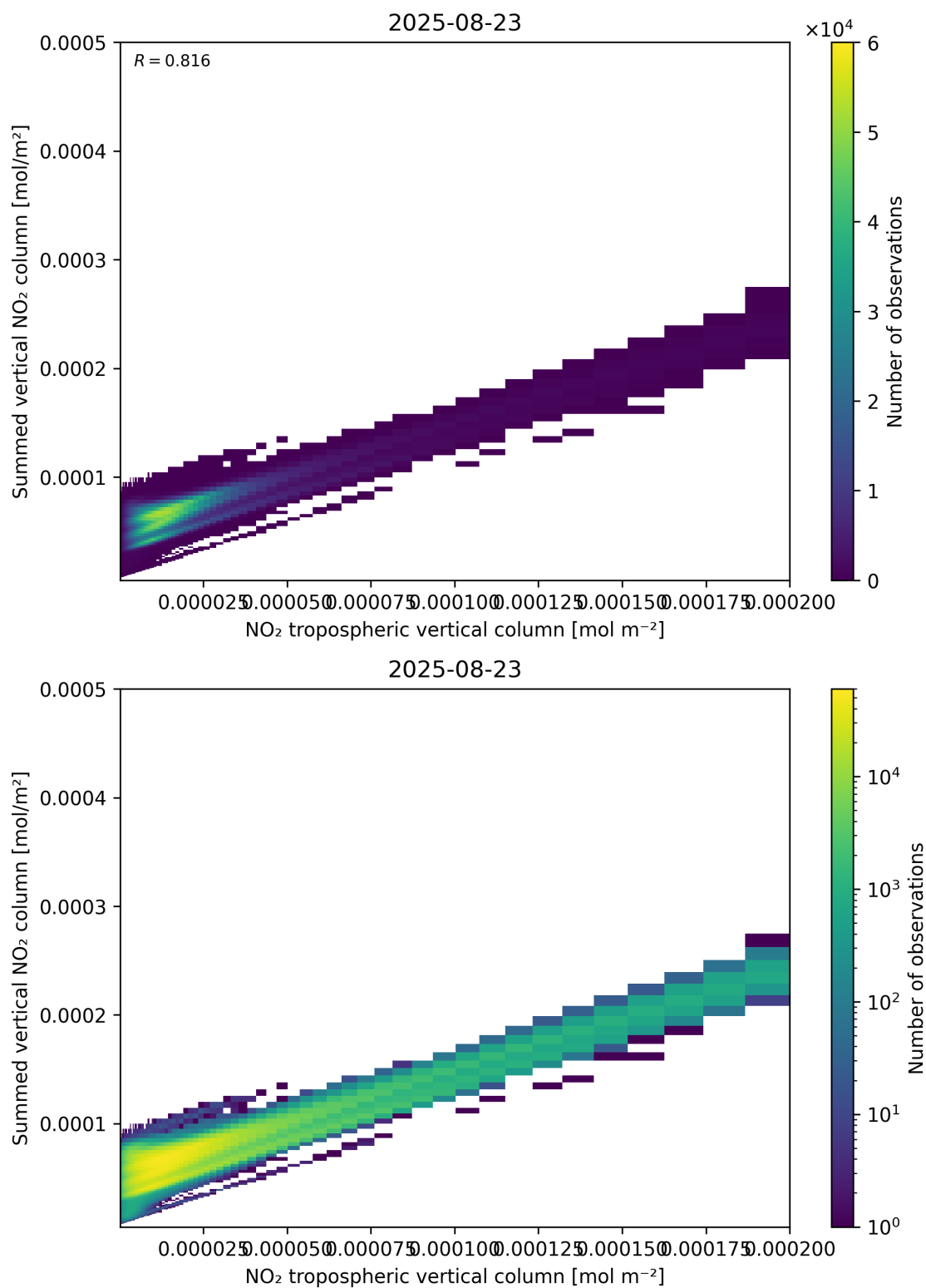
Figure 126: Scatter density plot of “NO 2 tropospheric vertical column” against “Summed vertical NO 2 column” for 2025-08-22 to 2025-08-24.
