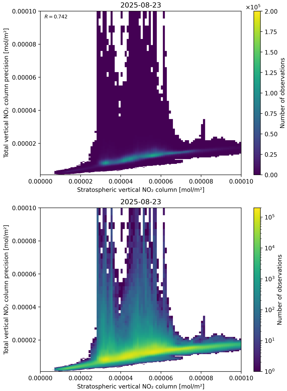
Figure 101: Scatter density plot of “Stratospheric vertical NO 2 column” against “Total vertical NO 2 column precision” for 2025-08-22 to 2025-08-24.
