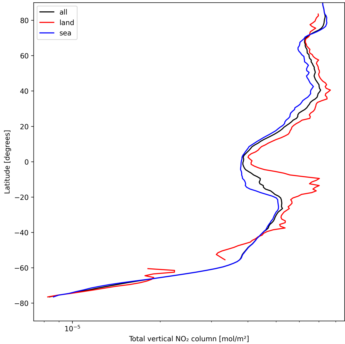
Figure 21: Zonal average of “Total vertical NO 2 column” for 2025-08-22 to 2025-08-24.
