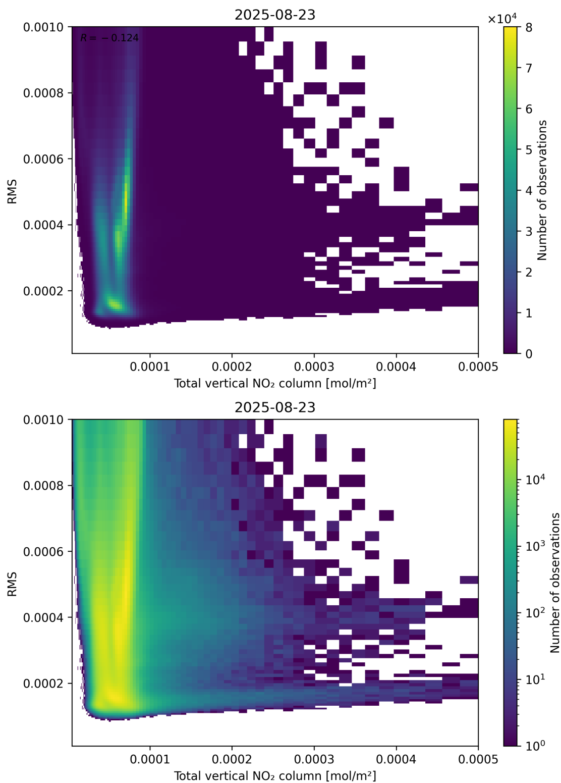
Figure 120: Scatter density plot of “Total vertical NO 2 column” against “RMS” for 2025-08-22 to 2025-08-24.
