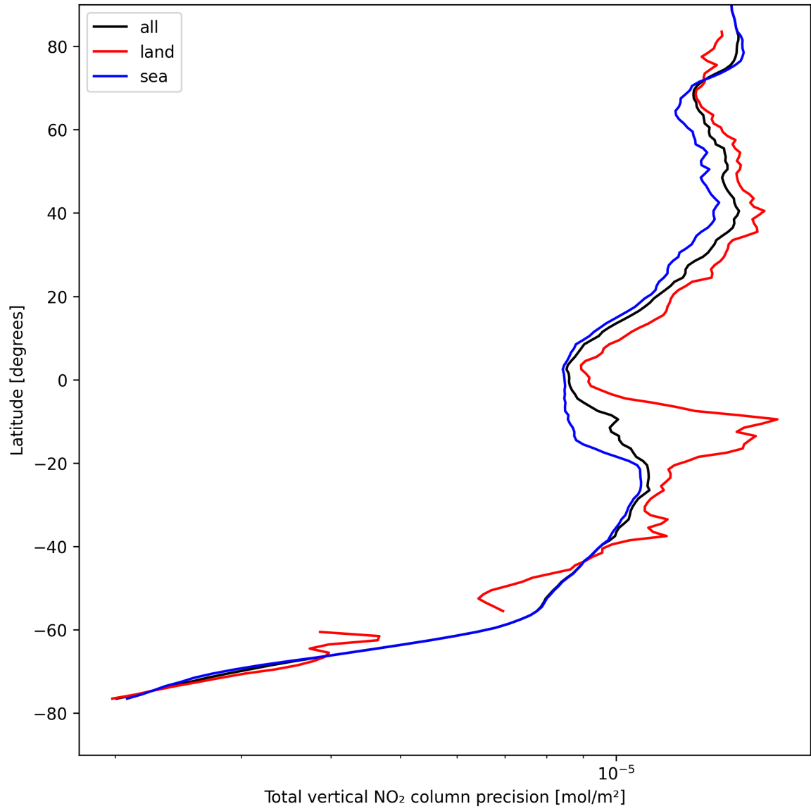
Figure 22: Zonal average of “Total vertical NO 2 column precision” for 2025-08-22 to 2025-08-24.
