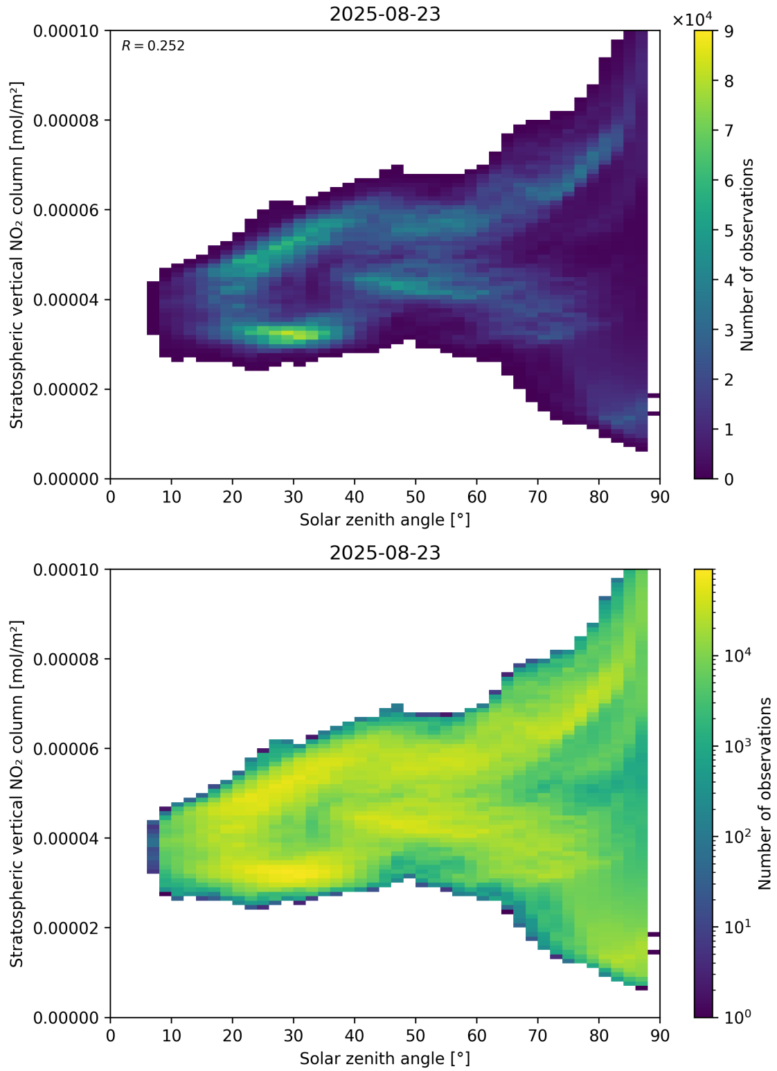
Figure 150: Scatter density plot of “Solar zenith angle” against “Stratospheric vertical NO 2 column” for 2025-08-22 to 2025-08-24.
