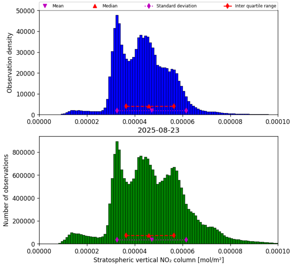
Figure 36: Histogram of “Stratospheric vertical NO 2 column” for 2025-08-22 to 2025-08-24
