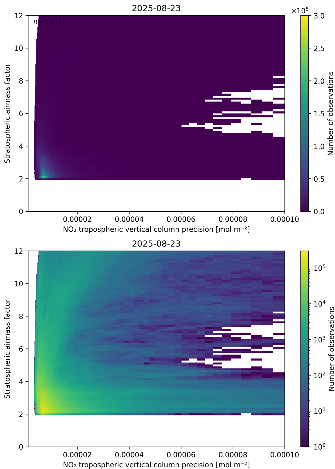
Figure 131: Scatter density plot of “NO 2 tropospheric vertical column precision” against “Stratospheric airmass factor” for 2025-08-22 to 2025-08-24.
