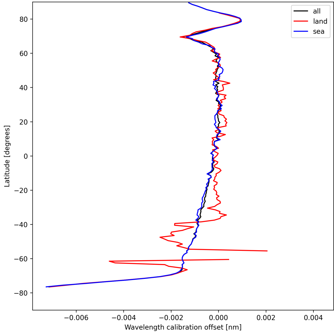
Figure 18: Zonal average of “Wavelength calibration offset” for 2025-08-22 to 2025-08-24.
