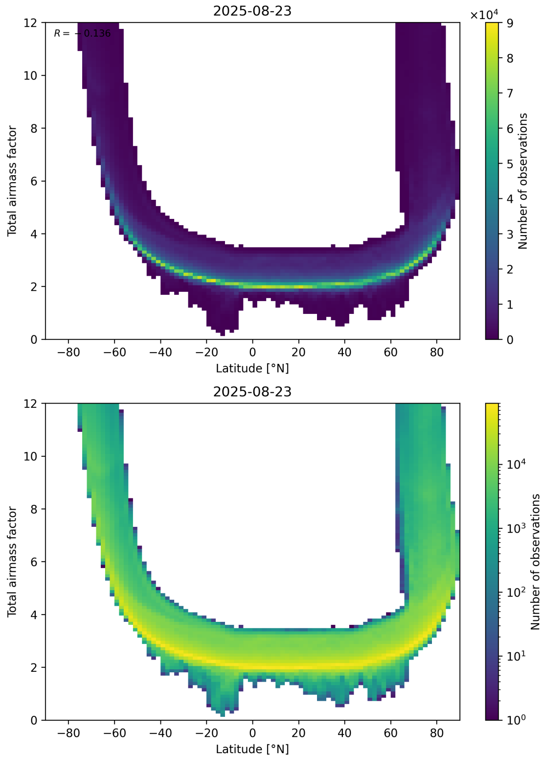
Figure 84: Scatter density plot of “Latitude” against “Total airmass factor” for 2025-08-22 to 2025-08-24.
