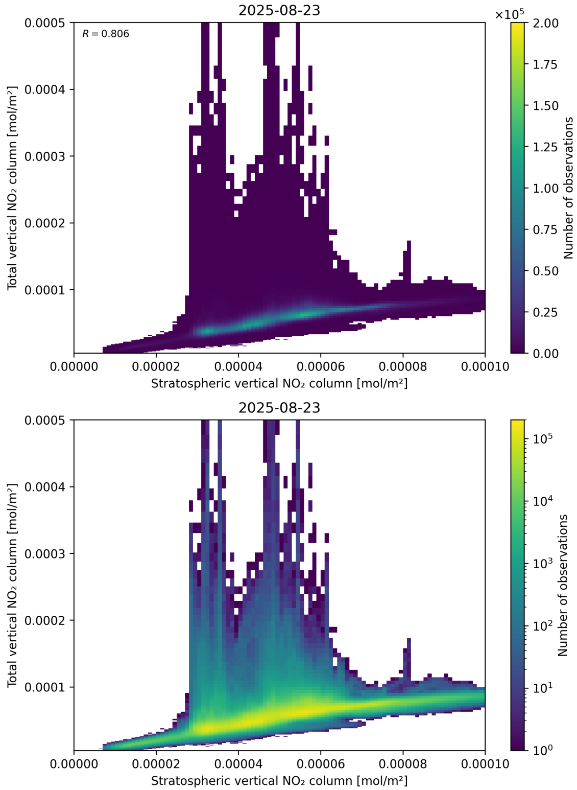
Figure 100: Scatter density plot of “Stratospheric vertical NO 2 column” against “Total vertical NO 2 column” for 2025-08-22 to 2025-08-24.
