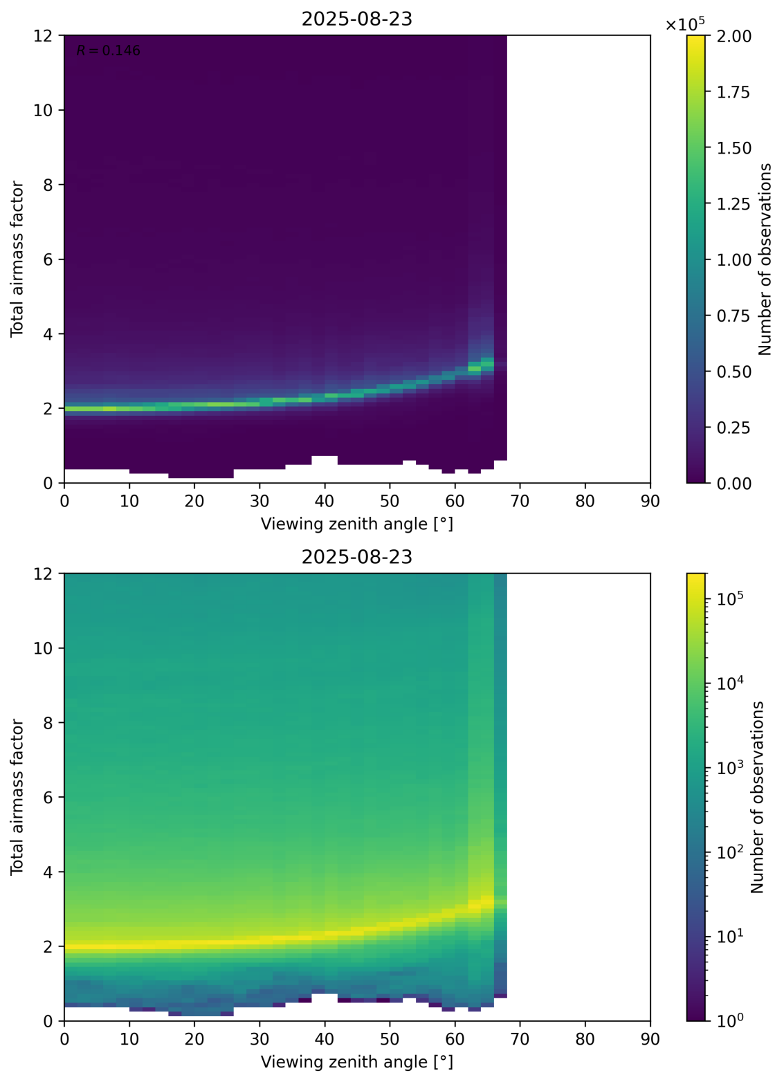
Figure 160: Scatter density plot of “Viewing zenith angle” against “Total airmass factor” for 2025-08-22 to 2025-08-24.
