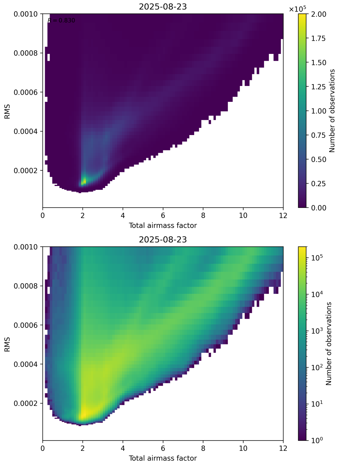
Figure 69: Scatter density plot of “Total airmass factor” against “RMS” for 2025-08-22 to 2025-08-24.
