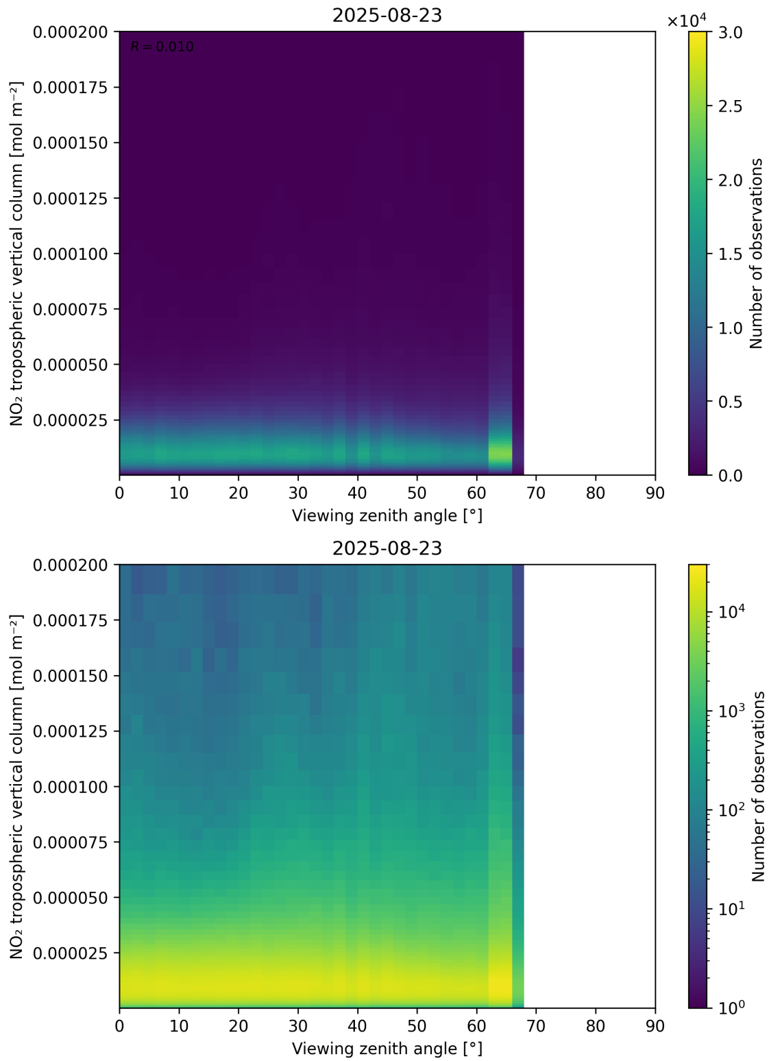
Figure 169: Scatter density plot of “Viewing zenith angle” against “NO 2 tropospheric vertical column” for 2025-08-22 to 2025-08-24.
