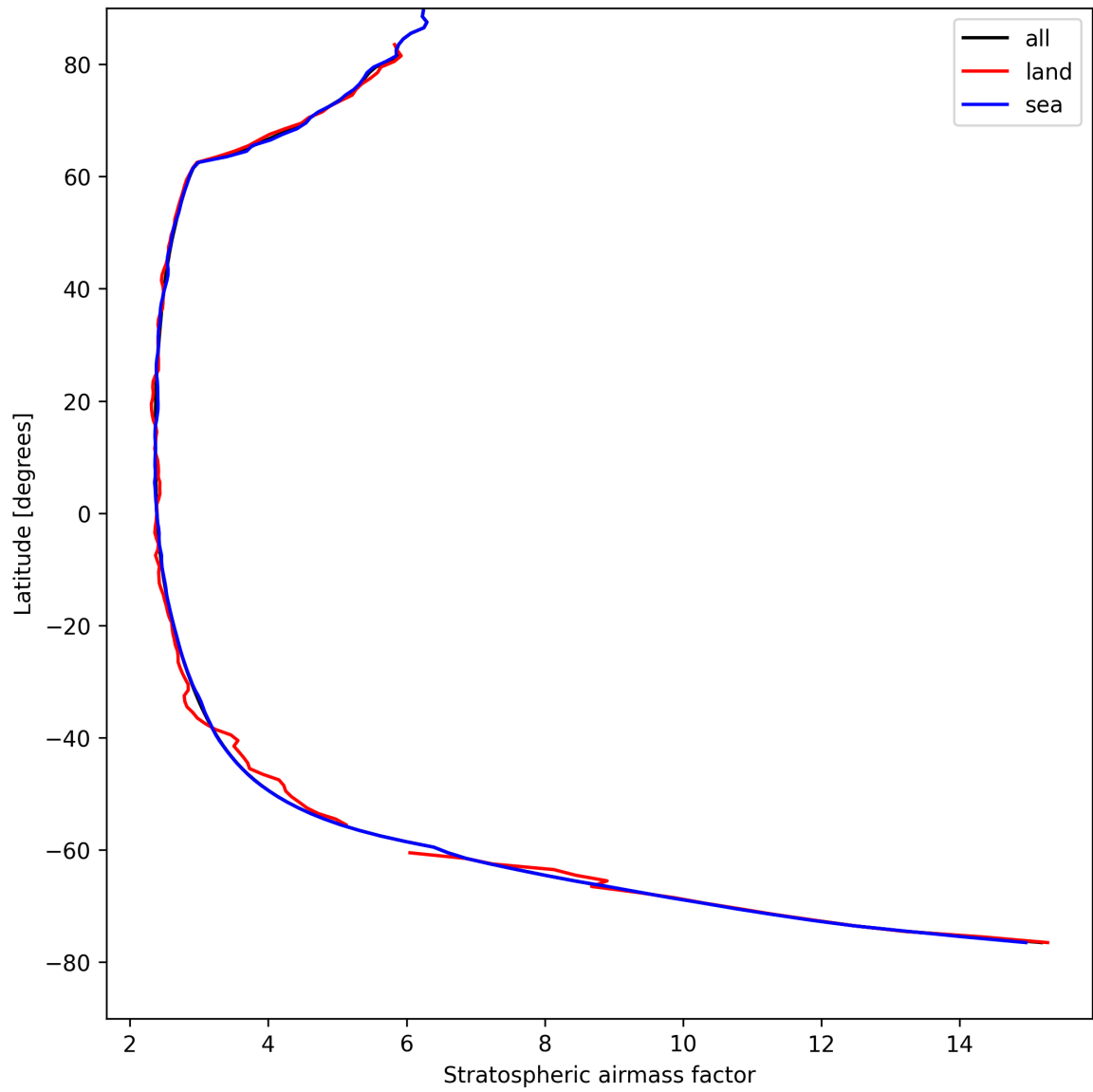
Figure 27: Zonal average of “Stratospheric air mass factor” for 2025-08-22 to 2025-08-24.
