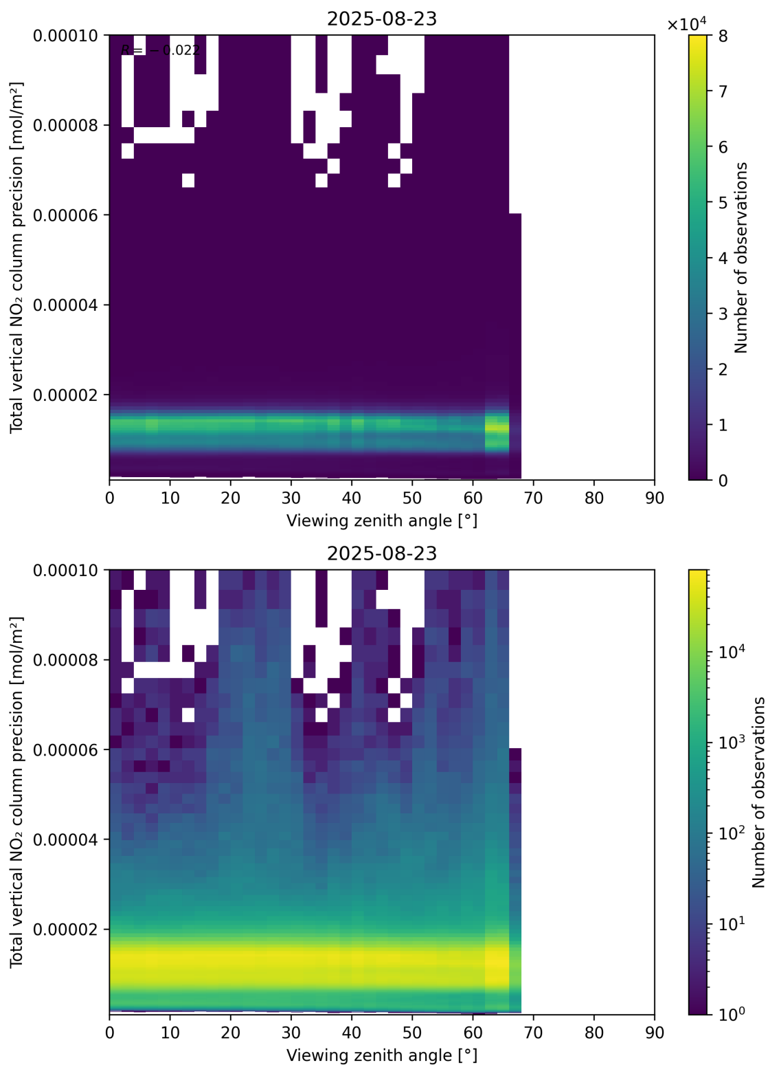
Figure 168: Scatter density plot of “Viewing zenith angle” against “Total vertical NO 2 column precision” for 2025-08-22 to 2025-08-24.
