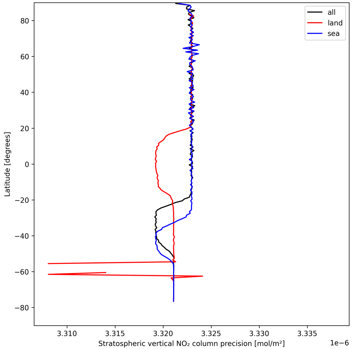
Figure 20: Zonal average of “Stratospheric vertical NO 2 column precision” for 2025-08-22 to 2025-08-24.
