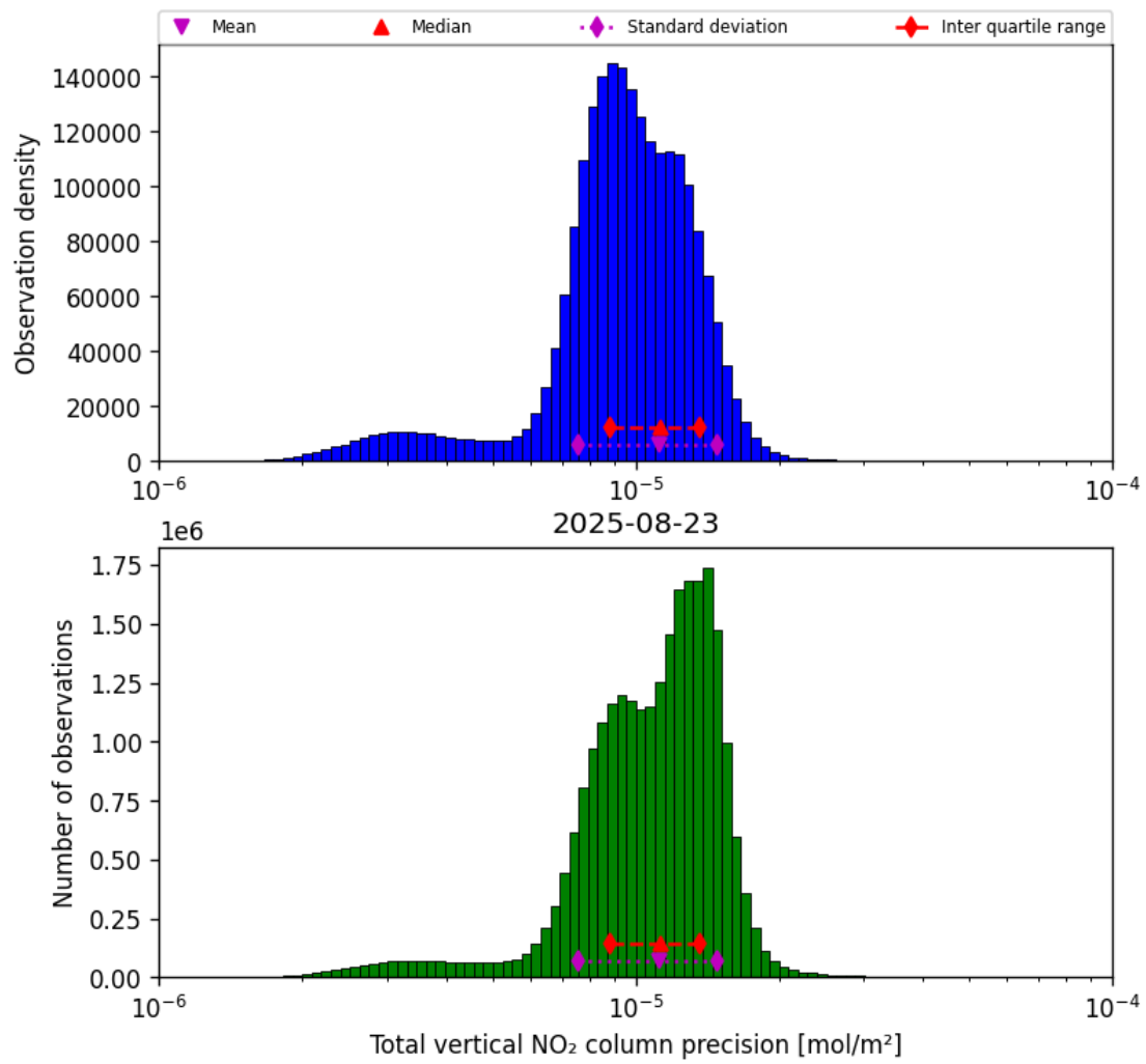
Figure 39: Histogram of “Total vertical NO 2 column precision” for 2025-08-22 to 2025-08-24
