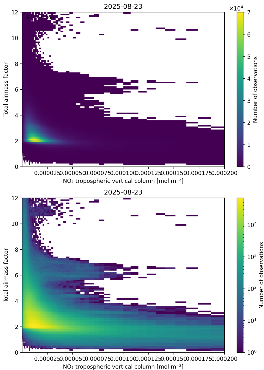
Figure 122: Scatter density plot of “NO 2 tropospheric vertical column” against “Total air mass factor” for 2025-08-22 to 2025-08-24.
