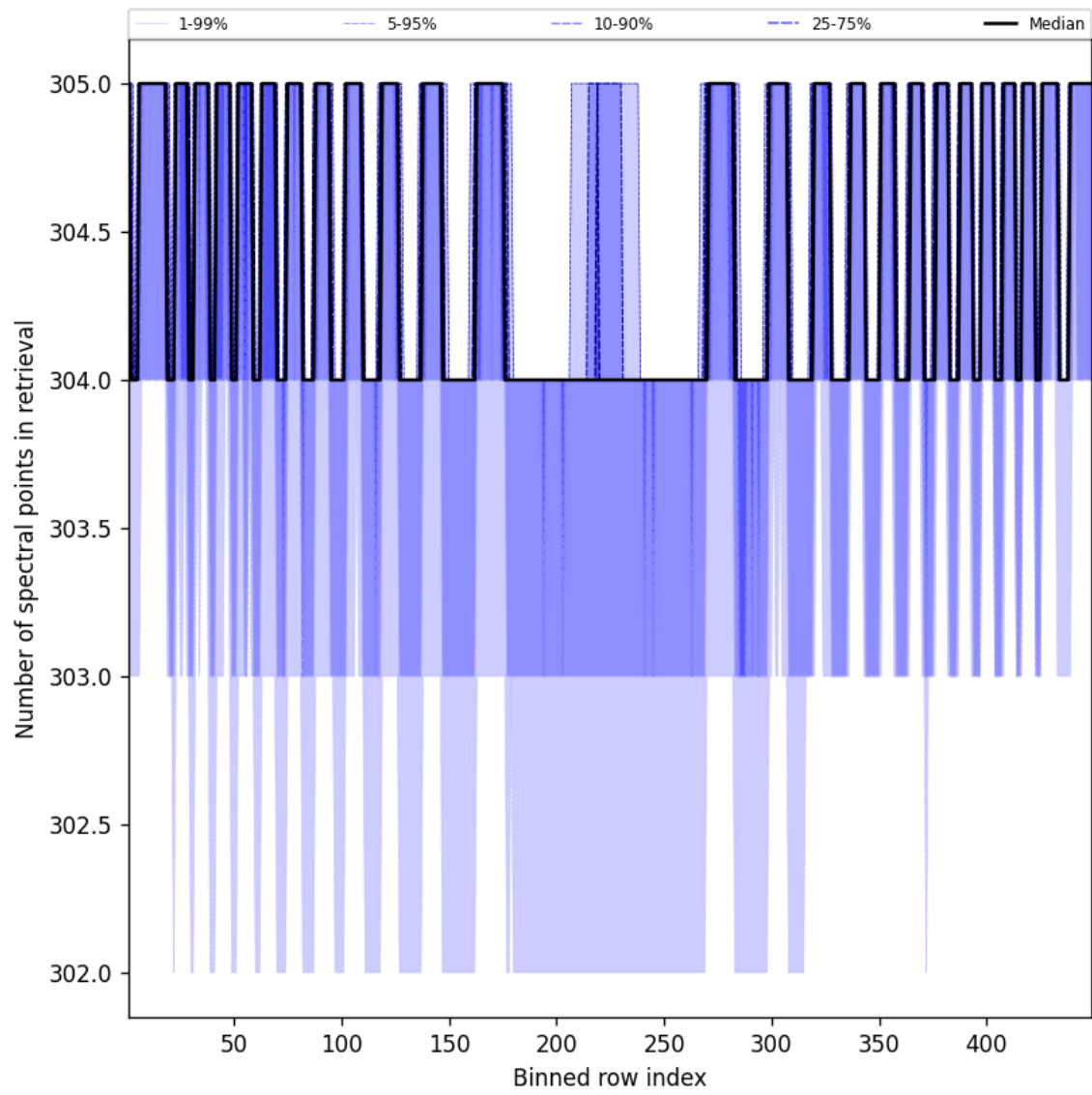
Figure 50: Along track statistics of “Number of spectral points in retrieval” for 2025-08-22 to 2025-08-24
