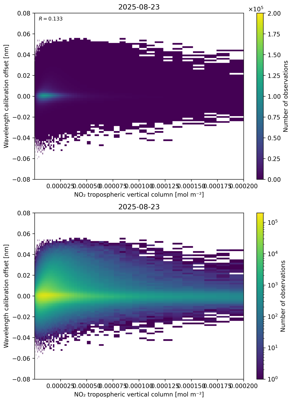
Figure 143: Scatter density plot of “NO 2 tropospheric vertical column” against “Wavelength calibration offset” for 2025-08-22 to 2025-08-24.
