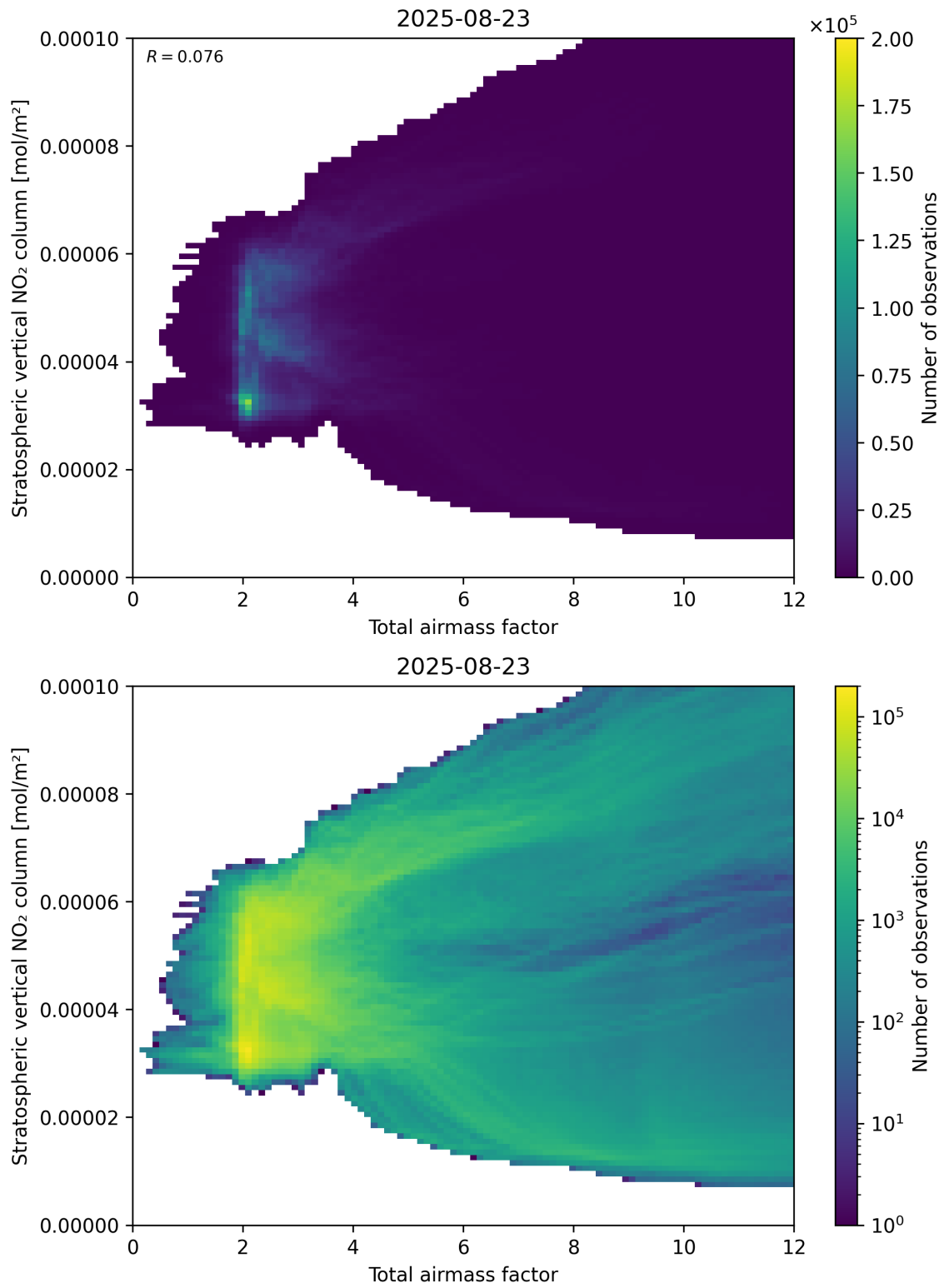
Figure 64: Scatter density plot of “Total airmass factor” against “Stratospheric vertical \text{NO}_2 column” for 2025-08-22 to 2025-08-24.
