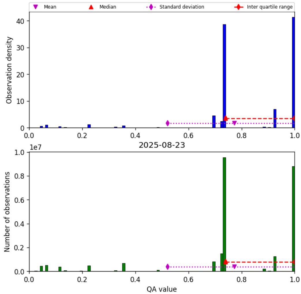
Figure 28: Histogram of “QA value” for 2025-08-22 to 2025-08-24
