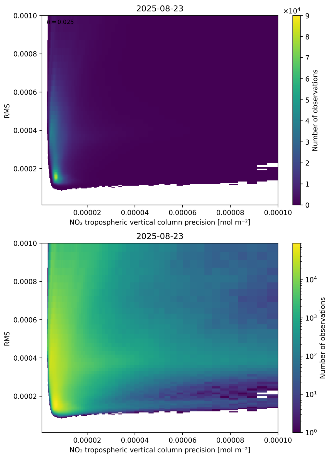
Figure 140: Scatter density plot of “NO 2 tropospheric vertical column precision” against “RMS” for 2025-08-22 to 2025-08-24.
