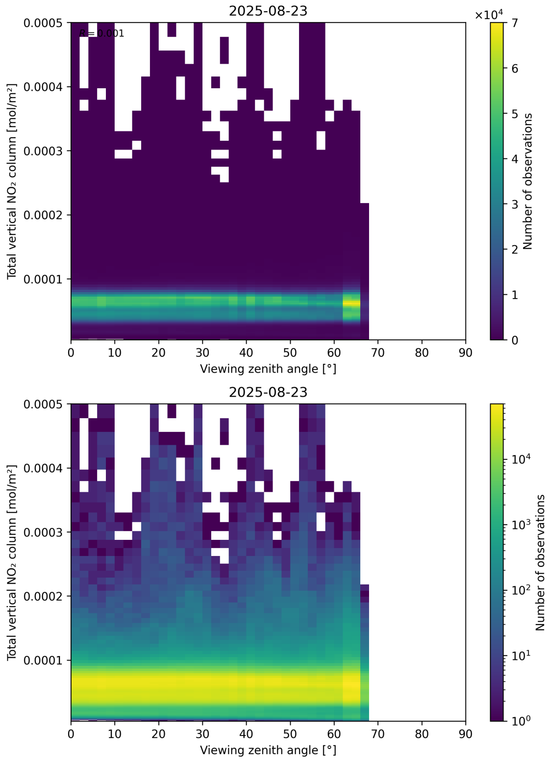
Figure 167: Scatter density plot of “Viewing zenith angle” against “Total vertical NO 2 column” for 2025-08-22 to 2025-08-24.
