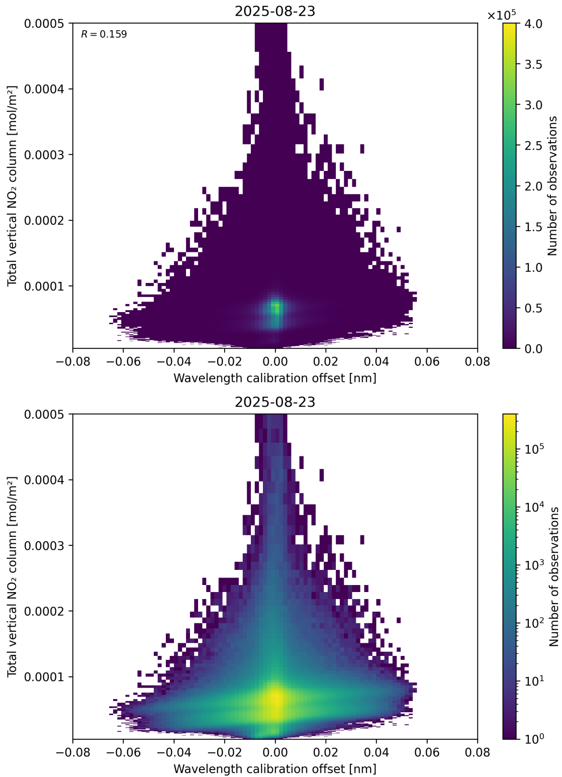
Figure 179: Scatter density plot of “Wavelength calibration offset” against “Total vertical NO 2 column” for 2025-08-22 to 2025-08-24.
