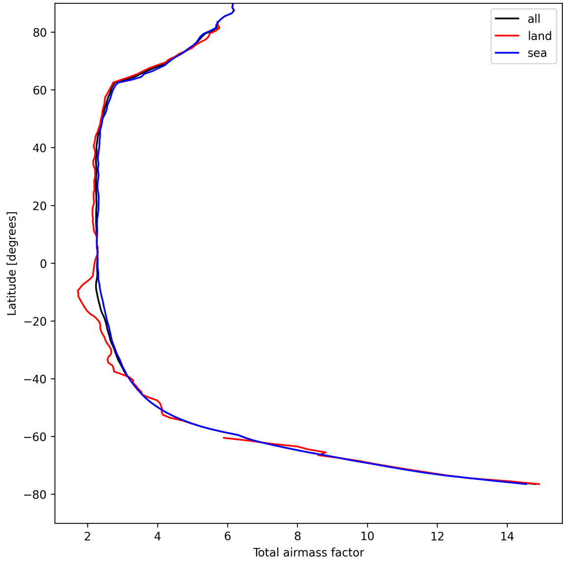
Figure 15: Zonal average of “Total airmass factor” for 2025-08-22 to 2025-08-24.
