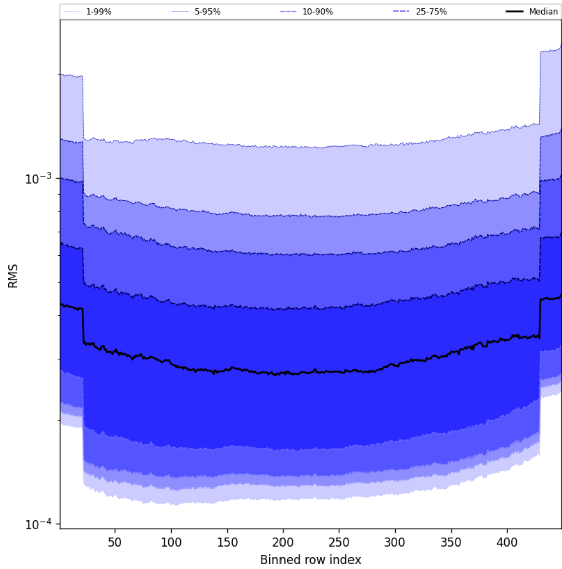
Figure 60: Along track statistics of “RMS” for 2025-08-22 to 2025-08-24
