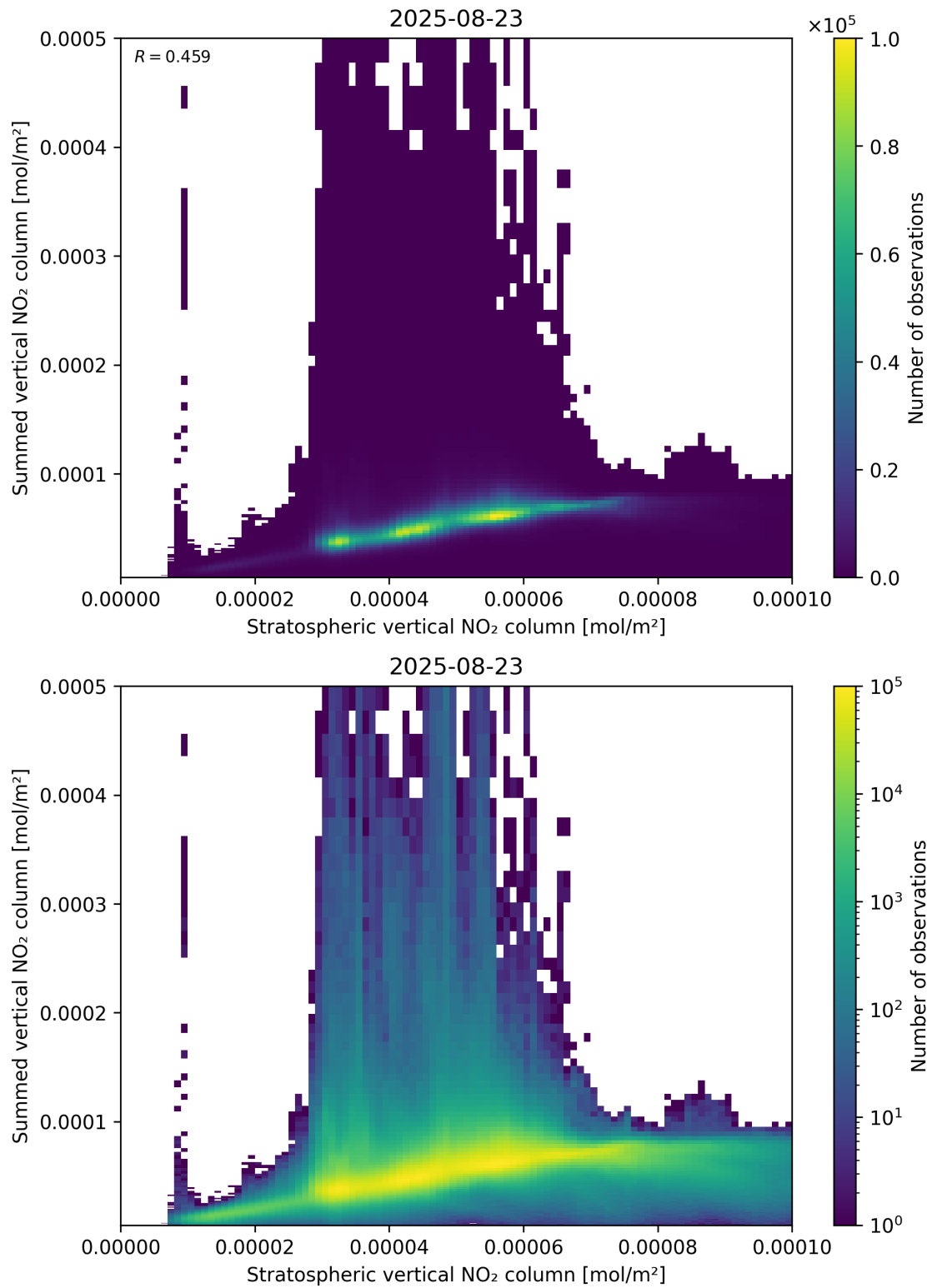
Figure 98: Scatter density plot of “Stratospheric vertical NO 2 column” against “Summed vertical NO 2 column” for 2025-08-22 to 2025-08-24.
