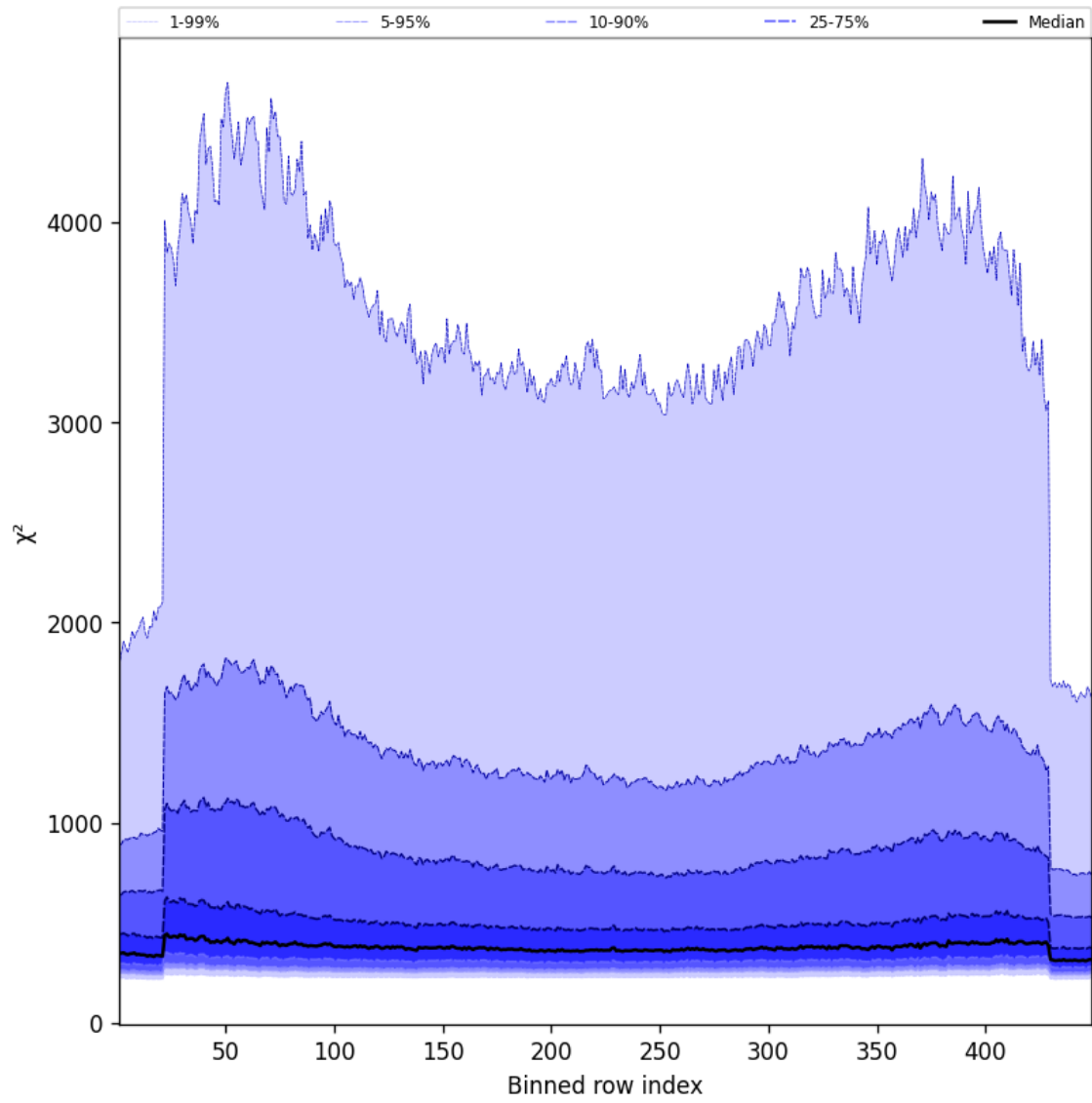
Figure 59: Along track statistics of “ \chi^2 ” for 2025-08-22 to 2025-08-24
