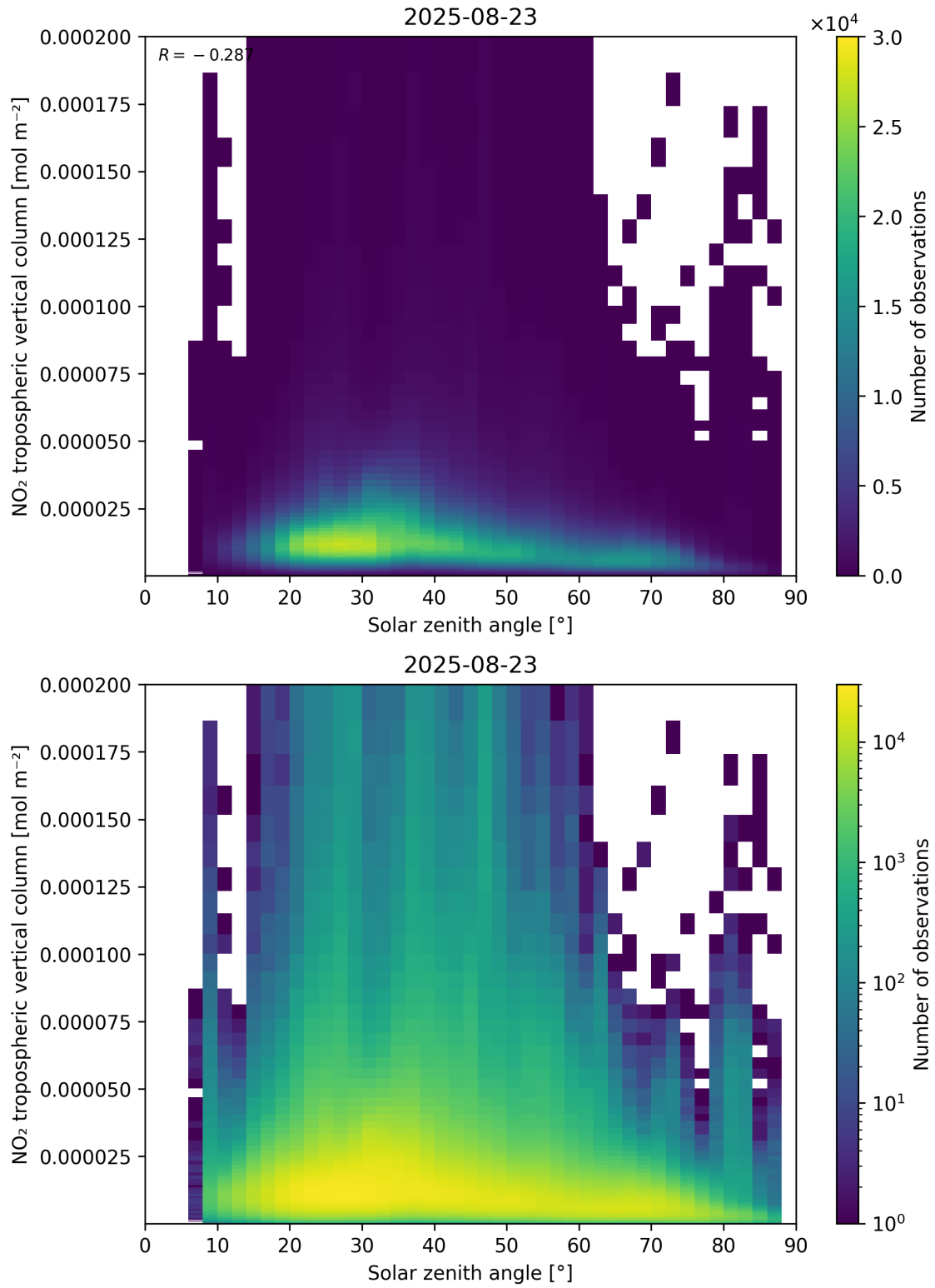
Figure 155: Scatter density plot of “Solar zenith angle” against “NO 2 tropospheric vertical column” for 2025-08-22 to 2025-08-24.
