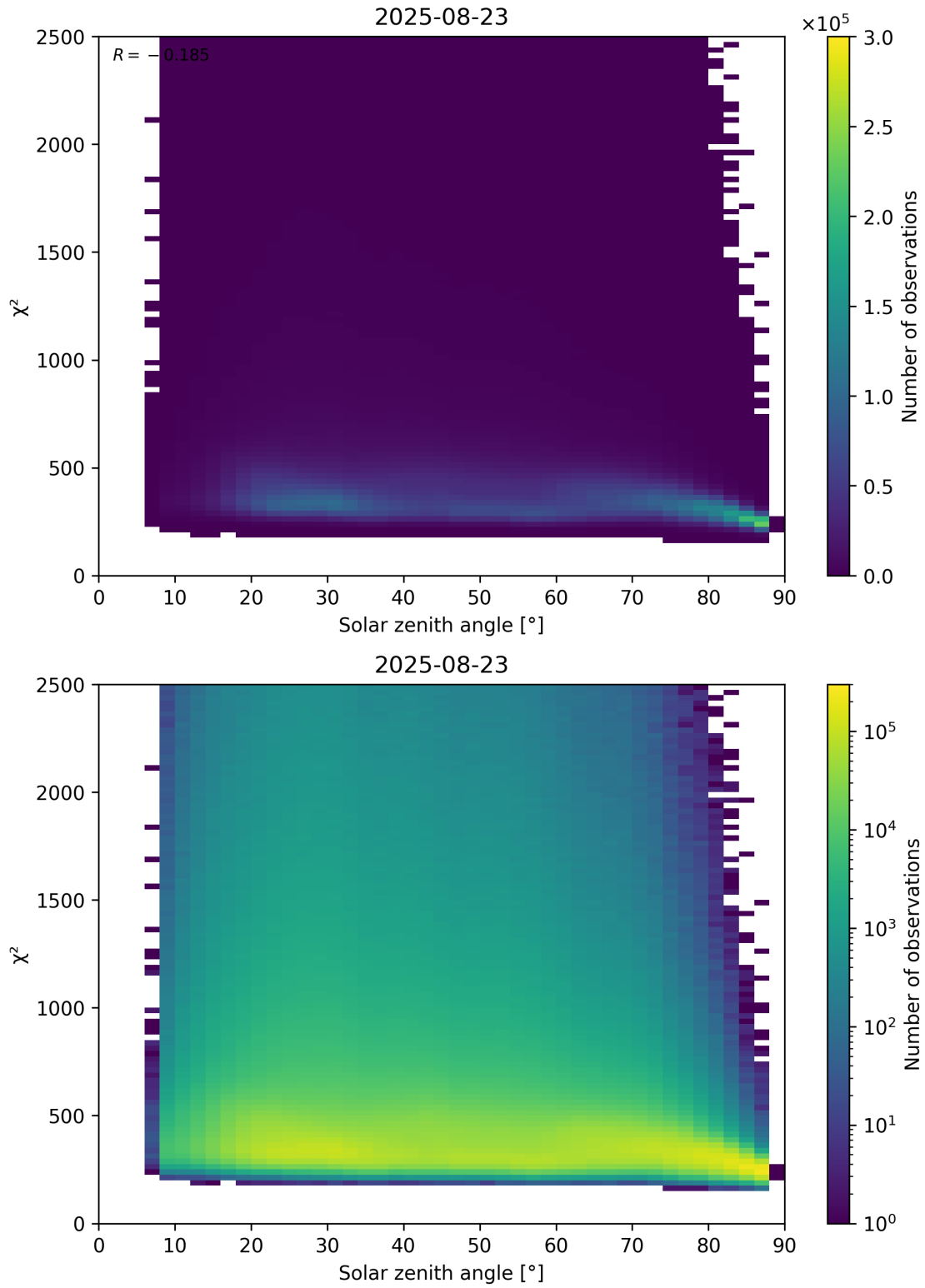
Figure 148: Scatter density plot of “Solar zenith angle” against “ \chi^2 ” for 2025-08-22 to 2025-08-24.
