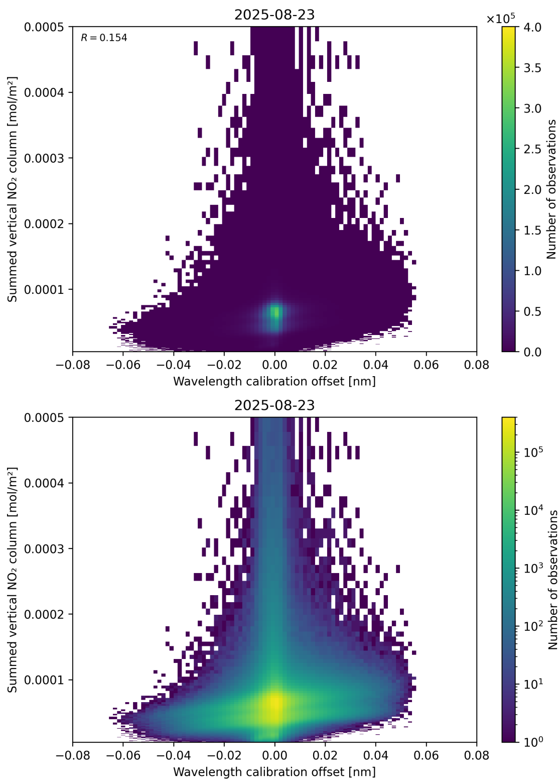
Figure 177: Scatter density plot of “Wavelength calibration offset” against “Summed vertical NO 2 column” for 2025-08-22 to 2025-08-24.
