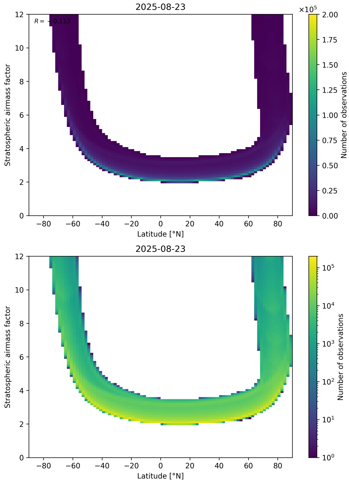
Figure 83: Scatter density plot of “Latitude” against “Stratospheric air mass factor” for 2025-08-22 to 2025-08-24.
