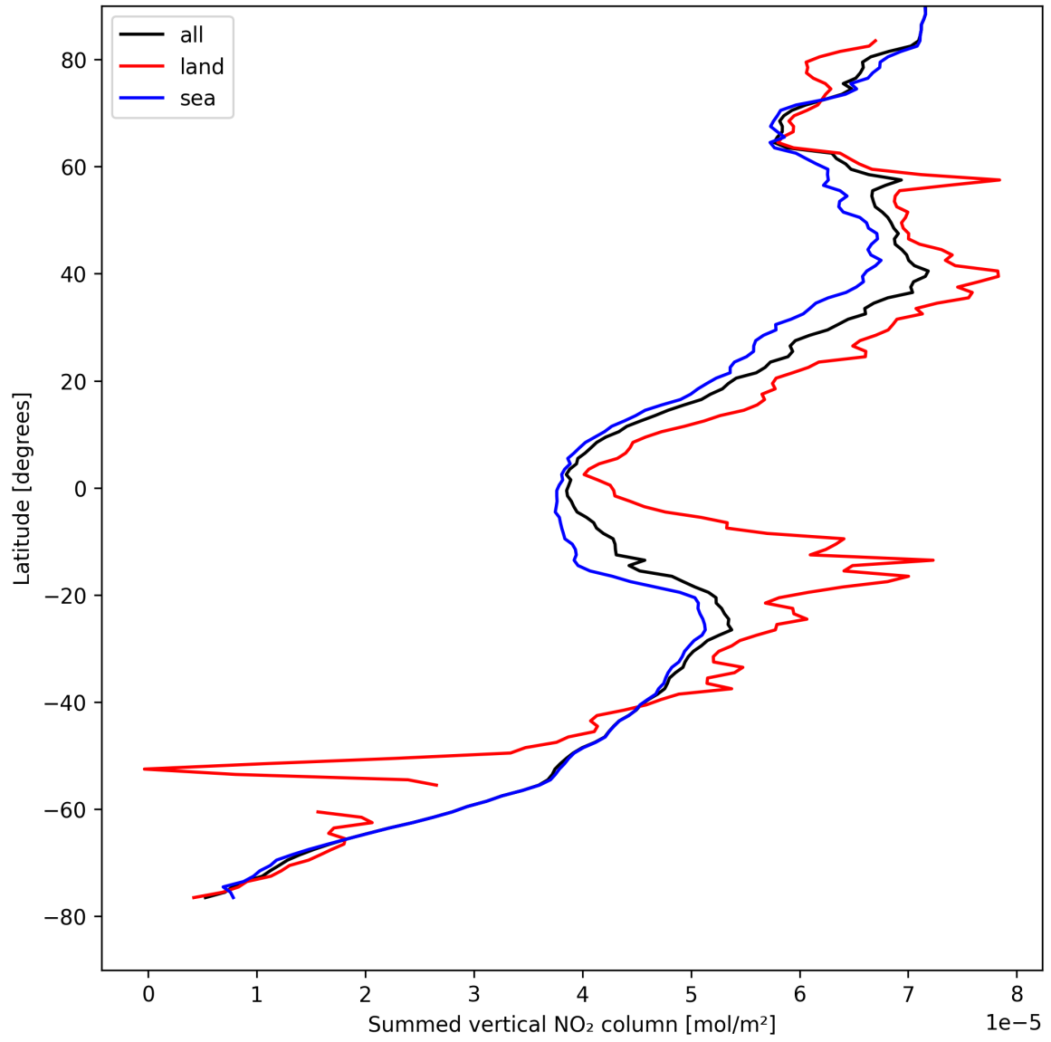
Figure 23: Zonal average of “Summed vertical NO 2 column” for 2025-08-22 to 2025-08-24.
