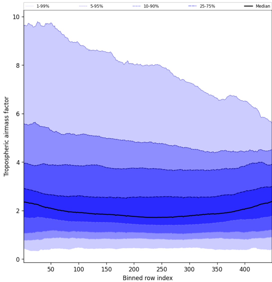
Figure 48: Along track statistics of “Tropospheric airmass factor” for 2025-08-22 to 2025-08-24
