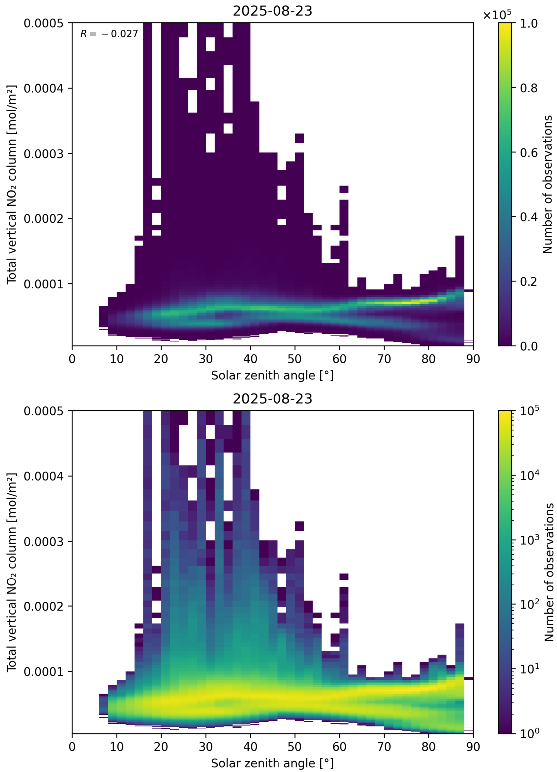
Figure 153: Scatter density plot of “Solar zenith angle” against “Total vertical NO 2 column” for 2025-08-22 to 2025-08-24.
