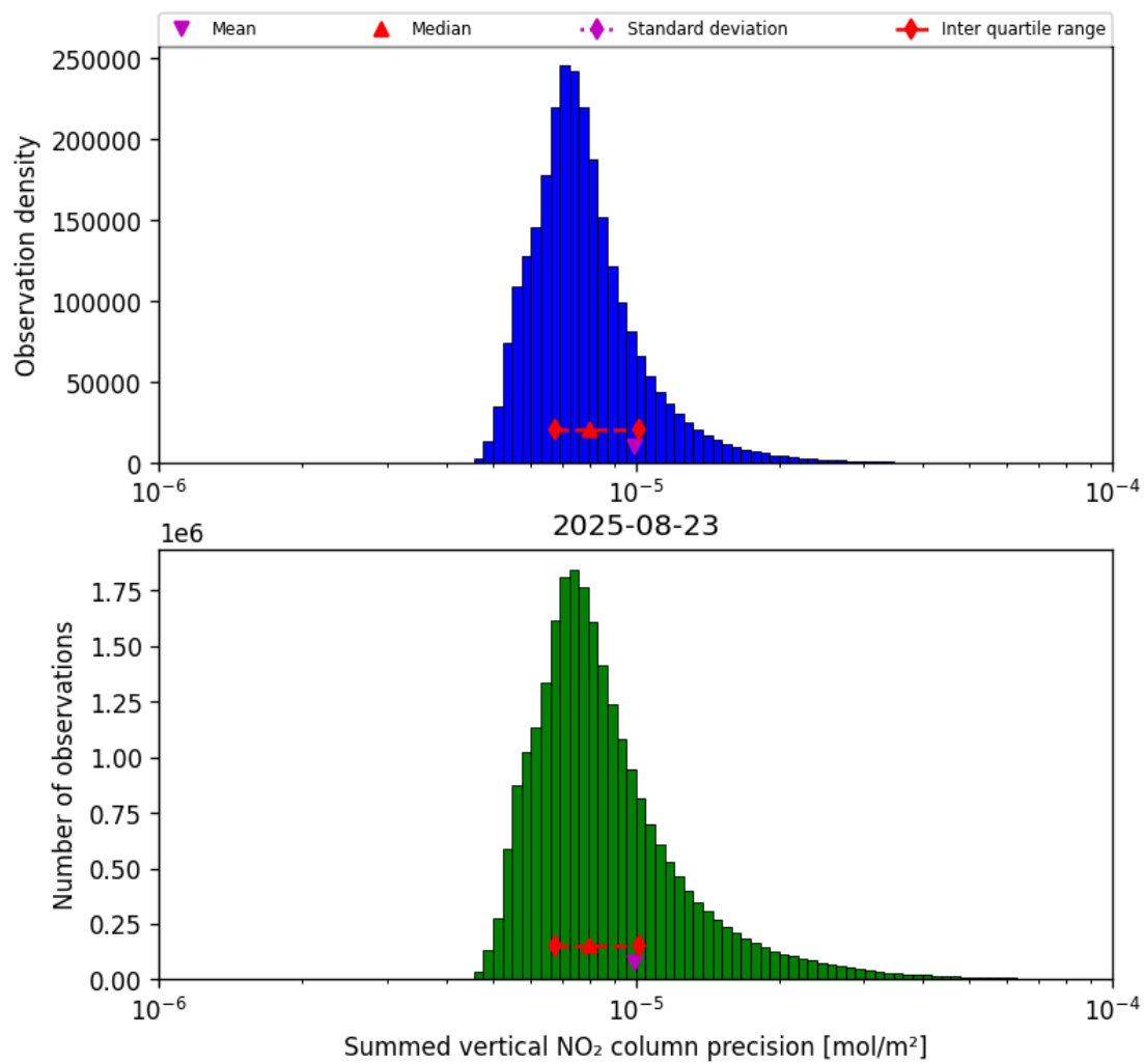
Figure 41: Histogram of “Summed vertical NO 2 column precision” for 2025-08-22 to 2025-08-24
