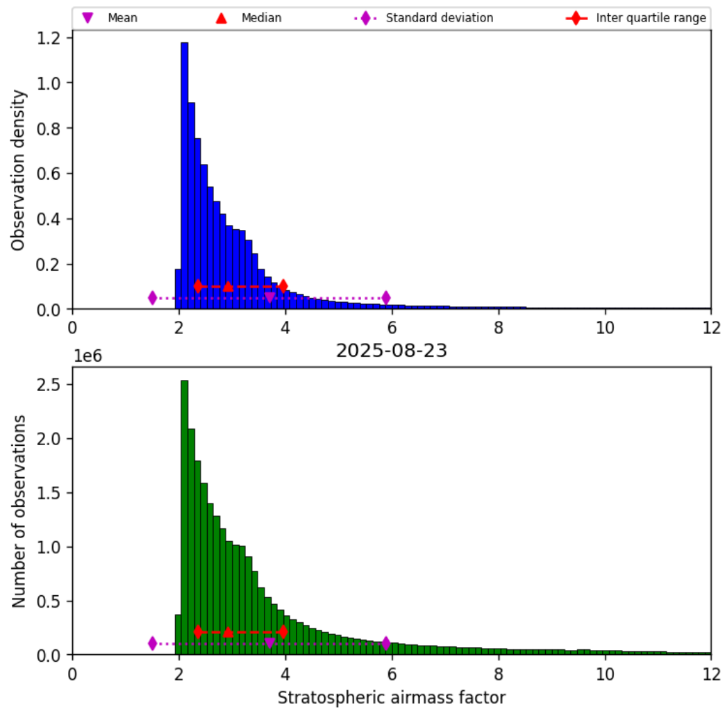
Figure 44: Histogram of “Stratospheric airmass factor” for 2025-08-22 to 2025-08-24
