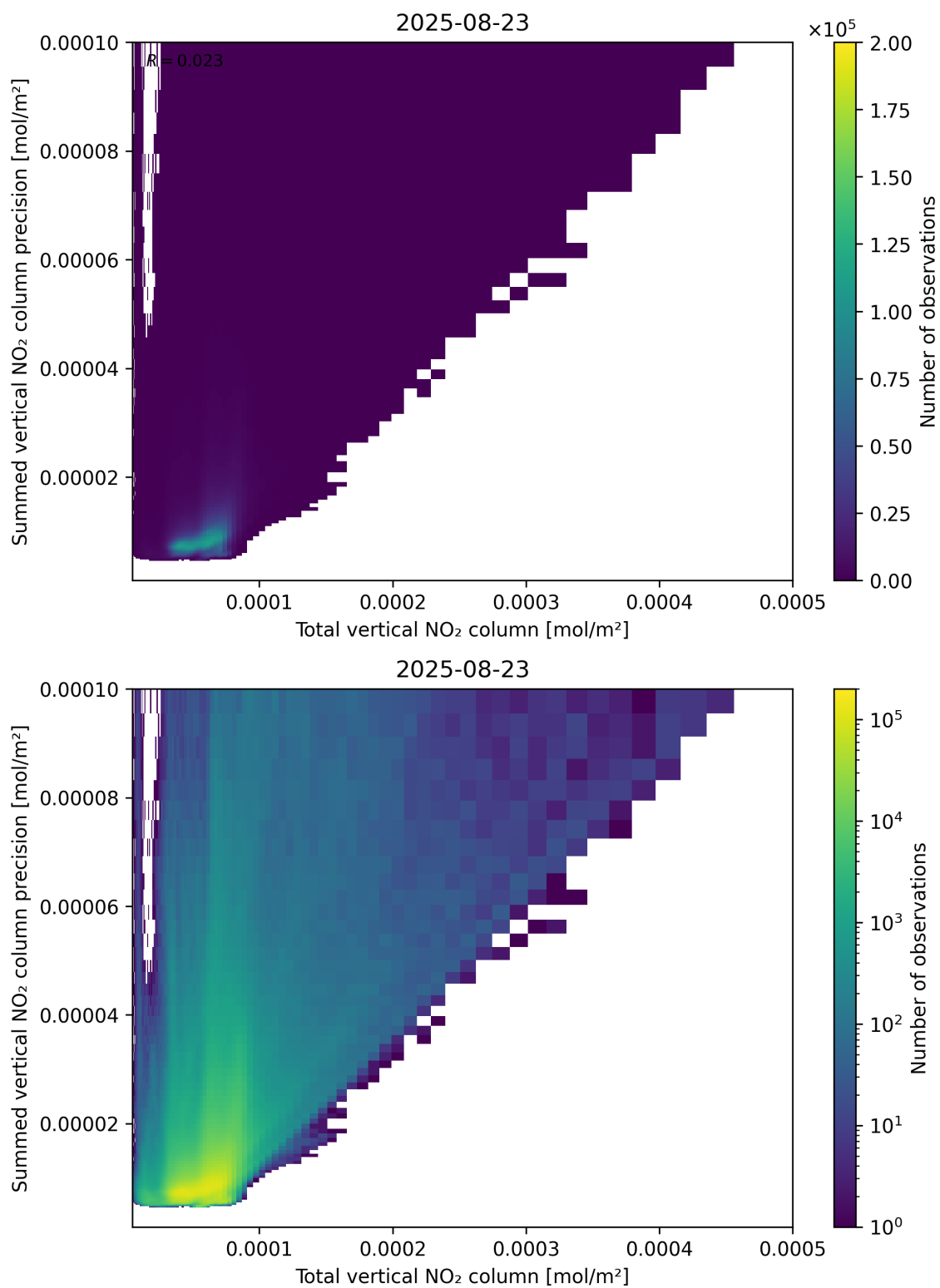
Figure 113: Scatter density plot of “Total vertical NO 2 column” against “Summed vertical NO 2 column precision” for 2025-08-22 to 2025-08-24.
