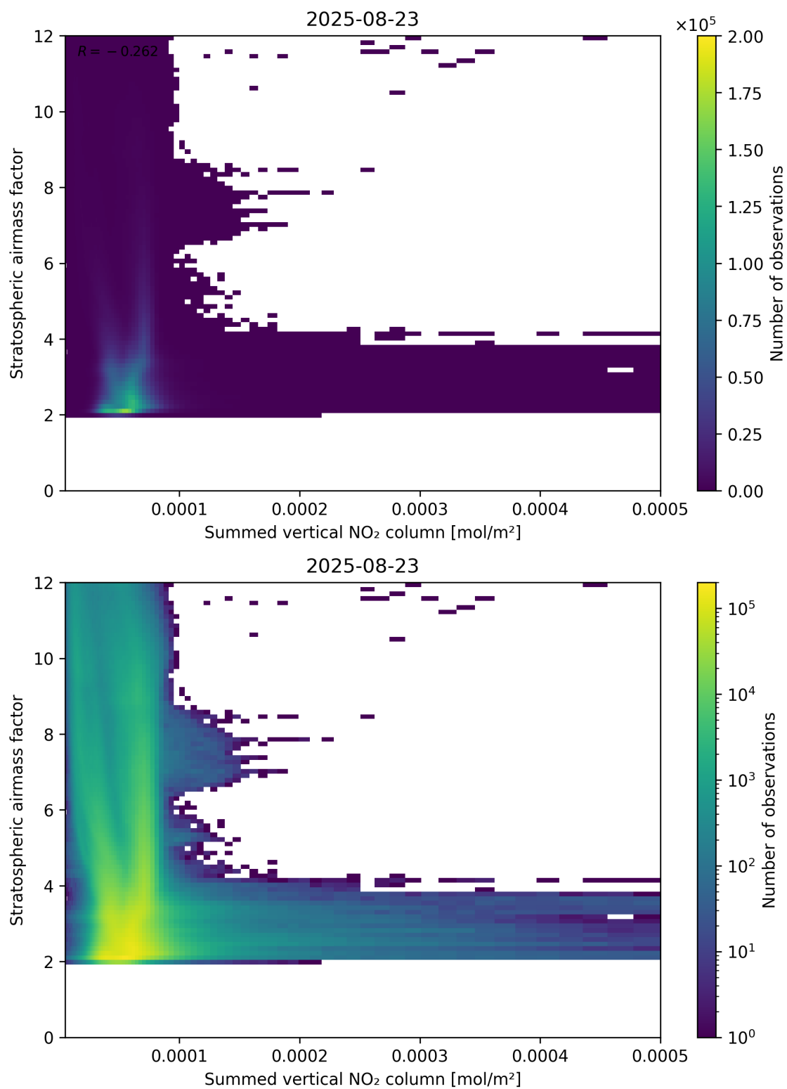
Figure 103: Scatter density plot of “Summed vertical NO 2 column” against “Stratospheric airmass factor” for 2025-08-22 to 2025-08-24.
