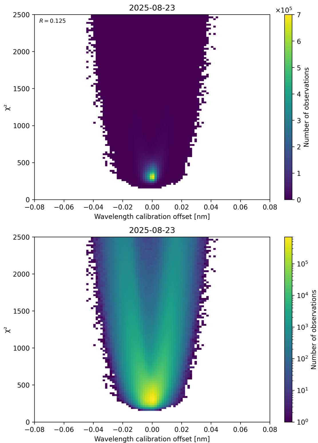
Figure 175: Scatter density plot of “Wavelength calibration offset” against “ \chi^2 ” for 2025-08-22 to 2025-08-24.
