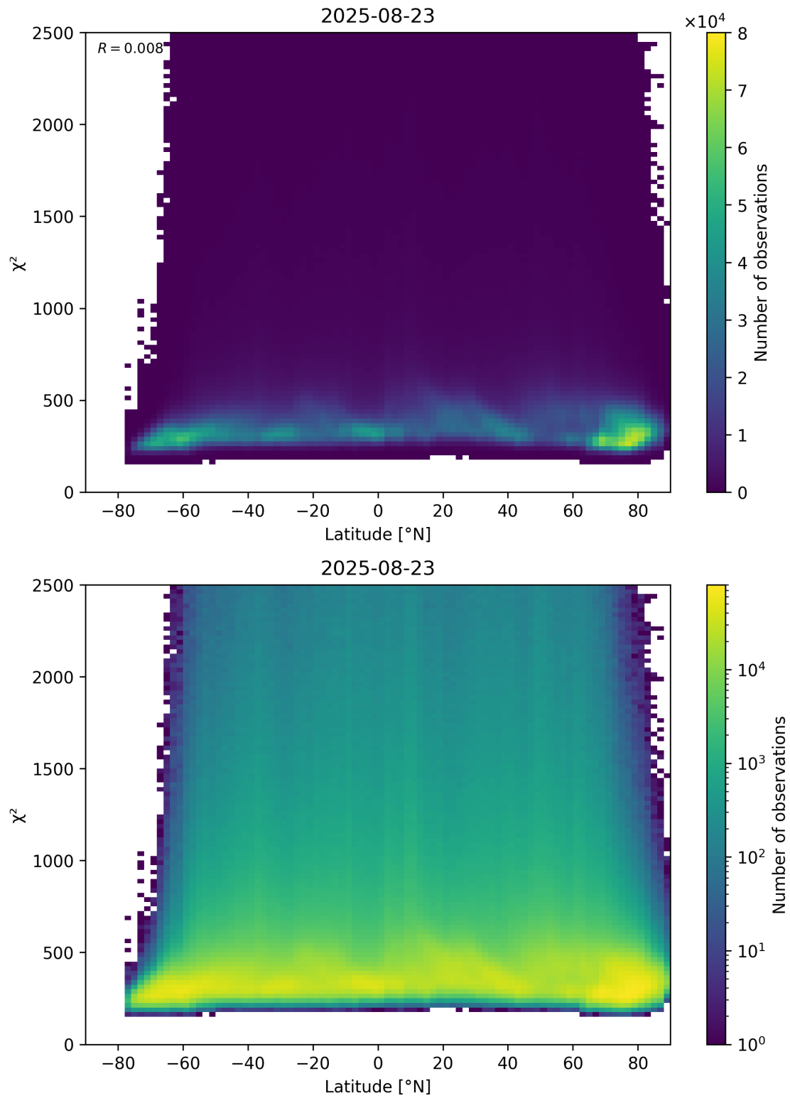
Figure 86: Scatter density plot of “Latitude” against “ \chi^2 ” for 2025-08-22 to 2025-08-24.
