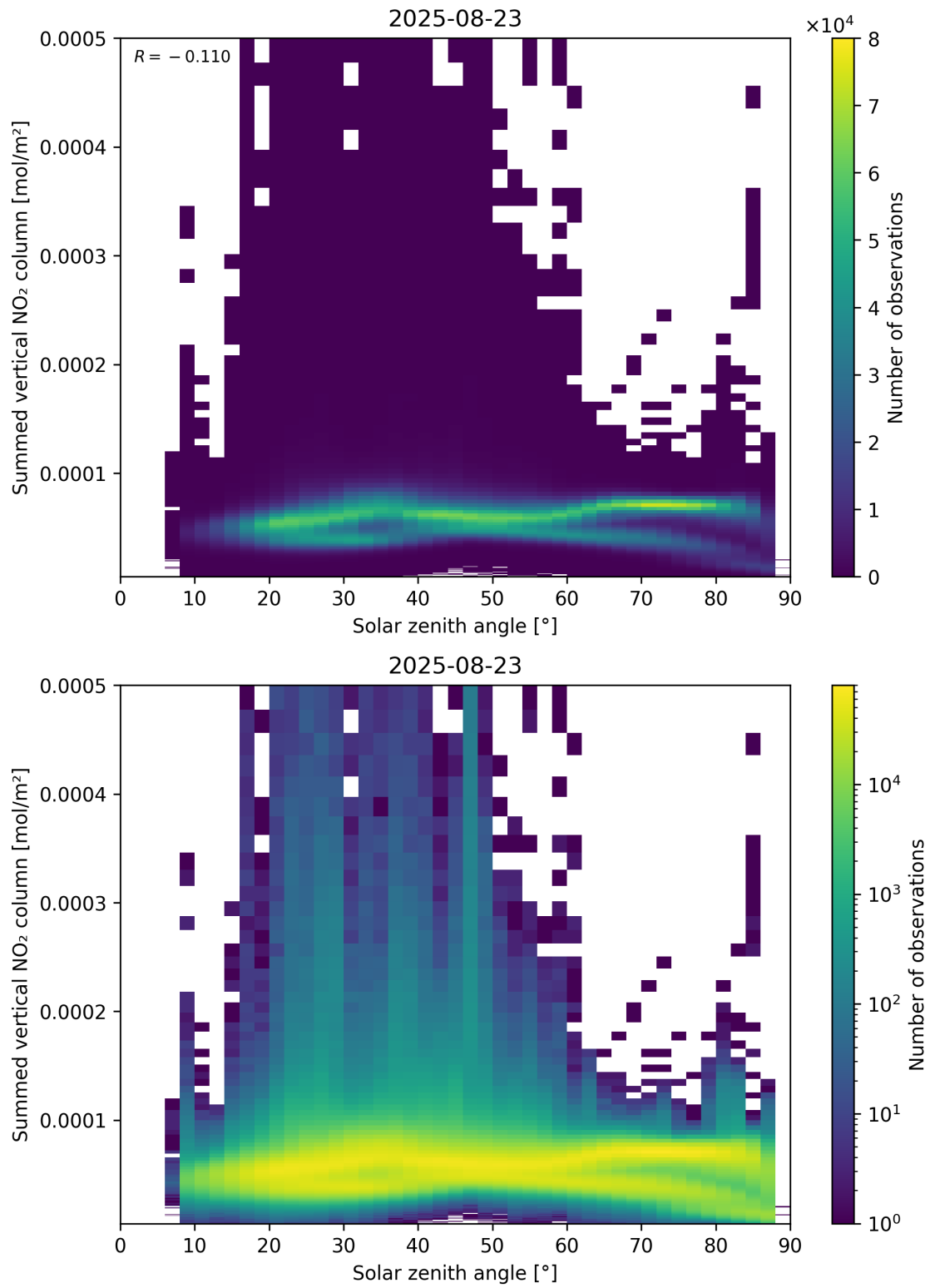
Figure 151: Scatter density plot of “Solar zenith angle” against “Summed vertical NO 2 column” for 2025-08-22 to 2025-08-24.
