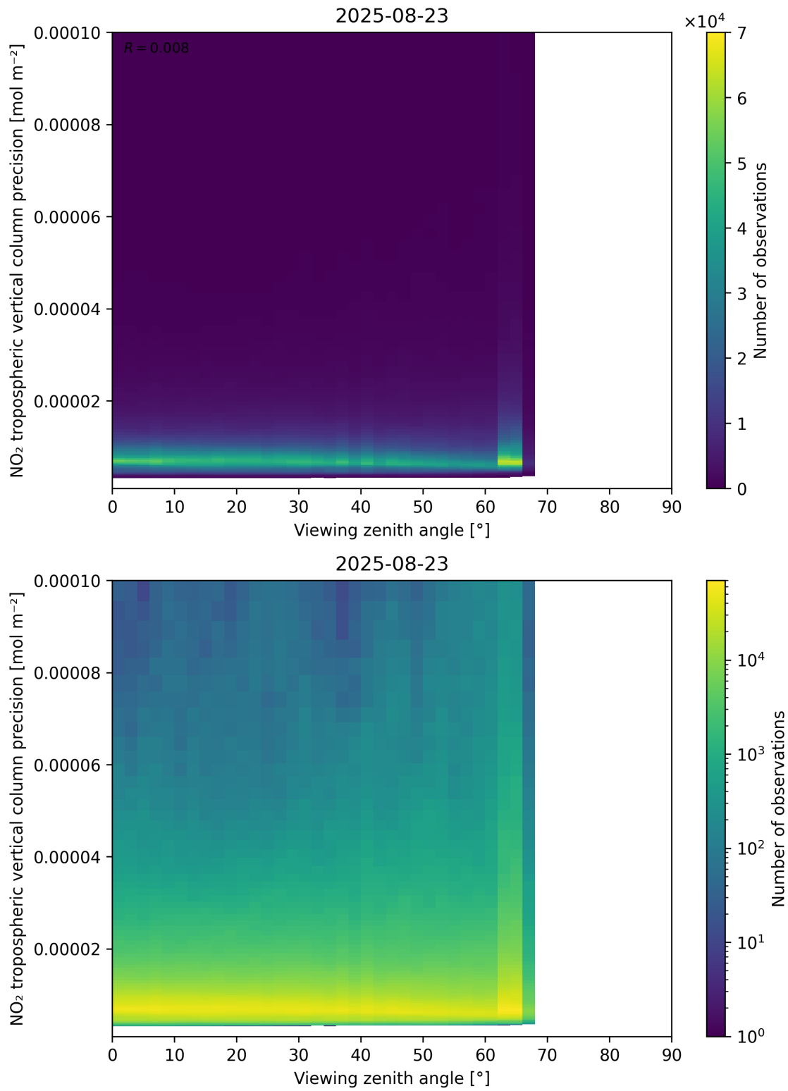
Figure 170: Scatter density plot of “Viewing zenith angle” against “NO 2 tropospheric vertical column precision” for 2025-08-22 to 2025-08-24.
