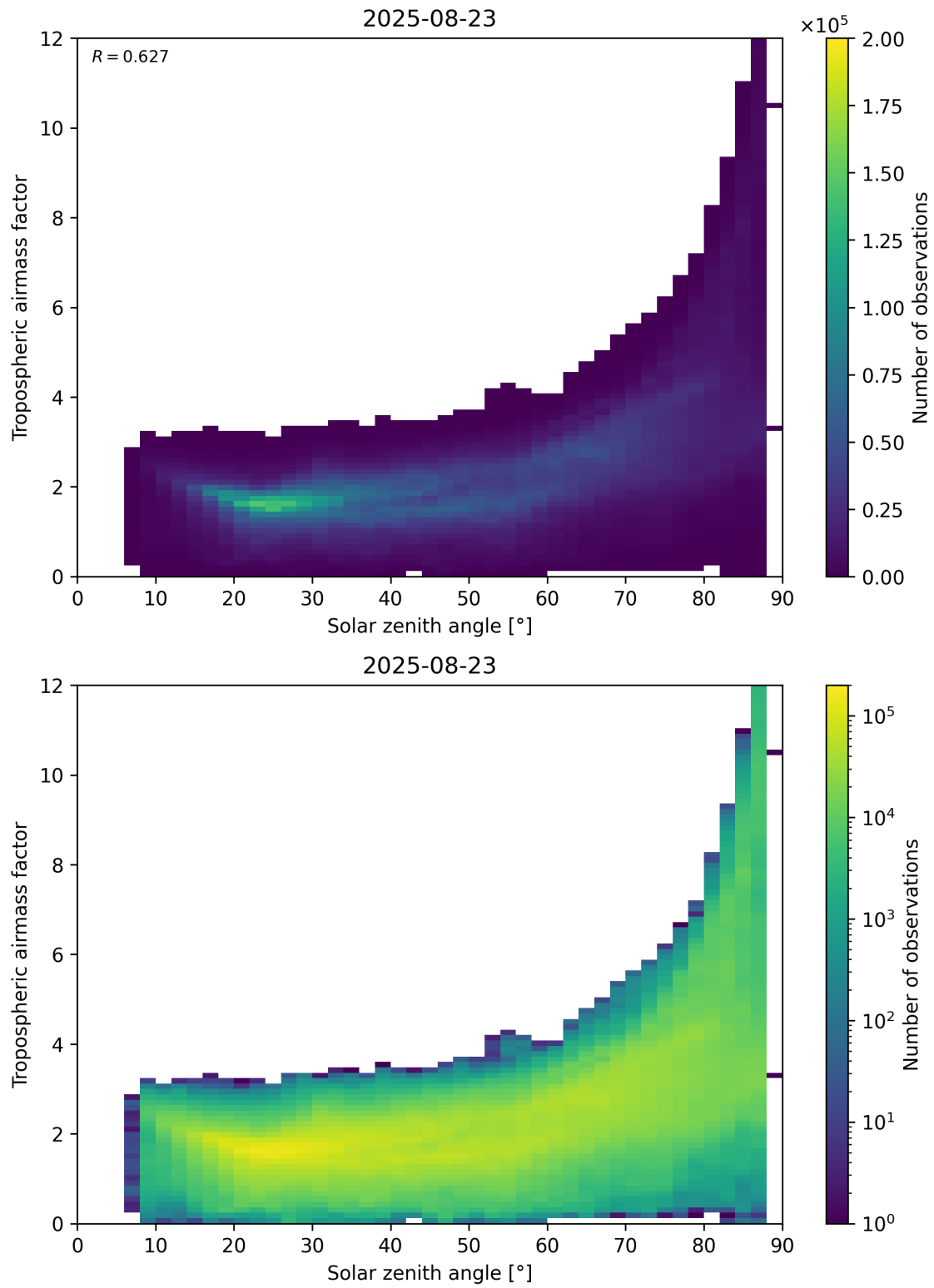
Figure 147: Scatter density plot of “Solar zenith angle” against “Tropospheric airmass factor” for 2025-08-22 to 2025-08-24.
