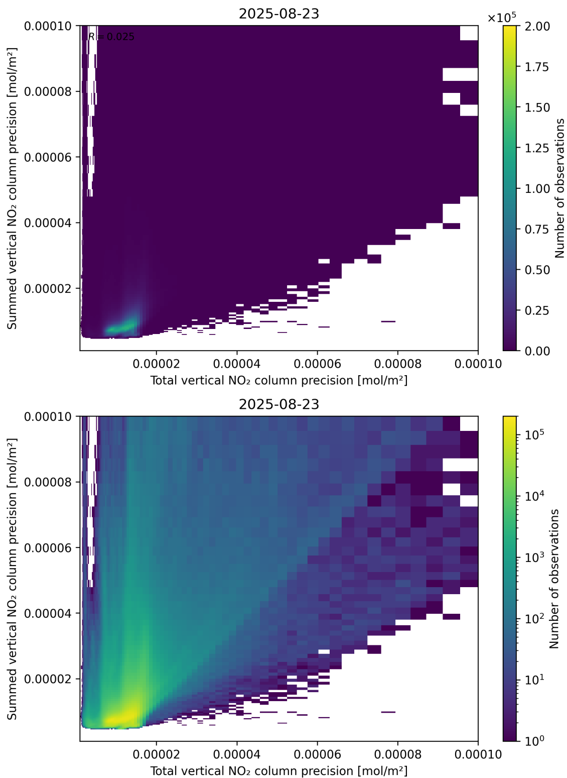
Figure 118: Scatter density plot of “Total vertical NO 2 column precision” against “Summed vertical NO 2 column precision” for 2025-08-22 to 2025-08-24.
