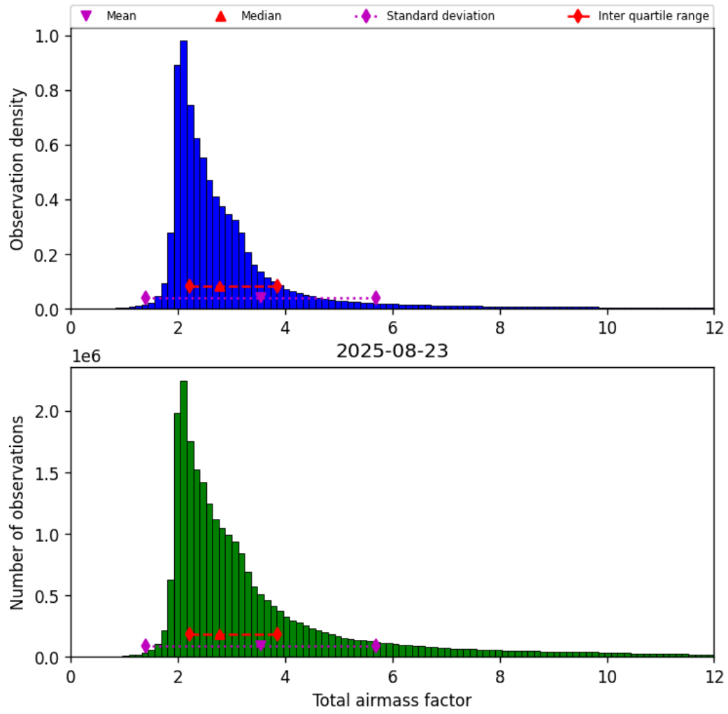
Figure 32: Histogram of “Total airmass factor” for 2025-08-22 to 2025-08-24
