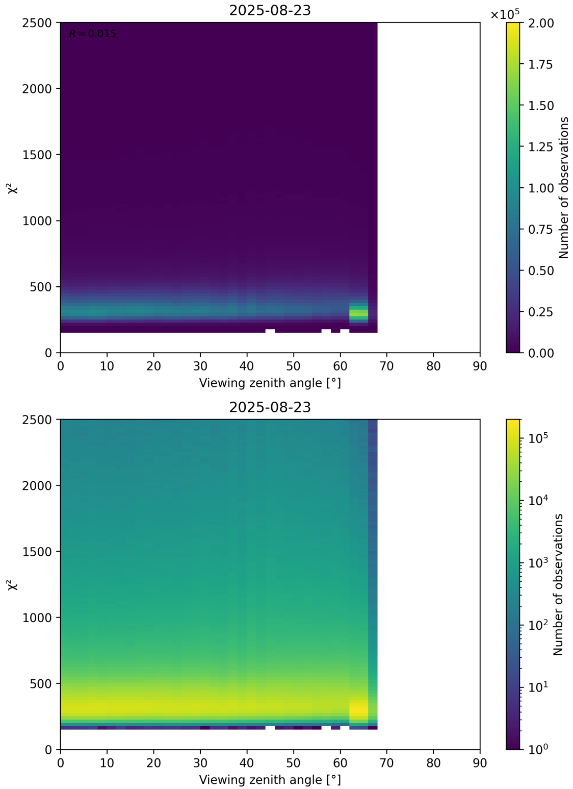
Figure 162: Scatter density plot of “Viewing zenith angle” against “ \chi^2 ” for 2025-08-22 to 2025-08-24.
