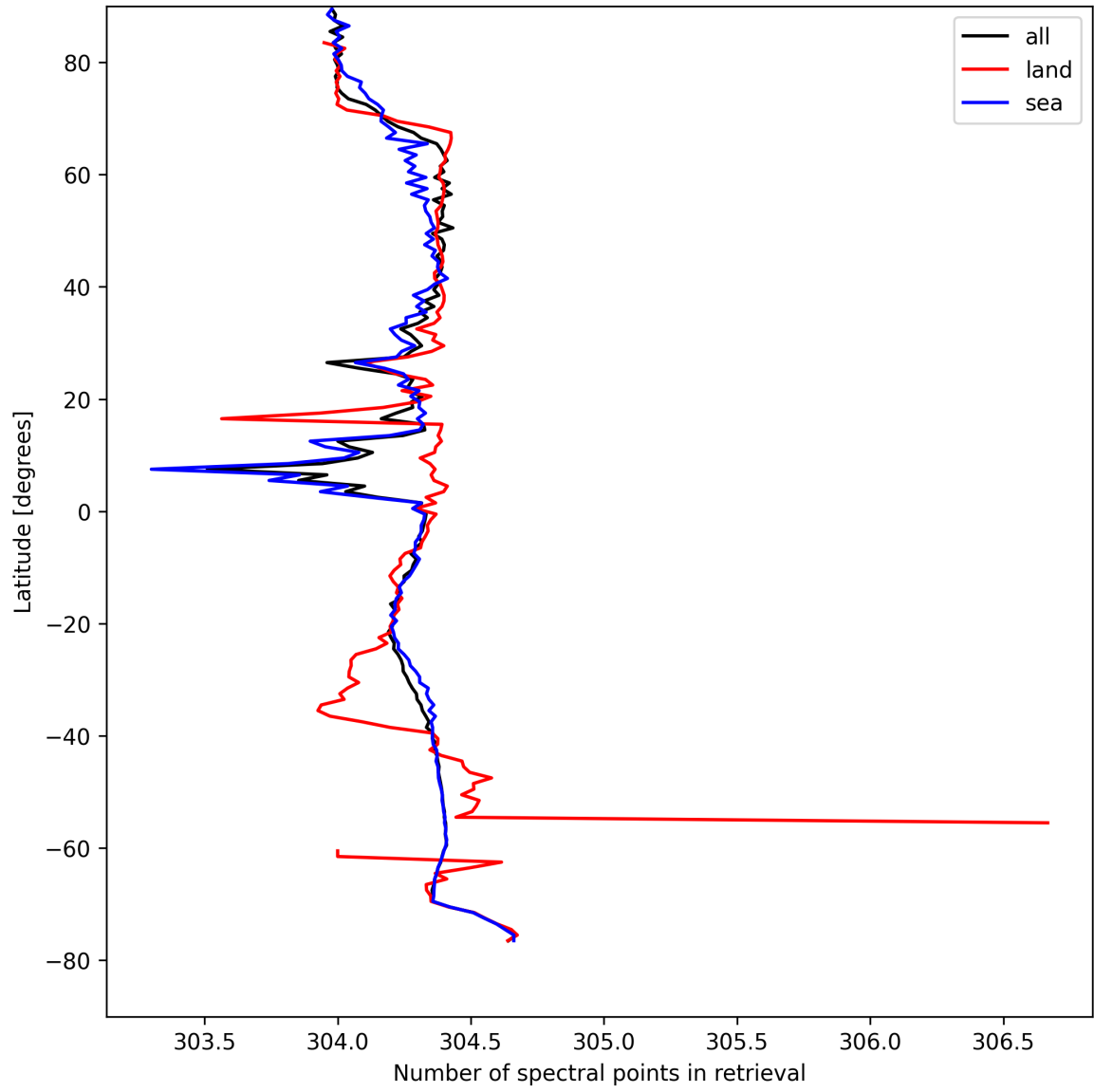
Figure 16: Zonal average of “Number of spectral points in retrieval” for 2025-08-22 to 2025-08-24.
