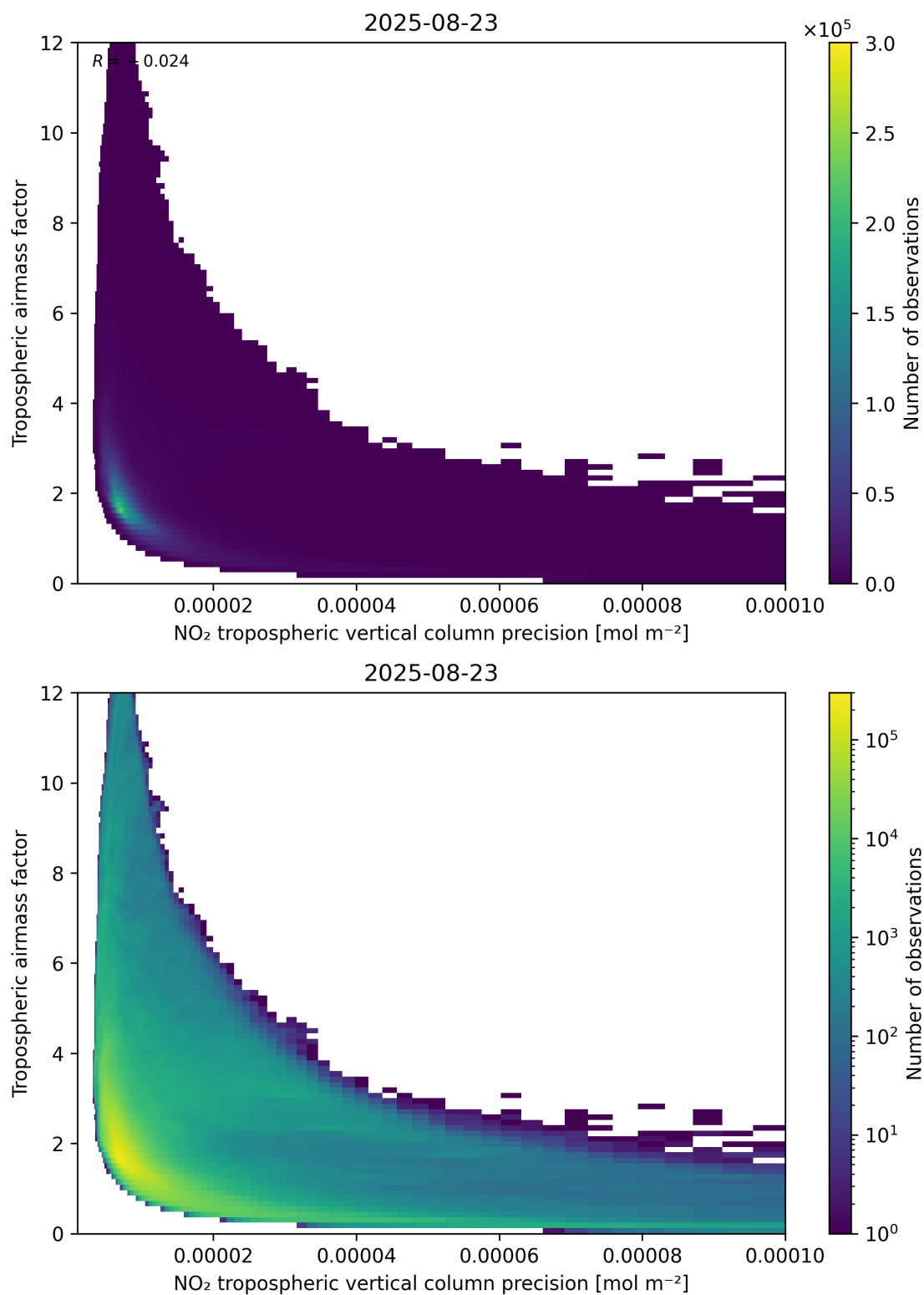
Figure 133: Scatter density plot of “NO 2 tropospheric vertical column precision” against “Tropospheric airmass factor” for 2025-08-22 to 2025-08-24.
