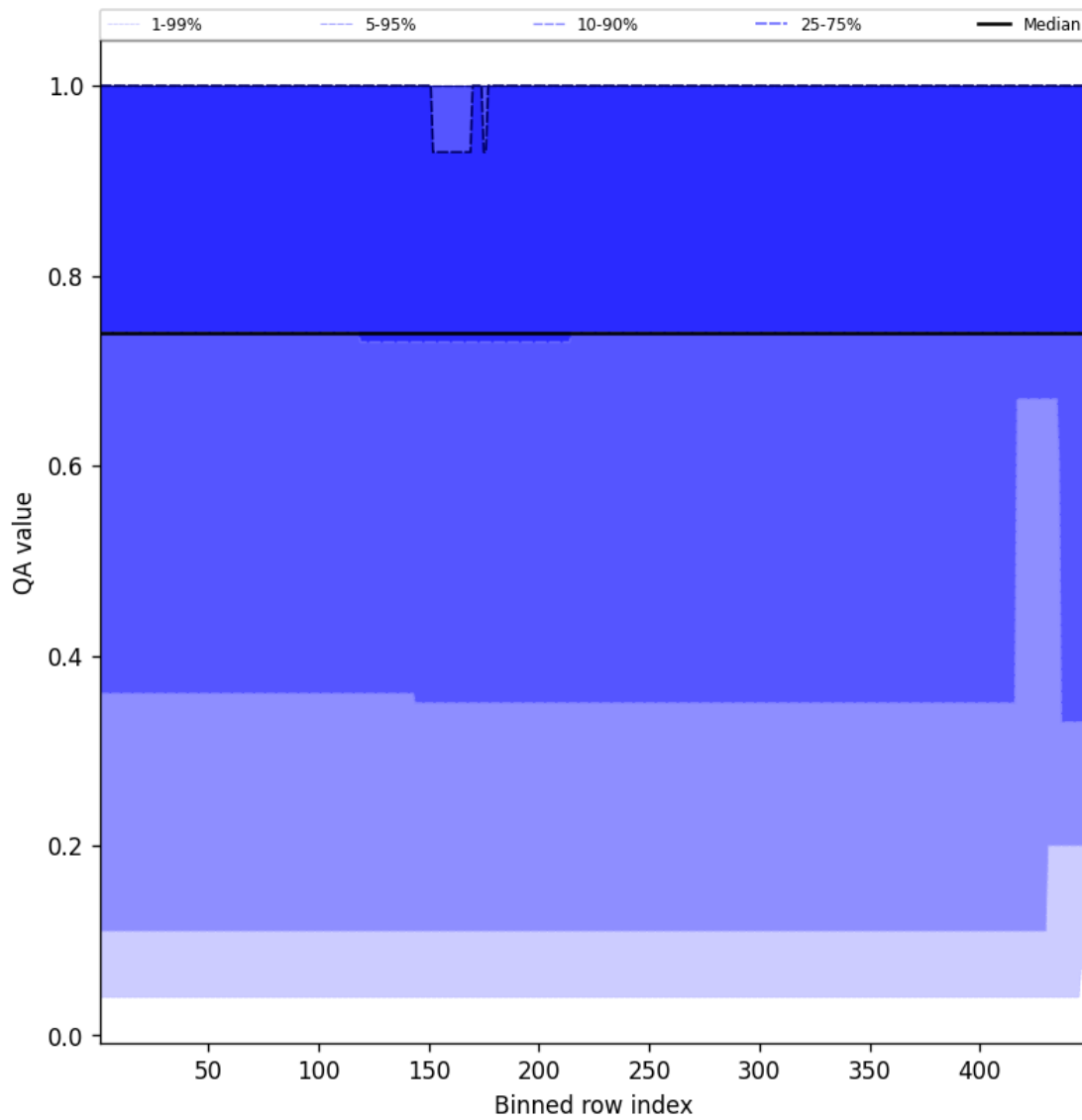
Figure 45: Along track statistics of “QA value” for 2025-08-22 to 2025-08-24
