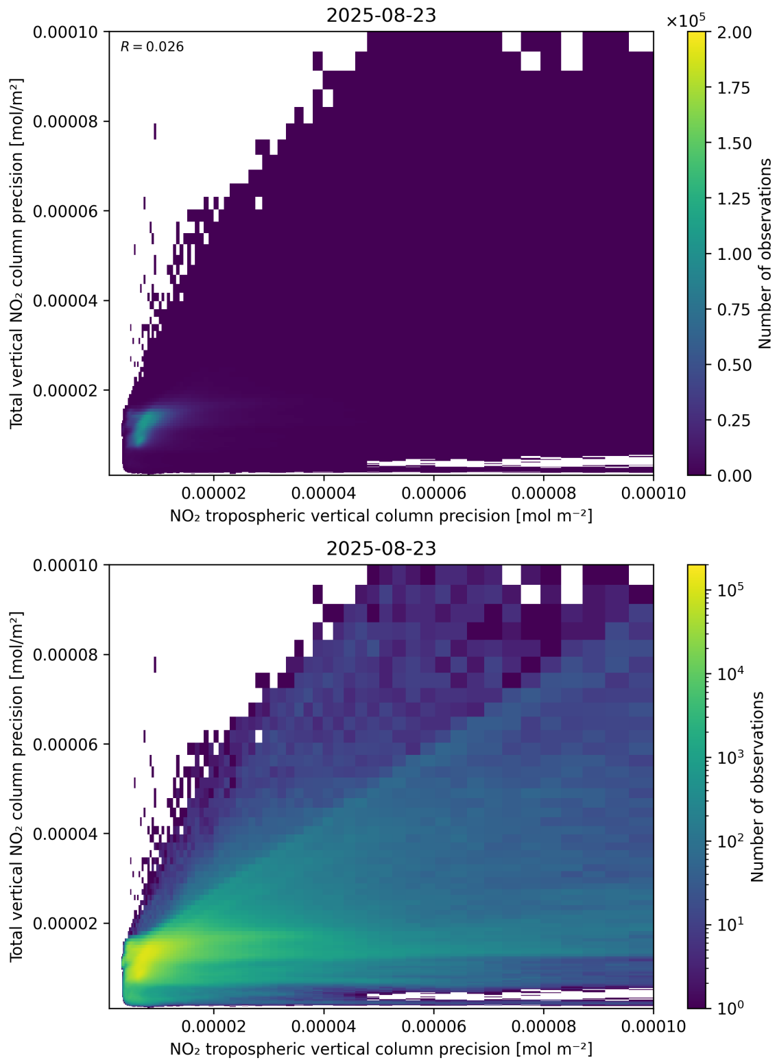
Figure 139: Scatter density plot of “NO 2 tropospheric vertical column precision” against “Total vertical NO 2 column precision” for 2025-08-22 to 2025-08-24.
