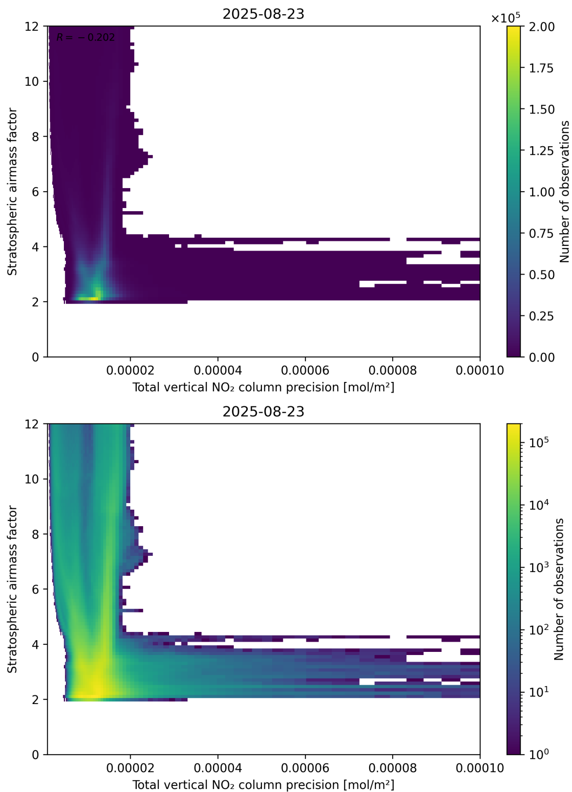
Figure 115: Scatter density plot of “Total vertical NO 2 column precision” against “Stratospheric air mass factor” for 2025-08-22 to 2025-08-24.
