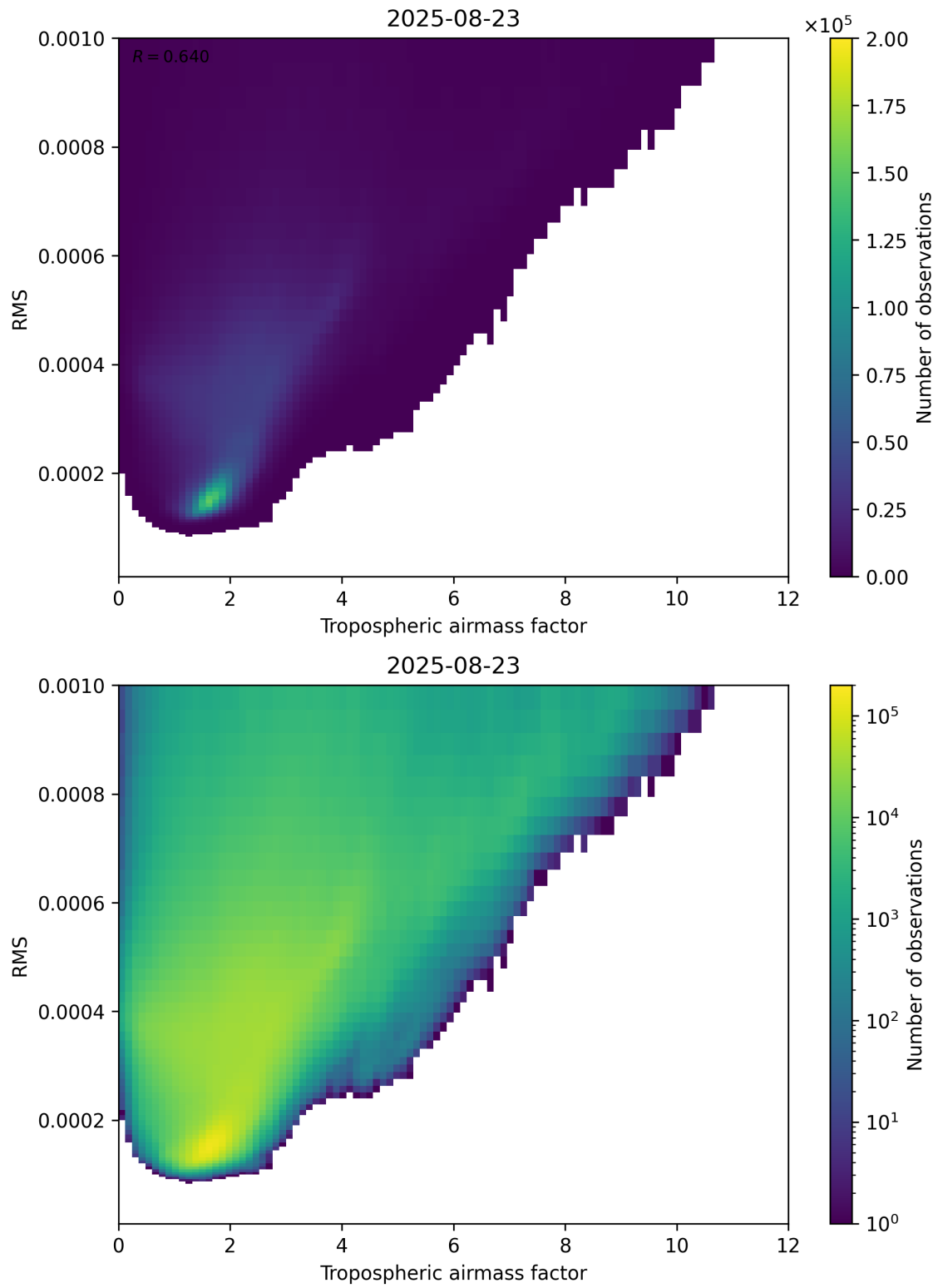
Figure 79: Scatter density plot of “Tropospheric airmass factor” against “RMS” for 2025-08-22 to 2025-08-24.
