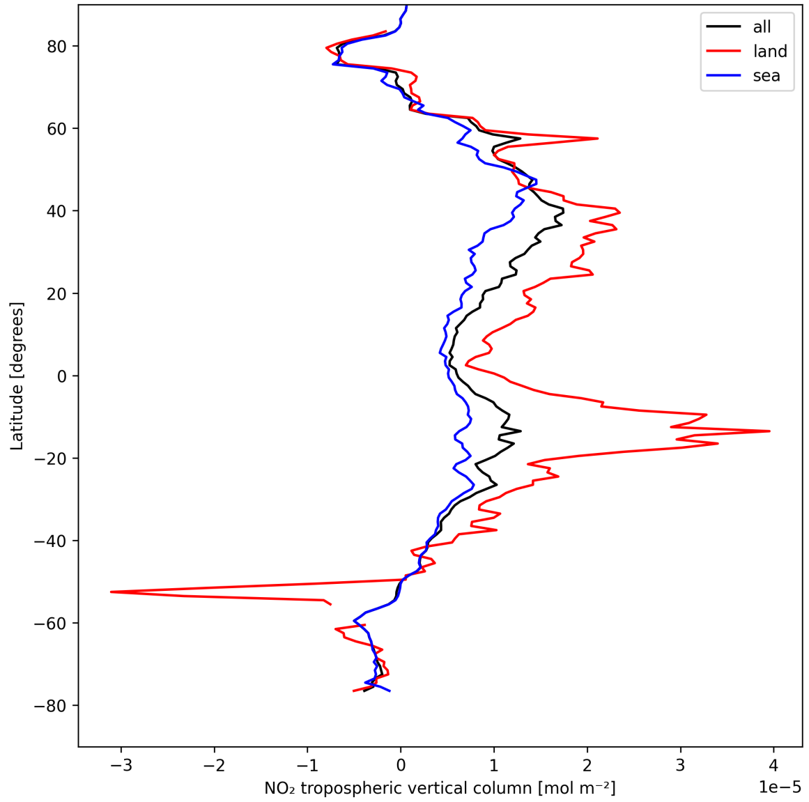
Figure 12: Zonal average of “NO 2 tropospheric vertical column” for 2025-08-22 to 2025-08-24.
