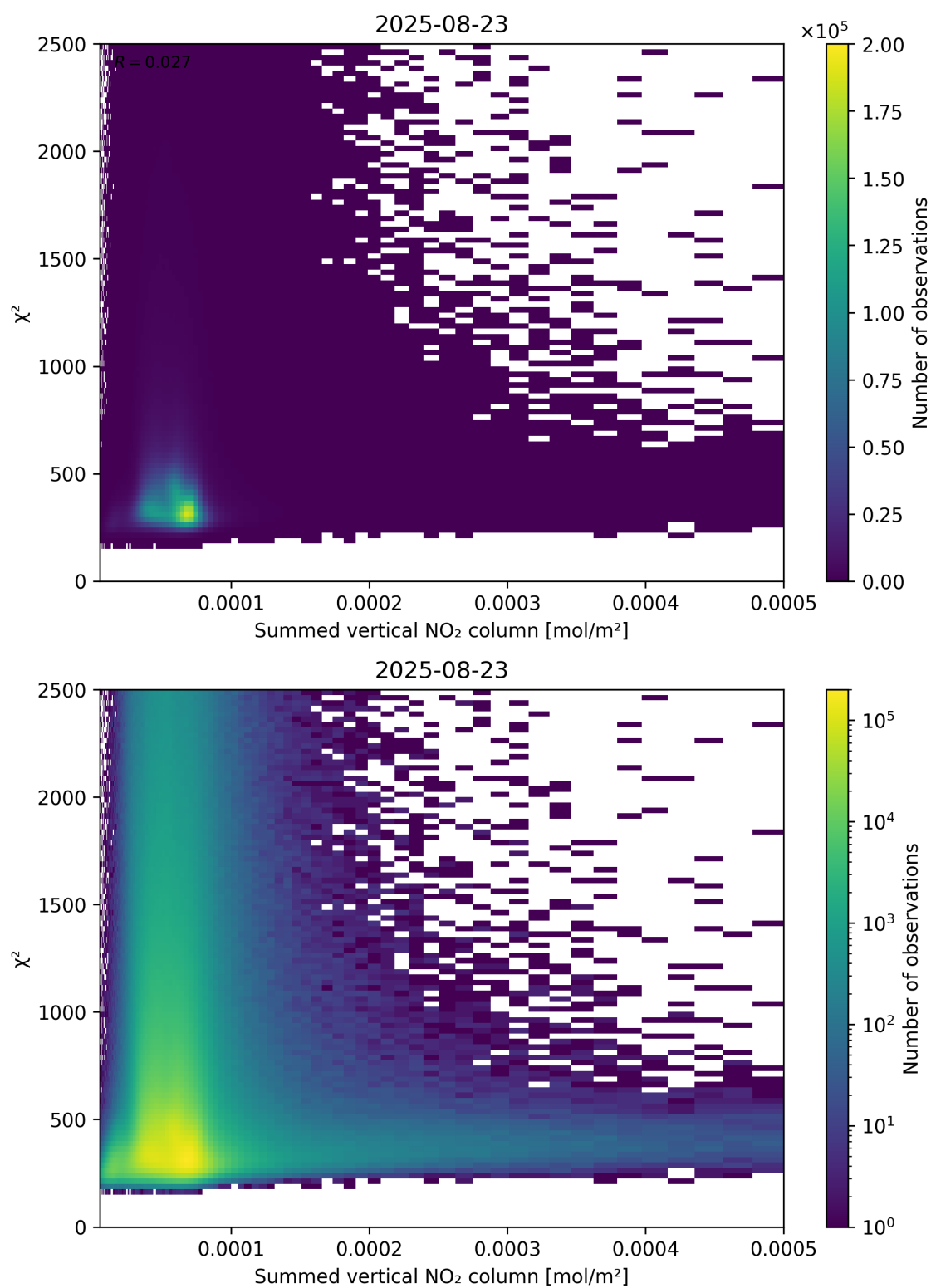
Figure 104: Scatter density plot of “Summed vertical NO 2 column” against “ \chi^2 ” for 2025-08-22 to 2025-08-24.
