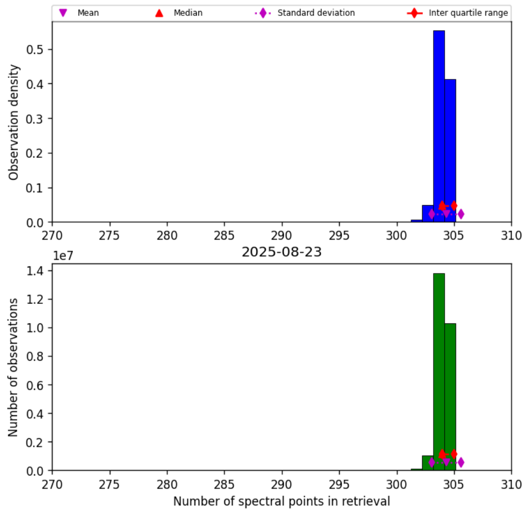
Figure 33: Histogram of “Number of spectral points in retrieval” for 2025-08-22 to 2025-08-24
