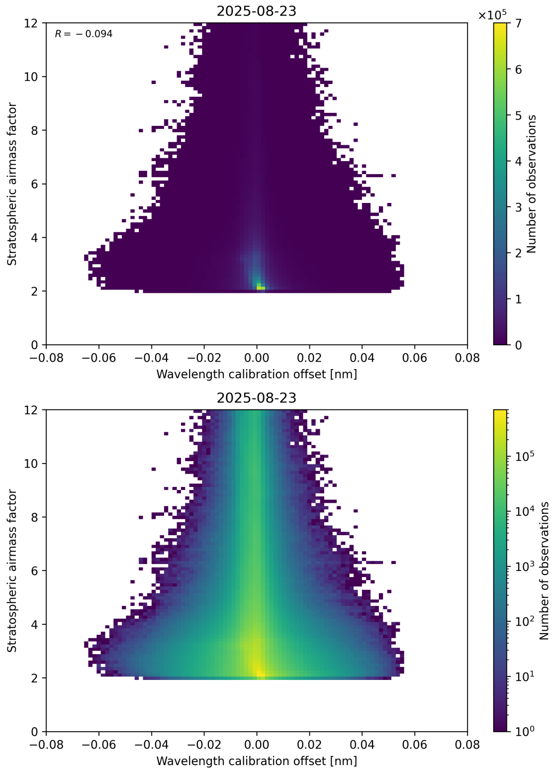
Figure 174: Scatter density plot of “Wavelength calibration offset” against “Stratospheric airmass factor” for 2025-08-22 to 2025-08-24.
