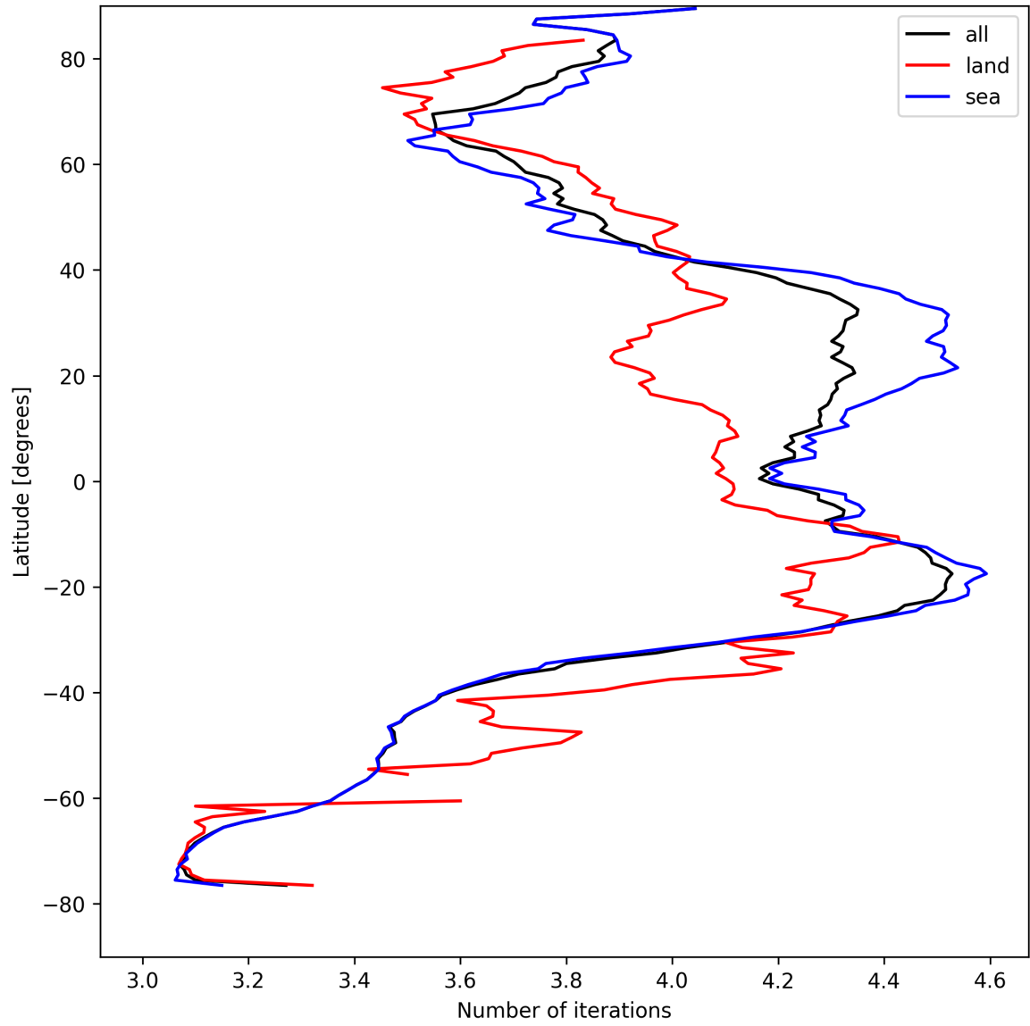
Figure 17: Zonal average of “Number of iterations” for 2025-08-22 to 2025-08-24.
