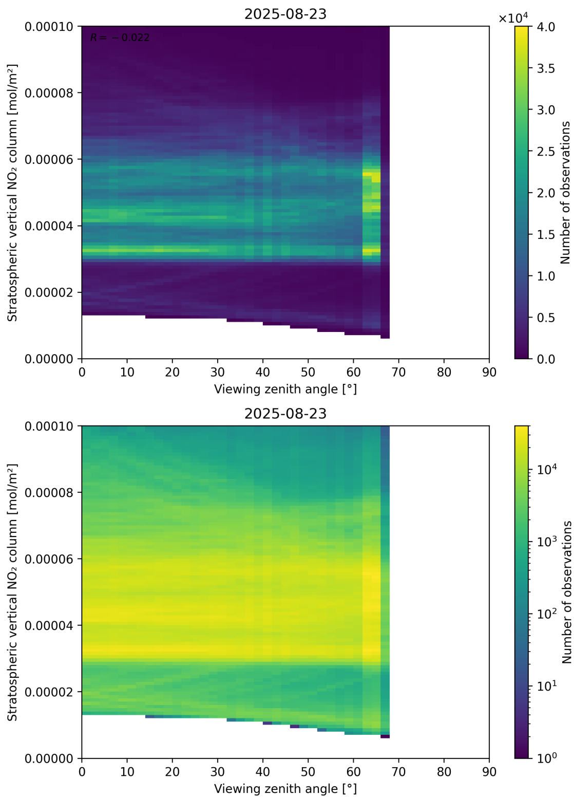
Figure 164: Scatter density plot of “Viewing zenith angle” against “Stratospheric vertical NO 2 column” for 2025-08-22 to 2025-08-24.
