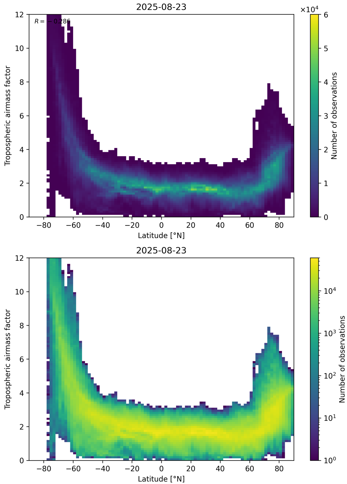
Figure 85: Scatter density plot of “Latitude” against “Tropospheric air mass factor” for 2025-08-22 to 2025-08-24.
