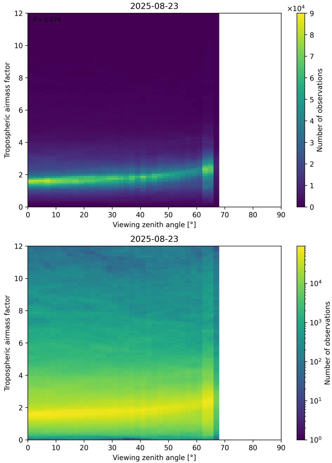
Figure 161: Scatter density plot of “Viewing zenith angle” against “Tropospheric airmass factor” for 2025-08-22 to 2025-08-24.
