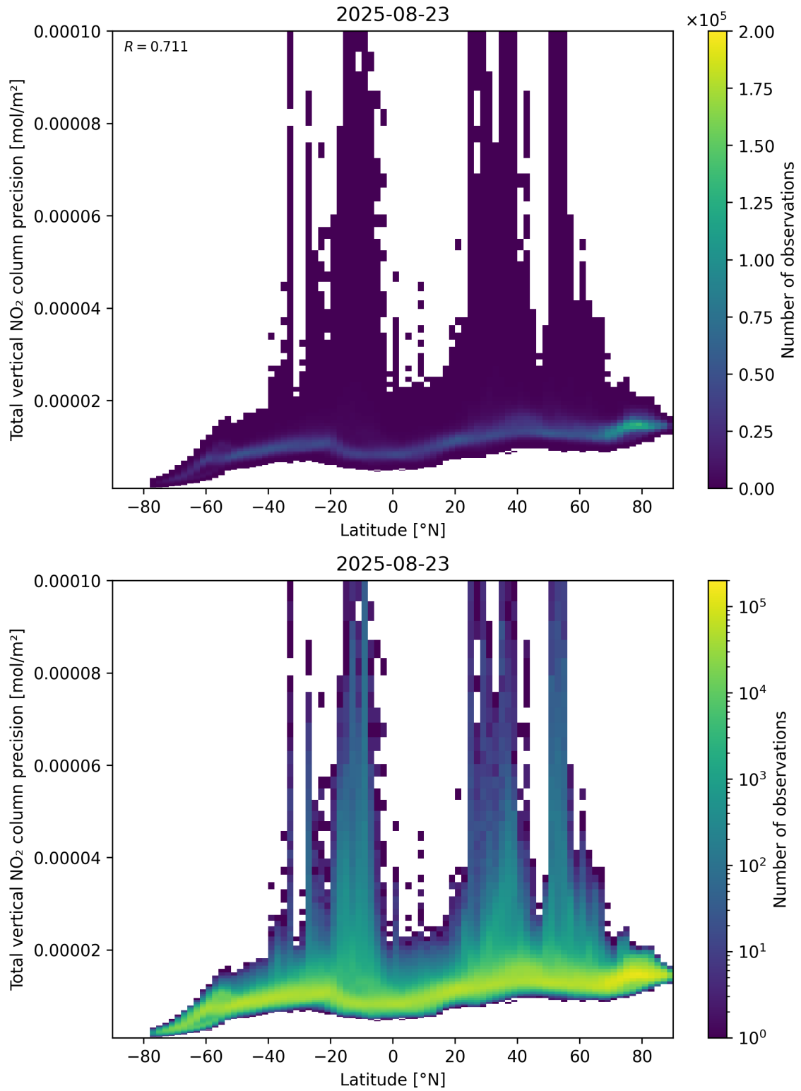
Figure 91: Scatter density plot of “Latitude” against “Total vertical NO 2 column precision” for 2025-08-22 to 2025-08-24.
