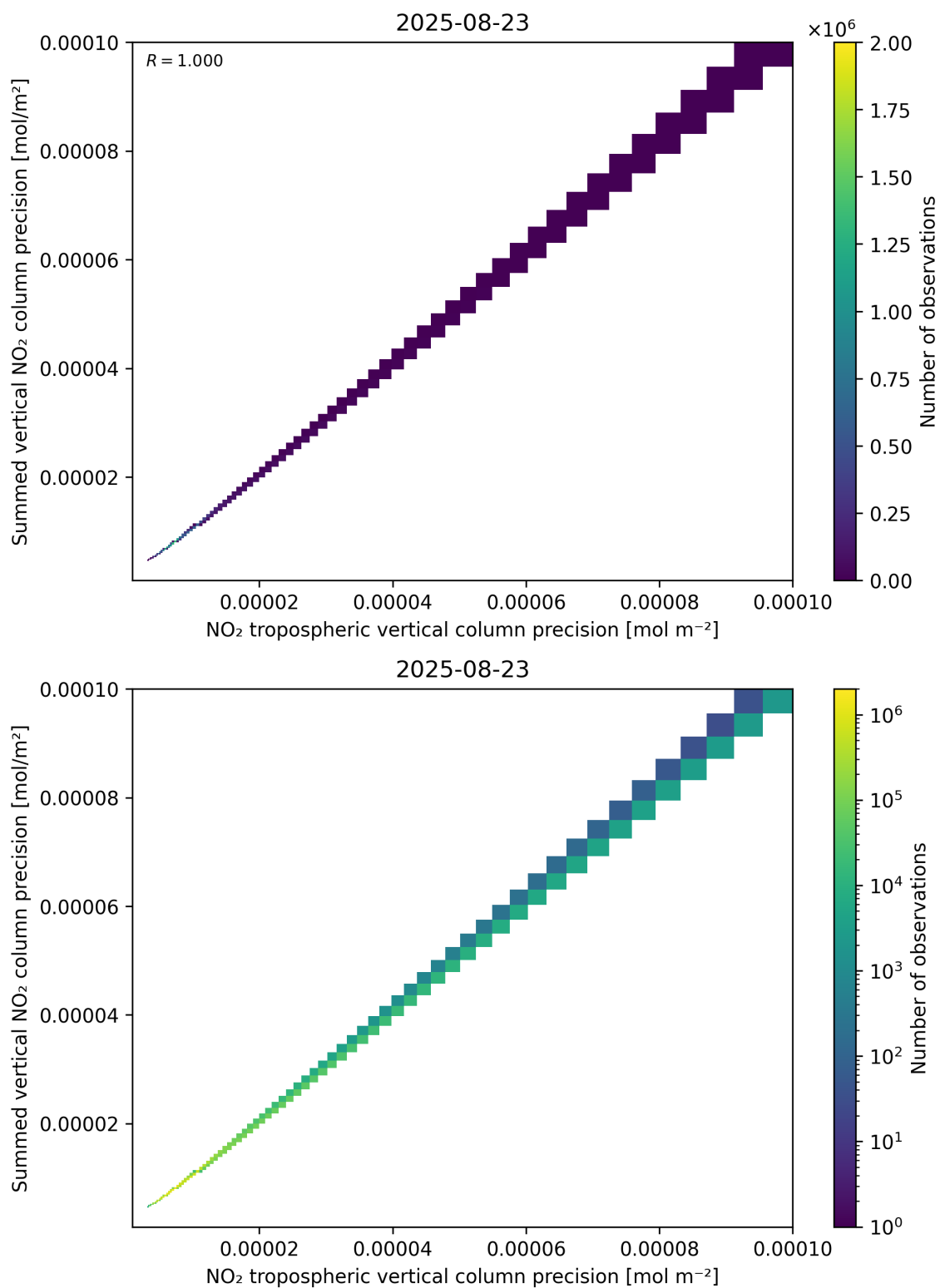
Figure 137: Scatter density plot of “NO 2 tropospheric vertical column precision” against “Summed vertical NO 2 column precision” for 2025-08-22 to 2025-08-24.
