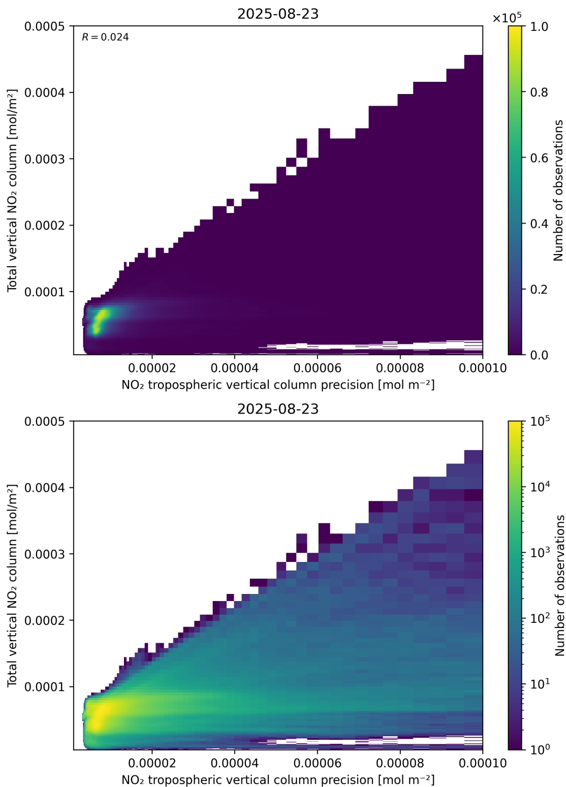
Figure 138: Scatter density plot of “NO 2 tropospheric vertical column precision” against “Total vertical NO 2 column” for 2025-08-22 to 2025-08-24.
