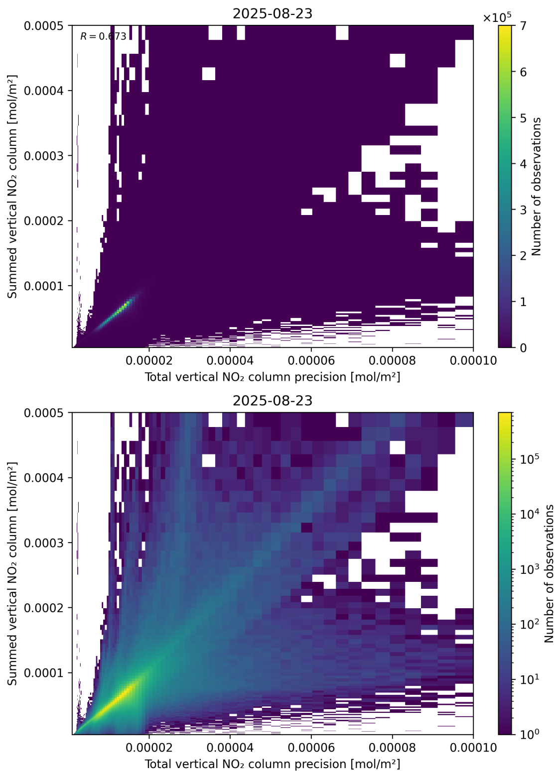
Figure 117: Scatter density plot of “Total vertical NO 2 column precision” against “Summed vertical NO 2 column” for 2025-08-22 to 2025-08-24.
