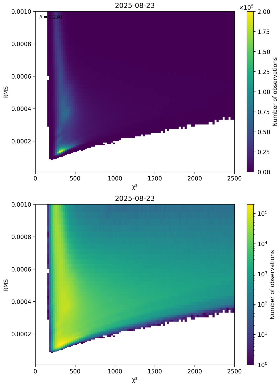
Figure 82: Scatter density plot of “ \chi^2 ” against “RMS” for 2025-08-22 to 2025-08-24.
