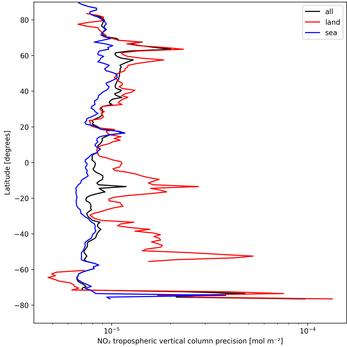
Figure 13: Zonal average of “NO 2 tropospheric vertical column precision” for 2025-08-22 to 2025-08-24.
