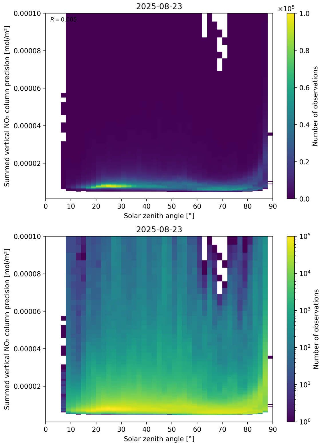
Figure 152: Scatter density plot of “Solar zenith angle” against “Summed vertical NO 2 column precision” for 2025-08-22 to 2025-08-24.
