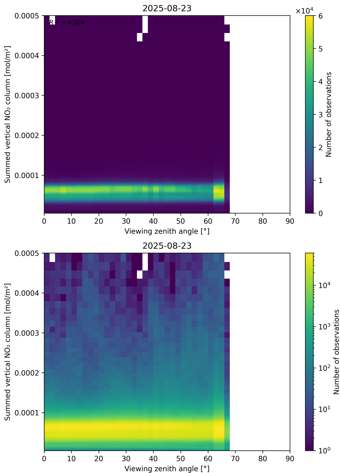
Figure 165: Scatter density plot of “Viewing zenith angle” against “Summed vertical NO 2 column” for 2025-08-22 to 2025-08-24.
