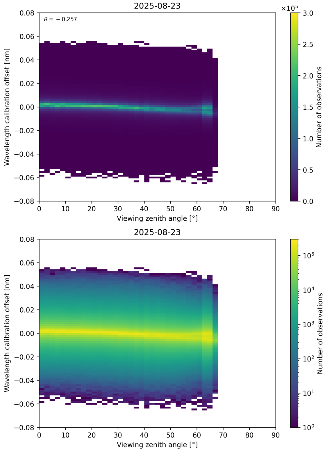
Figure 173: Scatter density plot of “Viewing zenith angle” against “Wavelength calibration offset” for 2025-08-22 to 2025-08-24.
