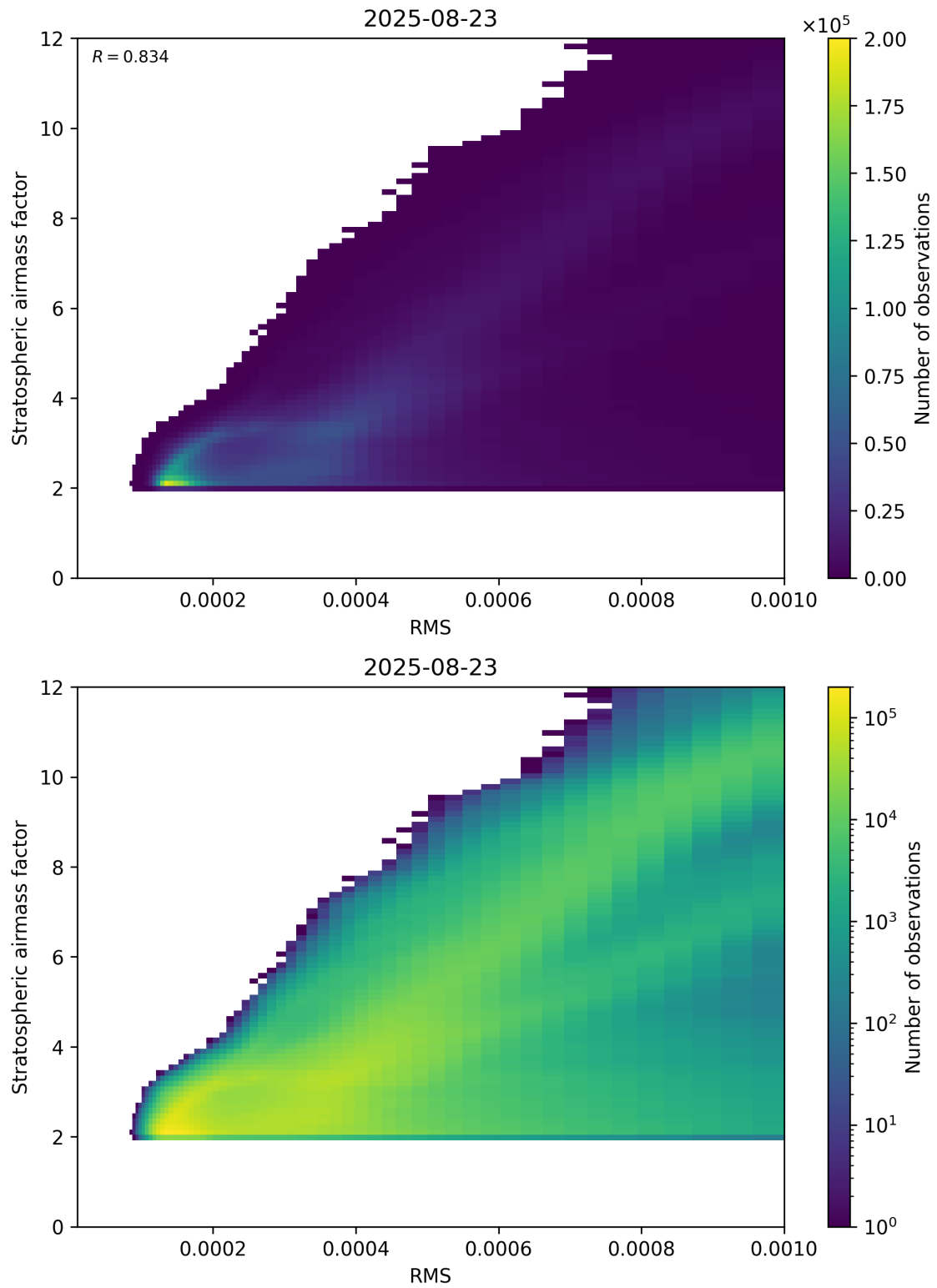
Figure 144: Scatter density plot of “RMS” against “Stratospheric airmass factor” for 2025-08-22 to 2025-08-24.
