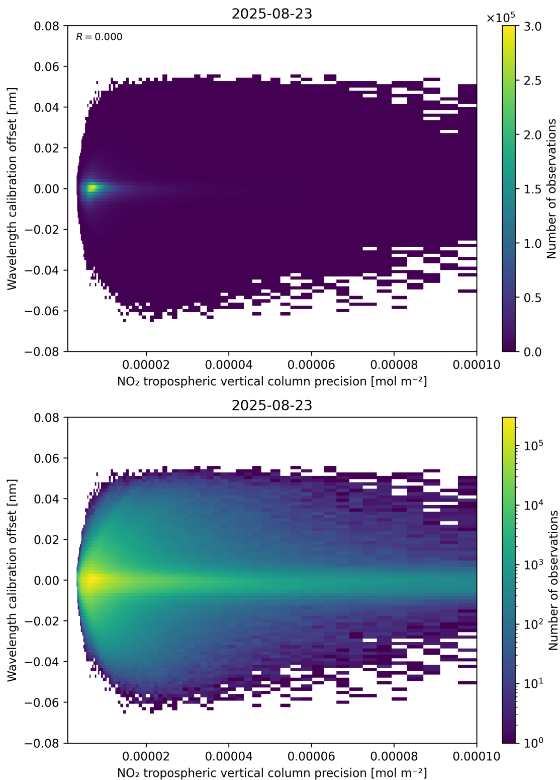
Figure 141: Scatter density plot of “NO 2 tropospheric vertical column precision” against “Wavelength calibration offset” for 2025-08-22 to 2025-08-24.
