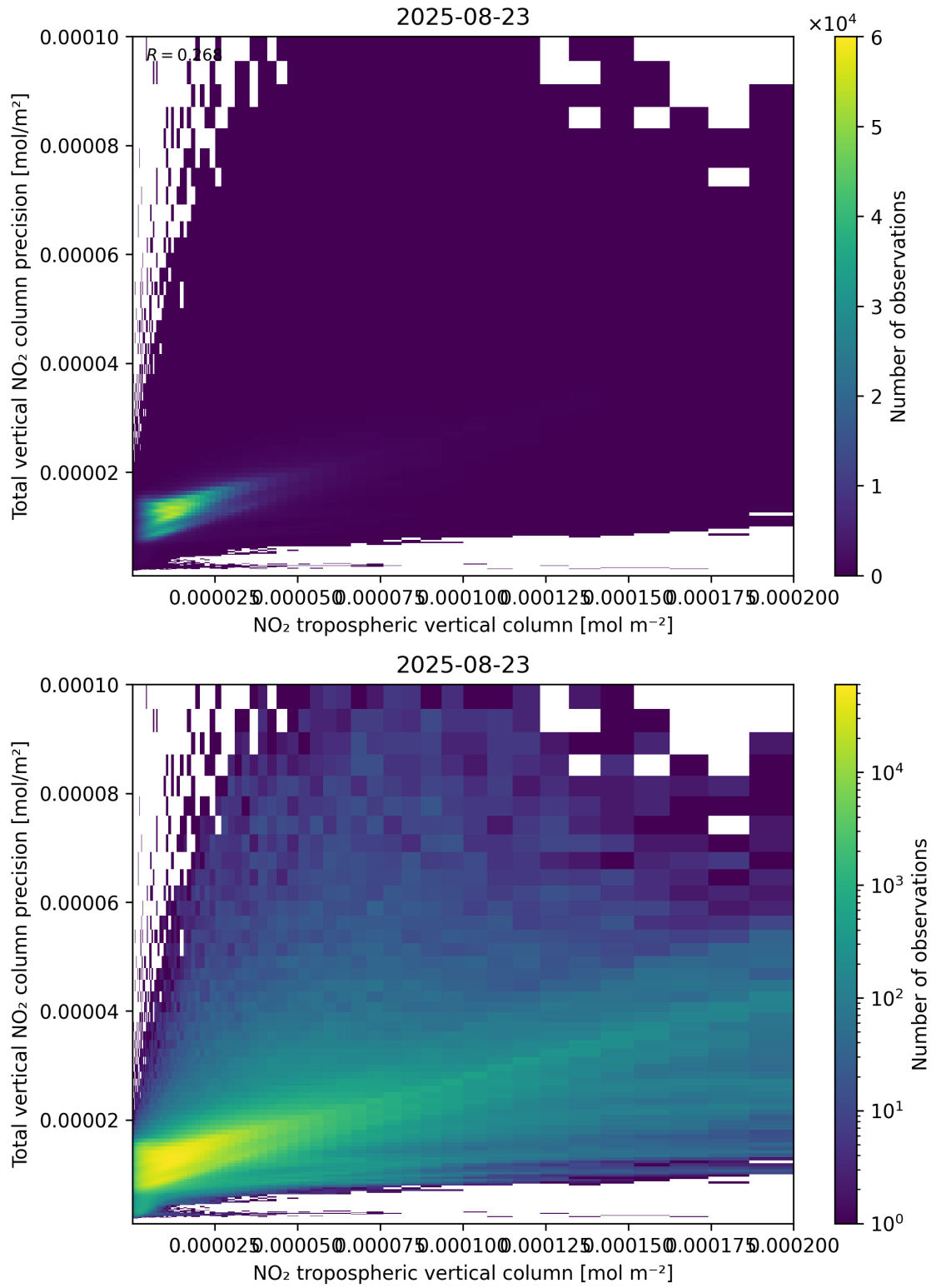
Figure 129: Scatter density plot of “NO 2 tropospheric vertical column” against “Total vertical NO 2 column precision” for 2025-08-22 to 2025-08-24.
