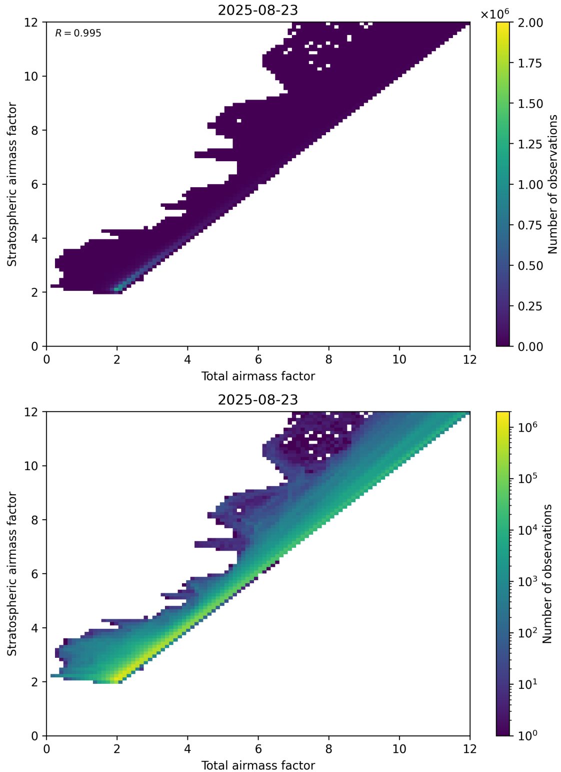
Figure 62: Scatter density plot of “Total airmass factor” against “Stratospheric airmass factor” for 2025-08-22 to 2025-08-24.
