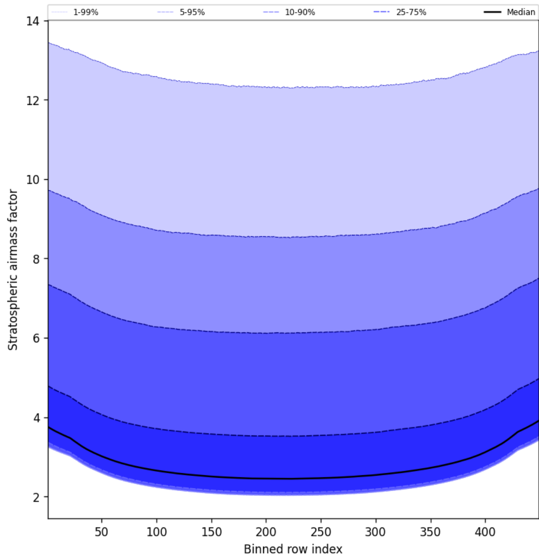
Figure 61: Along track statistics of “Stratospheric airmass factor” for 2025-08-22 to 2025-08-24
