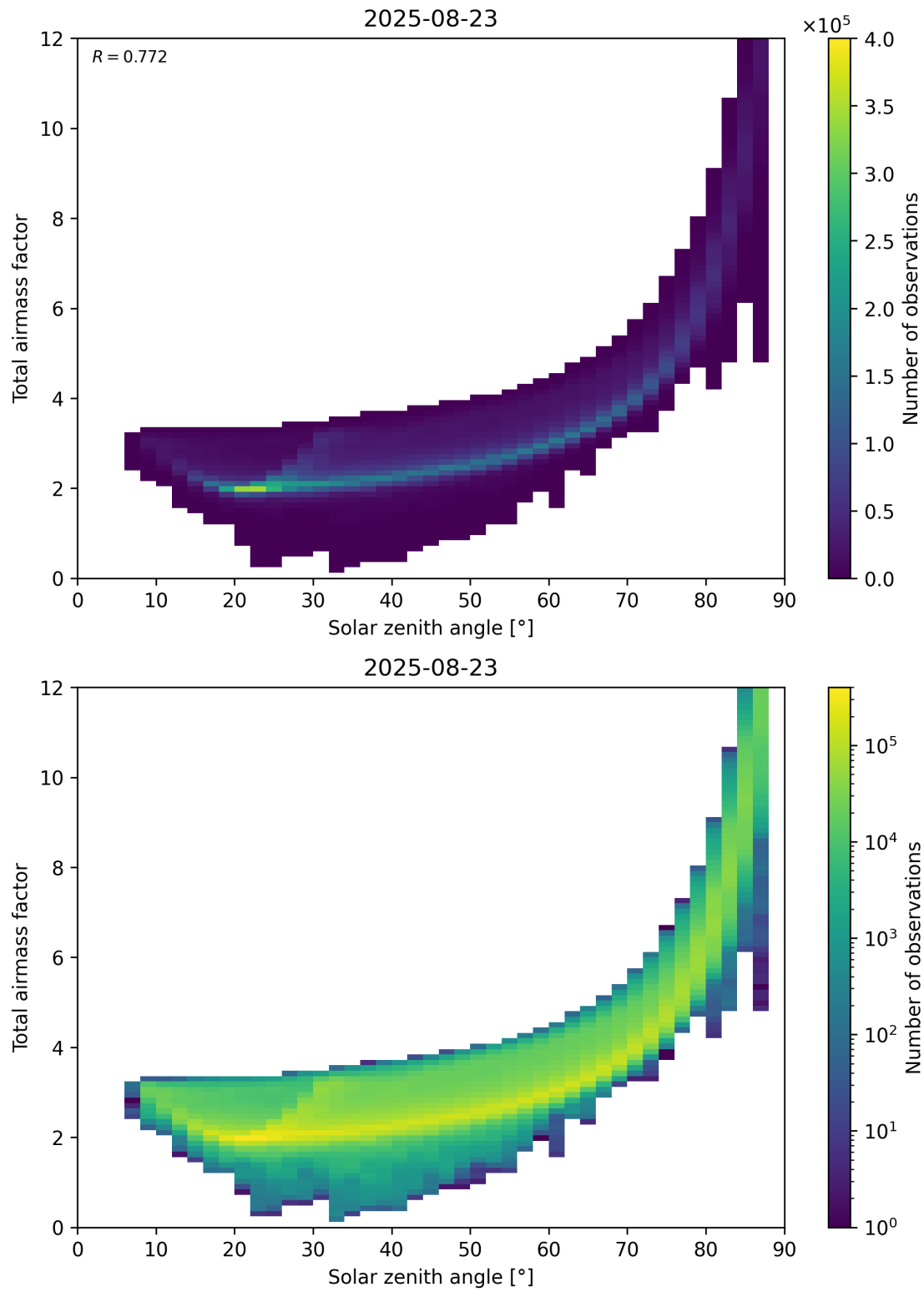
Figure 146: Scatter density plot of “Solar zenith angle” against “Total air mass factor” for 2025-08-22 to 2025-08-24.
