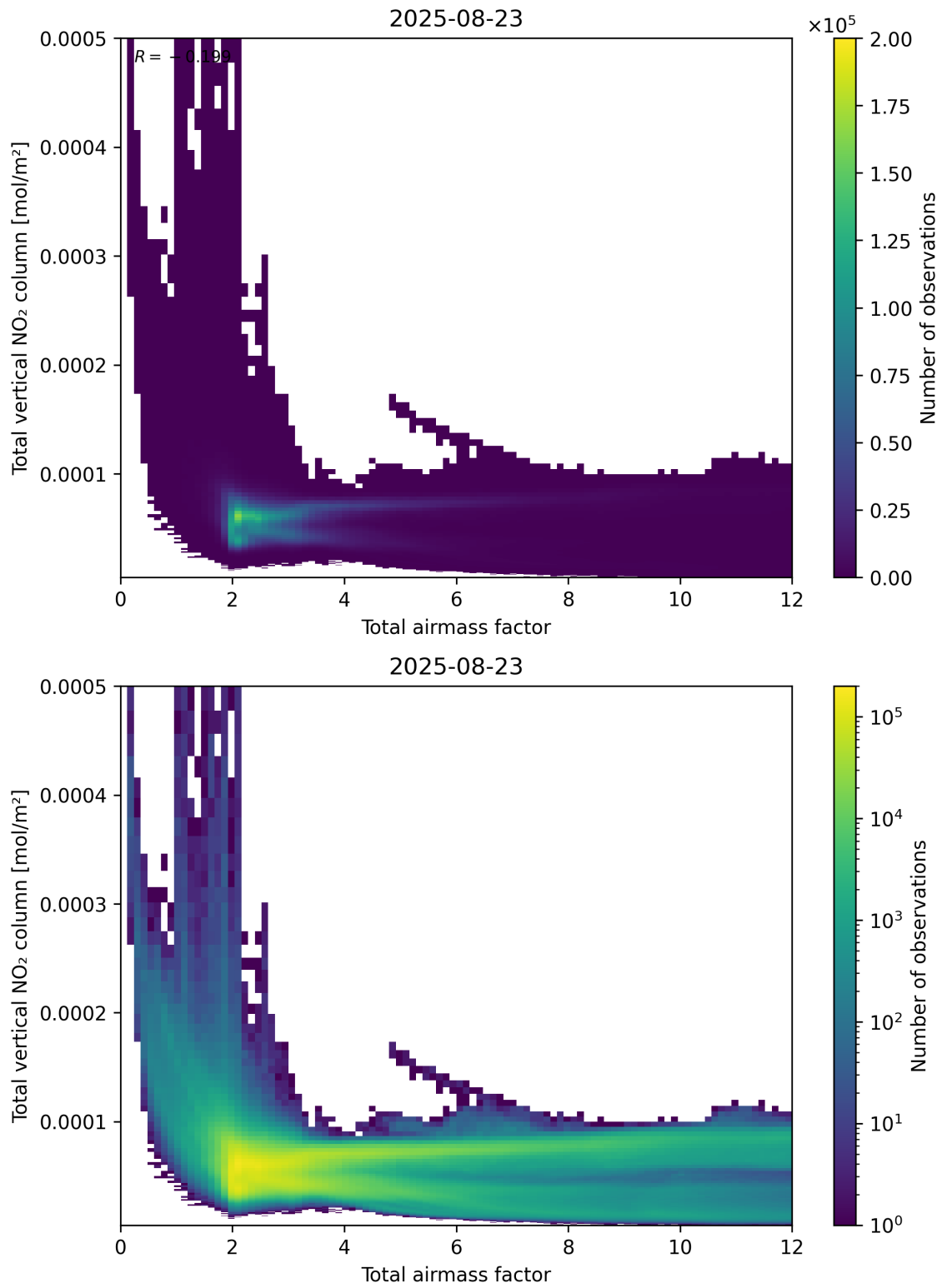
Figure 67: Scatter density plot of “Total airmass factor” against “Total vertical NO 2 column” for 2025-08-22 to 2025-08-24.
