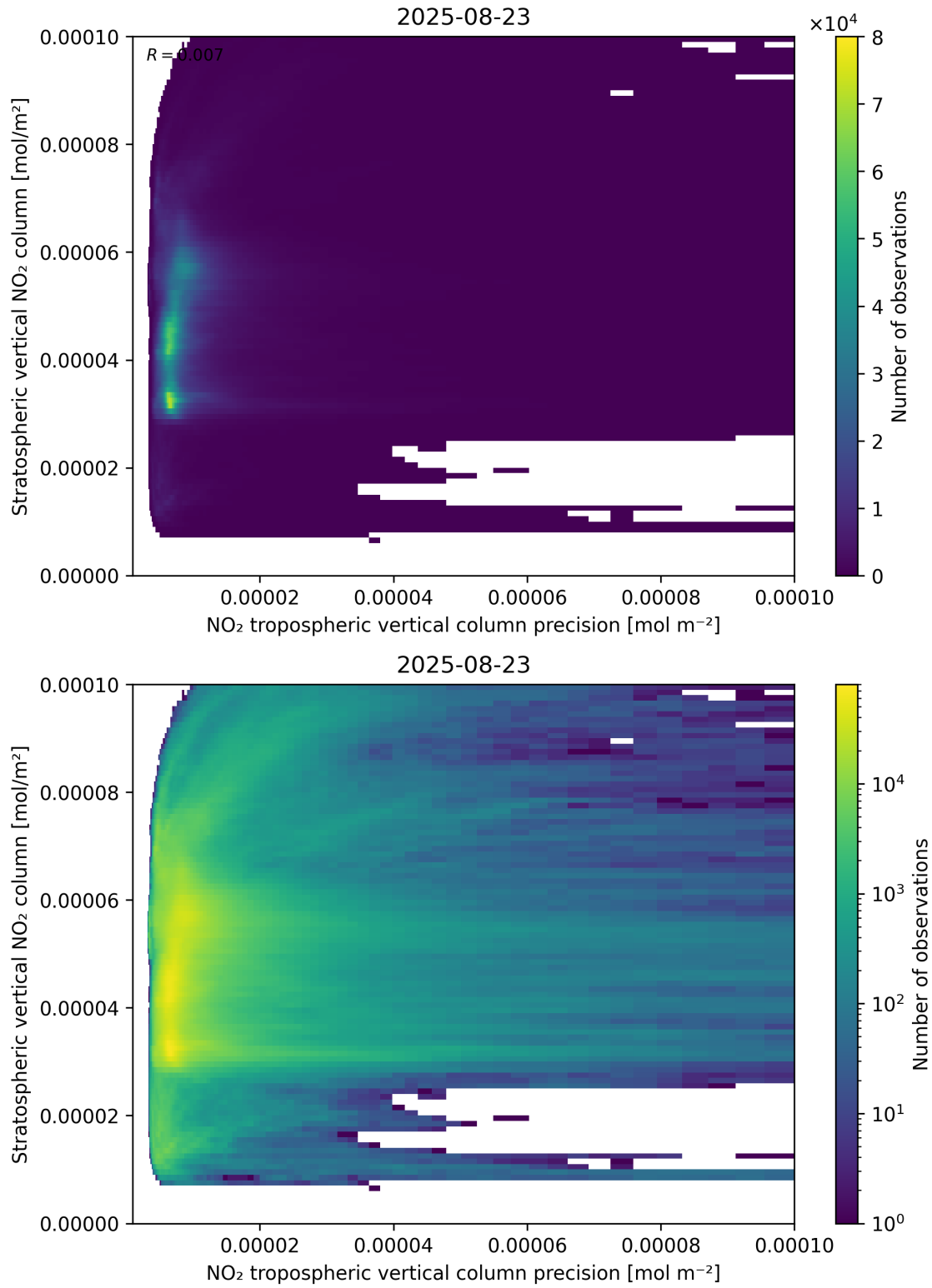
Figure 135: Scatter density plot of “NO 2 tropospheric vertical column precision” against “Stratospheric vertical NO 2 column” for 2025-08-22 to 2025-08-24.
