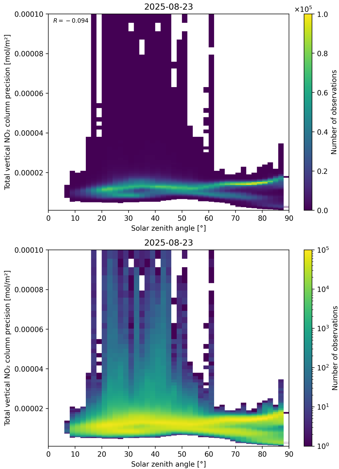
Figure 154: Scatter density plot of “Solar zenith angle” against “Total vertical NO 2 column precision” for 2025-08-22 to 2025-08-24.
