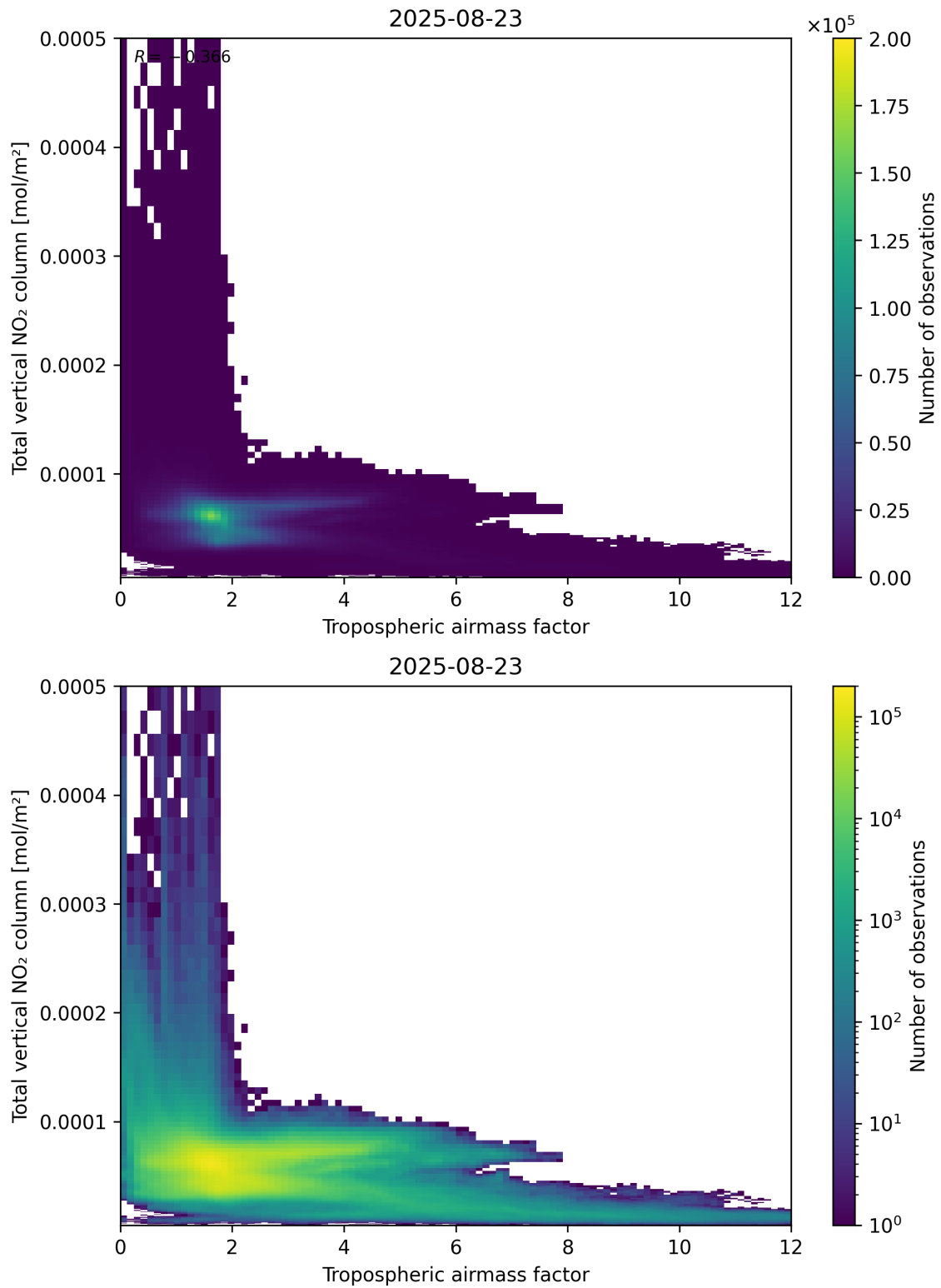
Figure 77: Scatter density plot of “Tropospheric airmass factor” against “Total vertical NO 2 column” for 2025-08-22 to 2025-08-24.
