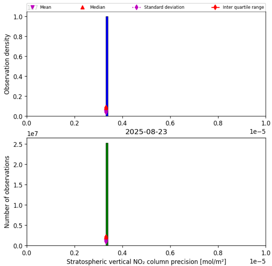
Figure 37: Histogram of “Stratospheric vertical NO 2 column precision” for 2025-08-22 to 2025-08-24
