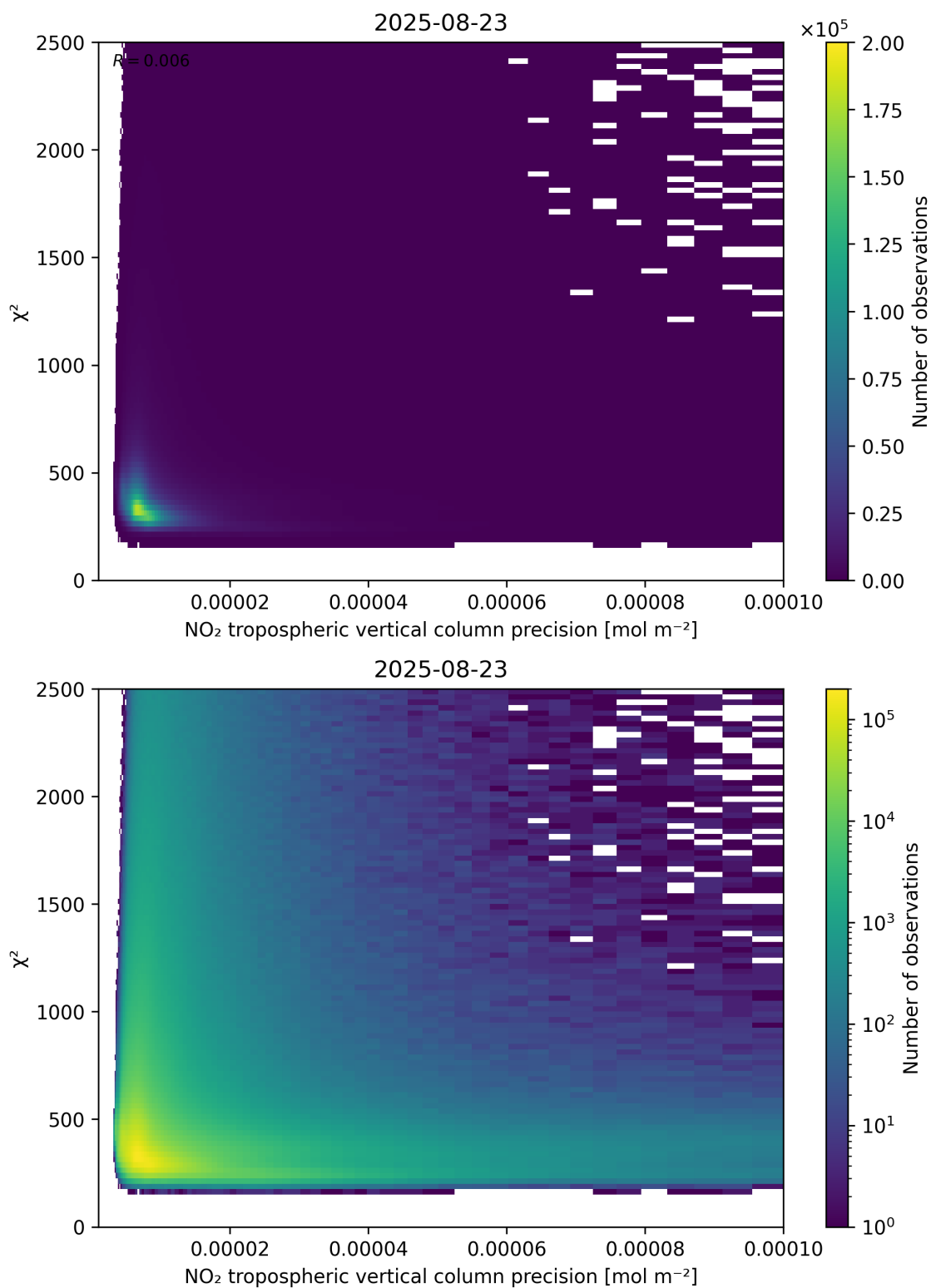
Figure 134: Scatter density plot of “NO 2 tropospheric vertical column precision” against “ \chi^2 ” for 2025-08-22 to 2025-08-24.
