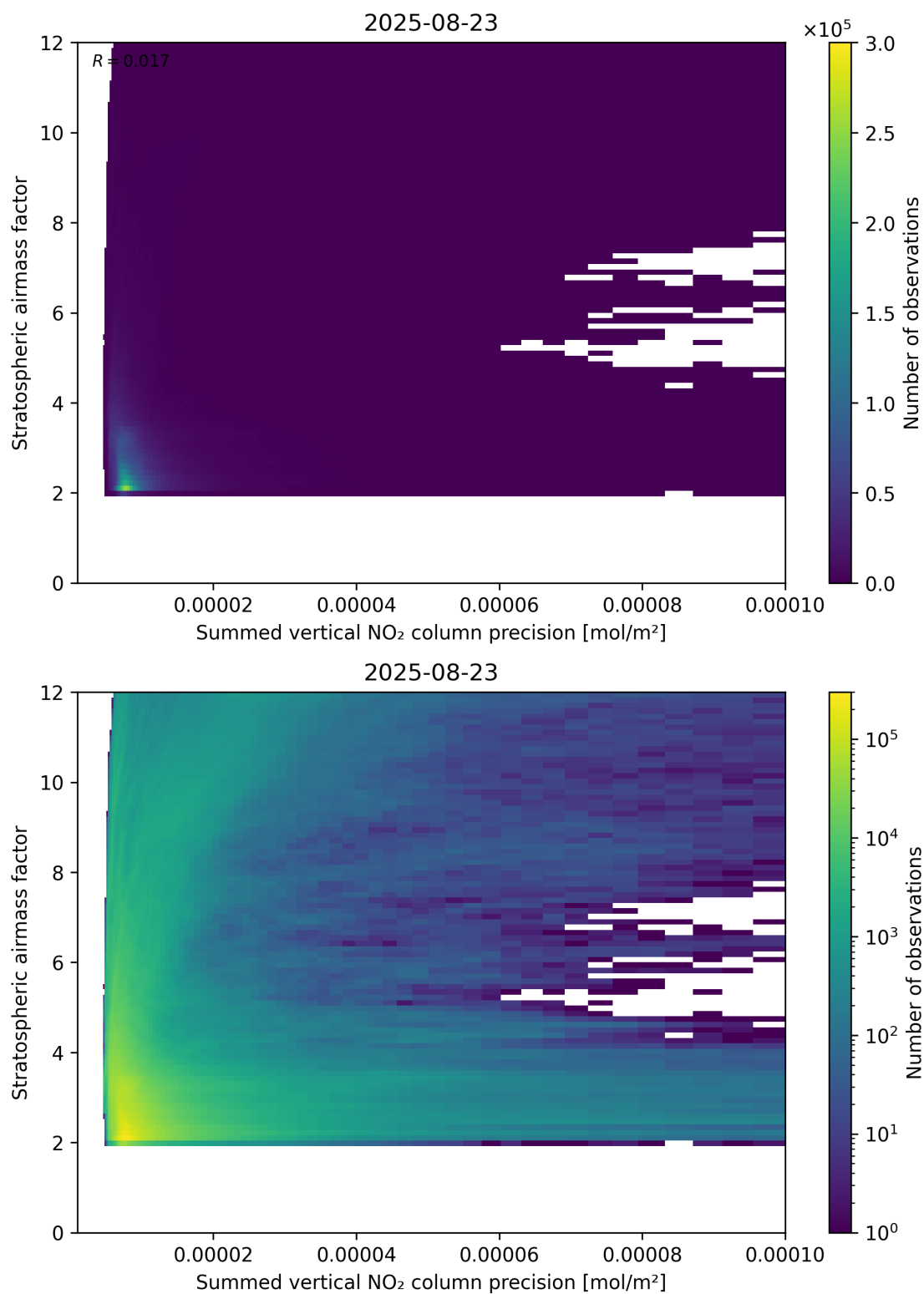
Figure 106: Scatter density plot of “Summed vertical NO 2 column precision” against “Stratospheric airmass factor” for 2025-08-22 to 2025-08-24.
