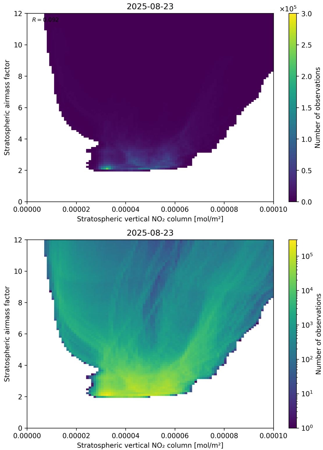
Figure 96: Scatter density plot of “Stratospheric vertical NO 2 column” against “Stratospheric airmass factor” for 2025-08-22 to 2025-08-24.
