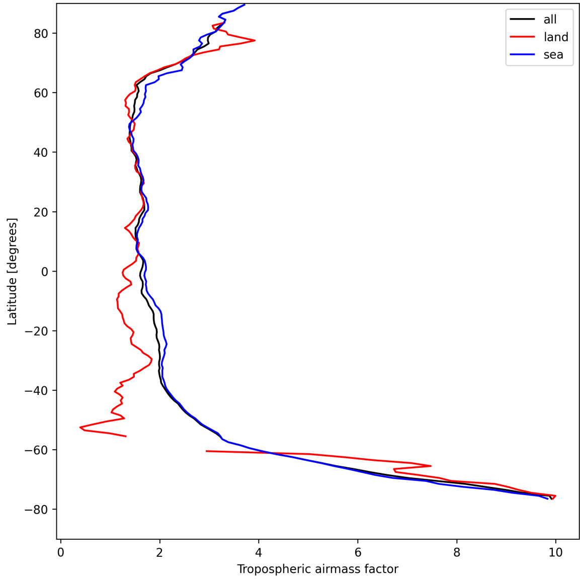
Figure 14: Zonal average of “Tropospheric airmass factor” for 2025-08-22 to 2025-08-24.
