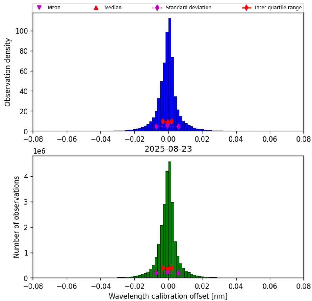
Figure 35: Histogram of “Wavelength calibration offset” for 2025-08-22 to 2025-08-24
