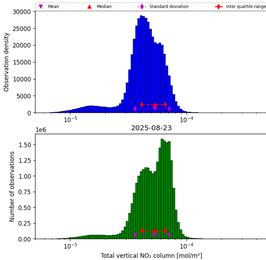
Figure 38: Histogram of “Total vertical NO 2 column” for 2025-08-22 to 2025-08-24
