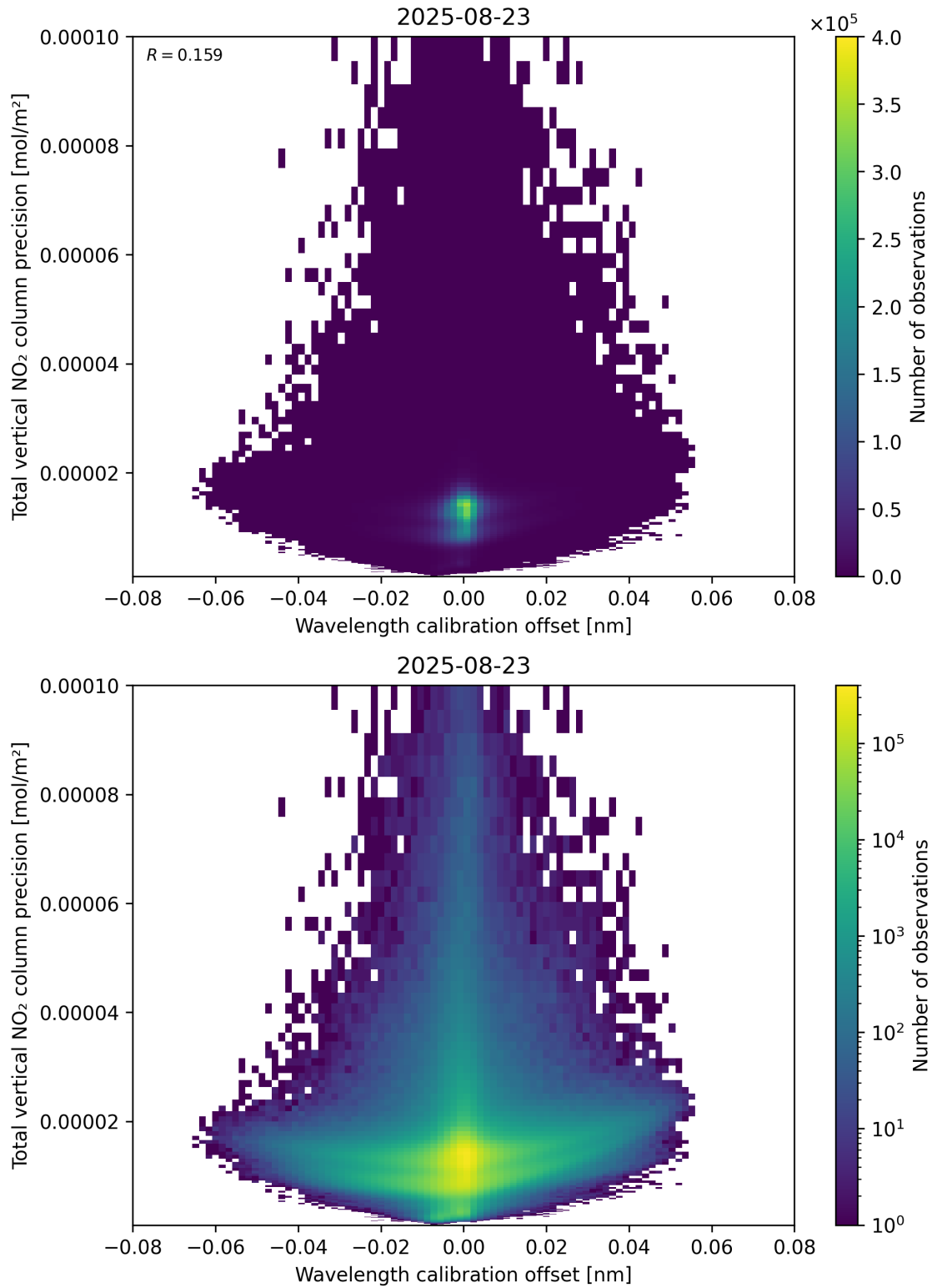
Figure 180: Scatter density plot of “Wavelength calibration offset” against “Total vertical NO 2 column precision” for 2025-08-22 to 2025-08-24.
