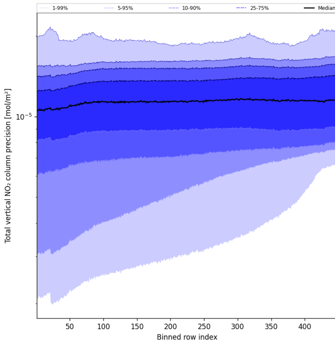
Figure 56: Along track statistics of “Total vertical NO 2 column precision” for 2025-08-22 to 2025-08-24
