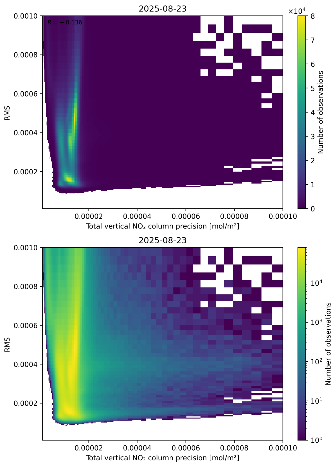
Figure 119: Scatter density plot of “Total vertical NO 2 column precision” against “RMS” for 2025-08-22 to 2025-08-24.
