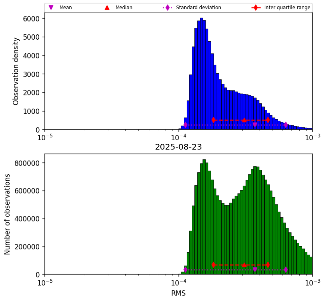
Figure 43: Histogram of “RMS” for 2025-08-22 to 2025-08-24
