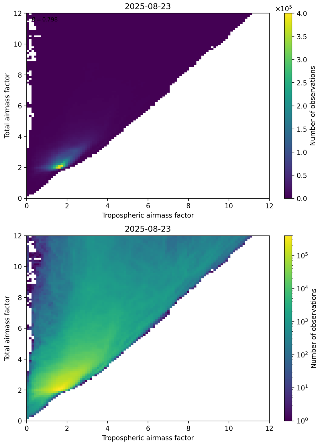
Figure 72: Scatter density plot of “Tropospheric airmass factor” against “Total airmass factor” for 2025-08-22 to 2025-08-24.
