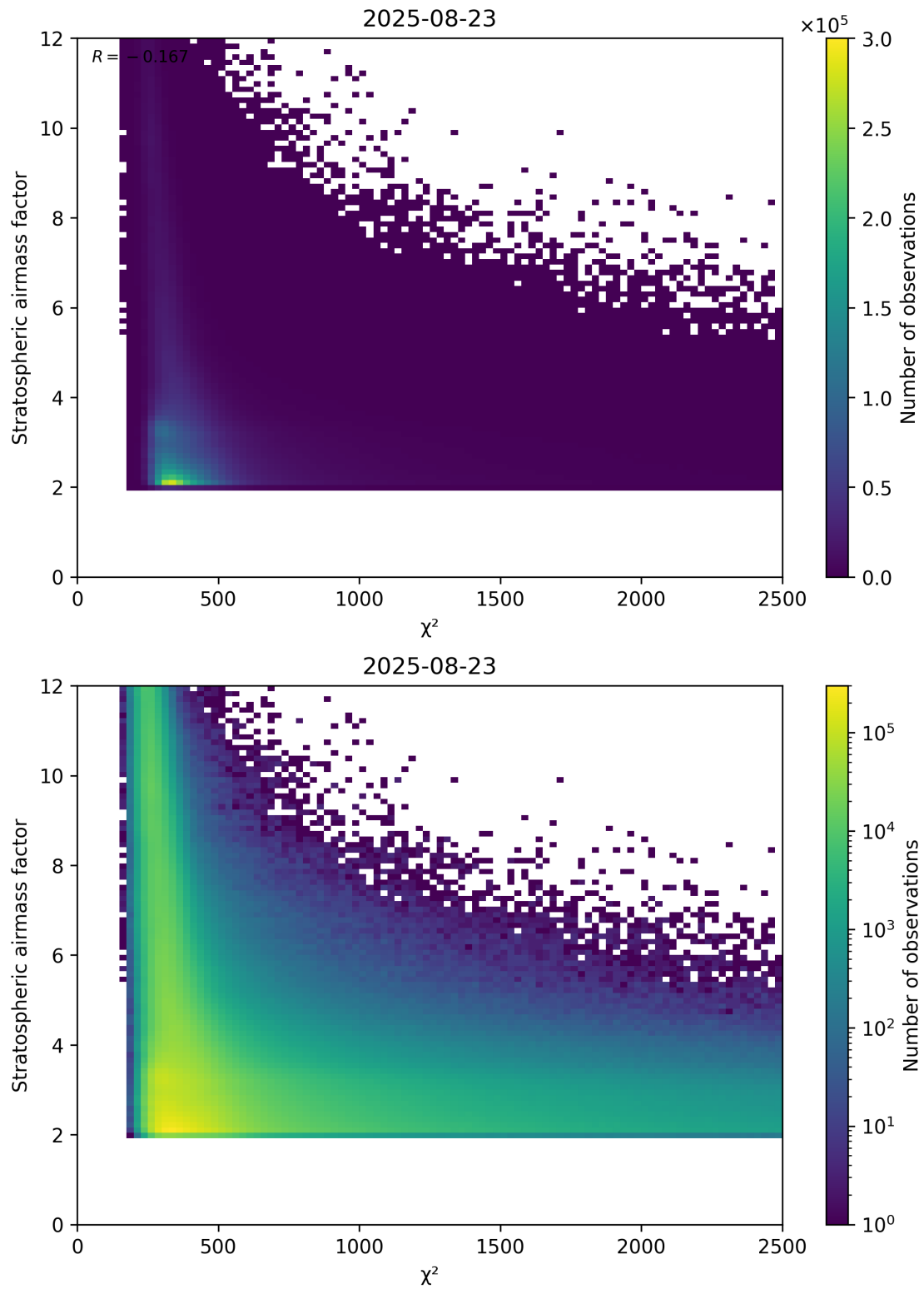
Figure 81: Scatter density plot of “ \chi^2 ” against “Stratospheric airmass factor” for 2025-08-22 to 2025-08-24.
