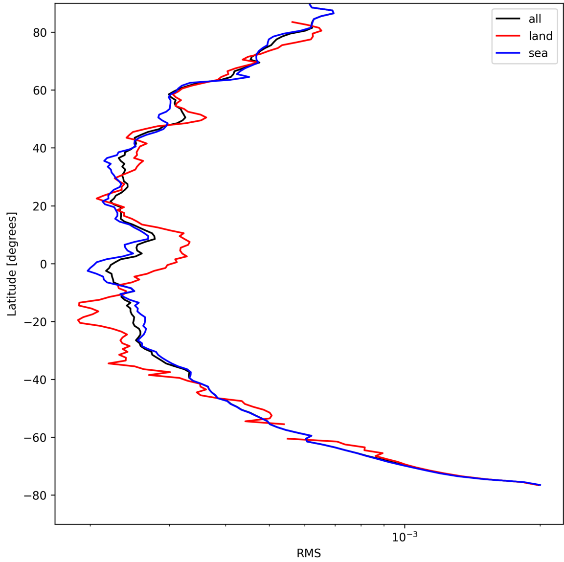
Figure 26: Zonal average of “RMS” for 2025-08-22 to 2025-08-24.
