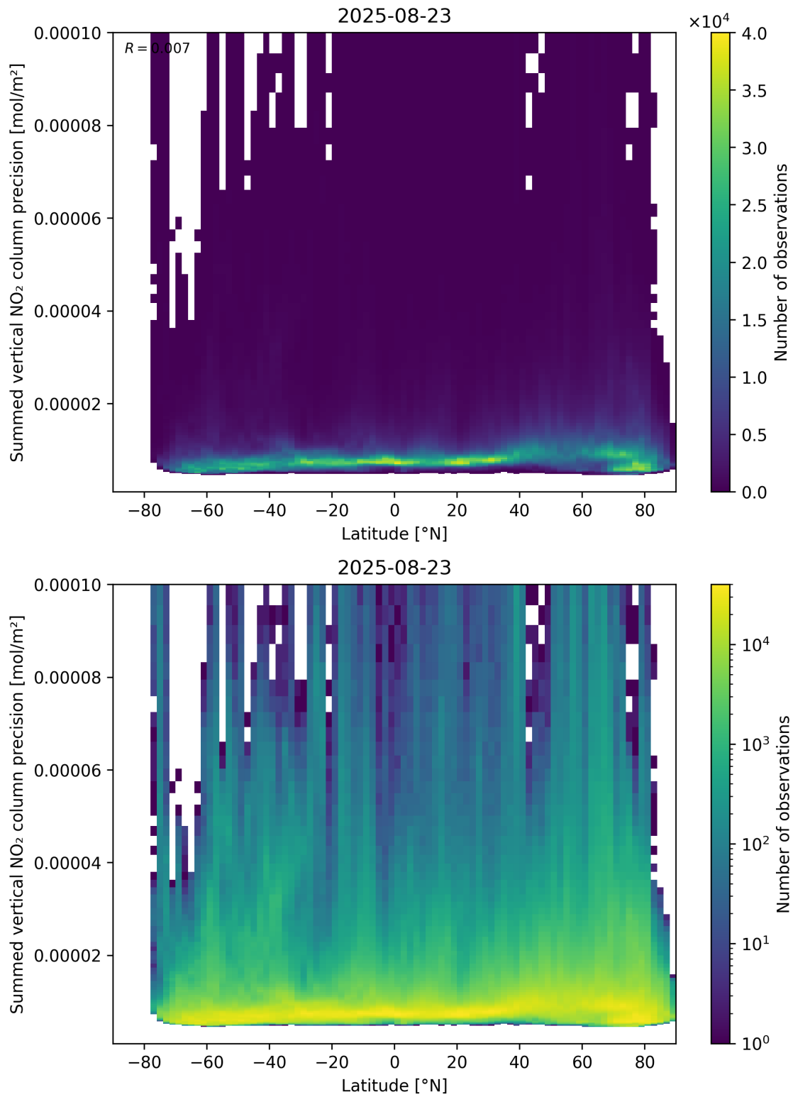
Figure 89: Scatter density plot of “Latitude” against “Summed vertical NO 2 column precision” for 2025-08-22 to 2025-08-24.
