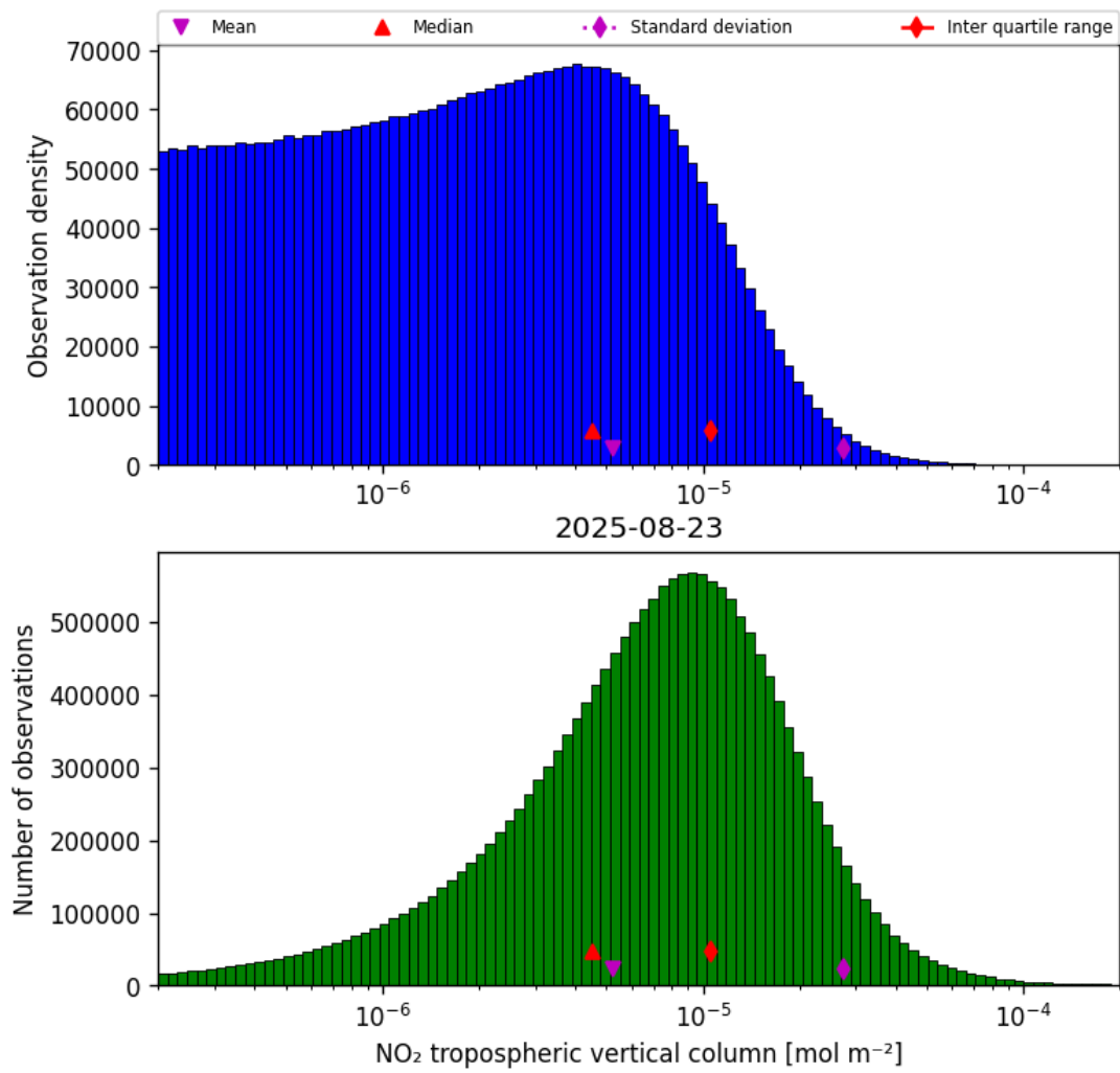
Figure 29: Histogram of “NO 2 tropospheric vertical column” for 2025-08-22 to 2025-08-24
