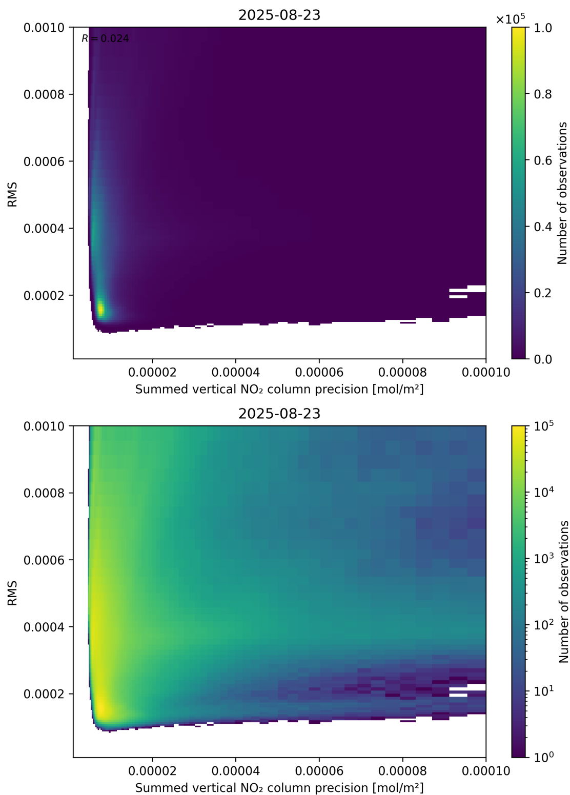
Figure 108: Scatter density plot of “Summed vertical NO 2 column precision” against “RMS” for 2025-08-22 to 2025-08-24.
