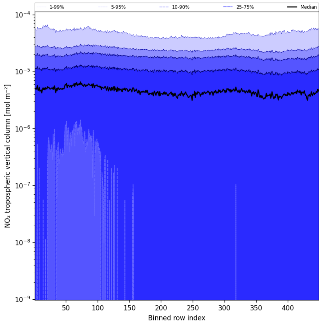
Figure 46: Along track statistics of “NO 2 tropospheric vertical column” for 2025-08-22 to 2025-08-24
