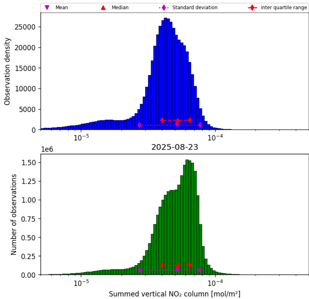
Figure 40: Histogram of “Summed vertical NO 2 column” for 2025-08-22 to 2025-08-24
