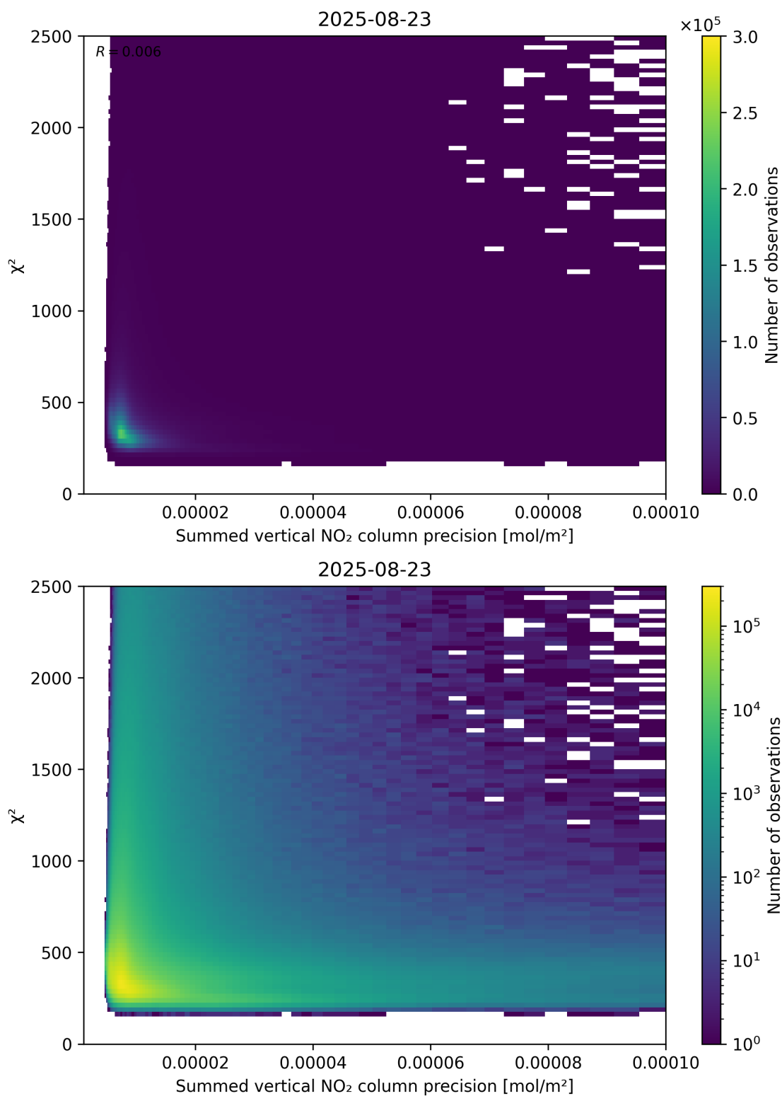
Figure 107: Scatter density plot of “Summed vertical NO 2 column precision” against “ \chi^2 ” for 2025-08-22 to 2025-08-24.
