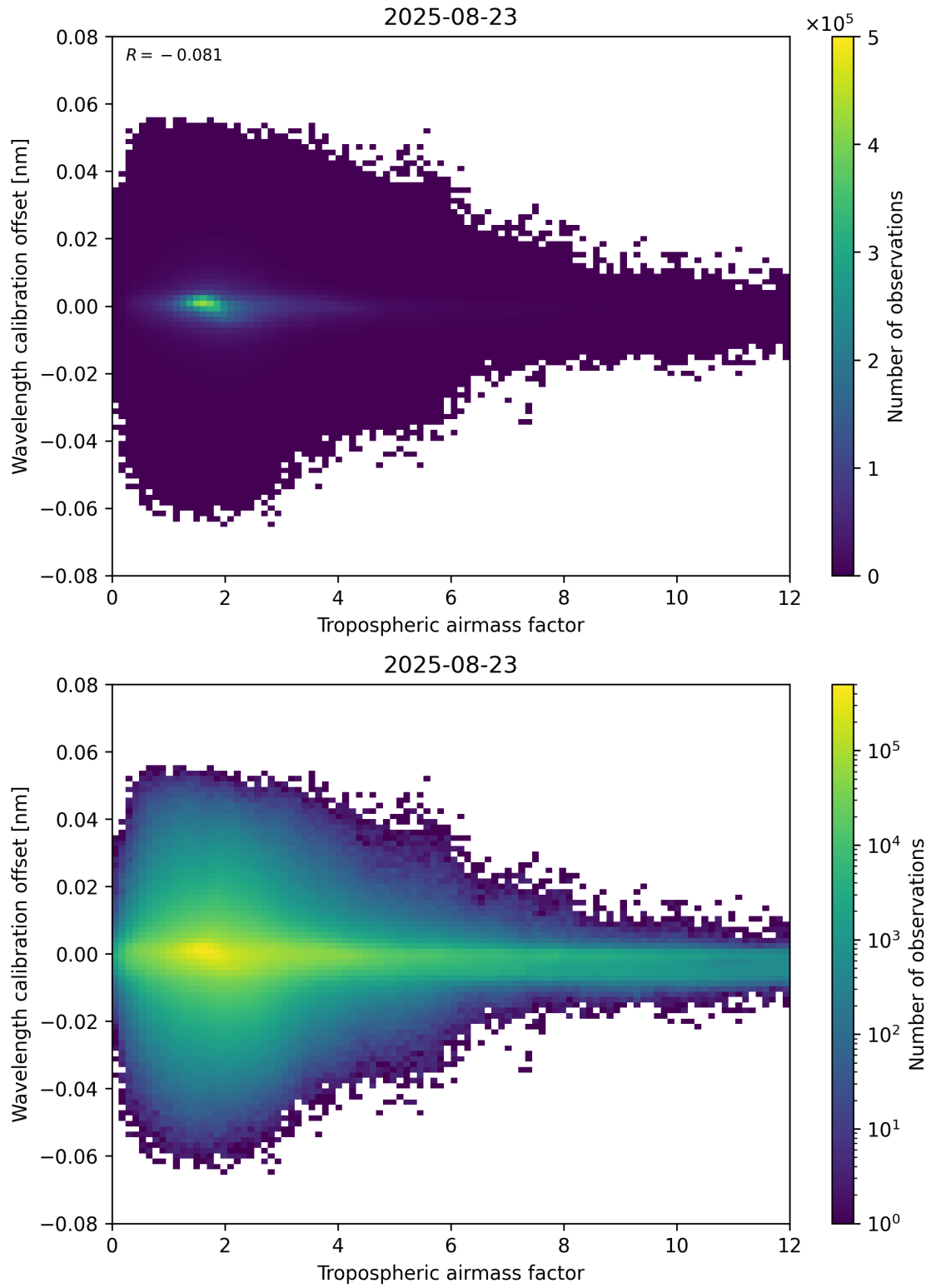
Figure 80: Scatter density plot of “Tropospheric airmass factor” against “Wavelength calibration offset” for 2025-08-22 to 2025-08-24.
