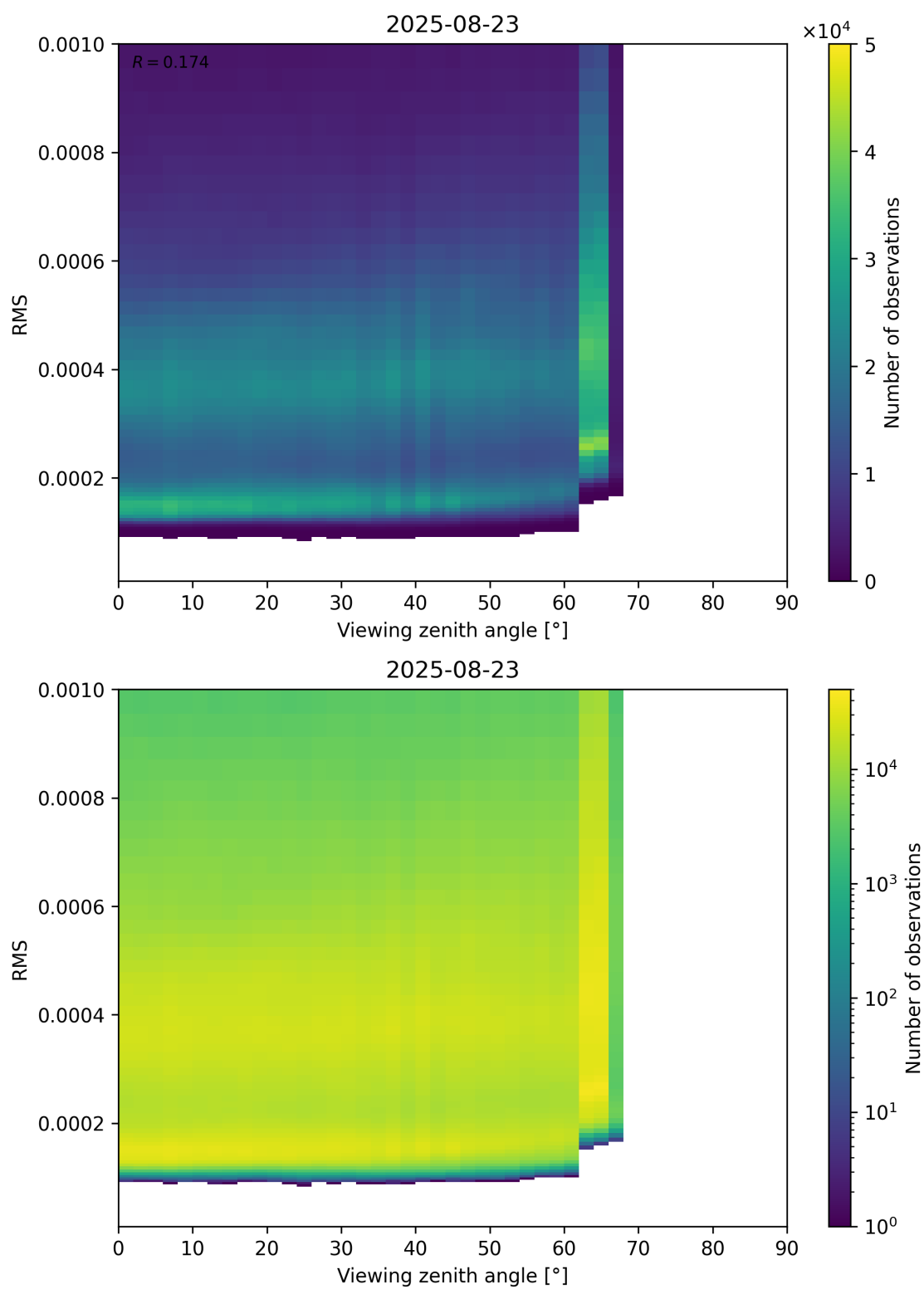
Figure 171: Scatter density plot of “Viewing zenith angle” against “RMS” for 2025-08-22 to 2025-08-24.
