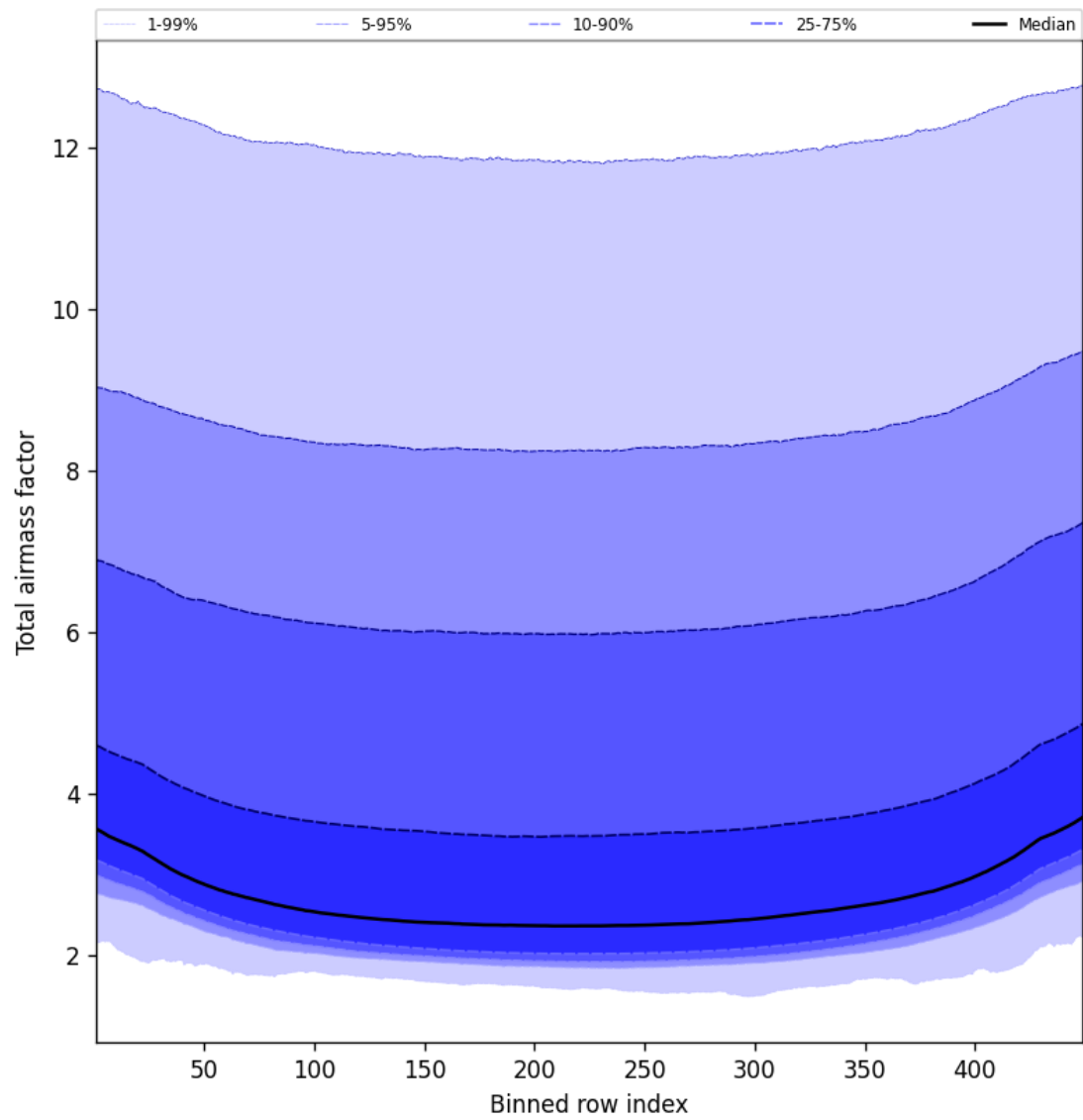
Figure 49: Along track statistics of “Total airmass factor” for 2025-08-22 to 2025-08-24
