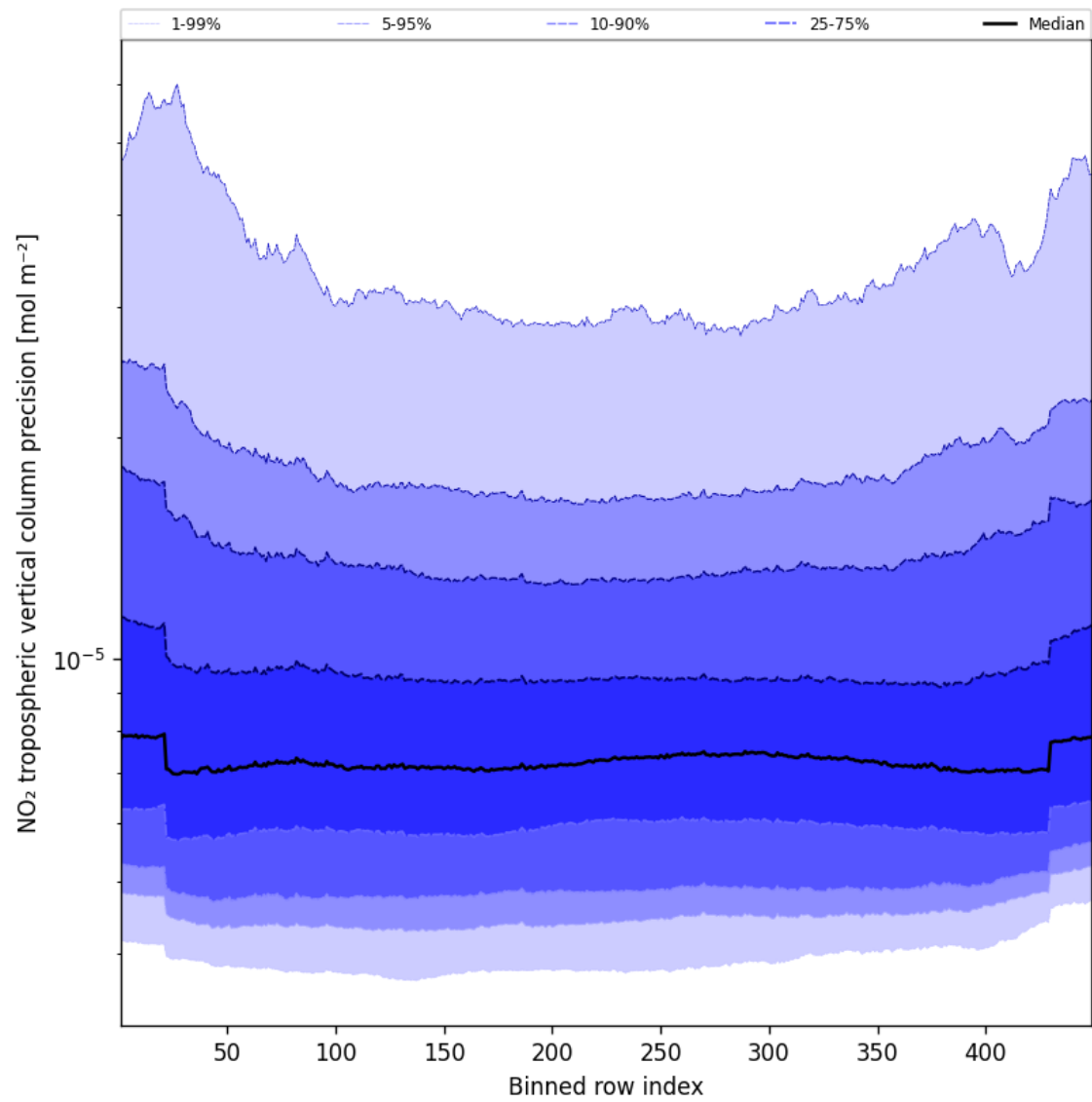
Figure 47: Along track statistics of “NO 2 tropospheric vertical column precision” for 2025-08-22 to 2025-08-24
