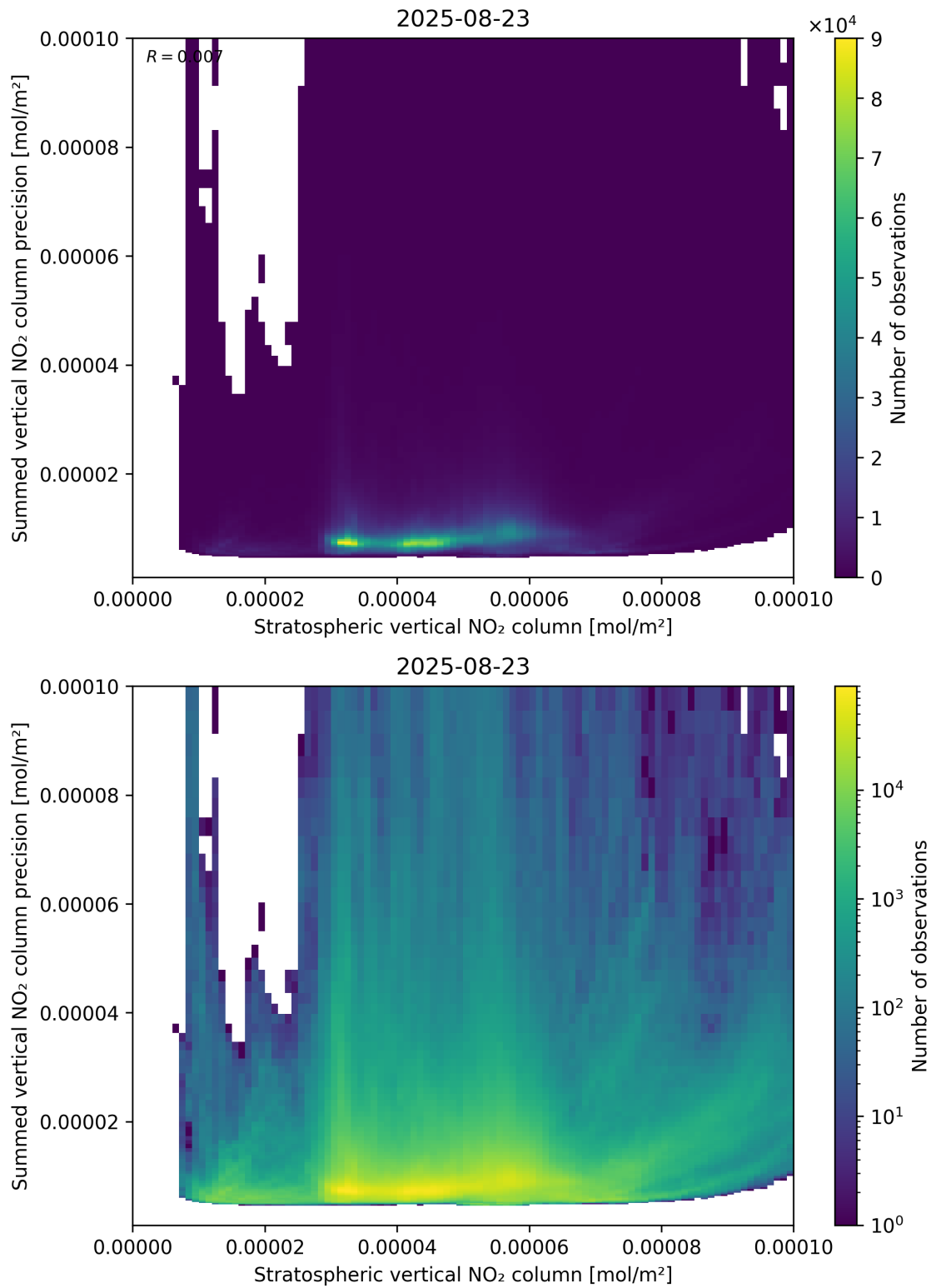
Figure 99: Scatter density plot of “Stratospheric vertical NO 2 column” against “Summed vertical NO 2 column precision” for 2025-08-22 to 2025-08-24.
