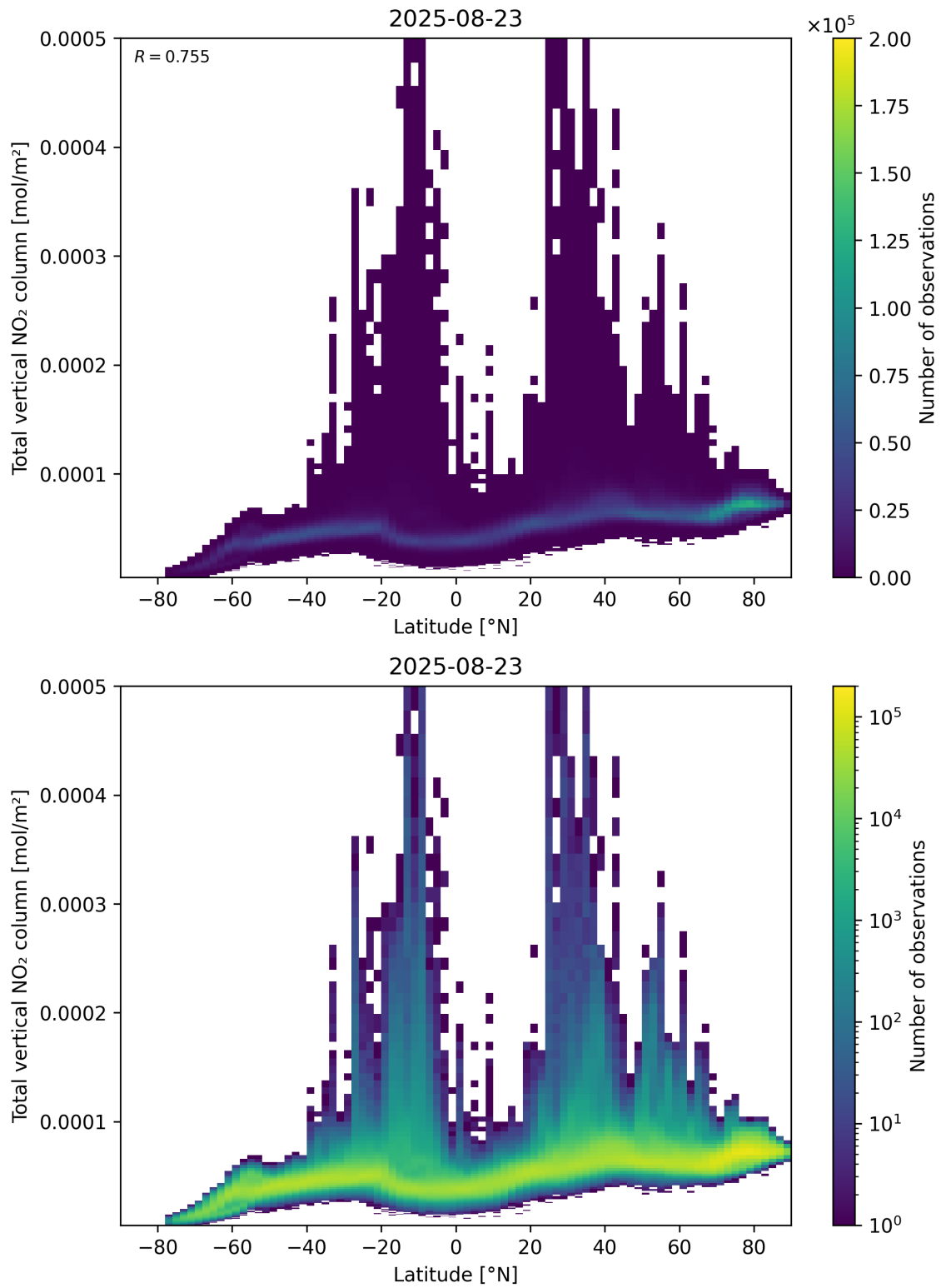
Figure 90: Scatter density plot of “Latitude” against “Total vertical NO 2 column” for 2025-08-22 to 2025-08-24.
