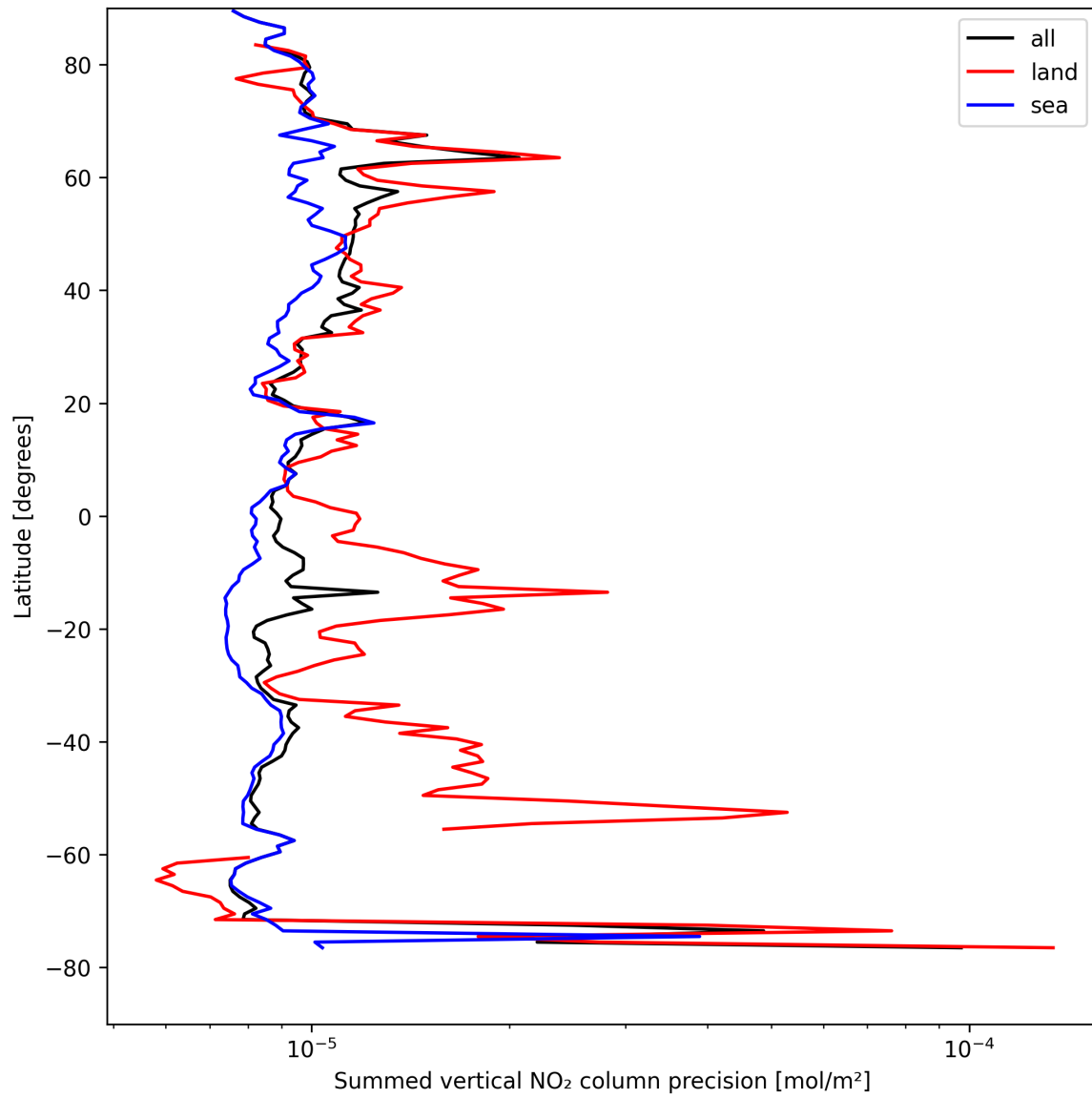
Figure 24: Zonal average of “Summed vertical NO 2 column precision” for 2025-08-22 to 2025-08-24.
