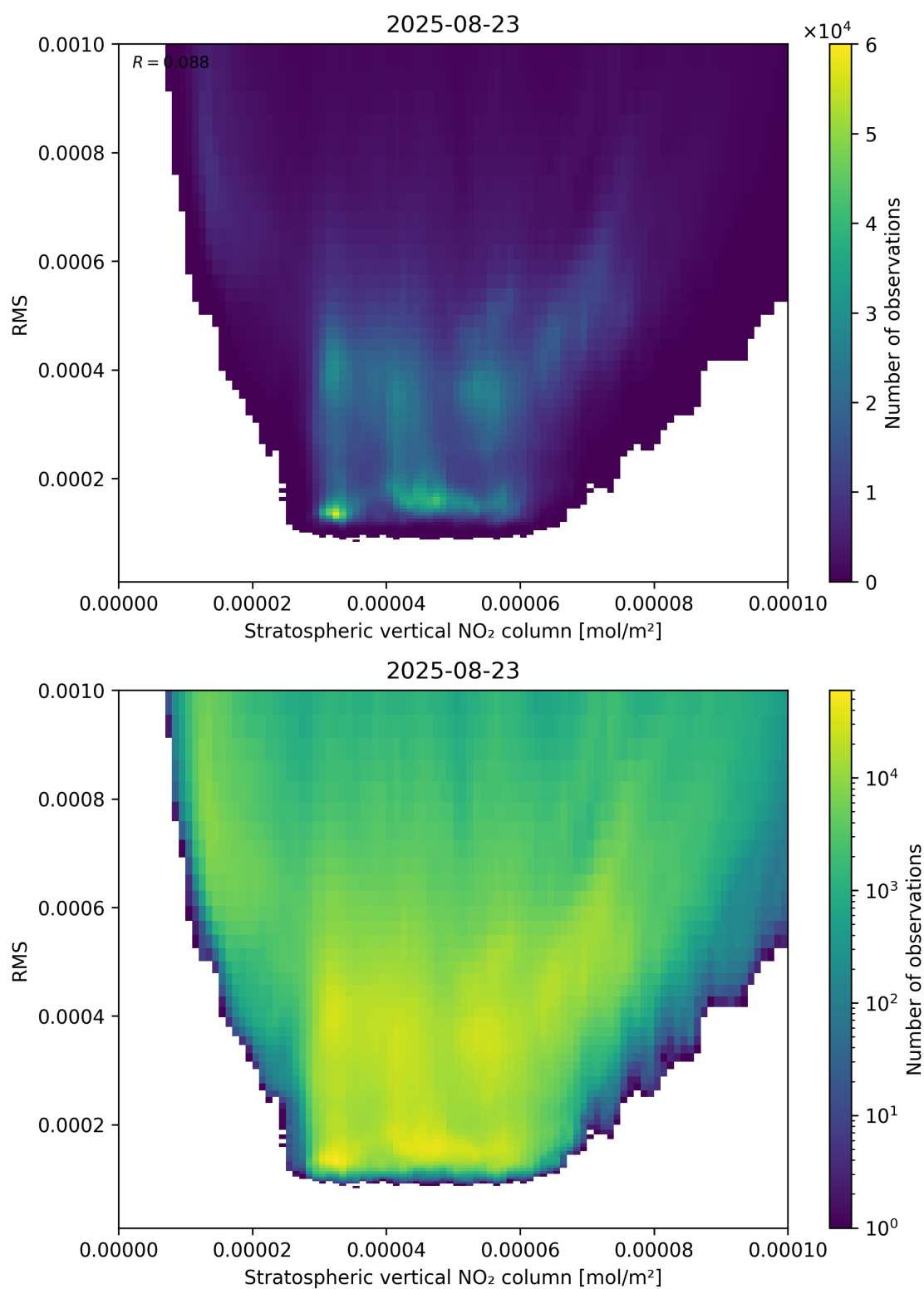
Figure 102: Scatter density plot of “Stratospheric vertical NO 2 column” against “RMS” for 2025-08-22 to 2025-08-24.
