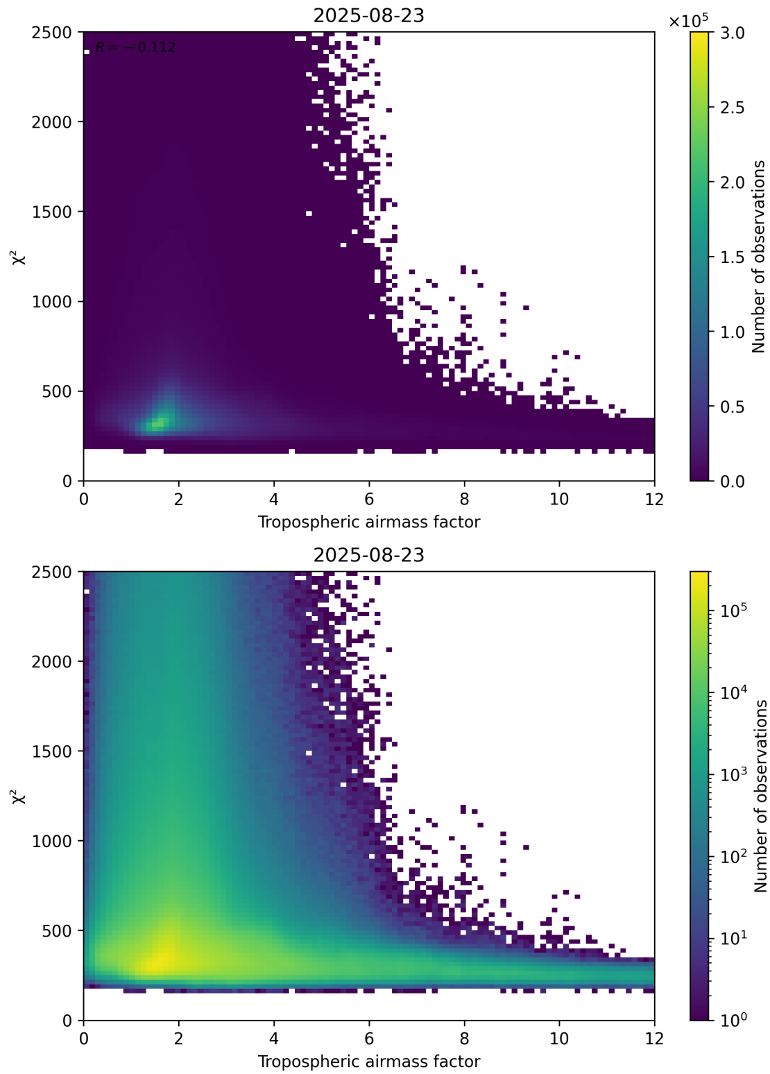
Figure 73: Scatter density plot of “Tropospheric airmass factor” against “ \chi^2 ” for 2025-08-22 to 2025-08-24.
