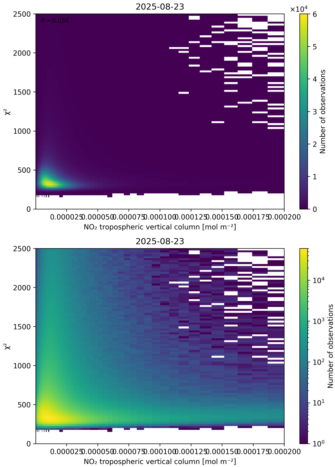
Figure 124: Scatter density plot of “NO 2 tropospheric vertical column” against “ \chi^2 ” for 2025-08-22 to 2025-08-24.
