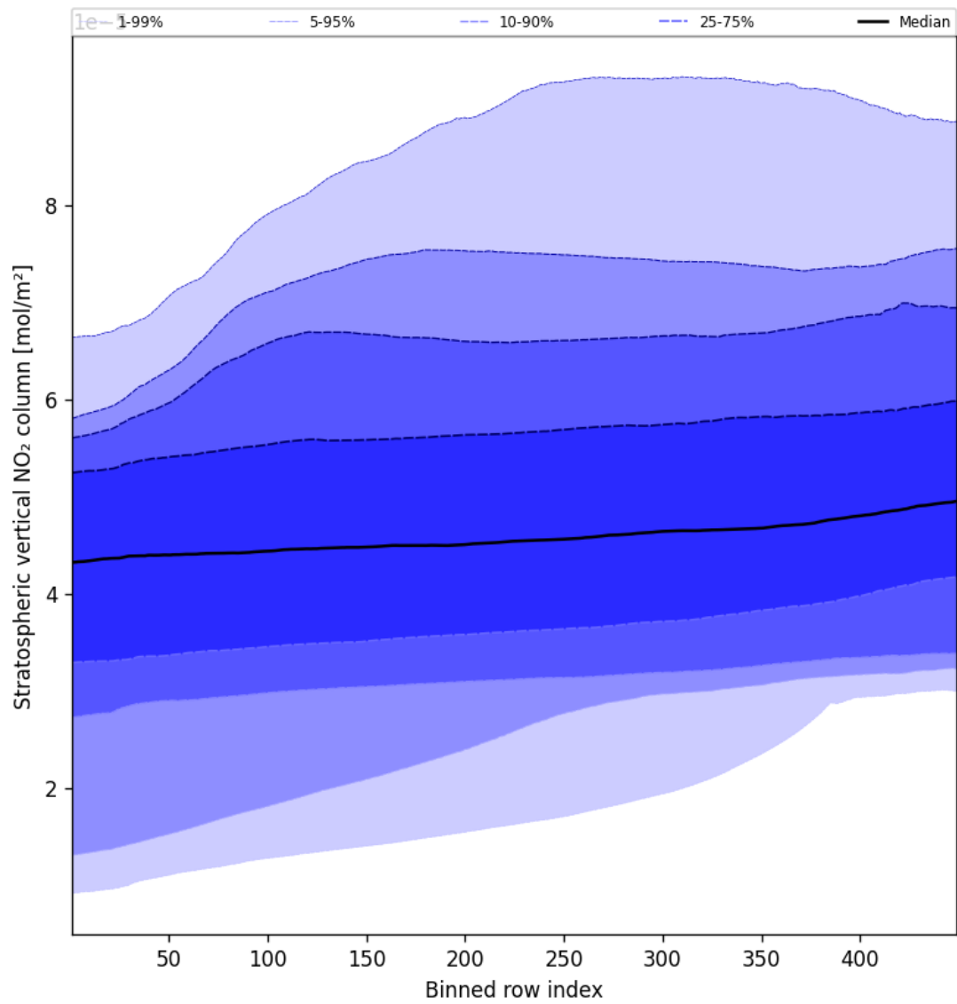
Figure 53: Along track statistics of “Stratospheric vertical NO 2 column” for 2025-08-22 to 2025-08-24
