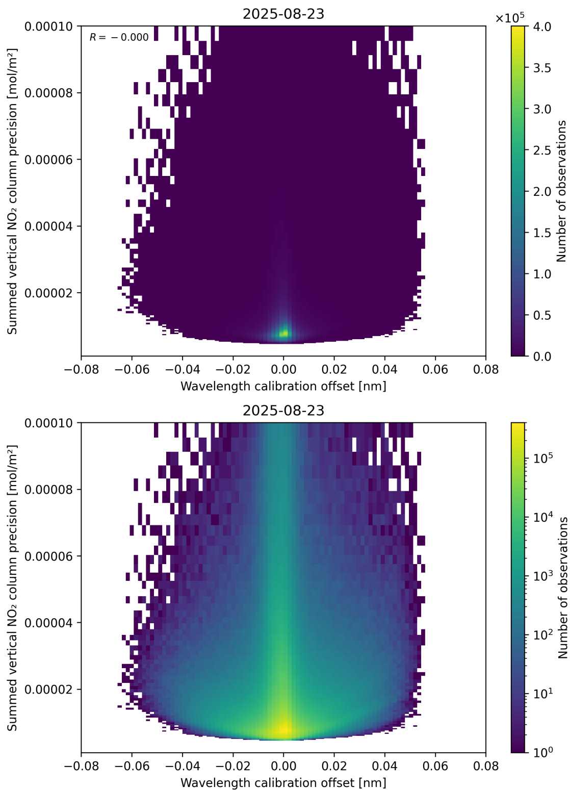
Figure 178: Scatter density plot of “Wavelength calibration offset” against “Summed vertical NO 2 column precision” for 2025-08-22 to 2025-08-24.
