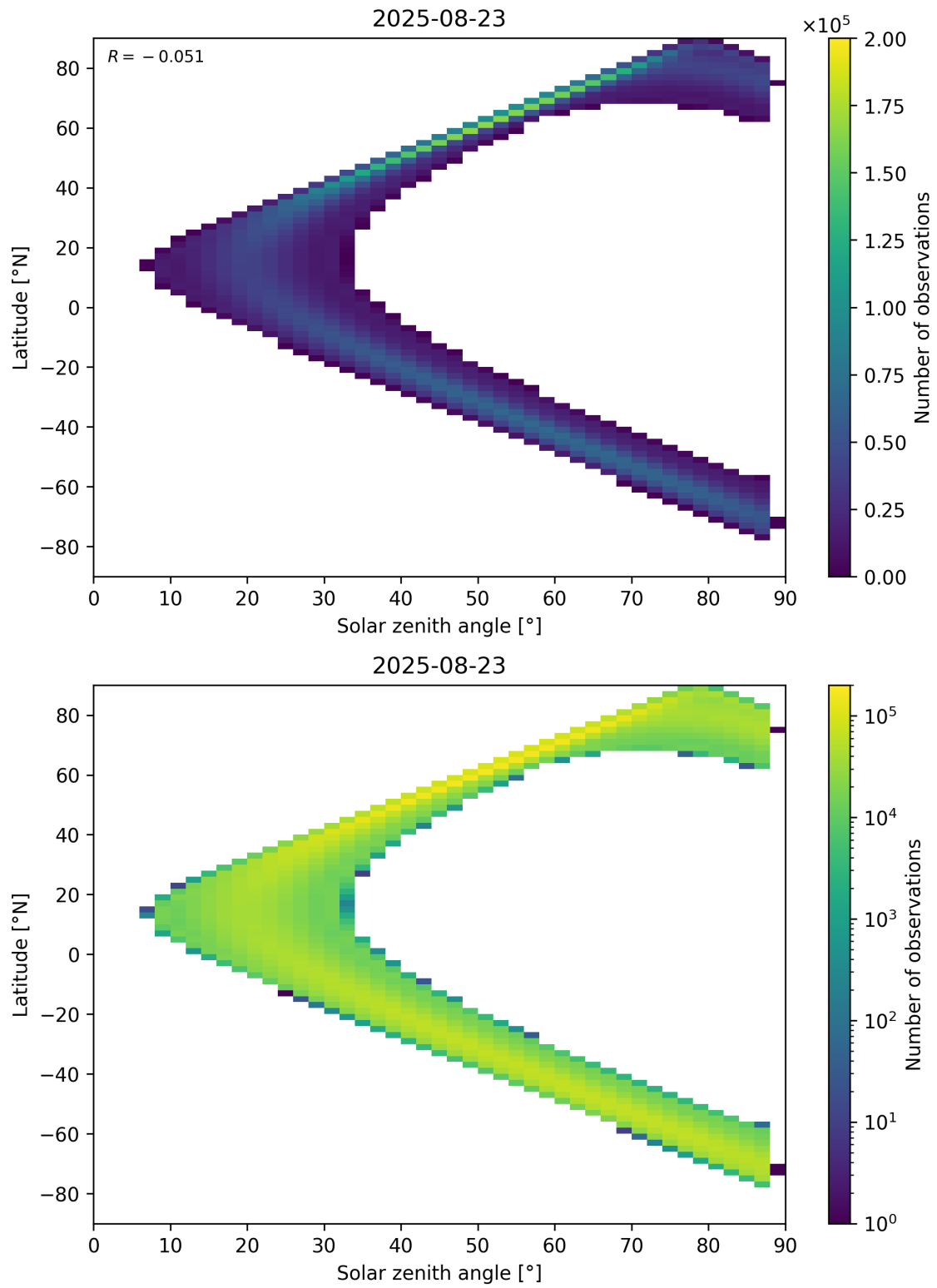
Figure 149: Scatter density plot of “Solar zenith angle” against “Latitude” for 2025-08-22 to 2025-08-24.
