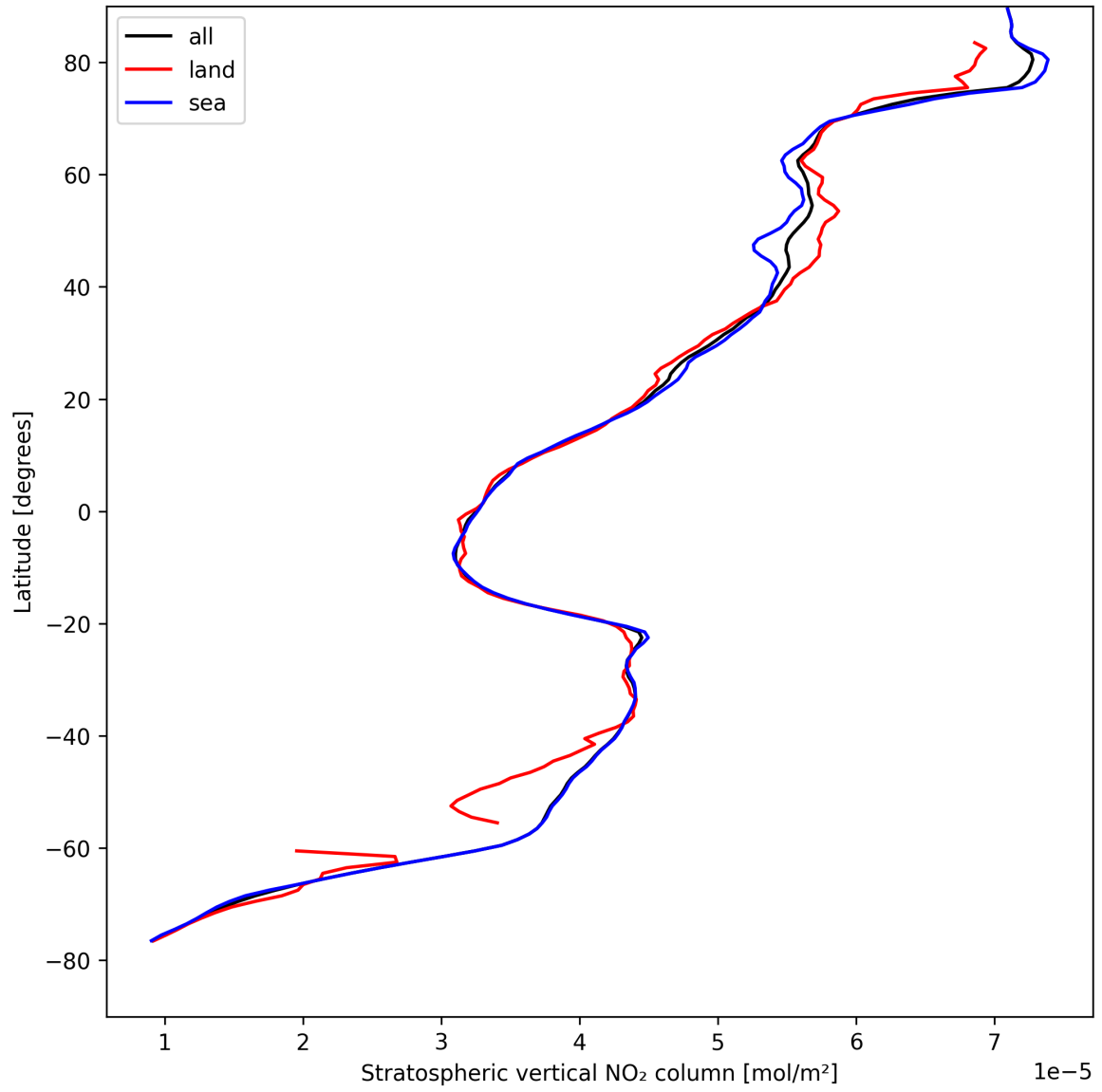
Figure 19: Zonal average of “Stratospheric vertical NO 2 column” for 2025-08-22 to 2025-08-24.
