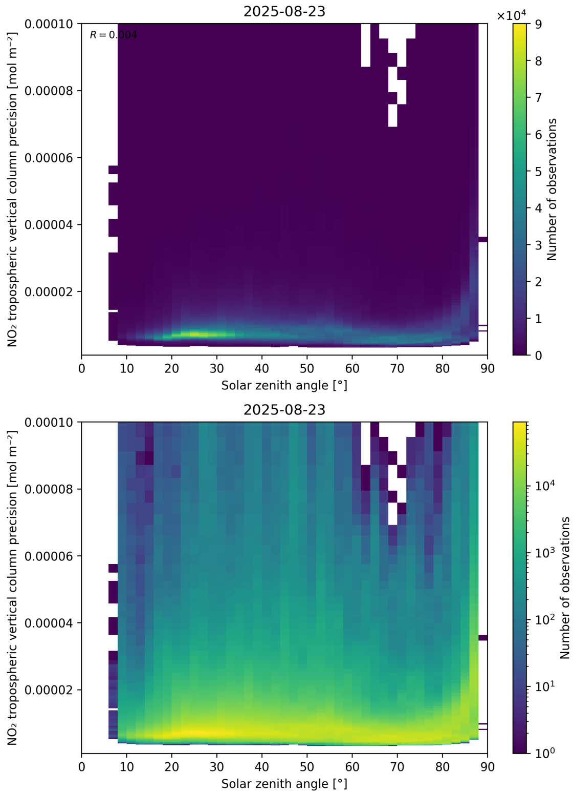
Figure 156: Scatter density plot of “Solar zenith angle” against “NO 2 tropospheric vertical column precision” for 2025-08-22 to 2025-08-24.
