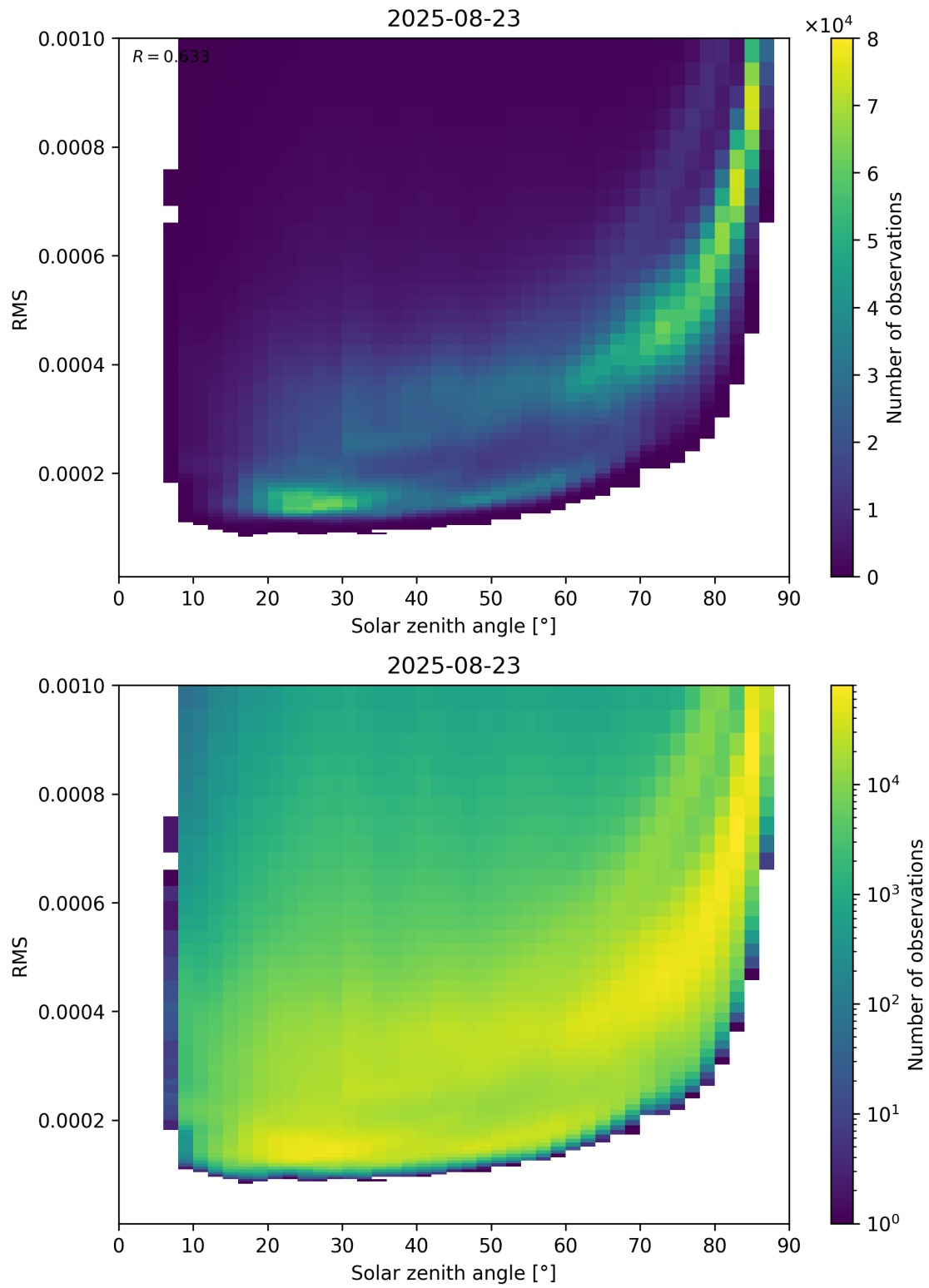
Figure 157: Scatter density plot of “Solar zenith angle” against “RMS” for 2025-08-22 to 2025-08-24.
