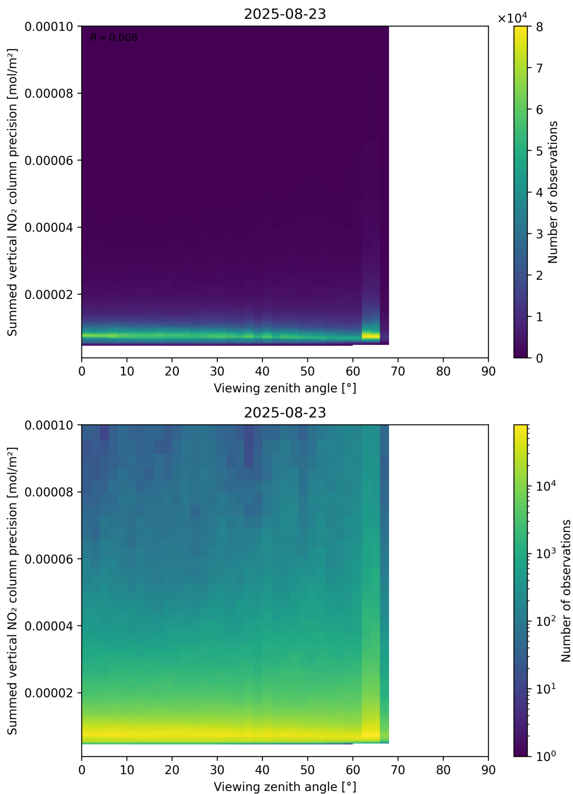
Figure 166: Scatter density plot of “Viewing zenith angle” against “Summed vertical NO 2 column precision” for 2025-08-22 to 2025-08-24.
