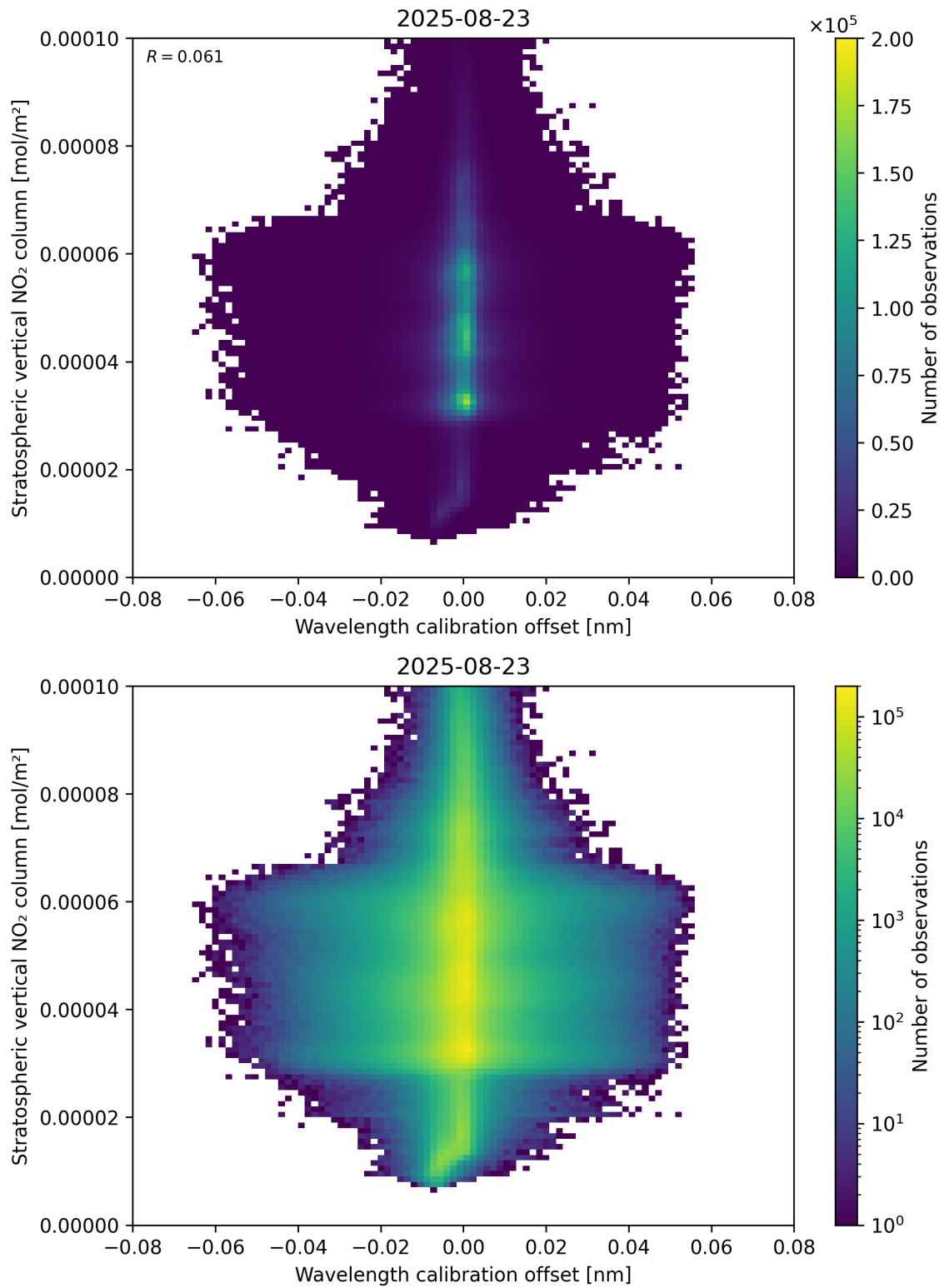
Figure 176: Scatter density plot of “Wavelength calibration offset” against “Stratospheric vertical NO 2 column” for 2025-08-22 to 2025-08-24.
