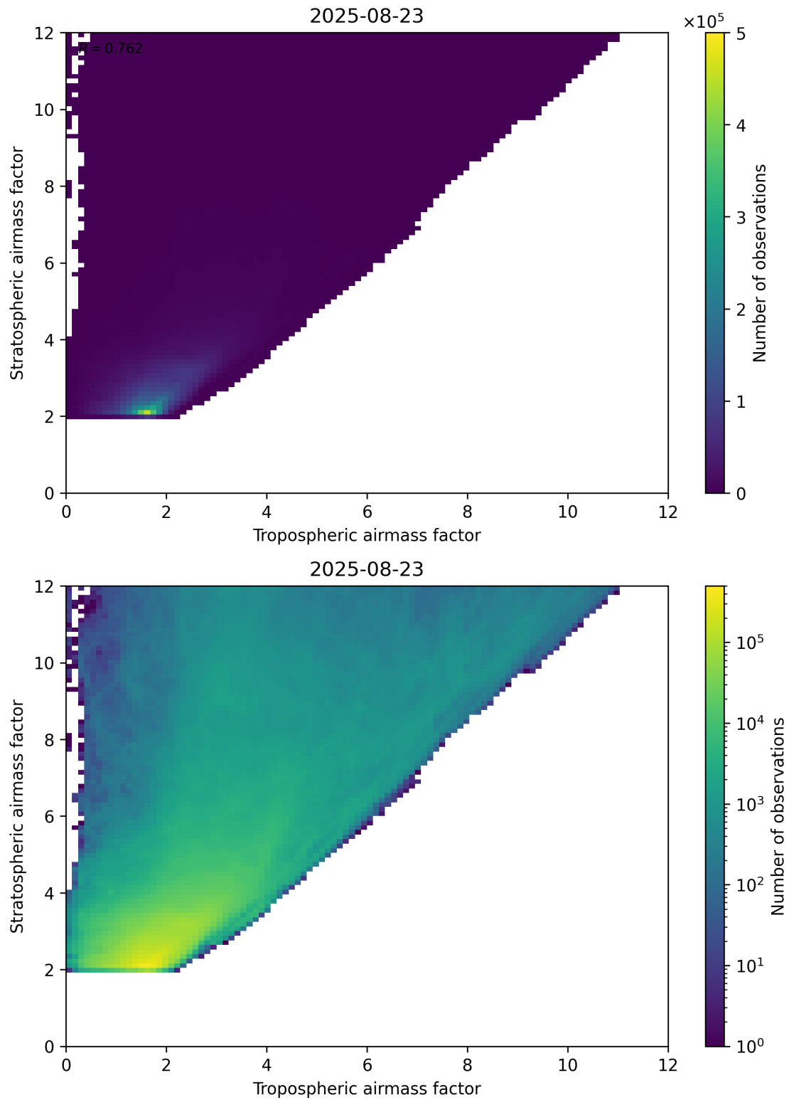
Figure 71: Scatter density plot of “Tropospheric airmass factor” against “Stratospheric airmass factor” for 2025-08-22 to 2025-08-24.
