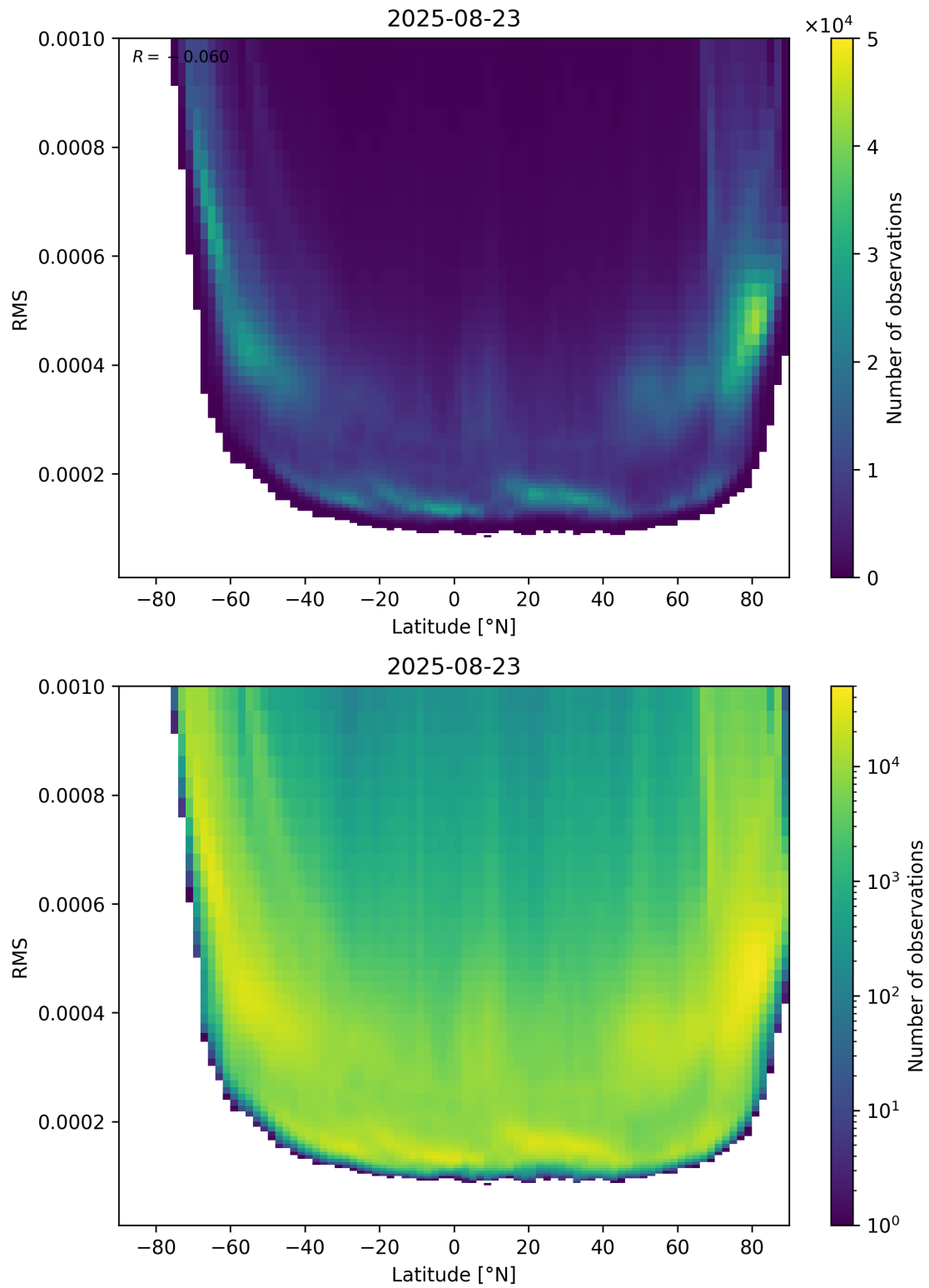
Figure 94: Scatter density plot of “Latitude” against “RMS” for 2025-08-22 to 2025-08-24.
