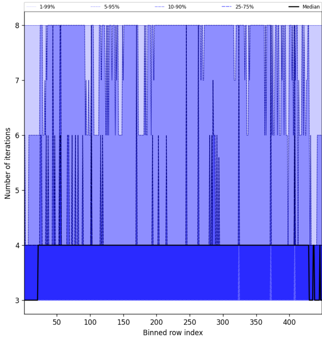
Figure 51: Along track statistics of “Number of iterations” for 2025-08-22 to 2025-08-24
