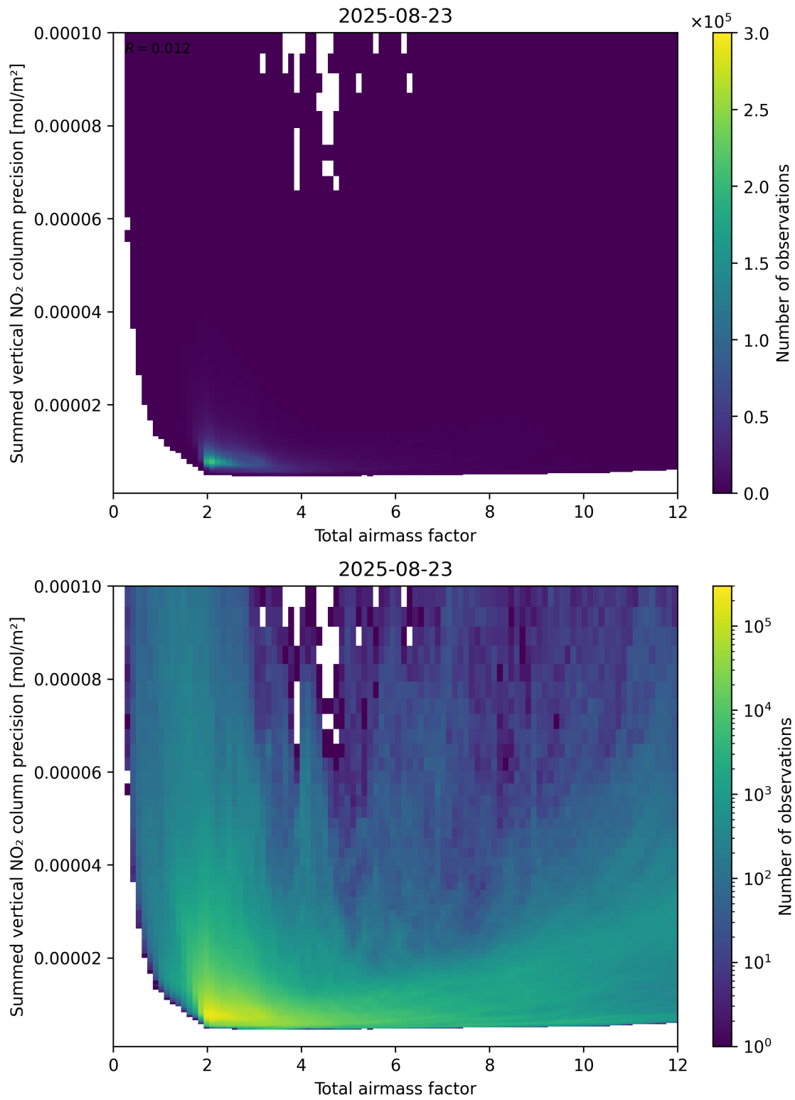
Figure 66: Scatter density plot of “Total airmass factor” against “Summed vertical NO 2 column precision” for 2025-08-22 to 2025-08-24.
