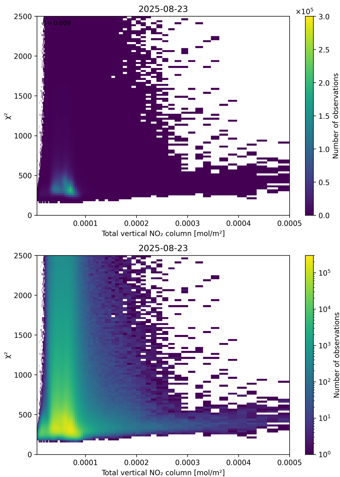
Figure 111: Scatter density plot of “Total vertical NO 2 column” against “ \chi^2 ” for 2025-08-22 to 2025-08-24.
