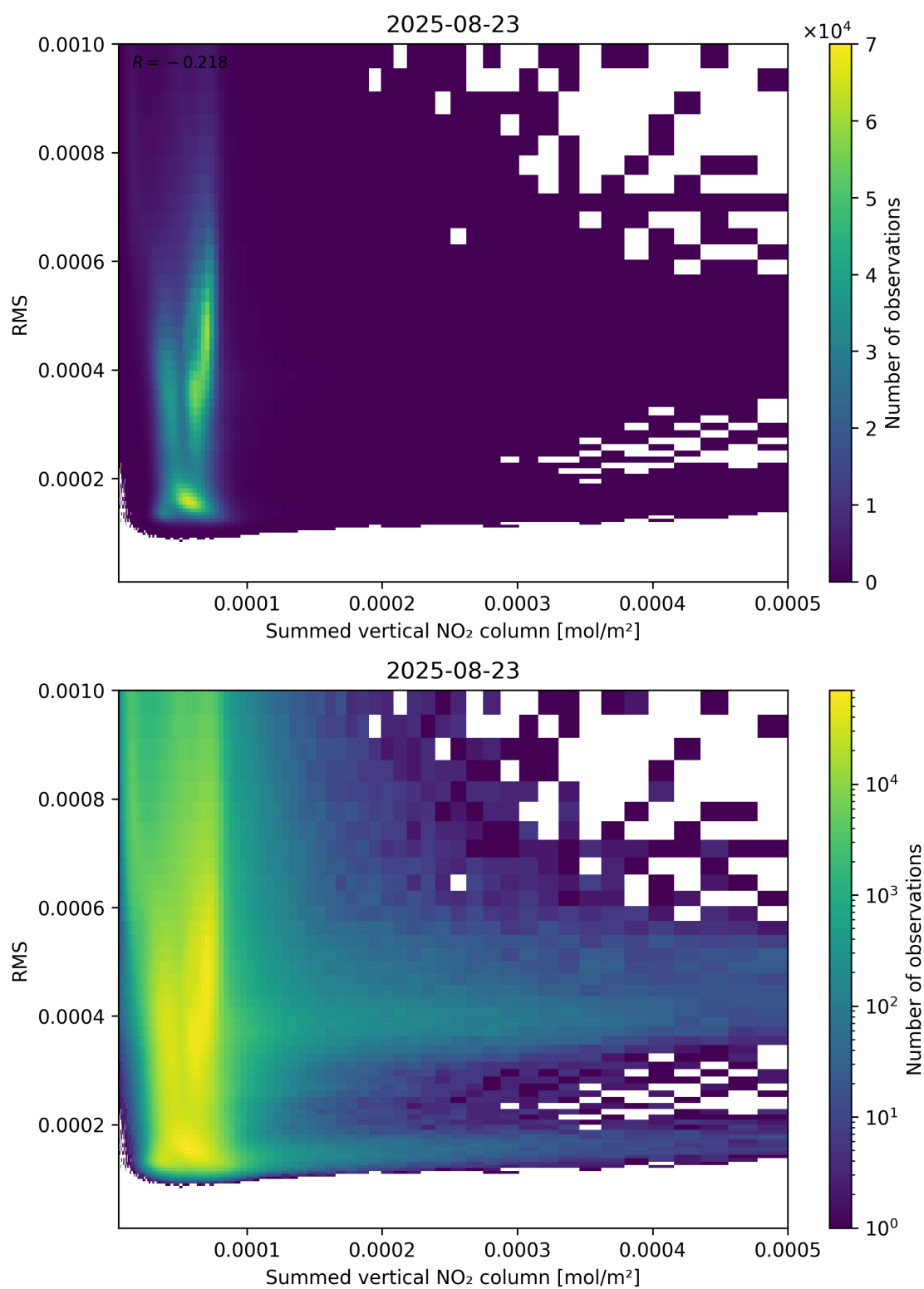
Figure 109: Scatter density plot of “Summed vertical NO 2 column” against “RMS” for 2025-08-22 to 2025-08-24.
