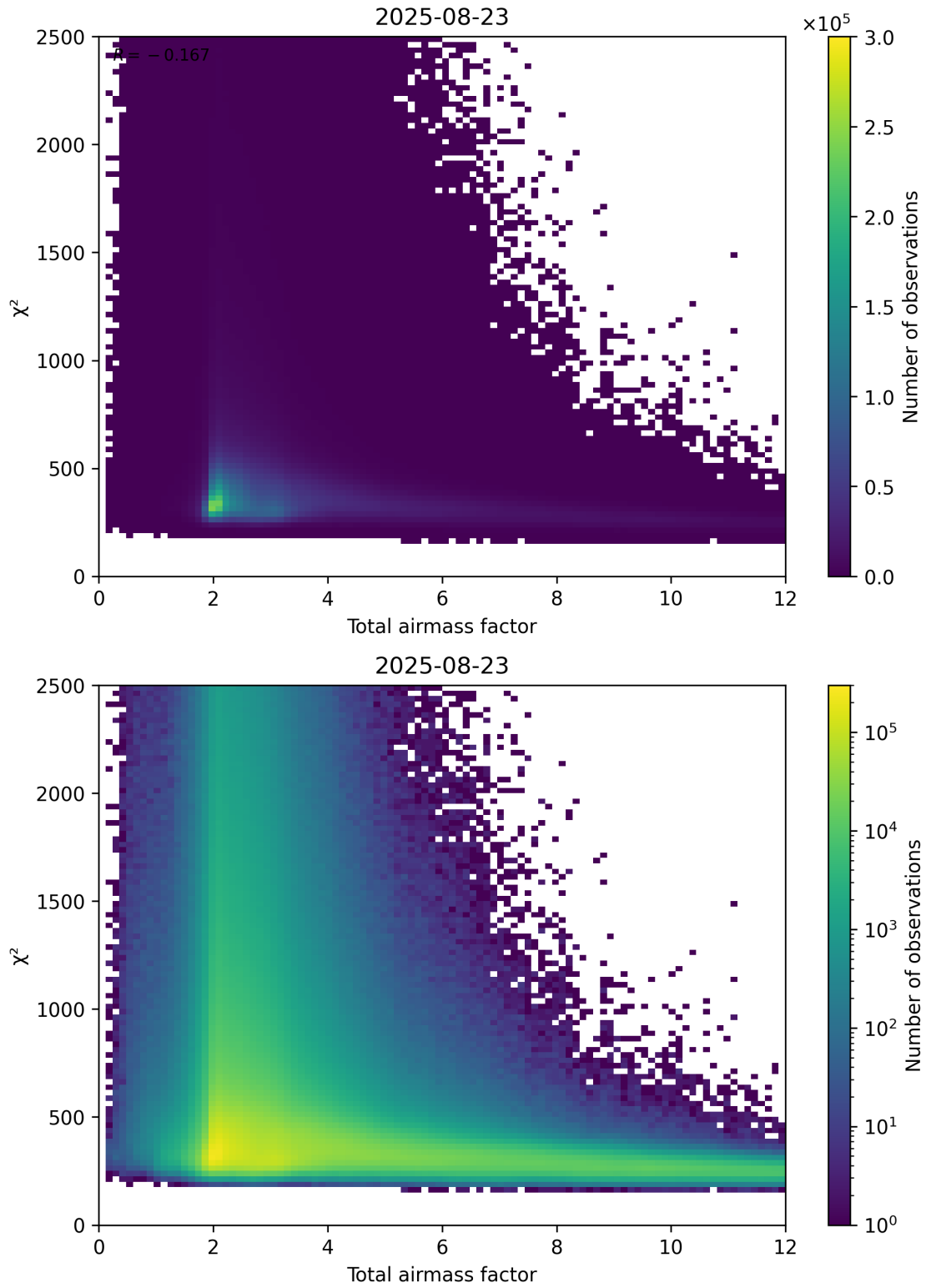
Figure 63: Scatter density plot of “Total airmass factor” against “ \chi^2 ” for 2025-08-22 to 2025-08-24.
