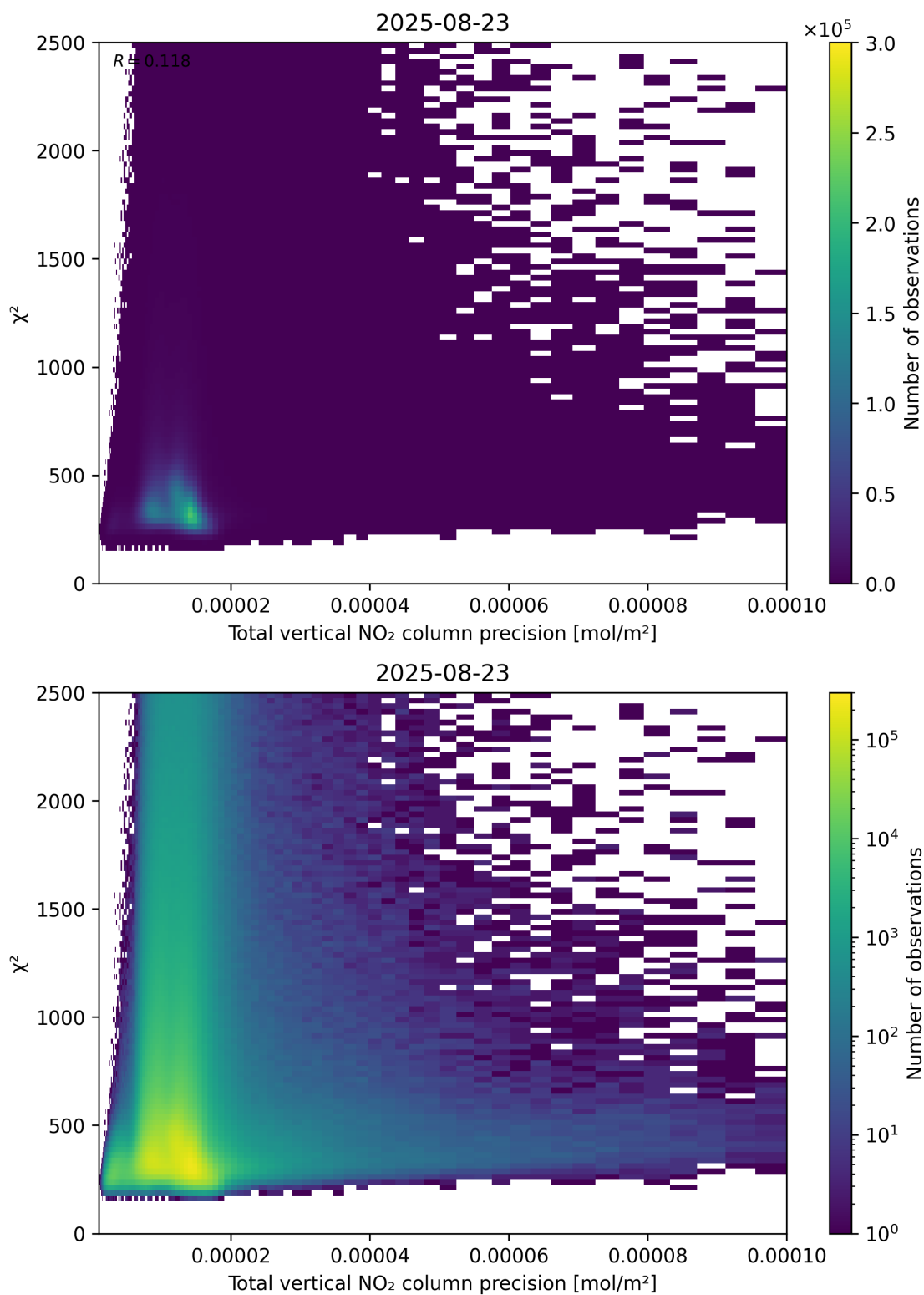
Figure 116: Scatter density plot of “Total vertical NO 2 column precision” against “ \chi^2 ” for 2025-08-22 to 2025-08-24.
