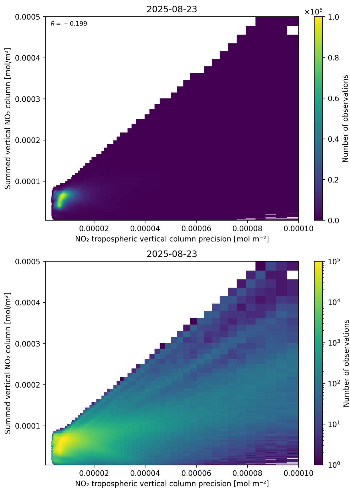
Figure 136: Scatter density plot of “NO 2 tropospheric vertical column precision” against “Summed vertical NO 2 column” for 2025-08-22 to 2025-08-24.
