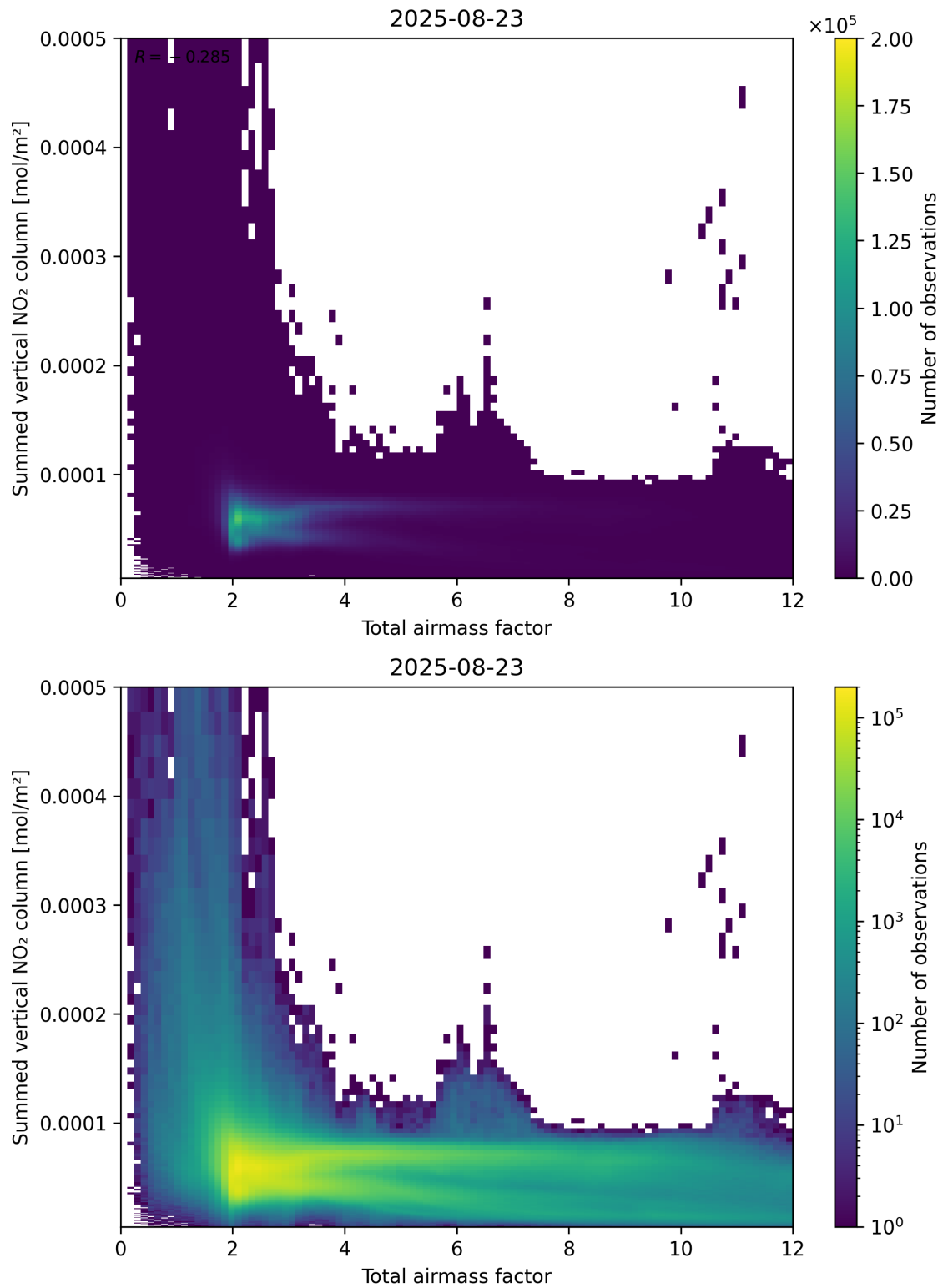
Figure 65: Scatter density plot of “Total airmass factor” against “Summed vertical NO 2 column” for 2025-08-22 to 2025-08-24.
