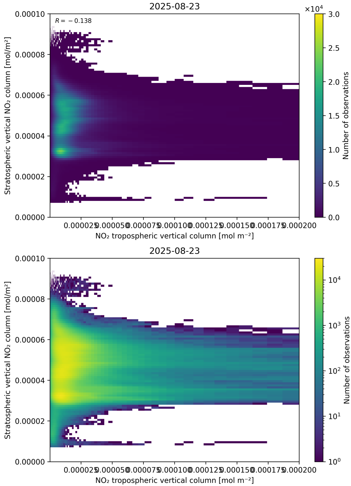
Figure 125: Scatter density plot of “NO 2 tropospheric vertical column” against “Stratospheric vertical NO 2 column” for 2025-08-22 to 2025-08-24.
