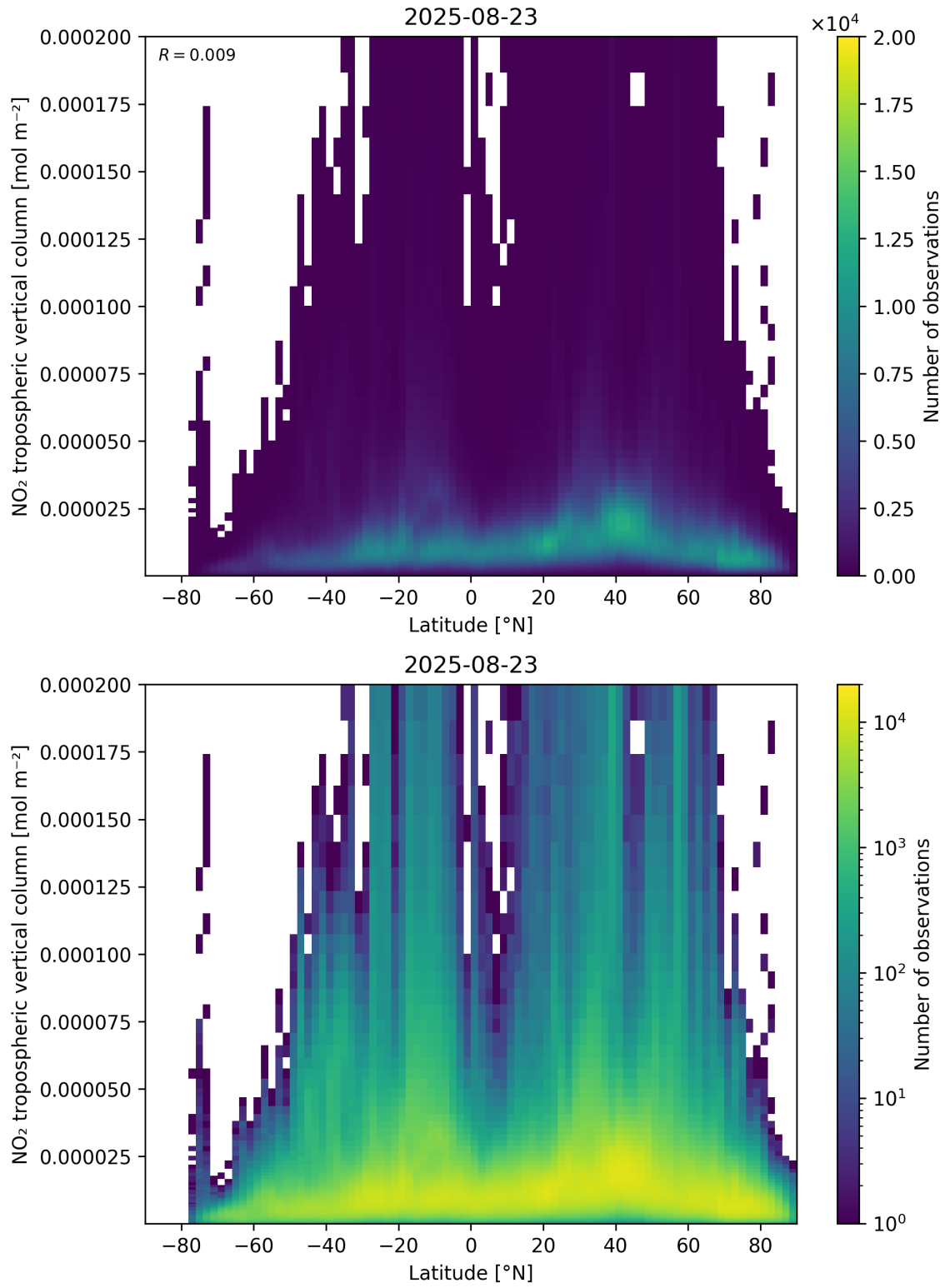
Figure 92: Scatter density plot of “Latitude” against “NO 2 tropospheric vertical column” for 2025-08-22 to 2025-08-24.
