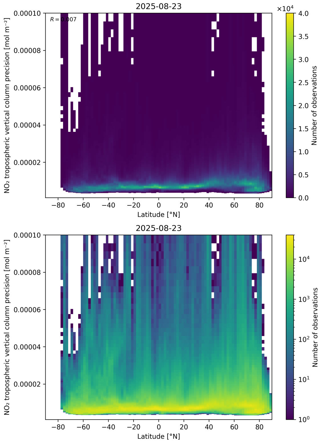
Figure 93: Scatter density plot of “Latitude” against “NO 2 tropospheric vertical column precision” for 2025-08-22 to 2025-08-24.
