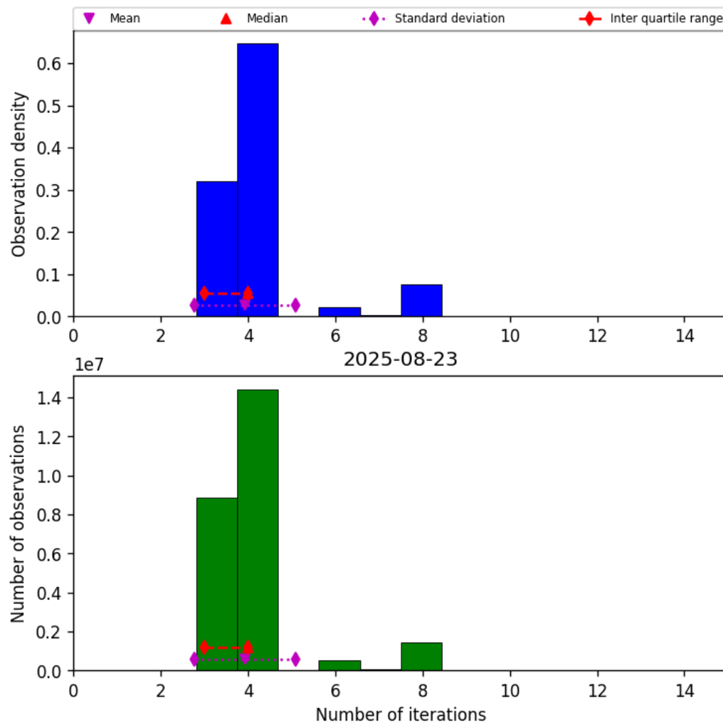
Figure 34: Histogram of “Number of iterations” for 2025-08-22 to 2025-08-24
