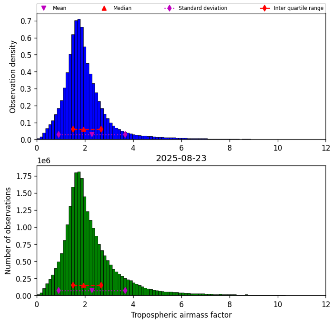
Figure 31: Histogram of “Tropospheric airmass factor” for 2025-08-22 to 2025-08-24
