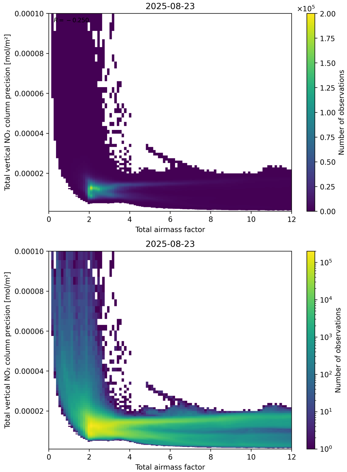
Figure 68: Scatter density plot of “Total airmass factor” against “Total vertical NO 2 column precision” for 2025-08-22 to 2025-08-24.
