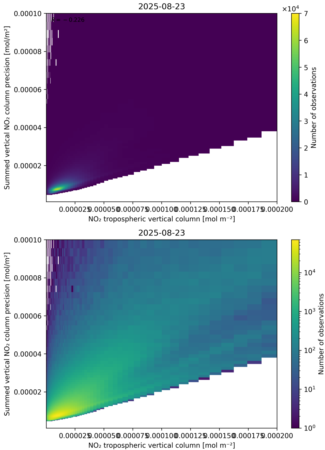
Figure 127: Scatter density plot of “NO 2 tropospheric vertical column” against “Summed vertical NO 2 column precision” for 2025-08-22 to 2025-08-24.
