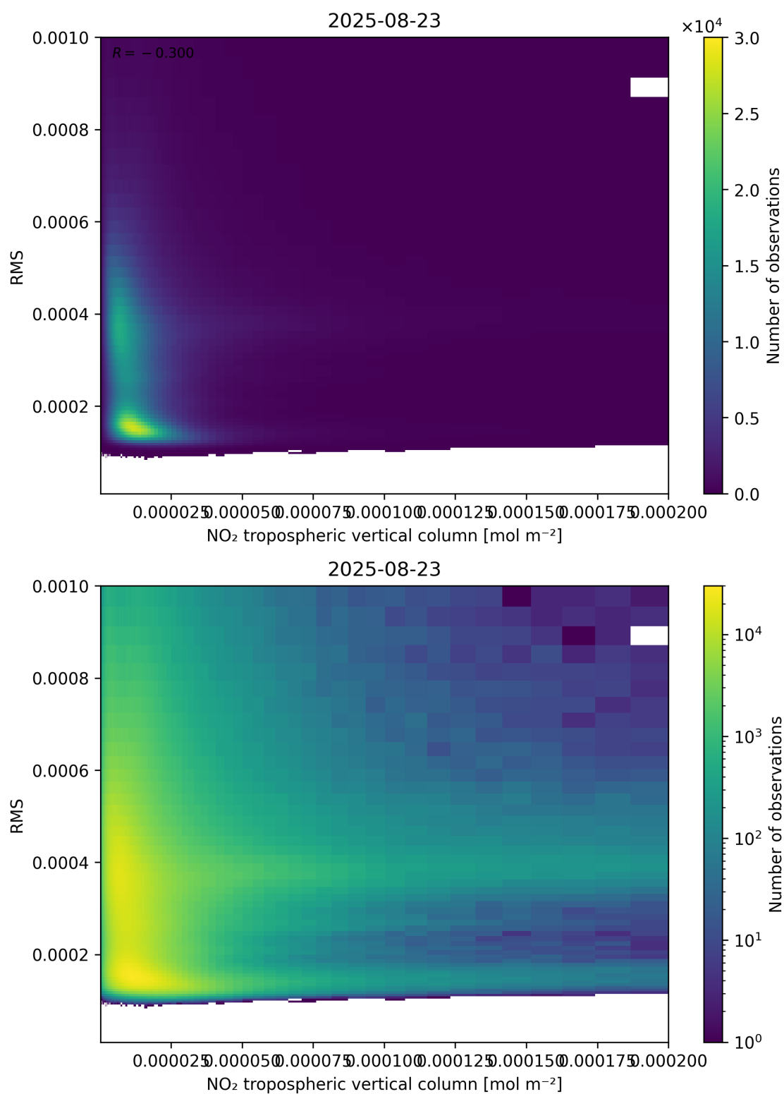
Figure 142: Scatter density plot of “NO 2 tropospheric vertical column” against “RMS” for 2025-08-22 to 2025-08-24.
