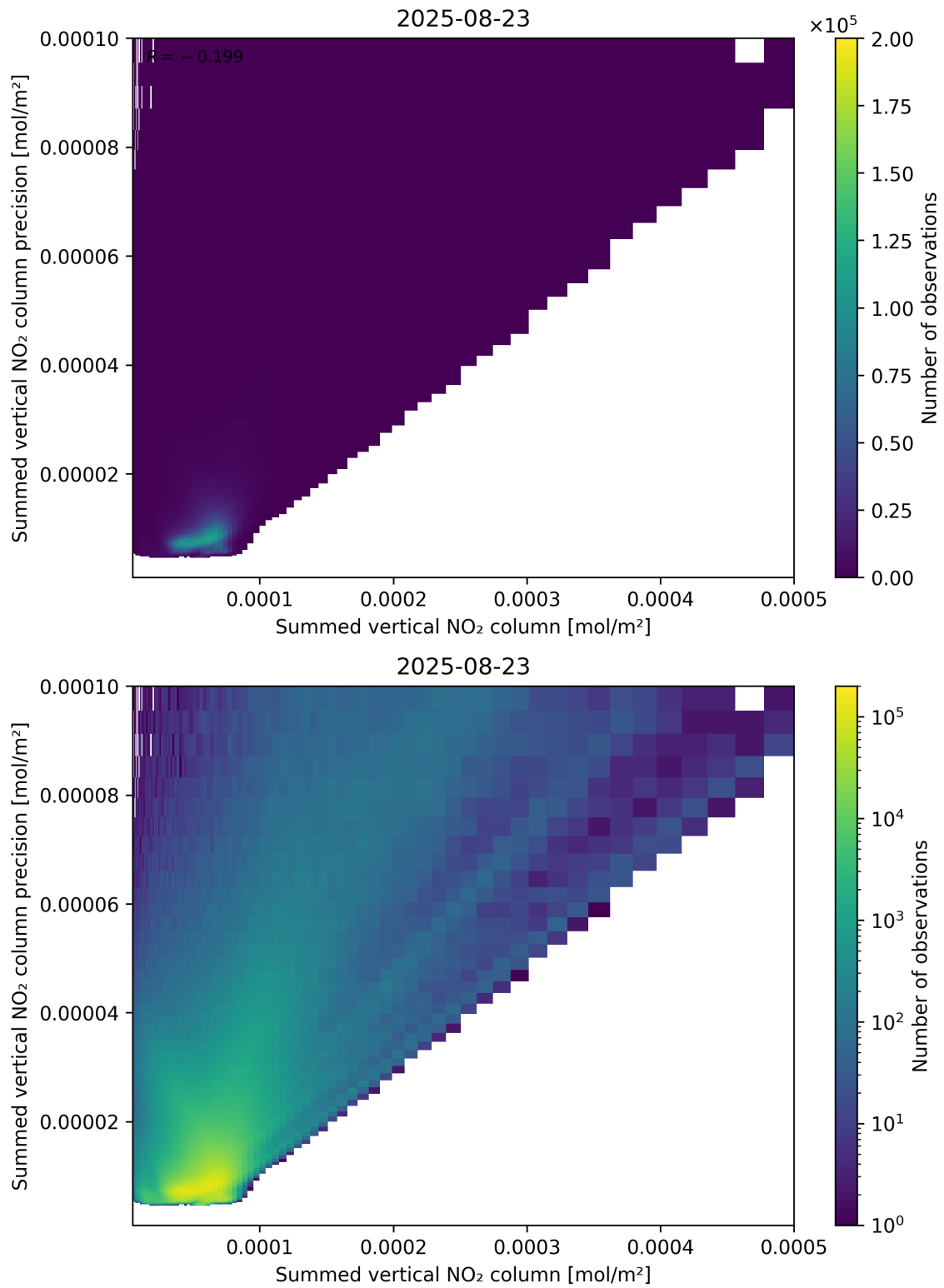
Figure 105: Scatter density plot of “Summed vertical NO 2 column” against “Summed vertical NO 2 column precision” for 2025-08-22 to 2025-08-24.
