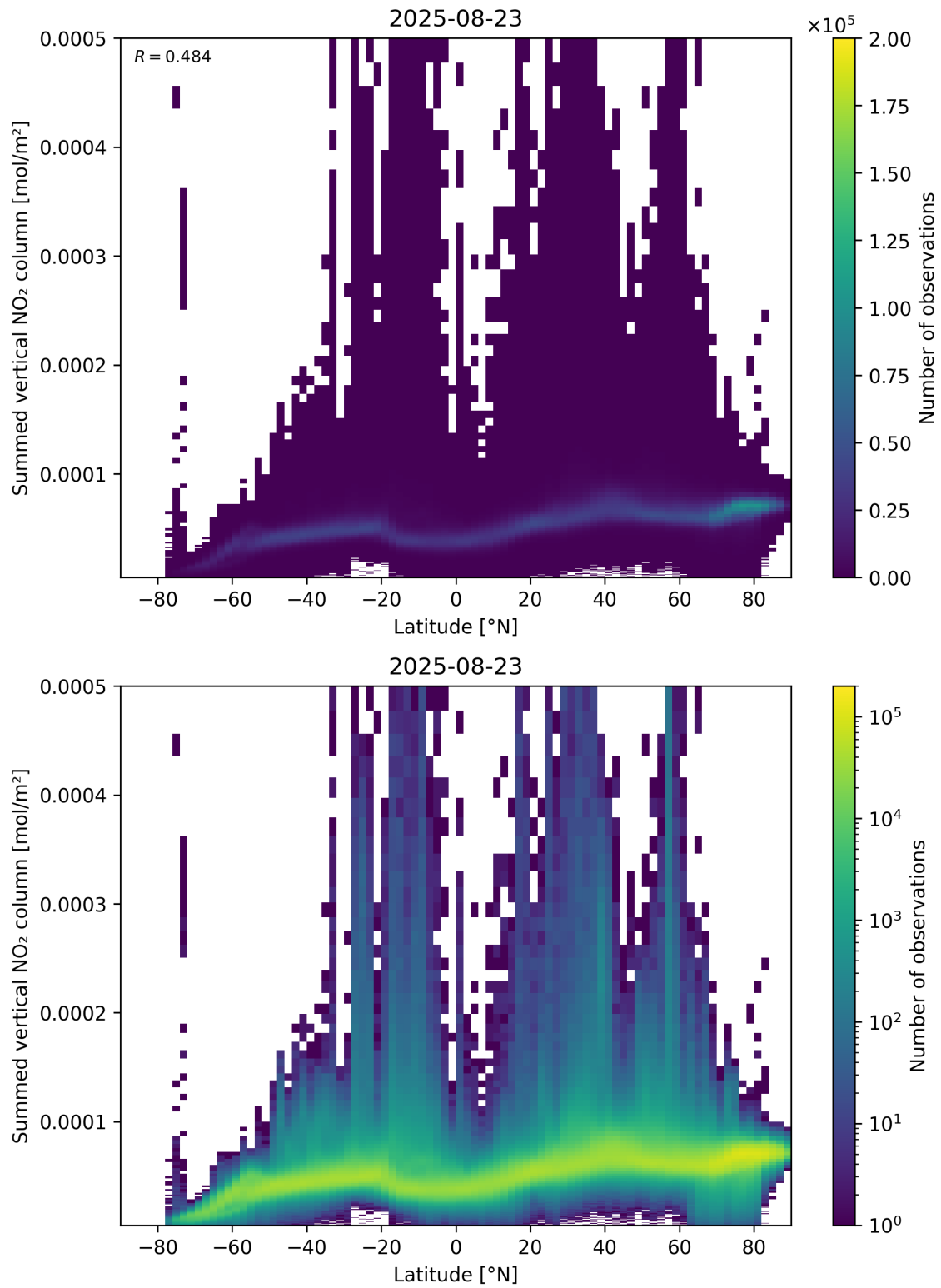
Figure 88: Scatter density plot of “Latitude” against “Summed vertical NO 2 column” for 2025-08-22 to 2025-08-24.
