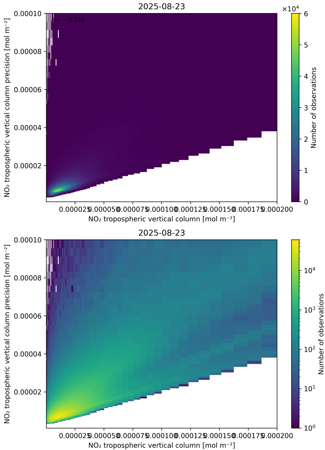
Figure 130: Scatter density plot of “NO 2 tropospheric vertical column” against “NO 2 tropospheric vertical column precision” for 2025-08-22 to 2025-08-24.
