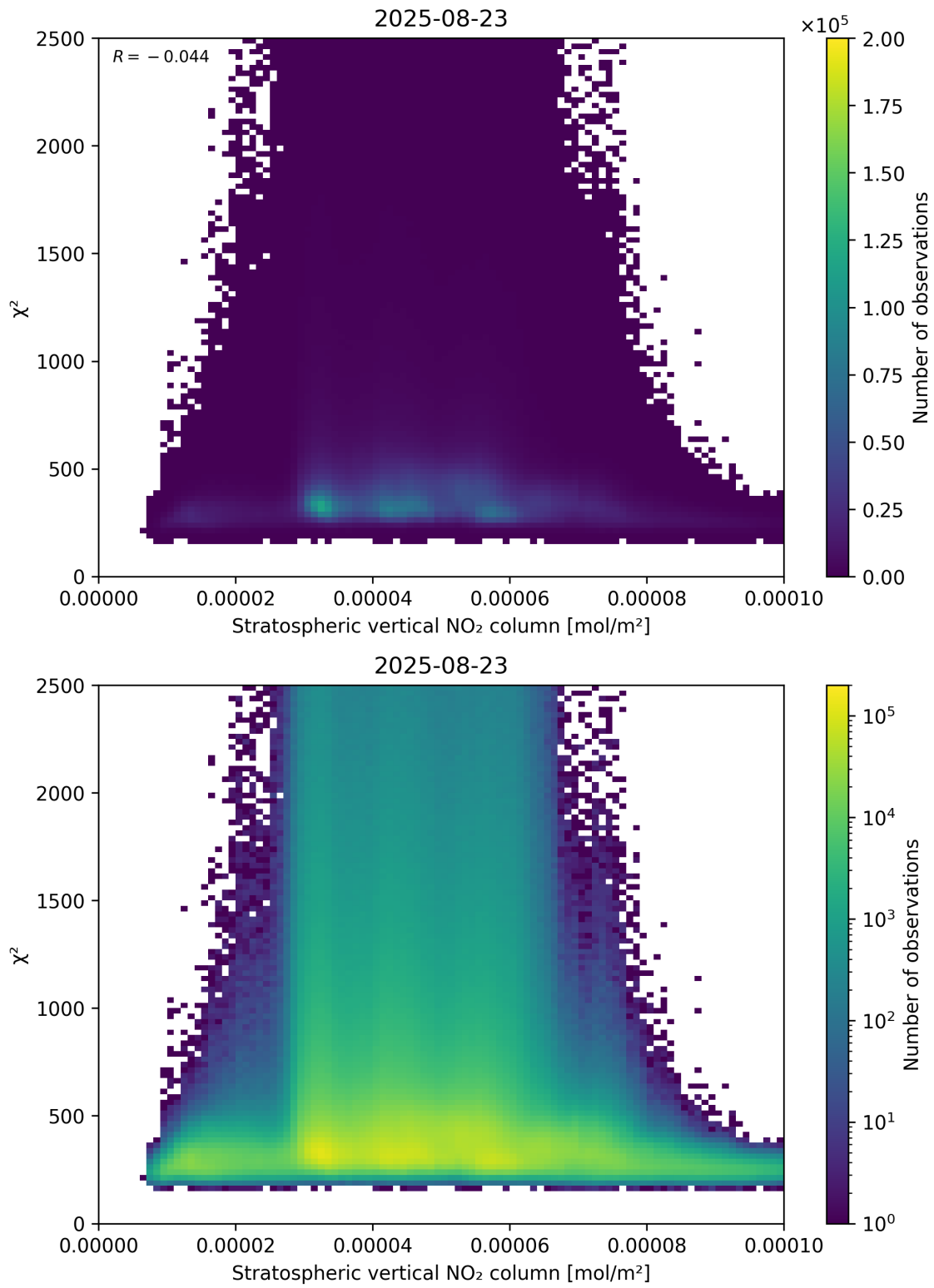
Figure 97: Scatter density plot of “Stratospheric vertical NO 2 column” against “ \chi^2 ” for 2025-08-22 to 2025-08-24.
