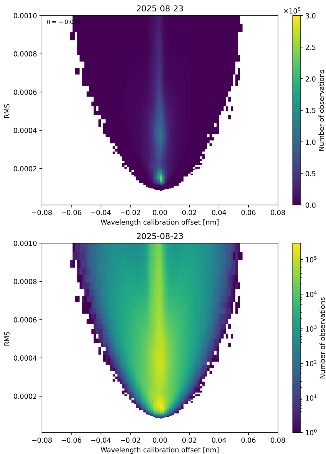
Figure 181: Scatter density plot of “Wavelength calibration offset” against “RMS” for 2025-08-22 to 2025-08-24.
