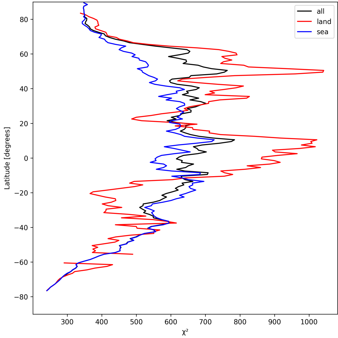
Figure 25: Zonal average of “ \chi^2 ” for 2025-08-22 to 2025-08-24.
