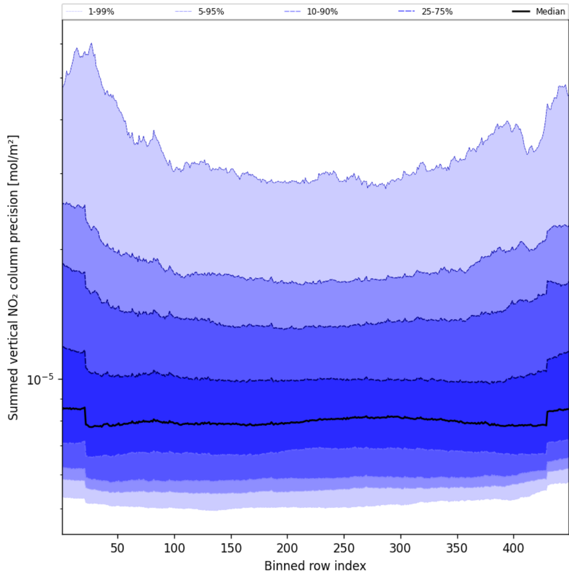
Figure 58: Along track statistics of “Summed vertical NO 2 column precision” for 2025-08-22 to 2025-08-24
