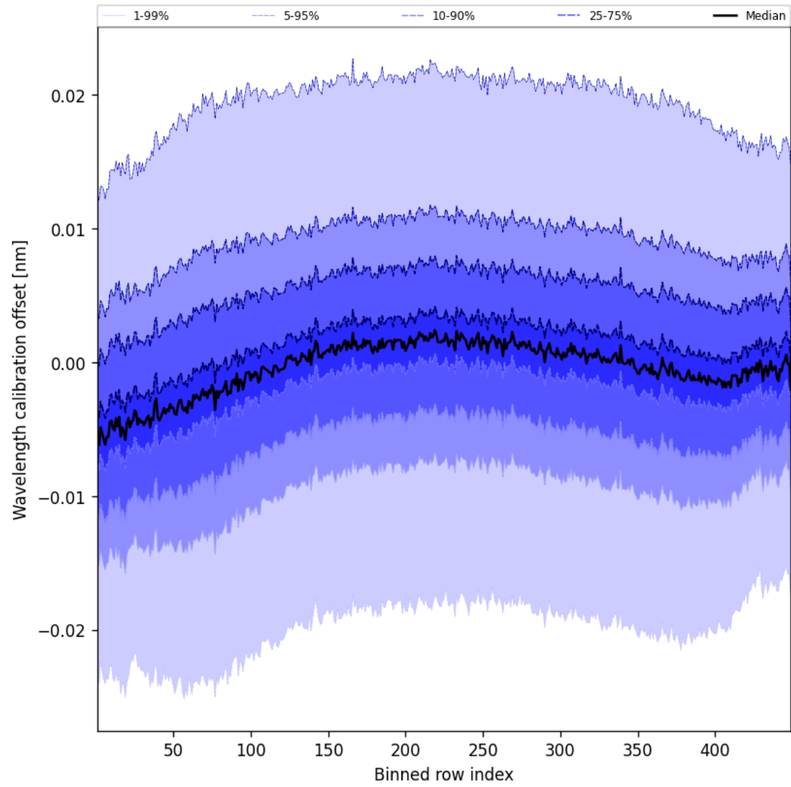
Figure 52: Along track statistics of “Wavelength calibration offset” for 2025-08-22 to 2025-08-24
