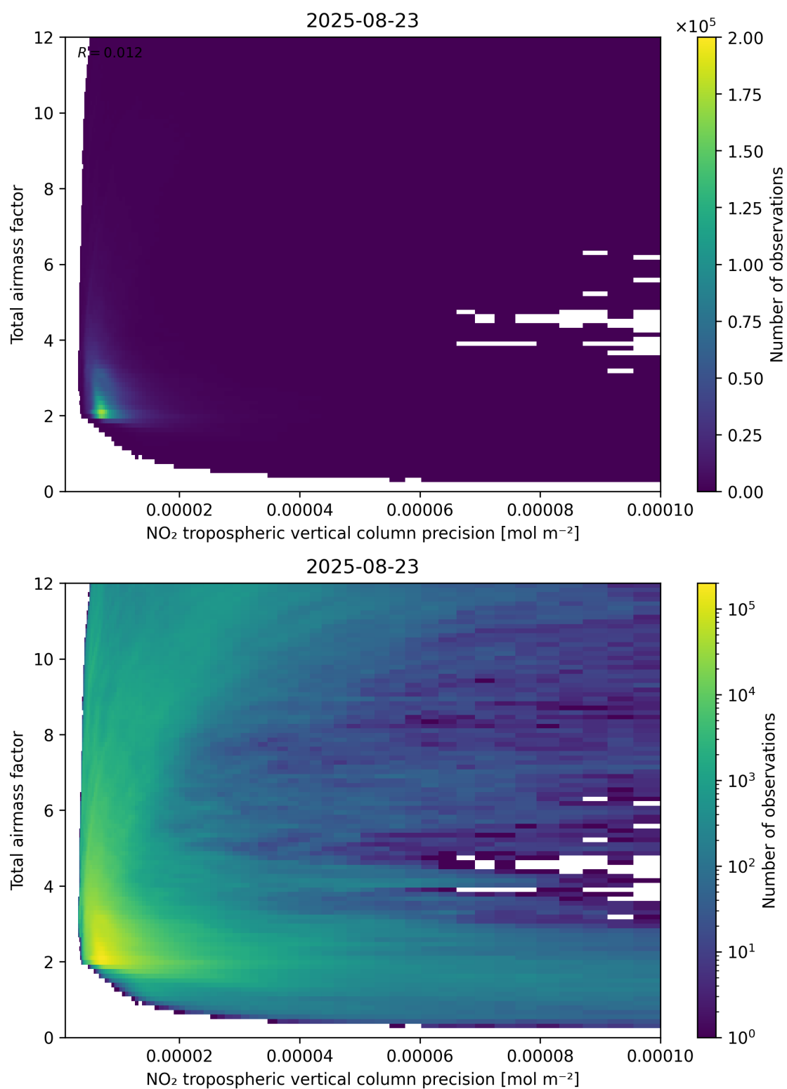
Figure 132: Scatter density plot of “NO 2 tropospheric vertical column precision” against “Total air mass factor” for 2025-08-22 to 2025-08-24.
