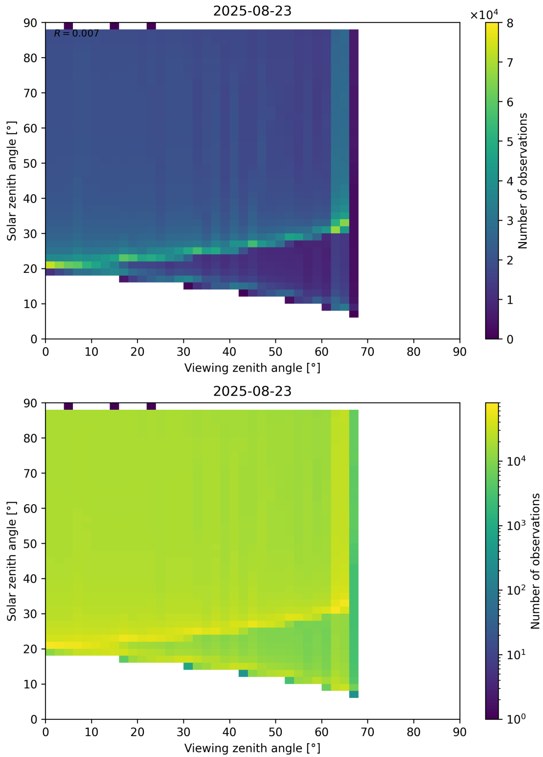
Figure 172: Scatter density plot of “Viewing zenith angle” against “Solar zenith angle” for 2025-08-22 to 2025-08-24.
