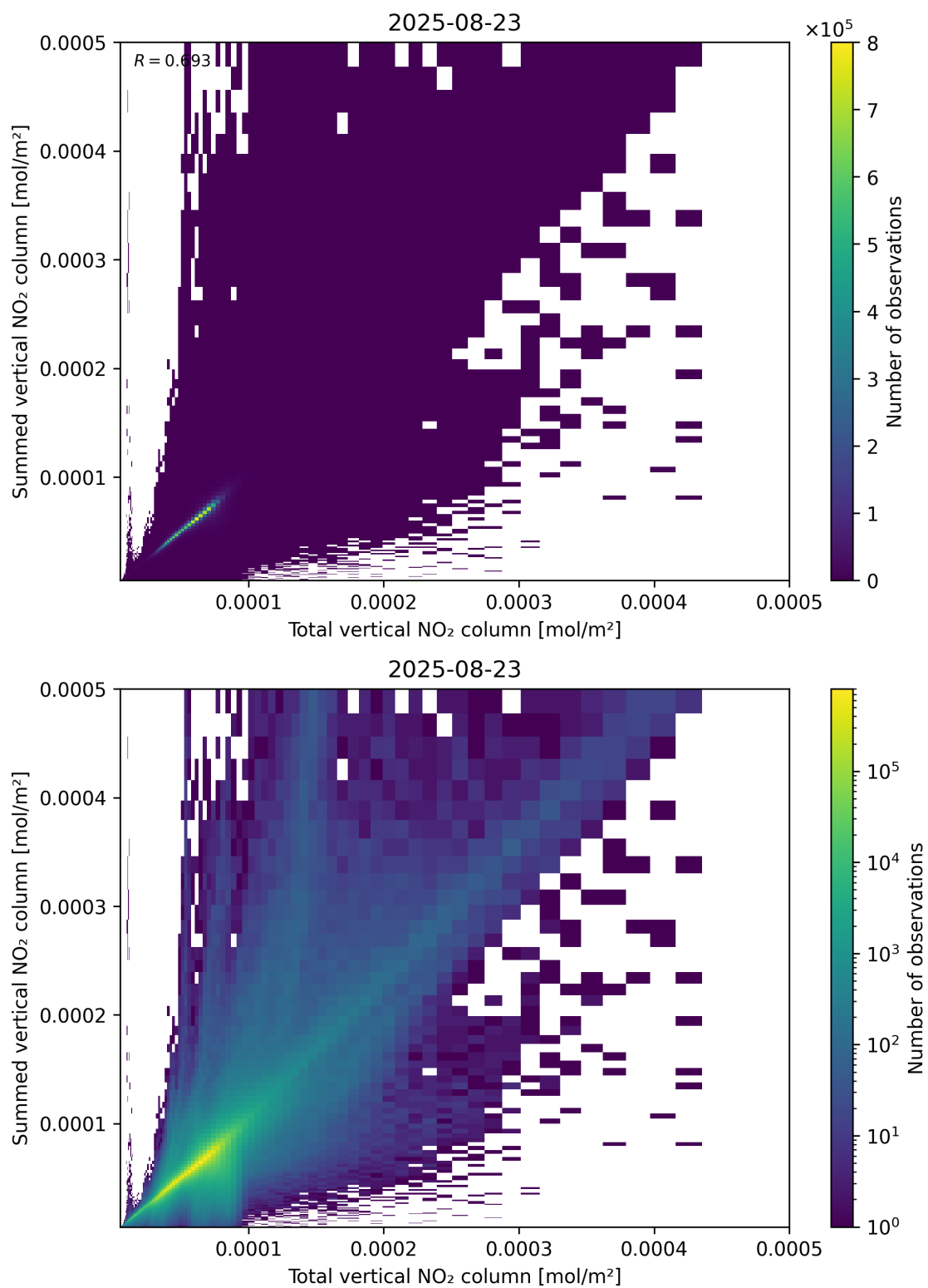
Figure 112: Scatter density plot of “Total vertical NO 2 column” against “Summed vertical NO 2 column” for 2025-08-22 to 2025-08-24.
