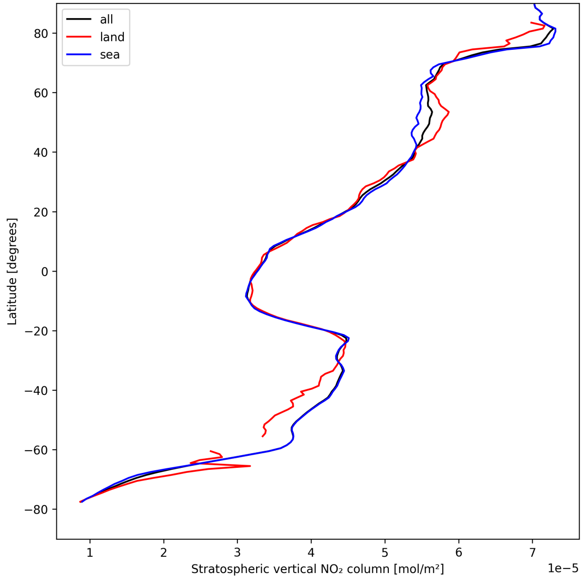
Figure 19: Zonal average of “Stratospheric vertical NO 2 column” for 2025-08-23 to 2025-08-25.
