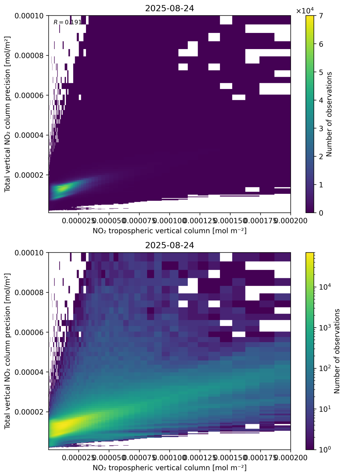
Figure 129: Scatter density plot of “NO 2 tropospheric vertical column” against “Total vertical NO 2 column precision” for 2025-08-23 to 2025-08-25.
