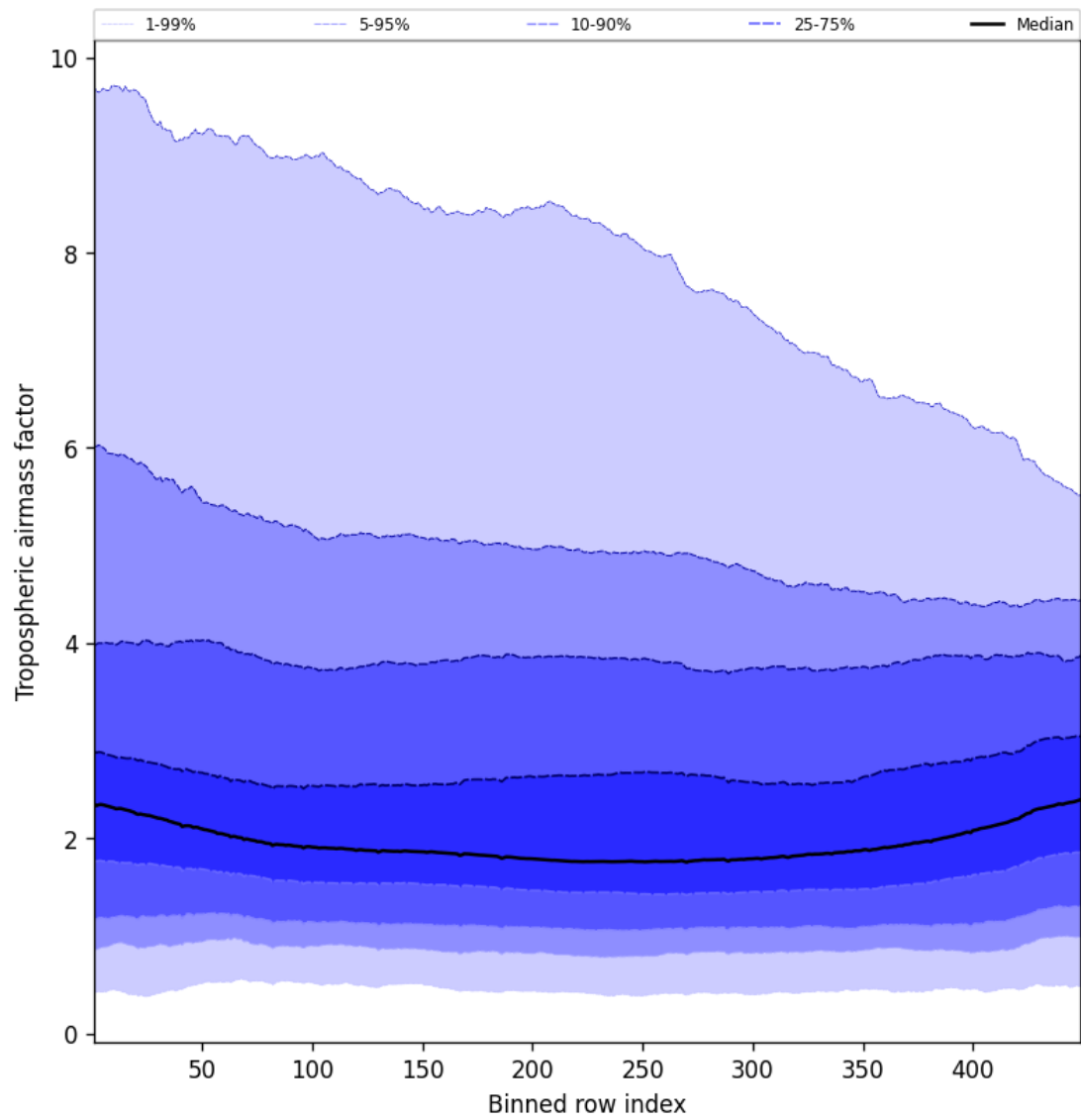
Figure 48: Along track statistics of “Tropospheric airmass factor” for 2025-08-23 to 2025-08-25
