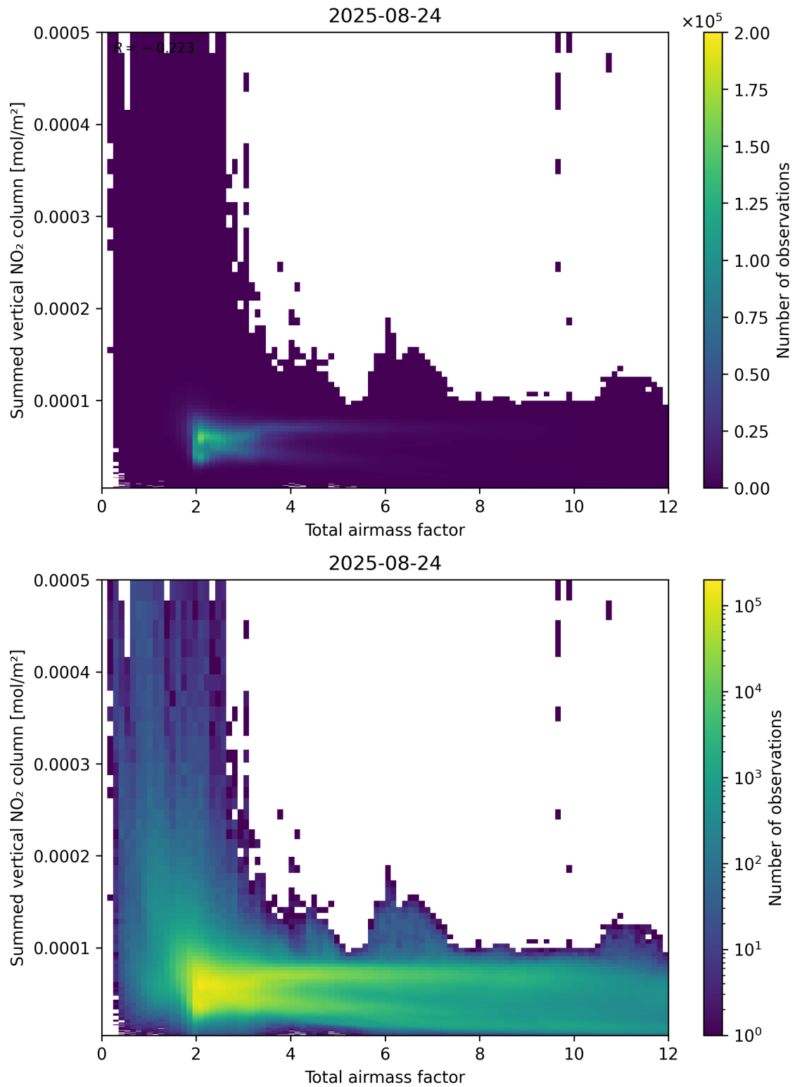
Figure 65: Scatter density plot of “Total airmass factor” against “Summed vertical NO 2 column” for 2025-08-23 to 2025-08-25.
