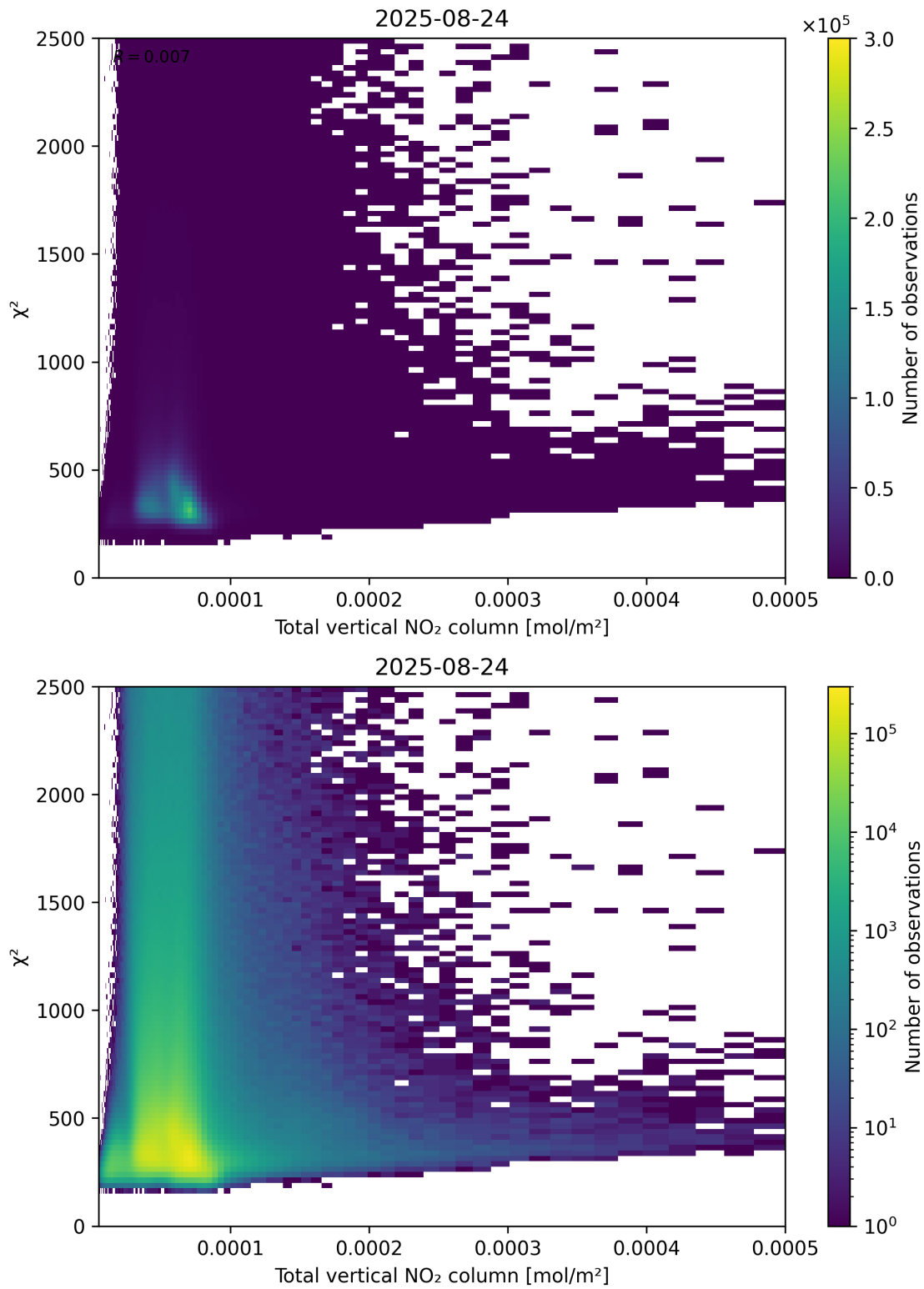
Figure 111: Scatter density plot of “Total vertical NO 2 column” against “ \chi^2 ” for 2025-08-23 to 2025-08-25.
