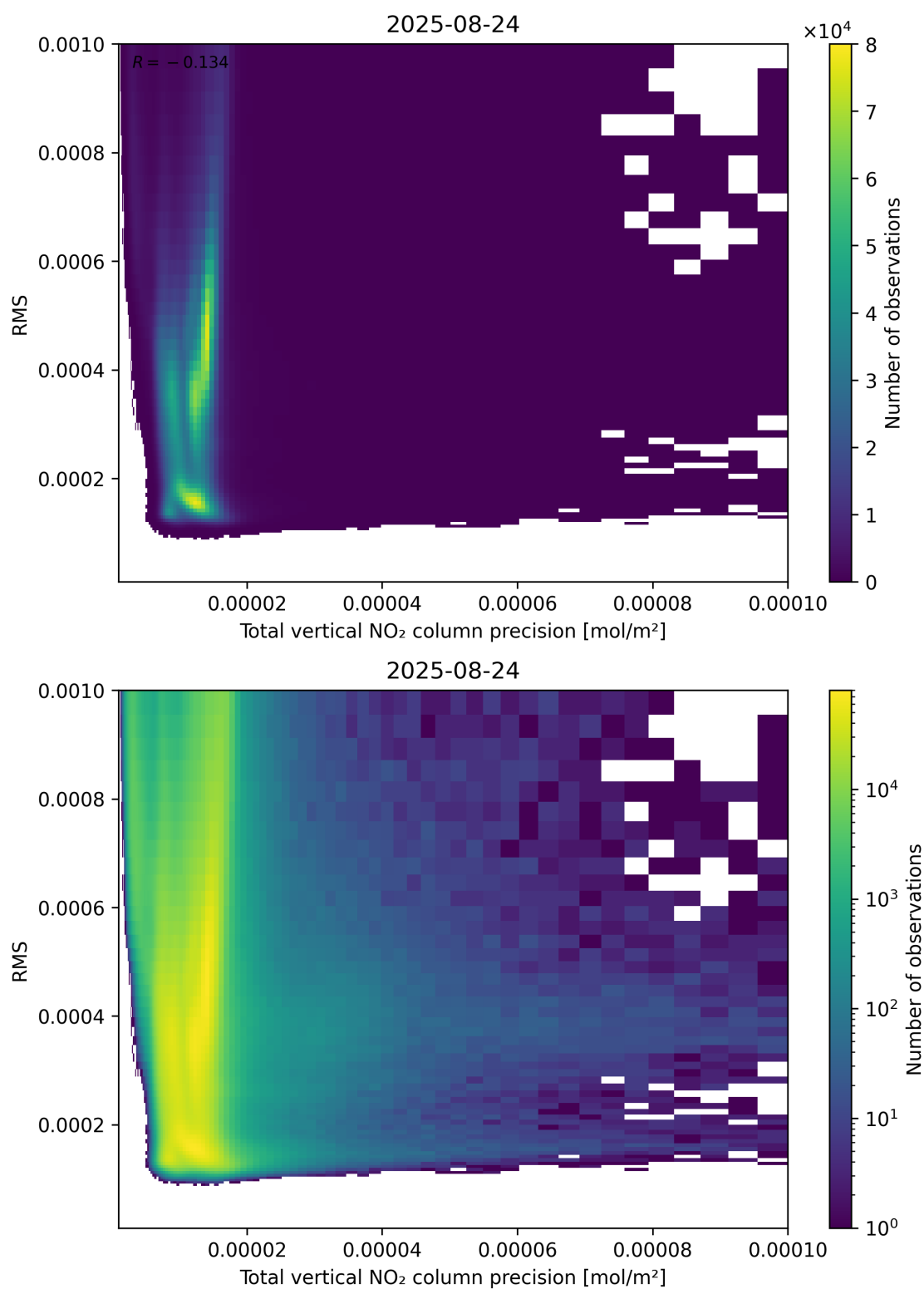
Figure 119: Scatter density plot of “Total vertical NO 2 column precision” against “RMS” for 2025-08-23 to 2025-08-25.
