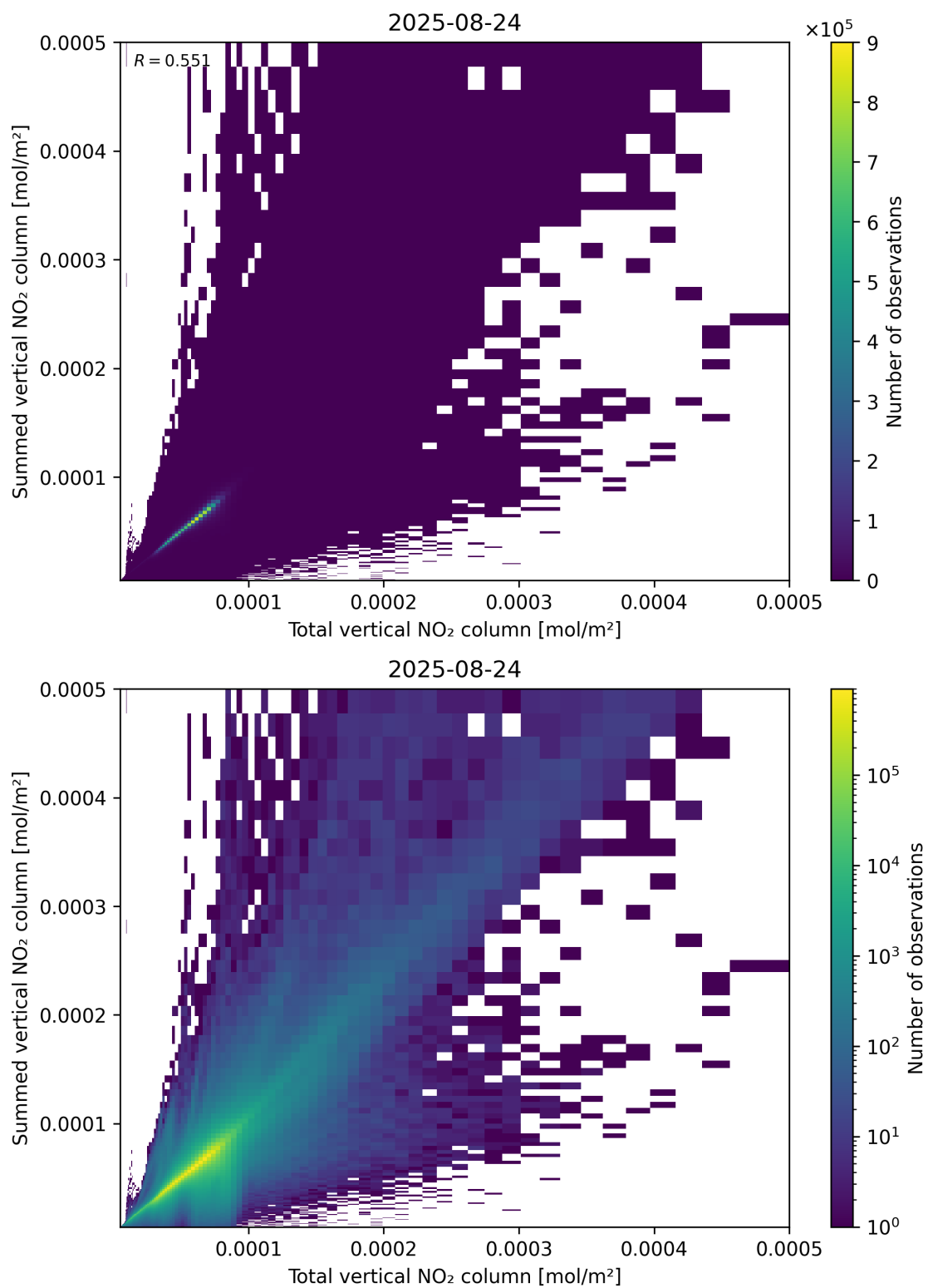
Figure 112: Scatter density plot of “Total vertical NO 2 column” against “Summed vertical NO 2 column” for 2025-08-23 to 2025-08-25.
