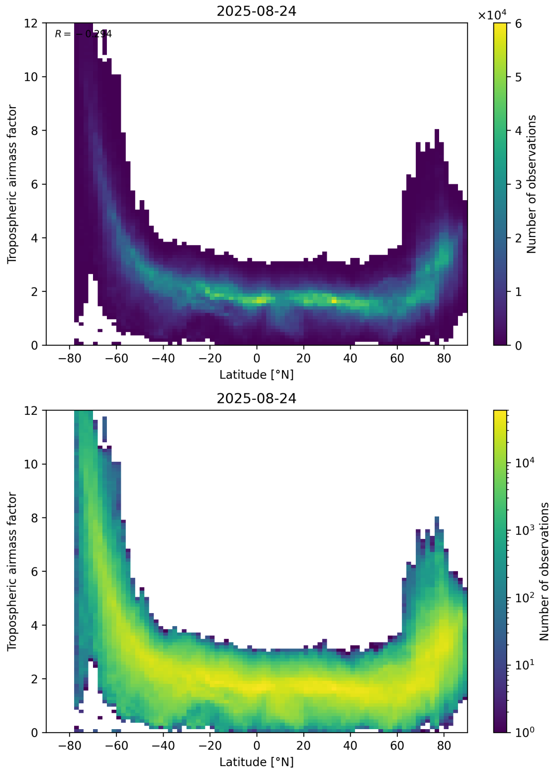
Figure 85: Scatter density plot of “Latitude” against “Tropospheric air mass factor” for 2025-08-23 to 2025-08-25.
