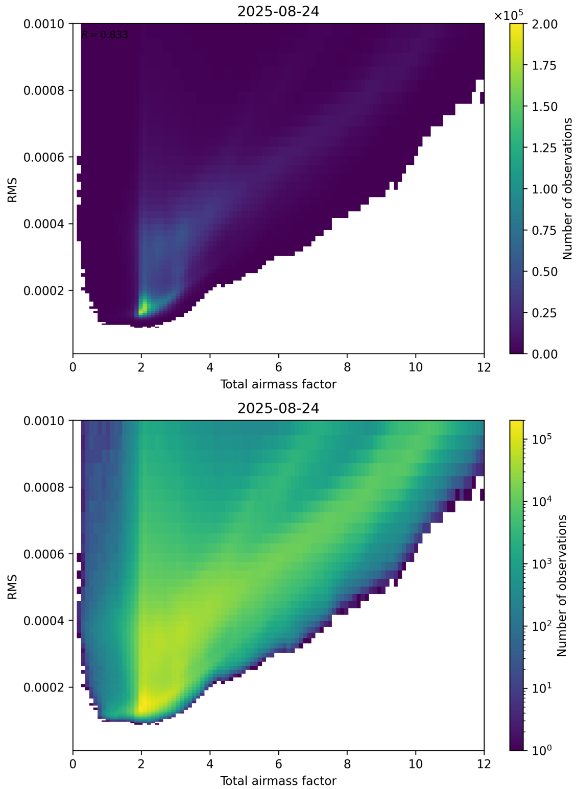
Figure 69: Scatter density plot of “Total airmass factor” against “RMS” for 2025-08-23 to 2025-08-25.
