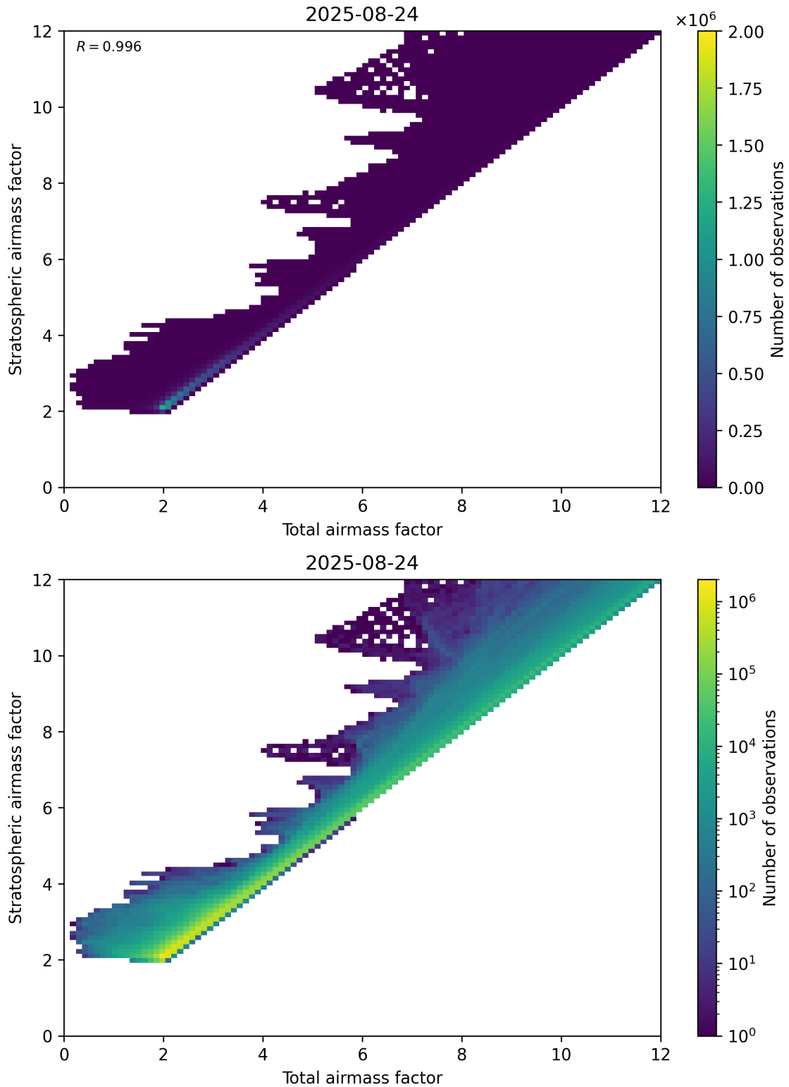
Figure 62: Scatter density plot of “Total airmass factor” against “Stratospheric airmass factor” for 2025-08-23 to 2025-08-25.
