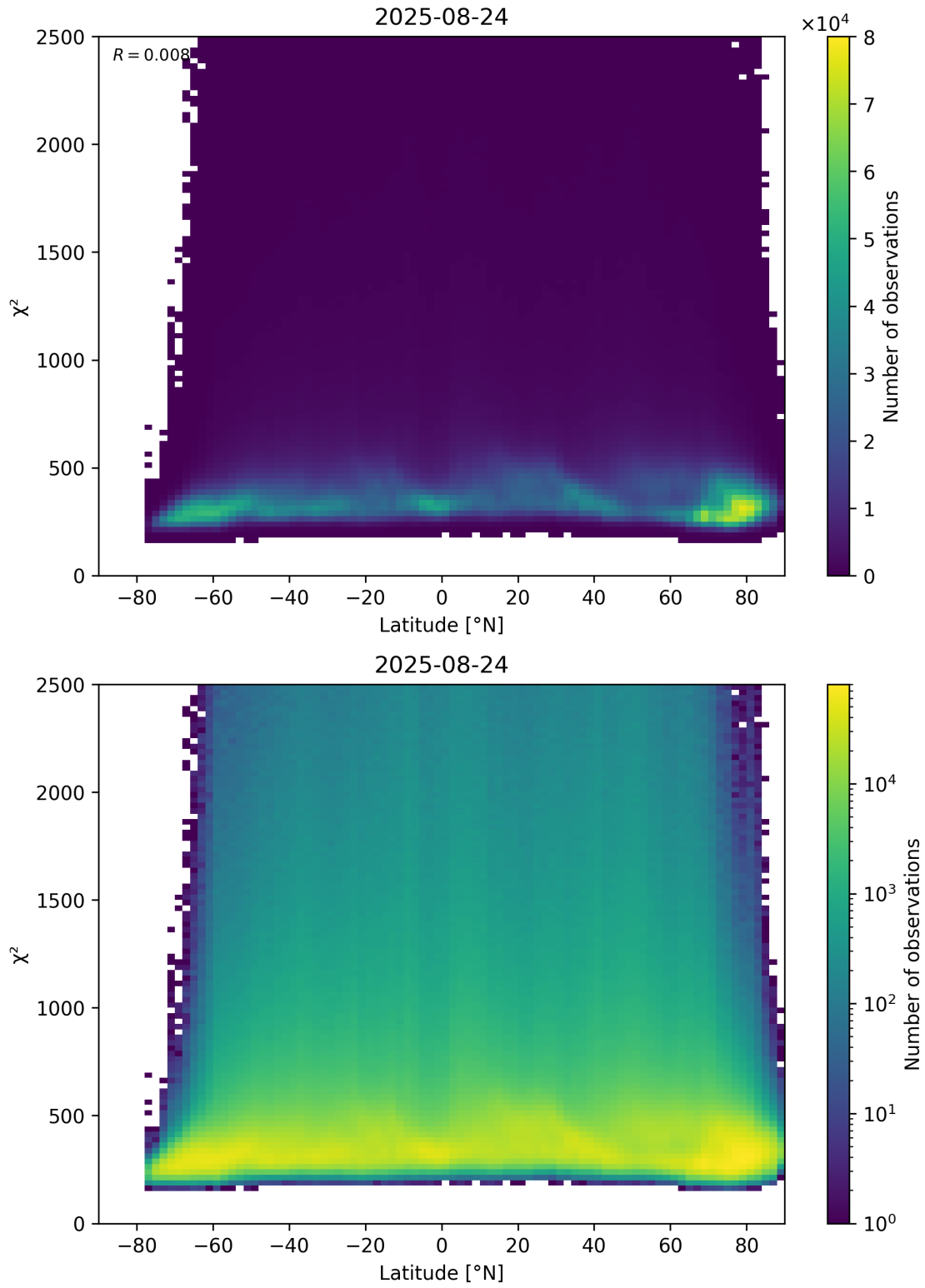
Figure 86: Scatter density plot of “Latitude” against “ \chi^2 ” for 2025-08-23 to 2025-08-25.
