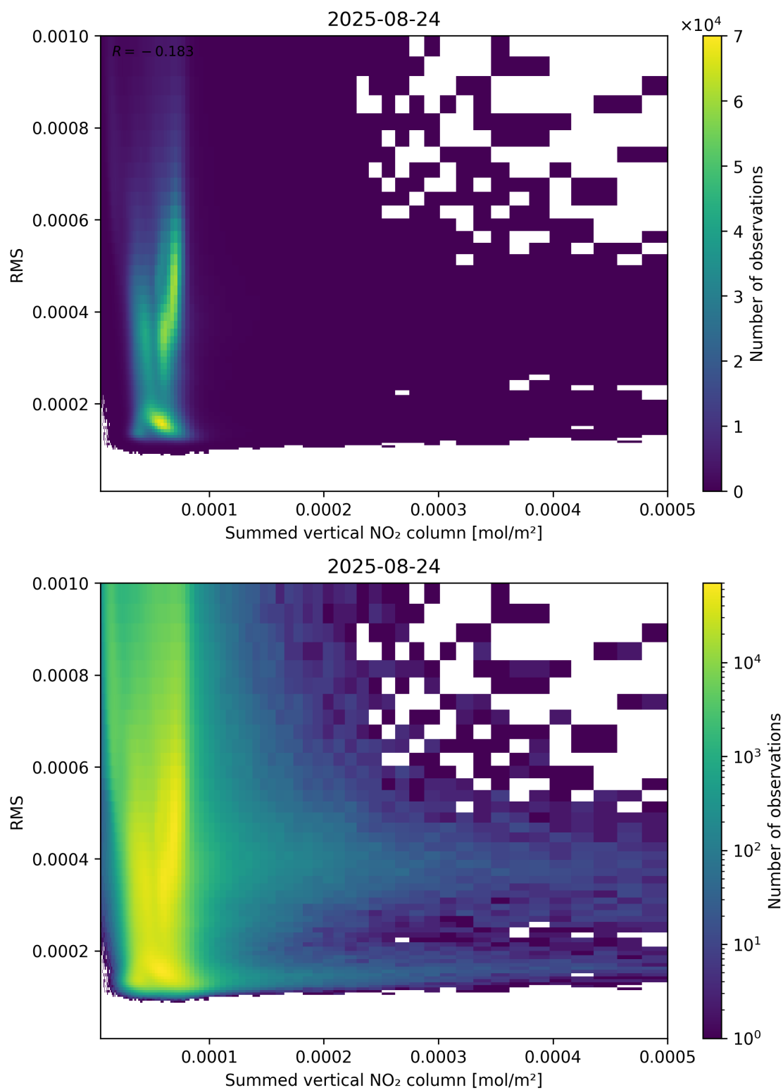
Figure 109: Scatter density plot of “Summed vertical NO 2 column” against “RMS” for 2025-08-23 to 2025-08-25.
