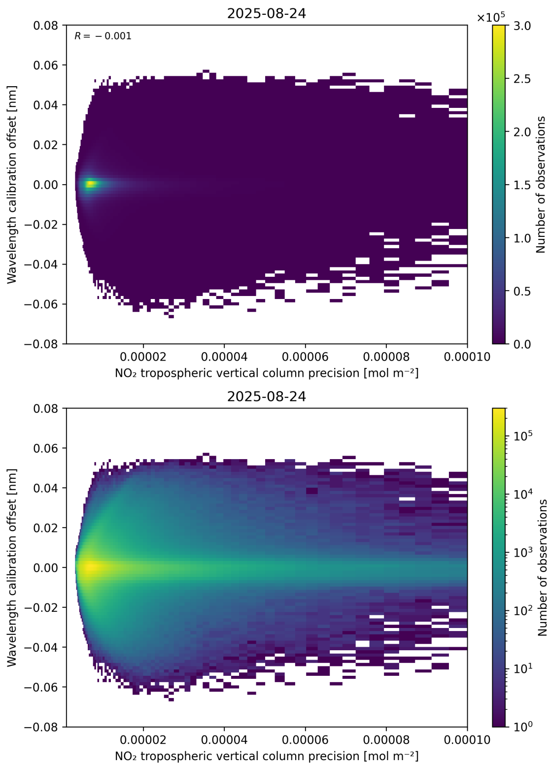
Figure 141: Scatter density plot of “NO 2 tropospheric vertical column precision” against “Wavelength calibration offset” for 2025-08-23 to 2025-08-25.
