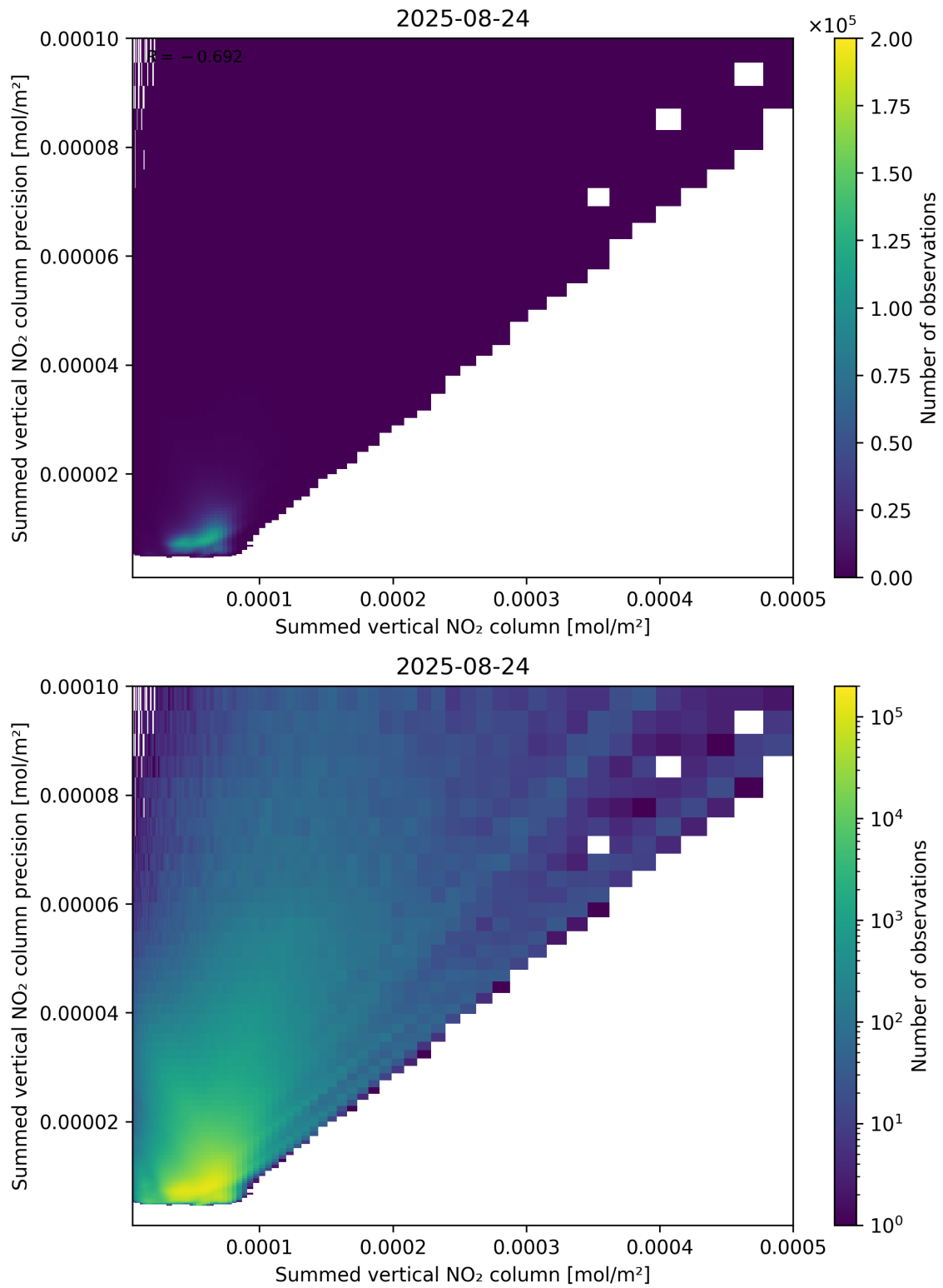
Figure 105: Scatter density plot of “Summed vertical NO 2 column” against “Summed vertical NO 2 column precision” for 2025-08-23 to 2025-08-25.
