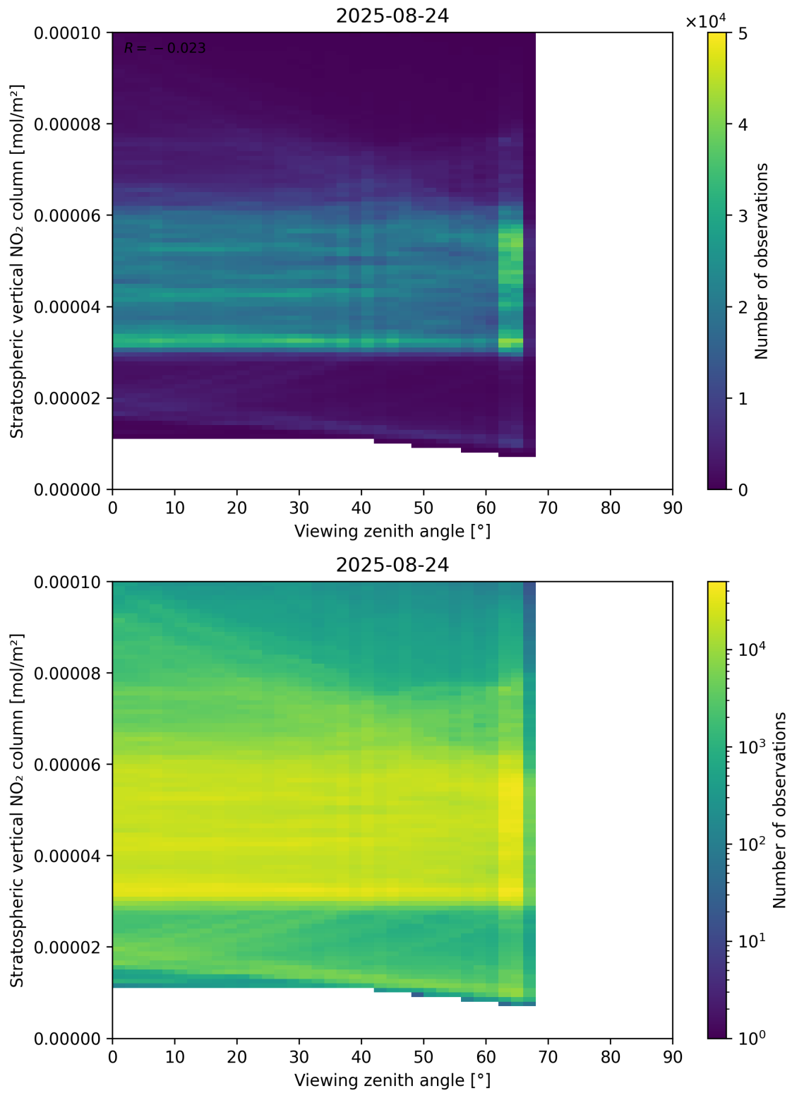
Figure 164: Scatter density plot of “Viewing zenith angle” against “Stratospheric vertical NO 2 column” for 2025-08-23 to 2025-08-25.
