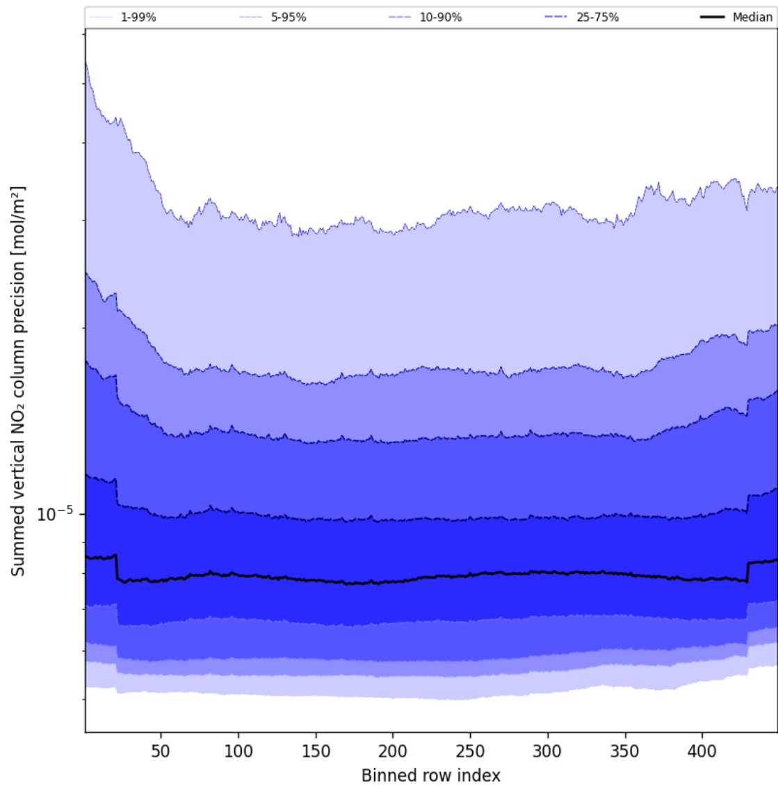
Figure 58: Along track statistics of “Summed vertical NO 2 column precision” for 2025-08-23 to 2025-08-25
