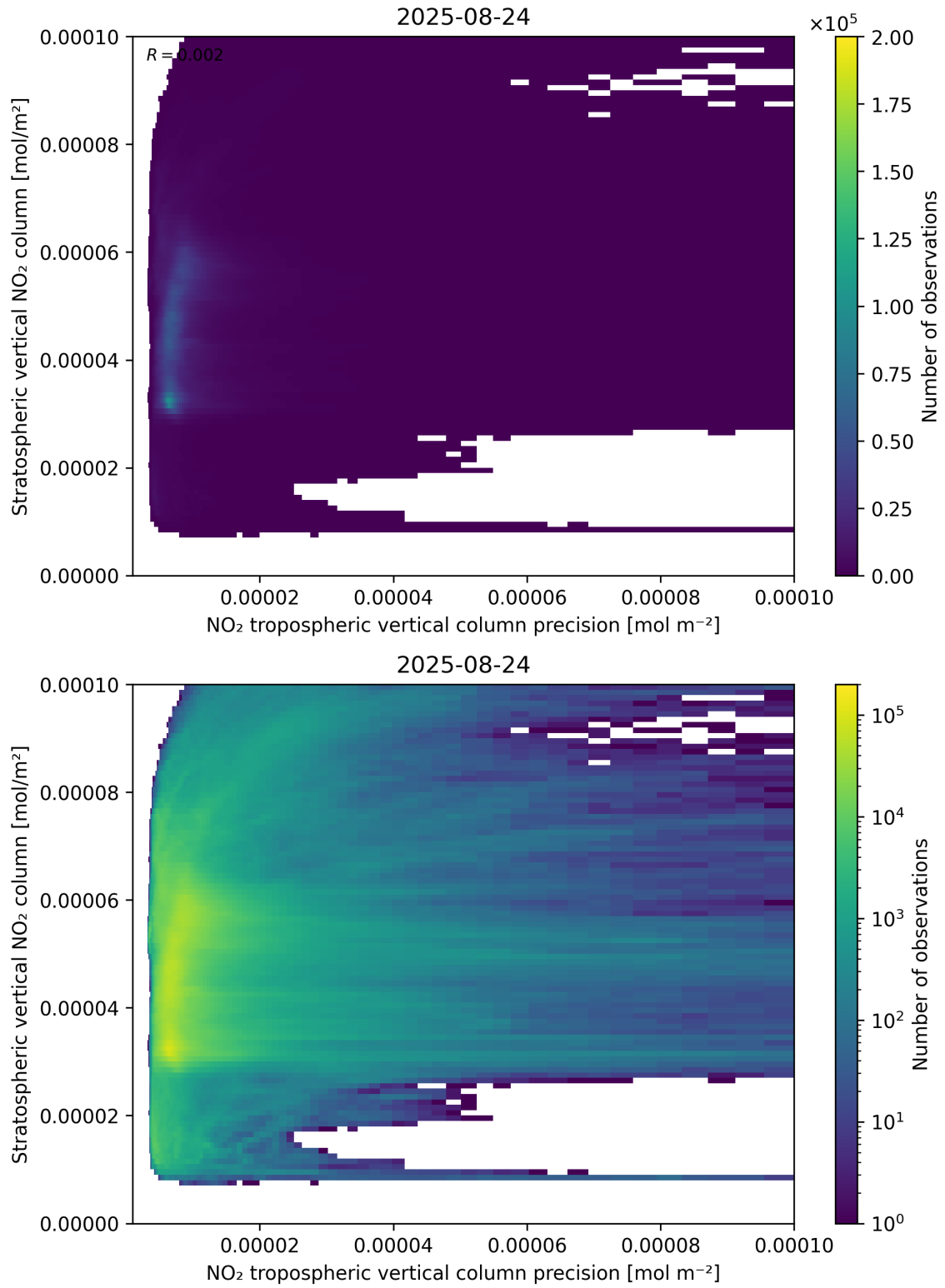
Figure 135: Scatter density plot of “NO 2 tropospheric vertical column precision” against “Stratospheric vertical NO 2 column” for 2025-08-23 to 2025-08-25.
