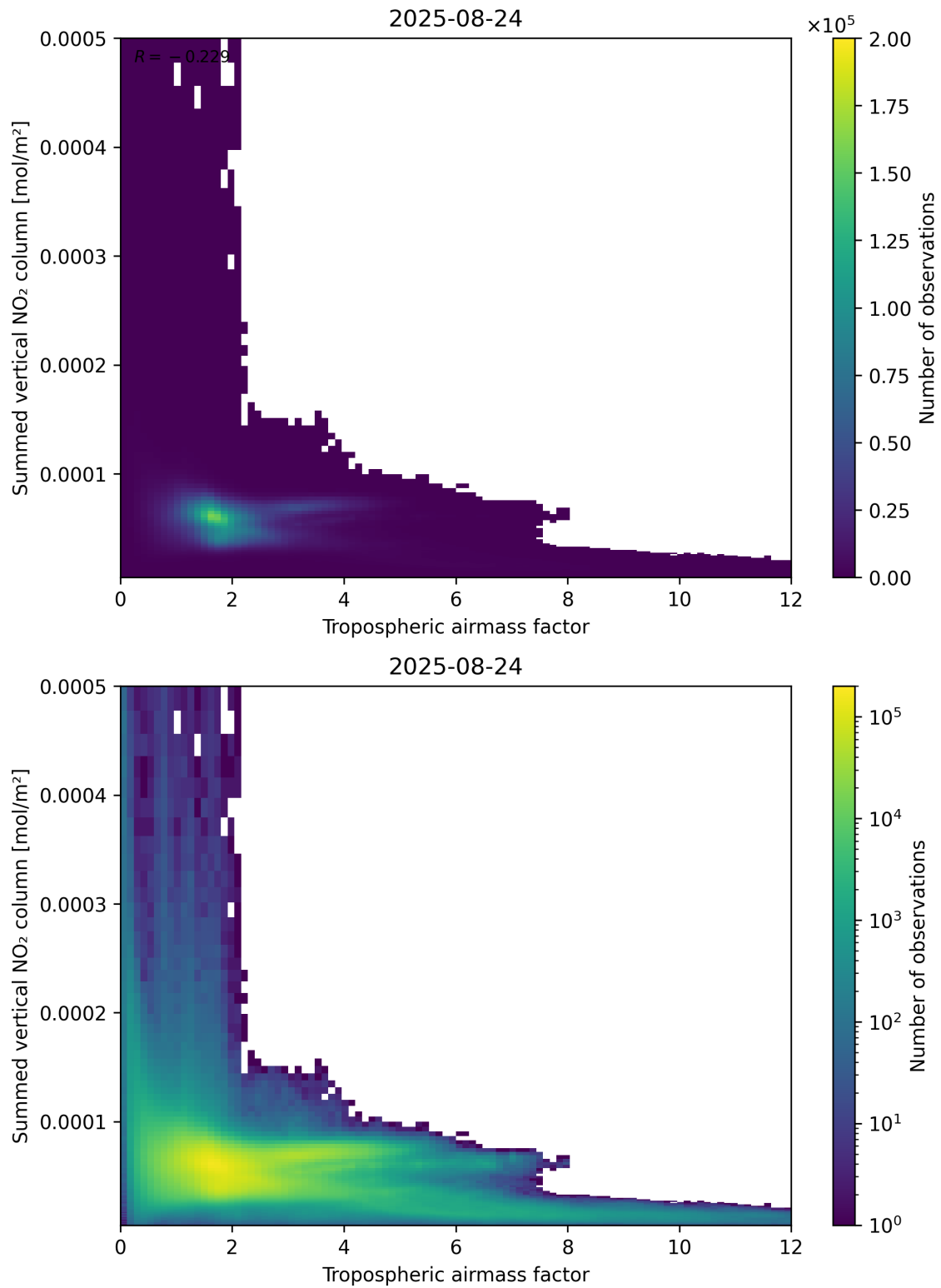
Figure 75: Scatter density plot of “Tropospheric air mass factor” against “Summed vertical NO 2 column” for 2025-08-23 to 2025-08-25.
