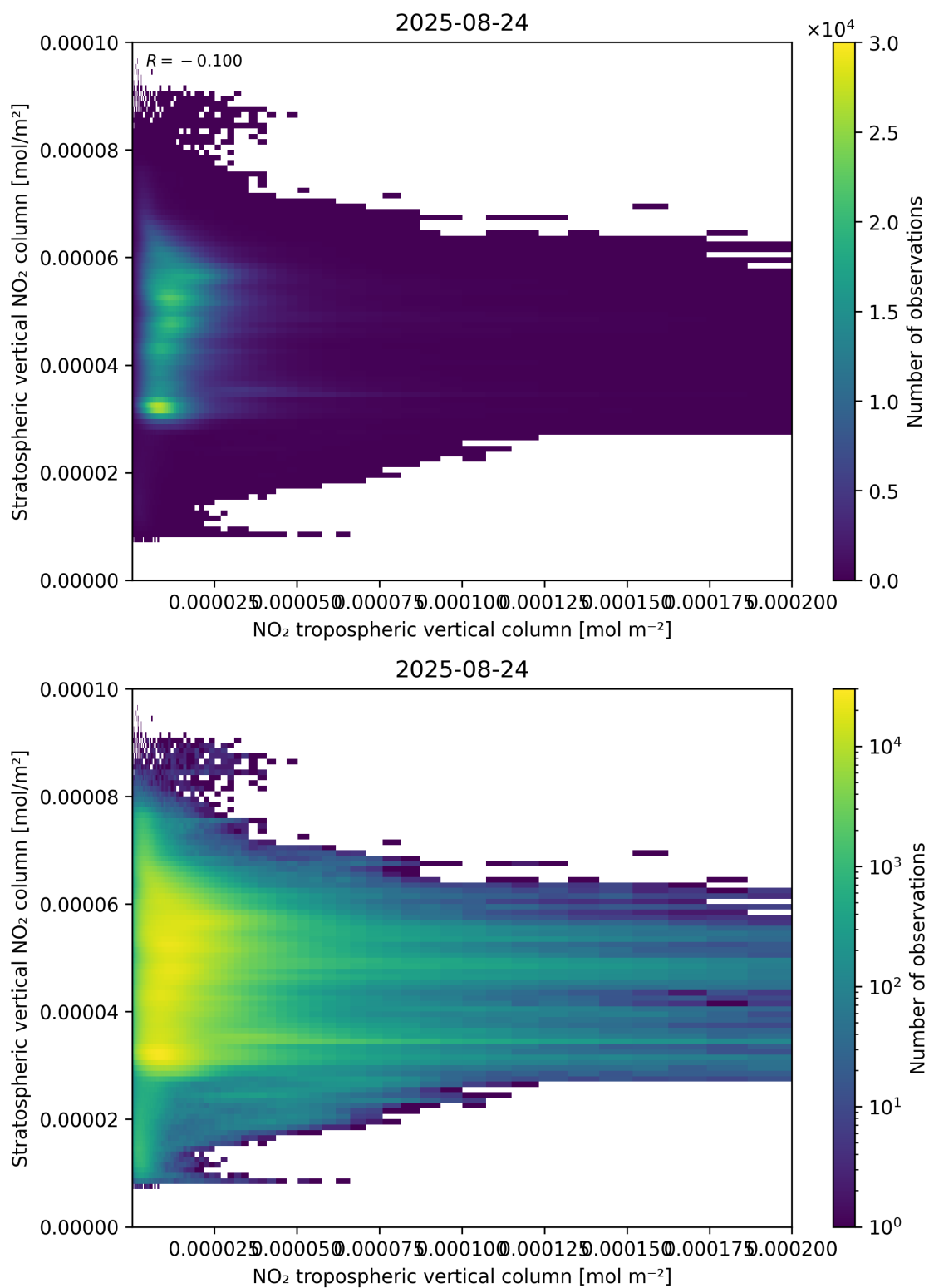
Figure 125: Scatter density plot of “NO 2 tropospheric vertical column” against “Stratospheric vertical NO 2 column” for 2025-08-23 to 2025-08-25.
