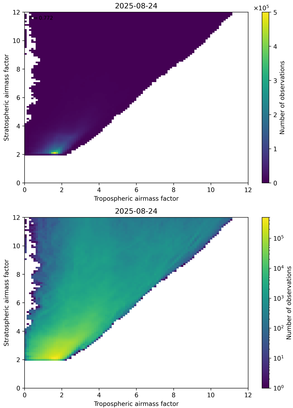
Figure 71: Scatter density plot of “Tropospheric airmass factor” against “Stratospheric airmass factor” for 2025-08-23 to 2025-08-25.
