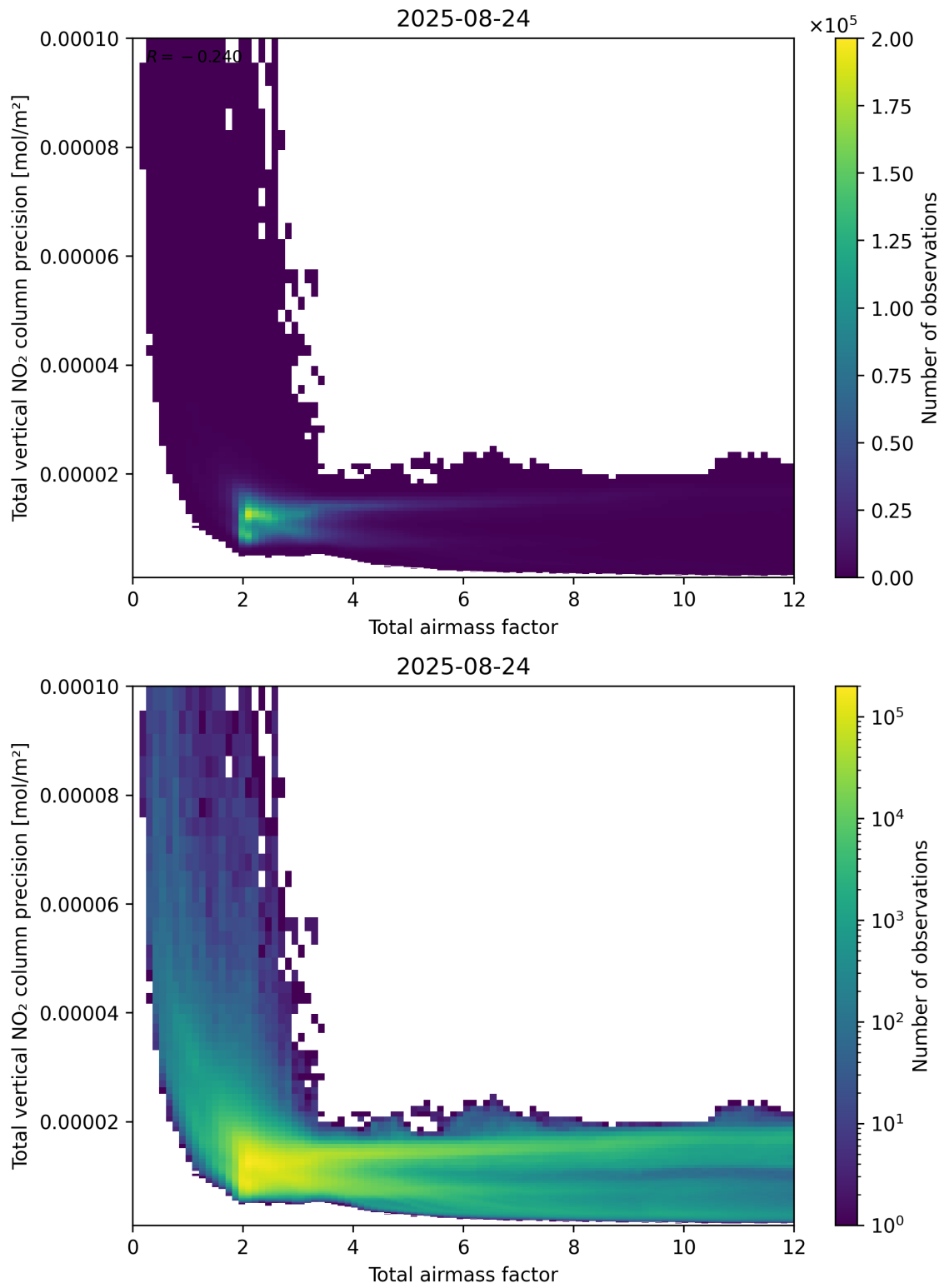
Figure 68: Scatter density plot of “Total airmass factor” against “Total vertical NO 2 column precision” for 2025-08-23 to 2025-08-25.
