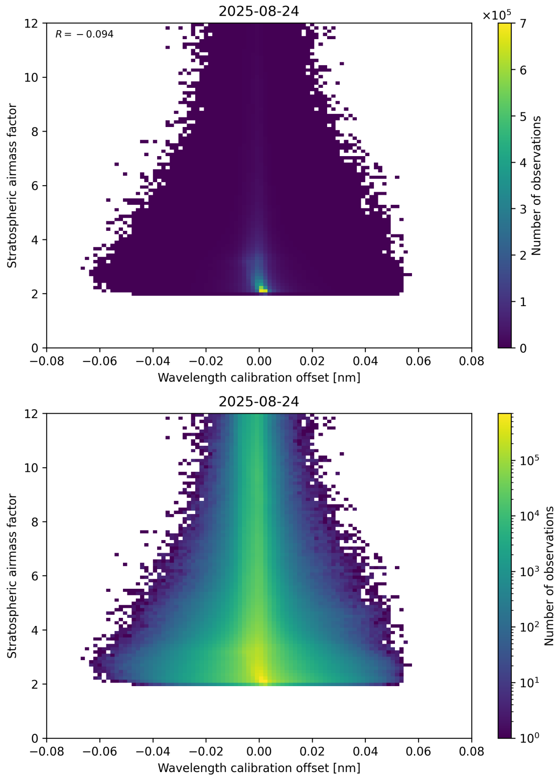
Figure 174: Scatter density plot of “Wavelength calibration offset” against “Stratospheric airmass factor” for 2025-08-23 to 2025-08-25.
