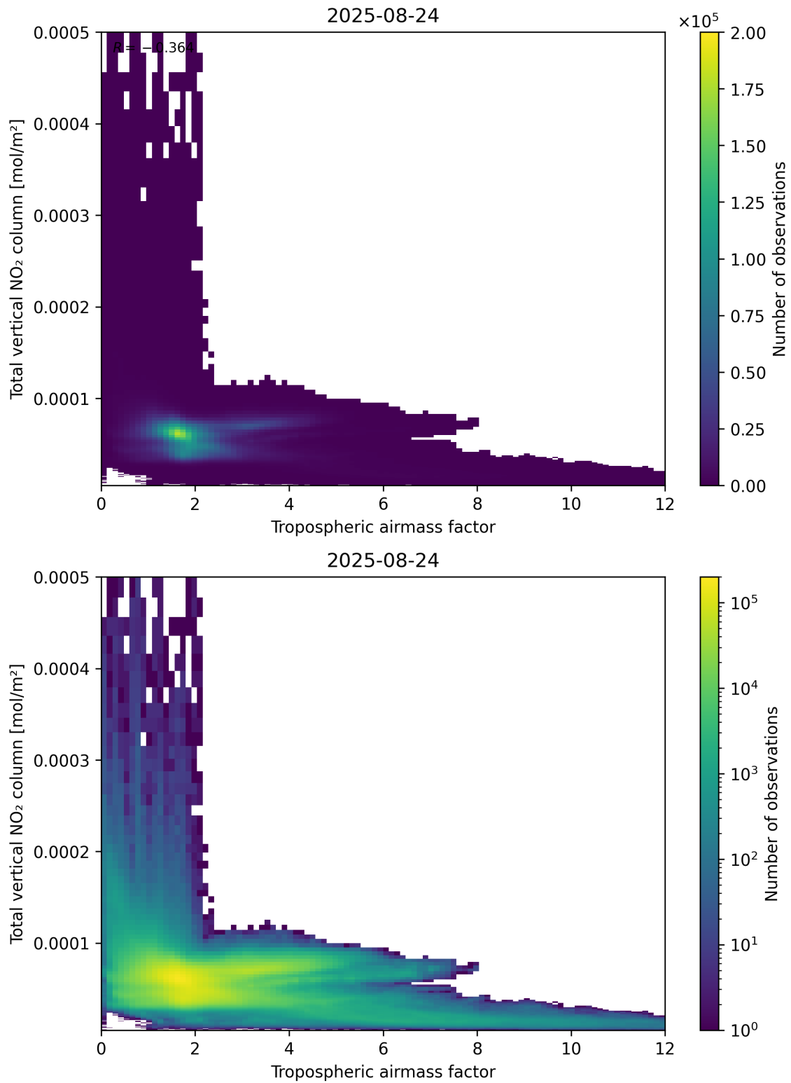
Figure 77: Scatter density plot of “Tropospheric airmass factor” against “Total vertical NO 2 column” for 2025-08-23 to 2025-08-25.
