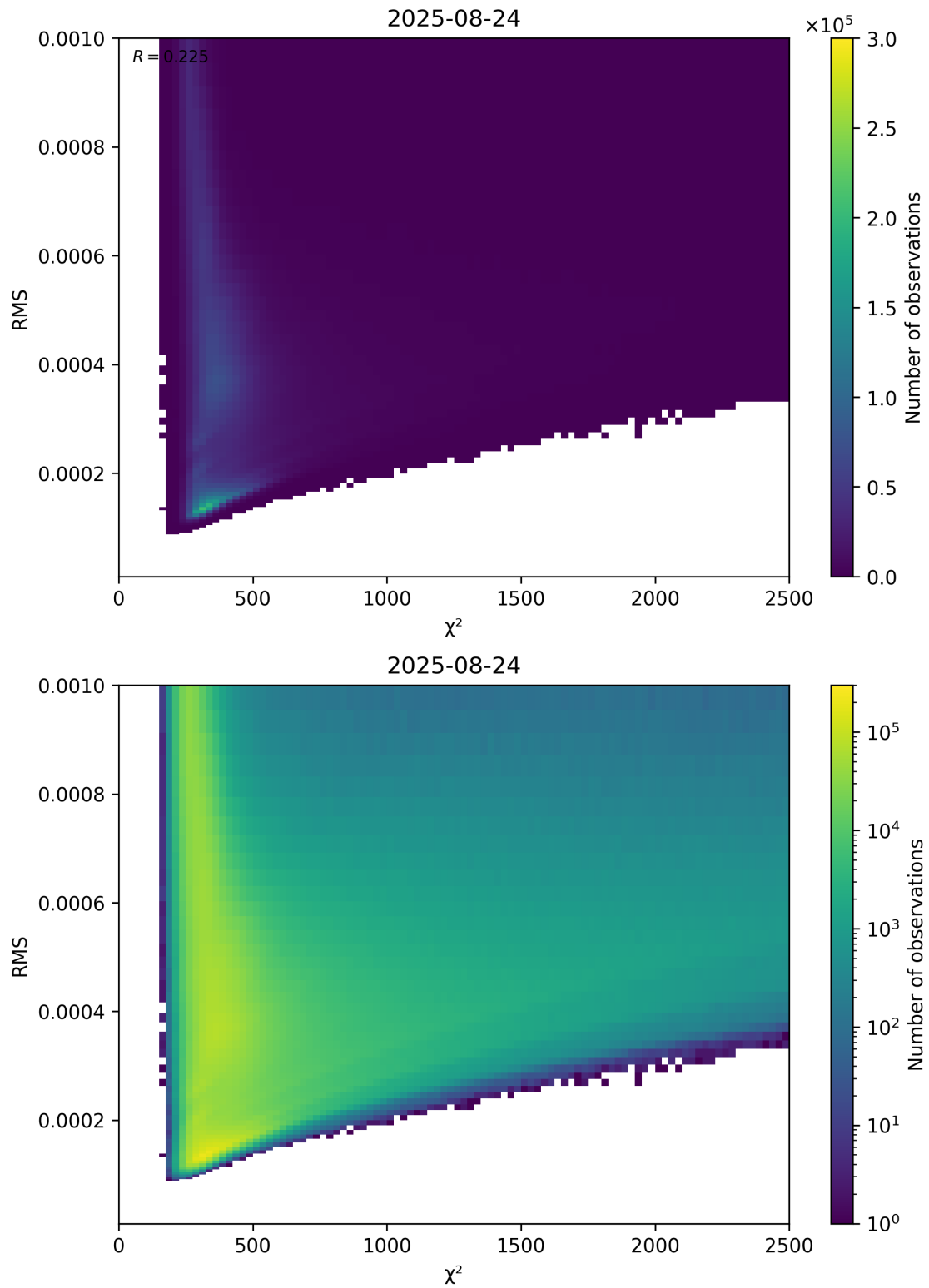
Figure 82: Scatter density plot of “ \chi^2 ” against “RMS” for 2025-08-23 to 2025-08-25.
