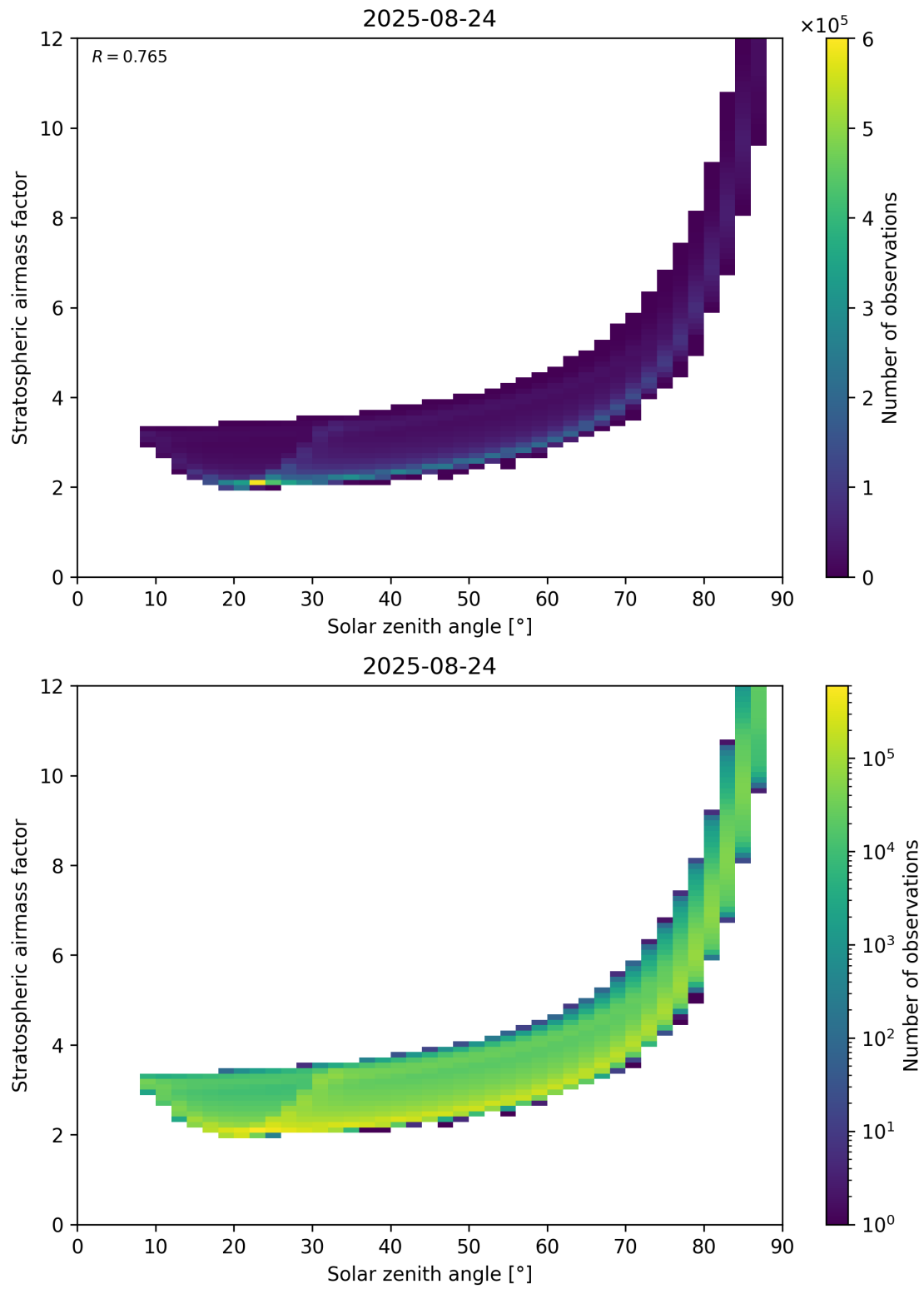
Figure 145: Scatter density plot of “Solar zenith angle” against “Stratospheric airmass factor” for 2025-08-23 to 2025-08-25.
