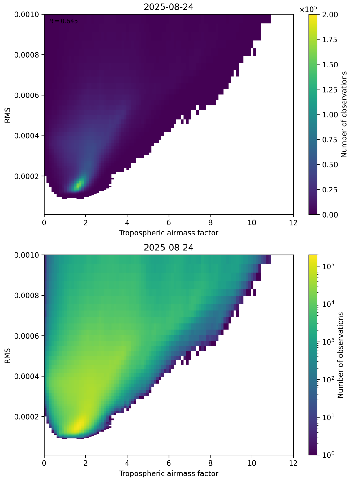
Figure 79: Scatter density plot of “Tropospheric airmass factor” against “RMS” for 2025-08-23 to 2025-08-25.
