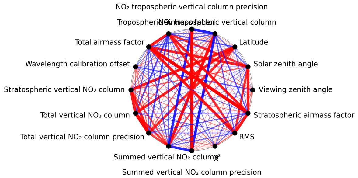
Figure 1: Map of correlation graph for 2025-08-23 to 2025-08-25.
