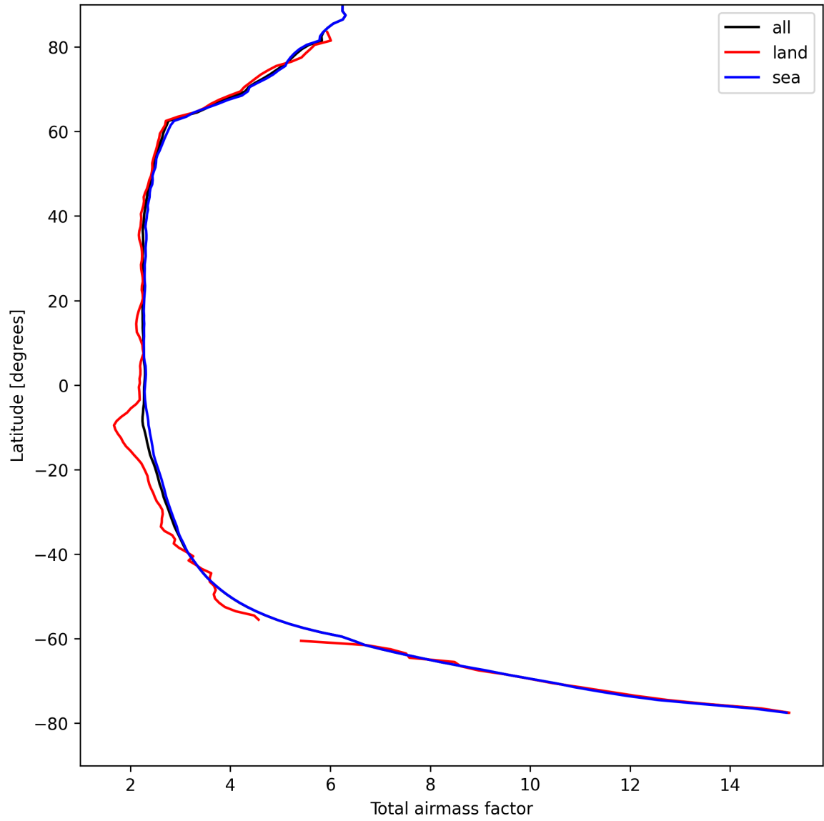
Figure 15: Zonal average of “Total airmass factor” for 2025-08-23 to 2025-08-25.
