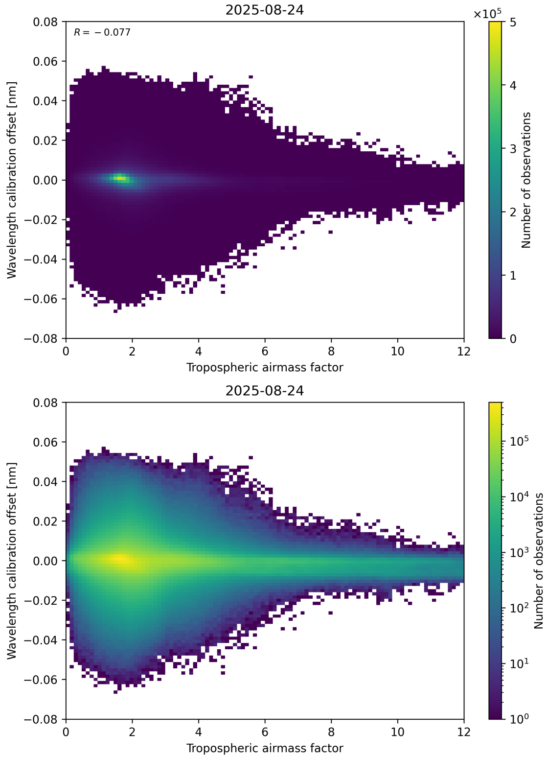
Figure 80: Scatter density plot of “Tropospheric airmass factor” against “Wavelength calibration offset” for 2025-08-23 to 2025-08-25.
