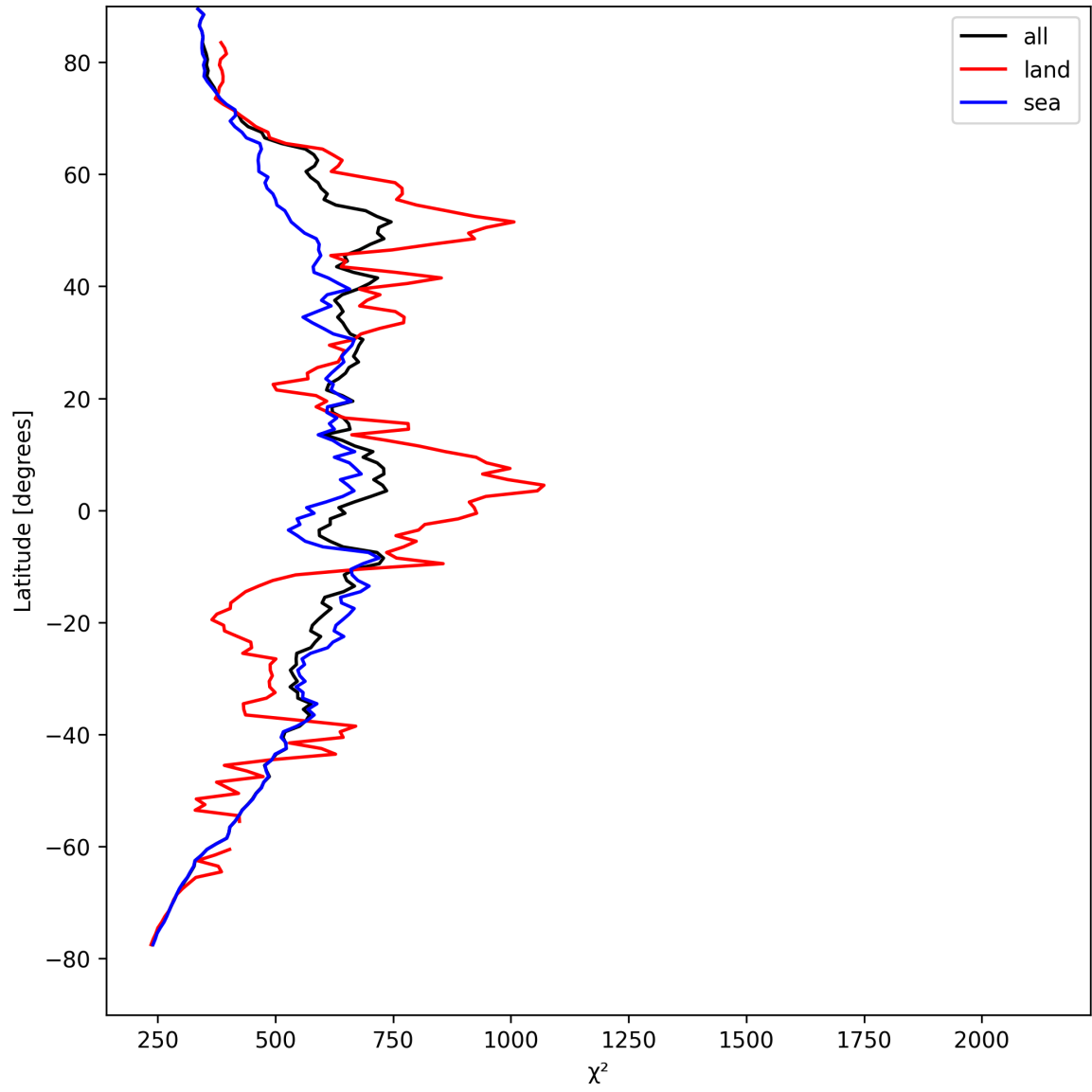
Figure 25: Zonal average of “ \chi^2 ” for 2025-08-23 to 2025-08-25.
