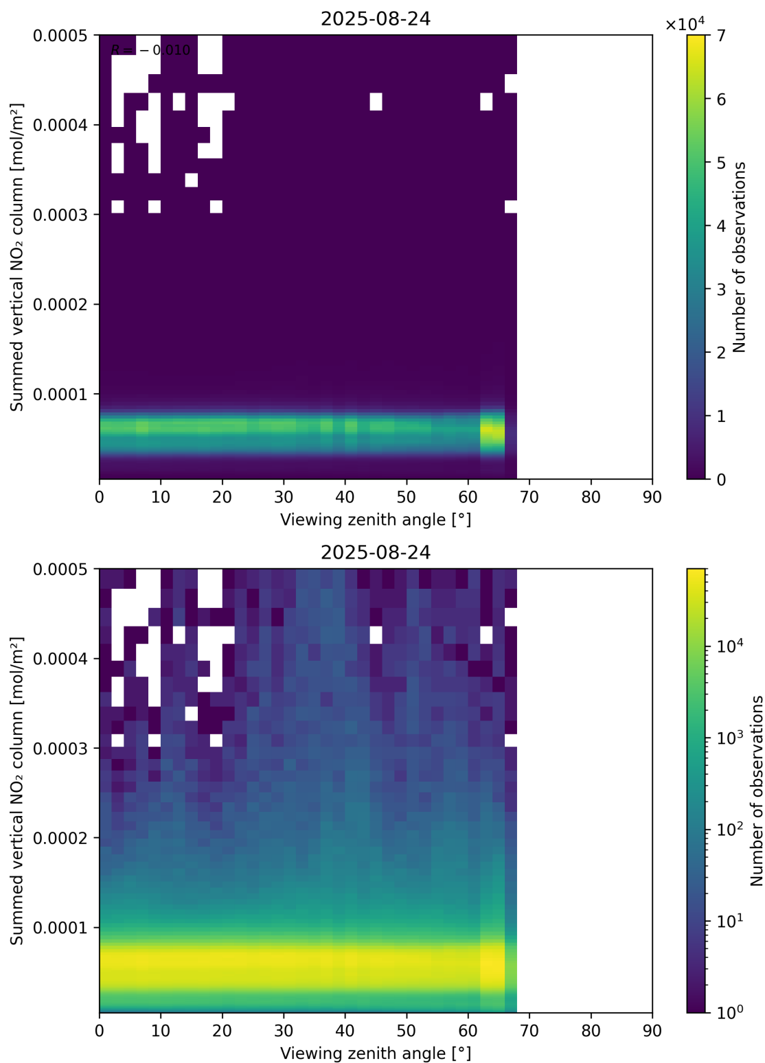
Figure 165: Scatter density plot of “Viewing zenith angle” against “Summed vertical NO 2 column” for 2025-08-23 to 2025-08-25.
