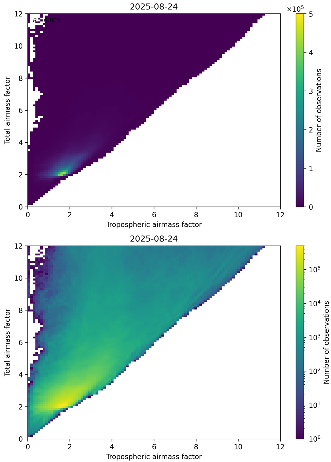
Figure 72: Scatter density plot of “Tropospheric airmass factor” against “Total airmass factor” for 2025-08-23 to 2025-08-25.
