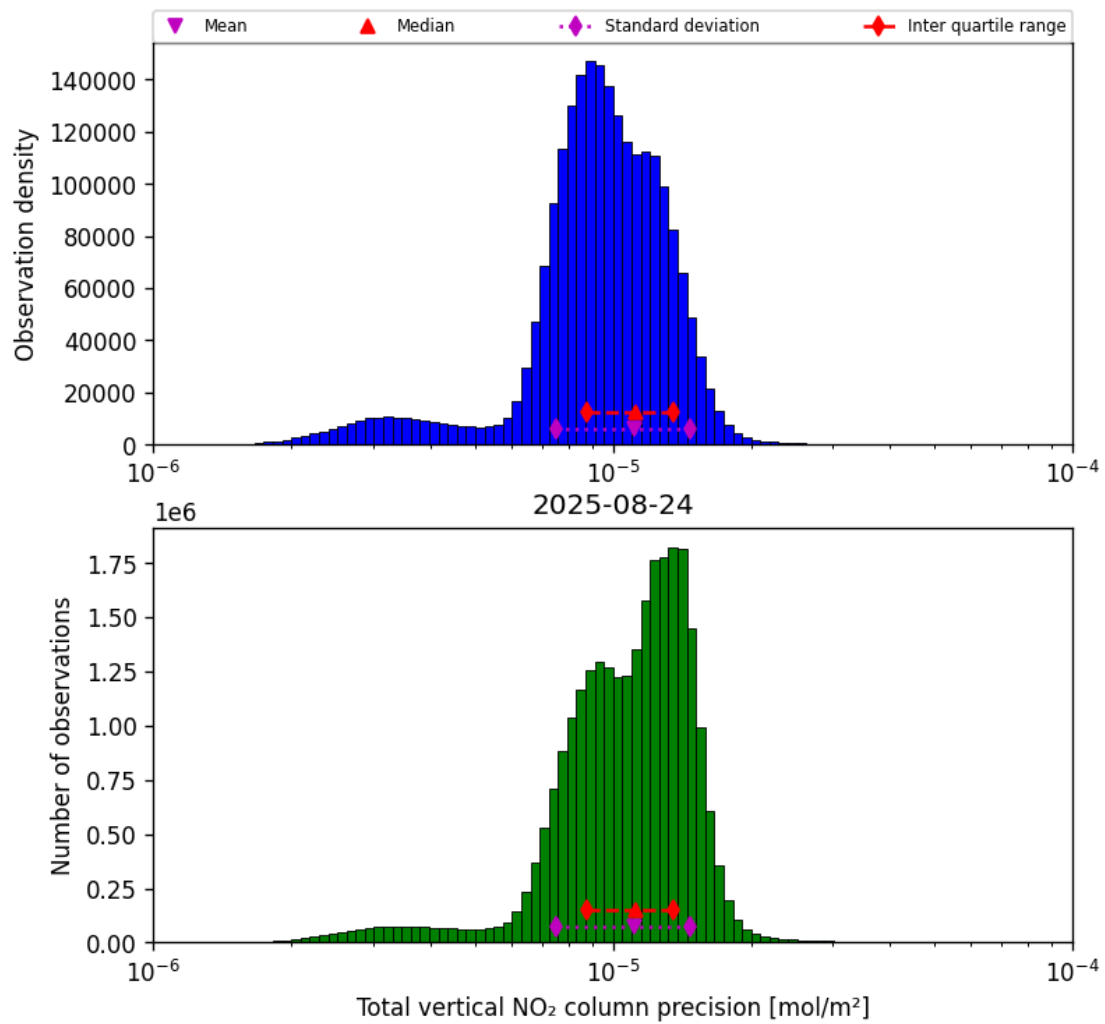
Figure 39: Histogram of “Total vertical NO 2 column precision” for 2025-08-23 to 2025-08-25
