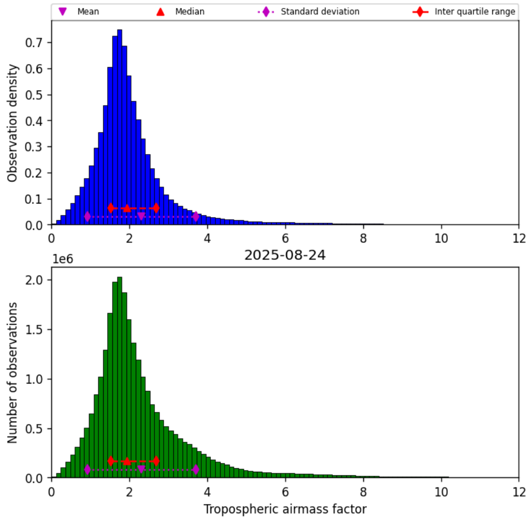
Figure 31: Histogram of “Tropospheric airmass factor” for 2025-08-23 to 2025-08-25
