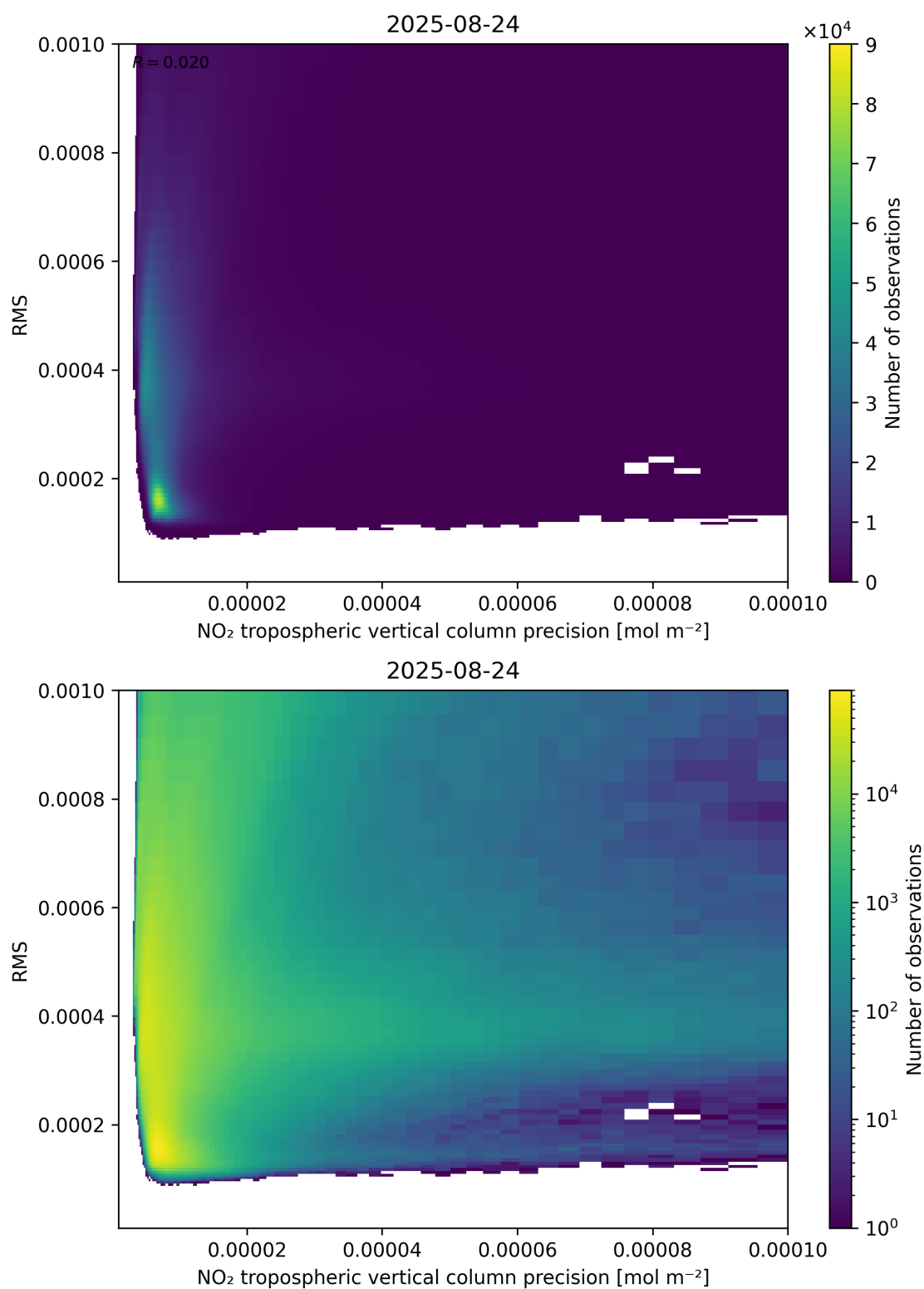
Figure 140: Scatter density plot of “NO 2 tropospheric vertical column precision” against “RMS” for 2025-08-23 to 2025-08-25.
