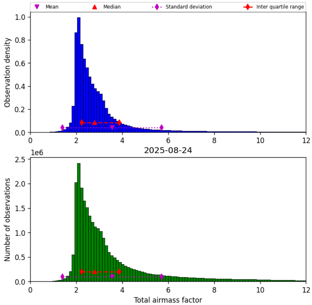
Figure 32: Histogram of “Total airmass factor” for 2025-08-23 to 2025-08-25
