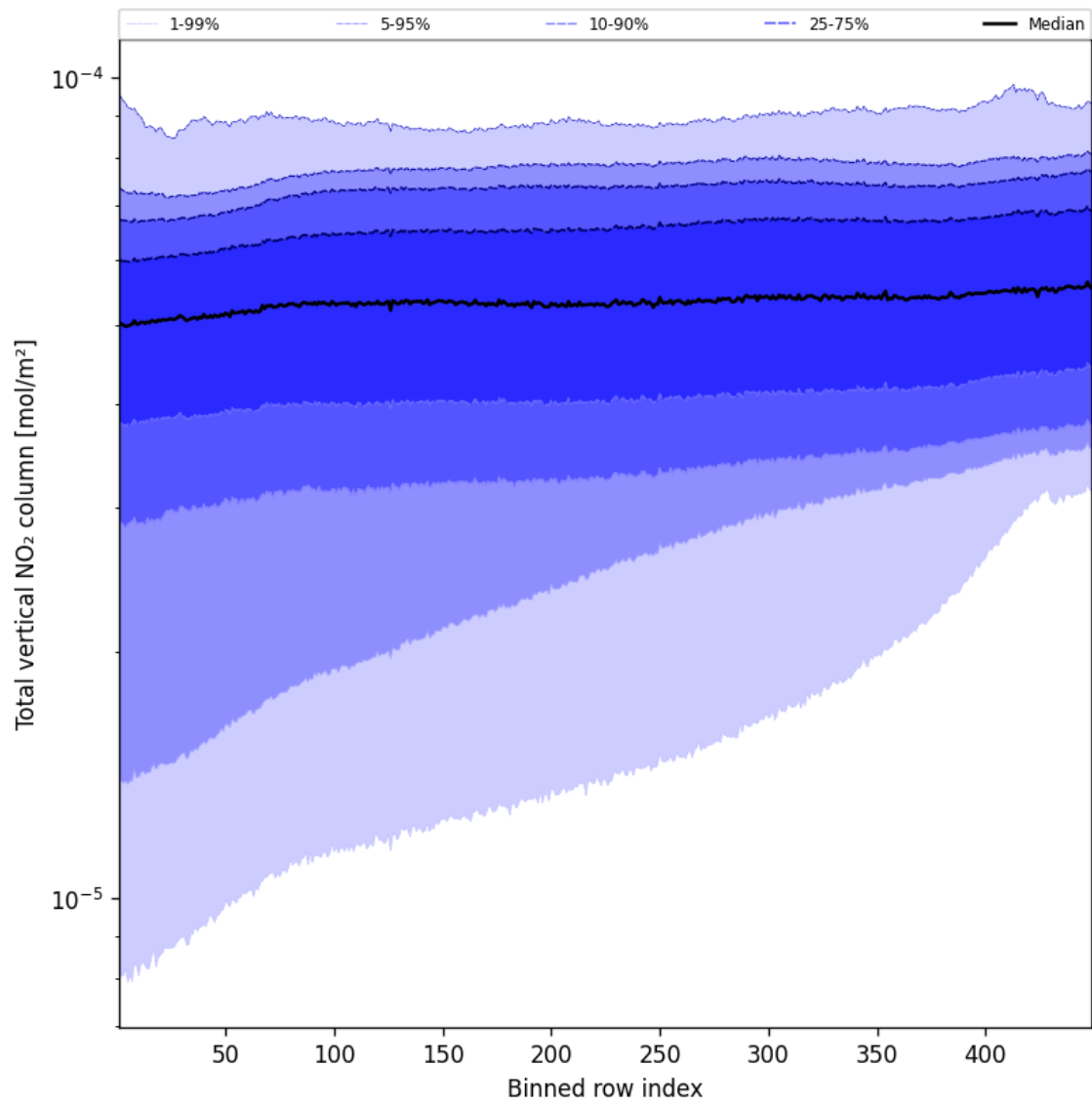
Figure 55: Along track statistics of “Total vertical NO 2 column” for 2025-08-23 to 2025-08-25
