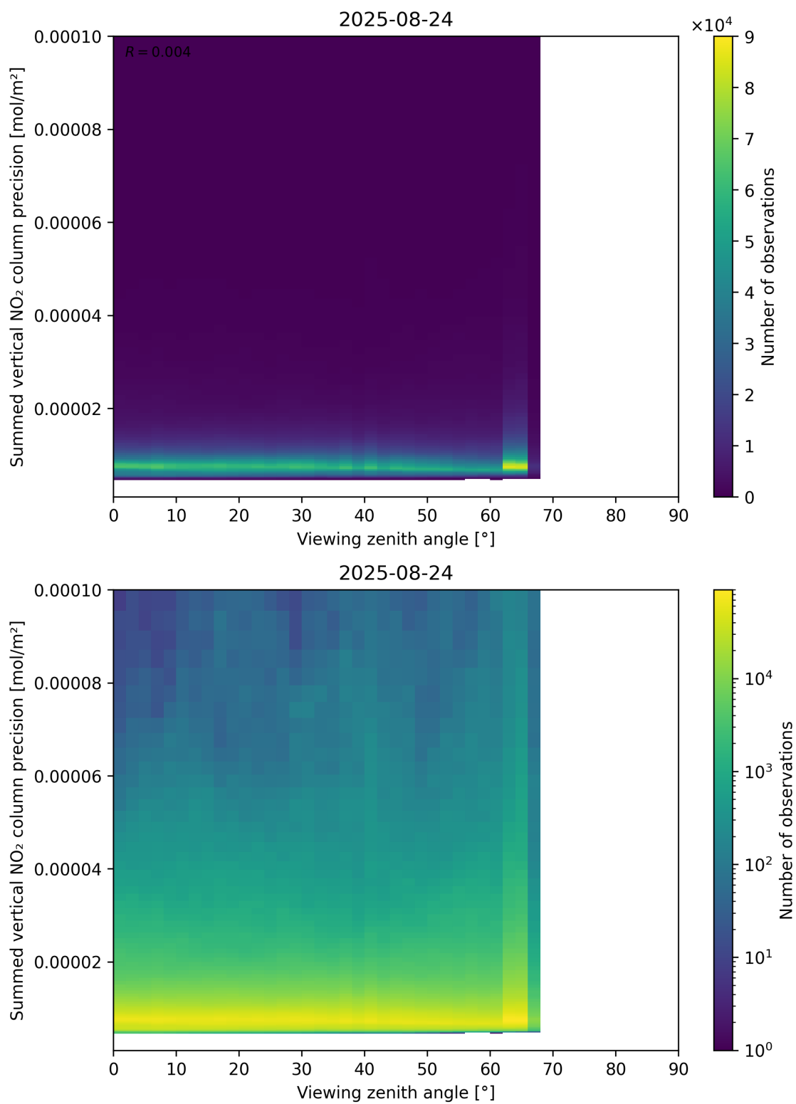
Figure 166: Scatter density plot of “Viewing zenith angle” against “Summed vertical NO 2 column precision” for 2025-08-23 to 2025-08-25.
