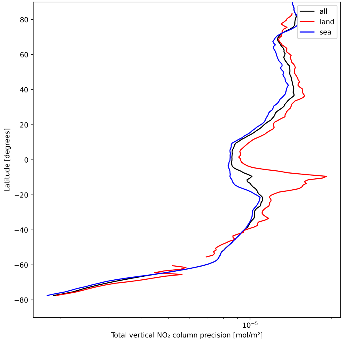
Figure 22: Zonal average of “Total vertical NO 2 column precision” for 2025-08-23 to 2025-08-25.
