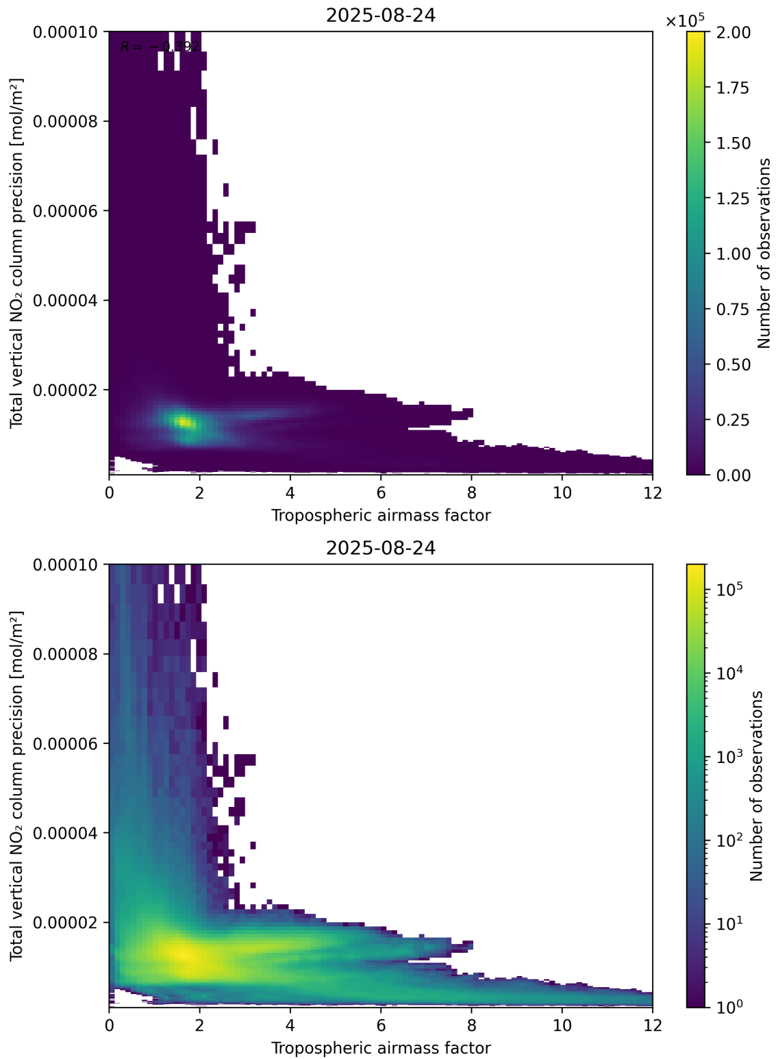
Figure 78: Scatter density plot of “Tropospheric air mass factor” against “Total vertical NO 2 column precision” for 2025-08-23 to 2025-08-25.
