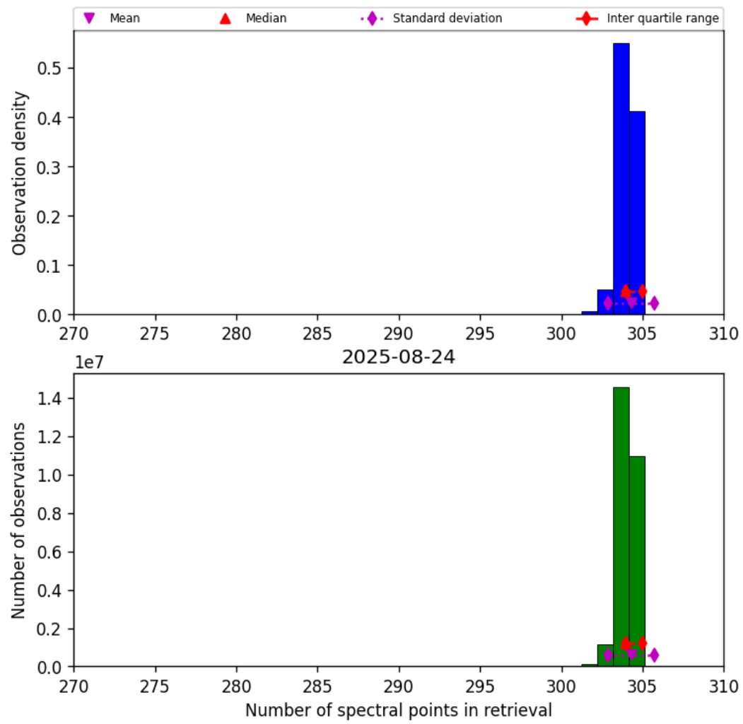
Figure 33: Histogram of “Number of spectral points in retrieval” for 2025-08-23 to 2025-08-25
