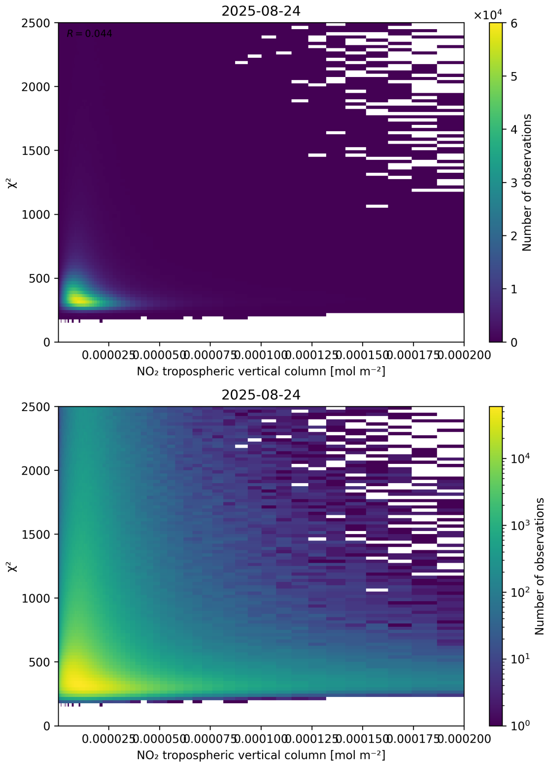
Figure 124: Scatter density plot of “NO 2 tropospheric vertical column” against “ \chi^2 ” for 2025-08-23 to 2025-08-25.
