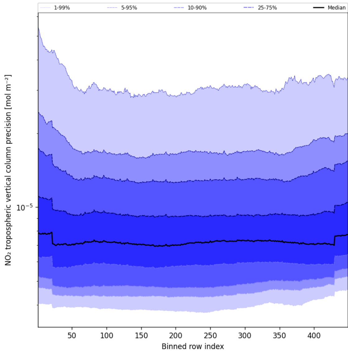
Figure 47: Along track statistics of “NO 2 tropospheric vertical column precision” for 2025-08-23 to 2025-08-25
