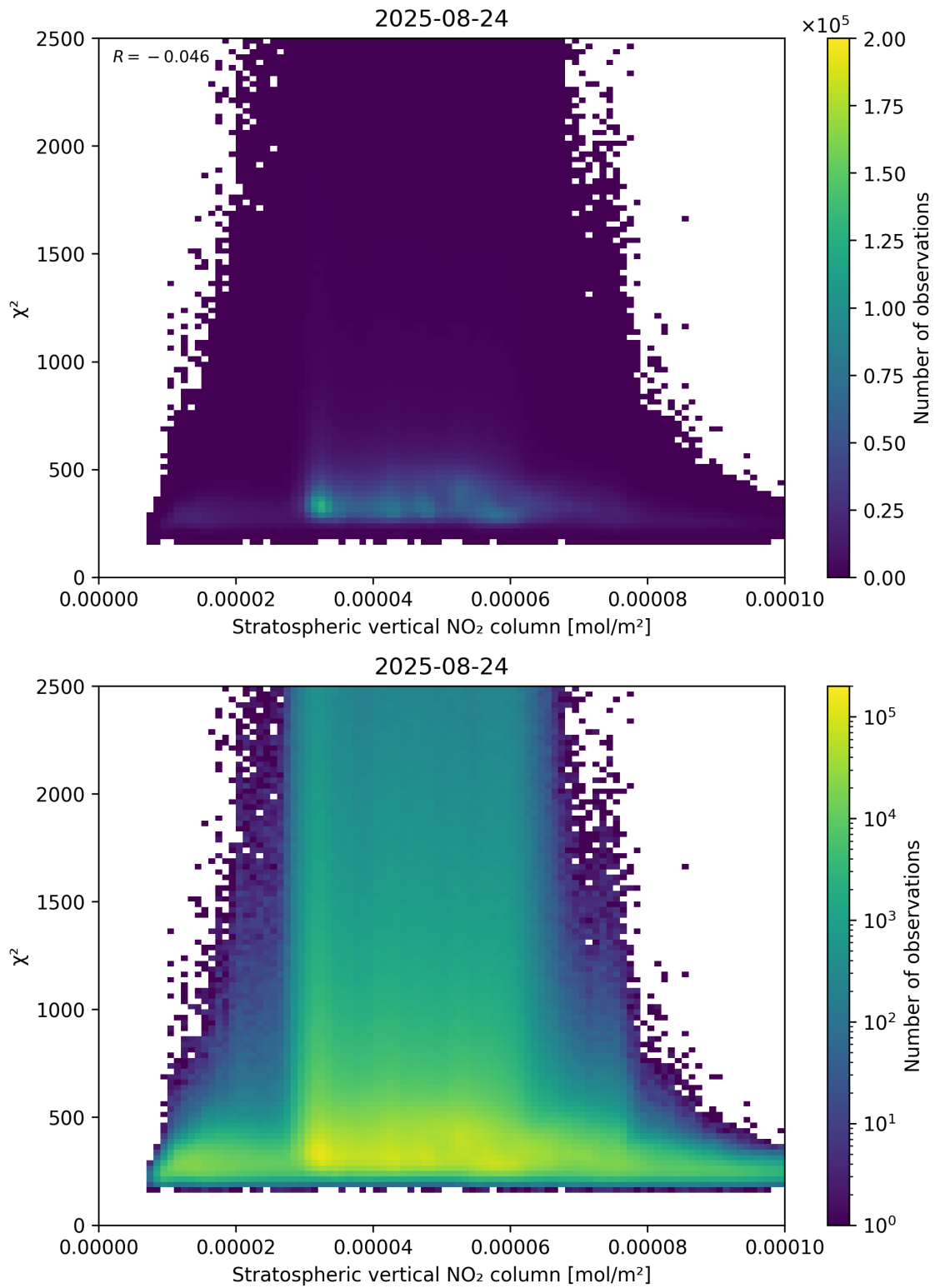
Figure 97: Scatter density plot of “Stratospheric vertical NO 2 column” against “ \chi^2 ” for 2025-08-23 to 2025-08-25.
