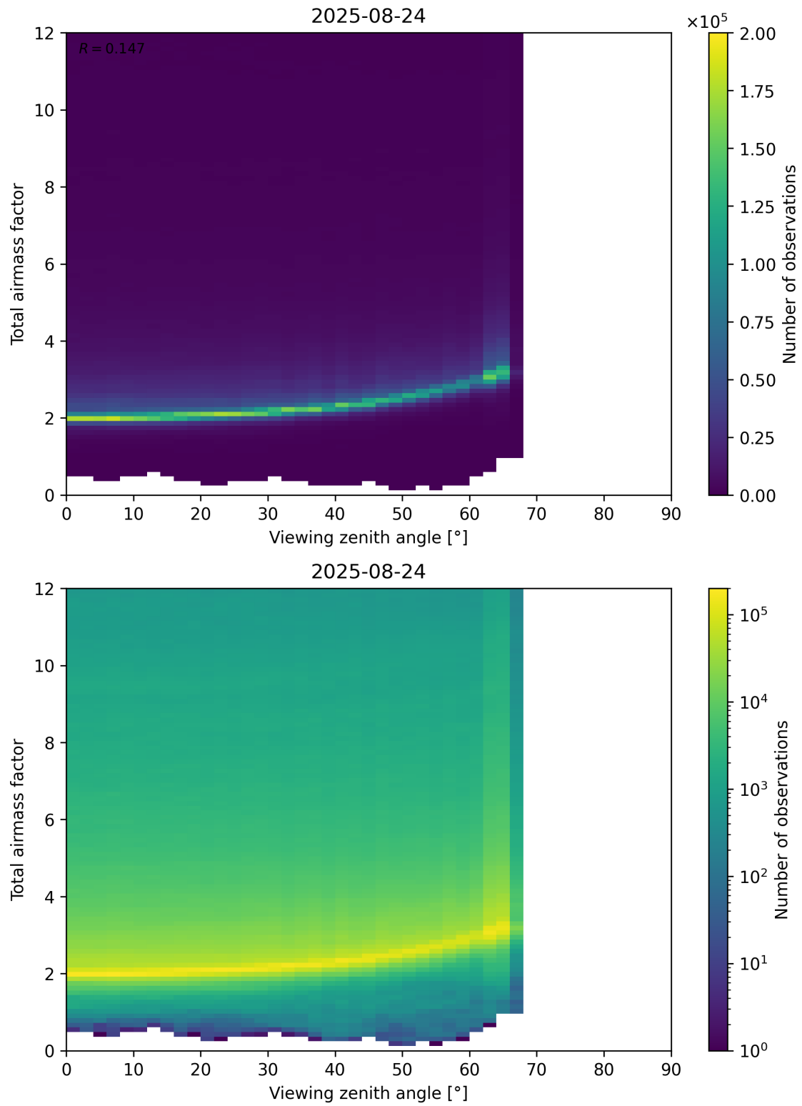
Figure 160: Scatter density plot of “Viewing zenith angle” against “Total airmass factor” for 2025-08-23 to 2025-08-25.
