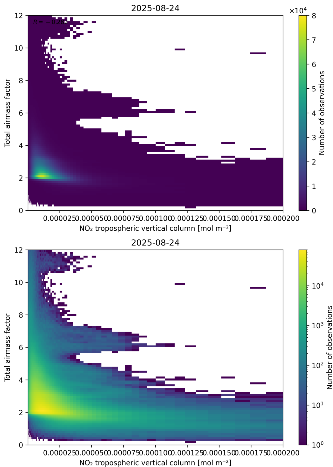
Figure 122: Scatter density plot of “NO 2 tropospheric vertical column” against “Total air mass factor” for 2025-08-23 to 2025-08-25.
