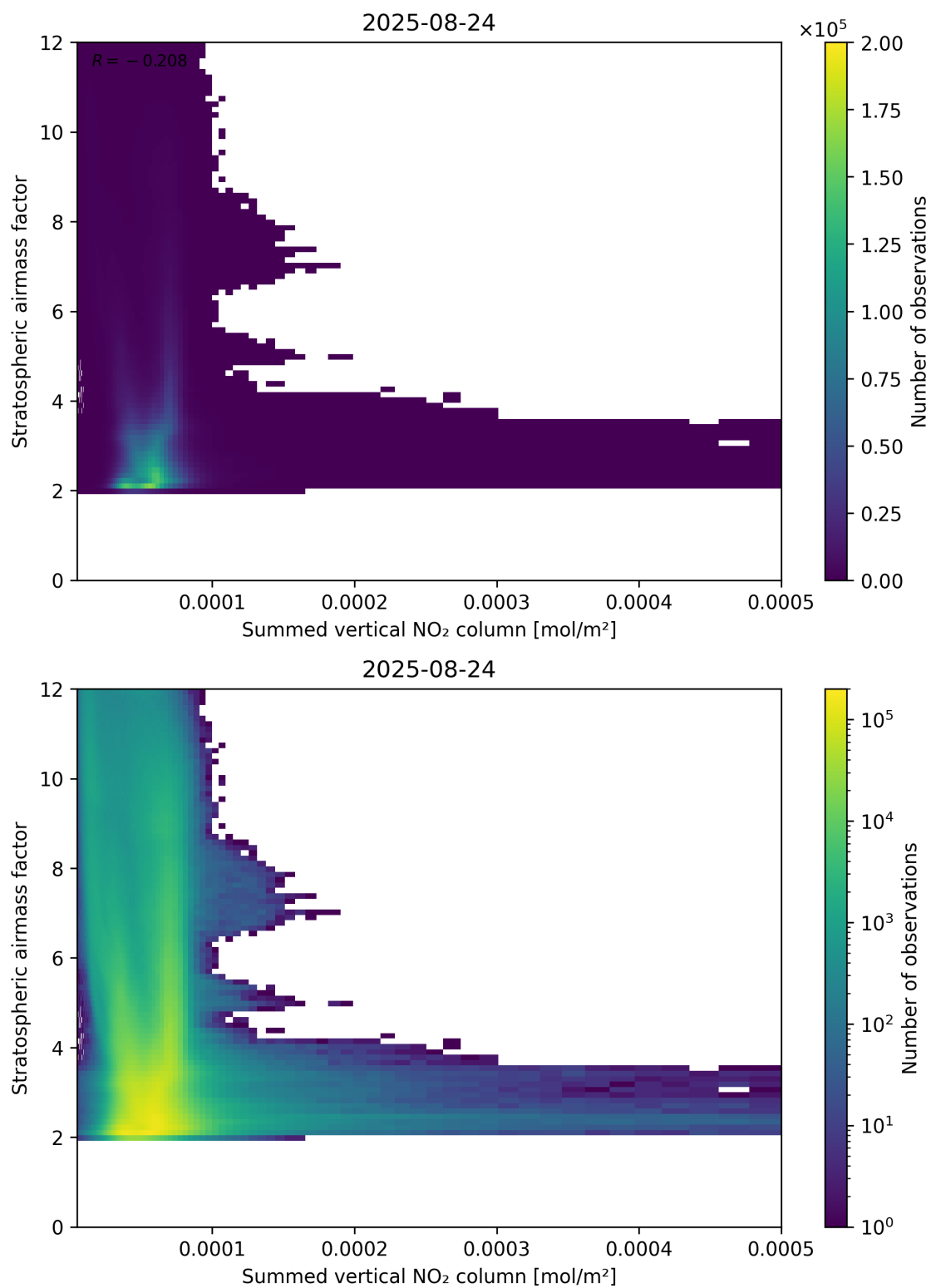
Figure 103: Scatter density plot of “Summed vertical NO 2 column” against “Stratospheric airmass factor” for 2025-08-23 to 2025-08-25.
