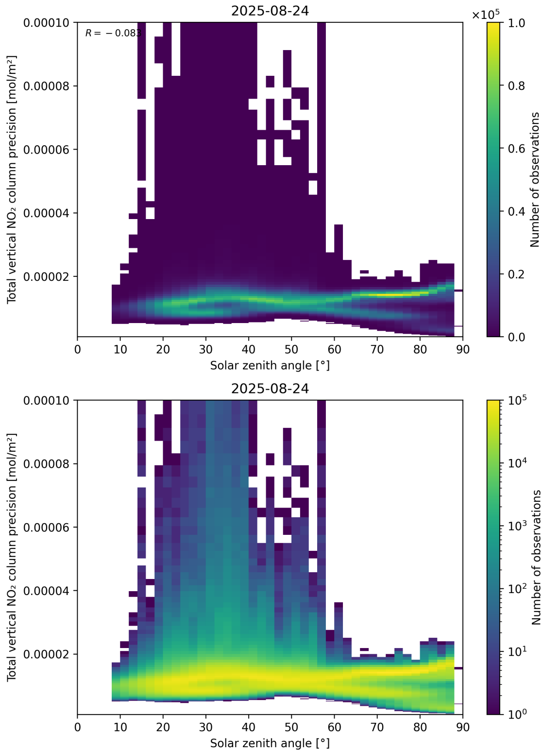
Figure 154: Scatter density plot of “Solar zenith angle” against “Total vertical NO 2 column precision” for 2025-08-23 to 2025-08-25.
