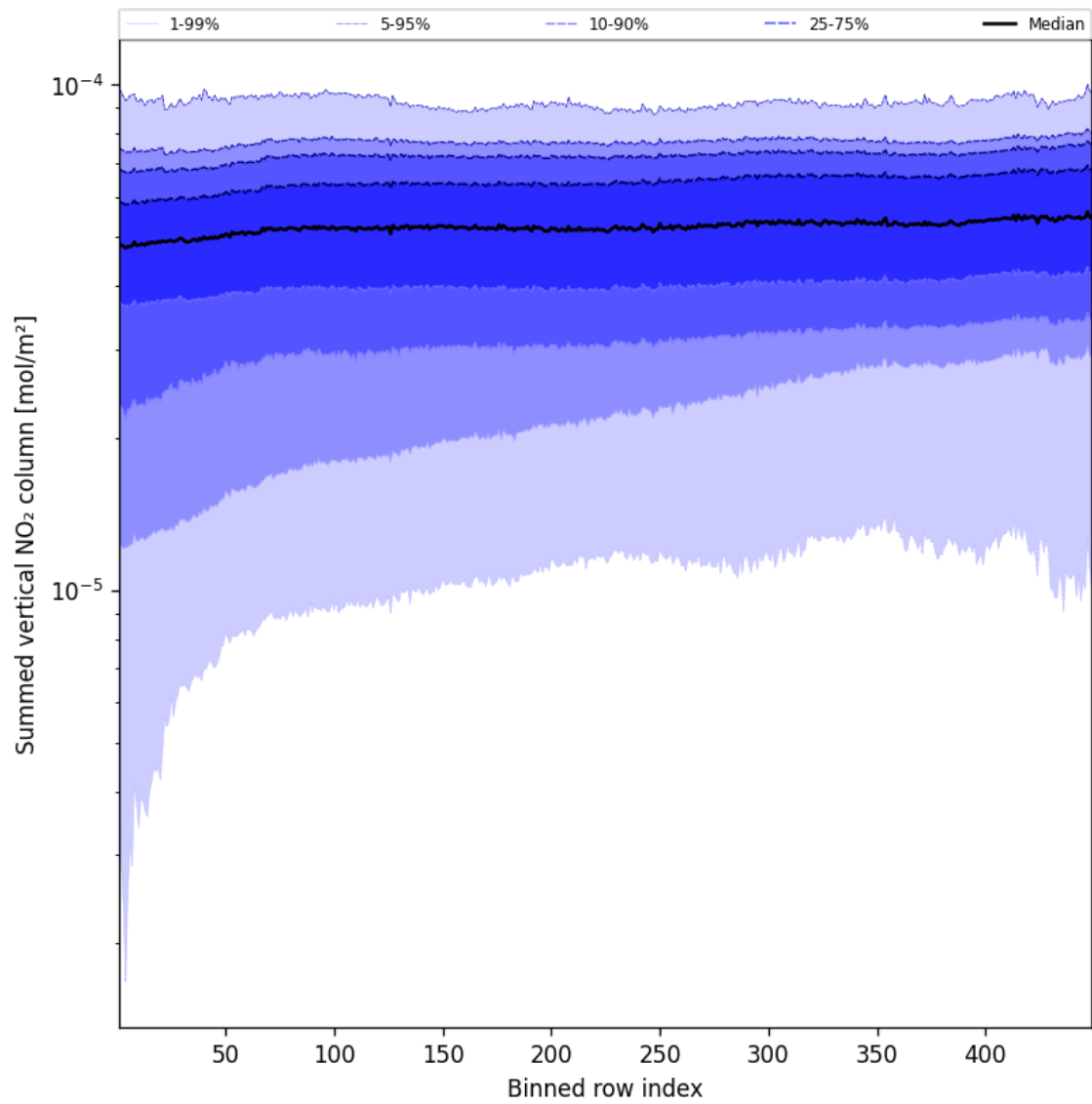
Figure 57: Along track statistics of “Summed vertical NO 2 column” for 2025-08-23 to 2025-08-25
