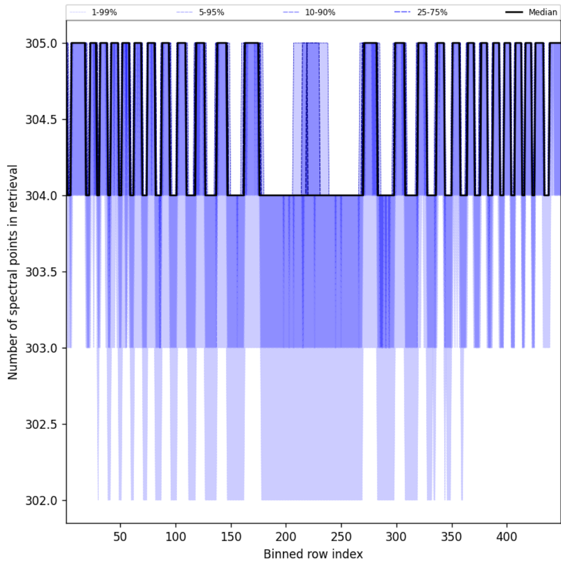
Figure 50: Along track statistics of “Number of spectral points in retrieval” for 2025-08-23 to 2025-08-25
