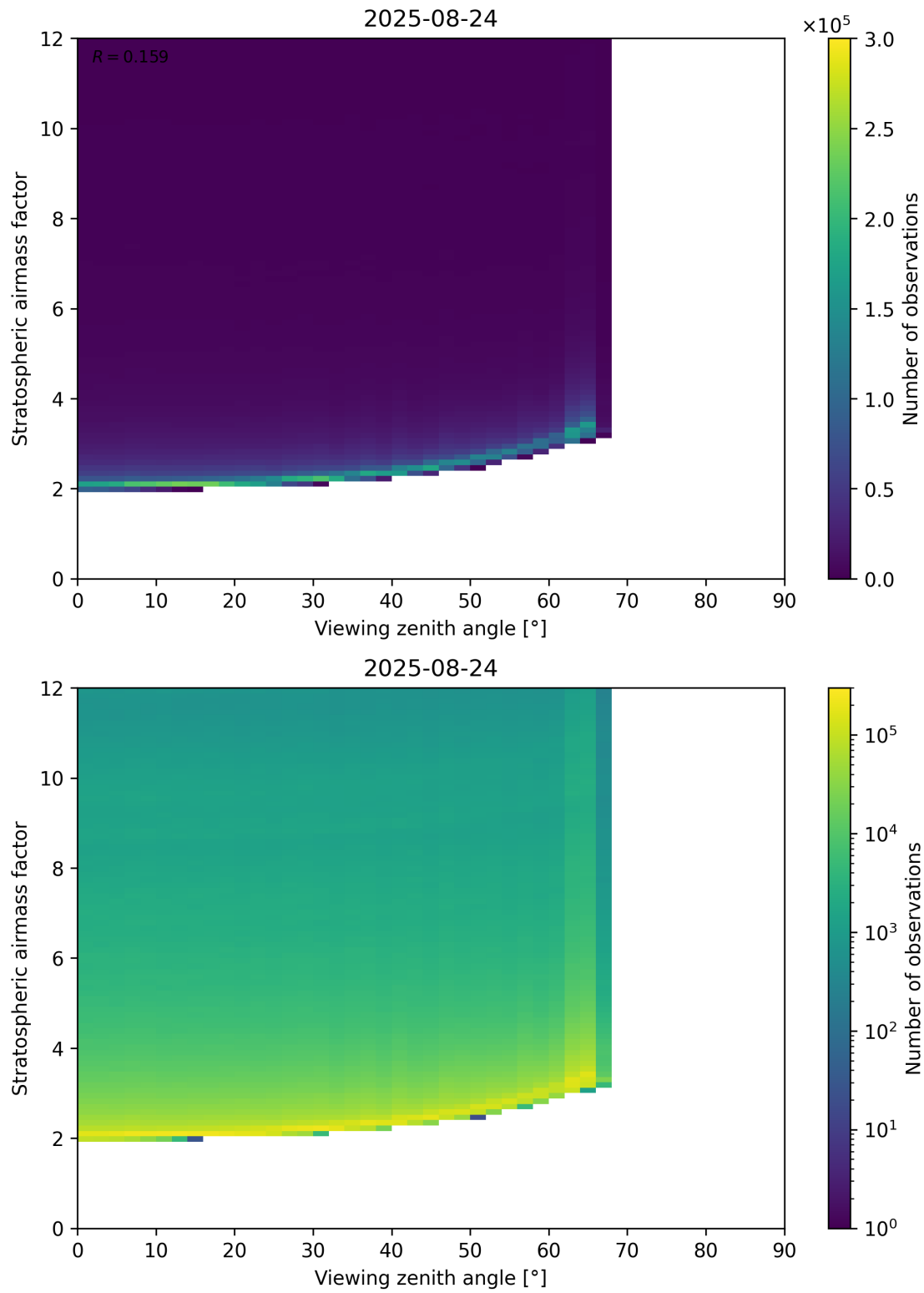
Figure 159: Scatter density plot of “Viewing zenith angle” against “Stratospheric airmass factor” for 2025-08-23 to 2025-08-25.
