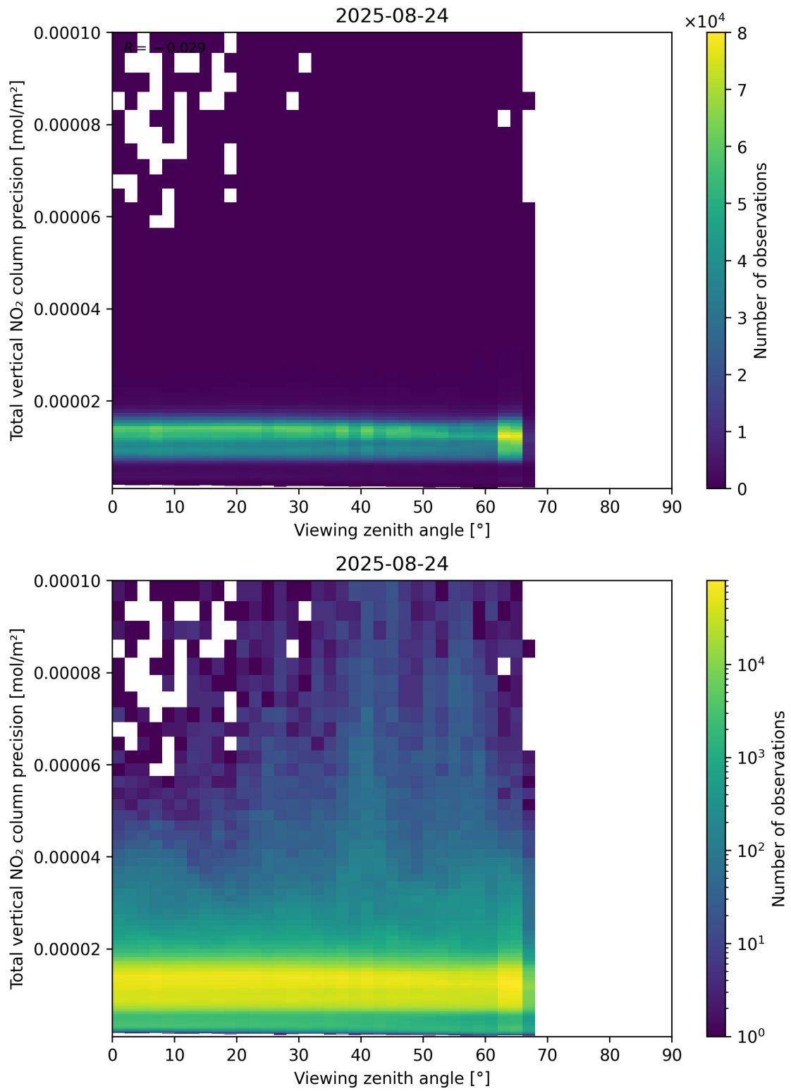
Figure 168: Scatter density plot of “Viewing zenith angle” against “Total vertical NO 2 column precision” for 2025-08-23 to 2025-08-25.
