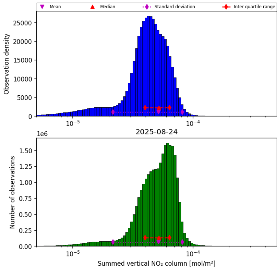
Figure 40: Histogram of “Summed vertical NO 2 column” for 2025-08-23 to 2025-08-25
