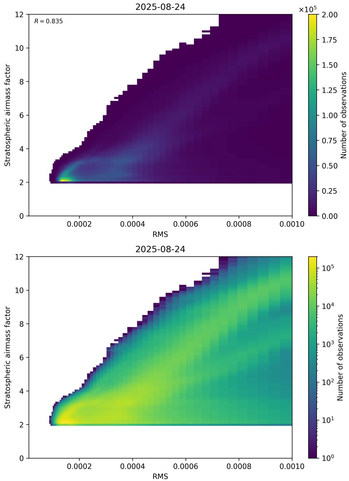
Figure 144: Scatter density plot of “RMS” against “Stratospheric airmass factor” for 2025-08-23 to 2025-08-25.
