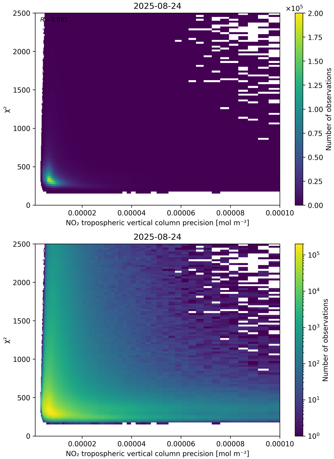
Figure 134: Scatter density plot of “NO 2 tropospheric vertical column precision” against “ \chi^2 ” for 2025-08-23 to 2025-08-25.
