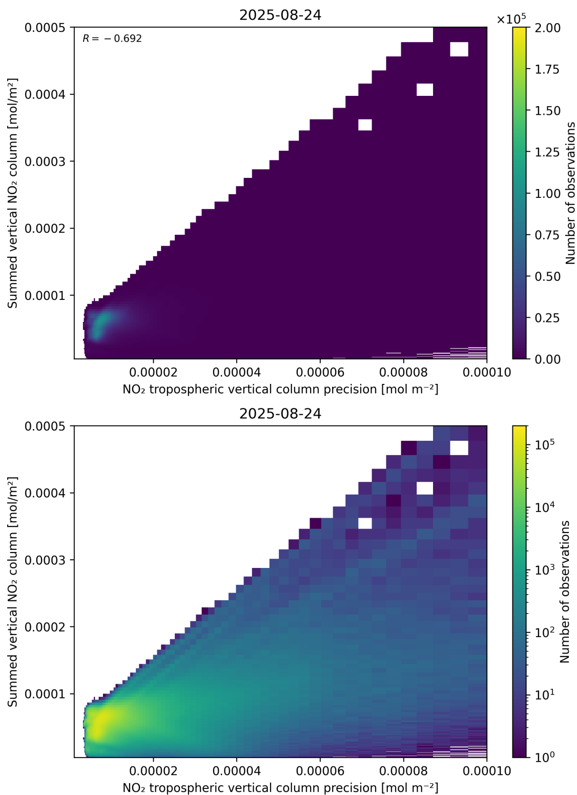
Figure 136: Scatter density plot of “NO 2 tropospheric vertical column precision” against “Summed vertical NO 2 column” for 2025-08-23 to 2025-08-25.
