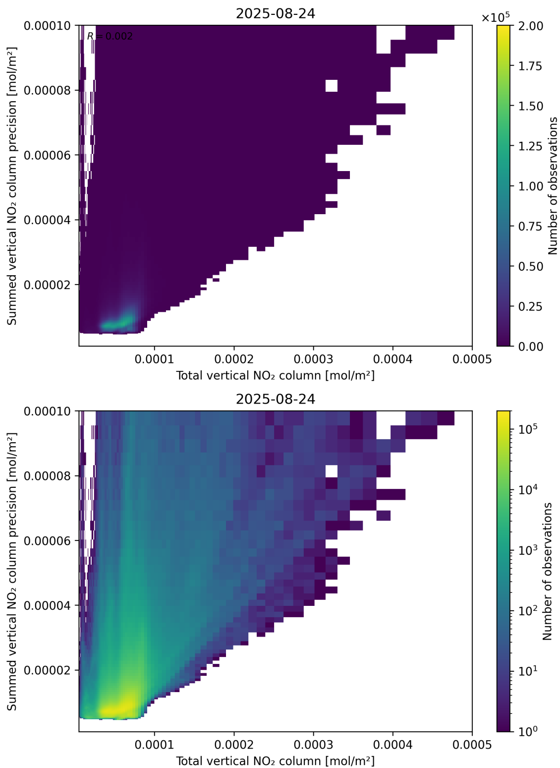
Figure 113: Scatter density plot of “Total vertical NO 2 column” against “Summed vertical NO 2 column precision” for 2025-08-23 to 2025-08-25.
