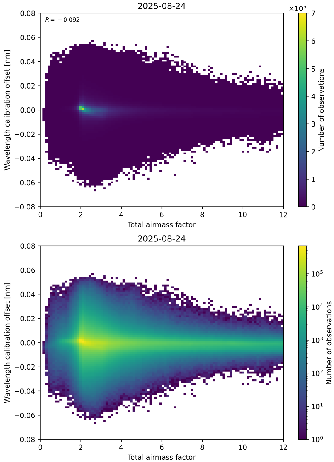
Figure 70: Scatter density plot of “Total airmass factor” against “Wavelength calibration offset” for 2025-08-23 to 2025-08-25.
