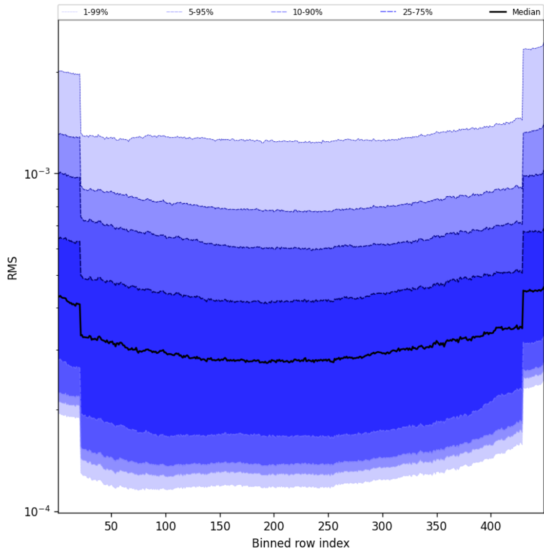
Figure 60: Along track statistics of “RMS” for 2025-08-23 to 2025-08-25
