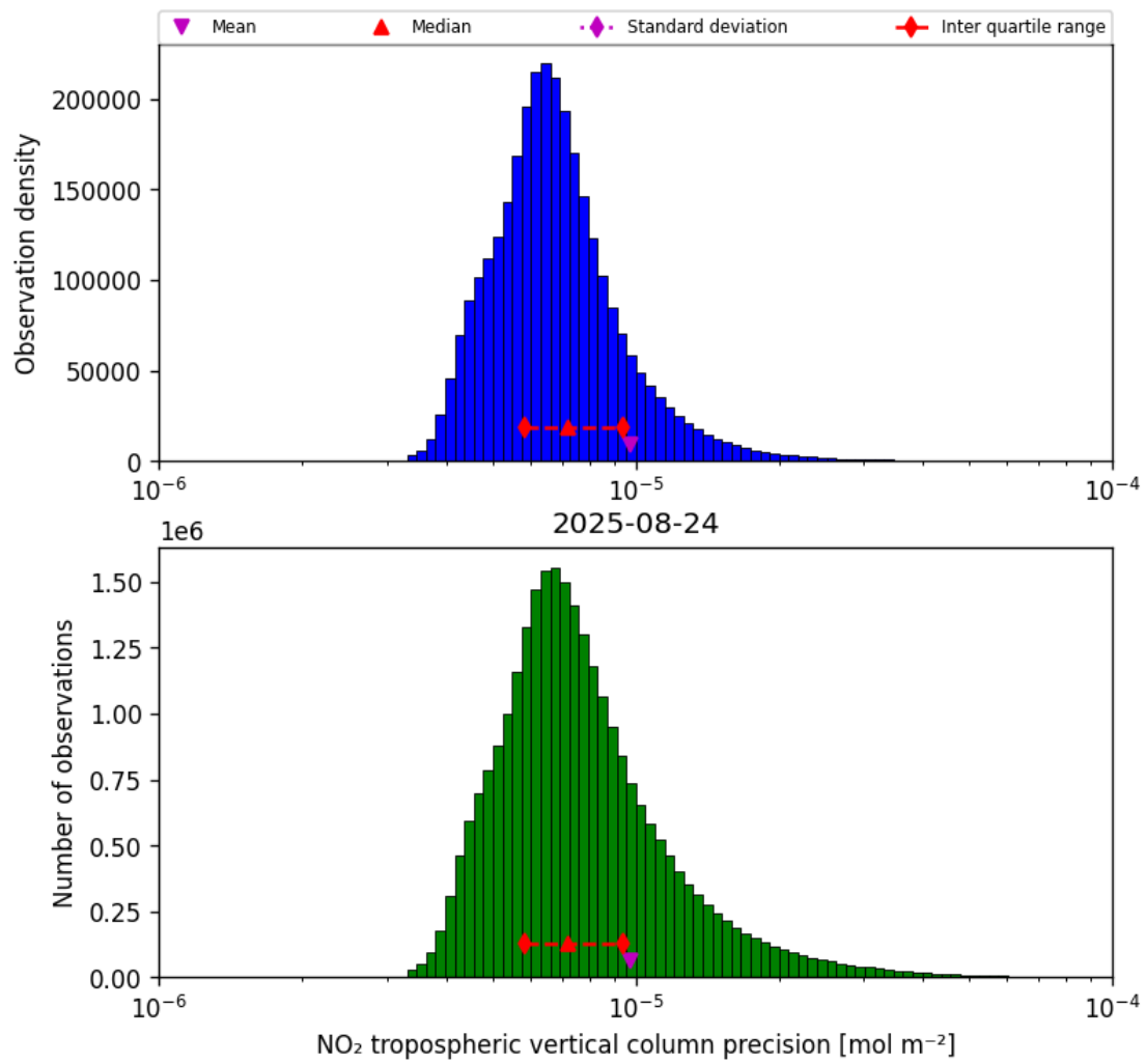
Figure 30: Histogram of “NO 2 tropospheric vertical column precision” for 2025-08-23 to 2025-08-25
