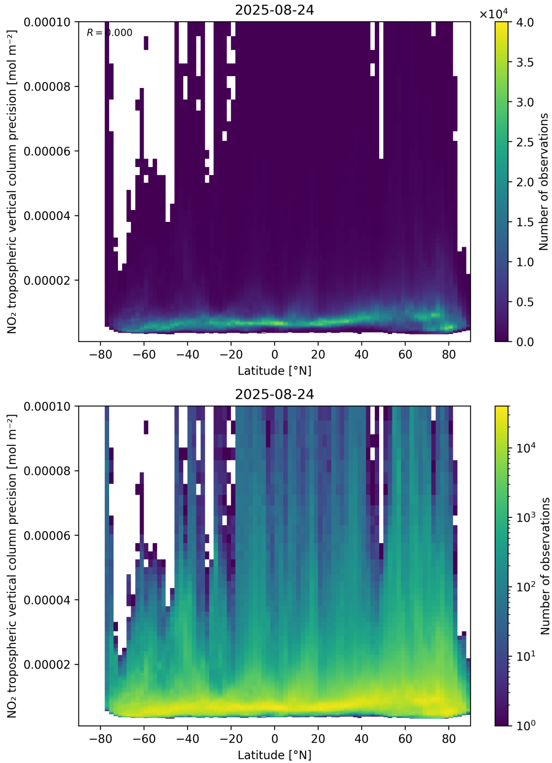
Figure 93: Scatter density plot of “Latitude” against “NO 2 tropospheric vertical column precision” for 2025-08-23 to 2025-08-25.
