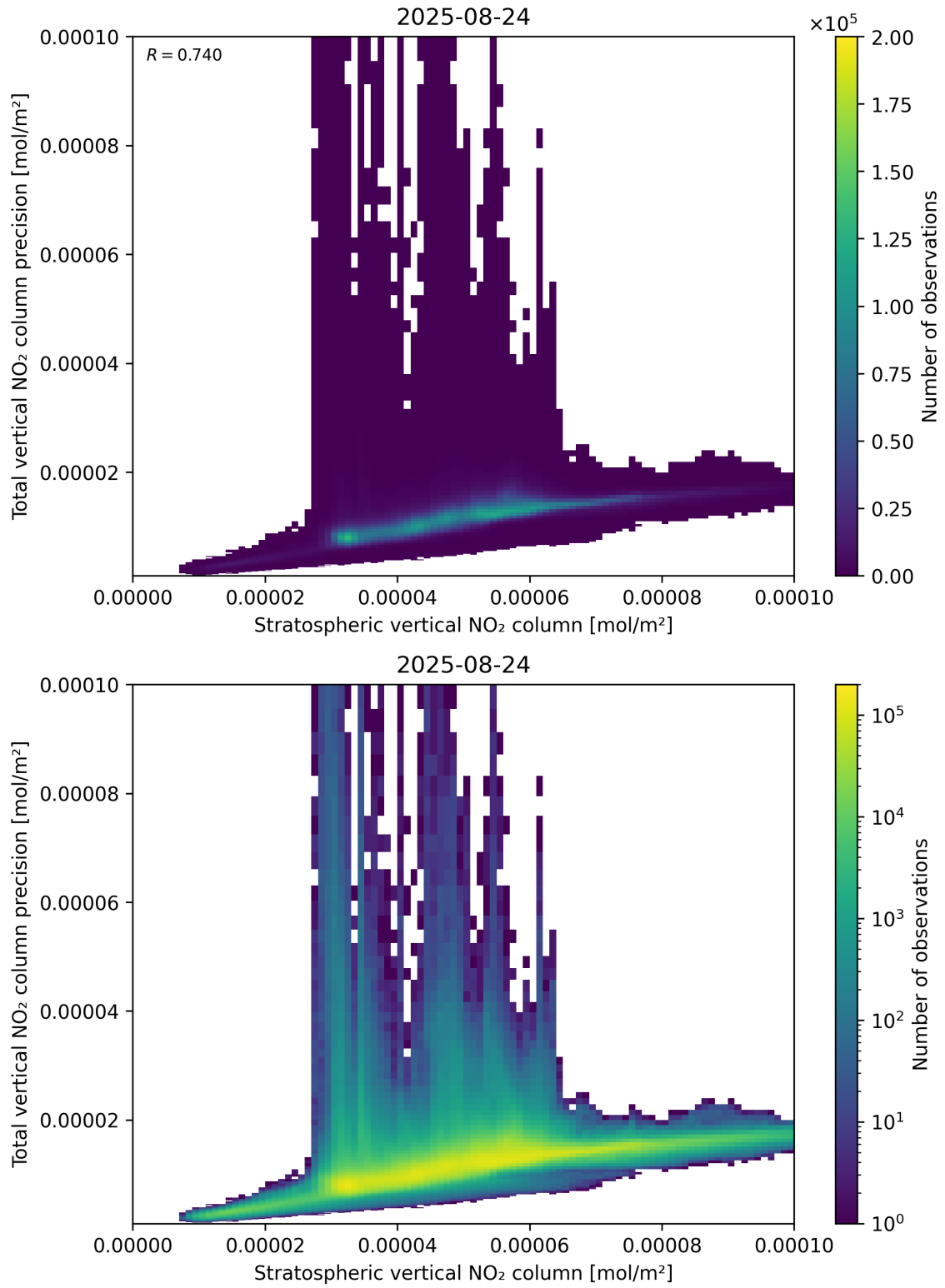
Figure 101: Scatter density plot of “Stratospheric vertical NO 2 column” against “Total vertical NO 2 column precision” for 2025-08-23 to 2025-08-25.
