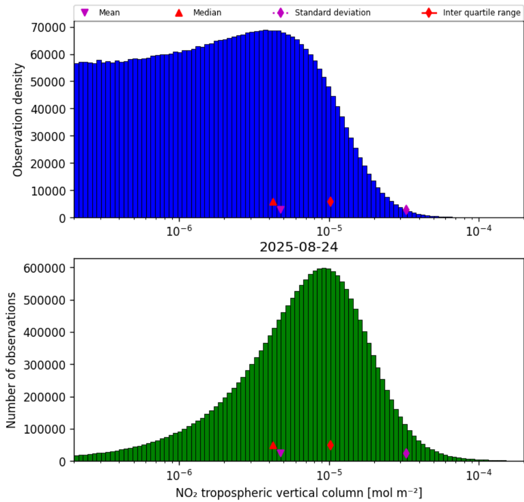
Figure 29: Histogram of “NO 2 tropospheric vertical column” for 2025-08-23 to 2025-08-25
