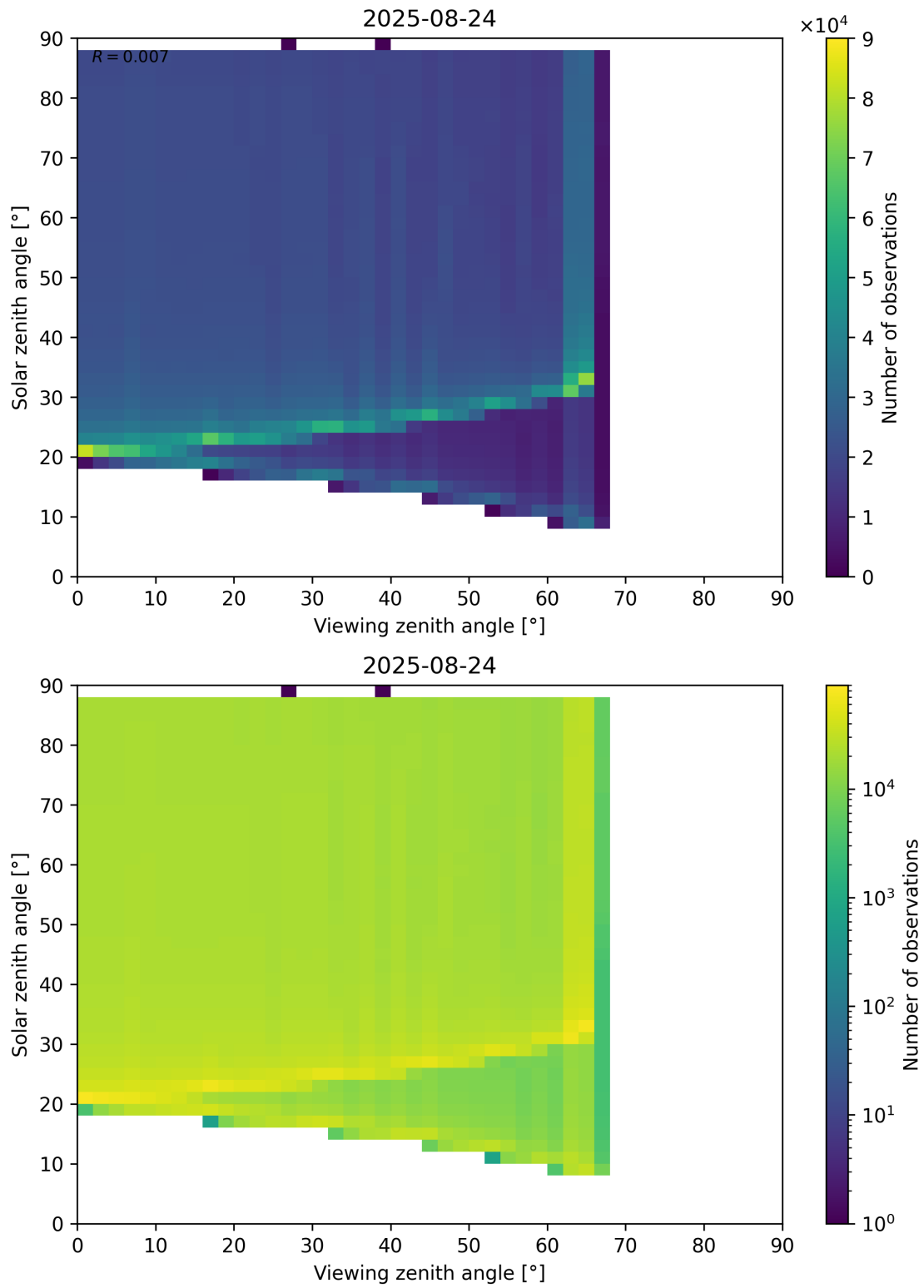
Figure 172: Scatter density plot of “Viewing zenith angle” against “Solar zenith angle” for 2025-08-23 to 2025-08-25.
