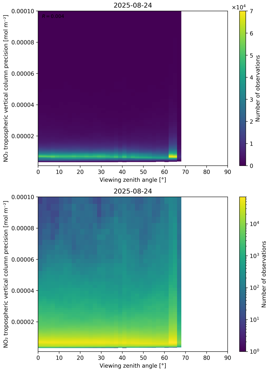
Figure 170: Scatter density plot of “Viewing zenith angle” against “NO 2 tropospheric vertical column precision” for 2025-08-23 to 2025-08-25.
