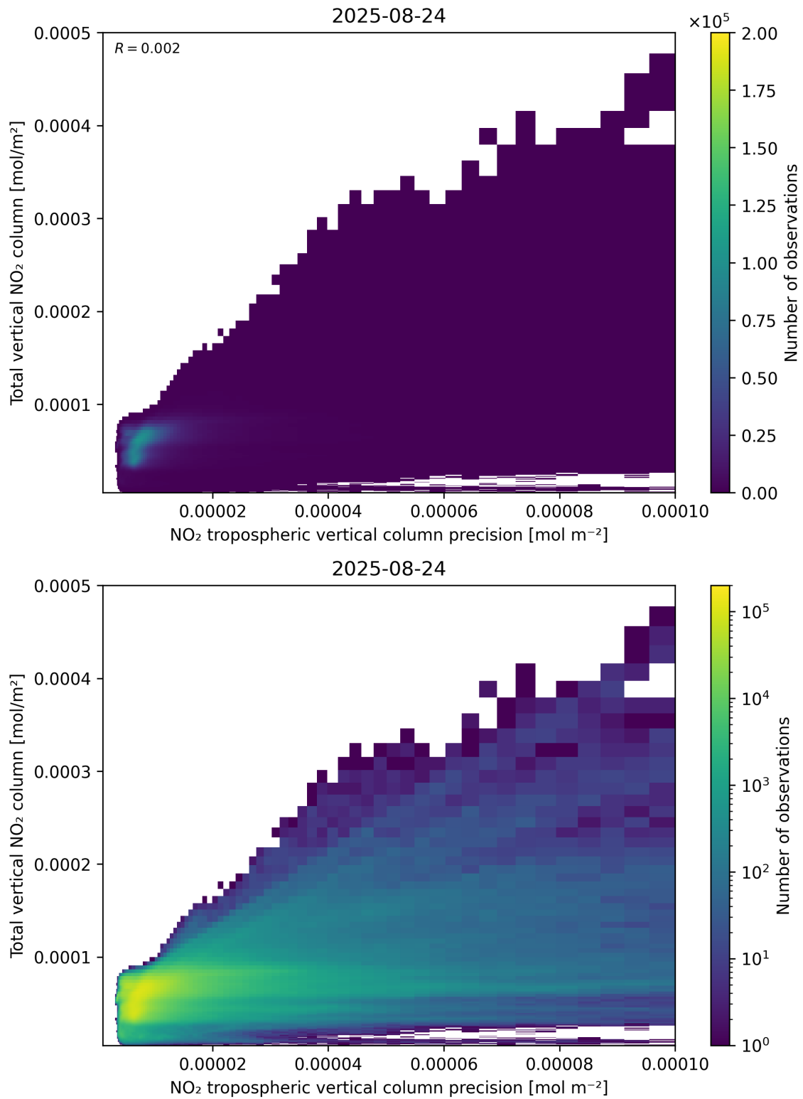
Figure 138: Scatter density plot of “NO 2 tropospheric vertical column precision” against “Total vertical NO 2 column” for 2025-08-23 to 2025-08-25.
