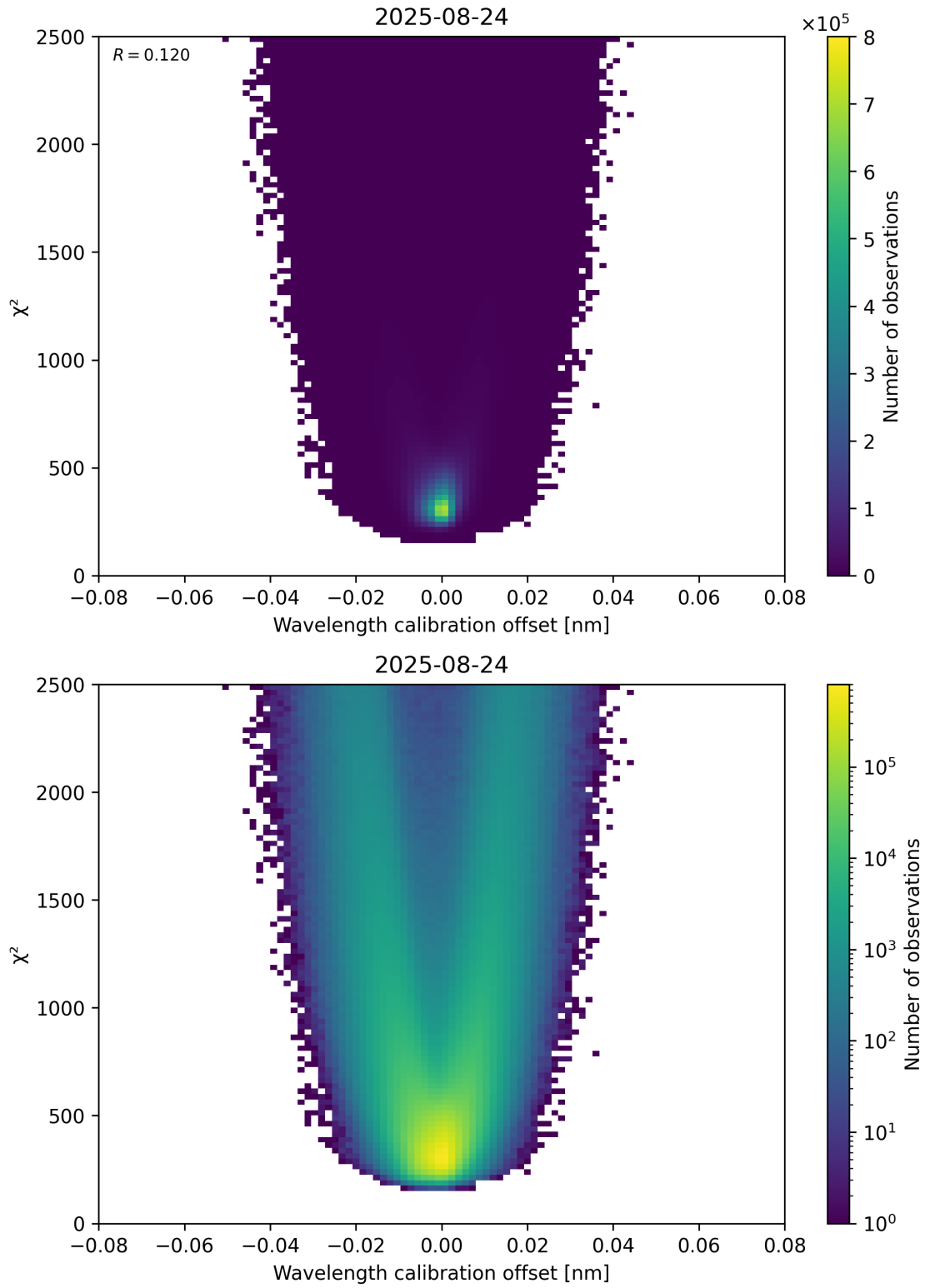
Figure 175: Scatter density plot of “Wavelength calibration offset” against “ \chi^2 ” for 2025-08-23 to 2025-08-25.
