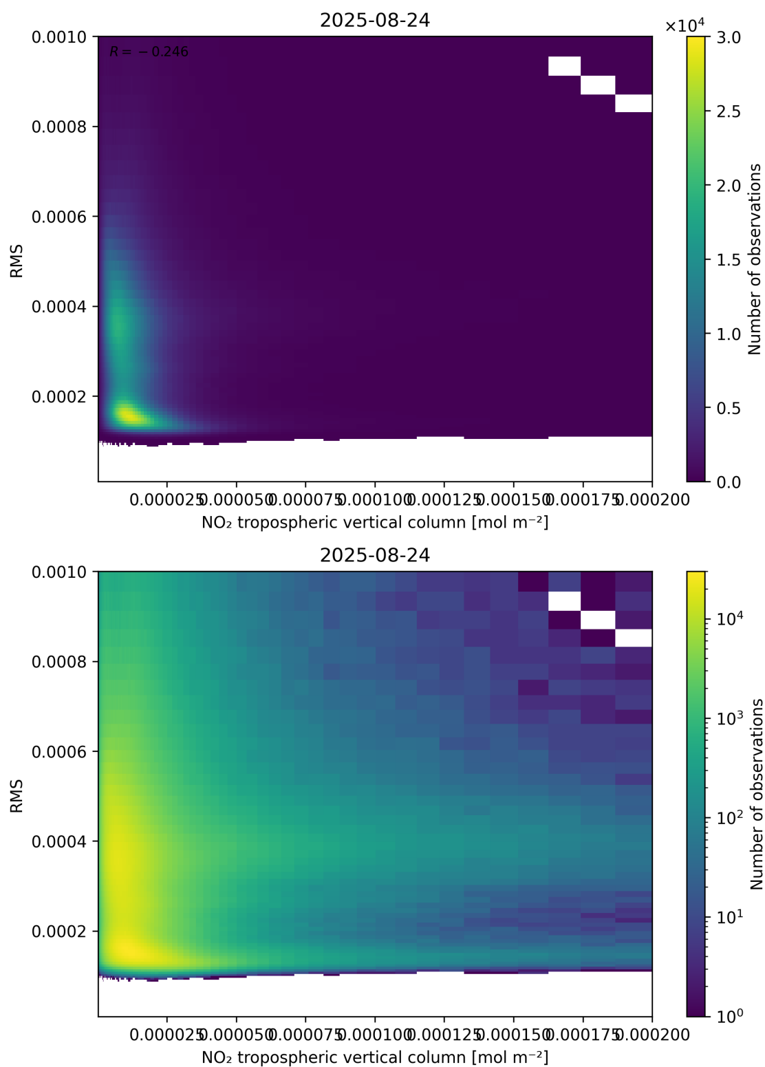
Figure 142: Scatter density plot of “NO 2 tropospheric vertical column” against “RMS” for 2025-08-23 to 2025-08-25.
