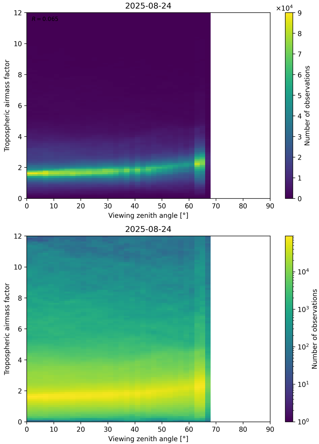
Figure 161: Scatter density plot of “Viewing zenith angle” against “Tropospheric airmass factor” for 2025-08-23 to 2025-08-25.
