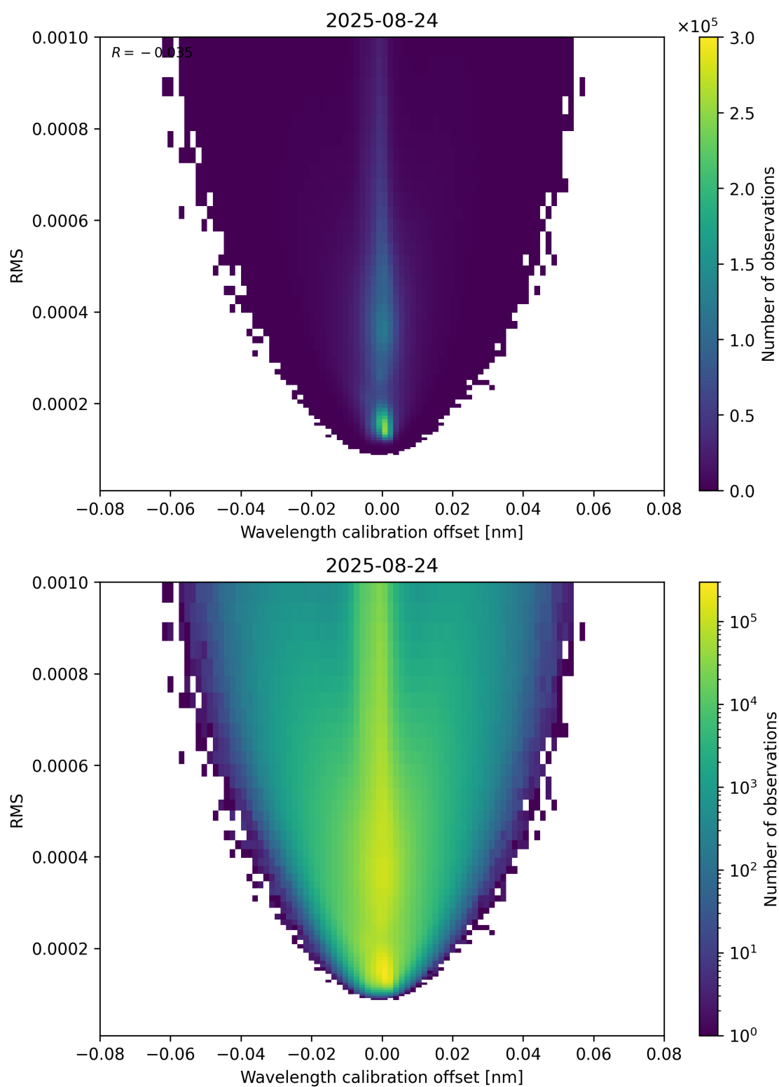
Figure 181: Scatter density plot of “Wavelength calibration offset” against “RMS” for 2025-08-23 to 2025-08-25.
