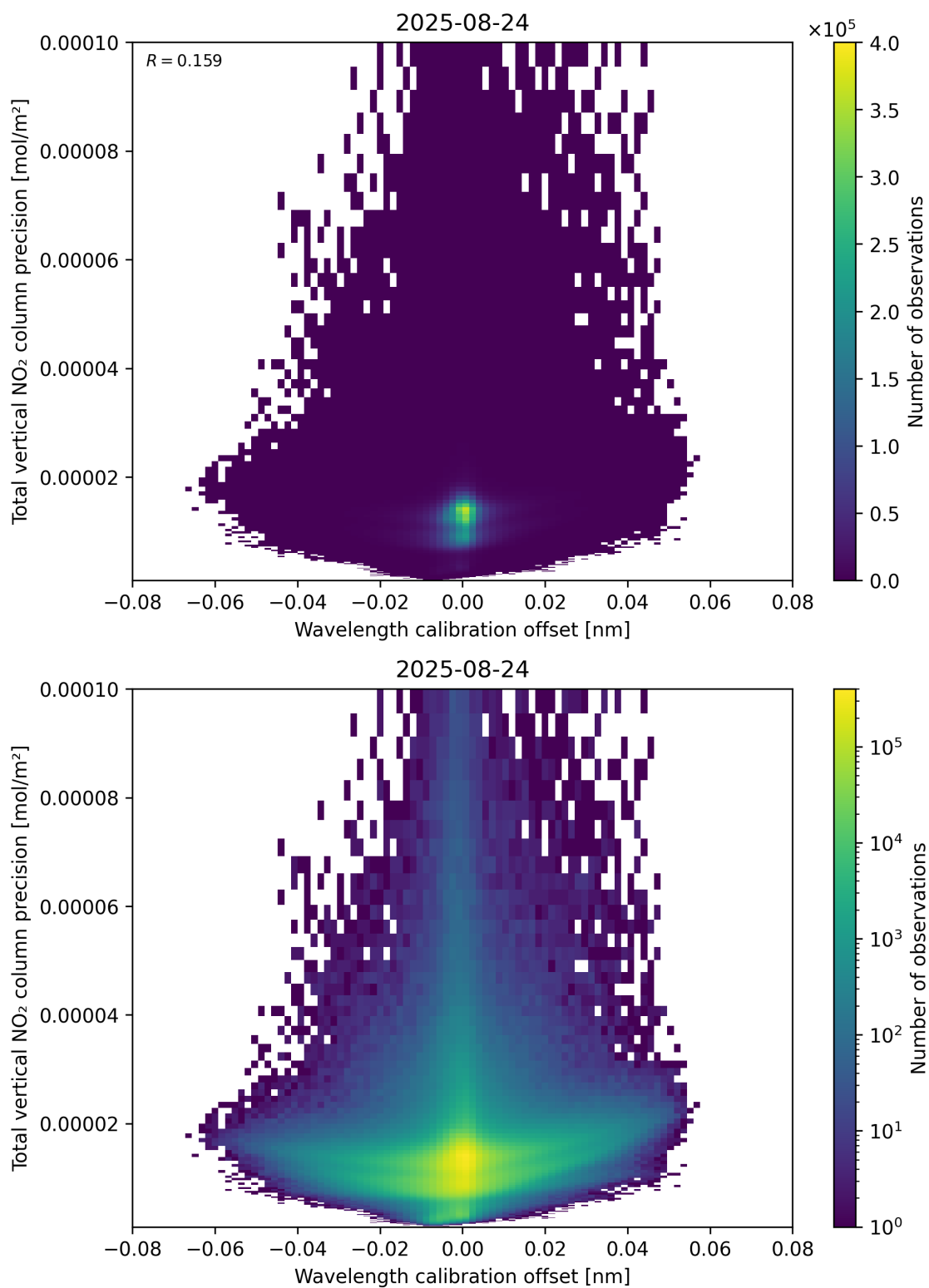
Figure 180: Scatter density plot of “Wavelength calibration offset” against “Total vertical NO 2 column precision” for 2025-08-23 to 2025-08-25.
