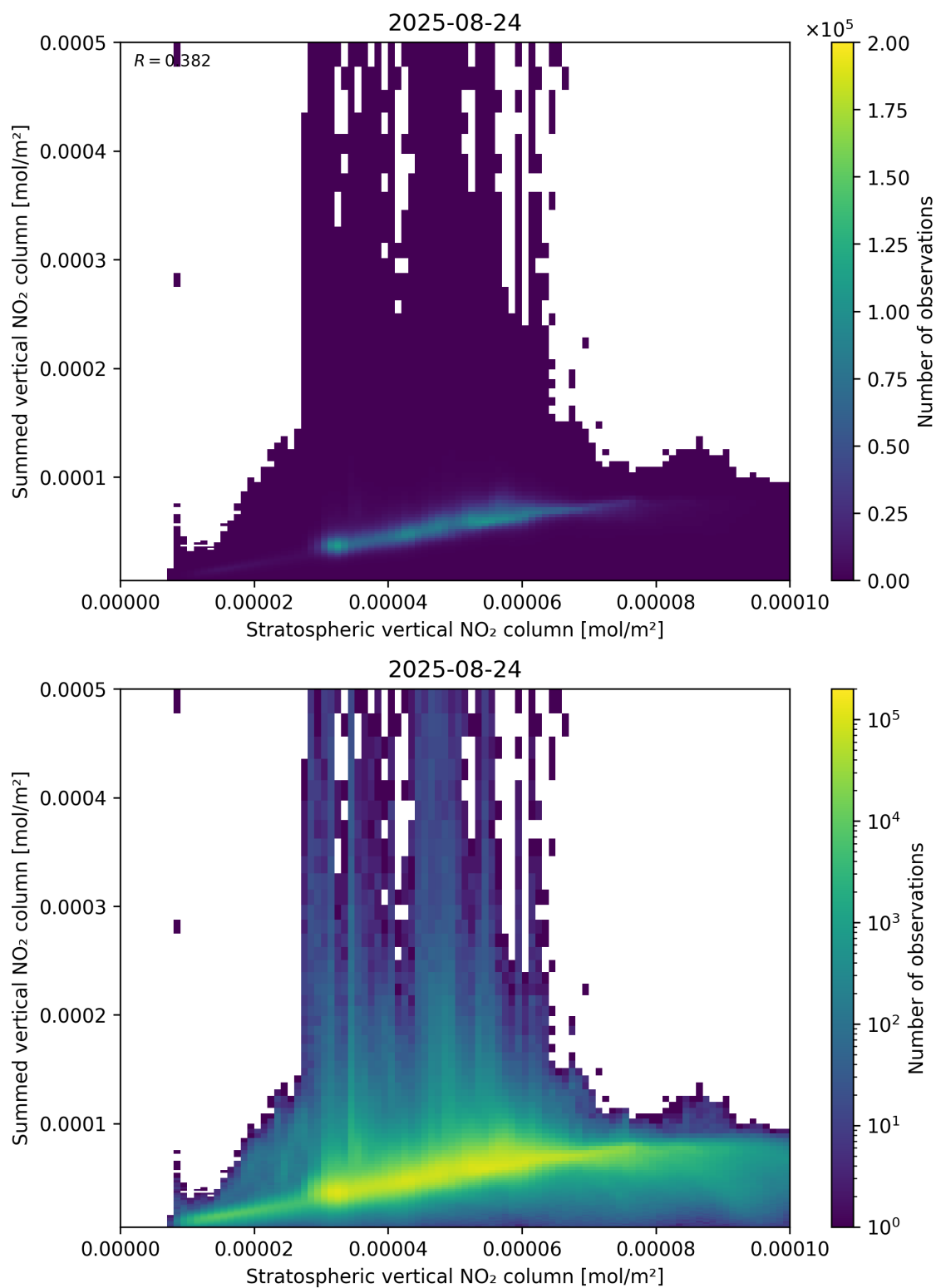
Figure 98: Scatter density plot of “Stratospheric vertical NO 2 column” against “Summed vertical NO 2 column” for 2025-08-23 to 2025-08-25.
