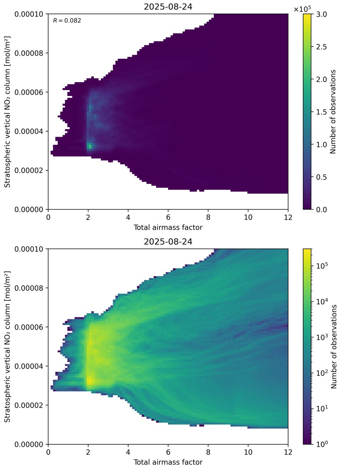
Figure 64: Scatter density plot of “Total airmass factor” against “Stratospheric vertical \text{NO}_2 column” for 2025-08-23 to 2025-08-25.
