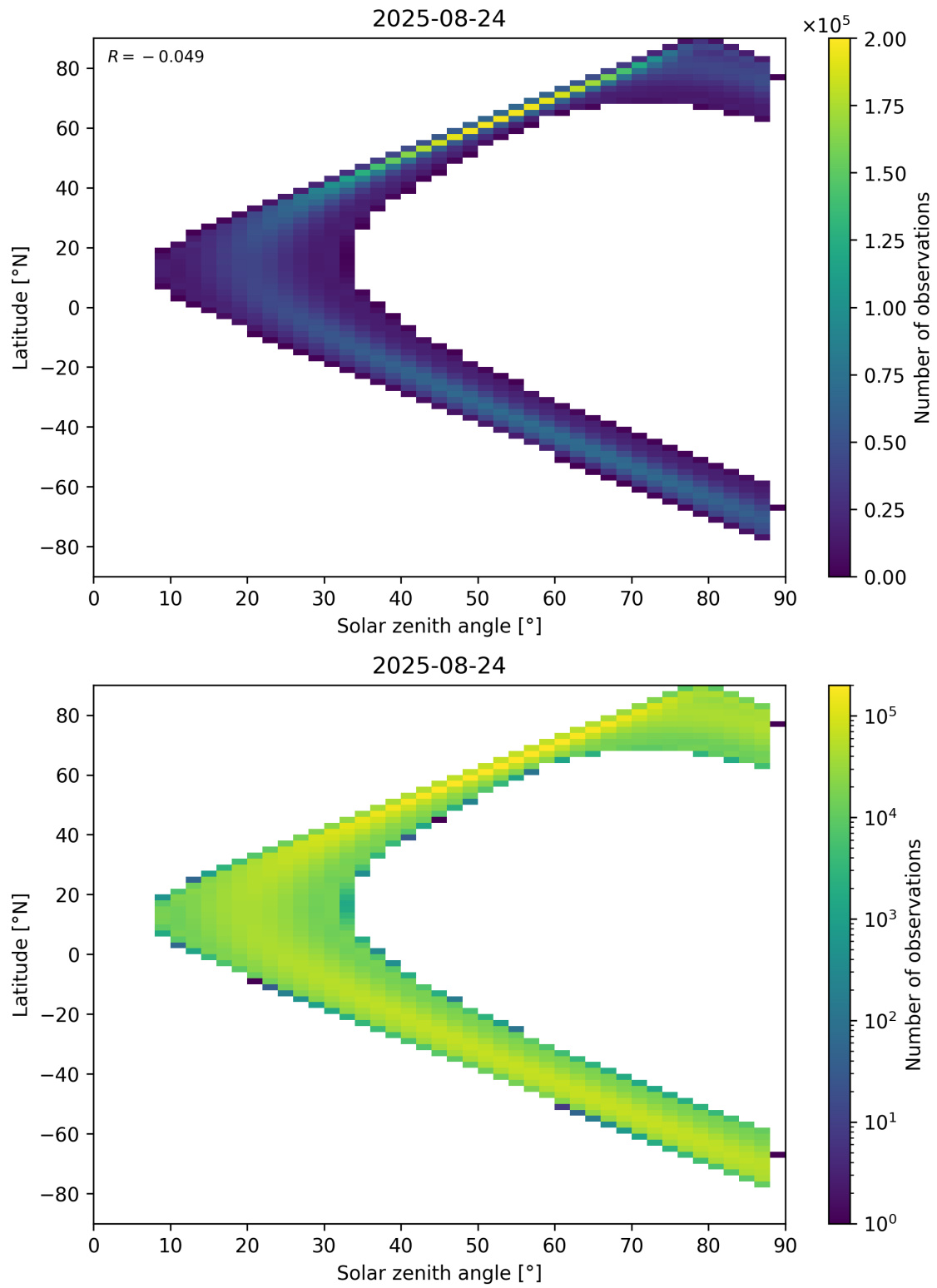
Figure 149: Scatter density plot of “Solar zenith angle” against “Latitude” for 2025-08-23 to 2025-08-25.
