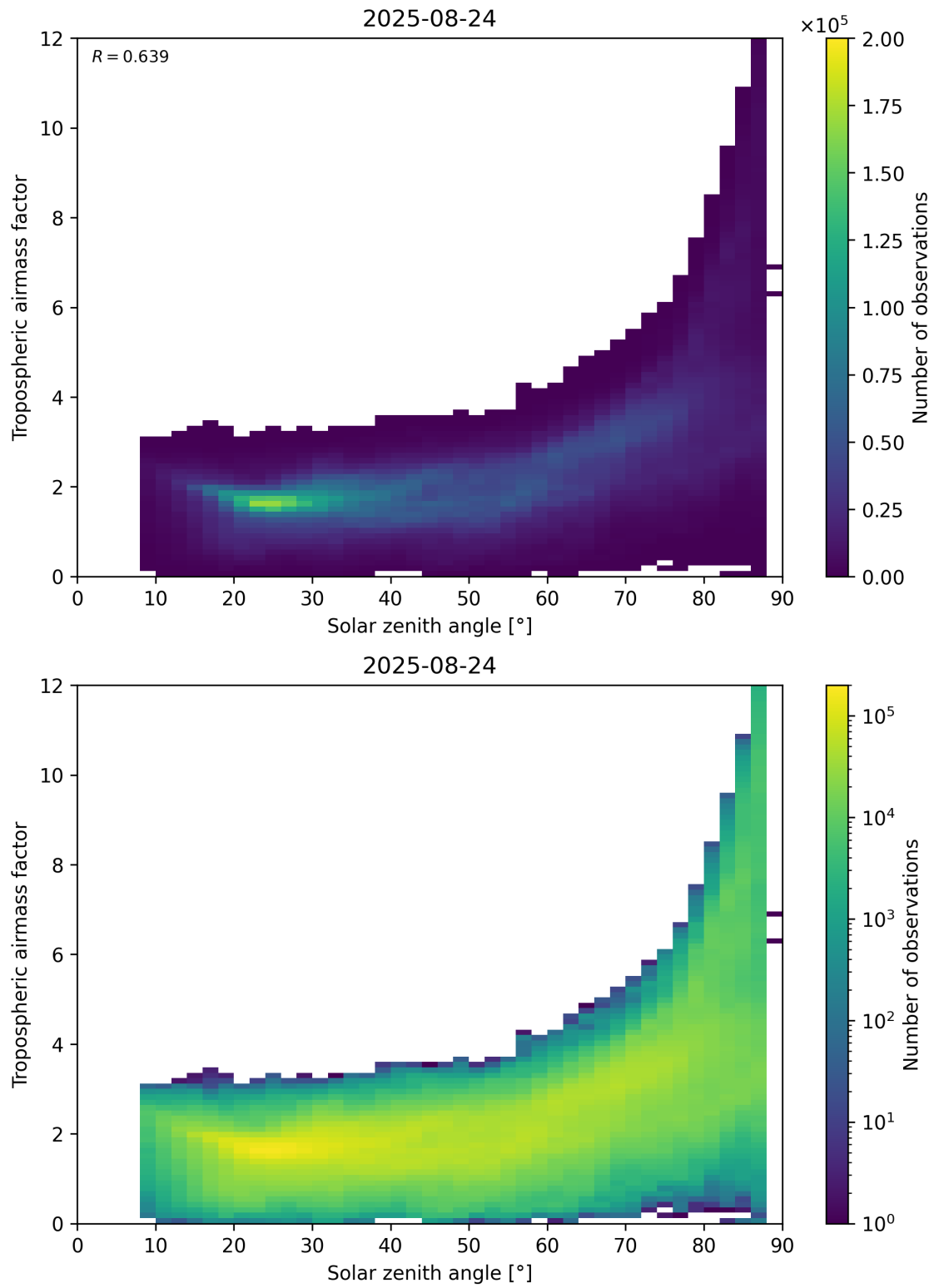
Figure 147: Scatter density plot of “Solar zenith angle” against “Tropospheric airmass factor” for 2025-08-23 to 2025-08-25.
