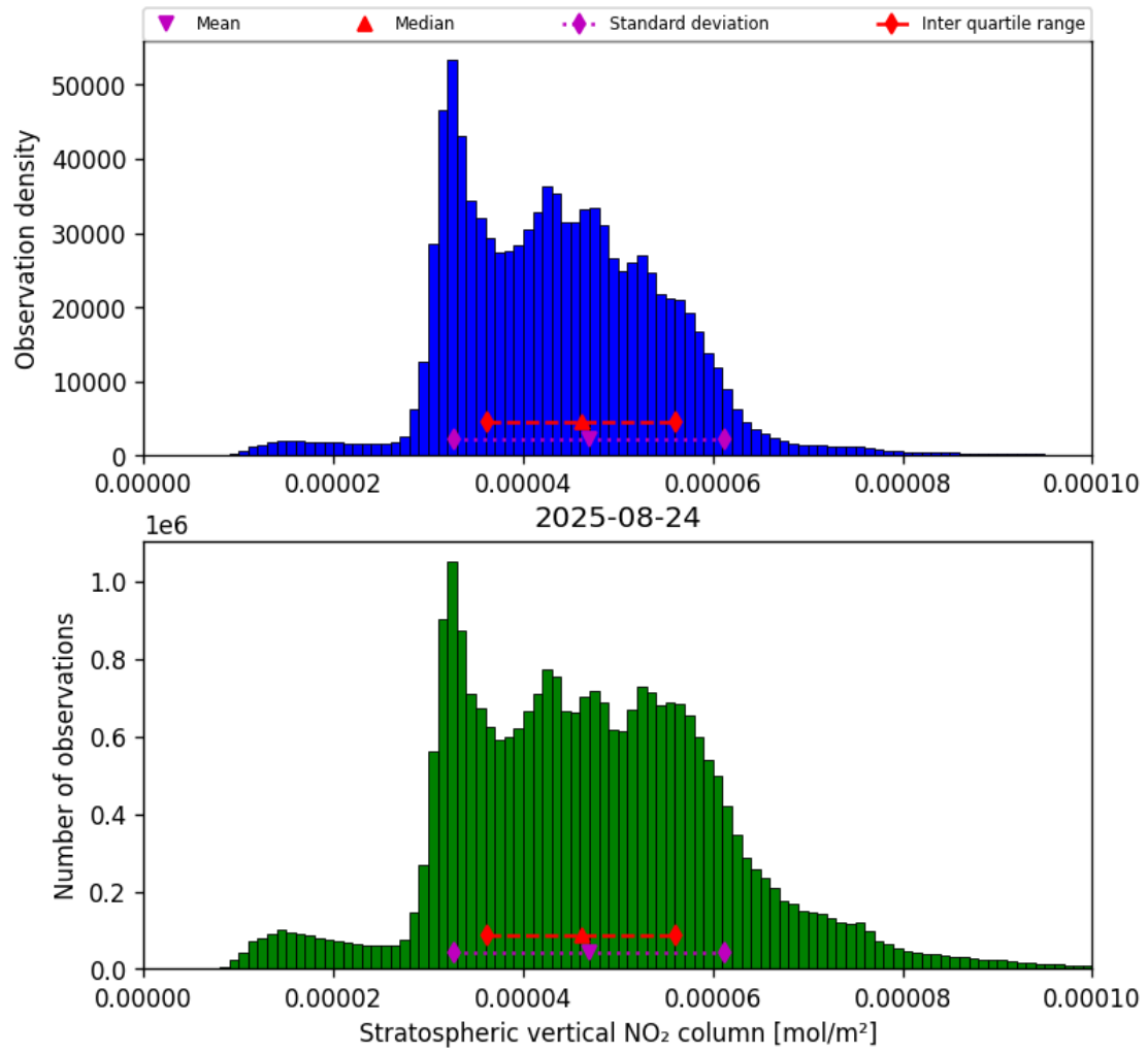
Figure 36: Histogram of “Stratospheric vertical NO 2 column” for 2025-08-23 to 2025-08-25
