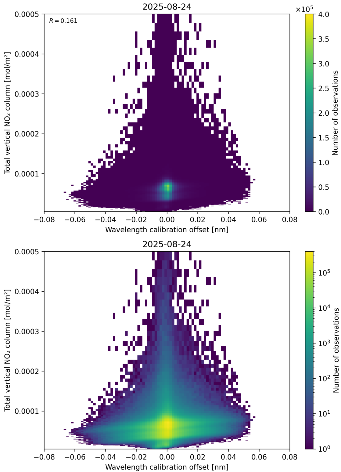
Figure 179: Scatter density plot of “Wavelength calibration offset” against “Total vertical NO 2 column” for 2025-08-23 to 2025-08-25.
