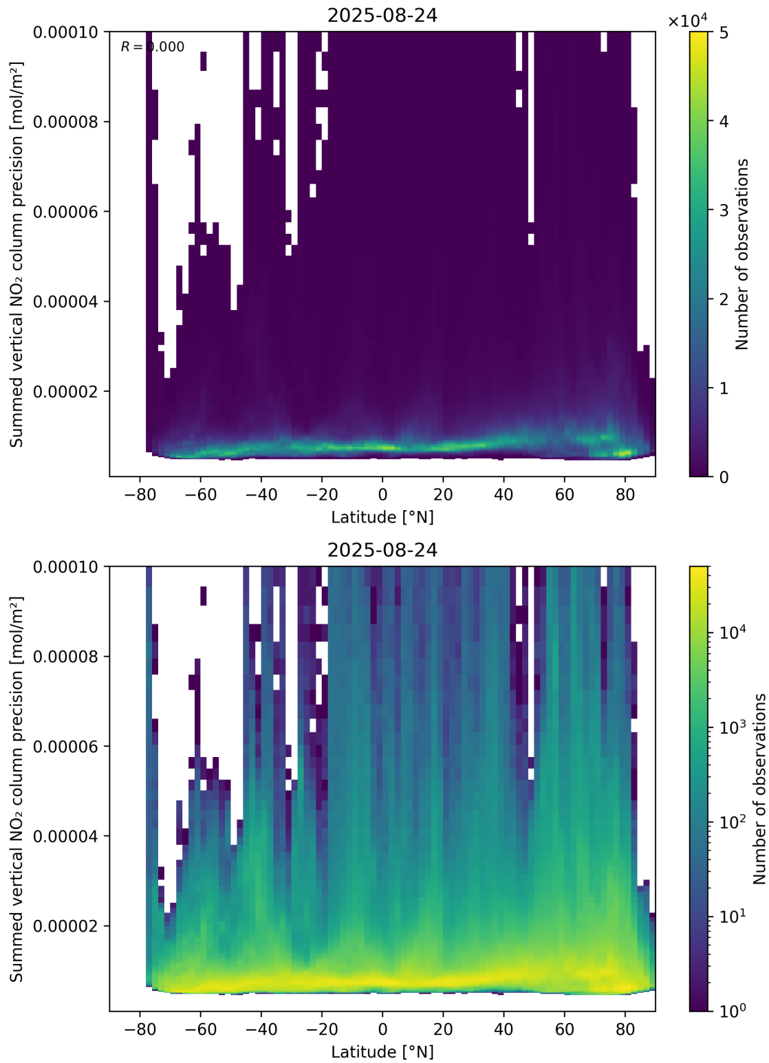
Figure 89: Scatter density plot of “Latitude” against “Summed vertical NO 2 column precision” for 2025-08-23 to 2025-08-25.
