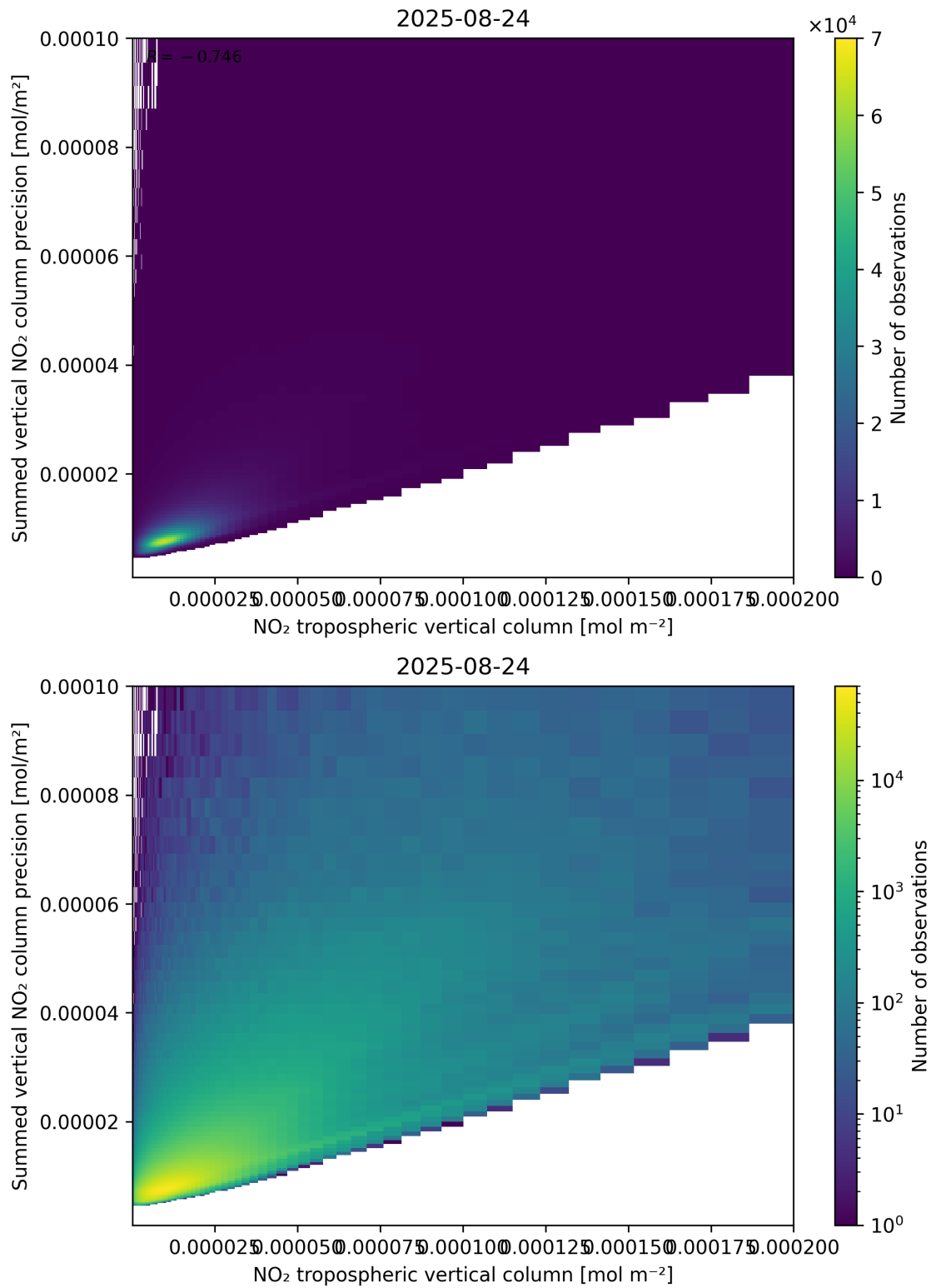
Figure 127: Scatter density plot of “NO 2 tropospheric vertical column” against “Summed vertical NO 2 column precision” for 2025-08-23 to 2025-08-25.
