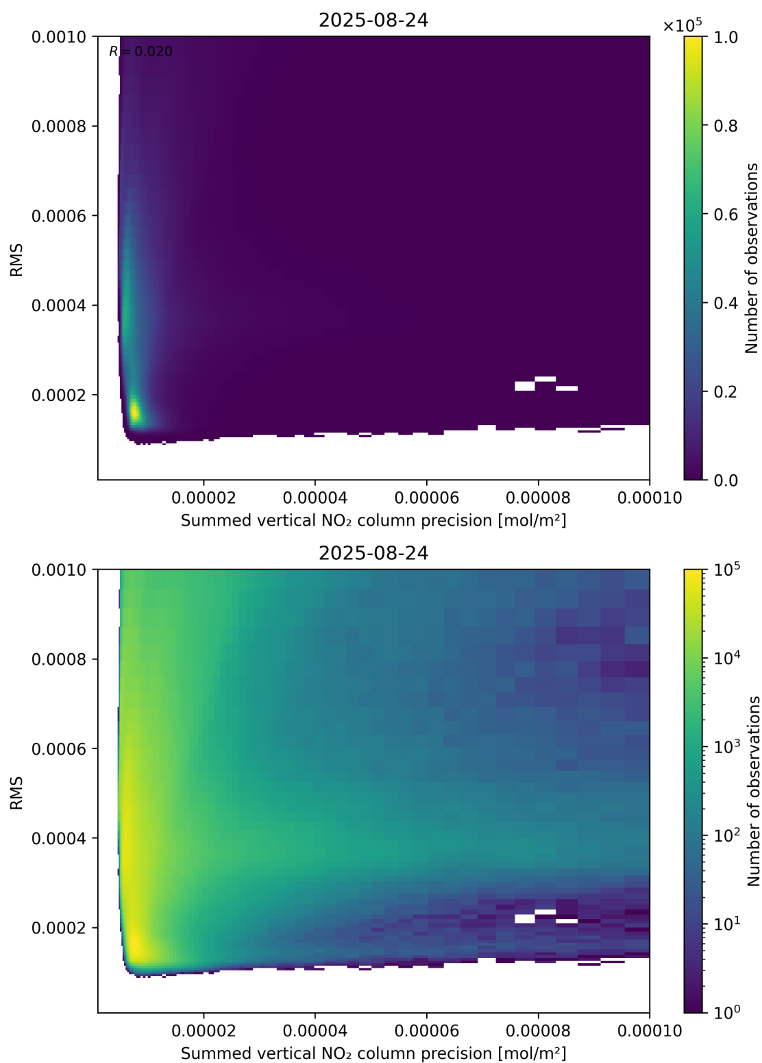
Figure 108: Scatter density plot of “Summed vertical NO 2 column precision” against “RMS” for 2025-08-23 to 2025-08-25.
