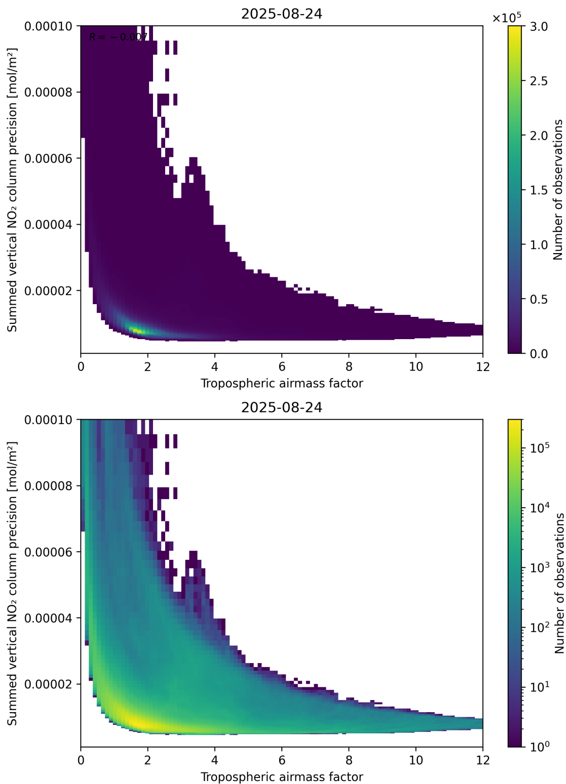
Figure 76: Scatter density plot of “Tropospheric air mass factor” against “Summed vertical NO 2 column precision” for 2025-08-23 to 2025-08-25.
