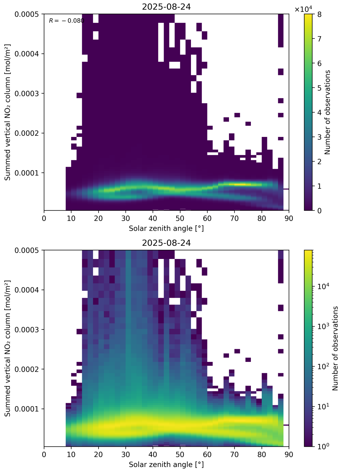
Figure 151: Scatter density plot of “Solar zenith angle” against “Summed vertical NO 2 column” for 2025-08-23 to 2025-08-25.
