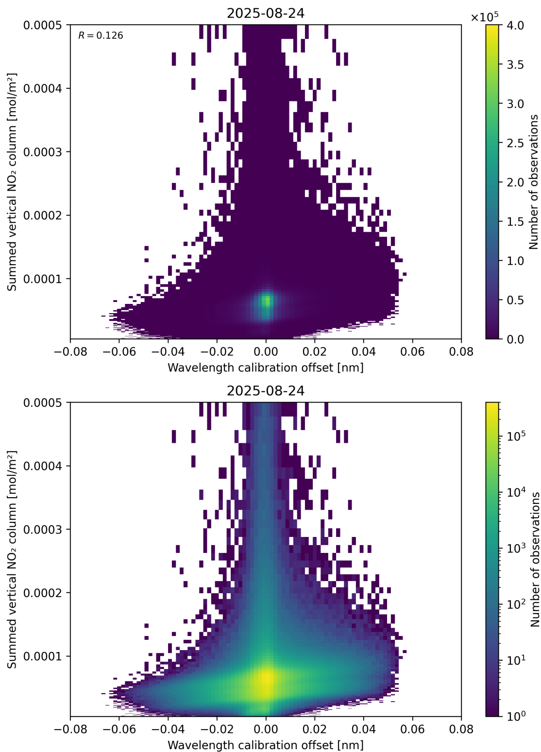
Figure 177: Scatter density plot of “Wavelength calibration offset” against “Summed vertical NO 2 column” for 2025-08-23 to 2025-08-25.
