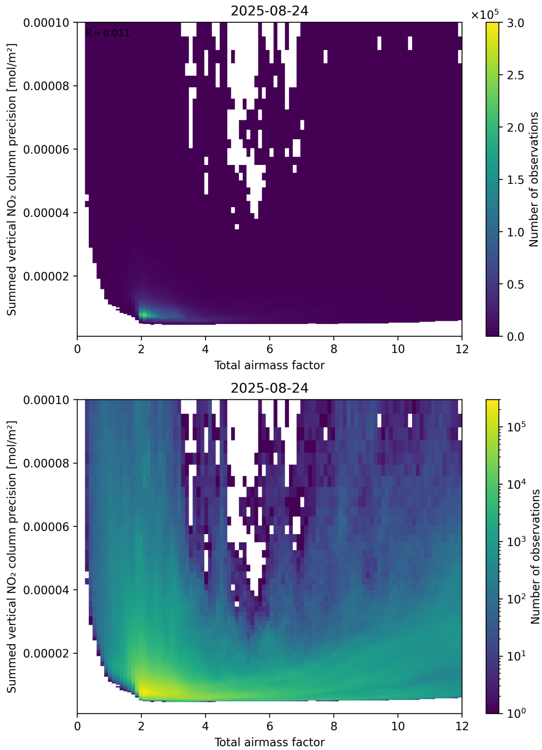
Figure 66: Scatter density plot of “Total airmass factor” against “Summed vertical NO 2 column precision” for 2025-08-23 to 2025-08-25.
