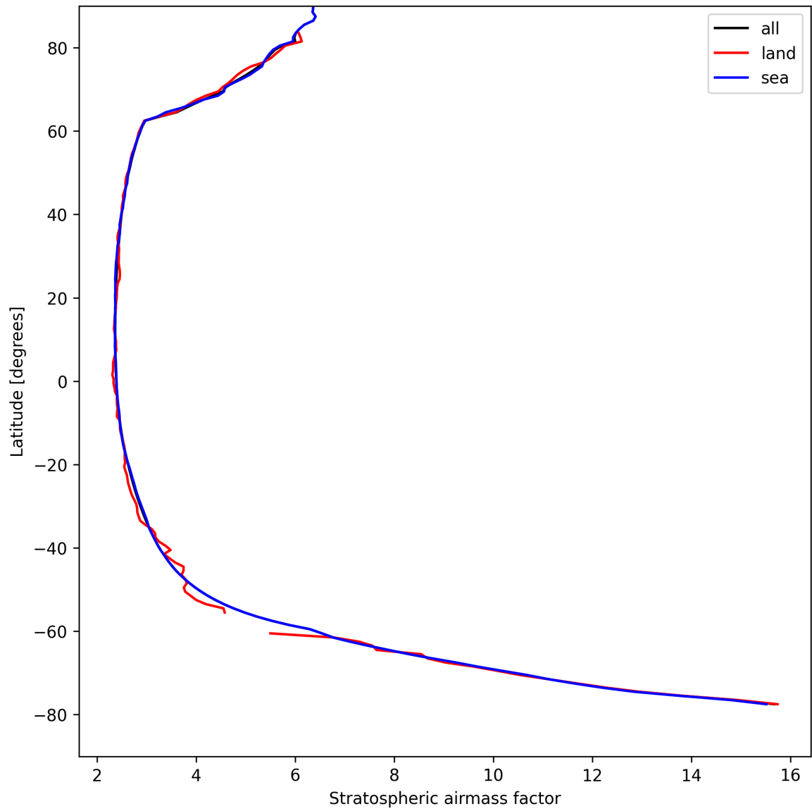
Figure 27: Zonal average of “Stratospheric air mass factor” for 2025-08-23 to 2025-08-25.
