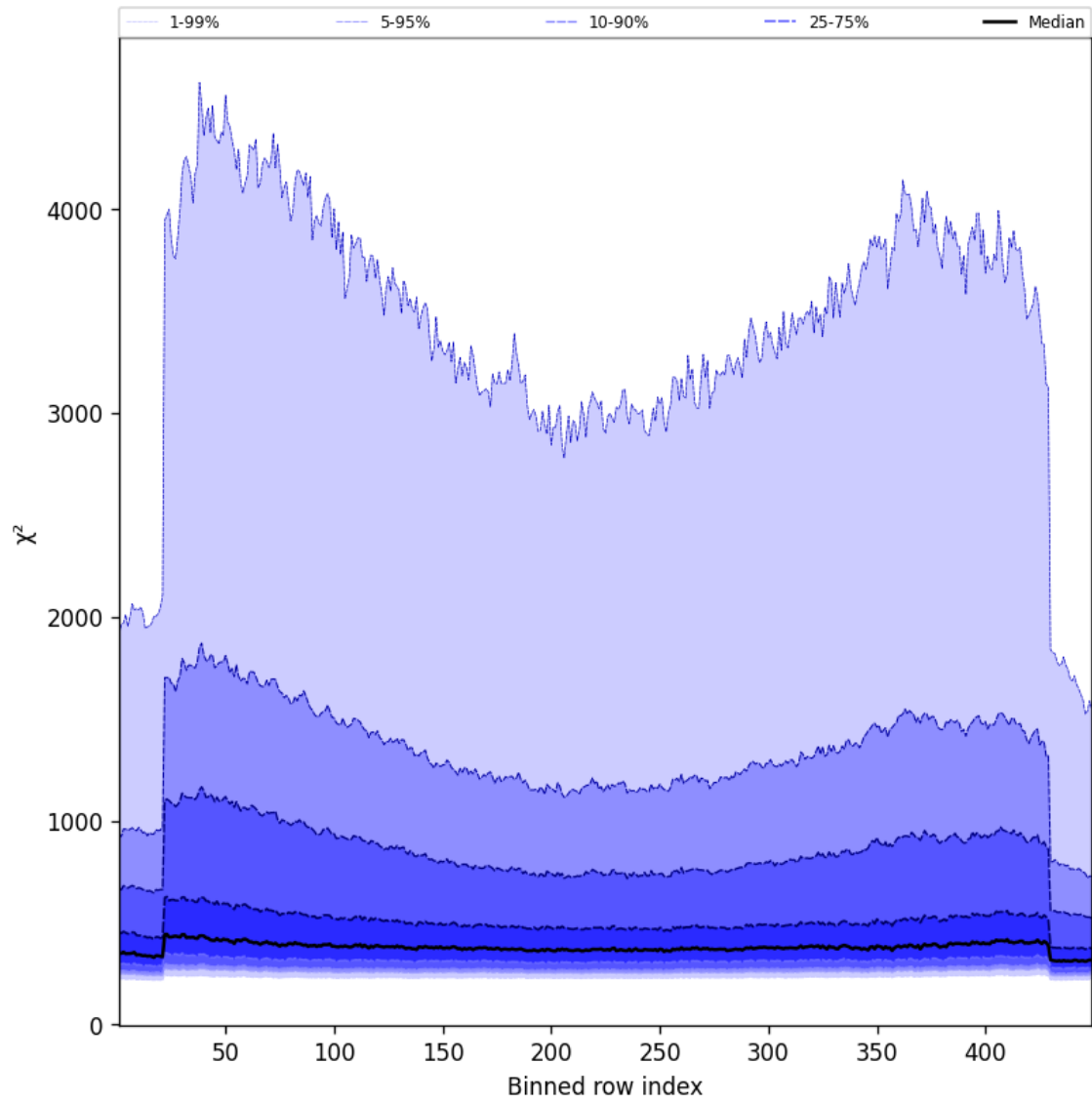
Figure 59: Along track statistics of “ \chi^2 ” for 2025-08-23 to 2025-08-25
