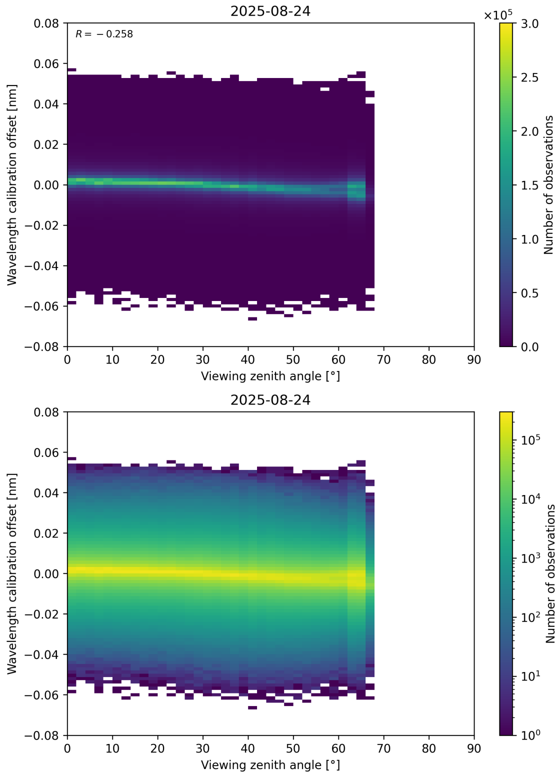
Figure 173: Scatter density plot of “Viewing zenith angle” against “Wavelength calibration offset” for 2025-08-23 to 2025-08-25.
