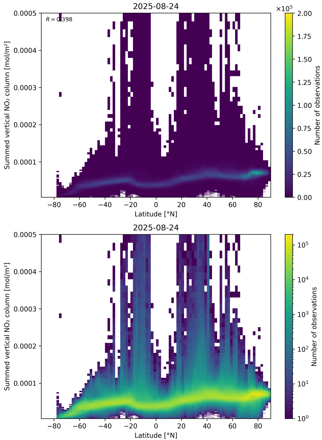
Figure 88: Scatter density plot of “Latitude” against “Summed vertical NO 2 column” for 2025-08-23 to 2025-08-25.
