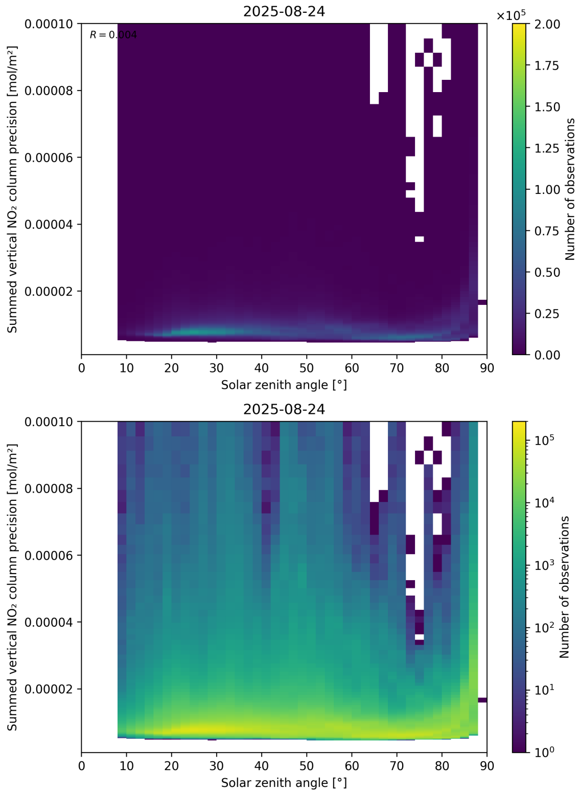
Figure 152: Scatter density plot of “Solar zenith angle” against “Summed vertical NO 2 column precision” for 2025-08-23 to 2025-08-25.
