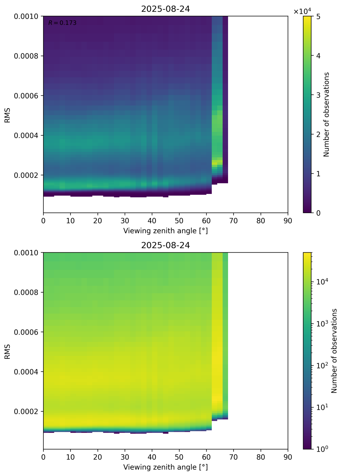
Figure 171: Scatter density plot of “Viewing zenith angle” against “RMS” for 2025-08-23 to 2025-08-25.
