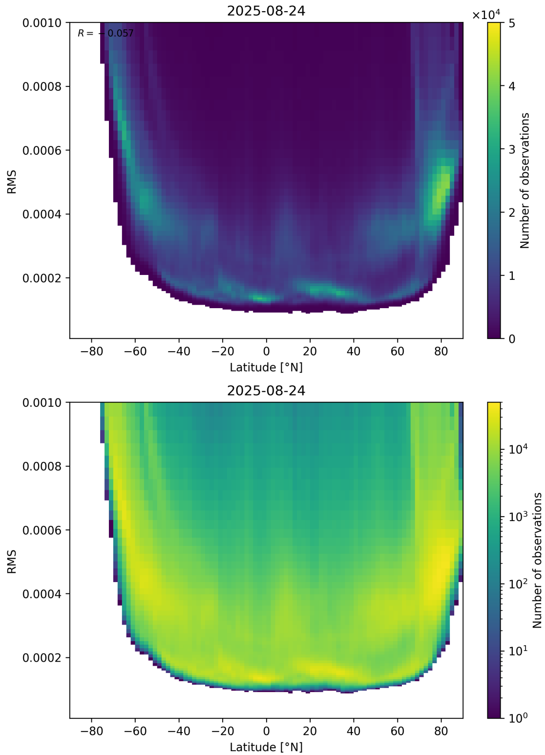
Figure 94: Scatter density plot of “Latitude” against “RMS” for 2025-08-23 to 2025-08-25.
