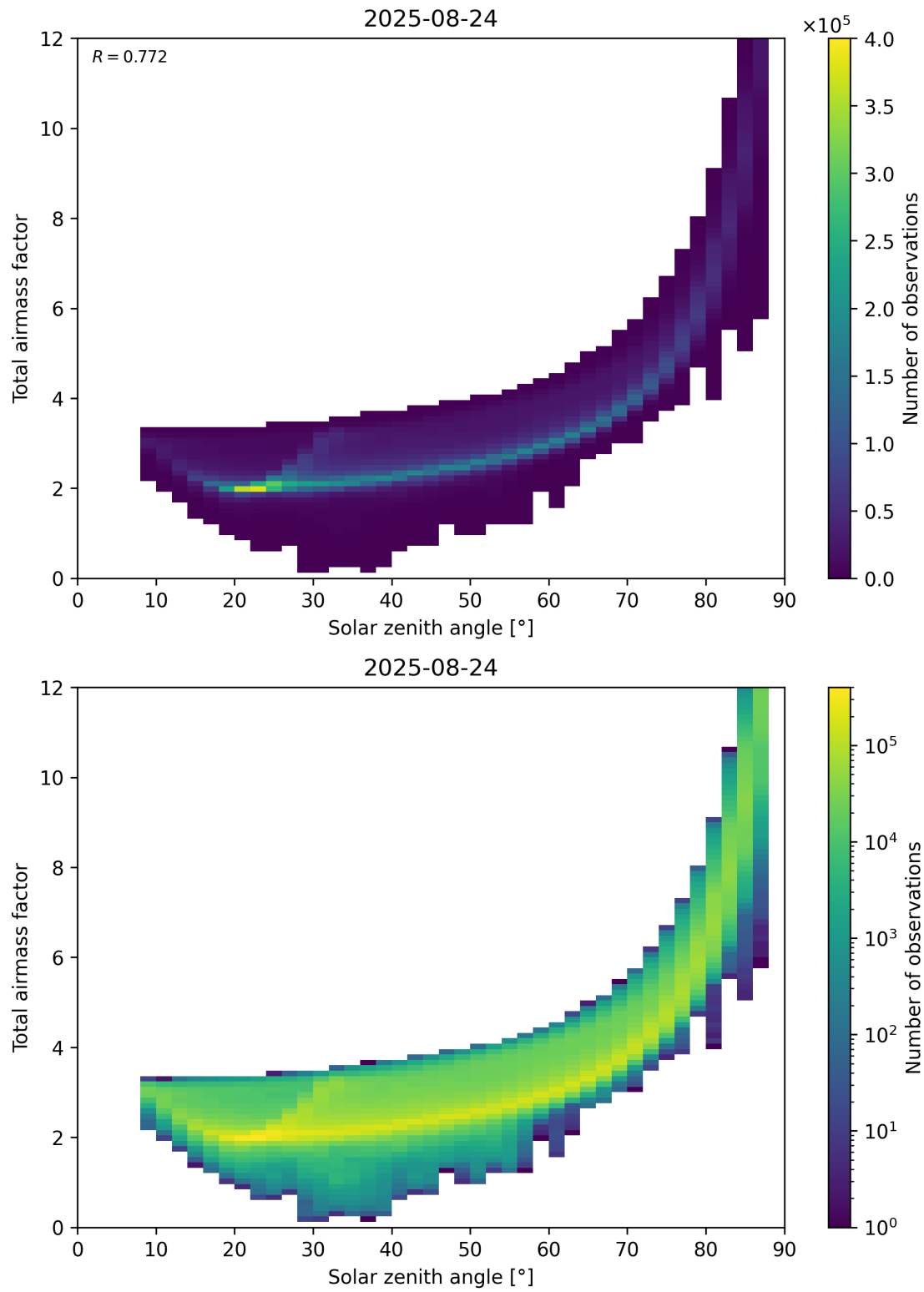
Figure 146: Scatter density plot of “Solar zenith angle” against “Total air mass factor” for 2025-08-23 to 2025-08-25.
