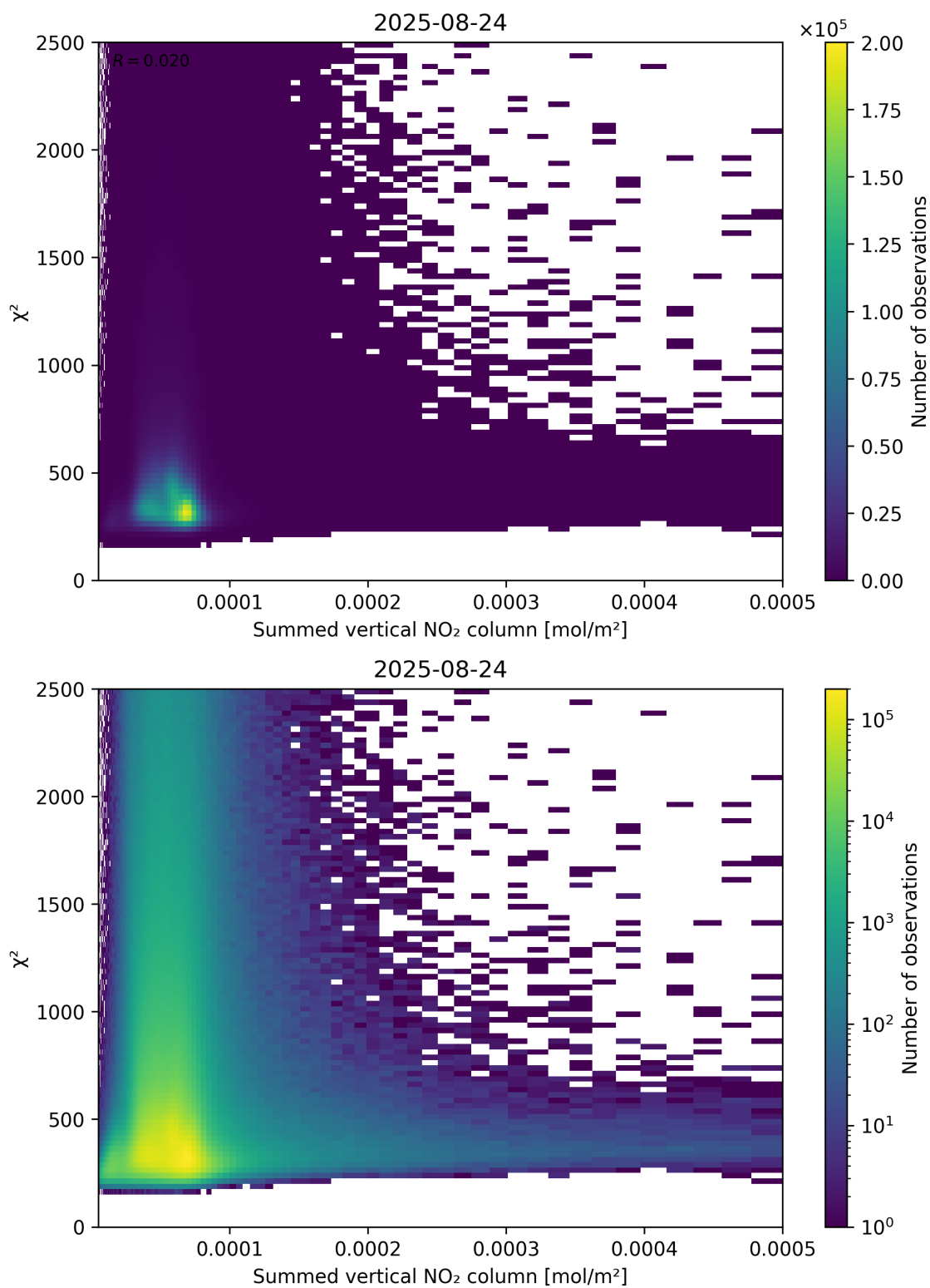
Figure 104: Scatter density plot of “Summed vertical NO 2 column” against “ \chi^2 ” for 2025-08-23 to 2025-08-25.
