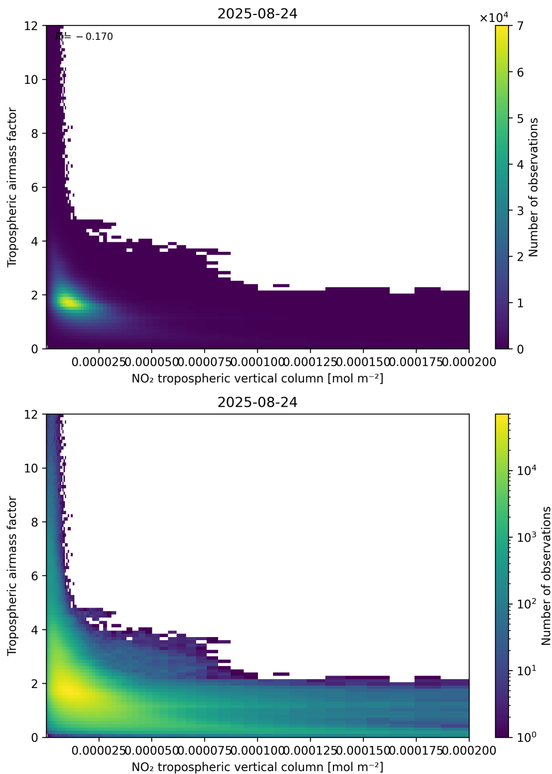
Figure 123: Scatter density plot of “NO 2 tropospheric vertical column” against “Tropospheric air mass factor” for 2025-08-23 to 2025-08-25.
