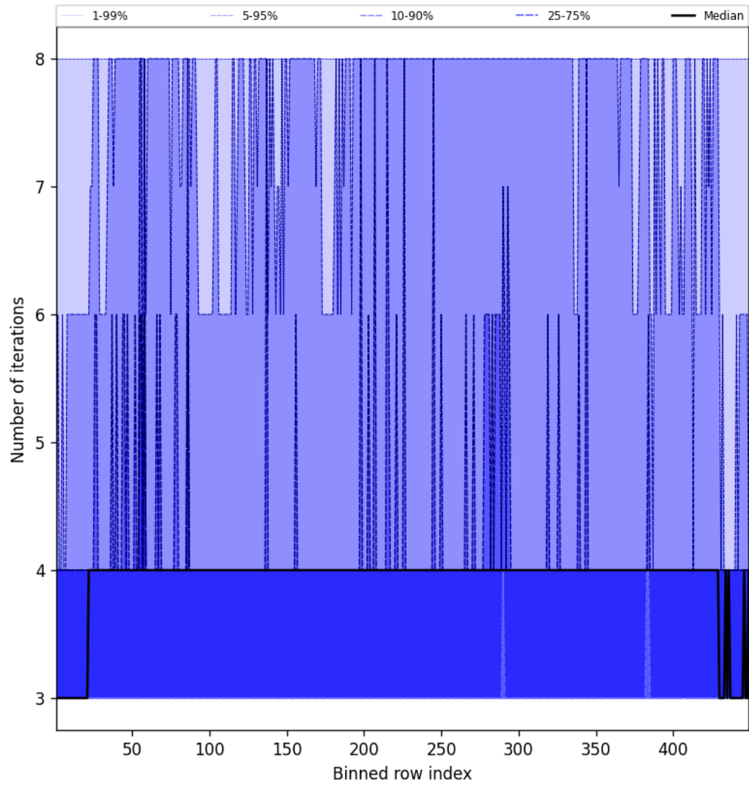
Figure 51: Along track statistics of “Number of iterations” for 2025-08-23 to 2025-08-25
