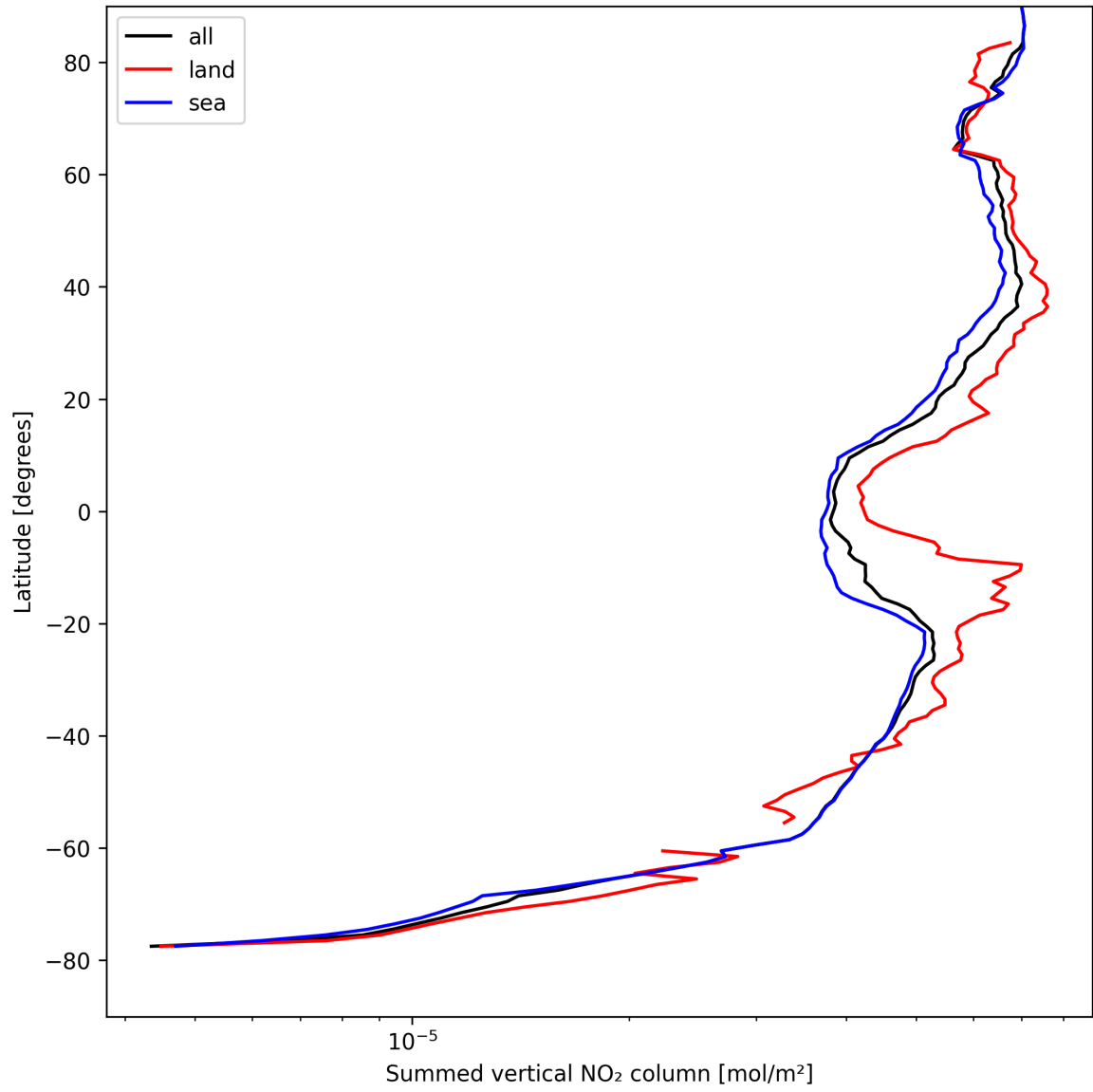
Figure 23: Zonal average of “Summed vertical NO 2 column” for 2025-08-23 to 2025-08-25.
