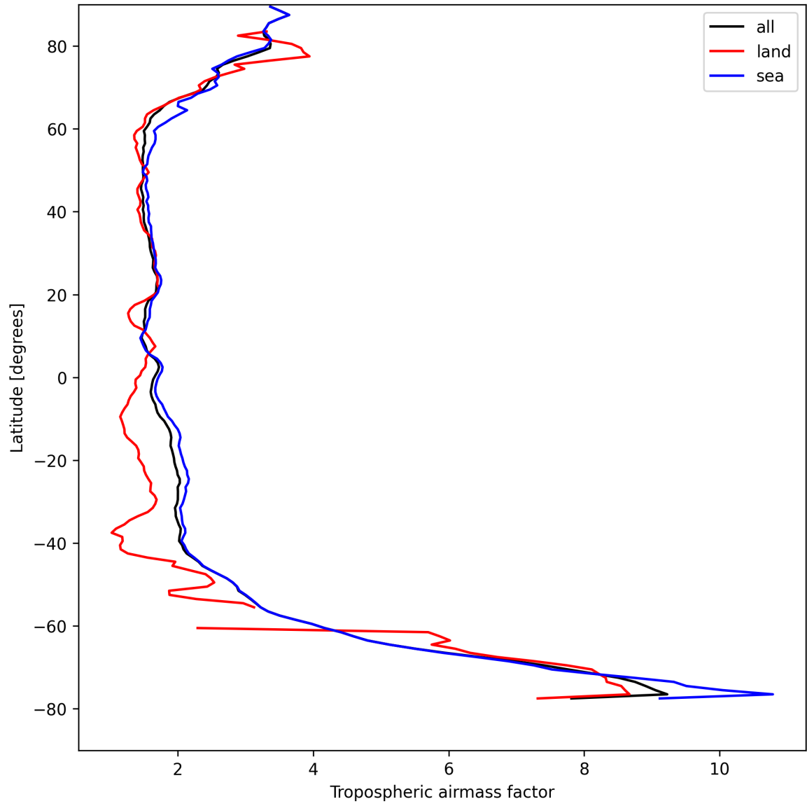
Figure 14: Zonal average of “Tropospheric airmass factor” for 2025-08-23 to 2025-08-25.
