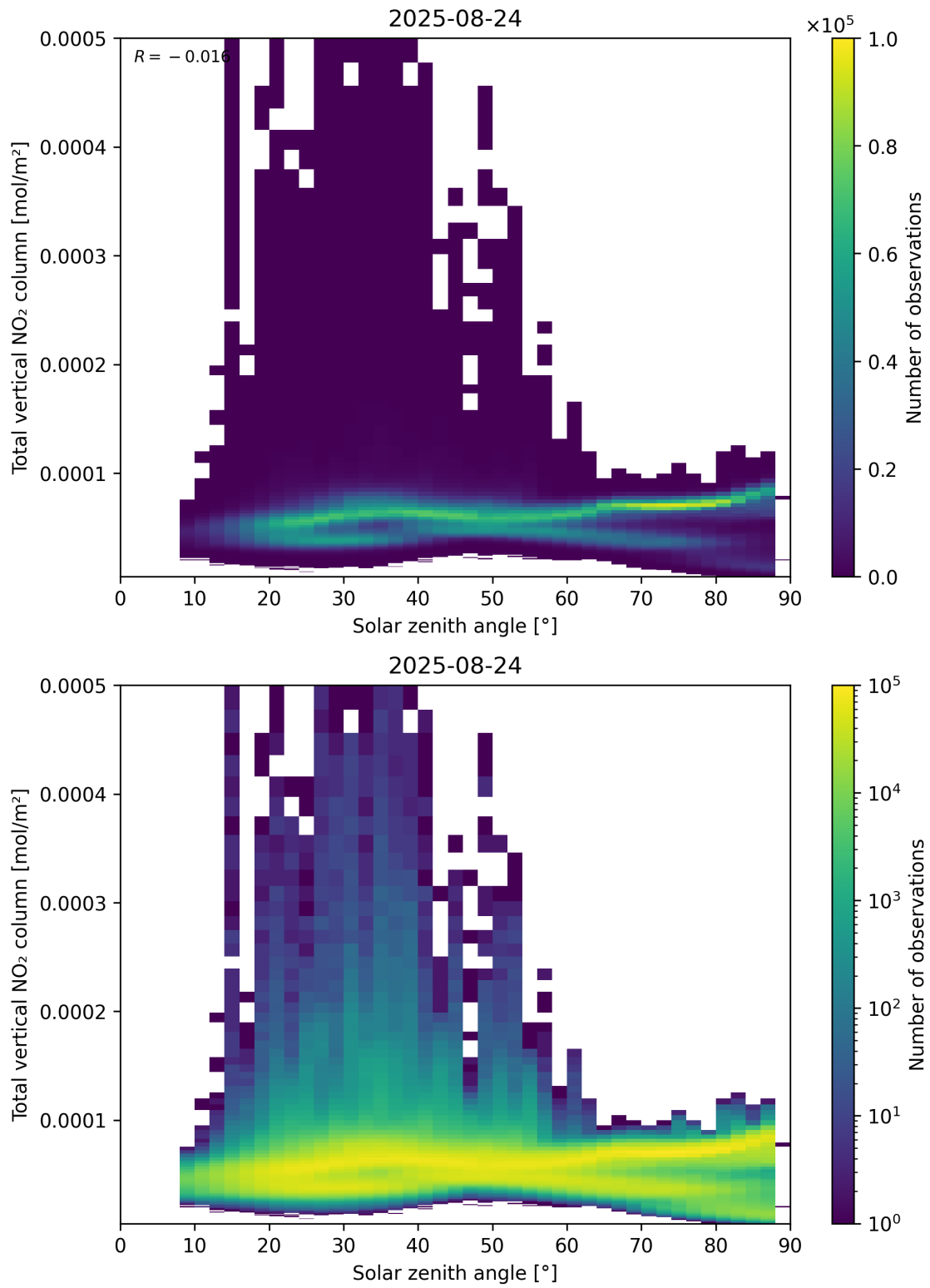
Figure 153: Scatter density plot of “Solar zenith angle” against “Total vertical NO 2 column” for 2025-08-23 to 2025-08-25.
