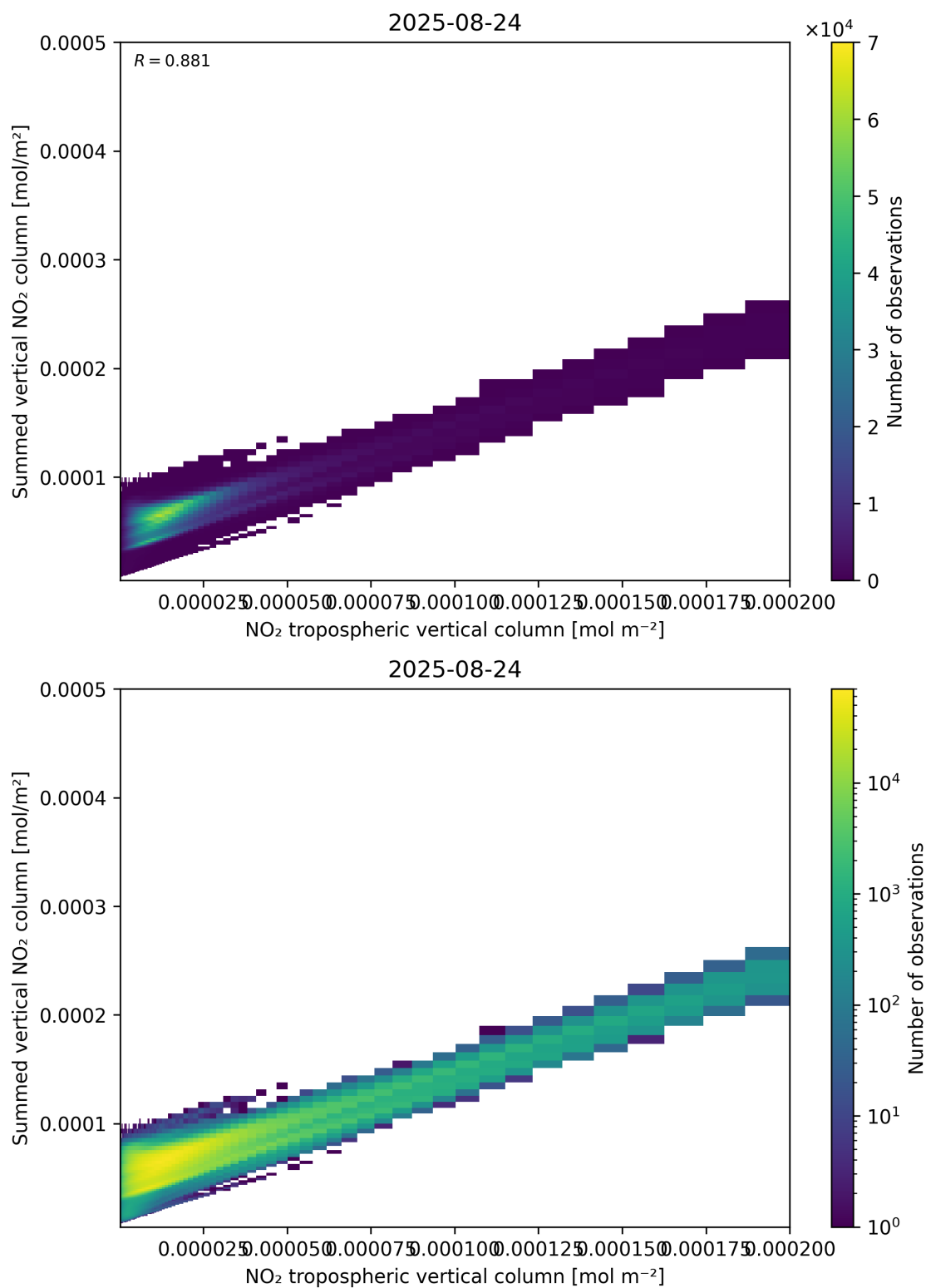
Figure 126: Scatter density plot of “NO 2 tropospheric vertical column” against “Summed vertical NO 2 column” for 2025-08-23 to 2025-08-25.
