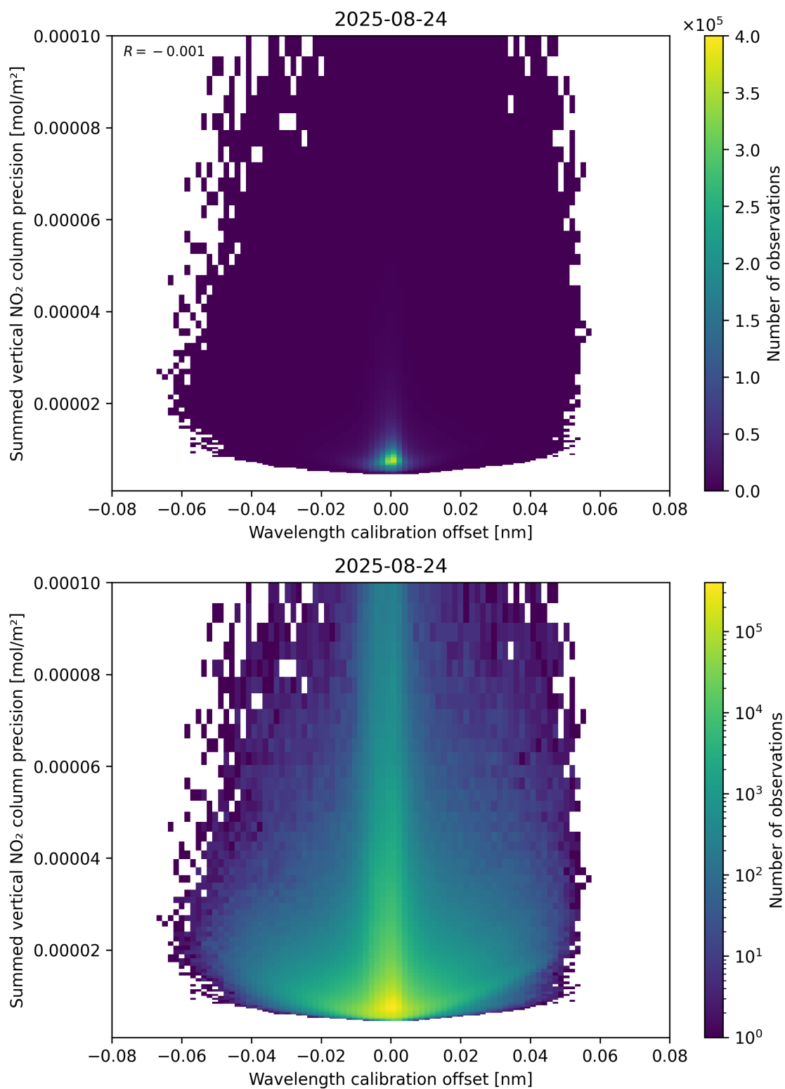
Figure 178: Scatter density plot of “Wavelength calibration offset” against “Summed vertical NO 2 column precision” for 2025-08-23 to 2025-08-25.
