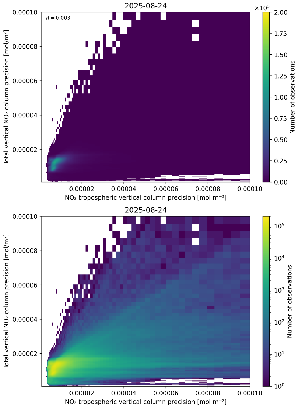
Figure 139: Scatter density plot of “NO 2 tropospheric vertical column precision” against “Total vertical NO 2 column precision” for 2025-08-23 to 2025-08-25.
