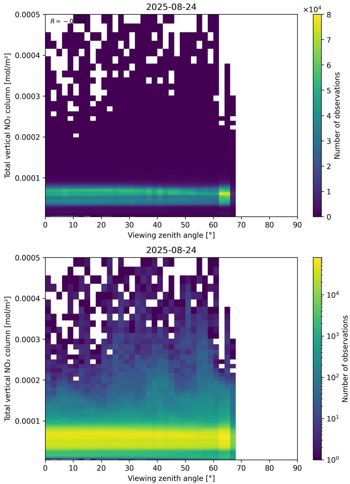
Figure 167: Scatter density plot of “Viewing zenith angle” against “Total vertical NO 2 column” for 2025-08-23 to 2025-08-25.
