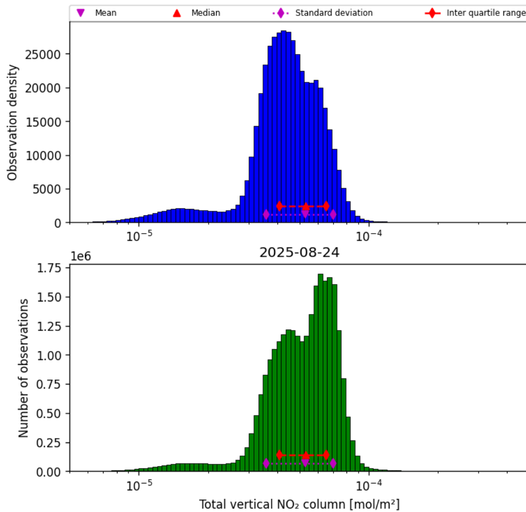
Figure 38: Histogram of “Total vertical NO 2 column” for 2025-08-23 to 2025-08-25
