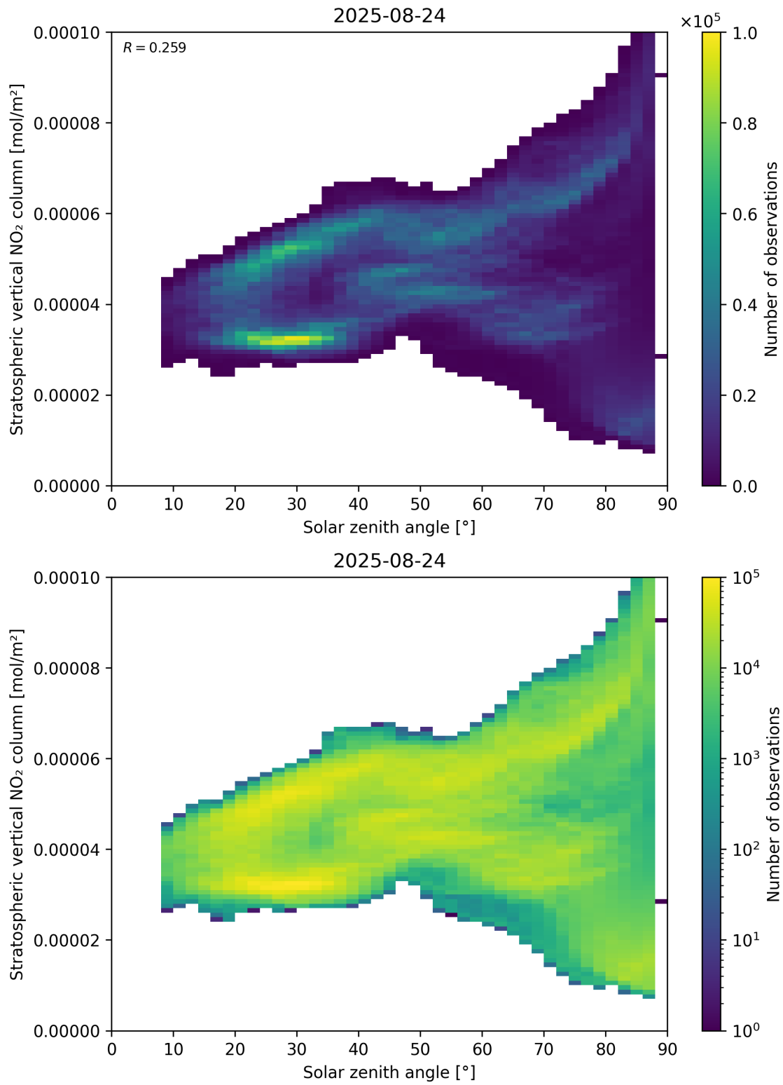
Figure 150: Scatter density plot of “Solar zenith angle” against “Stratospheric vertical NO 2 column” for 2025-08-23 to 2025-08-25.
