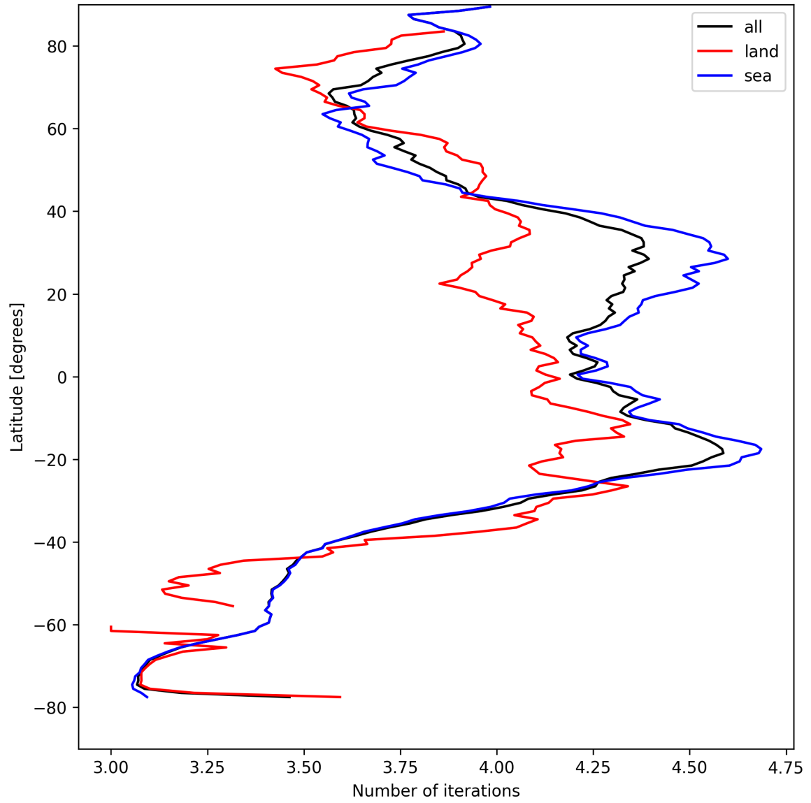
Figure 17: Zonal average of “Number of iterations” for 2025-08-23 to 2025-08-25.
