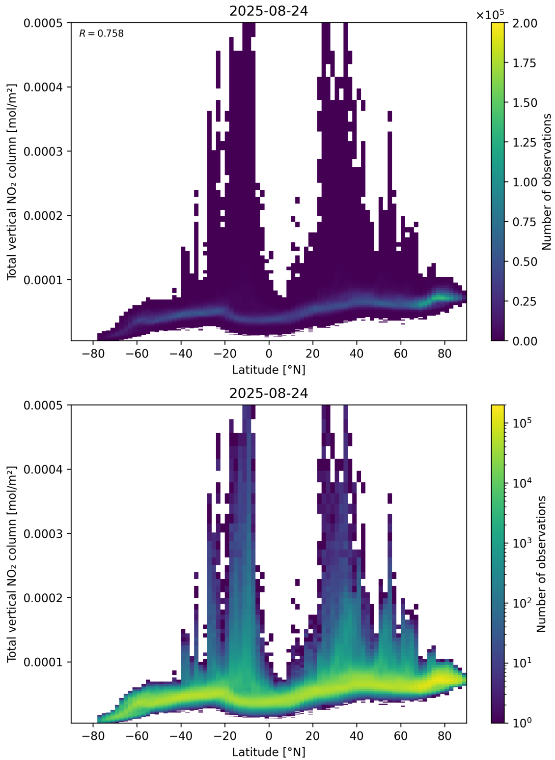
Figure 90: Scatter density plot of “Latitude” against “Total vertical NO 2 column” for 2025-08-23 to 2025-08-25.
