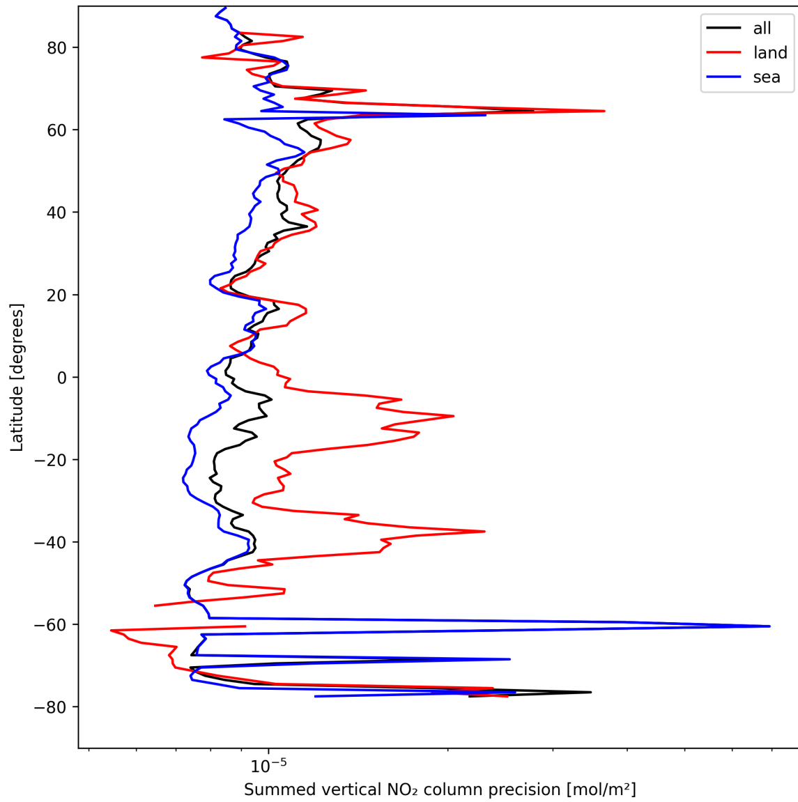
Figure 24: Zonal average of "Summed vertical NO 2 column precision" for 2025-08-23 to 2025-08-25.
