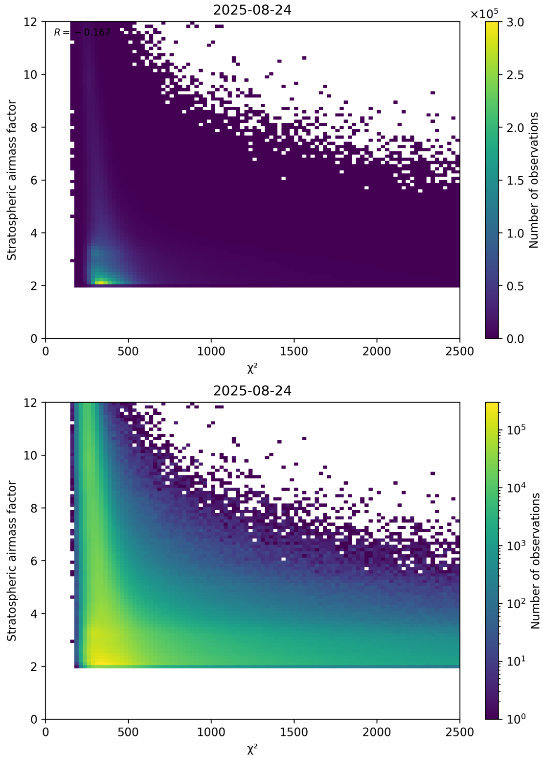
Figure 81: Scatter density plot of “ \chi^2 ” against “Stratospheric airmass factor” for 2025-08-23 to 2025-08-25.
