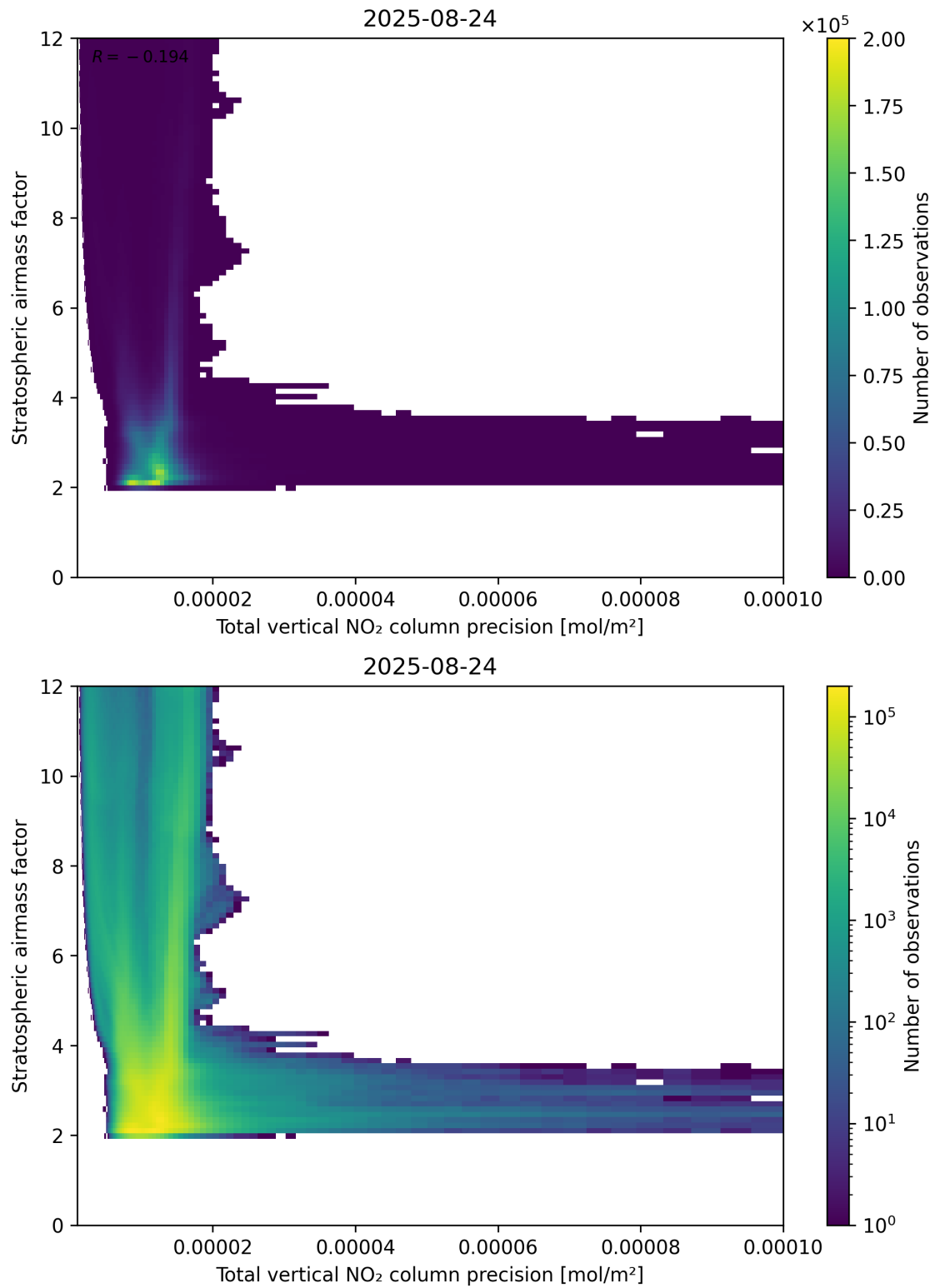
Figure 115: Scatter density plot of “Total vertical NO 2 column precision” against “Stratospheric air mass factor” for 2025-08-23 to 2025-08-25.
