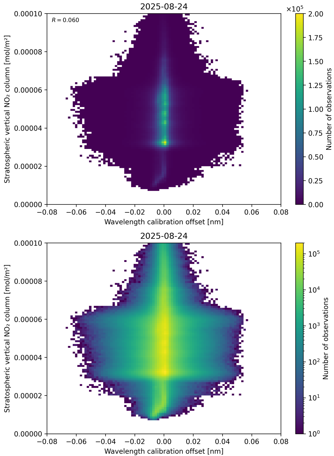
Figure 176: Scatter density plot of “Wavelength calibration offset” against “Stratospheric vertical NO 2 column” for 2025-08-23 to 2025-08-25.
