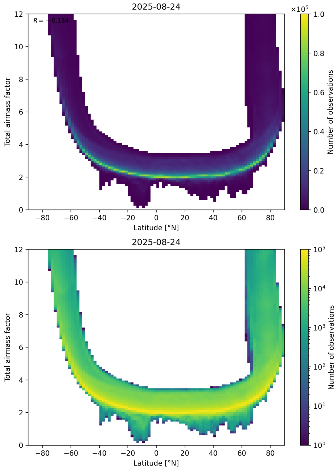
Figure 84: Scatter density plot of “Latitude” against “Total airmass factor” for 2025-08-23 to 2025-08-25.
