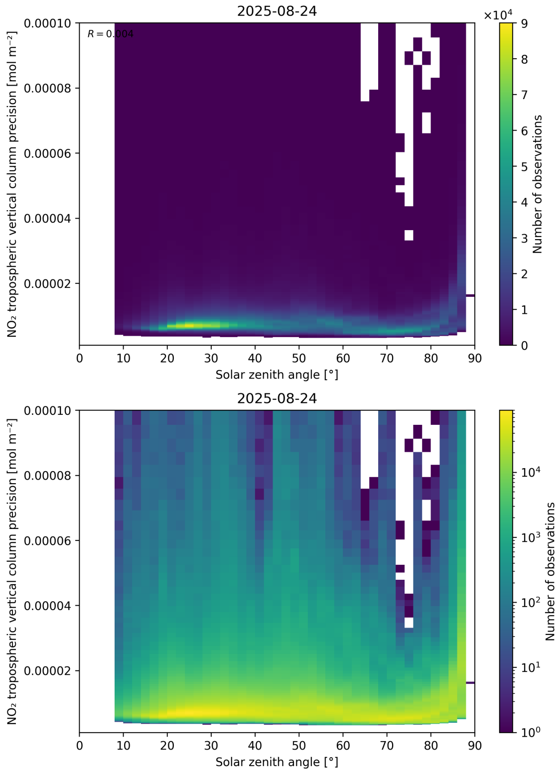
Figure 156: Scatter density plot of “Solar zenith angle” against “NO 2 tropospheric vertical column precision” for 2025-08-23 to 2025-08-25.
