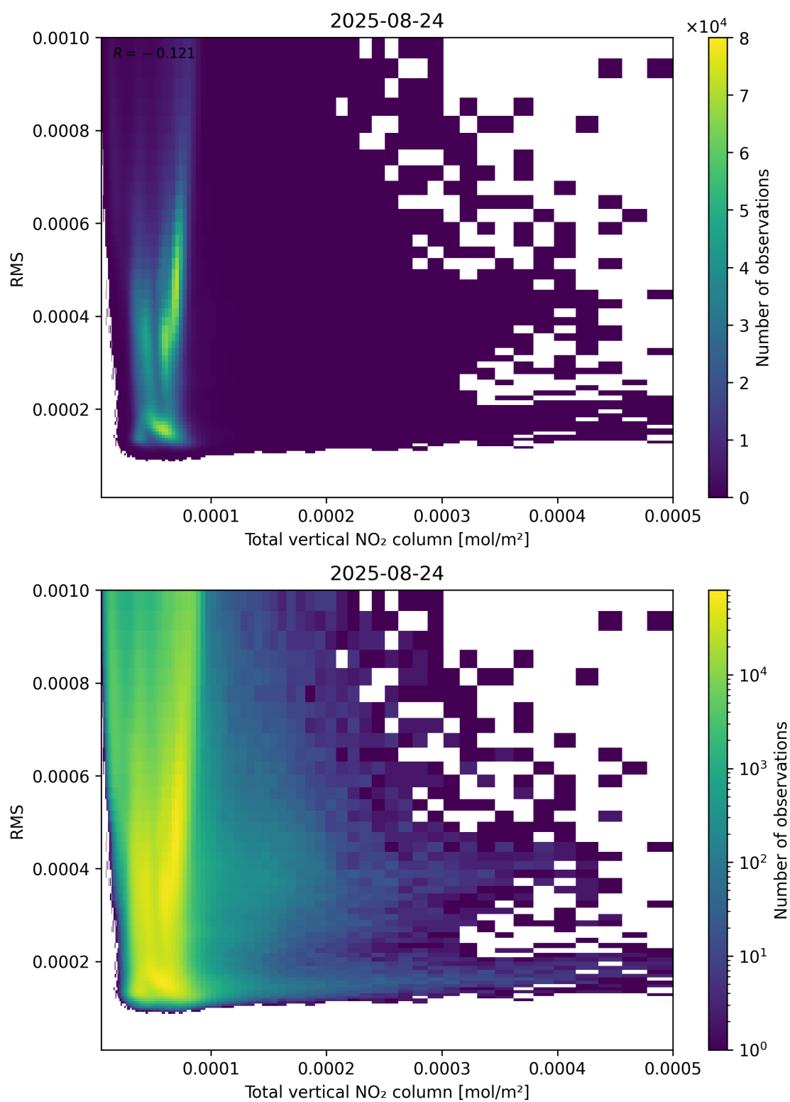
Figure 120: Scatter density plot of “Total vertical NO 2 column” against “RMS” for 2025-08-23 to 2025-08-25.
