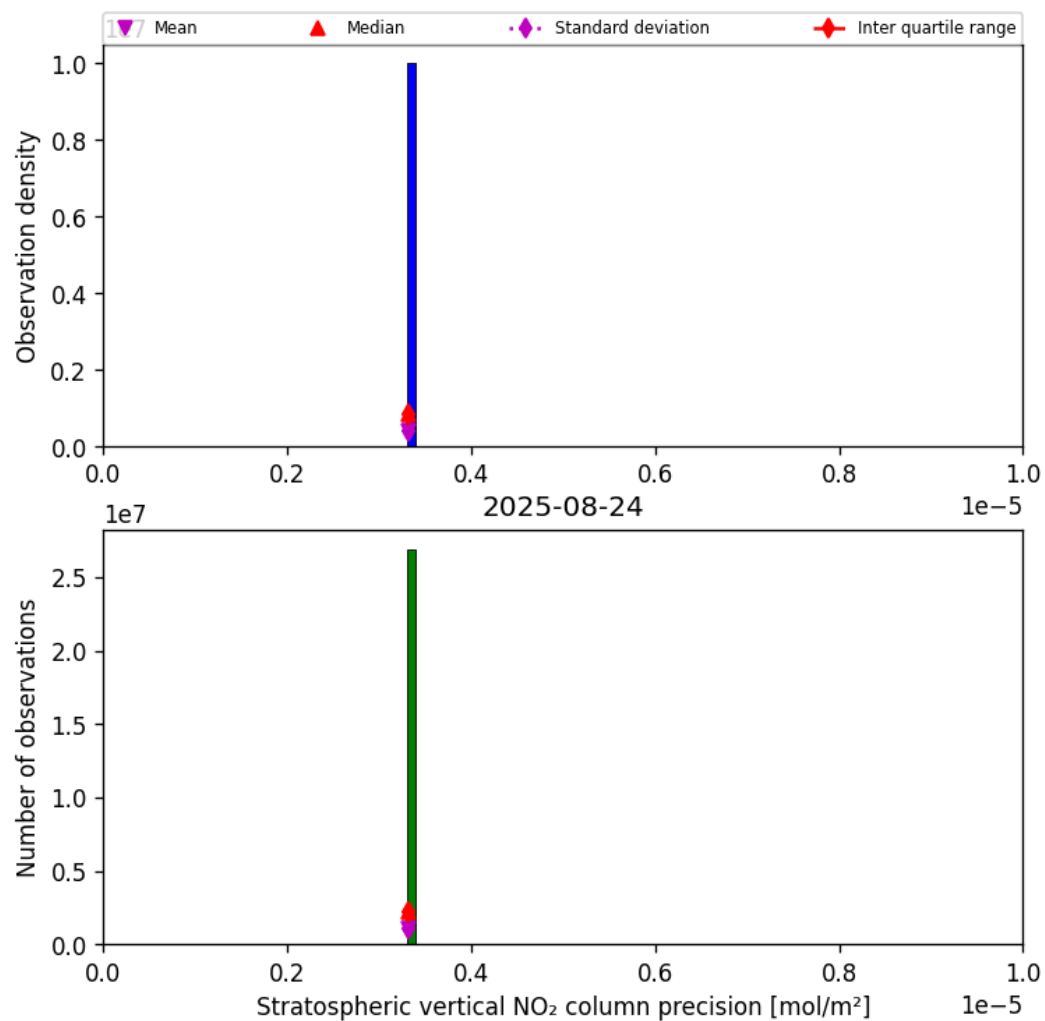
Figure 37: Histogram of “Stratospheric vertical NO 2 column precision” for 2025-08-23 to 2025-08-25
