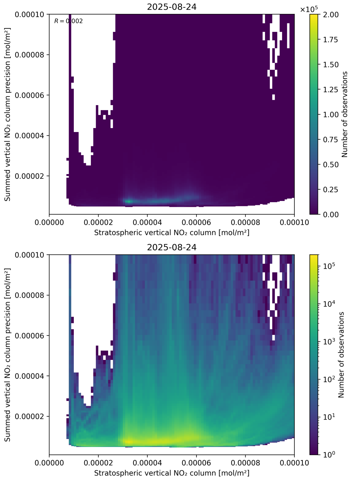
Figure 99: Scatter density plot of “Stratospheric vertical NO 2 column” against “Summed vertical NO 2 column precision” for 2025-08-23 to 2025-08-25.
