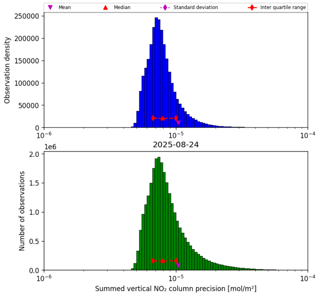
Figure 41: Histogram of "Summed vertical NO 2 column precision" for 2025-08-23 to 2025-08-25
