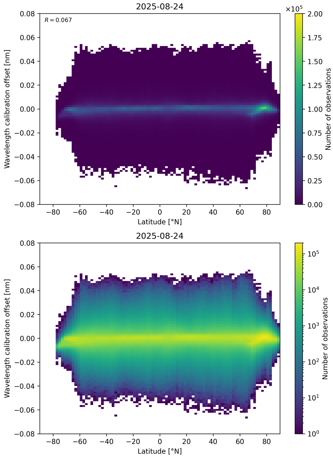
Figure 95: Scatter density plot of “Latitude” against “Wavelength calibration offset” for 2025-08-23 to 2025-08-25.
