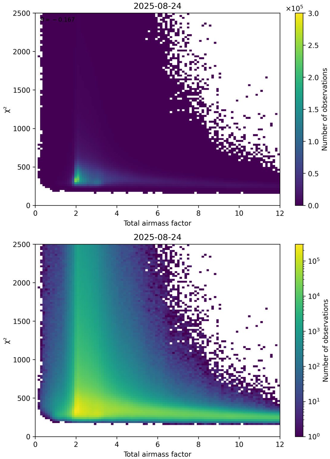
Figure 63: Scatter density plot of “Total airmass factor” against “ \chi^2 ” for 2025-08-23 to 2025-08-25.
