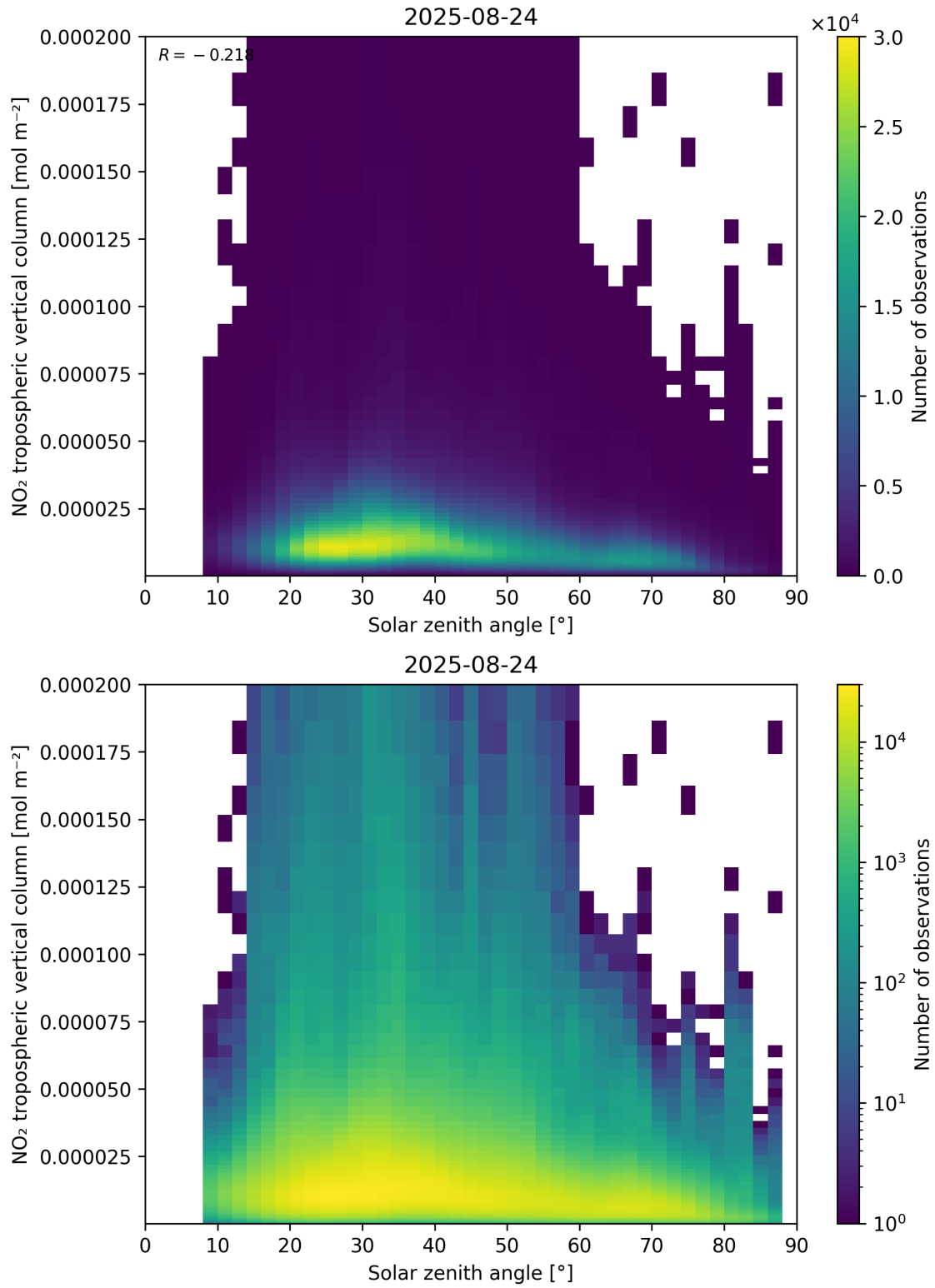
Figure 155: Scatter density plot of “Solar zenith angle” against “NO 2 tropospheric vertical column” for 2025-08-23 to 2025-08-25.
