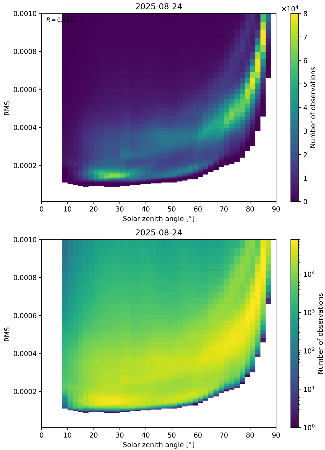
Figure 157: Scatter density plot of “Solar zenith angle” against “RMS” for 2025-08-23 to 2025-08-25.
