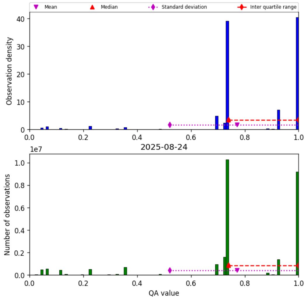
Figure 28: Histogram of “QA value” for 2025-08-23 to 2025-08-25
