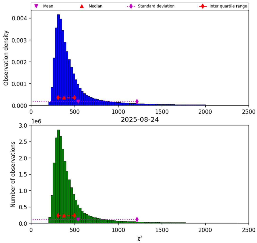
Figure 42: Histogram of “ \chi^2 ” for 2025-08-23 to 2025-08-25
