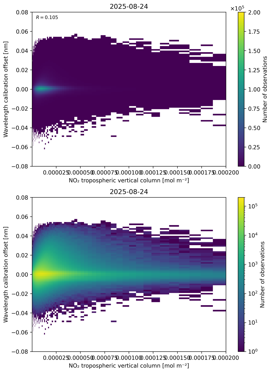
Figure 143: Scatter density plot of “NO 2 tropospheric vertical column” against “Wavelength calibration offset” for 2025-08-23 to 2025-08-25.
