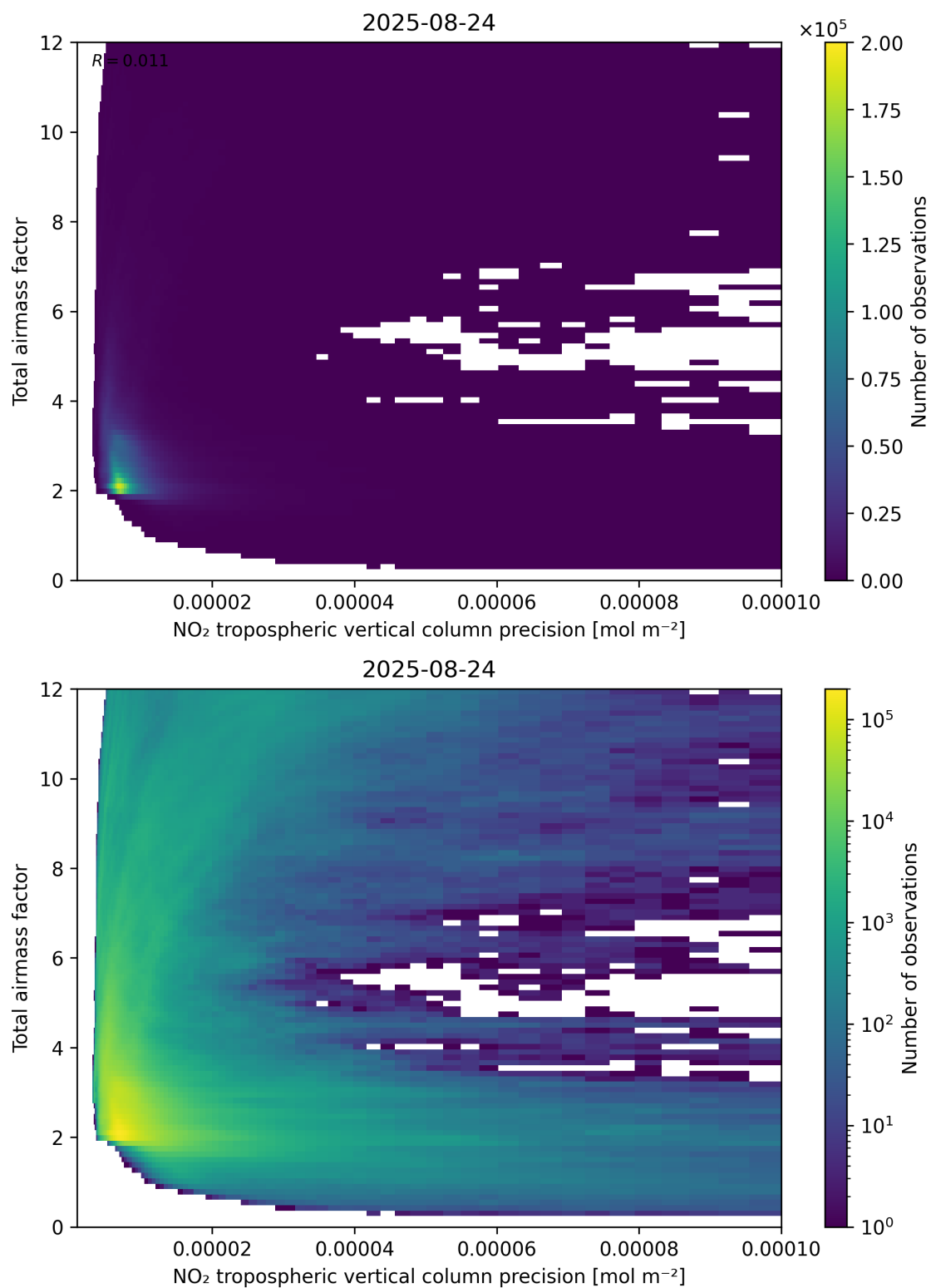
Figure 132: Scatter density plot of “NO 2 tropospheric vertical column precision” against “Total air mass factor” for 2025-08-23 to 2025-08-25.
