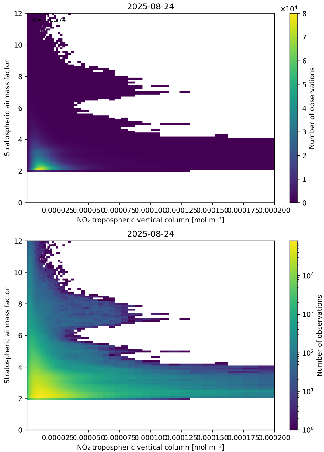
Figure 121: Scatter density plot of “NO 2 tropospheric vertical column” against “Stratospheric air mass factor” for 2025-08-23 to 2025-08-25.
