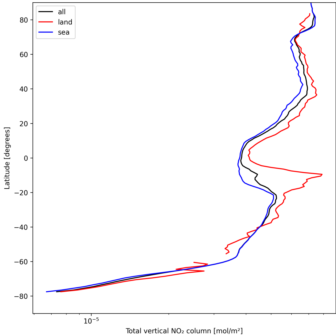
Figure 21: Zonal average of “Total vertical NO 2 column” for 2025-08-23 to 2025-08-25.
