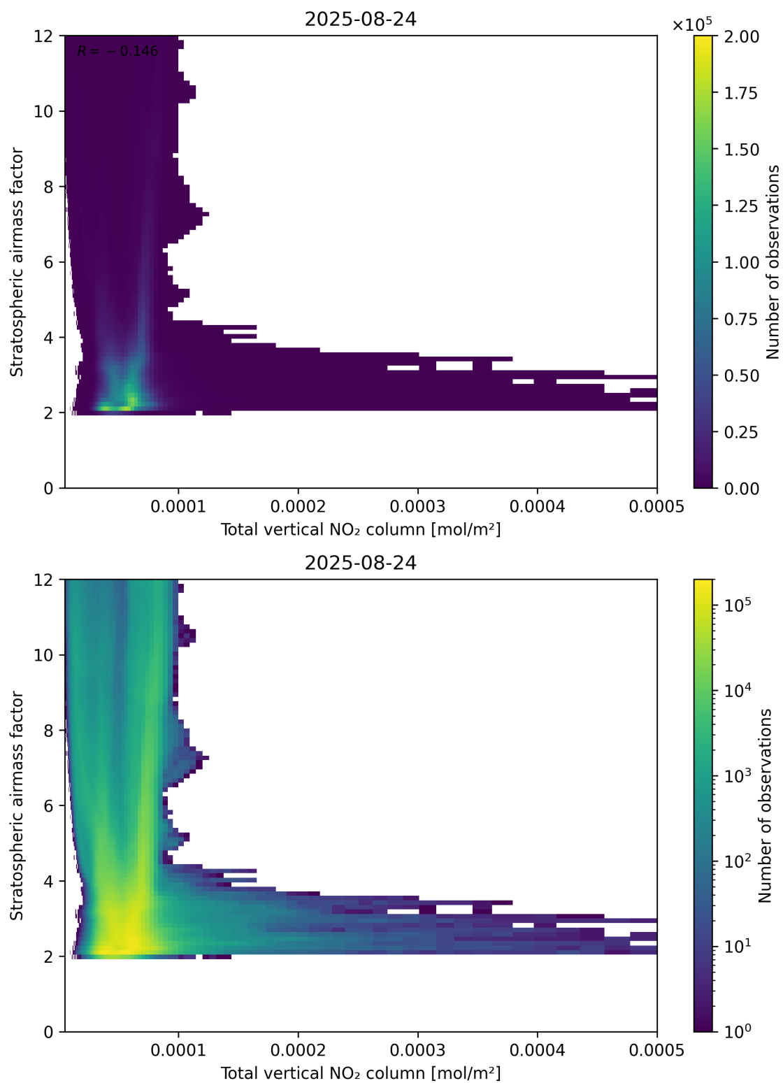
Figure 110: Scatter density plot of “Total vertical NO 2 column” against “Stratospheric airmass factor” for 2025-08-23 to 2025-08-25.
