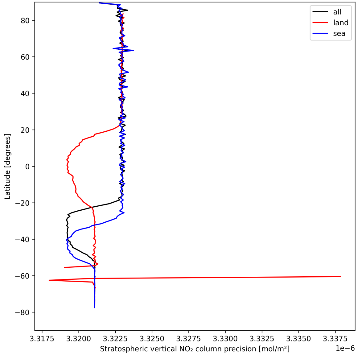
Figure 20: Zonal average of “Stratospheric vertical NO 2 column precision” for 2025-08-23 to 2025-08-25.
