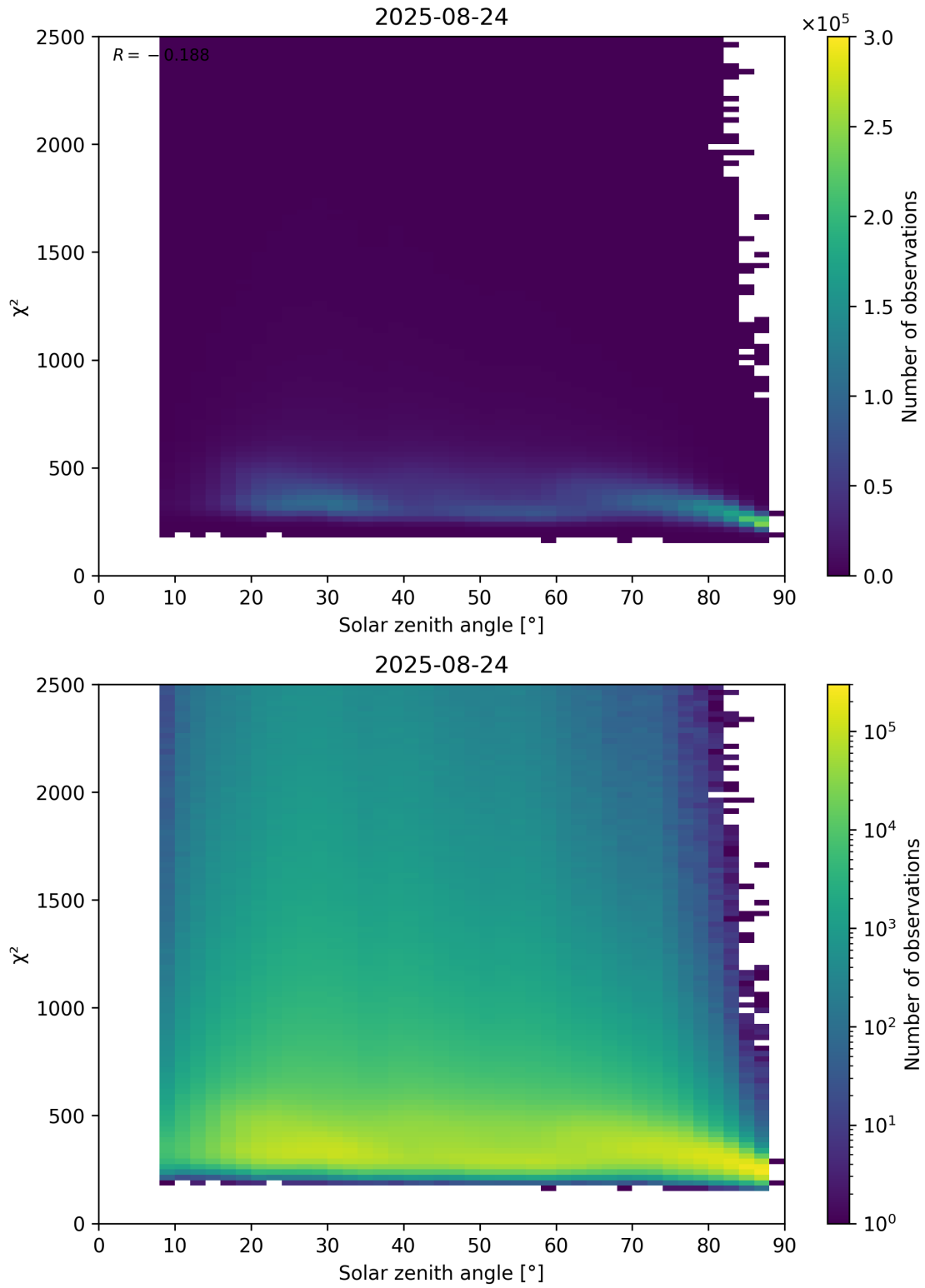
Figure 148: Scatter density plot of “Solar zenith angle” against “ \chi^2 ” for 2025-08-23 to 2025-08-25.
