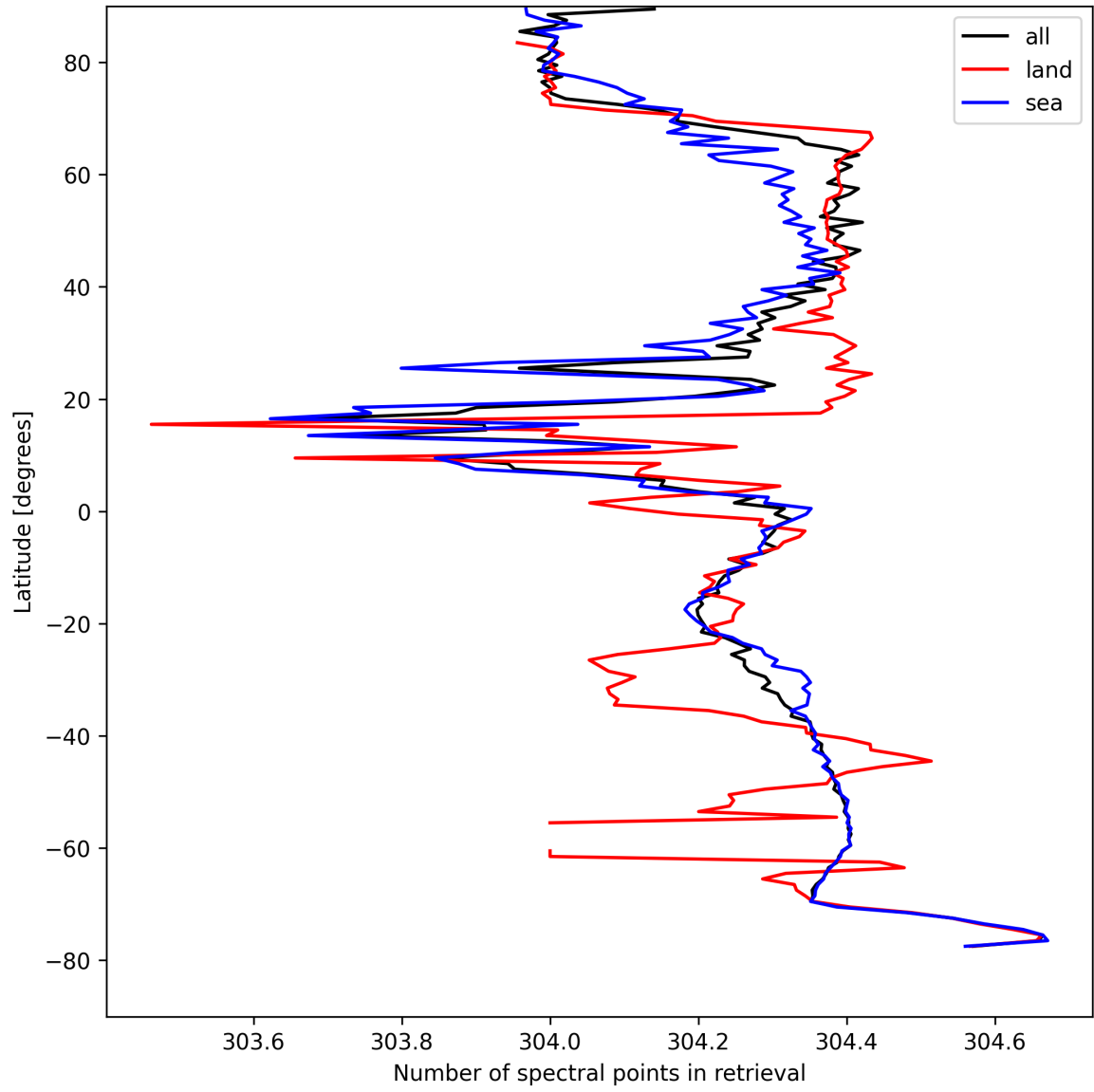
Figure 16: Zonal average of “Number of spectral points in retrieval” for 2025-08-23 to 2025-08-25.
