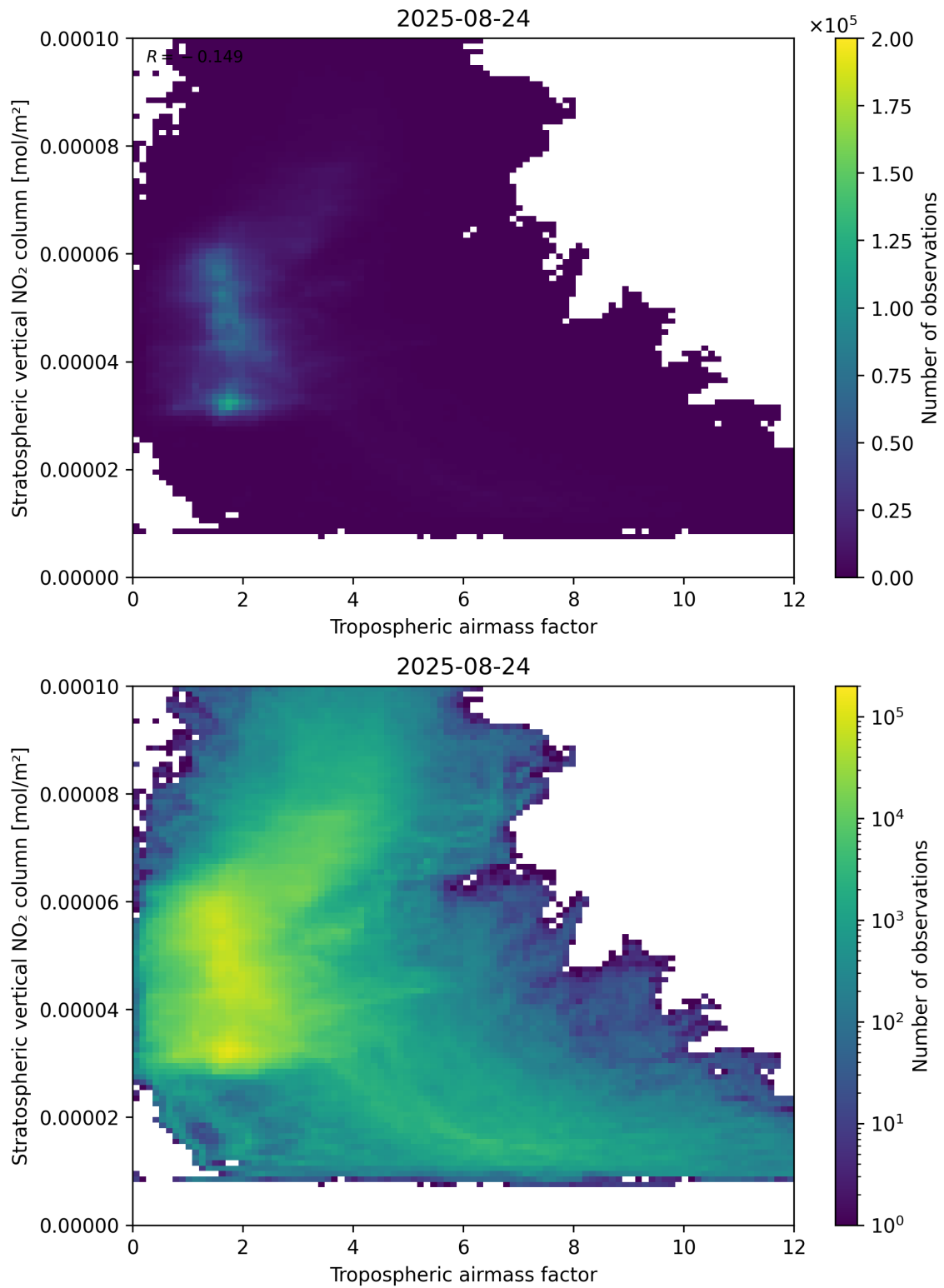
Figure 74: Scatter density plot of “Tropospheric air mass factor” against “Stratospheric vertical NO 2 column” for 2025-08-23 to 2025-08-25.
