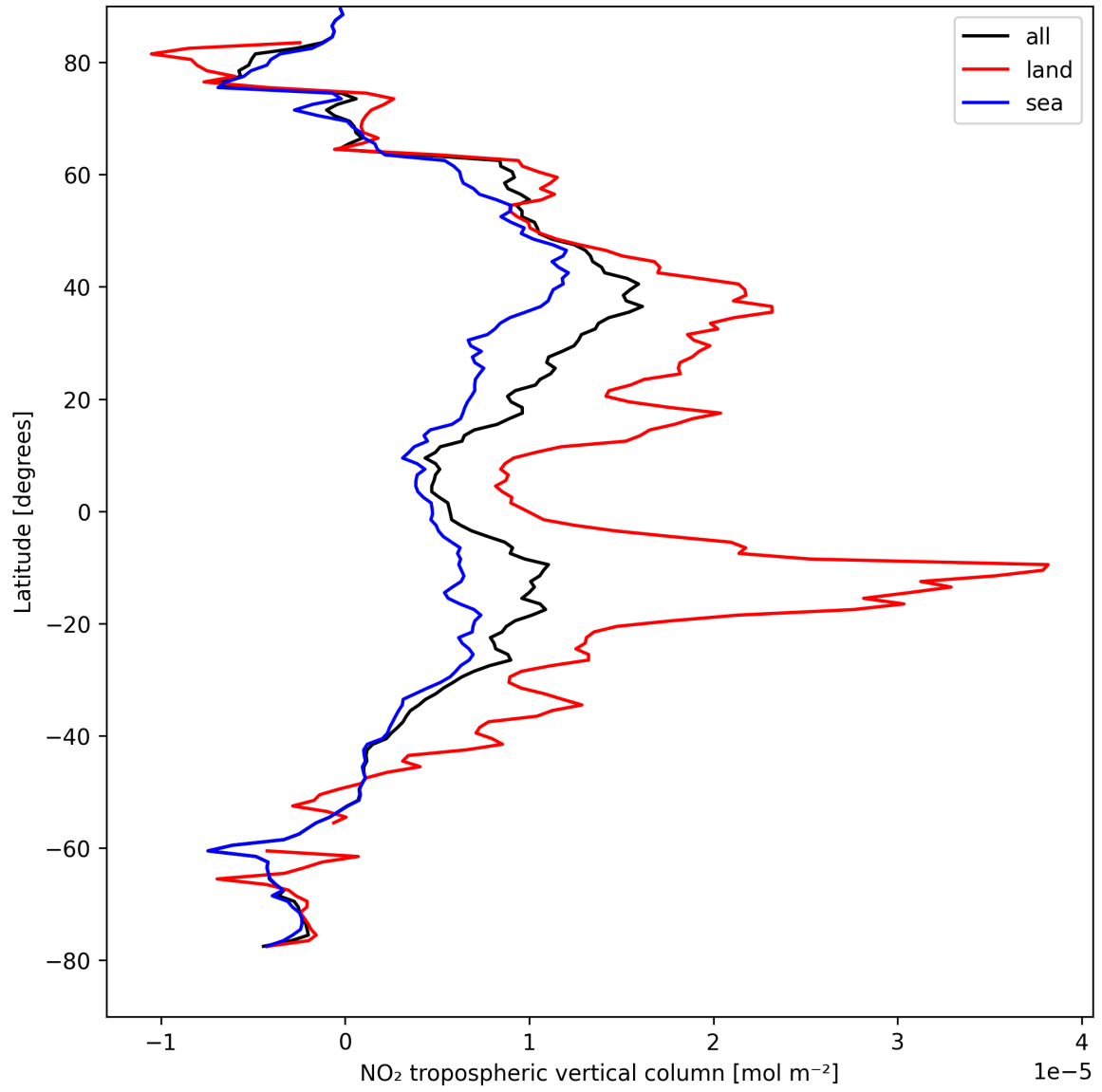
Figure 12: Zonal average of “NO 2 tropospheric vertical column” for 2025-08-23 to 2025-08-25.
