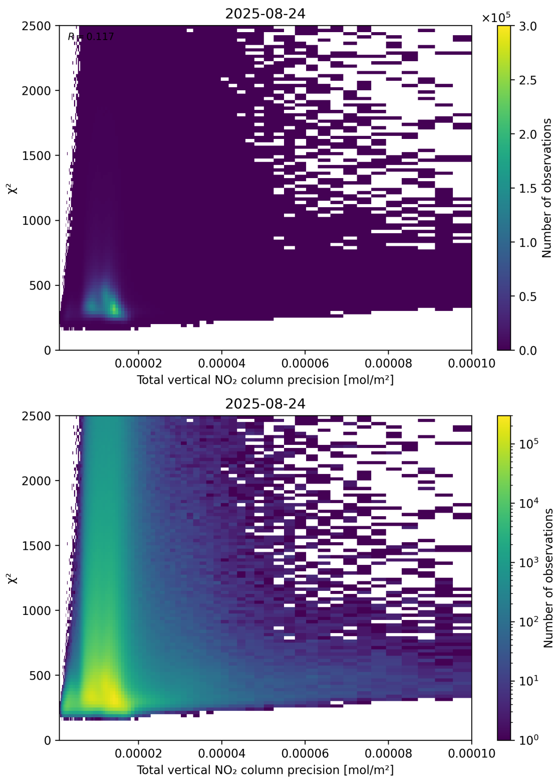
Figure 116: Scatter density plot of “Total vertical NO 2 column precision” against “ \chi^2 ” for 2025-08-23 to 2025-08-25.
