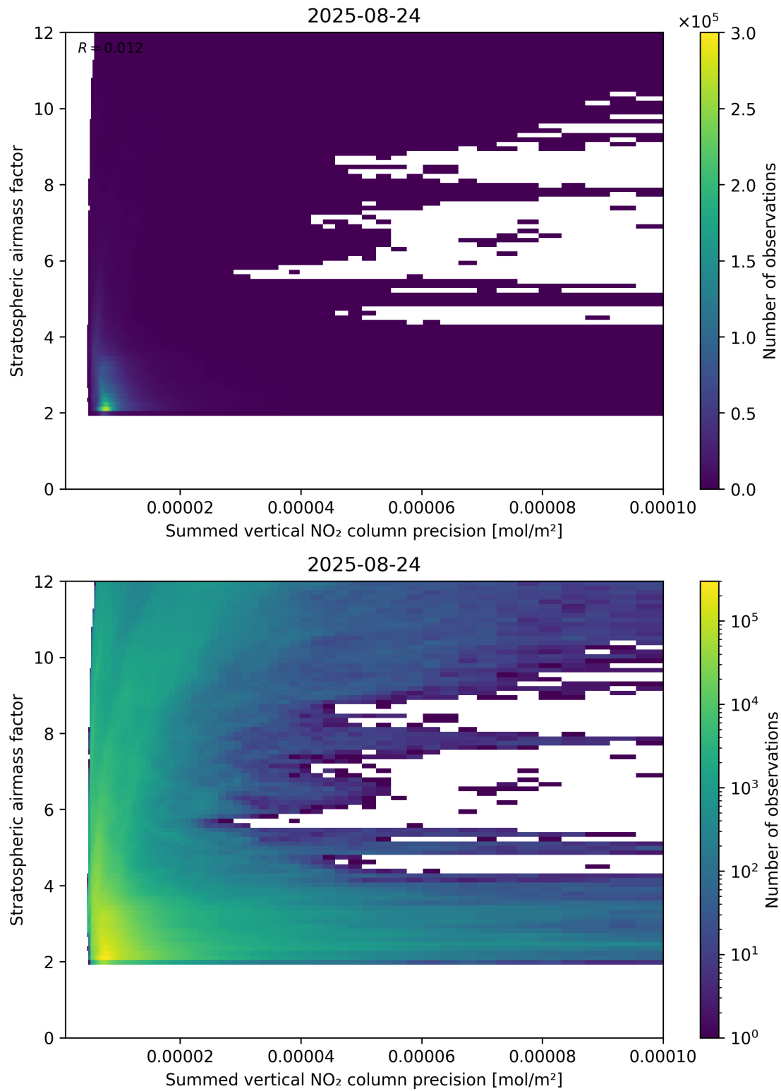
Figure 106: Scatter density plot of “Summed vertical NO 2 column precision” against “Stratospheric airmass factor” for 2025-08-23 to 2025-08-25.
