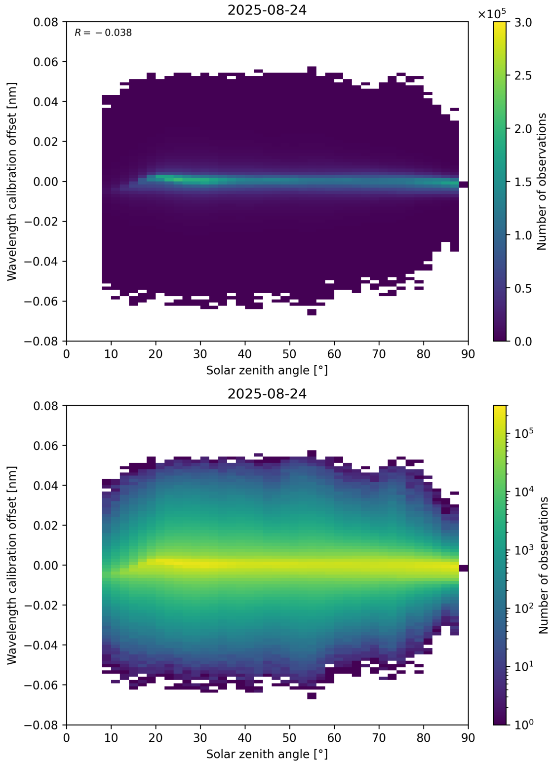
Figure 158: Scatter density plot of “Solar zenith angle” against “Wavelength calibration offset” for 2025-08-23 to 2025-08-25.
