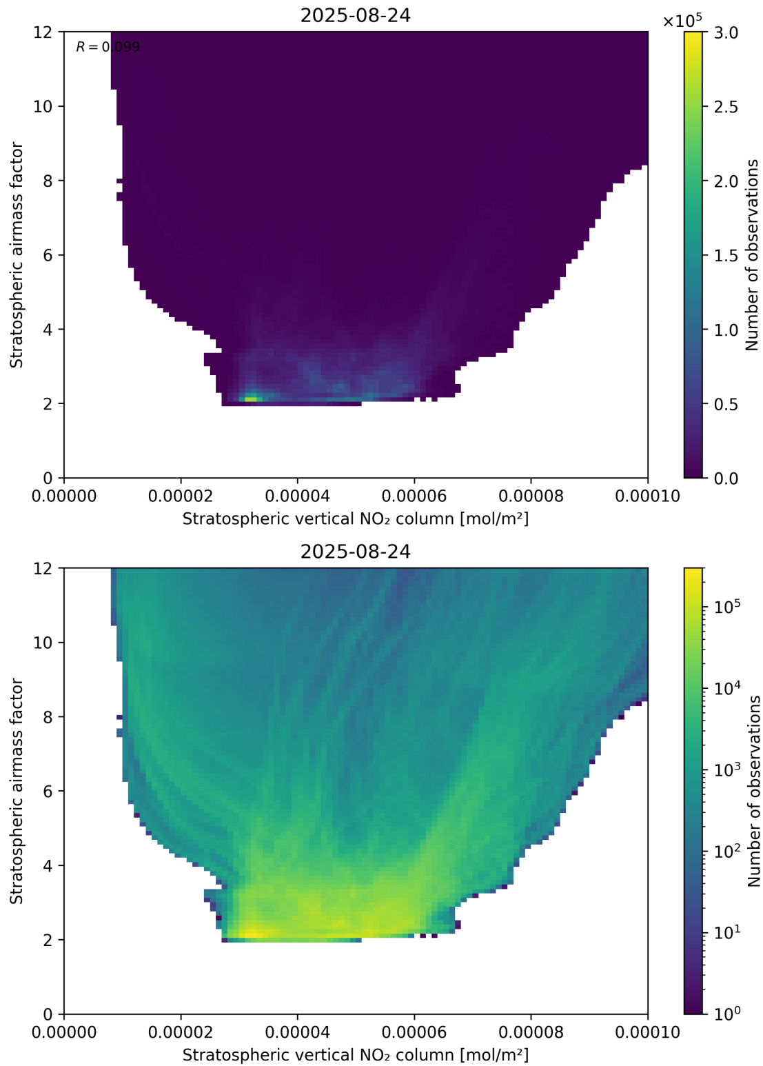
Figure 96: Scatter density plot of “Stratospheric vertical NO 2 column” against “Stratospheric airmass factor” for 2025-08-23 to 2025-08-25.
