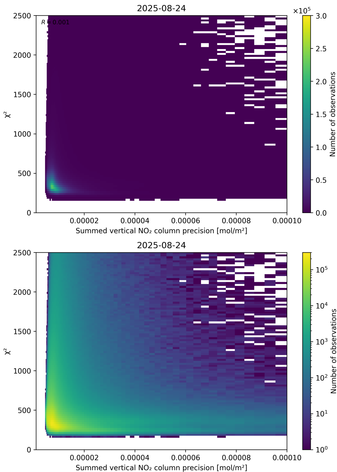
Figure 107: Scatter density plot of “Summed vertical NO 2 column precision” against “ \chi^2 ” for 2025-08-23 to 2025-08-25.
