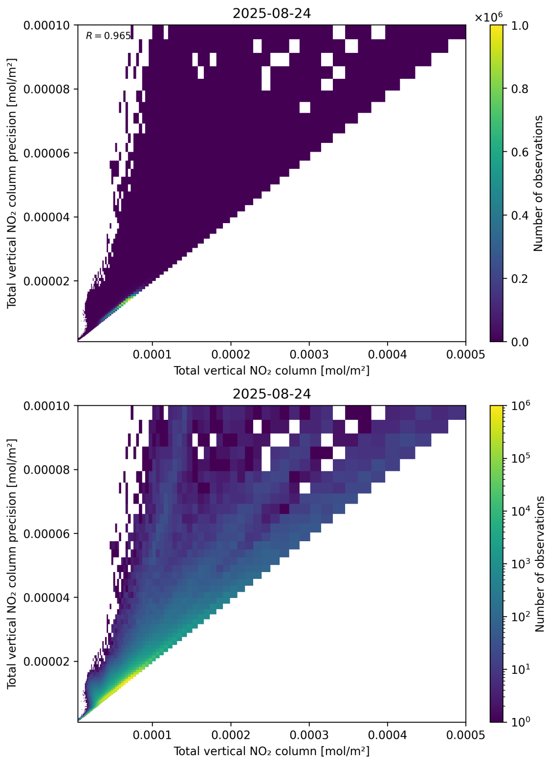
Figure 114: Scatter density plot of “Total vertical NO 2 column” against “Total vertical NO 2 column precision” for 2025-08-23 to 2025-08-25.
