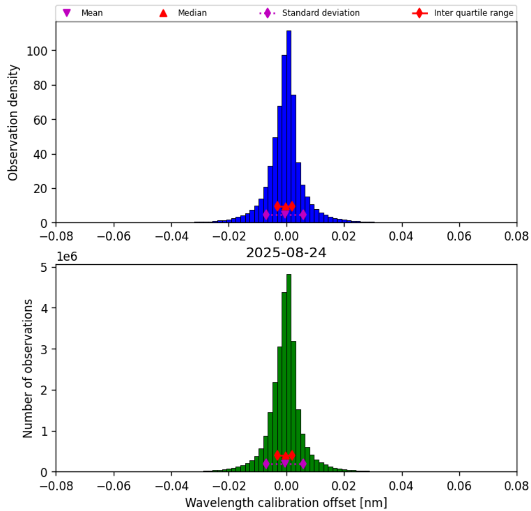
Figure 35: Histogram of “Wavelength calibration offset” for 2025-08-23 to 2025-08-25
