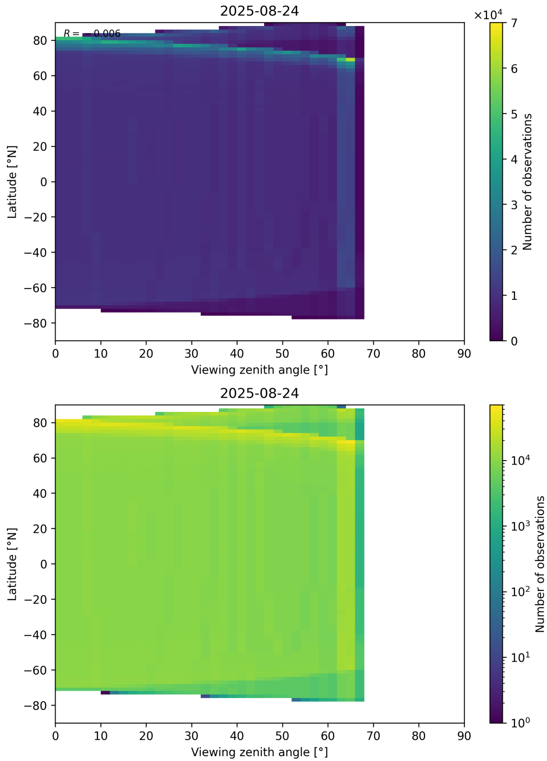
Figure 163: Scatter density plot of “Viewing zenith angle” against “Latitude” for 2025-08-23 to 2025-08-25.
