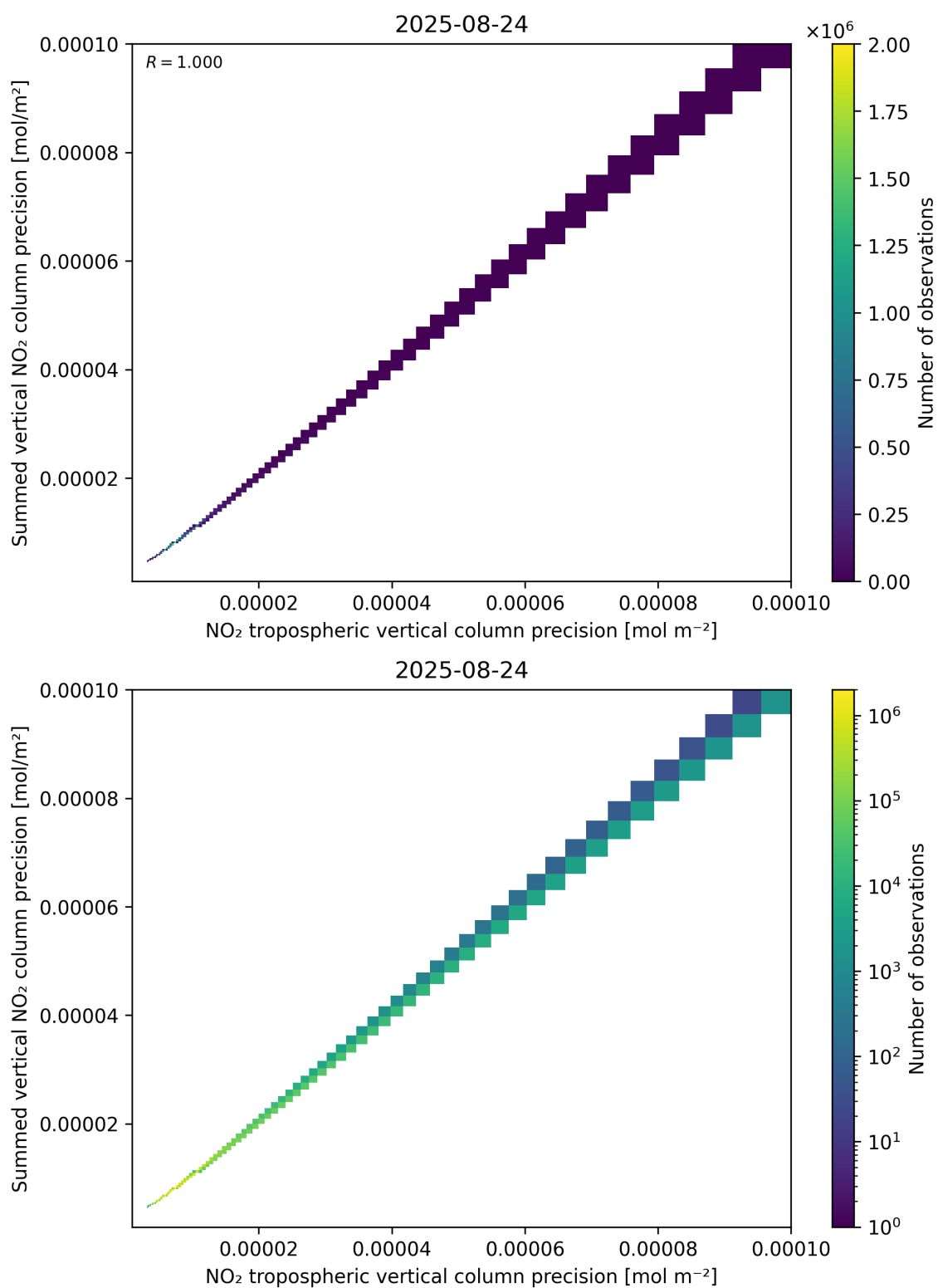
Figure 137: Scatter density plot of “NO 2 tropospheric vertical column precision” against “Summed vertical NO 2 column precision” for 2025-08-23 to 2025-08-25.
