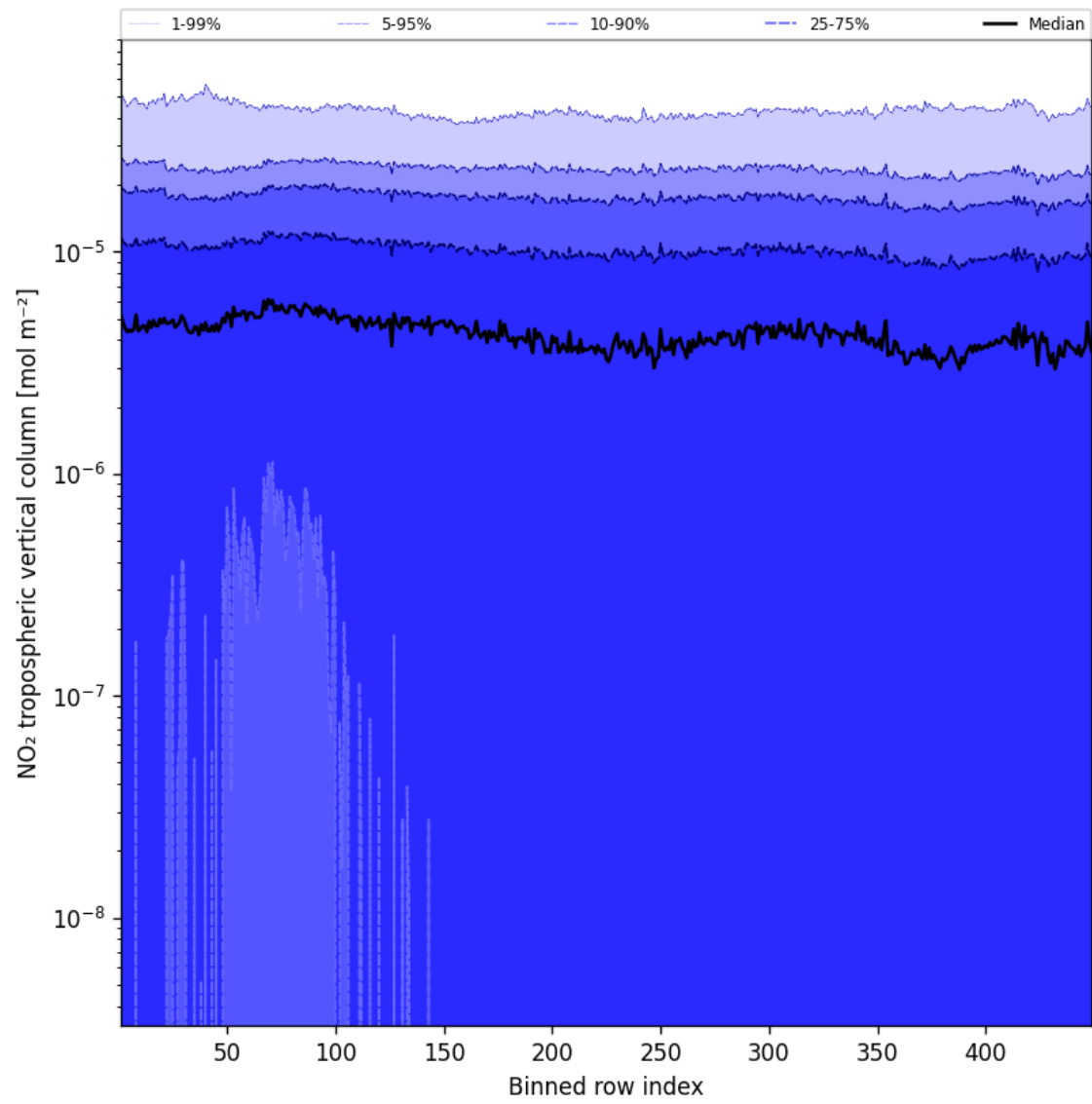
Figure 46: Along track statistics of “ \text{NO}_2 tropospheric vertical column” for 2025-08-23 to 2025-08-25
