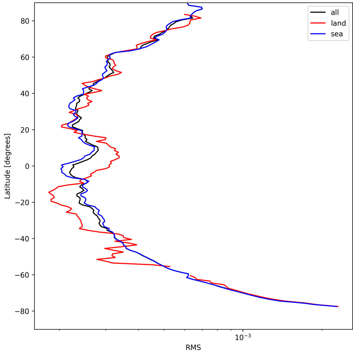
Figure 26: Zonal average of “RMS” for 2025-08-23 to 2025-08-25.
