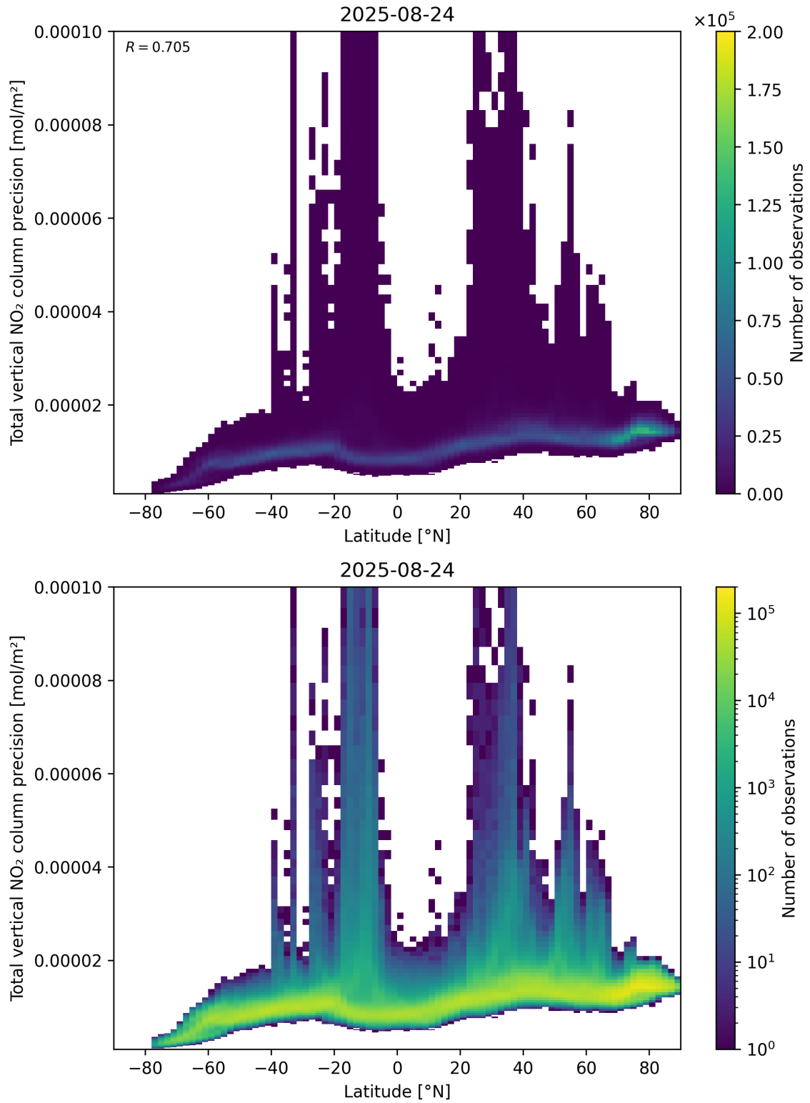
Figure 91: Scatter density plot of “Latitude” against “Total vertical NO 2 column precision” for 2025-08-23 to 2025-08-25.
