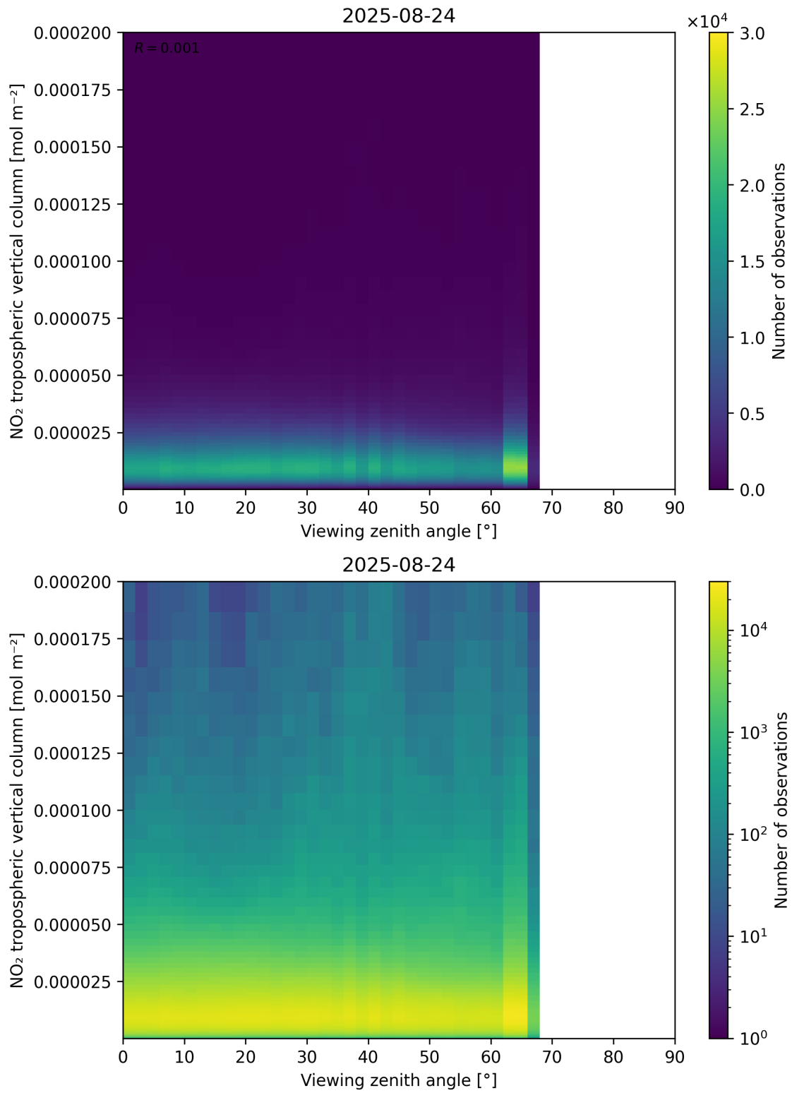
Figure 169: Scatter density plot of “Viewing zenith angle” against “NO 2 tropospheric vertical column” for 2025-08-23 to 2025-08-25.
