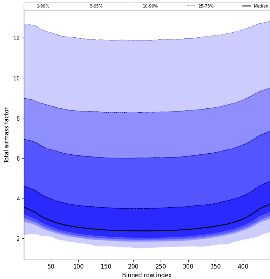
Figure 49: Along track statistics of “Total airmass factor” for 2025-08-23 to 2025-08-25
