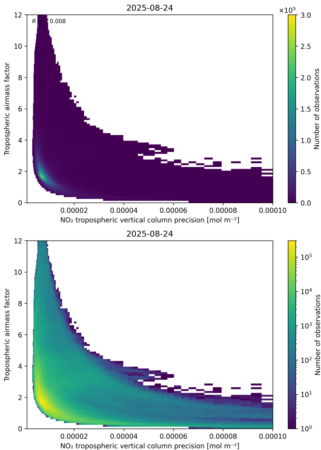
Figure 133: Scatter density plot of “NO 2 tropospheric vertical column precision” against “Tropospheric air mass factor” for 2025-08-23 to 2025-08-25.
