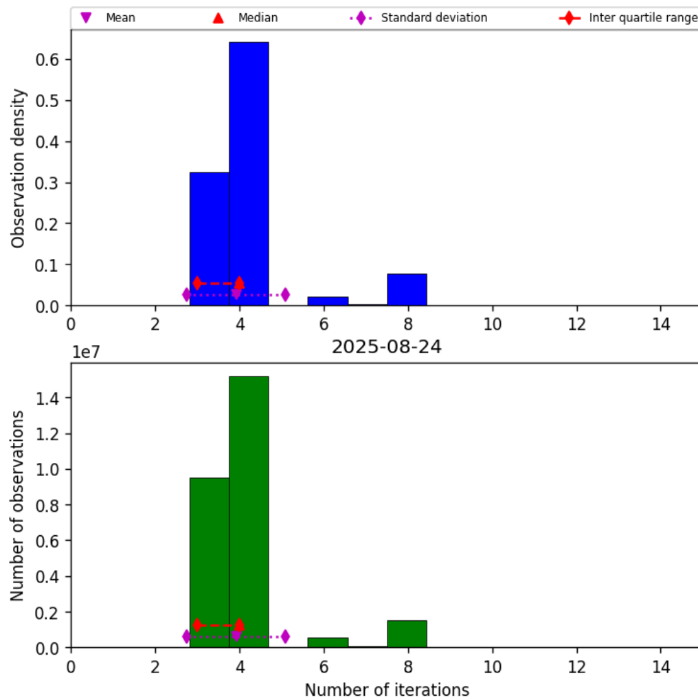
Figure 34: Histogram of “Number of iterations” for 2025-08-23 to 2025-08-25
