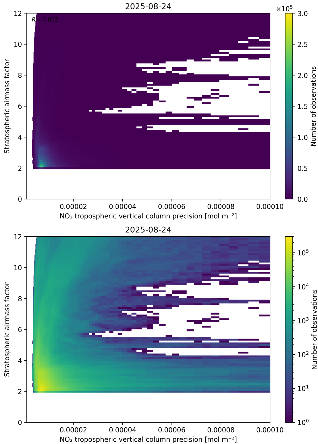
Figure 131: Scatter density plot of “NO 2 tropospheric vertical column precision” against “Stratospheric airmass factor” for 2025-08-23 to 2025-08-25.
