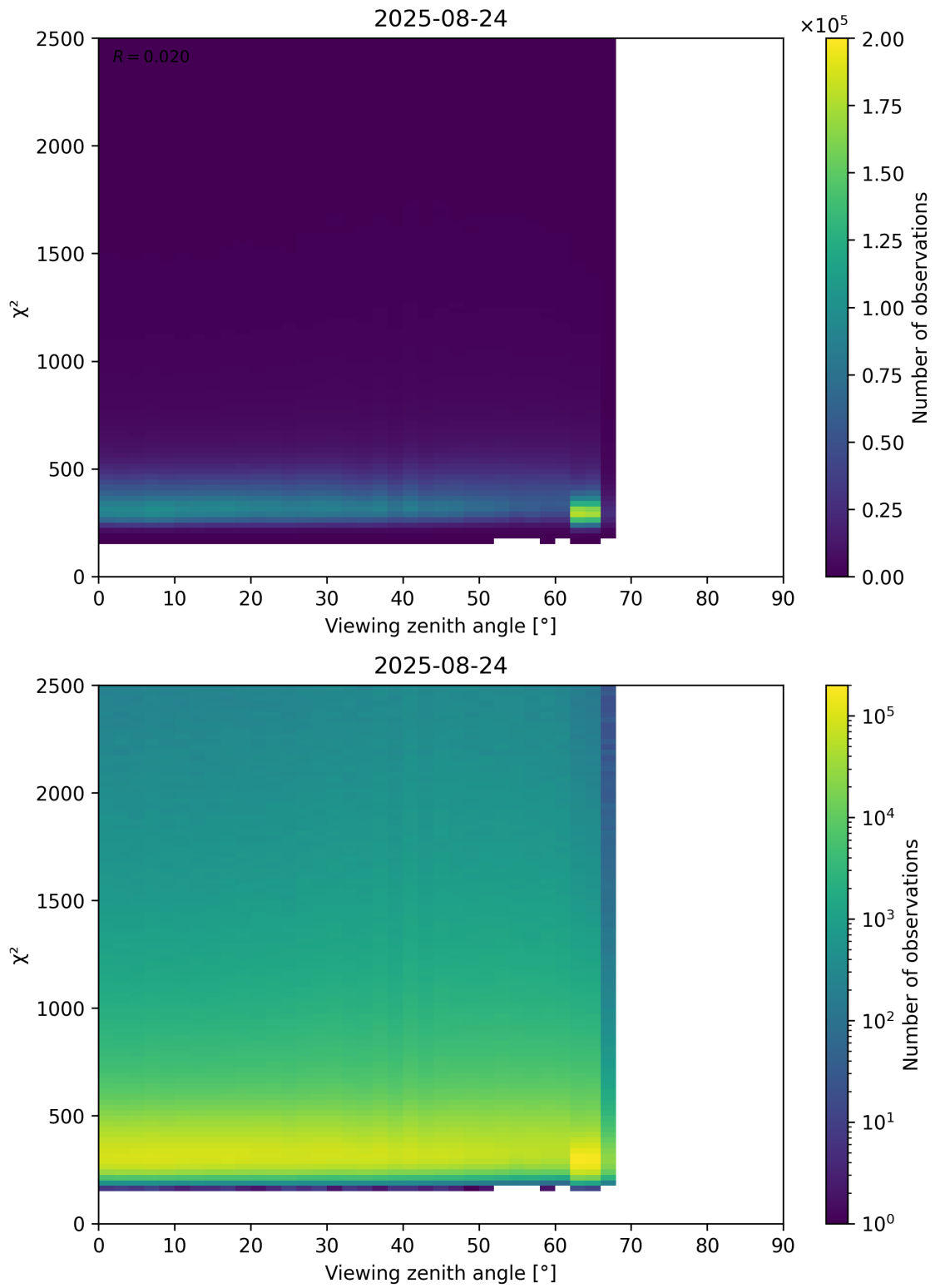
Figure 162: Scatter density plot of “Viewing zenith angle” against “ \chi^2 ” for 2025-08-23 to 2025-08-25.
