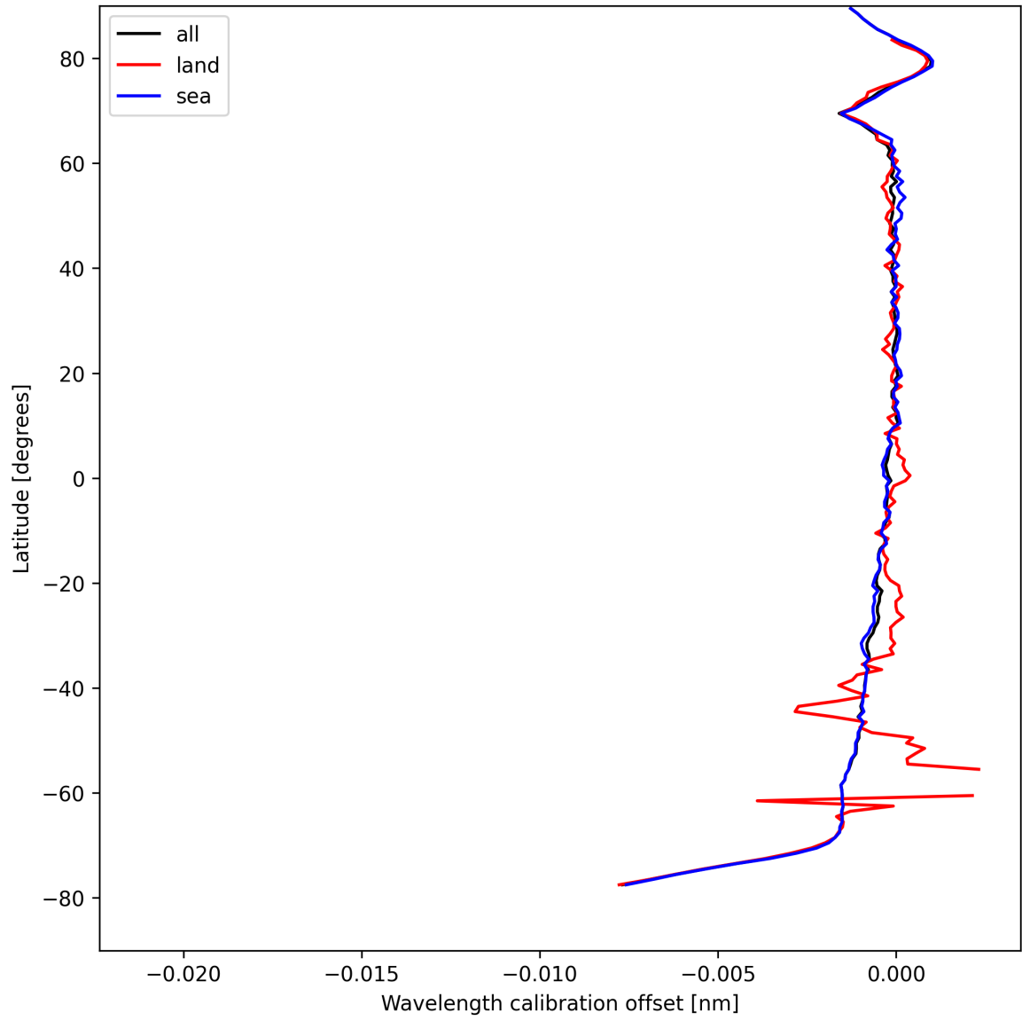
Figure 18: Zonal average of “Wavelength calibration offset” for 2025-08-23 to 2025-08-25.
