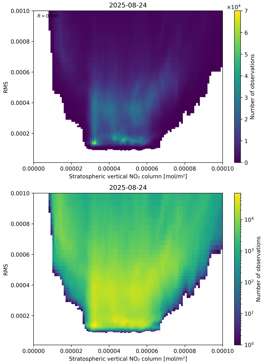
Figure 102: Scatter density plot of “Stratospheric vertical NO 2 column” against “RMS” for 2025-08-23 to 2025-08-25.
