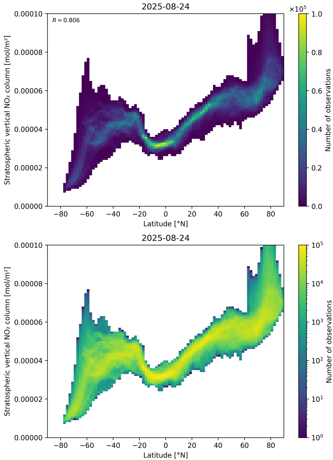
Figure 87: Scatter density plot of “Latitude” against “Stratospheric vertical \text{NO}_2 column” for 2025-08-23 to 2025-08-25.
