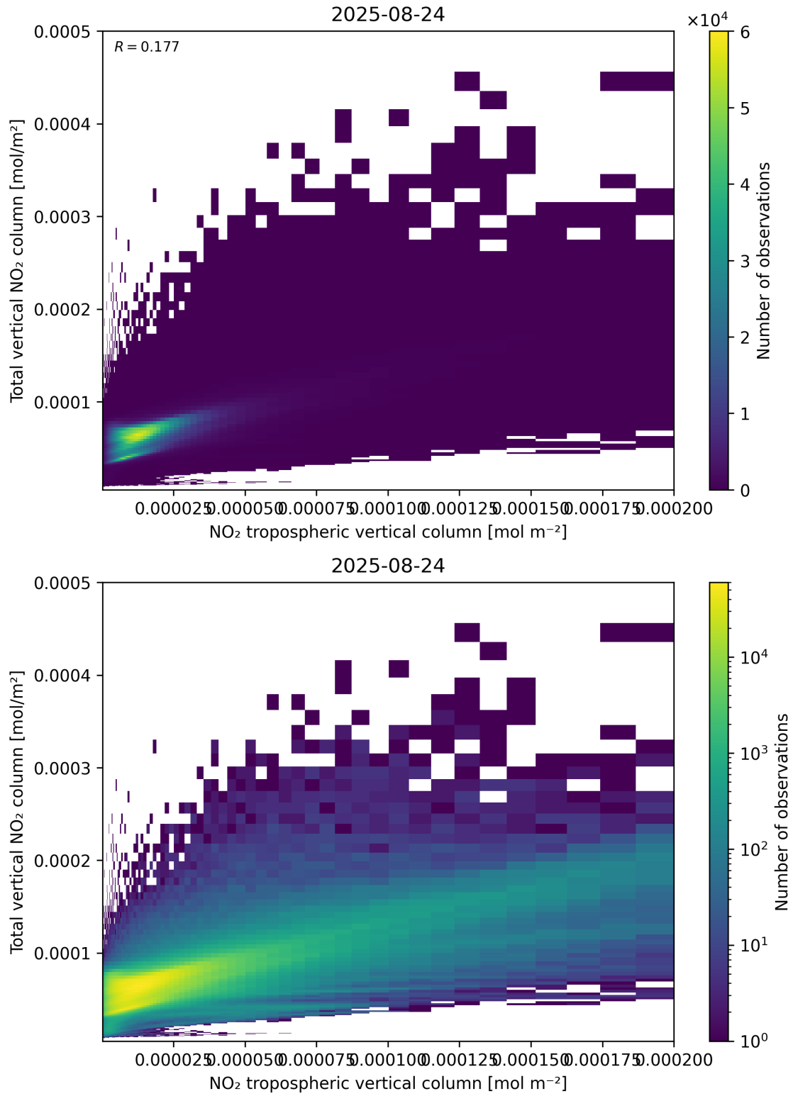
Figure 128: Scatter density plot of “NO 2 tropospheric vertical column” against “Total vertical NO 2 column” for 2025-08-23 to 2025-08-25.
