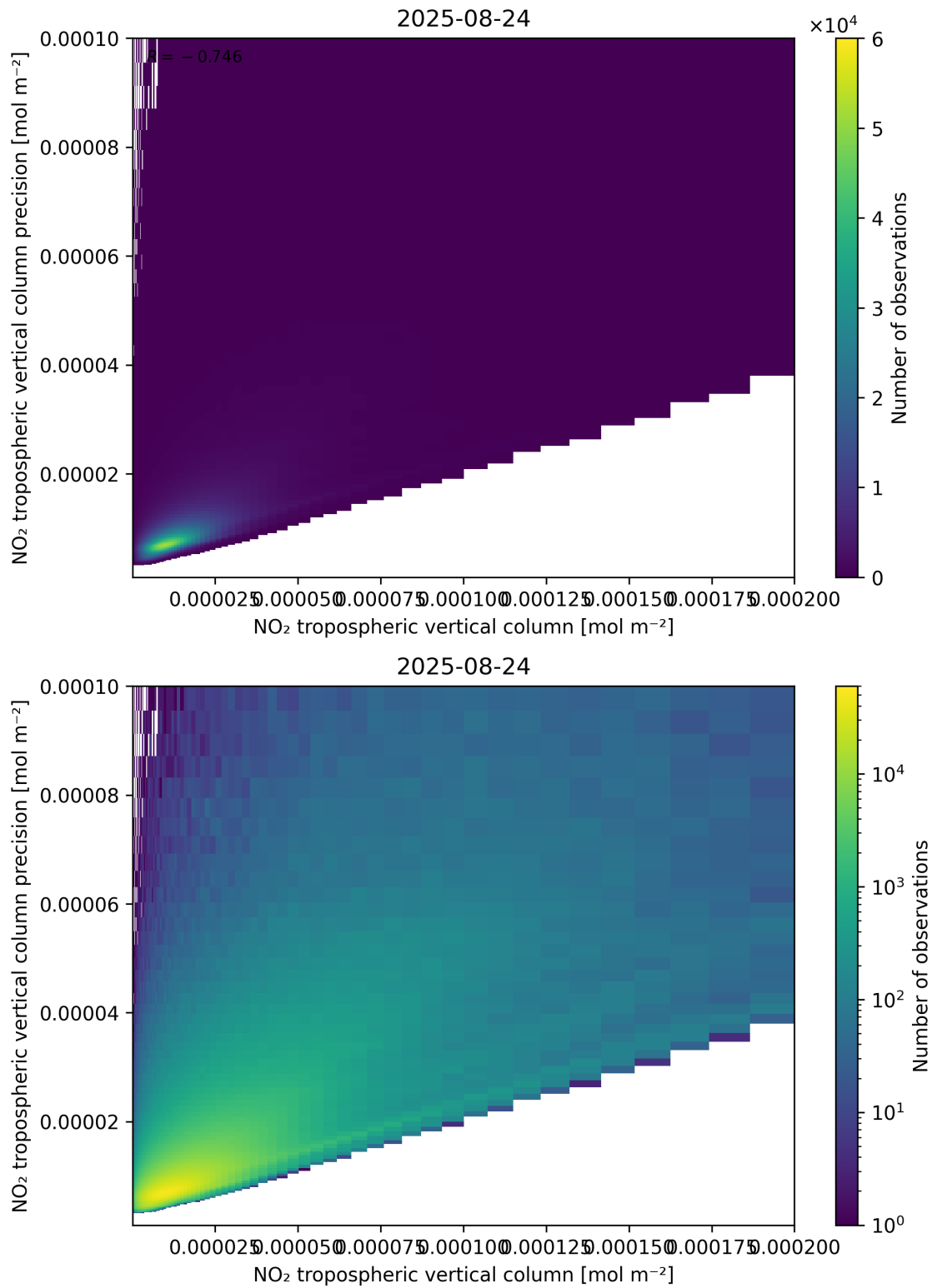
Figure 130: Scatter density plot of “NO 2 tropospheric vertical column” against “NO 2 tropospheric vertical column precision” for 2025-08-23 to 2025-08-25.
