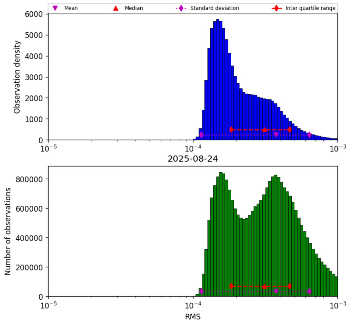
Figure 43: Histogram of “RMS” for 2025-08-23 to 2025-08-25
