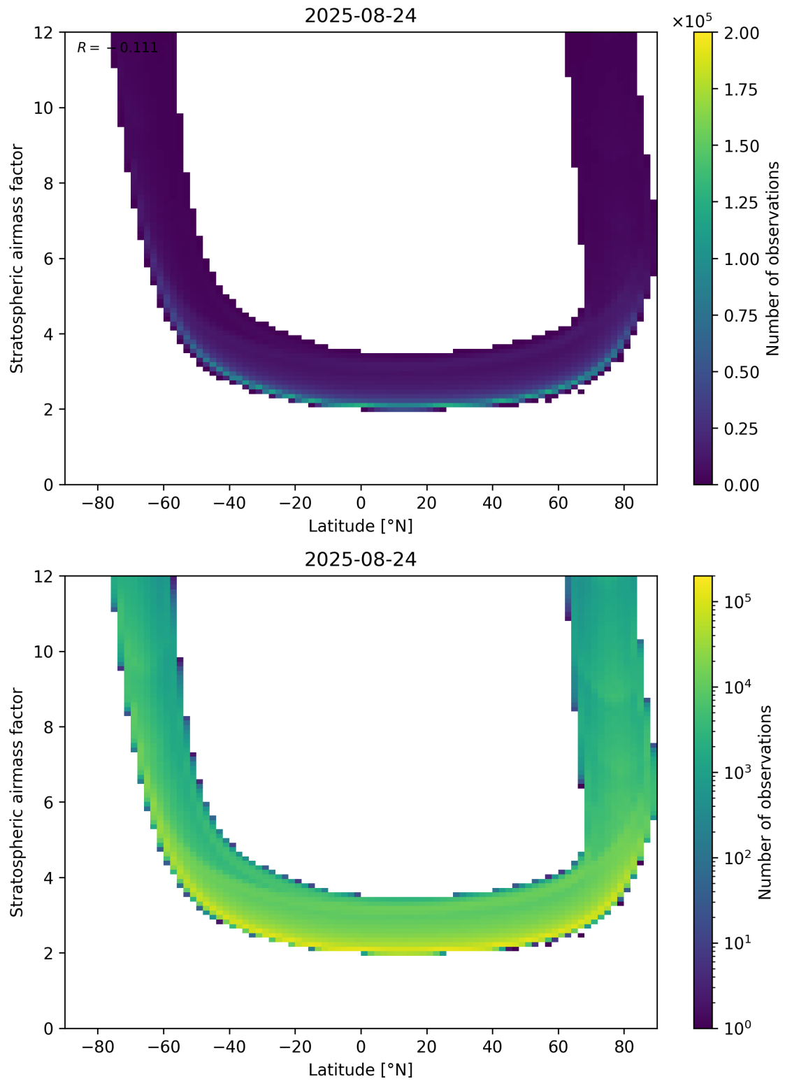
Figure 83: Scatter density plot of “Latitude” against “Stratospheric air mass factor” for 2025-08-23 to 2025-08-25.
