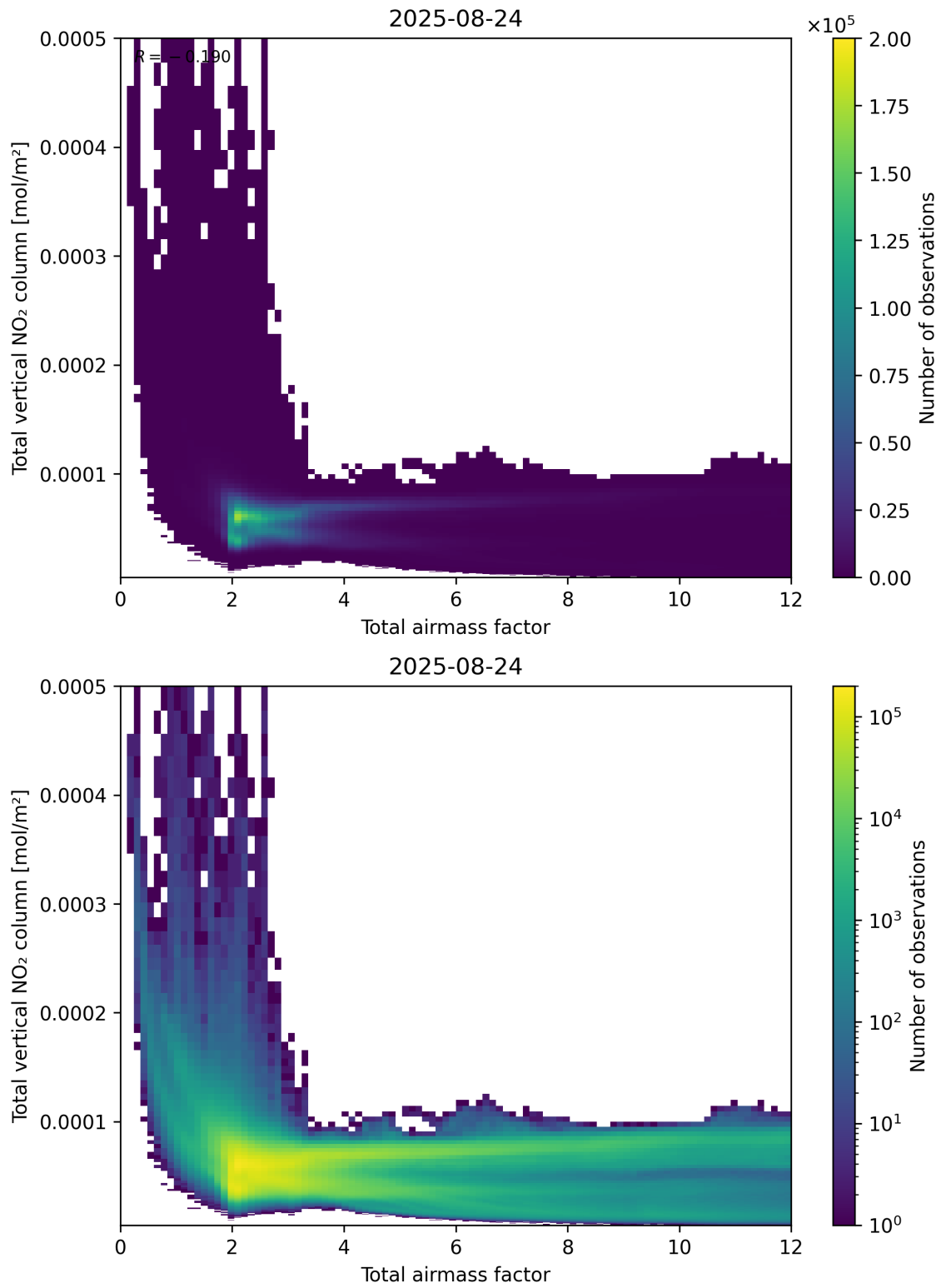
Figure 67: Scatter density plot of “Total airmass factor” against “Total vertical NO 2 column” for 2025-08-23 to 2025-08-25.
