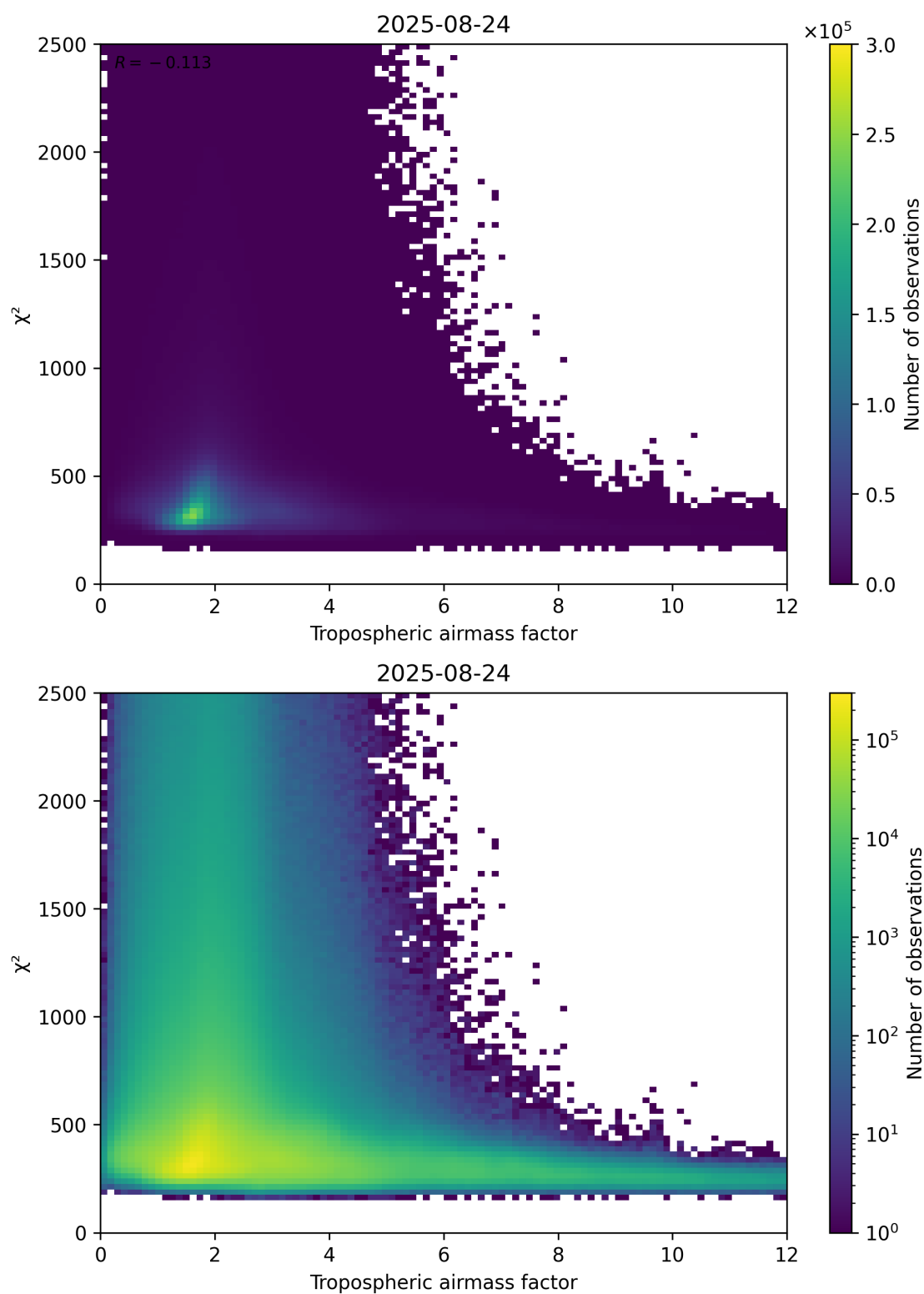
Figure 73: Scatter density plot of “Tropospheric airmass factor” against “ \chi^2 ” for 2025-08-23 to 2025-08-25.
