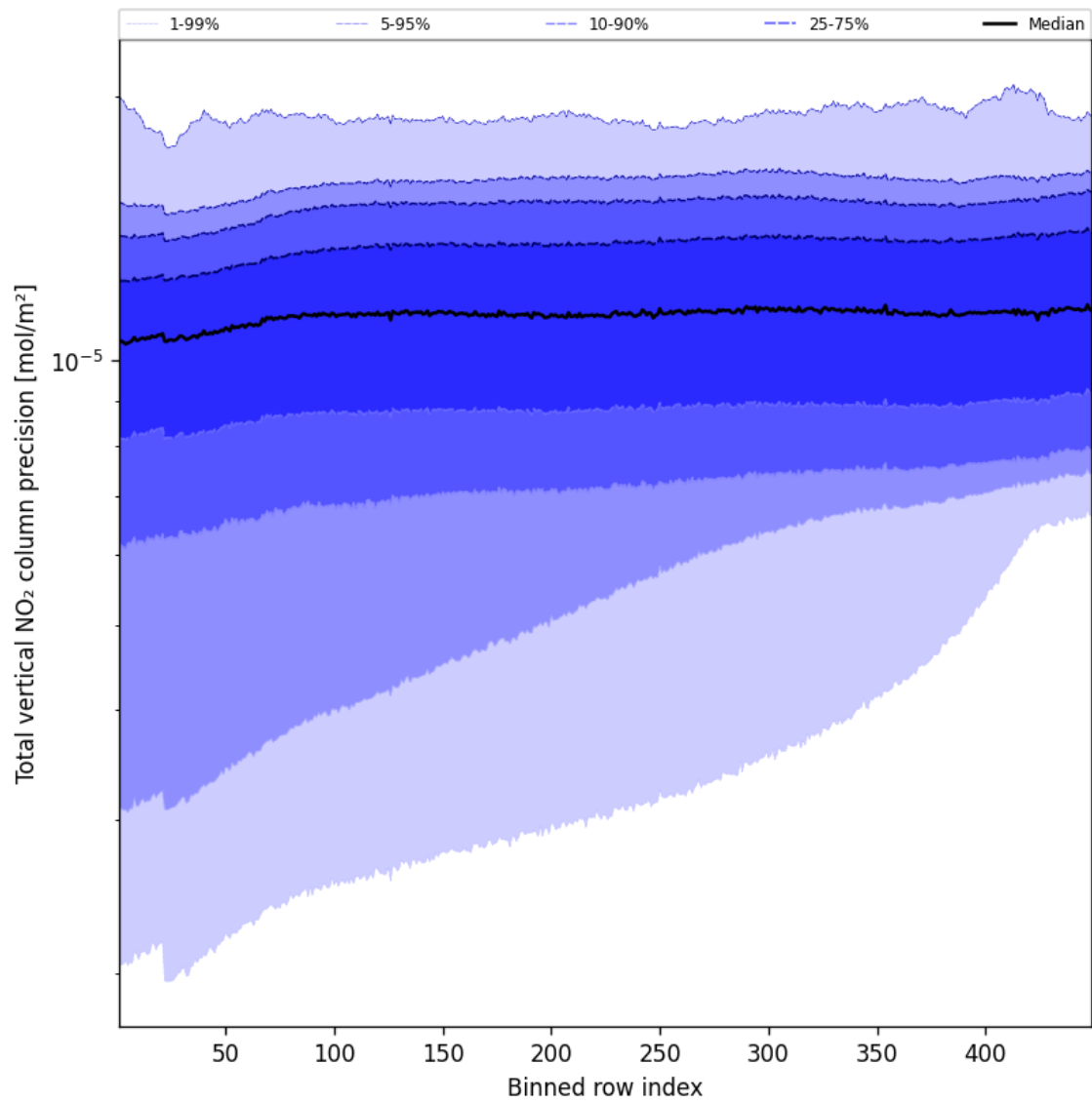
Figure 56: Along track statistics of “Total vertical NO 2 column precision” for 2025-08-23 to 2025-08-25
