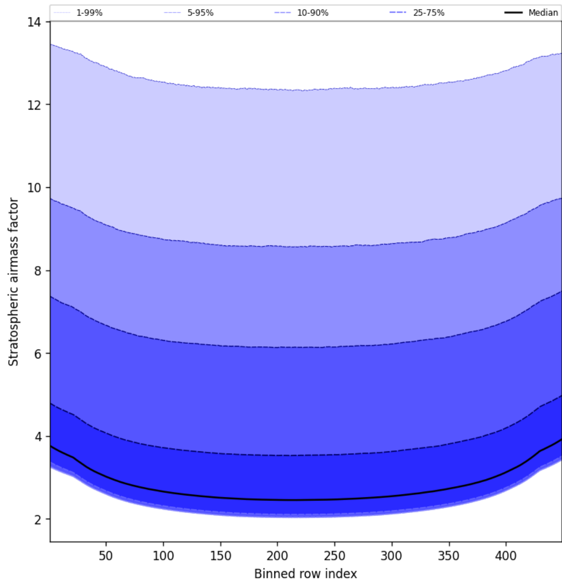
Figure 61: Along track statistics of “Stratospheric airmass factor” for 2025-08-23 to 2025-08-25
