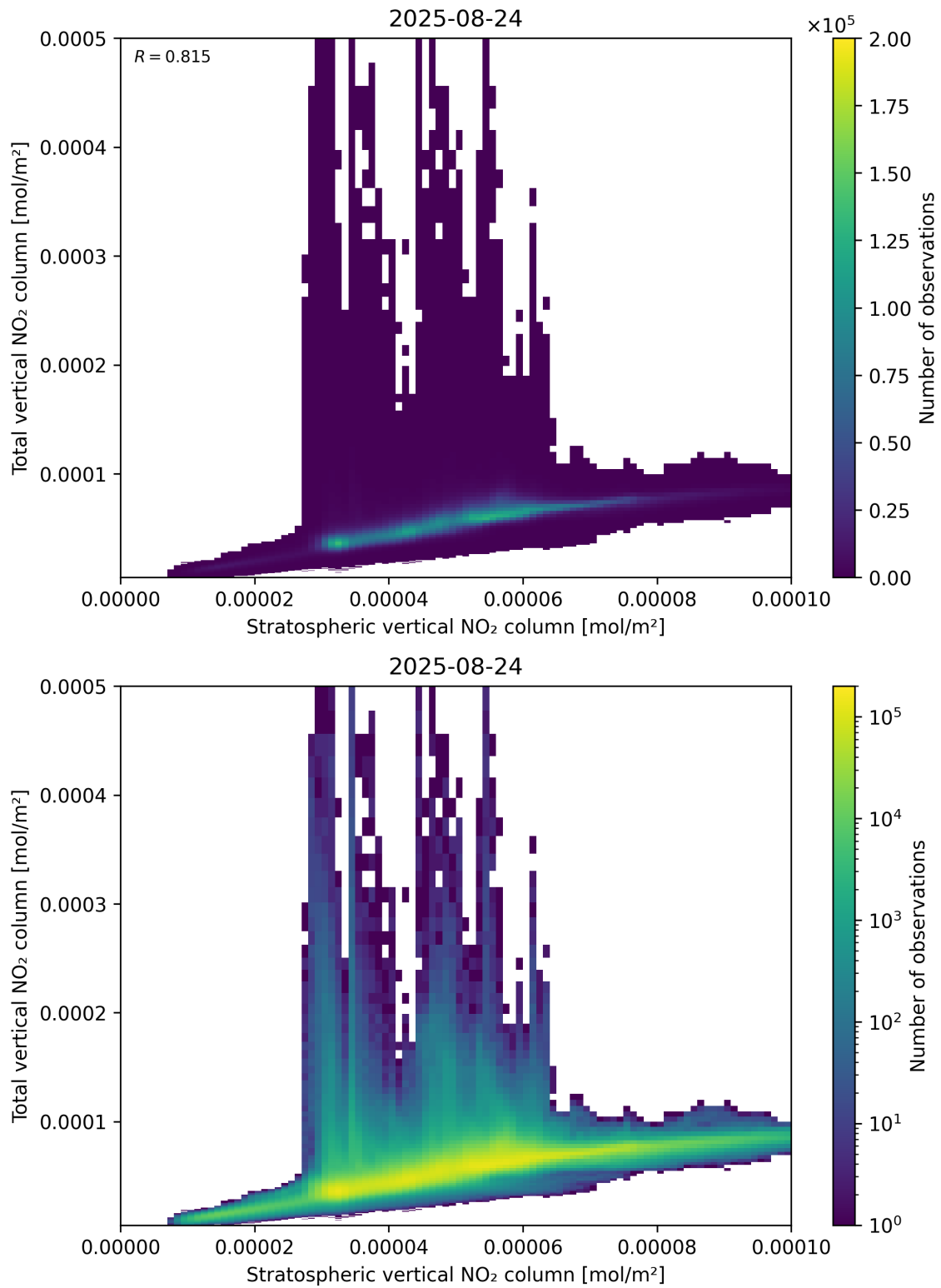
Figure 100: Scatter density plot of “Stratospheric vertical NO 2 column” against “Total vertical NO 2 column” for 2025-08-23 to 2025-08-25.
