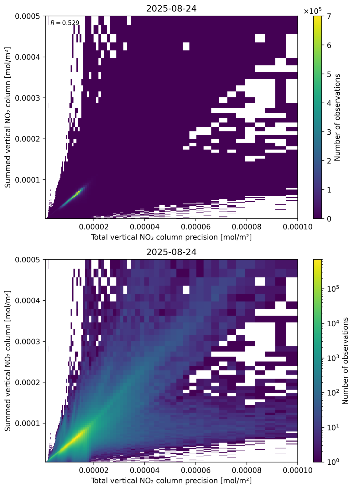
Figure 117: Scatter density plot of “Total vertical NO 2 column precision” against “Summed vertical NO 2 column” for 2025-08-23 to 2025-08-25.
