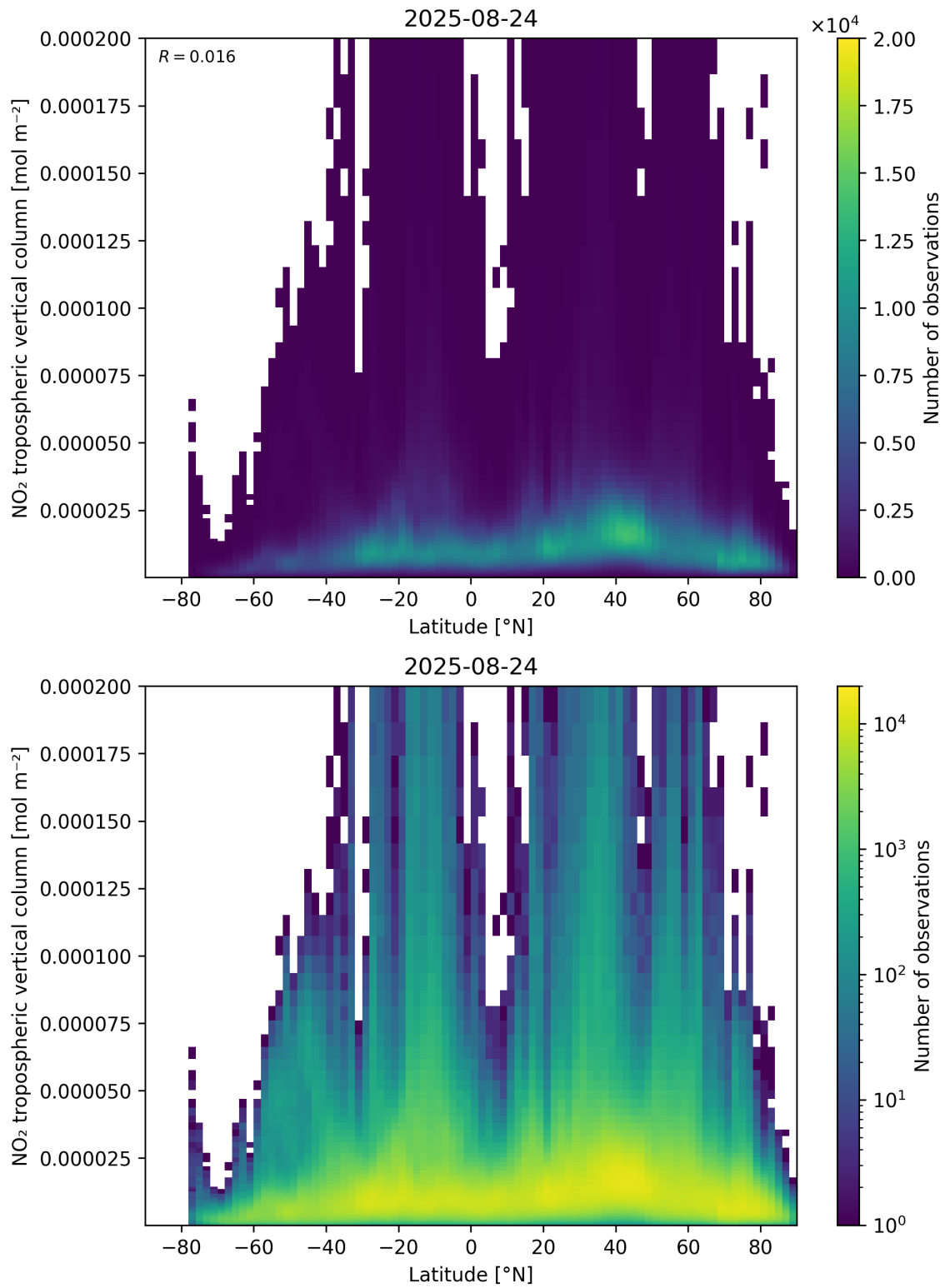
Figure 92: Scatter density plot of “Latitude” against “NO 2 tropospheric vertical column” for 2025-08-23 to 2025-08-25.
