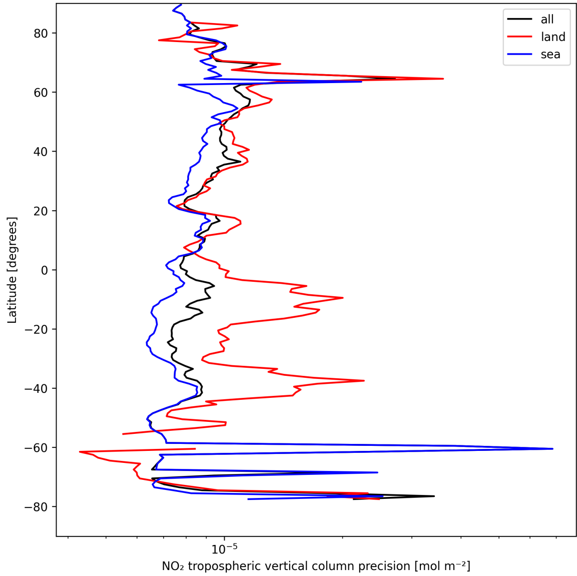
Figure 13: Zonal average of “NO 2 tropospheric vertical column precision” for 2025-08-23 to 2025-08-25.
