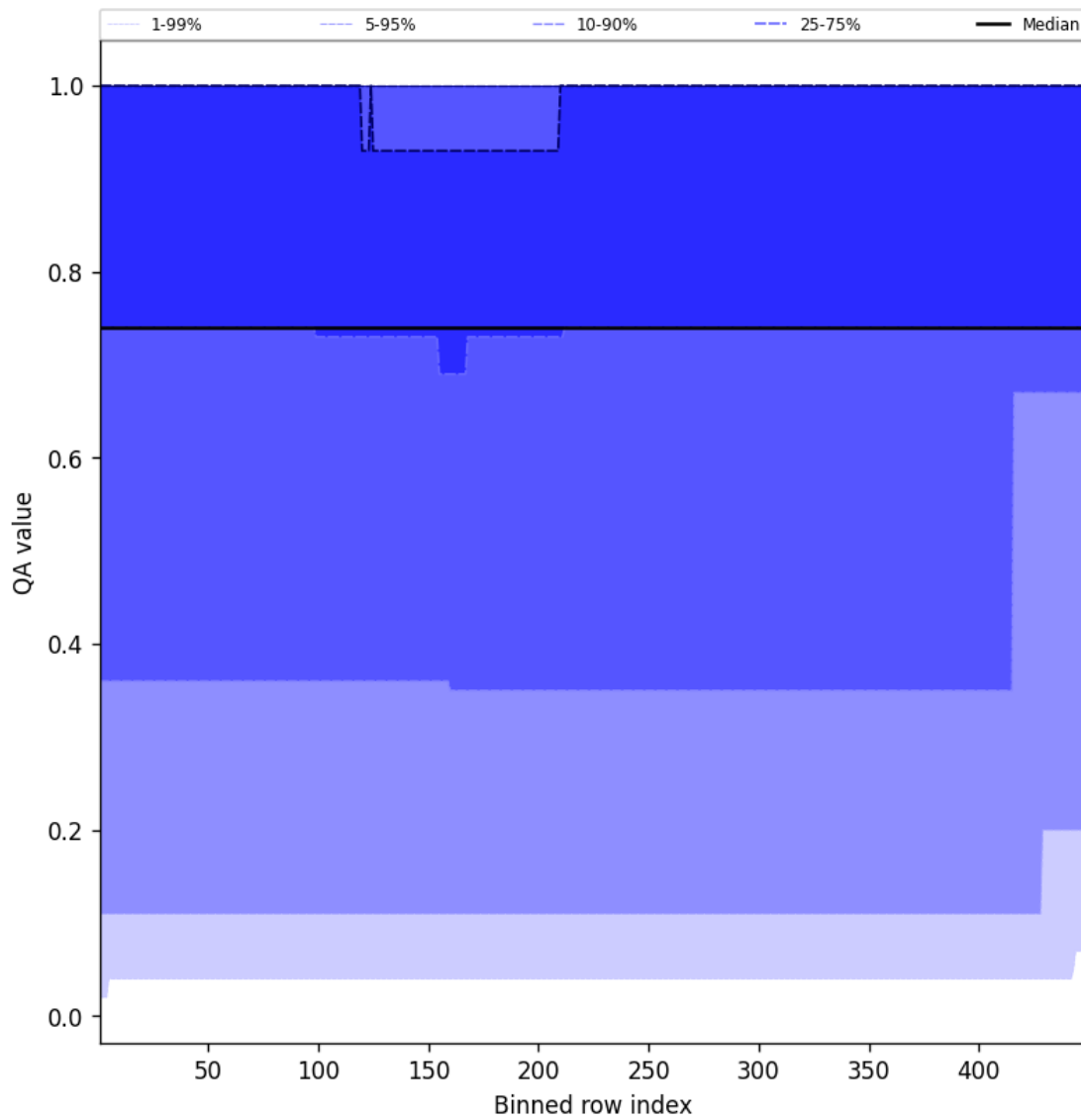
Figure 45: Along track statistics of “QA value” for 2025-08-23 to 2025-08-25
