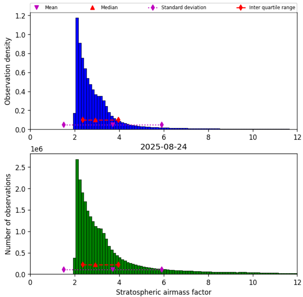
Figure 44: Histogram of “Stratospheric airmass factor” for 2025-08-23 to 2025-08-25
