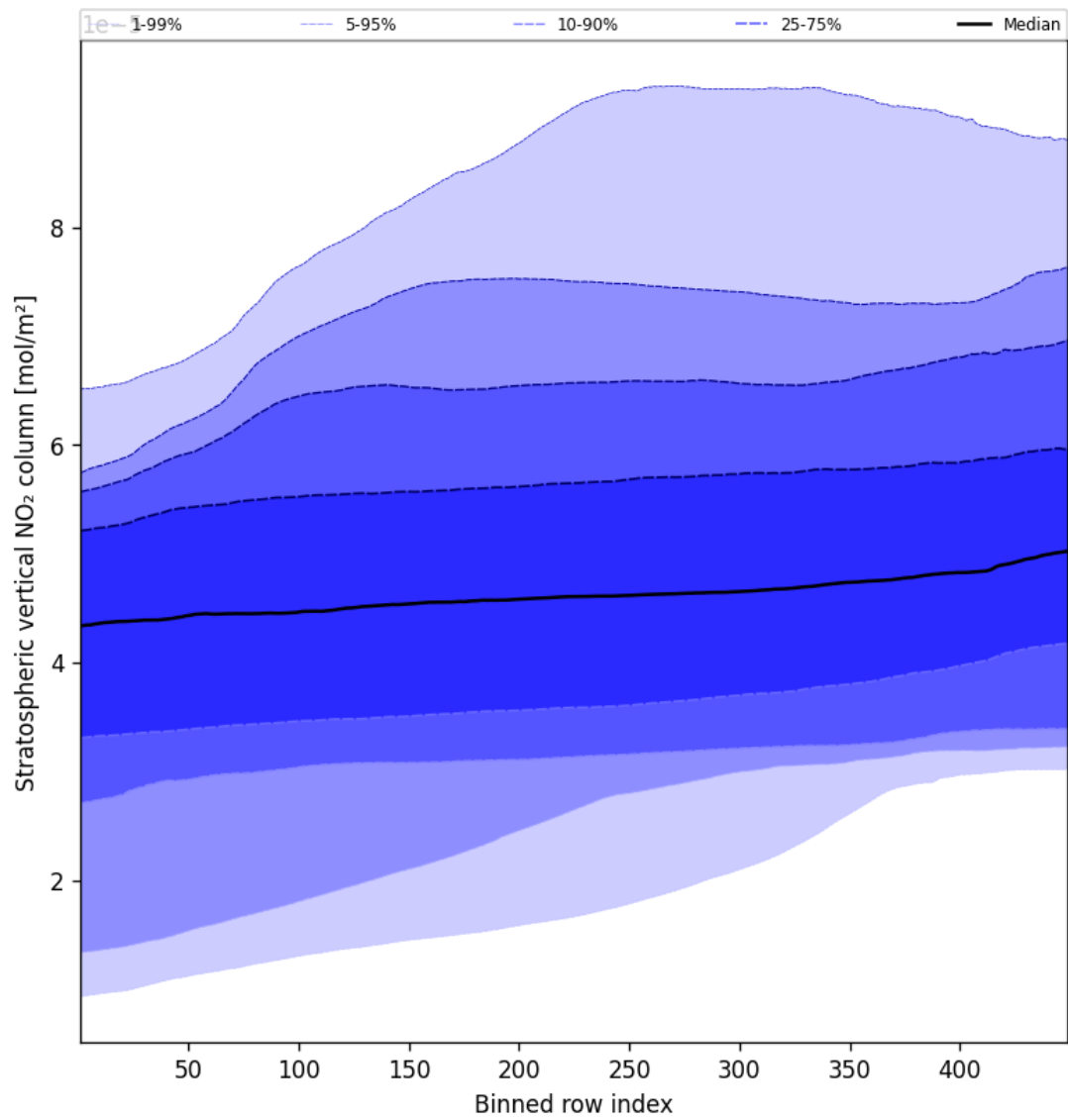
Figure 53: Along track statistics of “Stratospheric vertical NO 2 column” for 2025-08-23 to 2025-08-25
