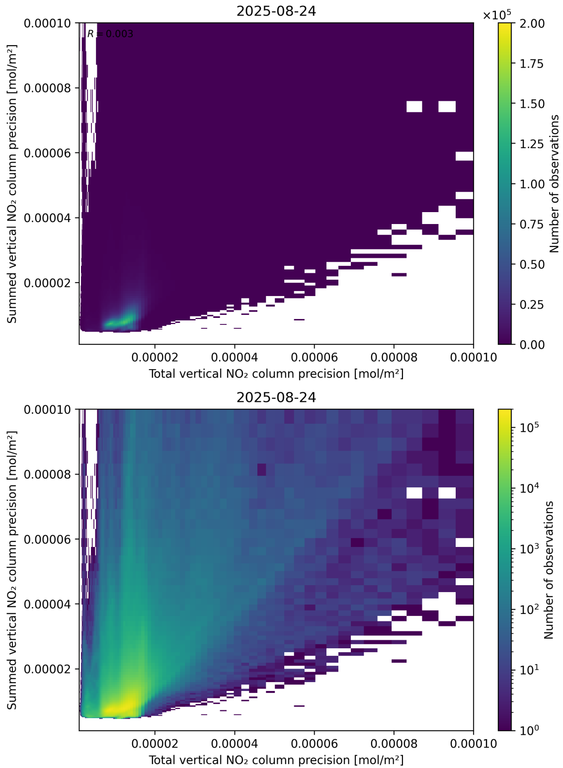
Figure 118: Scatter density plot of “Total vertical NO 2 column precision” against “Summed vertical NO 2 column precision” for 2025-08-23 to 2025-08-25.
