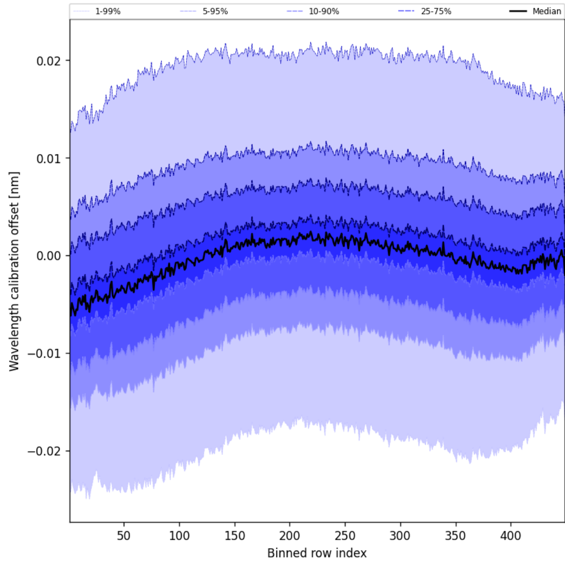
Figure 52: Along track statistics of “Wavelength calibration offset” for 2025-08-23 to 2025-08-25
