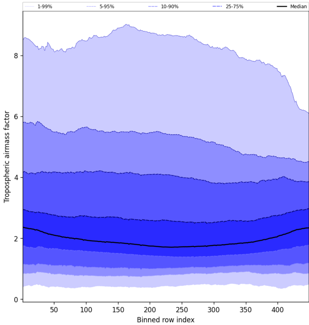
Figure 48: Along track statistics of “Tropospheric air mass factor” for 2025-08-25 to 2025-08-27
