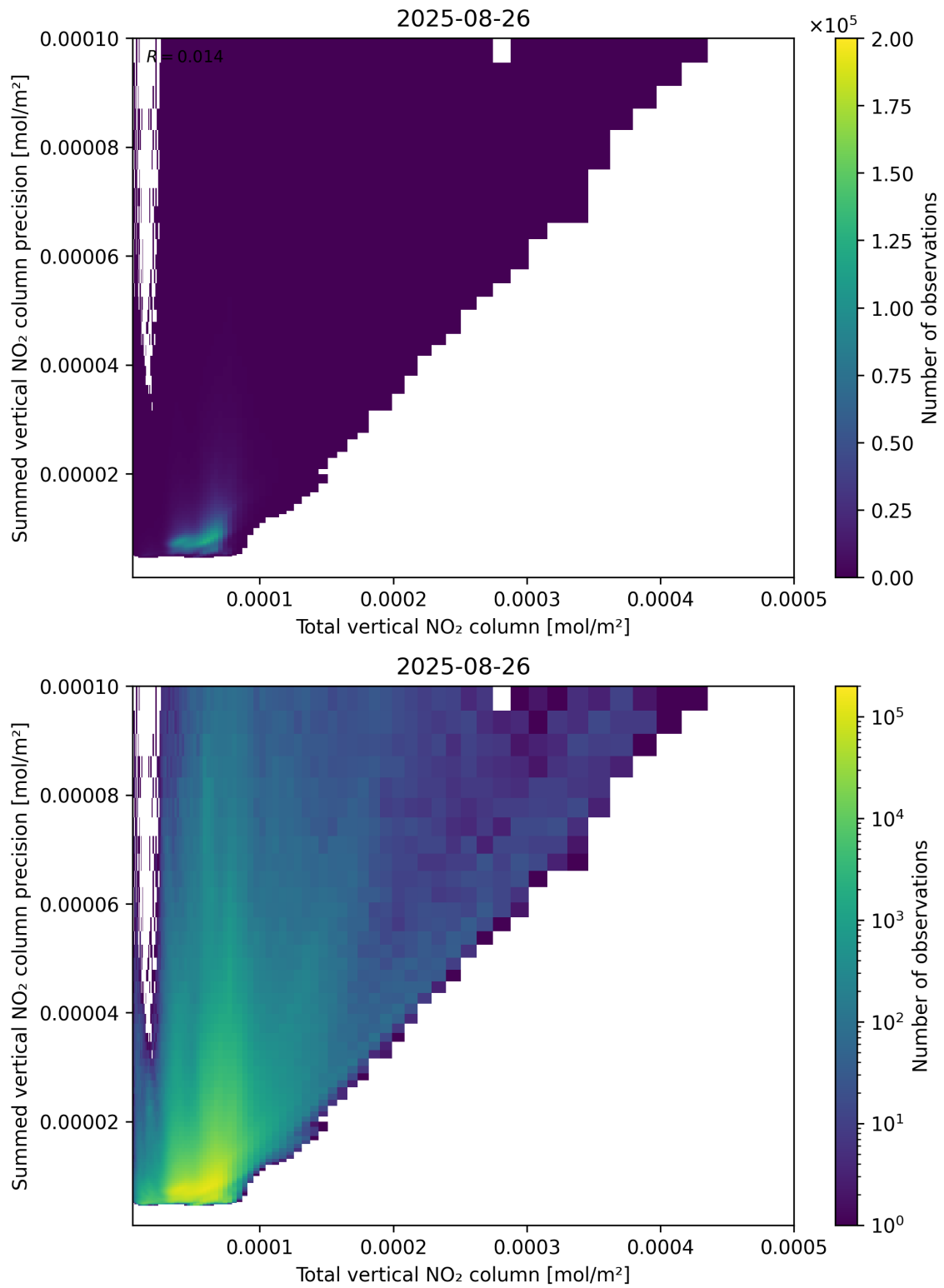
Figure 113: Scatter density plot of “Total vertical NO 2 column” against “Summed vertical NO 2 column precision” for 2025-08-25 to 2025-08-27.
