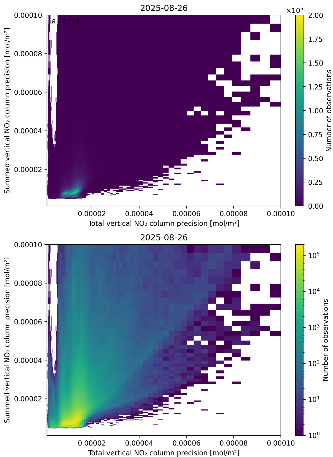
Figure 118: Scatter density plot of “Total vertical NO 2 column precision” against “Summed vertical NO 2 column precision” for 2025-08-25 to 2025-08-27.
