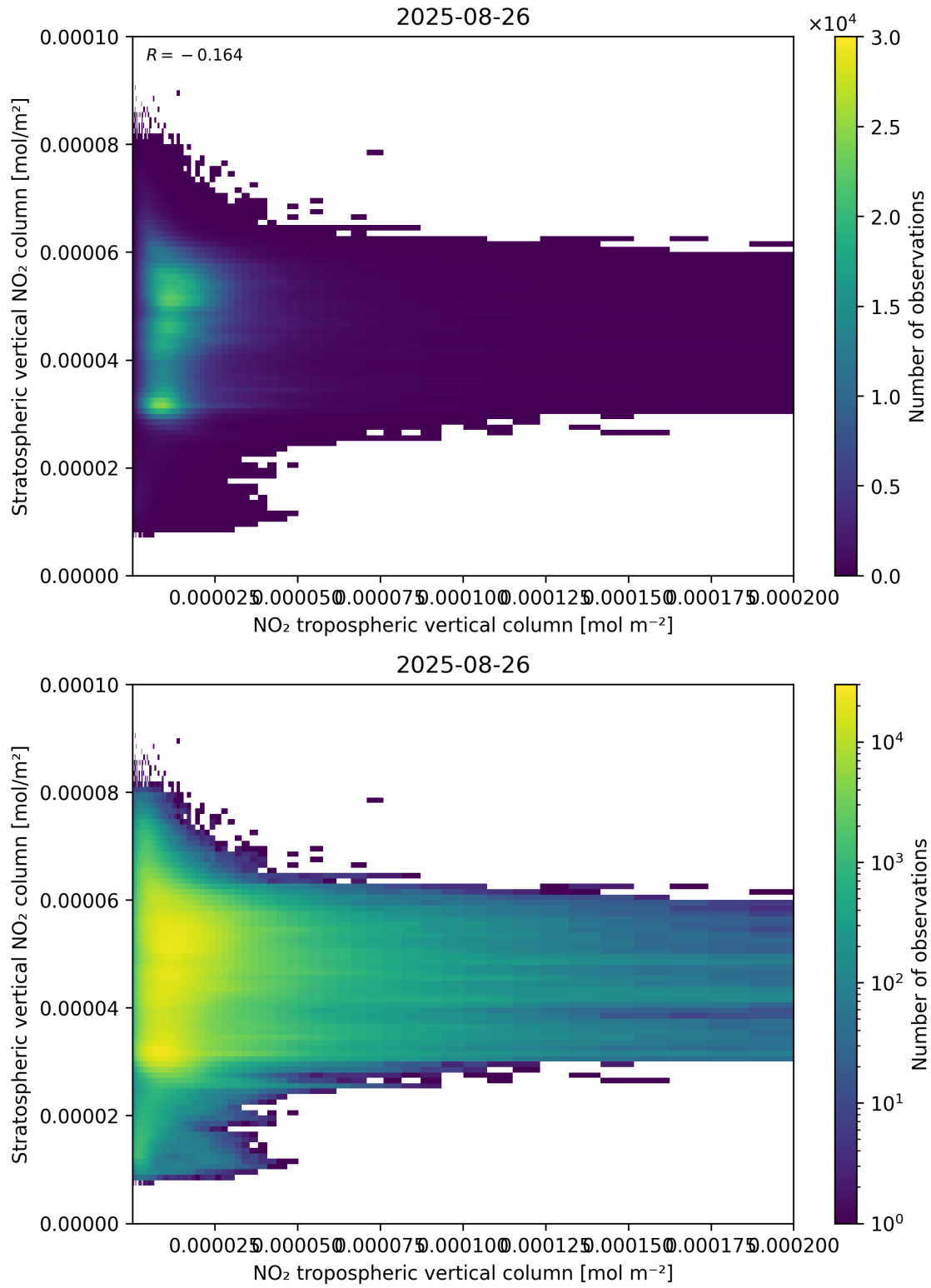
Figure 125: Scatter density plot of “NO 2 tropospheric vertical column” against “Stratospheric vertical NO 2 column” for 2025-08-25 to 2025-08-27.
