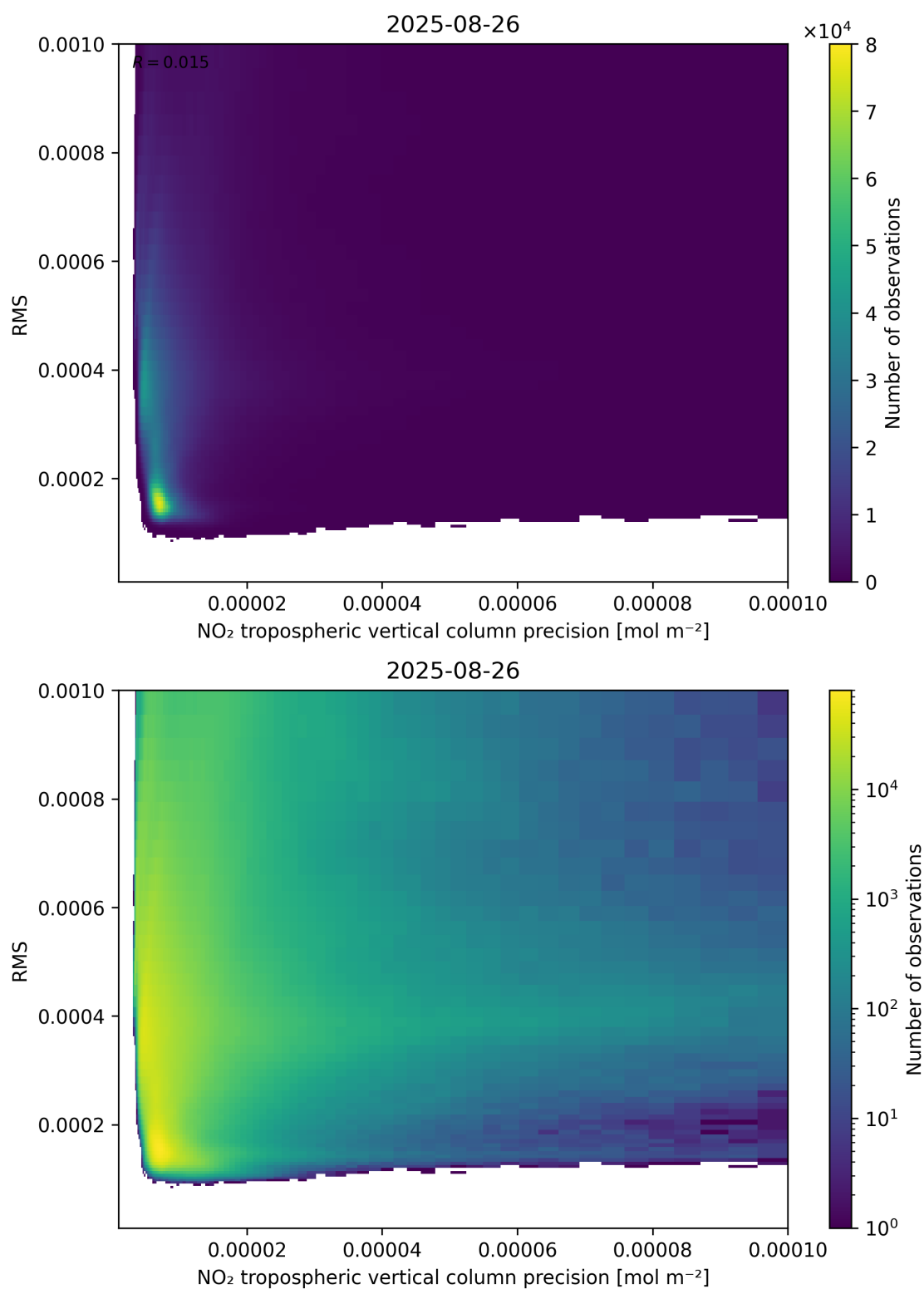
Figure 140: Scatter density plot of “NO 2 tropospheric vertical column precision” against “RMS” for 2025-08-25 to 2025-08-27.
