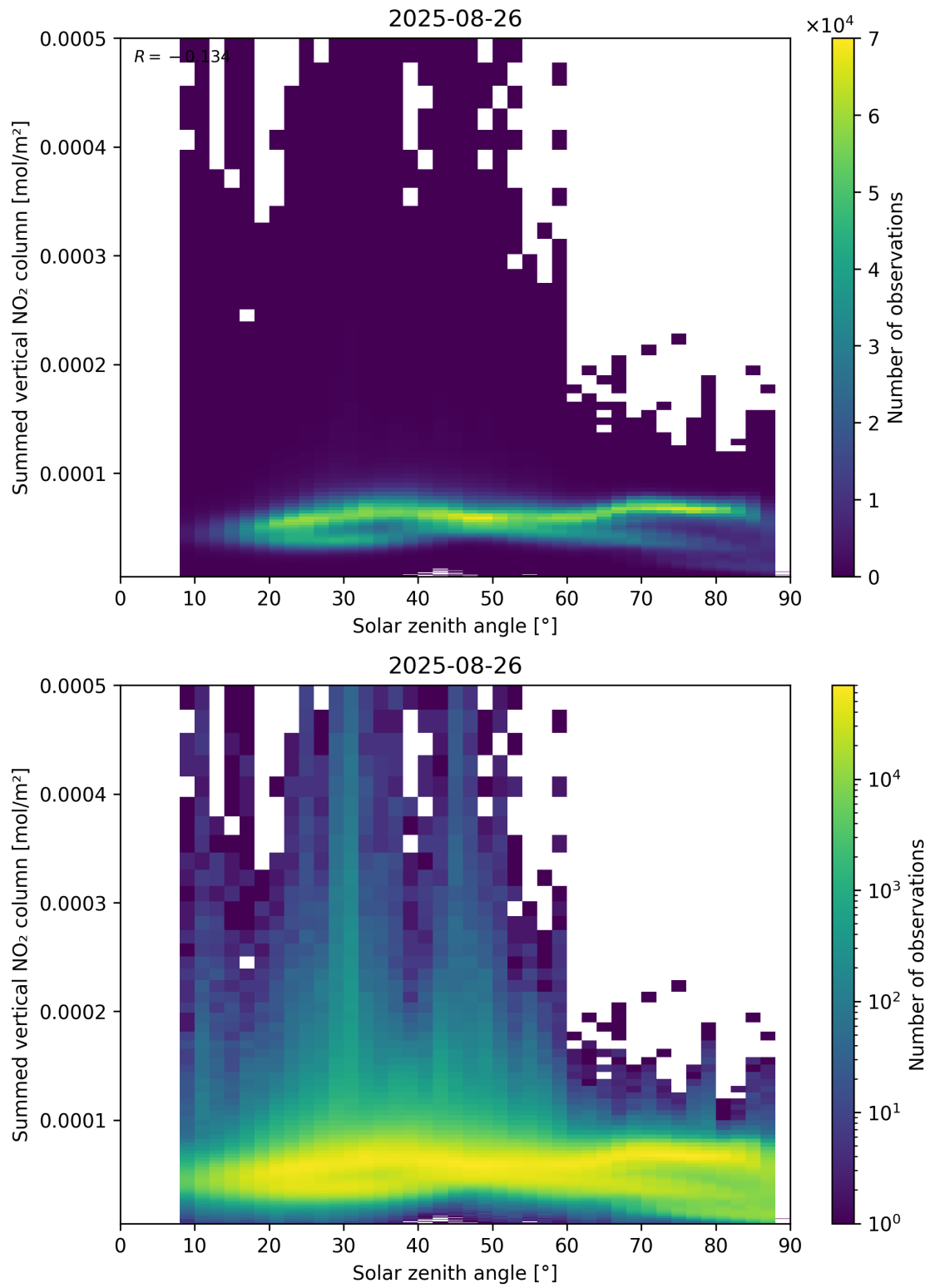
Figure 151: Scatter density plot of “Solar zenith angle” against “Summed vertical NO 2 column” for 2025-08-25 to 2025-08-27.
