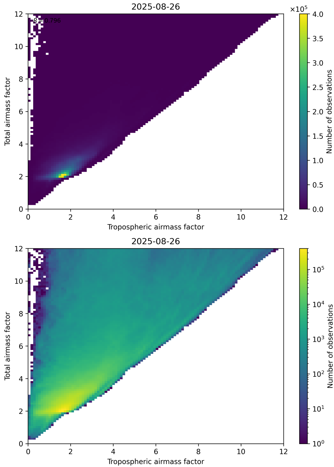
Figure 72: Scatter density plot of “Tropospheric airmass factor” against “Total airmass factor” for 2025-08-25 to 2025-08-27.
