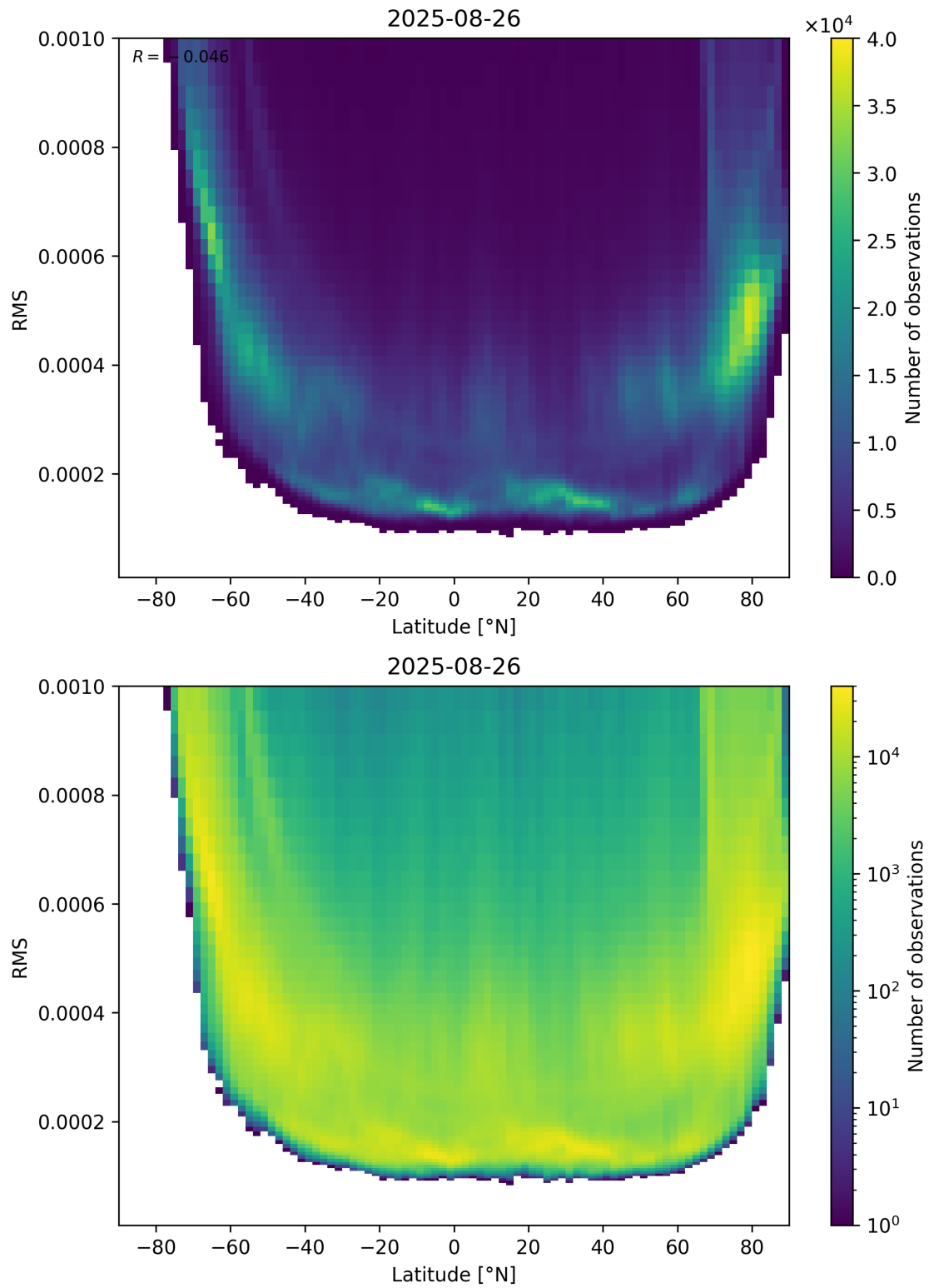
Figure 94: Scatter density plot of “Latitude” against “RMS” for 2025-08-25 to 2025-08-27.
