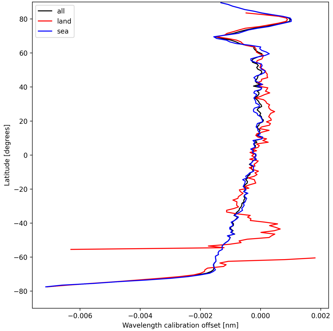
Figure 18: Zonal average of “Wavelength calibration offset” for 2025-08-25 to 2025-08-27.
