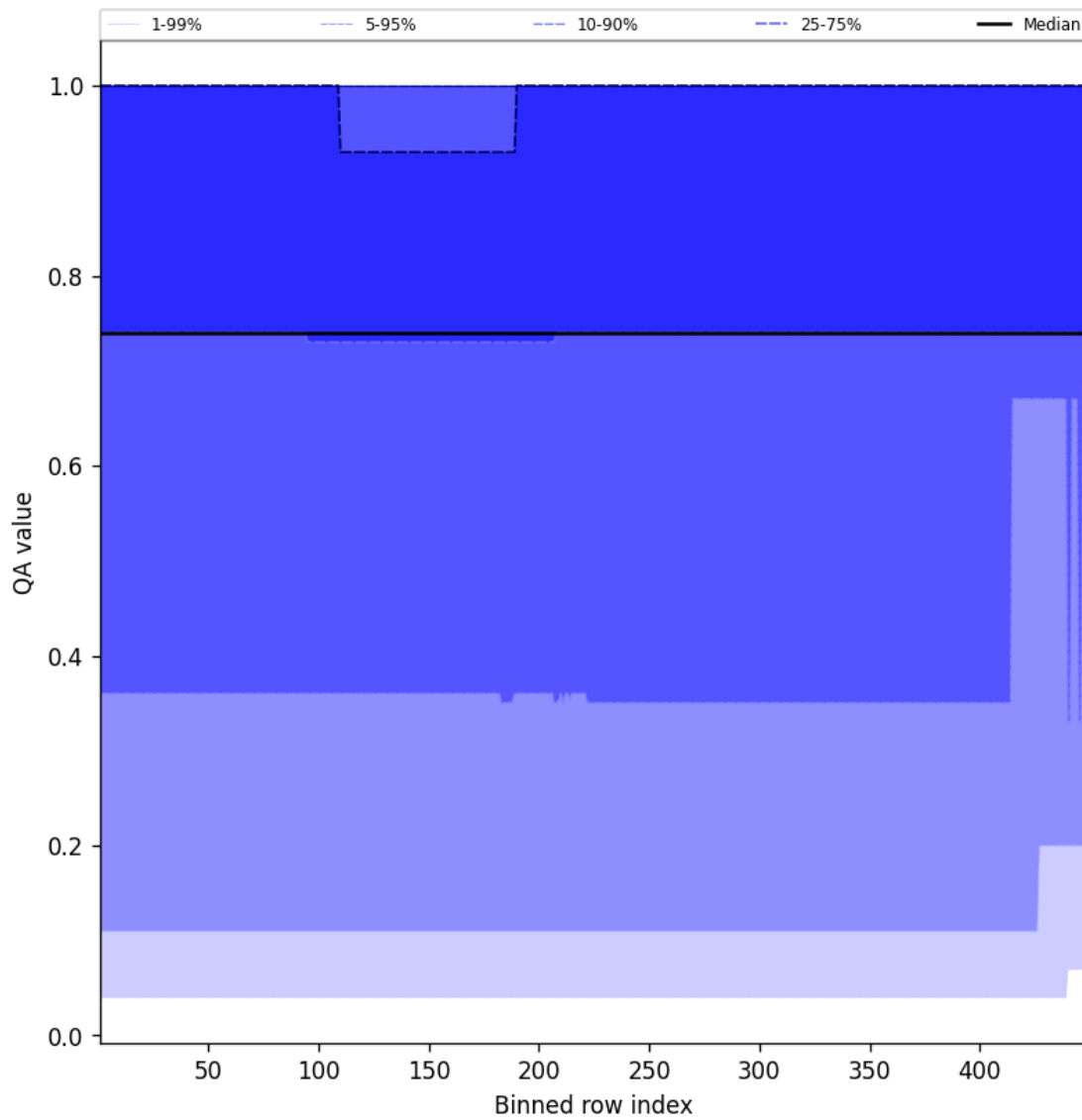
Figure 45: Along track statistics of “QA value” for 2025-08-25 to 2025-08-27
