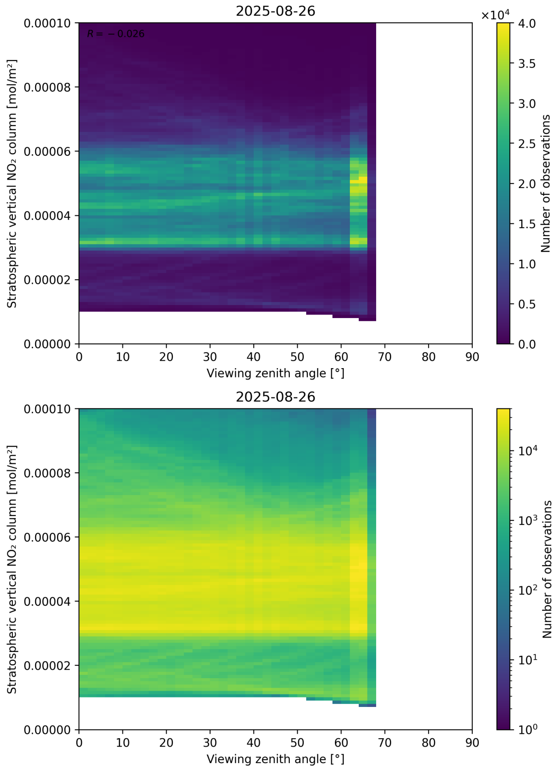
Figure 164: Scatter density plot of “Viewing zenith angle” against “Stratospheric vertical NO 2 column” for 2025-08-25 to 2025-08-27.
