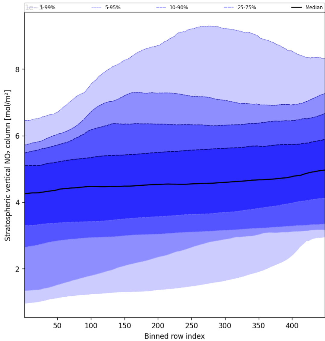
Figure 53: Along track statistics of “Stratospheric vertical NO 2 column” for 2025-08-25 to 2025-08-27
