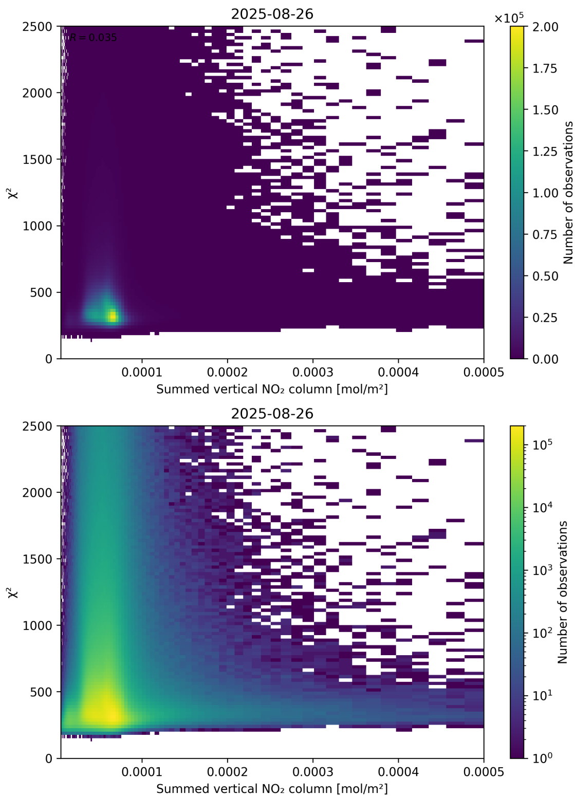
Figure 104: Scatter density plot of “Summed vertical NO 2 column” against “ \chi^2 ” for 2025-08-25 to 2025-08-27.
