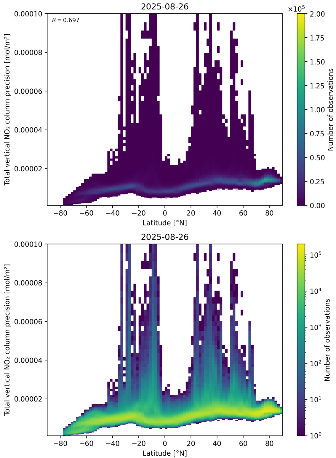
Figure 91: Scatter density plot of “Latitude” against “Total vertical NO 2 column precision” for 2025-08-25 to 2025-08-27.
