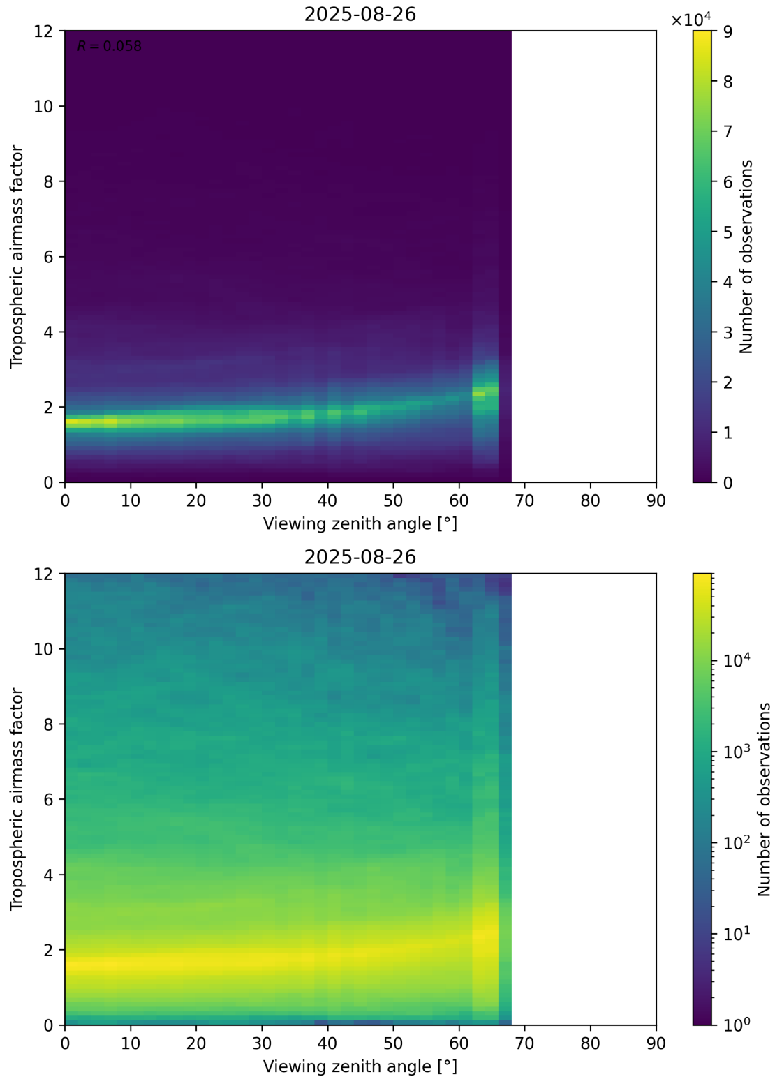
Figure 161: Scatter density plot of “Viewing zenith angle” against “Tropospheric airmass factor” for 2025-08-25 to 2025-08-27.
