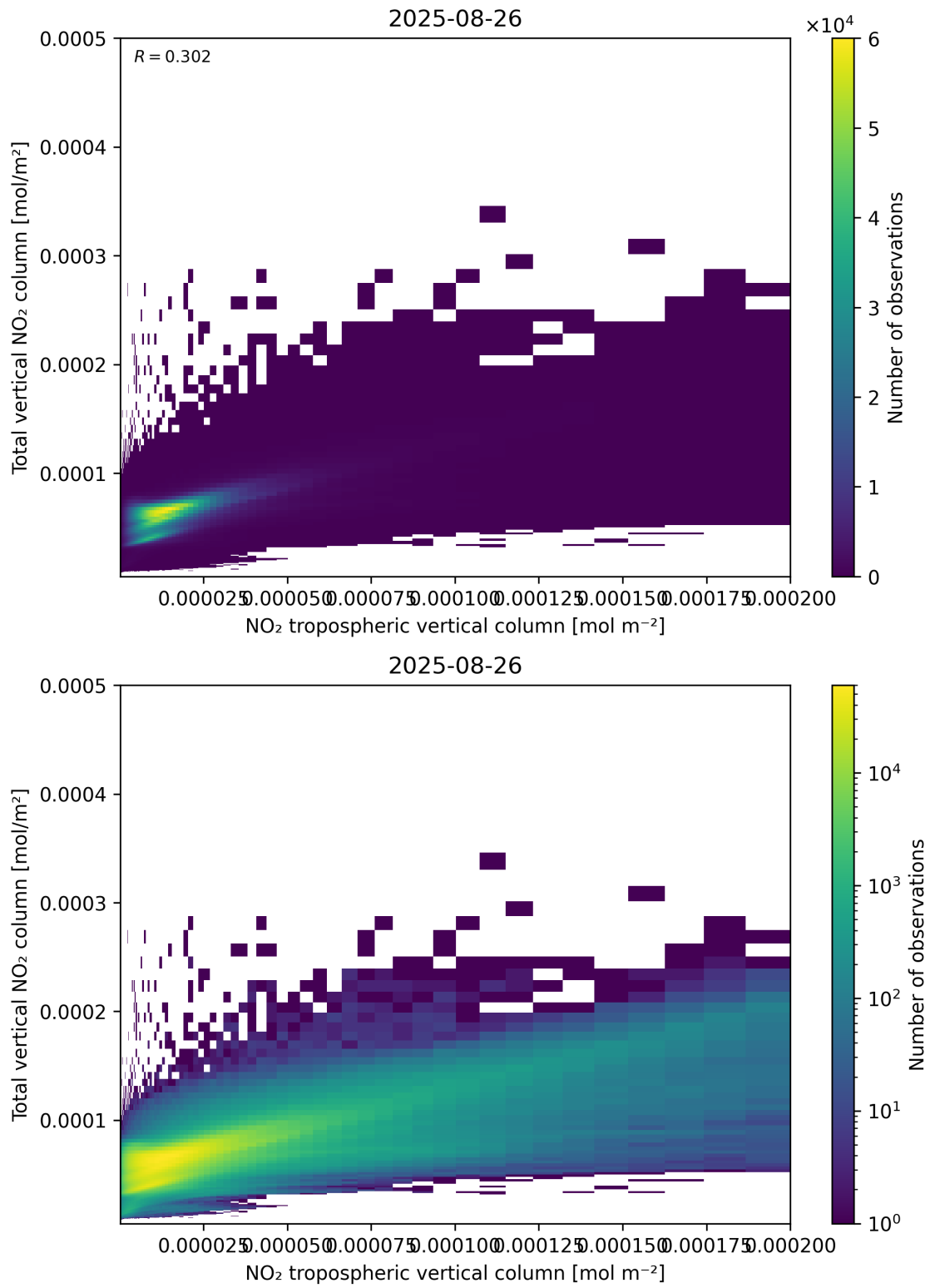
Figure 128: Scatter density plot of “NO 2 tropospheric vertical column” against “Total vertical NO 2 column” for 2025-08-25 to 2025-08-27.
