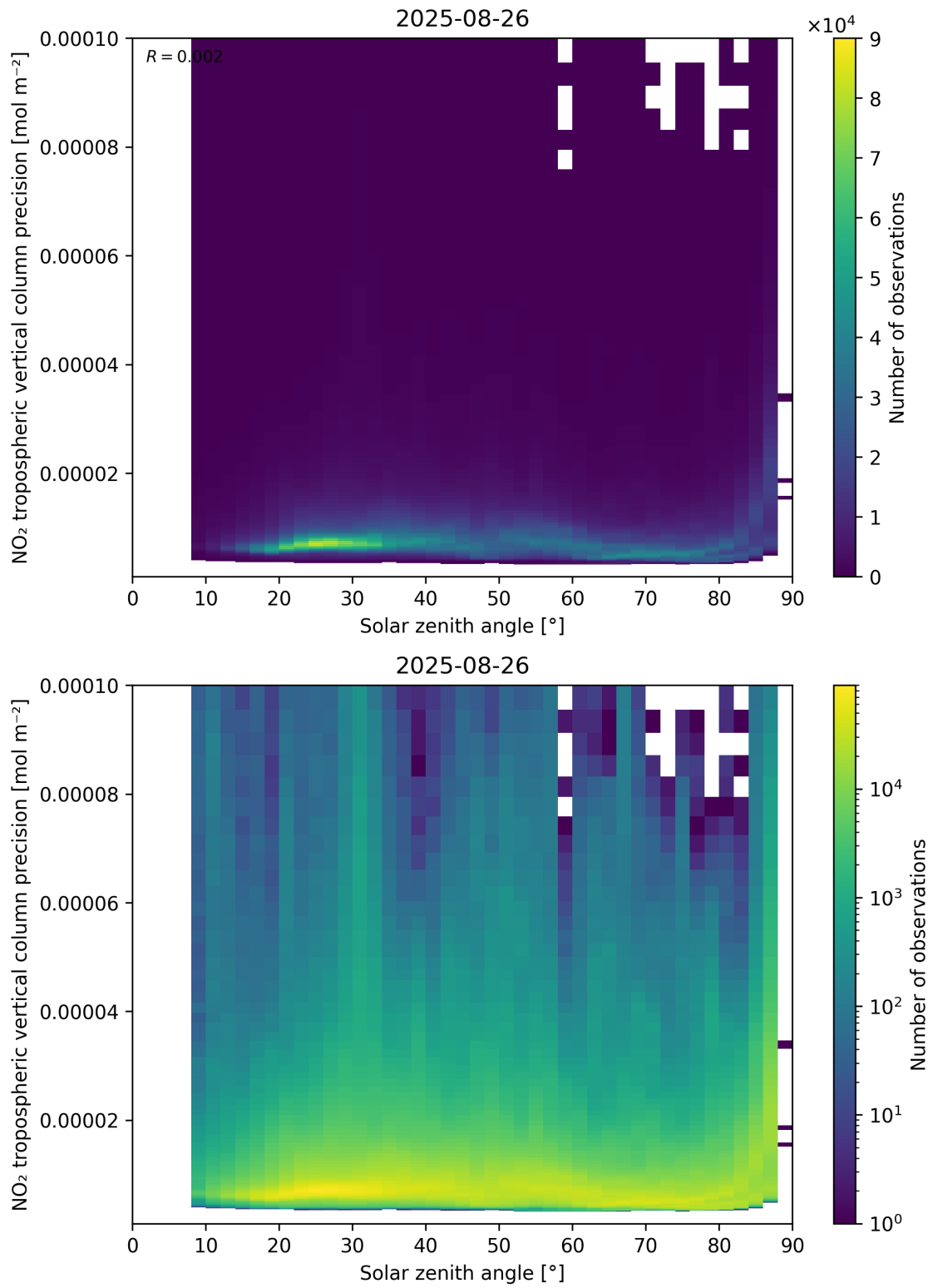
Figure 156: Scatter density plot of “Solar zenith angle” against “NO 2 tropospheric vertical column precision” for 2025-08-25 to 2025-08-27.
