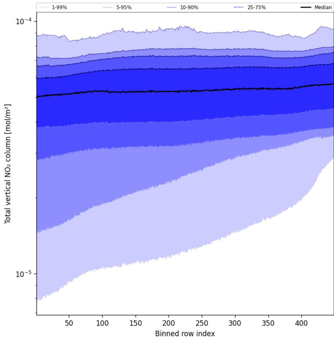
Figure 55: Along track statistics of “Total vertical NO 2 column” for 2025-08-25 to 2025-08-27
