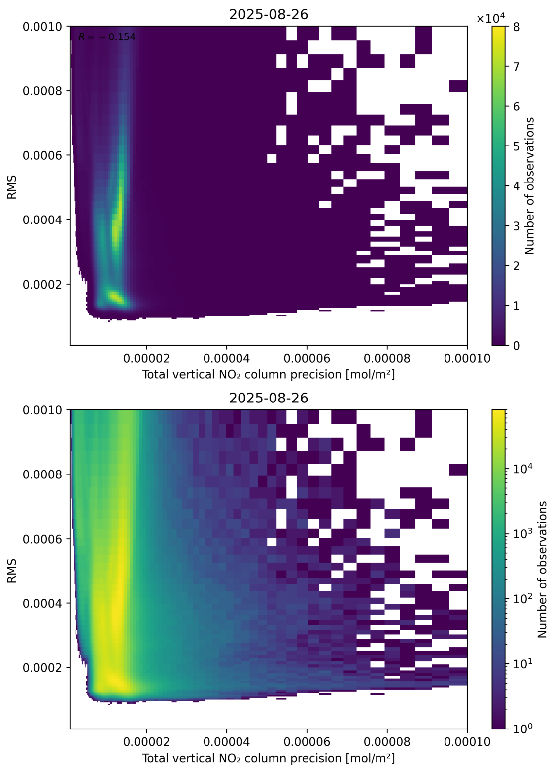
Figure 119: Scatter density plot of “Total vertical NO 2 column precision” against “RMS” for 2025-08-25 to 2025-08-27.
