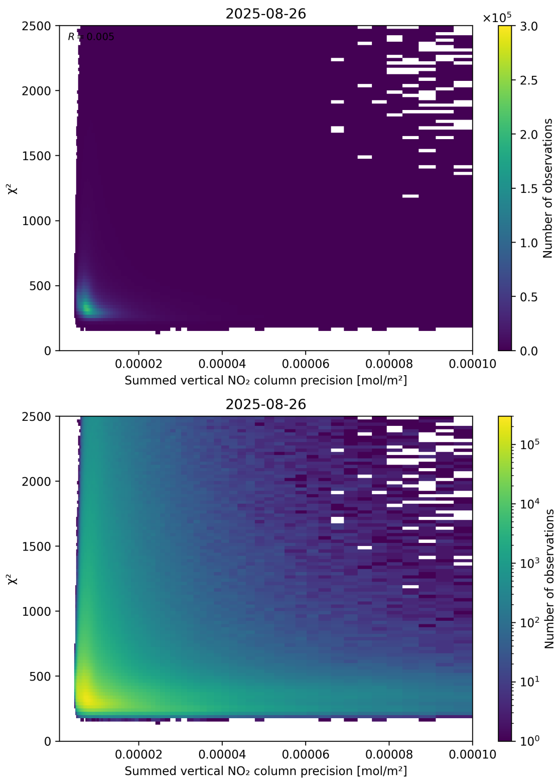
Figure 107: Scatter density plot of “Summed vertical NO 2 column precision” against “ \chi^2 ” for 2025-08-25 to 2025-08-27.
