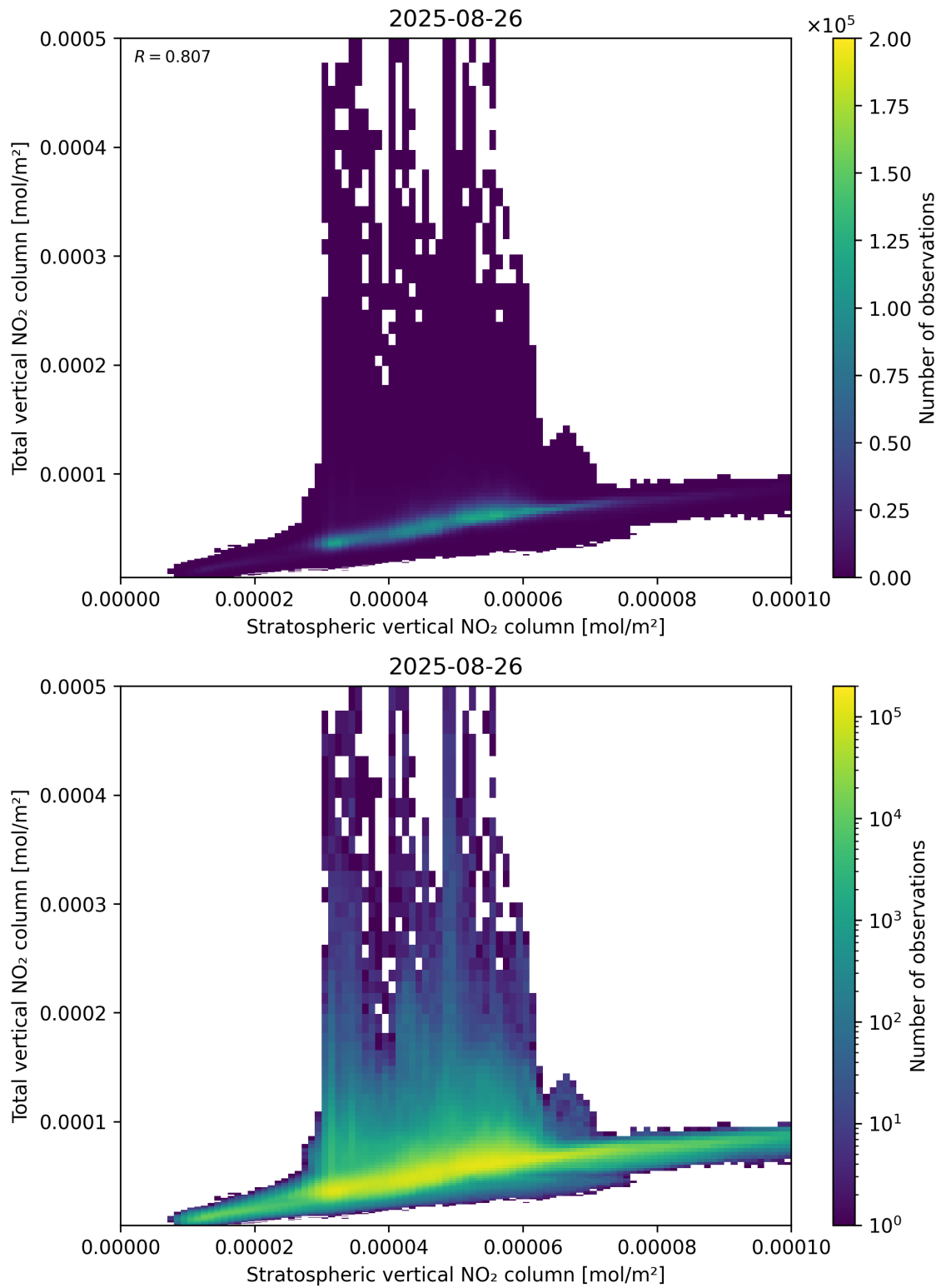
Figure 100: Scatter density plot of “Stratospheric vertical NO 2 column” against “Total vertical NO 2 column” for 2025-08-25 to 2025-08-27.
