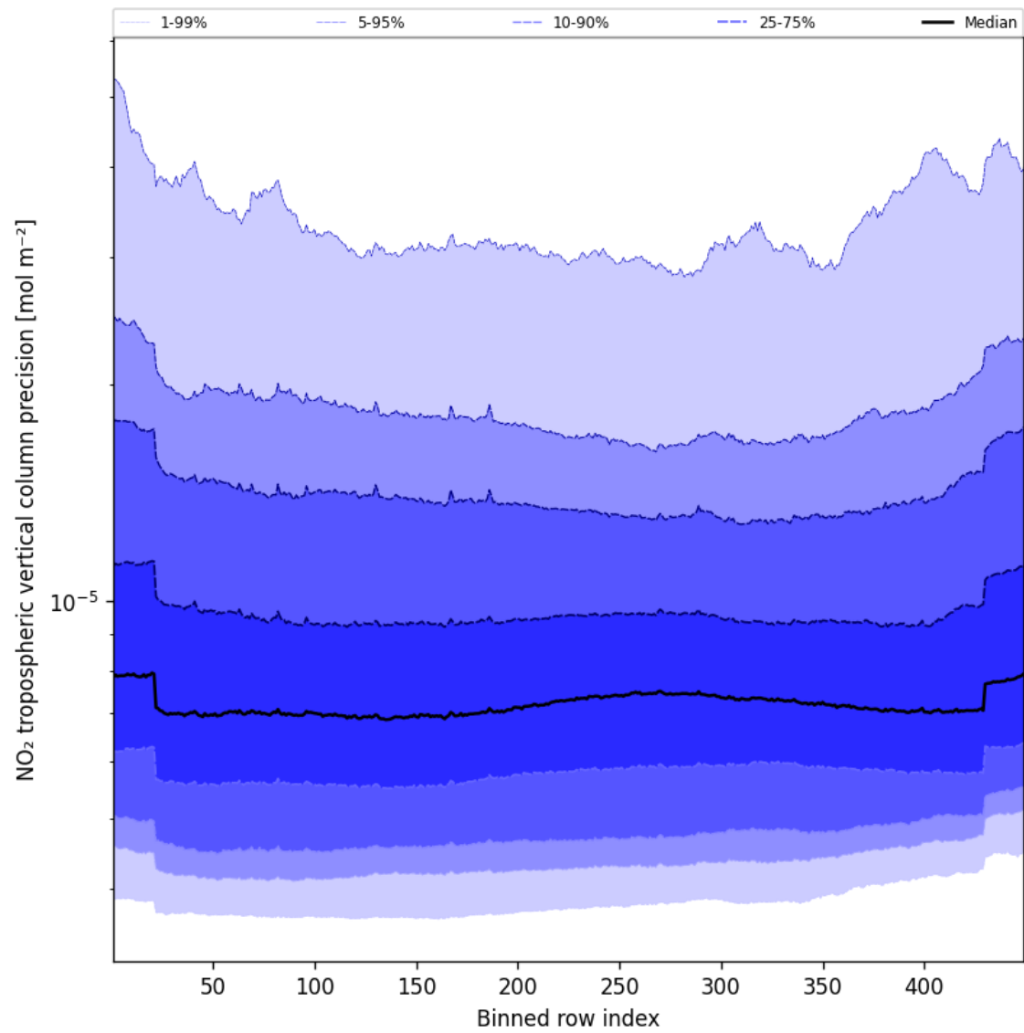
Figure 47: Along track statistics of “NO 2 tropospheric vertical column precision” for 2025-08-25 to 2025-08-27
