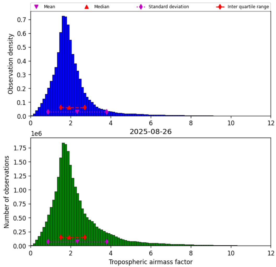
Figure 31: Histogram of “Tropospheric airmass factor” for 2025-08-25 to 2025-08-27
