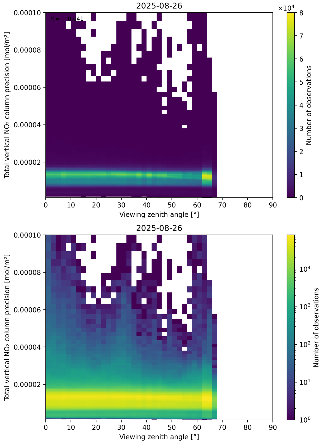
Figure 168: Scatter density plot of “Viewing zenith angle” against “Total vertical NO 2 column precision” for 2025-08-25 to 2025-08-27.
