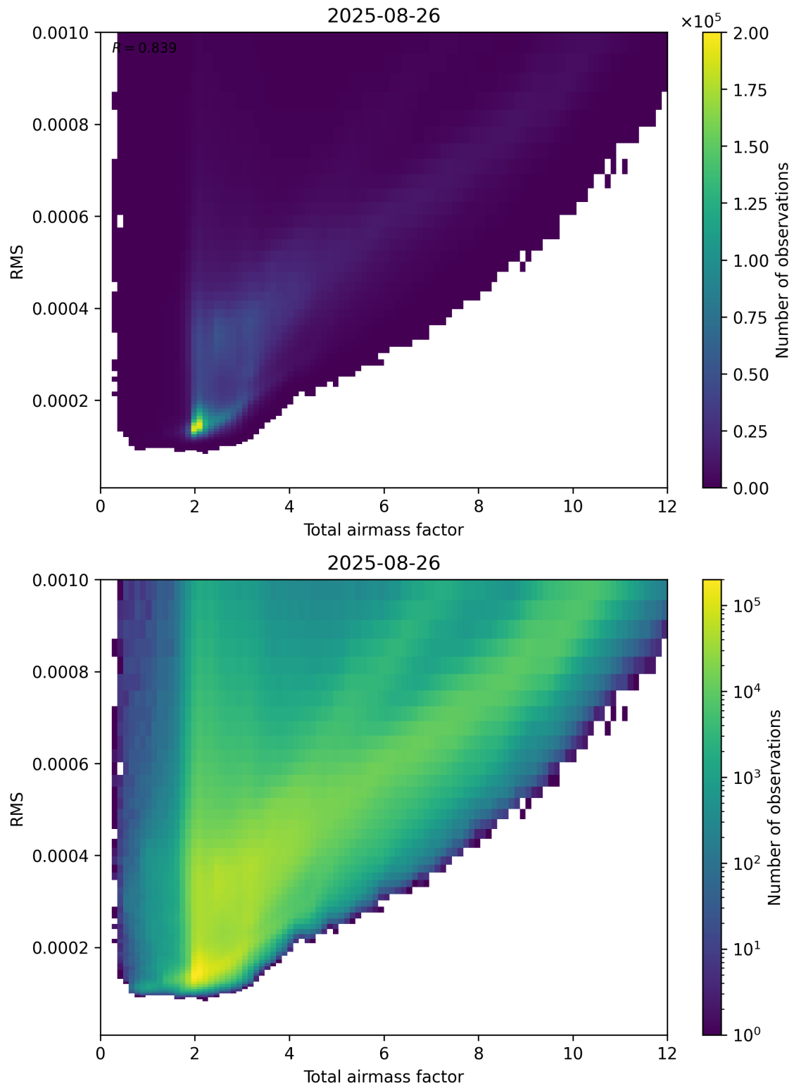
Figure 69: Scatter density plot of “Total airmass factor” against “RMS” for 2025-08-25 to 2025-08-27.
