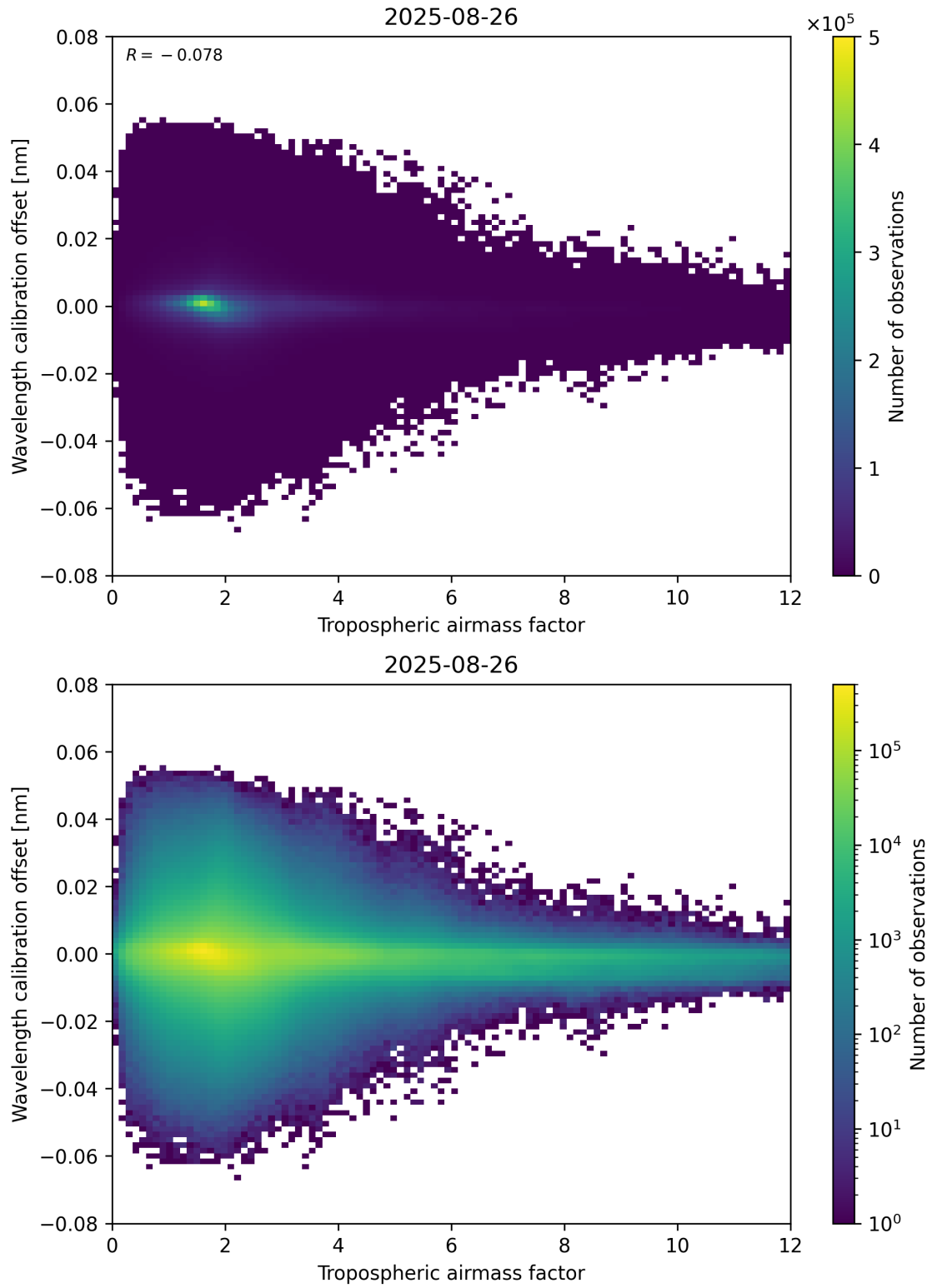
Figure 80: Scatter density plot of “Tropospheric airmass factor” against “Wavelength calibration offset” for 2025-08-25 to 2025-08-27.
