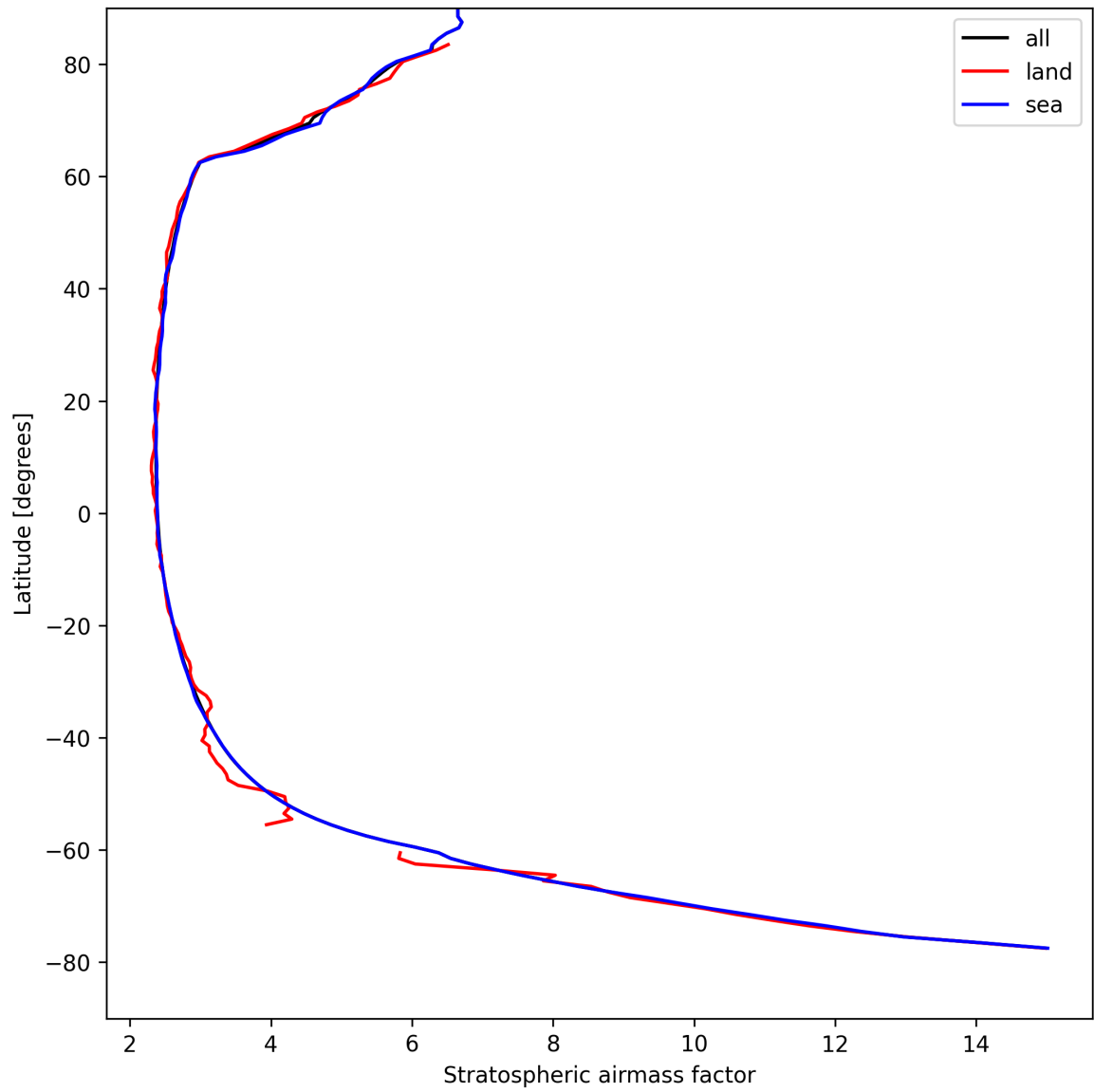
Figure 27: Zonal average of “Stratospheric airmass factor” for 2025-08-25 to 2025-08-27.
