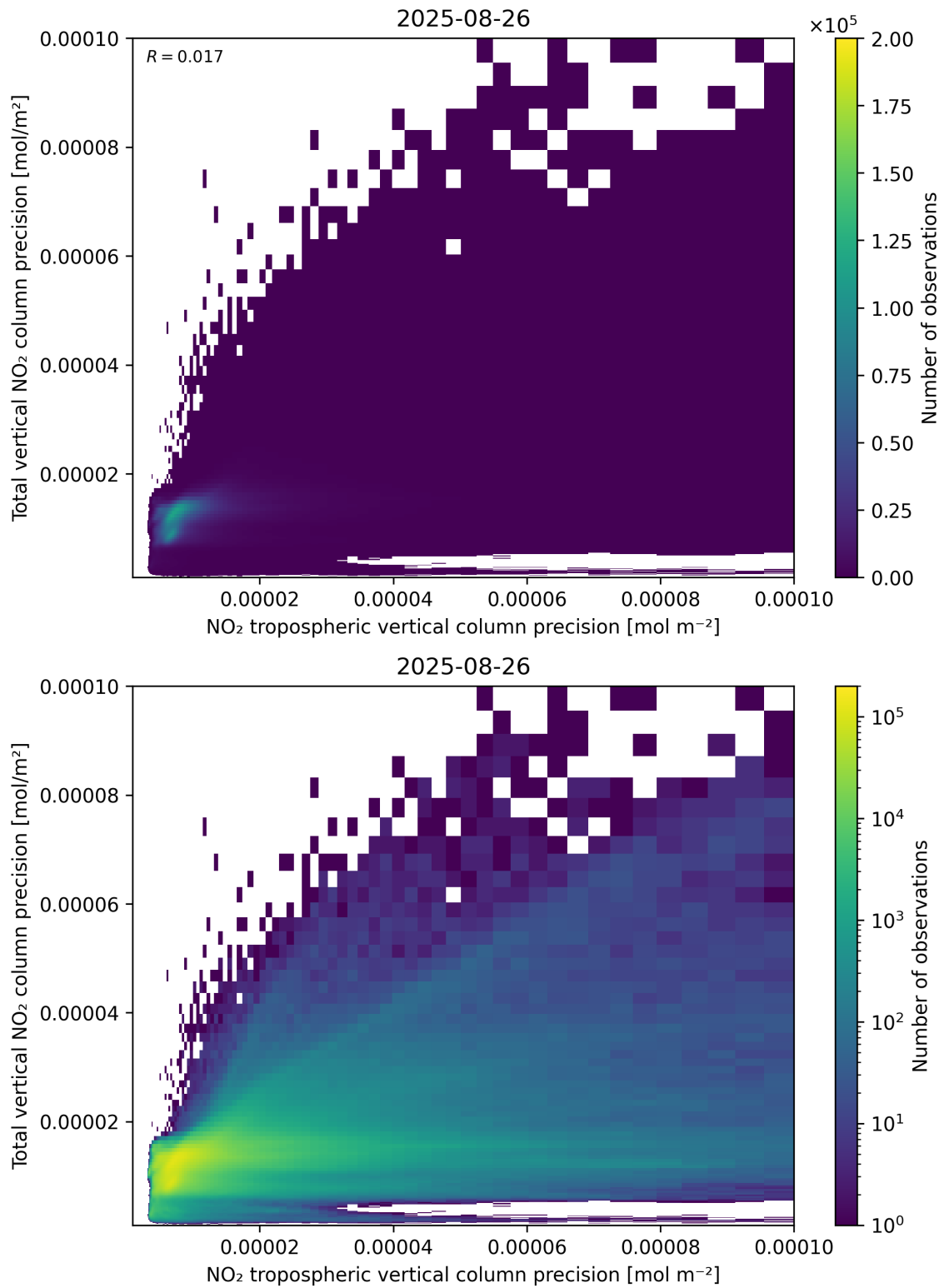
Figure 139: Scatter density plot of “NO 2 tropospheric vertical column precision” against “Total vertical NO 2 column precision” for 2025-08-25 to 2025-08-27.
