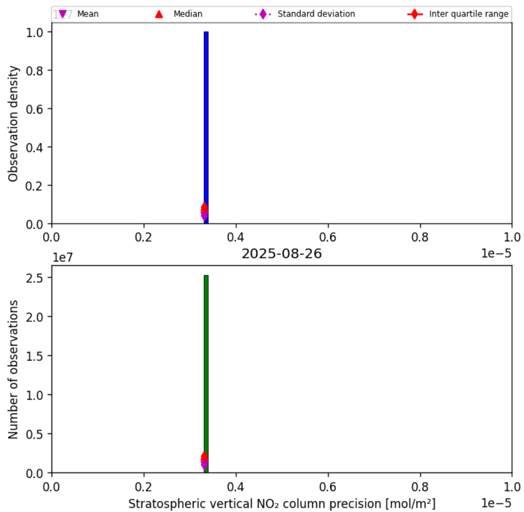
Figure 37: Histogram of “Stratospheric vertical NO 2 column precision” for 2025-08-25 to 2025-08-27
