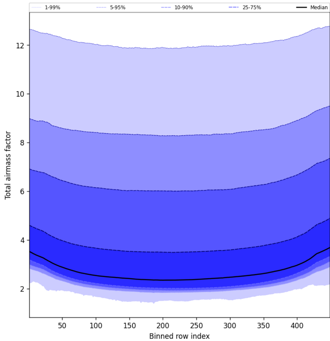
Figure 49: Along track statistics of “Total airmass factor” for 2025-08-25 to 2025-08-27
