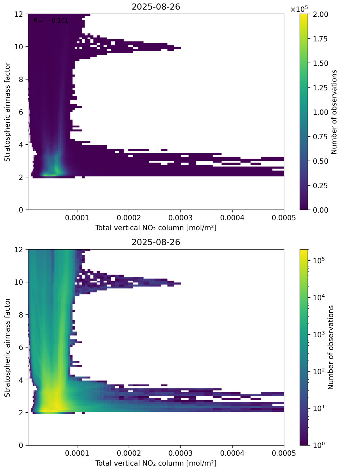
Figure 110: Scatter density plot of “Total vertical NO 2 column” against “Stratospheric airmass factor” for 2025-08-25 to 2025-08-27.
