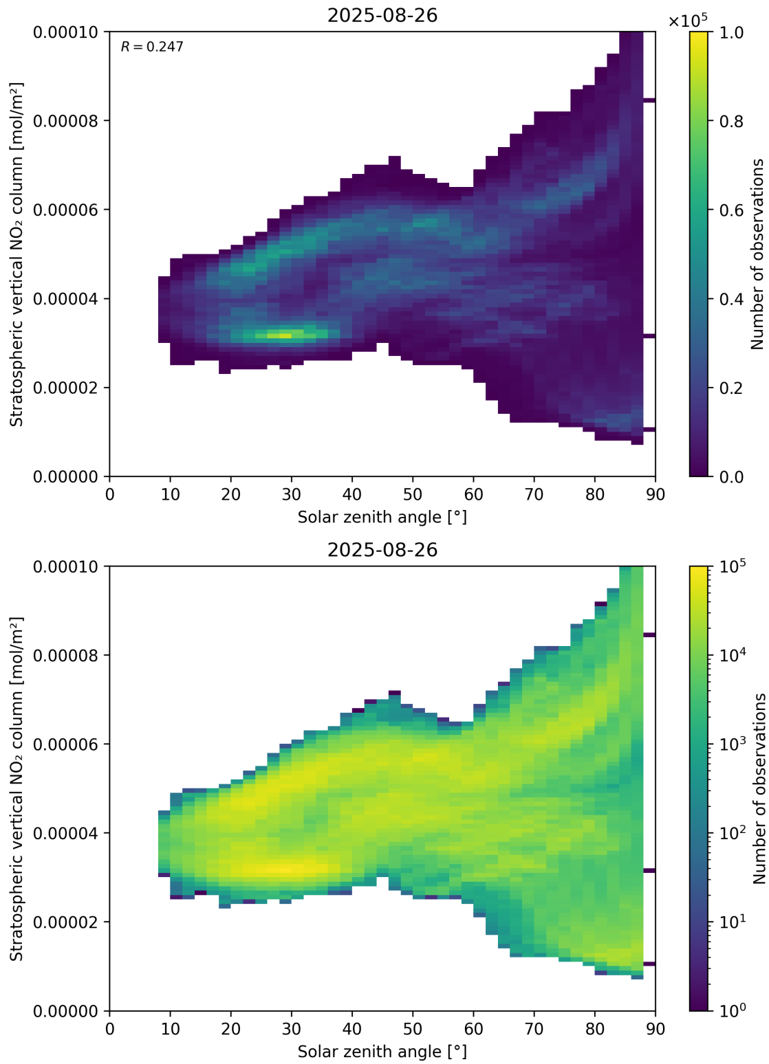
Figure 150: Scatter density plot of “Solar zenith angle” against “Stratospheric vertical NO 2 column” for 2025-08-25 to 2025-08-27.
