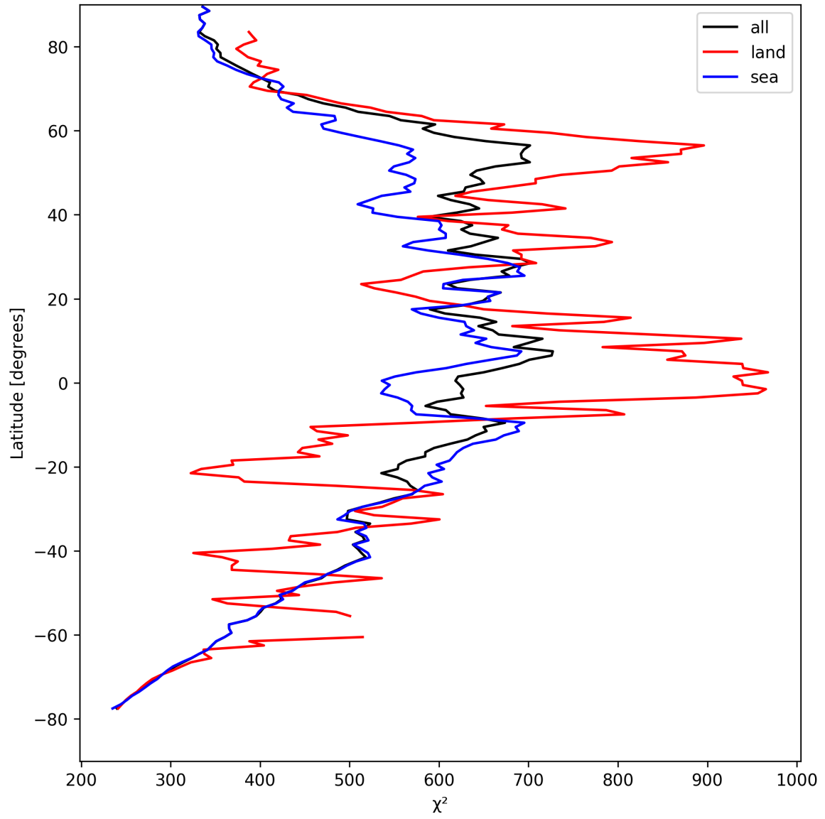
Figure 25: Zonal average of “ \chi^2 ” for 2025-08-25 to 2025-08-27.
