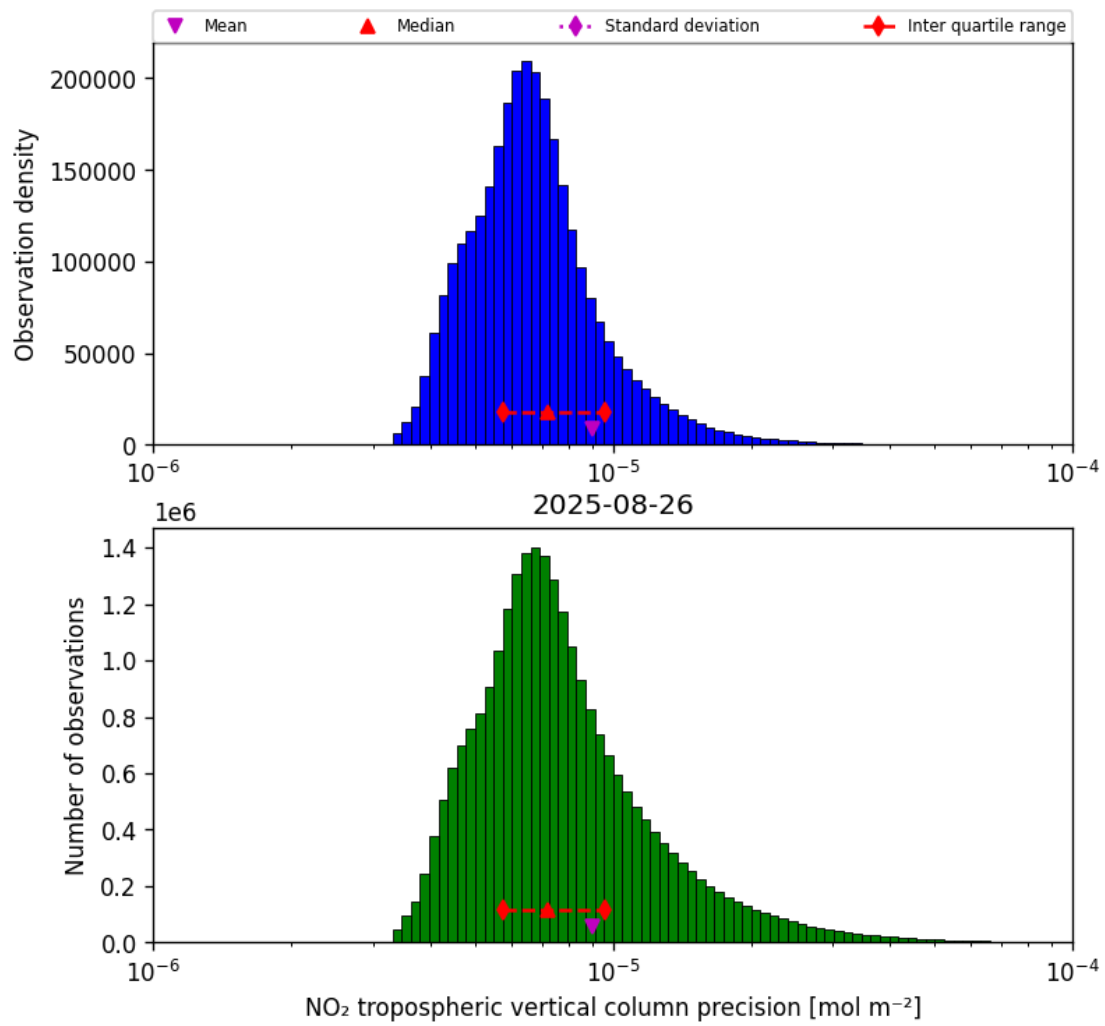
Figure 30: Histogram of “NO 2 tropospheric vertical column precision” for 2025-08-25 to 2025-08-27
