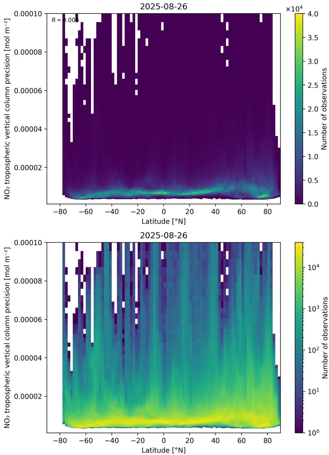
Figure 93: Scatter density plot of “Latitude” against “NO 2 tropospheric vertical column precision” for 2025-08-25 to 2025-08-27.
