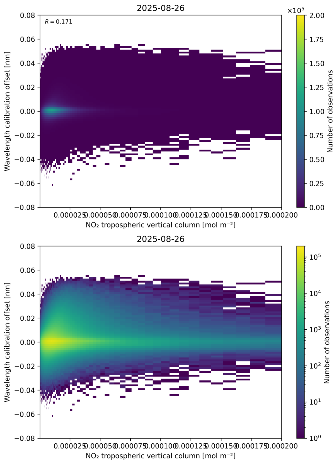
Figure 143: Scatter density plot of “NO 2 tropospheric vertical column” against “Wavelength calibration offset” for 2025-08-25 to 2025-08-27.
