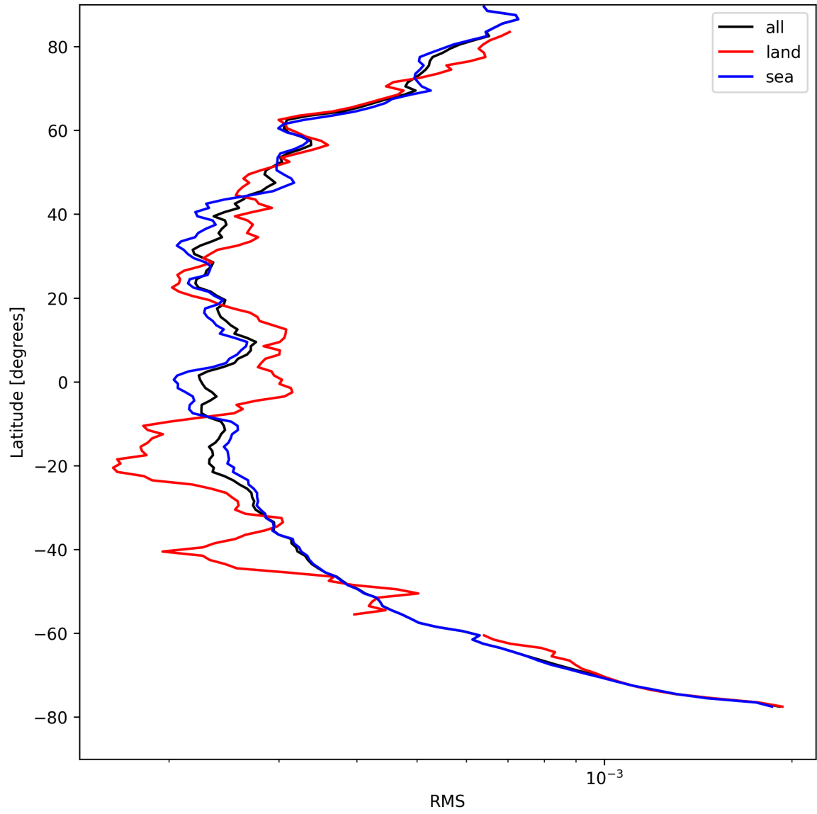
Figure 26: Zonal average of “RMS” for 2025-08-25 to 2025-08-27.
