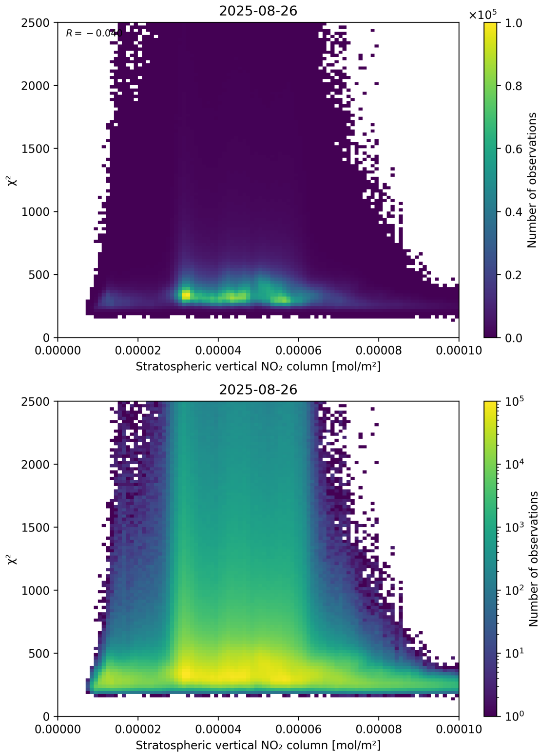
Figure 97: Scatter density plot of “Stratospheric vertical NO 2 column” against “ \chi^2 ” for 2025-08-25 to 2025-08-27.
