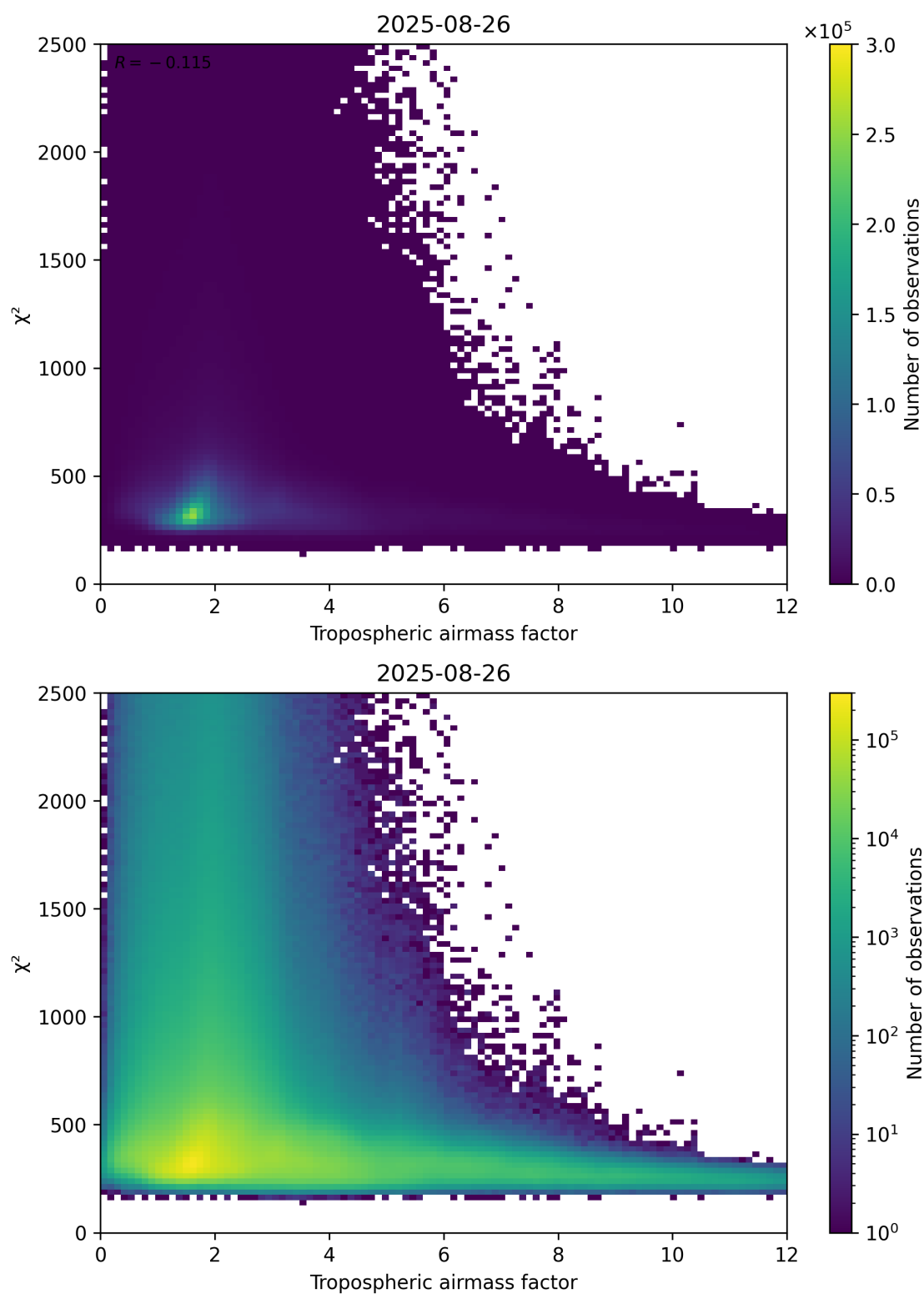
Figure 73: Scatter density plot of “Tropospheric airmass factor” against “ \chi^2 ” for 2025-08-25 to 2025-08-27.
