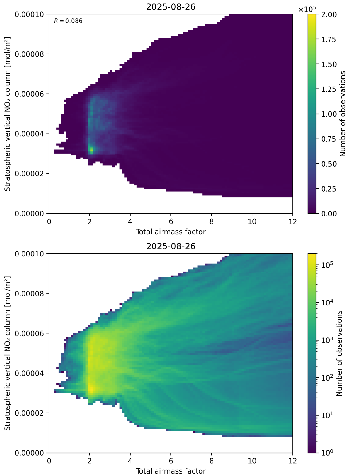
Figure 64: Scatter density plot of “Total airmass factor” against “Stratospheric vertical NO 2 column” for 2025-08-25 to 2025-08-27.
