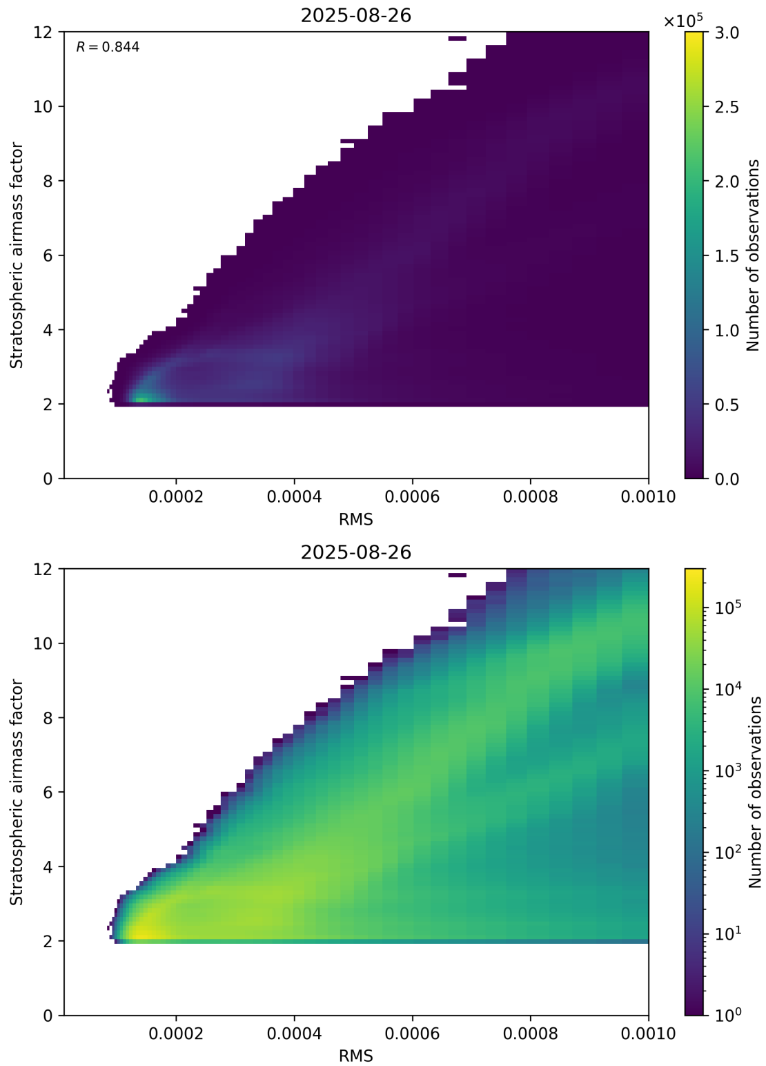
Figure 144: Scatter density plot of “RMS” against “Stratospheric airmass factor” for 2025-08-25 to 2025-08-27.
