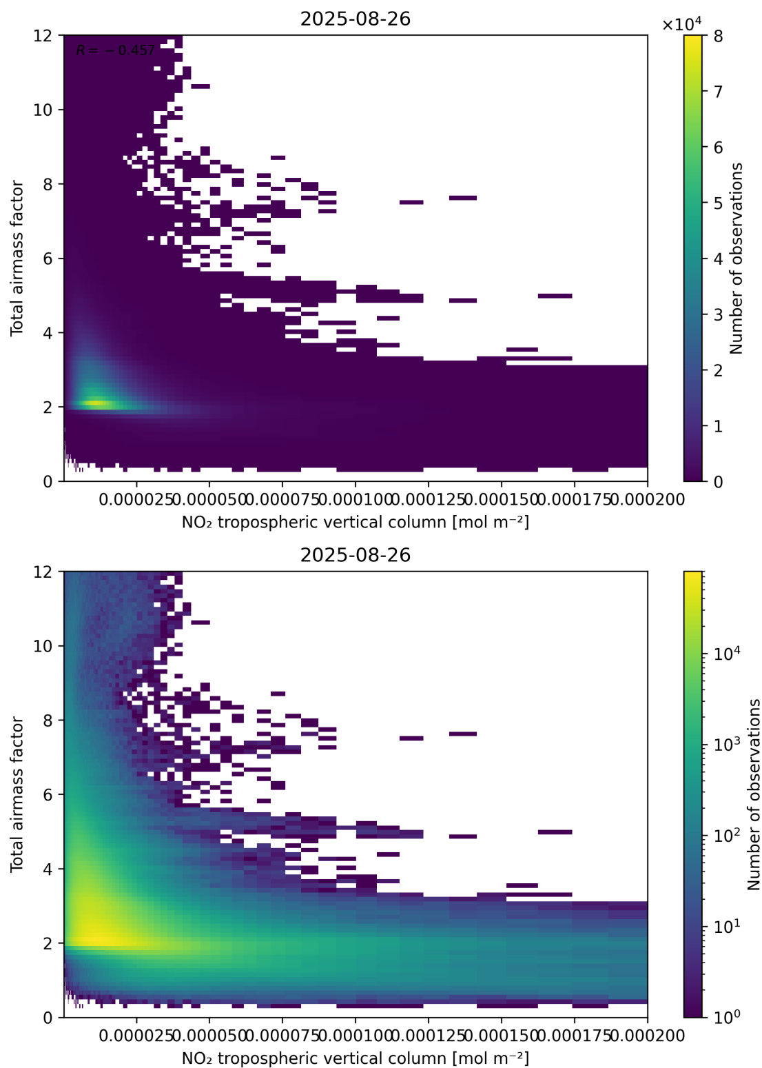
Figure 122: Scatter density plot of “NO 2 tropospheric vertical column” against “Total air mass factor” for 2025-08-25 to 2025-08-27.
