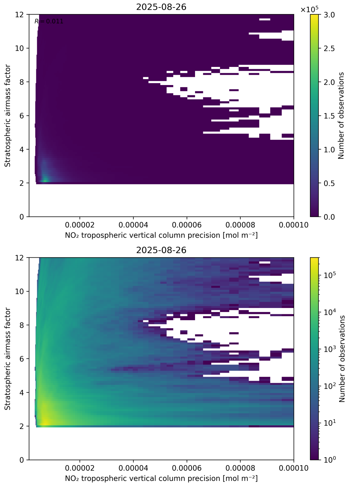
Figure 131: Scatter density plot of “NO 2 tropospheric vertical column precision” against “Stratospheric airmass factor” for 2025-08-25 to 2025-08-27.
