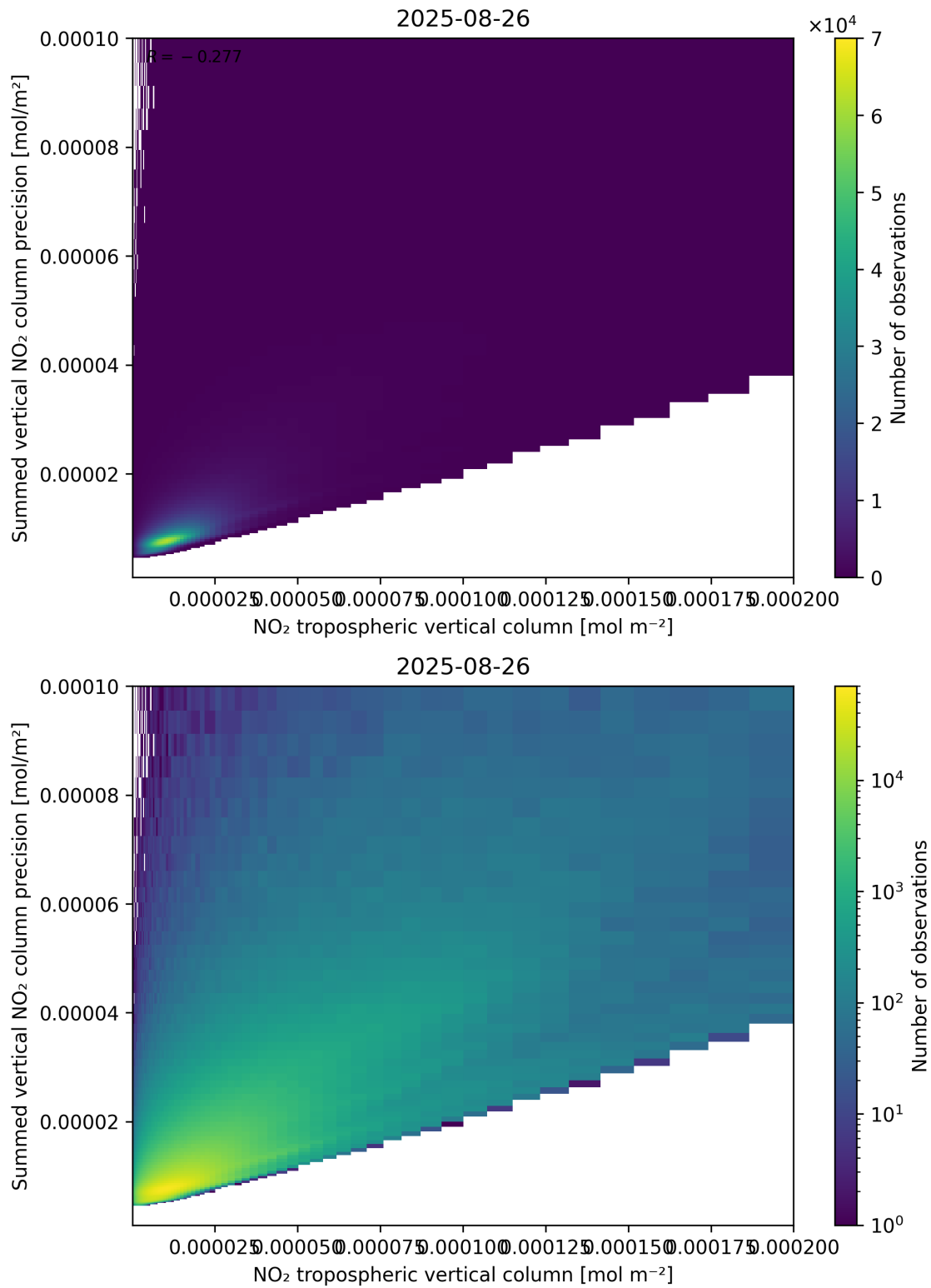
Figure 127: Scatter density plot of “NO 2 tropospheric vertical column” against “Summed vertical NO 2 column precision” for 2025-08-25 to 2025-08-27.
