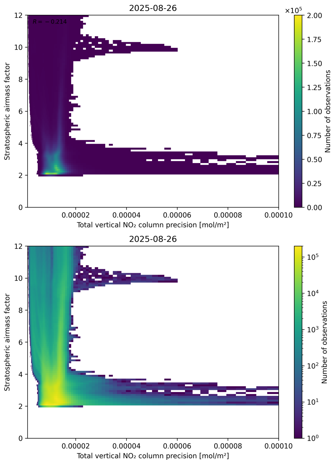
Figure 115: Scatter density plot of “Total vertical NO 2 column precision” against “Stratospheric air mass factor” for 2025-08-25 to 2025-08-27.
