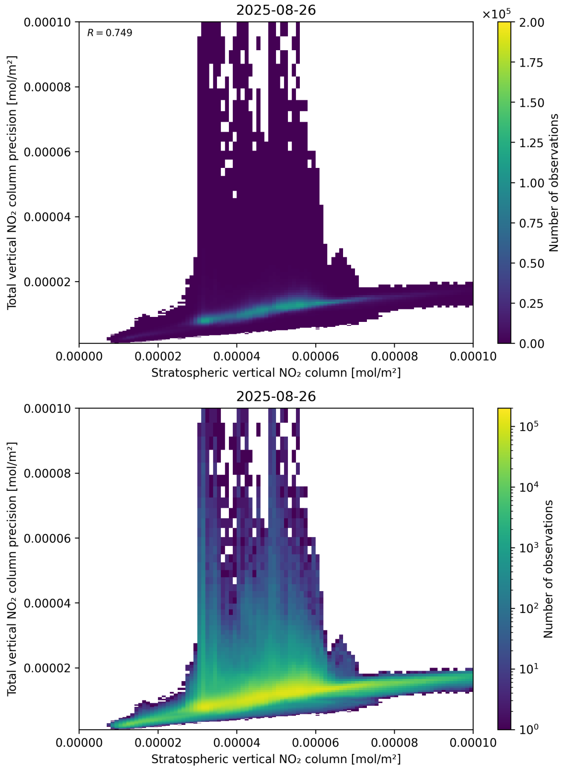
Figure 101: Scatter density plot of “Stratospheric vertical NO 2 column” against “Total vertical NO 2 column precision” for 2025-08-25 to 2025-08-27.
