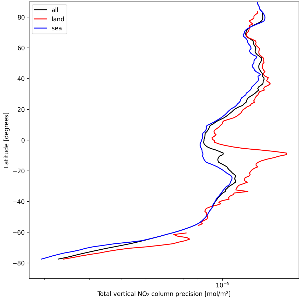
Figure 22: Zonal average of “Total vertical NO 2 column precision” for 2025-08-25 to 2025-08-27.
