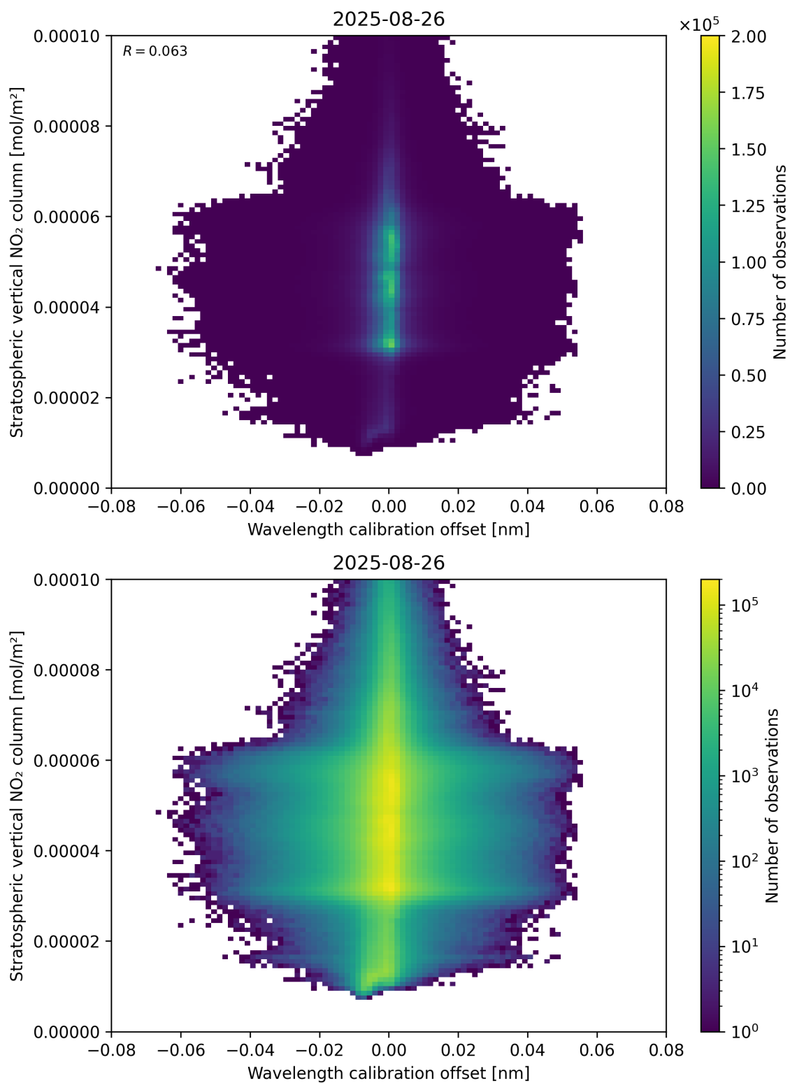
Figure 176: Scatter density plot of “Wavelength calibration offset” against “Stratospheric vertical NO 2 column” for 2025-08-25 to 2025-08-27.
