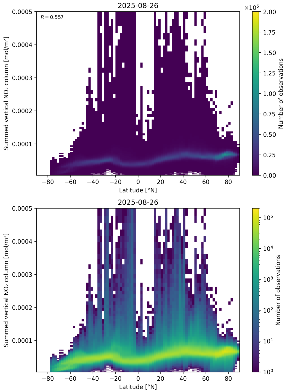
Figure 88: Scatter density plot of “Latitude” against “Summed vertical NO 2 column” for 2025-08-25 to 2025-08-27.
