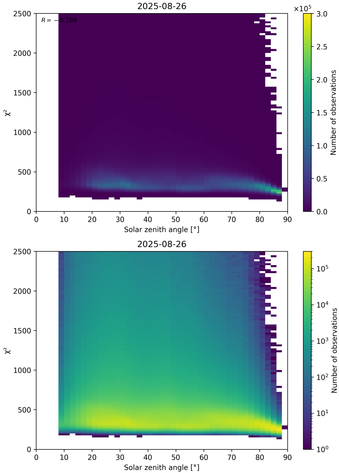
Figure 148: Scatter density plot of “Solar zenith angle” against “ \chi^2 ” for 2025-08-25 to 2025-08-27.
