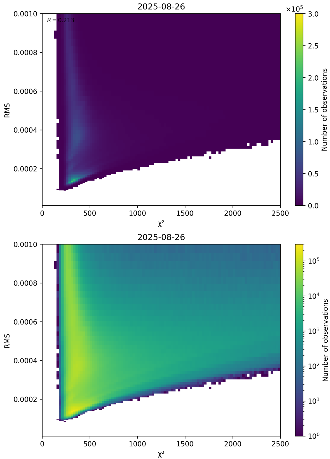
Figure 82: Scatter density plot of “ \chi^2 ” against “RMS” for 2025-08-25 to 2025-08-27.
