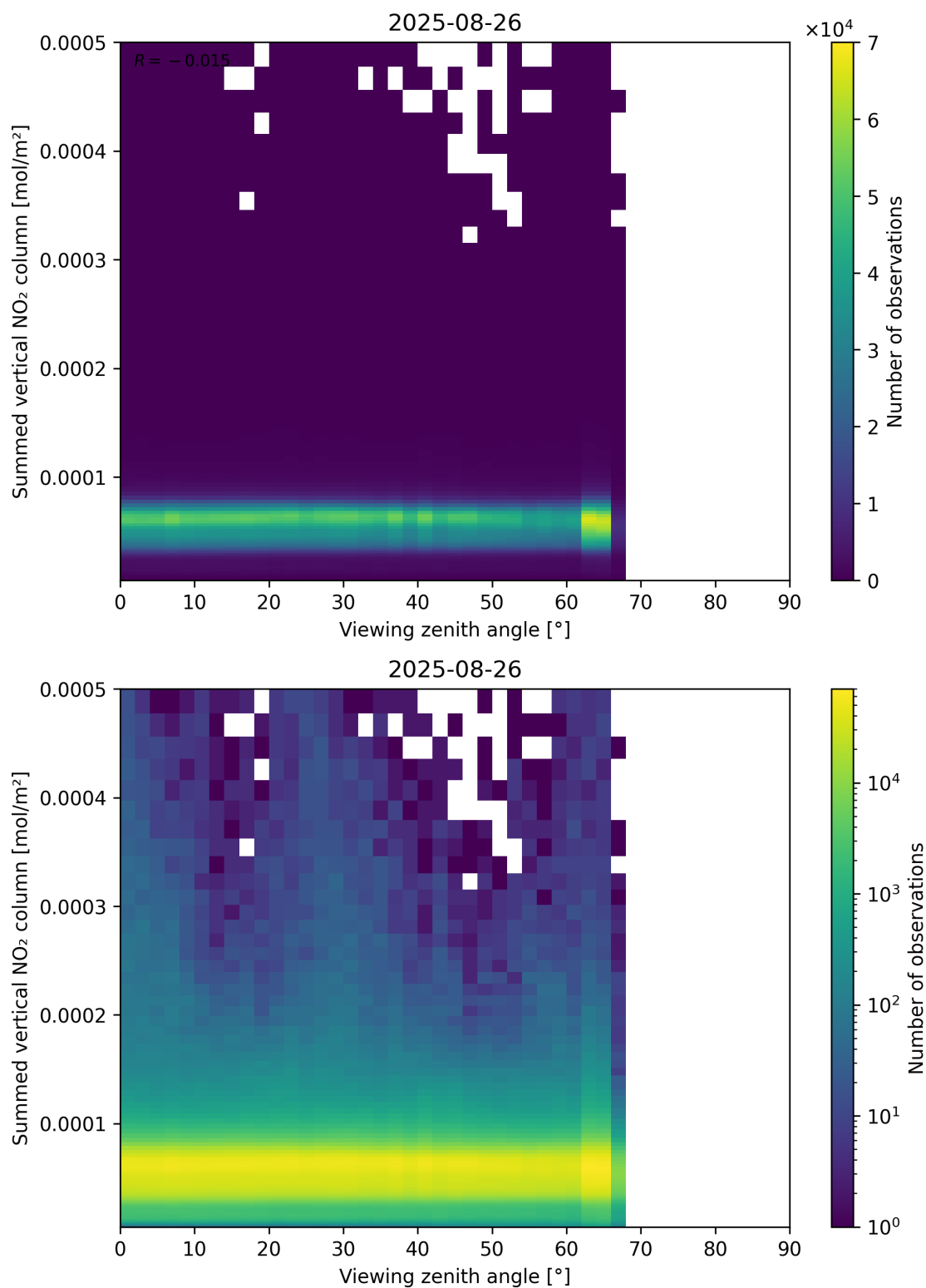
Figure 165: Scatter density plot of “Viewing zenith angle” against “Summed vertical NO 2 column” for 2025-08-25 to 2025-08-27.
