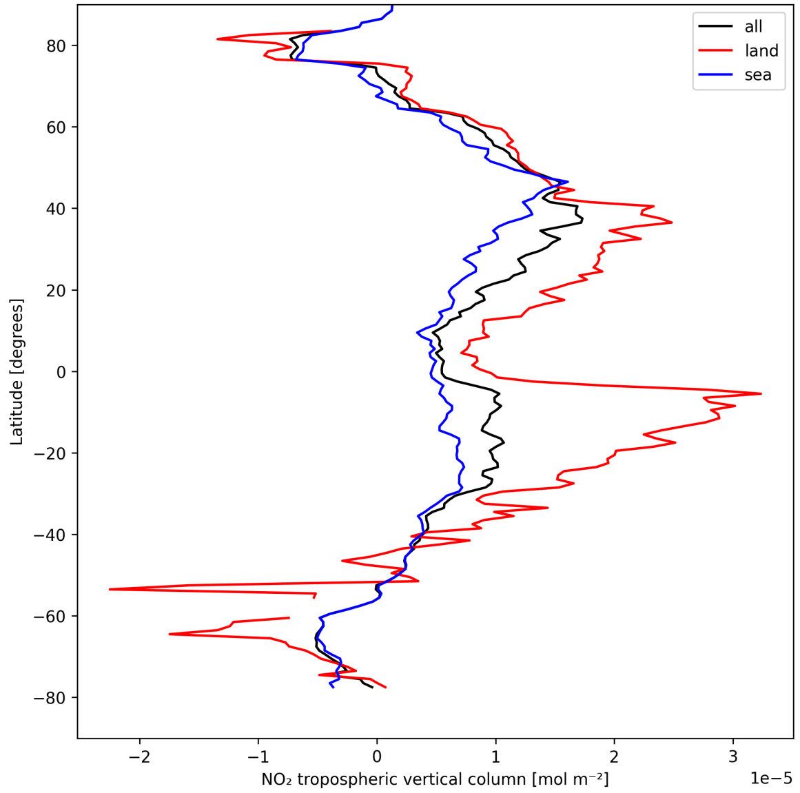
Figure 12: Zonal average of “NO 2 tropospheric vertical column” for 2025-08-25 to 2025-08-27.
