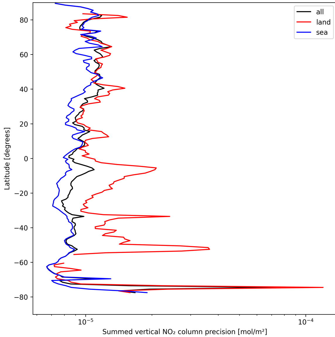
Figure 24: Zonal average of "Summed vertical NO 2 column precision" for 2025-08-25 to 2025-08-27.
