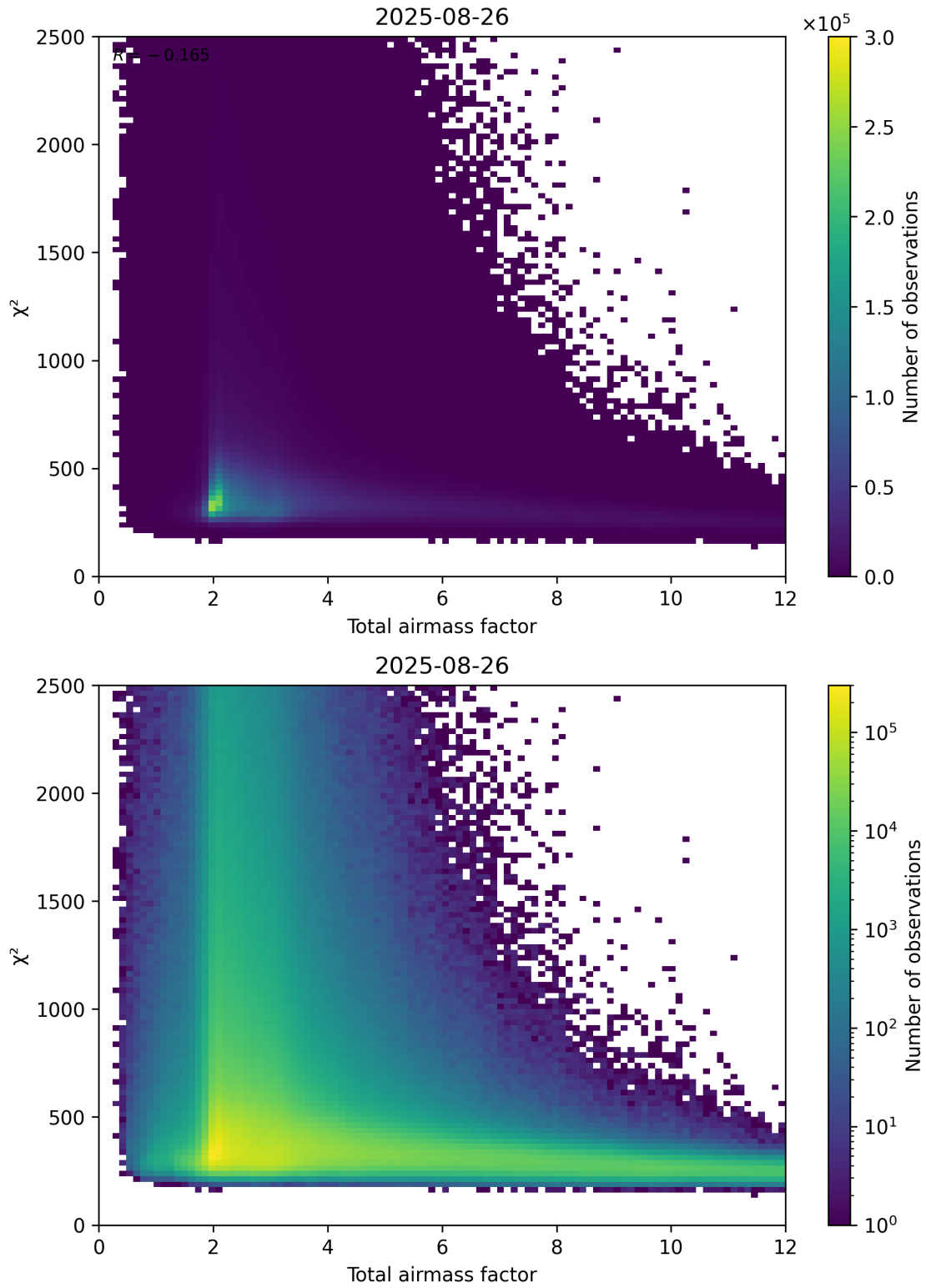
Figure 63: Scatter density plot of “Total airmass factor” against “ \chi^2 ” for 2025-08-25 to 2025-08-27.
