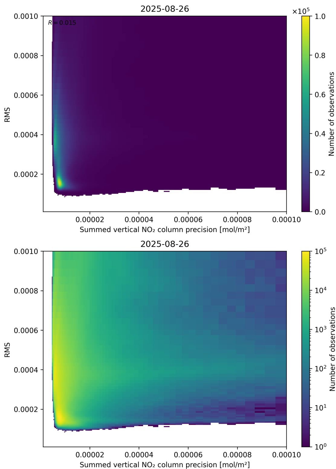
Figure 108: Scatter density plot of “Summed vertical NO 2 column precision” against “RMS” for 2025-08-25 to 2025-08-27.
