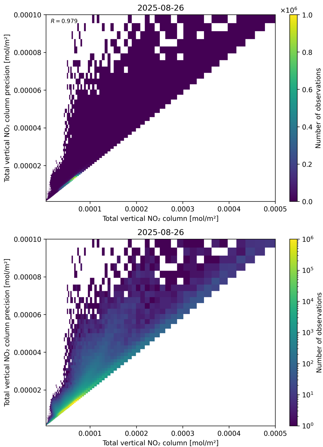
Figure 114: Scatter density plot of “Total vertical NO 2 column” against “Total vertical NO 2 column precision” for 2025-08-25 to 2025-08-27.
