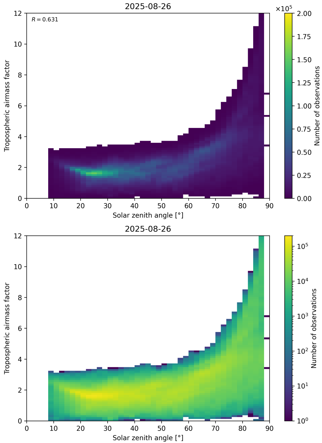
Figure 147: Scatter density plot of “Solar zenith angle” against “Tropospheric airmass factor” for 2025-08-25 to 2025-08-27.
