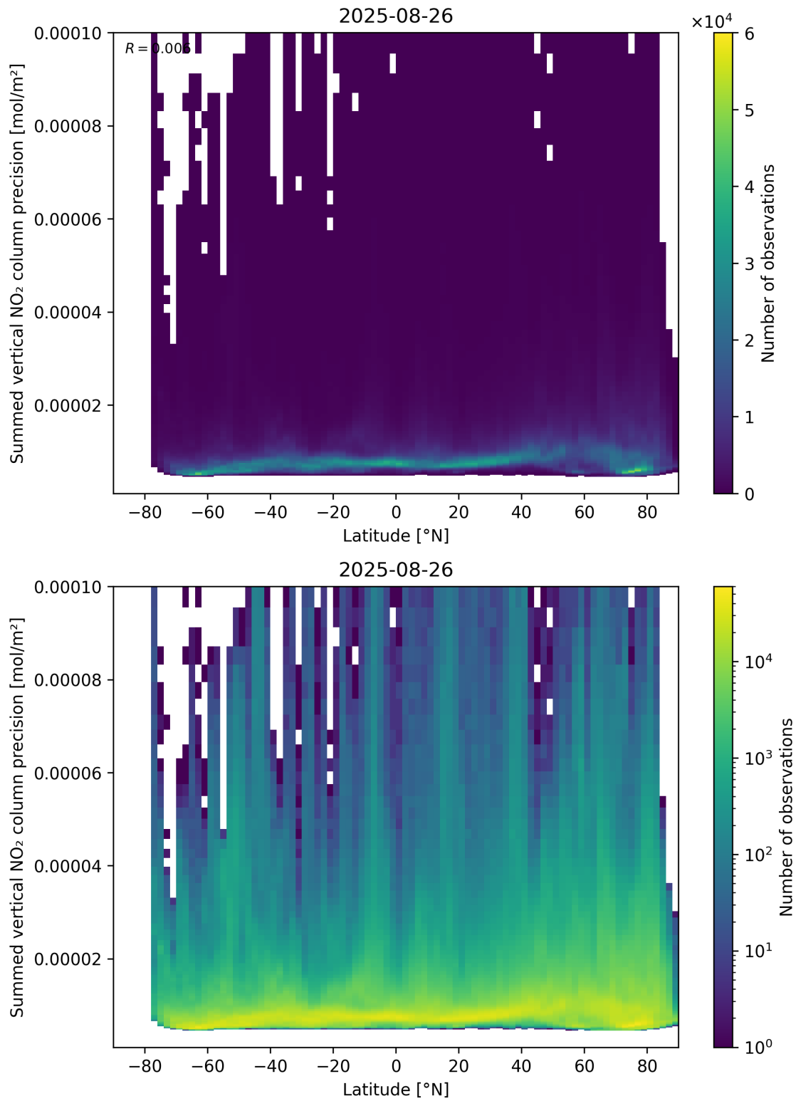
Figure 89: Scatter density plot of “Latitude” against “Summed vertical NO 2 column precision” for 2025-08-25 to 2025-08-27.
