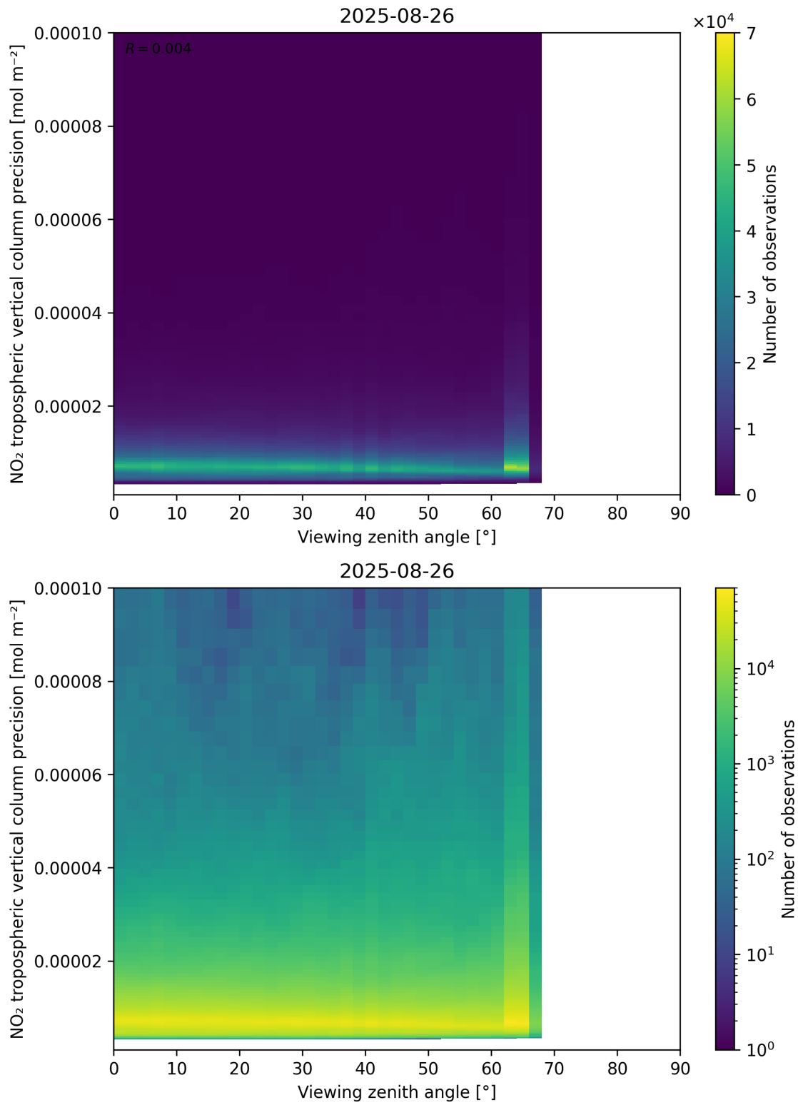
Figure 170: Scatter density plot of “Viewing zenith angle” against “NO 2 tropospheric vertical column precision” for 2025-08-25 to 2025-08-27.
