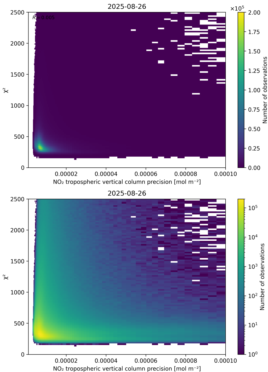
Figure 134: Scatter density plot of “NO 2 tropospheric vertical column precision” against “ \chi^2 ” for 2025-08-25 to 2025-08-27.
