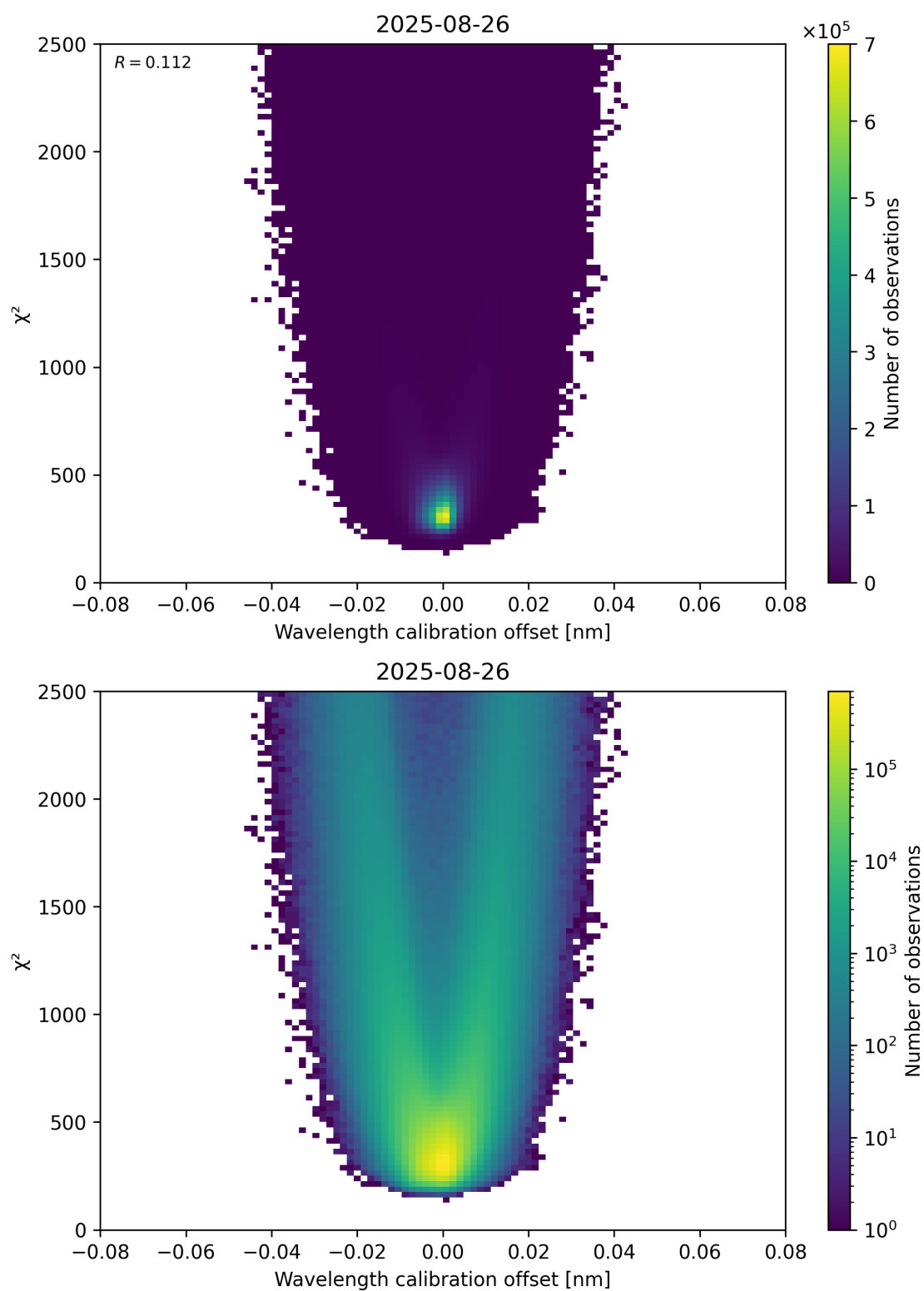
Figure 175: Scatter density plot of “Wavelength calibration offset” against “ \chi^2 ” for 2025-08-25 to 2025-08-27.
