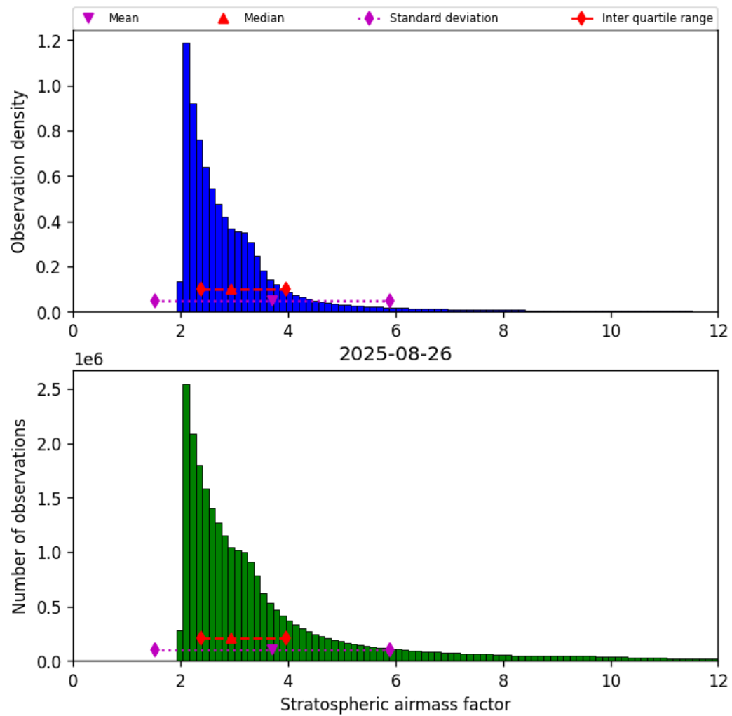
Figure 44: Histogram of “Stratospheric airmass factor” for 2025-08-25 to 2025-08-27
