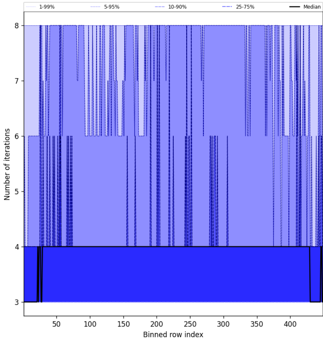
Figure 51: Along track statistics of “Number of iterations” for 2025-08-25 to 2025-08-27
