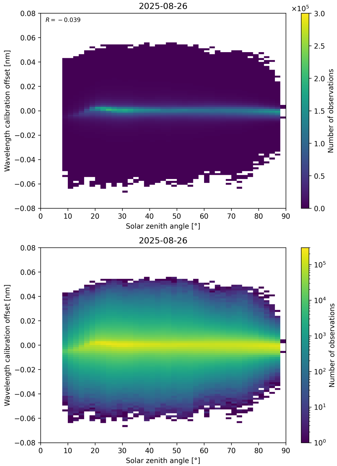
Figure 158: Scatter density plot of “Solar zenith angle” against “Wavelength calibration offset” for 2025-08-25 to 2025-08-27.
