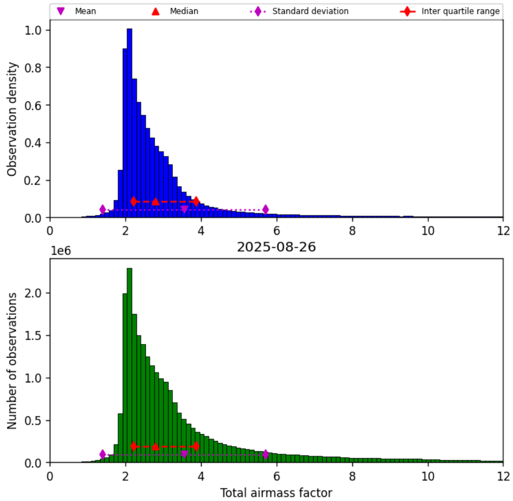
Figure 32: Histogram of “Total airmass factor” for 2025-08-25 to 2025-08-27
