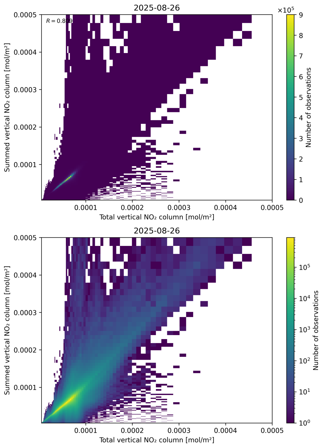
Figure 112: Scatter density plot of “Total vertical NO 2 column” against “Summed vertical NO 2 column” for 2025-08-25 to 2025-08-27.
