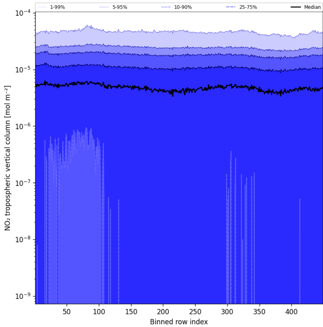
Figure 46: Along track statistics of “NO 2 tropospheric vertical column” for 2025-08-25 to 2025-08-27
