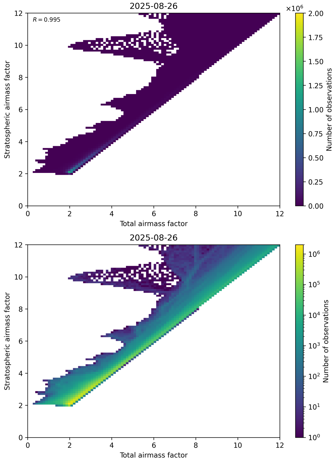
Figure 62: Scatter density plot of “Total airmass factor” against “Stratospheric airmass factor” for 2025-08-25 to 2025-08-27.
