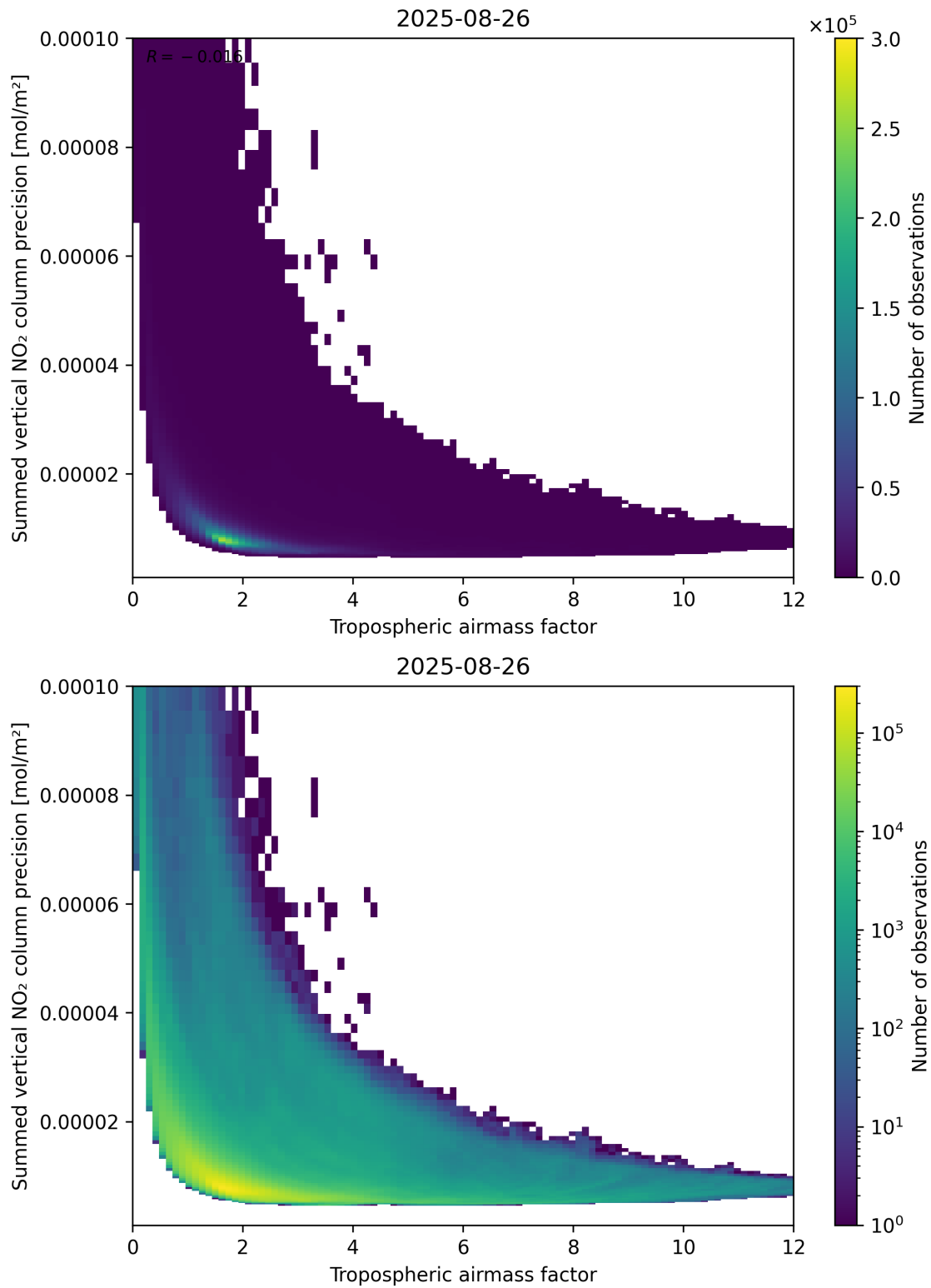
Figure 76: Scatter density plot of “Tropospheric air mass factor” against “Summed vertical NO 2 column precision” for 2025-08-25 to 2025-08-27.
