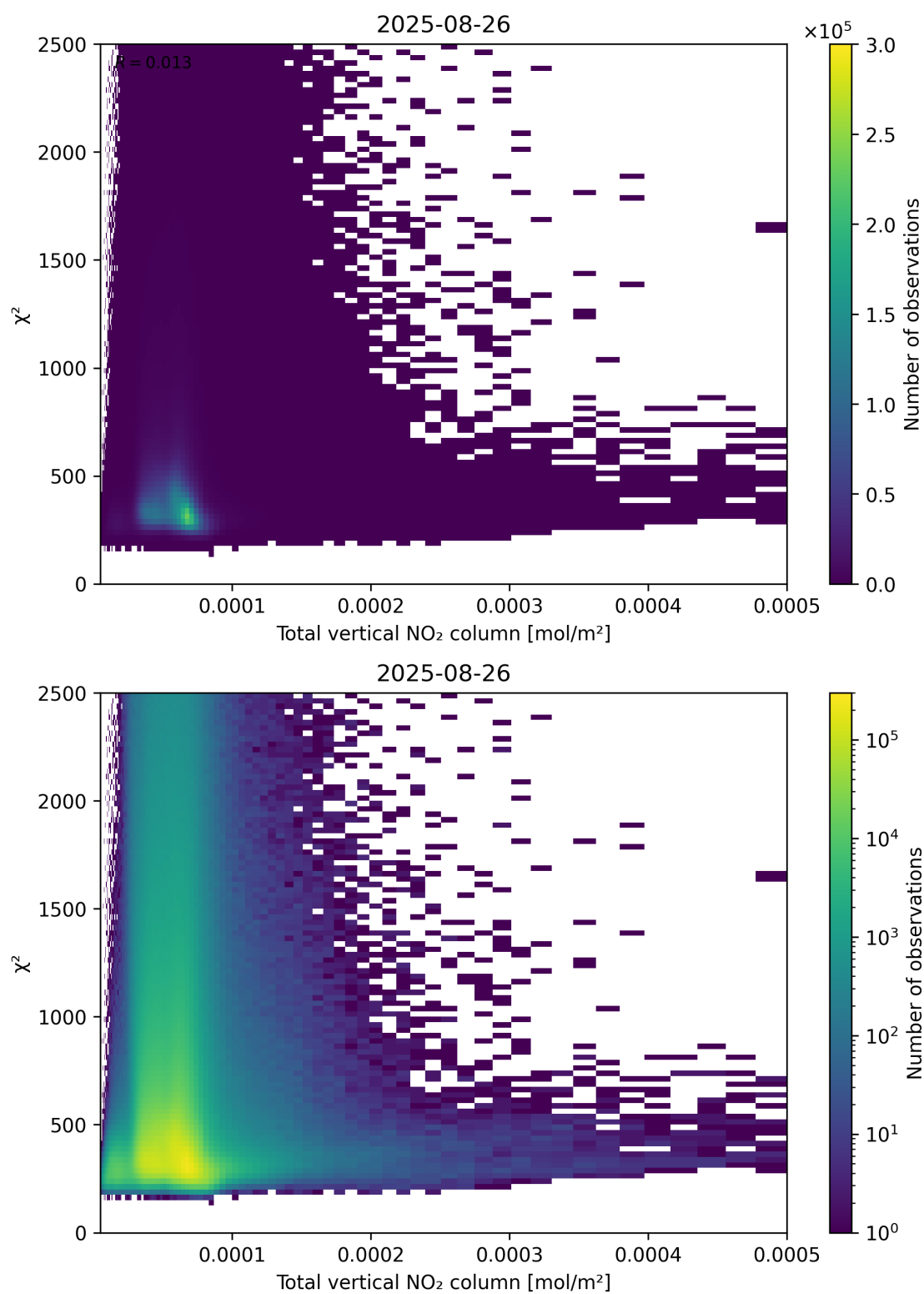
Figure 111: Scatter density plot of “Total vertical NO 2 column” against “ \chi^2 ” for 2025-08-25 to 2025-08-27.
