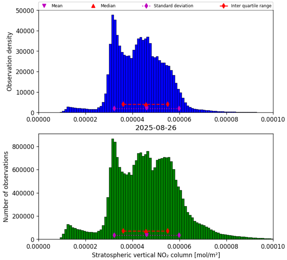
Figure 36: Histogram of “Stratospheric vertical NO 2 column” for 2025-08-25 to 2025-08-27
