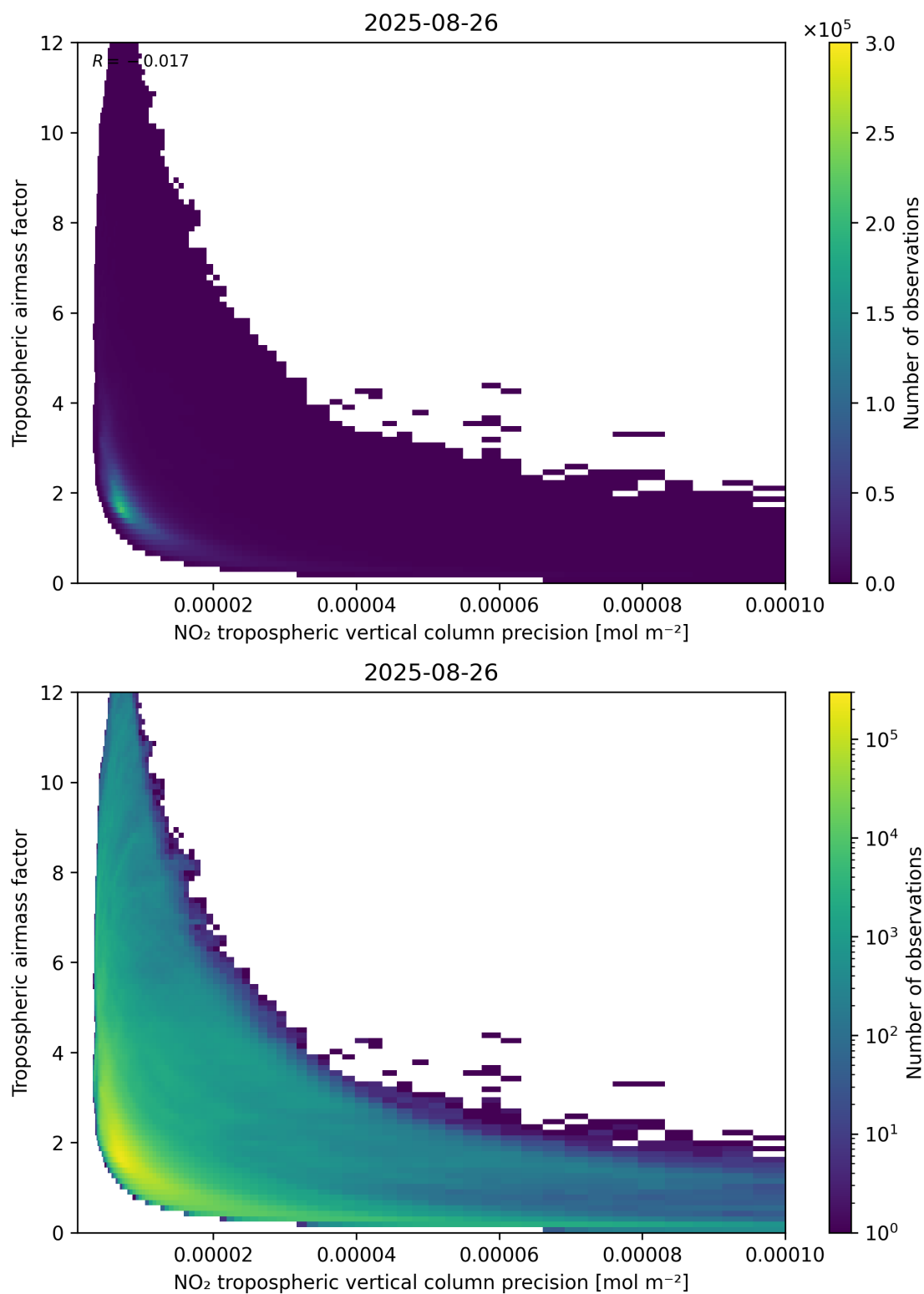
Figure 133: Scatter density plot of “NO 2 tropospheric vertical column precision” against “Tropospheric airmass factor” for 2025-08-25 to 2025-08-27.
