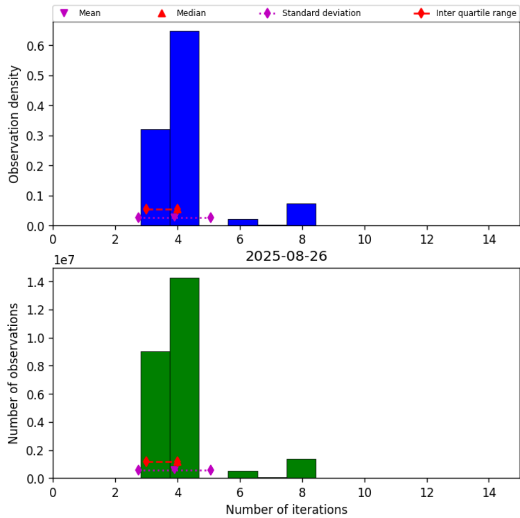
Figure 34: Histogram of “Number of iterations” for 2025-08-25 to 2025-08-27
