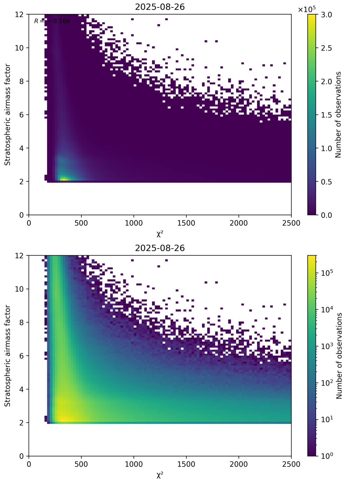
Figure 81: Scatter density plot of “ \chi^2 ” against “Stratospheric airmass factor” for 2025-08-25 to 2025-08-27.
