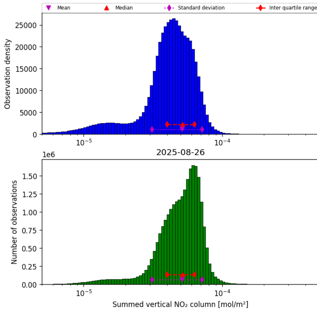
Figure 40: Histogram of “Summed vertical NO 2 column” for 2025-08-25 to 2025-08-27
