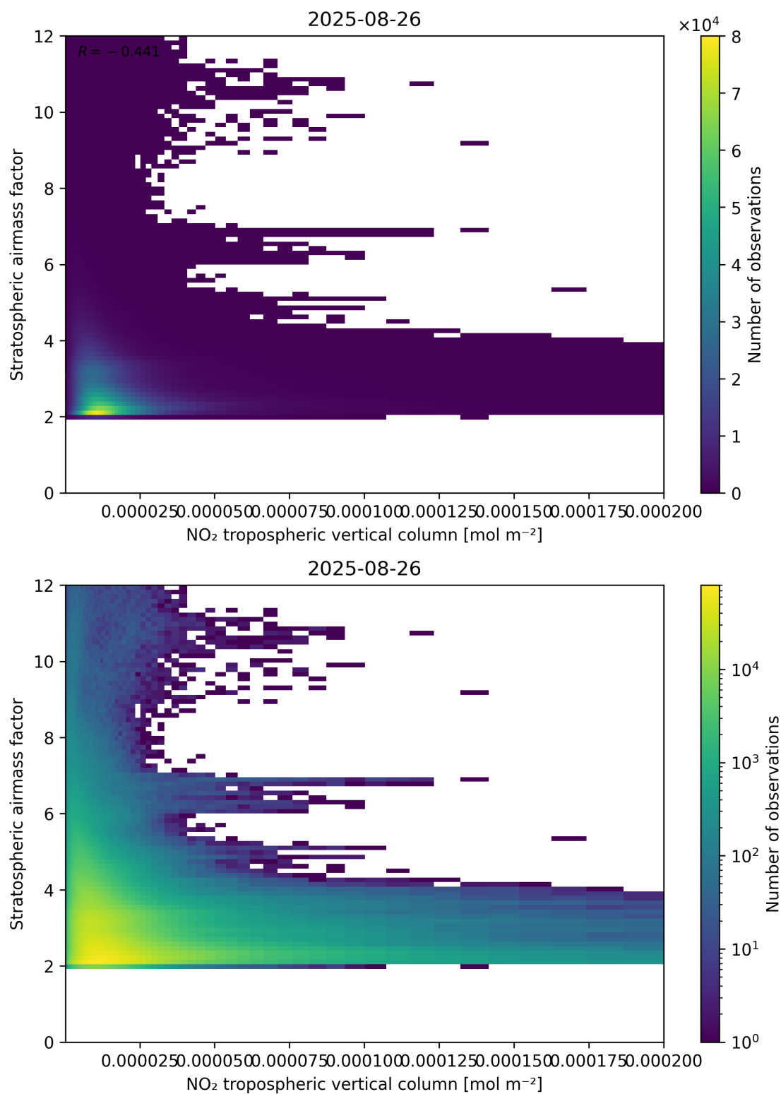
Figure 121: Scatter density plot of “NO 2 tropospheric vertical column” against “Stratospheric air mass factor” for 2025-08-25 to 2025-08-27.
