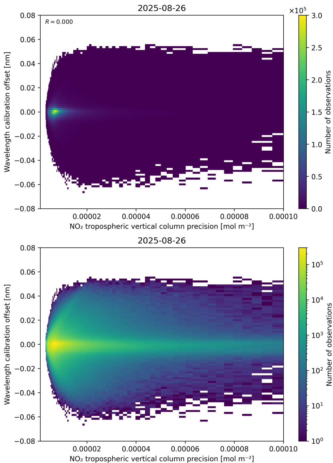
Figure 141: Scatter density plot of “NO 2 tropospheric vertical column precision” against “Wavelength calibration offset” for 2025-08-25 to 2025-08-27.
