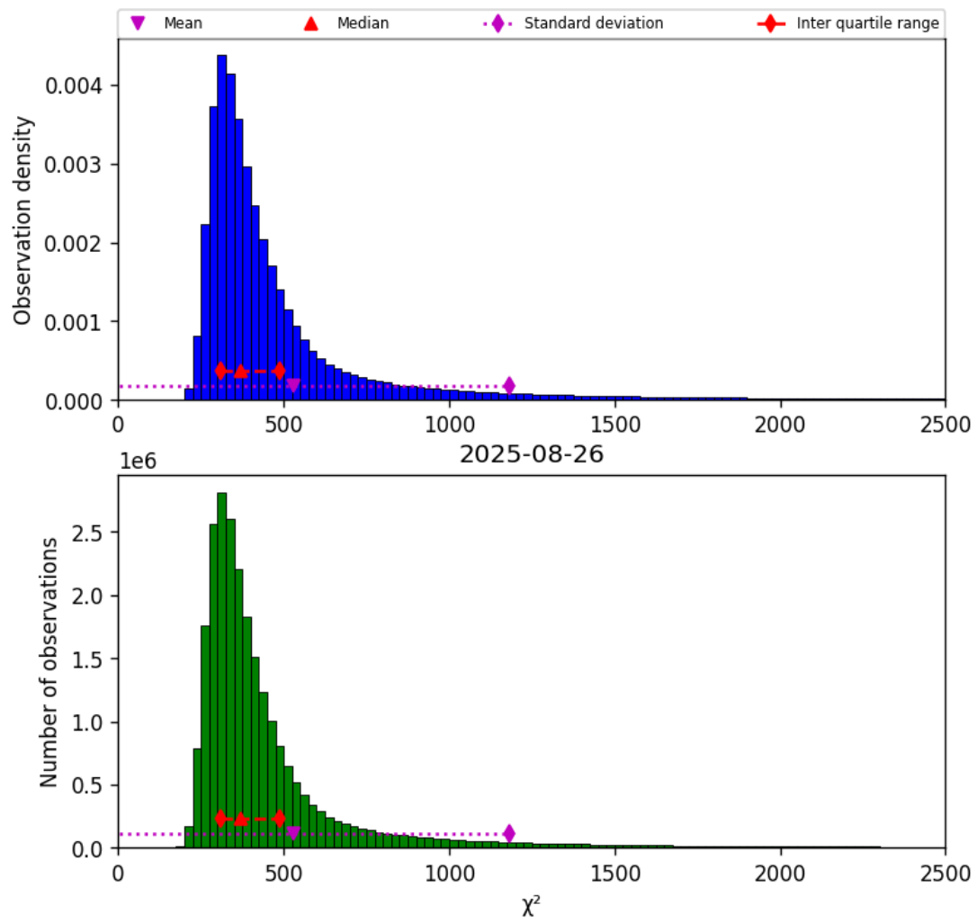
Figure 42: Histogram of “ \chi^2 ” for 2025-08-25 to 2025-08-27
