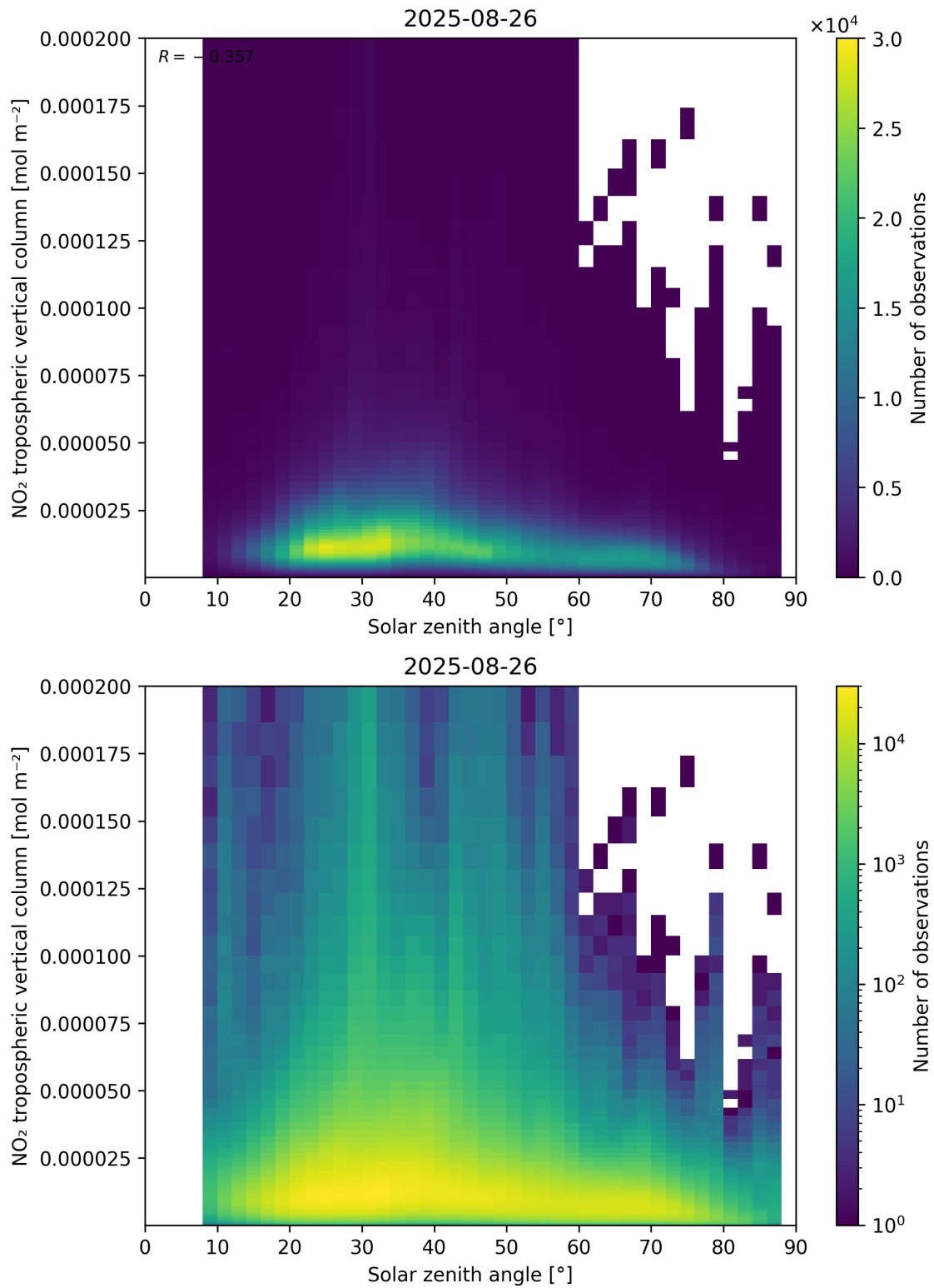
Figure 155: Scatter density plot of “Solar zenith angle” against “NO 2 tropospheric vertical column” for 2025-08-25 to 2025-08-27.
