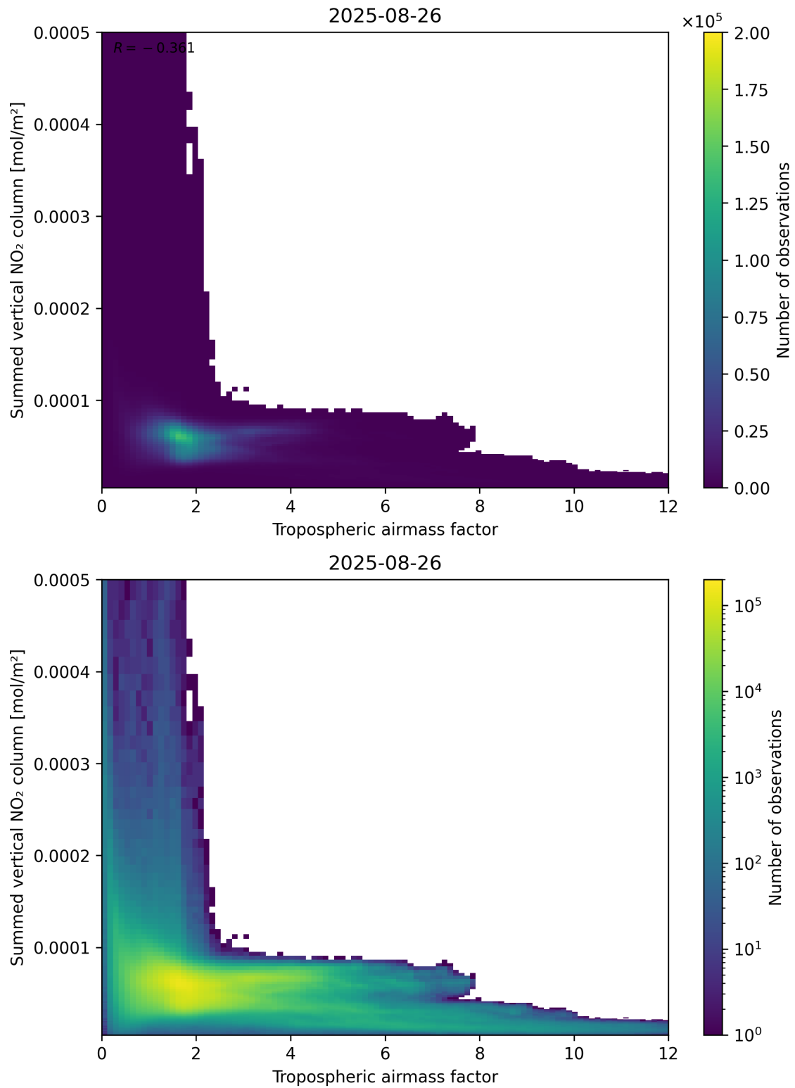
Figure 75: Scatter density plot of “Tropospheric air mass factor” against “Summed vertical NO 2 column” for 2025-08-25 to 2025-08-27.
