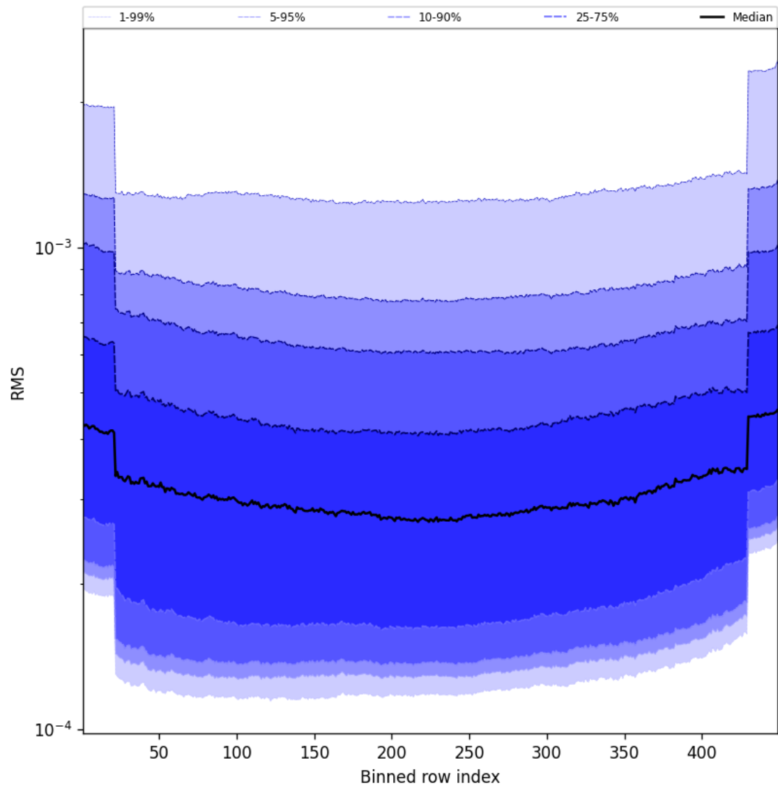
Figure 60: Along track statistics of “RMS” for 2025-08-25 to 2025-08-27
