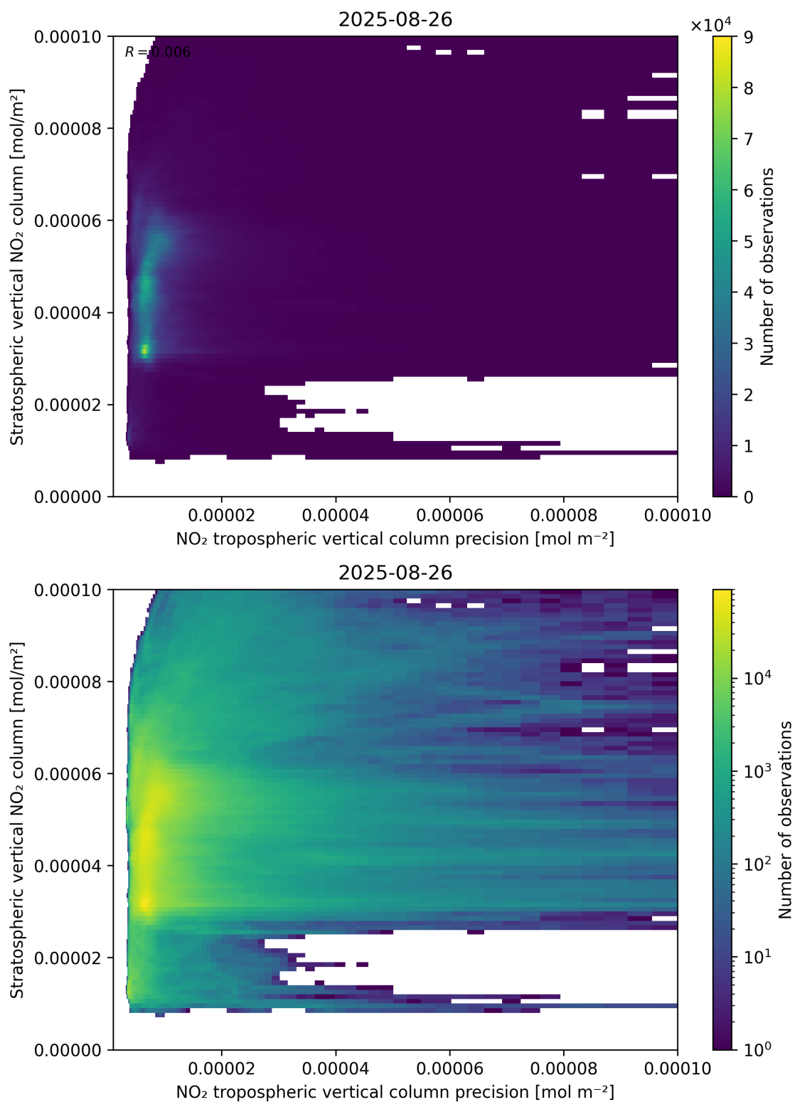
Figure 135: Scatter density plot of “NO 2 tropospheric vertical column precision” against “Stratospheric vertical NO 2 column” for 2025-08-25 to 2025-08-27.
