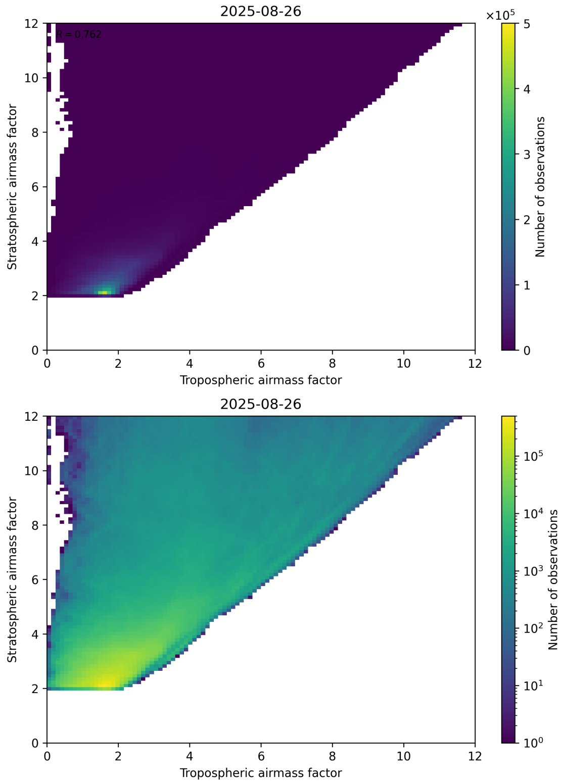
Figure 71: Scatter density plot of “Tropospheric airmass factor” against “Stratospheric airmass factor” for 2025-08-25 to 2025-08-27.
