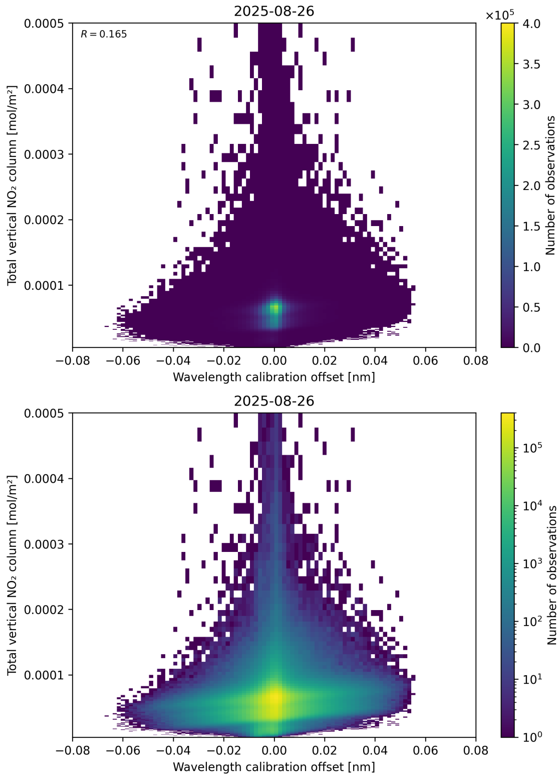
Figure 179: Scatter density plot of “Wavelength calibration offset” against “Total vertical NO 2 column” for 2025-08-25 to 2025-08-27.
