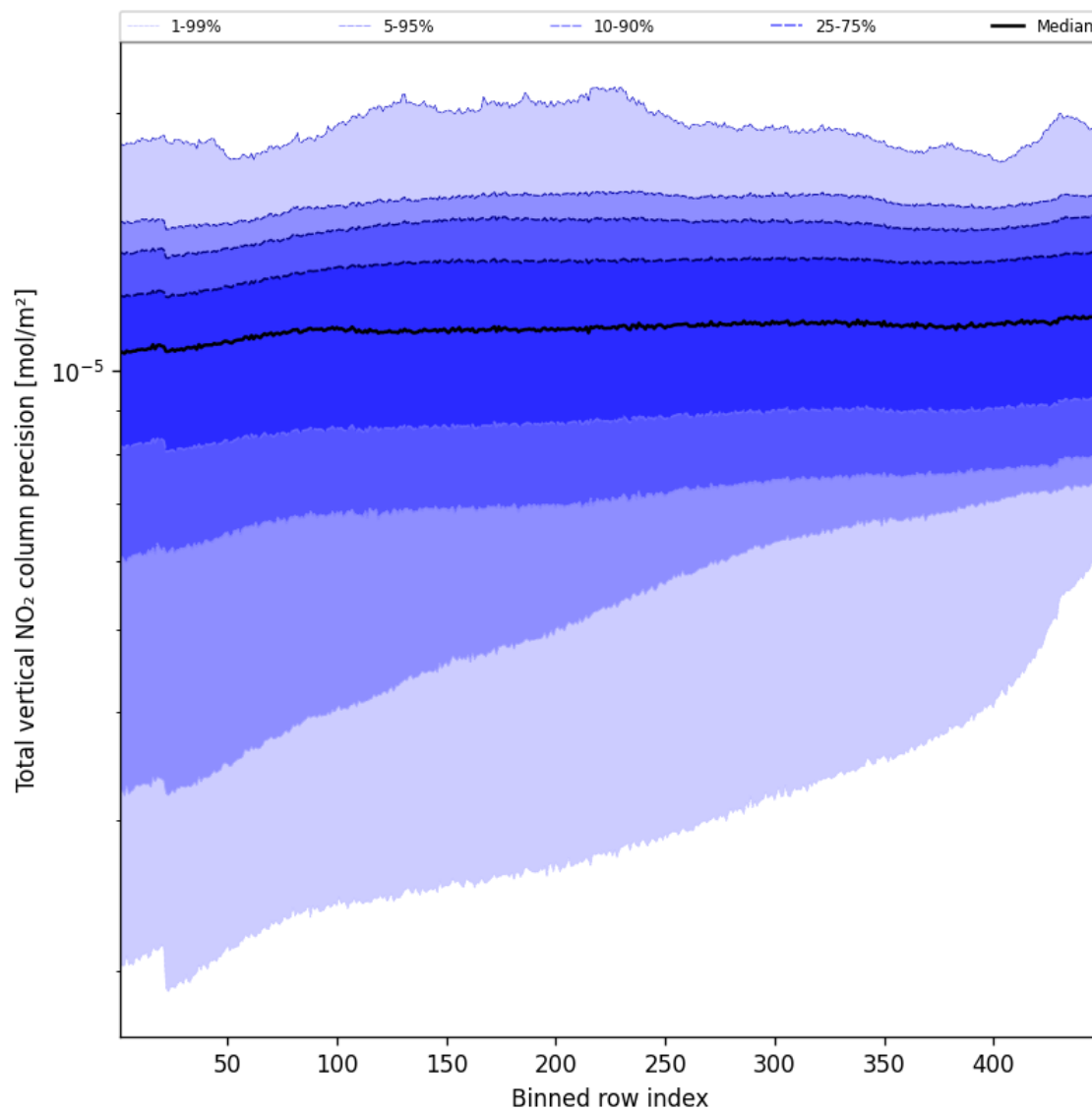
Figure 56: Along track statistics of “Total vertical NO 2 column precision” for 2025-08-25 to 2025-08-27
