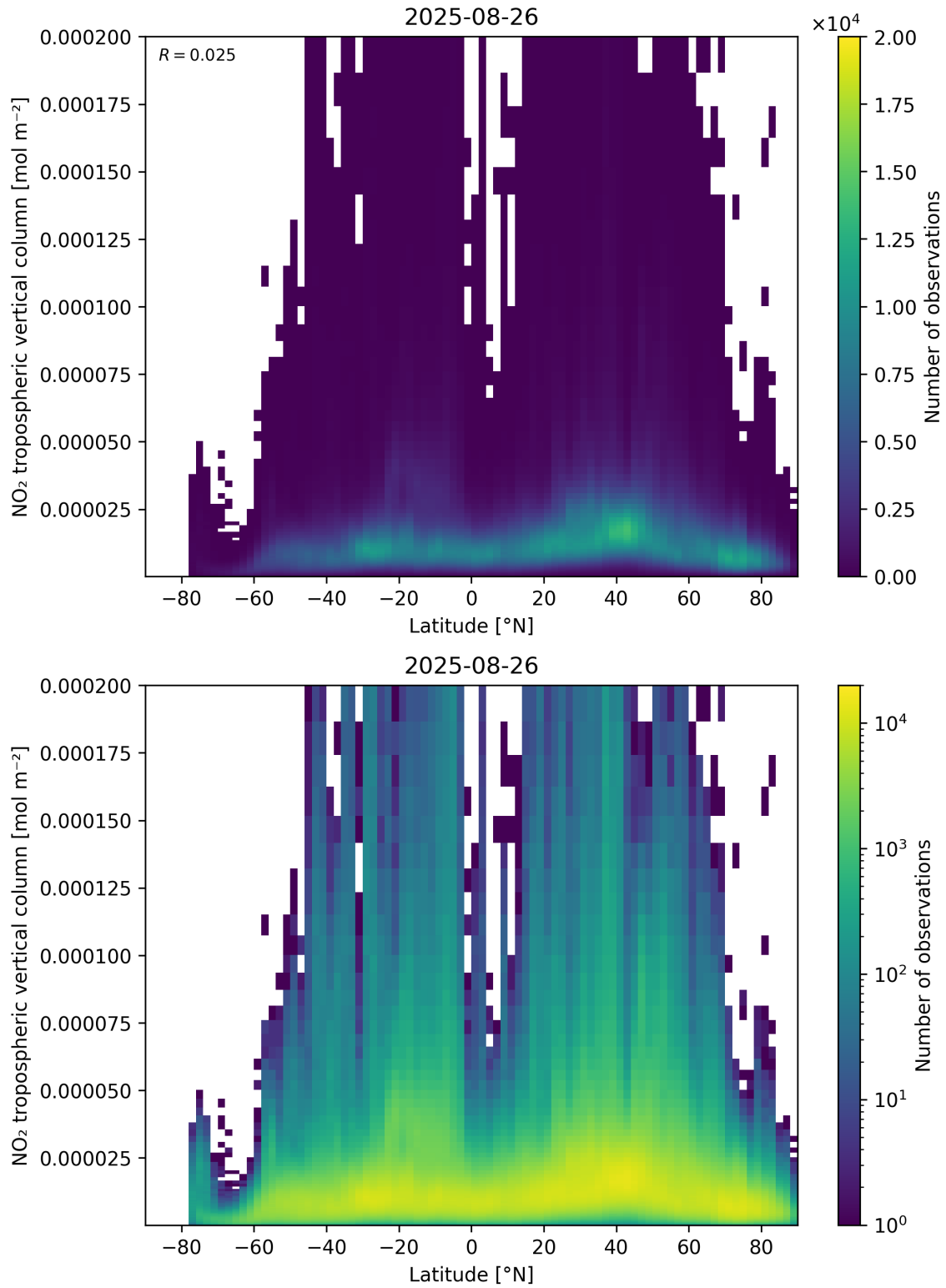
Figure 92: Scatter density plot of “Latitude” against “NO 2 tropospheric vertical column” for 2025-08-25 to 2025-08-27.
