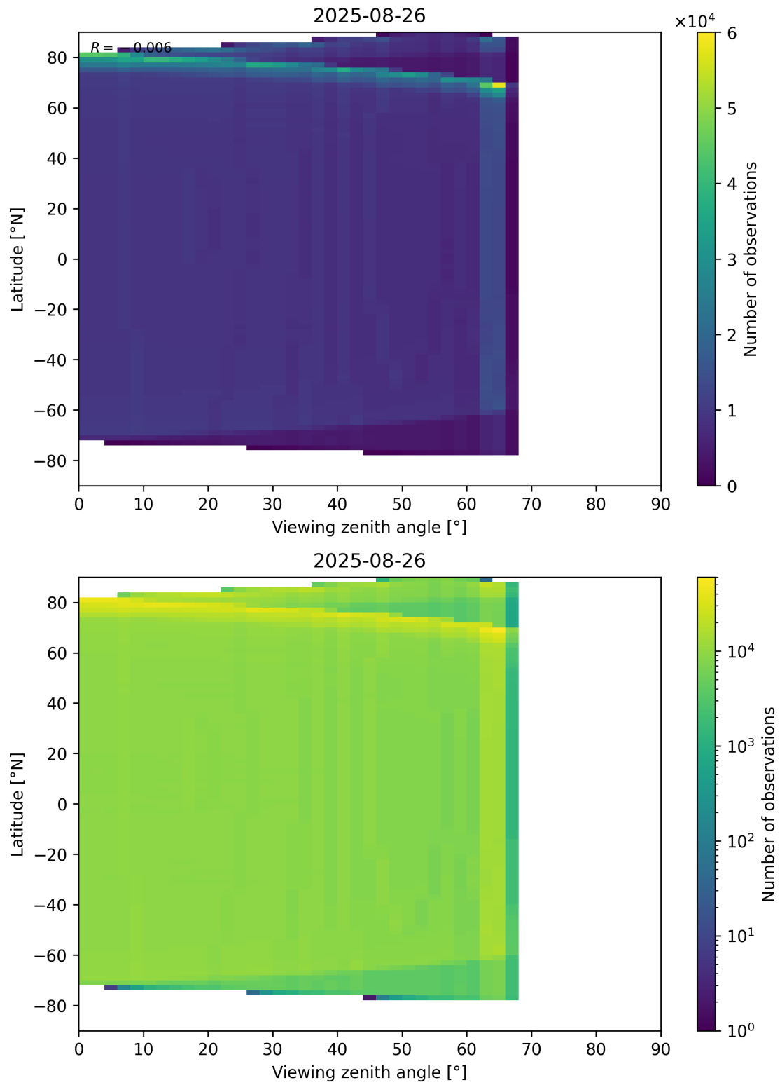
Figure 163: Scatter density plot of “Viewing zenith angle” against “Latitude” for 2025-08-25 to 2025-08-27.
