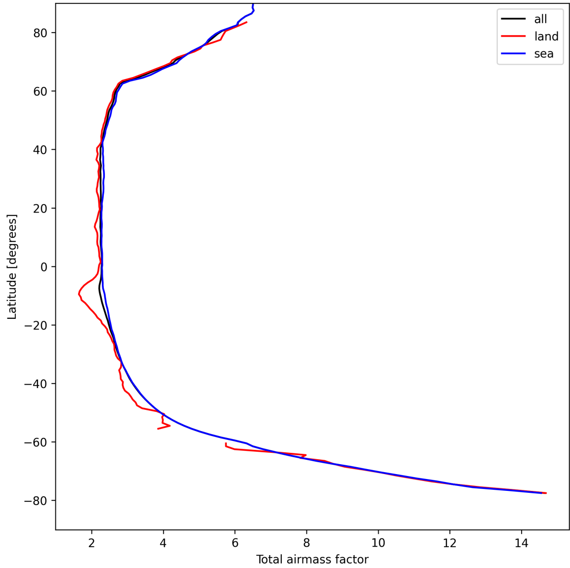
Figure 15: Zonal average of “Total airmass factor” for 2025-08-25 to 2025-08-27.
