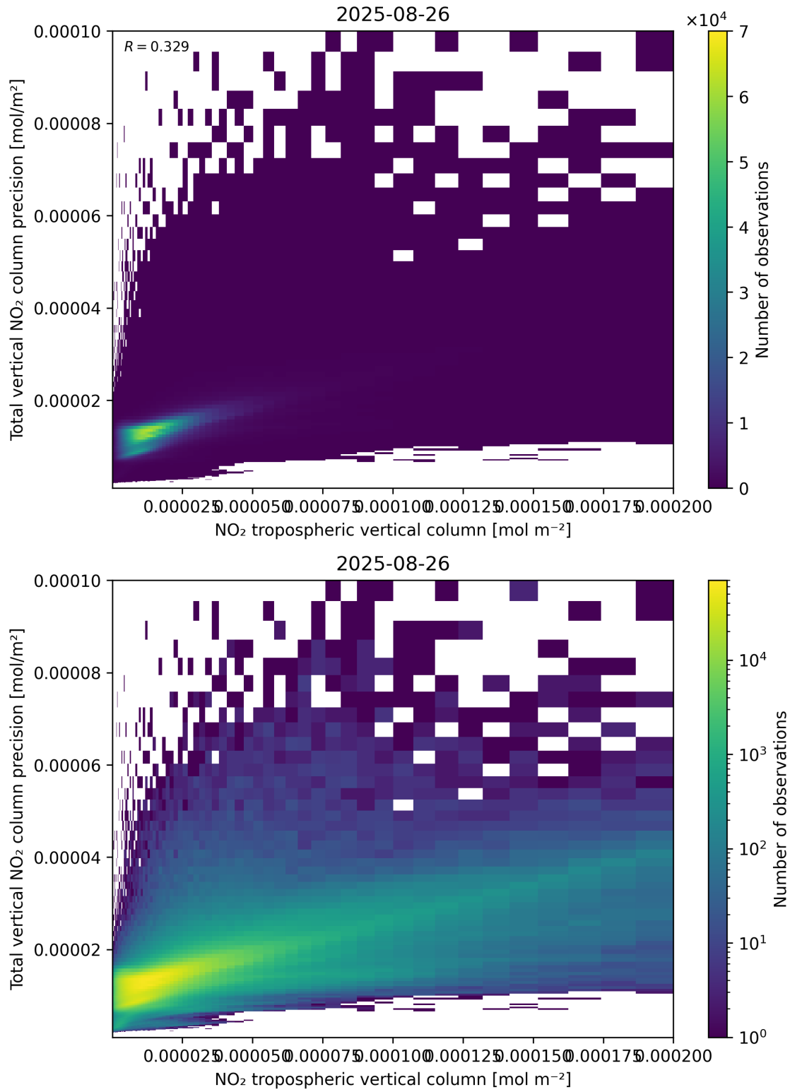
Figure 129: Scatter density plot of “NO 2 tropospheric vertical column” against “Total vertical NO 2 column precision” for 2025-08-25 to 2025-08-27.
