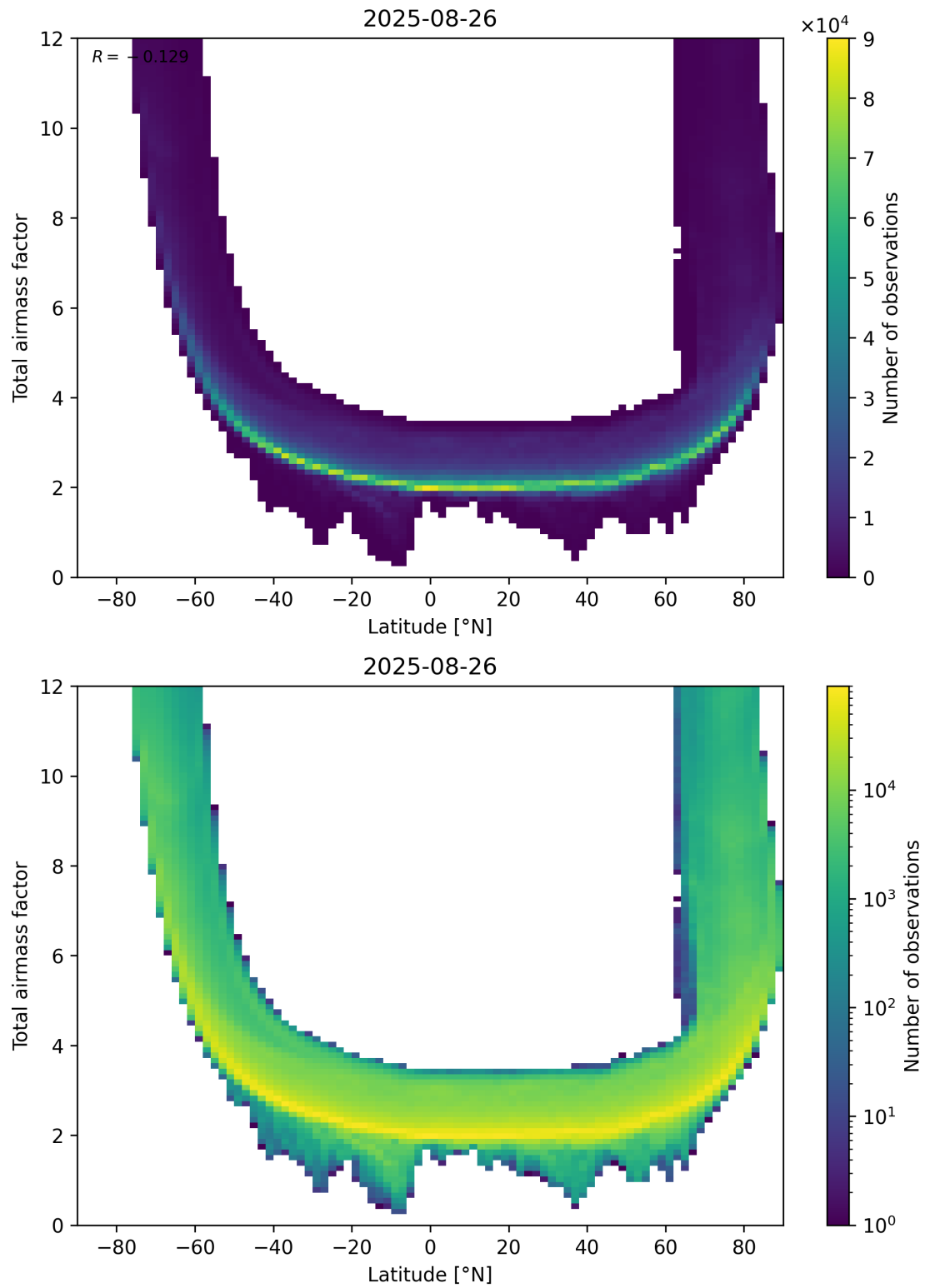
Figure 84: Scatter density plot of “Latitude” against “Total airmass factor” for 2025-08-25 to 2025-08-27.
