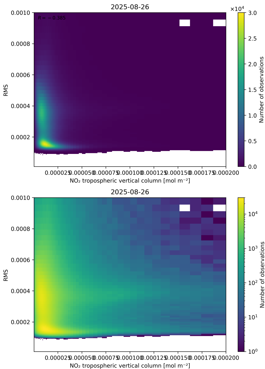
Figure 142: Scatter density plot of “NO 2 tropospheric vertical column” against “RMS” for 2025-08-25 to 2025-08-27.
