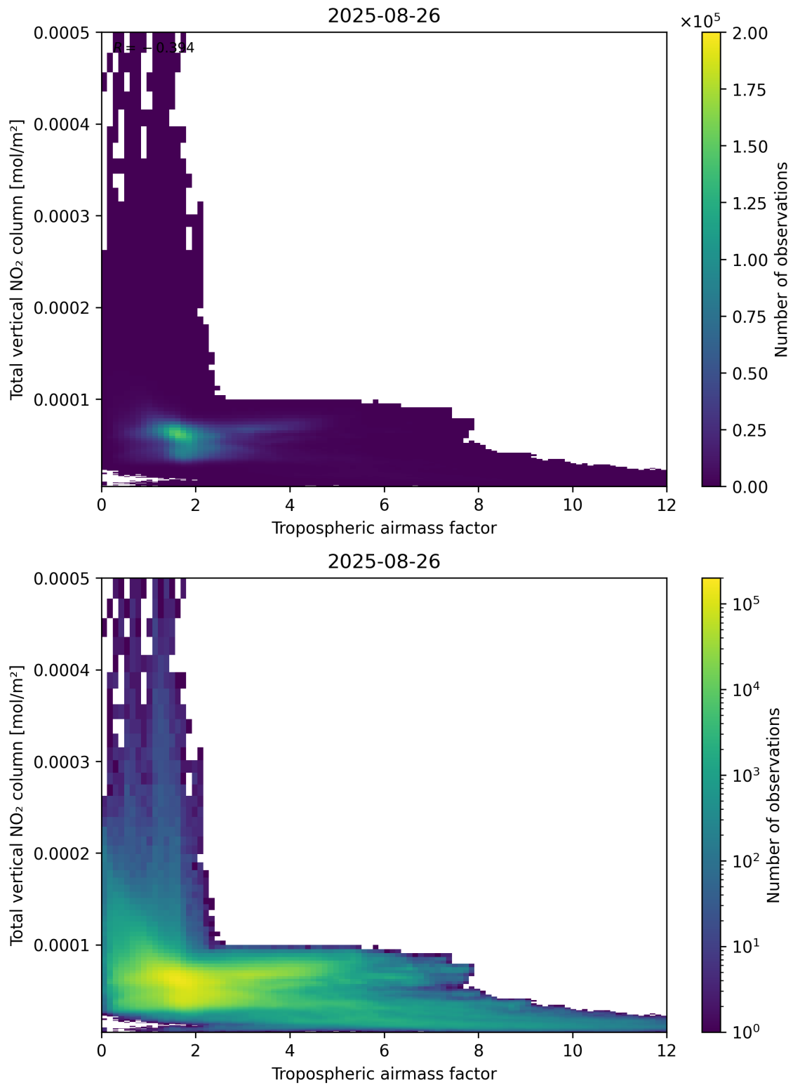
Figure 77: Scatter density plot of “Tropospheric airmass factor” against “Total vertical NO 2 column” for 2025-08-25 to 2025-08-27.
