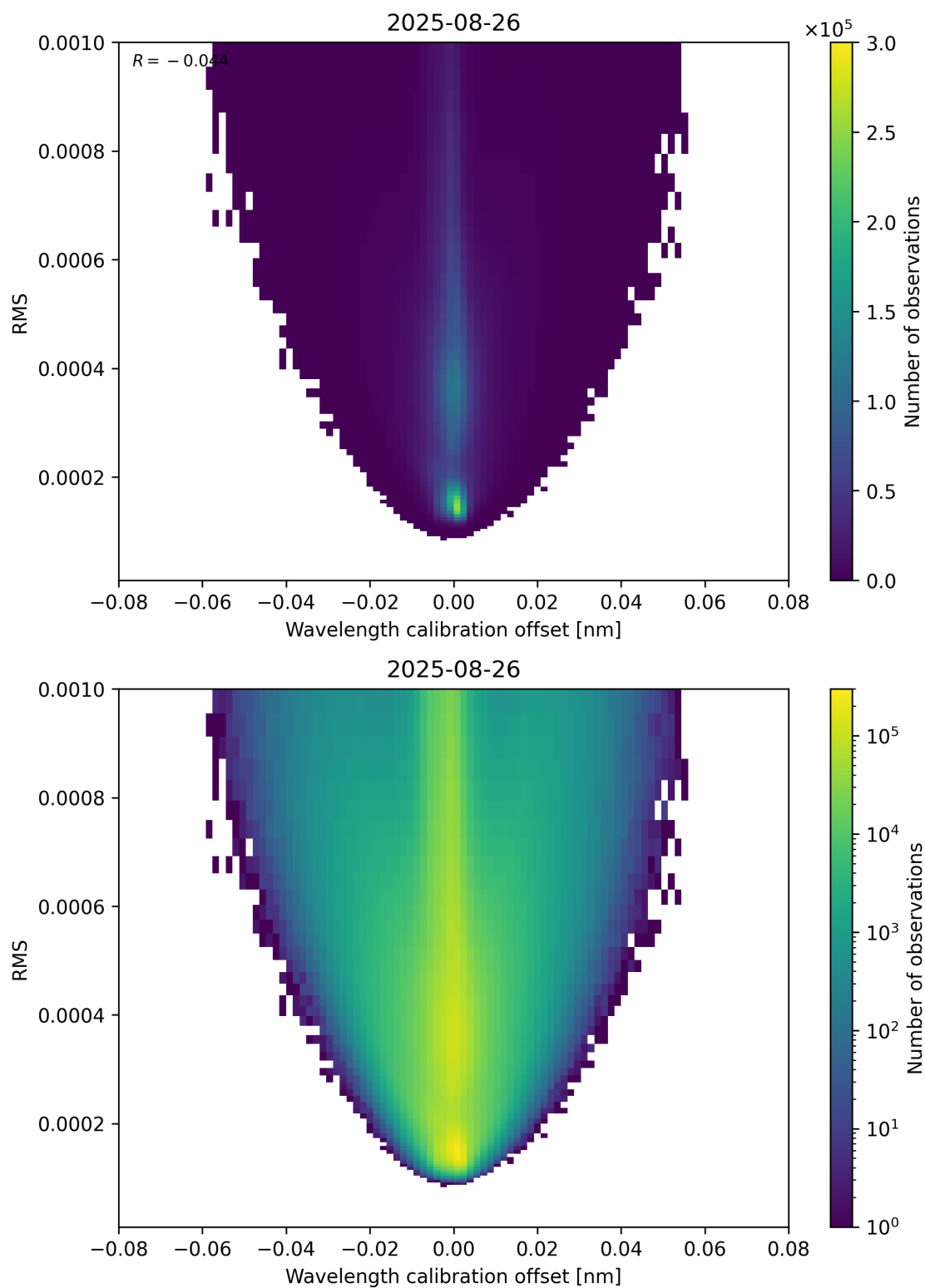
Figure 181: Scatter density plot of “Wavelength calibration offset” against “RMS” for 2025-08-25 to 2025-08-27.
