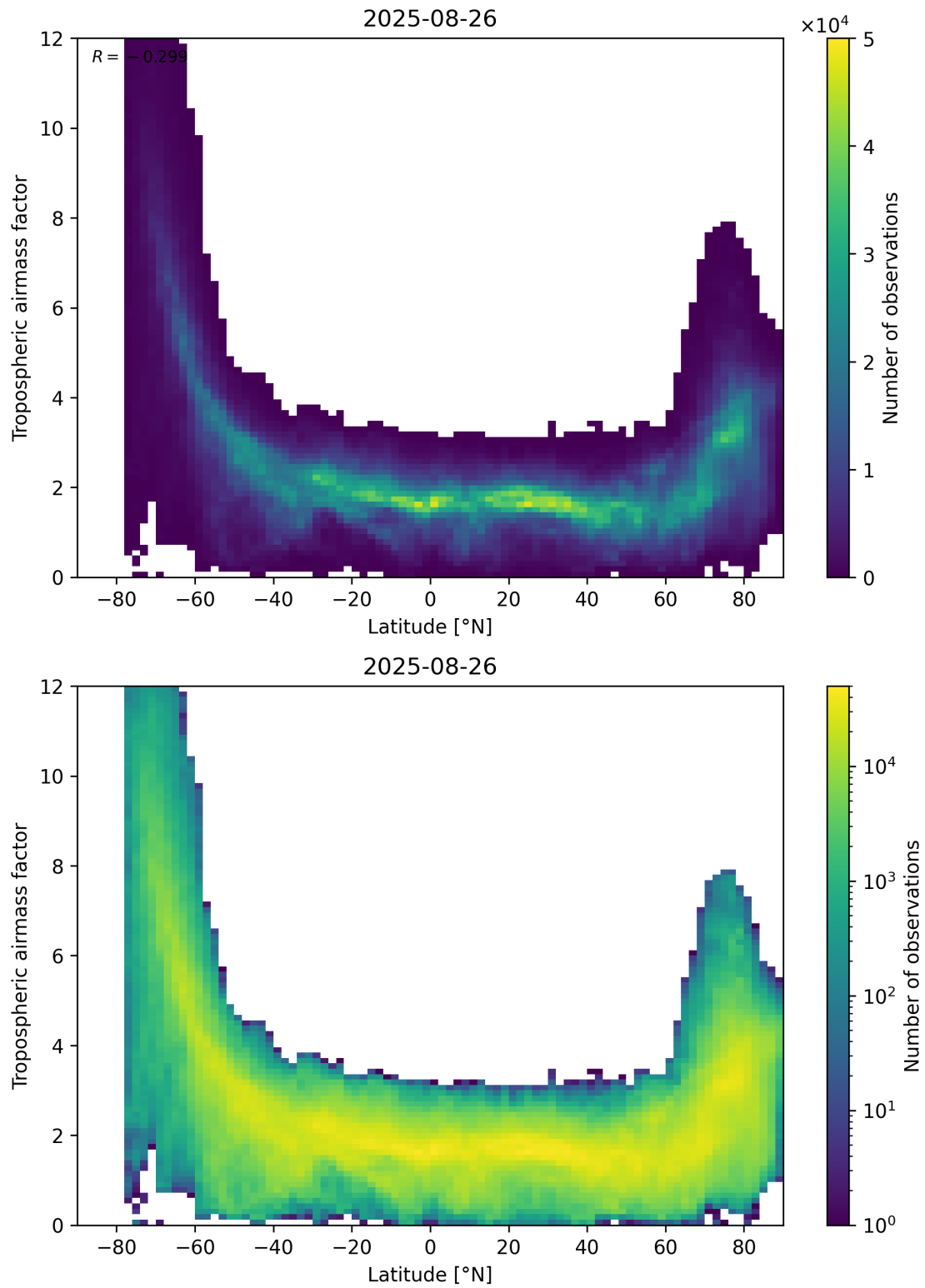
Figure 85: Scatter density plot of “Latitude” against “Tropospheric airmass factor” for 2025-08-25 to 2025-08-27.
