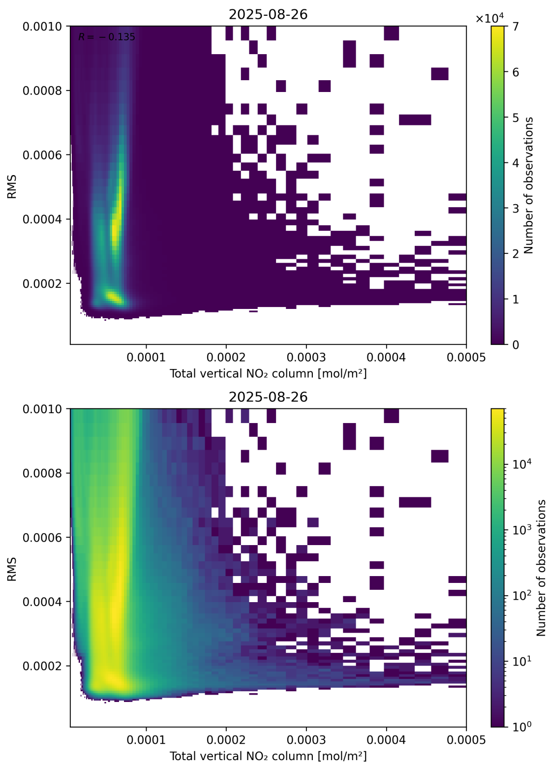
Figure 120: Scatter density plot of “Total vertical NO 2 column” against “RMS” for 2025-08-25 to 2025-08-27.
