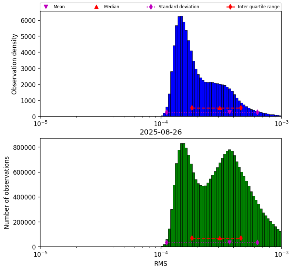
Figure 43: Histogram of “RMS” for 2025-08-25 to 2025-08-27
