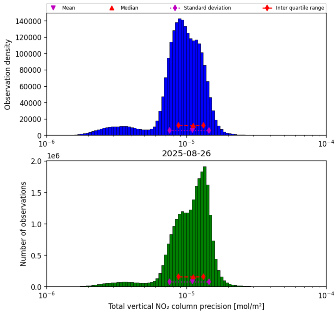
Figure 39: Histogram of “Total vertical NO 2 column precision” for 2025-08-25 to 2025-08-27
