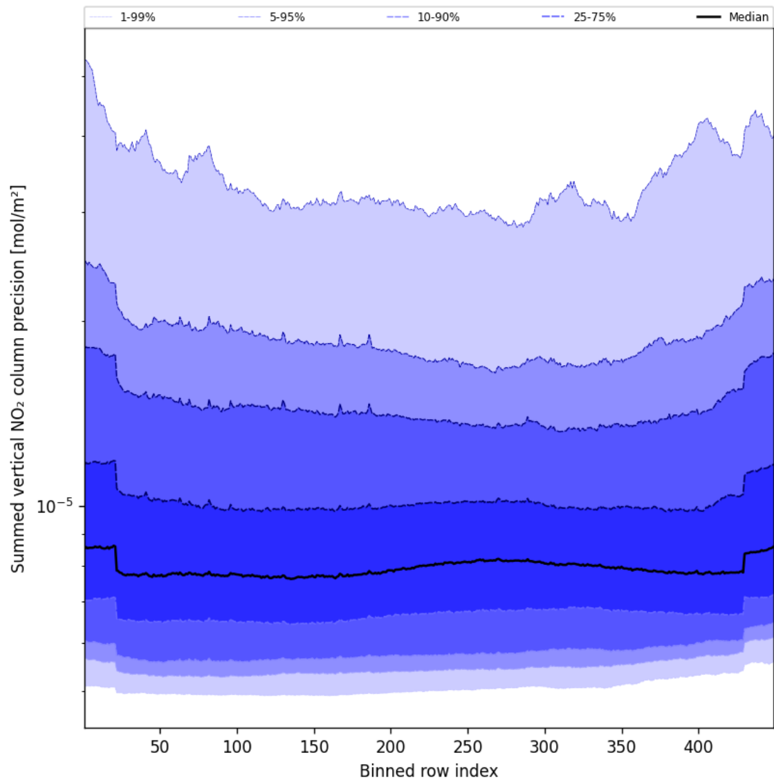
Figure 58: Along track statistics of “Summed vertical NO 2 column precision” for 2025-08-25 to 2025-08-27
