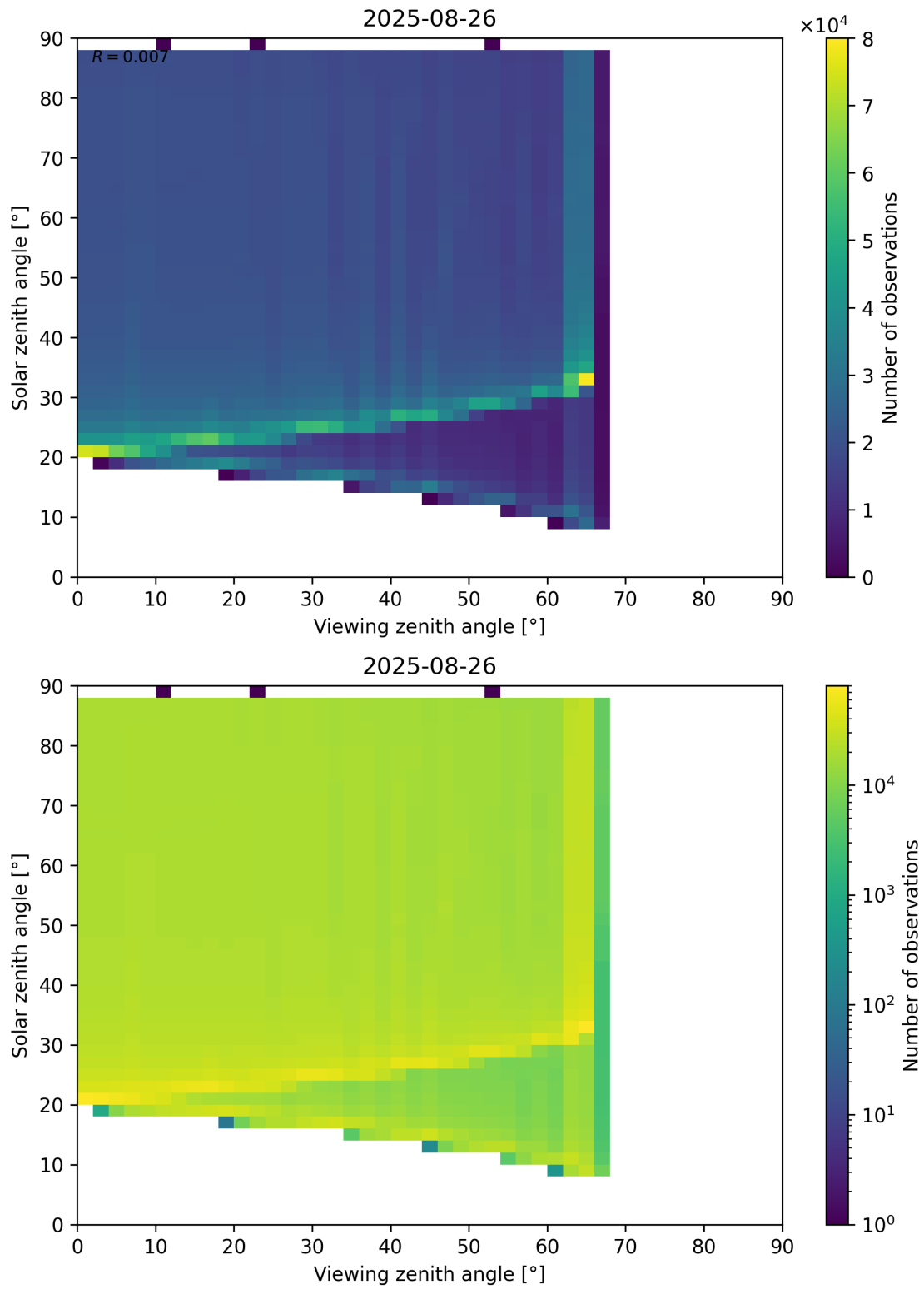
Figure 172: Scatter density plot of “Viewing zenith angle” against “Solar zenith angle” for 2025-08-25 to 2025-08-27.
