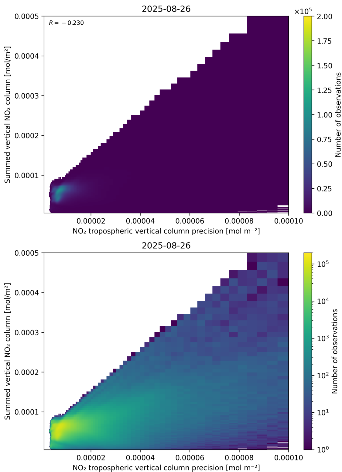
Figure 136: Scatter density plot of “NO 2 tropospheric vertical column precision” against “Summed vertical NO 2 column” for 2025-08-25 to 2025-08-27.
