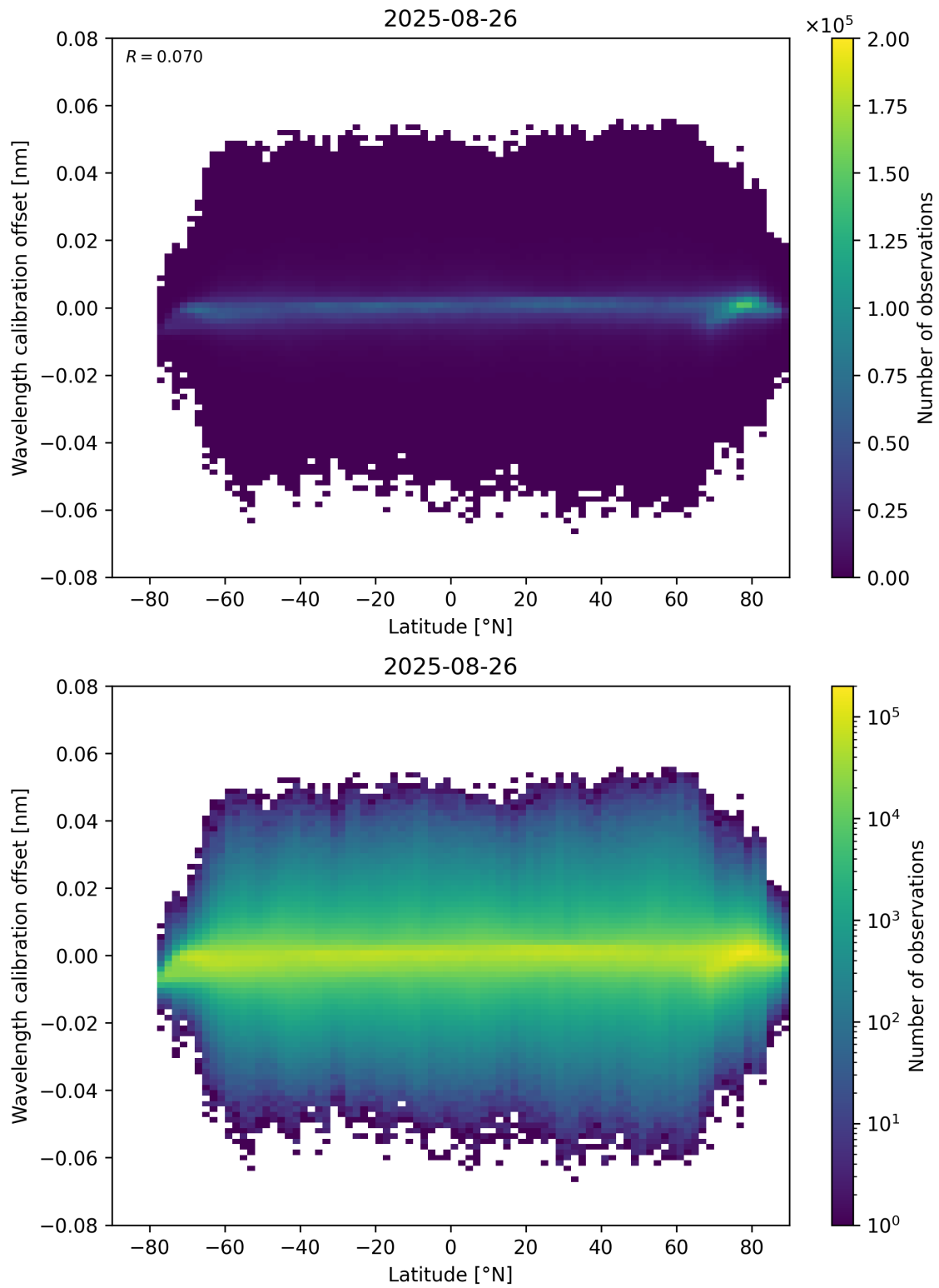
Figure 95: Scatter density plot of “Latitude” against “Wavelength calibration offset” for 2025-08-25 to 2025-08-27.
