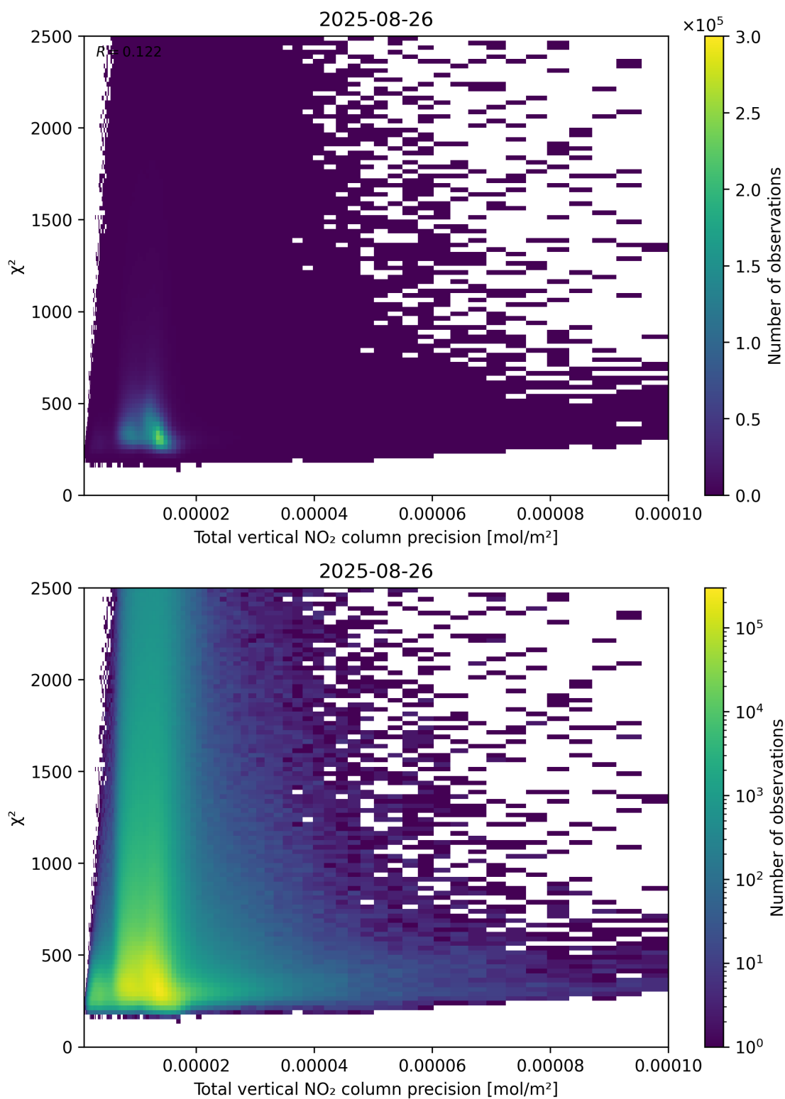
Figure 116: Scatter density plot of “Total vertical NO 2 column precision” against “ \chi^2 ” for 2025-08-25 to 2025-08-27.
