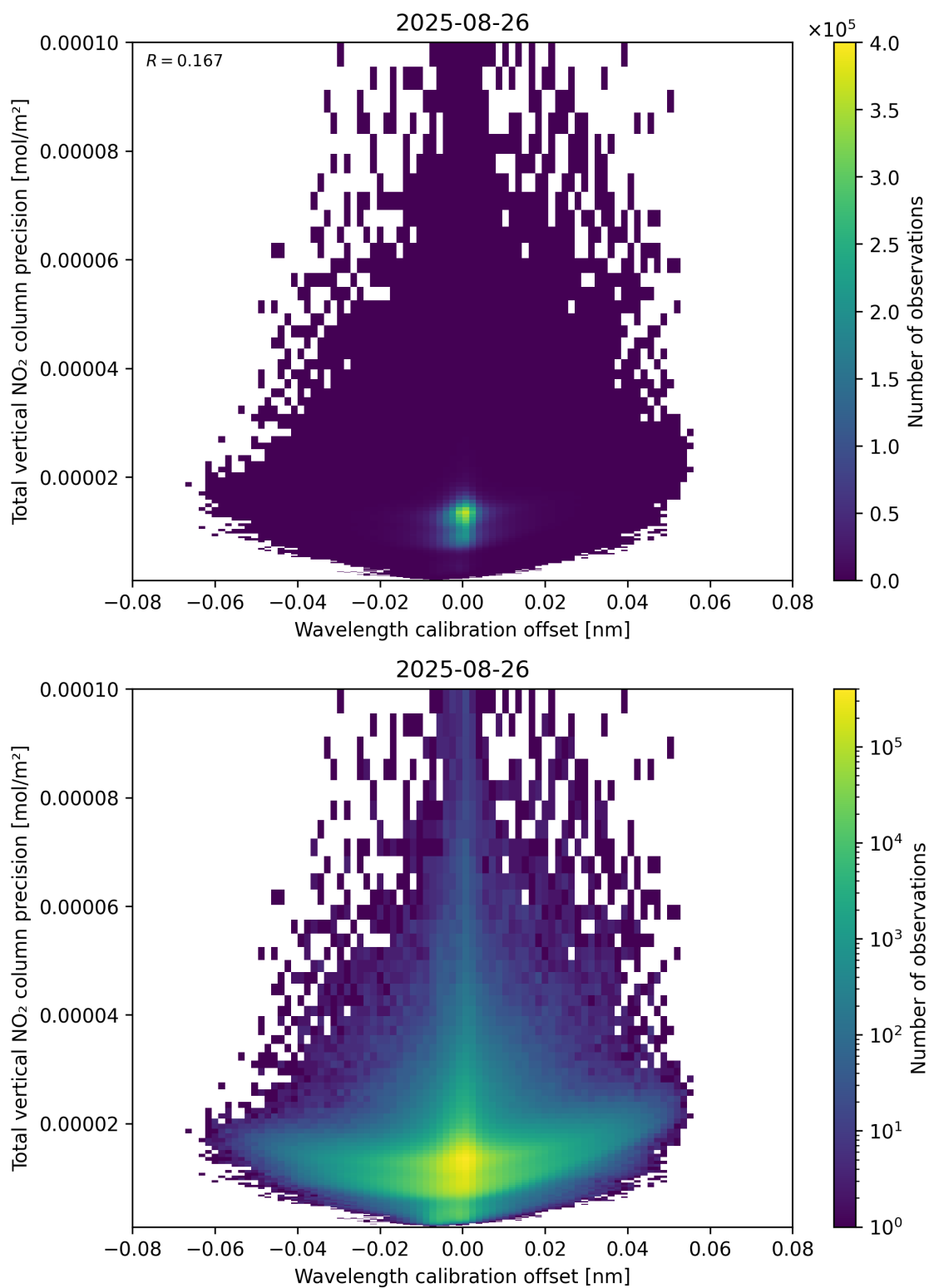
Figure 180: Scatter density plot of “Wavelength calibration offset” against “Total vertical NO 2 column precision” for 2025-08-25 to 2025-08-27.
