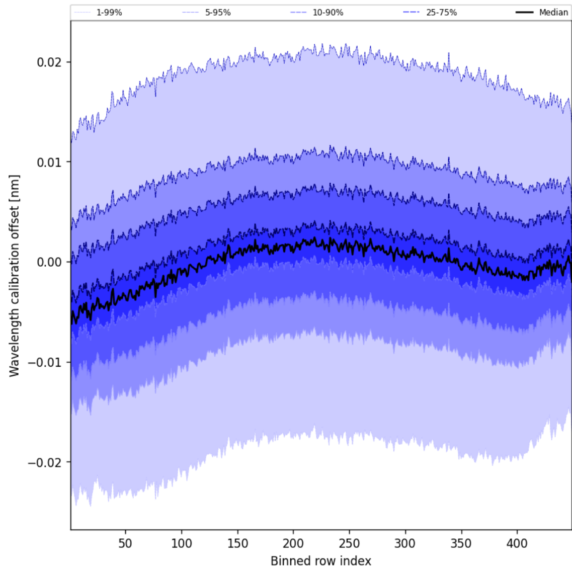
Figure 52: Along track statistics of “Wavelength calibration offset” for 2025-08-25 to 2025-08-27
