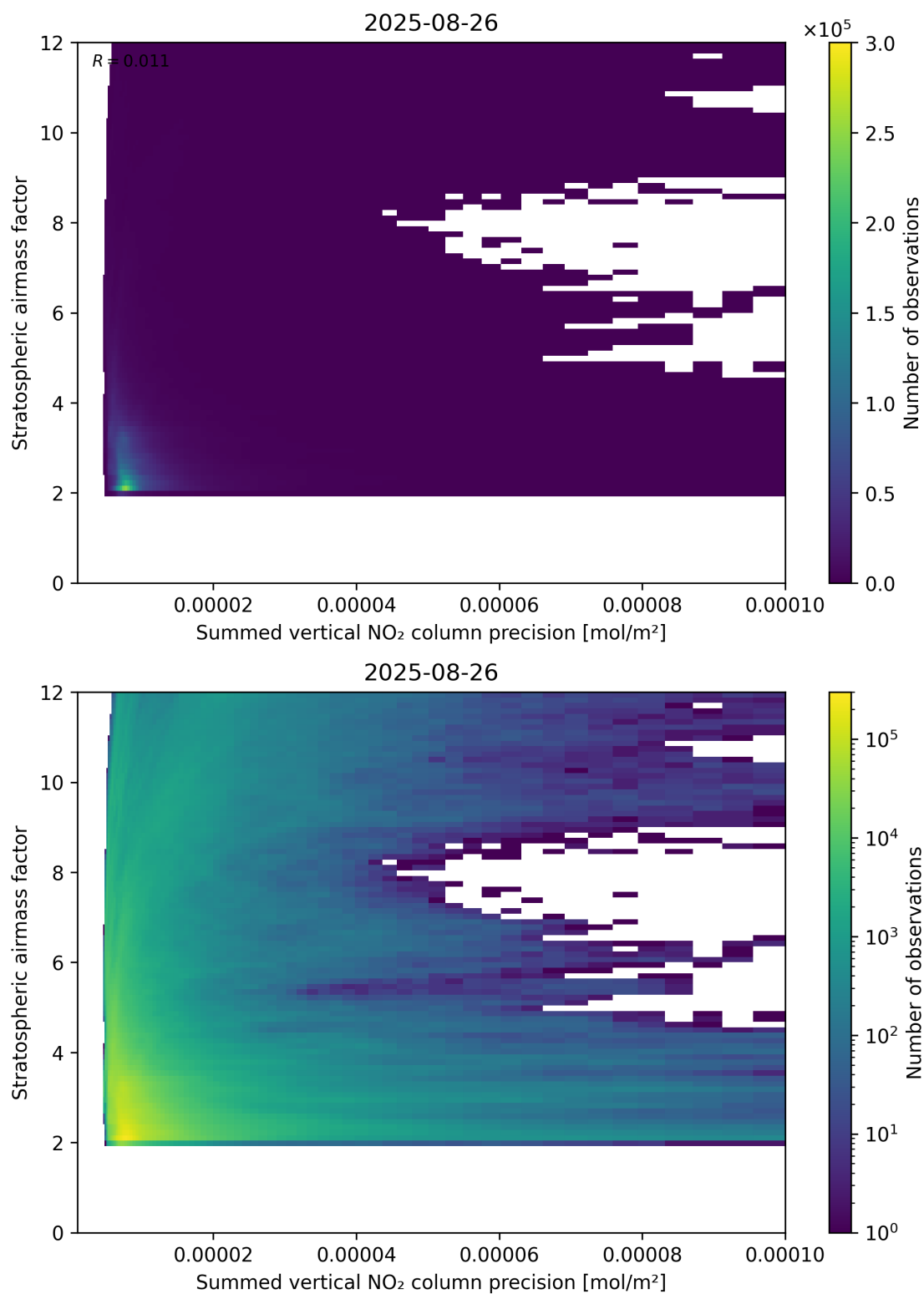
Figure 106: Scatter density plot of “Summed vertical NO 2 column precision” against “Stratospheric airmass factor” for 2025-08-25 to 2025-08-27.
