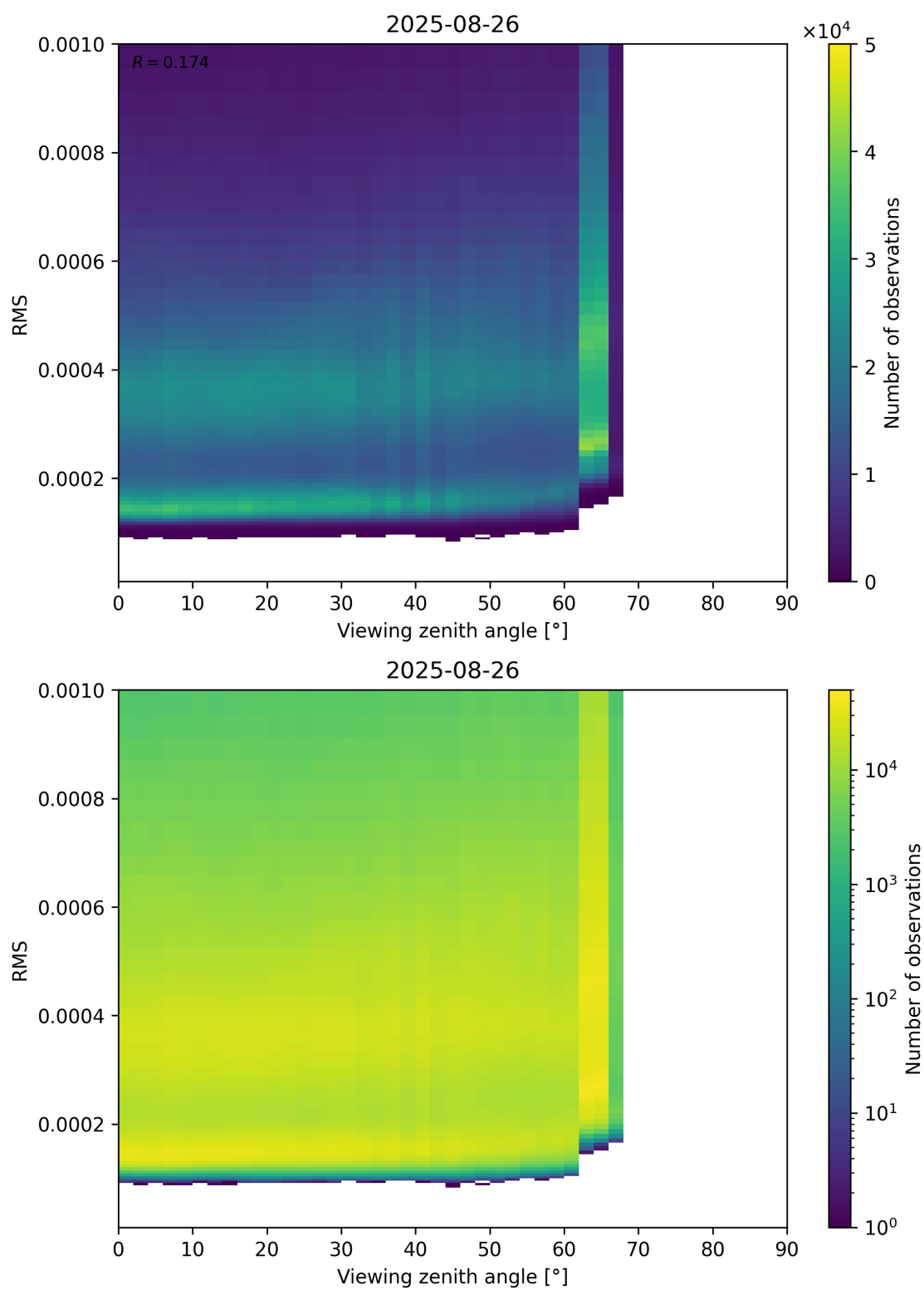
Figure 171: Scatter density plot of “Viewing zenith angle” against “RMS” for 2025-08-25 to 2025-08-27.
