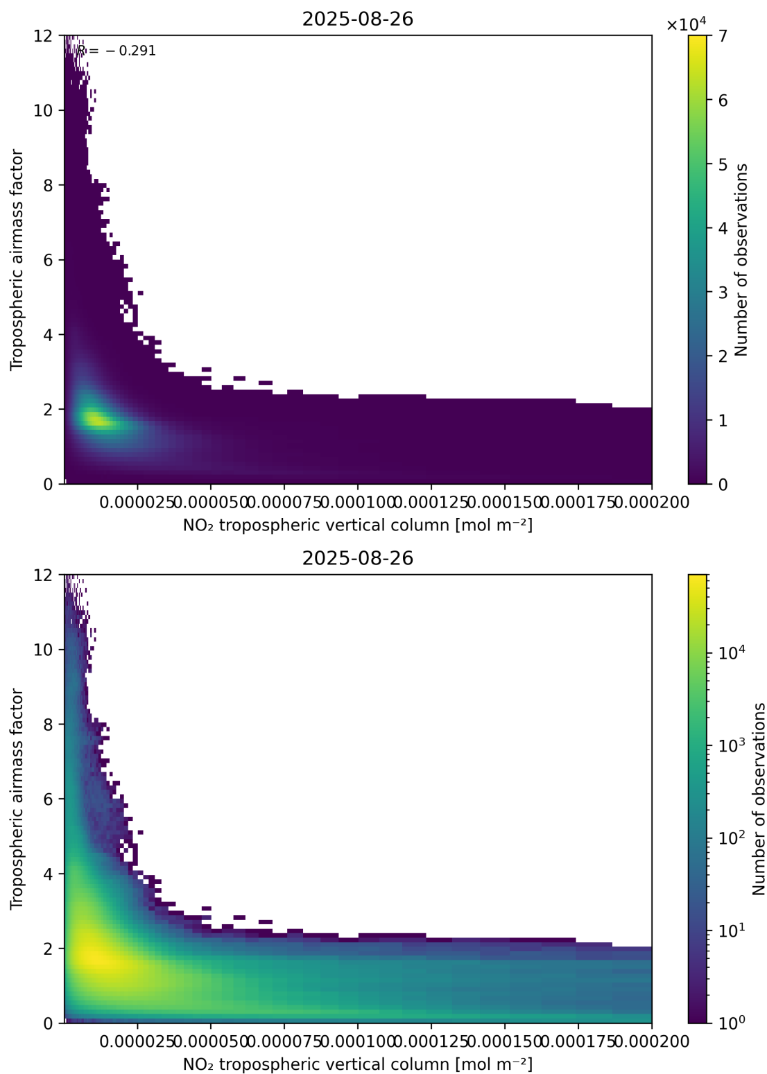
Figure 123: Scatter density plot of “NO 2 tropospheric vertical column” against “Tropospheric air mass factor” for 2025-08-25 to 2025-08-27.
