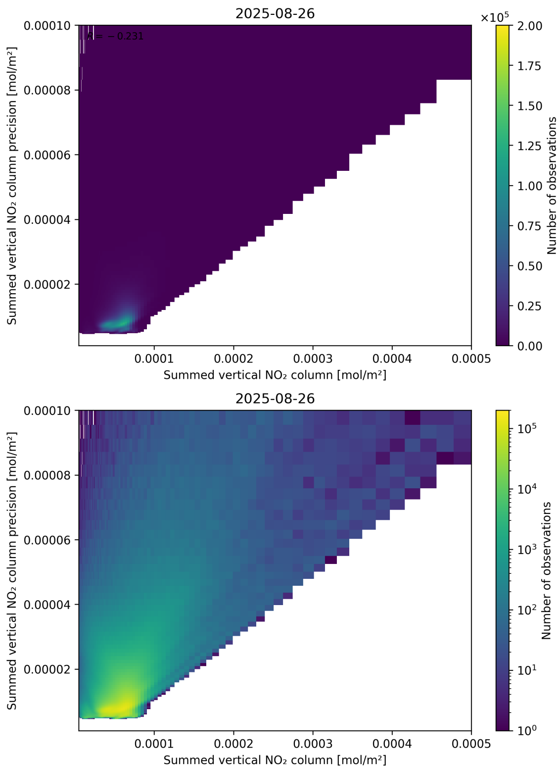
Figure 105: Scatter density plot of “Summed vertical NO 2 column” against “Summed vertical NO 2 column precision” for 2025-08-25 to 2025-08-27.
