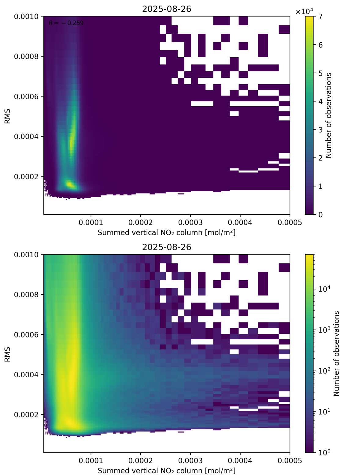
Figure 109: Scatter density plot of “Summed vertical NO 2 column” against “RMS” for 2025-08-25 to 2025-08-27.
