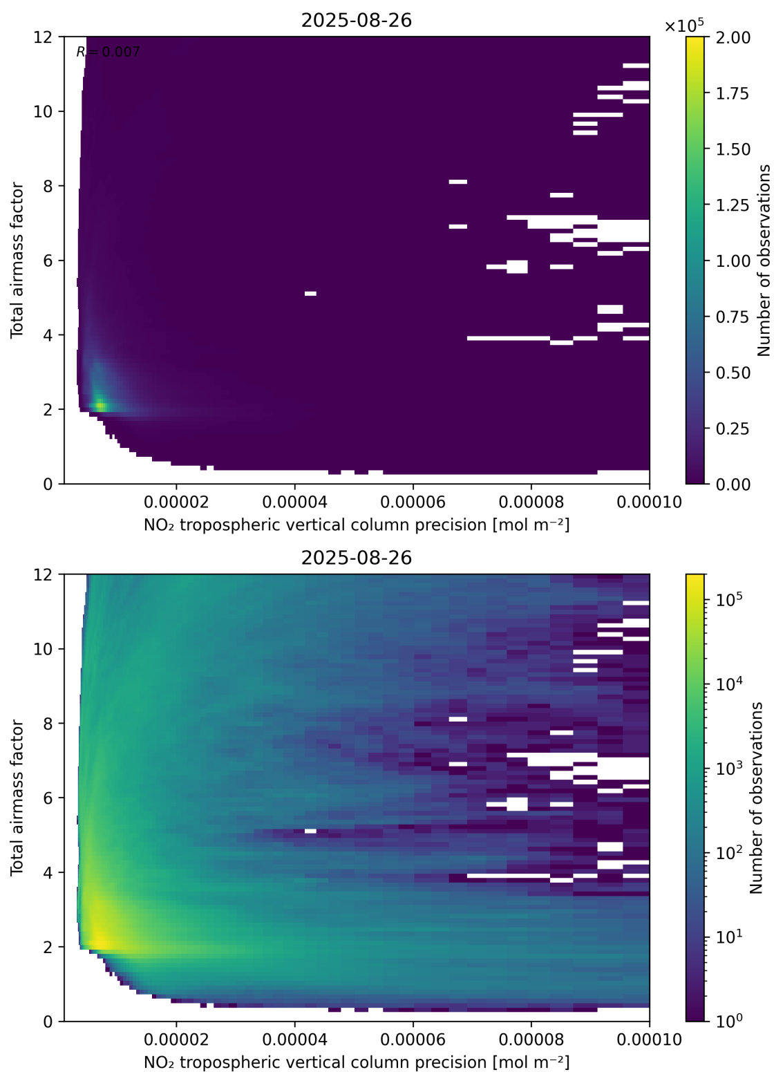
Figure 132: Scatter density plot of “NO 2 tropospheric vertical column precision” against “Total air mass factor” for 2025-08-25 to 2025-08-27.
