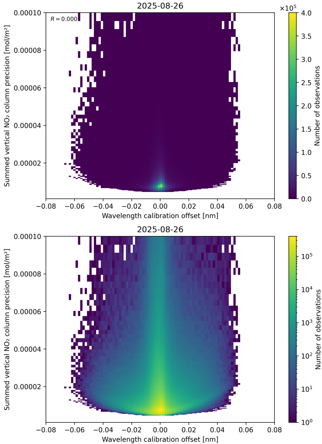
Figure 178: Scatter density plot of “Wavelength calibration offset” against “Summed vertical NO 2 column precision” for 2025-08-25 to 2025-08-27.
