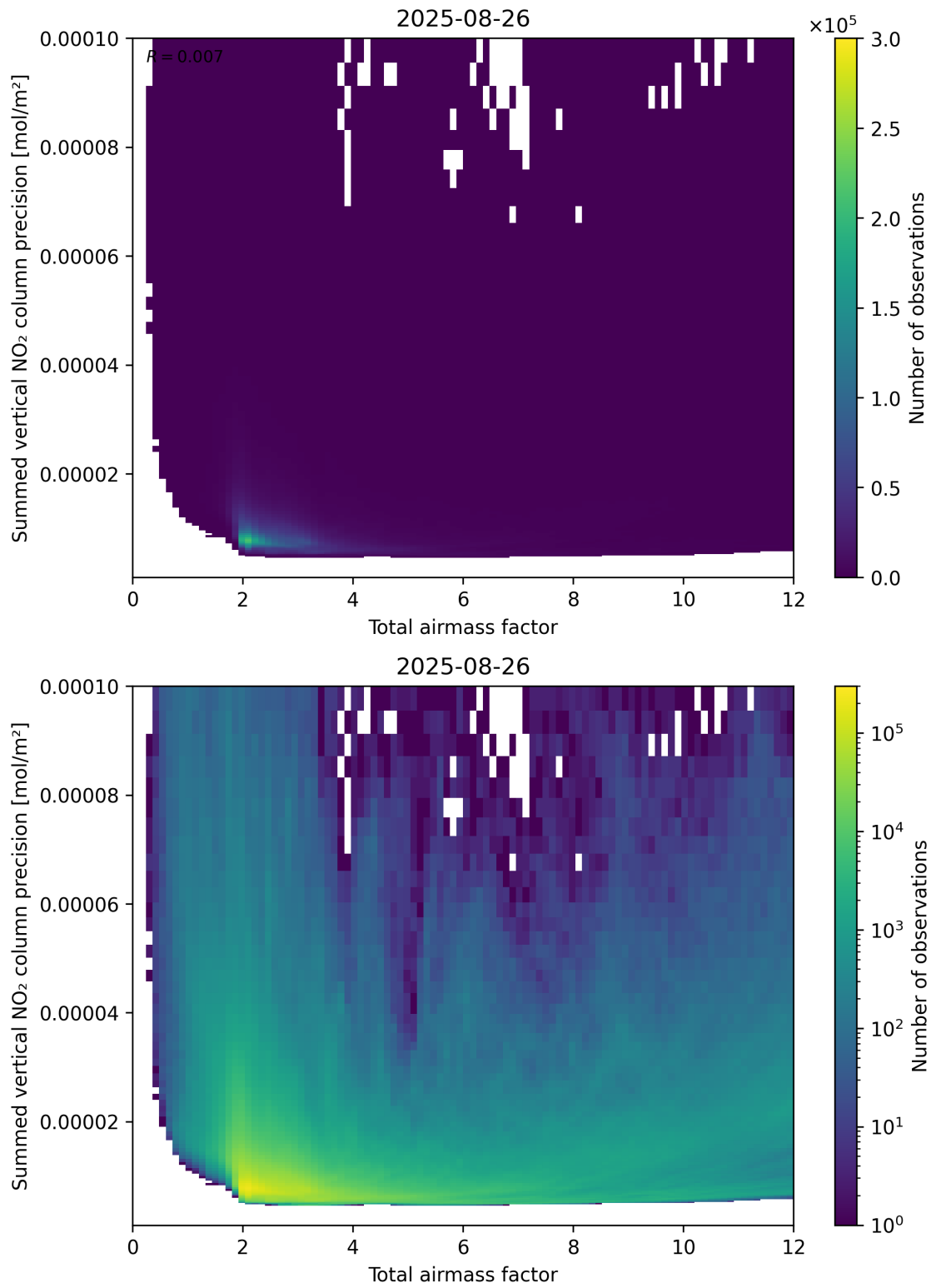
Figure 66: Scatter density plot of “Total airmass factor” against “Summed vertical NO 2 column precision” for 2025-08-25 to 2025-08-27.
