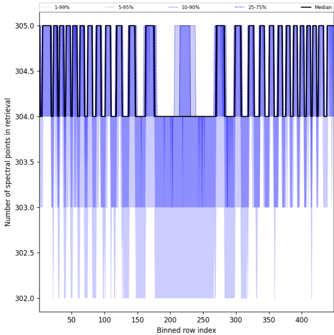
Figure 50: Along track statistics of “Number of spectral points in retrieval” for 2025-08-25 to 2025-08-27
