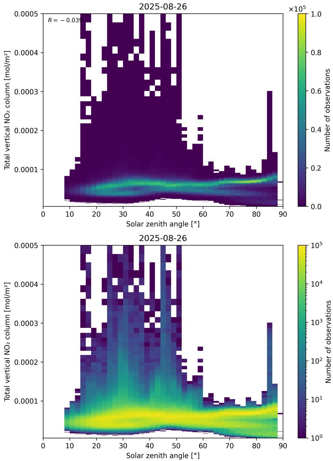
Figure 153: Scatter density plot of “Solar zenith angle” against “Total vertical NO 2 column” for 2025-08-25 to 2025-08-27.
