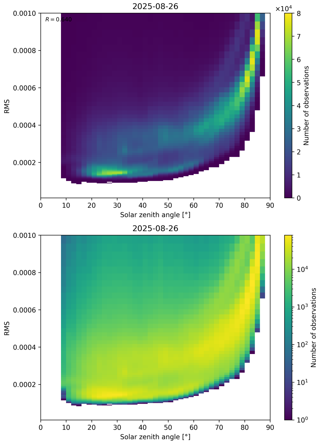
Figure 157: Scatter density plot of “Solar zenith angle” against “RMS” for 2025-08-25 to 2025-08-27.
