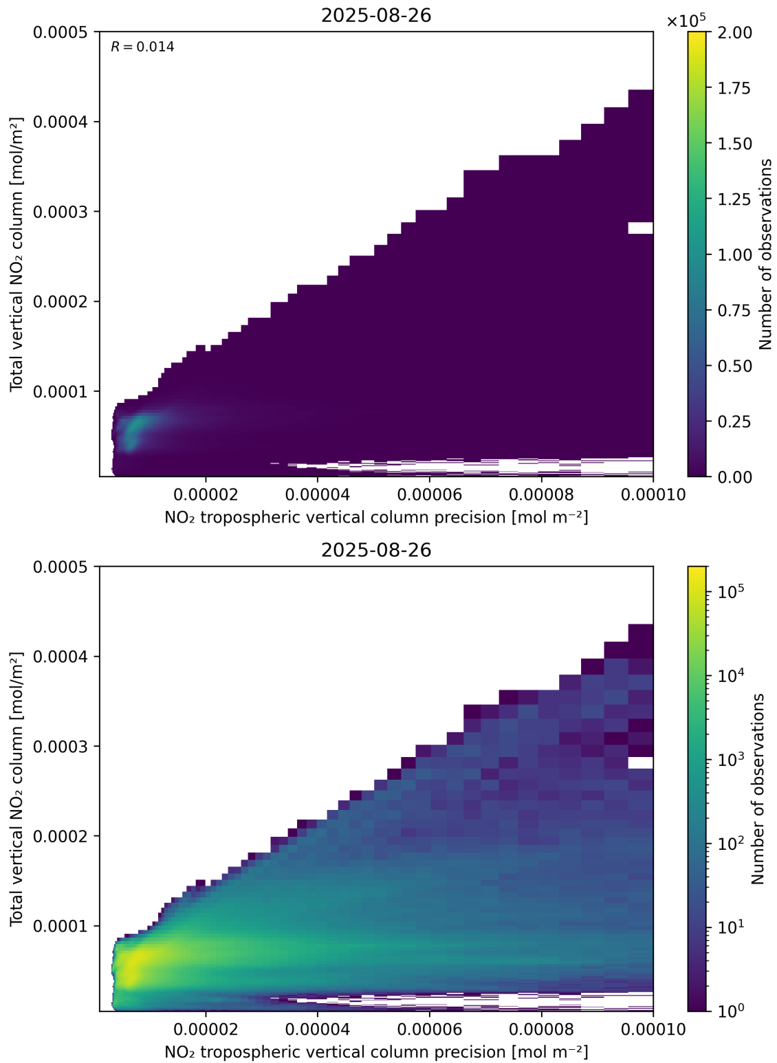
Figure 138: Scatter density plot of “NO 2 tropospheric vertical column precision” against “Total vertical NO 2 column” for 2025-08-25 to 2025-08-27.
