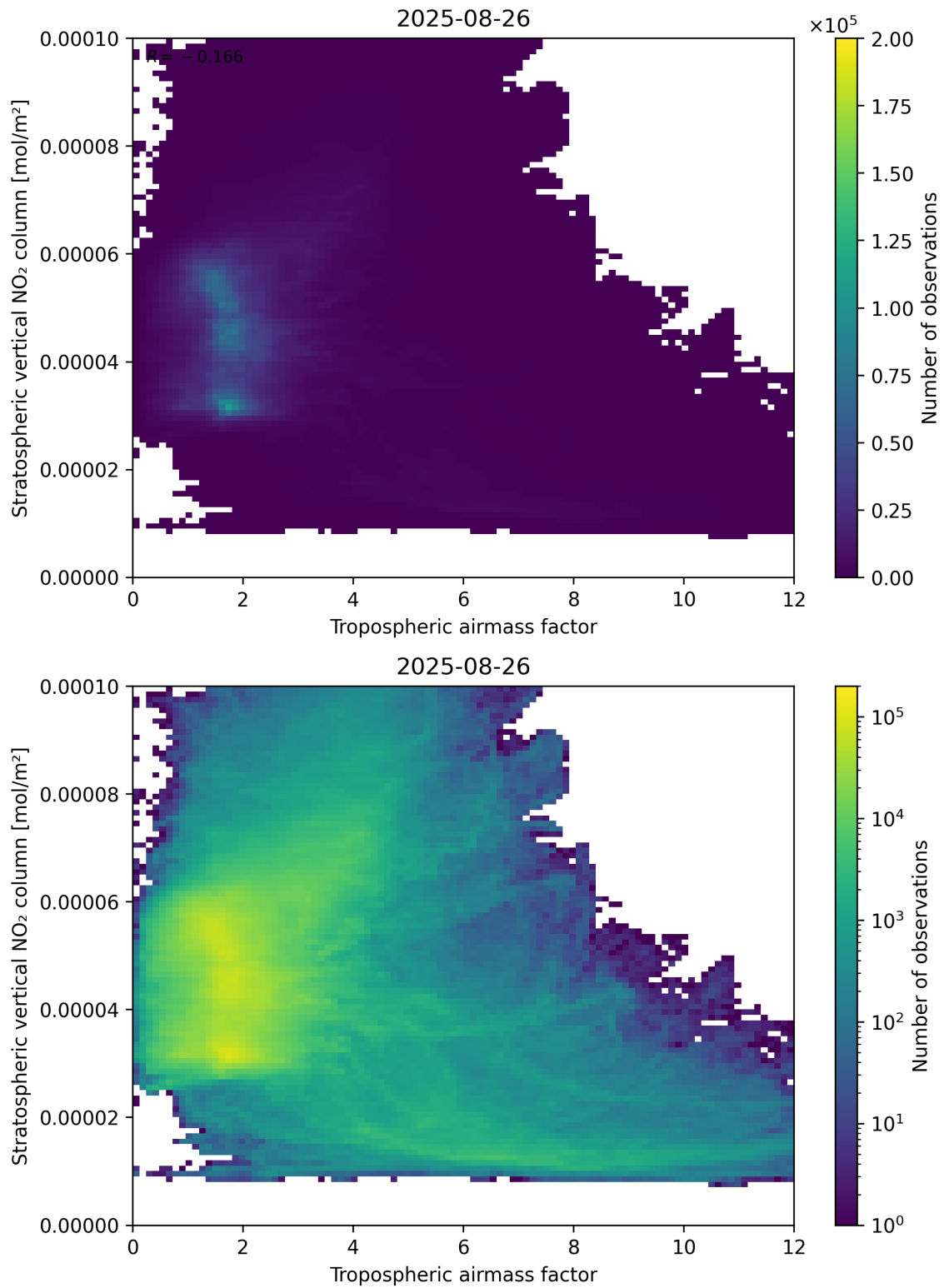
Figure 74: Scatter density plot of “Tropospheric air mass factor” against “Stratospheric vertical NO 2 column” for 2025-08-25 to 2025-08-27.
