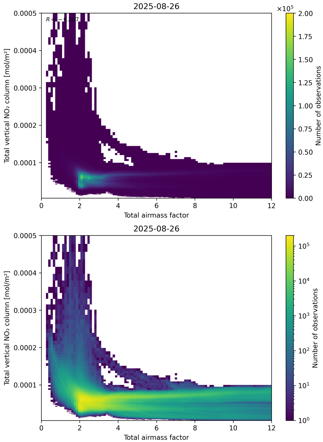
Figure 67: Scatter density plot of “Total airmass factor” against “Total vertical NO 2 column” for 2025-08-25 to 2025-08-27.
