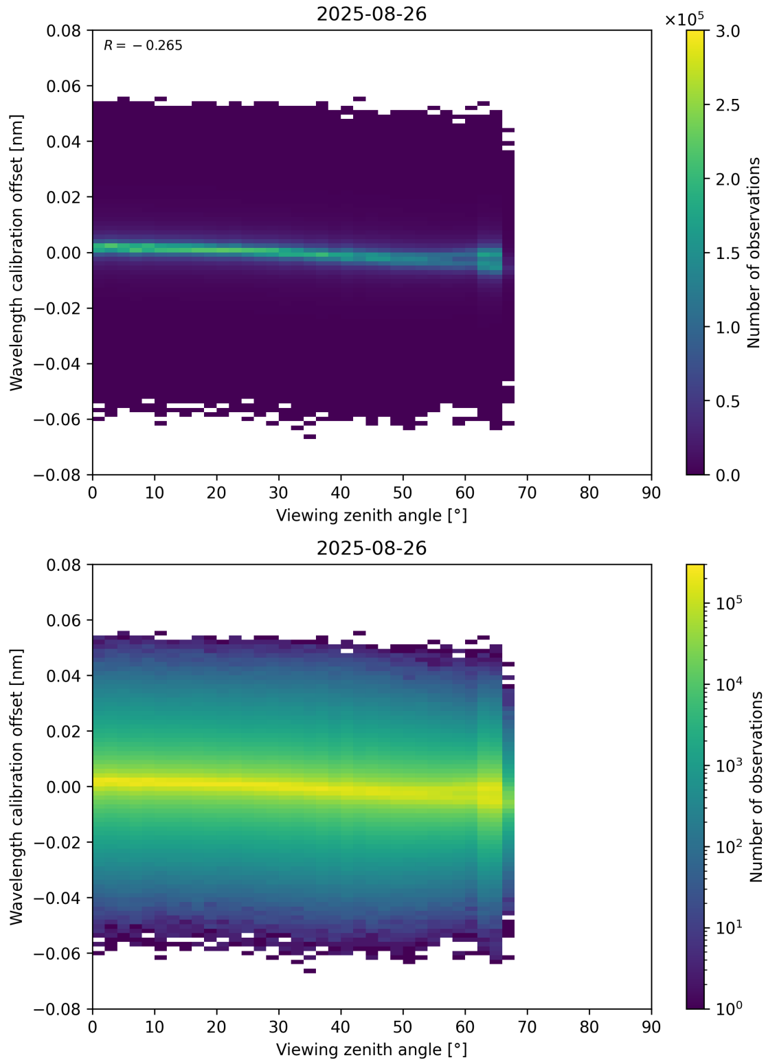
Figure 173: Scatter density plot of “Viewing zenith angle” against “Wavelength calibration offset” for 2025-08-25 to 2025-08-27.
