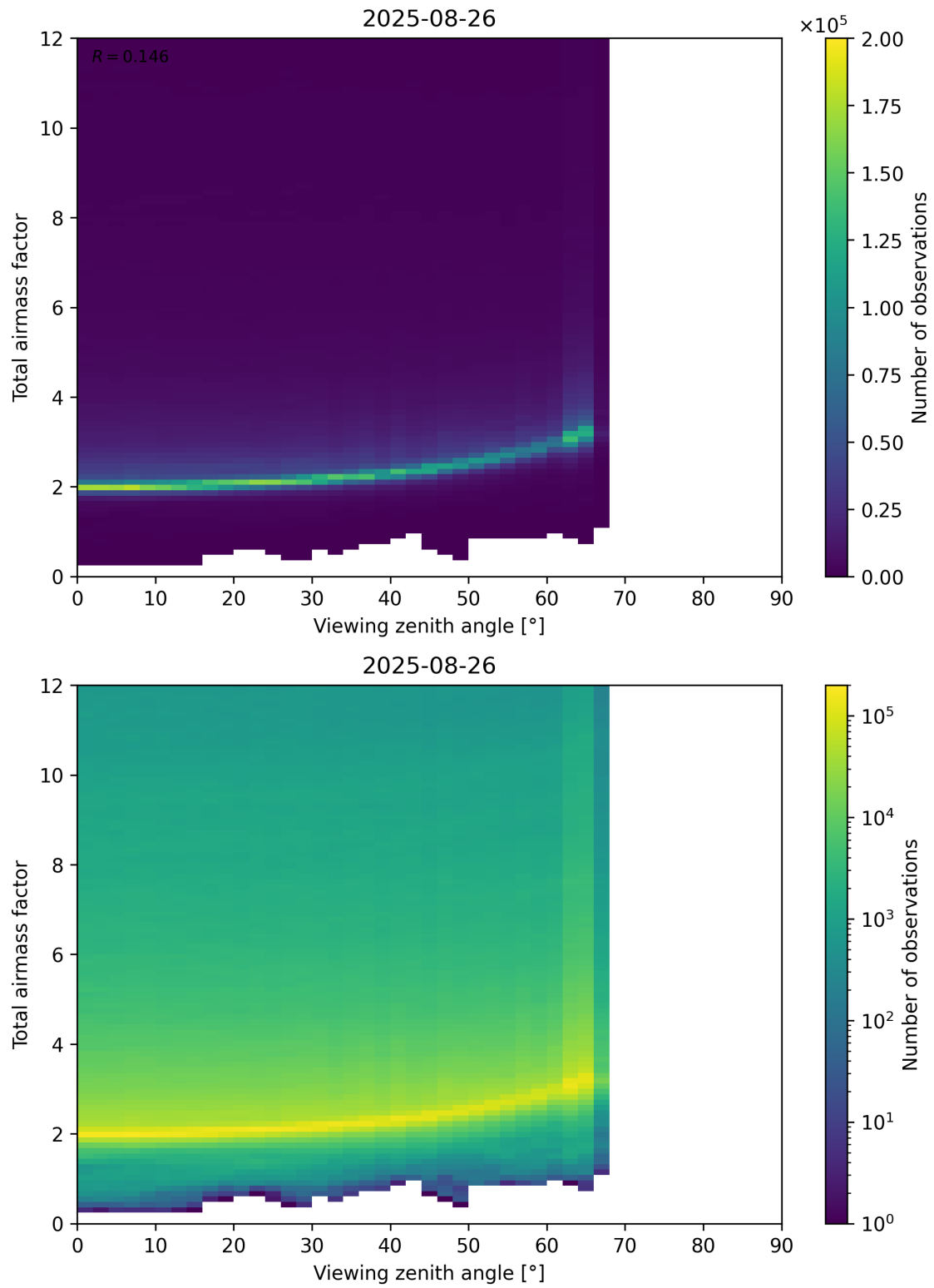
Figure 160: Scatter density plot of “Viewing zenith angle” against “Total airmass factor” for 2025-08-25 to 2025-08-27.
