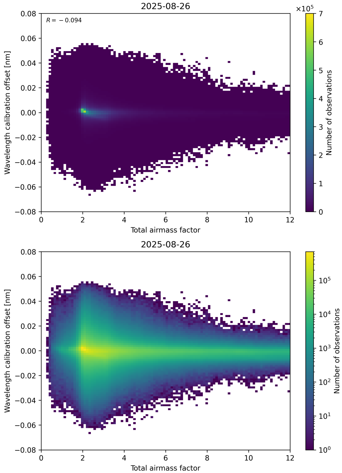
Figure 70: Scatter density plot of “Total airmass factor” against “Wavelength calibration offset” for 2025-08-25 to 2025-08-27.
