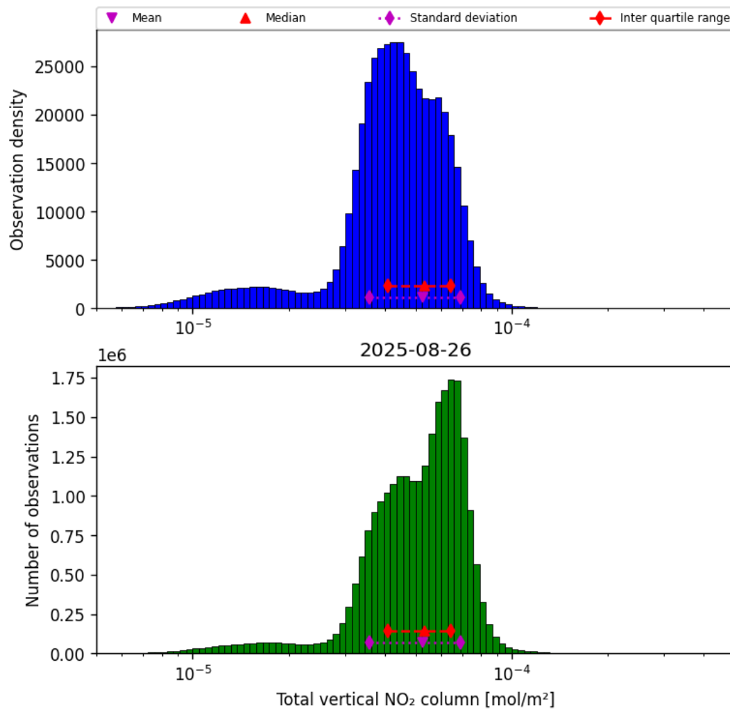
Figure 38: Histogram of “Total vertical NO 2 column” for 2025-08-25 to 2025-08-27
