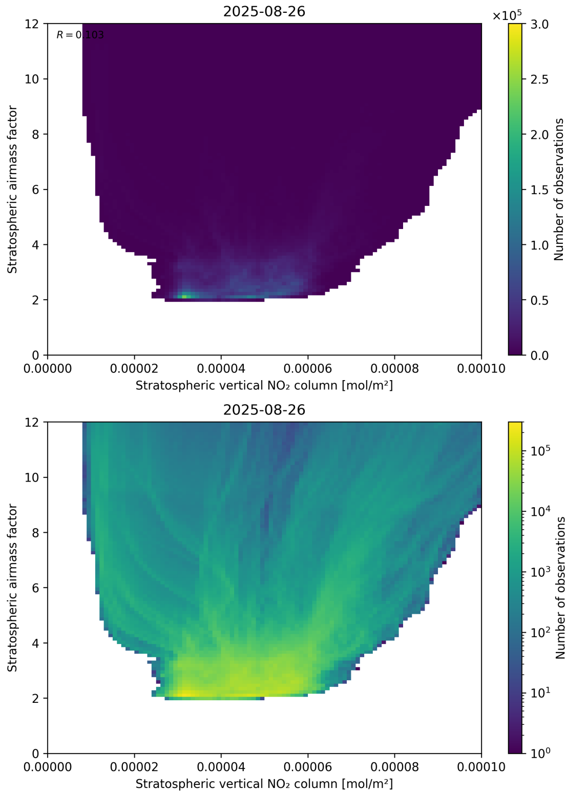
Figure 96: Scatter density plot of “Stratospheric vertical NO 2 column” against “Stratospheric airmass factor” for 2025-08-25 to 2025-08-27.
