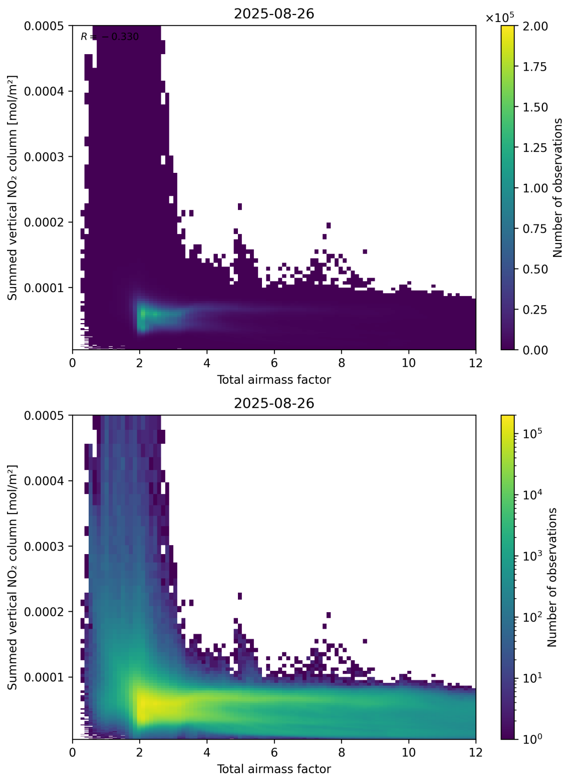
Figure 65: Scatter density plot of “Total airmass factor” against “Summed vertical NO 2 column” for 2025-08-25 to 2025-08-27.
