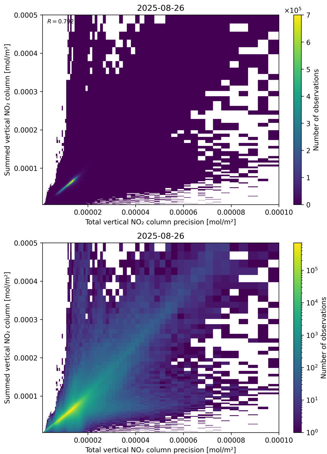
Figure 117: Scatter density plot of “Total vertical NO 2 column precision” against “Summed vertical NO 2 column” for 2025-08-25 to 2025-08-27.
