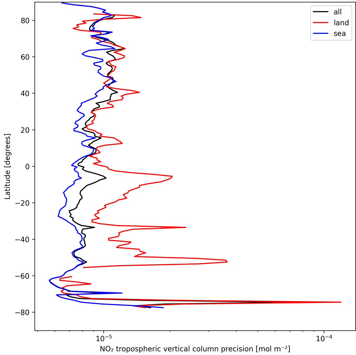
Figure 13: Zonal average of "NO 2 tropospheric vertical column precision" for 2025-08-25 to 2025-08-27.
