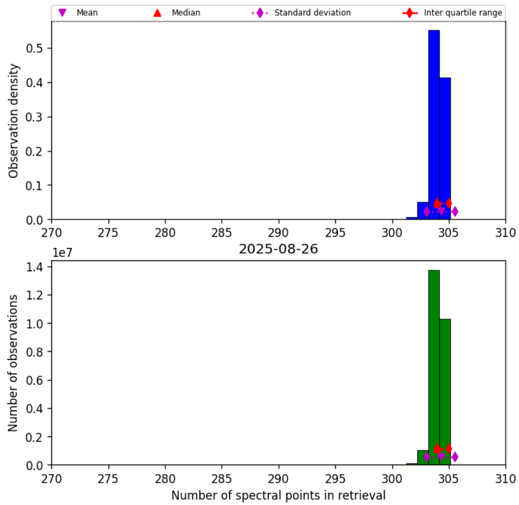
Figure 33: Histogram of “Number of spectral points in retrieval” for 2025-08-25 to 2025-08-27
