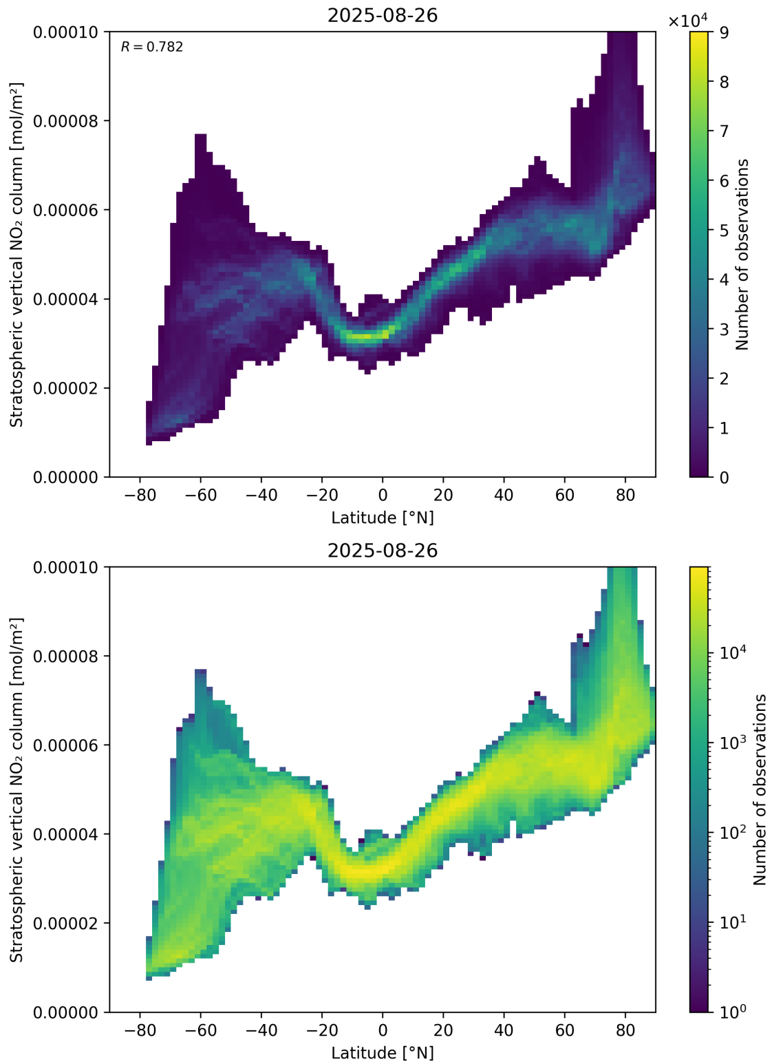
Figure 87: Scatter density plot of “Latitude” against “Stratospheric vertical NO 2 column” for 2025-08-25 to 2025-08-27.
