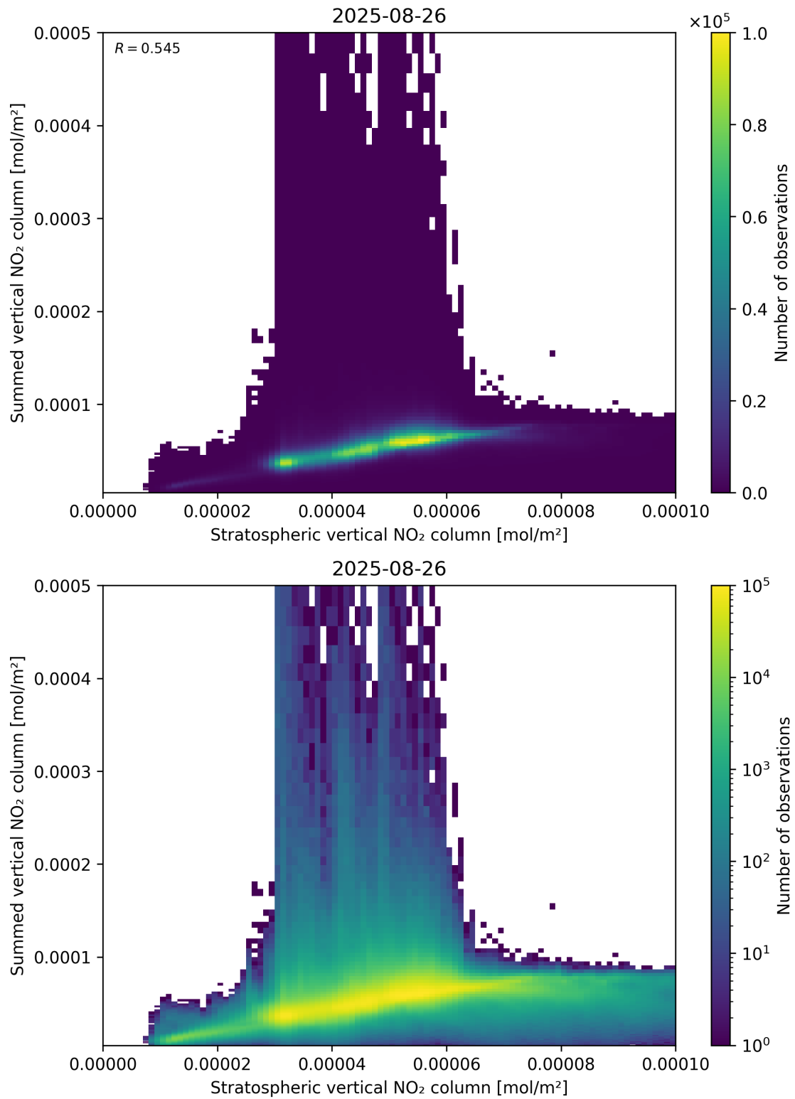
Figure 98: Scatter density plot of “Stratospheric vertical NO 2 column” against “Summed vertical NO 2 column” for 2025-08-25 to 2025-08-27.
