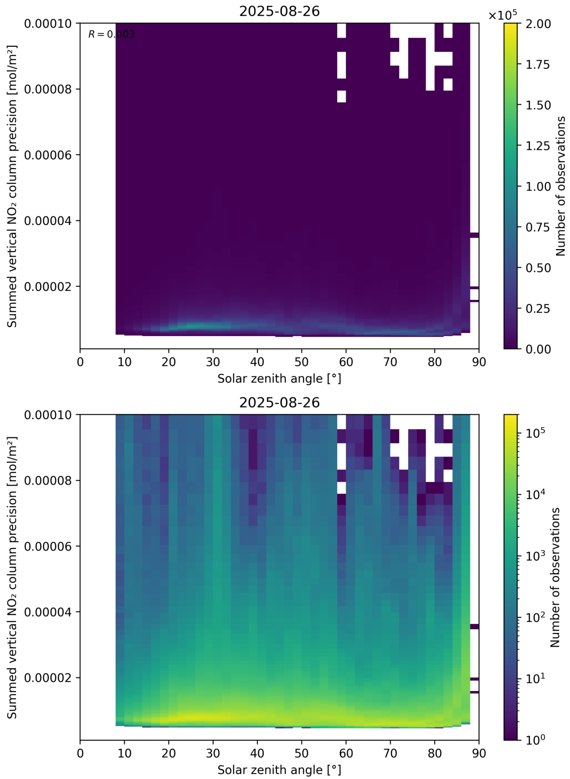
Figure 152: Scatter density plot of “Solar zenith angle” against “Summed vertical NO 2 column precision” for 2025-08-25 to 2025-08-27.
