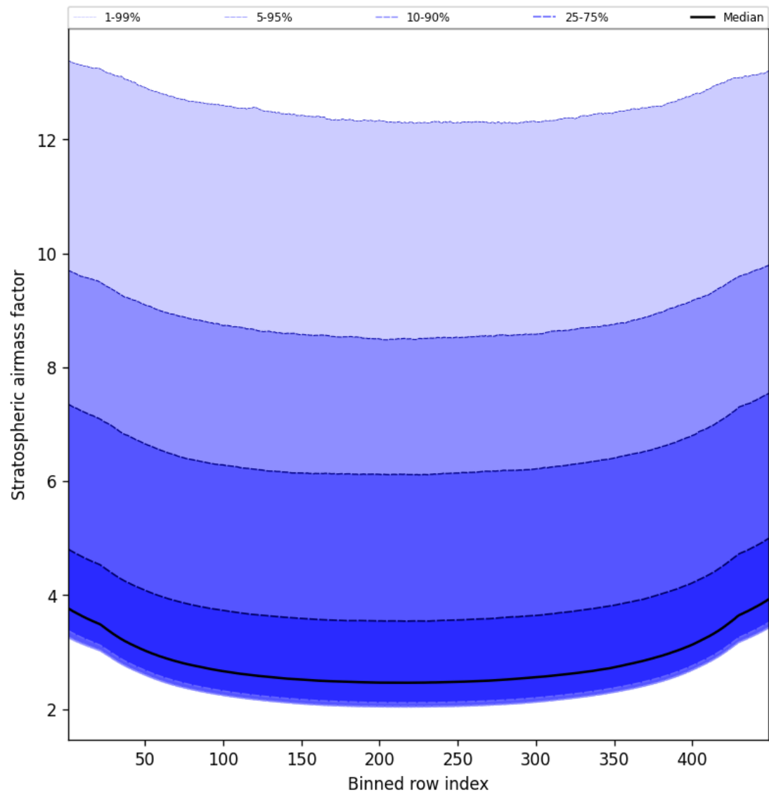
Figure 61: Along track statistics of “Stratospheric airmass factor” for 2025-08-25 to 2025-08-27
