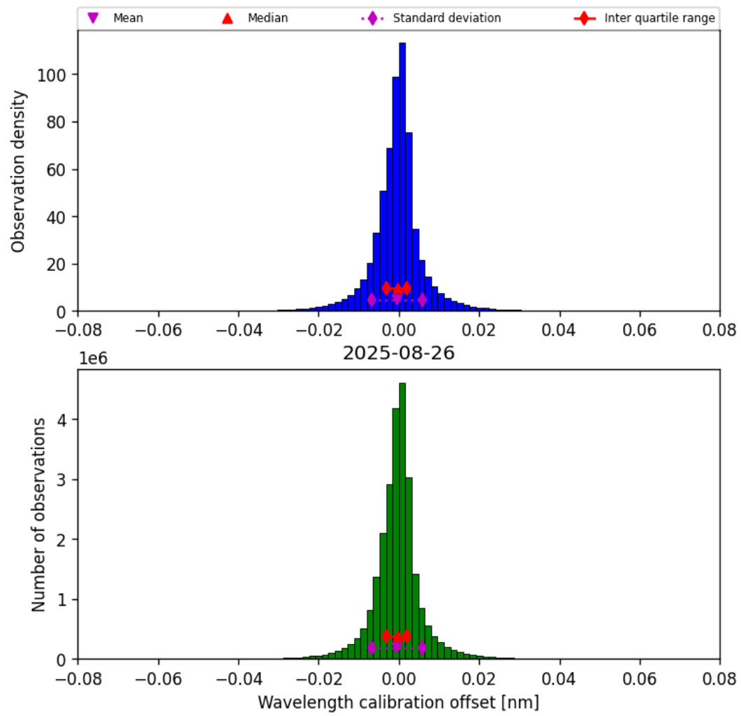
Figure 35: Histogram of “Wavelength calibration offset” for 2025-08-25 to 2025-08-27
