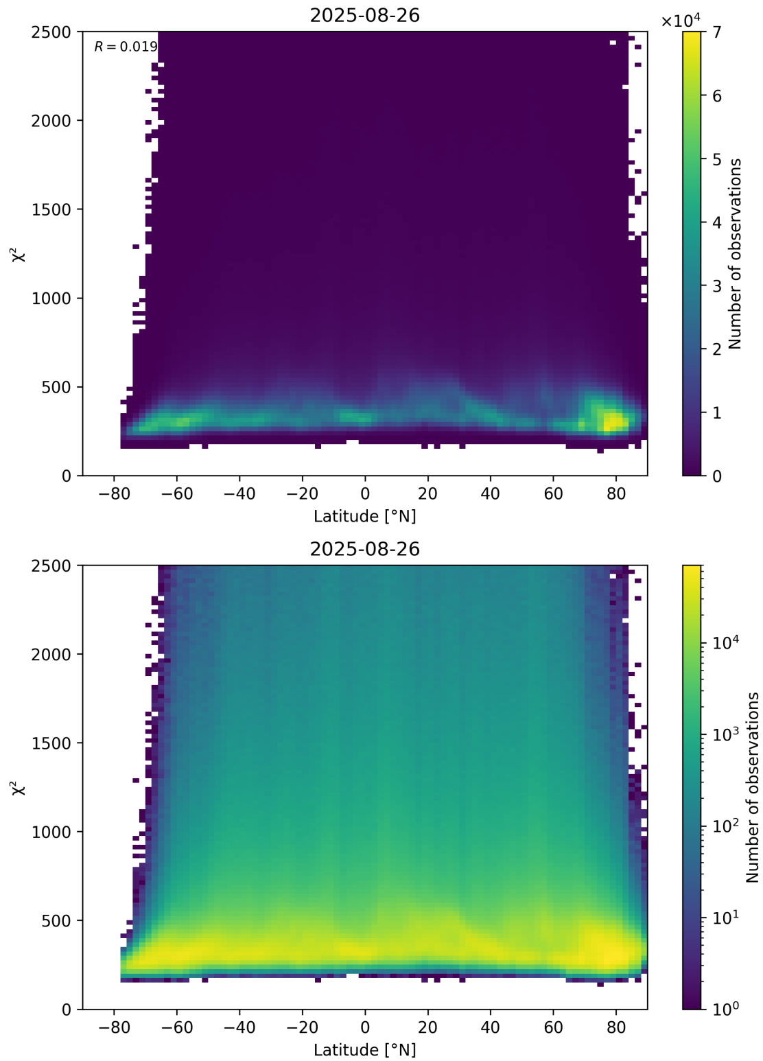
Figure 86: Scatter density plot of “Latitude” against “ \chi^2 ” for 2025-08-25 to 2025-08-27.
