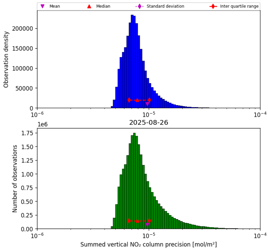
Figure 41: Histogram of "Summed vertical NO 2 column precision" for 2025-08-25 to 2025-08-27
