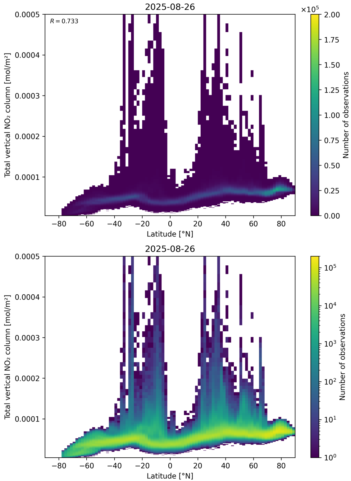
Figure 90: Scatter density plot of “Latitude” against “Total vertical NO 2 column” for 2025-08-25 to 2025-08-27.
