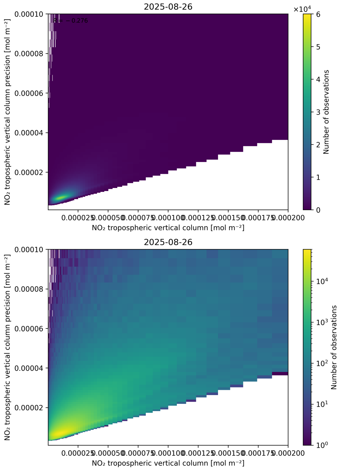
Figure 130: Scatter density plot of “NO 2 tropospheric vertical column” against “NO 2 tropospheric vertical column precision” for 2025-08-25 to 2025-08-27.
