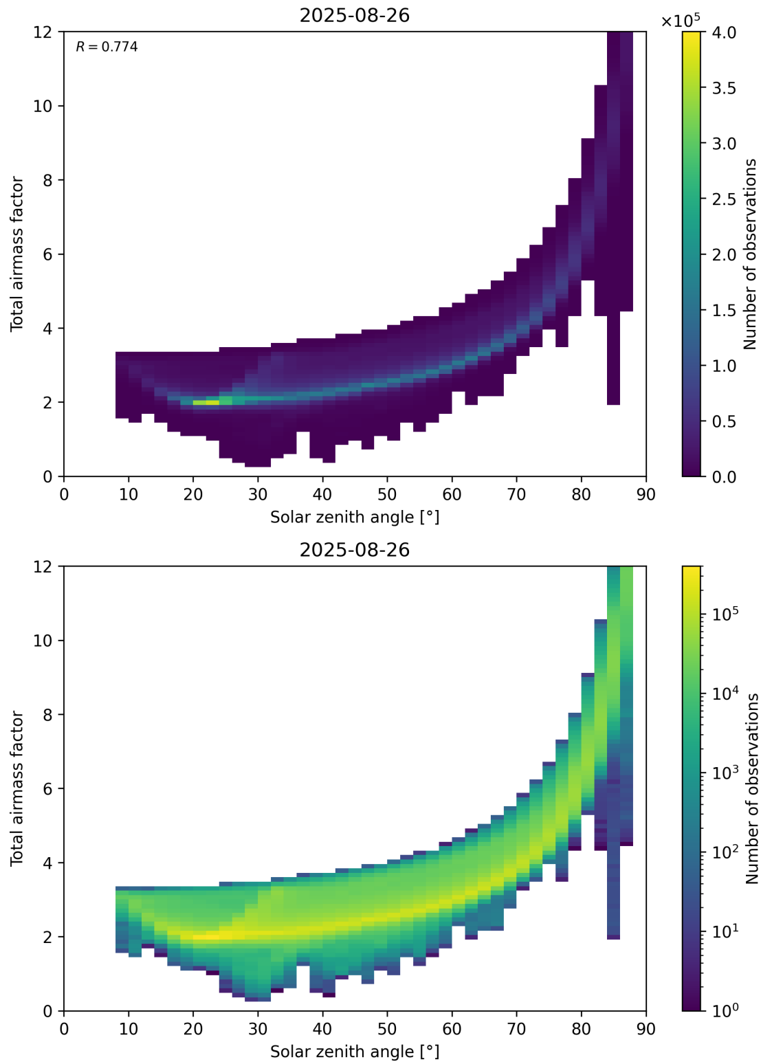
Figure 146: Scatter density plot of “Solar zenith angle” against “Total air mass factor” for 2025-08-25 to 2025-08-27.
