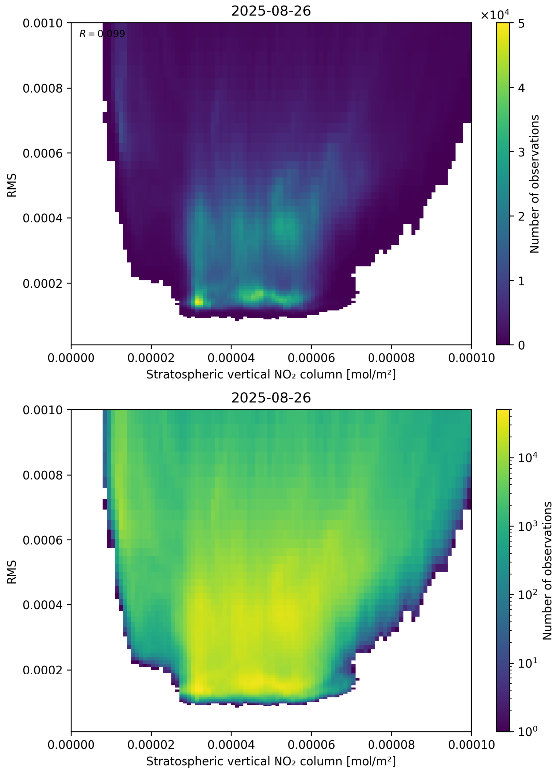
Figure 102: Scatter density plot of “Stratospheric vertical NO 2 column” against “RMS” for 2025-08-25 to 2025-08-27.
