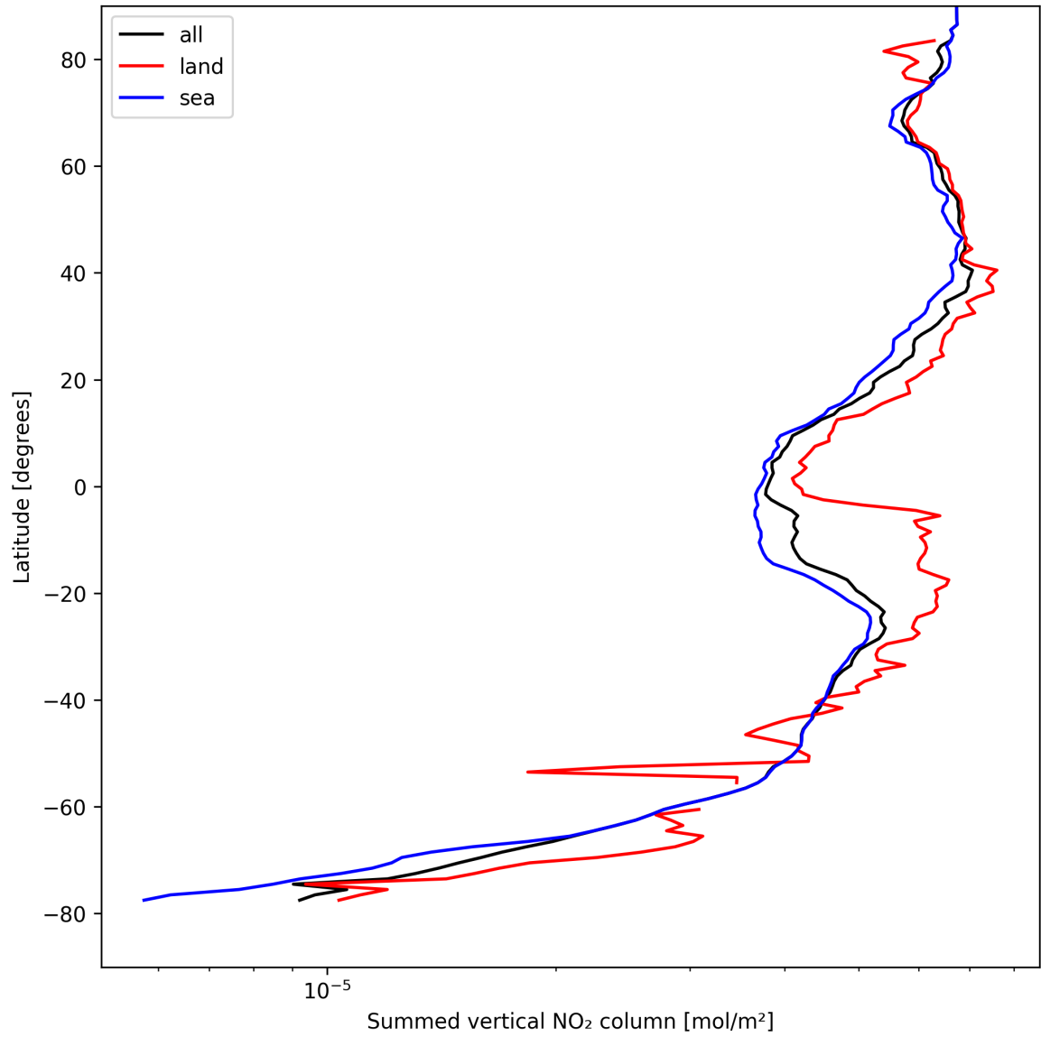
Figure 23: Zonal average of “Summed vertical NO 2 column” for 2025-08-25 to 2025-08-27.
