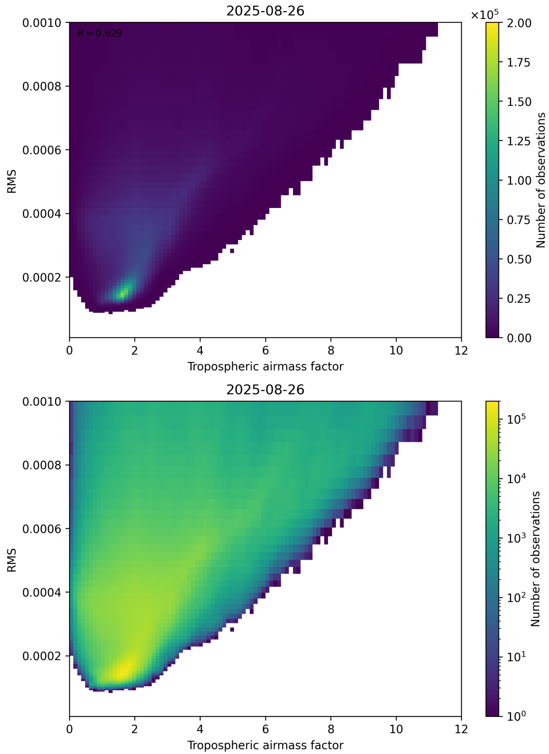
Figure 79: Scatter density plot of “Tropospheric airmass factor” against “RMS” for 2025-08-25 to 2025-08-27.
