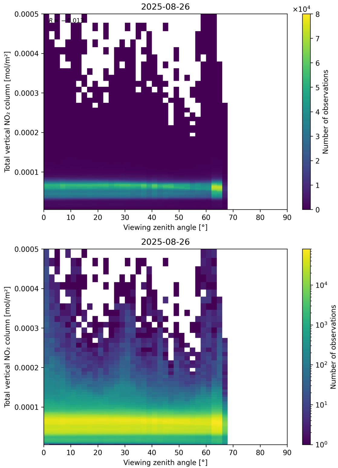
Figure 167: Scatter density plot of “Viewing zenith angle” against “Total vertical NO 2 column” for 2025-08-25 to 2025-08-27.
