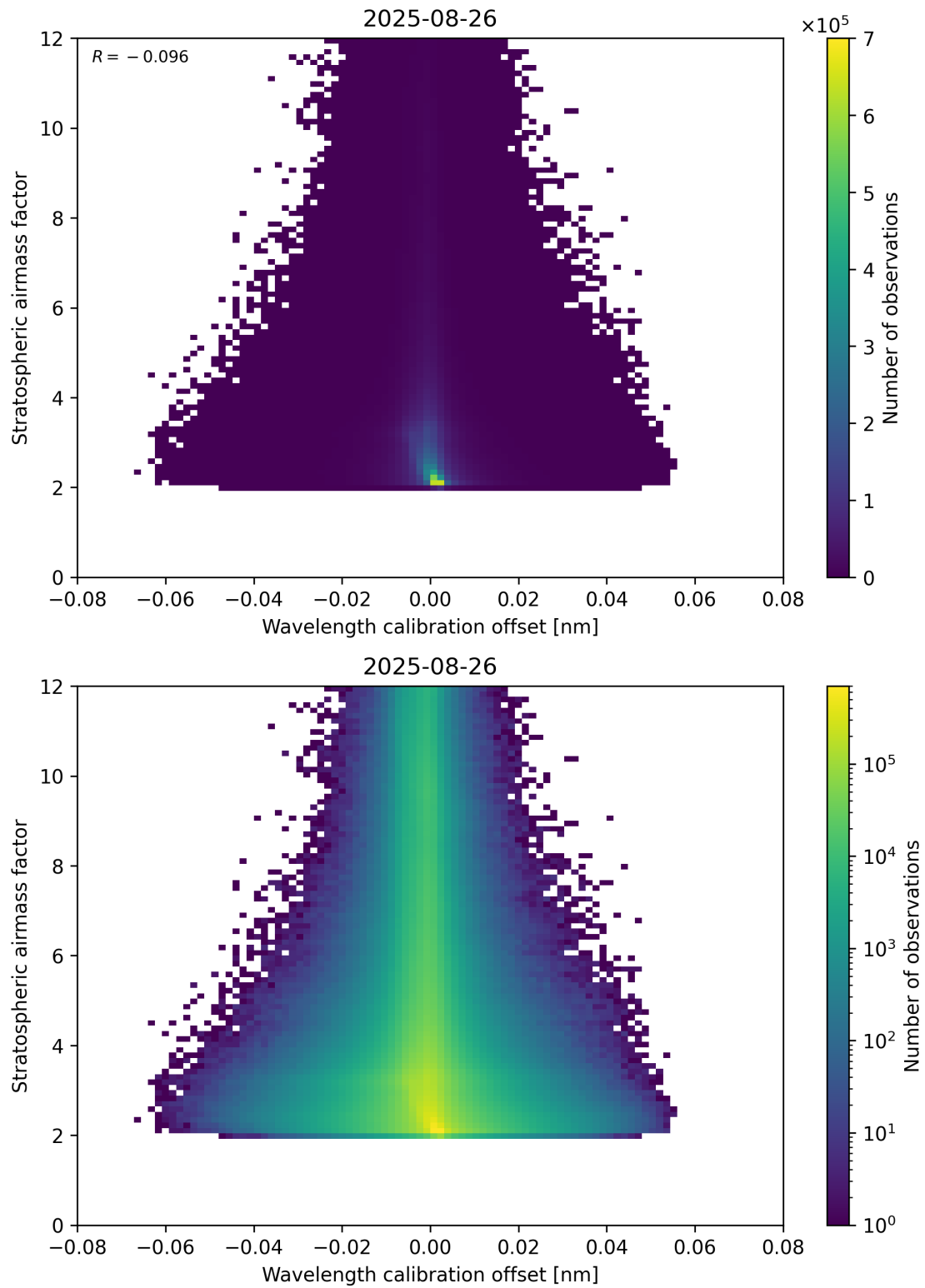
Figure 174: Scatter density plot of “Wavelength calibration offset” against “Stratospheric airmass factor” for 2025-08-25 to 2025-08-27.
