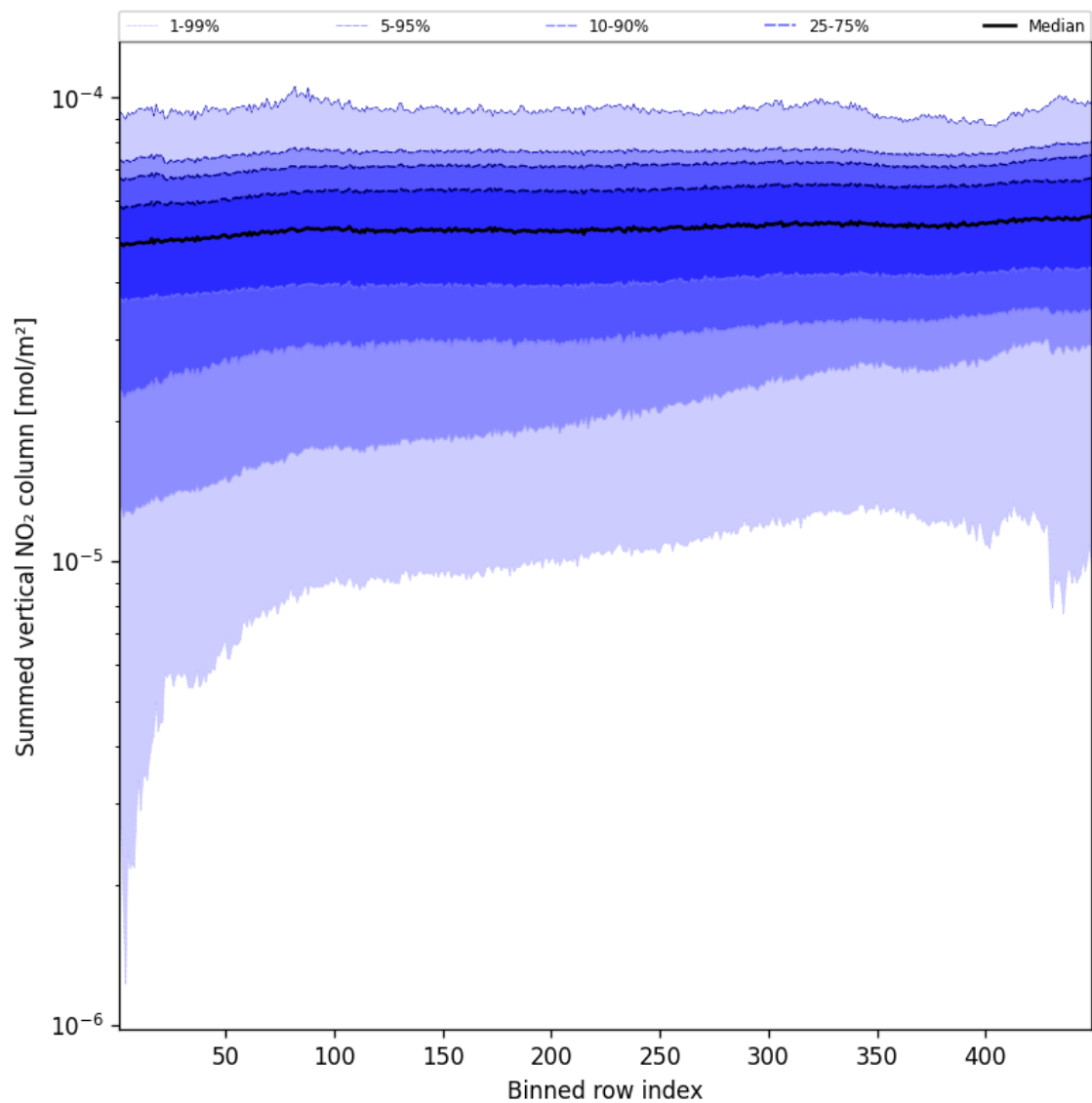
Figure 57: Along track statistics of “Summed vertical NO 2 column” for 2025-08-25 to 2025-08-27
