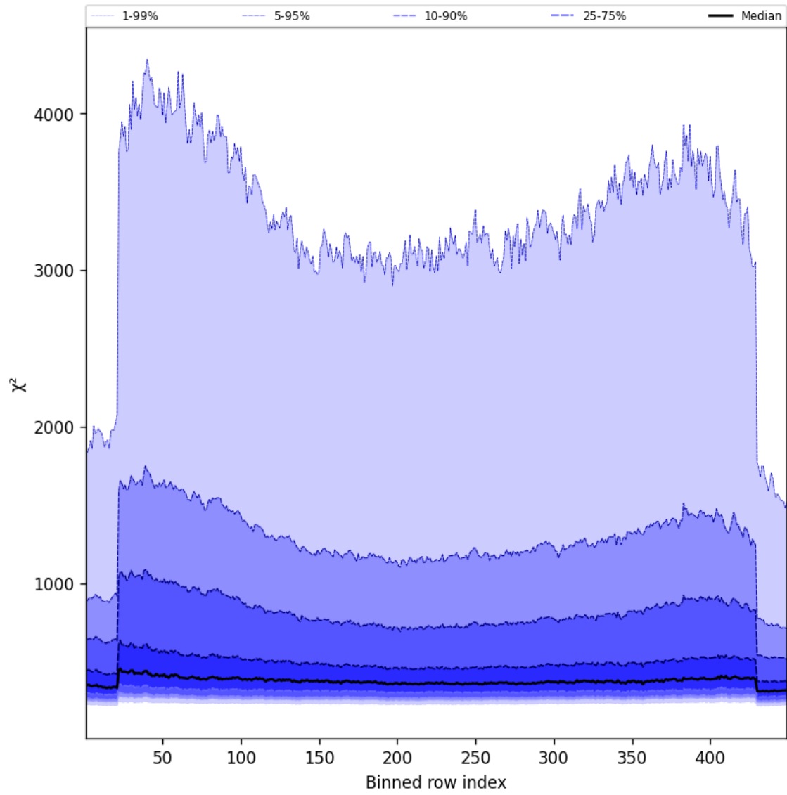
Figure 59: Along track statistics of “ \chi^2 ” for 2025-08-25 to 2025-08-27
