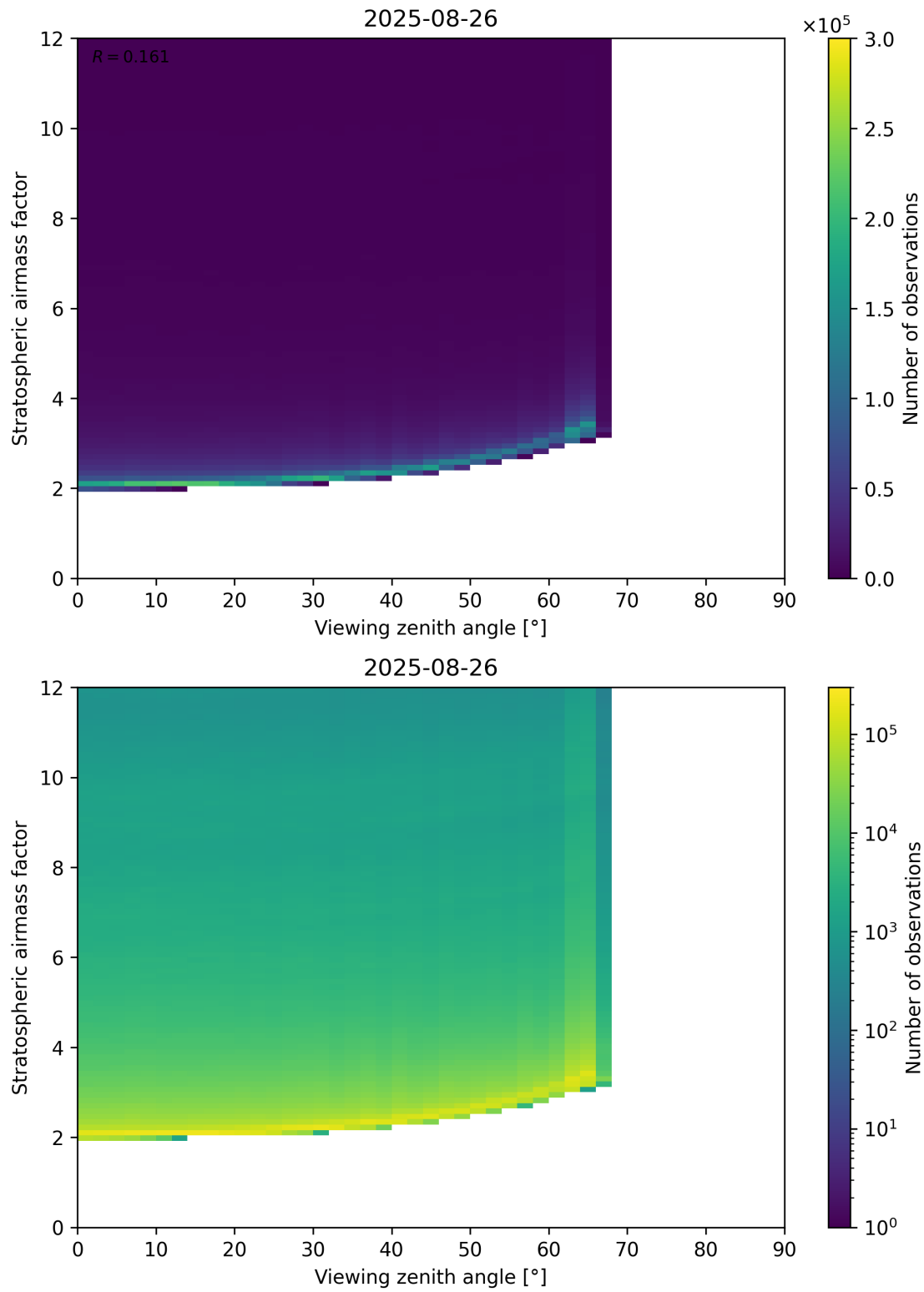
Figure 159: Scatter density plot of “Viewing zenith angle” against “Stratospheric airmass factor” for 2025-08-25 to 2025-08-27.
