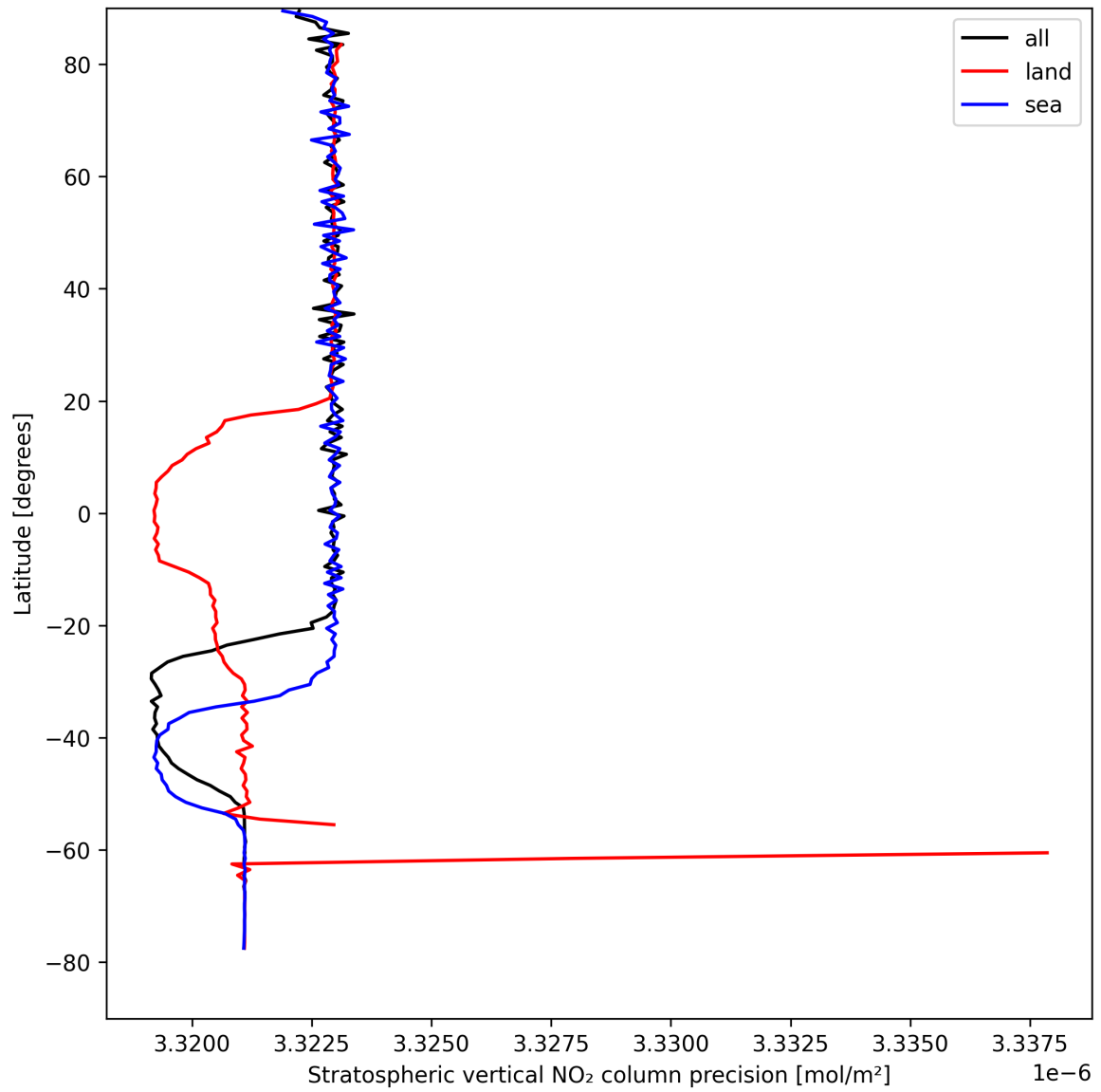
Figure 20: Zonal average of “Stratospheric vertical NO 2 column precision” for 2025-08-25 to 2025-08-27.
