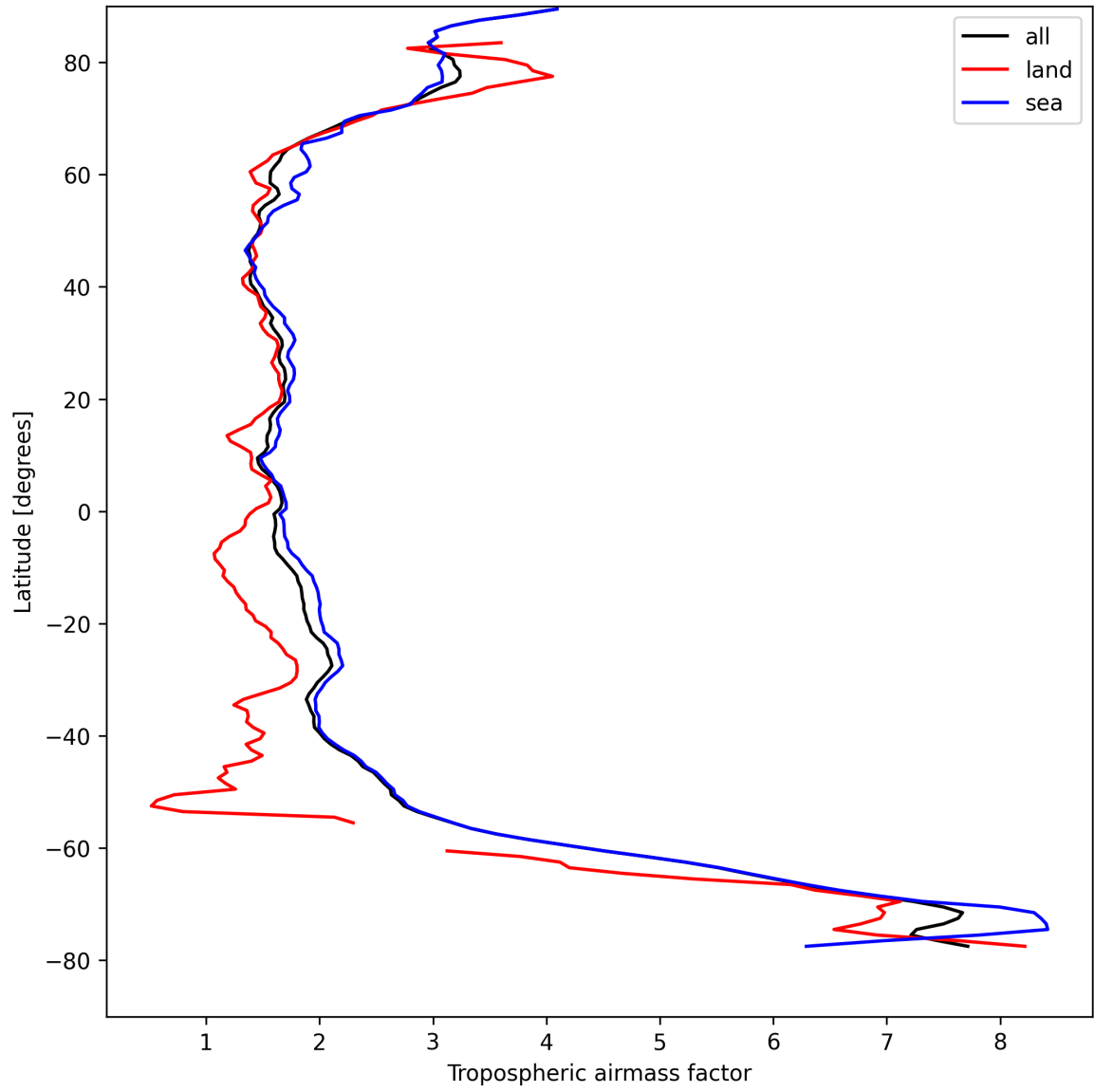
Figure 14: Zonal average of “Tropospheric airmass factor” for 2025-08-25 to 2025-08-27.
