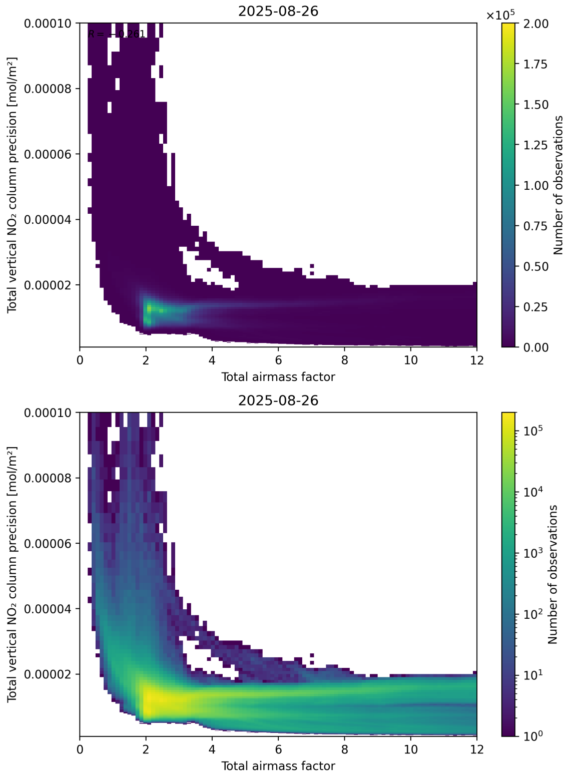
Figure 68: Scatter density plot of “Total airmass factor” against “Total vertical NO 2 column precision” for 2025-08-25 to 2025-08-27.
