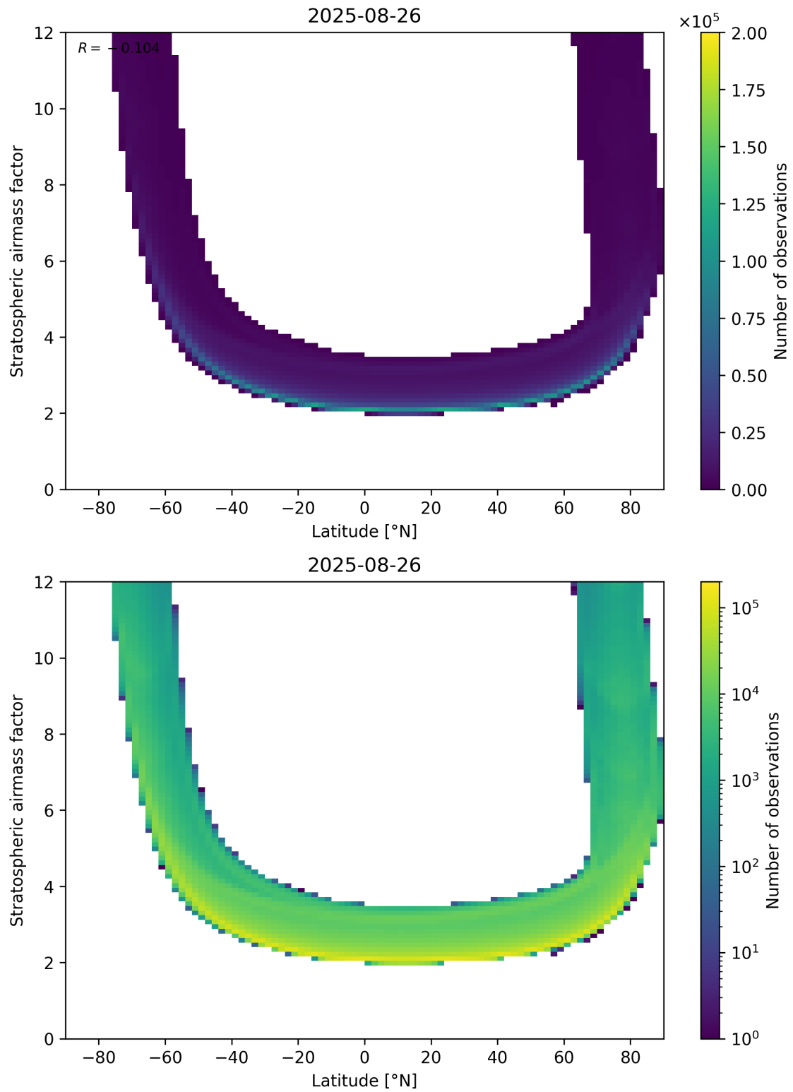
Figure 83: Scatter density plot of “Latitude” against “Stratospheric air mass factor” for 2025-08-25 to 2025-08-27.
