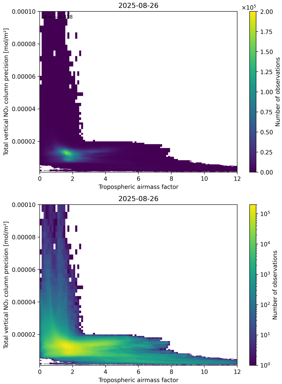
Figure 78: Scatter density plot of “Tropospheric airmass factor” against “Total vertical NO 2 column precision” for 2025-08-25 to 2025-08-27.
