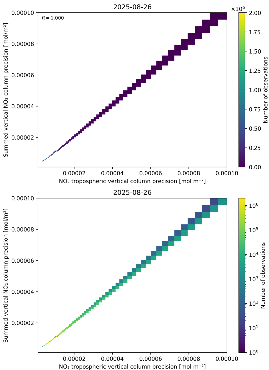
Figure 137: Scatter density plot of “NO 2 tropospheric vertical column precision” against “Summed vertical NO 2 column precision” for 2025-08-25 to 2025-08-27.
