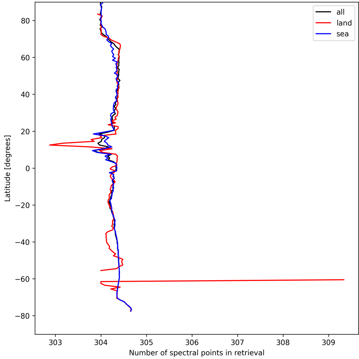
Figure 16: Zonal average of “Number of spectral points in retrieval” for 2025-08-25 to 2025-08-27.
