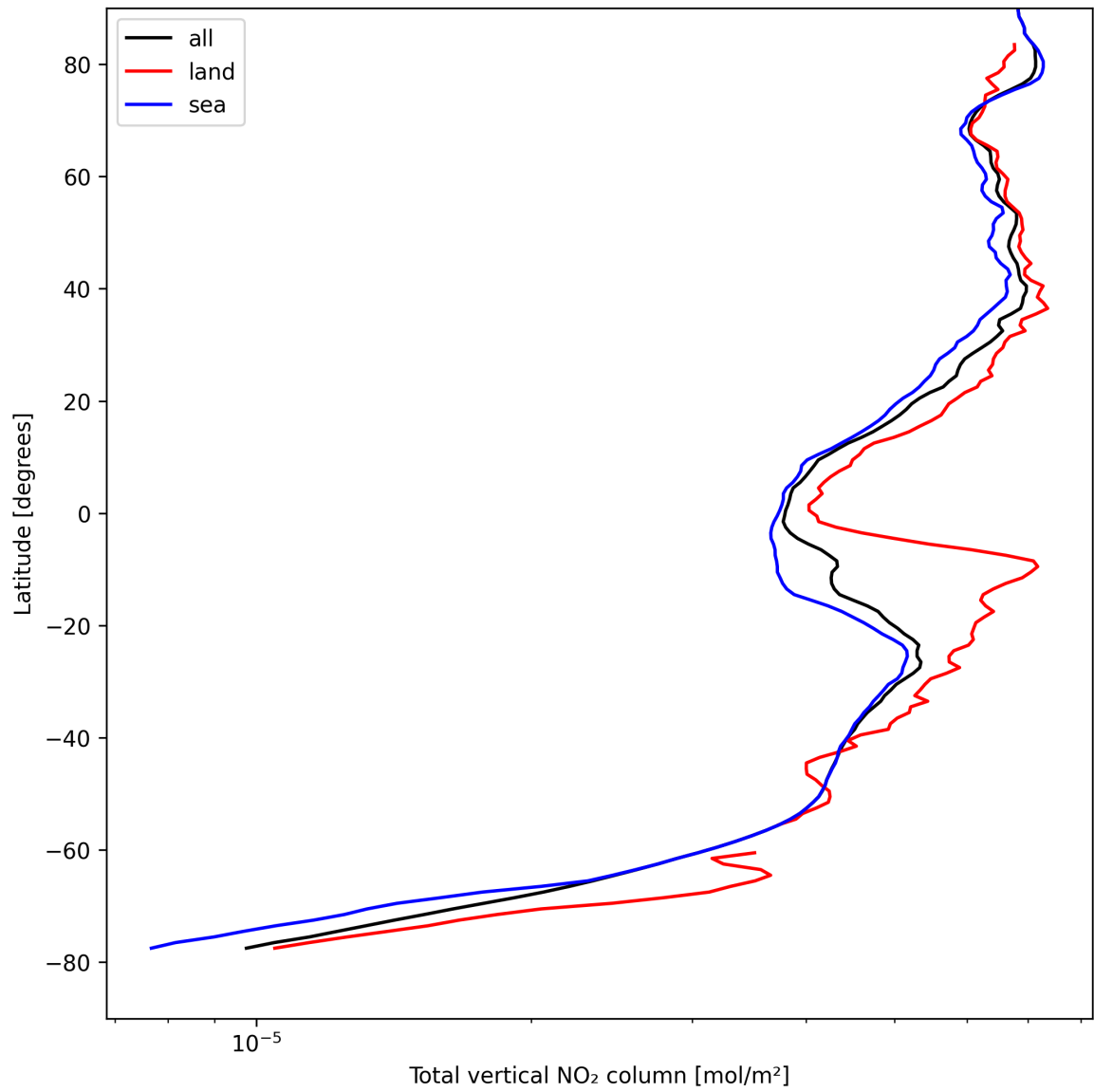
Figure 21: Zonal average of “Total vertical NO 2 column” for 2025-08-25 to 2025-08-27.
