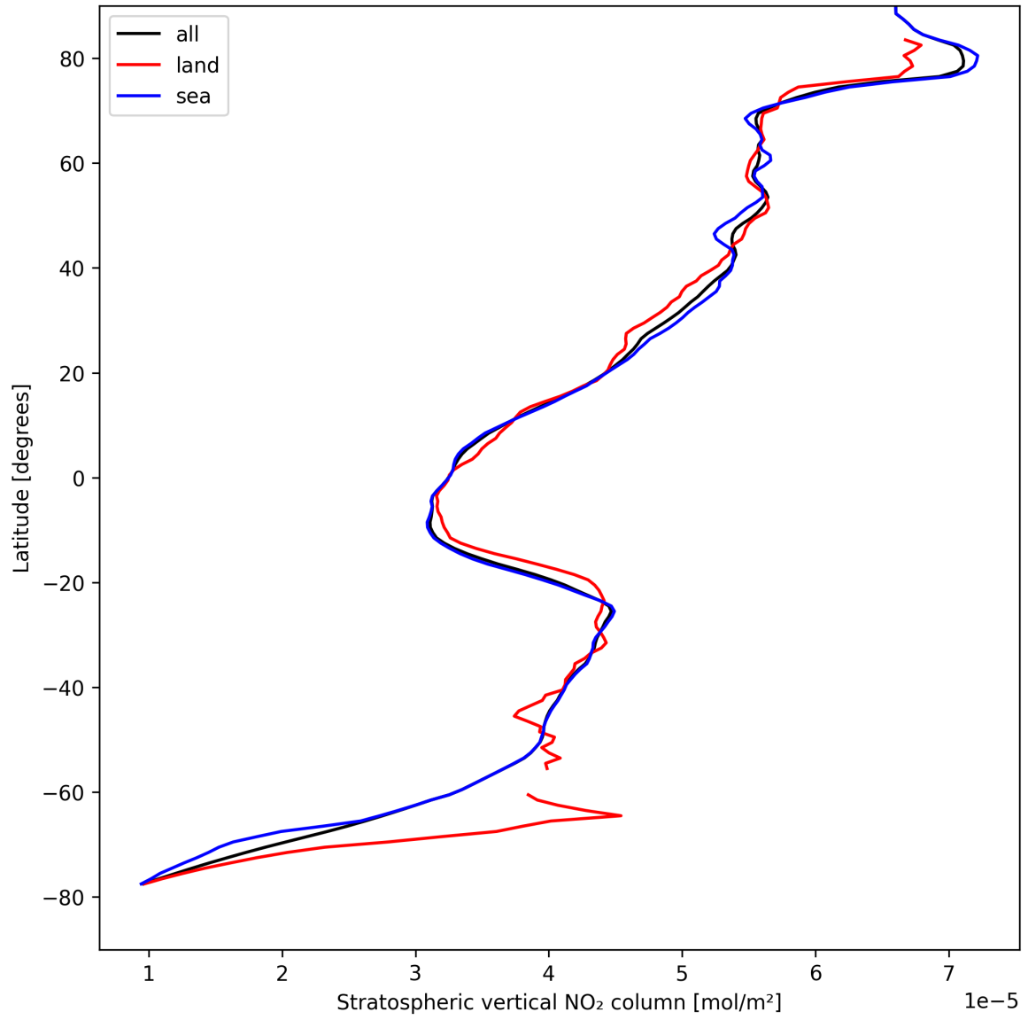
Figure 19: Zonal average of “Stratospheric vertical NO 2 column” for 2025-08-25 to 2025-08-27.
