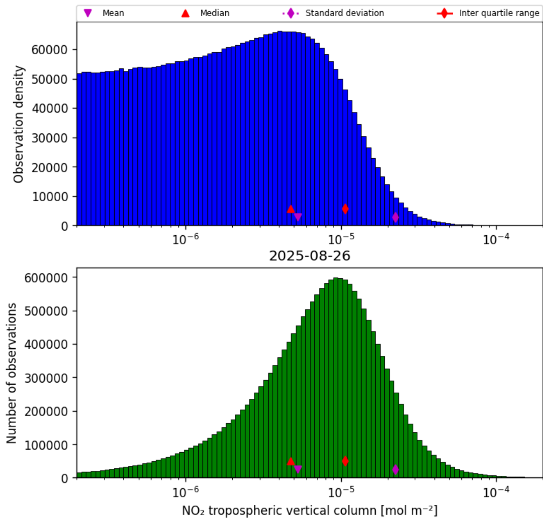
Figure 29: Histogram of “NO 2 tropospheric vertical column” for 2025-08-25 to 2025-08-27
