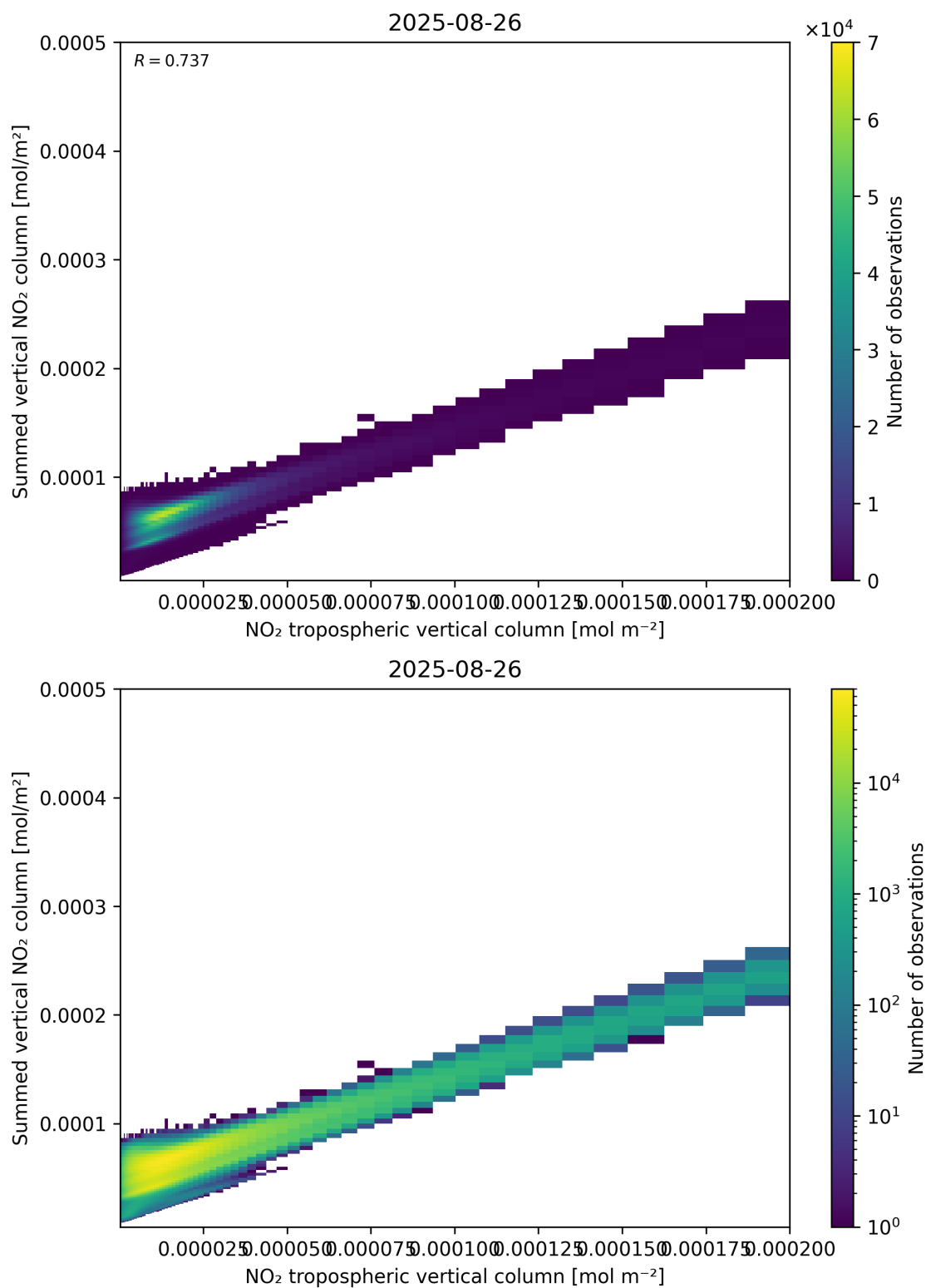
Figure 126: Scatter density plot of “NO 2 tropospheric vertical column” against “Summed vertical NO 2 column” for 2025-08-25 to 2025-08-27.
