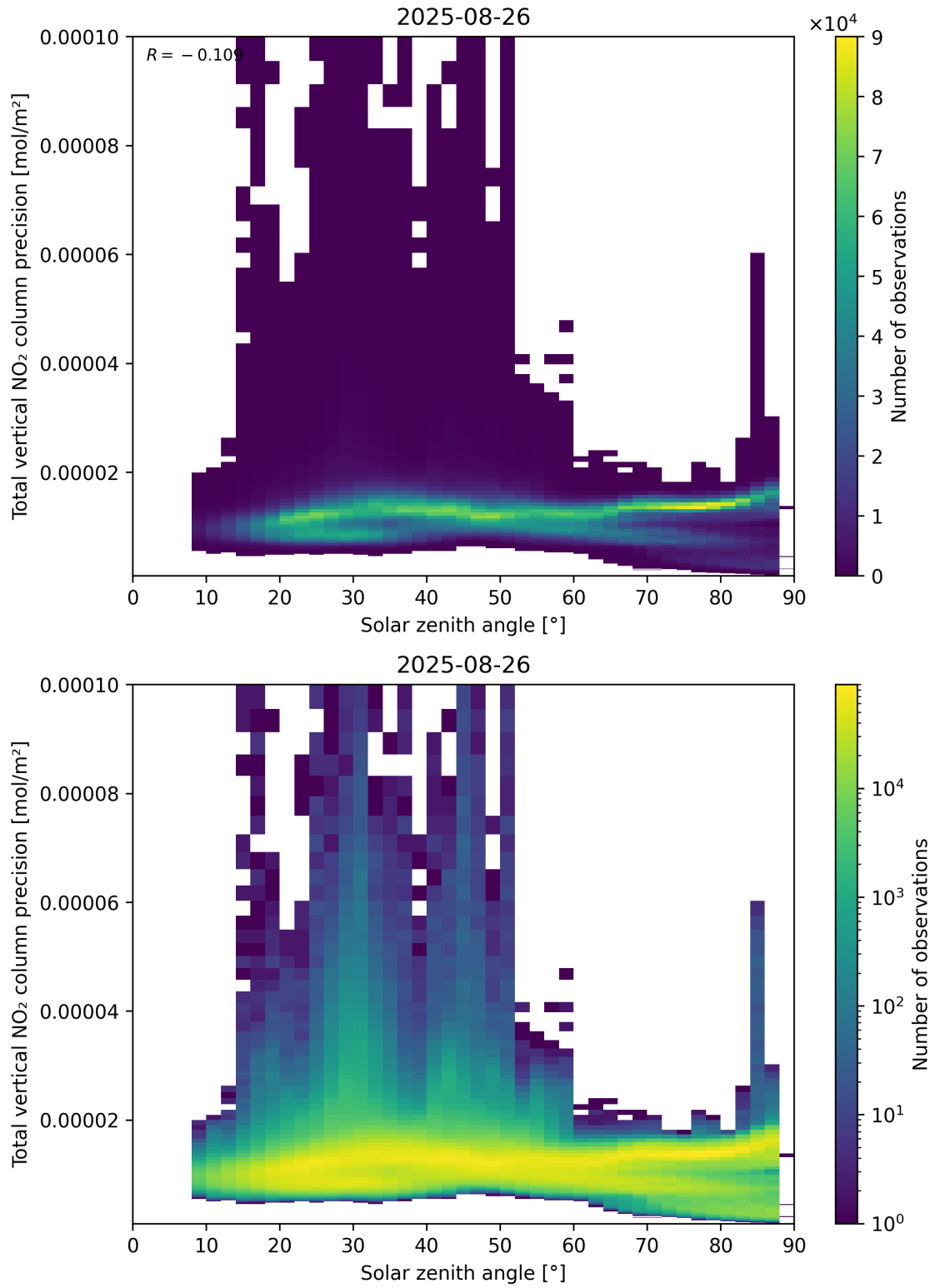
Figure 154: Scatter density plot of “Solar zenith angle” against “Total vertical NO 2 column precision” for 2025-08-25 to 2025-08-27.
