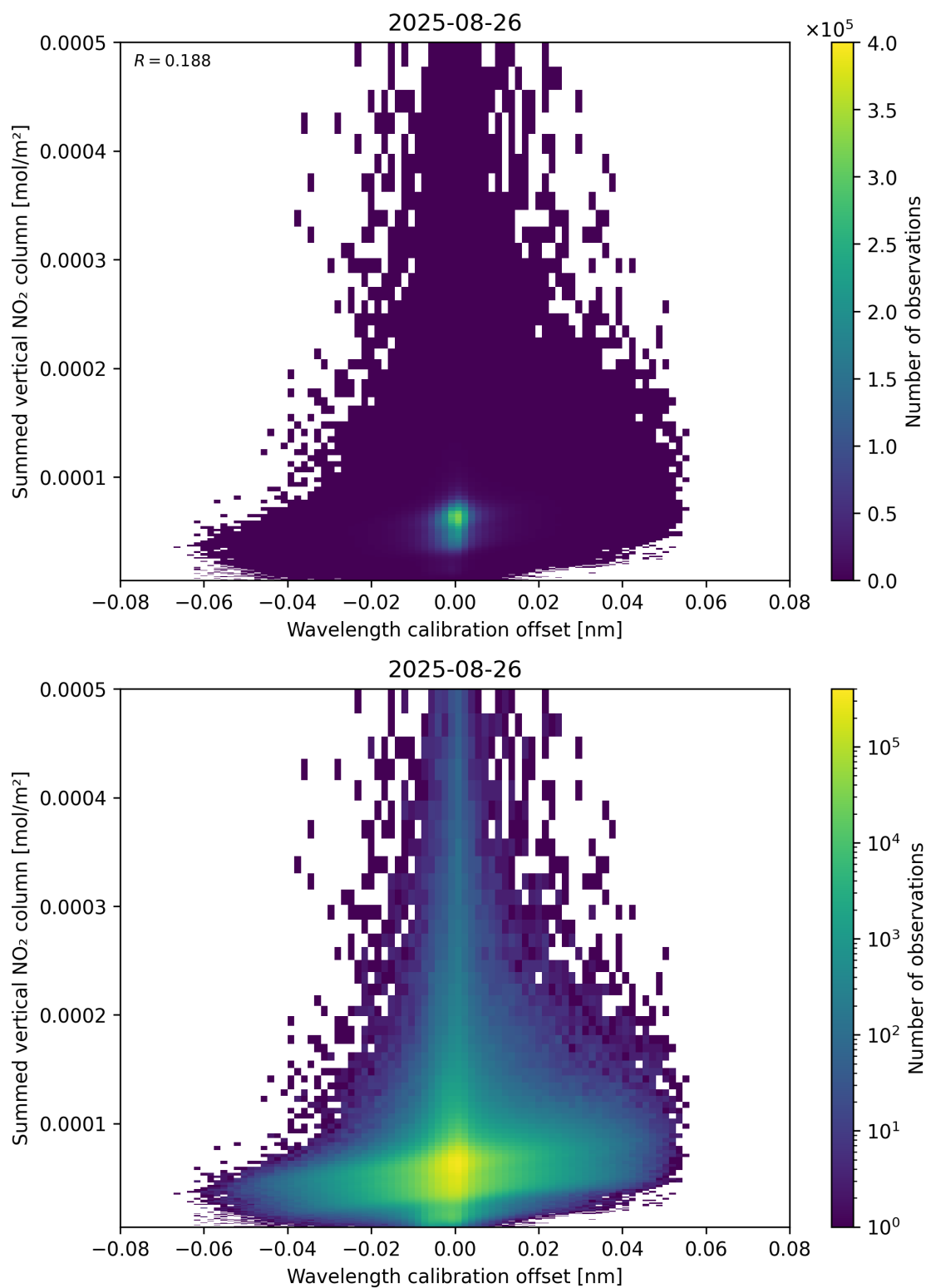
Figure 177: Scatter density plot of “Wavelength calibration offset” against “Summed vertical NO 2 column” for 2025-08-25 to 2025-08-27.
