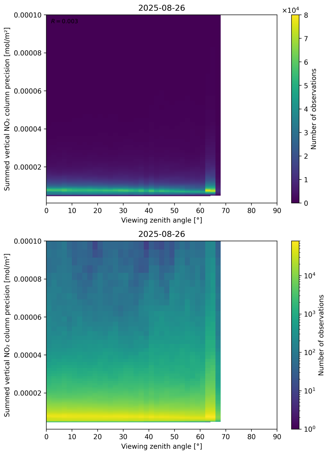
Figure 166: Scatter density plot of “Viewing zenith angle” against “Summed vertical NO 2 column precision” for 2025-08-25 to 2025-08-27.
