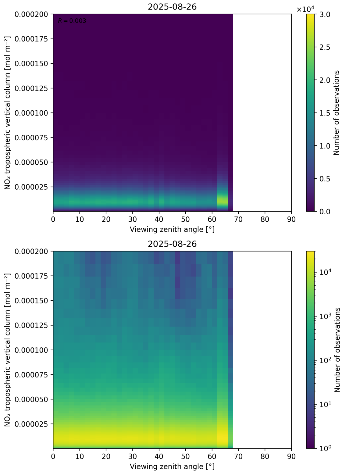
Figure 169: Scatter density plot of “Viewing zenith angle” against “NO 2 tropospheric vertical column” for 2025-08-25 to 2025-08-27.
