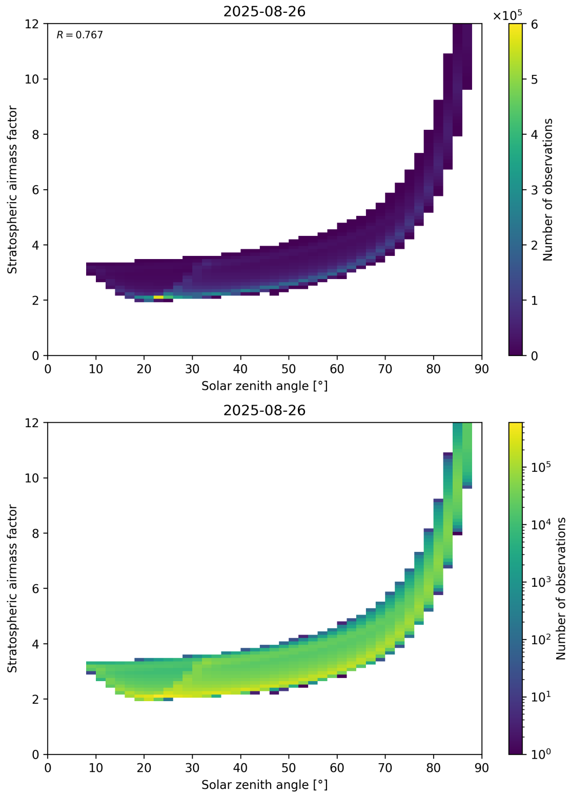
Figure 145: Scatter density plot of “Solar zenith angle” against “Stratospheric airmass factor” for 2025-08-25 to 2025-08-27.
