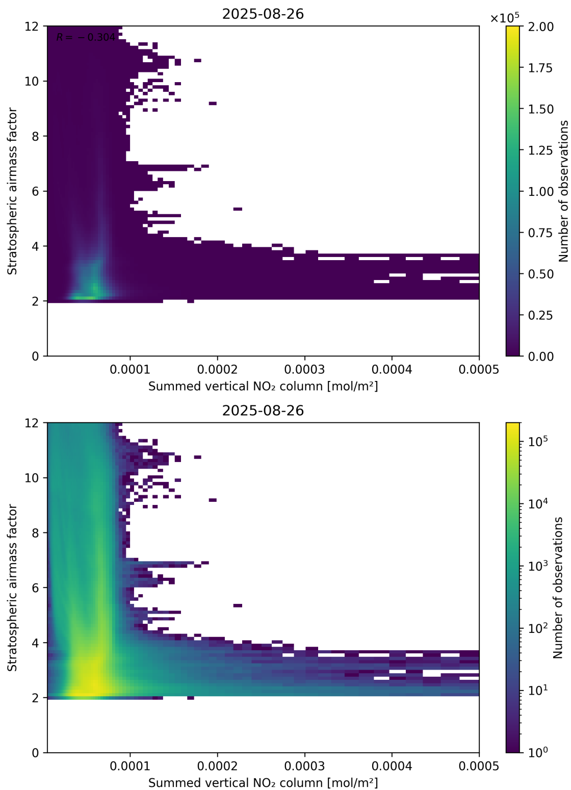
Figure 103: Scatter density plot of “Summed vertical NO 2 column” against “Stratospheric airmass factor” for 2025-08-25 to 2025-08-27.
