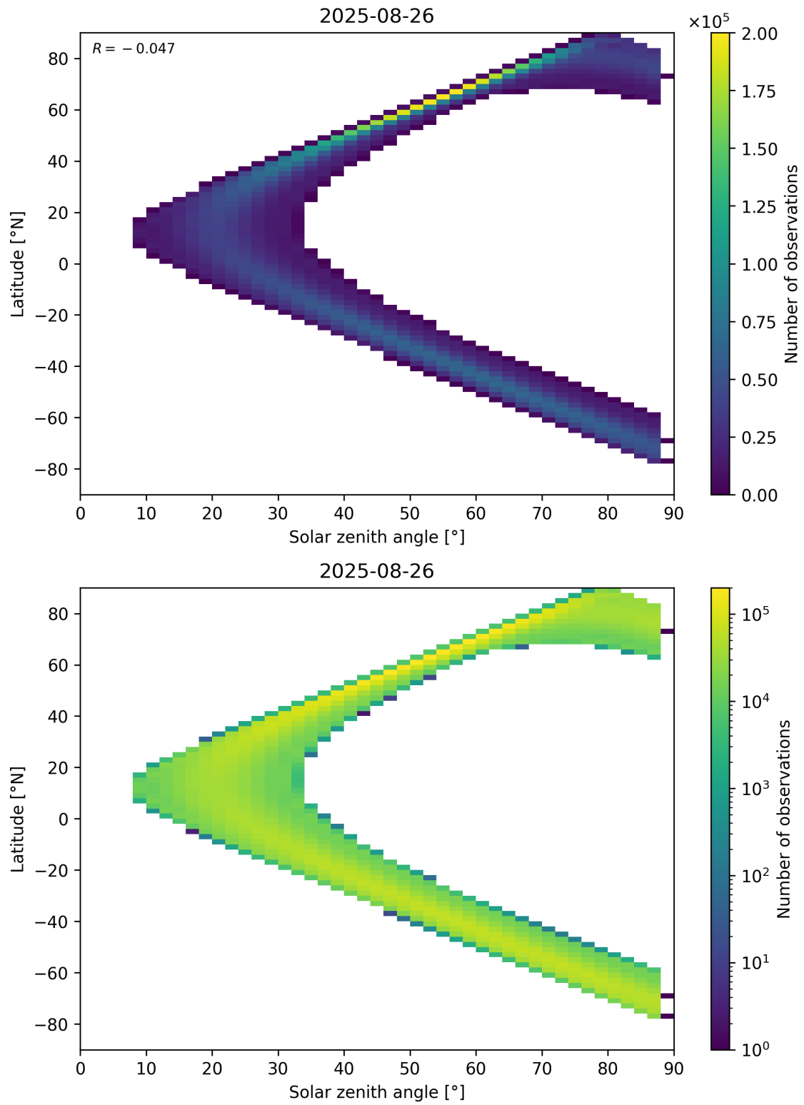
Figure 149: Scatter density plot of “Solar zenith angle” against “Latitude” for 2025-08-25 to 2025-08-27.
