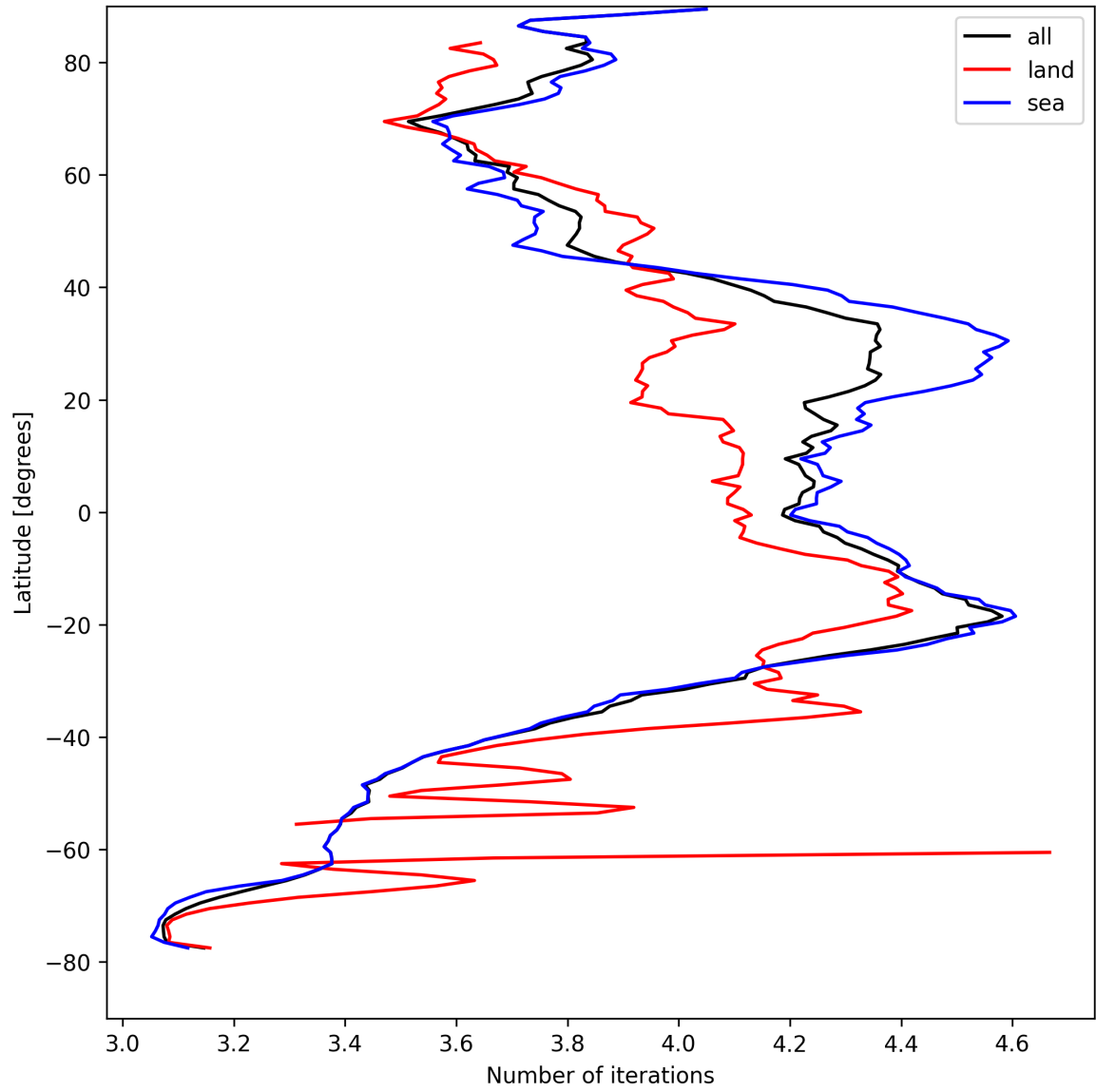
Figure 17: Zonal average of “Number of iterations” for 2025-08-25 to 2025-08-27.
