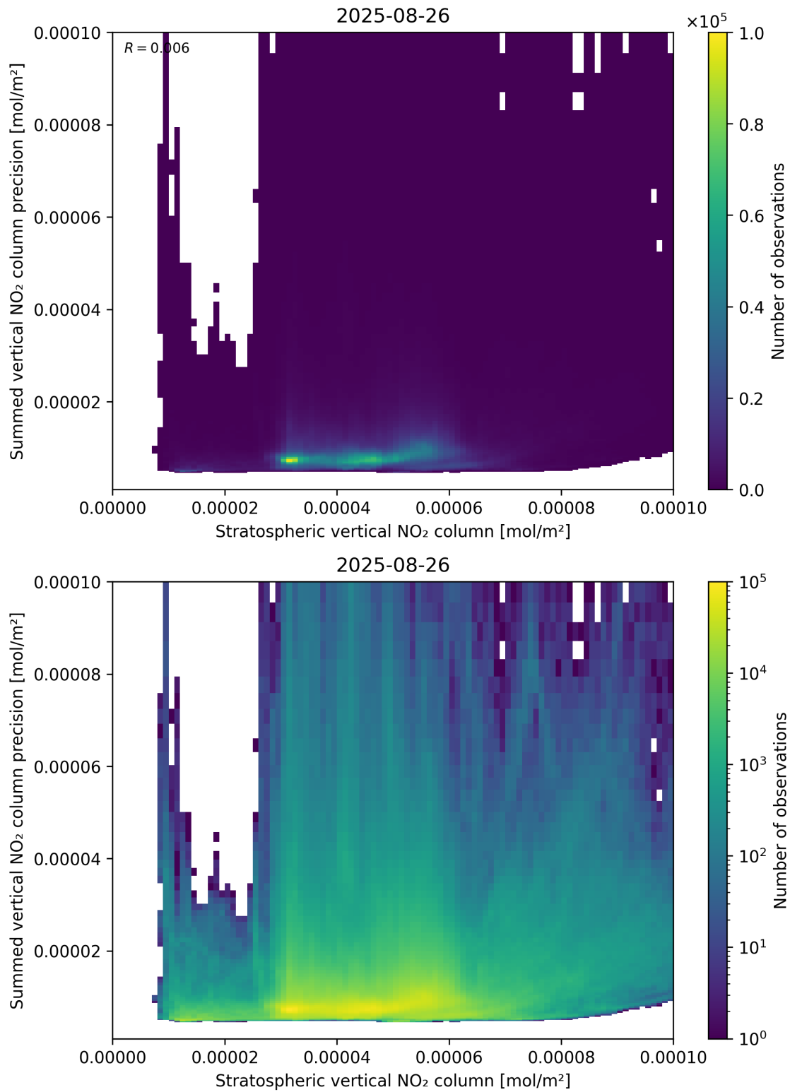
Figure 99: Scatter density plot of “Stratospheric vertical NO 2 column” against “Summed vertical NO 2 column precision” for 2025-08-25 to 2025-08-27.
