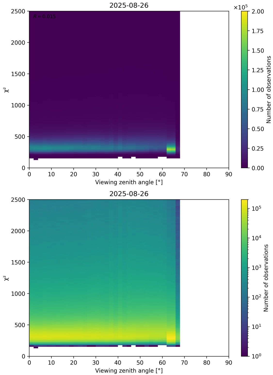
Figure 162: Scatter density plot of “Viewing zenith angle” against “ \chi^2 ” for 2025-08-25 to 2025-08-27.
