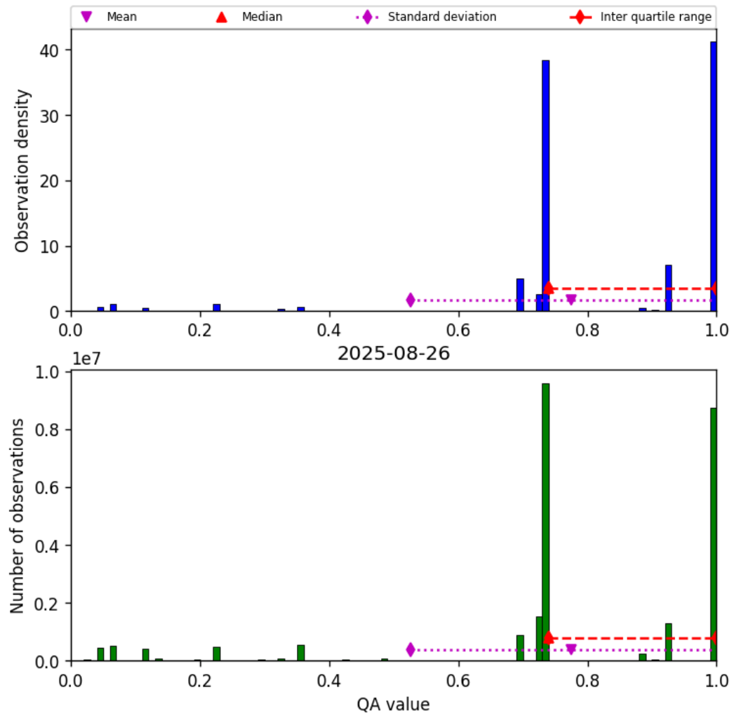
Figure 28: Histogram of “QA value” for 2025-08-25 to 2025-08-27
