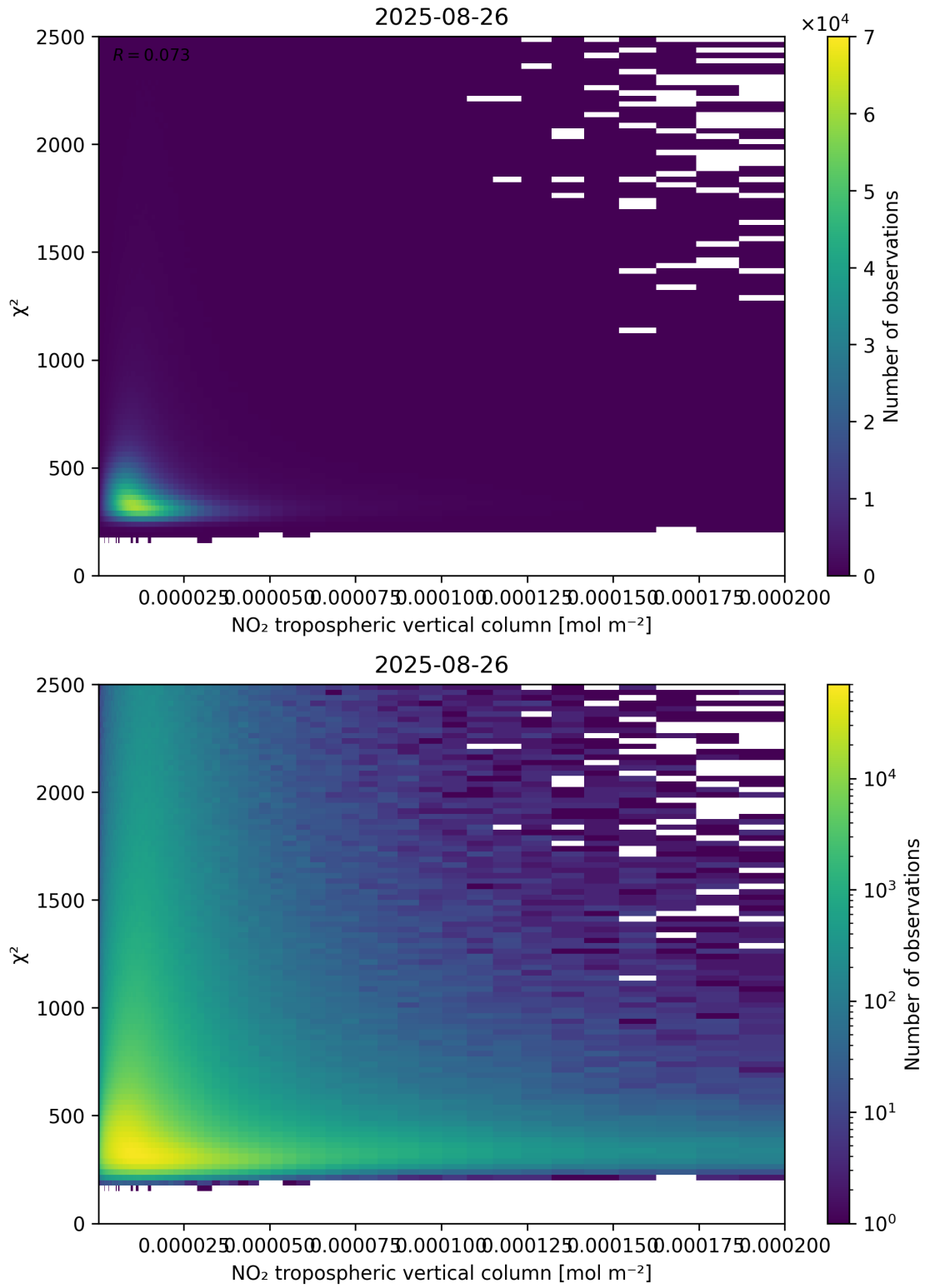
Figure 124: Scatter density plot of “NO 2 tropospheric vertical column” against “ \chi^2 ” for 2025-08-25 to 2025-08-27.
