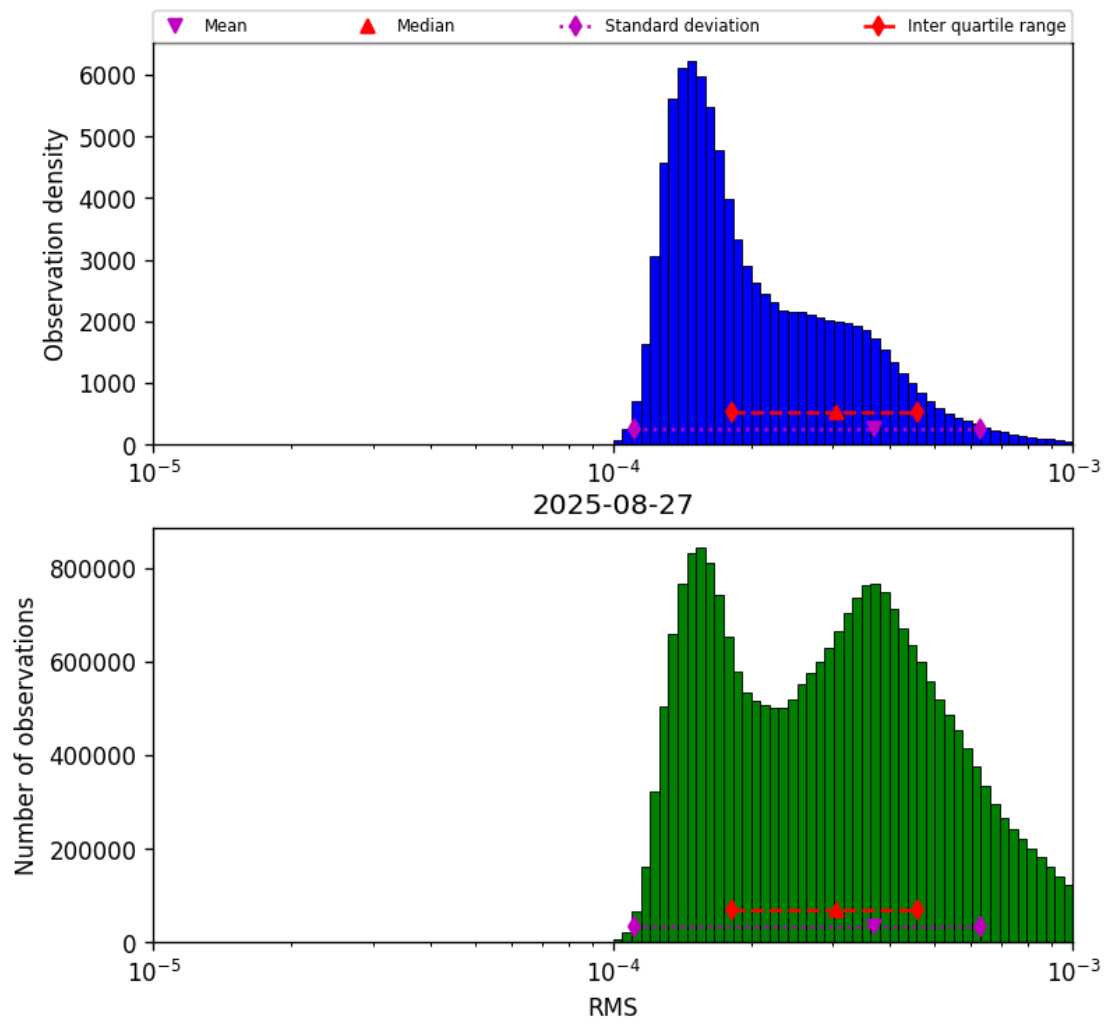
Figure 43: Histogram of “RMS” for 2025-08-26 to 2025-08-28
