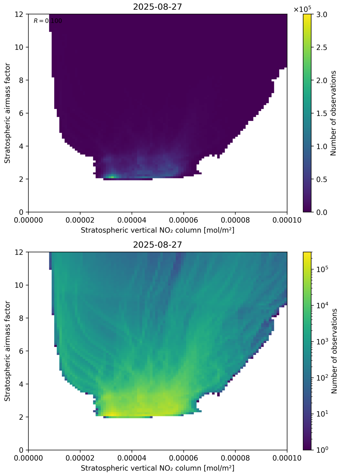
Figure 96: Scatter density plot of “Stratospheric vertical NO 2 column” against “Stratospheric airmass factor” for 2025-08-26 to 2025-08-28.
