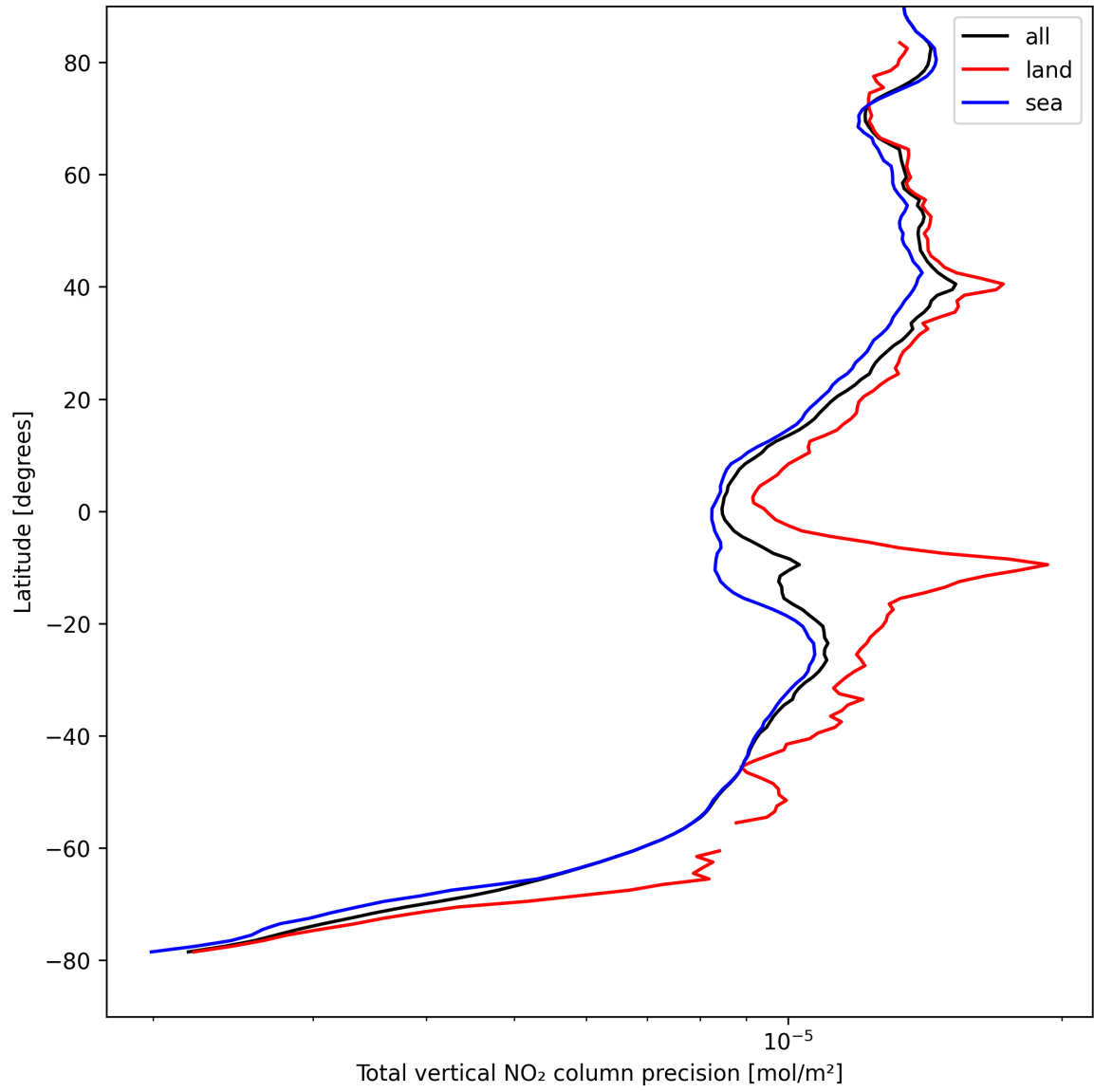
Figure 22: Zonal average of “Total vertical NO 2 column precision” for 2025-08-26 to 2025-08-28.
