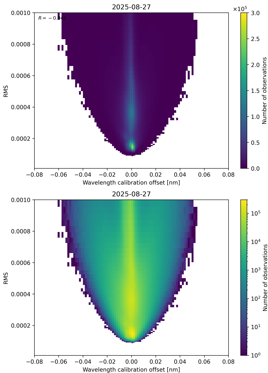
Figure 181: Scatter density plot of “Wavelength calibration offset” against “RMS” for 2025-08-26 to 2025-08-28.
