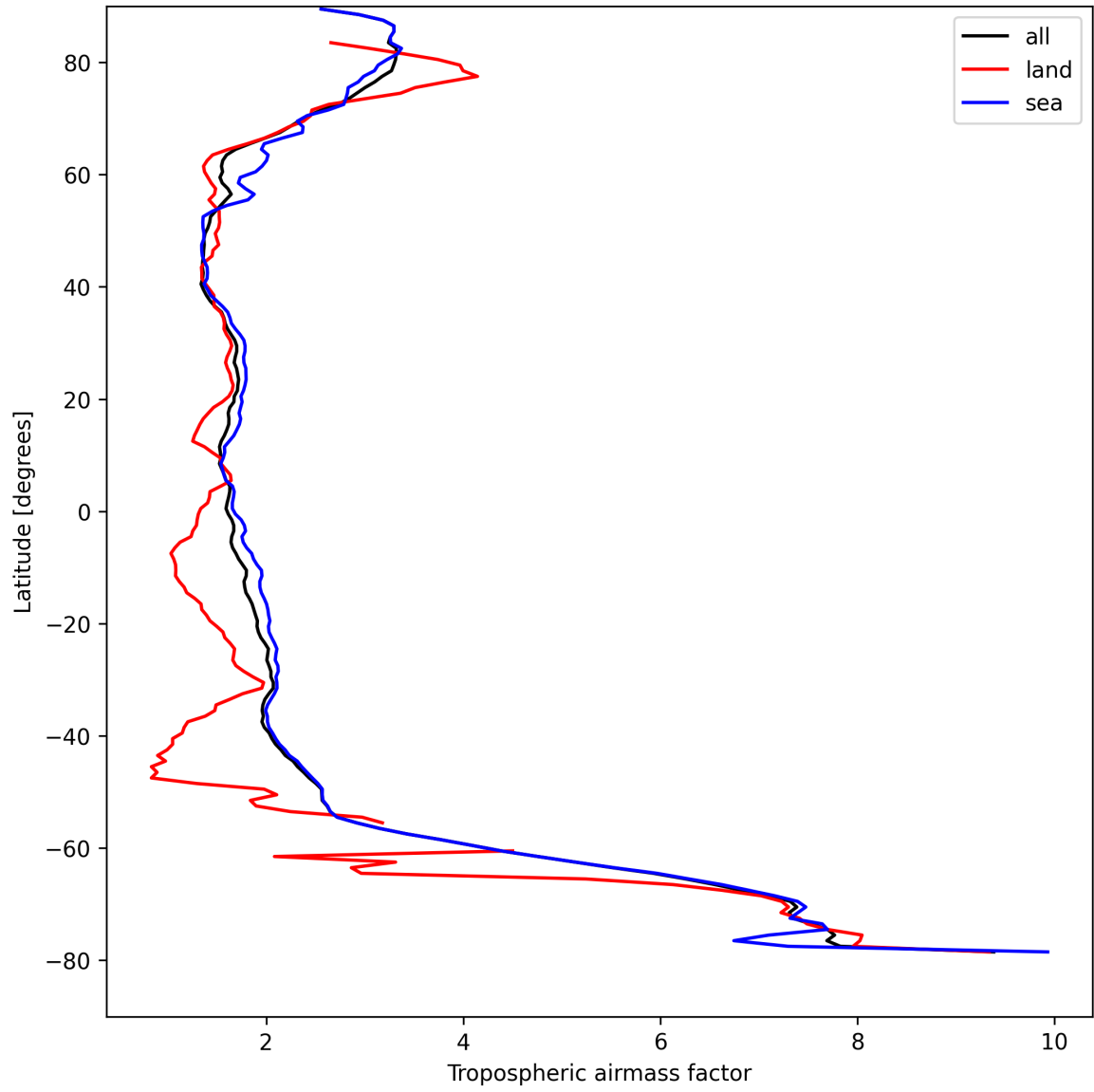
Figure 14: Zonal average of “Tropospheric airmass factor” for 2025-08-26 to 2025-08-28.
