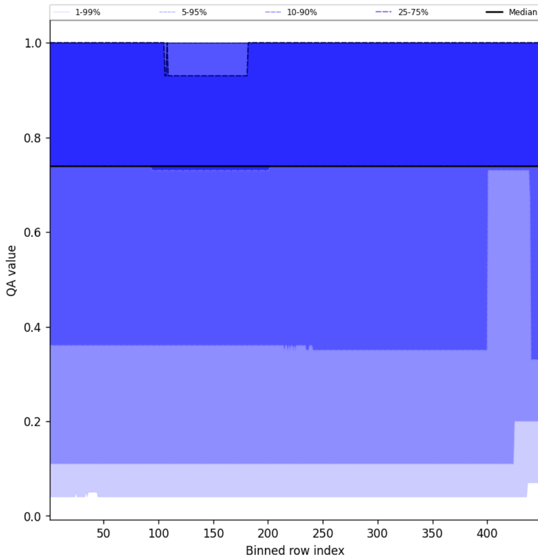
Figure 45: Along track statistics of “QA value” for 2025-08-26 to 2025-08-28
