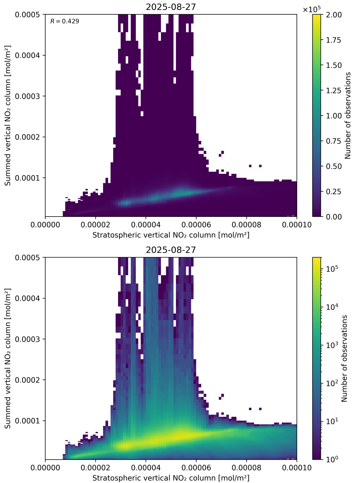
Figure 98: Scatter density plot of “Stratospheric vertical NO 2 column” against “Summed vertical NO 2 column” for 2025-08-26 to 2025-08-28.
