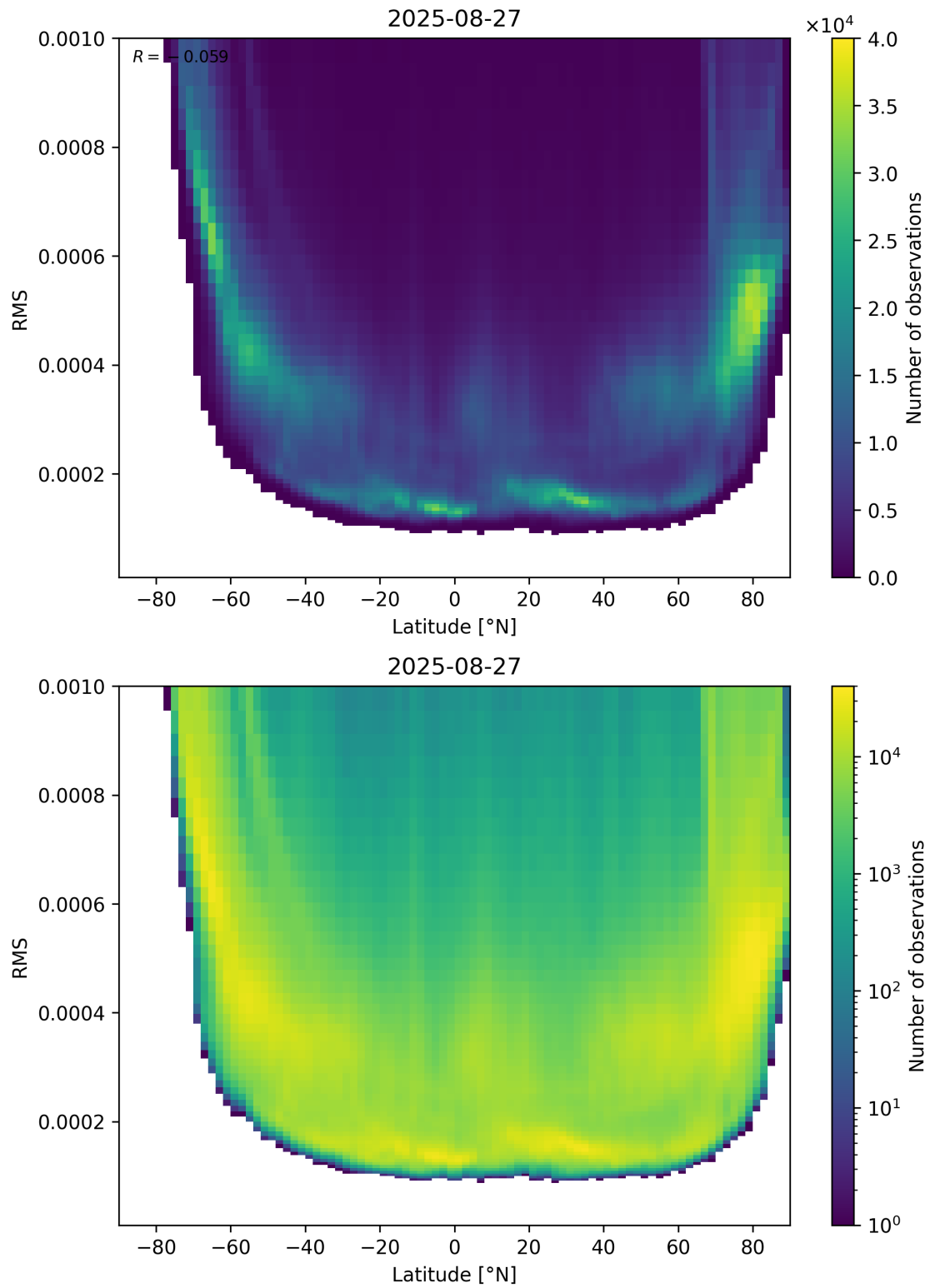
Figure 94: Scatter density plot of “Latitude” against “RMS” for 2025-08-26 to 2025-08-28.
