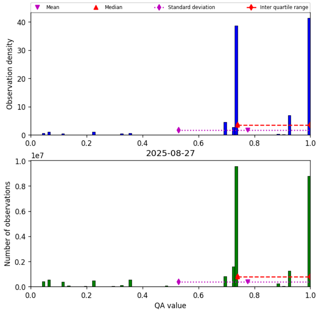
Figure 28: Histogram of “QA value” for 2025-08-26 to 2025-08-28
