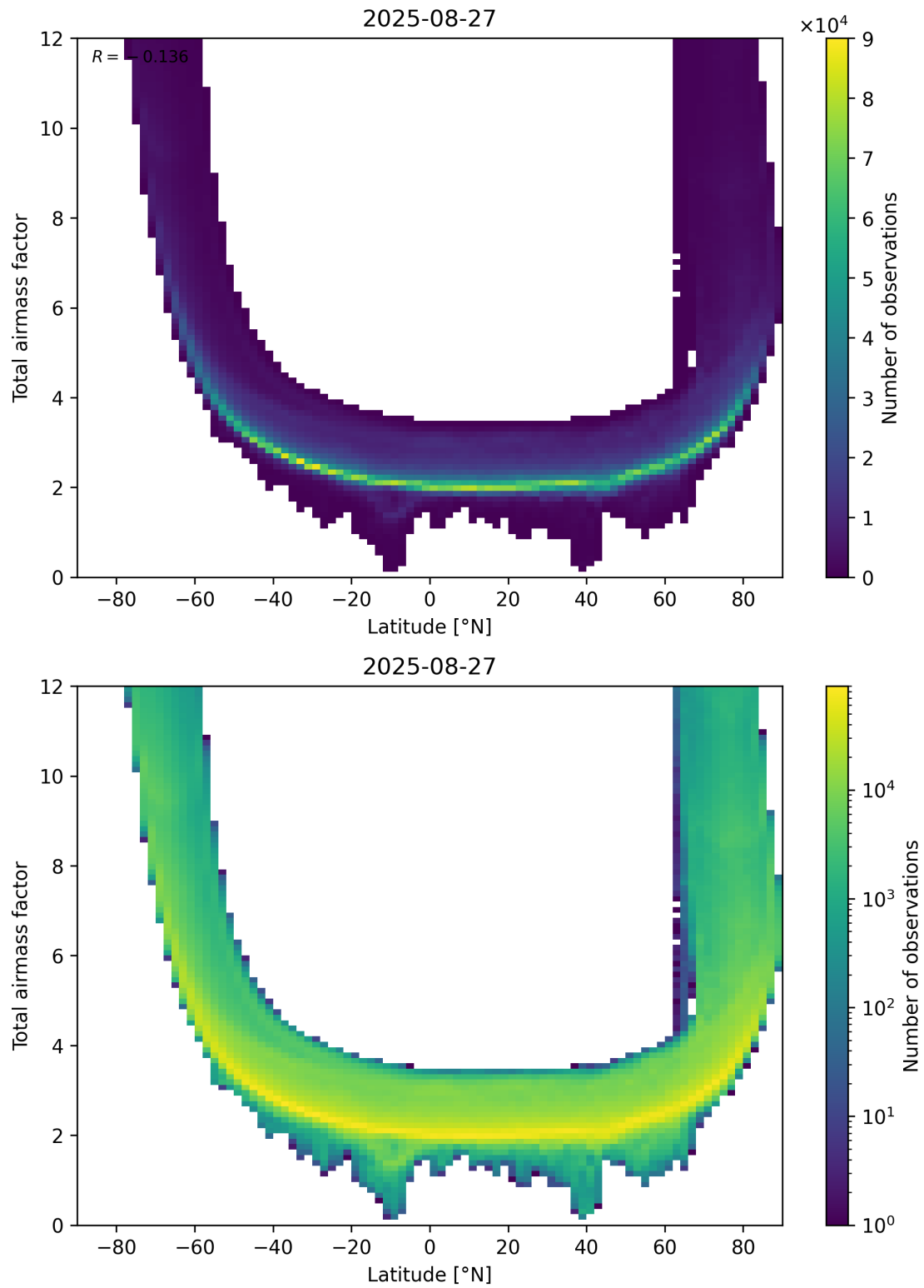
Figure 84: Scatter density plot of “Latitude” against “Total airmass factor” for 2025-08-26 to 2025-08-28.
