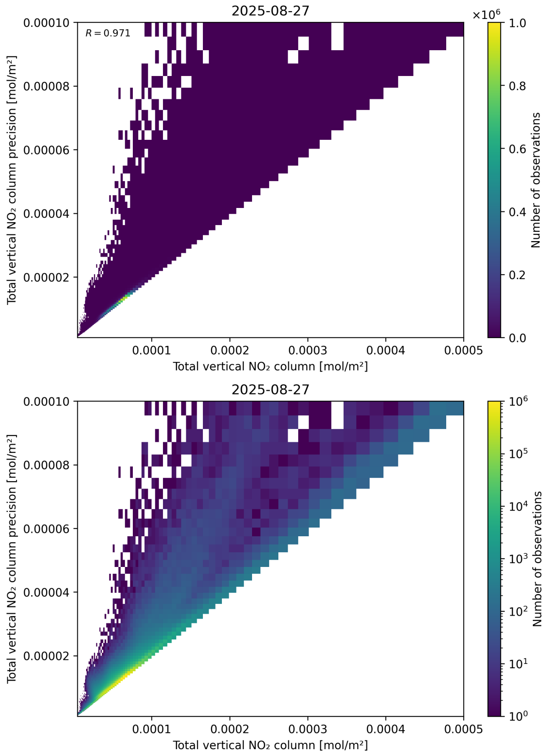
Figure 114: Scatter density plot of “Total vertical NO 2 column” against “Total vertical NO 2 column precision” for 2025-08-26 to 2025-08-28.
