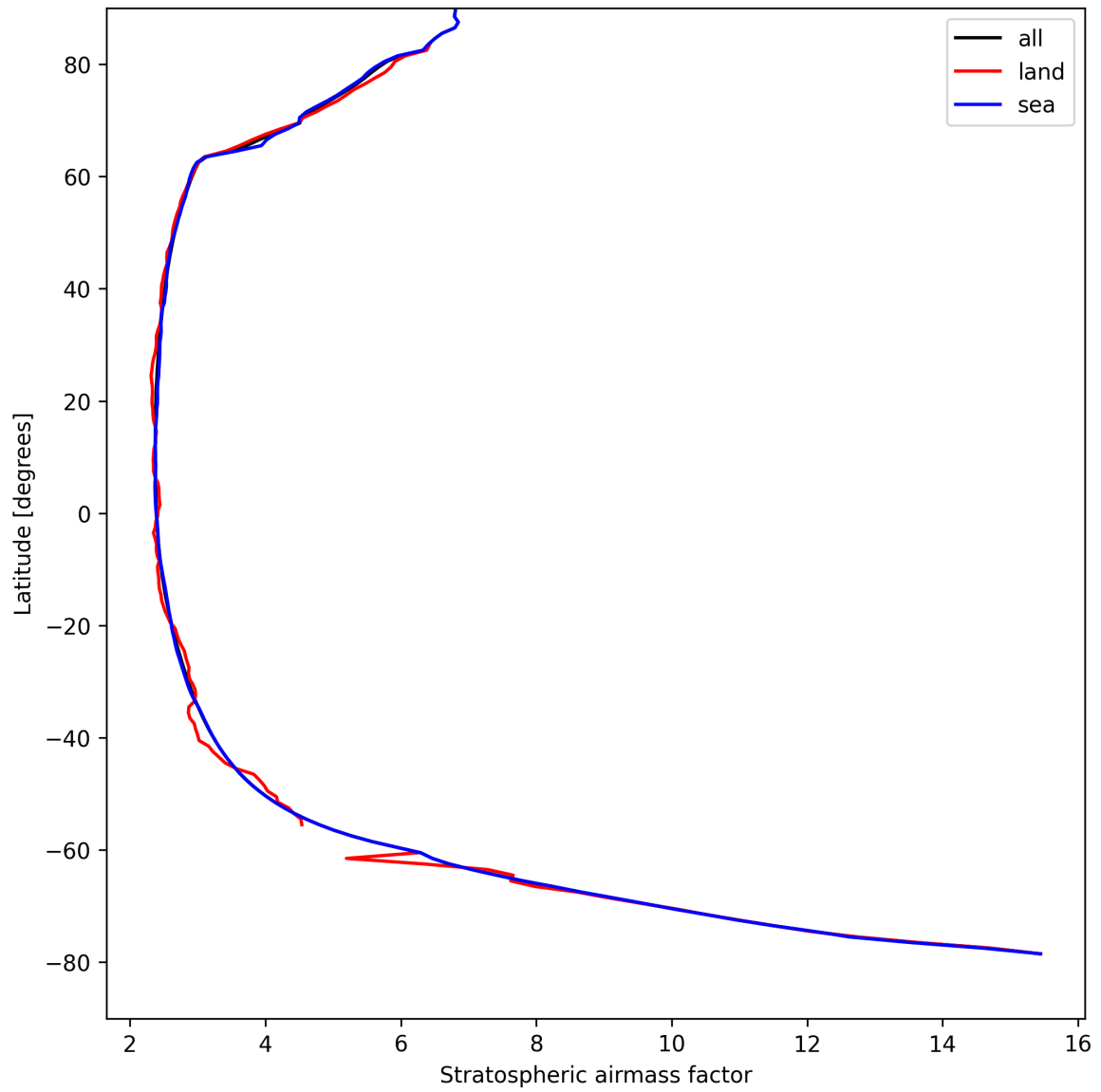
Figure 27: Zonal average of “Stratospheric airmass factor” for 2025-08-26 to 2025-08-28.
