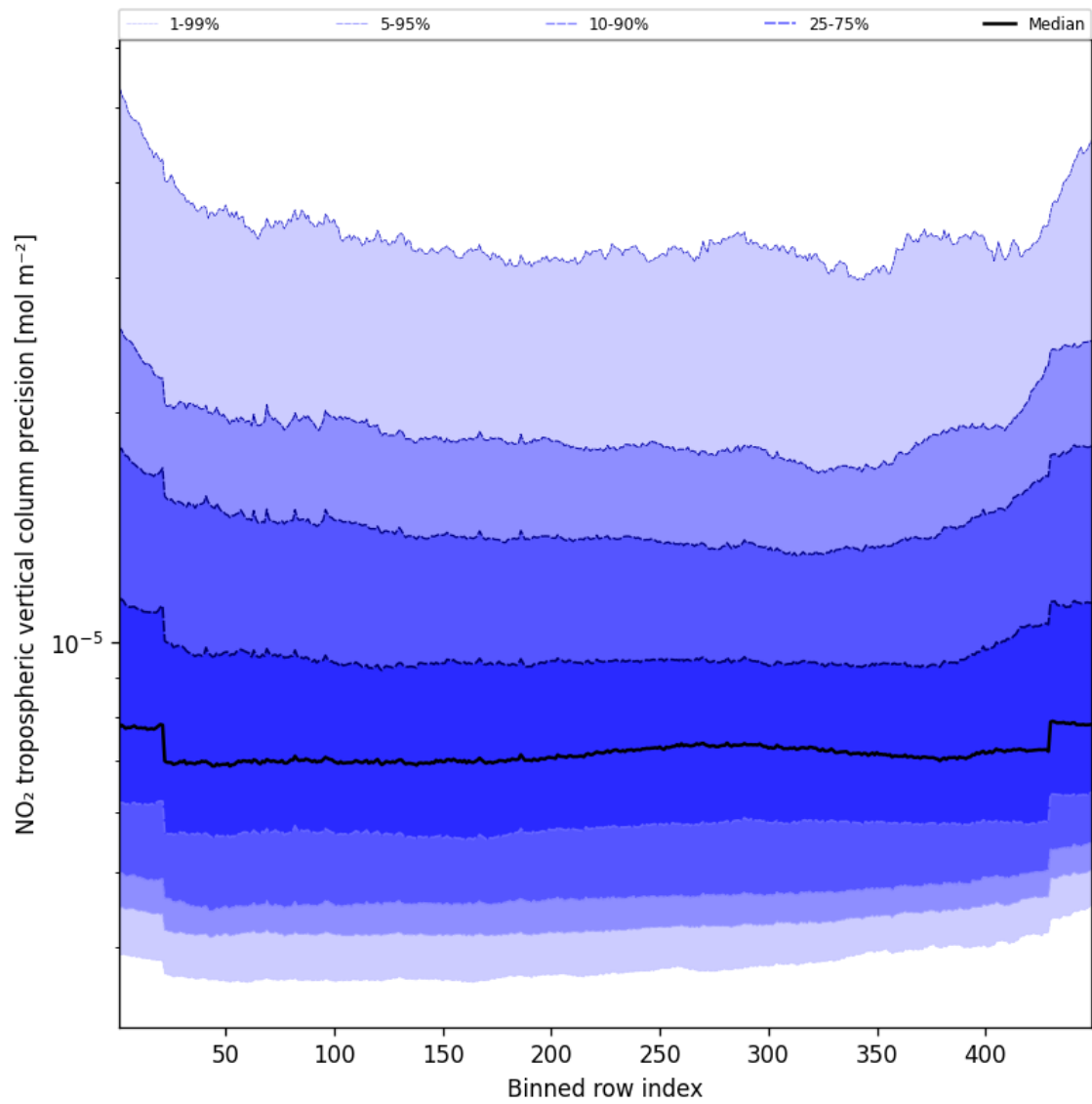
Figure 47: Along track statistics of “NO 2 tropospheric vertical column precision” for 2025-08-26 to 2025-08-28
