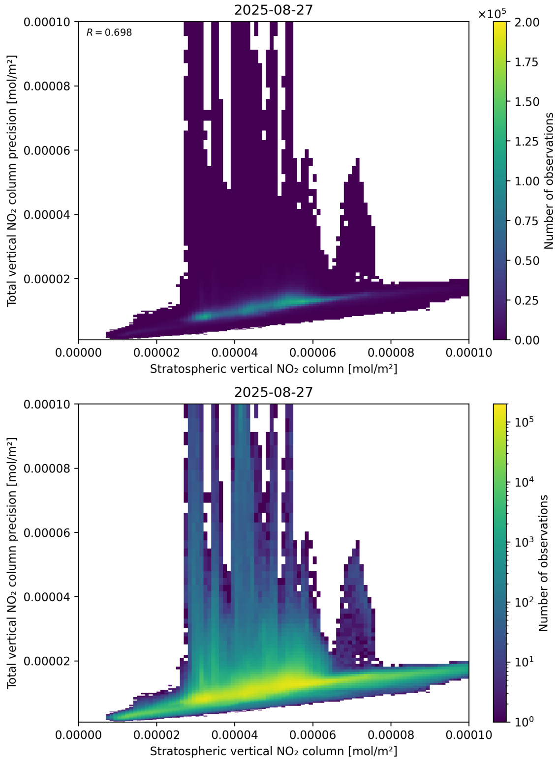
Figure 101: Scatter density plot of “Stratospheric vertical NO 2 column” against “Total vertical NO 2 column precision” for 2025-08-26 to 2025-08-28.
