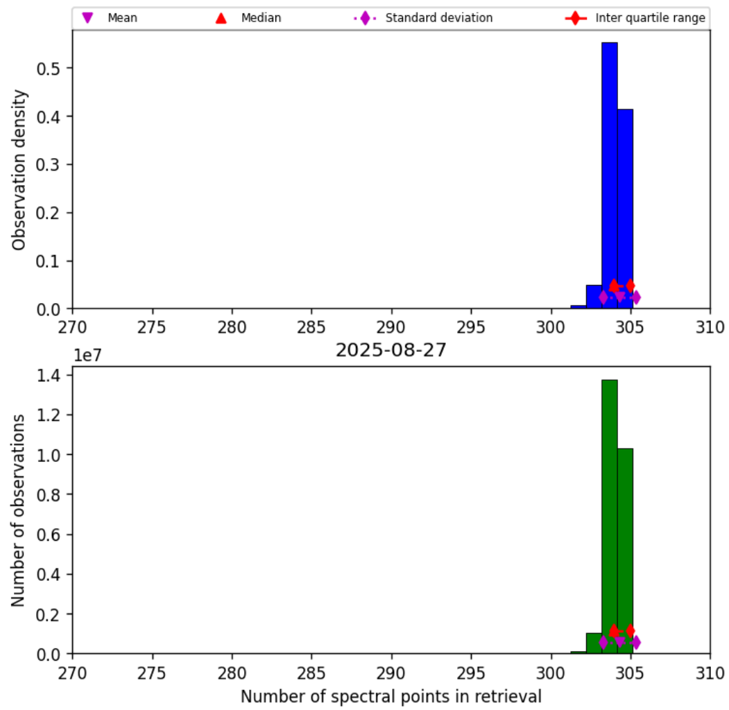
Figure 33: Histogram of “Number of spectral points in retrieval” for 2025-08-26 to 2025-08-28
