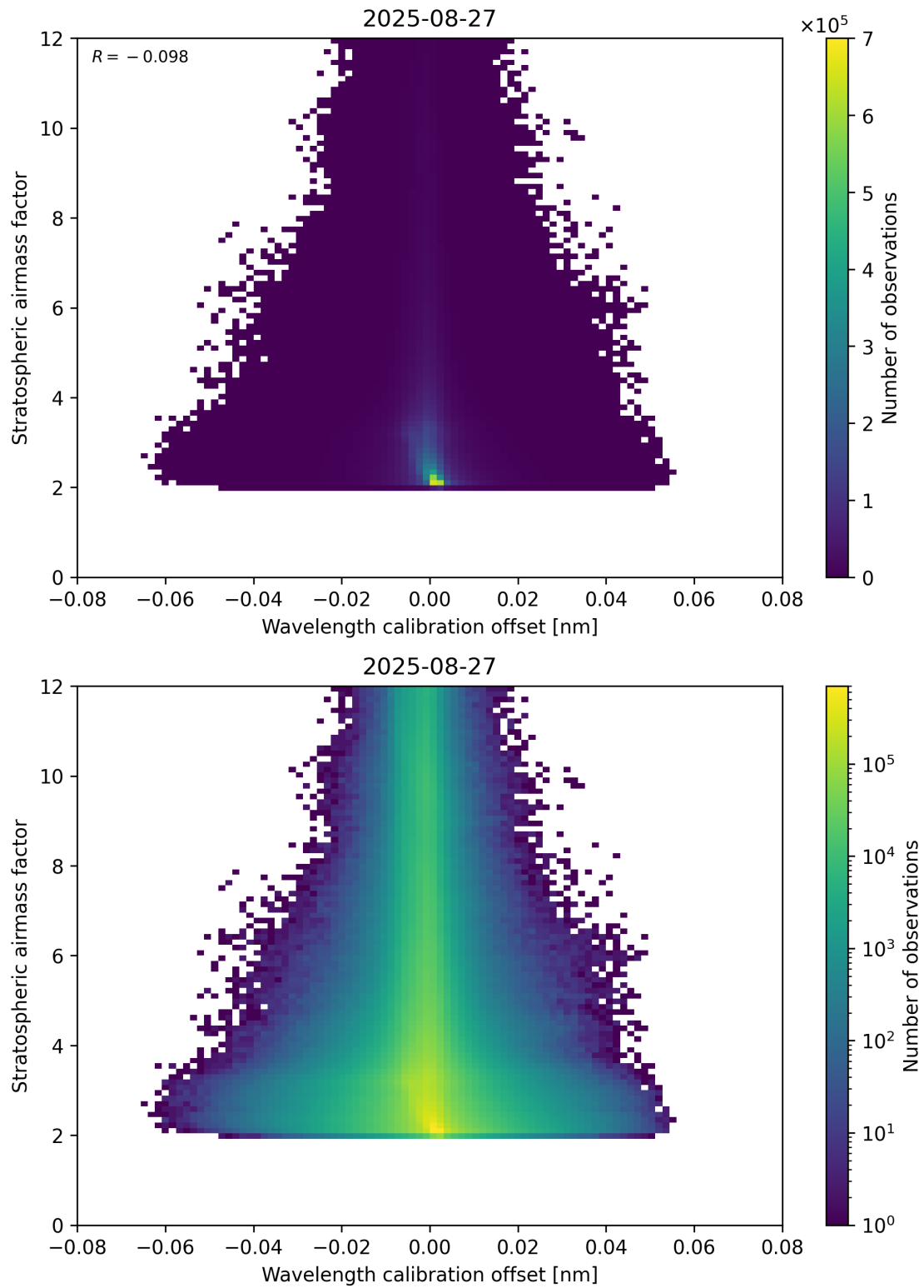
Figure 174: Scatter density plot of “Wavelength calibration offset” against “Stratospheric airmass factor” for 2025-08-26 to 2025-08-28.
