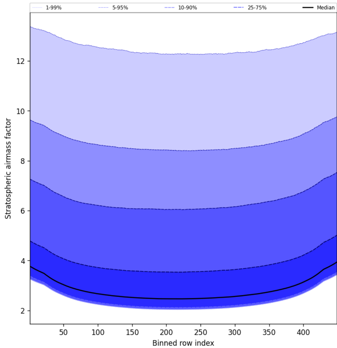
Figure 61: Along track statistics of “Stratospheric airmass factor” for 2025-08-26 to 2025-08-28
