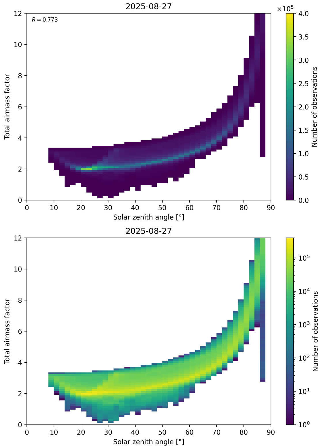
Figure 146: Scatter density plot of “Solar zenith angle” against “Total air mass factor” for 2025-08-26 to 2025-08-28.
