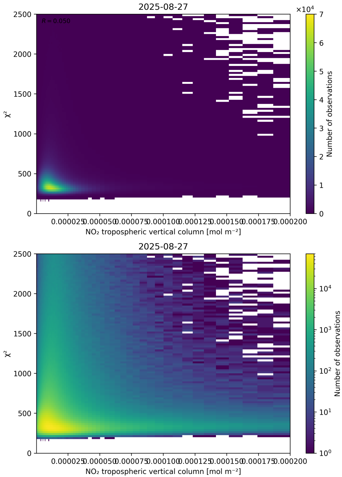
Figure 124: Scatter density plot of “NO 2 tropospheric vertical column” against “ \chi^2 ” for 2025-08-26 to 2025-08-28.
