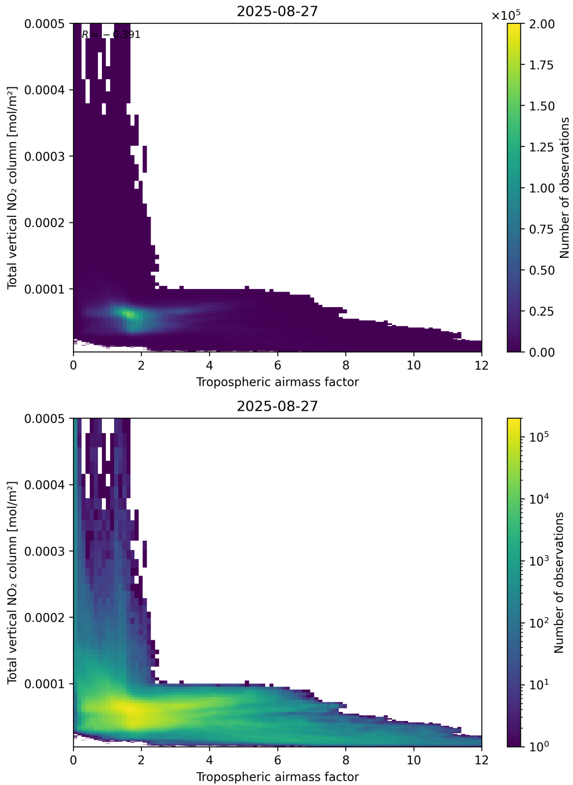
Figure 77: Scatter density plot of “Tropospheric airmass factor” against “Total vertical NO 2 column” for 2025-08-26 to 2025-08-28.
