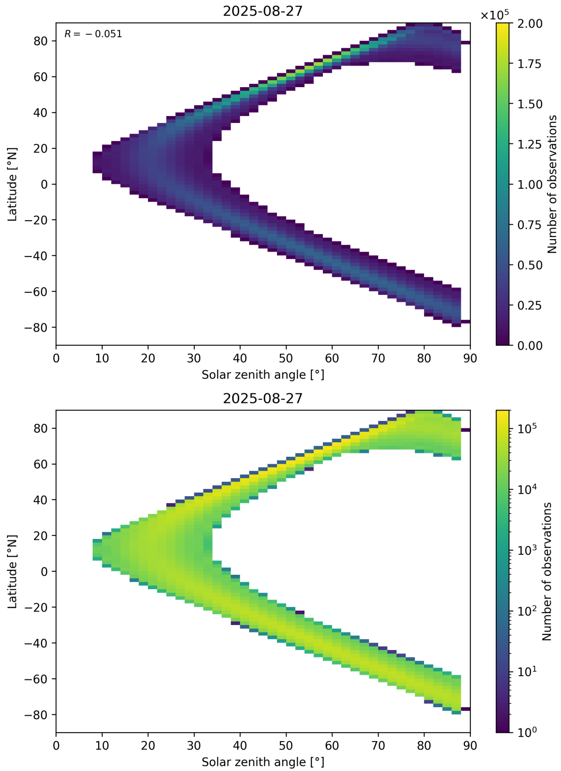
Figure 149: Scatter density plot of “Solar zenith angle” against “Latitude” for 2025-08-26 to 2025-08-28.
