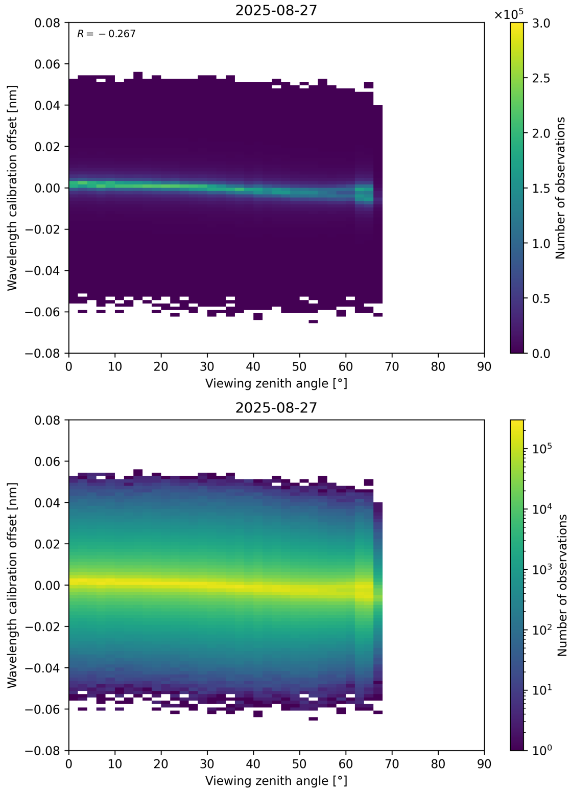
Figure 173: Scatter density plot of “Viewing zenith angle” against “Wavelength calibration offset” for 2025-08-26 to 2025-08-28.
