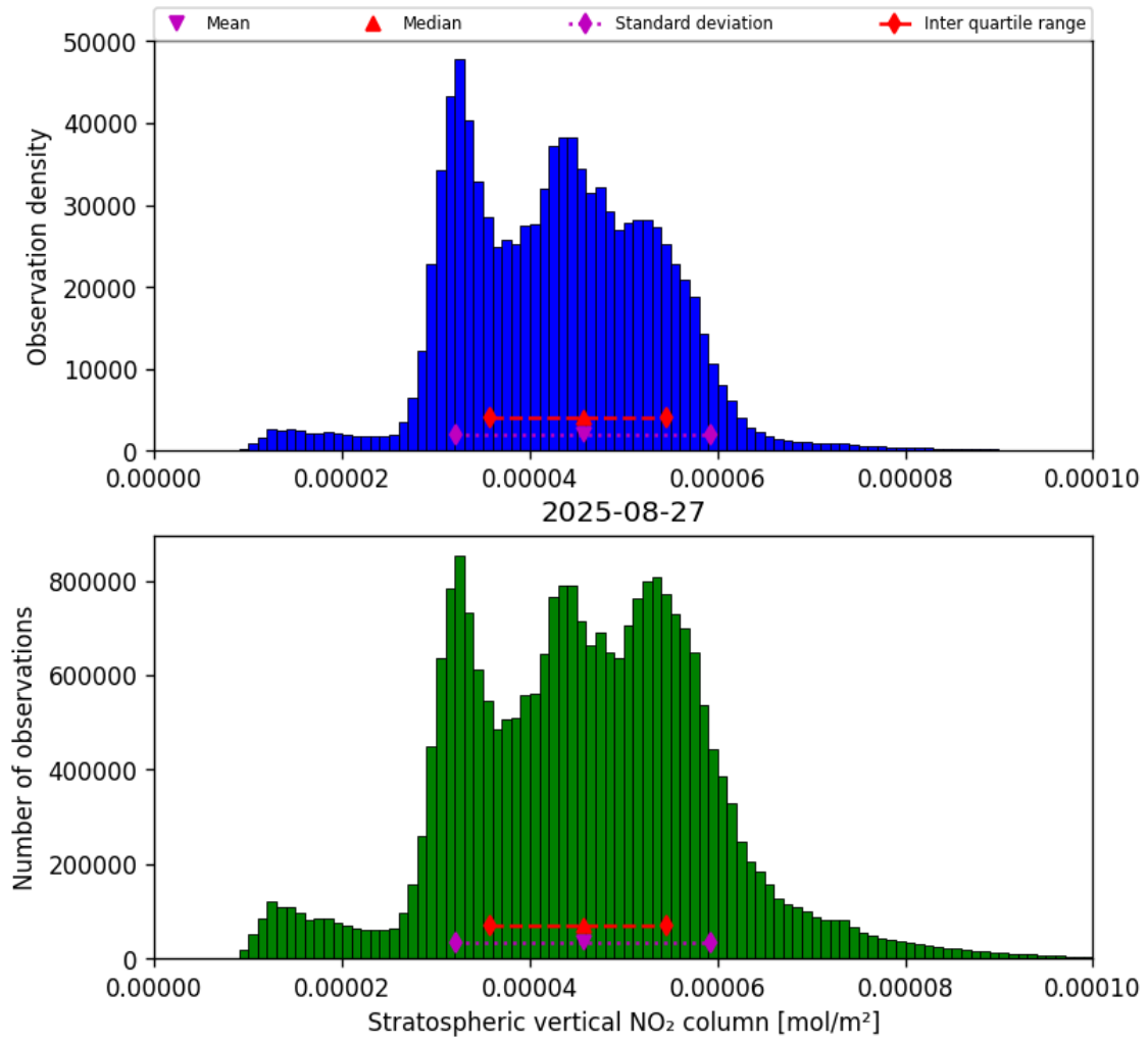
Figure 36: Histogram of “Stratospheric vertical NO 2 column” for 2025-08-26 to 2025-08-28
