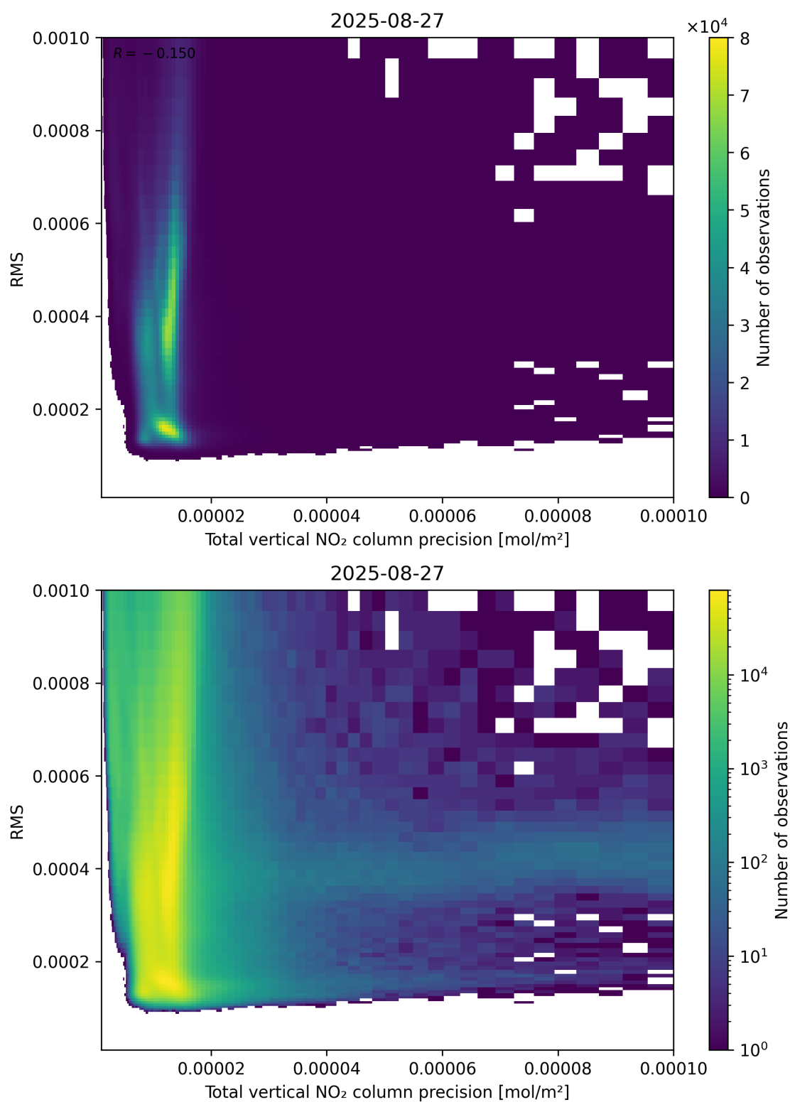
Figure 119: Scatter density plot of “Total vertical NO 2 column precision” against “RMS” for 2025-08-26 to 2025-08-28.
