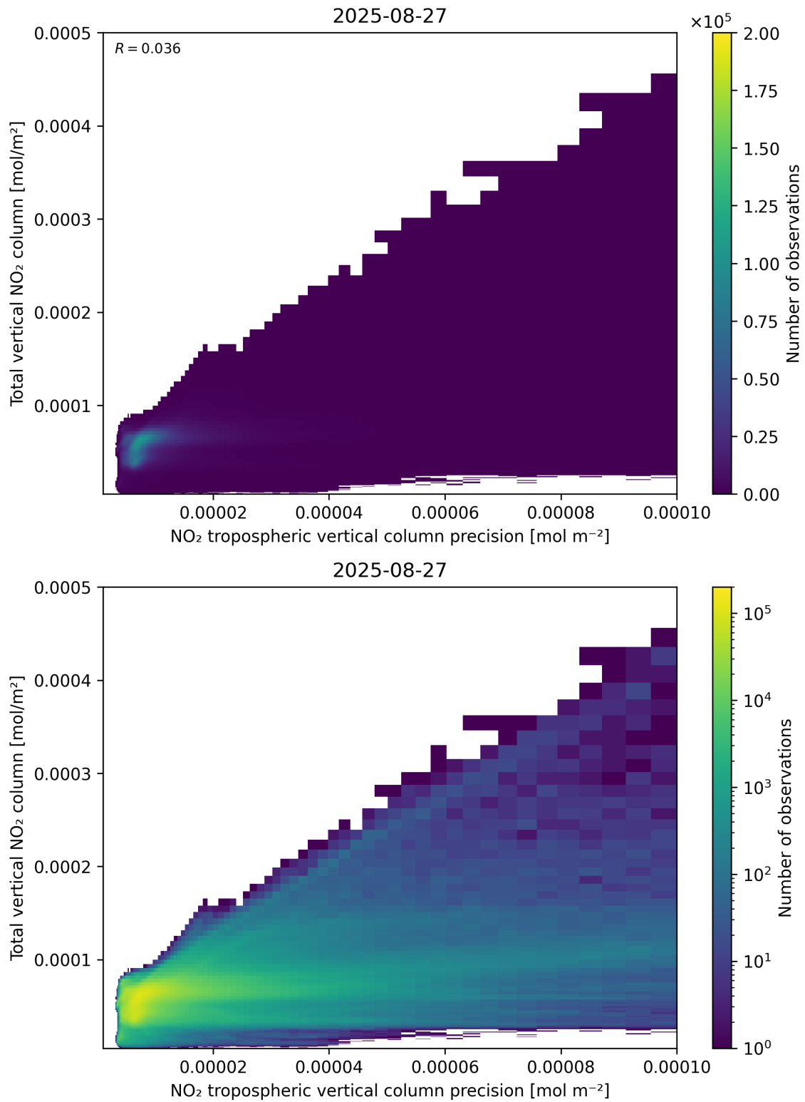
Figure 138: Scatter density plot of “NO 2 tropospheric vertical column precision” against “Total vertical NO 2 column” for 2025-08-26 to 2025-08-28.
