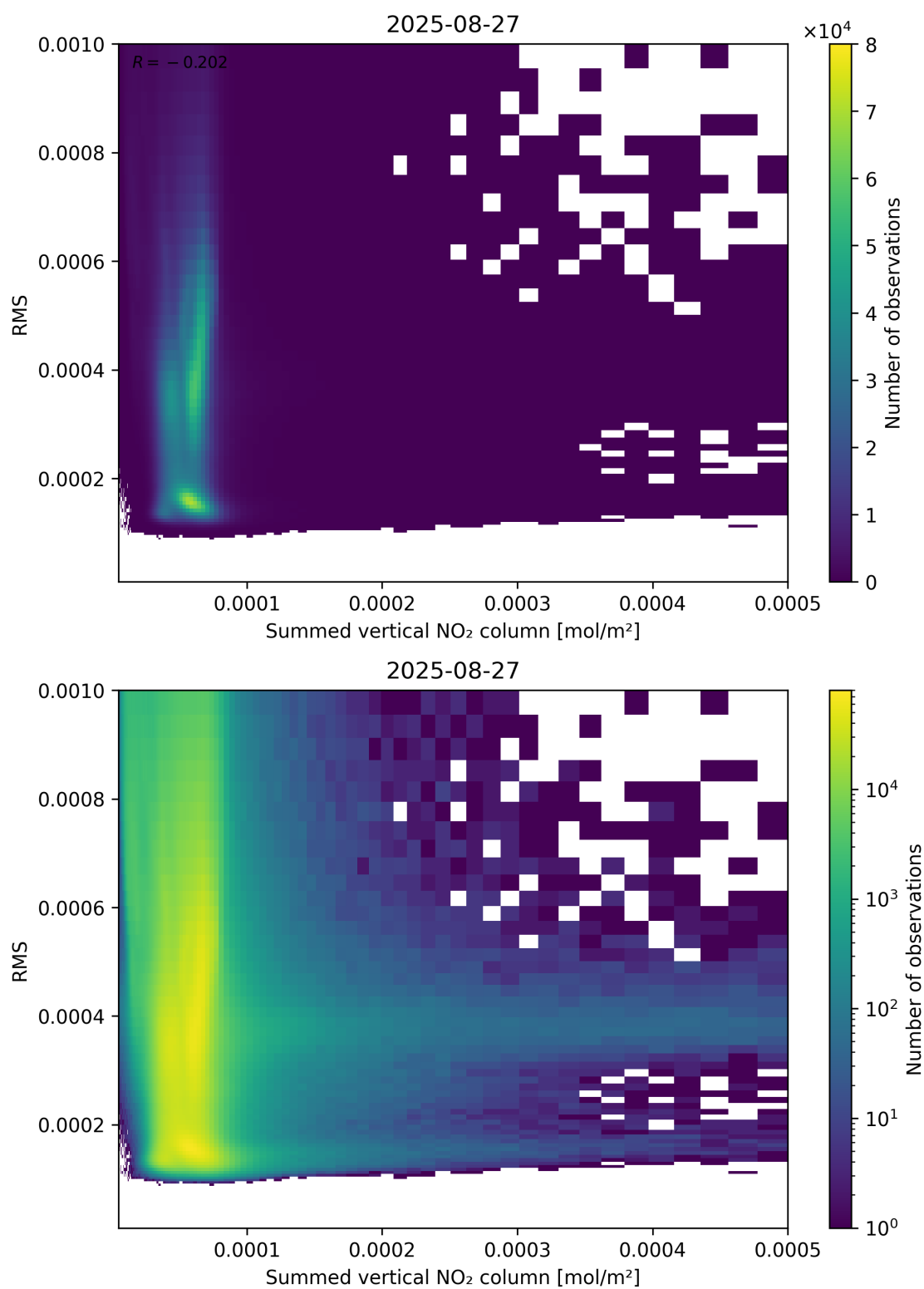
Figure 109: Scatter density plot of “Summed vertical NO 2 column” against “RMS” for 2025-08-26 to 2025-08-28.
