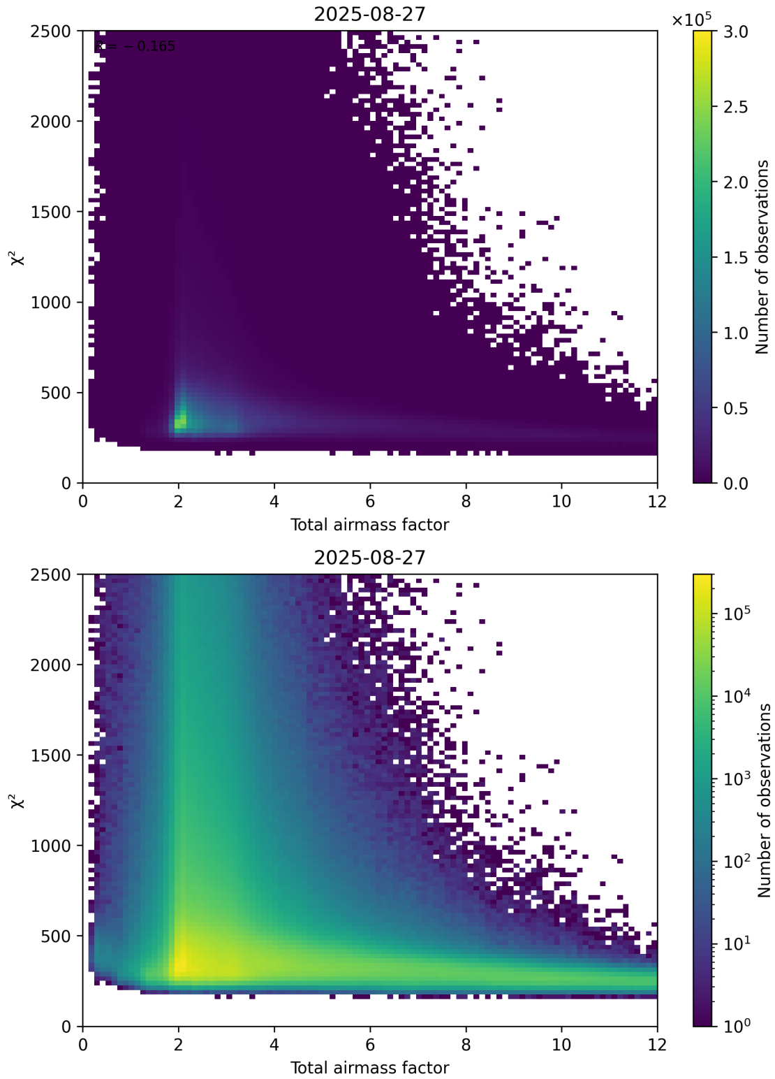
Figure 63: Scatter density plot of “Total airmass factor” against “ \chi^2 ” for 2025-08-26 to 2025-08-28.
