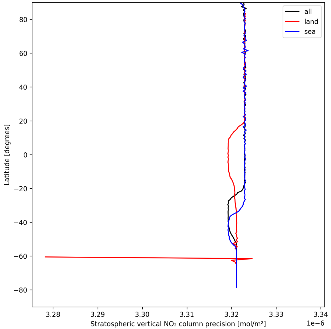
Figure 20: Zonal average of “Stratospheric vertical NO 2 column precision” for 2025-08-26 to 2025-08-28.
