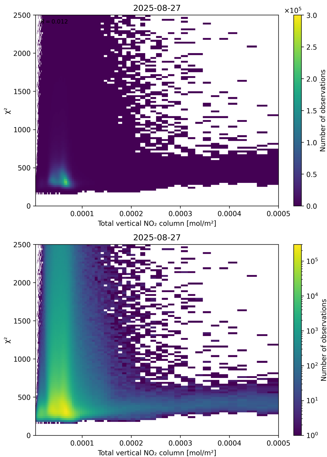
Figure 111: Scatter density plot of “Total vertical NO 2 column” against “ \chi^2 ” for 2025-08-26 to 2025-08-28.
