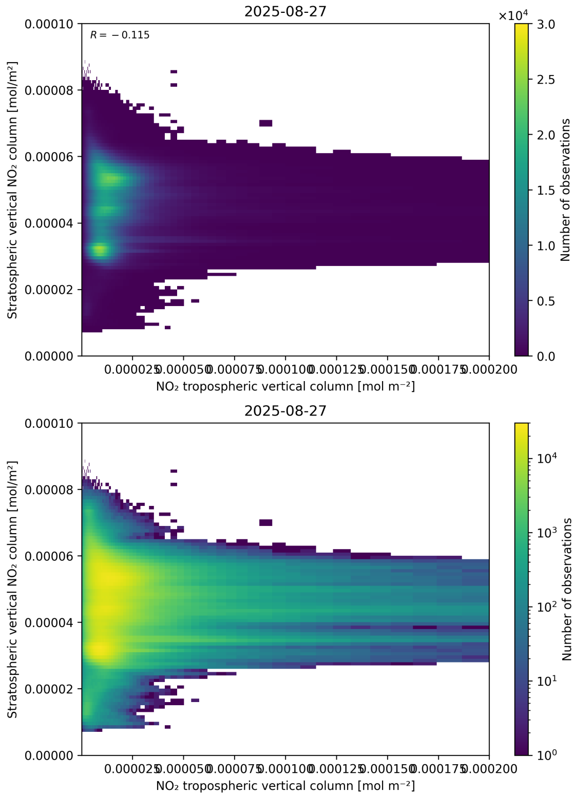
Figure 125: Scatter density plot of “NO 2 tropospheric vertical column” against “Stratospheric vertical NO 2 column” for 2025-08-26 to 2025-08-28.
