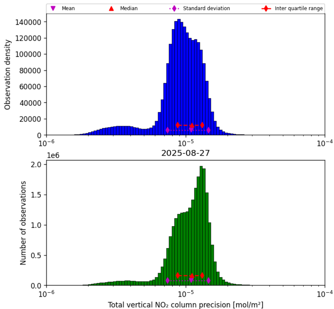
Figure 39: Histogram of “Total vertical NO 2 column precision” for 2025-08-26 to 2025-08-28
