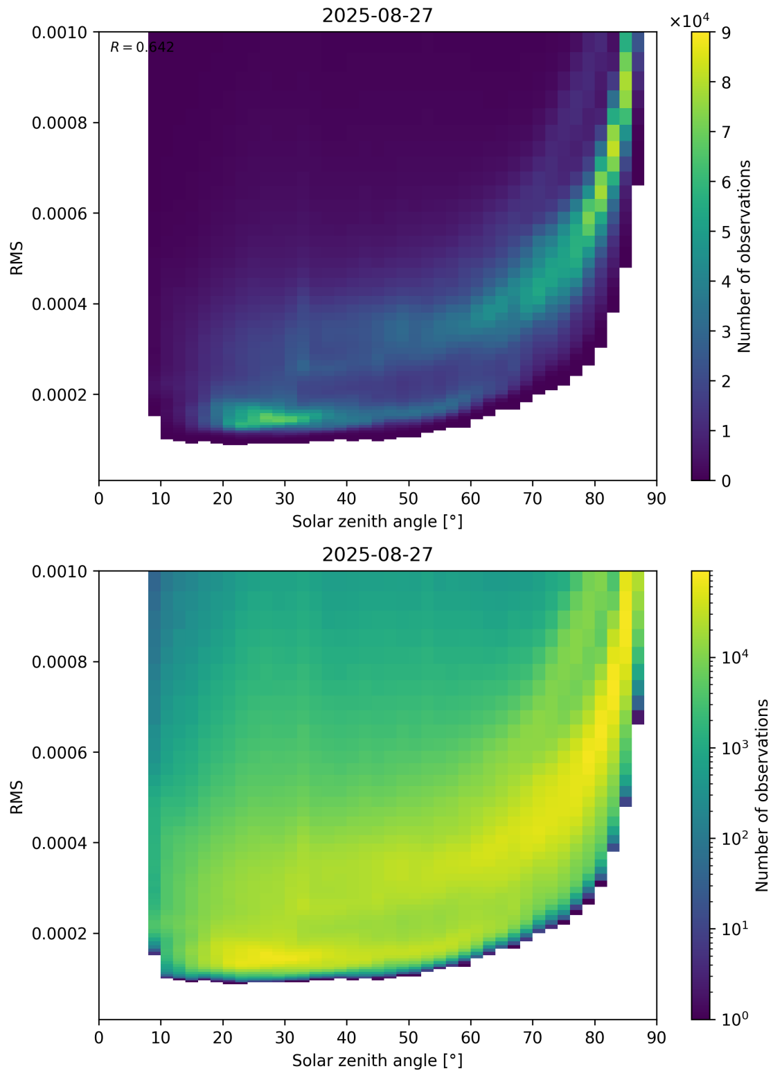
Figure 157: Scatter density plot of “Solar zenith angle” against “RMS” for 2025-08-26 to 2025-08-28.
