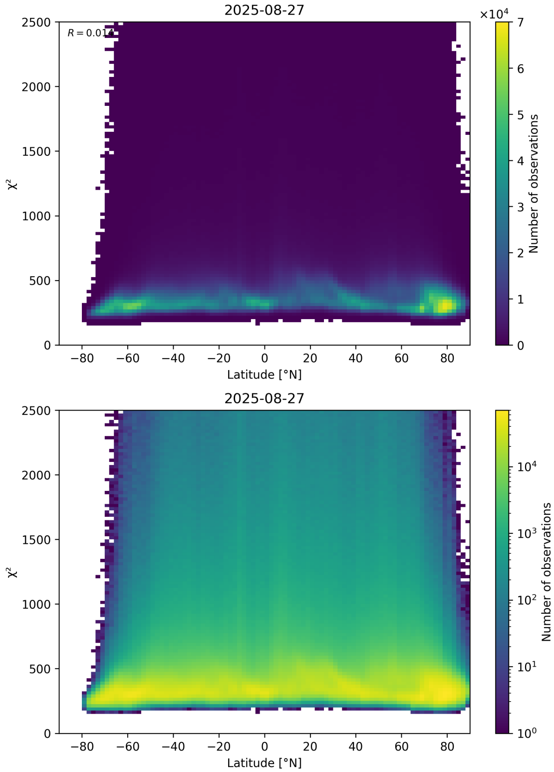
Figure 86: Scatter density plot of “Latitude” against “ \chi^2 ” for 2025-08-26 to 2025-08-28.
