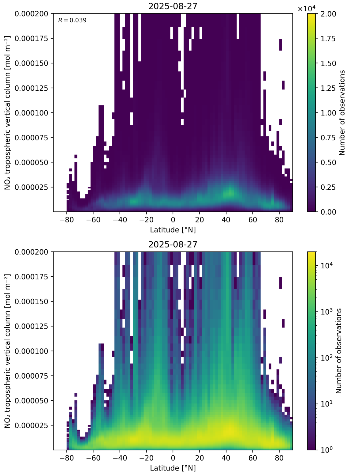
Figure 92: Scatter density plot of “Latitude” against “NO 2 tropospheric vertical column” for 2025-08-26 to 2025-08-28.
