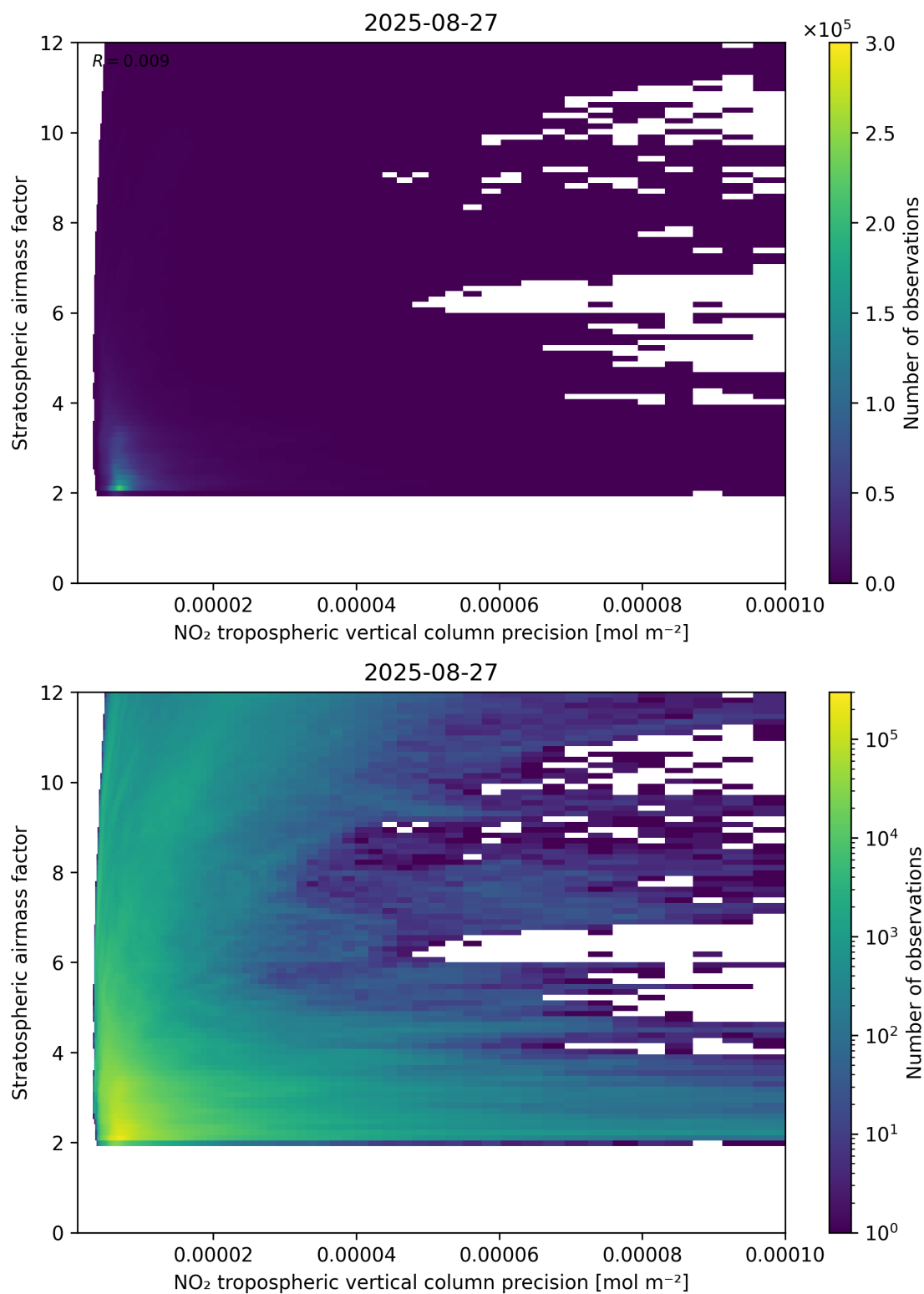
Figure 131: Scatter density plot of “NO 2 tropospheric vertical column precision” against “Stratospheric airmass factor” for 2025-08-26 to 2025-08-28.
