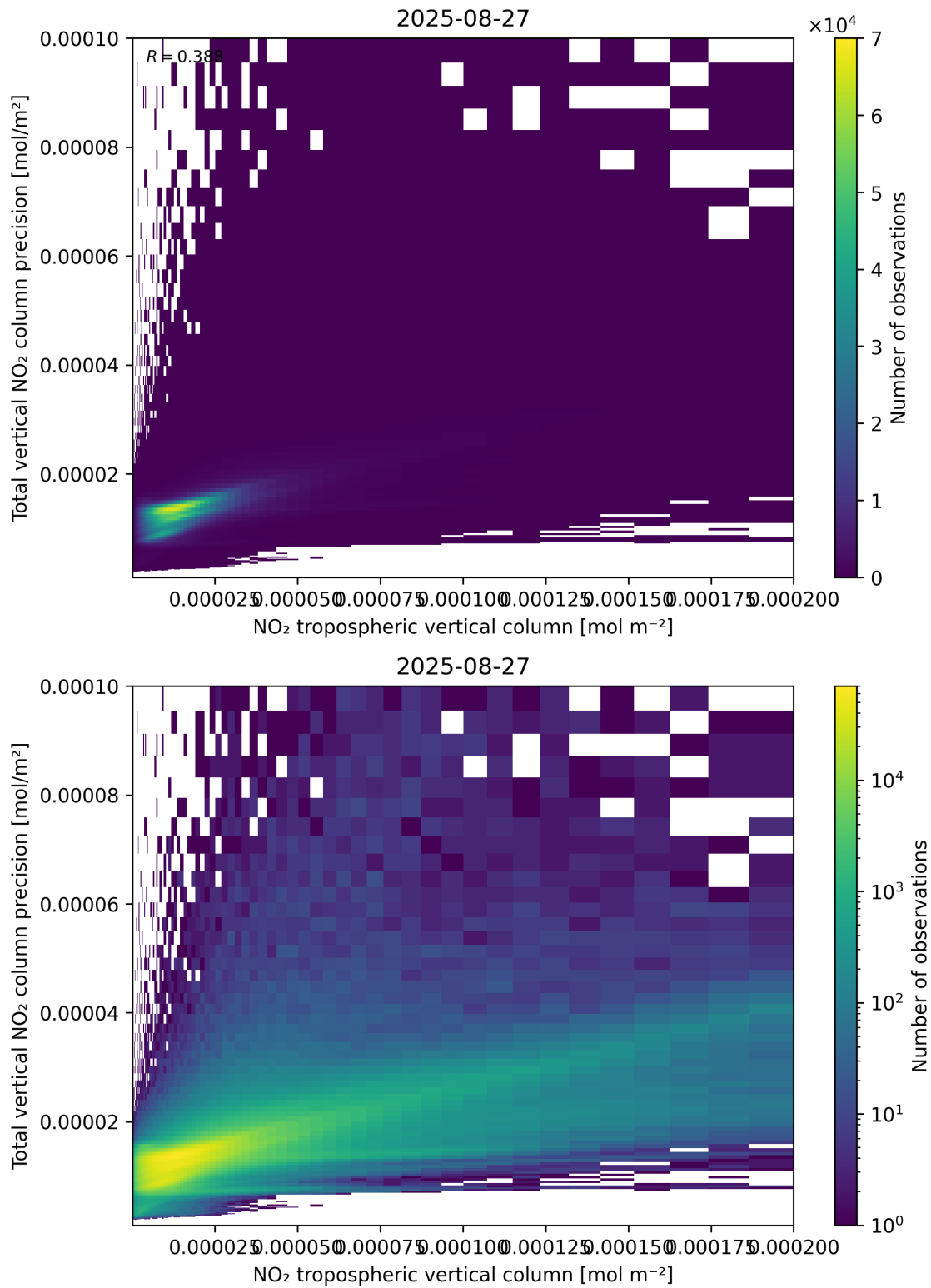
Figure 129: Scatter density plot of “NO 2 tropospheric vertical column” against “Total vertical NO 2 column precision” for 2025-08-26 to 2025-08-28.
