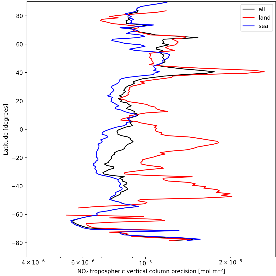
Figure 13: Zonal average of “NO 2 tropospheric vertical column precision” for 2025-08-26 to 2025-08-28.
