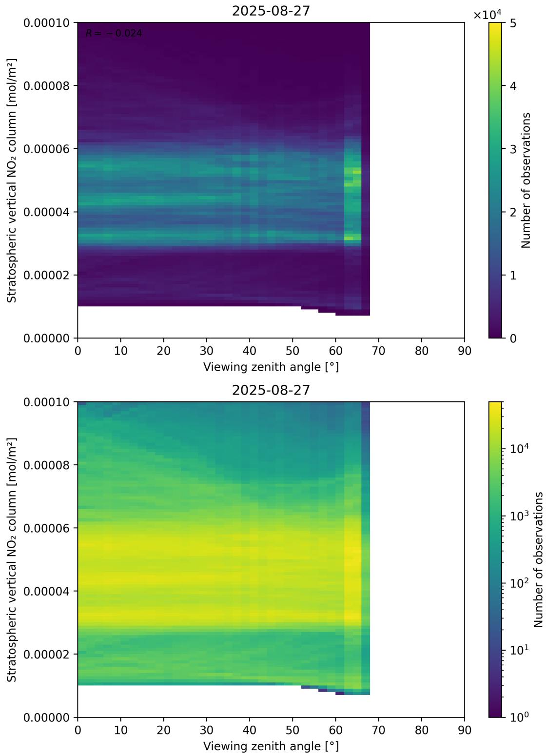
Figure 164: Scatter density plot of “Viewing zenith angle” against “Stratospheric vertical NO 2 column” for 2025-08-26 to 2025-08-28.
