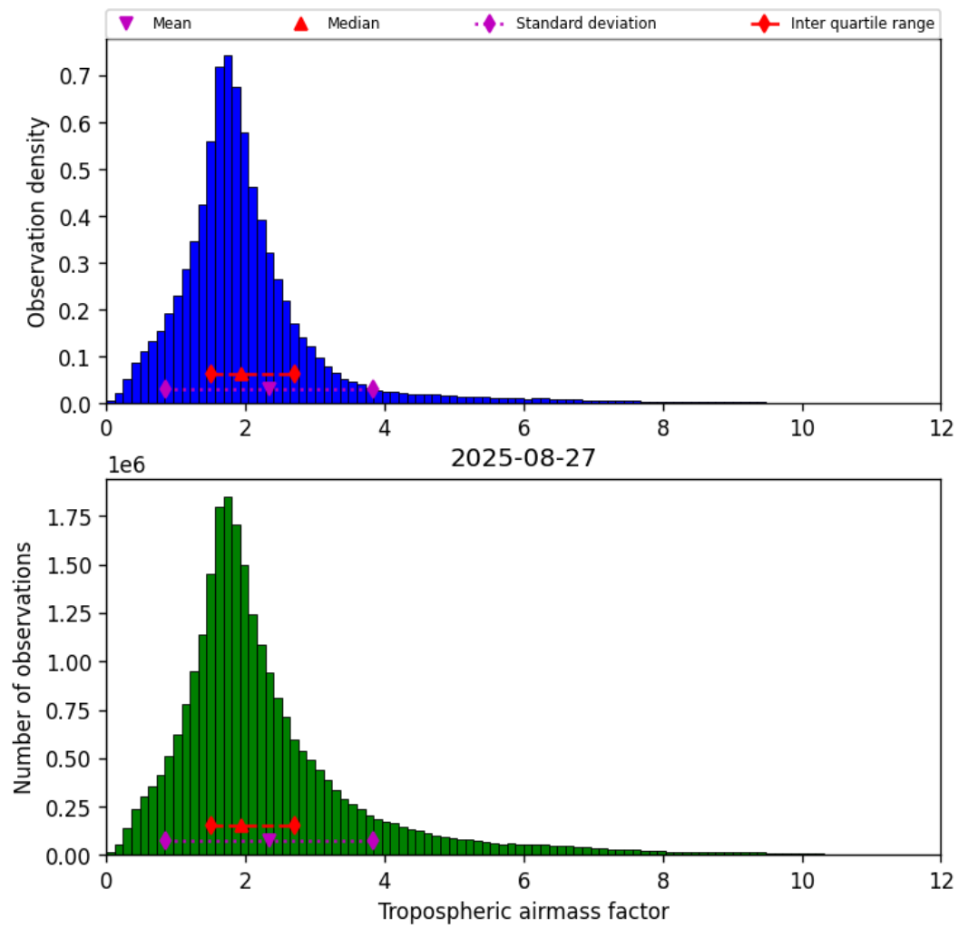
Figure 31: Histogram of “Tropospheric airmass factor” for 2025-08-26 to 2025-08-28
