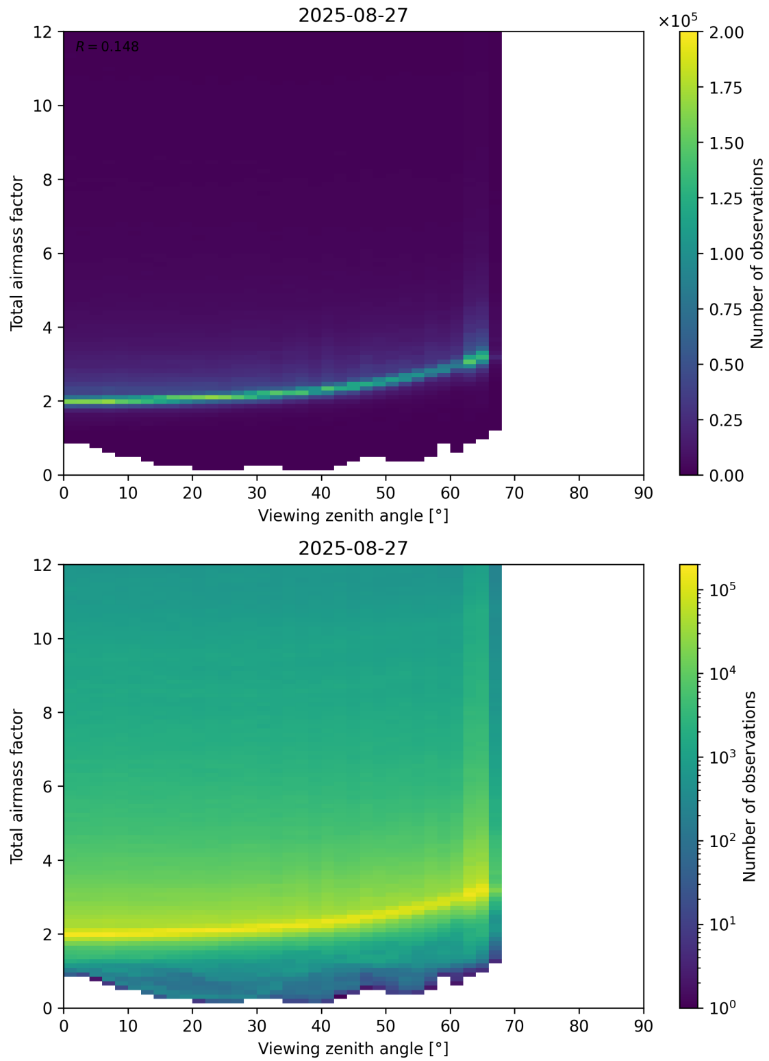
Figure 160: Scatter density plot of “Viewing zenith angle” against “Total airmass factor” for 2025-08-26 to 2025-08-28.
