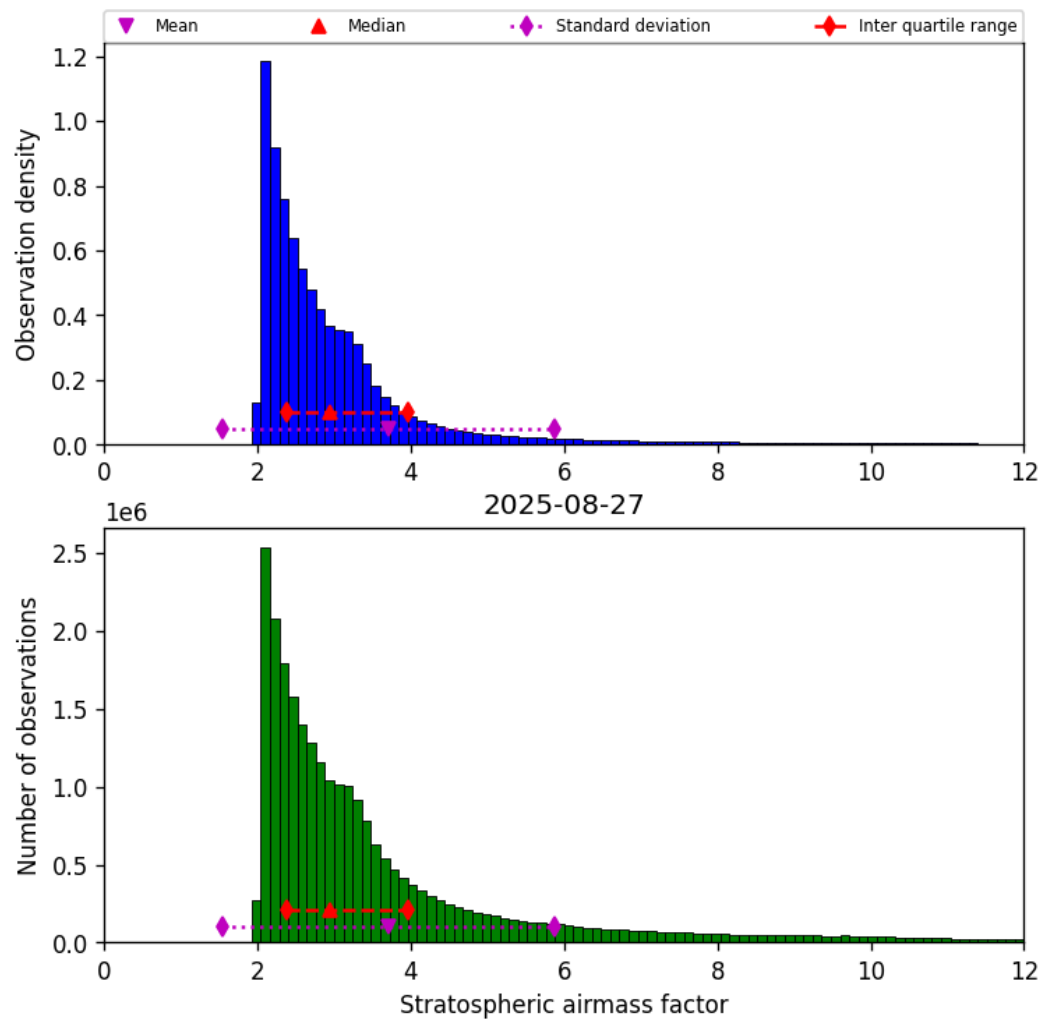
Figure 44: Histogram of “Stratospheric airmass factor” for 2025-08-26 to 2025-08-28
