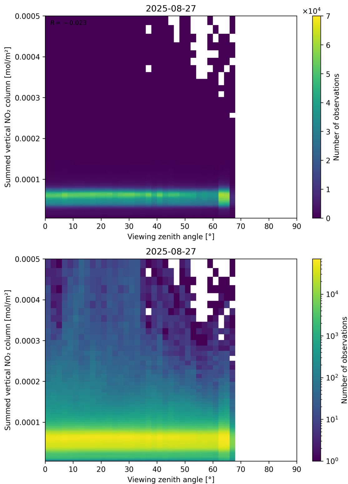
Figure 165: Scatter density plot of “Viewing zenith angle” against “Summed vertical NO 2 column” for 2025-08-26 to 2025-08-28.
