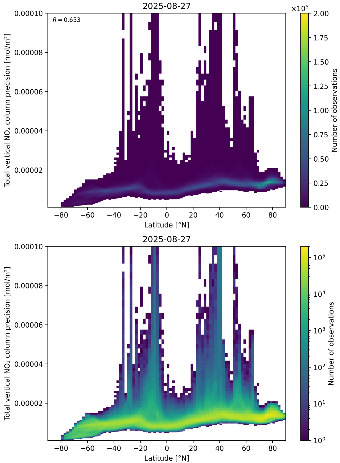
Figure 91: Scatter density plot of “Latitude” against “Total vertical NO 2 column precision” for 2025-08-26 to 2025-08-28.
