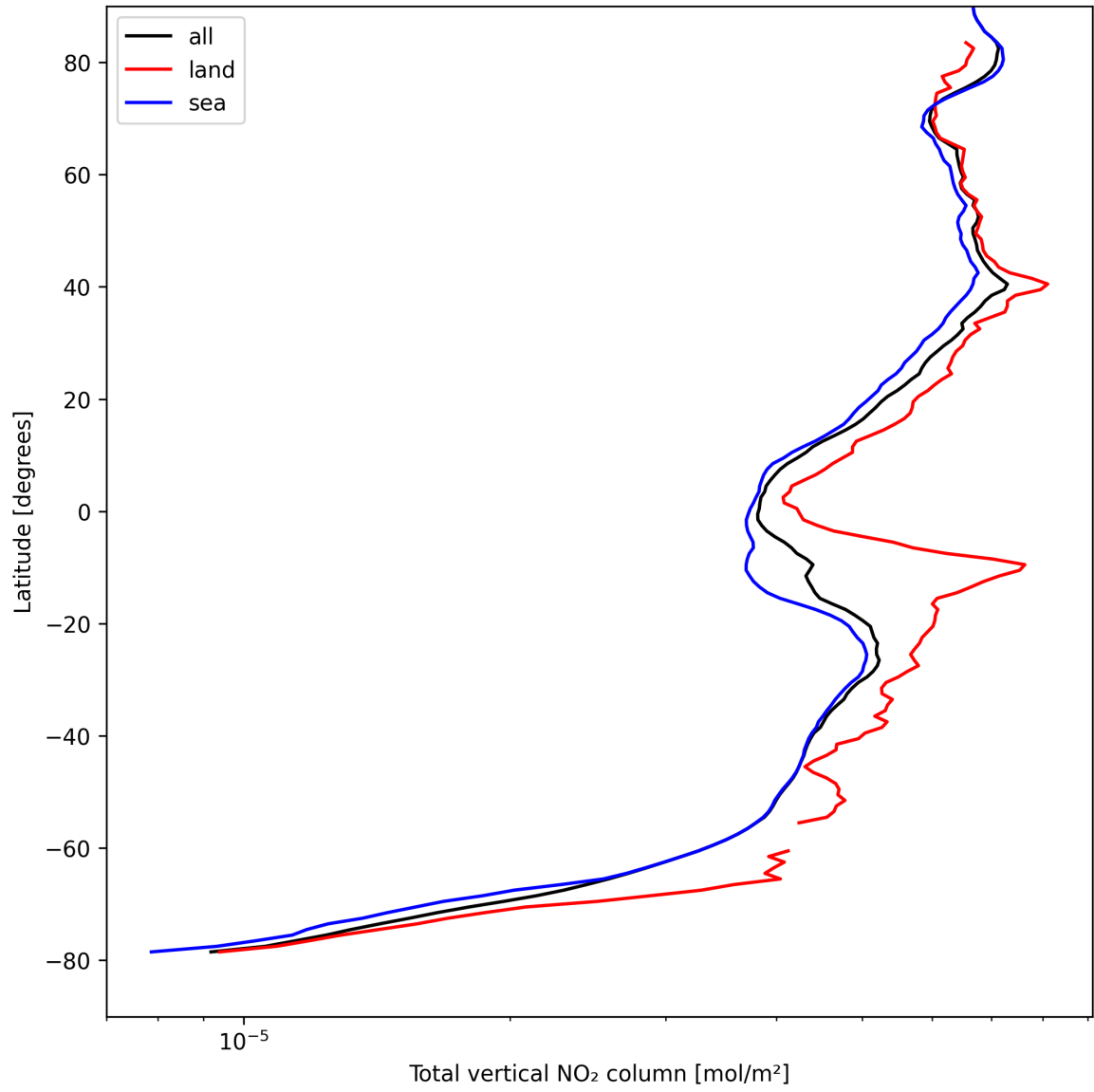
Figure 21: Zonal average of “Total vertical NO 2 column” for 2025-08-26 to 2025-08-28.
