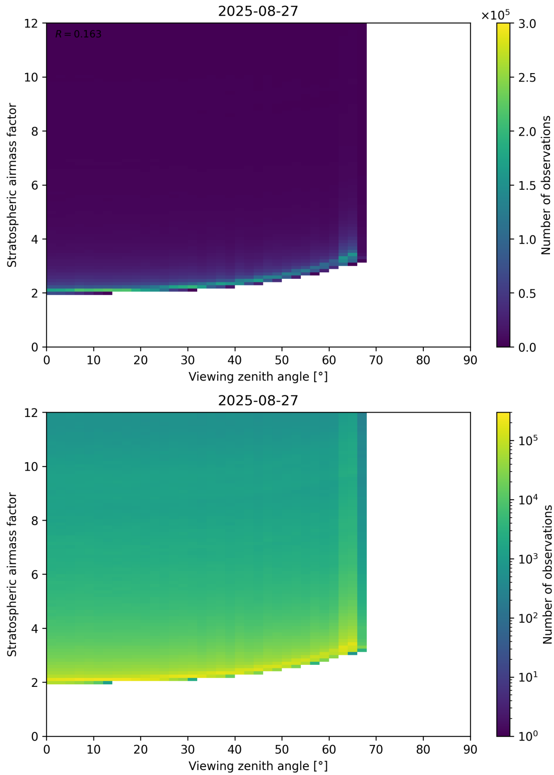
Figure 159: Scatter density plot of “Viewing zenith angle” against “Stratospheric airmass factor” for 2025-08-26 to 2025-08-28.
