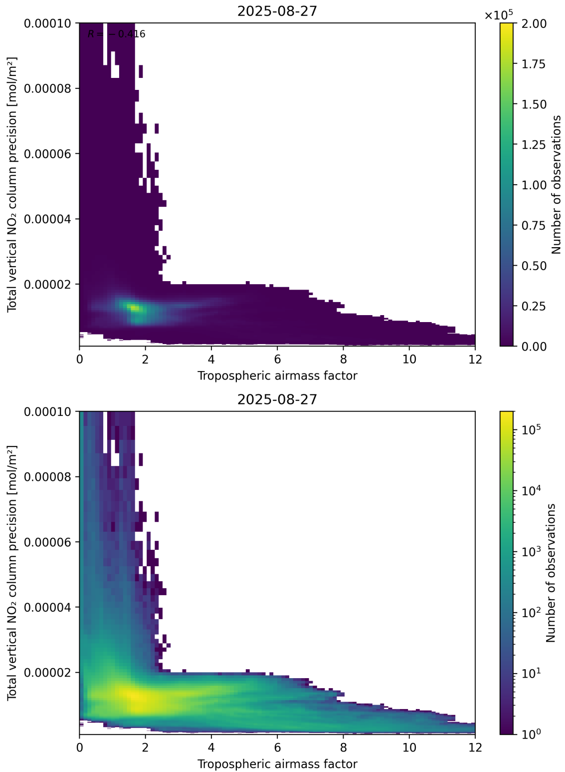
Figure 78: Scatter density plot of “Tropospheric airmass factor” against “Total vertical NO 2 column precision” for 2025-08-26 to 2025-08-28.
