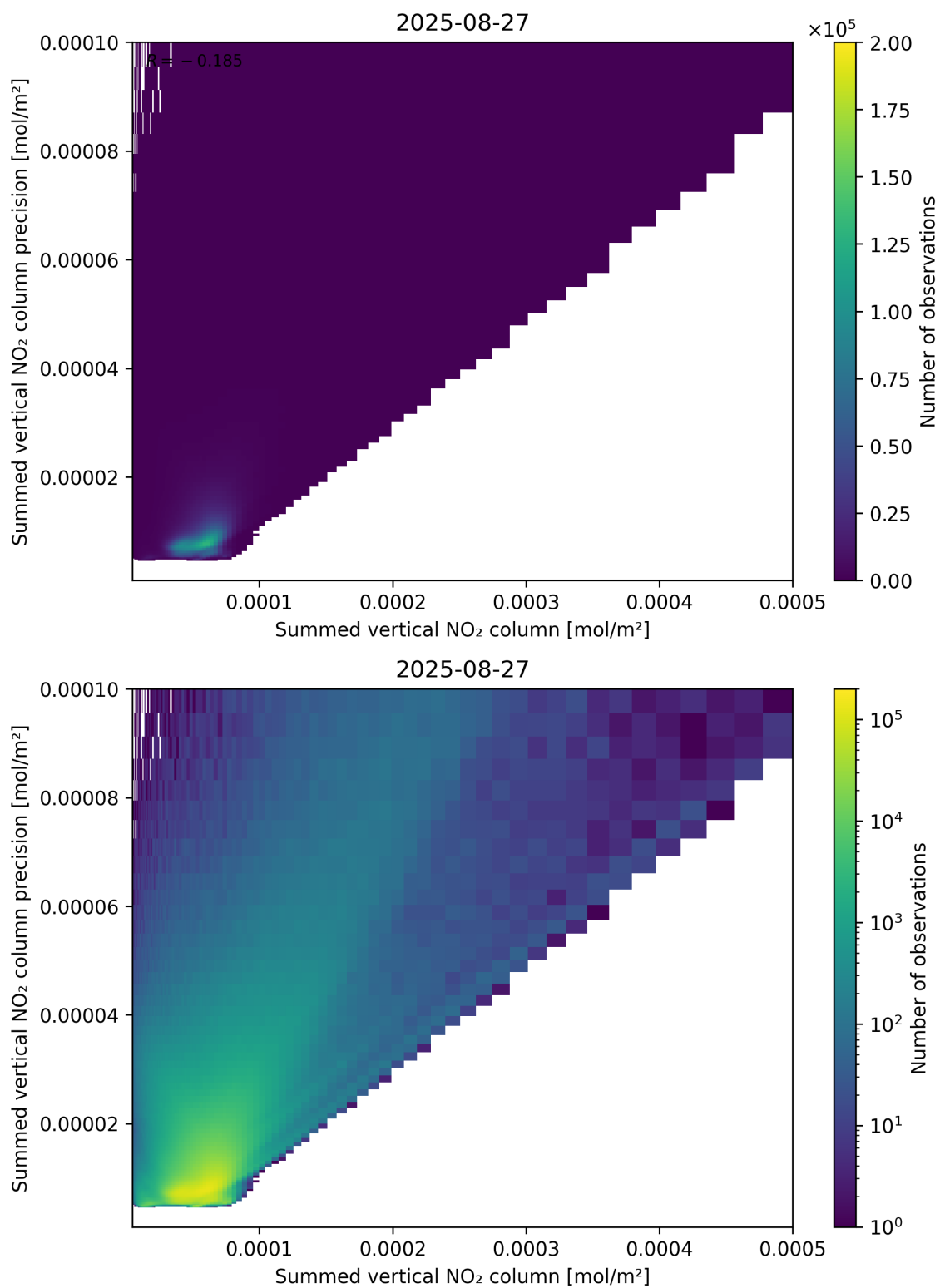
Figure 105: Scatter density plot of “Summed vertical NO 2 column” against “Summed vertical NO 2 column precision” for 2025-08-26 to 2025-08-28.
