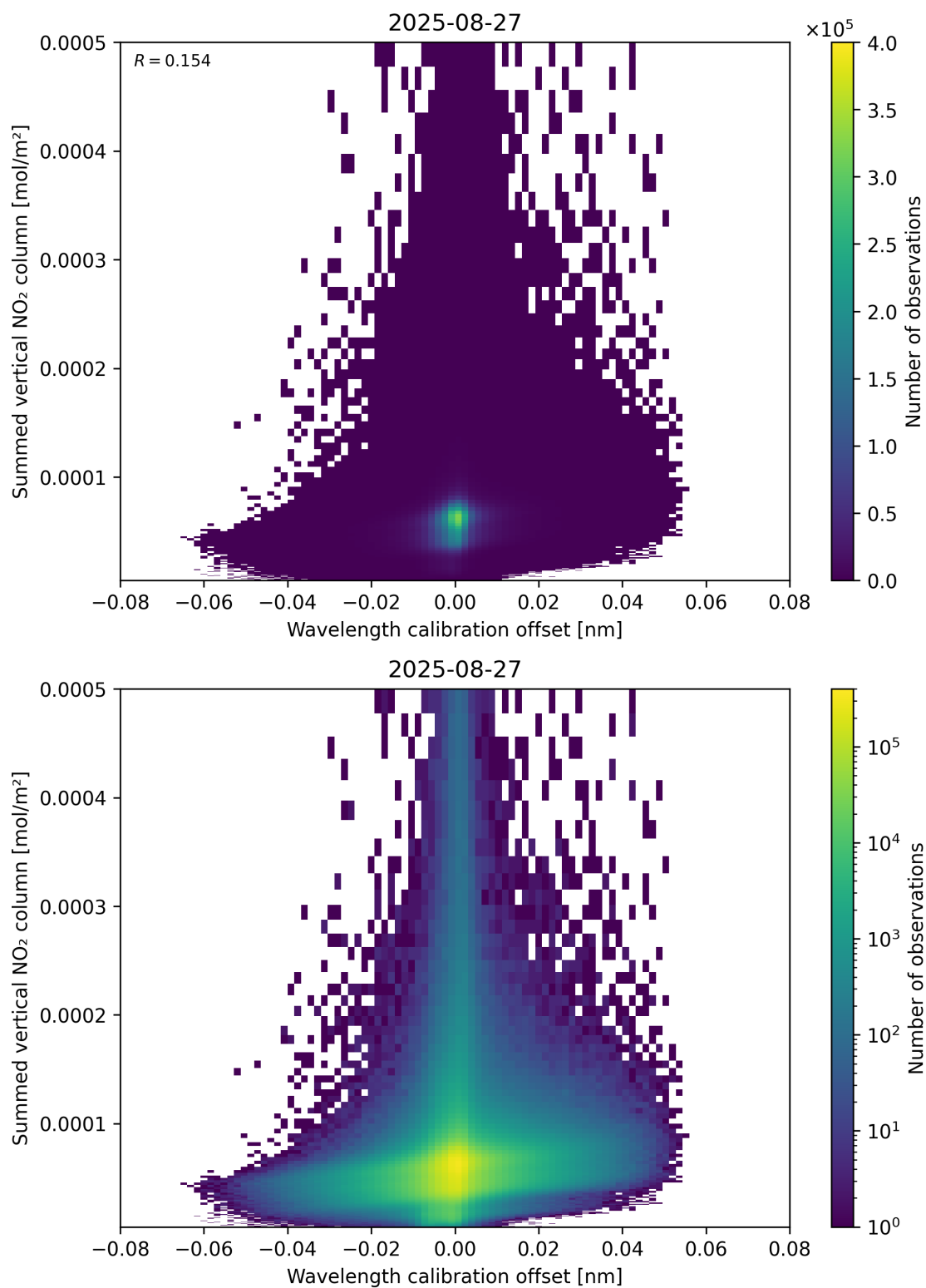
Figure 177: Scatter density plot of “Wavelength calibration offset” against “Summed vertical NO 2 column” for 2025-08-26 to 2025-08-28.
