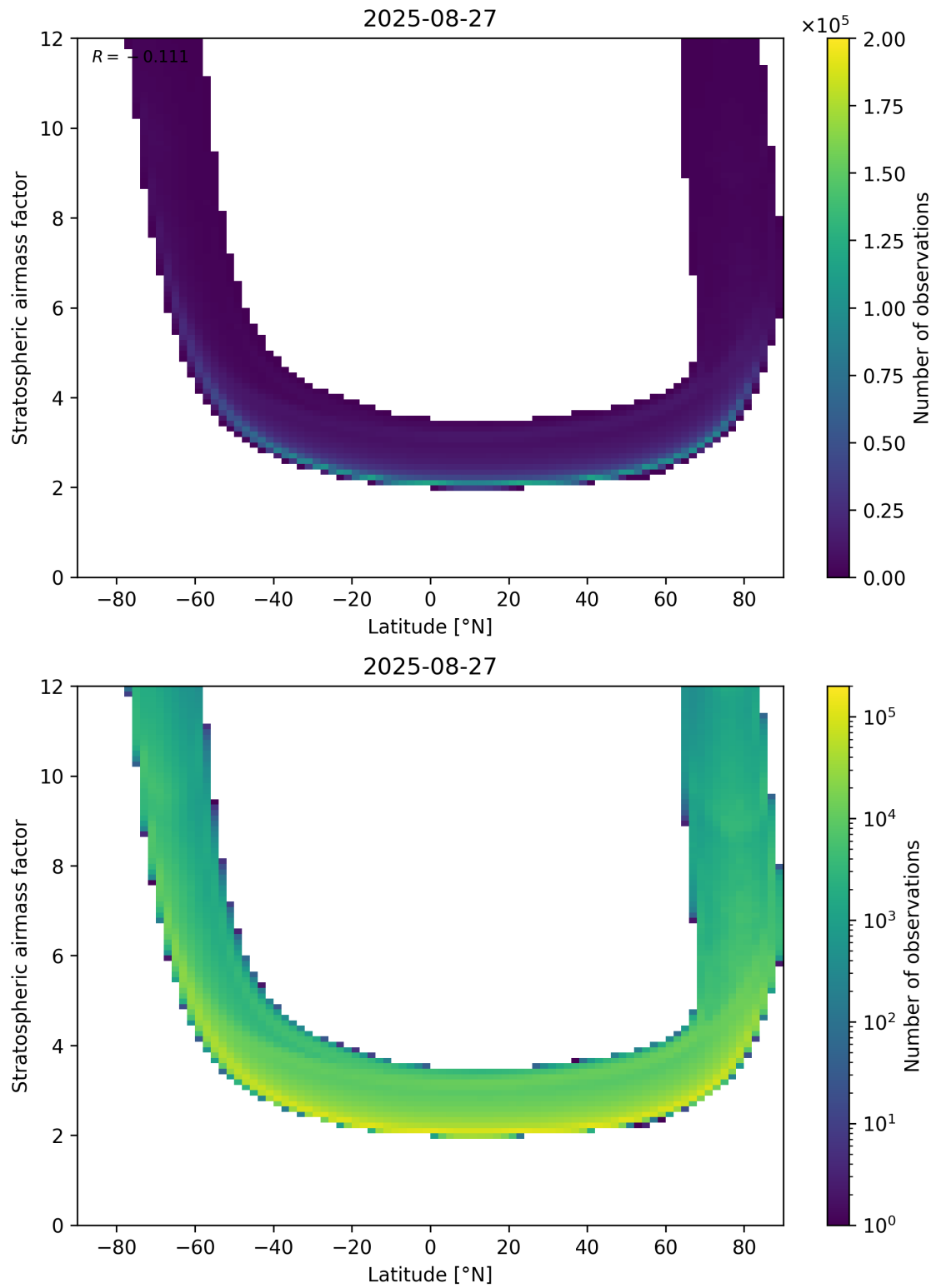
Figure 83: Scatter density plot of “Latitude” against “Stratospheric air mass factor” for 2025-08-26 to 2025-08-28.
