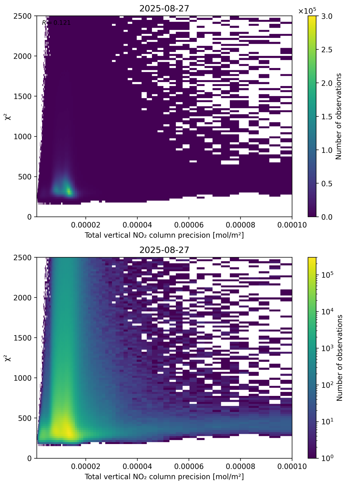
Figure 116: Scatter density plot of “Total vertical NO 2 column precision” against “ \chi^2 ” for 2025-08-26 to 2025-08-28.
