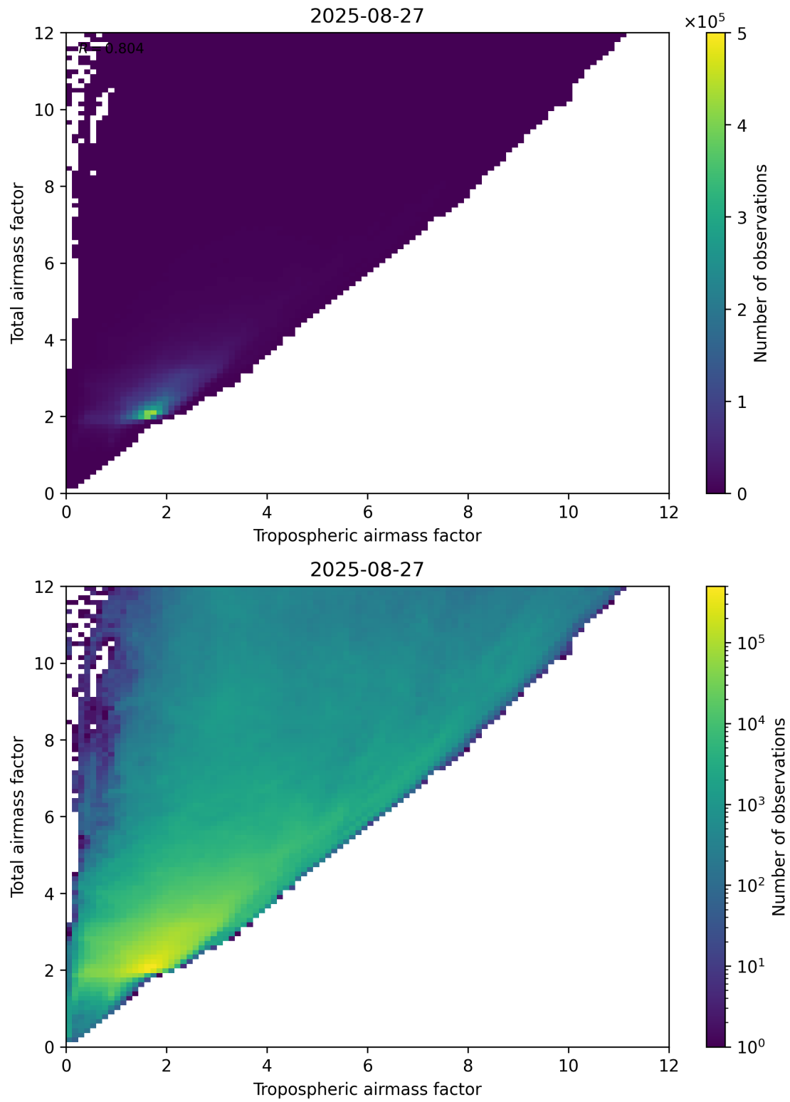
Figure 72: Scatter density plot of “Tropospheric airmass factor” against “Total airmass factor” for 2025-08-26 to 2025-08-28.
