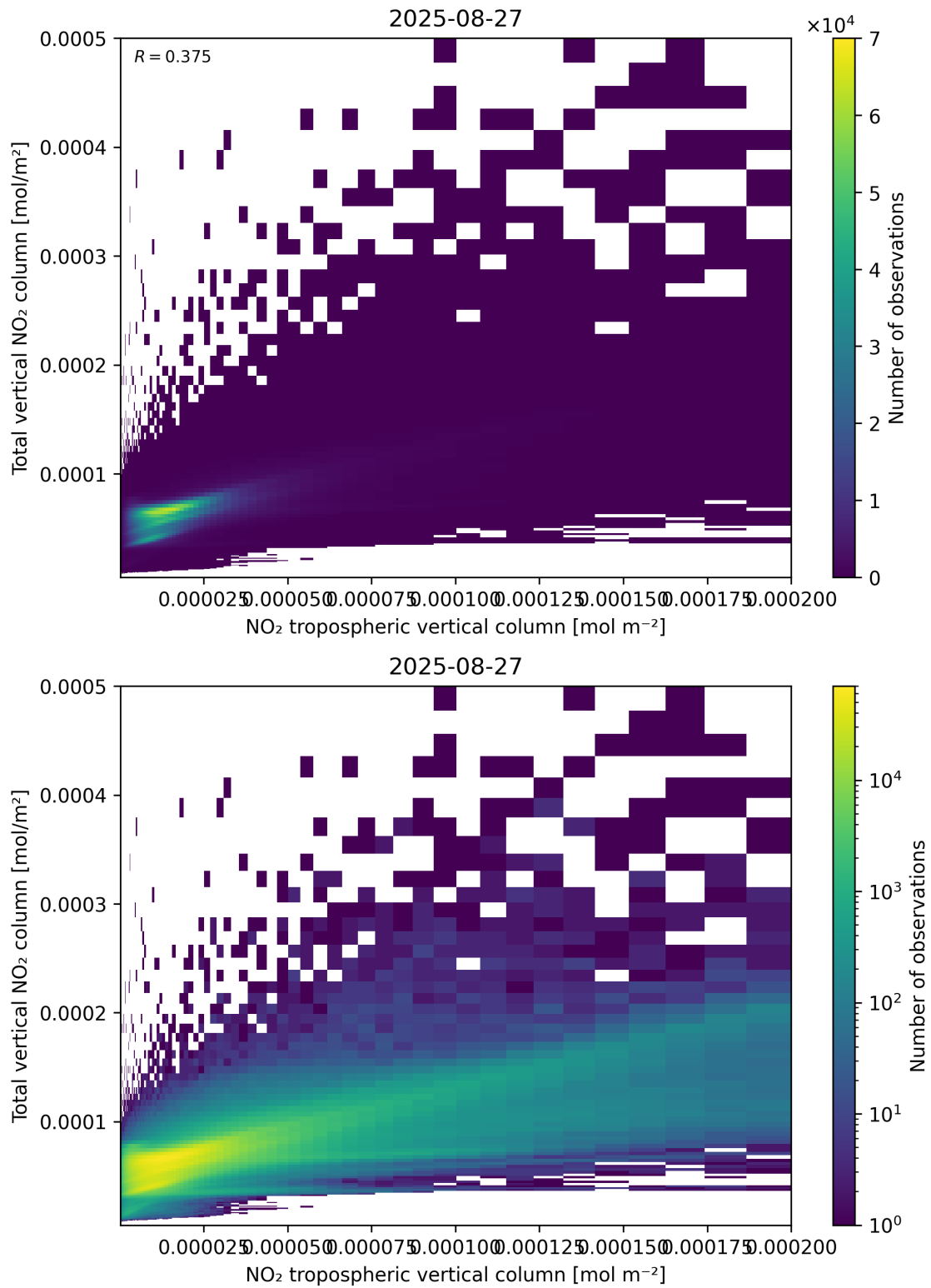
Figure 128: Scatter density plot of “NO 2 tropospheric vertical column” against “Total vertical NO 2 column” for 2025-08-26 to 2025-08-28.
