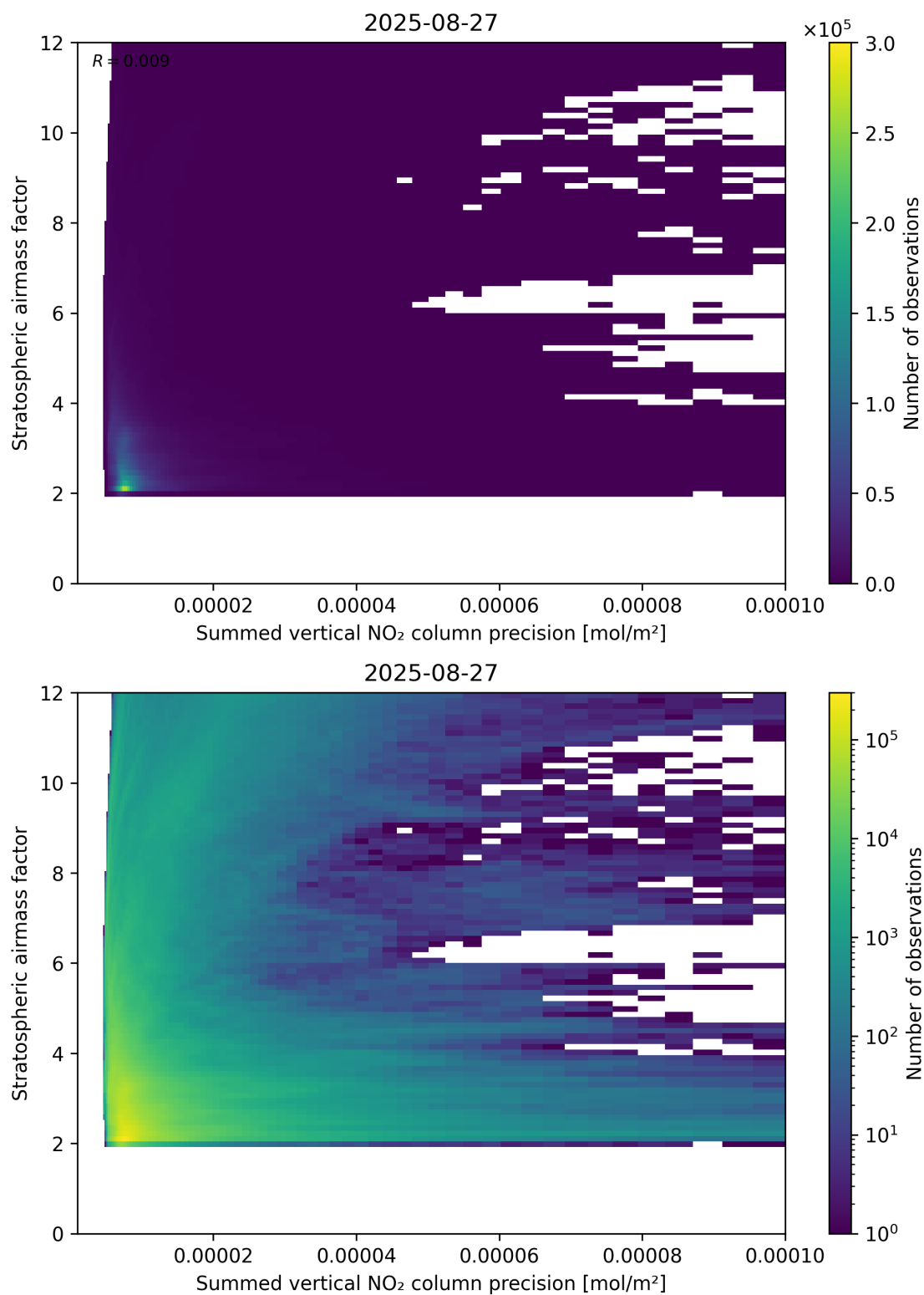
Figure 106: Scatter density plot of “Summed vertical NO 2 column precision” against “Stratospheric airmass factor” for 2025-08-26 to 2025-08-28.
