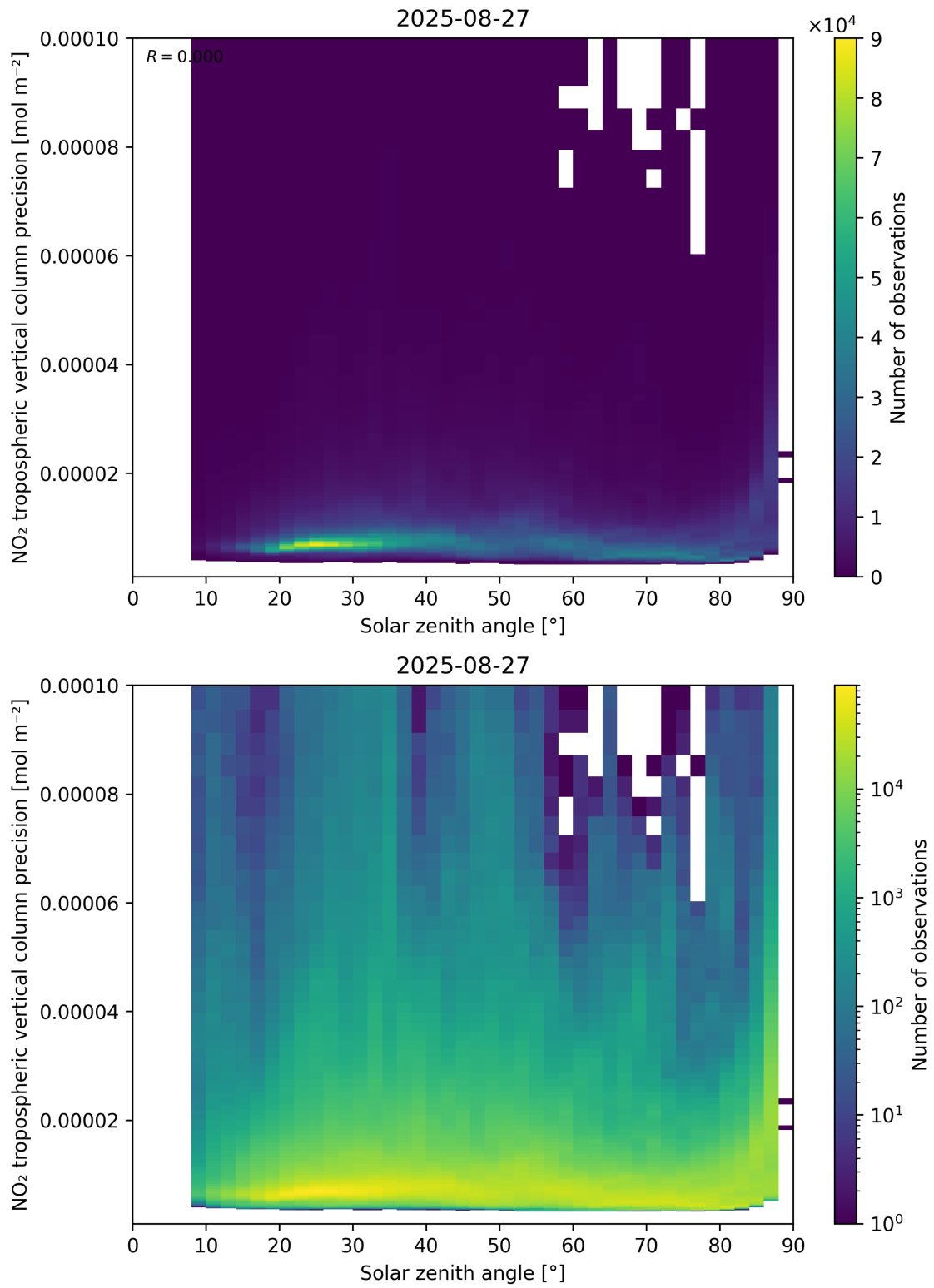
Figure 156: Scatter density plot of “Solar zenith angle” against “NO 2 tropospheric vertical column precision” for 2025-08-26 to 2025-08-28.
