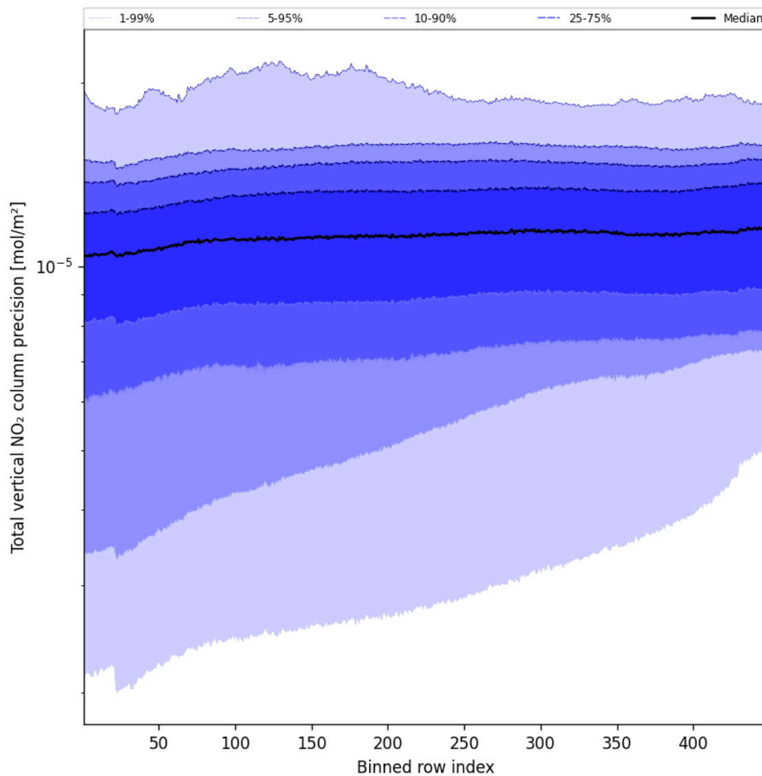
Figure 56: Along track statistics of “Total vertical NO 2 column precision” for 2025-08-26 to 2025-08-28
