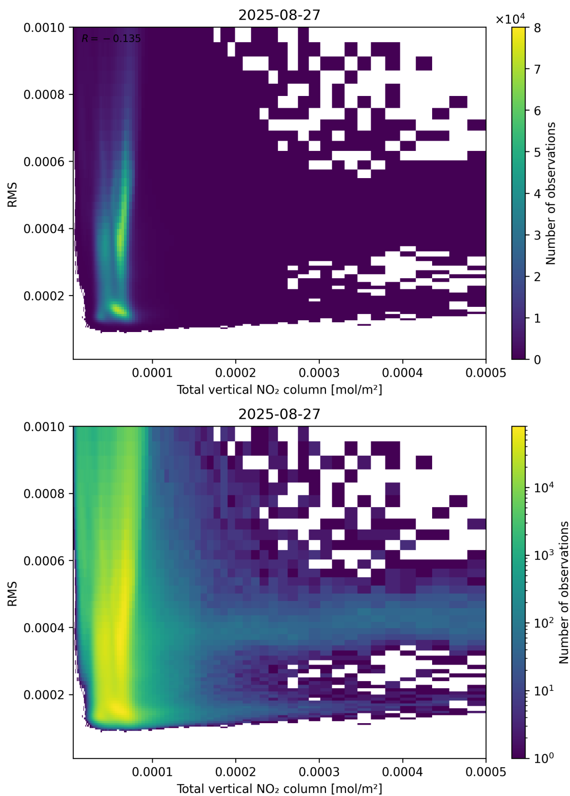
Figure 120: Scatter density plot of “Total vertical NO 2 column” against “RMS” for 2025-08-26 to 2025-08-28.
