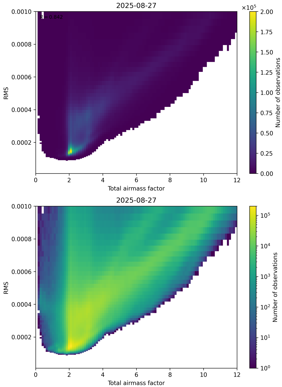
Figure 69: Scatter density plot of “Total airmass factor” against “RMS” for 2025-08-26 to 2025-08-28.
