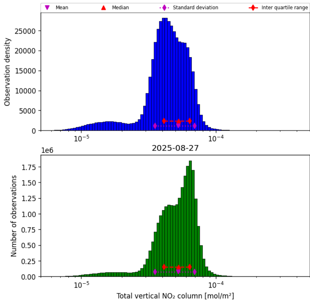
Figure 38: Histogram of “Total vertical NO 2 column” for 2025-08-26 to 2025-08-28
