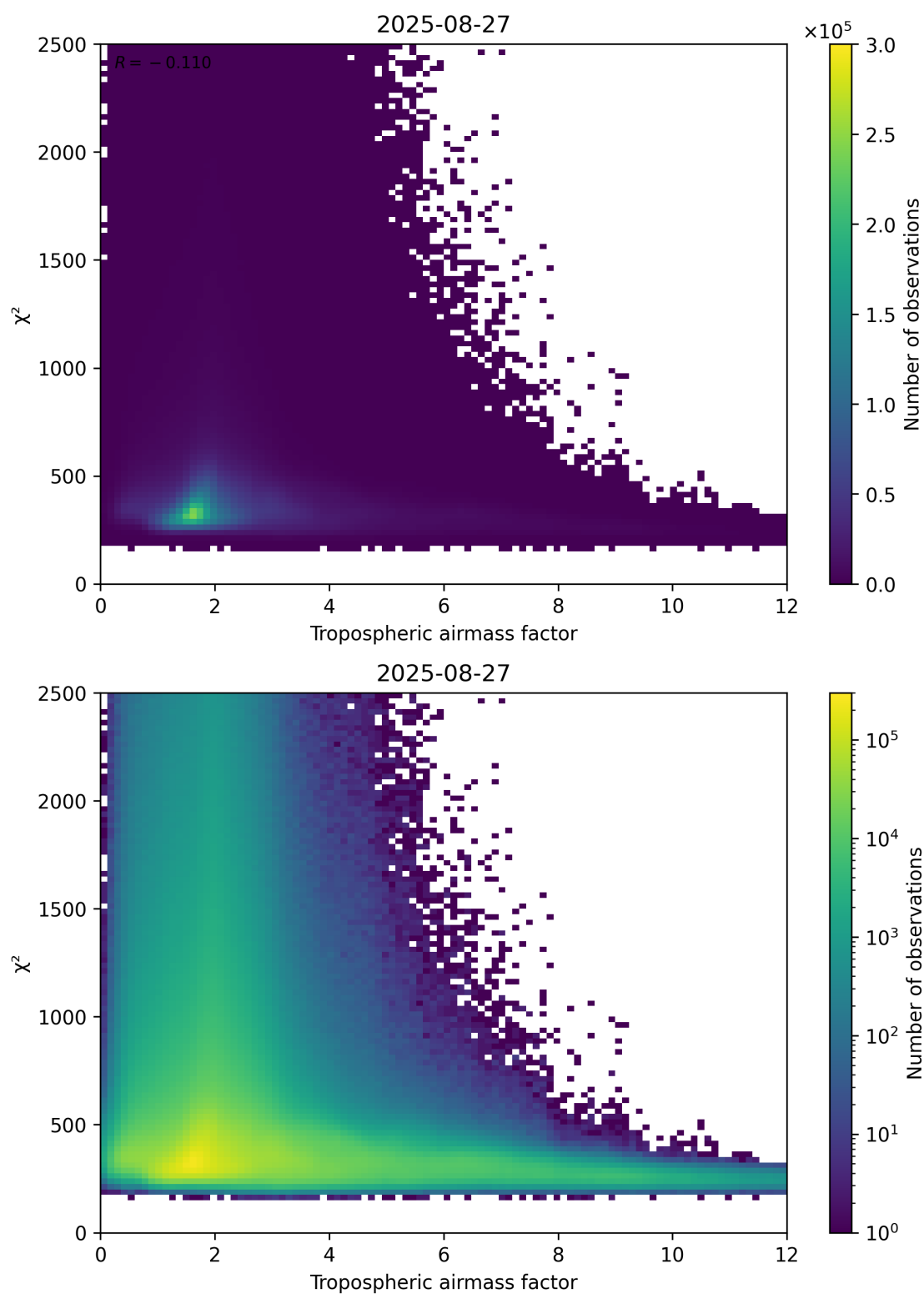
Figure 73: Scatter density plot of “Tropospheric airmass factor” against “ \chi^2 ” for 2025-08-26 to 2025-08-28.
