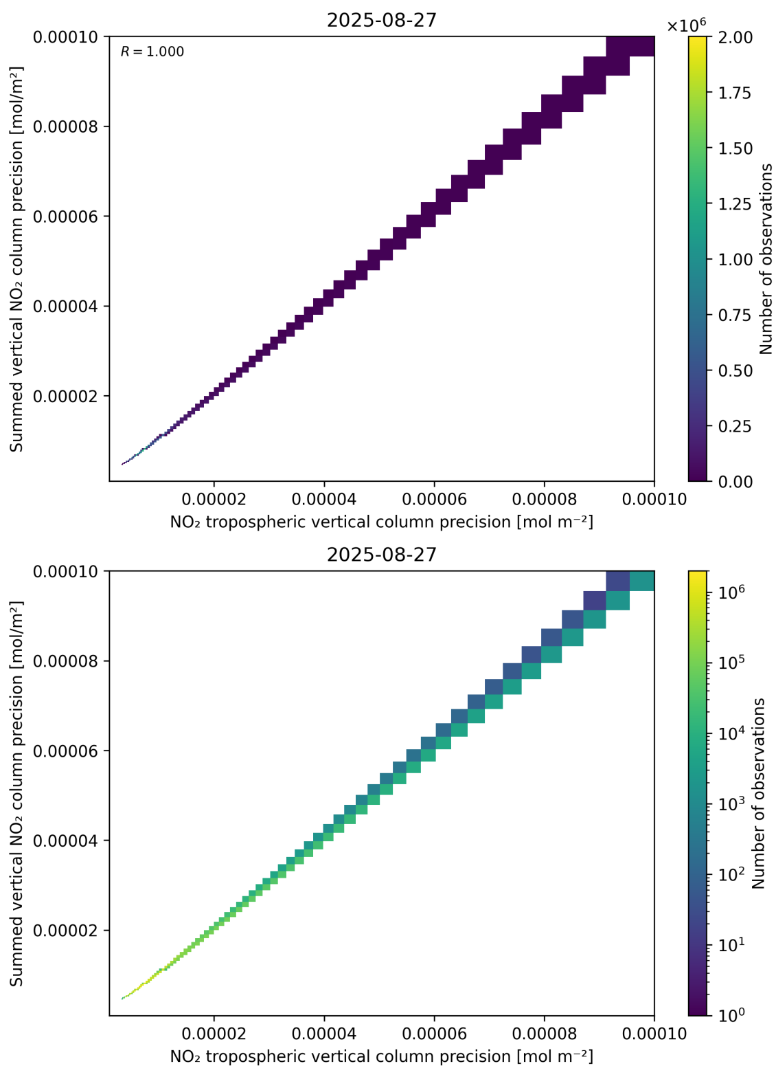
Figure 137: Scatter density plot of “NO 2 tropospheric vertical column precision” against “Summed vertical NO 2 column precision” for 2025-08-26 to 2025-08-28.
