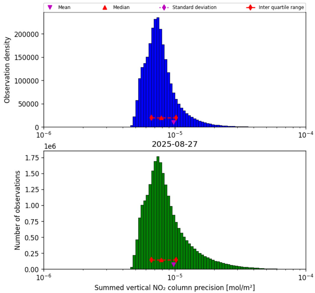
Figure 41: Histogram of "Summed vertical NO 2 column precision" for 2025-08-26 to 2025-08-28
