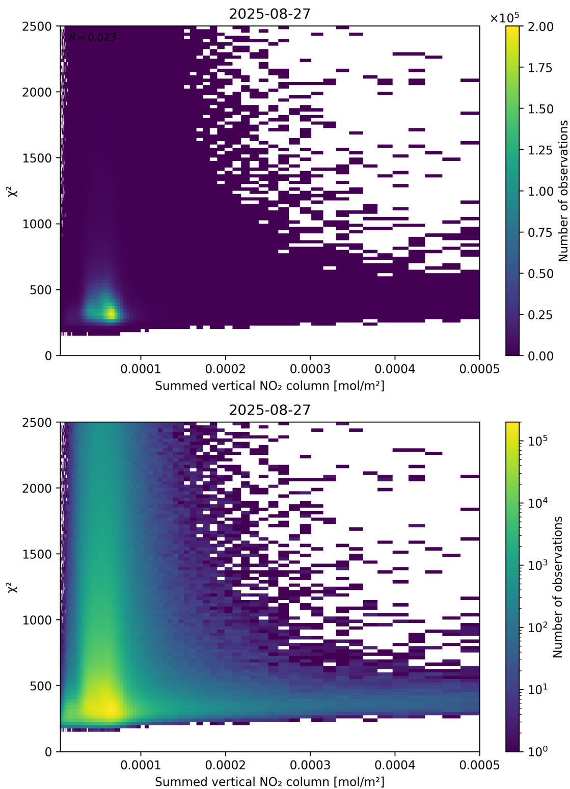
Figure 104: Scatter density plot of “Summed vertical NO 2 column” against “ \chi^2 ” for 2025-08-26 to 2025-08-28.
