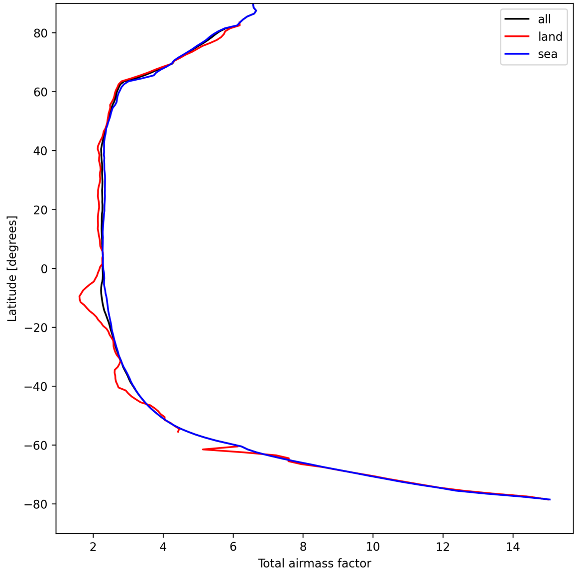
Figure 15: Zonal average of “Total airmass factor” for 2025-08-26 to 2025-08-28.
