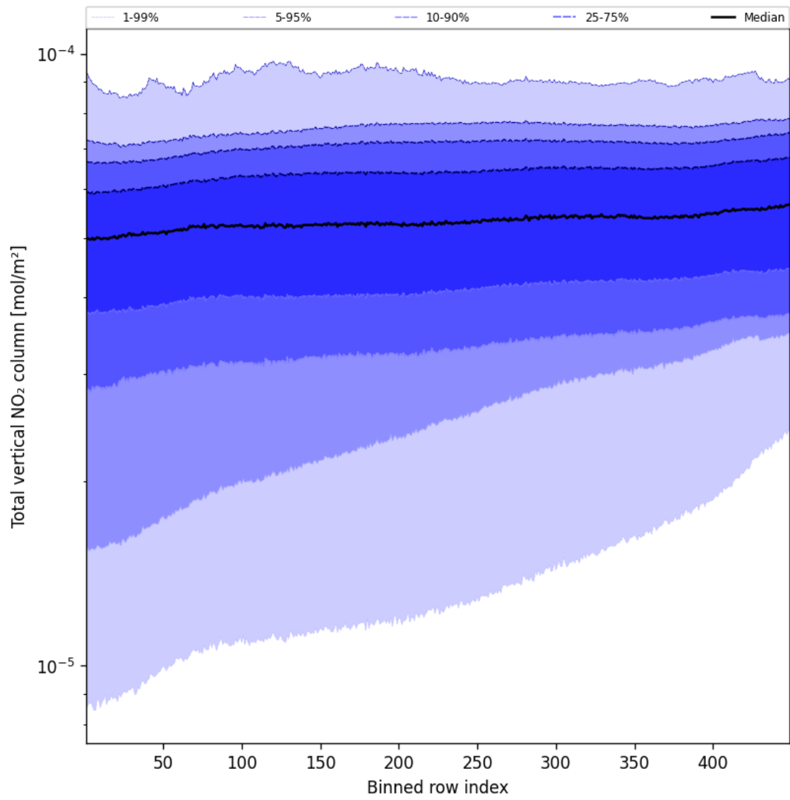
Figure 55: Along track statistics of “Total vertical NO 2 column” for 2025-08-26 to 2025-08-28
