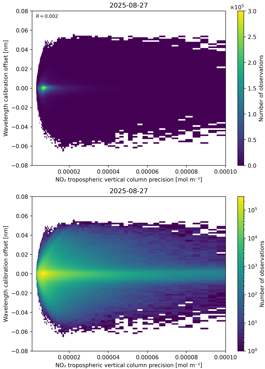
Figure 141: Scatter density plot of “NO 2 tropospheric vertical column precision” against “Wavelength calibration offset” for 2025-08-26 to 2025-08-28.
