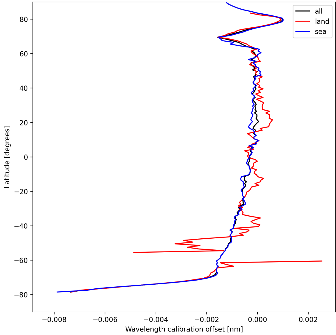
Figure 18: Zonal average of “Wavelength calibration offset” for 2025-08-26 to 2025-08-28.
