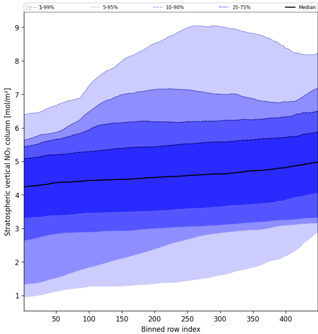
Figure 53: Along track statistics of “Stratospheric vertical NO 2 column” for 2025-08-26 to 2025-08-28
