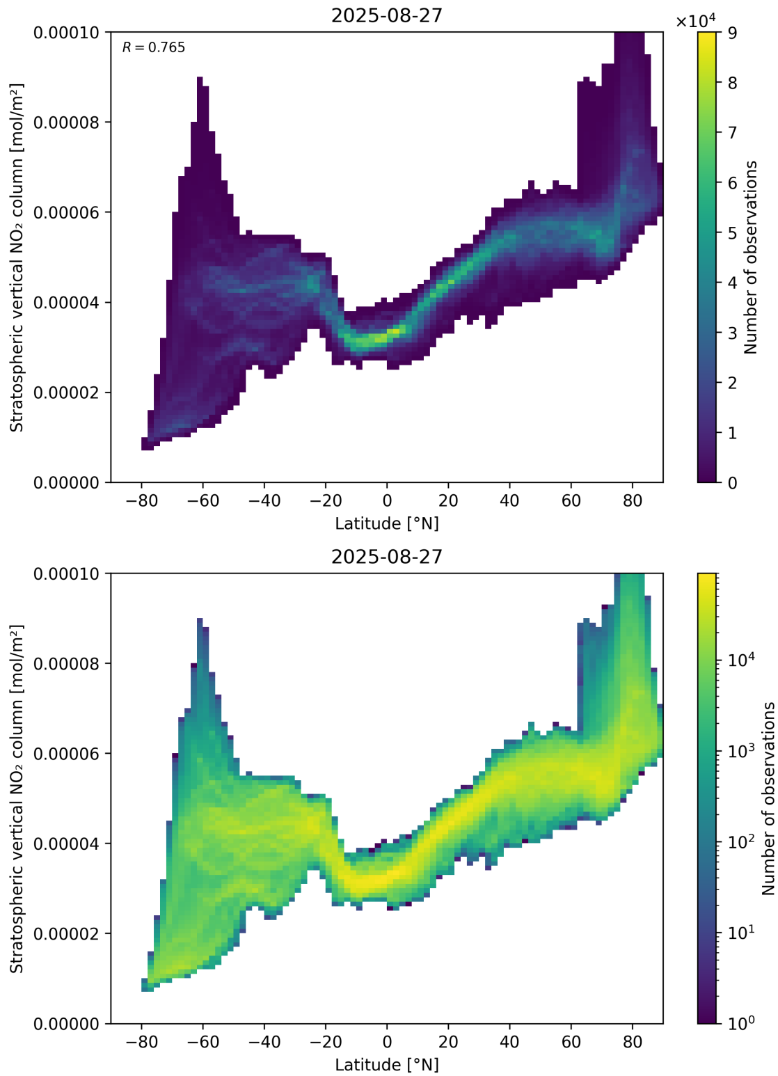
Figure 87: Scatter density plot of “Latitude” against “Stratospheric vertical NO 2 column” for 2025-08-26 to 2025-08-28.
