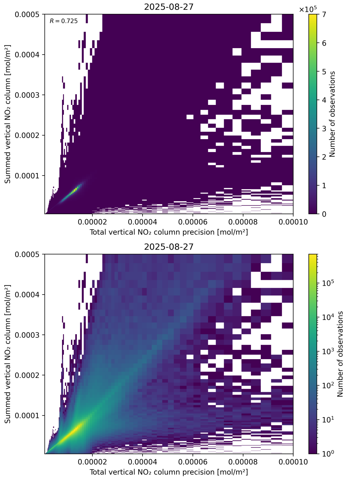
Figure 117: Scatter density plot of “Total vertical NO 2 column precision” against “Summed vertical NO 2 column” for 2025-08-26 to 2025-08-28.
