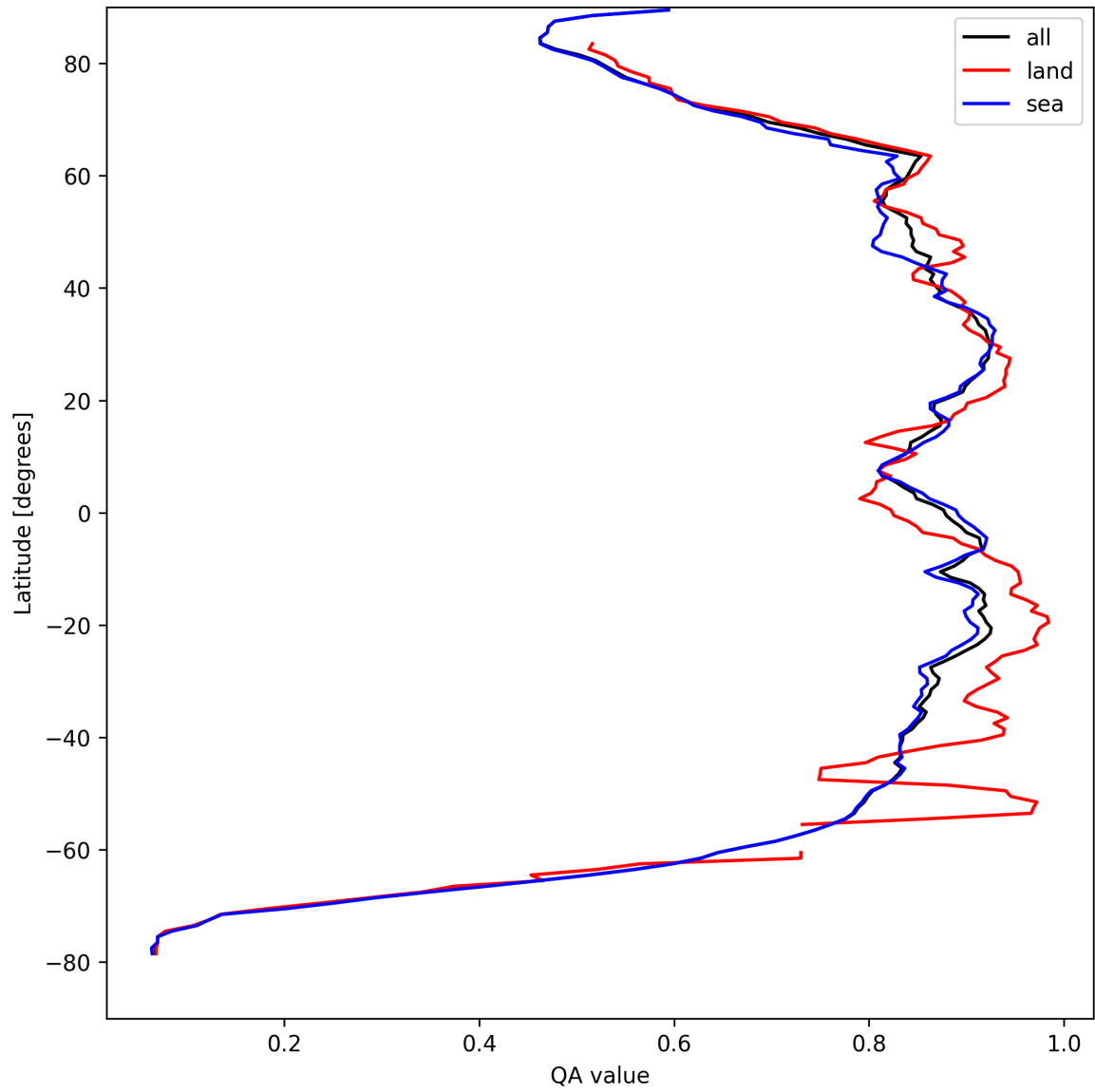
Figure 11: Zonal average of “QA value” for 2025-08-26 to 2025-08-28.
