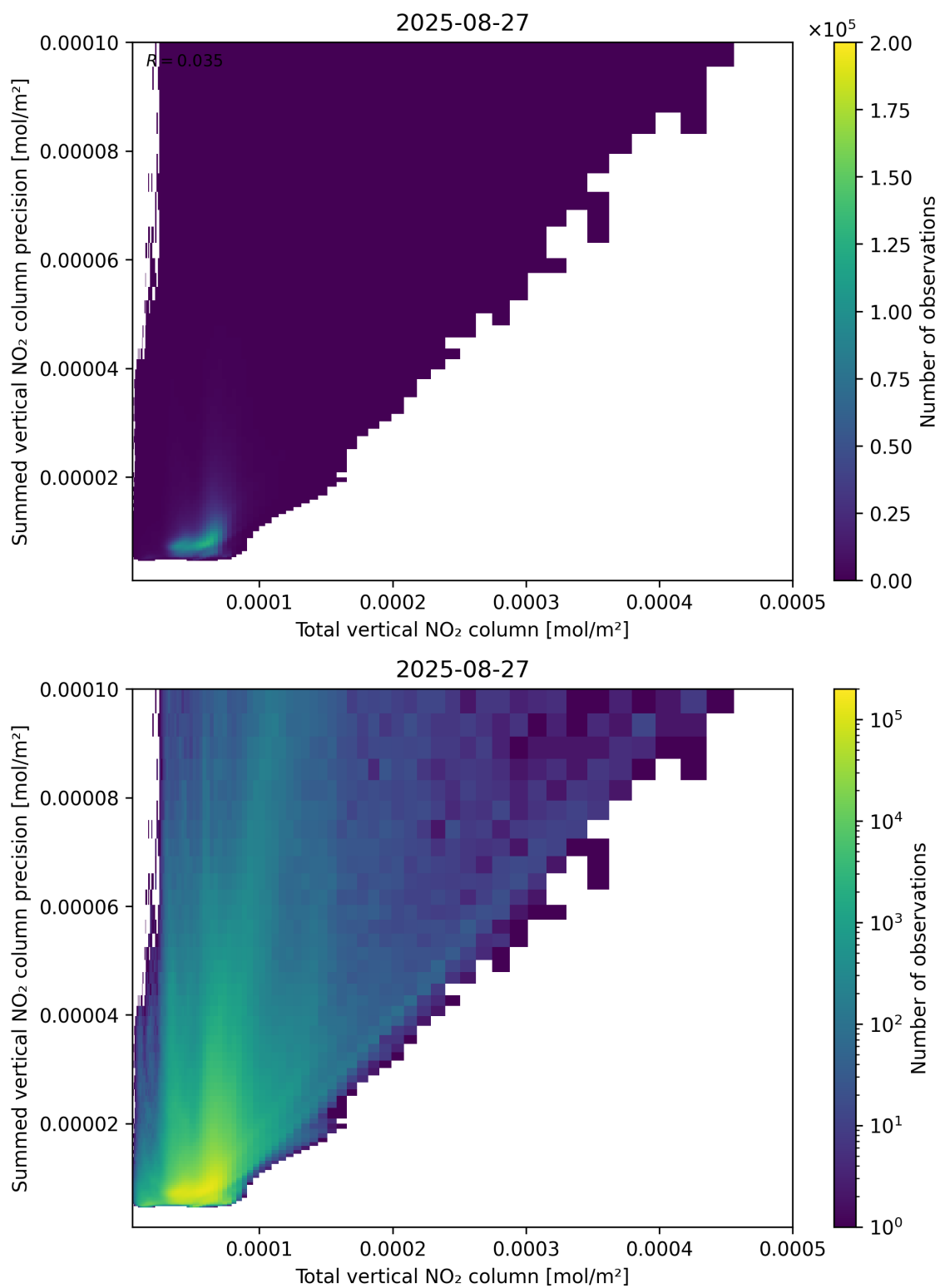
Figure 113: Scatter density plot of “Total vertical NO 2 column” against “Summed vertical NO 2 column precision” for 2025-08-26 to 2025-08-28.
