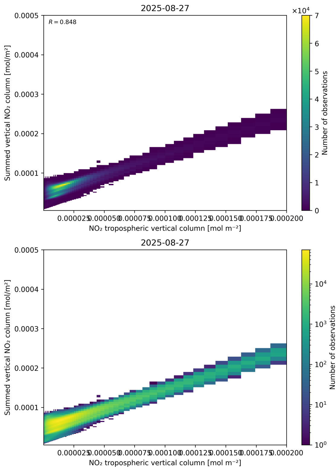
Figure 126: Scatter density plot of “NO 2 tropospheric vertical column” against “Summed vertical NO 2 column” for 2025-08-26 to 2025-08-28.
