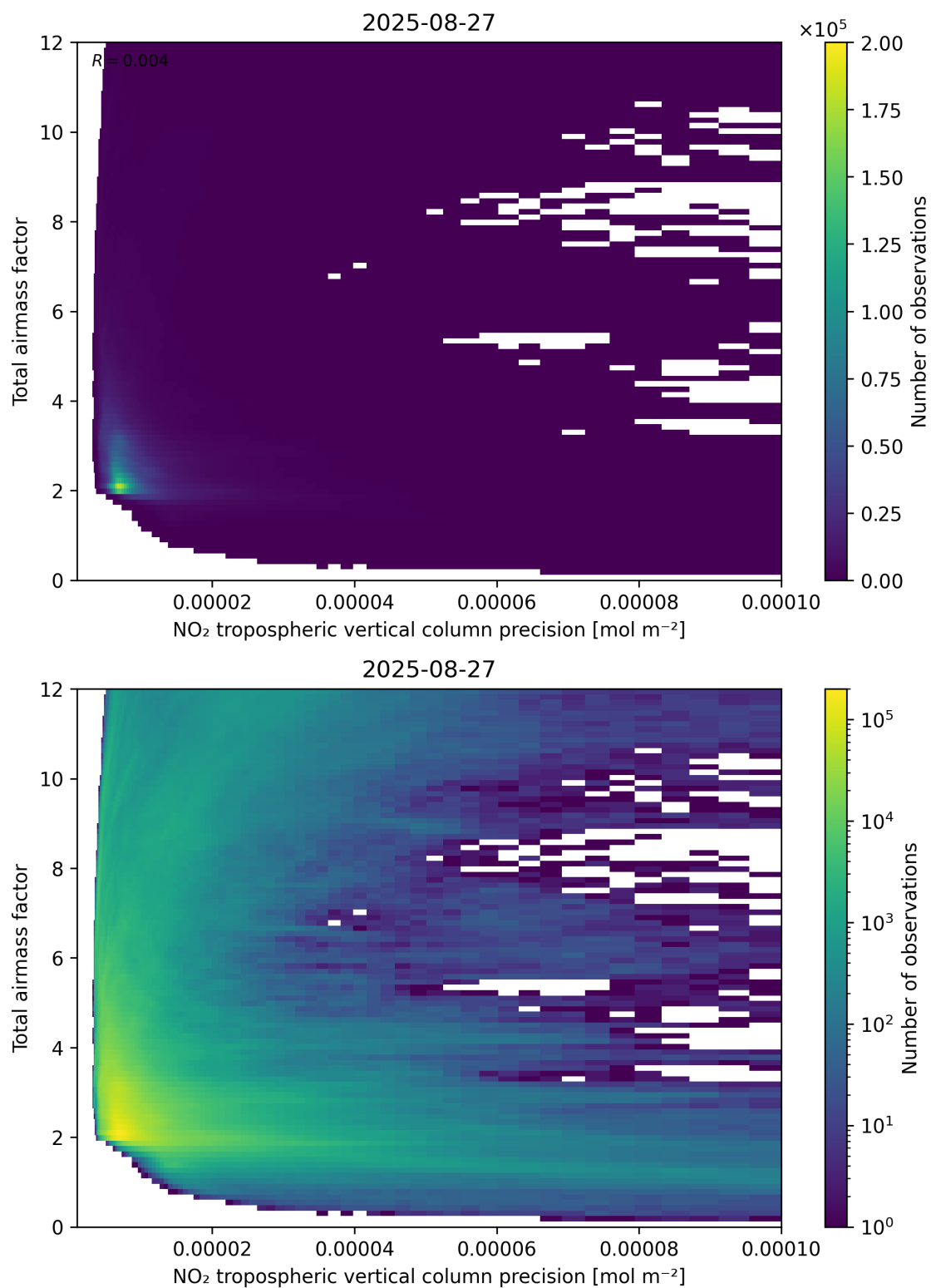
Figure 132: Scatter density plot of “NO 2 tropospheric vertical column precision” against “Total air mass factor” for 2025-08-26 to 2025-08-28.
