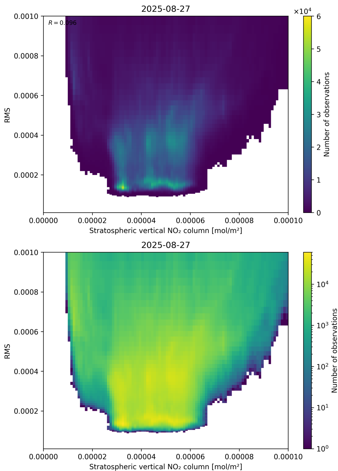
Figure 102: Scatter density plot of “Stratospheric vertical NO 2 column” against “RMS” for 2025-08-26 to 2025-08-28.
