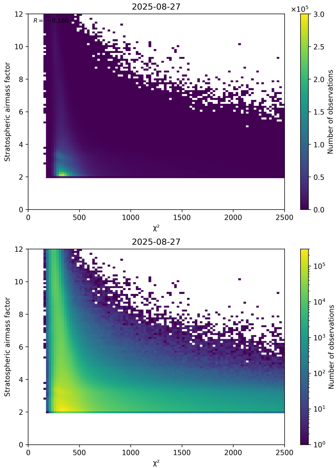
Figure 81: Scatter density plot of “ \chi^2 ” against “Stratospheric airmass factor” for 2025-08-26 to 2025-08-28.
