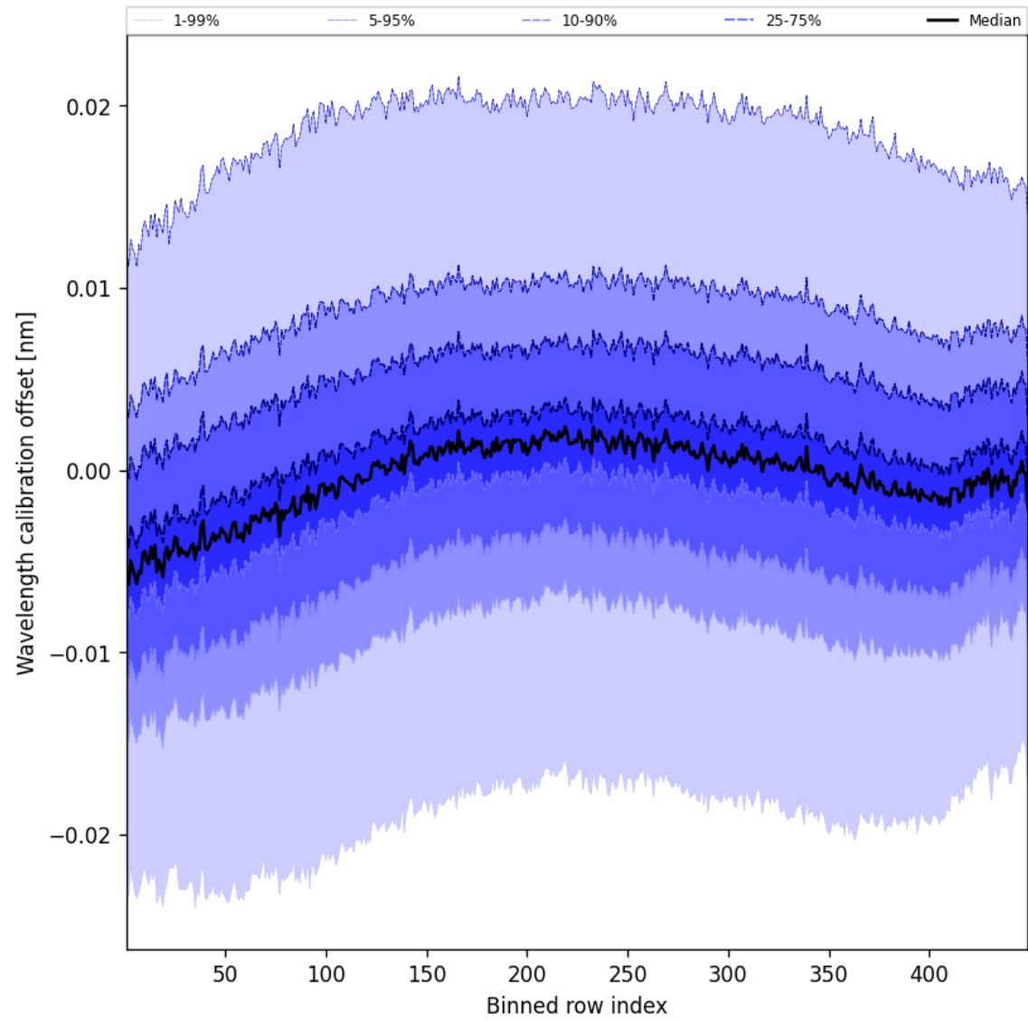
Figure 52: Along track statistics of “Wavelength calibration offset” for 2025-08-26 to 2025-08-28
