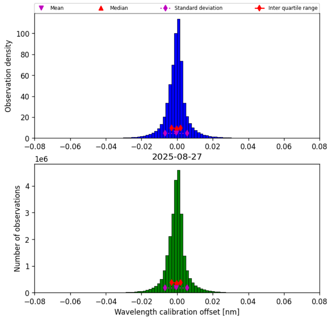
Figure 35: Histogram of “Wavelength calibration offset” for 2025-08-26 to 2025-08-28
