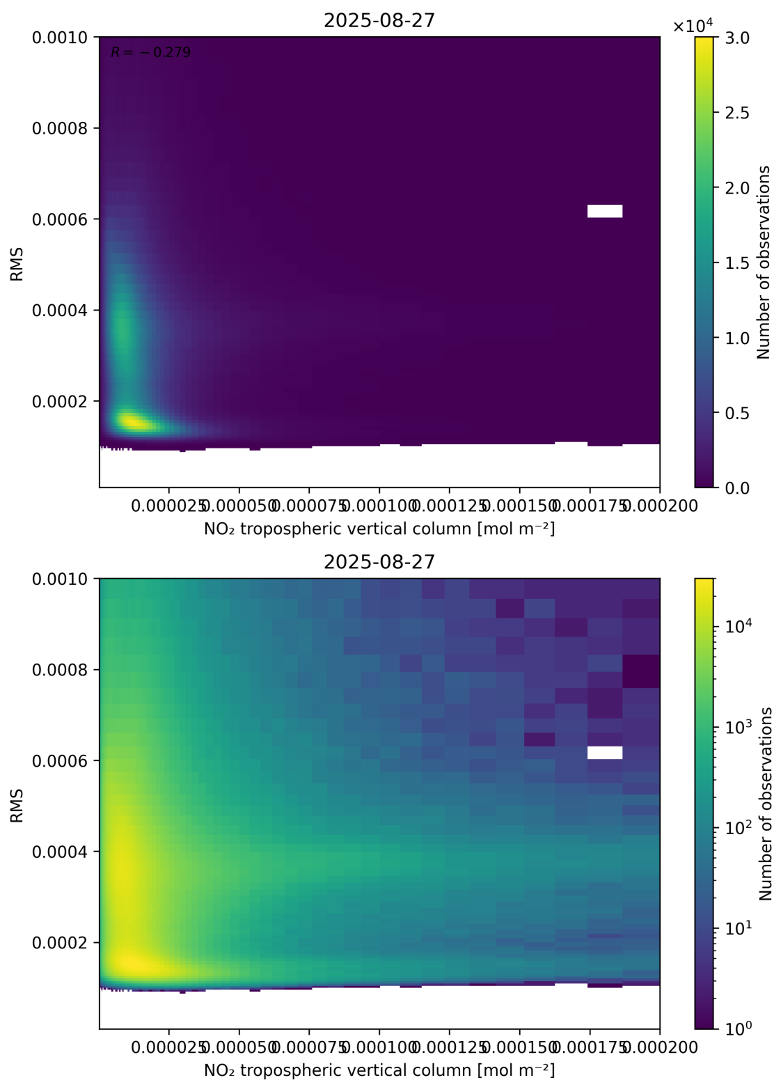
Figure 142: Scatter density plot of “NO 2 tropospheric vertical column” against “RMS” for 2025-08-26 to 2025-08-28.
