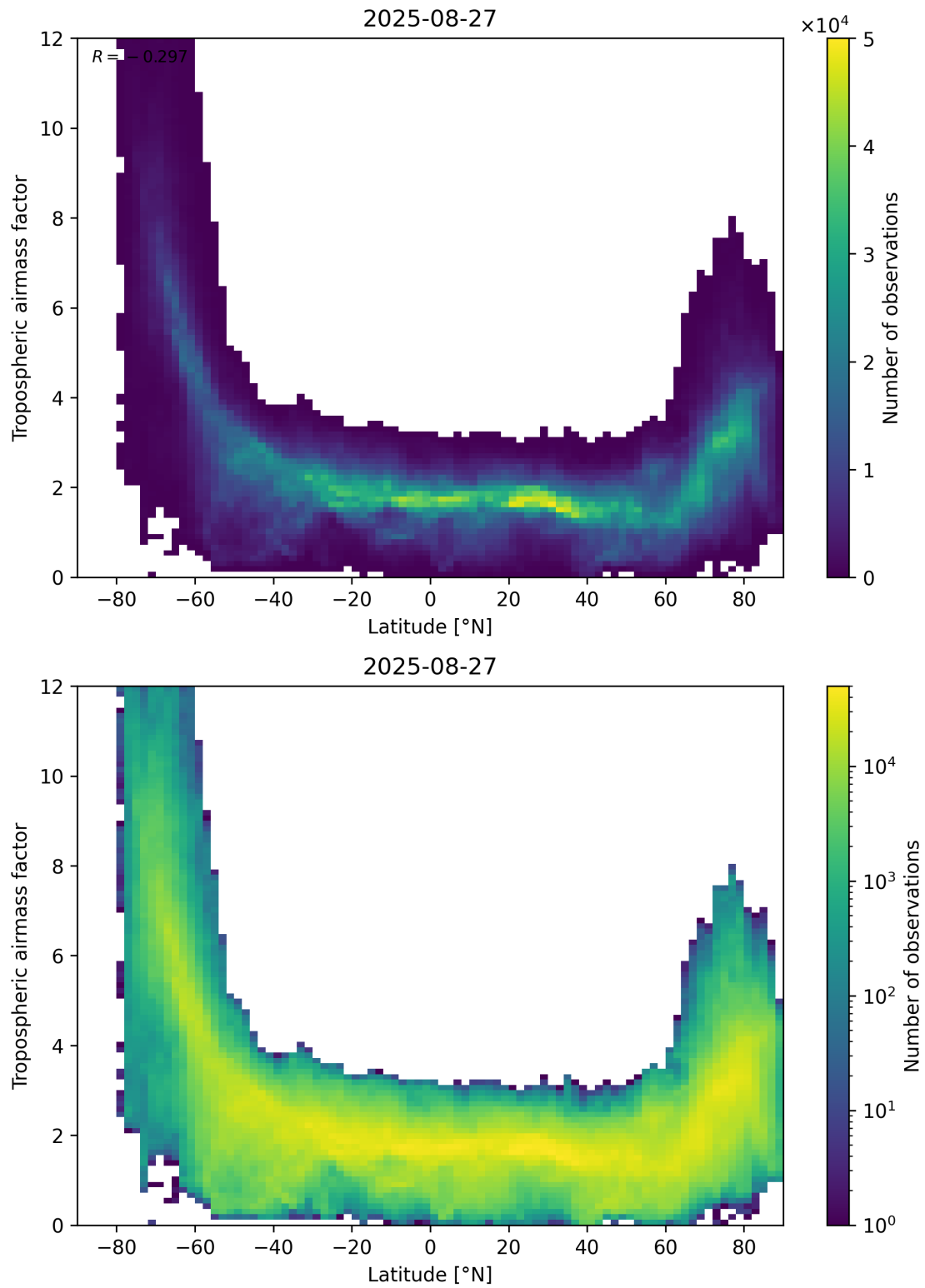
Figure 85: Scatter density plot of “Latitude” against “Tropospheric airmass factor” for 2025-08-26 to 2025-08-28.
