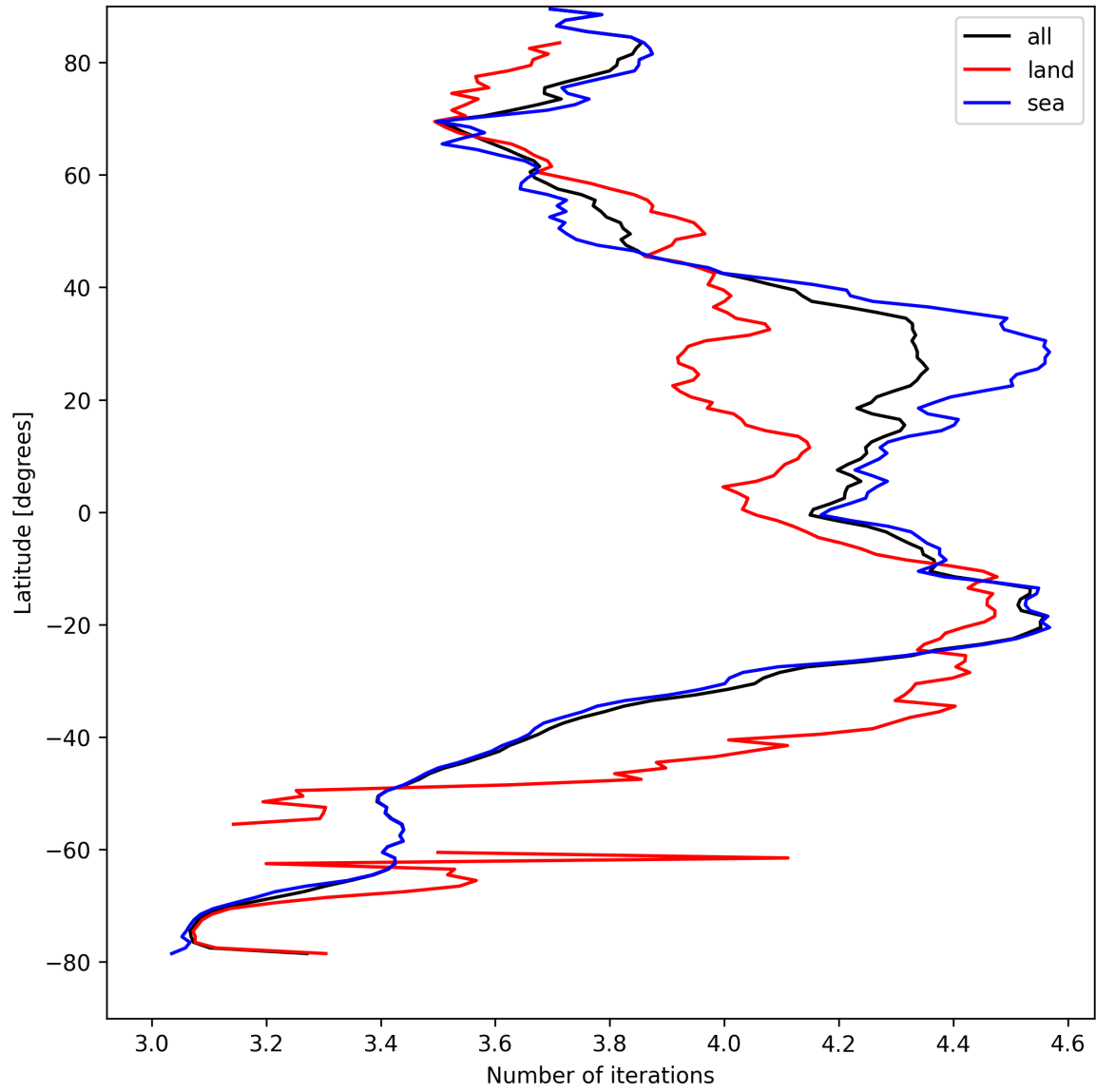
Figure 17: Zonal average of “Number of iterations” for 2025-08-26 to 2025-08-28.
