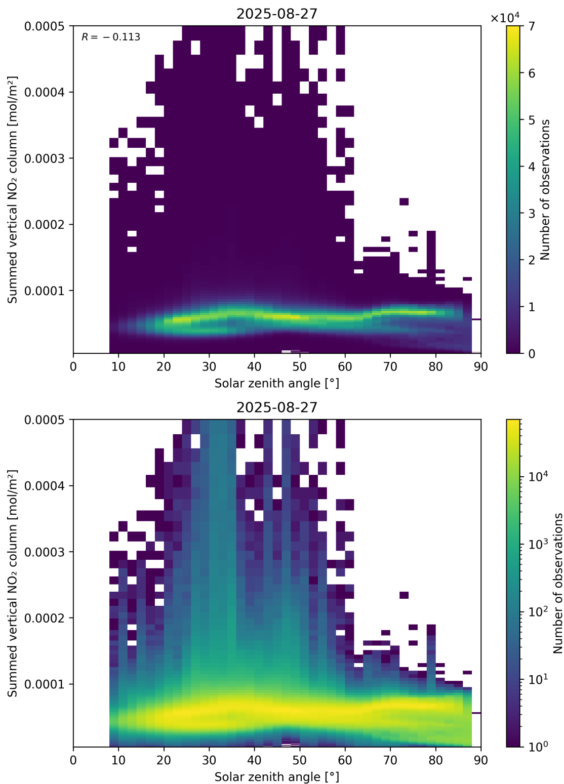
Figure 151: Scatter density plot of “Solar zenith angle” against “Summed vertical NO 2 column” for 2025-08-26 to 2025-08-28.
