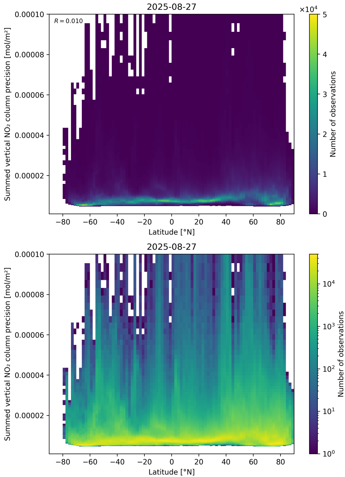
Figure 89: Scatter density plot of “Latitude” against “Summed vertical NO 2 column precision” for 2025-08-26 to 2025-08-28.
