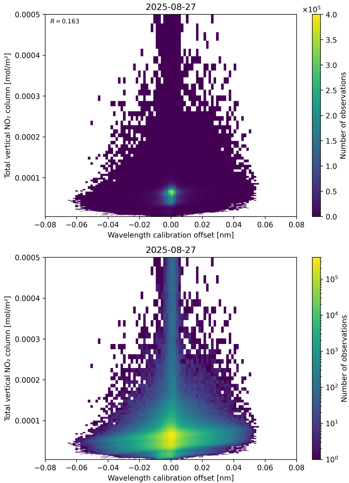
Figure 179: Scatter density plot of “Wavelength calibration offset” against “Total vertical NO 2 column” for 2025-08-26 to 2025-08-28.
