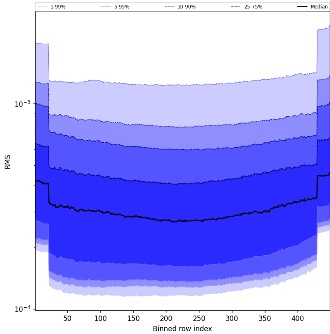
Figure 60: Along track statistics of “RMS” for 2025-08-26 to 2025-08-28
