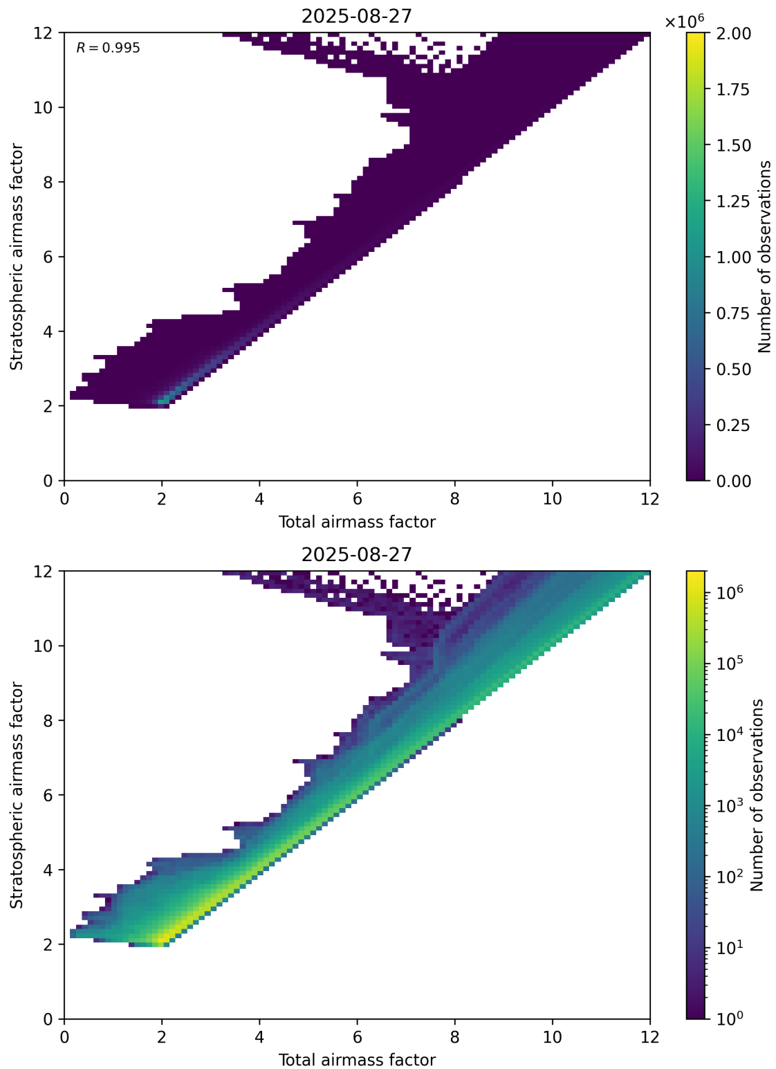
Figure 62: Scatter density plot of “Total airmass factor” against “Stratospheric airmass factor” for 2025-08-26 to 2025-08-28.
