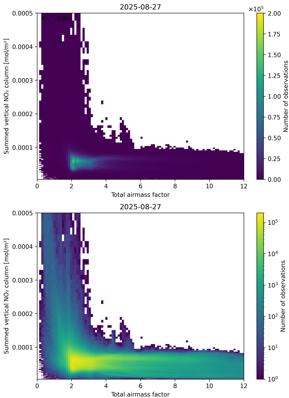
Figure 65: Scatter density plot of “Total airmass factor” against “Summed vertical NO 2 column” for 2025-08-26 to 2025-08-28.
