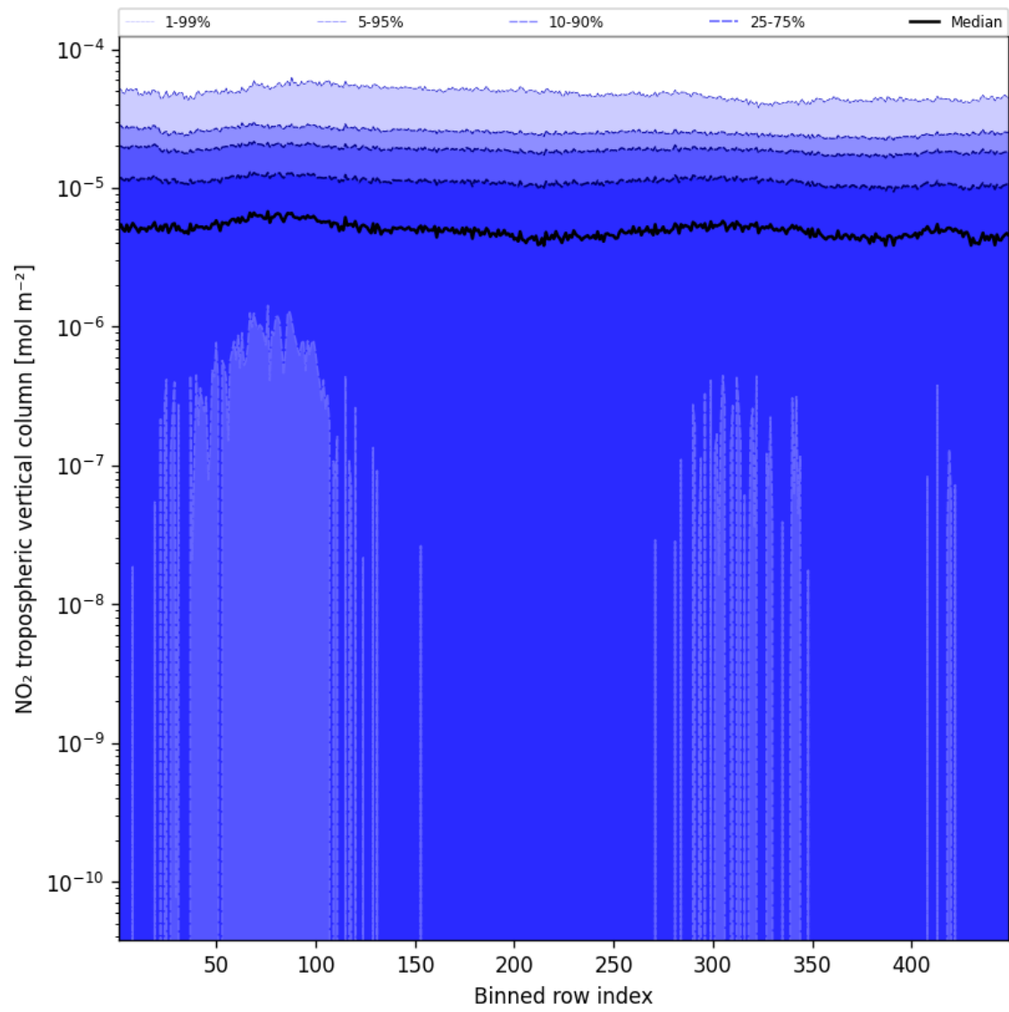
Figure 46: Along track statistics of “NO 2 tropospheric vertical column” for 2025-08-26 to 2025-08-28
