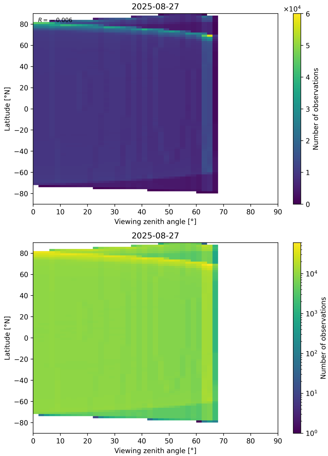
Figure 163: Scatter density plot of “Viewing zenith angle” against “Latitude” for 2025-08-26 to 2025-08-28.
