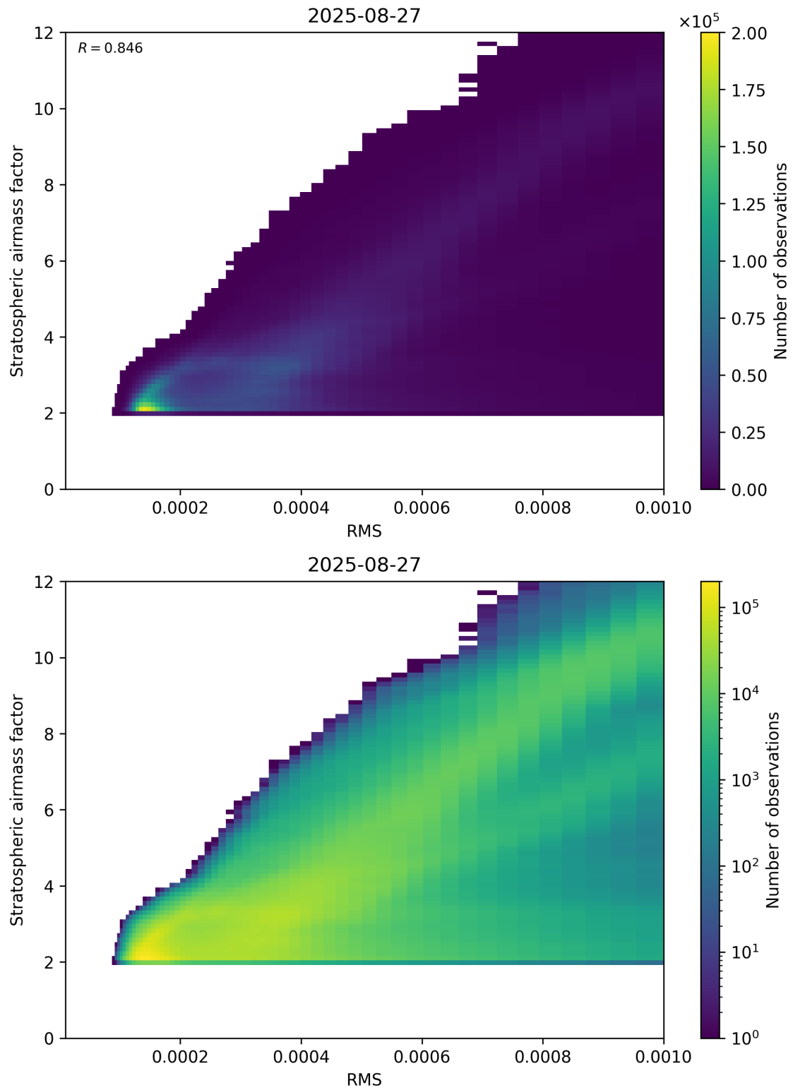
Figure 144: Scatter density plot of “RMS” against “Stratospheric airmass factor” for 2025-08-26 to 2025-08-28.
