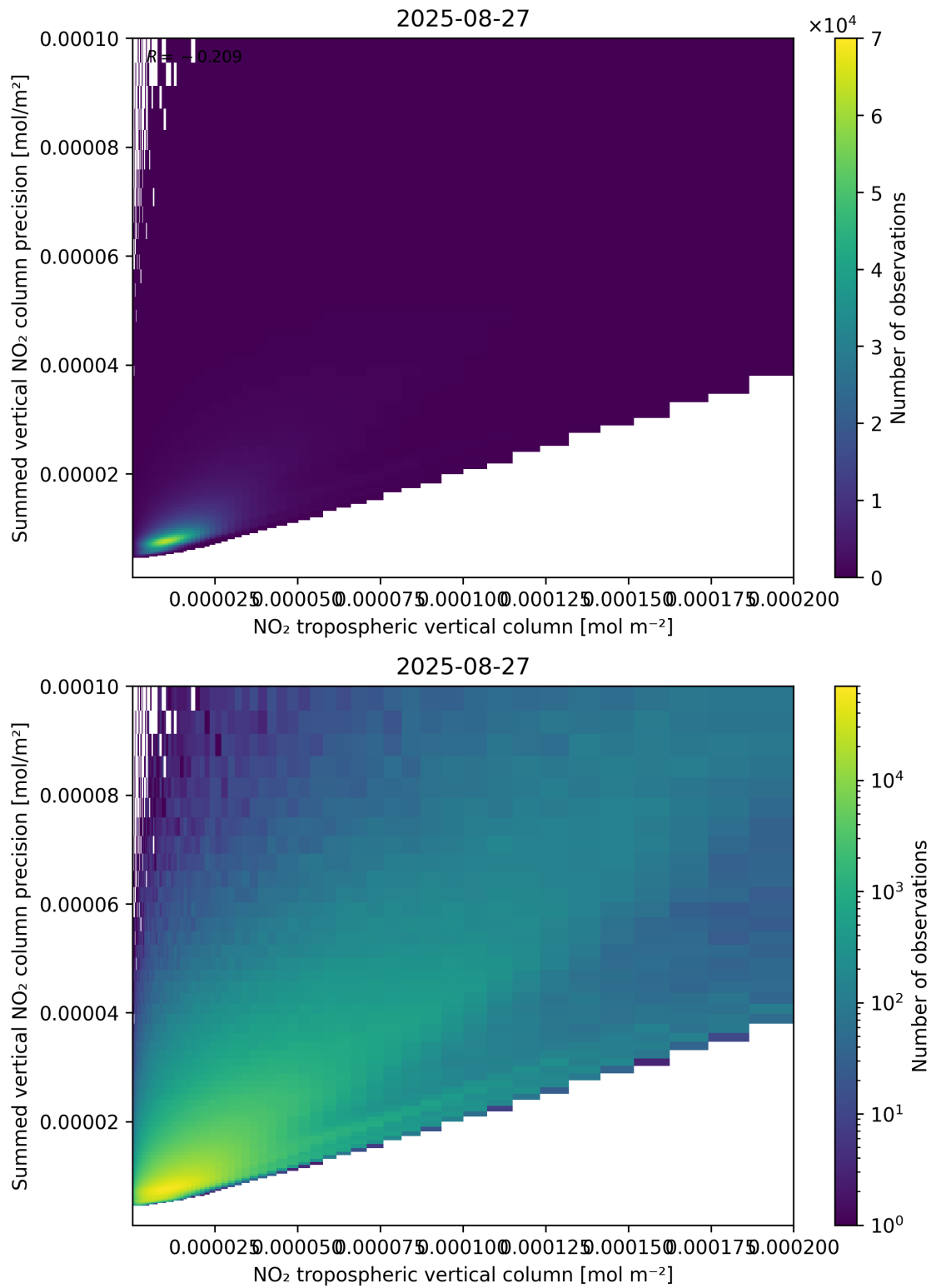
Figure 127: Scatter density plot of “NO 2 tropospheric vertical column” against “Summed vertical NO 2 column precision” for 2025-08-26 to 2025-08-28.
