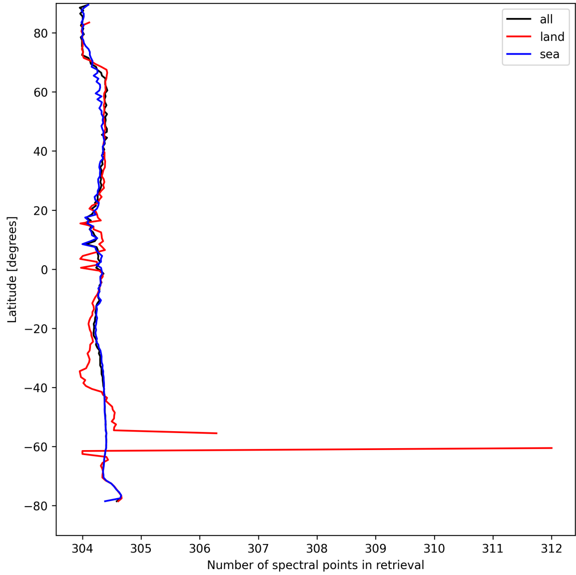
Figure 16: Zonal average of “Number of spectral points in retrieval” for 2025-08-26 to 2025-08-28.
