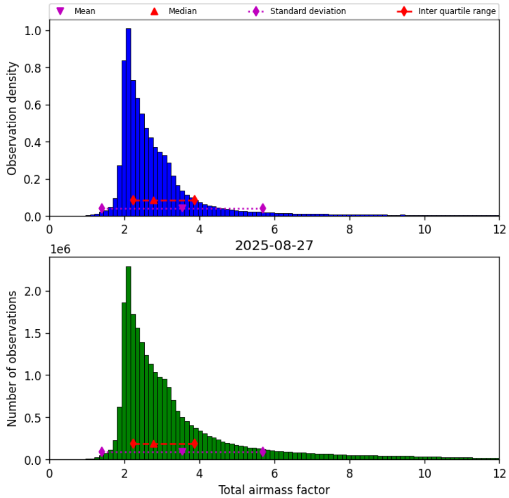
Figure 32: Histogram of “Total airmass factor” for 2025-08-26 to 2025-08-28
