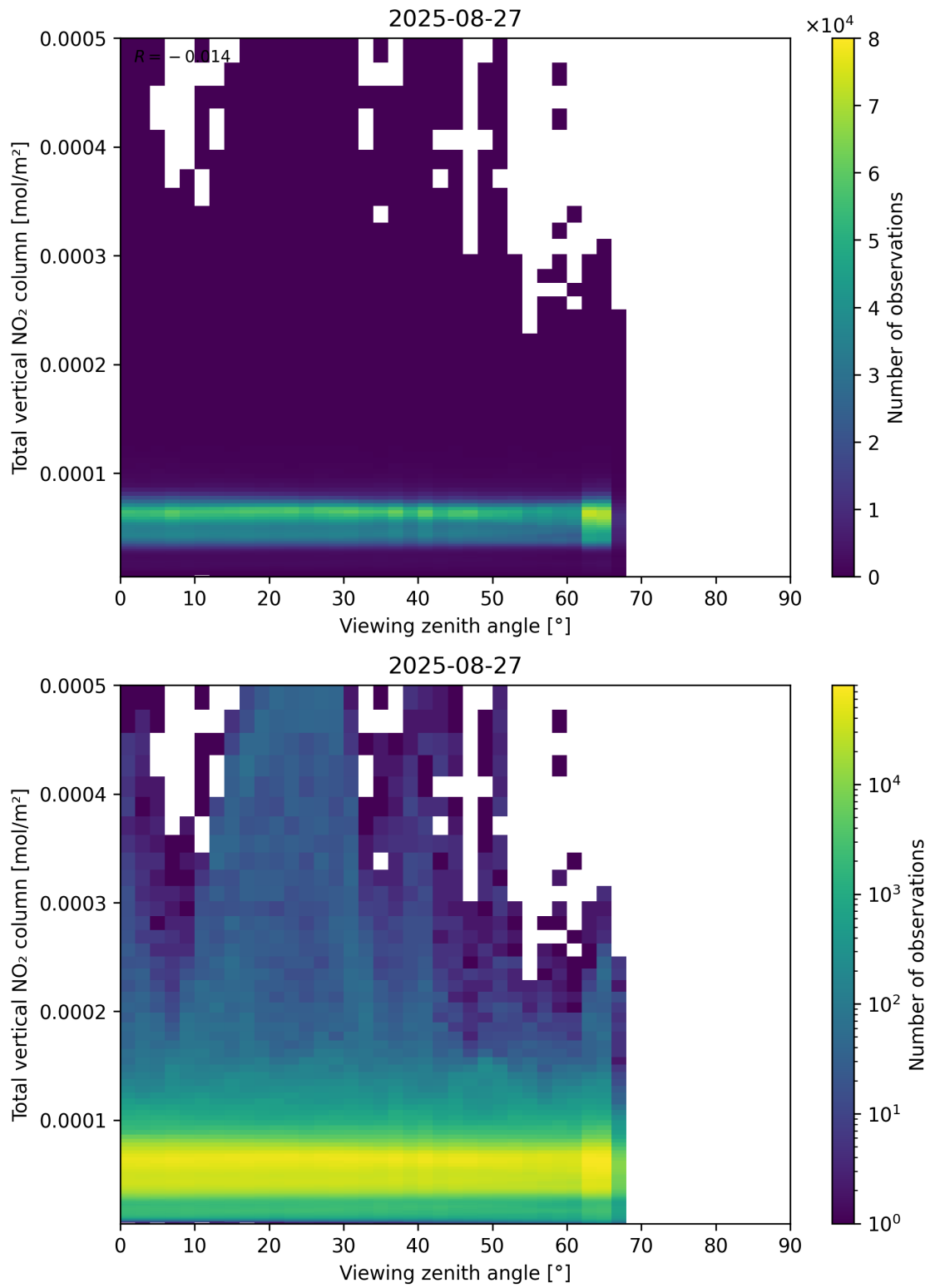
Figure 167: Scatter density plot of “Viewing zenith angle” against “Total vertical NO 2 column” for 2025-08-26 to 2025-08-28.
