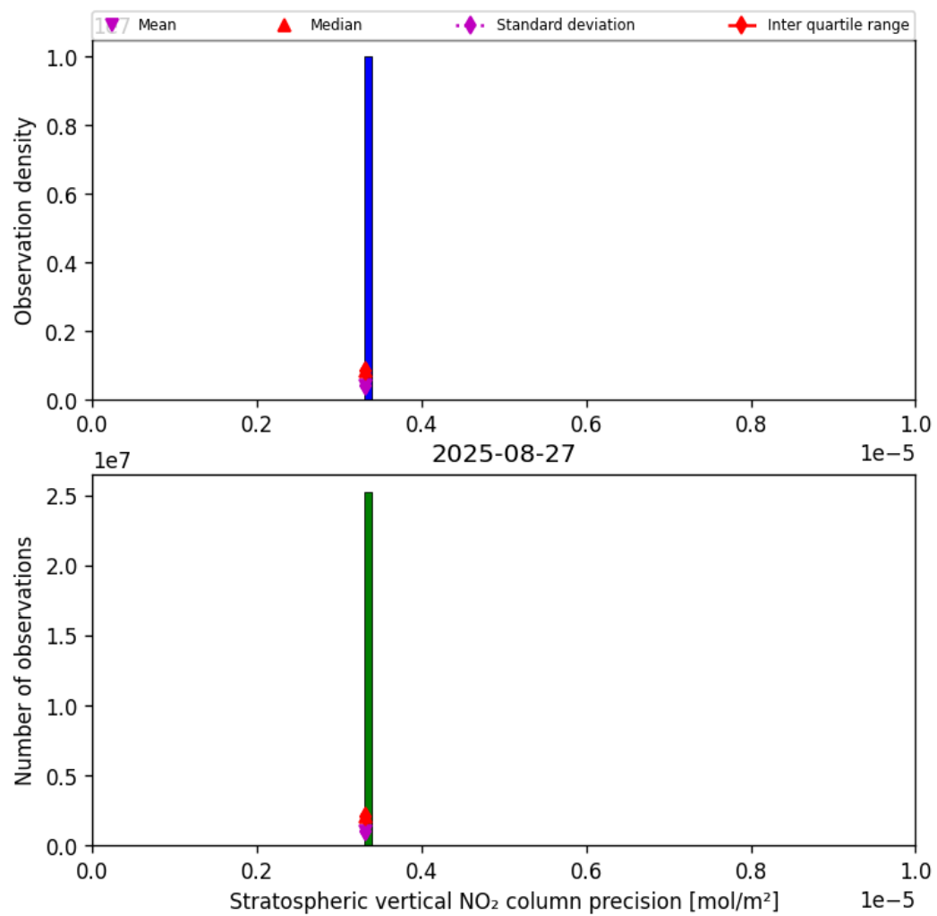
Figure 37: Histogram of “Stratospheric vertical NO 2 column precision” for 2025-08-26 to 2025-08-28
