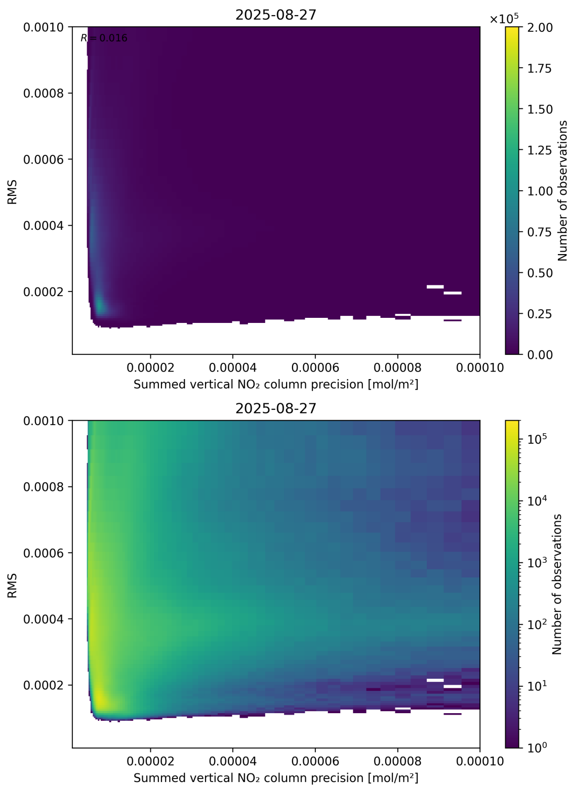
Figure 108: Scatter density plot of “Summed vertical NO 2 column precision” against “RMS” for 2025-08-26 to 2025-08-28.
