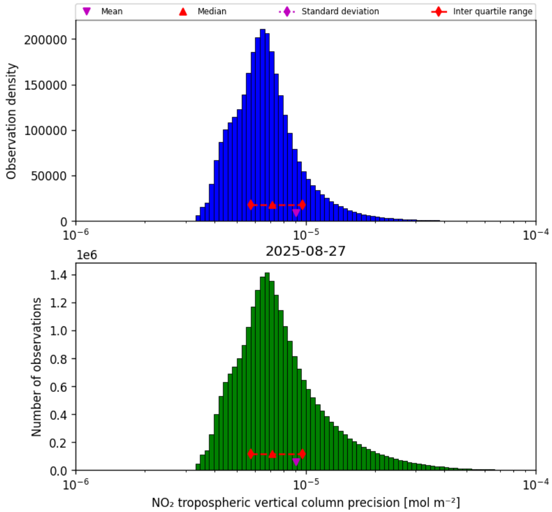
Figure 30: Histogram of “NO 2 tropospheric vertical column precision” for 2025-08-26 to 2025-08-28
