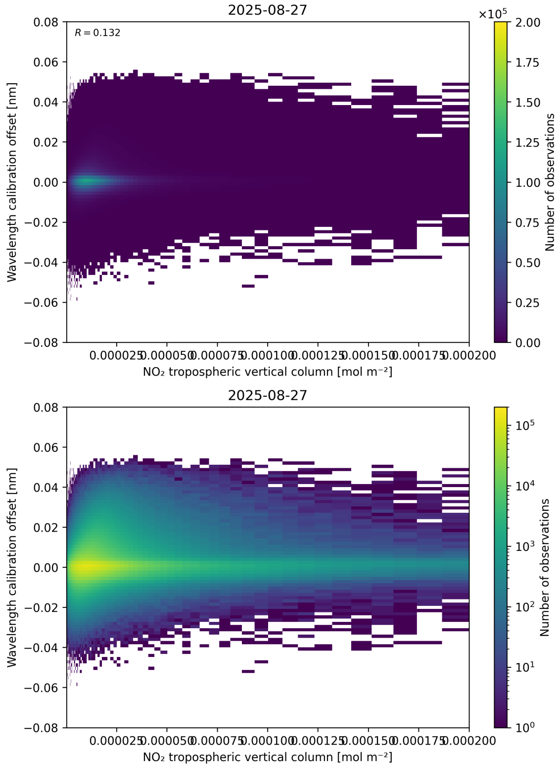
Figure 143: Scatter density plot of “NO 2 tropospheric vertical column” against “Wavelength calibration offset” for 2025-08-26 to 2025-08-28.
