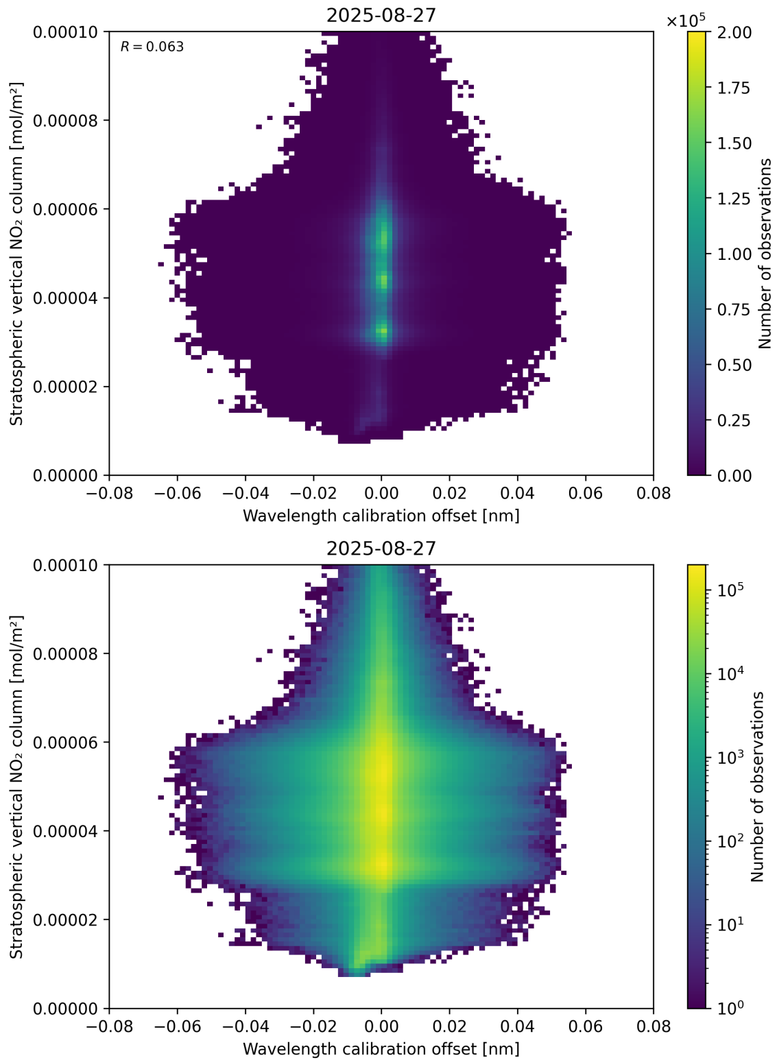
Figure 176: Scatter density plot of “Wavelength calibration offset” against “Stratospheric vertical NO 2 column” for 2025-08-26 to 2025-08-28.
