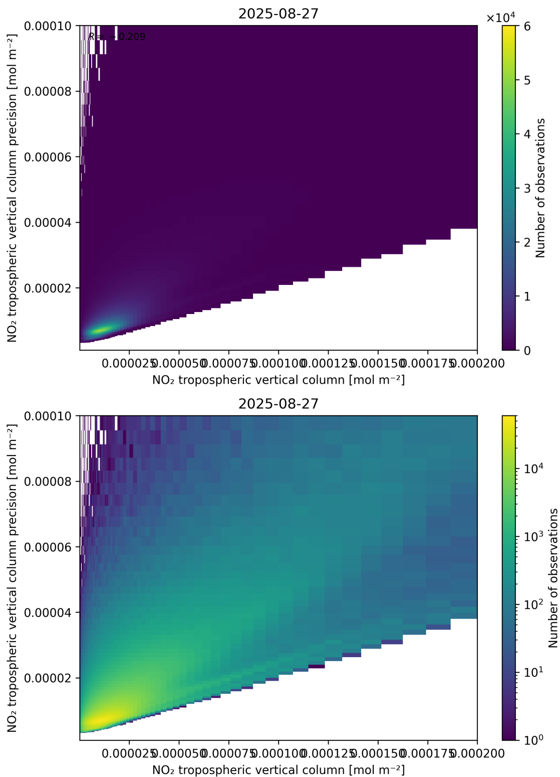
Figure 130: Scatter density plot of “NO 2 tropospheric vertical column” against “NO 2 tropospheric vertical column precision” for 2025-08-26 to 2025-08-28.
