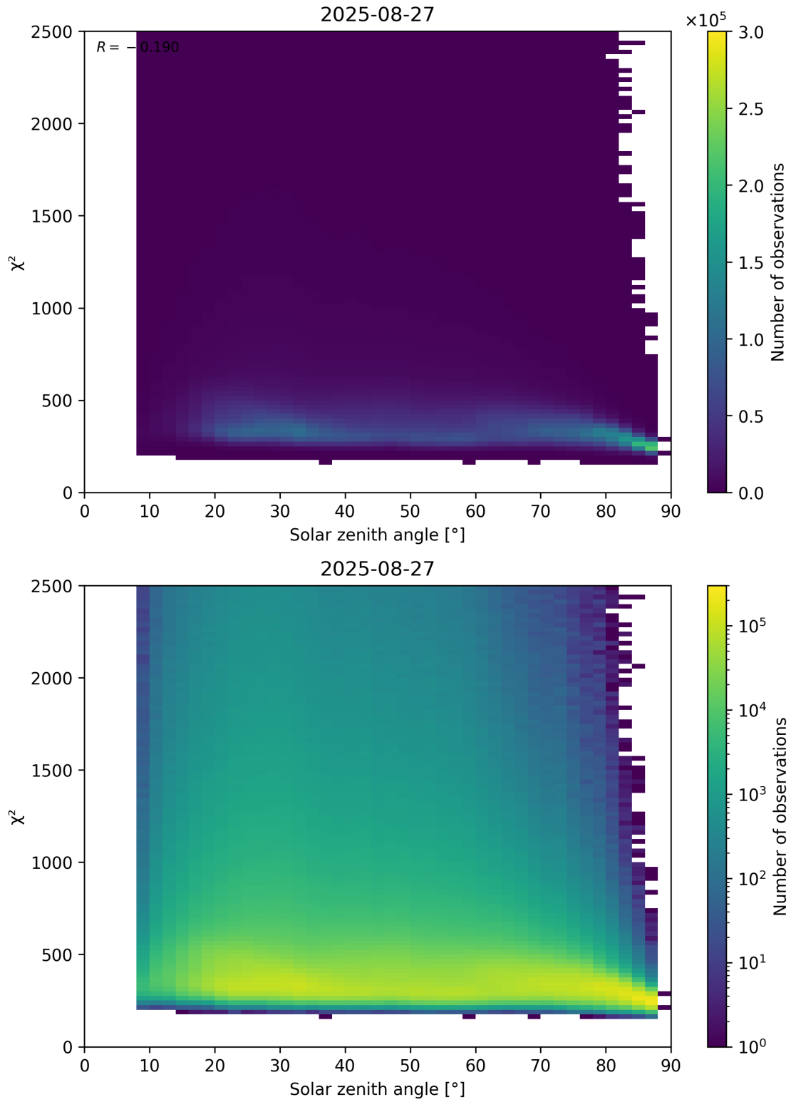
Figure 148: Scatter density plot of “Solar zenith angle” against “ \chi^2 ” for 2025-08-26 to 2025-08-28.
