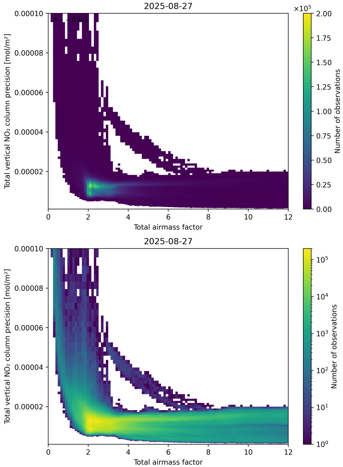
Figure 68: Scatter density plot of “Total airmass factor” against “Total vertical NO 2 column precision” for 2025-08-26 to 2025-08-28.
