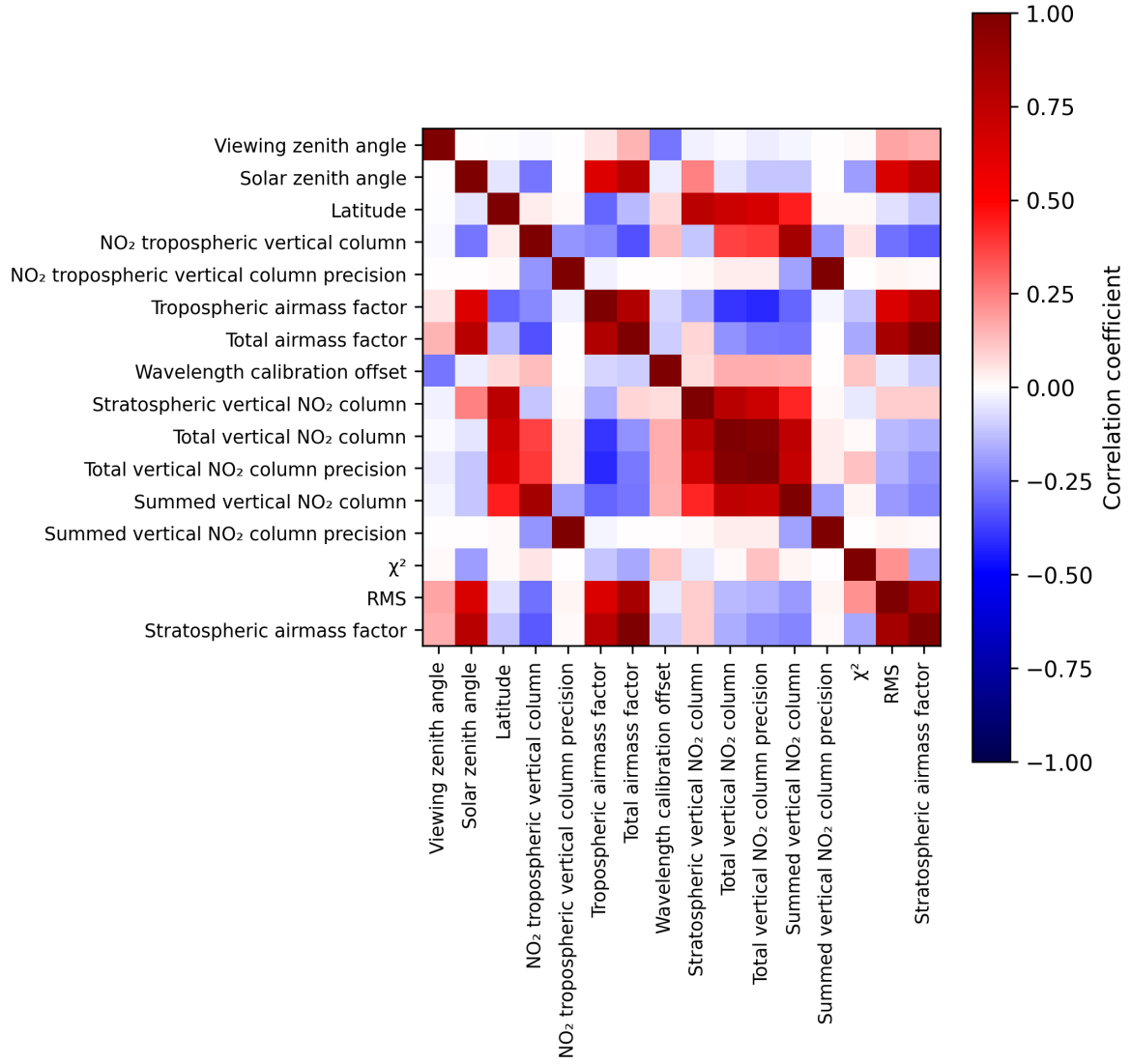
Figure 2: Map of correlation matrix for 2025-08-26 to 2025-08-28.
