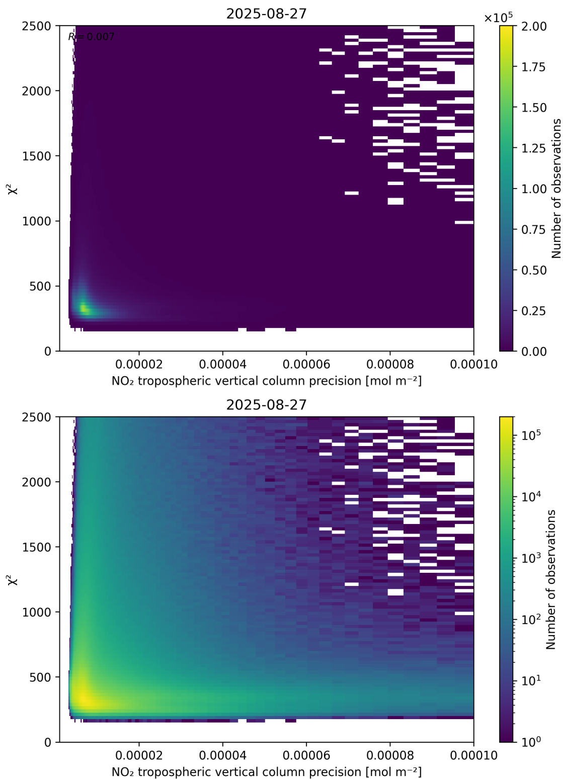
Figure 134: Scatter density plot of “NO 2 tropospheric vertical column precision” against “ \chi^2 ” for 2025-08-26 to 2025-08-28.
