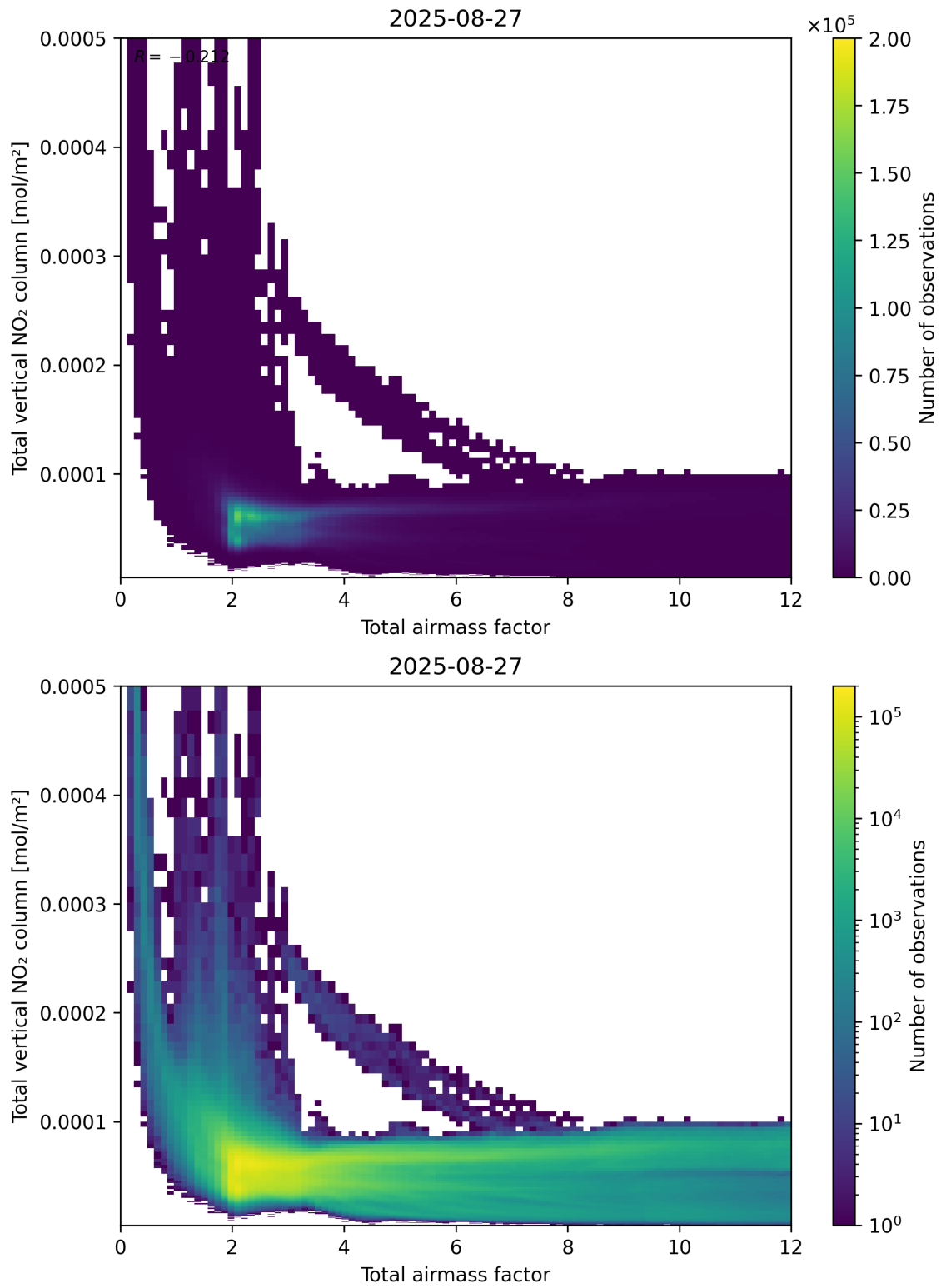
Figure 67: Scatter density plot of “Total airmass factor” against “Total vertical NO 2 column” for 2025-08-26 to 2025-08-28.
