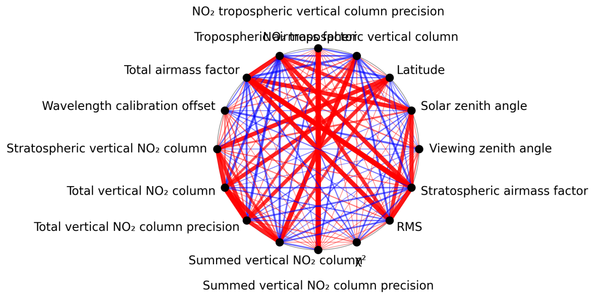
Figure 1: Map of correlation graph for 2025-08-26 to 2025-08-28.
