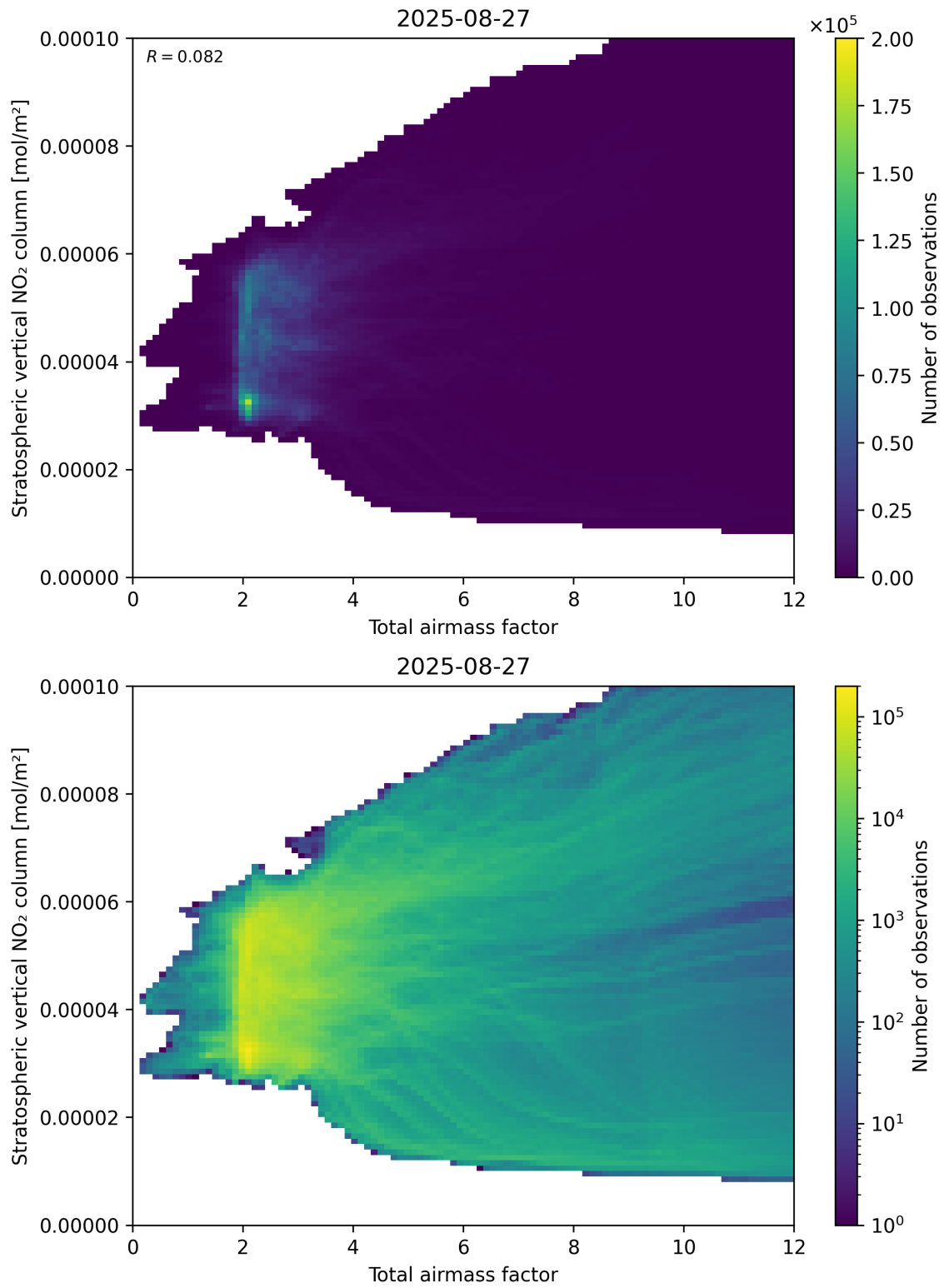
Figure 64: Scatter density plot of “Total airmass factor” against “Stratospheric vertical \text{NO}_2 column” for 2025-08-26 to 2025-08-28.
