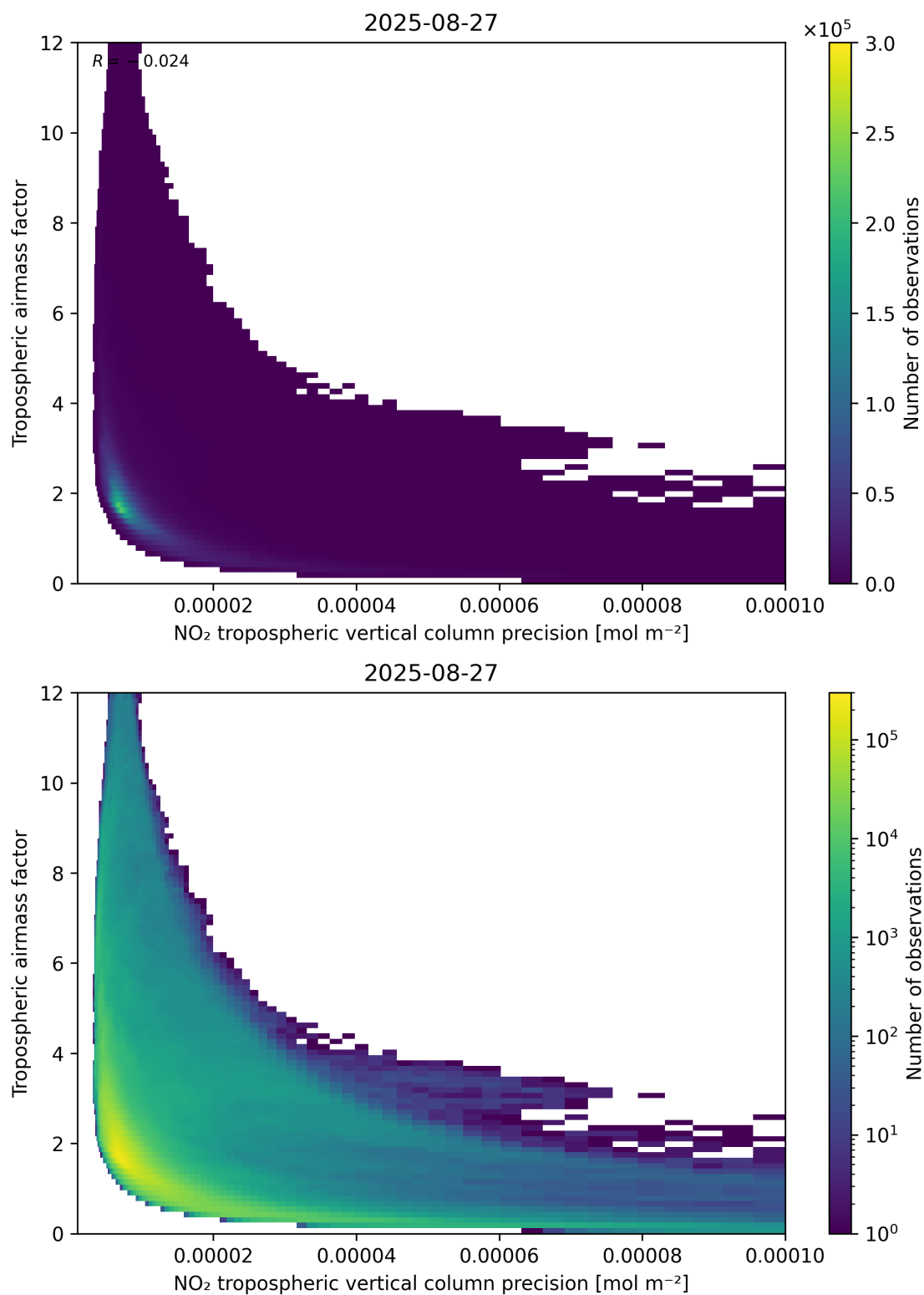
Figure 133: Scatter density plot of “NO 2 tropospheric vertical column precision” against “Tropospheric airmass factor” for 2025-08-26 to 2025-08-28.
