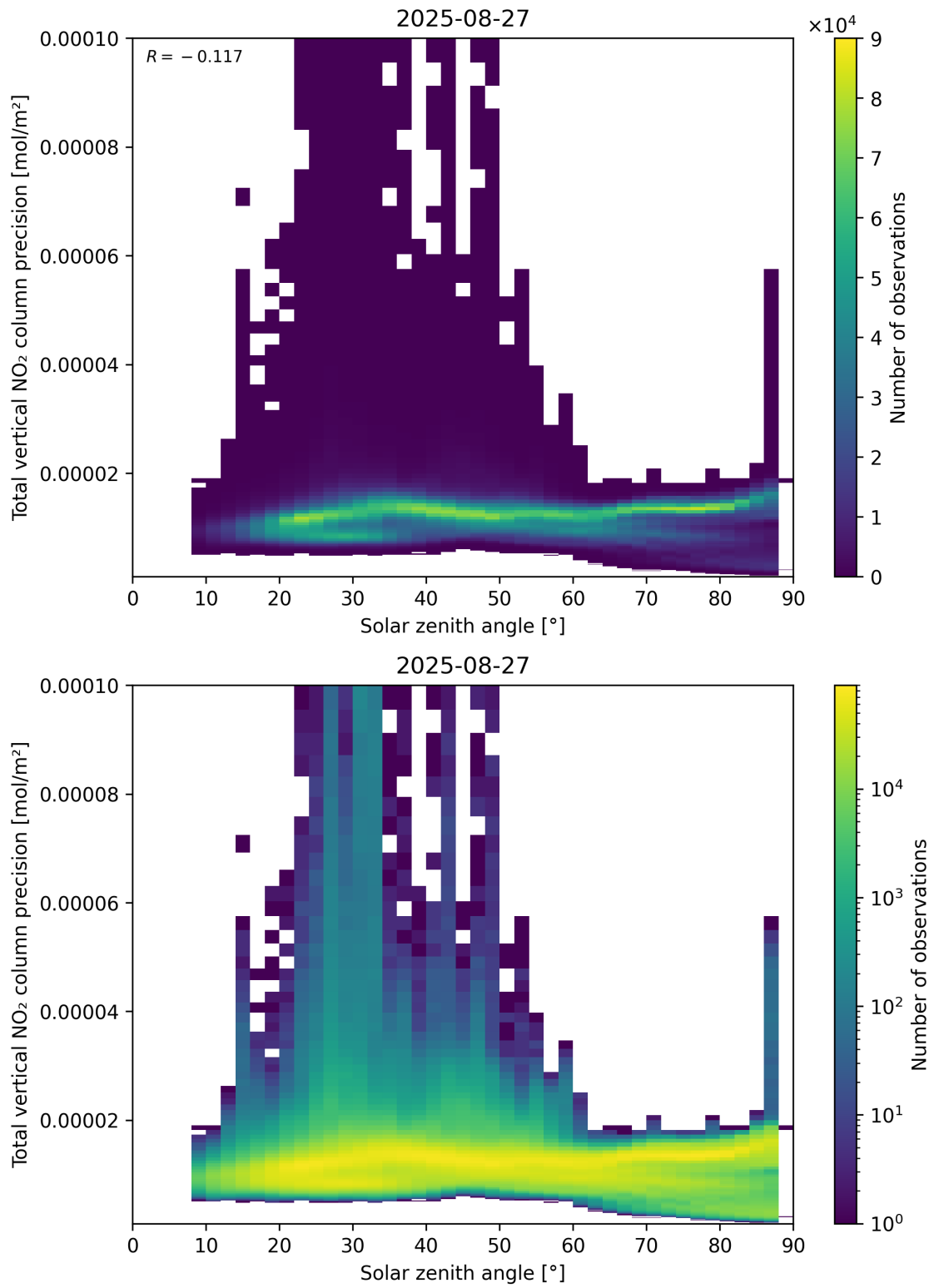
Figure 154: Scatter density plot of “Solar zenith angle” against “Total vertical NO 2 column precision” for 2025-08-26 to 2025-08-28.
