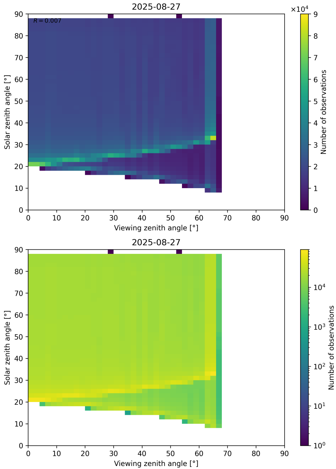
Figure 172: Scatter density plot of “Viewing zenith angle” against “Solar zenith angle” for 2025-08-26 to 2025-08-28.
