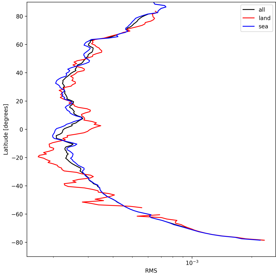
Figure 26: Zonal average of “RMS” for 2025-08-26 to 2025-08-28.
