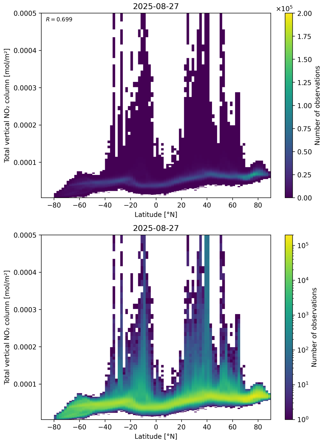
Figure 90: Scatter density plot of “Latitude” against “Total vertical NO 2 column” for 2025-08-26 to 2025-08-28.
