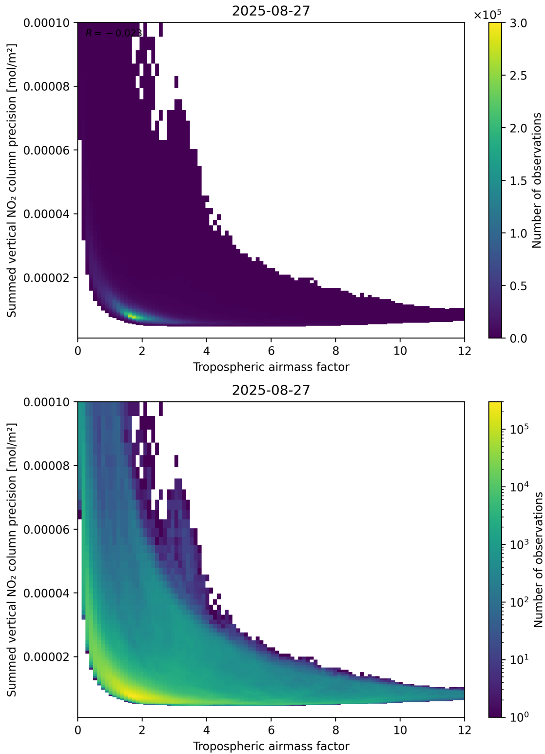
Figure 76: Scatter density plot of “Tropospheric air mass factor” against “Summed vertical NO 2 column precision” for 2025-08-26 to 2025-08-28.
