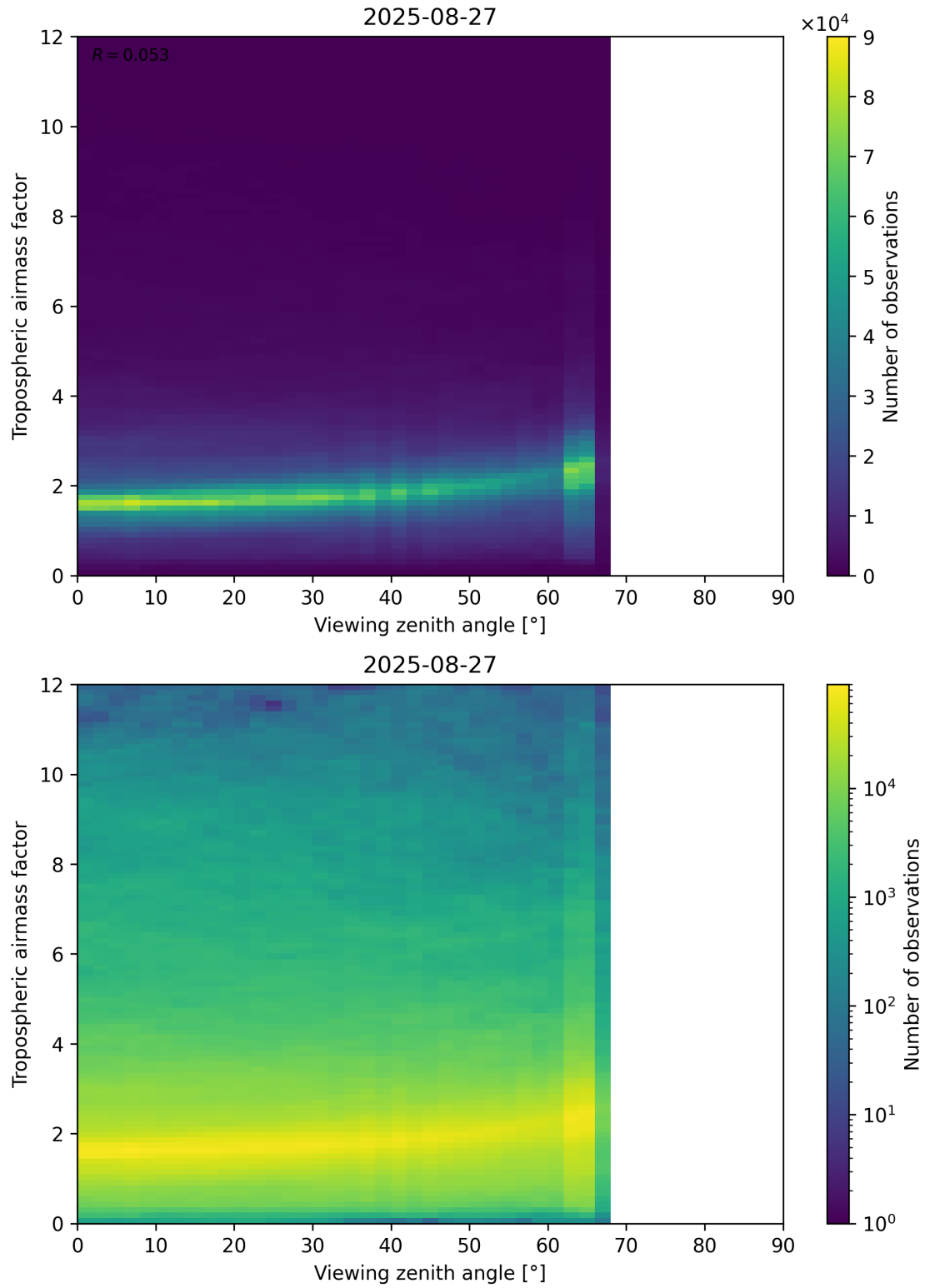
Figure 161: Scatter density plot of “Viewing zenith angle” against “Tropospheric airmass factor” for 2025-08-26 to 2025-08-28.
