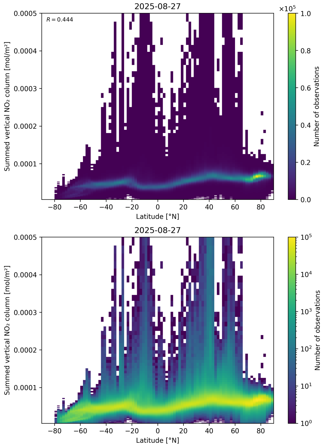
Figure 88: Scatter density plot of “Latitude” against “Summed vertical NO 2 column” for 2025-08-26 to 2025-08-28.
