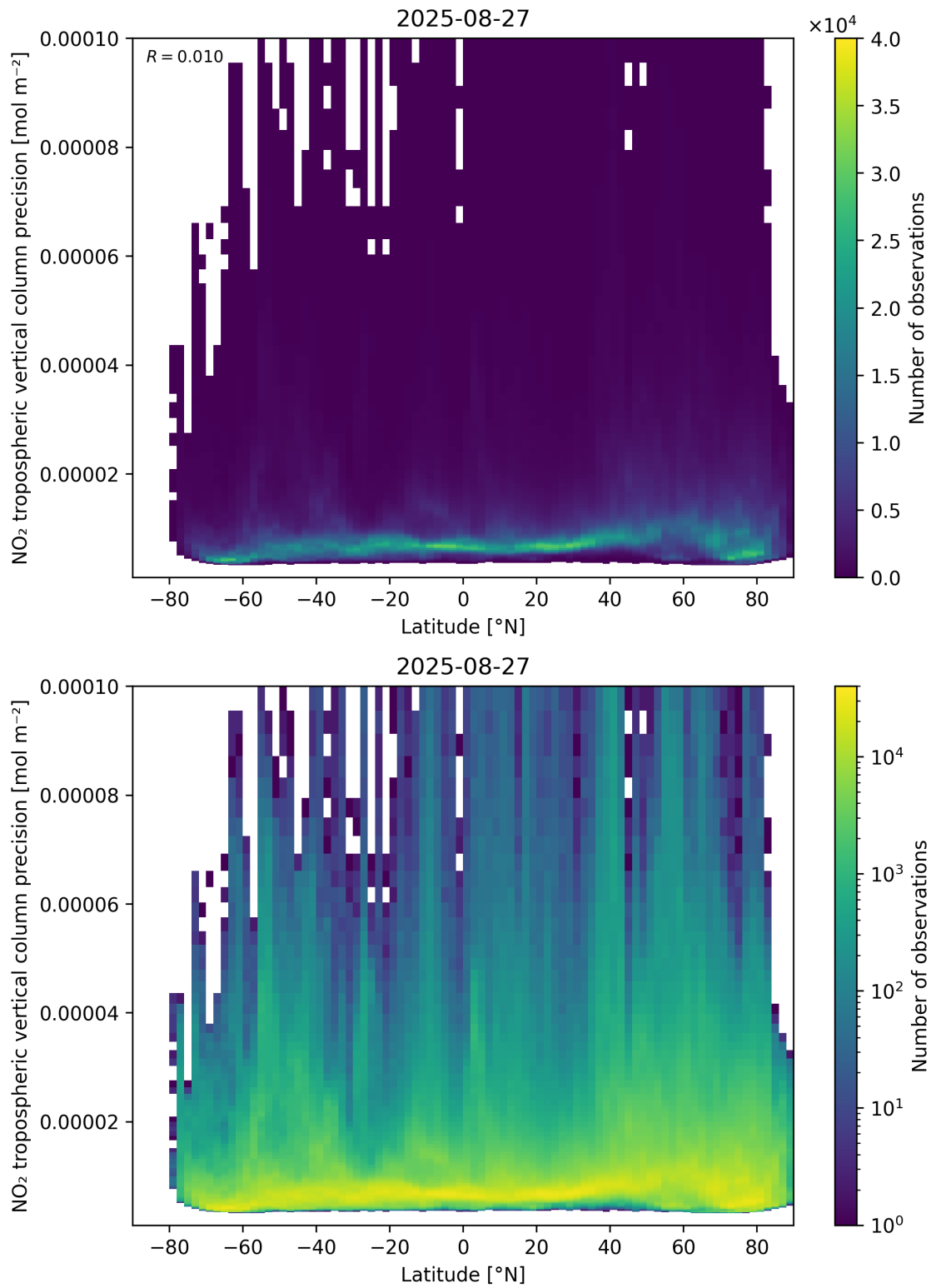
Figure 93: Scatter density plot of “Latitude” against “NO 2 tropospheric vertical column precision” for 2025-08-26 to 2025-08-28.
