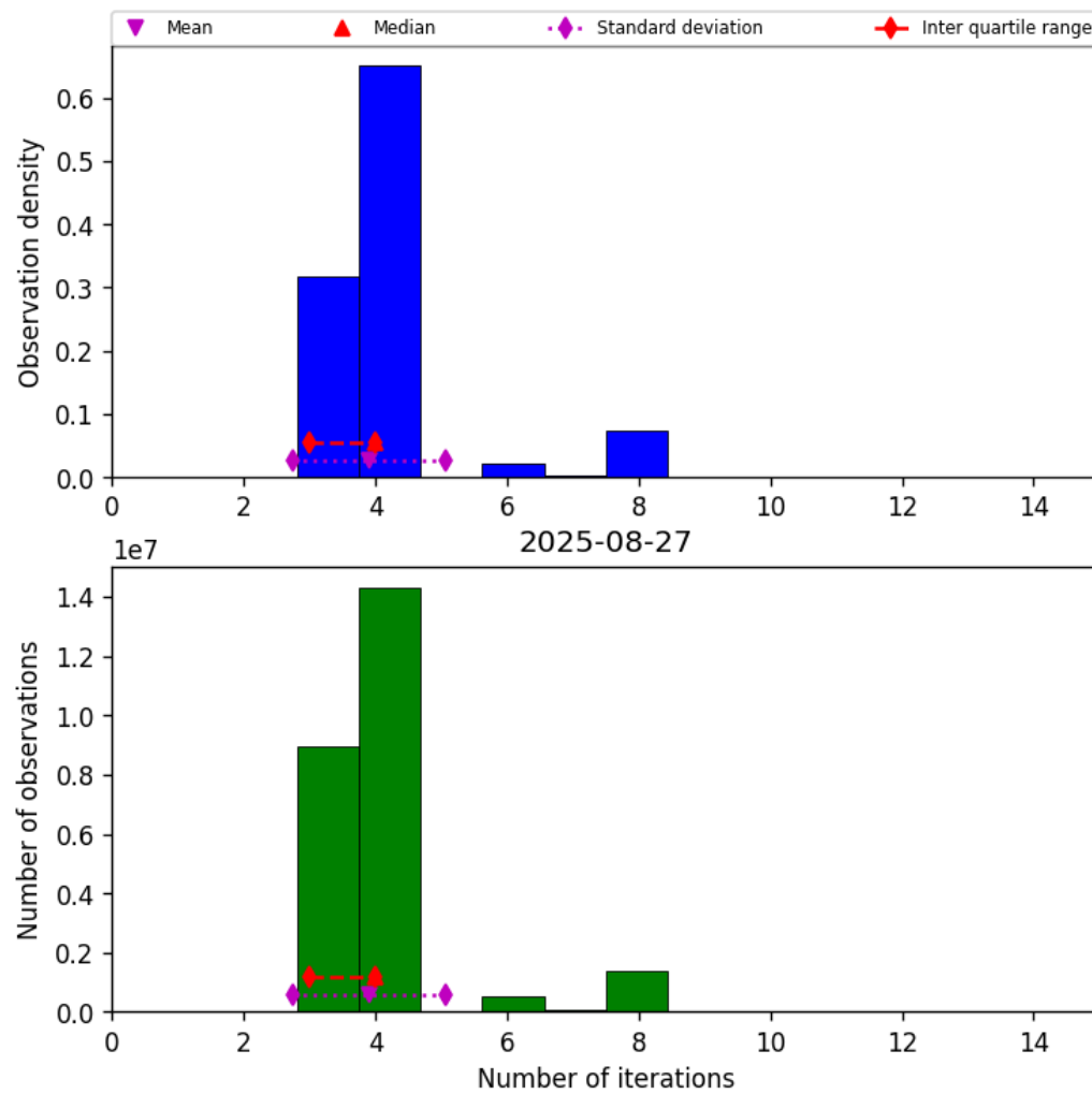
Figure 34: Histogram of “Number of iterations” for 2025-08-26 to 2025-08-28
