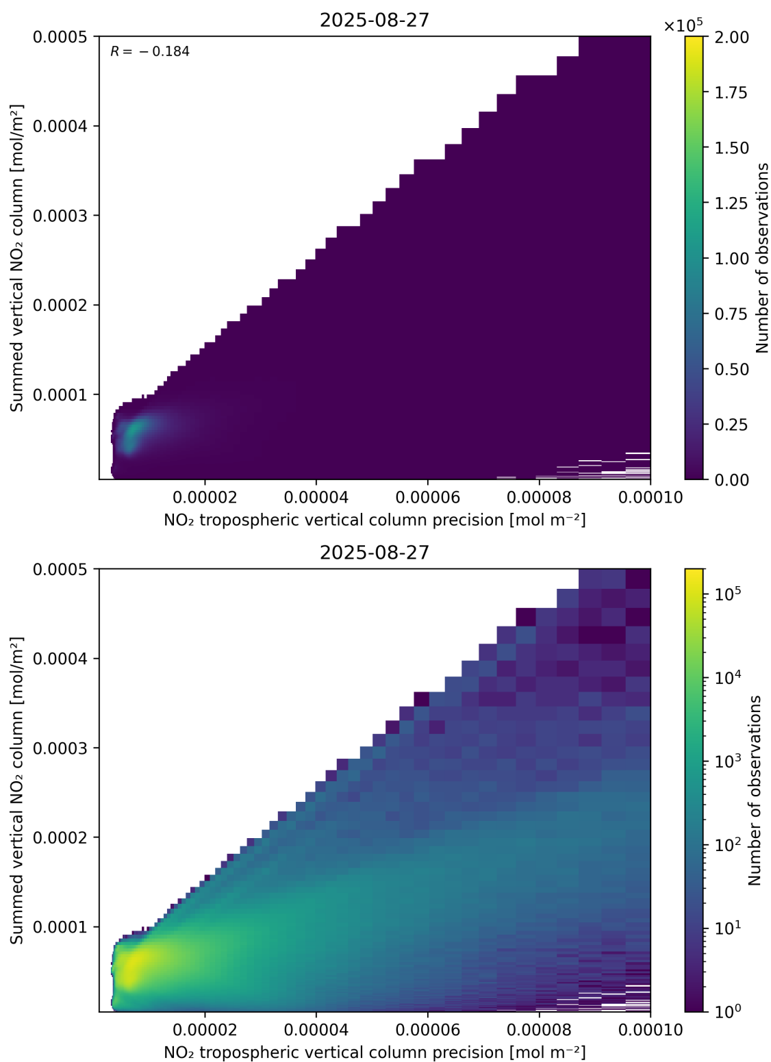
Figure 136: Scatter density plot of “NO 2 tropospheric vertical column precision” against “Summed vertical NO 2 column” for 2025-08-26 to 2025-08-28.
