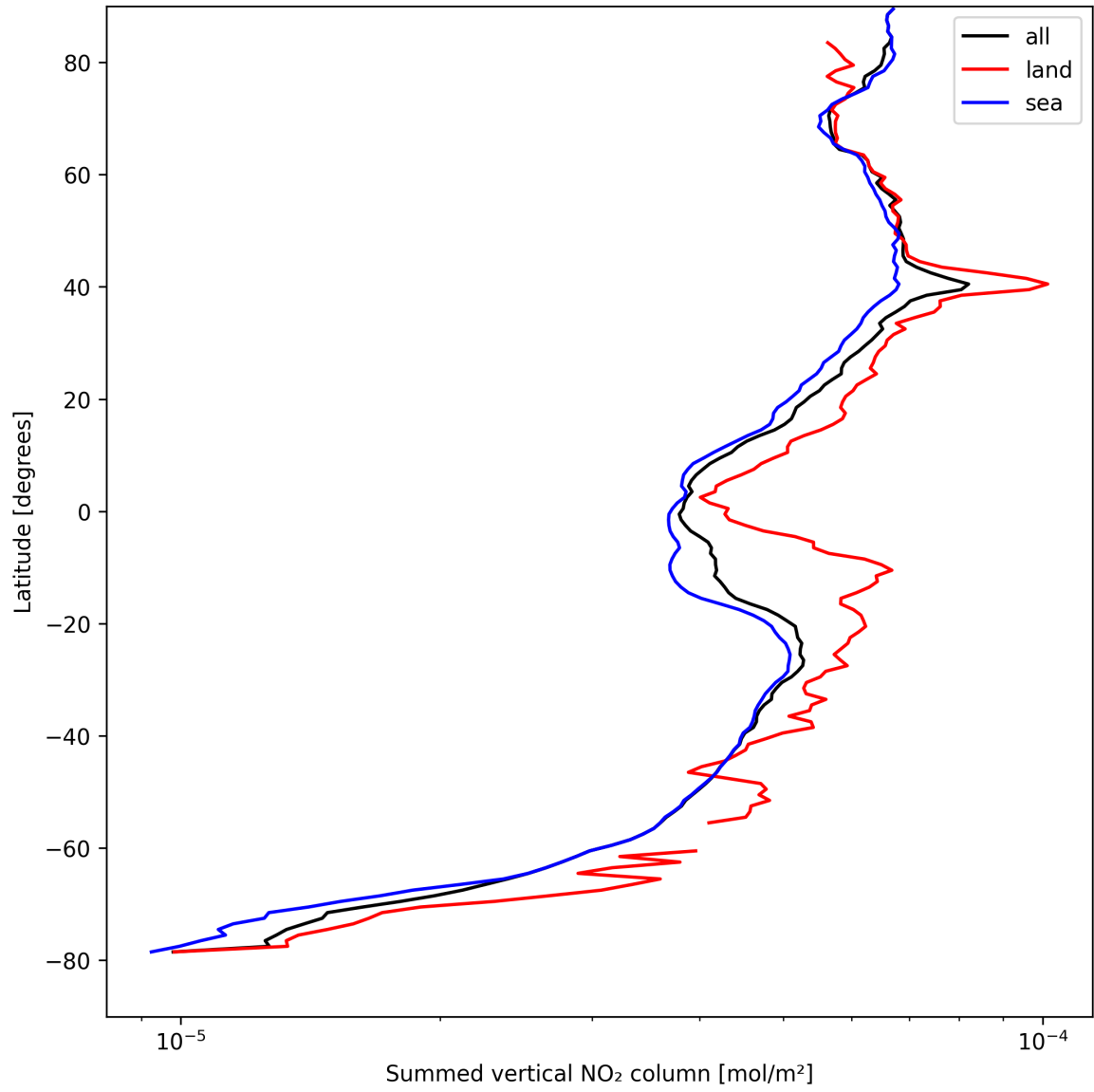
Figure 23: Zonal average of “Summed vertical NO 2 column” for 2025-08-26 to 2025-08-28.
