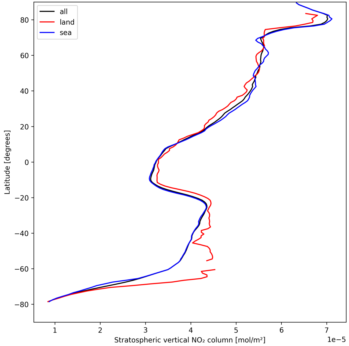
Figure 19: Zonal average of “Stratospheric vertical NO 2 column” for 2025-08-26 to 2025-08-28.
