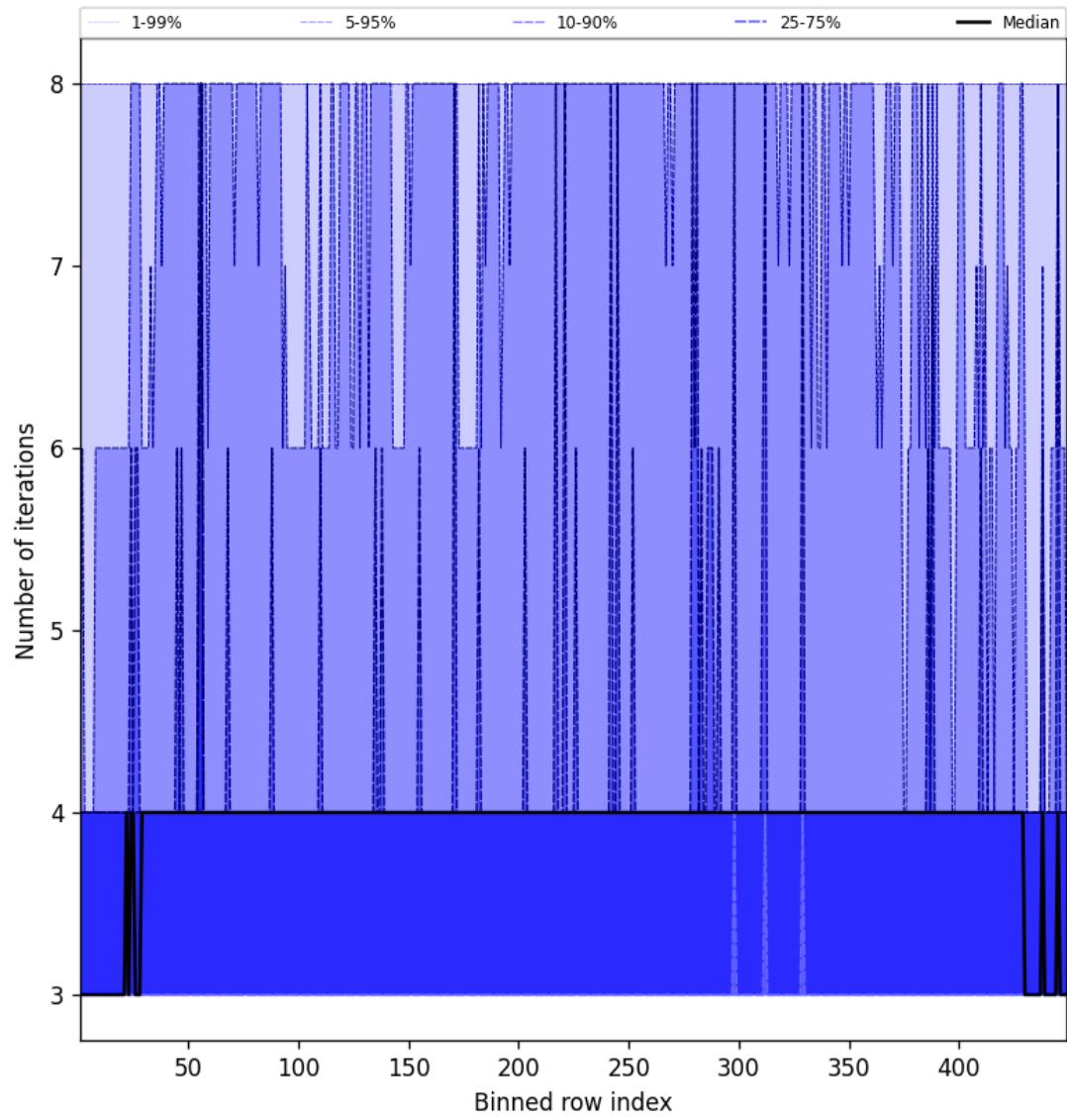
Figure 51: Along track statistics of “Number of iterations” for 2025-08-26 to 2025-08-28
