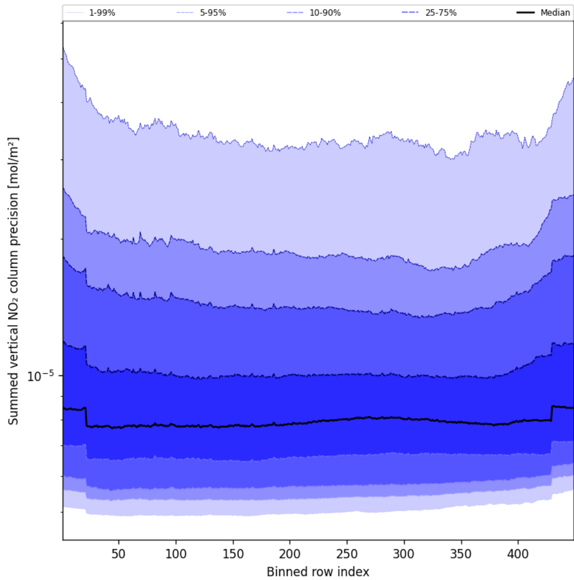
Figure 58: Along track statistics of “Summed vertical NO 2 column precision” for 2025-08-26 to 2025-08-28
