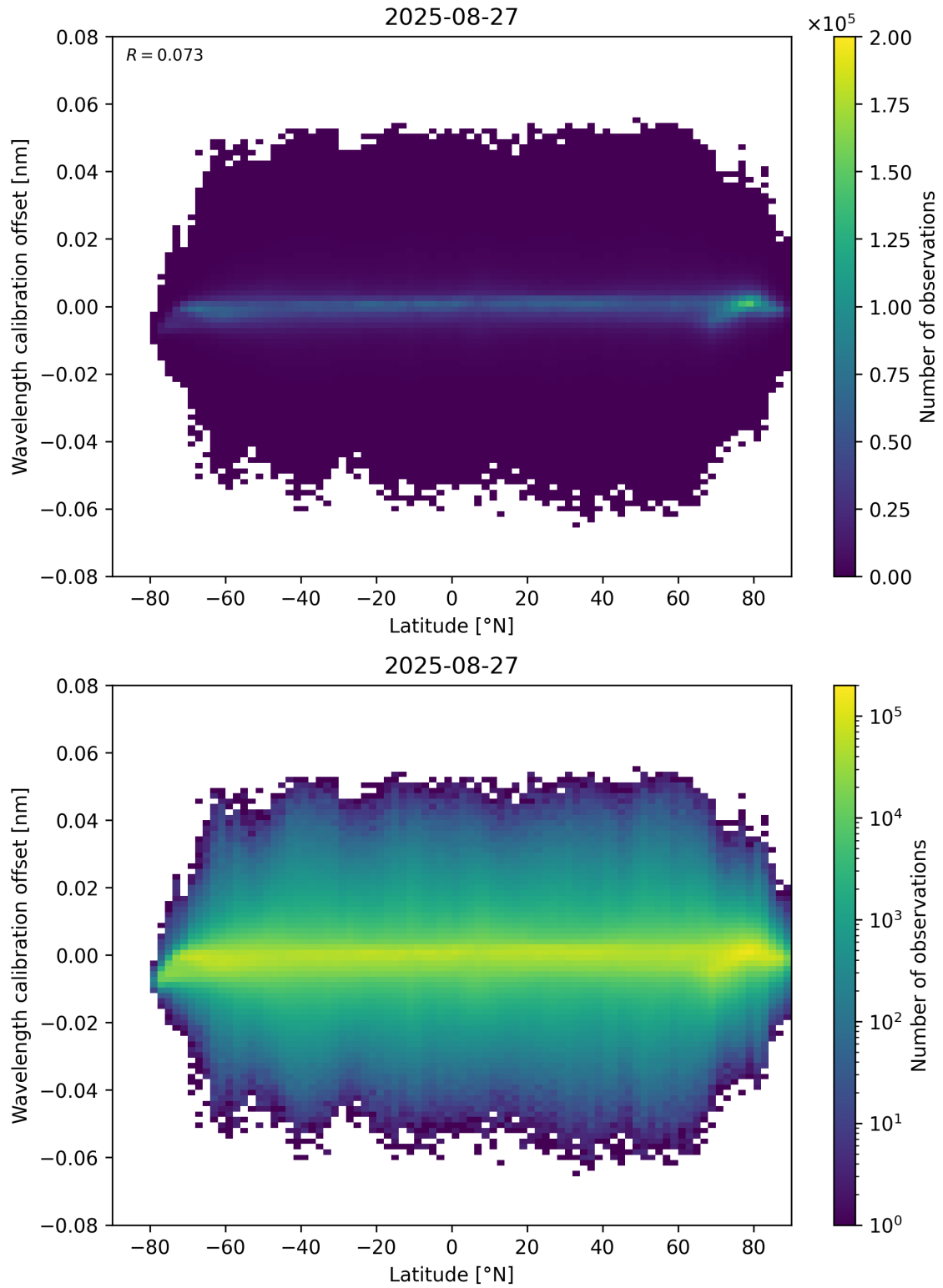
Figure 95: Scatter density plot of “Latitude” against “Wavelength calibration offset” for 2025-08-26 to 2025-08-28.
