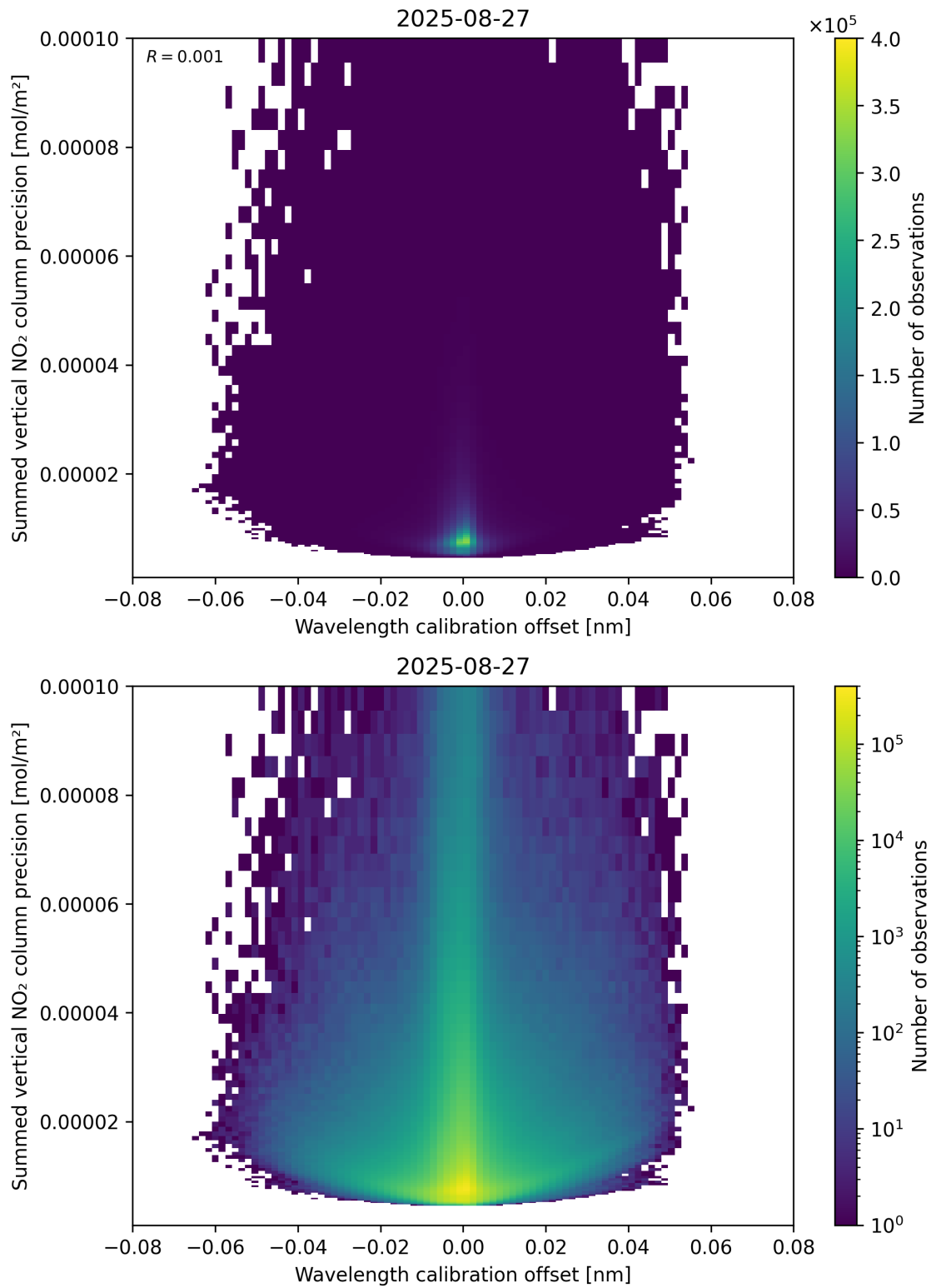
Figure 178: Scatter density plot of “Wavelength calibration offset” against “Summed vertical NO 2 column precision” for 2025-08-26 to 2025-08-28.
