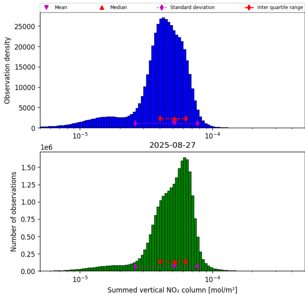
Figure 40: Histogram of “Summed vertical NO 2 column” for 2025-08-26 to 2025-08-28
