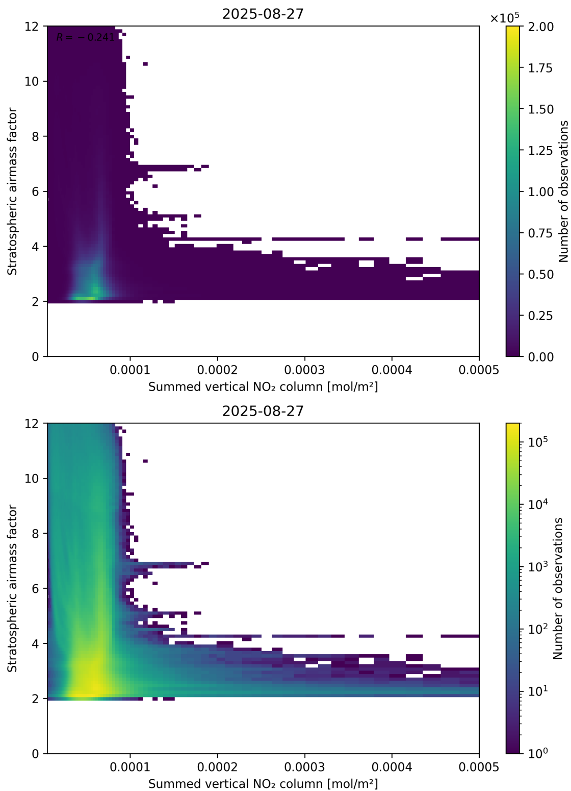
Figure 103: Scatter density plot of “Summed vertical NO 2 column” against “Stratospheric airmass factor” for 2025-08-26 to 2025-08-28.
