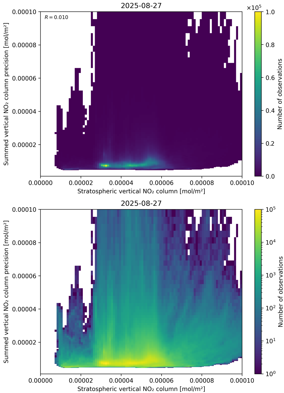
Figure 99: Scatter density plot of “Stratospheric vertical NO 2 column” against “Summed vertical NO 2 column precision” for 2025-08-26 to 2025-08-28.
