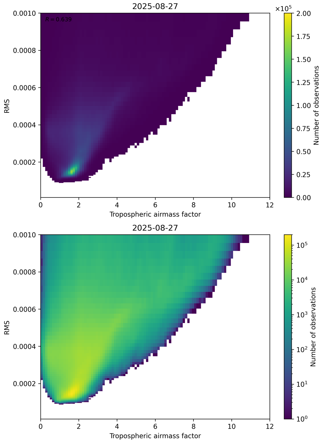
Figure 79: Scatter density plot of “Tropospheric airmass factor” against “RMS” for 2025-08-26 to 2025-08-28.
