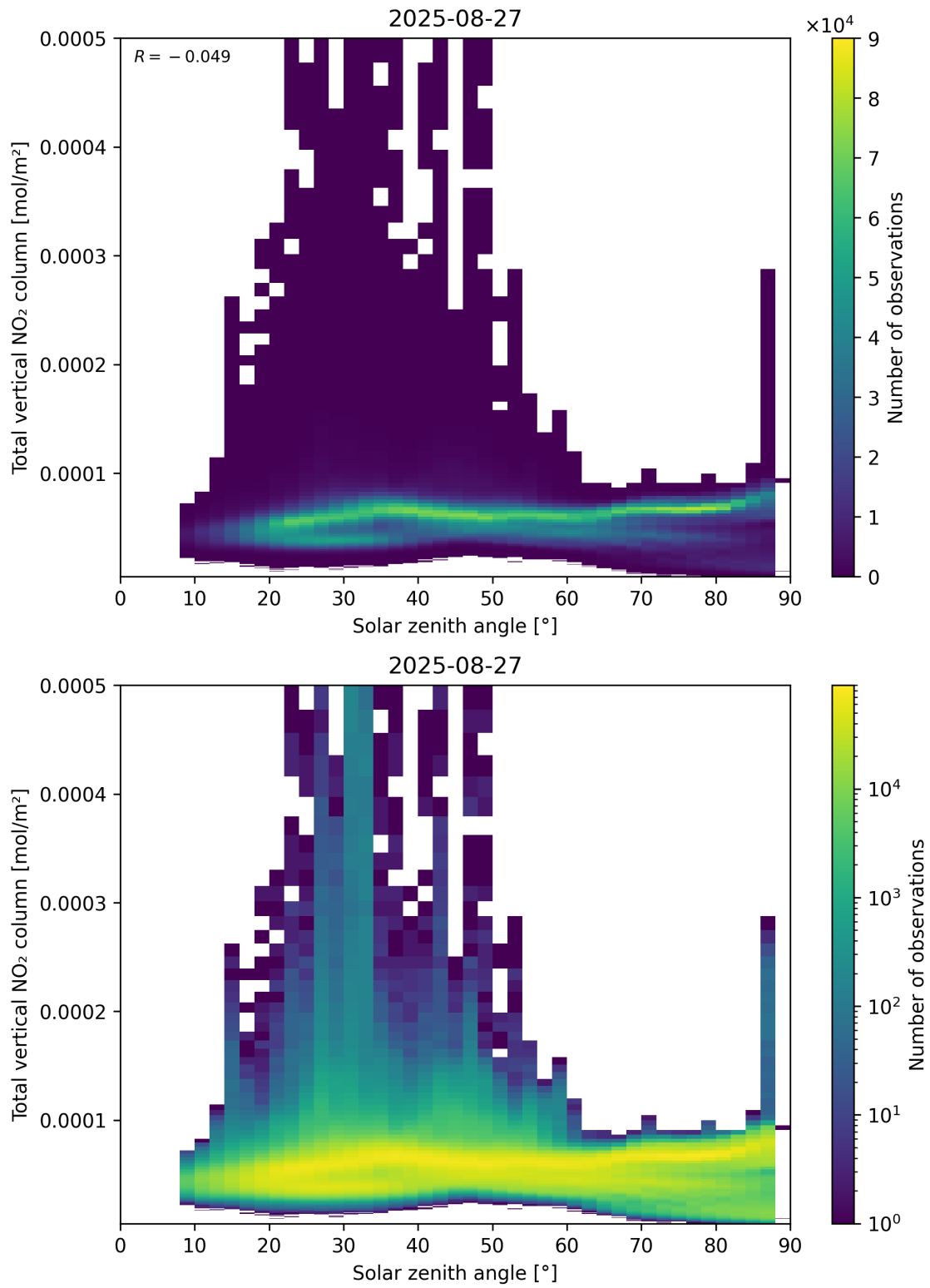
Figure 153: Scatter density plot of “Solar zenith angle” against “Total vertical NO 2 column” for 2025-08-26 to 2025-08-28.
