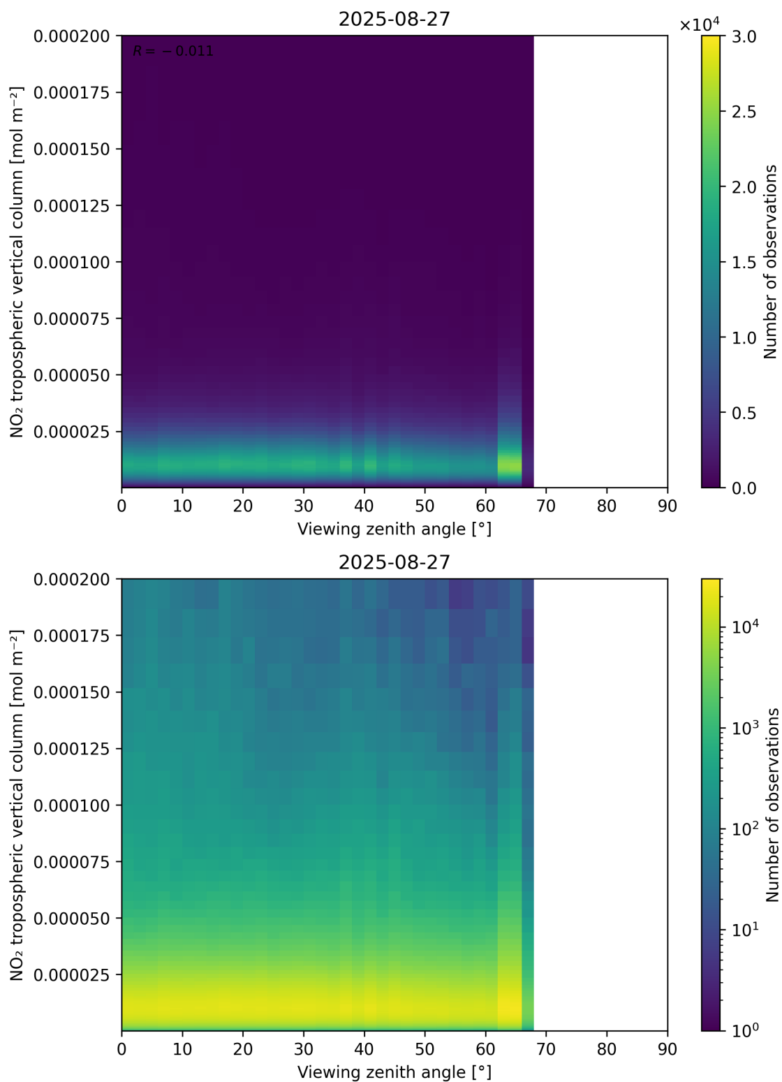
Figure 169: Scatter density plot of “Viewing zenith angle” against “NO 2 tropospheric vertical column” for 2025-08-26 to 2025-08-28.
