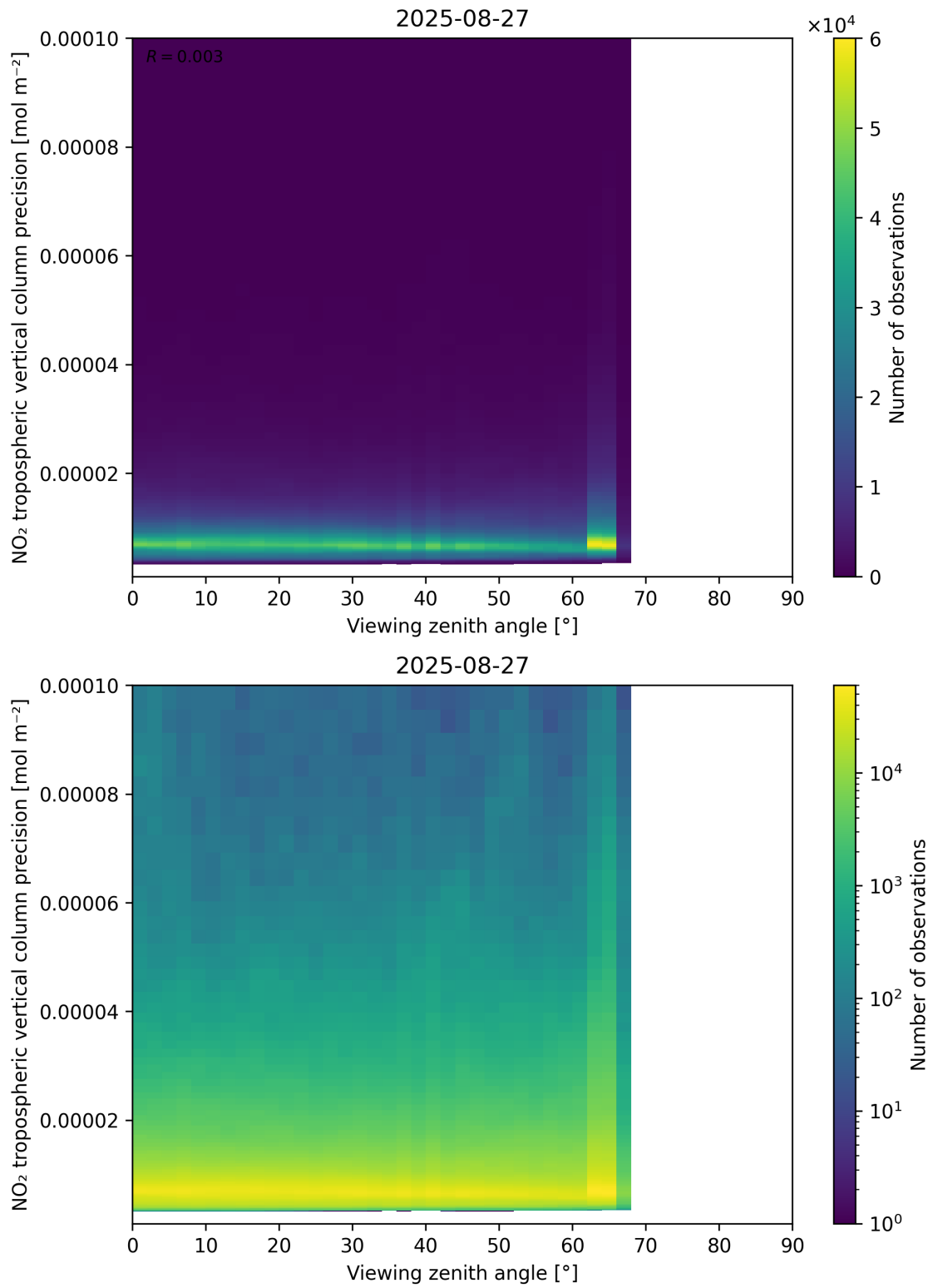
Figure 170: Scatter density plot of “Viewing zenith angle” against “NO 2 tropospheric vertical column precision” for 2025-08-26 to 2025-08-28.
