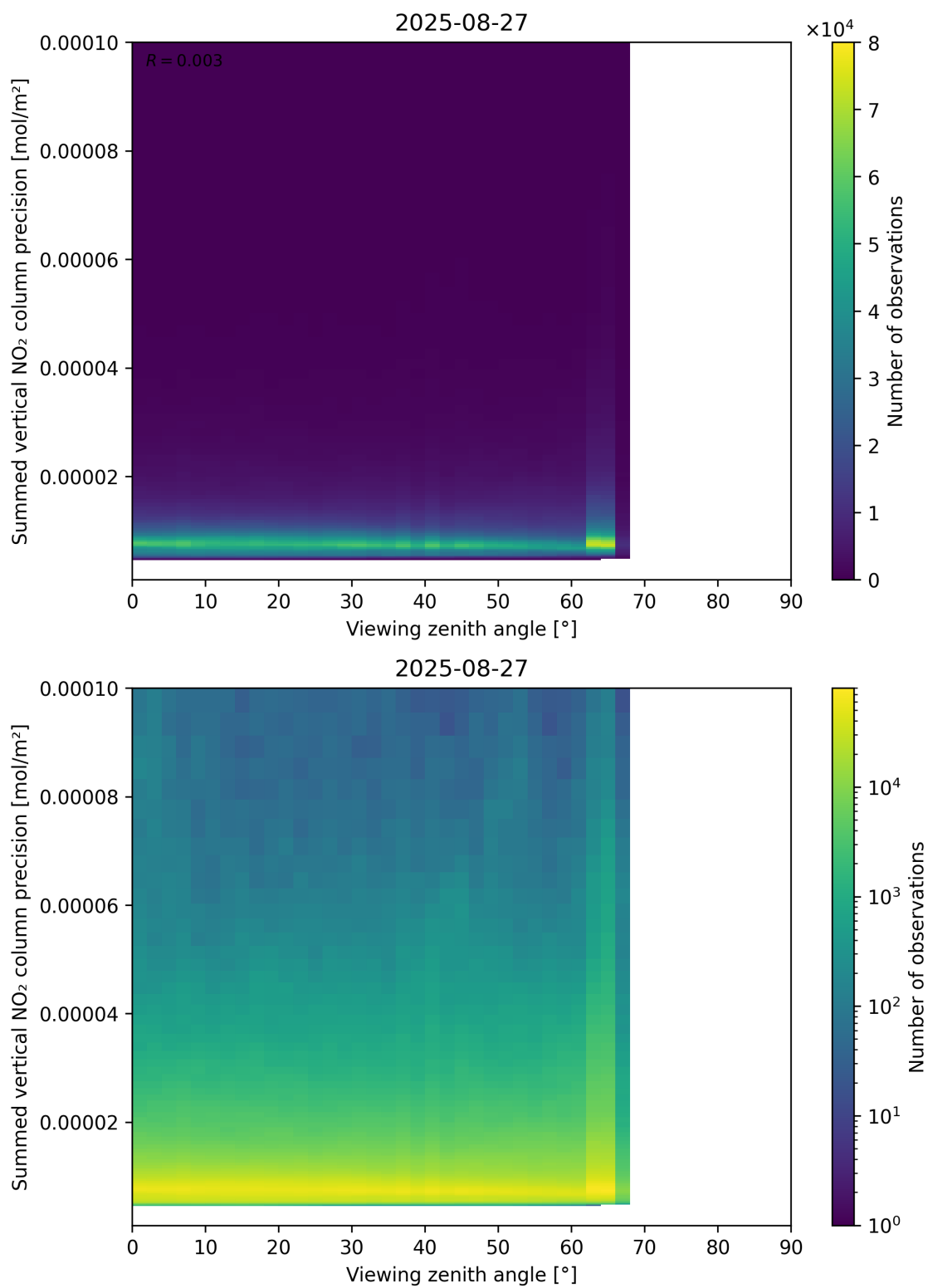
Figure 166: Scatter density plot of “Viewing zenith angle” against “Summed vertical NO 2 column precision” for 2025-08-26 to 2025-08-28.
