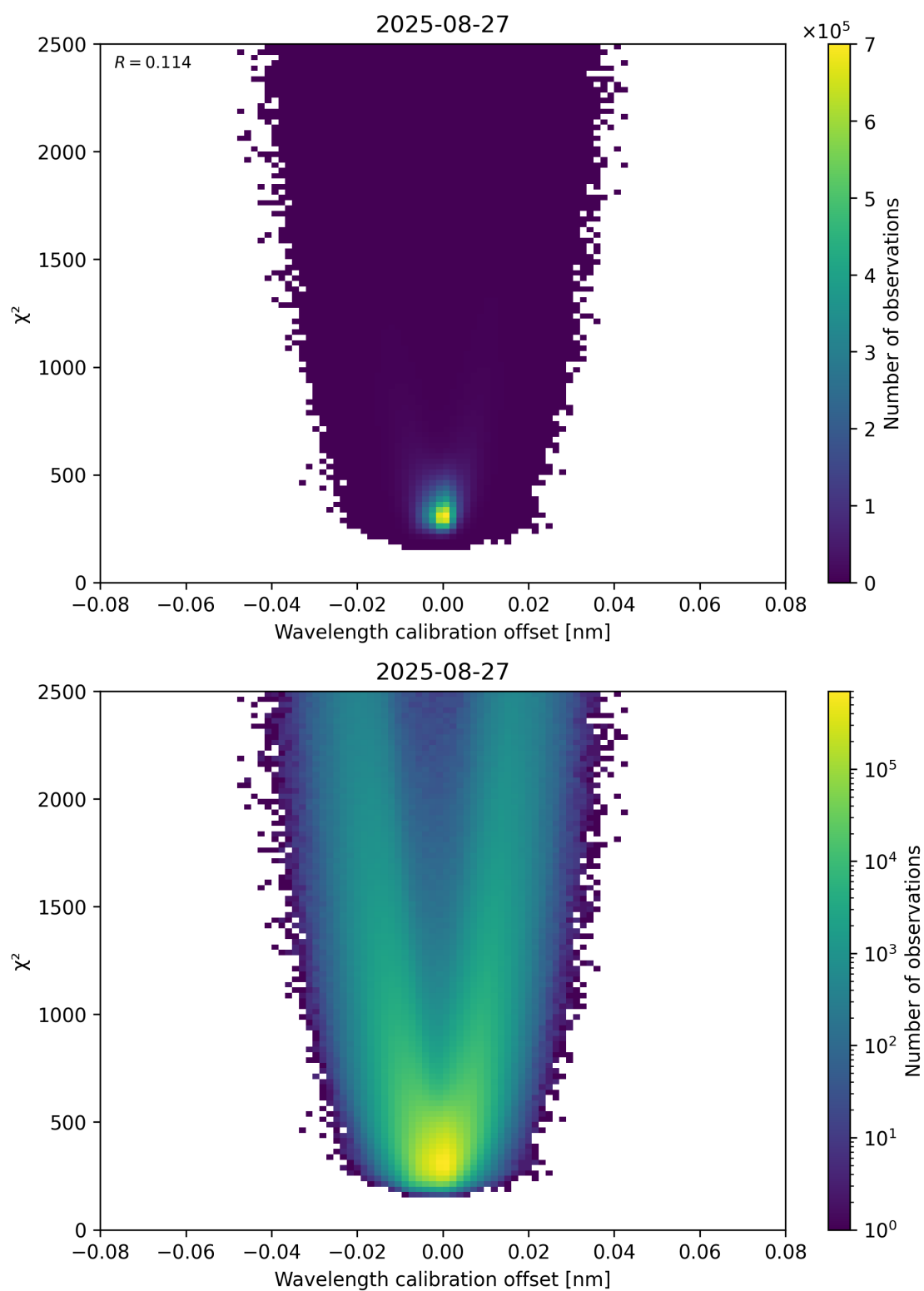
Figure 175: Scatter density plot of “Wavelength calibration offset” against “ \chi^2 ” for 2025-08-26 to 2025-08-28.
