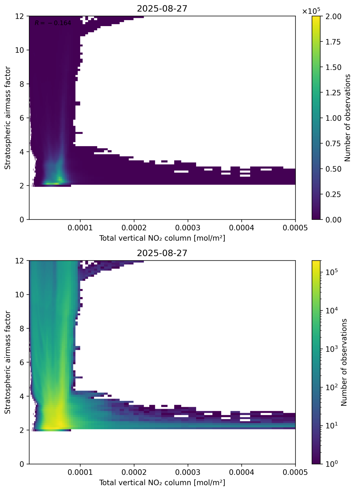
Figure 110: Scatter density plot of “Total vertical NO 2 column” against “Stratospheric airmass factor” for 2025-08-26 to 2025-08-28.
