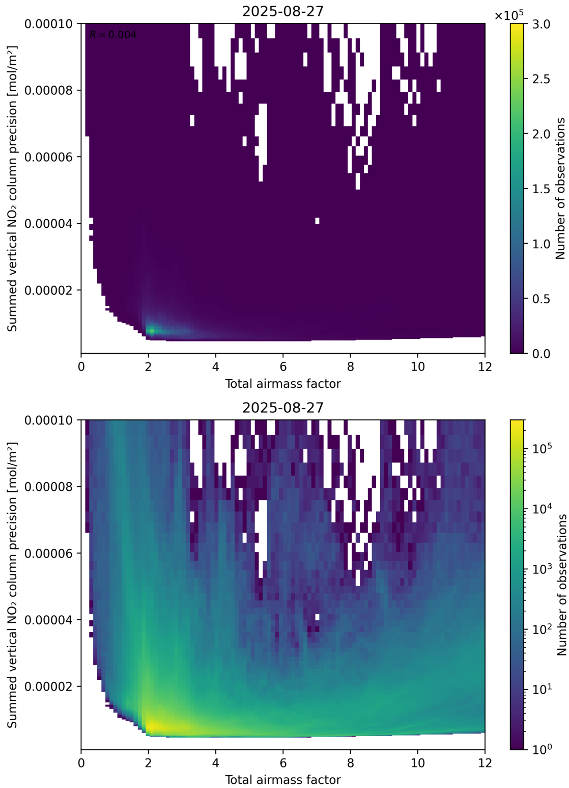
Figure 66: Scatter density plot of “Total airmass factor” against “Summed vertical NO 2 column precision” for 2025-08-26 to 2025-08-28.
