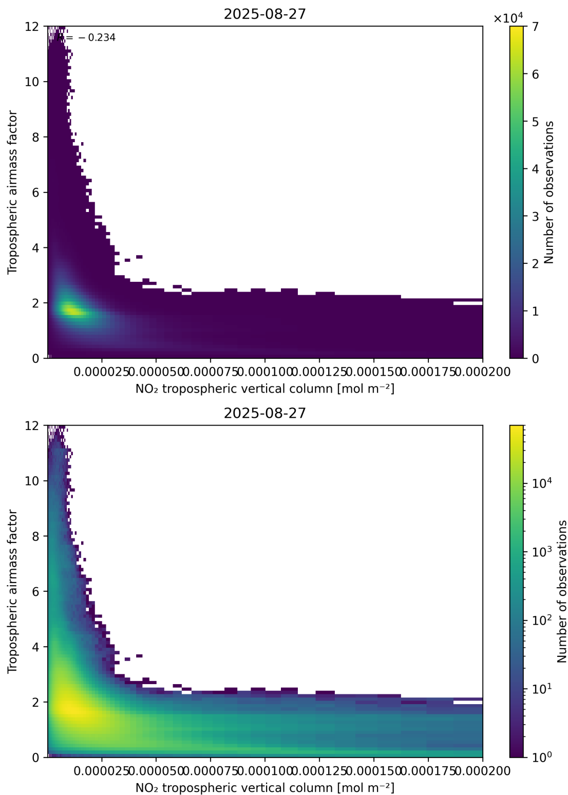
Figure 123: Scatter density plot of “NO 2 tropospheric vertical column” against “Tropospheric air mass factor” for 2025-08-26 to 2025-08-28.
