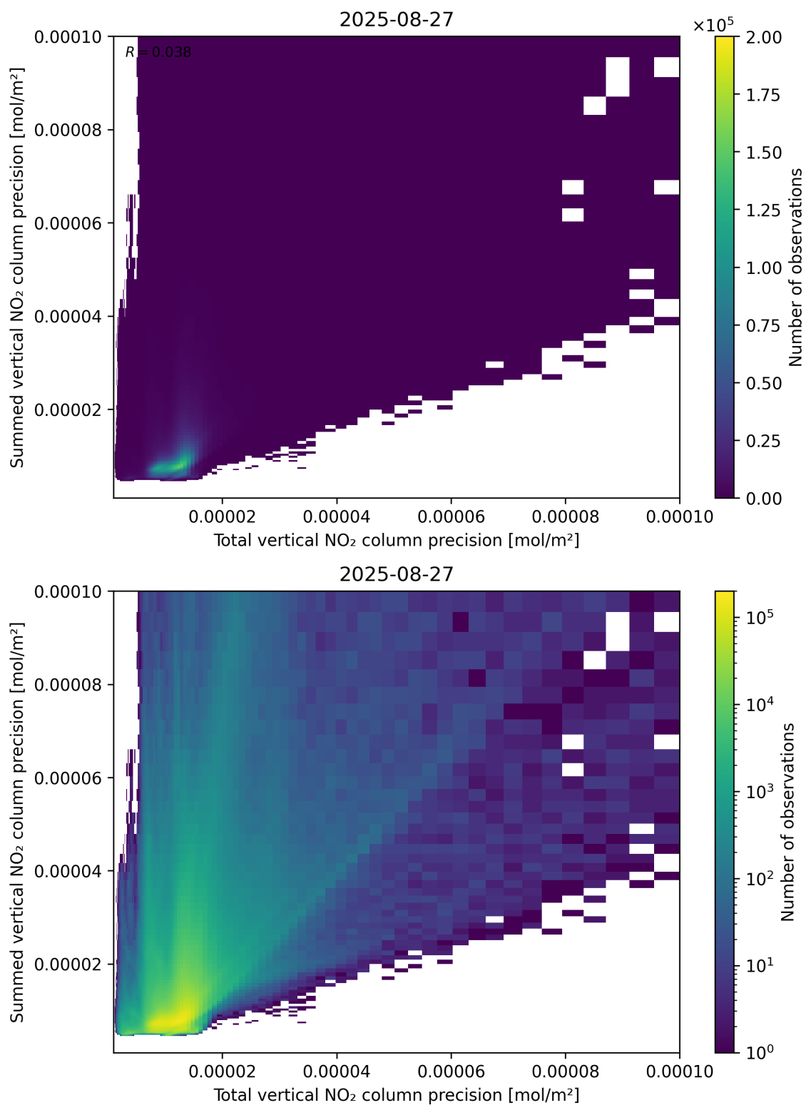
Figure 118: Scatter density plot of “Total vertical NO 2 column precision” against “Summed vertical NO 2 column precision” for 2025-08-26 to 2025-08-28.
