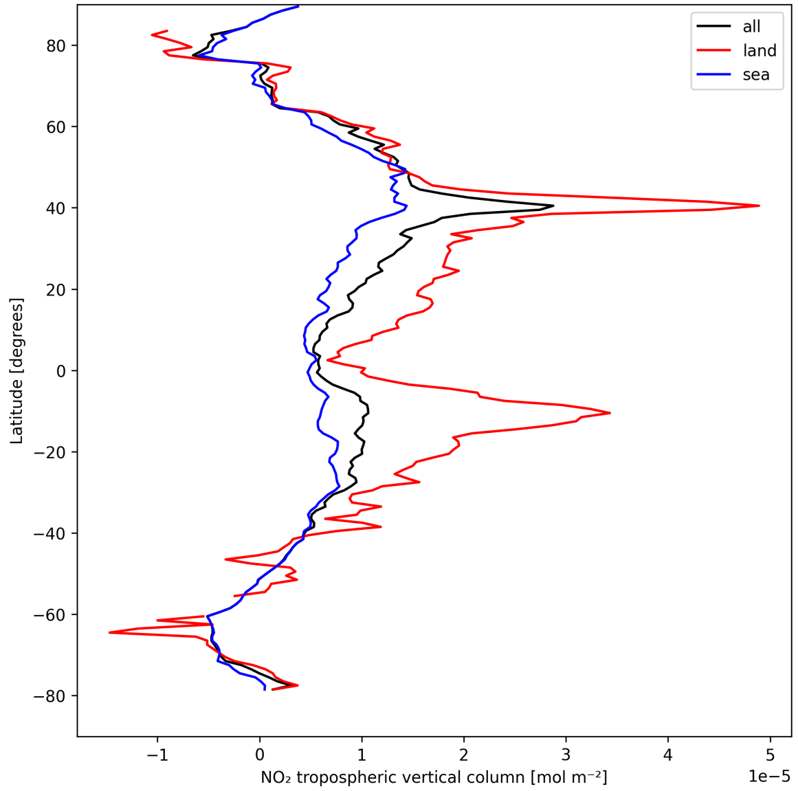
Figure 12: Zonal average of “NO 2 tropospheric vertical column” for 2025-08-26 to 2025-08-28.
