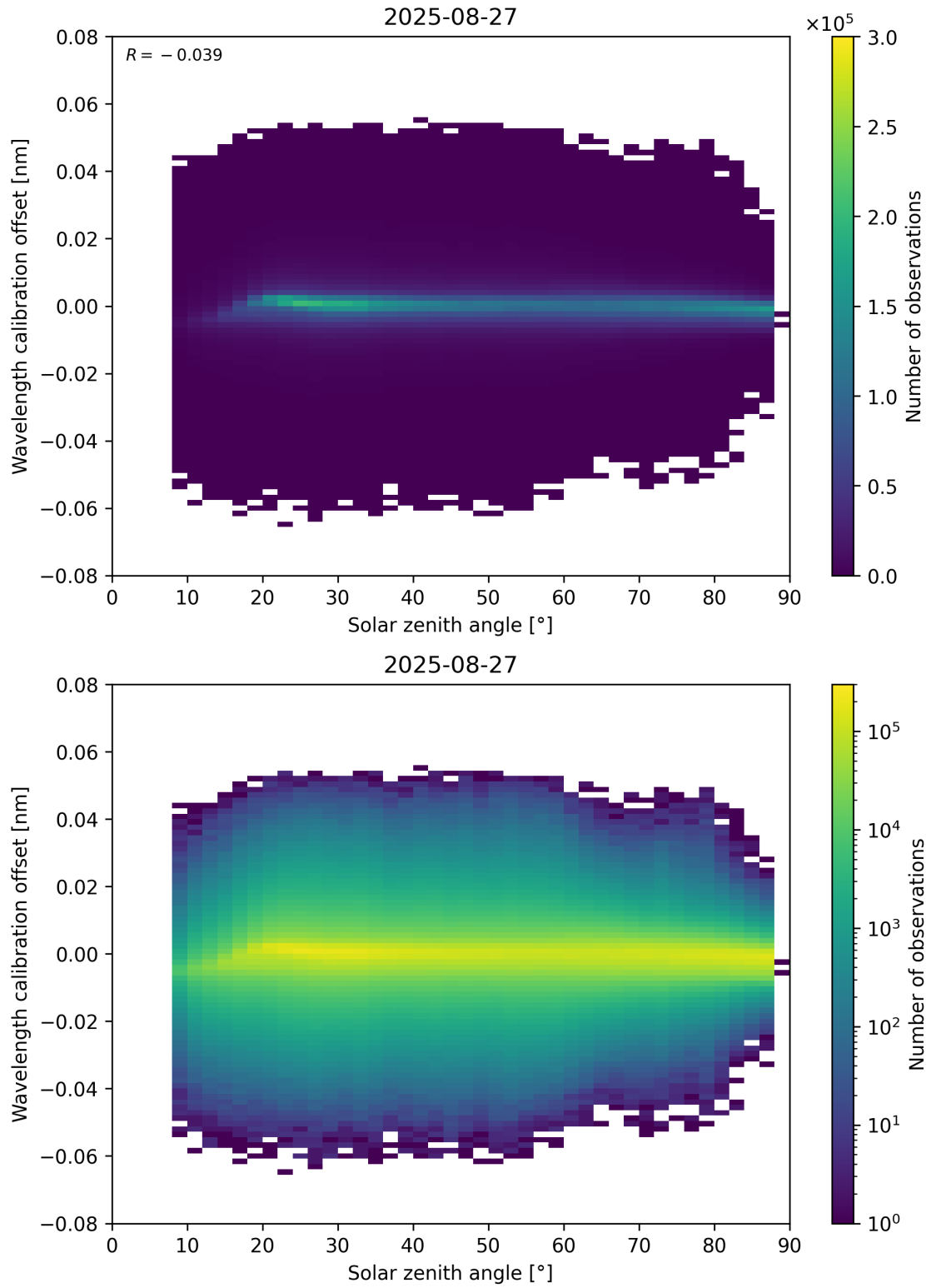
Figure 158: Scatter density plot of “Solar zenith angle” against “Wavelength calibration offset” for 2025-08-26 to 2025-08-28.
