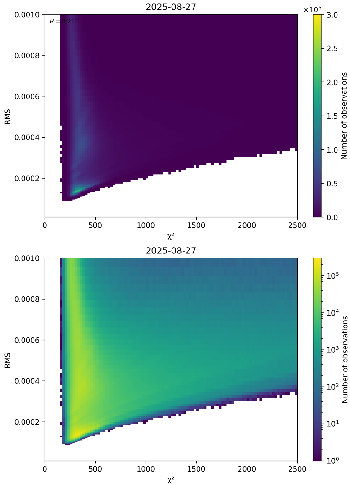
Figure 82: Scatter density plot of “ \chi^2 ” against “RMS” for 2025-08-26 to 2025-08-28.
