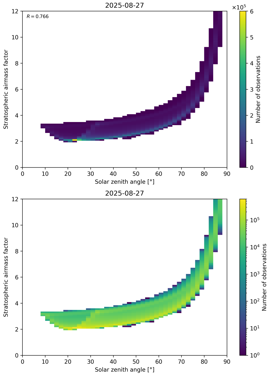
Figure 145: Scatter density plot of “Solar zenith angle” against “Stratospheric airmass factor” for 2025-08-26 to 2025-08-28.
