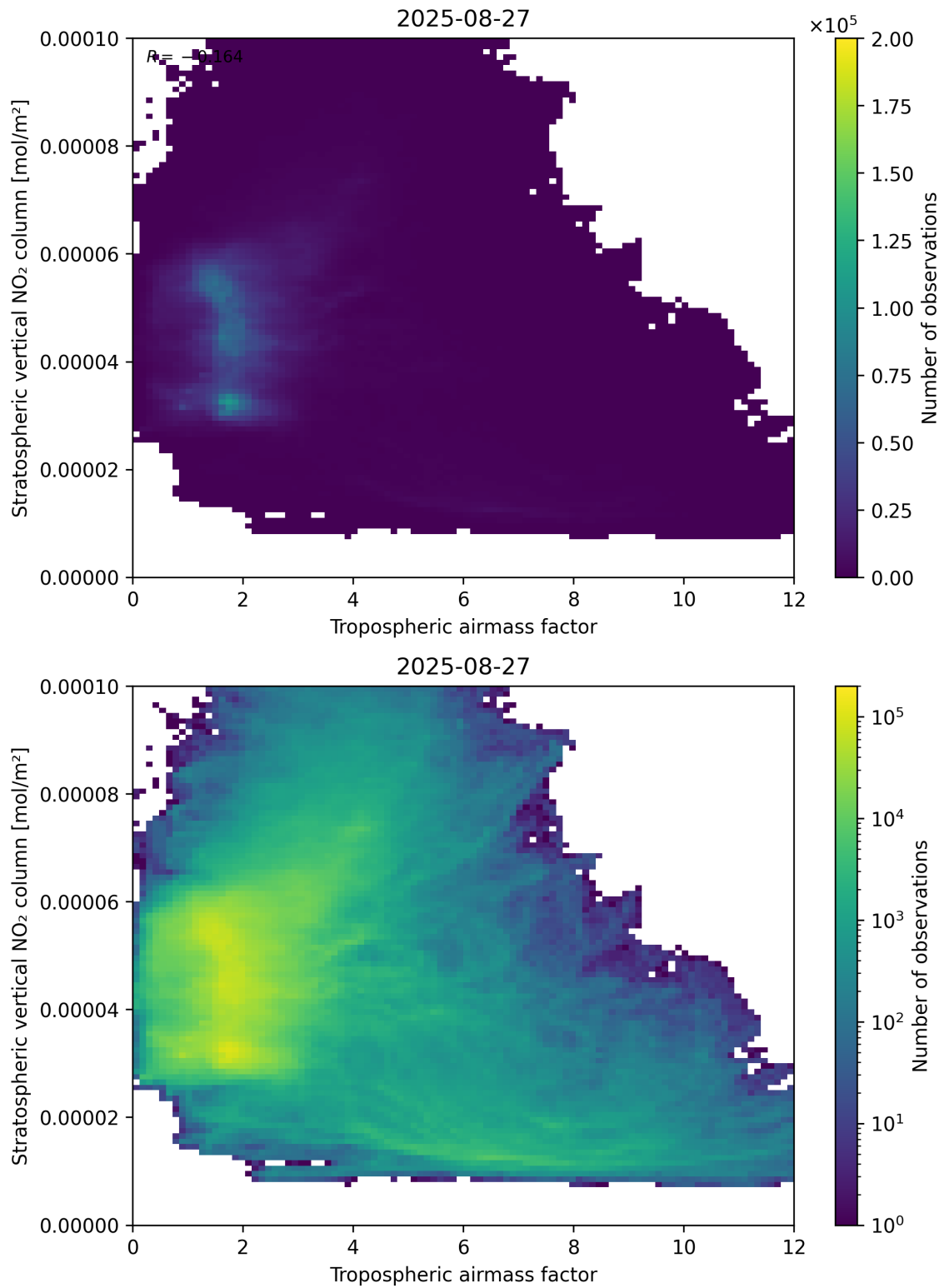
Figure 74: Scatter density plot of “Tropospheric air mass factor” against “Stratospheric vertical NO 2 column” for 2025-08-26 to 2025-08-28.
