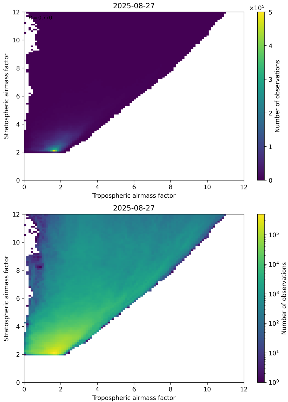
Figure 71: Scatter density plot of “Tropospheric airmass factor” against “Stratospheric airmass factor” for 2025-08-26 to 2025-08-28.
