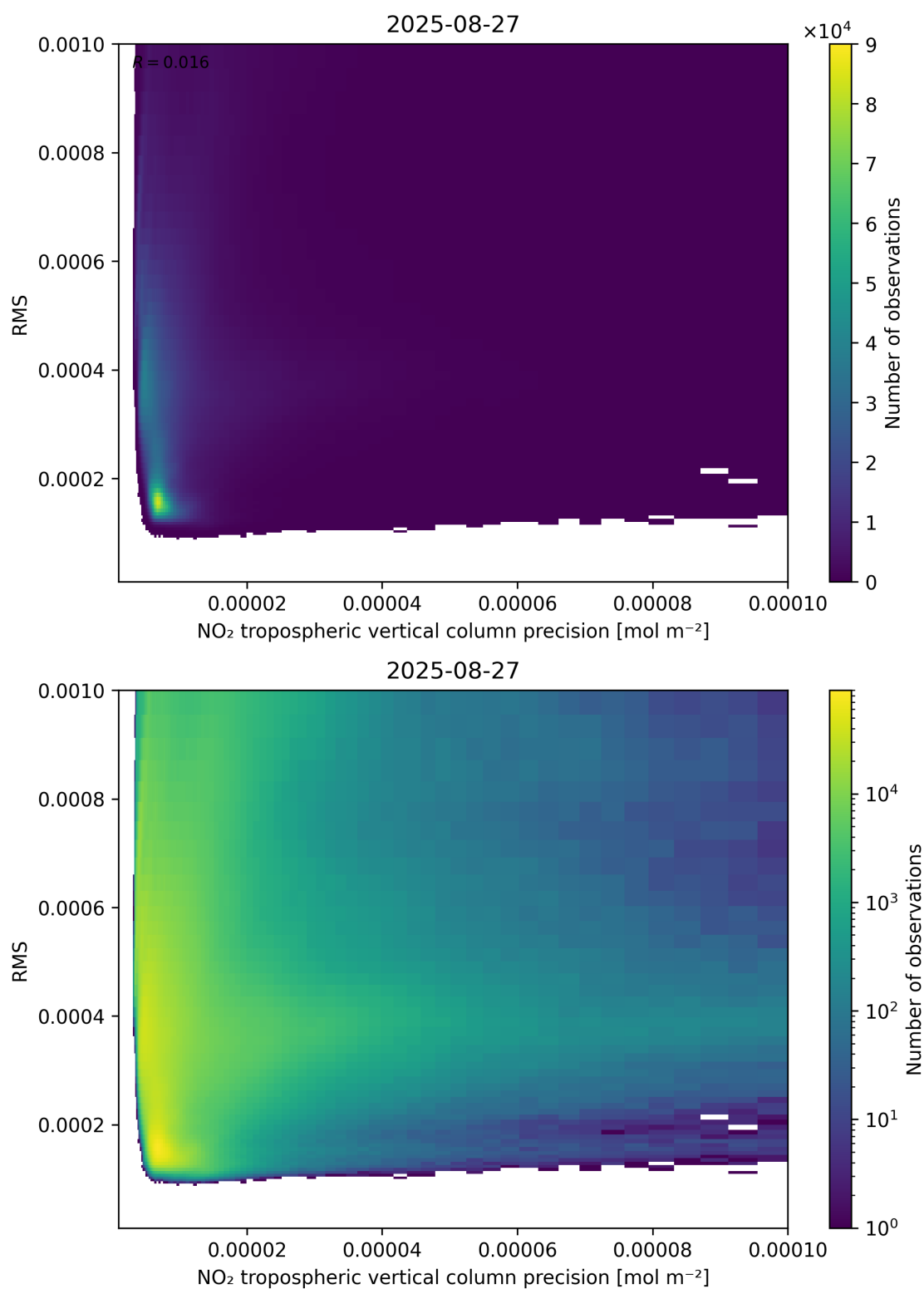
Figure 140: Scatter density plot of “NO 2 tropospheric vertical column precision” against “RMS” for 2025-08-26 to 2025-08-28.
