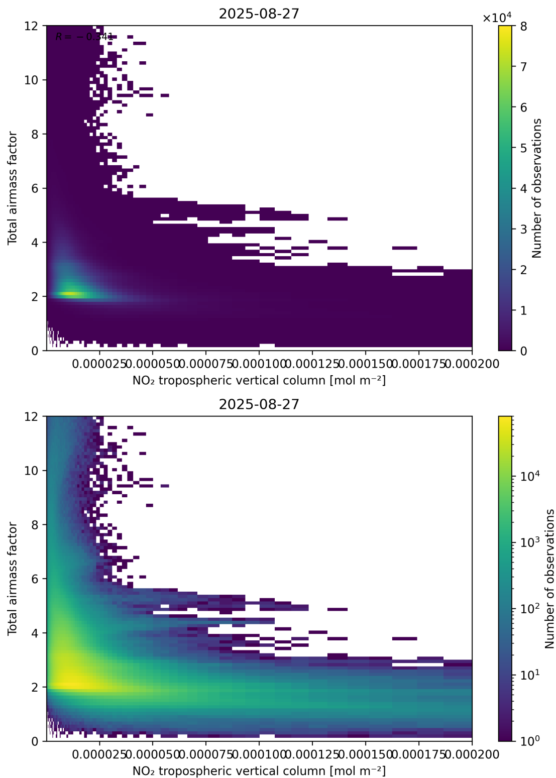
Figure 122: Scatter density plot of “NO 2 tropospheric vertical column” against “Total air mass factor” for 2025-08-26 to 2025-08-28.
