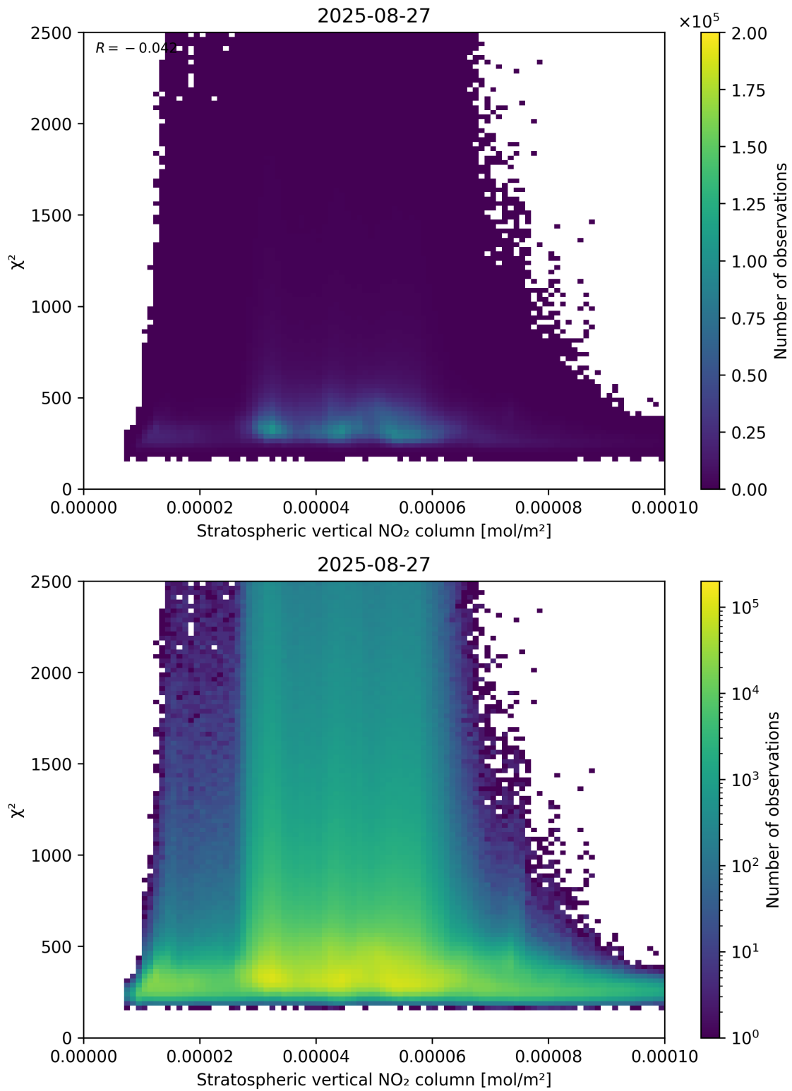
Figure 97: Scatter density plot of “Stratospheric vertical NO 2 column” against “ \chi^2 ” for 2025-08-26 to 2025-08-28.
