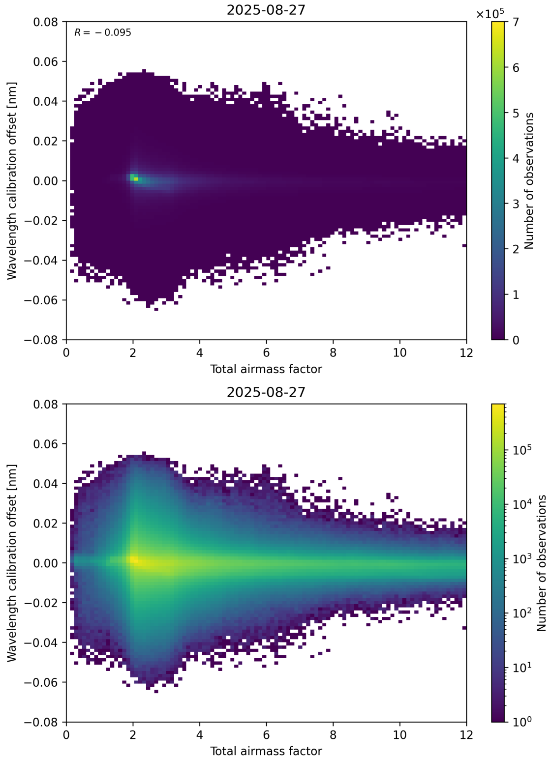
Figure 70: Scatter density plot of “Total airmass factor” against “Wavelength calibration offset” for 2025-08-26 to 2025-08-28.
