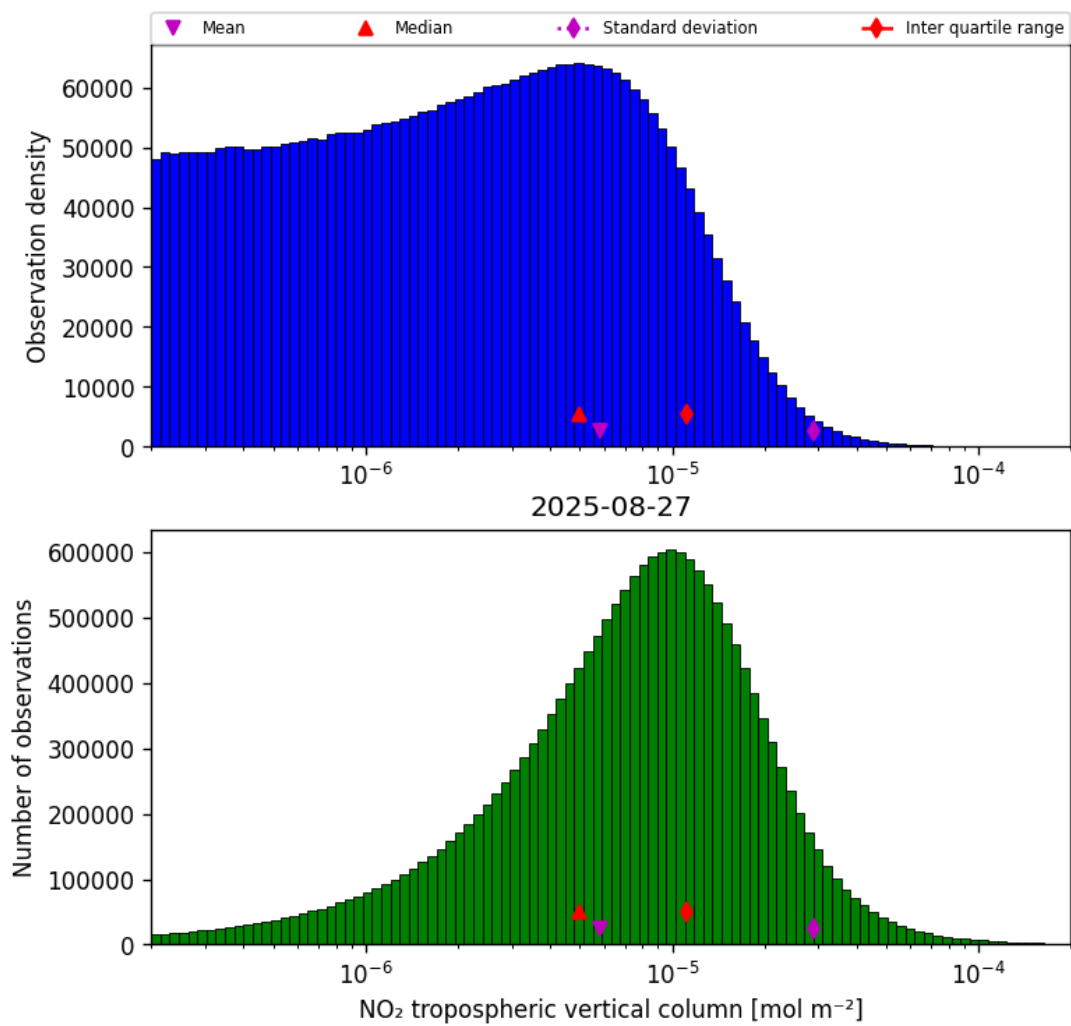
Figure 29: Histogram of “NO 2 tropospheric vertical column” for 2025-08-26 to 2025-08-28
