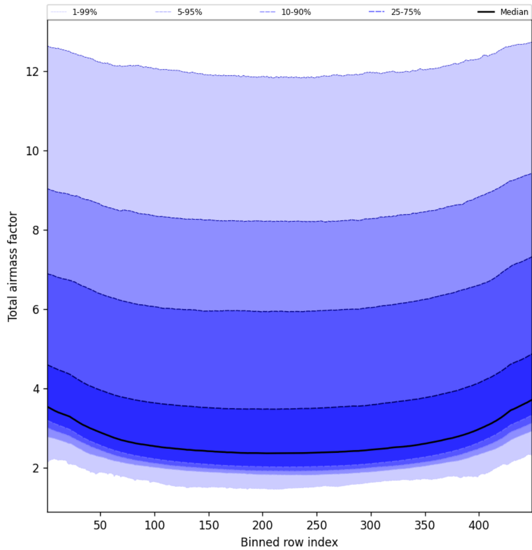
Figure 49: Along track statistics of “Total airmass factor” for 2025-08-26 to 2025-08-28
