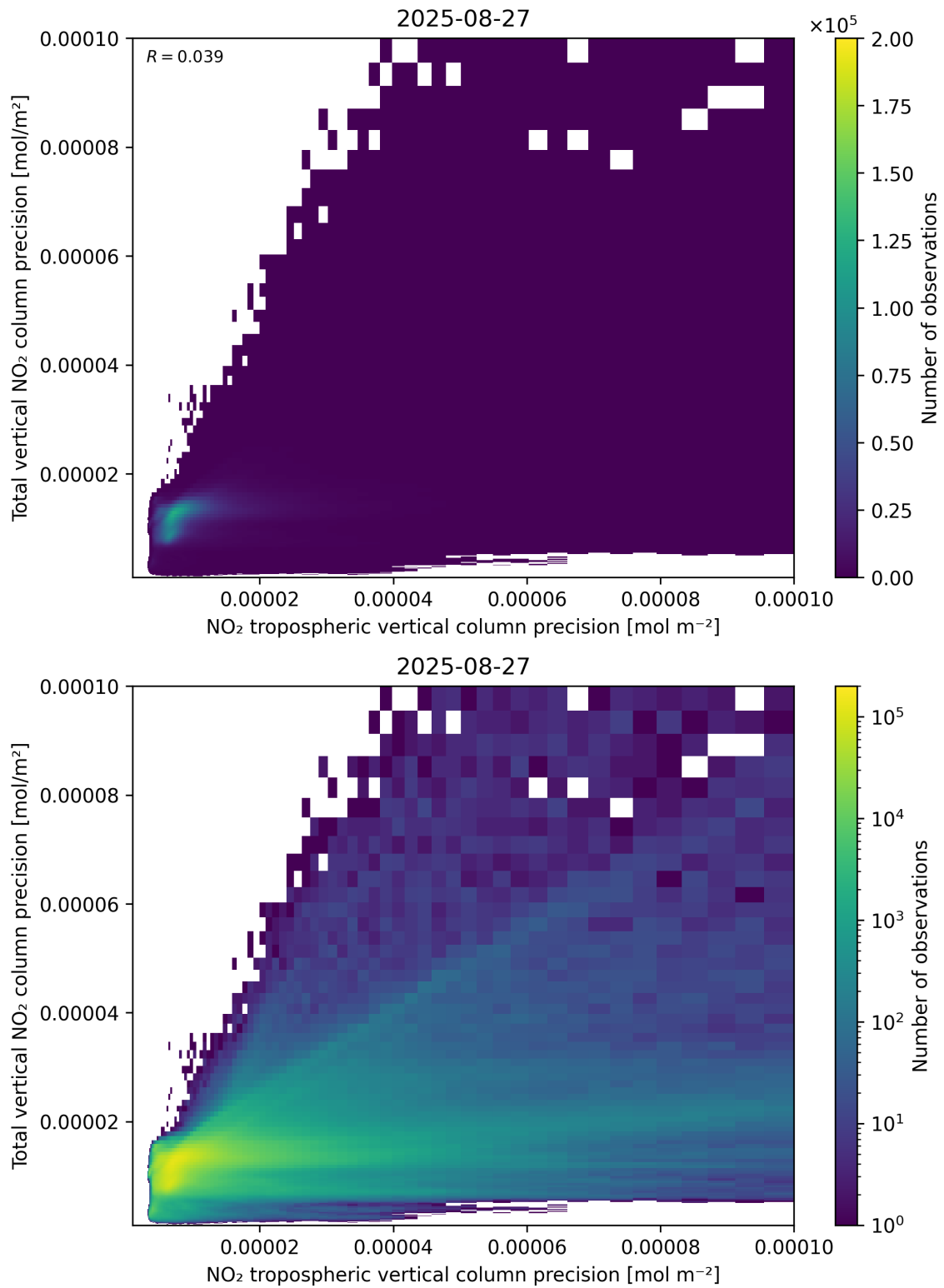
Figure 139: Scatter density plot of “NO 2 tropospheric vertical column precision” against “Total vertical NO 2 column precision” for 2025-08-26 to 2025-08-28.
