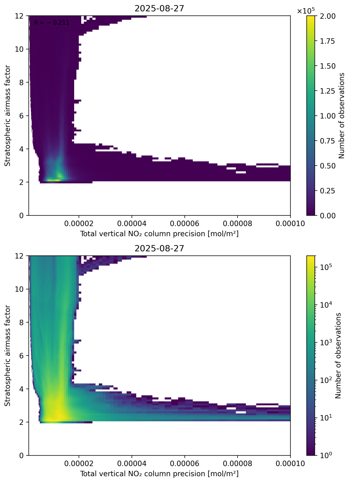
Figure 115: Scatter density plot of “Total vertical NO 2 column precision” against “Stratospheric air mass factor” for 2025-08-26 to 2025-08-28.
