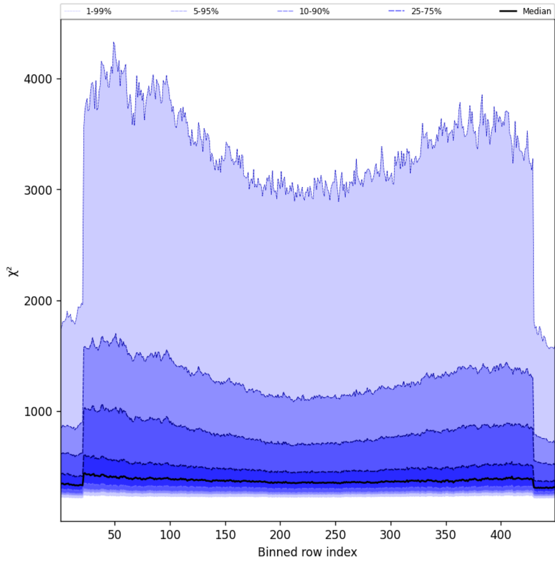
Figure 59: Along track statistics of “ \chi^2 ” for 2025-08-26 to 2025-08-28
