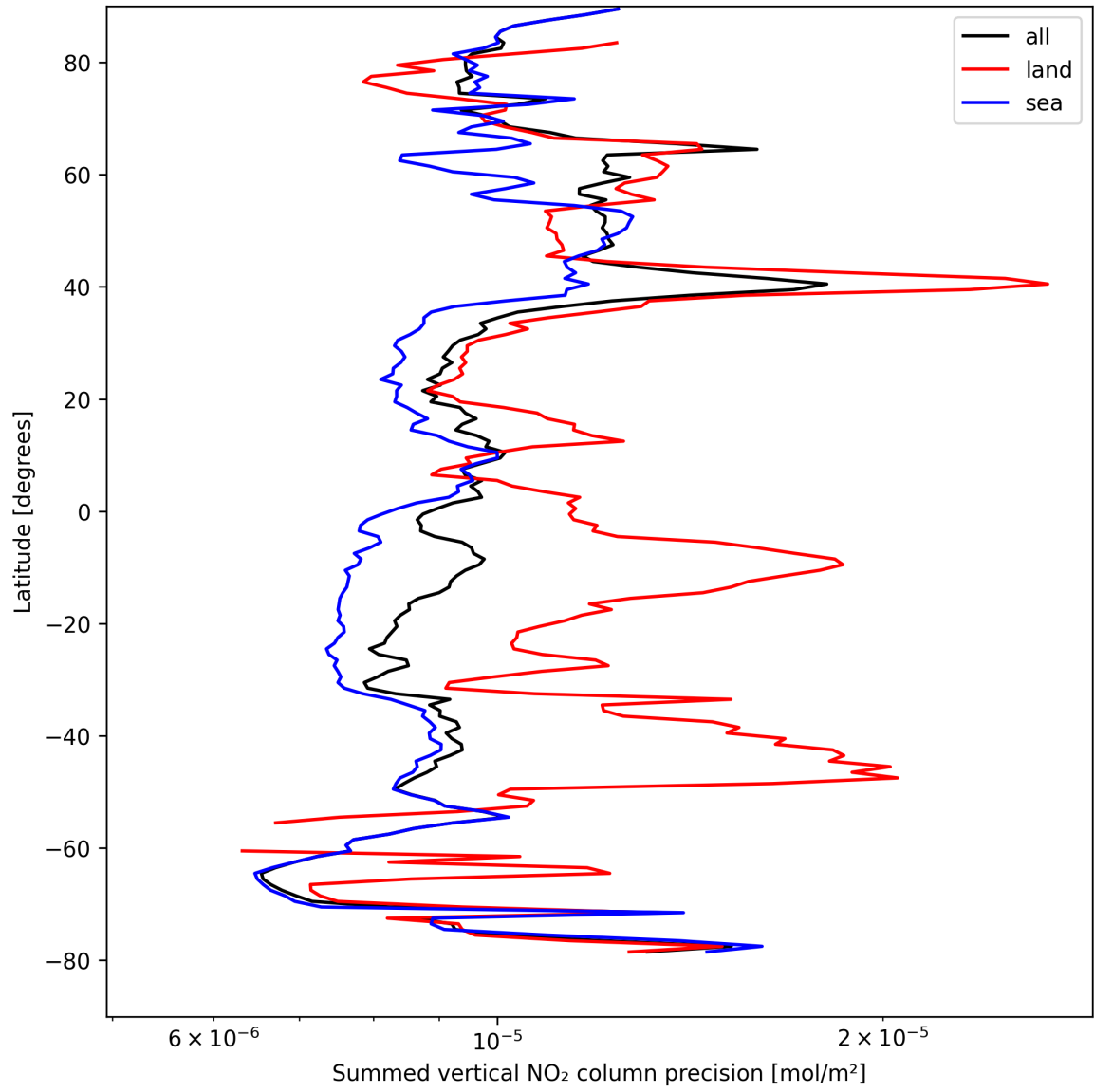
Figure 24: Zonal average of “Summed vertical NO 2 column precision” for 2025-08-26 to 2025-08-28.
