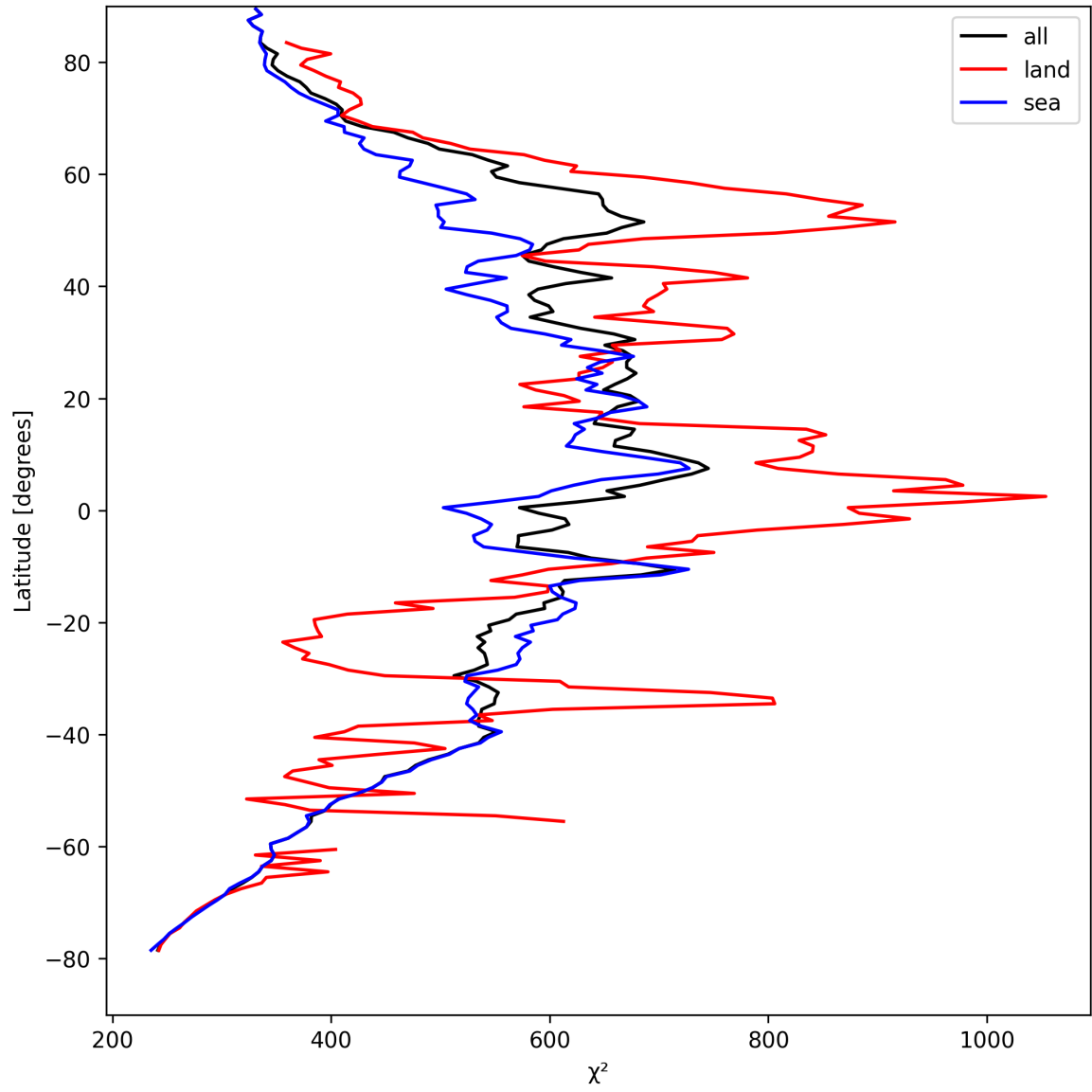
Figure 25: Zonal average of “ \chi^2 ” for 2025-08-26 to 2025-08-28.
