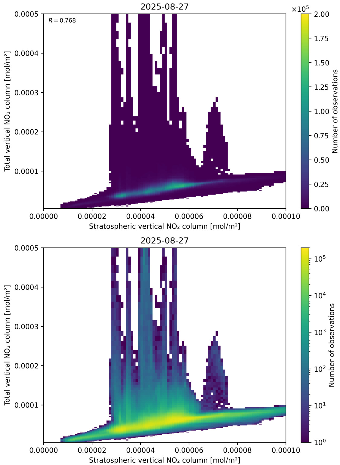
Figure 100: Scatter density plot of “Stratospheric vertical NO 2 column” against “Total vertical NO 2 column” for 2025-08-26 to 2025-08-28.
