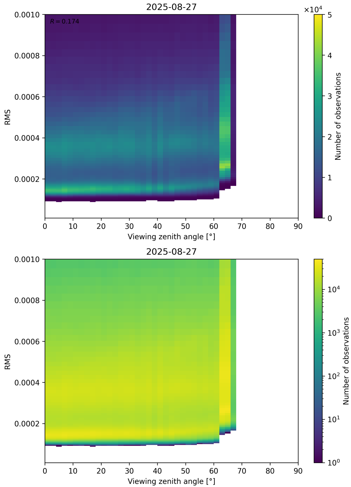
Figure 171: Scatter density plot of “Viewing zenith angle” against “RMS” for 2025-08-26 to 2025-08-28.
