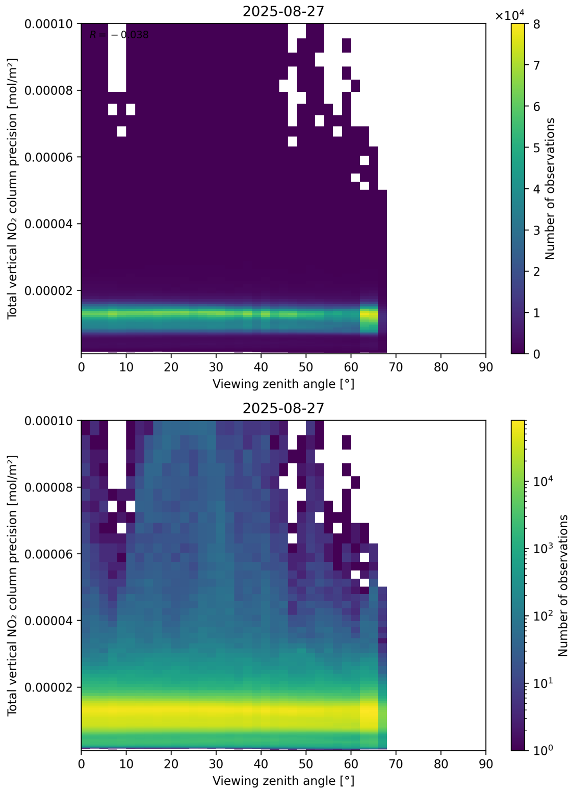
Figure 168: Scatter density plot of “Viewing zenith angle” against “Total vertical NO 2 column precision” for 2025-08-26 to 2025-08-28.
