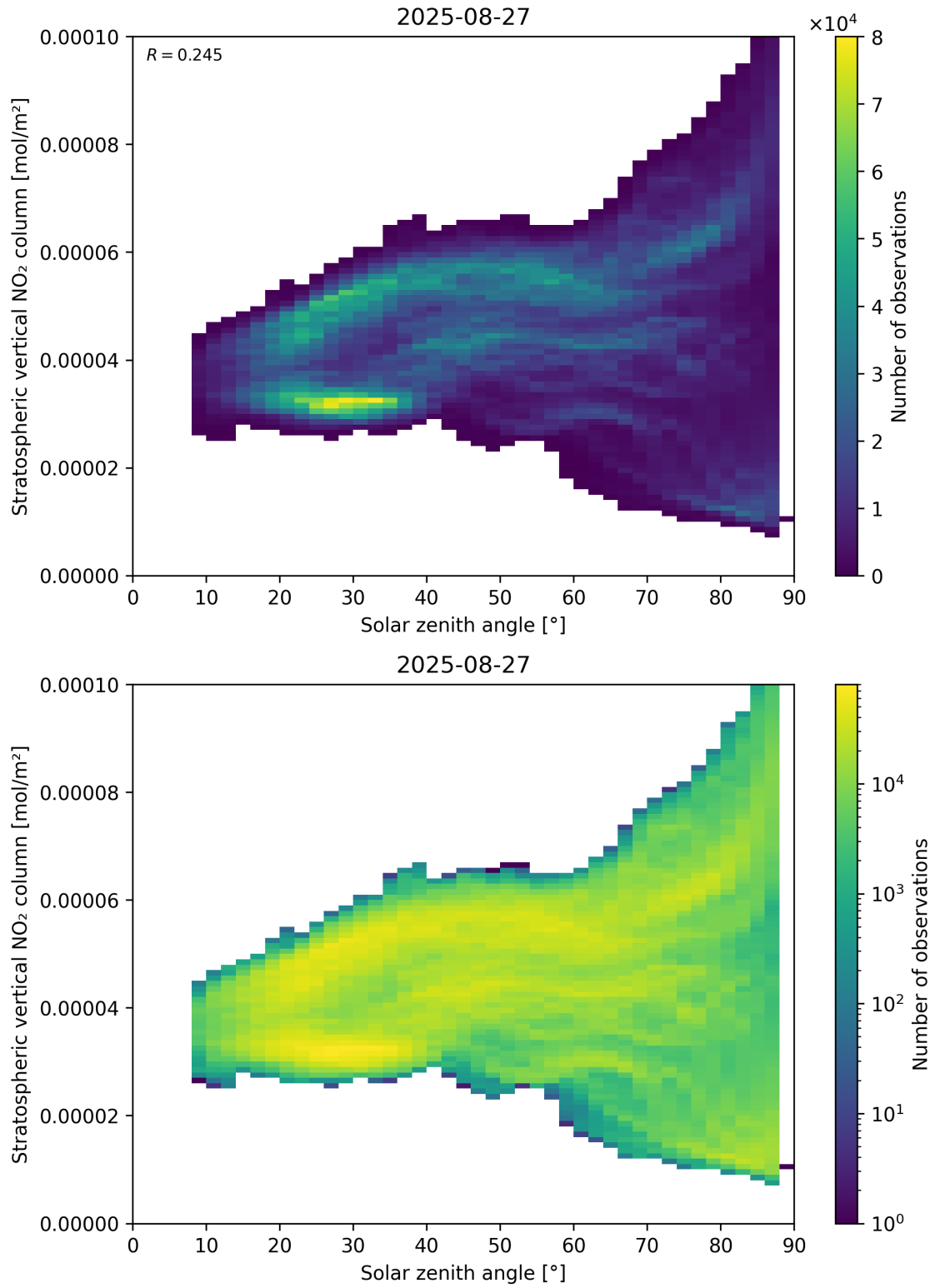
Figure 150: Scatter density plot of “Solar zenith angle” against “Stratospheric vertical \text{NO}_2 column” for 2025-08-26 to 2025-08-28.
