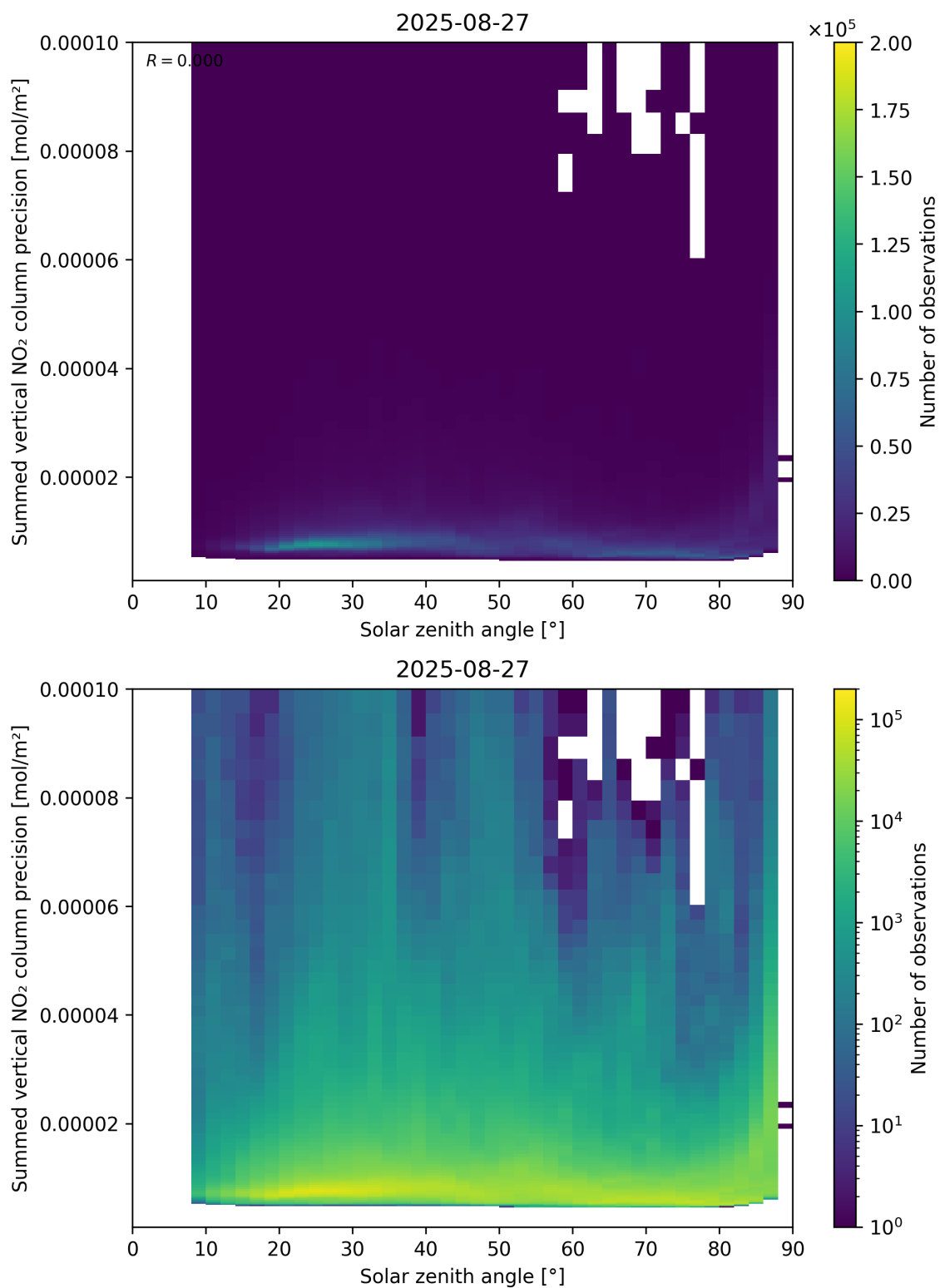
Figure 152: Scatter density plot of “Solar zenith angle” against “Summed vertical NO 2 column precision” for 2025-08-26 to 2025-08-28.
