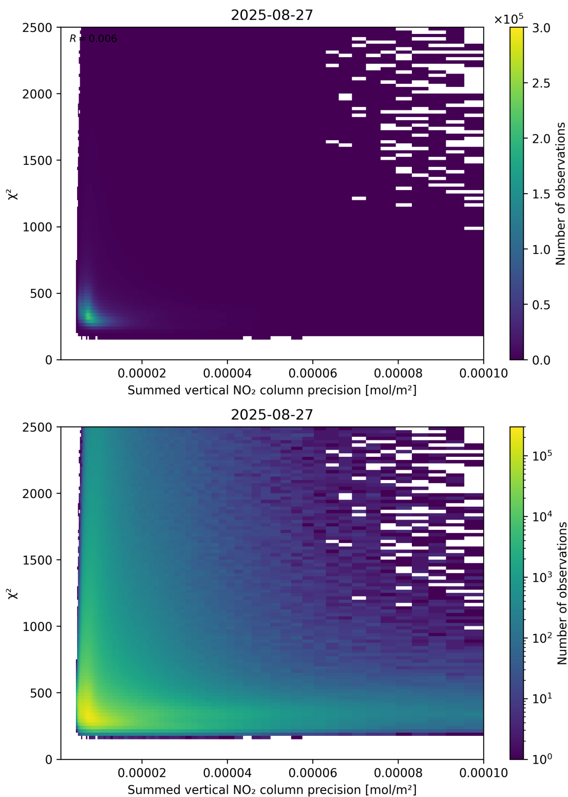
Figure 107: Scatter density plot of “Summed vertical NO 2 column precision” against “ \chi^2 ” for 2025-08-26 to 2025-08-28.
