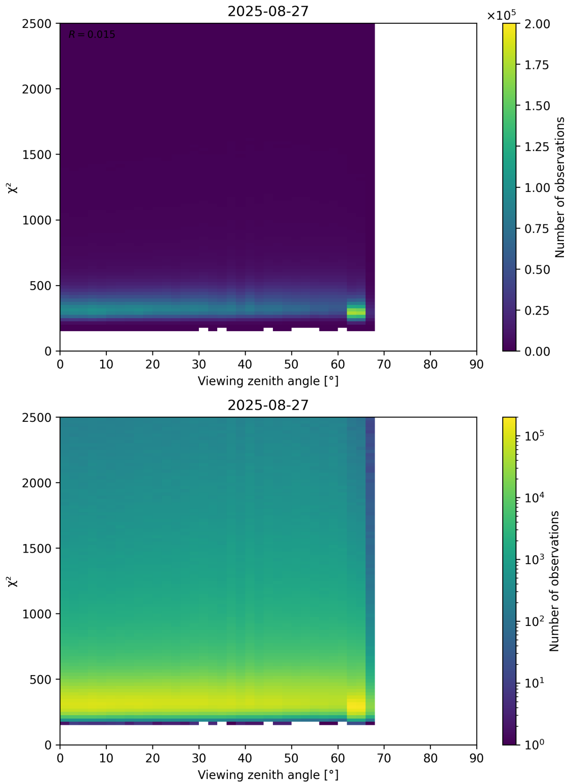
Figure 162: Scatter density plot of “Viewing zenith angle” against “ \chi^2 ” for 2025-08-26 to 2025-08-28.
