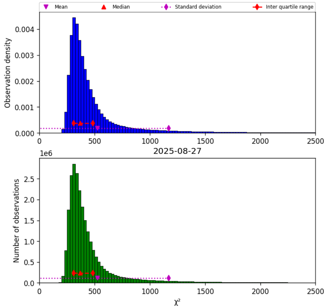
Figure 42: Histogram of “ \chi^2 ” for 2025-08-26 to 2025-08-28
