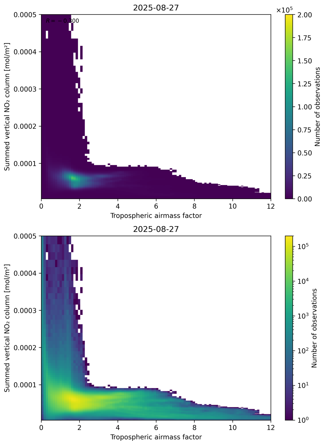
Figure 75: Scatter density plot of “Tropospheric air mass factor” against “Summed vertical NO 2 column” for 2025-08-26 to 2025-08-28.
