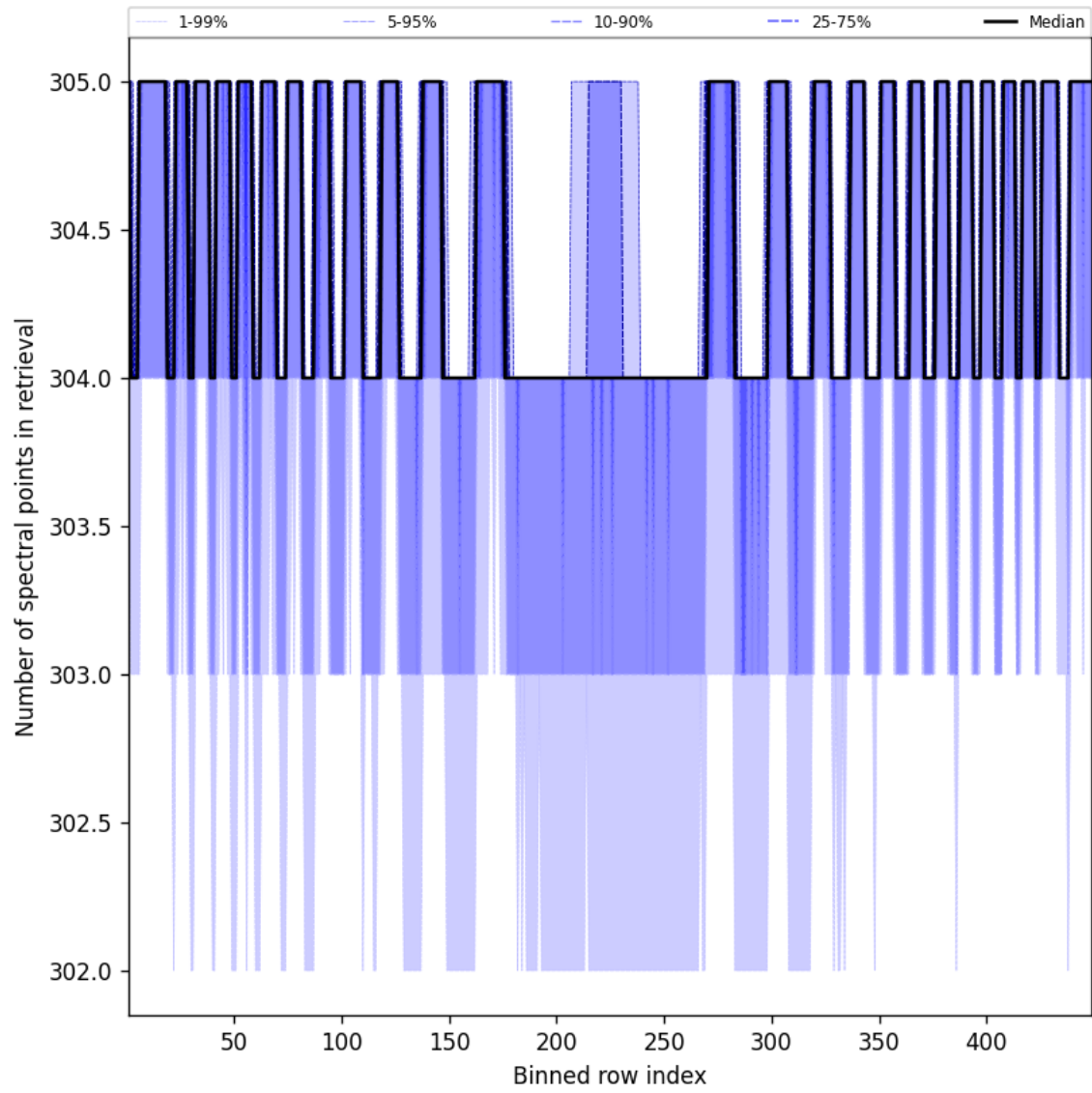
Figure 50: Along track statistics of “Number of spectral points in retrieval” for 2025-08-26 to 2025-08-28
