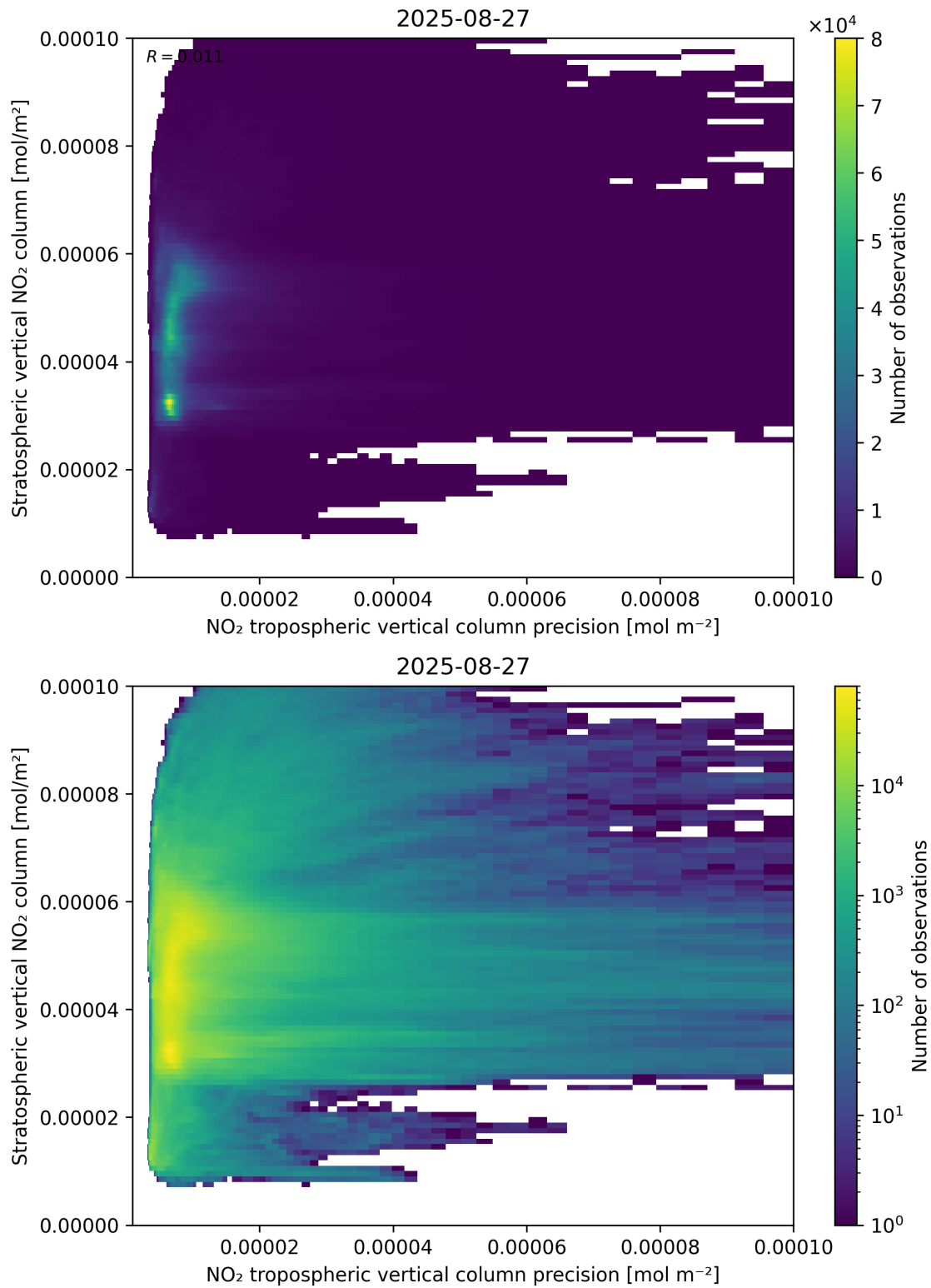
Figure 135: Scatter density plot of “NO 2 tropospheric vertical column precision” against “Stratospheric vertical NO 2 column” for 2025-08-26 to 2025-08-28.
