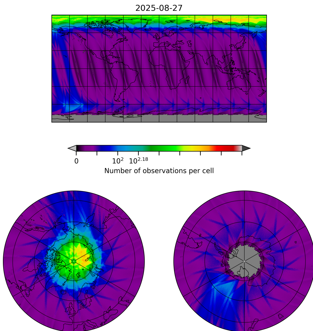
Figure 10: Map of the number of observations for 2025-08-26 to 2025-08-28
