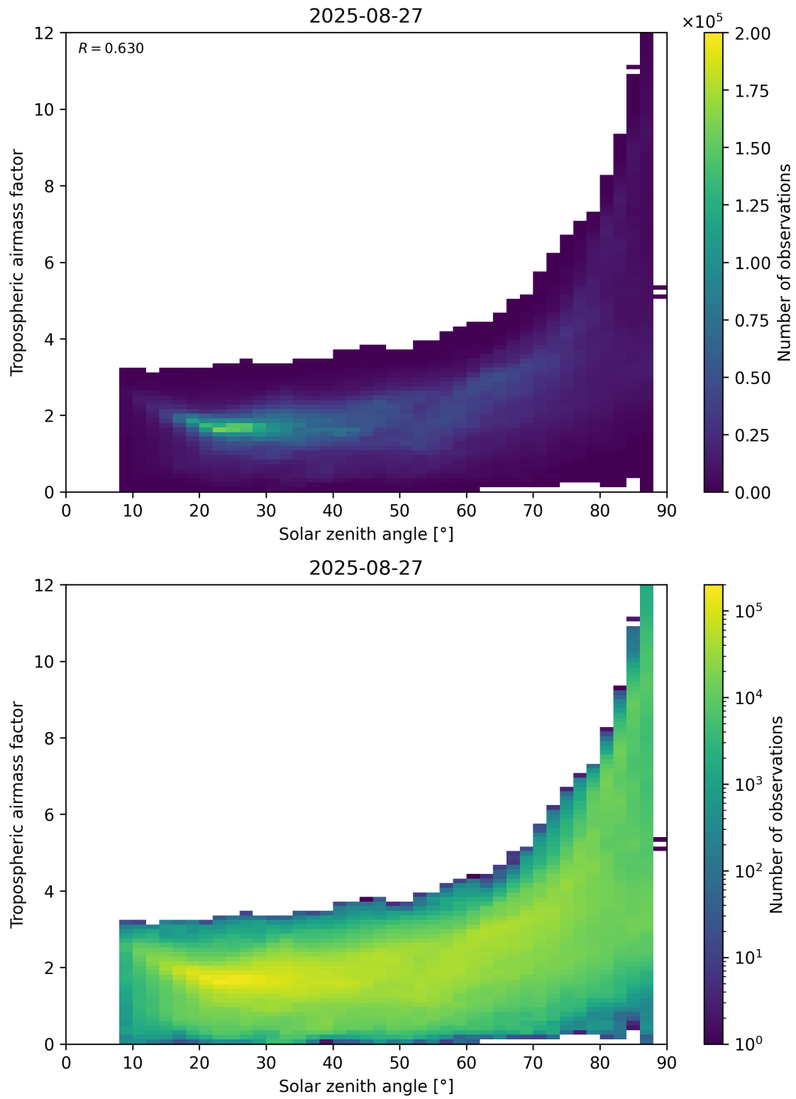
Figure 147: Scatter density plot of “Solar zenith angle” against “Tropospheric airmass factor” for 2025-08-26 to 2025-08-28.
