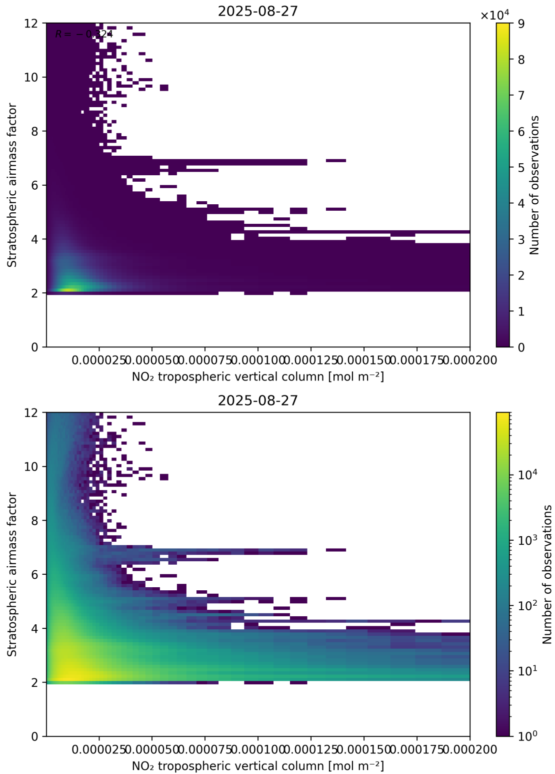
Figure 121: Scatter density plot of “NO 2 tropospheric vertical column” against “Stratospheric air mass factor” for 2025-08-26 to 2025-08-28.
