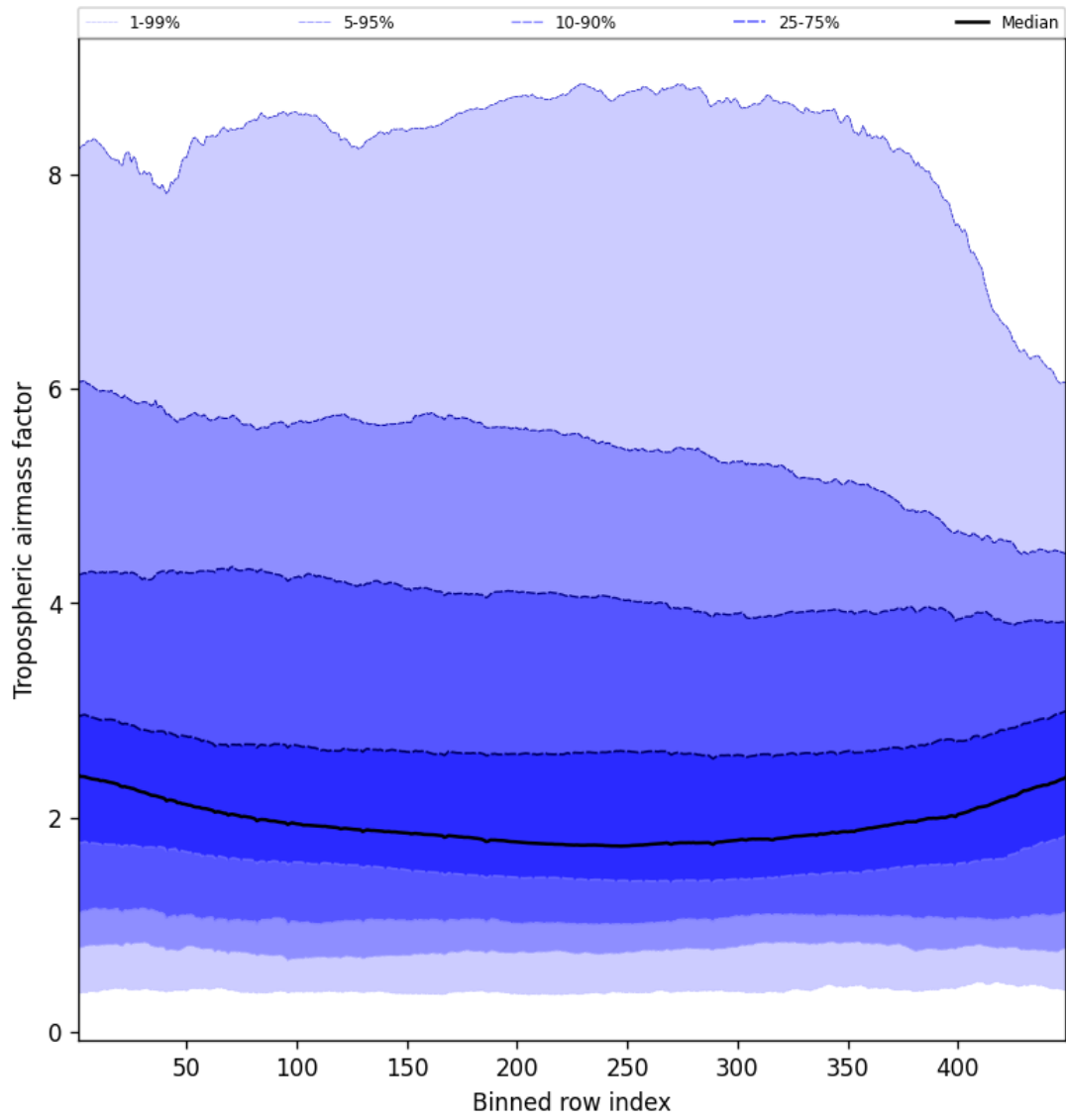
Figure 48: Along track statistics of “Tropospheric airmass factor” for 2025-08-26 to 2025-08-28
