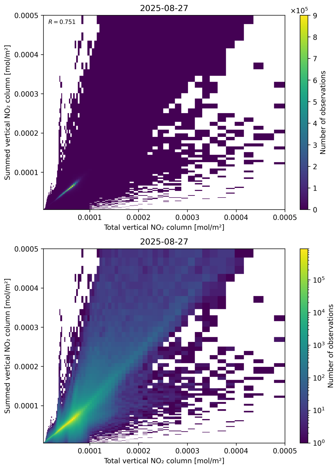
Figure 112: Scatter density plot of “Total vertical NO 2 column” against “Summed vertical NO 2 column” for 2025-08-26 to 2025-08-28.
