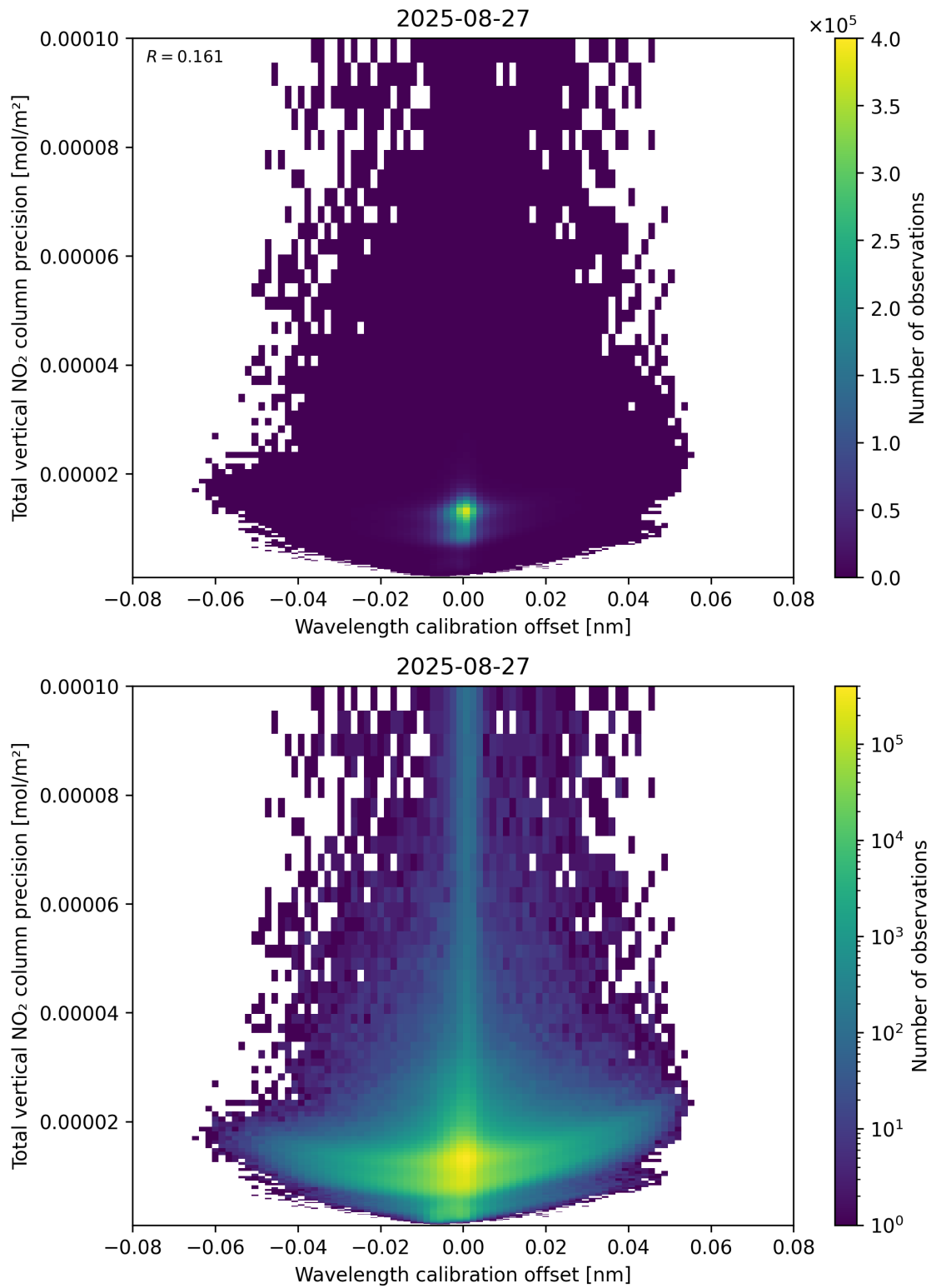
Figure 180: Scatter density plot of “Wavelength calibration offset” against “Total vertical NO 2 column precision” for 2025-08-26 to 2025-08-28.
