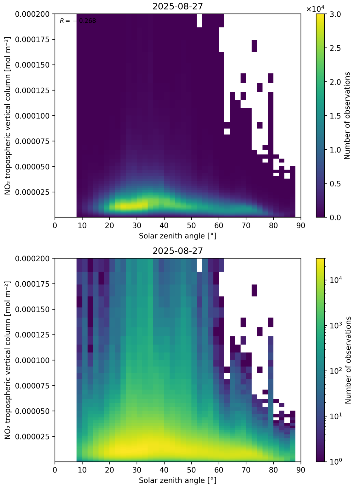
Figure 155: Scatter density plot of “Solar zenith angle” against “NO 2 tropospheric vertical column” for 2025-08-26 to 2025-08-28.
