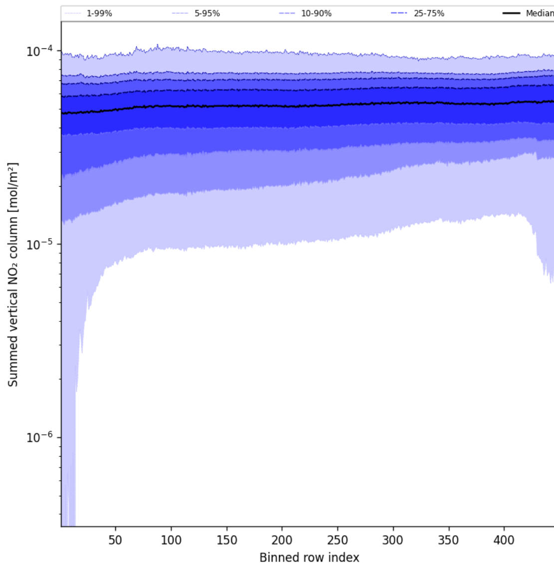
Figure 57: Along track statistics of “Summed vertical NO 2 column” for 2025-08-26 to 2025-08-28
