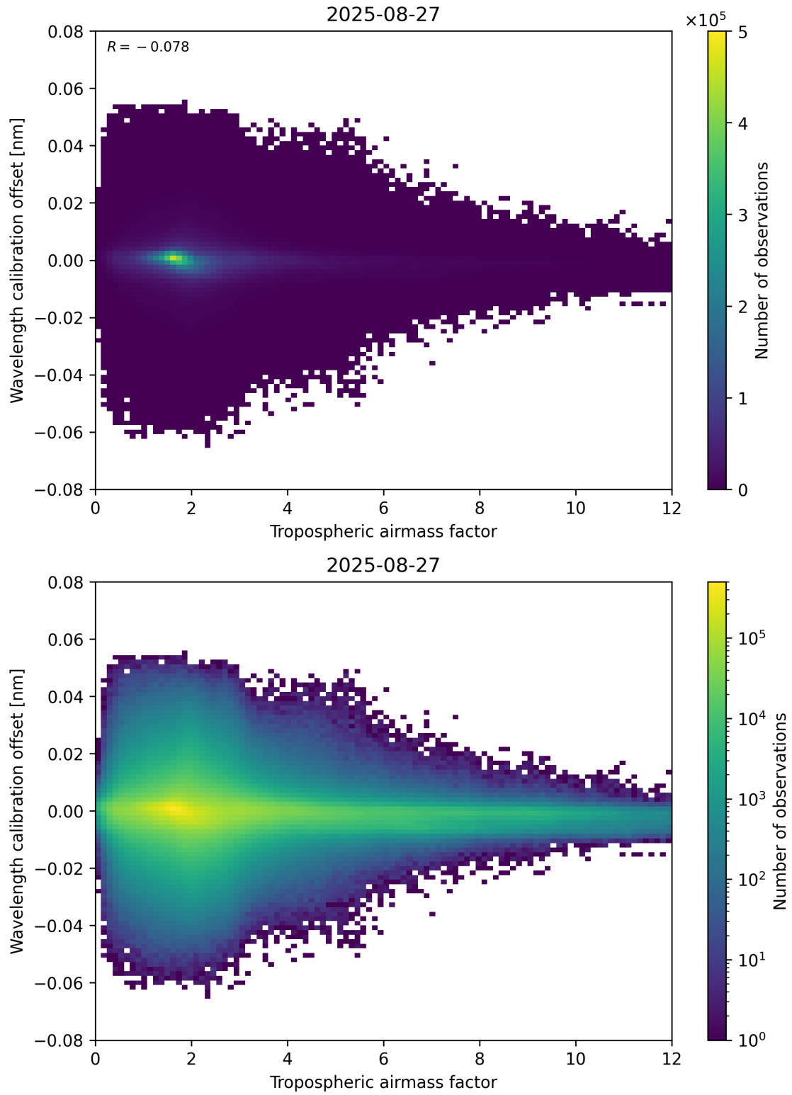
Figure 80: Scatter density plot of “Tropospheric airmass factor” against “Wavelength calibration offset” for 2025-08-26 to 2025-08-28.
