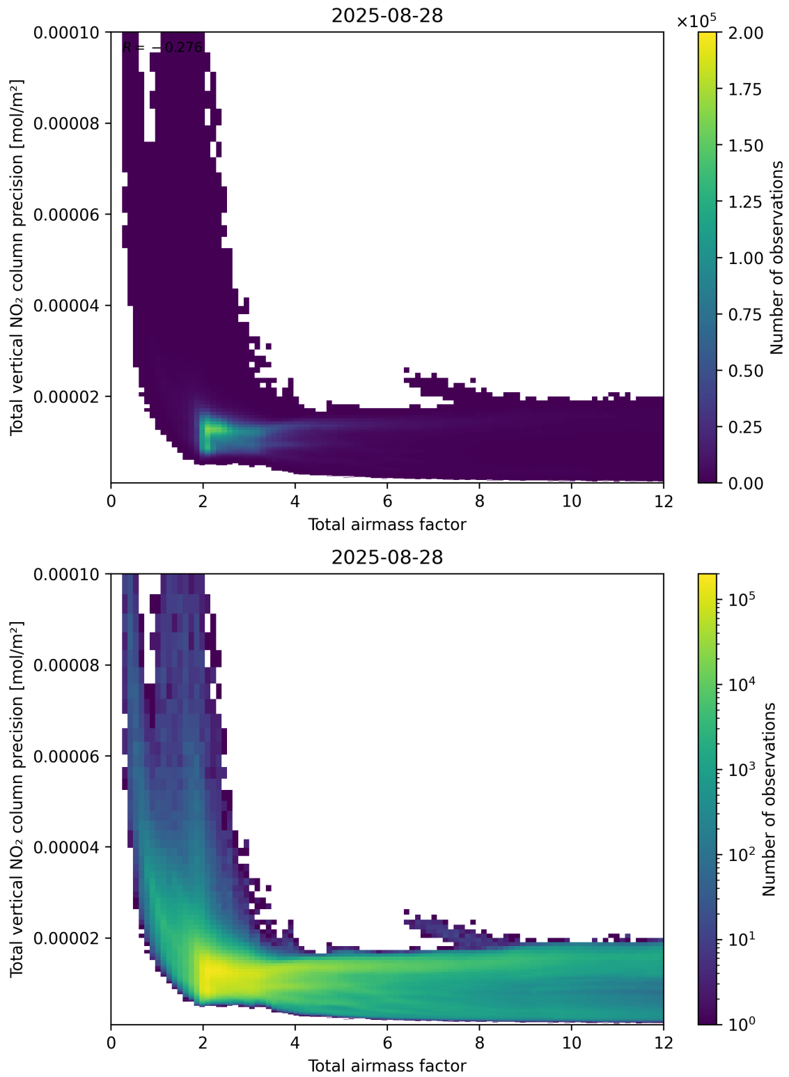
Figure 68: Scatter density plot of “Total airmass factor” against “Total vertical NO 2 column precision” for 2025-08-27 to 2025-08-29.
