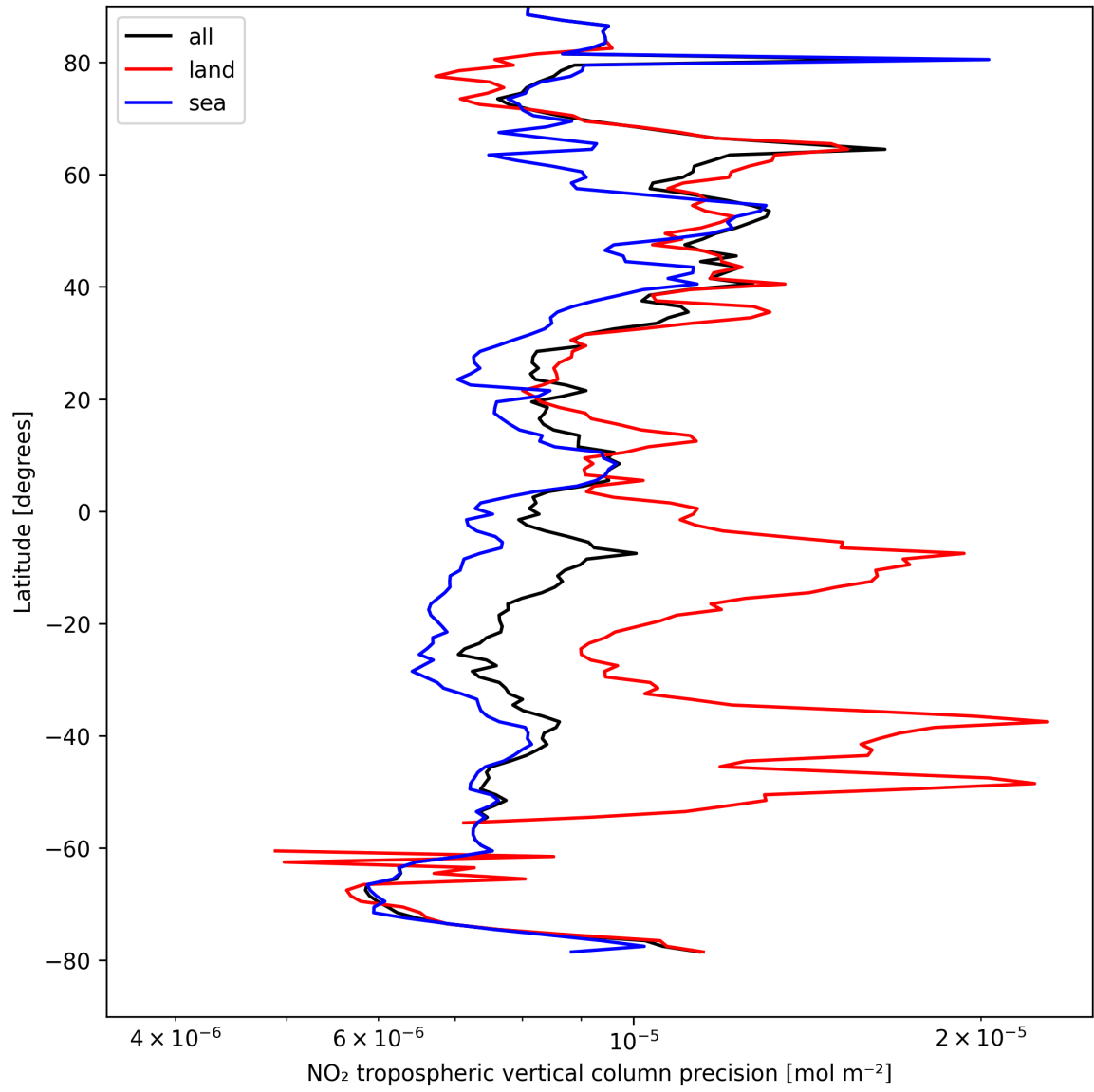
Figure 13: Zonal average of “NO 2 tropospheric vertical column precision” for 2025-08-27 to 2025-08-29.
