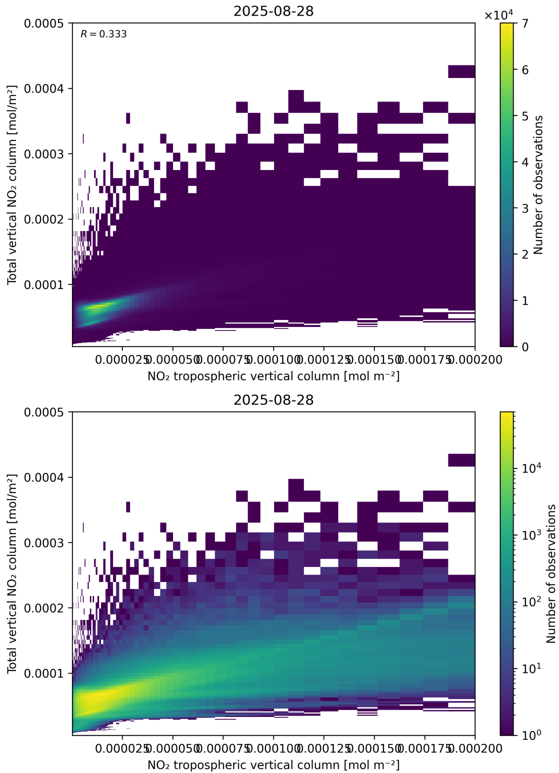
Figure 128: Scatter density plot of “NO 2 tropospheric vertical column” against “Total vertical NO 2 column” for 2025-08-27 to 2025-08-29.
