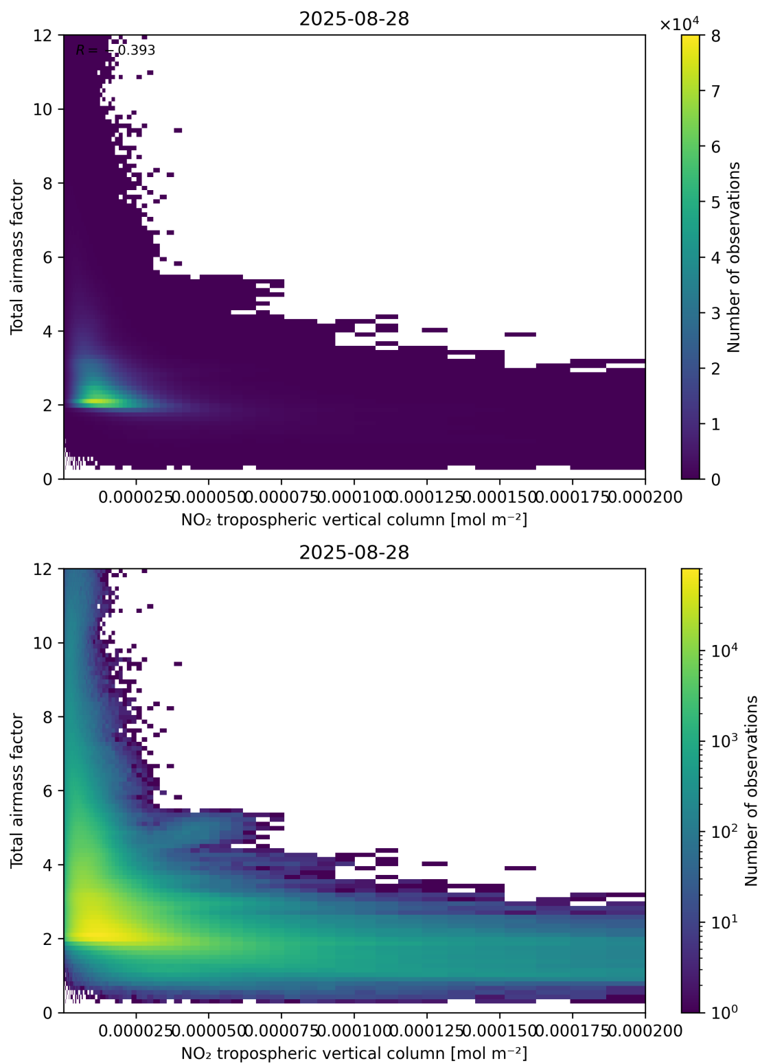
Figure 122: Scatter density plot of “NO 2 tropospheric vertical column” against “Total air mass factor” for 2025-08-27 to 2025-08-29.
