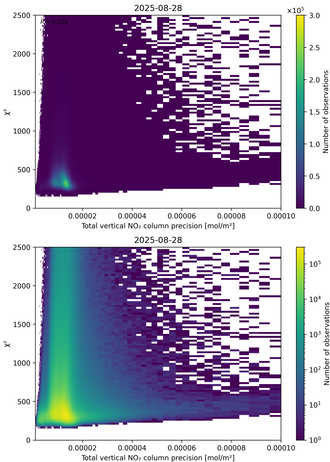
Figure 116: Scatter density plot of “Total vertical NO 2 column precision” against “ \chi^2 ” for 2025-08-27 to 2025-08-29.
