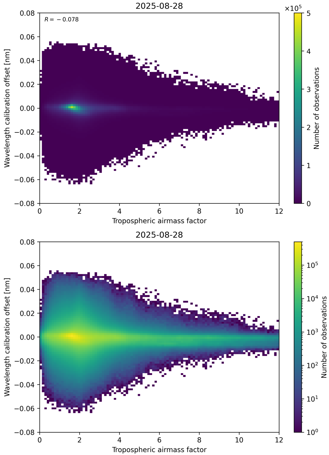
Figure 80: Scatter density plot of “Tropospheric airmass factor” against “Wavelength calibration offset” for 2025-08-27 to 2025-08-29.
