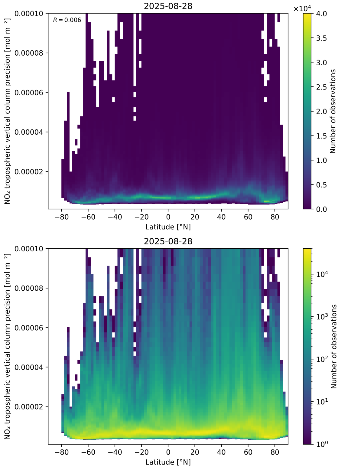
Figure 93: Scatter density plot of “Latitude” against “NO 2 tropospheric vertical column precision” for 2025-08-27 to 2025-08-29.
