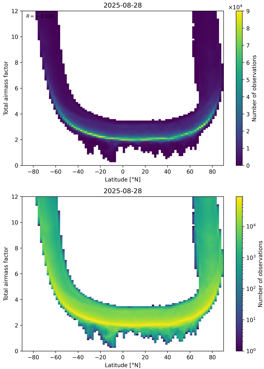
Figure 84: Scatter density plot of “Latitude” against “Total airmass factor” for 2025-08-27 to 2025-08-29.
