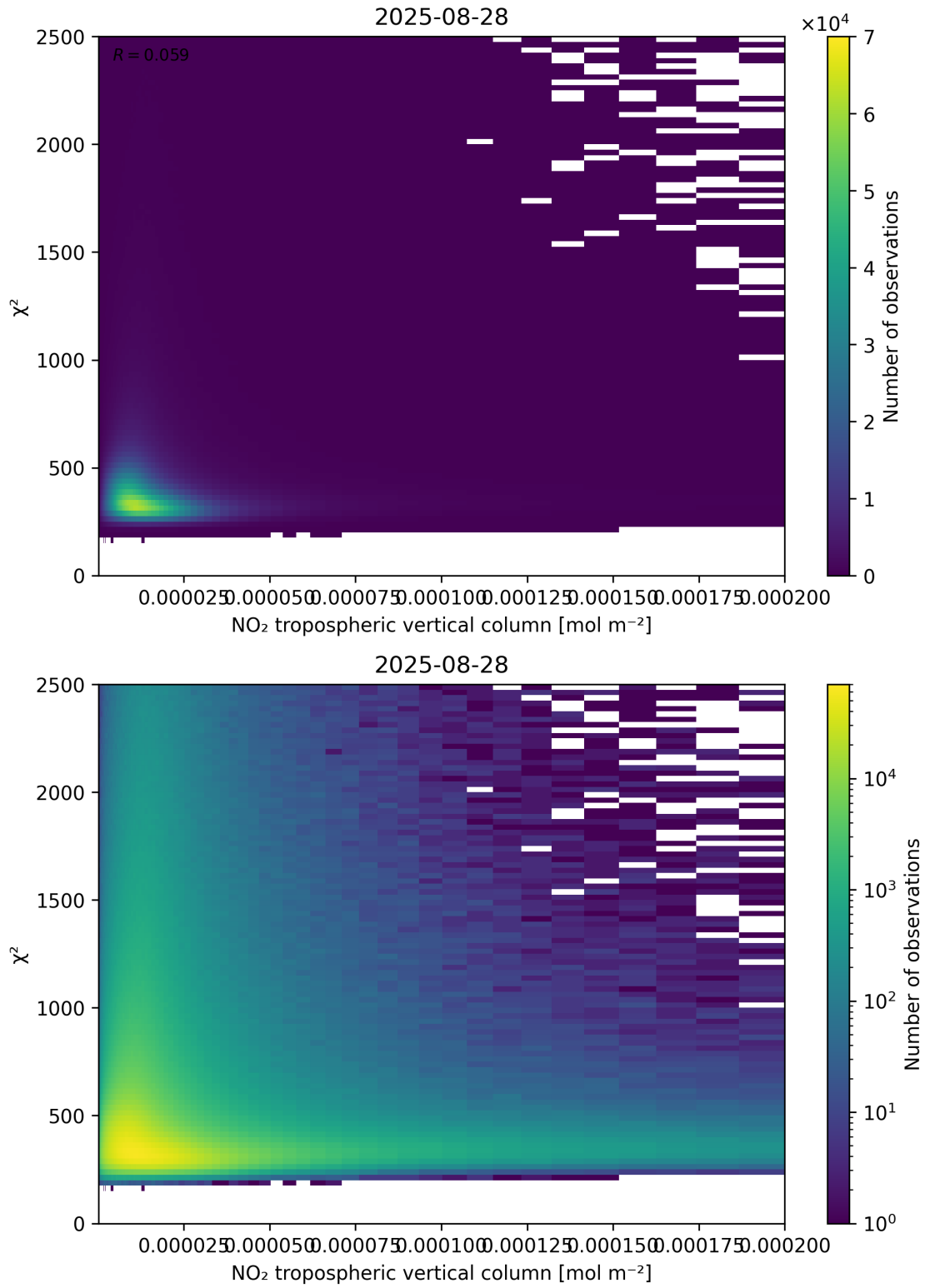
Figure 124: Scatter density plot of “NO 2 tropospheric vertical column” against “ \chi^2 ” for 2025-08-27 to 2025-08-29.
