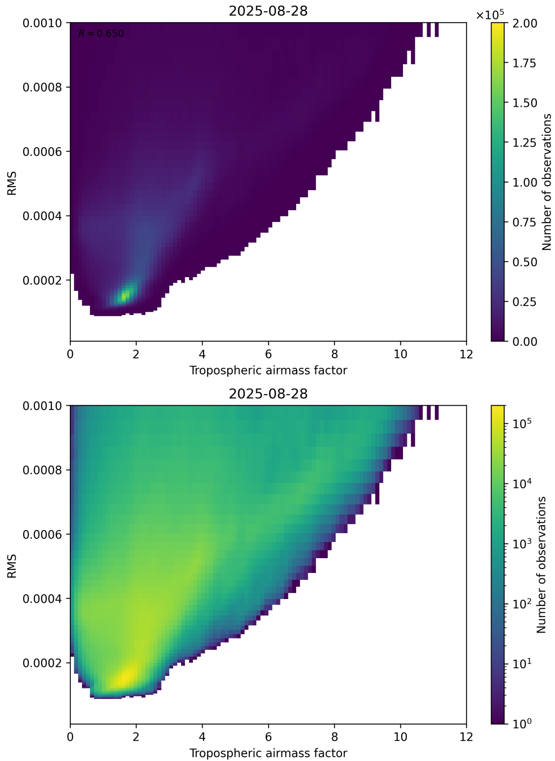
Figure 79: Scatter density plot of “Tropospheric airmass factor” against “RMS” for 2025-08-27 to 2025-08-29.
