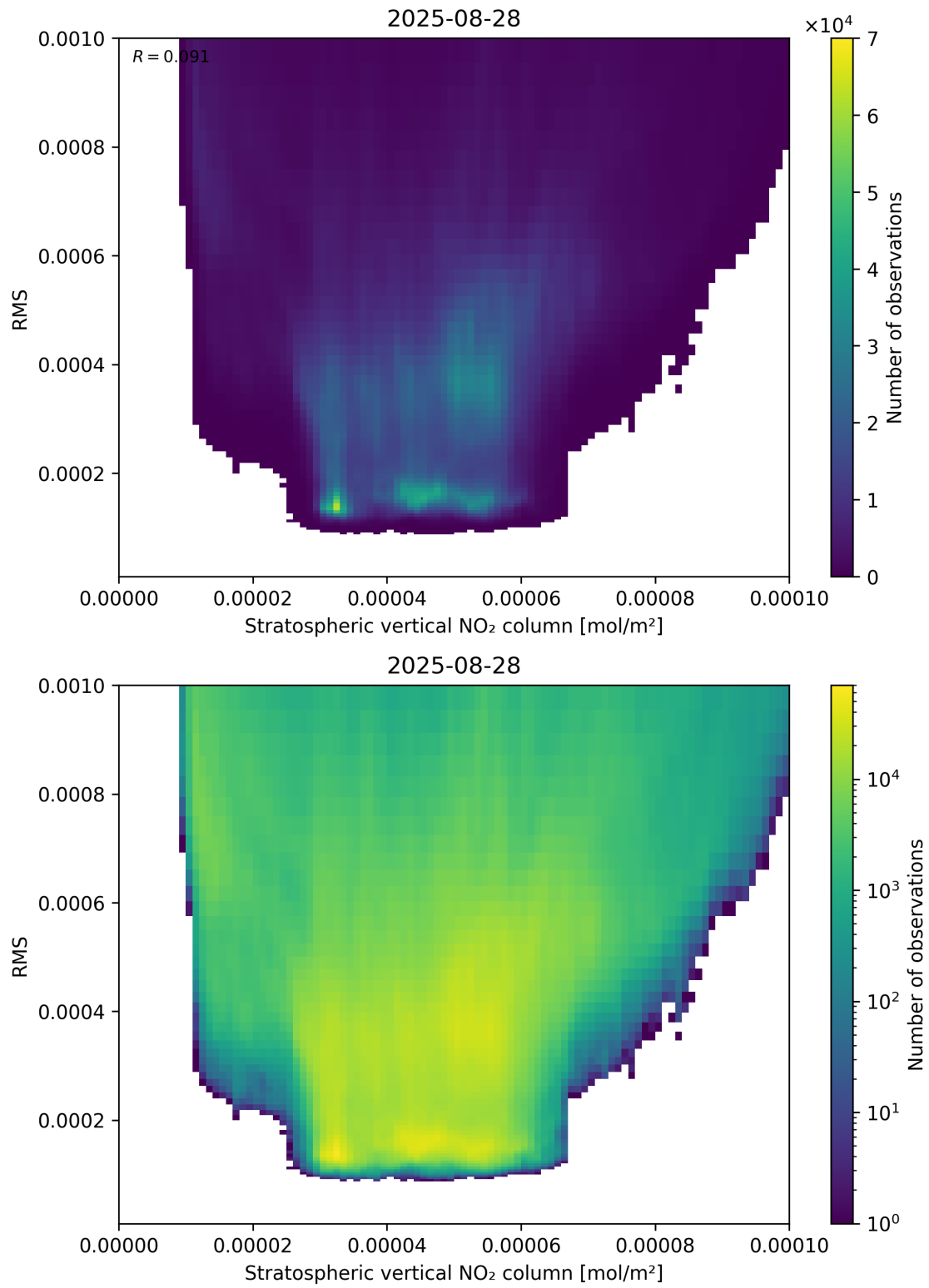
Figure 102: Scatter density plot of “Stratospheric vertical NO 2 column” against “RMS” for 2025-08-27 to 2025-08-29.
