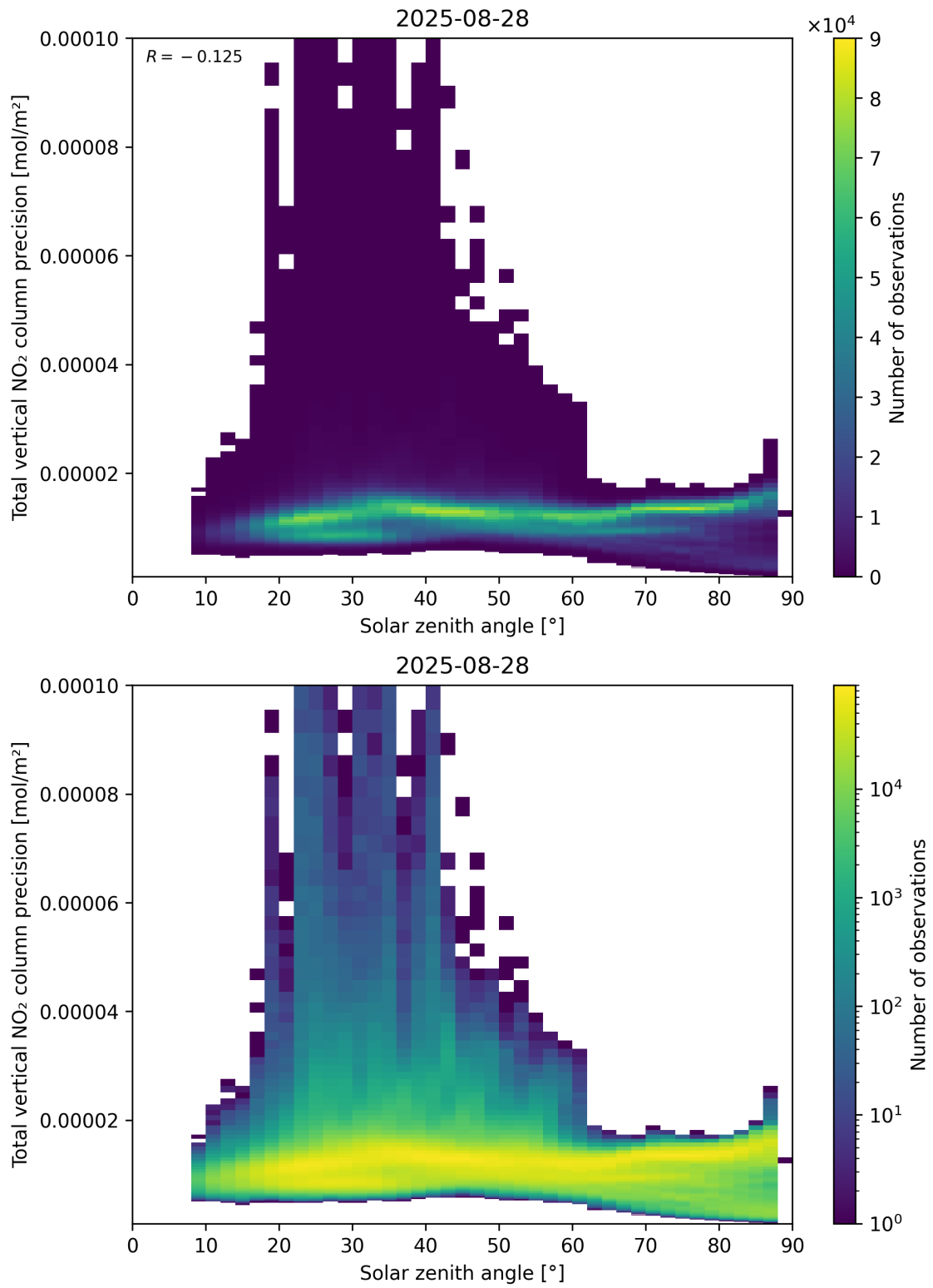
Figure 154: Scatter density plot of “Solar zenith angle” against “Total vertical NO 2 column precision” for 2025-08-27 to 2025-08-29.
