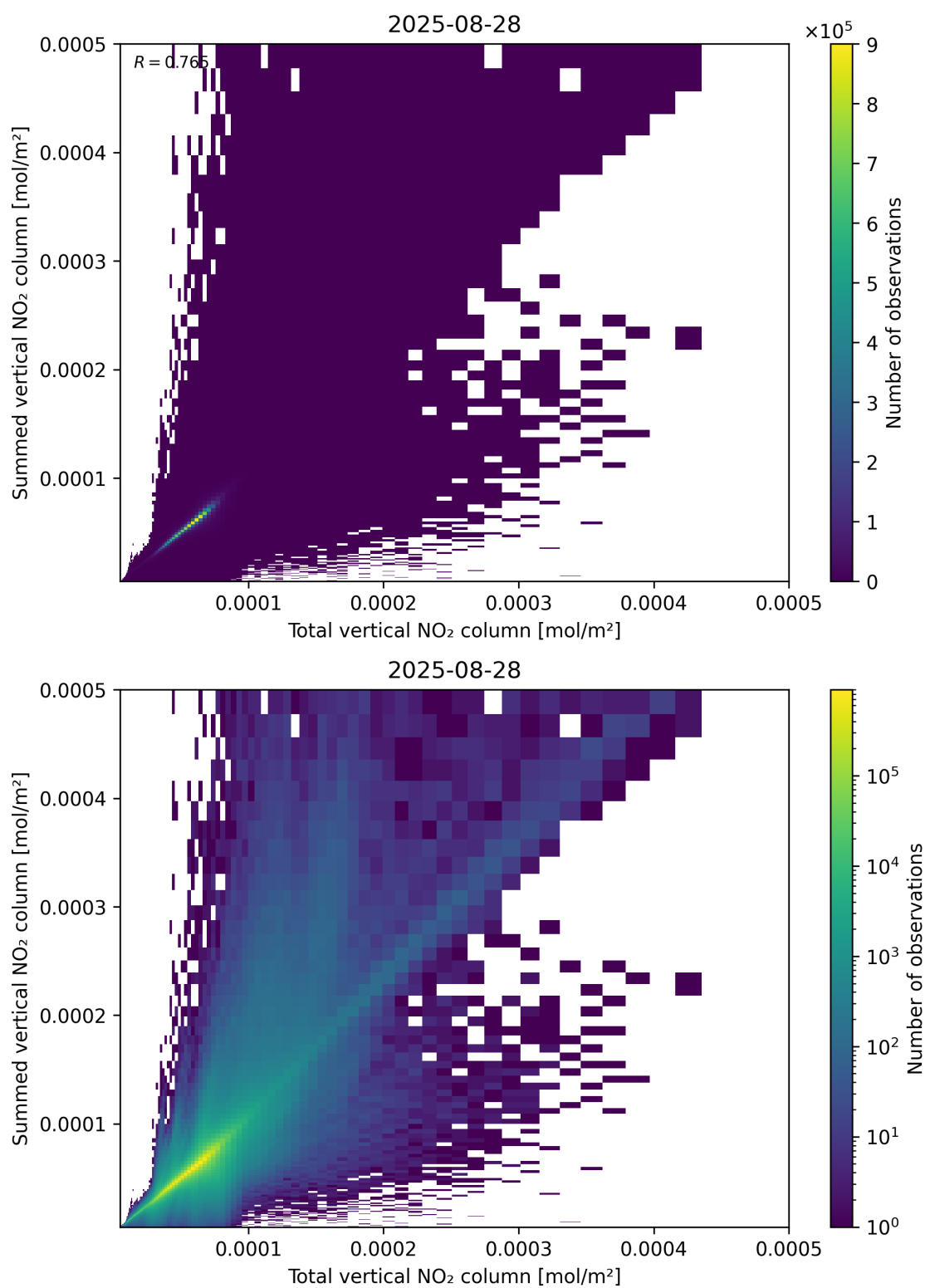
Figure 112: Scatter density plot of “Total vertical NO 2 column” against “Summed vertical NO 2 column” for 2025-08-27 to 2025-08-29.
