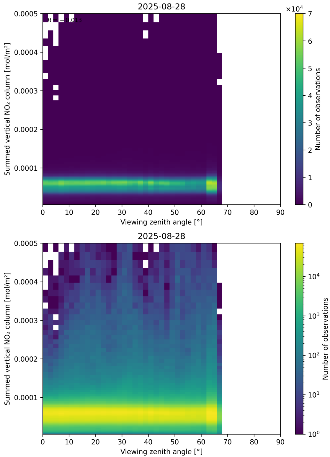
Figure 165: Scatter density plot of “Viewing zenith angle” against “Summed vertical NO 2 column” for 2025-08-27 to 2025-08-29.
