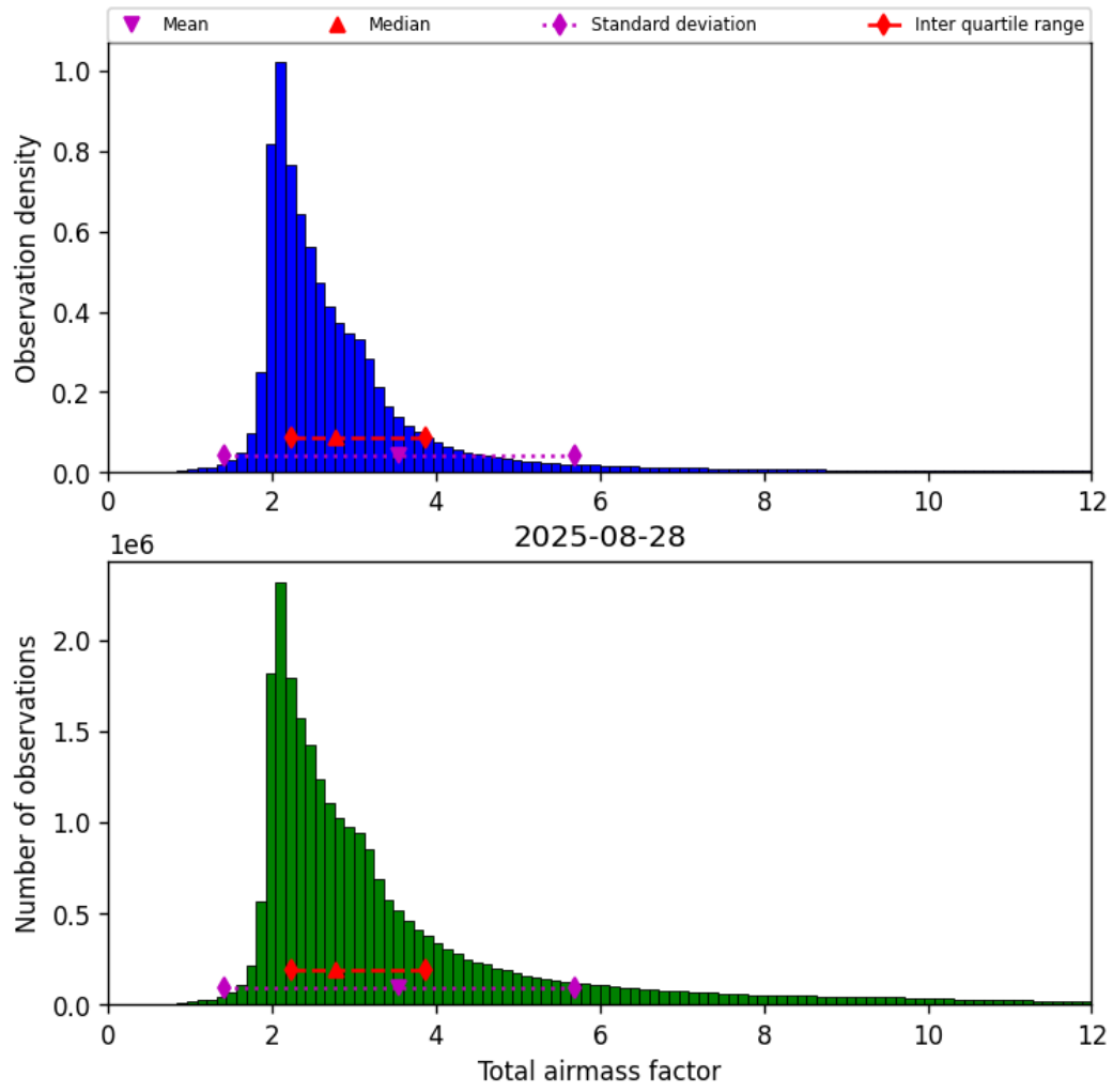
Figure 32: Histogram of “Total airmass factor” for 2025-08-27 to 2025-08-29
