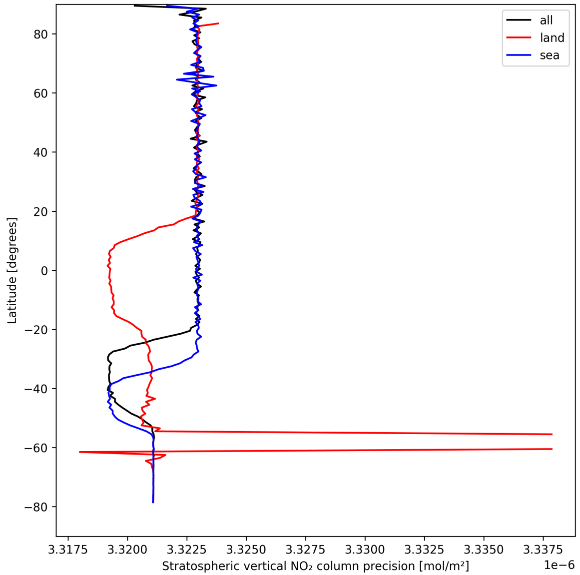
Figure 20: Zonal average of “Stratospheric vertical NO 2 column precision” for 2025-08-27 to 2025-08-29.
