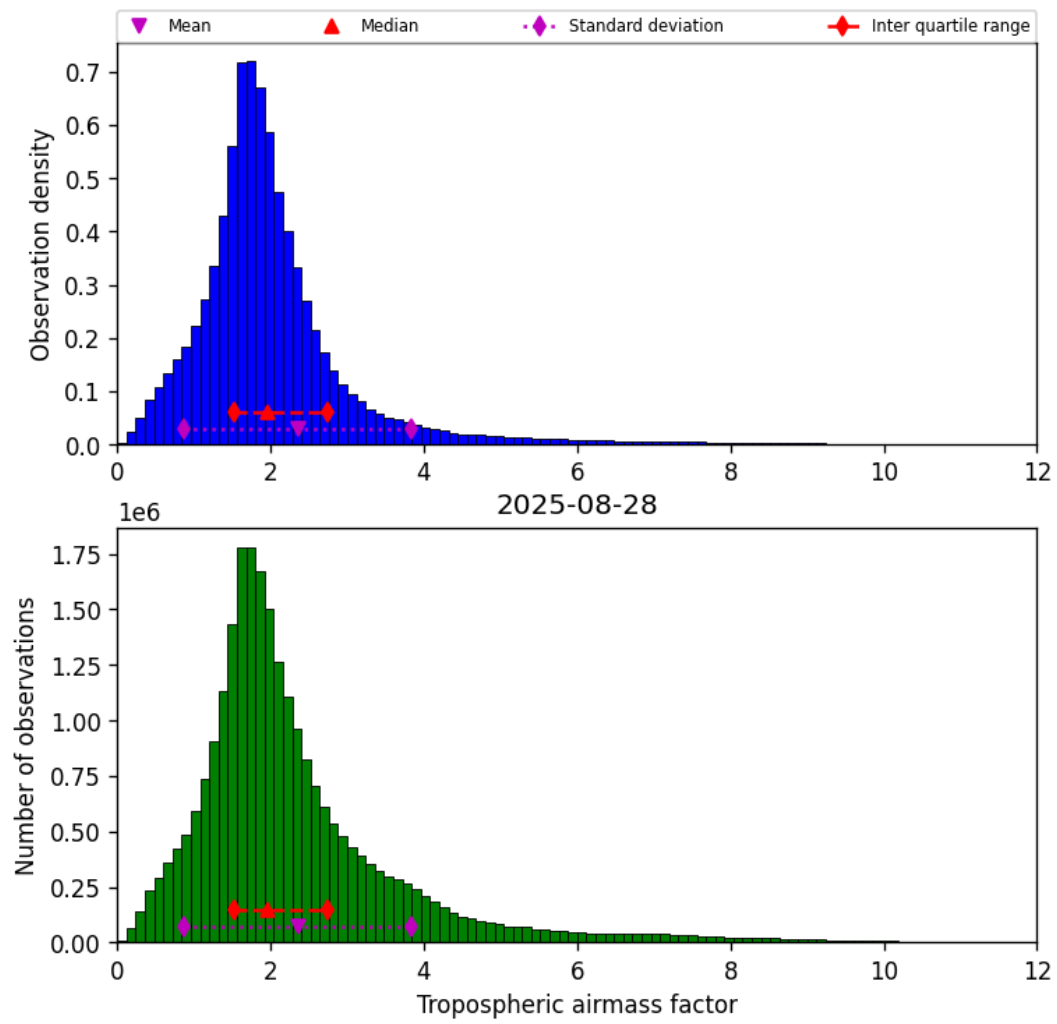
Figure 31: Histogram of “Tropospheric airmass factor” for 2025-08-27 to 2025-08-29
