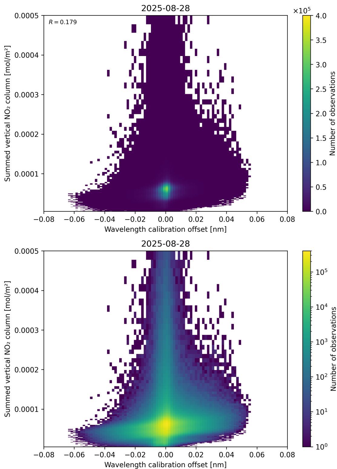
Figure 177: Scatter density plot of “Wavelength calibration offset” against “Summed vertical NO 2 column” for 2025-08-27 to 2025-08-29.
