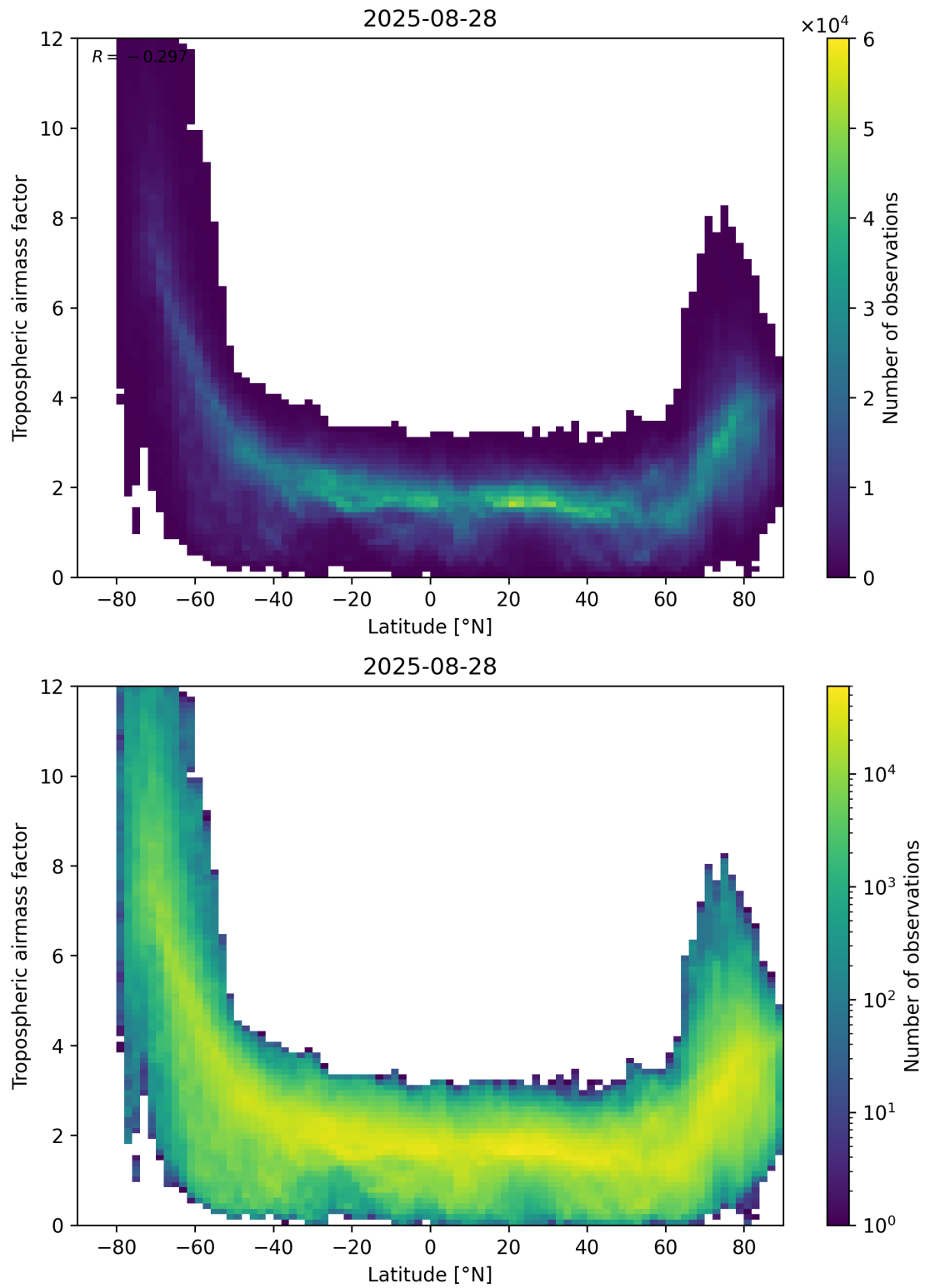
Figure 85: Scatter density plot of “Latitude” against “Tropospheric airmass factor” for 2025-08-27 to 2025-08-29.
