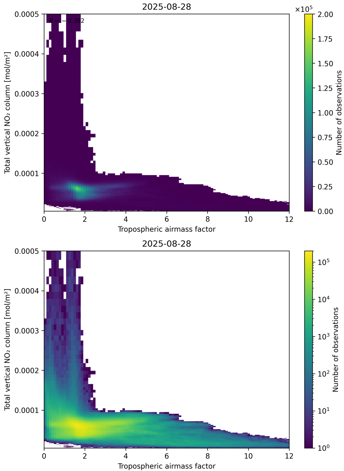
Figure 77: Scatter density plot of “Tropospheric airmass factor” against “Total vertical NO 2 column” for 2025-08-27 to 2025-08-29.
