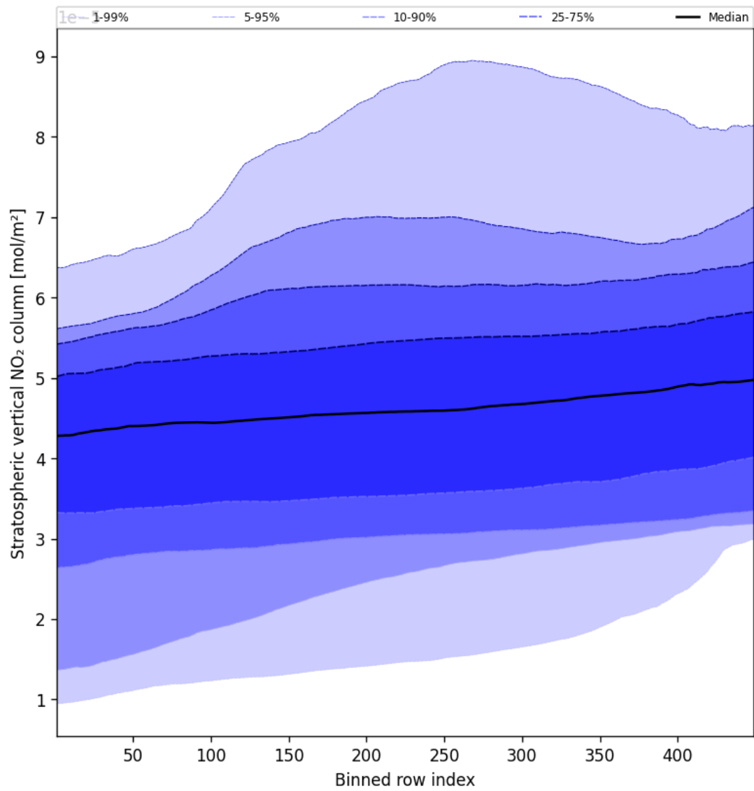
Figure 53: Along track statistics of “Stratospheric vertical NO 2 column” for 2025-08-27 to 2025-08-29
