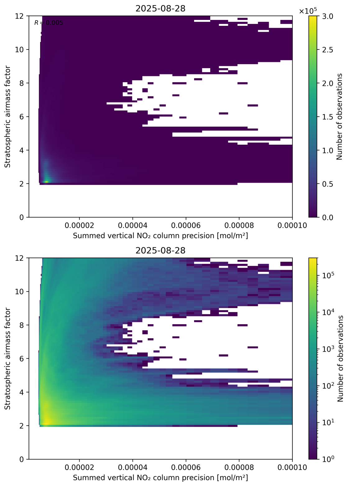
Figure 106: Scatter density plot of “Summed vertical NO 2 column precision” against “Stratospheric airmass factor” for 2025-08-27 to 2025-08-29.
