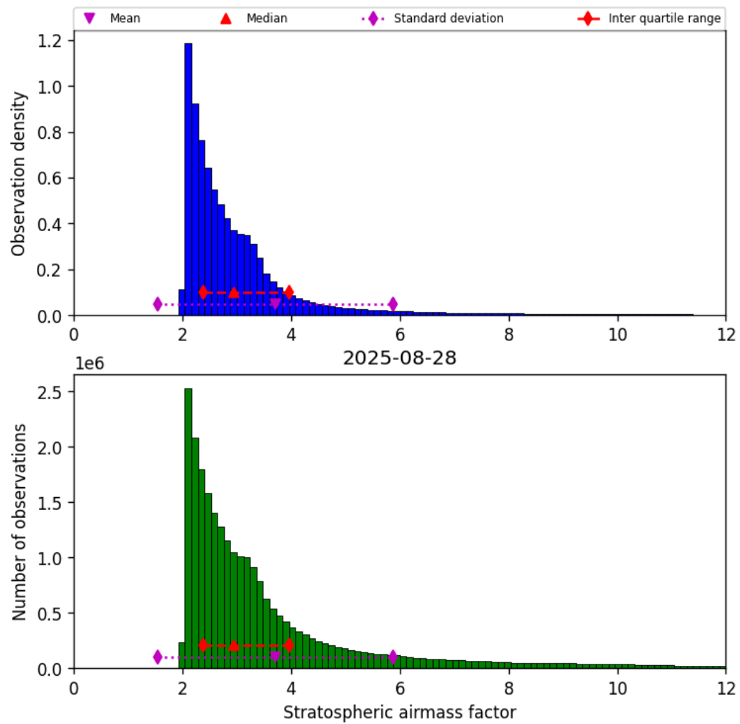
Figure 44: Histogram of “Stratospheric airmass factor” for 2025-08-27 to 2025-08-29
