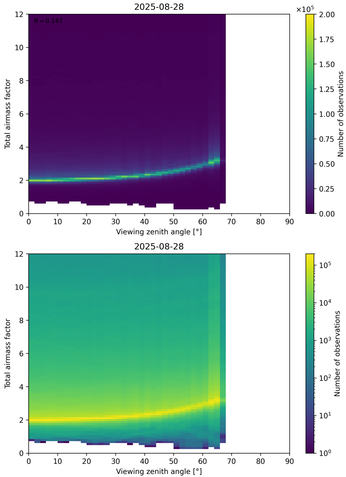
Figure 160: Scatter density plot of “Viewing zenith angle” against “Total airmass factor” for 2025-08-27 to 2025-08-29.
