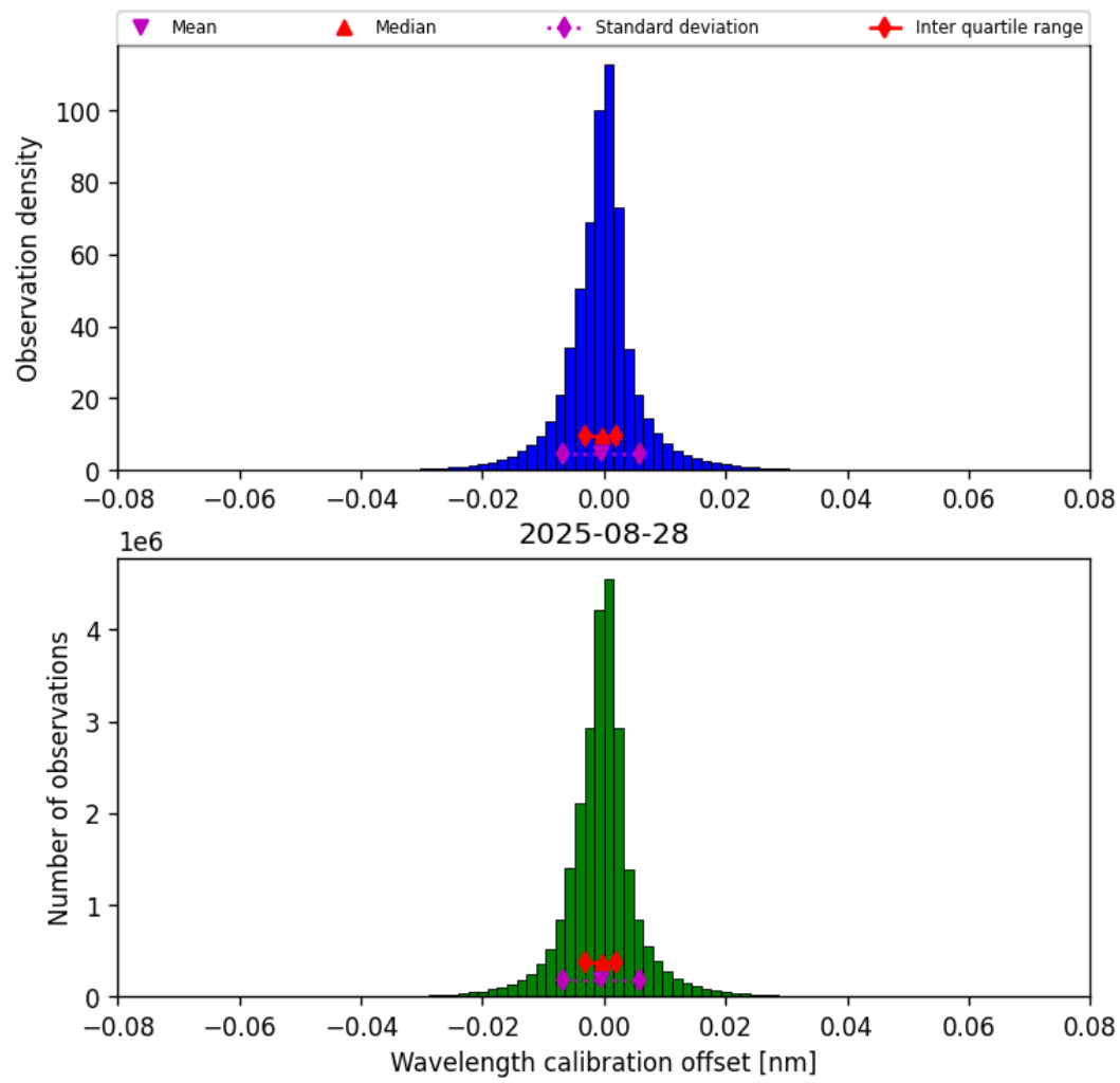
Figure 35: Histogram of “Wavelength calibration offset” for 2025-08-27 to 2025-08-29
