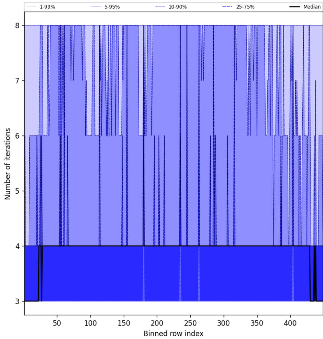
Figure 51: Along track statistics of “Number of iterations” for 2025-08-27 to 2025-08-29
