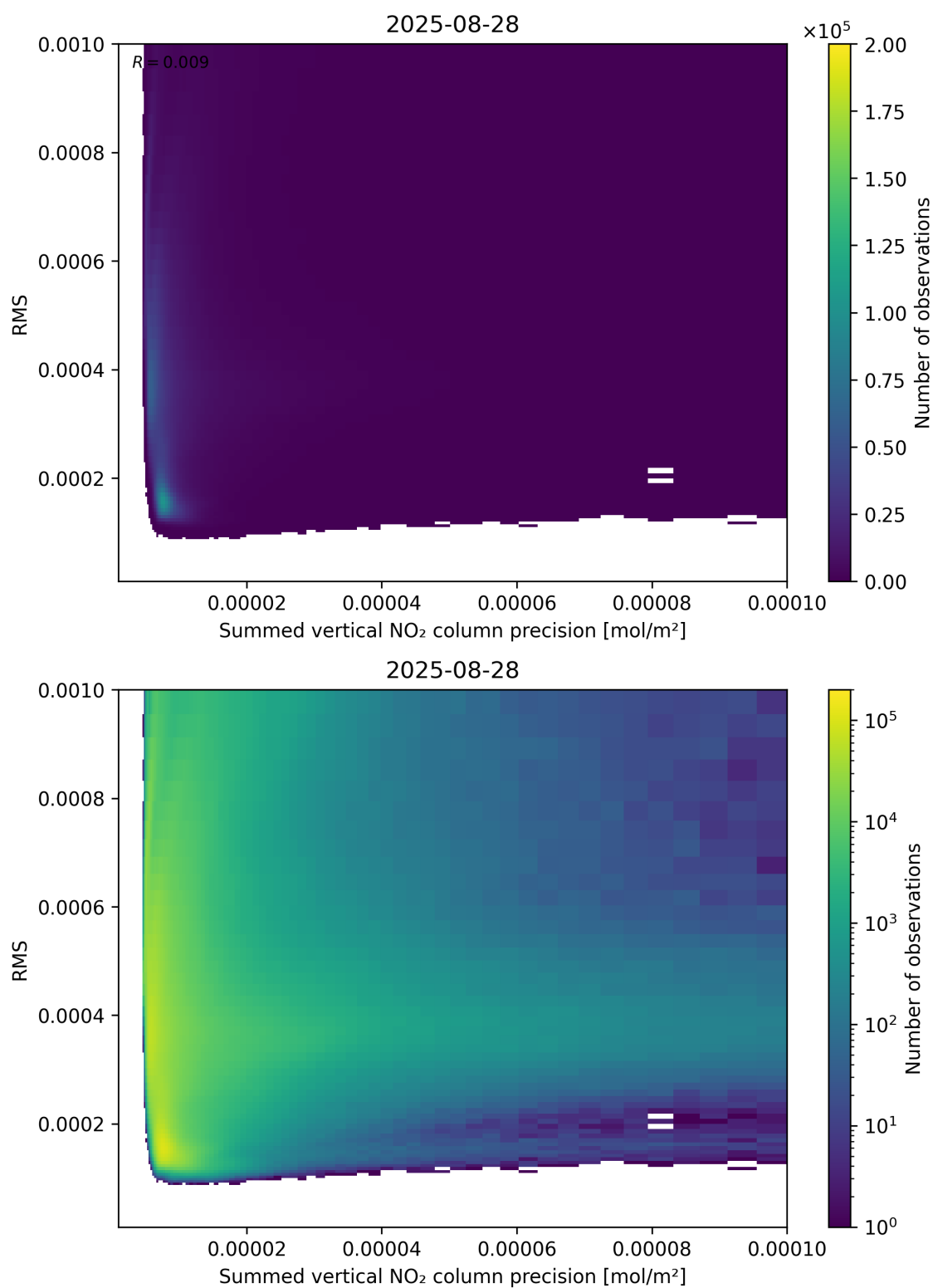
Figure 108: Scatter density plot of “Summed vertical NO 2 column precision” against “RMS” for 2025-08-27 to 2025-08-29.
