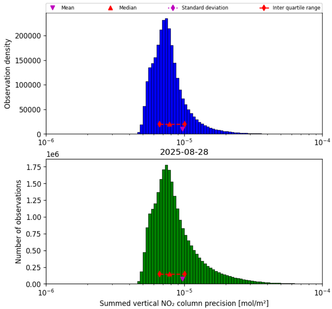
Figure 41: Histogram of “Summed vertical NO 2 column precision” for 2025-08-27 to 2025-08-29
