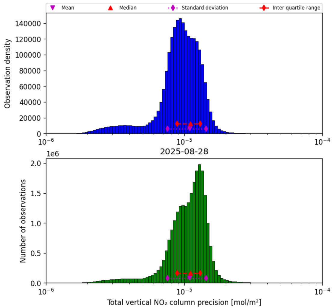
Figure 39: Histogram of “Total vertical NO 2 column precision” for 2025-08-27 to 2025-08-29
