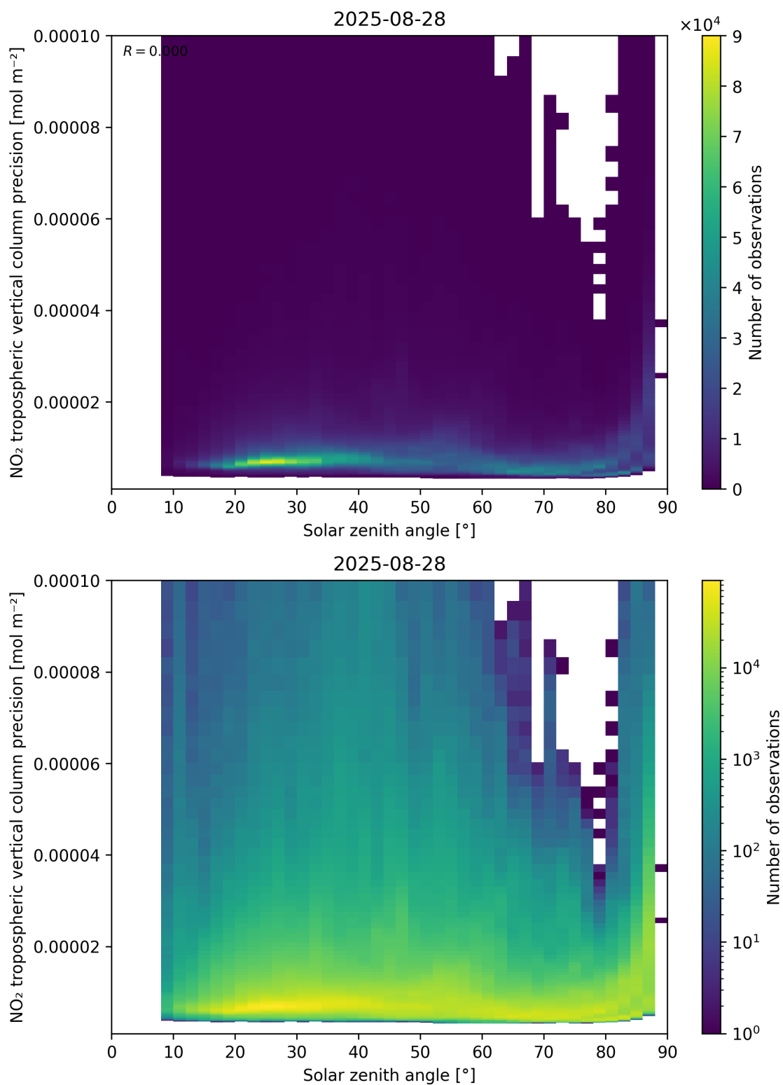
Figure 156: Scatter density plot of “Solar zenith angle” against “NO 2 tropospheric vertical column precision” for 2025-08-27 to 2025-08-29.
