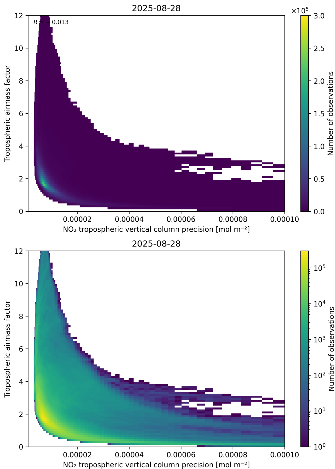
Figure 133: Scatter density plot of “NO 2 tropospheric vertical column precision” against “Tropospheric air mass factor” for 2025-08-27 to 2025-08-29.
