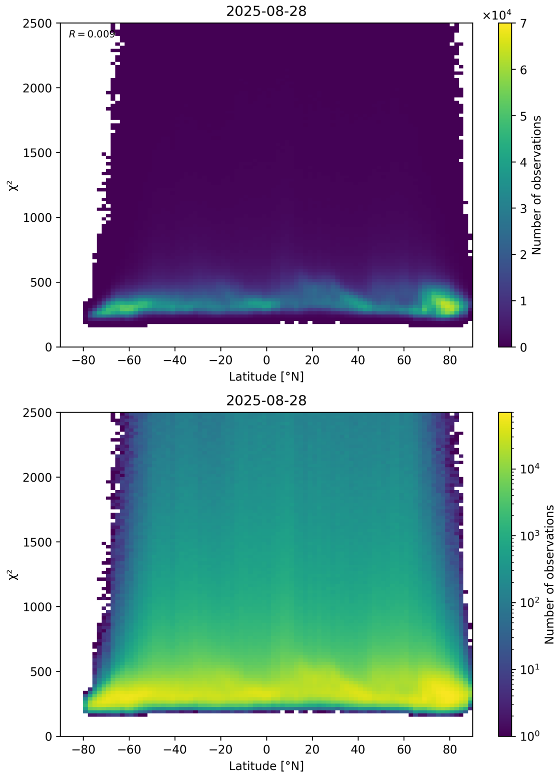
Figure 86: Scatter density plot of “Latitude” against “ \chi^2 ” for 2025-08-27 to 2025-08-29.
