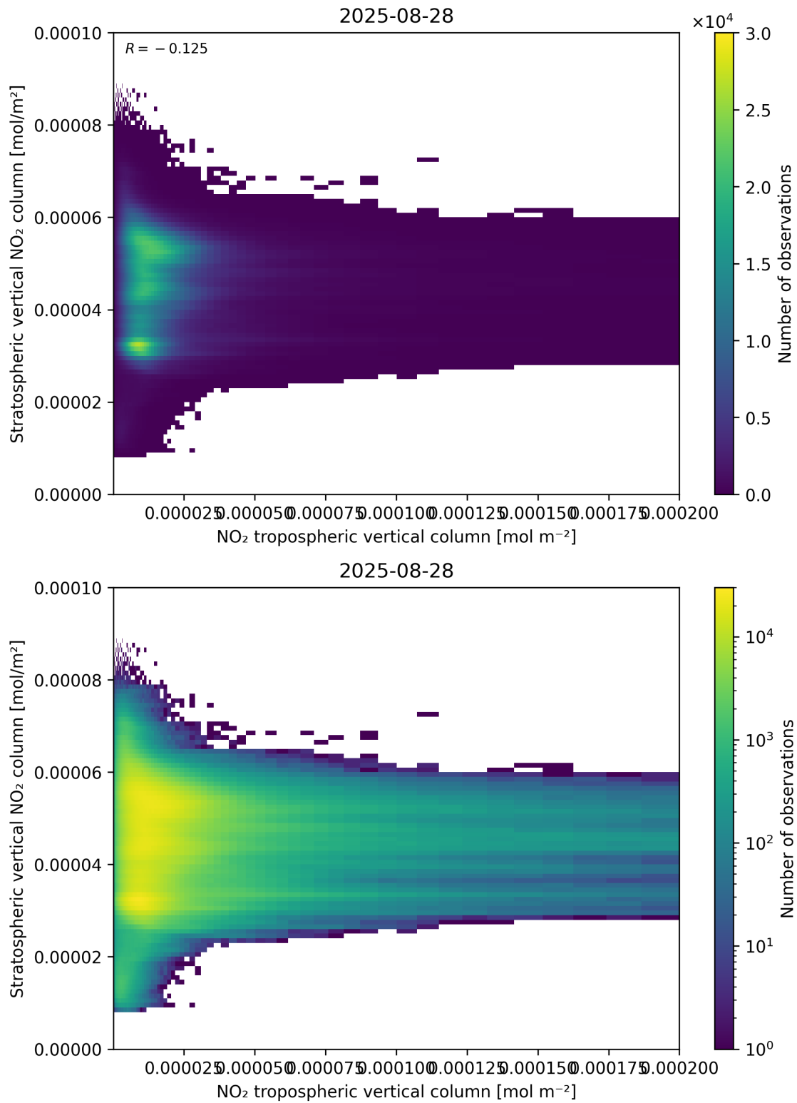
Figure 125: Scatter density plot of “NO 2 tropospheric vertical column” against “Stratospheric vertical NO 2 column” for 2025-08-27 to 2025-08-29.
