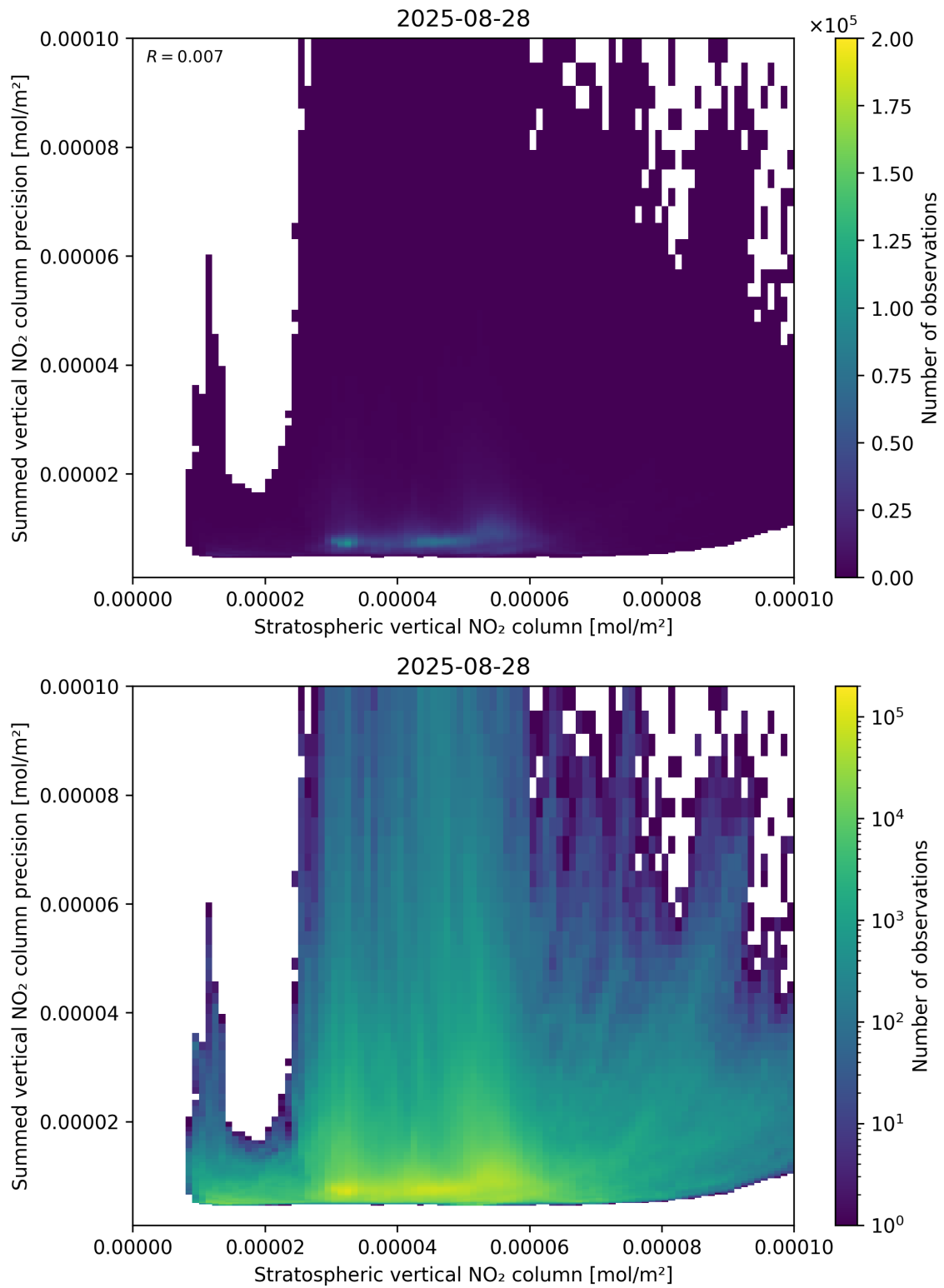
Figure 99: Scatter density plot of “Stratospheric vertical NO 2 column” against “Summed vertical NO 2 column precision” for 2025-08-27 to 2025-08-29.
