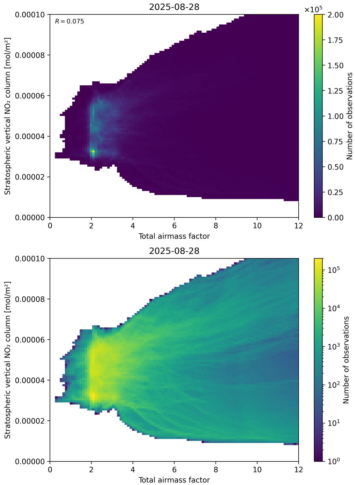
Figure 64: Scatter density plot of “Total airmass factor” against “Stratospheric vertical \text{NO}_2 column” for 2025-08-27 to 2025-08-29.
