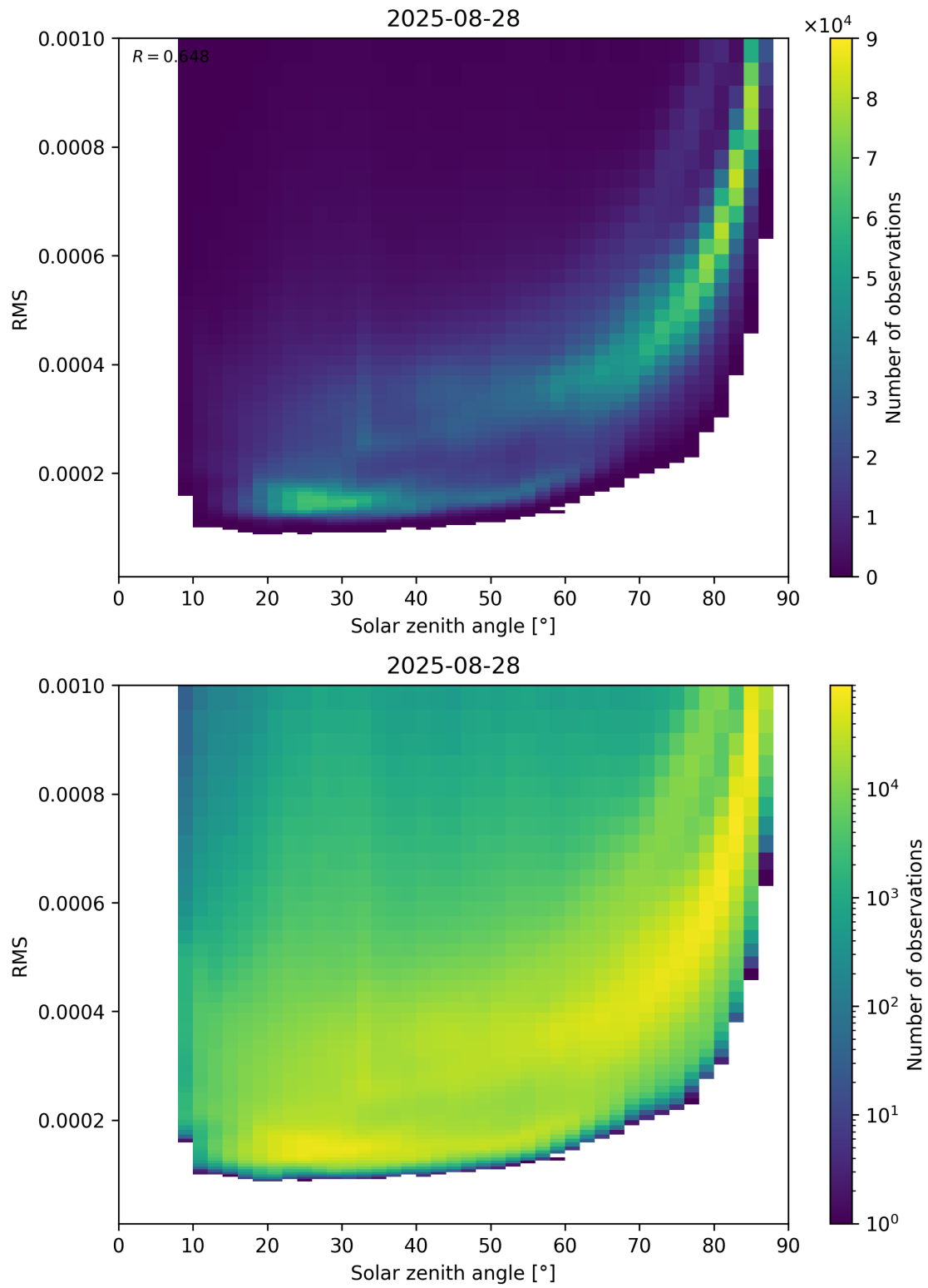
Figure 157: Scatter density plot of “Solar zenith angle” against “RMS” for 2025-08-27 to 2025-08-29.
