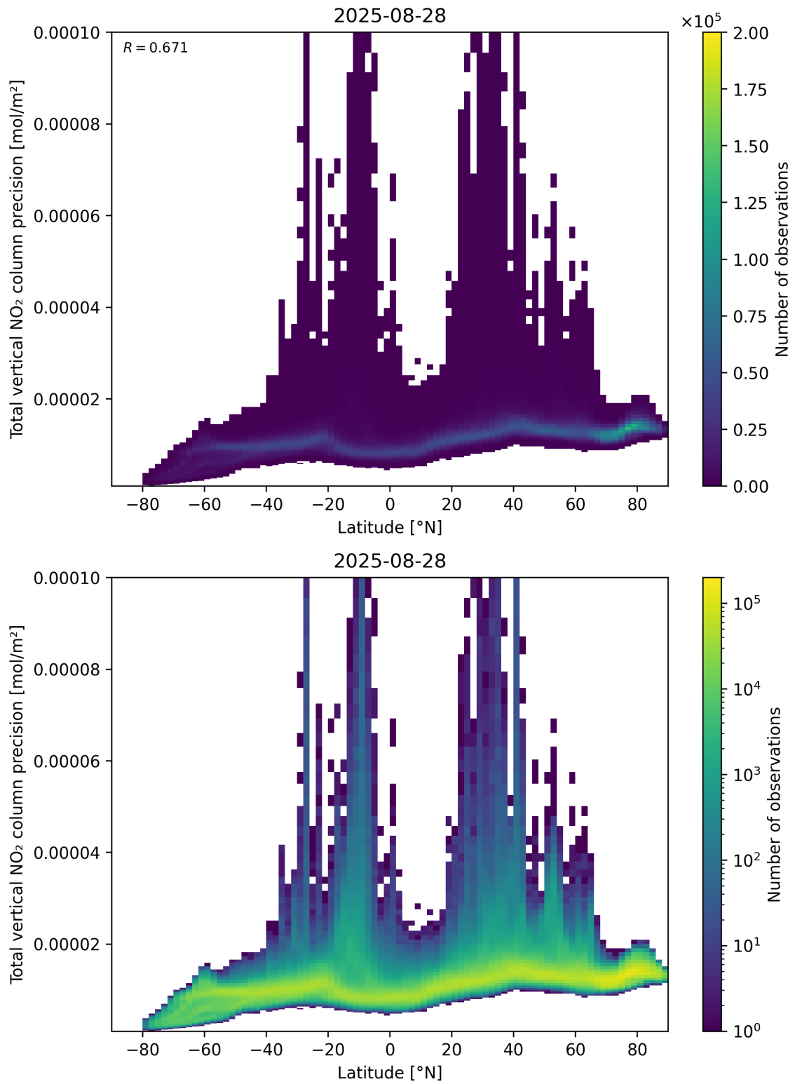
Figure 91: Scatter density plot of “Latitude” against “Total vertical NO 2 column precision” for 2025-08-27 to 2025-08-29.
