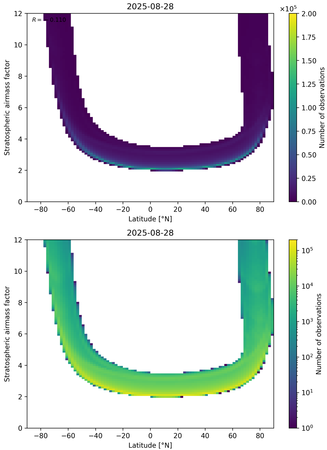
Figure 83: Scatter density plot of “Latitude” against “Stratospheric air mass factor” for 2025-08-27 to 2025-08-29.
