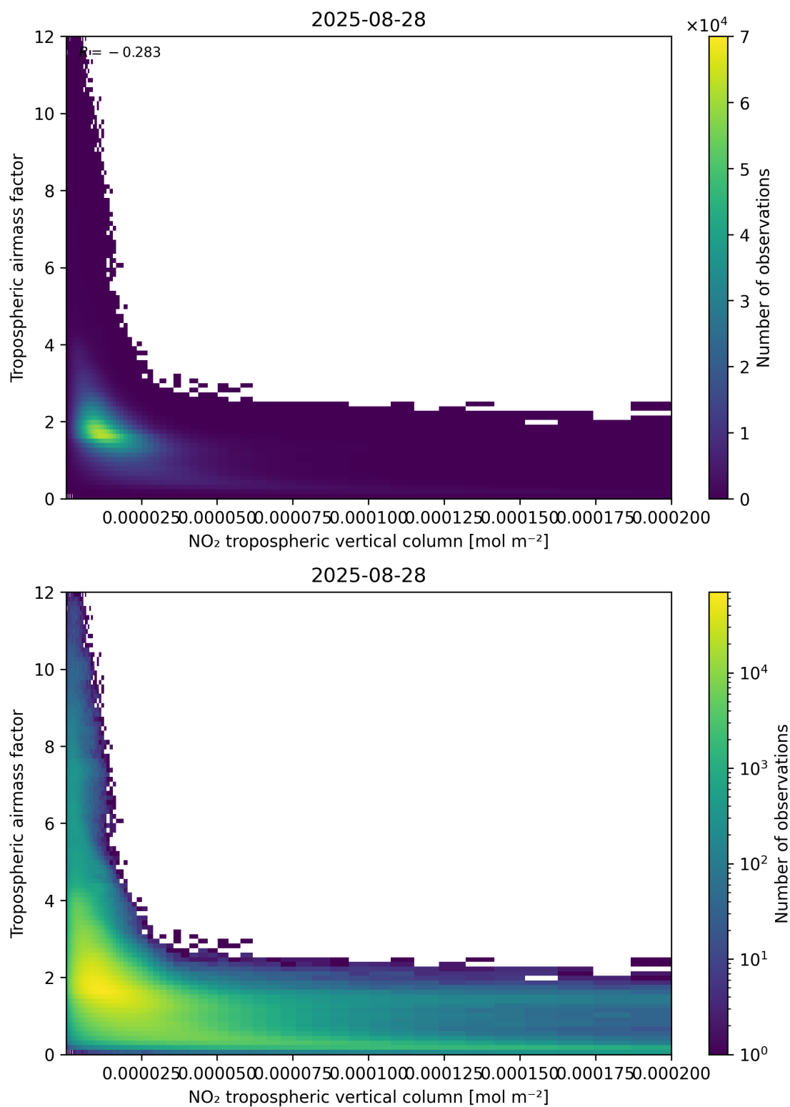
Figure 123: Scatter density plot of “NO 2 tropospheric vertical column” against “Tropospheric air mass factor” for 2025-08-27 to 2025-08-29.
