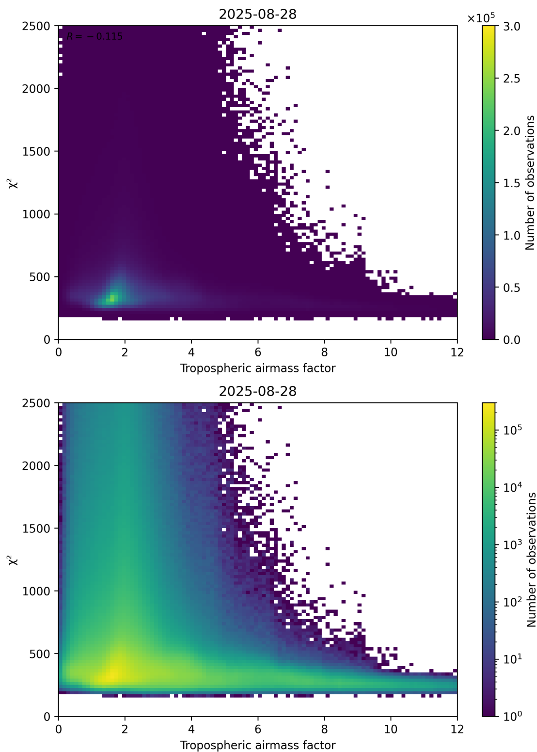
Figure 73: Scatter density plot of “Tropospheric airmass factor” against “ \chi^2 ” for 2025-08-27 to 2025-08-29.
