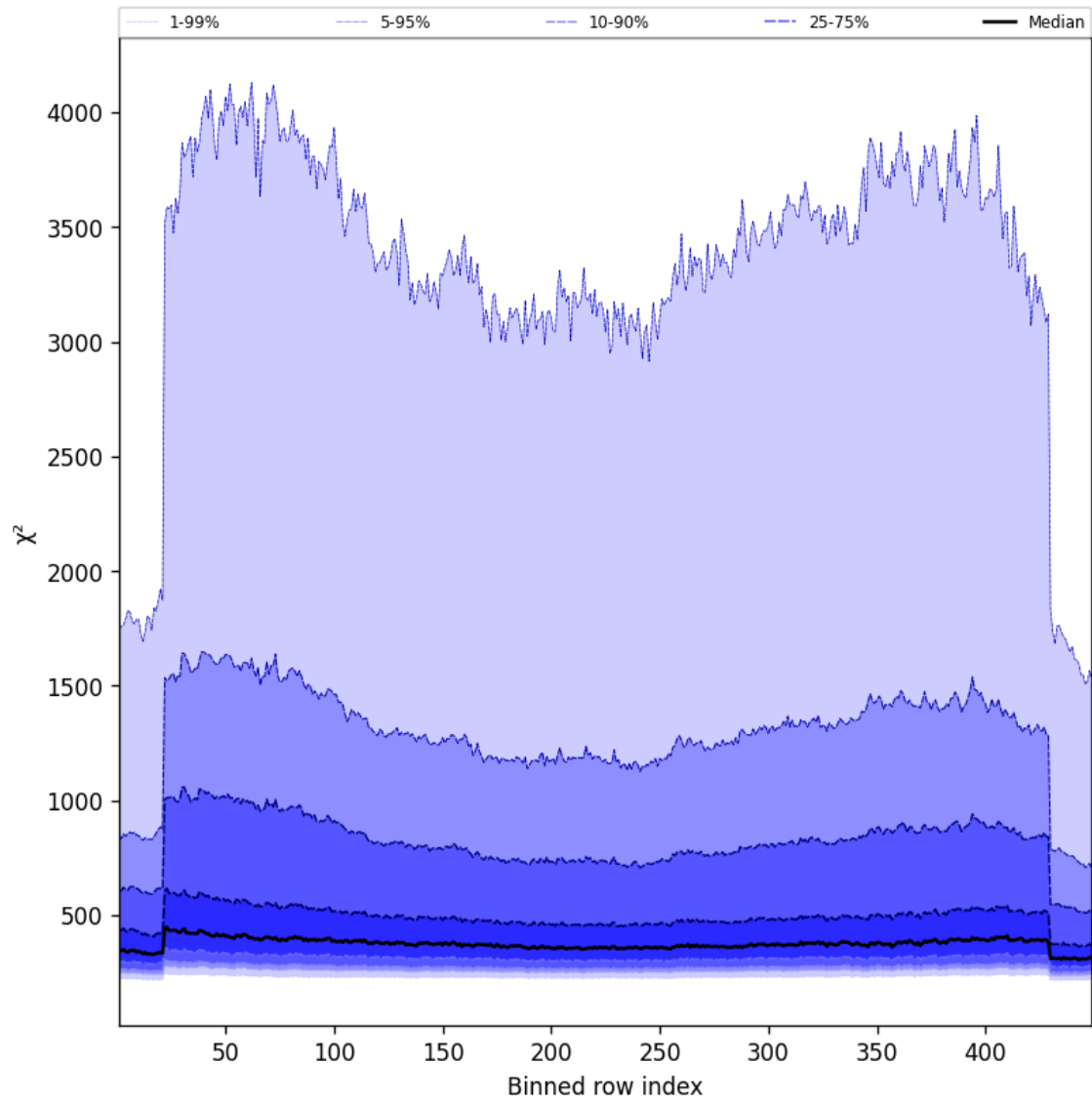
Figure 59: Along track statistics of “ \chi^2 ” for 2025-08-27 to 2025-08-29
