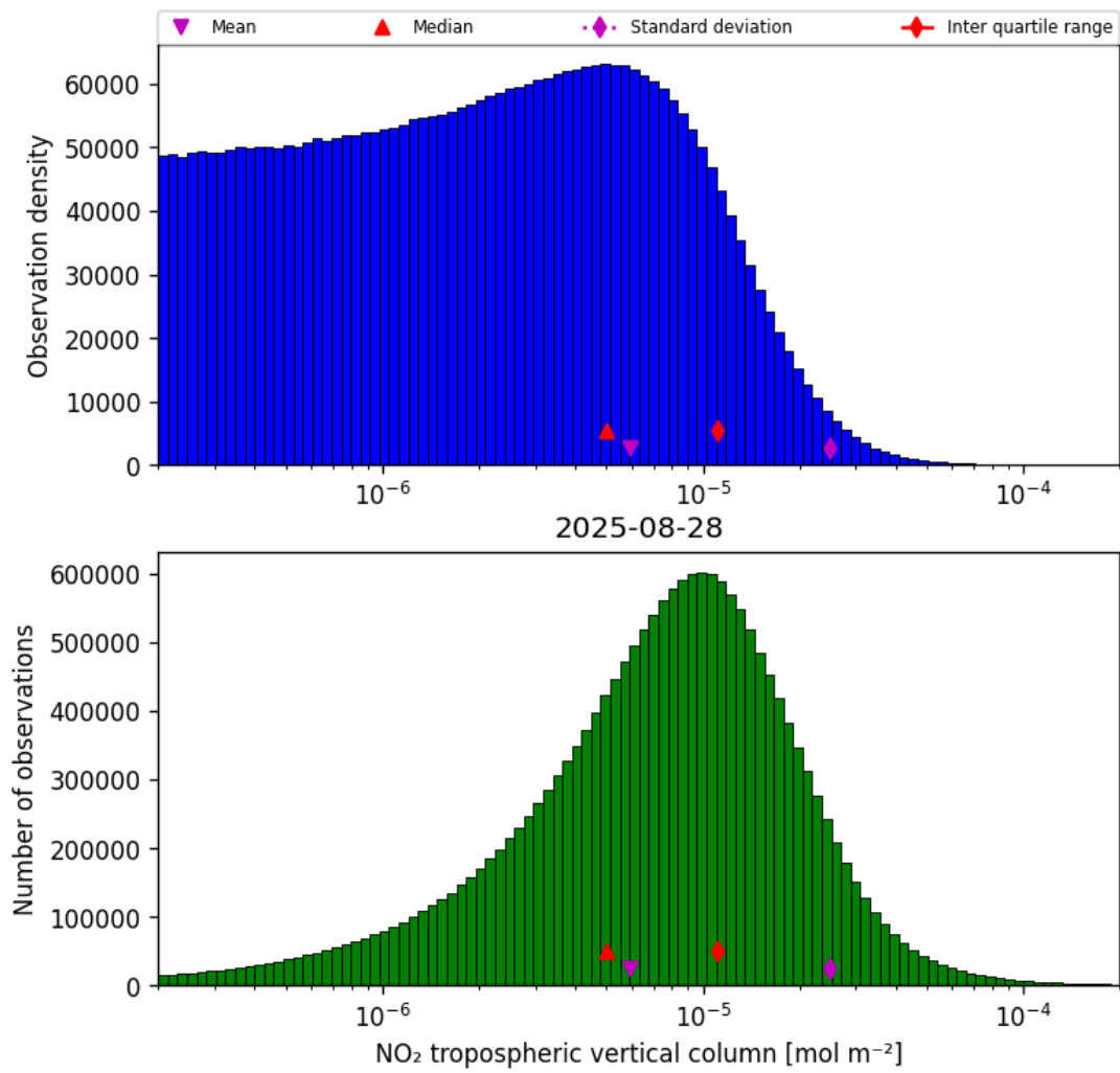
Figure 29: Histogram of “NO 2 tropospheric vertical column” for 2025-08-27 to 2025-08-29
