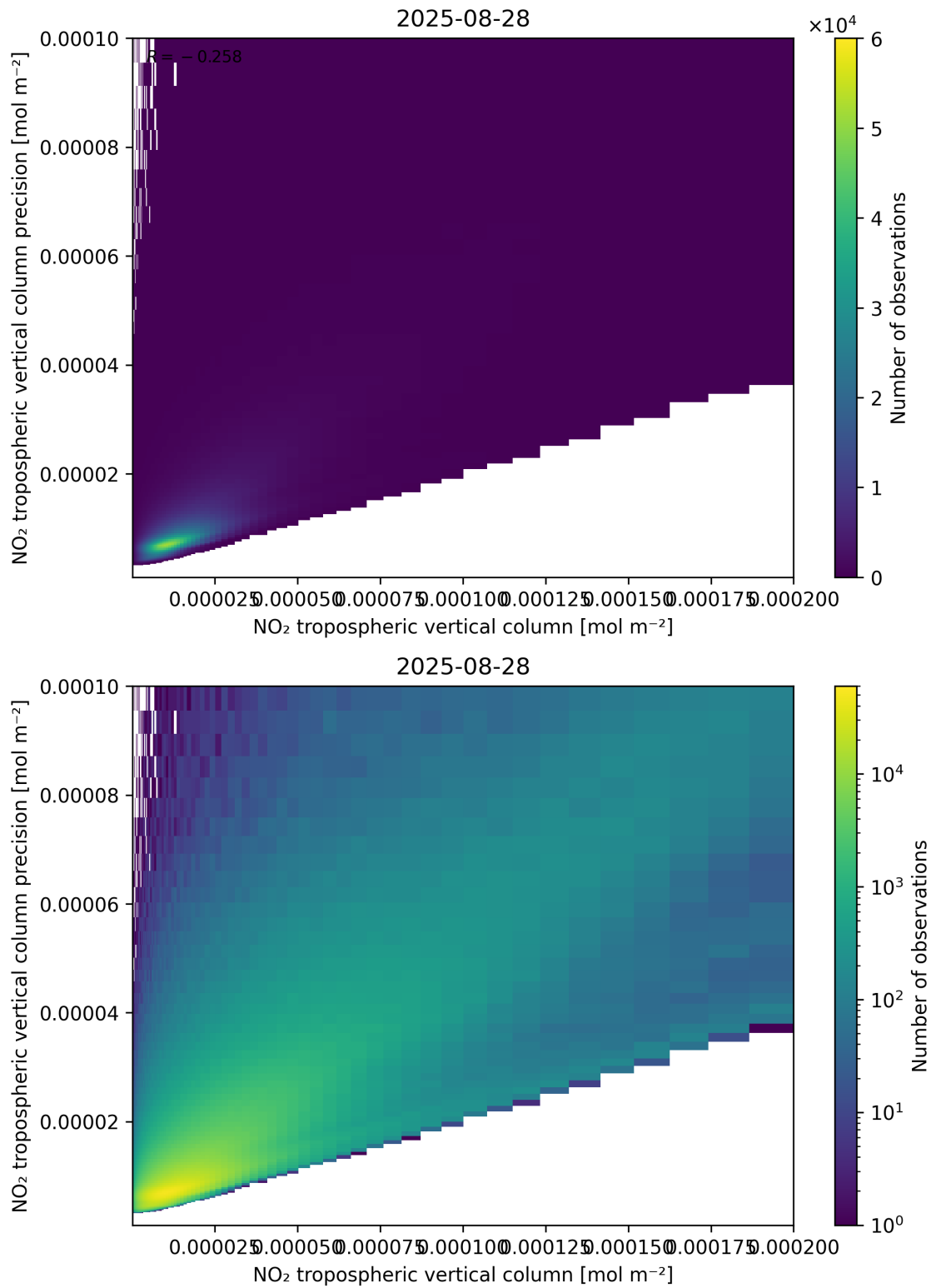
Figure 130: Scatter density plot of “NO 2 tropospheric vertical column” against “NO 2 tropospheric vertical column precision” for 2025-08-27 to 2025-08-29.
