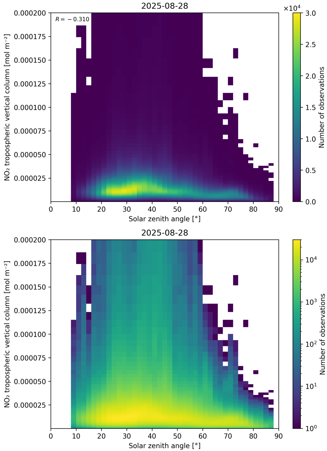
Figure 155: Scatter density plot of “Solar zenith angle” against “NO 2 tropospheric vertical column” for 2025-08-27 to 2025-08-29.
