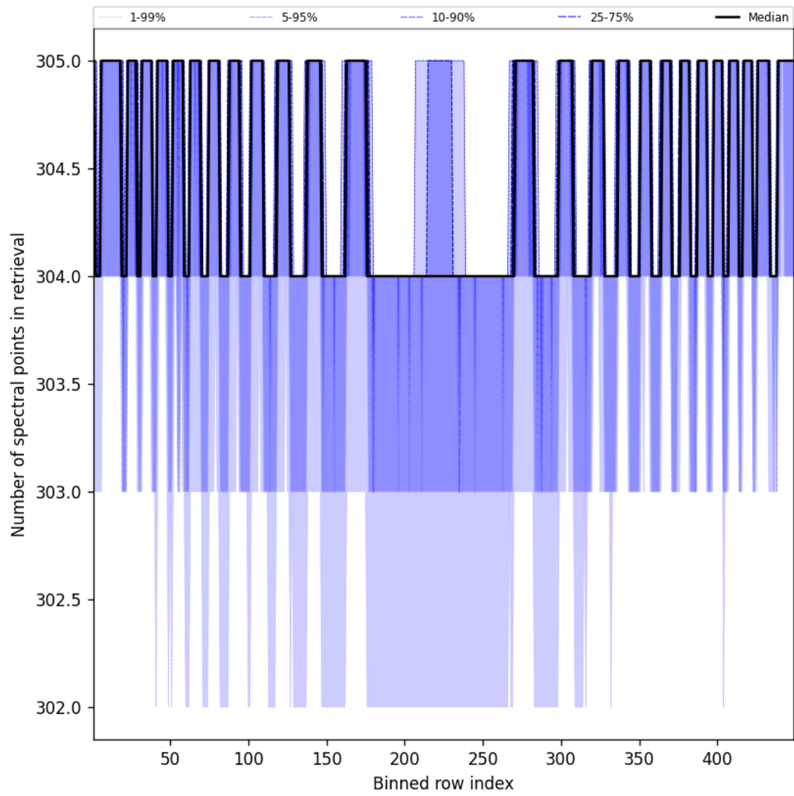
Figure 50: Along track statistics of “Number of spectral points in retrieval” for 2025-08-27 to 2025-08-29
