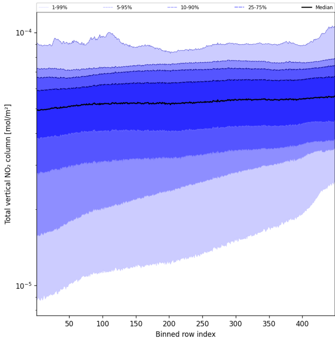
Figure 55: Along track statistics of “Total vertical NO 2 column” for 2025-08-27 to 2025-08-29
