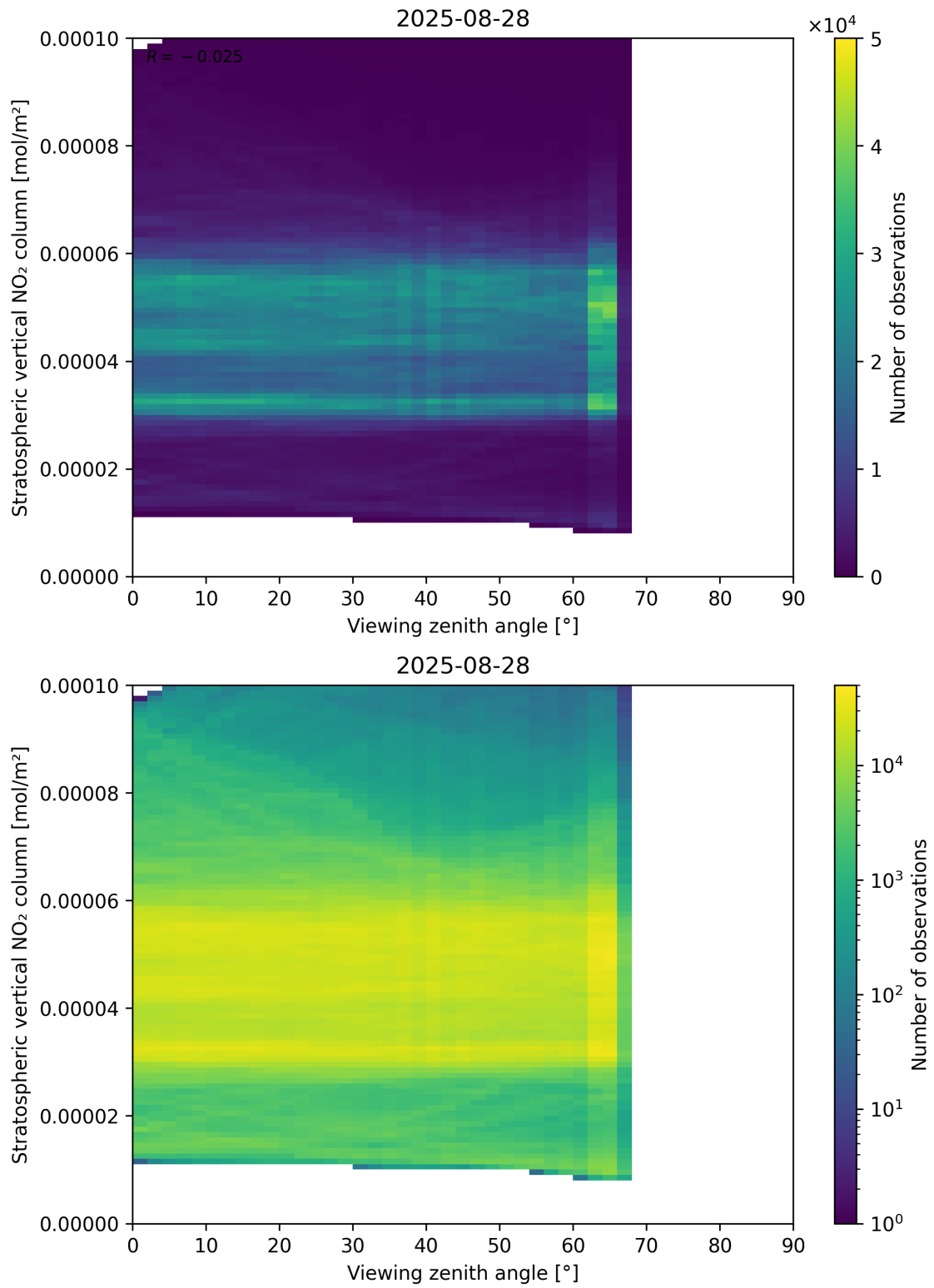
Figure 164: Scatter density plot of “Viewing zenith angle” against “Stratospheric vertical NO 2 column” for 2025-08-27 to 2025-08-29.
