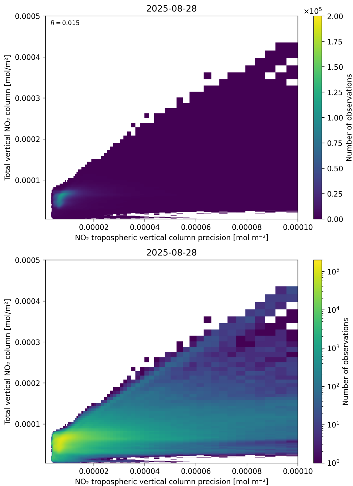
Figure 138: Scatter density plot of “NO 2 tropospheric vertical column precision” against “Total vertical NO 2 column” for 2025-08-27 to 2025-08-29.
