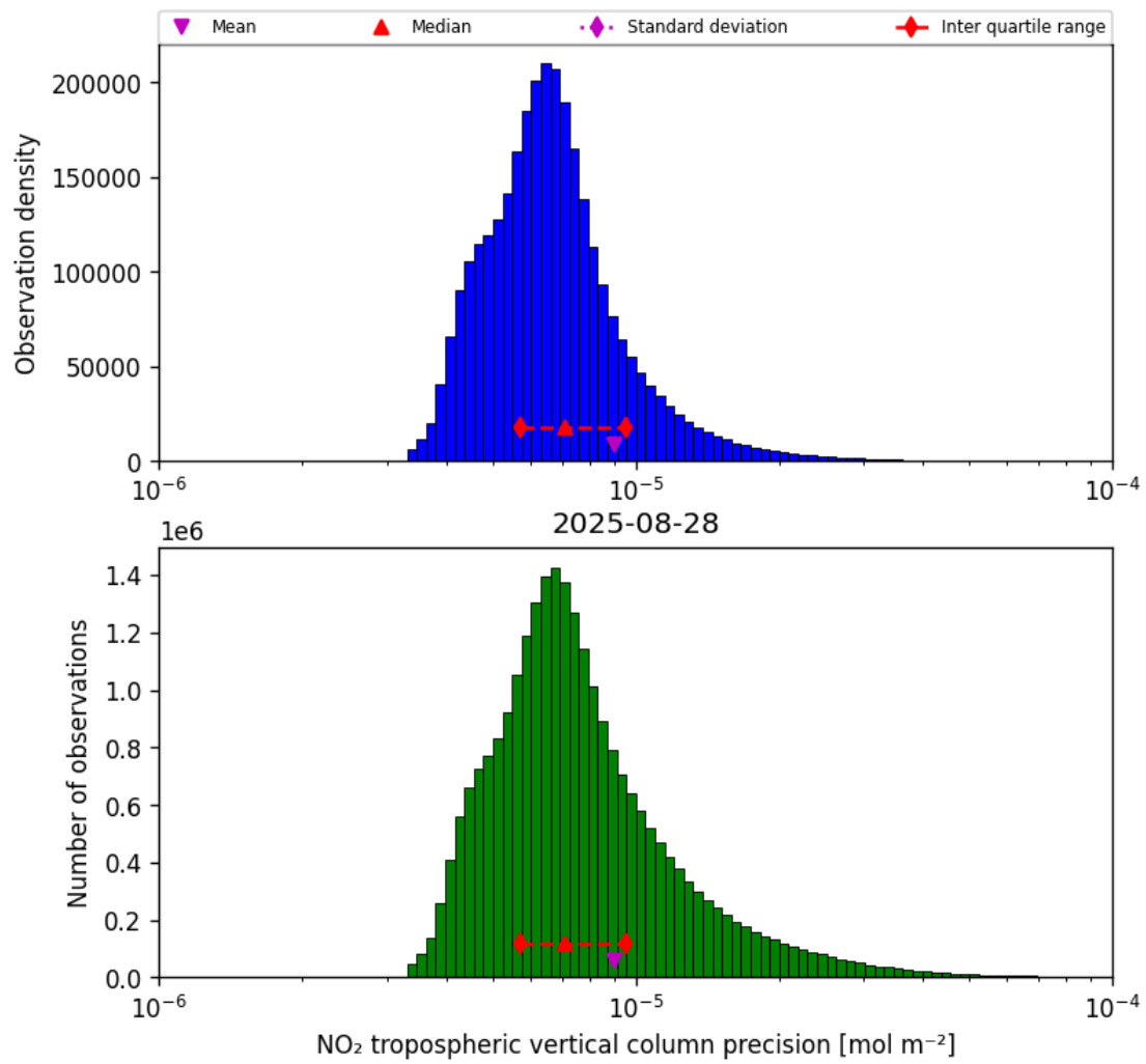
Figure 30: Histogram of “NO 2 tropospheric vertical column precision” for 2025-08-27 to 2025-08-29
