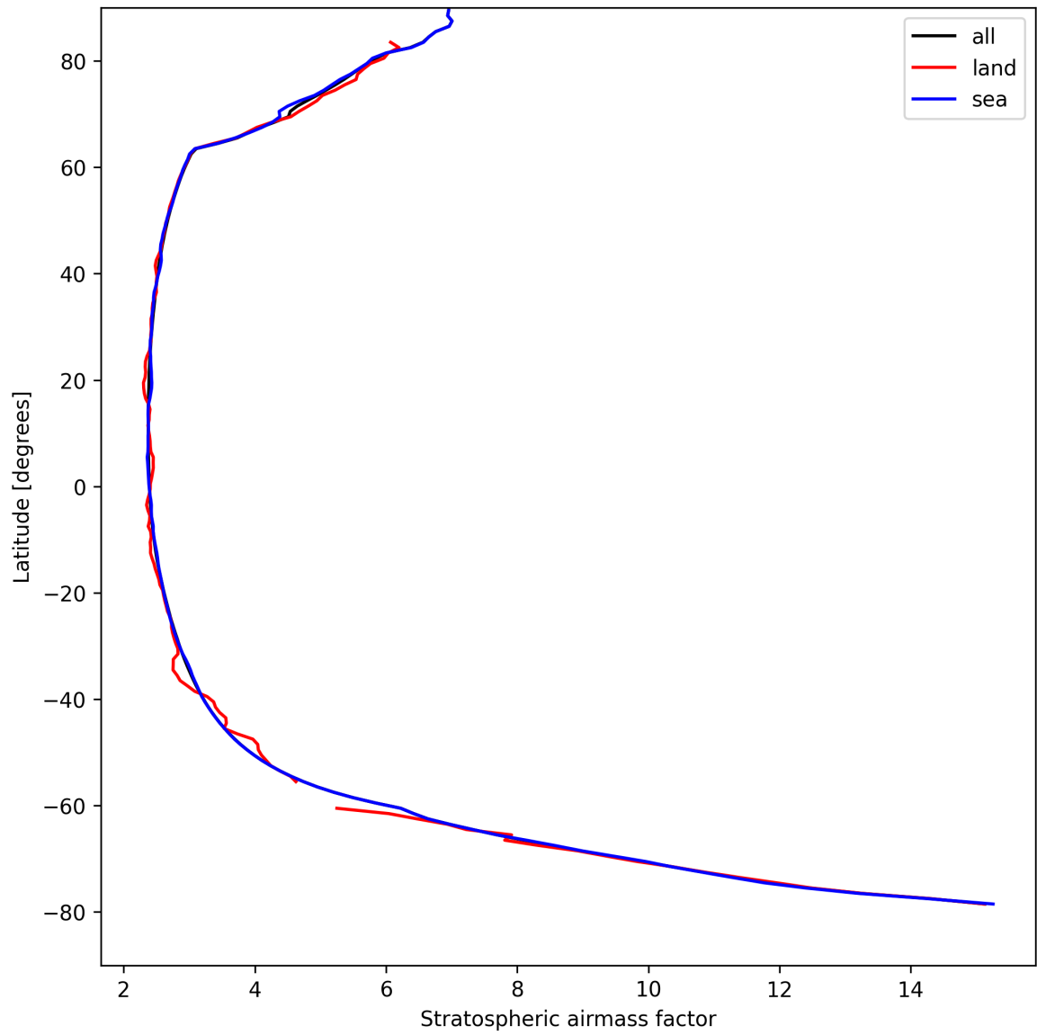
Figure 27: Zonal average of “Stratospheric airmass factor” for 2025-08-27 to 2025-08-29.
