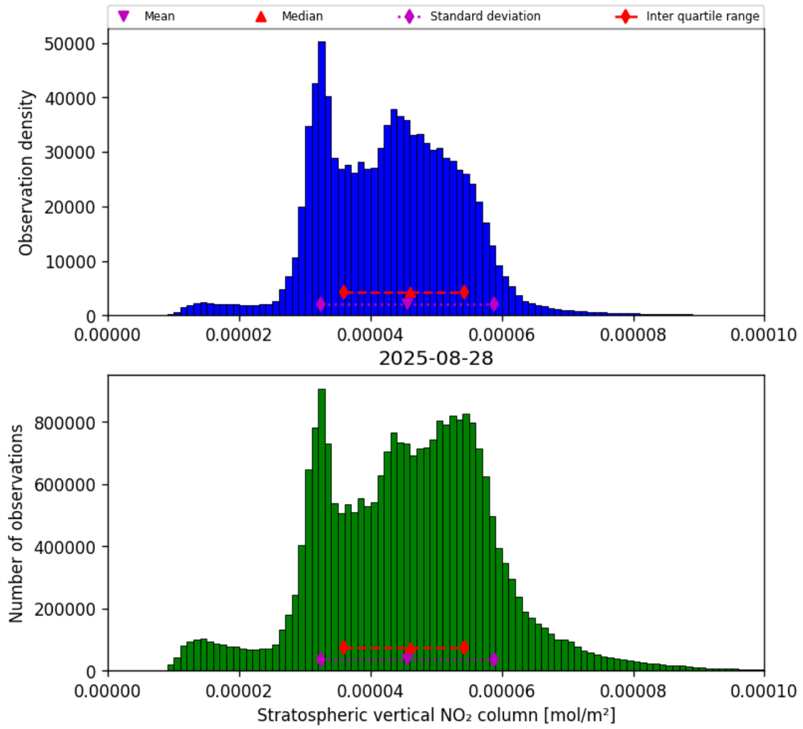
Figure 36: Histogram of “Stratospheric vertical NO 2 column” for 2025-08-27 to 2025-08-29
