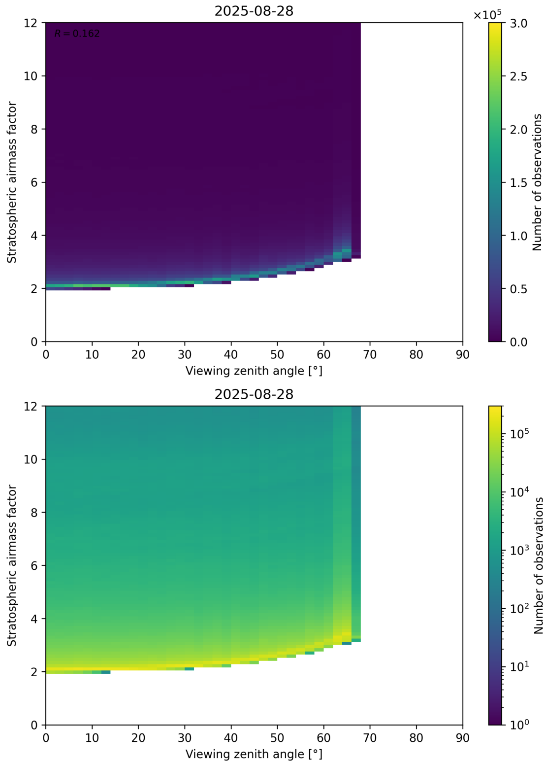
Figure 159: Scatter density plot of “Viewing zenith angle” against “Stratospheric airmass factor” for 2025-08-27 to 2025-08-29.
