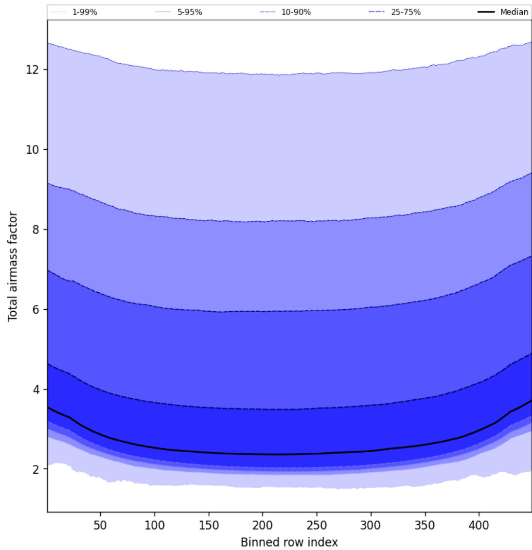
Figure 49: Along track statistics of “Total airmass factor” for 2025-08-27 to 2025-08-29
