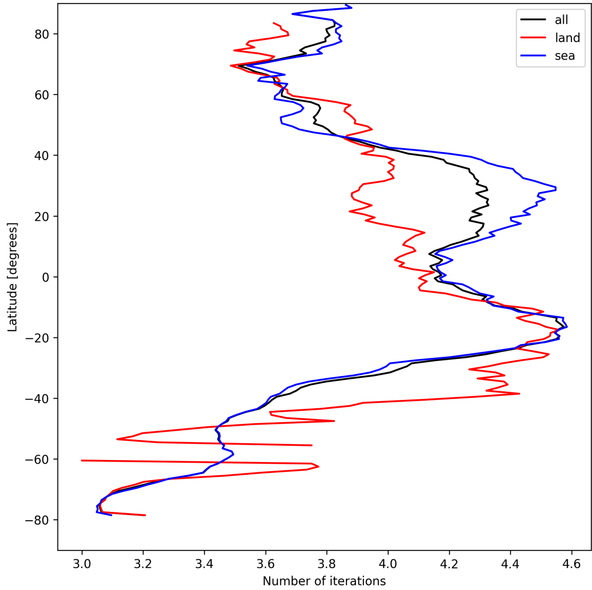
Figure 17: Zonal average of “Number of iterations” for 2025-08-27 to 2025-08-29.
