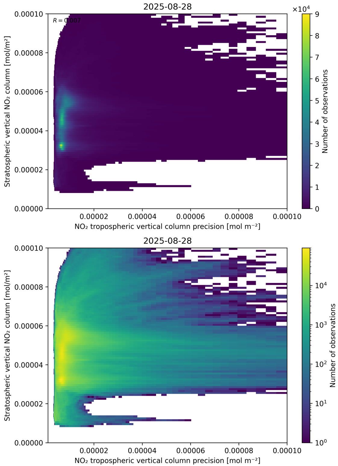
Figure 135: Scatter density plot of “NO 2 tropospheric vertical column precision” against “Stratospheric vertical NO 2 column” for 2025-08-27 to 2025-08-29.
