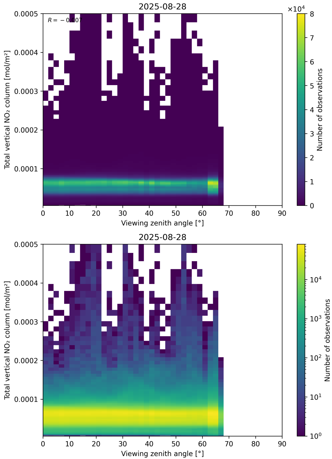
Figure 167: Scatter density plot of “Viewing zenith angle” against “Total vertical NO 2 column” for 2025-08-27 to 2025-08-29.
