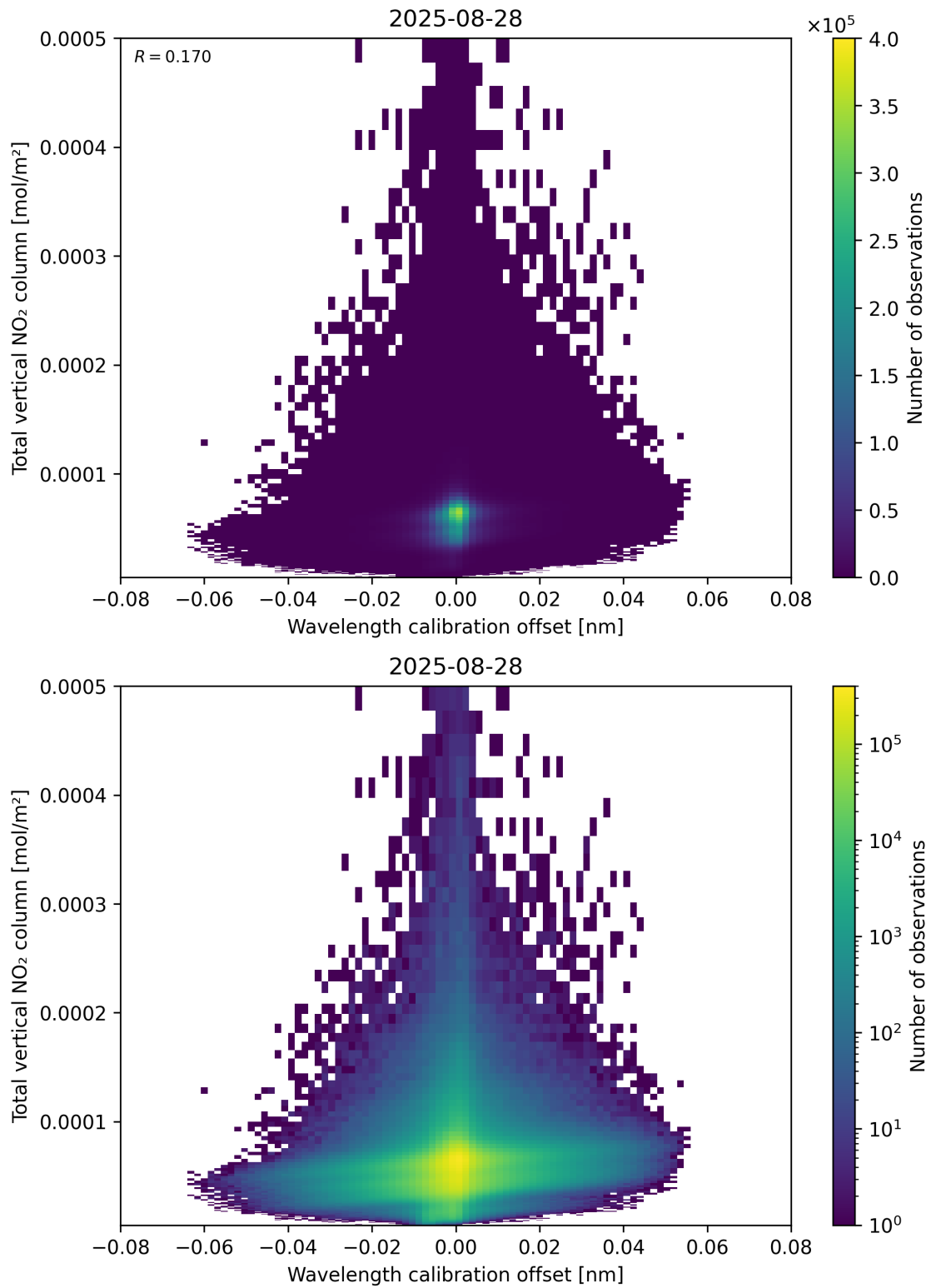
Figure 179: Scatter density plot of “Wavelength calibration offset” against “Total vertical NO 2 column” for 2025-08-27 to 2025-08-29.
