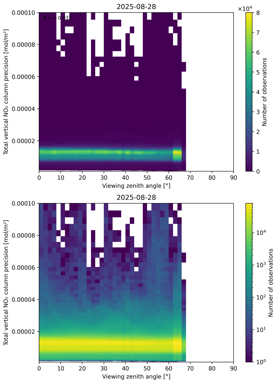
Figure 168: Scatter density plot of “Viewing zenith angle” against “Total vertical NO 2 column precision” for 2025-08-27 to 2025-08-29.
