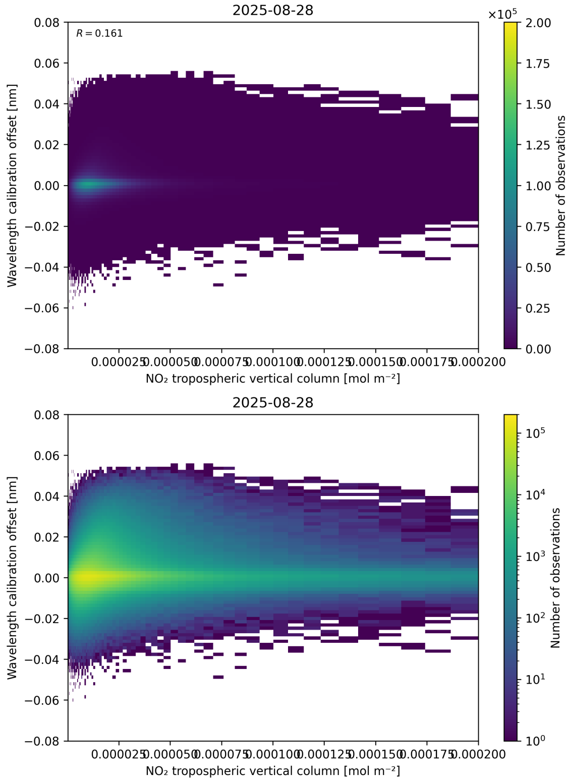
Figure 143: Scatter density plot of “NO 2 tropospheric vertical column” against “Wavelength calibration offset” for 2025-08-27 to 2025-08-29.
