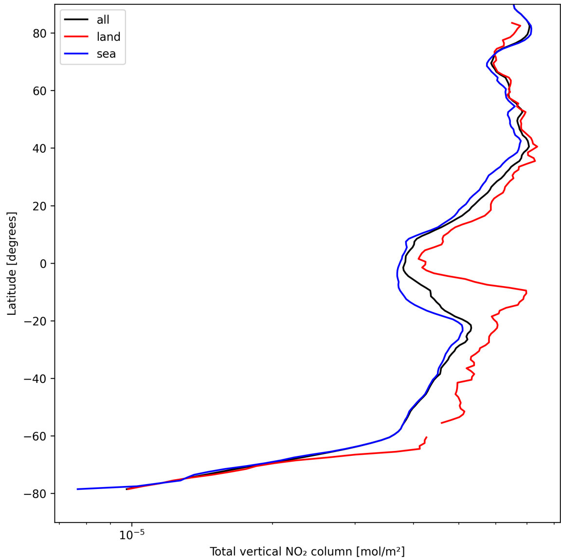
Figure 21: Zonal average of “Total vertical NO 2 column” for 2025-08-27 to 2025-08-29.
