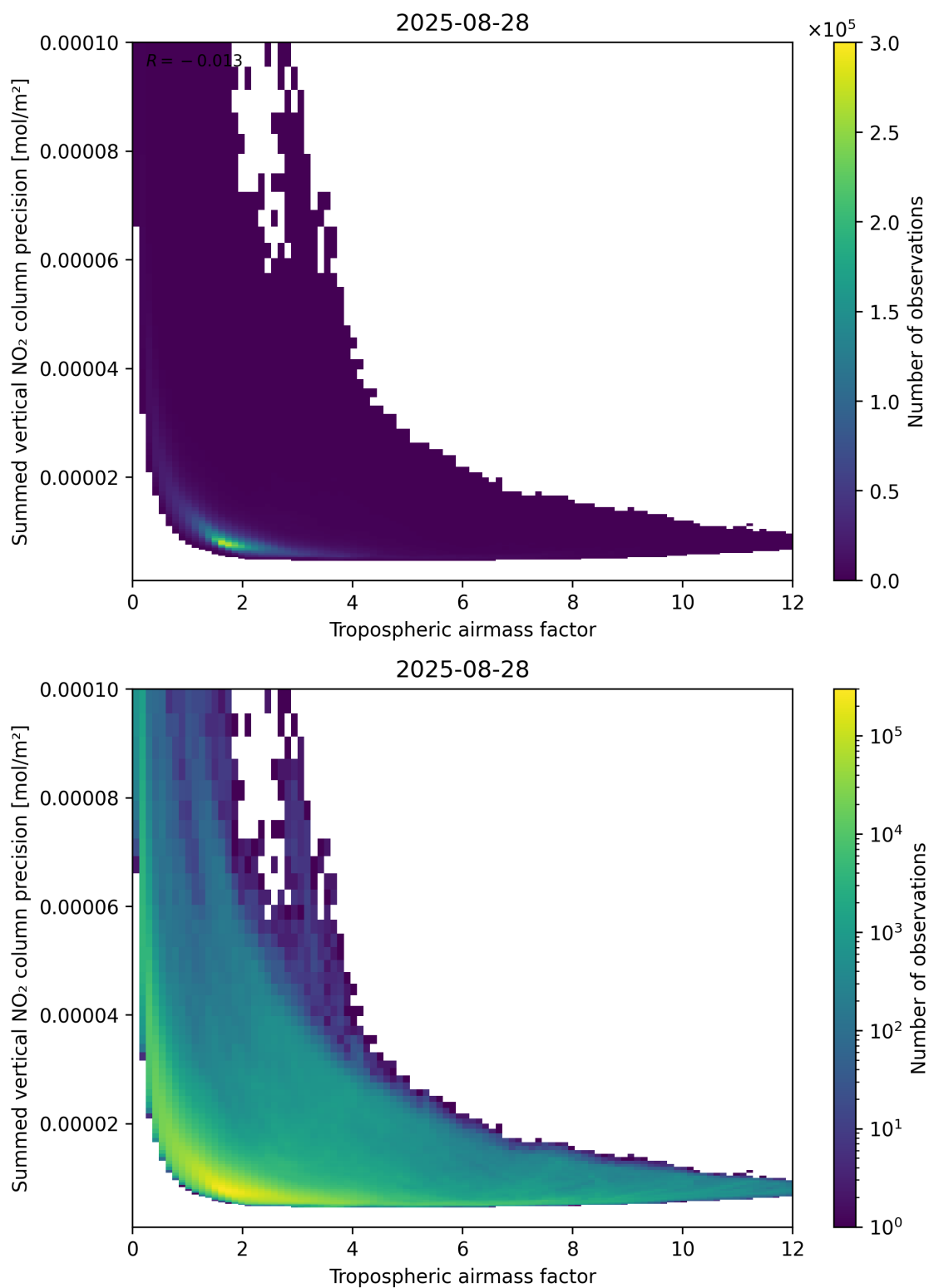
Figure 76: Scatter density plot of “Tropospheric airmass factor” against “Summed vertical NO 2 column precision” for 2025-08-27 to 2025-08-29.
