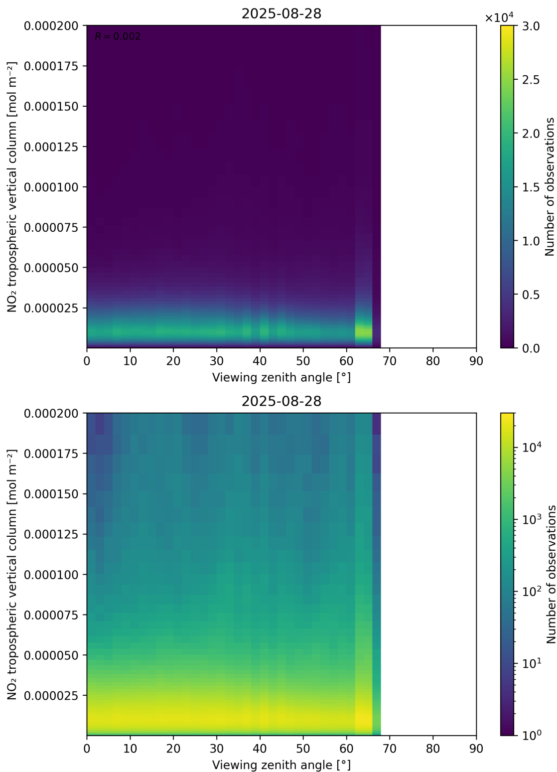
Figure 169: Scatter density plot of “Viewing zenith angle” against “NO 2 tropospheric vertical column” for 2025-08-27 to 2025-08-29.
