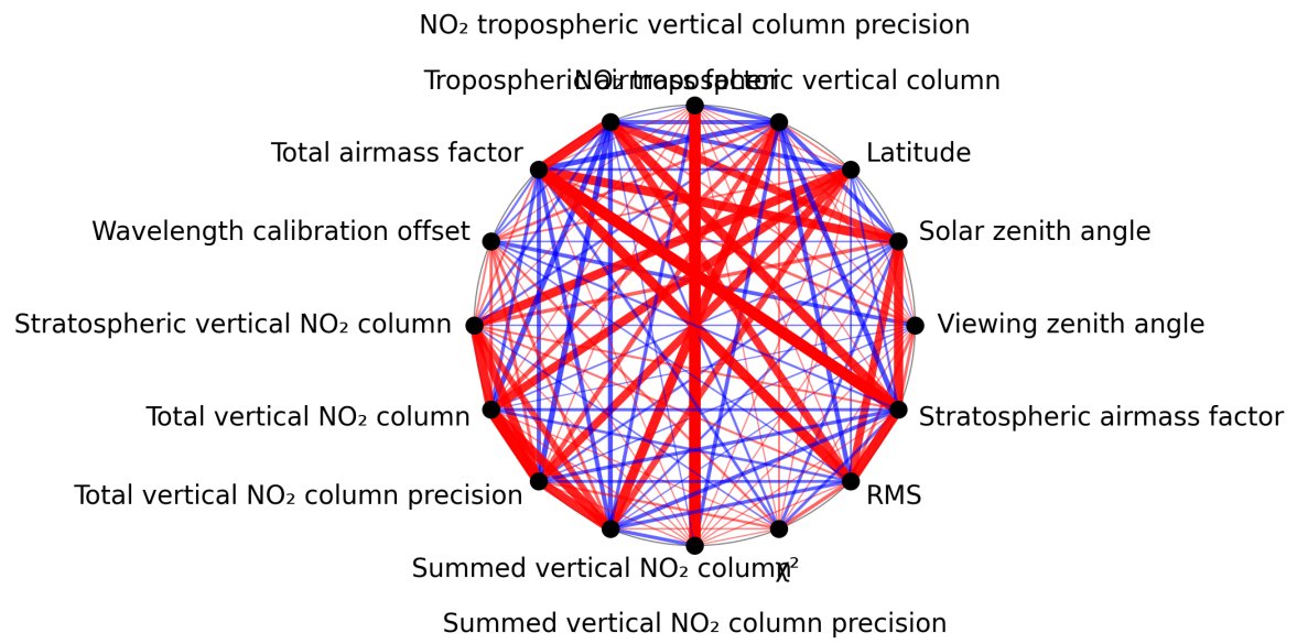
Figure 1: Map of correlation graph for 2025-08-27 to 2025-08-29.
