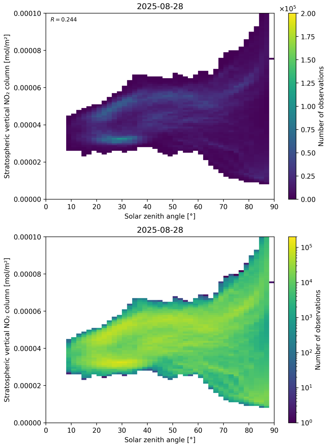
Figure 150: Scatter density plot of “Solar zenith angle” against “Stratospheric vertical NO 2 column” for 2025-08-27 to 2025-08-29.
