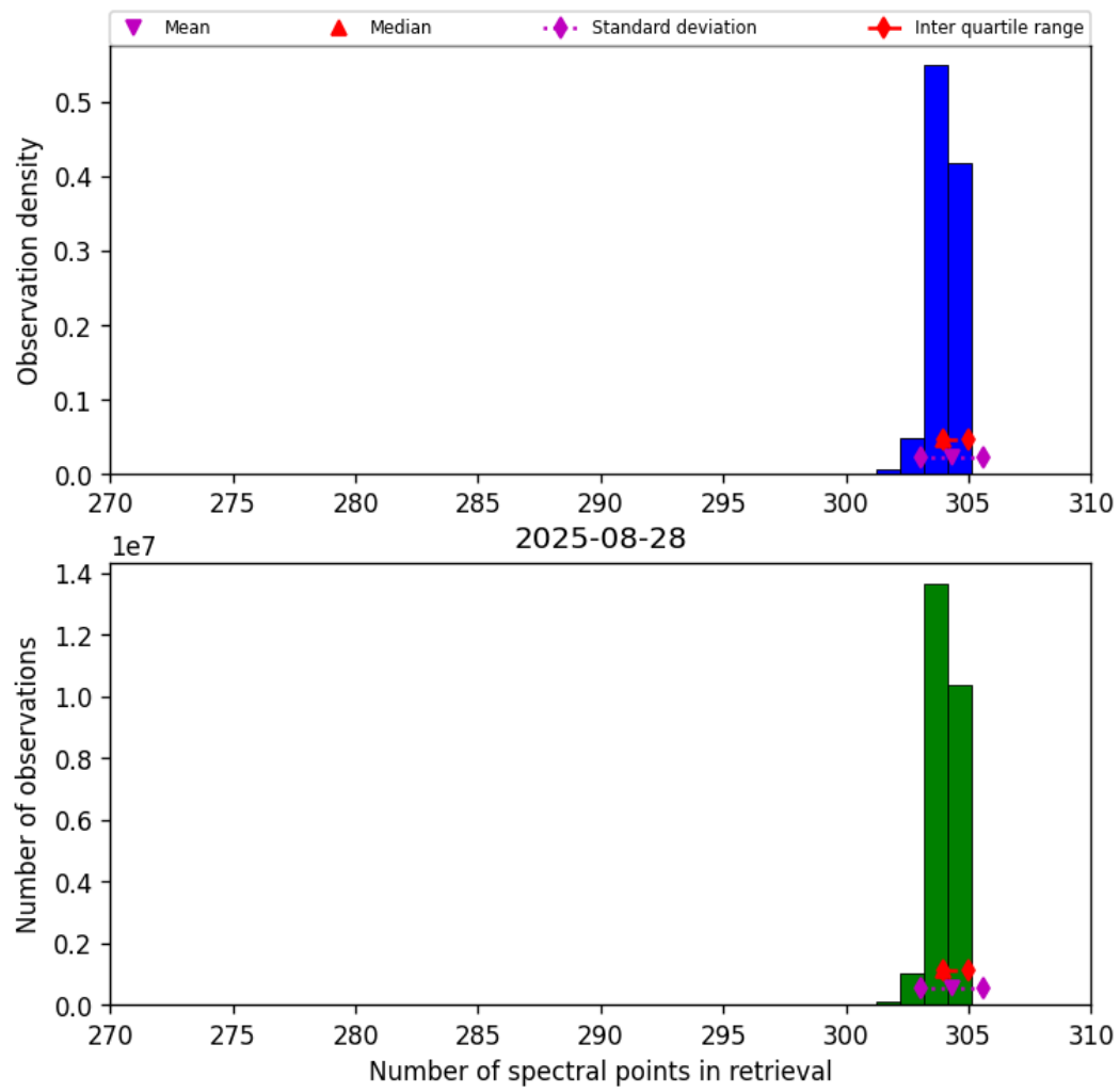
Figure 33: Histogram of “Number of spectral points in retrieval” for 2025-08-27 to 2025-08-29
