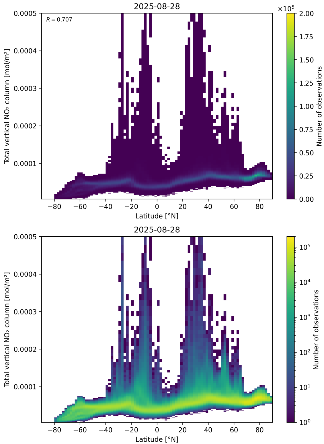
Figure 90: Scatter density plot of “Latitude” against “Total vertical NO 2 column” for 2025-08-27 to 2025-08-29.
