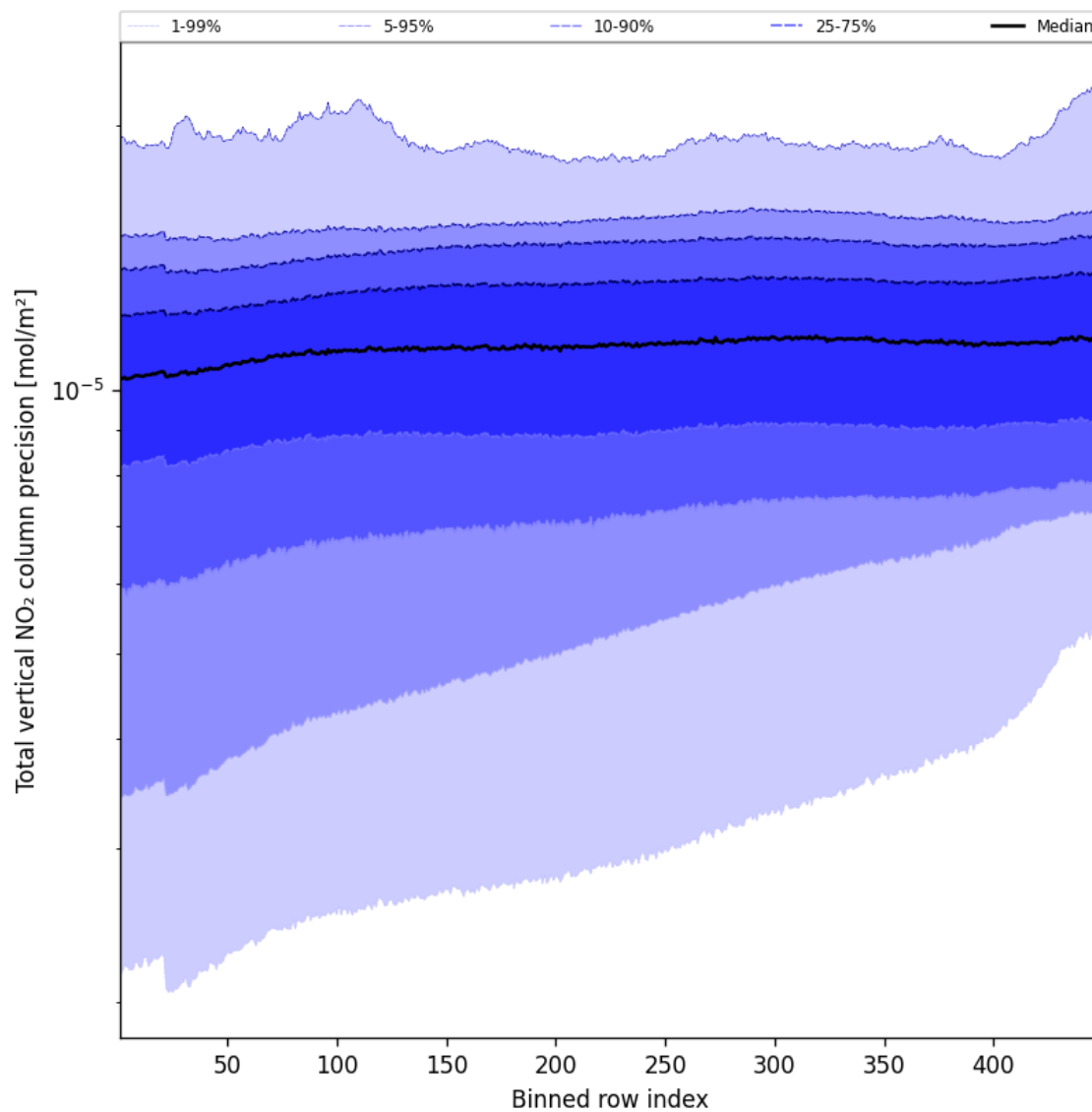
Figure 56: Along track statistics of “Total vertical NO 2 column precision” for 2025-08-27 to 2025-08-29
