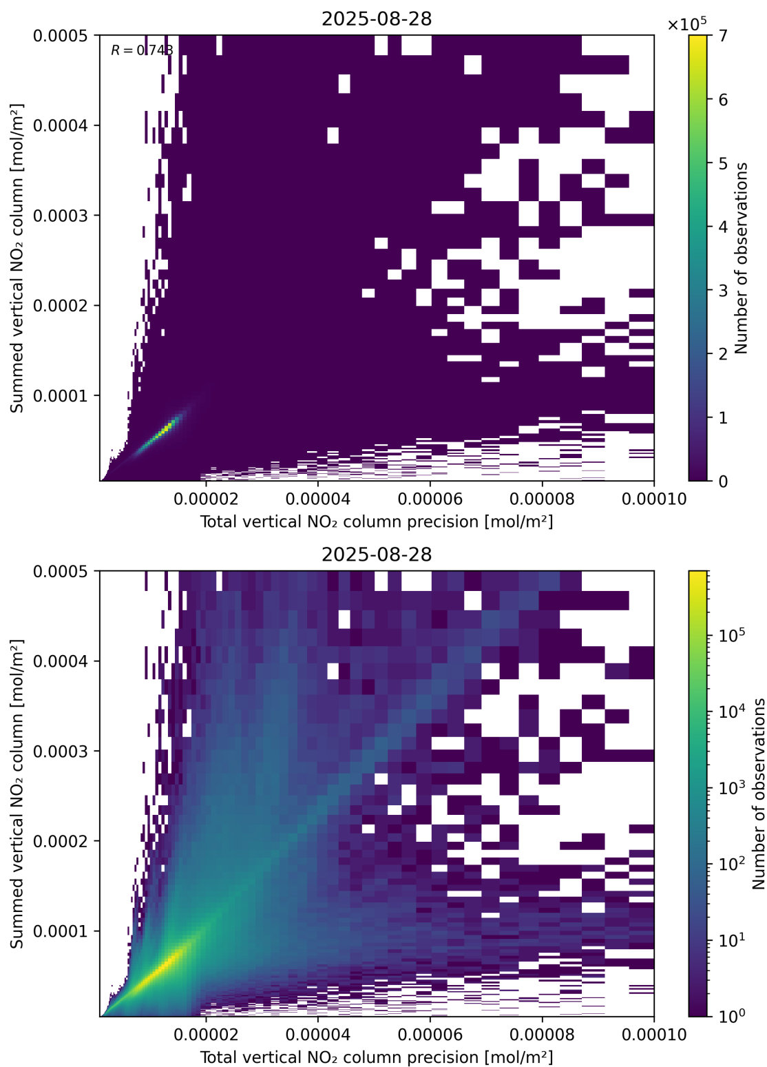
Figure 117: Scatter density plot of “Total vertical NO 2 column precision” against “Summed vertical NO 2 column” for 2025-08-27 to 2025-08-29.
