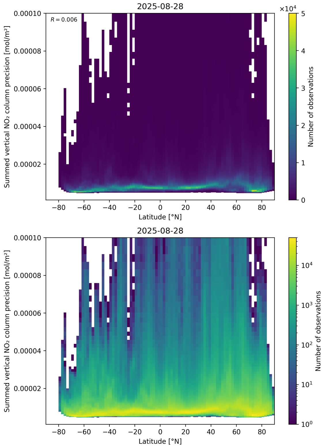
Figure 89: Scatter density plot of “Latitude” against “Summed vertical NO 2 column precision” for 2025-08-27 to 2025-08-29.
