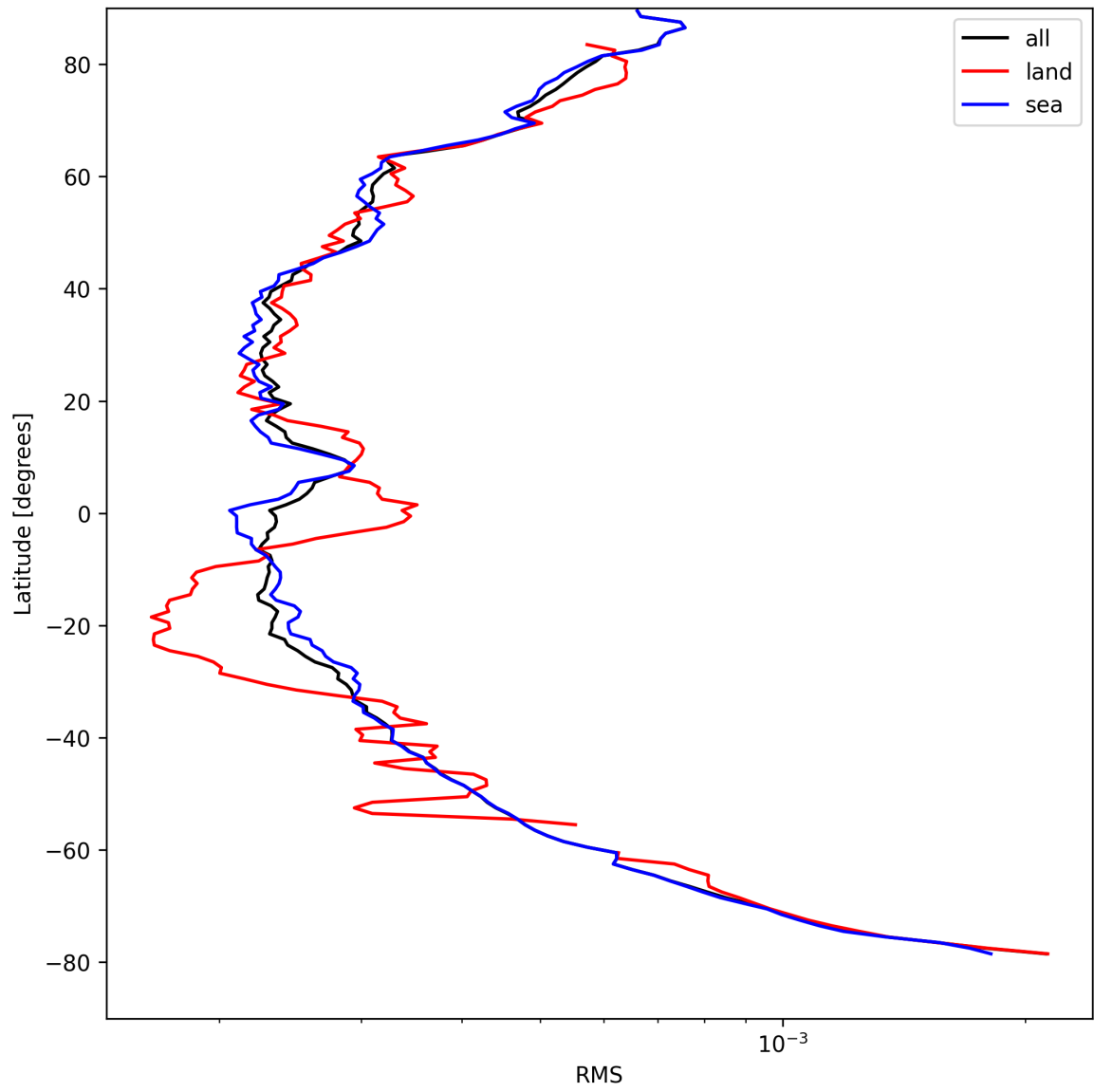
Figure 26: Zonal average of “RMS” for 2025-08-27 to 2025-08-29.
