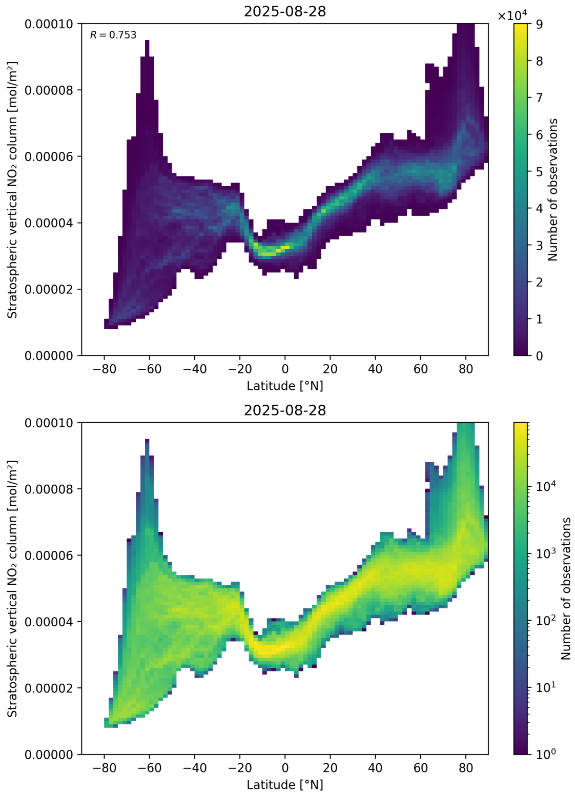
Figure 87: Scatter density plot of “Latitude” against “Stratospheric vertical NO 2 column” for 2025-08-27 to 2025-08-29.
