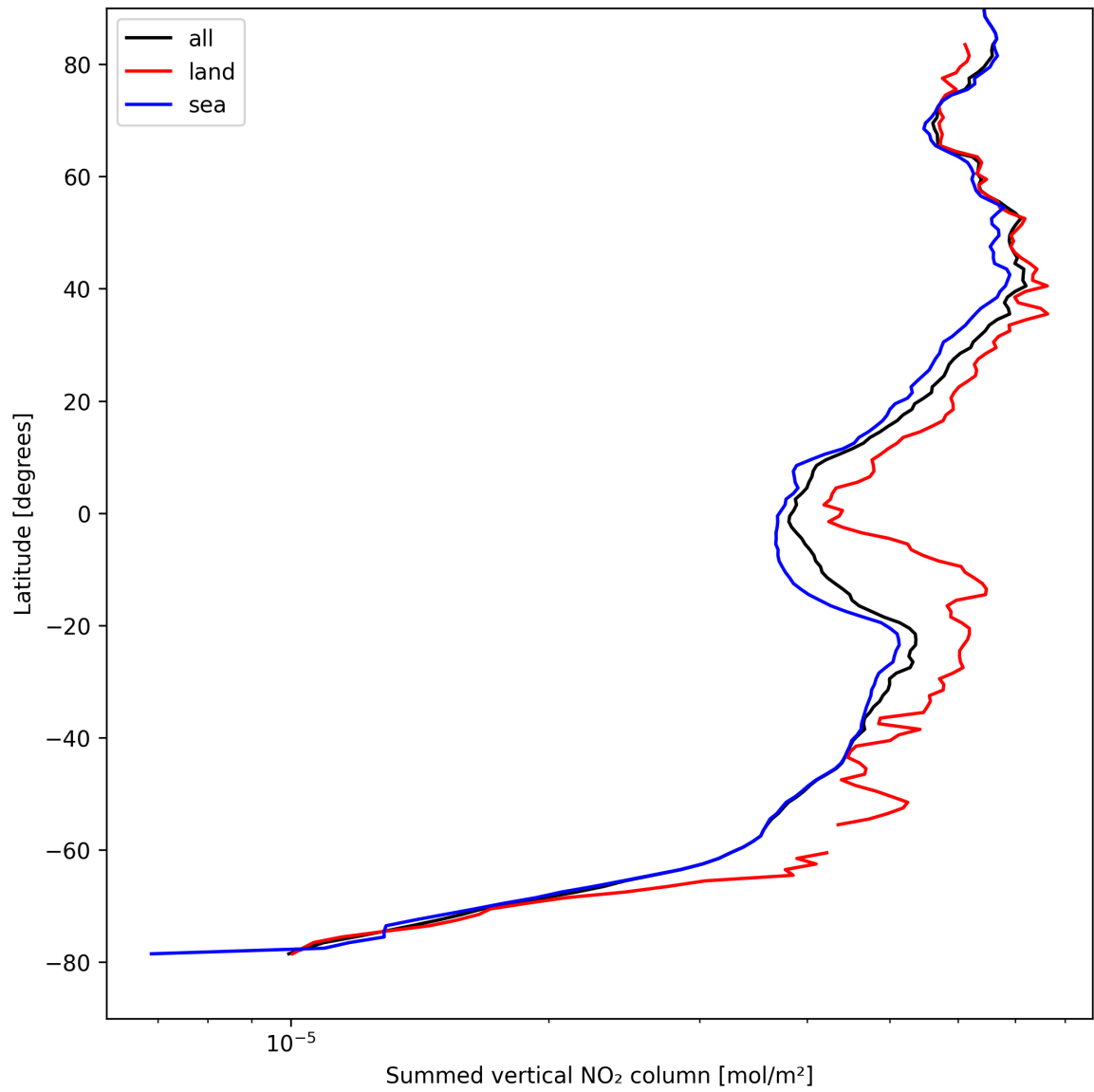
Figure 23: Zonal average of “Summed vertical NO 2 column” for 2025-08-27 to 2025-08-29.
