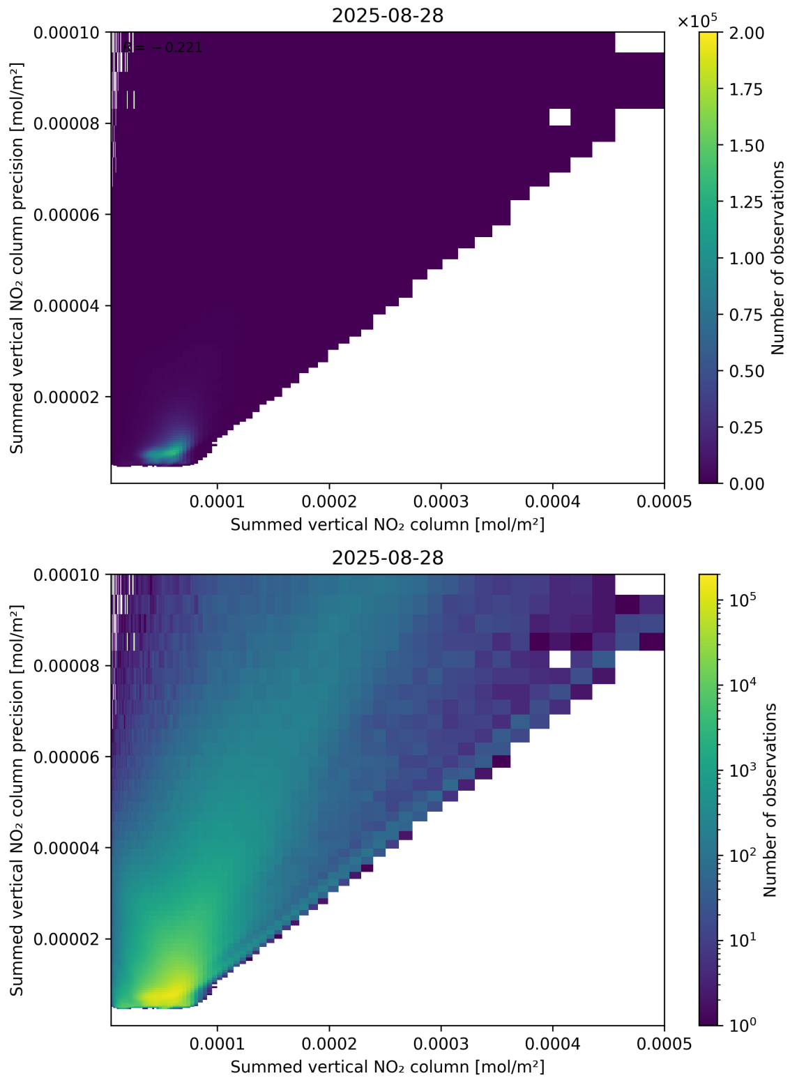
Figure 105: Scatter density plot of “Summed vertical NO 2 column” against “Summed vertical NO 2 column precision” for 2025-08-27 to 2025-08-29.
