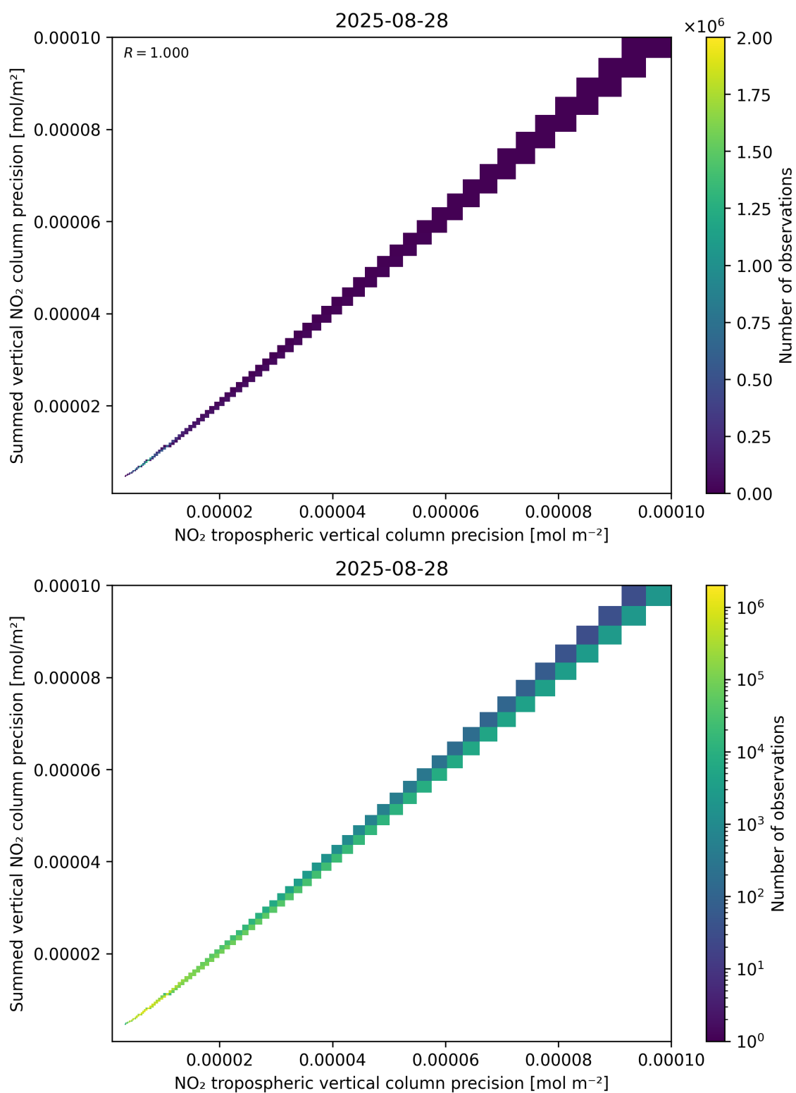
Figure 137: Scatter density plot of “NO 2 tropospheric vertical column precision” against “Summed vertical NO 2 column precision” for 2025-08-27 to 2025-08-29.
