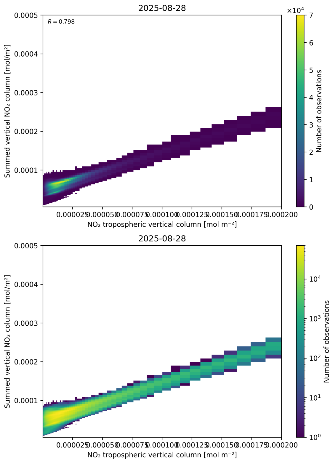
Figure 126: Scatter density plot of “NO 2 tropospheric vertical column” against “Summed vertical NO 2 column” for 2025-08-27 to 2025-08-29.
