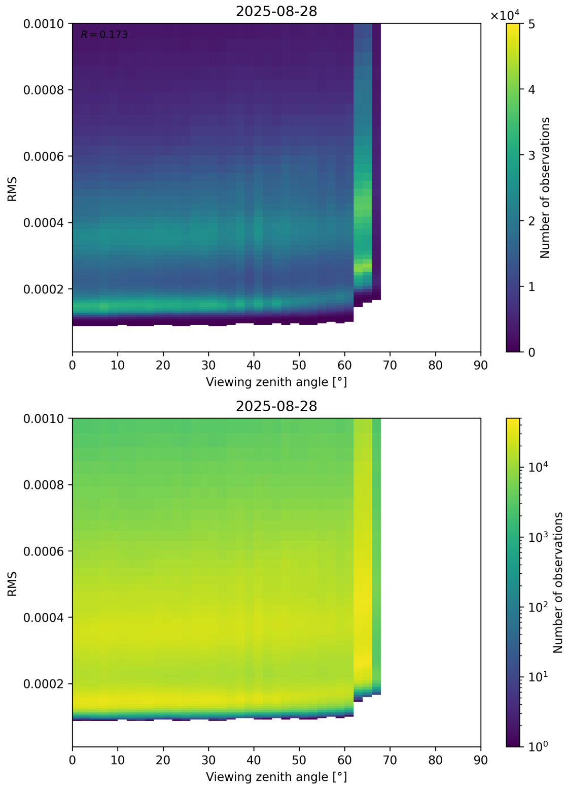
Figure 171: Scatter density plot of “Viewing zenith angle” against “RMS” for 2025-08-27 to 2025-08-29.
