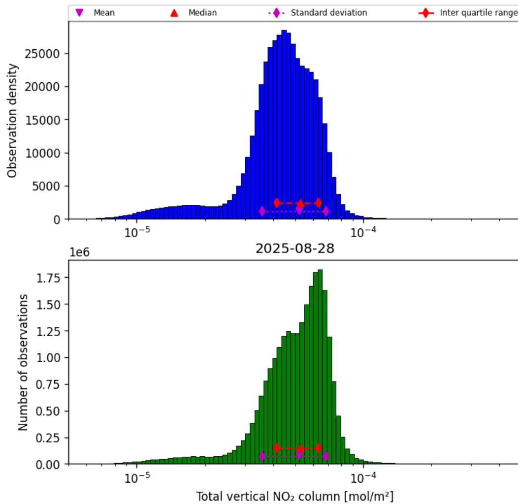
Figure 38: Histogram of “Total vertical NO 2 column” for 2025-08-27 to 2025-08-29
