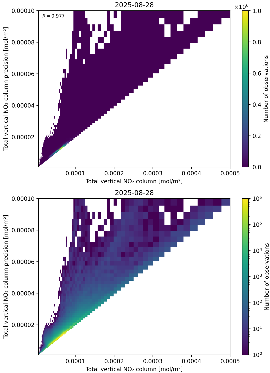
Figure 114: Scatter density plot of “Total vertical NO 2 column” against “Total vertical NO 2 column precision” for 2025-08-27 to 2025-08-29.
