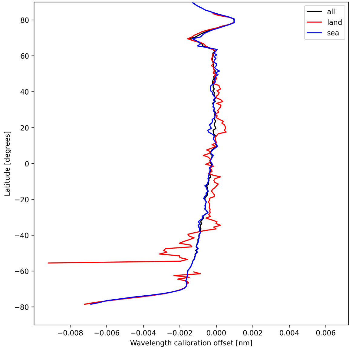
Figure 18: Zonal average of “Wavelength calibration offset” for 2025-08-27 to 2025-08-29.
