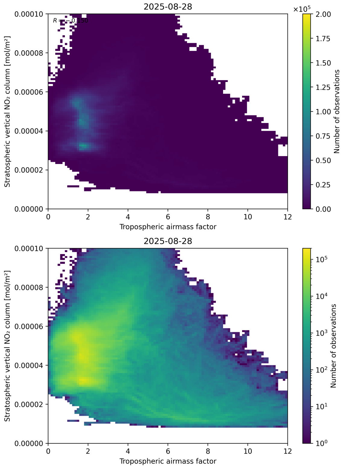
Figure 74: Scatter density plot of “Tropospheric airmass factor” against “Stratospheric vertical NO 2 column” for 2025-08-27 to 2025-08-29.
