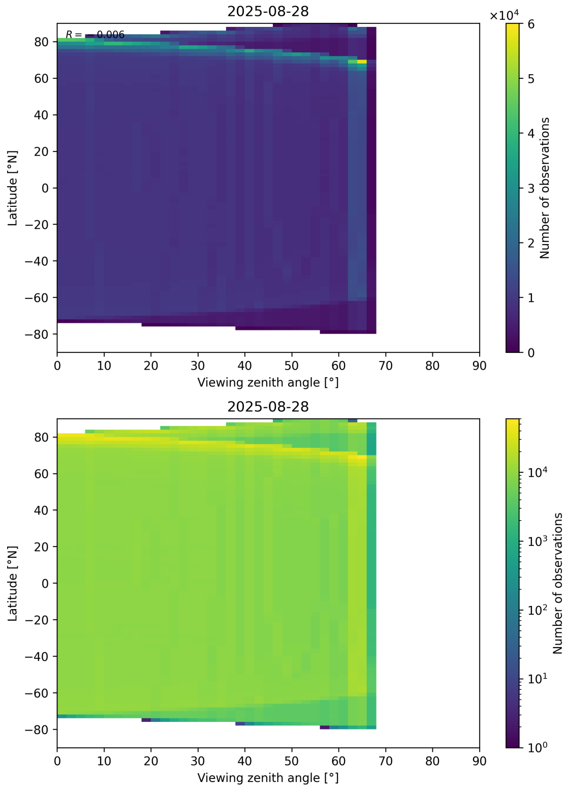
Figure 163: Scatter density plot of “Viewing zenith angle” against “Latitude” for 2025-08-27 to 2025-08-29.
