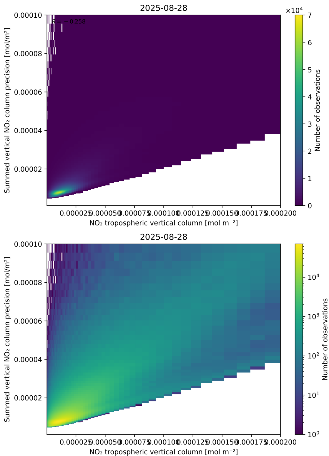
Figure 127: Scatter density plot of “NO 2 tropospheric vertical column” against “Summed vertical NO 2 column precision” for 2025-08-27 to 2025-08-29.
