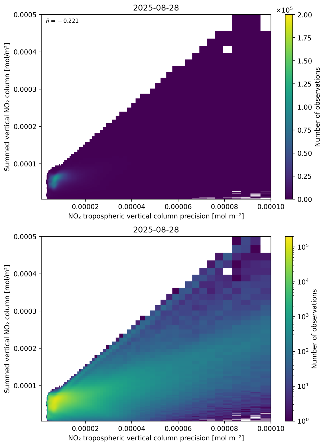
Figure 136: Scatter density plot of “NO 2 tropospheric vertical column precision” against “Summed vertical NO 2 column” for 2025-08-27 to 2025-08-29.
