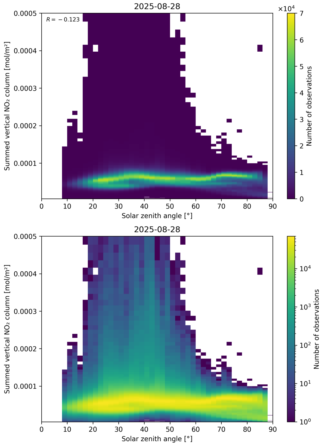
Figure 151: Scatter density plot of “Solar zenith angle” against “Summed vertical NO 2 column” for 2025-08-27 to 2025-08-29.
