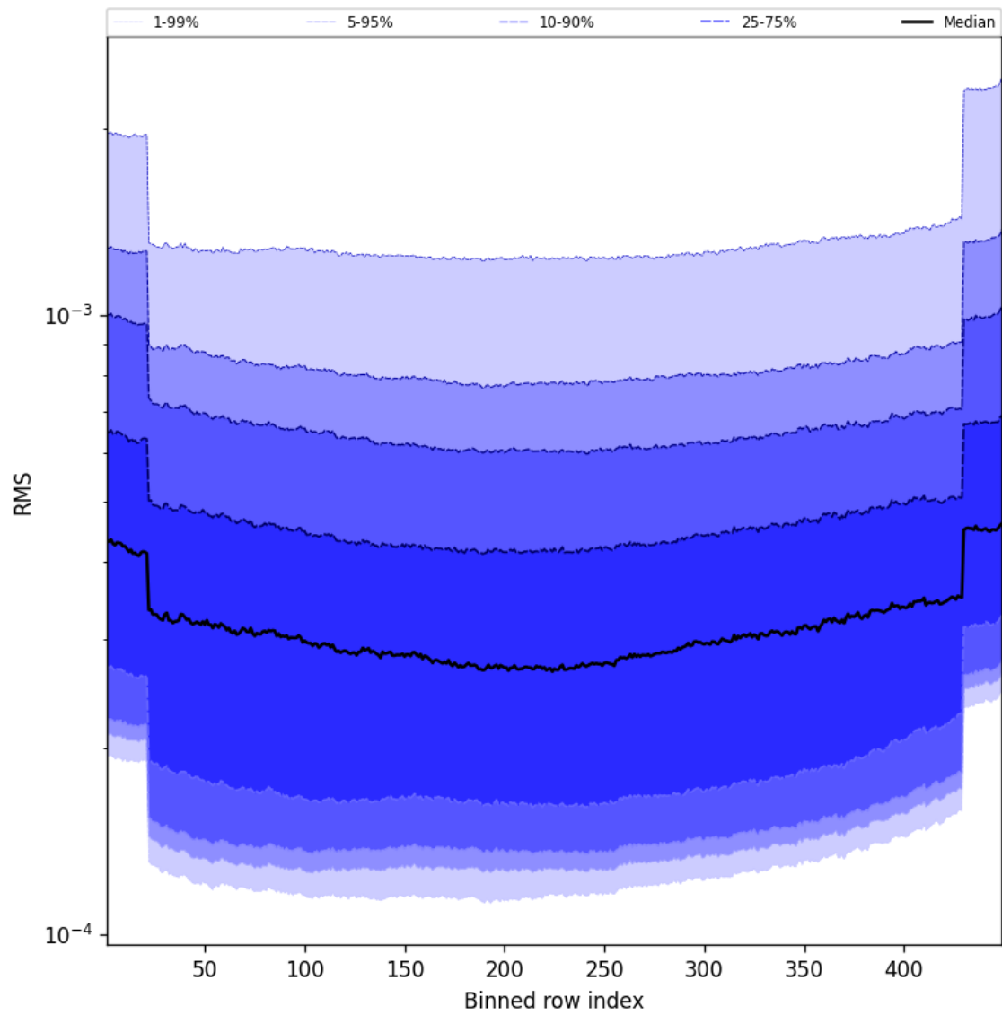
Figure 60: Along track statistics of “RMS” for 2025-08-27 to 2025-08-29
