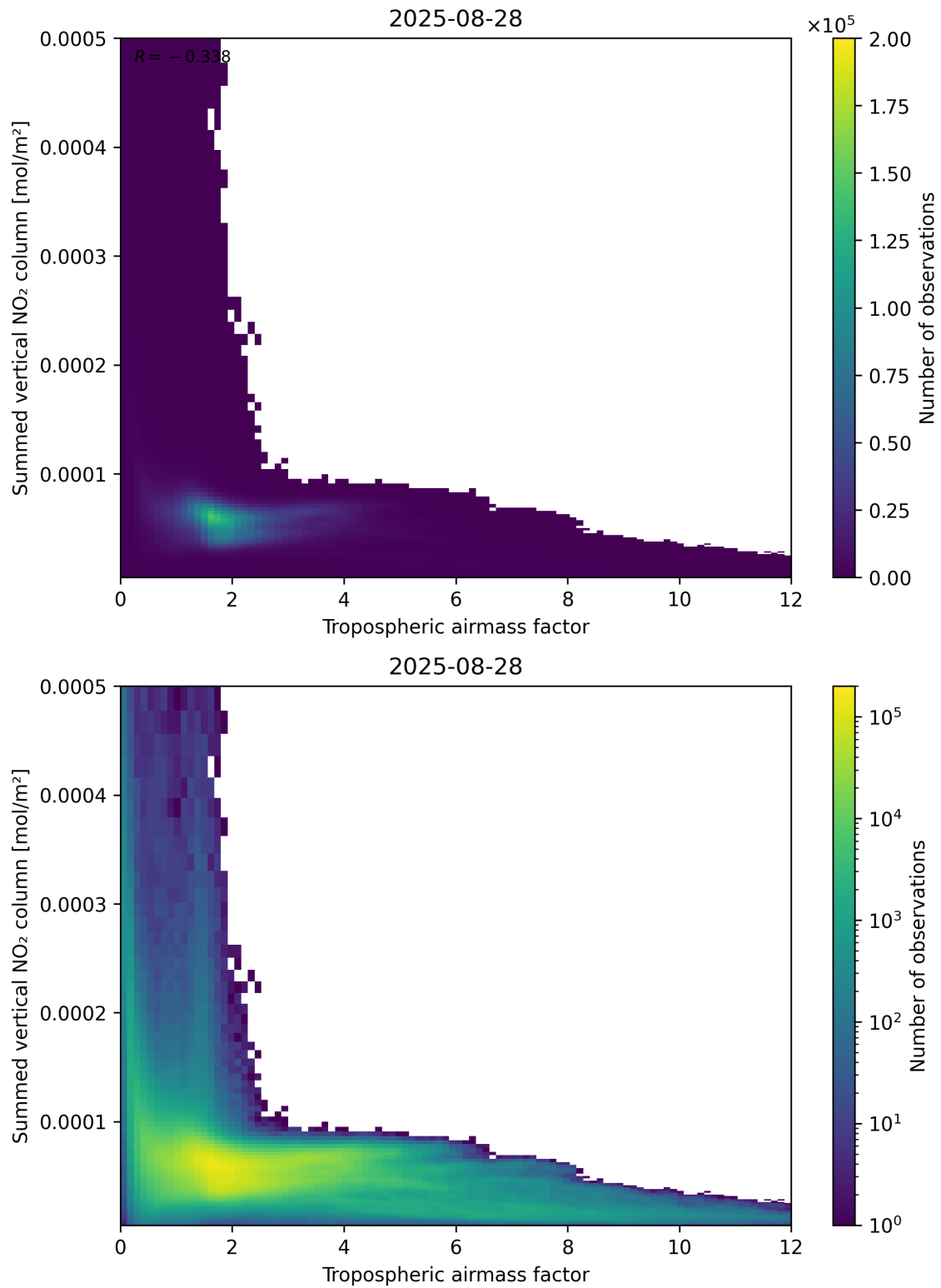
Figure 75: Scatter density plot of “Tropospheric air mass factor” against “Summed vertical NO 2 column” for 2025-08-27 to 2025-08-29.
