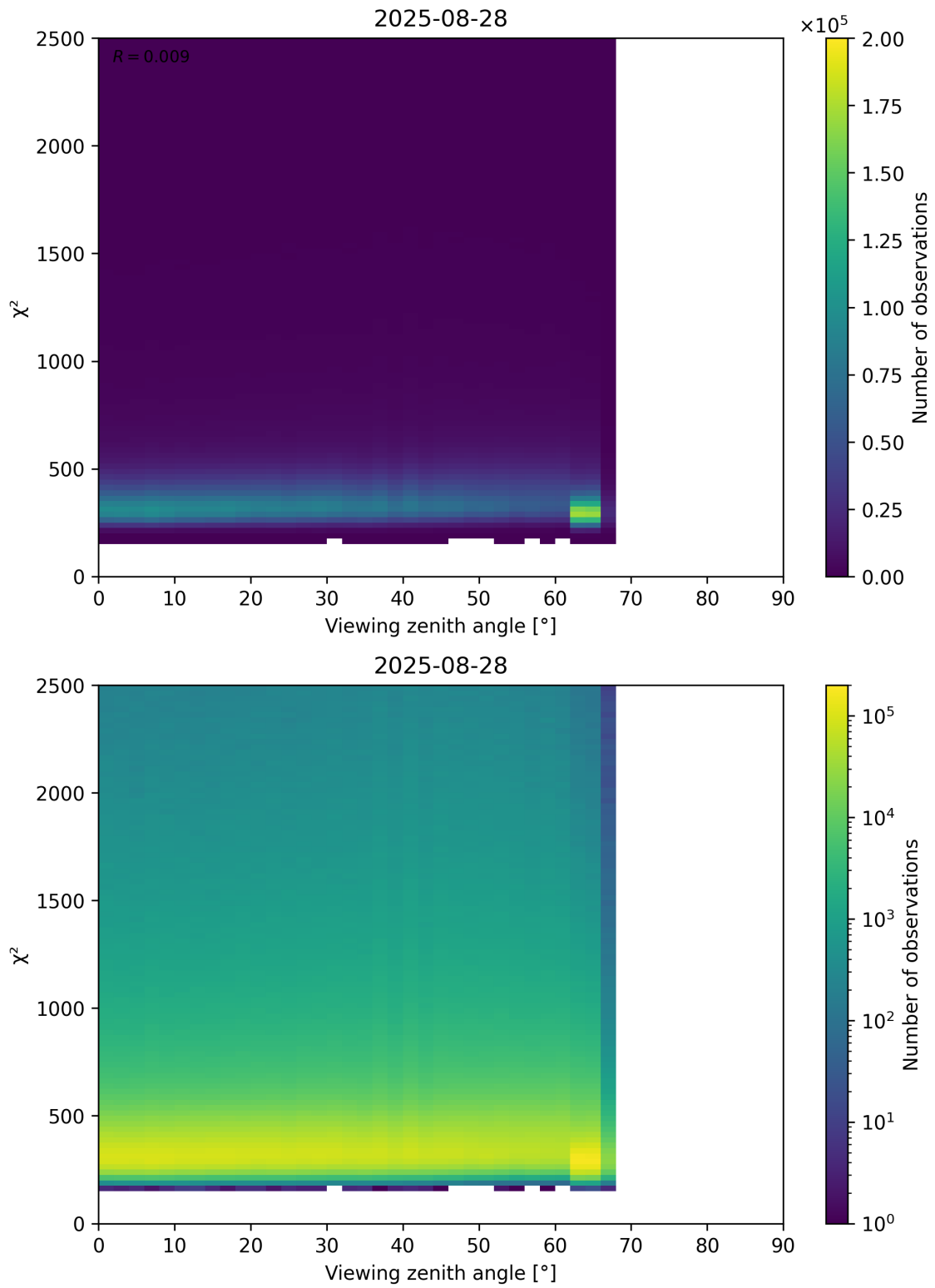
Figure 162: Scatter density plot of “Viewing zenith angle” against “ \chi^2 ” for 2025-08-27 to 2025-08-29.
