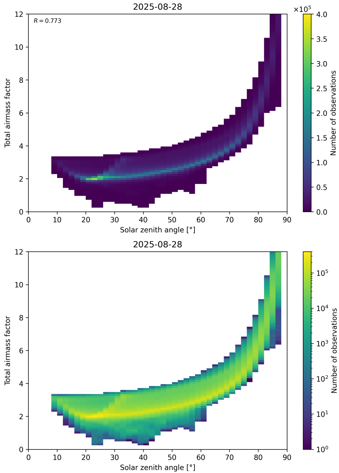
Figure 146: Scatter density plot of “Solar zenith angle” against “Total air mass factor” for 2025-08-27 to 2025-08-29.
