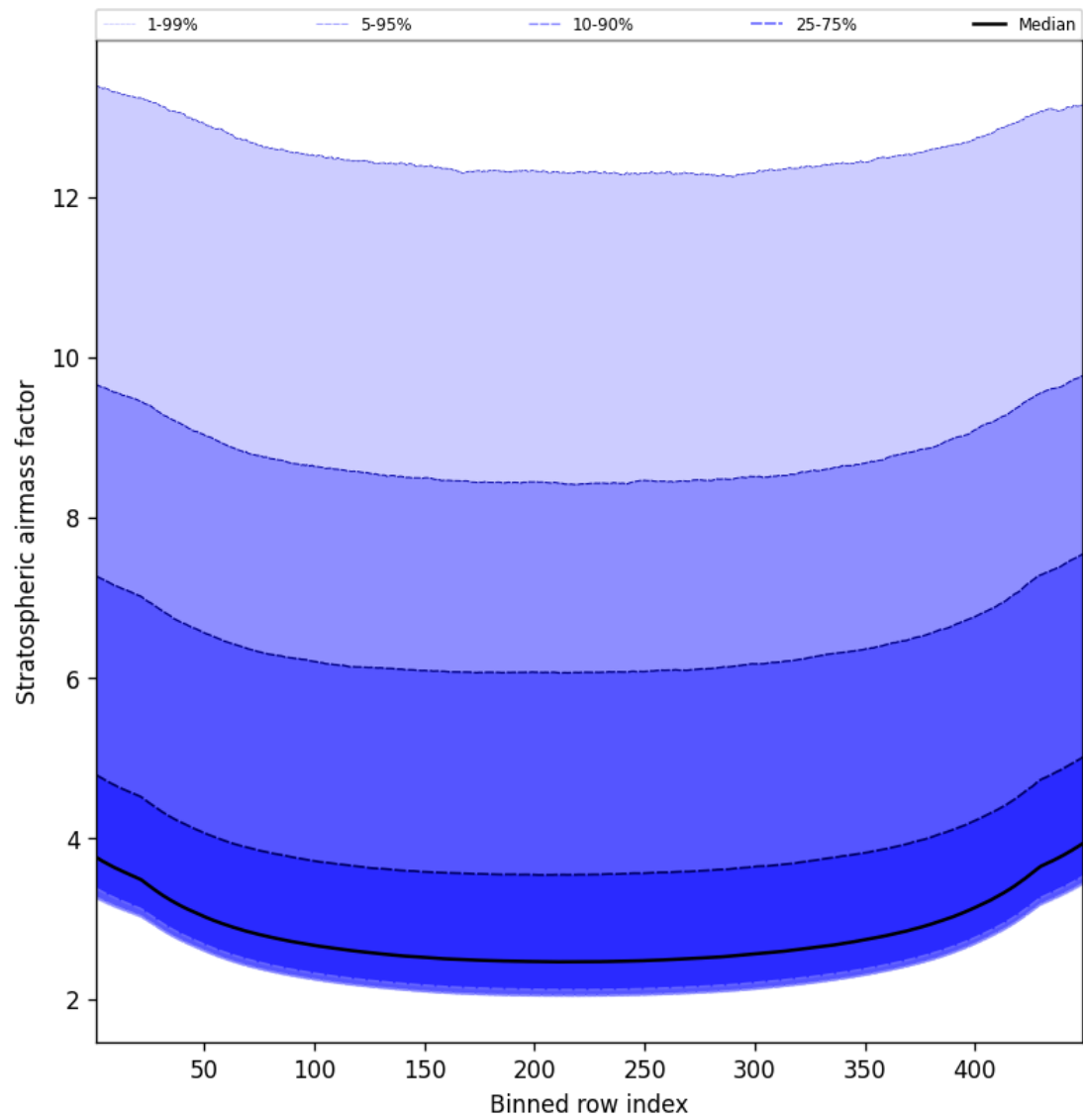
Figure 61: Along track statistics of “Stratospheric airmass factor” for 2025-08-27 to 2025-08-29
