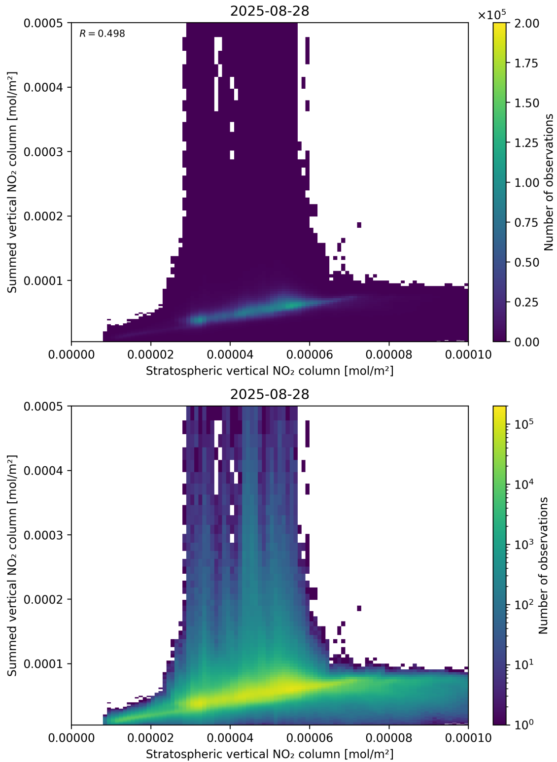
Figure 98: Scatter density plot of “Stratospheric vertical NO 2 column” against “Summed vertical NO 2 column” for 2025-08-27 to 2025-08-29.
