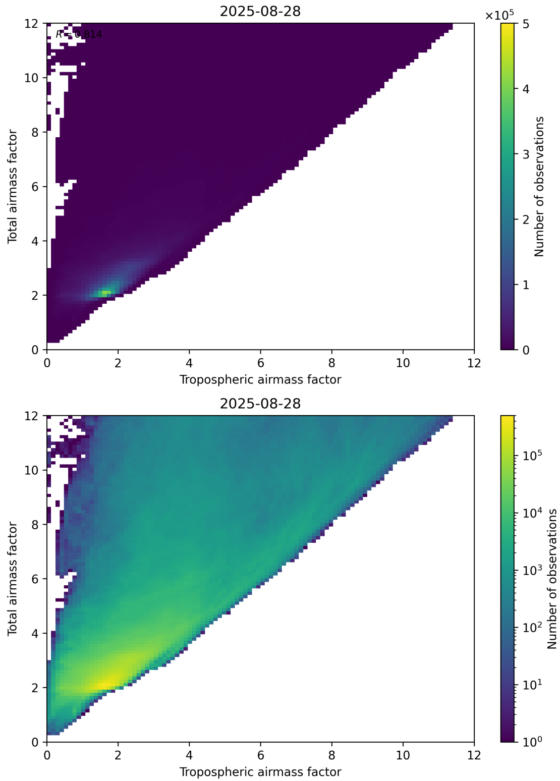
Figure 72: Scatter density plot of “Tropospheric airmass factor” against “Total airmass factor” for 2025-08-27 to 2025-08-29.
