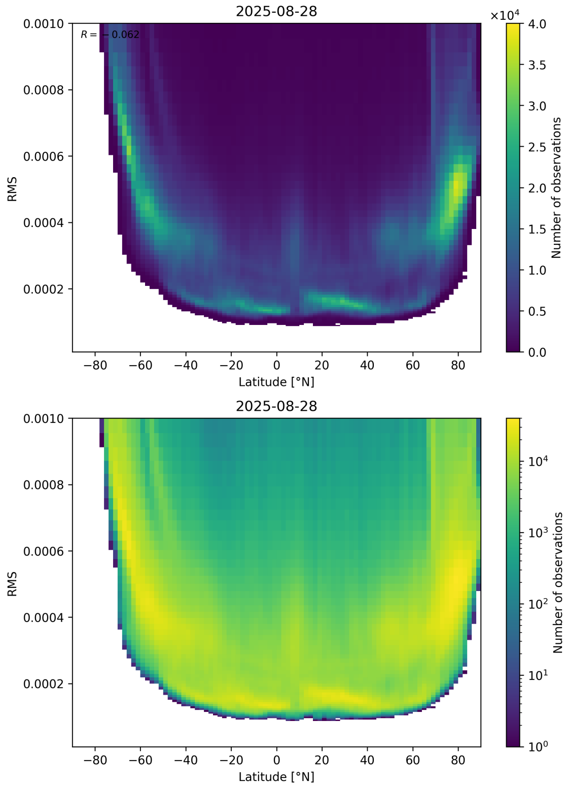
Figure 94: Scatter density plot of “Latitude” against “RMS” for 2025-08-27 to 2025-08-29.
