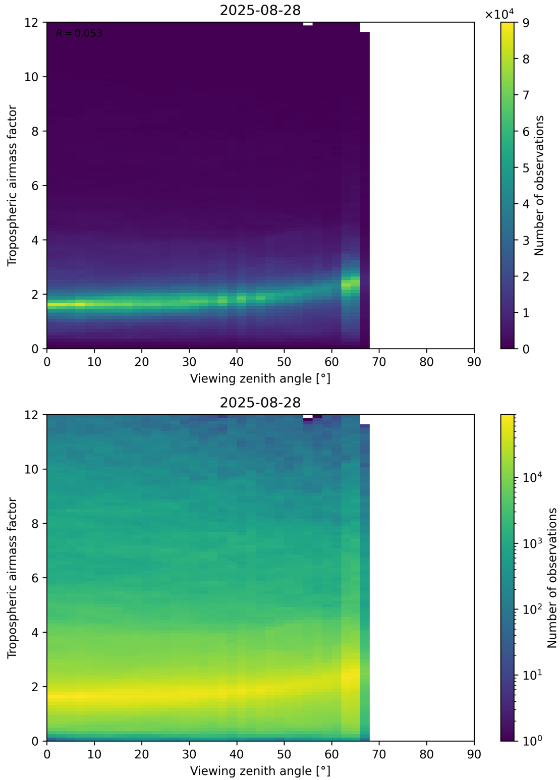
Figure 161: Scatter density plot of “Viewing zenith angle” against “Tropospheric airmass factor” for 2025-08-27 to 2025-08-29.
