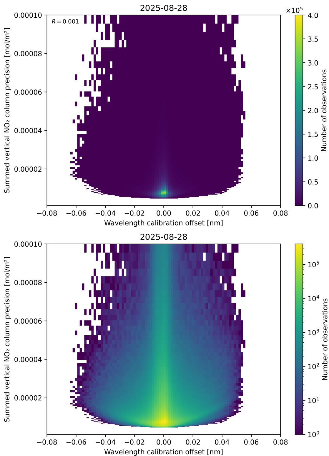
Figure 178: Scatter density plot of “Wavelength calibration offset” against “Summed vertical NO 2 column precision” for 2025-08-27 to 2025-08-29.
