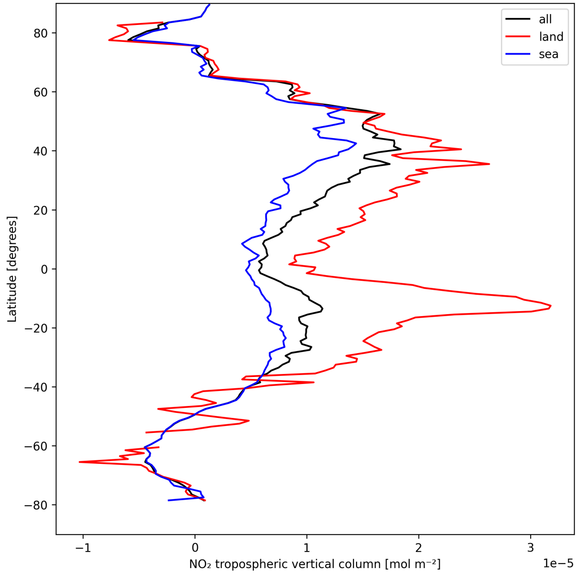
Figure 12: Zonal average of “NO 2 tropospheric vertical column” for 2025-08-27 to 2025-08-29.
