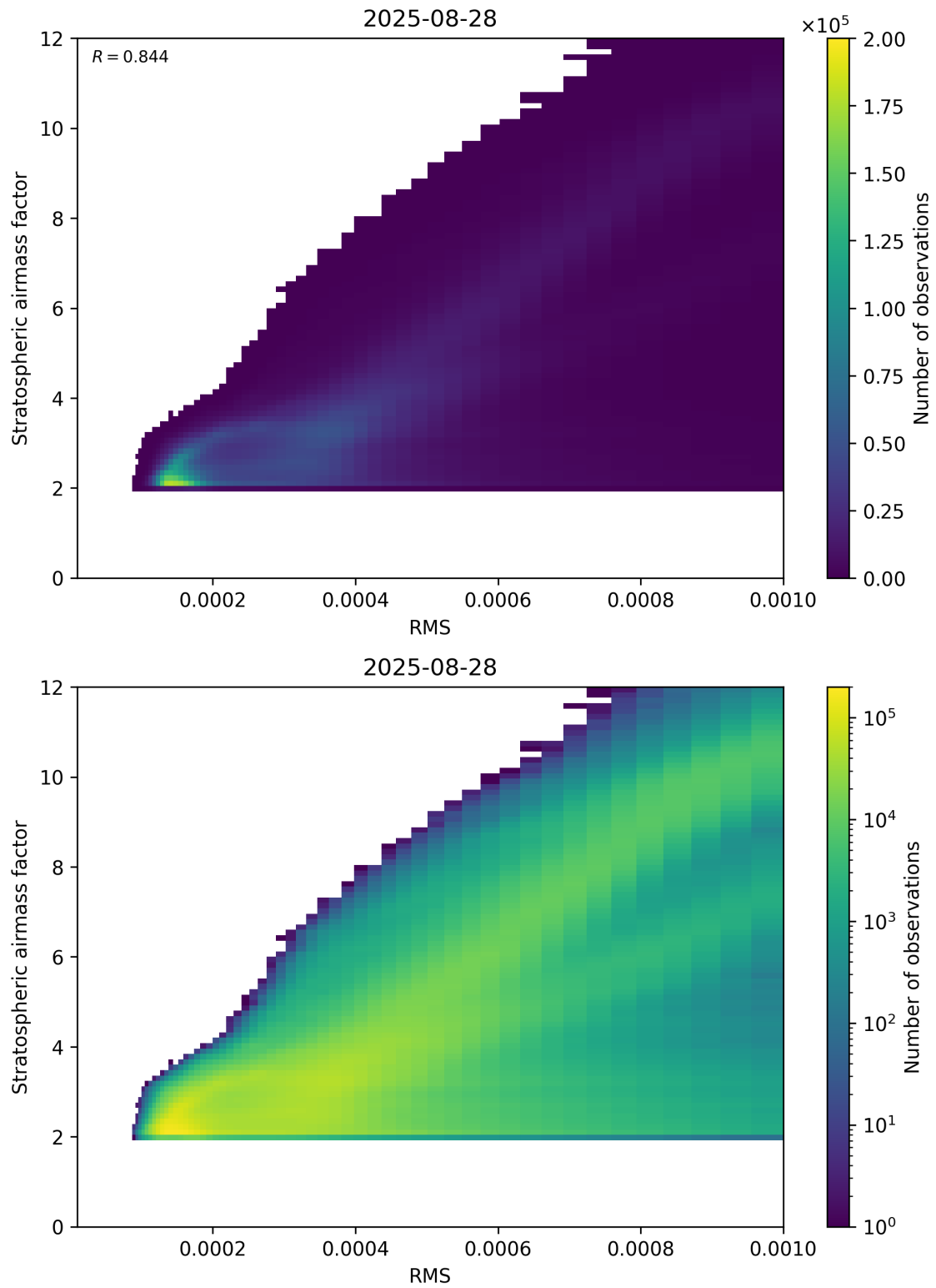
Figure 144: Scatter density plot of “RMS” against “Stratospheric airmass factor” for 2025-08-27 to 2025-08-29.
