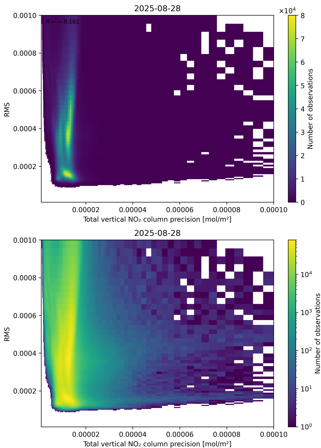
Figure 119: Scatter density plot of “Total vertical NO 2 column precision” against “RMS” for 2025-08-27 to 2025-08-29.
