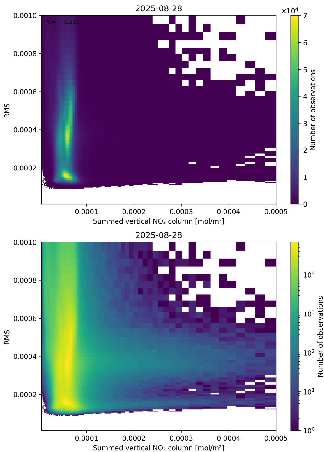
Figure 109: Scatter density plot of “Summed vertical NO 2 column” against “RMS” for 2025-08-27 to 2025-08-29.
