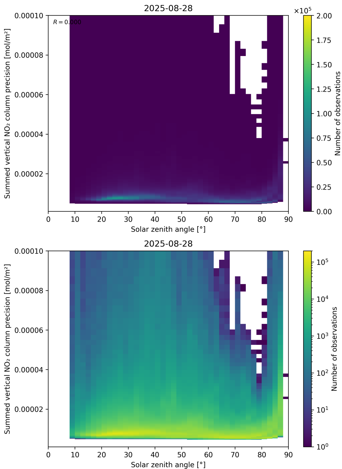
Figure 152: Scatter density plot of “Solar zenith angle” against “Summed vertical NO 2 column precision” for 2025-08-27 to 2025-08-29.
