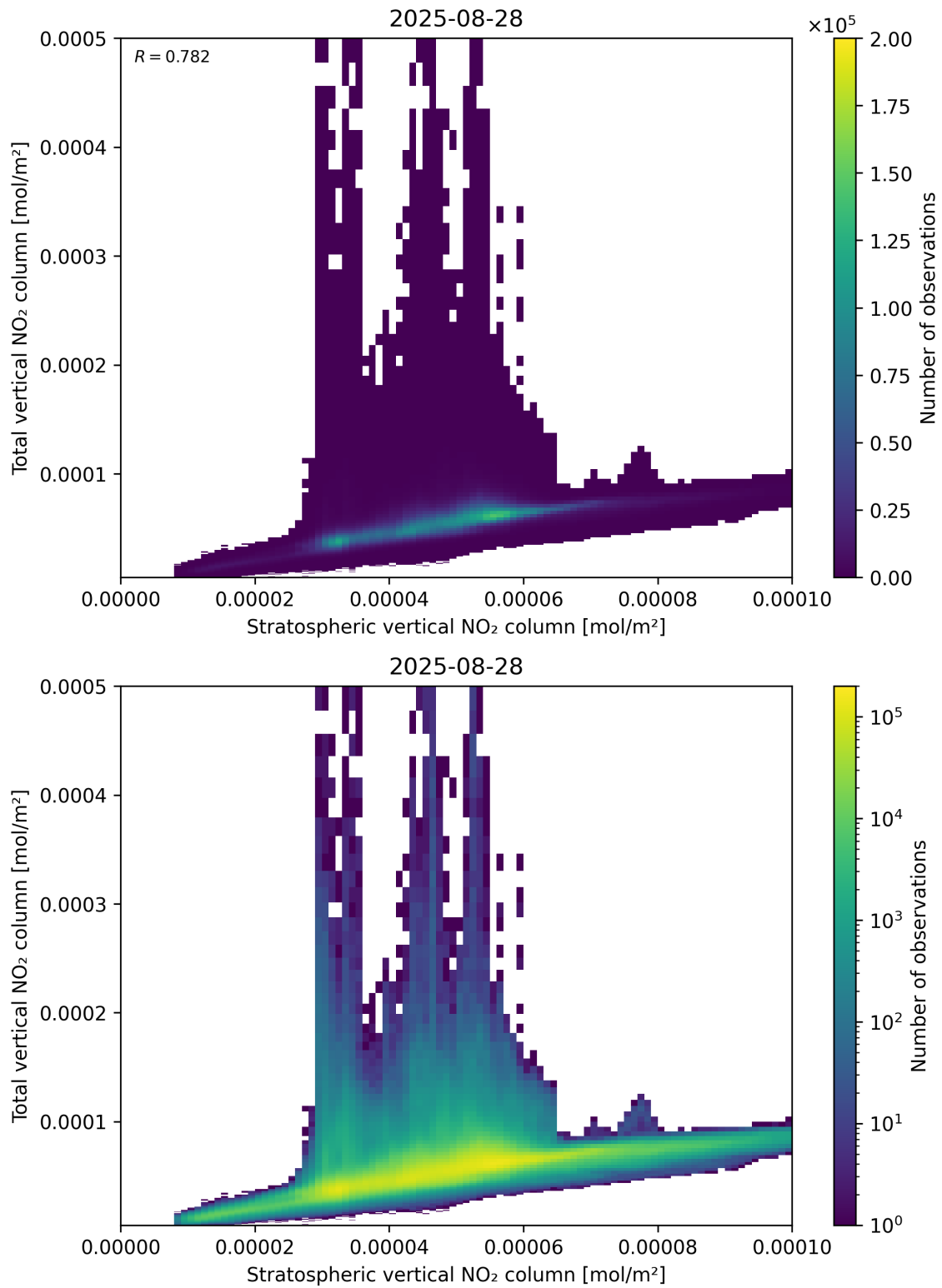
Figure 100: Scatter density plot of “Stratospheric vertical NO 2 column” against “Total vertical NO 2 column” for 2025-08-27 to 2025-08-29.
