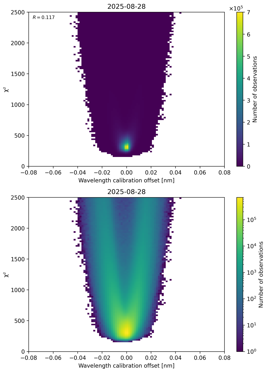
Figure 175: Scatter density plot of “Wavelength calibration offset” against “ \chi^2 ” for 2025-08-27 to 2025-08-29.
