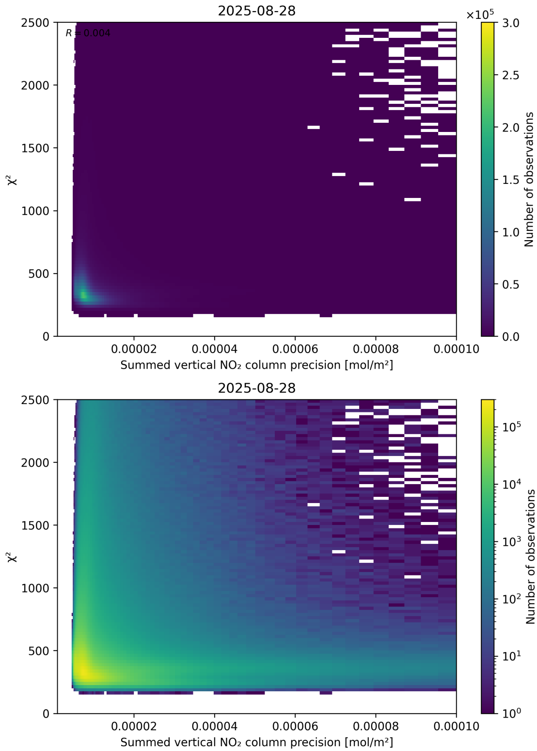
Figure 107: Scatter density plot of “Summed vertical NO 2 column precision” against “ \chi^2 ” for 2025-08-27 to 2025-08-29.
