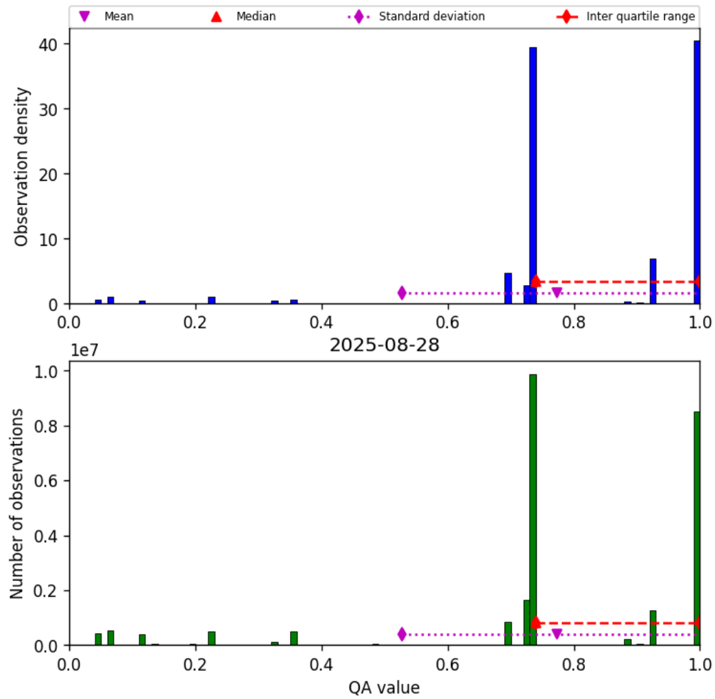
Figure 28: Histogram of “QA value” for 2025-08-27 to 2025-08-29
