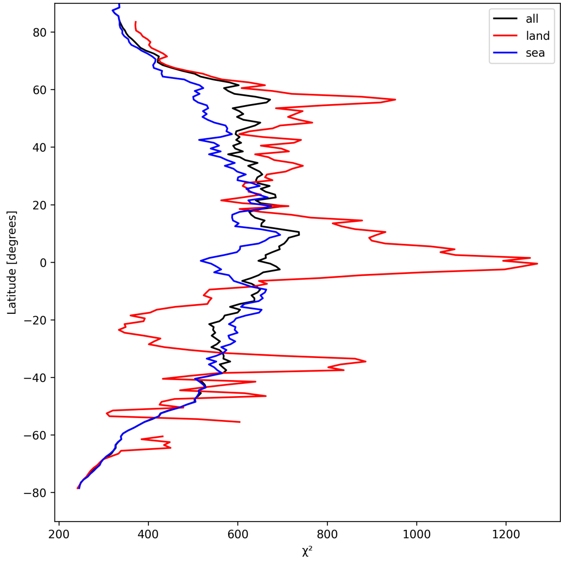
Figure 25: Zonal average of “ \chi^2 ” for 2025-08-27 to 2025-08-29.
