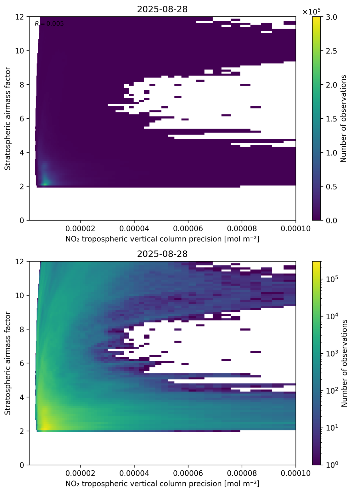
Figure 131: Scatter density plot of “NO 2 tropospheric vertical column precision” against “Stratospheric airmass factor” for 2025-08-27 to 2025-08-29.
