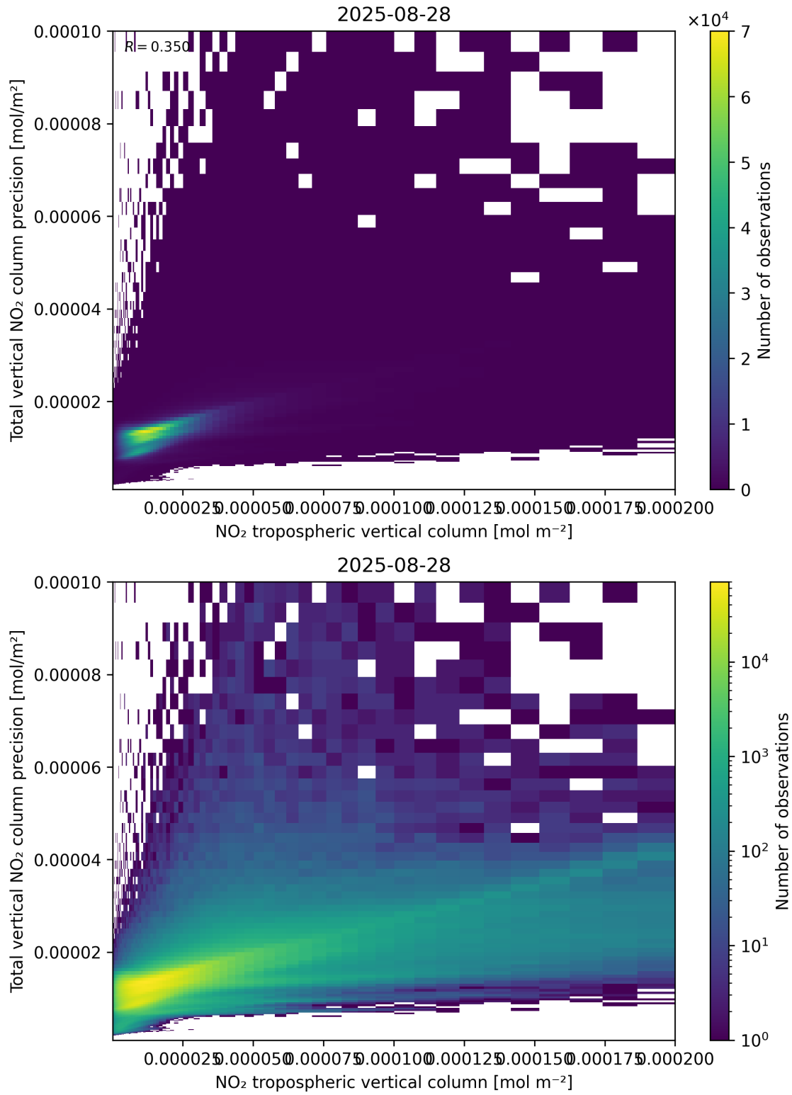
Figure 129: Scatter density plot of “NO 2 tropospheric vertical column” against “Total vertical NO 2 column precision” for 2025-08-27 to 2025-08-29.
