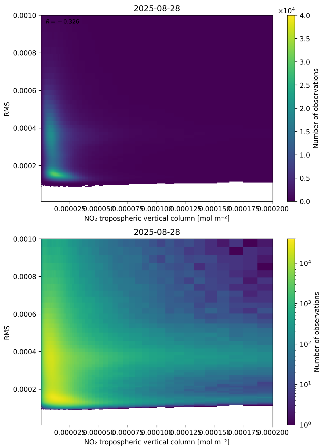
Figure 142: Scatter density plot of “NO 2 tropospheric vertical column” against “RMS” for 2025-08-27 to 2025-08-29.
