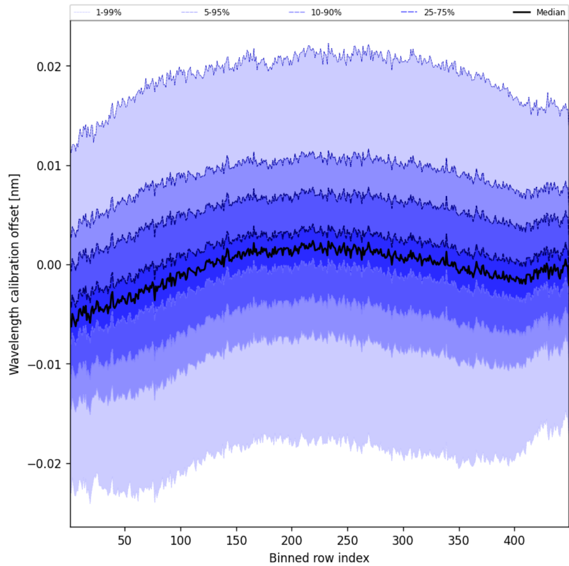
Figure 52: Along track statistics of “Wavelength calibration offset” for 2025-08-27 to 2025-08-29
