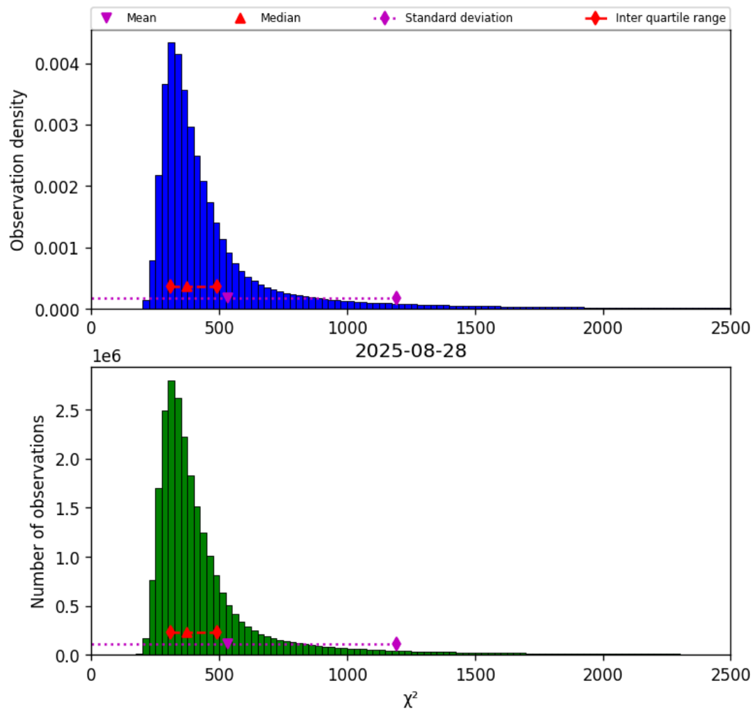
Figure 42: Histogram of “ \chi^2 ” for 2025-08-27 to 2025-08-29
