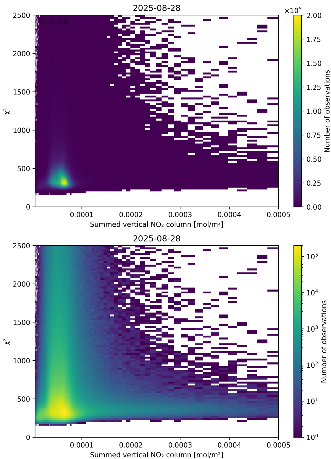
Figure 104: Scatter density plot of “Summed vertical NO 2 column” against “ \chi^2 ” for 2025-08-27 to 2025-08-29.
