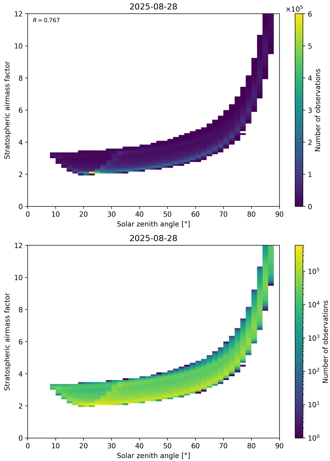
Figure 145: Scatter density plot of “Solar zenith angle” against “Stratospheric airmass factor” for 2025-08-27 to 2025-08-29.
