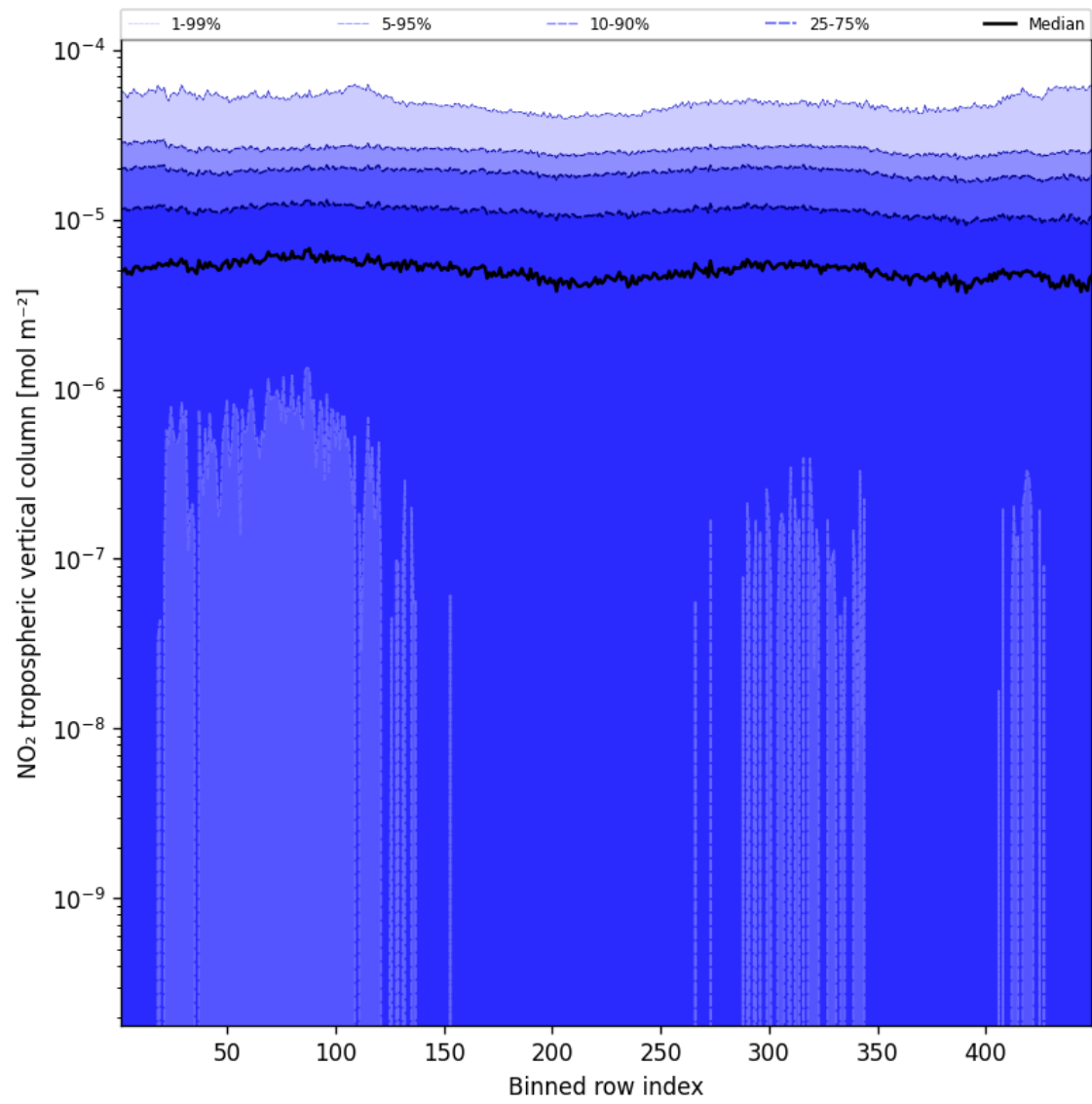
Figure 46: Along track statistics of "NO 2 tropospheric vertical column" for 2025-08-27 to 2025-08-29
