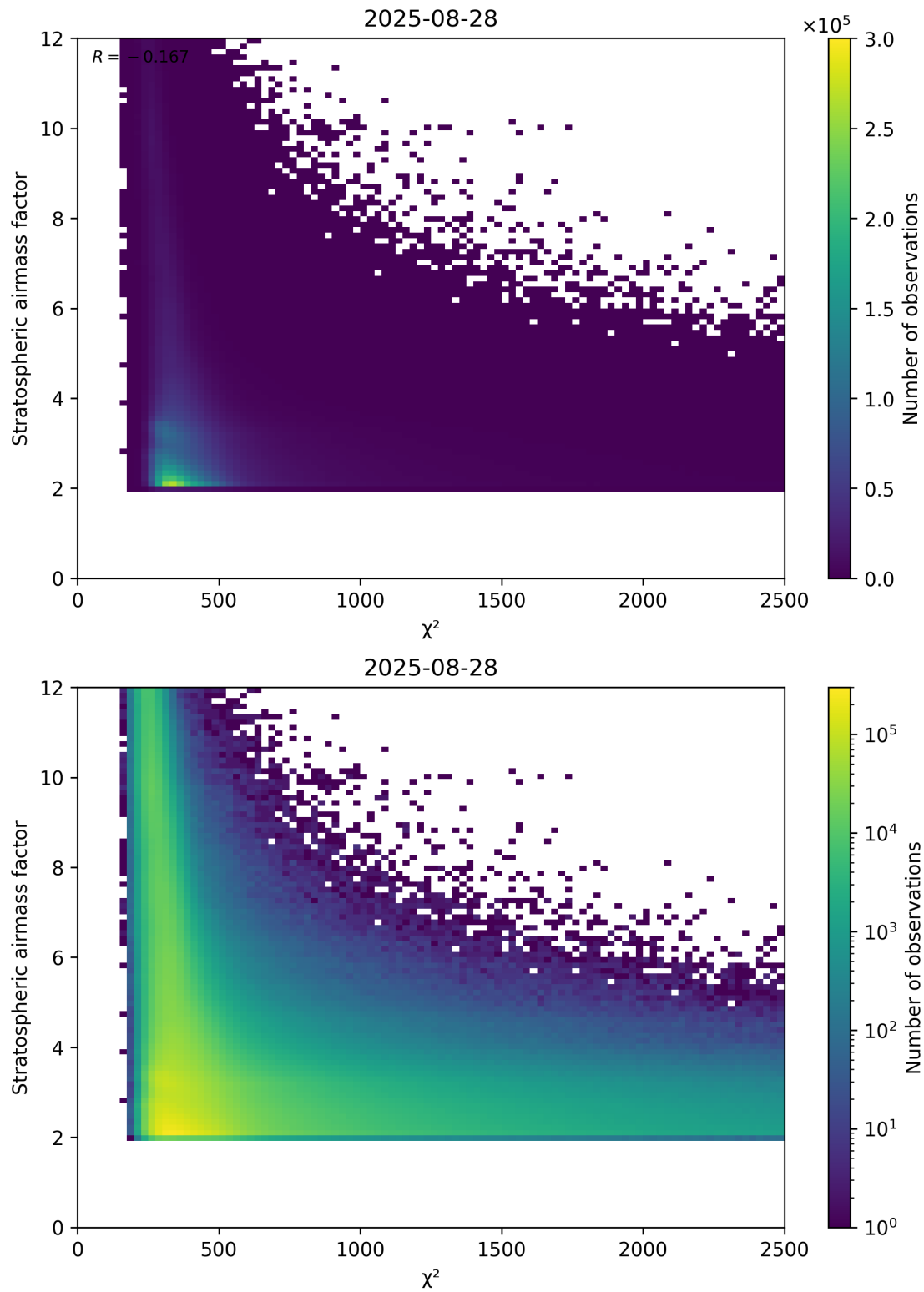
Figure 81: Scatter density plot of “ \chi^2 ” against “Stratospheric air mass factor” for 2025-08-27 to 2025-08-29.
