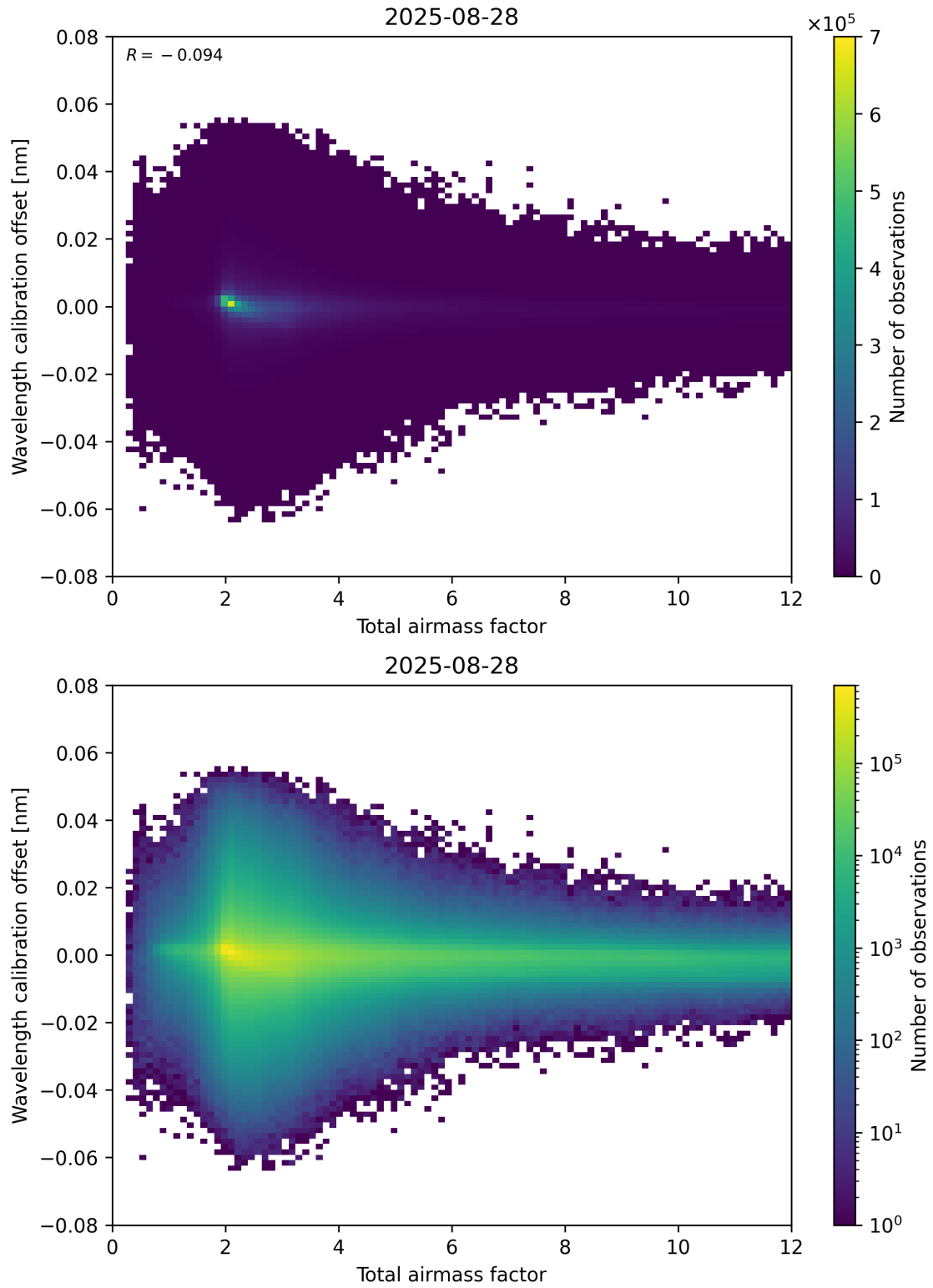
Figure 70: Scatter density plot of “Total airmass factor” against “Wavelength calibration offset” for 2025-08-27 to 2025-08-29.
