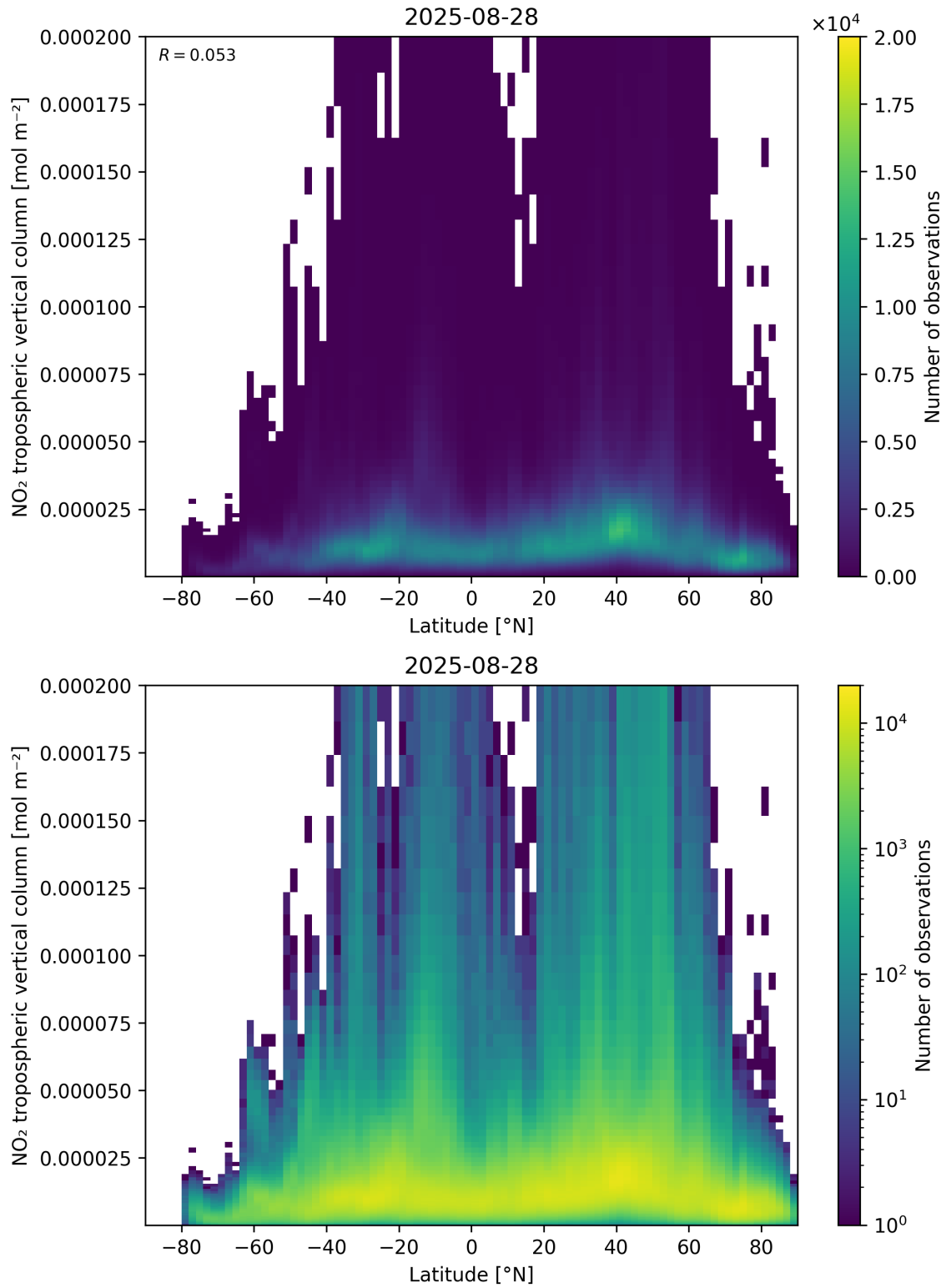
Figure 92: Scatter density plot of “Latitude” against “NO 2 tropospheric vertical column” for 2025-08-27 to 2025-08-29.
