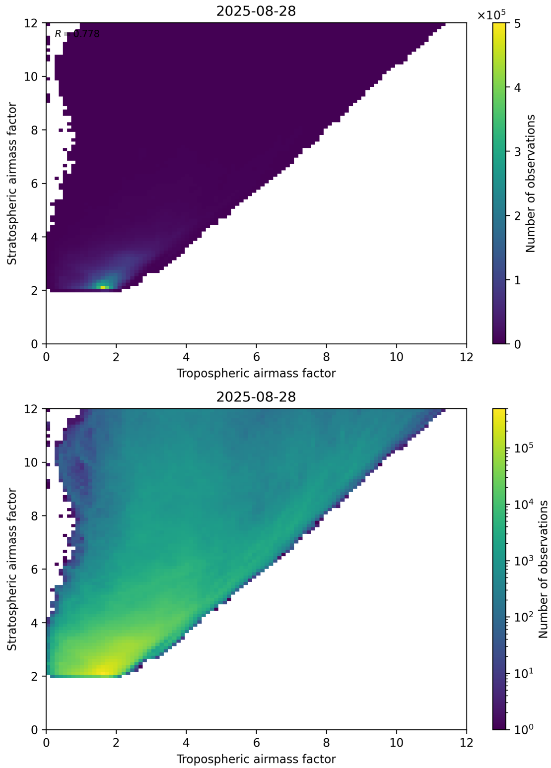
Figure 71: Scatter density plot of “Tropospheric airmass factor” against “Stratospheric airmass factor” for 2025-08-27 to 2025-08-29.
