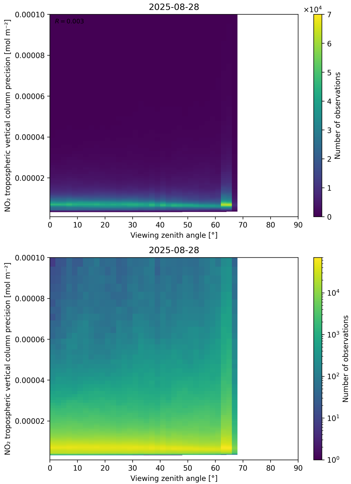
Figure 170: Scatter density plot of “Viewing zenith angle” against “NO 2 tropospheric vertical column precision” for 2025-08-27 to 2025-08-29.
