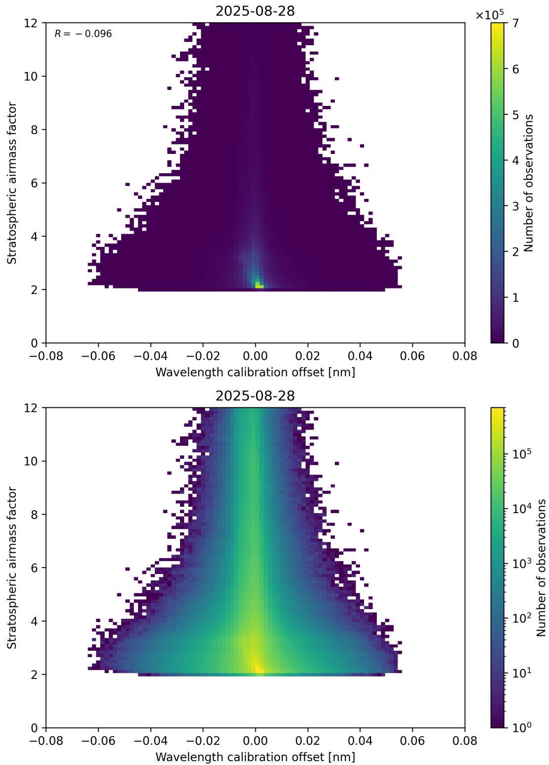
Figure 174: Scatter density plot of “Wavelength calibration offset” against “Stratospheric airmass factor” for 2025-08-27 to 2025-08-29.
