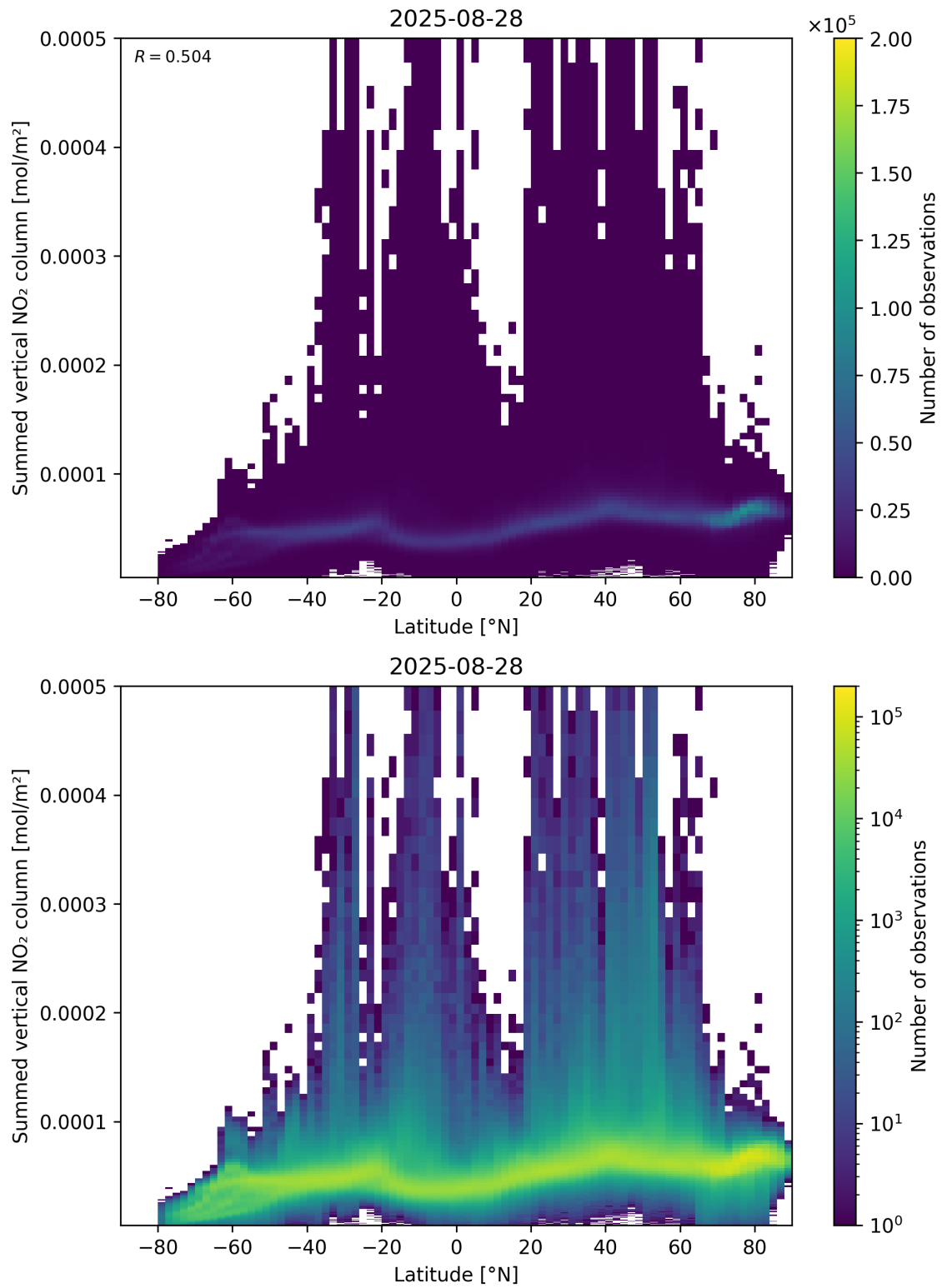
Figure 88: Scatter density plot of “Latitude” against “Summed vertical NO 2 column” for 2025-08-27 to 2025-08-29.
