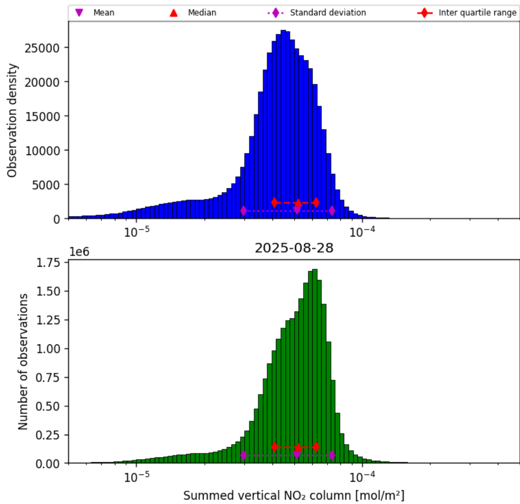
Figure 40: Histogram of “Summed vertical NO 2 column” for 2025-08-27 to 2025-08-29
