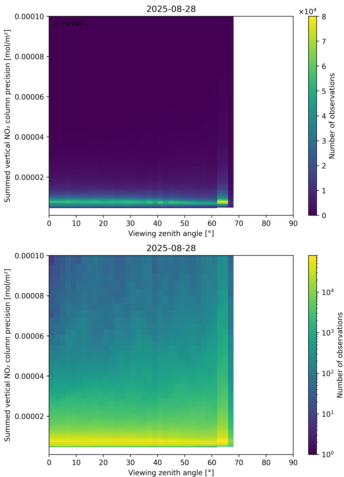
Figure 166: Scatter density plot of “Viewing zenith angle” against “Summed vertical NO 2 column precision” for 2025-08-27 to 2025-08-29.
