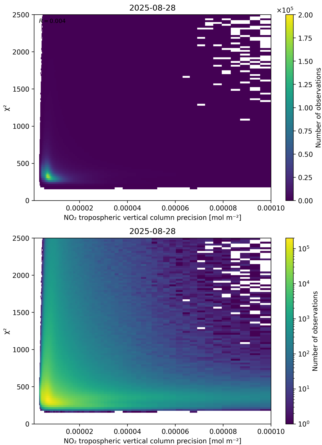
Figure 134: Scatter density plot of “NO 2 tropospheric vertical column precision” against “ \chi^2 ” for 2025-08-27 to 2025-08-29.
