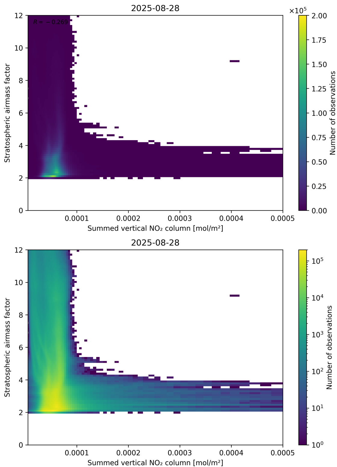
Figure 103: Scatter density plot of “Summed vertical NO 2 column” against “Stratospheric air mass factor” for 2025-08-27 to 2025-08-29.
