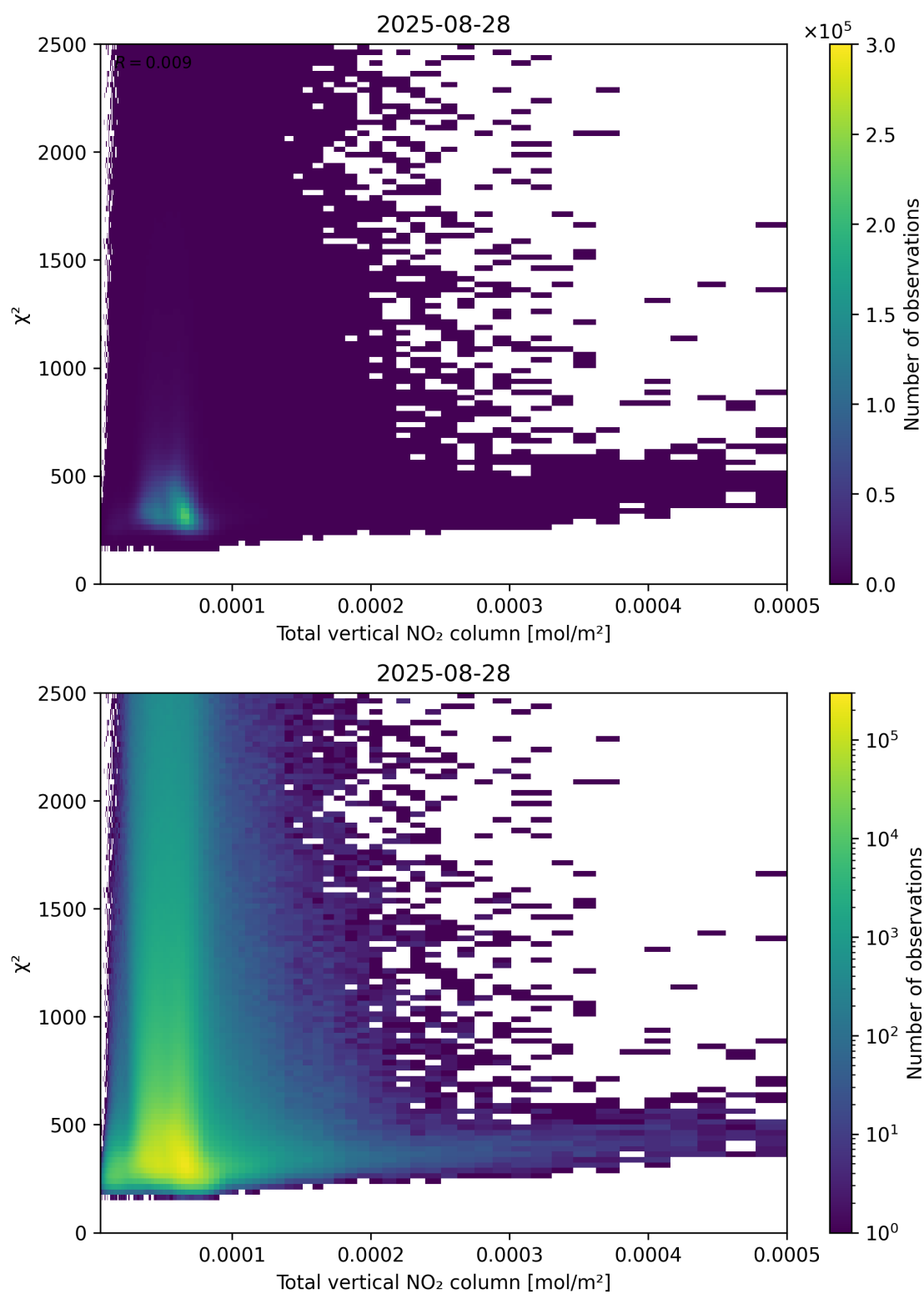
Figure 111: Scatter density plot of “Total vertical NO 2 column” against “ \chi^2 ” for 2025-08-27 to 2025-08-29.
