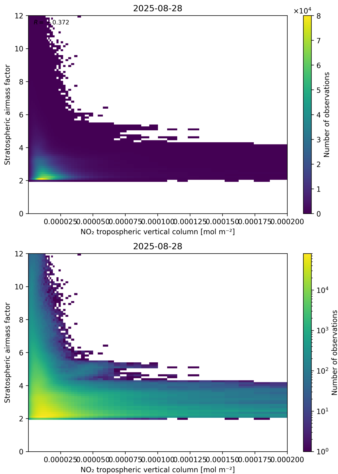
Figure 121: Scatter density plot of “NO 2 tropospheric vertical column” against “Stratospheric air mass factor” for 2025-08-27 to 2025-08-29.
