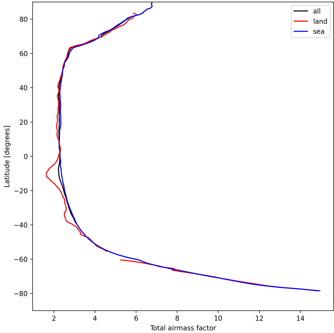
Figure 15: Zonal average of “Total airmass factor” for 2025-08-27 to 2025-08-29.
