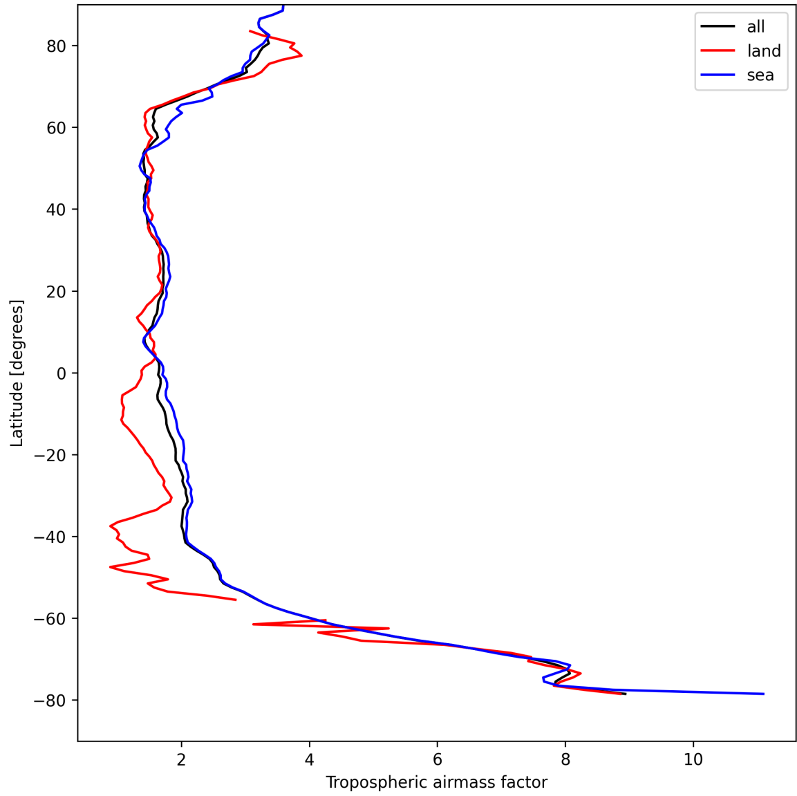
Figure 14: Zonal average of “Tropospheric airmass factor” for 2025-08-27 to 2025-08-29.
