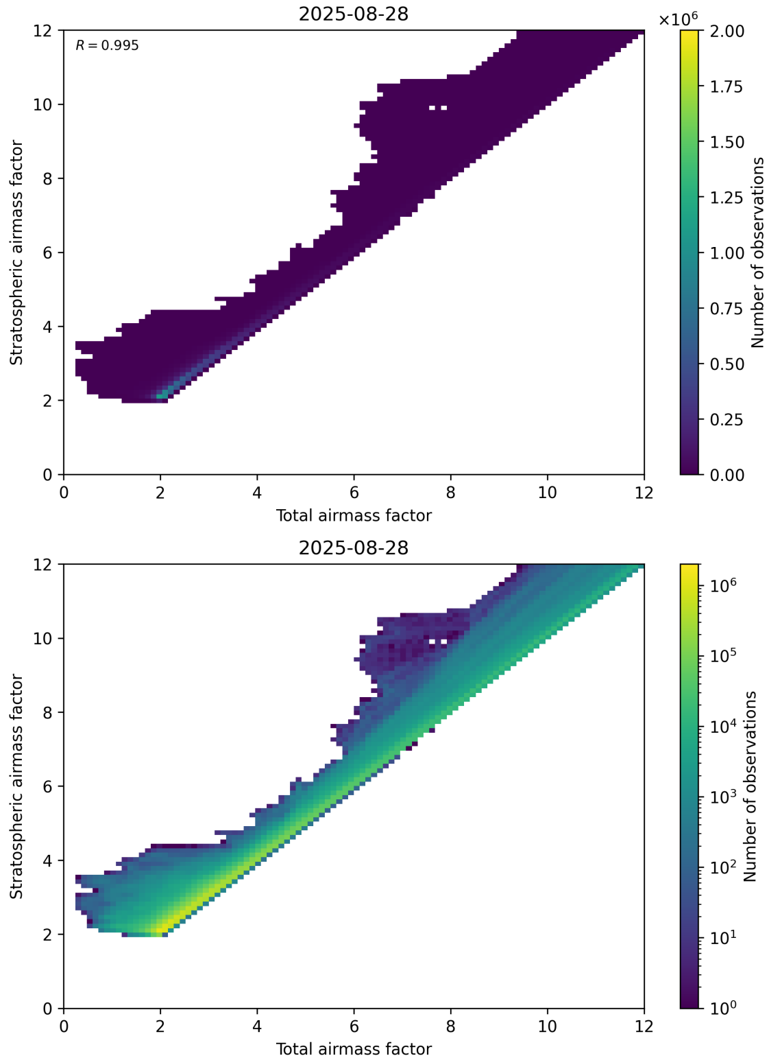
Figure 62: Scatter density plot of “Total airmass factor” against “Stratospheric airmass factor” for 2025-08-27 to 2025-08-29.
