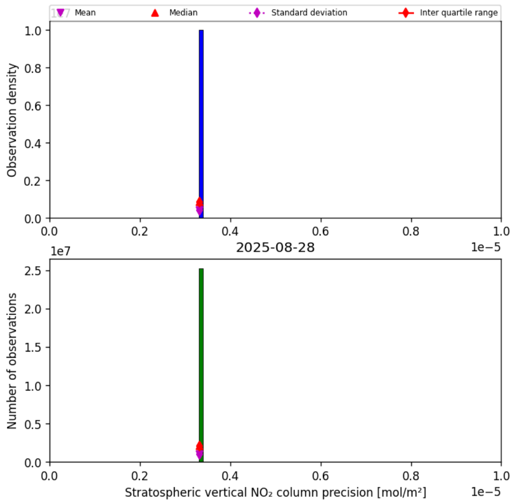
Figure 37: Histogram of “Stratospheric vertical NO 2 column precision” for 2025-08-27 to 2025-08-29
