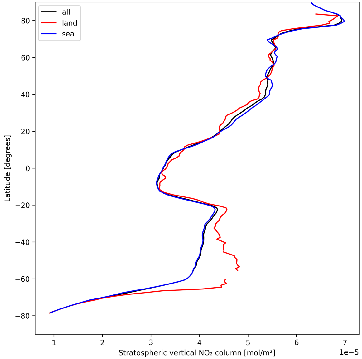
Figure 19: Zonal average of “Stratospheric vertical NO 2 column” for 2025-08-27 to 2025-08-29.
