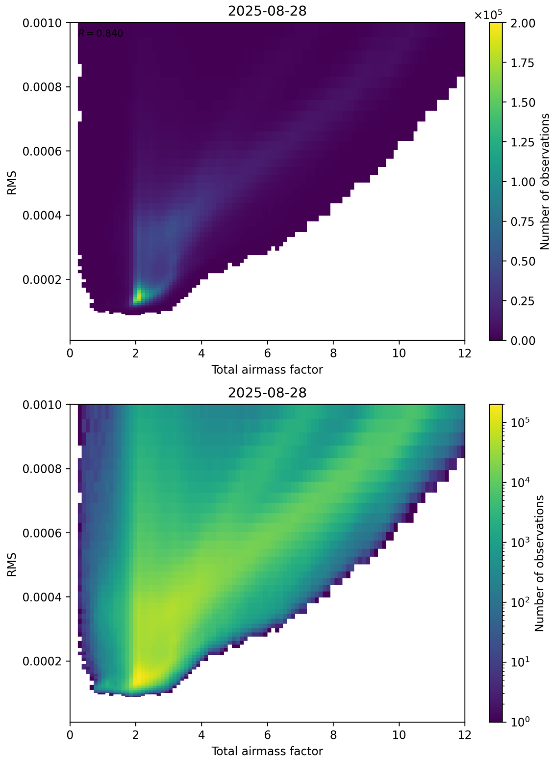
Figure 69: Scatter density plot of “Total airmass factor” against “RMS” for 2025-08-27 to 2025-08-29.
