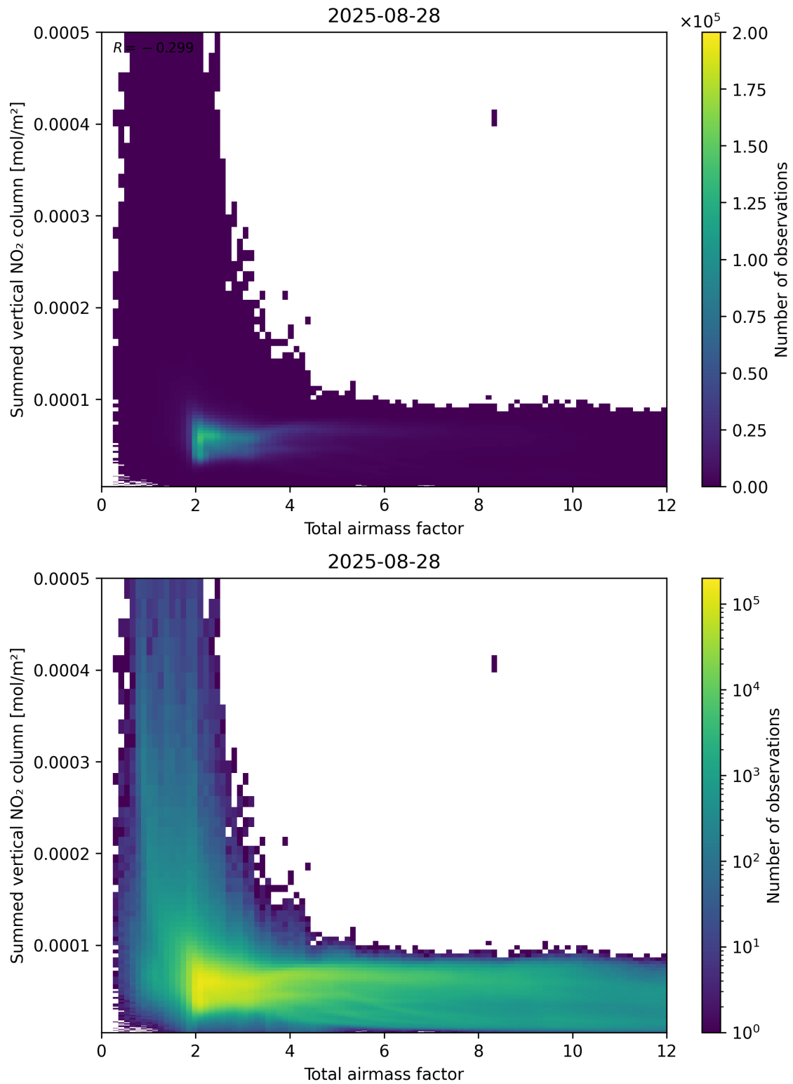
Figure 65: Scatter density plot of “Total airmass factor” against “Summed vertical NO 2 column” for 2025-08-27 to 2025-08-29.
