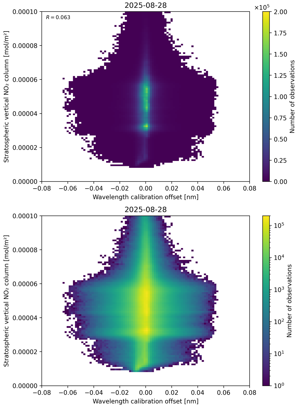
Figure 176: Scatter density plot of “Wavelength calibration offset” against “Stratospheric vertical NO 2 column” for 2025-08-27 to 2025-08-29.
