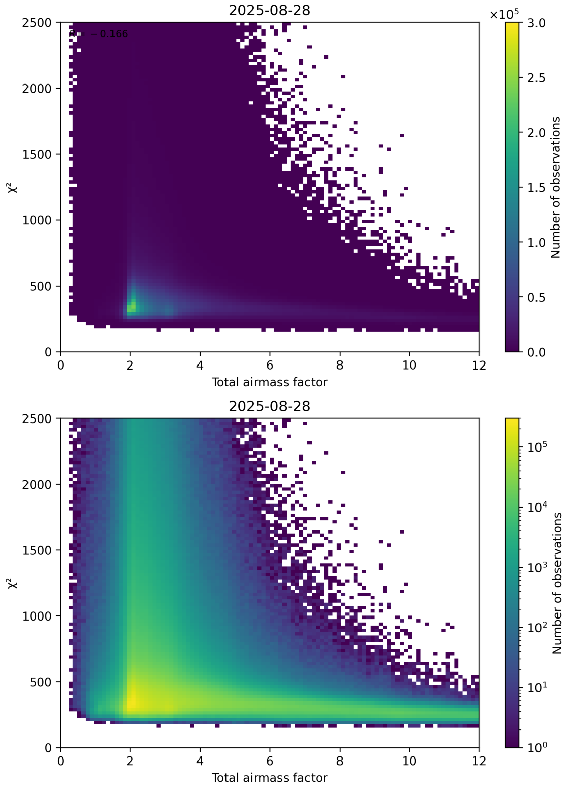
Figure 63: Scatter density plot of “Total airmass factor” against “ \chi^2 ” for 2025-08-27 to 2025-08-29.
