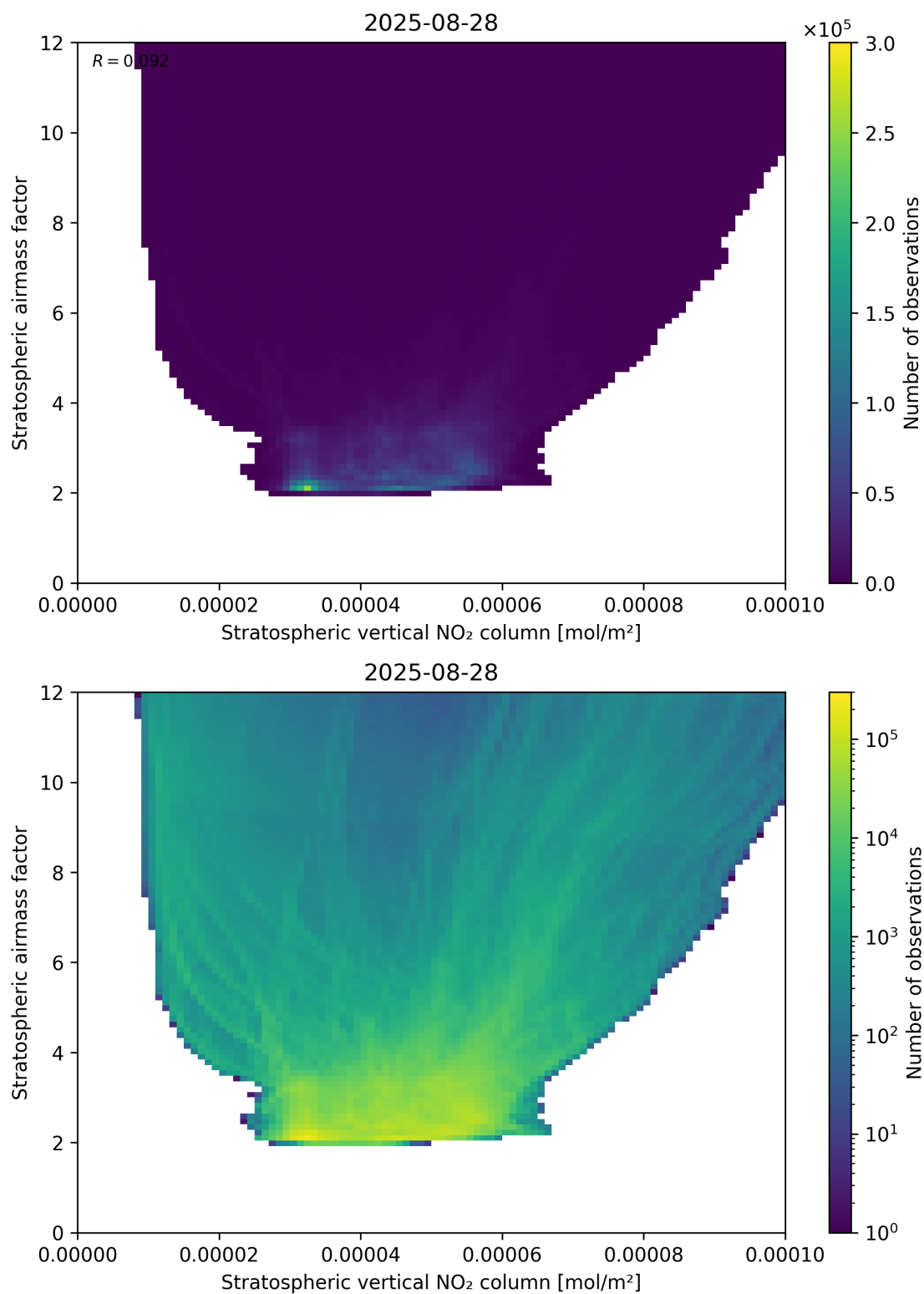
Figure 96: Scatter density plot of “Stratospheric vertical NO 2 column” against “Stratospheric airmass factor” for 2025-08-27 to 2025-08-29.
