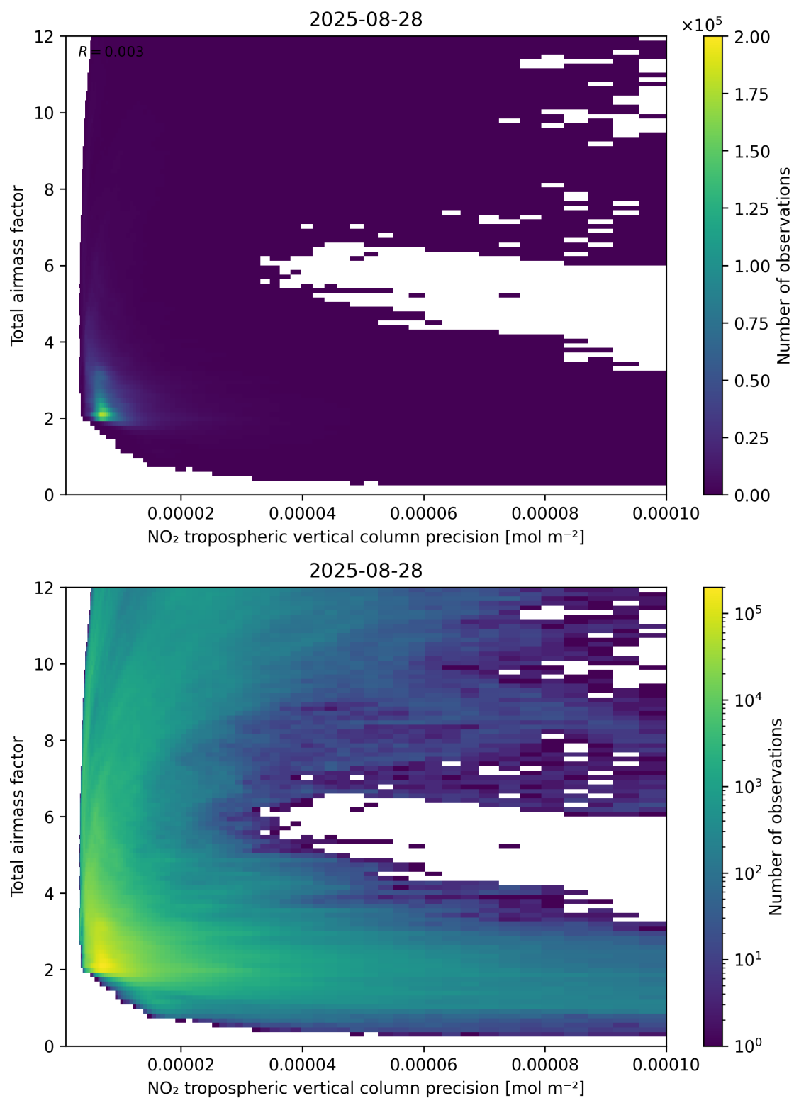
Figure 132: Scatter density plot of “NO 2 tropospheric vertical column precision” against “Total air mass factor” for 2025-08-27 to 2025-08-29.
