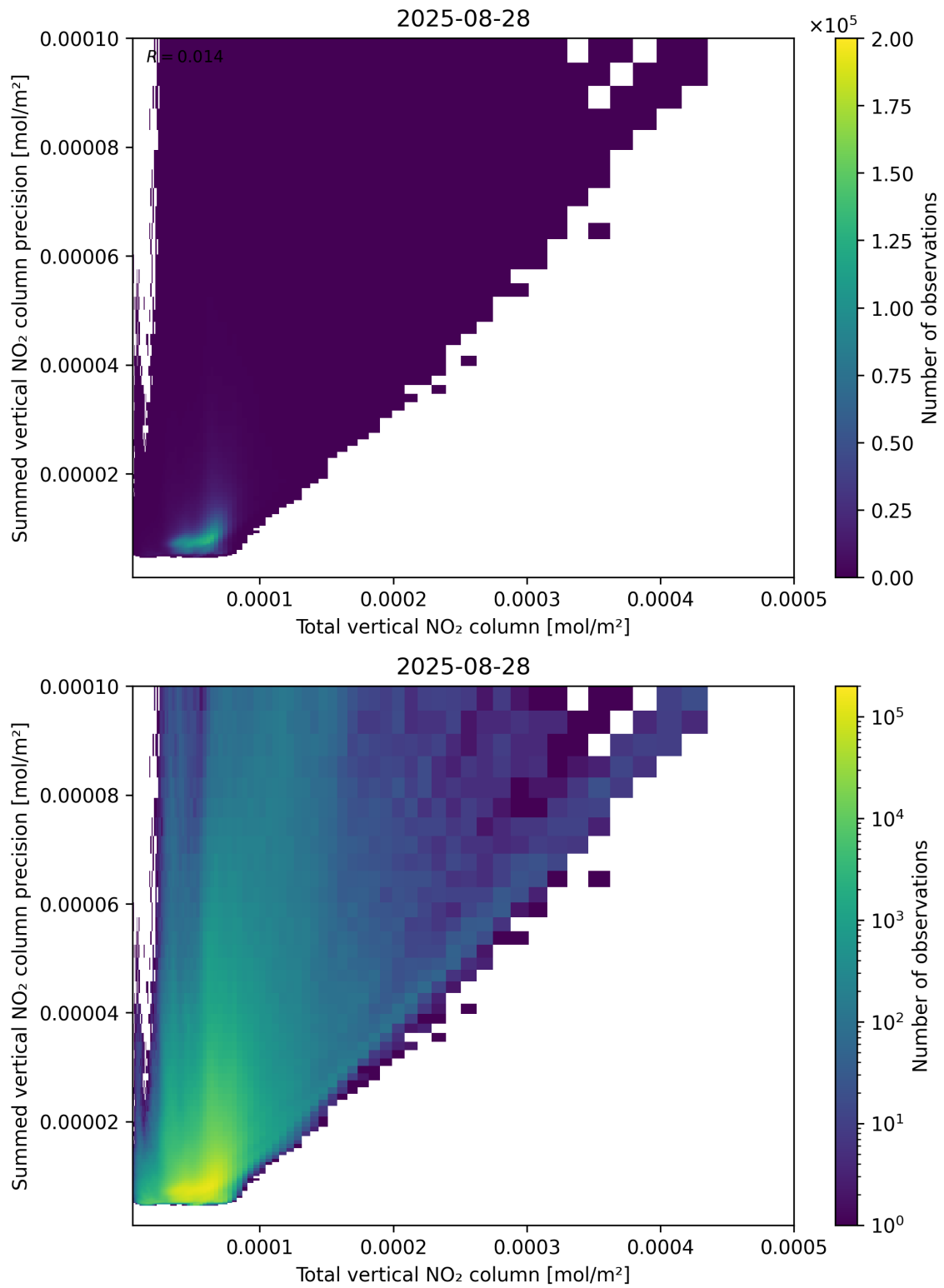
Figure 113: Scatter density plot of “Total vertical NO 2 column” against “Summed vertical NO 2 column precision” for 2025-08-27 to 2025-08-29.
