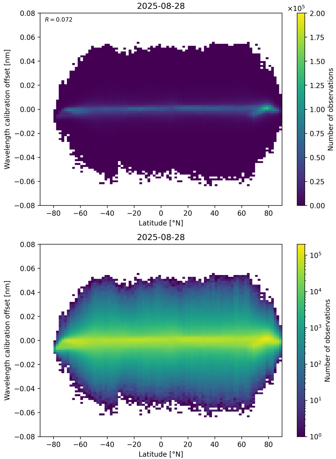
Figure 95: Scatter density plot of “Latitude” against “Wavelength calibration offset” for 2025-08-27 to 2025-08-29.
