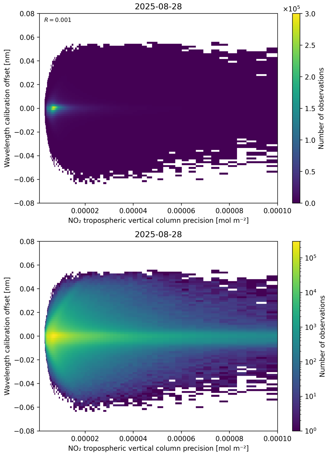
Figure 141: Scatter density plot of “NO 2 tropospheric vertical column precision” against “Wavelength calibration offset” for 2025-08-27 to 2025-08-29.
