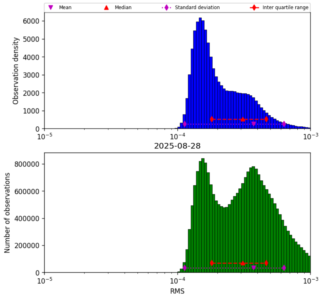
Figure 43: Histogram of “RMS” for 2025-08-27 to 2025-08-29
