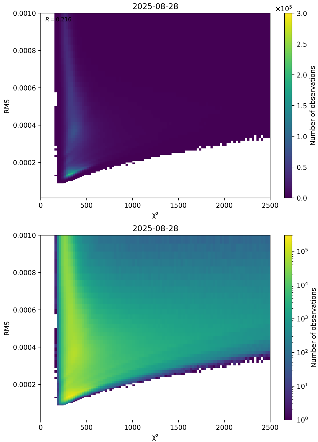
Figure 82: Scatter density plot of “ \chi^2 ” against “RMS” for 2025-08-27 to 2025-08-29.
