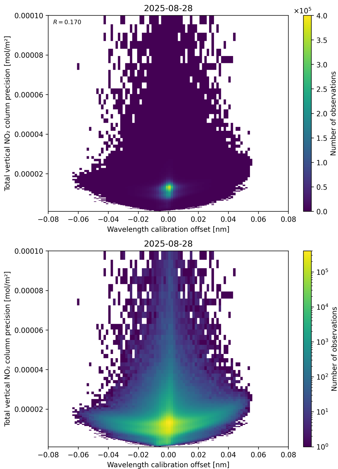
Figure 180: Scatter density plot of “Wavelength calibration offset” against “Total vertical NO 2 column precision” for 2025-08-27 to 2025-08-29.
