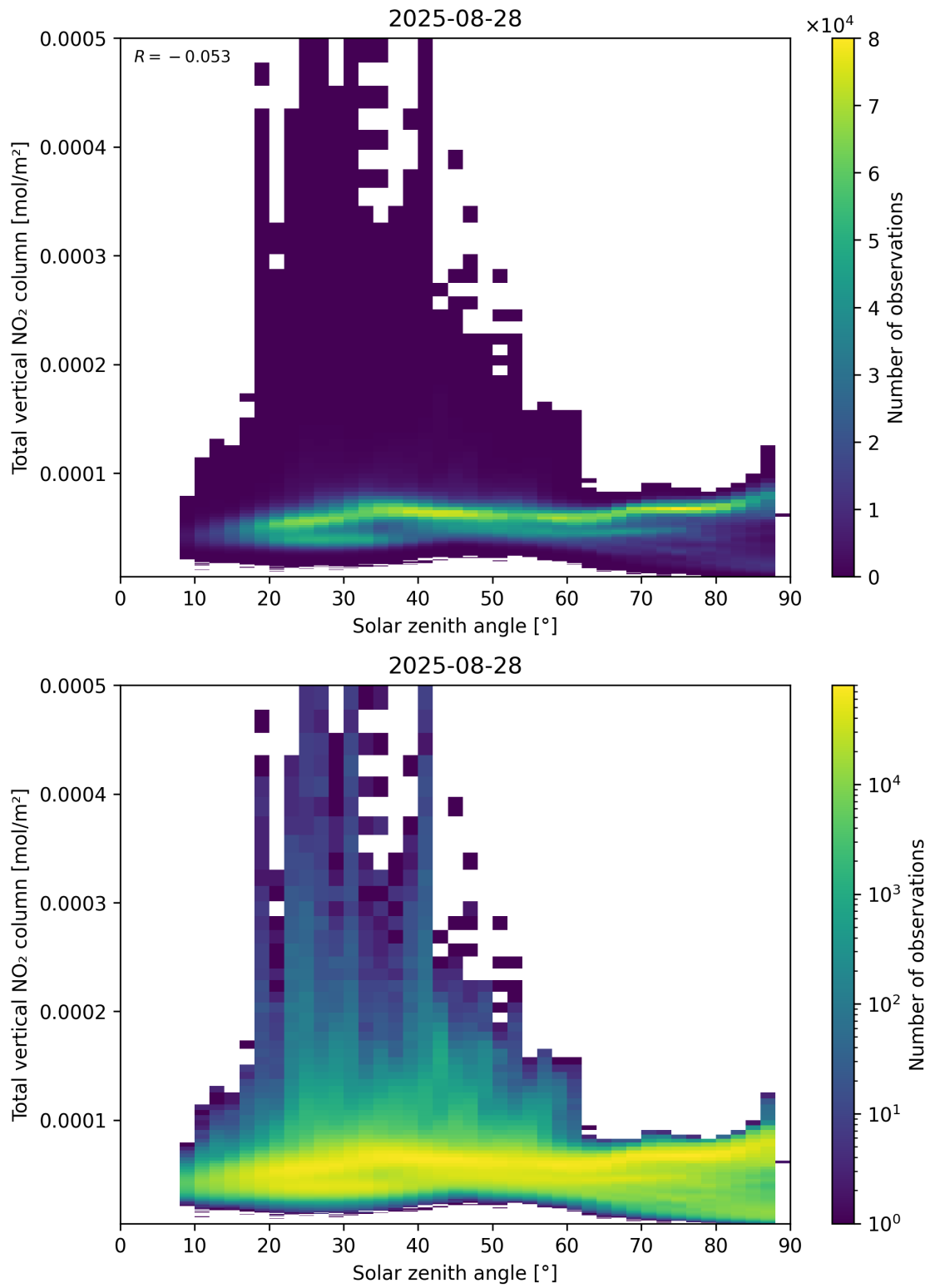
Figure 153: Scatter density plot of “Solar zenith angle” against “Total vertical NO 2 column” for 2025-08-27 to 2025-08-29.
