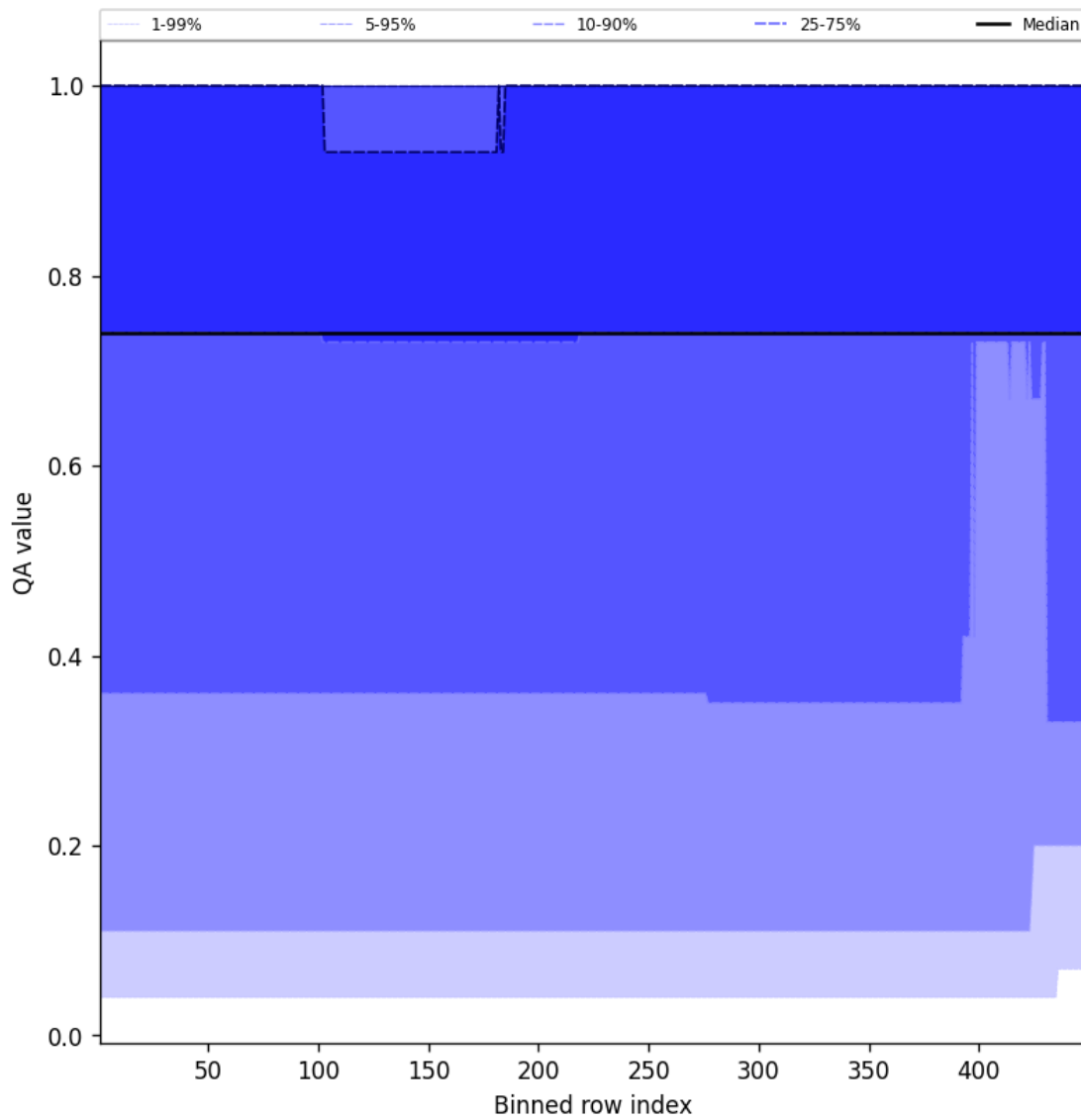
Figure 45: Along track statistics of “QA value” for 2025-08-27 to 2025-08-29
