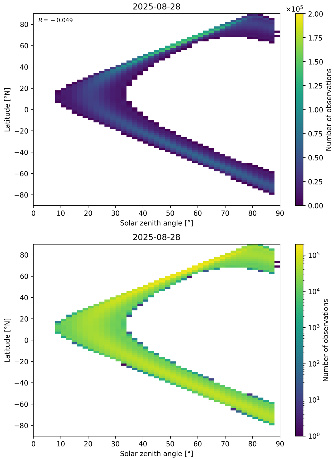
Figure 149: Scatter density plot of “Solar zenith angle” against “Latitude” for 2025-08-27 to 2025-08-29.
