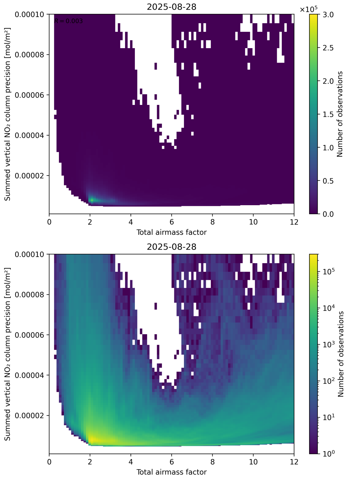
Figure 66: Scatter density plot of “Total airmass factor” against “Summed vertical NO 2 column precision” for 2025-08-27 to 2025-08-29.
