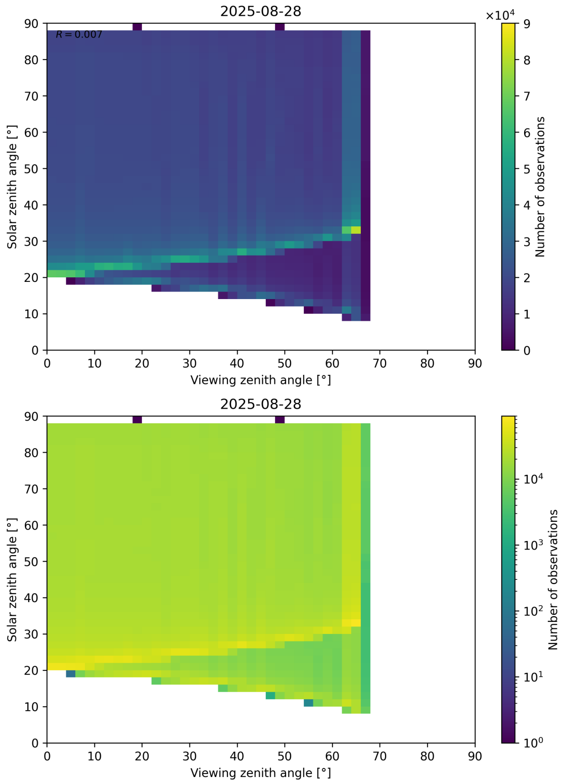
Figure 172: Scatter density plot of “Viewing zenith angle” against “Solar zenith angle” for 2025-08-27 to 2025-08-29.
