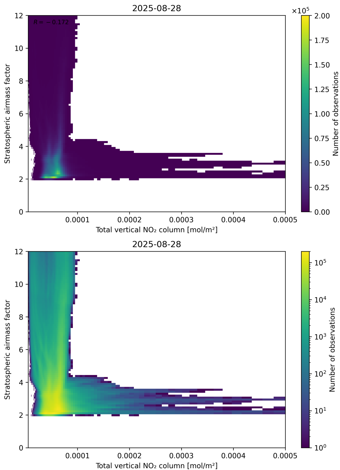
Figure 110: Scatter density plot of “Total vertical NO 2 column” against “Stratospheric air mass factor” for 2025-08-27 to 2025-08-29.
