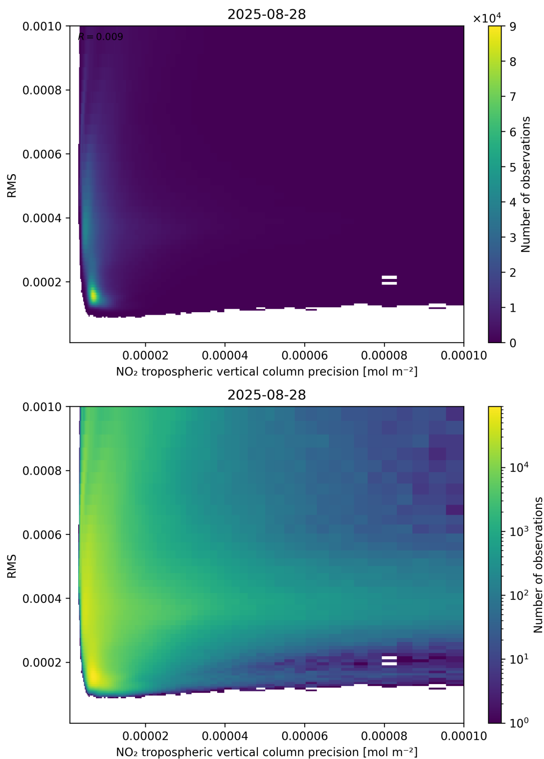
Figure 140: Scatter density plot of “NO 2 tropospheric vertical column precision” against “RMS” for 2025-08-27 to 2025-08-29.
