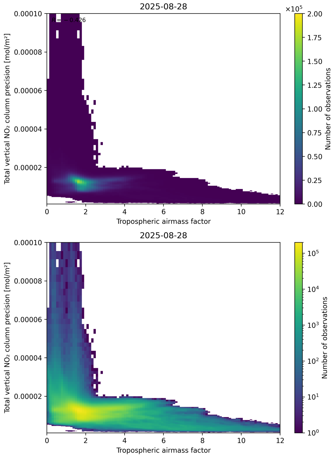
Figure 78: Scatter density plot of “Tropospheric air mass factor” against “Total vertical NO 2 column precision” for 2025-08-27 to 2025-08-29.
