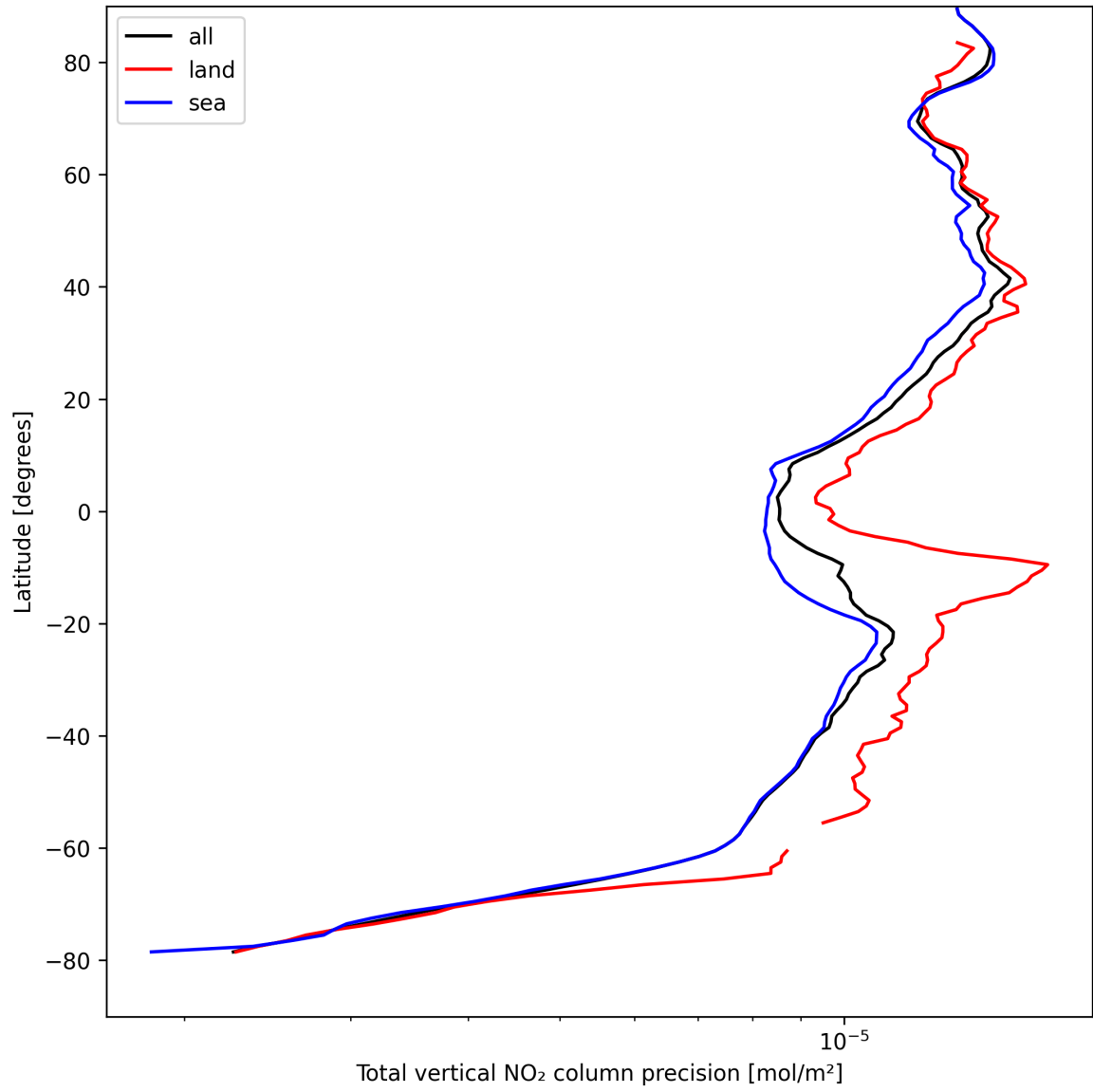
Figure 22: Zonal average of “Total vertical NO 2 column precision” for 2025-08-27 to 2025-08-29.
