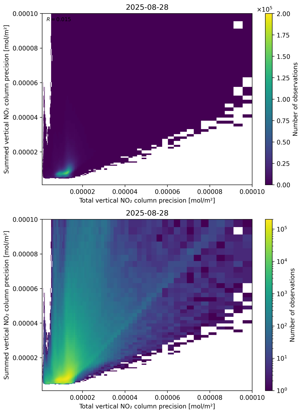
Figure 118: Scatter density plot of “Total vertical NO 2 column precision” against “Summed vertical NO 2 column precision” for 2025-08-27 to 2025-08-29.
