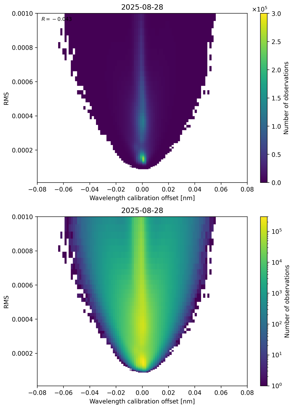
Figure 181: Scatter density plot of “Wavelength calibration offset” against “RMS” for 2025-08-27 to 2025-08-29.
