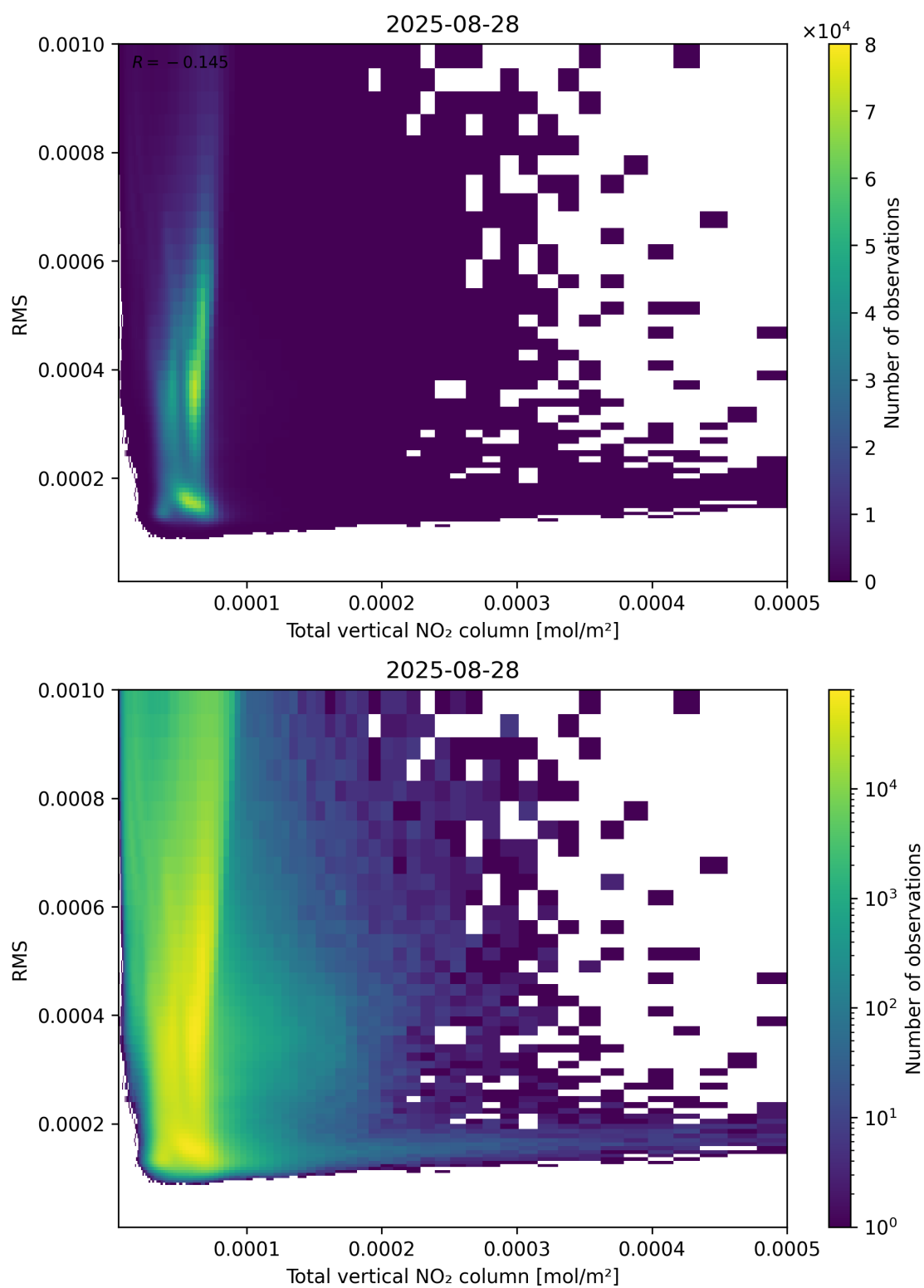
Figure 120: Scatter density plot of “Total vertical NO 2 column” against “RMS” for 2025-08-27 to 2025-08-29.
