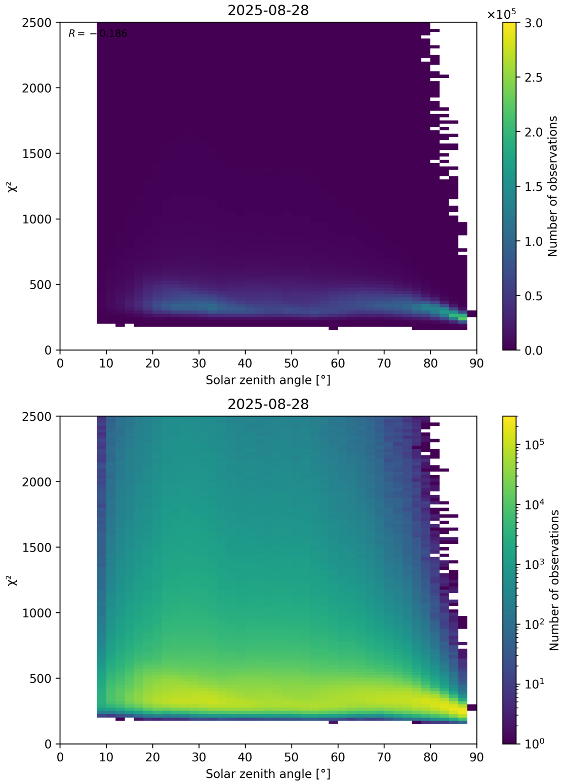
Figure 148: Scatter density plot of “Solar zenith angle” against “ \chi^2 ” for 2025-08-27 to 2025-08-29.
