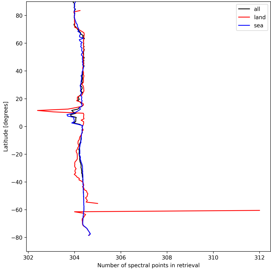
Figure 16: Zonal average of “Number of spectral points in retrieval” for 2025-08-27 to 2025-08-29.
