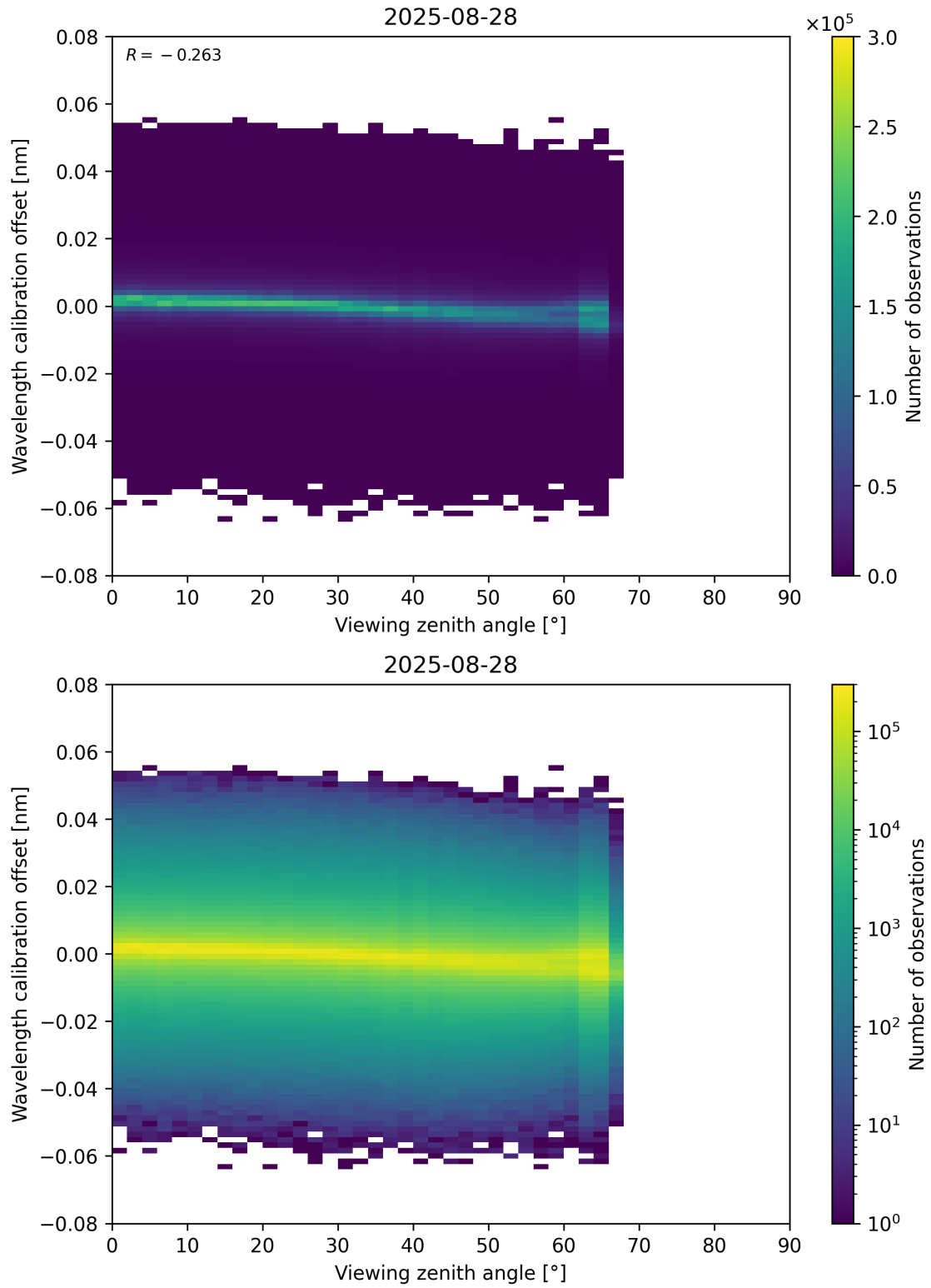
Figure 173: Scatter density plot of “Viewing zenith angle” against “Wavelength calibration offset” for 2025-08-27 to 2025-08-29.
