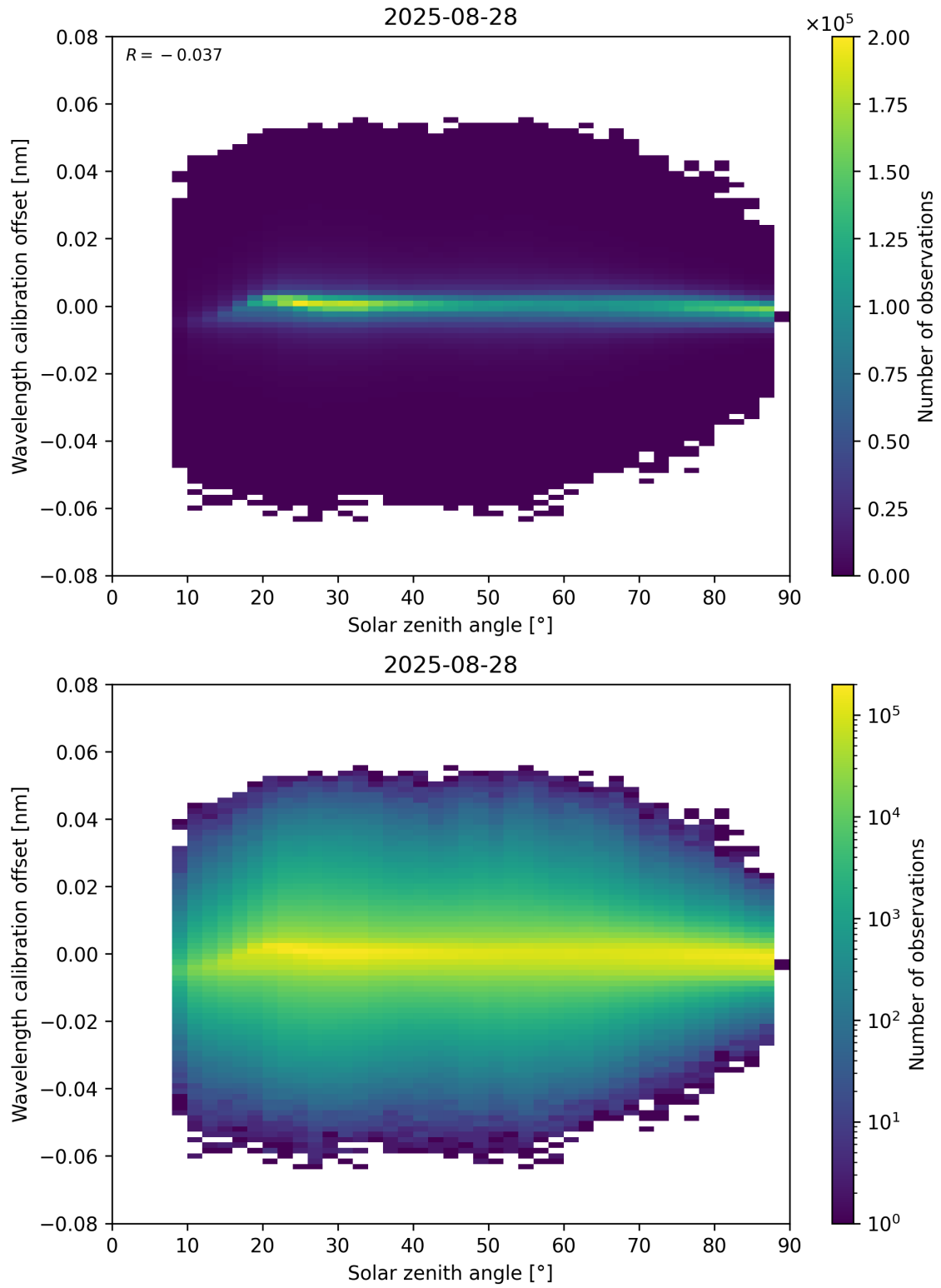
Figure 158: Scatter density plot of “Solar zenith angle” against “Wavelength calibration offset” for 2025-08-27 to 2025-08-29.
