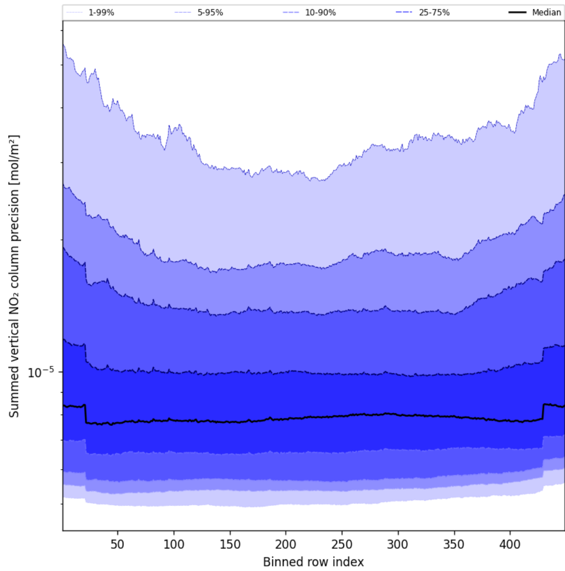
Figure 58: Along track statistics of “Summed vertical NO 2 column precision” for 2025-08-27 to 2025-08-29
