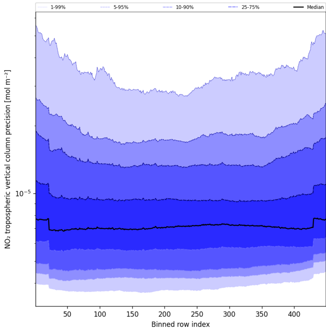
Figure 47: Along track statistics of “NO 2 tropospheric vertical column precision” for 2025-08-27 to 2025-08-29
