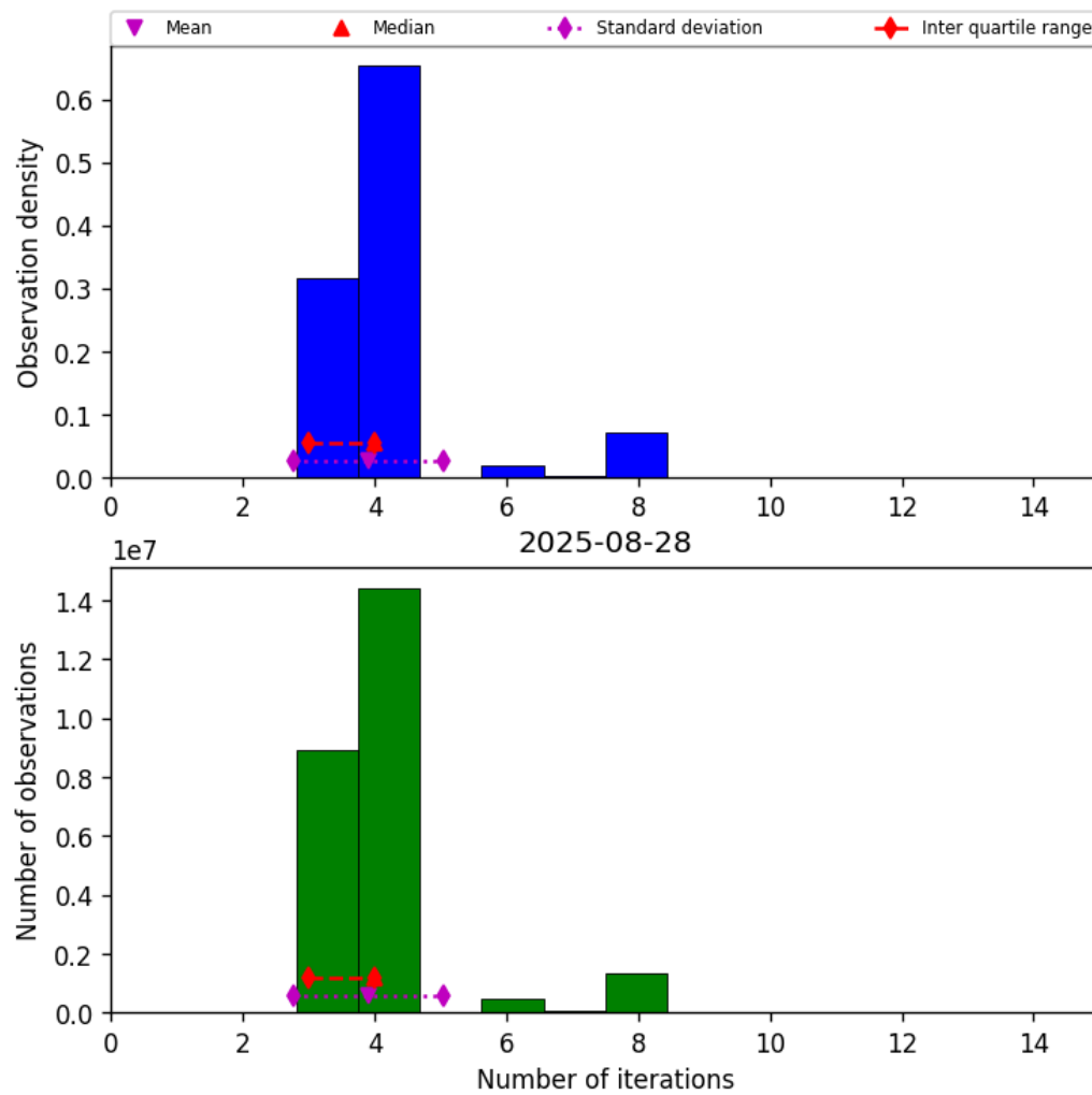
Figure 34: Histogram of “Number of iterations” for 2025-08-27 to 2025-08-29
