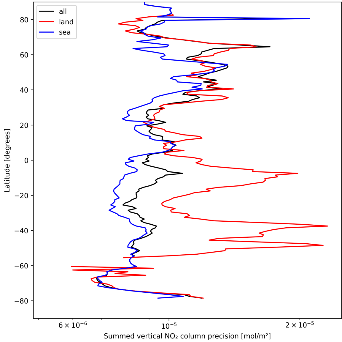
Figure 24: Zonal average of “Summed vertical NO 2 column precision” for 2025-08-27 to 2025-08-29.
