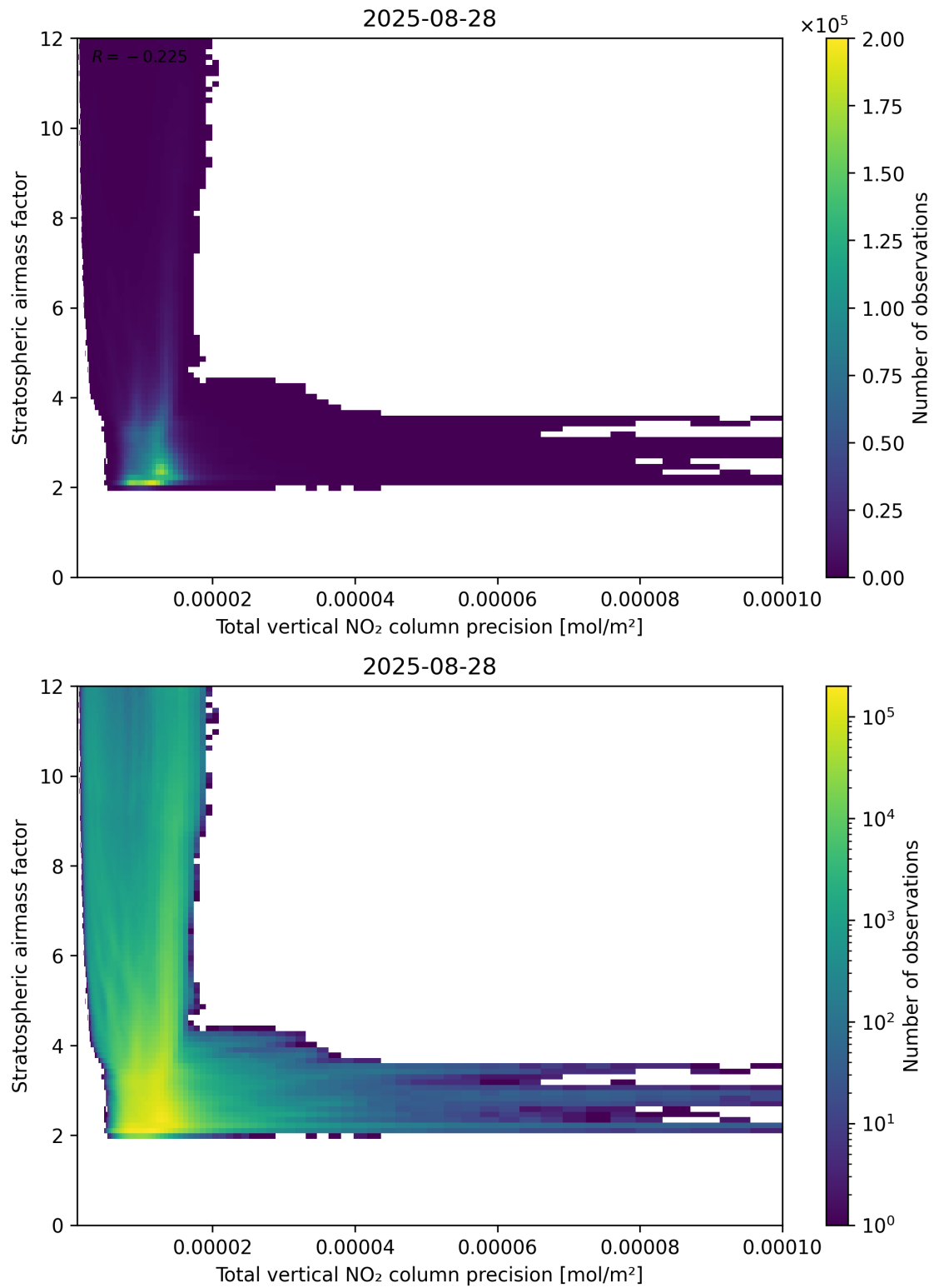
Figure 115: Scatter density plot of “Total vertical NO 2 column precision” against “Stratospheric air mass factor” for 2025-08-27 to 2025-08-29.
