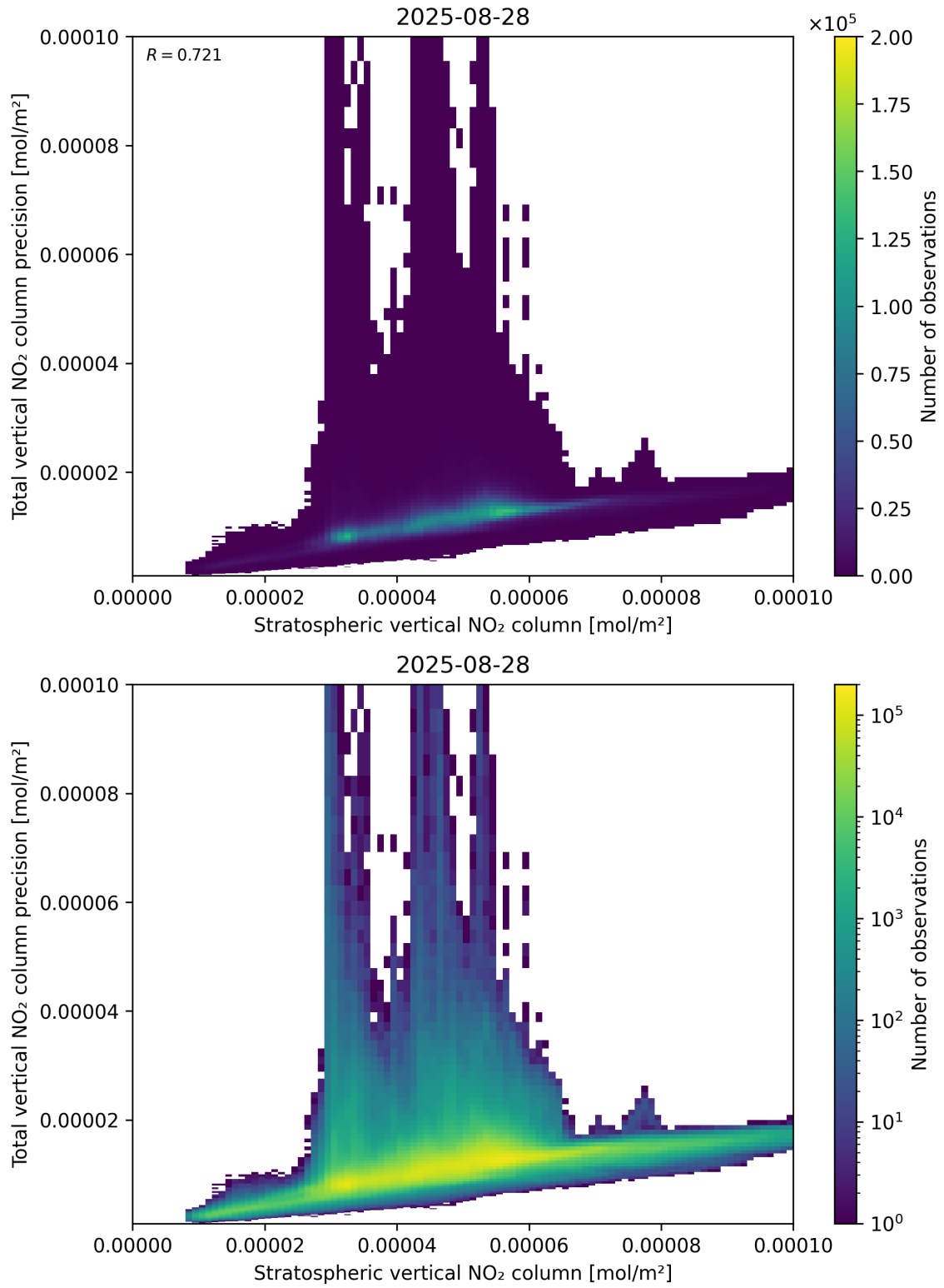
Figure 101: Scatter density plot of “Stratospheric vertical NO 2 column” against “Total vertical NO 2 column precision” for 2025-08-27 to 2025-08-29.
