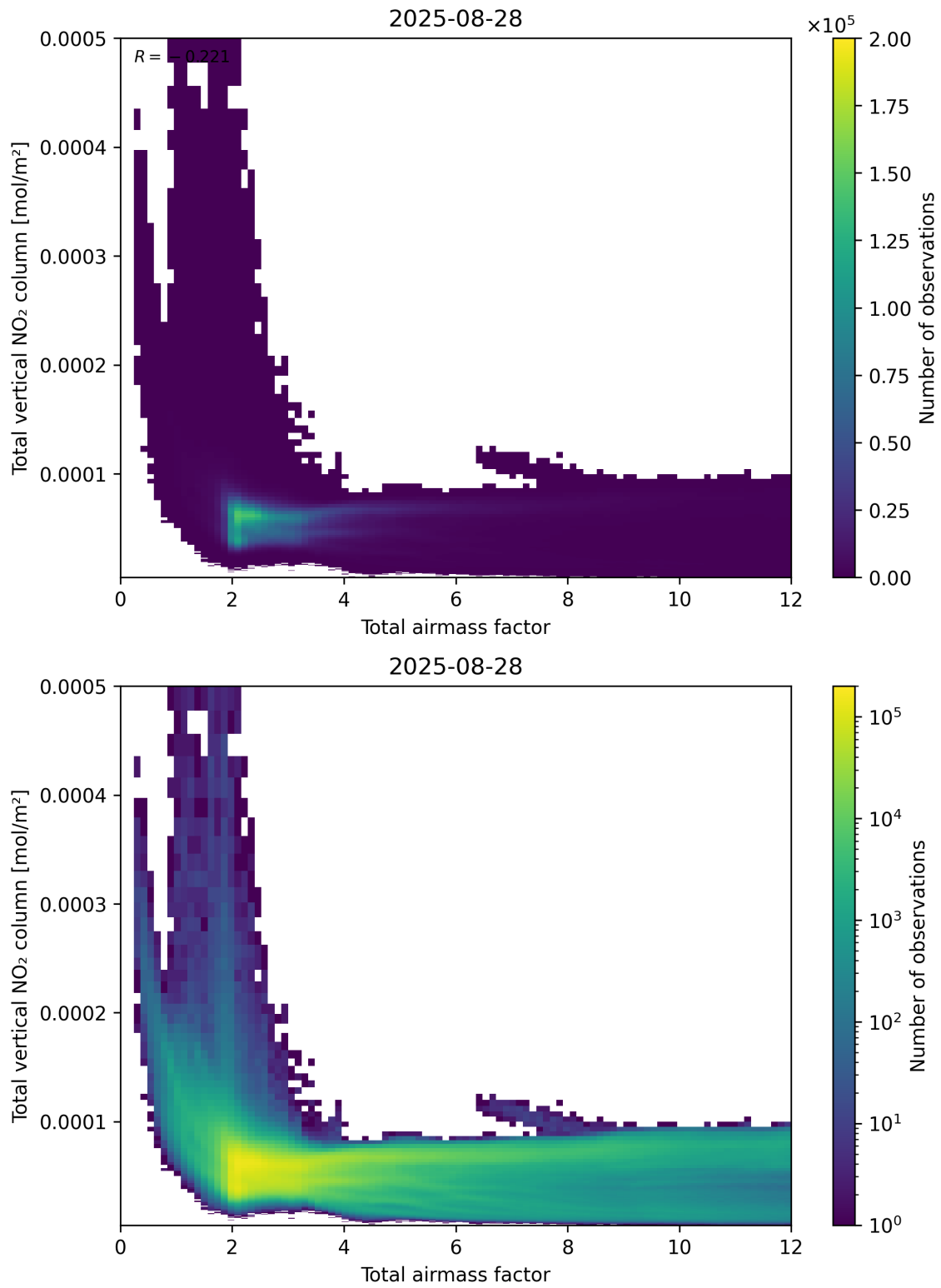
Figure 67: Scatter density plot of “Total airmass factor” against “Total vertical NO 2 column” for 2025-08-27 to 2025-08-29.
