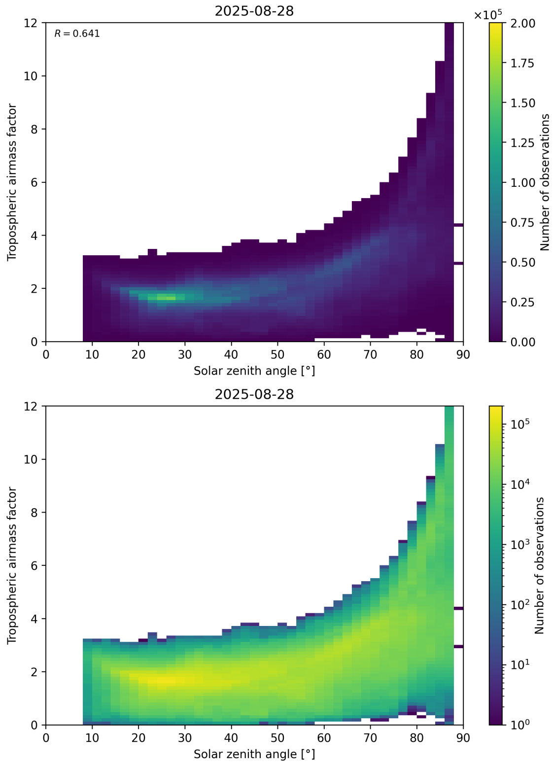
Figure 147: Scatter density plot of “Solar zenith angle” against “Tropospheric airmass factor” for 2025-08-27 to 2025-08-29.
