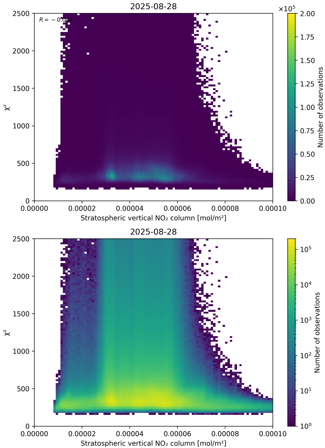
Figure 97: Scatter density plot of “Stratospheric vertical NO 2 column” against “ \chi^2 ” for 2025-08-27 to 2025-08-29.
