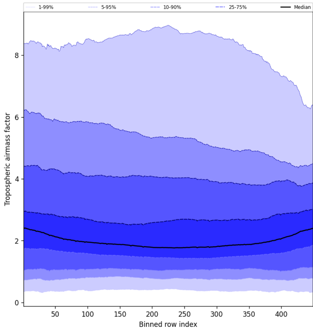
Figure 48: Along track statistics of “Tropospheric air mass factor” for 2025-08-27 to 2025-08-29
