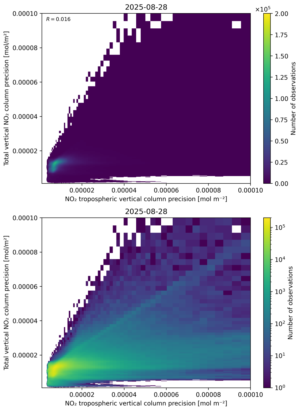
Figure 139: Scatter density plot of “NO 2 tropospheric vertical column precision” against “Total vertical NO 2 column precision” for 2025-08-27 to 2025-08-29.
