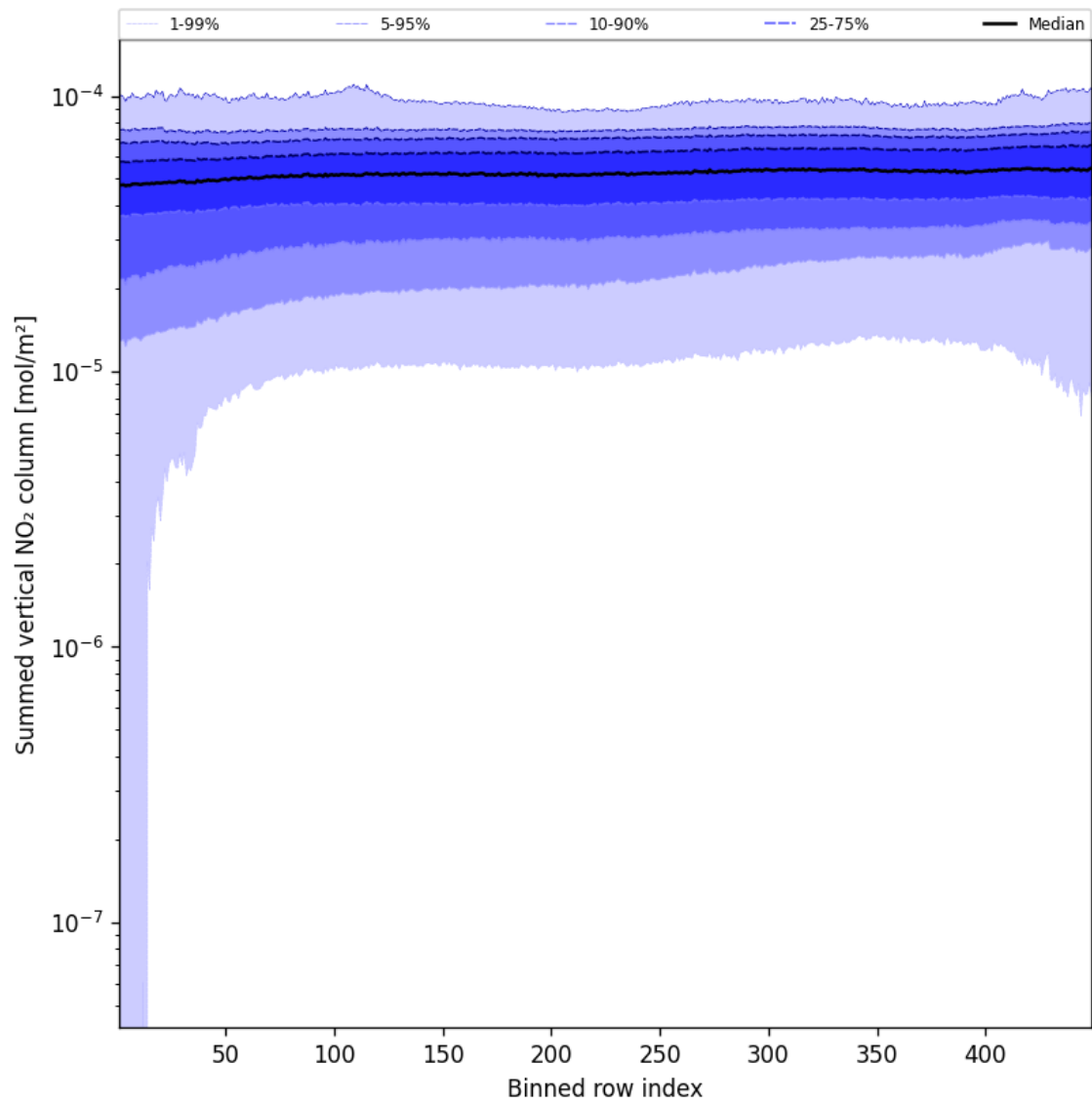
Figure 57: Along track statistics of “Summed vertical NO 2 column” for 2025-08-27 to 2025-08-29
